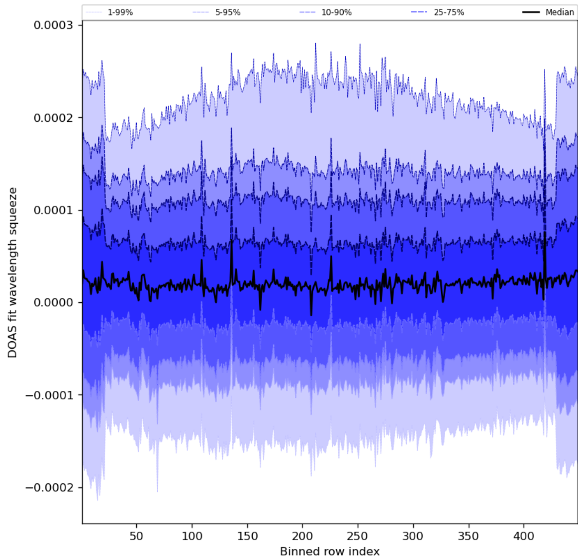
Figure 59: Along track statistics of “DOAS fit wavelength squeeze” for 2023-07-05 to 2023-07-07
