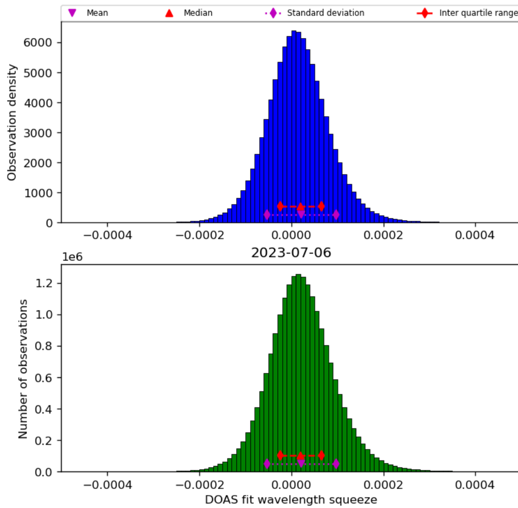
Figure 45: Histogram of “DOAS fit wavelength squeeze” for 2023-07-05 to 2023-07-07
