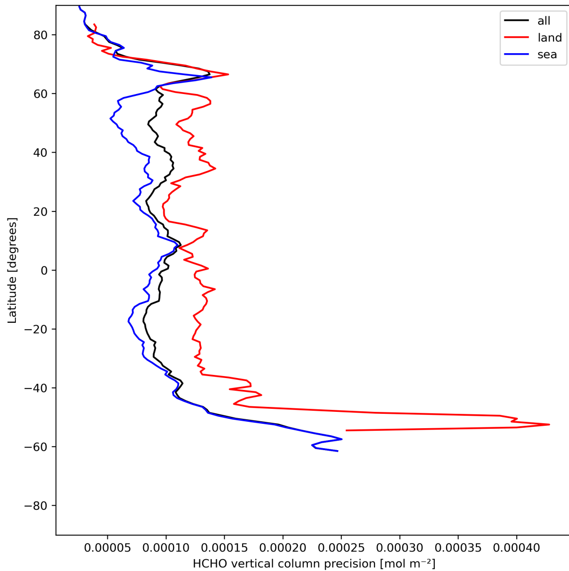
Figure 22: Zonal average of “HCHO vertical column precision” for 2023-07-05 to 2023-07-07.
