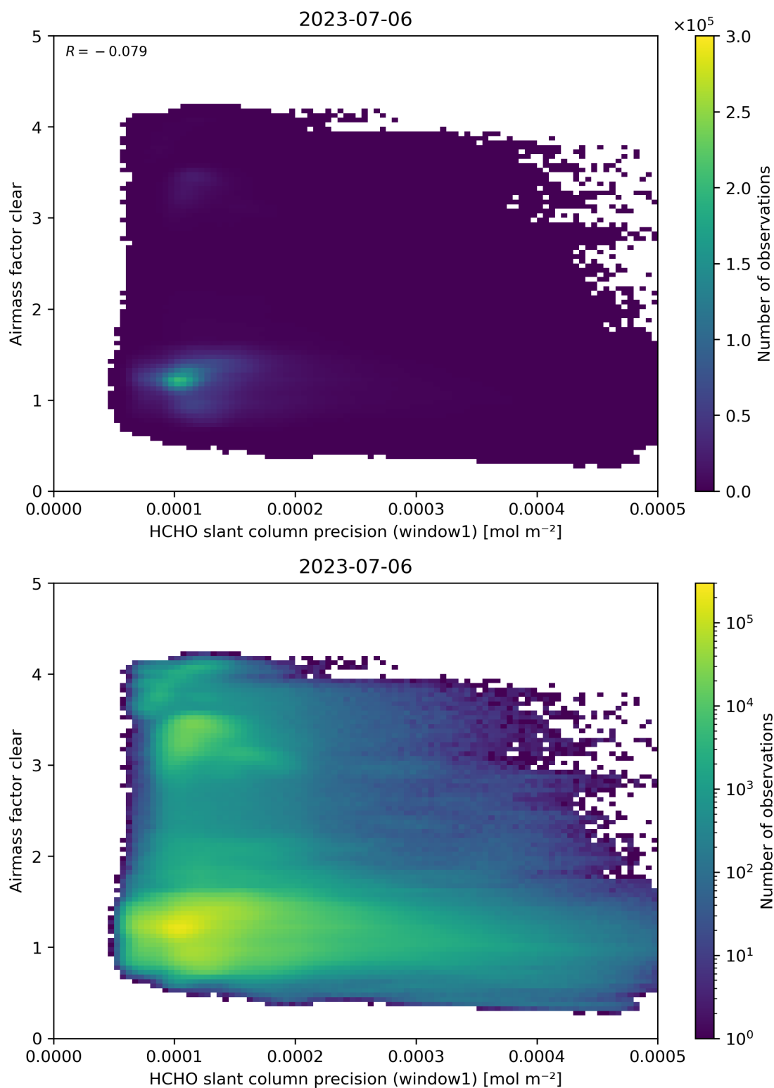
Figure 91: Scatter density plot of “HCHO slant column precision (window1)” against “Airmass factor clear” for 2023-07-05 to 2023-07-07.
