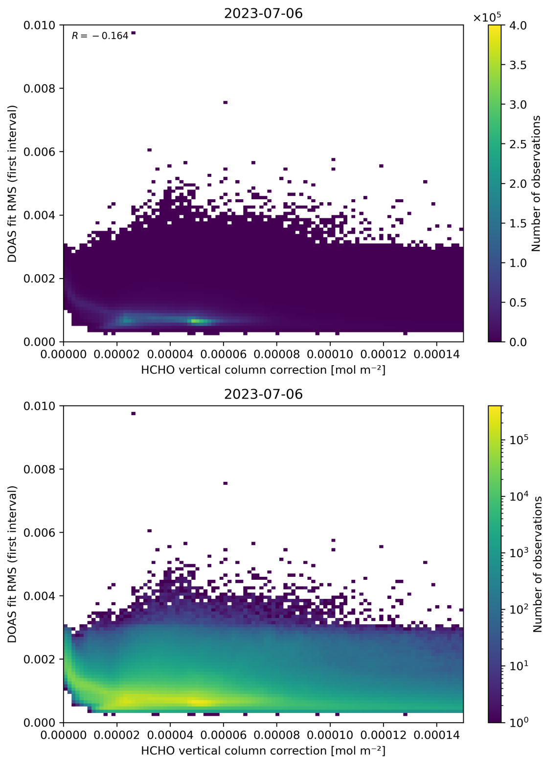
Figure 112: Scatter density plot of “HCHO vertical column correction” against “DOAS fit RMS (first interval)” for 2023-07-05 to 2023-07-07.
