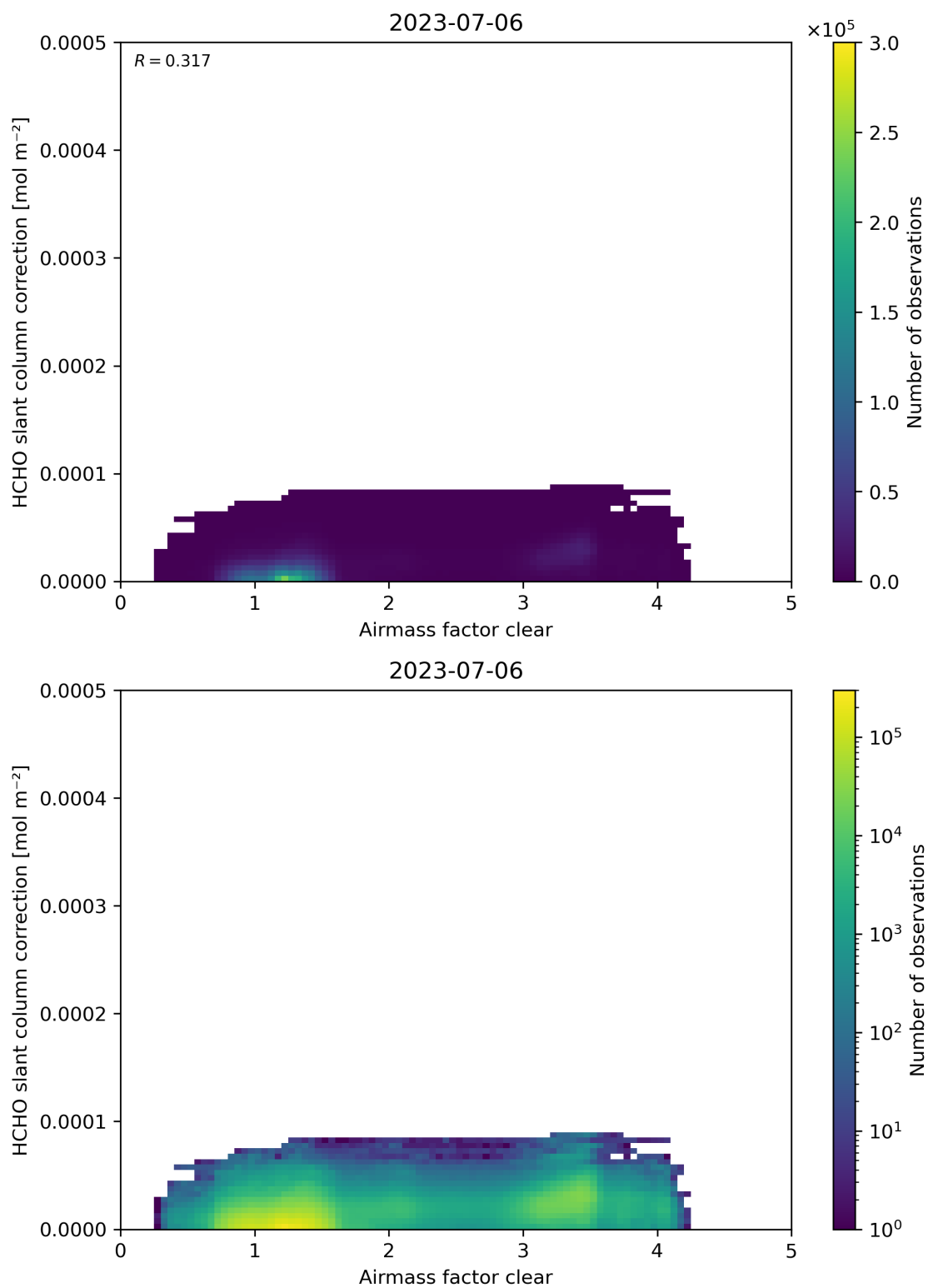
Figure 75: Scatter density plot of “Airmass factor clear” against “HCHO slant column correction” for 2023-07-05 to 2023-07-07.
