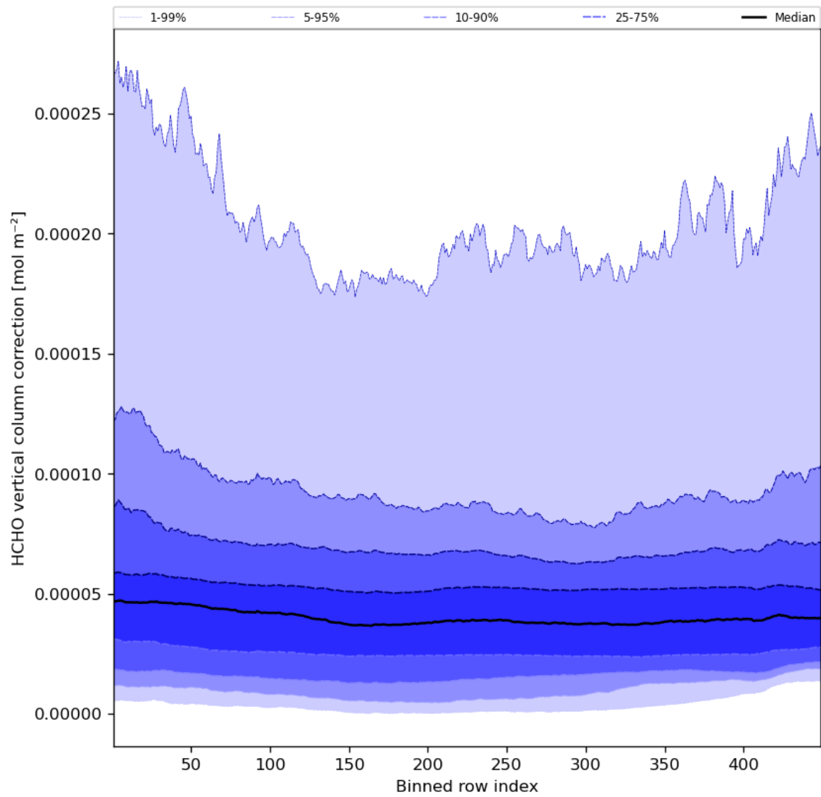
Figure 51: Along track statistics of “HCHO vertical column correction” for 2023-07-05 to 2023-07-07
