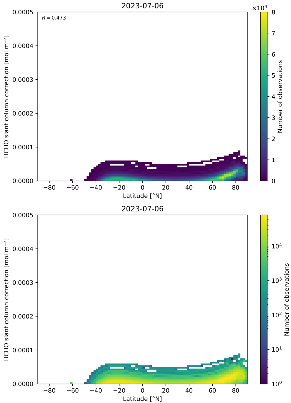
Figure 158: Scatter density plot of “Latitude” against “HCHO slant column correction” for 2023-07-05 to 2023-07-07.
