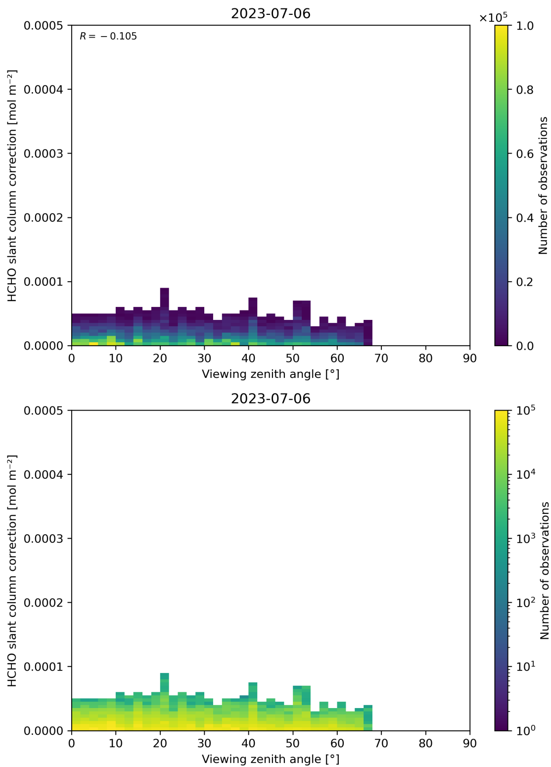
Figure 187: Scatter density plot of “Viewing zenith angle” against “HCHO slant column correction” for 2023-07-05 to 2023-07-07.
