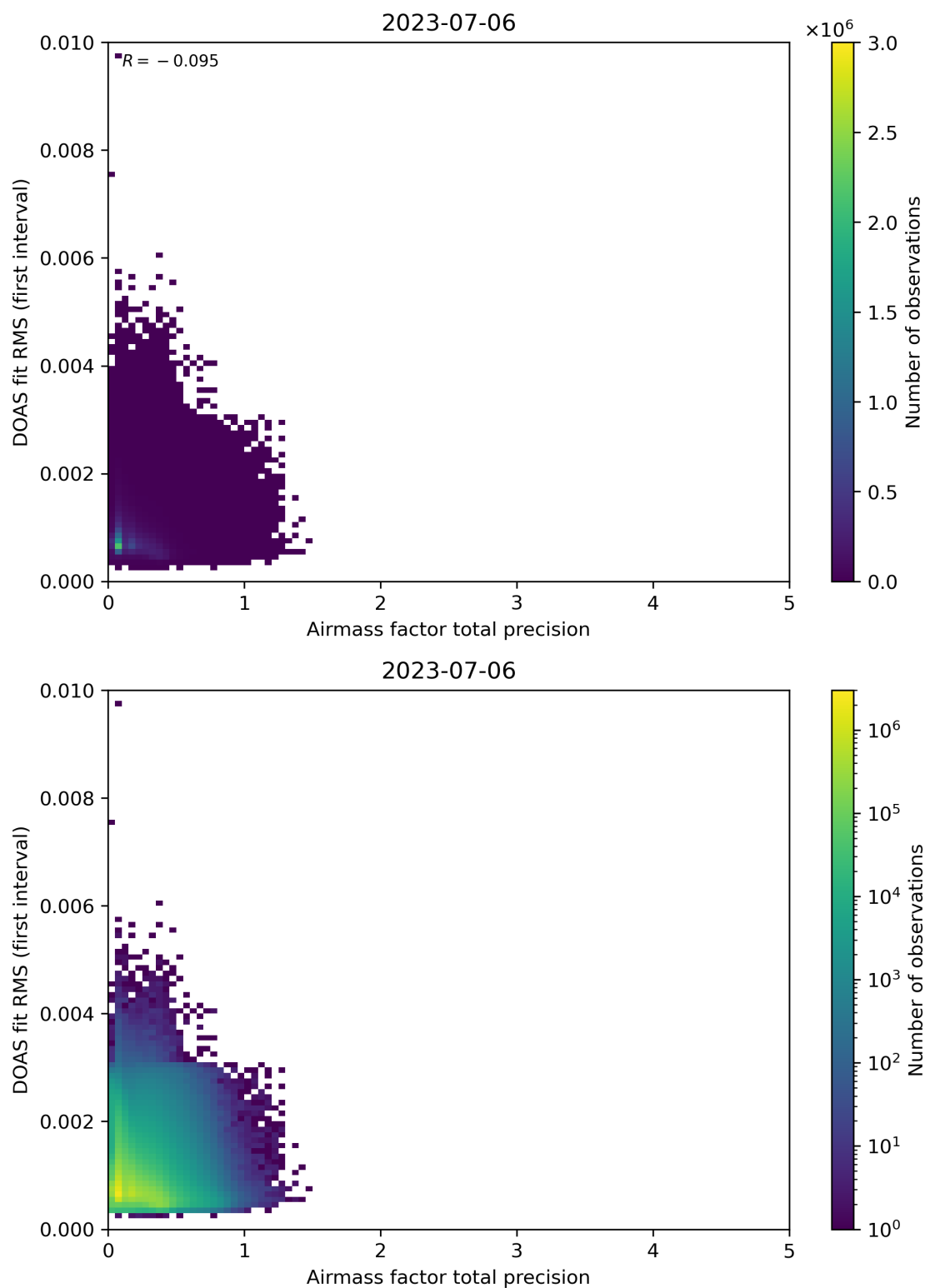
Figure 105: Scatter density plot of “Airmass factor total precision” against “DOAS fit RMS (first interval)” for 2023-07-05 to 2023-07-07.
