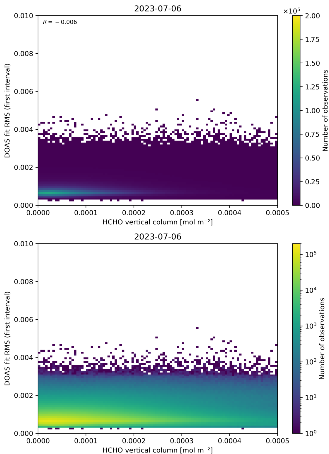
Figure 123: Scatter density plot of “HCHO vertical column” against “DOAS fit RMS (first interval)” for 2023-07-05 to 2023-07-07.
