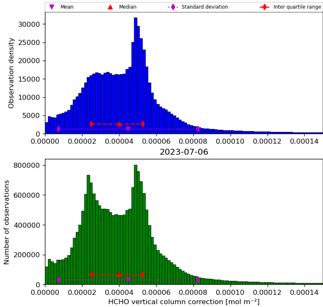
Figure 37: Histogram of “HCHO vertical column correction” for 2023-07-05 to 2023-07-07
