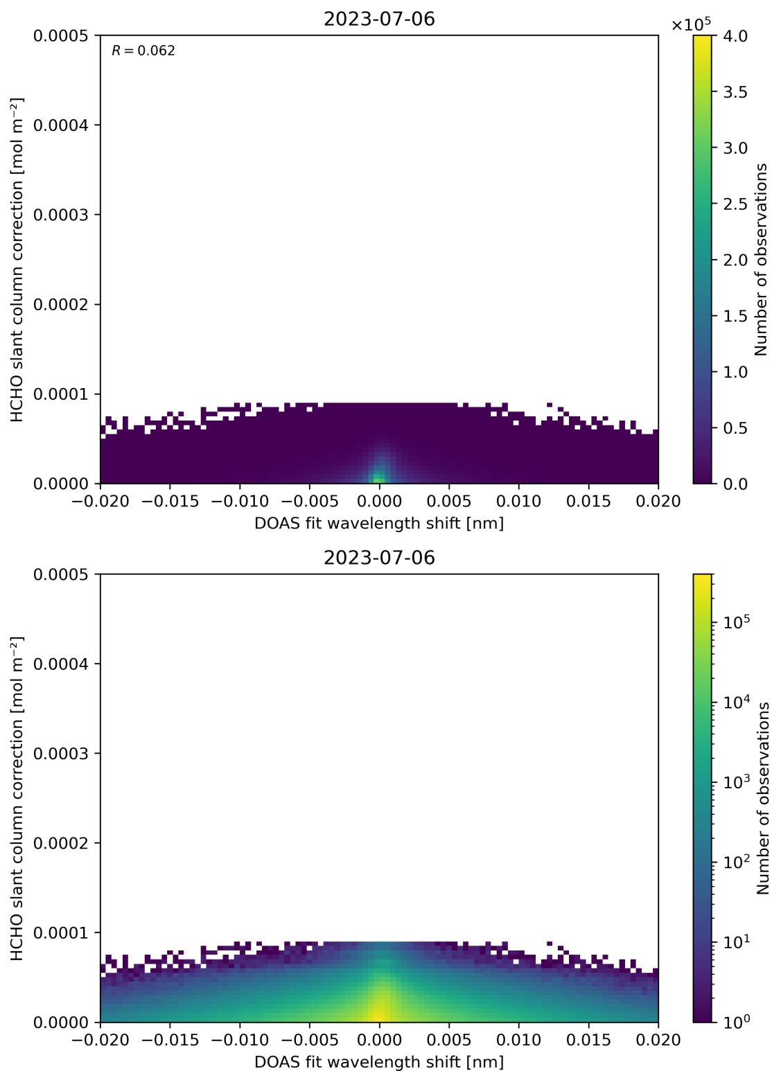
Figure 67: Scatter density plot of “DOAS fit wavelength shift” against “HCHO slant column correction” for 2023-07-05 to 2023-07-07.
