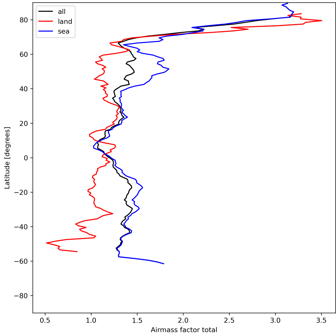
Figure 26: Zonal average of “Airmass factor total” for 2023-07-05 to 2023-07-07.
