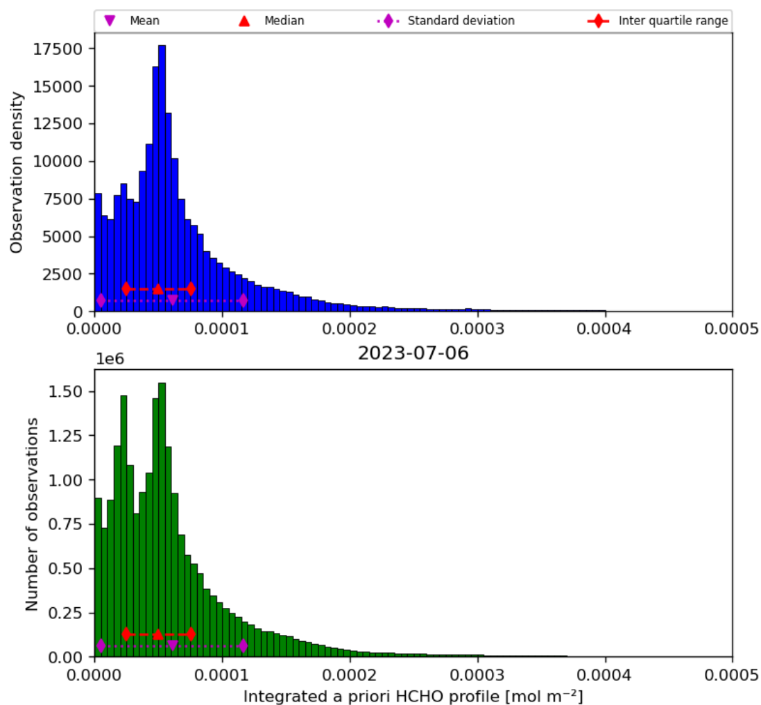
Figure 43: Histogram of “Integrated a priori HCHO profile” for 2023-07-05 to 2023-07-07
