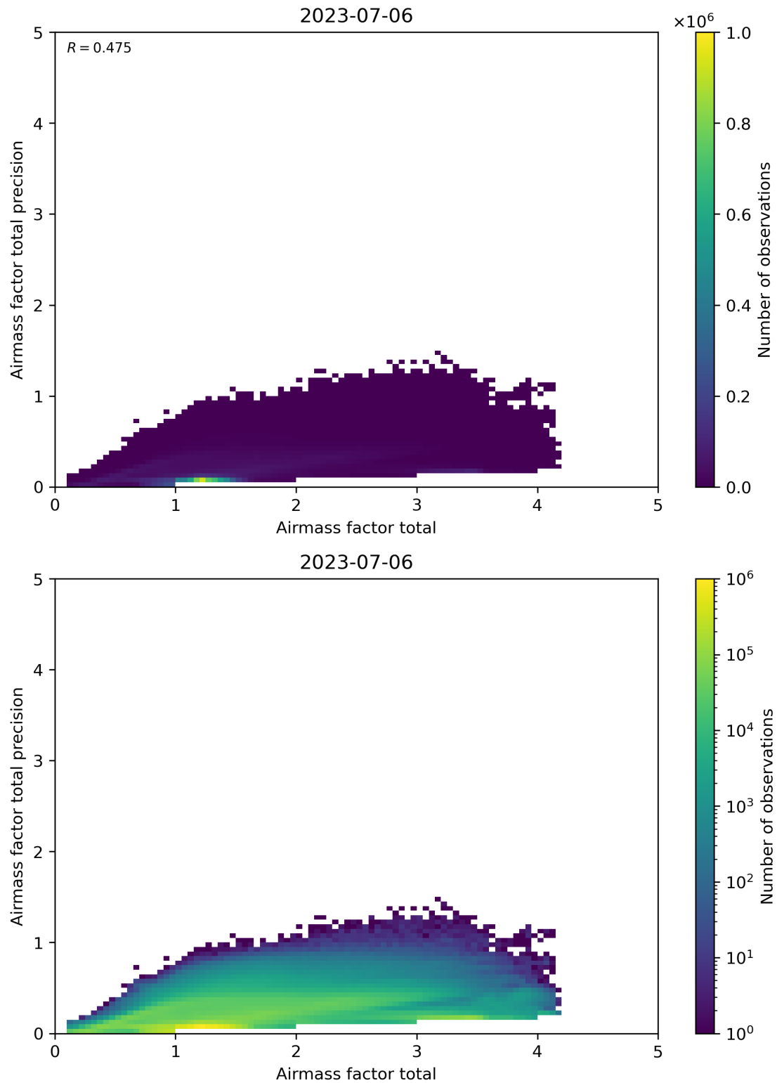
Figure 103: Scatter density plot of “Airmass factor total” against “Airmass factor total precision” for 2023-07-05 to 2023-07-07.
