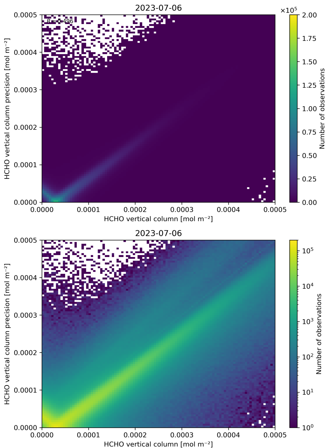
Figure 134: Scatter density plot of “HCHO vertical column” against “HCHO vertical column precision” for 2023-07-05 to 2023-07-07.
