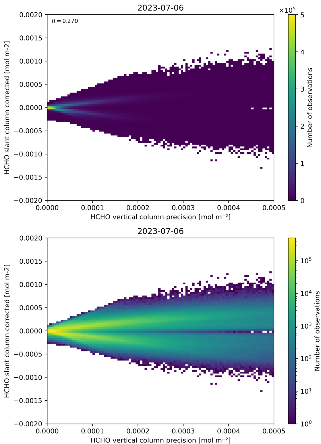
Figure 140: Scatter density plot of “HCHO vertical column precision” against “HCHO slant column corrected” for 2023-07-05 to 2023-07-07.
