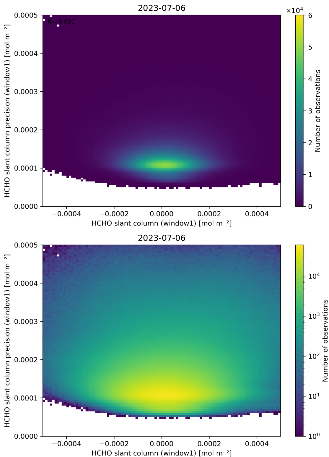
Figure 84: Scatter density plot of “HCHO slant column (window1)” against “HCHO slant column precision (window1)” for 2023-07-05 to 2023-07-07.
