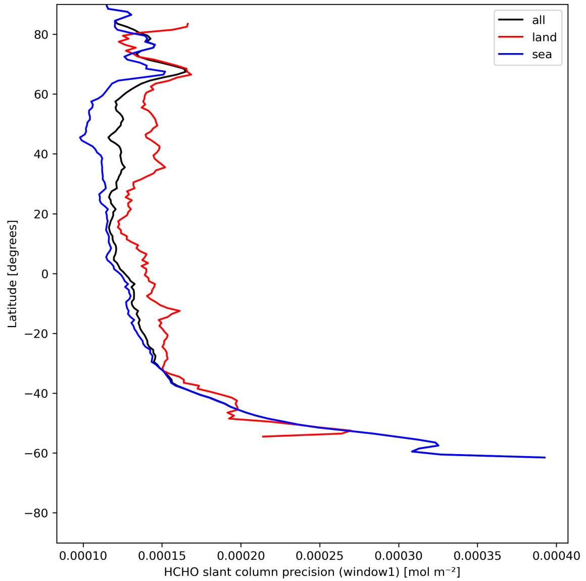
Figure 25: Zonal average of "HCHO slant column precision (window1)" for 2023-07-05 to 2023-07-07.
