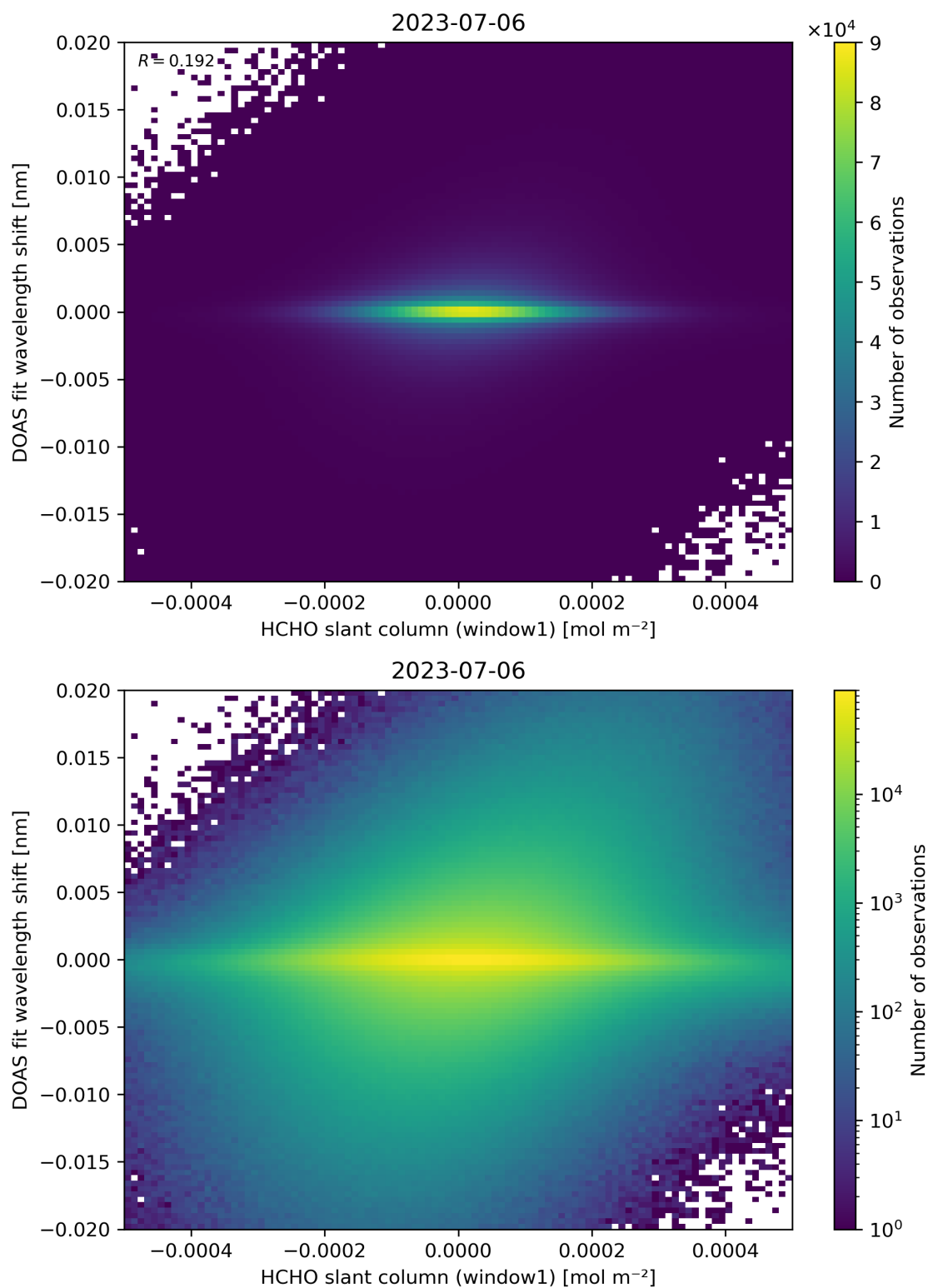
Figure 79: Scatter density plot of “HCHO slant column (window1)” against “DOAS fit wavelength shift” for 2023-07-05 to 2023-07-07.
