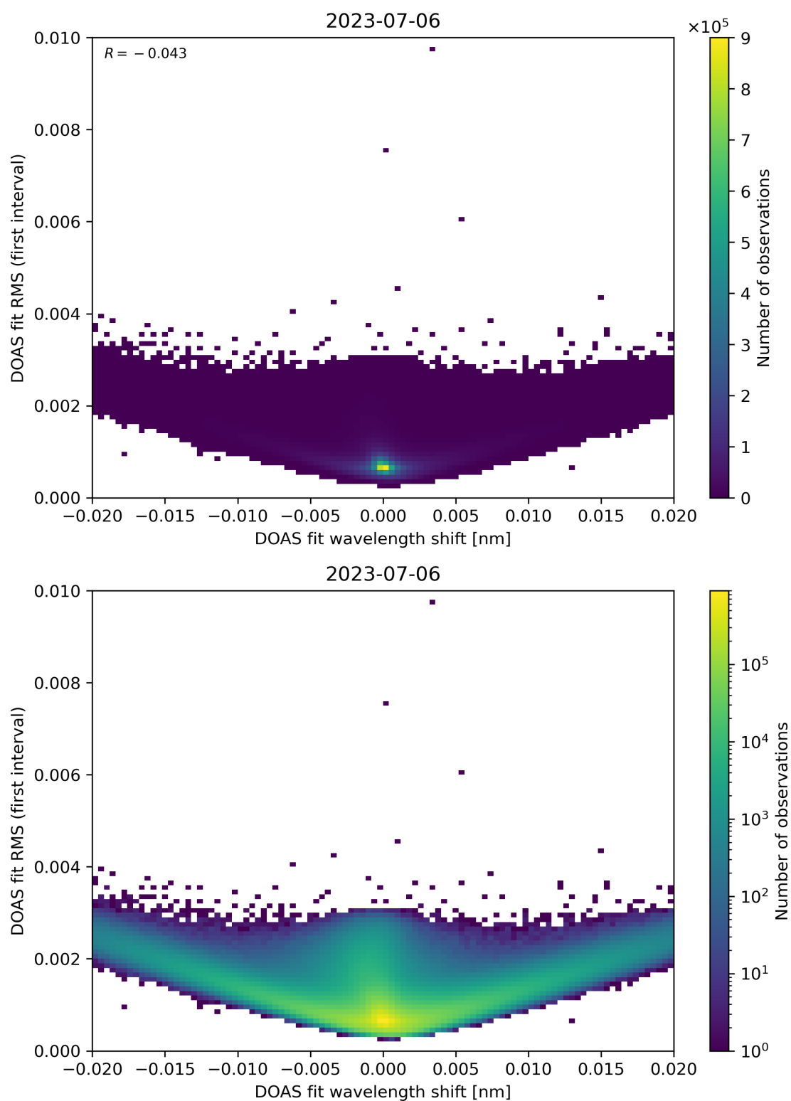
Figure 64: Scatter density plot of “DOAS fit wavelength shift” against “DOAS fit RMS (first interval)” for 2023-07-05 to 2023-07-07.
