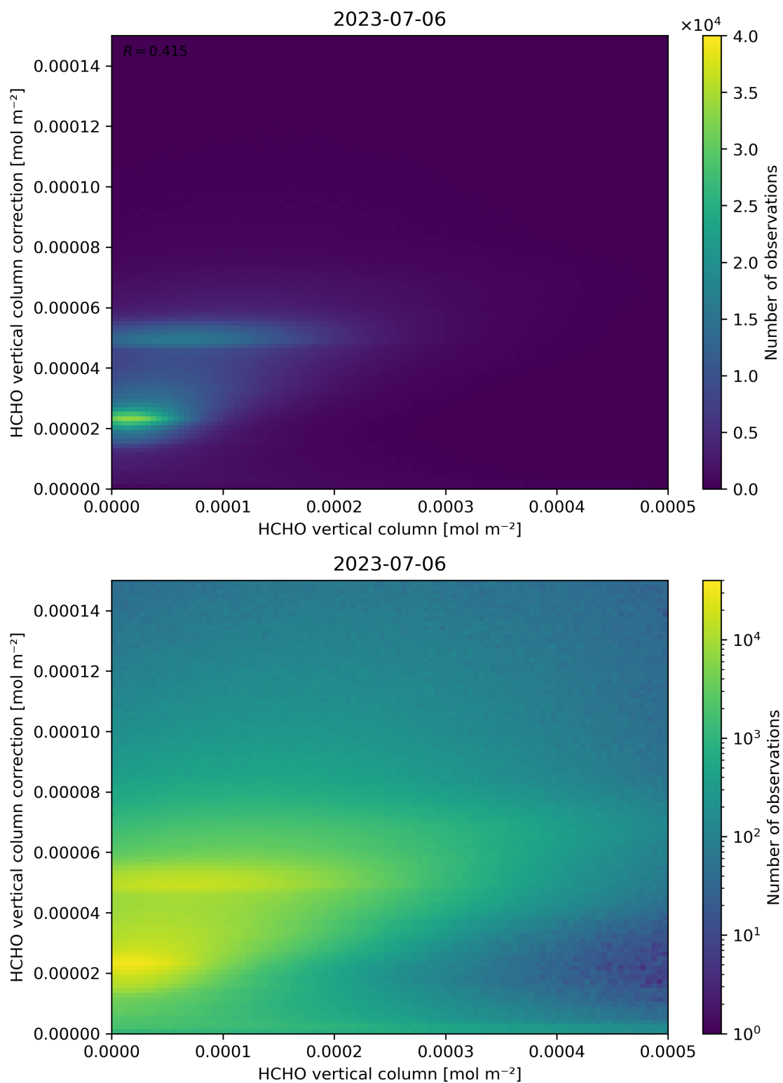
Figure 133: Scatter density plot of “HCHO vertical column” against “HCHO vertical column correction” for 2023-07-05 to 2023-07-07.
