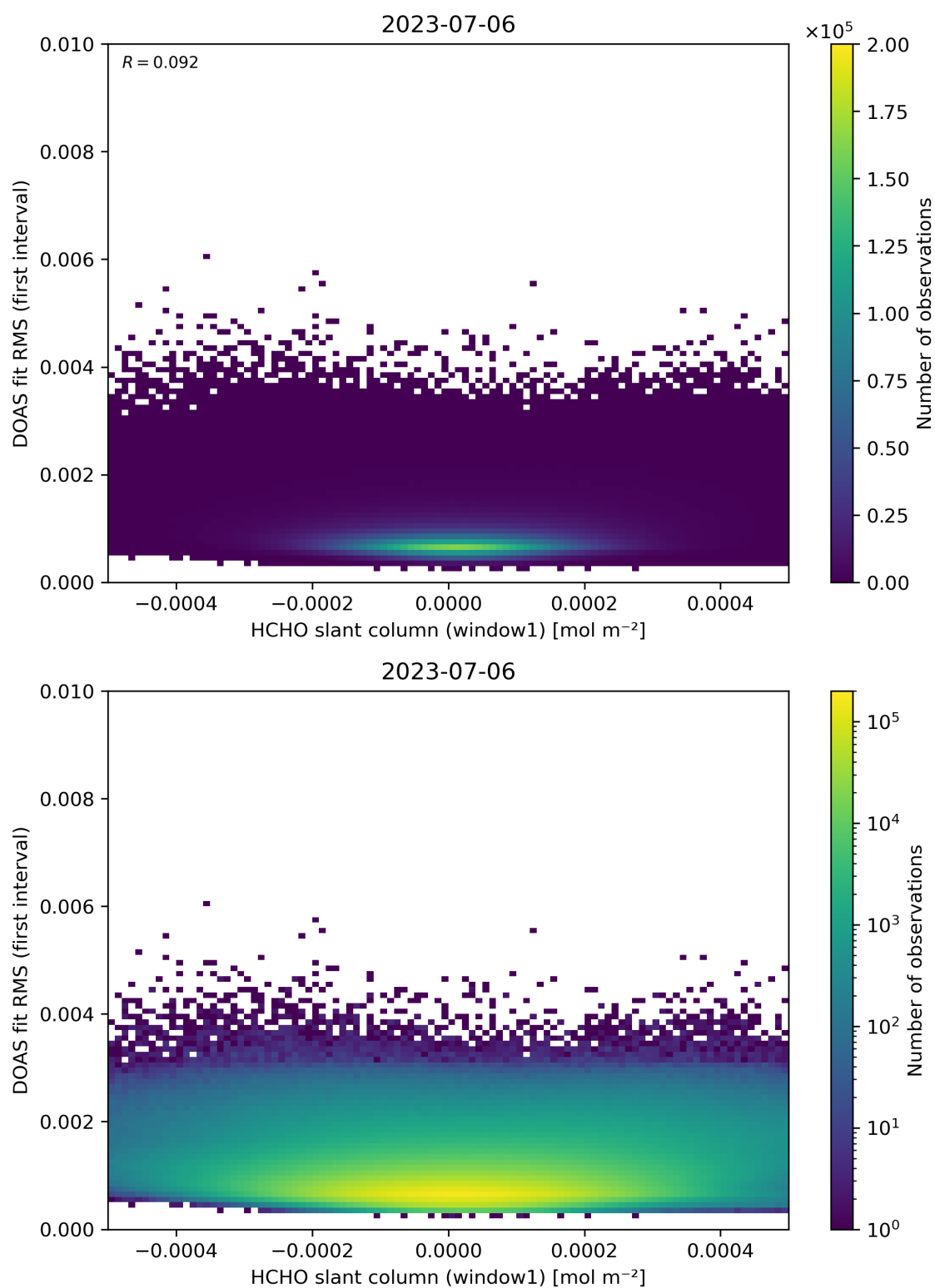
Figure 78: Scatter density plot of “HCHO slant column (window1)” against “DOAS fit RMS (first interval)” for 2023-07-05 to 2023-07-07.
