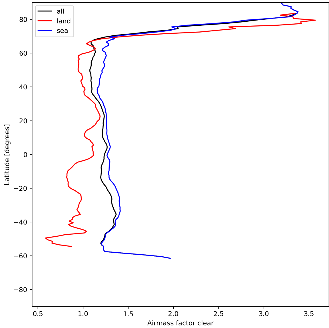
Figure 28: Zonal average of “Airmass factor clear” for 2023-07-05 to 2023-07-07.
