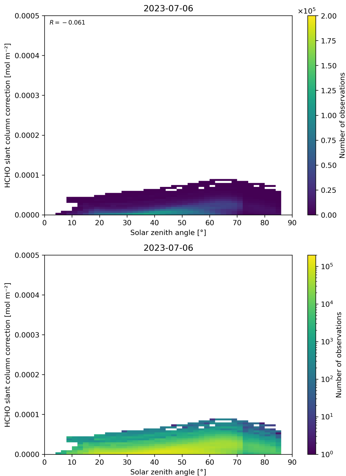
Figure 172: Scatter density plot of “Solar zenith angle” against “HCHO slant column correction” for 2023-07-05 to 2023-07-07.
