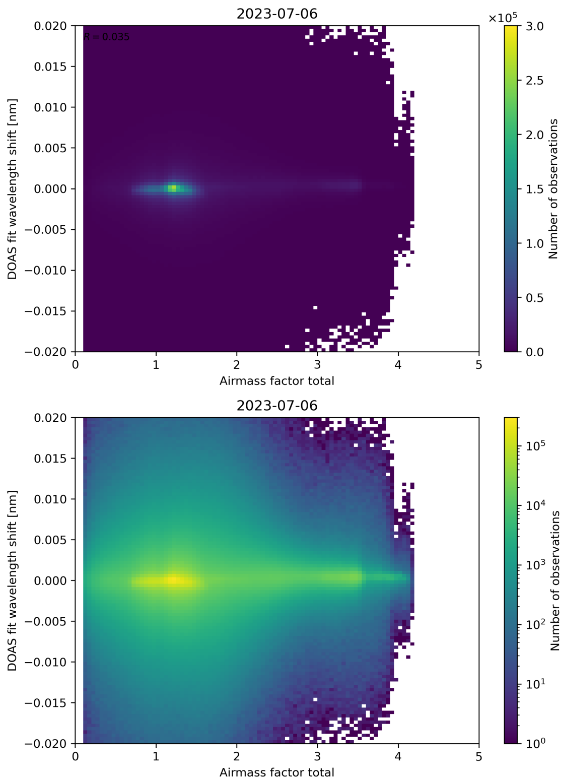
Figure 98: Scatter density plot of “Airmass factor total” against “DOAS fit wavelength shift” for 2023-07-05 to 2023-07-07.
