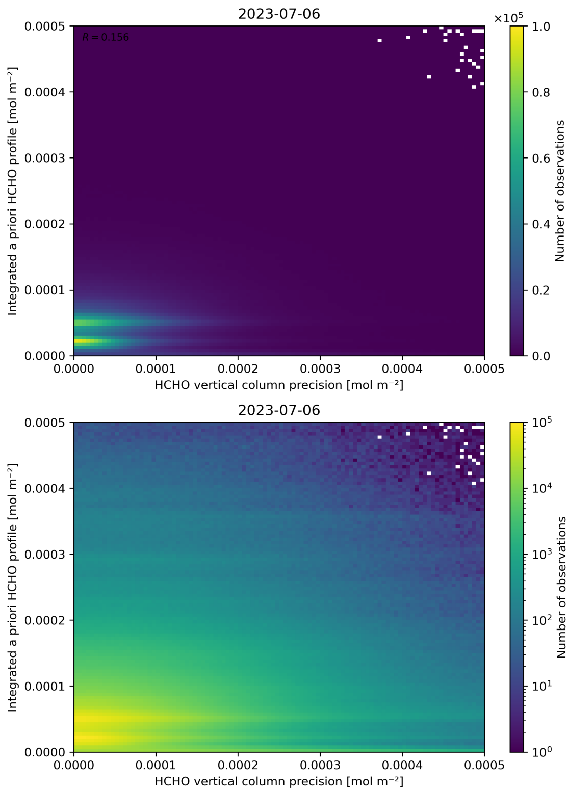
Figure 147: Scatter density plot of “HCHO vertical column precision” against “Integrated a priori HCHO profile” for 2023-07-05 to 2023-07-07.
