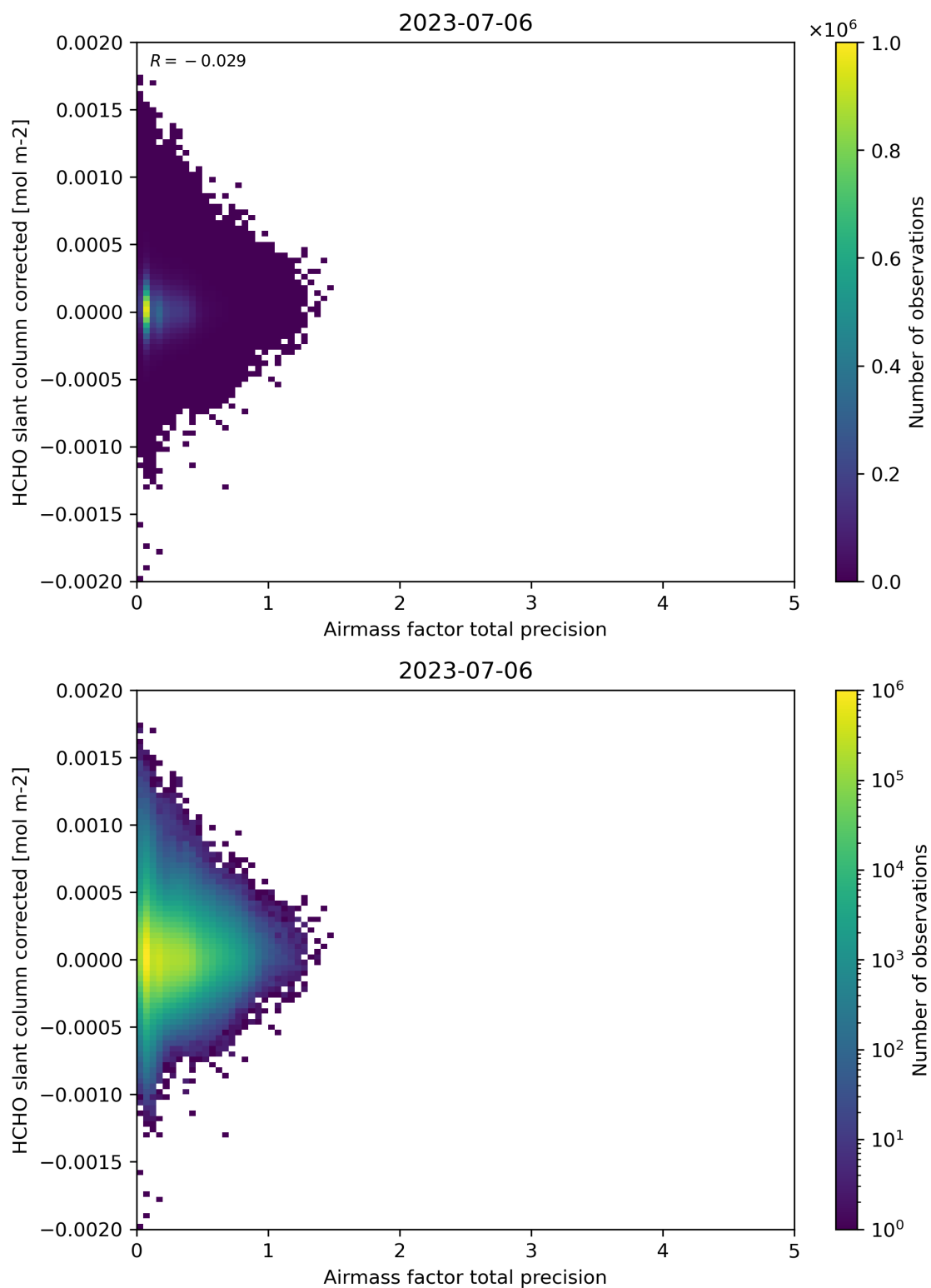
Figure 109: Scatter density plot of “Airmass factor total precision” against “HCHO slant column corrected” for 2023-07-05 to 2023-07-07.
