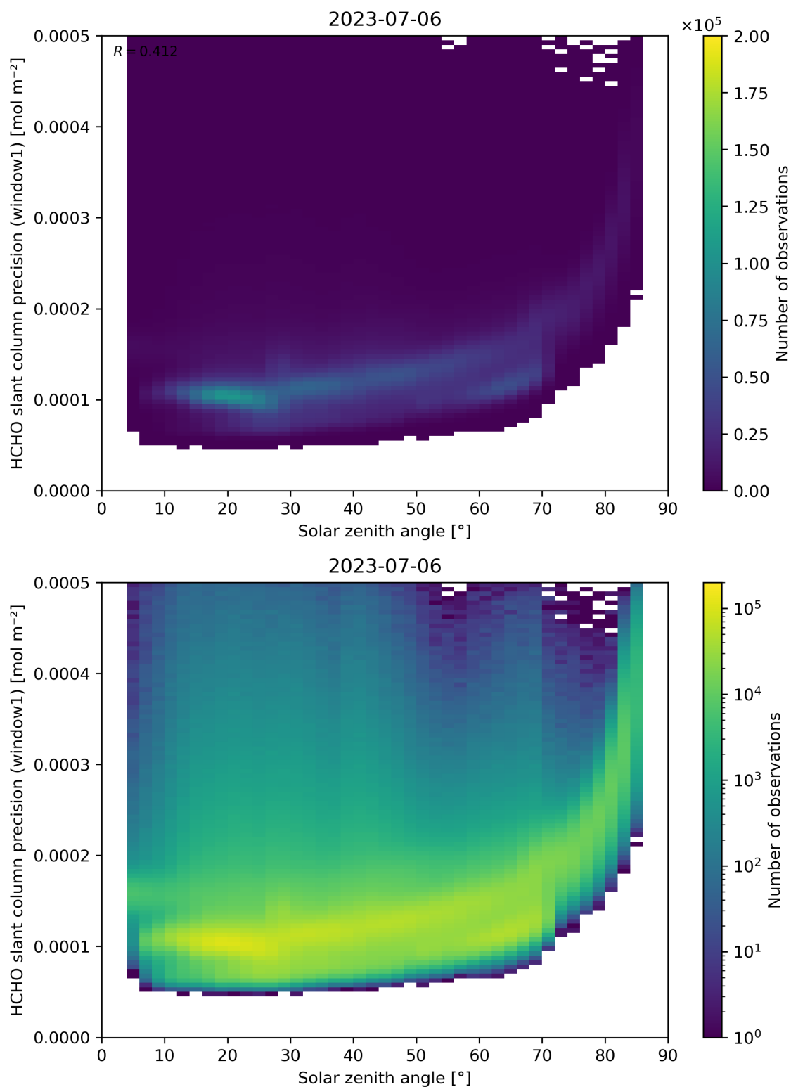
Figure 174: Scatter density plot of “Solar zenith angle” against “HCHO slant column precision (window1)” for 2023-07-05 to 2023-07-07.
