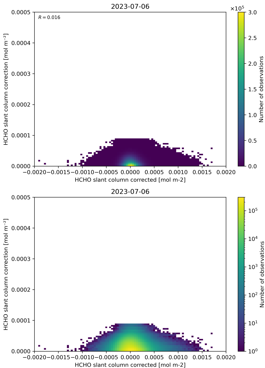
Figure 77: Scatter density plot of “HCHO slant column corrected” against “HCHO slant column correction” for 2023-07-05 to 2023-07-07.
