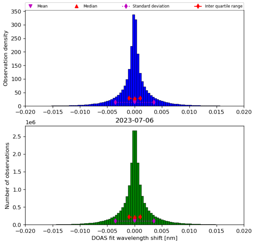
Figure 44: Histogram of “DOAS fit wavelength shift” for 2023-07-05 to 2023-07-07
