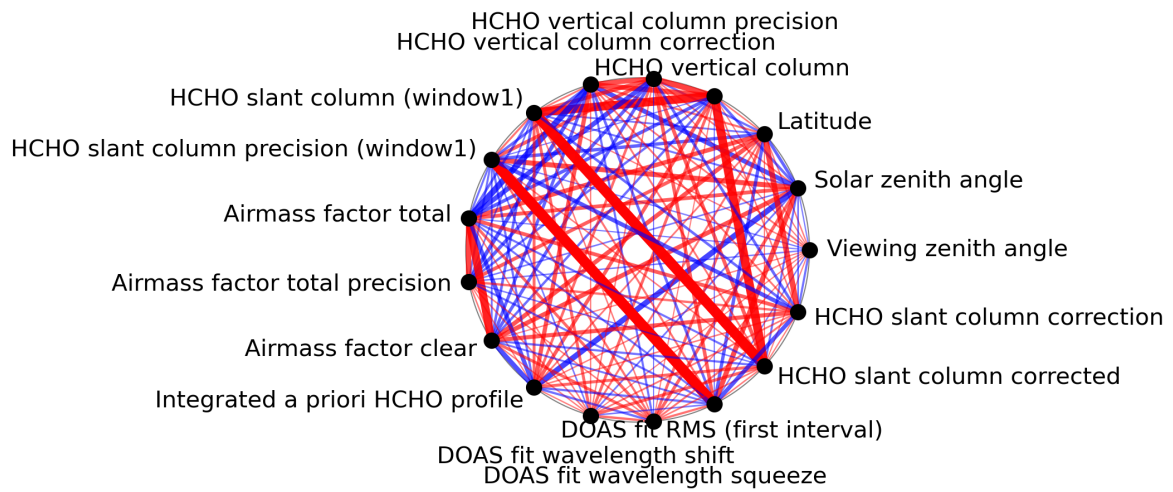
Figure 1: Map of correlation graph for 2023-07-05 to 2023-07-07.
