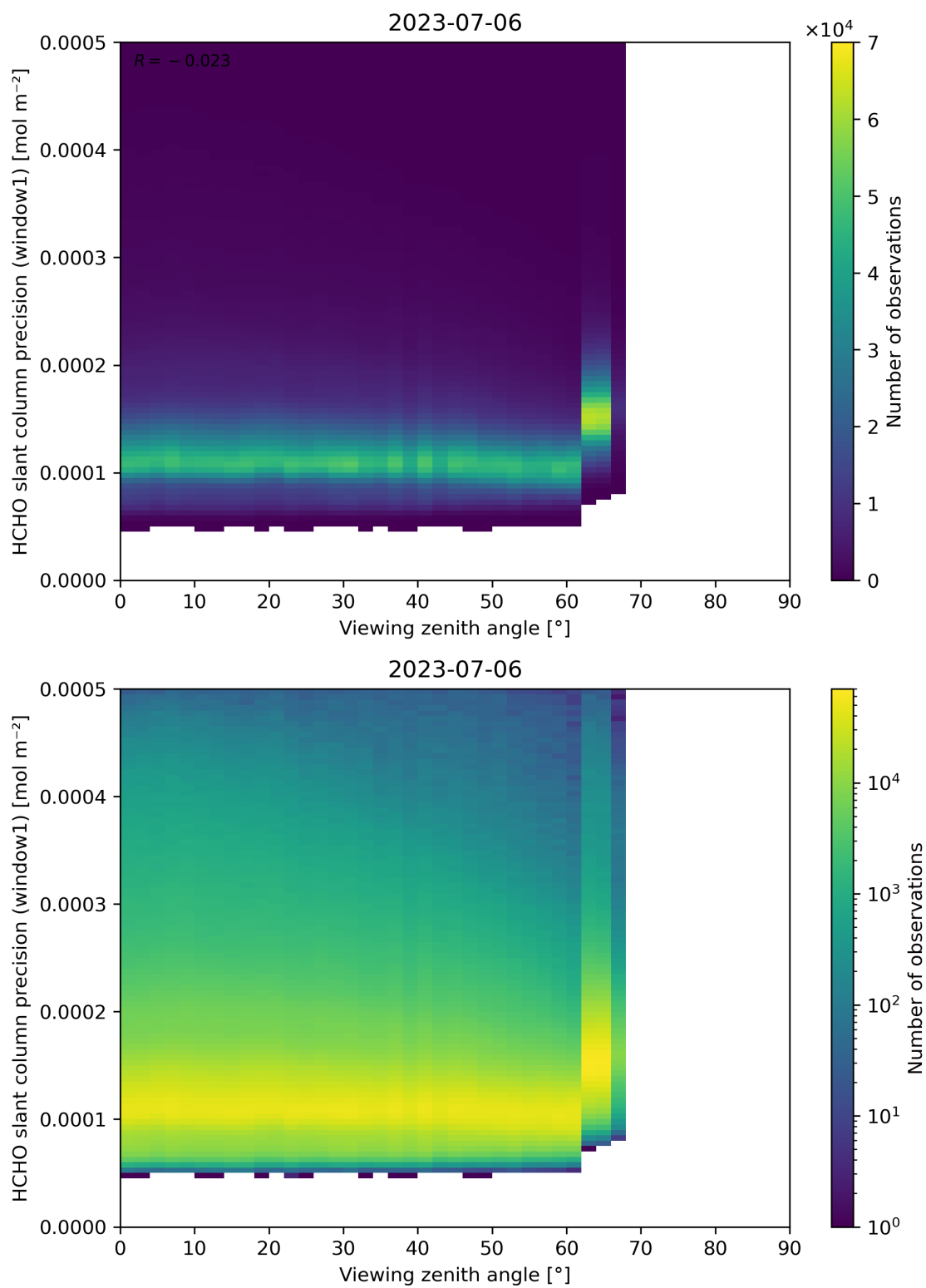
Figure 189: Scatter density plot of “Viewing zenith angle” against “HCHO slant column precision (window1)” for 2023-07-05 to 2023-07-07.
