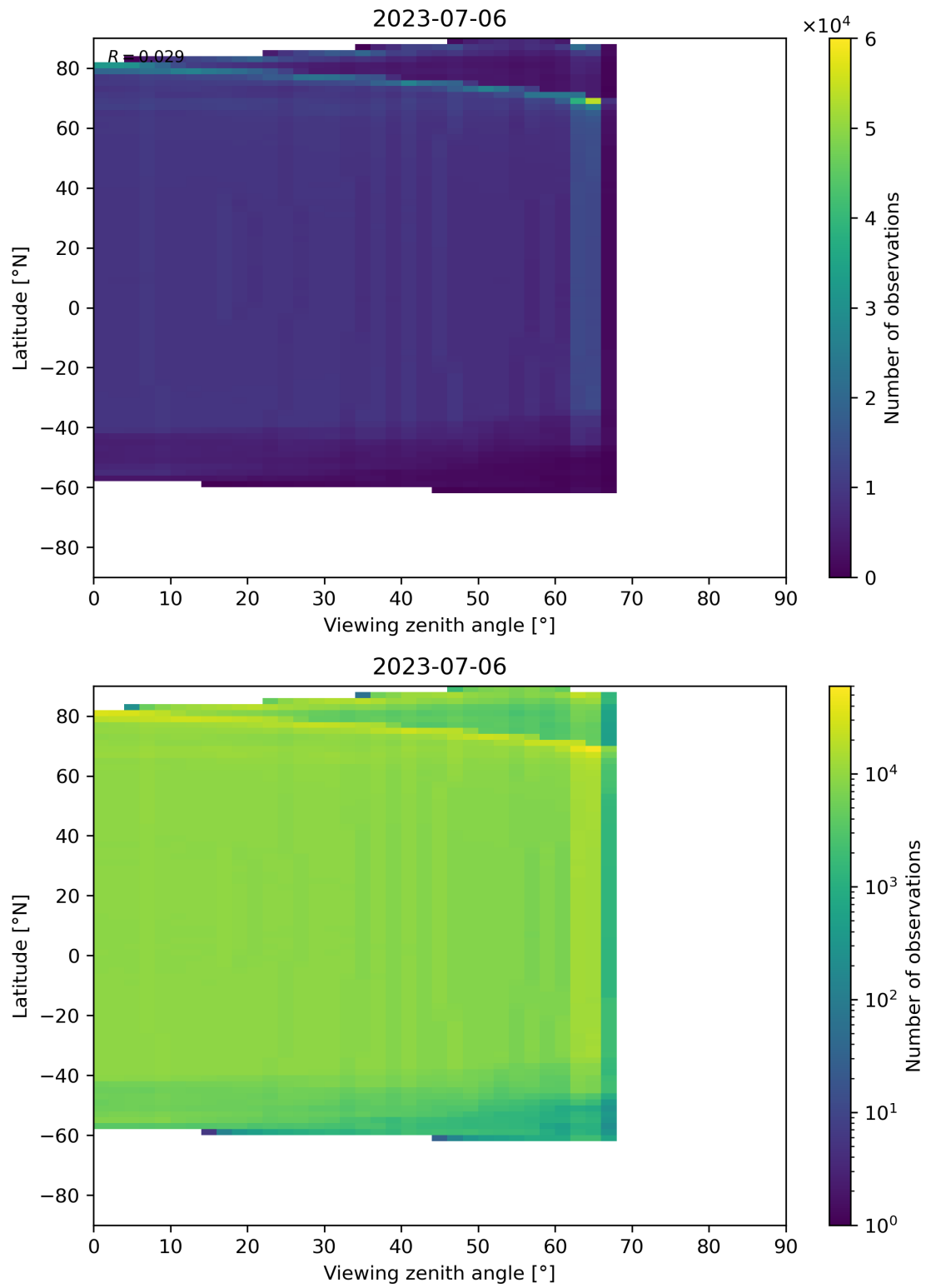
Figure 196: Scatter density plot of “Viewing zenith angle” against “Latitude” for 2023-07-05 to 2023-07-07.
