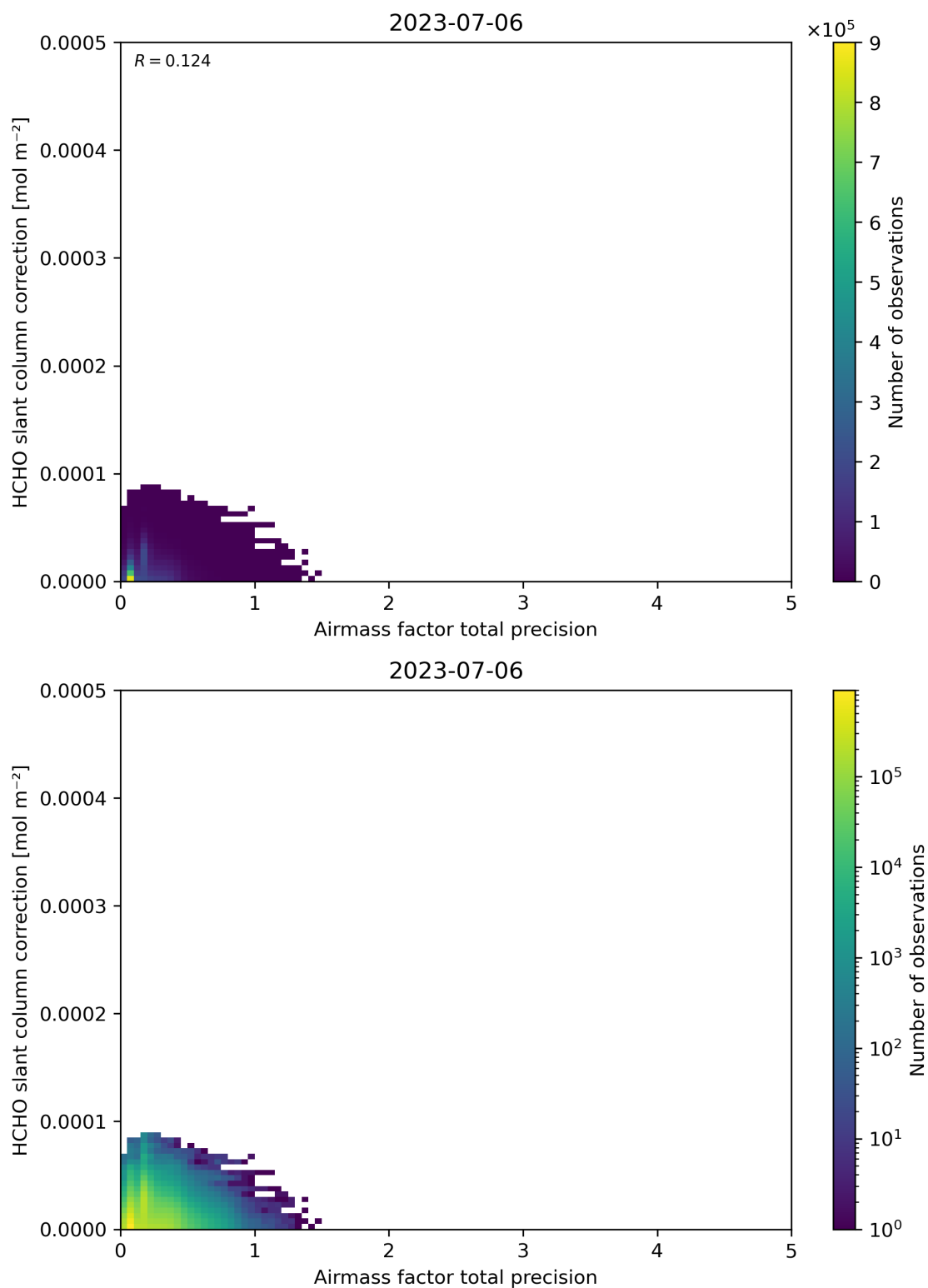
Figure 110: Scatter density plot of “Airmass factor total precision” against “HCHO slant column correction” for 2023-07-05 to 2023-07-07.
