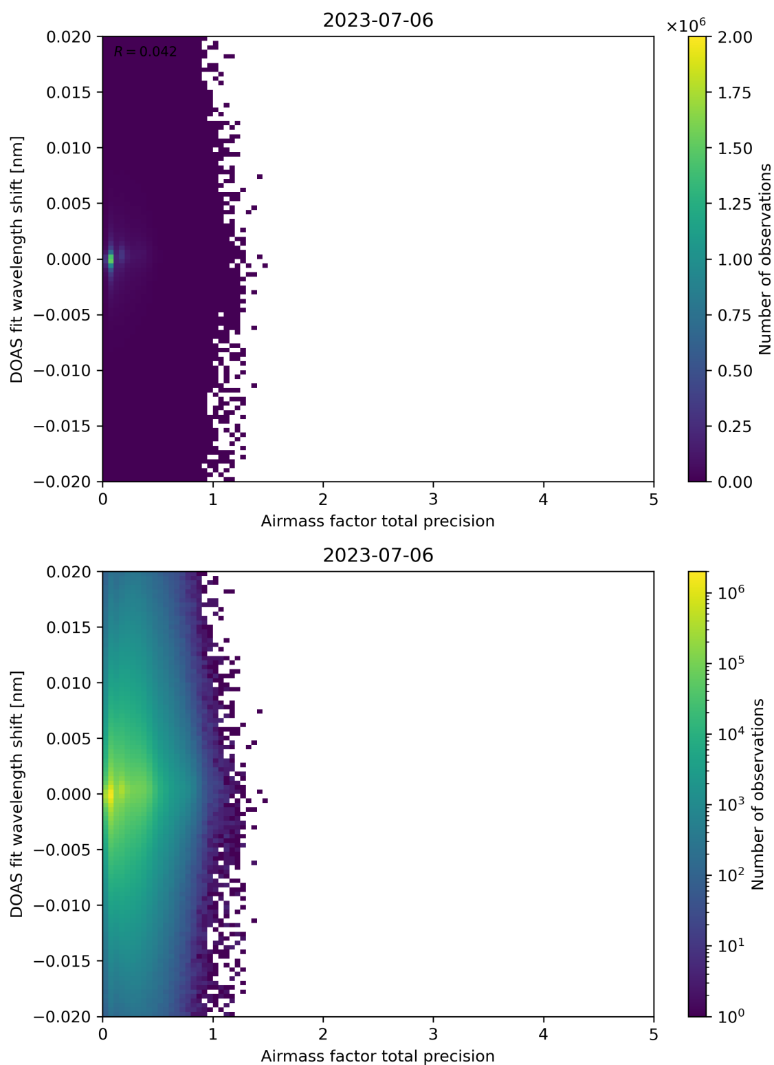
Figure 106: Scatter density plot of “Airmass factor total precision” against “DOAS fit wavelength shift” for 2023-07-05 to 2023-07-07.
