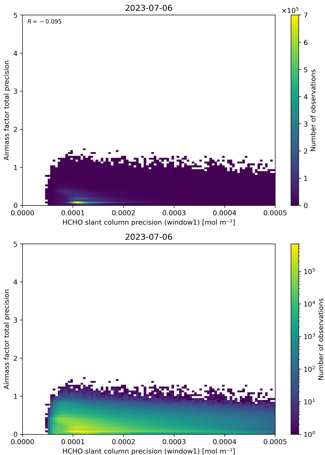
Figure 95: Scatter density plot of “HCHO slant column precision (window1)” against “Airmass factor total precision” for 2023-07-05 to 2023-07-07.
