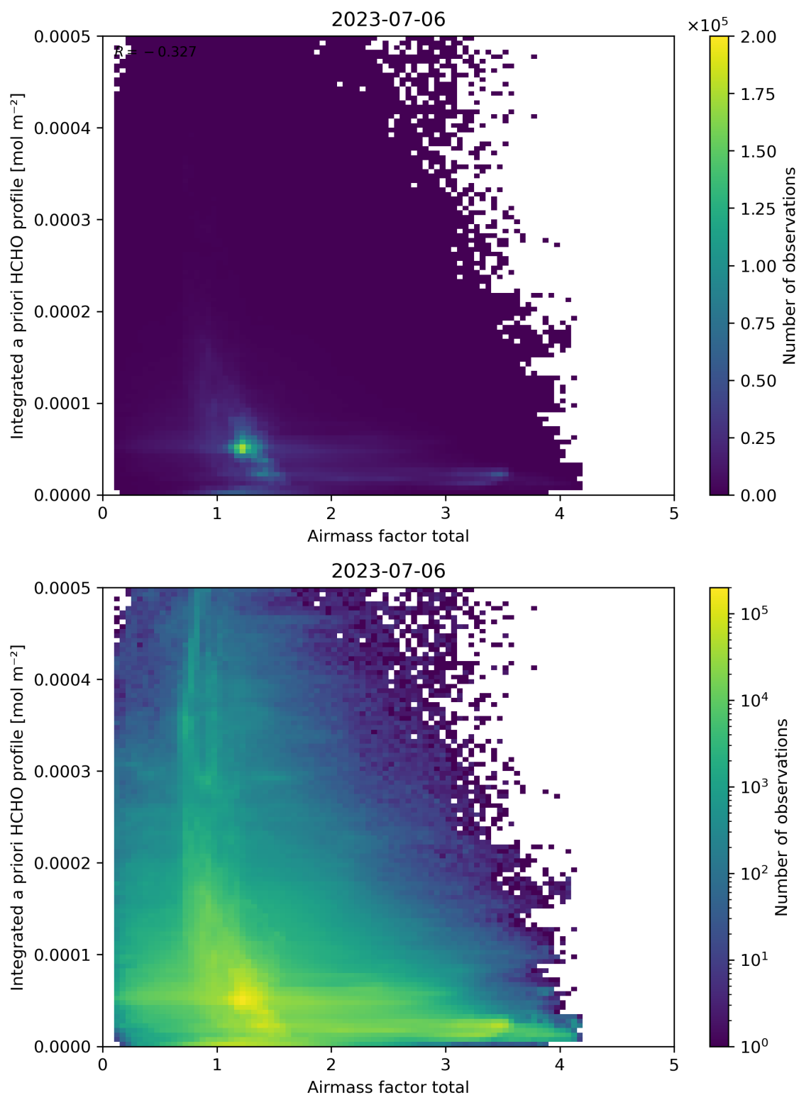
Figure 104: Scatter density plot of “Airmass factor total” against “Integrated a priori HCHO profile” for 2023-07-05 to 2023-07-07.
