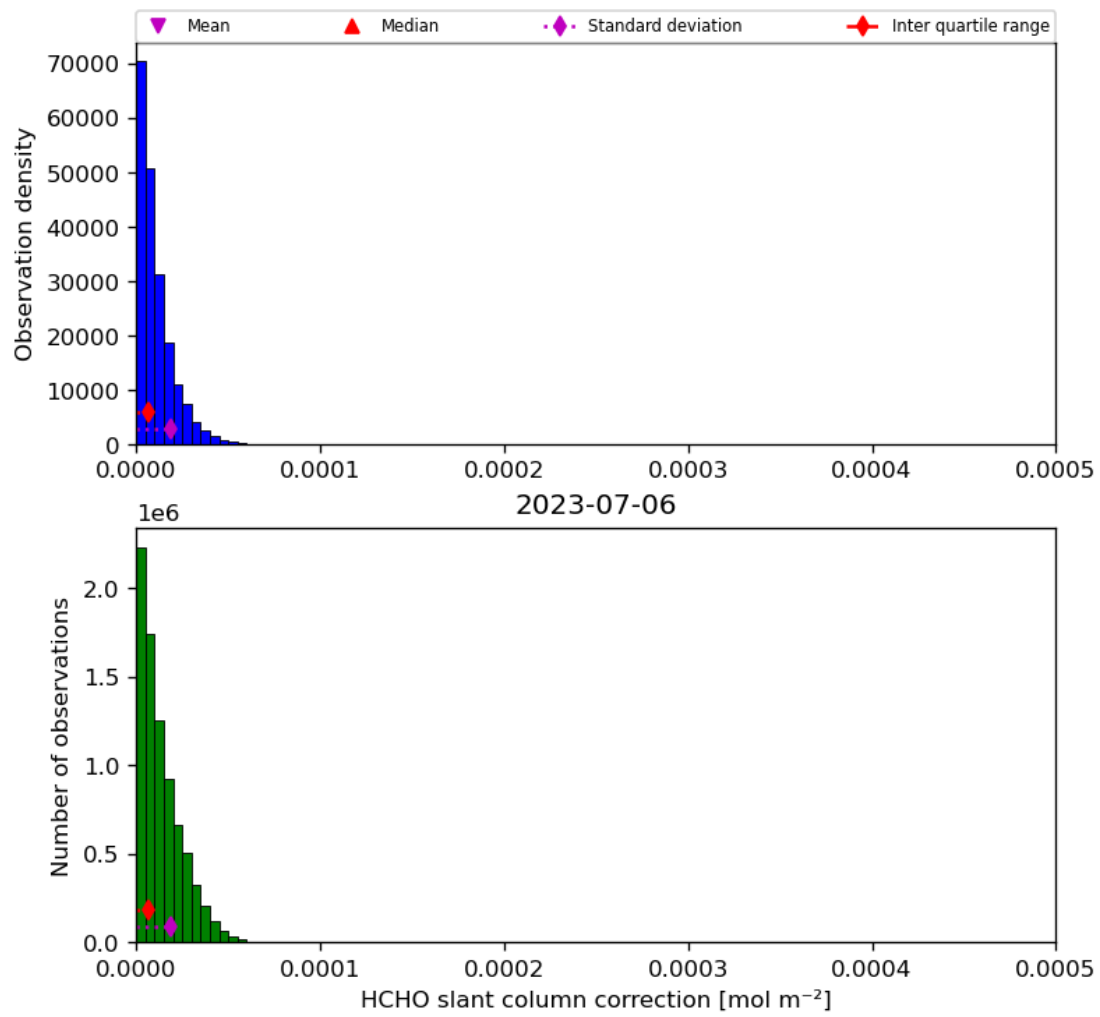
Figure 47: Histogram of “HCHO slant column correction” for 2023-07-05 to 2023-07-07
