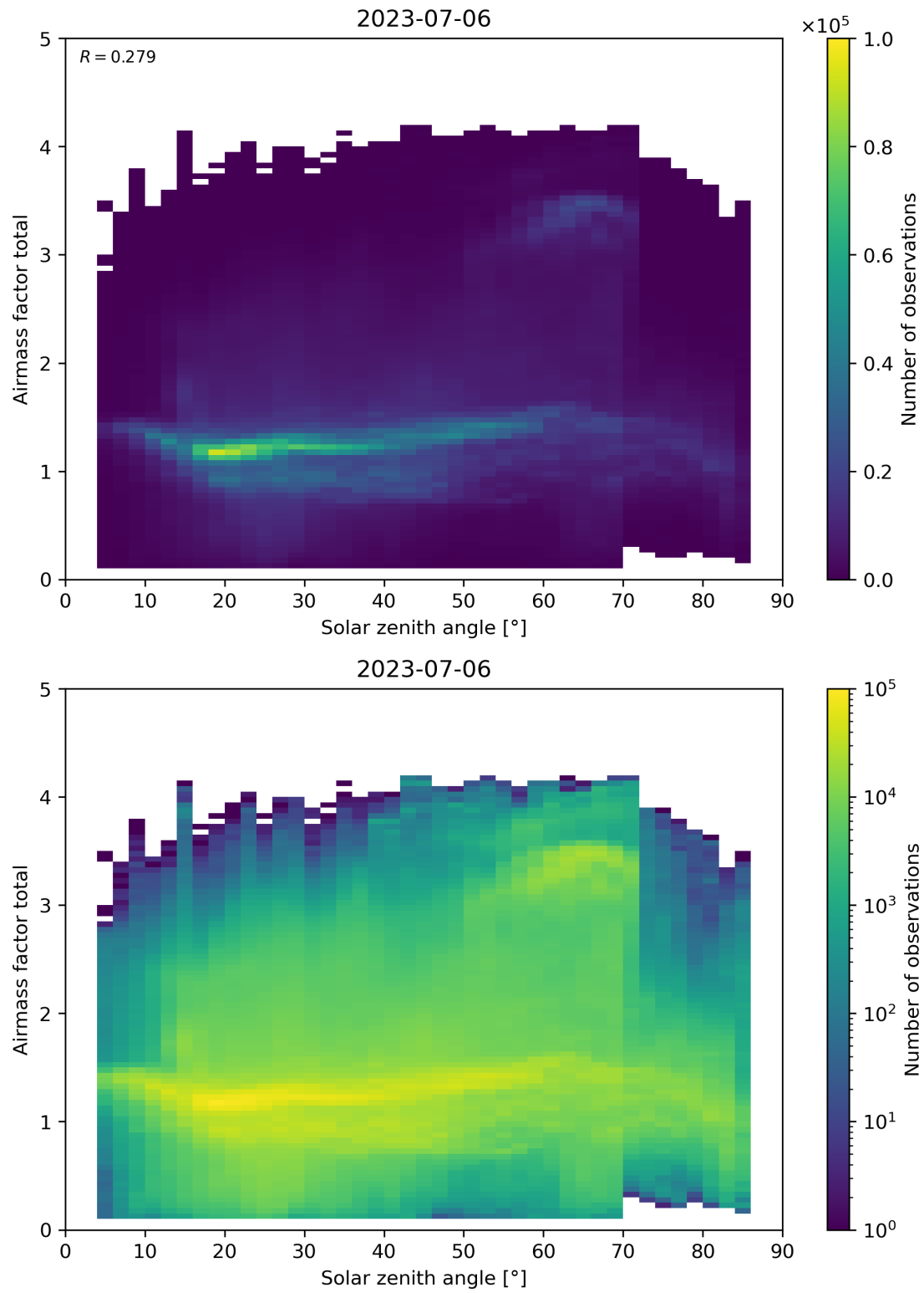
Figure 175: Scatter density plot of “Solar zenith angle” against “Airmass factor total” for 2023-07-05 to 2023-07-07.
