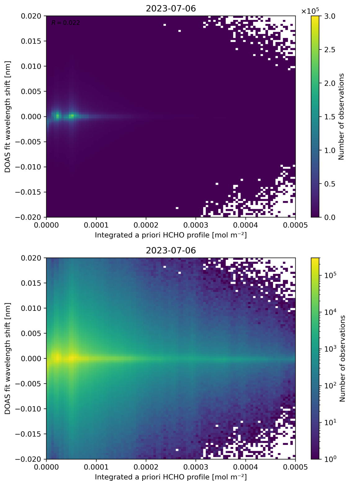
Figure 149: Scatter density plot of “Integrated a priori HCHO profile” against “DOAS fit wavelength shift” for 2023-07-05 to 2023-07-07.
