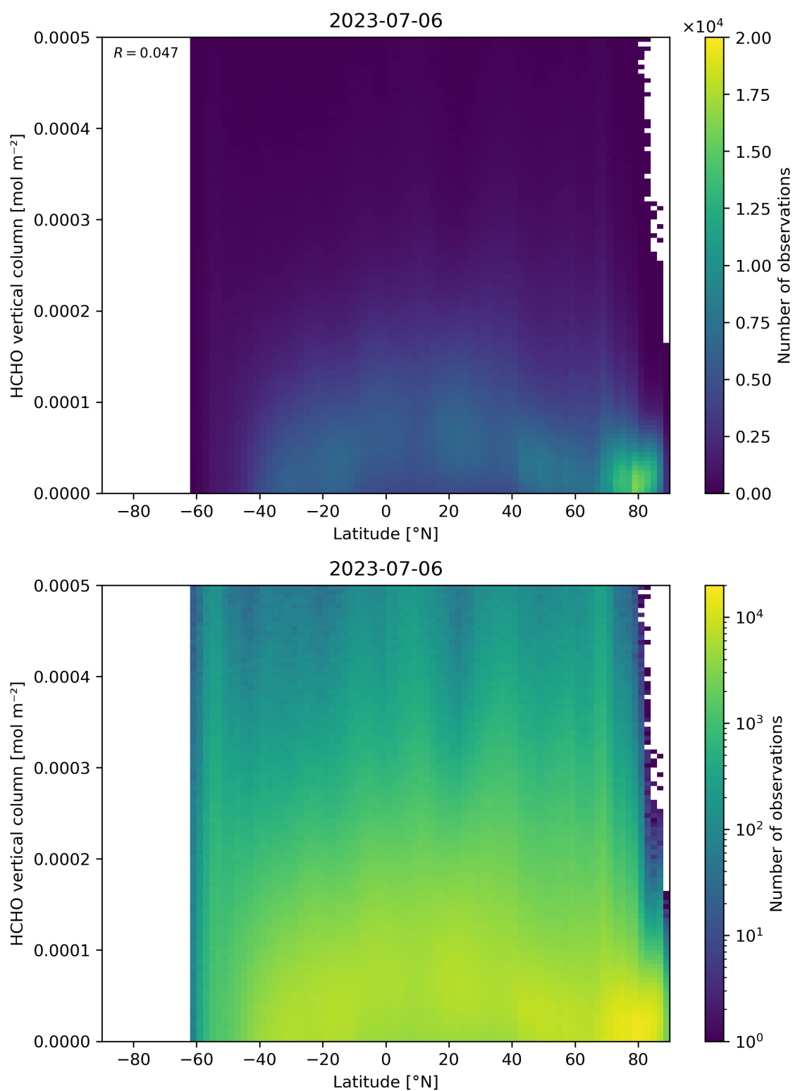
Figure 163: Scatter density plot of “Latitude” against “HCHO vertical column” for 2023-07-05 to 2023-07-07.
