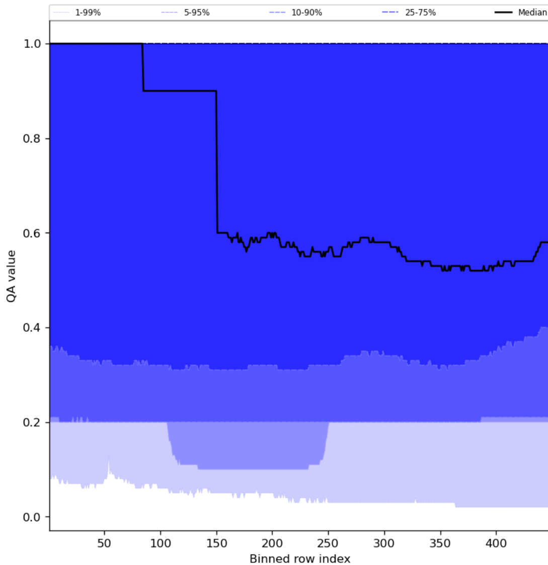
Figure 48: Along track statistics of “QA value” for 2023-07-05 to 2023-07-07
