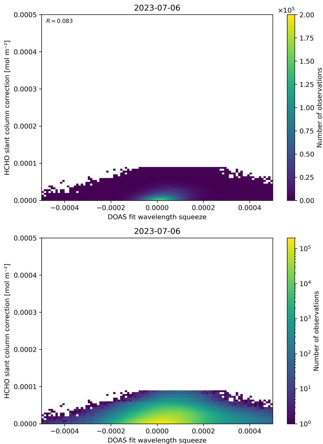
Figure 70: Scatter density plot of “DOAS fit wavelength squeeze” against “HCHO slant column correction” for 2023-07-05 to 2023-07-07.
