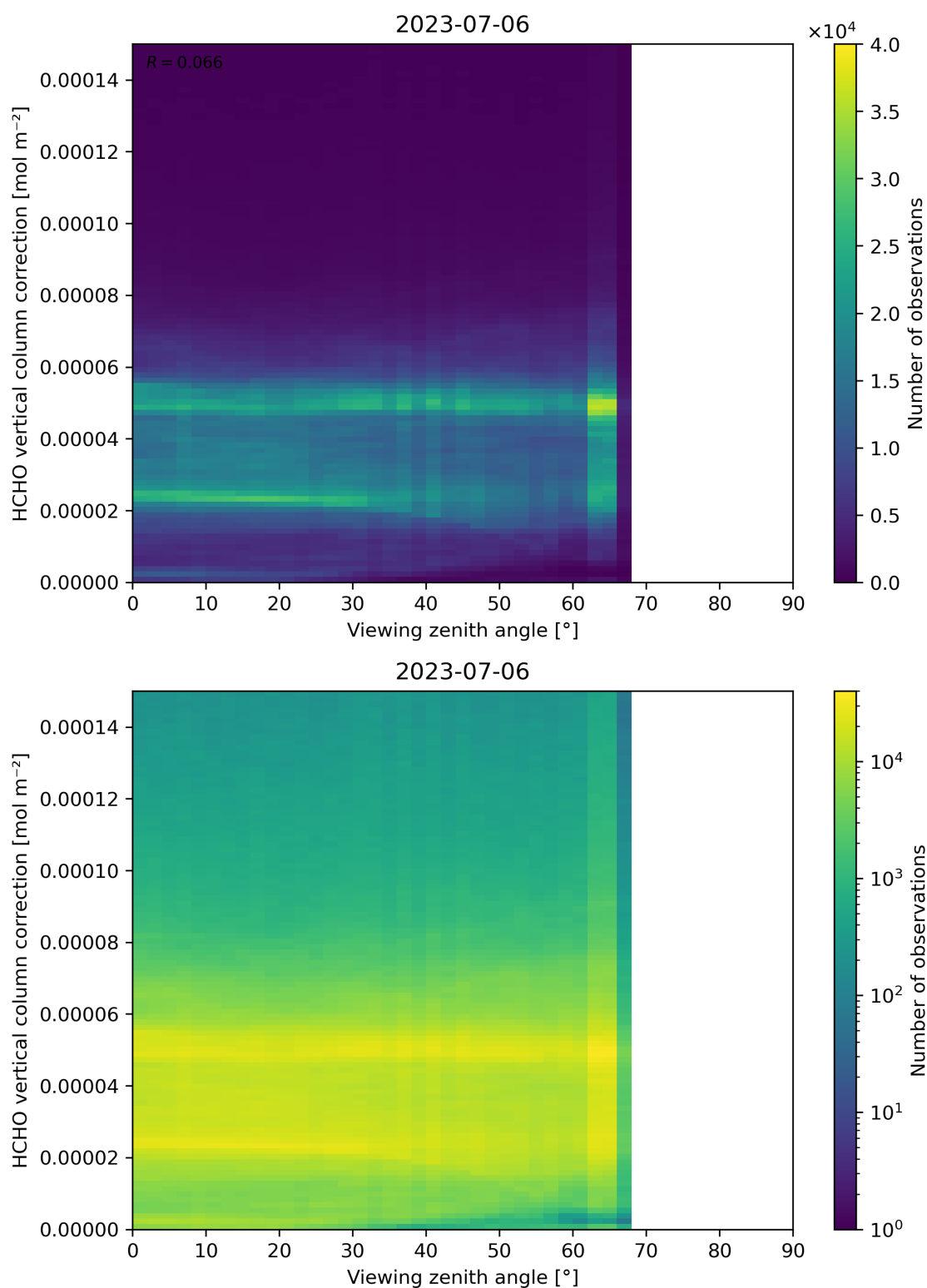
Figure 193: Scatter density plot of “Viewing zenith angle” against “HCHO vertical column correction” for 2023-07-05 to 2023-07-07.
