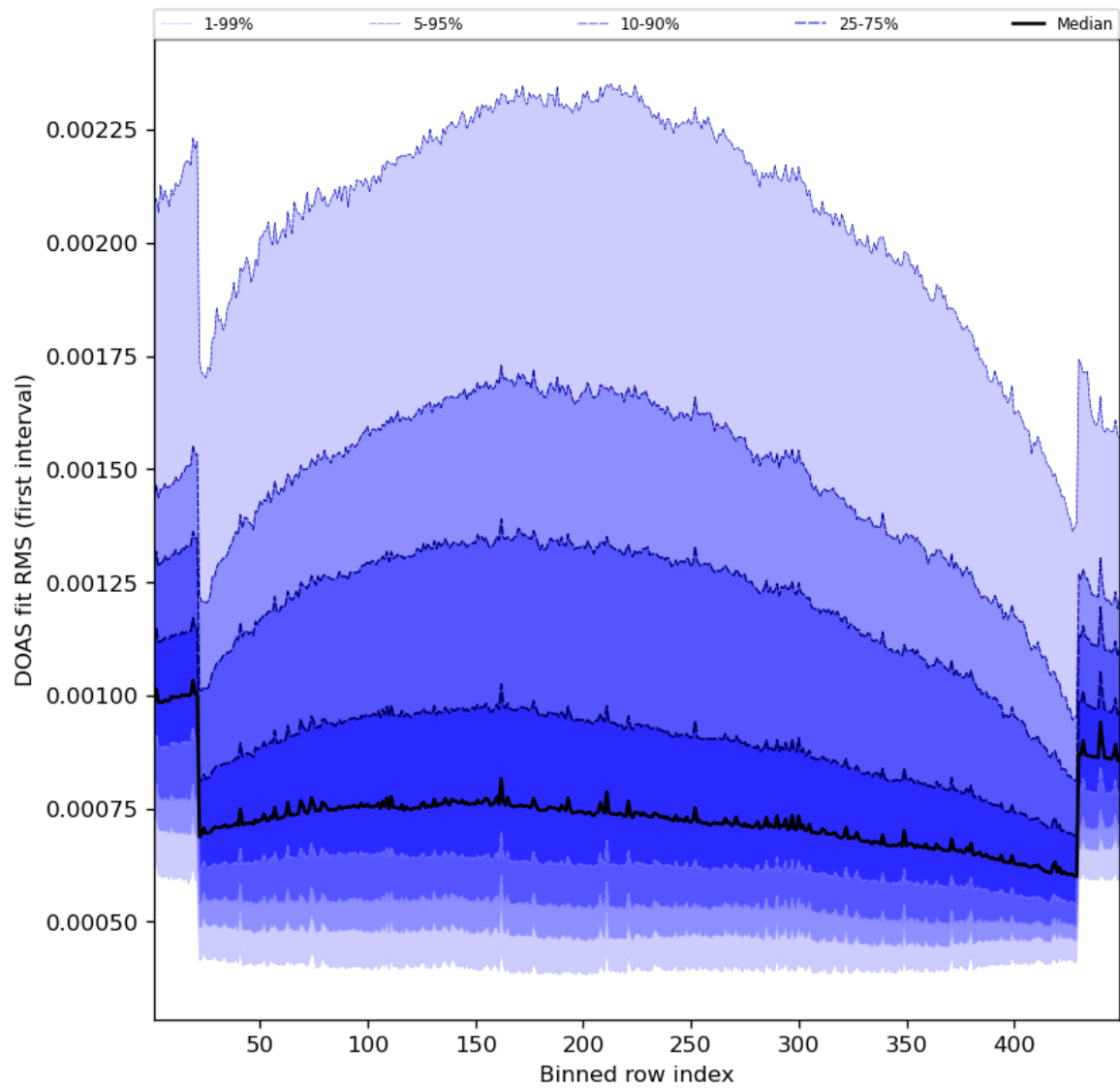
Figure 60: Along track statistics of “DOAS fit RMS (first interval)” for 2023-07-05 to 2023-07-07
