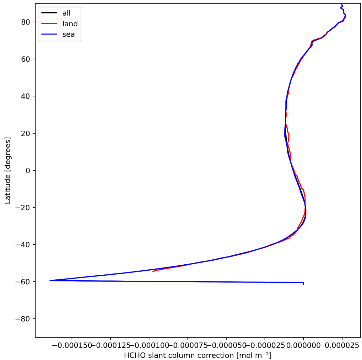
Figure 33: Zonal average of “HCHO slant column correction” for 2023-07-05 to 2023-07-07.
