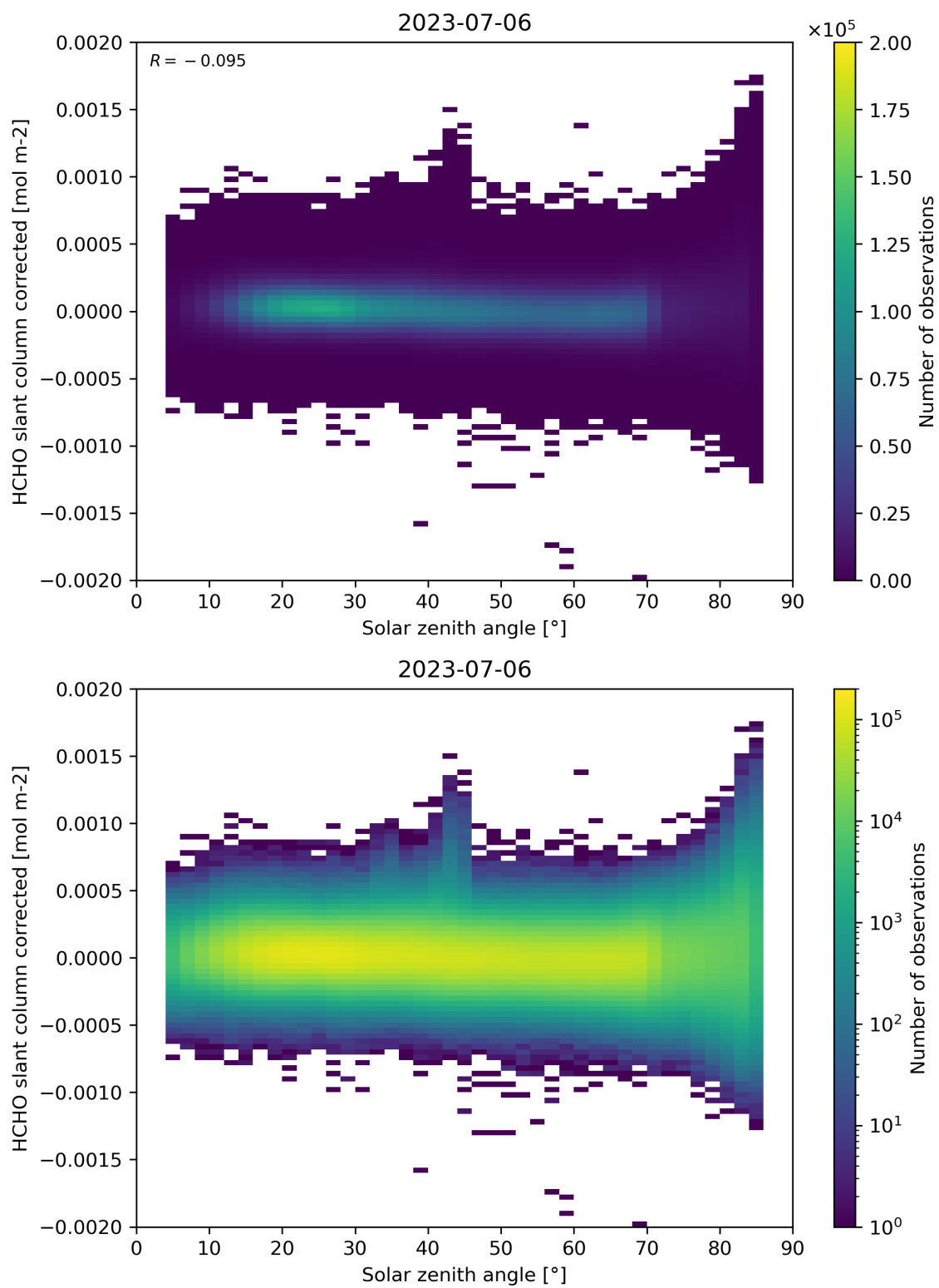
Figure 171: Scatter density plot of “Solar zenith angle” against “HCHO slant column corrected” for 2023-07-05 to 2023-07-07.
