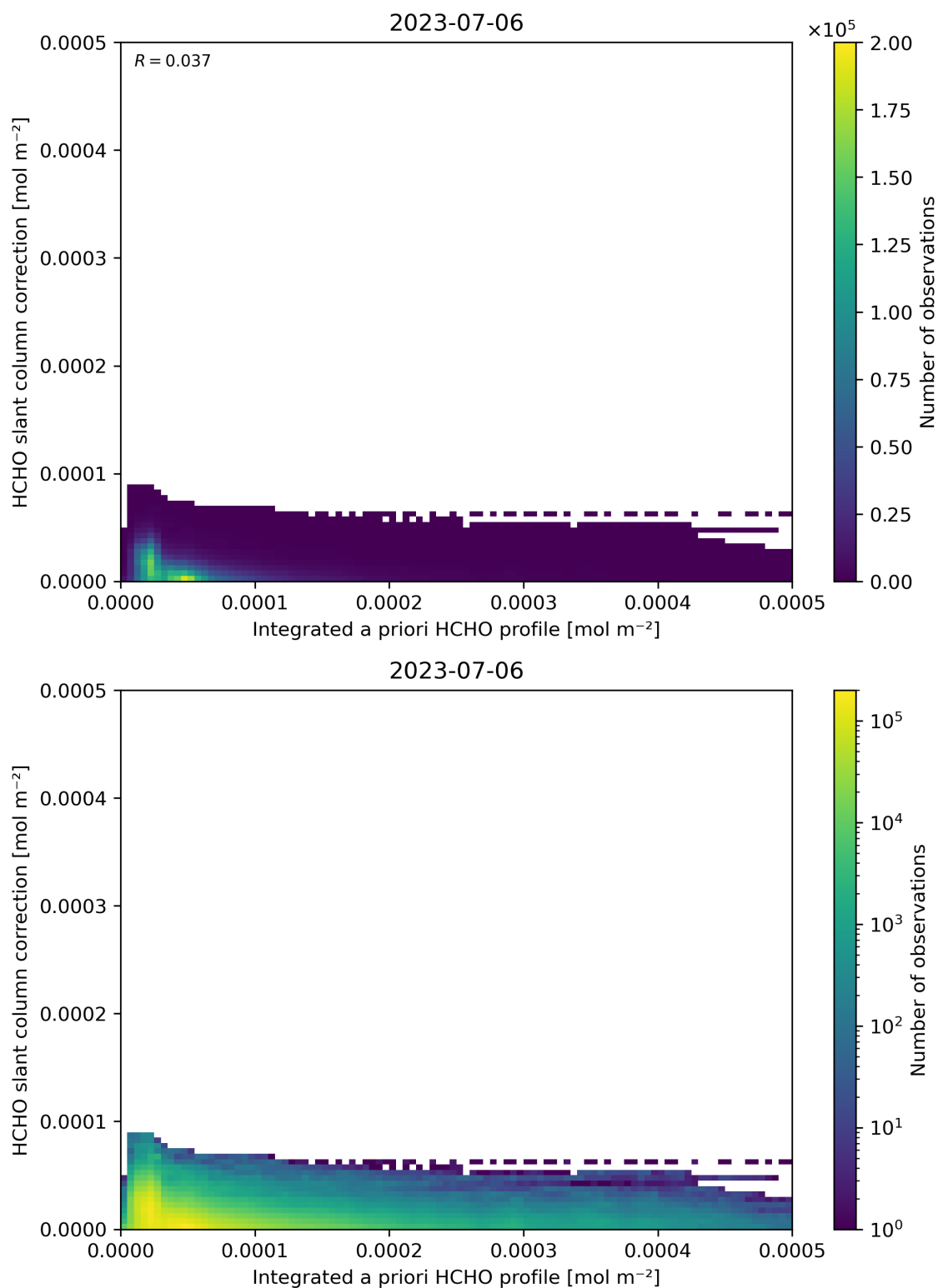
Figure 152: Scatter density plot of “Integrated a priori HCHO profile” against “HCHO slant column correction” for 2023-07-05 to 2023-07-07.
