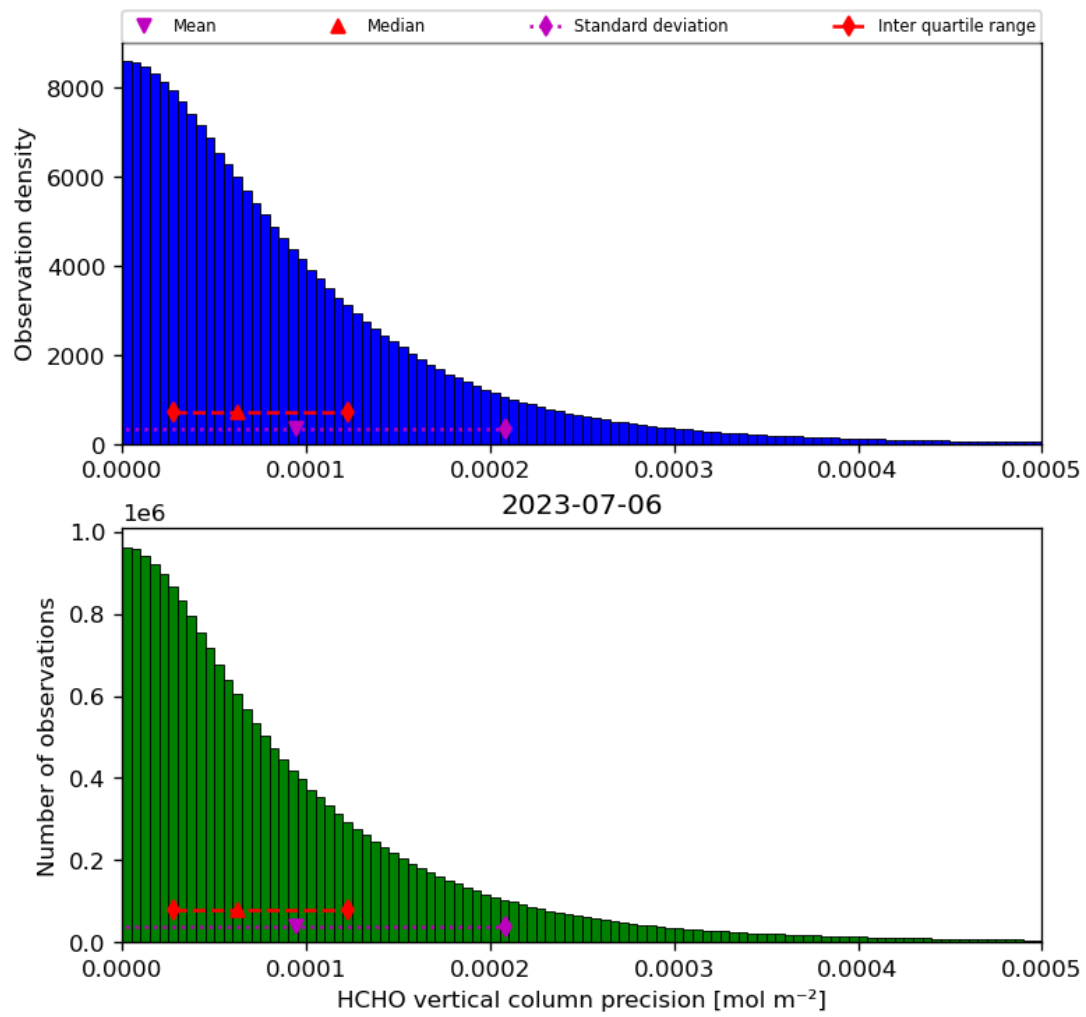
Figure 36: Histogram of “HCHO vertical column precision” for 2023-07-05 to 2023-07-07
