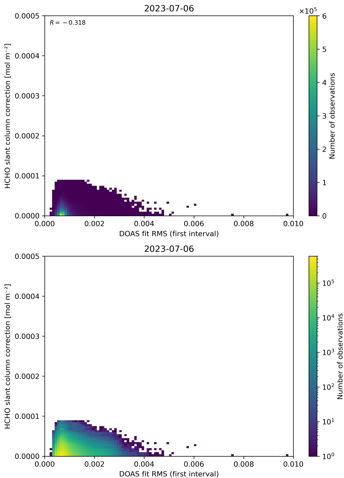
Figure 63: Scatter density plot of “DOAS fit RMS (first interval)” against “HCHO slant column correction” for 2023-07-05 to 2023-07-07.
