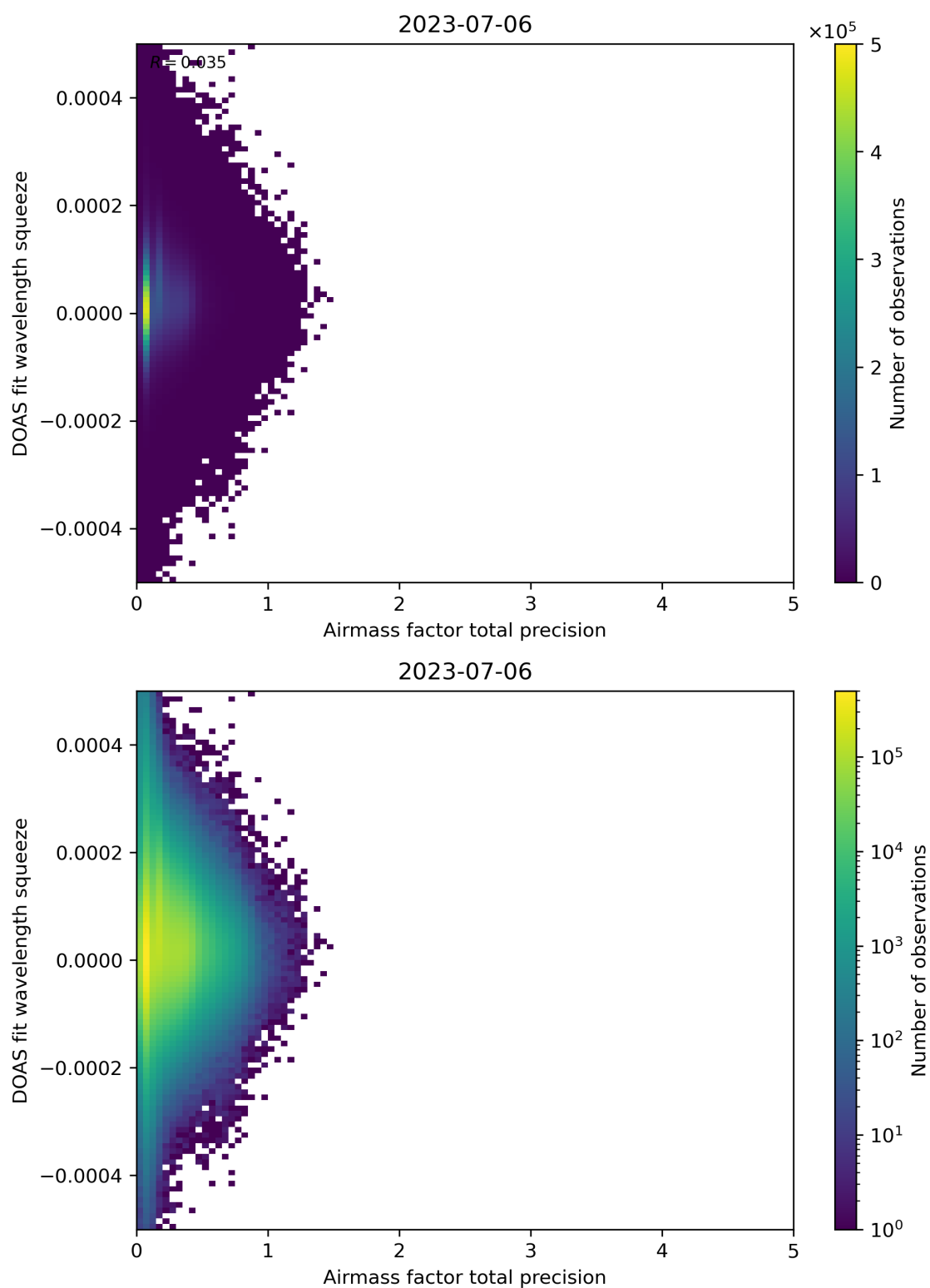
Figure 107: Scatter density plot of “Airmass factor total precision” against “DOAS fit wavelength squeeze” for 2023-07-05 to 2023-07-07.
