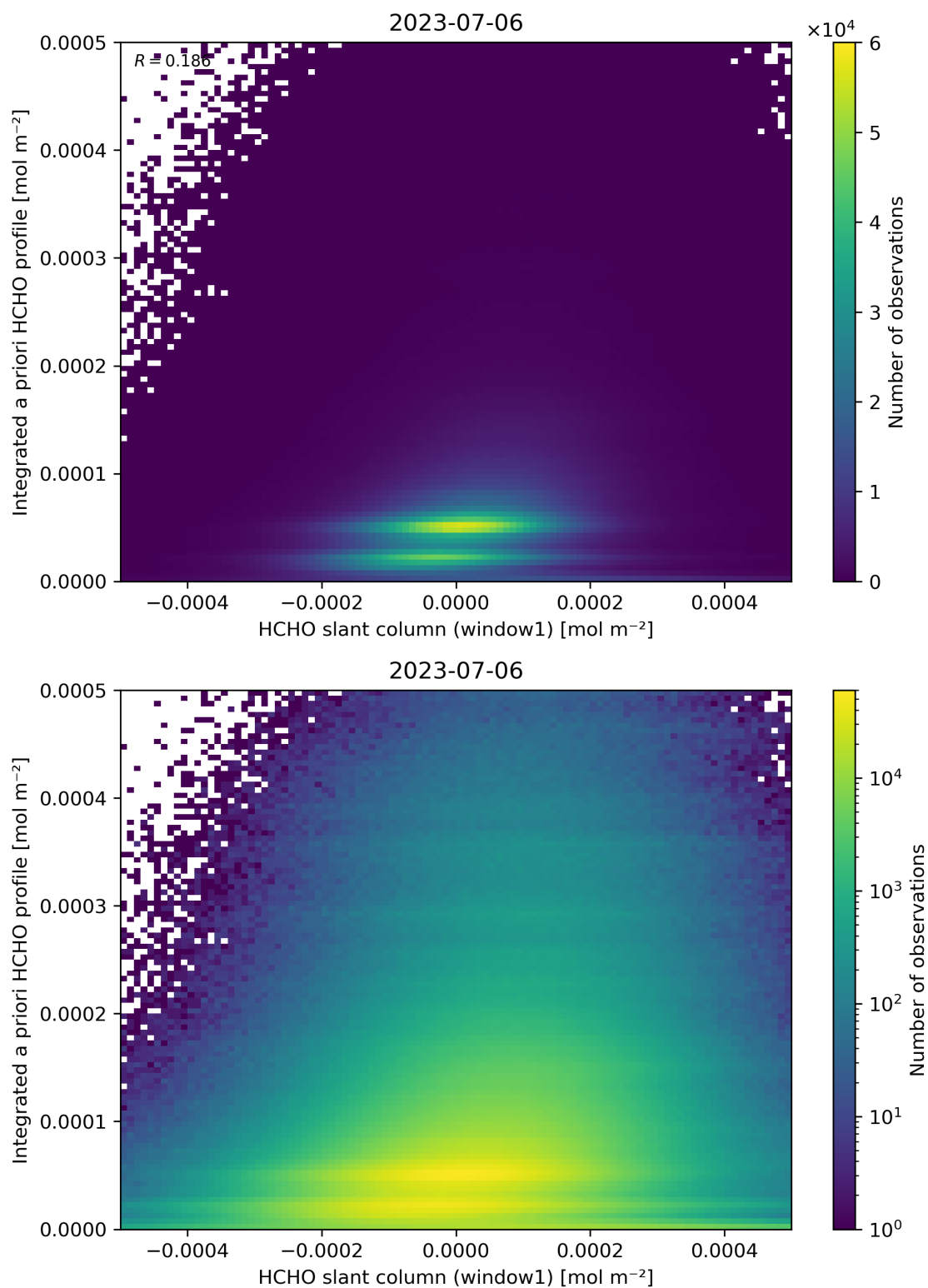
Figure 87: Scatter density plot of “HCHO slant column (window1)” against “Integrated a priori HCHO profile” for 2023-07-05 to 2023-07-07.
