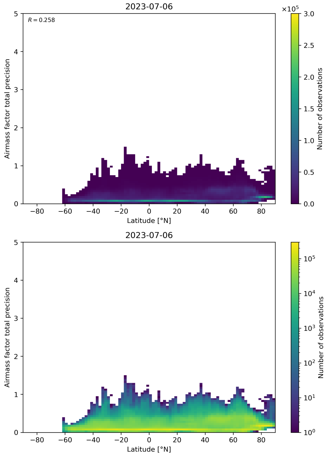
Figure 162: Scatter density plot of “Latitude” against “Airmass factor total precision” for 2023-07-05 to 2023-07-07.
