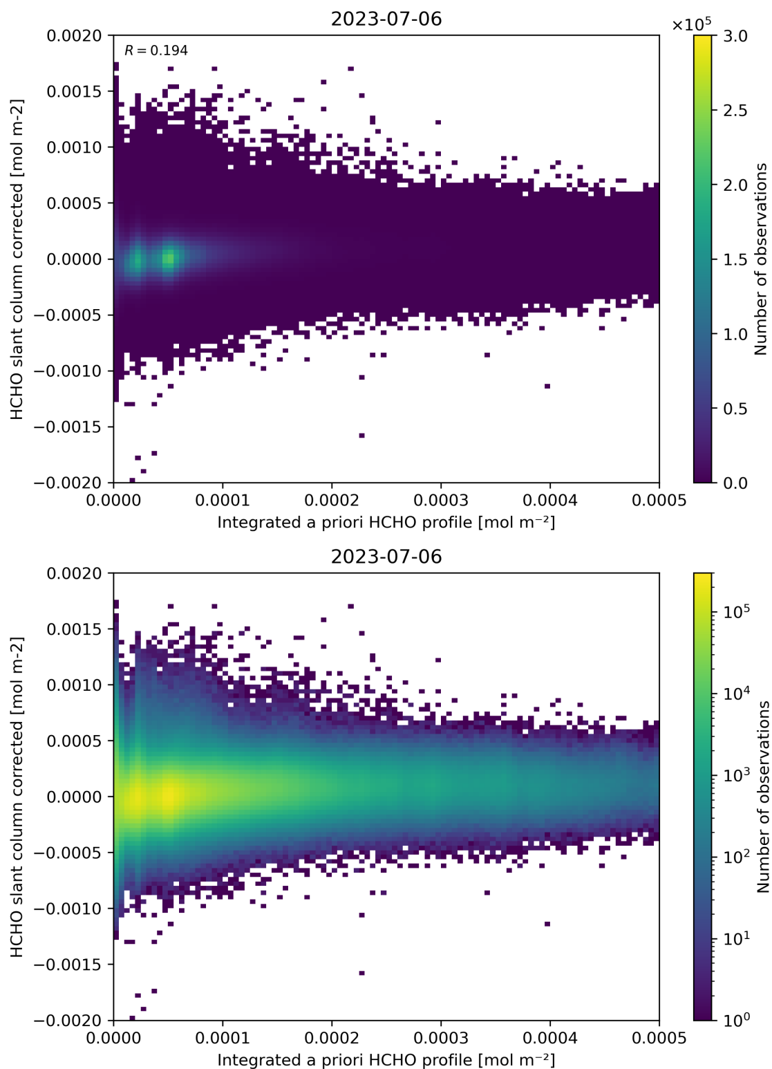
Figure 151: Scatter density plot of “Integrated a priori HCHO profile” against “HCHO slant column corrected” for 2023-07-05 to 2023-07-07.
