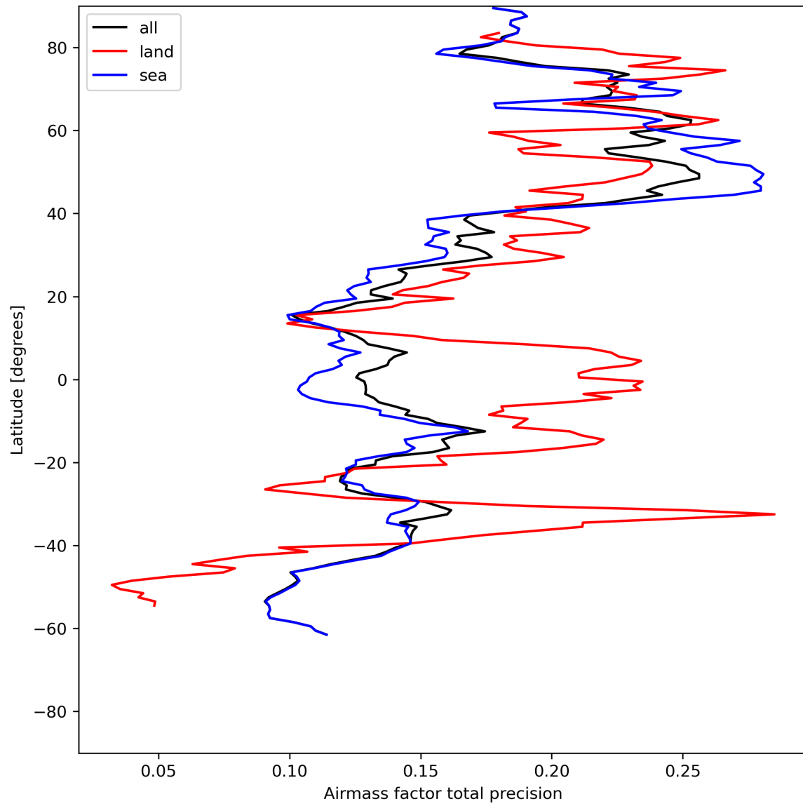
Figure 27: Zonal average of “Airmass factor total precision” for 2023-07-05 to 2023-07-07.
