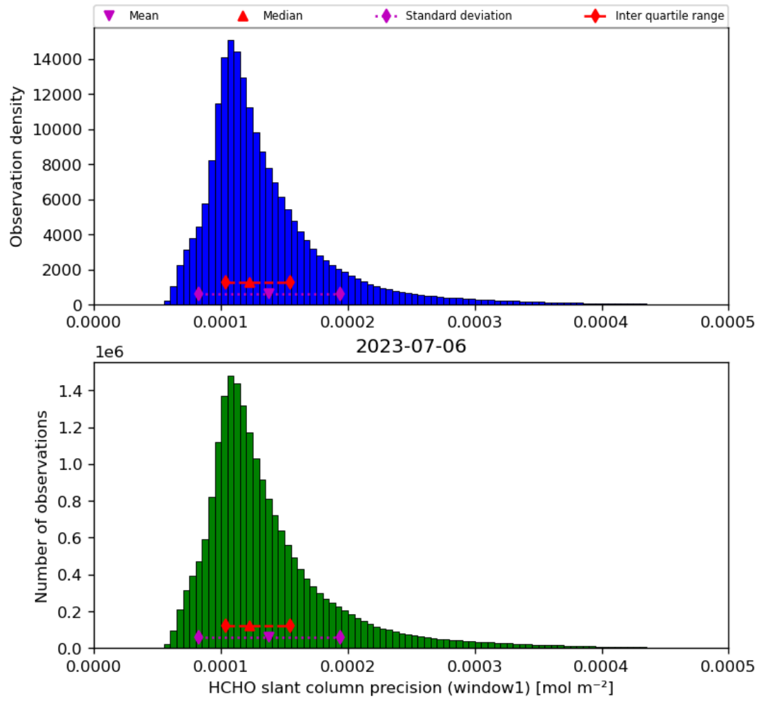
Figure 39: Histogram of “HCHO slant column precision (window1)” for 2023-07-05 to 2023-07-07
