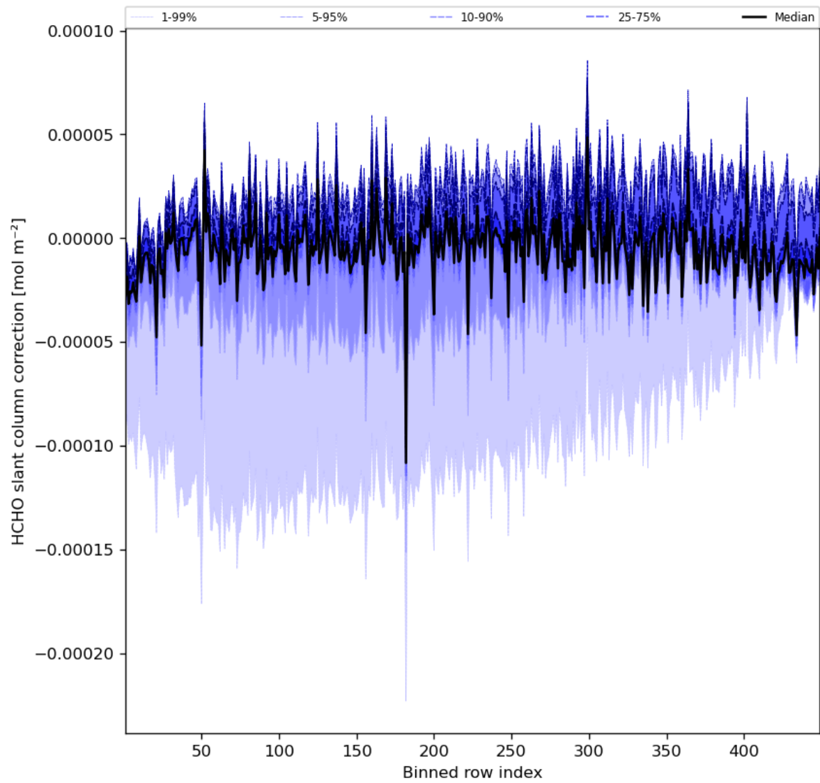
Figure 61: Along track statistics of “HCHO slant column correction” for 2023-07-05 to 2023-07-07
