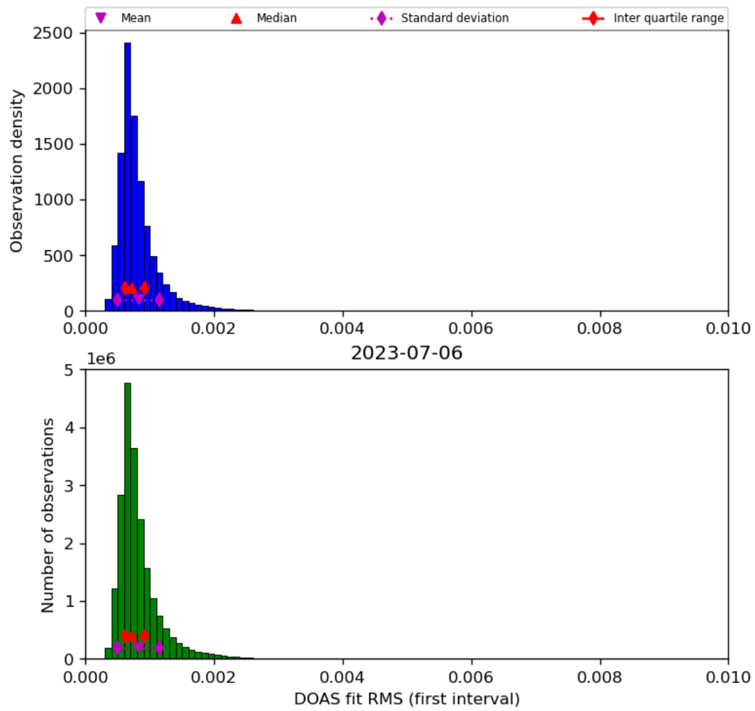
Figure 46: Histogram of “DOAS fit RMS (first interval)” for 2023-07-05 to 2023-07-07
