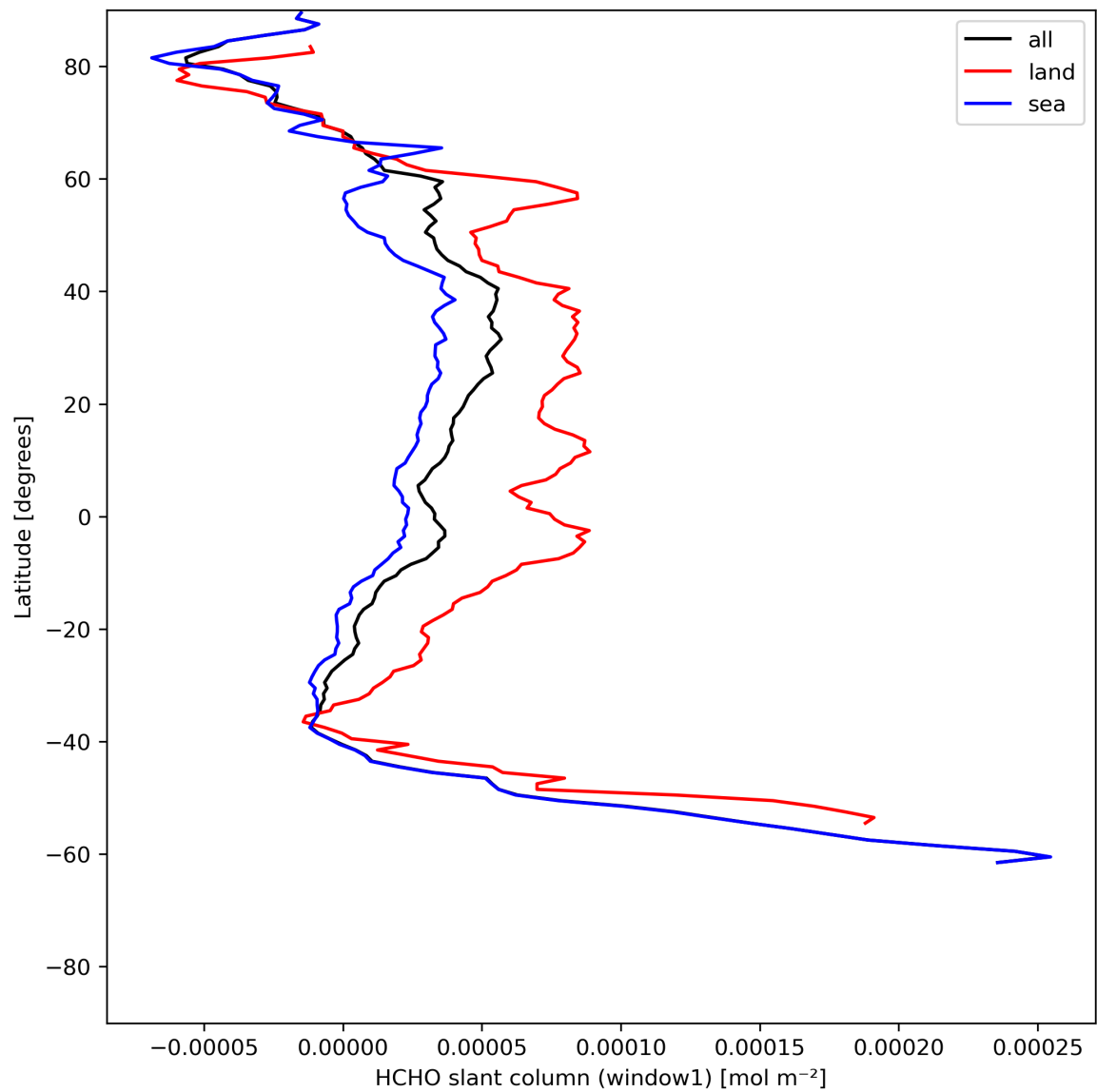
Figure 24: Zonal average of “HCHO slant column (window1)” for 2023-07-05 to 2023-07-07.
