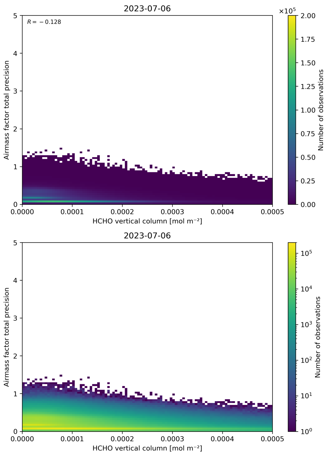
Figure 132: Scatter density plot of “HCHO vertical column” against “Airmass factor total precision” for 2023-07-05 to 2023-07-07.
