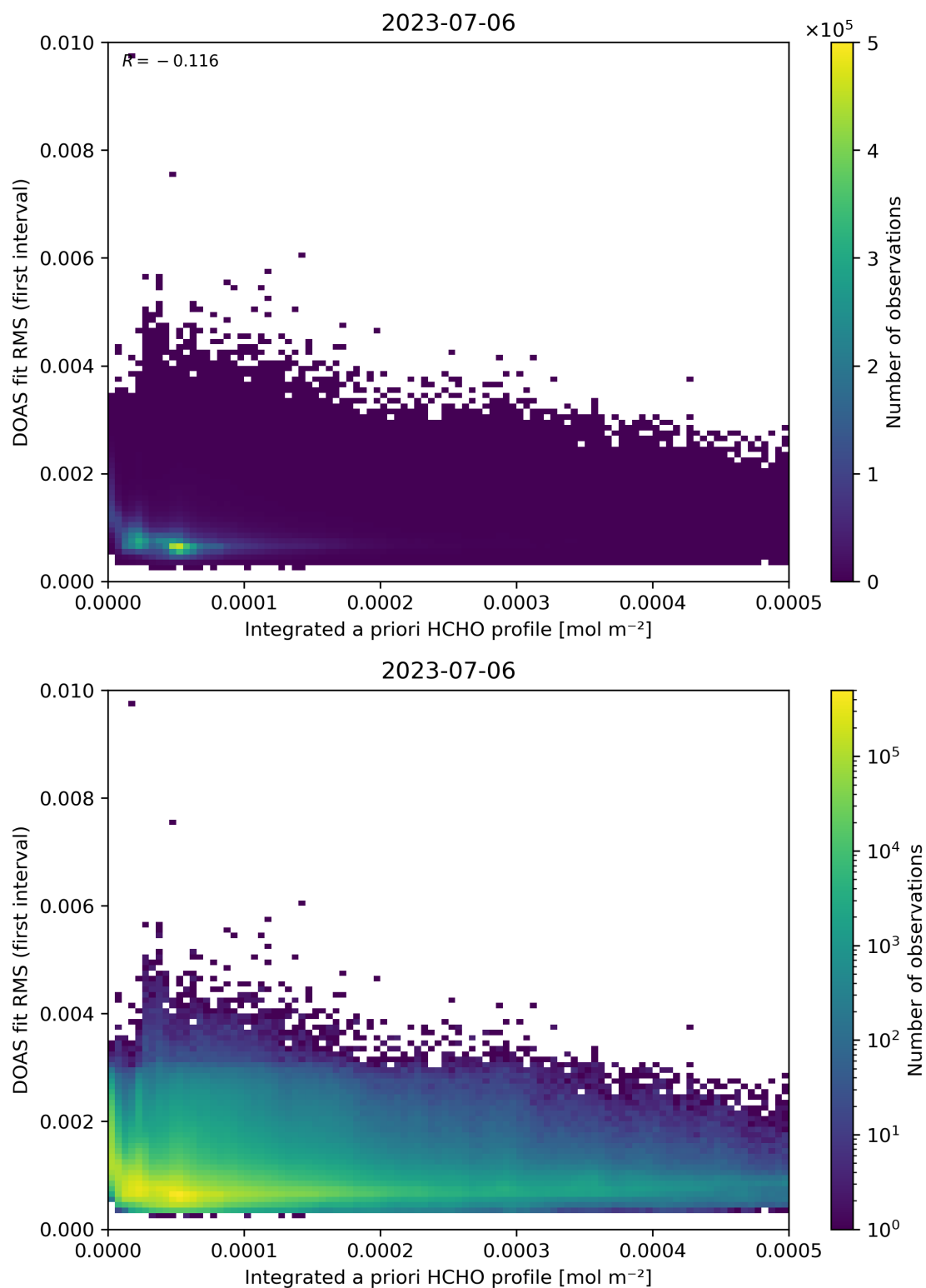
Figure 148: Scatter density plot of “Integrated a priori HCHO profile” against “DOAS fit RMS (first interval)” for 2023-07-05 to 2023-07-07.
