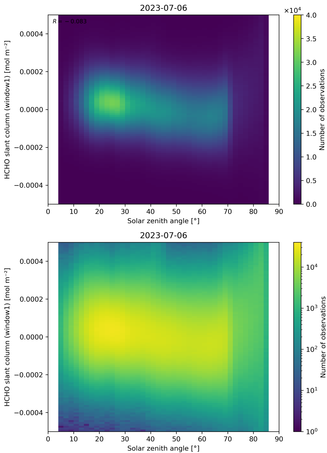
Figure 173: Scatter density plot of “Solar zenith angle” against “HCHO slant column (window1)” for 2023-07-05 to 2023-07-07.
