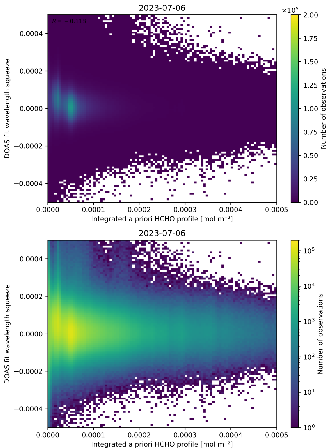
Figure 150: Scatter density plot of “Integrated a priori HCHO profile” against “DOAS fit wavelength squeeze” for 2023-07-05 to 2023-07-07.
