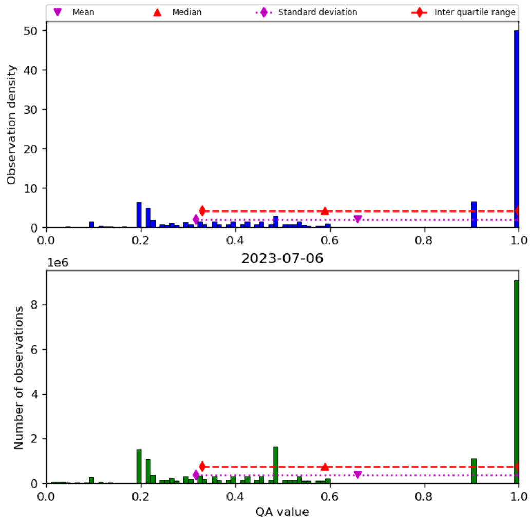
Figure 34: Histogram of “QA value” for 2023-07-05 to 2023-07-07
