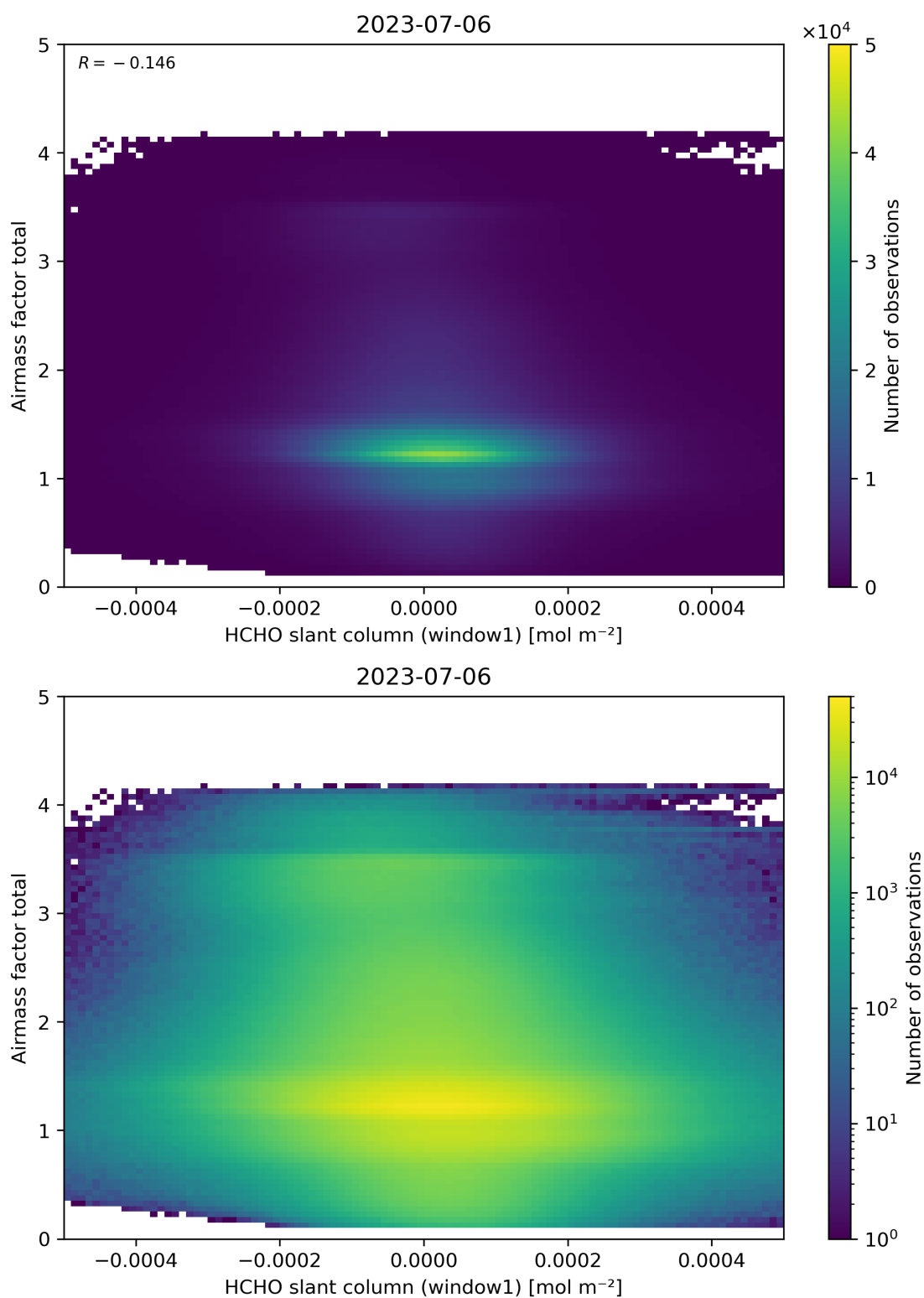
Figure 85: Scatter density plot of “HCHO slant column (window1)” against “Airmass factor total” for 2023-07-05 to 2023-07-07.
