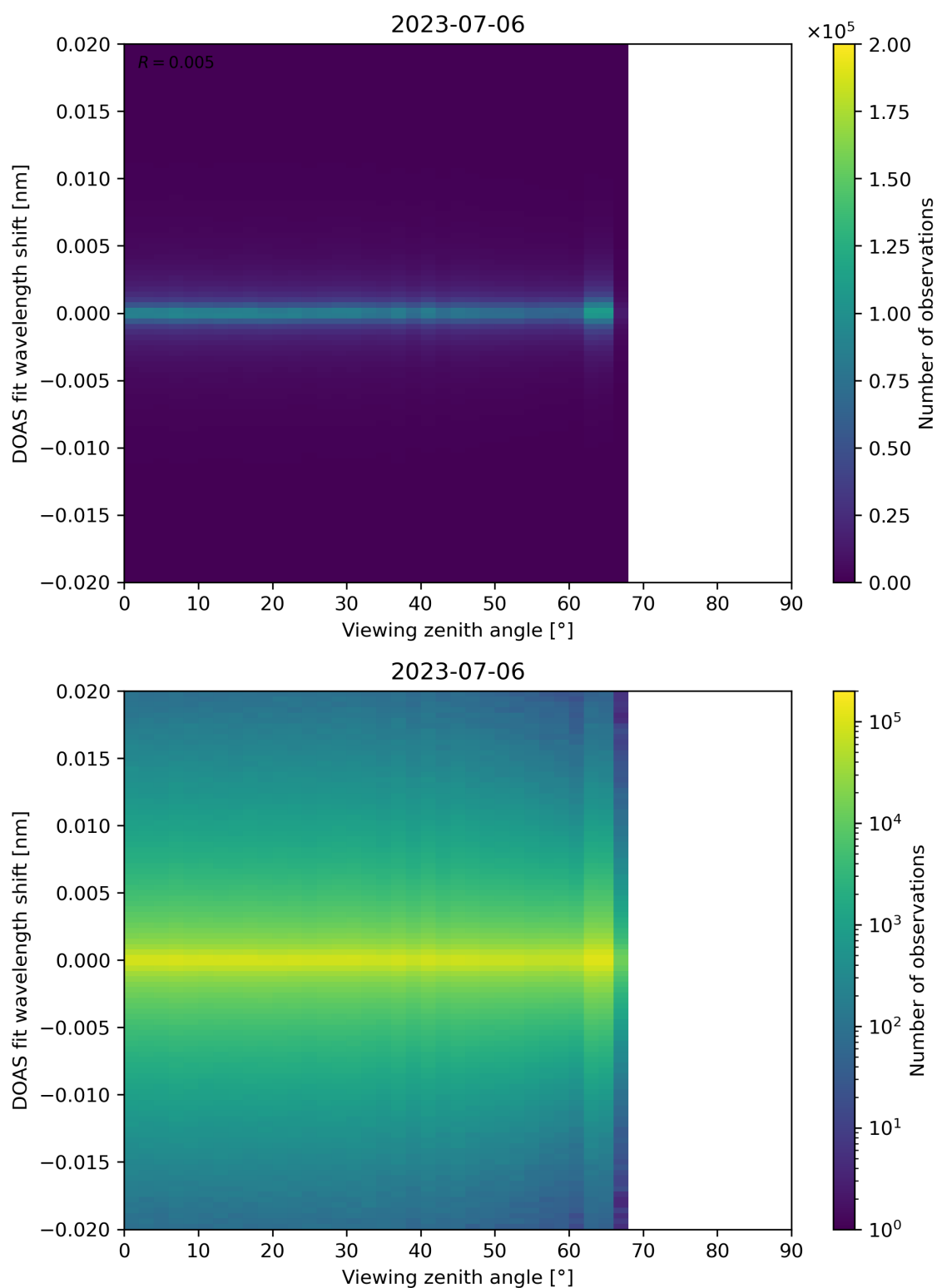
Figure 183: Scatter density plot of “Viewing zenith angle” against “DOAS fit wavelength shift” for 2023-07-05 to 2023-07-07.
