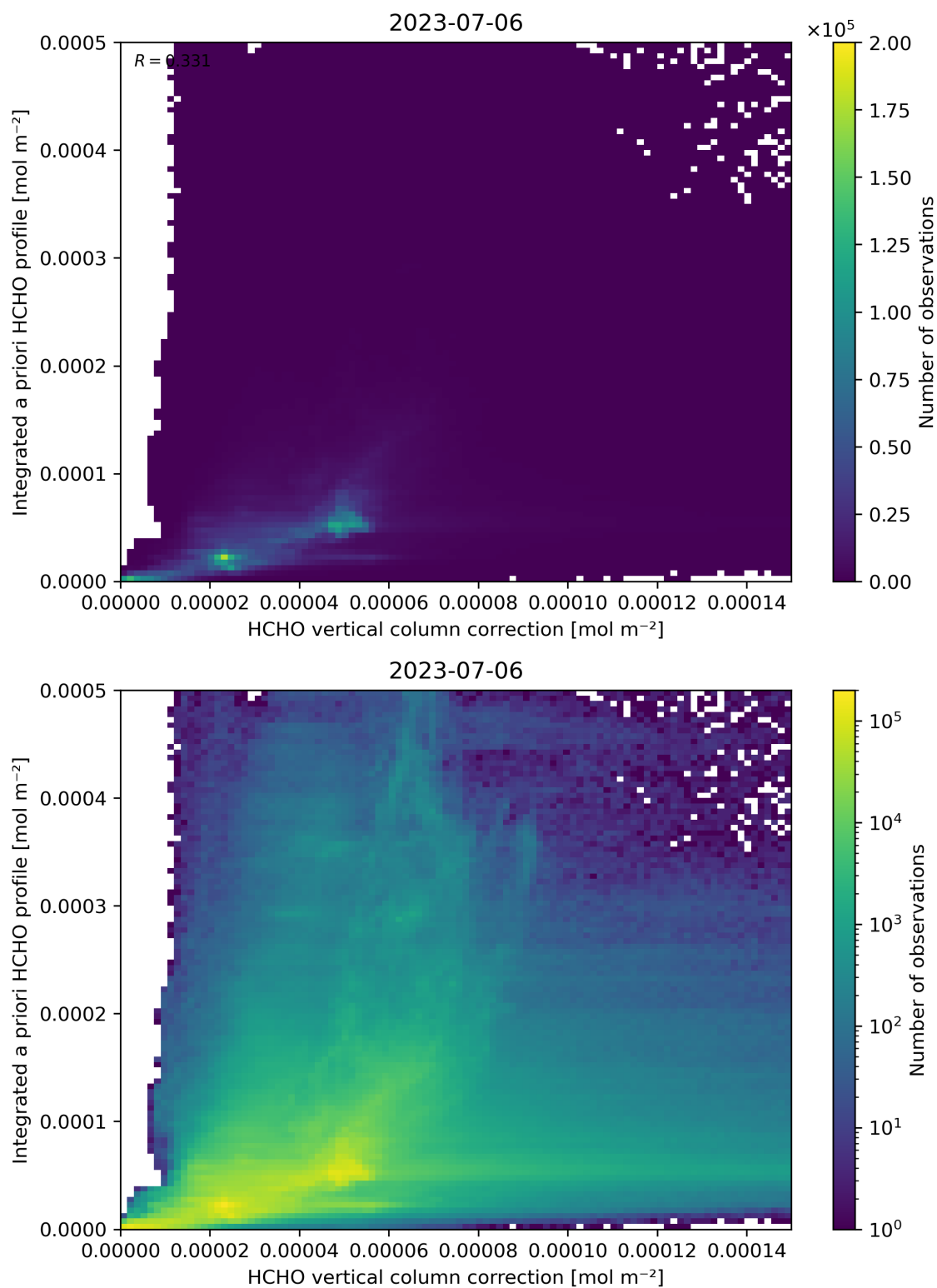
Figure 122: Scatter density plot of “HCHO vertical column correction” against “Integrated a priori HCHO profile” for 2023-07-05 to 2023-07-07.
