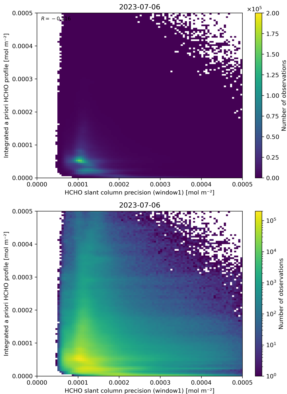
Figure 96: Scatter density plot of “HCHO slant column precision (window1)” against “Integrated a priori HCHO profile” for 2023-07-05 to 2023-07-07.
