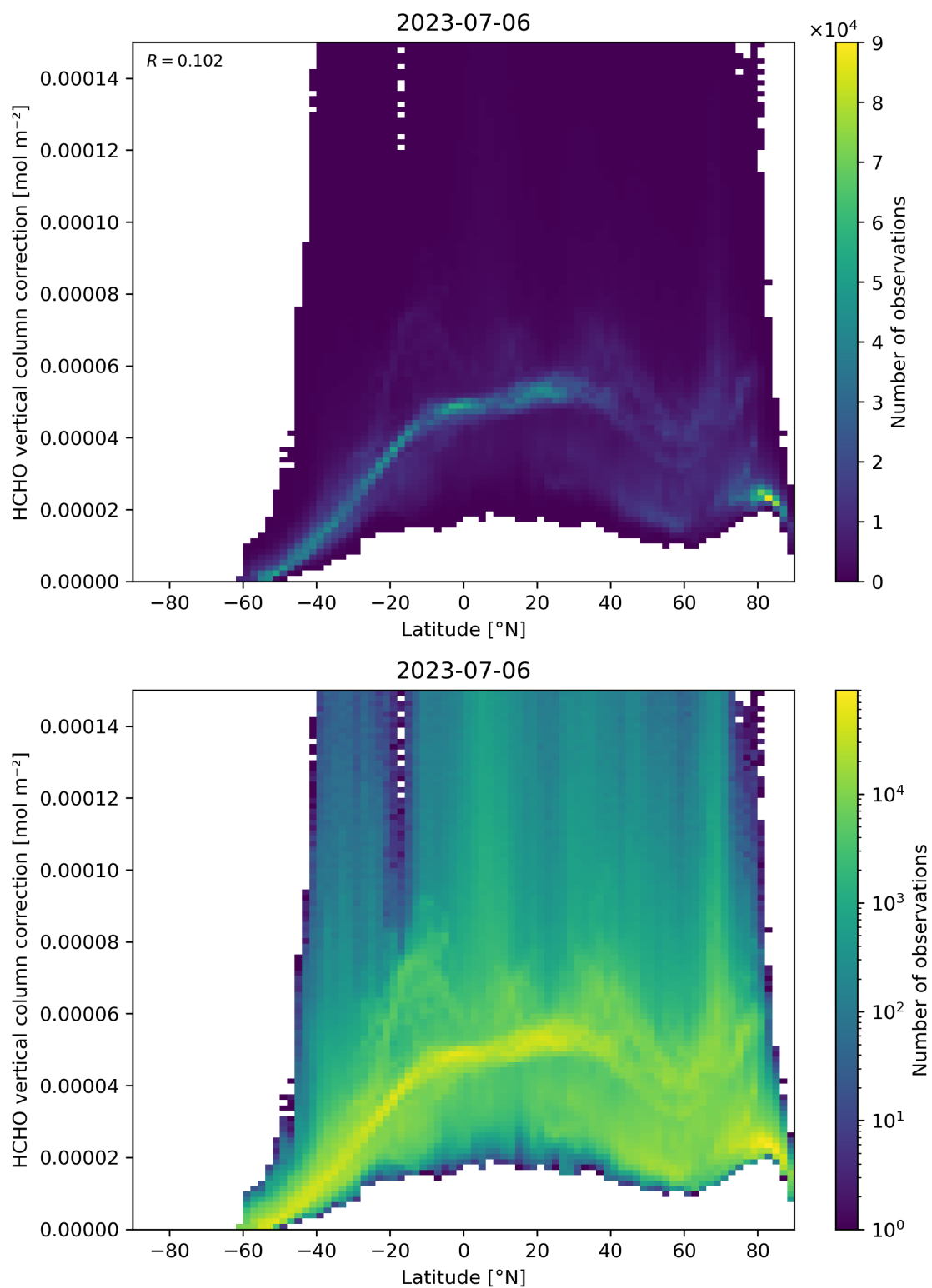
Figure 164: Scatter density plot of “Latitude” against “HCHO vertical column correction” for 2023-07-05 to 2023-07-07.
