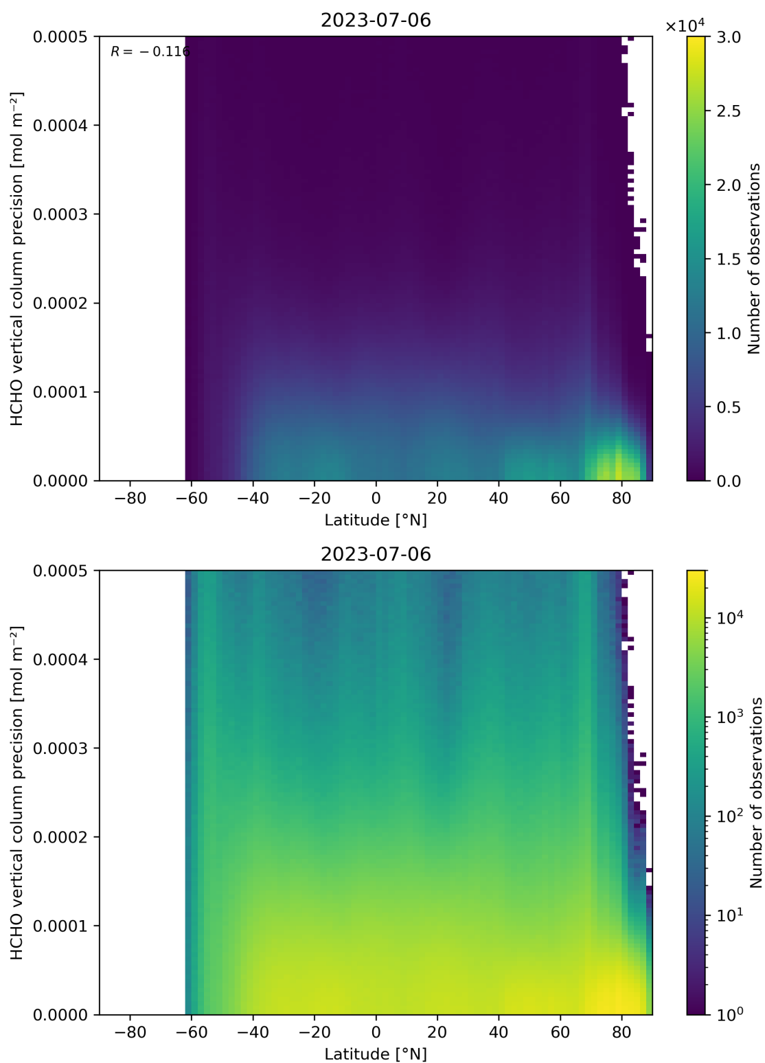
Figure 165: Scatter density plot of “Latitude” against “HCHO vertical column precision” for 2023-07-05 to 2023-07-07.
