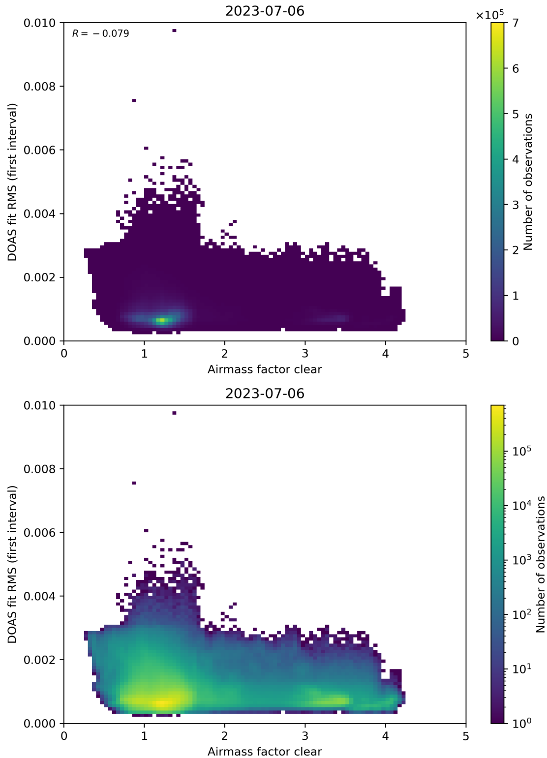
Figure 71: Scatter density plot of “Airmass factor clear” against “DOAS fit RMS (first interval)” for 2023-07-05 to 2023-07-07.
