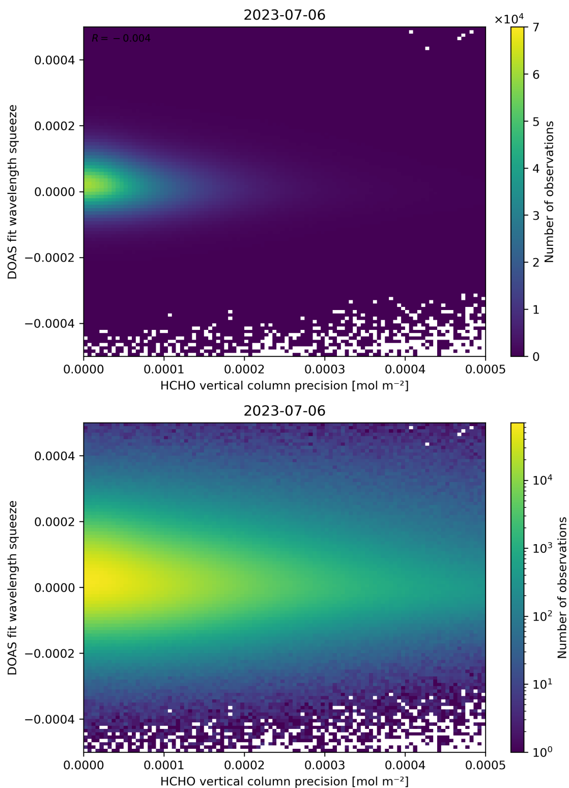
Figure 138: Scatter density plot of “HCHO vertical column precision” against “DOAS fit wavelength squeeze” for 2023-07-05 to 2023-07-07.
