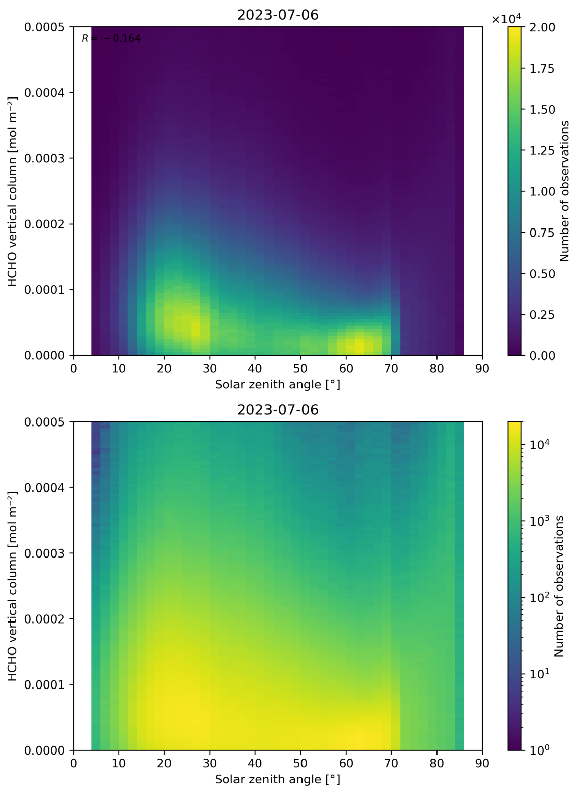
Figure 177: Scatter density plot of “Solar zenith angle” against “HCHO vertical column” for 2023-07-05 to 2023-07-07.
