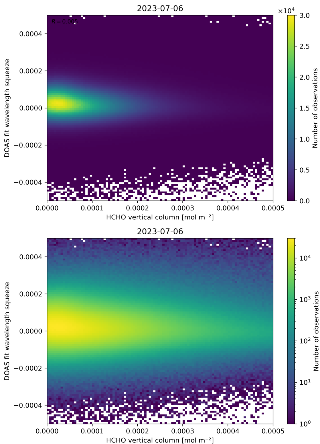
Figure 125: Scatter density plot of “HCHO vertical column” against “DOAS fit wavelength squeeze” for 2023-07-05 to 2023-07-07.
