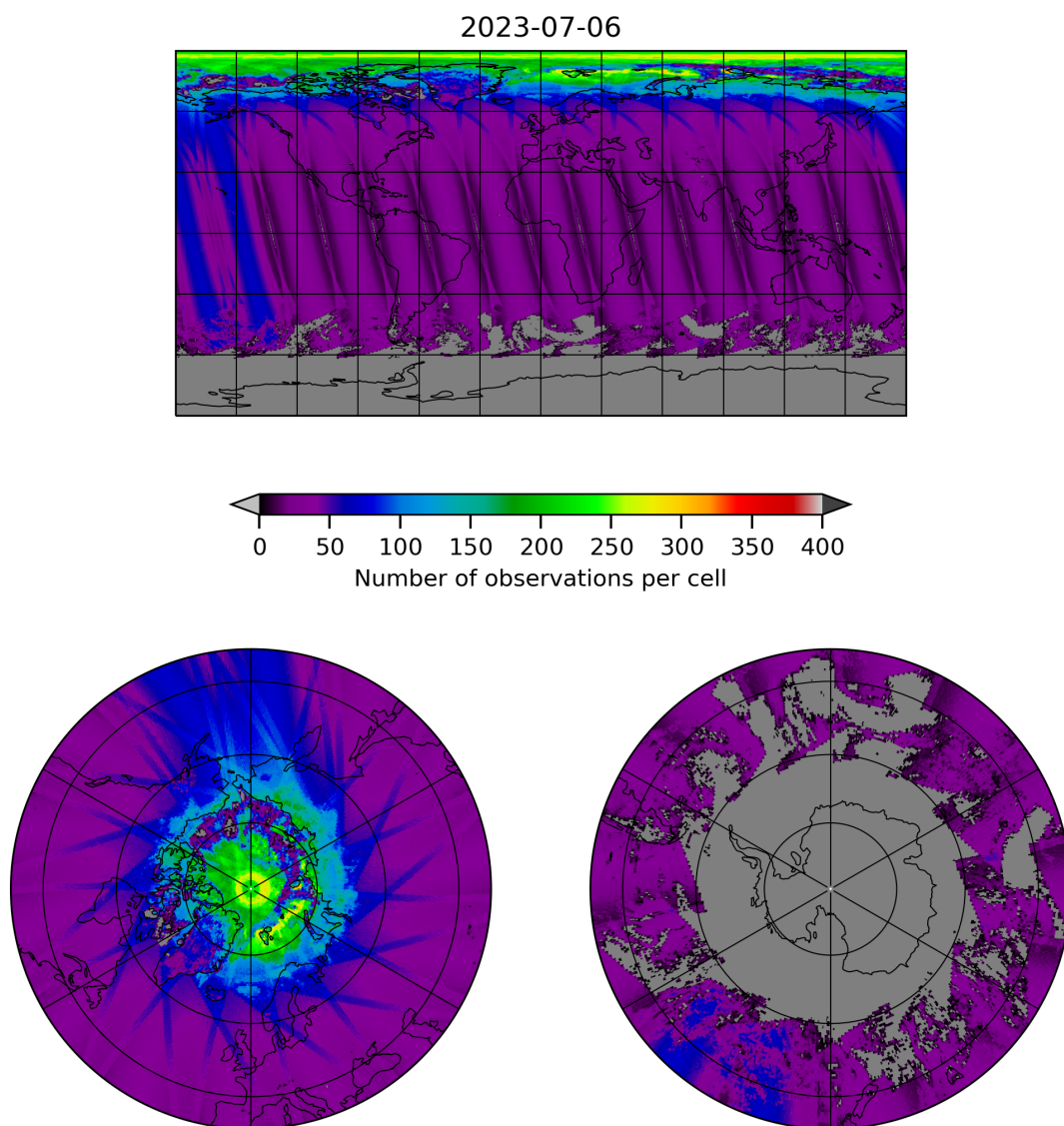
Figure 19: Map of the number of observations for 2023-07-05 to 2023-07-07
