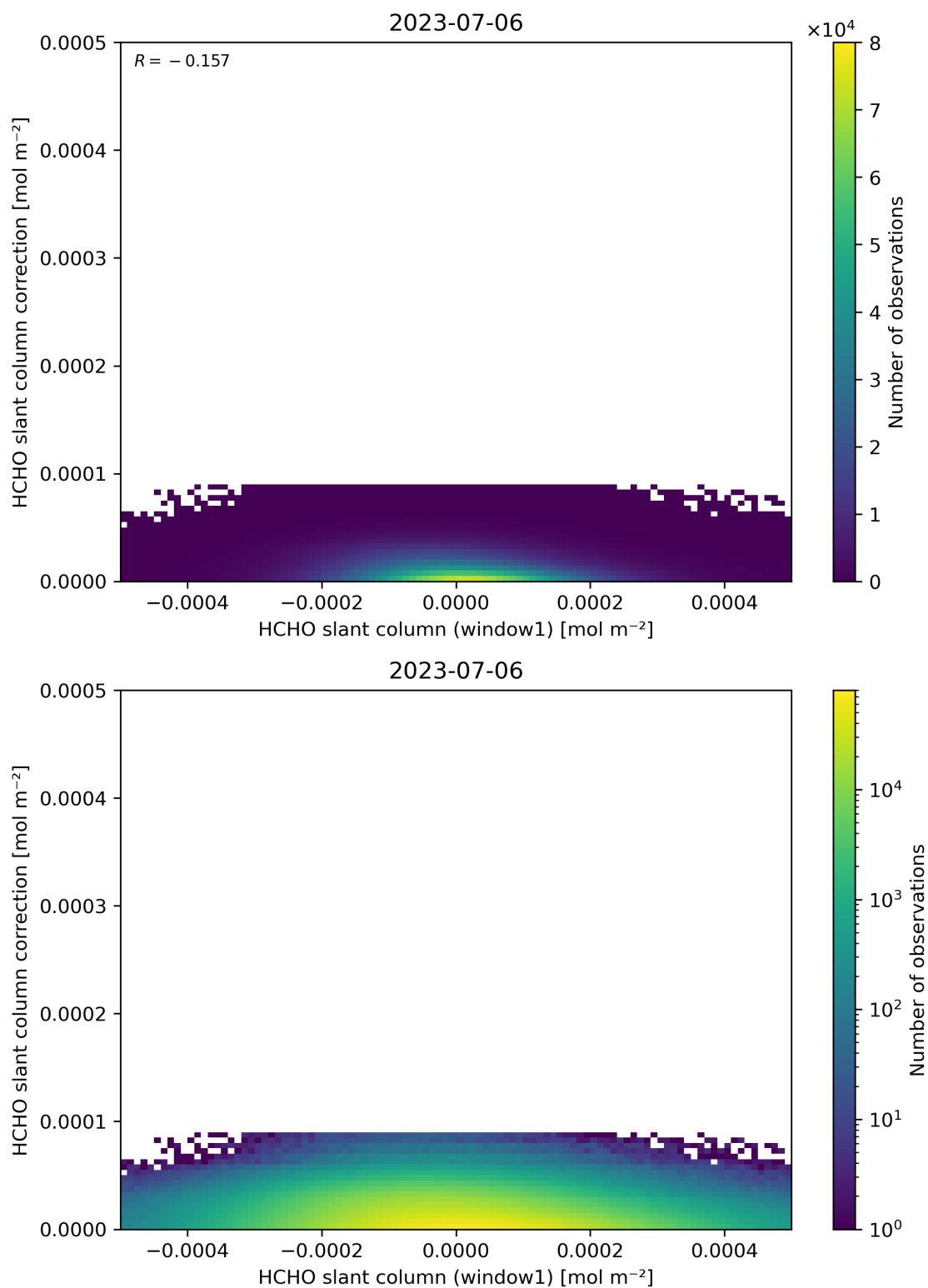
Figure 83: Scatter density plot of “HCHO slant column (window1)” against “HCHO slant column correction” for 2023-07-05 to 2023-07-07.
