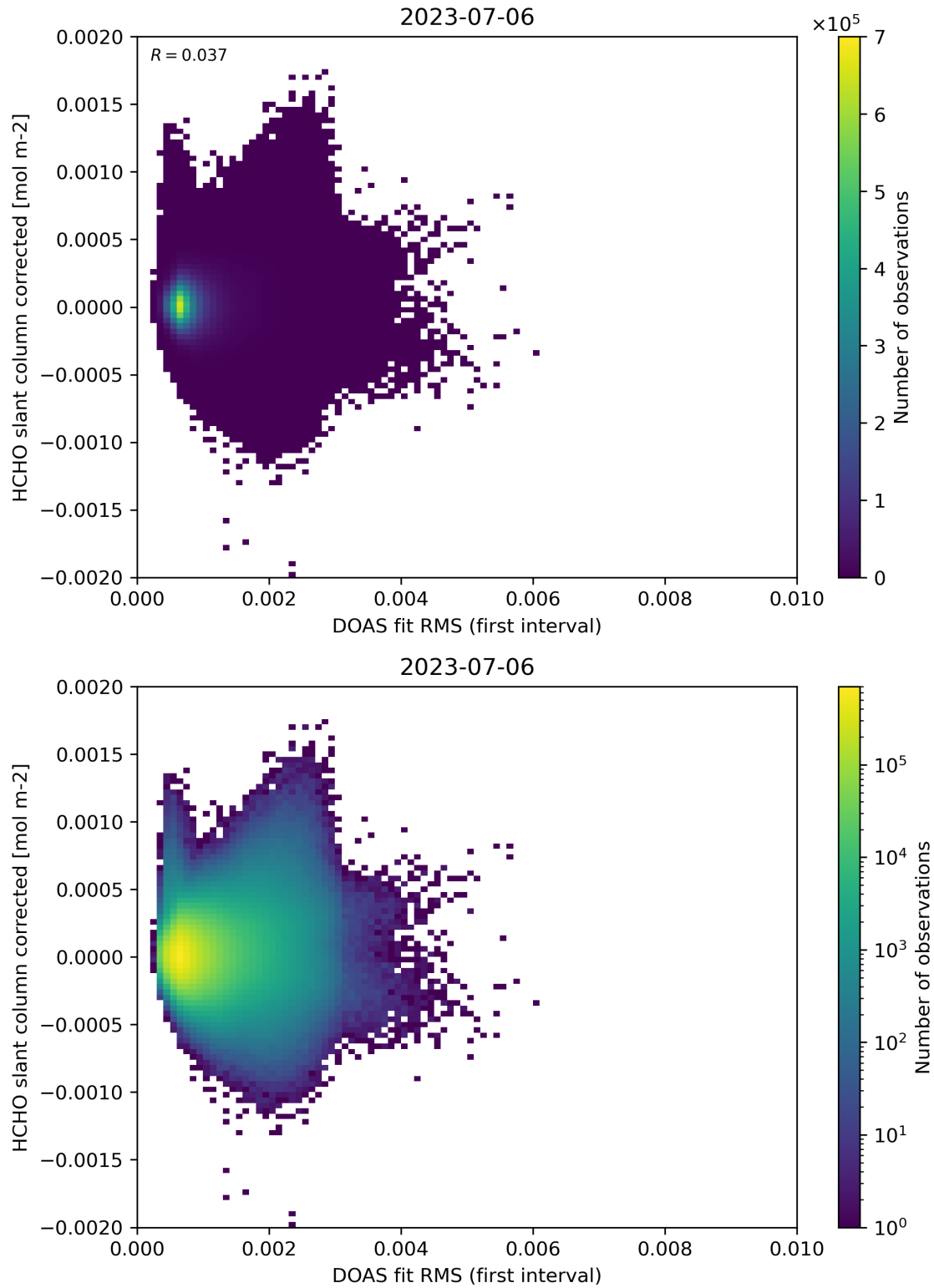
Figure 62: Scatter density plot of “DOAS fit RMS (first interval)” against “HCHO slant column corrected” for 2023-07-05 to 2023-07-07.
