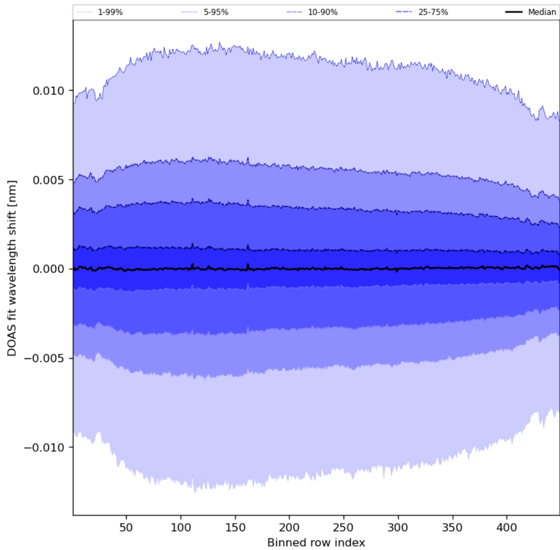
Figure 58: Along track statistics of “DOAS fit wavelength shift” for 2023-07-05 to 2023-07-07
