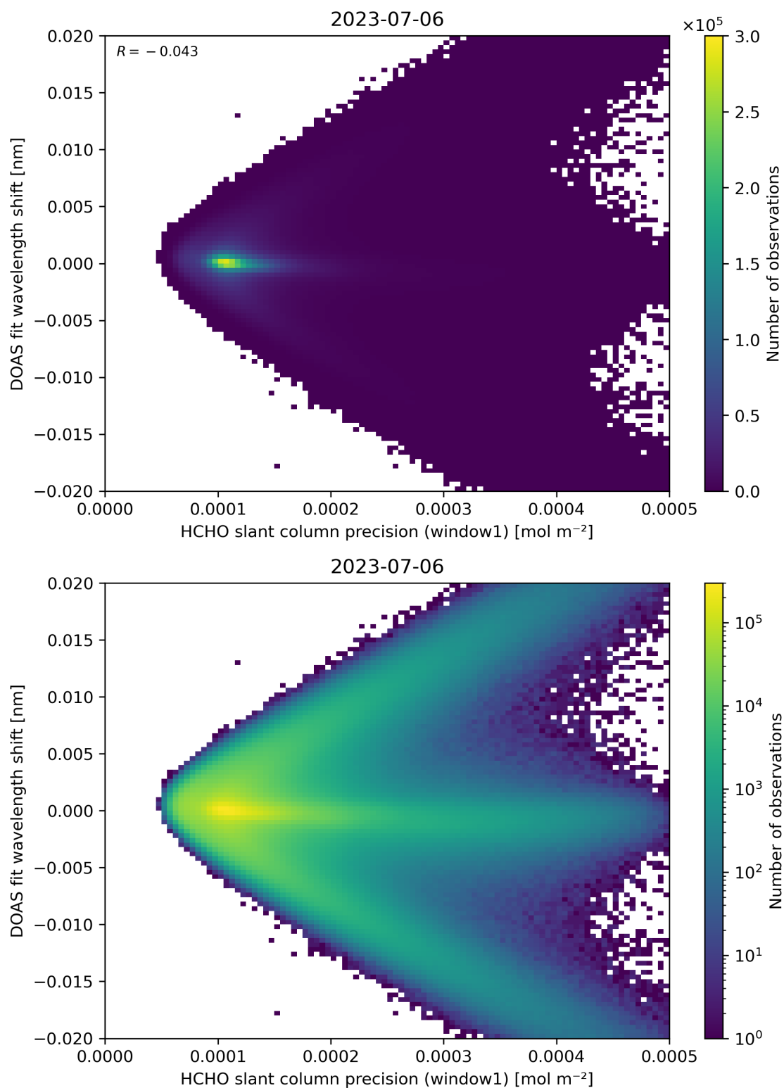
Figure 89: Scatter density plot of “HCHO slant column precision (window1)” against “DOAS fit wavelength shift” for 2023-07-05 to 2023-07-07.
