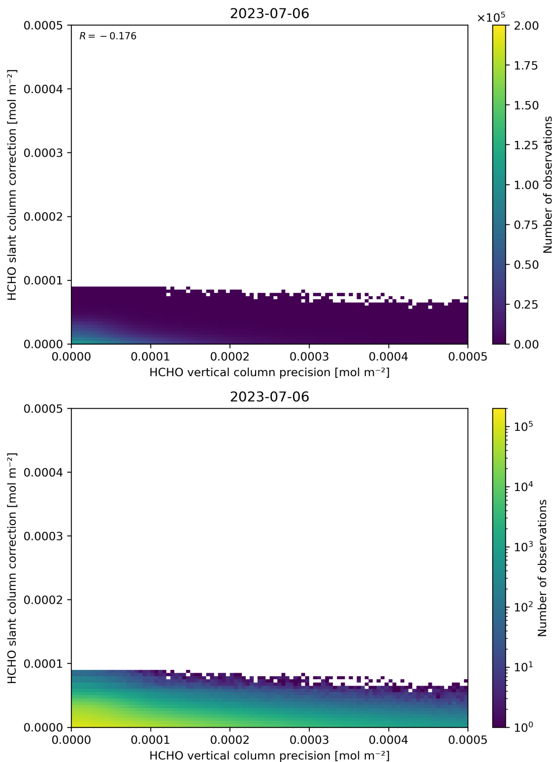
Figure 141: Scatter density plot of “HCHO vertical column precision” against “HCHO slant column correction” for 2023-07-05 to 2023-07-07.
