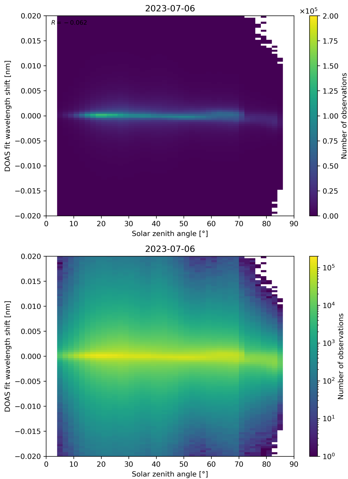
Figure 168: Scatter density plot of “Solar zenith angle” against “DOAS fit wavelength shift” for 2023-07-05 to 2023-07-07.
