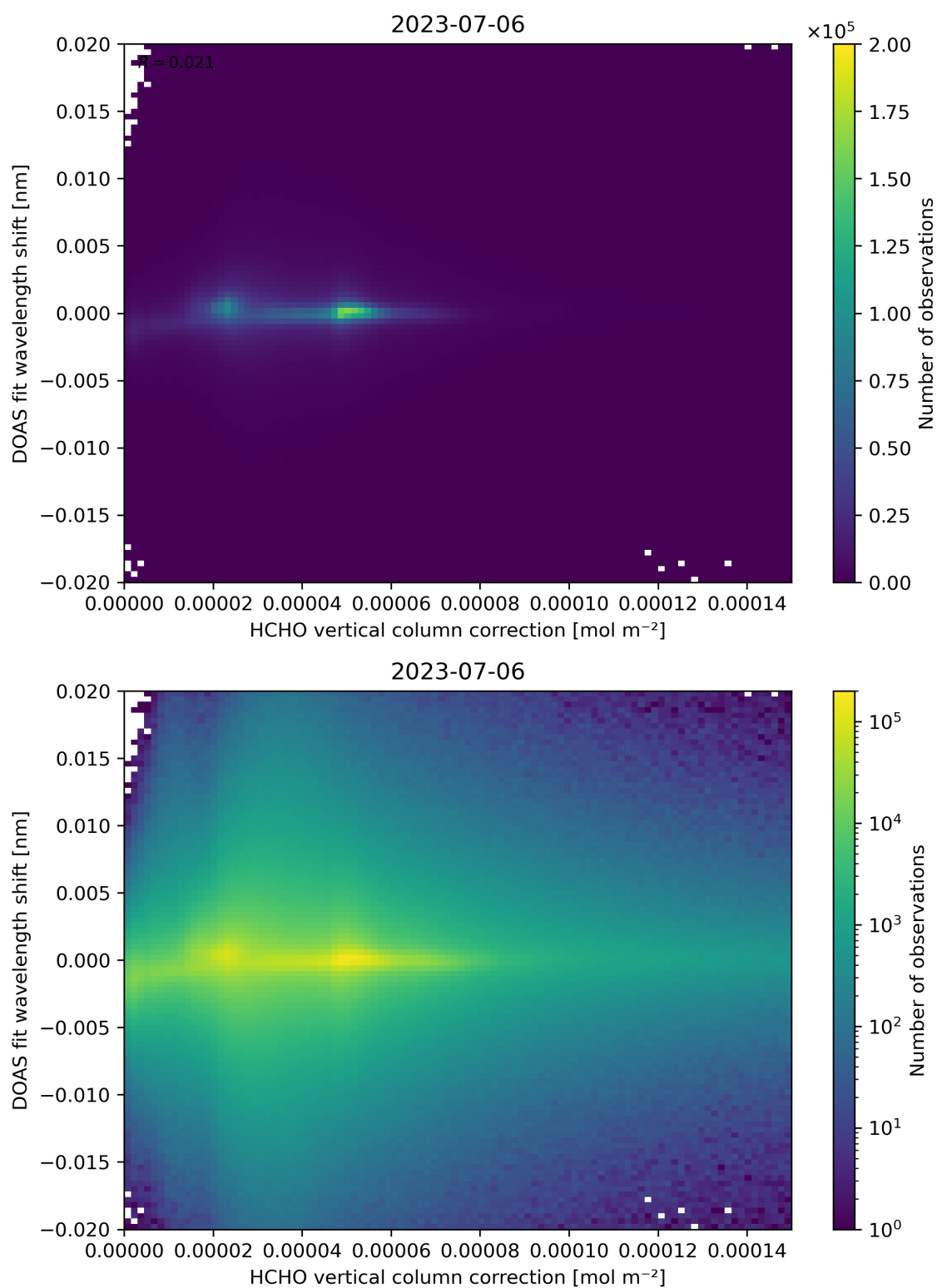
Figure 113: Scatter density plot of “HCHO vertical column correction” against “DOAS fit wavelength shift” for 2023-07-05 to 2023-07-07.
