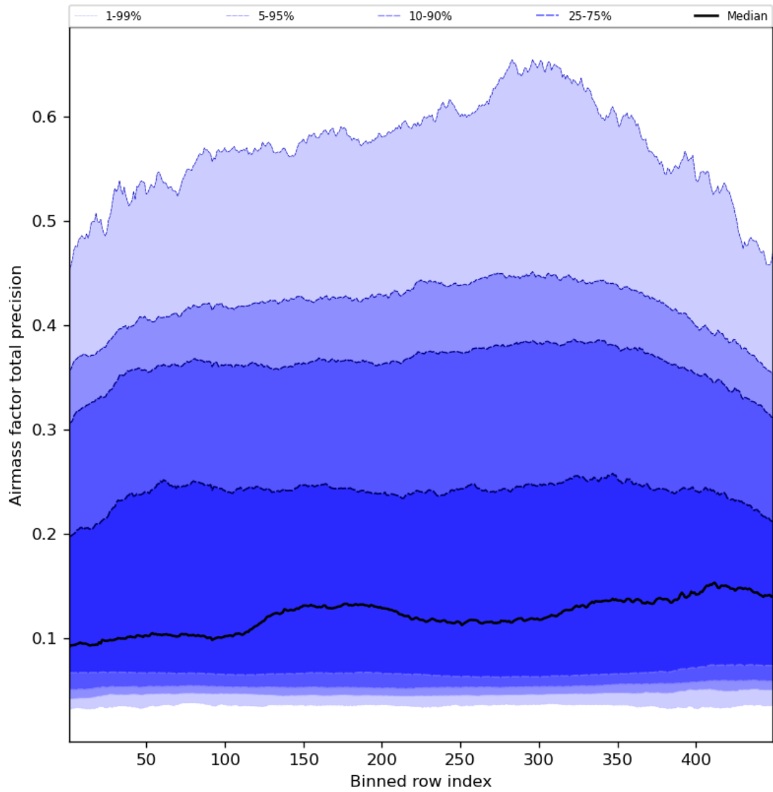
Figure 55: Along track statistics of “Airmass factor total precision” for 2023-07-05 to 2023-07-07
