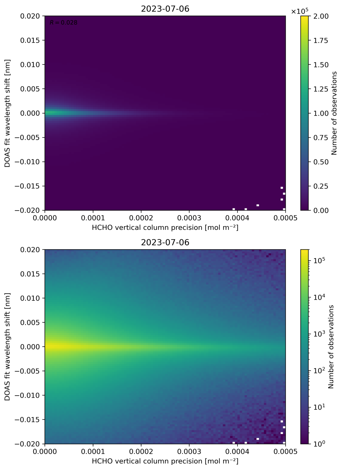
Figure 137: Scatter density plot of “HCHO vertical column precision” against “DOAS fit wavelength shift” for 2023-07-05 to 2023-07-07.
