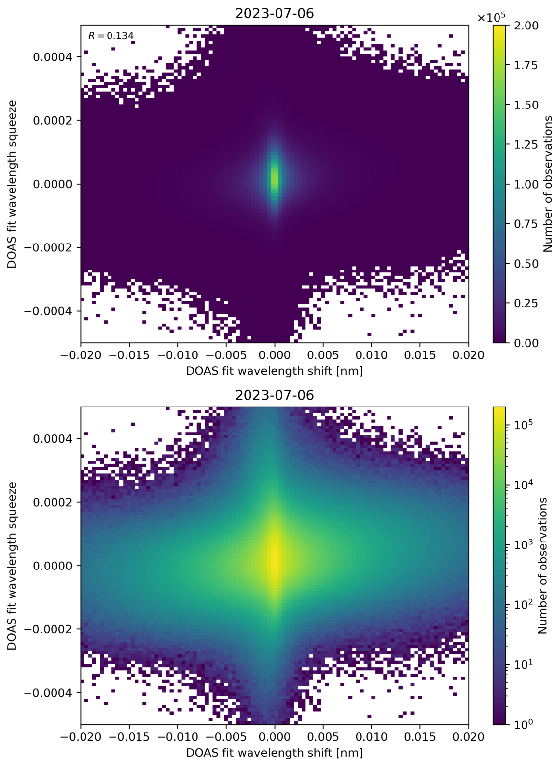
Figure 65: Scatter density plot of “DOAS fit wavelength shift” against “DOAS fit wavelength squeeze” for 2023-07-05 to 2023-07-07.
