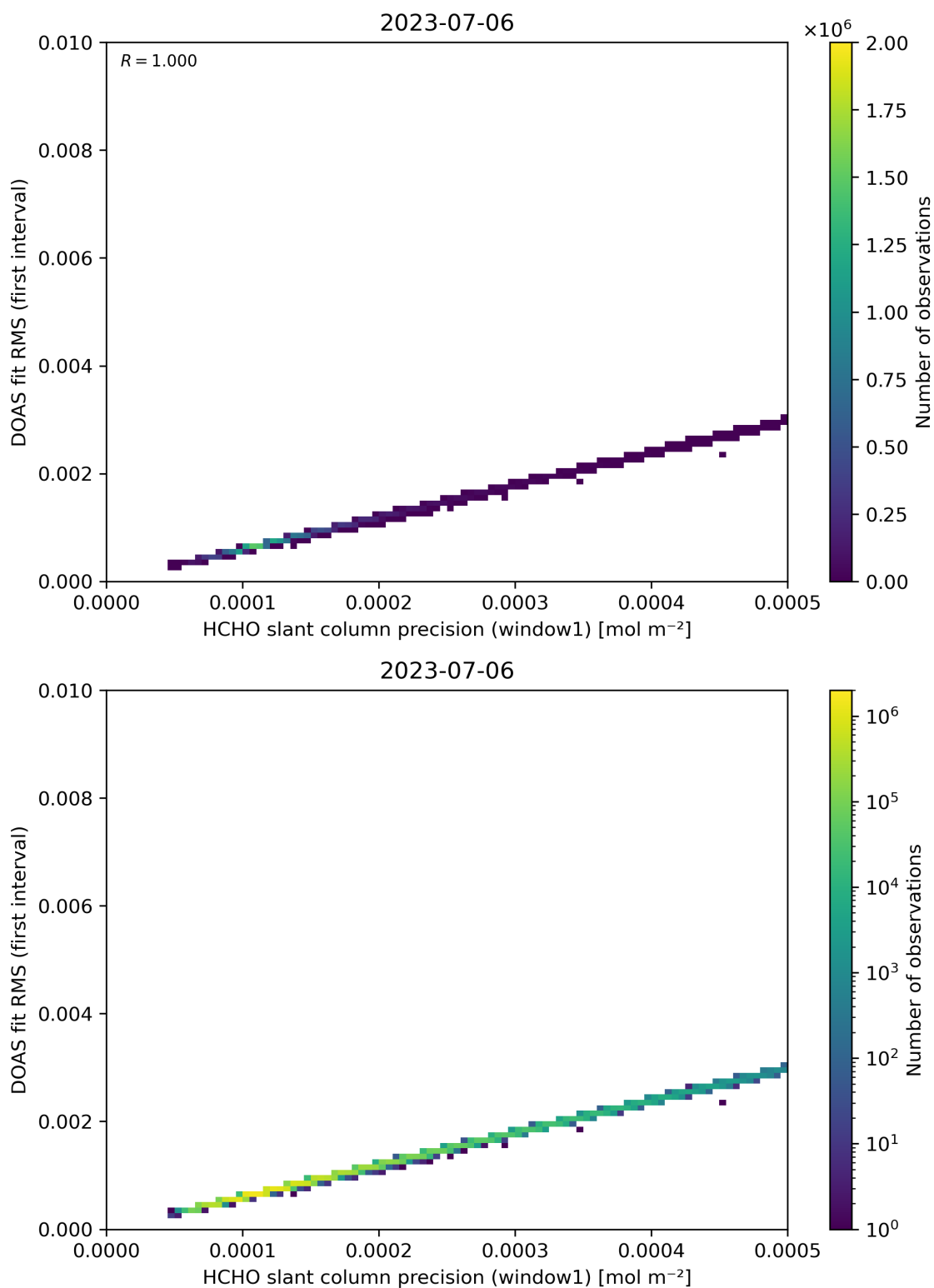
Figure 88: Scatter density plot of “HCHO slant column precision (window1)” against “DOAS fit RMS (first interval)” for 2023-07-05 to 2023-07-07.
