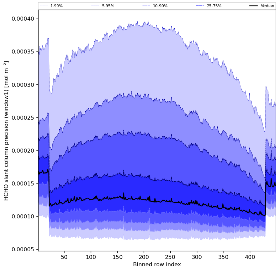
Figure 53: Along track statistics of “HCHO slant column precision (window1)” for 2023-07-05 to 2023-07-07
