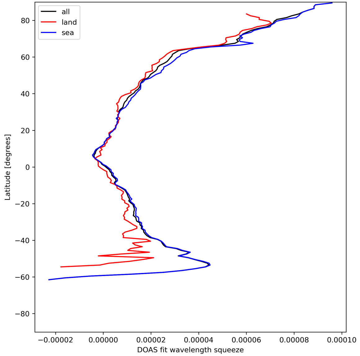
Figure 31: Zonal average of “DOAS fit wavelength squeeze” for 2023-07-05 to 2023-07-07.
