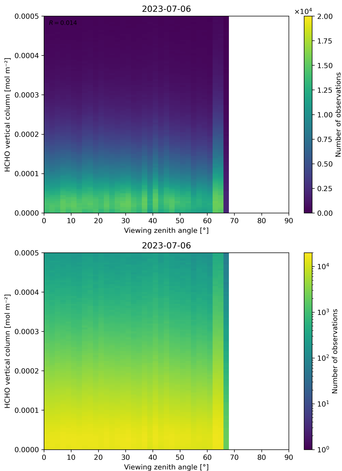
Figure 192: Scatter density plot of “Viewing zenith angle” against “HCHO vertical column” for 2023-07-05 to 2023-07-07.
