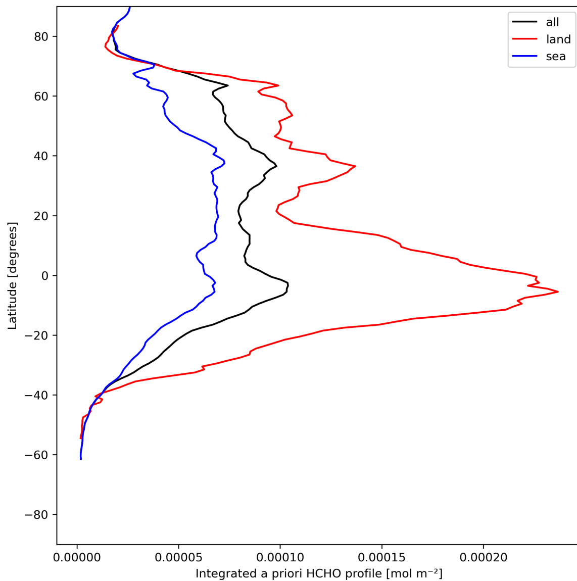
Figure 29: Zonal average of “Integrated a priori HCHO profile” for 2023-07-05 to 2023-07-07.
