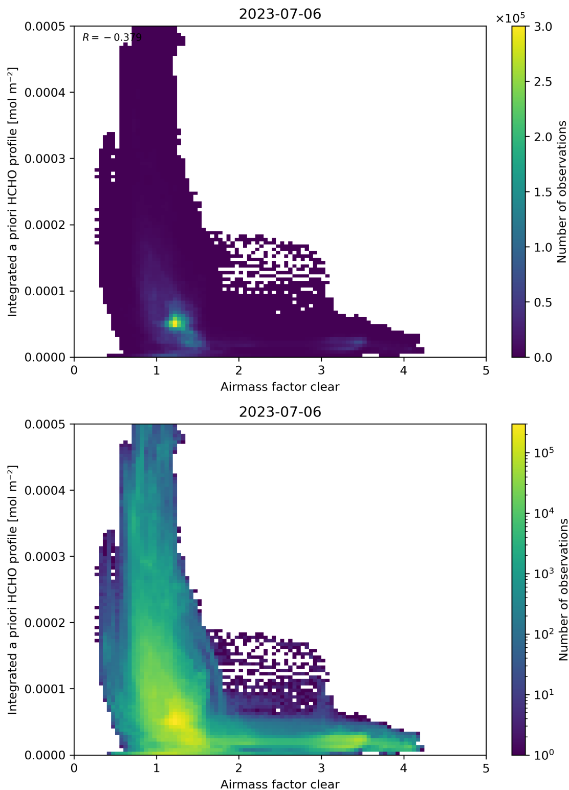
Figure 76: Scatter density plot of “Airmass factor clear” against “Integrated a priori HCHO profile” for 2023-07-05 to 2023-07-07.
