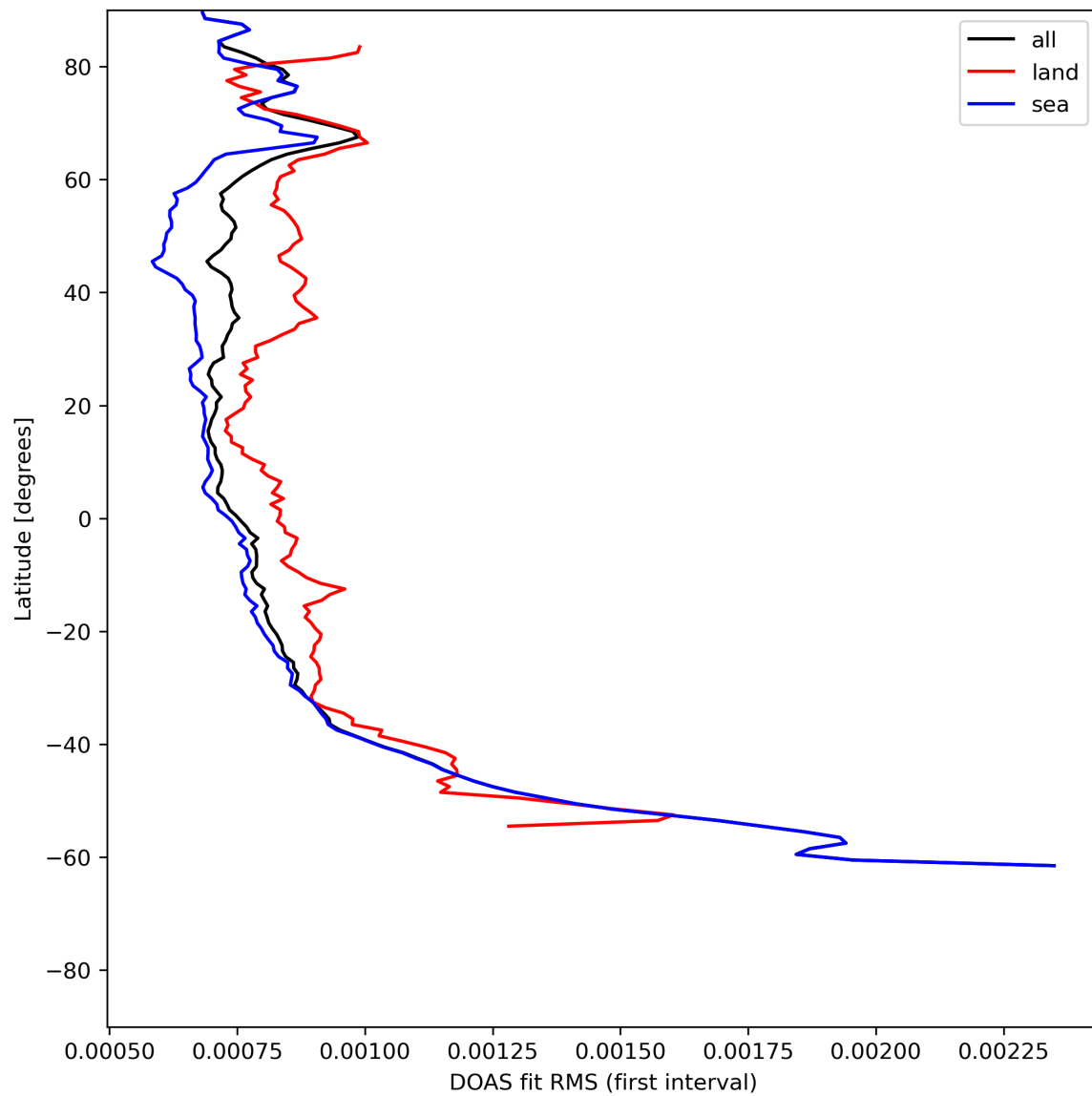
Figure 32: Zonal average of "DOAS fit RMS (first interval)" for 2023-07-05 to 2023-07-07.
