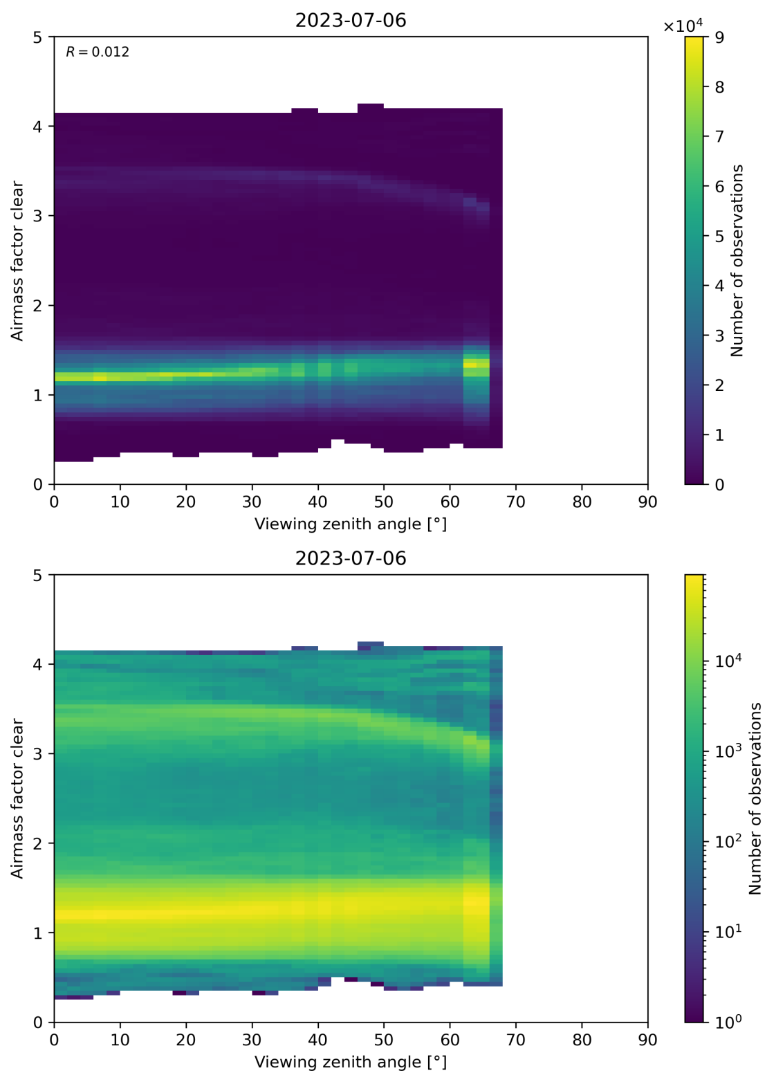
Figure 185: Scatter density plot of “Viewing zenith angle” against “Airmass factor clear” for 2023-07-05 to 2023-07-07.
