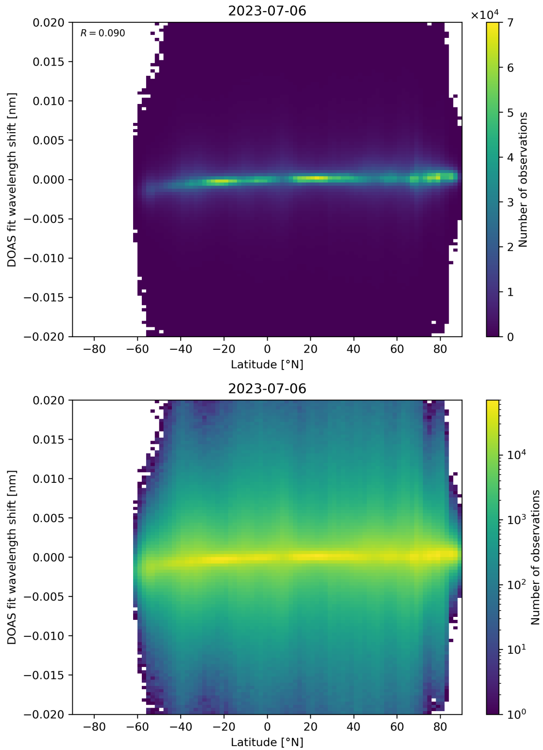
Figure 154: Scatter density plot of “Latitude” against “DOAS fit wavelength shift” for 2023-07-05 to 2023-07-07.
