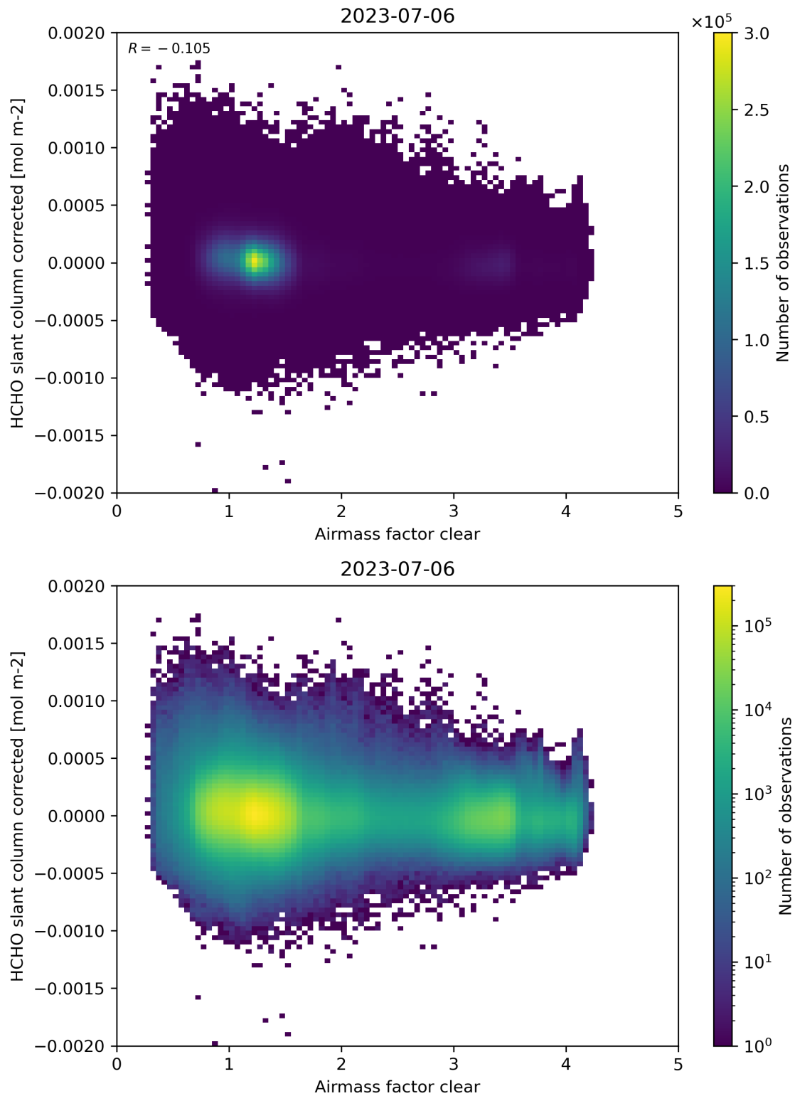
Figure 74: Scatter density plot of “Airmass factor clear” against “HCHO slant column corrected” for 2023-07-05 to 2023-07-07.
