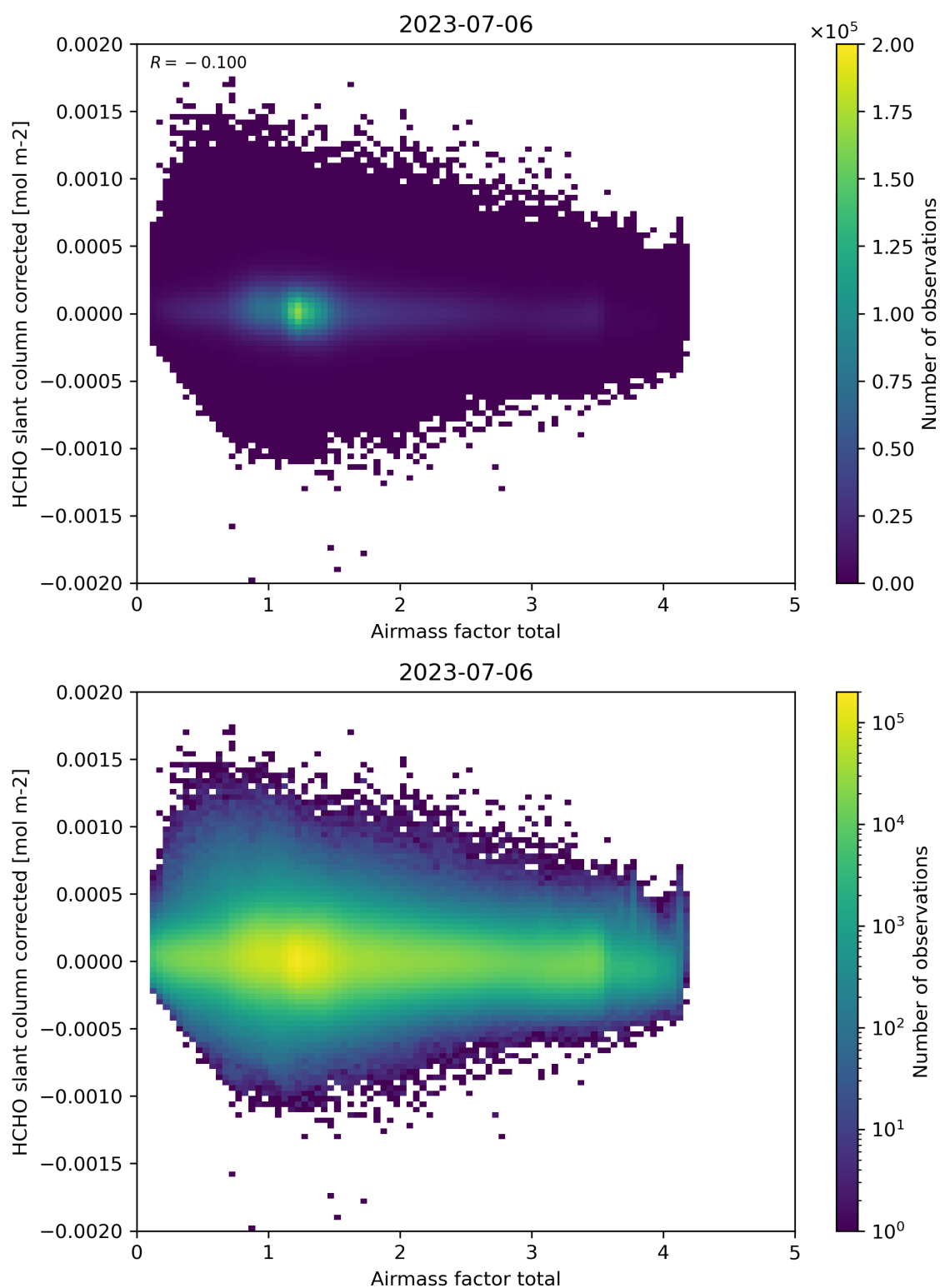
Figure 101: Scatter density plot of “Airmass factor total” against “HCHO slant column corrected” for 2023-07-05 to 2023-07-07.
