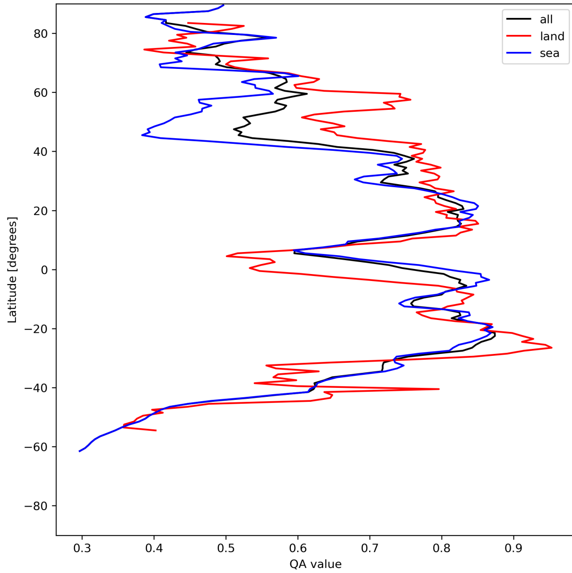
Figure 20: Zonal average of “QA value” for 2023-07-05 to 2023-07-07.
