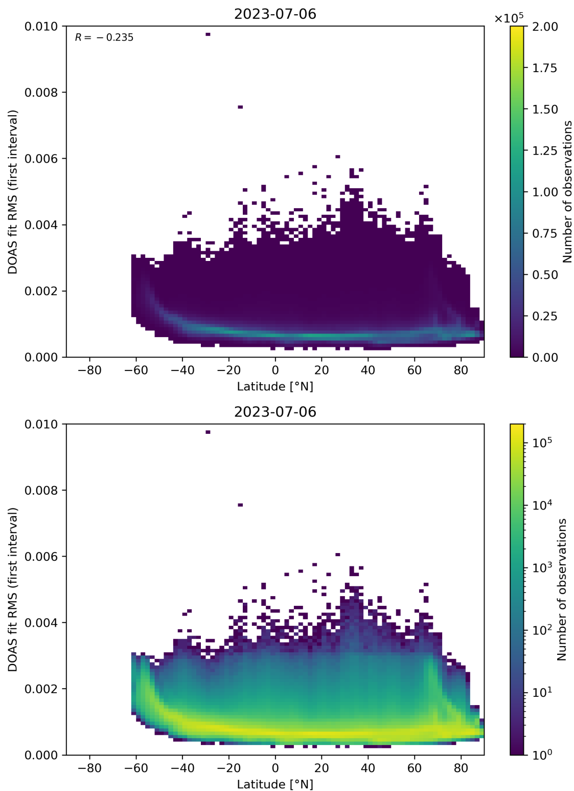
Figure 153: Scatter density plot of “Latitude” against “DOAS fit RMS (first interval)” for 2023-07-05 to 2023-07-07.
