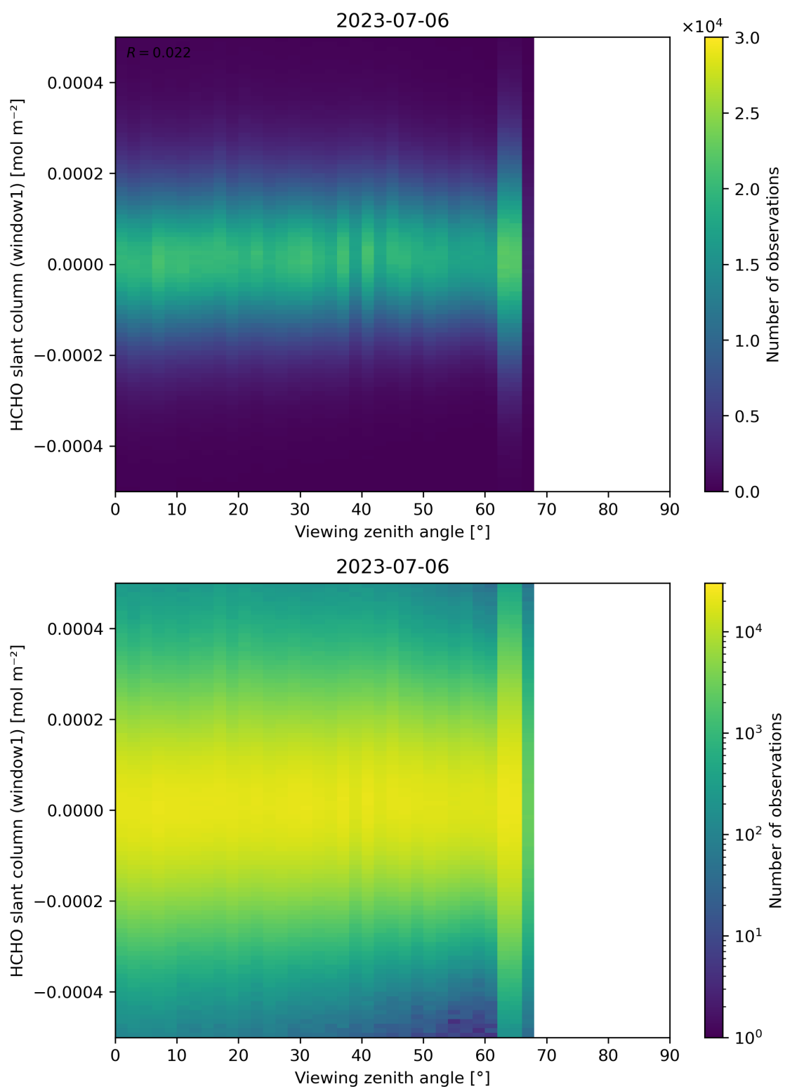
Figure 188: Scatter density plot of “Viewing zenith angle” against “HCHO slant column (window1)” for 2023-07-05 to 2023-07-07.
