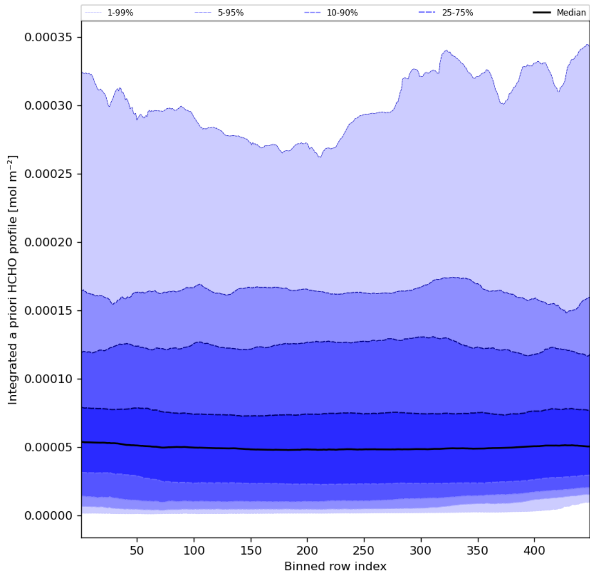
Figure 57: Along track statistics of "Integrated a priori HCHO profile" for 2023-07-05 to 2023-07-07
