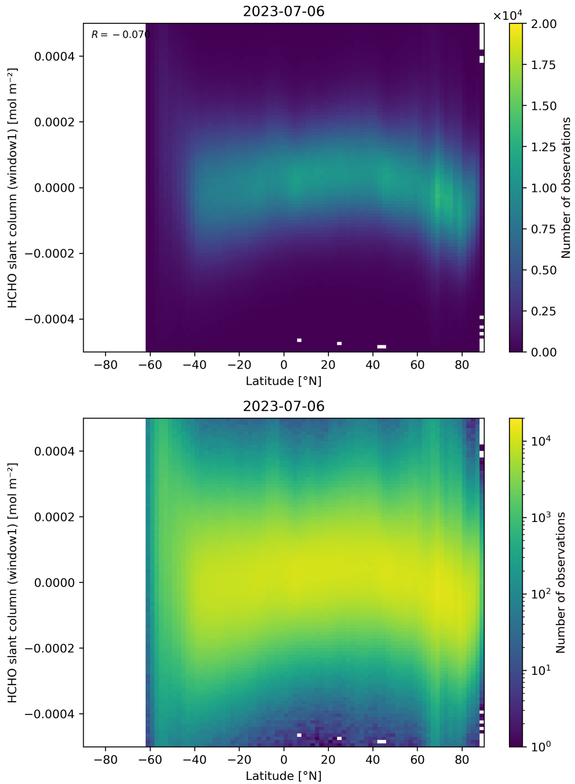
Figure 159: Scatter density plot of “Latitude” against “HCHO slant column (window1)” for 2023-07-05 to 2023-07-07.
