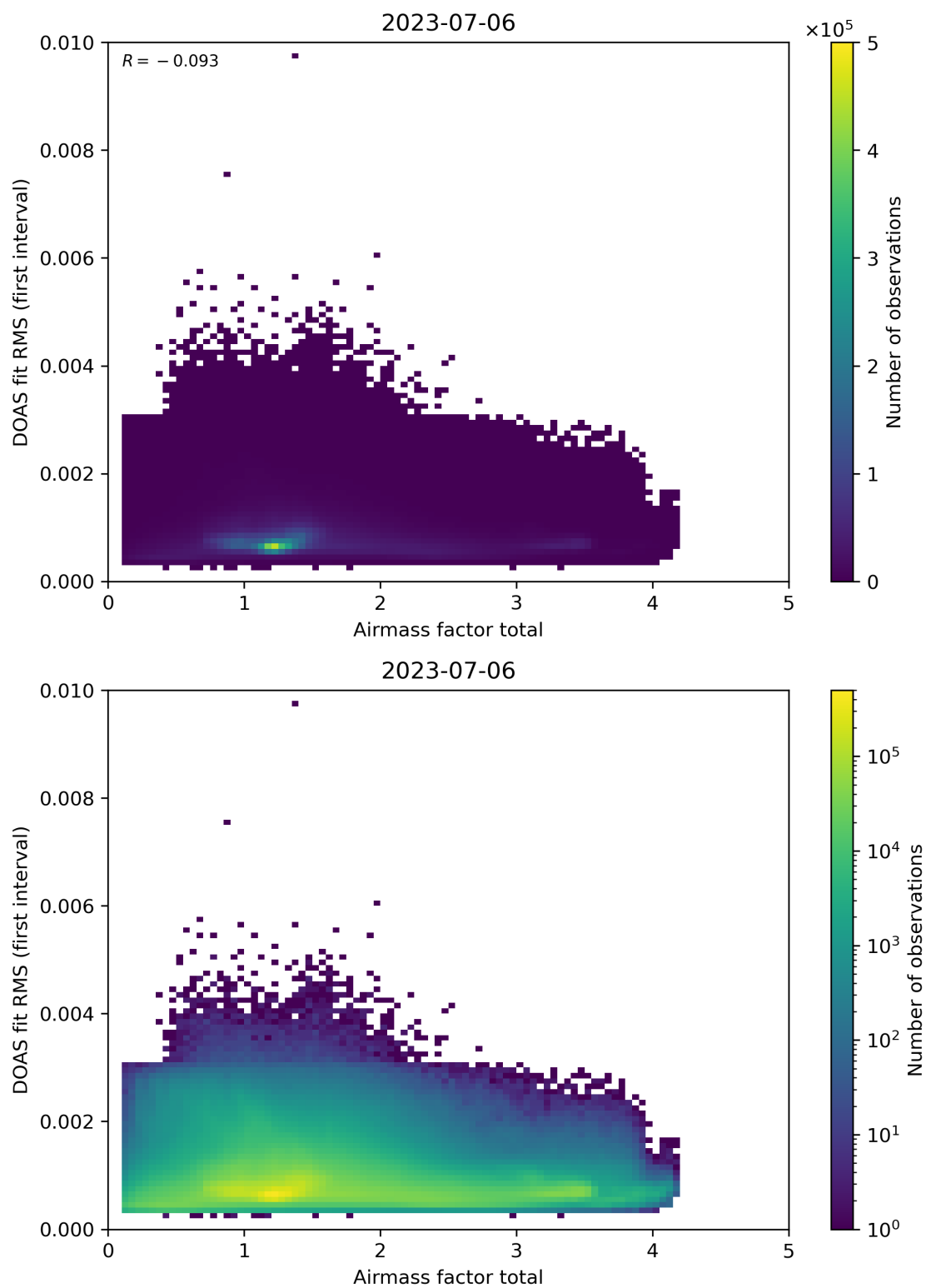
Figure 97: Scatter density plot of “Airmass factor total” against “DOAS fit RMS (first interval)” for 2023-07-05 to 2023-07-07.
