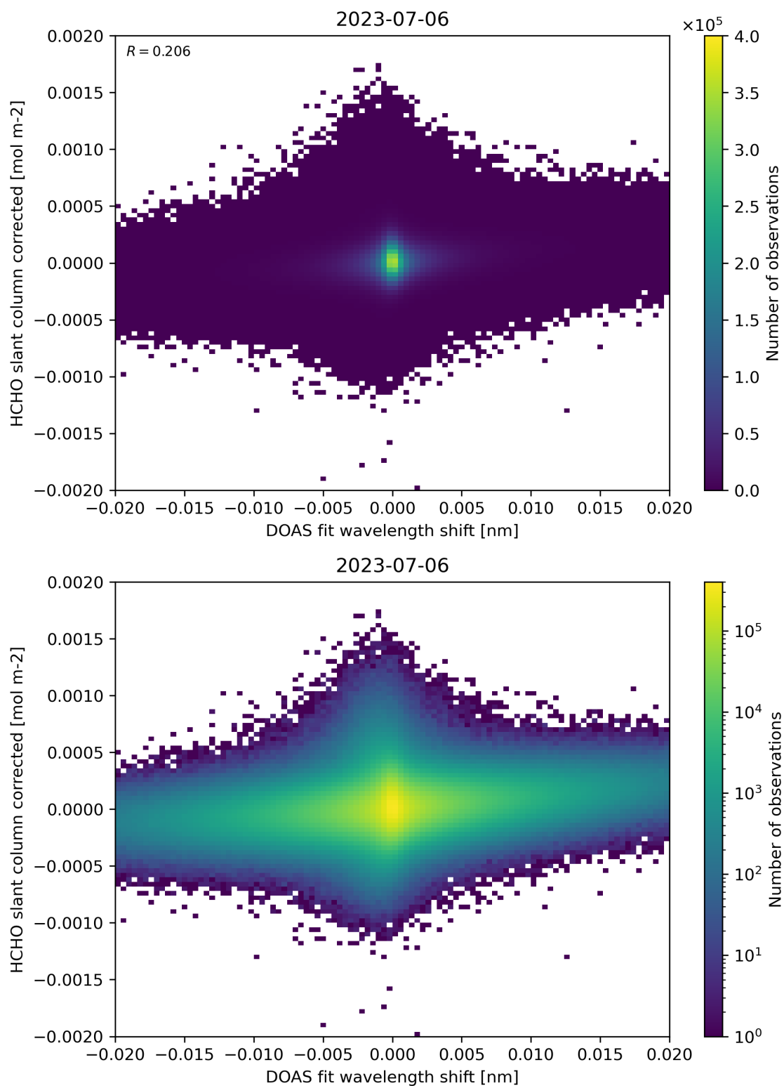
Figure 66: Scatter density plot of “DOAS fit wavelength shift” against “HCHO slant column corrected” for 2023-07-05 to 2023-07-07.
