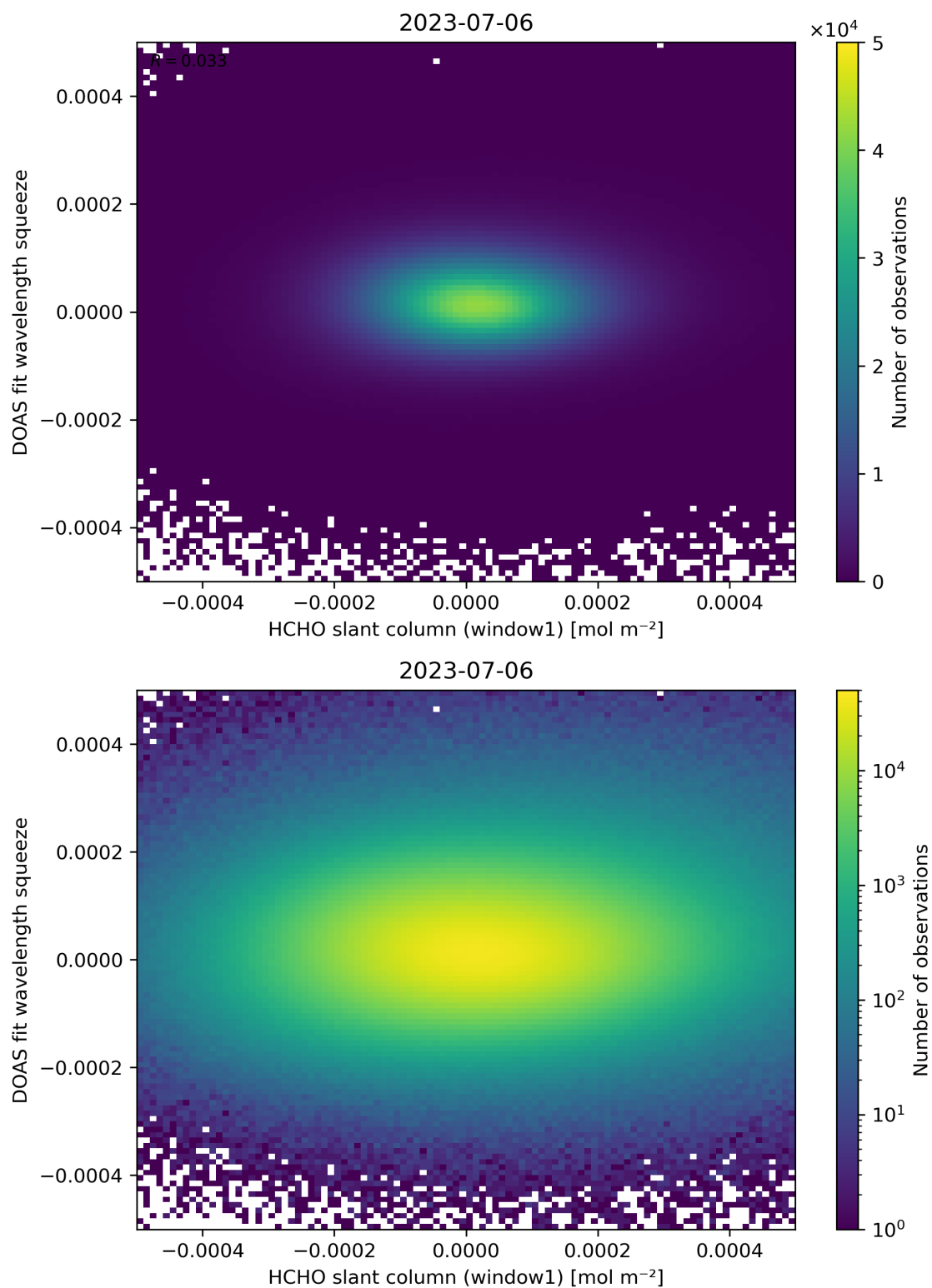
Figure 80: Scatter density plot of “HCHO slant column (window1)” against “DOAS fit wavelength squeeze” for 2023-07-05 to 2023-07-07.
