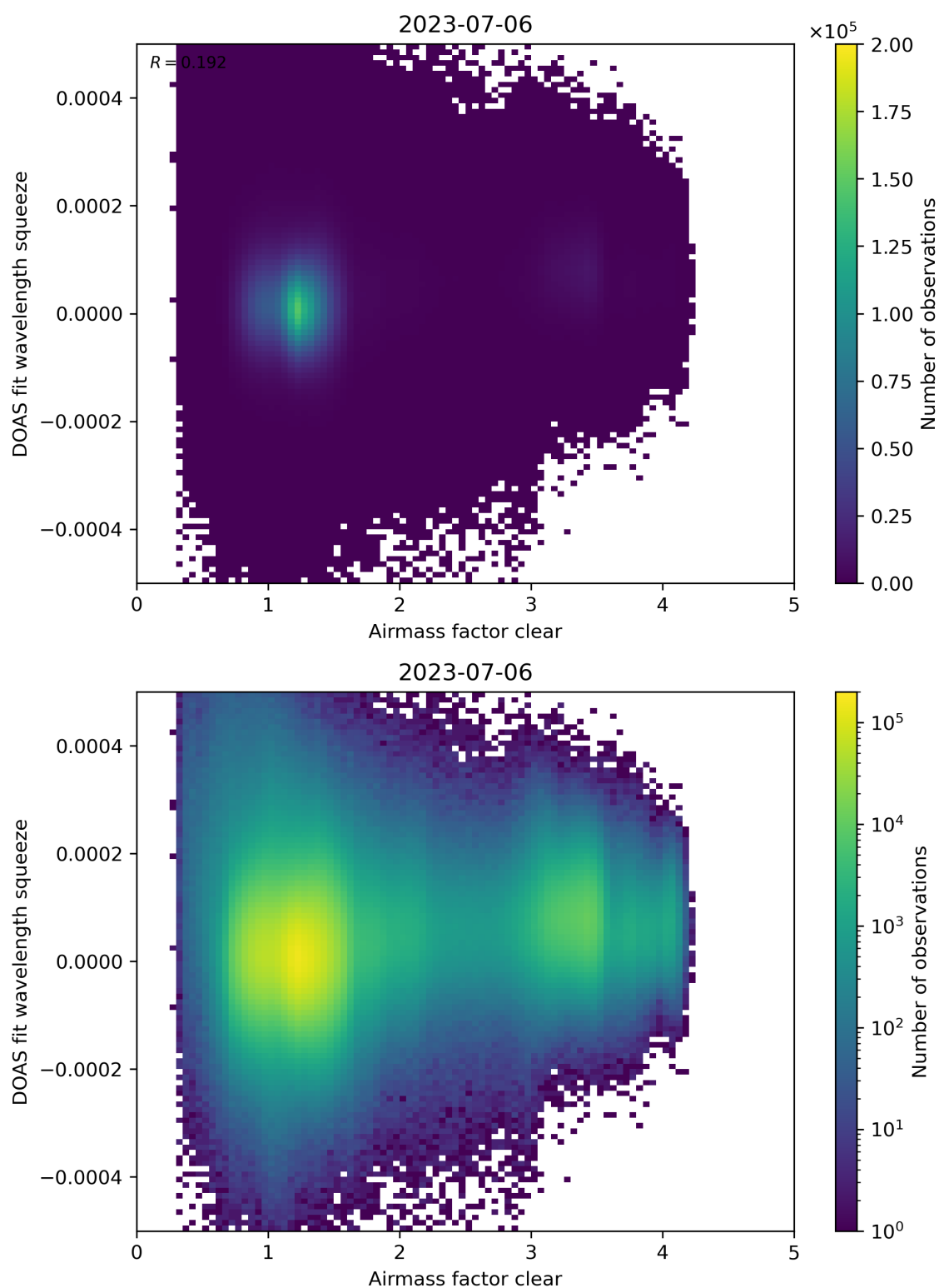
Figure 73: Scatter density plot of “Airmass factor clear” against “DOAS fit wavelength squeeze” for 2023-07-05 to 2023-07-07.
