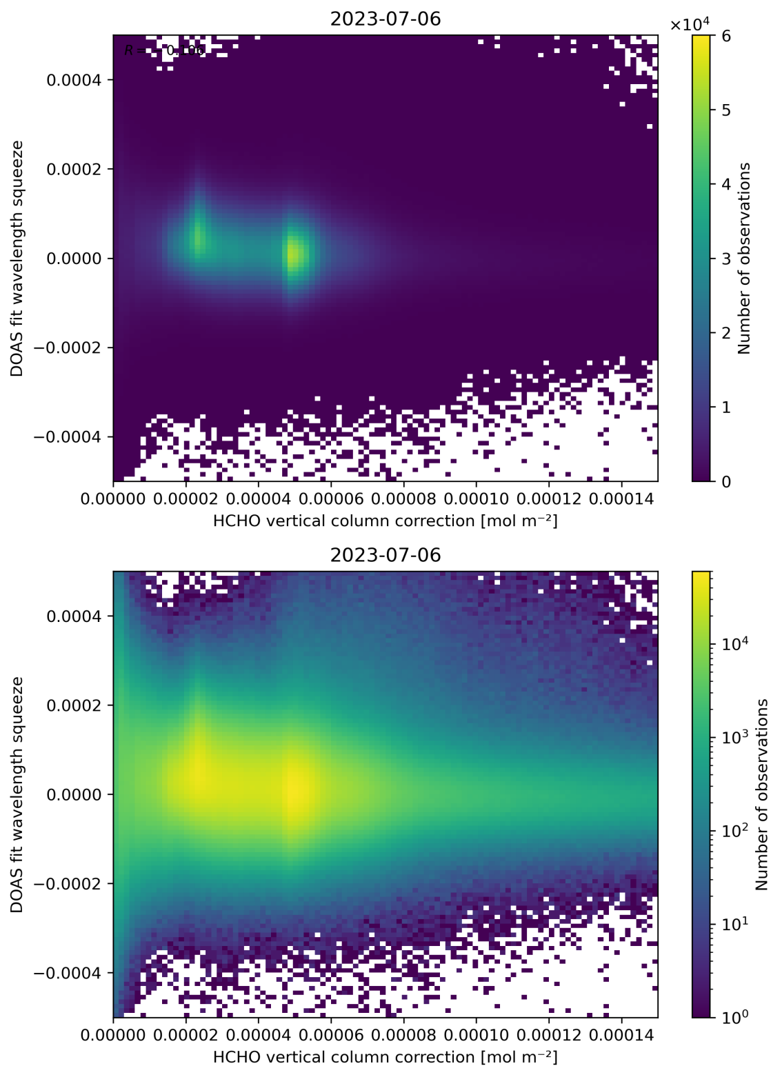
Figure 114: Scatter density plot of “HCHO vertical column correction” against “DOAS fit wavelength squeeze” for 2023-07-05 to 2023-07-07.
