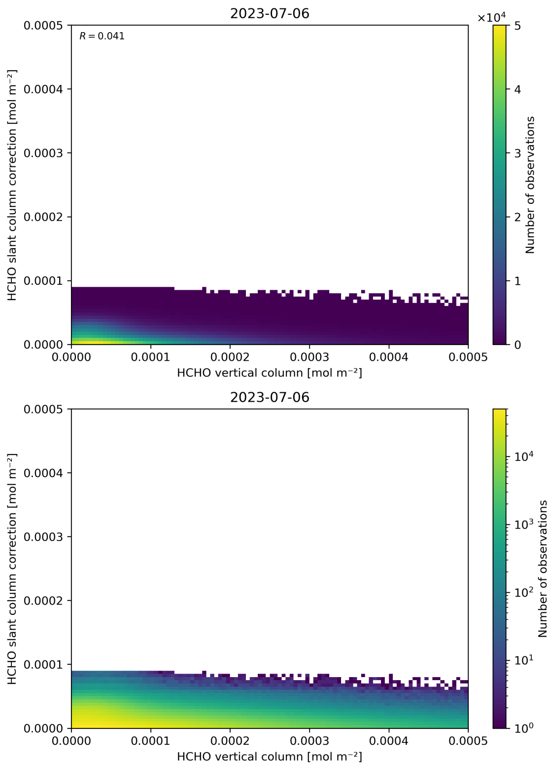
Figure 128: Scatter density plot of “HCHO vertical column” against “HCHO slant column correction” for 2023-07-05 to 2023-07-07.
