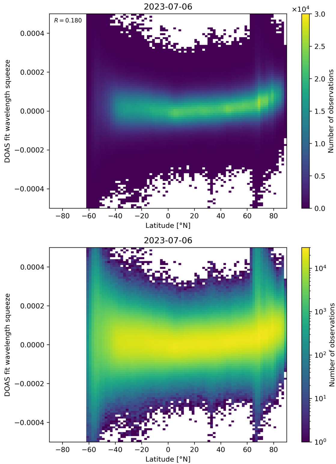
Figure 155: Scatter density plot of “Latitude” against “DOAS fit wavelength squeeze” for 2023-07-05 to 2023-07-07.
