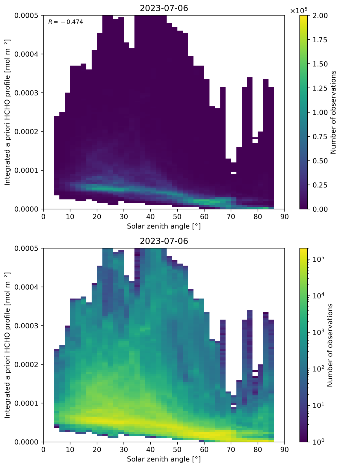
Figure 180: Scatter density plot of “Solar zenith angle” against “Integrated a priori HCHO profile” for 2023-07-05 to 2023-07-07.
