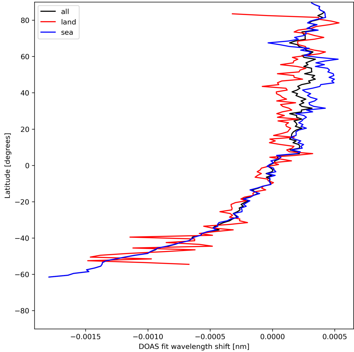
Figure 30: Zonal average of "DOAS fit wavelength shift" for 2023-07-05 to 2023-07-07.
