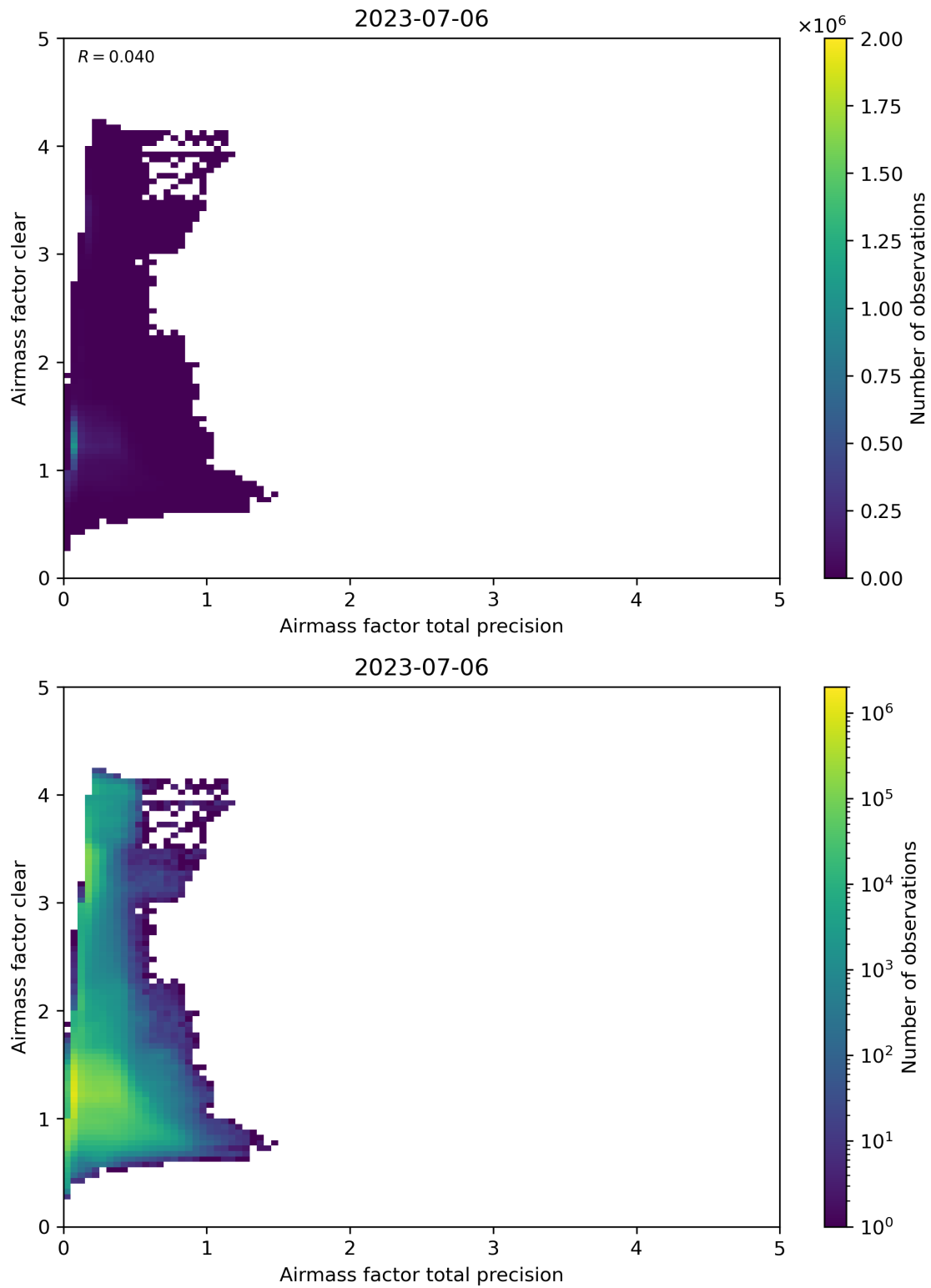
Figure 108: Scatter density plot of “Airmass factor total precision” against “Airmass factor clear” for 2023-07-05 to 2023-07-07.
