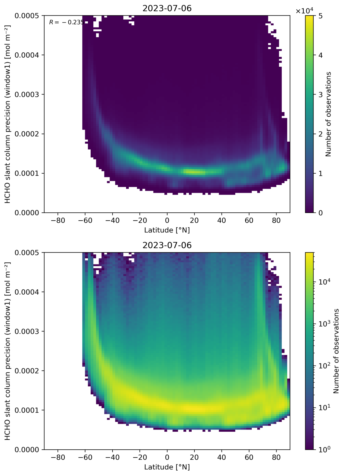
Figure 160: Scatter density plot of “Latitude” against “HCHO slant column precision (window1)” for 2023-07-05 to 2023-07-07.
