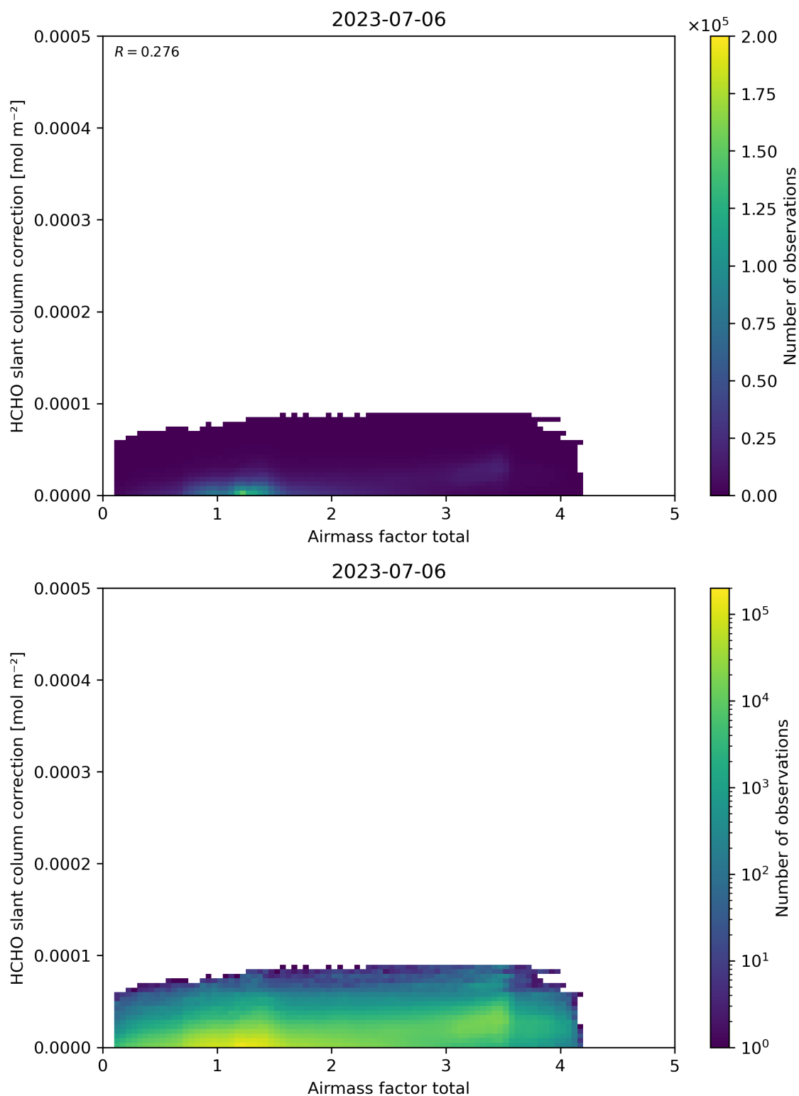
Figure 102: Scatter density plot of “Airmass factor total” against “HCHO slant column correction” for 2023-07-05 to 2023-07-07.
