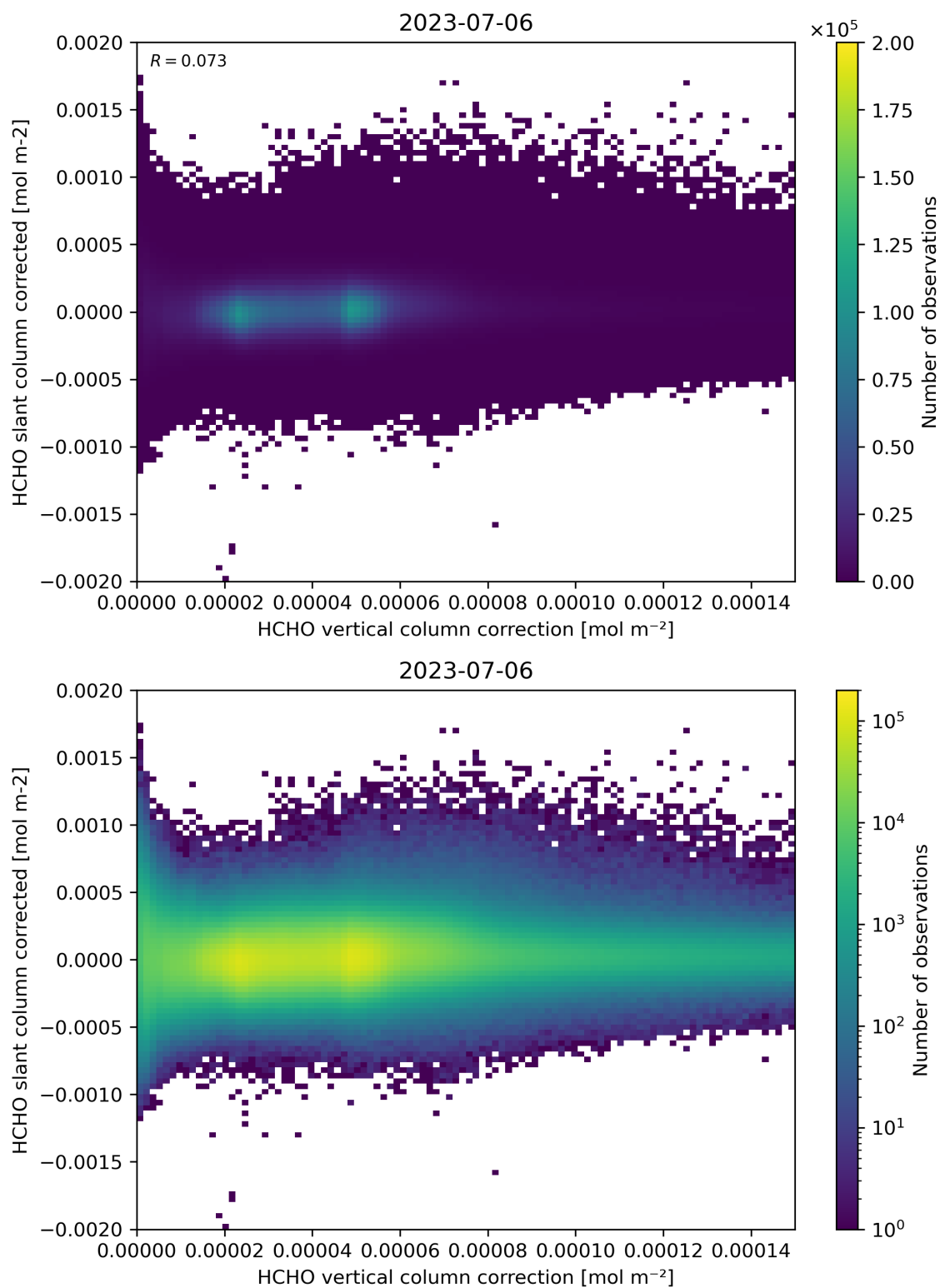
Figure 116: Scatter density plot of “HCHO vertical column correction” against “HCHO slant column corrected” for 2023-07-05 to 2023-07-07.
