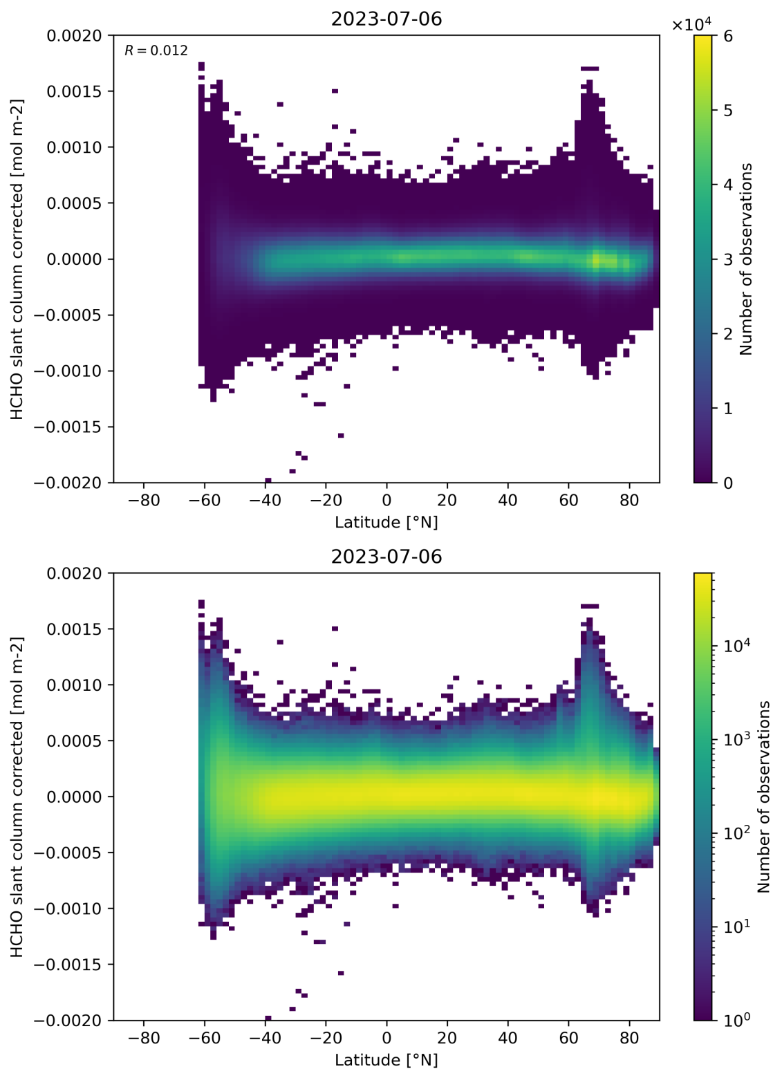
Figure 157: Scatter density plot of “Latitude” against “HCHO slant column corrected” for 2023-07-05 to 2023-07-07.
