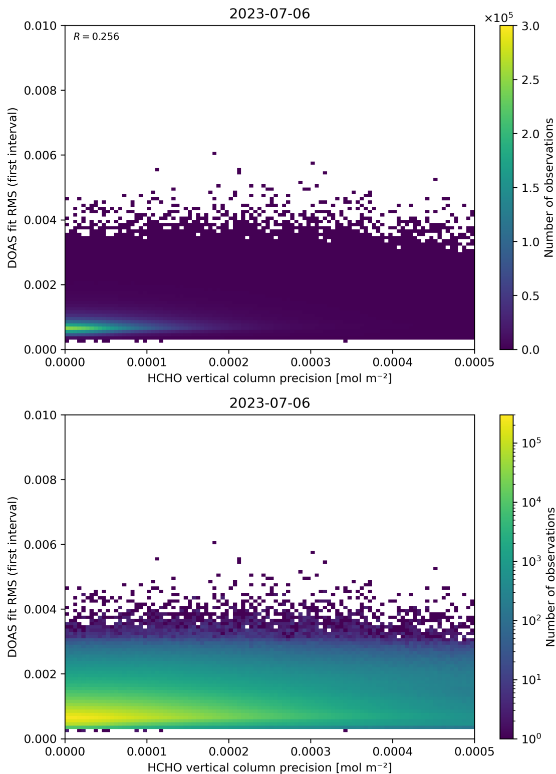
Figure 136: Scatter density plot of “HCHO vertical column precision” against “DOAS fit RMS (first interval)” for 2023-07-05 to 2023-07-07.
