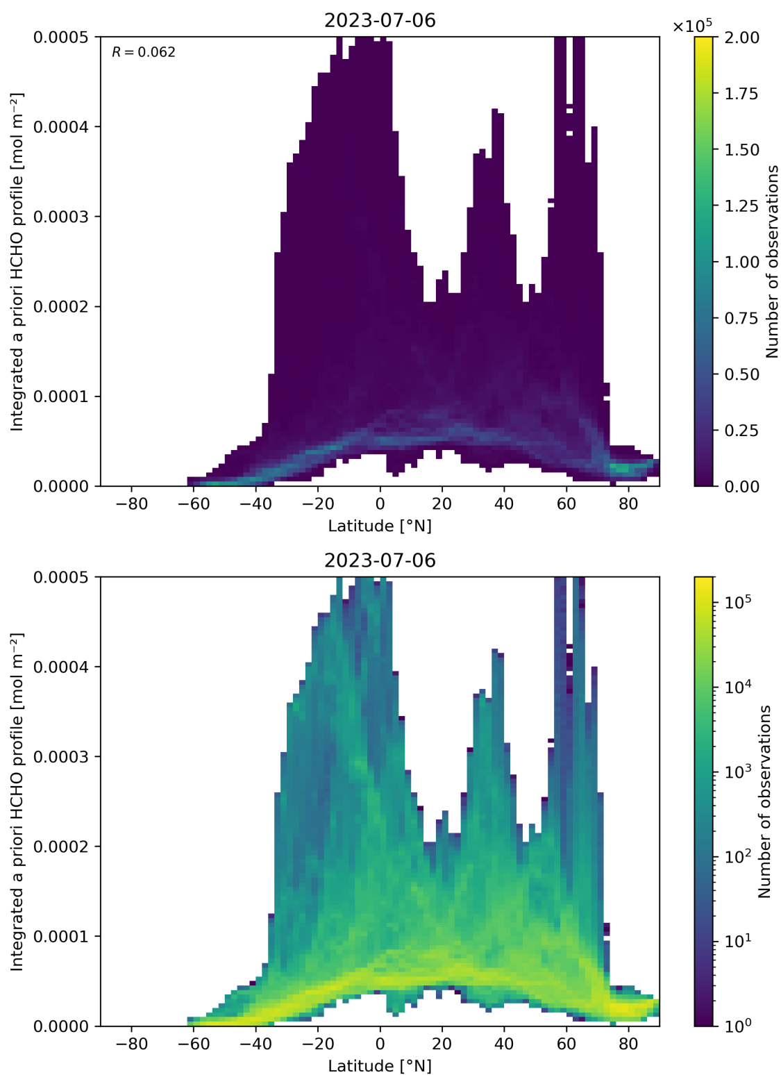
Figure 166: Scatter density plot of “Latitude” against “Integrated a priori HCHO profile” for 2023-07-05 to 2023-07-07.
