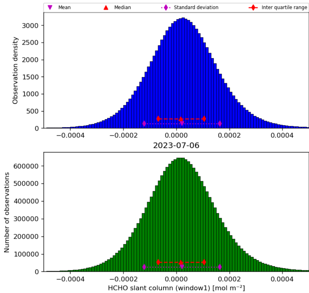
Figure 38: Histogram of “HCHO slant column (window1)” for 2023-07-05 to 2023-07-07
