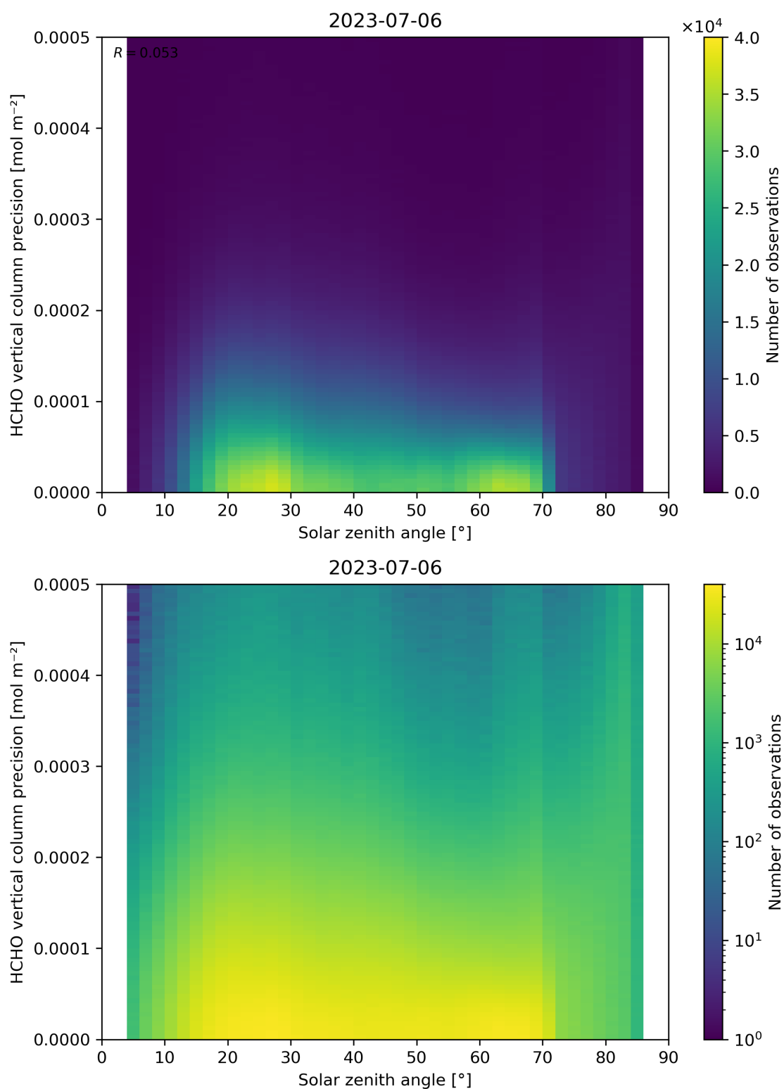
Figure 179: Scatter density plot of “Solar zenith angle” against “HCHO vertical column precision” for 2023-07-05 to 2023-07-07.
