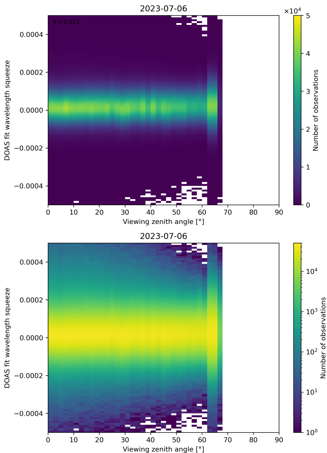
Figure 184: Scatter density plot of “Viewing zenith angle” against “DOAS fit wavelength squeeze” for 2023-07-05 to 2023-07-07.
