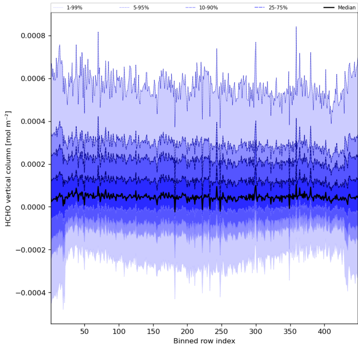
Figure 49: Along track statistics of “HCHO vertical column” for 2023-07-05 to 2023-07-07
