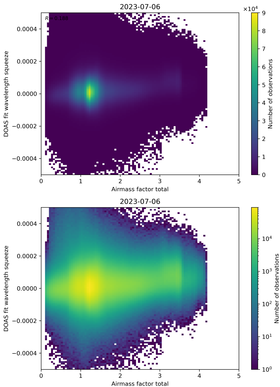
Figure 99: Scatter density plot of “Airmass factor total” against “DOAS fit wavelength squeeze” for 2023-07-05 to 2023-07-07.
