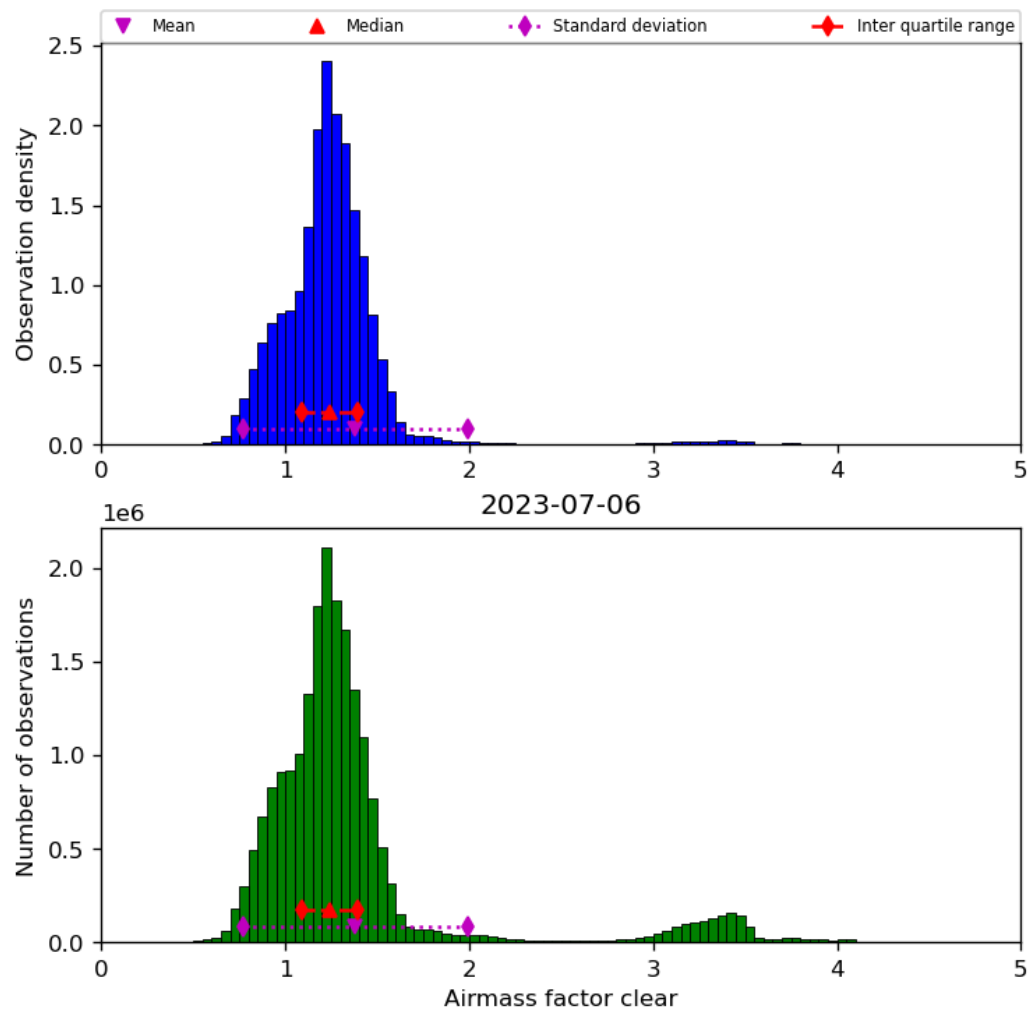
Figure 42: Histogram of “Airmass factor clear” for 2023-07-05 to 2023-07-07
