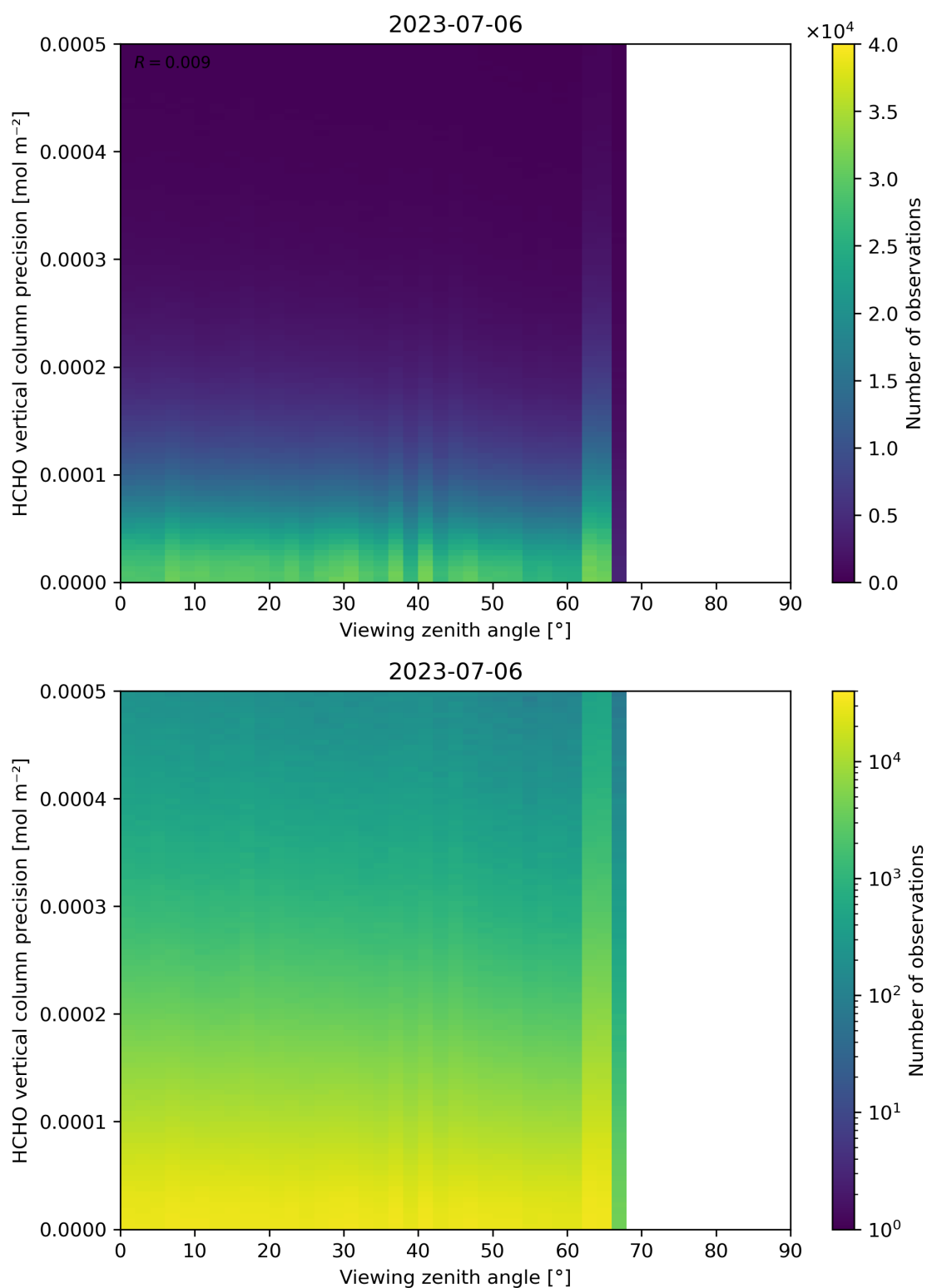
Figure 194: Scatter density plot of “Viewing zenith angle” against “HCHO vertical column precision” for 2023-07-05 to 2023-07-07.
