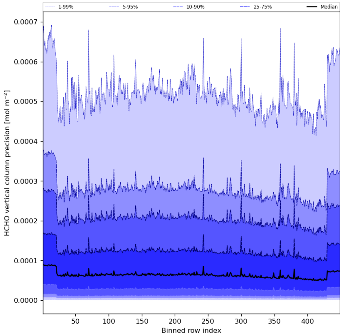
Figure 50: Along track statistics of “HCHO vertical column precision” for 2023-07-05 to 2023-07-07
