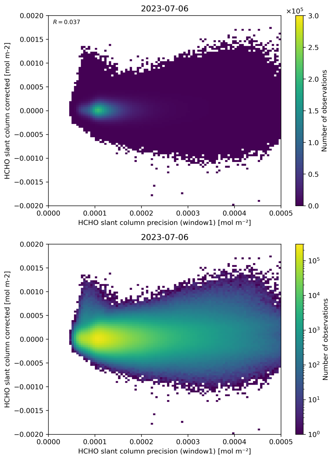
Figure 92: Scatter density plot of “HCHO slant column precision (window1)” against “HCHO slant column corrected” for 2023-07-05 to 2023-07-07.
