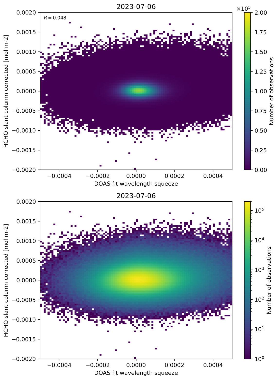
Figure 69: Scatter density plot of “DOAS fit wavelength squeeze” against “HCHO slant column corrected” for 2023-07-05 to 2023-07-07.
