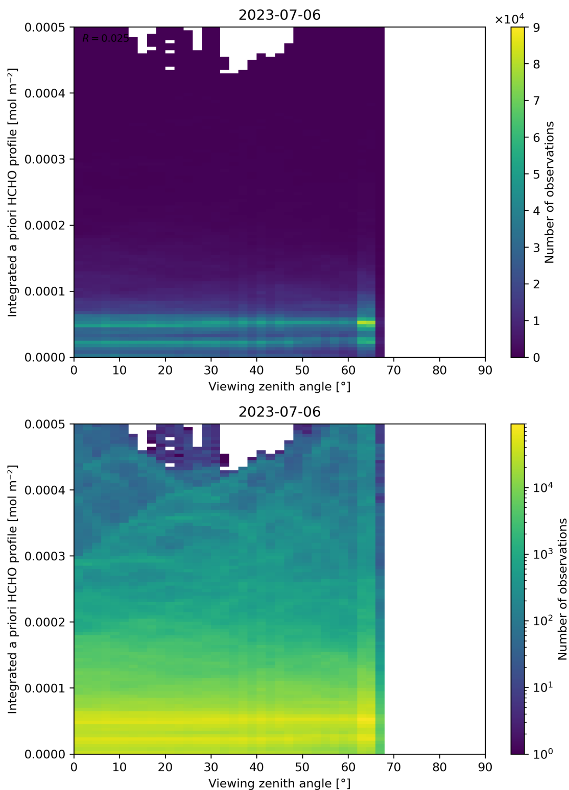
Figure 195: Scatter density plot of “Viewing zenith angle” against “Integrated a priori HCHO profile” for 2023-07-05 to 2023-07-07.
