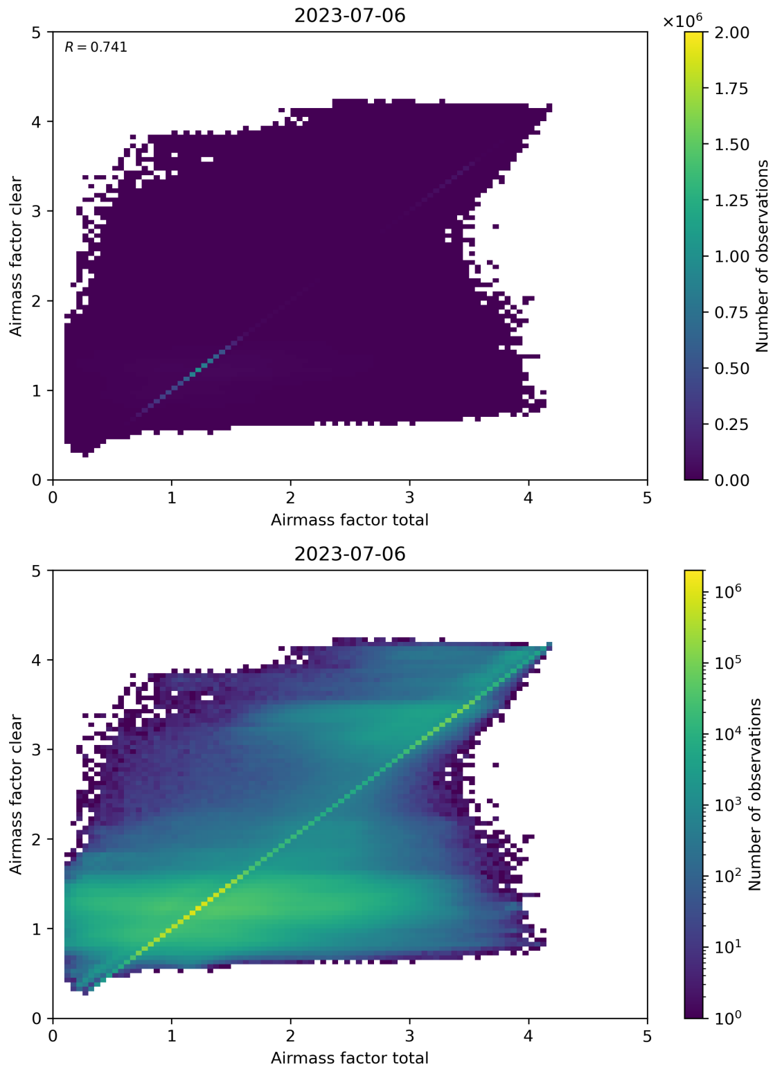
Figure 100: Scatter density plot of “Airmass factor total” against “Airmass factor clear” for 2023-07-05 to 2023-07-07.
