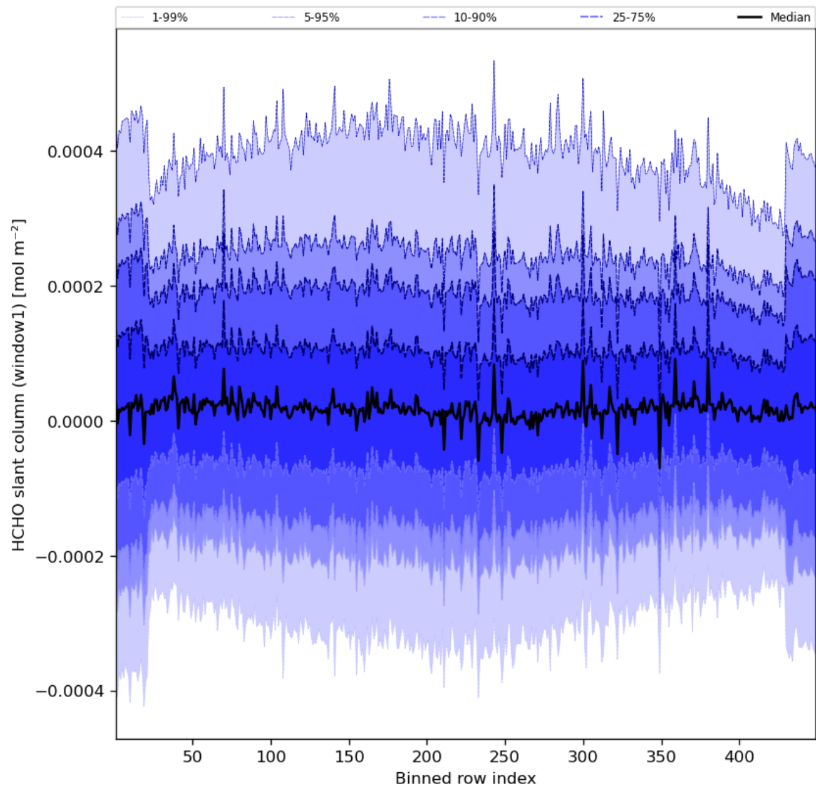
Figure 52: Along track statistics of “HCHO slant column (window1)” for 2023-07-05 to 2023-07-07
