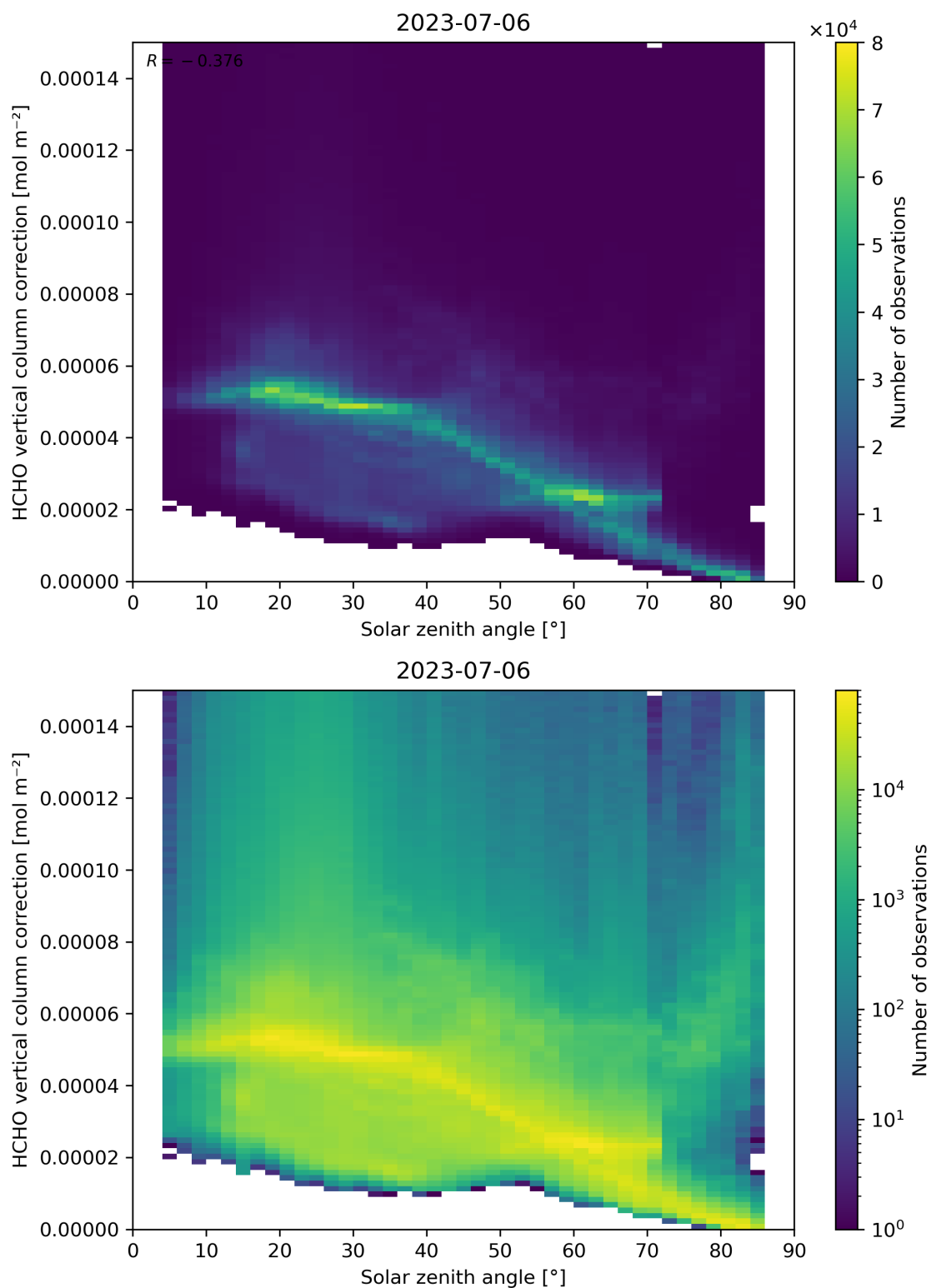
Figure 178: Scatter density plot of “Solar zenith angle” against “HCHO vertical column correction” for 2023-07-05 to 2023-07-07.
