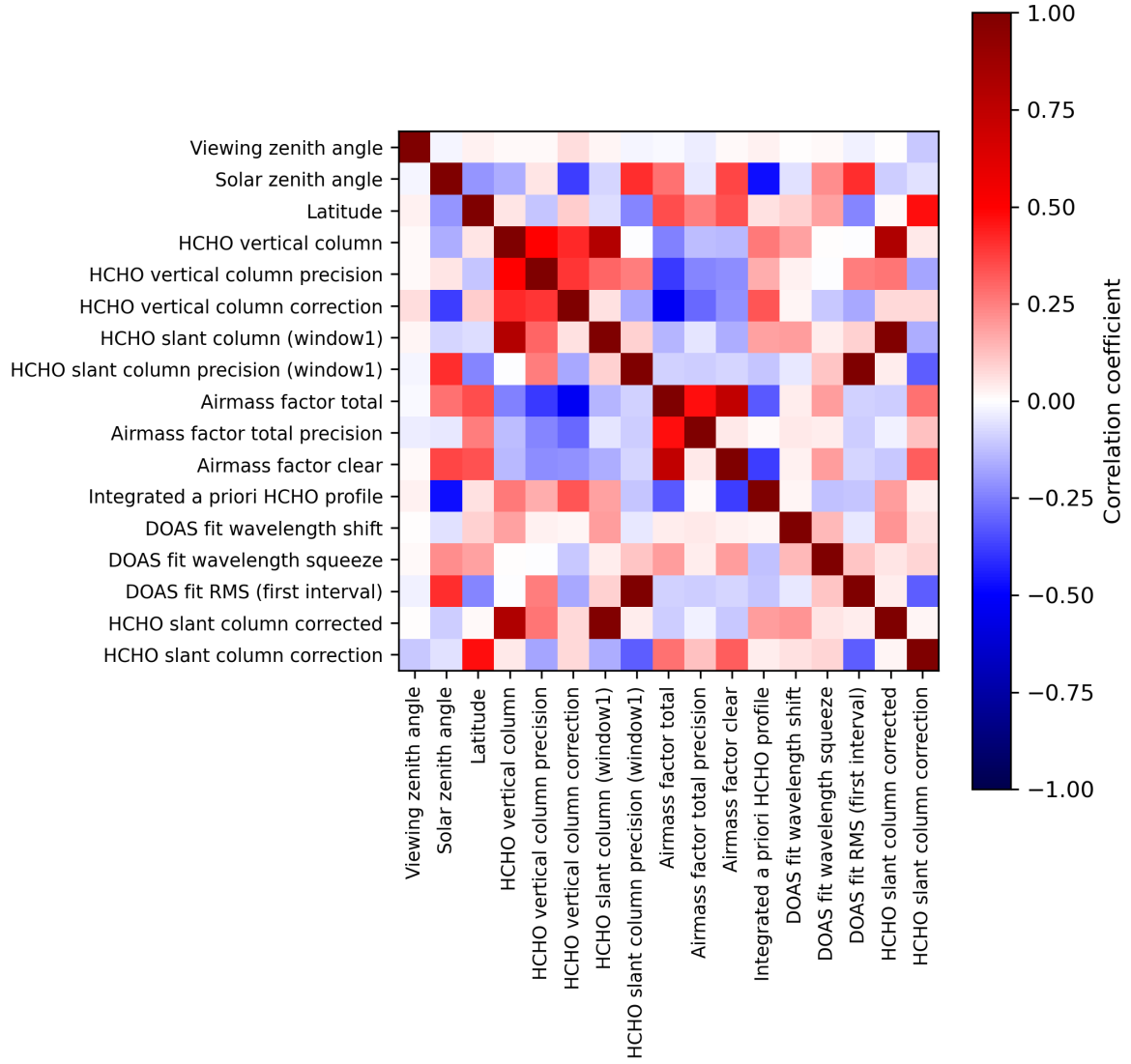
Figure 2: Map of correlation matrix for 2023-07-05 to 2023-07-07.
