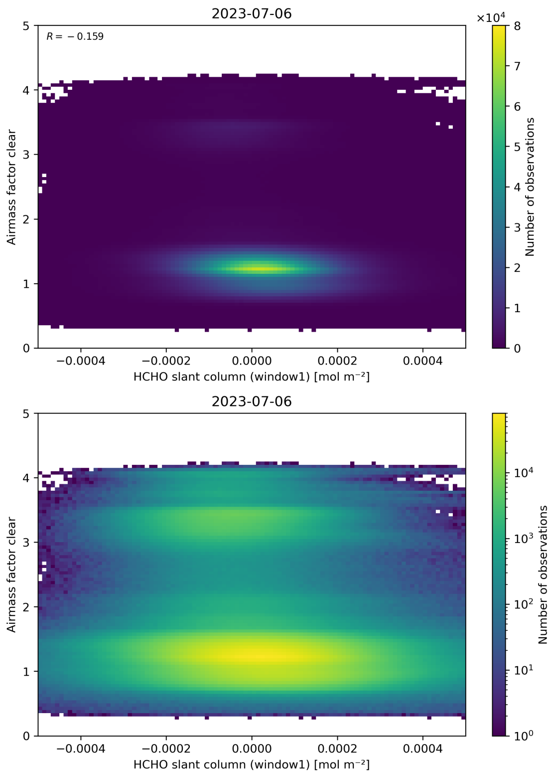
Figure 81: Scatter density plot of “HCHO slant column (window1)” against “Airmass factor clear” for 2023-07-05 to 2023-07-07.
