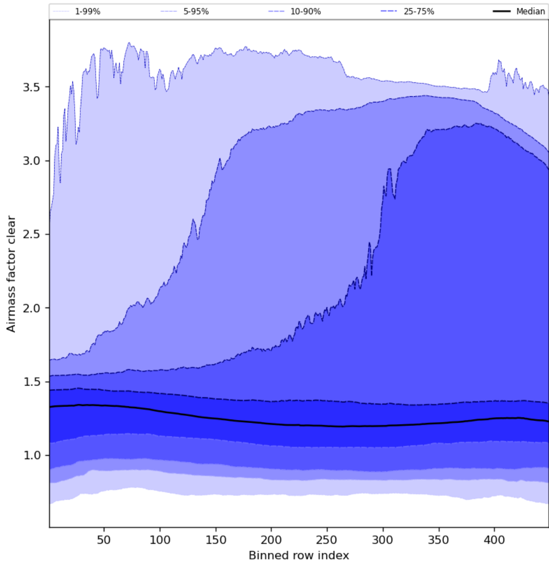
Figure 56: Along track statistics of “Airmass factor clear” for 2023-07-05 to 2023-07-07
