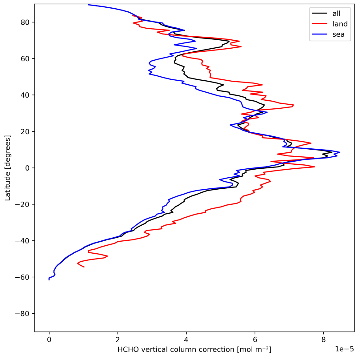
Figure 23: Zonal average of “HCHO vertical column correction” for 2023-07-05 to 2023-07-07.
