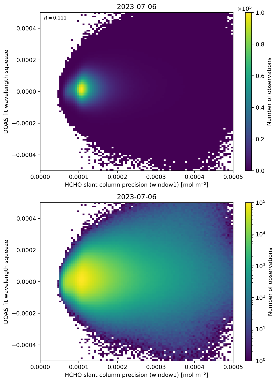
Figure 90: Scatter density plot of “HCHO slant column precision (window1)” against “DOAS fit wavelength squeeze” for 2023-07-05 to 2023-07-07.
