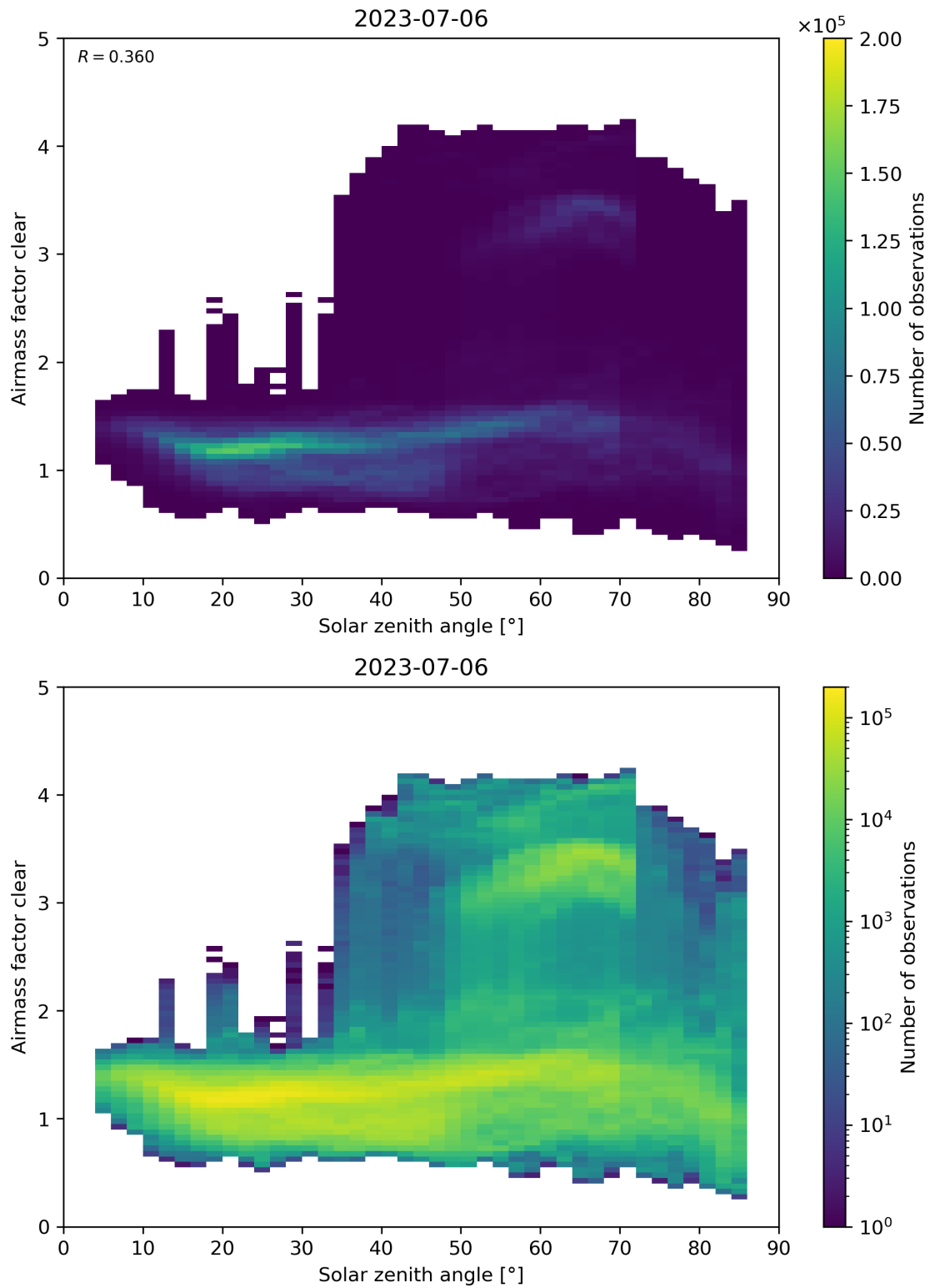
Figure 170: Scatter density plot of “Solar zenith angle” against “Airmass factor clear” for 2023-07-05 to 2023-07-07.
