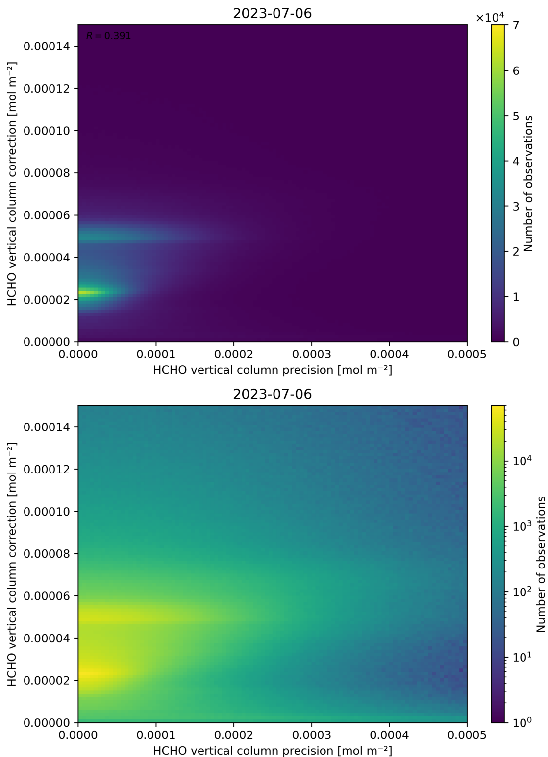
Figure 146: Scatter density plot of “HCHO vertical column precision” against “HCHO vertical column correction” for 2023-07-05 to 2023-07-07.
