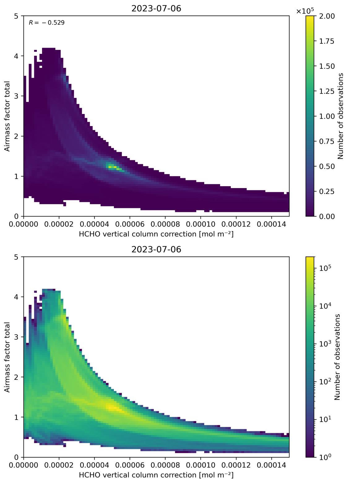
Figure 120: Scatter density plot of “HCHO vertical column correction” against “Airmass factor total” for 2023-07-05 to 2023-07-07.
