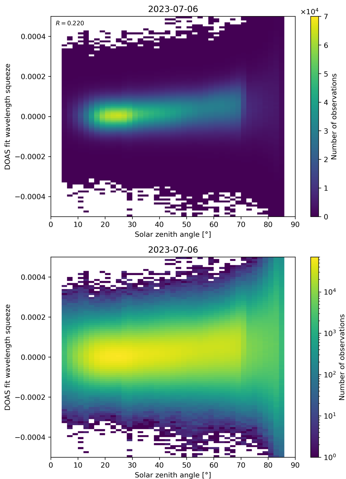
Figure 169: Scatter density plot of “Solar zenith angle” against “DOAS fit wavelength squeeze” for 2023-07-05 to 2023-07-07.
