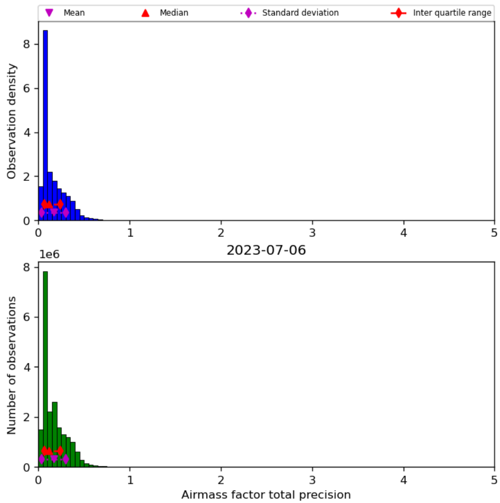
Figure 41: Histogram of “Airmass factor total precision” for 2023-07-05 to 2023-07-07
