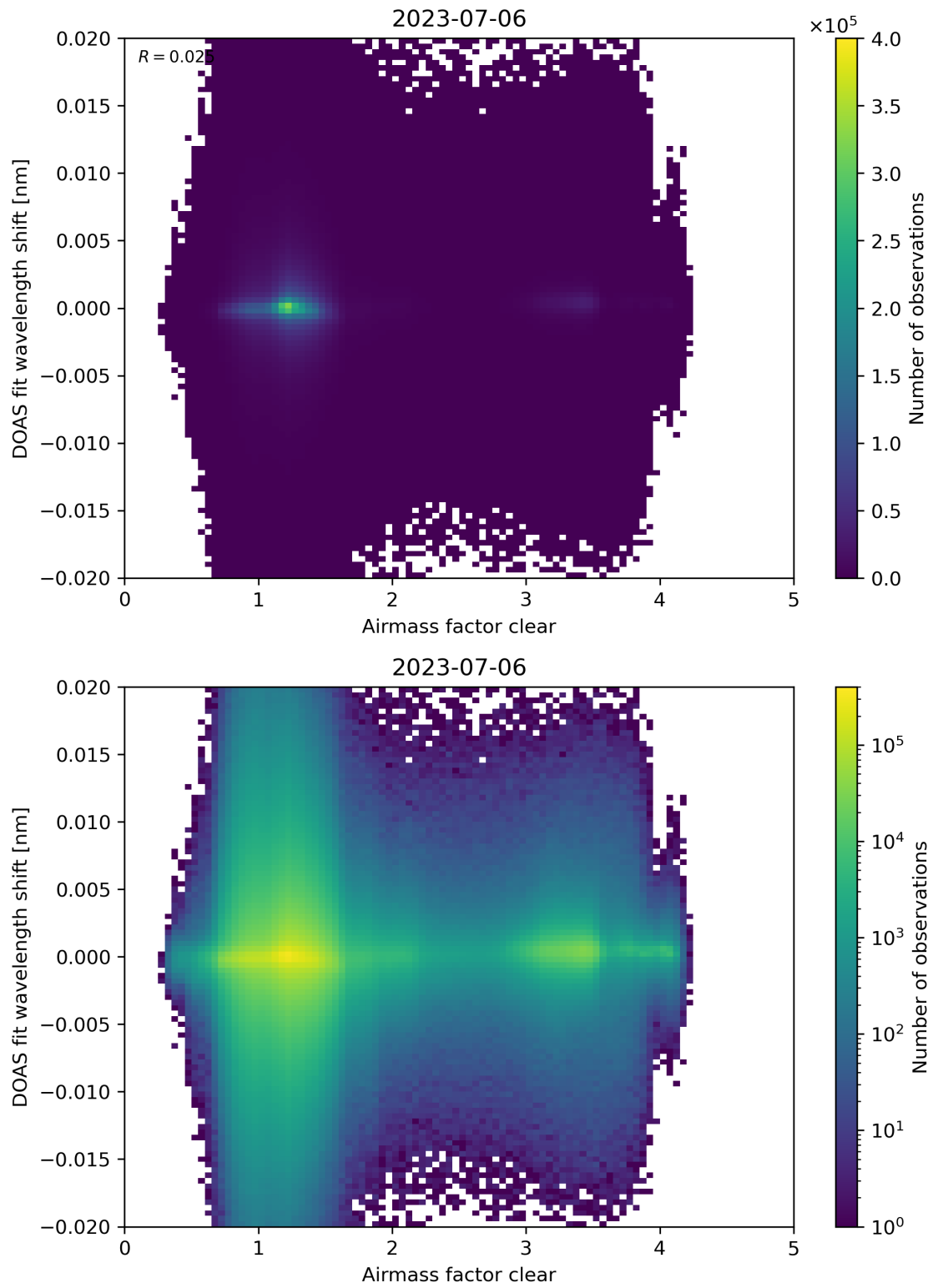
Figure 72: Scatter density plot of “Airmass factor clear” against “DOAS fit wavelength shift” for 2023-07-05 to 2023-07-07.
