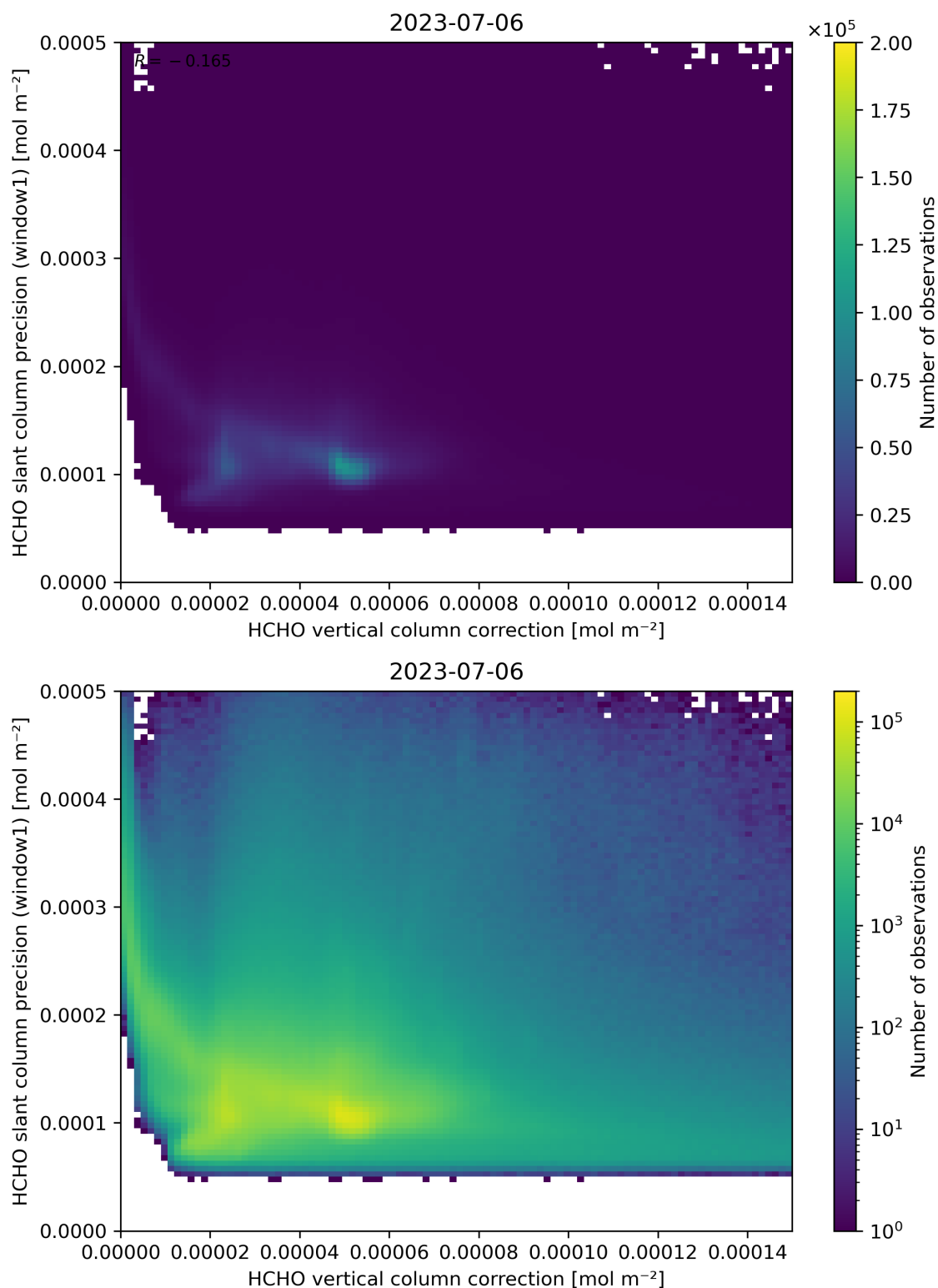
Figure 119: Scatter density plot of “HCHO vertical column correction” against “HCHO slant column precision (window1)” for 2023-07-05 to 2023-07-07.
