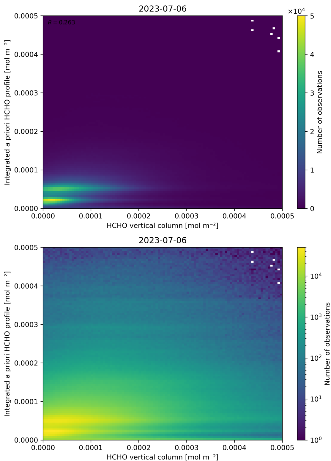
Figure 135: Scatter density plot of “HCHO vertical column” against “Integrated a priori HCHO profile” for 2023-07-05 to 2023-07-07.
