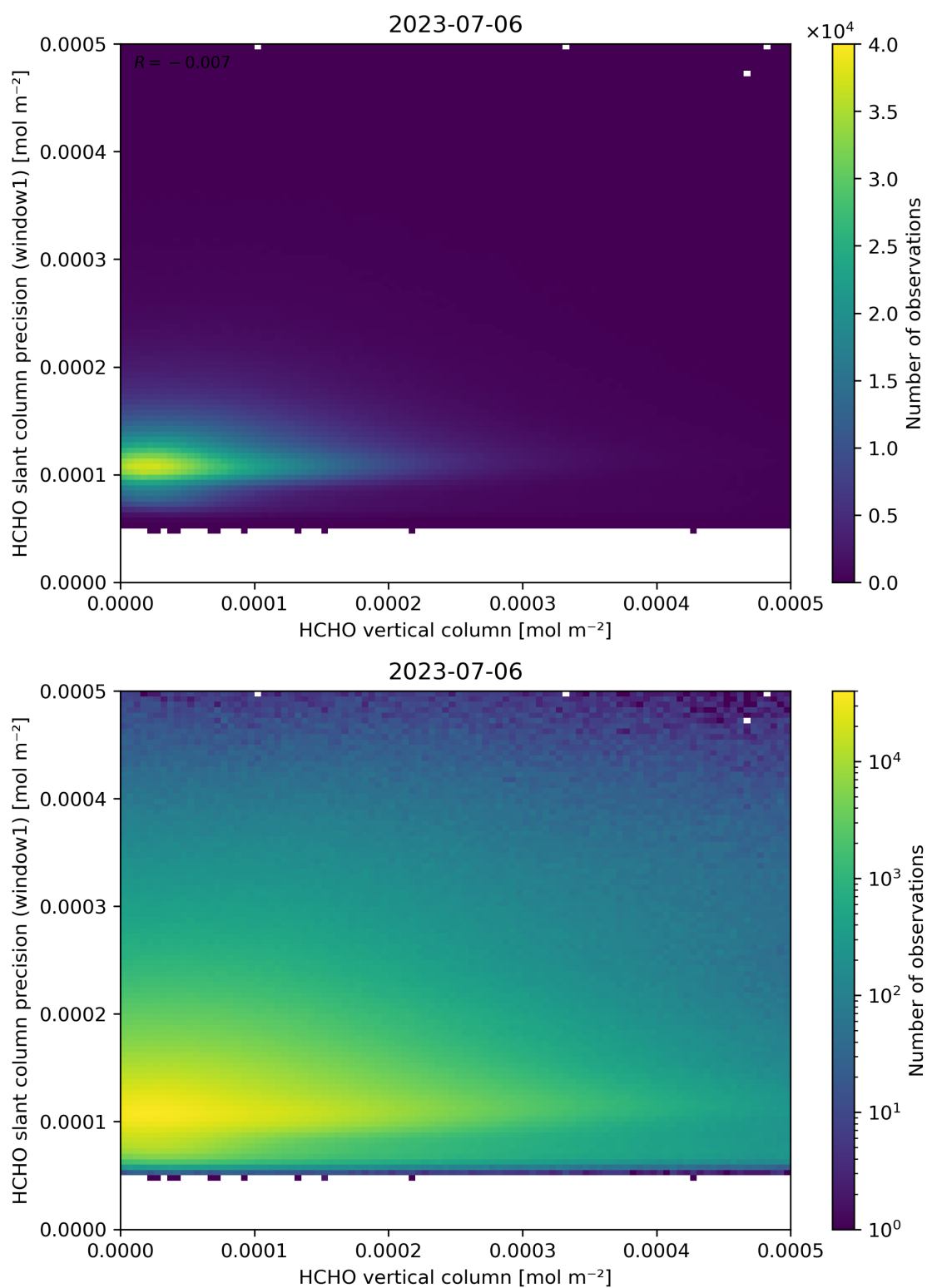
Figure 130: Scatter density plot of “HCHO vertical column” against “HCHO slant column precision (window1)” for 2023-07-05 to 2023-07-07.
