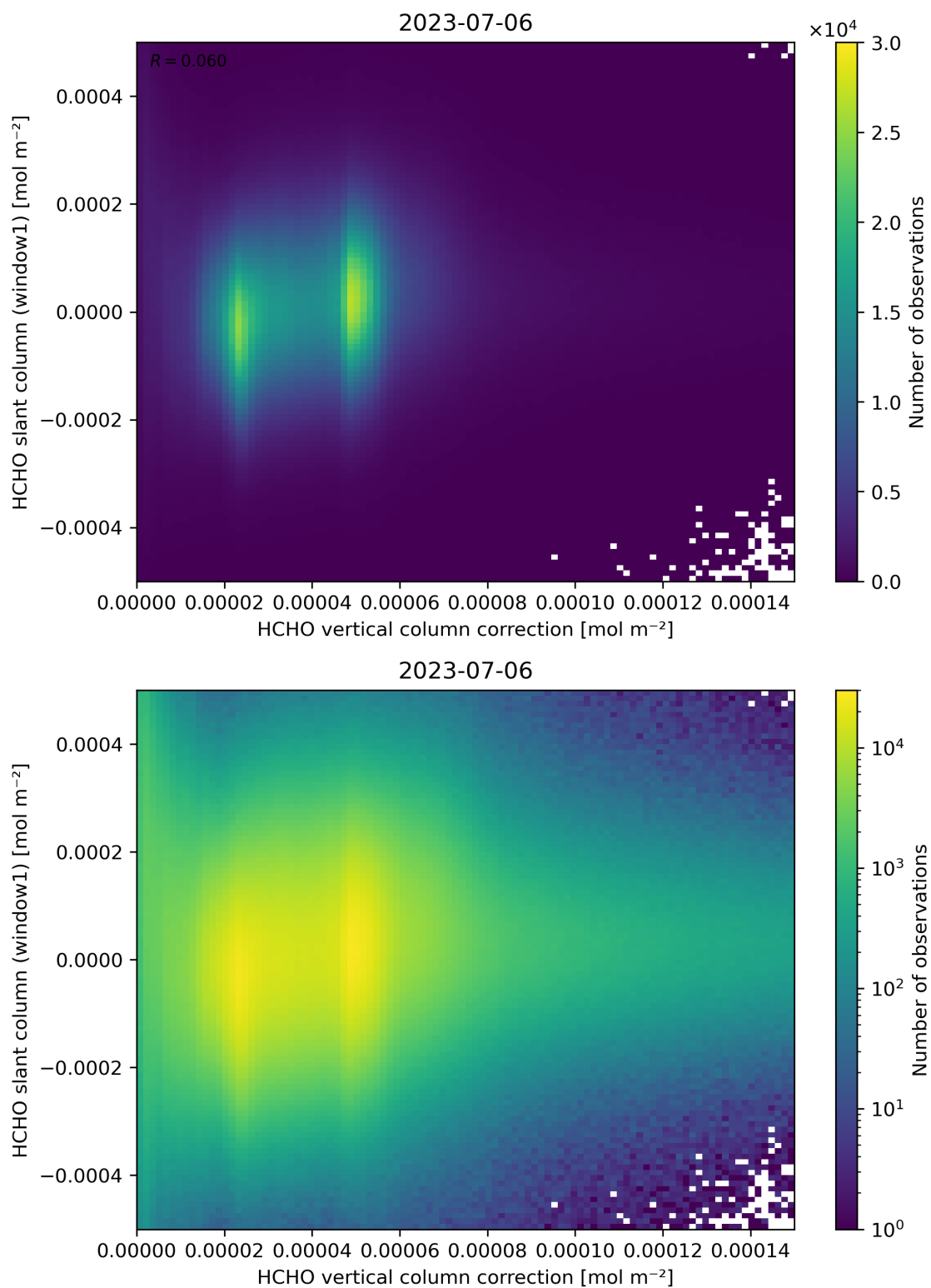
Figure 118: Scatter density plot of “HCHO vertical column correction” against “HCHO slant column (window1)” for 2023-07-05 to 2023-07-07.
