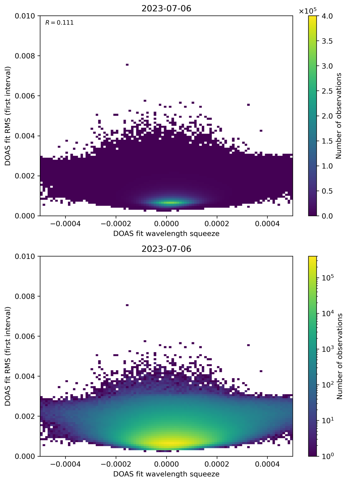
Figure 68: Scatter density plot of “DOAS fit wavelength squeeze” against “DOAS fit RMS (first interval)” for 2023-07-05 to 2023-07-07.
