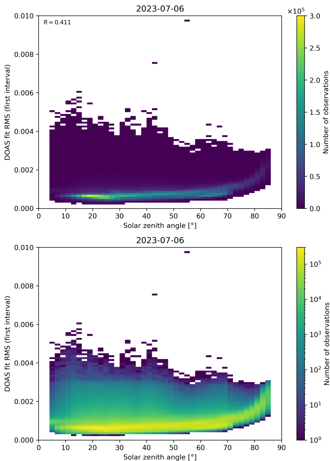
Figure 167: Scatter density plot of “Solar zenith angle” against “DOAS fit RMS (first interval)” for 2023-07-05 to 2023-07-07.
