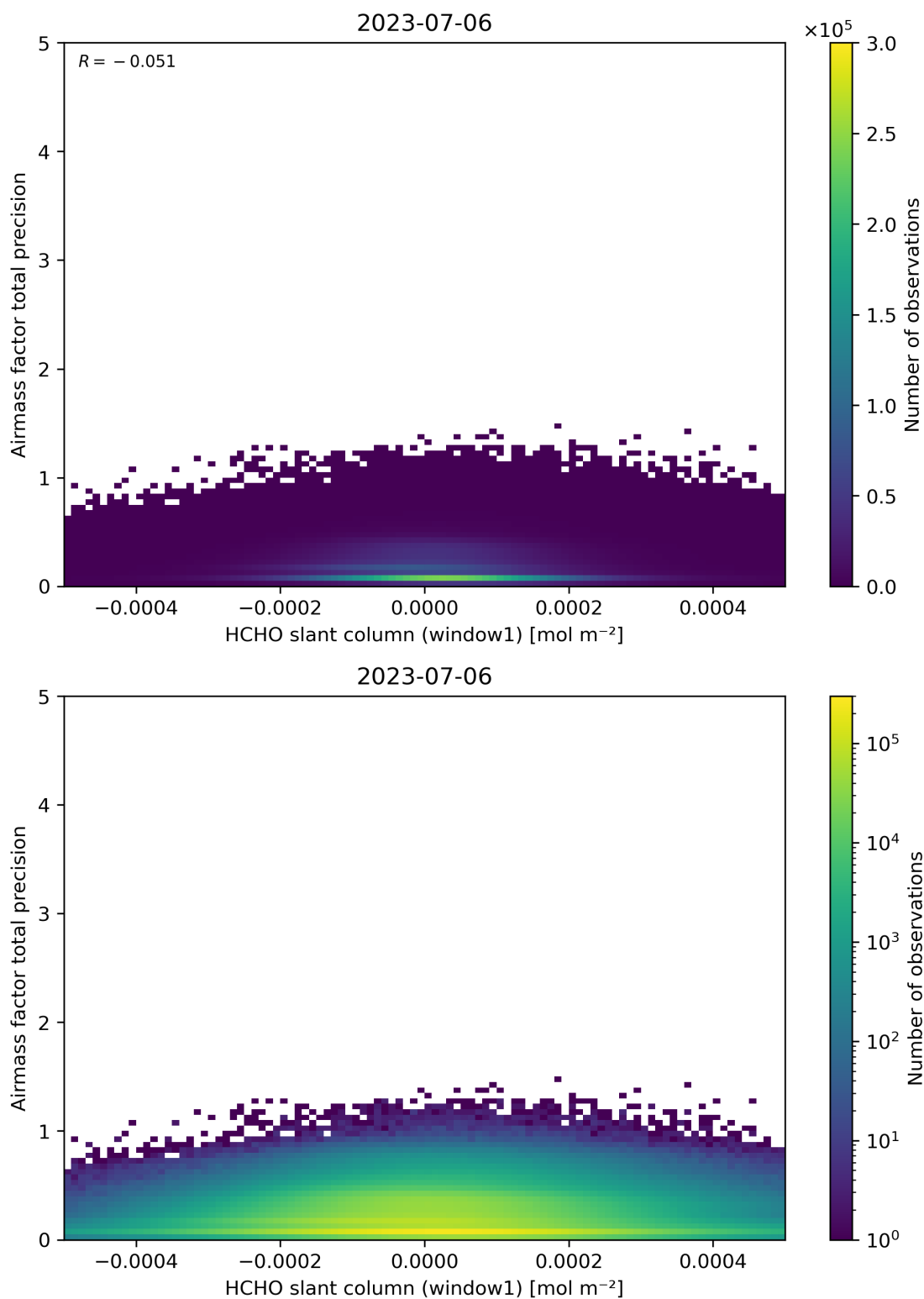
Figure 86: Scatter density plot of “HCHO slant column (window1)” against “Airmass factor total precision” for 2023-07-05 to 2023-07-07.
