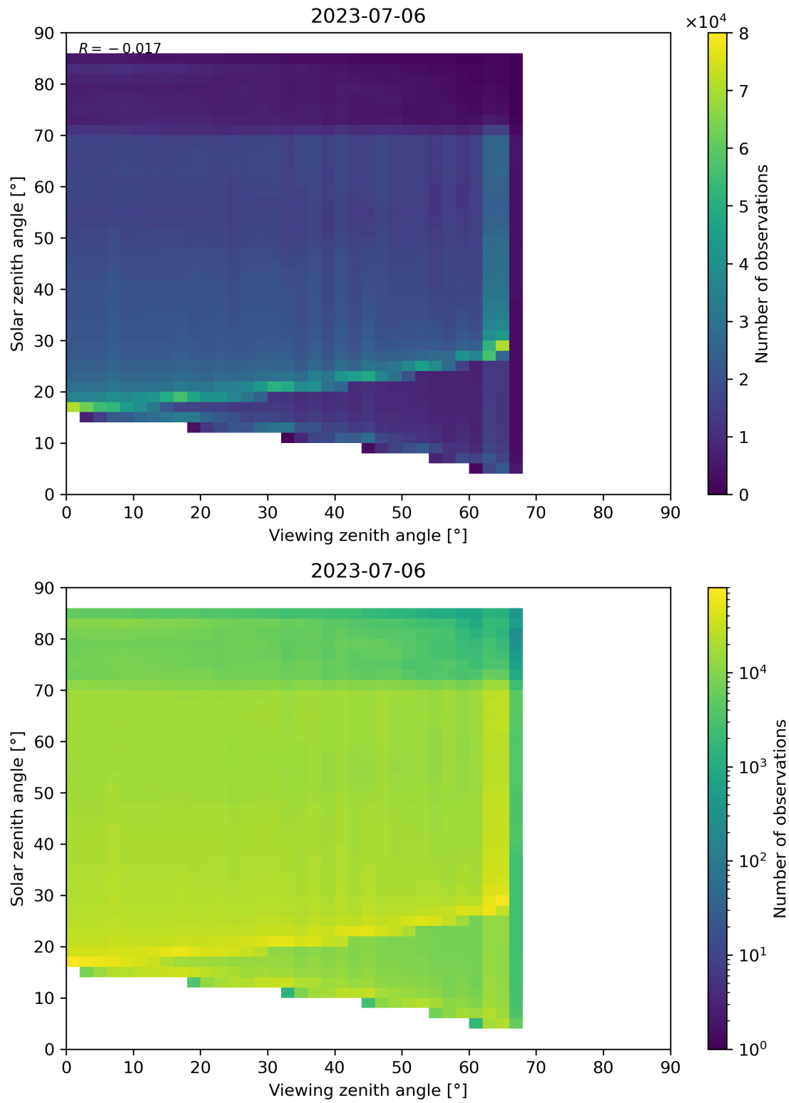
Figure 197: Scatter density plot of “Viewing zenith angle” against “Solar zenith angle” for 2023-07-05 to 2023-07-07.
