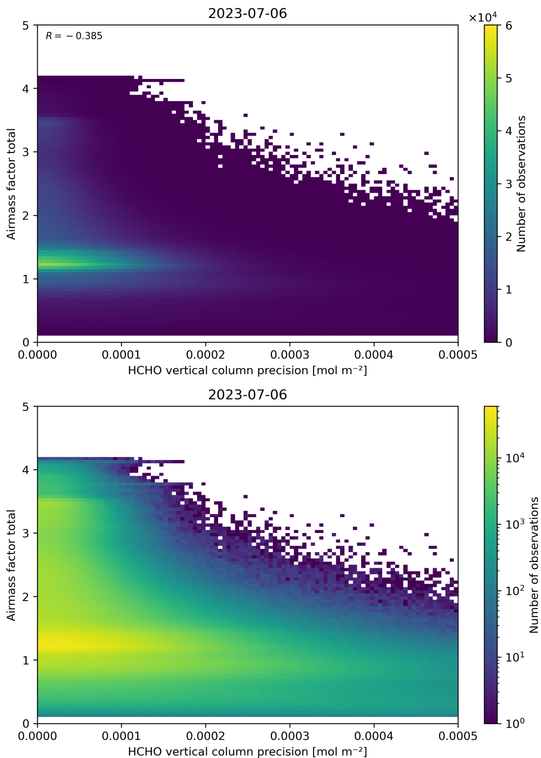
Figure 144: Scatter density plot of “HCHO vertical column precision” against “Airmass factor total” for 2023-07-05 to 2023-07-07.
