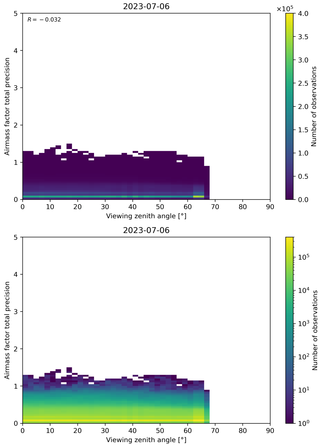
Figure 191: Scatter density plot of “Viewing zenith angle” against “Airmass factor total precision” for 2023-07-05 to 2023-07-07.
