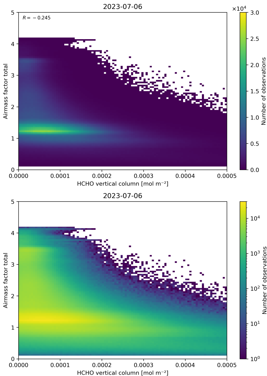
Figure 131: Scatter density plot of “HCHO vertical column” against “Airmass factor total” for 2023-07-05 to 2023-07-07.
