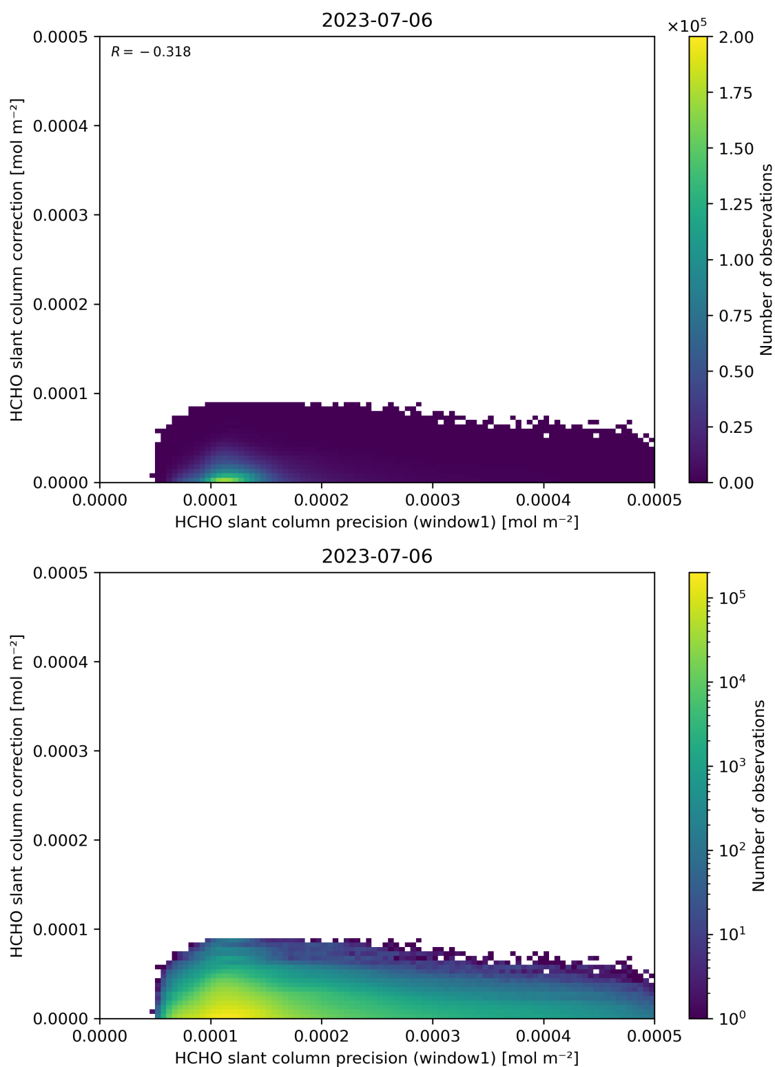
Figure 93: Scatter density plot of “HCHO slant column precision (window1)” against “HCHO slant column correction” for 2023-07-05 to 2023-07-07.
