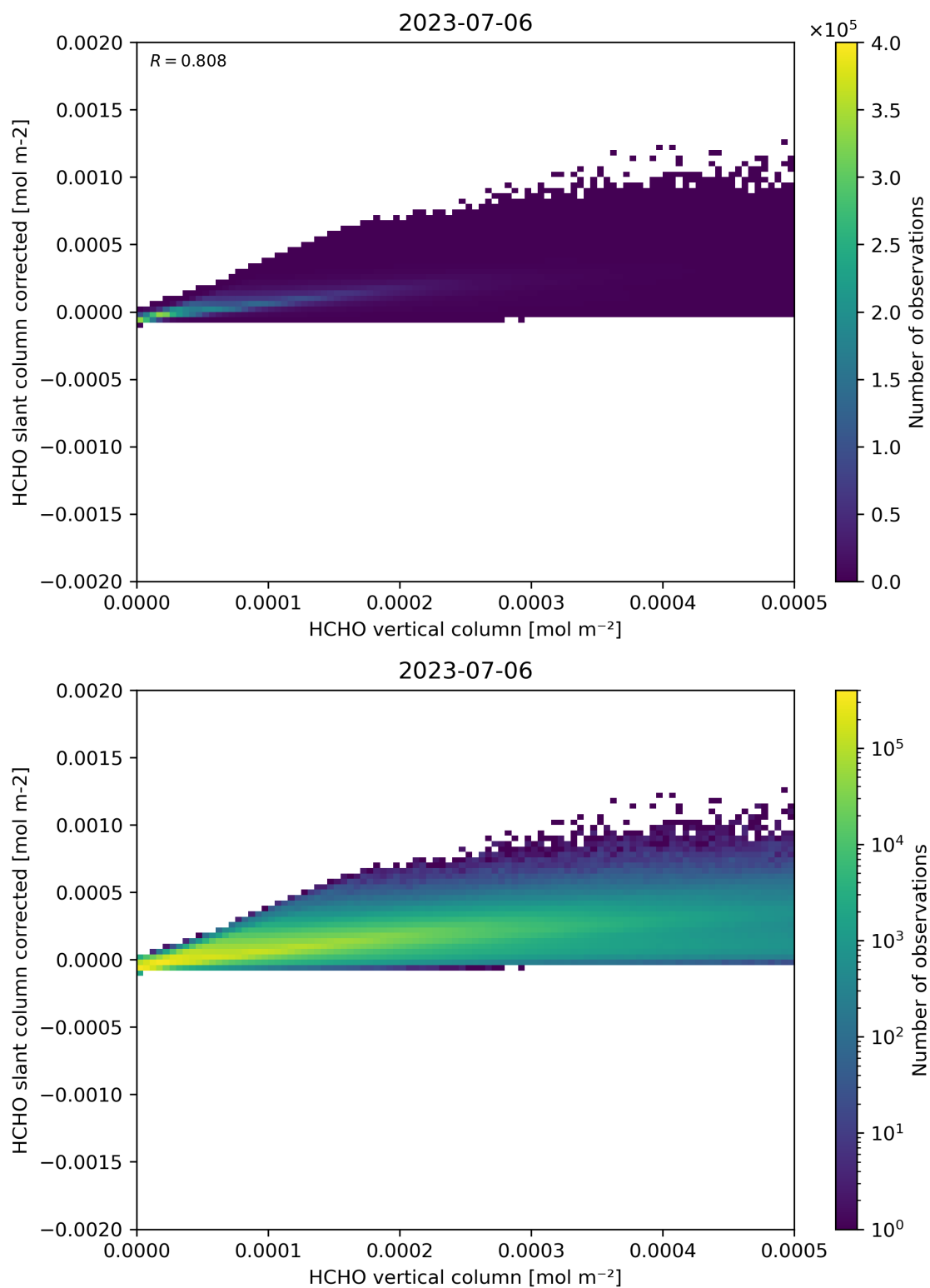
Figure 127: Scatter density plot of “HCHO vertical column” against “HCHO slant column corrected” for 2023-07-05 to 2023-07-07.
