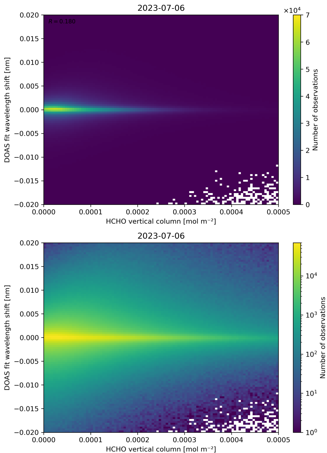
Figure 124: Scatter density plot of “HCHO vertical column” against “DOAS fit wavelength shift” for 2023-07-05 to 2023-07-07.
