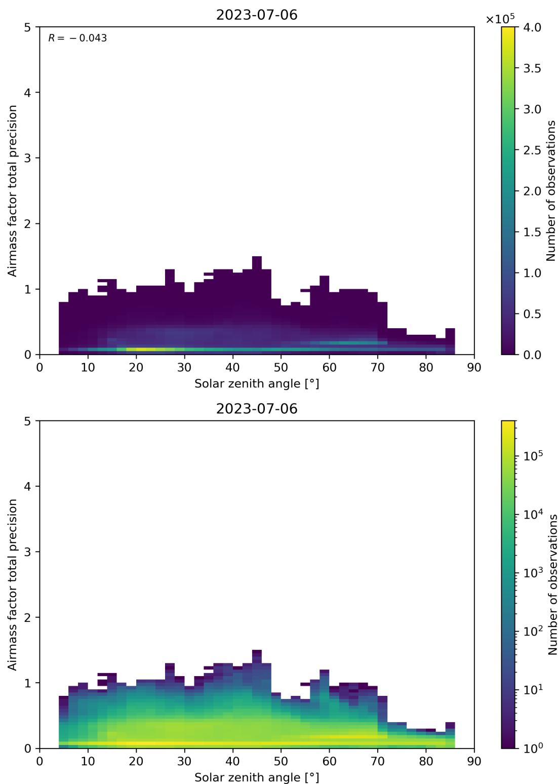
Figure 176: Scatter density plot of “Solar zenith angle” against “Airmass factor total precision” for 2023-07-05 to 2023-07-07.
