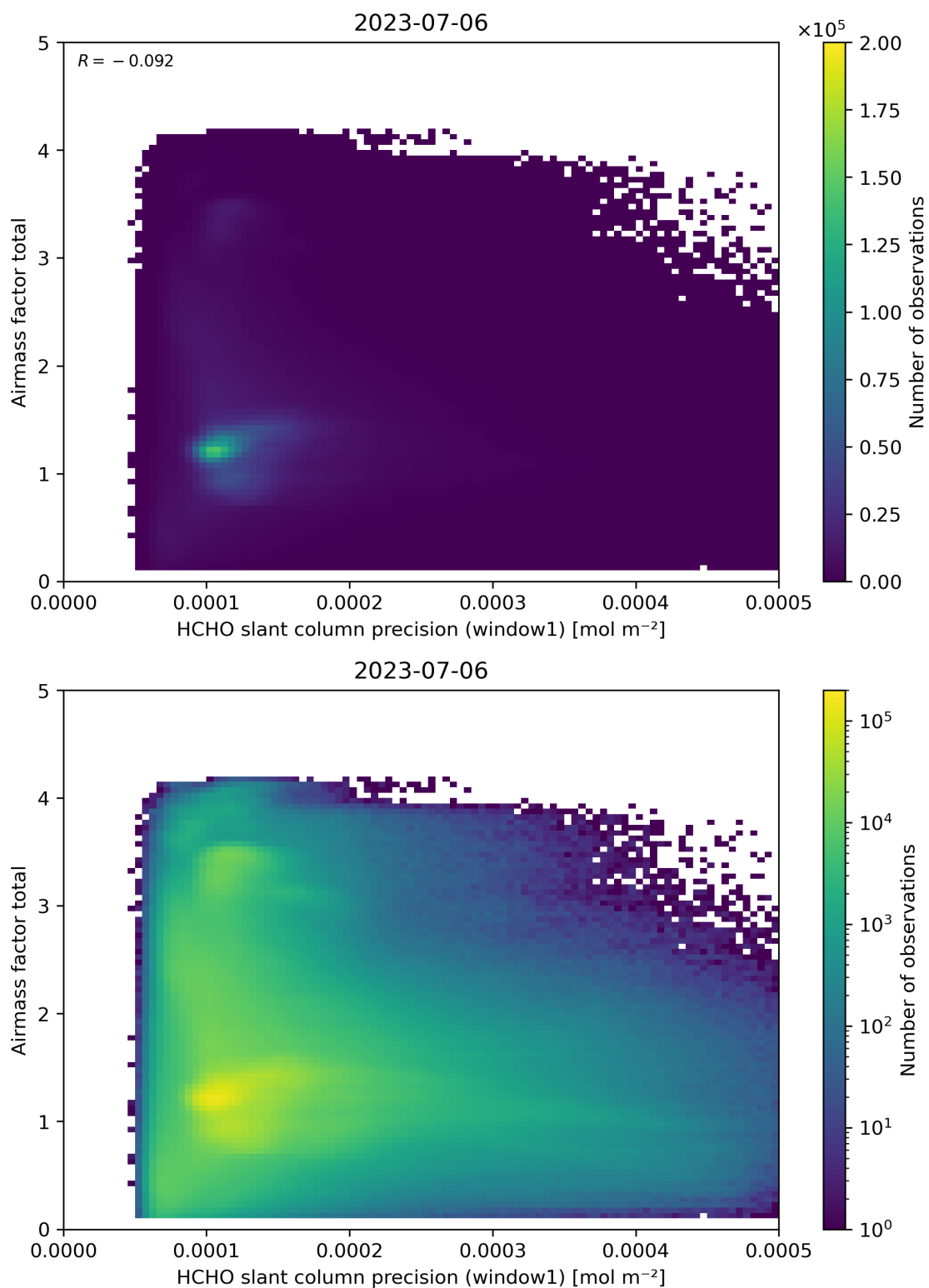
Figure 94: Scatter density plot of “HCHO slant column precision (window1)” against “Airmass factor total” for 2023-07-05 to 2023-07-07.
