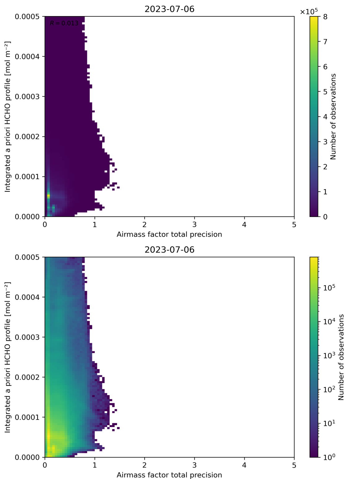
Figure 111: Scatter density plot of “Airmass factor total precision” against “Integrated a priori HCHO profile” for 2023-07-05 to 2023-07-07.
