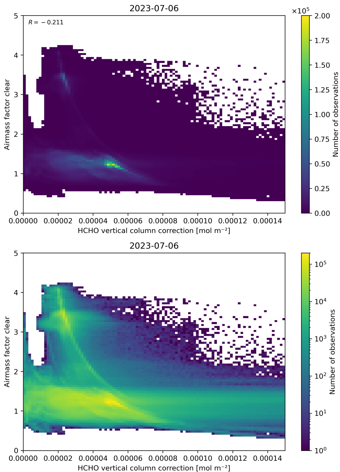
Figure 115: Scatter density plot of “HCHO vertical column correction” against “Airmass factor clear” for 2023-07-05 to 2023-07-07.
