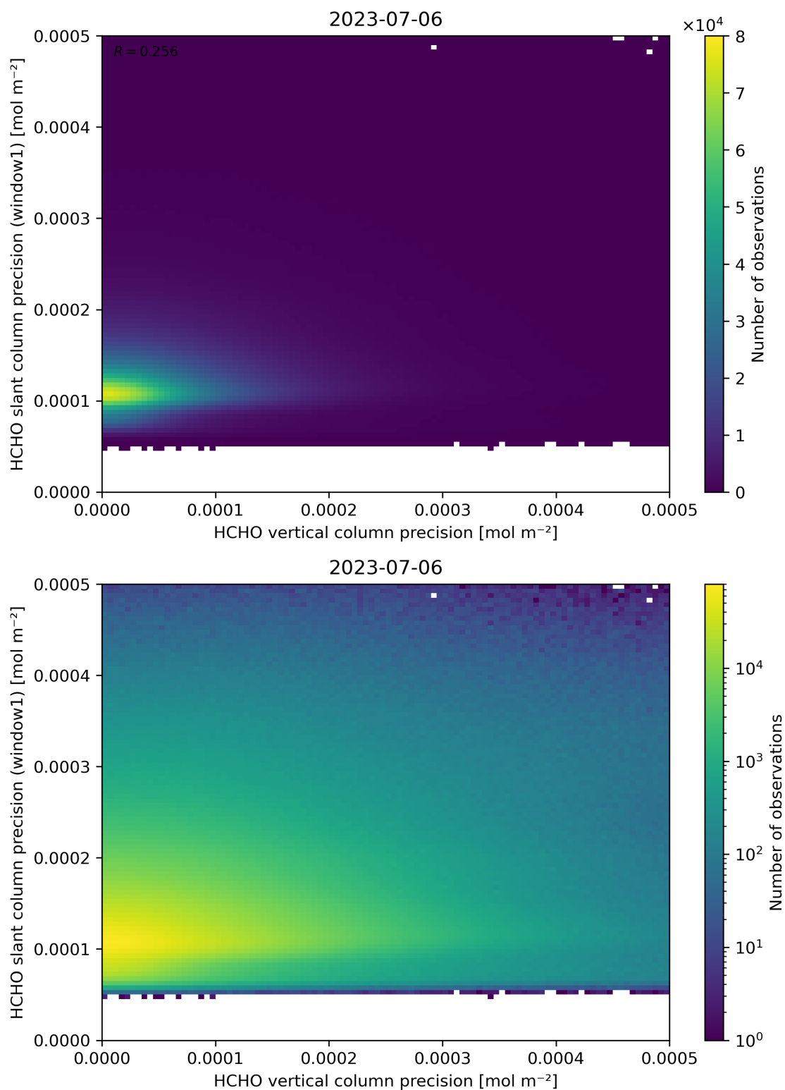
Figure 143: Scatter density plot of “HCHO vertical column precision” against “HCHO slant column precision (window1)” for 2023-07-05 to 2023-07-07.
