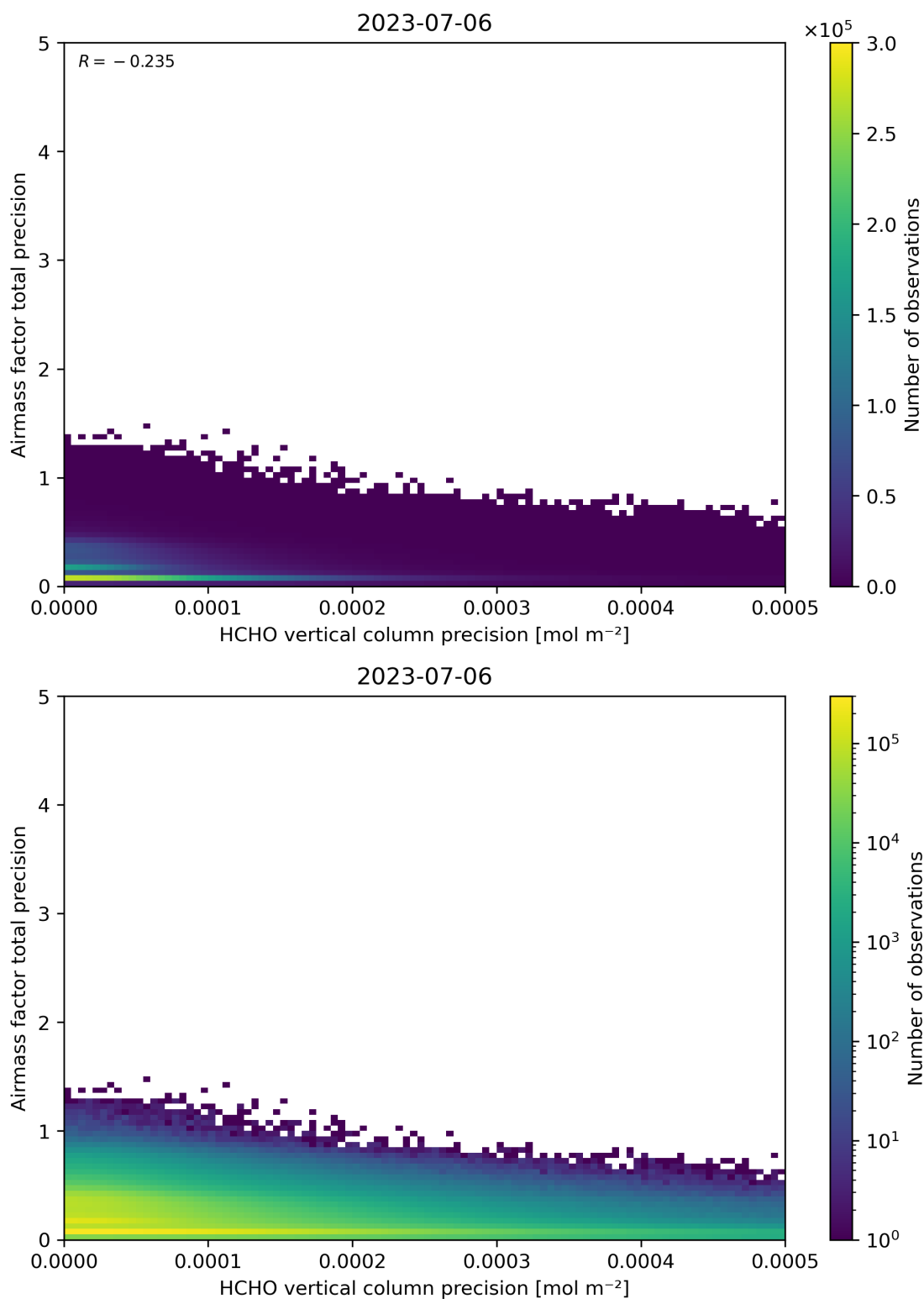
Figure 145: Scatter density plot of “HCHO vertical column precision” against “Airmass factor total precision” for 2023-07-05 to 2023-07-07.
