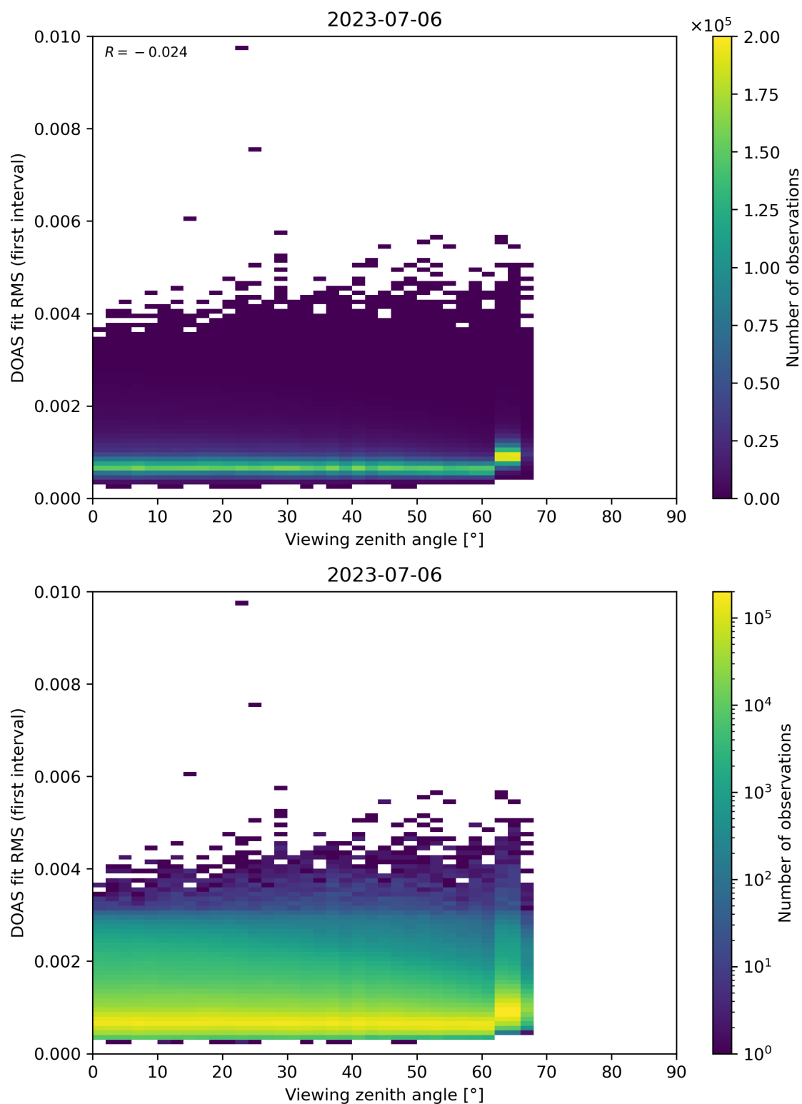
Figure 182: Scatter density plot of “Viewing zenith angle” against “DOAS fit RMS (first interval)” for 2023-07-05 to 2023-07-07.
