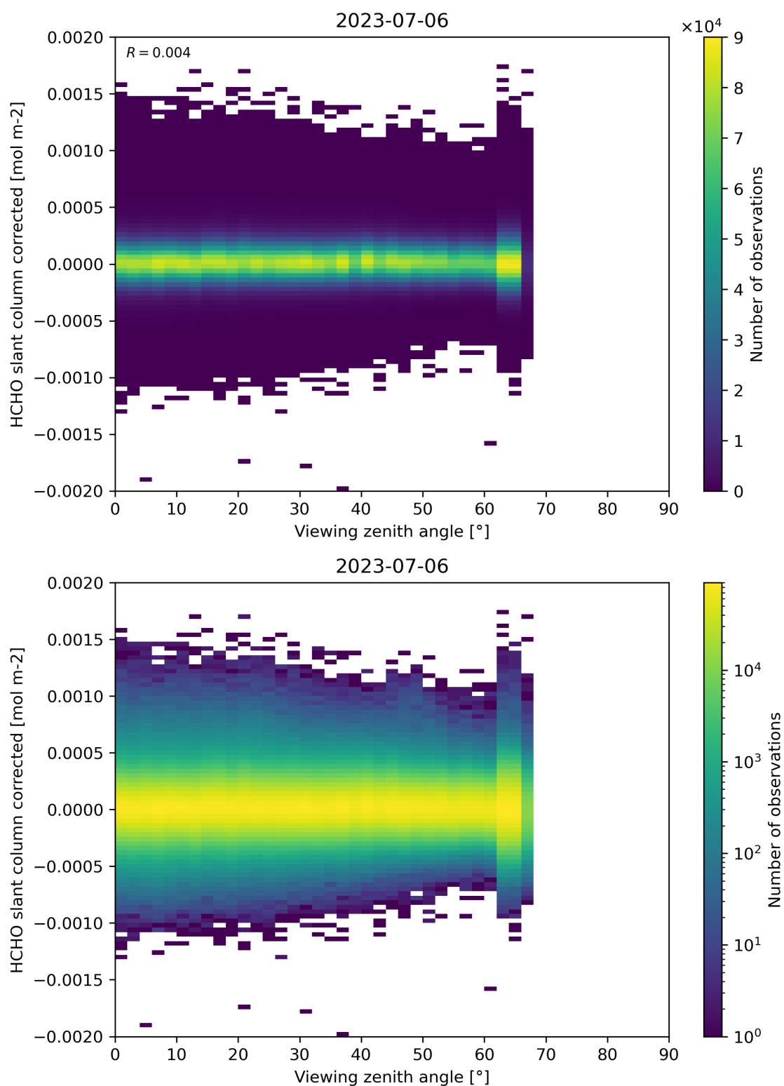
Figure 186: Scatter density plot of “Viewing zenith angle” against “HCHO slant column corrected” for 2023-07-05 to 2023-07-07.
