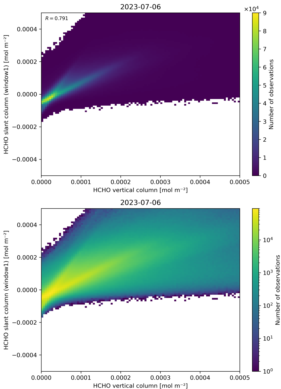
Figure 129: Scatter density plot of “HCHO vertical column” against “HCHO slant column (window1)” for 2023-07-05 to 2023-07-07.
