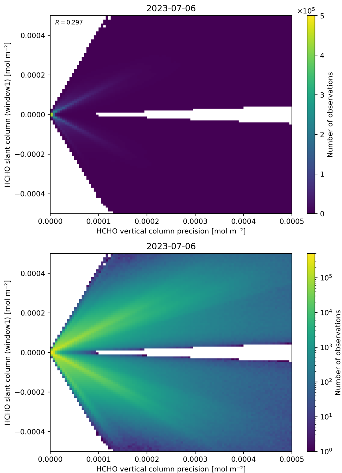
Figure 142: Scatter density plot of “HCHO vertical column precision” against “HCHO slant column (window1)” for 2023-07-05 to 2023-07-07.
