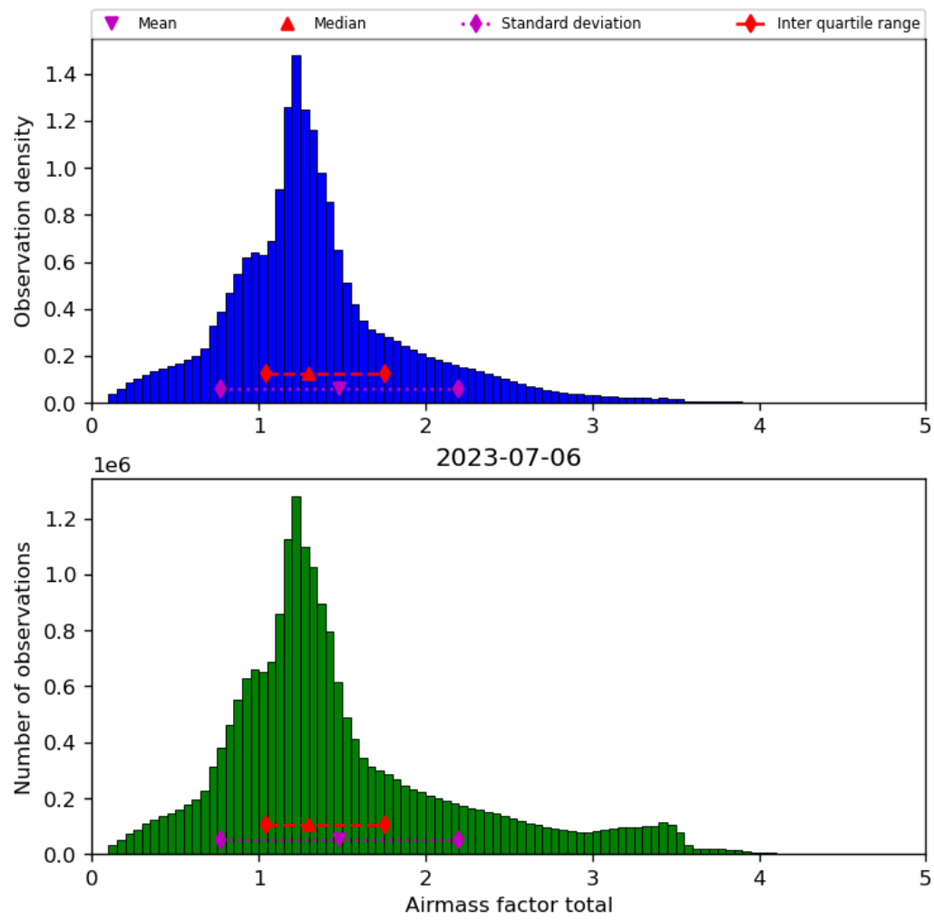
Figure 40: Histogram of “Airmass factor total” for 2023-07-05 to 2023-07-07
