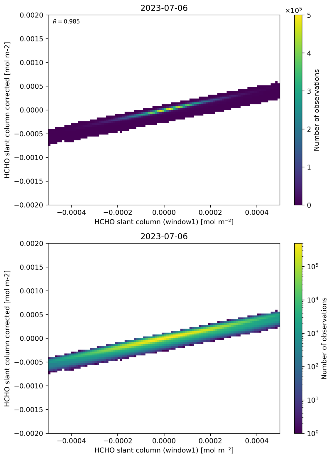
Figure 82: Scatter density plot of “HCHO slant column (window1)” against “HCHO slant column corrected” for 2023-07-05 to 2023-07-07.
