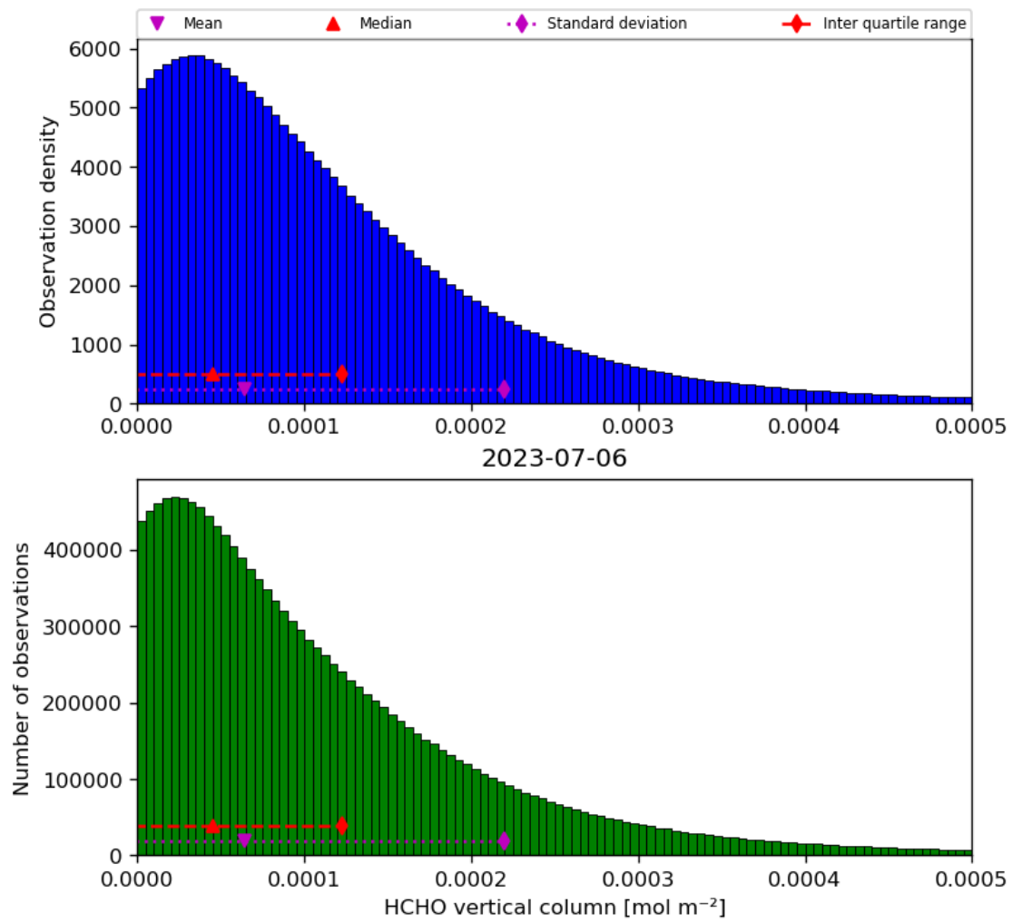
Figure 35: Histogram of “HCHO vertical column” for 2023-07-05 to 2023-07-07
