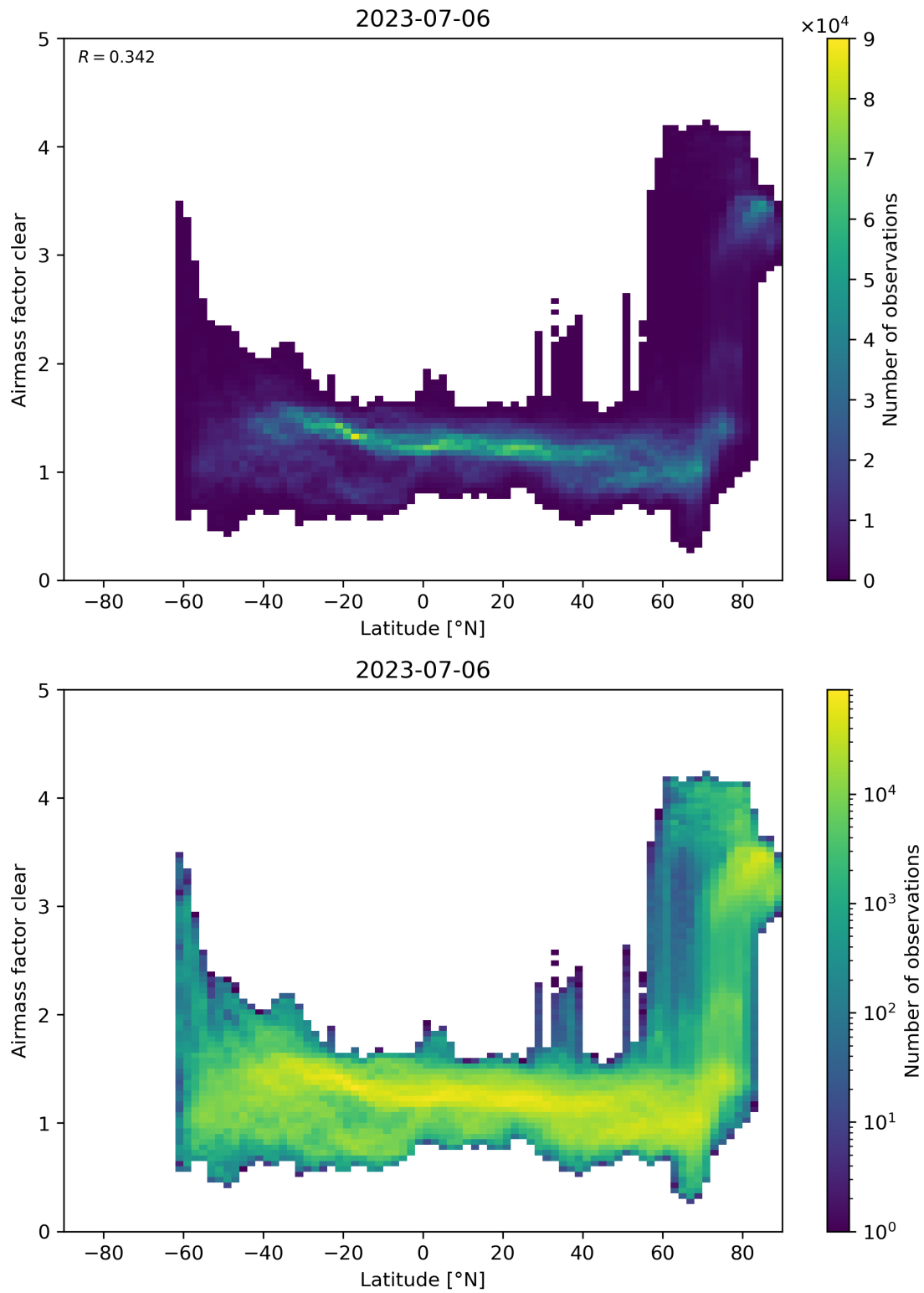
Figure 156: Scatter density plot of “Latitude” against “Airmass factor clear” for 2023-07-05 to 2023-07-07.
