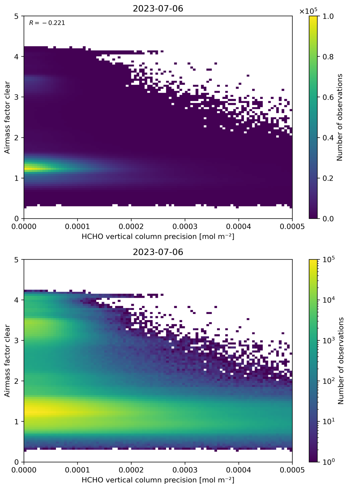
Figure 139: Scatter density plot of “HCHO vertical column precision” against “Airmass factor clear” for 2023-07-05 to 2023-07-07.
