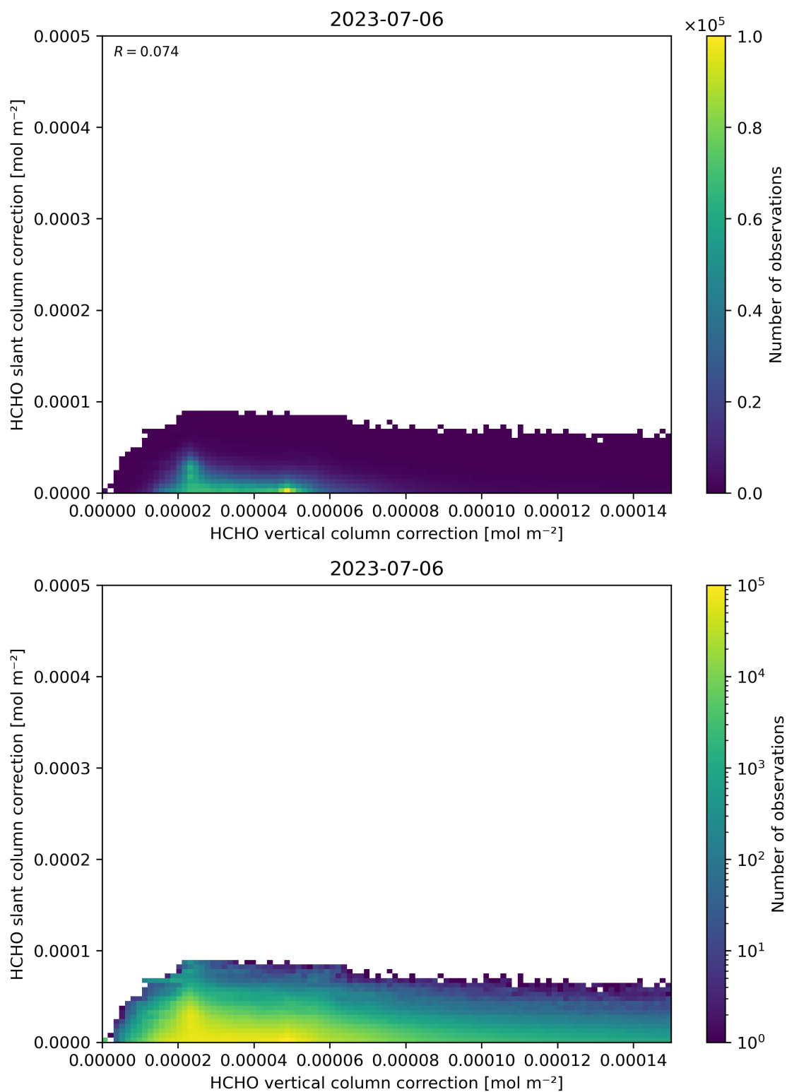
Figure 117: Scatter density plot of “HCHO vertical column correction” against “HCHO slant column correction” for 2023-07-05 to 2023-07-07.
