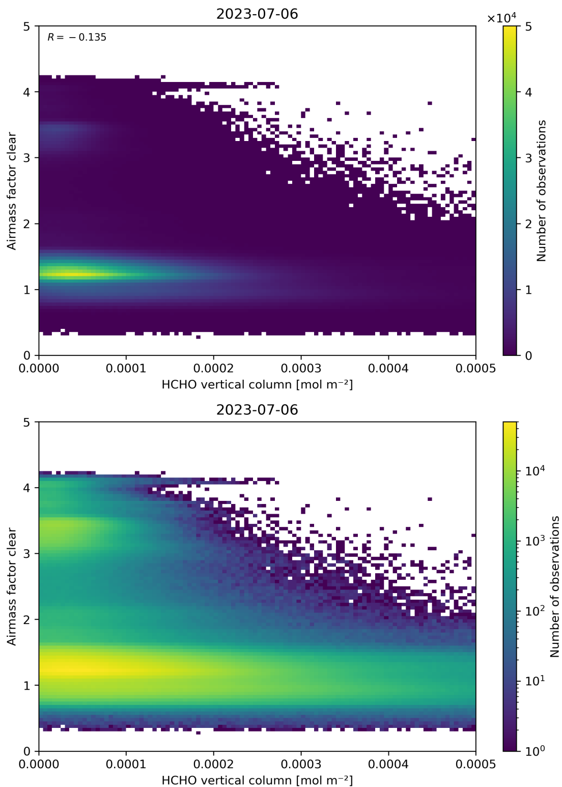
Figure 126: Scatter density plot of “HCHO vertical column” against “Airmass factor clear” for 2023-07-05 to 2023-07-07.
