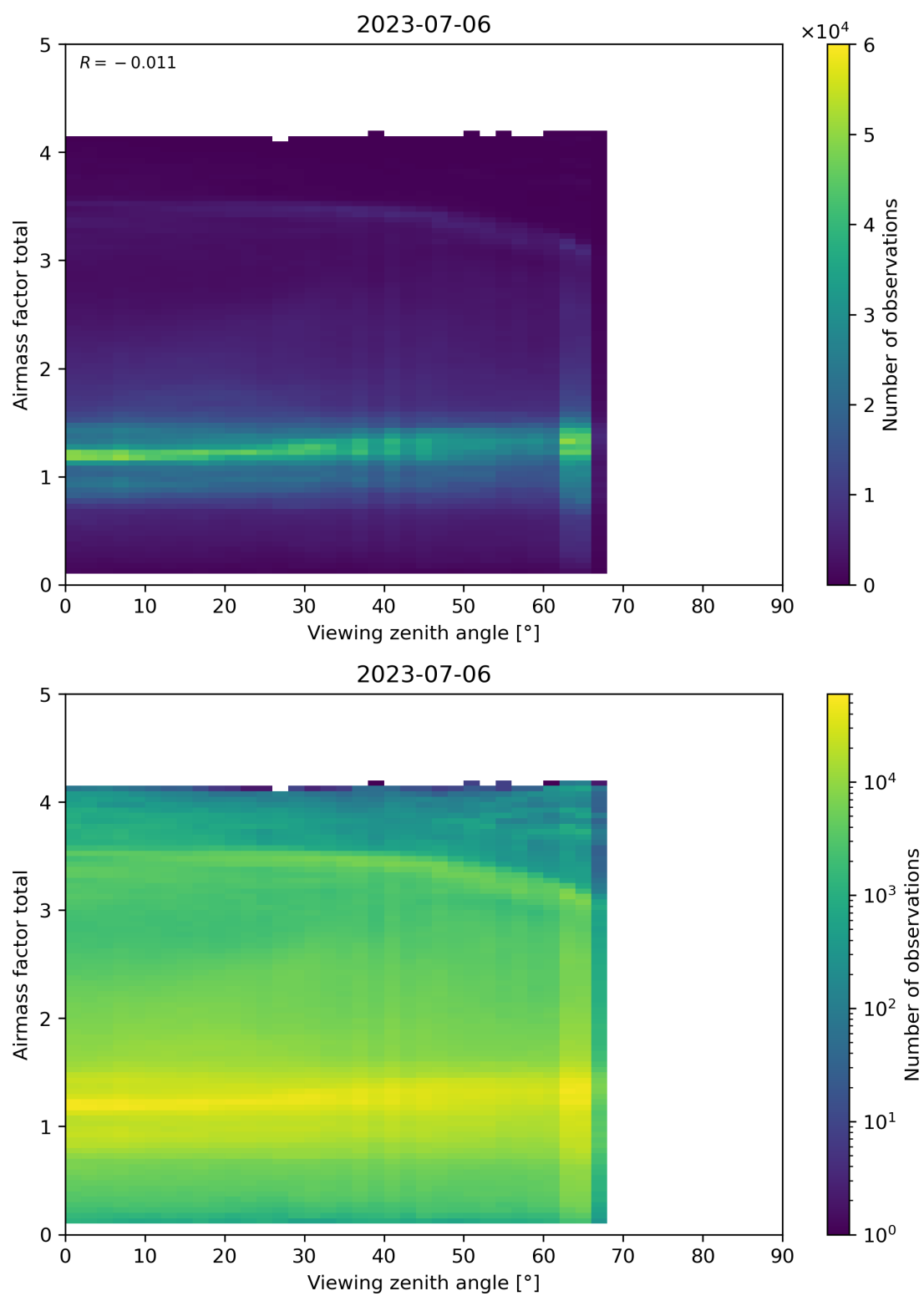
Figure 190: Scatter density plot of “Viewing zenith angle” against “Airmass factor total” for 2023-07-05 to 2023-07-07.
