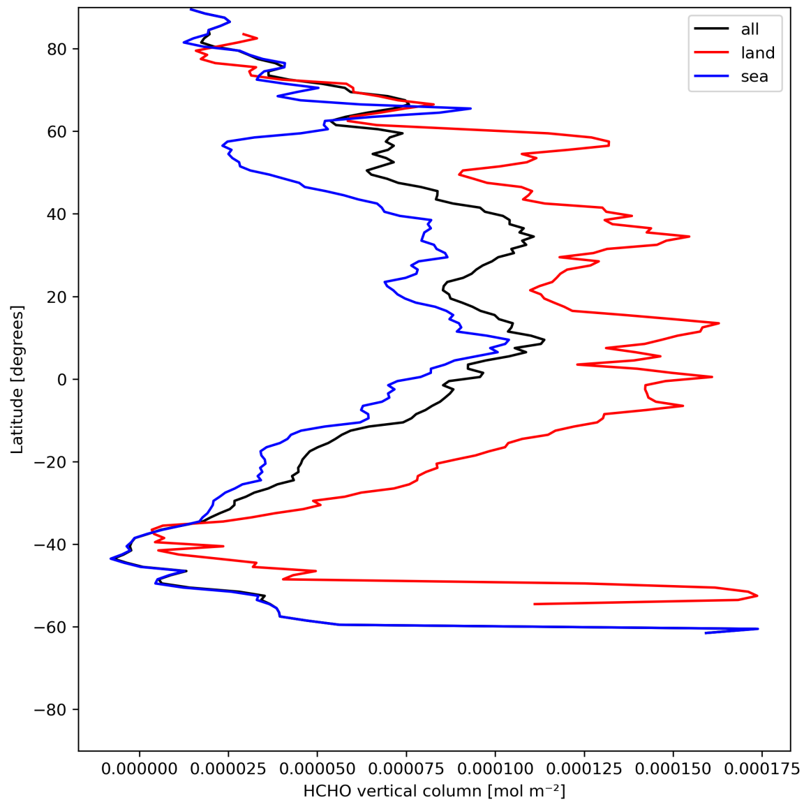
Figure 21: Zonal average of “HCHO vertical column” for 2023-07-05 to 2023-07-07.
