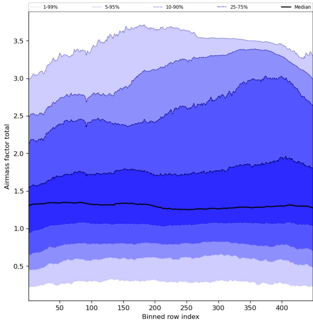
Figure 54: Along track statistics of “Airmass factor total” for 2023-07-05 to 2023-07-07
