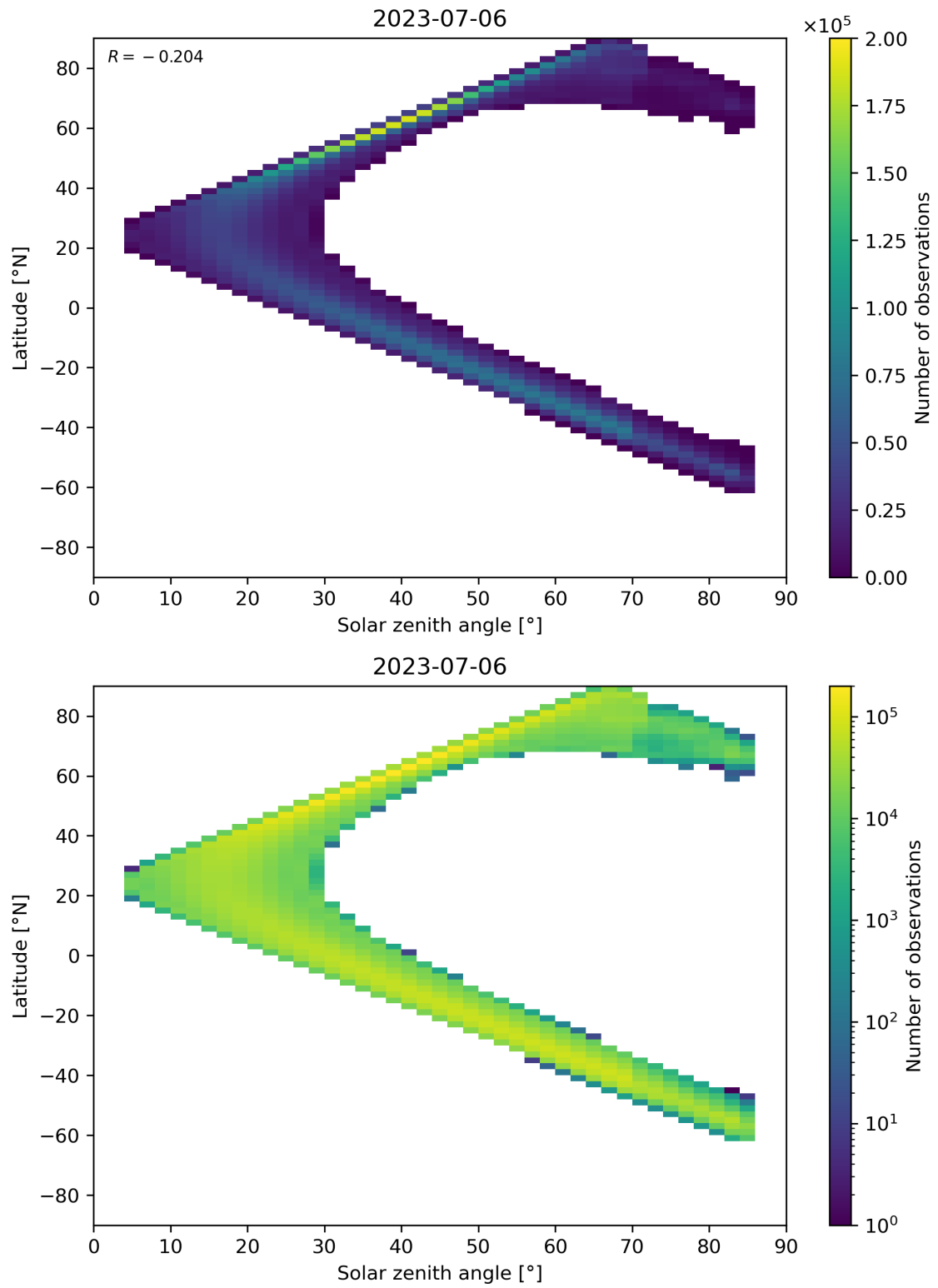
Figure 181: Scatter density plot of “Solar zenith angle” against “Latitude” for 2023-07-05 to 2023-07-07.
