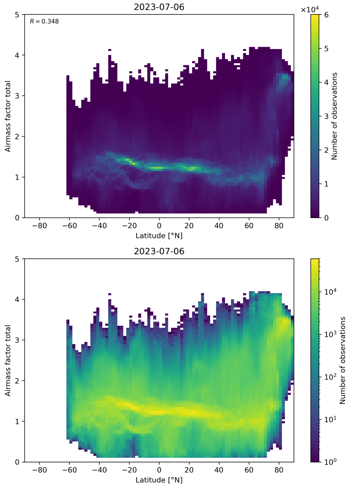
Figure 161: Scatter density plot of “Latitude” against “Airmass factor total” for 2023-07-05 to 2023-07-07.
