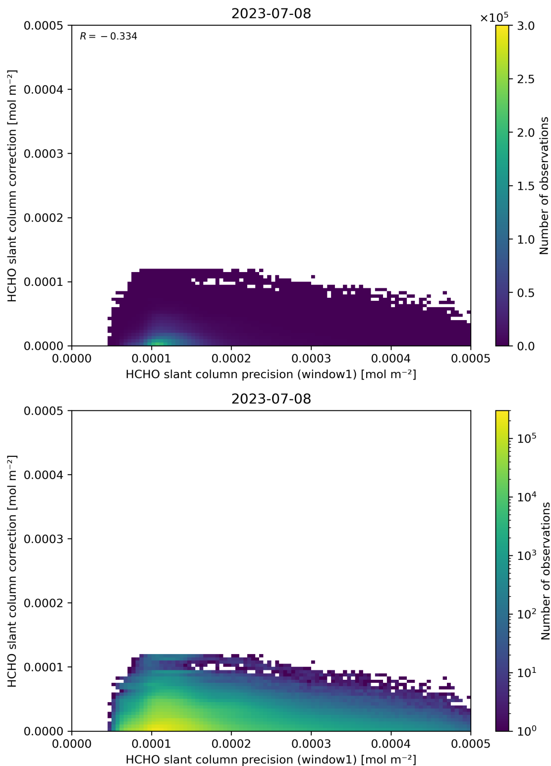
Figure 93: Scatter density plot of “HCHO slant column precision (window1)” against “HCHO slant column correction” for 2023-07-08 to 2023-07-09.
