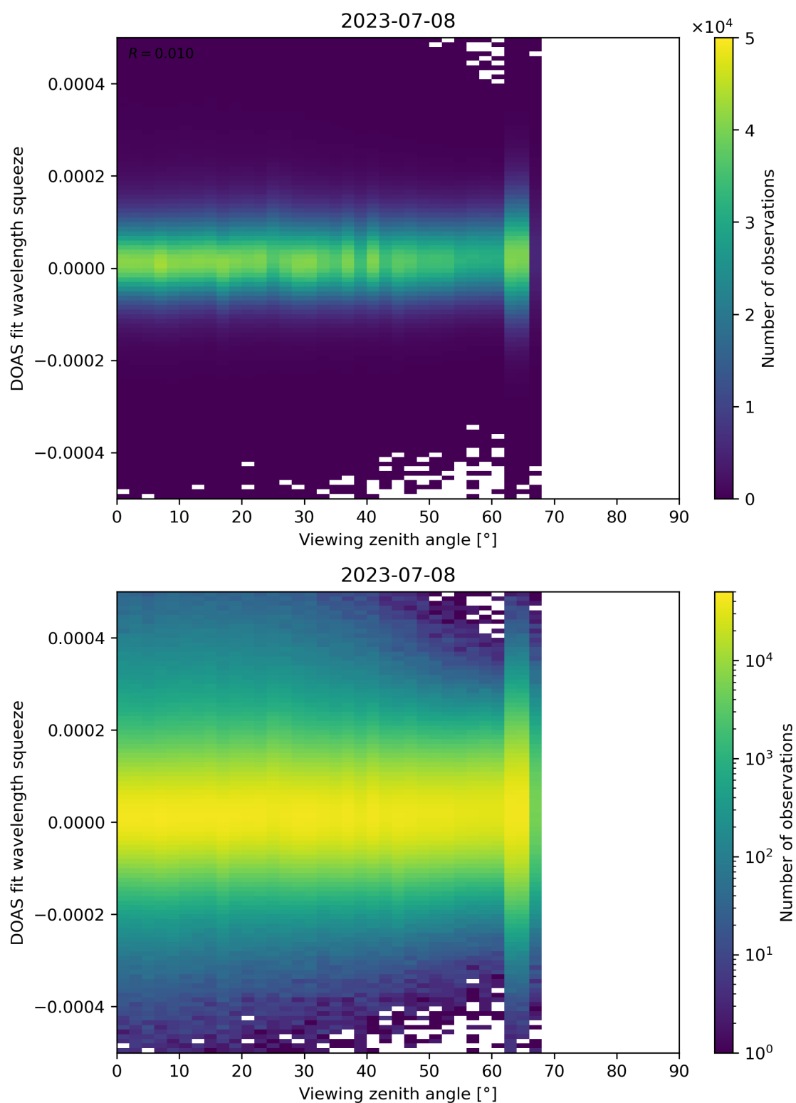
Figure 184: Scatter density plot of “Viewing zenith angle” against “DOAS fit wavelength squeeze” for 2023-07-08 to 2023-07-09.
