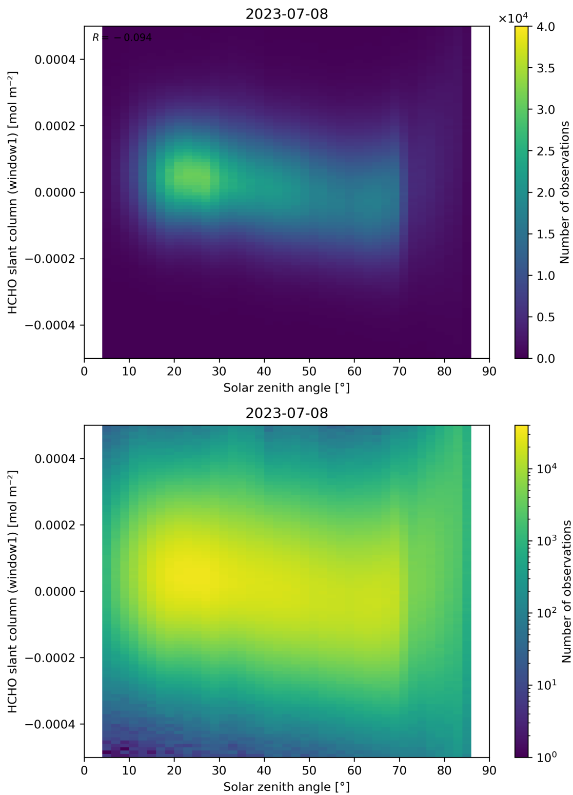
Figure 173: Scatter density plot of “Solar zenith angle” against “HCHO slant column (window1)” for 2023-07-08 to 2023-07-09.
