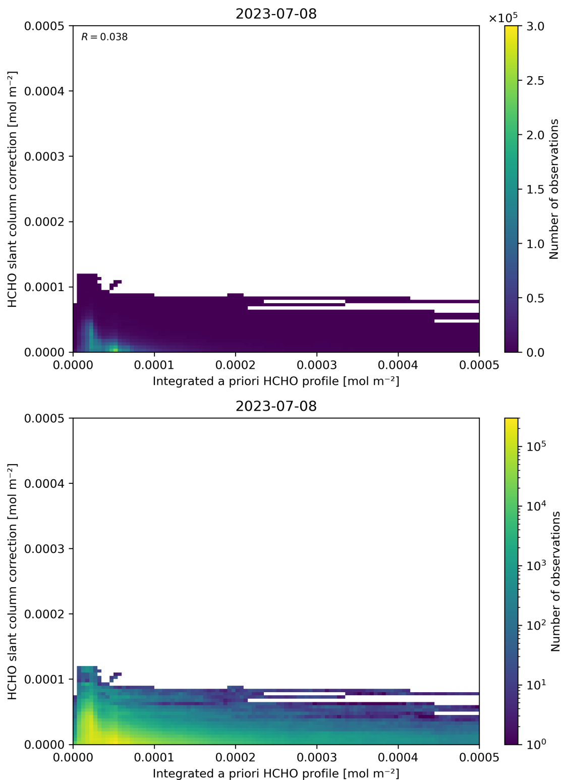
Figure 152: Scatter density plot of “Integrated a priori HCHO profile” against “HCHO slant column correction” for 2023-07-08 to 2023-07-09.
