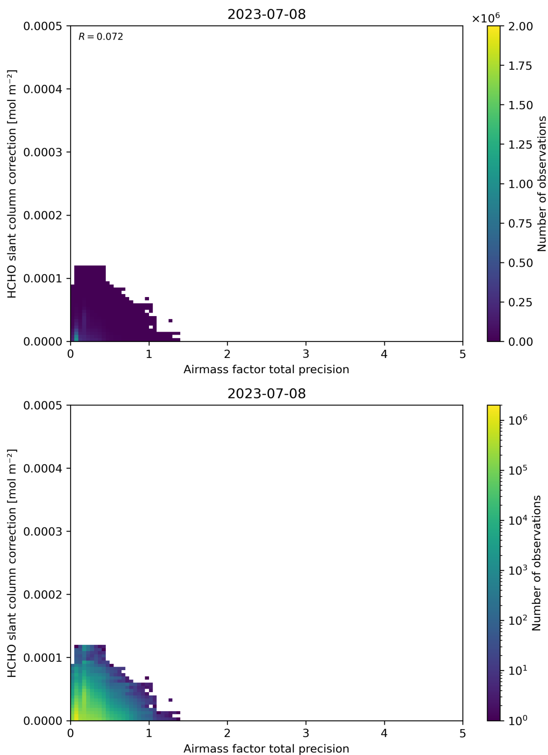
Figure 110: Scatter density plot of “Airmass factor total precision” against “HCHO slant column correction” for 2023-07-08 to 2023-07-09.
