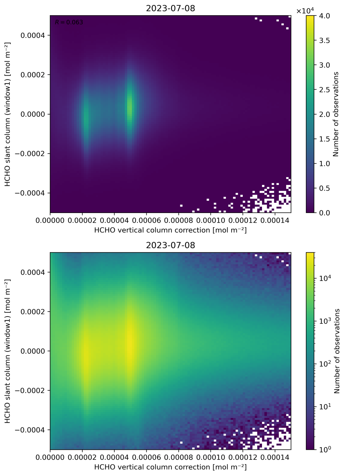
Figure 118: Scatter density plot of “HCHO vertical column correction” against “HCHO slant column (window1)” for 2023-07-08 to 2023-07-09.
