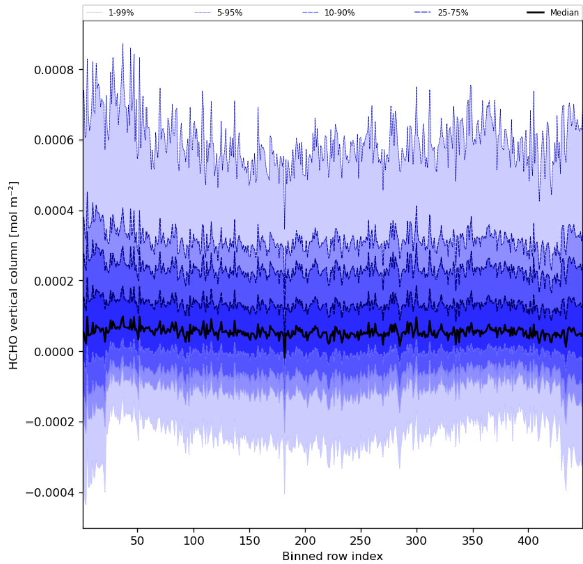
Figure 49: Along track statistics of “HCHO vertical column” for 2023-07-08 to 2023-07-09
