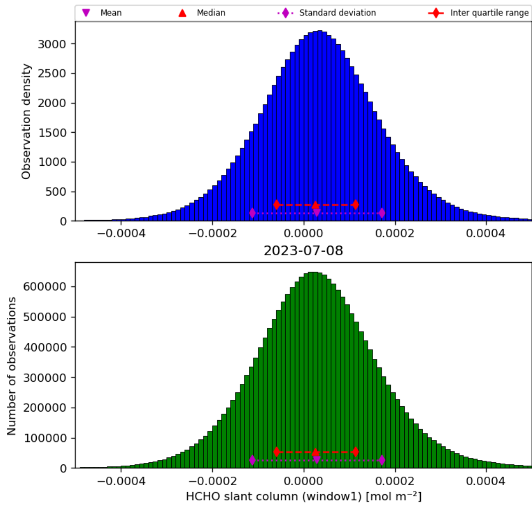
Figure 38: Histogram of “HCHO slant column (window1)” for 2023-07-08 to 2023-07-09
