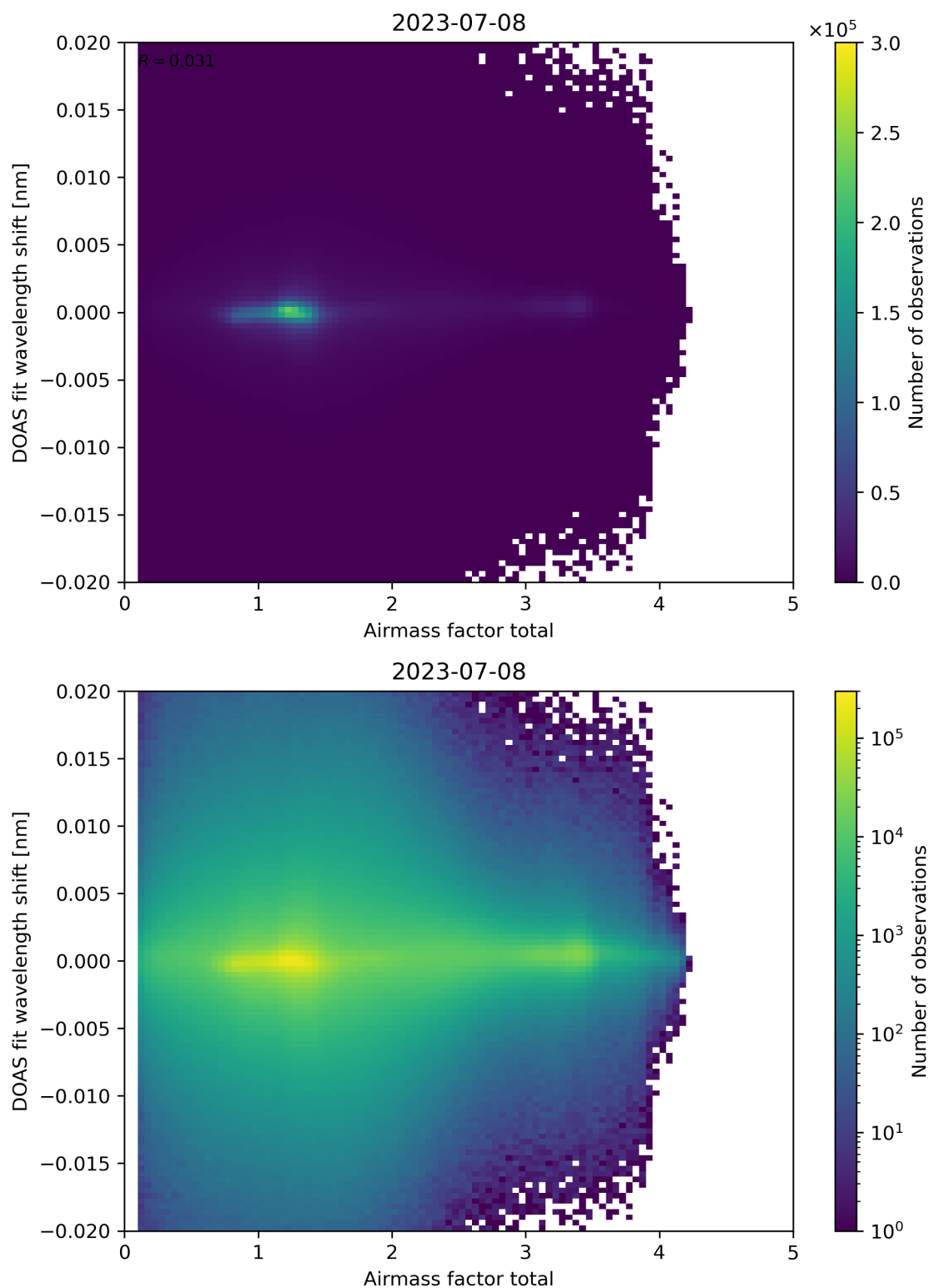
Figure 98: Scatter density plot of “Airmass factor total” against “DOAS fit wavelength shift” for 2023-07-08 to 2023-07-09.
