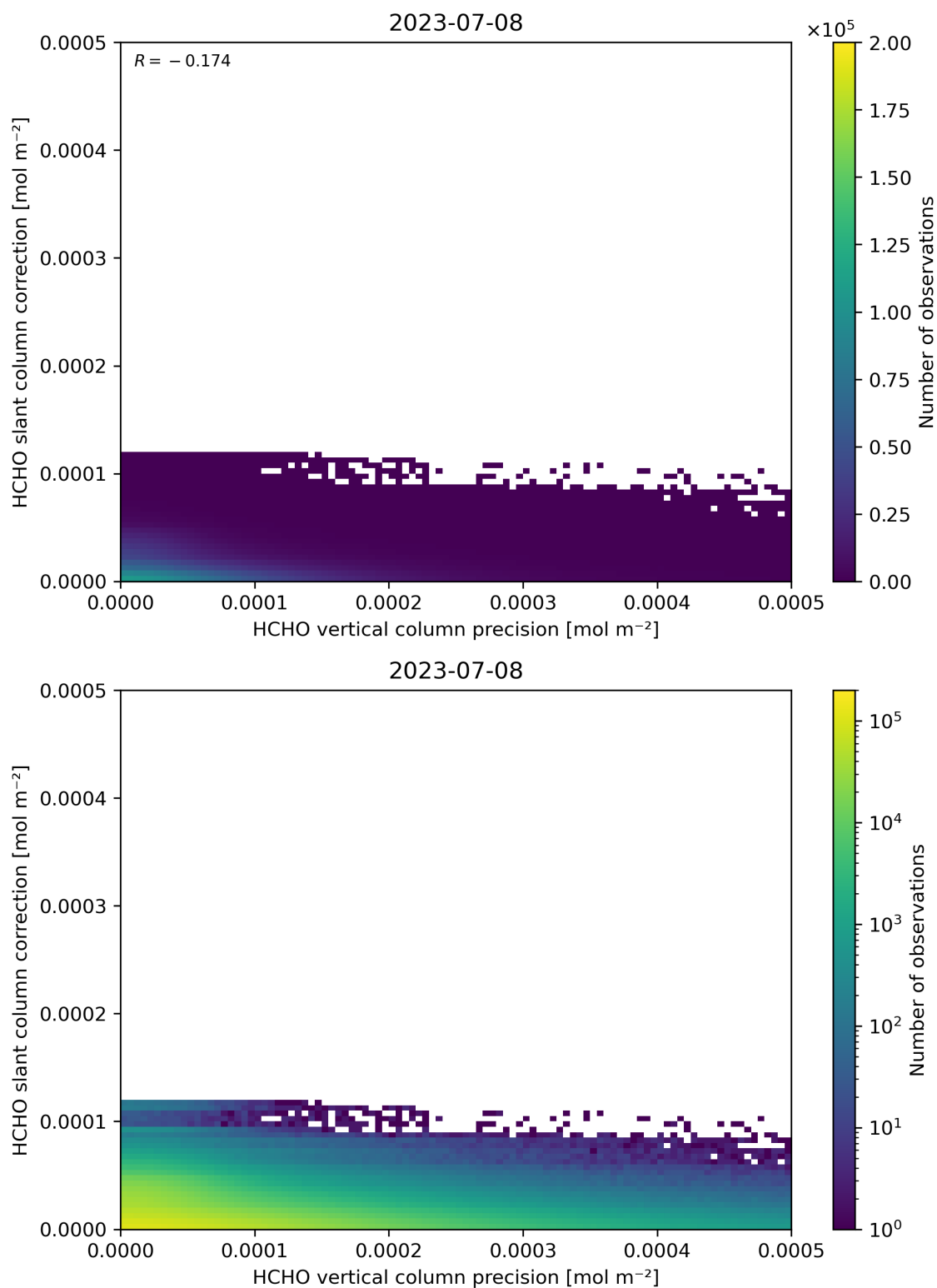
Figure 141: Scatter density plot of “HCHO vertical column precision” against “HCHO slant column correction” for 2023-07-08 to 2023-07-09.
