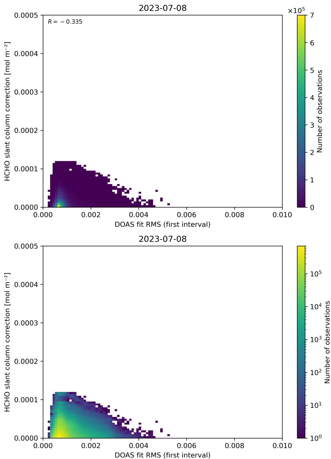
Figure 63: Scatter density plot of “DOAS fit RMS (first interval)” against “HCHO slant column correction” for 2023-07-08 to 2023-07-09.
