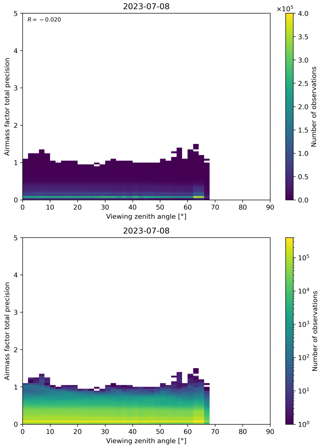
Figure 191: Scatter density plot of “Viewing zenith angle” against “Airmass factor total precision” for 2023-07-08 to 2023-07-09.
