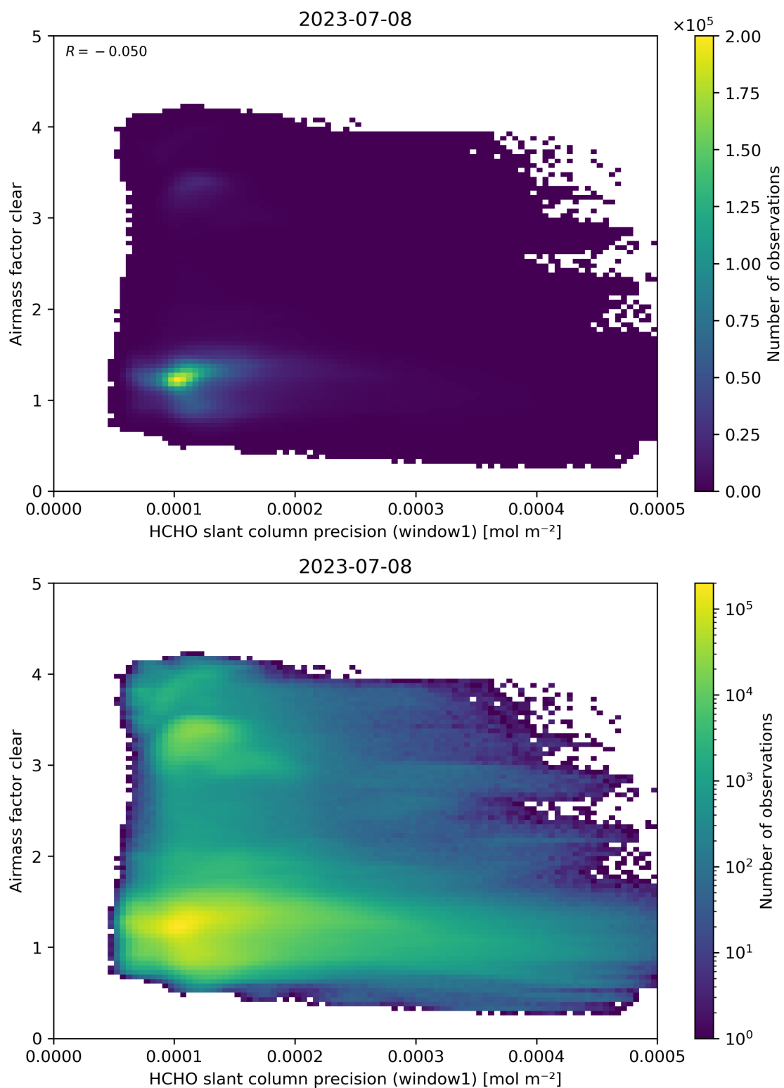
Figure 91: Scatter density plot of “HCHO slant column precision (window1)” against “Airmass factor clear” for 2023-07-08 to 2023-07-09.
