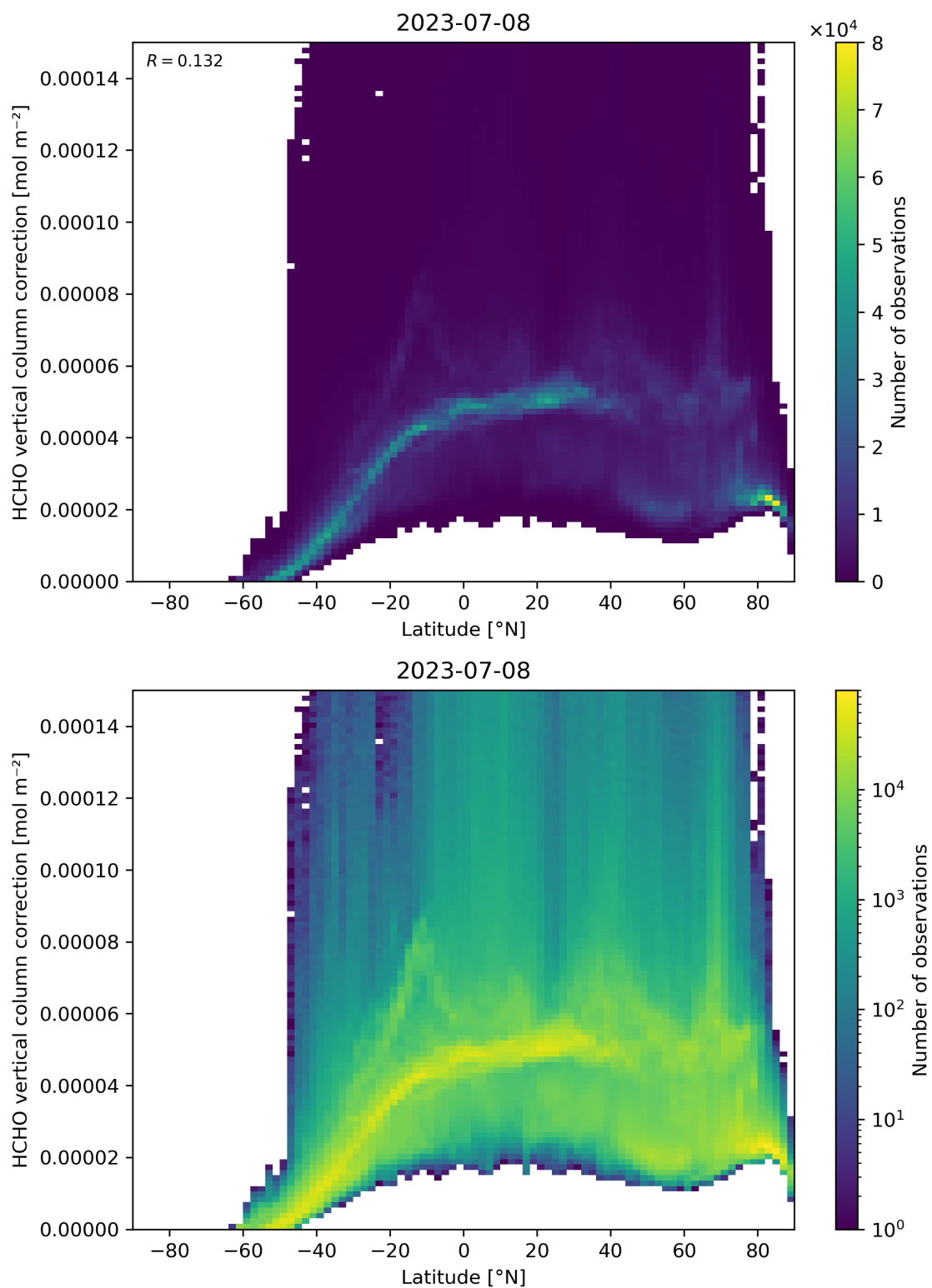
Figure 164: Scatter density plot of “Latitude” against “HCHO vertical column correction” for 2023-07-08 to 2023-07-09.
