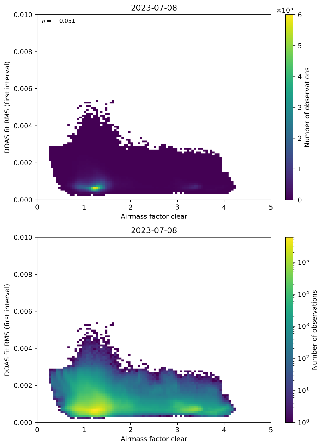
Figure 71: Scatter density plot of “Airmass factor clear” against “DOAS fit RMS (first interval)” for 2023-07-08 to 2023-07-09.
