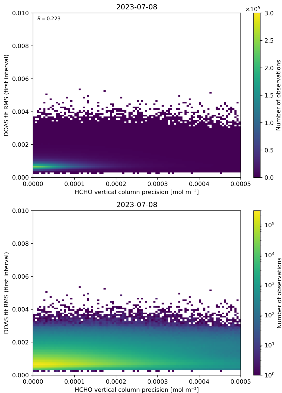
Figure 136: Scatter density plot of “HCHO vertical column precision” against “DOAS fit RMS (first interval)” for 2023-07-08 to 2023-07-09.
