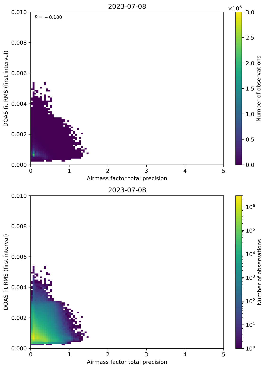
Figure 105: Scatter density plot of “Airmass factor total precision” against “DOAS fit RMS (first interval)” for 2023-07-08 to 2023-07-09.
