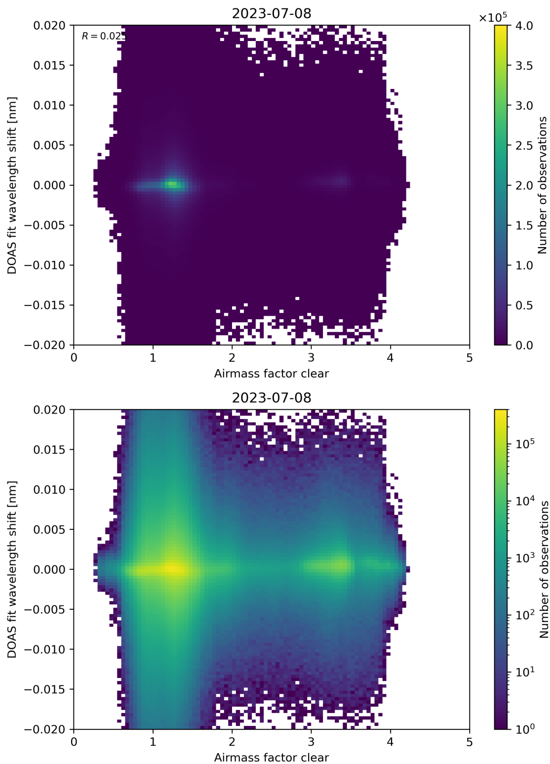
Figure 72: Scatter density plot of “Airmass factor clear” against “DOAS fit wavelength shift” for 2023-07-08 to 2023-07-09.
