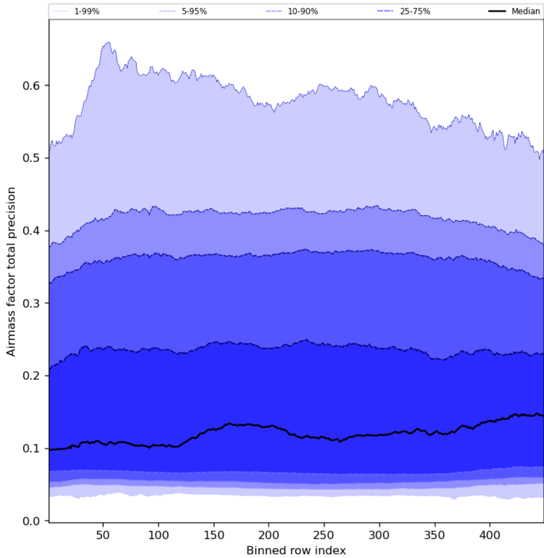
Figure 55: Along track statistics of “Airmass factor total precision” for 2023-07-08 to 2023-07-09
