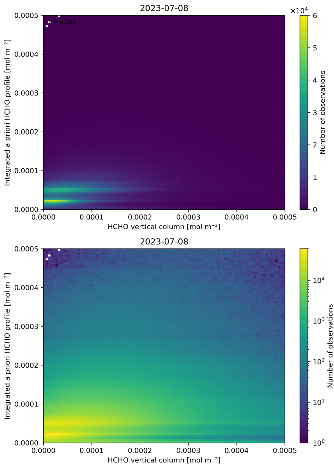
Figure 135: Scatter density plot of “HCHO vertical column” against “Integrated a priori HCHO profile” for 2023-07-08 to 2023-07-09.
