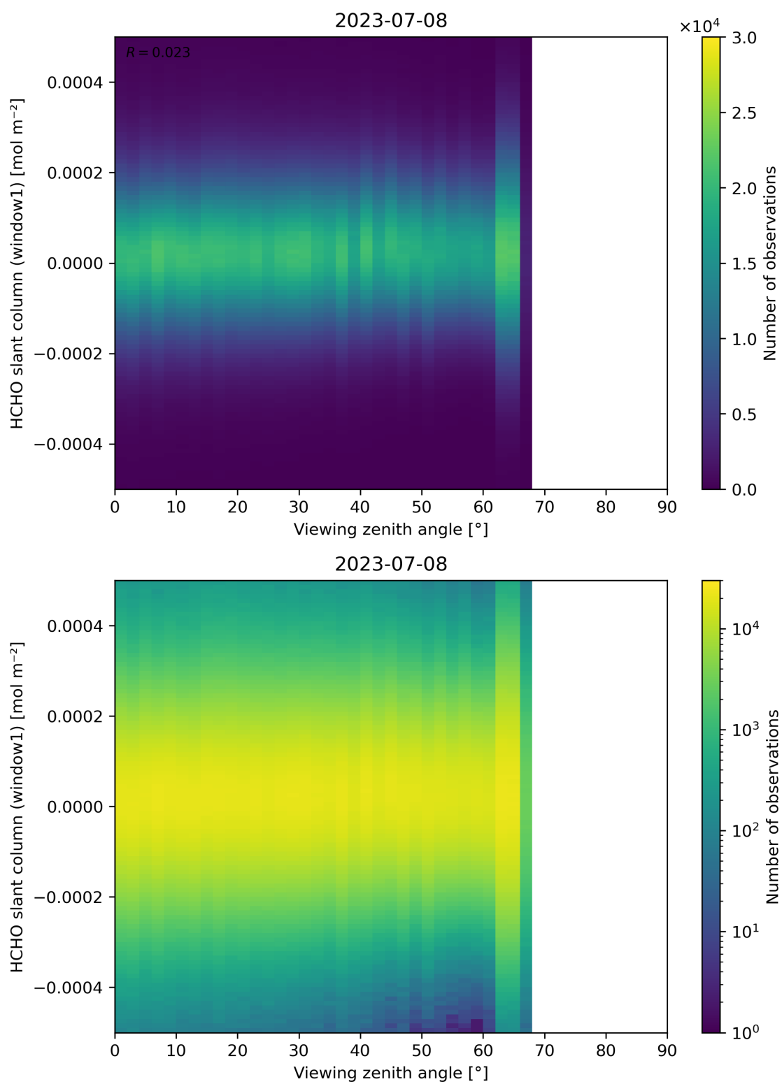
Figure 188: Scatter density plot of “Viewing zenith angle” against “HCHO slant column (window1)” for 2023-07-08 to 2023-07-09.
