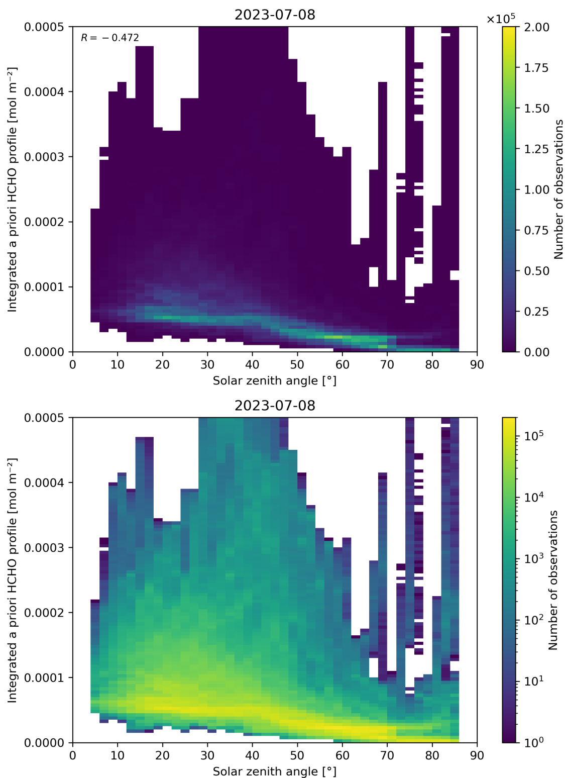
Figure 180: Scatter density plot of “Solar zenith angle” against “Integrated a priori HCHO profile” for 2023-07-08 to 2023-07-09.
