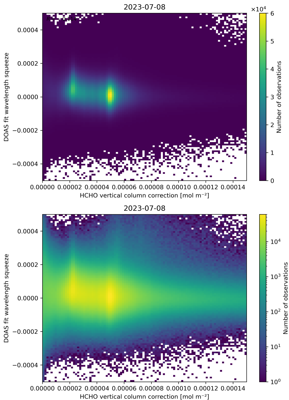
Figure 114: Scatter density plot of “HCHO vertical column correction” against “DOAS fit wavelength squeeze” for 2023-07-08 to 2023-07-09.
