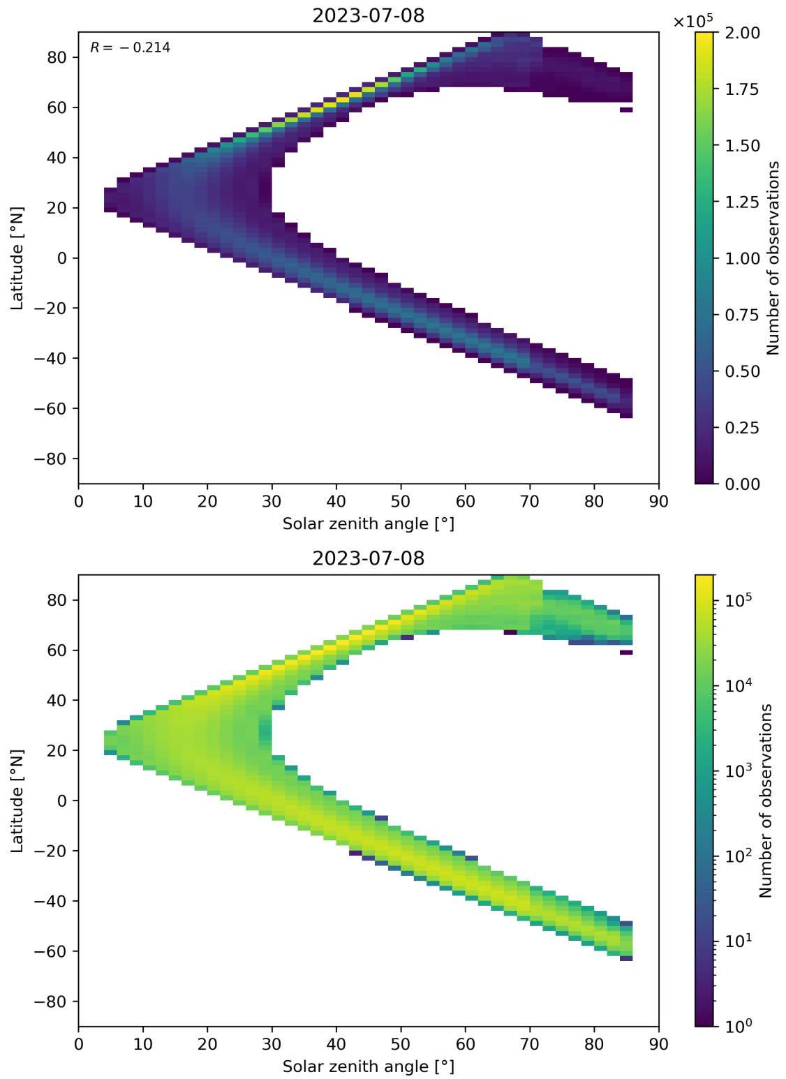
Figure 181: Scatter density plot of “Solar zenith angle” against “Latitude” for 2023-07-08 to 2023-07-09.
