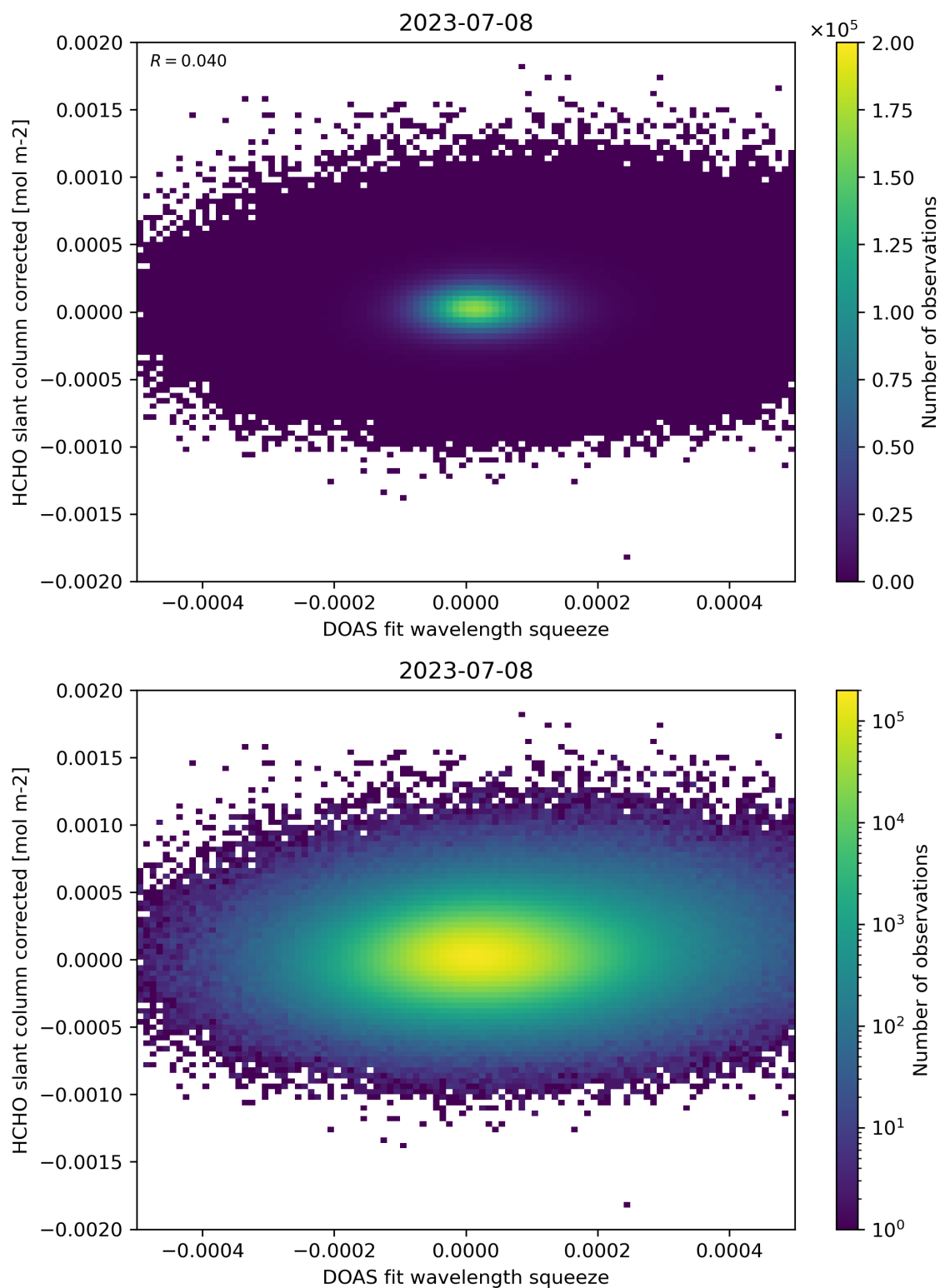
Figure 69: Scatter density plot of “DOAS fit wavelength squeeze” against “HCHO slant column corrected” for 2023-07-08 to 2023-07-09.
