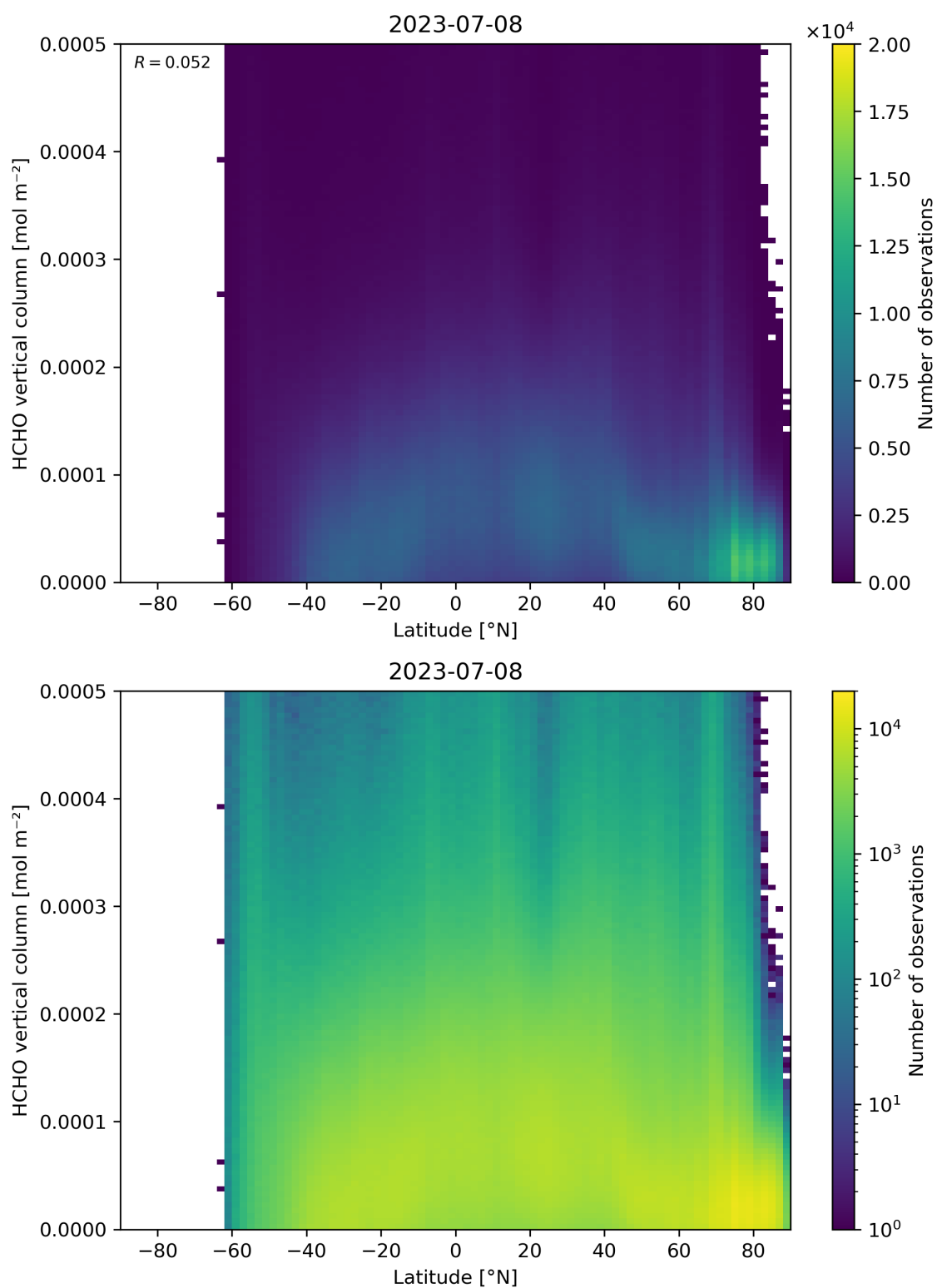
Figure 163: Scatter density plot of “Latitude” against “HCHO vertical column” for 2023-07-08 to 2023-07-09.
