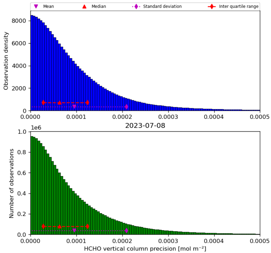
Figure 36: Histogram of “HCHO vertical column precision” for 2023-07-08 to 2023-07-09
