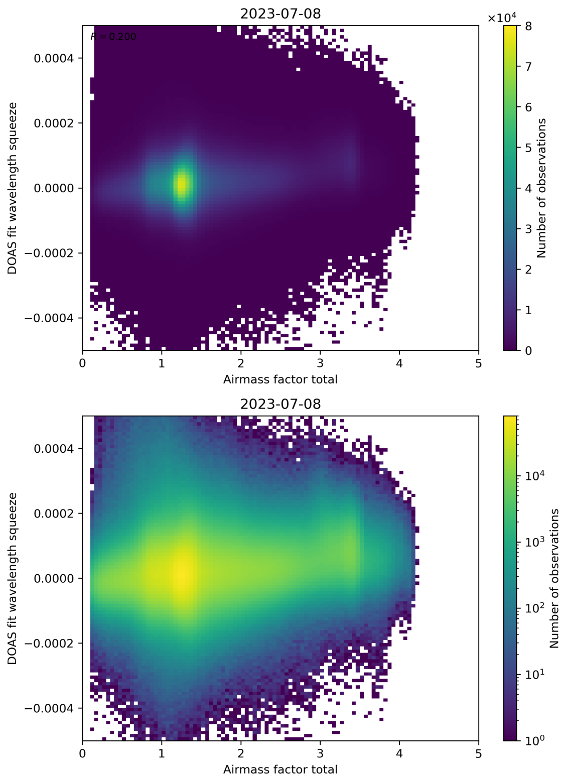
Figure 99: Scatter density plot of “Airmass factor total” against “DOAS fit wavelength squeeze” for 2023-07-08 to 2023-07-09.
