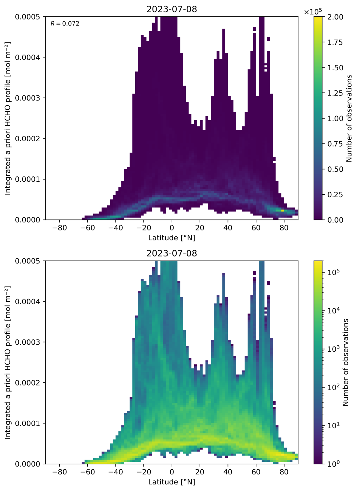
Figure 166: Scatter density plot of “Latitude” against “Integrated a priori HCHO profile” for 2023-07-08 to 2023-07-09.
