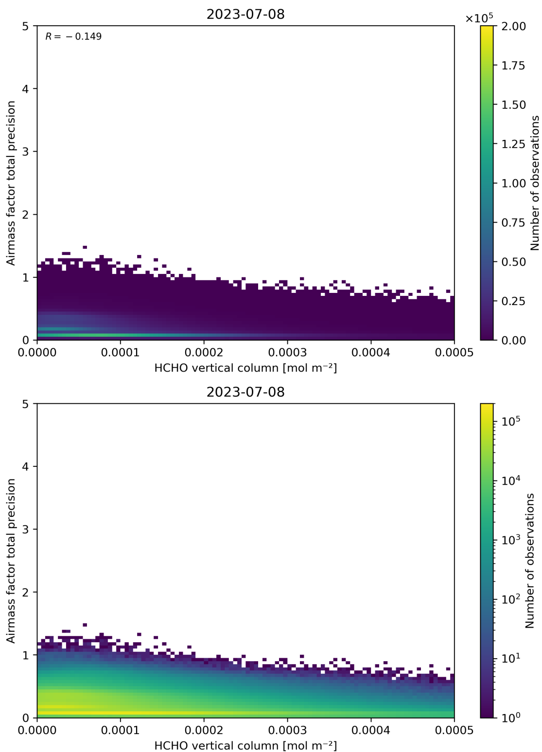
Figure 132: Scatter density plot of “HCHO vertical column” against “Airmass factor total precision” for 2023-07-08 to 2023-07-09.
