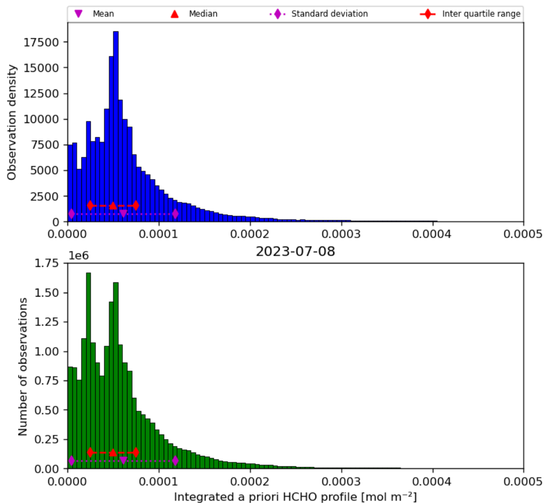
Figure 43: Histogram of “Integrated a priori HCHO profile” for 2023-07-08 to 2023-07-09
