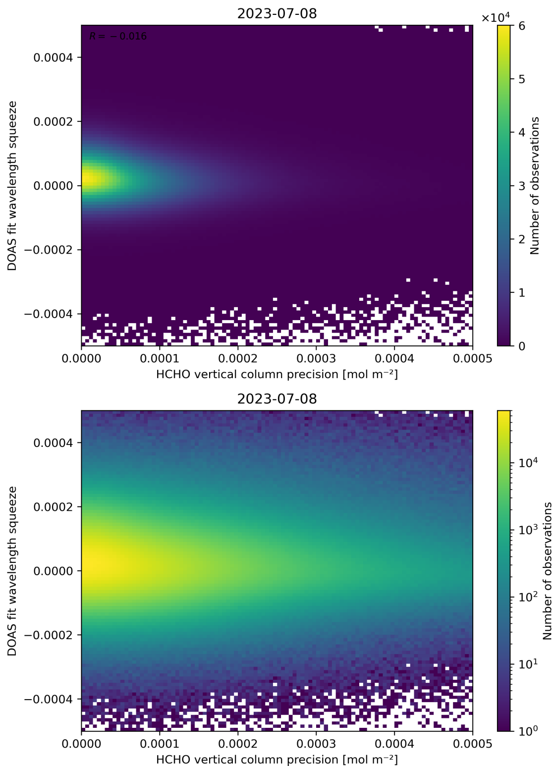
Figure 138: Scatter density plot of “HCHO vertical column precision” against “DOAS fit wavelength squeeze” for 2023-07-08 to 2023-07-09.
