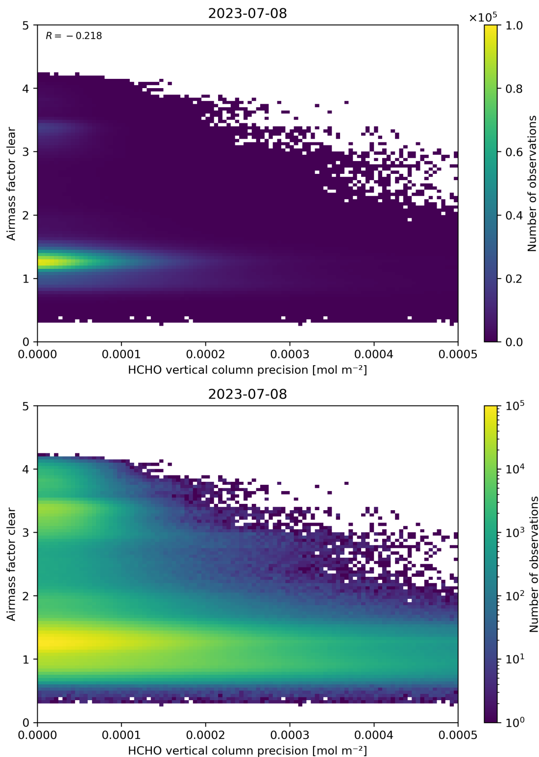
Figure 139: Scatter density plot of “HCHO vertical column precision” against “Airmass factor clear” for 2023-07-08 to 2023-07-09.
