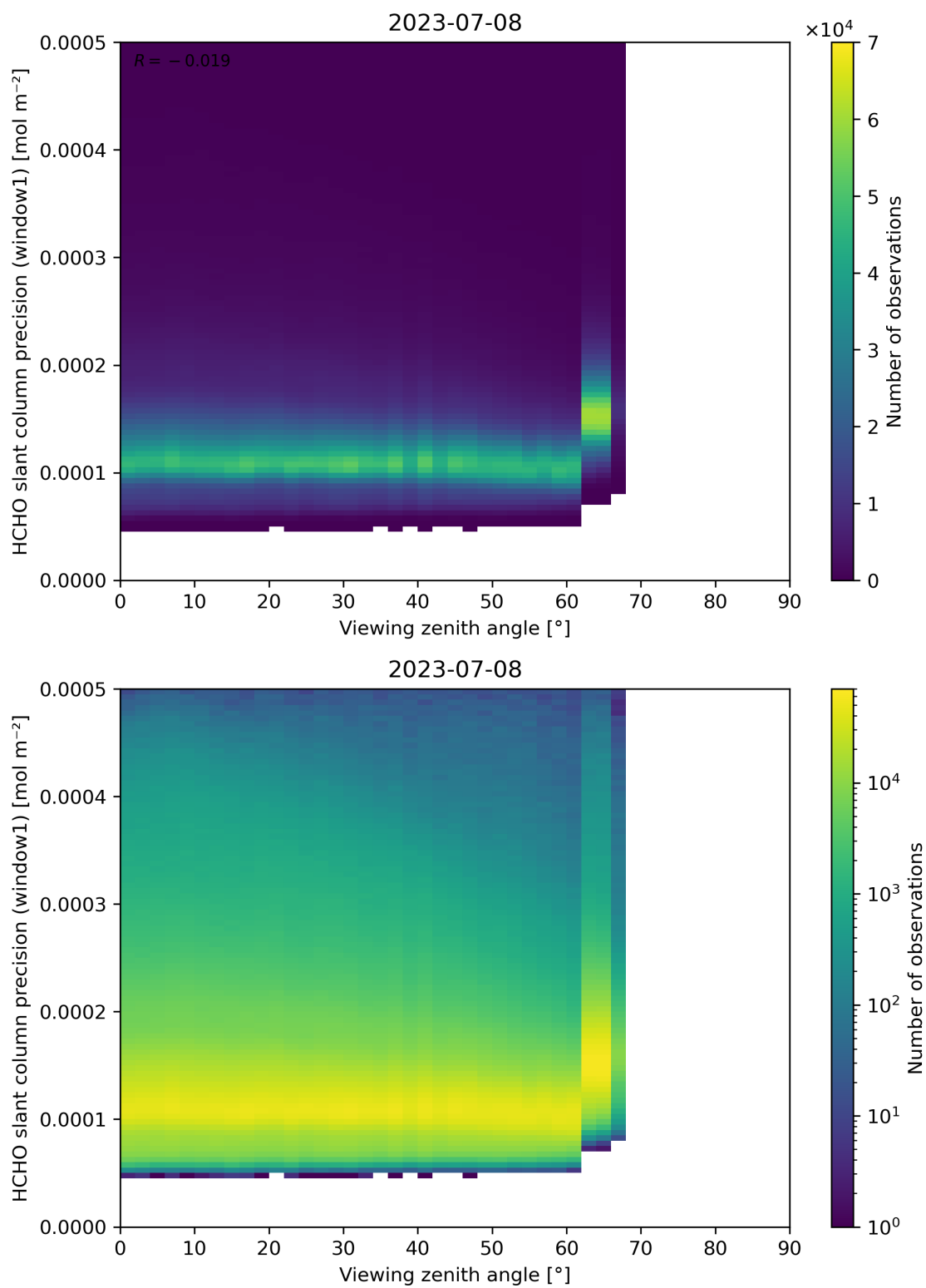
Figure 189: Scatter density plot of “Viewing zenith angle” against “HCHO slant column precision (window1)” for 2023-07-08 to 2023-07-09.
