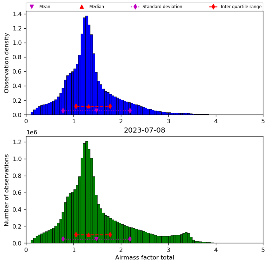
Figure 40: Histogram of “Airmass factor total” for 2023-07-08 to 2023-07-09
