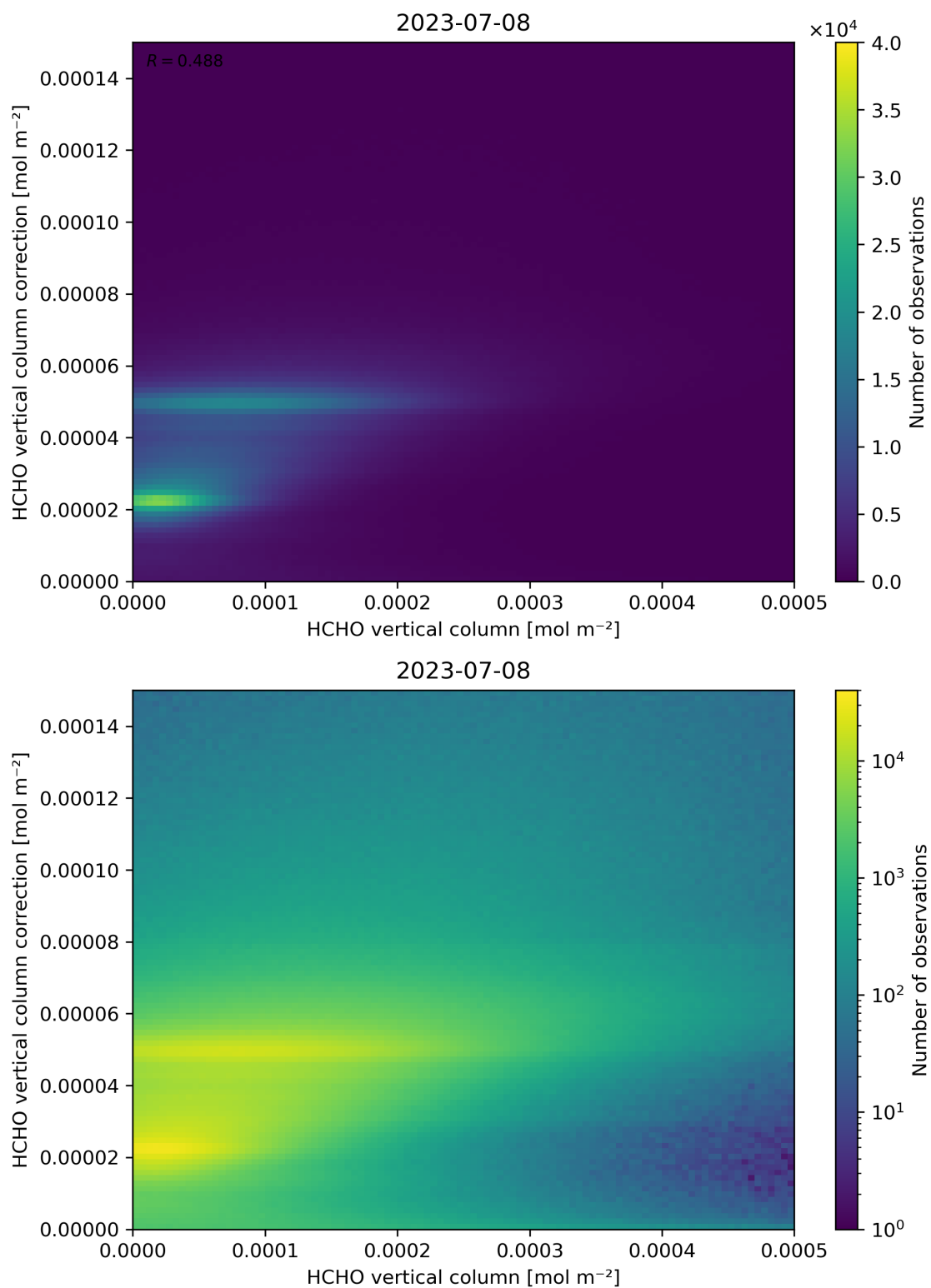
Figure 133: Scatter density plot of “HCHO vertical column” against “HCHO vertical column correction” for 2023-07-08 to 2023-07-09.
