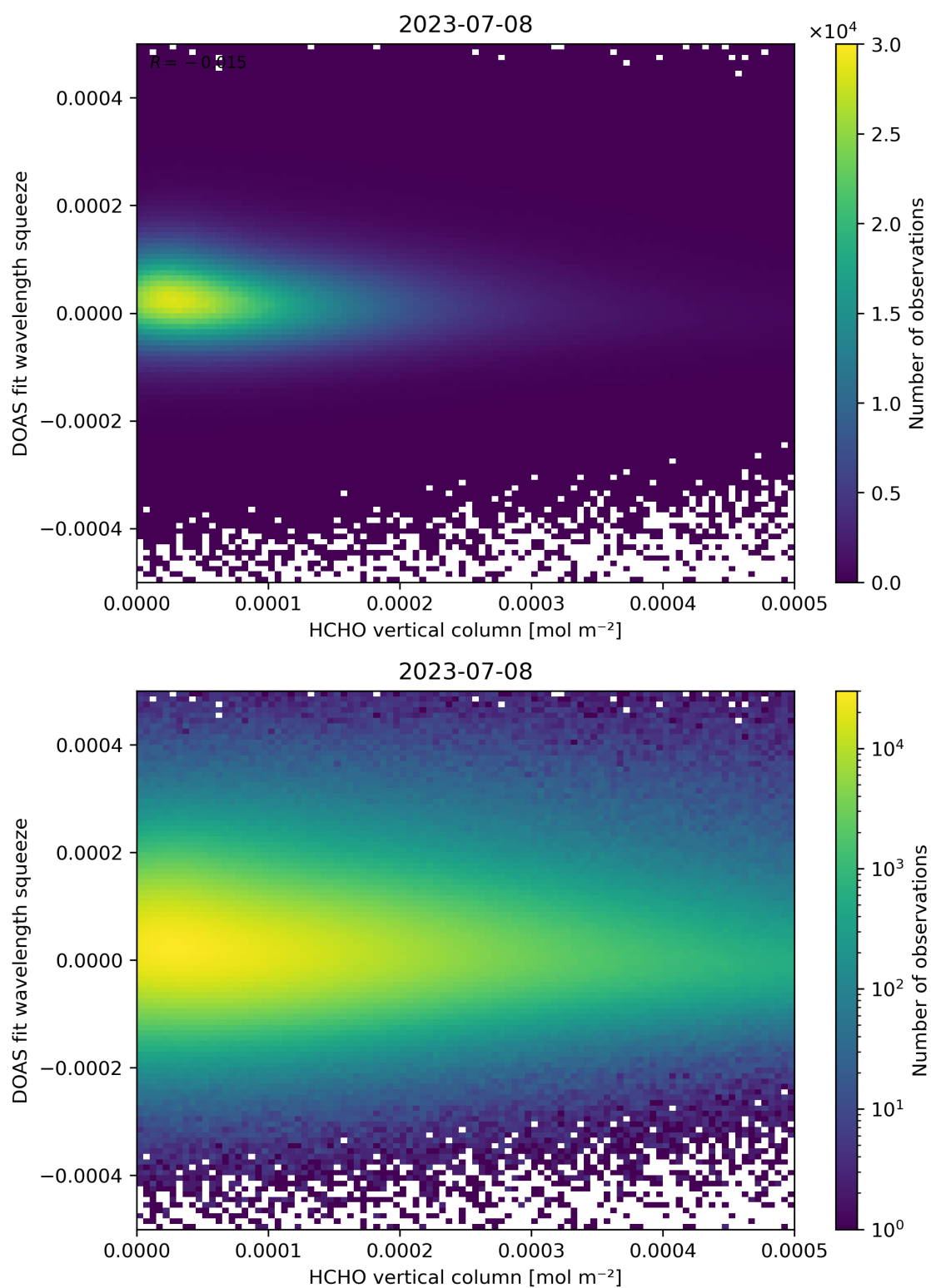
Figure 125: Scatter density plot of “HCHO vertical column” against “DOAS fit wavelength squeeze” for 2023-07-08 to 2023-07-09.
