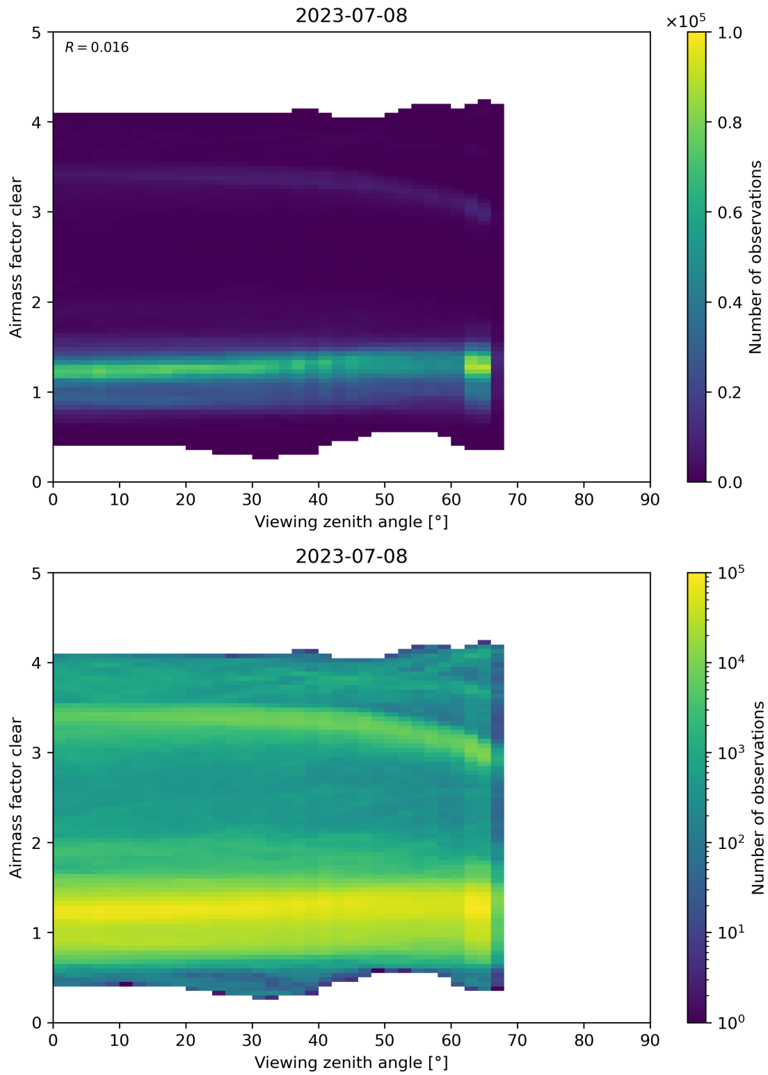
Figure 185: Scatter density plot of “Viewing zenith angle” against “Airmass factor clear” for 2023-07-08 to 2023-07-09.
