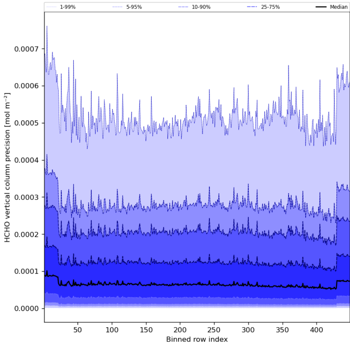
Figure 50: Along track statistics of “HCHO vertical column precision” for 2023-07-08 to 2023-07-09
