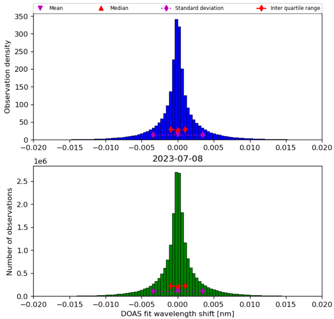
Figure 44: Histogram of “DOAS fit wavelength shift” for 2023-07-08 to 2023-07-09
