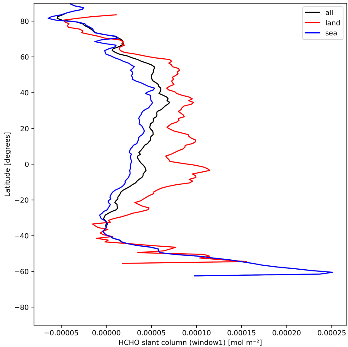
Figure 24: Zonal average of “HCHO slant column (window1)” for 2023-07-08 to 2023-07-09.
