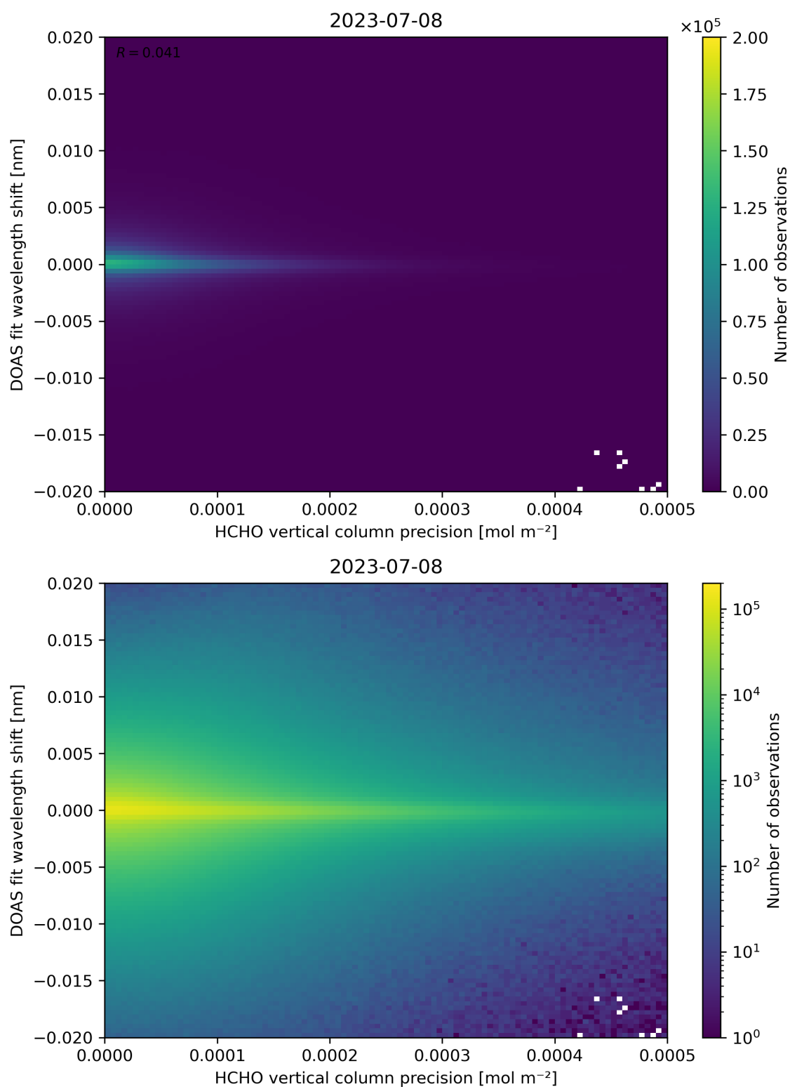
Figure 137: Scatter density plot of “HCHO vertical column precision” against “DOAS fit wavelength shift” for 2023-07-08 to 2023-07-09.
