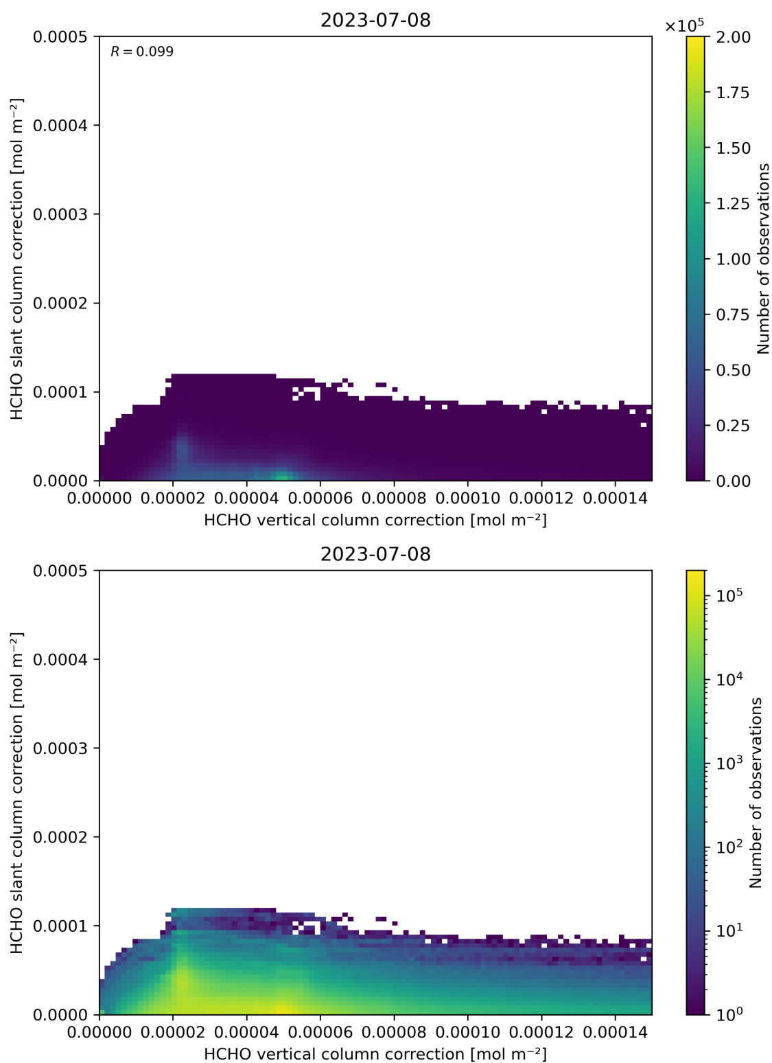
Figure 117: Scatter density plot of “HCHO vertical column correction” against “HCHO slant column correction” for 2023-07-08 to 2023-07-09.
