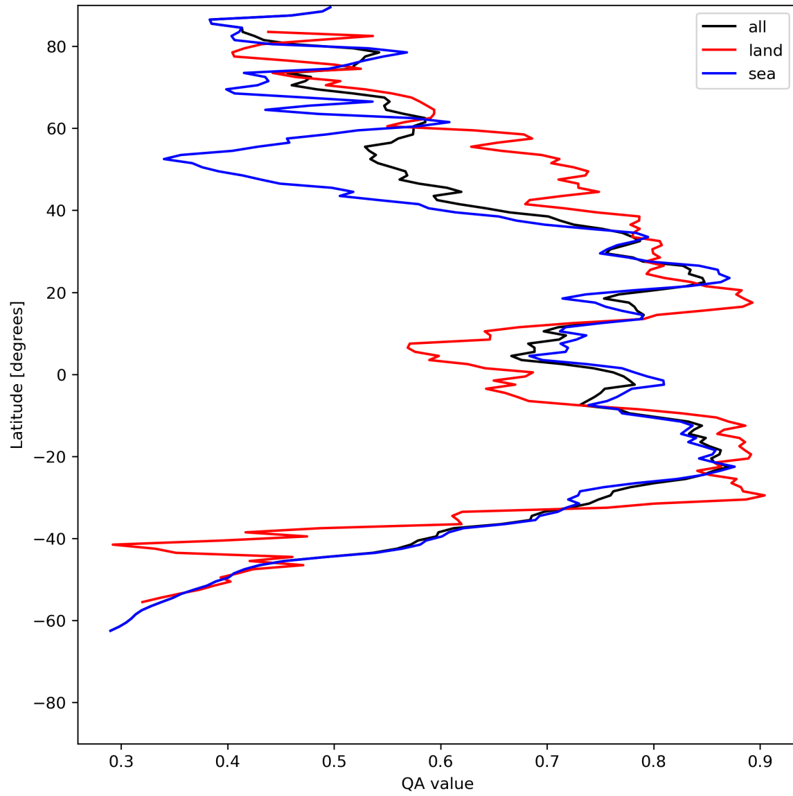
Figure 20: Zonal average of “QA value” for 2023-07-08 to 2023-07-09.
