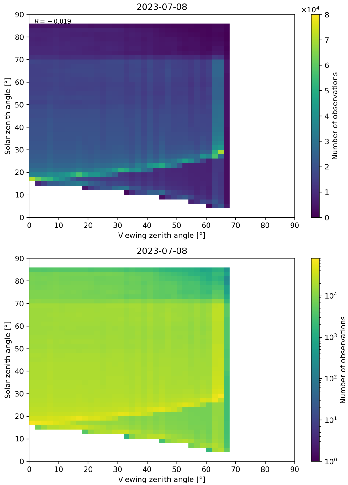
Figure 197: Scatter density plot of “Viewing zenith angle” against “Solar zenith angle” for 2023-07-08 to 2023-07-09.
