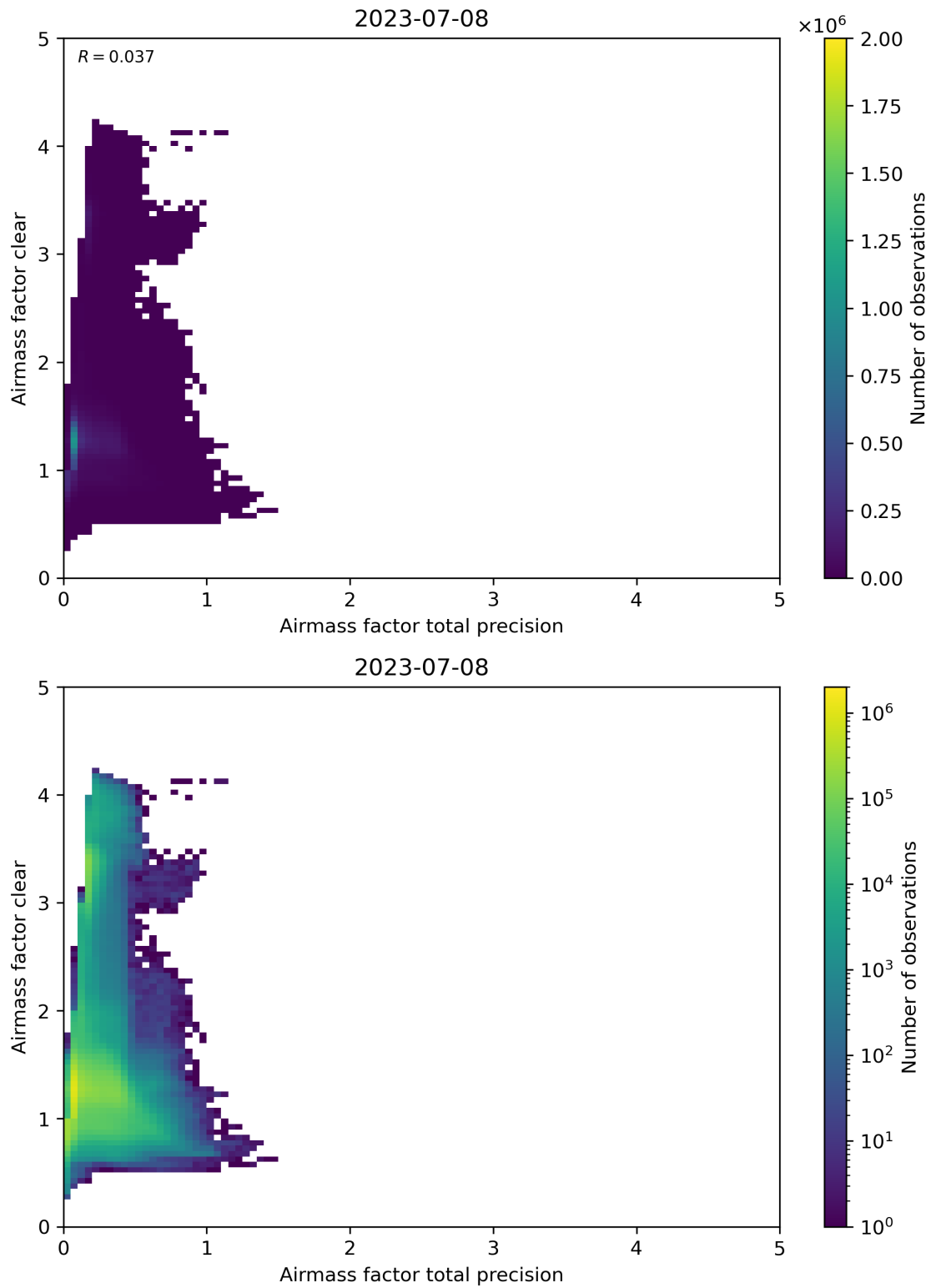
Figure 108: Scatter density plot of “Airmass factor total precision” against “Airmass factor clear” for 2023-07-08 to 2023-07-09.
