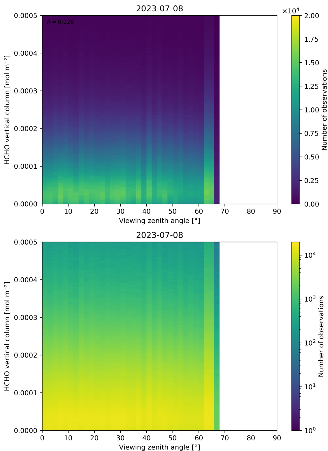
Figure 192: Scatter density plot of “Viewing zenith angle” against “HCHO vertical column” for 2023-07-08 to 2023-07-09.
