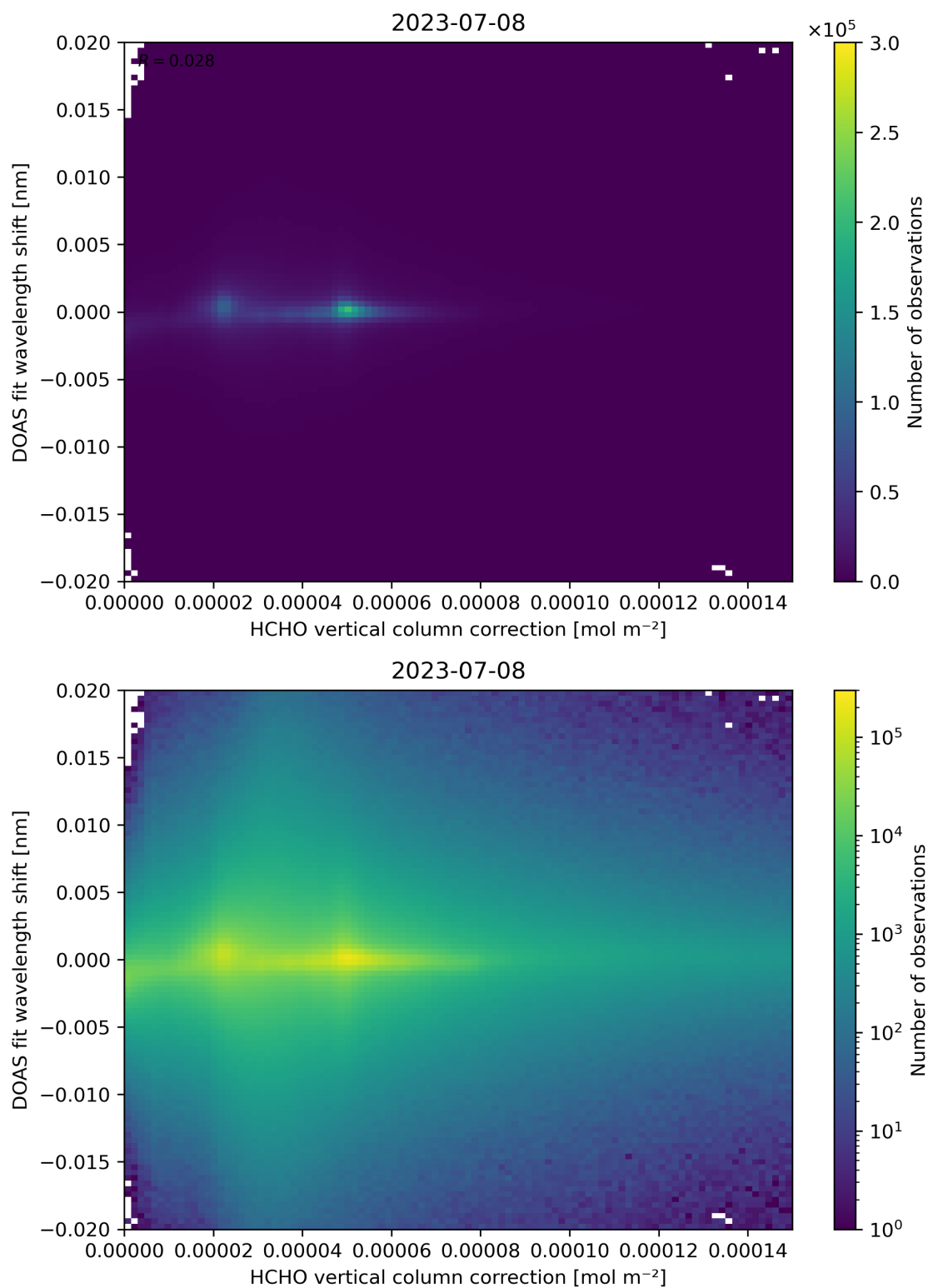
Figure 113: Scatter density plot of “HCHO vertical column correction” against “DOAS fit wavelength shift” for 2023-07-08 to 2023-07-09.
