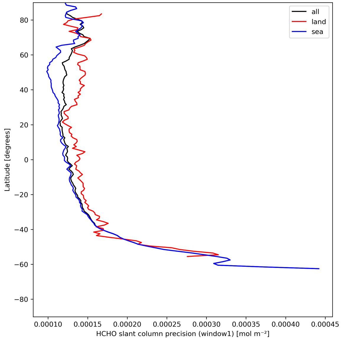
Figure 25: Zonal average of “HCHO slant column precision (window1)” for 2023-07-08 to 2023-07-09.
