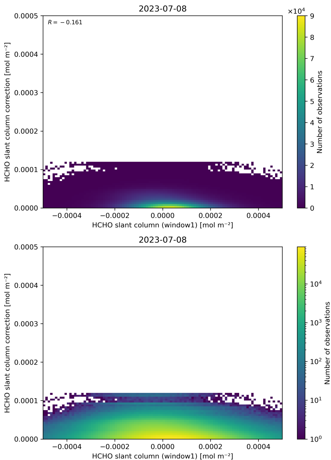
Figure 83: Scatter density plot of “HCHO slant column (window1)” against “HCHO slant column correction” for 2023-07-08 to 2023-07-09.
