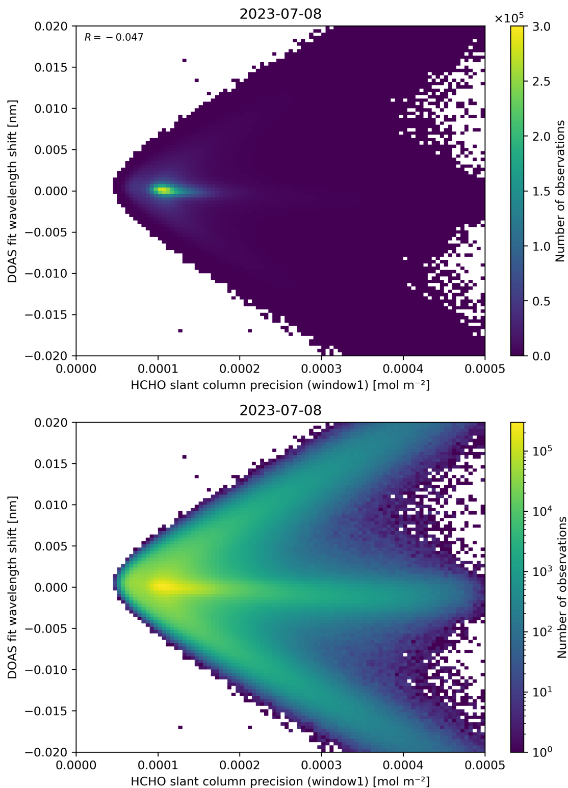
Figure 89: Scatter density plot of “HCHO slant column precision (window1)” against “DOAS fit wavelength shift” for 2023-07-08 to 2023-07-09.
