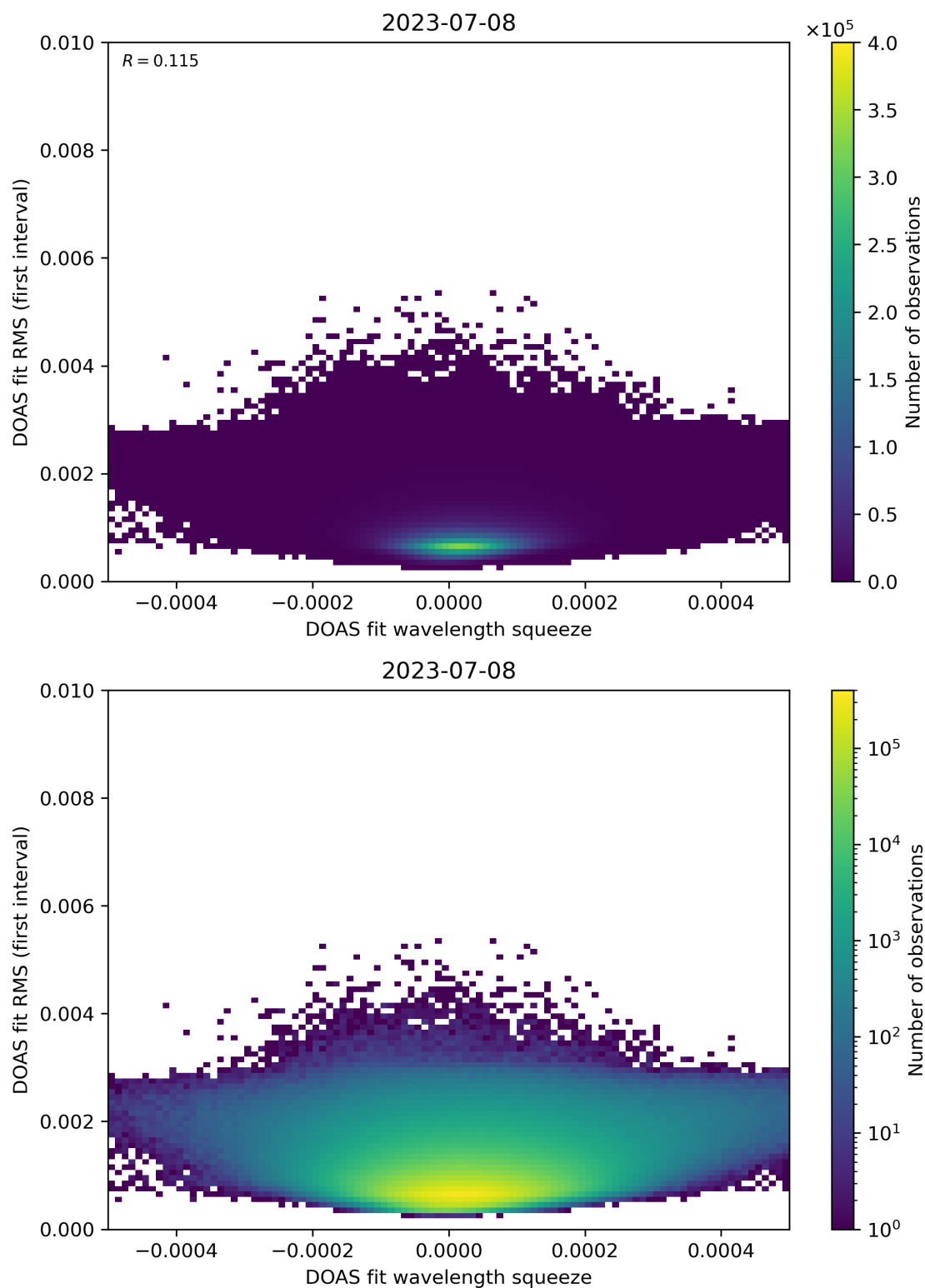
Figure 68: Scatter density plot of “DOAS fit wavelength squeeze” against “DOAS fit RMS (first interval)” for 2023-07-08 to 2023-07-09.
