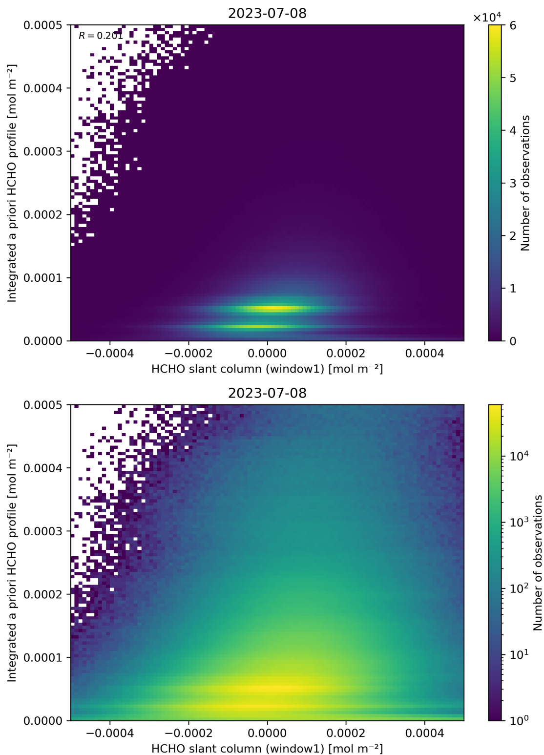
Figure 87: Scatter density plot of “HCHO slant column (window1)” against “Integrated a priori HCHO profile” for 2023-07-08 to 2023-07-09.
