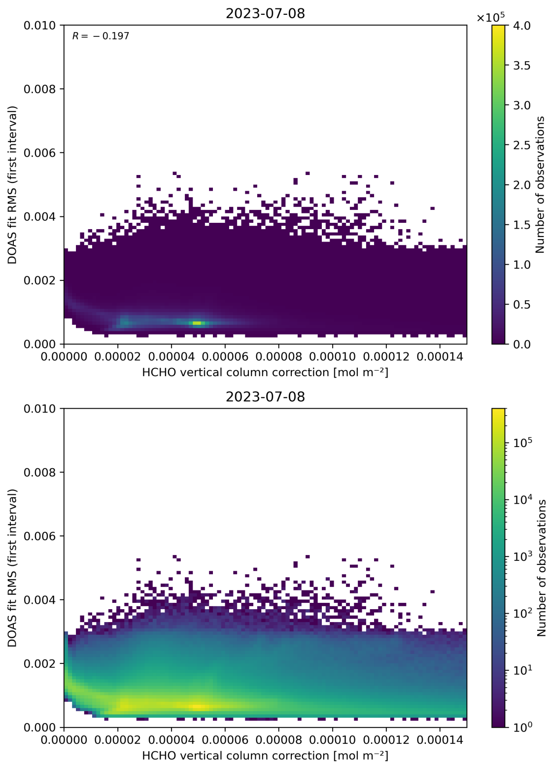
Figure 112: Scatter density plot of “HCHO vertical column correction” against “DOAS fit RMS (first interval)” for 2023-07-08 to 2023-07-09.
