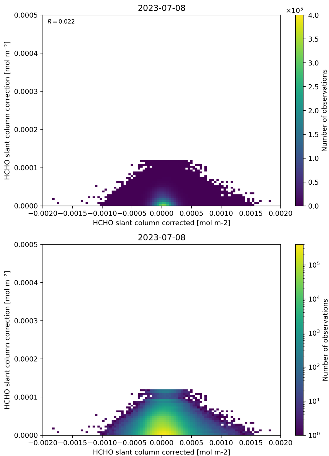
Figure 77: Scatter density plot of “HCHO slant column corrected” against “HCHO slant column correction” for 2023-07-08 to 2023-07-09.
