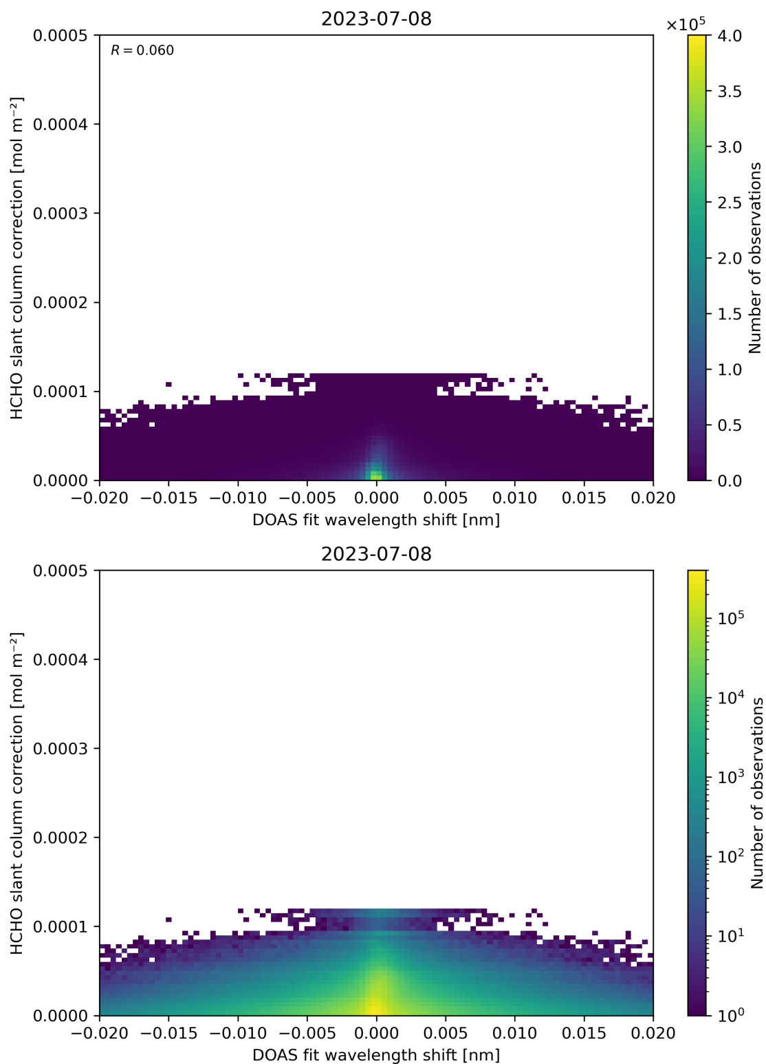
Figure 67: Scatter density plot of “DOAS fit wavelength shift” against “HCHO slant column correction” for 2023-07-08 to 2023-07-09.
