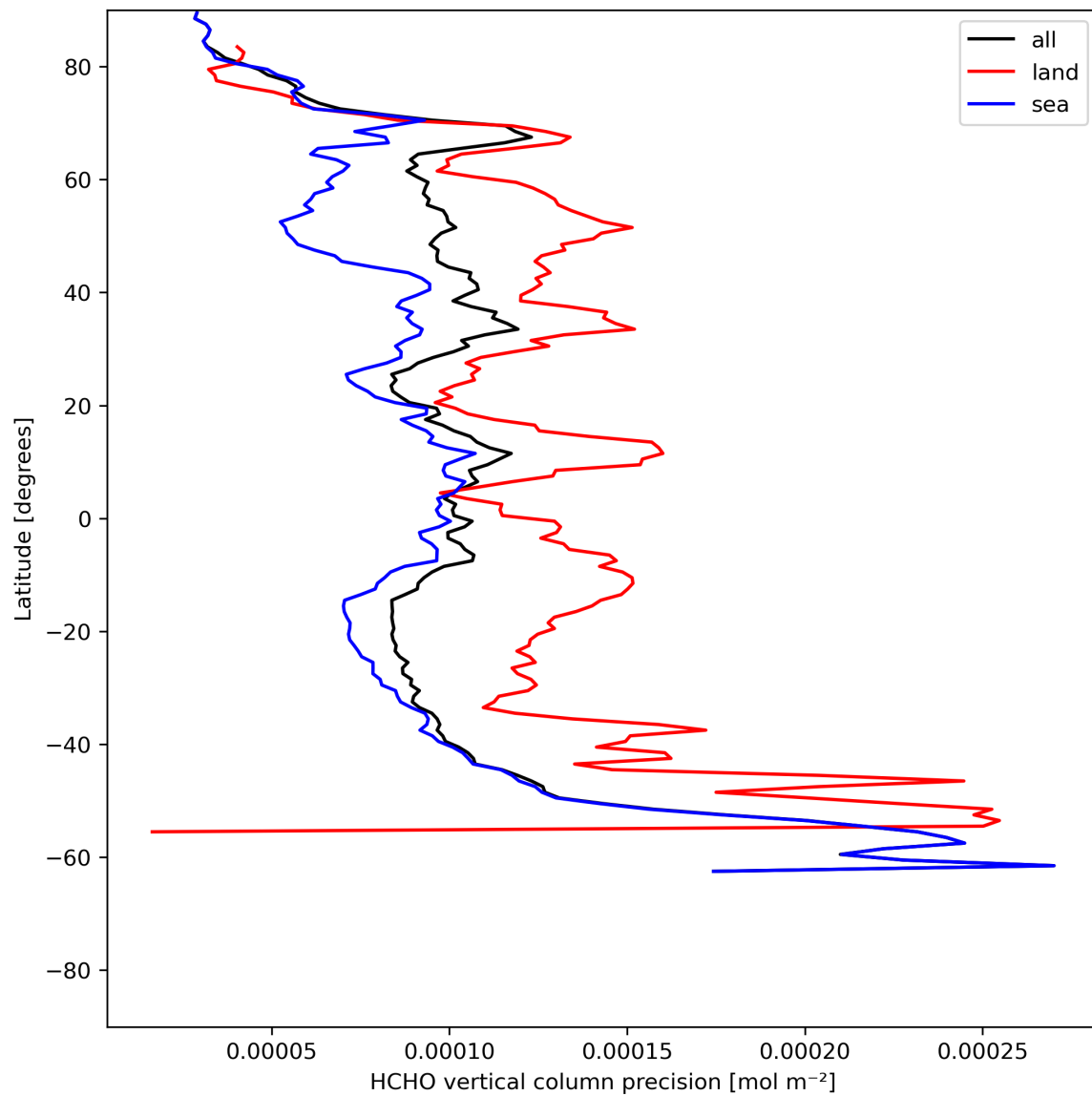
Figure 22: Zonal average of "HCHO vertical column precision" for 2023-07-08 to 2023-07-09.
