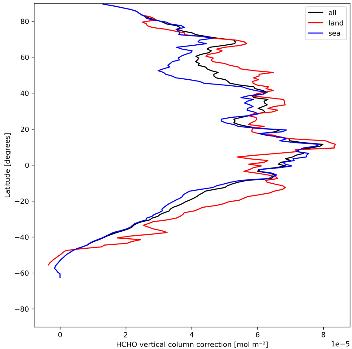
Figure 23: Zonal average of “HCHO vertical column correction” for 2023-07-08 to 2023-07-09.
