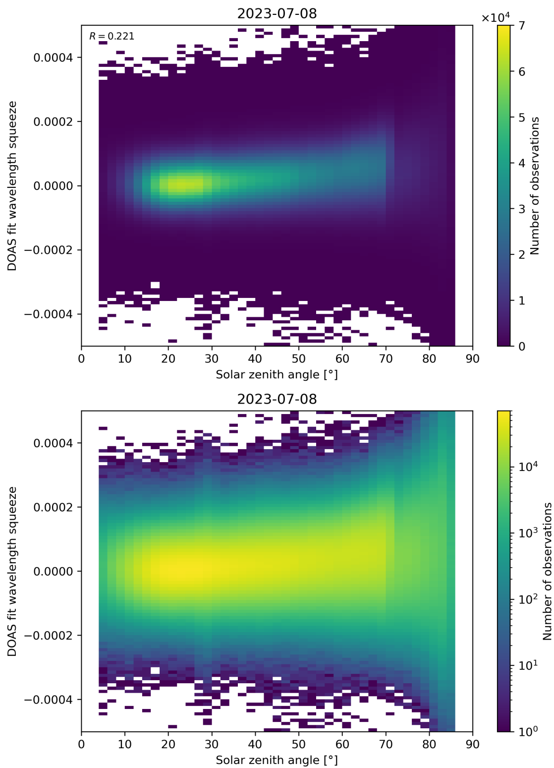
Figure 169: Scatter density plot of “Solar zenith angle” against “DOAS fit wavelength squeeze” for 2023-07-08 to 2023-07-09.
