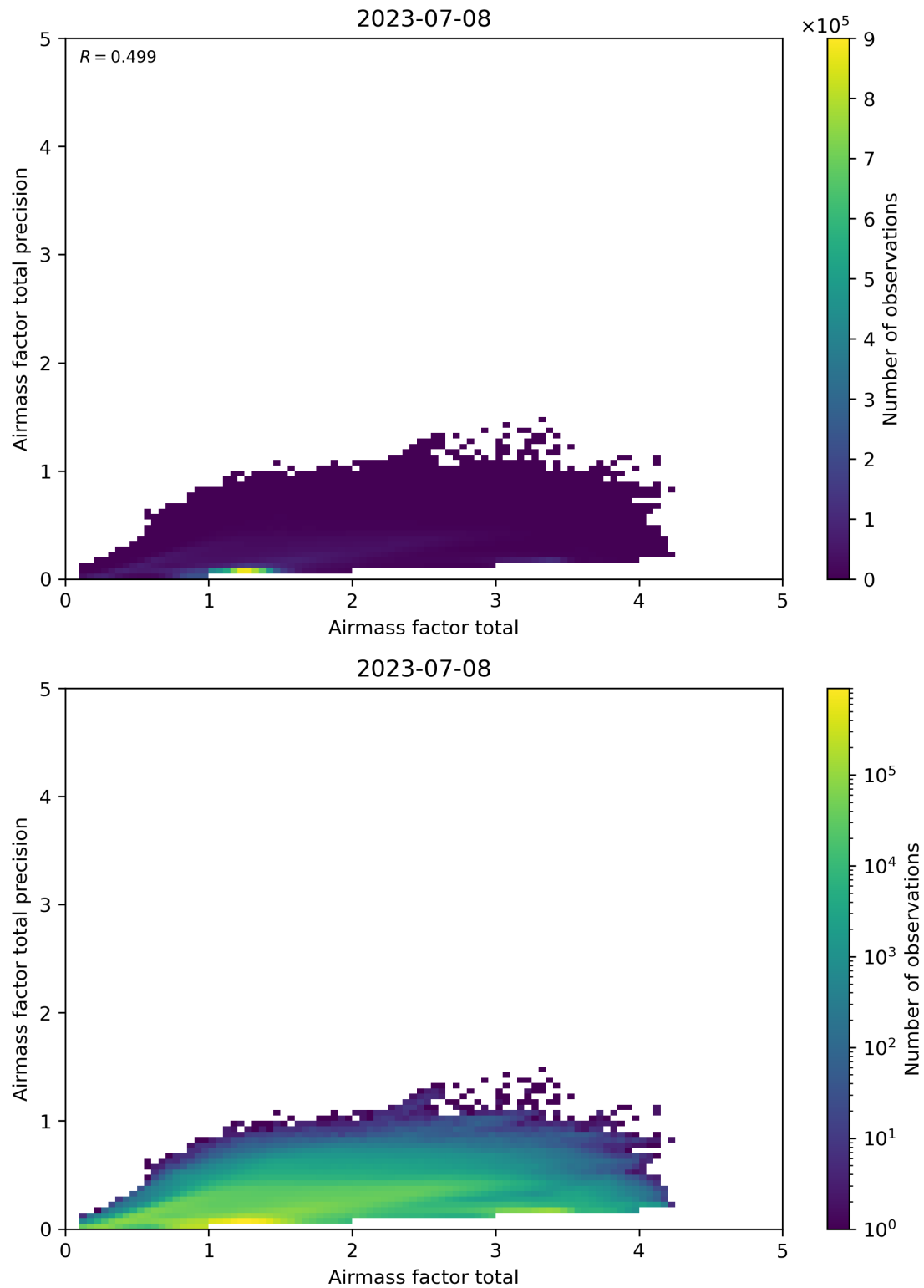
Figure 103: Scatter density plot of “Airmass factor total” against “Airmass factor total precision” for 2023-07-08 to 2023-07-09.
