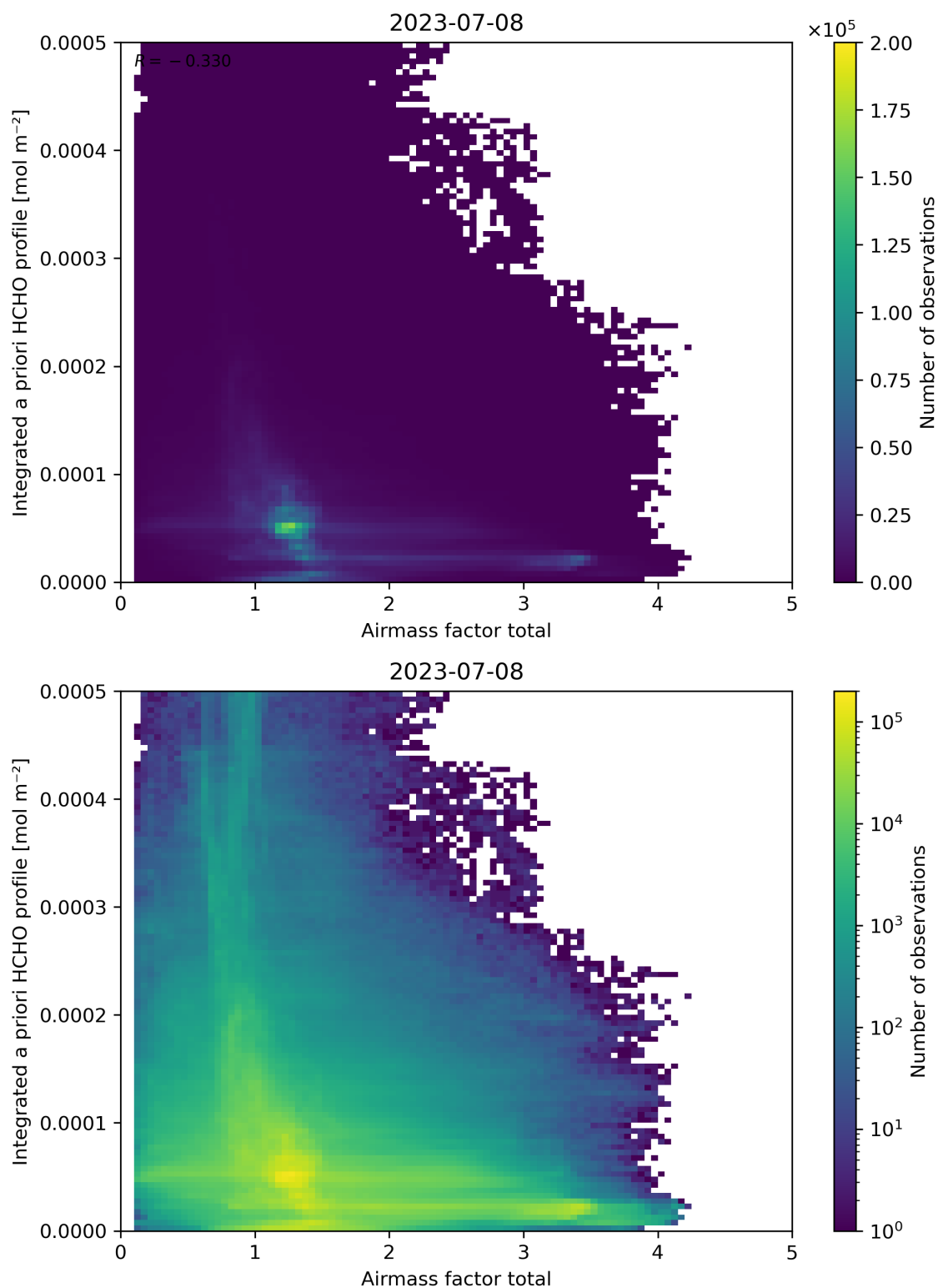
Figure 104: Scatter density plot of “Airmass factor total” against “Integrated a priori HCHO profile” for 2023-07-08 to 2023-07-09.
