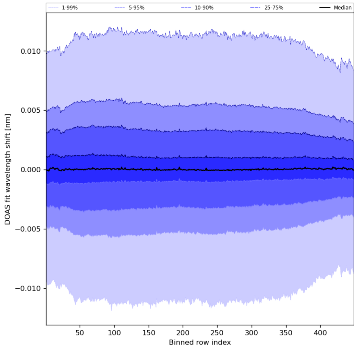
Figure 58: Along track statistics of “DOAS fit wavelength shift” for 2023-07-08 to 2023-07-09
