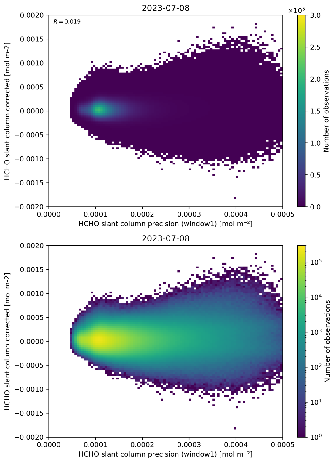
Figure 92: Scatter density plot of “HCHO slant column precision (window1)” against “HCHO slant column corrected” for 2023-07-08 to 2023-07-09.
