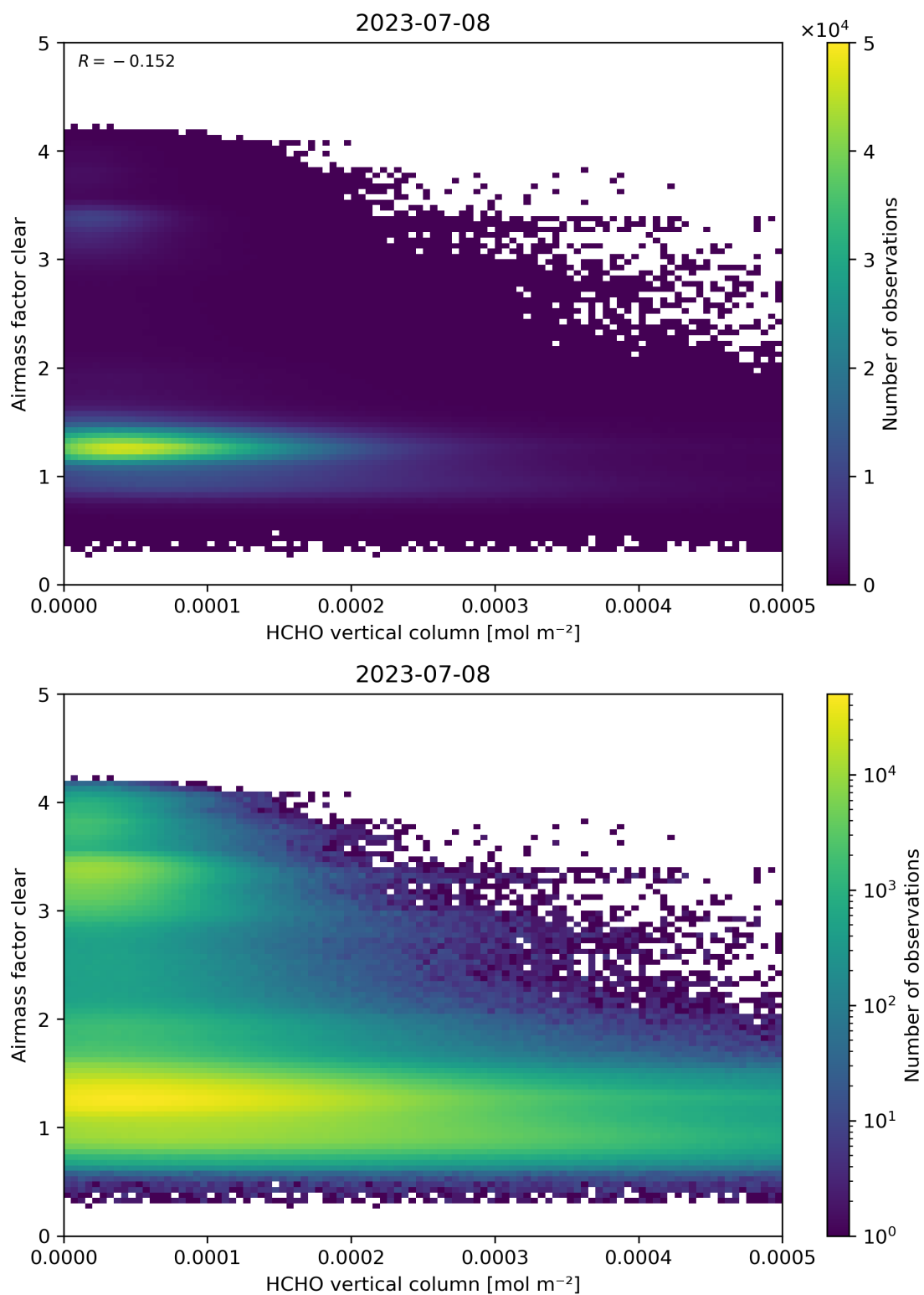
Figure 126: Scatter density plot of “HCHO vertical column” against “Airmass factor clear” for 2023-07-08 to 2023-07-09.
