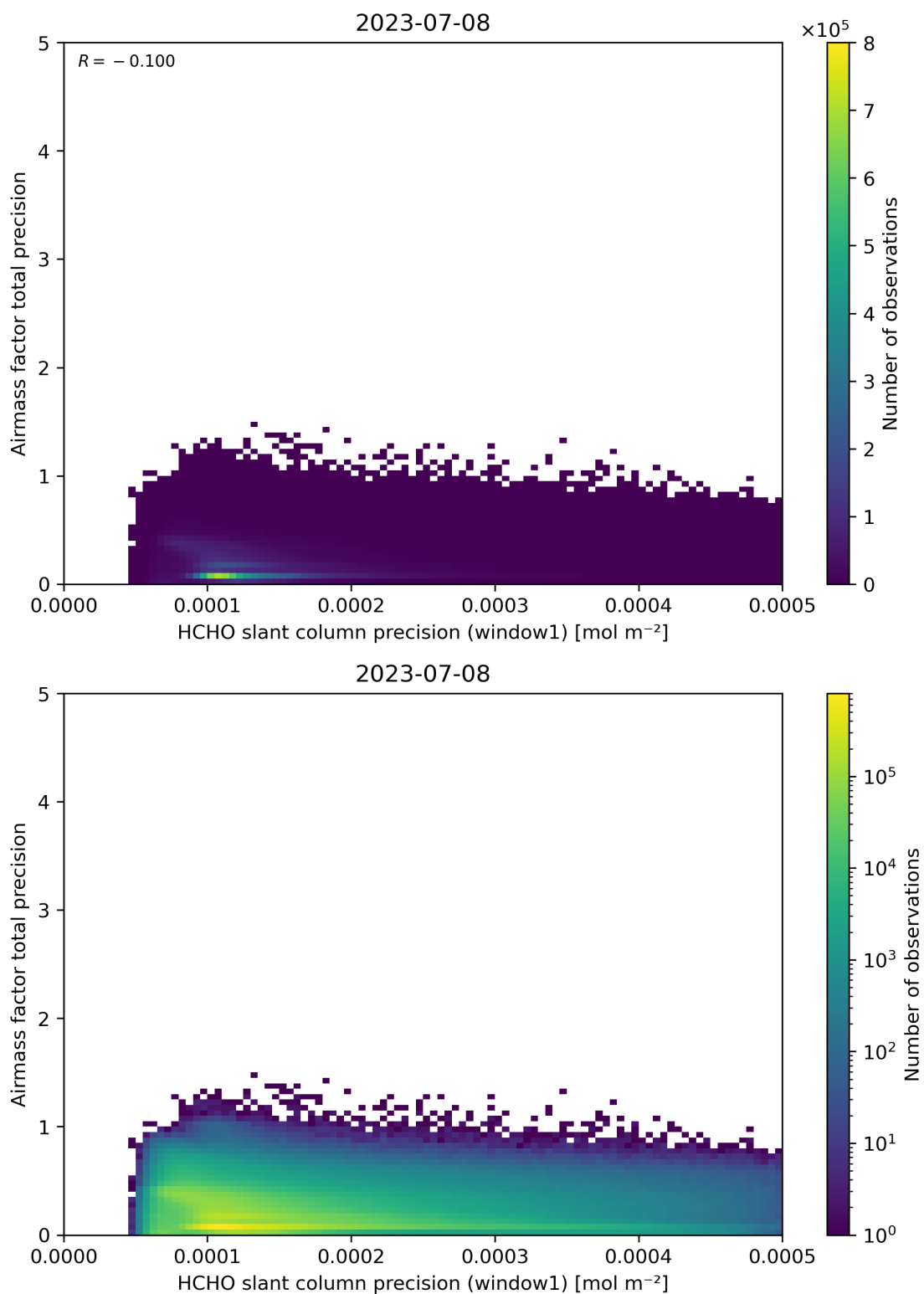
Figure 95: Scatter density plot of “HCHO slant column precision (window1)” against “Airmass factor total precision” for 2023-07-08 to 2023-07-09.
