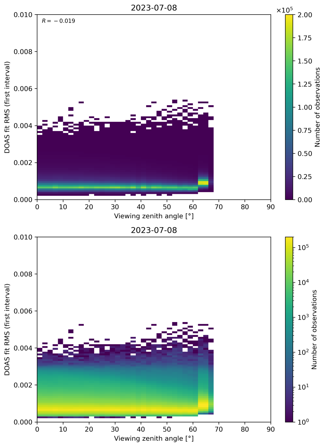
Figure 182: Scatter density plot of “Viewing zenith angle” against “DOAS fit RMS (first interval)” for 2023-07-08 to 2023-07-09.
