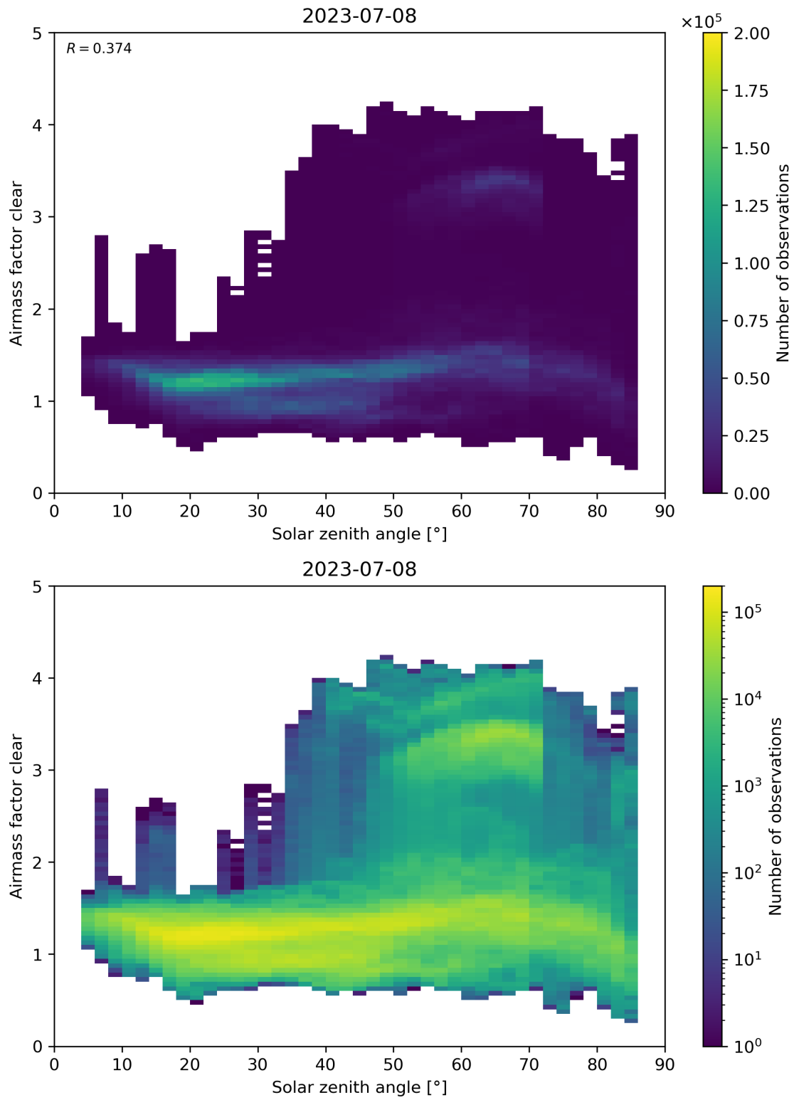
Figure 170: Scatter density plot of “Solar zenith angle” against “Airmass factor clear” for 2023-07-08 to 2023-07-09.
