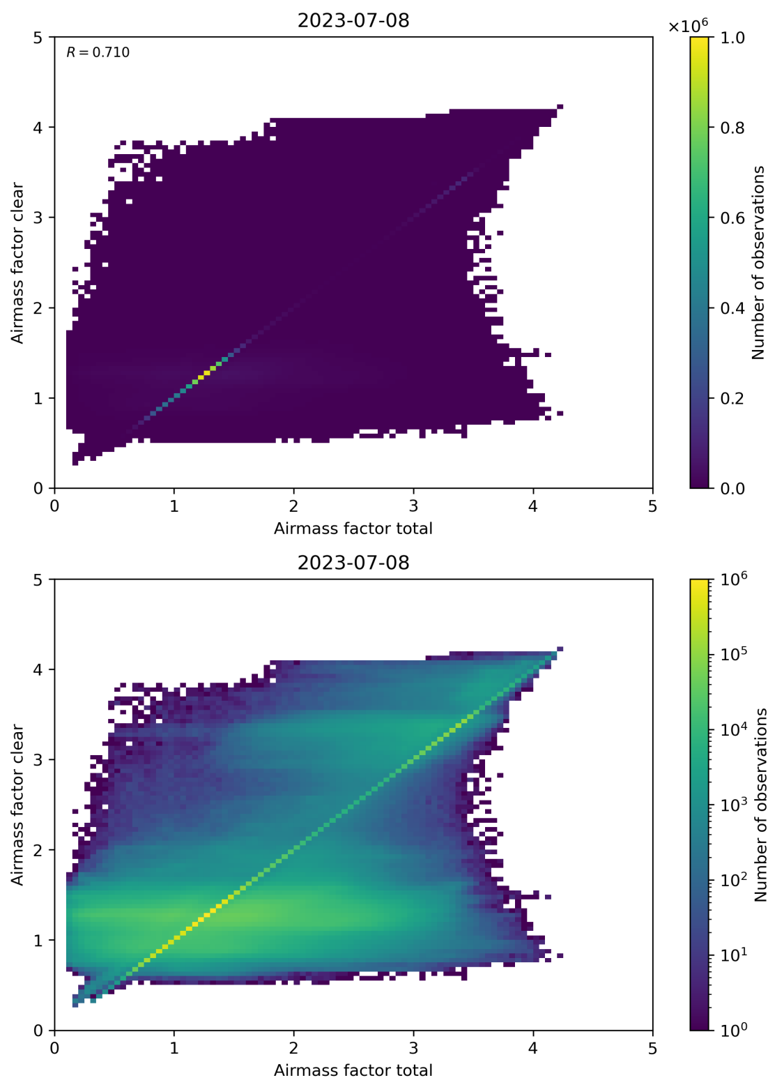
Figure 100: Scatter density plot of “Airmass factor total” against “Airmass factor clear” for 2023-07-08 to 2023-07-09.
