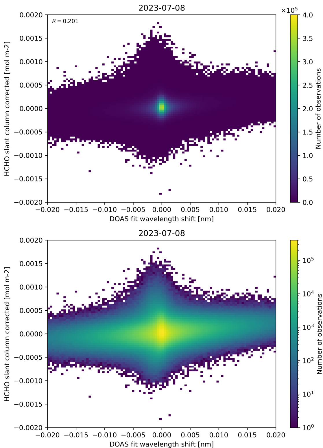
Figure 66: Scatter density plot of “DOAS fit wavelength shift” against “HCHO slant column corrected” for 2023-07-08 to 2023-07-09.
