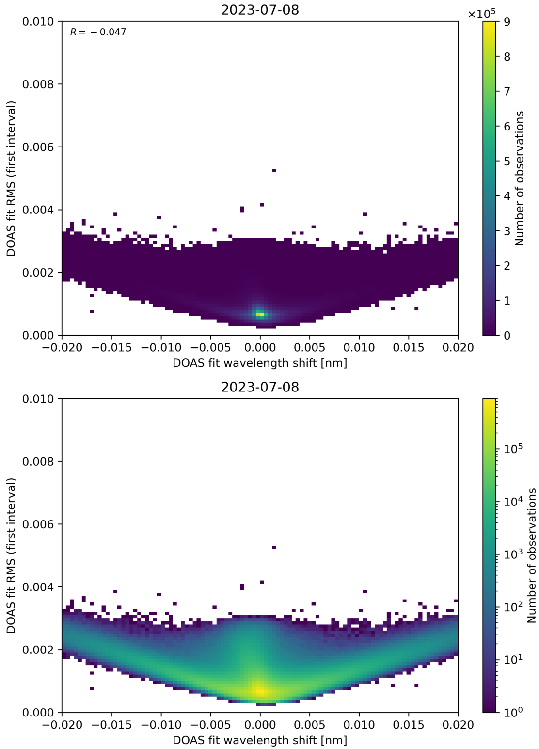
Figure 64: Scatter density plot of “DOAS fit wavelength shift” against “DOAS fit RMS (first interval)” for 2023-07-08 to 2023-07-09.
