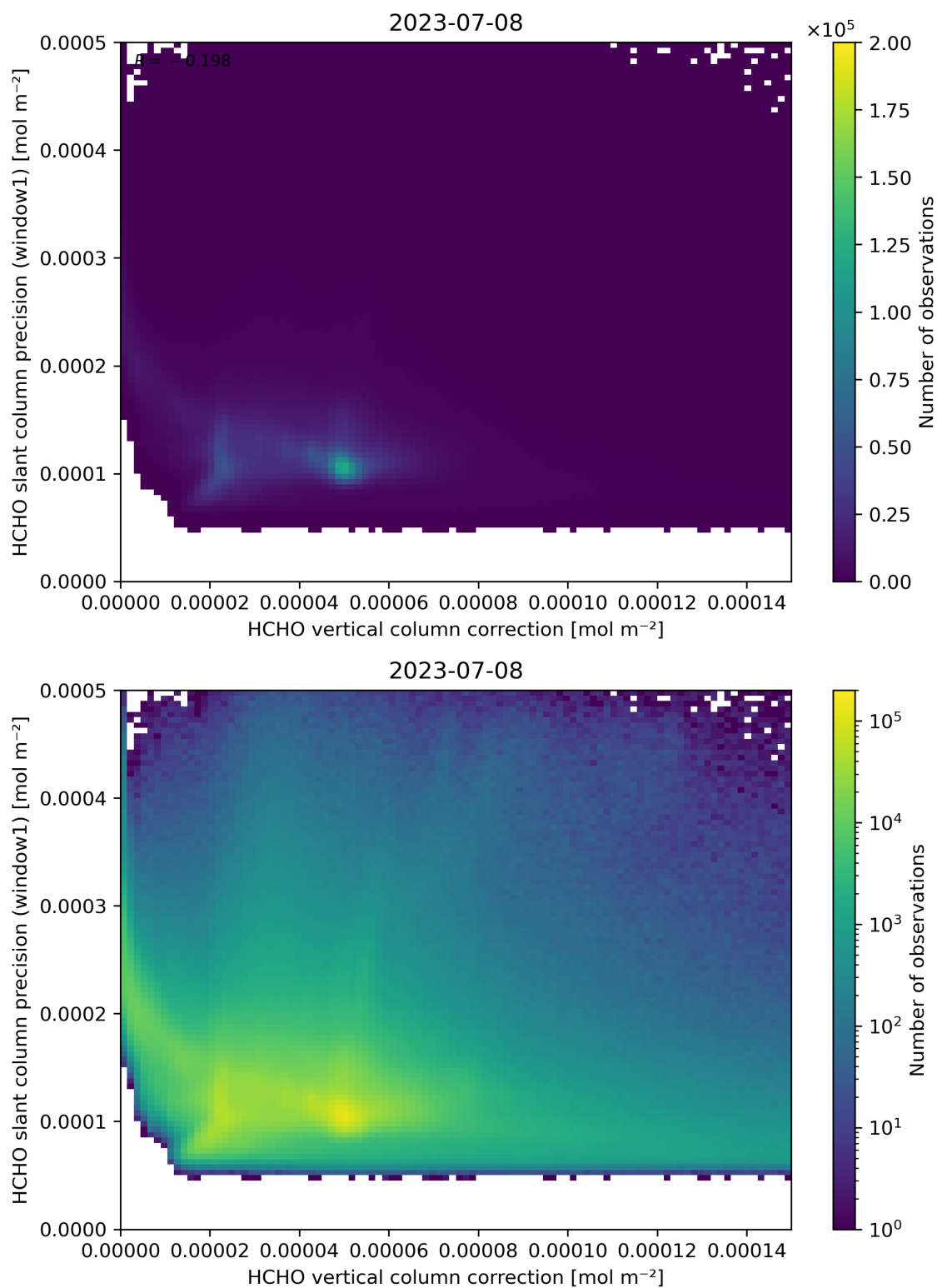
Figure 119: Scatter density plot of “HCHO vertical column correction” against “HCHO slant column precision (window1)” for 2023-07-08 to 2023-07-09.
