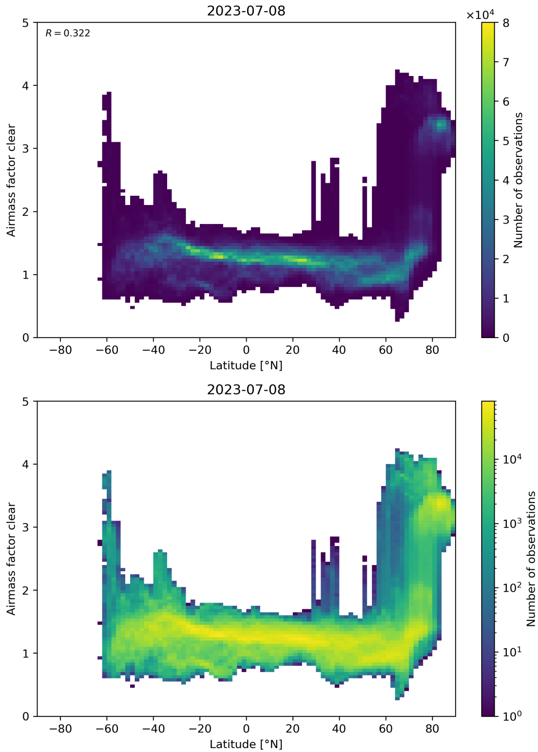
Figure 156: Scatter density plot of “Latitude” against “Airmass factor clear” for 2023-07-08 to 2023-07-09.
