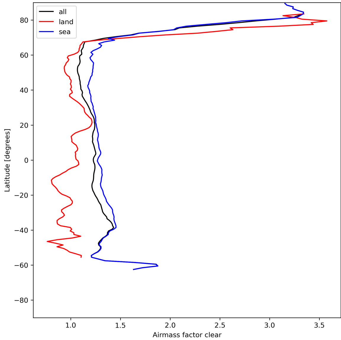
Figure 28: Zonal average of “Airmass factor clear” for 2023-07-08 to 2023-07-09.
