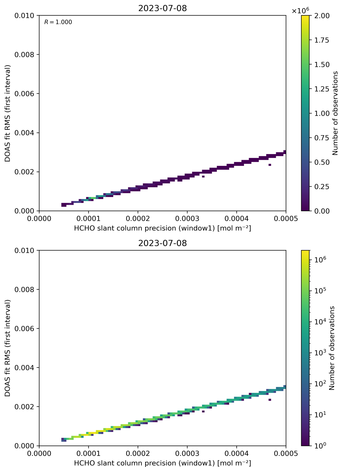
Figure 88: Scatter density plot of “HCHO slant column precision (window1)” against “DOAS fit RMS (first interval)” for 2023-07-08 to 2023-07-09.
