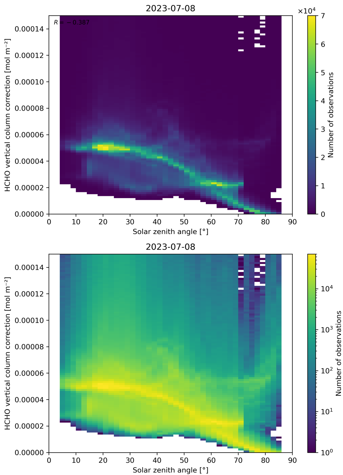
Figure 178: Scatter density plot of “Solar zenith angle” against “HCHO vertical column correction” for 2023-07-08 to 2023-07-09.
