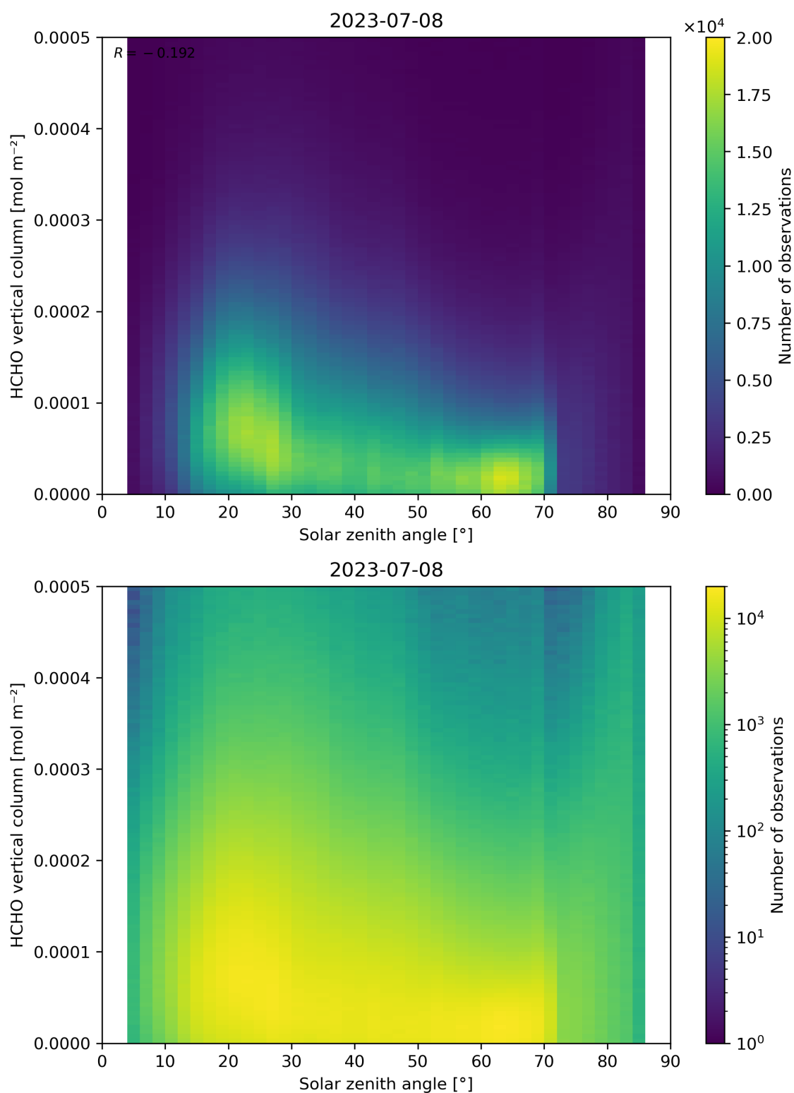
Figure 177: Scatter density plot of “Solar zenith angle” against “HCHO vertical column” for 2023-07-08 to 2023-07-09.
