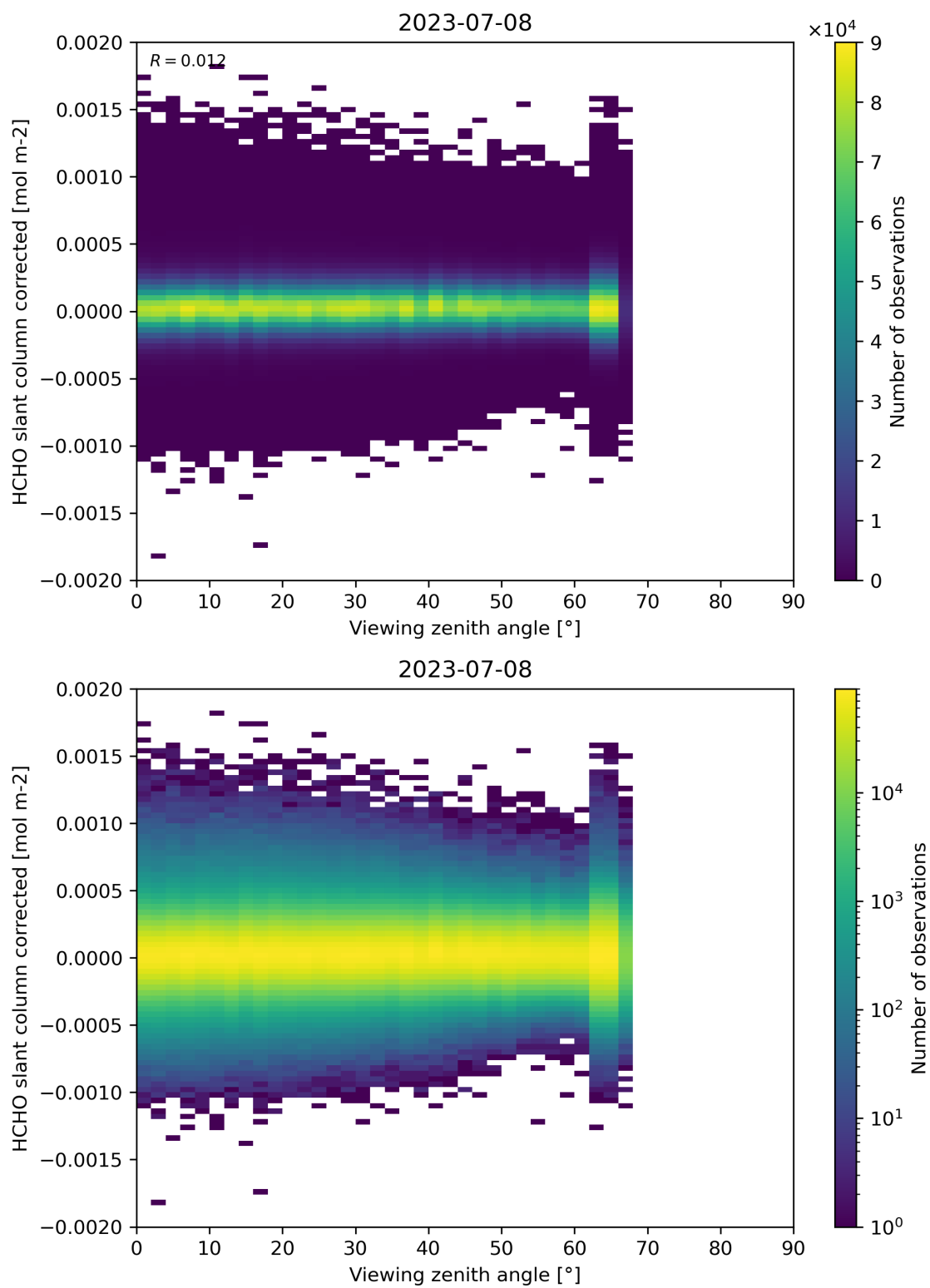
Figure 186: Scatter density plot of “Viewing zenith angle” against “HCHO slant column corrected” for 2023-07-08 to 2023-07-09.
