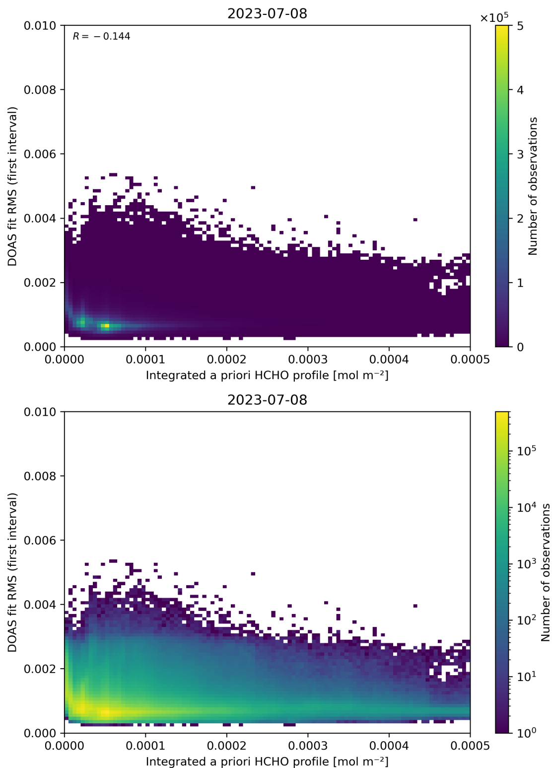
Figure 148: Scatter density plot of “Integrated a priori HCHO profile” against “DOAS fit RMS (first interval)” for 2023-07-08 to 2023-07-09.
