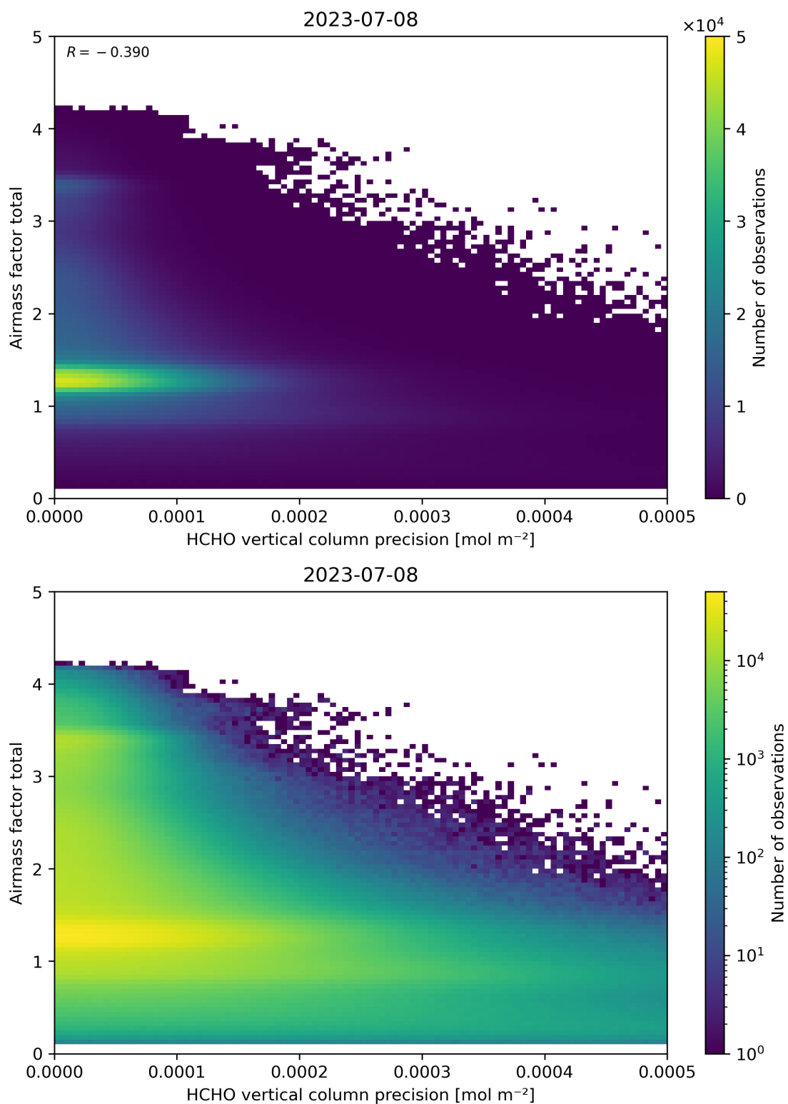
Figure 144: Scatter density plot of “HCHO vertical column precision” against “Airmass factor total” for 2023-07-08 to 2023-07-09.
