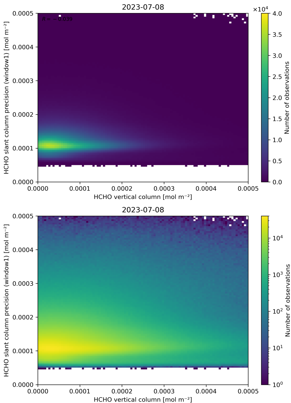
Figure 130: Scatter density plot of “HCHO vertical column” against “HCHO slant column precision (window1)” for 2023-07-08 to 2023-07-09.
