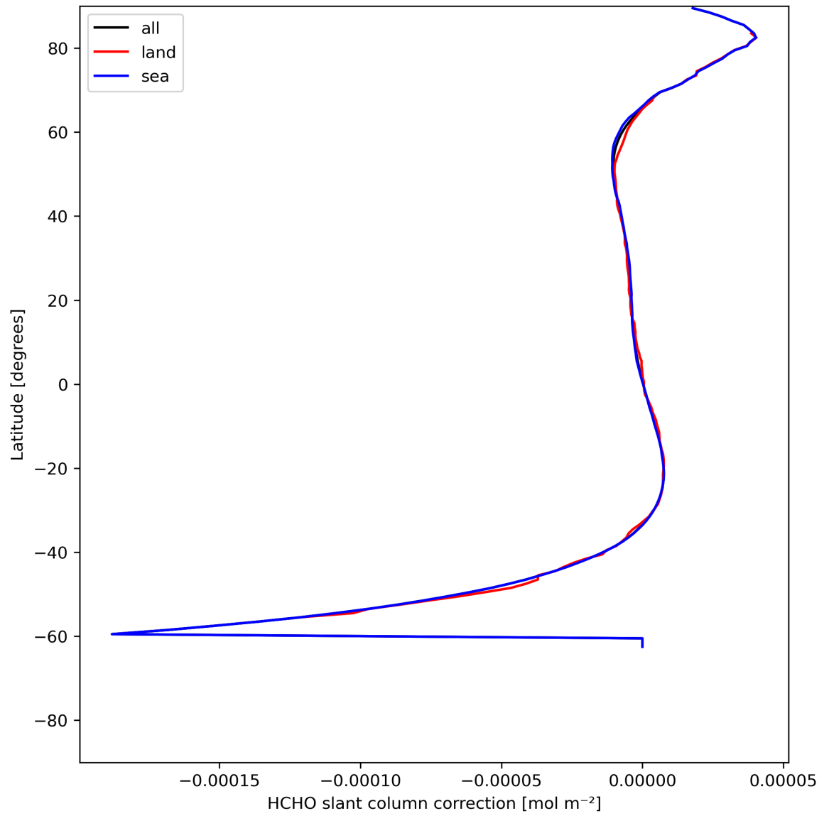
Figure 33: Zonal average of “HCHO slant column correction” for 2023-07-08 to 2023-07-09.
