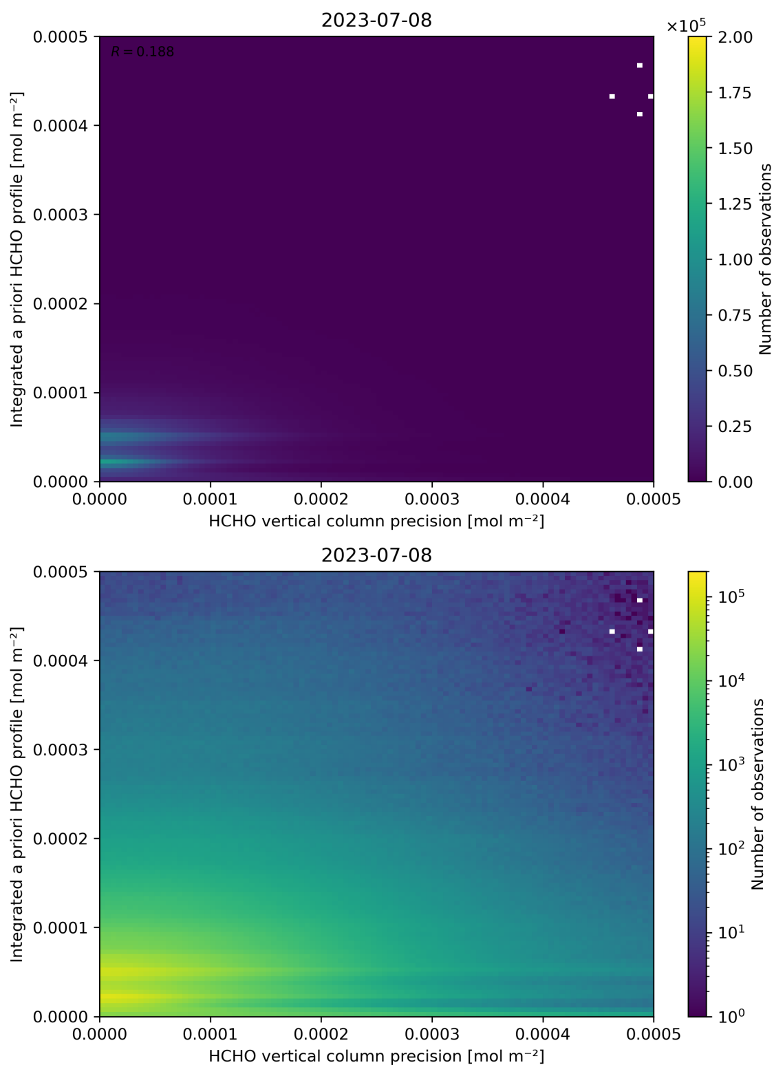
Figure 147: Scatter density plot of “HCHO vertical column precision” against “Integrated a priori HCHO profile” for 2023-07-08 to 2023-07-09.
