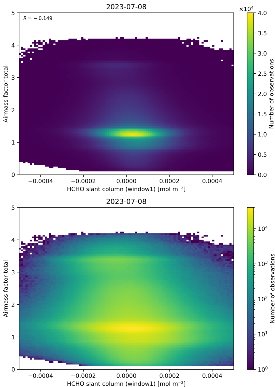
Figure 85: Scatter density plot of “HCHO slant column (window1)” against “Airmass factor total” for 2023-07-08 to 2023-07-09.
