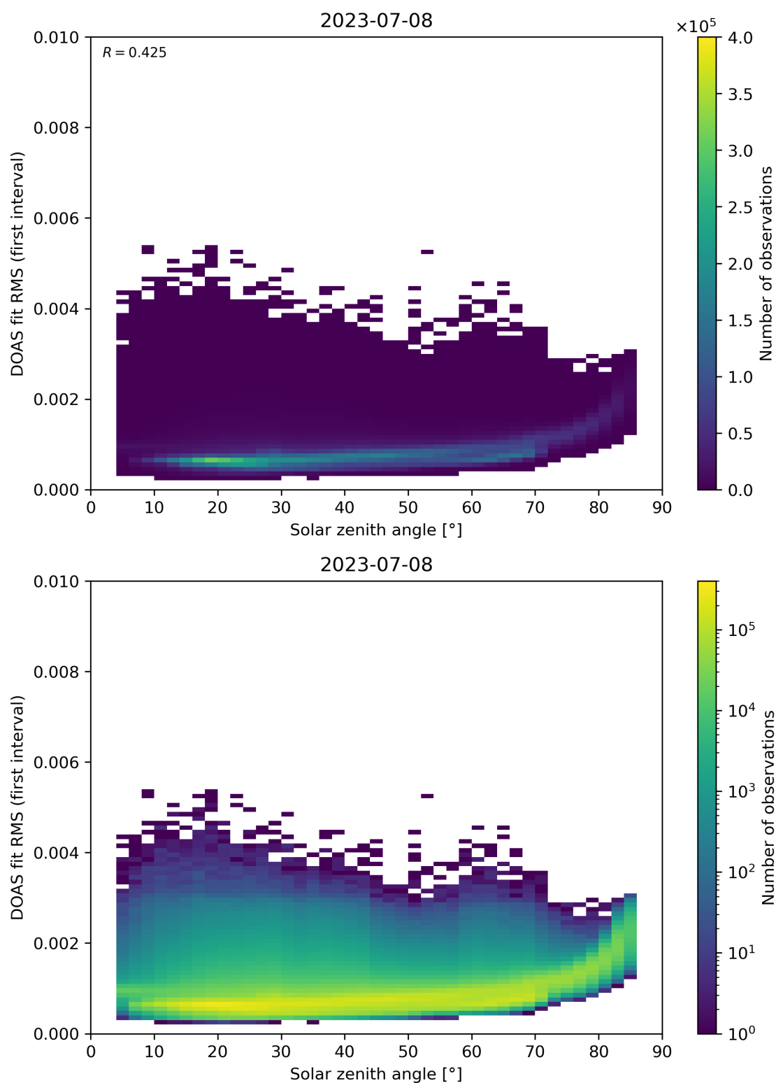
Figure 167: Scatter density plot of “Solar zenith angle” against “DOAS fit RMS (first interval)” for 2023-07-08 to 2023-07-09.
