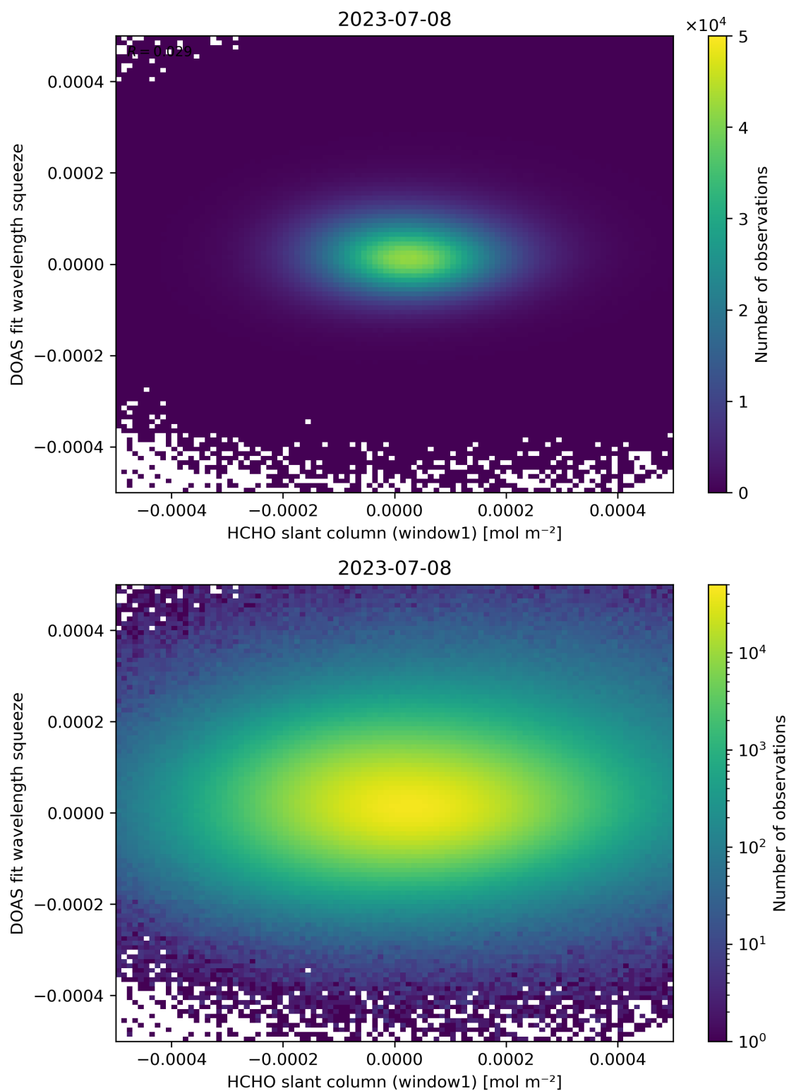
Figure 80: Scatter density plot of “HCHO slant column (window1)” against “DOAS fit wavelength squeeze” for 2023-07-08 to 2023-07-09.
