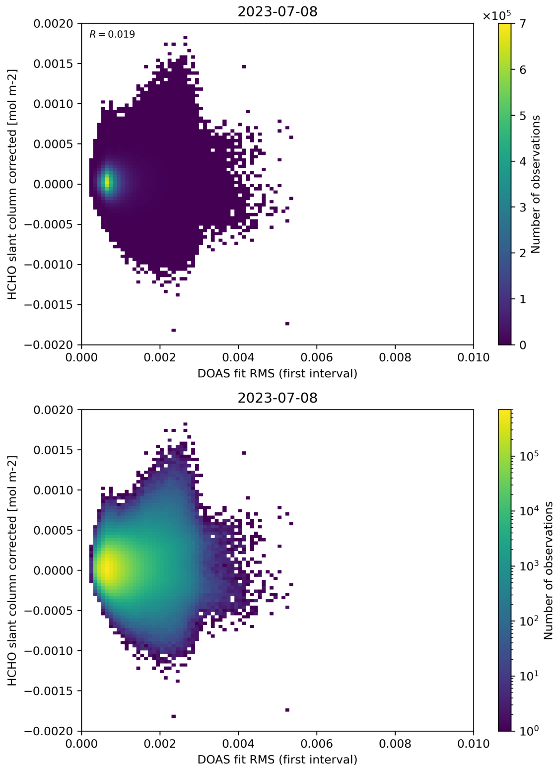
Figure 62: Scatter density plot of “DOAS fit RMS (first interval)” against “HCHO slant column corrected” for 2023-07-08 to 2023-07-09.
