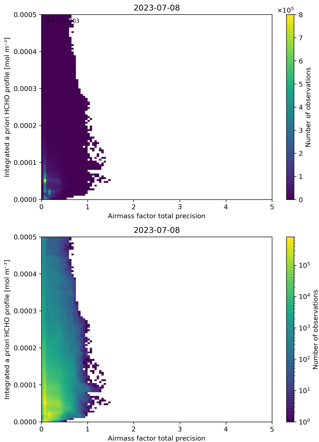
Figure 111: Scatter density plot of “Airmass factor total precision” against “Integrated a priori HCHO profile” for 2023-07-08 to 2023-07-09.
