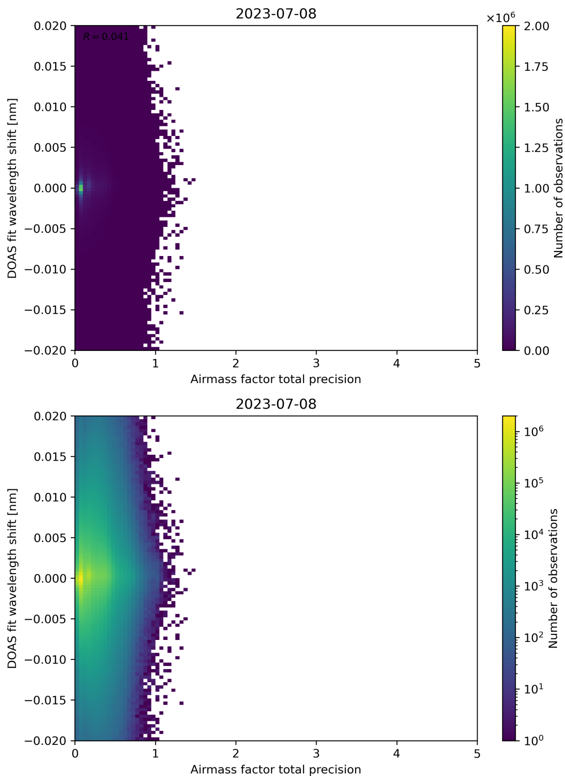
Figure 106: Scatter density plot of “Airmass factor total precision” against “DOAS fit wavelength shift” for 2023-07-08 to 2023-07-09.
