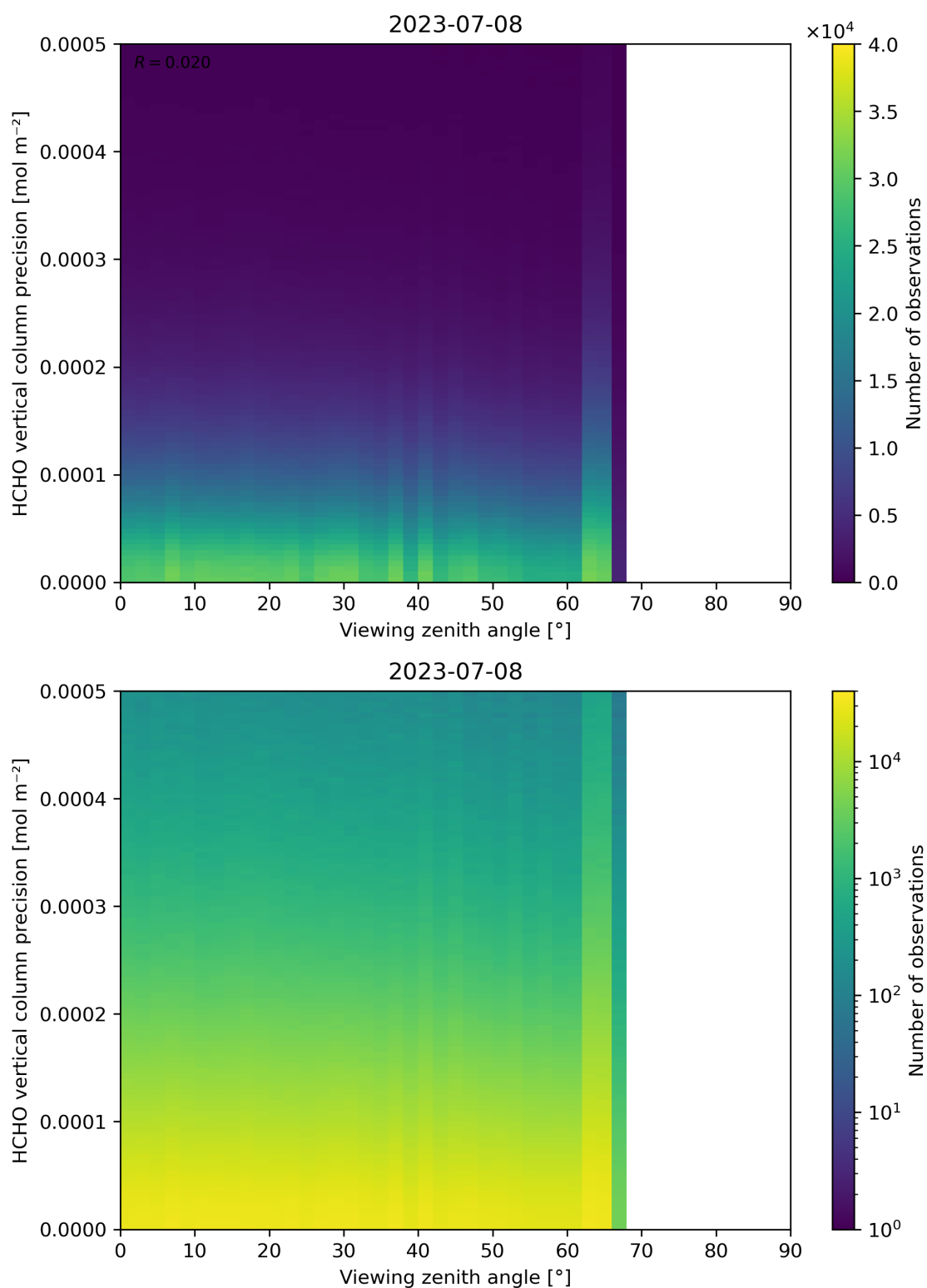
Figure 194: Scatter density plot of “Viewing zenith angle” against “HCHO vertical column precision” for 2023-07-08 to 2023-07-09.
