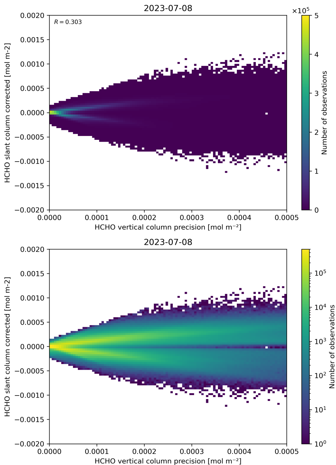
Figure 140: Scatter density plot of “HCHO vertical column precision” against “HCHO slant column corrected” for 2023-07-08 to 2023-07-09.
