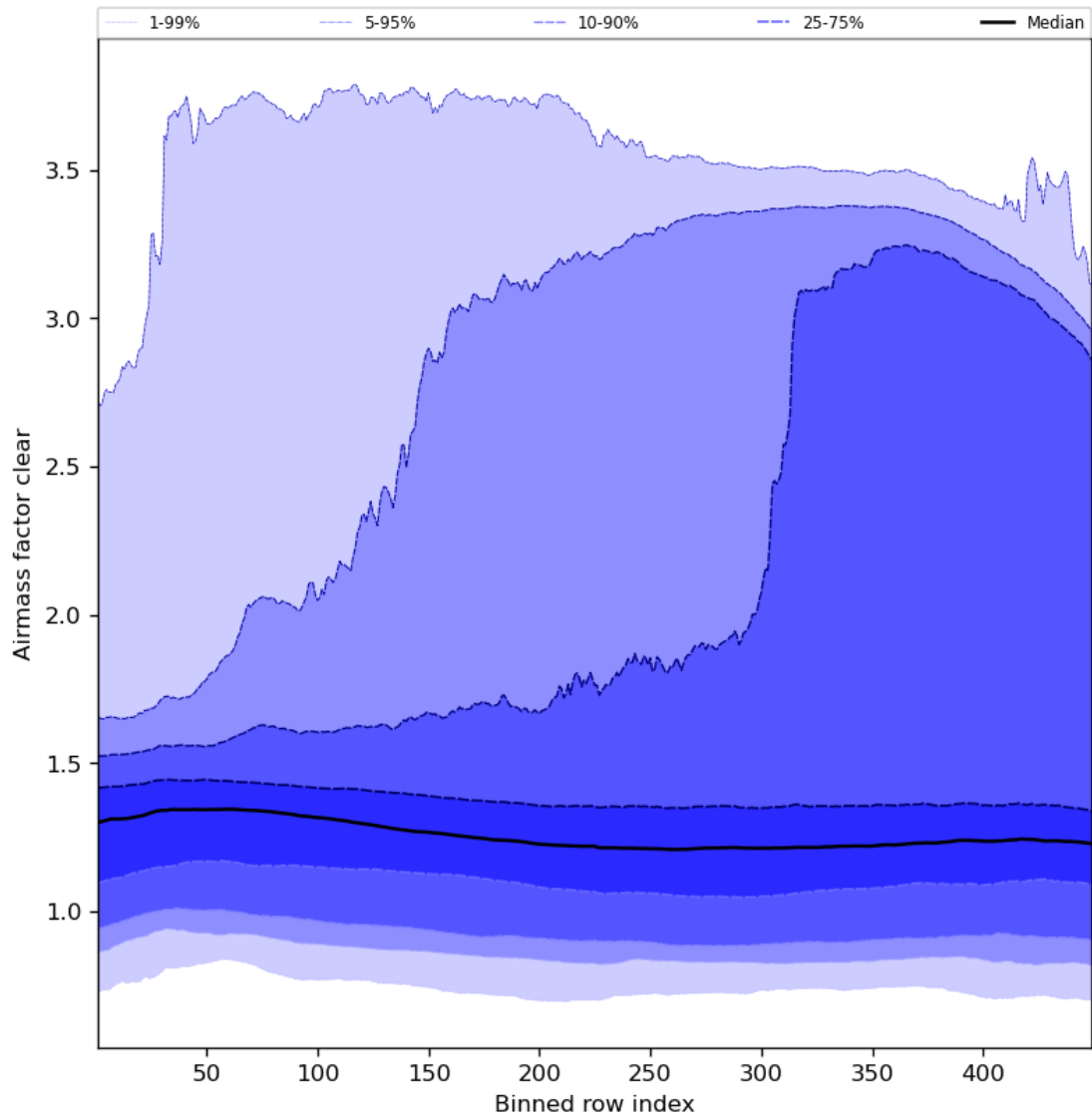
Figure 56: Along track statistics of “Airmass factor clear” for 2023-07-08 to 2023-07-09
