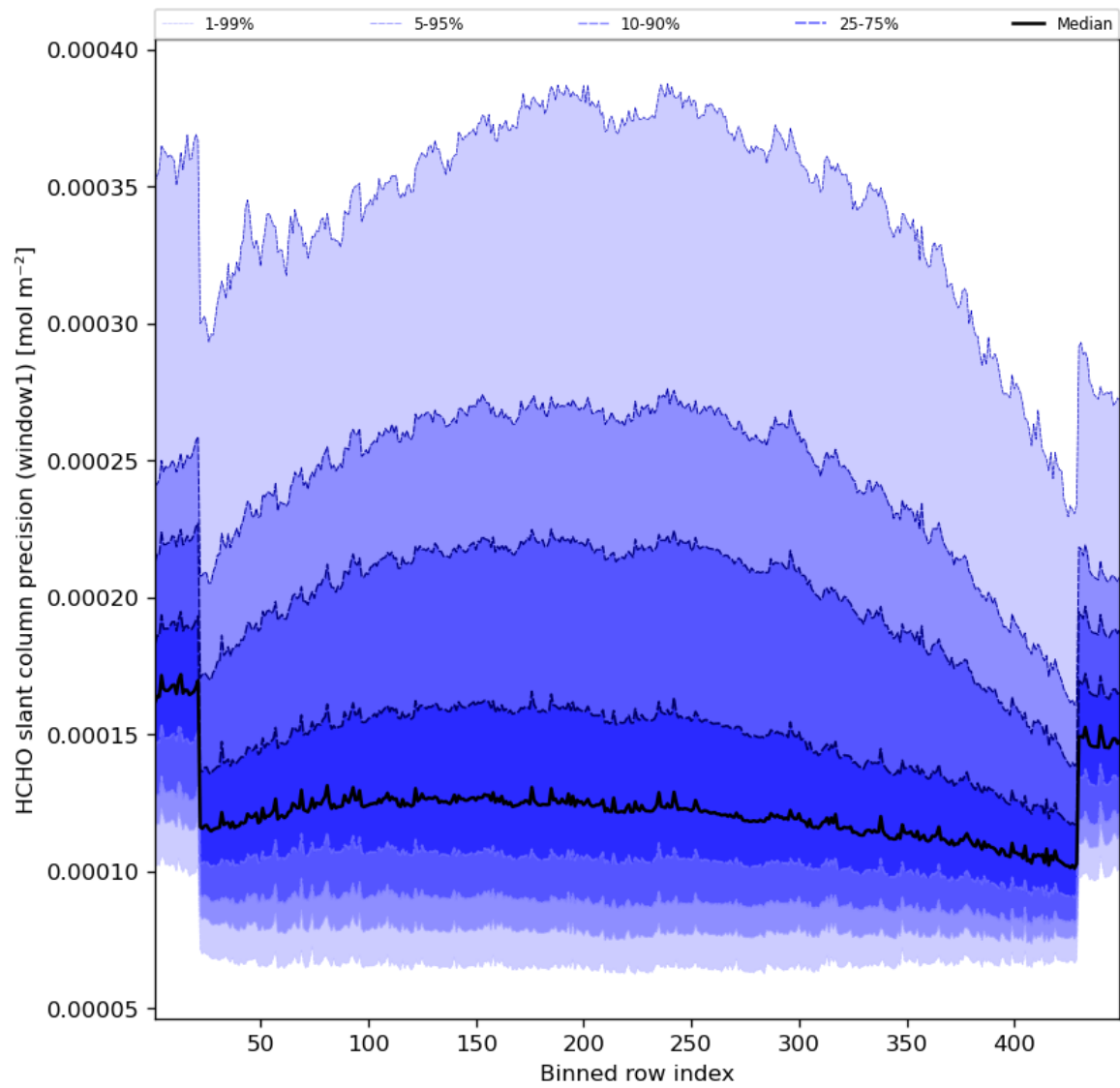
Figure 53: Along track statistics of “HCHO slant column precision (window1)” for 2023-07-08 to 2023-07-09
