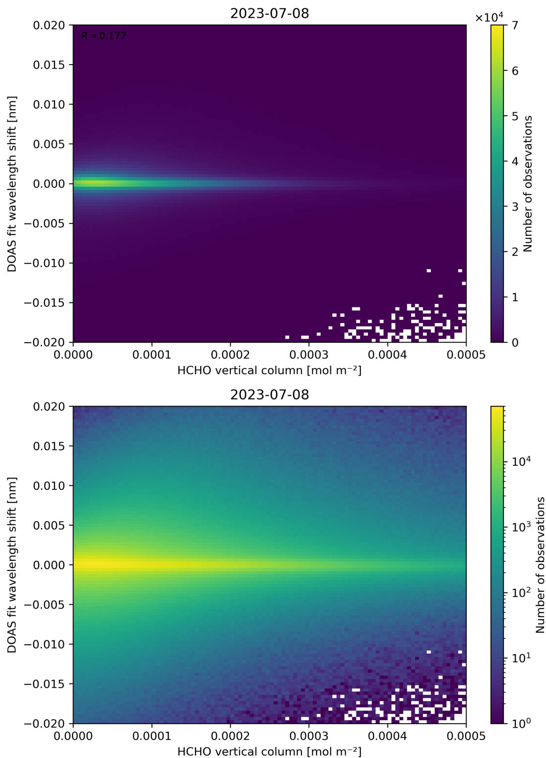
Figure 124: Scatter density plot of “HCHO vertical column” against “DOAS fit wavelength shift” for 2023-07-08 to 2023-07-09.
