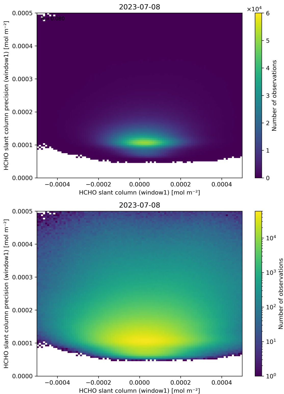
Figure 84: Scatter density plot of “HCHO slant column (window1)” against “HCHO slant column precision (window1)” for 2023-07-08 to 2023-07-09.
