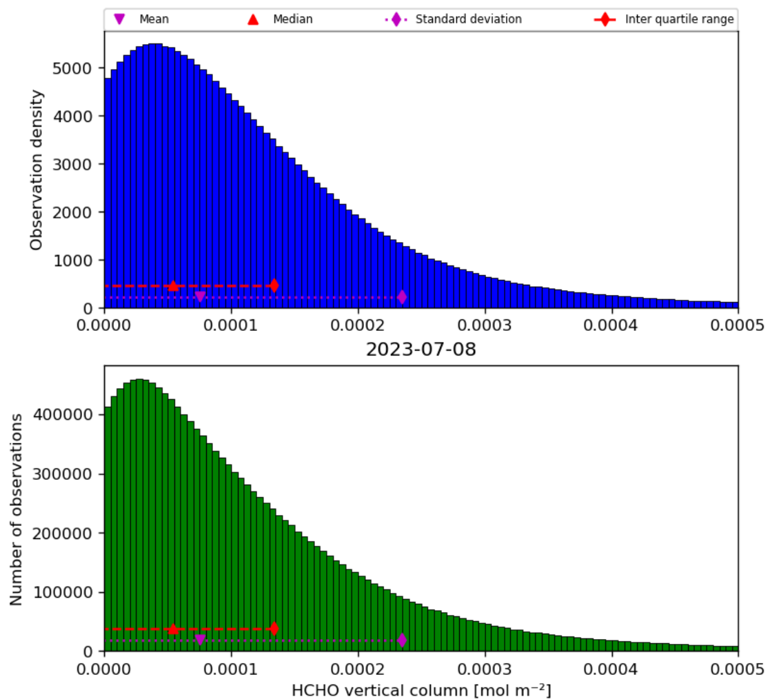
Figure 35: Histogram of “HCHO vertical column” for 2023-07-08 to 2023-07-09
