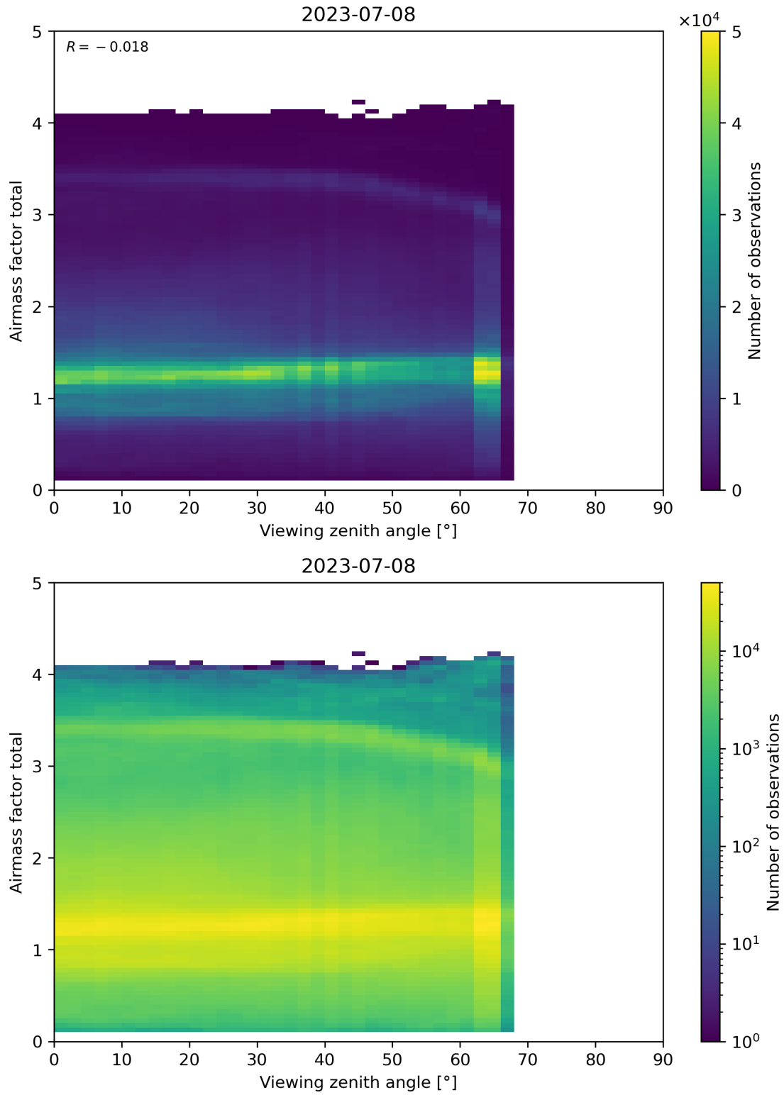
Figure 190: Scatter density plot of “Viewing zenith angle” against “Airmass factor total” for 2023-07-08 to 2023-07-09.
