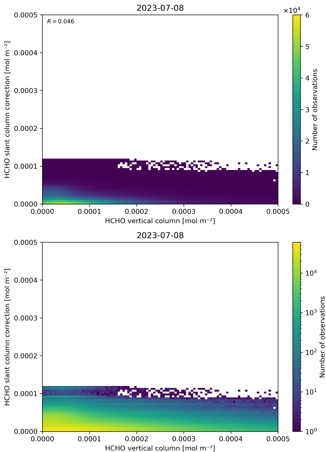
Figure 128: Scatter density plot of “HCHO vertical column” against “HCHO slant column correction” for 2023-07-08 to 2023-07-09.
