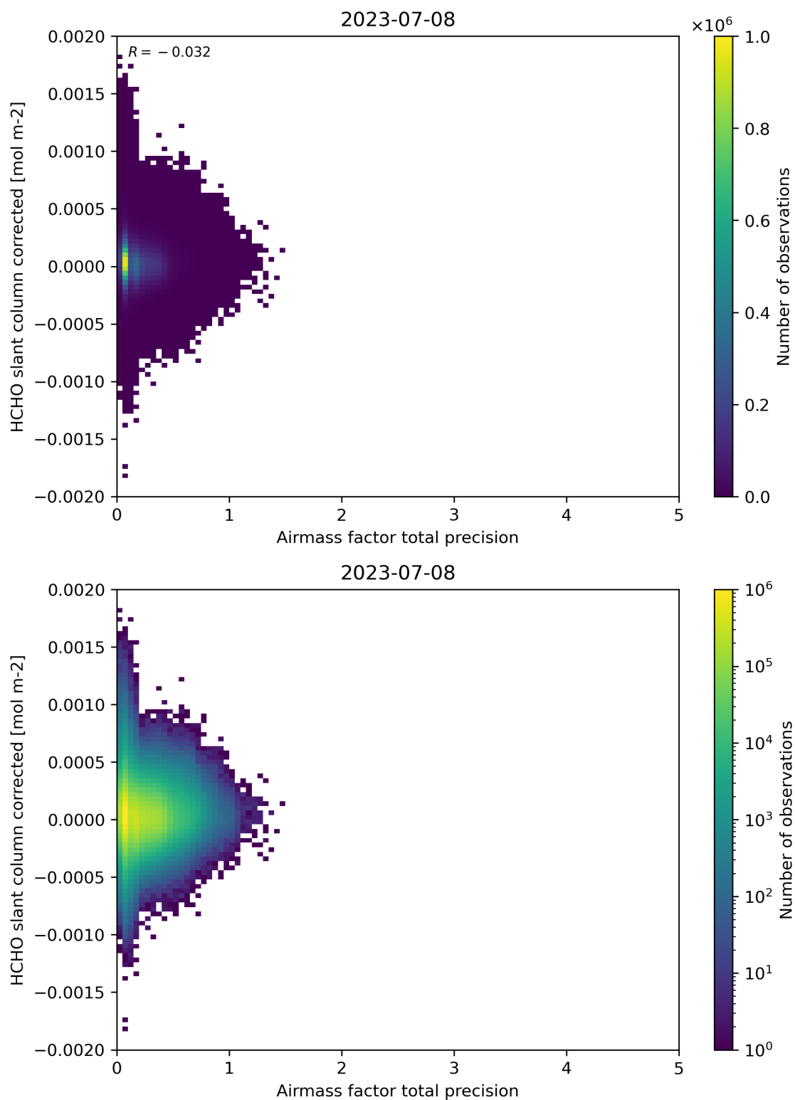
Figure 109: Scatter density plot of “Airmass factor total precision” against “HCHO slant column corrected” for 2023-07-08 to 2023-07-09.
