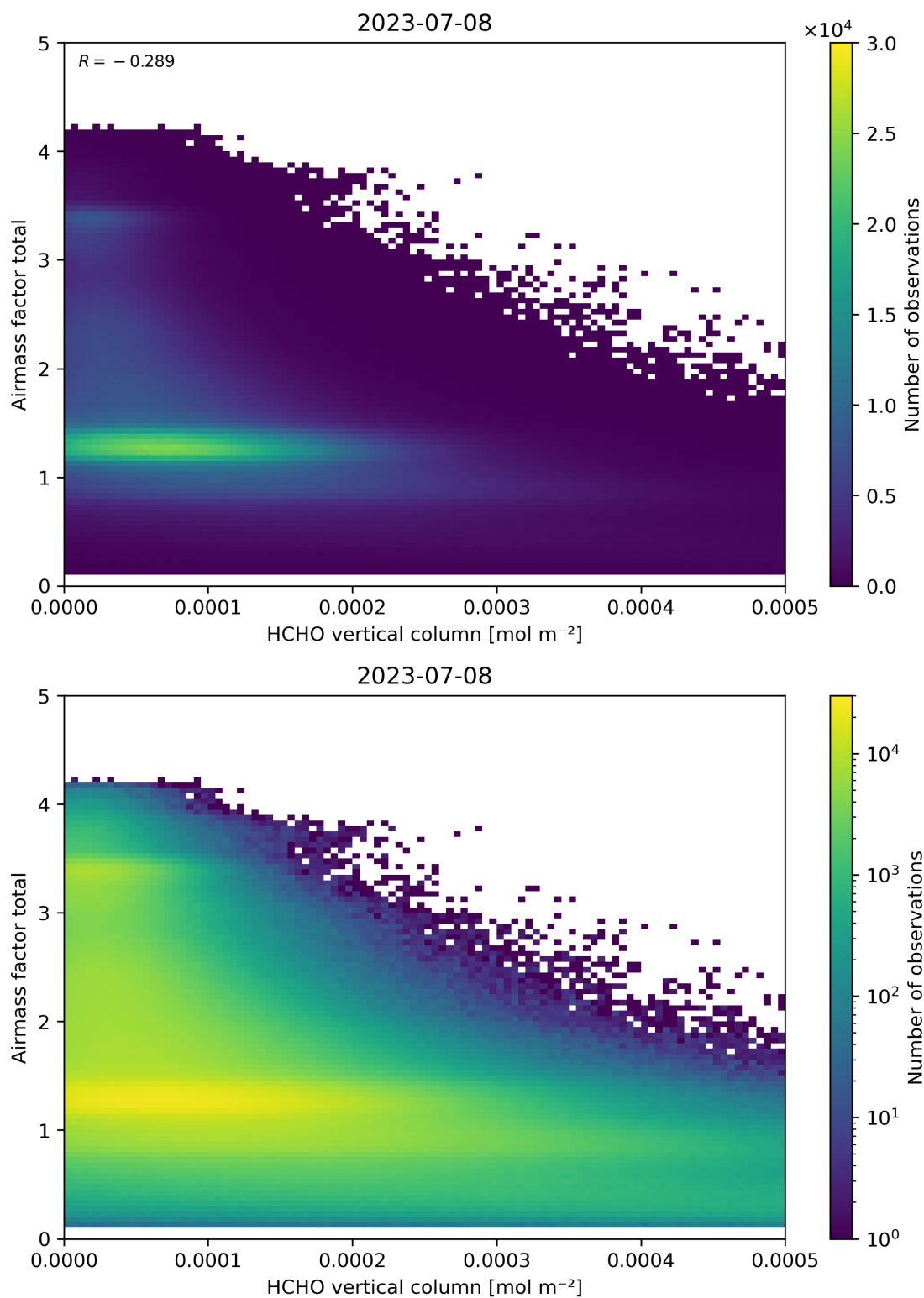
Figure 131: Scatter density plot of “HCHO vertical column” against “Airmass factor total” for 2023-07-08 to 2023-07-09.
