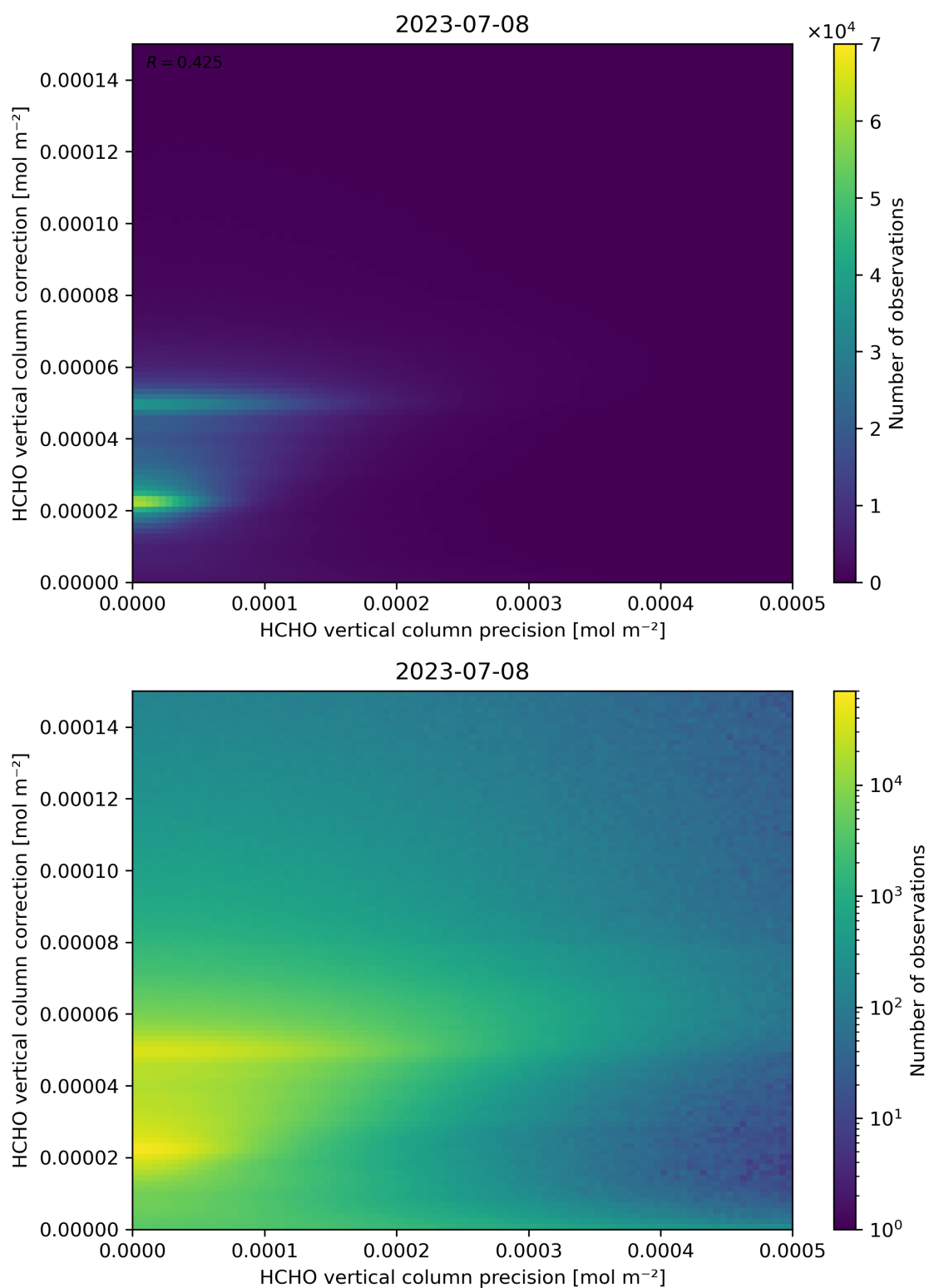
Figure 146: Scatter density plot of “HCHO vertical column precision” against “HCHO vertical column correction” for 2023-07-08 to 2023-07-09.
