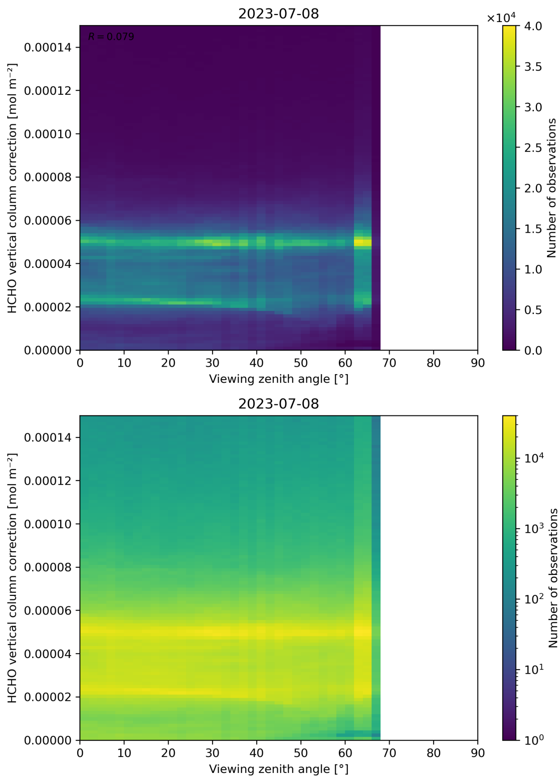
Figure 193: Scatter density plot of “Viewing zenith angle” against “HCHO vertical column correction” for 2023-07-08 to 2023-07-09.
