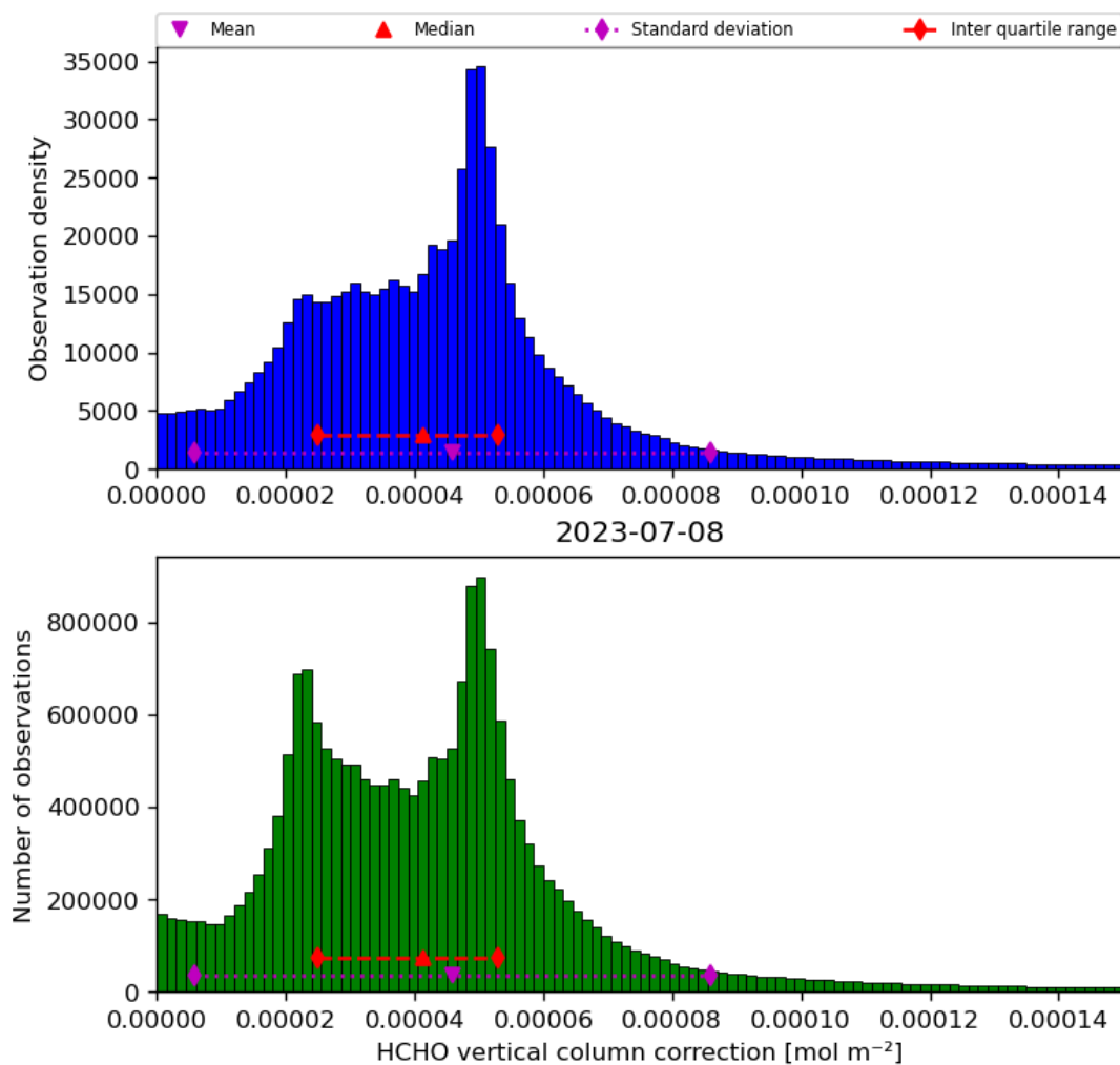
Figure 37: Histogram of “HCHO vertical column correction” for 2023-07-08 to 2023-07-09
