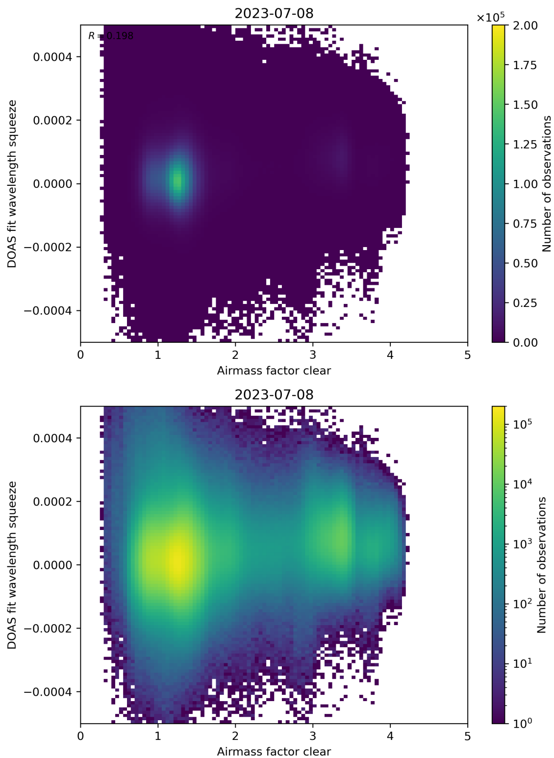
Figure 73: Scatter density plot of “Airmass factor clear” against “DOAS fit wavelength squeeze” for 2023-07-08 to 2023-07-09.
