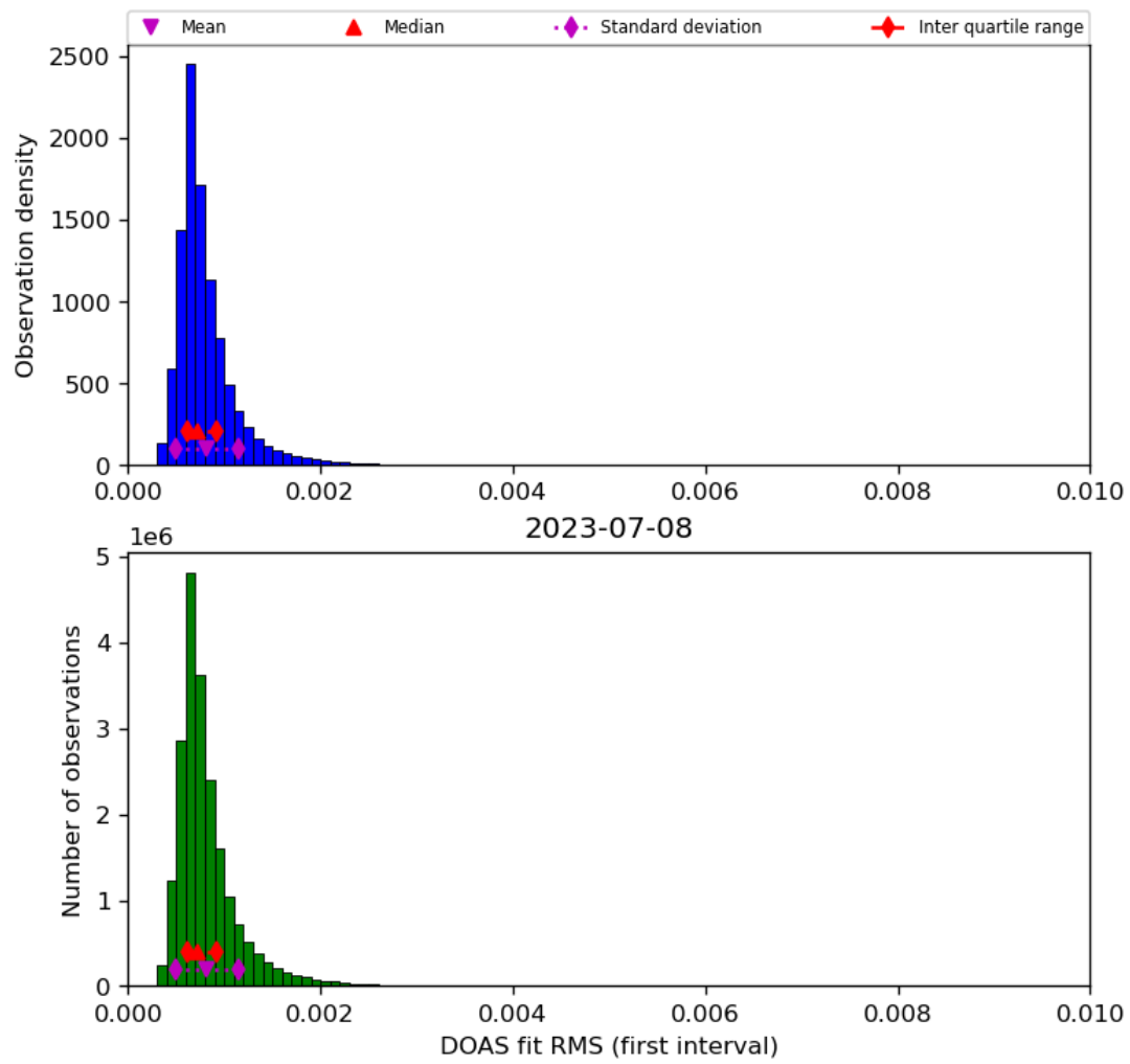
Figure 46: Histogram of “DOAS fit RMS (first interval)” for 2023-07-08 to 2023-07-09
