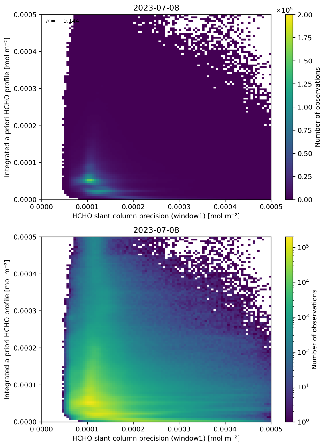
Figure 96: Scatter density plot of “HCHO slant column precision (window1)” against “Integrated a priori HCHO profile” for 2023-07-08 to 2023-07-09.
