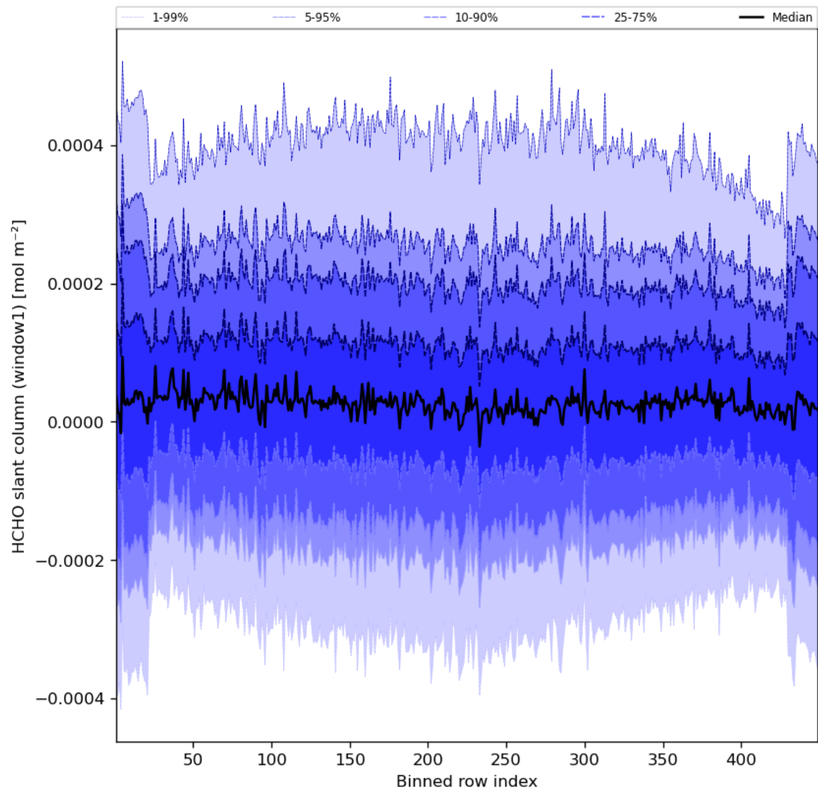
Figure 52: Along track statistics of “HCHO slant column (window1)” for 2023-07-08 to 2023-07-09
