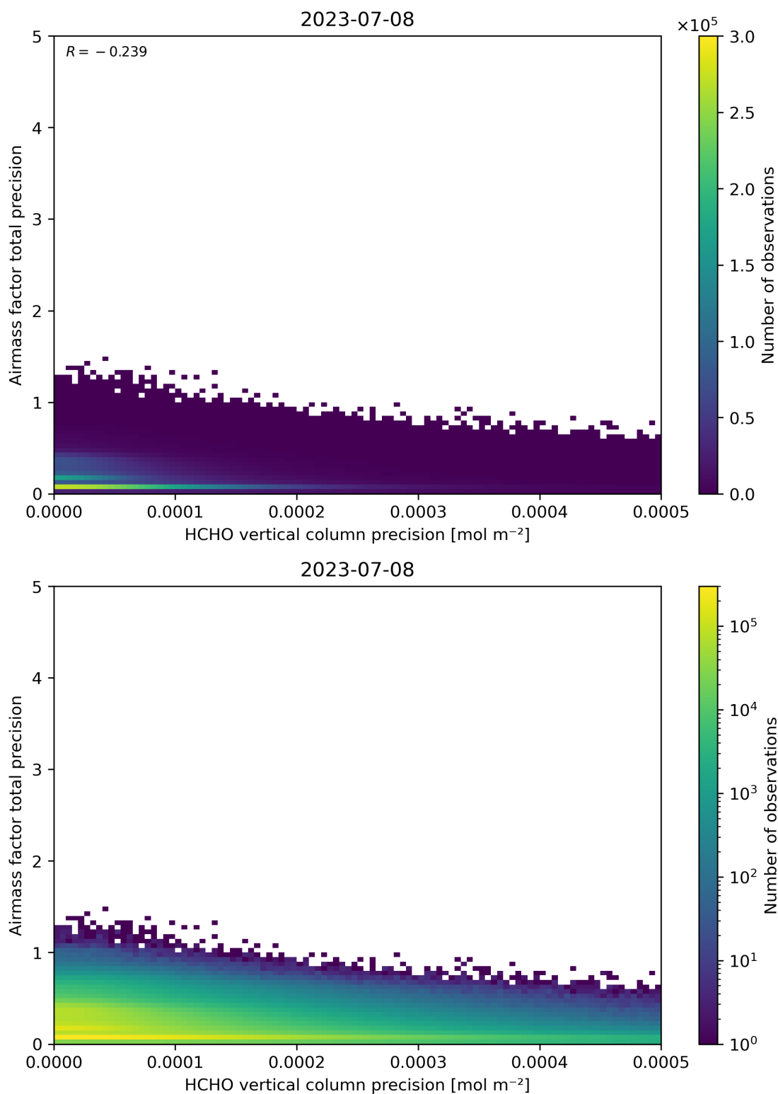
Figure 145: Scatter density plot of “HCHO vertical column precision” against “Airmass factor total precision” for 2023-07-08 to 2023-07-09.
