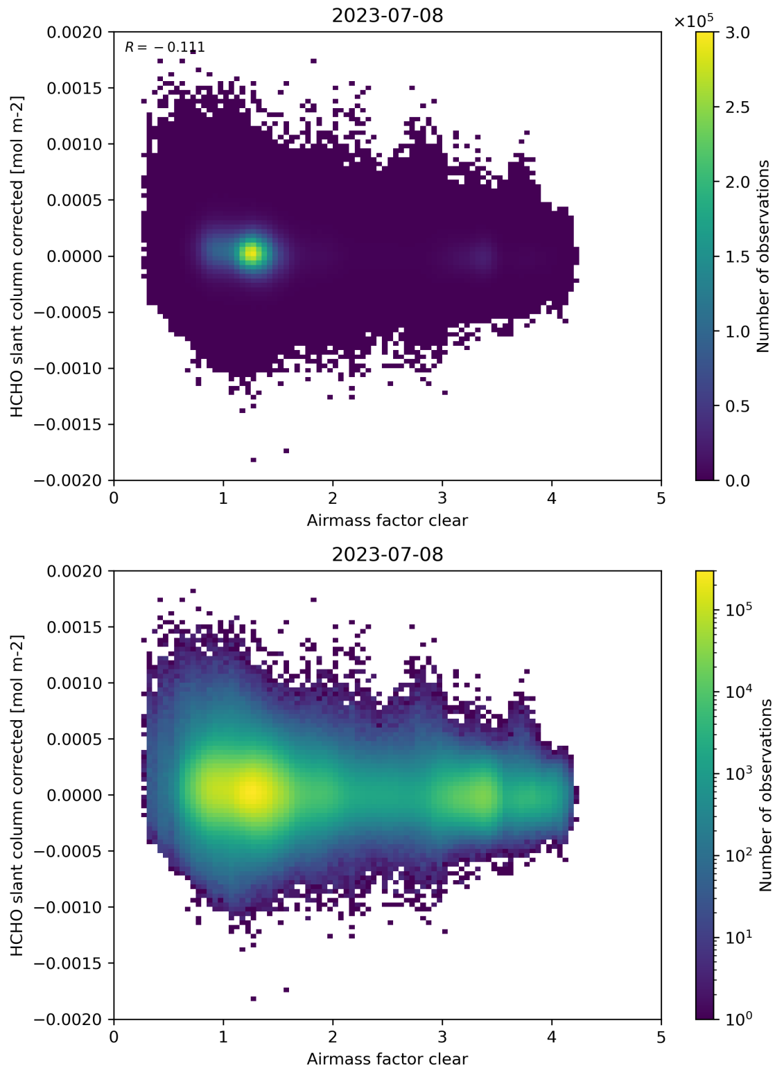
Figure 74: Scatter density plot of “Airmass factor clear” against “HCHO slant column corrected” for 2023-07-08 to 2023-07-09.
