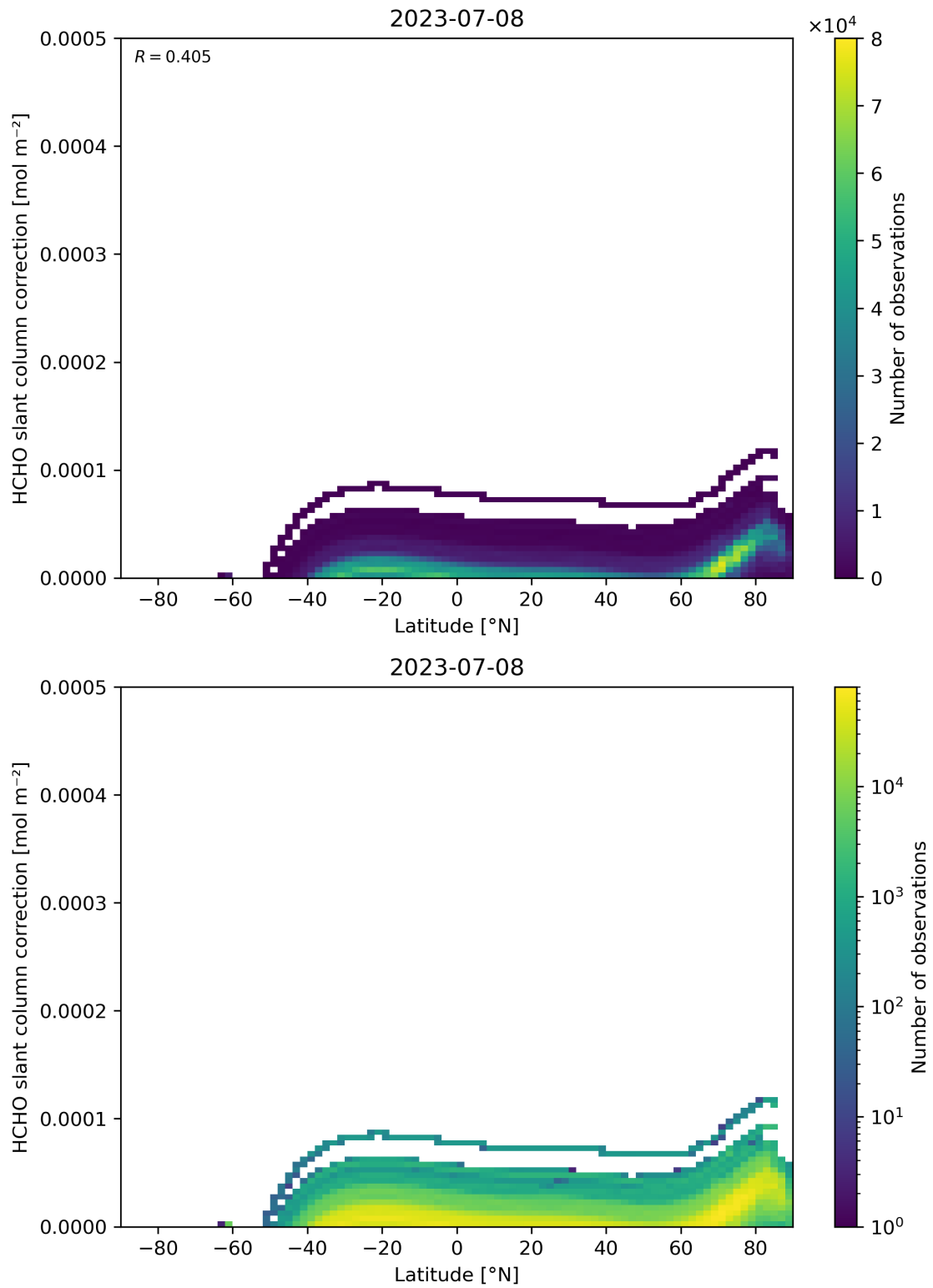
Figure 158: Scatter density plot of “Latitude” against “HCHO slant column correction” for 2023-07-08 to 2023-07-09.
