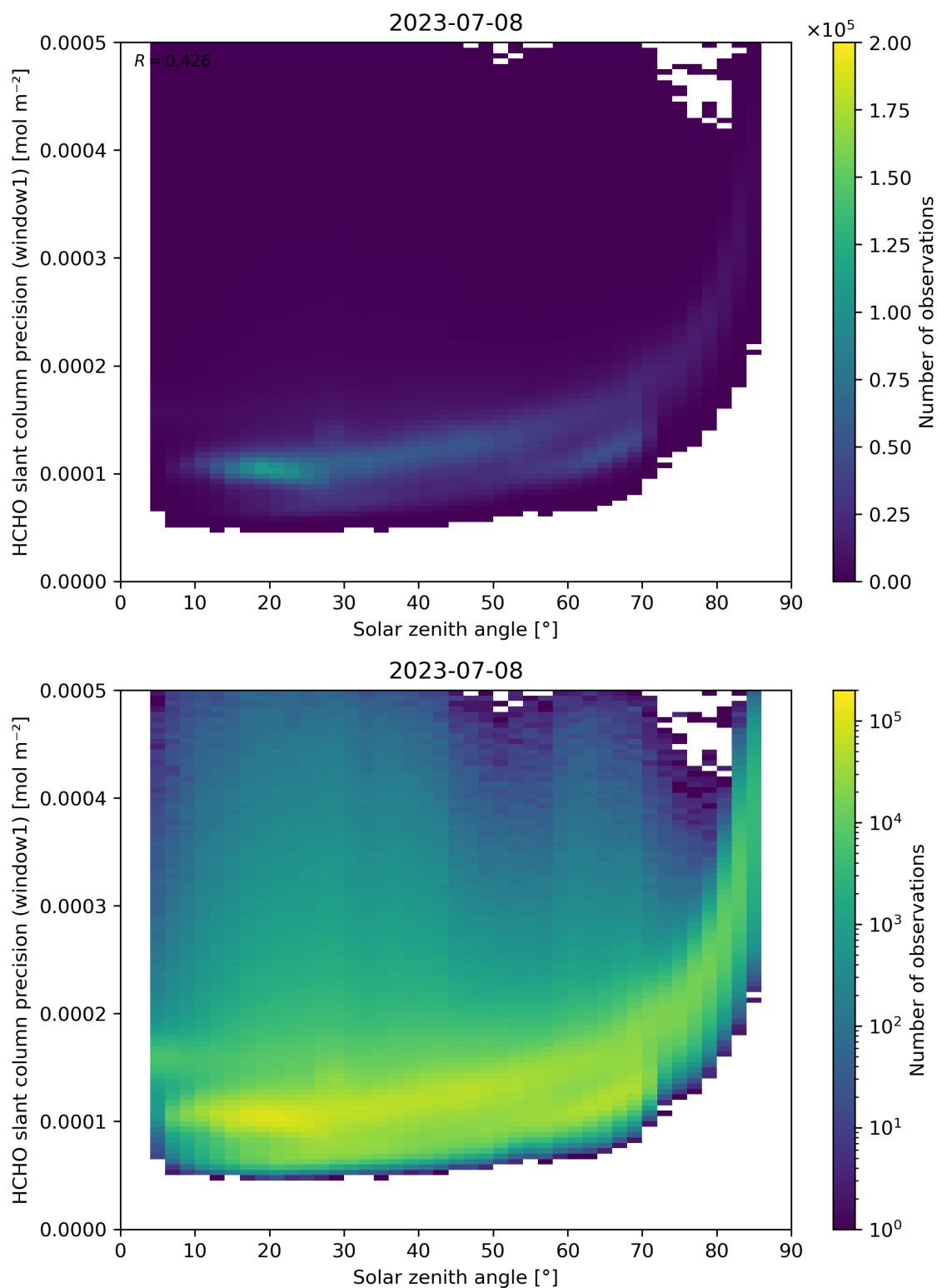
Figure 174: Scatter density plot of “Solar zenith angle” against “HCHO slant column precision (window1)” for 2023-07-08 to 2023-07-09.
