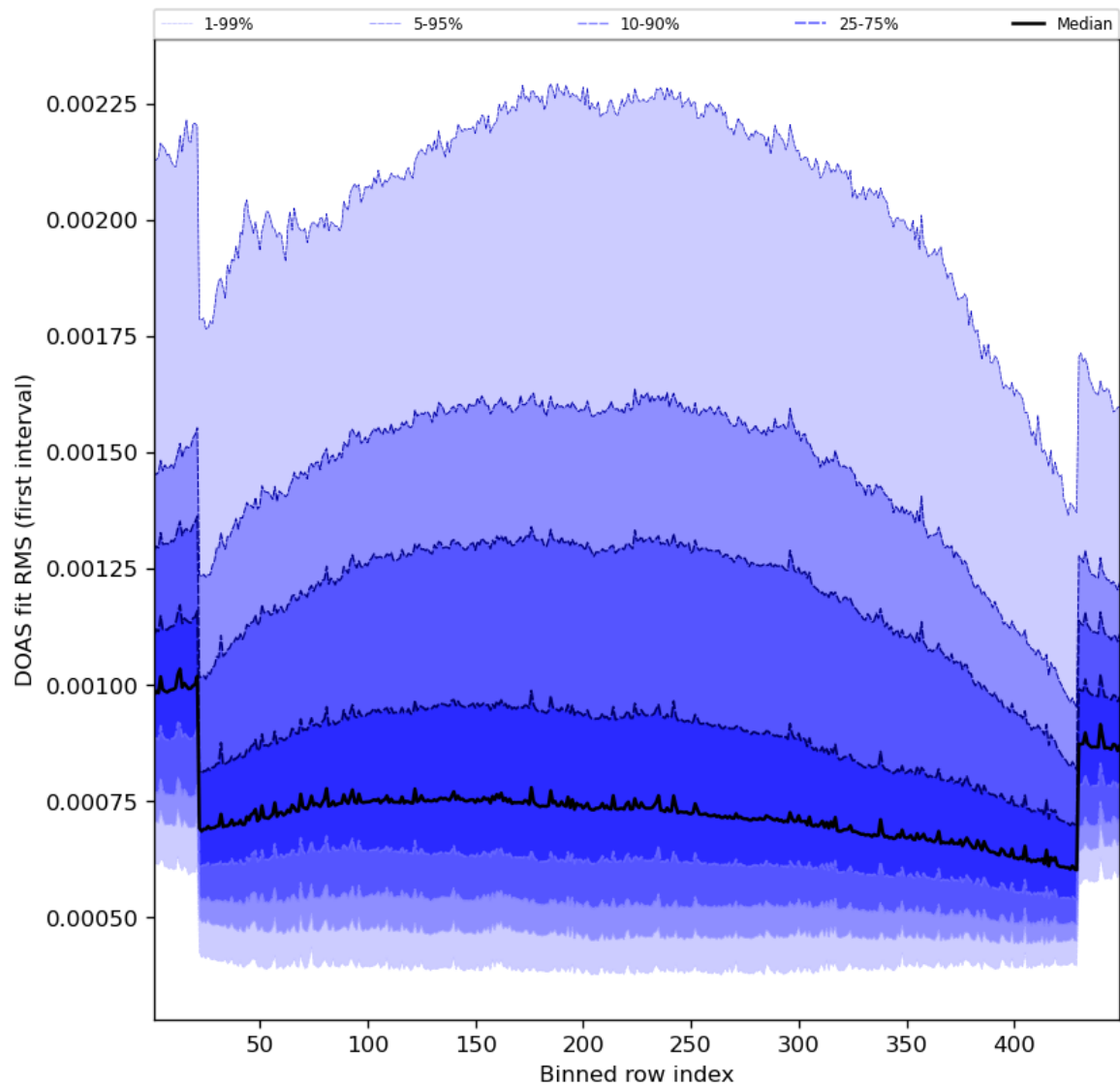
Figure 60: Along track statistics of “DOAS fit RMS (first interval)” for 2023-07-08 to 2023-07-09
