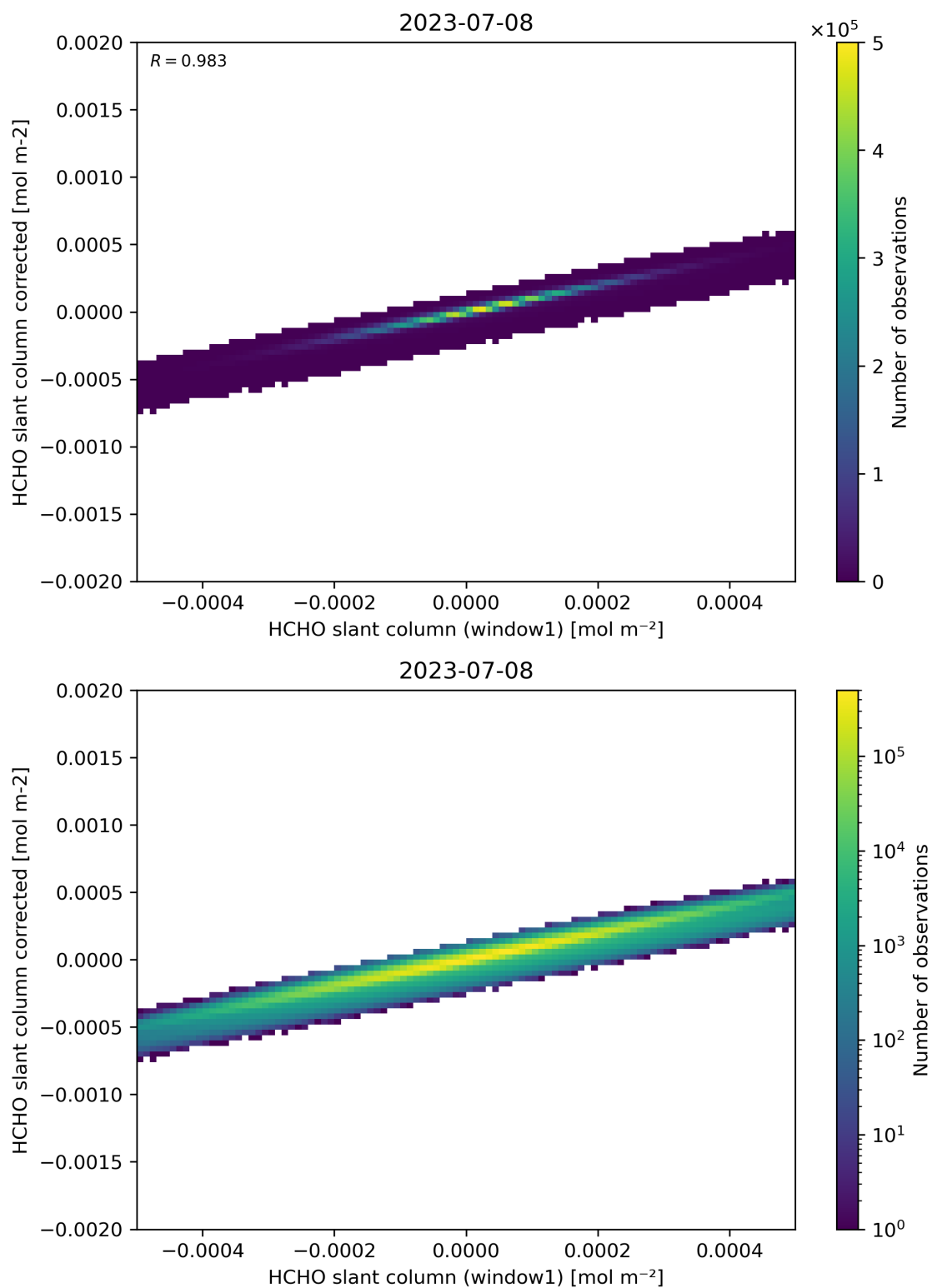
Figure 82: Scatter density plot of “HCHO slant column (window1)” against “HCHO slant column corrected” for 2023-07-08 to 2023-07-09.
