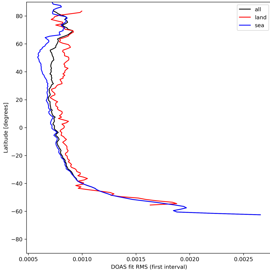
Figure 32: Zonal average of "DOAS fit RMS (first interval)" for 2023-07-08 to 2023-07-09.
