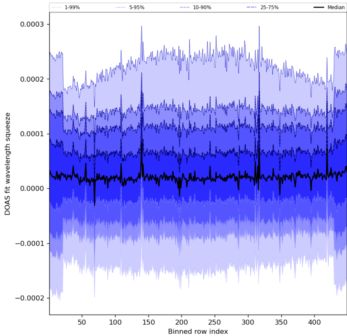
Figure 59: Along track statistics of “DOAS fit wavelength squeeze” for 2023-07-08 to 2023-07-09
