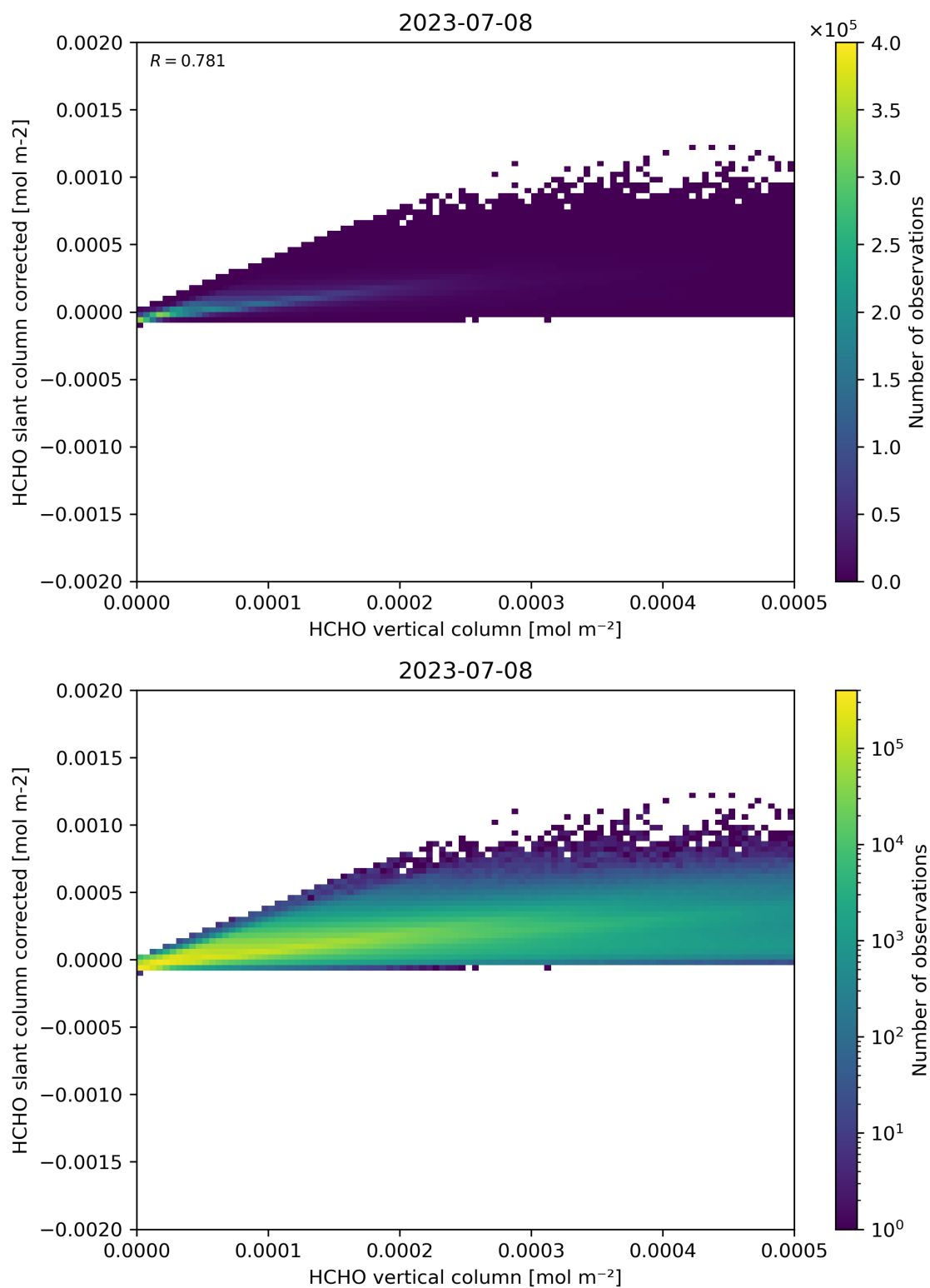
Figure 127: Scatter density plot of “HCHO vertical column” against “HCHO slant column corrected” for 2023-07-08 to 2023-07-09.
