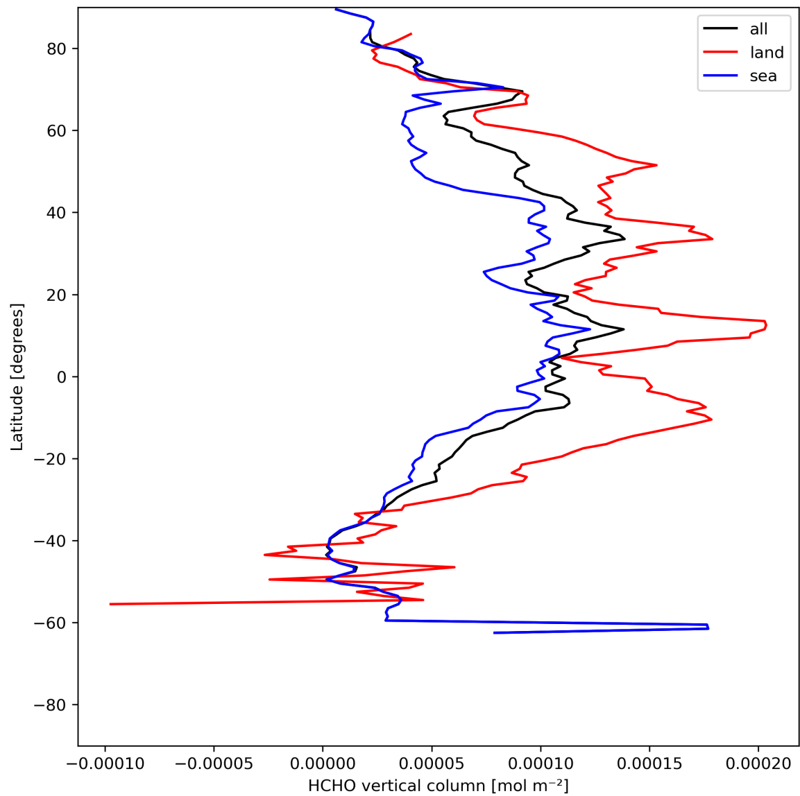
Figure 21: Zonal average of “HCHO vertical column” for 2023-07-08 to 2023-07-09.
