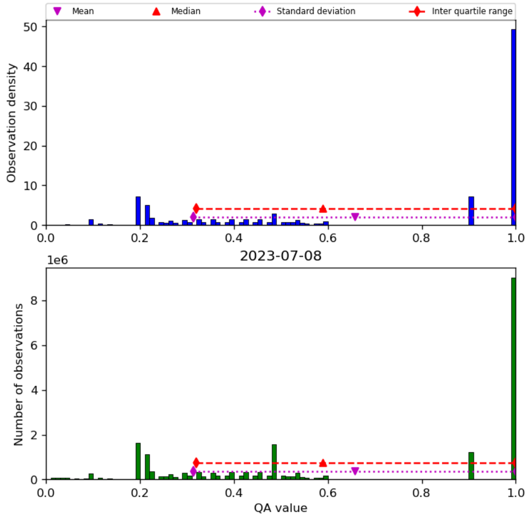
Figure 34: Histogram of “QA value” for 2023-07-08 to 2023-07-09
