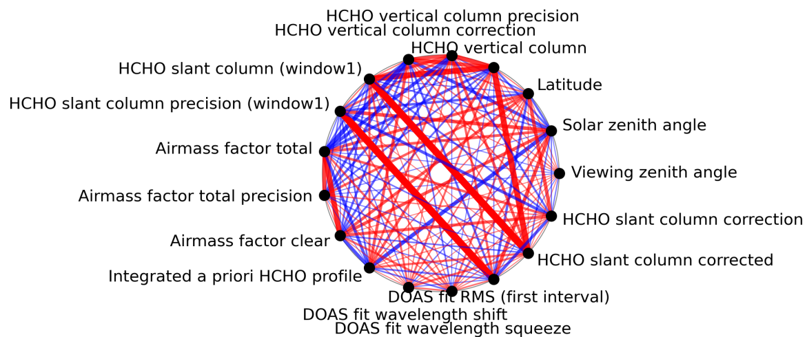
Figure 1: Map of correlation graph for 2023-07-08 to 2023-07-09.
