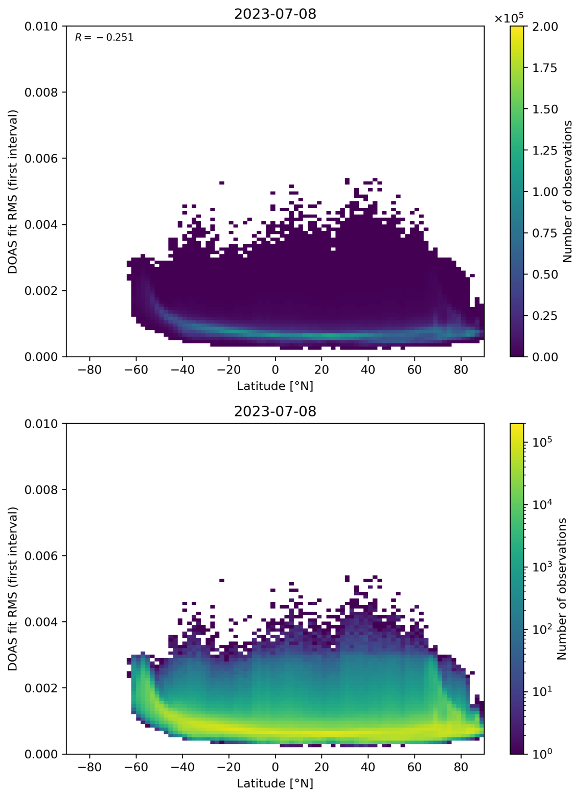
Figure 153: Scatter density plot of “Latitude” against “DOAS fit RMS (first interval)” for 2023-07-08 to 2023-07-09.
