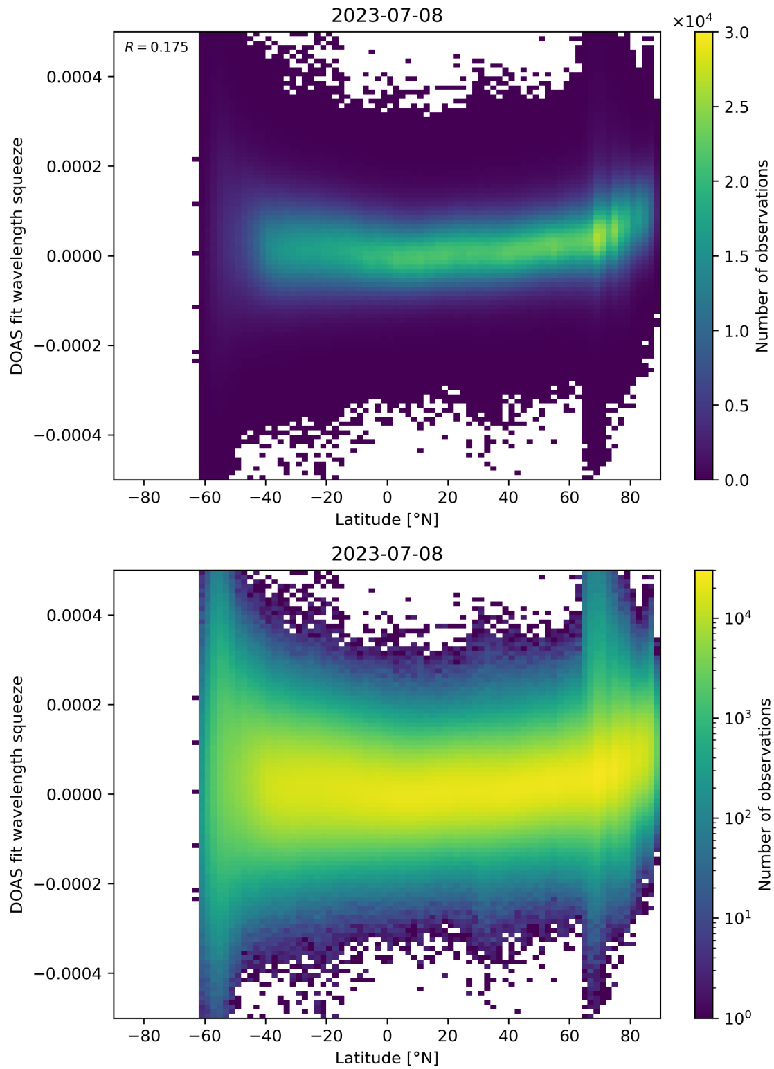
Figure 155: Scatter density plot of “Latitude” against “DOAS fit wavelength squeeze” for 2023-07-08 to 2023-07-09.
