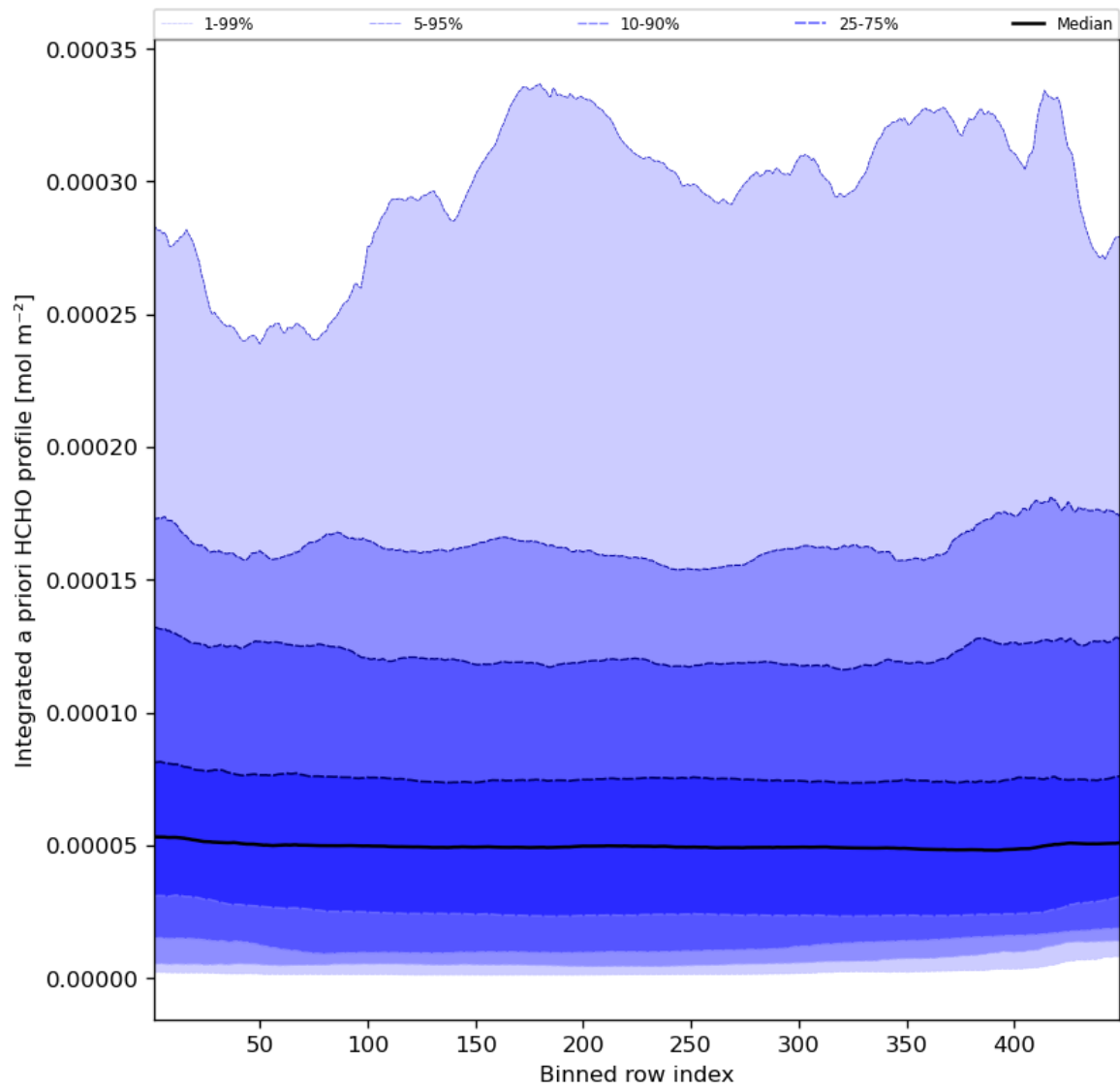
Figure 57: Along track statistics of “Integrated a priori HCHO profile” for 2023-07-08 to 2023-07-09
