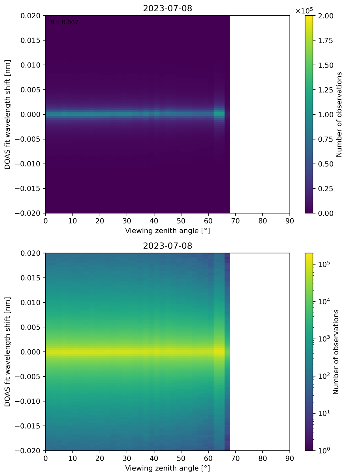
Figure 183: Scatter density plot of “Viewing zenith angle” against “DOAS fit wavelength shift” for 2023-07-08 to 2023-07-09.
