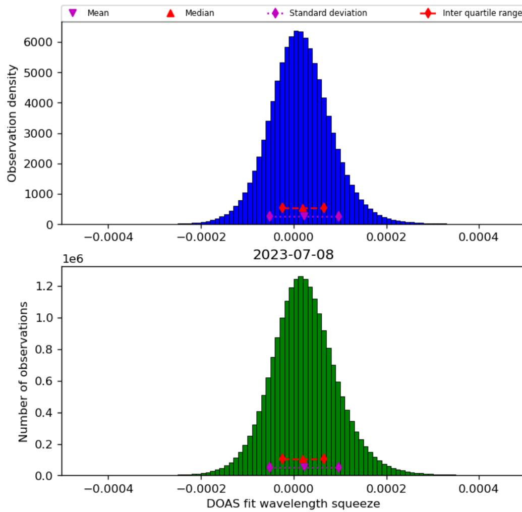
Figure 45: Histogram of “DOAS fit wavelength squeeze” for 2023-07-08 to 2023-07-09
