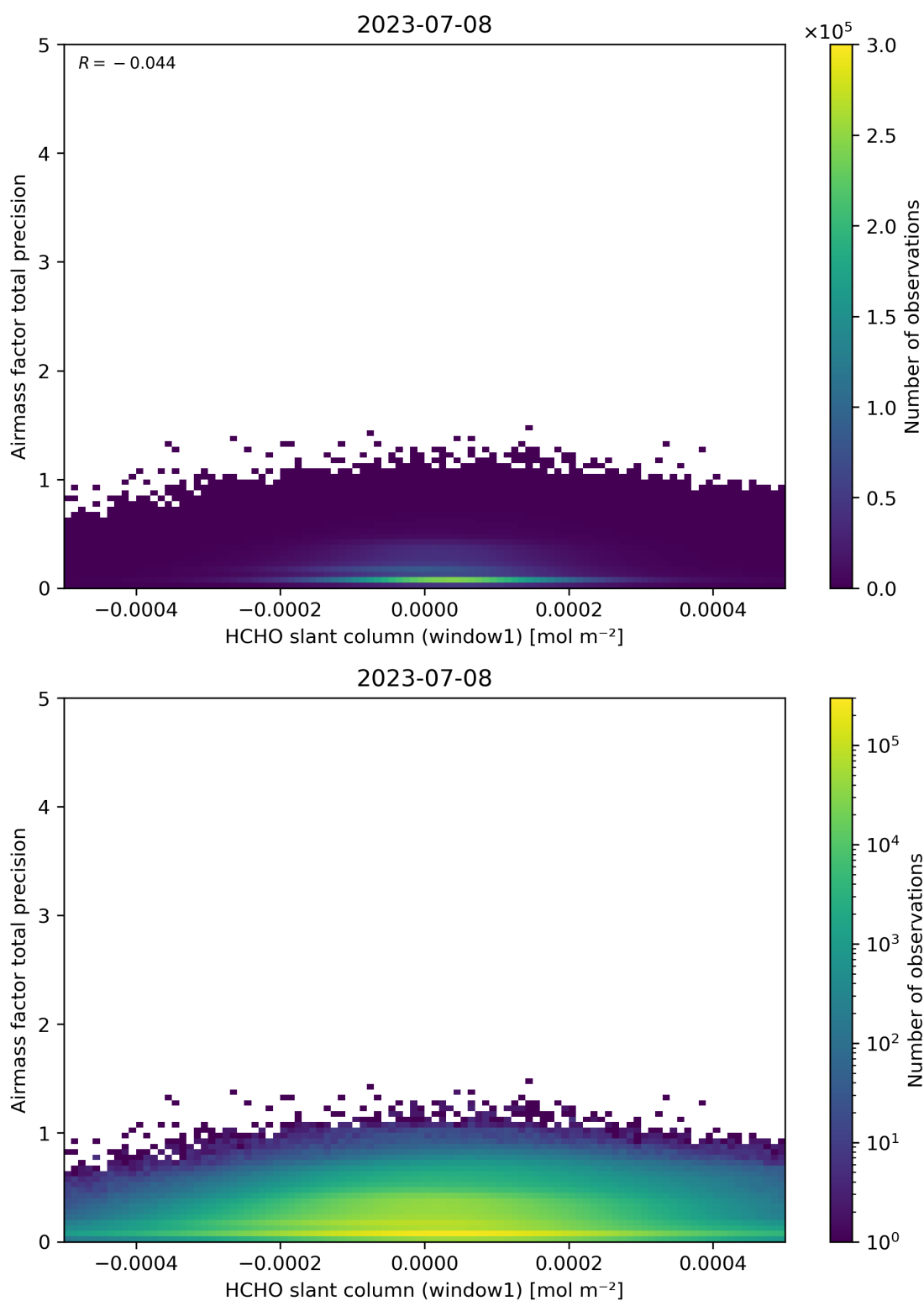
Figure 86: Scatter density plot of “HCHO slant column (window1)” against “Airmass factor total precision” for 2023-07-08 to 2023-07-09.
