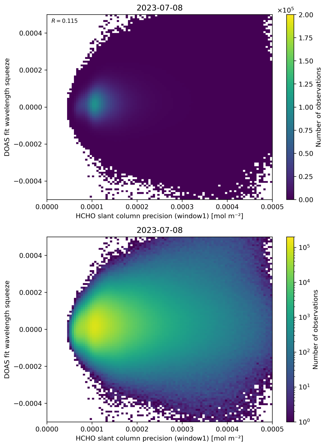
Figure 90: Scatter density plot of “HCHO slant column precision (window1)” against “DOAS fit wavelength squeeze” for 2023-07-08 to 2023-07-09.
