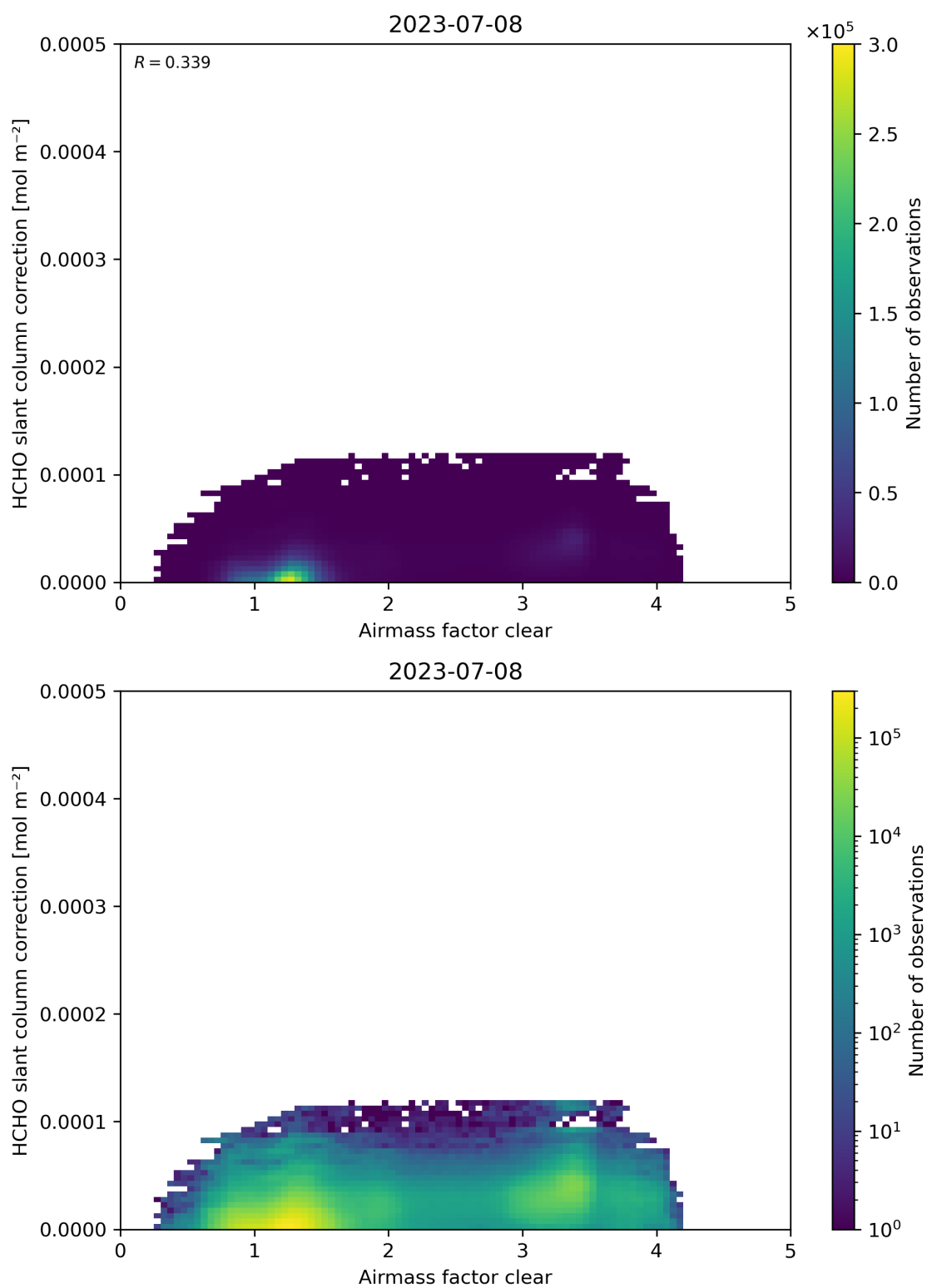
Figure 75: Scatter density plot of “Airmass factor clear” against “HCHO slant column correction” for 2023-07-08 to 2023-07-09.
