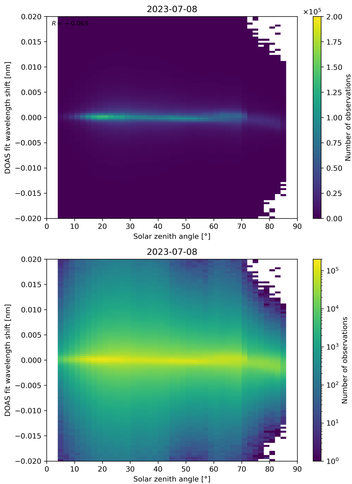
Figure 168: Scatter density plot of “Solar zenith angle” against “DOAS fit wavelength shift” for 2023-07-08 to 2023-07-09.
