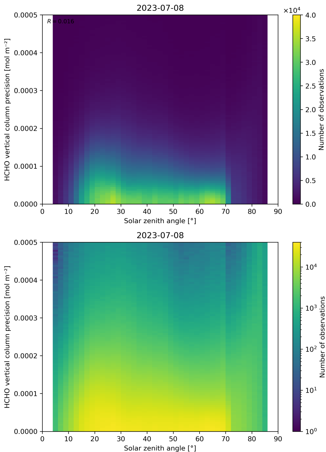
Figure 179: Scatter density plot of “Solar zenith angle” against “HCHO vertical column precision” for 2023-07-08 to 2023-07-09.
