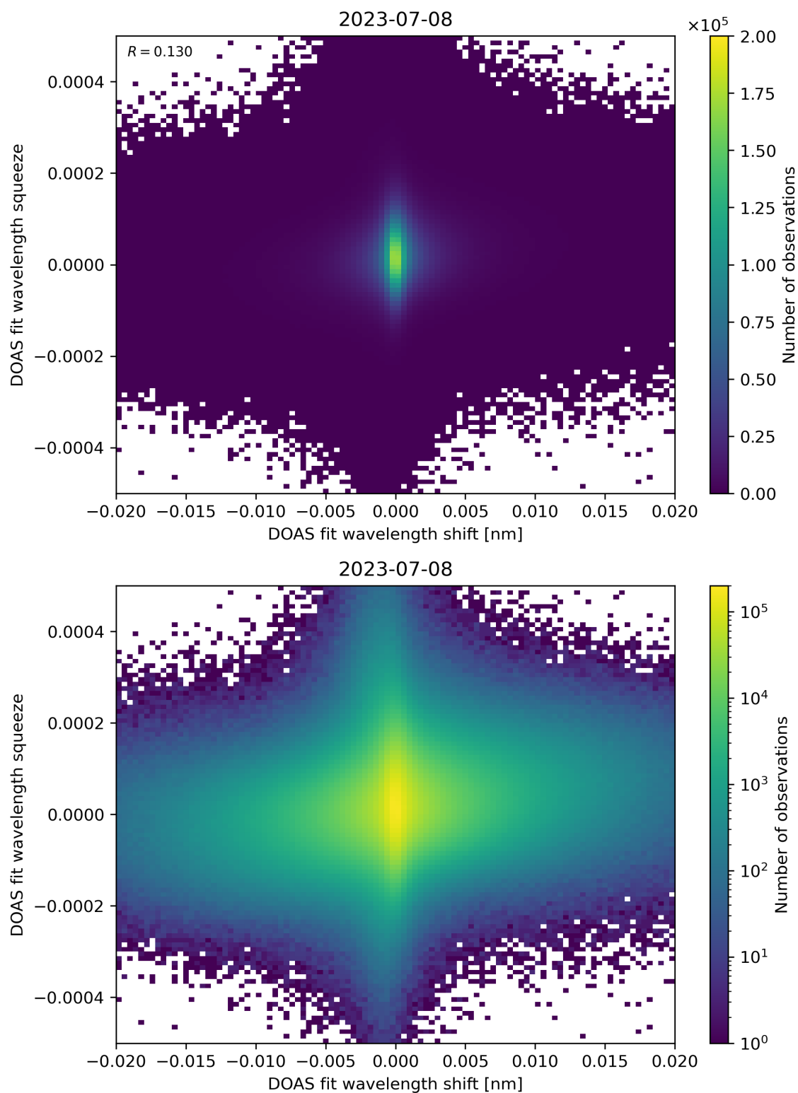
Figure 65: Scatter density plot of “DOAS fit wavelength shift” against “DOAS fit wavelength squeeze” for 2023-07-08 to 2023-07-09.
