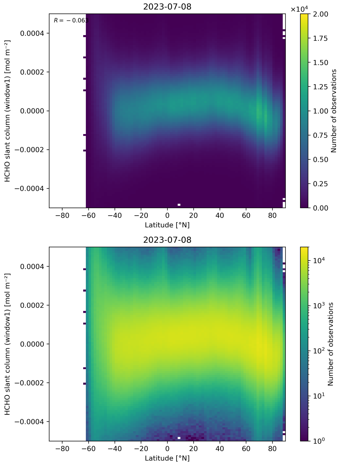
Figure 159: Scatter density plot of “Latitude” against “HCHO slant column (window1)” for 2023-07-08 to 2023-07-09.
