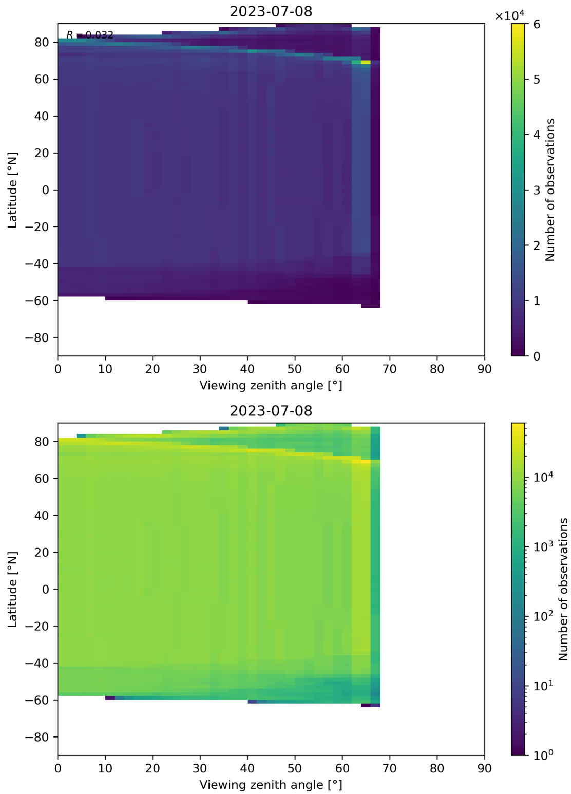
Figure 196: Scatter density plot of “Viewing zenith angle” against “Latitude” for 2023-07-08 to 2023-07-09.
