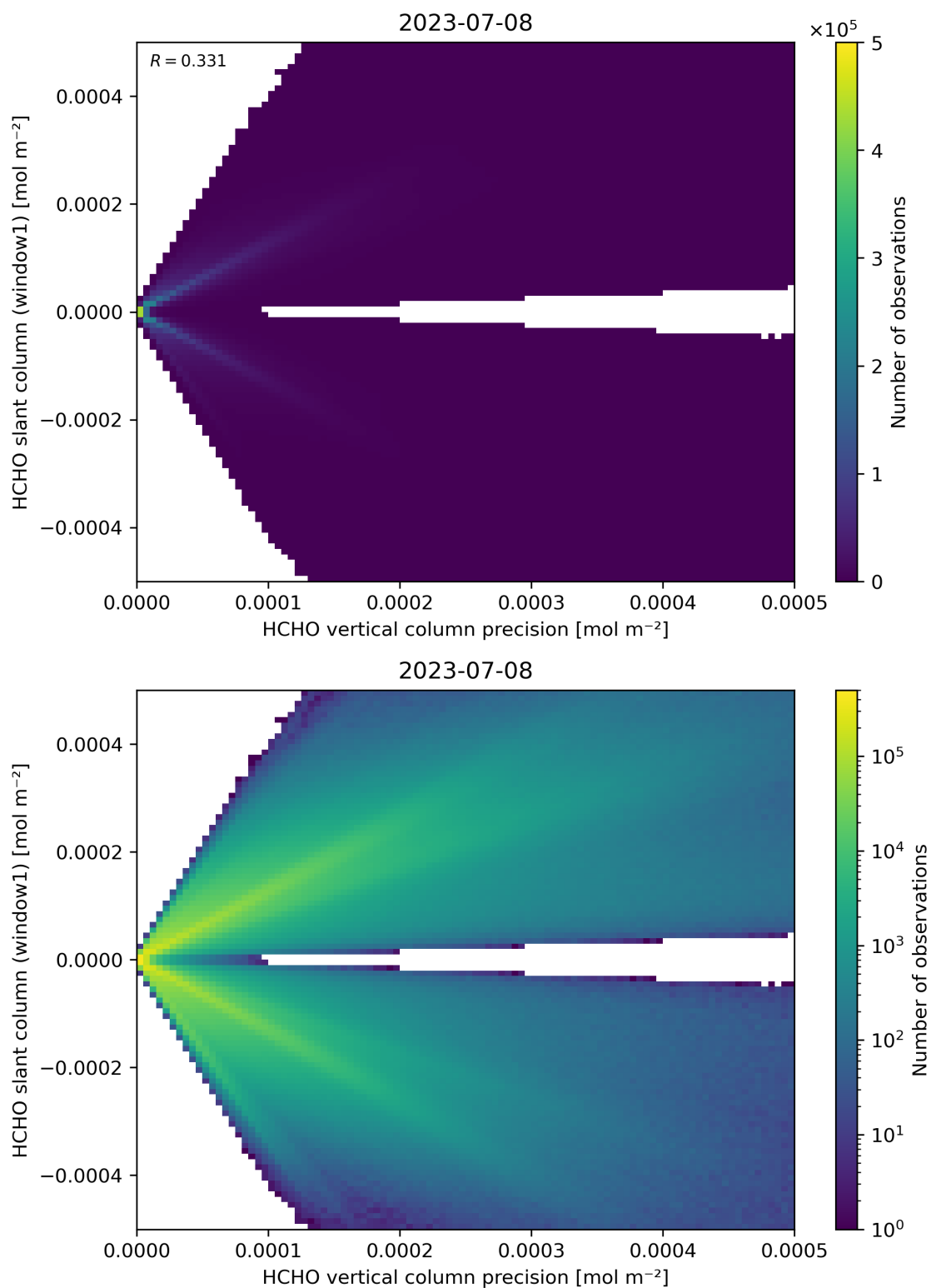
Figure 142: Scatter density plot of “HCHO vertical column precision” against “HCHO slant column (window1)” for 2023-07-08 to 2023-07-09.
