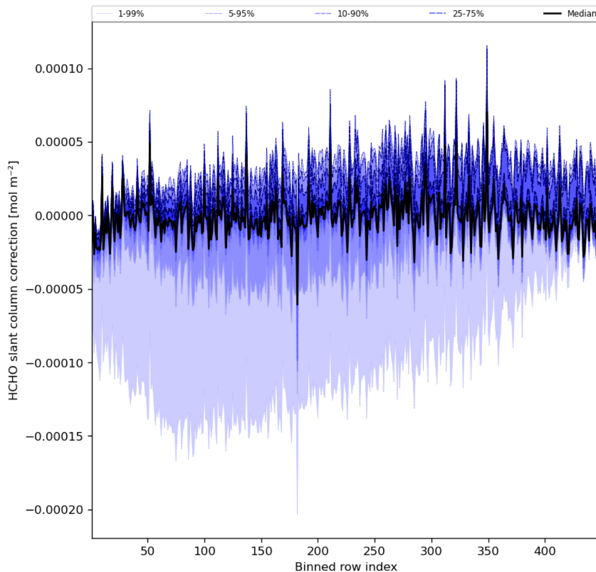
Figure 61: Along track statistics of “HCHO slant column correction” for 2023-07-08 to 2023-07-09
