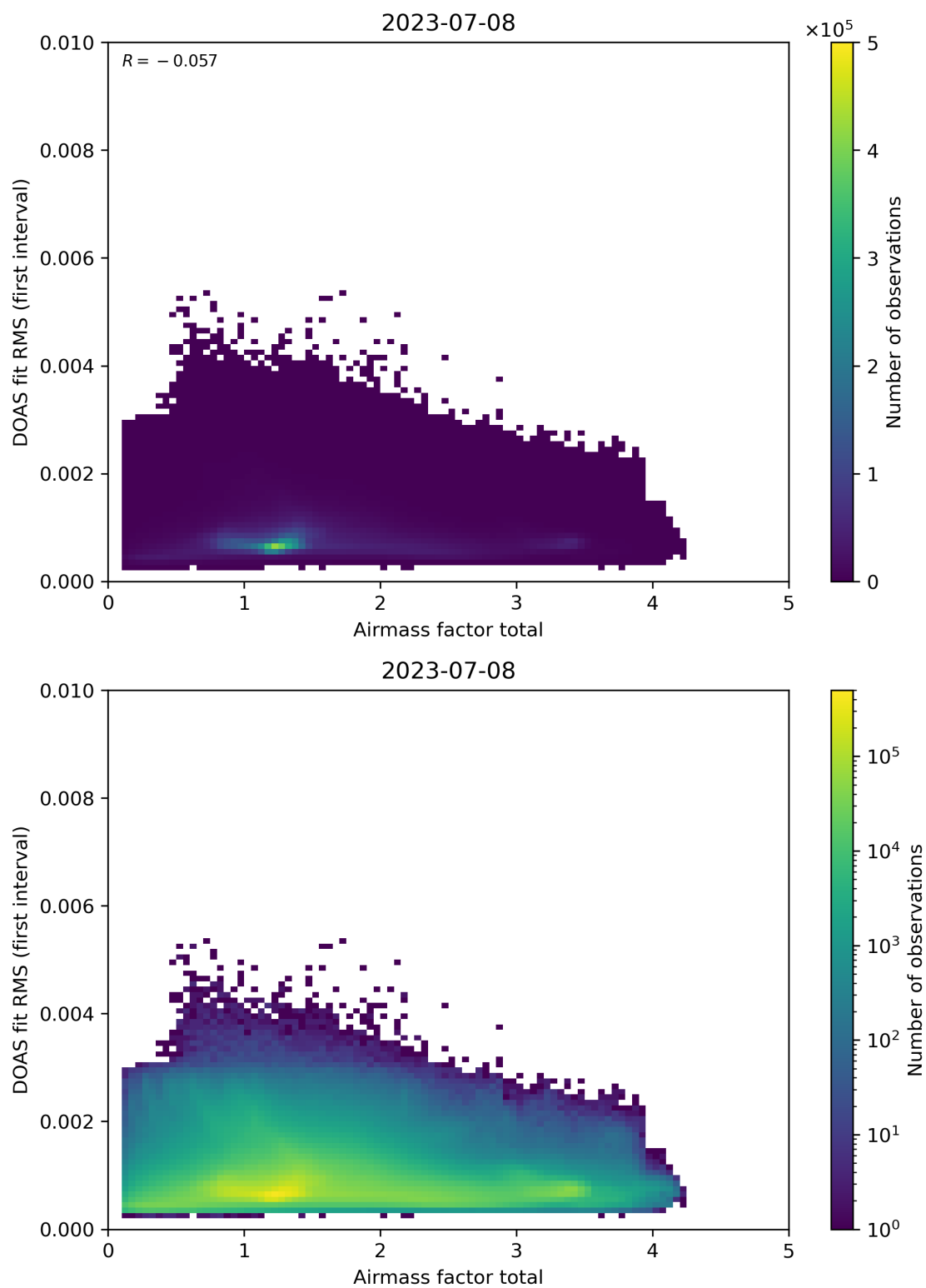
Figure 97: Scatter density plot of “Airmass factor total” against “DOAS fit RMS (first interval)” for 2023-07-08 to 2023-07-09.
