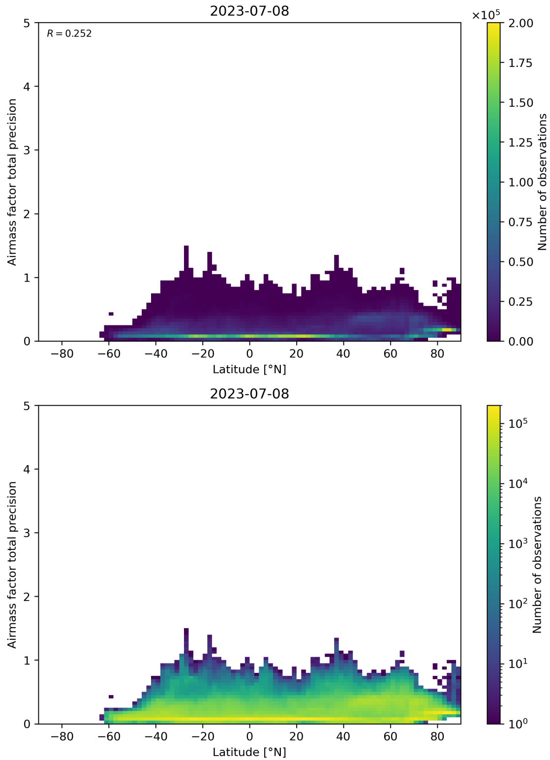
Figure 162: Scatter density plot of “Latitude” against “Airmass factor total precision” for 2023-07-08 to 2023-07-09.
