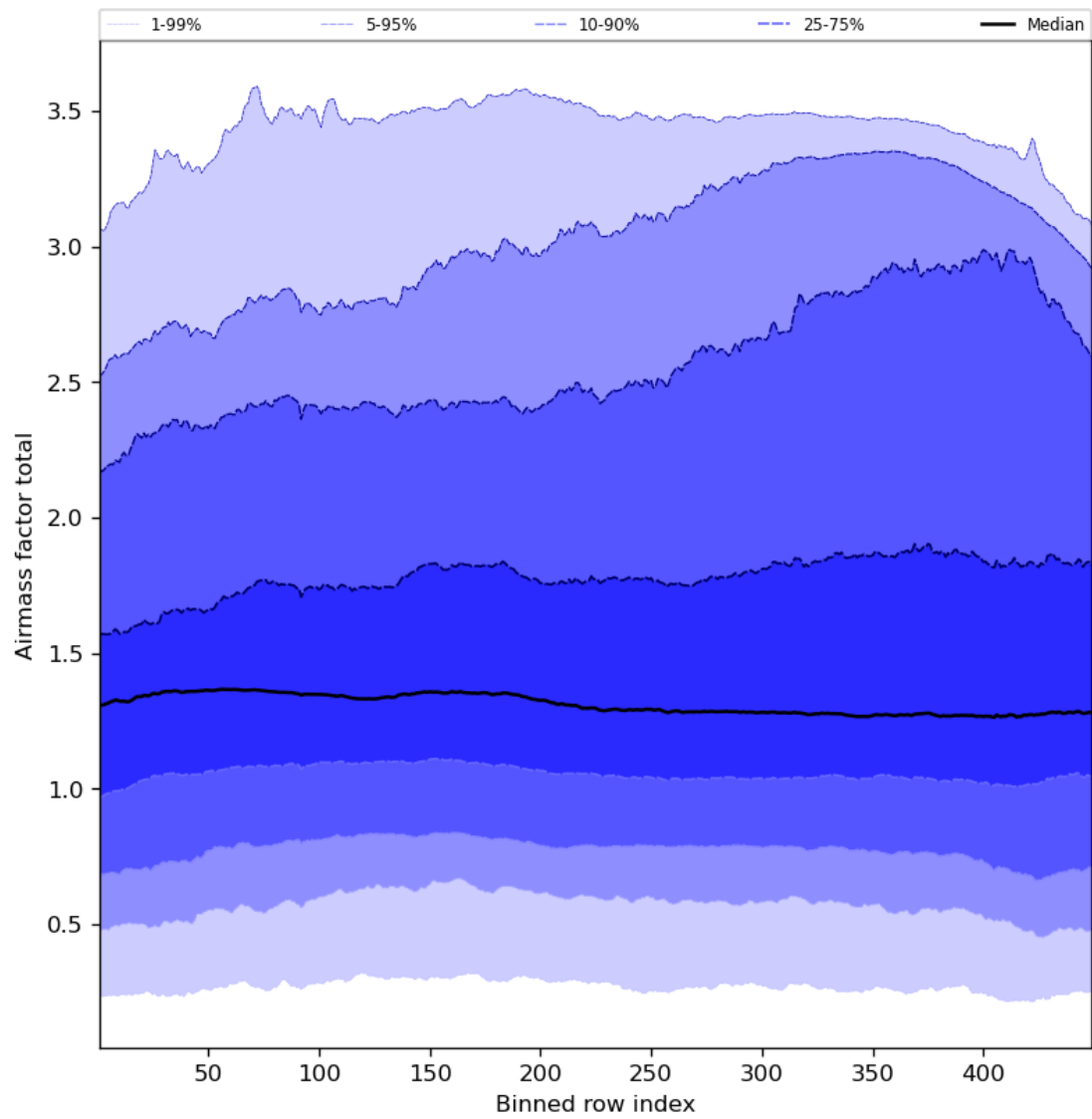
Figure 54: Along track statistics of “Airmass factor total” for 2023-07-08 to 2023-07-09
