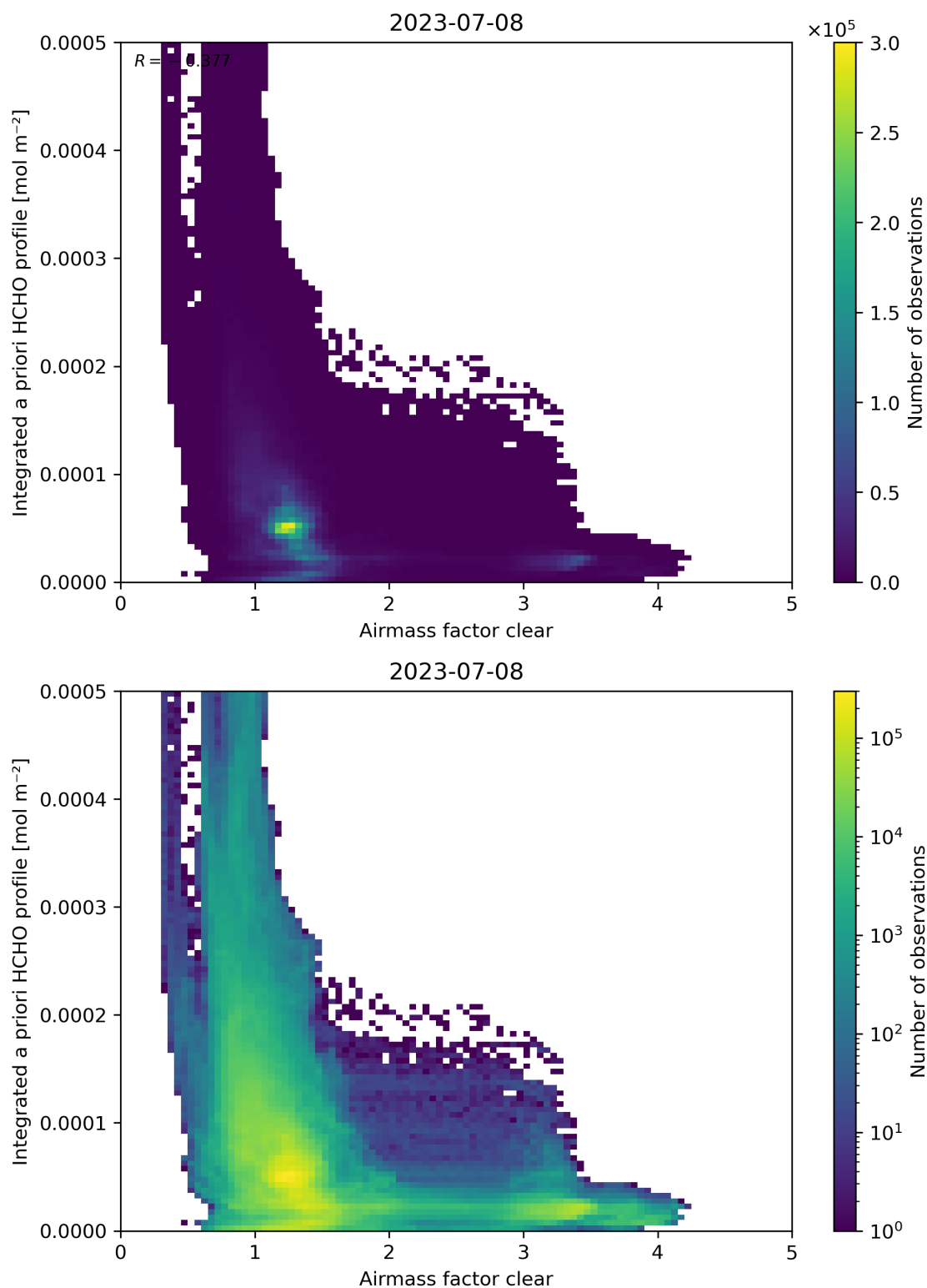
Figure 76: Scatter density plot of “Airmass factor clear” against “Integrated a priori HCHO profile” for 2023-07-08 to 2023-07-09.
