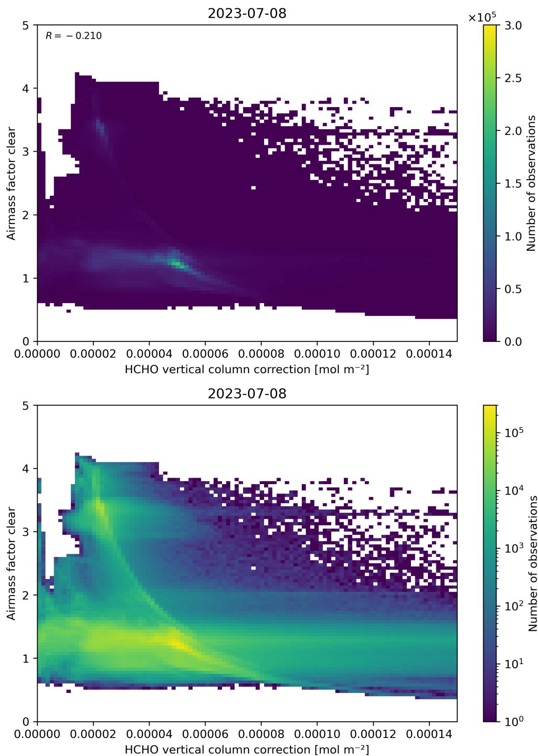
Figure 115: Scatter density plot of “HCHO vertical column correction” against “Airmass factor clear” for 2023-07-08 to 2023-07-09.
