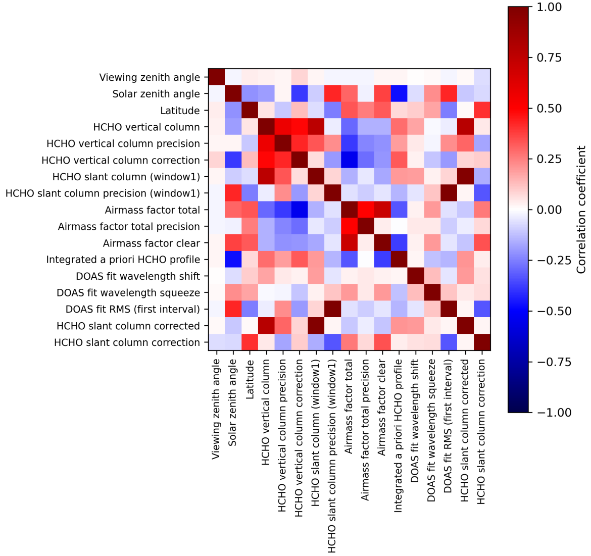
Figure 2: Map of correlation matrix for 2023-07-08 to 2023-07-09.
