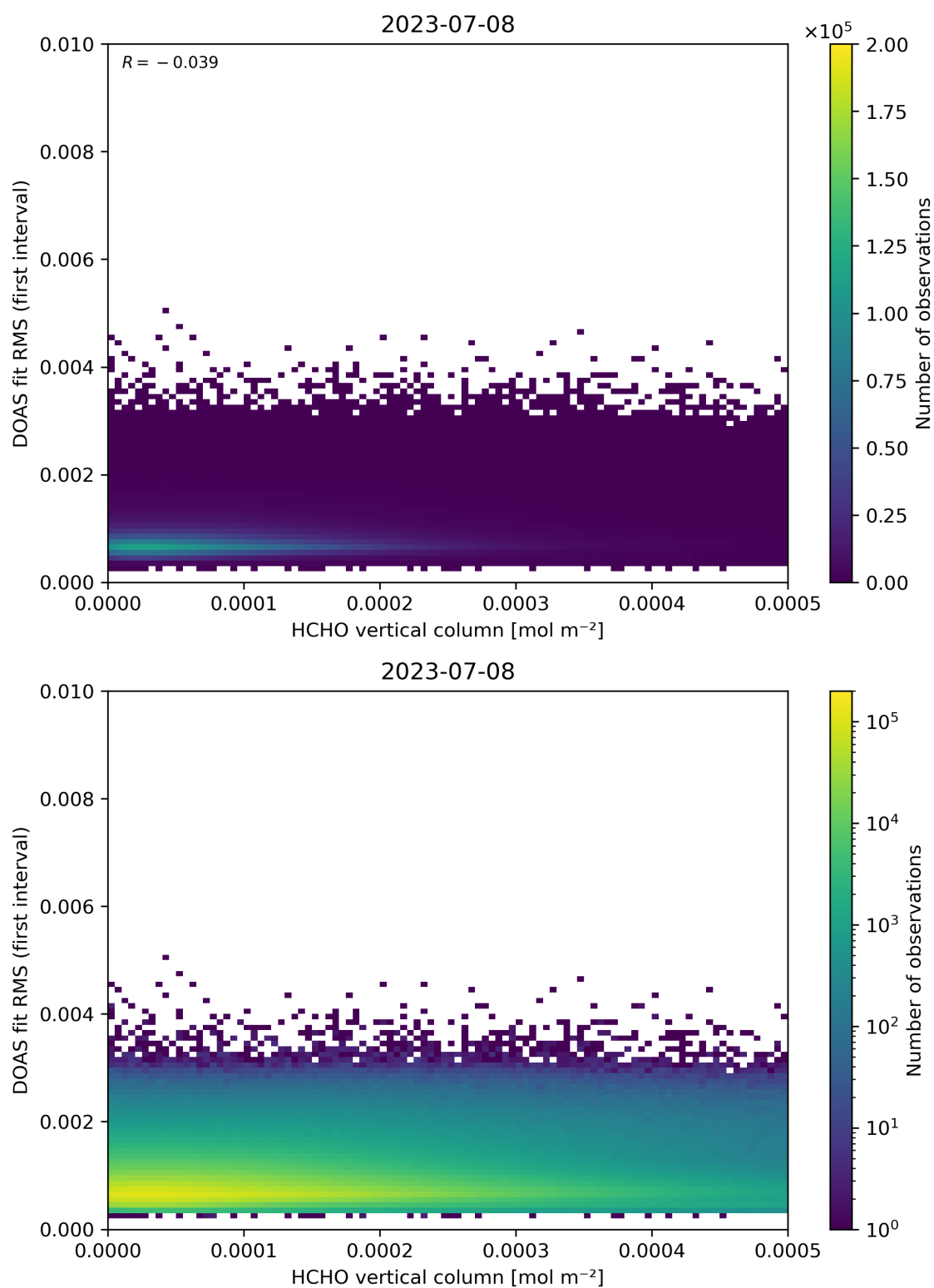
Figure 123: Scatter density plot of “HCHO vertical column” against “DOAS fit RMS (first interval)” for 2023-07-08 to 2023-07-09.
