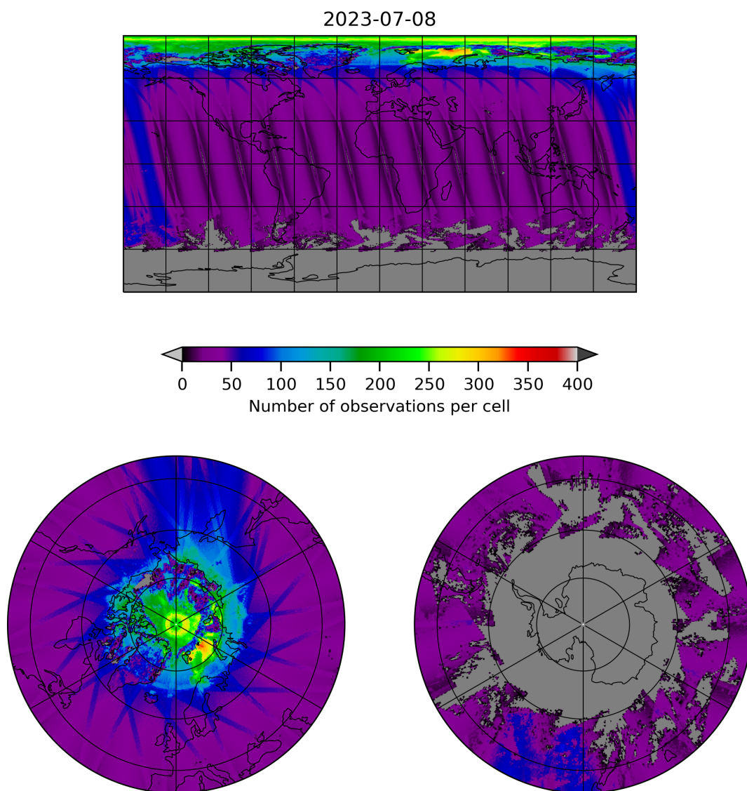
Figure 19: Map of the number of observations for 2023-07-08 to 2023-07-09
