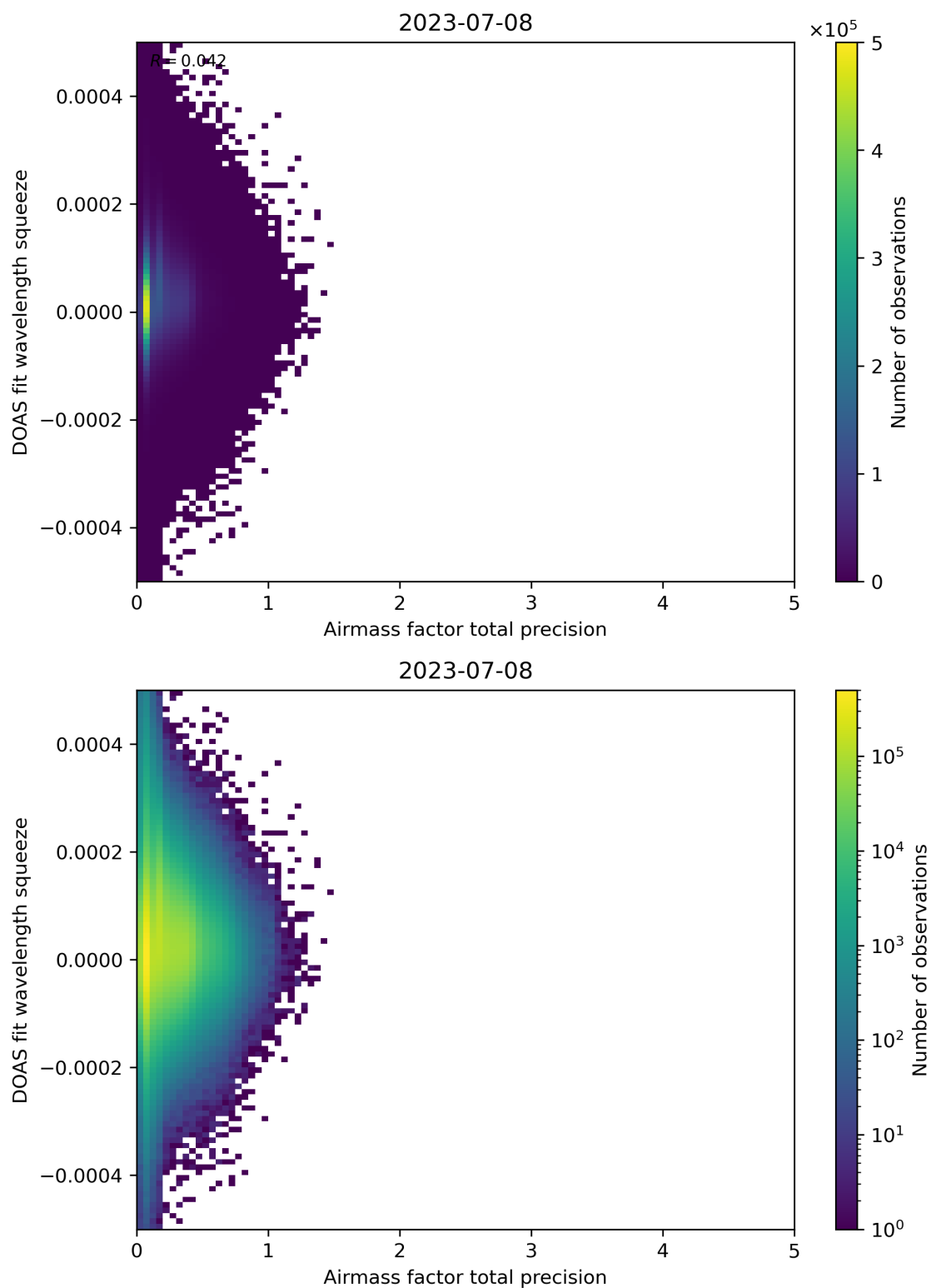
Figure 107: Scatter density plot of “Airmass factor total precision” against “DOAS fit wavelength squeeze” for 2023-07-08 to 2023-07-09.
