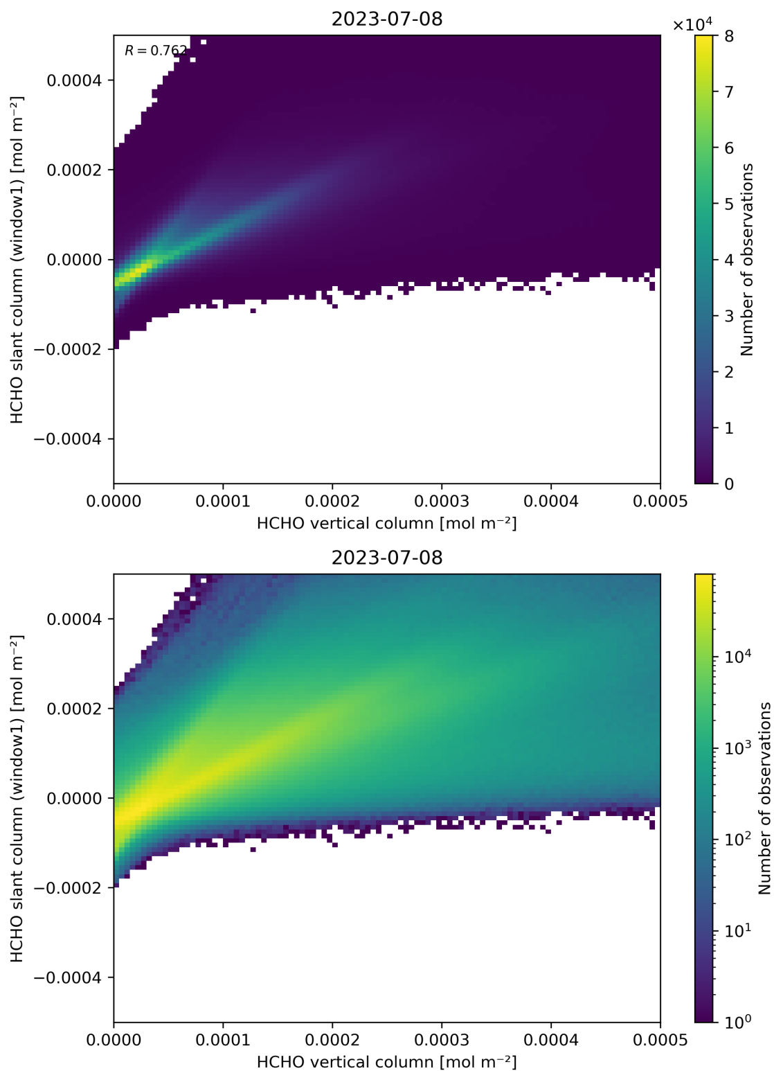
Figure 129: Scatter density plot of “HCHO vertical column” against “HCHO slant column (window1)” for 2023-07-08 to 2023-07-09.
