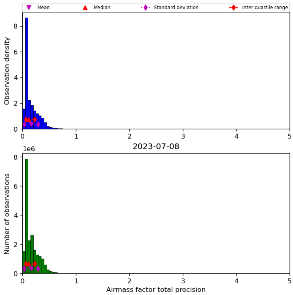
Figure 41: Histogram of “Airmass factor total precision” for 2023-07-08 to 2023-07-09
