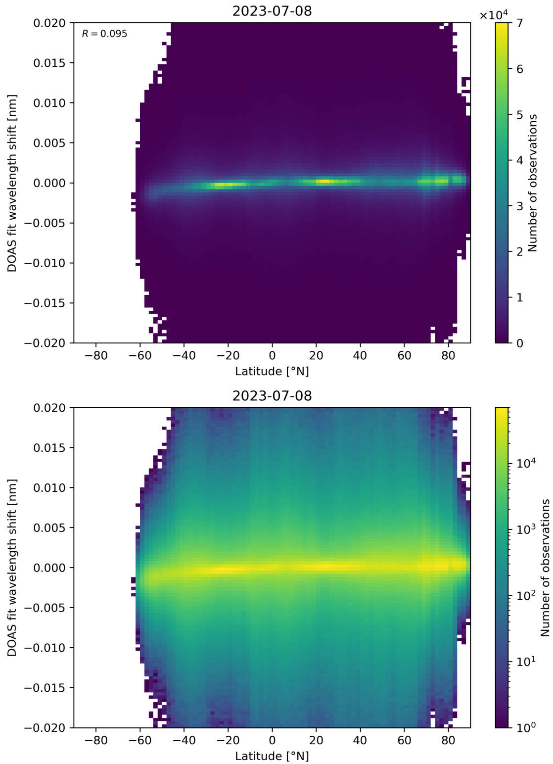
Figure 154: Scatter density plot of “Latitude” against “DOAS fit wavelength shift” for 2023-07-08 to 2023-07-09.
