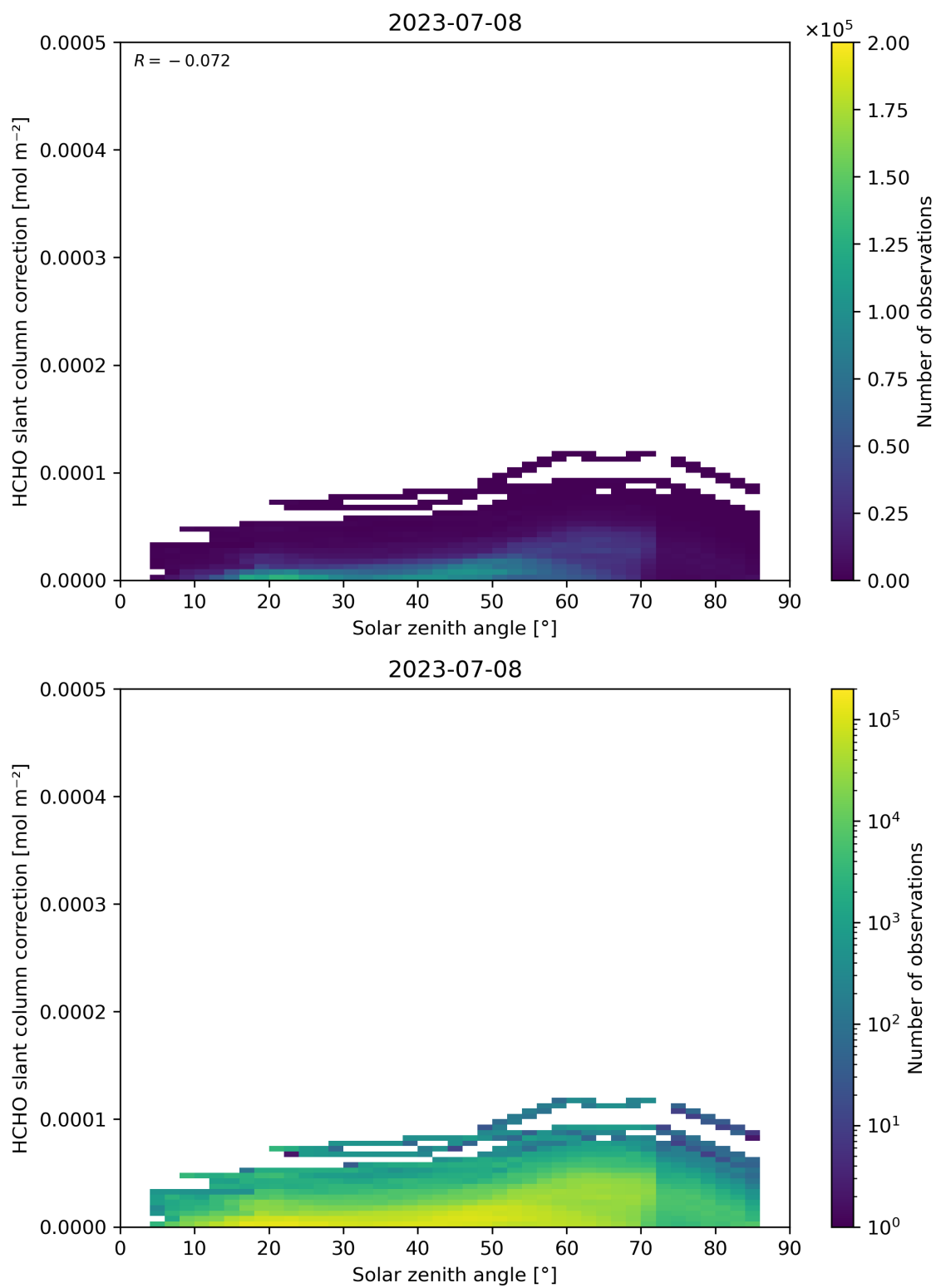
Figure 172: Scatter density plot of “Solar zenith angle” against “HCHO slant column correction” for 2023-07-08 to 2023-07-09.
