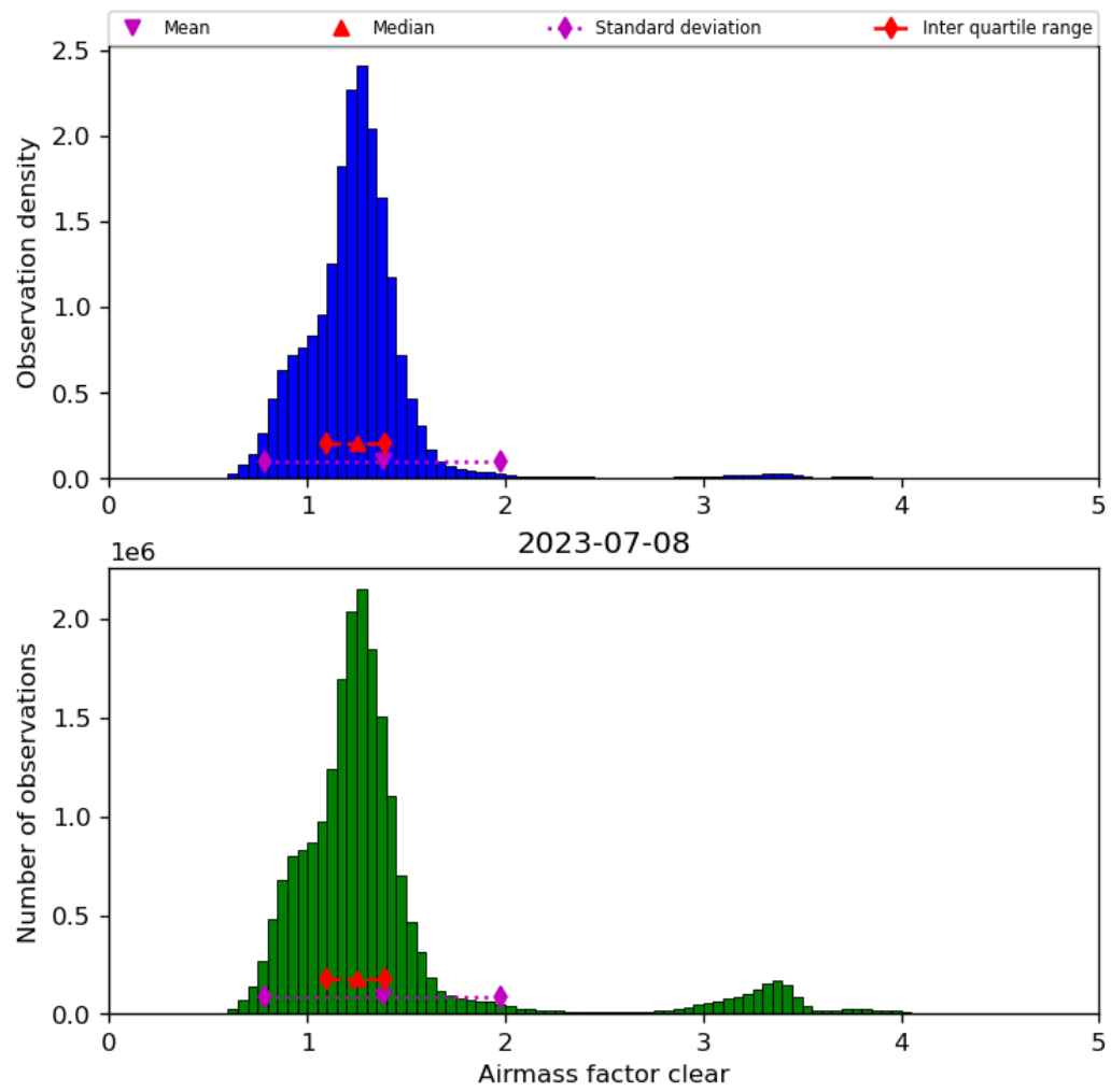
Figure 42: Histogram of “Airmass factor clear” for 2023-07-08 to 2023-07-09
