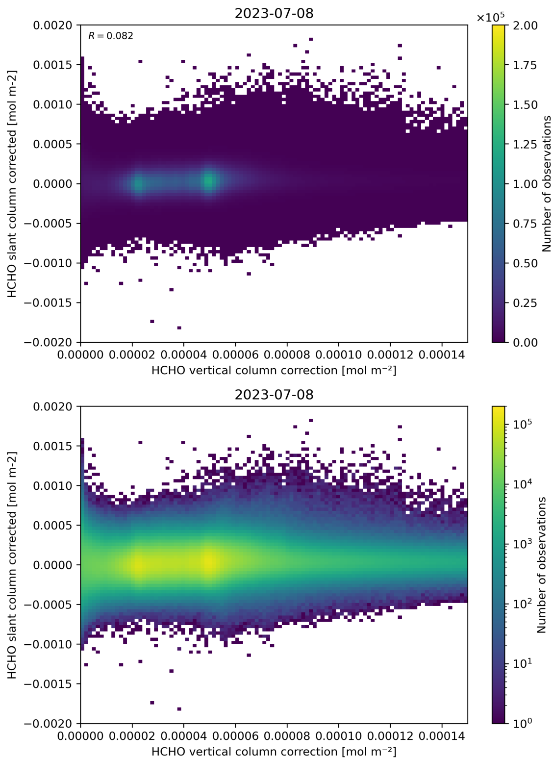
Figure 116: Scatter density plot of “HCHO vertical column correction” against “HCHO slant column corrected” for 2023-07-08 to 2023-07-09.
