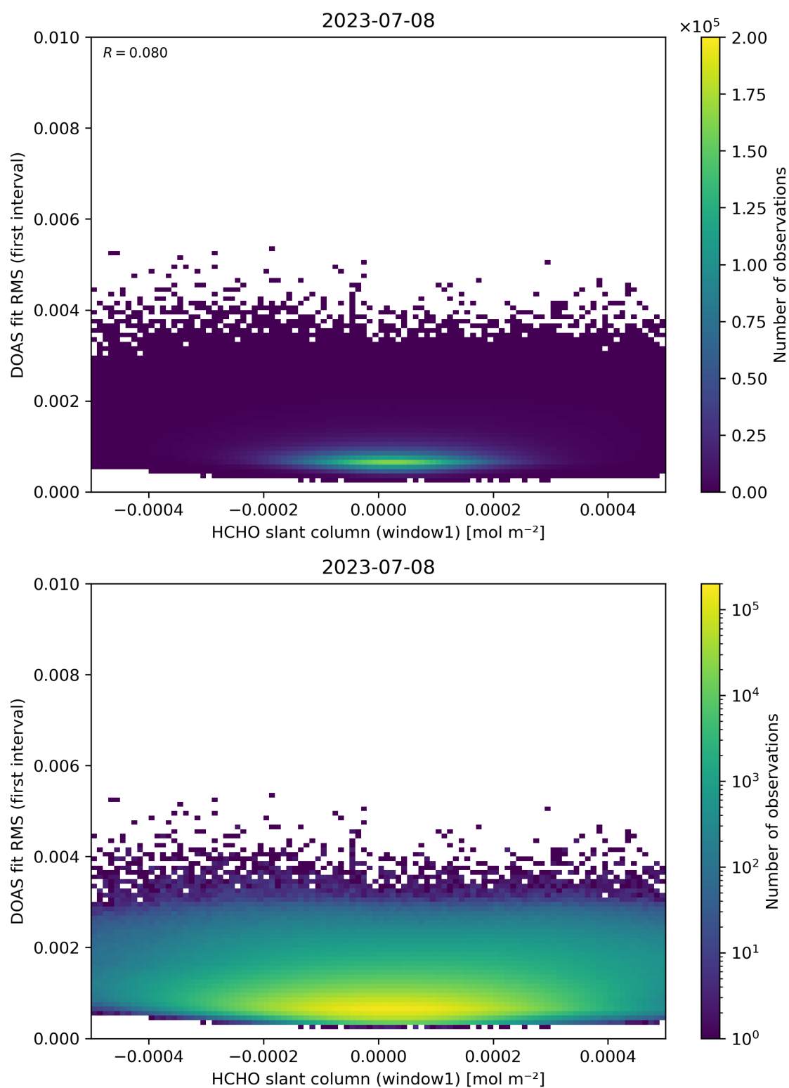
Figure 78: Scatter density plot of “HCHO slant column (window1)” against “DOAS fit RMS (first interval)” for 2023-07-08 to 2023-07-09.
