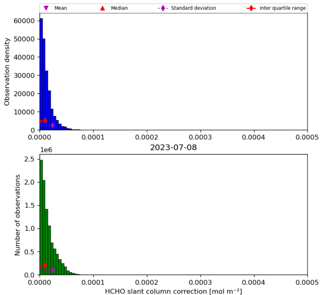
Figure 47: Histogram of “HCHO slant column correction” for 2023-07-08 to 2023-07-09
