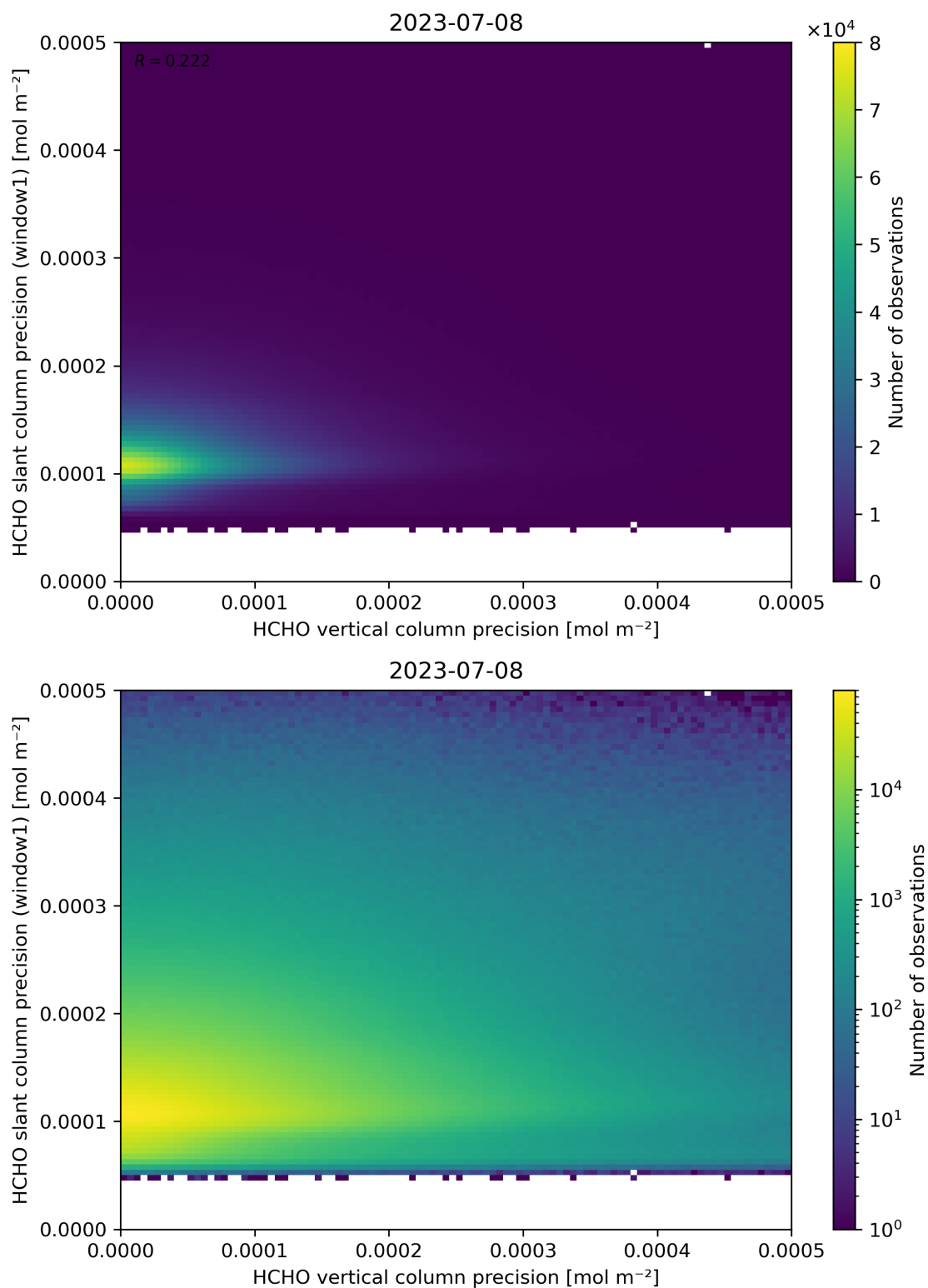
Figure 143: Scatter density plot of “HCHO vertical column precision” against “HCHO slant column precision (window1)” for 2023-07-08 to 2023-07-09.
