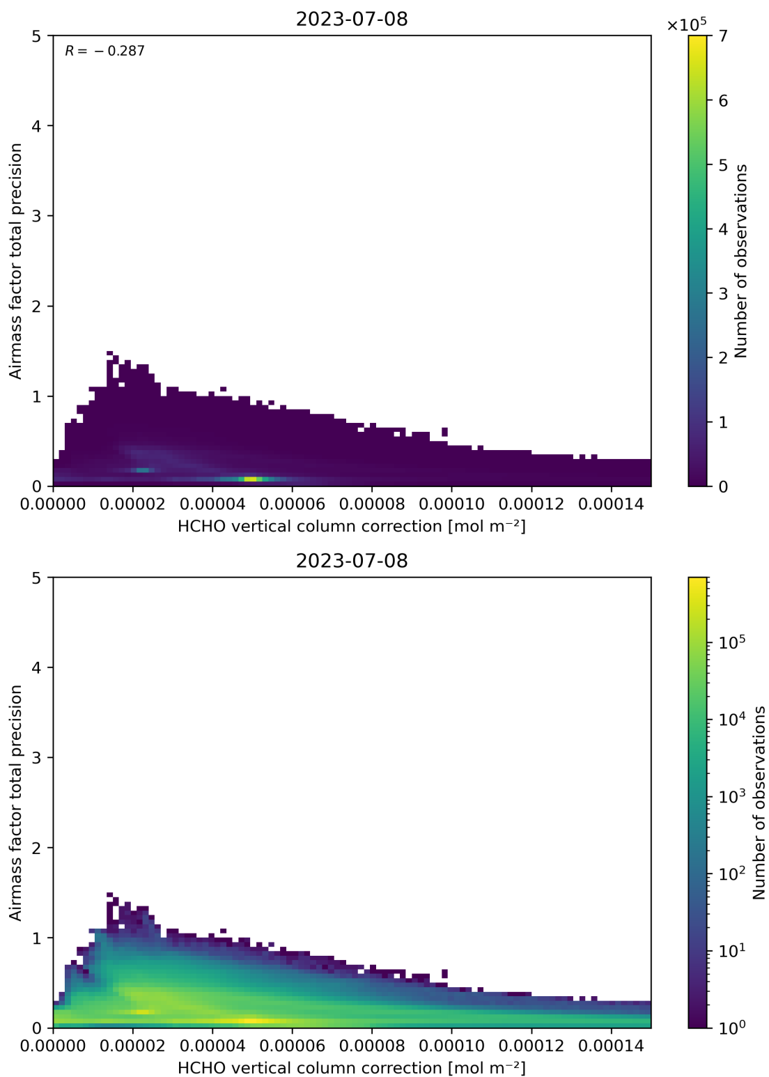
Figure 121: Scatter density plot of “HCHO vertical column correction” against “Airmass factor total precision” for 2023-07-08 to 2023-07-09.
