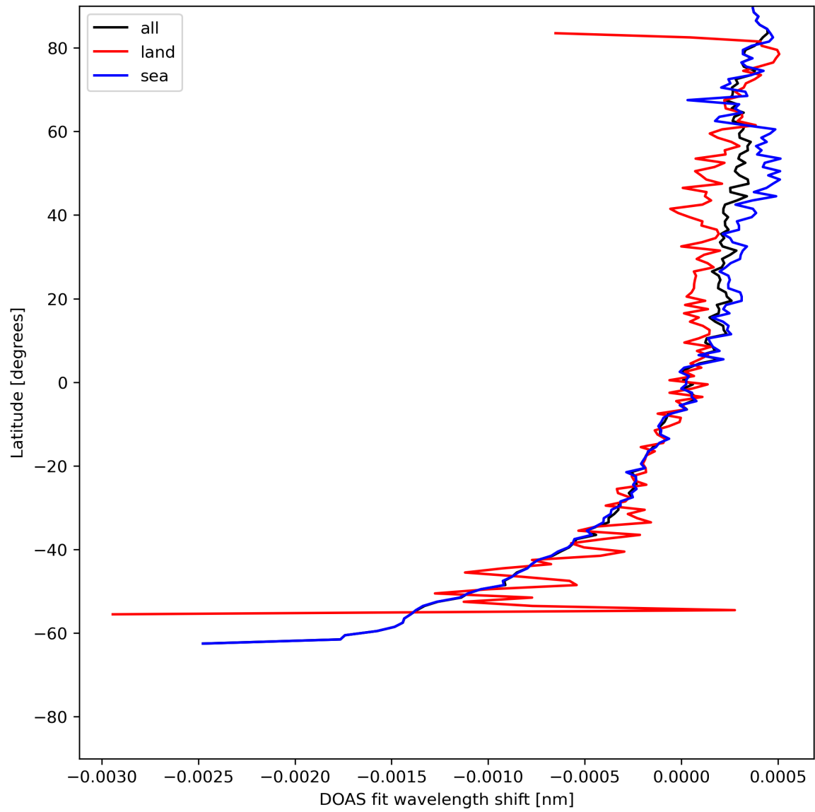
Figure 30: Zonal average of “DOAS fit wavelength shift” for 2023-07-08 to 2023-07-09.
