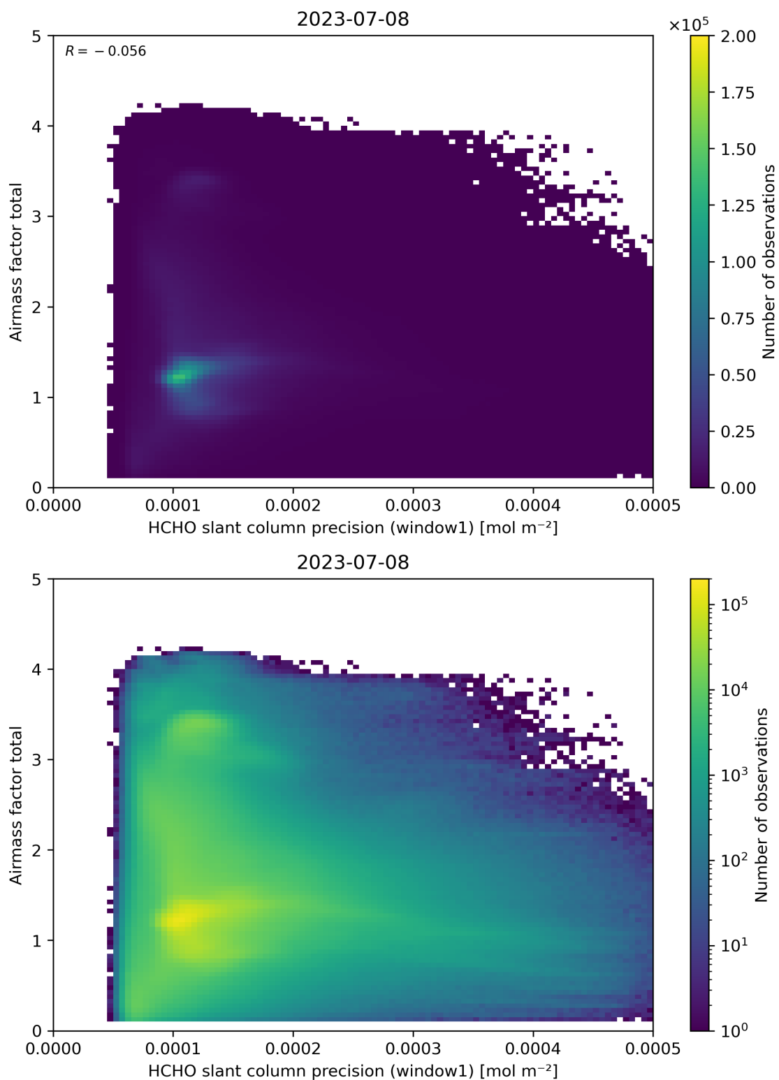
Figure 94: Scatter density plot of “HCHO slant column precision (window1)” against “Airmass factor total” for 2023-07-08 to 2023-07-09.
