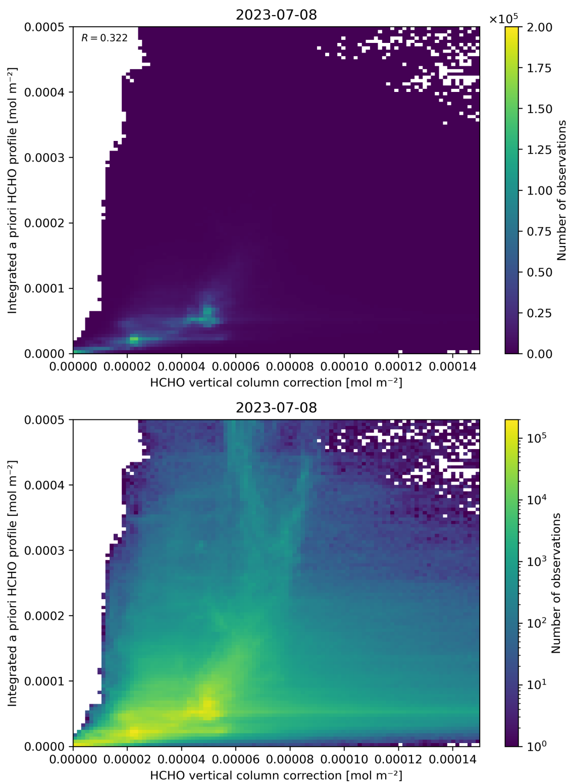
Figure 122: Scatter density plot of “HCHO vertical column correction” against “Integrated a priori HCHO profile” for 2023-07-08 to 2023-07-09.
