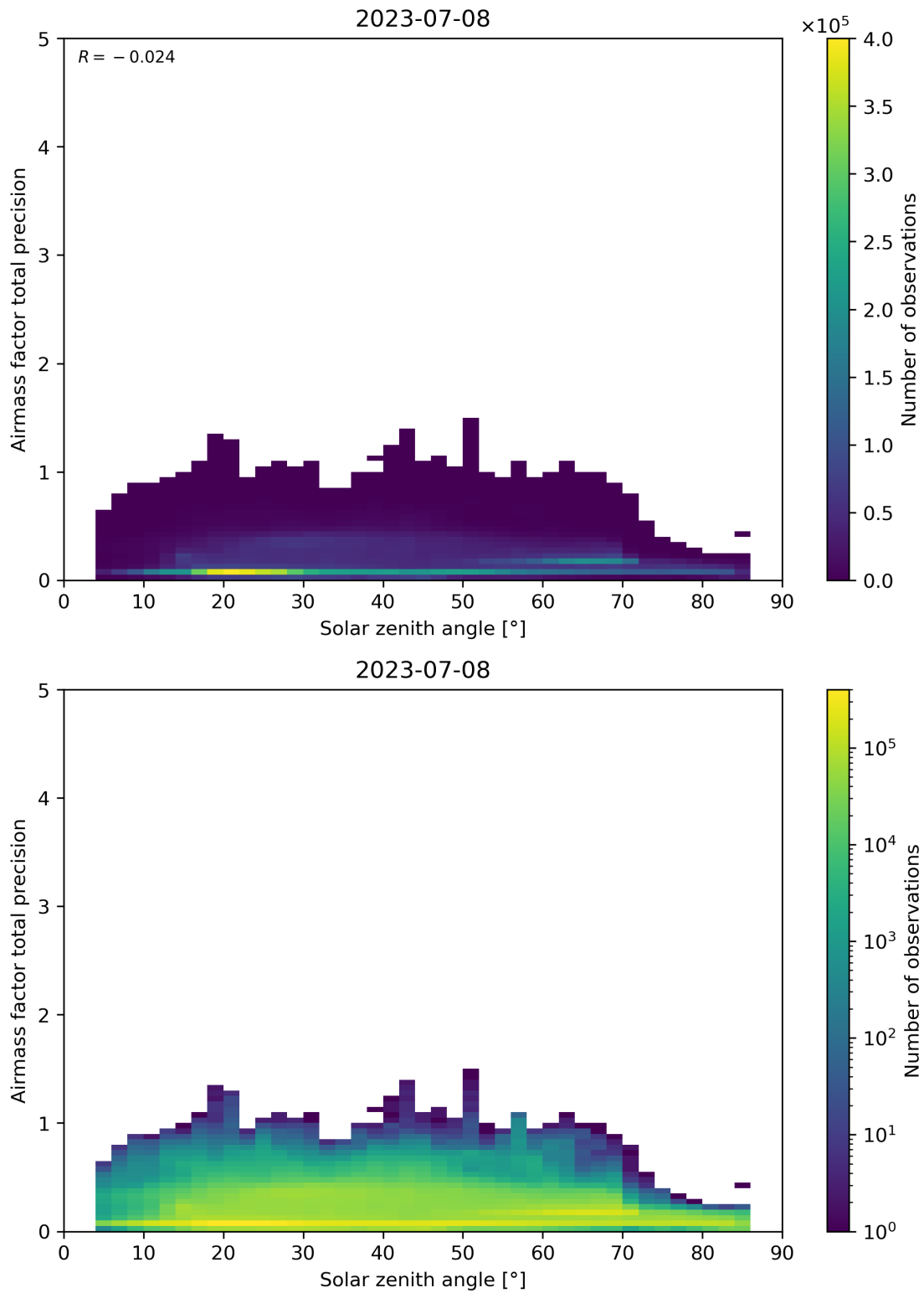
Figure 176: Scatter density plot of “Solar zenith angle” against “Airmass factor total precision” for 2023-07-08 to 2023-07-09.
