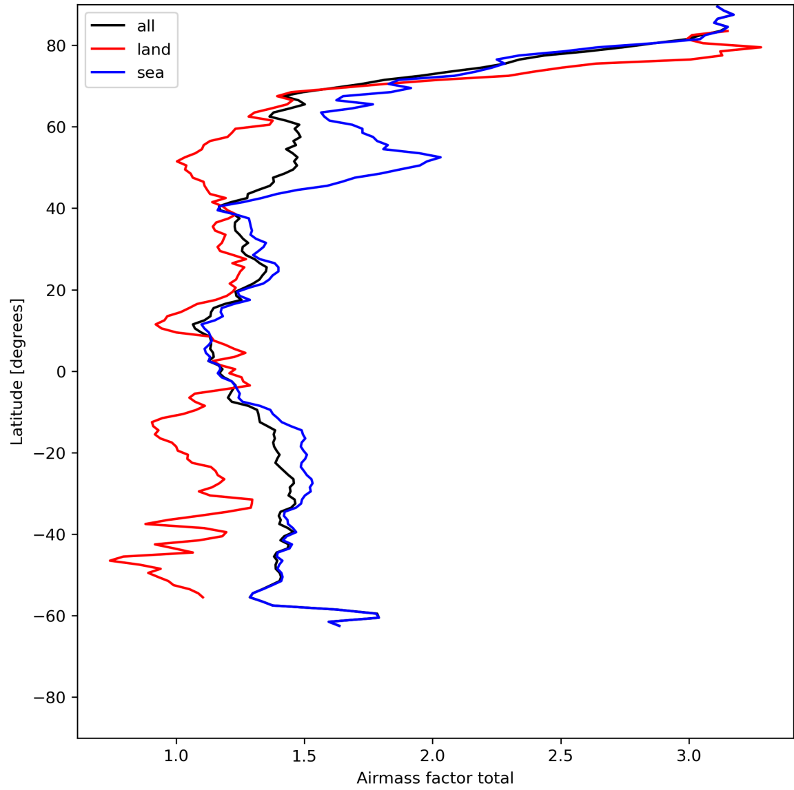
Figure 26: Zonal average of “Airmass factor total” for 2023-07-08 to 2023-07-09.
