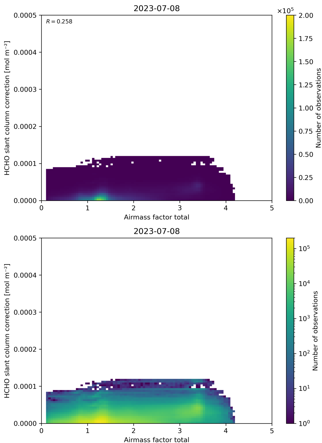
Figure 102: Scatter density plot of “Airmass factor total” against “HCHO slant column correction” for 2023-07-08 to 2023-07-09.
