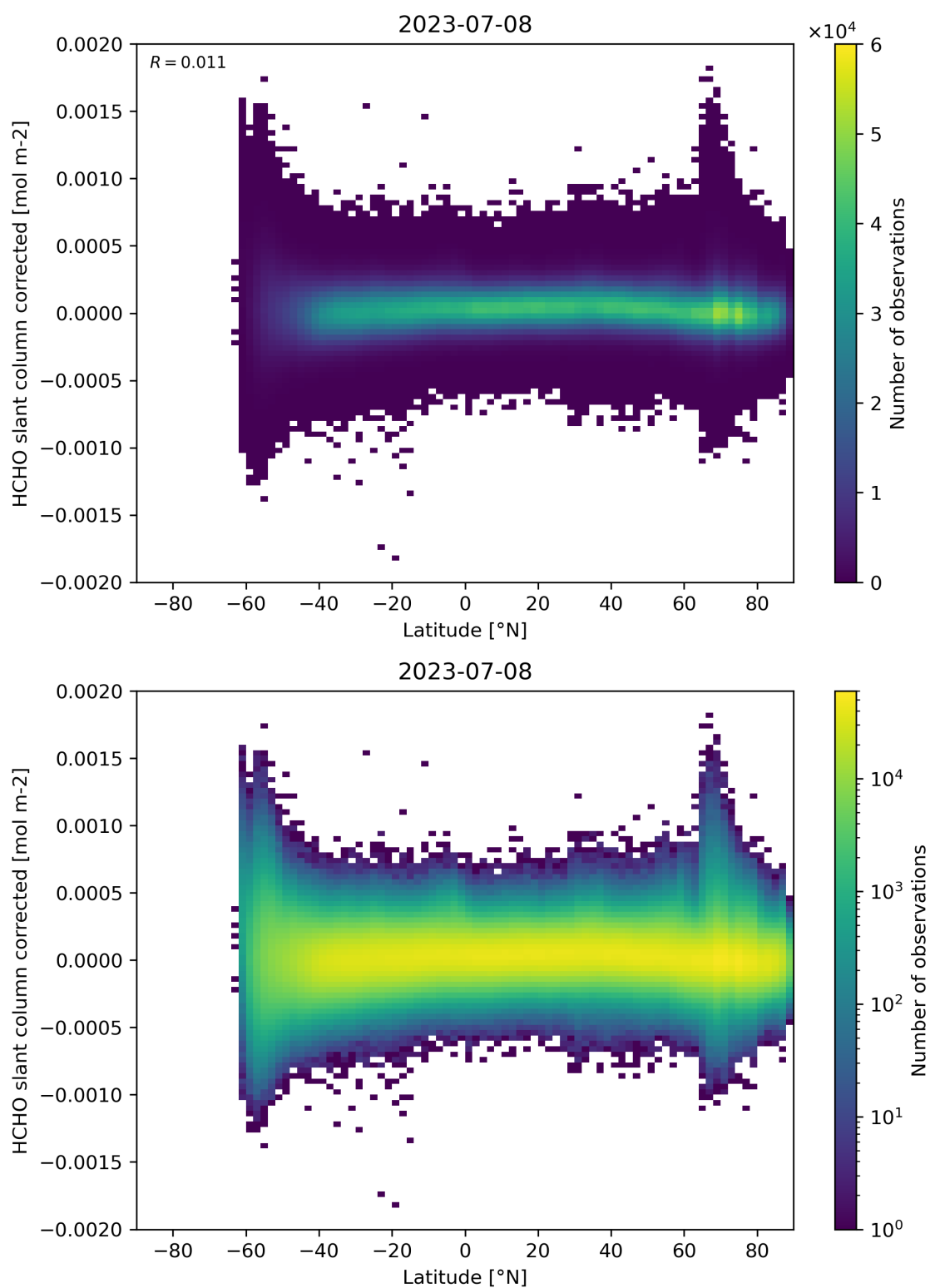
Figure 157: Scatter density plot of “Latitude” against “HCHO slant column corrected” for 2023-07-08 to 2023-07-09.
