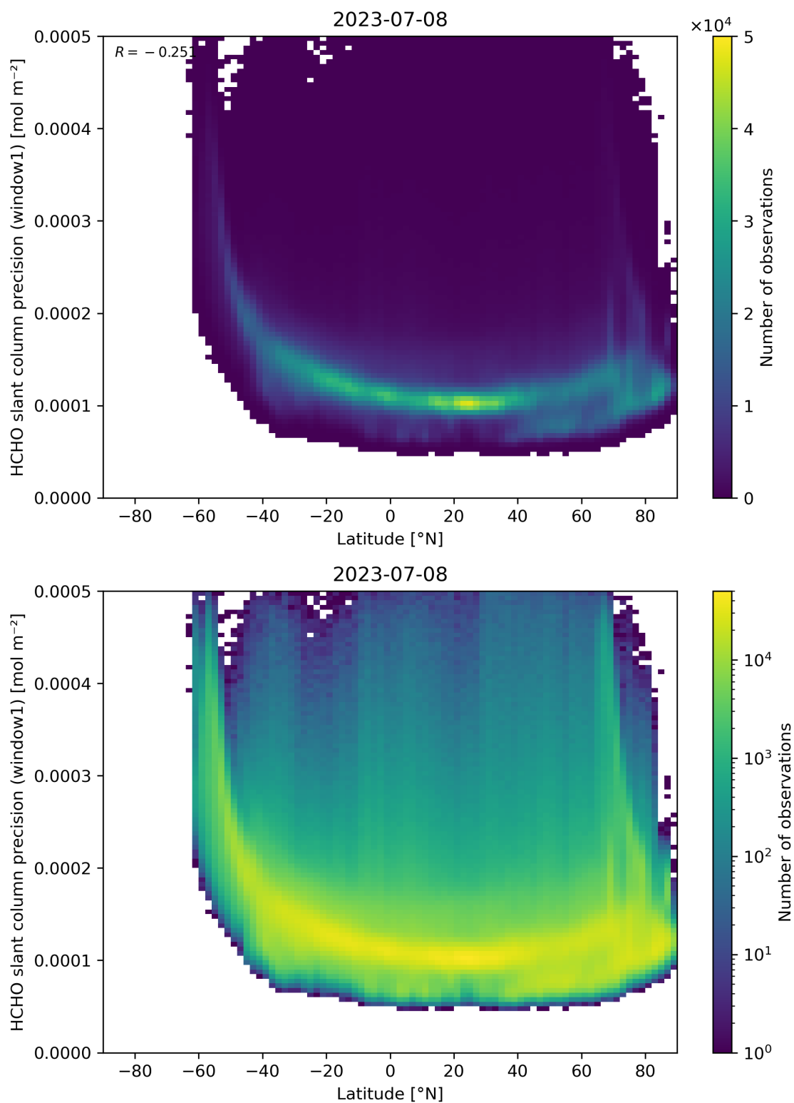
Figure 160: Scatter density plot of “Latitude” against “HCHO slant column precision (window1)” for 2023-07-08 to 2023-07-09.
