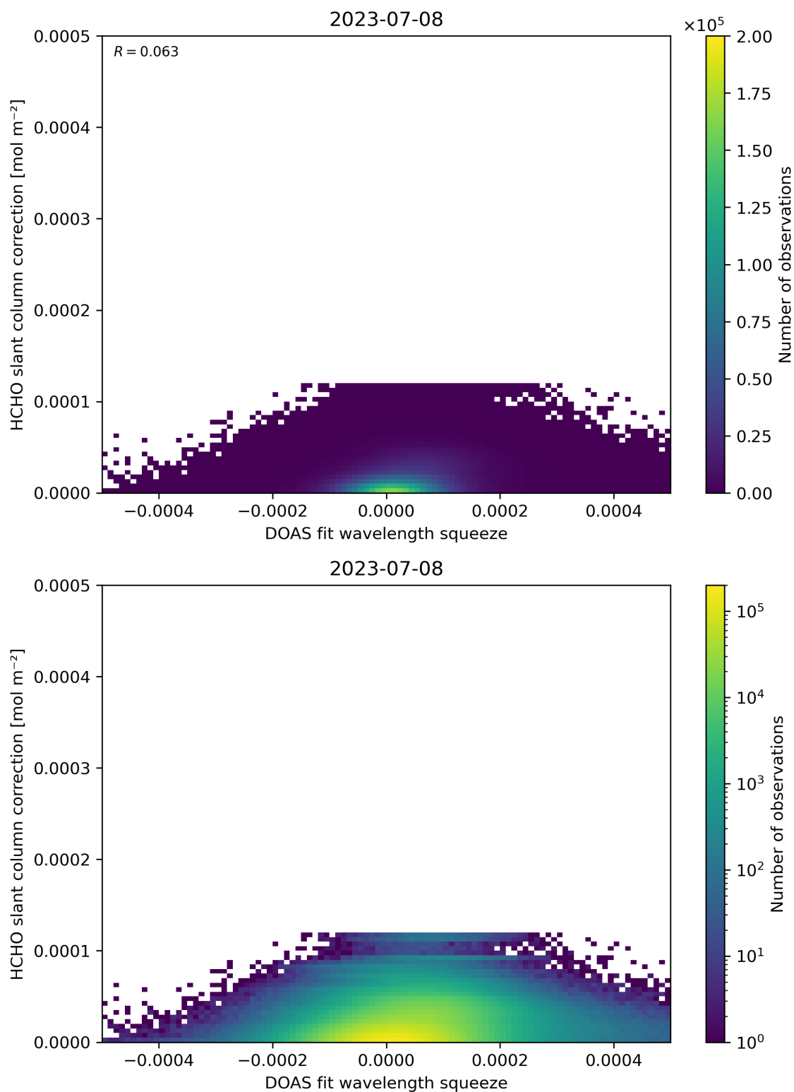
Figure 70: Scatter density plot of “DOAS fit wavelength squeeze” against “HCHO slant column correction” for 2023-07-08 to 2023-07-09.
