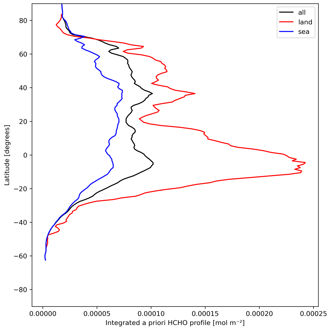
Figure 29: Zonal average of “Integrated a priori HCHO profile” for 2023-07-08 to 2023-07-09.
