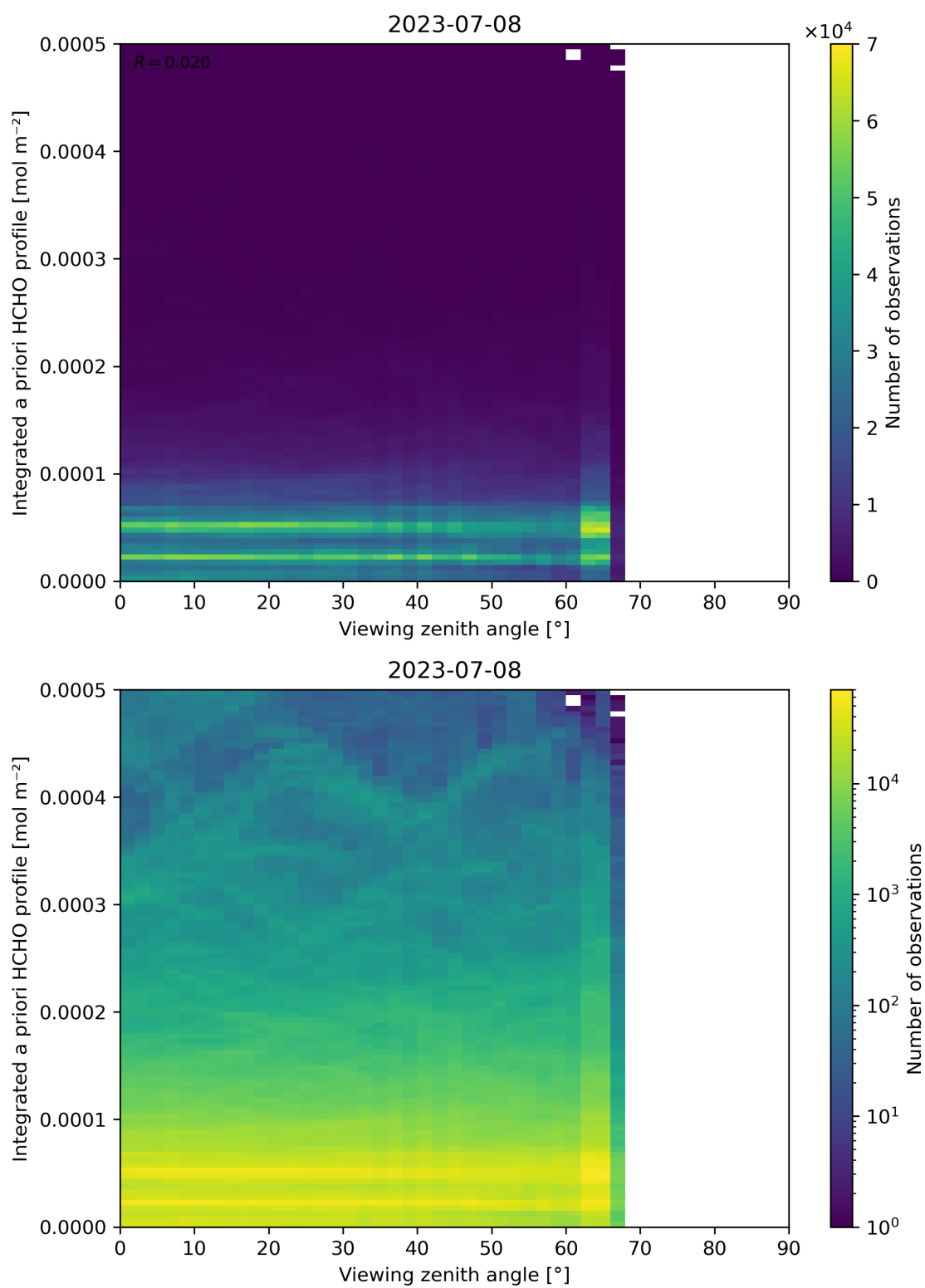
Figure 195: Scatter density plot of “Viewing zenith angle” against “Integrated a priori HCHO profile” for 2023-07-08 to 2023-07-09.
