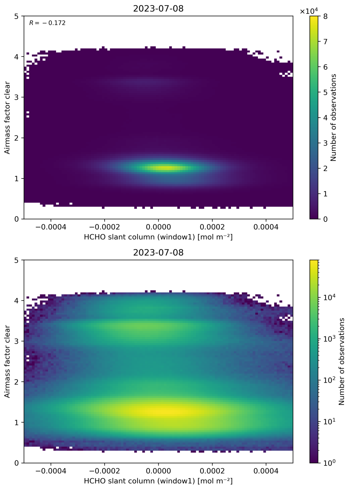
Figure 81: Scatter density plot of “HCHO slant column (window1)” against “Airmass factor clear” for 2023-07-08 to 2023-07-09.
