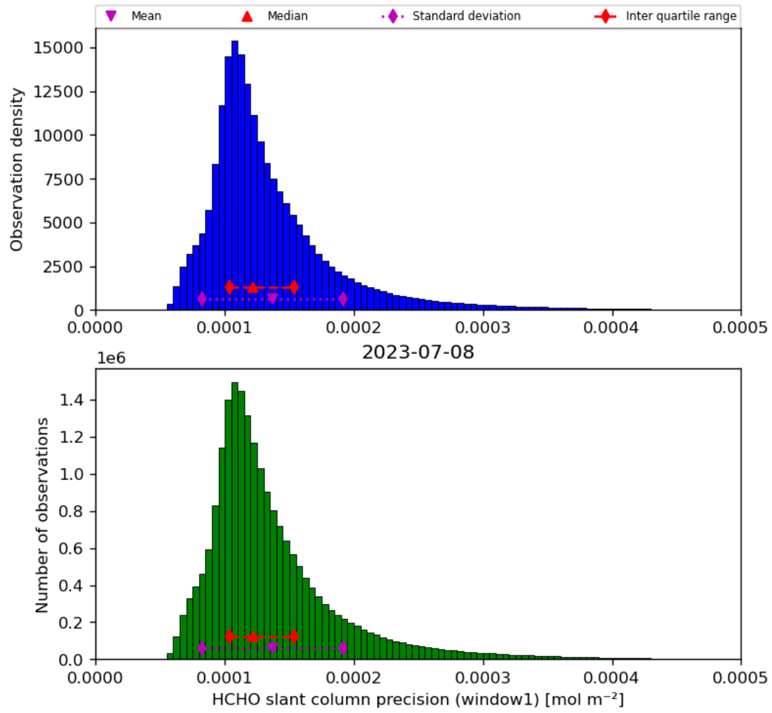
Figure 39: Histogram of “HCHO slant column precision (window1)” for 2023-07-08 to 2023-07-09
