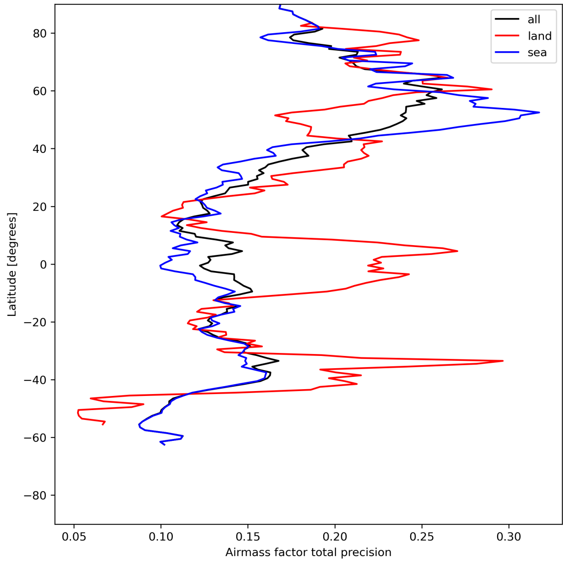
Figure 27: Zonal average of “Airmass factor total precision” for 2023-07-08 to 2023-07-09.
