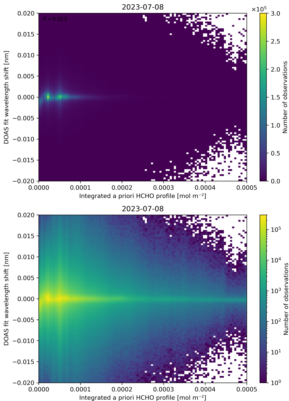
Figure 149: Scatter density plot of “Integrated a priori HCHO profile” against “DOAS fit wavelength shift” for 2023-07-08 to 2023-07-09.
