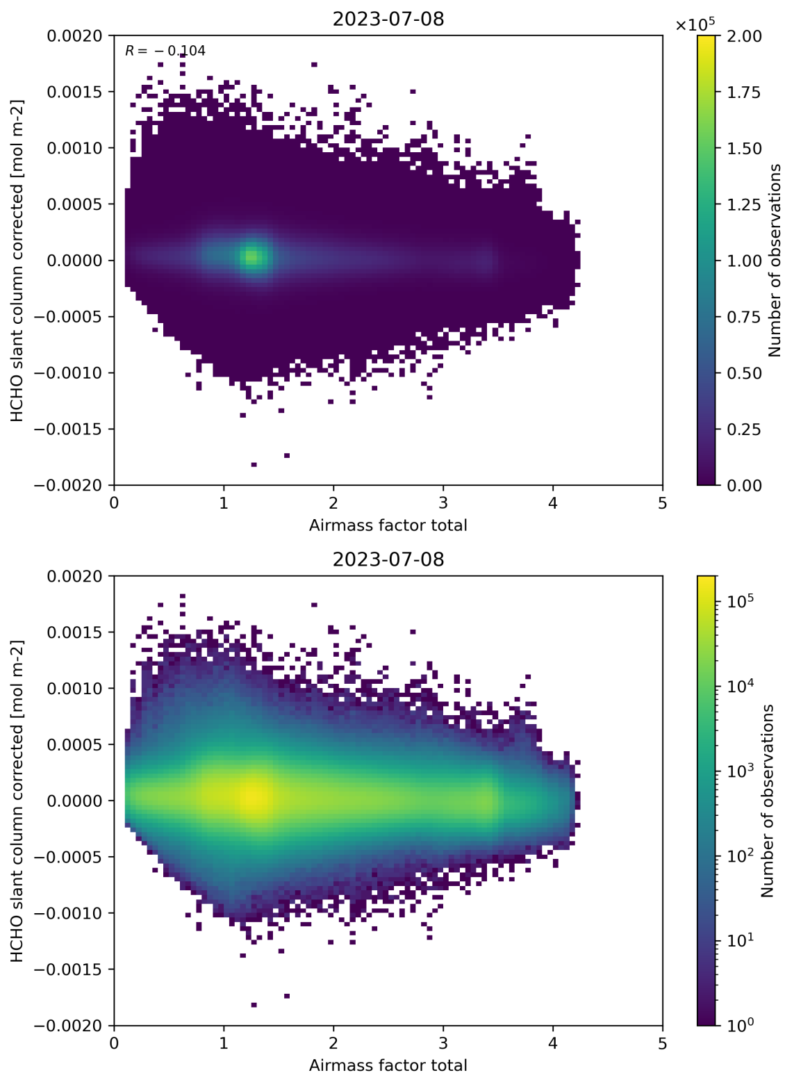
Figure 101: Scatter density plot of “Airmass factor total” against “HCHO slant column corrected” for 2023-07-08 to 2023-07-09.
