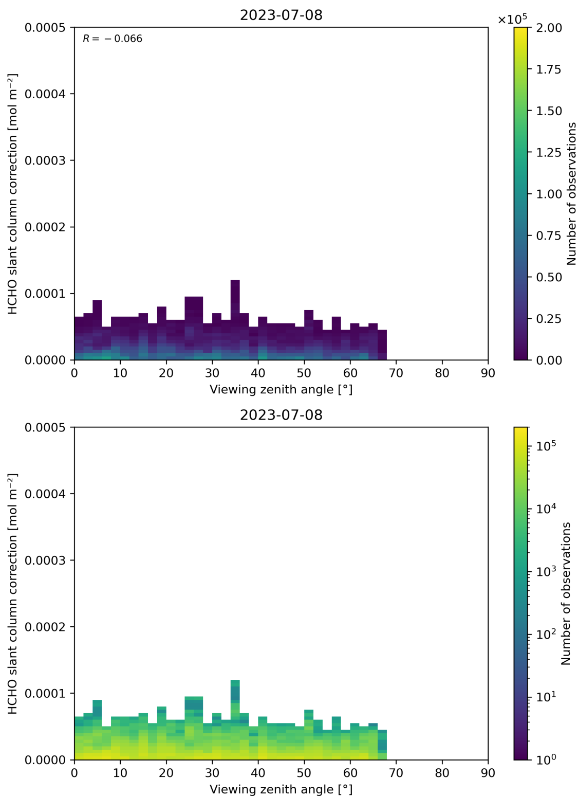
Figure 187: Scatter density plot of “Viewing zenith angle” against “HCHO slant column correction” for 2023-07-08 to 2023-07-09.
