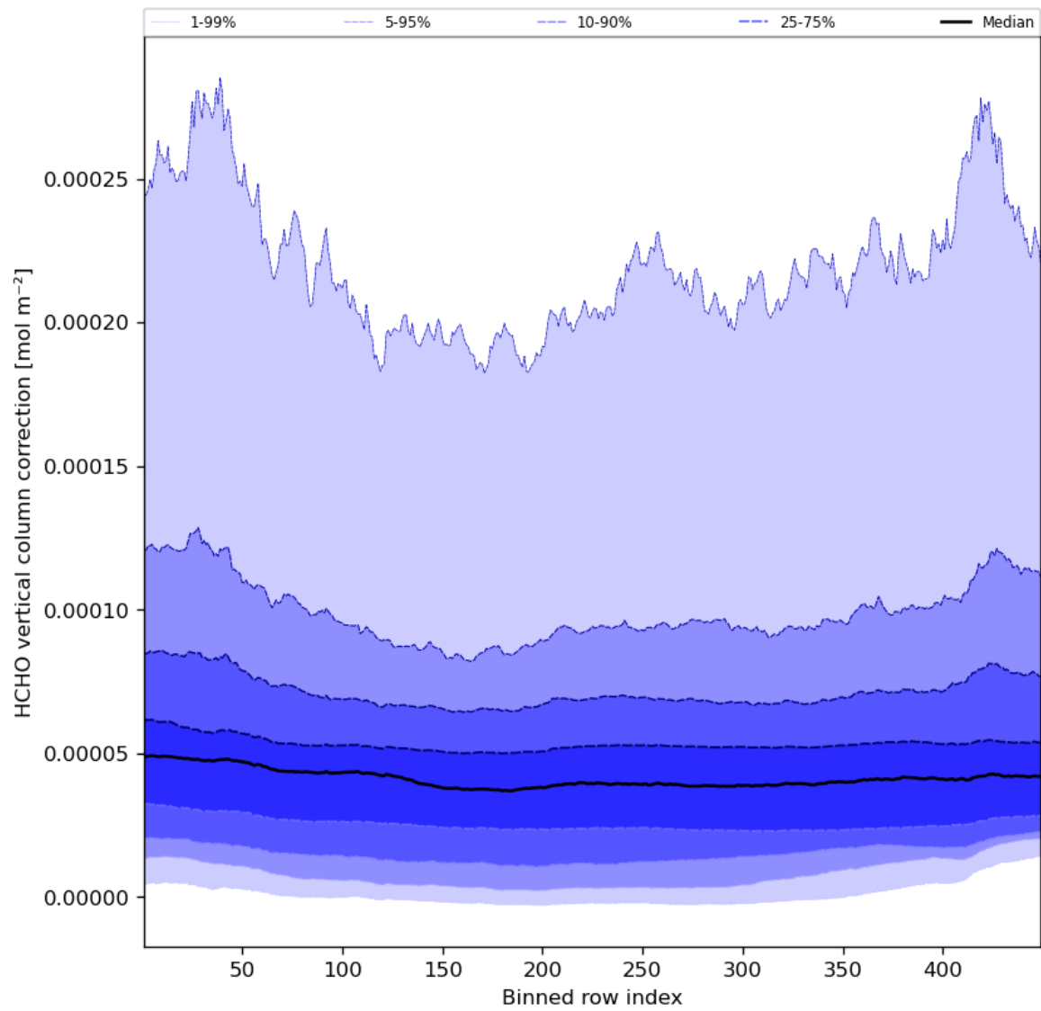
Figure 51: Along track statistics of “HCHO vertical column correction” for 2023-07-08 to 2023-07-09
