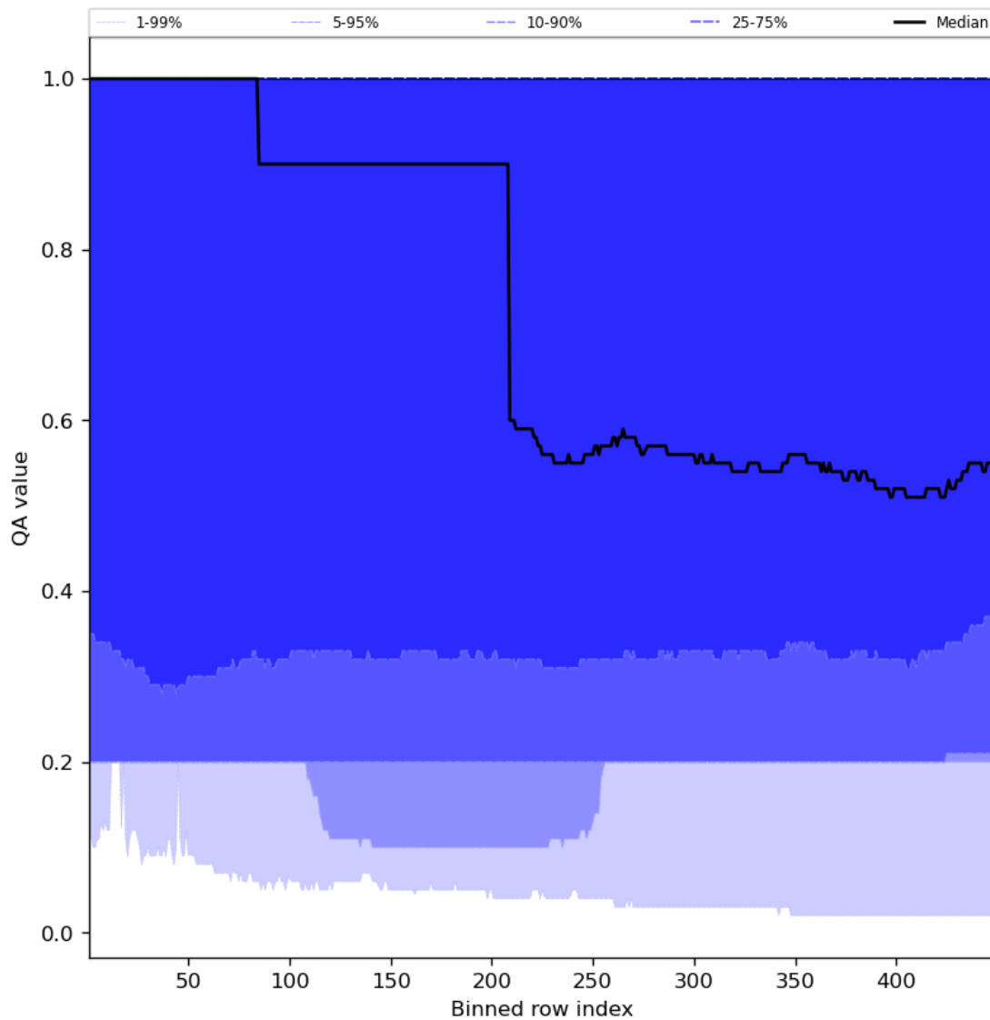
Figure 48: Along track statistics of “QA value” for 2023-07-08 to 2023-07-09
