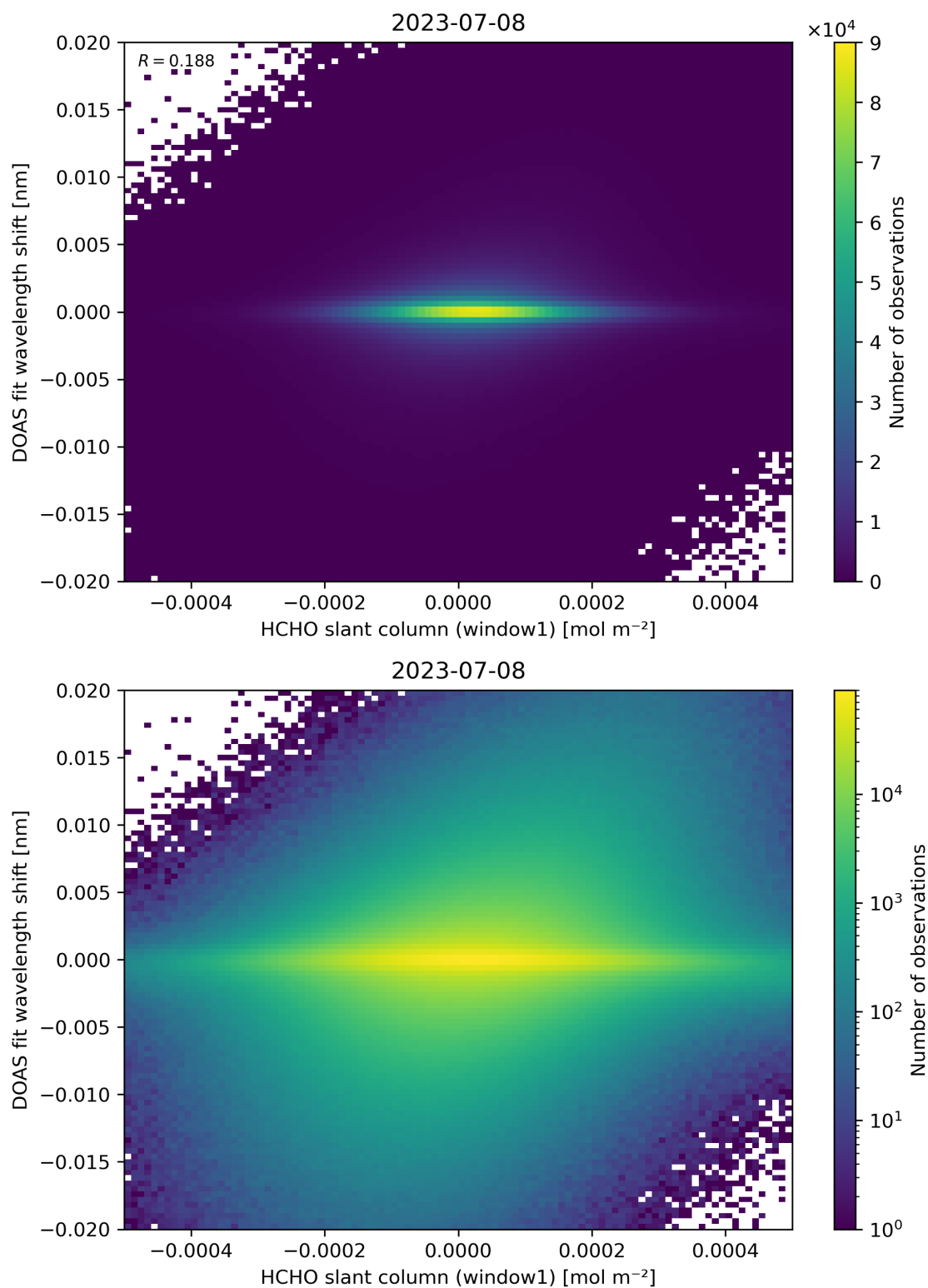
Figure 79: Scatter density plot of “HCHO slant column (window1)” against “DOAS fit wavelength shift” for 2023-07-08 to 2023-07-09.
