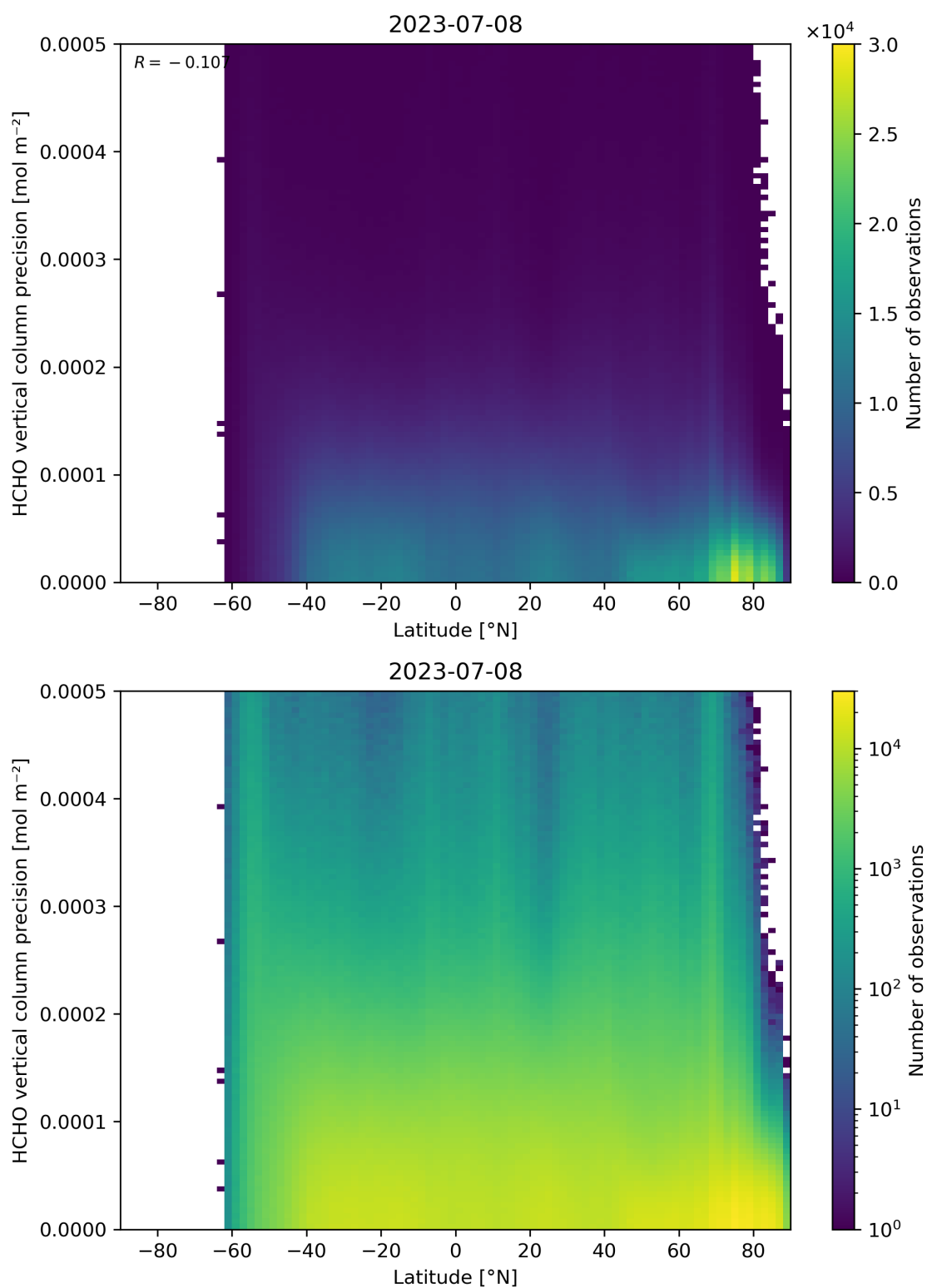
Figure 165: Scatter density plot of “Latitude” against “HCHO vertical column precision” for 2023-07-08 to 2023-07-09.
