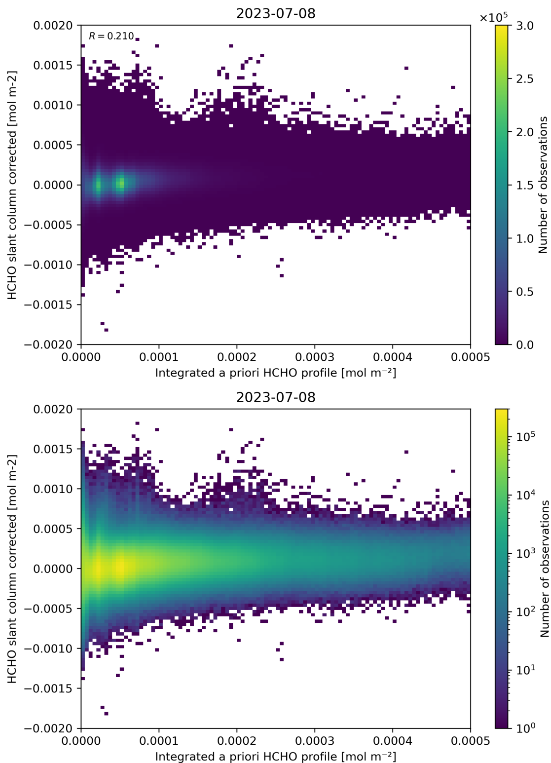
Figure 151: Scatter density plot of “Integrated a priori HCHO profile” against “HCHO slant column corrected” for 2023-07-08 to 2023-07-09.
