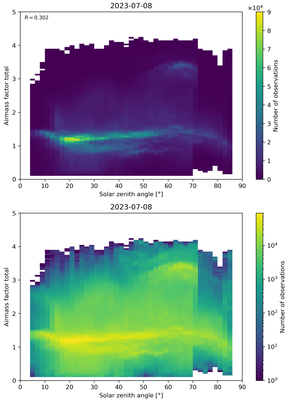
Figure 175: Scatter density plot of “Solar zenith angle” against “Airmass factor total” for 2023-07-08 to 2023-07-09.
