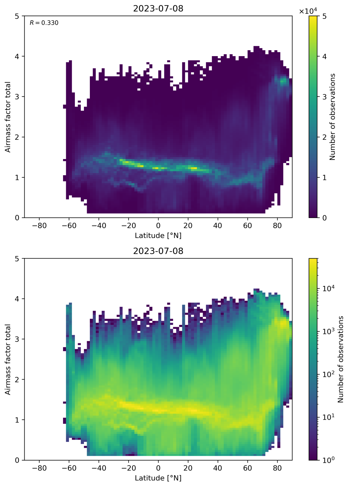
Figure 161: Scatter density plot of “Latitude” against “Airmass factor total” for 2023-07-08 to 2023-07-09.
