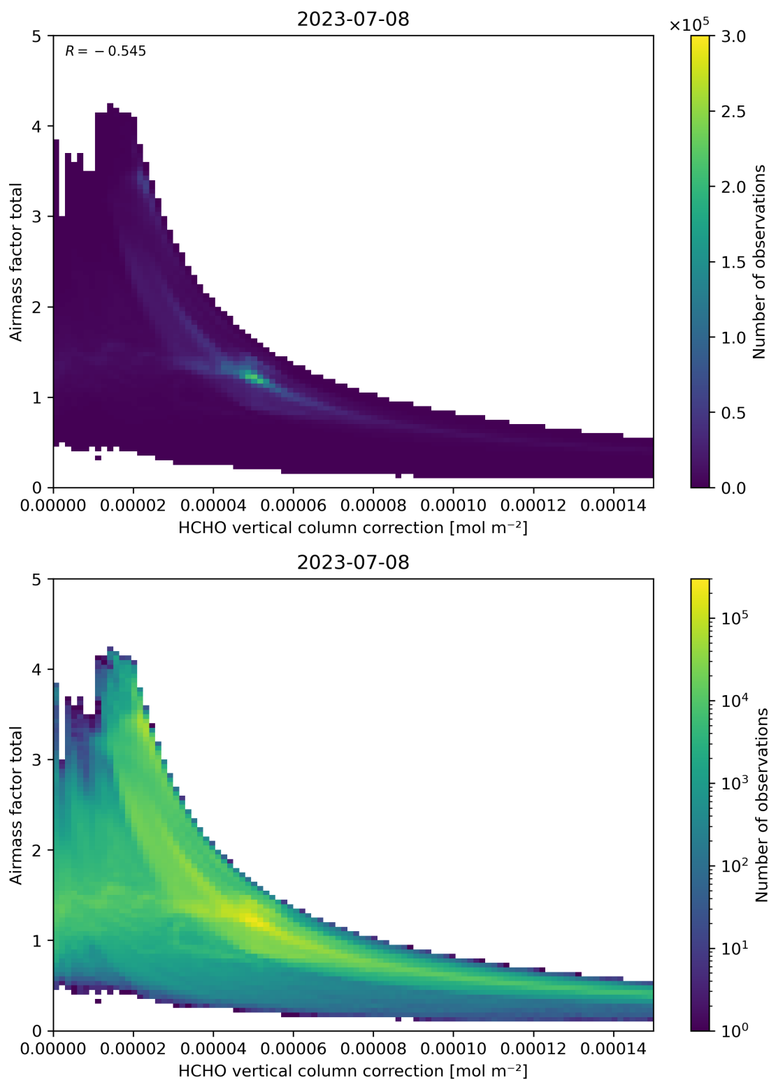
Figure 120: Scatter density plot of “HCHO vertical column correction” against “Airmass factor total” for 2023-07-08 to 2023-07-09.
