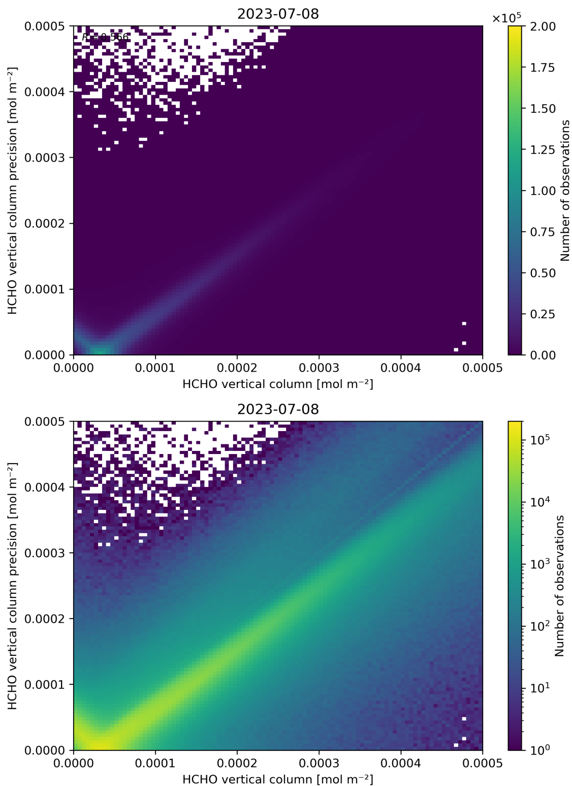
Figure 134: Scatter density plot of “HCHO vertical column” against “HCHO vertical column precision” for 2023-07-08 to 2023-07-09.
