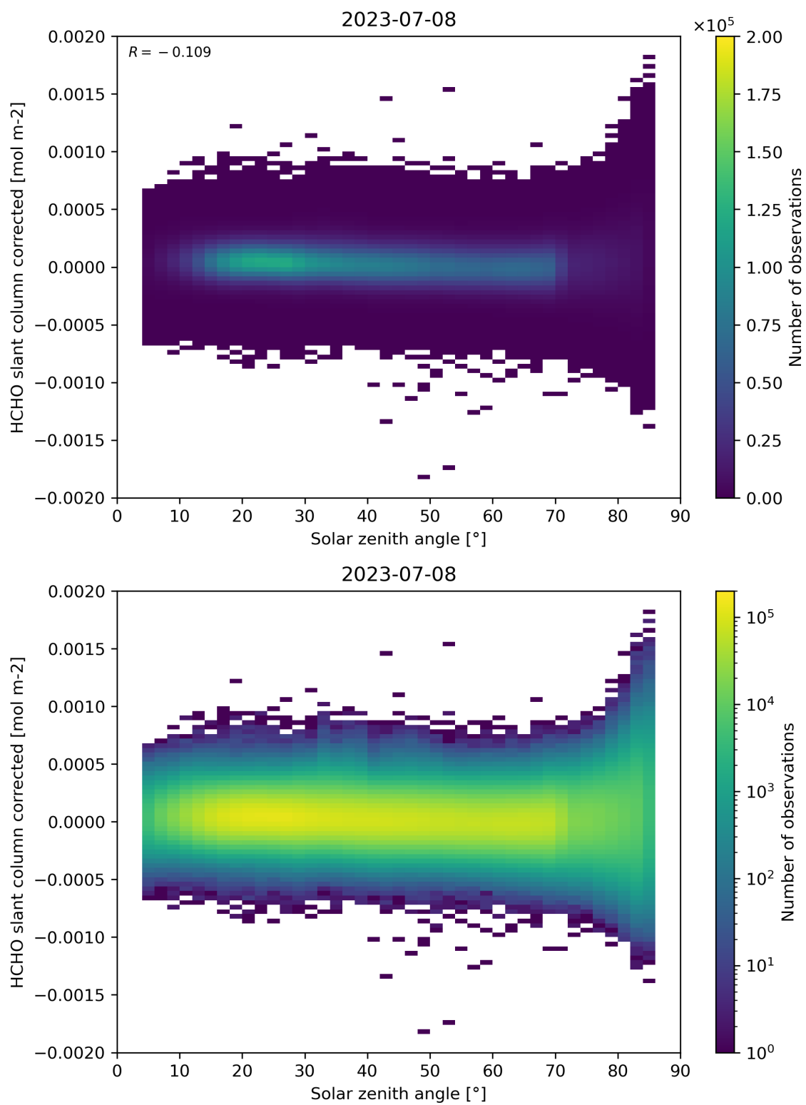
Figure 171: Scatter density plot of “Solar zenith angle” against “HCHO slant column corrected” for 2023-07-08 to 2023-07-09.
