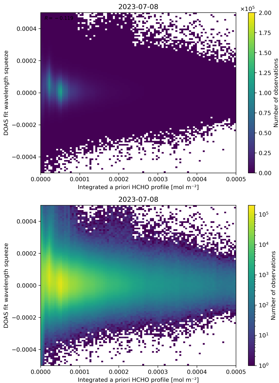
Figure 150: Scatter density plot of “Integrated a priori HCHO profile” against “DOAS fit wavelength squeeze” for 2023-07-08 to 2023-07-09.
