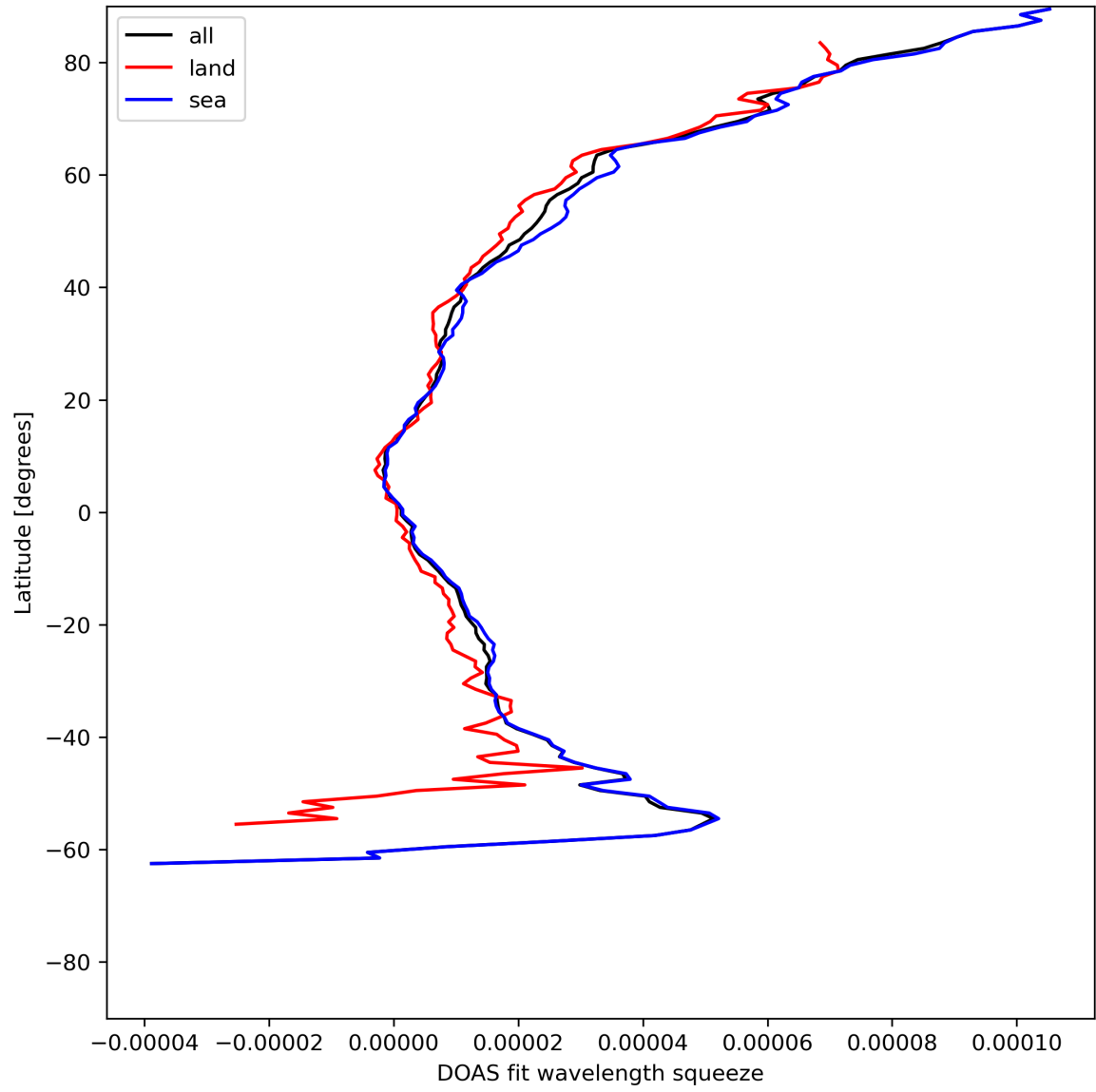
Figure 31: Zonal average of “DOAS fit wavelength squeeze” for 2023-07-08 to 2023-07-09.
