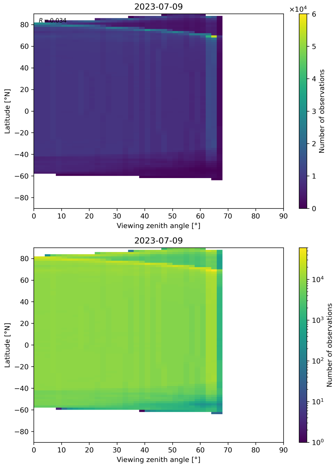
Figure 196: Scatter density plot of “Viewing zenith angle” against “Latitude” for 2023-07-08 to 2023-07-10.
