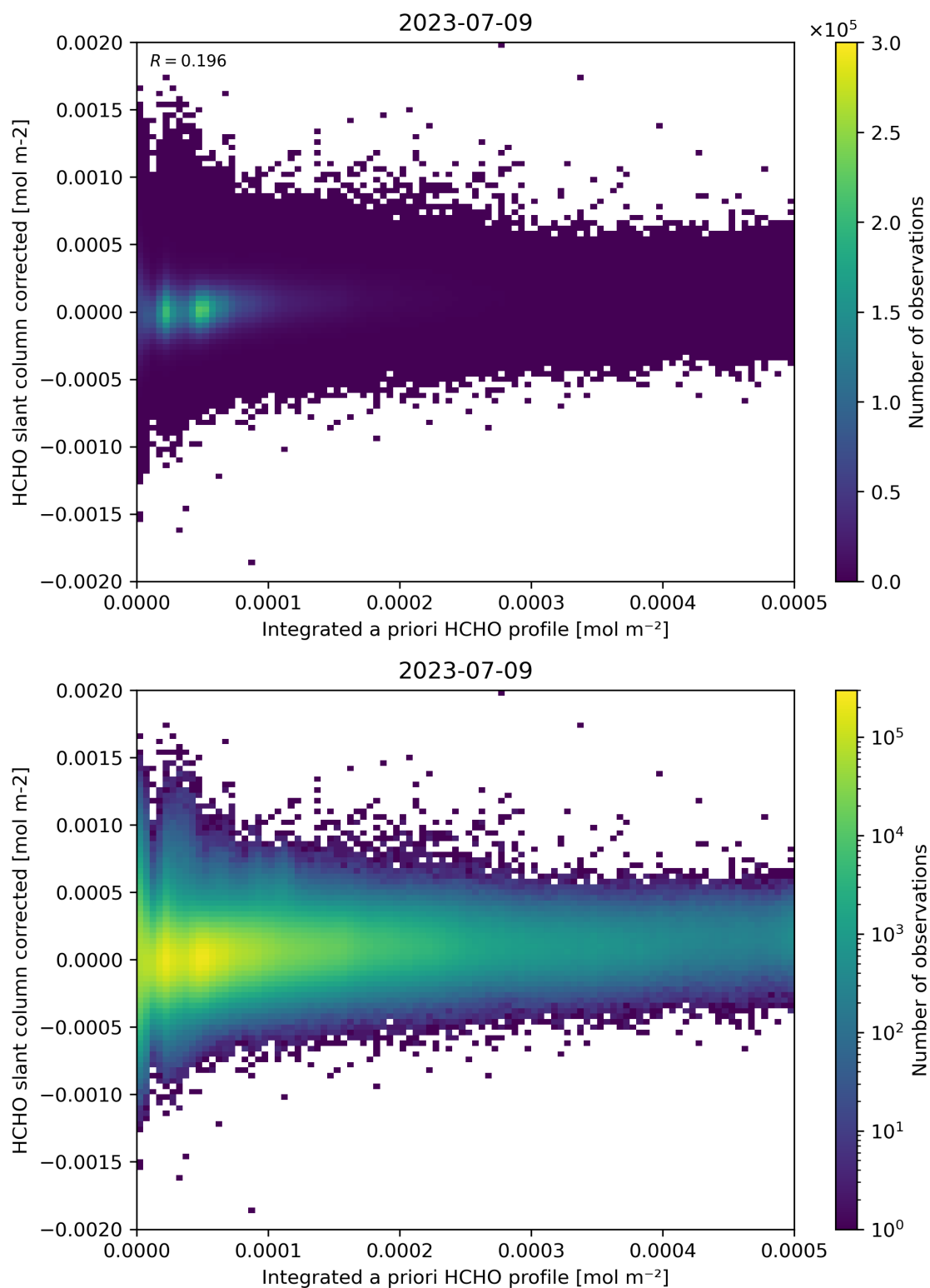
Figure 151: Scatter density plot of “Integrated a priori HCHO profile” against “HCHO slant column corrected” for 2023-07-08 to 2023-07-10.
