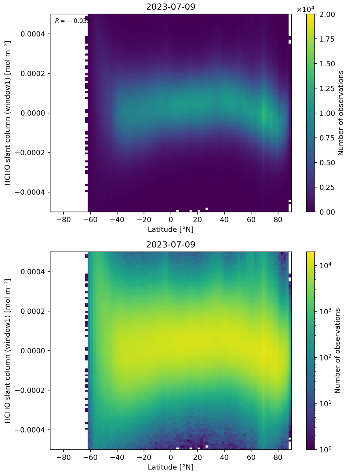
Figure 159: Scatter density plot of “Latitude” against “HCHO slant column (window1)” for 2023-07-08 to 2023-07-10.
