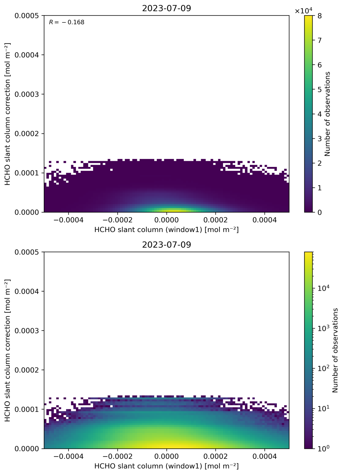
Figure 83: Scatter density plot of “HCHO slant column (window1)” against “HCHO slant column correction” for 2023-07-08 to 2023-07-10.
