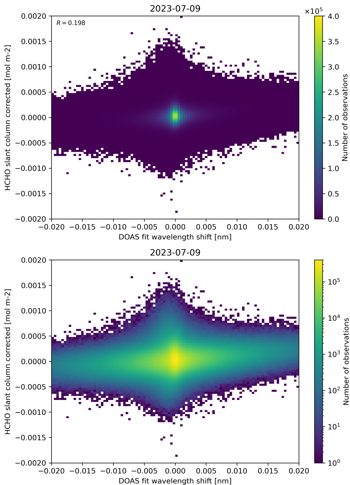
Figure 66: Scatter density plot of “DOAS fit wavelength shift” against “HCHO slant column corrected” for 2023-07-08 to 2023-07-10.
