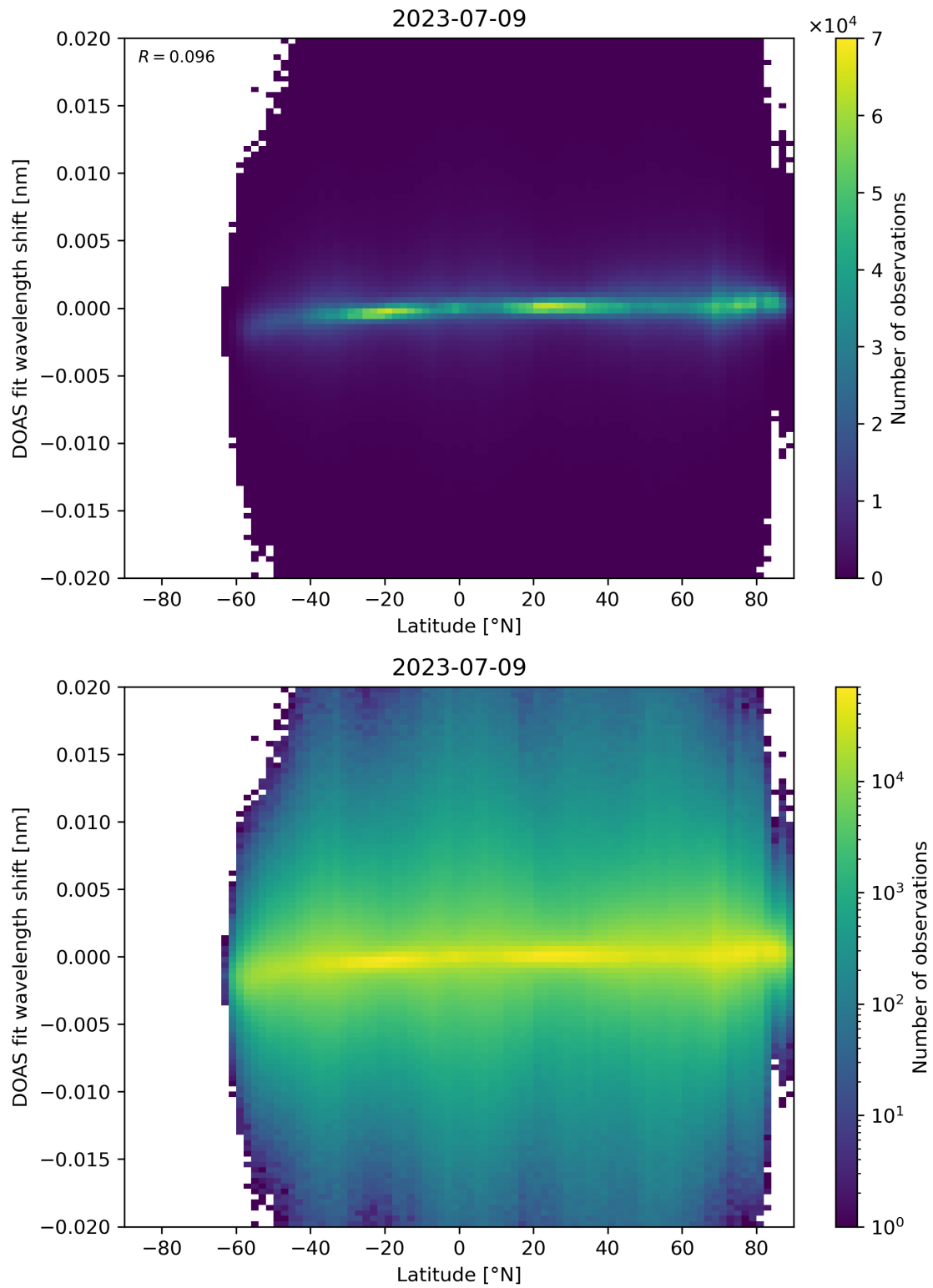
Figure 154: Scatter density plot of “Latitude” against “DOAS fit wavelength shift” for 2023-07-08 to 2023-07-10.
