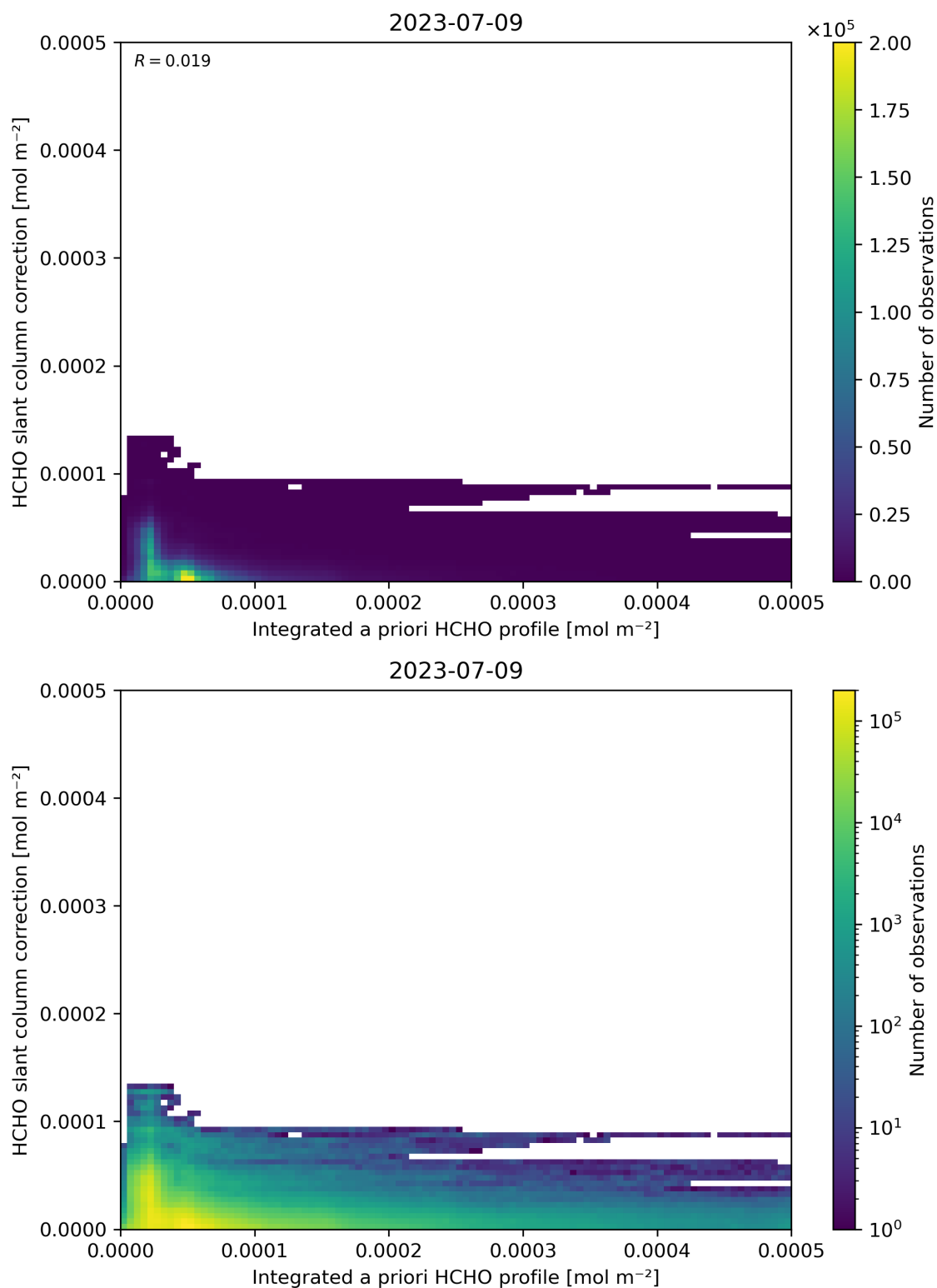
Figure 152: Scatter density plot of “Integrated a priori HCHO profile” against “HCHO slant column correction” for 2023-07-08 to 2023-07-10.
