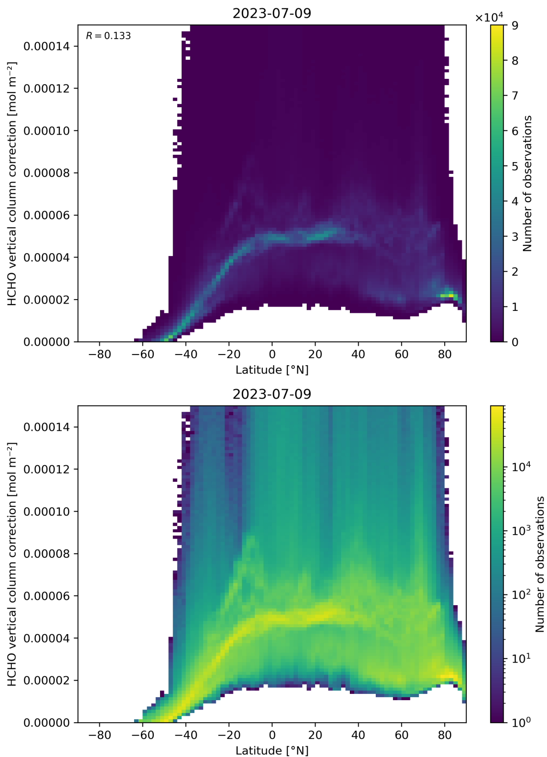
Figure 164: Scatter density plot of “Latitude” against “HCHO vertical column correction” for 2023-07-08 to 2023-07-10.
