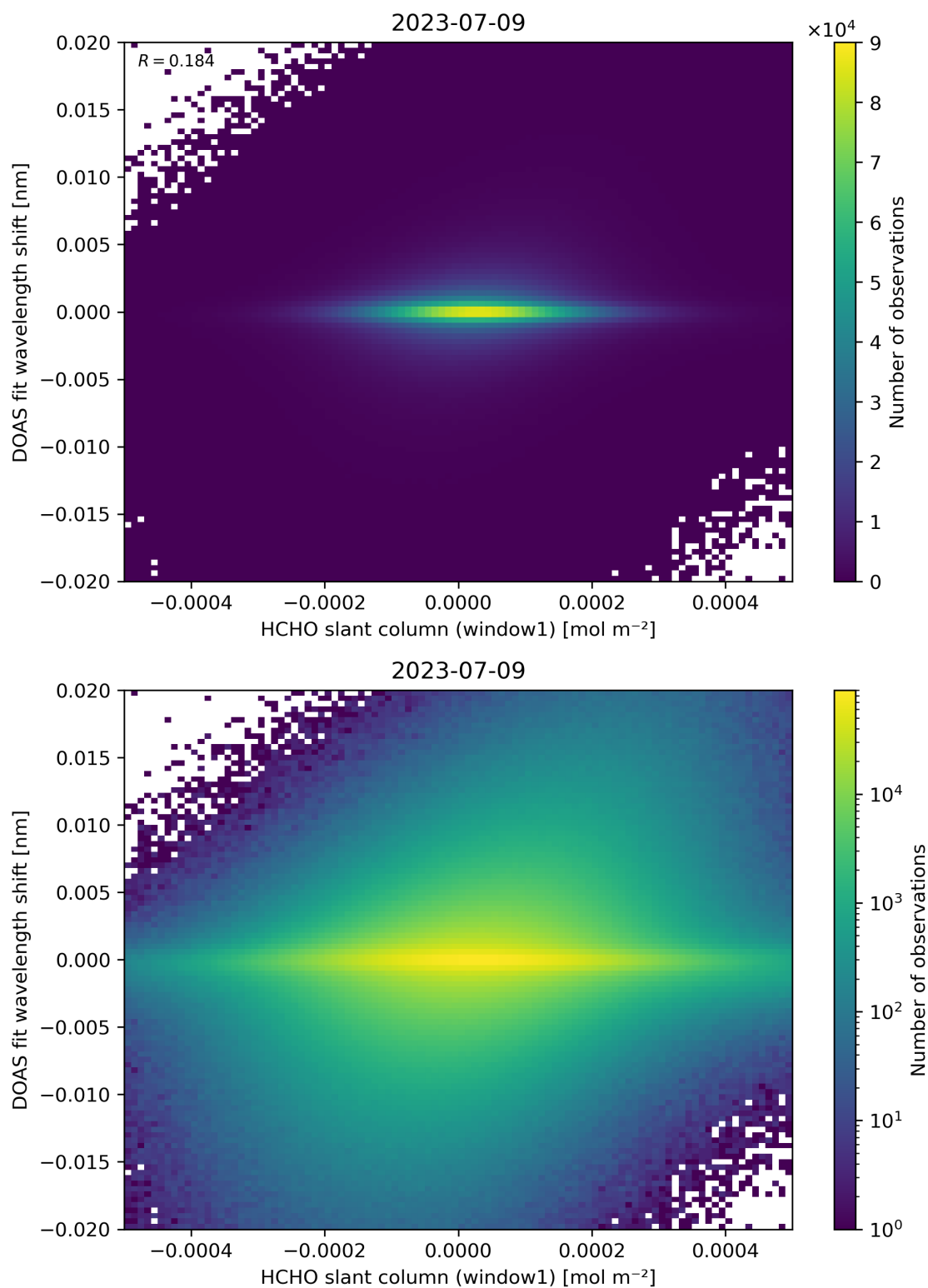
Figure 79: Scatter density plot of “HCHO slant column (window1)” against “DOAS fit wavelength shift” for 2023-07-08 to 2023-07-10.
