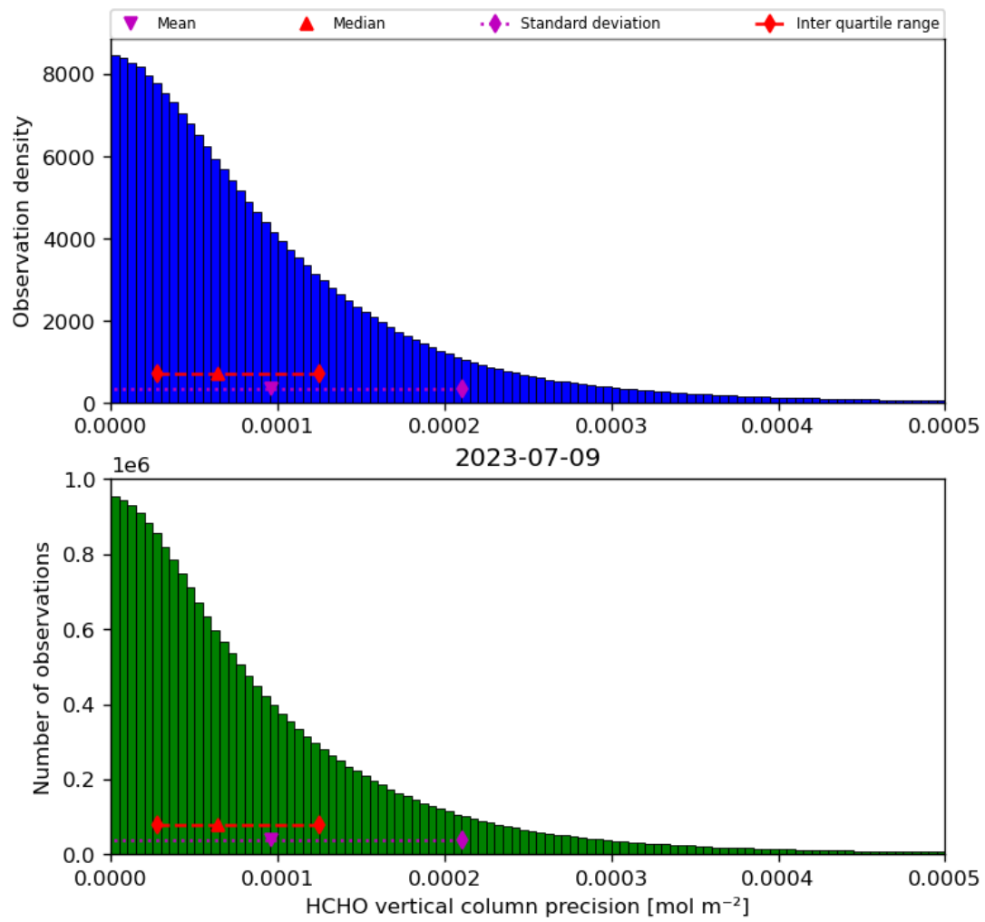
Figure 36: Histogram of “HCHO vertical column precision” for 2023-07-08 to 2023-07-10
