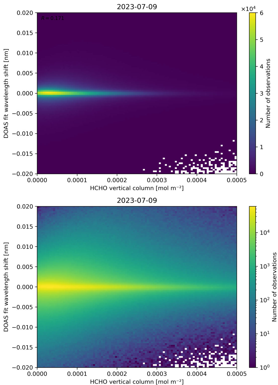
Figure 124: Scatter density plot of “HCHO vertical column” against “DOAS fit wavelength shift” for 2023-07-08 to 2023-07-10.
