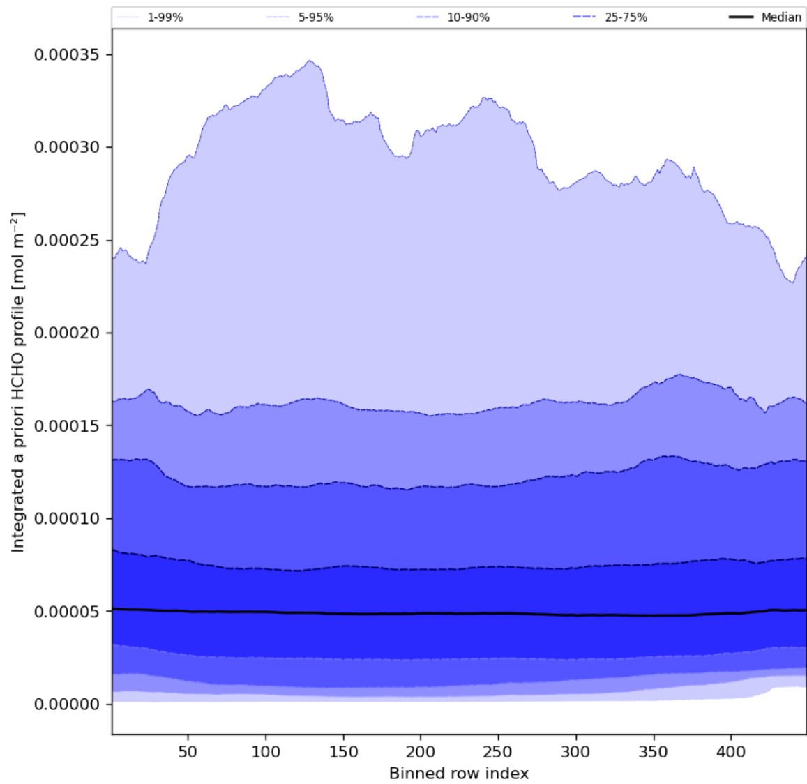
Figure 57: Along track statistics of “Integrated a priori HCHO profile” for 2023-07-08 to 2023-07-10
