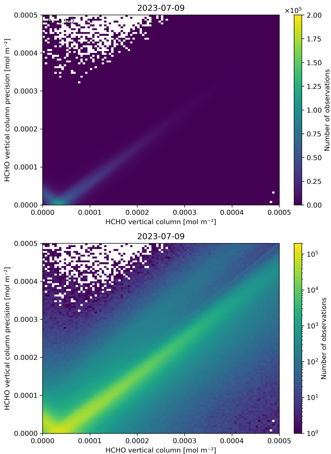
Figure 134: Scatter density plot of “HCHO vertical column” against “HCHO vertical column precision” for 2023-07-08 to 2023-07-10.
