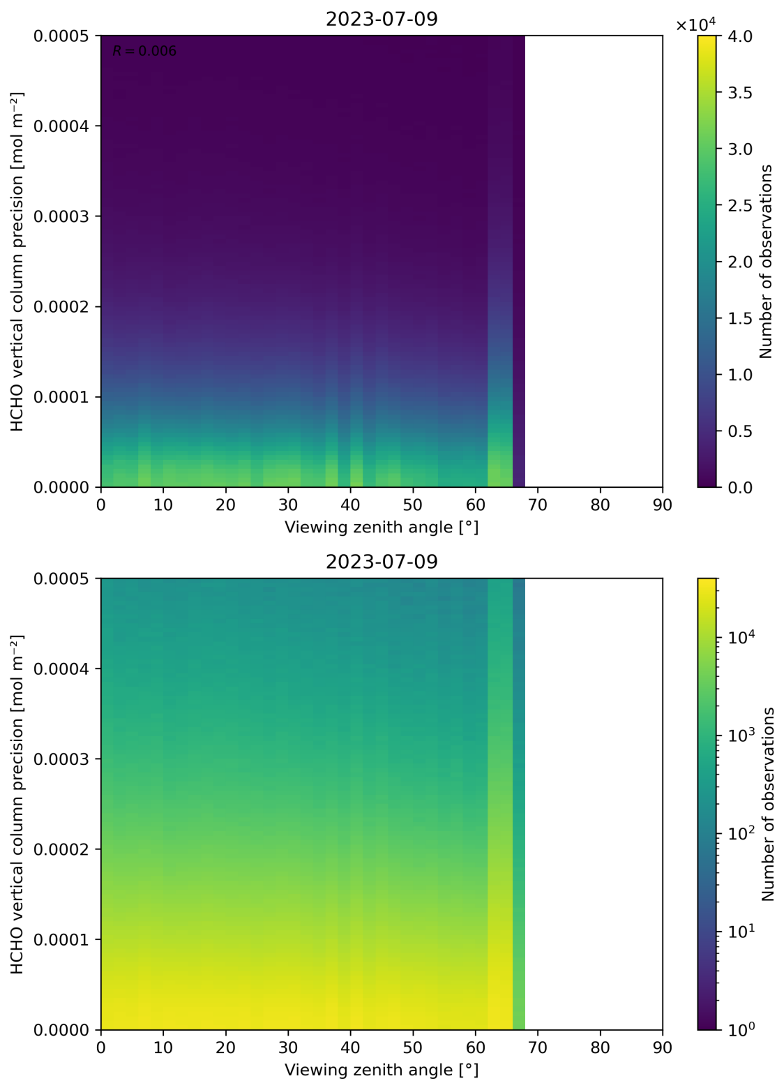
Figure 194: Scatter density plot of “Viewing zenith angle” against “HCHO vertical column precision” for 2023-07-08 to 2023-07-10.
