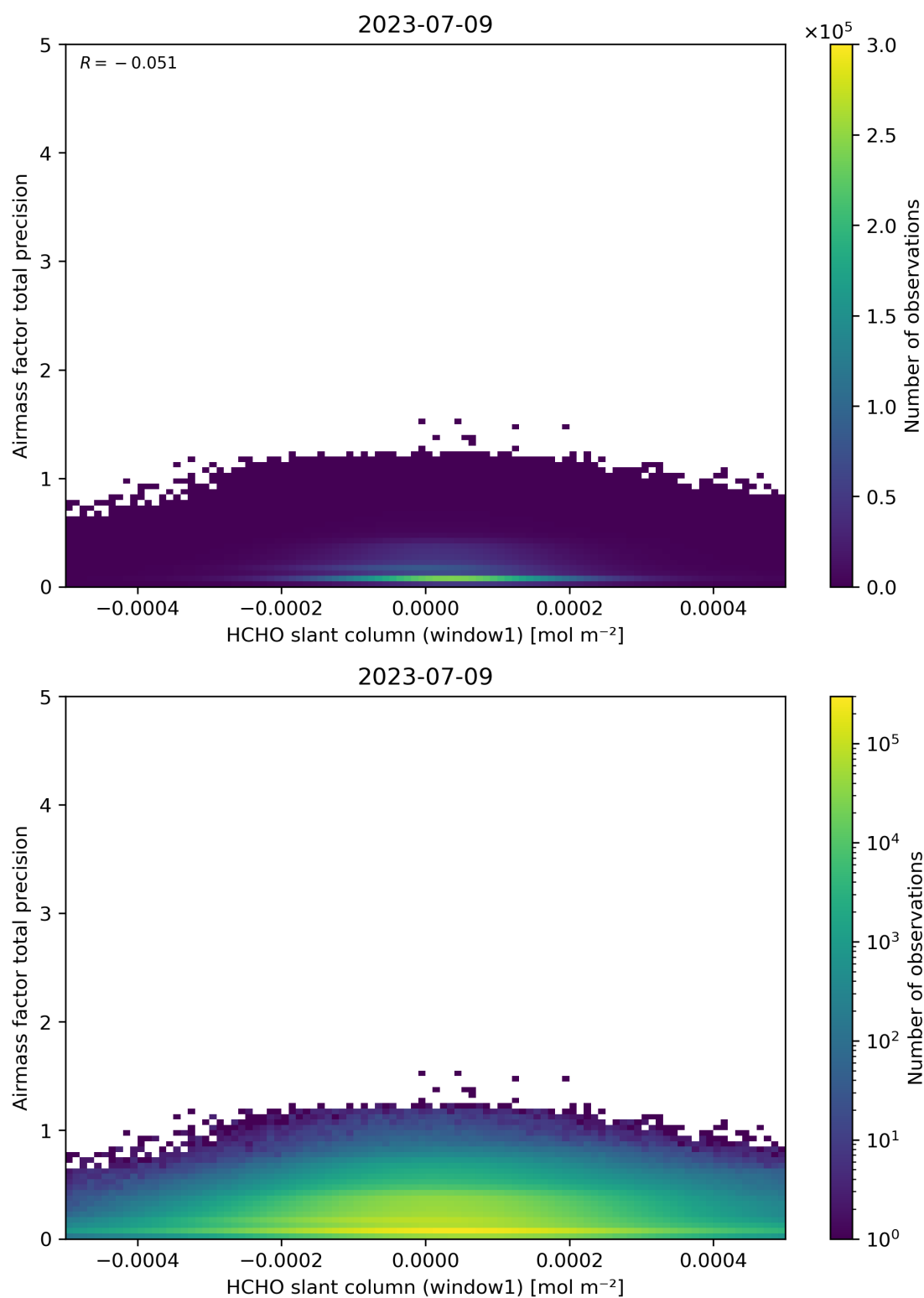
Figure 86: Scatter density plot of “HCHO slant column (window1)” against “Airmass factor total precision” for 2023-07-08 to 2023-07-10.
