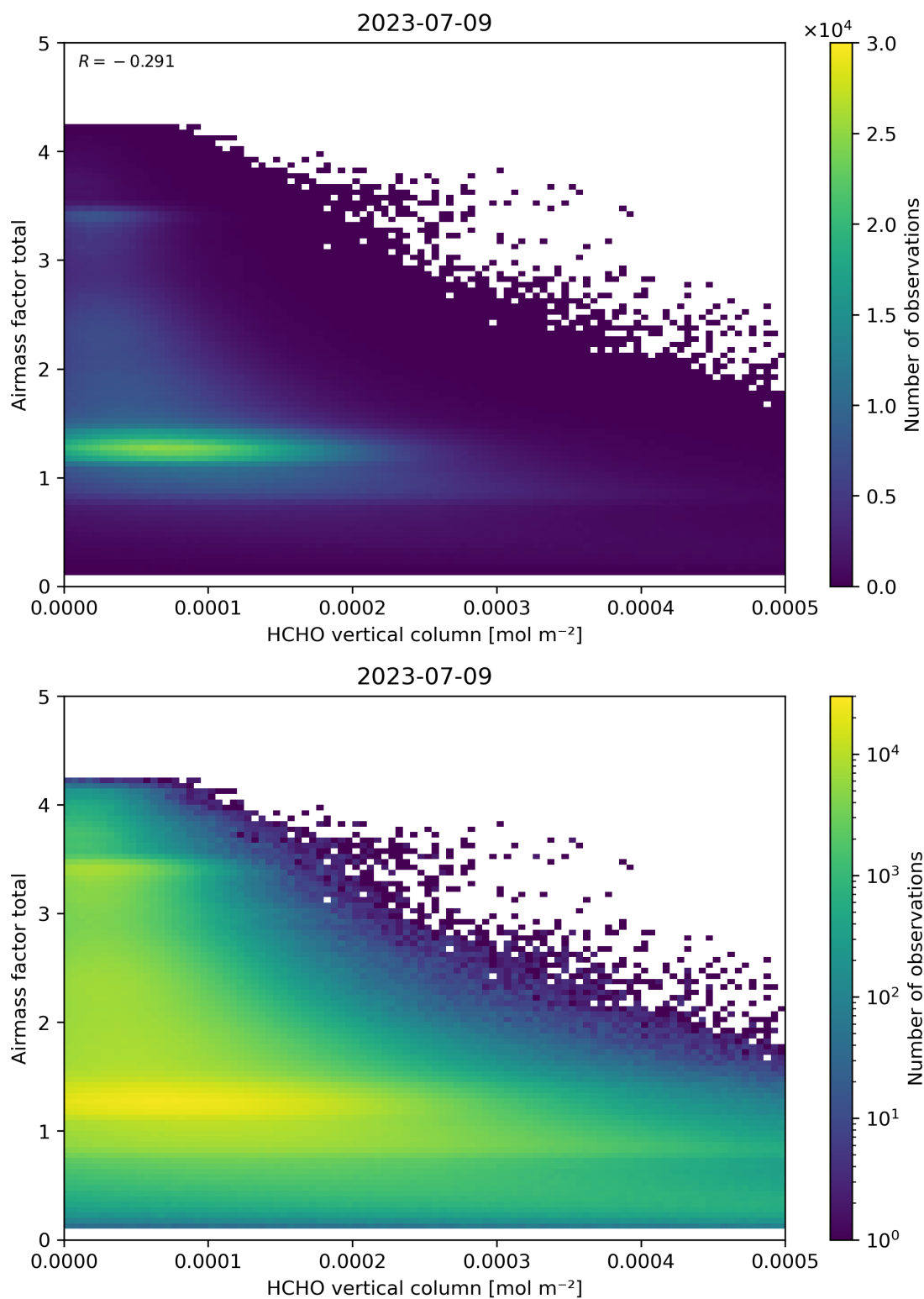
Figure 131: Scatter density plot of “HCHO vertical column” against “Airmass factor total” for 2023-07-08 to 2023-07-10.
