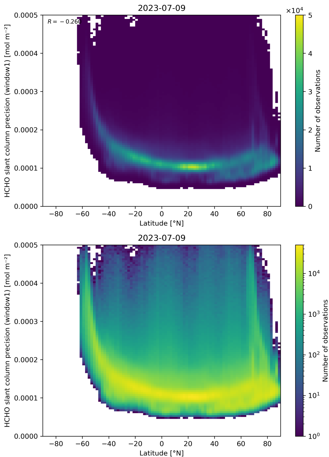
Figure 160: Scatter density plot of “Latitude” against “HCHO slant column precision (window1)” for 2023-07-08 to 2023-07-10.
