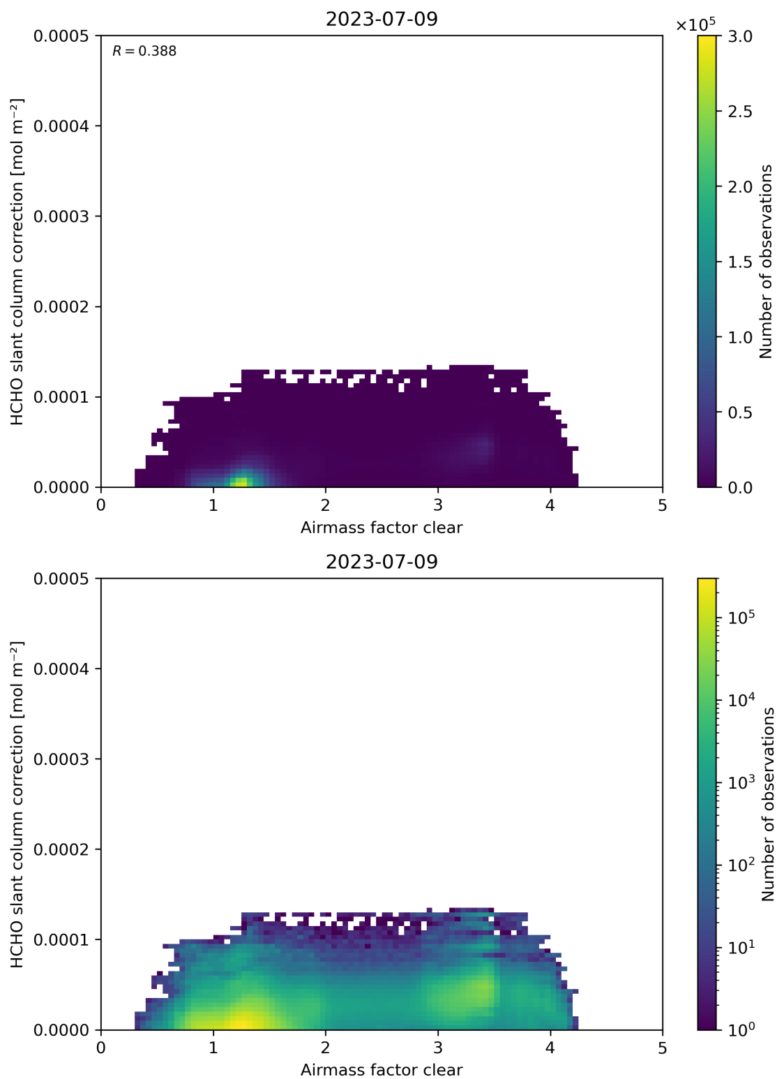
Figure 75: Scatter density plot of “Airmass factor clear” against “HCHO slant column correction” for 2023-07-08 to 2023-07-10.
