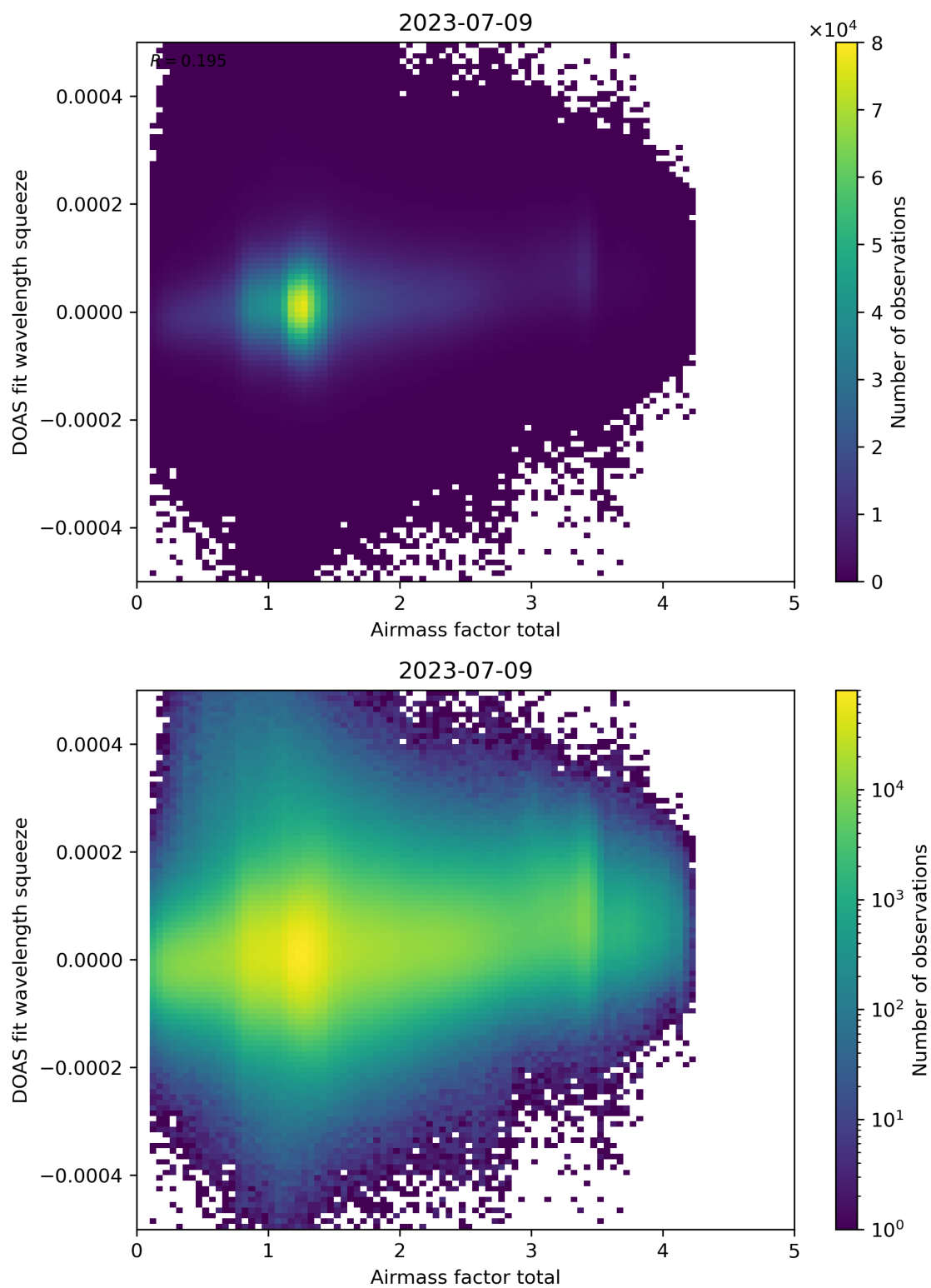
Figure 99: Scatter density plot of “Airmass factor total” against “DOAS fit wavelength squeeze” for 2023-07-08 to 2023-07-10.
