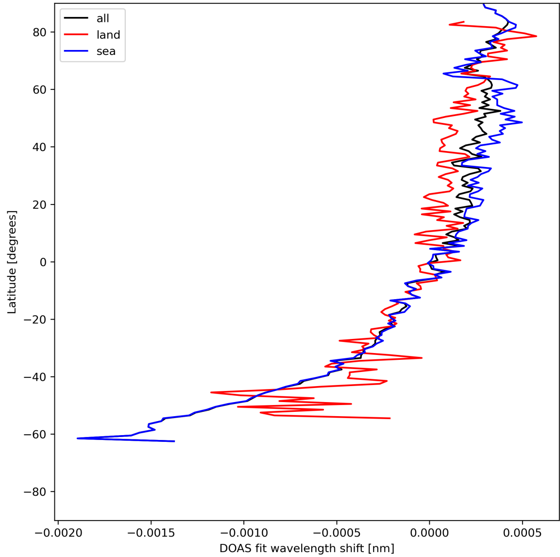
Figure 30: Zonal average of "DOAS fit wavelength shift" for 2023-07-08 to 2023-07-10.
