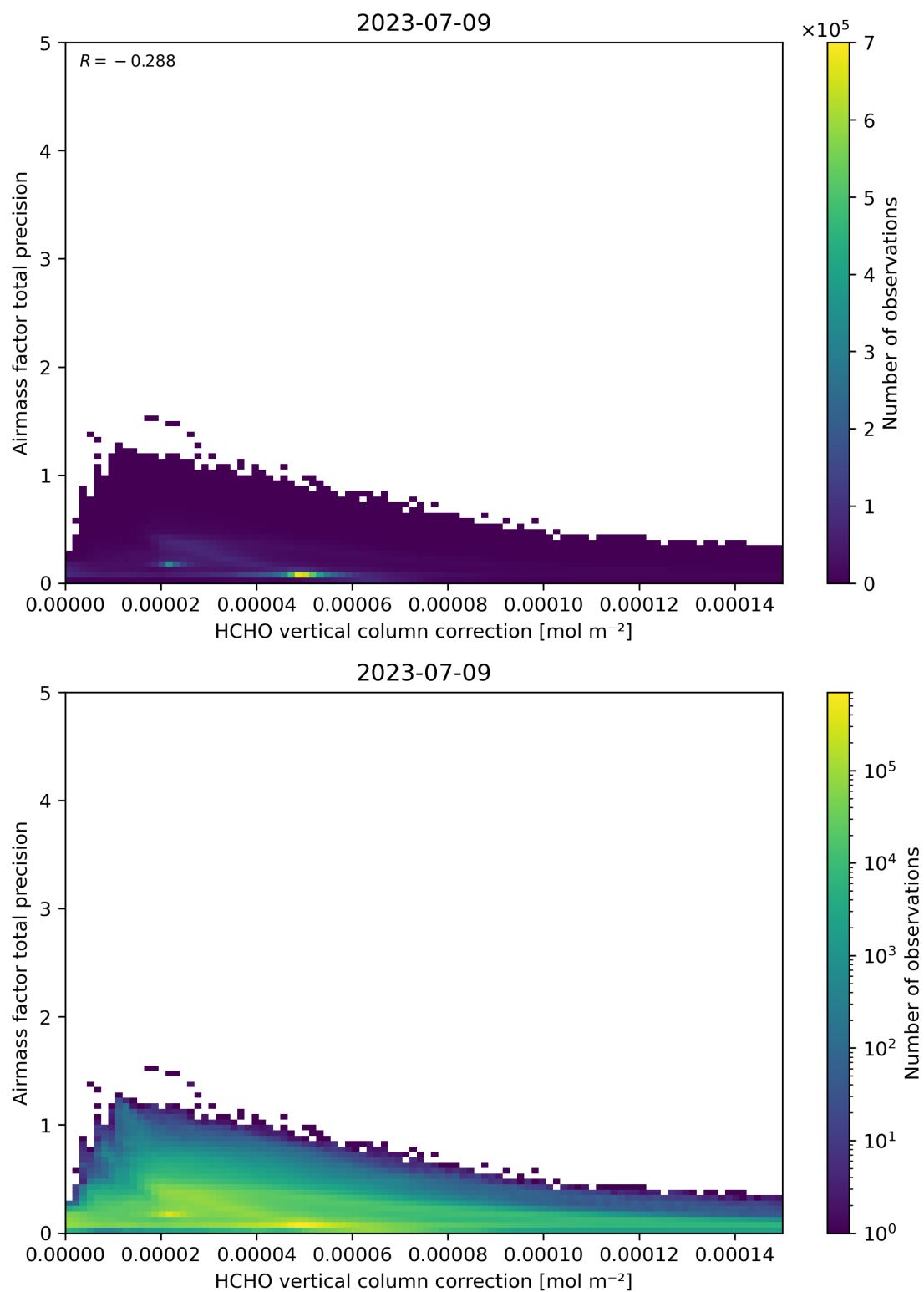
Figure 121: Scatter density plot of “HCHO vertical column correction” against “Airmass factor total precision” for 2023-07-08 to 2023-07-10.
