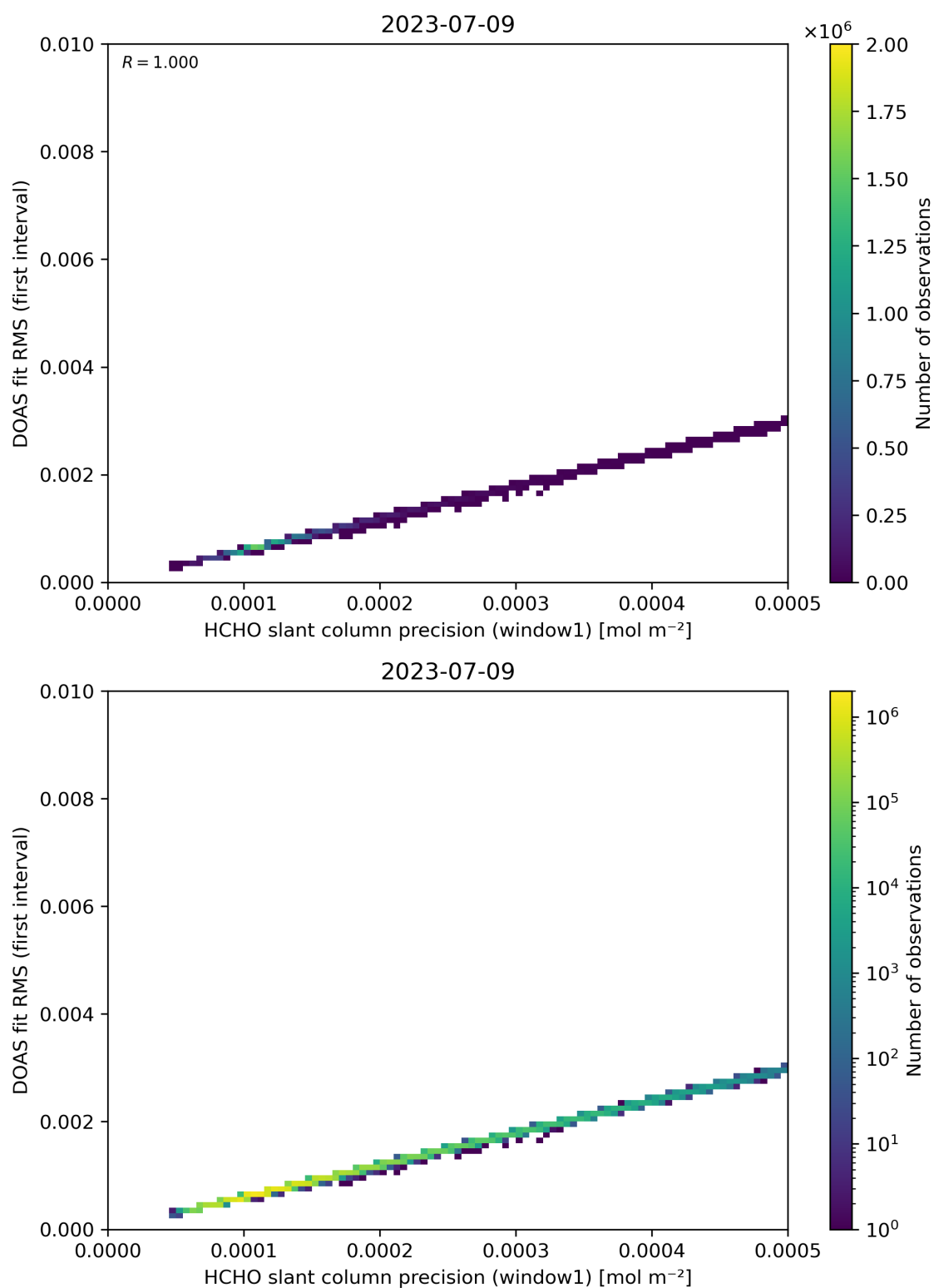
Figure 88: Scatter density plot of “HCHO slant column precision (window1)” against “DOAS fit RMS (first interval)” for 2023-07-08 to 2023-07-10.
