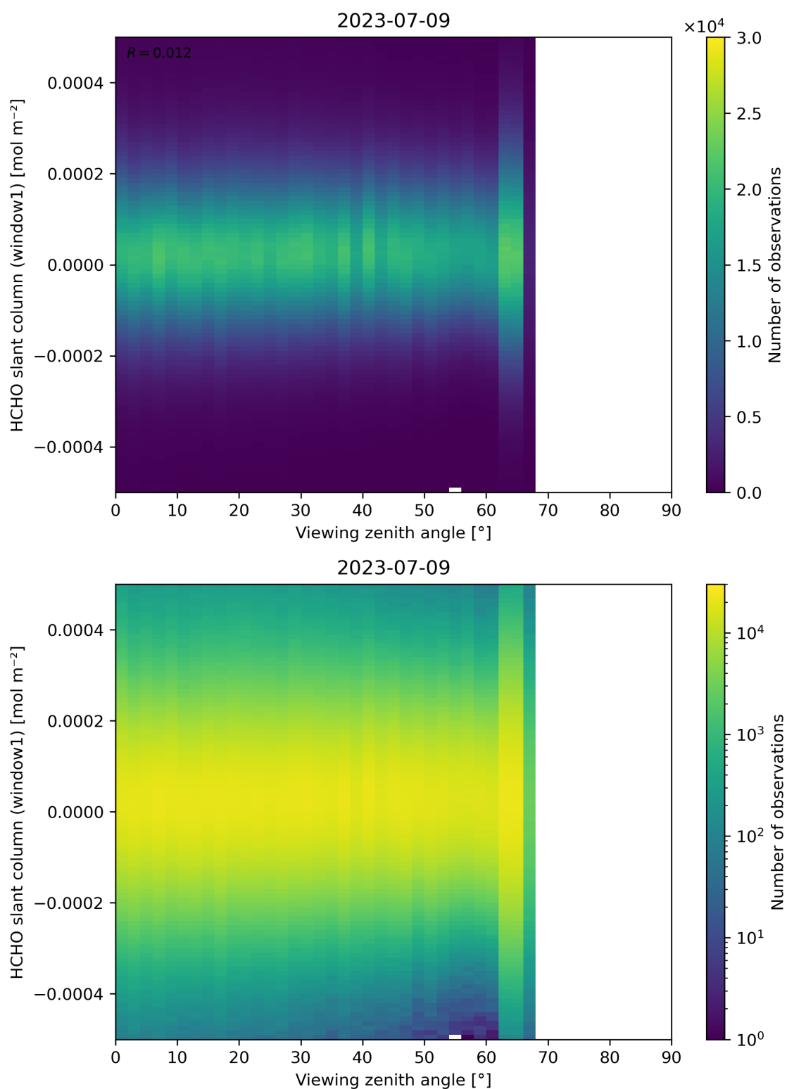
Figure 188: Scatter density plot of “Viewing zenith angle” against “HCHO slant column (window1)” for 2023-07-08 to 2023-07-10.
