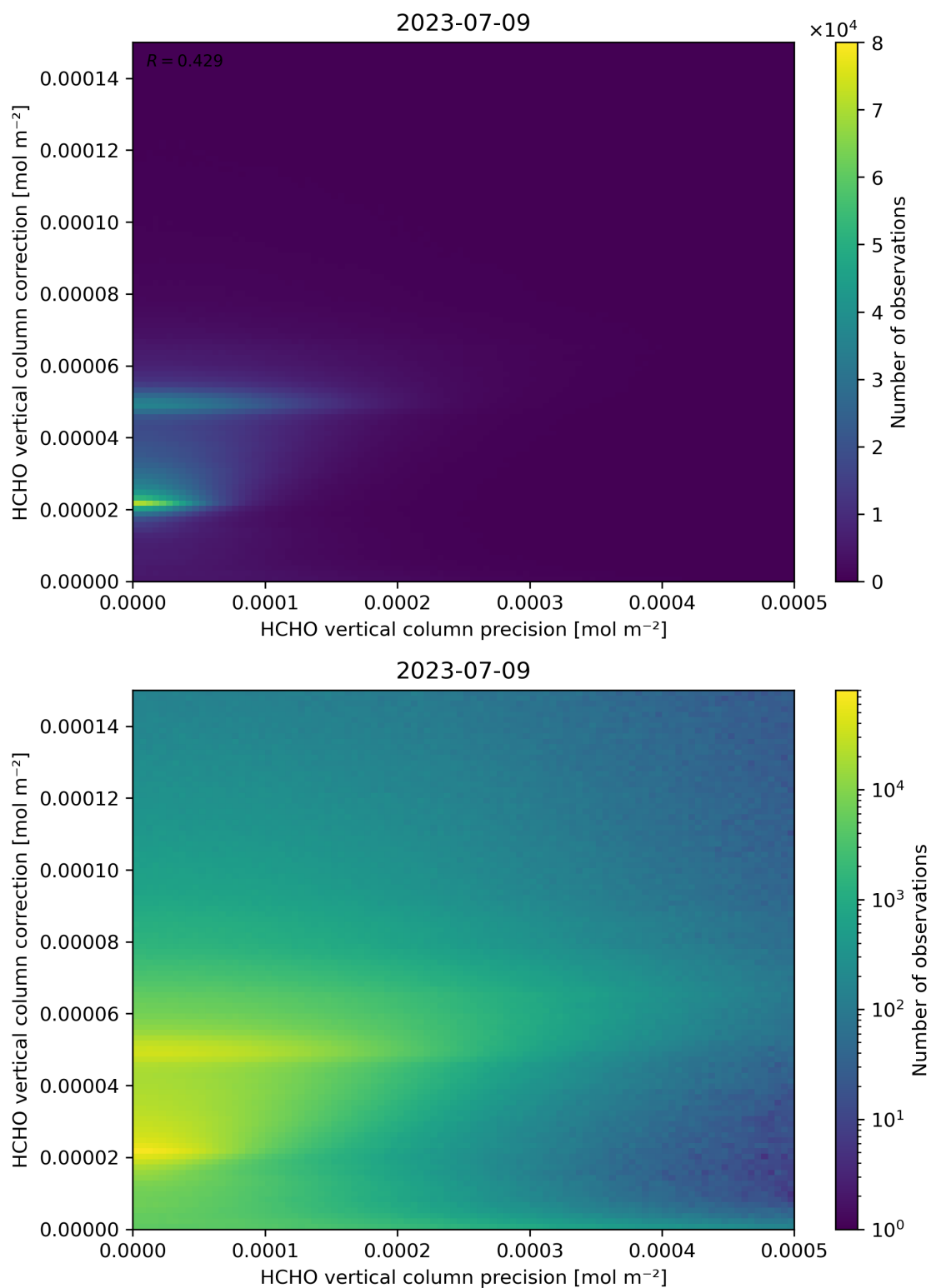
Figure 146: Scatter density plot of “HCHO vertical column precision” against “HCHO vertical column correction” for 2023-07-08 to 2023-07-10.
