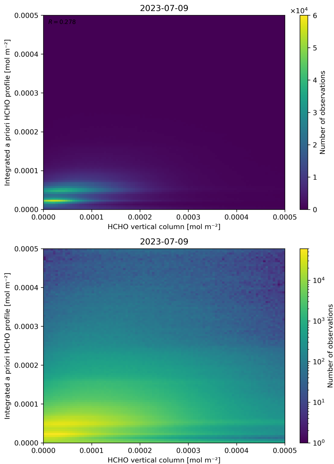
Figure 135: Scatter density plot of “HCHO vertical column” against “Integrated a priori HCHO profile” for 2023-07-08 to 2023-07-10.
