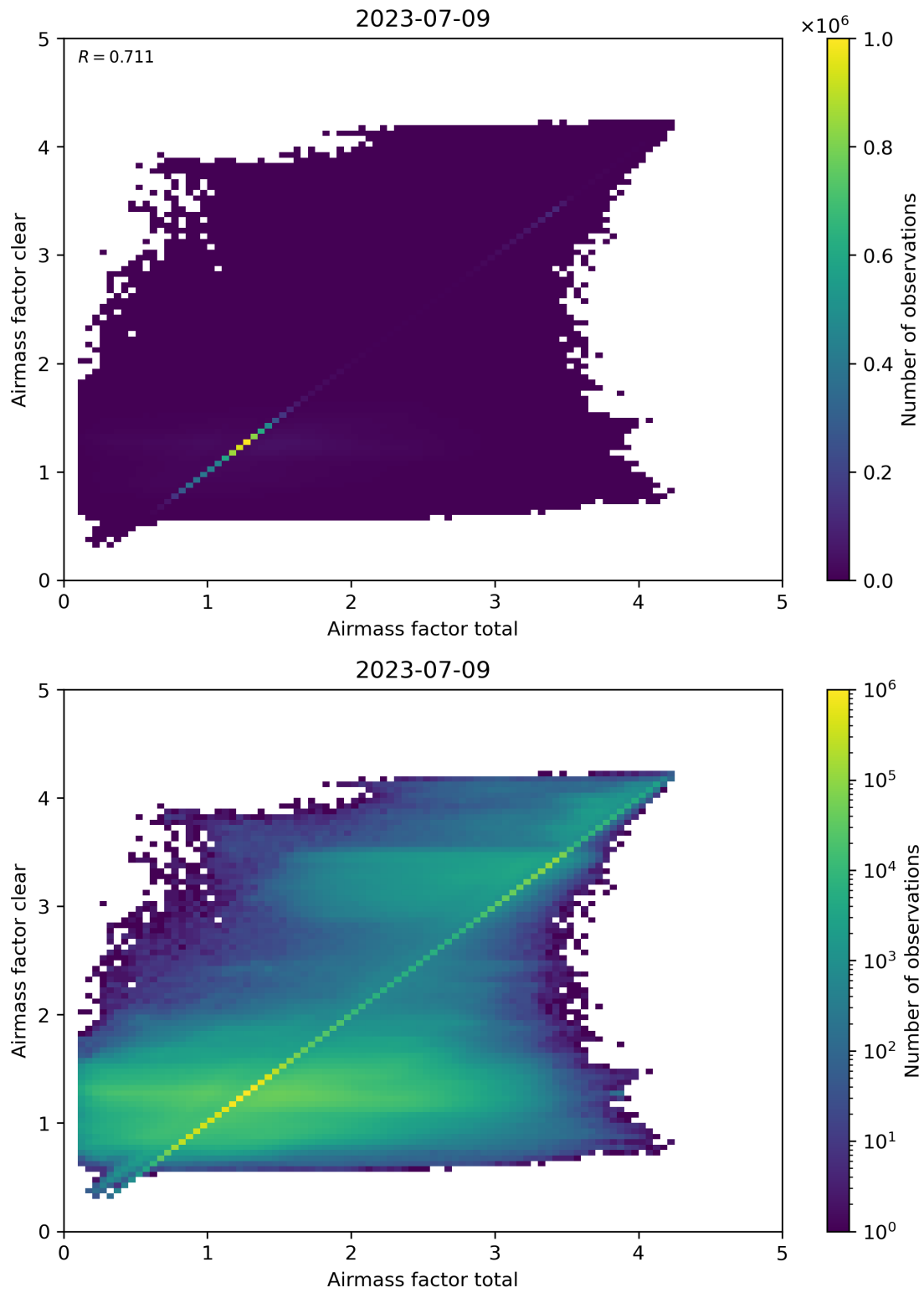
Figure 100: Scatter density plot of “Airmass factor total” against “Airmass factor clear” for 2023-07-08 to 2023-07-10.
