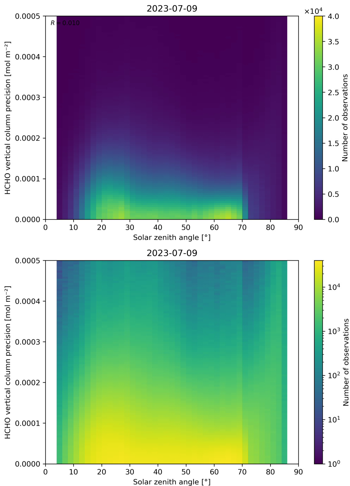
Figure 179: Scatter density plot of “Solar zenith angle” against “HCHO vertical column precision” for 2023-07-08 to 2023-07-10.
