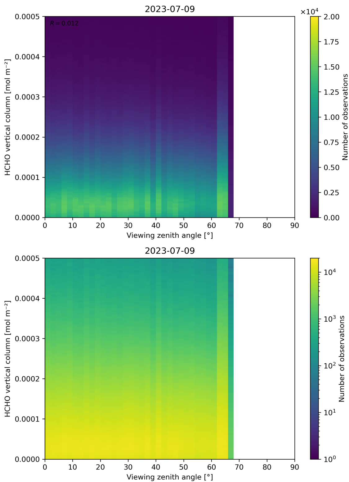
Figure 192: Scatter density plot of “Viewing zenith angle” against “HCHO vertical column” for 2023-07-08 to 2023-07-10.
