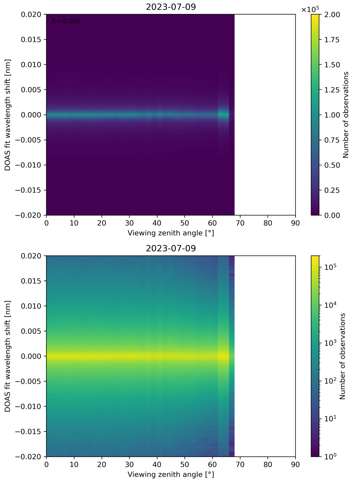
Figure 183: Scatter density plot of “Viewing zenith angle” against “DOAS fit wavelength shift” for 2023-07-08 to 2023-07-10.
