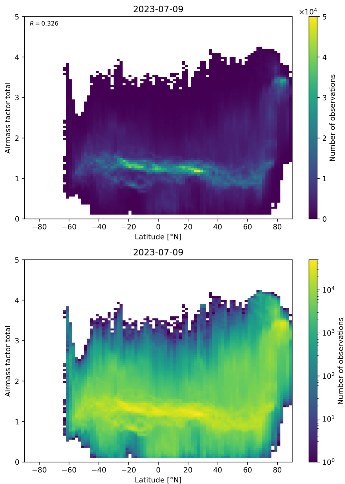
Figure 161: Scatter density plot of “Latitude” against “Airmass factor total” for 2023-07-08 to 2023-07-10.
