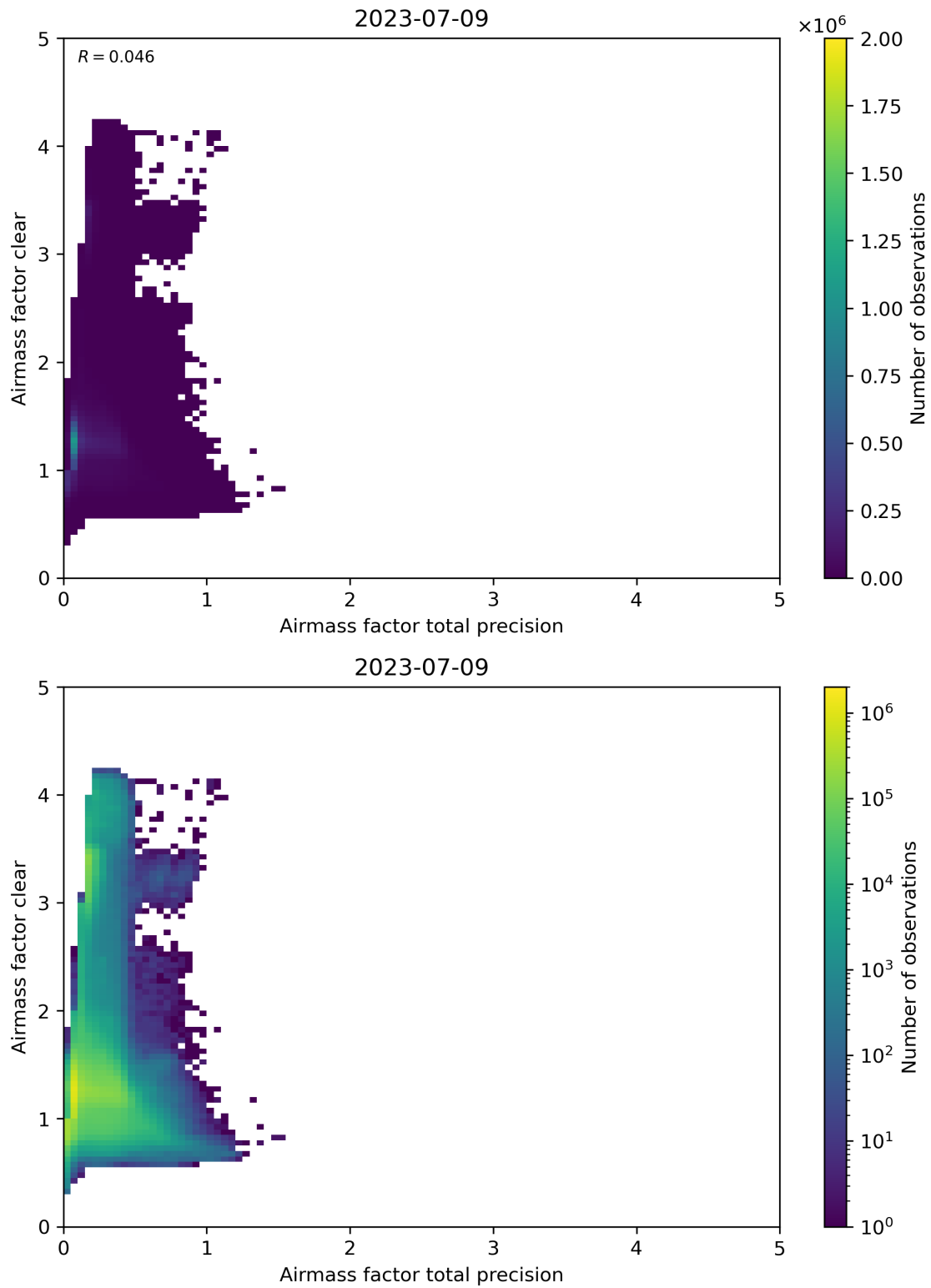
Figure 108: Scatter density plot of “Airmass factor total precision” against “Airmass factor clear” for 2023-07-08 to 2023-07-10.
