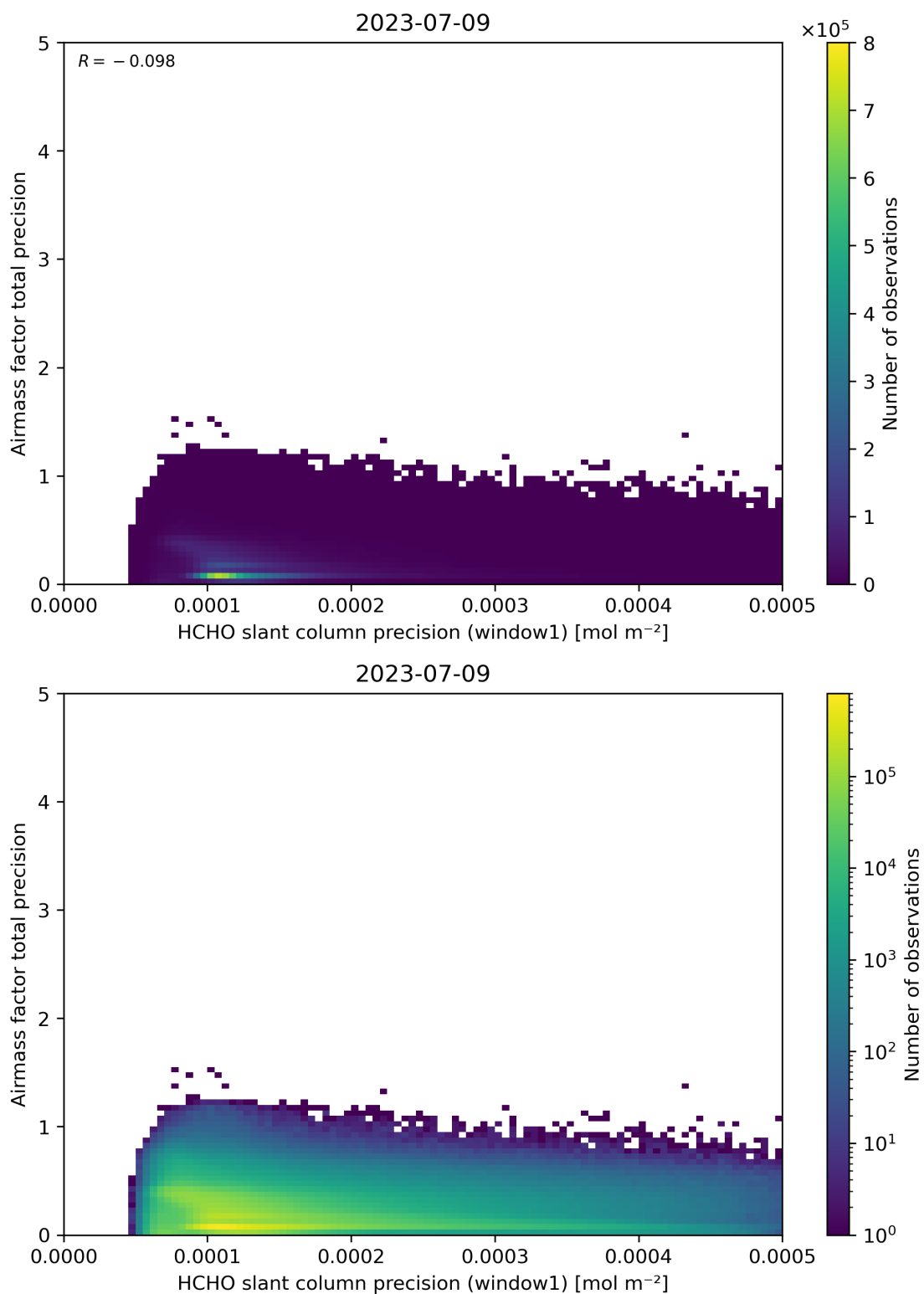
Figure 95: Scatter density plot of “HCHO slant column precision (window1)” against “Airmass factor total precision” for 2023-07-08 to 2023-07-10.
