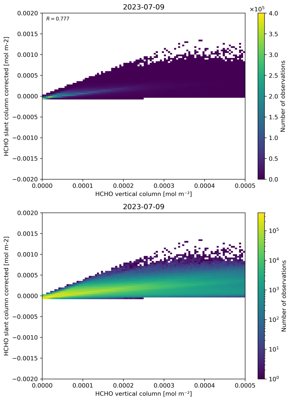
Figure 127: Scatter density plot of “HCHO vertical column” against “HCHO slant column corrected” for 2023-07-08 to 2023-07-10.
