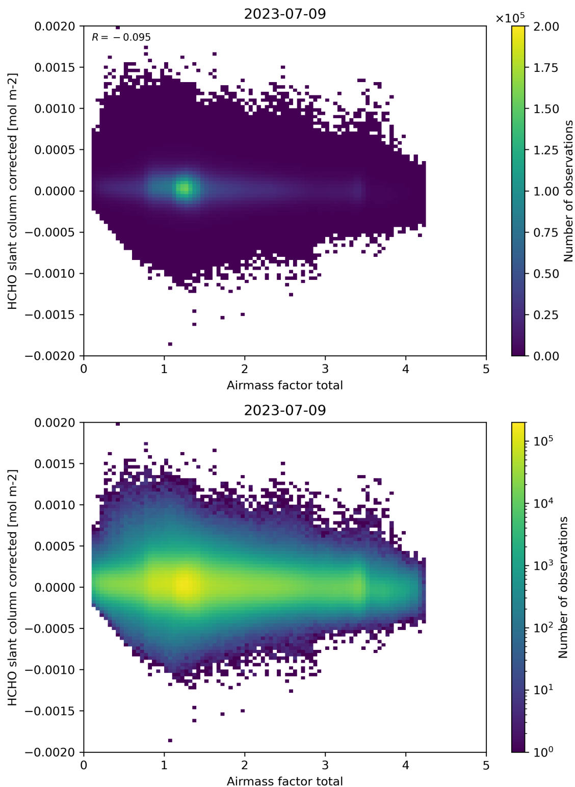
Figure 101: Scatter density plot of “Airmass factor total” against “HCHO slant column corrected” for 2023-07-08 to 2023-07-10.
