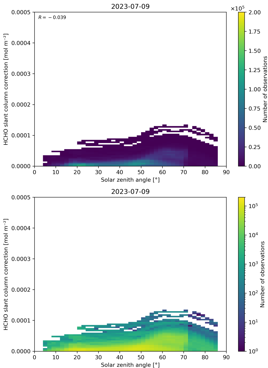
Figure 172: Scatter density plot of “Solar zenith angle” against “HCHO slant column correction” for 2023-07-08 to 2023-07-10.
