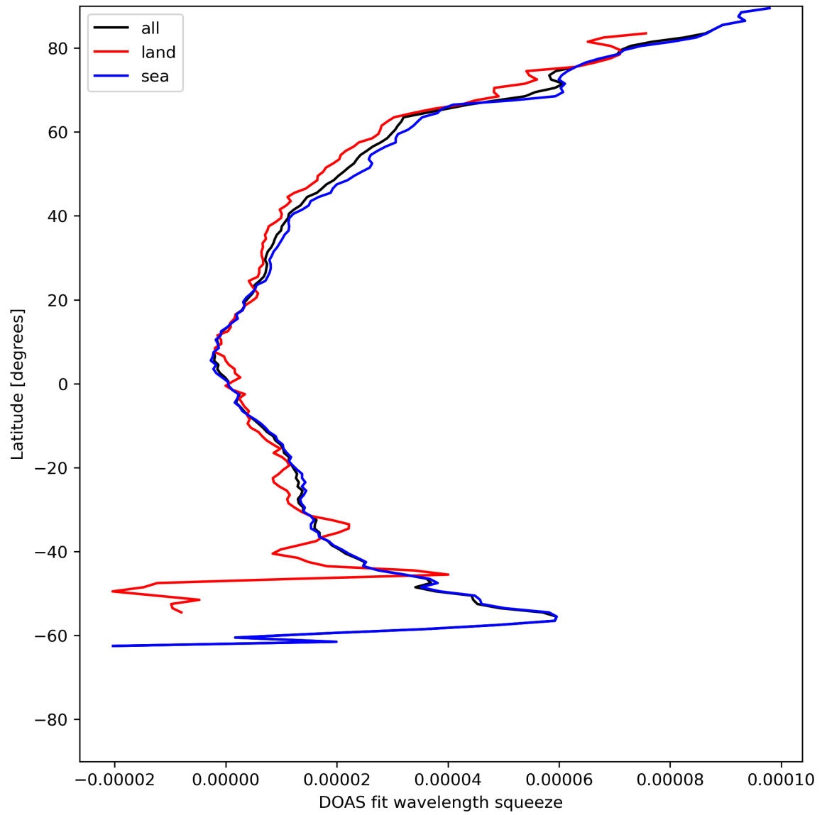
Figure 31: Zonal average of “DOAS fit wavelength squeeze” for 2023-07-08 to 2023-07-10.
