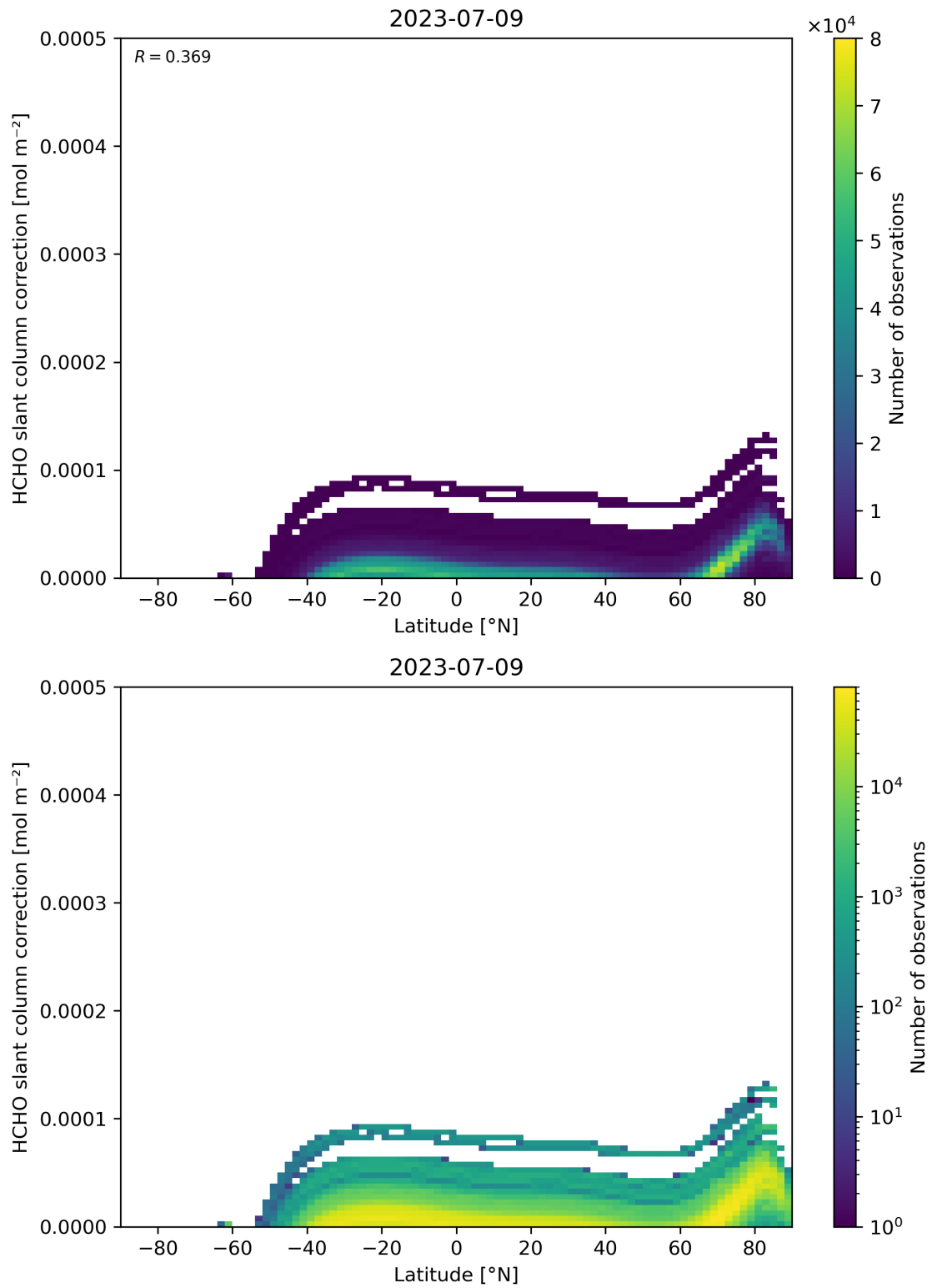
Figure 158: Scatter density plot of “Latitude” against “HCHO slant column correction” for 2023-07-08 to 2023-07-10.
