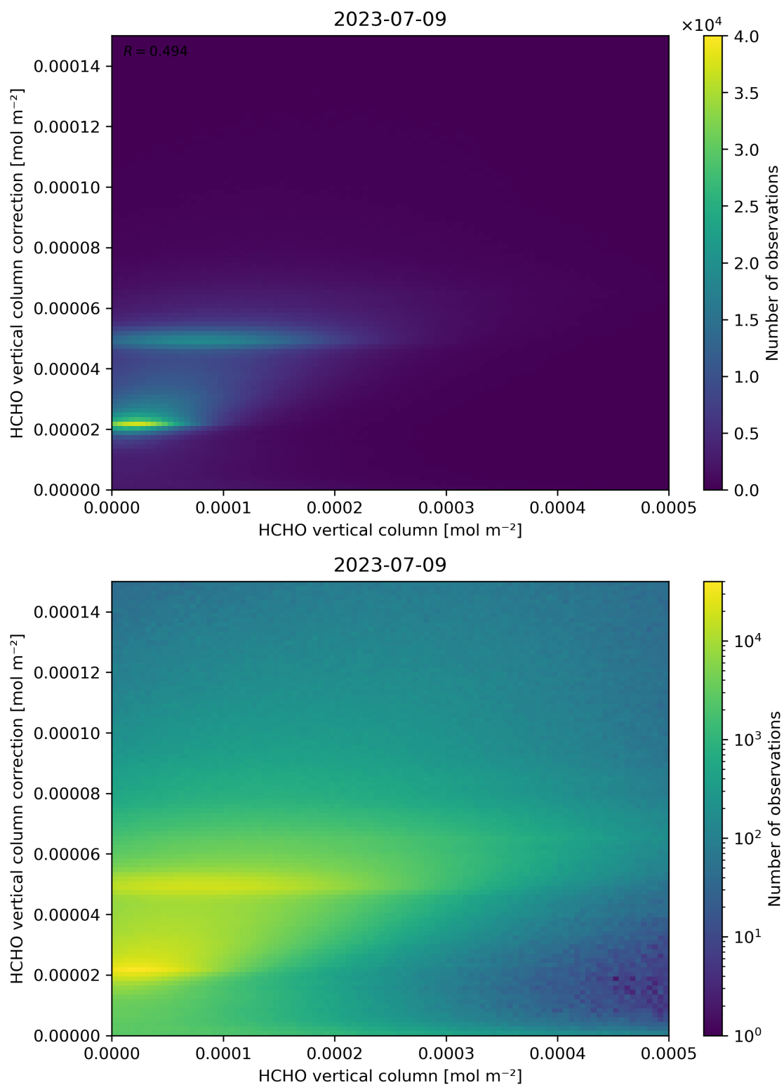
Figure 133: Scatter density plot of “HCHO vertical column” against “HCHO vertical column correction” for 2023-07-08 to 2023-07-10.
