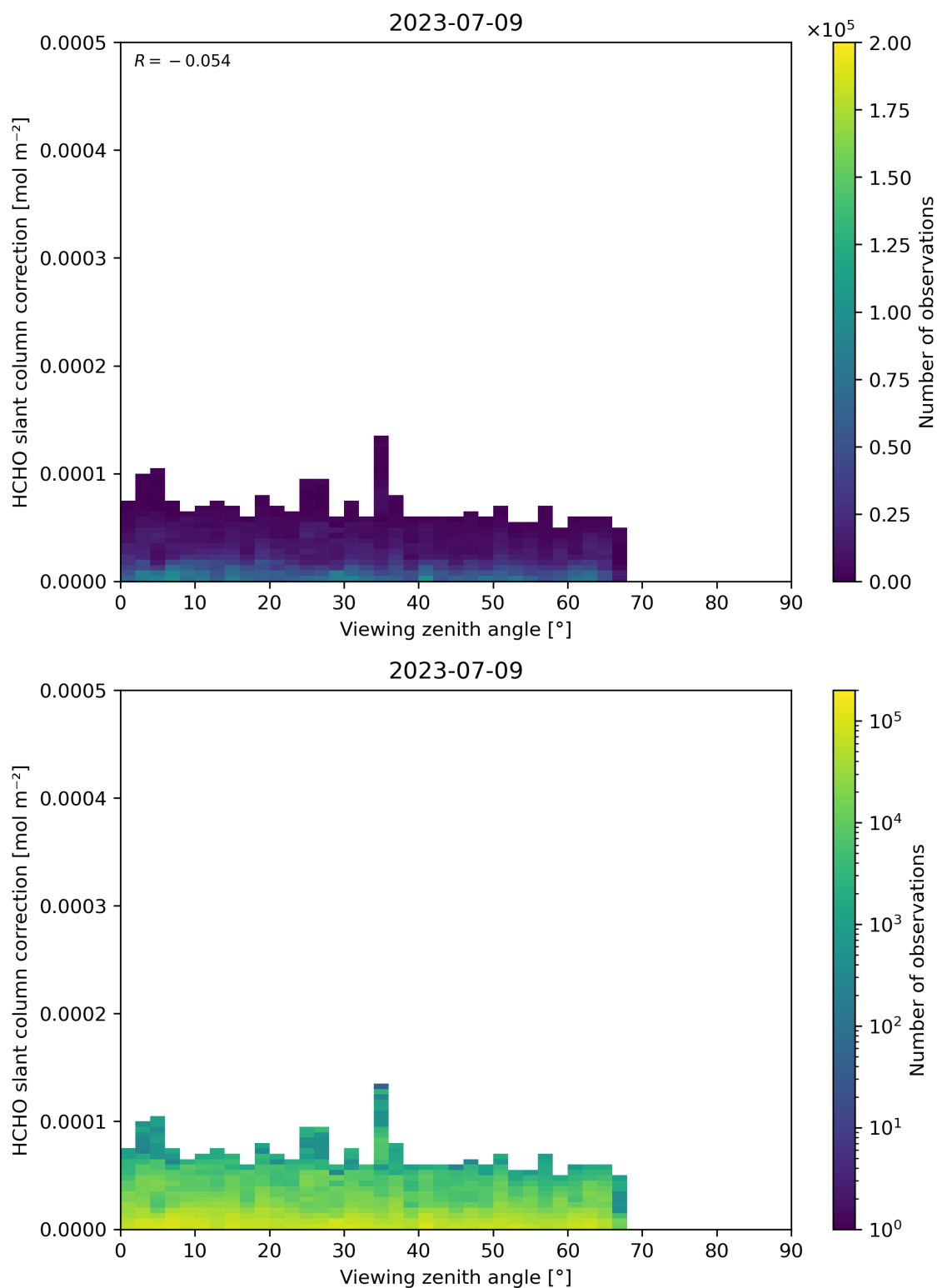
Figure 187: Scatter density plot of “Viewing zenith angle” against “HCHO slant column correction” for 2023-07-08 to 2023-07-10.
