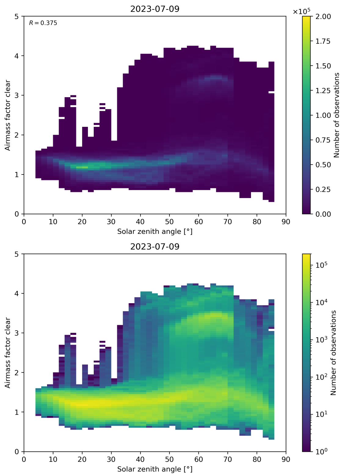
Figure 170: Scatter density plot of “Solar zenith angle” against “Airmass factor clear” for 2023-07-08 to 2023-07-10.
