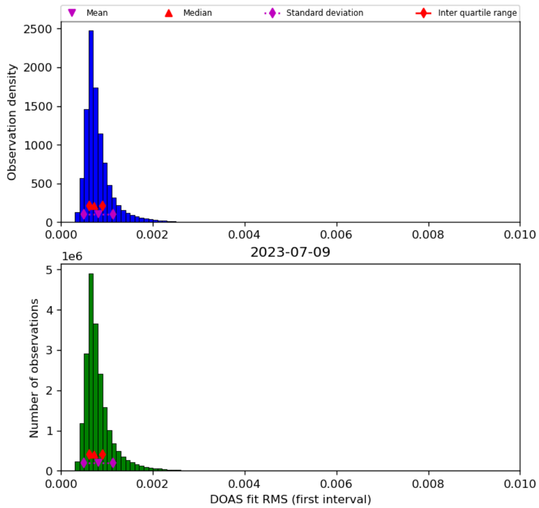
Figure 46: Histogram of “DOAS fit RMS (first interval)” for 2023-07-08 to 2023-07-10
