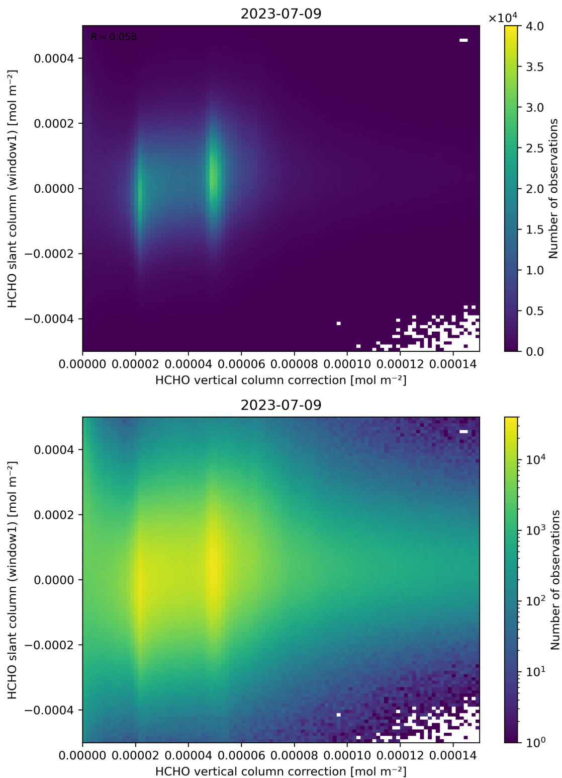
Figure 118: Scatter density plot of “HCHO vertical column correction” against “HCHO slant column (window1)” for 2023-07-08 to 2023-07-10.
