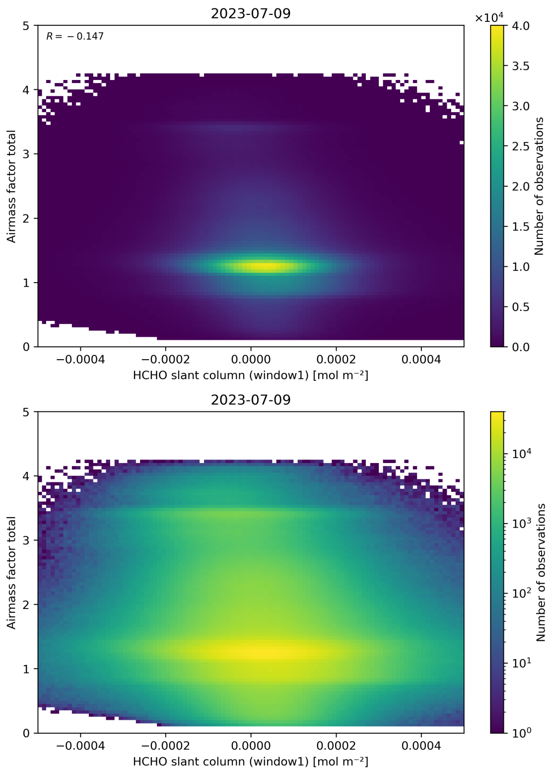
Figure 85: Scatter density plot of “HCHO slant column (window1)” against “Airmass factor total” for 2023-07-08 to 2023-07-10.
