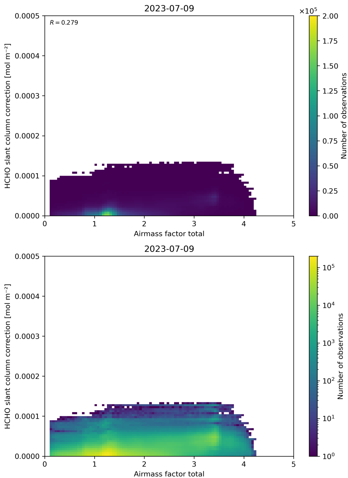
Figure 102: Scatter density plot of “Airmass factor total” against “HCHO slant column correction” for 2023-07-08 to 2023-07-10.
