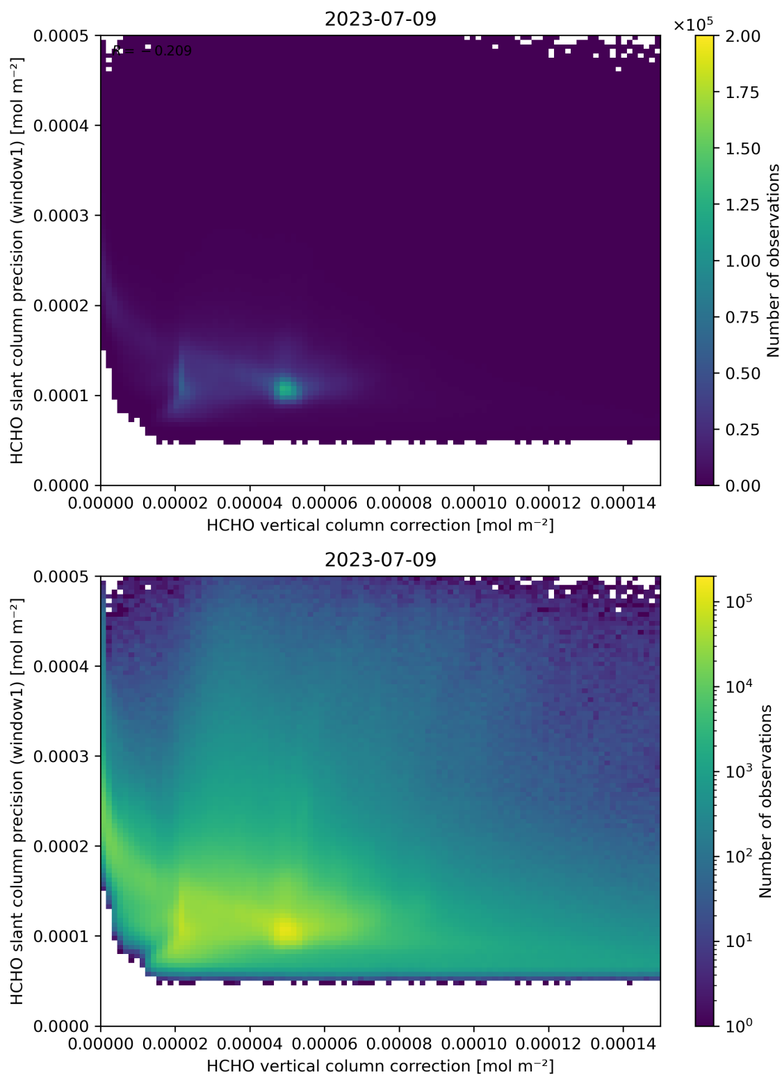
Figure 119: Scatter density plot of “HCHO vertical column correction” against “HCHO slant column precision (window1)” for 2023-07-08 to 2023-07-10.
