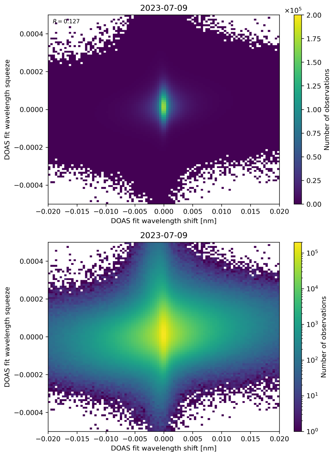
Figure 65: Scatter density plot of “DOAS fit wavelength shift” against “DOAS fit wavelength squeeze” for 2023-07-08 to 2023-07-10.
