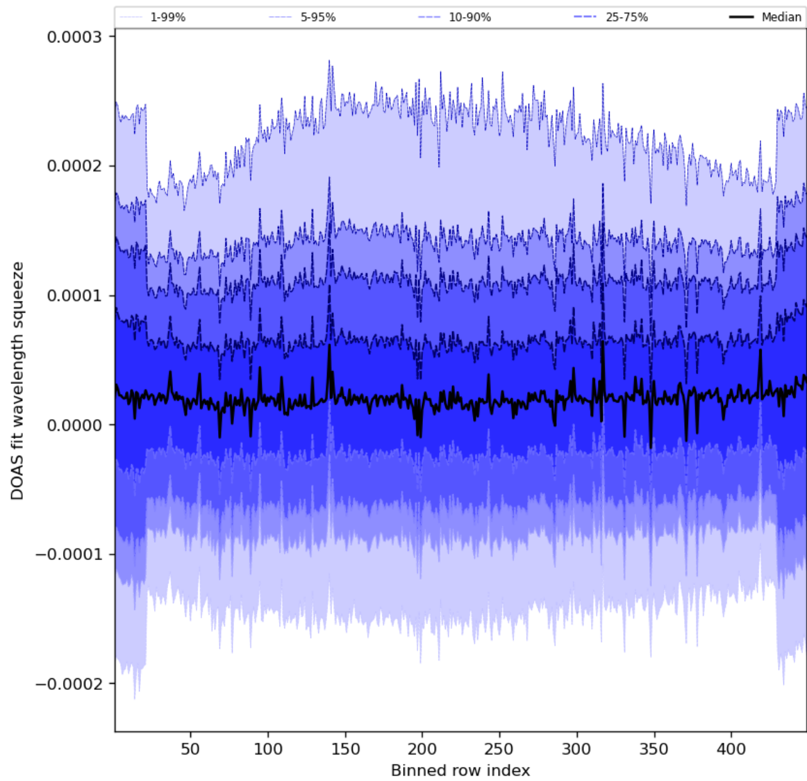
Figure 59: Along track statistics of “DOAS fit wavelength squeeze” for 2023-07-08 to 2023-07-10
