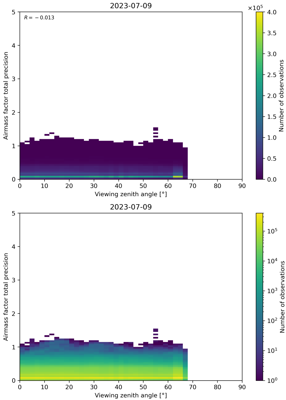
Figure 191: Scatter density plot of “Viewing zenith angle” against “Airmass factor total precision” for 2023-07-08 to 2023-07-10.
