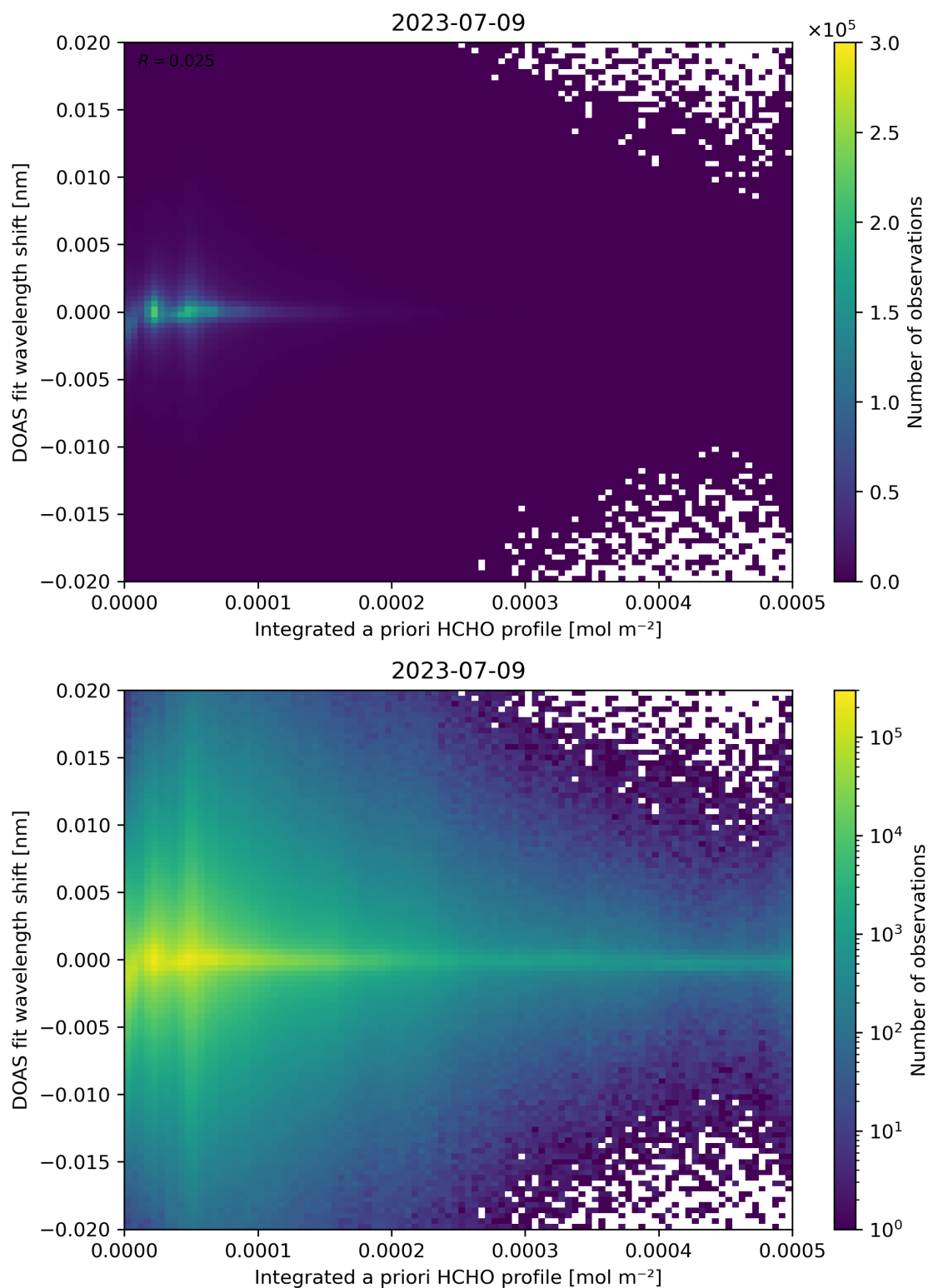
Figure 149: Scatter density plot of “Integrated a priori HCHO profile” against “DOAS fit wavelength shift” for 2023-07-08 to 2023-07-10.
