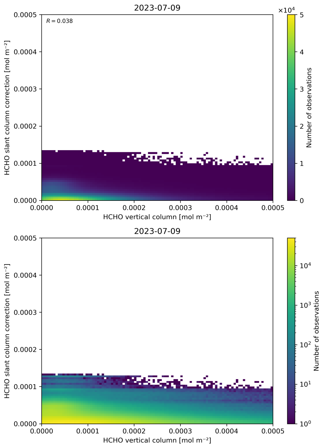
Figure 128: Scatter density plot of “HCHO vertical column” against “HCHO slant column correction” for 2023-07-08 to 2023-07-10.
