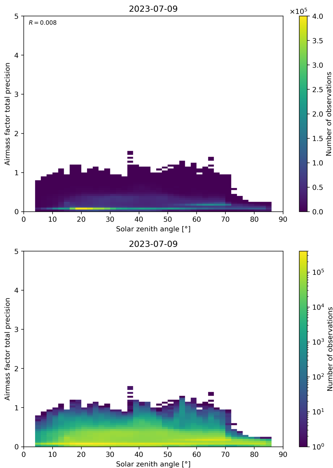
Figure 176: Scatter density plot of “Solar zenith angle” against “Airmass factor total precision” for 2023-07-08 to 2023-07-10.
