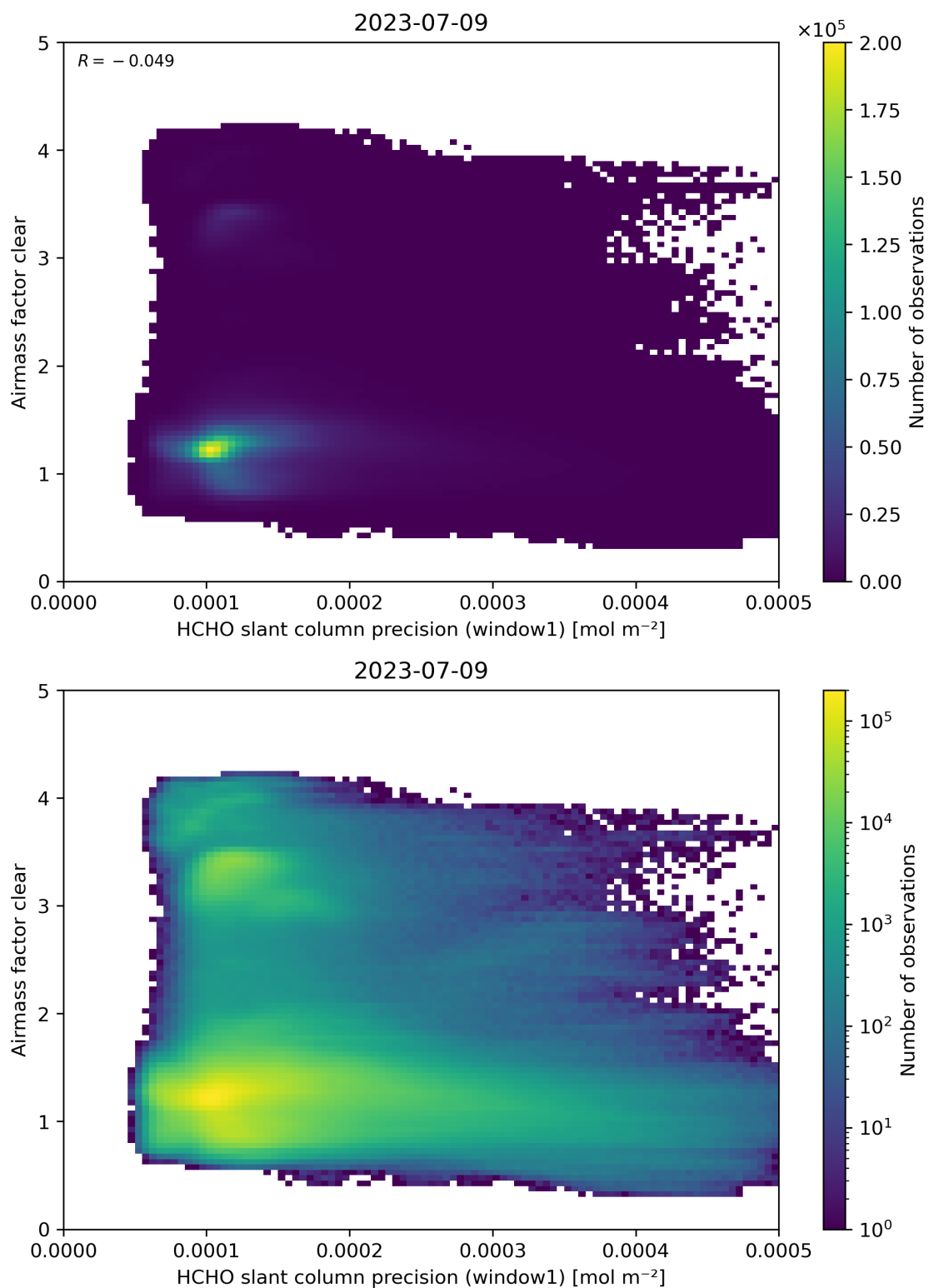
Figure 91: Scatter density plot of “HCHO slant column precision (window1)” against “Airmass factor clear” for 2023-07-08 to 2023-07-10.
