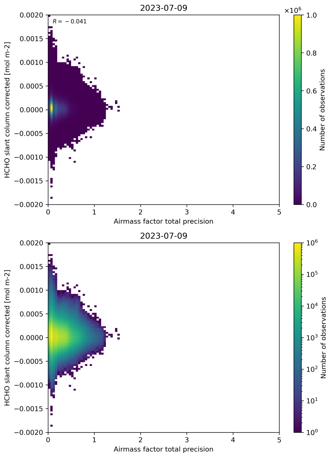
Figure 109: Scatter density plot of “Airmass factor total precision” against “HCHO slant column corrected” for 2023-07-08 to 2023-07-10.
