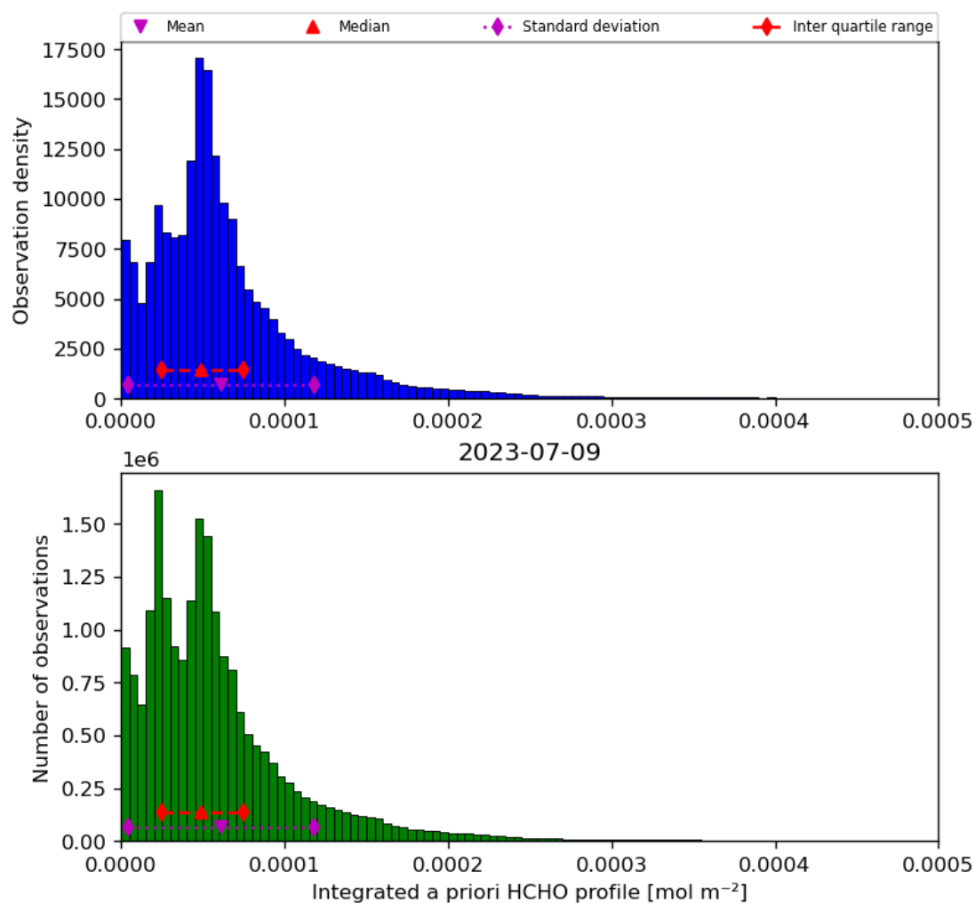
Figure 43: Histogram of “Integrated a priori HCHO profile” for 2023-07-08 to 2023-07-10
