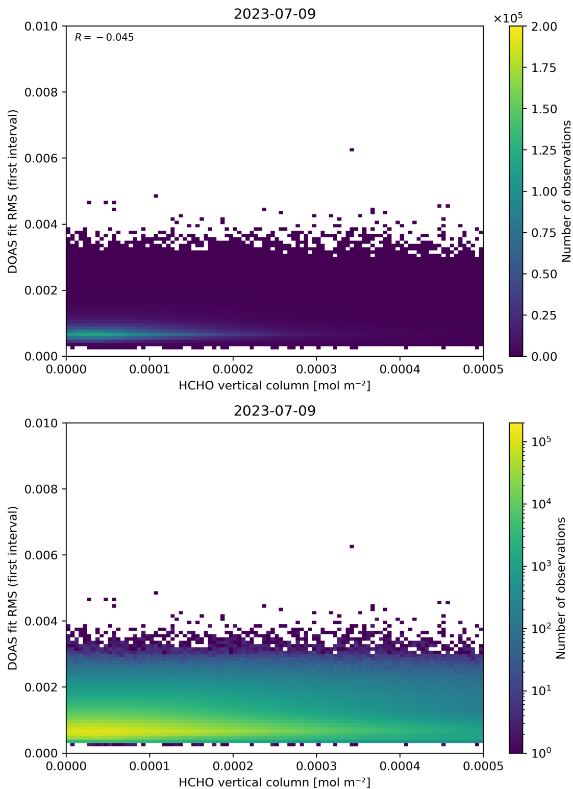
Figure 123: Scatter density plot of “HCHO vertical column” against “DOAS fit RMS (first interval)” for 2023-07-08 to 2023-07-10.
