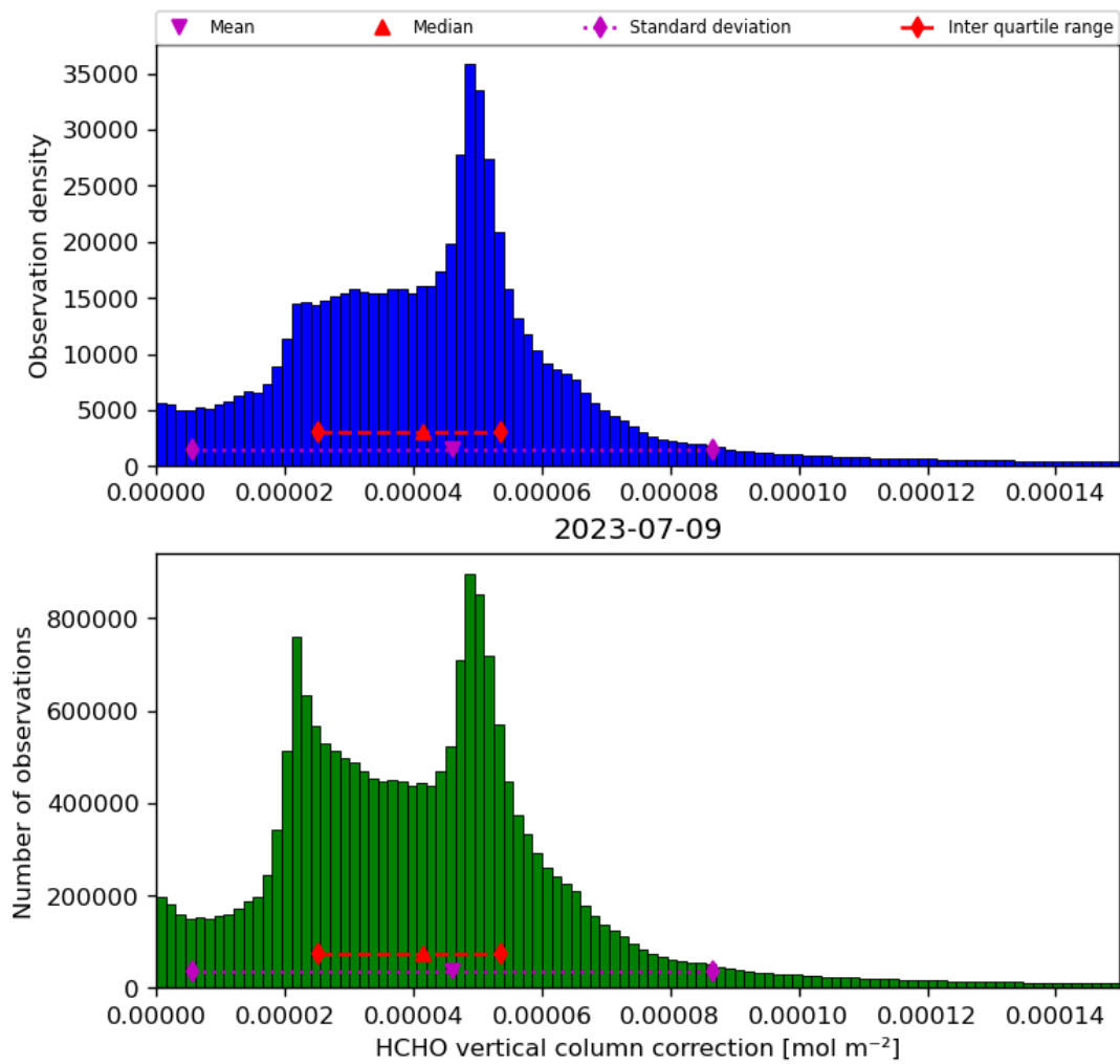
Figure 37: Histogram of “HCHO vertical column correction” for 2023-07-08 to 2023-07-10
