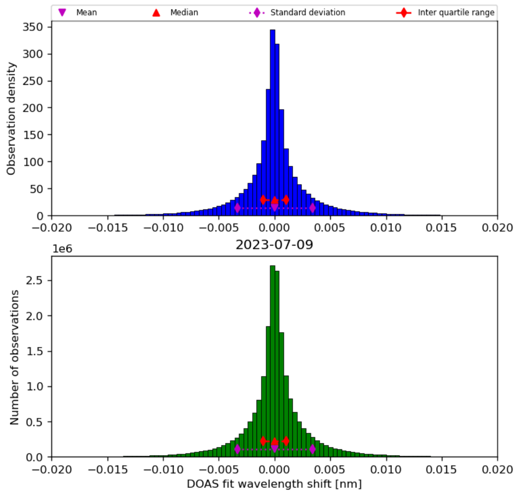
Figure 44: Histogram of “DOAS fit wavelength shift” for 2023-07-08 to 2023-07-10
