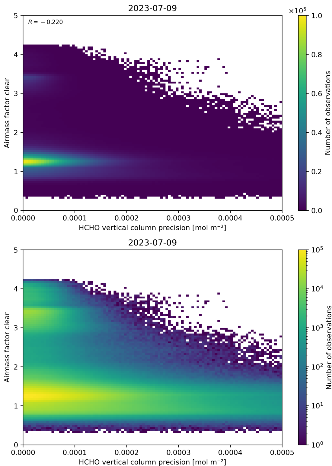
Figure 139: Scatter density plot of “HCHO vertical column precision” against “Airmass factor clear” for 2023-07-08 to 2023-07-10.
