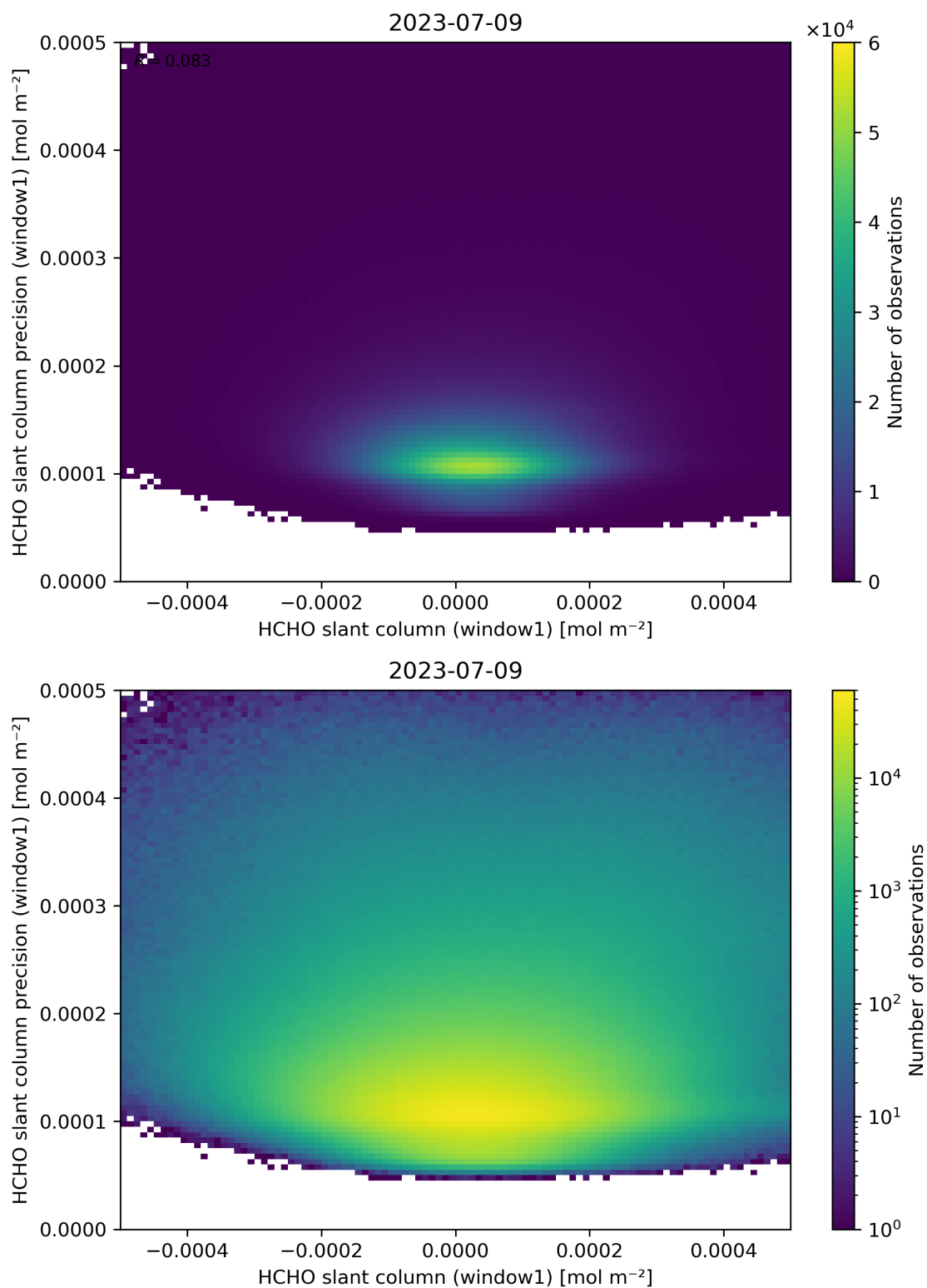
Figure 84: Scatter density plot of “HCHO slant column (window1)” against “HCHO slant column precision (window1)” for 2023-07-08 to 2023-07-10.
