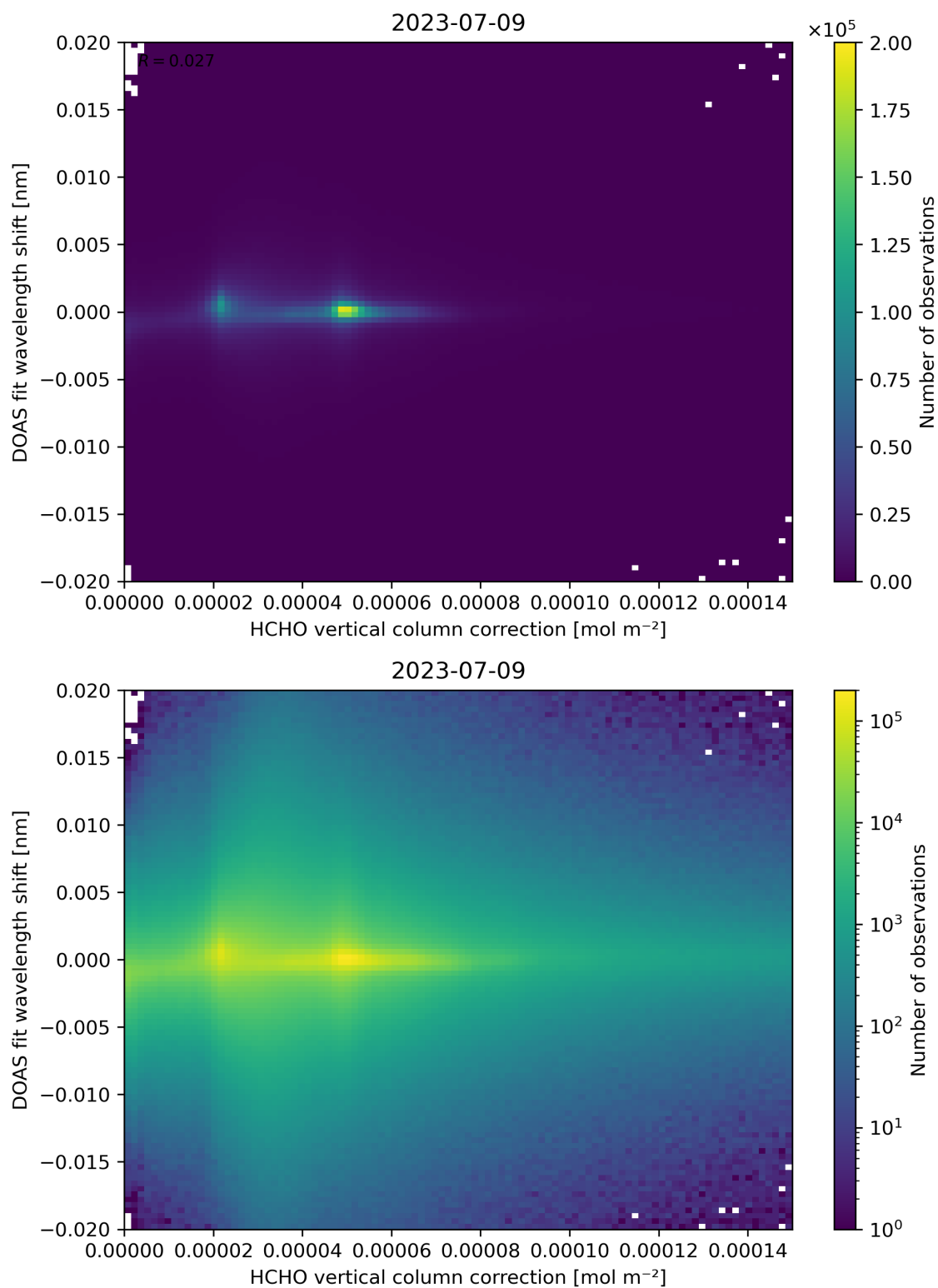
Figure 113: Scatter density plot of “HCHO vertical column correction” against “DOAS fit wavelength shift” for 2023-07-08 to 2023-07-10.
