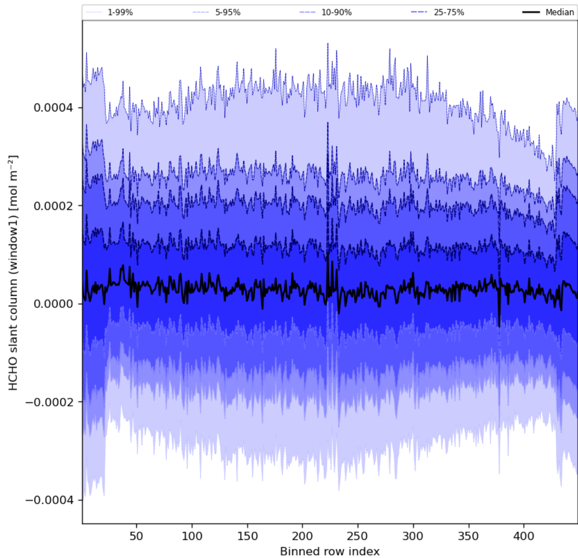
Figure 52: Along track statistics of “HCHO slant column (window1)” for 2023-07-08 to 2023-07-10
