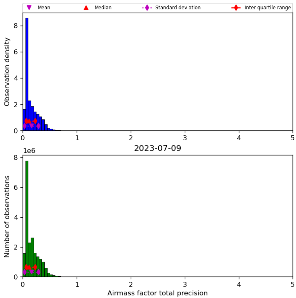
Figure 41: Histogram of “Airmass factor total precision” for 2023-07-08 to 2023-07-10
