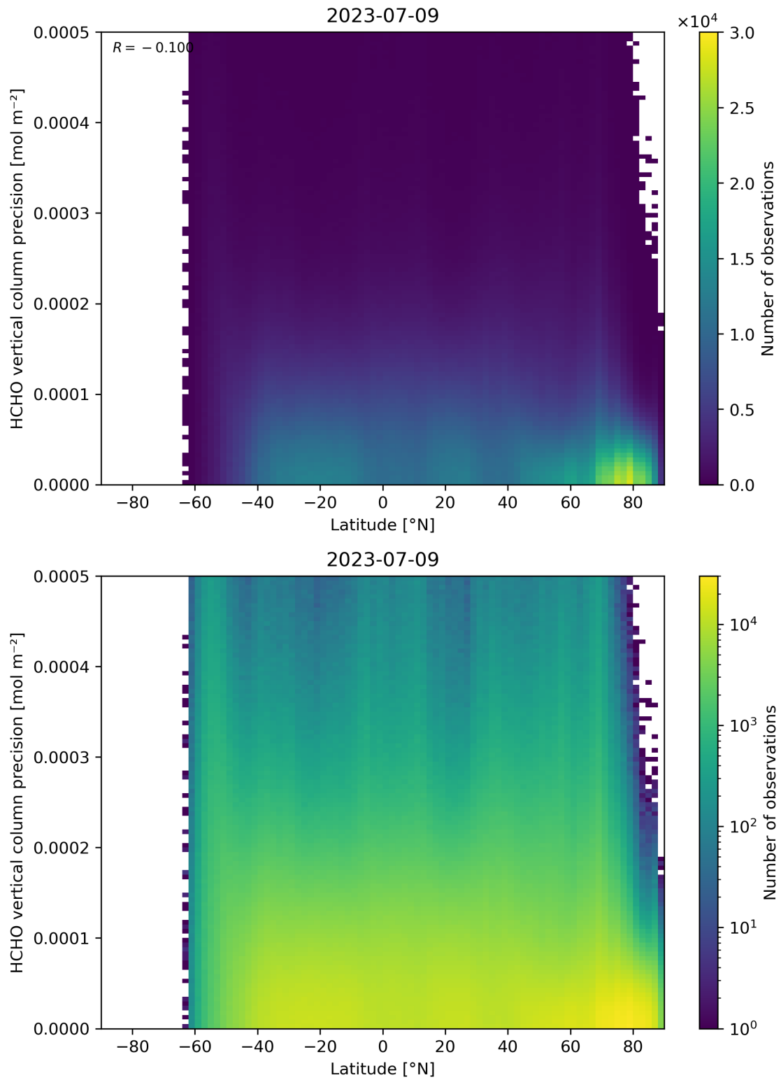
Figure 165: Scatter density plot of “Latitude” against “HCHO vertical column precision” for 2023-07-08 to 2023-07-10.
