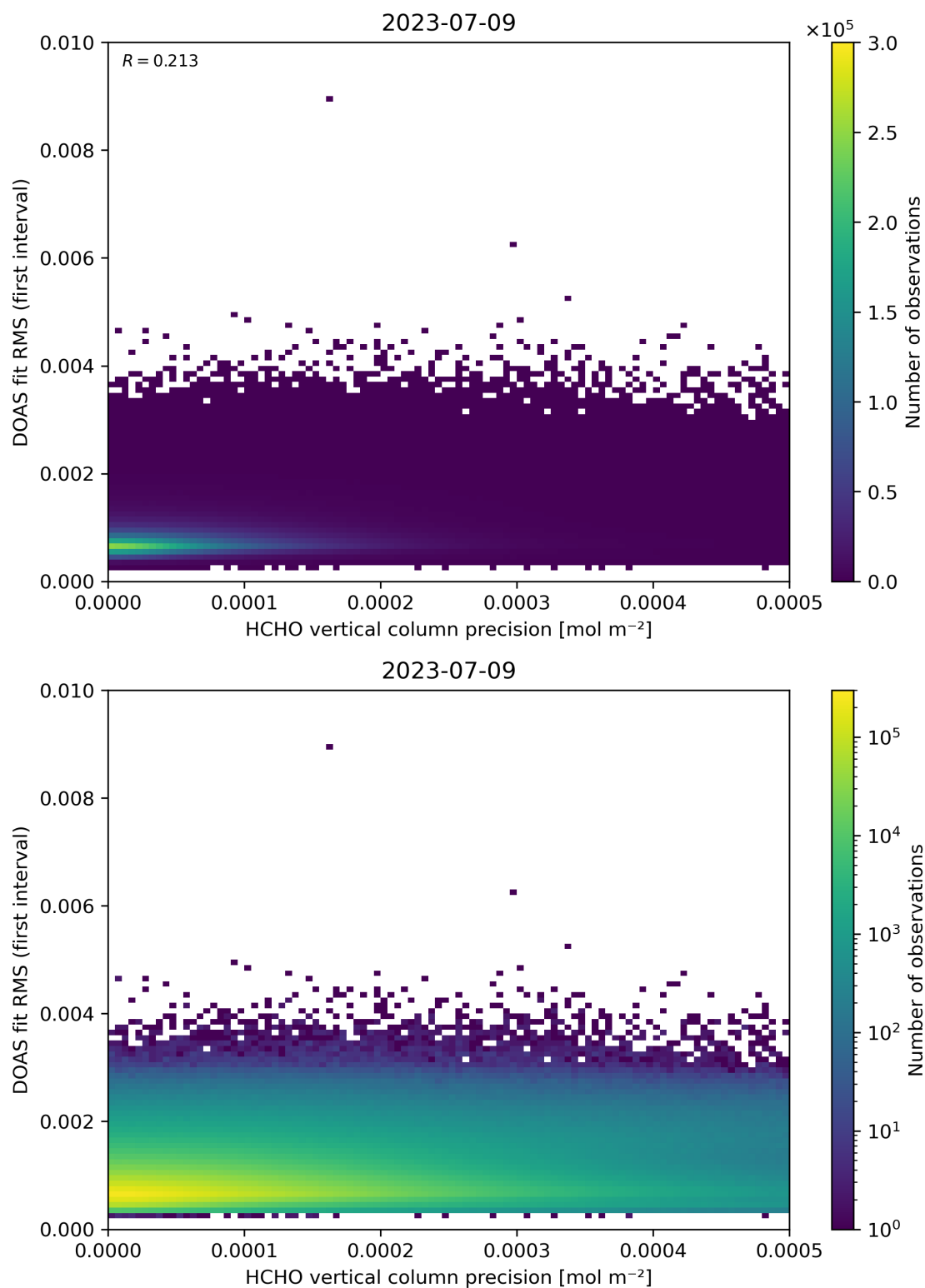
Figure 136: Scatter density plot of “HCHO vertical column precision” against “DOAS fit RMS (first interval)” for 2023-07-08 to 2023-07-10.
