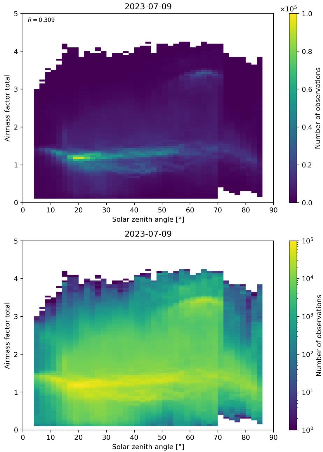
Figure 175: Scatter density plot of “Solar zenith angle” against “Airmass factor total” for 2023-07-08 to 2023-07-10.
