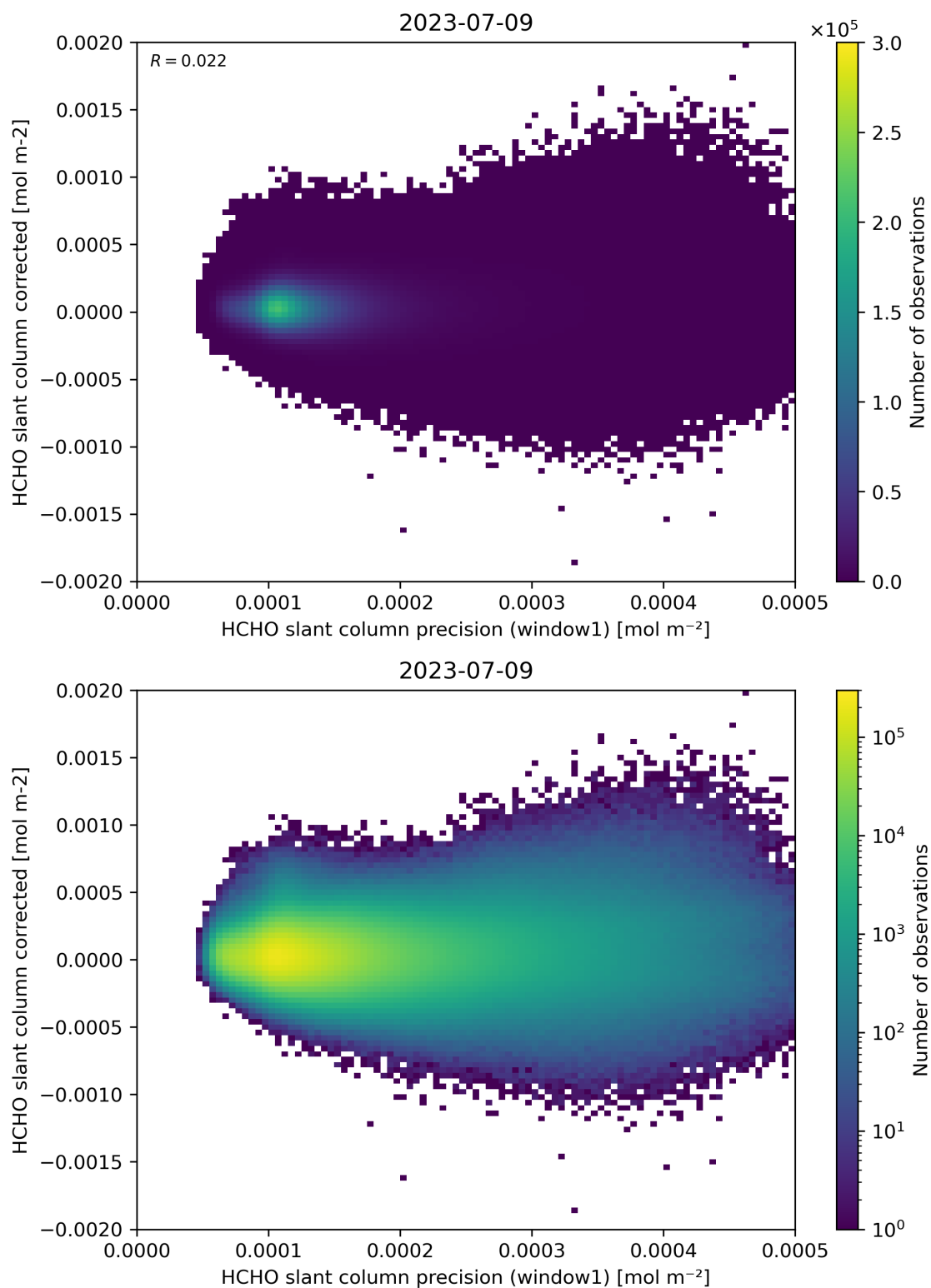
Figure 92: Scatter density plot of “HCHO slant column precision (window1)” against “HCHO slant column corrected” for 2023-07-08 to 2023-07-10.
