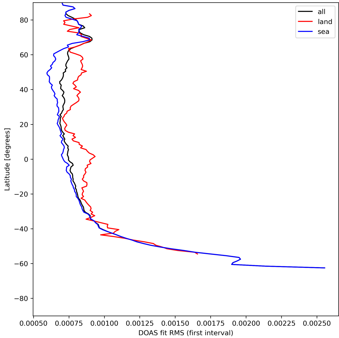
Figure 32: Zonal average of “DOAS fit RMS (first interval)” for 2023-07-08 to 2023-07-10.
