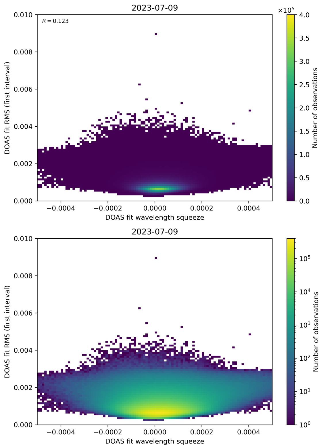
Figure 68: Scatter density plot of “DOAS fit wavelength squeeze” against “DOAS fit RMS (first interval)” for 2023-07-08 to 2023-07-10.
