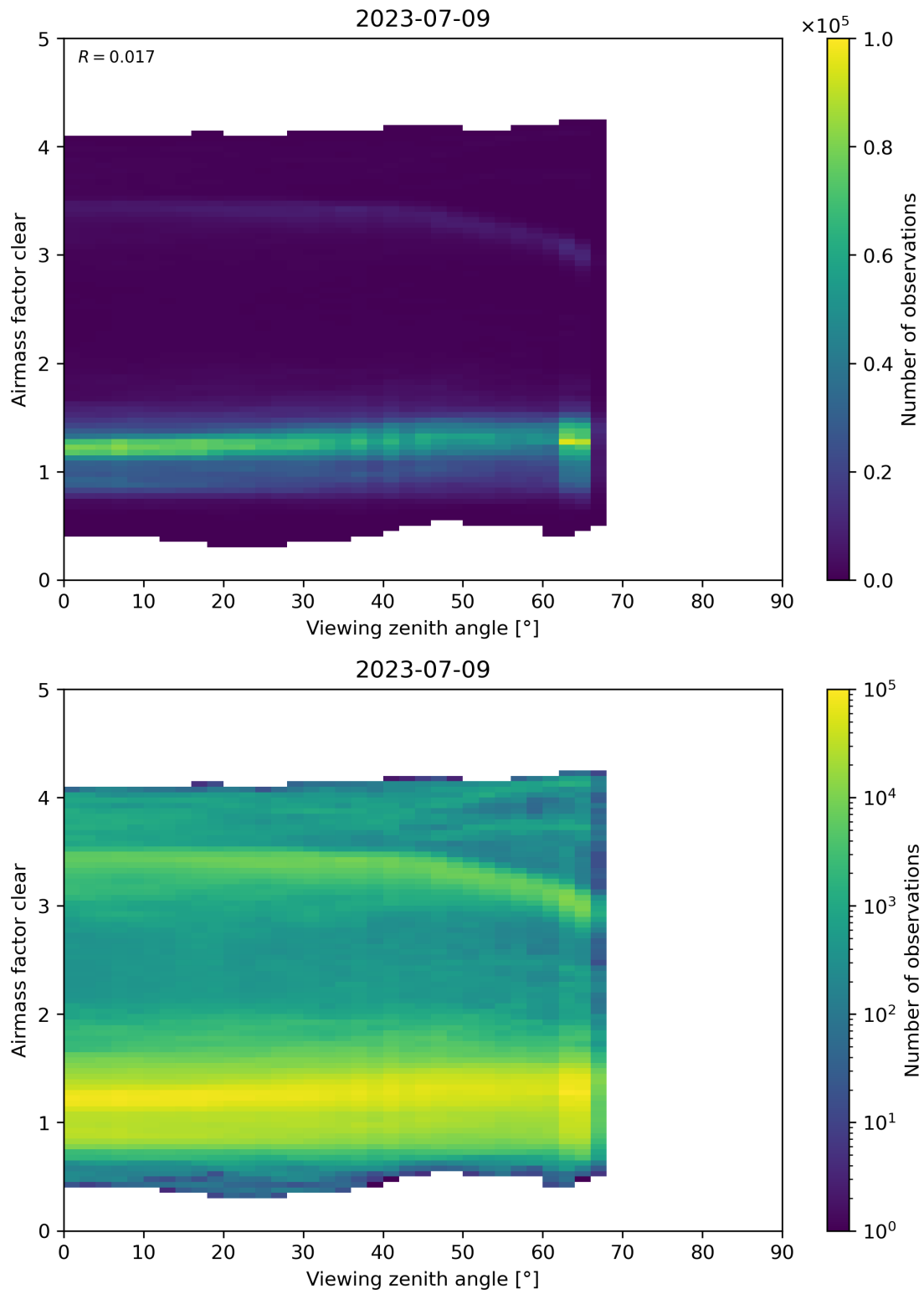
Figure 185: Scatter density plot of “Viewing zenith angle” against “Airmass factor clear” for 2023-07-08 to 2023-07-10.
