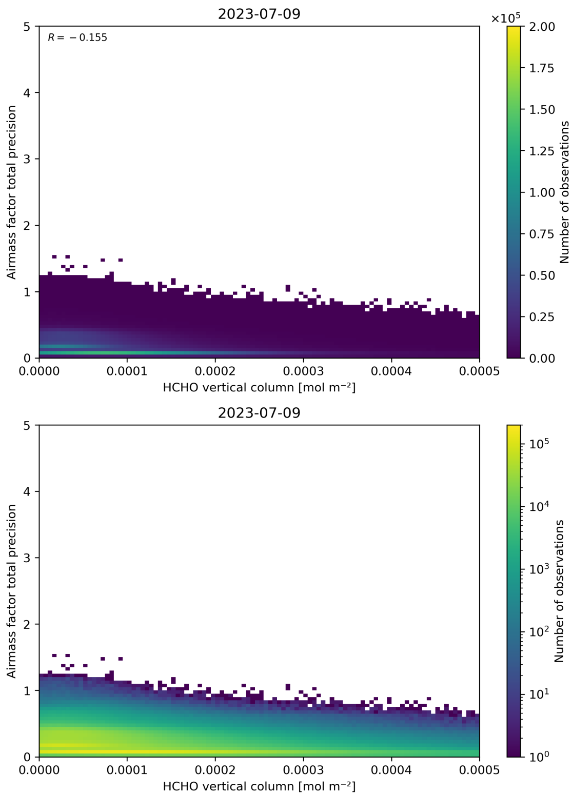
Figure 132: Scatter density plot of “HCHO vertical column” against “Airmass factor total precision” for 2023-07-08 to 2023-07-10.
