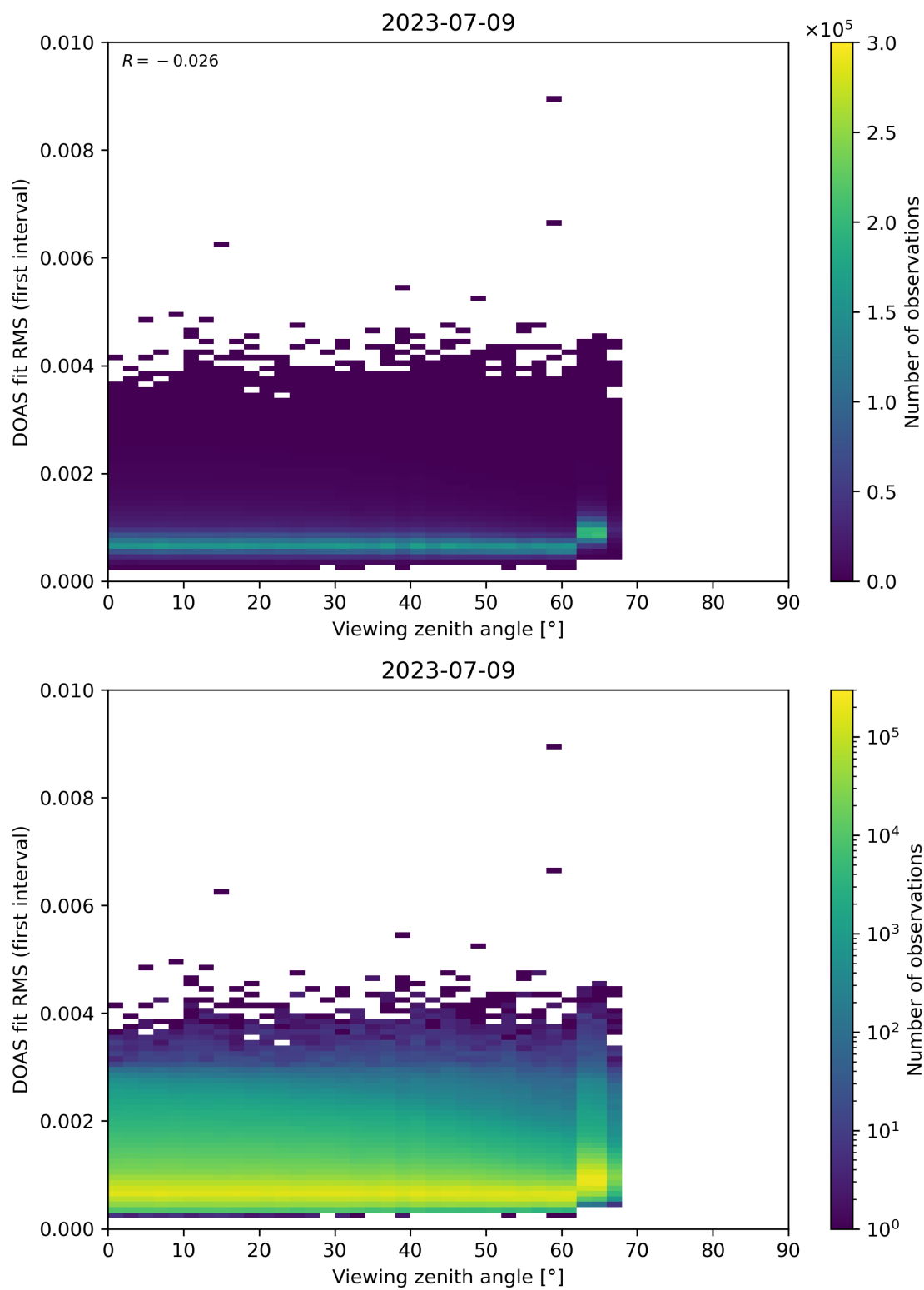
Figure 182: Scatter density plot of “Viewing zenith angle” against “DOAS fit RMS (first interval)” for 2023-07-08 to 2023-07-10.
