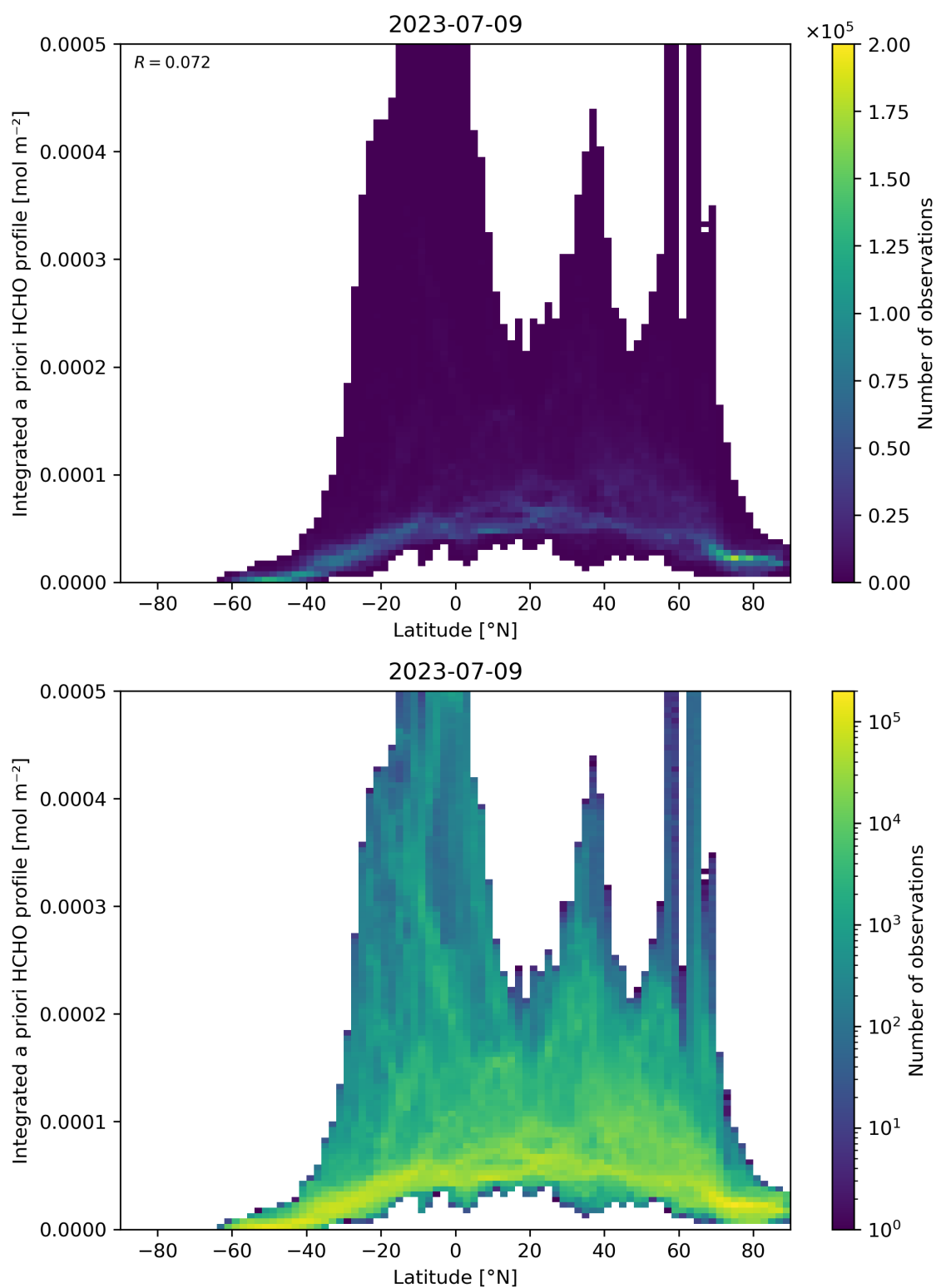
Figure 166: Scatter density plot of “Latitude” against “Integrated a priori HCHO profile” for 2023-07-08 to 2023-07-10.
