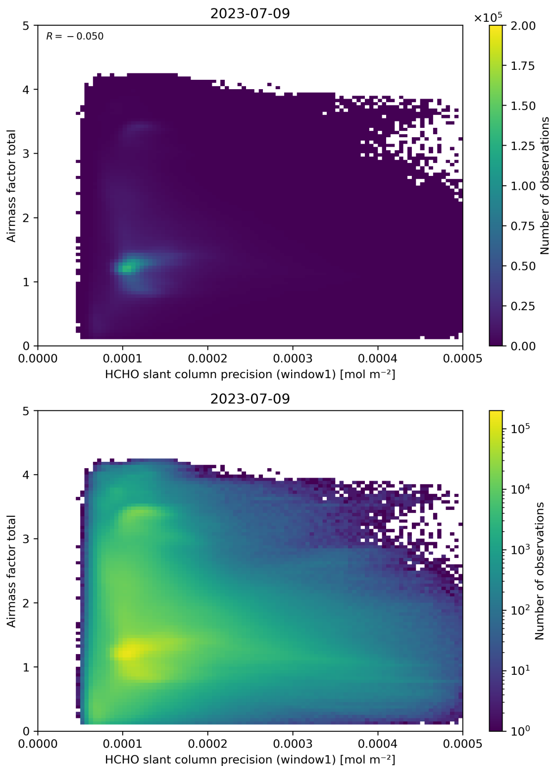
Figure 94: Scatter density plot of “HCHO slant column precision (window1)” against “Airmass factor total” for 2023-07-08 to 2023-07-10.
