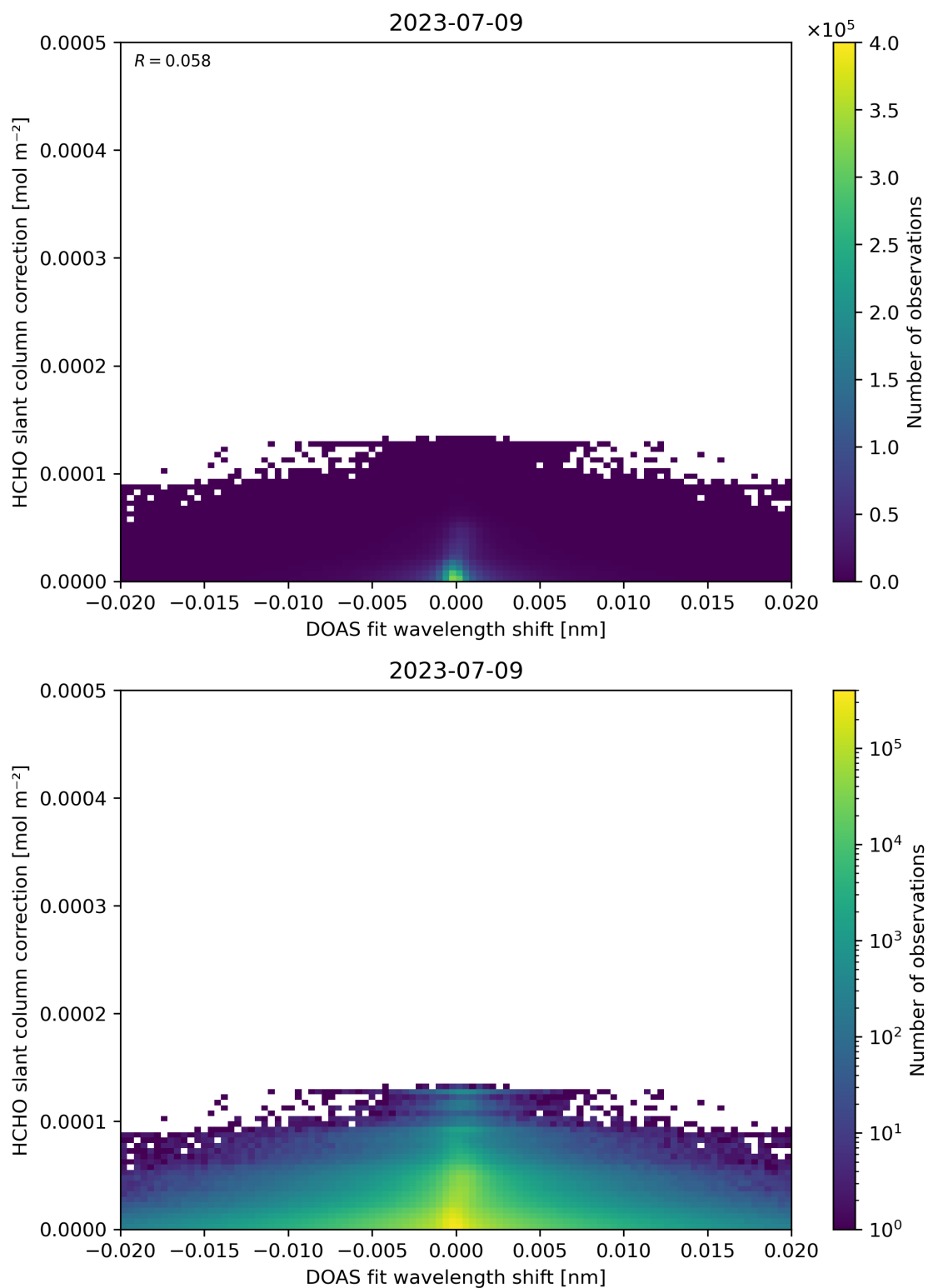
Figure 67: Scatter density plot of “DOAS fit wavelength shift” against “HCHO slant column correction” for 2023-07-08 to 2023-07-10.
