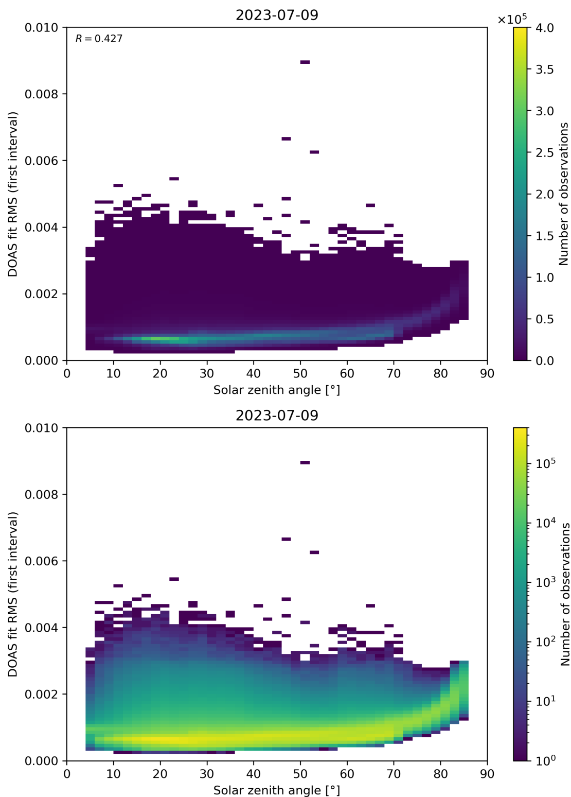
Figure 167: Scatter density plot of “Solar zenith angle” against “DOAS fit RMS (first interval)” for 2023-07-08 to 2023-07-10.
