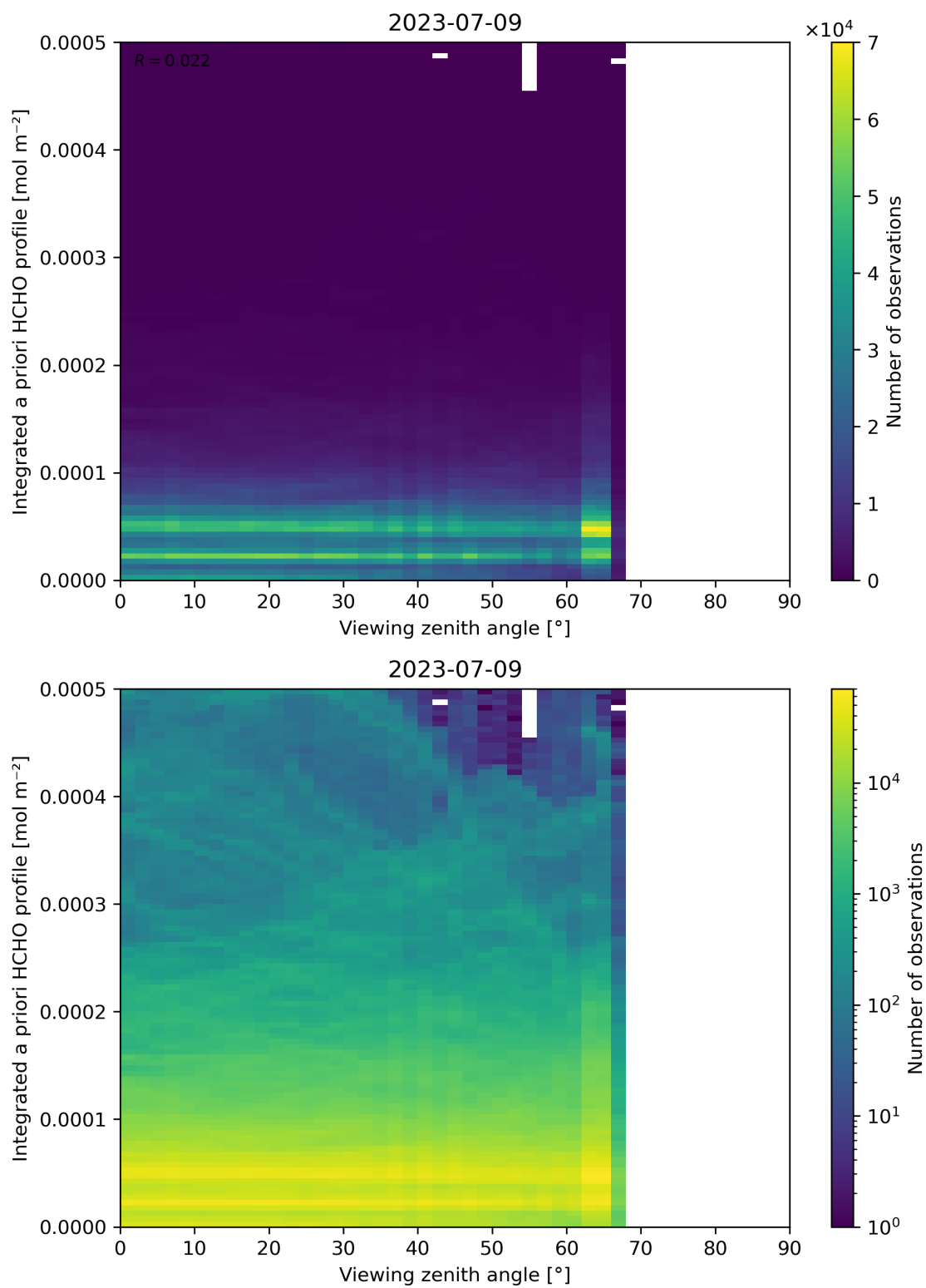
Figure 195: Scatter density plot of “Viewing zenith angle” against “Integrated a priori HCHO profile” for 2023-07-08 to 2023-07-10.
