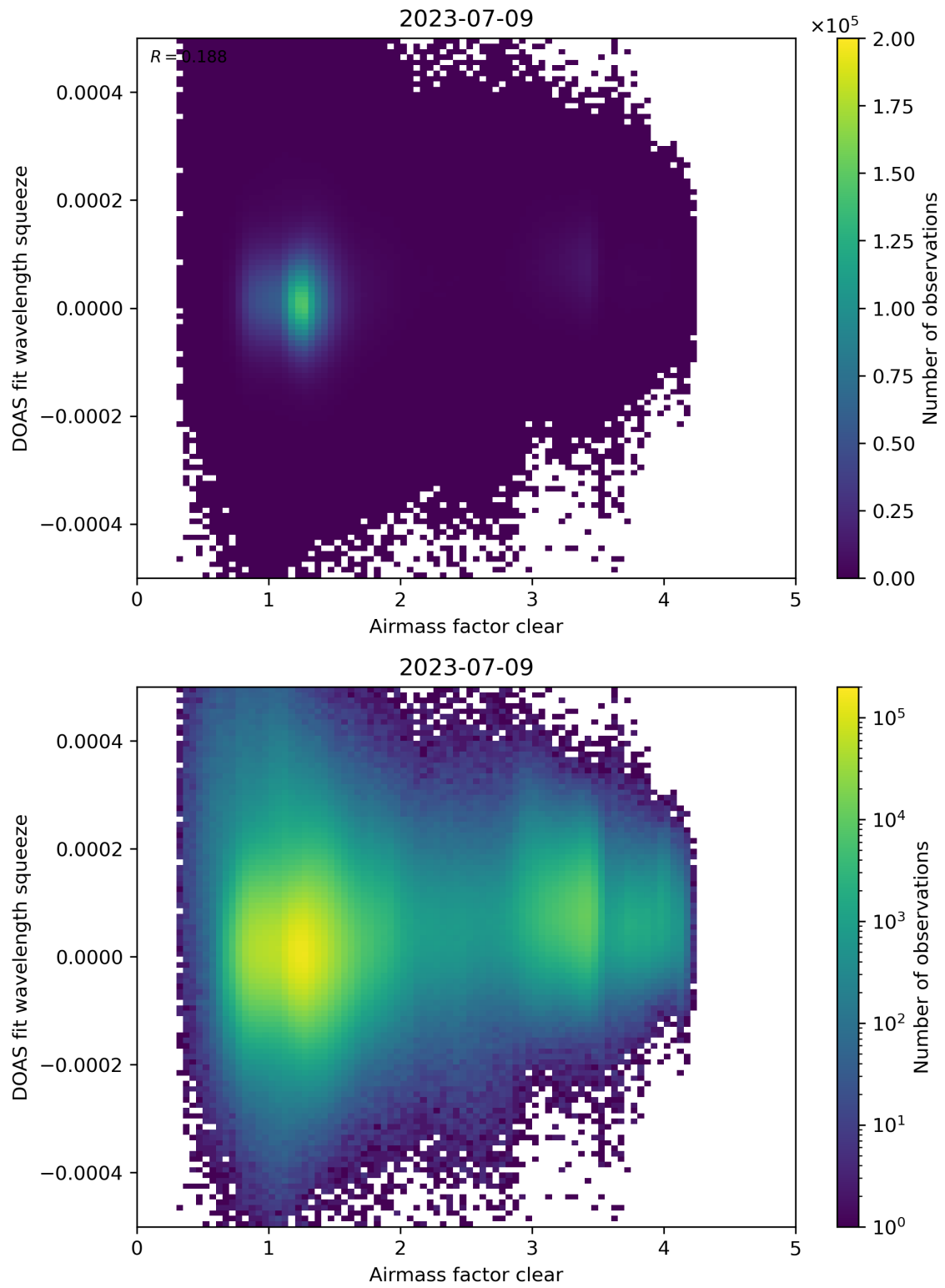
Figure 73: Scatter density plot of “Airmass factor clear” against “DOAS fit wavelength squeeze” for 2023-07-08 to 2023-07-10.
