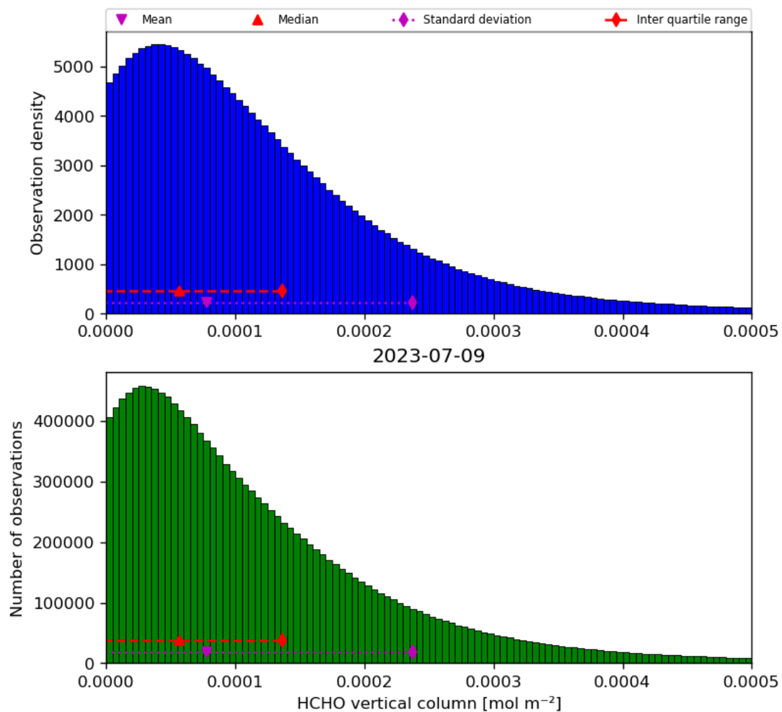
Figure 35: Histogram of “HCHO vertical column” for 2023-07-08 to 2023-07-10
