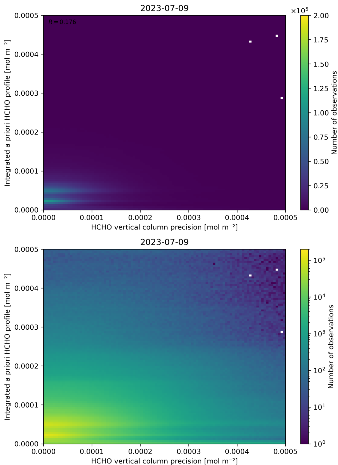
Figure 147: Scatter density plot of “HCHO vertical column precision” against “Integrated a priori HCHO profile” for 2023-07-08 to 2023-07-10.
