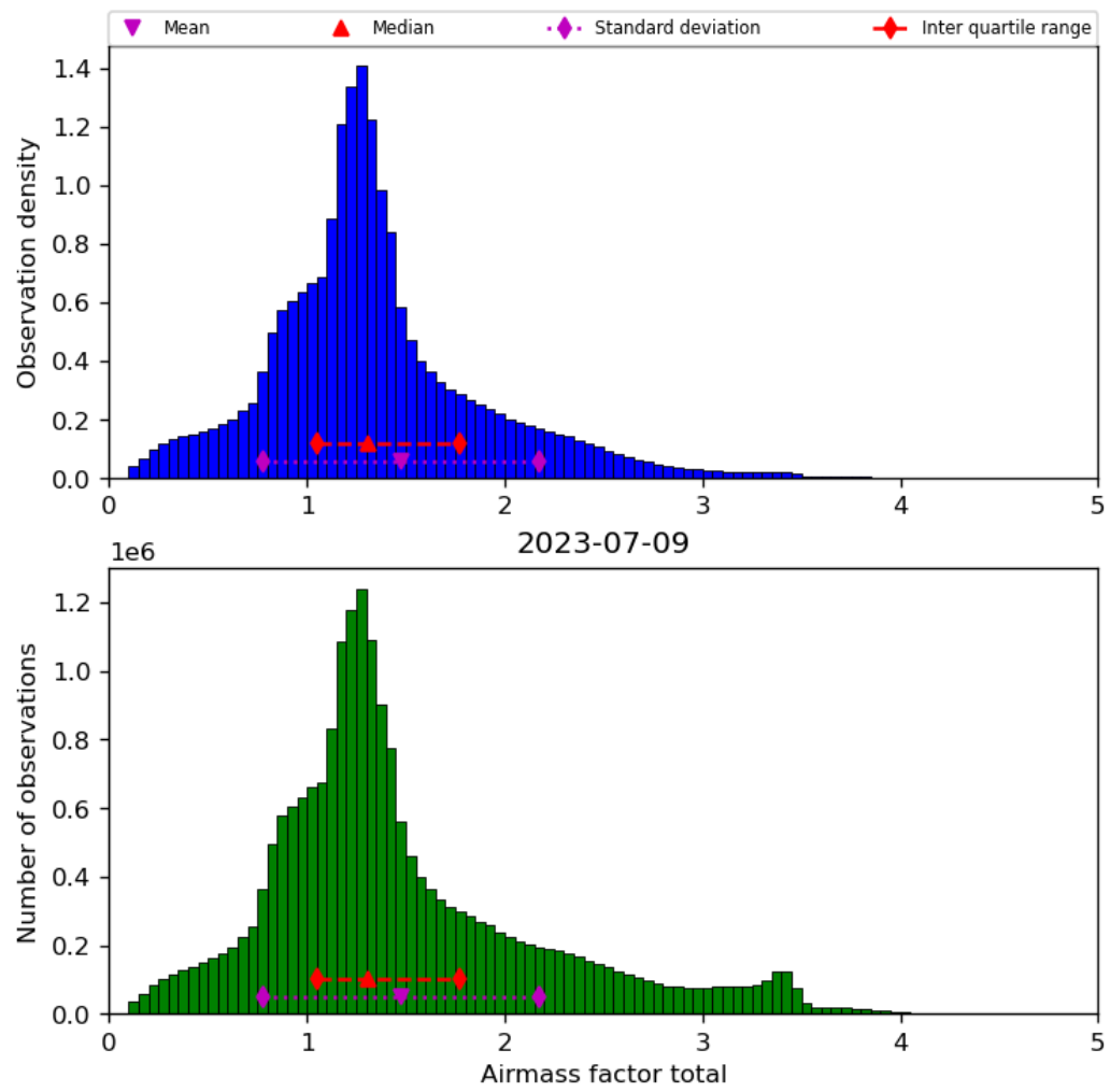
Figure 40: Histogram of “Airmass factor total” for 2023-07-08 to 2023-07-10
