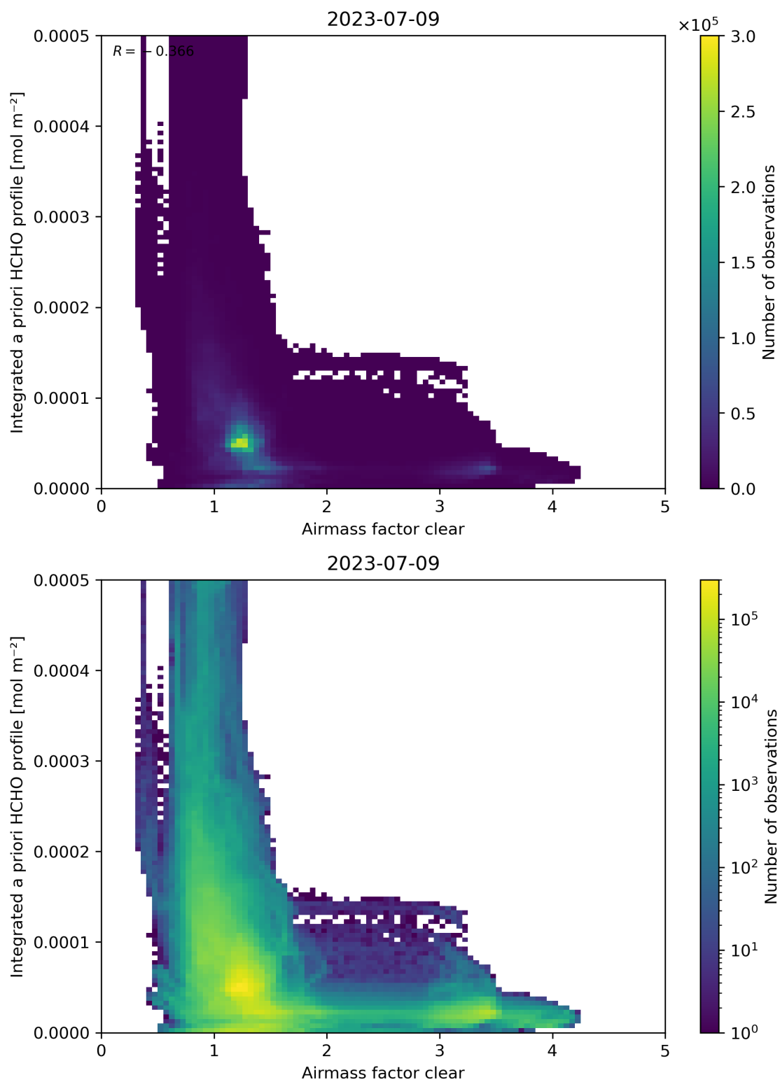
Figure 76: Scatter density plot of “Airmass factor clear” against “Integrated a priori HCHO profile” for 2023-07-08 to 2023-07-10.
