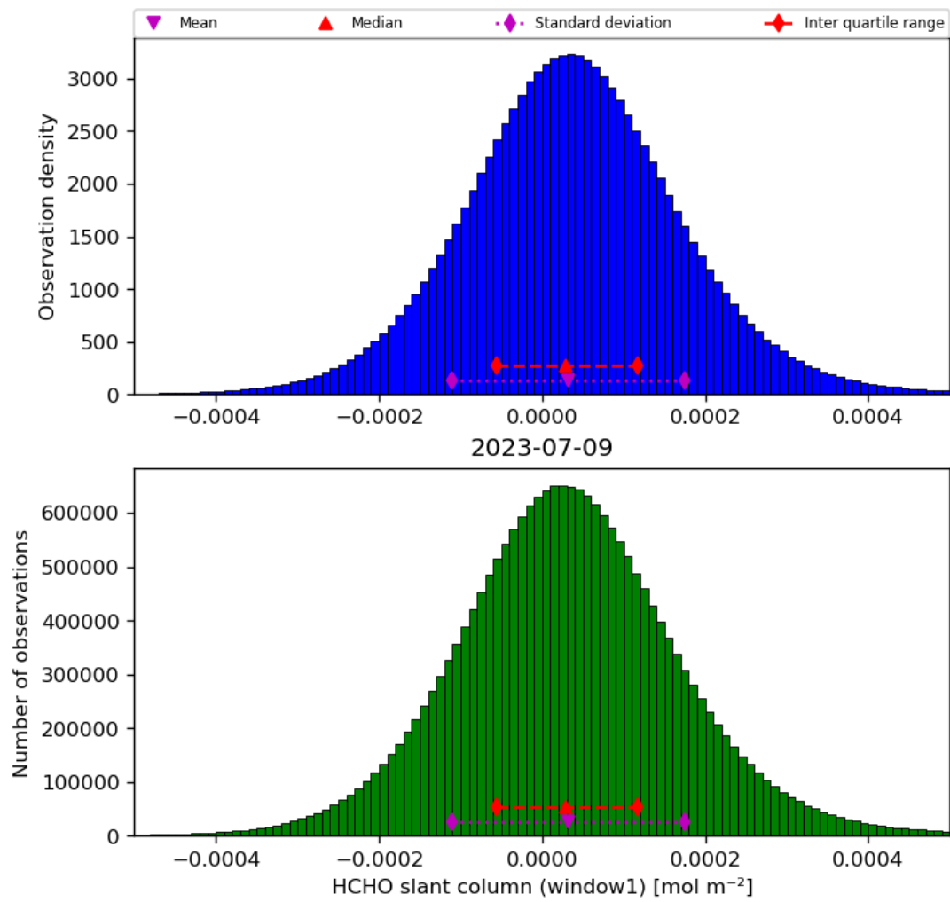
Figure 38: Histogram of “HCHO slant column (window1)” for 2023-07-08 to 2023-07-10
