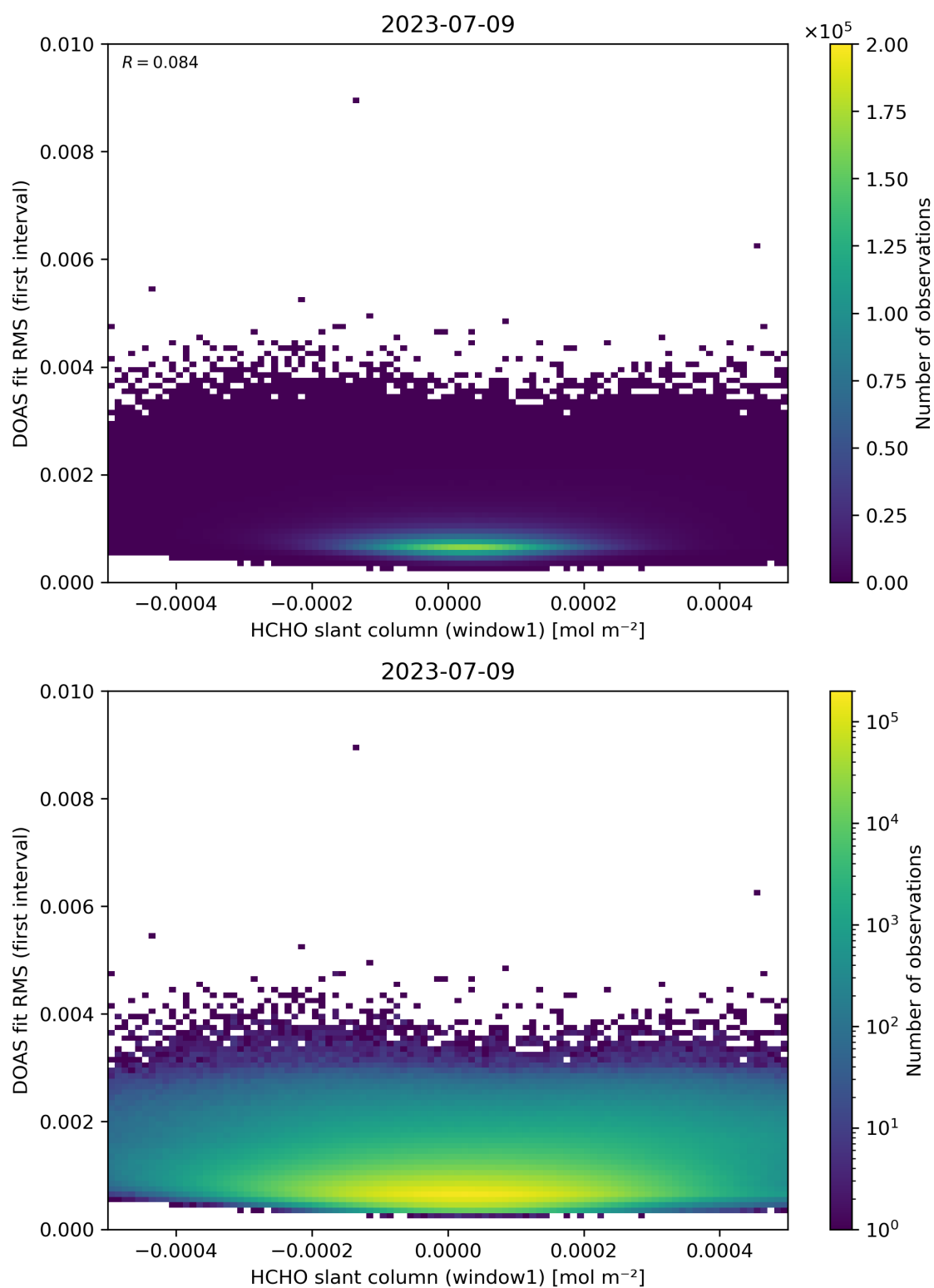
Figure 78: Scatter density plot of “HCHO slant column (window1)” against “DOAS fit RMS (first interval)” for 2023-07-08 to 2023-07-10.
