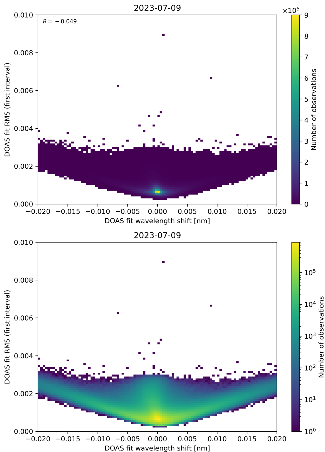
Figure 64: Scatter density plot of “DOAS fit wavelength shift” against “DOAS fit RMS (first interval)” for 2023-07-08 to 2023-07-10.
