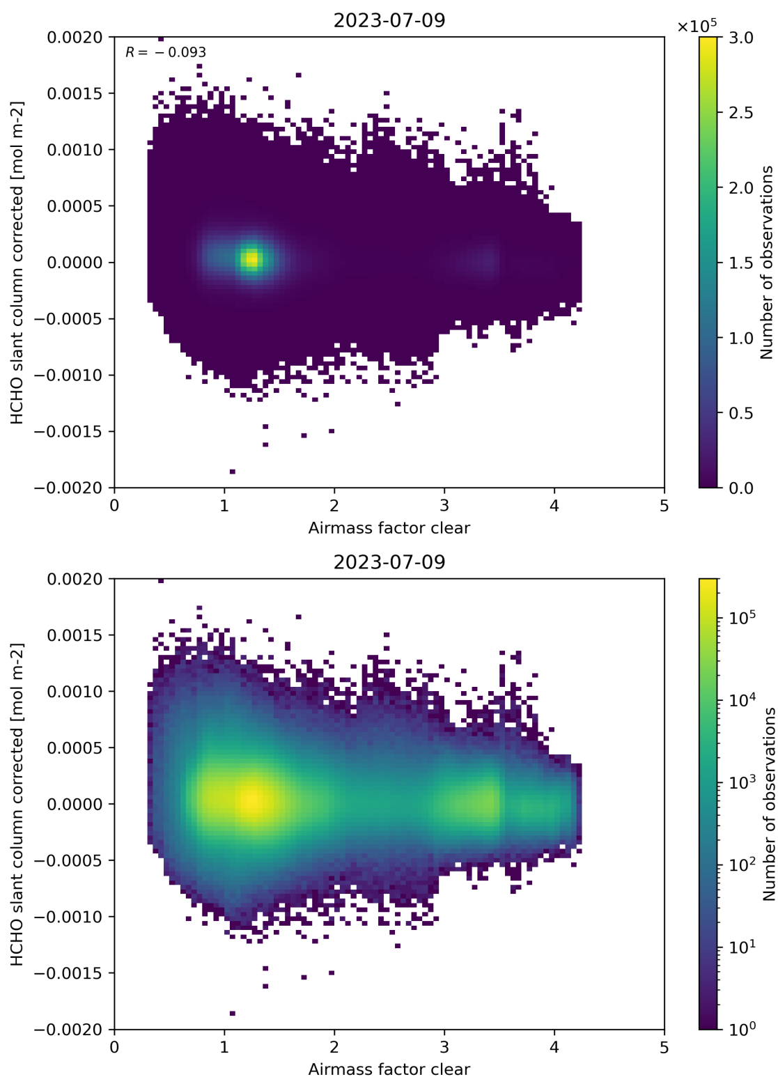
Figure 74: Scatter density plot of “Airmass factor clear” against “HCHO slant column corrected” for 2023-07-08 to 2023-07-10.
