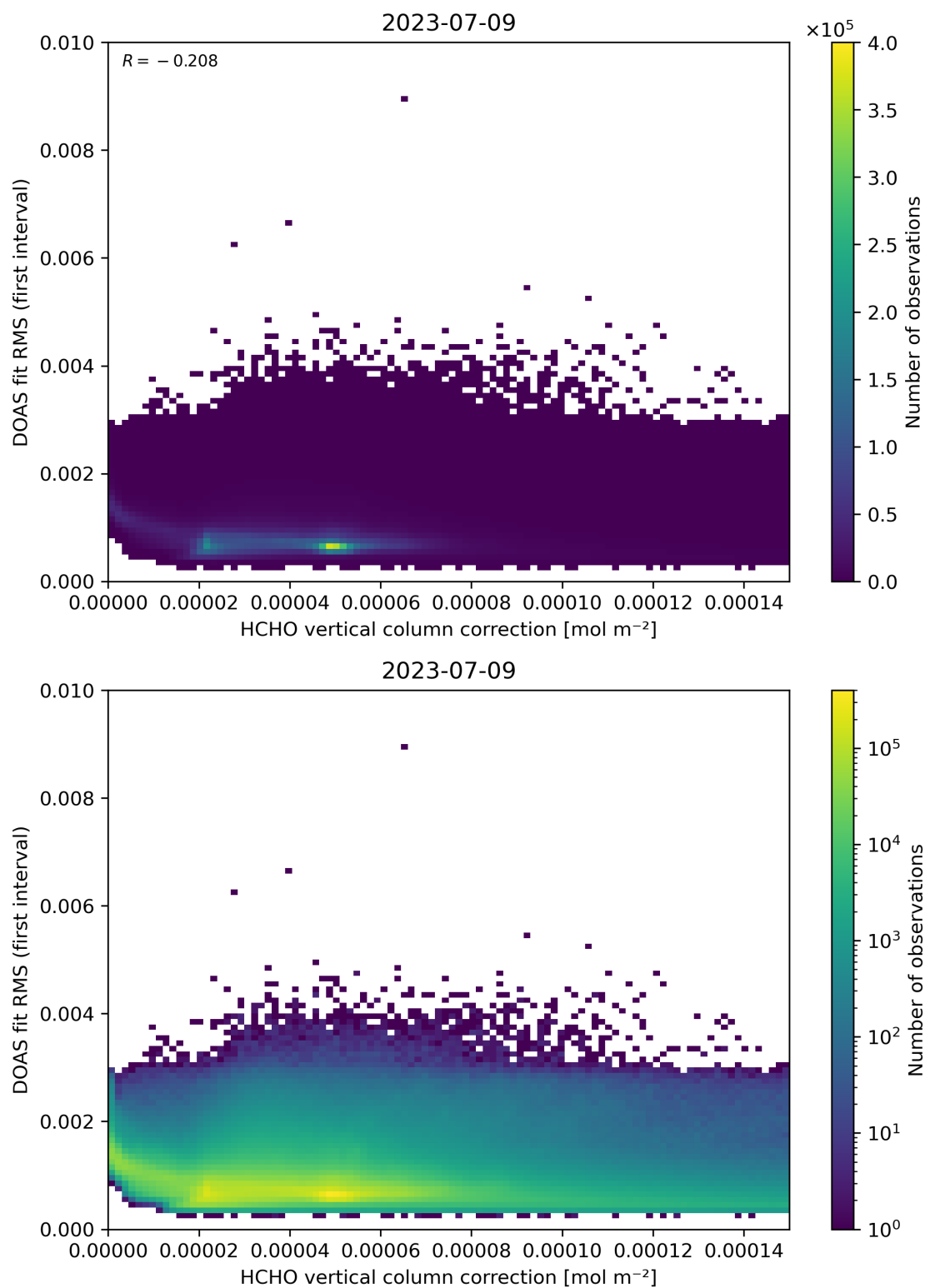
Figure 112: Scatter density plot of “HCHO vertical column correction” against “DOAS fit RMS (first interval)” for 2023-07-08 to 2023-07-10.
