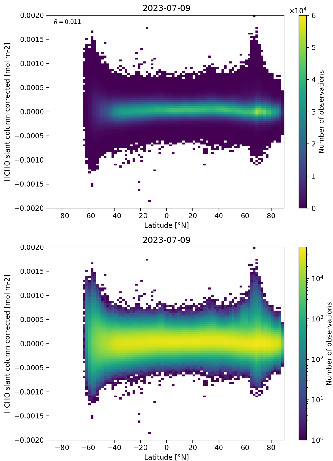
Figure 157: Scatter density plot of “Latitude” against “HCHO slant column corrected” for 2023-07-08 to 2023-07-10.
