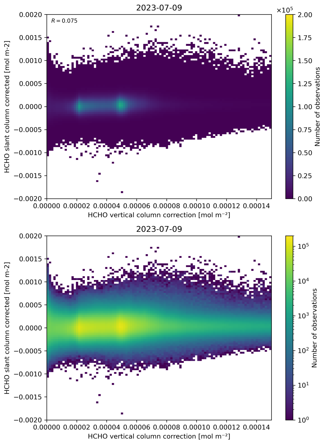
Figure 116: Scatter density plot of “HCHO vertical column correction” against “HCHO slant column corrected” for 2023-07-08 to 2023-07-10.
