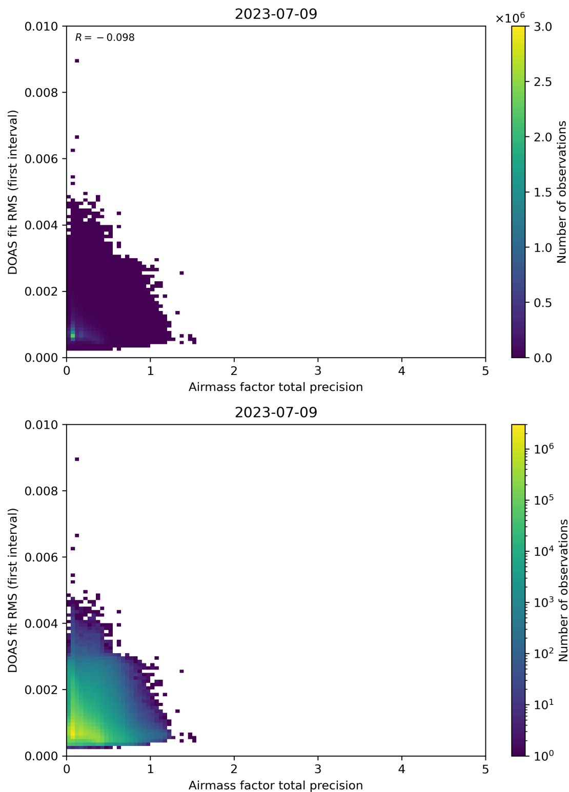
Figure 105: Scatter density plot of “Airmass factor total precision” against “DOAS fit RMS (first interval)” for 2023-07-08 to 2023-07-10.
