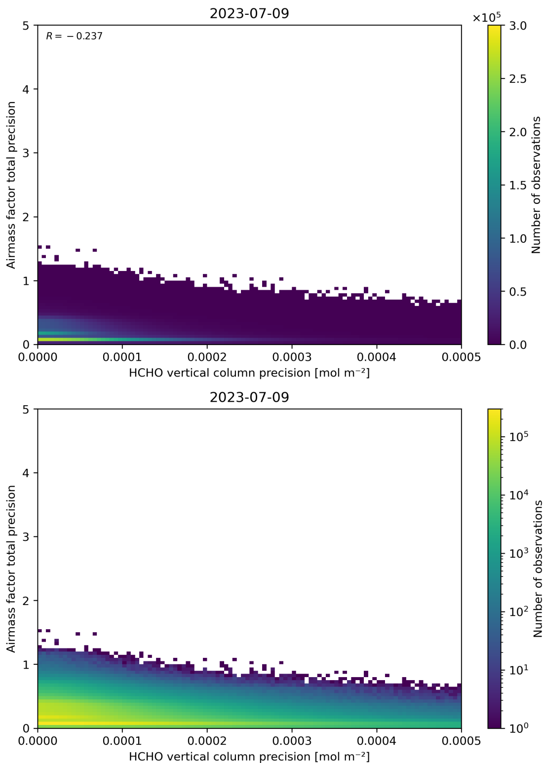
Figure 145: Scatter density plot of “HCHO vertical column precision” against “Airmass factor total precision” for 2023-07-08 to 2023-07-10.
