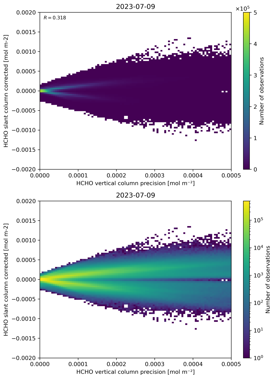
Figure 140: Scatter density plot of “HCHO vertical column precision” against “HCHO slant column corrected” for 2023-07-08 to 2023-07-10.
