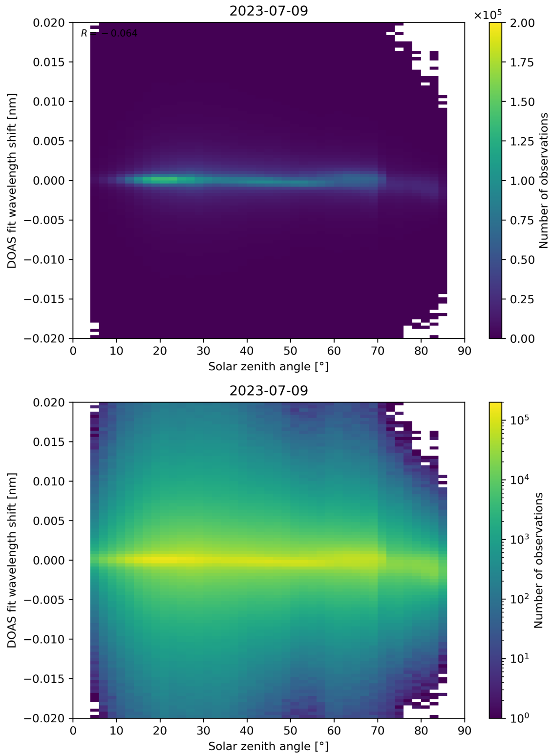
Figure 168: Scatter density plot of “Solar zenith angle” against “DOAS fit wavelength shift” for 2023-07-08 to 2023-07-10.
