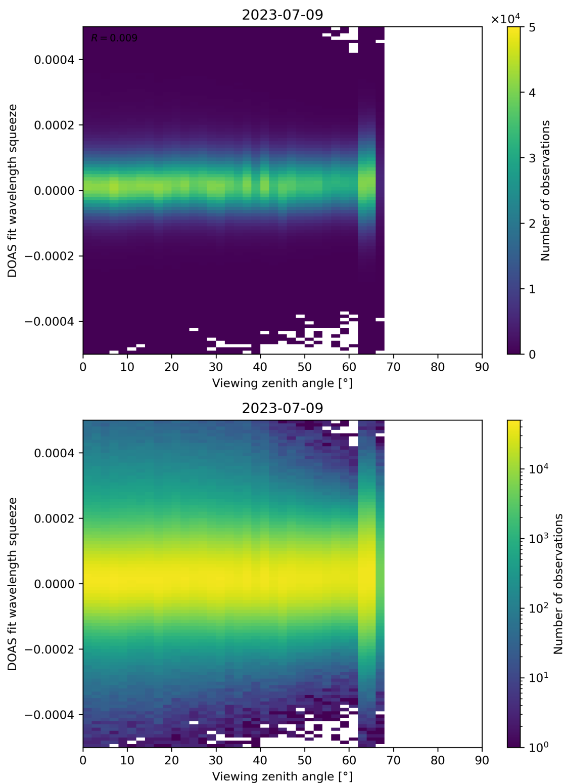
Figure 184: Scatter density plot of “Viewing zenith angle” against “DOAS fit wavelength squeeze” for 2023-07-08 to 2023-07-10.
