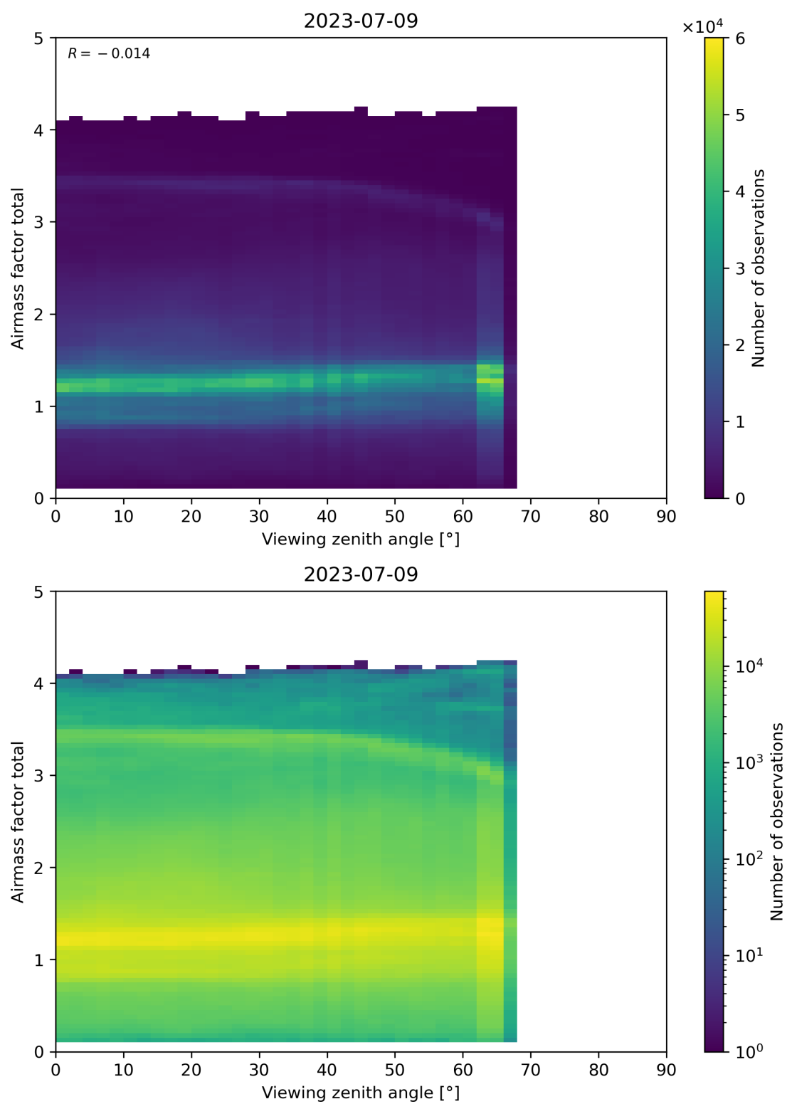
Figure 190: Scatter density plot of “Viewing zenith angle” against “Airmass factor total” for 2023-07-08 to 2023-07-10.
