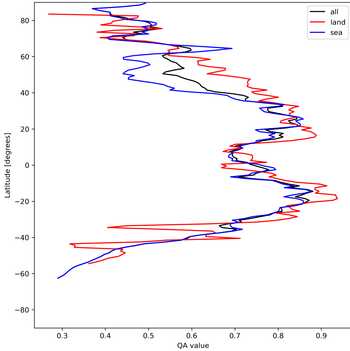
Figure 20: Zonal average of “QA value” for 2023-07-08 to 2023-07-10.
