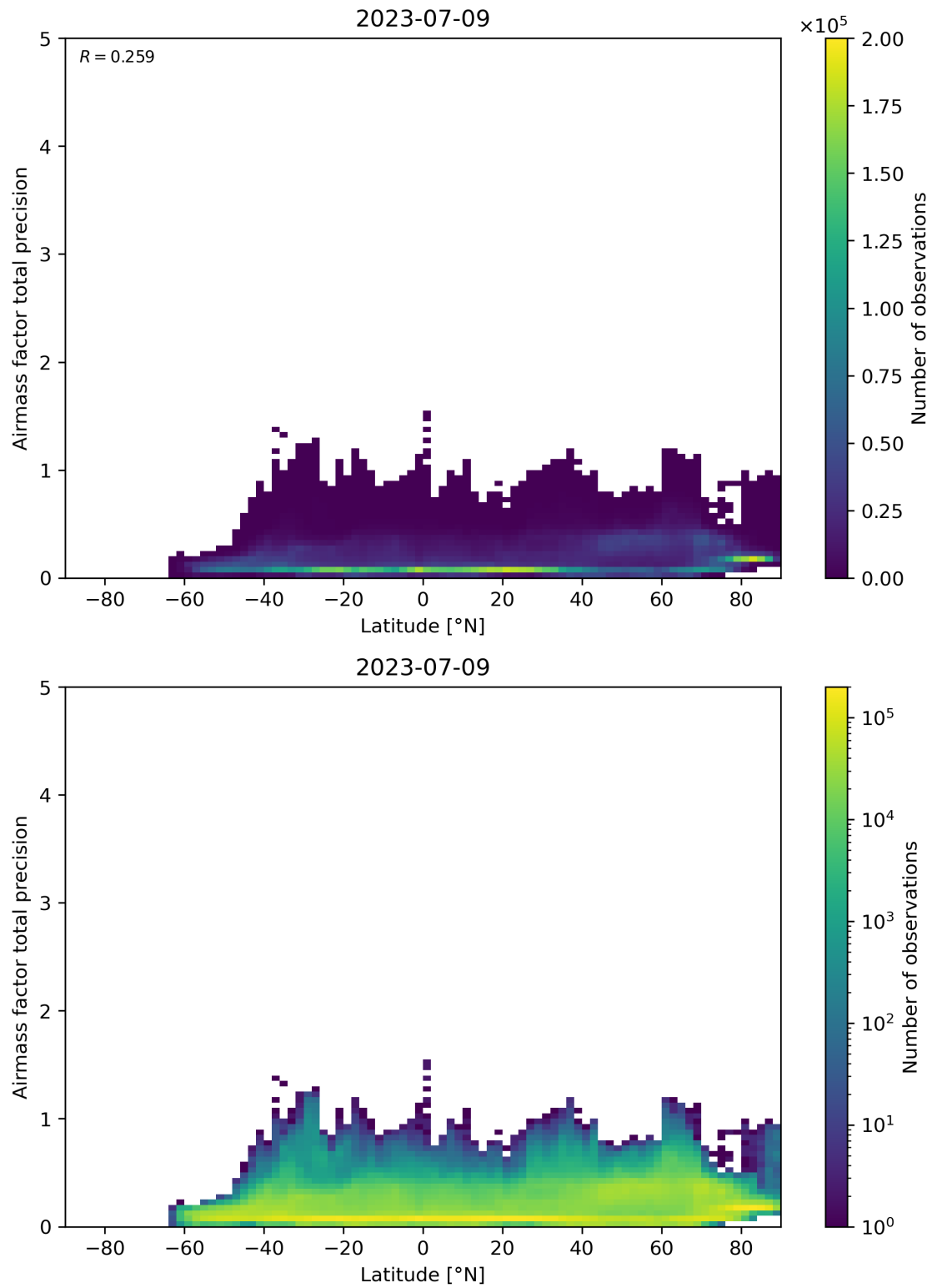
Figure 162: Scatter density plot of “Latitude” against “Airmass factor total precision” for 2023-07-08 to 2023-07-10.
