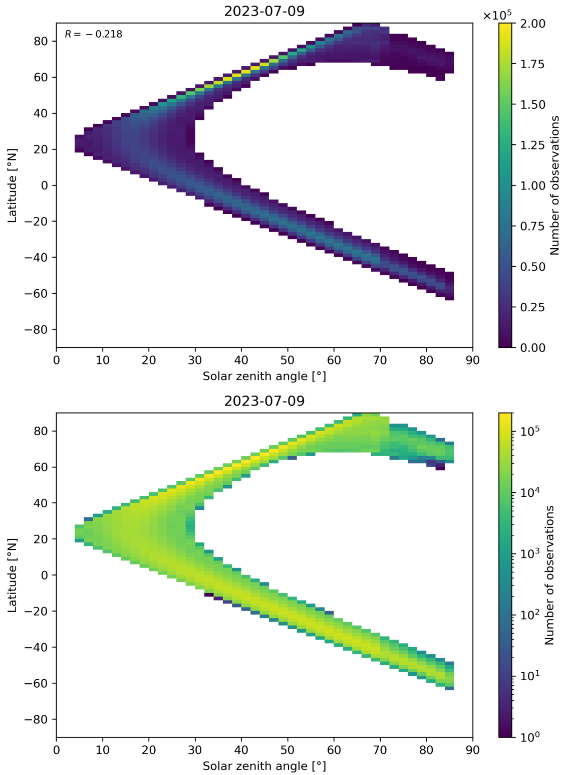
Figure 181: Scatter density plot of “Solar zenith angle” against “Latitude” for 2023-07-08 to 2023-07-10.
