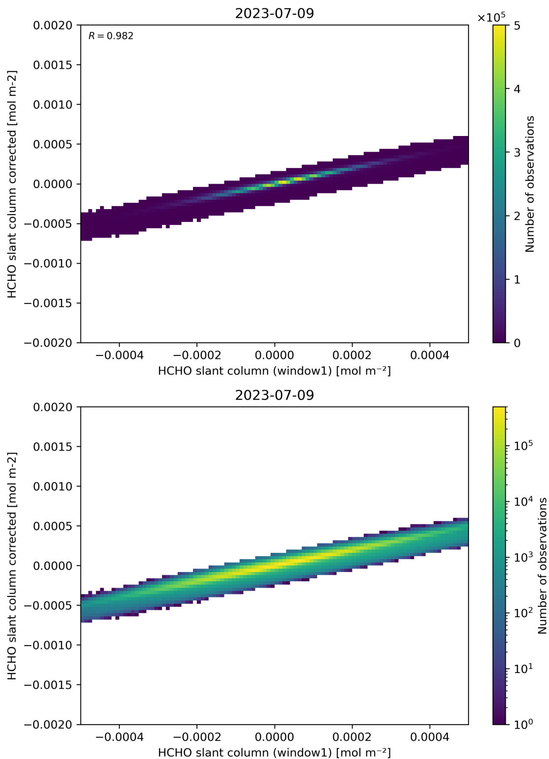
Figure 82: Scatter density plot of “HCHO slant column (window1)” against “HCHO slant column corrected” for 2023-07-08 to 2023-07-10.
