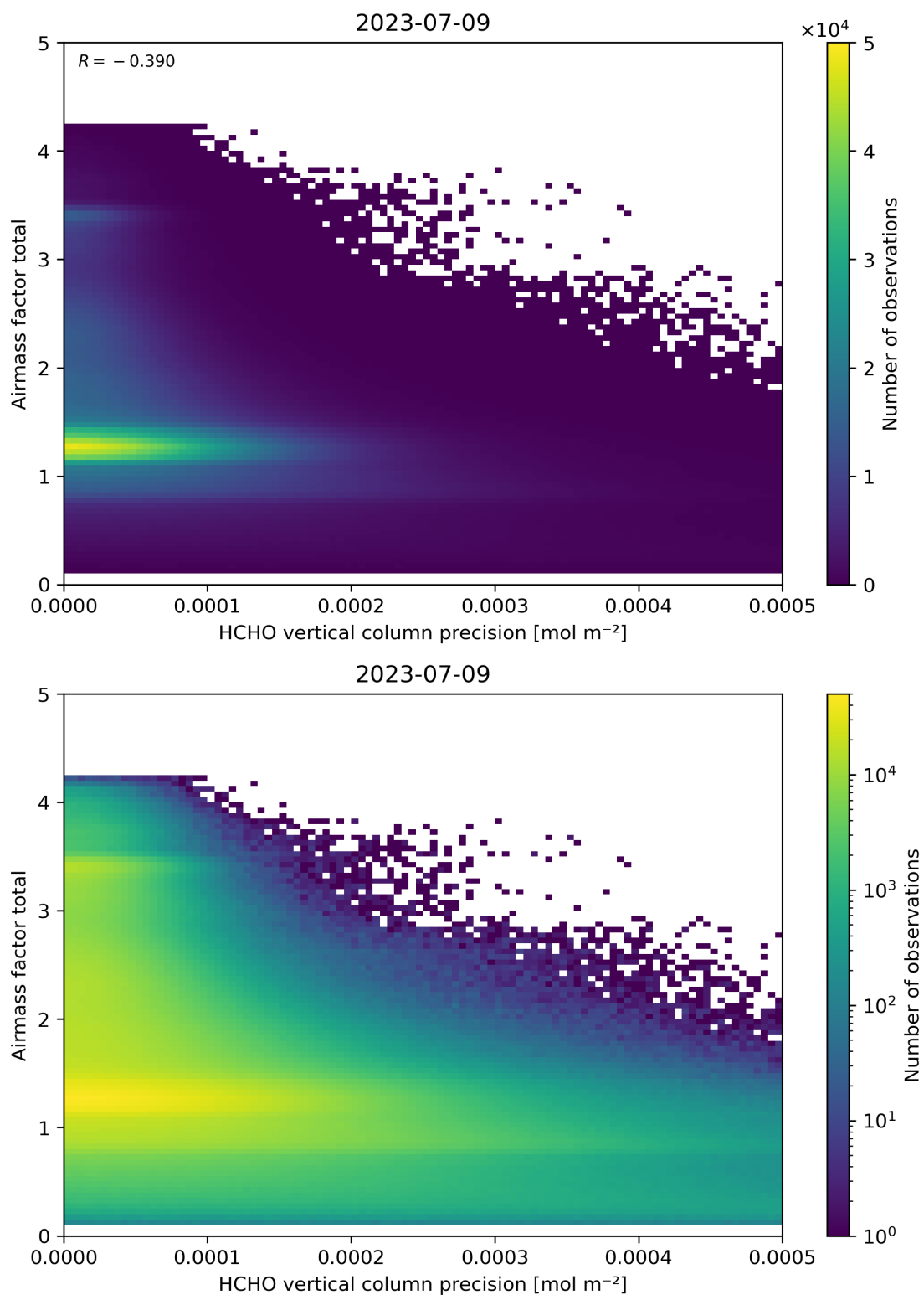
Figure 144: Scatter density plot of “HCHO vertical column precision” against “Airmass factor total” for 2023-07-08 to 2023-07-10.
