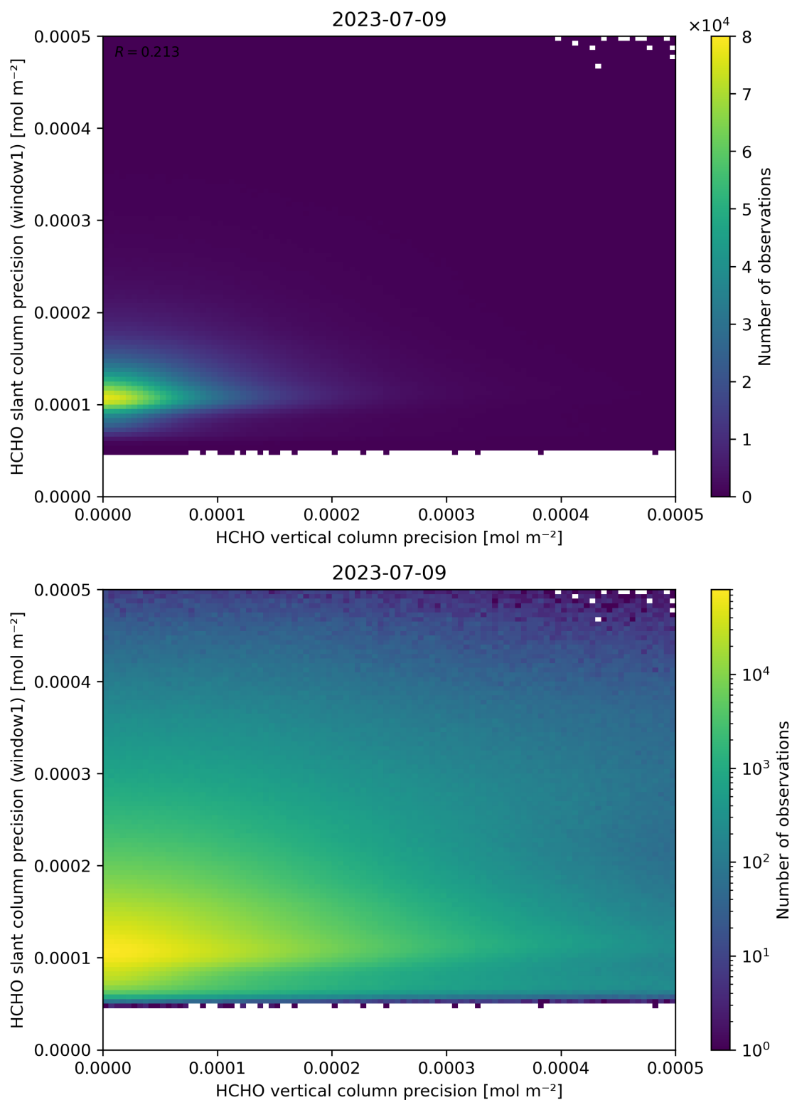
Figure 143: Scatter density plot of “HCHO vertical column precision” against “HCHO slant column precision (window1)” for 2023-07-08 to 2023-07-10.
