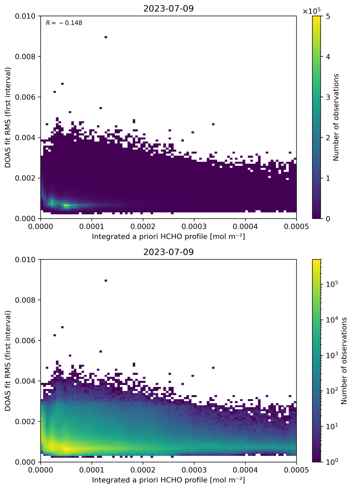
Figure 148: Scatter density plot of “Integrated a priori HCHO profile” against “DOAS fit RMS (first interval)” for 2023-07-08 to 2023-07-10.
