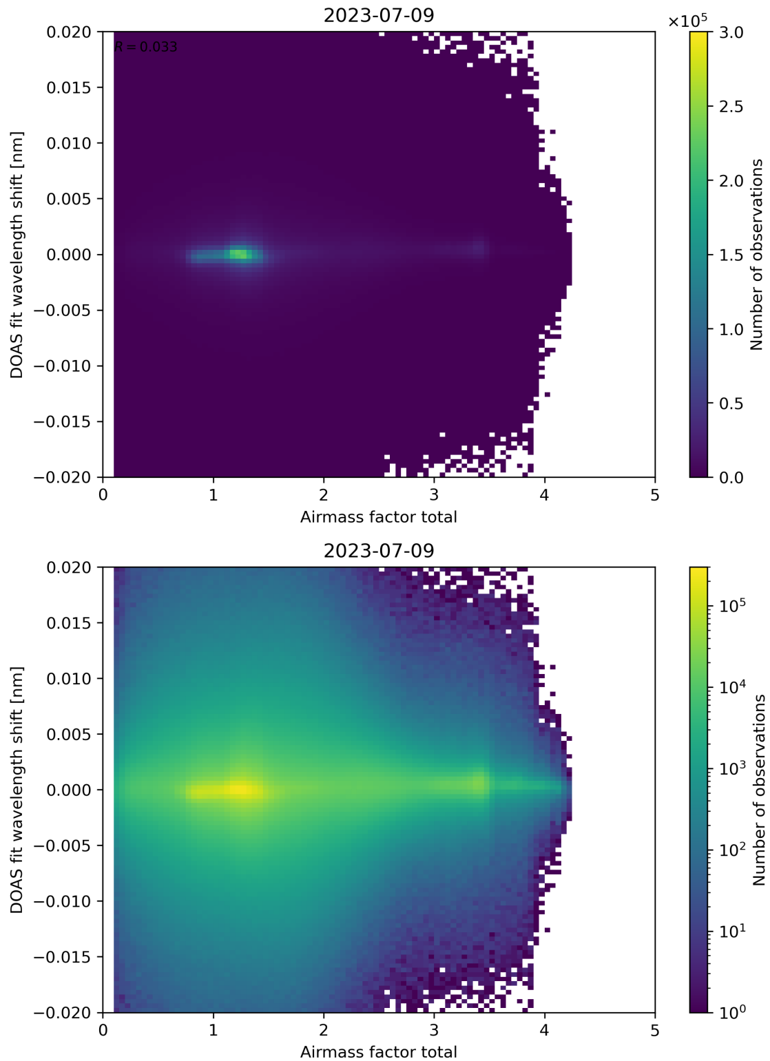
Figure 98: Scatter density plot of “Airmass factor total” against “DOAS fit wavelength shift” for 2023-07-08 to 2023-07-10.
