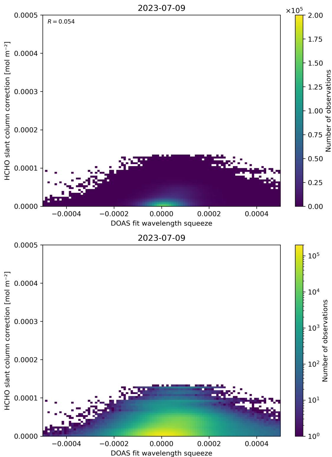
Figure 70: Scatter density plot of “DOAS fit wavelength squeeze” against “HCHO slant column correction” for 2023-07-08 to 2023-07-10.
