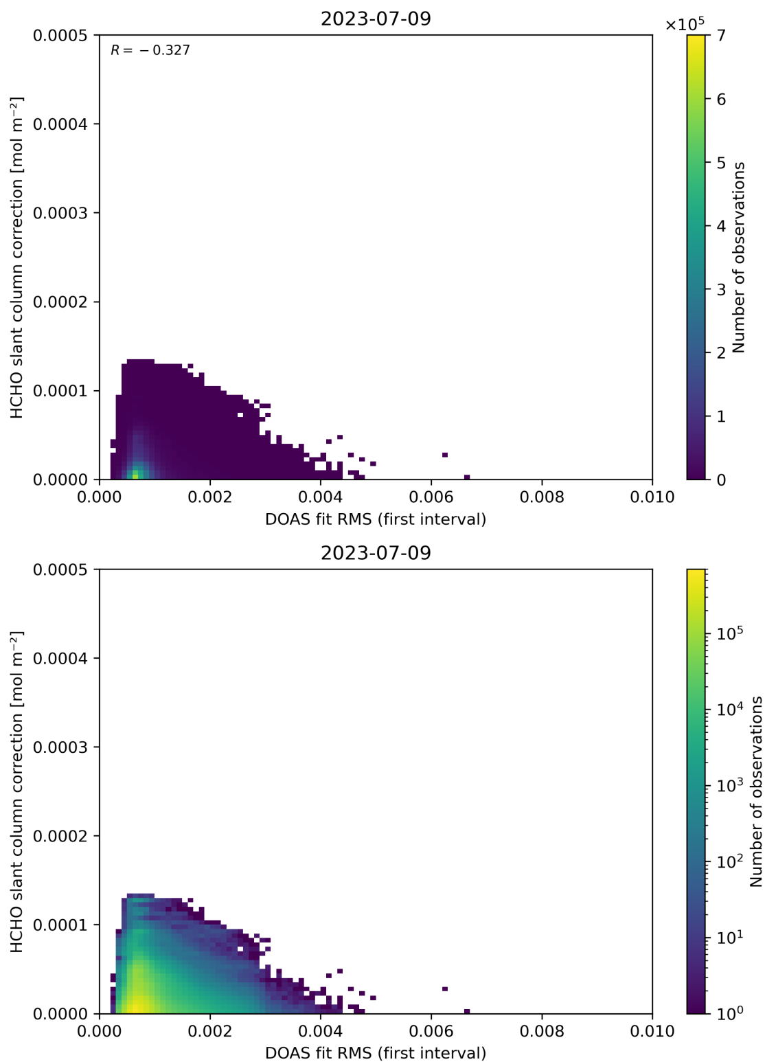
Figure 63: Scatter density plot of “DOAS fit RMS (first interval)” against “HCHO slant column correction” for 2023-07-08 to 2023-07-10.
