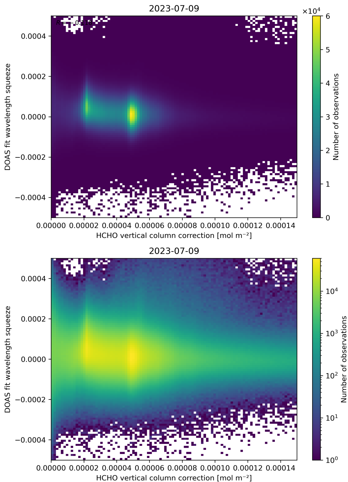
Figure 114: Scatter density plot of “HCHO vertical column correction” against “DOAS fit wavelength squeeze” for 2023-07-08 to 2023-07-10.
