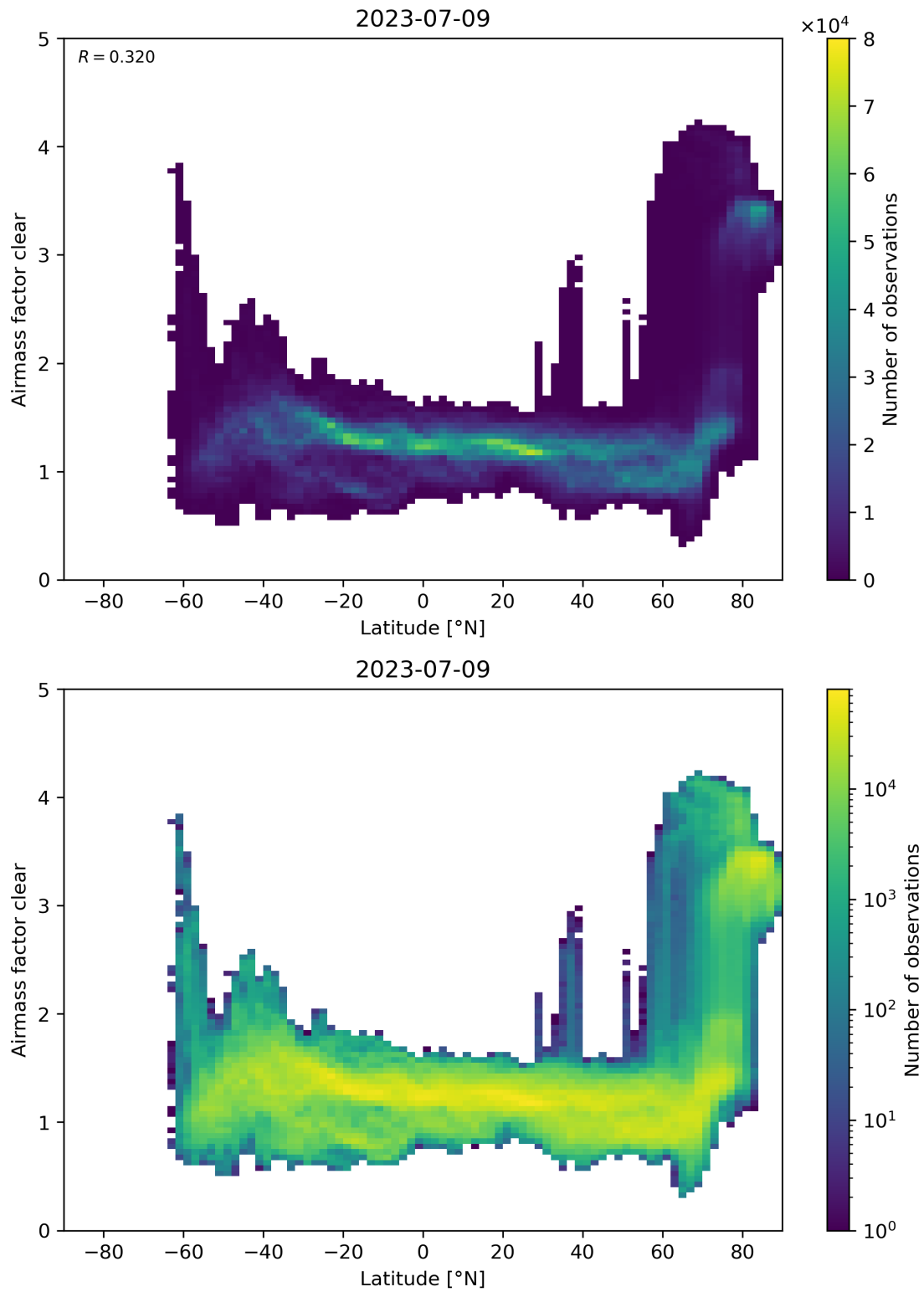
Figure 156: Scatter density plot of “Latitude” against “Airmass factor clear” for 2023-07-08 to 2023-07-10.
