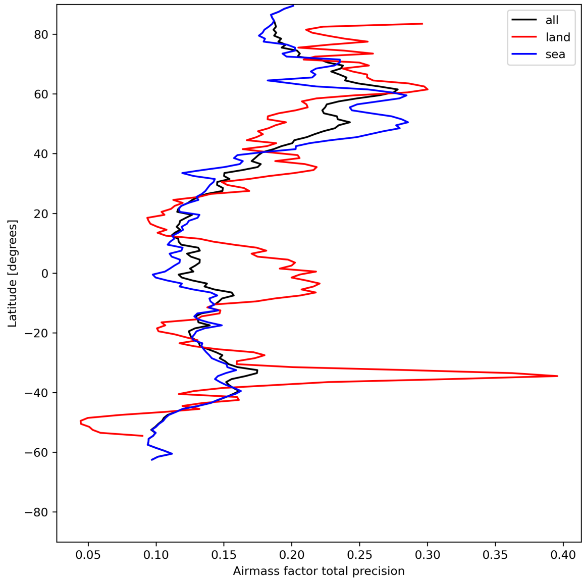
Figure 27: Zonal average of “Airmass factor total precision” for 2023-07-08 to 2023-07-10.
