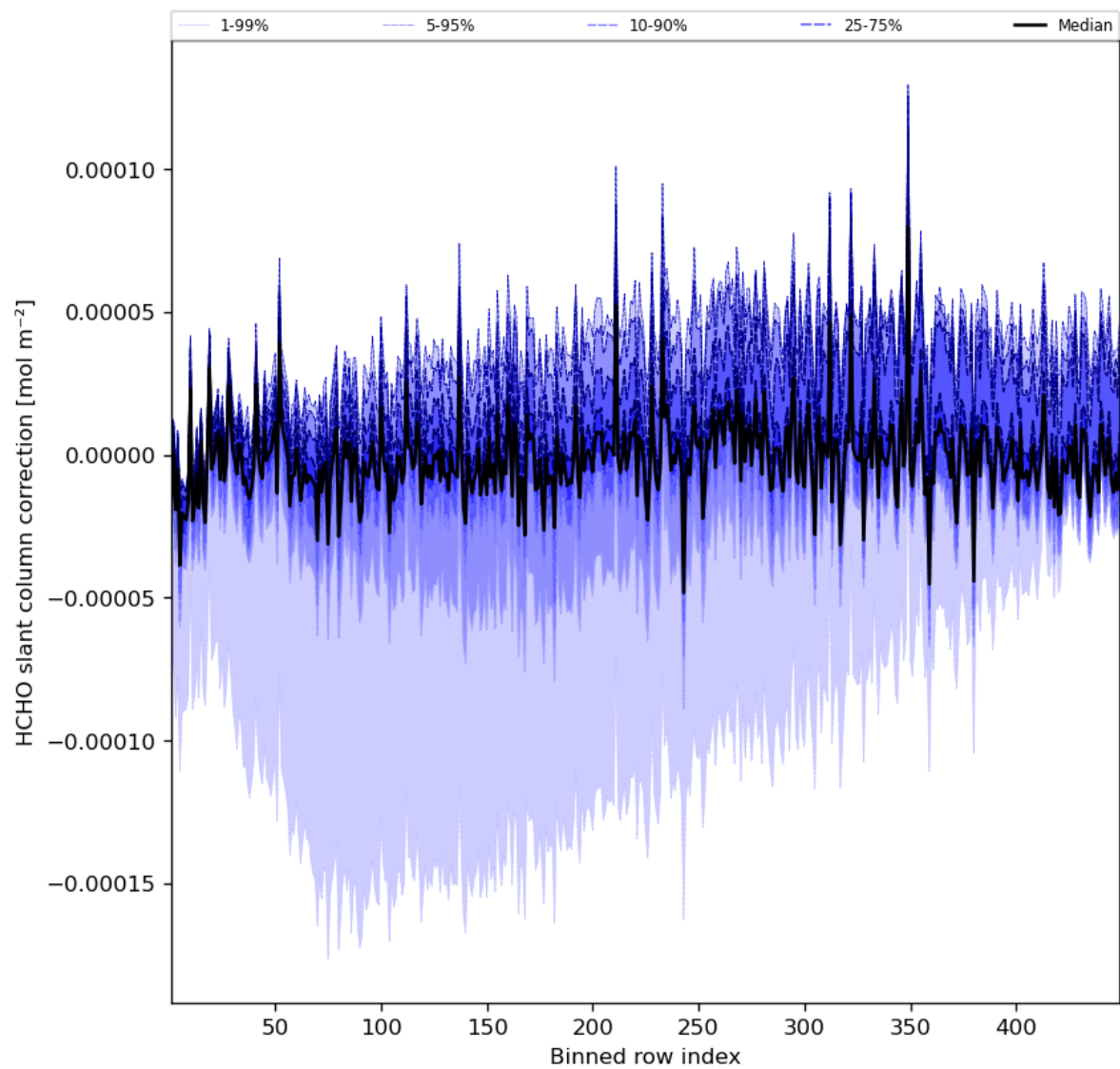
Figure 61: Along track statistics of “HCHO slant column correction” for 2023-07-08 to 2023-07-10
