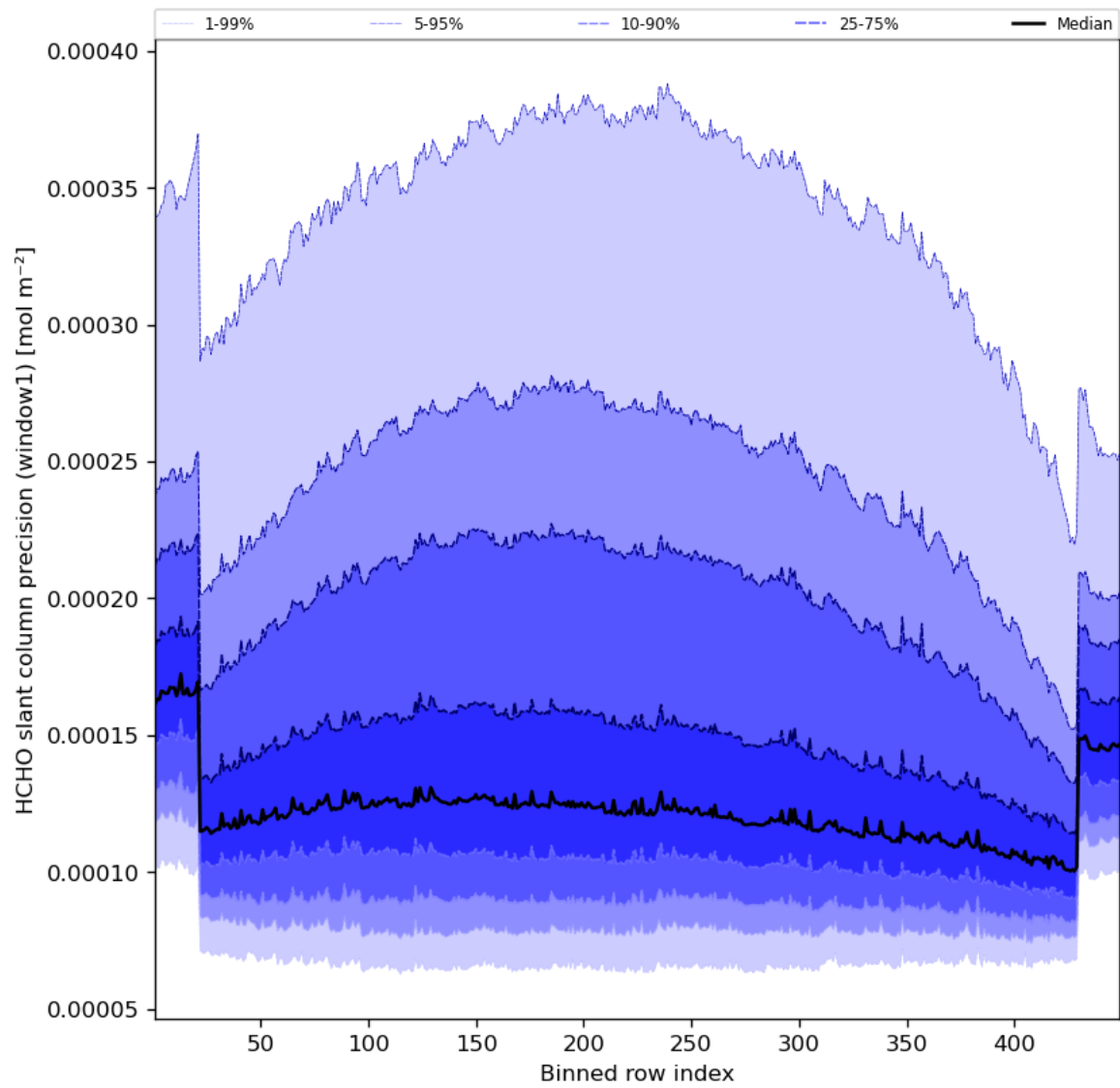
Figure 53: Along track statistics of “HCHO slant column precision (window1)” for 2023-07-08 to 2023-07-10
