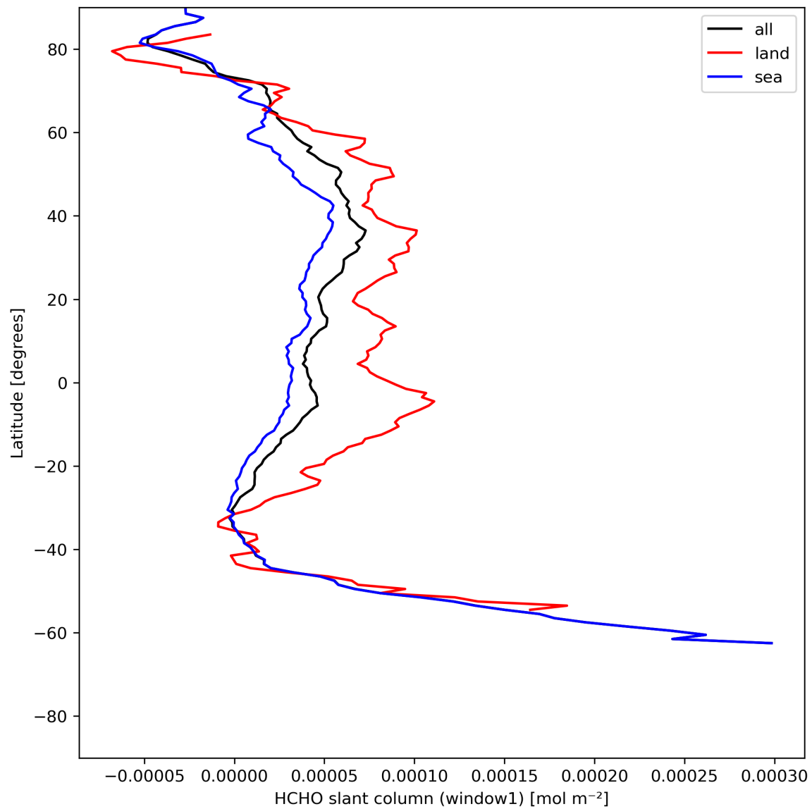
Figure 24: Zonal average of “HCHO slant column (window1)” for 2023-07-08 to 2023-07-10.
