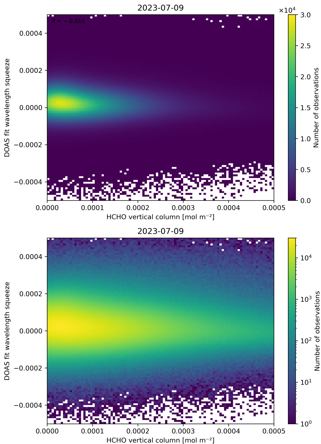
Figure 125: Scatter density plot of “HCHO vertical column” against “DOAS fit wavelength squeeze” for 2023-07-08 to 2023-07-10.
