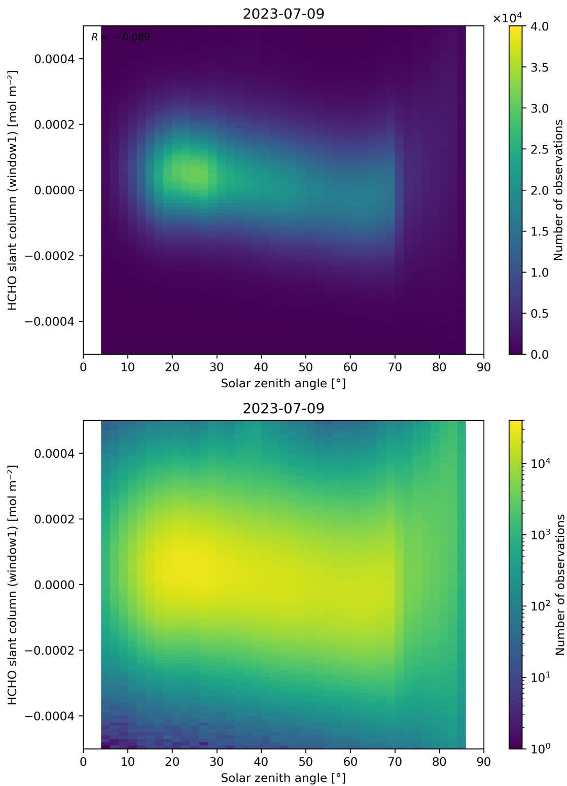
Figure 173: Scatter density plot of “Solar zenith angle” against “HCHO slant column (window1)” for 2023-07-08 to 2023-07-10.
