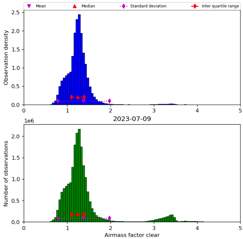
Figure 42: Histogram of “Airmass factor clear” for 2023-07-08 to 2023-07-10
