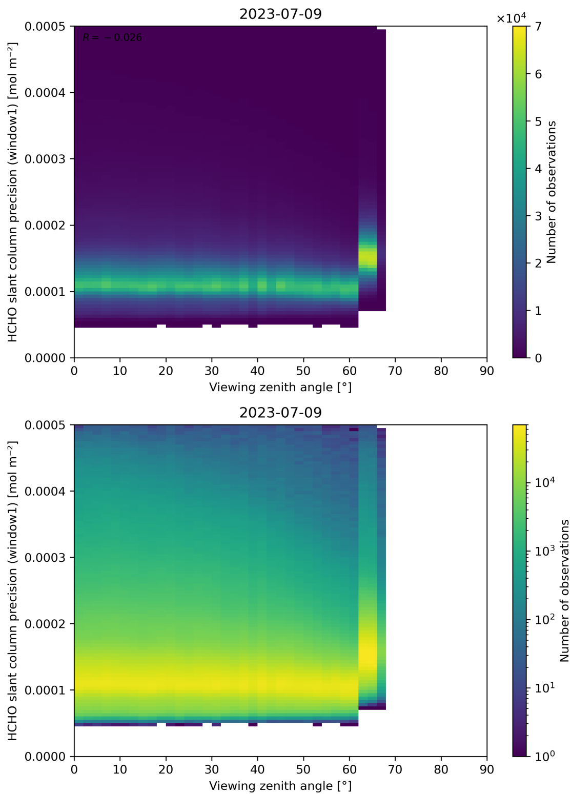
Figure 189: Scatter density plot of “Viewing zenith angle” against “HCHO slant column precision (window1)” for 2023-07-08 to 2023-07-10.
