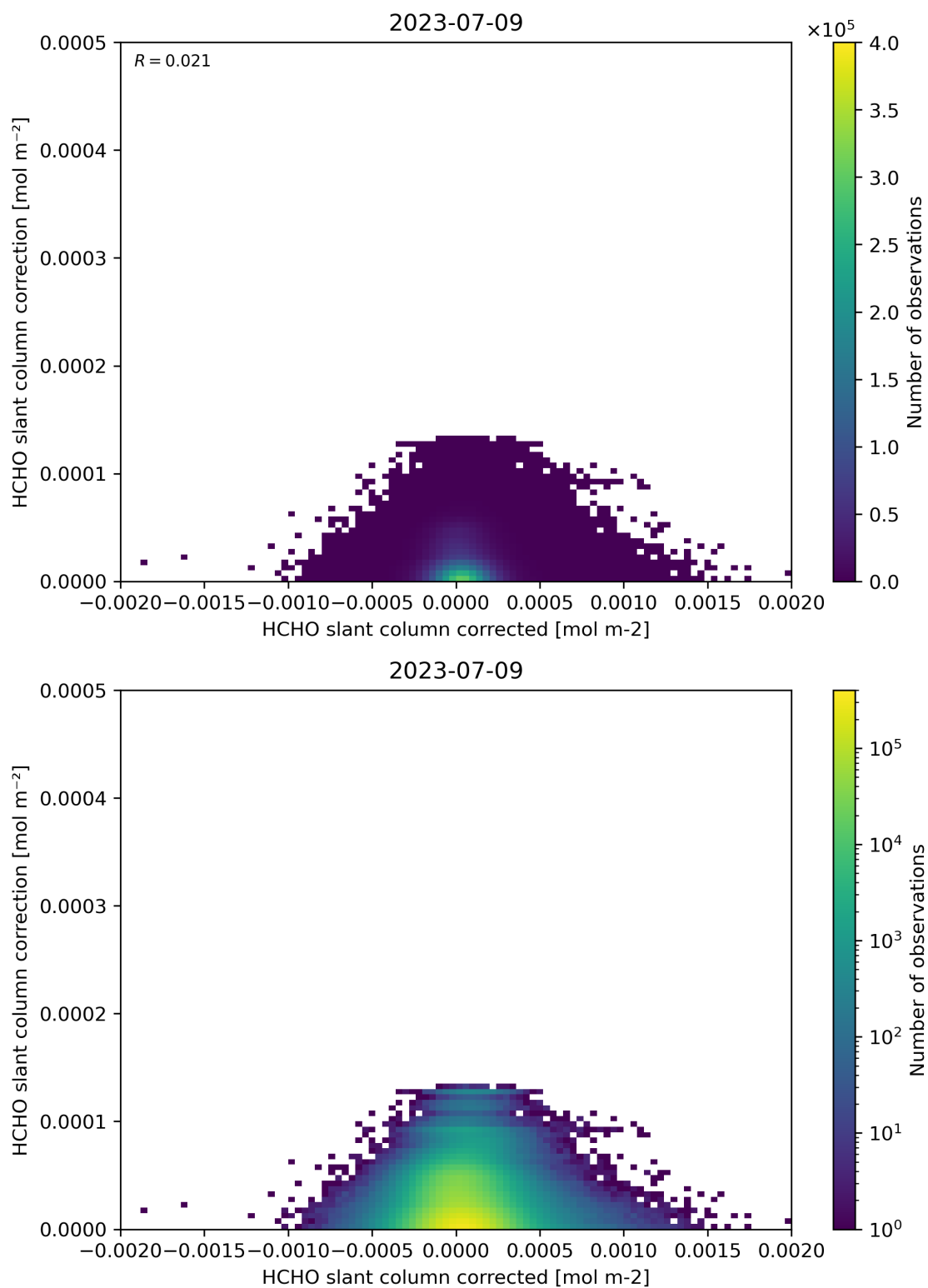
Figure 77: Scatter density plot of “HCHO slant column corrected” against “HCHO slant column correction” for 2023-07-08 to 2023-07-10.
