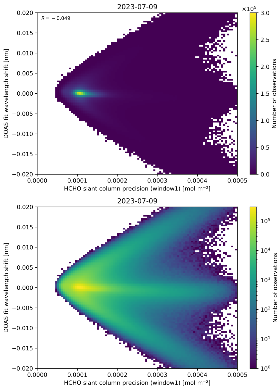
Figure 89: Scatter density plot of “HCHO slant column precision (window1)” against “DOAS fit wavelength shift” for 2023-07-08 to 2023-07-10.
