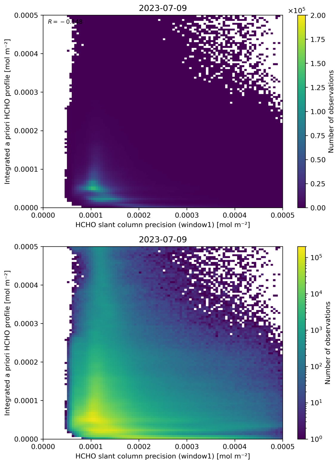
Figure 96: Scatter density plot of “HCHO slant column precision (window1)” against “Integrated a priori HCHO profile” for 2023-07-08 to 2023-07-10.
