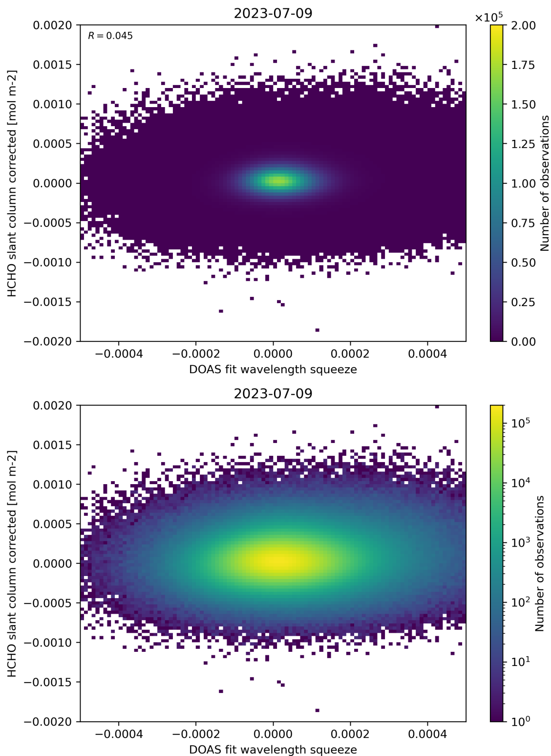
Figure 69: Scatter density plot of “DOAS fit wavelength squeeze” against “HCHO slant column corrected” for 2023-07-08 to 2023-07-10.
