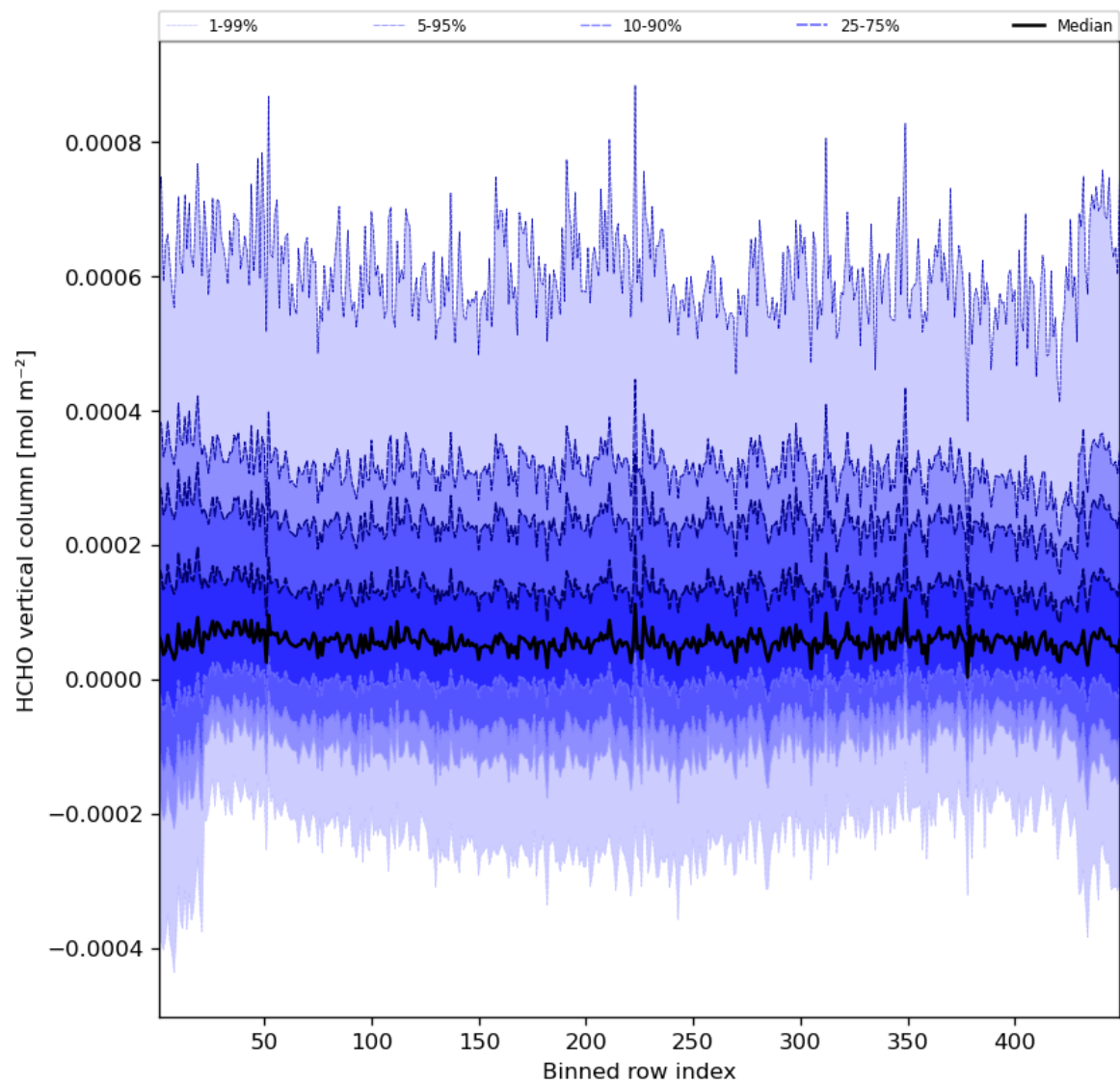
Figure 49: Along track statistics of “HCHO vertical column” for 2023-07-08 to 2023-07-10
