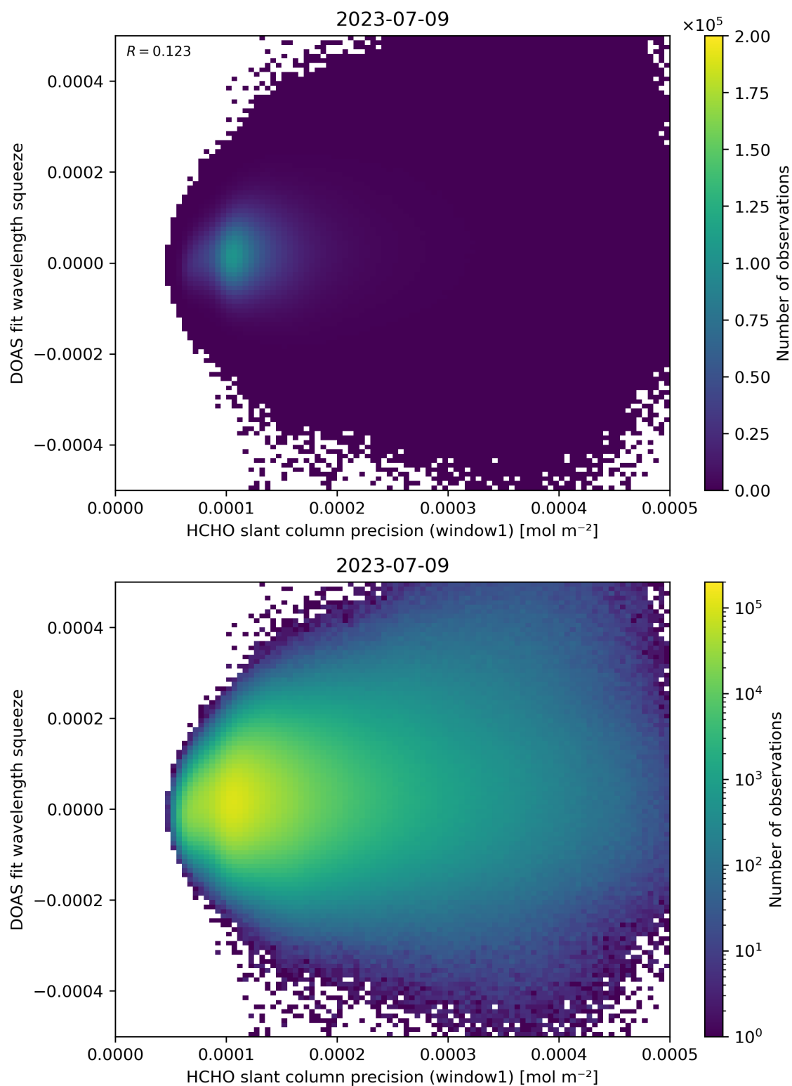
Figure 90: Scatter density plot of “HCHO slant column precision (window1)” against “DOAS fit wavelength squeeze” for 2023-07-08 to 2023-07-10.
