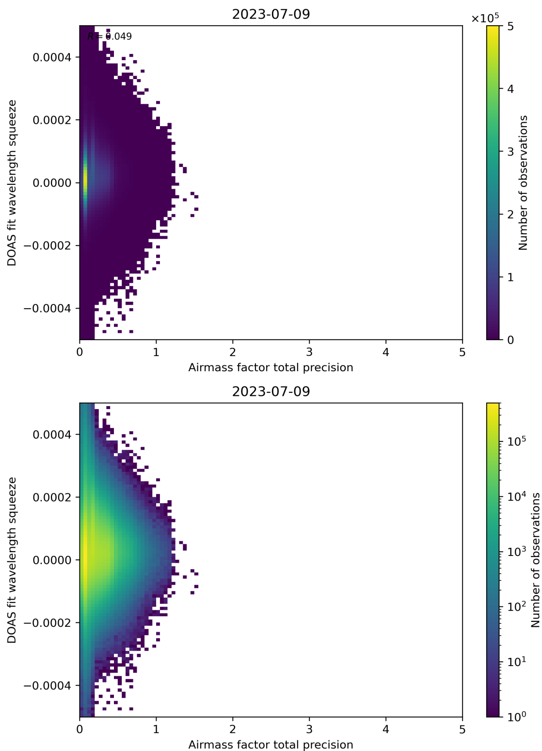
Figure 107: Scatter density plot of “Airmass factor total precision” against “DOAS fit wavelength squeeze” for 2023-07-08 to 2023-07-10.
