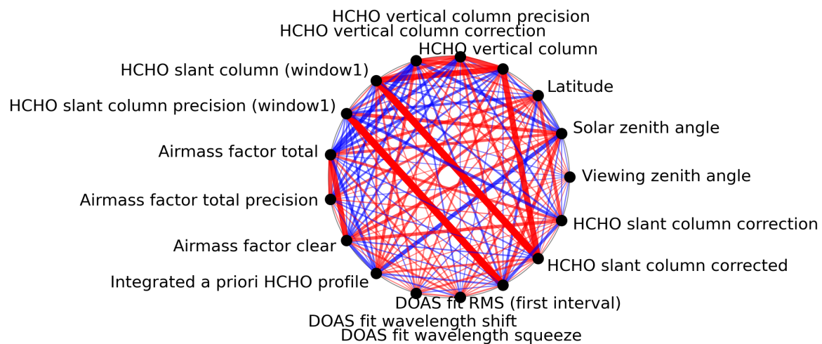
Figure 1: Map of correlation graph for 2023-07-08 to 2023-07-10.
