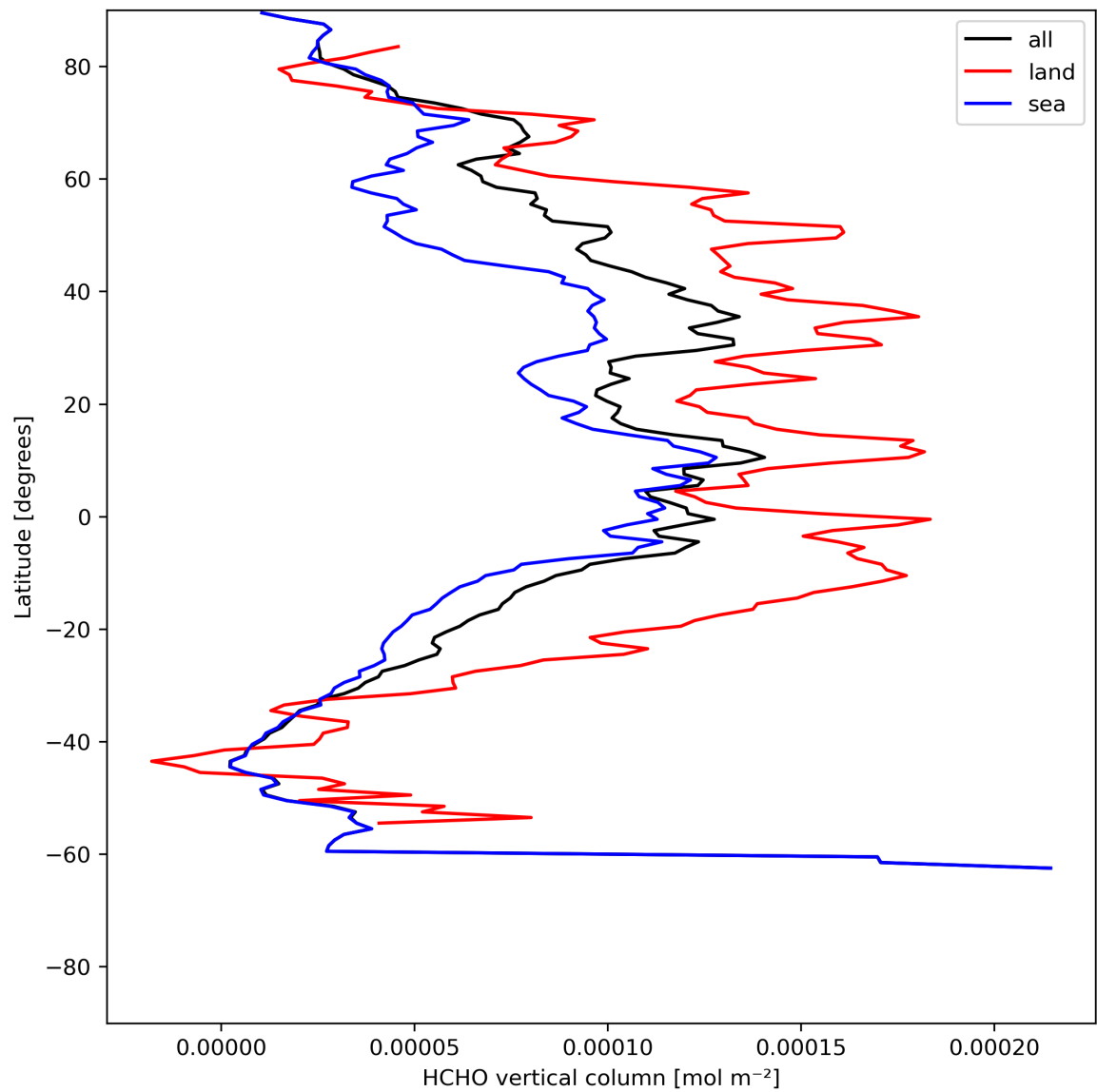
Figure 21: Zonal average of “HCHO vertical column” for 2023-07-08 to 2023-07-10.
