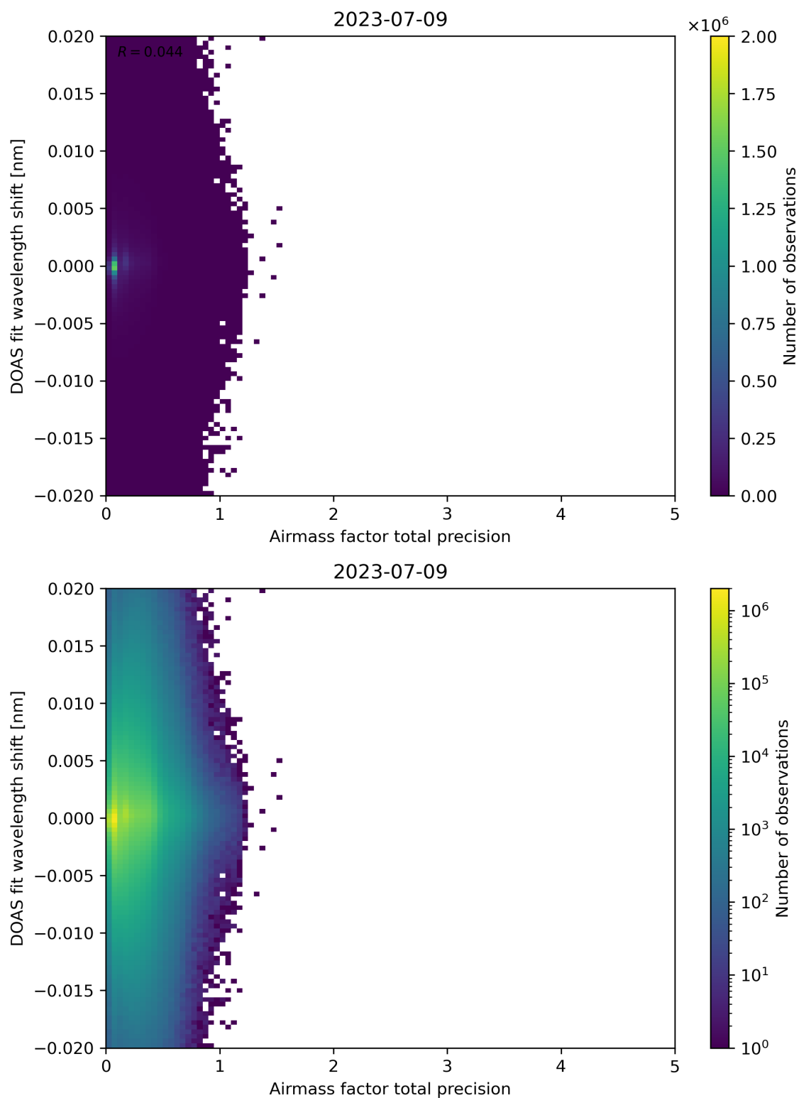
Figure 106: Scatter density plot of “Airmass factor total precision” against “DOAS fit wavelength shift” for 2023-07-08 to 2023-07-10.
