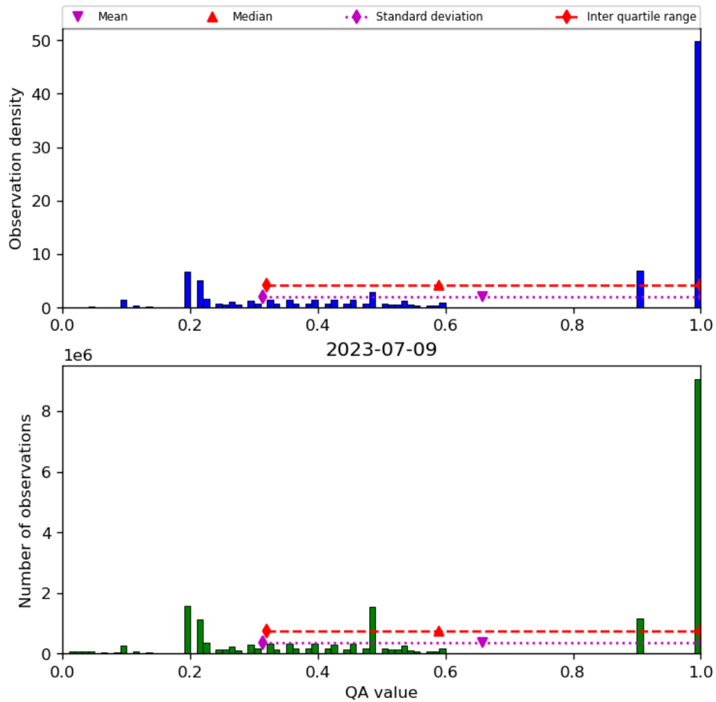
Figure 34: Histogram of “QA value” for 2023-07-08 to 2023-07-10
