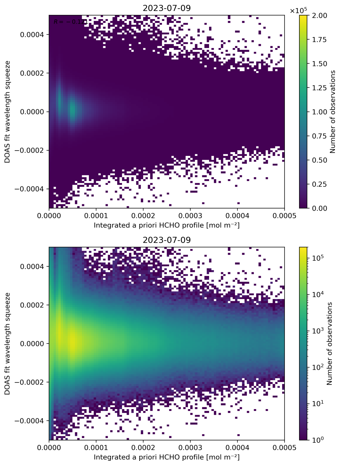
Figure 150: Scatter density plot of “Integrated a priori HCHO profile” against “DOAS fit wavelength squeeze” for 2023-07-08 to 2023-07-10.
