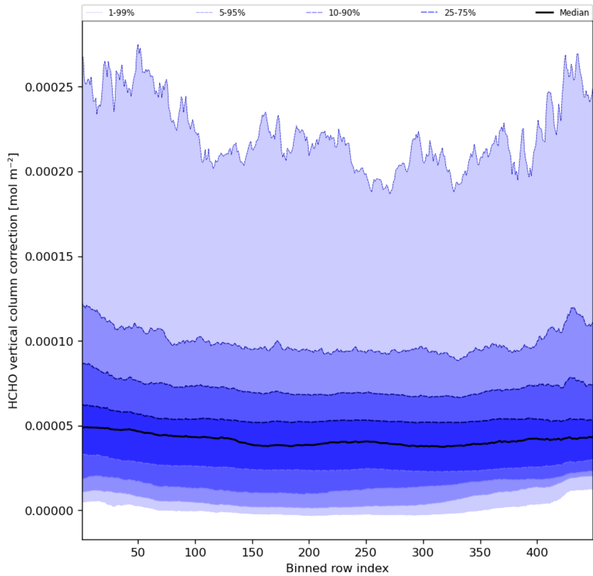
Figure 51: Along track statistics of “HCHO vertical column correction” for 2023-07-08 to 2023-07-10
