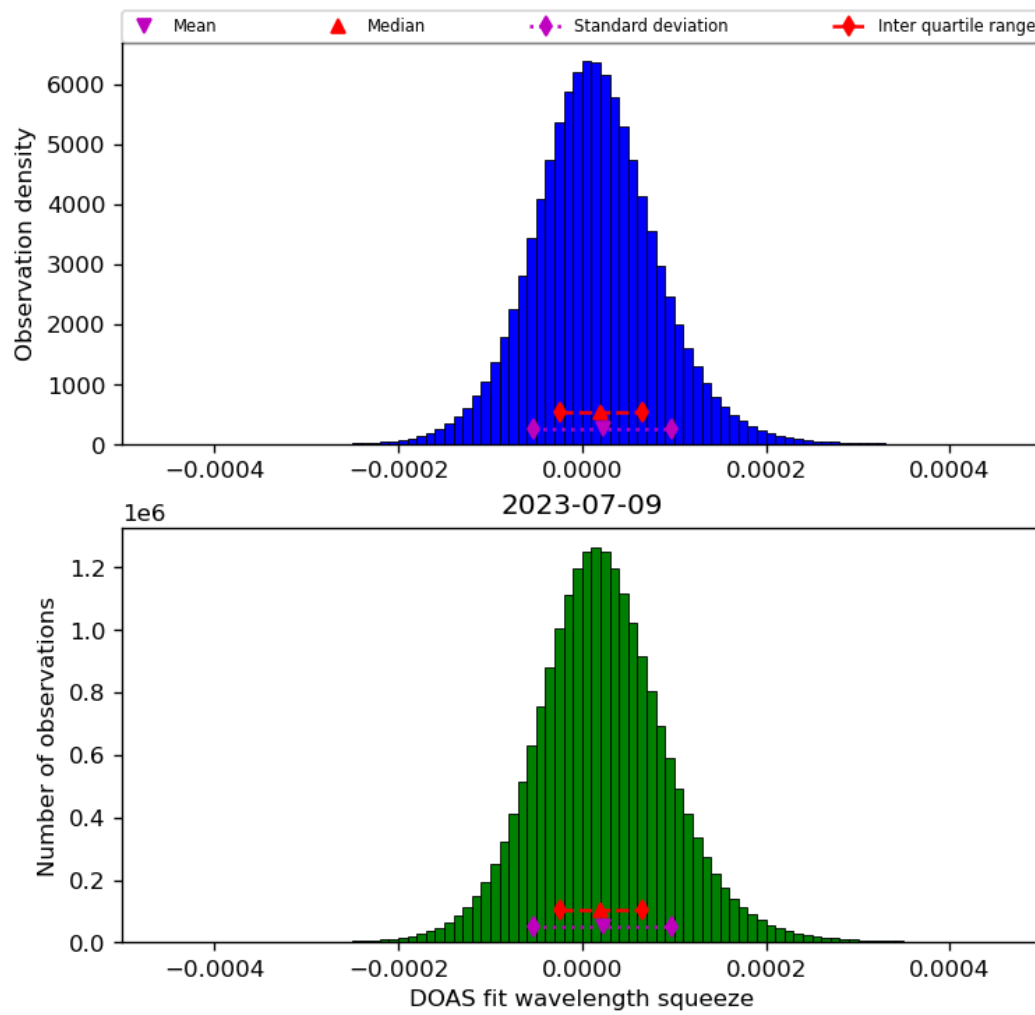
Figure 45: Histogram of “DOAS fit wavelength squeeze” for 2023-07-08 to 2023-07-10
