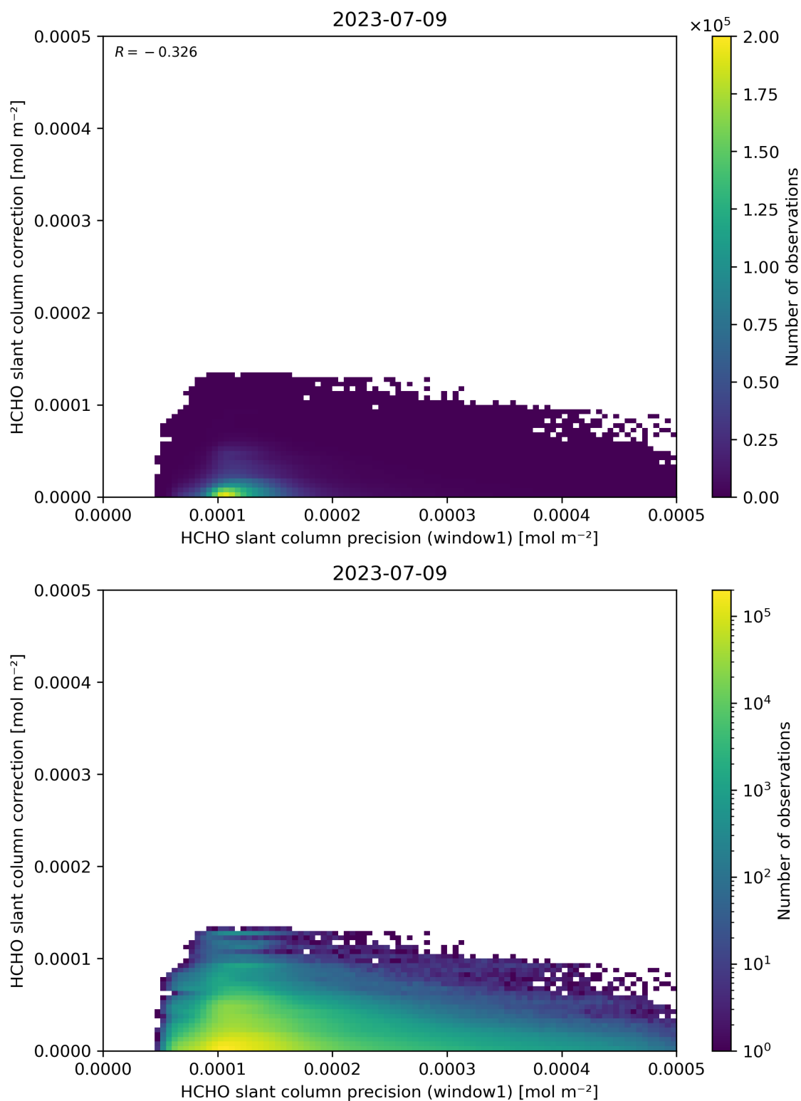
Figure 93: Scatter density plot of “HCHO slant column precision (window1)” against “HCHO slant column correction” for 2023-07-08 to 2023-07-10.
