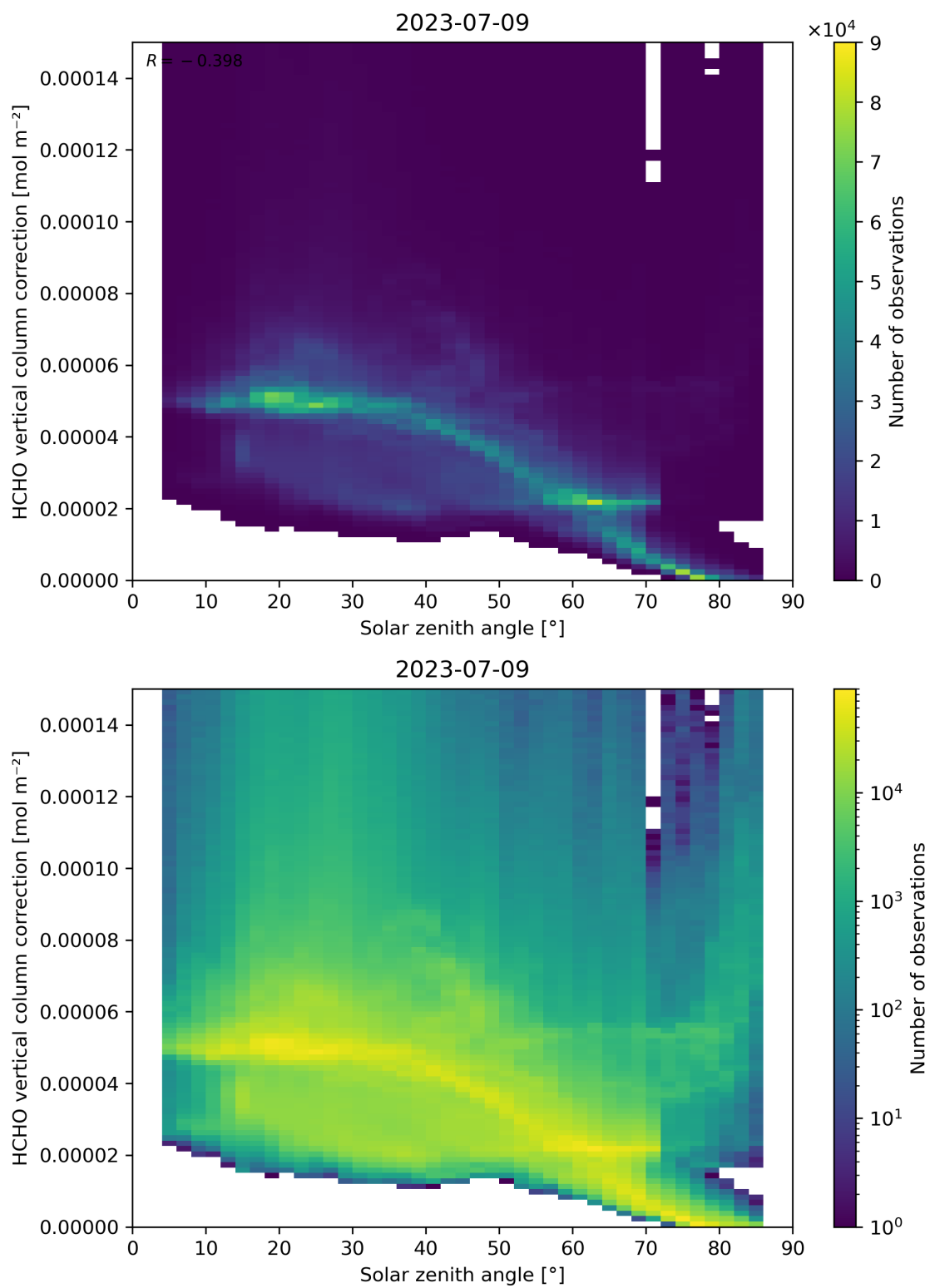
Figure 178: Scatter density plot of “Solar zenith angle” against “HCHO vertical column correction” for 2023-07-08 to 2023-07-10.
