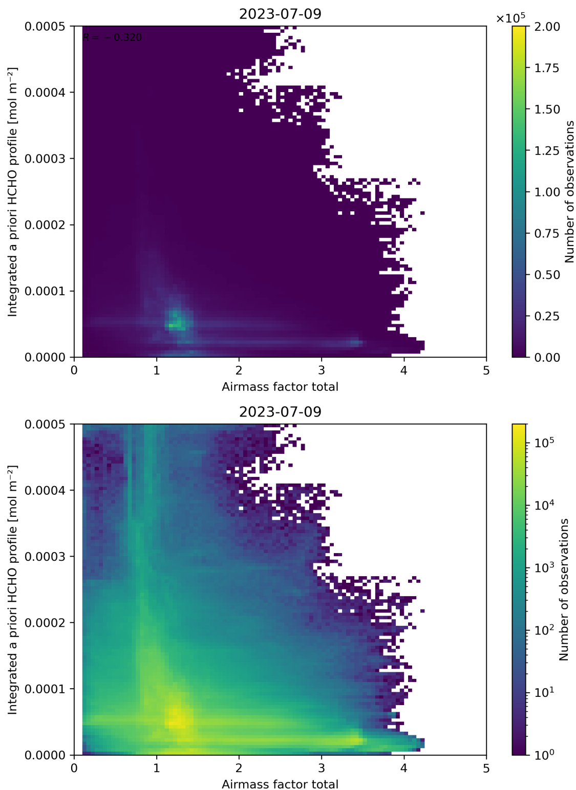
Figure 104: Scatter density plot of “Airmass factor total” against “Integrated a priori HCHO profile” for 2023-07-08 to 2023-07-10.
