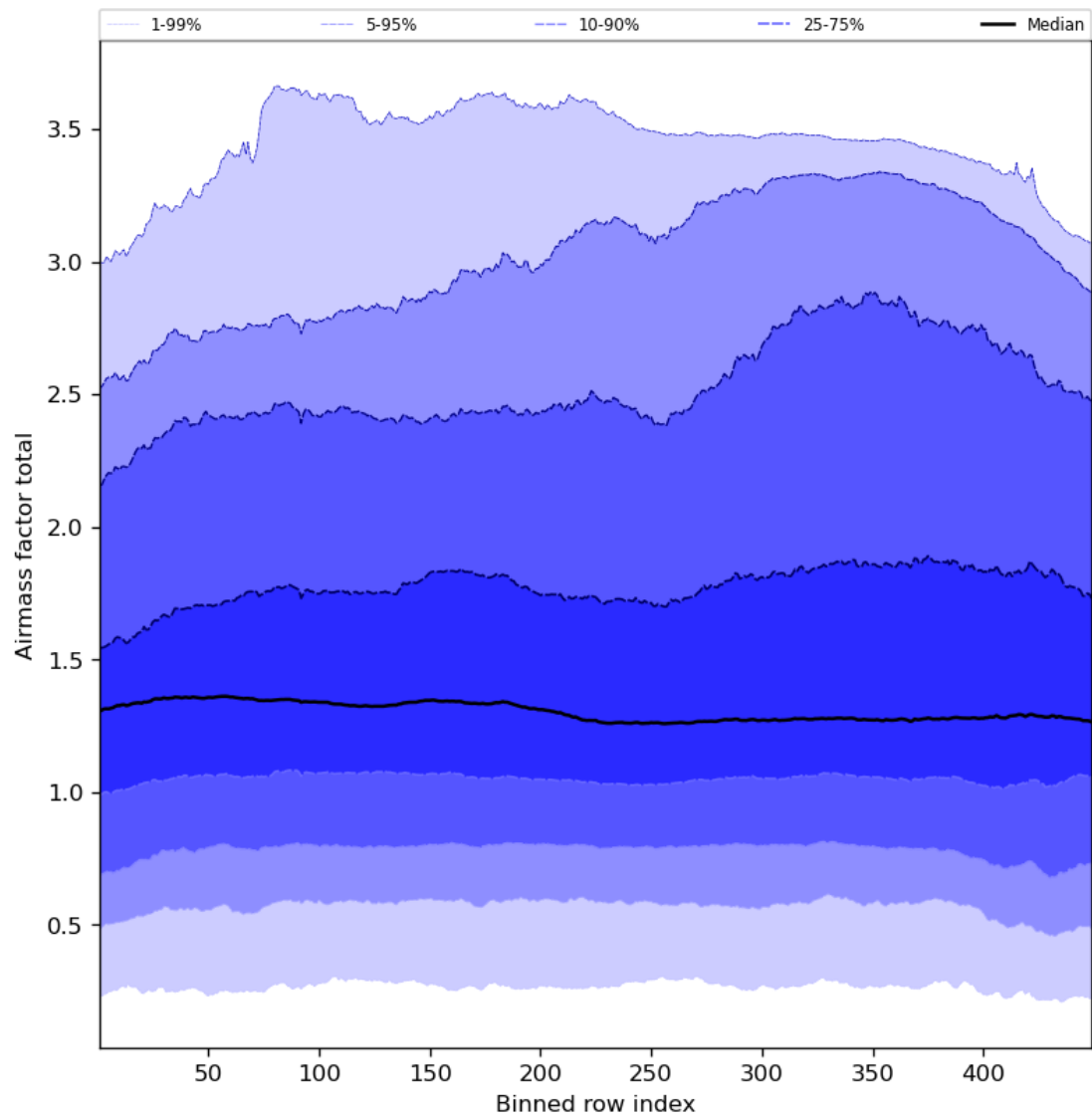
Figure 54: Along track statistics of “Airmass factor total” for 2023-07-08 to 2023-07-10
