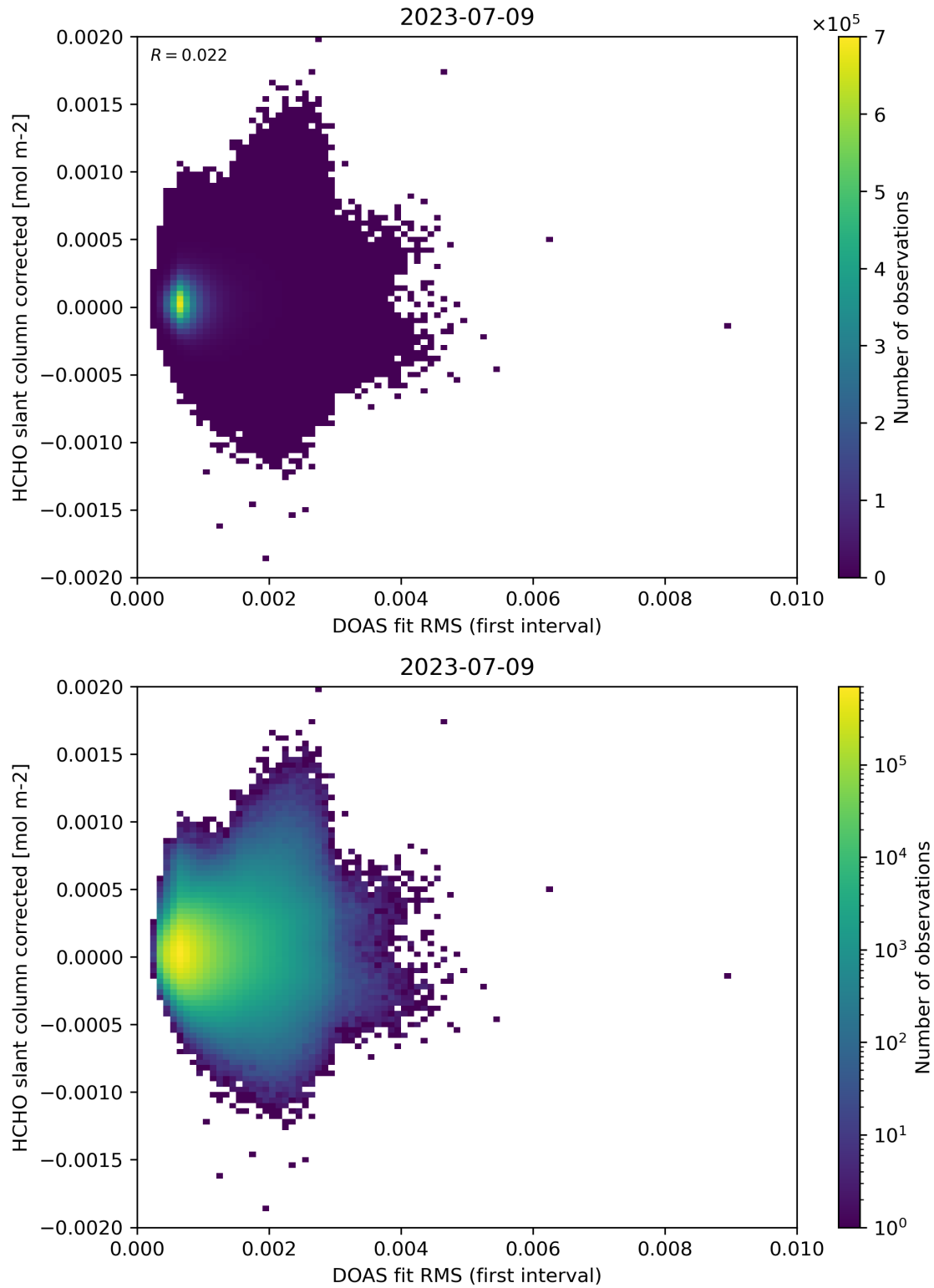
Figure 62: Scatter density plot of “DOAS fit RMS (first interval)” against “HCHO slant column corrected” for 2023-07-08 to 2023-07-10.
