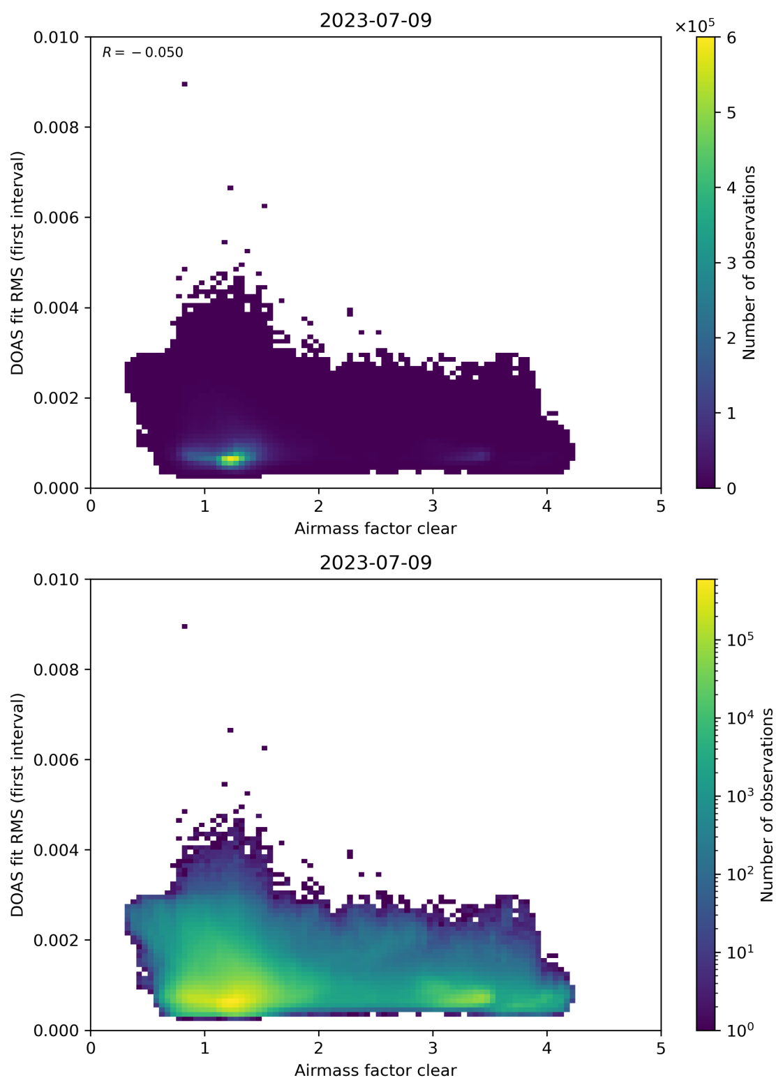
Figure 71: Scatter density plot of “Airmass factor clear” against “DOAS fit RMS (first interval)” for 2023-07-08 to 2023-07-10.
