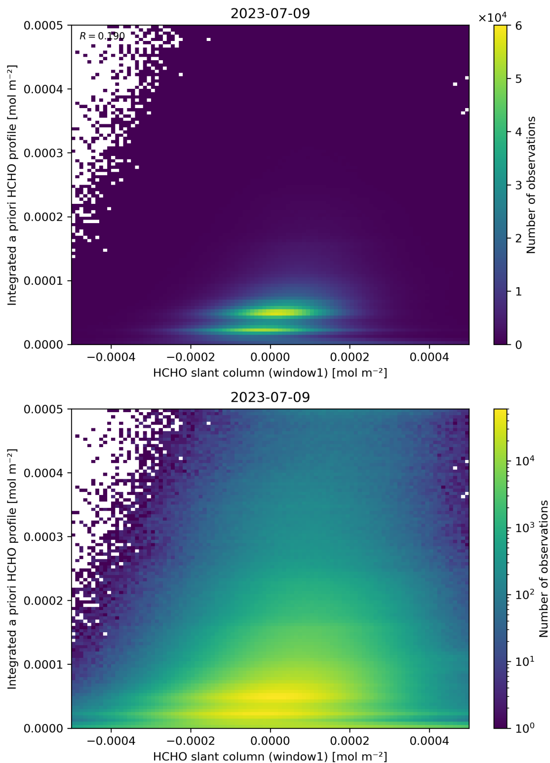
Figure 87: Scatter density plot of “HCHO slant column (window1)” against “Integrated a priori HCHO profile” for 2023-07-08 to 2023-07-10.
