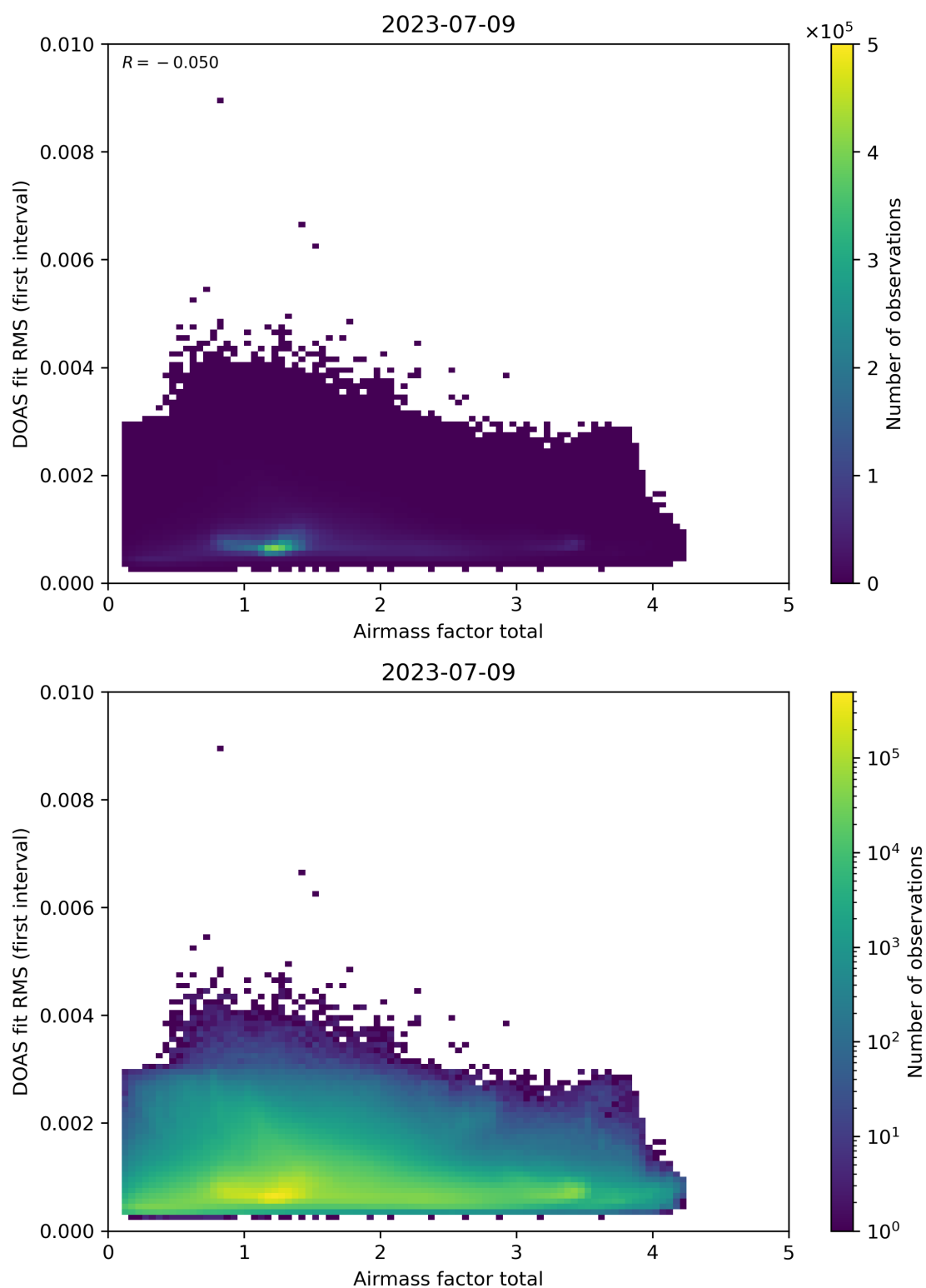
Figure 97: Scatter density plot of “Airmass factor total” against “DOAS fit RMS (first interval)” for 2023-07-08 to 2023-07-10.
