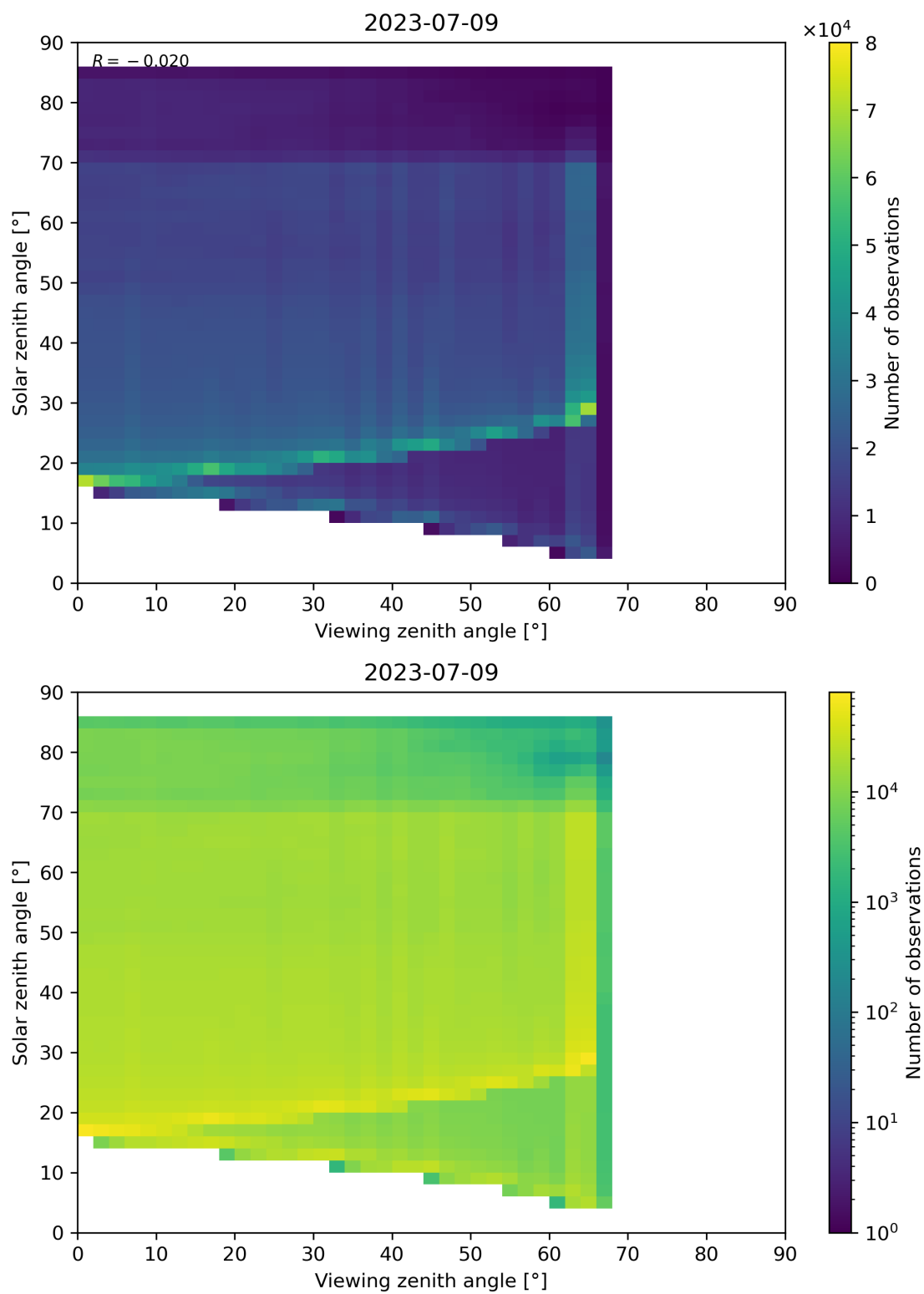
Figure 197: Scatter density plot of “Viewing zenith angle” against “Solar zenith angle” for 2023-07-08 to 2023-07-10.
