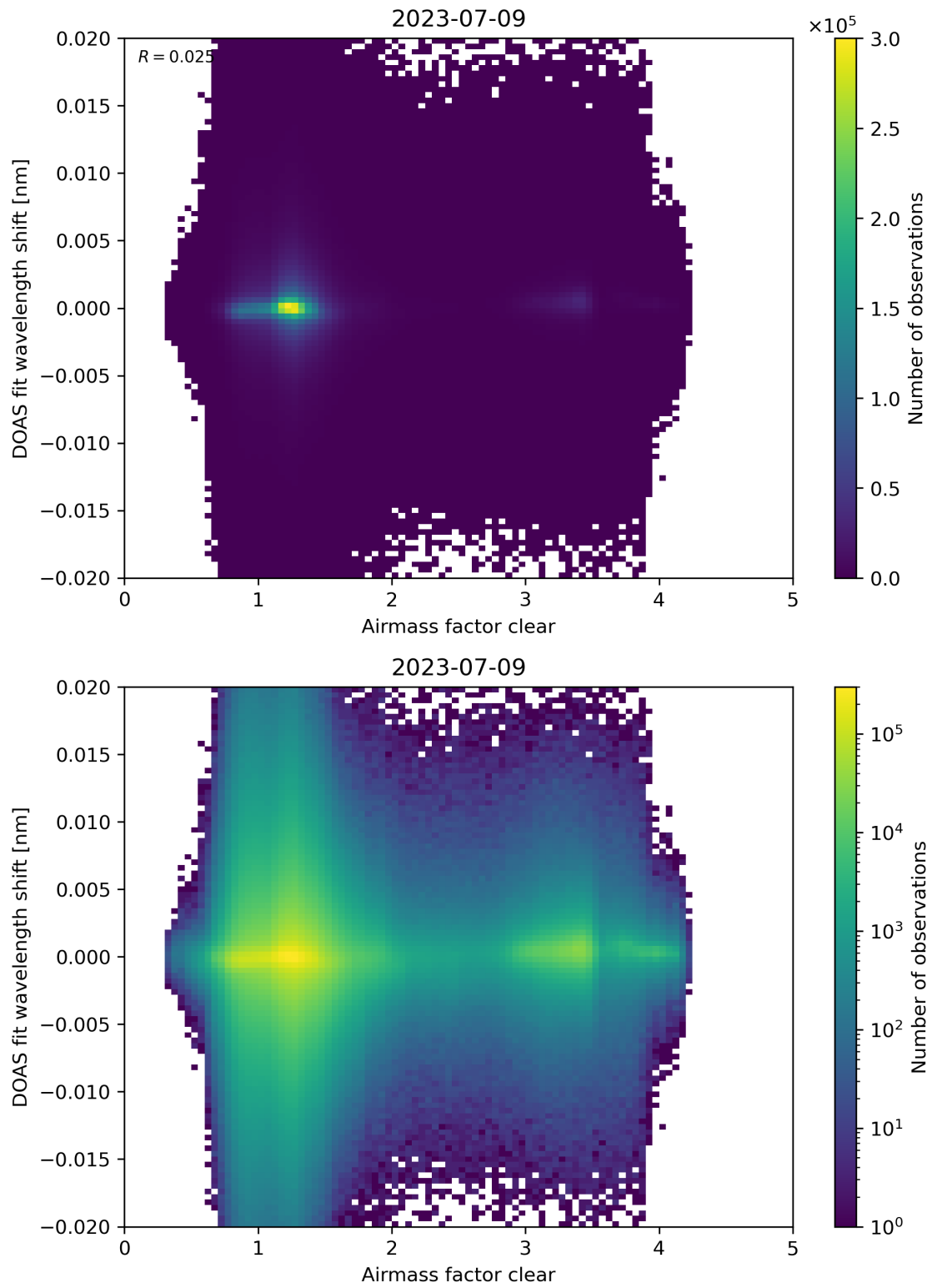
Figure 72: Scatter density plot of “Airmass factor clear” against “DOAS fit wavelength shift” for 2023-07-08 to 2023-07-10.
