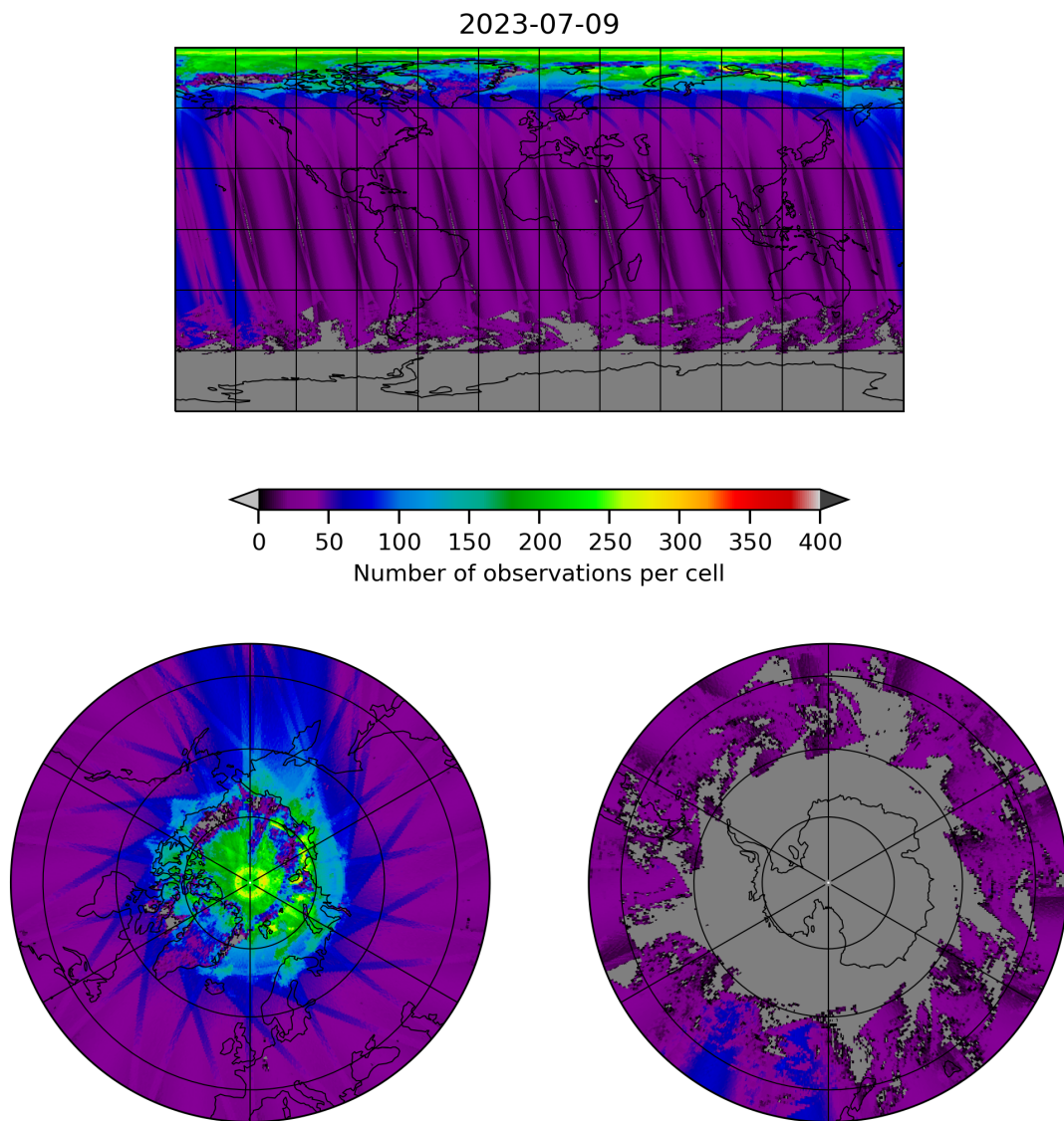
Figure 19: Map of the number of observations for 2023-07-08 to 2023-07-10
