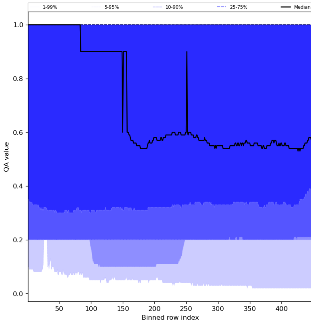
Figure 48: Along track statistics of “QA value” for 2023-07-08 to 2023-07-10
