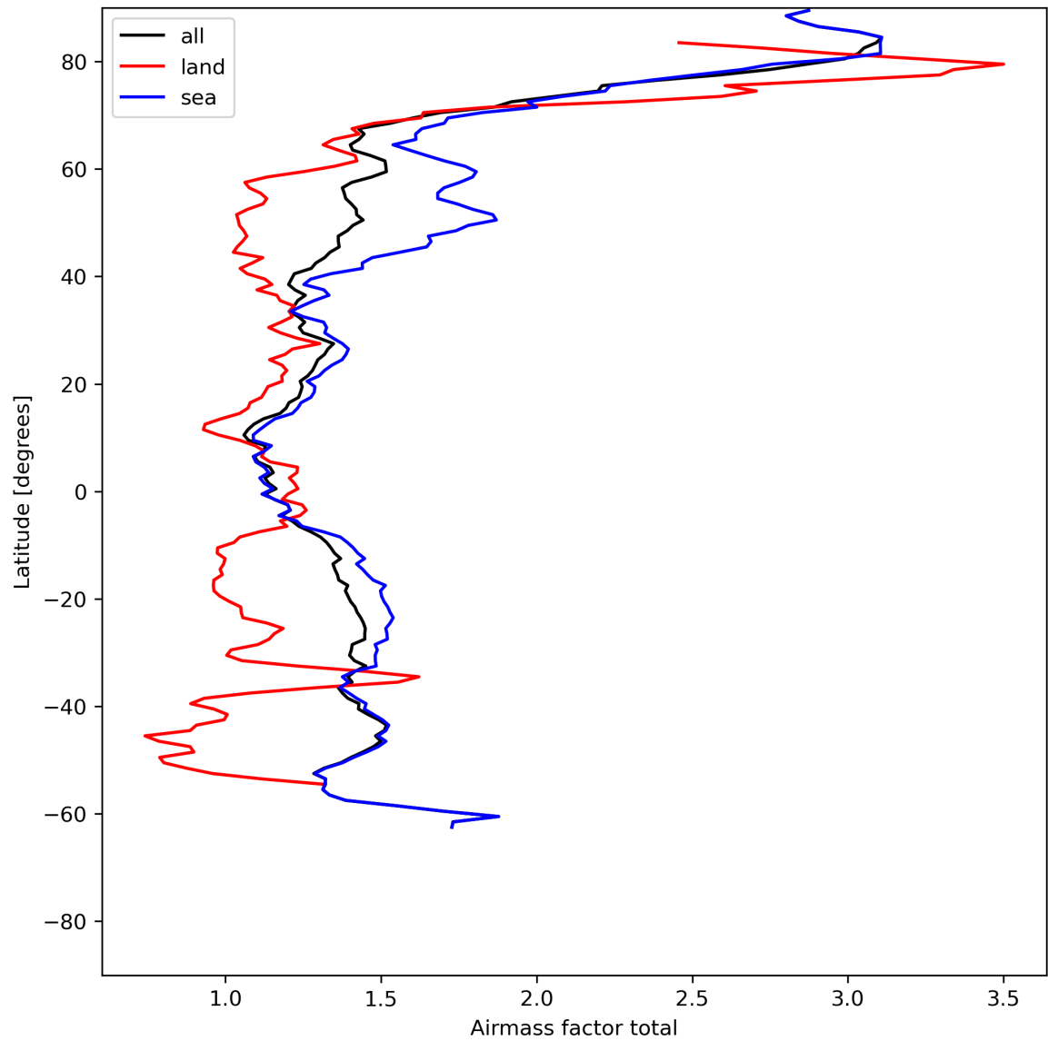
Figure 26: Zonal average of “Airmass factor total” for 2023-07-08 to 2023-07-10.
