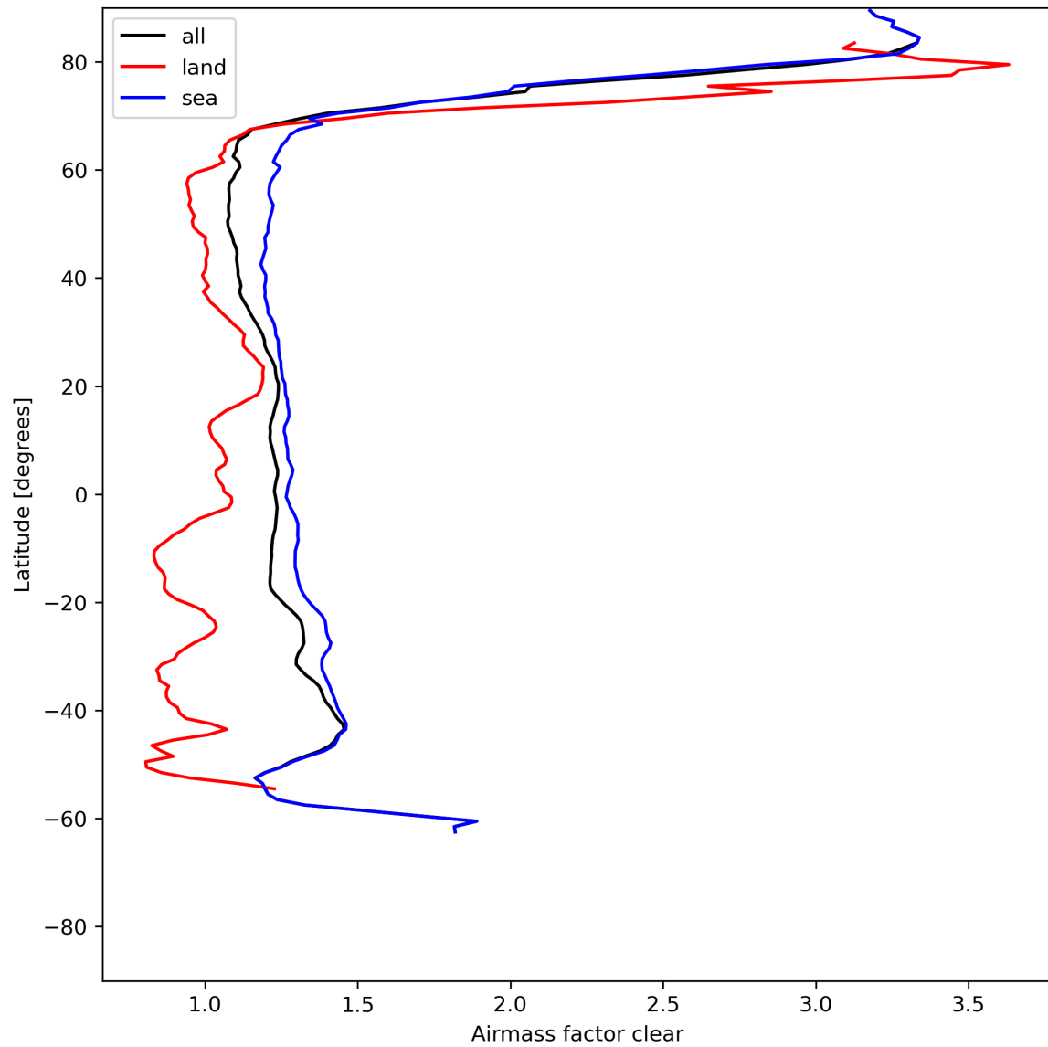
Figure 28: Zonal average of “Airmass factor clear” for 2023-07-08 to 2023-07-10.
