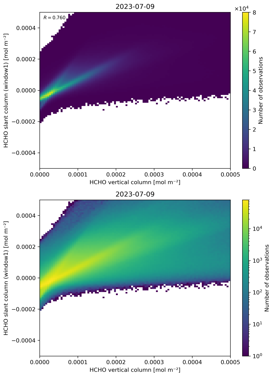
Figure 129: Scatter density plot of “HCHO vertical column” against “HCHO slant column (window1)” for 2023-07-08 to 2023-07-10.
