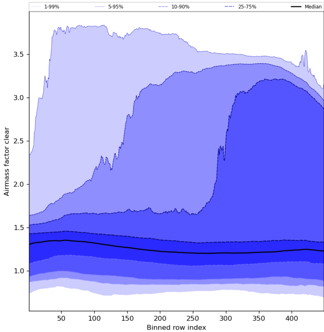
Figure 56: Along track statistics of “Airmass factor clear” for 2023-07-08 to 2023-07-10
