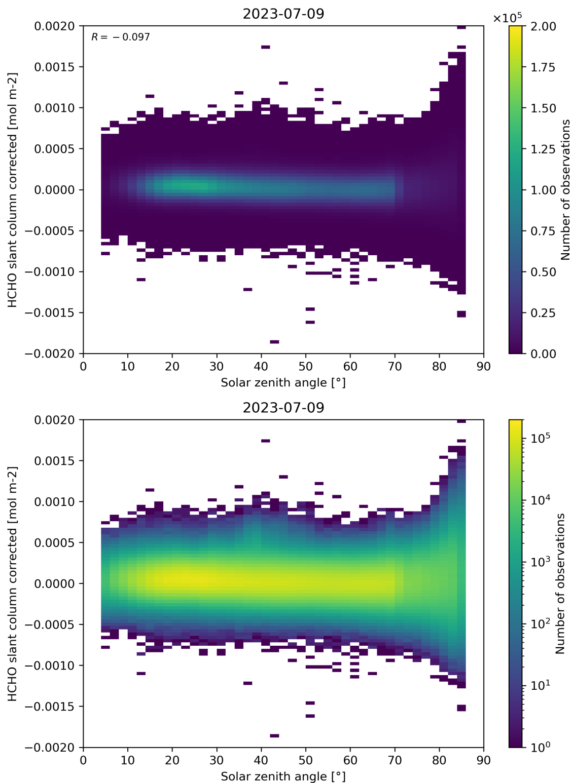
Figure 171: Scatter density plot of “Solar zenith angle” against “HCHO slant column corrected” for 2023-07-08 to 2023-07-10.
