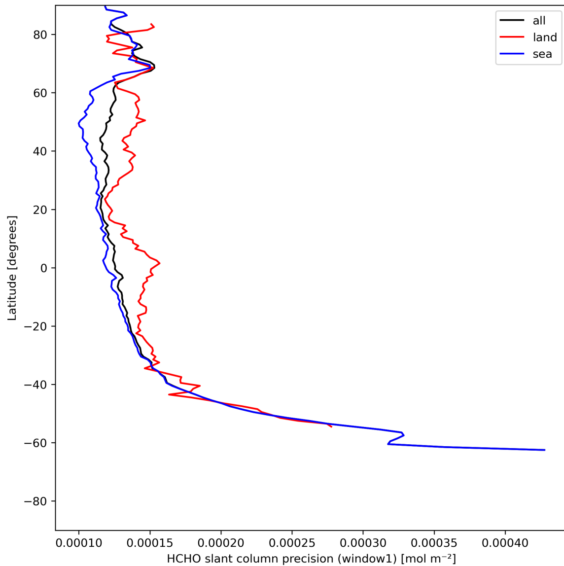
Figure 25: Zonal average of "HCHO slant column precision (window1)" for 2023-07-08 to 2023-07-10.
