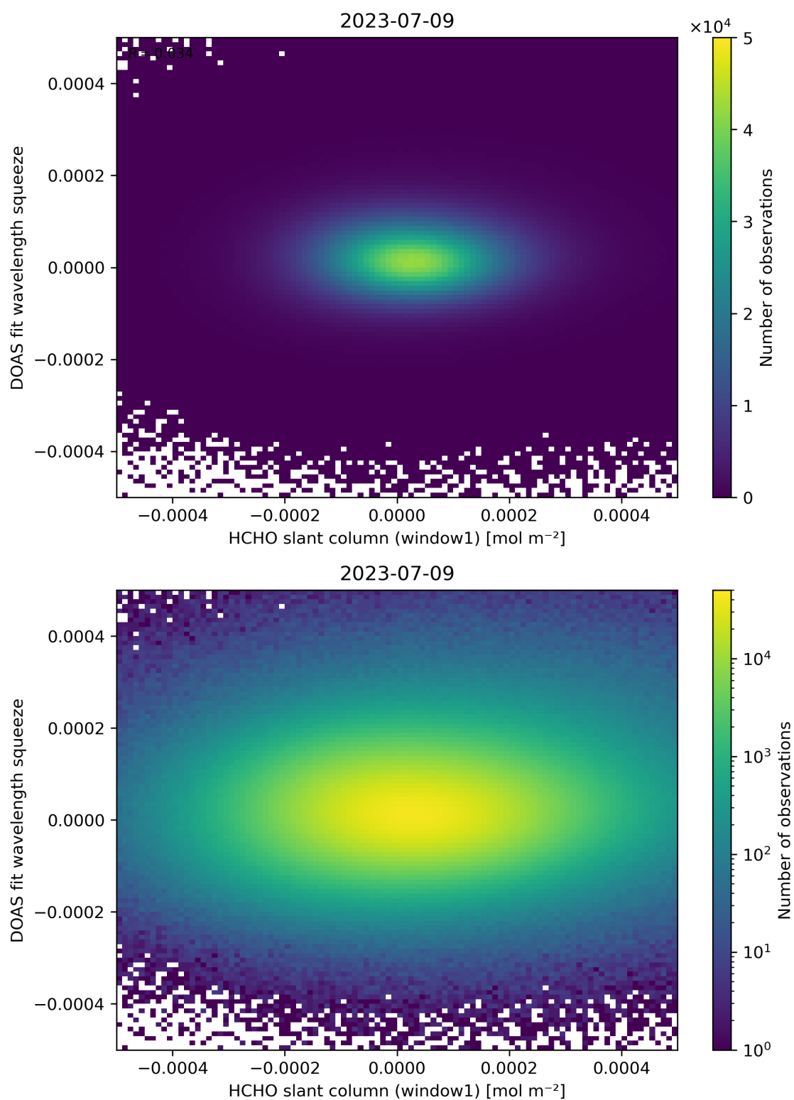
Figure 80: Scatter density plot of “HCHO slant column (window1)” against “DOAS fit wavelength squeeze” for 2023-07-08 to 2023-07-10.
