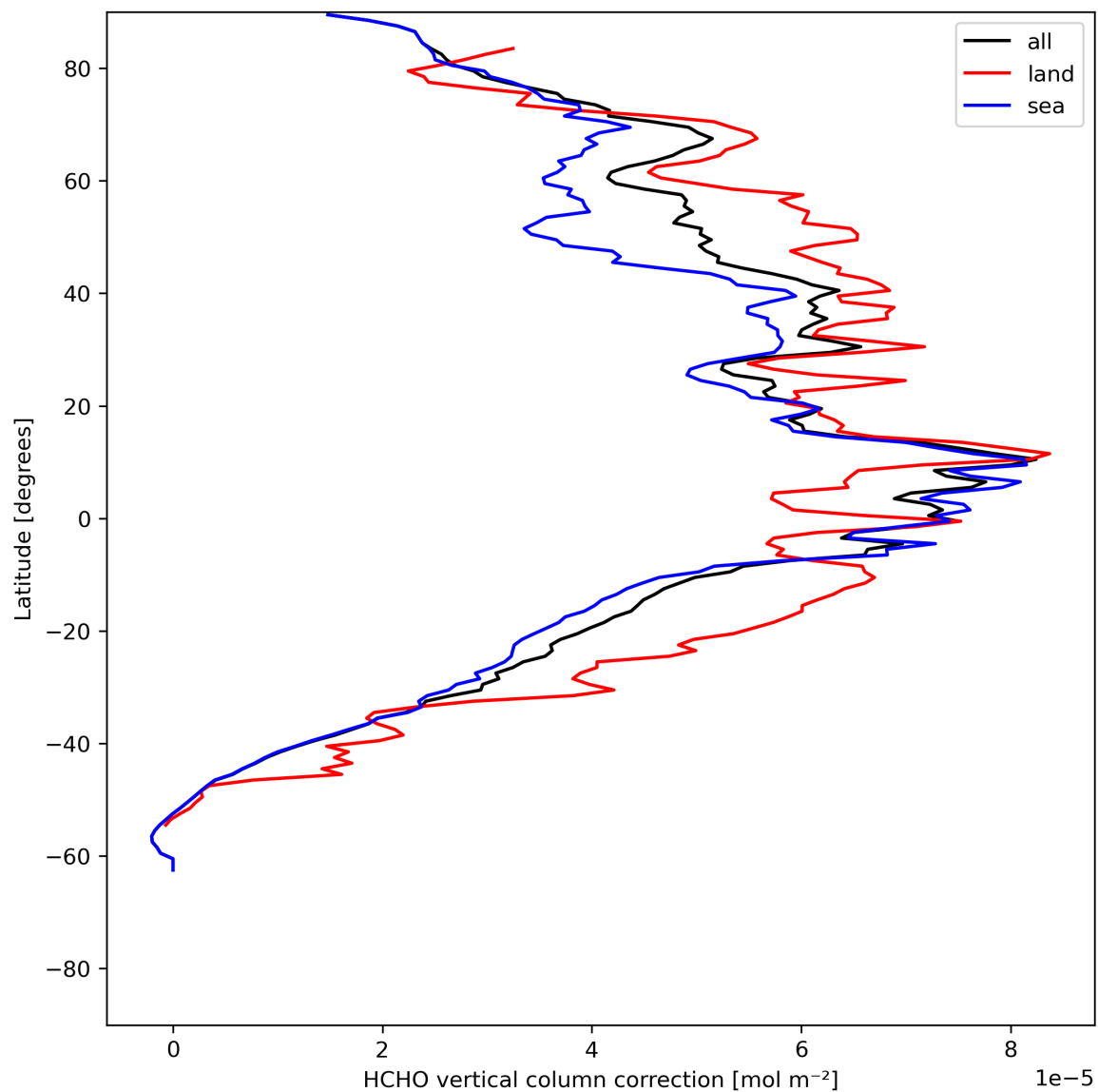
Figure 23: Zonal average of “HCHO vertical column correction” for 2023-07-08 to 2023-07-10.
