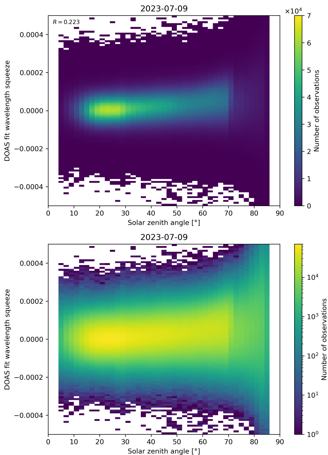
Figure 169: Scatter density plot of “Solar zenith angle” against “DOAS fit wavelength squeeze” for 2023-07-08 to 2023-07-10.
