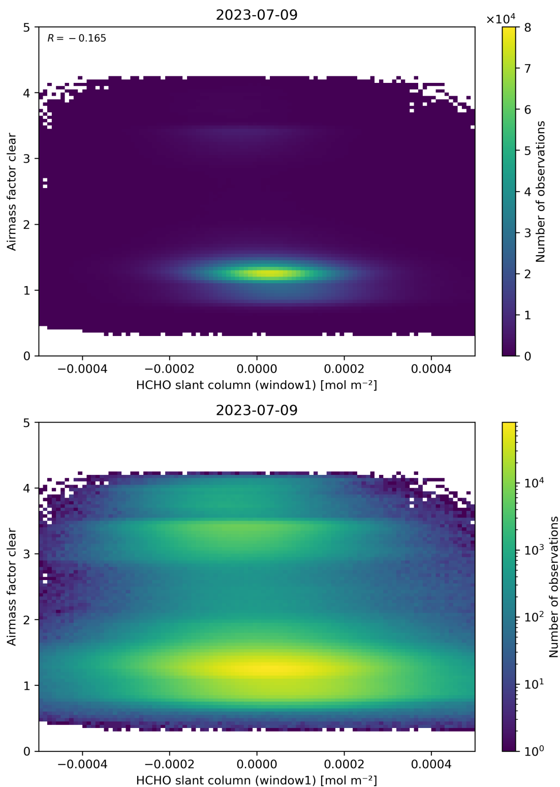
Figure 81: Scatter density plot of “HCHO slant column (window1)” against “Airmass factor clear” for 2023-07-08 to 2023-07-10.
