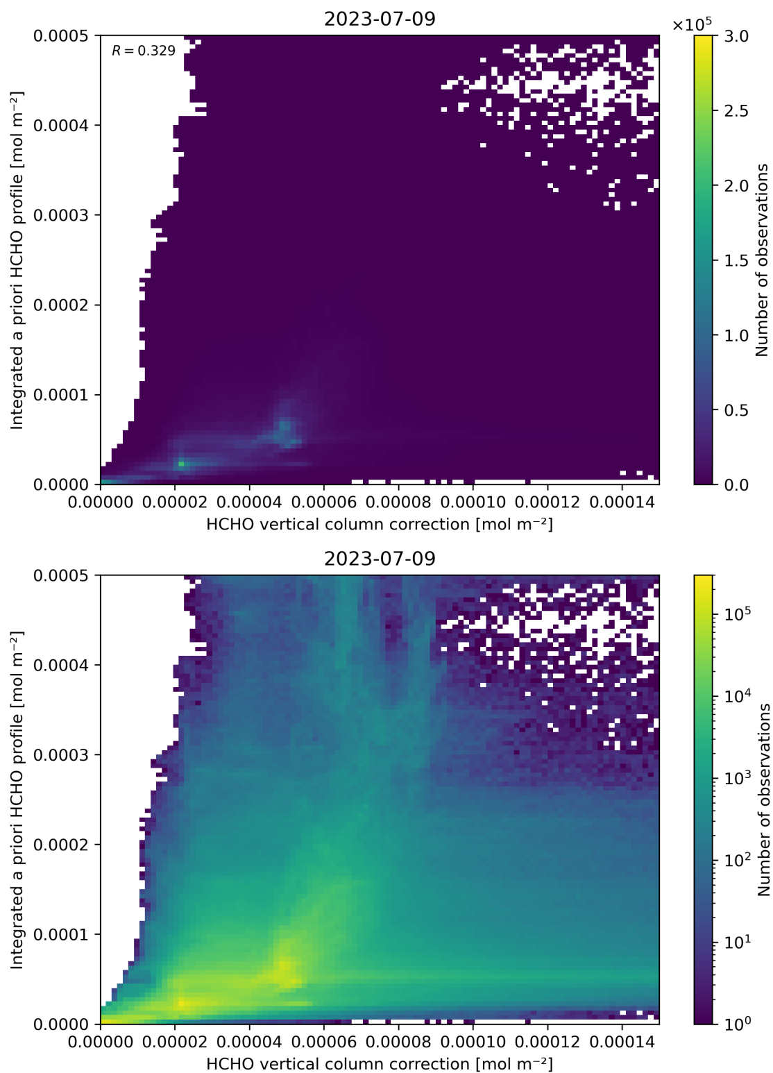
Figure 122: Scatter density plot of “HCHO vertical column correction” against “Integrated a priori HCHO profile” for 2023-07-08 to 2023-07-10.
