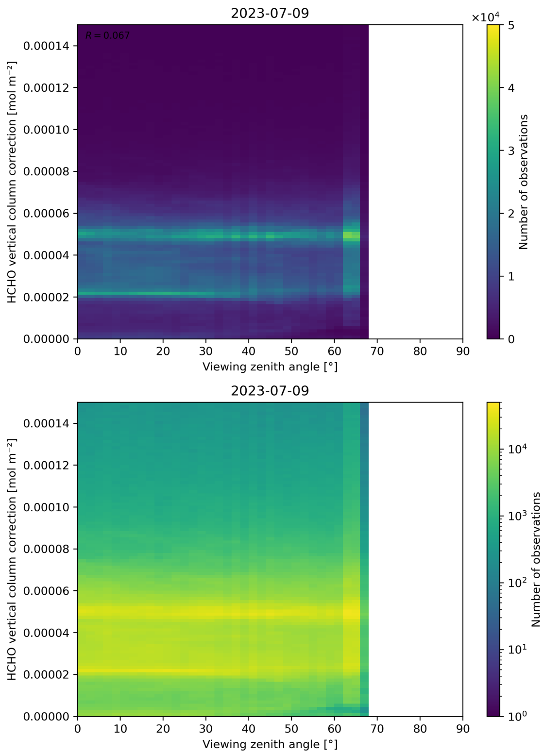
Figure 193: Scatter density plot of “Viewing zenith angle” against “HCHO vertical column correction” for 2023-07-08 to 2023-07-10.
