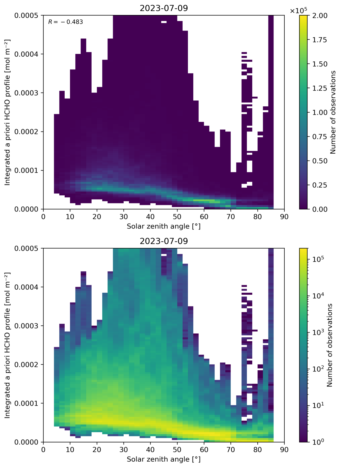
Figure 180: Scatter density plot of “Solar zenith angle” against “Integrated a priori HCHO profile” for 2023-07-08 to 2023-07-10.
