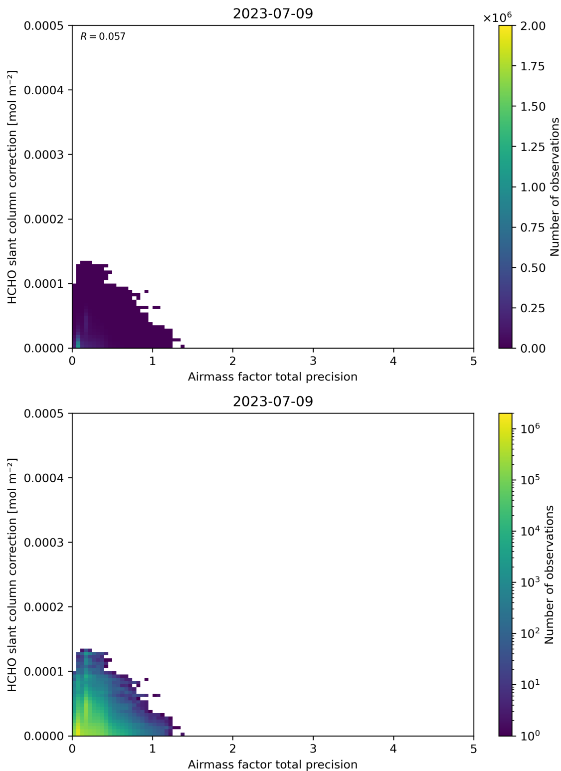
Figure 110: Scatter density plot of “Airmass factor total precision” against “HCHO slant column correction” for 2023-07-08 to 2023-07-10.
