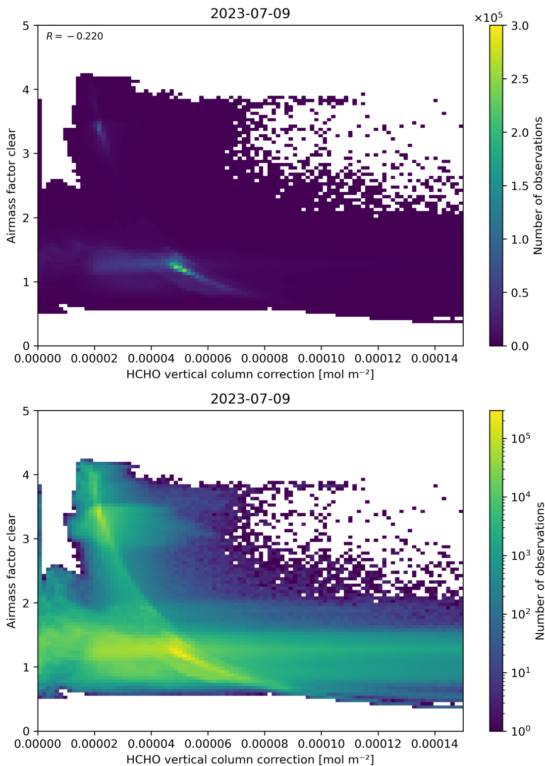
Figure 115: Scatter density plot of “HCHO vertical column correction” against “Airmass factor clear” for 2023-07-08 to 2023-07-10.
