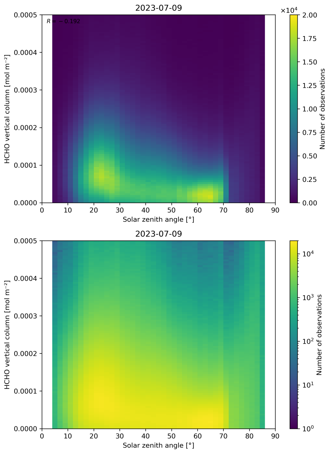
Figure 177: Scatter density plot of “Solar zenith angle” against “HCHO vertical column” for 2023-07-08 to 2023-07-10.
