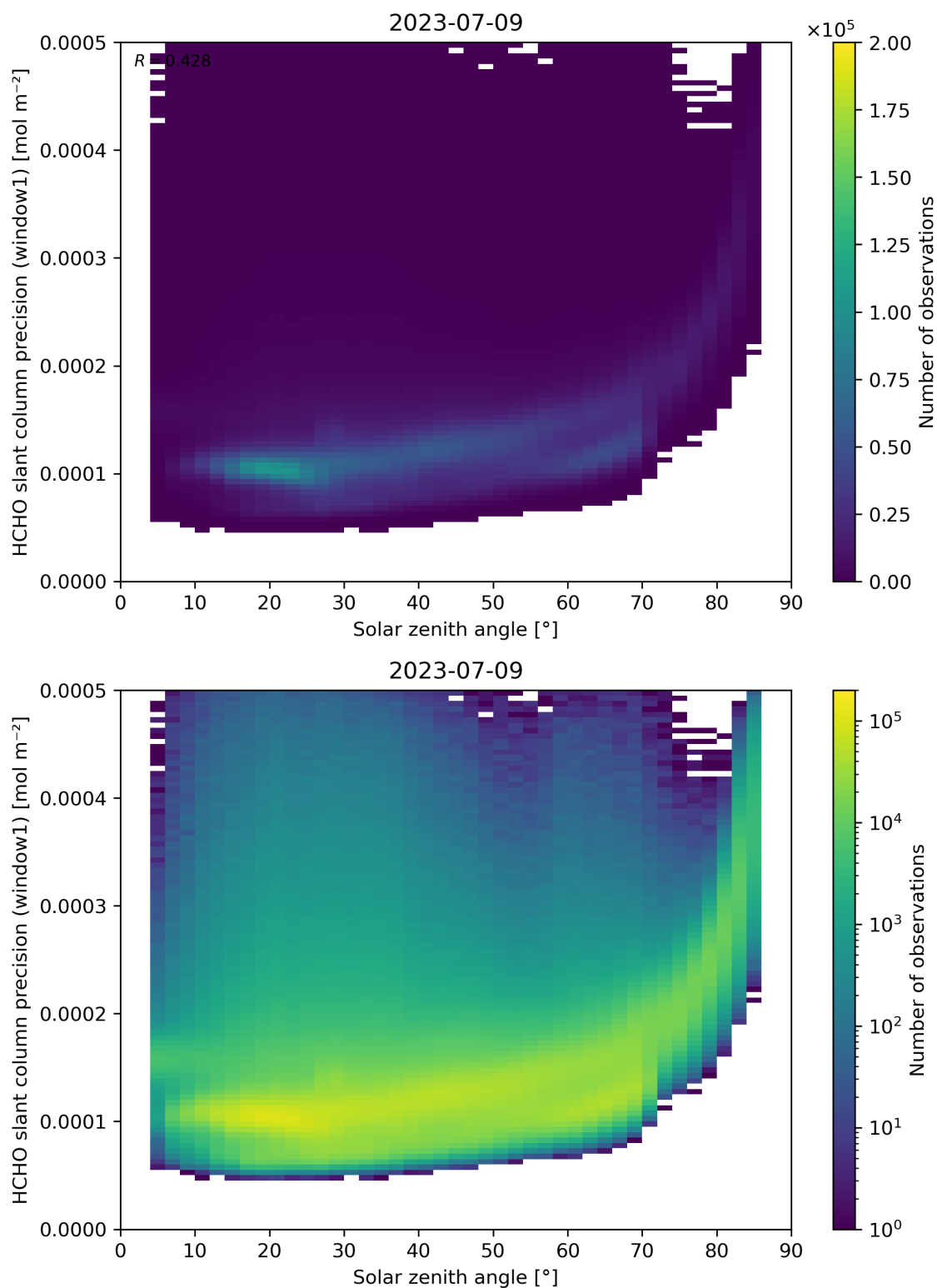
Figure 174: Scatter density plot of “Solar zenith angle” against “HCHO slant column precision (window1)” for 2023-07-08 to 2023-07-10.
