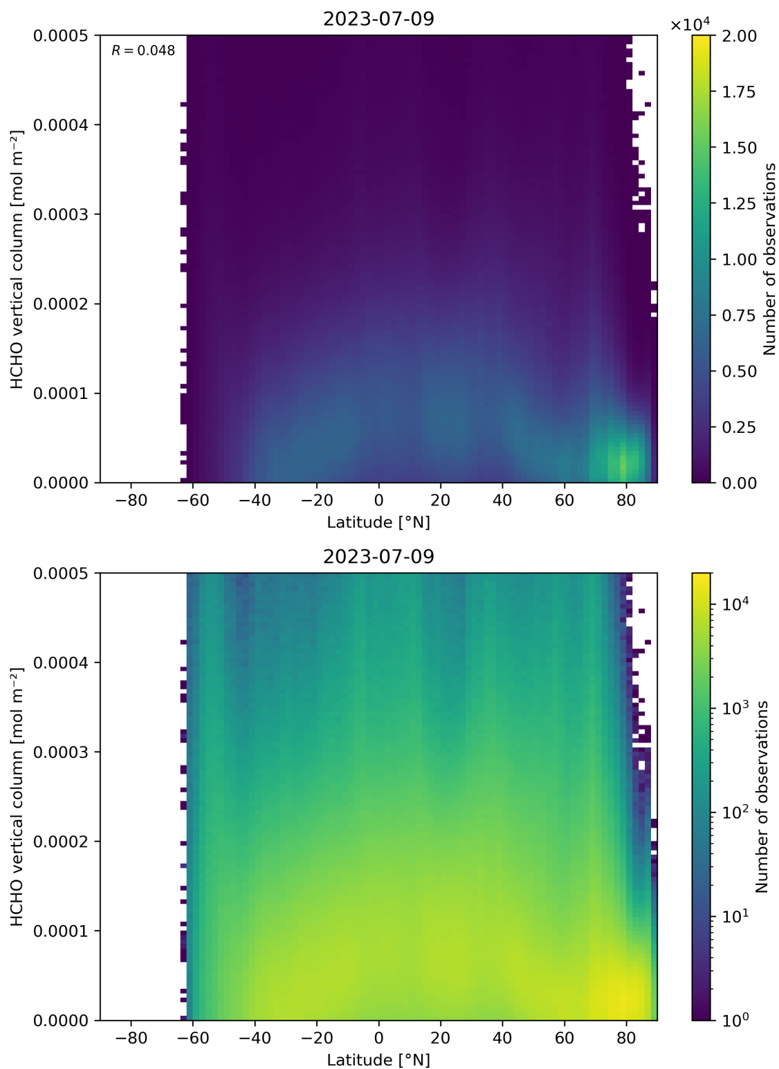
Figure 163: Scatter density plot of “Latitude” against “HCHO vertical column” for 2023-07-08 to 2023-07-10.
