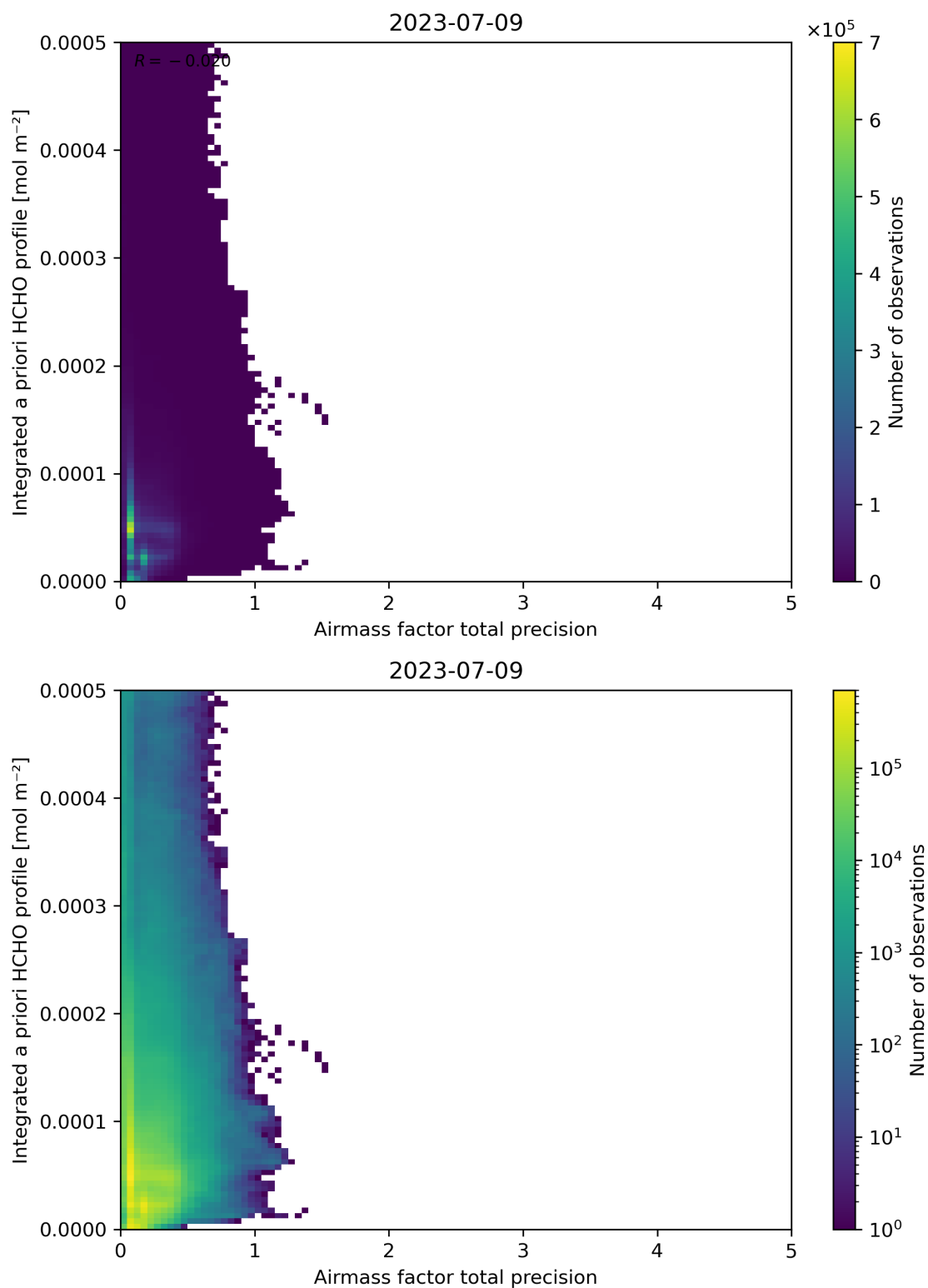
Figure 111: Scatter density plot of “Airmass factor total precision” against “Integrated a priori HCHO profile” for 2023-07-08 to 2023-07-10.
