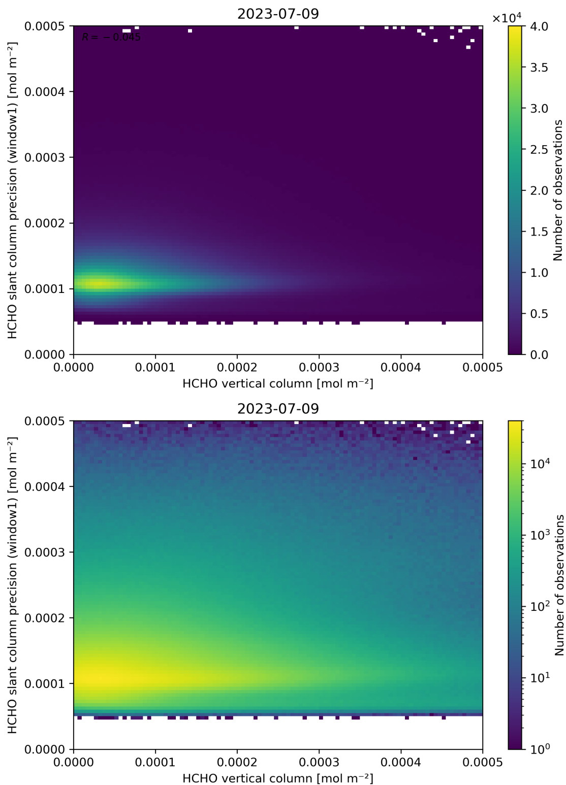
Figure 130: Scatter density plot of “HCHO vertical column” against “HCHO slant column precision (window1)” for 2023-07-08 to 2023-07-10.
