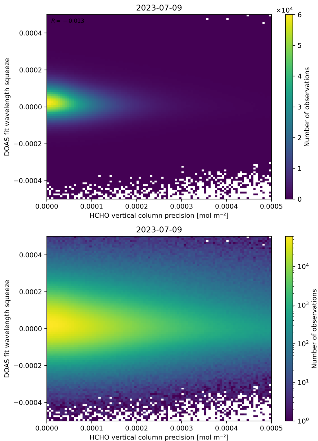
Figure 138: Scatter density plot of “HCHO vertical column precision” against “DOAS fit wavelength squeeze” for 2023-07-08 to 2023-07-10.
