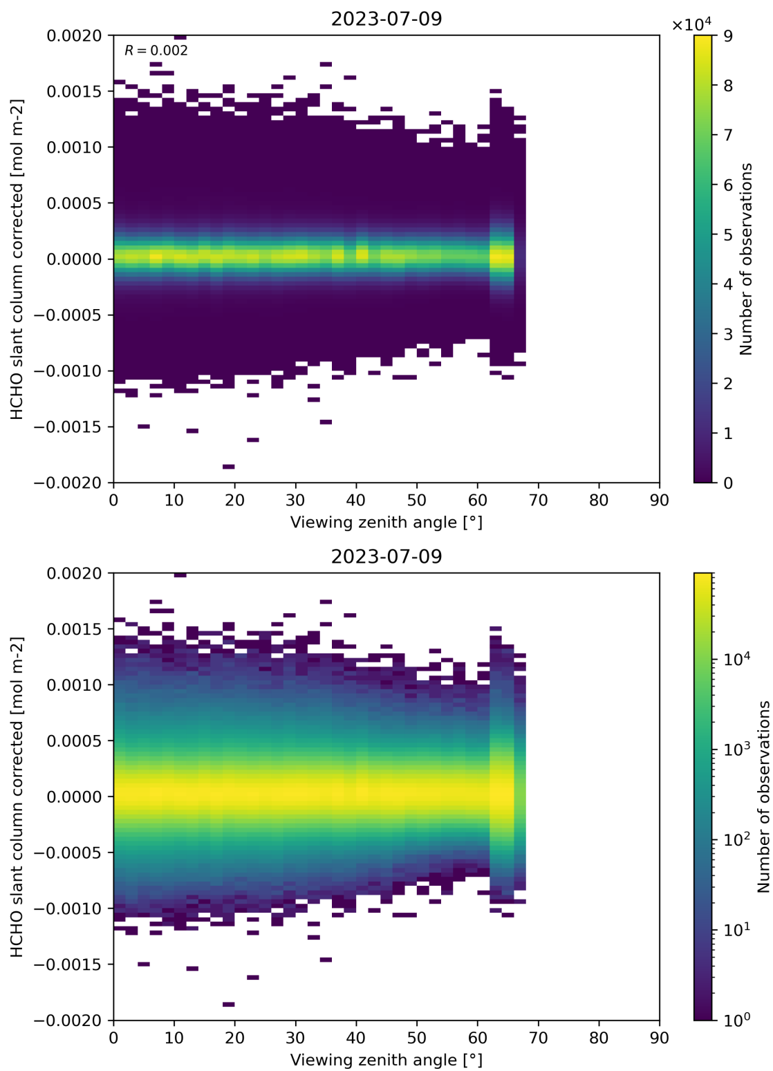
Figure 186: Scatter density plot of “Viewing zenith angle” against “HCHO slant column corrected” for 2023-07-08 to 2023-07-10.
