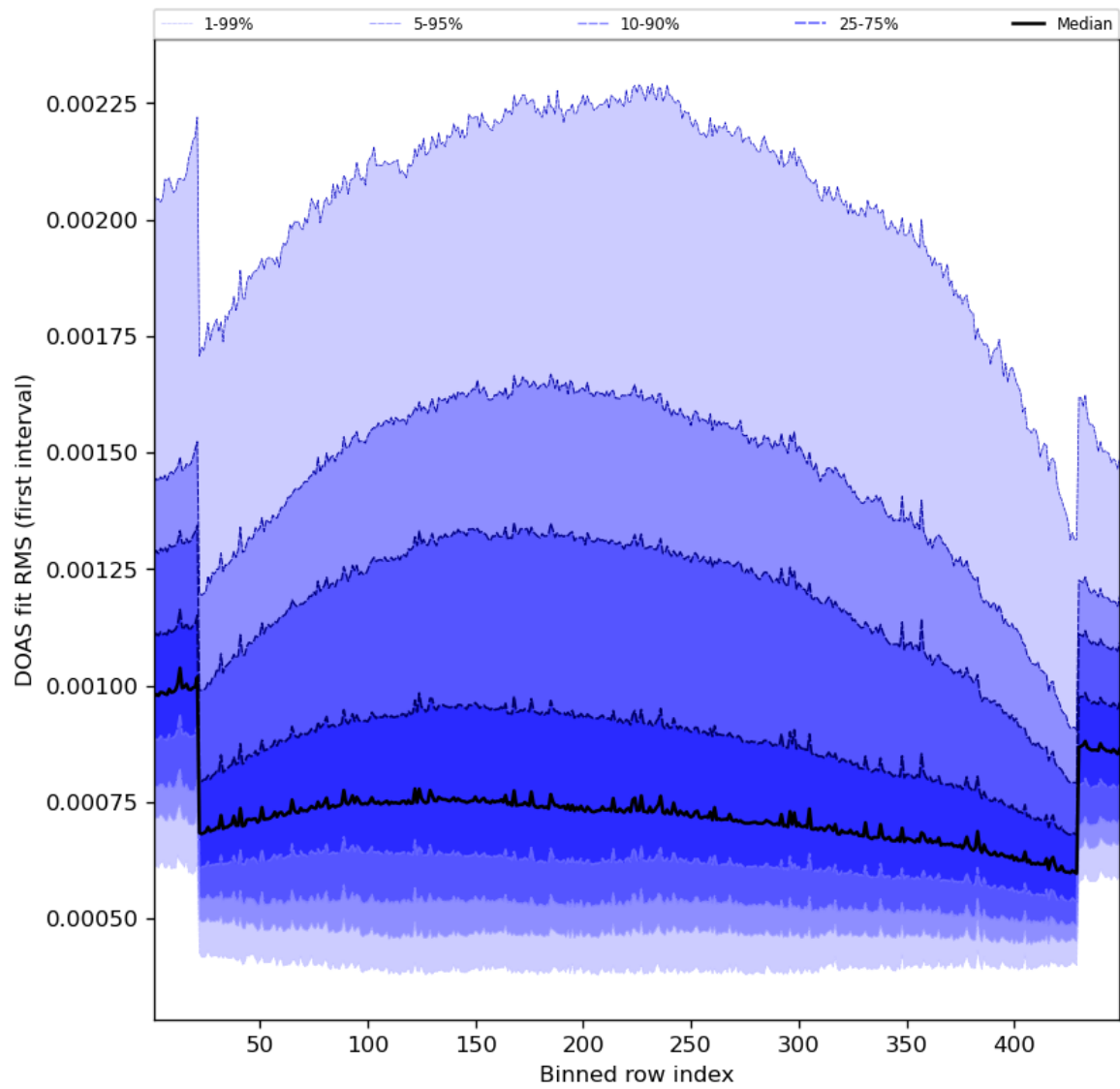
Figure 60: Along track statistics of “DOAS fit RMS (first interval)” for 2023-07-08 to 2023-07-10
