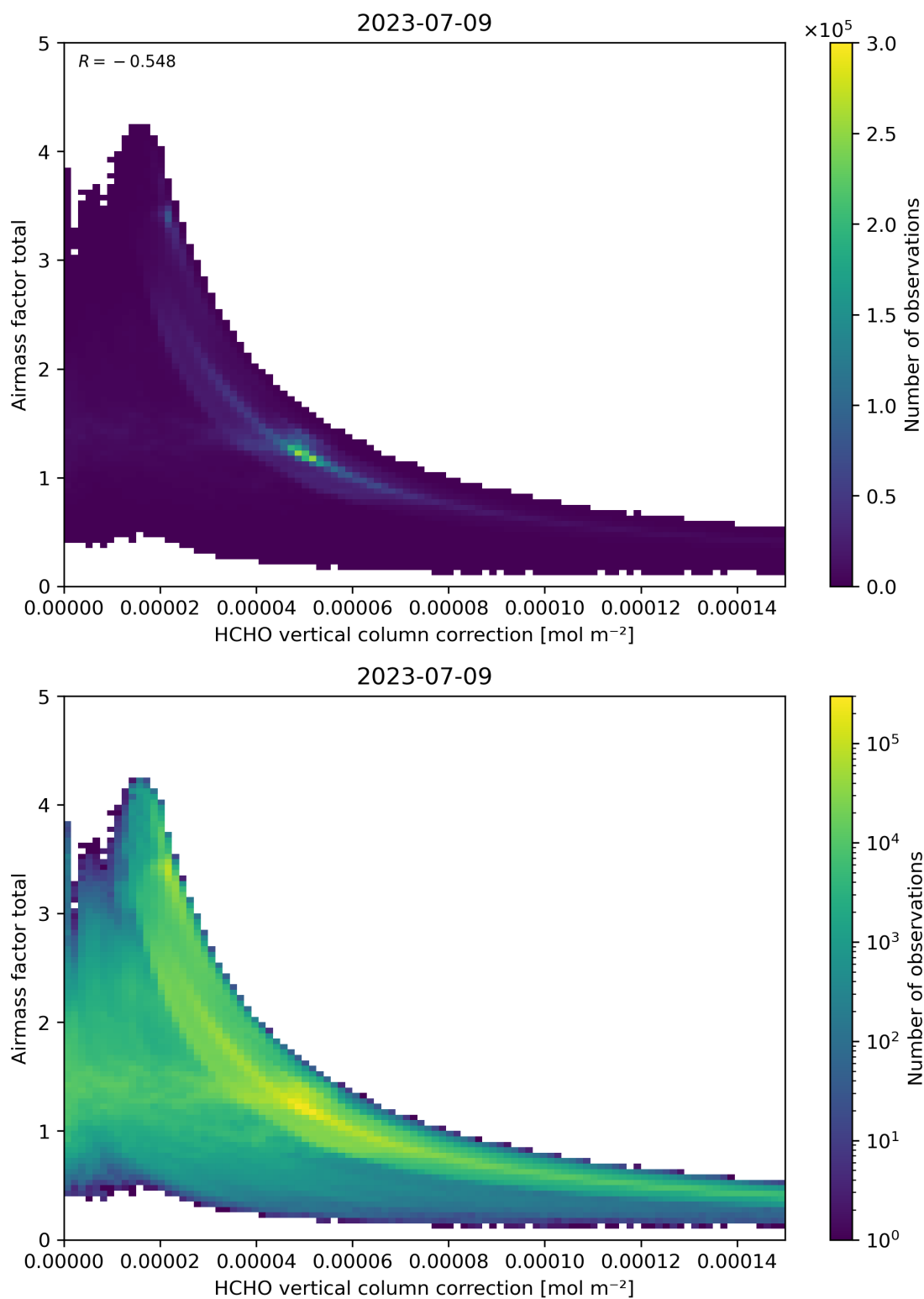
Figure 120: Scatter density plot of “HCHO vertical column correction” against “Airmass factor total” for 2023-07-08 to 2023-07-10.
