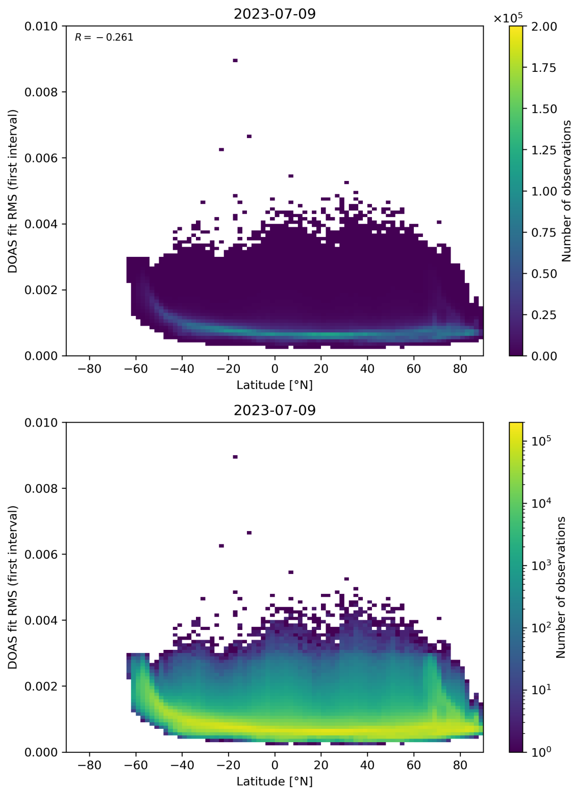
Figure 153: Scatter density plot of “Latitude” against “DOAS fit RMS (first interval)” for 2023-07-08 to 2023-07-10.
