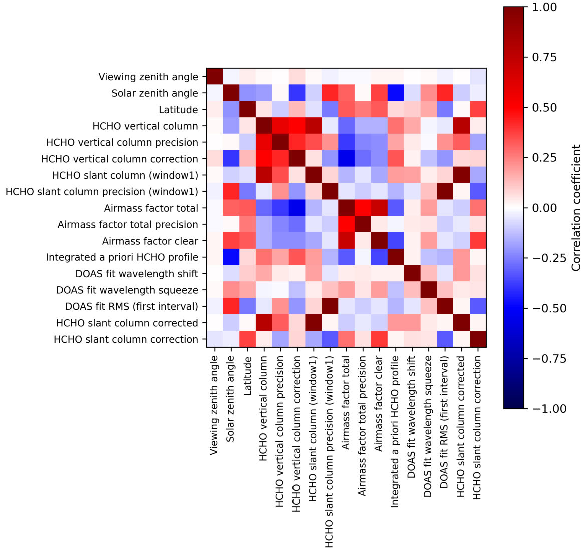
Figure 2: Map of correlation matrix for 2023-07-08 to 2023-07-10.
