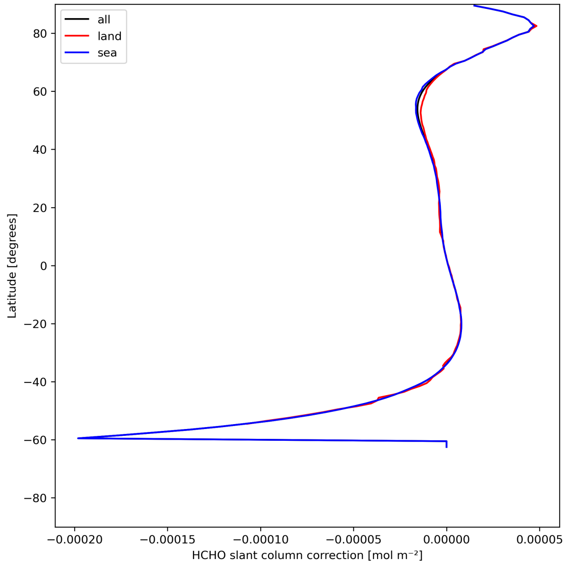
Figure 33: Zonal average of “HCHO slant column correction” for 2023-07-08 to 2023-07-10.
