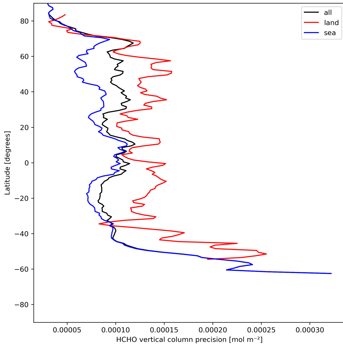
Figure 22: Zonal average of “HCHO vertical column precision” for 2023-07-08 to 2023-07-10.
