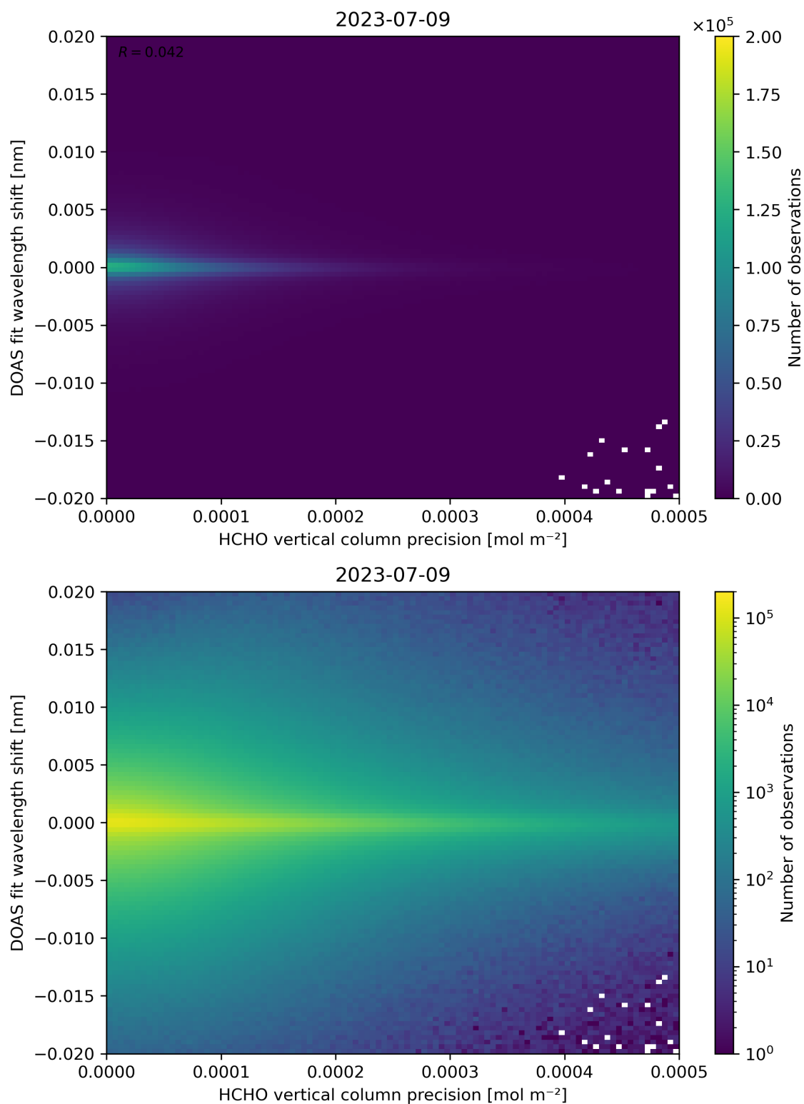
Figure 137: Scatter density plot of “HCHO vertical column precision” against “DOAS fit wavelength shift” for 2023-07-08 to 2023-07-10.
