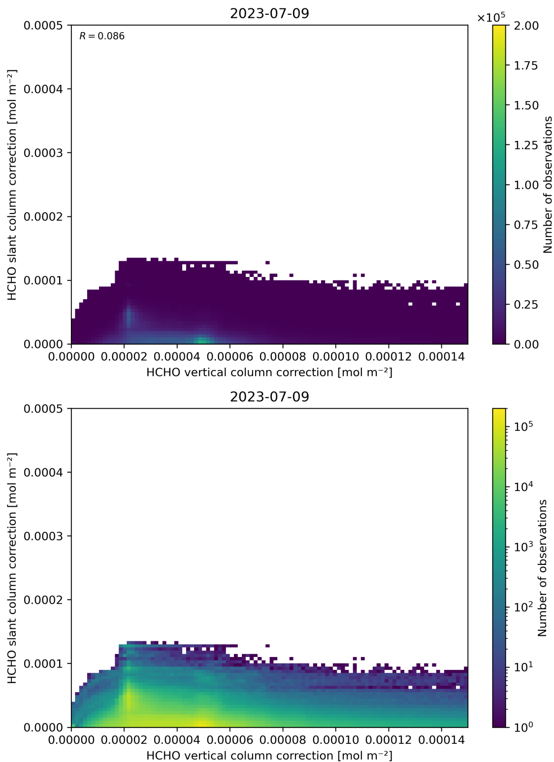
Figure 117: Scatter density plot of “HCHO vertical column correction” against “HCHO slant column correction” for 2023-07-08 to 2023-07-10.
