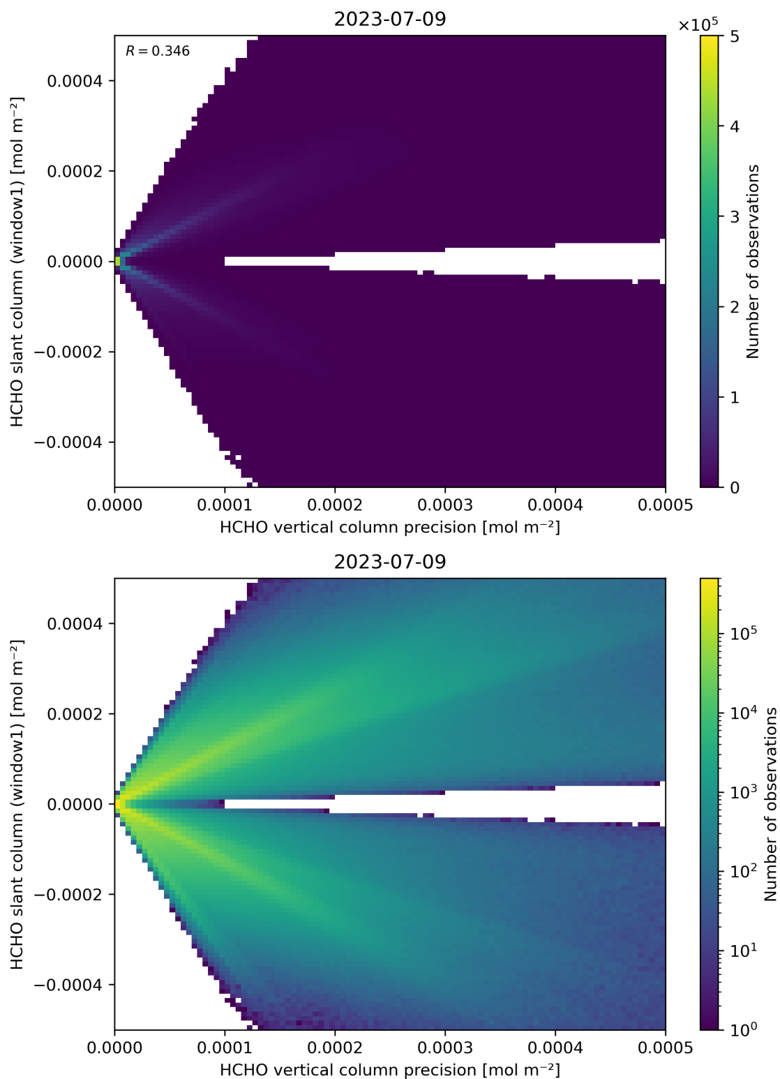
Figure 142: Scatter density plot of “HCHO vertical column precision” against “HCHO slant column (window1)” for 2023-07-08 to 2023-07-10.
