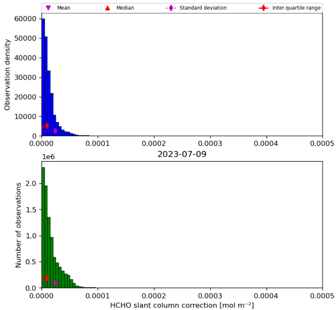
Figure 47: Histogram of “HCHO slant column correction” for 2023-07-08 to 2023-07-10
