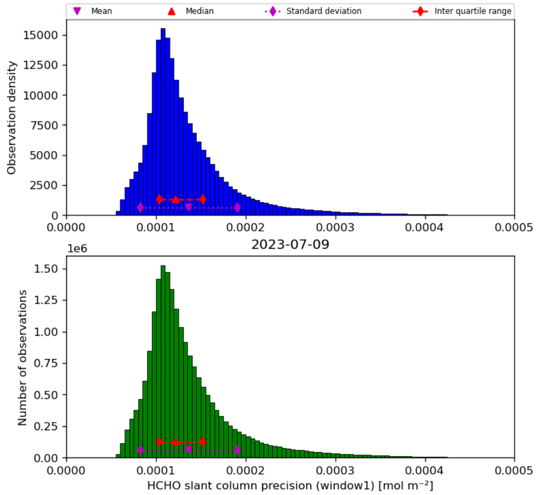
Figure 39: Histogram of “HCHO slant column precision (window1)” for 2023-07-08 to 2023-07-10
