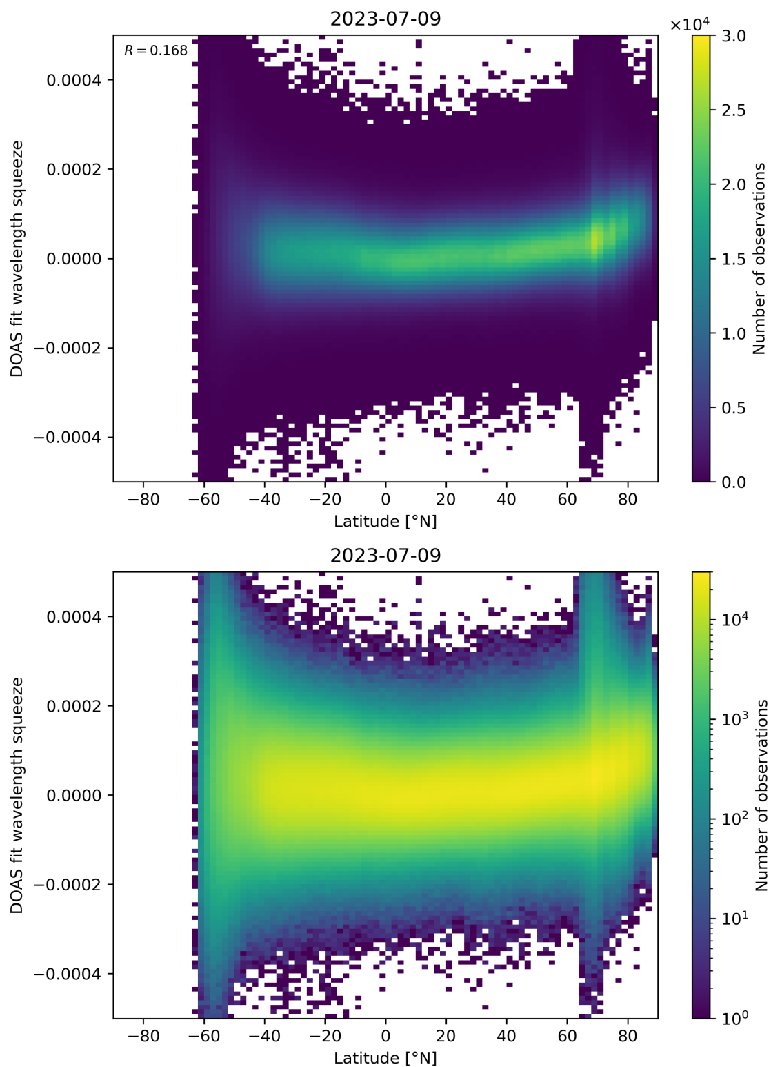
Figure 155: Scatter density plot of “Latitude” against “DOAS fit wavelength squeeze” for 2023-07-08 to 2023-07-10.
