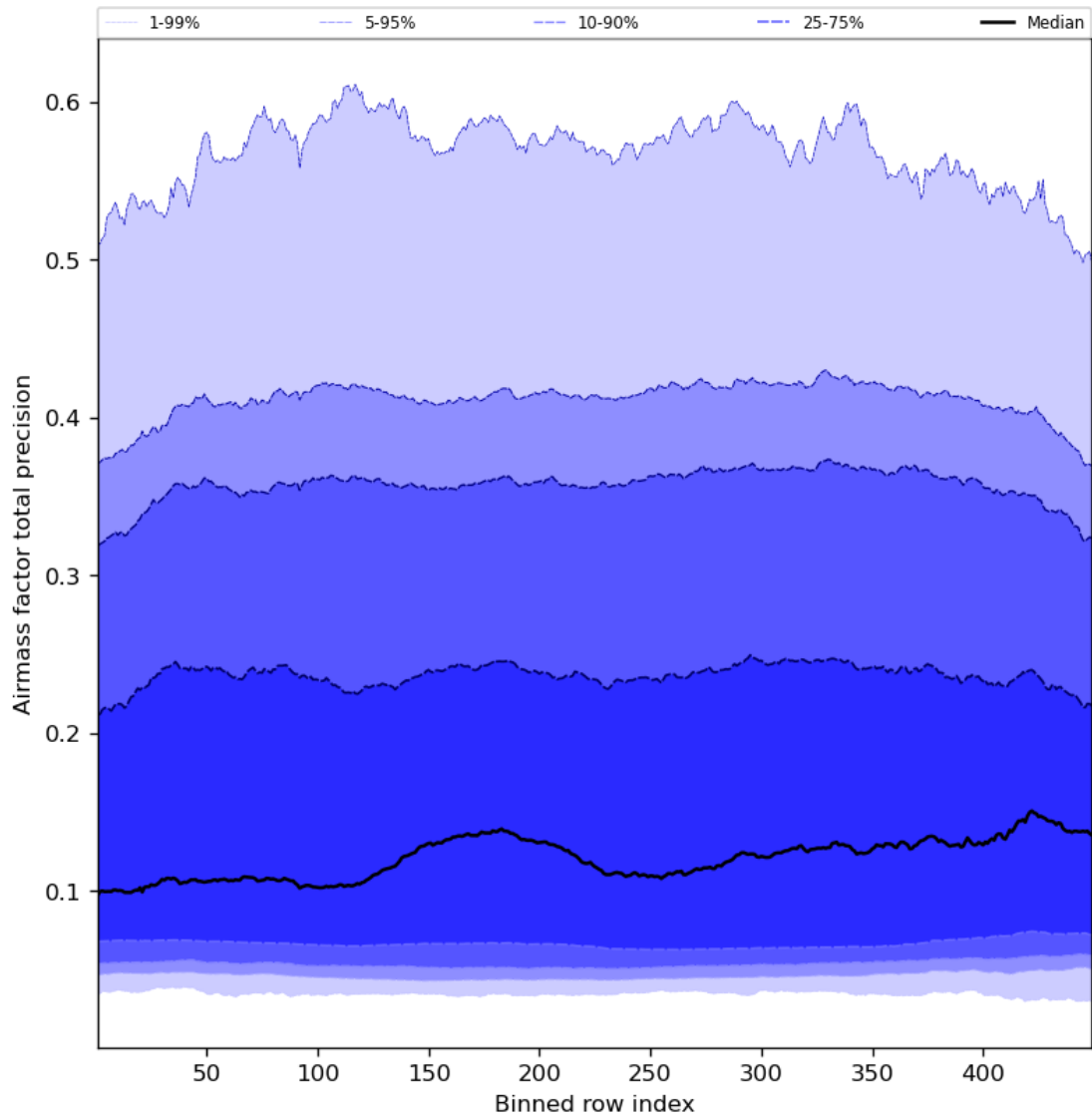
Figure 55: Along track statistics of “Airmass factor total precision” for 2023-07-08 to 2023-07-10
