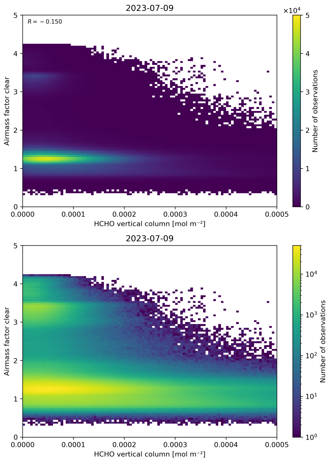
Figure 126: Scatter density plot of “HCHO vertical column” against “Airmass factor clear” for 2023-07-08 to 2023-07-10.
