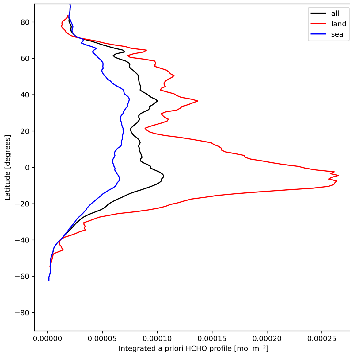
Figure 29: Zonal average of “Integrated a priori HCHO profile” for 2023-07-08 to 2023-07-10.
