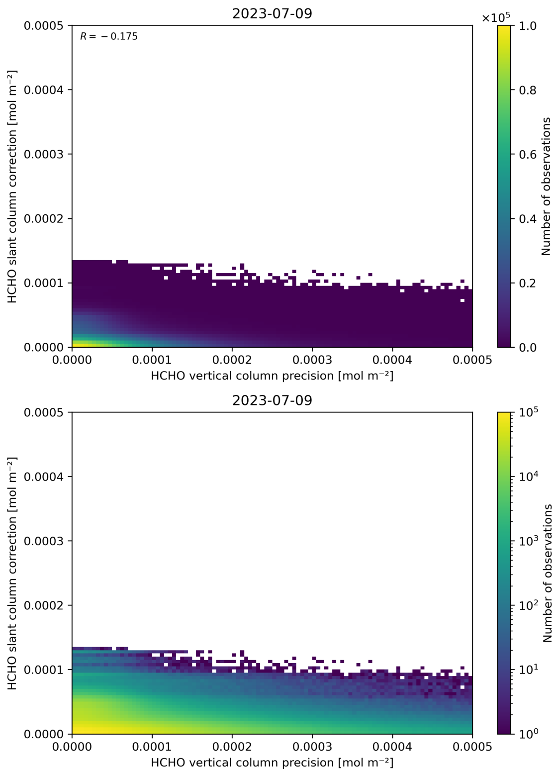
Figure 141: Scatter density plot of “HCHO vertical column precision” against “HCHO slant column correction” for 2023-07-08 to 2023-07-10.
