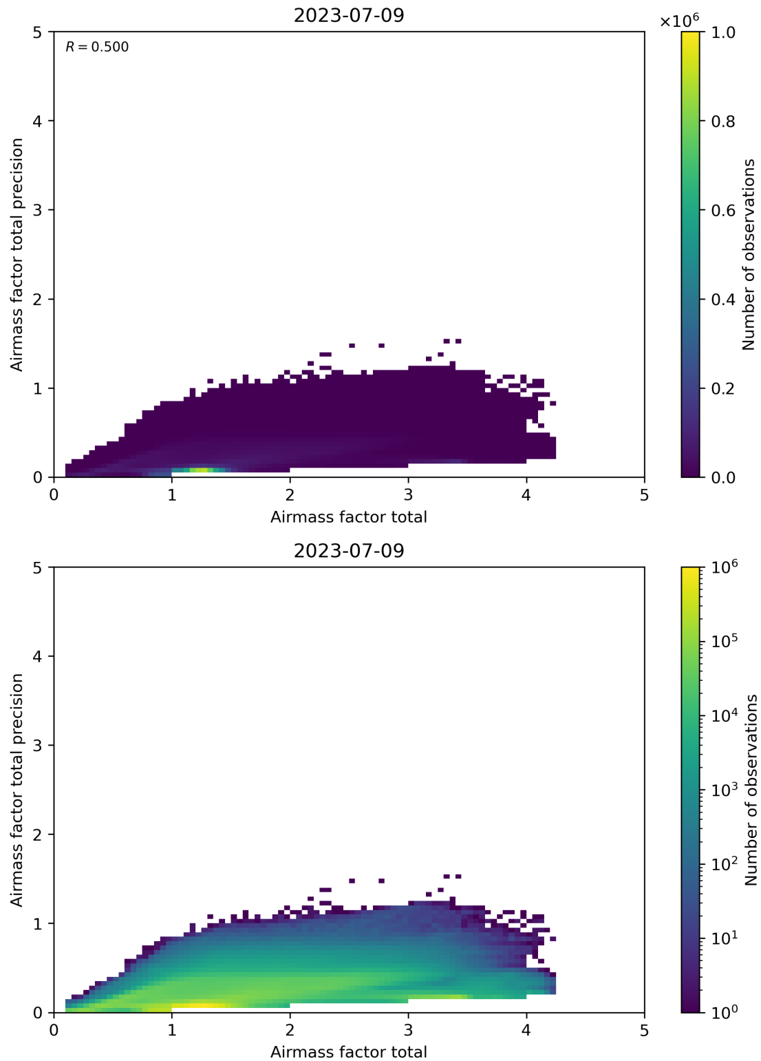
Figure 103: Scatter density plot of “Airmass factor total” against “Airmass factor total precision” for 2023-07-08 to 2023-07-10.
