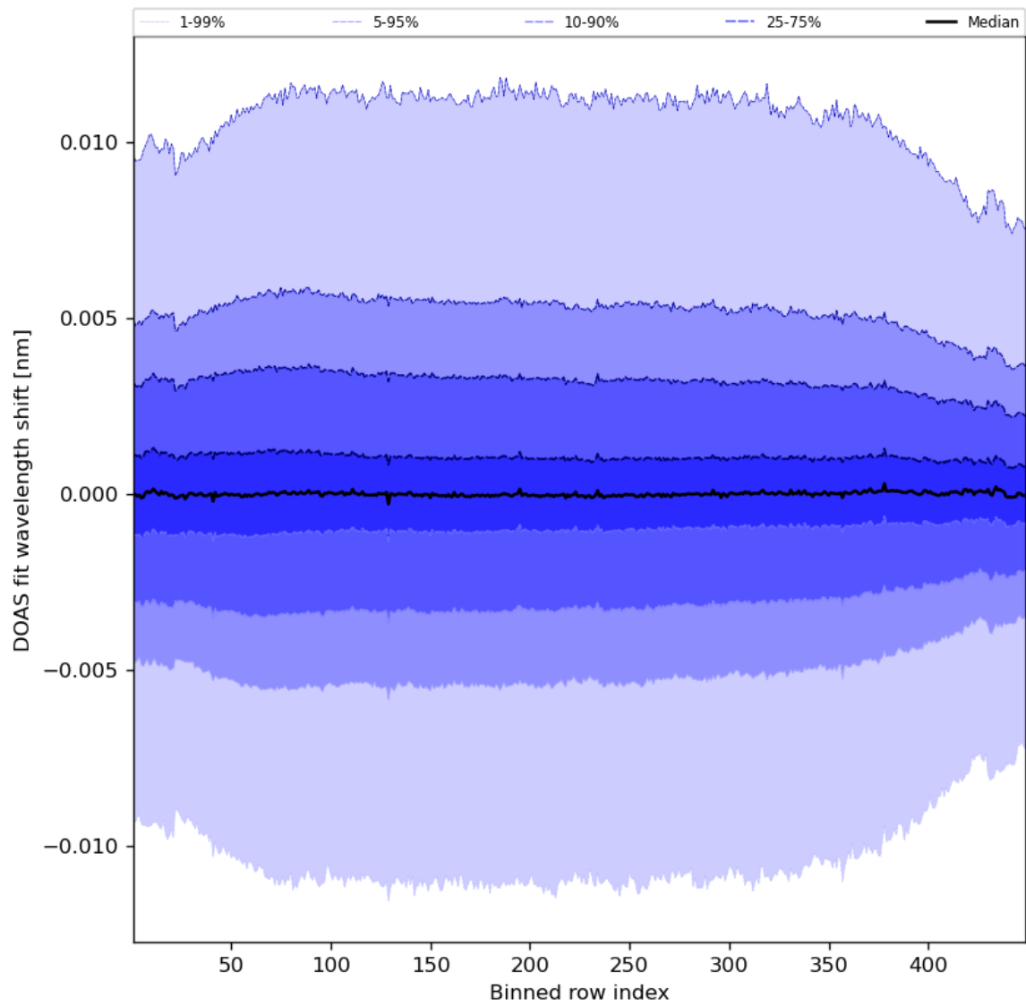
Figure 58: Along track statistics of “DOAS fit wavelength shift” for 2023-07-08 to 2023-07-10
