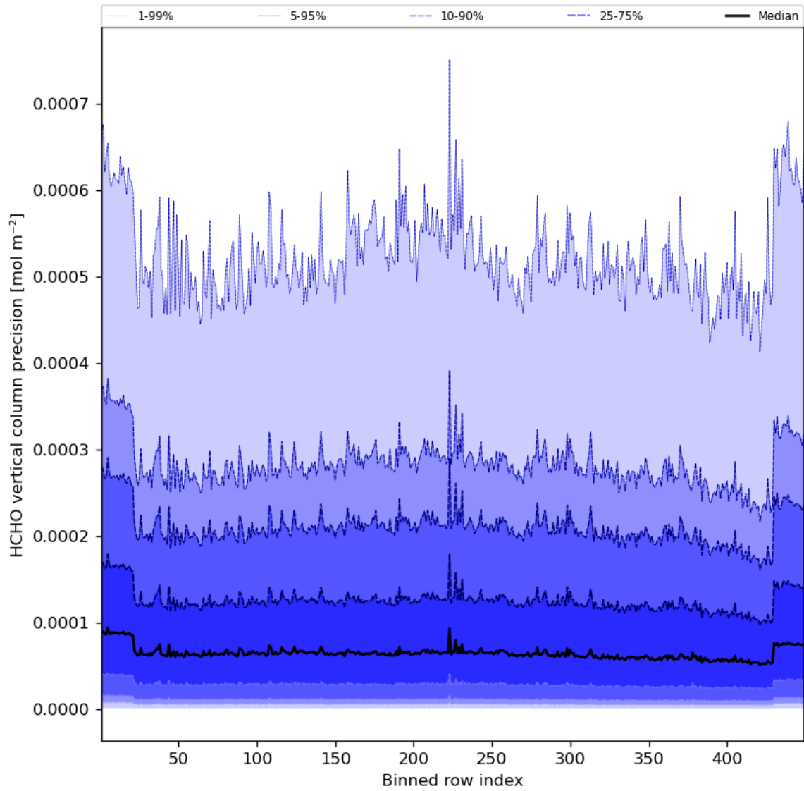
Figure 50: Along track statistics of “HCHO vertical column precision” for 2023-07-08 to 2023-07-10
