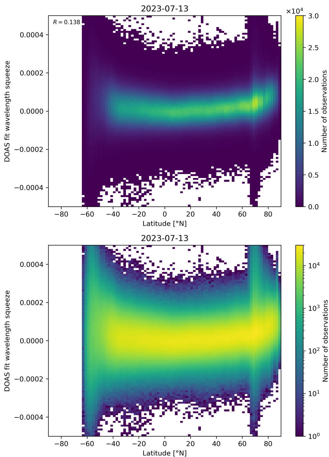
Figure 155: Scatter density plot of “Latitude” against “DOAS fit wavelength squeeze” for 2023-07-13 to 2023-07-14.
