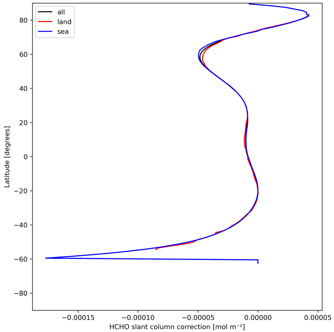
Figure 33: Zonal average of “HCHO slant column correction” for 2023-07-13 to 2023-07-14.
