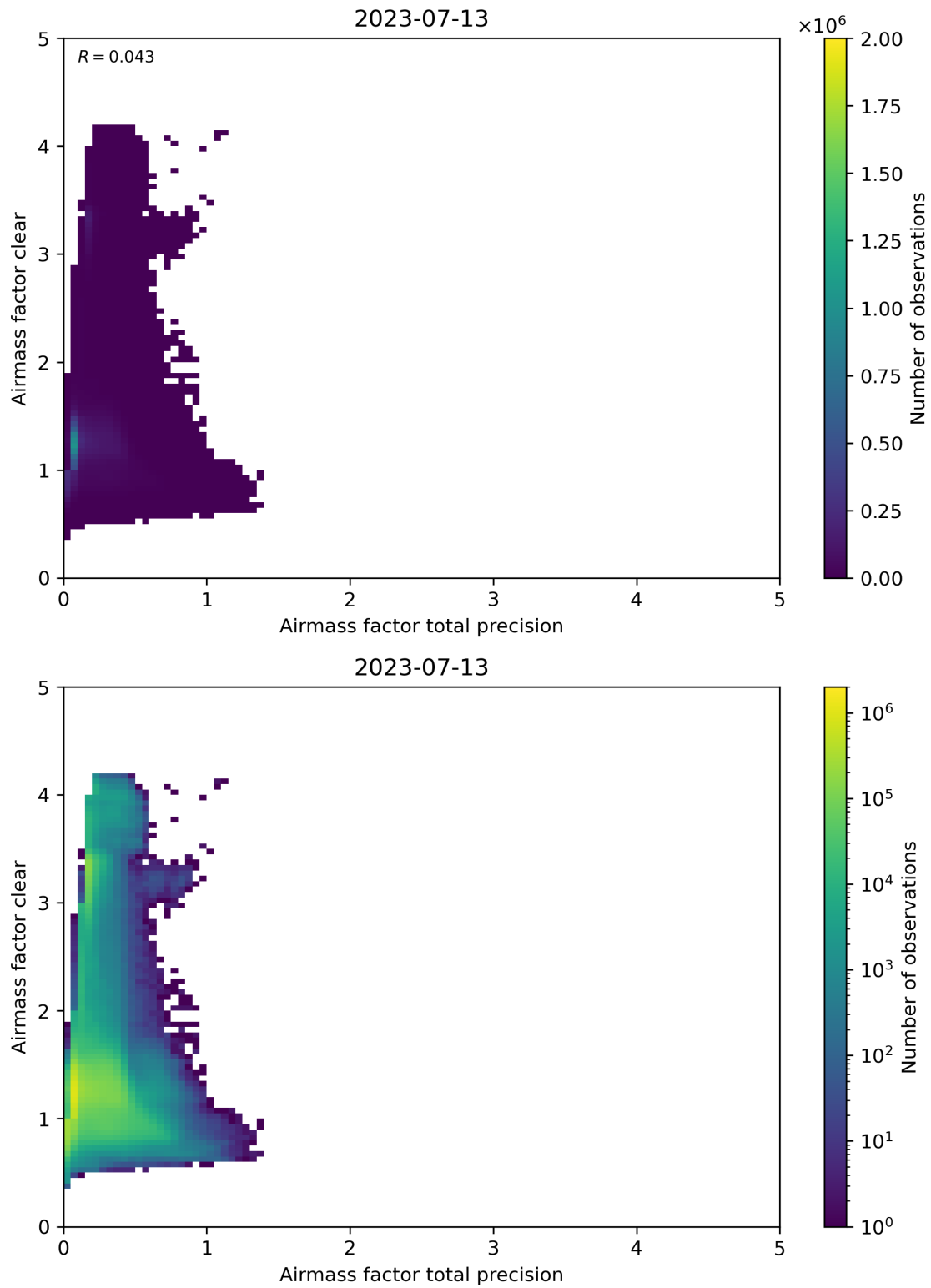
Figure 108: Scatter density plot of “Airmass factor total precision” against “Airmass factor clear” for 2023-07-13 to 2023-07-14.
