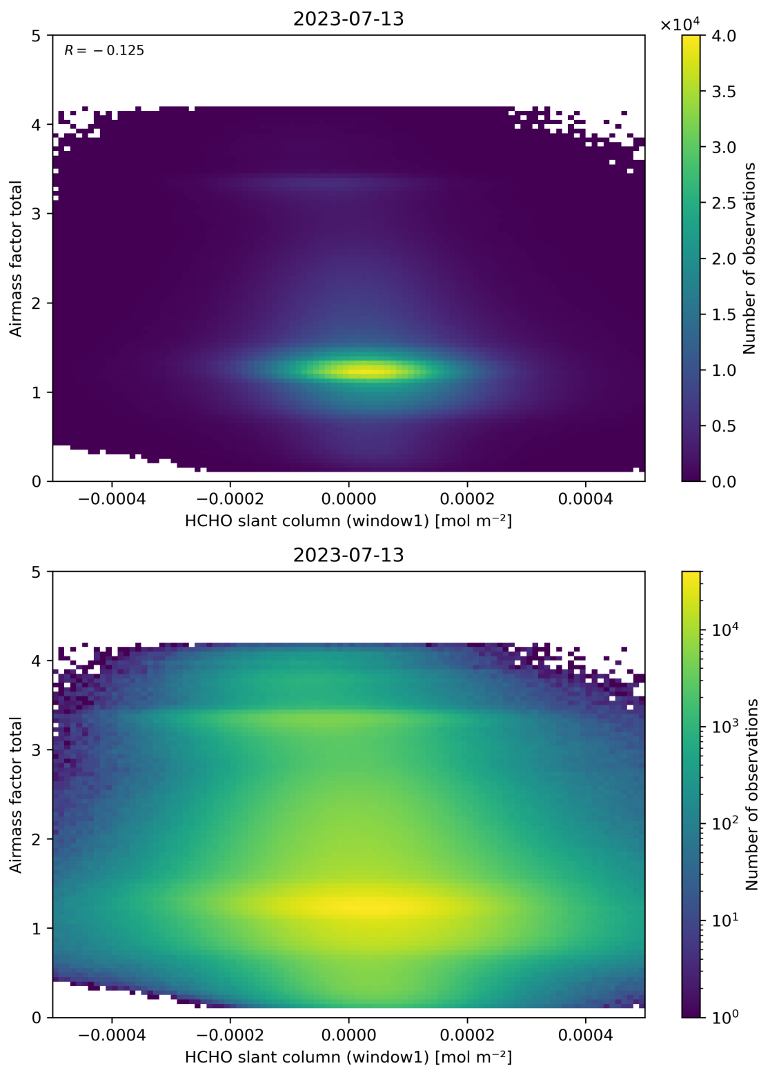
Figure 85: Scatter density plot of “HCHO slant column (window1)” against “Airmass factor total” for 2023-07-13 to 2023-07-14.
