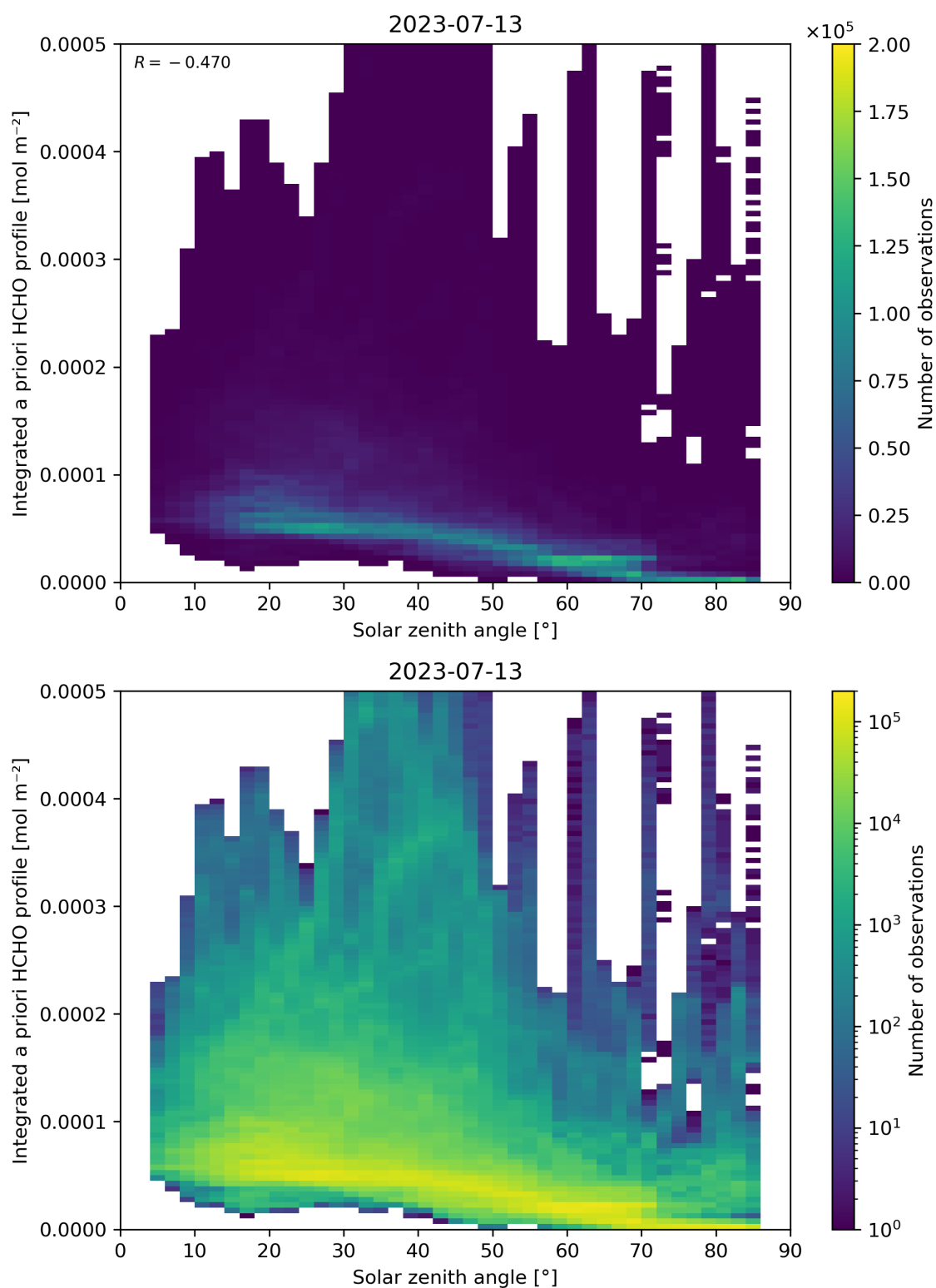
Figure 180: Scatter density plot of “Solar zenith angle” against “Integrated a priori HCHO profile” for 2023-07-13 to 2023-07-14.
