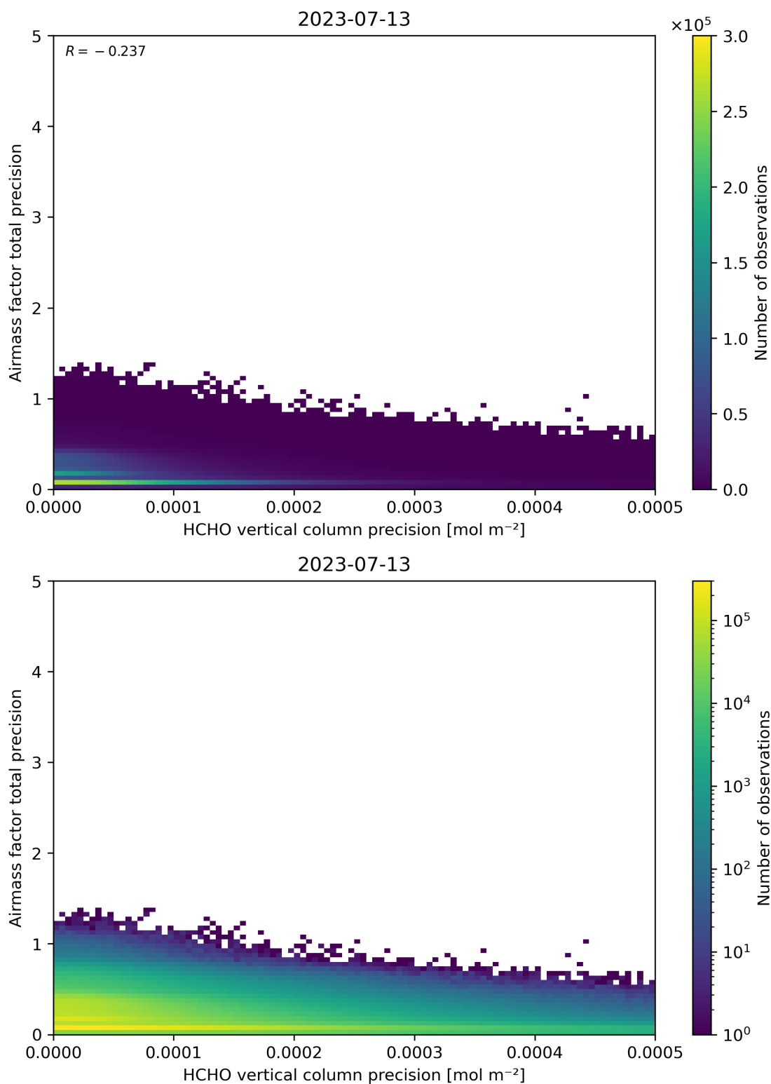
Figure 145: Scatter density plot of “HCHO vertical column precision” against “Airmass factor total precision” for 2023-07-13 to 2023-07-14.
