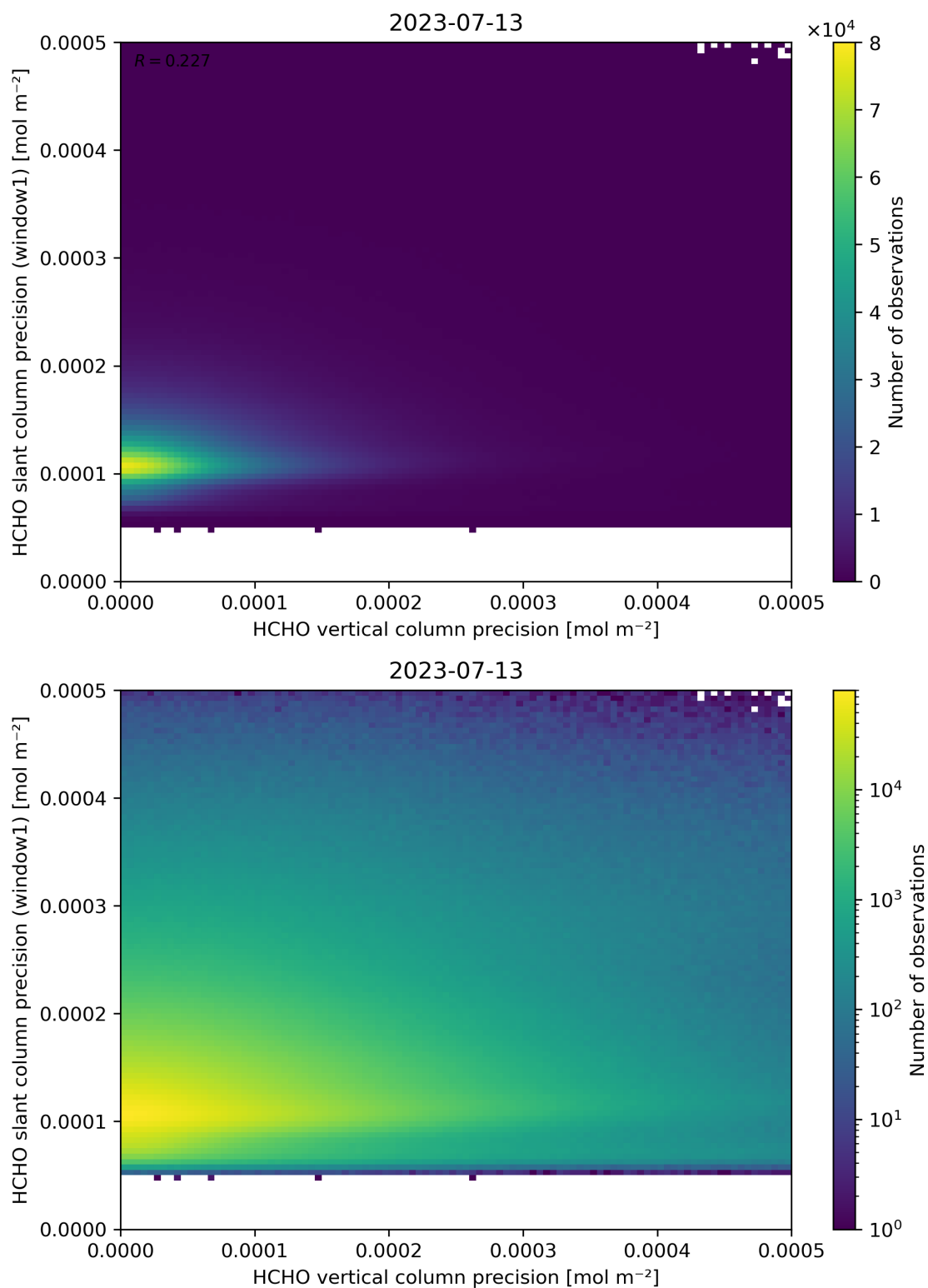
Figure 143: Scatter density plot of “HCHO vertical column precision” against “HCHO slant column precision (window1)” for 2023-07-13 to 2023-07-14.
