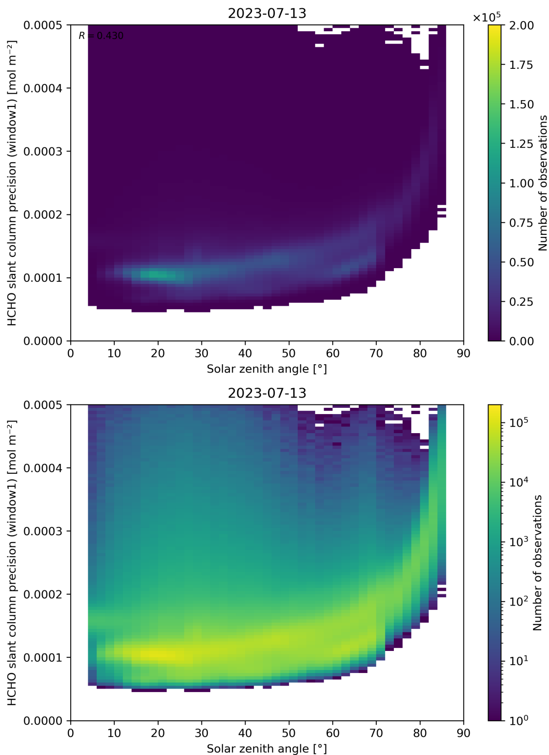
Figure 174: Scatter density plot of “Solar zenith angle” against “HCHO slant column precision (window1)” for 2023-07-13 to 2023-07-14.
