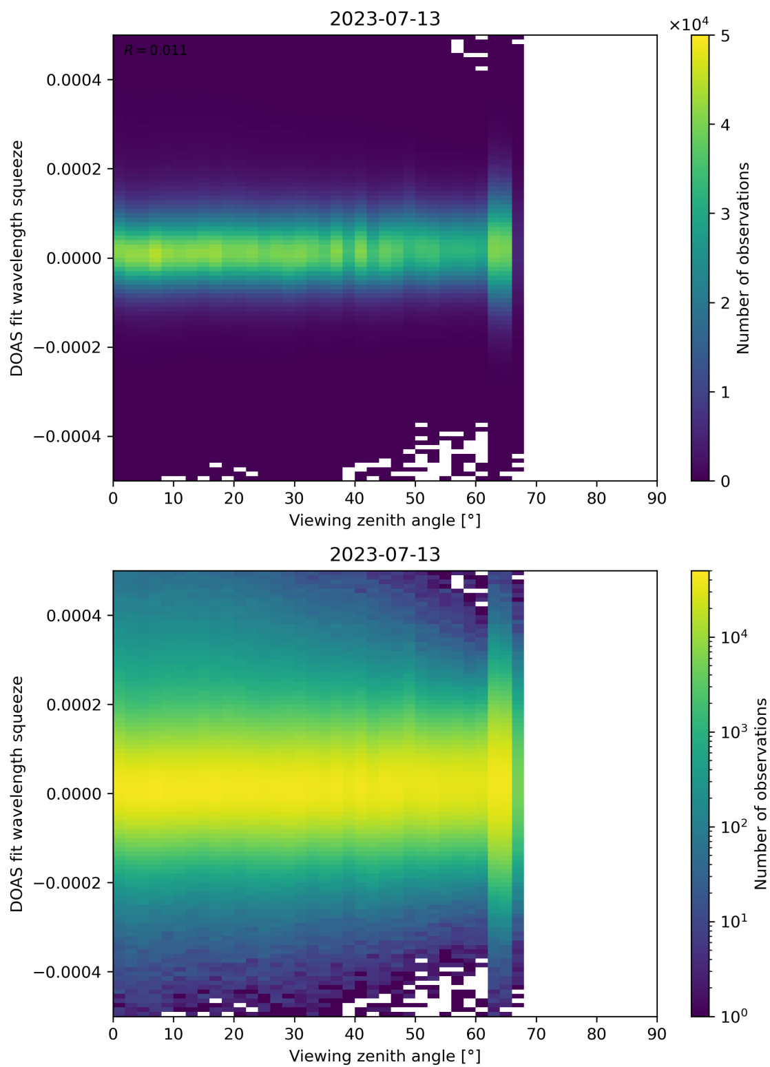
Figure 184: Scatter density plot of “Viewing zenith angle” against “DOAS fit wavelength squeeze” for 2023-07-13 to 2023-07-14.
