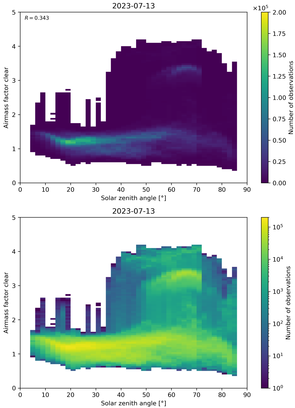
Figure 170: Scatter density plot of “Solar zenith angle” against “Airmass factor clear” for 2023-07-13 to 2023-07-14.
