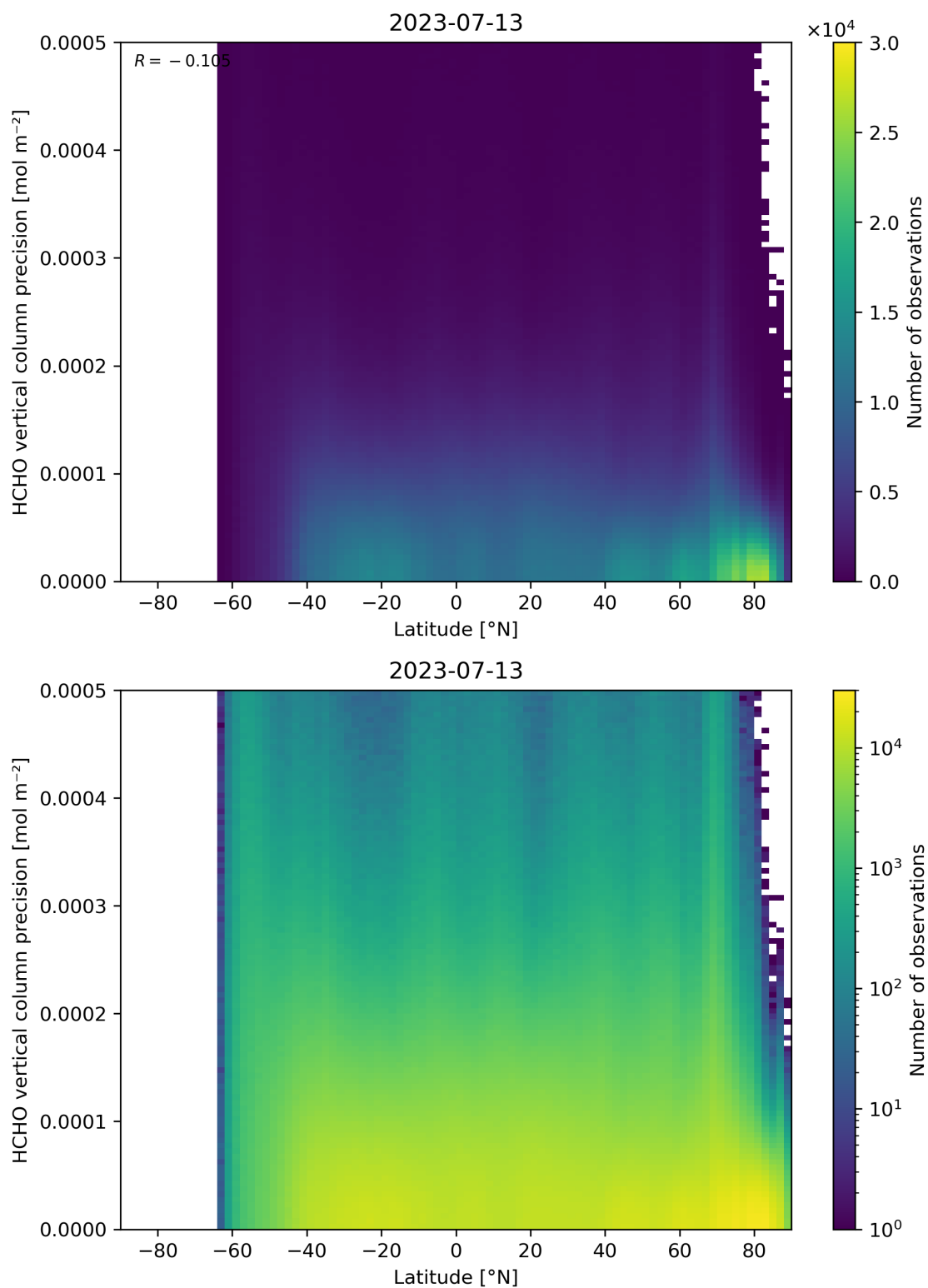
Figure 165: Scatter density plot of “Latitude” against “HCHO vertical column precision” for 2023-07-13 to 2023-07-14.
