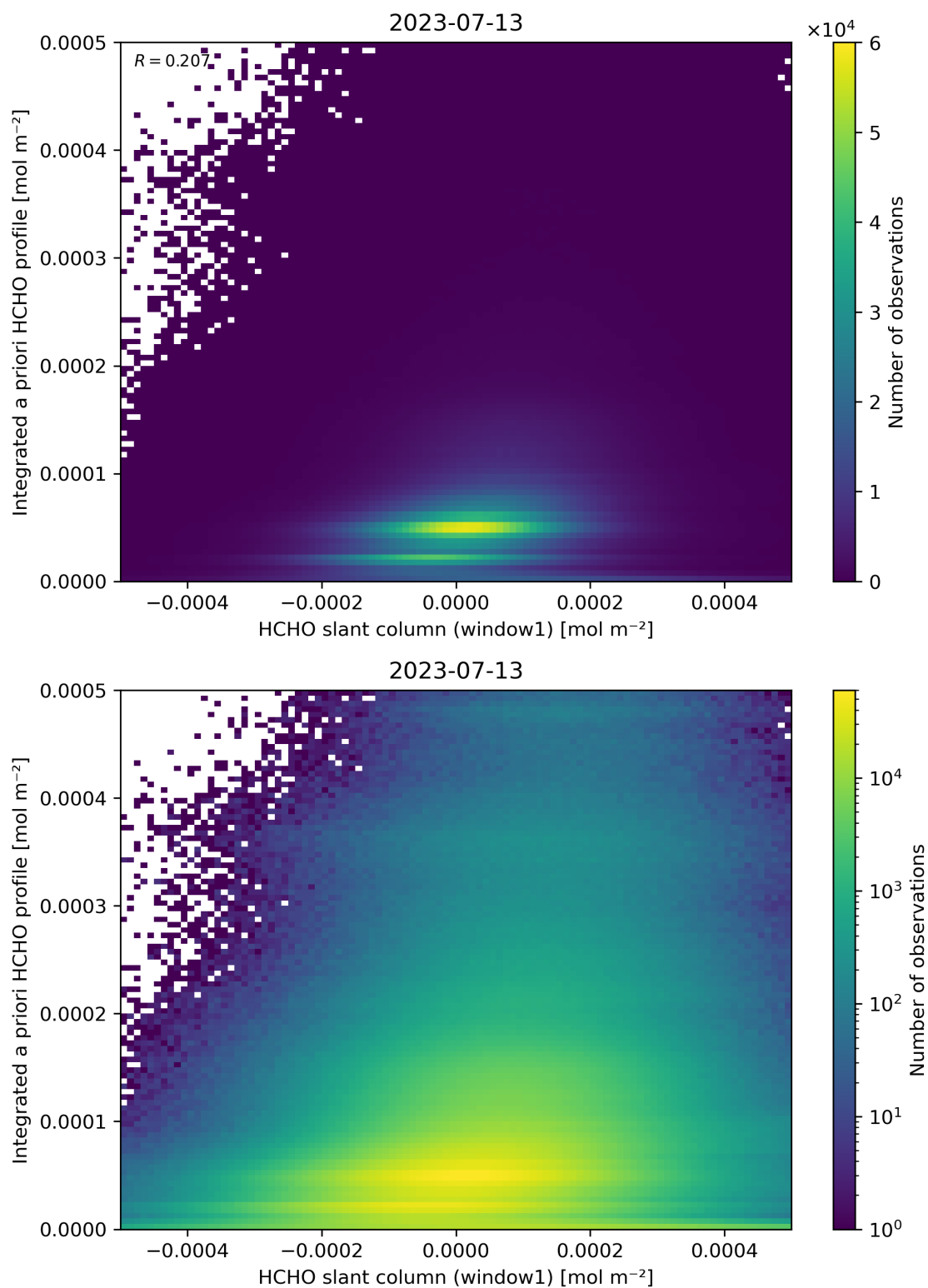
Figure 87: Scatter density plot of “HCHO slant column (window1)” against “Integrated a priori HCHO profile” for 2023-07-13 to 2023-07-14.
