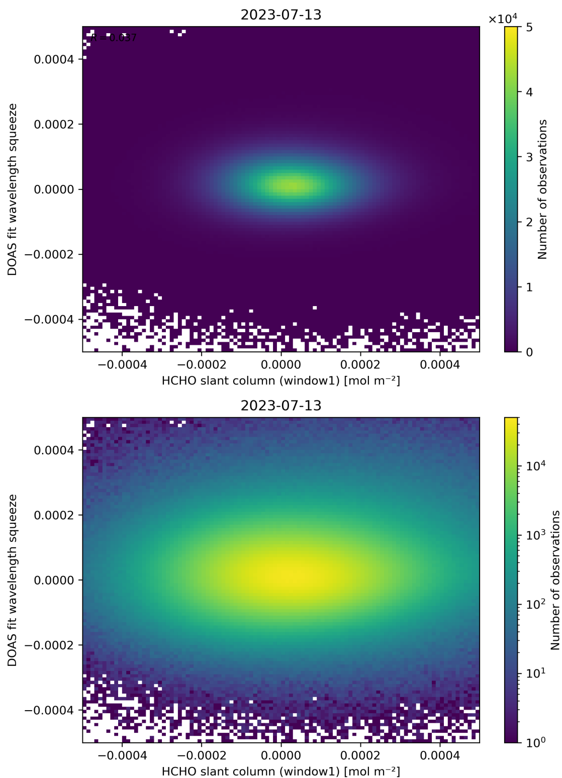
Figure 80: Scatter density plot of “HCHO slant column (window1)” against “DOAS fit wavelength squeeze” for 2023-07-13 to 2023-07-14.
