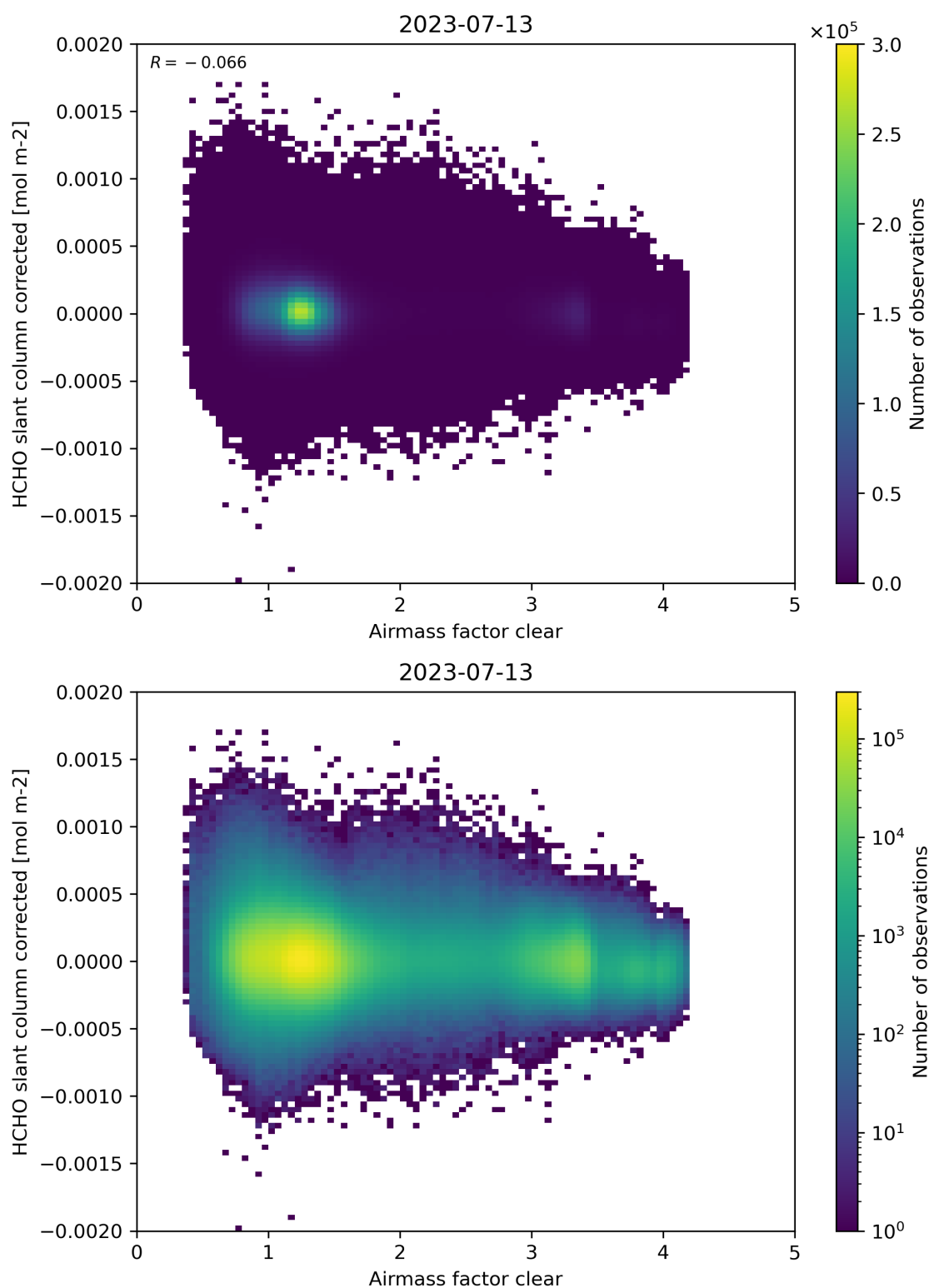
Figure 74: Scatter density plot of “Airmass factor clear” against “HCHO slant column corrected” for 2023-07-13 to 2023-07-14.
