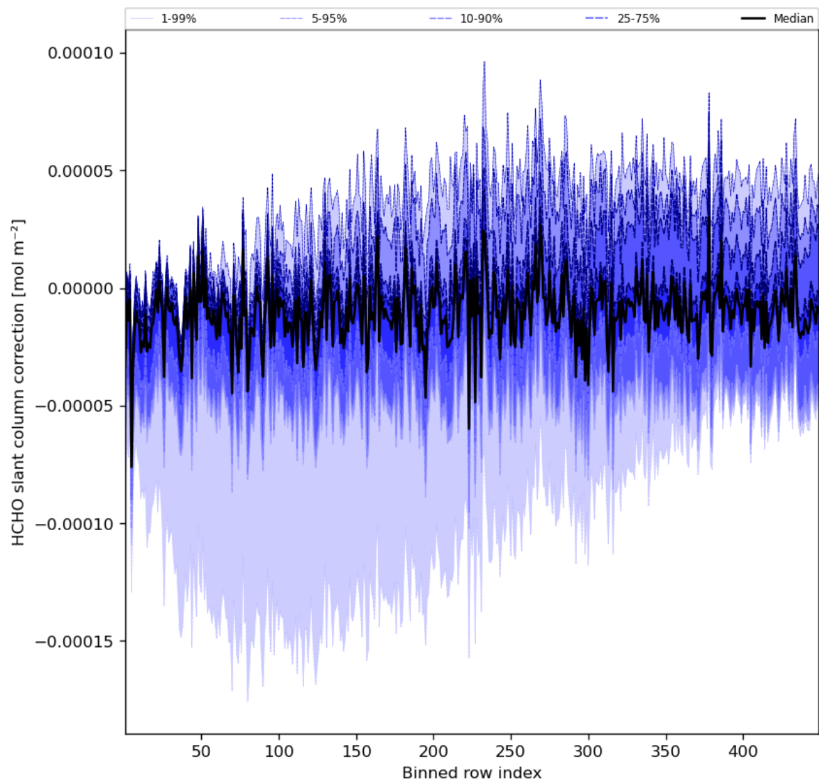
Figure 61: Along track statistics of “HCHO slant column correction” for 2023-07-13 to 2023-07-14
