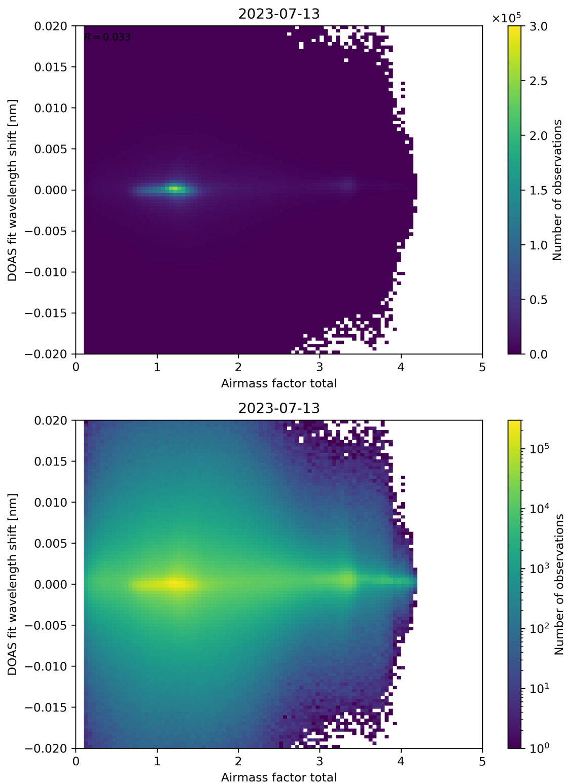
Figure 98: Scatter density plot of “Airmass factor total” against “DOAS fit wavelength shift” for 2023-07-13 to 2023-07-14.
