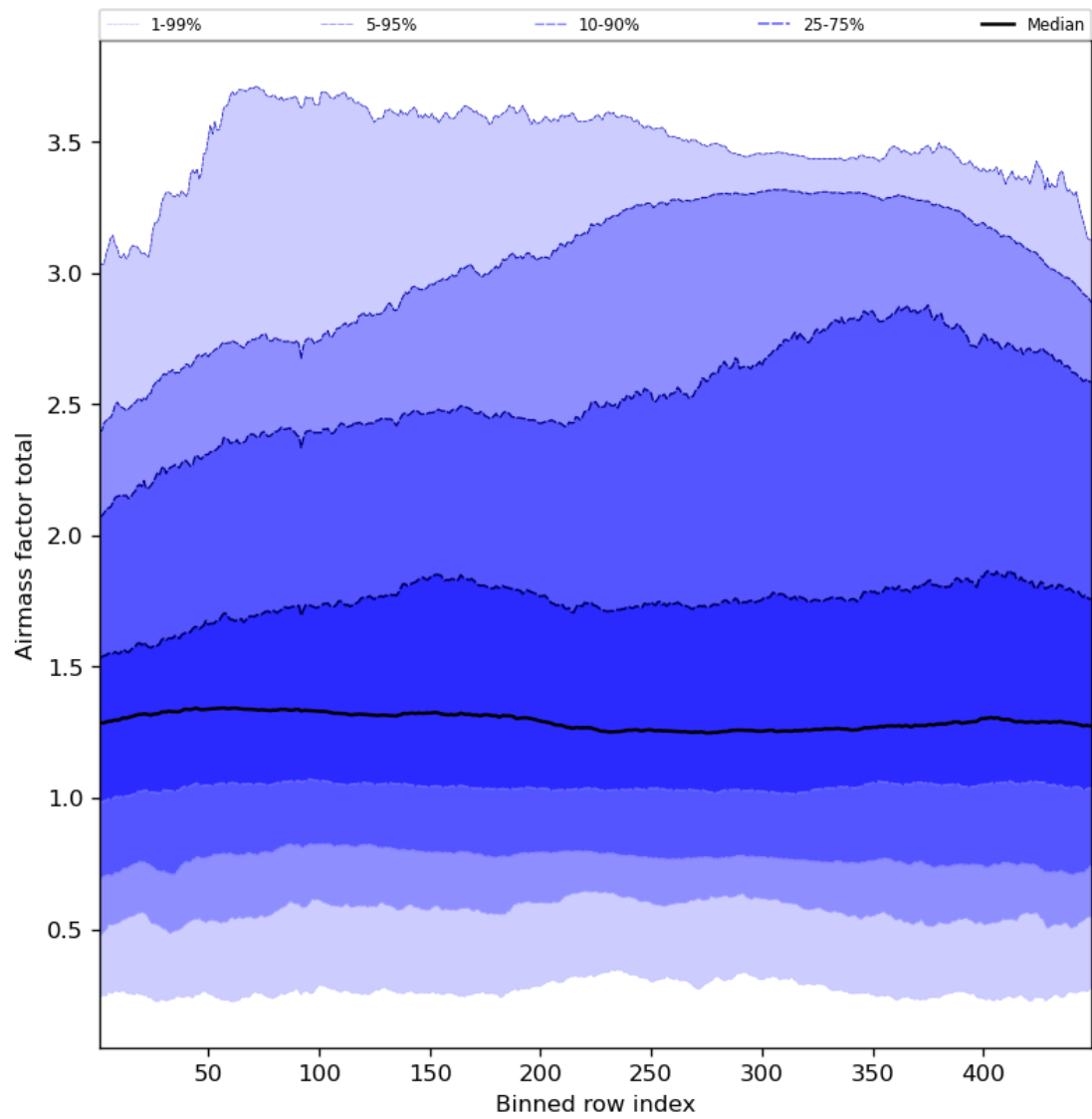
Figure 54: Along track statistics of “Airmass factor total” for 2023-07-13 to 2023-07-14
