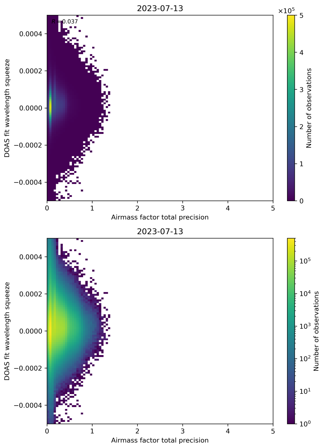
Figure 107: Scatter density plot of “Airmass factor total precision” against “DOAS fit wavelength squeeze” for 2023-07-13 to 2023-07-14.
