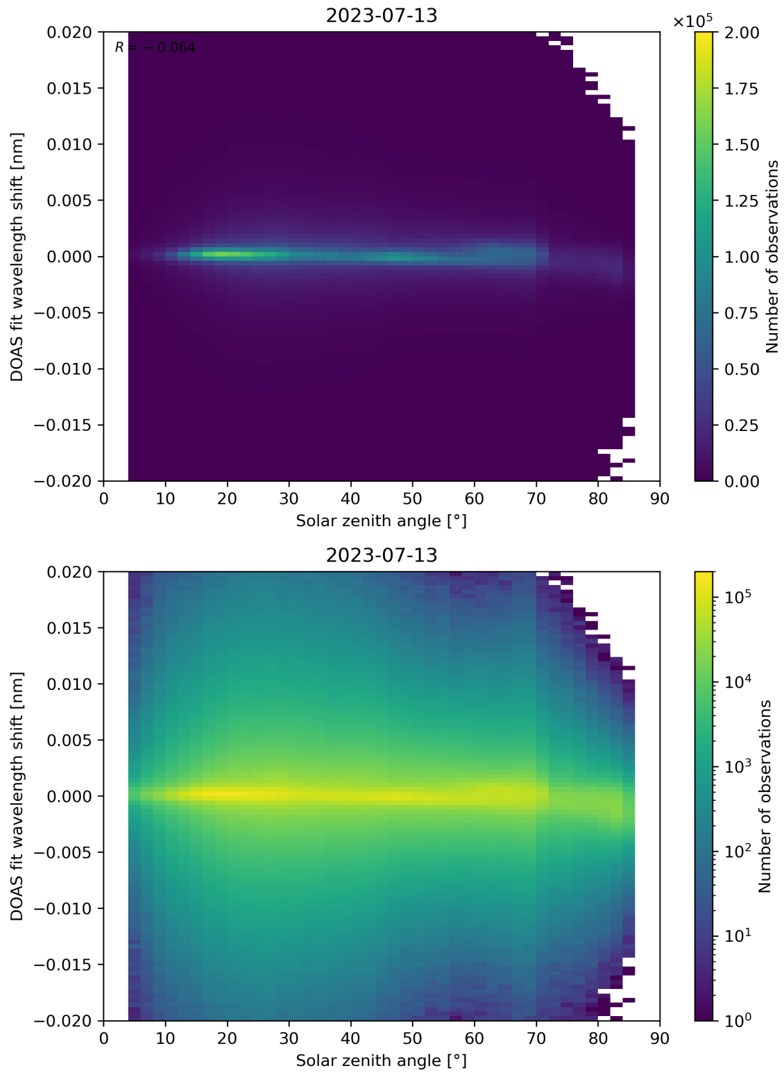
Figure 168: Scatter density plot of “Solar zenith angle” against “DOAS fit wavelength shift” for 2023-07-13 to 2023-07-14.
