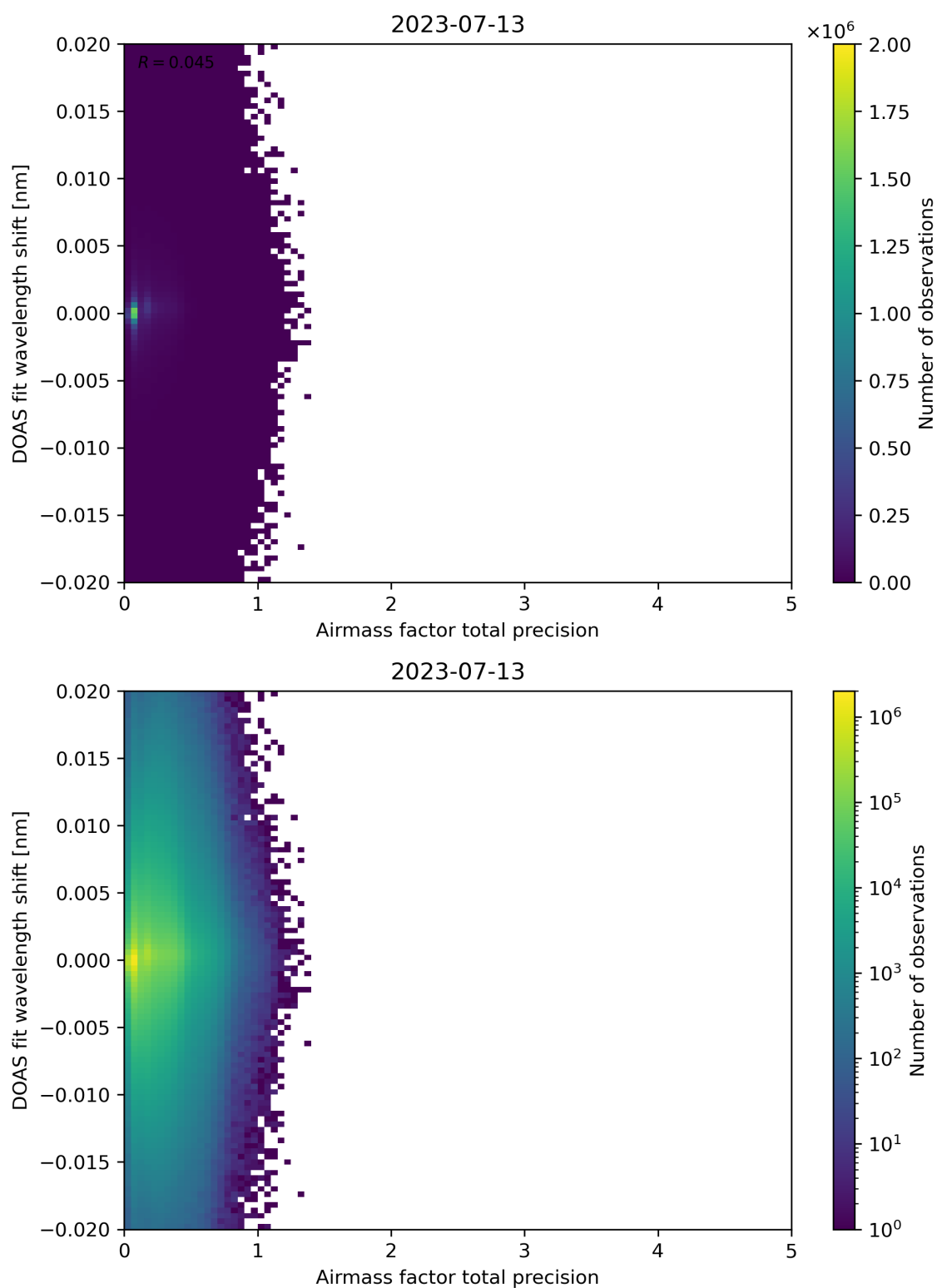
Figure 106: Scatter density plot of “Airmass factor total precision” against “DOAS fit wavelength shift” for 2023-07-13 to 2023-07-14.
