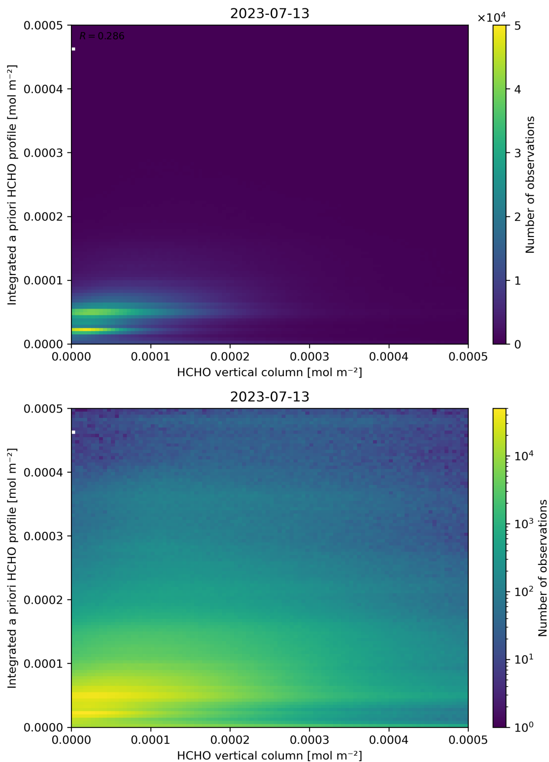
Figure 135: Scatter density plot of “HCHO vertical column” against “Integrated a priori HCHO profile” for 2023-07-13 to 2023-07-14.
