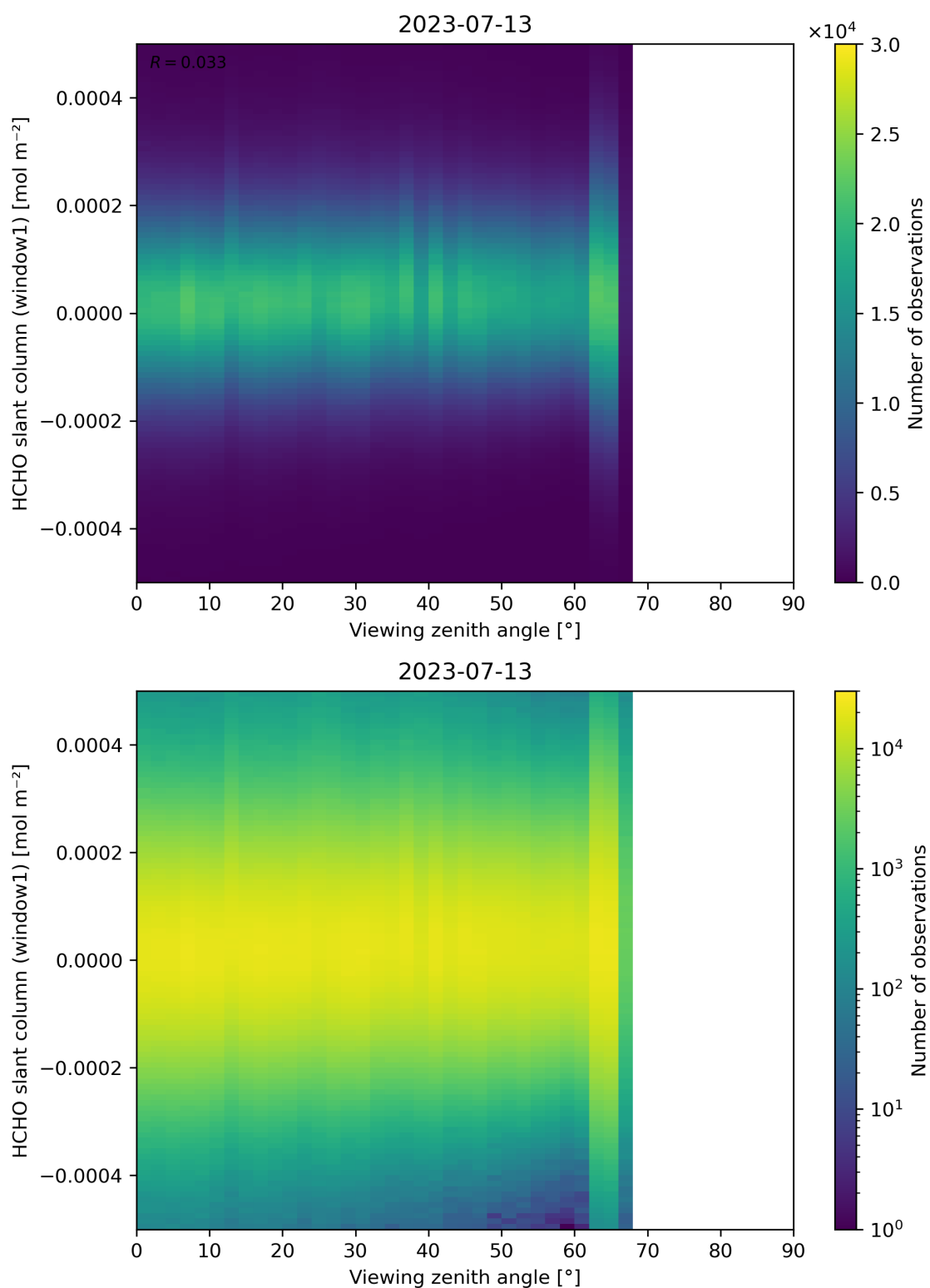
Figure 188: Scatter density plot of “Viewing zenith angle” against “HCHO slant column (window1)” for 2023-07-13 to 2023-07-14.
