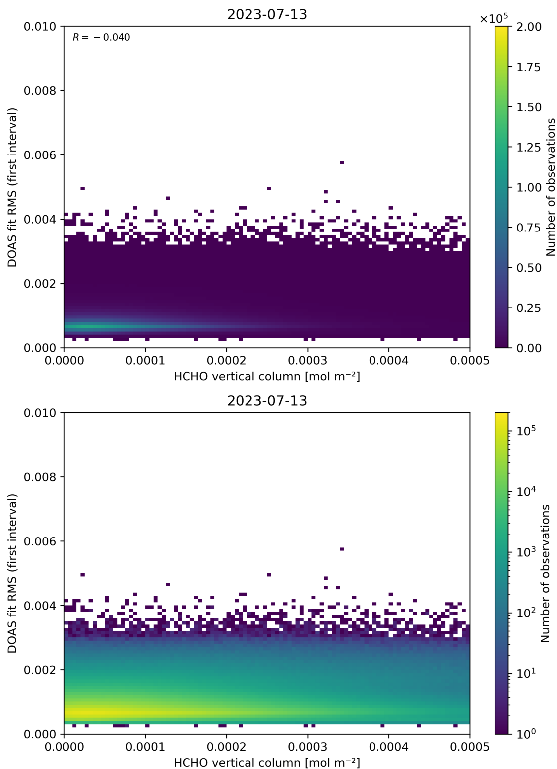
Figure 123: Scatter density plot of “HCHO vertical column” against “DOAS fit RMS (first interval)” for 2023-07-13 to 2023-07-14.
