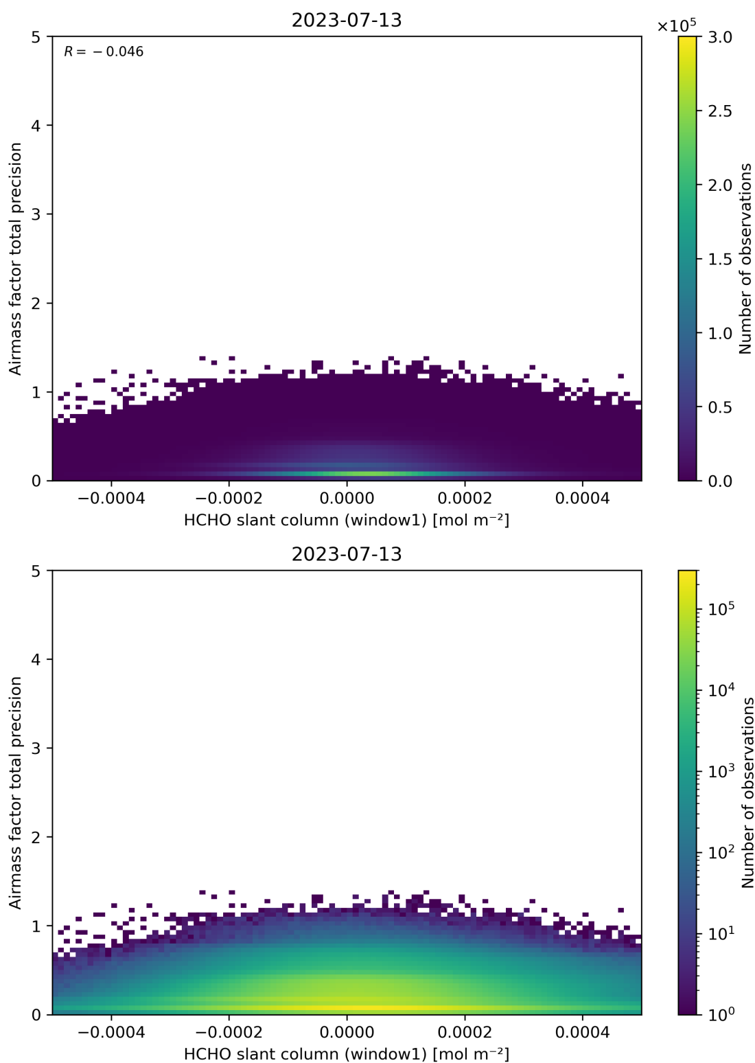
Figure 86: Scatter density plot of “HCHO slant column (window1)” against “Airmass factor total precision” for 2023-07-13 to 2023-07-14.
