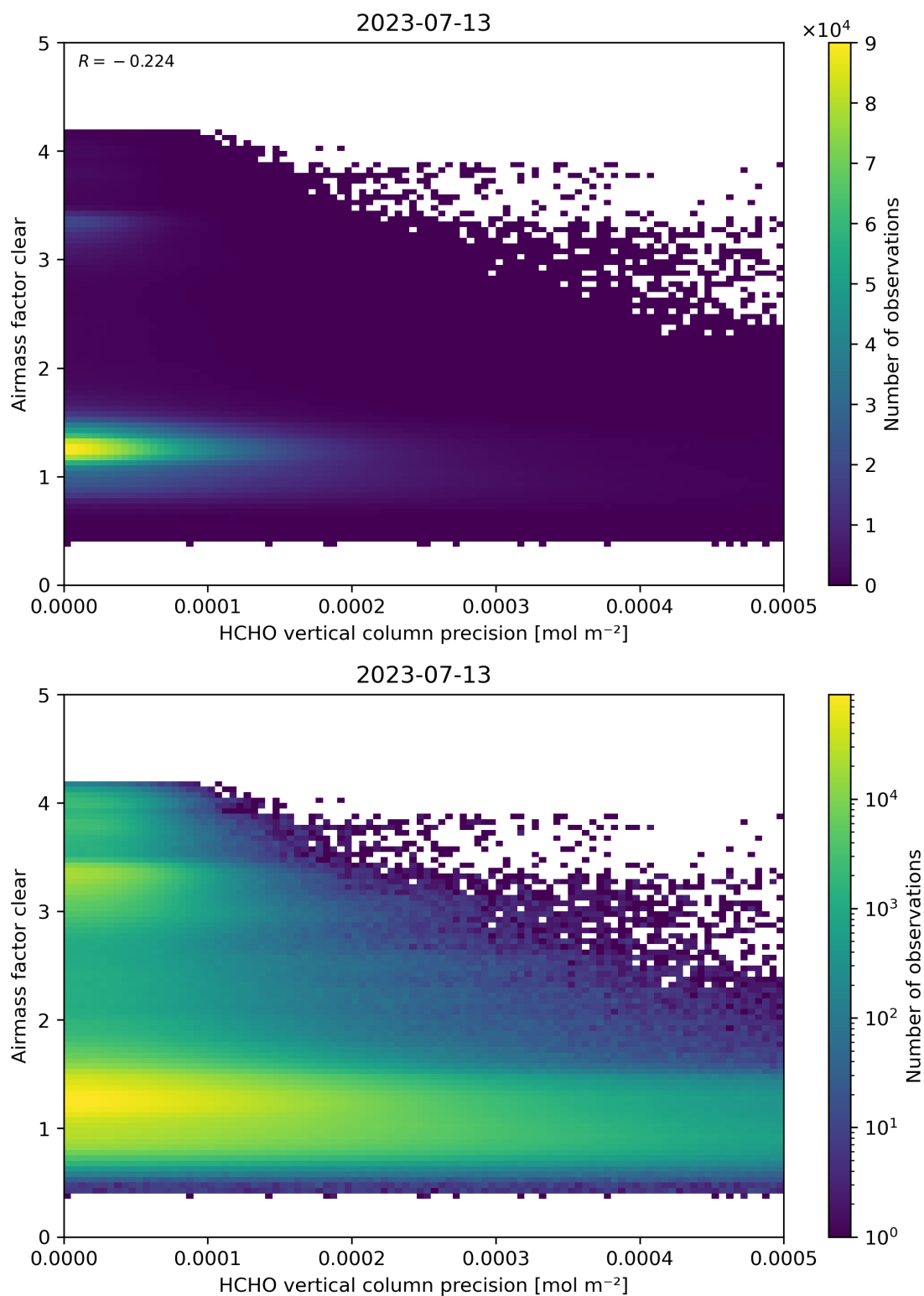
Figure 139: Scatter density plot of “HCHO vertical column precision” against “Airmass factor clear” for 2023-07-13 to 2023-07-14.
