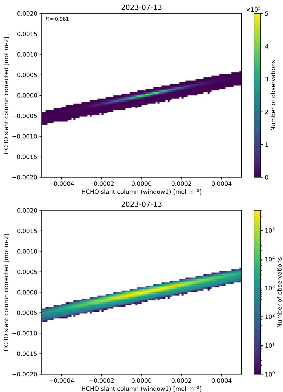
Figure 82: Scatter density plot of “HCHO slant column (window1)” against “HCHO slant column corrected” for 2023-07-13 to 2023-07-14.
