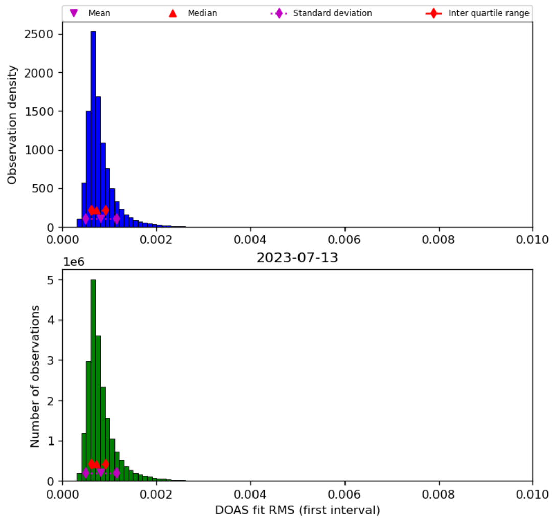
Figure 46: Histogram of “DOAS fit RMS (first interval)” for 2023-07-13 to 2023-07-14
