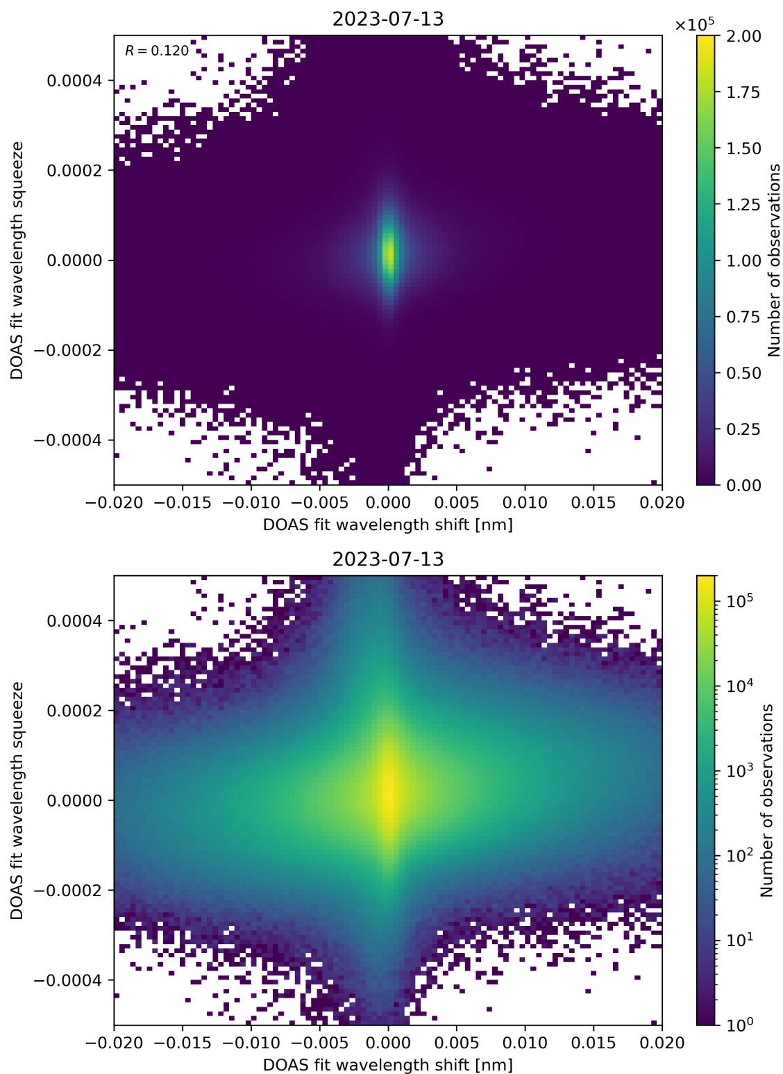
Figure 65: Scatter density plot of “DOAS fit wavelength shift” against “DOAS fit wavelength squeeze” for 2023-07-13 to 2023-07-14.
