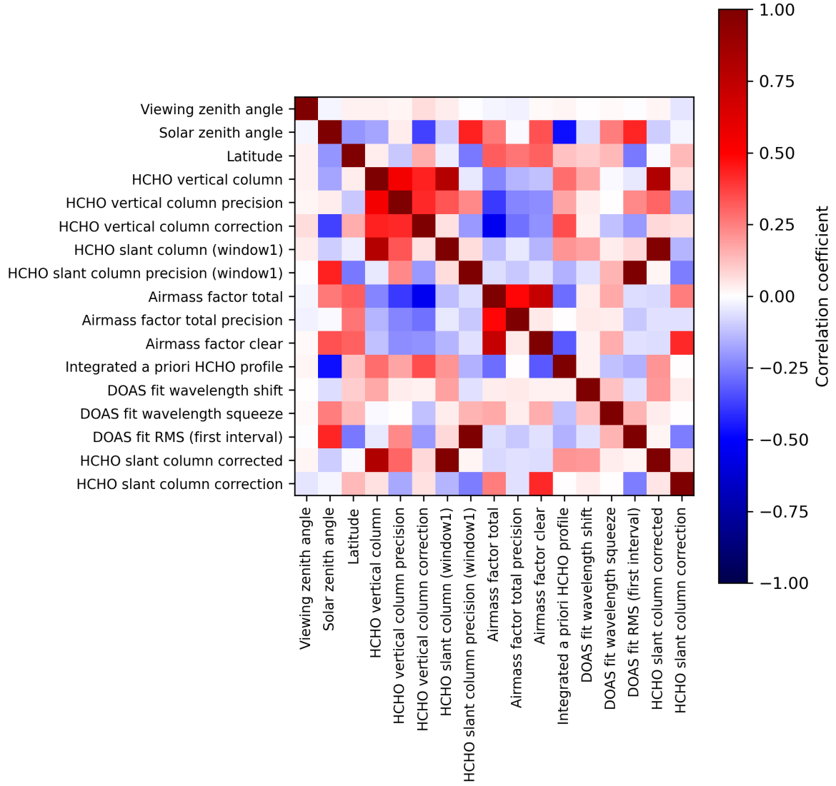
Figure 2: Map of correlation matrix for 2023-07-13 to 2023-07-14.
