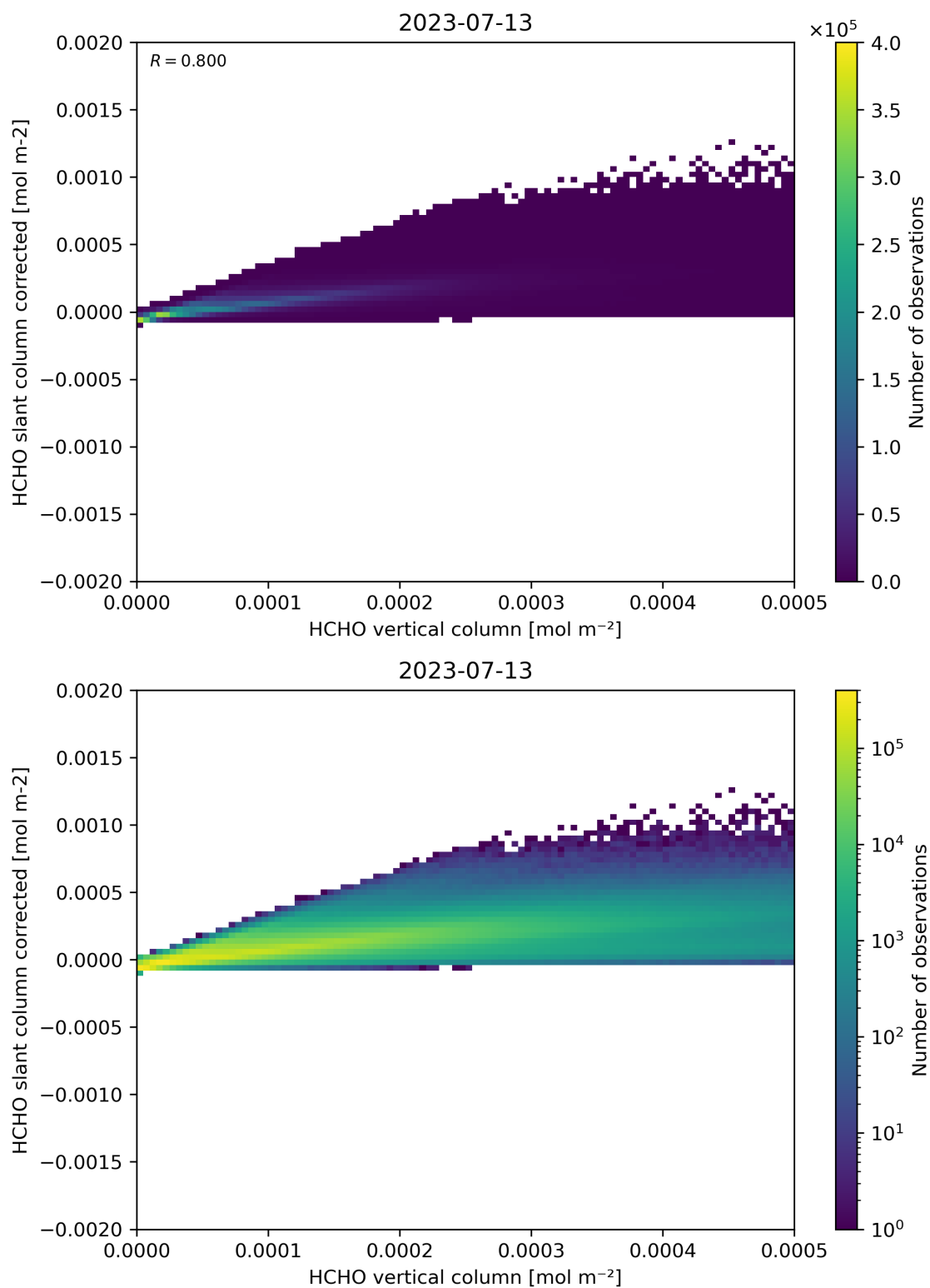
Figure 127: Scatter density plot of “HCHO vertical column” against “HCHO slant column corrected” for 2023-07-13 to 2023-07-14.
