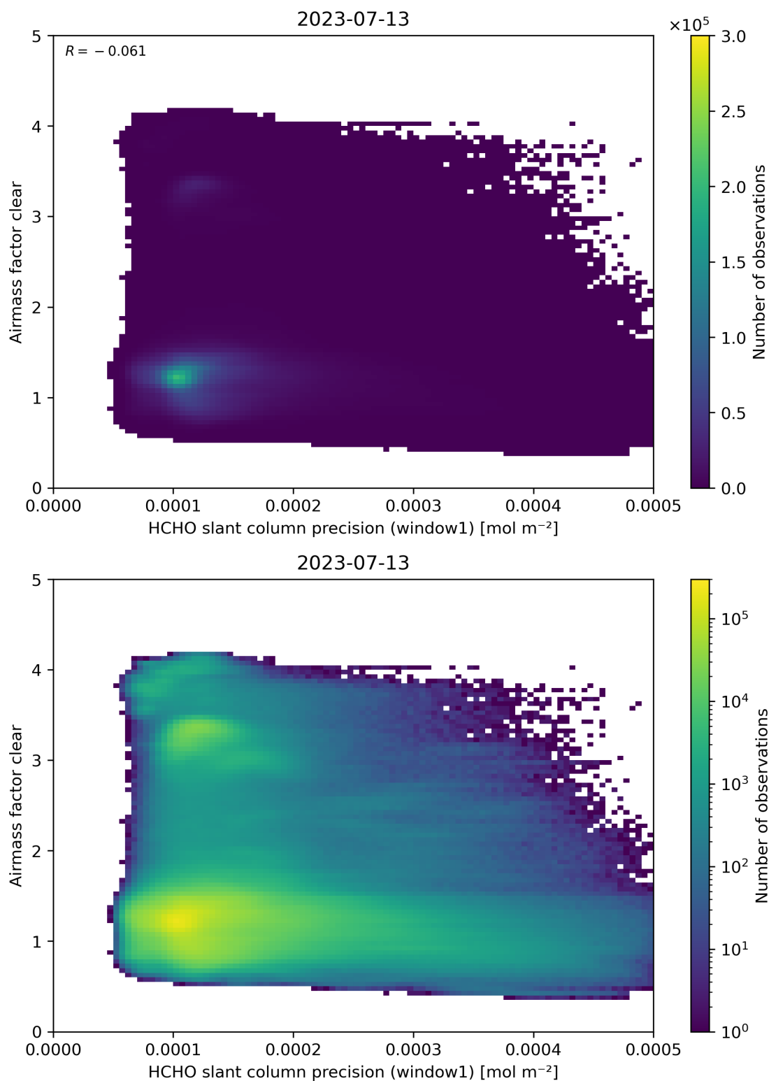
Figure 91: Scatter density plot of “HCHO slant column precision (window1)” against “Airmass factor clear” for 2023-07-13 to 2023-07-14.
