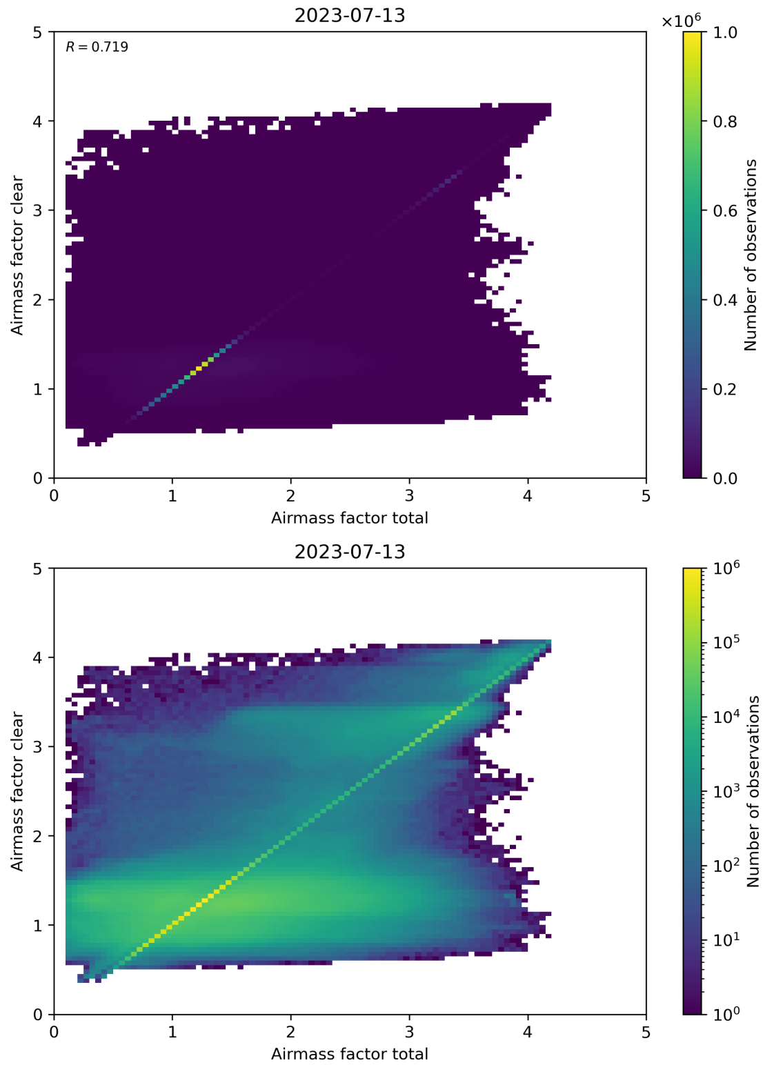
Figure 100: Scatter density plot of “Airmass factor total” against “Airmass factor clear” for 2023-07-13 to 2023-07-14.
