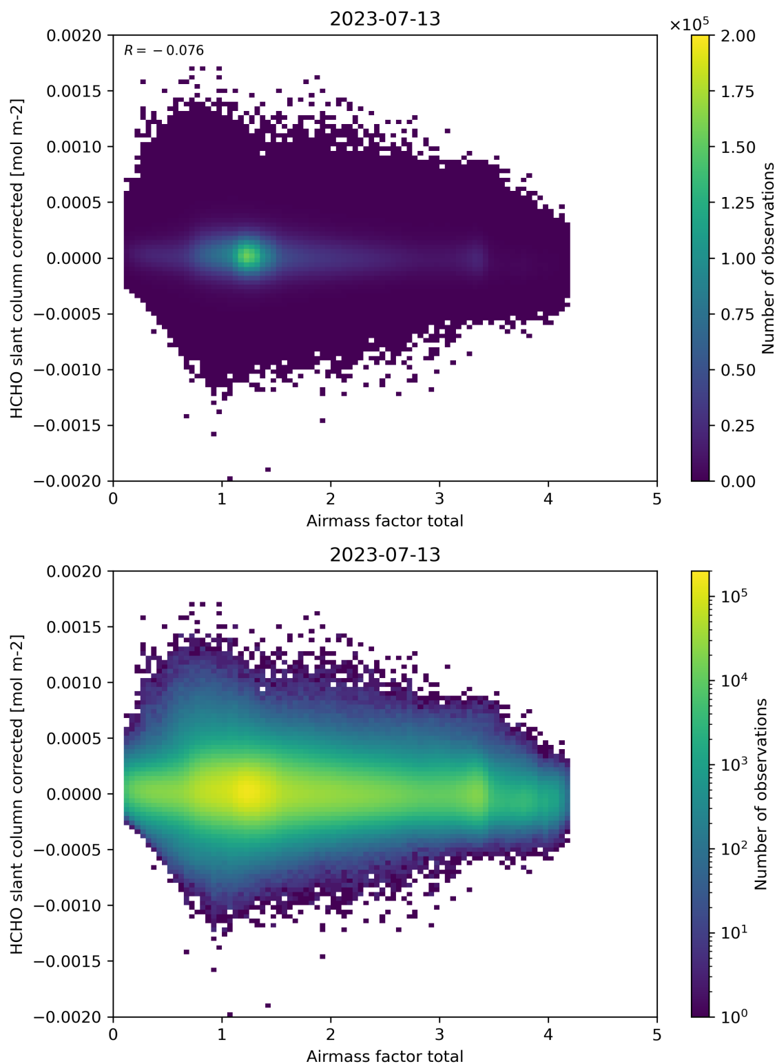
Figure 101: Scatter density plot of “Airmass factor total” against “HCHO slant column corrected” for 2023-07-13 to 2023-07-14.
