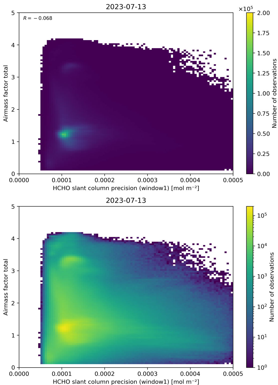
Figure 94: Scatter density plot of “HCHO slant column precision (window1)” against “Air mass factor total” for 2023-07-13 to 2023-07-14.
