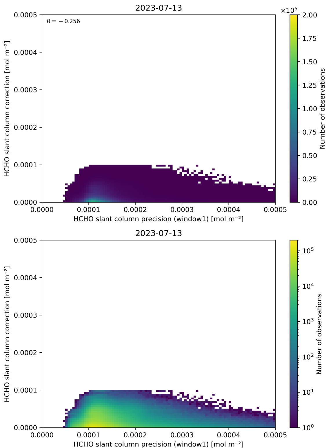
Figure 93: Scatter density plot of “HCHO slant column precision (window1)” against “HCHO slant column correction” for 2023-07-13 to 2023-07-14.
