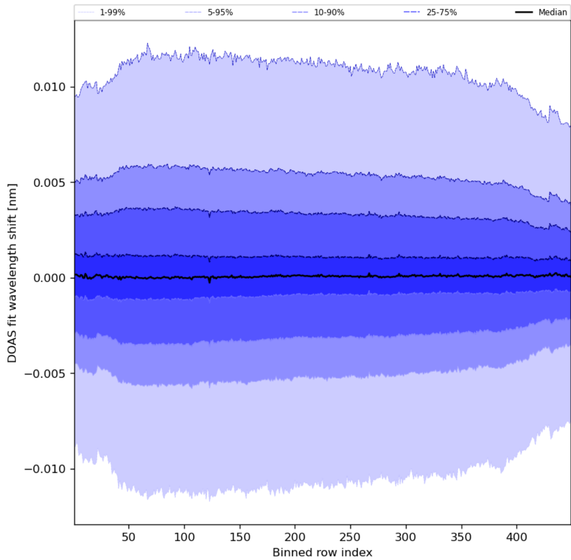
Figure 58: Along track statistics of “DOAS fit wavelength shift” for 2023-07-13 to 2023-07-14
