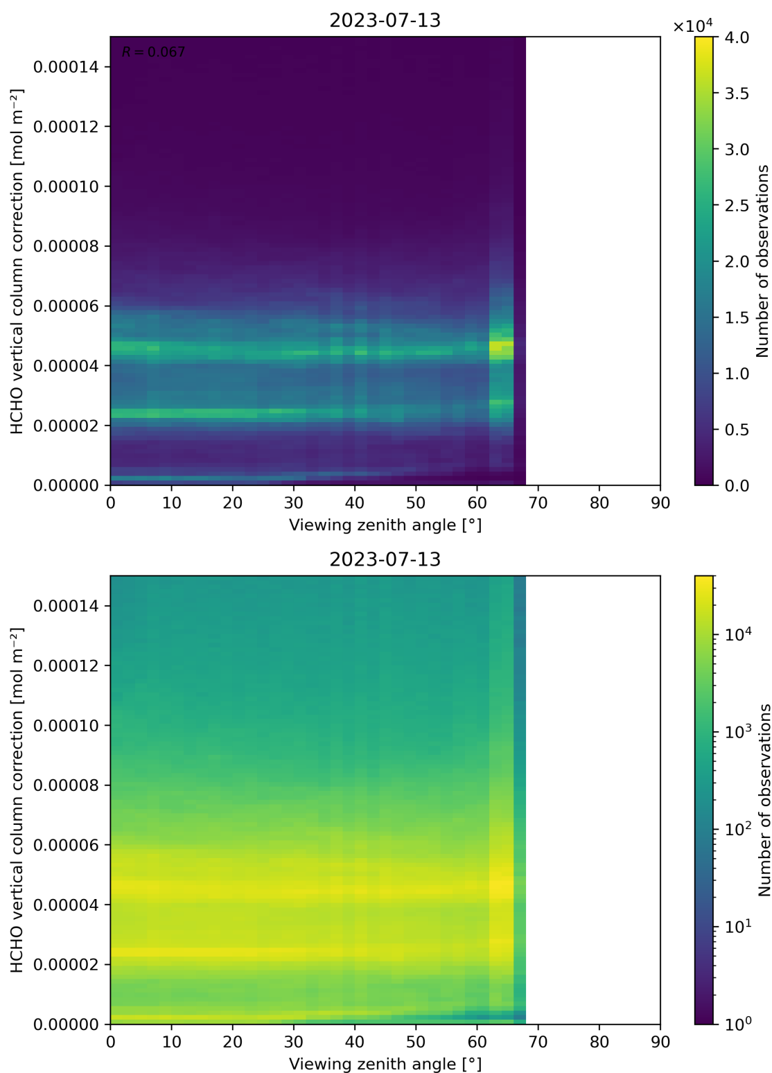
Figure 193: Scatter density plot of “Viewing zenith angle” against “HCHO vertical column correction” for 2023-07-13 to 2023-07-14.
