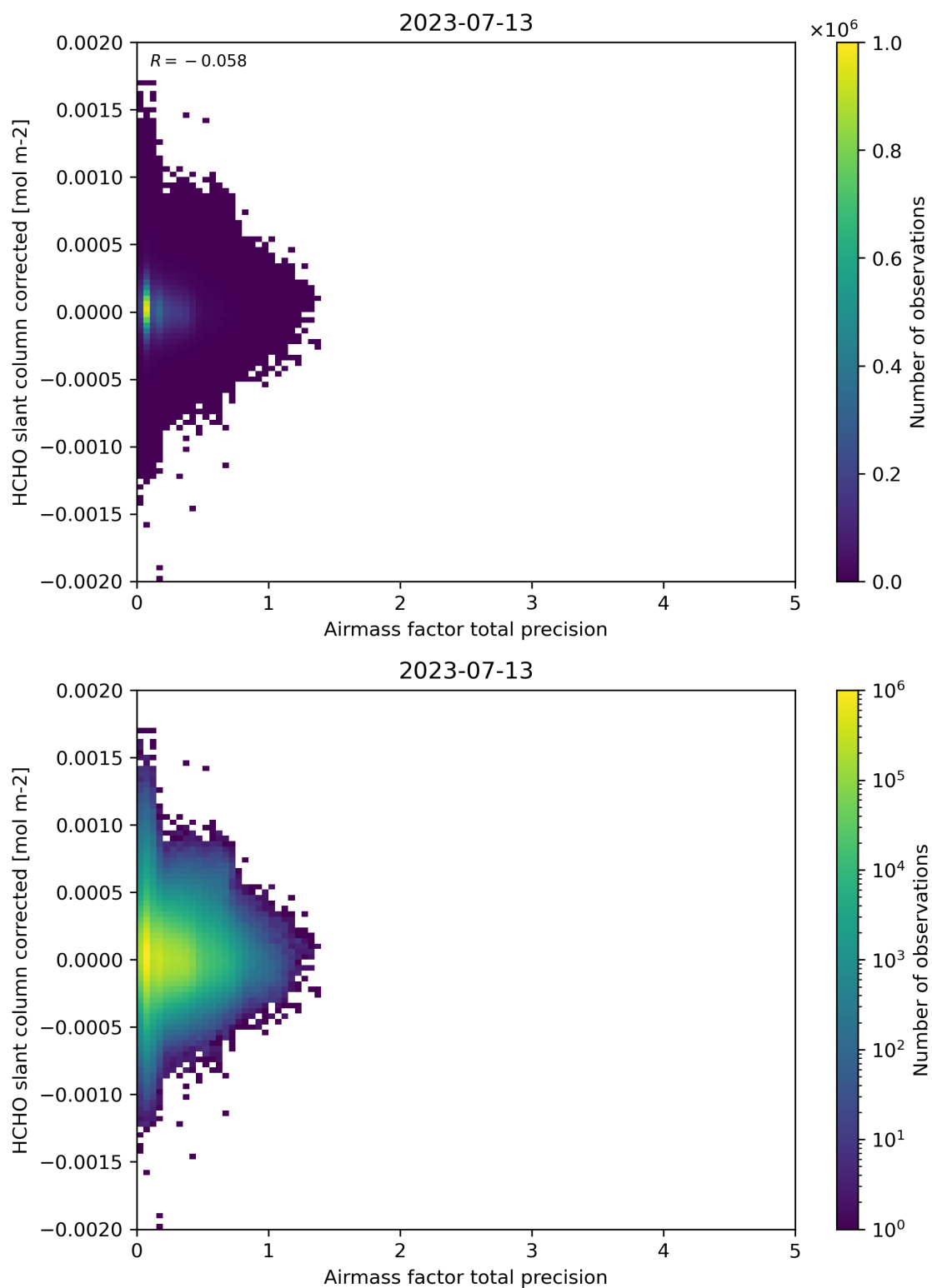
Figure 109: Scatter density plot of “Airmass factor total precision” against “HCHO slant column corrected” for 2023-07-13 to 2023-07-14.
