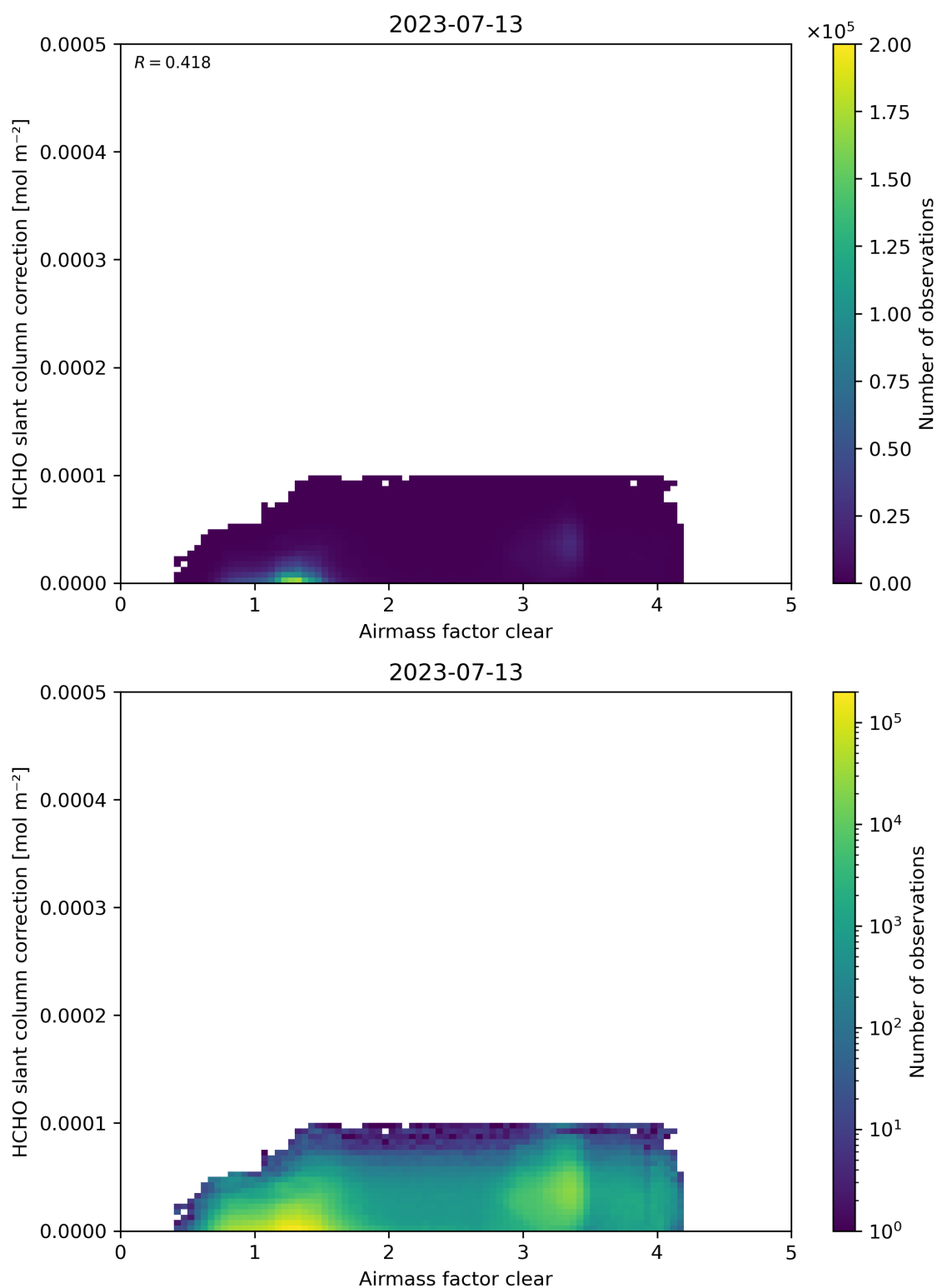
Figure 75: Scatter density plot of “Airmass factor clear” against “HCHO slant column correction” for 2023-07-13 to 2023-07-14.
