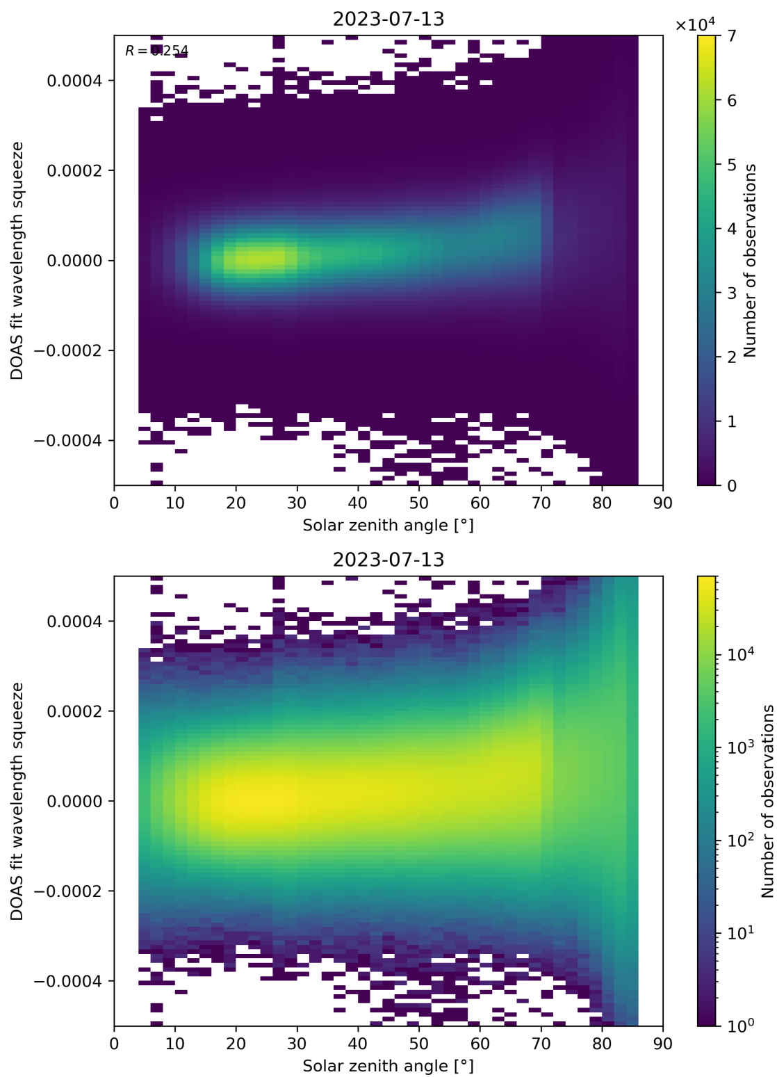
Figure 169: Scatter density plot of “Solar zenith angle” against “DOAS fit wavelength squeeze” for 2023-07-13 to 2023-07-14.
