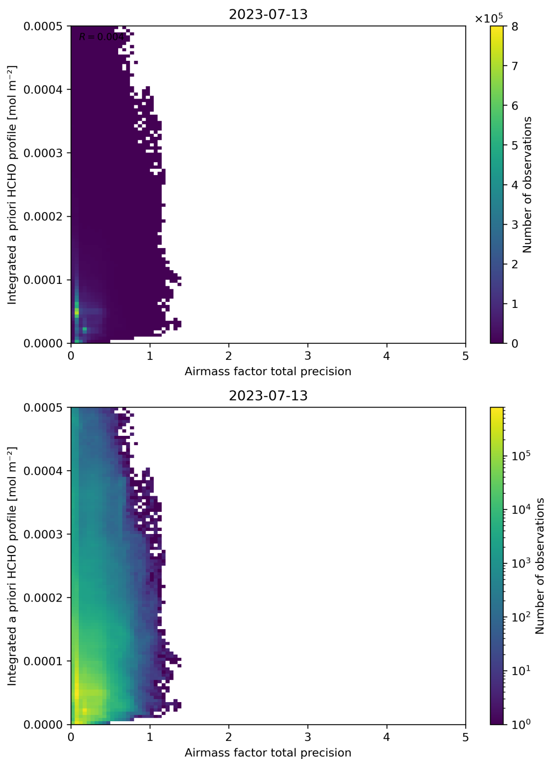
Figure 111: Scatter density plot of “Airmass factor total precision” against “Integrated a priori HCHO profile” for 2023-07-13 to 2023-07-14.
