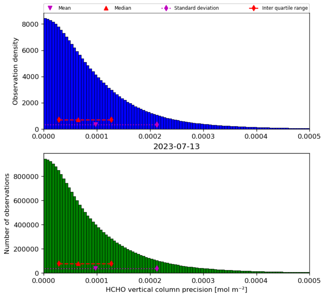
Figure 36: Histogram of “HCHO vertical column precision” for 2023-07-13 to 2023-07-14
