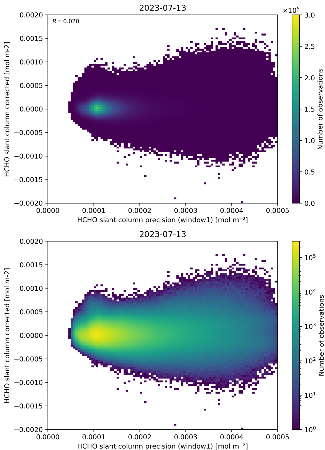
Figure 92: Scatter density plot of “HCHO slant column precision (window1)” against “HCHO slant column corrected” for 2023-07-13 to 2023-07-14.
