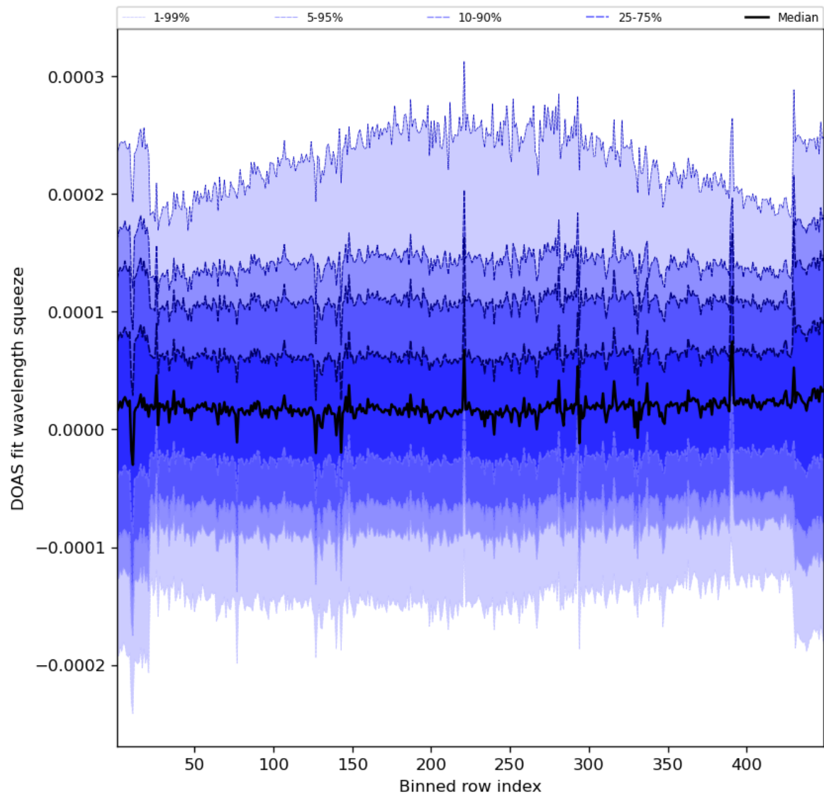
Figure 59: Along track statistics of “DOAS fit wavelength squeeze” for 2023-07-13 to 2023-07-14
