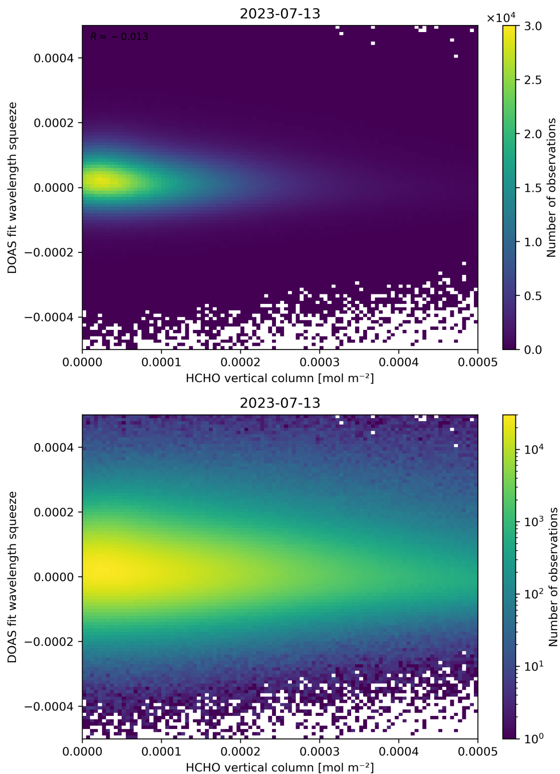
Figure 125: Scatter density plot of “HCHO vertical column” against “DOAS fit wavelength squeeze” for 2023-07-13 to 2023-07-14.
