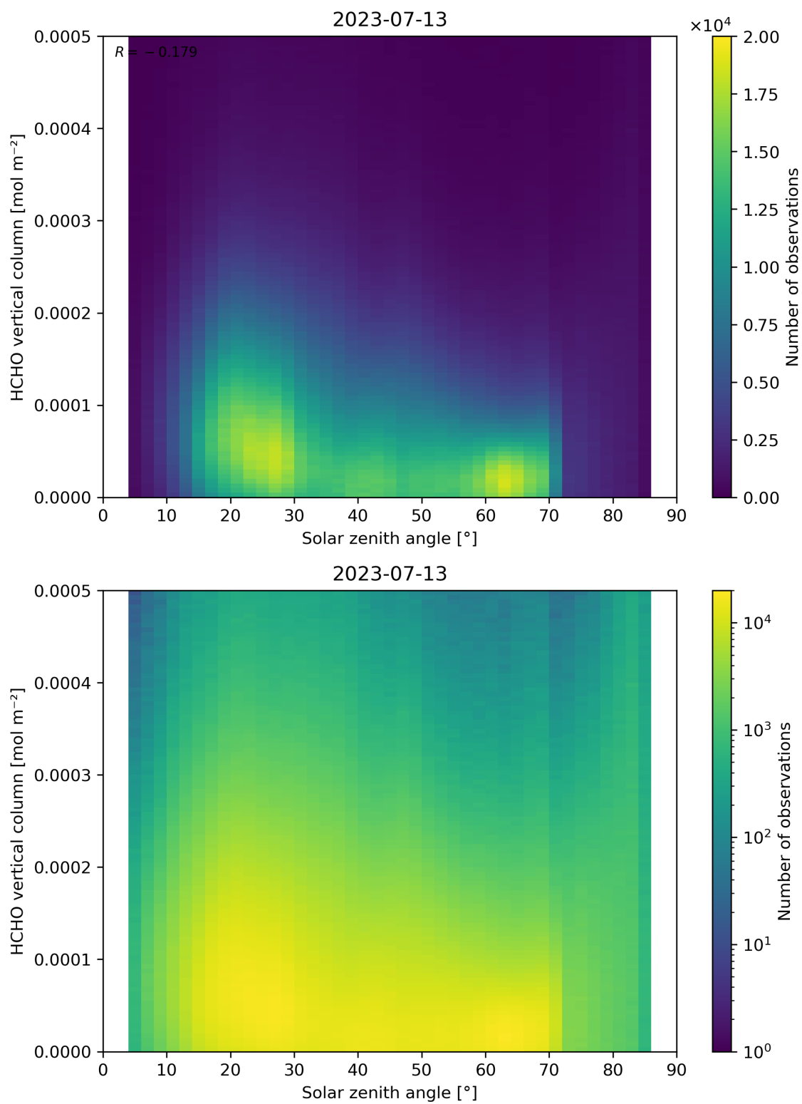
Figure 177: Scatter density plot of “Solar zenith angle” against “HCHO vertical column” for 2023-07-13 to 2023-07-14.
