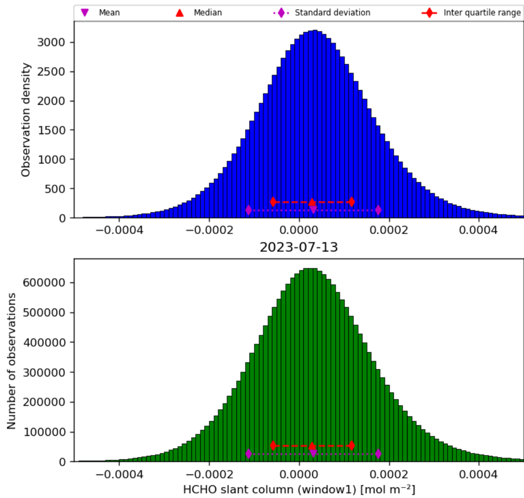
Figure 38: Histogram of “HCHO slant column (window1)” for 2023-07-13 to 2023-07-14
