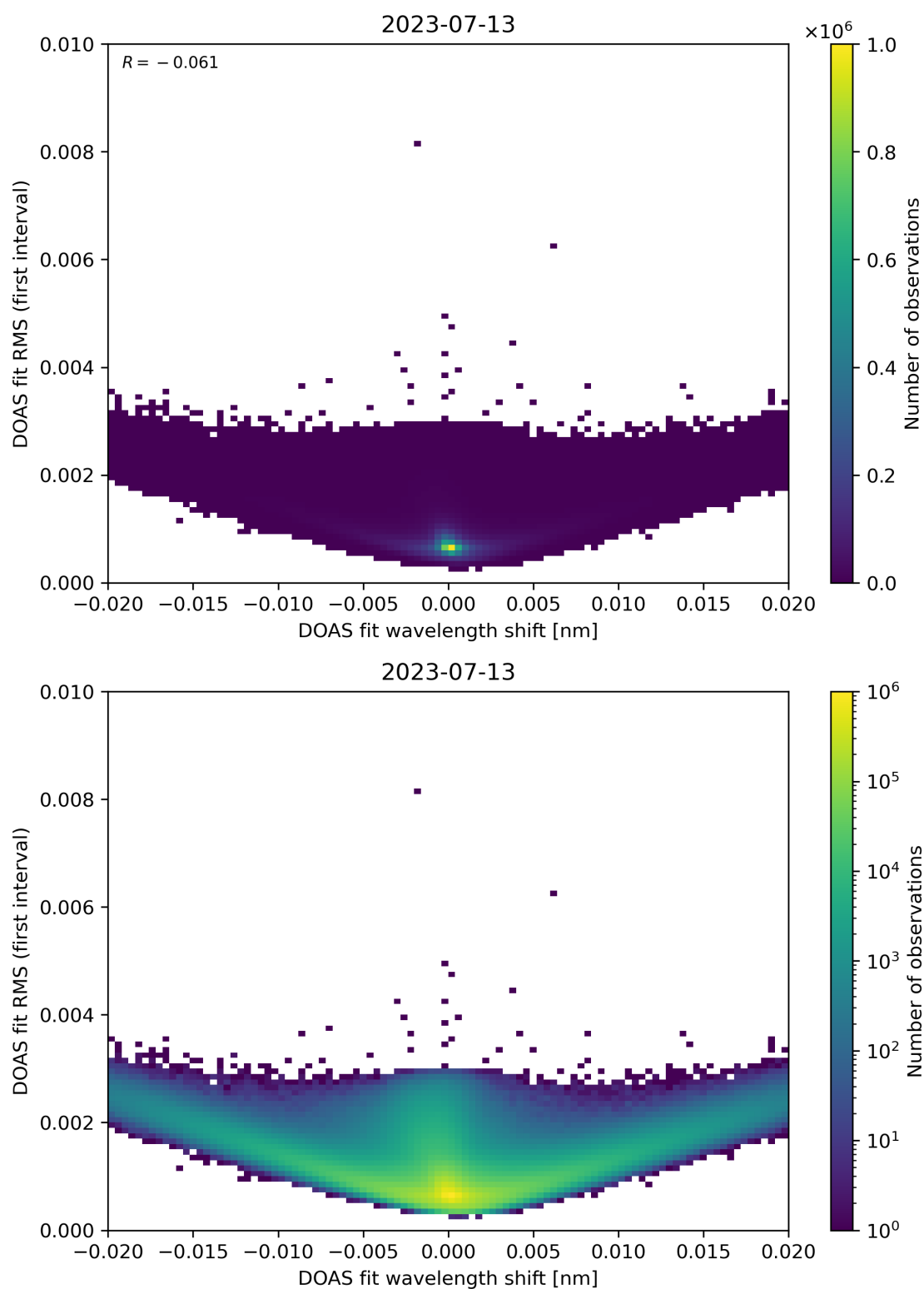
Figure 64: Scatter density plot of “DOAS fit wavelength shift” against “DOAS fit RMS (first interval)” for 2023-07-13 to 2023-07-14.
