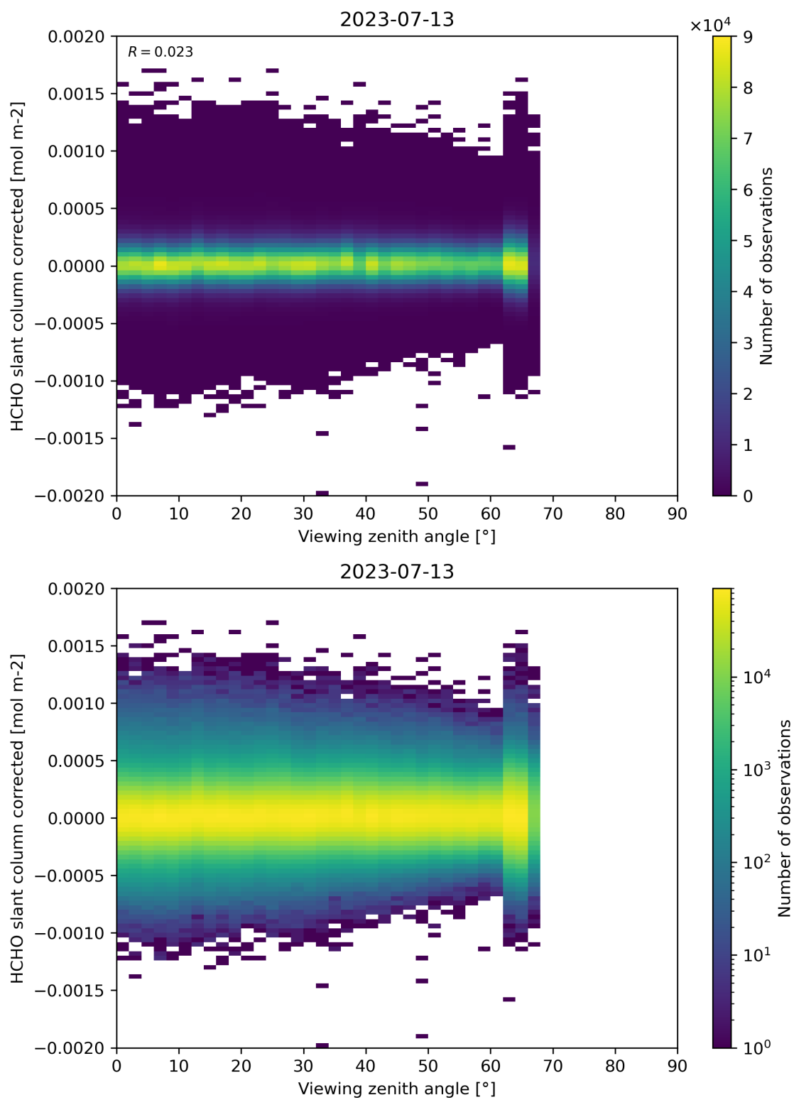
Figure 186: Scatter density plot of “Viewing zenith angle” against “HCHO slant column corrected” for 2023-07-13 to 2023-07-14.
