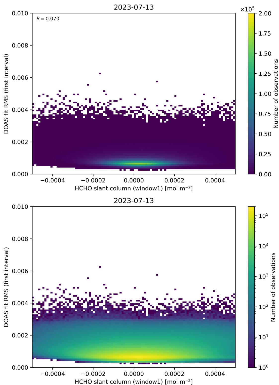
Figure 78: Scatter density plot of “HCHO slant column (window1)” against “DOAS fit RMS (first interval)” for 2023-07-13 to 2023-07-14.
