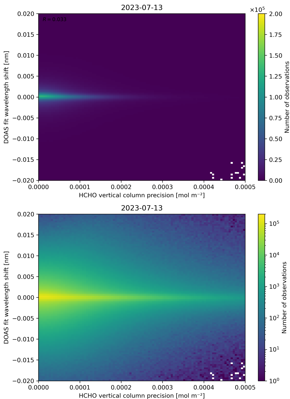
Figure 137: Scatter density plot of “HCHO vertical column precision” against “DOAS fit wavelength shift” for 2023-07-13 to 2023-07-14.
