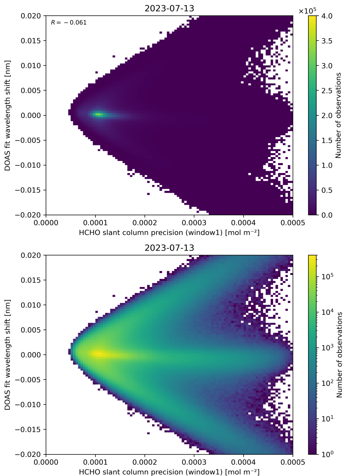
Figure 89: Scatter density plot of “HCHO slant column precision (window1)” against “DOAS fit wavelength shift” for 2023-07-13 to 2023-07-14.
