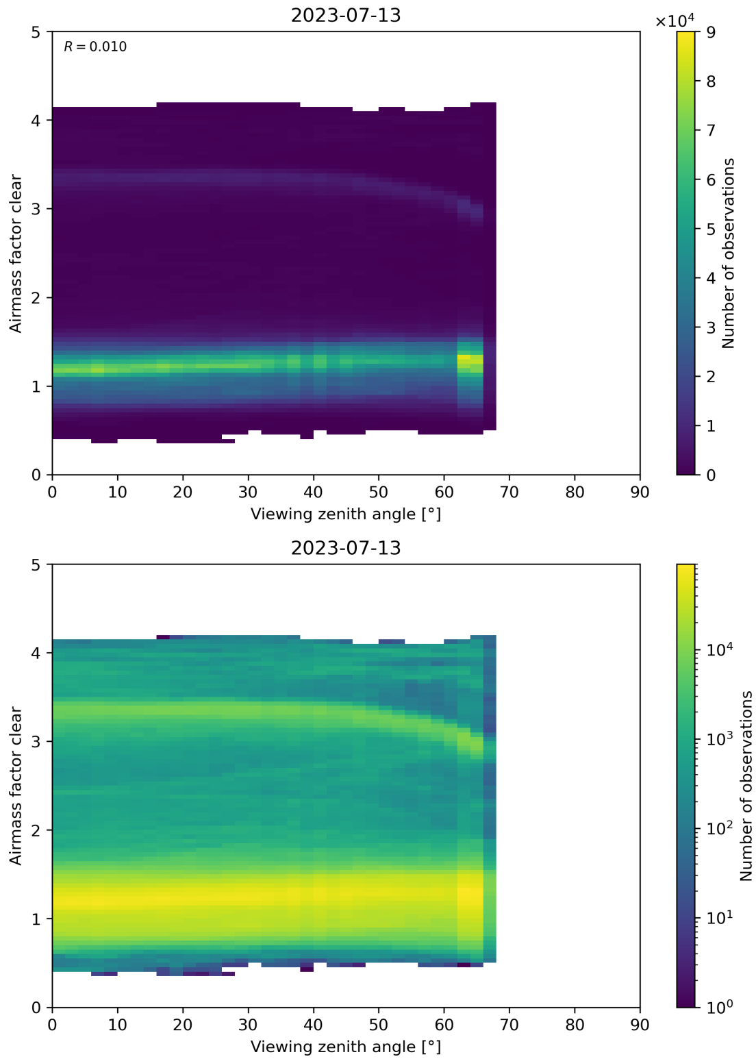
Figure 185: Scatter density plot of “Viewing zenith angle” against “Airmass factor clear” for 2023-07-13 to 2023-07-14.
