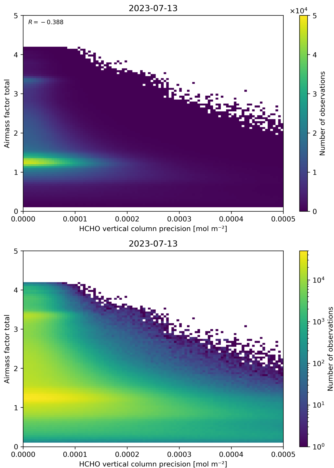
Figure 144: Scatter density plot of “HCHO vertical column precision” against “Airmass factor total” for 2023-07-13 to 2023-07-14.
