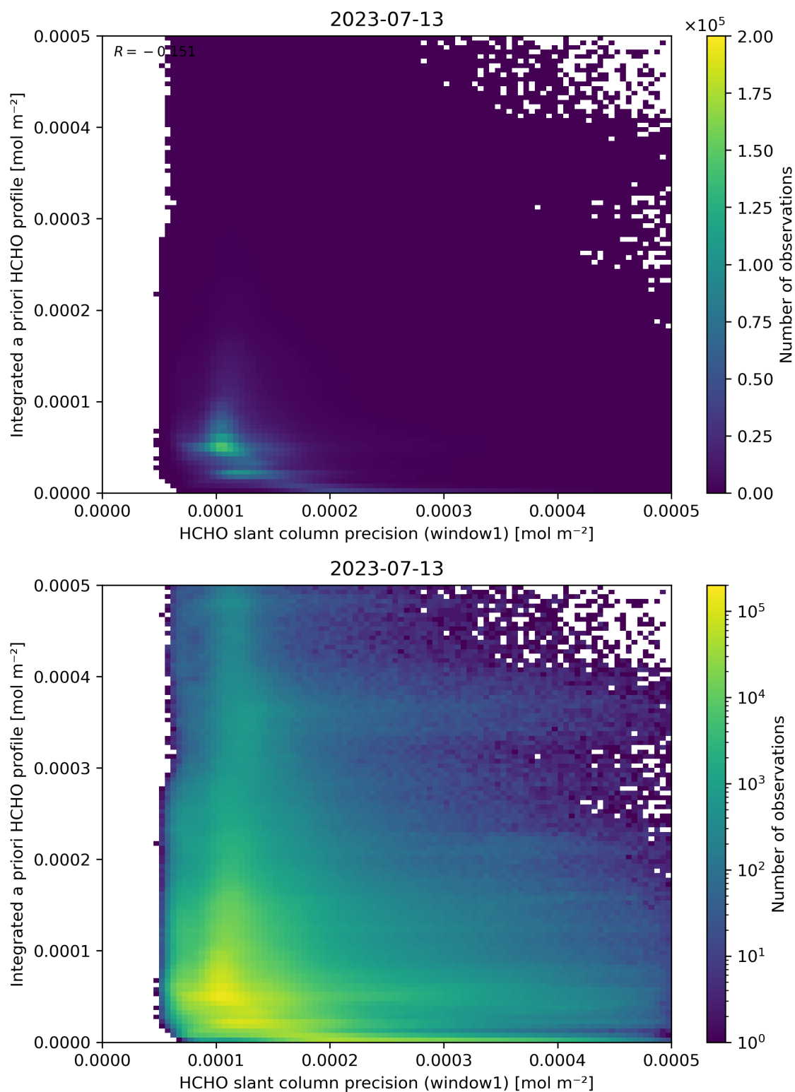
Figure 96: Scatter density plot of “HCHO slant column precision (window1)” against “Integrated a priori HCHO profile” for 2023-07-13 to 2023-07-14.
