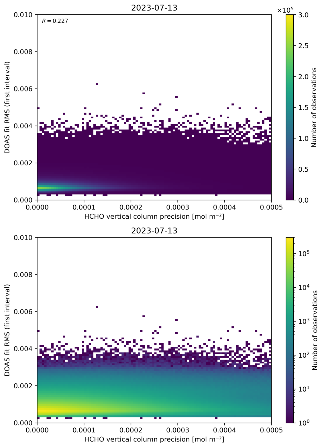
Figure 136: Scatter density plot of “HCHO vertical column precision” against “DOAS fit RMS (first interval)” for 2023-07-13 to 2023-07-14.
