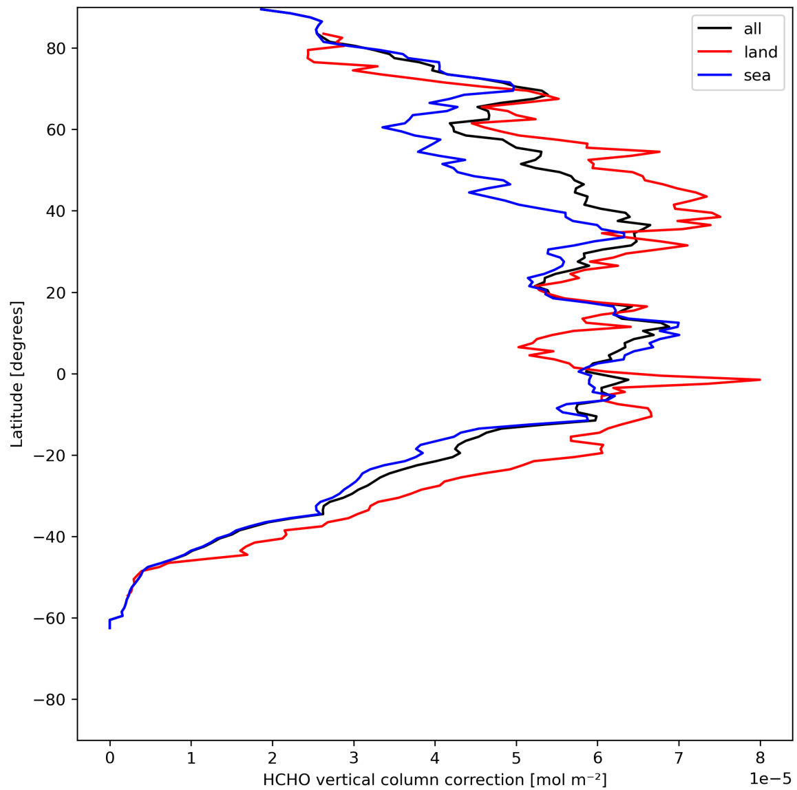
Figure 23: Zonal average of “HCHO vertical column correction” for 2023-07-13 to 2023-07-14.
