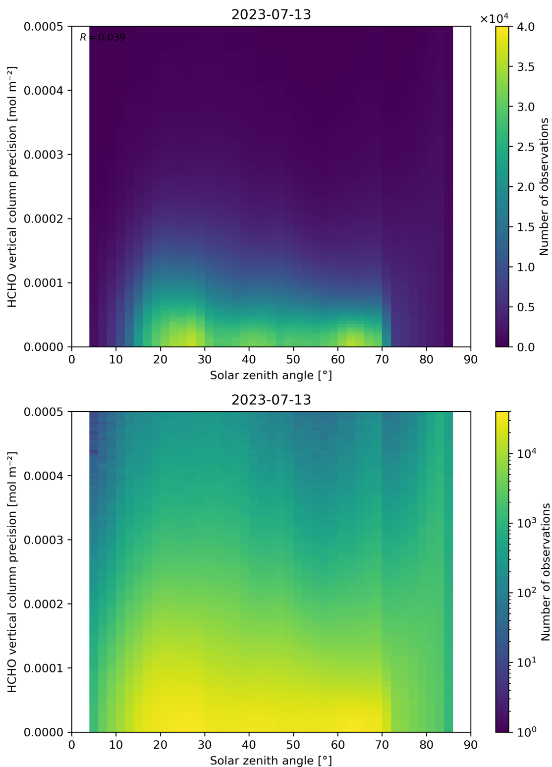
Figure 179: Scatter density plot of “Solar zenith angle” against “HCHO vertical column precision” for 2023-07-13 to 2023-07-14.
