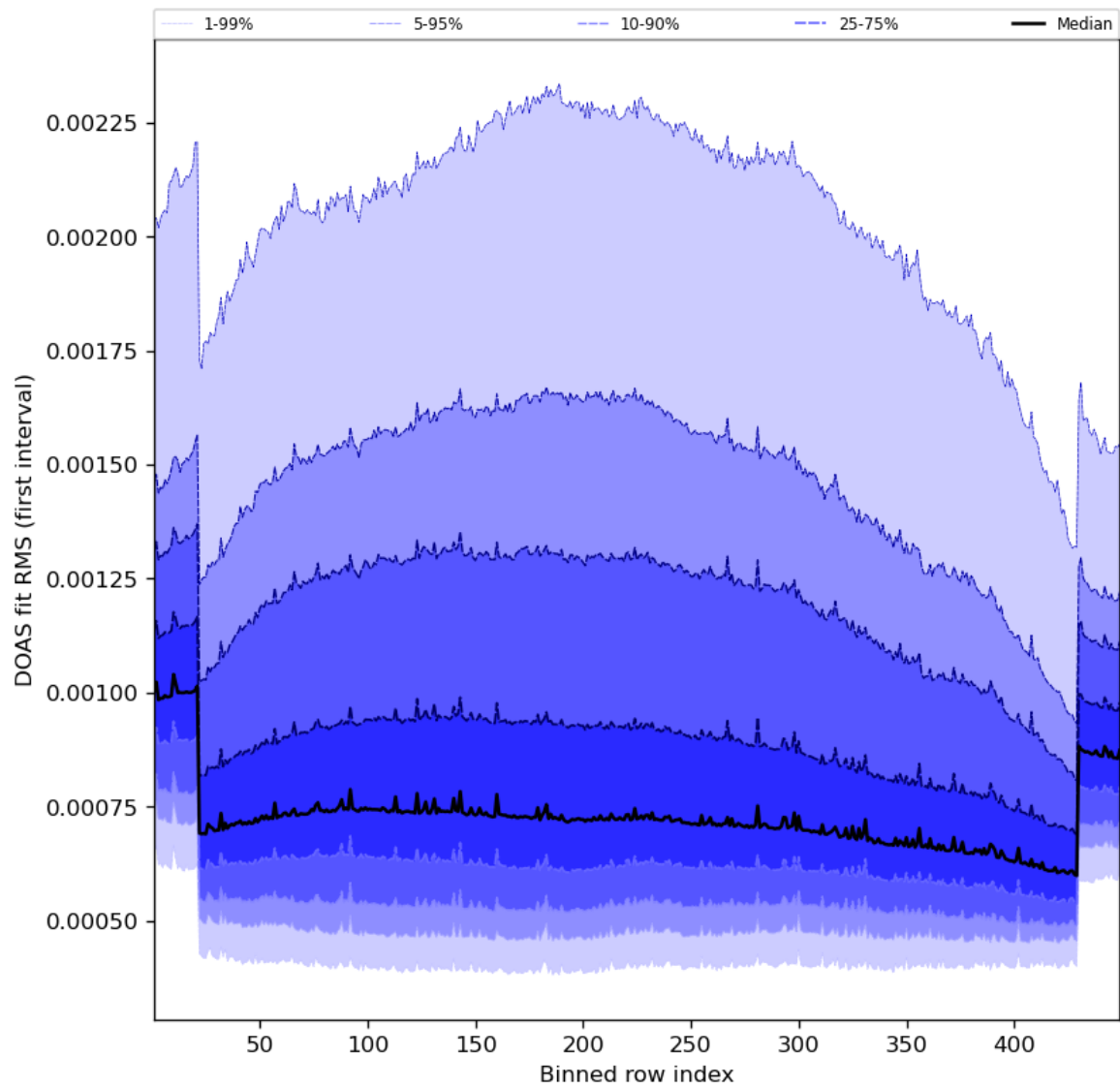
Figure 60: Along track statistics of “DOAS fit RMS (first interval)” for 2023-07-13 to 2023-07-14
