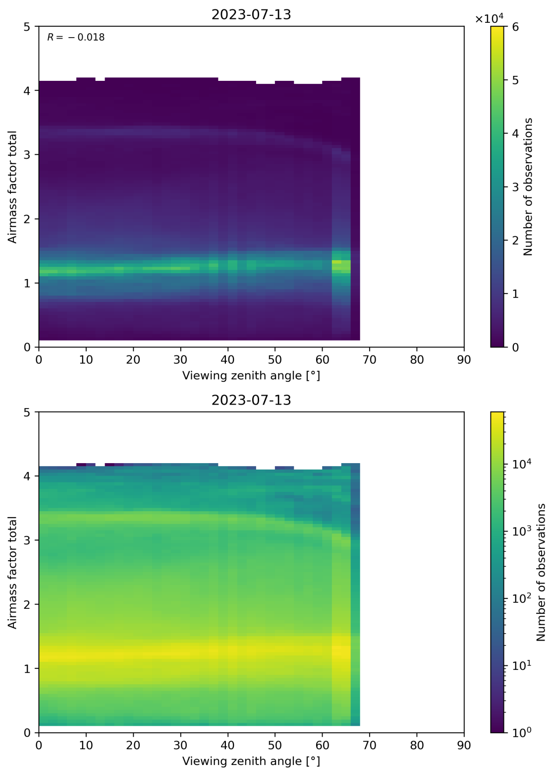
Figure 190: Scatter density plot of “Viewing zenith angle” against “Airmass factor total” for 2023-07-13 to 2023-07-14.
