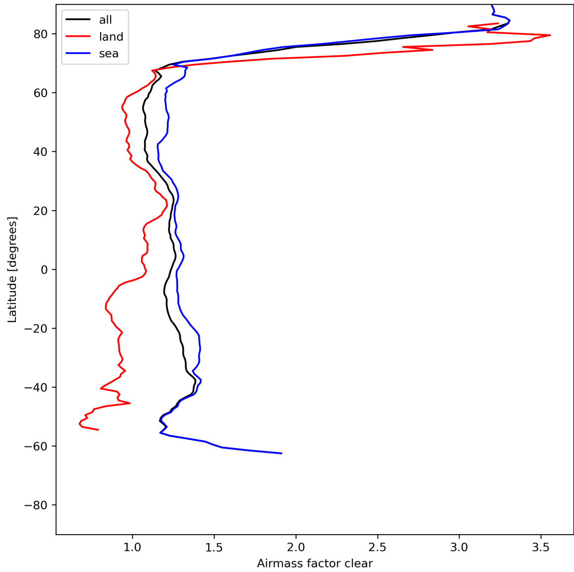
Figure 28: Zonal average of “Airmass factor clear” for 2023-07-13 to 2023-07-14.
