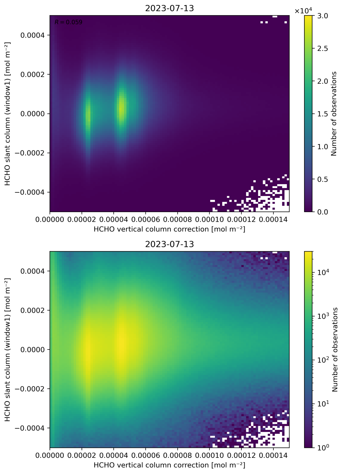
Figure 118: Scatter density plot of “HCHO vertical column correction” against “HCHO slant column (window1)” for 2023-07-13 to 2023-07-14.
