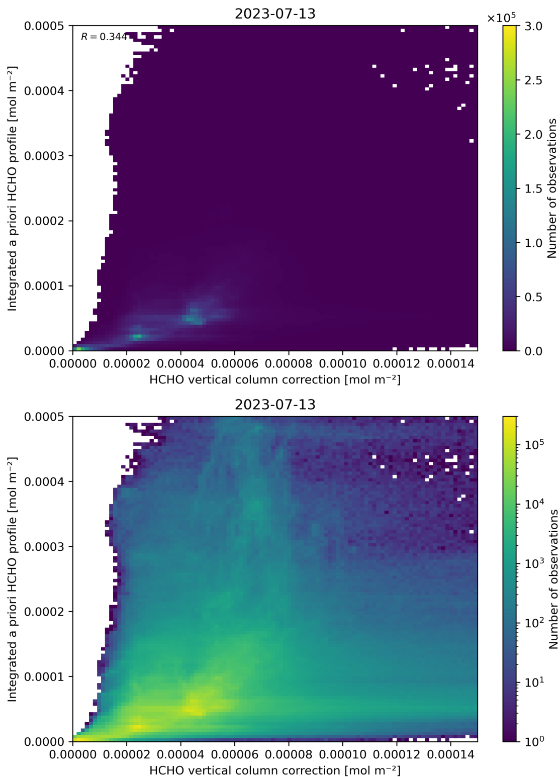
Figure 122: Scatter density plot of “HCHO vertical column correction” against “Integrated a priori HCHO profile” for 2023-07-13 to 2023-07-14.
