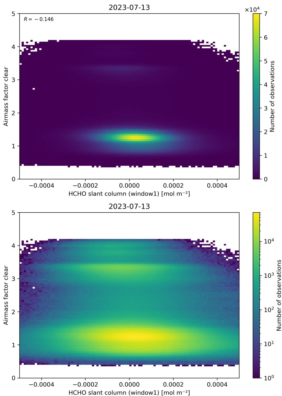
Figure 81: Scatter density plot of “HCHO slant column (window1)” against “Airmass factor clear” for 2023-07-13 to 2023-07-14.
