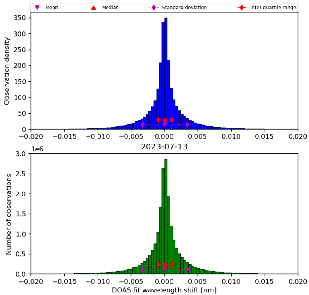
Figure 44: Histogram of “DOAS fit wavelength shift” for 2023-07-13 to 2023-07-14
