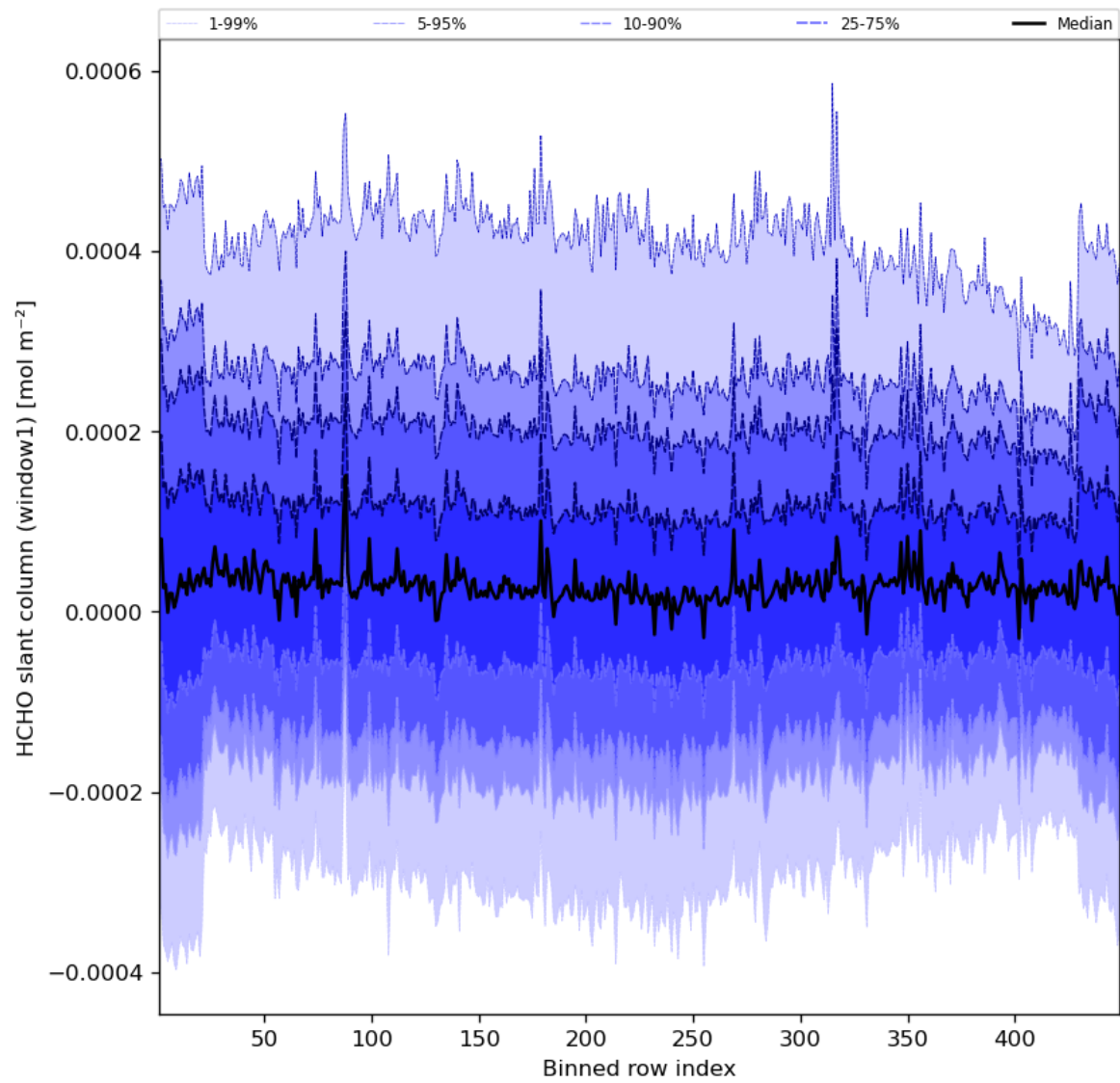
Figure 52: Along track statistics of “HCHO slant column (window1)” for 2023-07-13 to 2023-07-14
