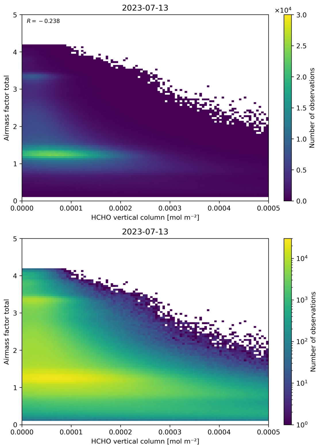
Figure 131: Scatter density plot of “HCHO vertical column” against “Airmass factor total” for 2023-07-13 to 2023-07-14.
