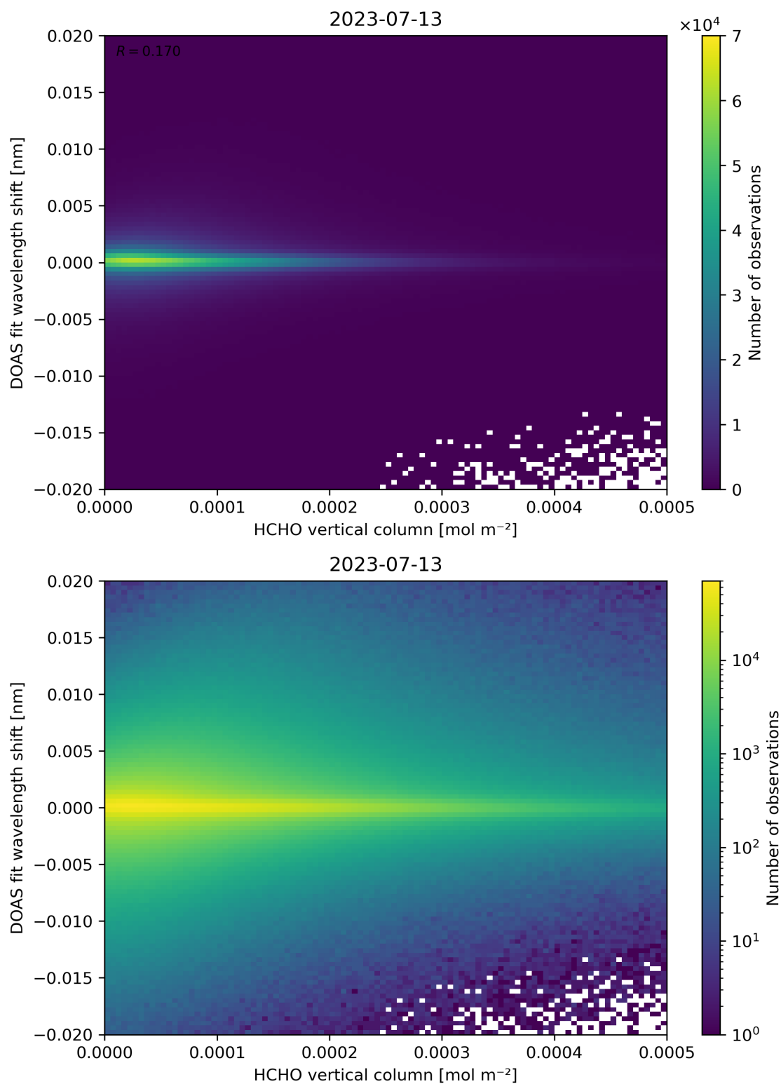
Figure 124: Scatter density plot of “HCHO vertical column” against “DOAS fit wavelength shift” for 2023-07-13 to 2023-07-14.
