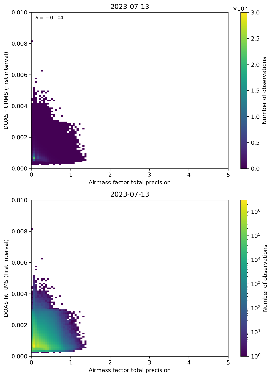
Figure 105: Scatter density plot of “Airmass factor total precision” against “DOAS fit RMS (first interval)” for 2023-07-13 to 2023-07-14.
