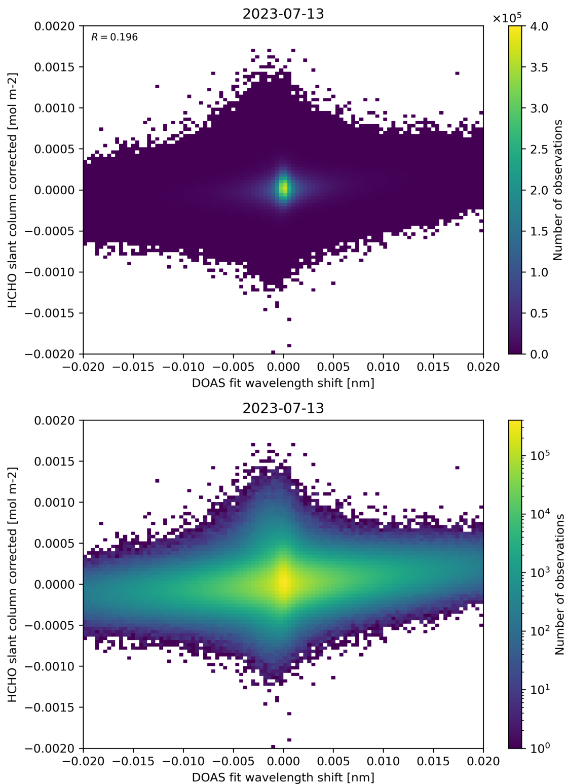
Figure 66: Scatter density plot of “DOAS fit wavelength shift” against “HCHO slant column corrected” for 2023-07-13 to 2023-07-14.
