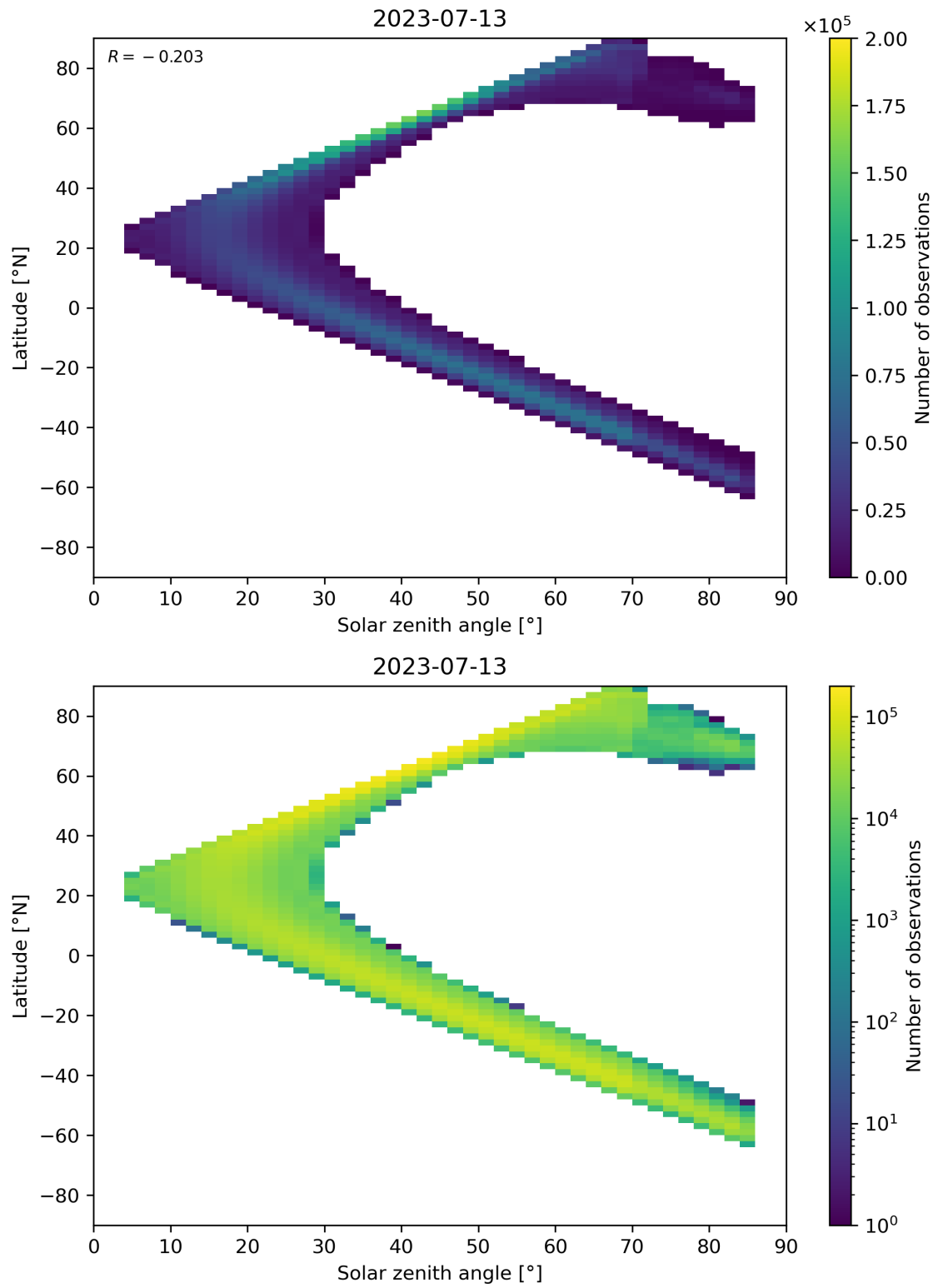
Figure 181: Scatter density plot of “Solar zenith angle” against “Latitude” for 2023-07-13 to 2023-07-14.
