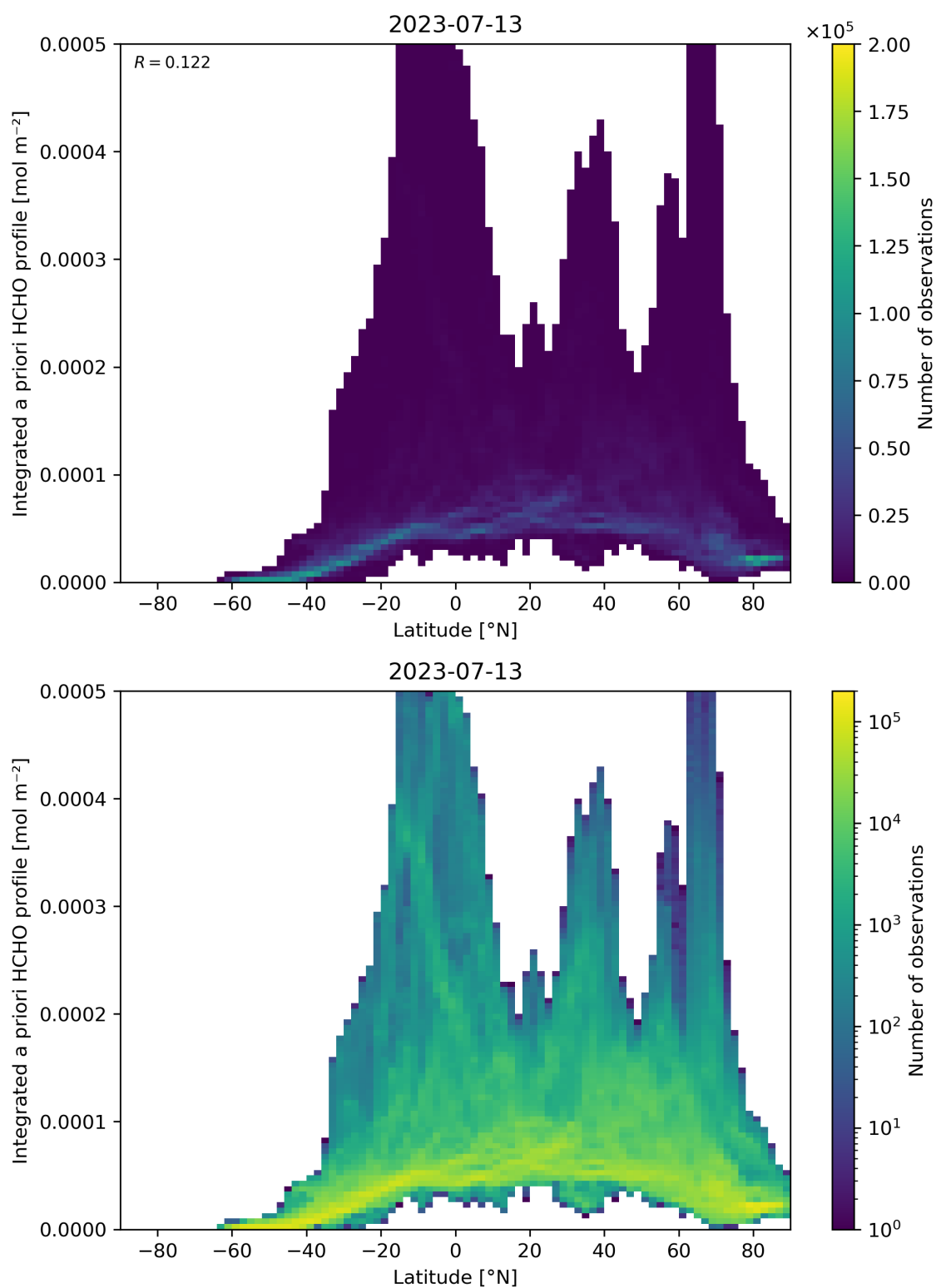
Figure 166: Scatter density plot of “Latitude” against “Integrated a priori HCHO profile” for 2023-07-13 to 2023-07-14.
