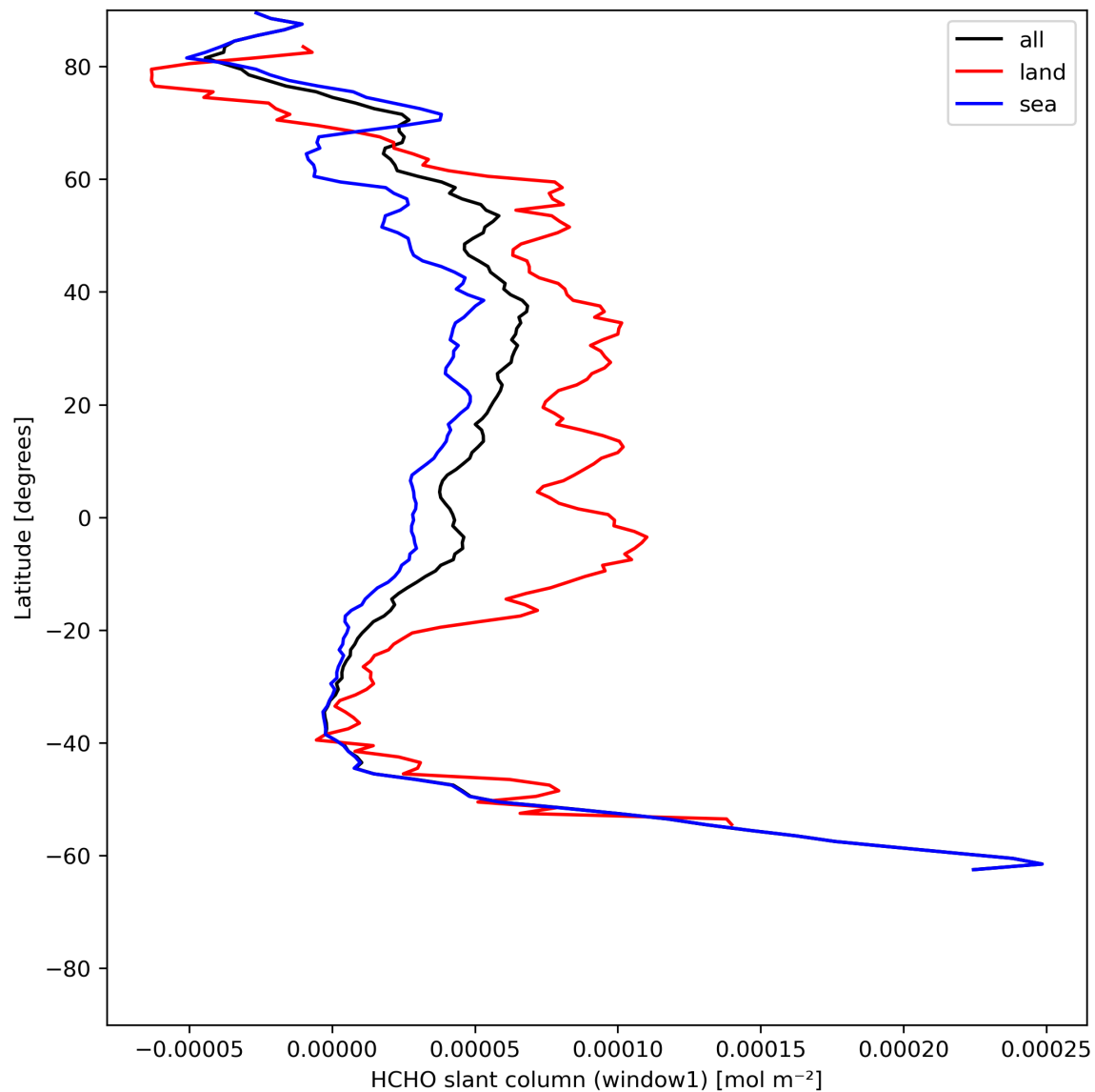
Figure 24: Zonal average of “HCHO slant column (window1)” for 2023-07-13 to 2023-07-14.
