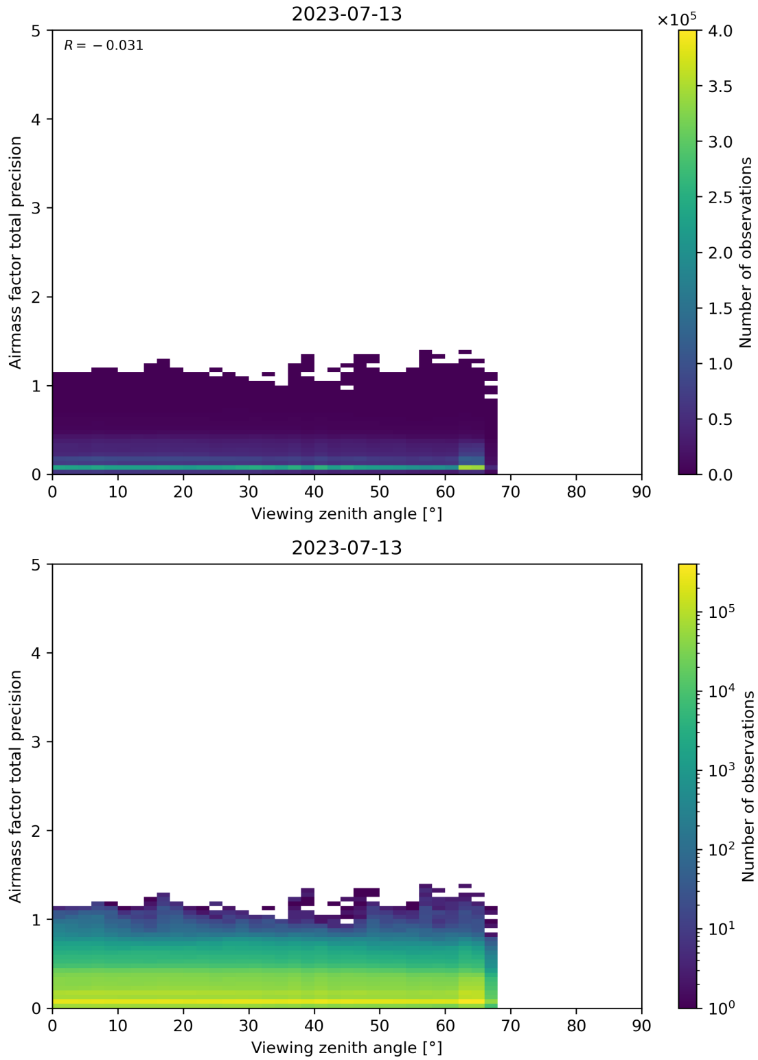
Figure 191: Scatter density plot of “Viewing zenith angle” against “Airmass factor total precision” for 2023-07-13 to 2023-07-14.
