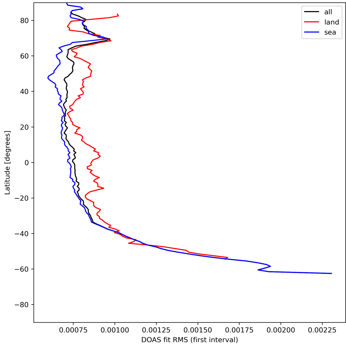
Figure 32: Zonal average of “DOAS fit RMS (first interval)” for 2023-07-13 to 2023-07-14.
