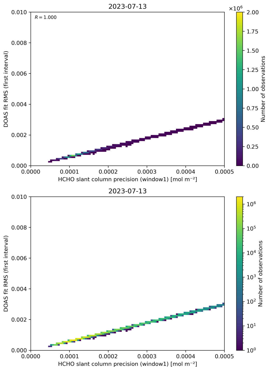
Figure 88: Scatter density plot of “HCHO slant column precision (window1)” against “DOAS fit RMS (first interval)” for 2023-07-13 to 2023-07-14.
