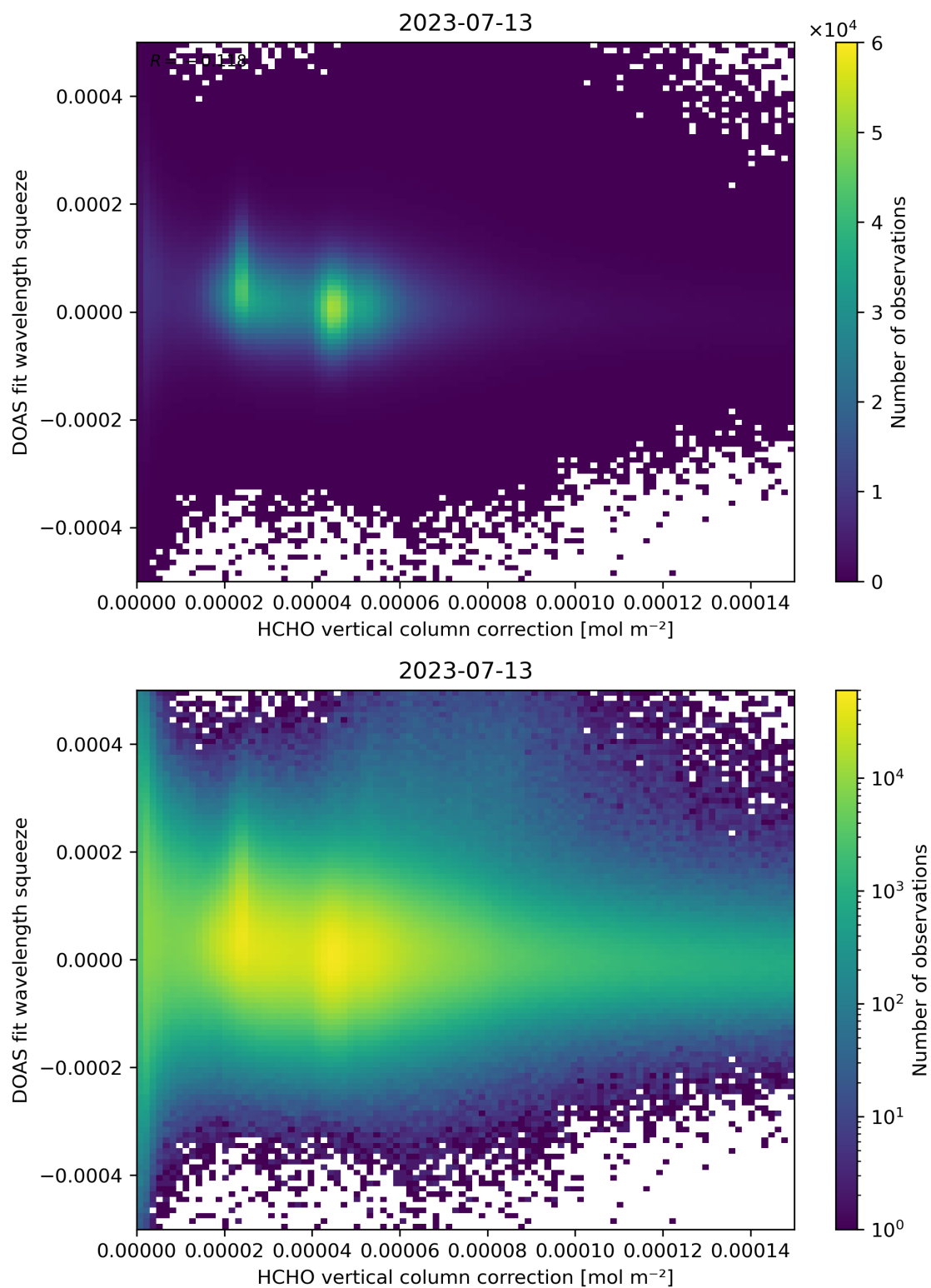
Figure 114: Scatter density plot of “HCHO vertical column correction” against “DOAS fit wavelength squeeze” for 2023-07-13 to 2023-07-14.
