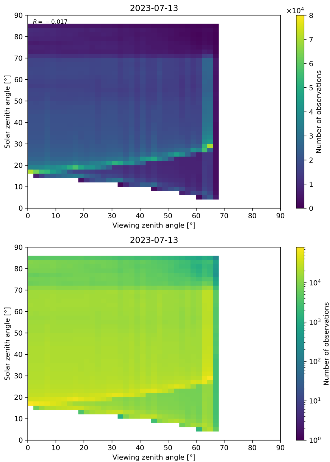
Figure 197: Scatter density plot of “Viewing zenith angle” against “Solar zenith angle” for 2023-07-13 to 2023-07-14.
