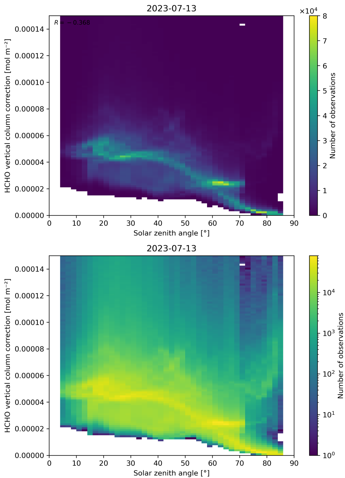
Figure 178: Scatter density plot of “Solar zenith angle” against “HCHO vertical column correction” for 2023-07-13 to 2023-07-14.
