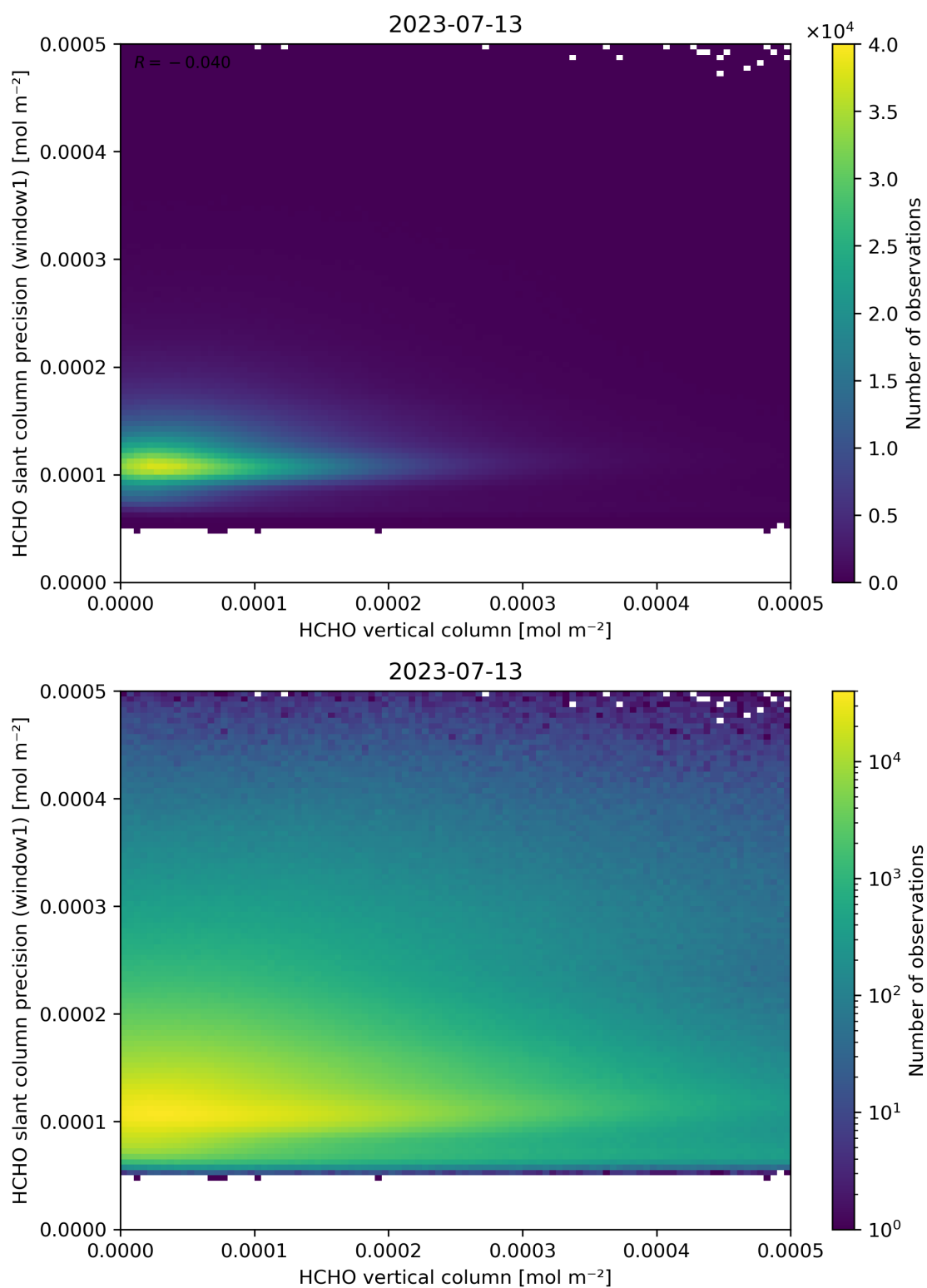
Figure 130: Scatter density plot of “HCHO vertical column” against “HCHO slant column precision (window1)” for 2023-07-13 to 2023-07-14.
