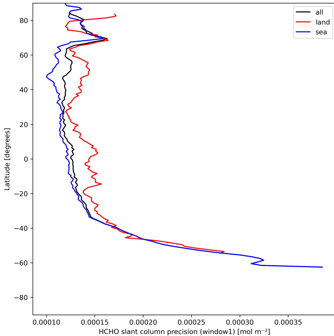
Figure 25: Zonal average of “HCHO slant column precision (window1)” for 2023-07-13 to 2023-07-14.
