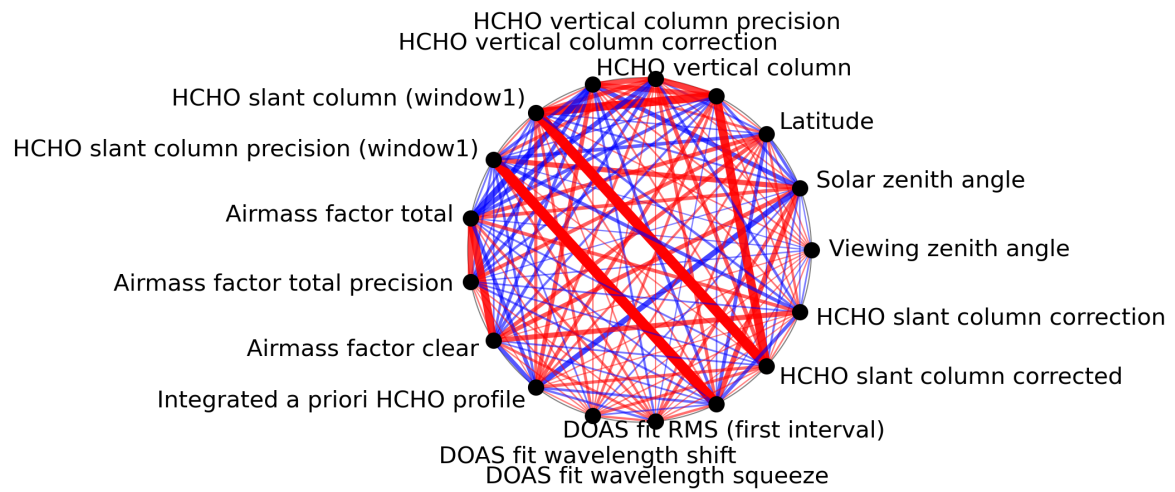
Figure 1: Map of correlation graph for 2023-07-13 to 2023-07-14.
