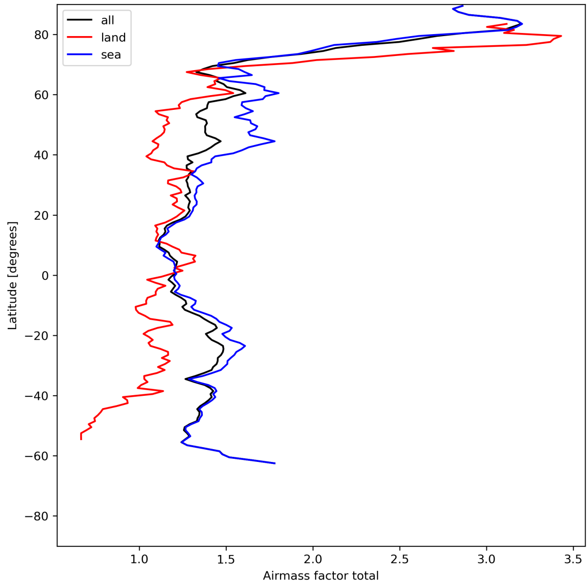
Figure 26: Zonal average of “Airmass factor total” for 2023-07-13 to 2023-07-14.
