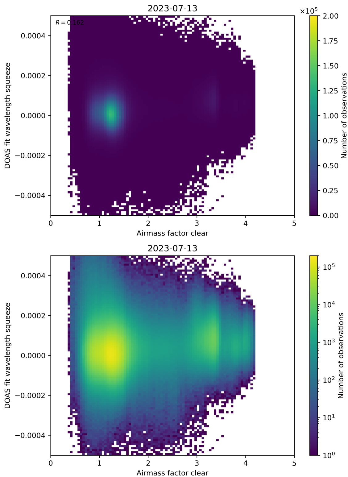
Figure 73: Scatter density plot of “Airmass factor clear” against “DOAS fit wavelength squeeze” for 2023-07-13 to 2023-07-14.
