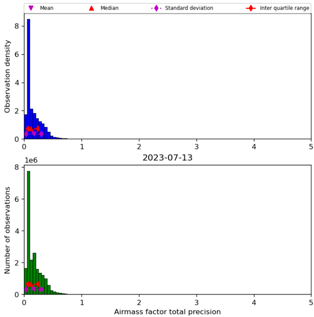
Figure 41: Histogram of “Airmass factor total precision” for 2023-07-13 to 2023-07-14
