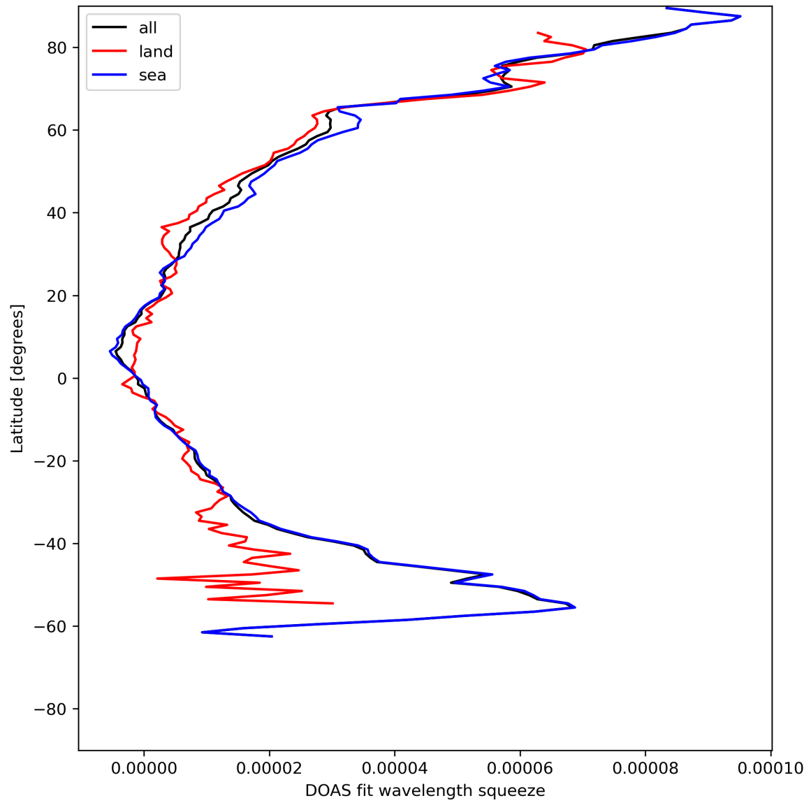
Figure 31: Zonal average of “DOAS fit wavelength squeeze” for 2023-07-13 to 2023-07-14.
