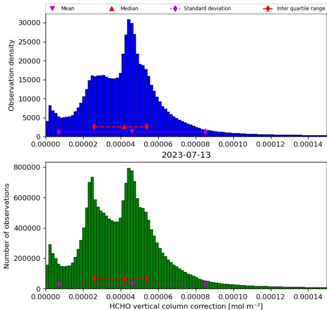
Figure 37: Histogram of “HCHO vertical column correction” for 2023-07-13 to 2023-07-14
