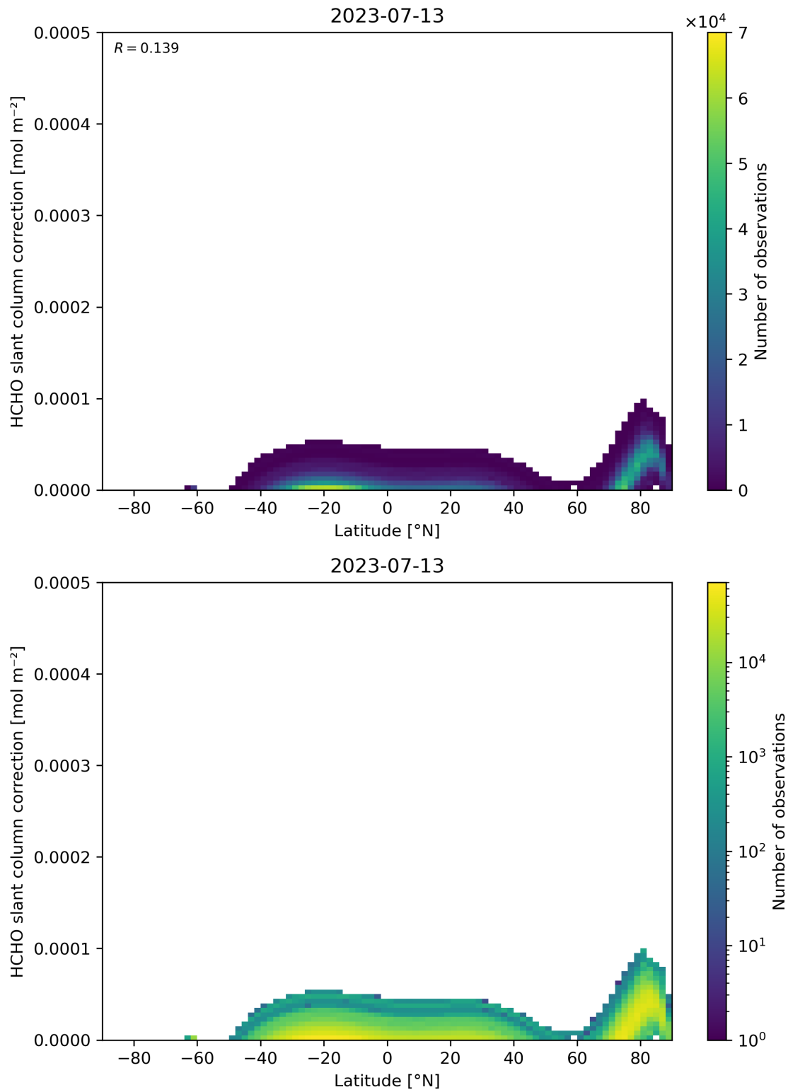
Figure 158: Scatter density plot of “Latitude” against “HCHO slant column correction” for 2023-07-13 to 2023-07-14.
