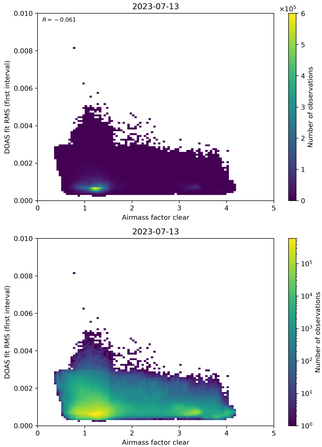
Figure 71: Scatter density plot of “Airmass factor clear” against “DOAS fit RMS (first interval)” for 2023-07-13 to 2023-07-14.
