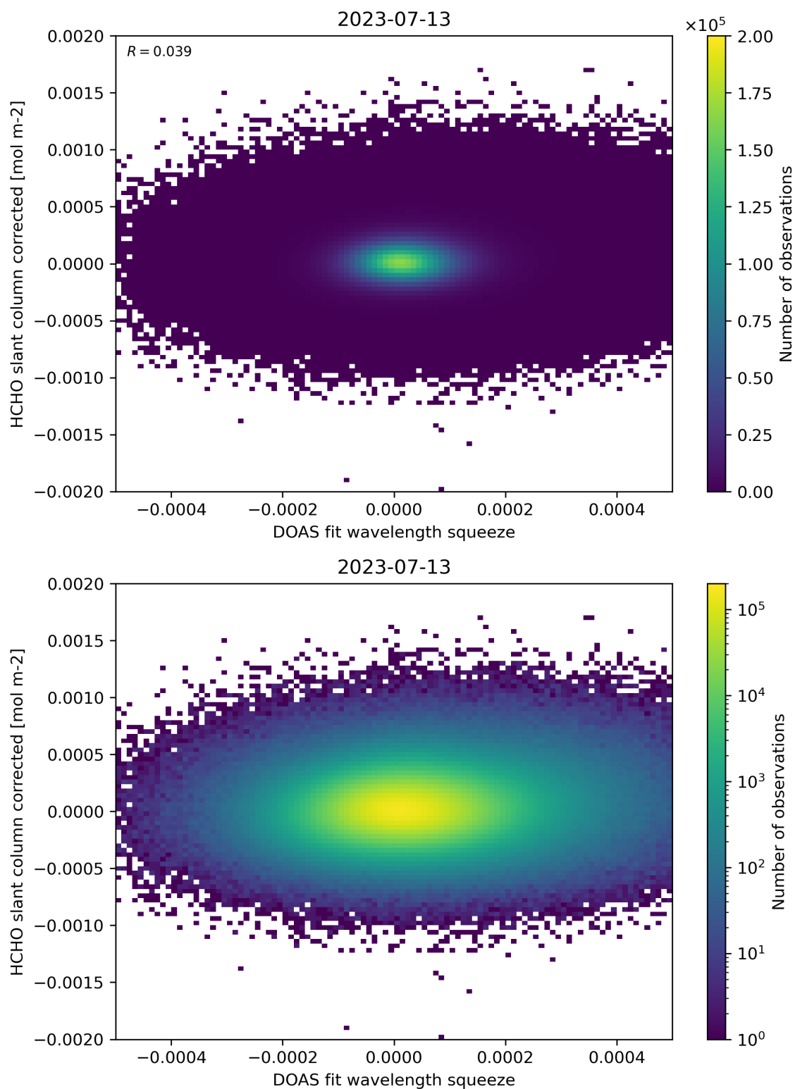
Figure 69: Scatter density plot of “DOAS fit wavelength squeeze” against “HCHO slant column corrected” for 2023-07-13 to 2023-07-14.
