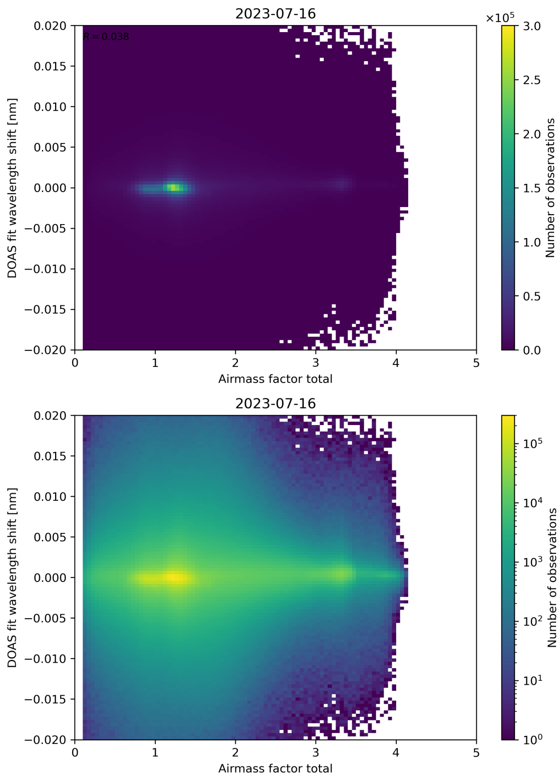
Figure 98: Scatter density plot of “Airmass factor total” against “DOAS fit wavelength shift” for 2023-07-15 to 2023-07-17.
