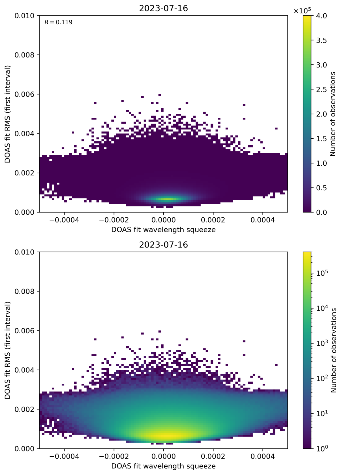
Figure 68: Scatter density plot of “DOAS fit wavelength squeeze” against “DOAS fit RMS (first interval)” for 2023-07-15 to 2023-07-17.
