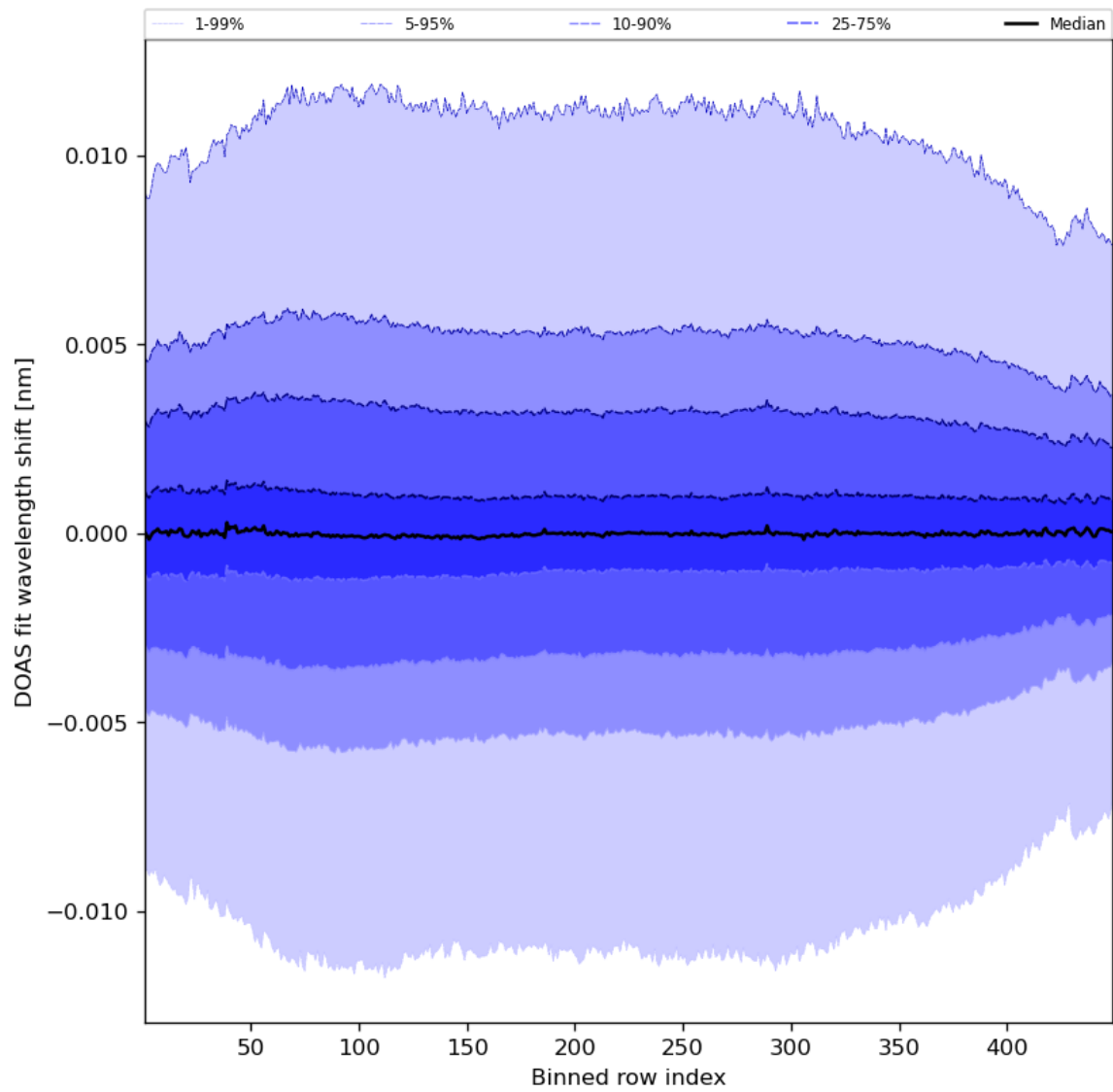
Figure 58: Along track statistics of “DOAS fit wavelength shift” for 2023-07-15 to 2023-07-17
