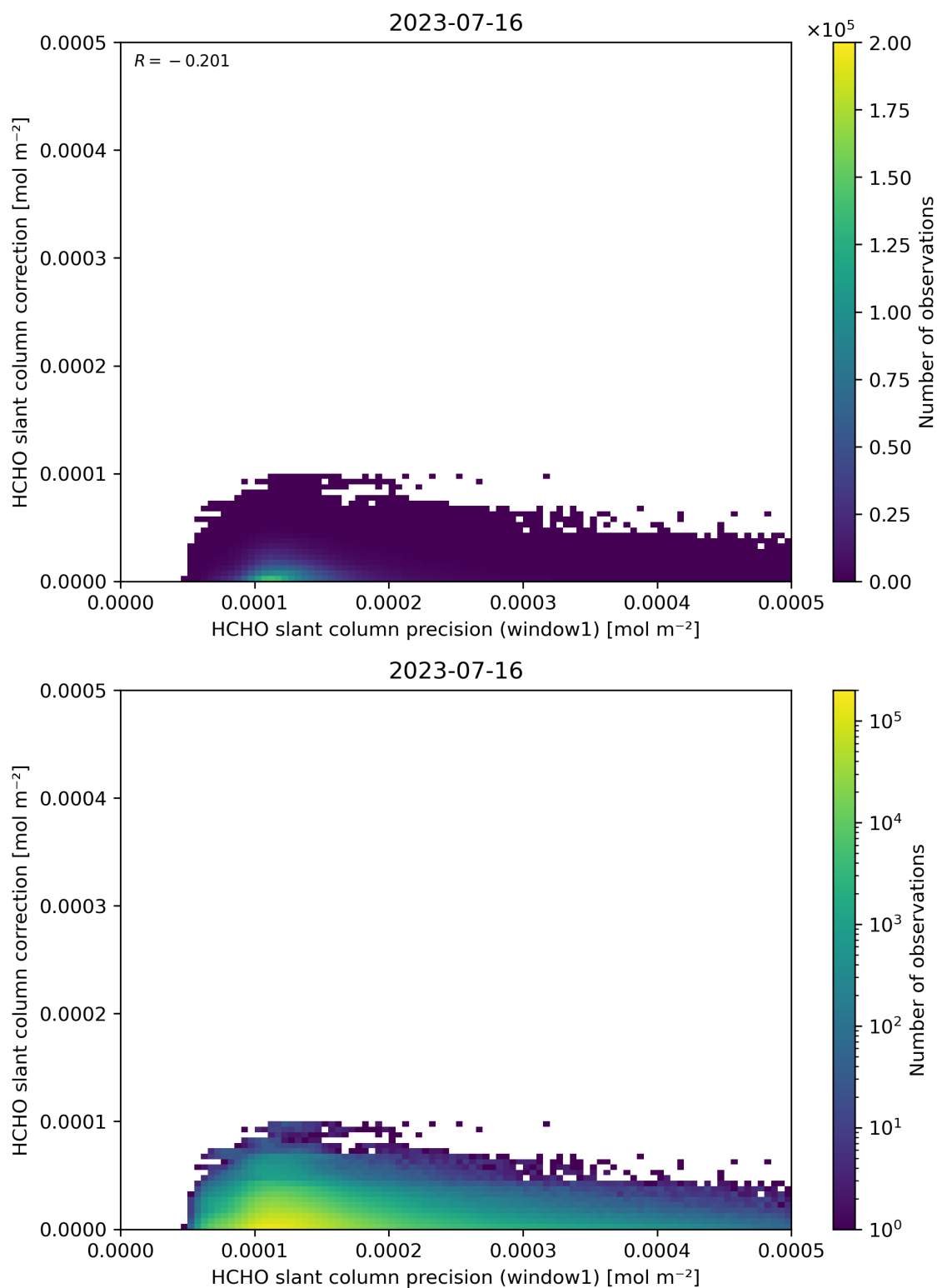
Figure 93: Scatter density plot of “HCHO slant column precision (window1)” against “HCHO slant column correction” for 2023-07-15 to 2023-07-17.
