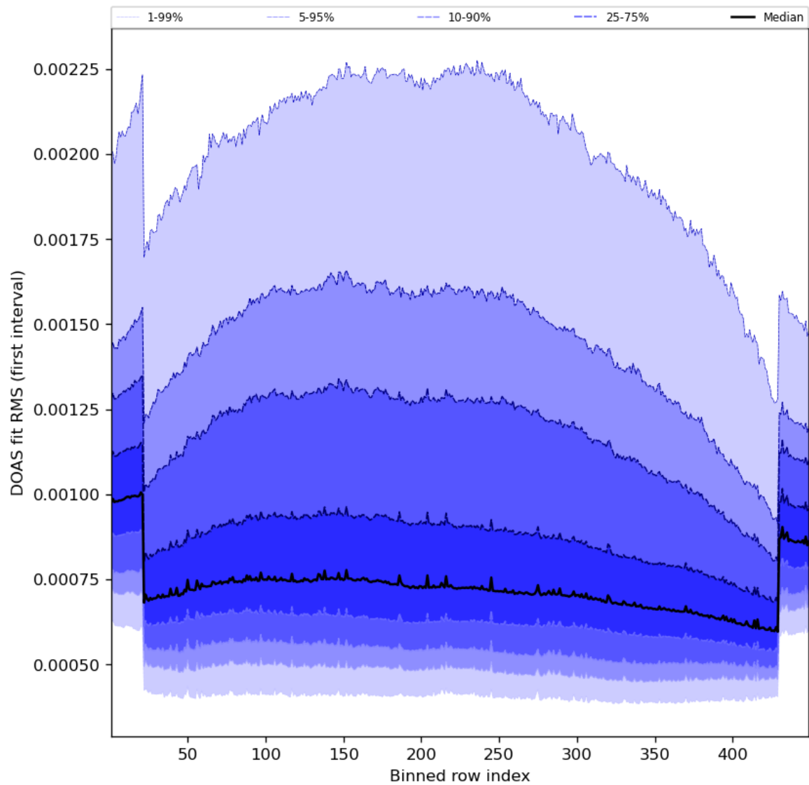
Figure 60: Along track statistics of “DOAS fit RMS (first interval)” for 2023-07-15 to 2023-07-17
