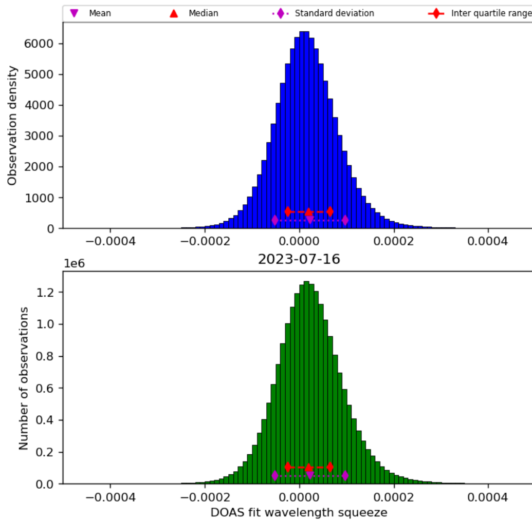
Figure 45: Histogram of “DOAS fit wavelength squeeze” for 2023-07-15 to 2023-07-17
