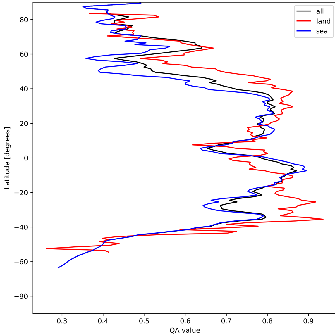
Figure 20: Zonal average of “QA value” for 2023-07-15 to 2023-07-17.
