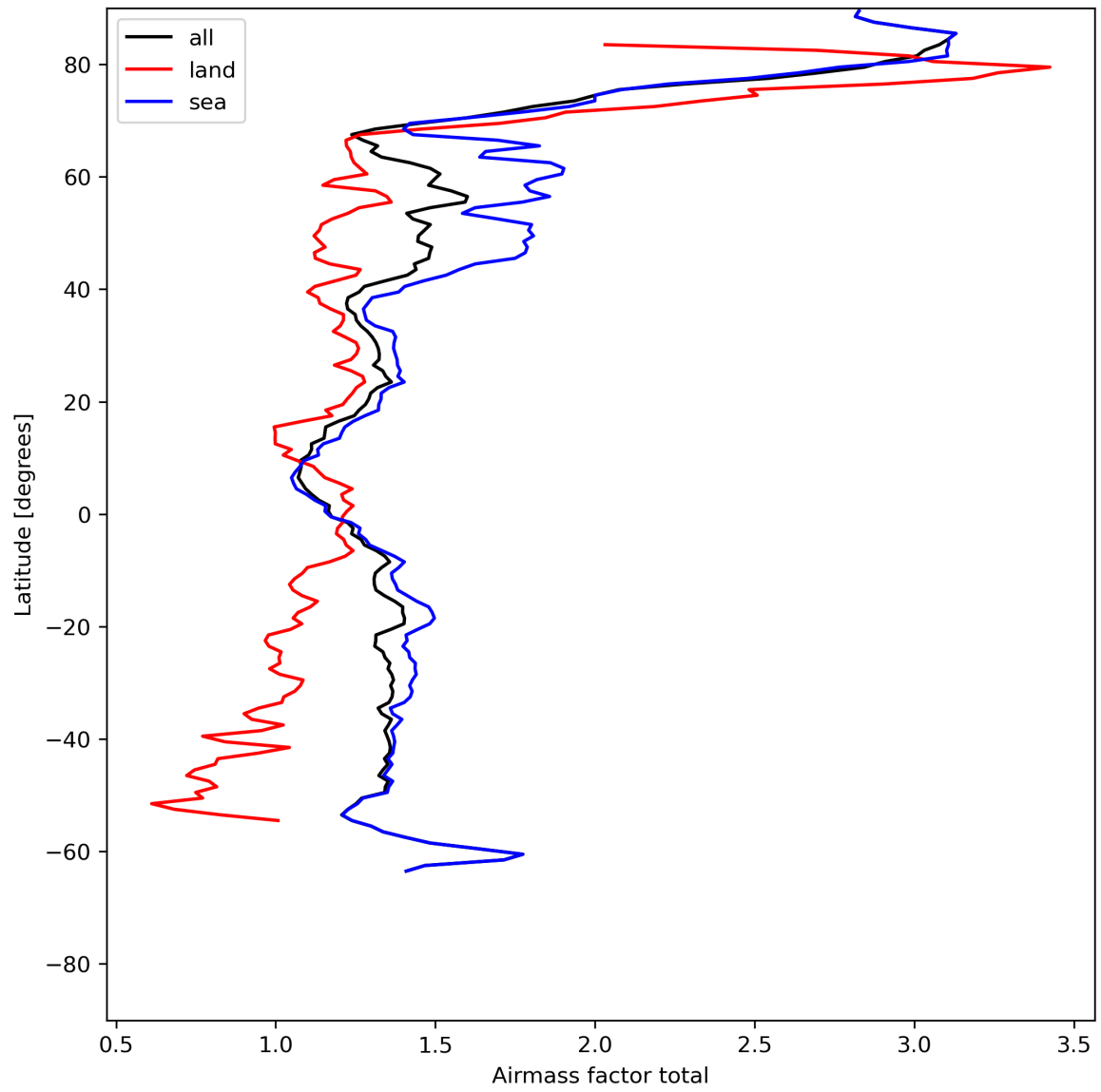
Figure 26: Zonal average of “Airmass factor total” for 2023-07-15 to 2023-07-17.
