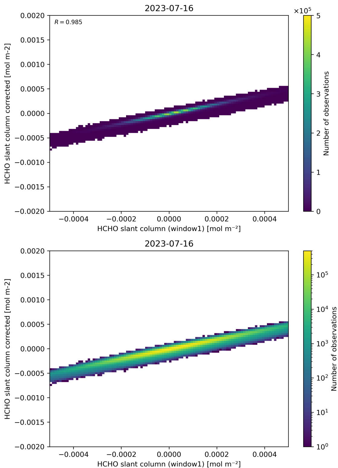
Figure 82: Scatter density plot of “HCHO slant column (window1)” against “HCHO slant column corrected” for 2023-07-15 to 2023-07-17.
