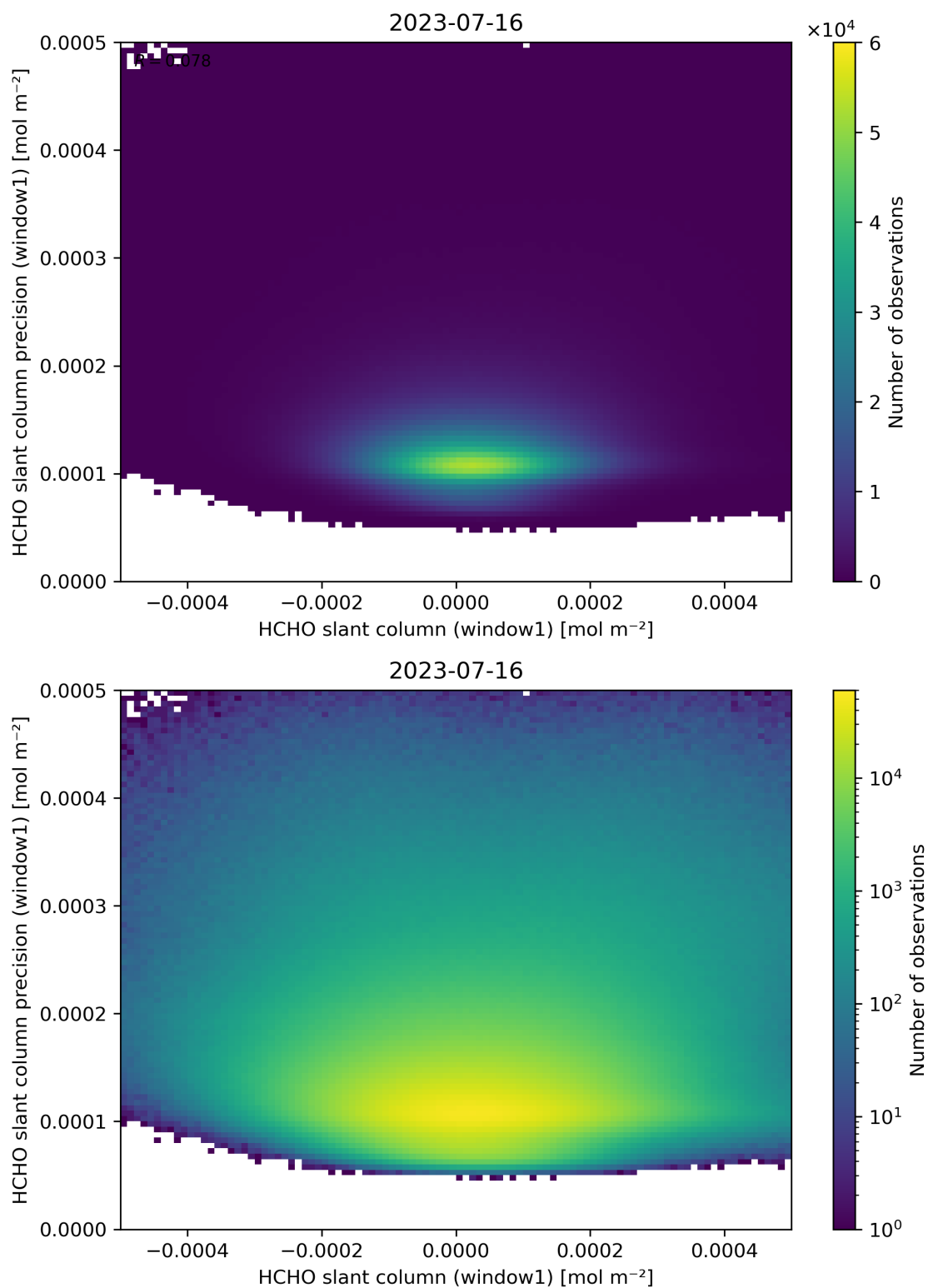
Figure 84: Scatter density plot of “HCHO slant column (window1)” against “HCHO slant column precision (window1)” for 2023-07-15 to 2023-07-17.
