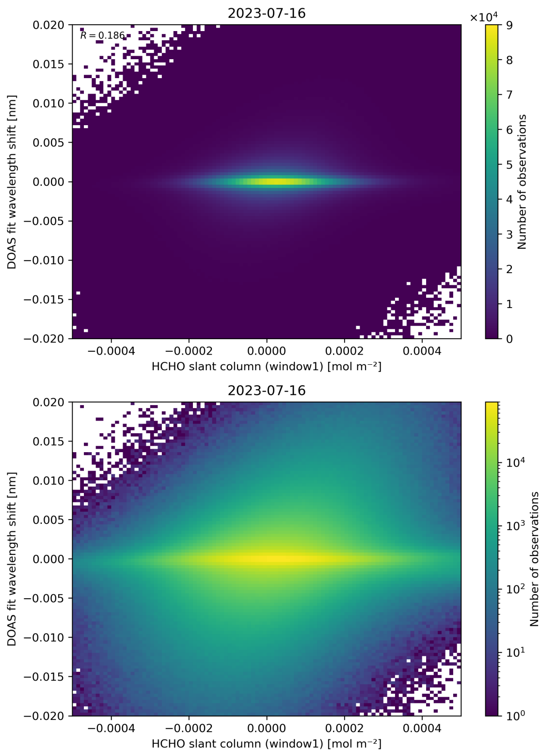
Figure 79: Scatter density plot of “HCHO slant column (window1)” against “DOAS fit wavelength shift” for 2023-07-15 to 2023-07-17.
