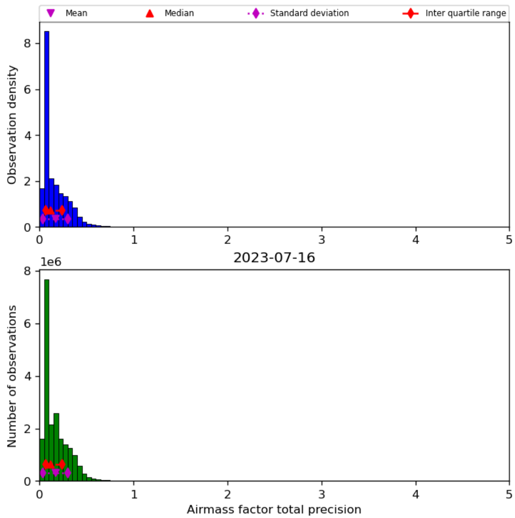
Figure 41: Histogram of “Airmass factor total precision” for 2023-07-15 to 2023-07-17
