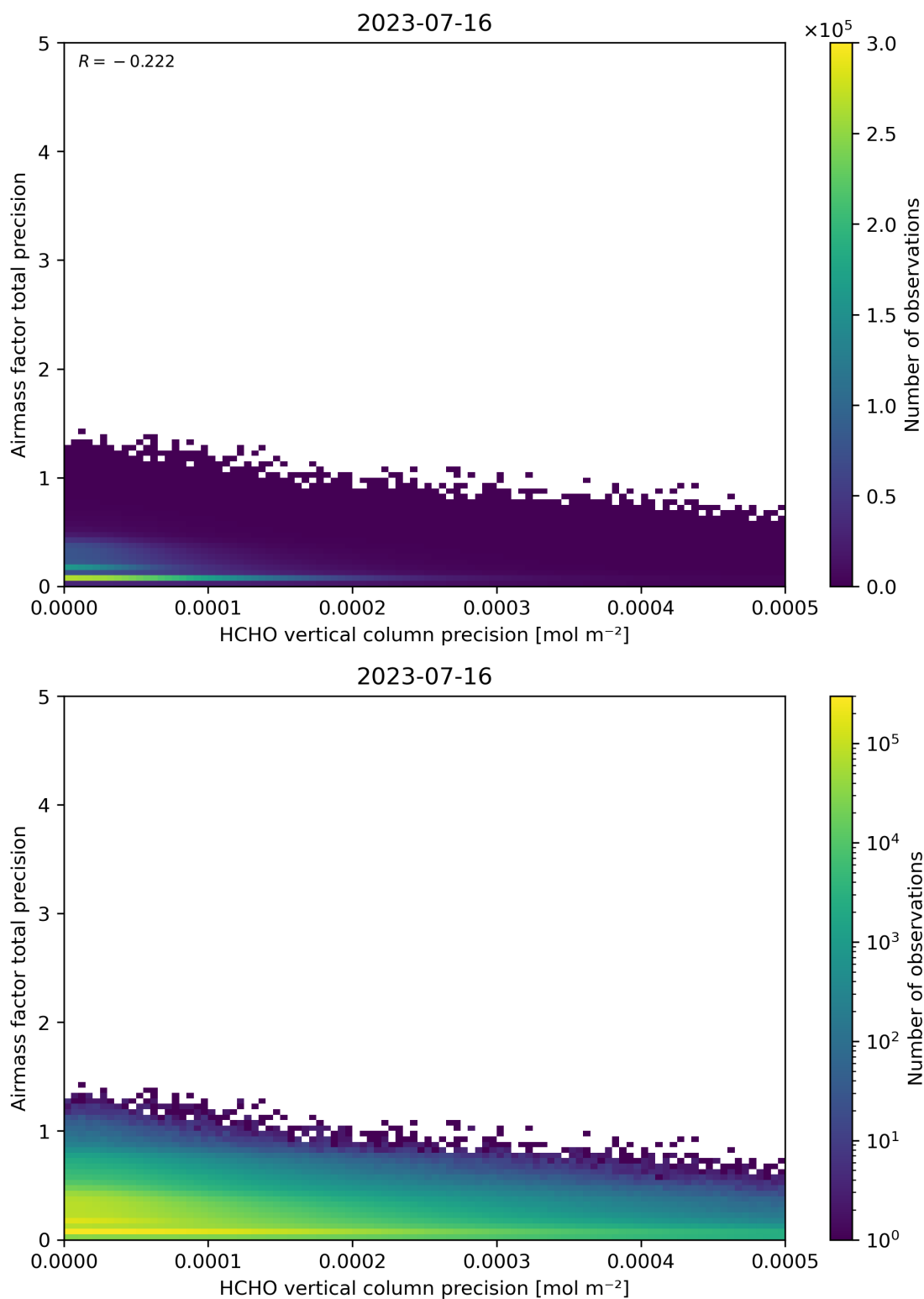
Figure 145: Scatter density plot of “HCHO vertical column precision” against “Airmass factor total precision” for 2023-07-15 to 2023-07-17.
