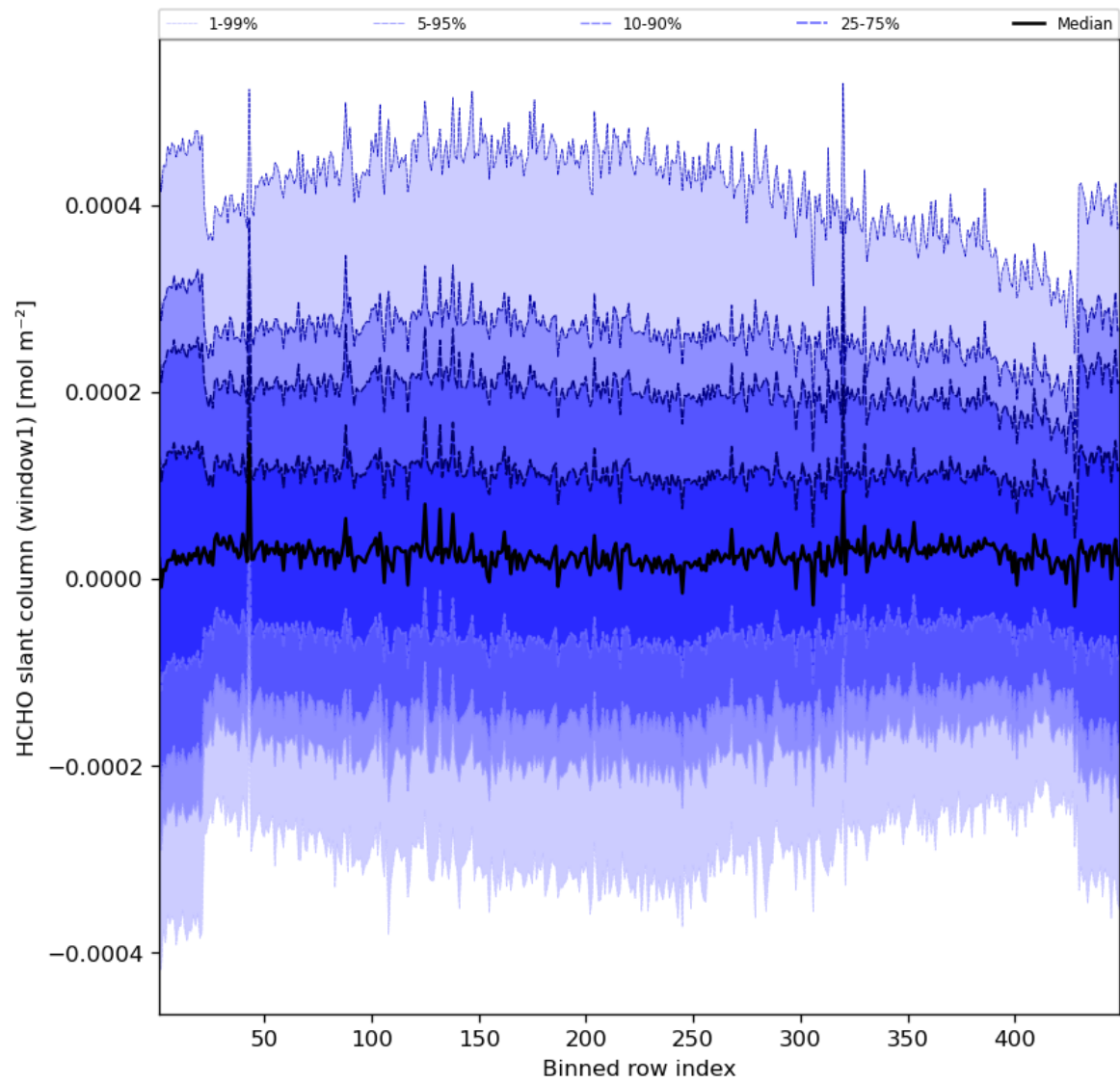
Figure 52: Along track statistics of “HCHO slant column (window1)” for 2023-07-15 to 2023-07-17
