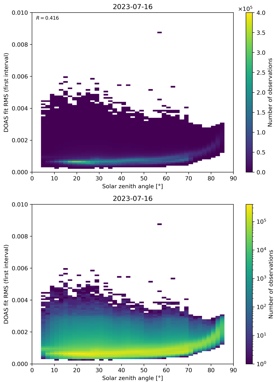
Figure 167: Scatter density plot of “Solar zenith angle” against “DOAS fit RMS (first interval)” for 2023-07-15 to 2023-07-17.
