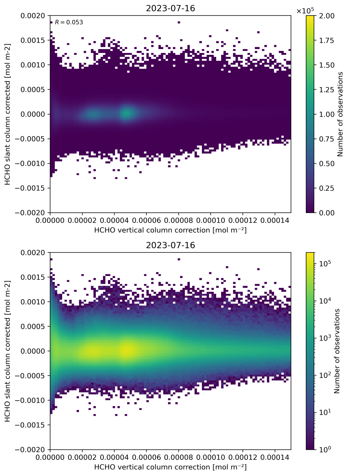
Figure 116: Scatter density plot of “HCHO vertical column correction” against “HCHO slant column corrected” for 2023-07-15 to 2023-07-17.
