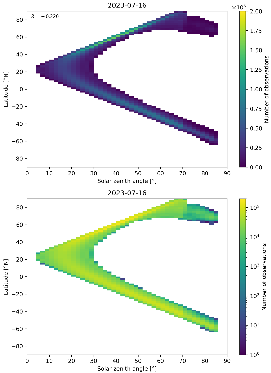
Figure 181: Scatter density plot of “Solar zenith angle” against “Latitude” for 2023-07-15 to 2023-07-17.
