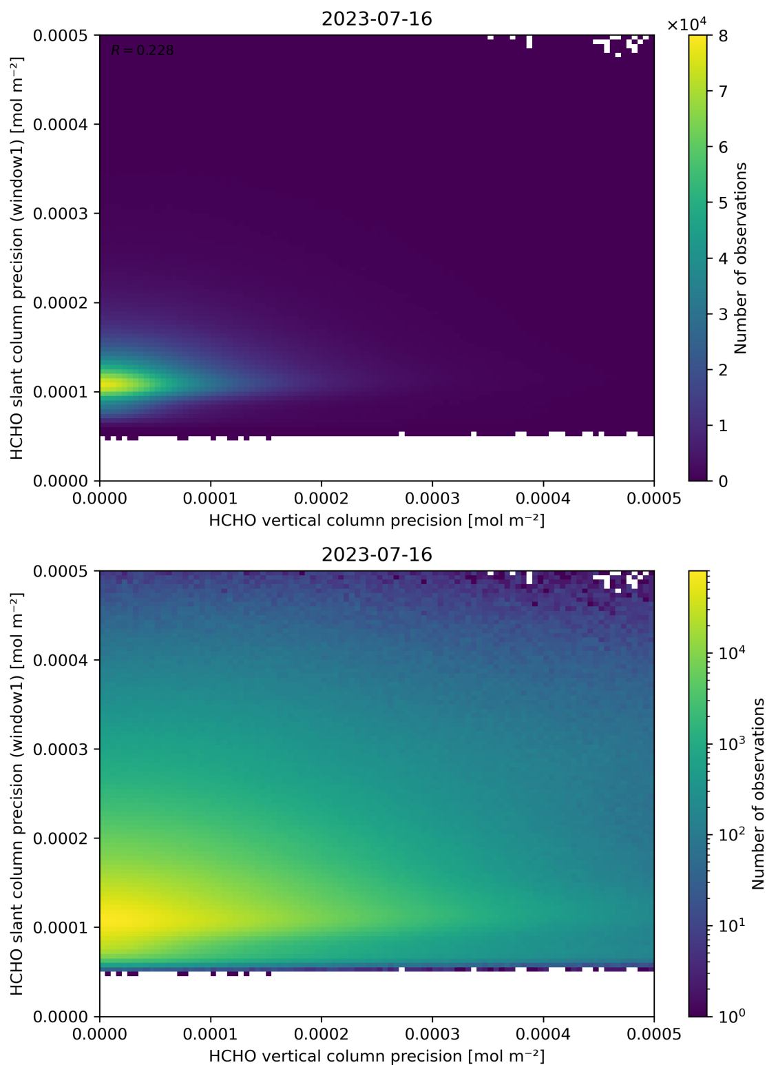
Figure 143: Scatter density plot of “HCHO vertical column precision” against “HCHO slant column precision (window1)” for 2023-07-15 to 2023-07-17.
