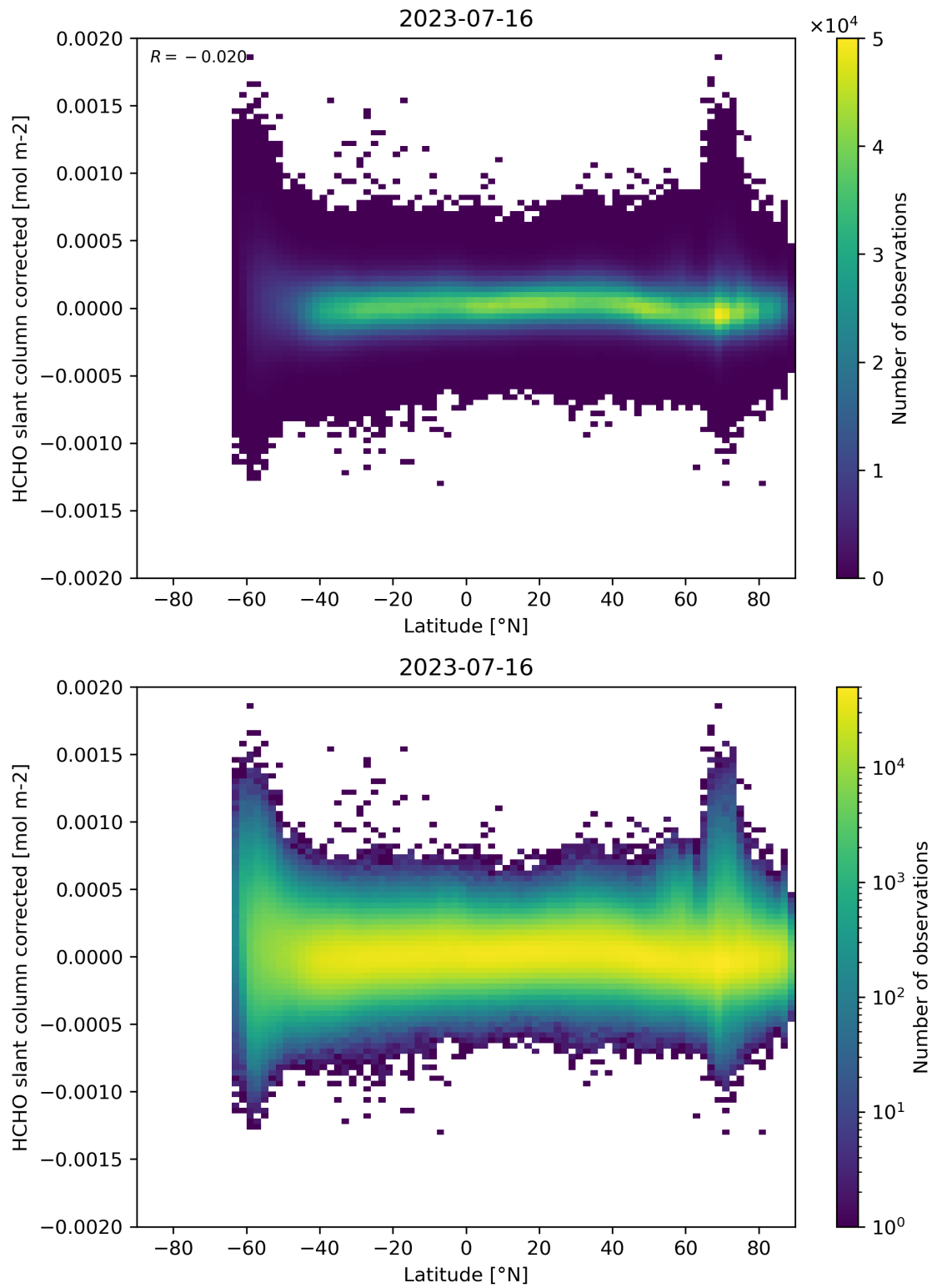
Figure 157: Scatter density plot of “Latitude” against “HCHO slant column corrected” for 2023-07-15 to 2023-07-17.
