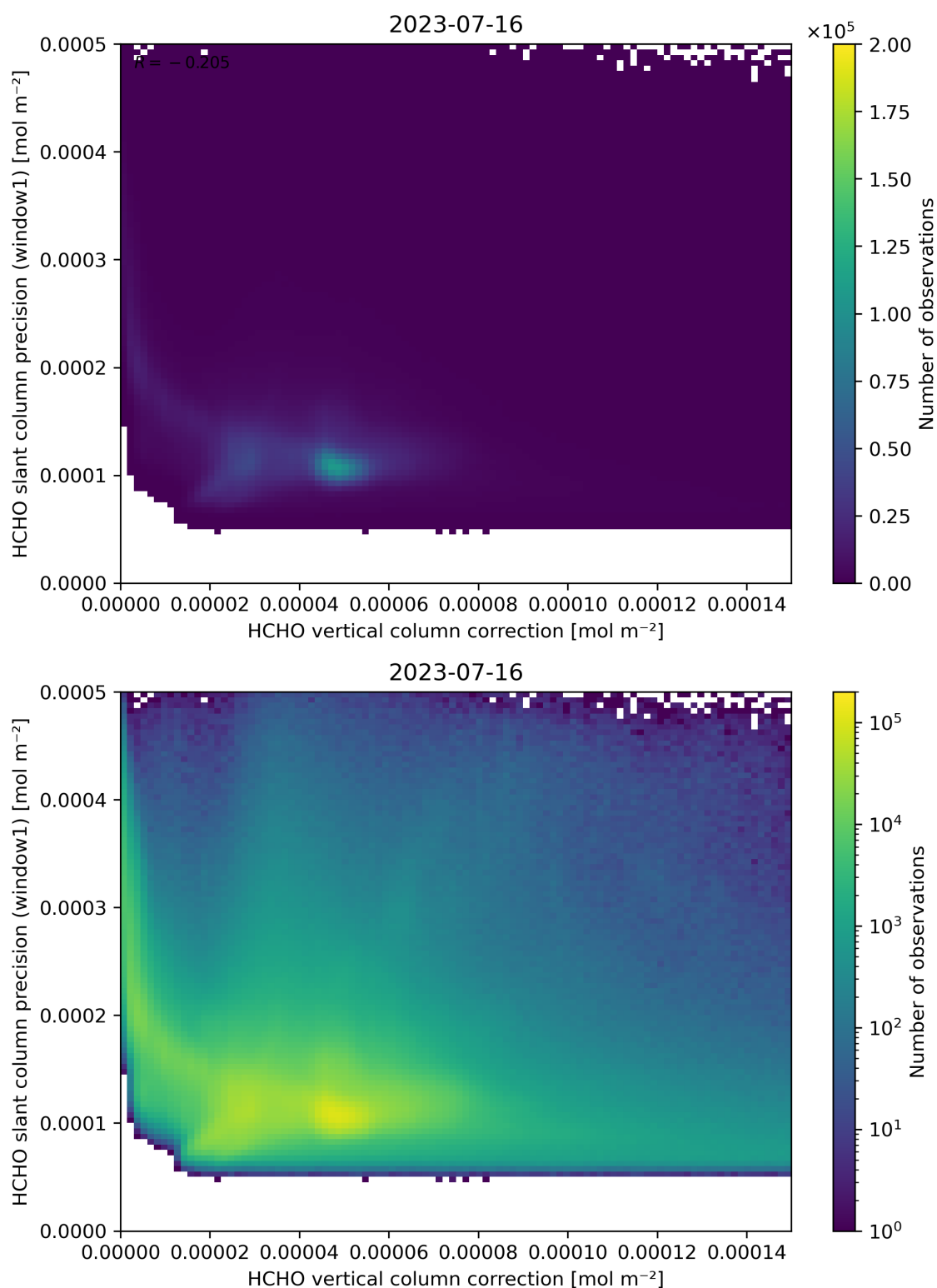
Figure 119: Scatter density plot of “HCHO vertical column correction” against “HCHO slant column precision (window1)” for 2023-07-15 to 2023-07-17.
