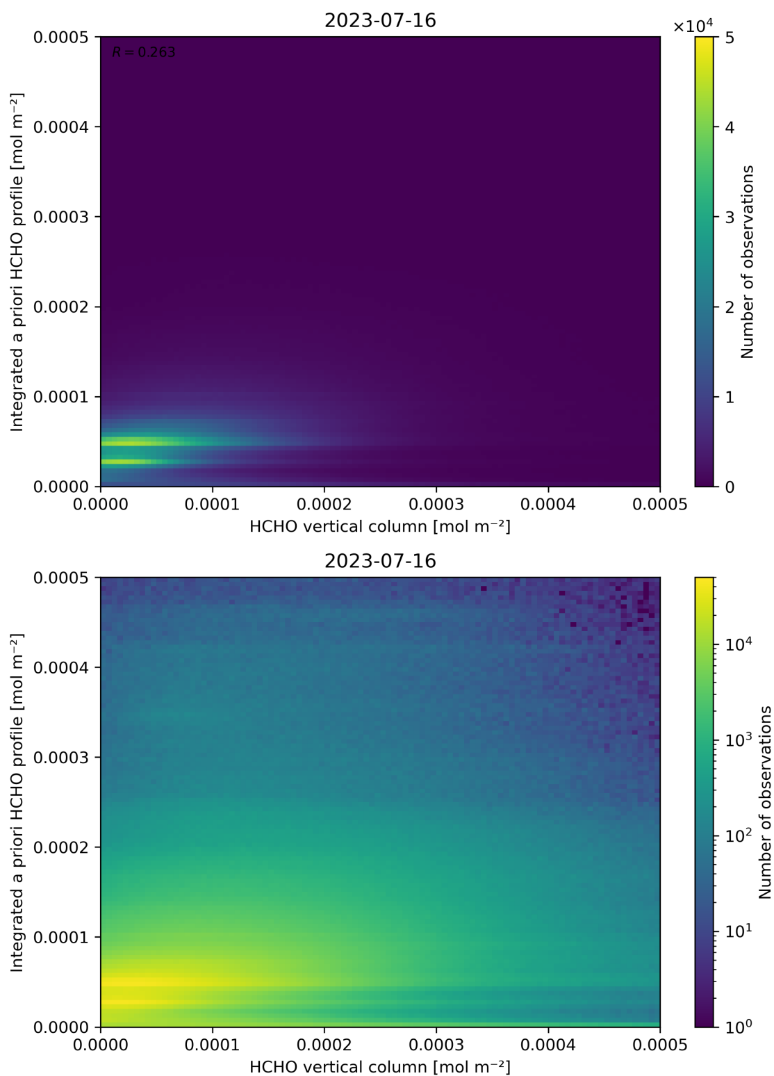
Figure 135: Scatter density plot of “HCHO vertical column” against “Integrated a priori HCHO profile” for 2023-07-15 to 2023-07-17.
