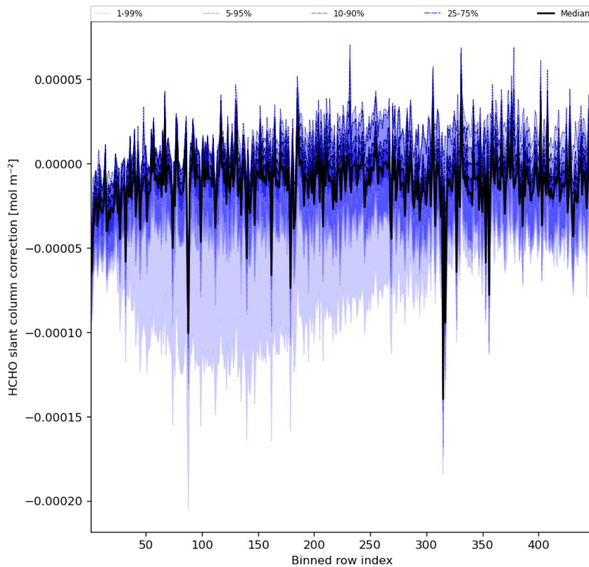
Figure 61: Along track statistics of “HCHO slant column correction” for 2023-07-15 to 2023-07-17
