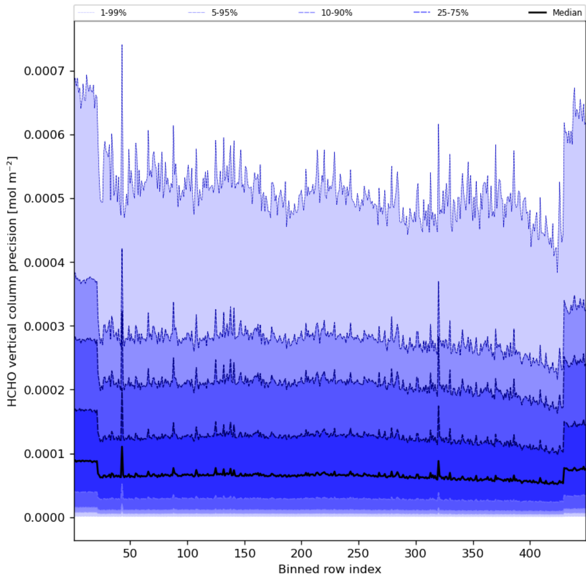
Figure 50: Along track statistics of “HCHO vertical column precision” for 2023-07-15 to 2023-07-17
