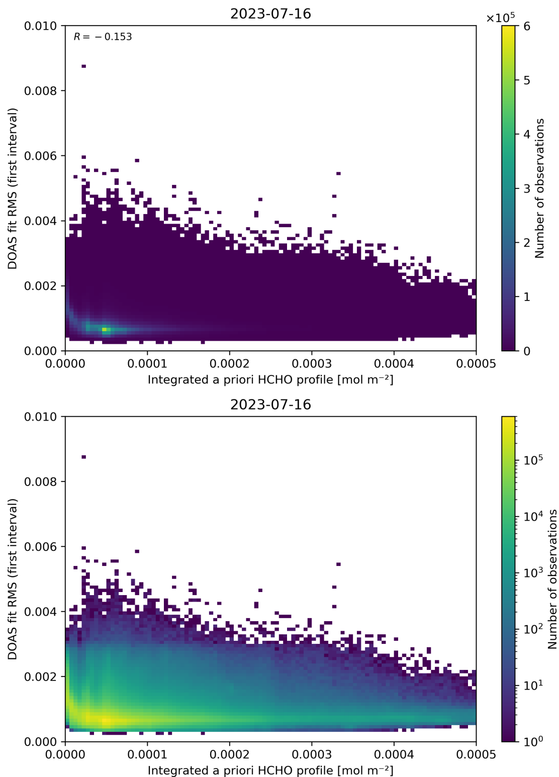
Figure 148: Scatter density plot of “Integrated a priori HCHO profile” against “DOAS fit RMS (first interval)” for 2023-07-15 to 2023-07-17.
