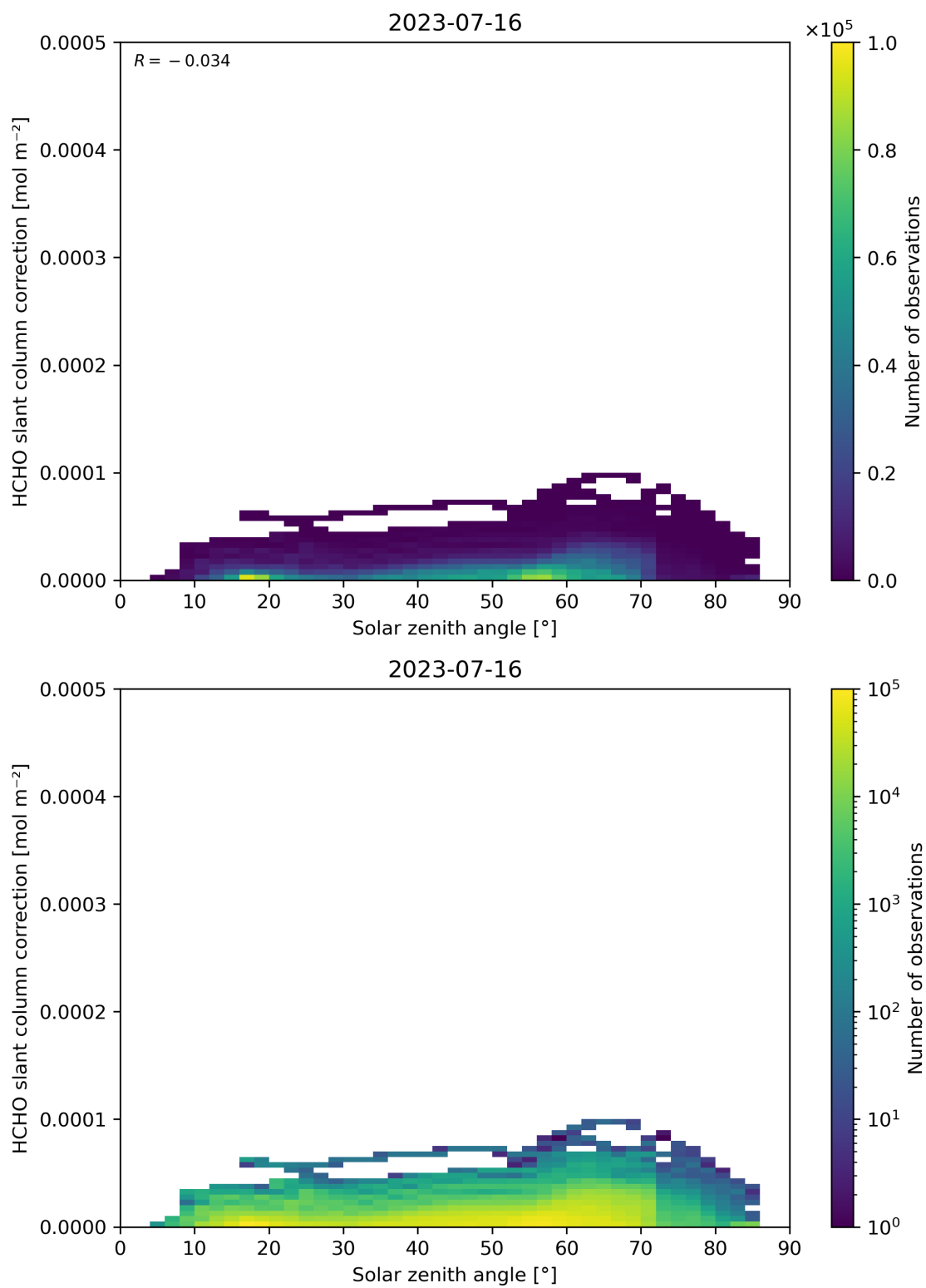
Figure 172: Scatter density plot of “Solar zenith angle” against “HCHO slant column correction” for 2023-07-15 to 2023-07-17.
