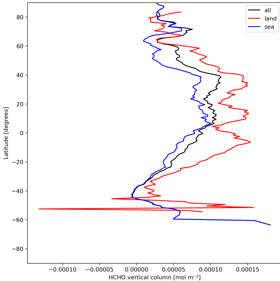
Figure 21: Zonal average of “HCHO vertical column” for 2023-07-15 to 2023-07-17.
