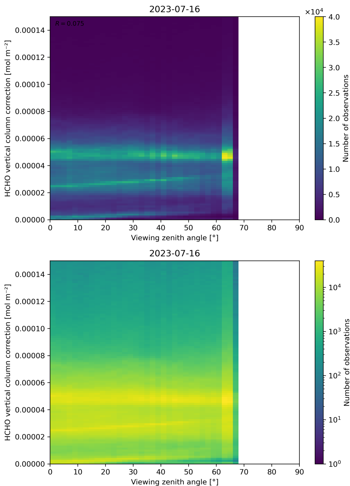
Figure 193: Scatter density plot of “Viewing zenith angle” against “HCHO vertical column correction” for 2023-07-15 to 2023-07-17.
