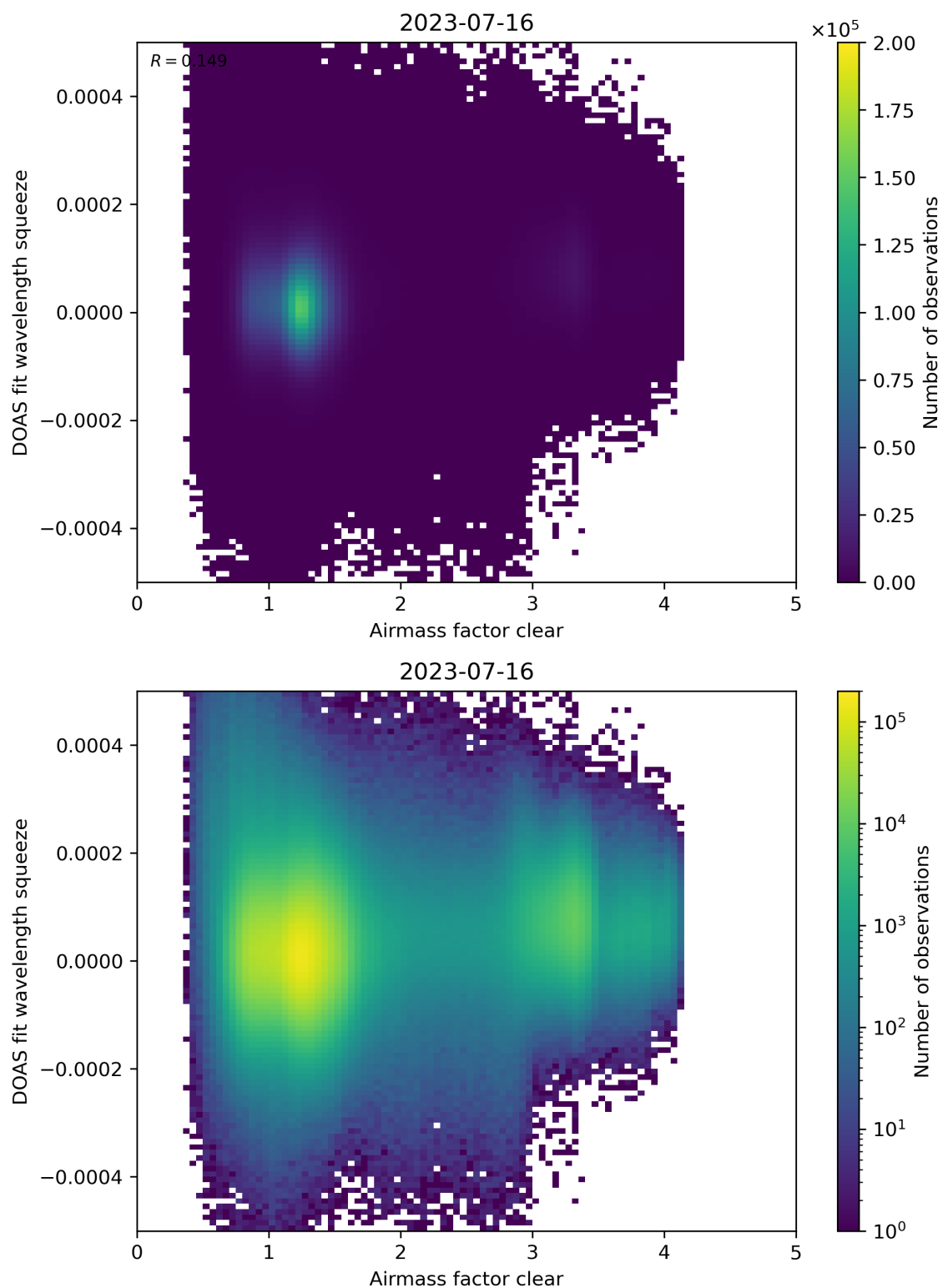
Figure 73: Scatter density plot of “Airmass factor clear” against “DOAS fit wavelength squeeze” for 2023-07-15 to 2023-07-17.
