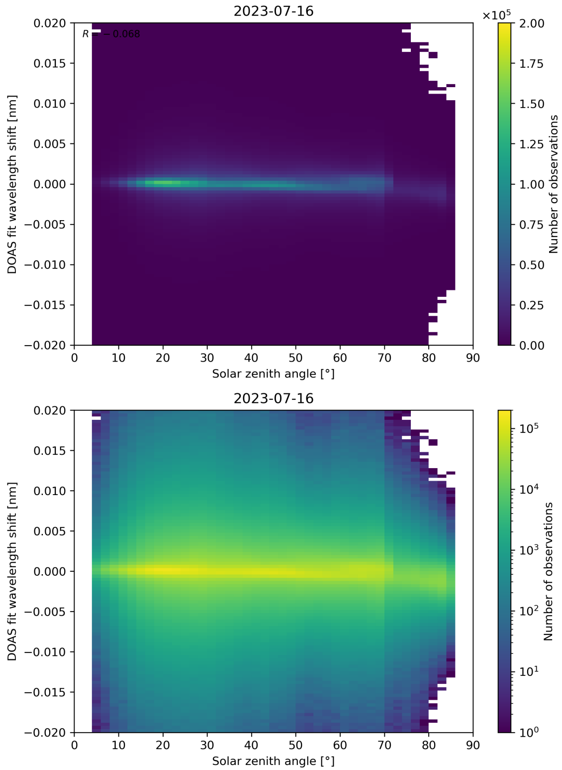
Figure 168: Scatter density plot of “Solar zenith angle” against “DOAS fit wavelength shift” for 2023-07-15 to 2023-07-17.
