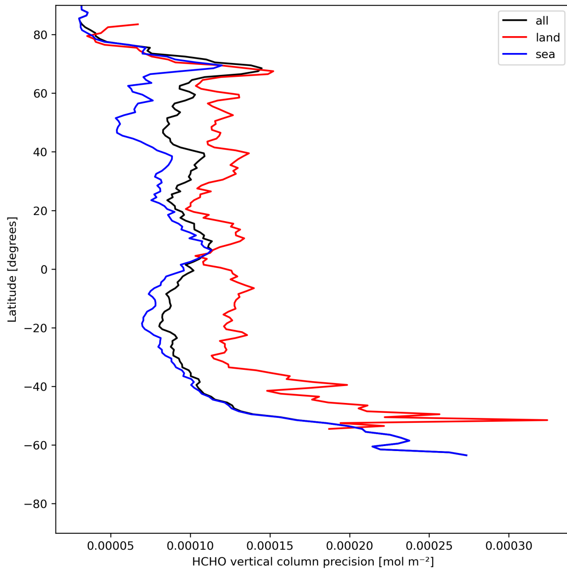
Figure 22: Zonal average of “HCHO vertical column precision” for 2023-07-15 to 2023-07-17.
