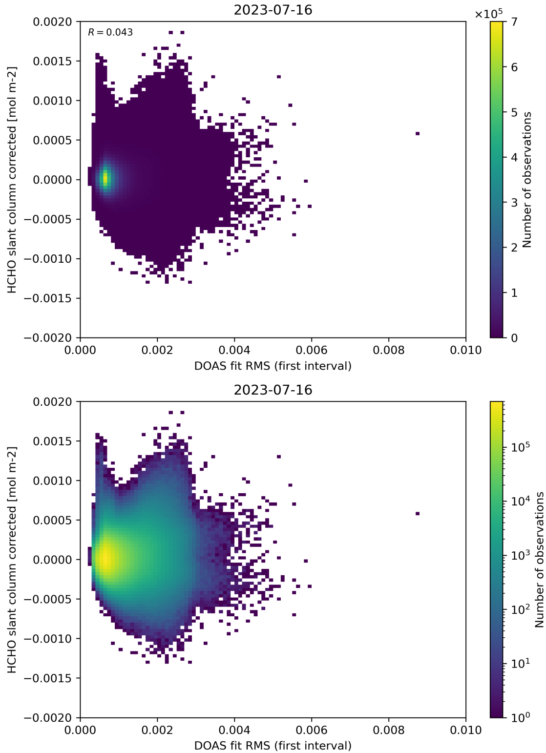
Figure 62: Scatter density plot of “DOAS fit RMS (first interval)” against “HCHO slant column corrected” for 2023-07-15 to 2023-07-17.
