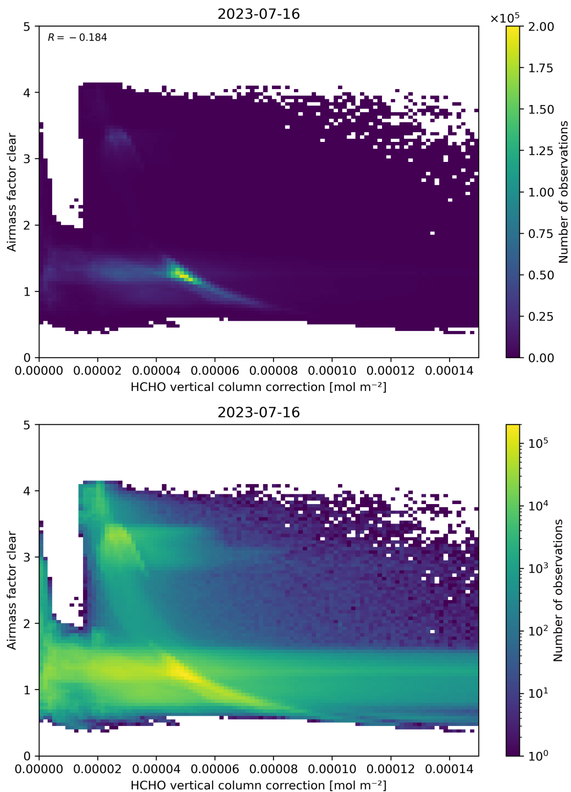
Figure 115: Scatter density plot of “HCHO vertical column correction” against “Airmass factor clear” for 2023-07-15 to 2023-07-17.
