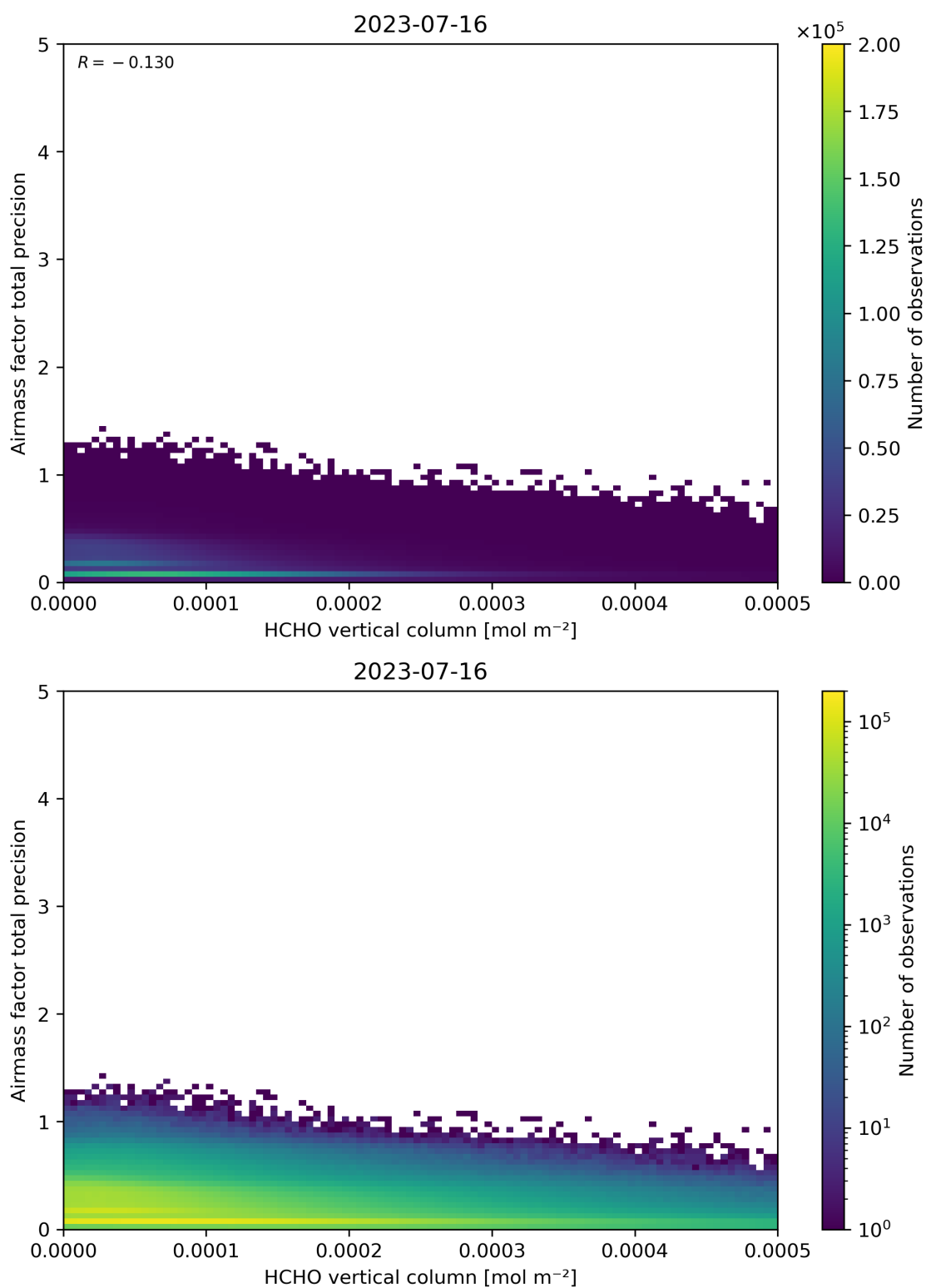
Figure 132: Scatter density plot of “HCHO vertical column” against “Airmass factor total precision” for 2023-07-15 to 2023-07-17.
