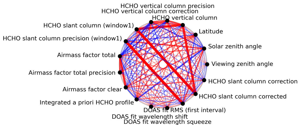
Figure 1: Map of correlation graph for 2023-07-15 to 2023-07-17.
