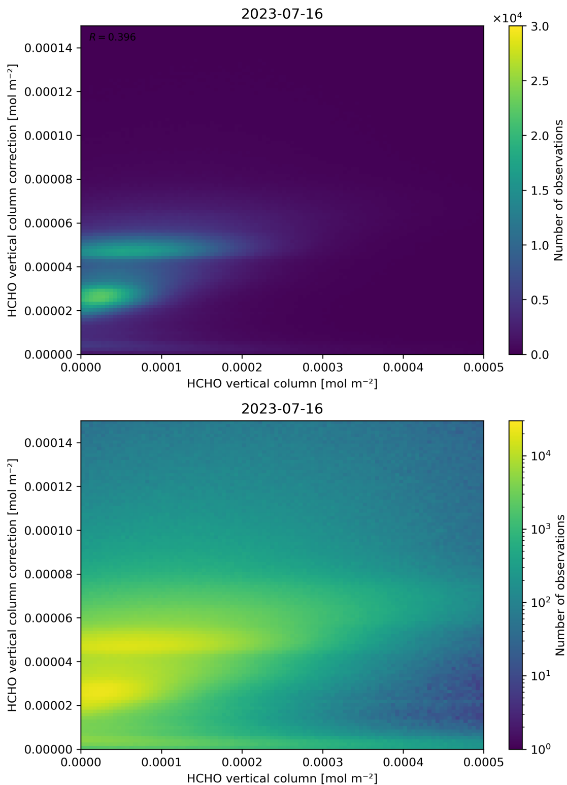
Figure 133: Scatter density plot of “HCHO vertical column” against “HCHO vertical column correction” for 2023-07-15 to 2023-07-17.
