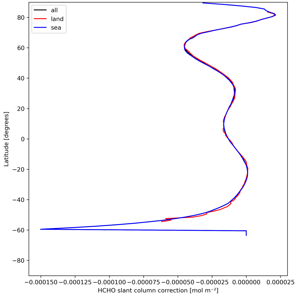
Figure 33: Zonal average of “HCHO slant column correction” for 2023-07-15 to 2023-07-17.
