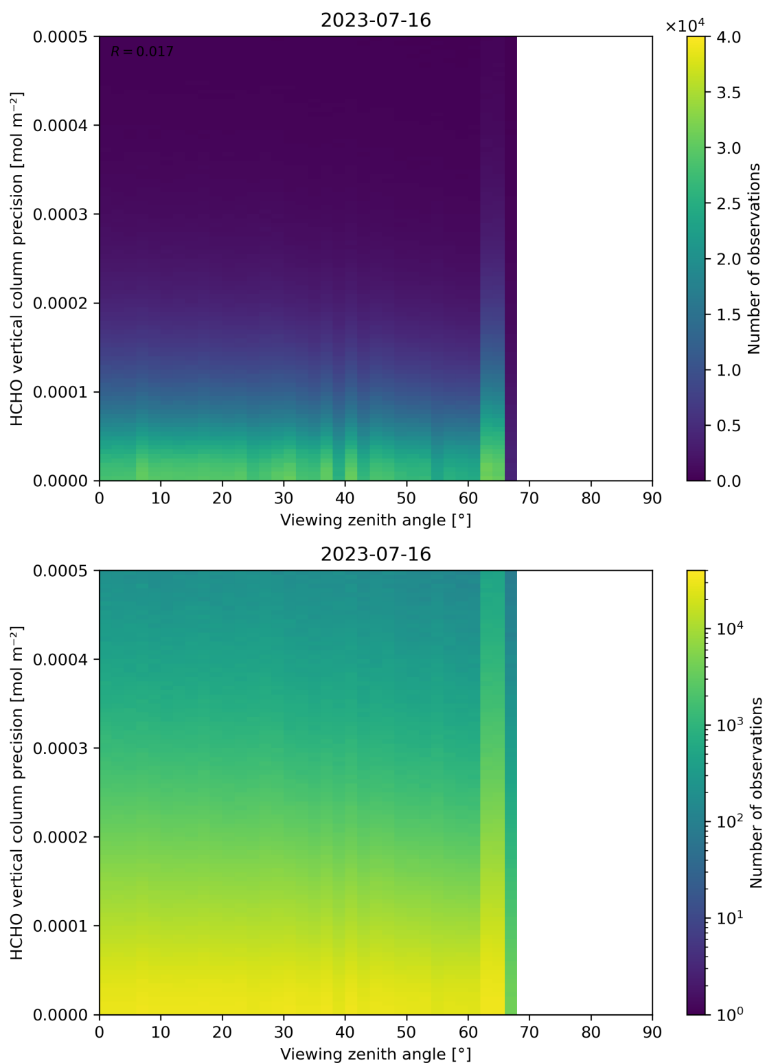
Figure 194: Scatter density plot of “Viewing zenith angle” against “HCHO vertical column precision” for 2023-07-15 to 2023-07-17.
