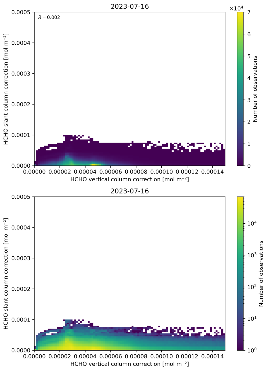
Figure 117: Scatter density plot of “HCHO vertical column correction” against “HCHO slant column correction” for 2023-07-15 to 2023-07-17.
