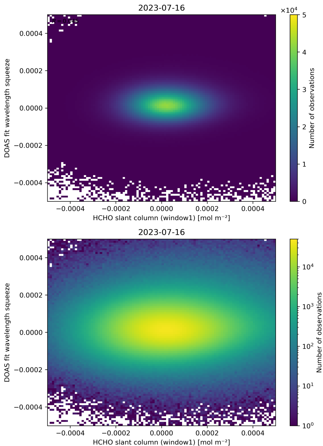
Figure 80: Scatter density plot of “HCHO slant column (window1)” against “DOAS fit wavelength squeeze” for 2023-07-15 to 2023-07-17.
