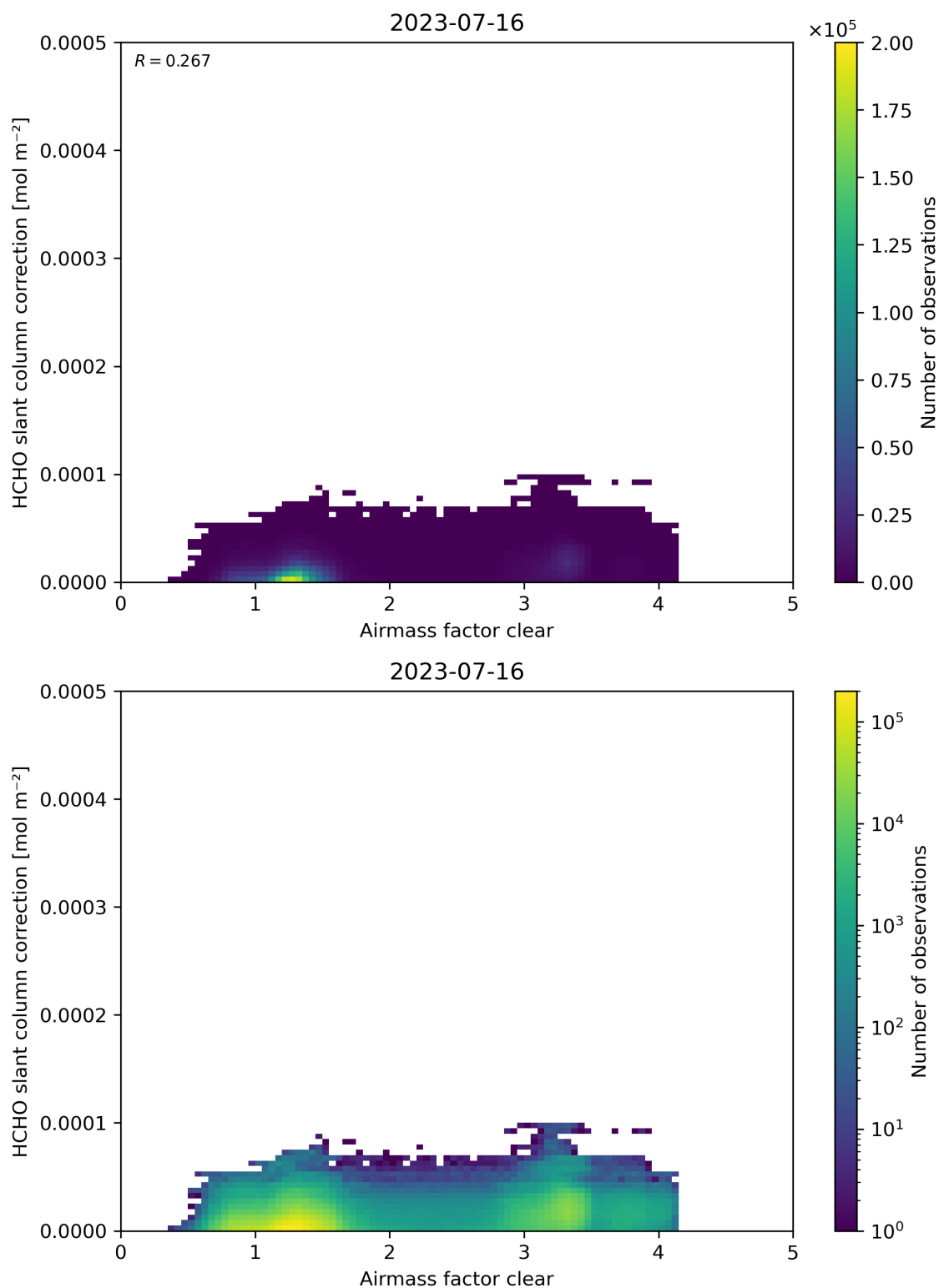
Figure 75: Scatter density plot of “Airmass factor clear” against “HCHO slant column correction” for 2023-07-15 to 2023-07-17.
