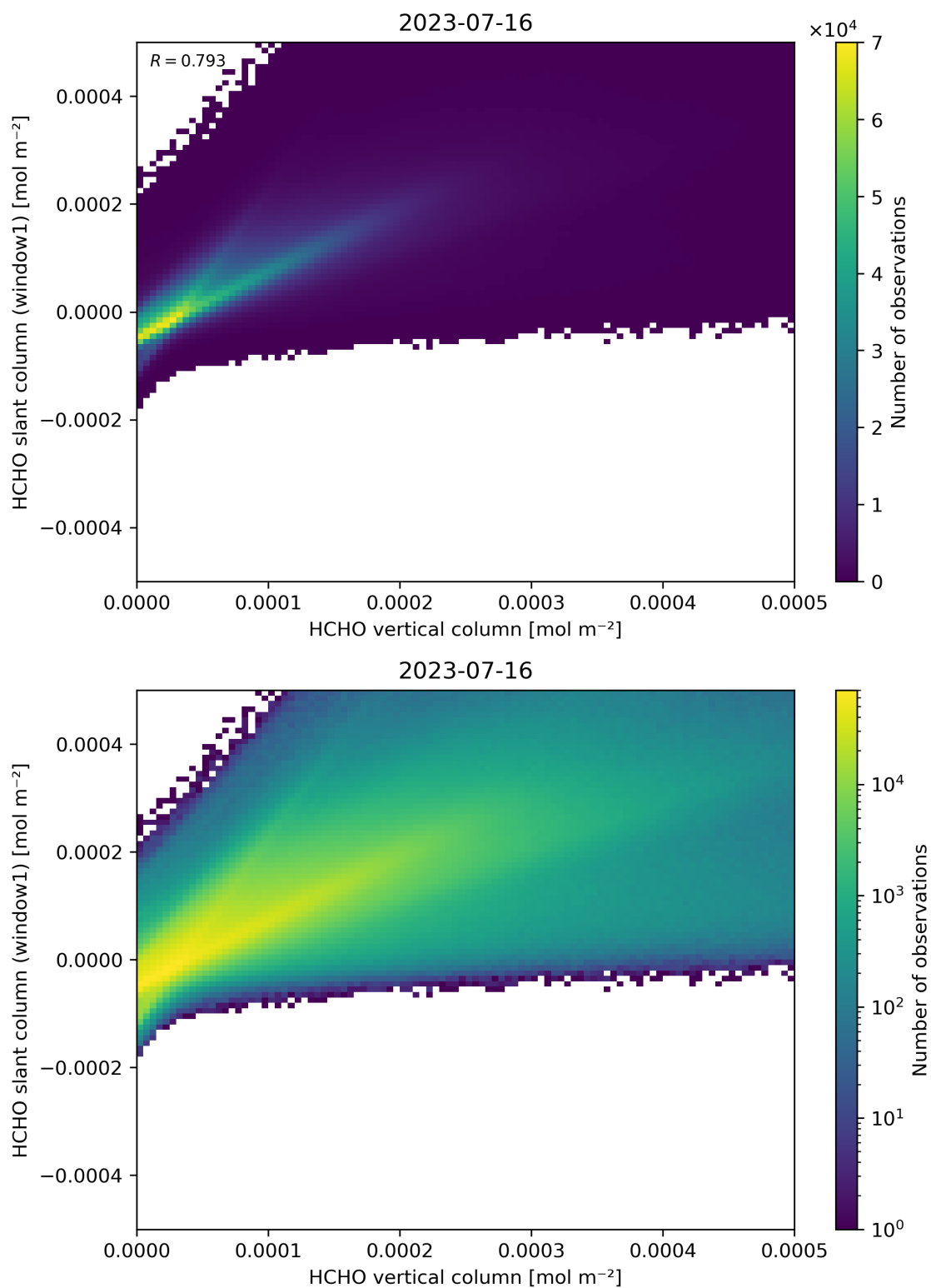
Figure 129: Scatter density plot of “HCHO vertical column” against “HCHO slant column (window1)” for 2023-07-15 to 2023-07-17.
