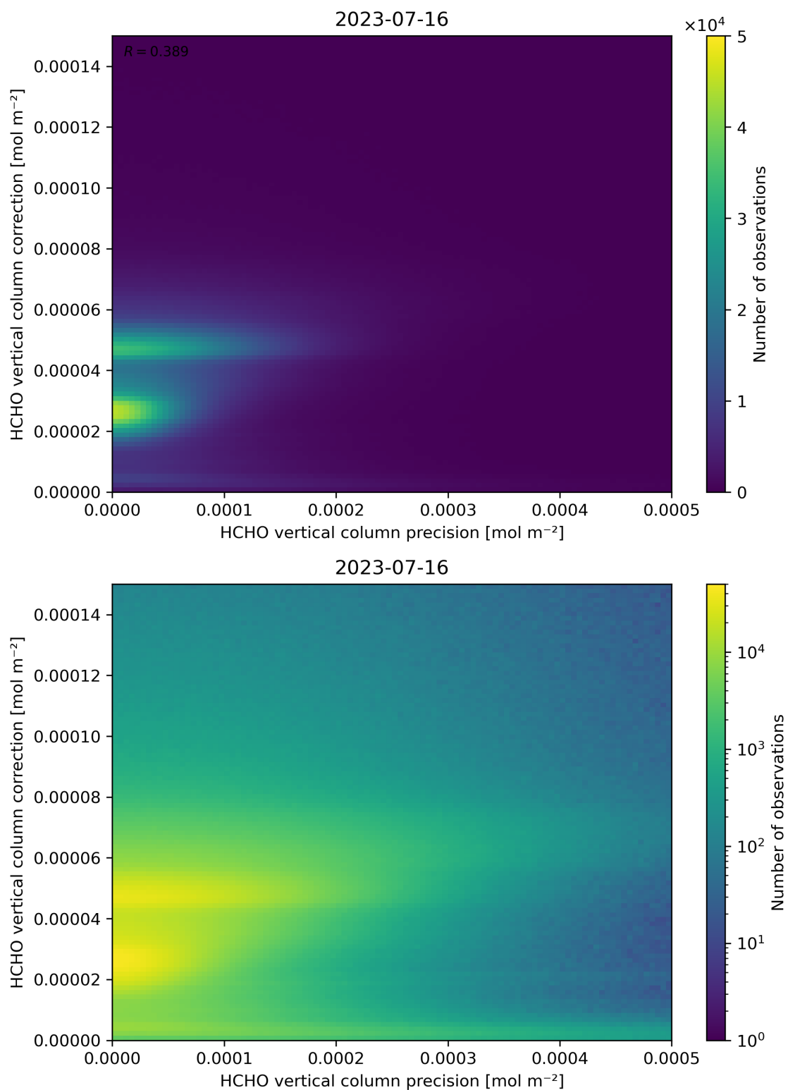
Figure 146: Scatter density plot of “HCHO vertical column precision” against “HCHO vertical column correction” for 2023-07-15 to 2023-07-17.
