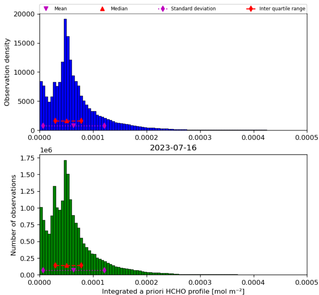
Figure 43: Histogram of “Integrated a priori HCHO profile” for 2023-07-15 to 2023-07-17
