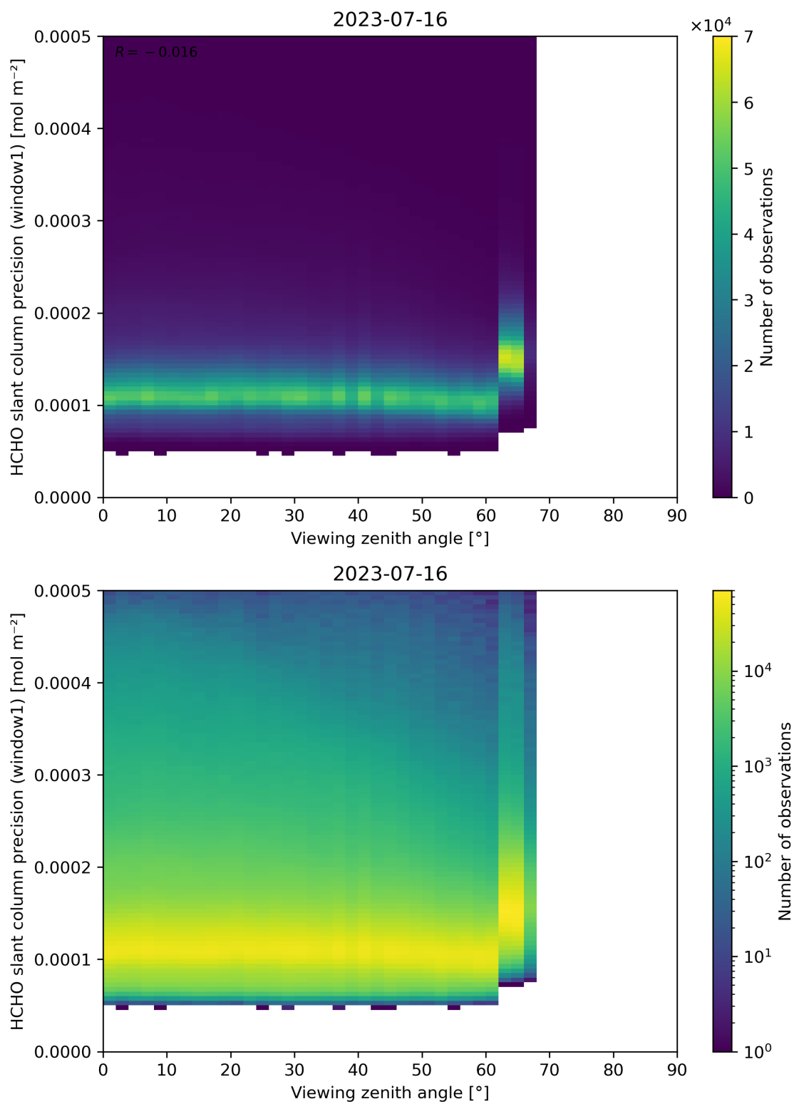
Figure 189: Scatter density plot of “Viewing zenith angle” against “HCHO slant column precision (window1)” for 2023-07-15 to 2023-07-17.
