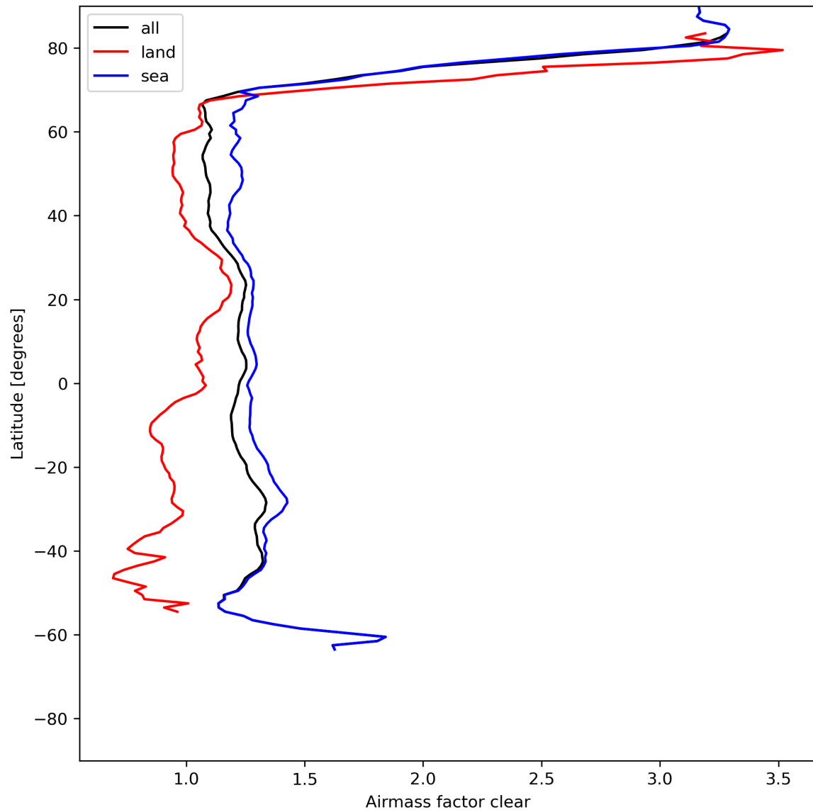
Figure 28: Zonal average of “Airmass factor clear” for 2023-07-15 to 2023-07-17.
