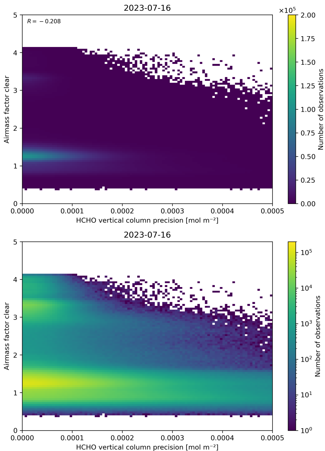
Figure 139: Scatter density plot of “HCHO vertical column precision” against “Airmass factor clear” for 2023-07-15 to 2023-07-17.
