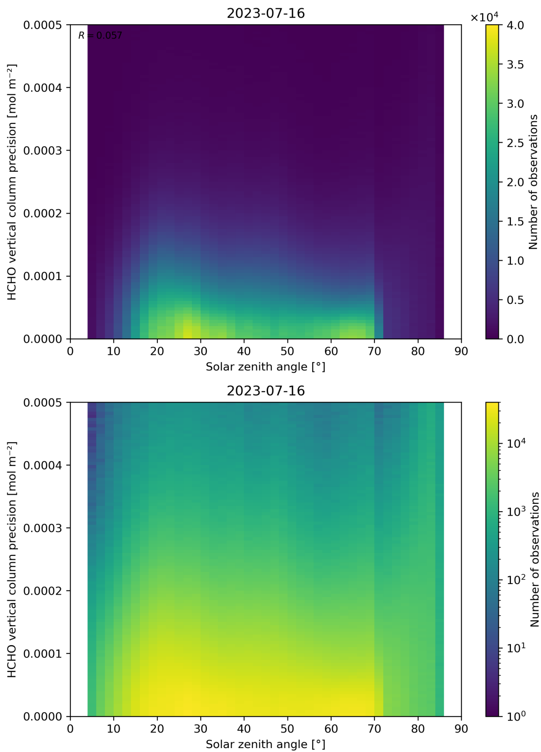
Figure 179: Scatter density plot of “Solar zenith angle” against “HCHO vertical column precision” for 2023-07-15 to 2023-07-17.
