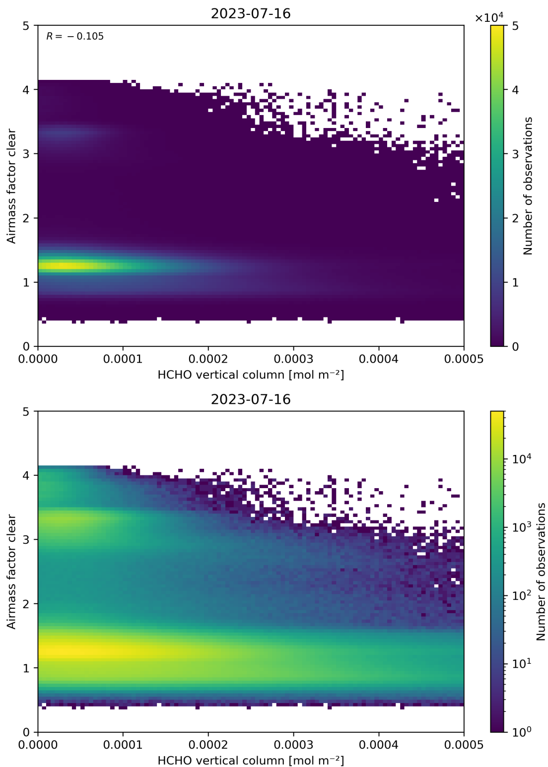
Figure 126: Scatter density plot of “HCHO vertical column” against “Airmass factor clear” for 2023-07-15 to 2023-07-17.
