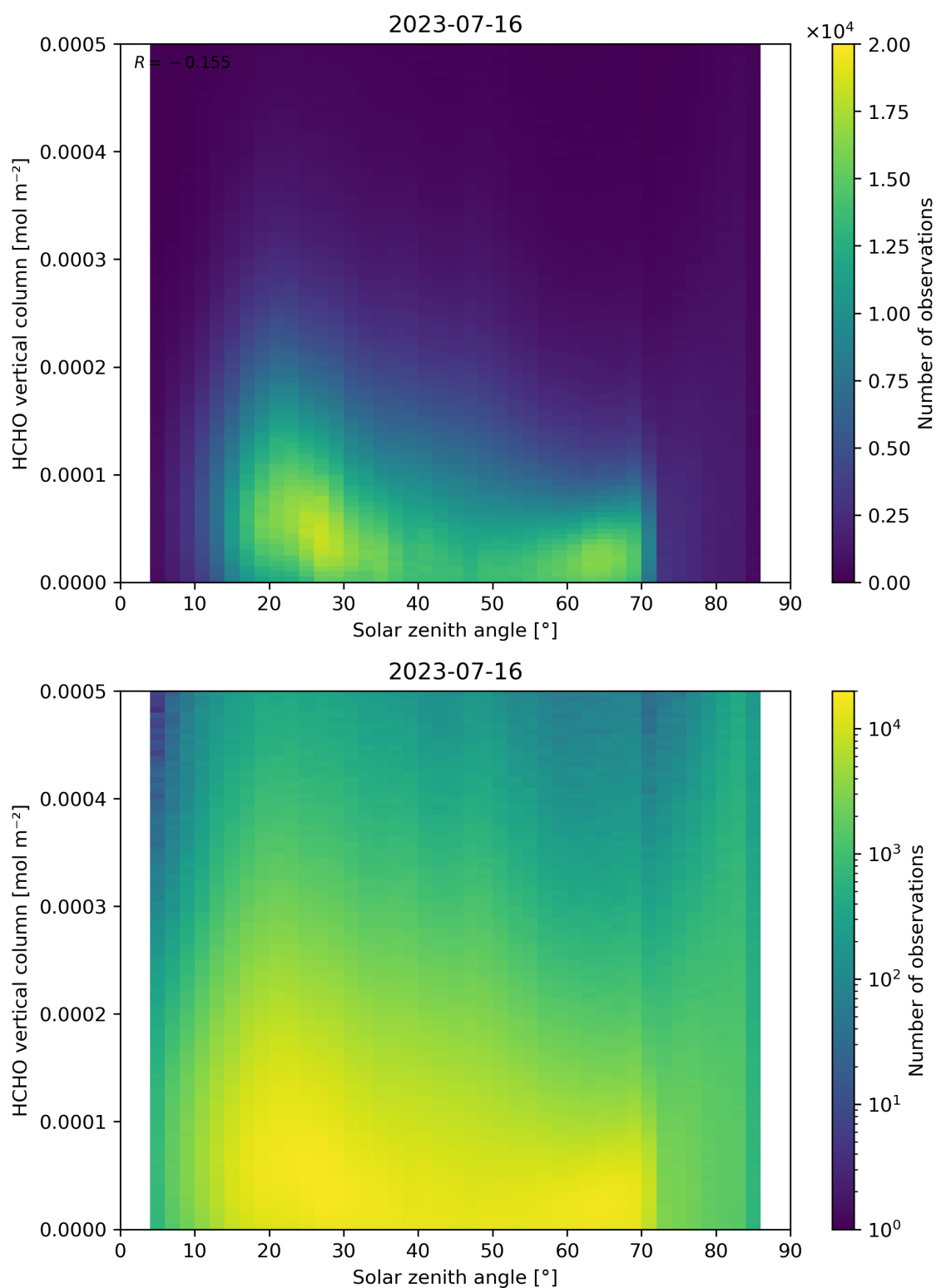
Figure 177: Scatter density plot of “Solar zenith angle” against “HCHO vertical column” for 2023-07-15 to 2023-07-17.
