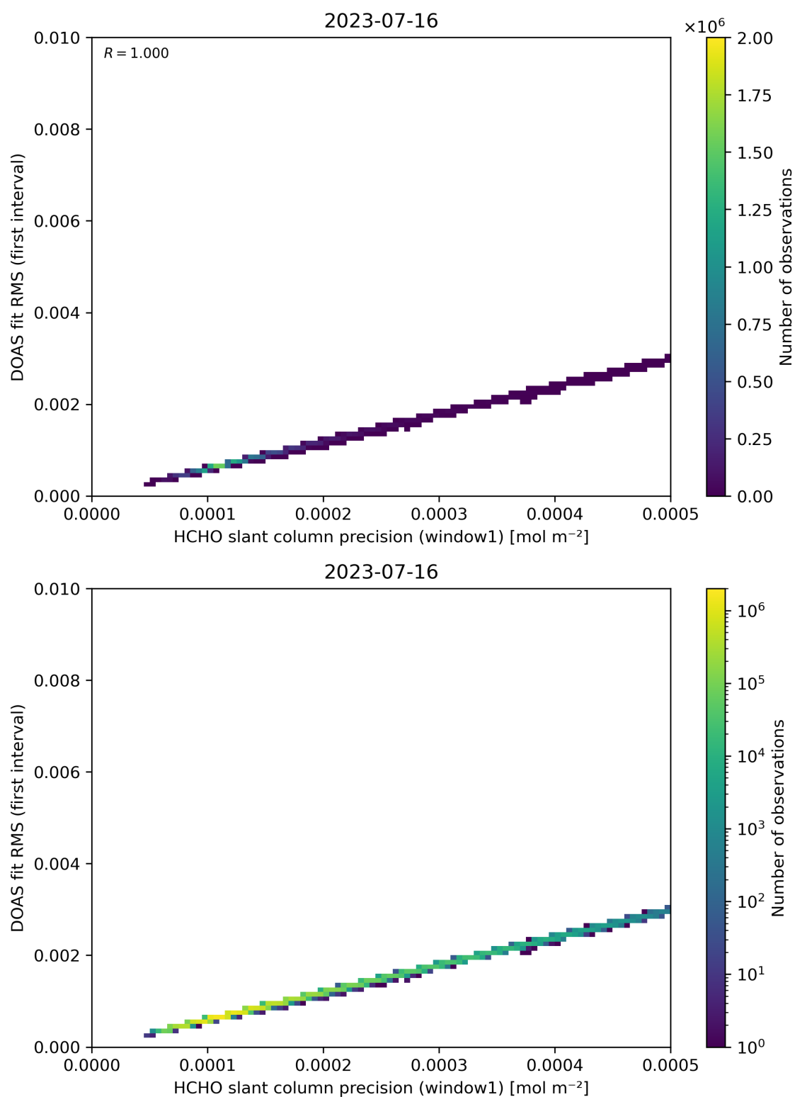
Figure 88: Scatter density plot of “HCHO slant column precision (window1)” against “DOAS fit RMS (first interval)” for 2023-07-15 to 2023-07-17.
