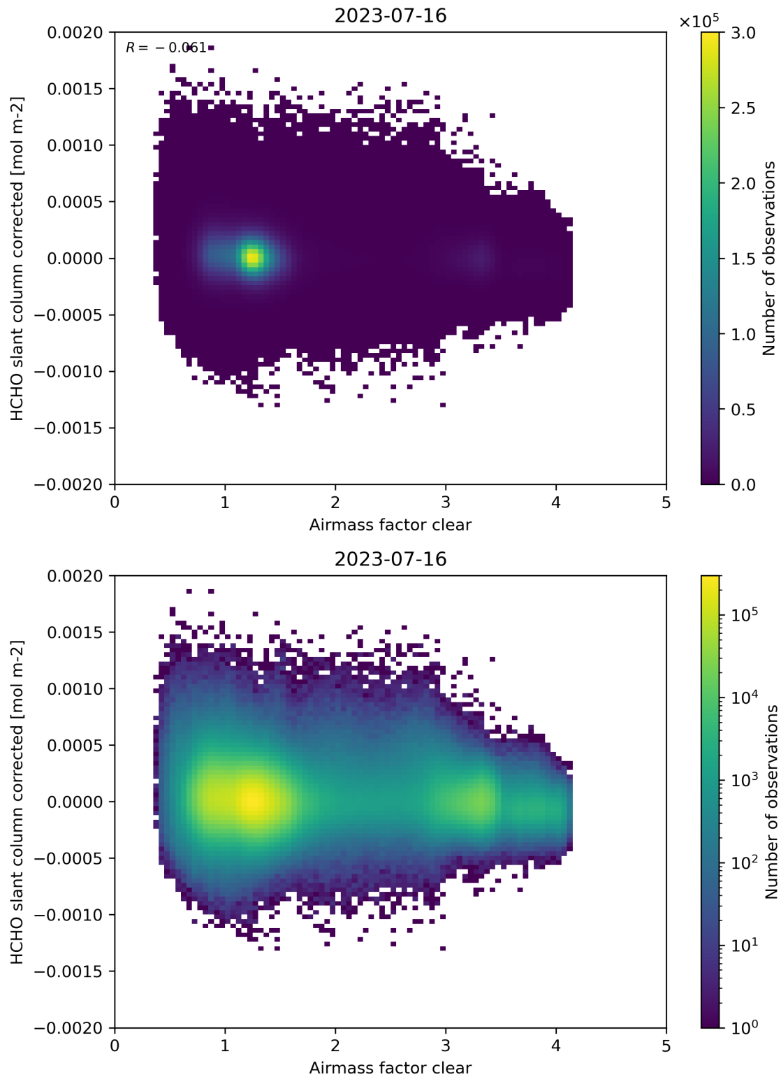
Figure 74: Scatter density plot of “Airmass factor clear” against “HCHO slant column corrected” for 2023-07-15 to 2023-07-17.
