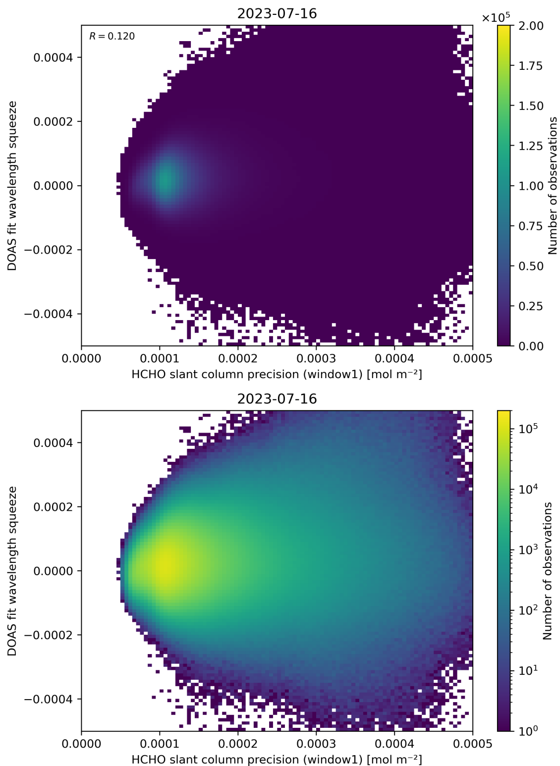
Figure 90: Scatter density plot of “HCHO slant column precision (window1)” against “DOAS fit wavelength squeeze” for 2023-07-15 to 2023-07-17.
