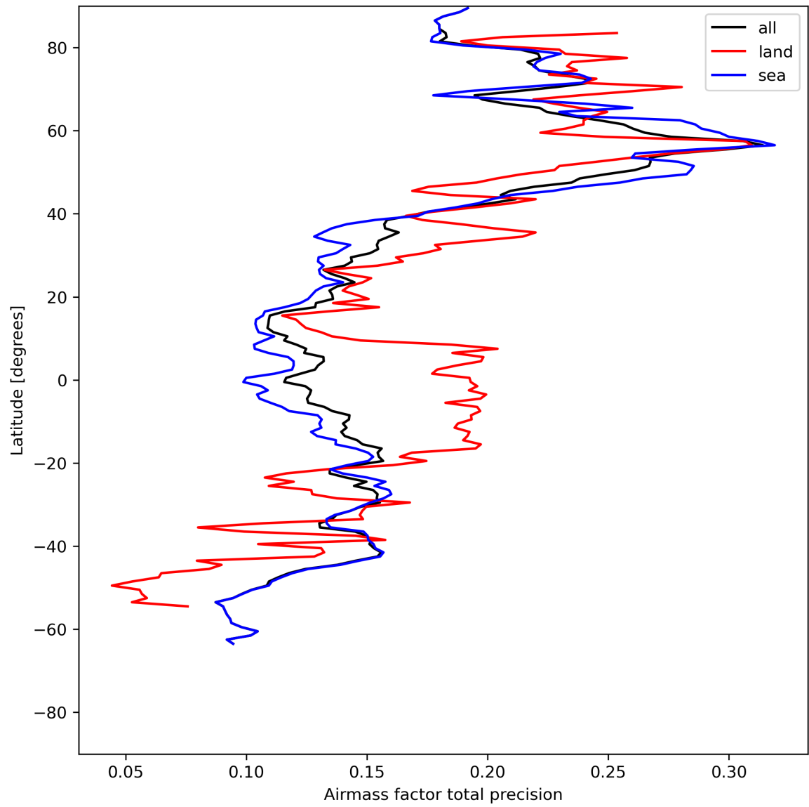
Figure 27: Zonal average of “Airmass factor total precision” for 2023-07-15 to 2023-07-17.
