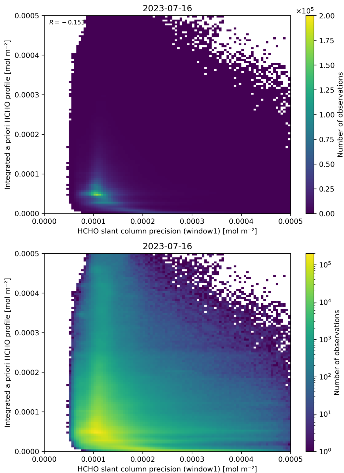
Figure 96: Scatter density plot of “HCHO slant column precision (window1)” against “Integrated a priori HCHO profile” for 2023-07-15 to 2023-07-17.
