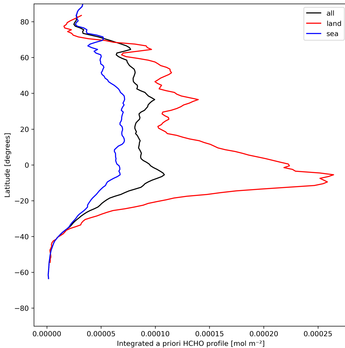
Figure 29: Zonal average of “Integrated a priori HCHO profile” for 2023-07-15 to 2023-07-17.
