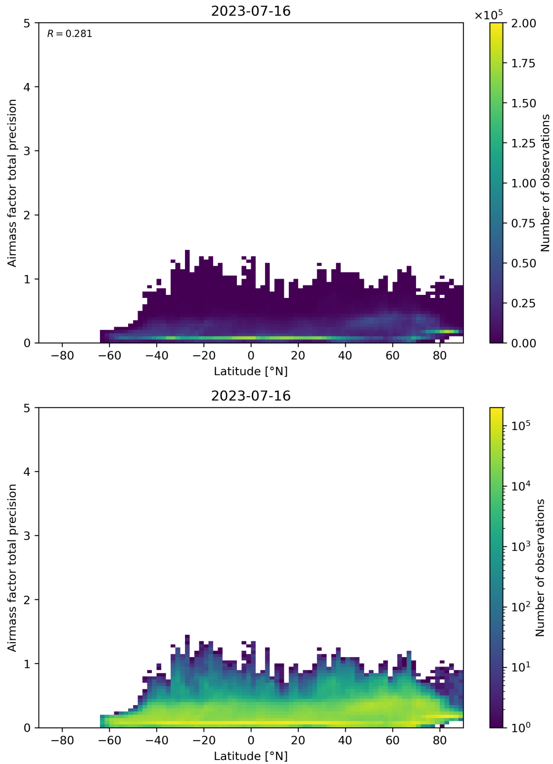
Figure 162: Scatter density plot of “Latitude” against “Airmass factor total precision” for 2023-07-15 to 2023-07-17.
