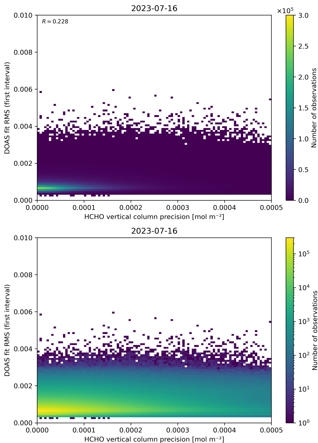
Figure 136: Scatter density plot of “HCHO vertical column precision” against “DOAS fit RMS (first interval)” for 2023-07-15 to 2023-07-17.
