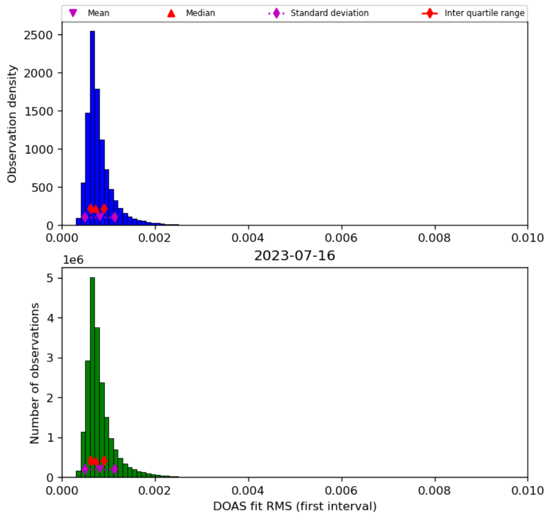
Figure 46: Histogram of “DOAS fit RMS (first interval)” for 2023-07-15 to 2023-07-17
