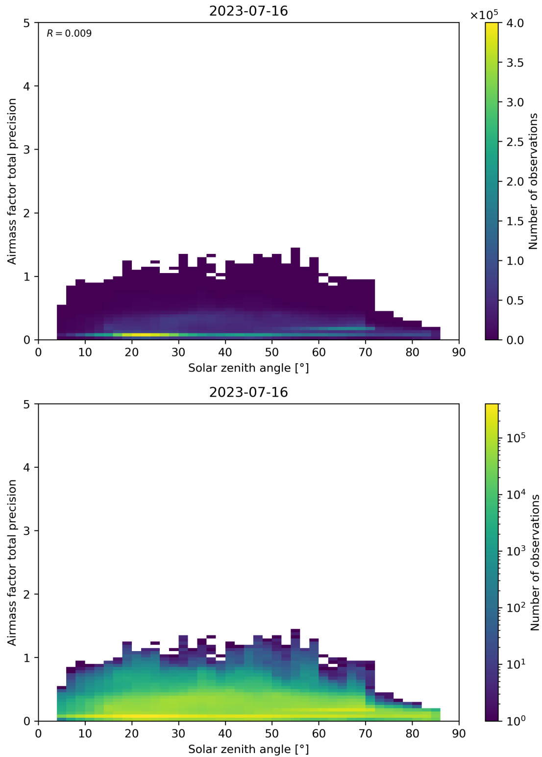
Figure 176: Scatter density plot of “Solar zenith angle” against “Airmass factor total precision” for 2023-07-15 to 2023-07-17.
