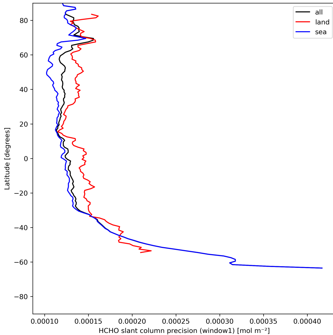
Figure 25: Zonal average of “HCHO slant column precision (window1)” for 2023-07-15 to 2023-07-17.
