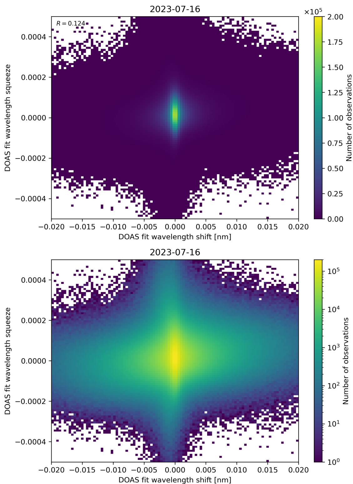
Figure 65: Scatter density plot of “DOAS fit wavelength shift” against “DOAS fit wavelength squeeze” for 2023-07-15 to 2023-07-17.
