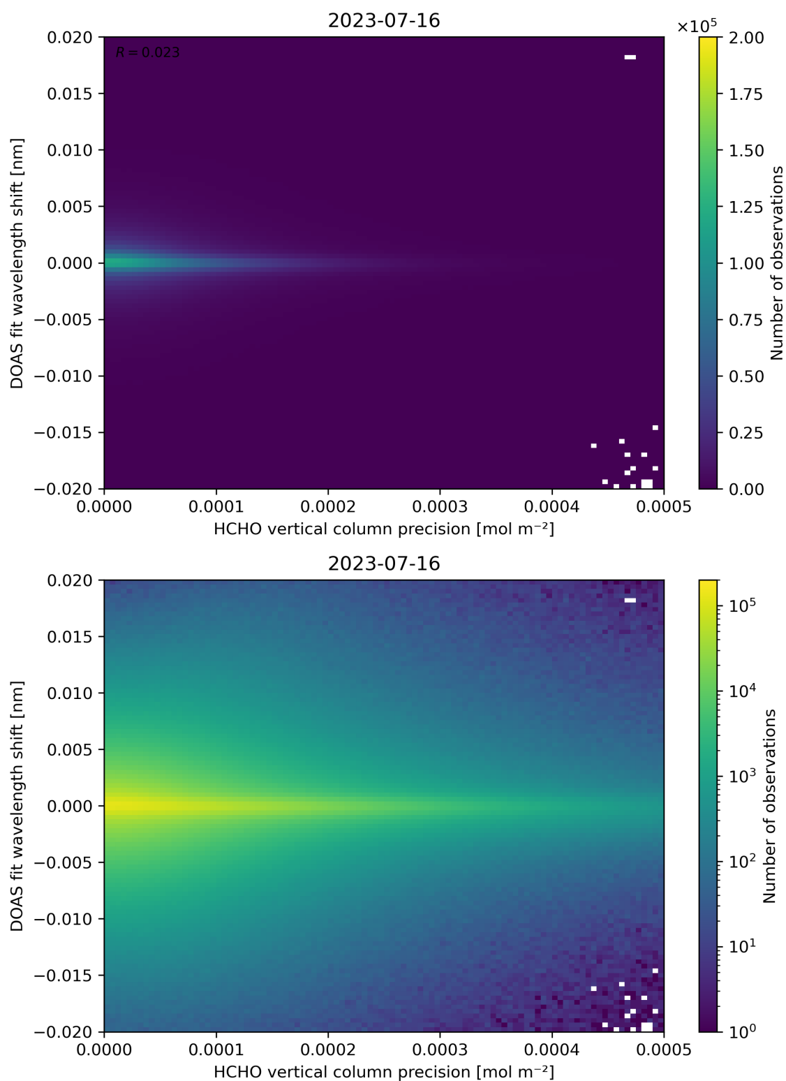
Figure 137: Scatter density plot of “HCHO vertical column precision” against “DOAS fit wavelength shift” for 2023-07-15 to 2023-07-17.
