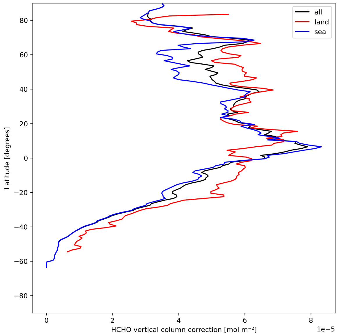
Figure 23: Zonal average of “HCHO vertical column correction” for 2023-07-15 to 2023-07-17.
