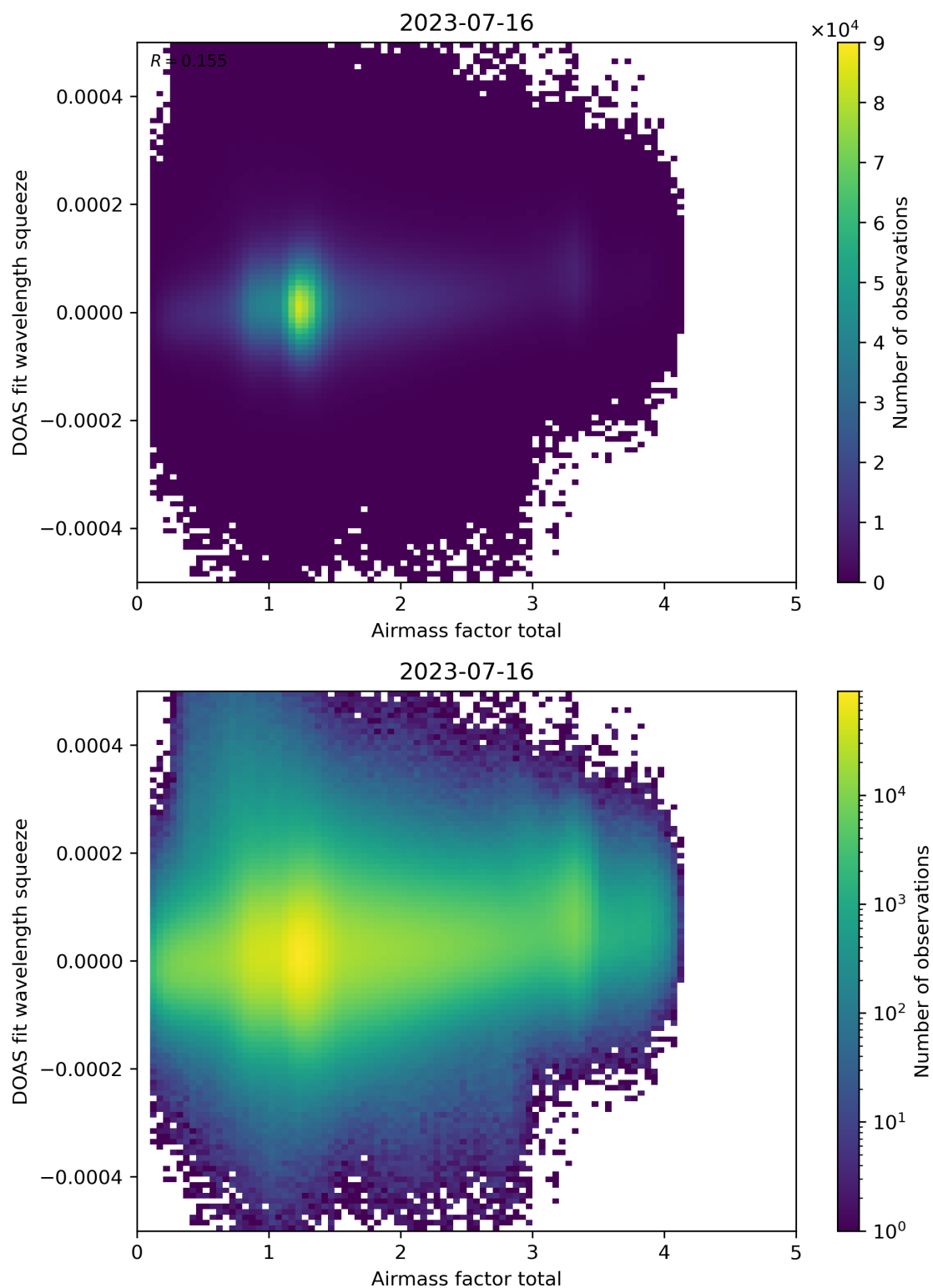
Figure 99: Scatter density plot of “Airmass factor total” against “DOAS fit wavelength squeeze” for 2023-07-15 to 2023-07-17.
