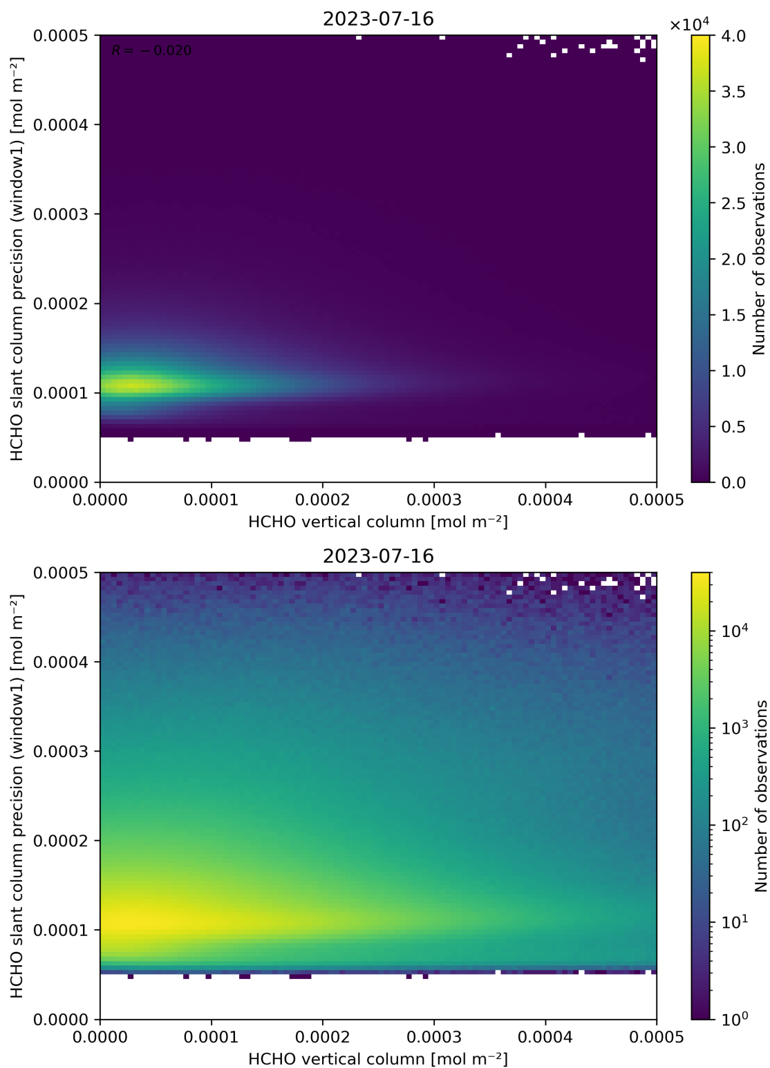
Figure 130: Scatter density plot of “HCHO vertical column” against “HCHO slant column precision (window1)” for 2023-07-15 to 2023-07-17.
