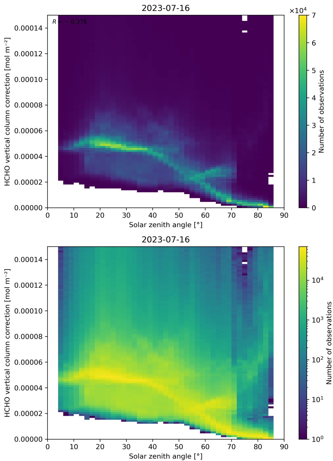
Figure 178: Scatter density plot of “Solar zenith angle” against “HCHO vertical column correction” for 2023-07-15 to 2023-07-17.
