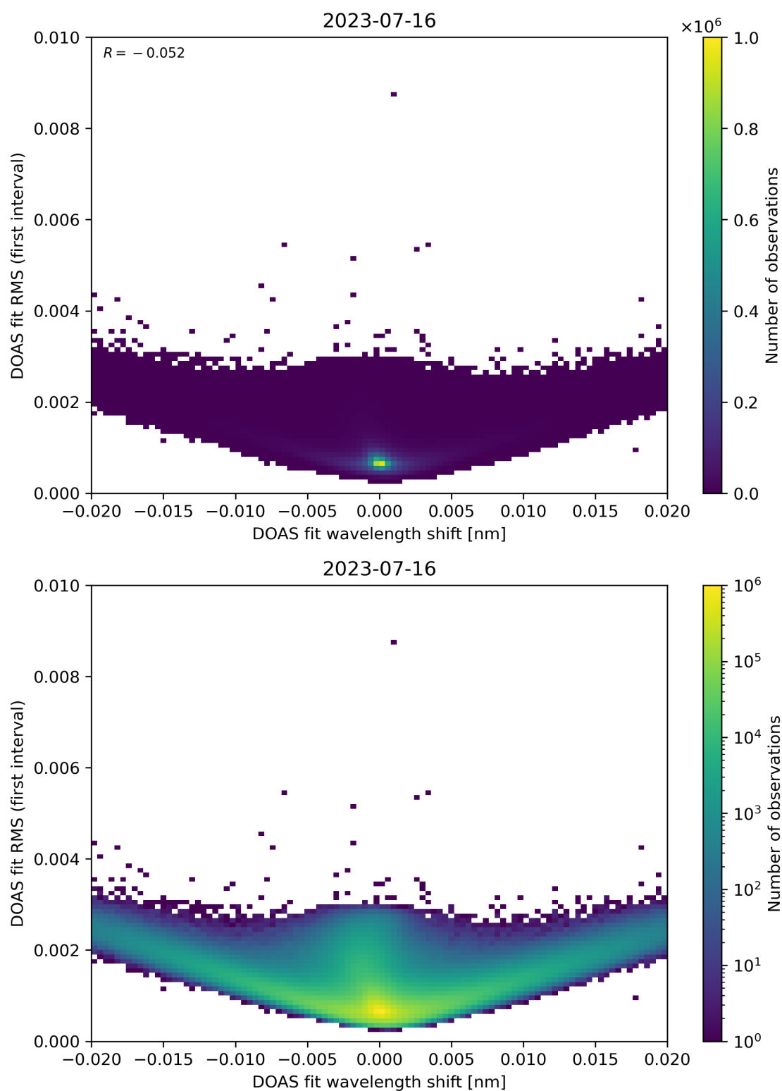
Figure 64: Scatter density plot of “DOAS fit wavelength shift” against “DOAS fit RMS (first interval)” for 2023-07-15 to 2023-07-17.
