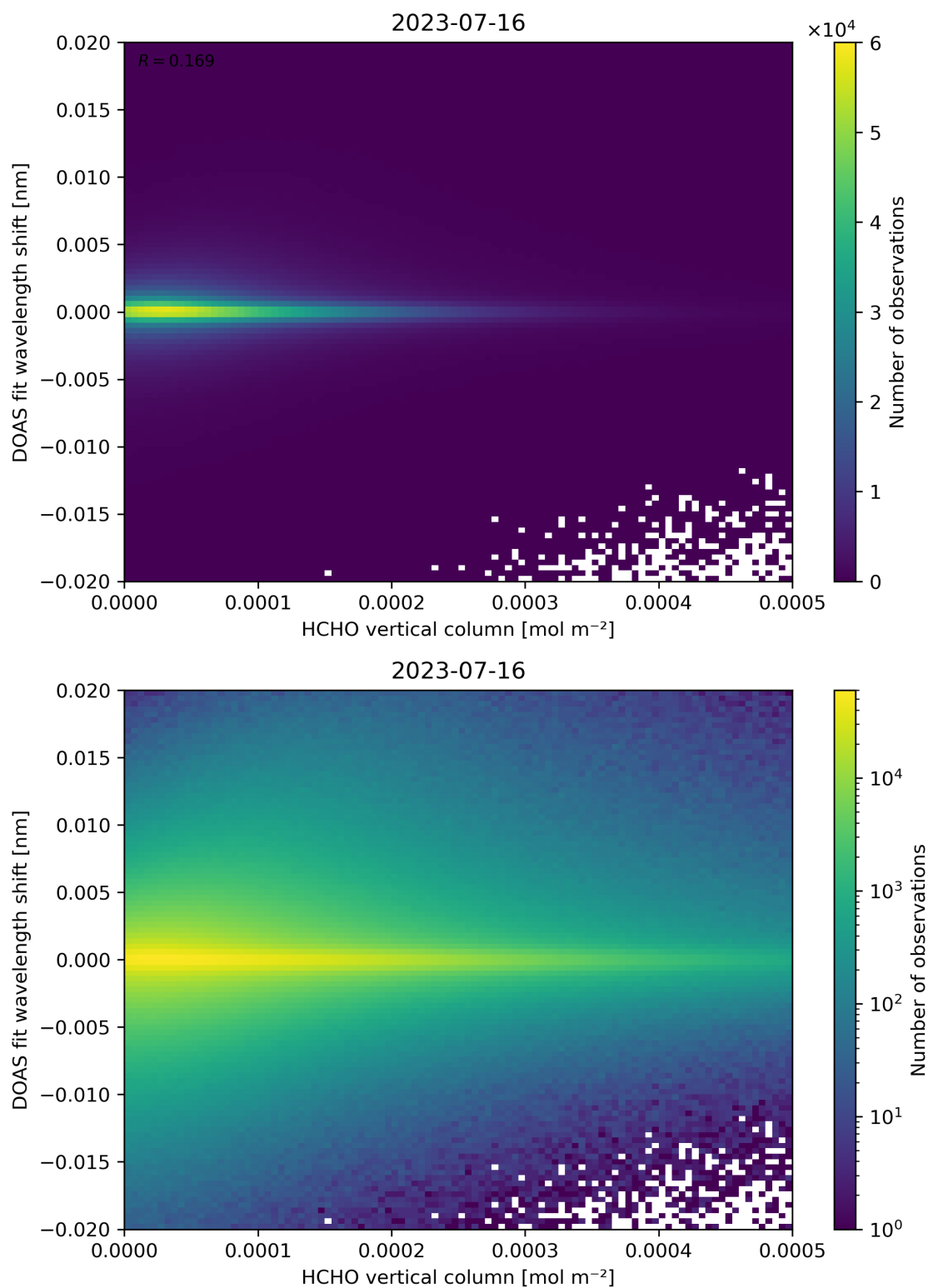
Figure 124: Scatter density plot of “HCHO vertical column” against “DOAS fit wavelength shift” for 2023-07-15 to 2023-07-17.
