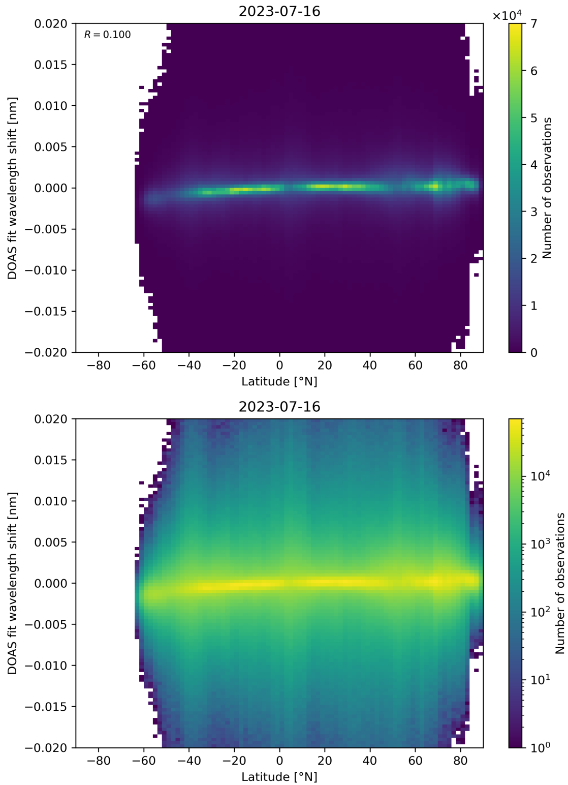
Figure 154: Scatter density plot of “Latitude” against “DOAS fit wavelength shift” for 2023-07-15 to 2023-07-17.
