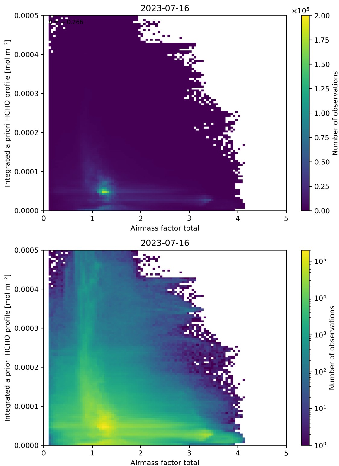
Figure 104: Scatter density plot of “Airmass factor total” against “Integrated a priori HCHO profile” for 2023-07-15 to 2023-07-17.
