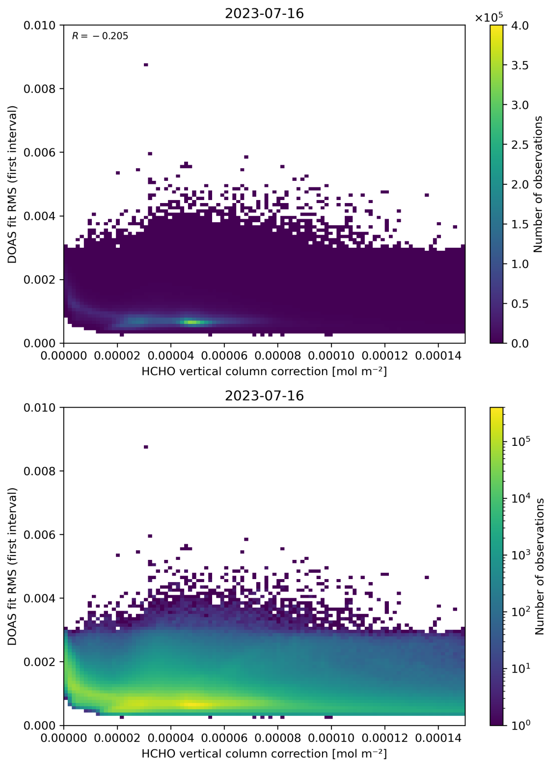
Figure 112: Scatter density plot of “HCHO vertical column correction” against “DOAS fit RMS (first interval)” for 2023-07-15 to 2023-07-17.
