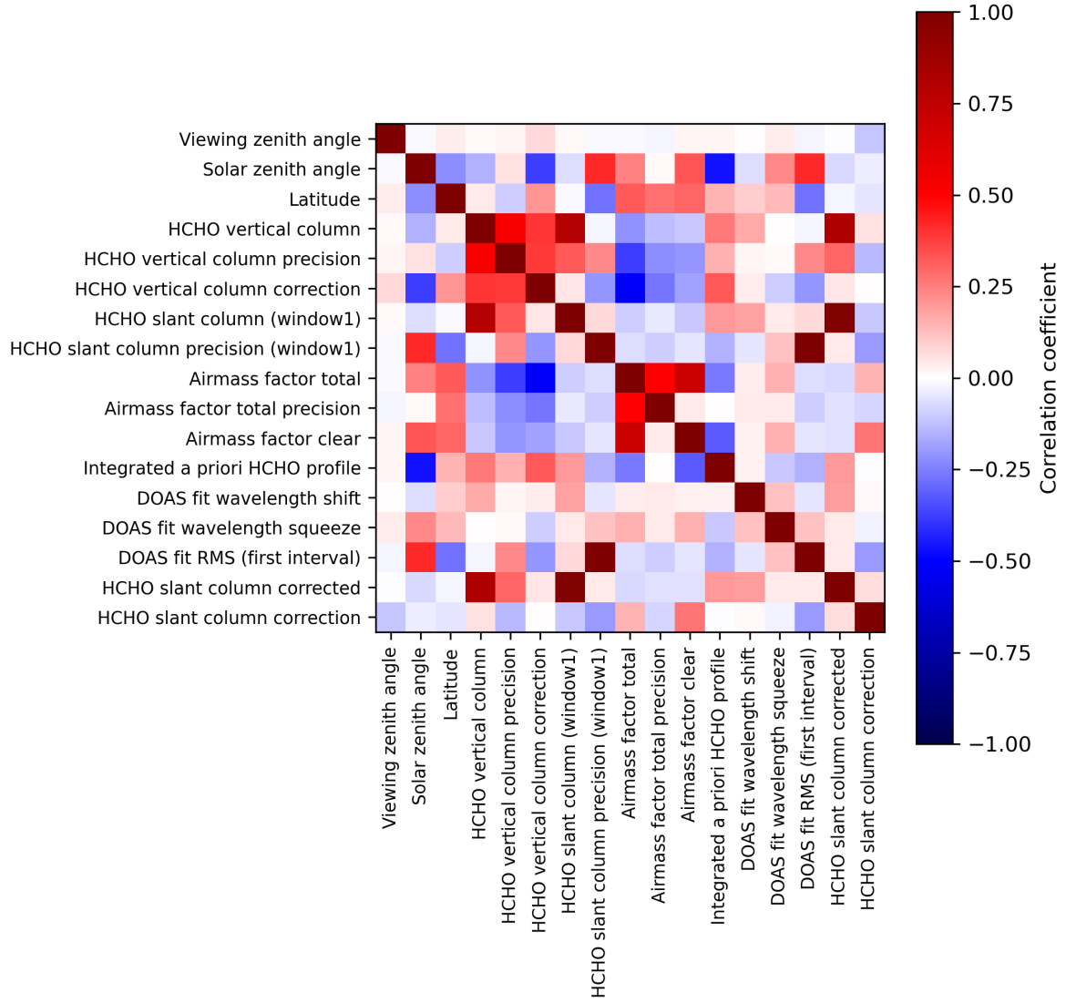
Figure 2: Map of correlation matrix for 2023-07-15 to 2023-07-17.
