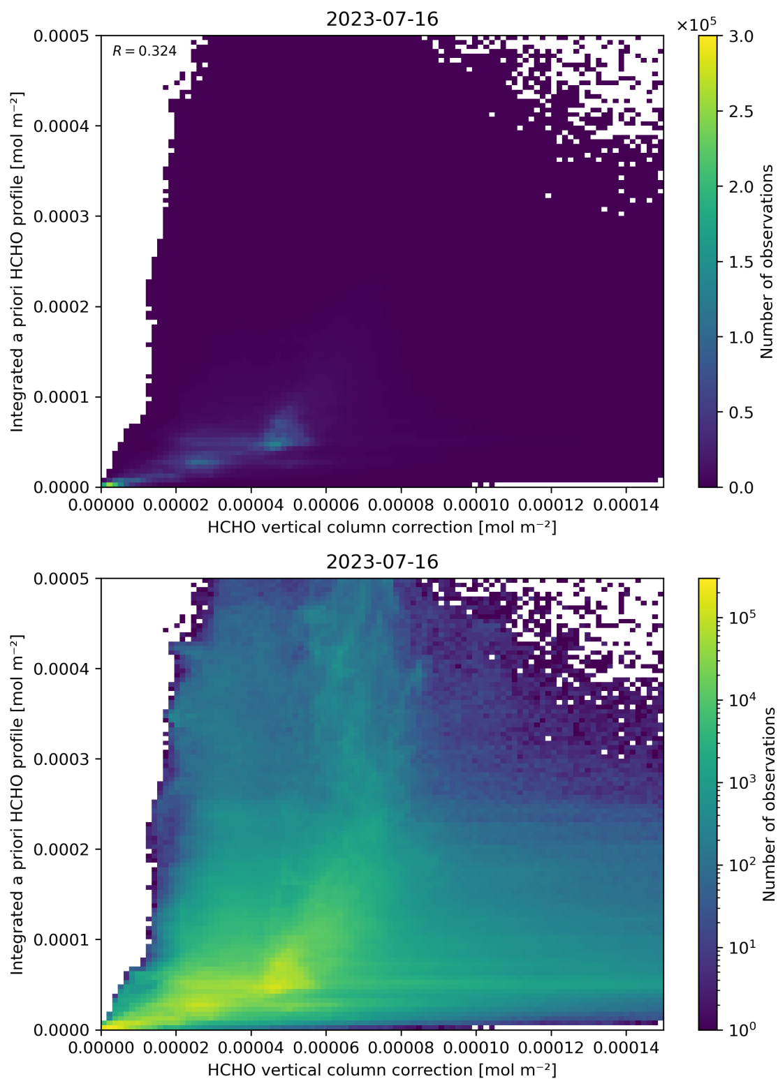
Figure 122: Scatter density plot of “HCHO vertical column correction” against “Integrated a priori HCHO profile” for 2023-07-15 to 2023-07-17.
