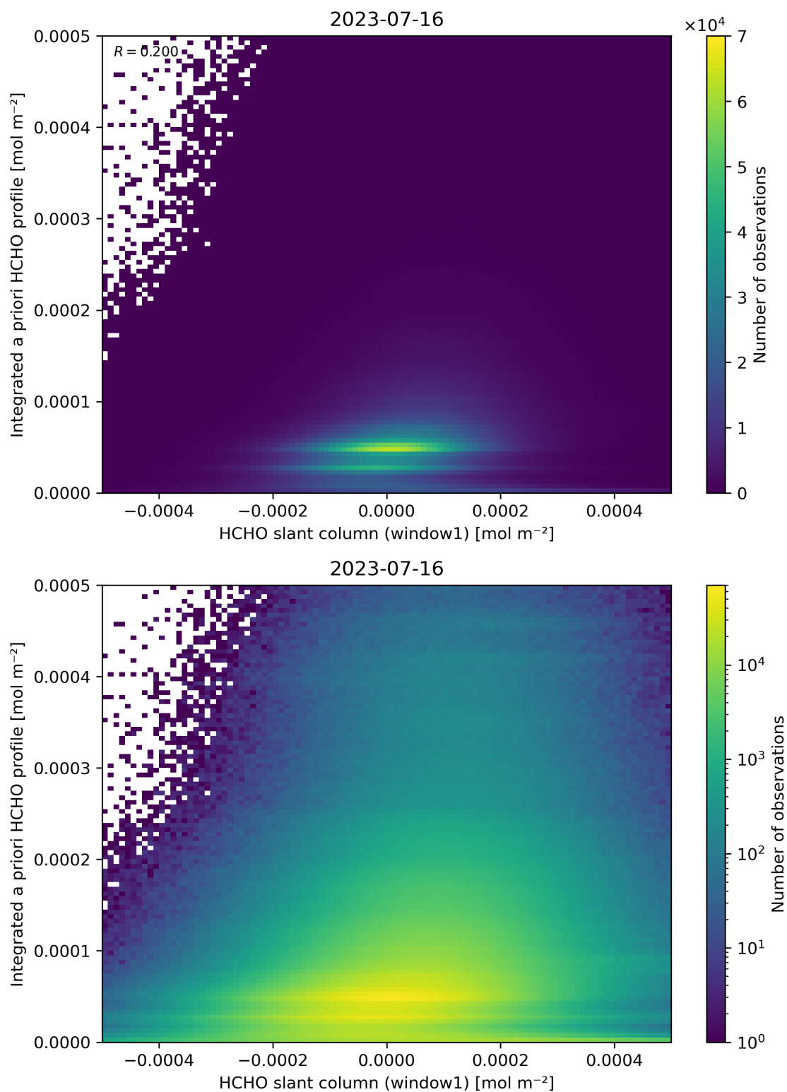
Figure 87: Scatter density plot of “HCHO slant column (window1)” against “Integrated a priori HCHO profile” for 2023-07-15 to 2023-07-17.
