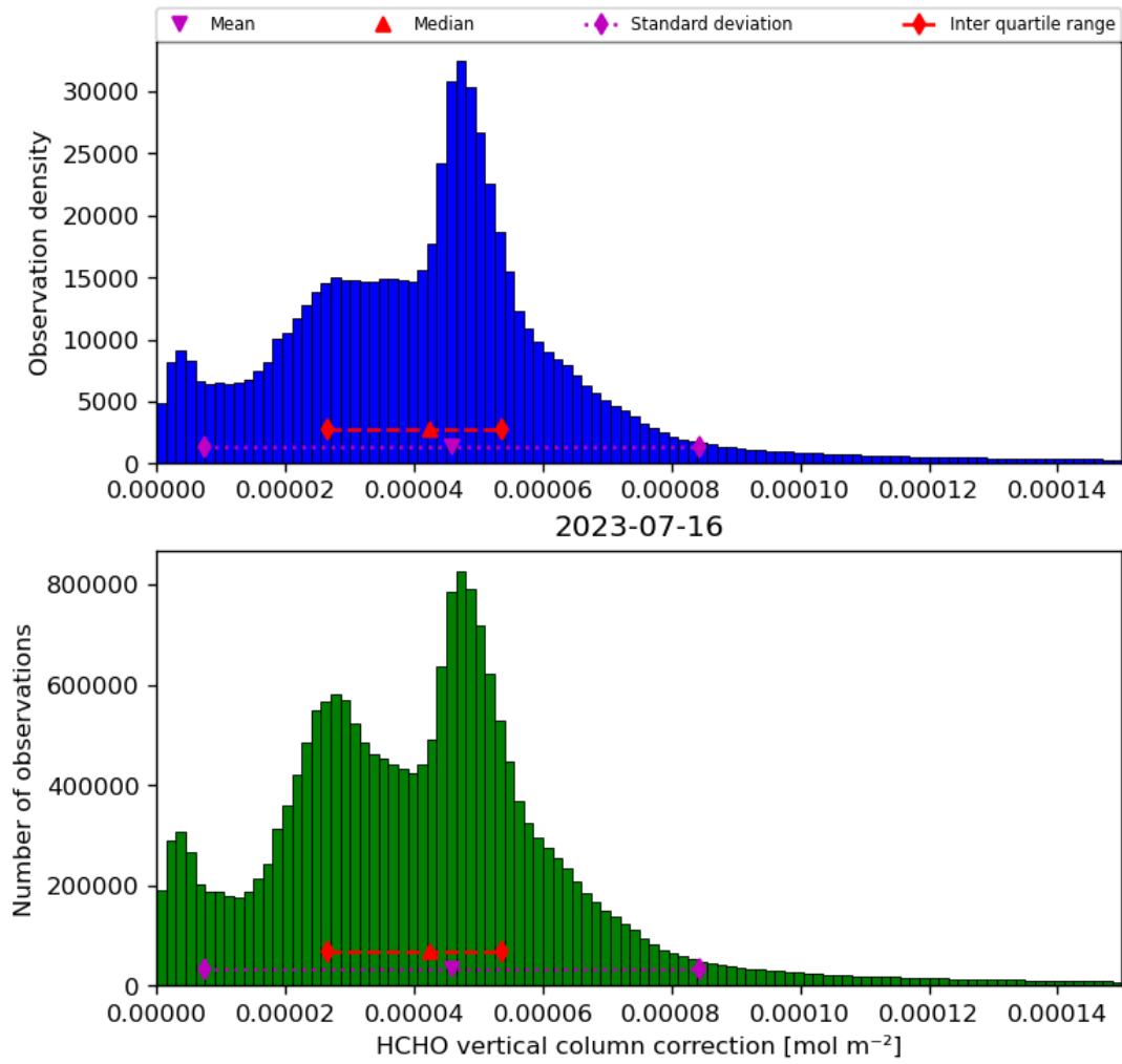
Figure 37: Histogram of “HCHO vertical column correction” for 2023-07-15 to 2023-07-17
