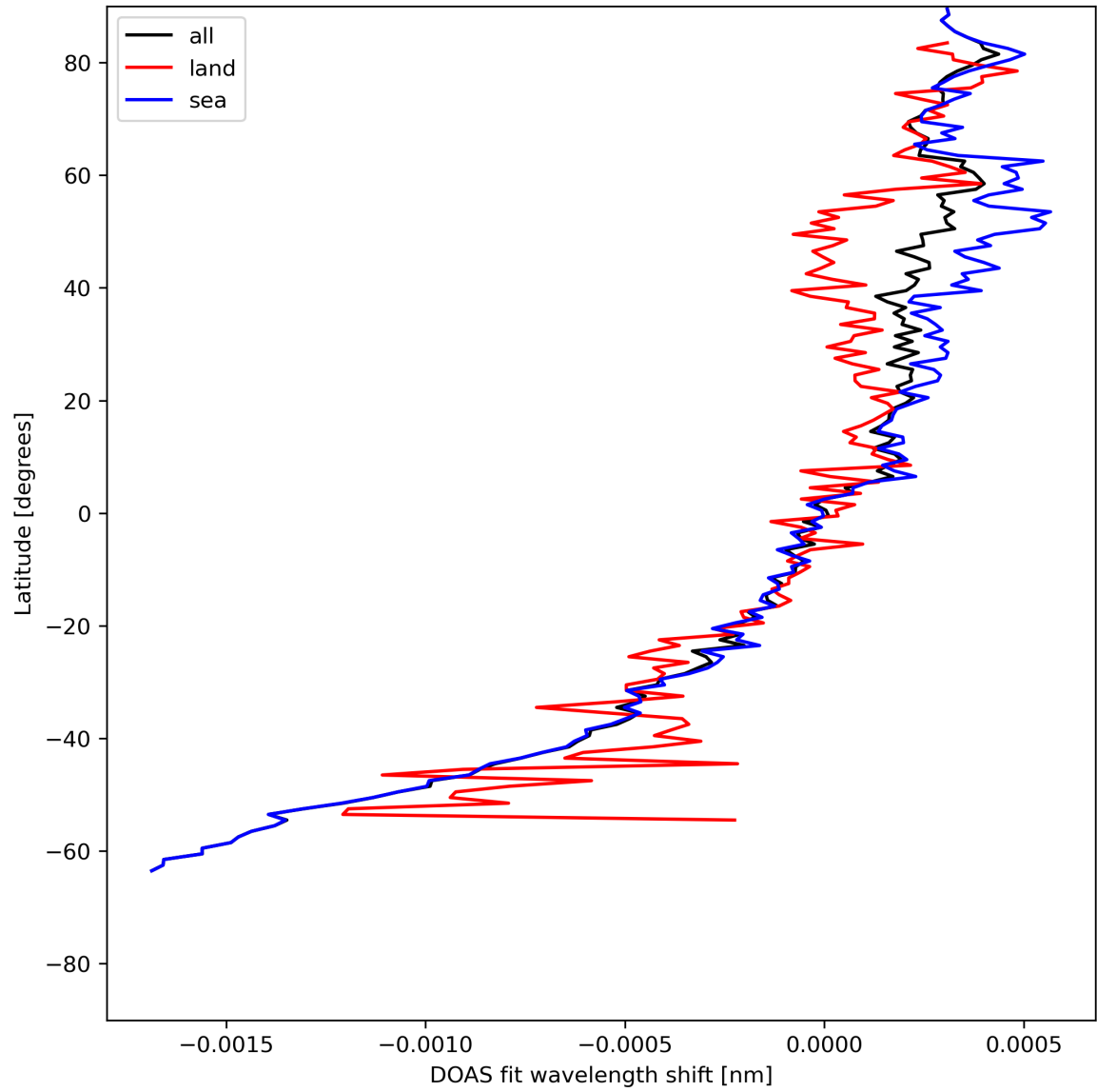
Figure 30: Zonal average of “DOAS fit wavelength shift” for 2023-07-15 to 2023-07-17.
