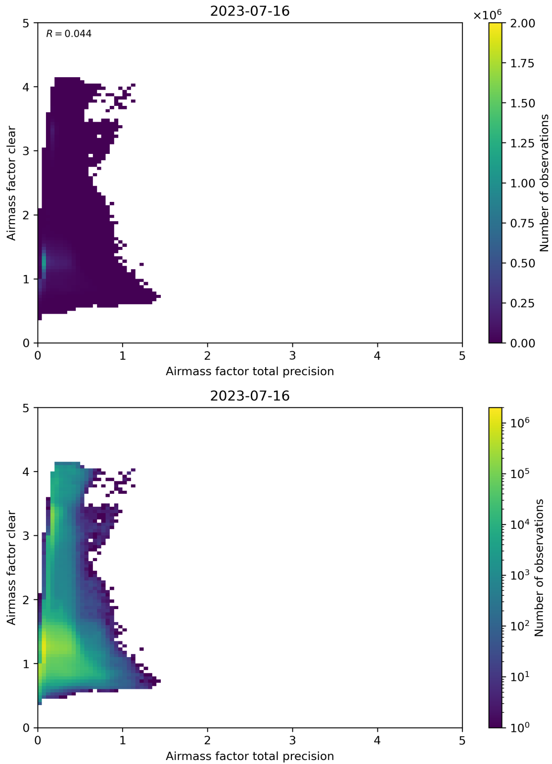
Figure 108: Scatter density plot of “Airmass factor total precision” against “Airmass factor clear” for 2023-07-15 to 2023-07-17.
