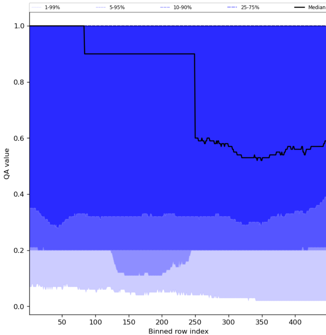
Figure 48: Along track statistics of “QA value” for 2023-07-15 to 2023-07-17
