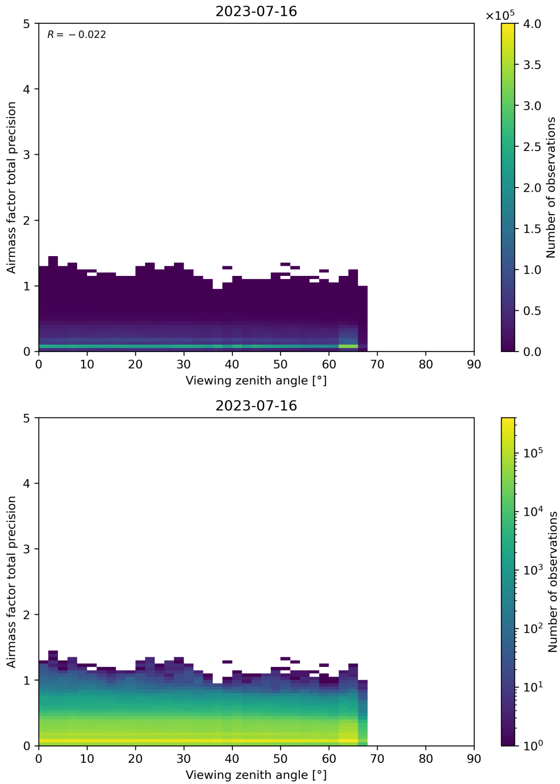
Figure 191: Scatter density plot of “Viewing zenith angle” against “Airmass factor total precision” for 2023-07-15 to 2023-07-17.
