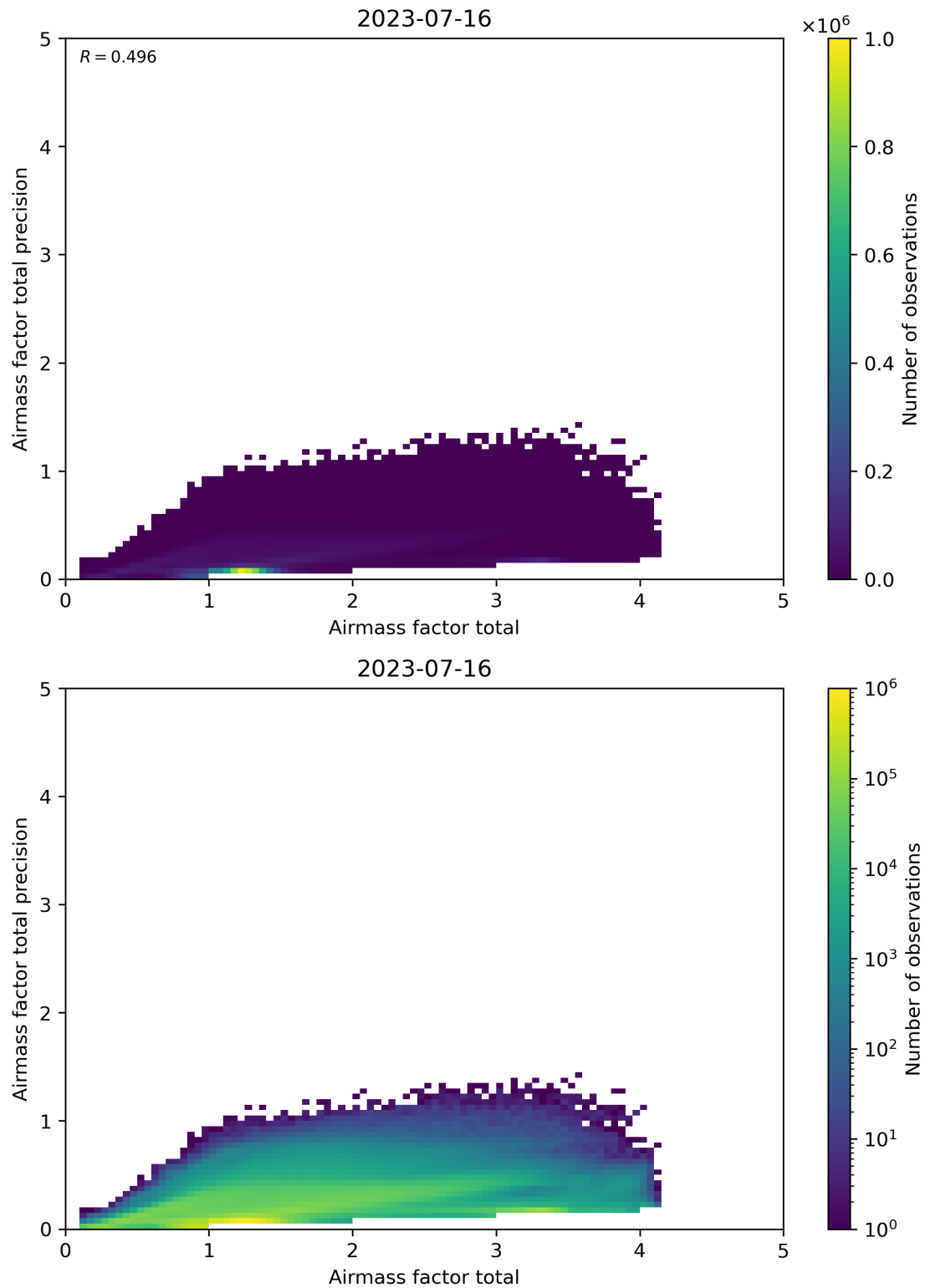
Figure 103: Scatter density plot of “Airmass factor total” against “Airmass factor total precision” for 2023-07-15 to 2023-07-17.
