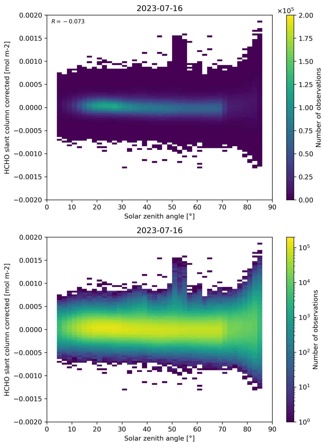
Figure 171: Scatter density plot of “Solar zenith angle” against “HCHO slant column corrected” for 2023-07-15 to 2023-07-17.
