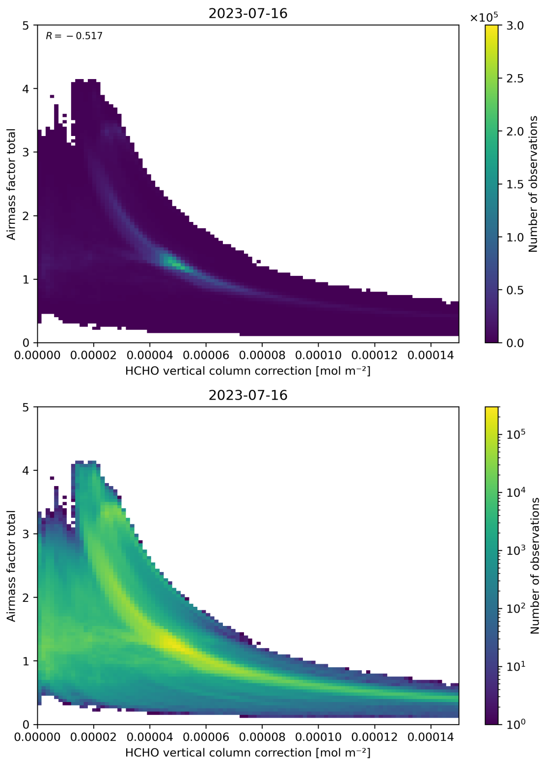
Figure 120: Scatter density plot of “HCHO vertical column correction” against “Airmass factor total” for 2023-07-15 to 2023-07-17.
