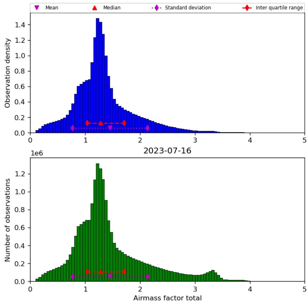
Figure 40: Histogram of “Airmass factor total” for 2023-07-15 to 2023-07-17
