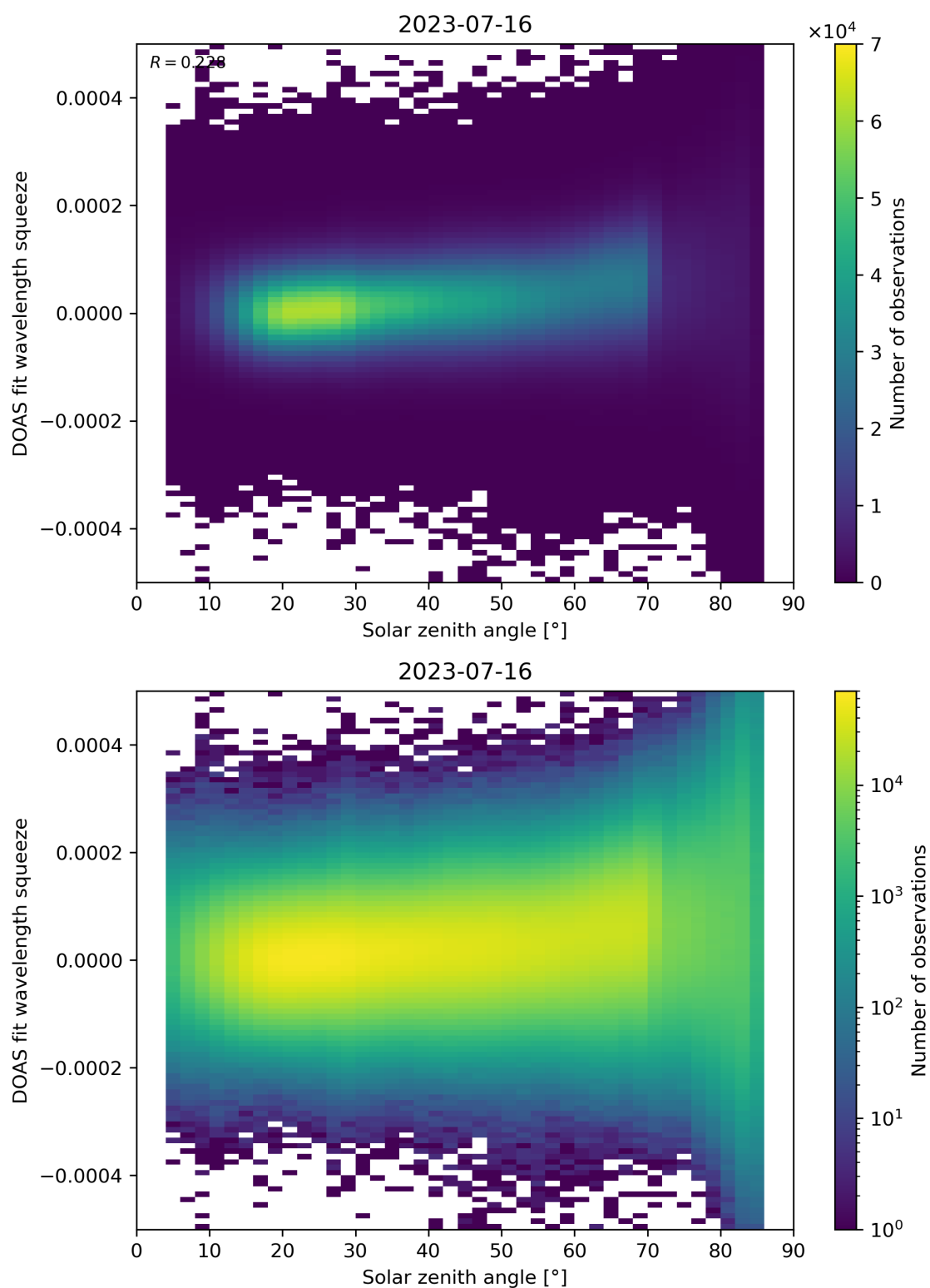
Figure 169: Scatter density plot of “Solar zenith angle” against “DOAS fit wavelength squeeze” for 2023-07-15 to 2023-07-17.
