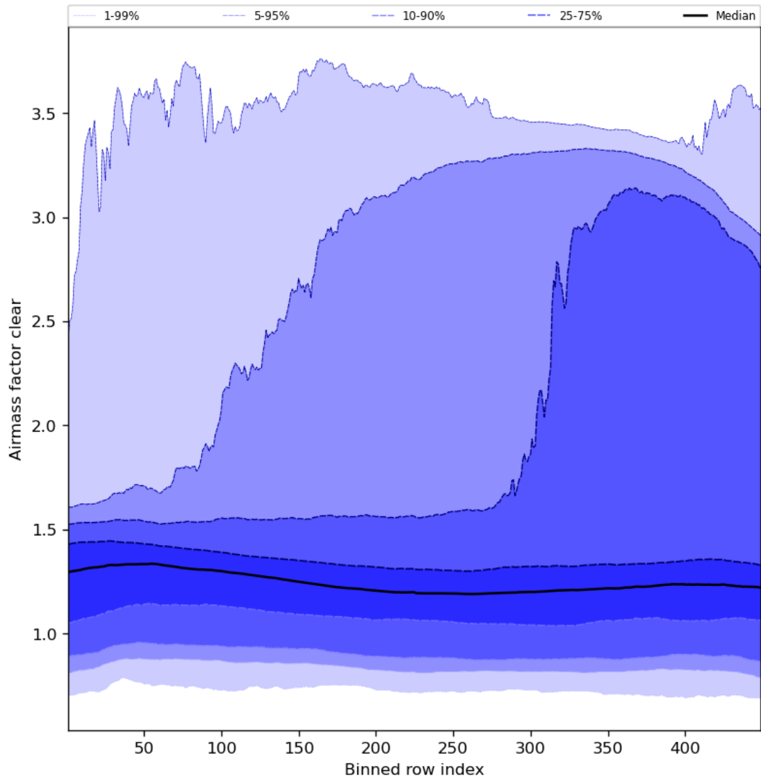
Figure 56: Along track statistics of “Airmass factor clear” for 2023-07-15 to 2023-07-17
