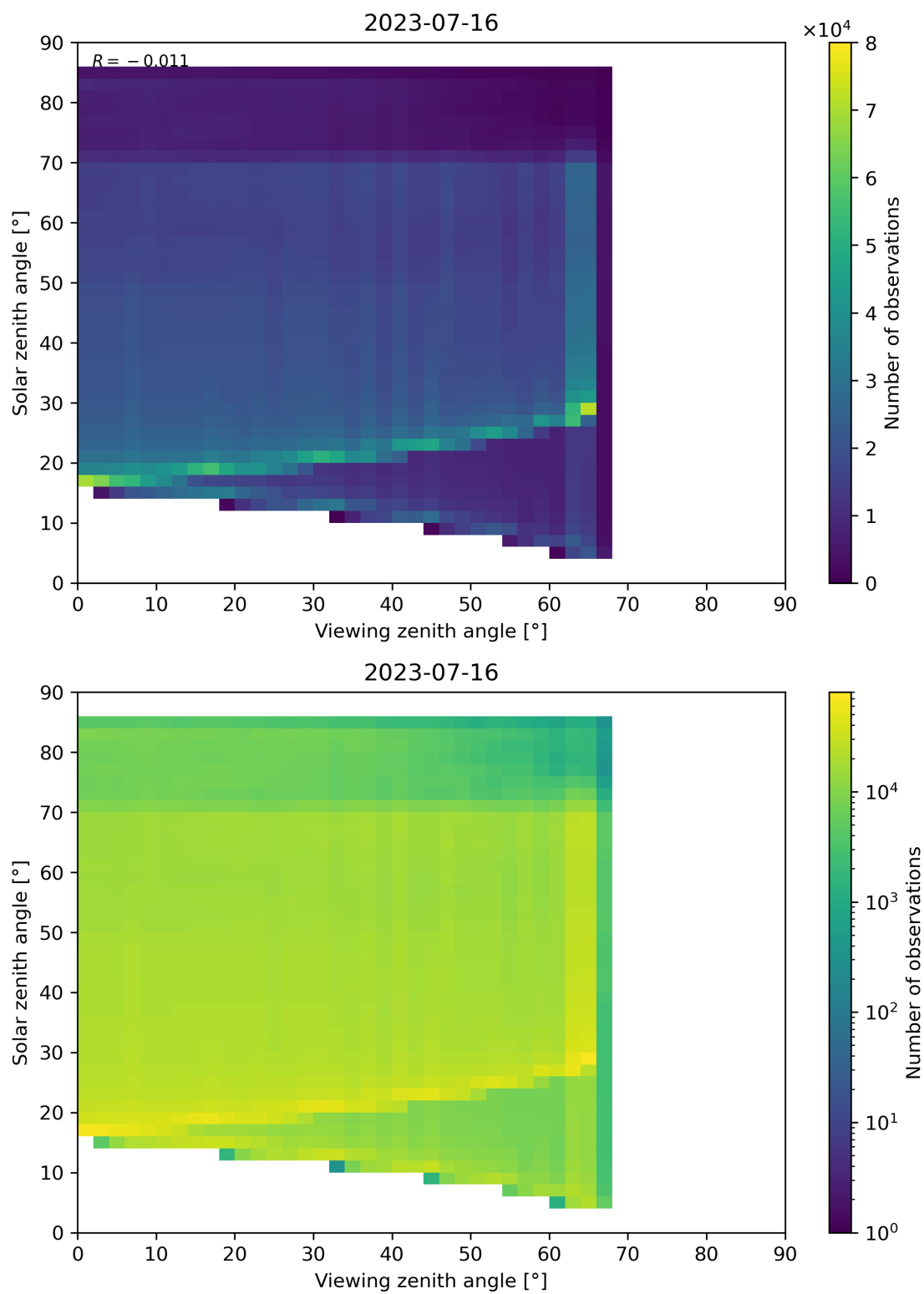
Figure 197: Scatter density plot of “Viewing zenith angle” against “Solar zenith angle” for 2023-07-15 to 2023-07-17.
