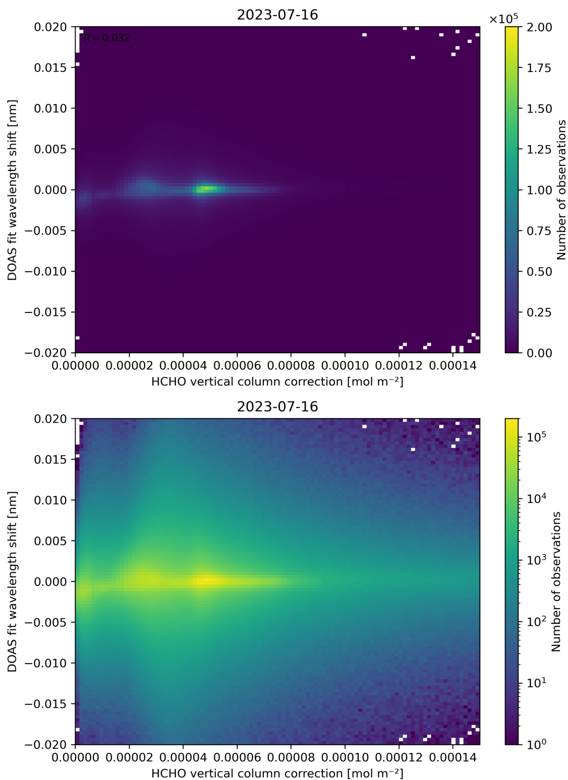
Figure 113: Scatter density plot of “HCHO vertical column correction” against “DOAS fit wavelength shift” for 2023-07-15 to 2023-07-17.
