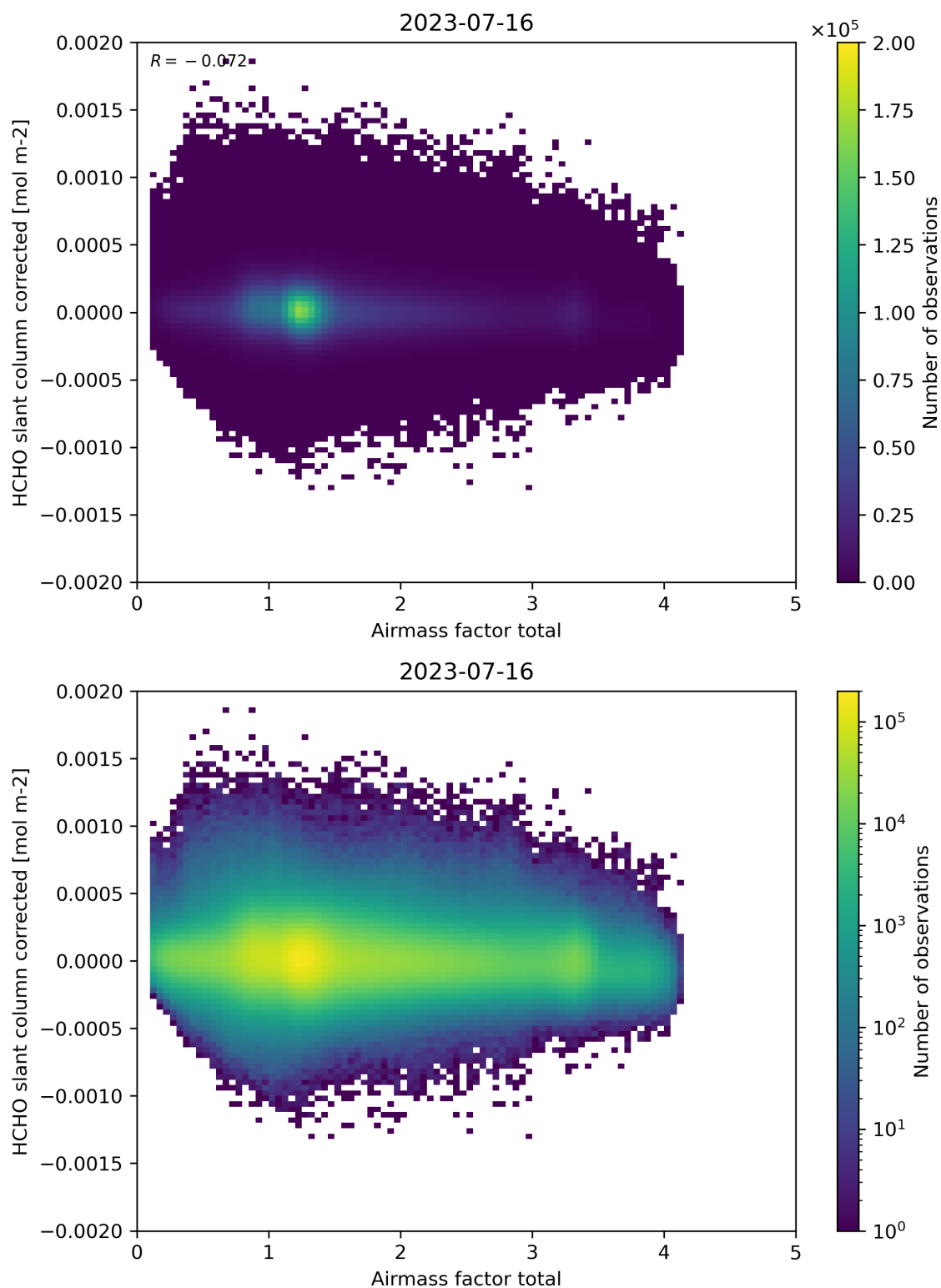
Figure 101: Scatter density plot of “Airmass factor total” against “HCHO slant column corrected” for 2023-07-15 to 2023-07-17.
