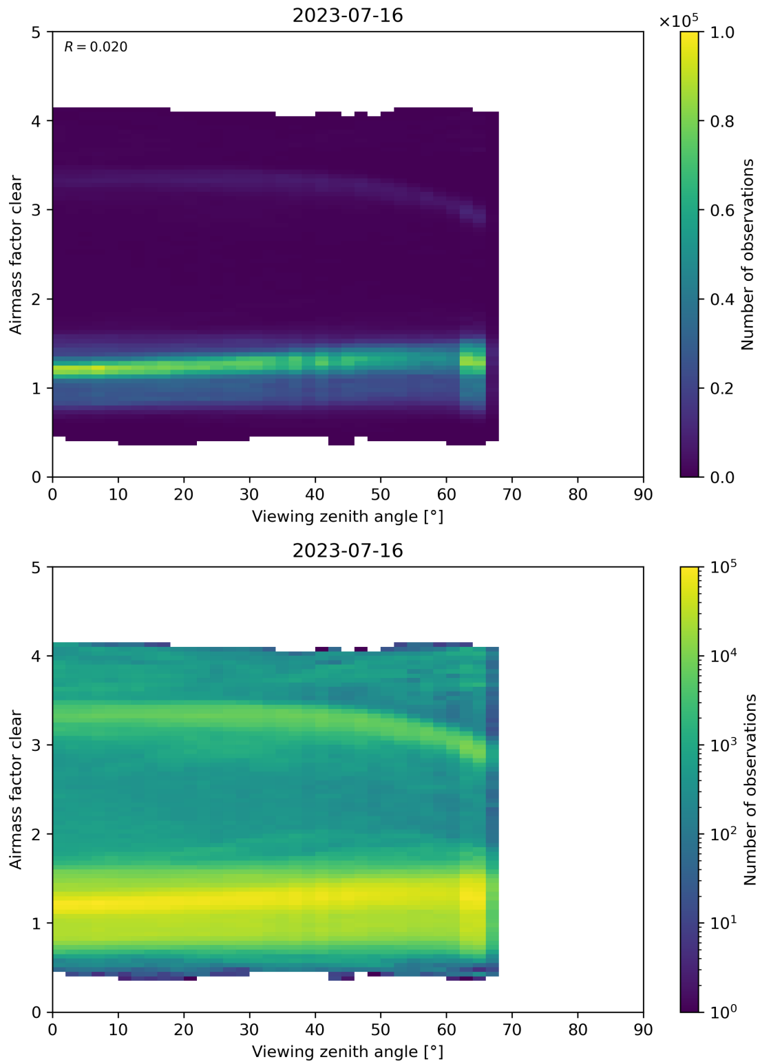
Figure 185: Scatter density plot of “Viewing zenith angle” against “Airmass factor clear” for 2023-07-15 to 2023-07-17.
