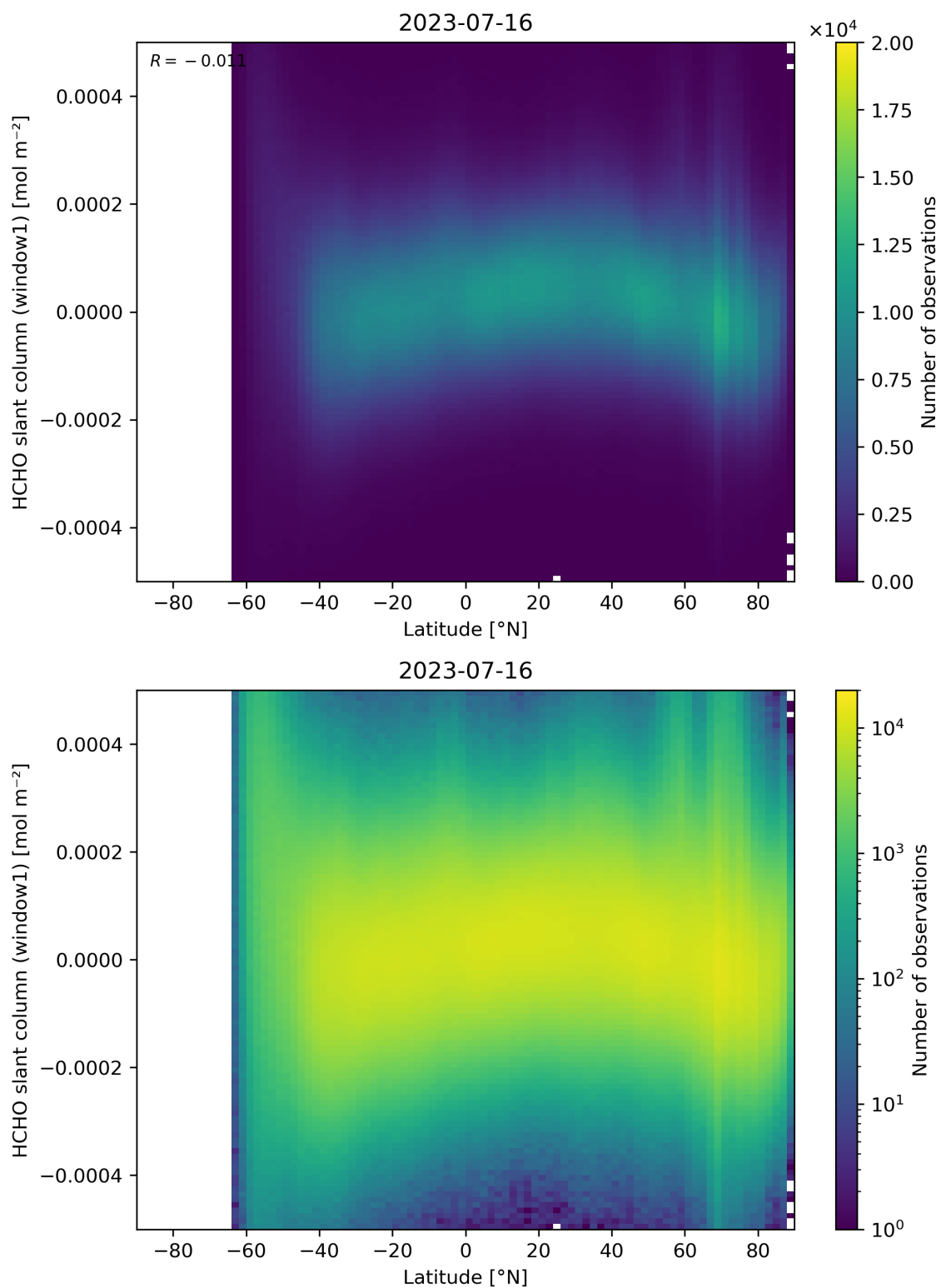
Figure 159: Scatter density plot of “Latitude” against “HCHO slant column (window1)” for 2023-07-15 to 2023-07-17.
