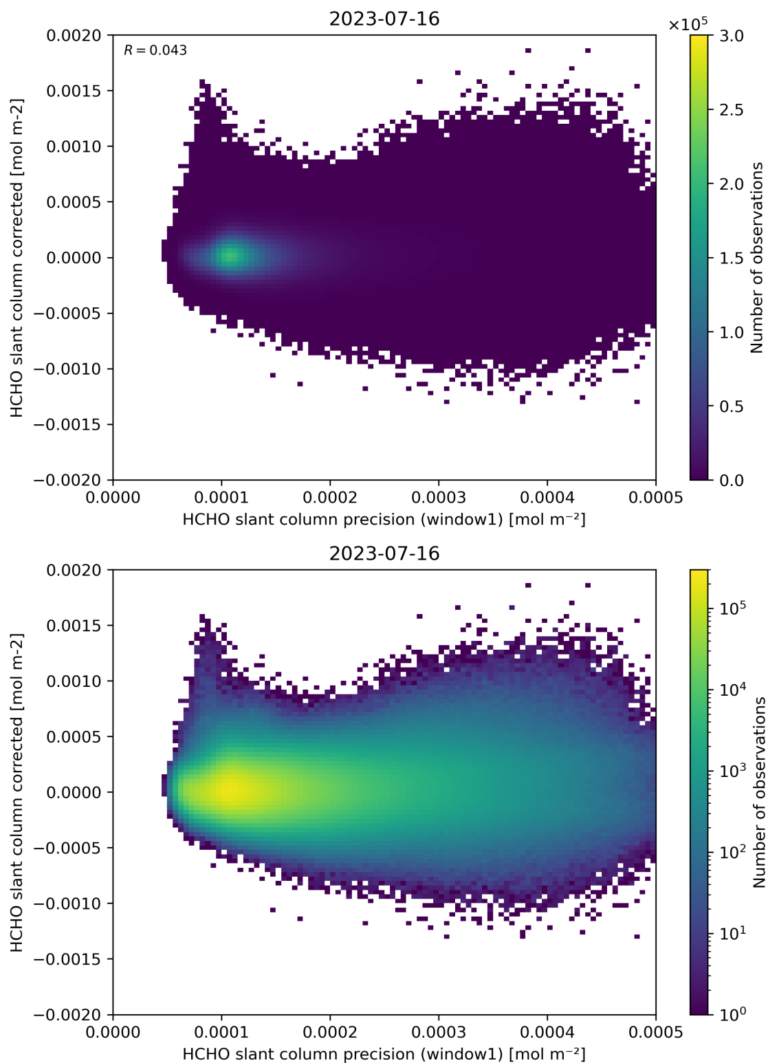
Figure 92: Scatter density plot of “HCHO slant column precision (window1)” against “HCHO slant column corrected” for 2023-07-15 to 2023-07-17.
