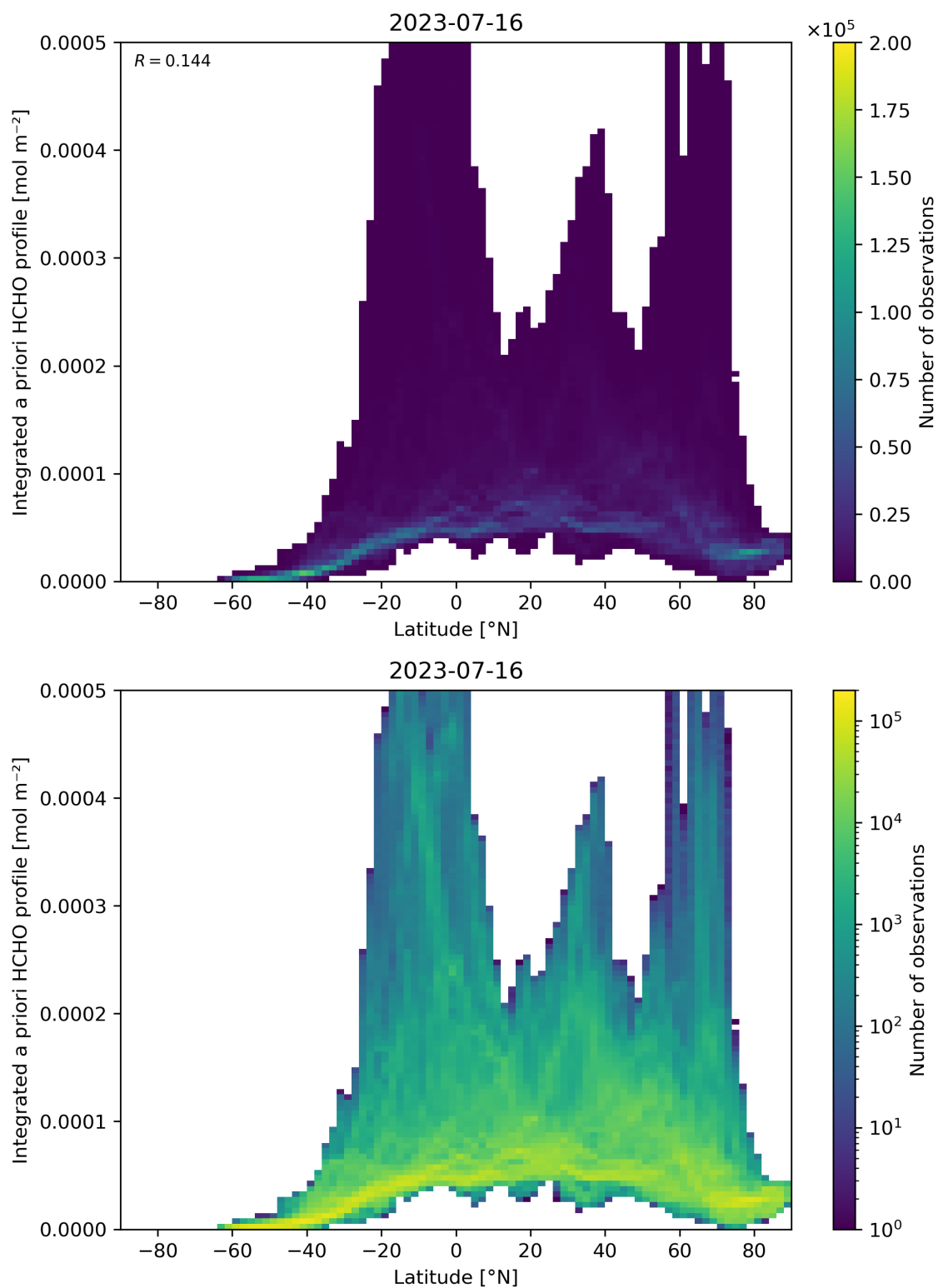
Figure 166: Scatter density plot of “Latitude” against “Integrated a priori HCHO profile” for 2023-07-15 to 2023-07-17.
