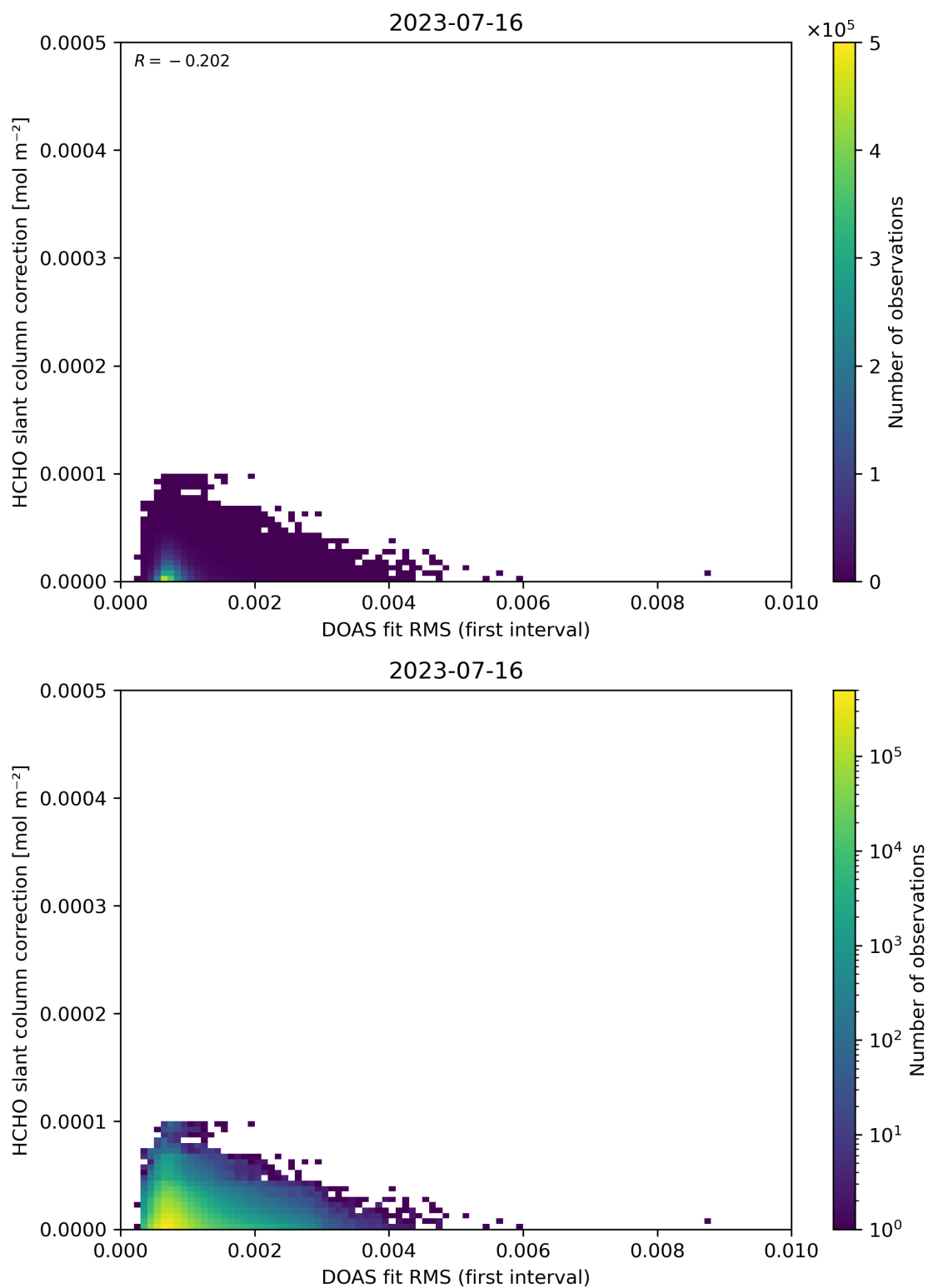
Figure 63: Scatter density plot of “DOAS fit RMS (first interval)” against “HCHO slant column correction” for 2023-07-15 to 2023-07-17.
