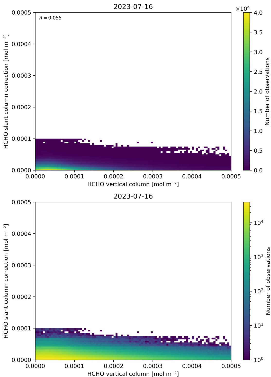
Figure 128: Scatter density plot of “HCHO vertical column” against “HCHO slant column correction” for 2023-07-15 to 2023-07-17.
