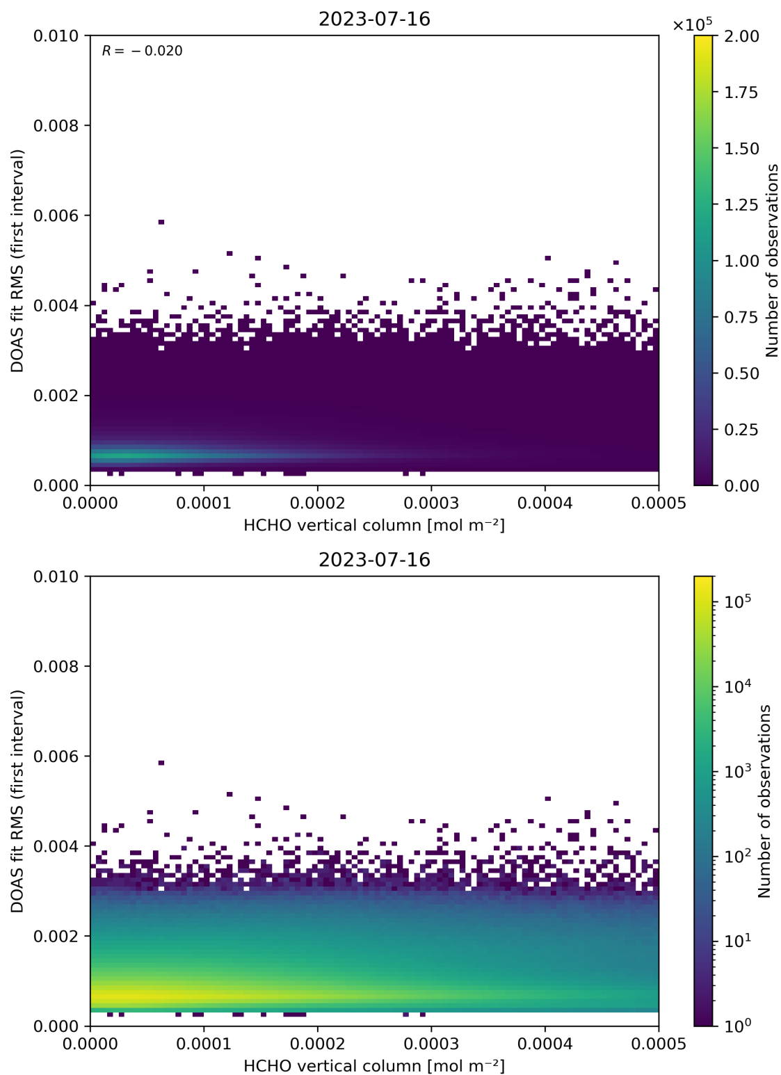
Figure 123: Scatter density plot of “HCHO vertical column” against “DOAS fit RMS (first interval)” for 2023-07-15 to 2023-07-17.
