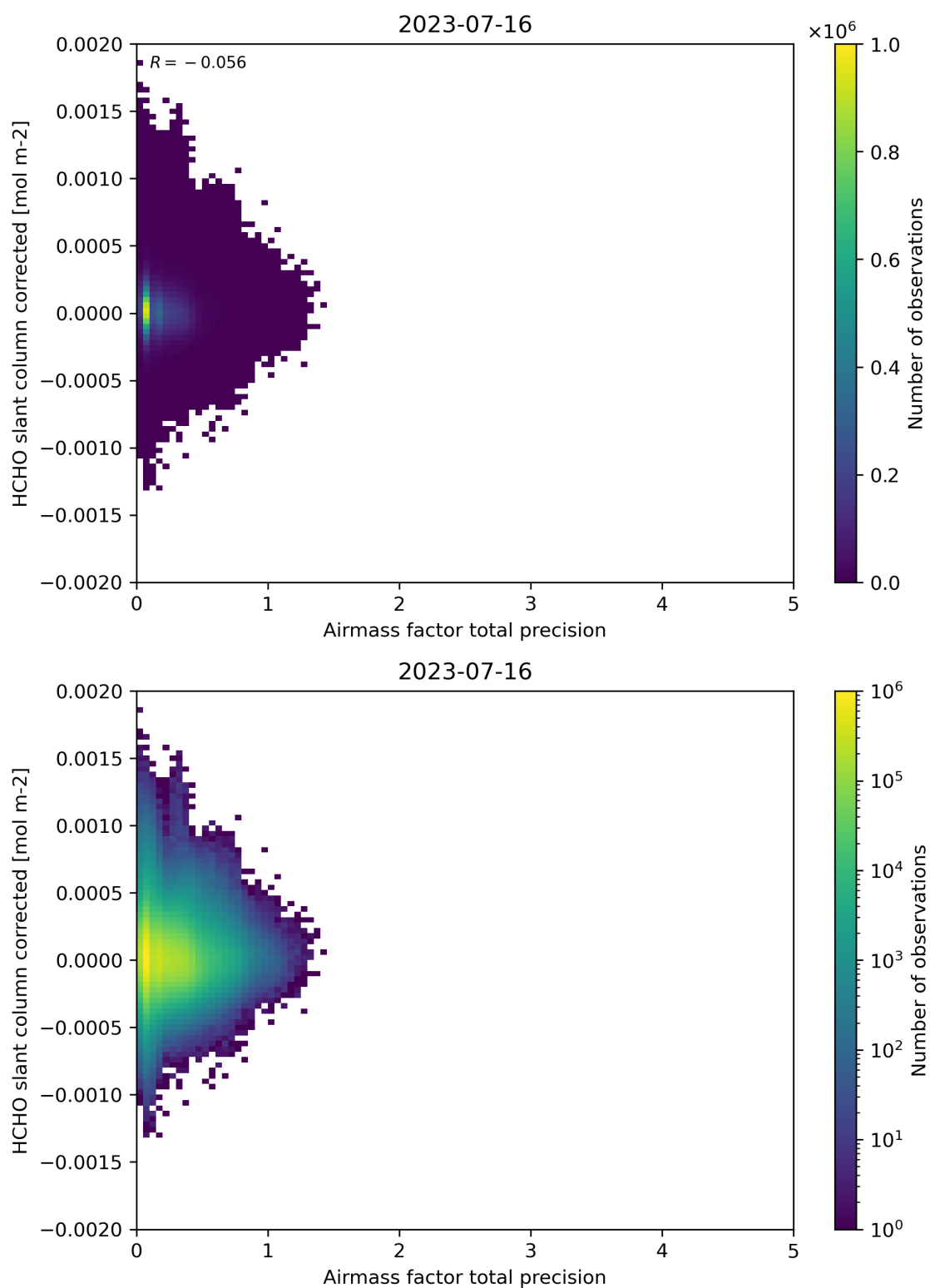
Figure 109: Scatter density plot of “Airmass factor total precision” against “HCHO slant column corrected” for 2023-07-15 to 2023-07-17.
