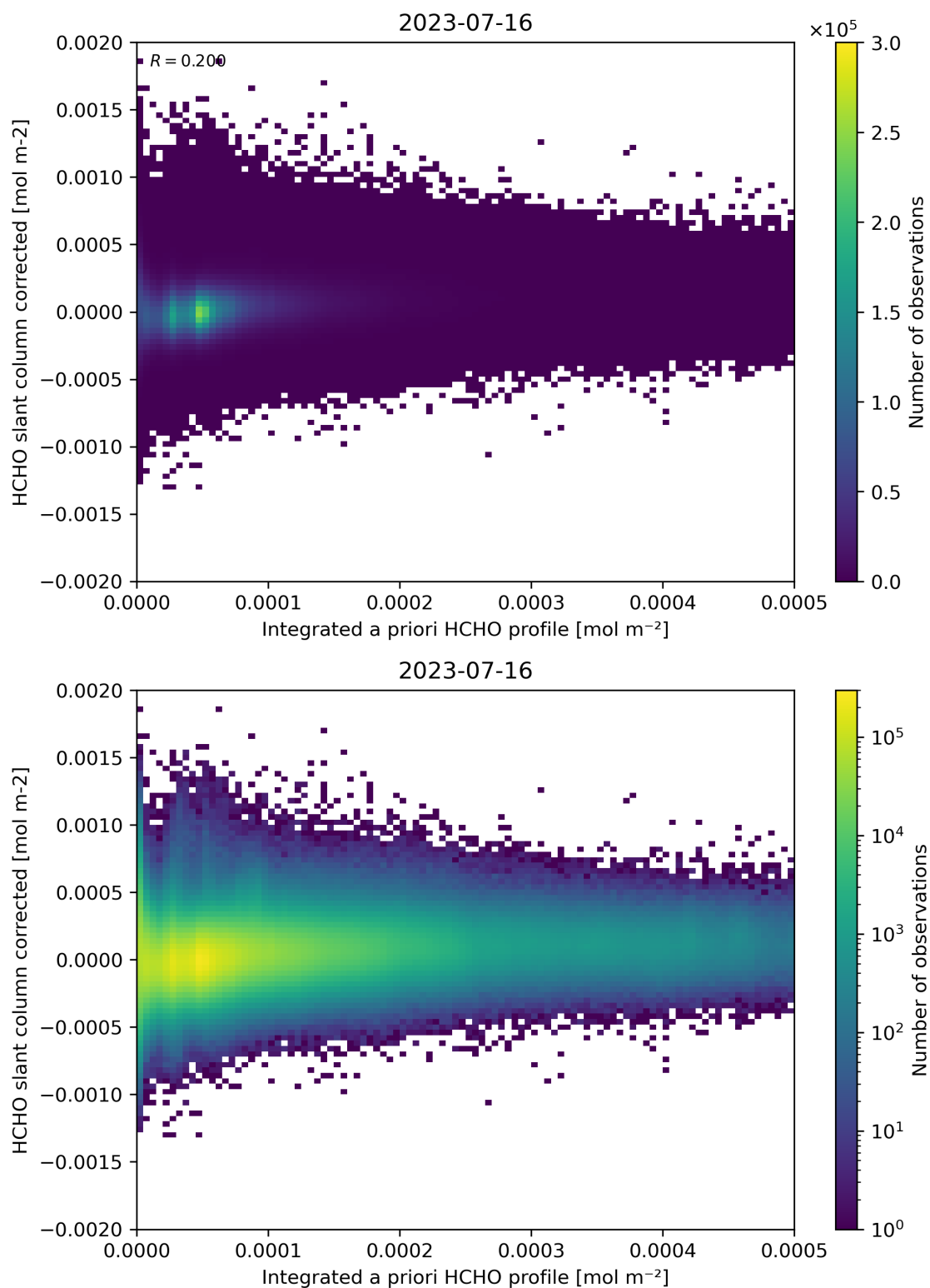
Figure 151: Scatter density plot of “Integrated a priori HCHO profile” against “HCHO slant column corrected” for 2023-07-15 to 2023-07-17.
