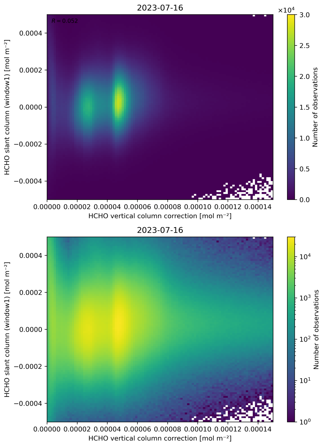
Figure 118: Scatter density plot of “HCHO vertical column correction” against “HCHO slant column (window1)” for 2023-07-15 to 2023-07-17.
