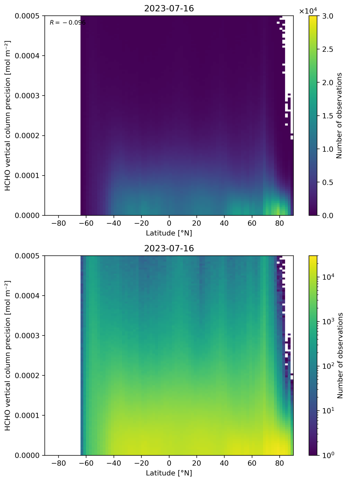
Figure 165: Scatter density plot of “Latitude” against “HCHO vertical column precision” for 2023-07-15 to 2023-07-17.
