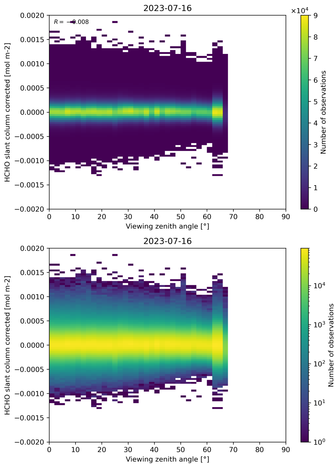
Figure 186: Scatter density plot of “Viewing zenith angle” against “HCHO slant column corrected” for 2023-07-15 to 2023-07-17.
