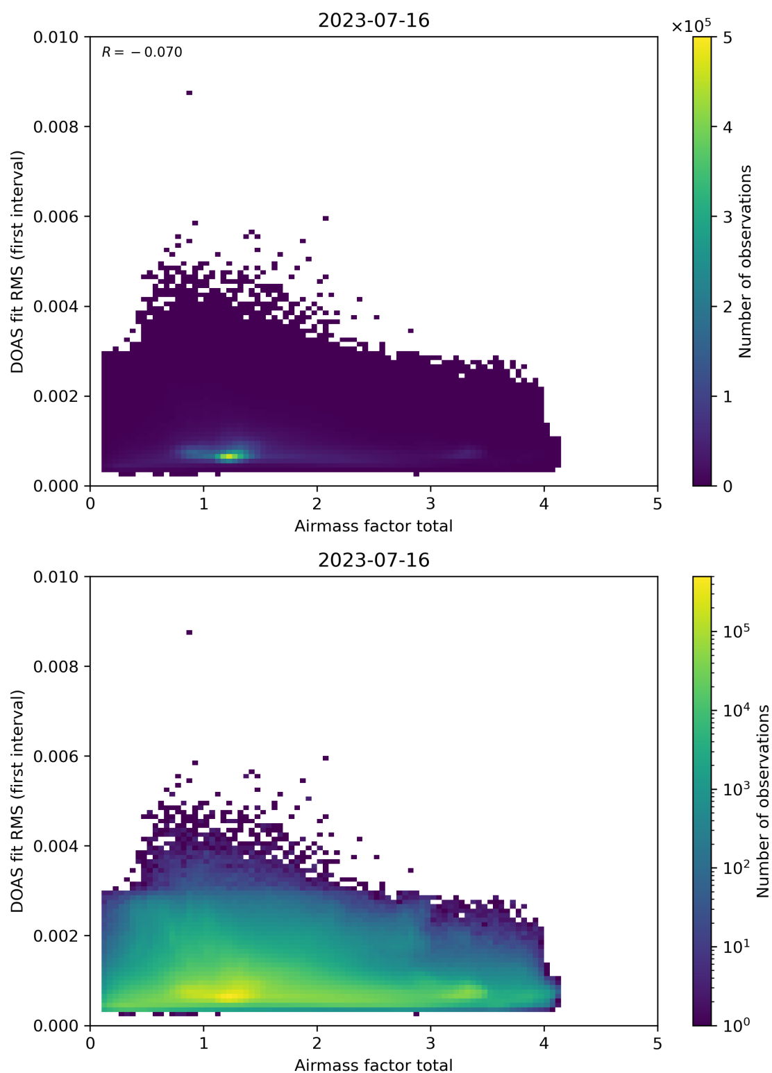
Figure 97: Scatter density plot of “Airmass factor total” against “DOAS fit RMS (first interval)” for 2023-07-15 to 2023-07-17.
