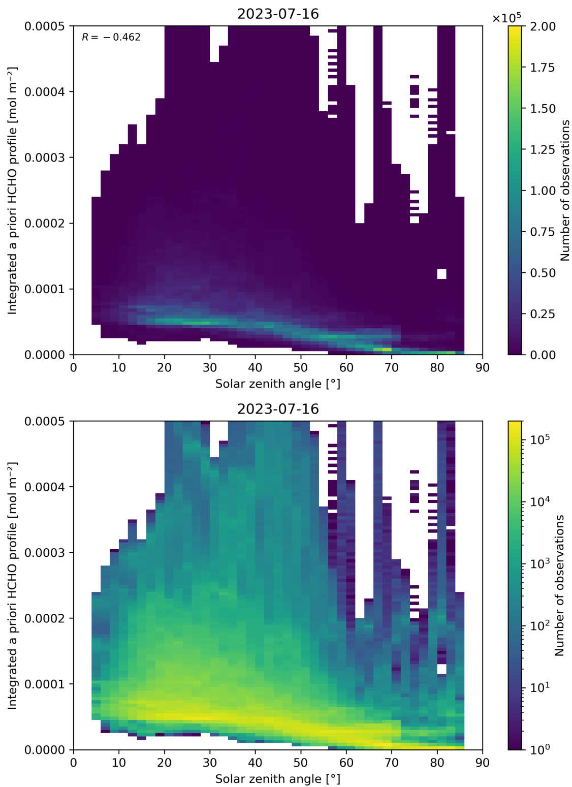
Figure 180: Scatter density plot of “Solar zenith angle” against “Integrated a priori HCHO profile” for 2023-07-15 to 2023-07-17.
