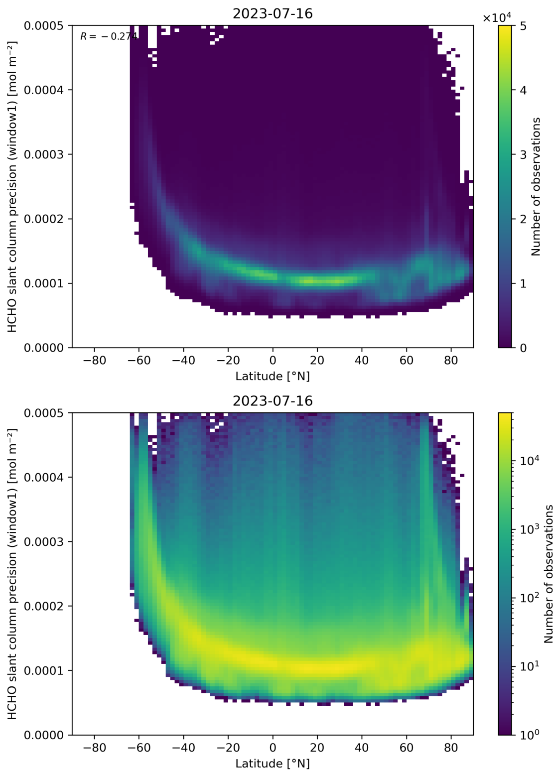
Figure 160: Scatter density plot of “Latitude” against “HCHO slant column precision (window1)” for 2023-07-15 to 2023-07-17.
