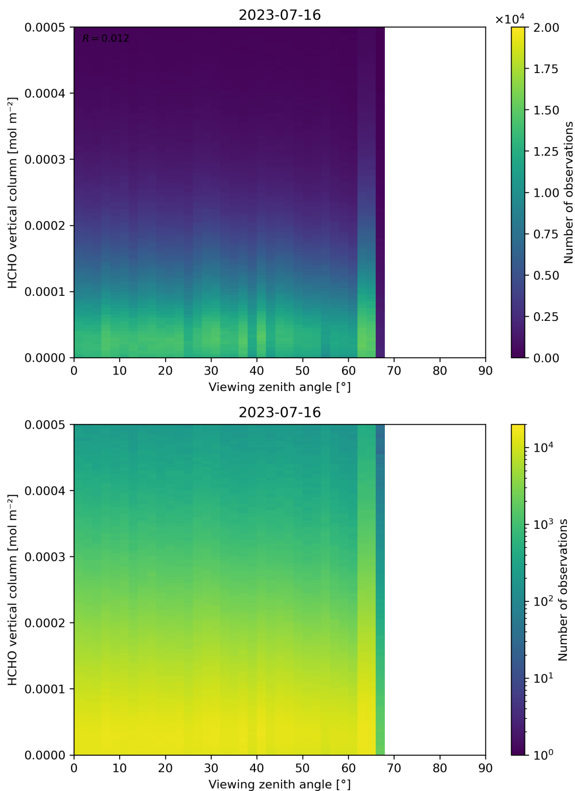
Figure 192: Scatter density plot of “Viewing zenith angle” against “HCHO vertical column” for 2023-07-15 to 2023-07-17.
