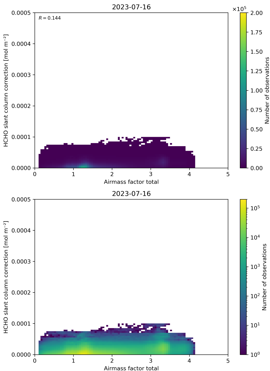
Figure 102: Scatter density plot of “Airmass factor total” against “HCHO slant column correction” for 2023-07-15 to 2023-07-17.
