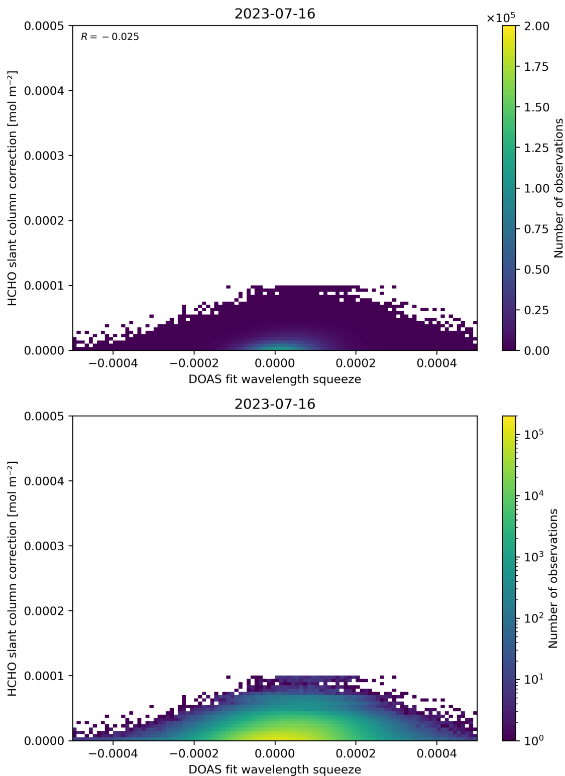
Figure 70: Scatter density plot of “DOAS fit wavelength squeeze” against “HCHO slant column correction” for 2023-07-15 to 2023-07-17.
