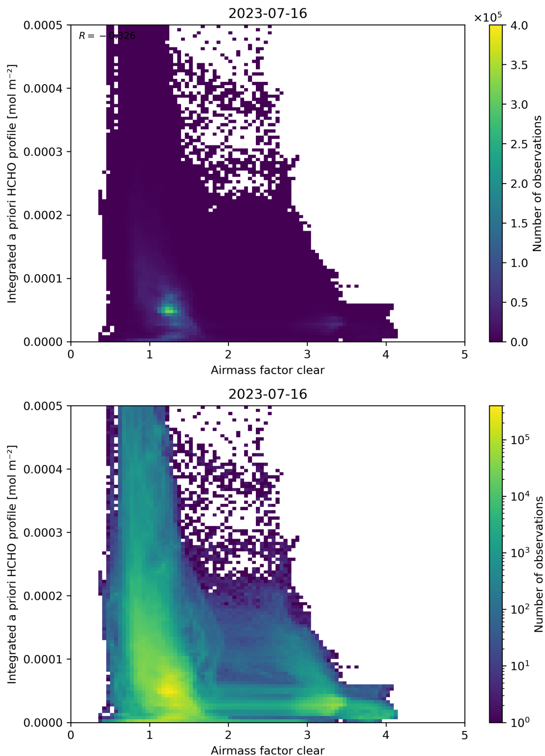
Figure 76: Scatter density plot of “Airmass factor clear” against “Integrated a priori HCHO profile” for 2023-07-15 to 2023-07-17.
