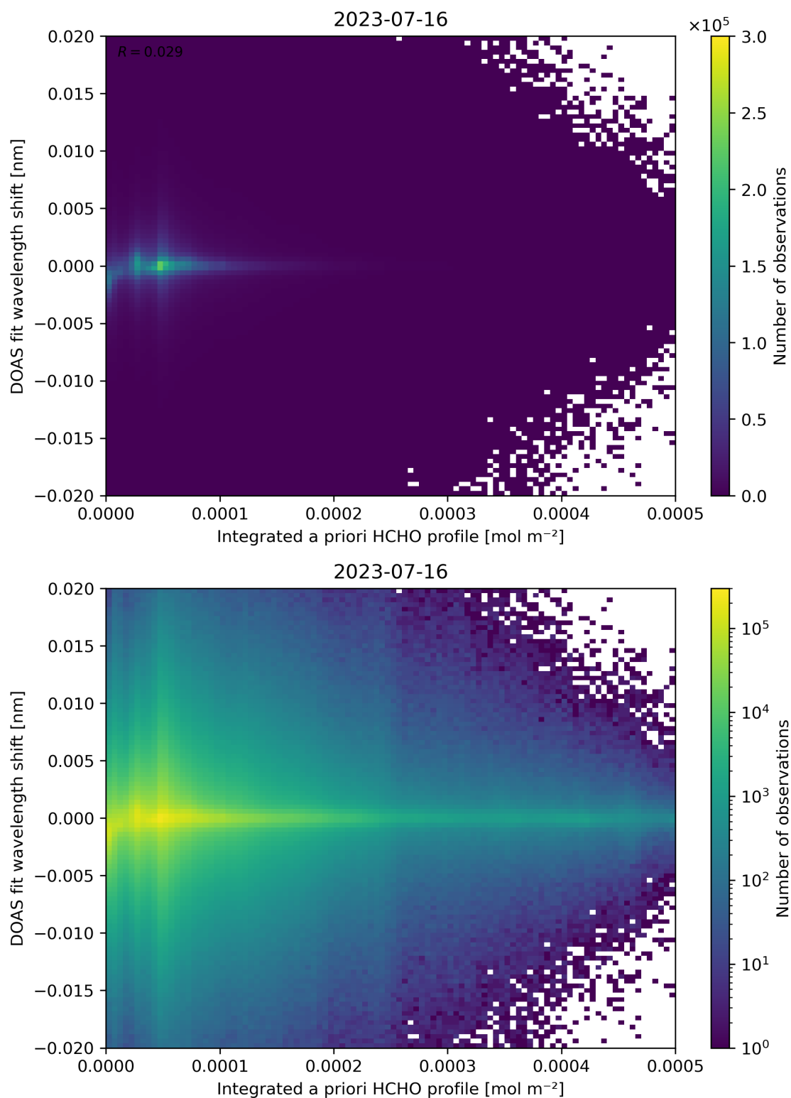
Figure 149: Scatter density plot of “Integrated a priori HCHO profile” against “DOAS fit wavelength shift” for 2023-07-15 to 2023-07-17.
