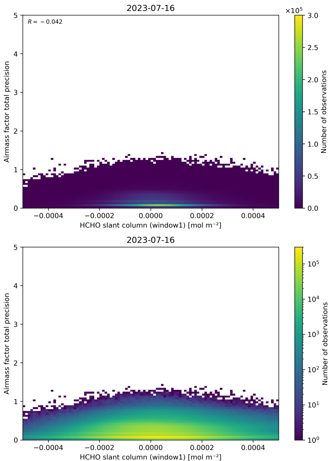
Figure 86: Scatter density plot of “HCHO slant column (window1)” against “Airmass factor total precision” for 2023-07-15 to 2023-07-17.
