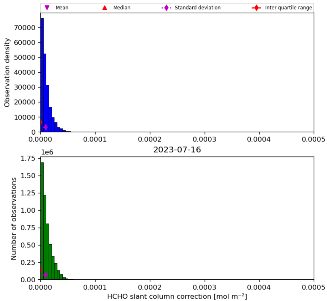
Figure 47: Histogram of “HCHO slant column correction” for 2023-07-15 to 2023-07-17
