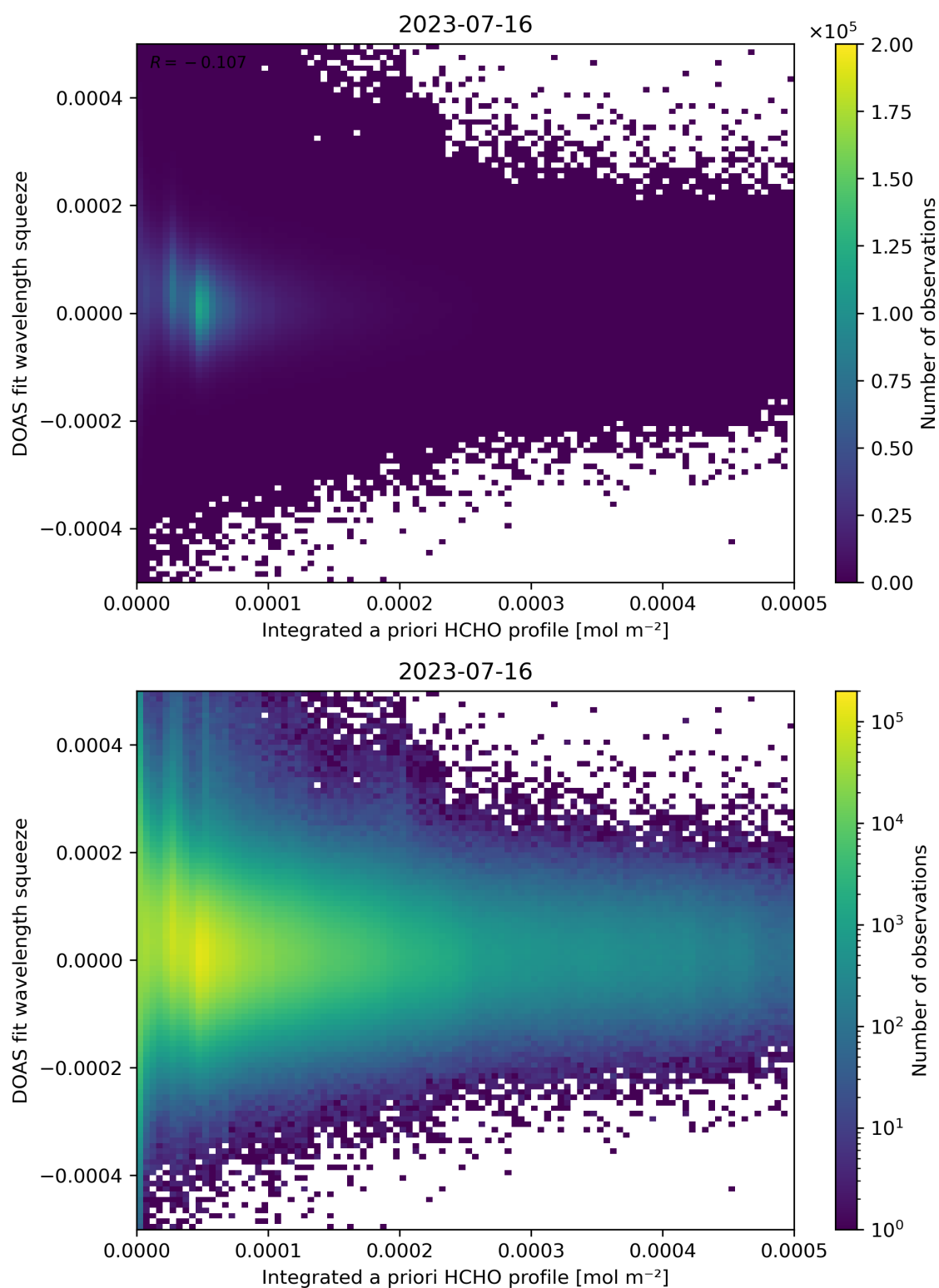
Figure 150: Scatter density plot of “Integrated a priori HCHO profile” against “DOAS fit wavelength squeeze” for 2023-07-15 to 2023-07-17.
