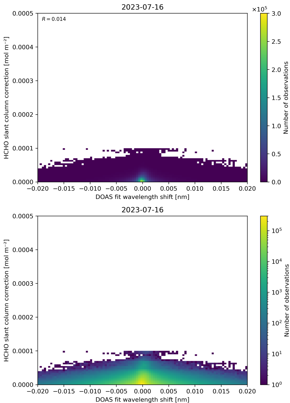
Figure 67: Scatter density plot of “DOAS fit wavelength shift” against “HCHO slant column correction” for 2023-07-15 to 2023-07-17.
