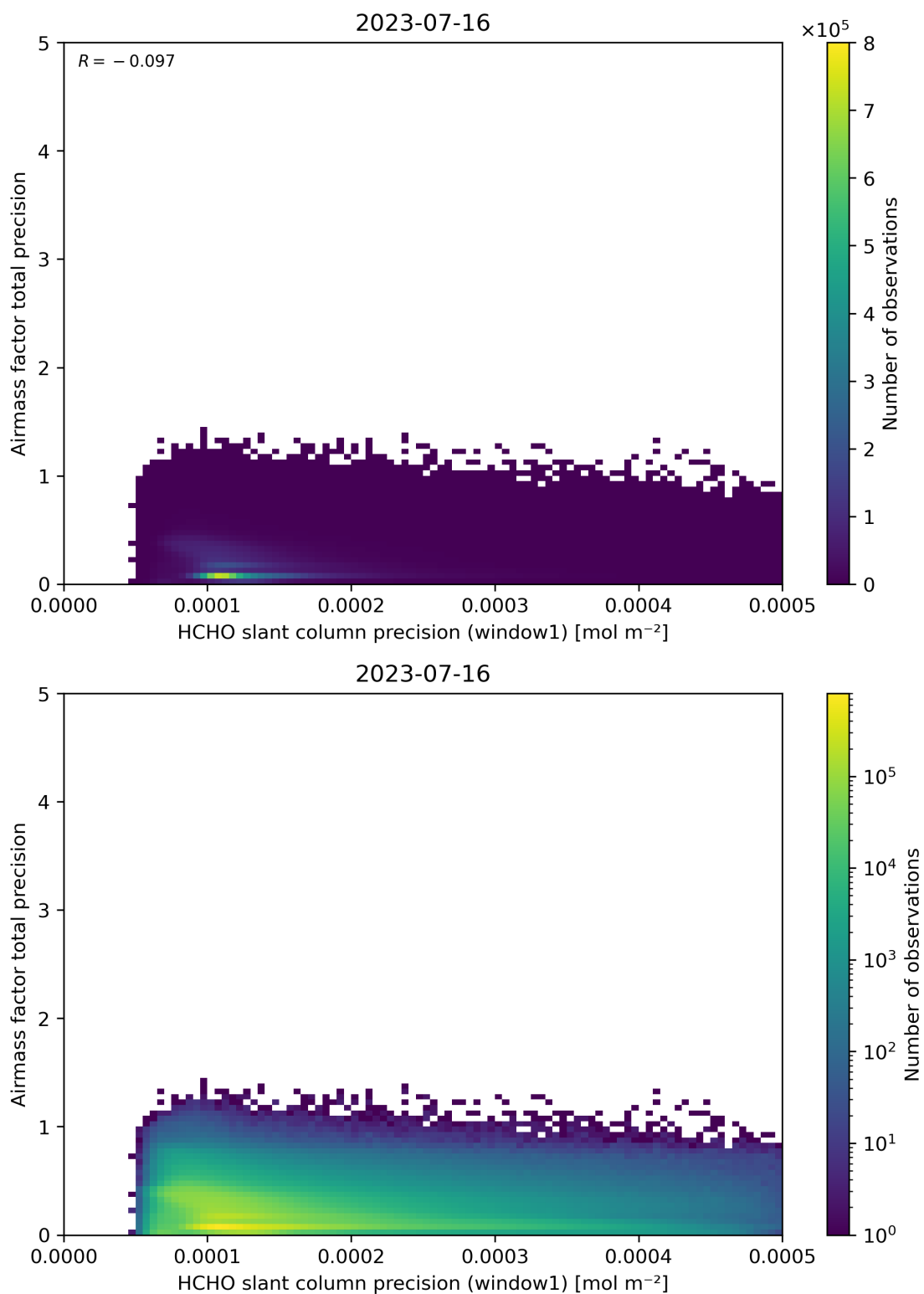
Figure 95: Scatter density plot of “HCHO slant column precision (window1)” against “Airmass factor total precision” for 2023-07-15 to 2023-07-17.
