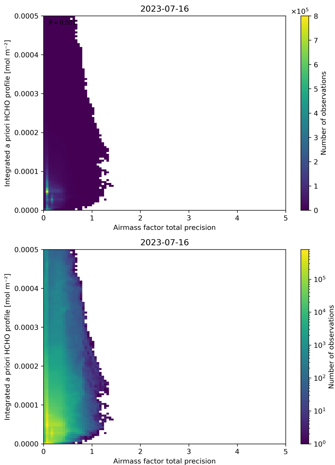
Figure 111: Scatter density plot of “Airmass factor total precision” against “Integrated a priori HCHO profile” for 2023-07-15 to 2023-07-17.
