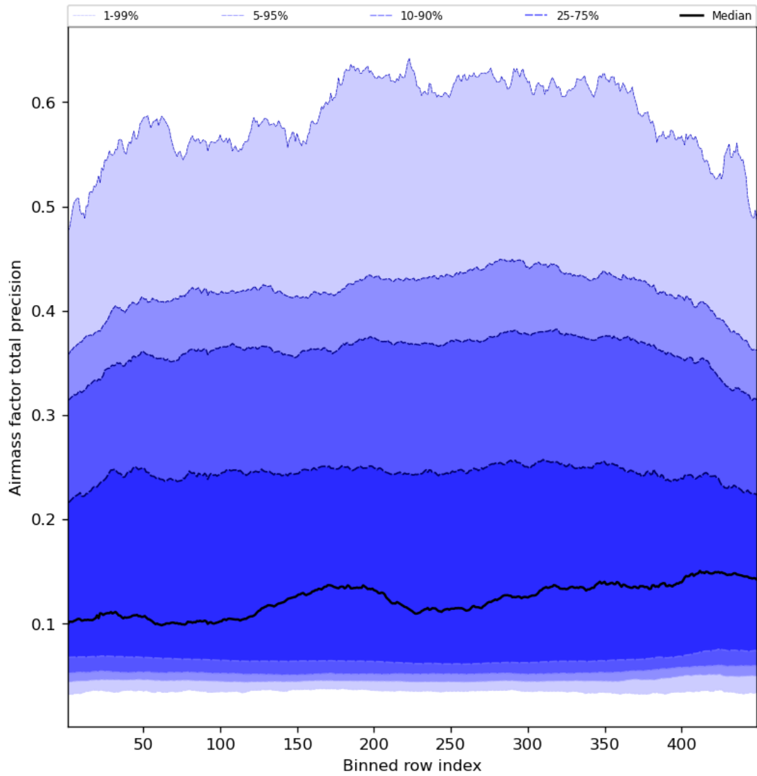
Figure 55: Along track statistics of “Airmass factor total precision” for 2023-07-15 to 2023-07-17
