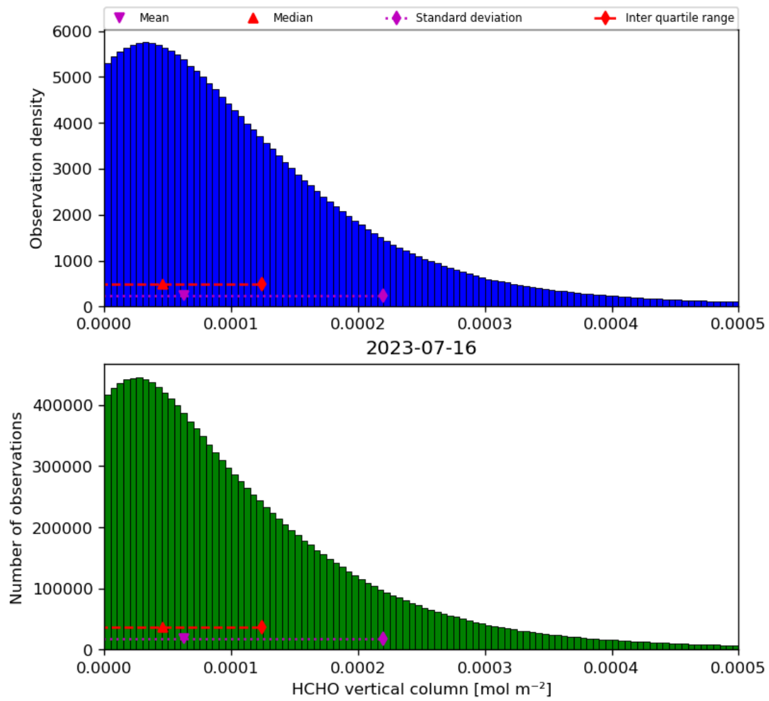
Figure 35: Histogram of “HCHO vertical column” for 2023-07-15 to 2023-07-17
