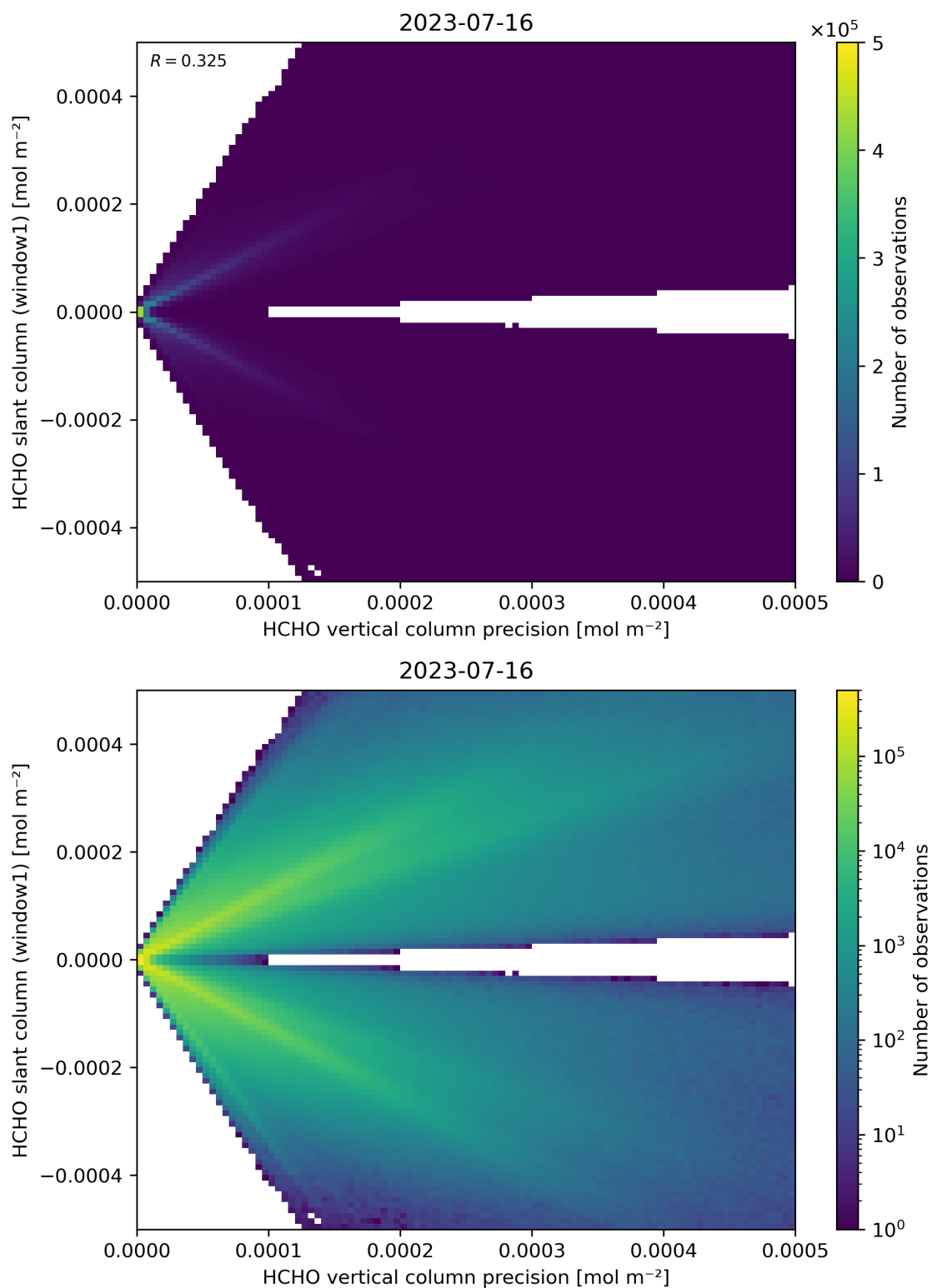
Figure 142: Scatter density plot of “HCHO vertical column precision” against “HCHO slant column (window1)” for 2023-07-15 to 2023-07-17.
