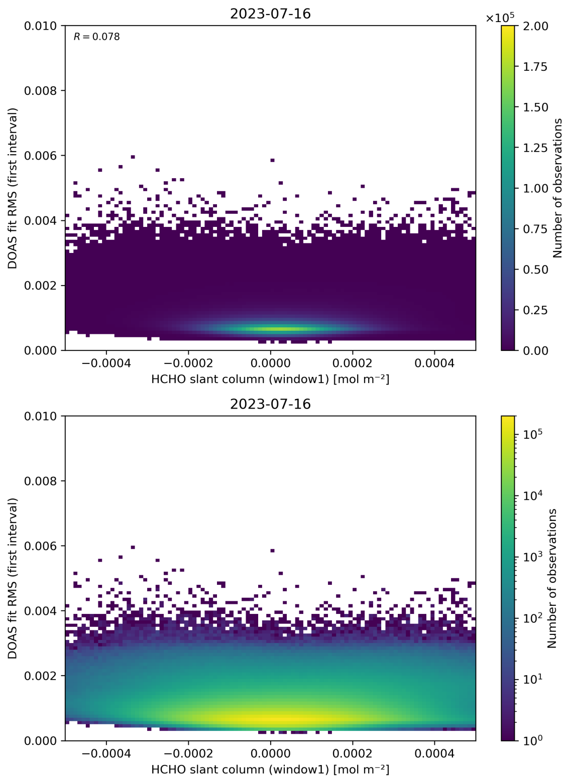
Figure 78: Scatter density plot of “HCHO slant column (window1)” against “DOAS fit RMS (first interval)” for 2023-07-15 to 2023-07-17.
