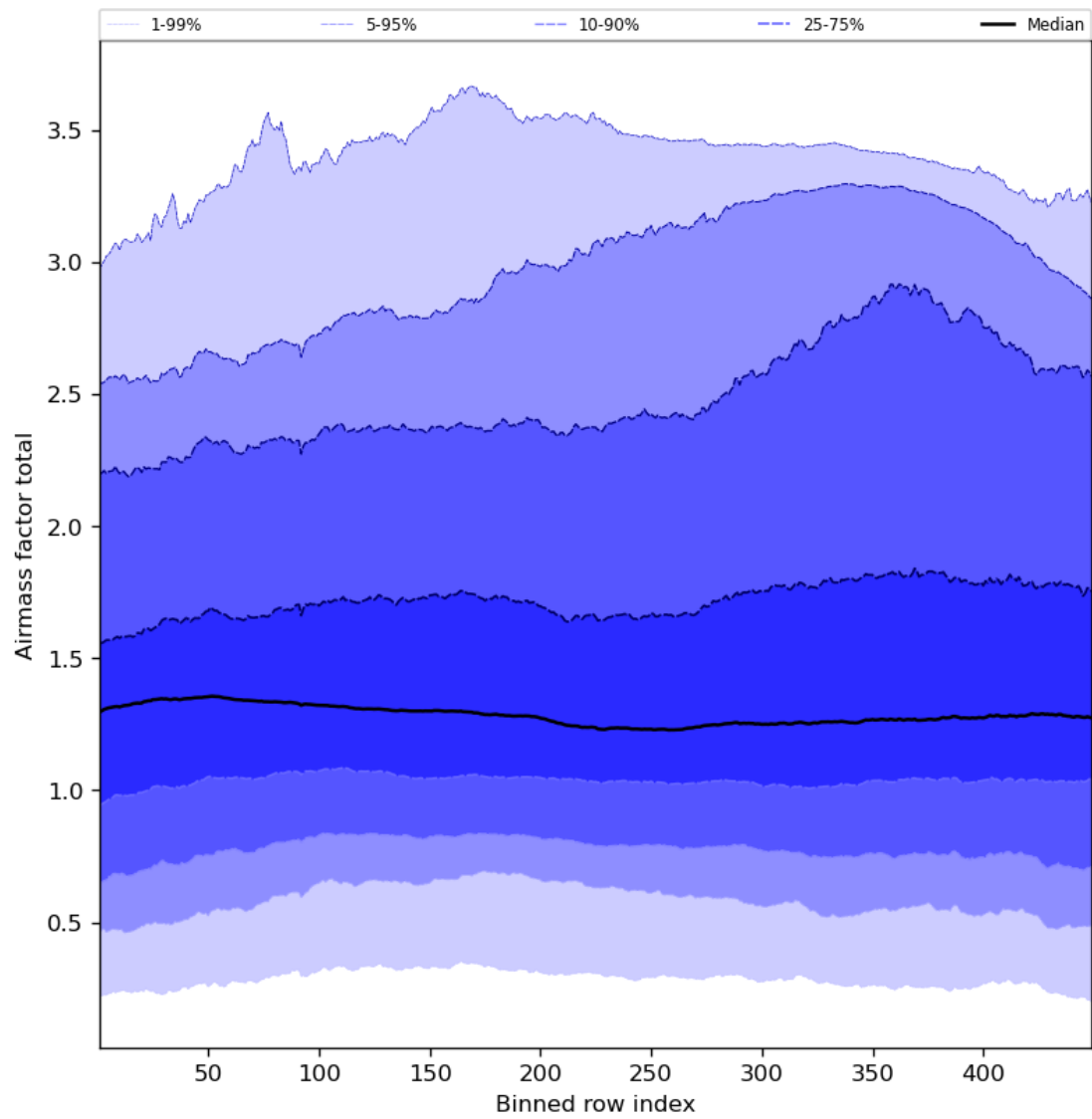
Figure 54: Along track statistics of “Airmass factor total” for 2023-07-15 to 2023-07-17
