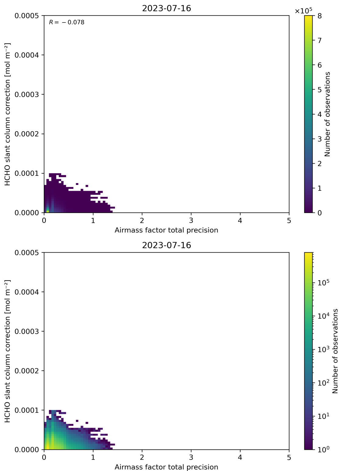
Figure 110: Scatter density plot of “Airmass factor total precision” against “HCHO slant column correction” for 2023-07-15 to 2023-07-17.
