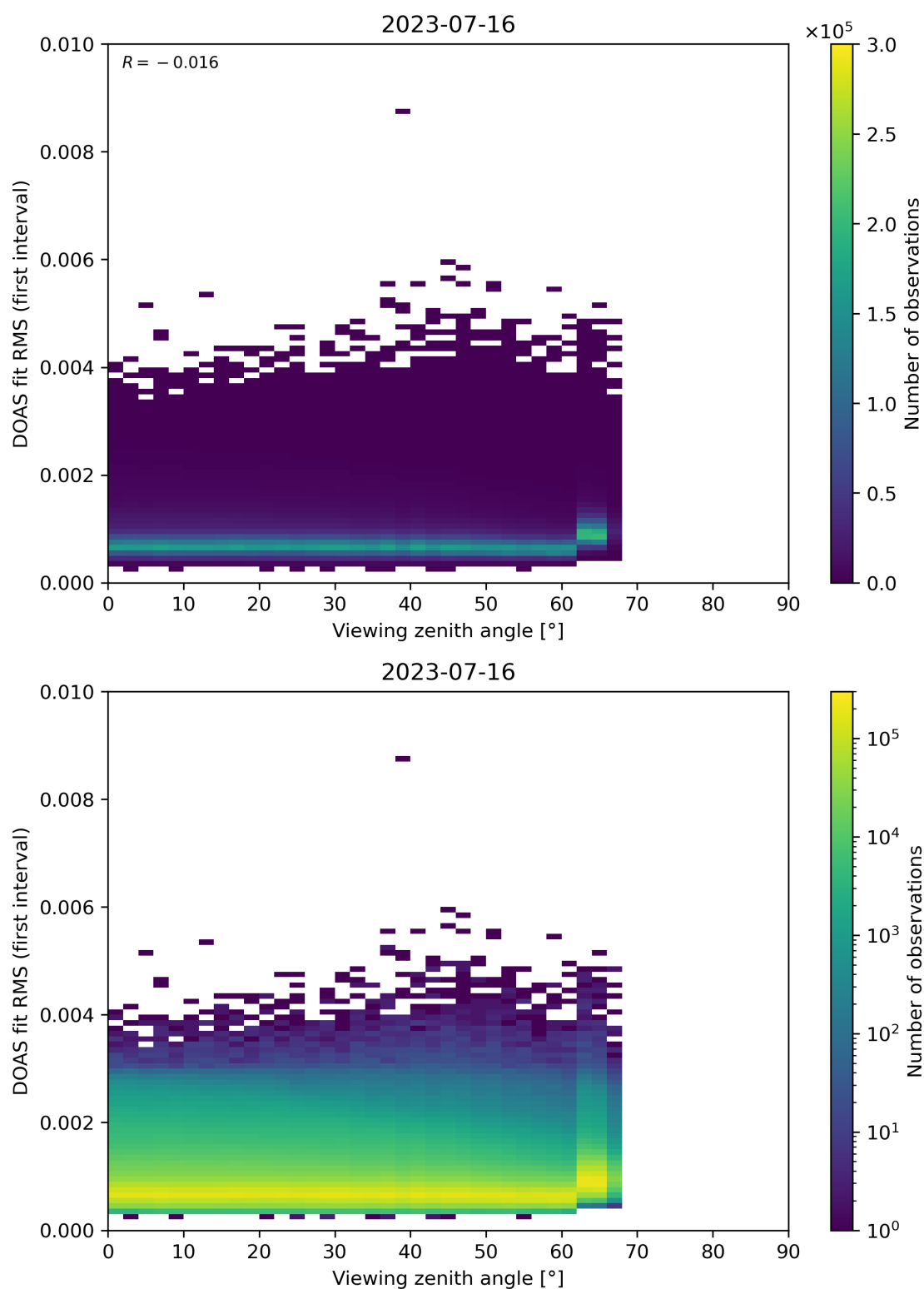
Figure 182: Scatter density plot of “Viewing zenith angle” against “DOAS fit RMS (first interval)” for 2023-07-15 to 2023-07-17.
