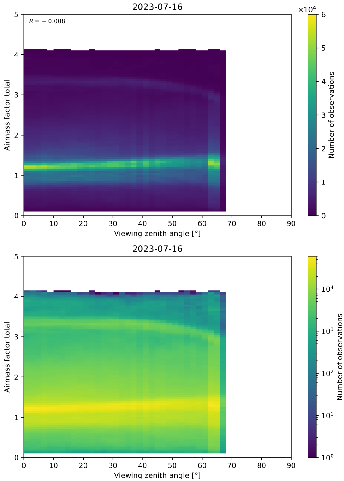
Figure 190: Scatter density plot of “Viewing zenith angle” against “Airmass factor total” for 2023-07-15 to 2023-07-17.
