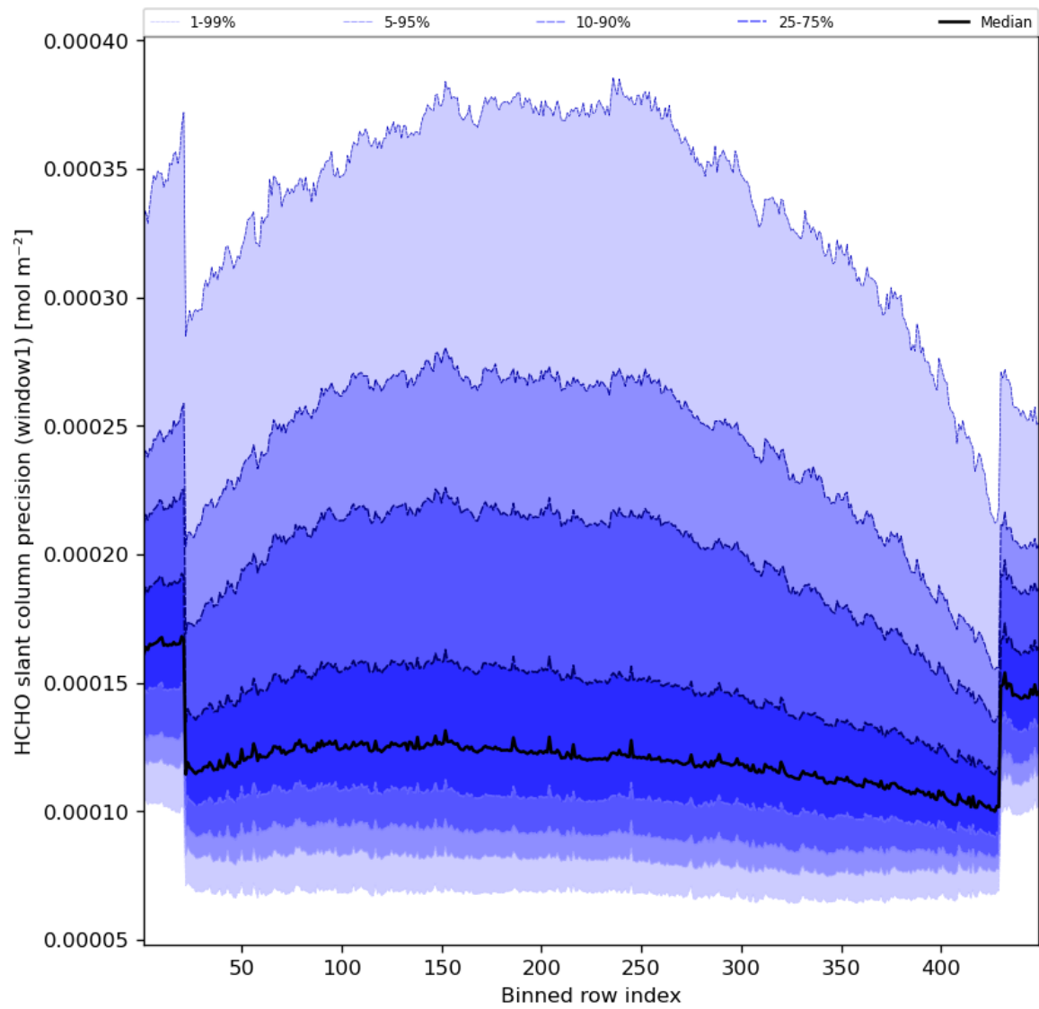
Figure 53: Along track statistics of “HCHO slant column precision (window1)” for 2023-07-15 to 2023-07-17
