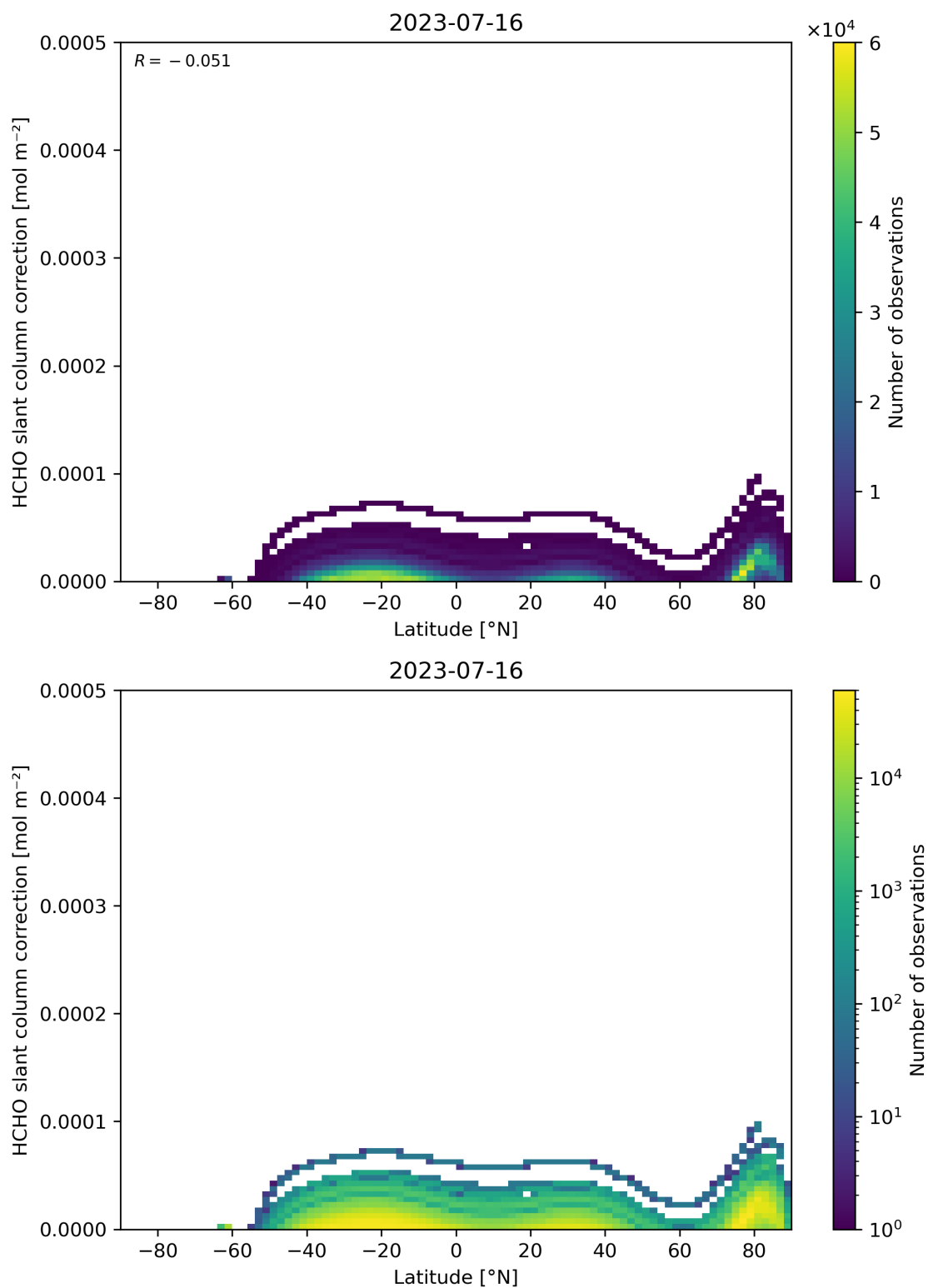
Figure 158: Scatter density plot of “Latitude” against “HCHO slant column correction” for 2023-07-15 to 2023-07-17.
