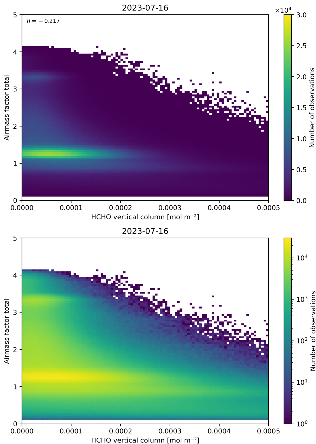
Figure 131: Scatter density plot of “HCHO vertical column” against “Airmass factor total” for 2023-07-15 to 2023-07-17.
