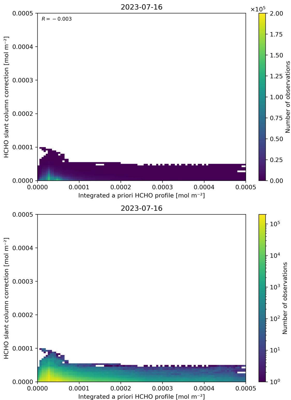
Figure 152: Scatter density plot of “Integrated a priori HCHO profile” against “HCHO slant column correction” for 2023-07-15 to 2023-07-17.
