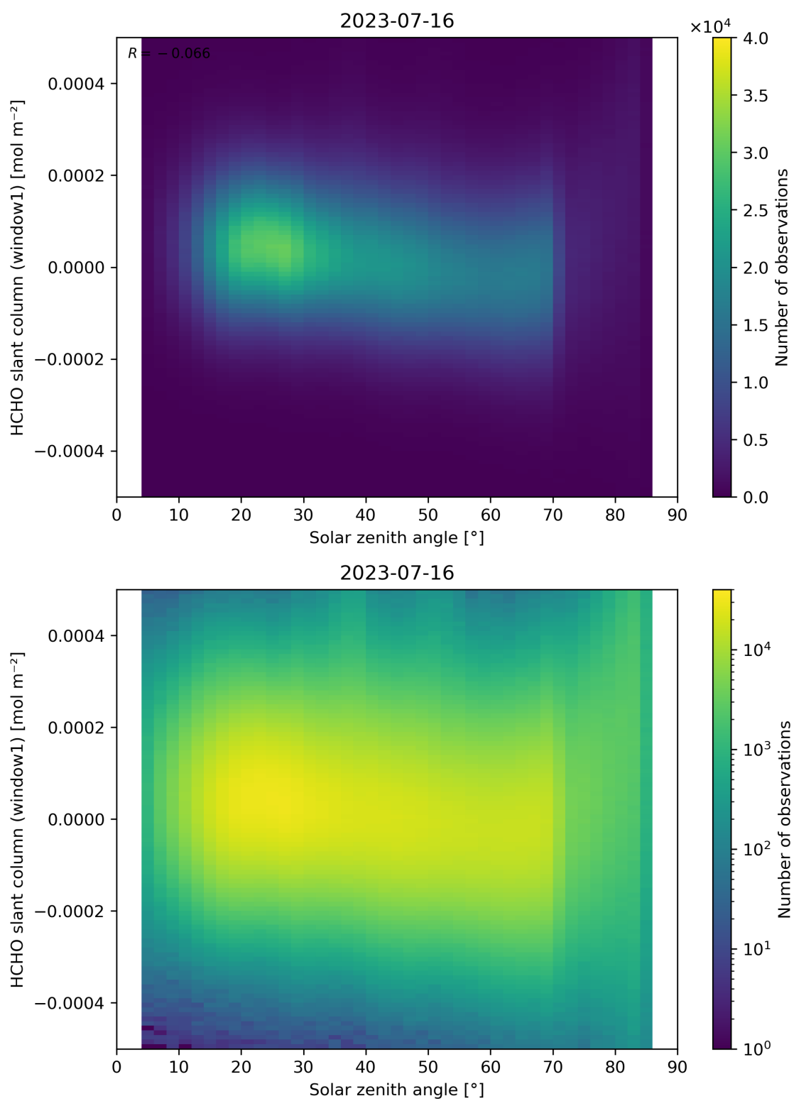
Figure 173: Scatter density plot of “Solar zenith angle” against “HCHO slant column (window1)” for 2023-07-15 to 2023-07-17.
