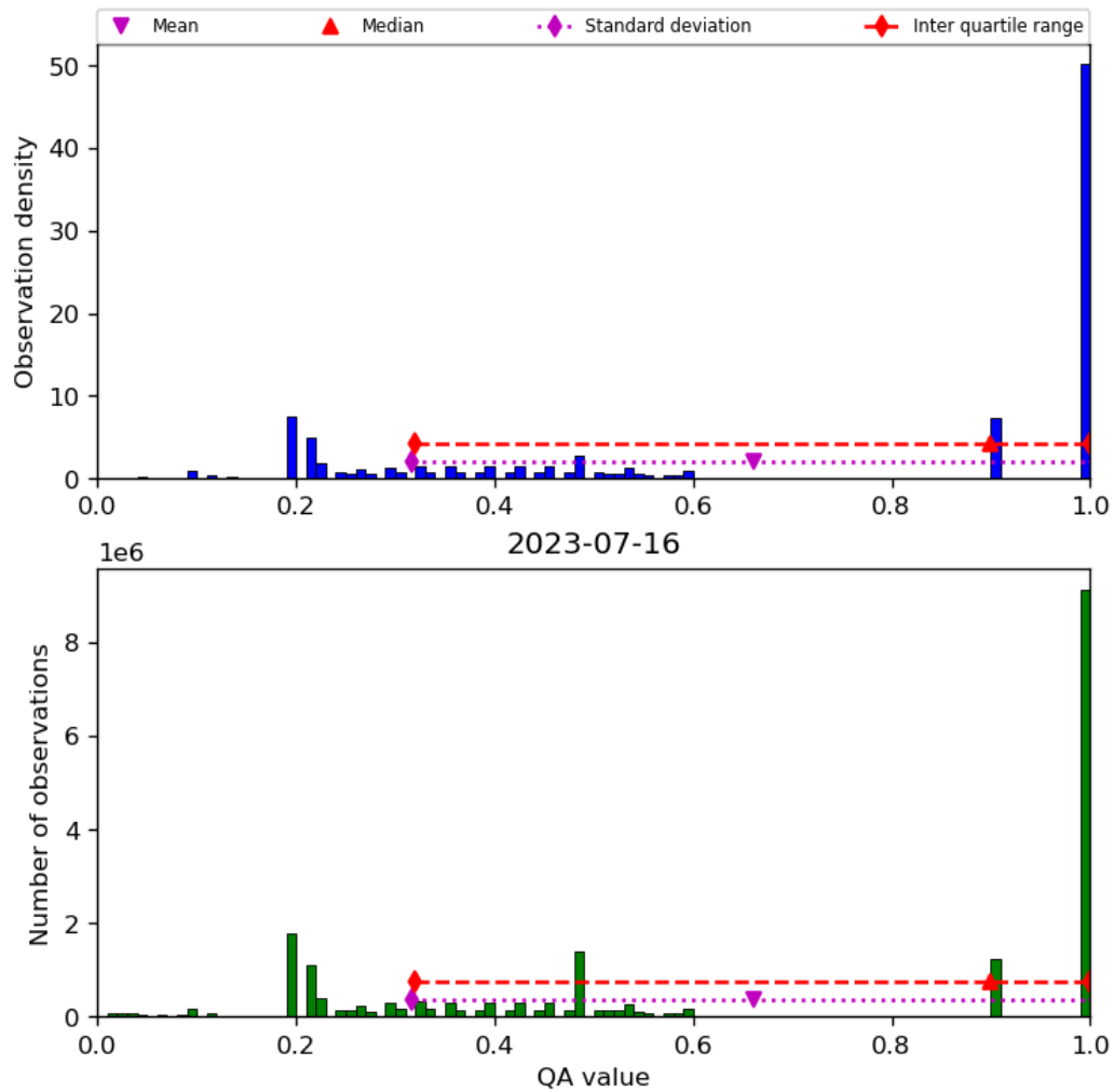
Figure 34: Histogram of “QA value” for 2023-07-15 to 2023-07-17
