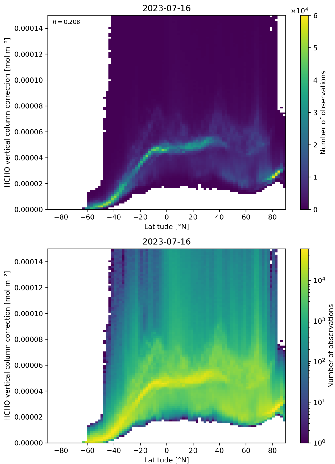
Figure 164: Scatter density plot of “Latitude” against “HCHO vertical column correction” for 2023-07-15 to 2023-07-17.
