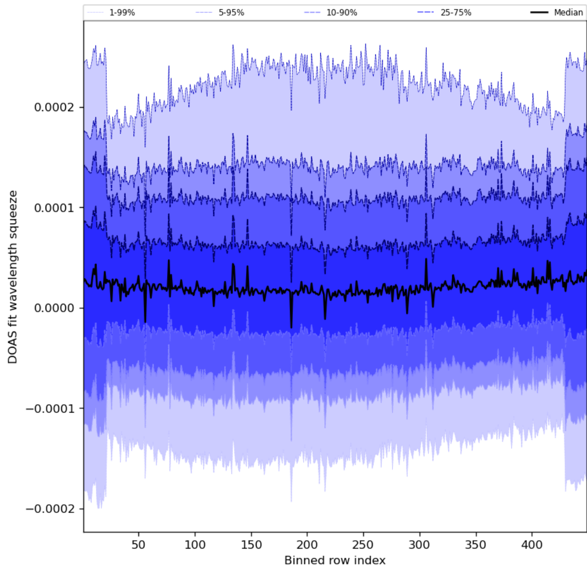
Figure 59: Along track statistics of “DOAS fit wavelength squeeze” for 2023-07-15 to 2023-07-17
