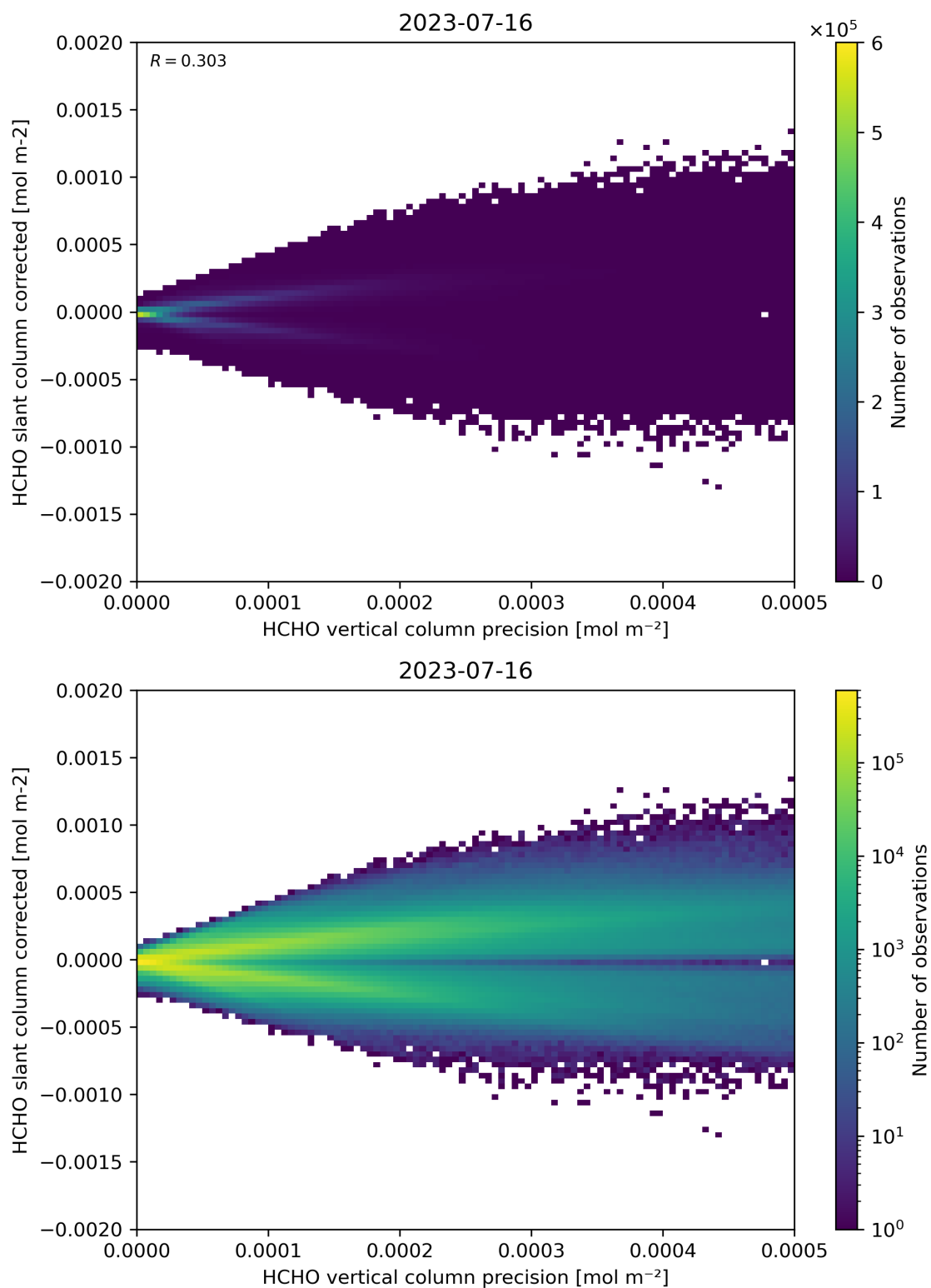
Figure 140: Scatter density plot of “HCHO vertical column precision” against “HCHO slant column corrected” for 2023-07-15 to 2023-07-17.
