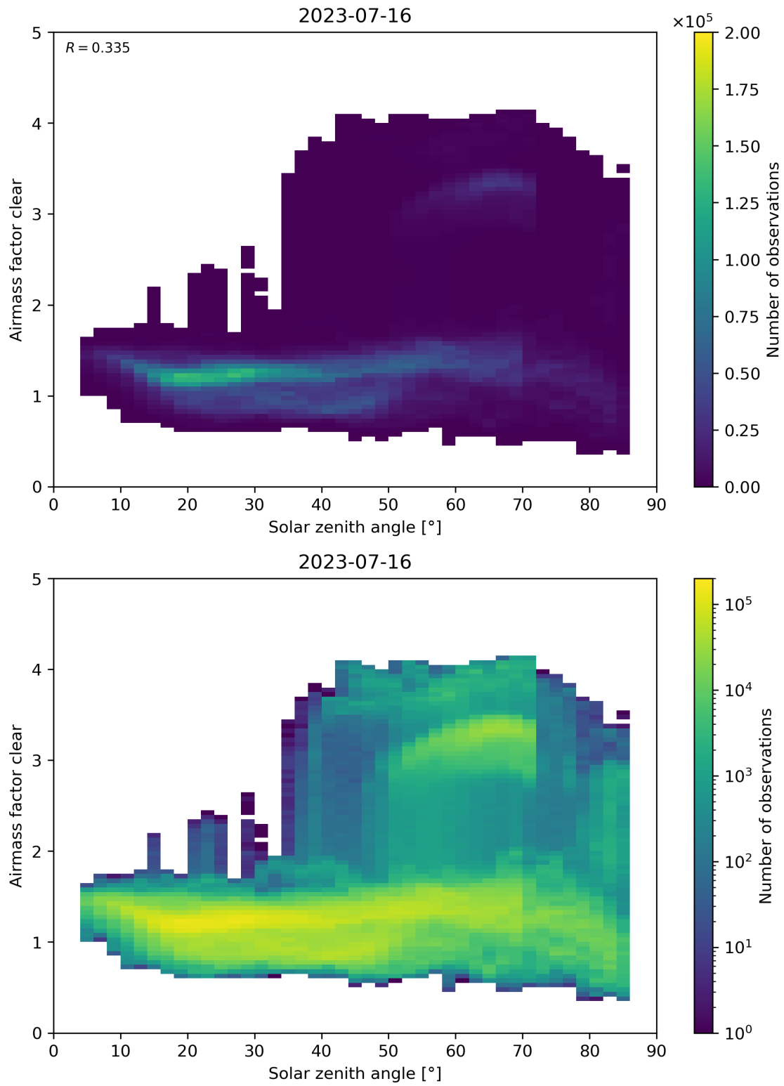
Figure 170: Scatter density plot of “Solar zenith angle” against “Airmass factor clear” for 2023-07-15 to 2023-07-17.
