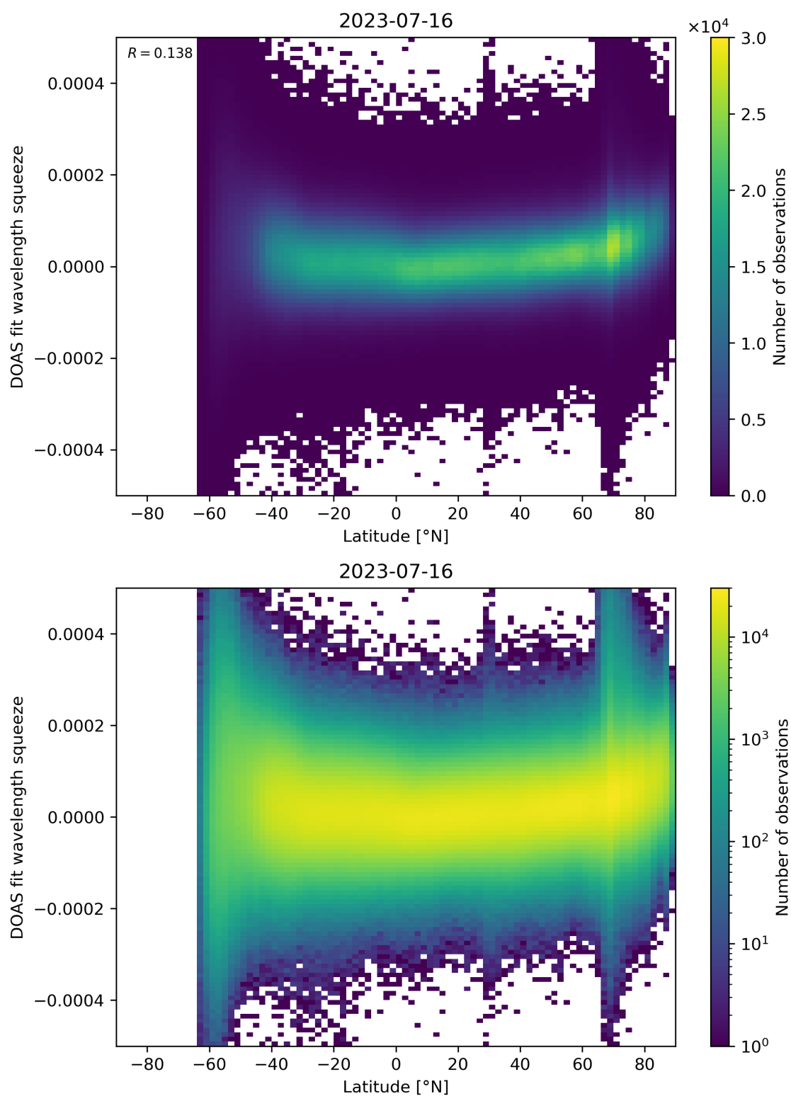
Figure 155: Scatter density plot of “Latitude” against “DOAS fit wavelength squeeze” for 2023-07-15 to 2023-07-17.
