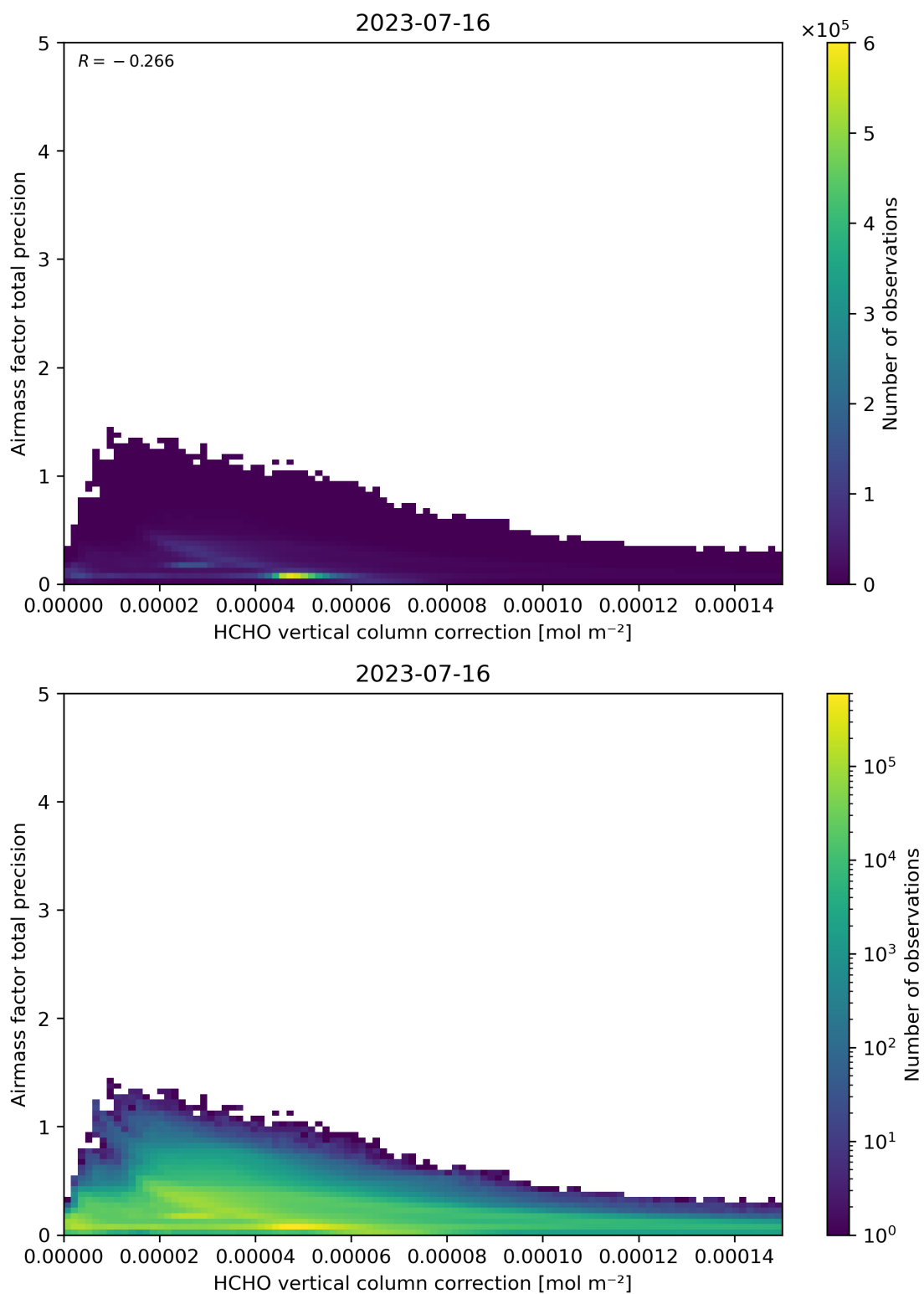
Figure 121: Scatter density plot of “HCHO vertical column correction” against “Airmass factor total precision” for 2023-07-15 to 2023-07-17.
