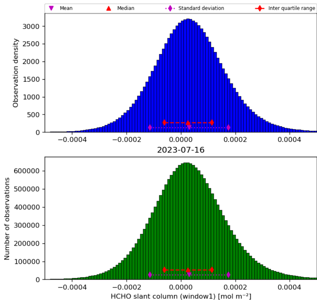
Figure 38: Histogram of “HCHO slant column (window1)” for 2023-07-15 to 2023-07-17
