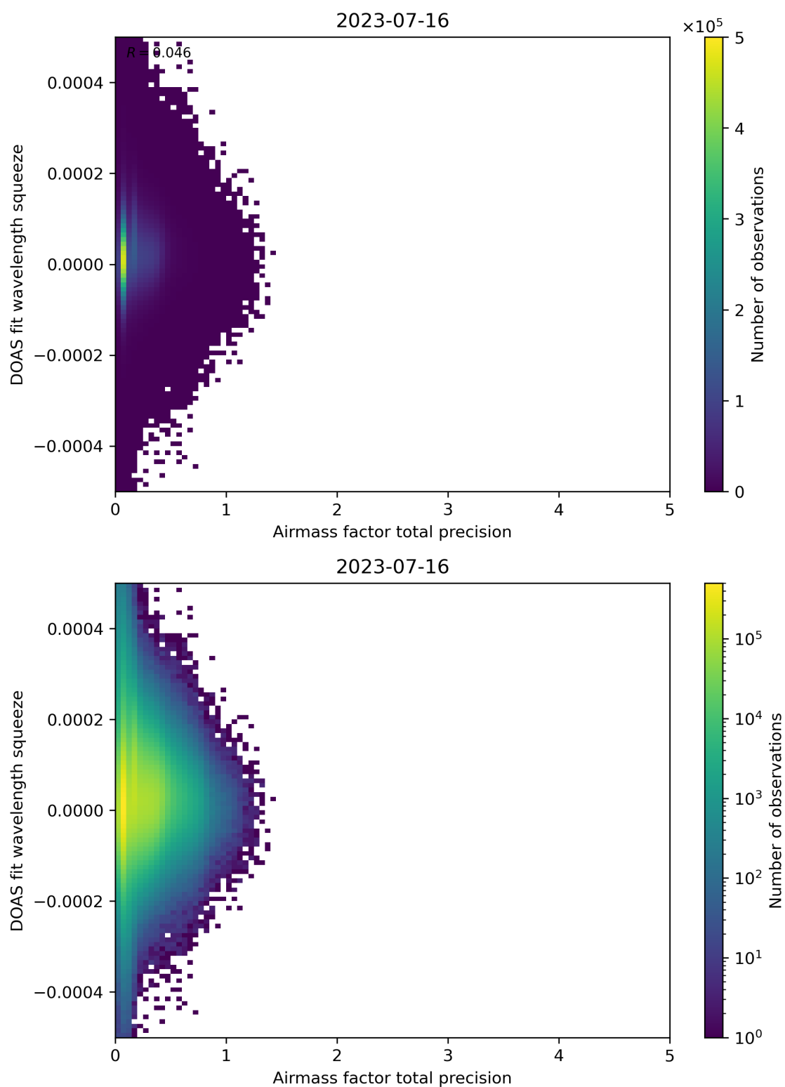
Figure 107: Scatter density plot of “Airmass factor total precision” against “DOAS fit wavelength squeeze” for 2023-07-15 to 2023-07-17.
