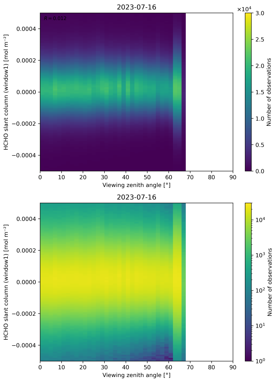
Figure 188: Scatter density plot of “Viewing zenith angle” against “HCHO slant column (window1)” for 2023-07-15 to 2023-07-17.
