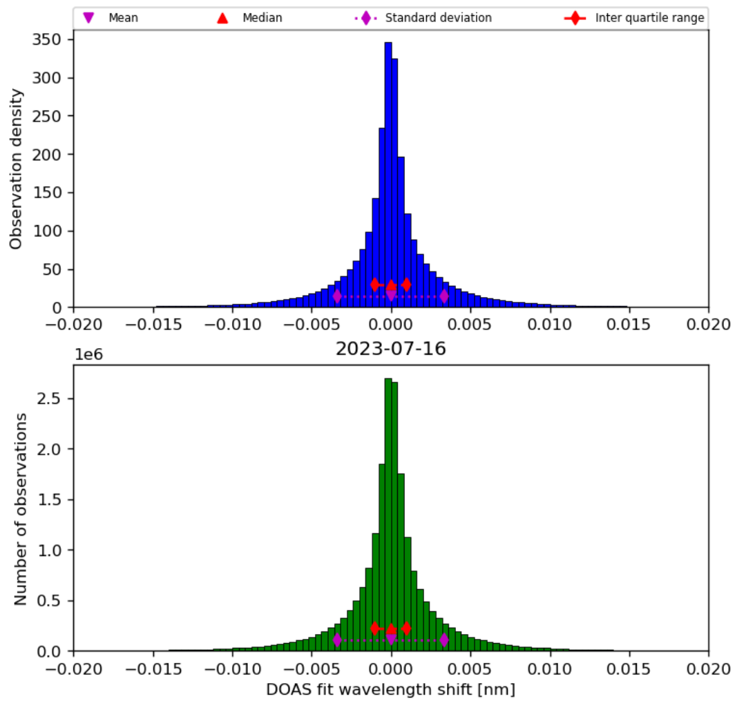
Figure 44: Histogram of “DOAS fit wavelength shift” for 2023-07-15 to 2023-07-17
