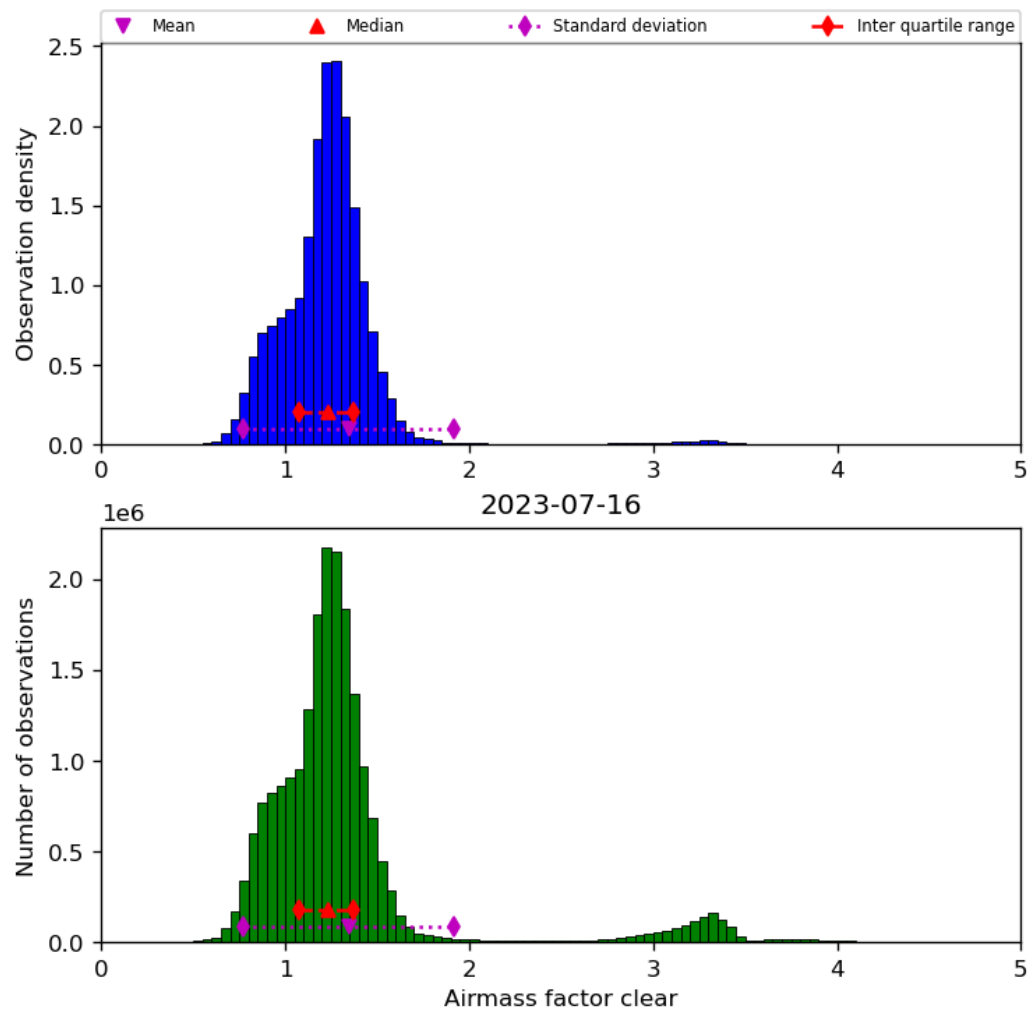
Figure 42: Histogram of “Airmass factor clear” for 2023-07-15 to 2023-07-17
