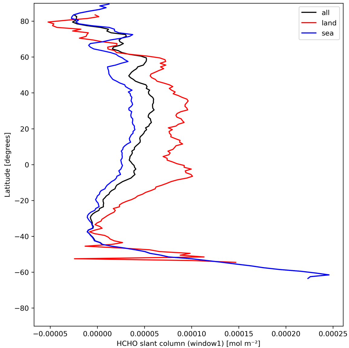
Figure 24: Zonal average of “HCHO slant column (window1)” for 2023-07-15 to 2023-07-17.
