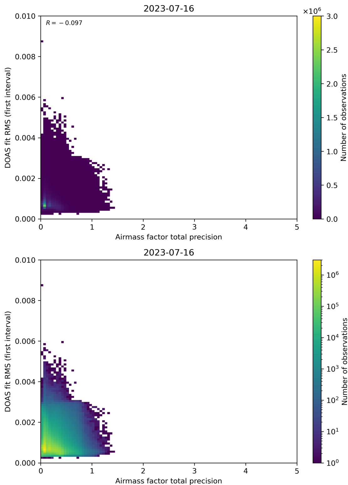
Figure 105: Scatter density plot of “Airmass factor total precision” against “DOAS fit RMS (first interval)” for 2023-07-15 to 2023-07-17.
