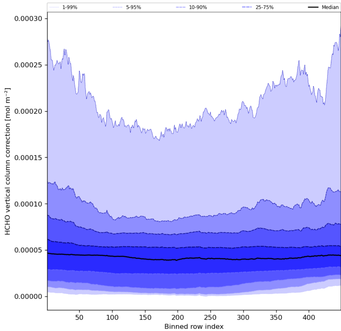
Figure 51: Along track statistics of “HCHO vertical column correction” for 2023-07-15 to 2023-07-17
