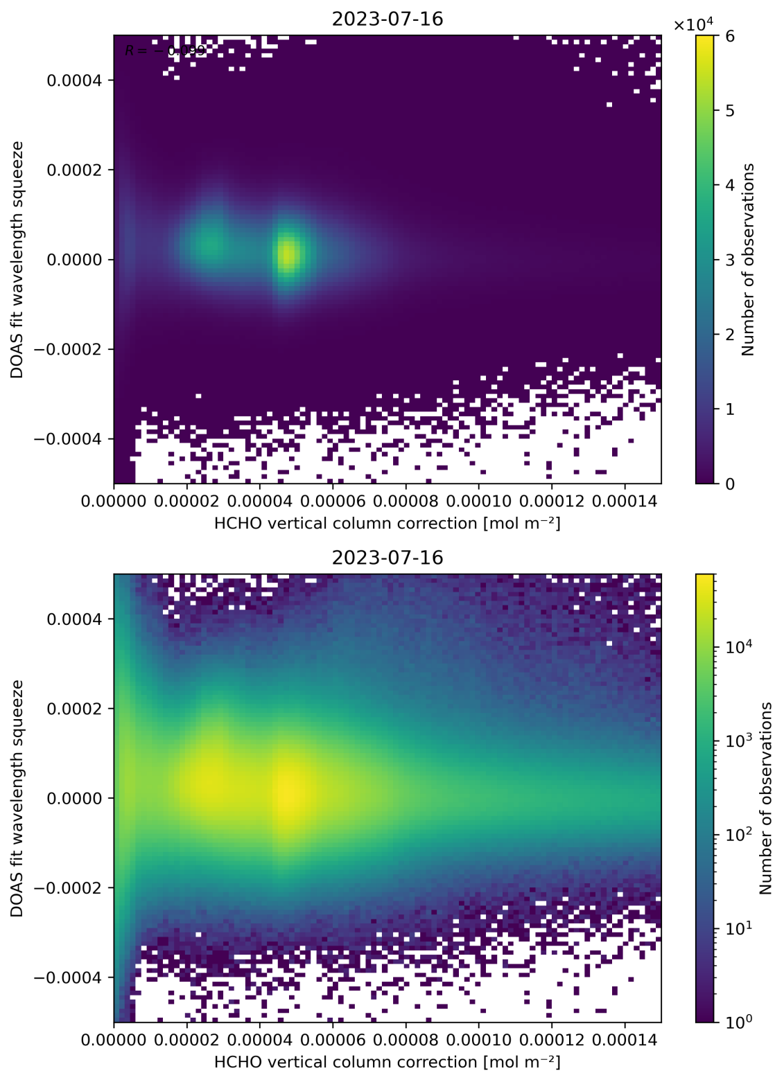
Figure 114: Scatter density plot of “HCHO vertical column correction” against “DOAS fit wavelength squeeze” for 2023-07-15 to 2023-07-17.
