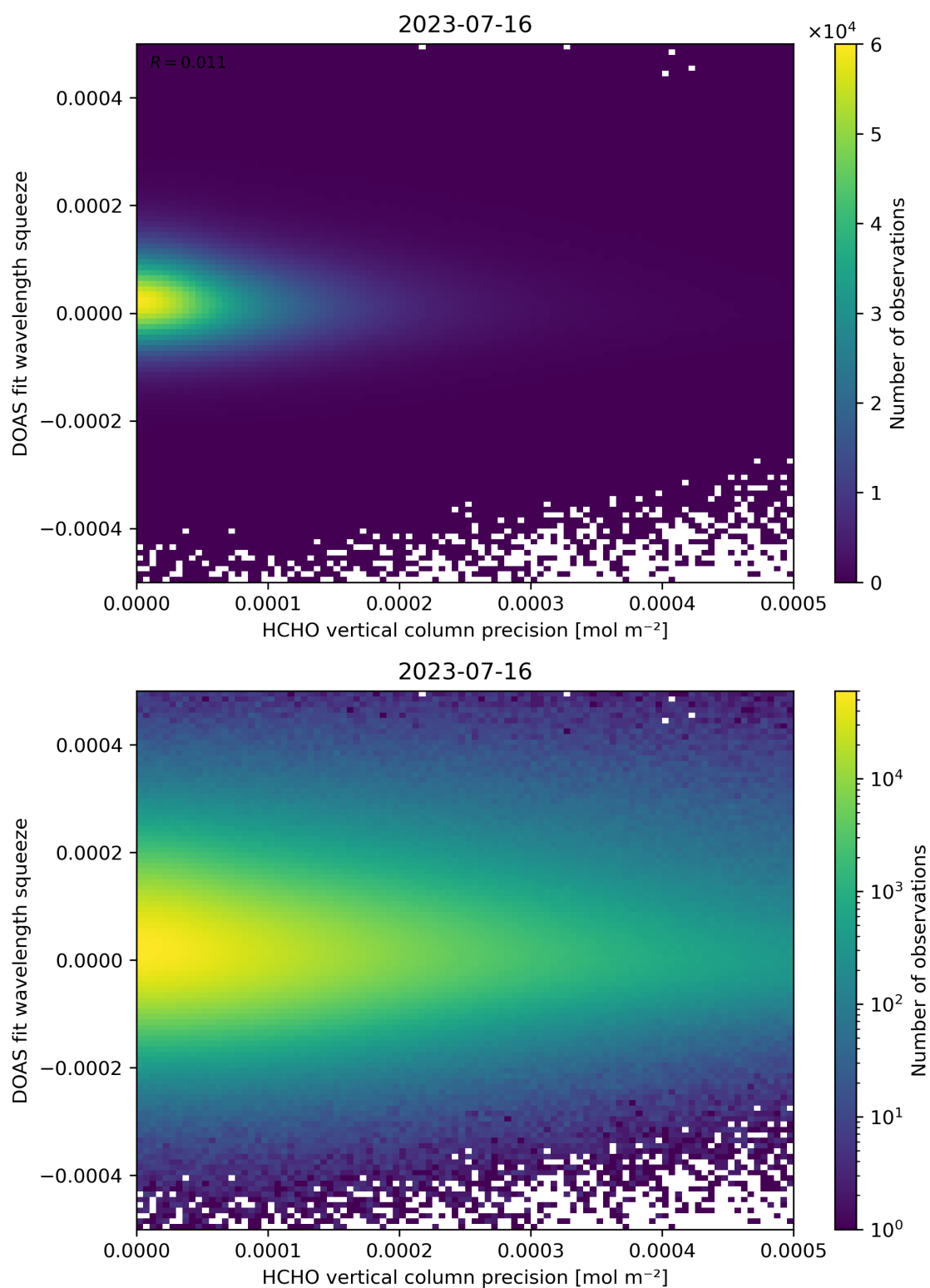
Figure 138: Scatter density plot of “HCHO vertical column precision” against “DOAS fit wavelength squeeze” for 2023-07-15 to 2023-07-17.
