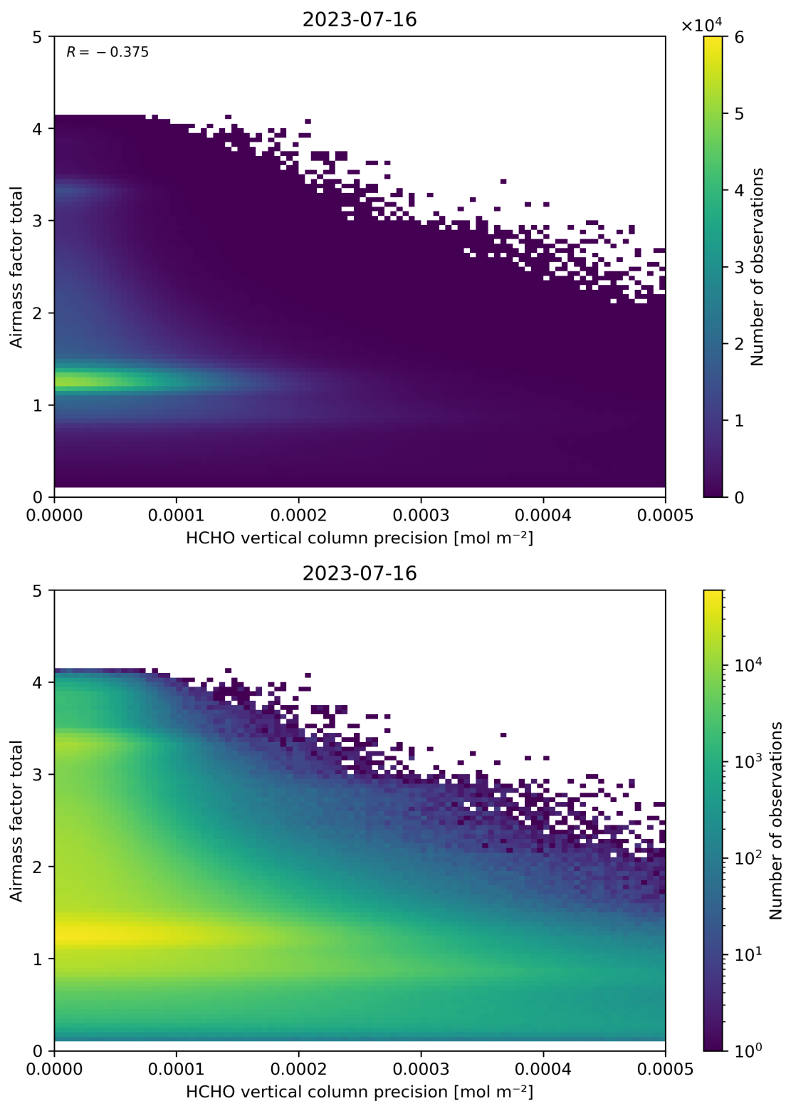
Figure 144: Scatter density plot of “HCHO vertical column precision” against “Airmass factor total” for 2023-07-15 to 2023-07-17.
