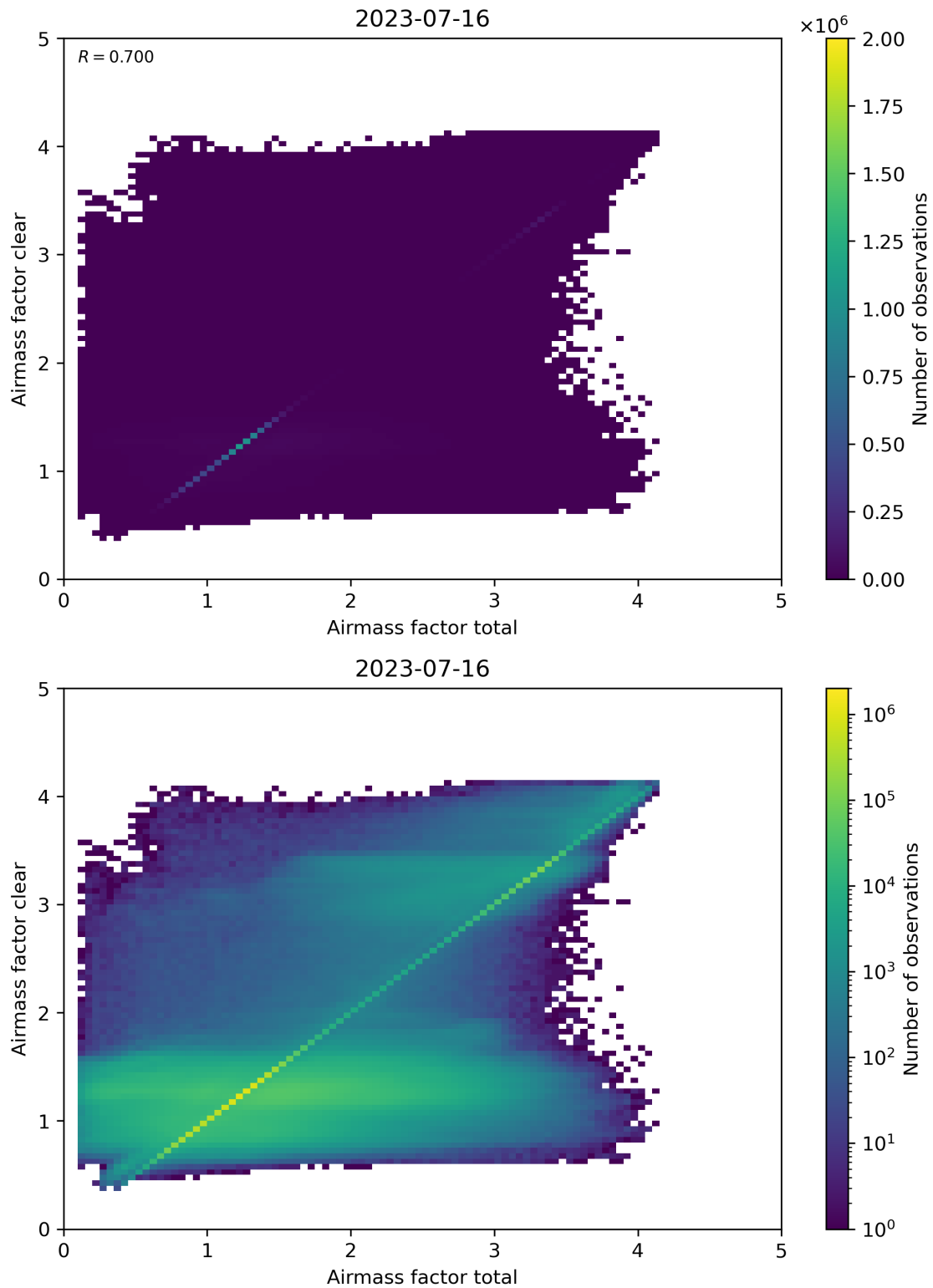
Figure 100: Scatter density plot of “Airmass factor total” against “Airmass factor clear” for 2023-07-15 to 2023-07-17.
