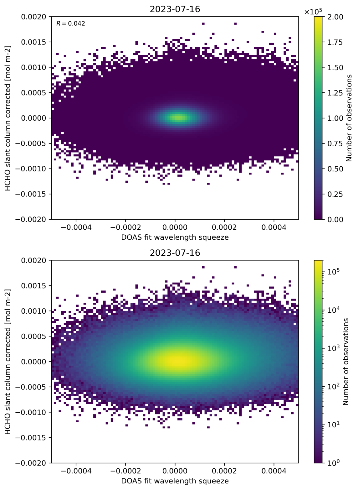
Figure 69: Scatter density plot of “DOAS fit wavelength squeeze” against “HCHO slant column corrected” for 2023-07-15 to 2023-07-17.
