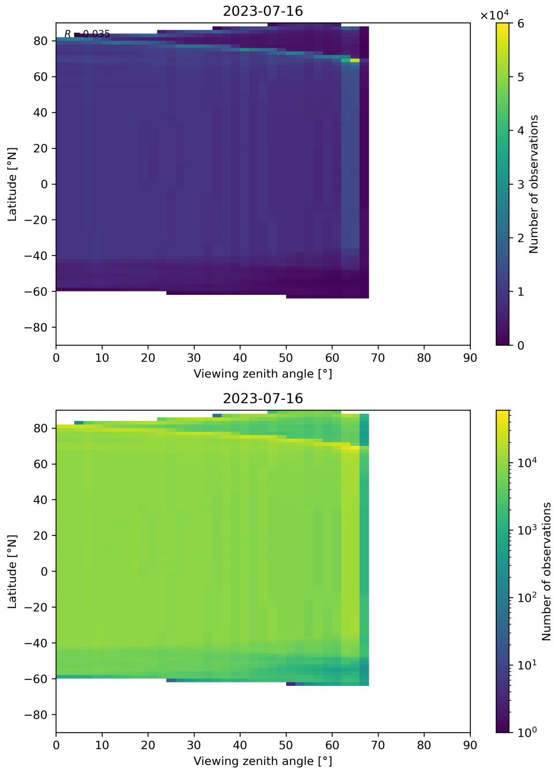
Figure 196: Scatter density plot of “Viewing zenith angle” against “Latitude” for 2023-07-15 to 2023-07-17.
