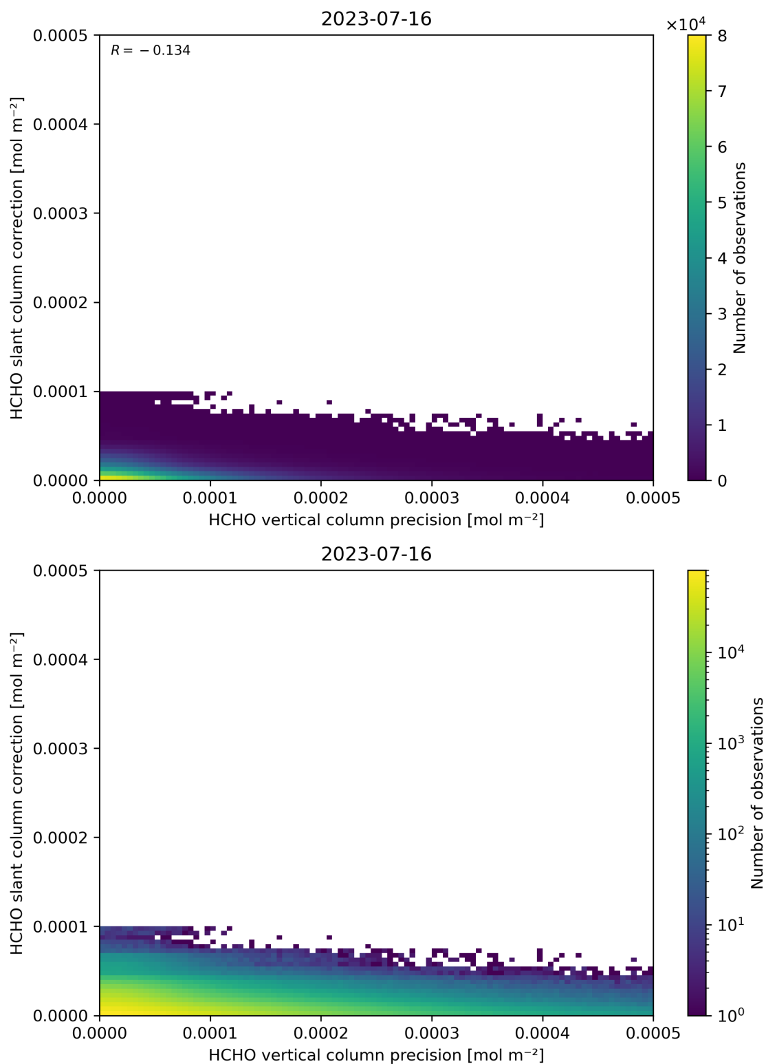
Figure 141: Scatter density plot of “HCHO vertical column precision” against “HCHO slant column correction” for 2023-07-15 to 2023-07-17.
