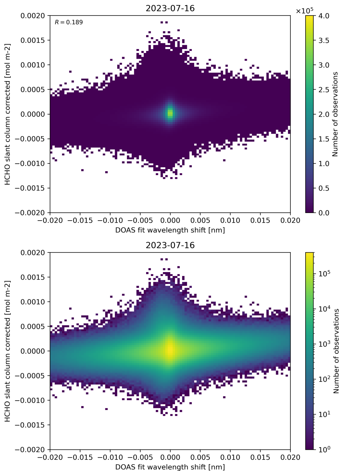
Figure 66: Scatter density plot of “DOAS fit wavelength shift” against “HCHO slant column corrected” for 2023-07-15 to 2023-07-17.
