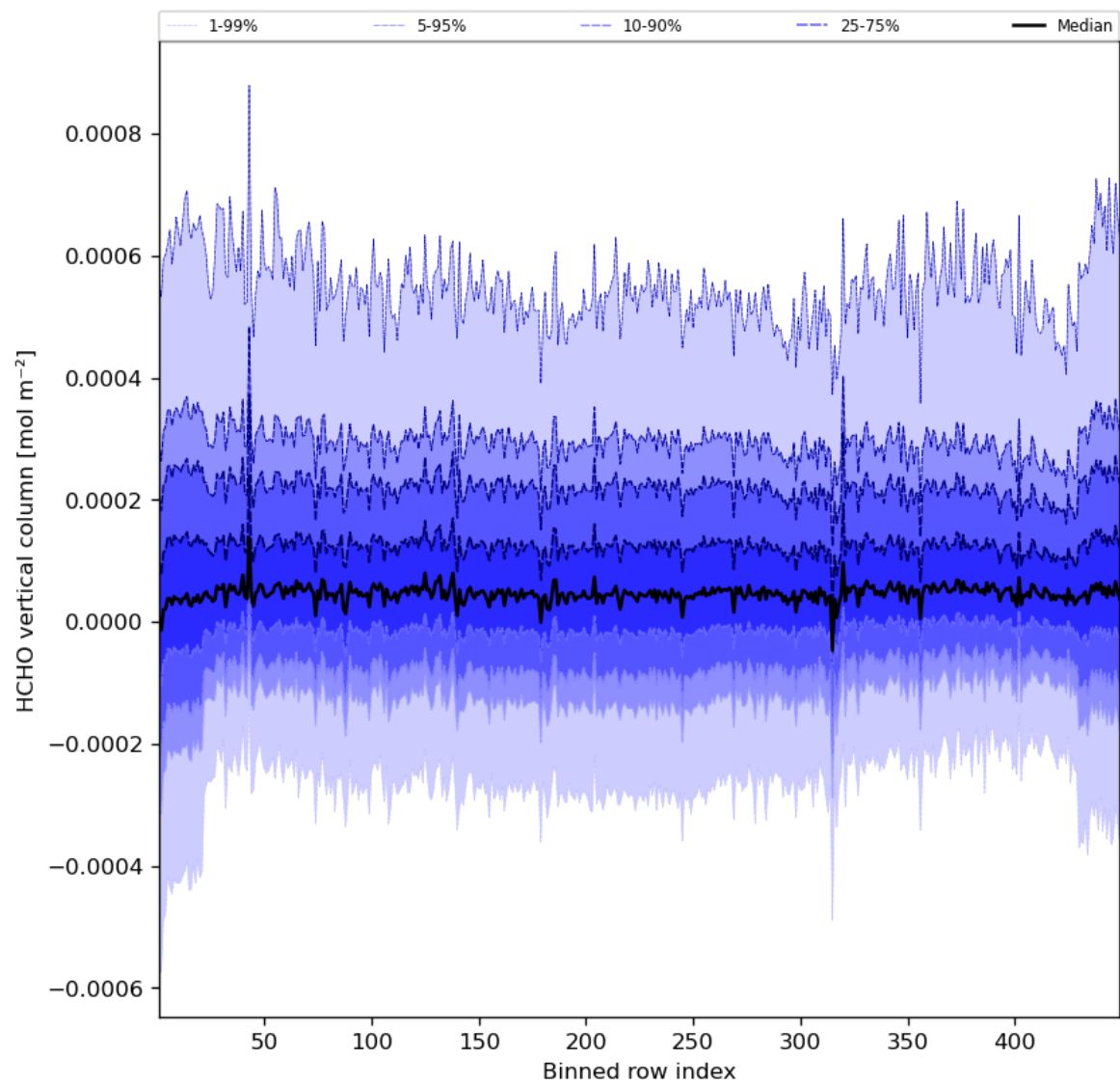
Figure 49: Along track statistics of “HCHO vertical column” for 2023-07-15 to 2023-07-17
