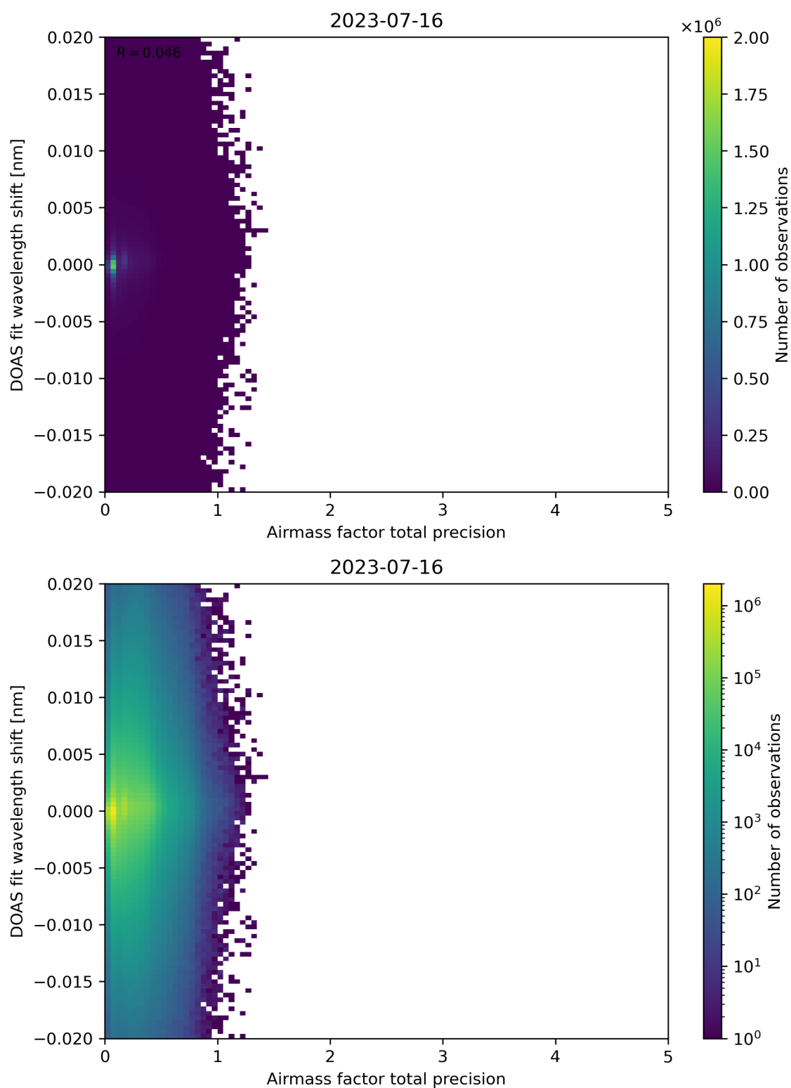
Figure 106: Scatter density plot of “Airmass factor total precision” against “DOAS fit wavelength shift” for 2023-07-15 to 2023-07-17.
