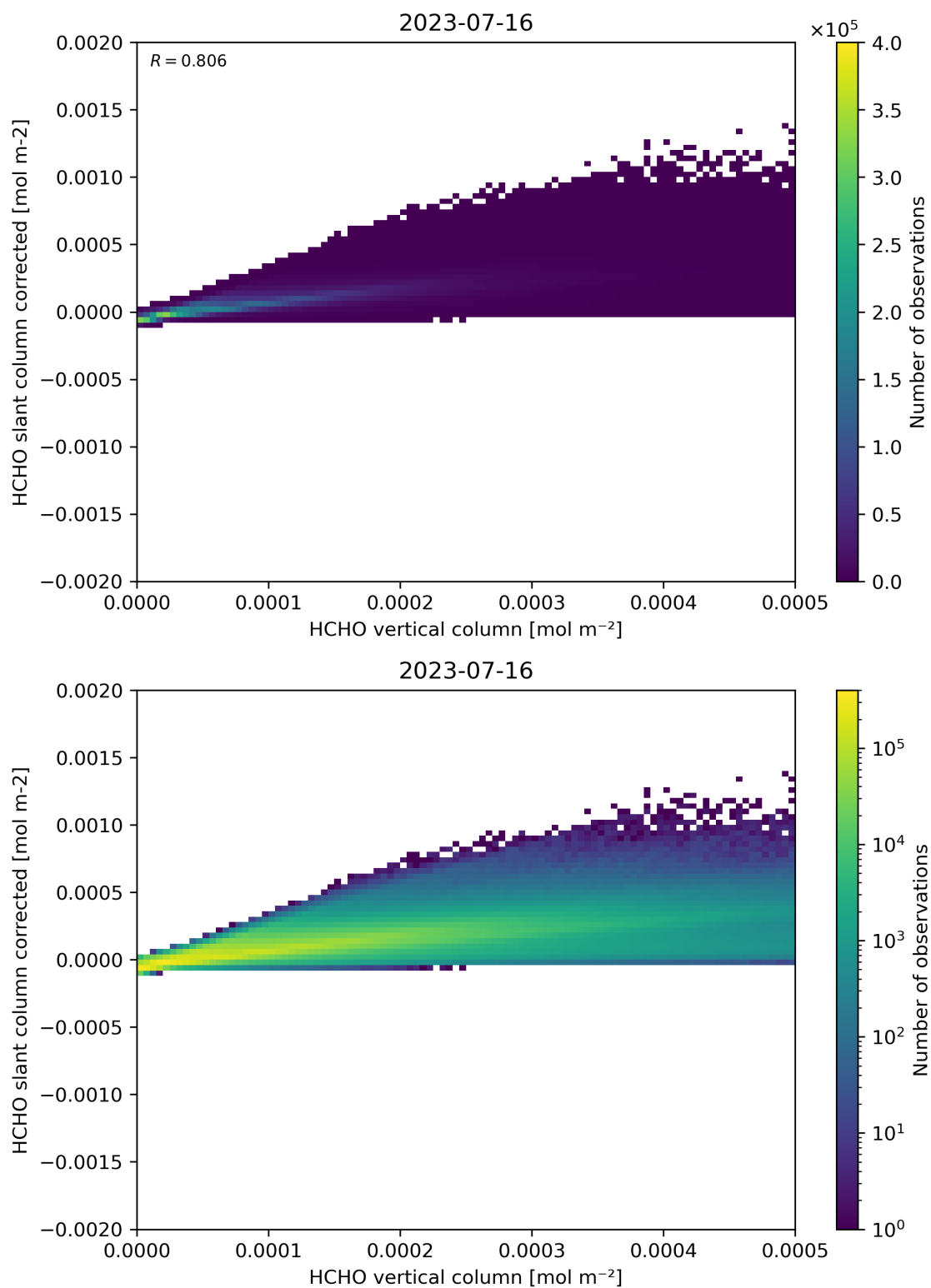
Figure 127: Scatter density plot of “HCHO vertical column” against “HCHO slant column corrected” for 2023-07-15 to 2023-07-17.
