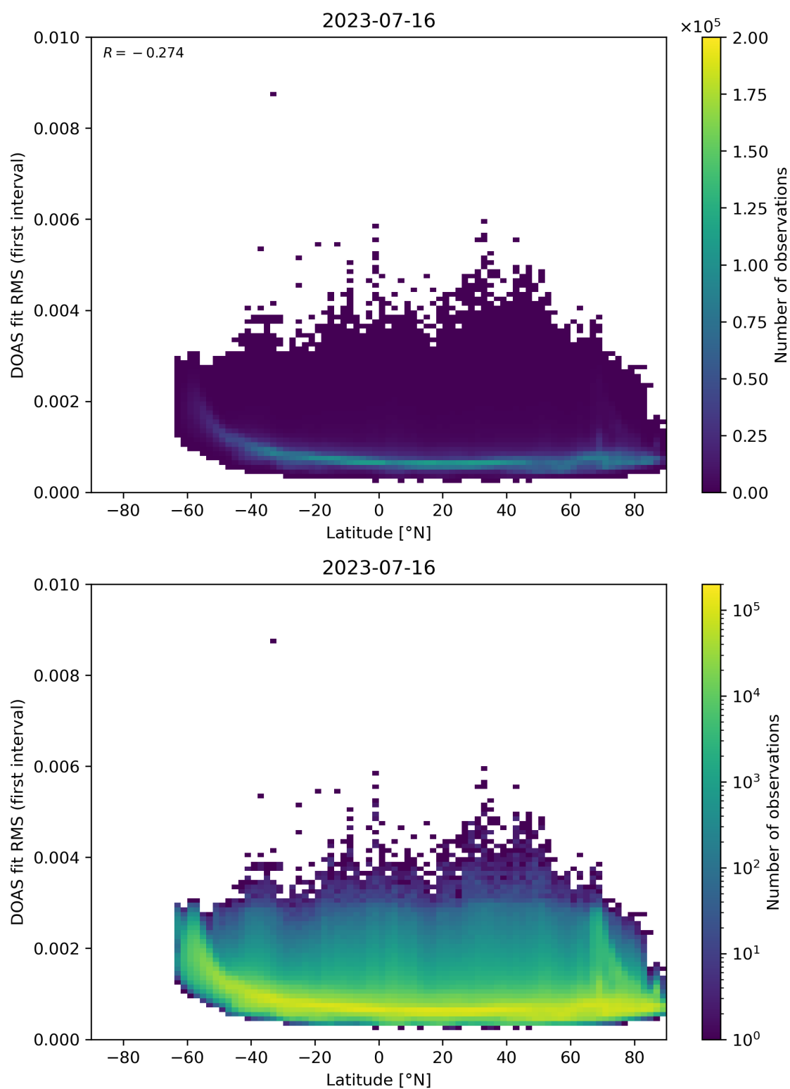
Figure 153: Scatter density plot of “Latitude” against “DOAS fit RMS (first interval)” for 2023-07-15 to 2023-07-17.
