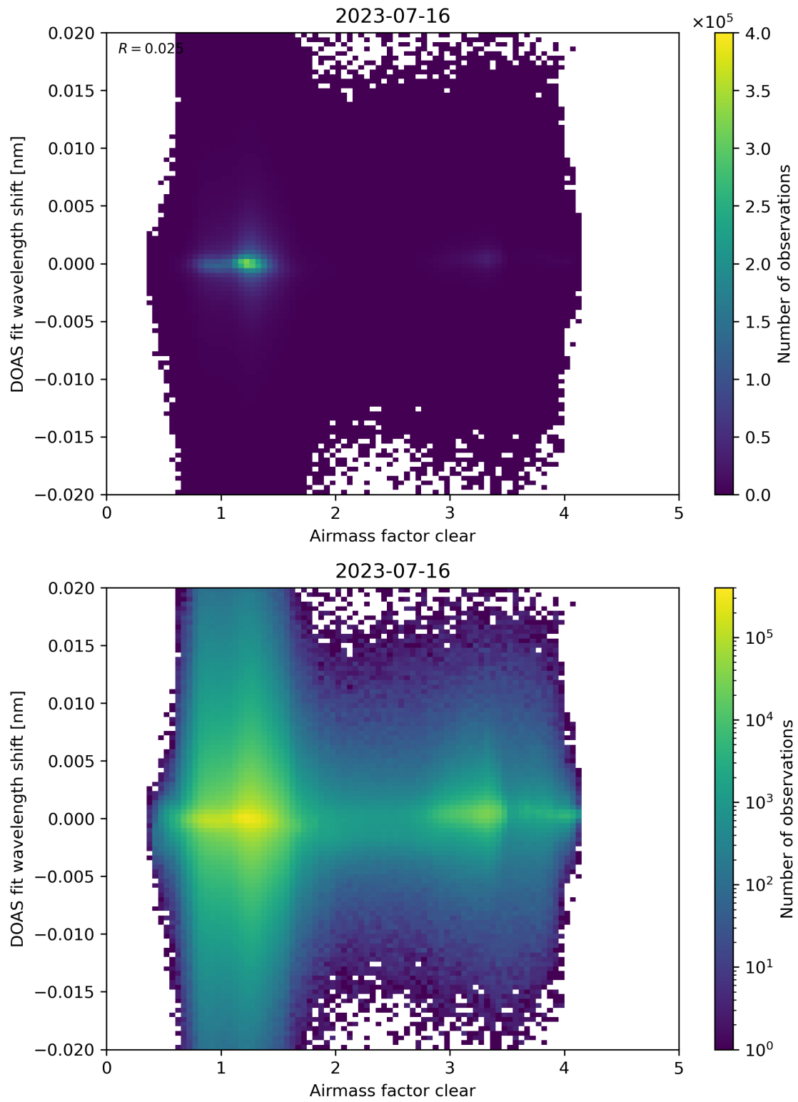
Figure 72: Scatter density plot of “Airmass factor clear” against “DOAS fit wavelength shift” for 2023-07-15 to 2023-07-17.
