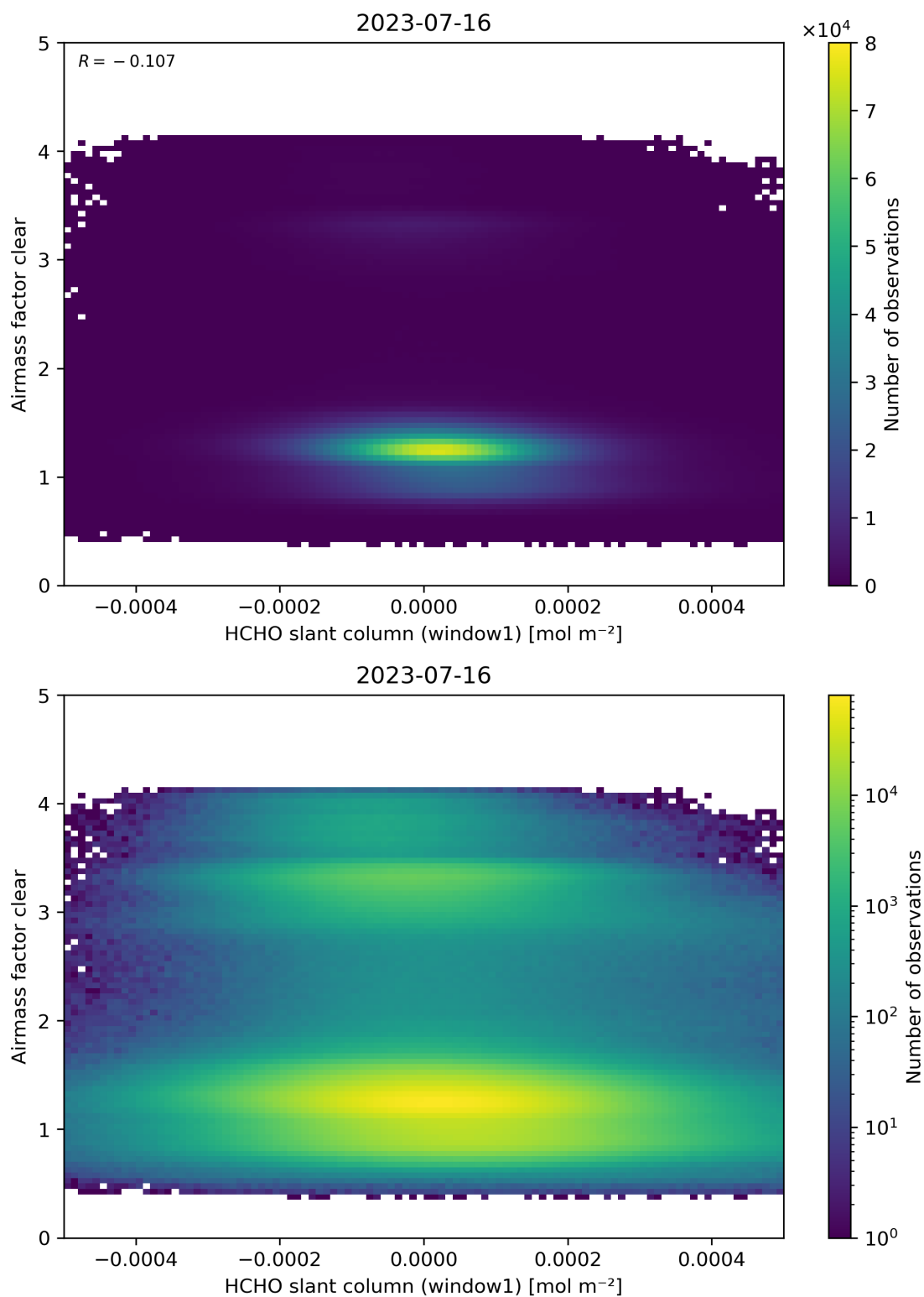
Figure 81: Scatter density plot of “HCHO slant column (window1)” against “Airmass factor clear” for 2023-07-15 to 2023-07-17.
