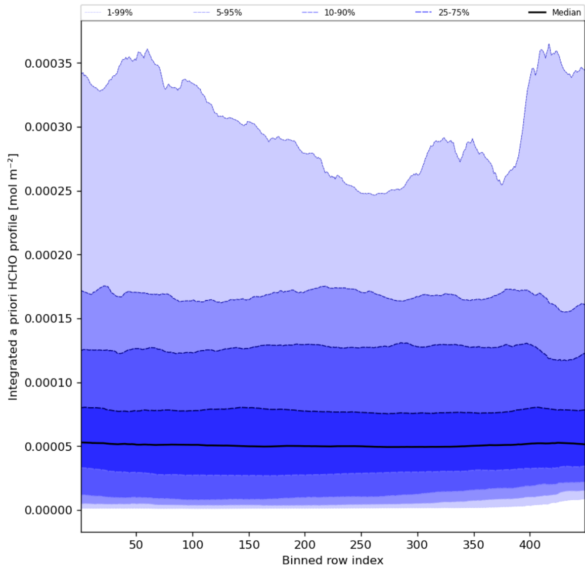
Figure 57: Along track statistics of “Integrated a priori HCHO profile” for 2023-07-15 to 2023-07-17
