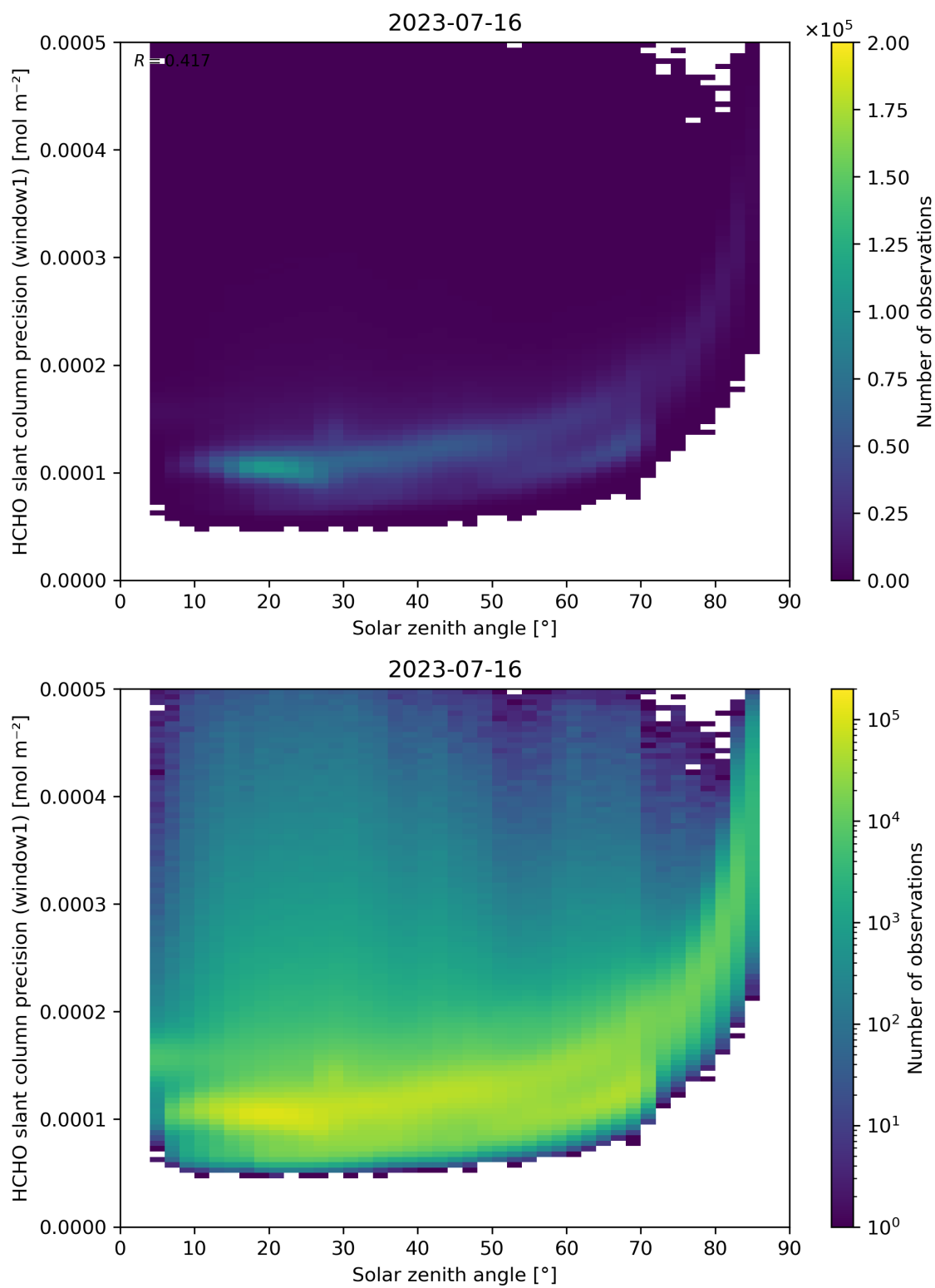
Figure 174: Scatter density plot of “Solar zenith angle” against “HCHO slant column precision (window1)” for 2023-07-15 to 2023-07-17.
