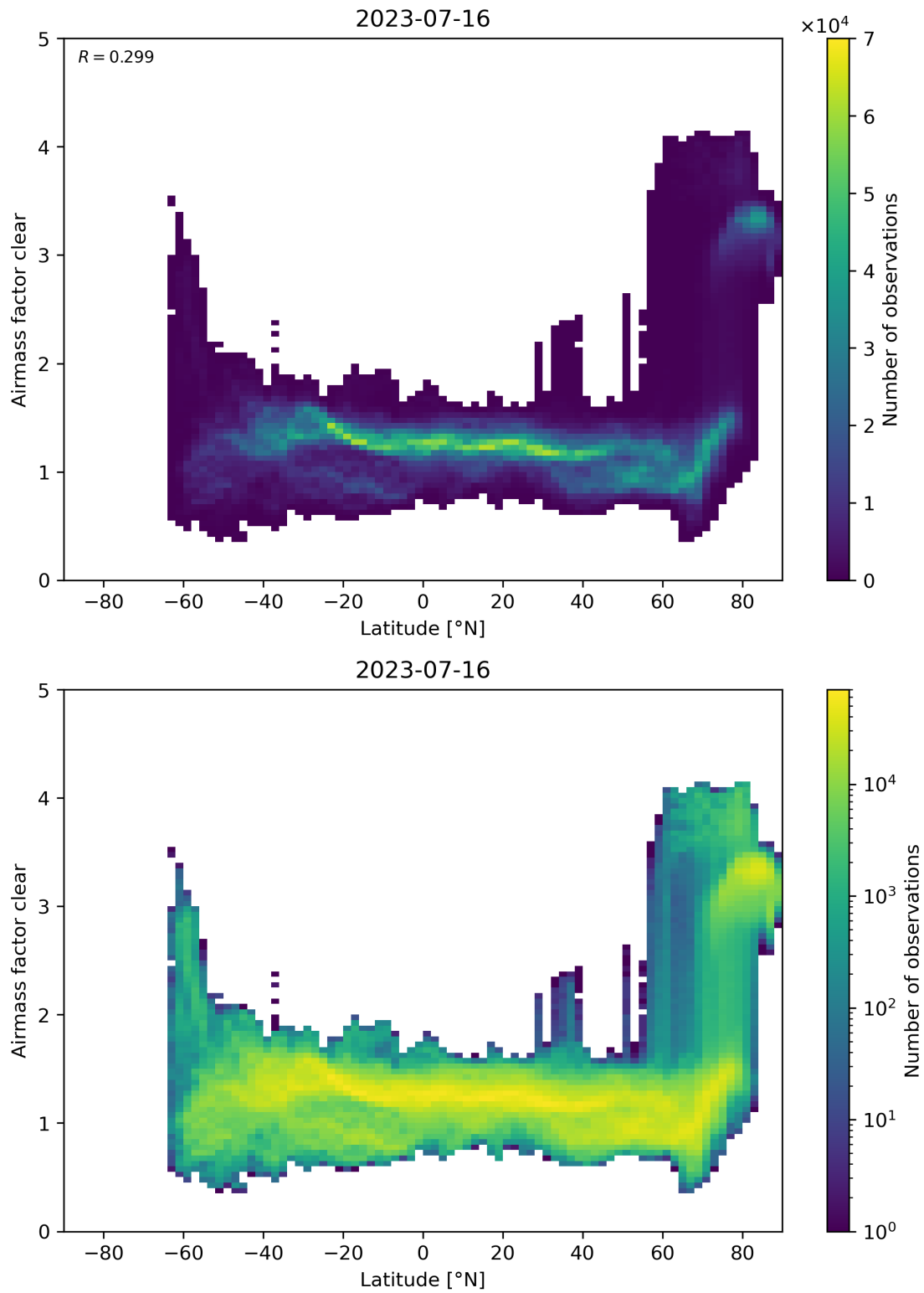
Figure 156: Scatter density plot of “Latitude” against “Airmass factor clear” for 2023-07-15 to 2023-07-17.
