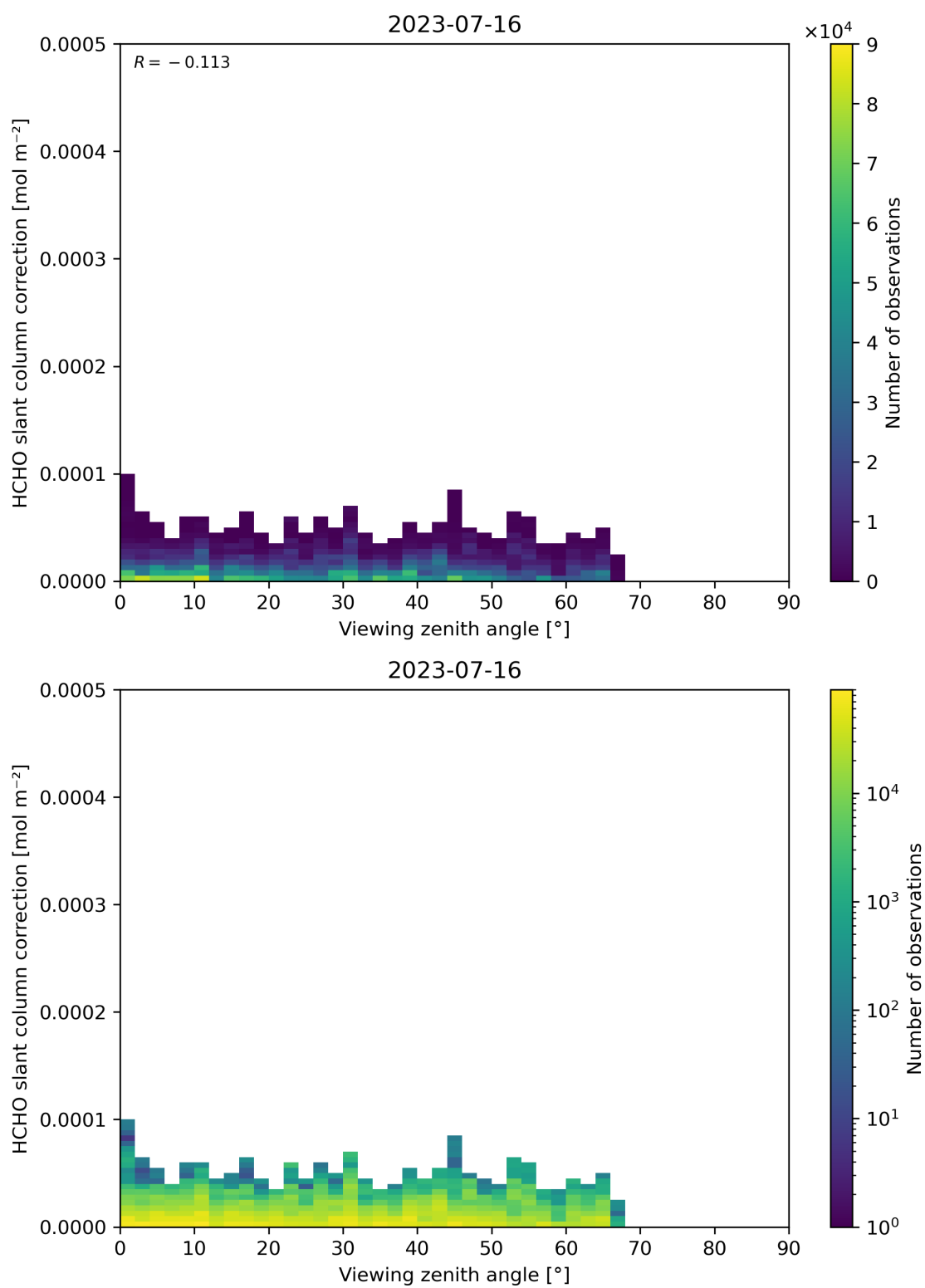
Figure 187: Scatter density plot of “Viewing zenith angle” against “HCHO slant column correction” for 2023-07-15 to 2023-07-17.
