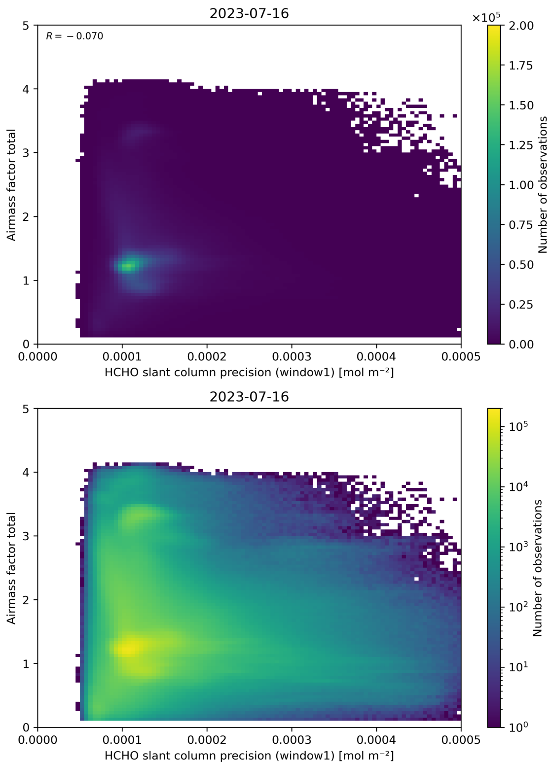
Figure 94: Scatter density plot of “HCHO slant column precision (window1)” against “Airmass factor total” for 2023-07-15 to 2023-07-17.
