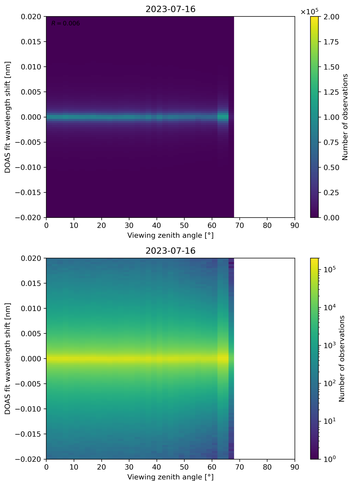
Figure 183: Scatter density plot of “Viewing zenith angle” against “DOAS fit wavelength shift” for 2023-07-15 to 2023-07-17.
