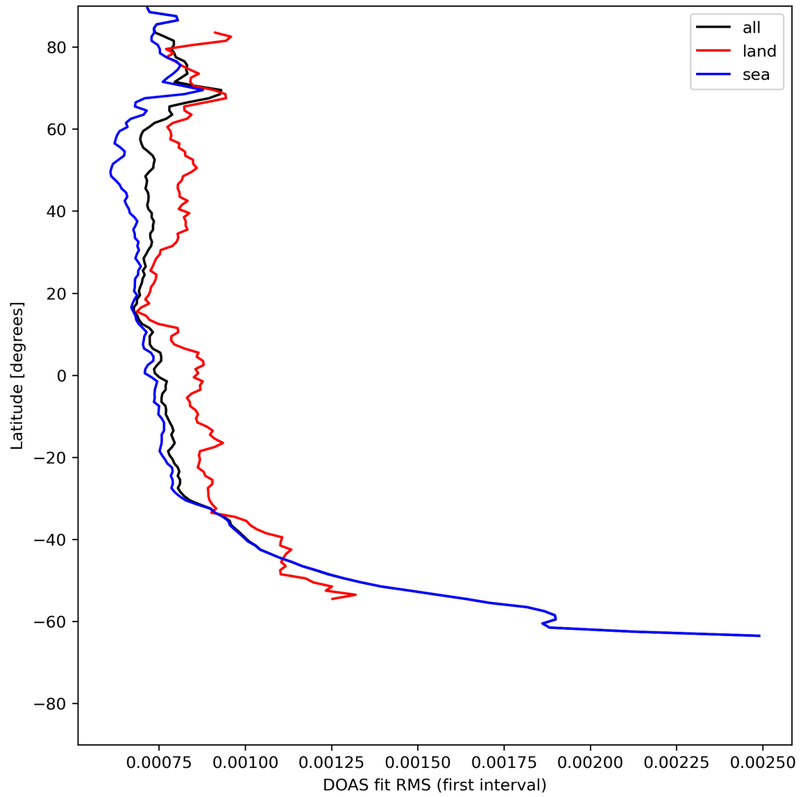
Figure 32: Zonal average of “DOAS fit RMS (first interval)” for 2023-07-15 to 2023-07-17.
