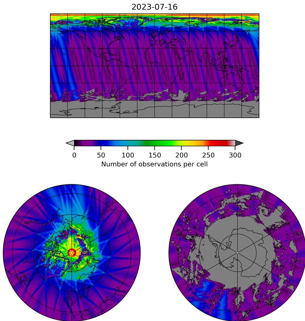
Figure 19: Map of the number of observations for 2023-07-15 to 2023-07-17
