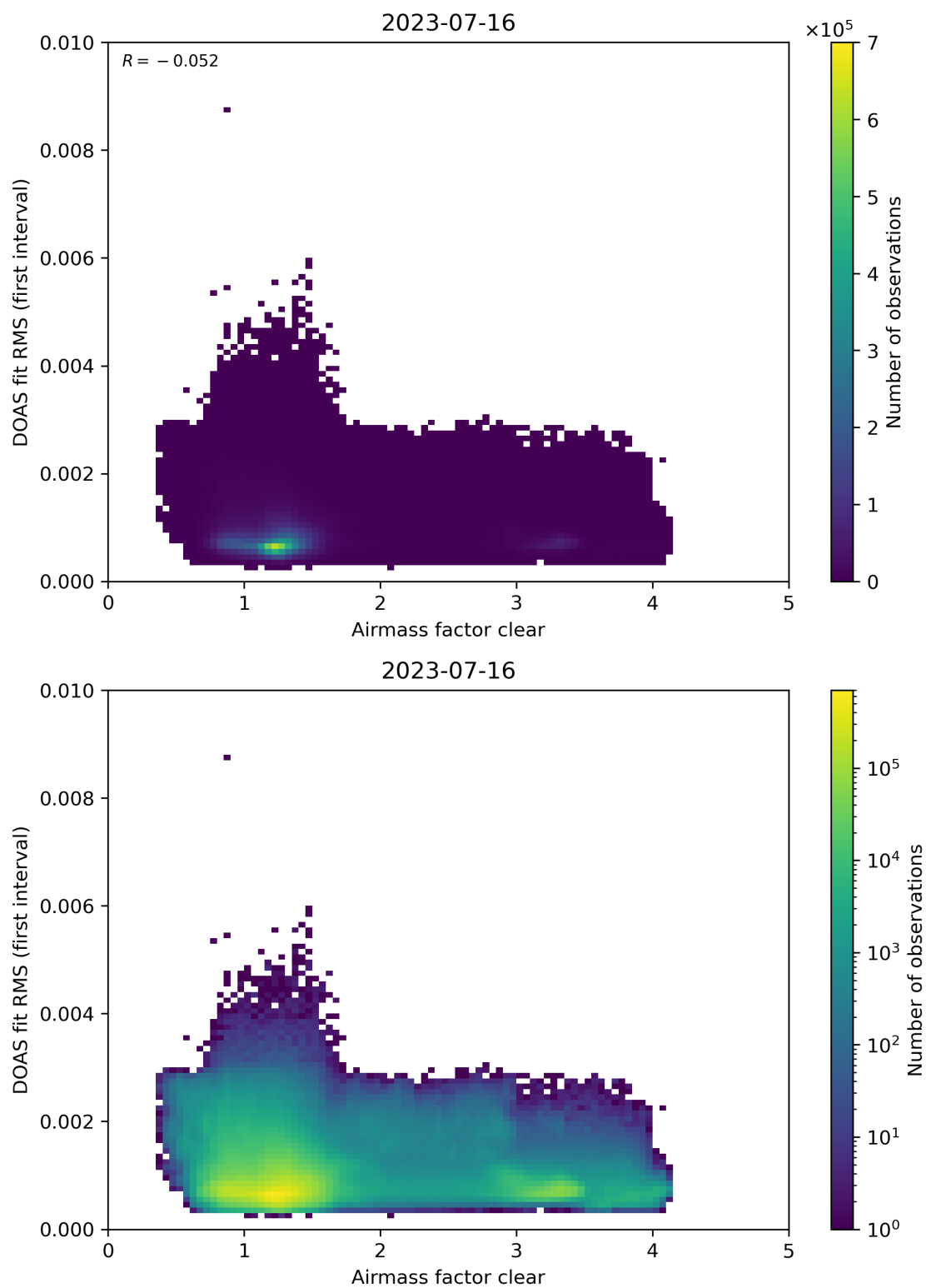
Figure 71: Scatter density plot of “Airmass factor clear” against “DOAS fit RMS (first interval)” for 2023-07-15 to 2023-07-17.
