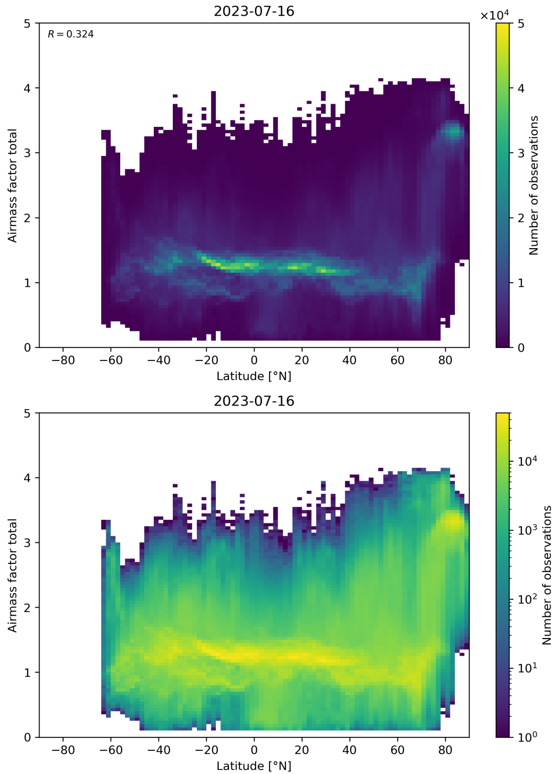
Figure 161: Scatter density plot of “Latitude” against “Airmass factor total” for 2023-07-15 to 2023-07-17.
