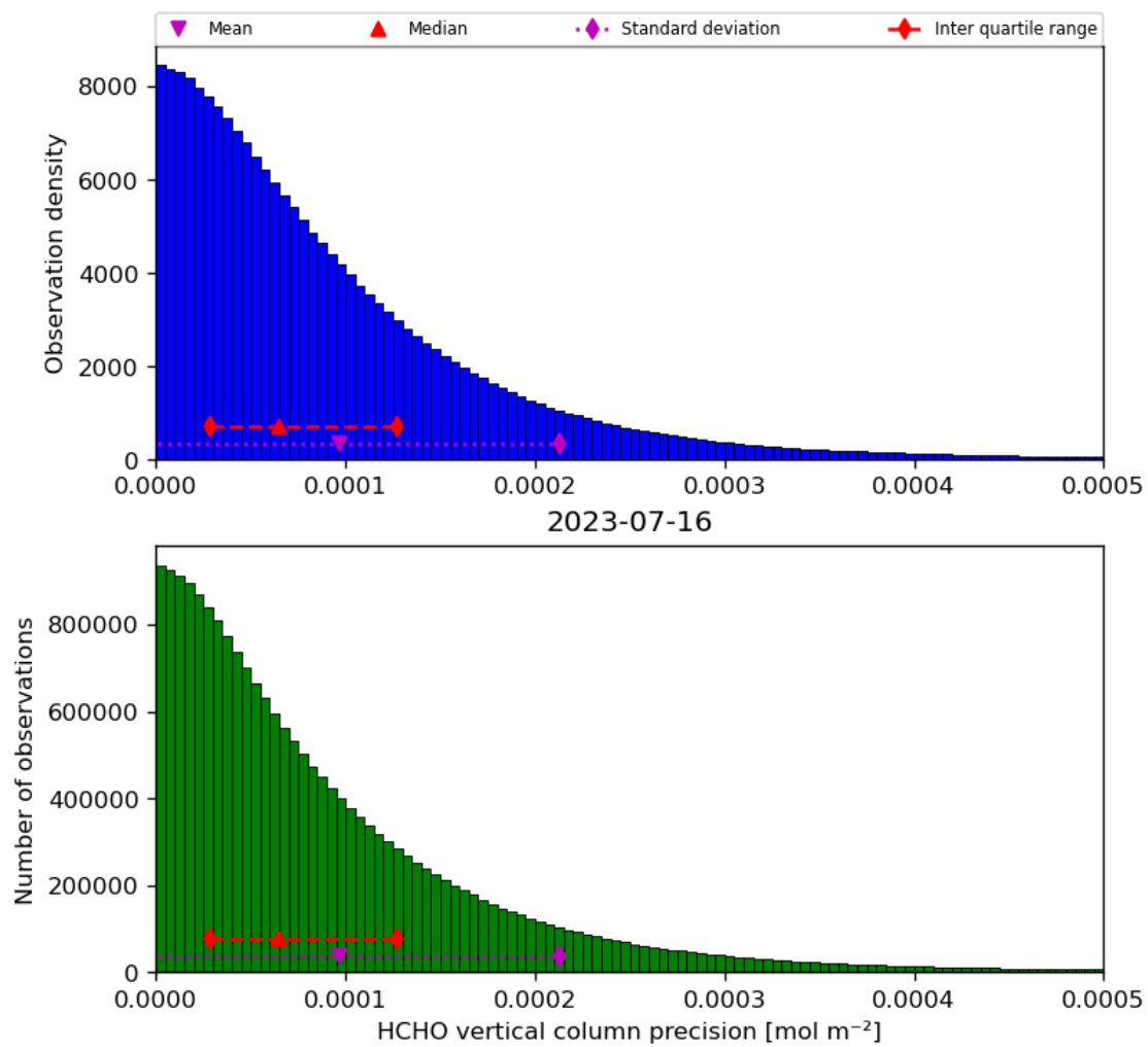
Figure 36: Histogram of “HCHO vertical column precision” for 2023-07-15 to 2023-07-17
