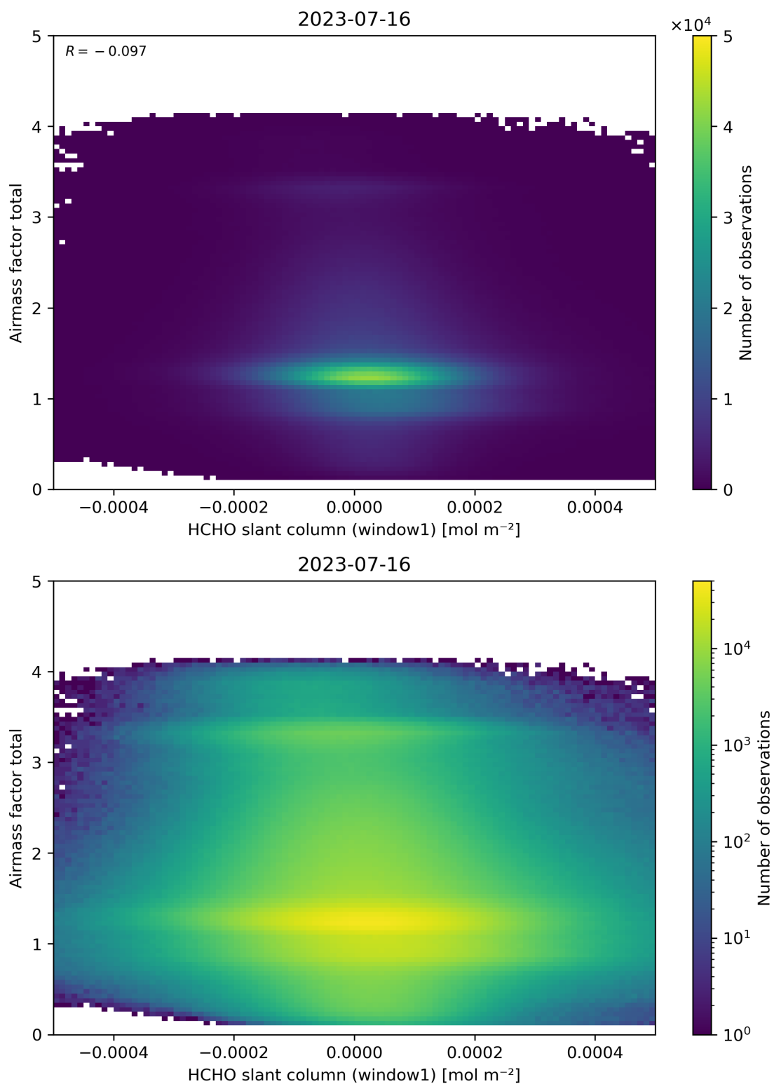
Figure 85: Scatter density plot of “HCHO slant column (window1)” against “Airmass factor total” for 2023-07-15 to 2023-07-17.
