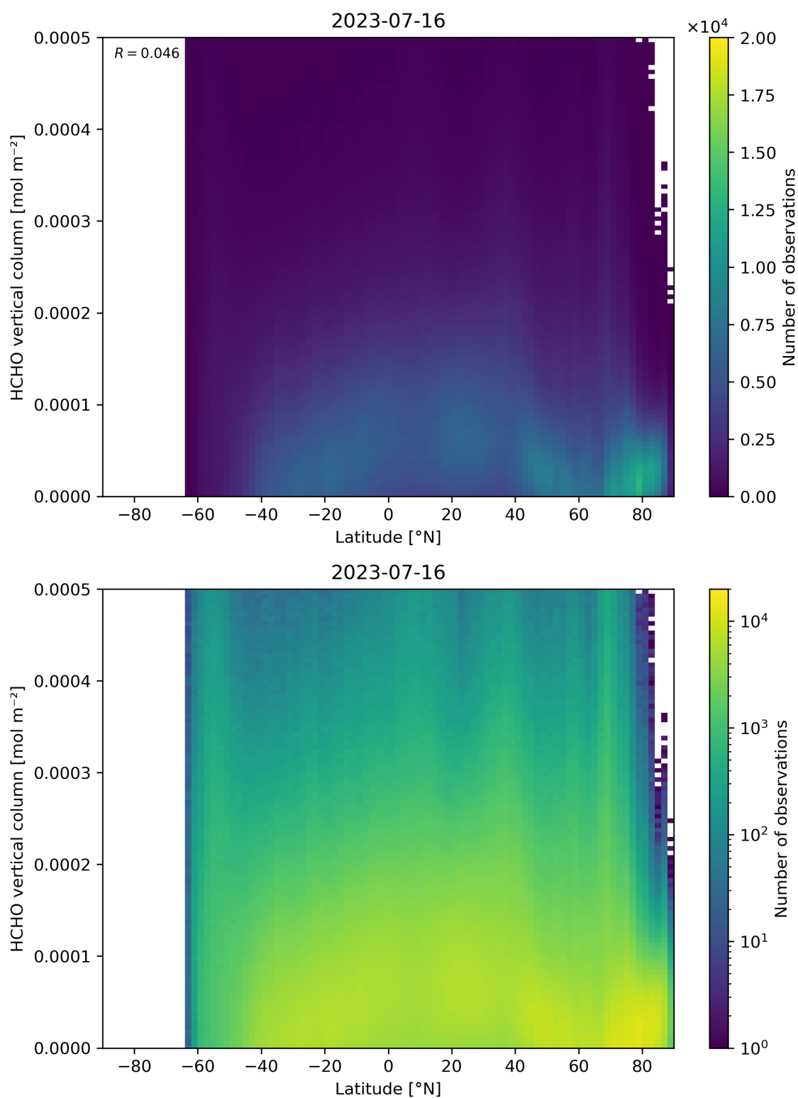
Figure 163: Scatter density plot of “Latitude” against “HCHO vertical column” for 2023-07-15 to 2023-07-17.
