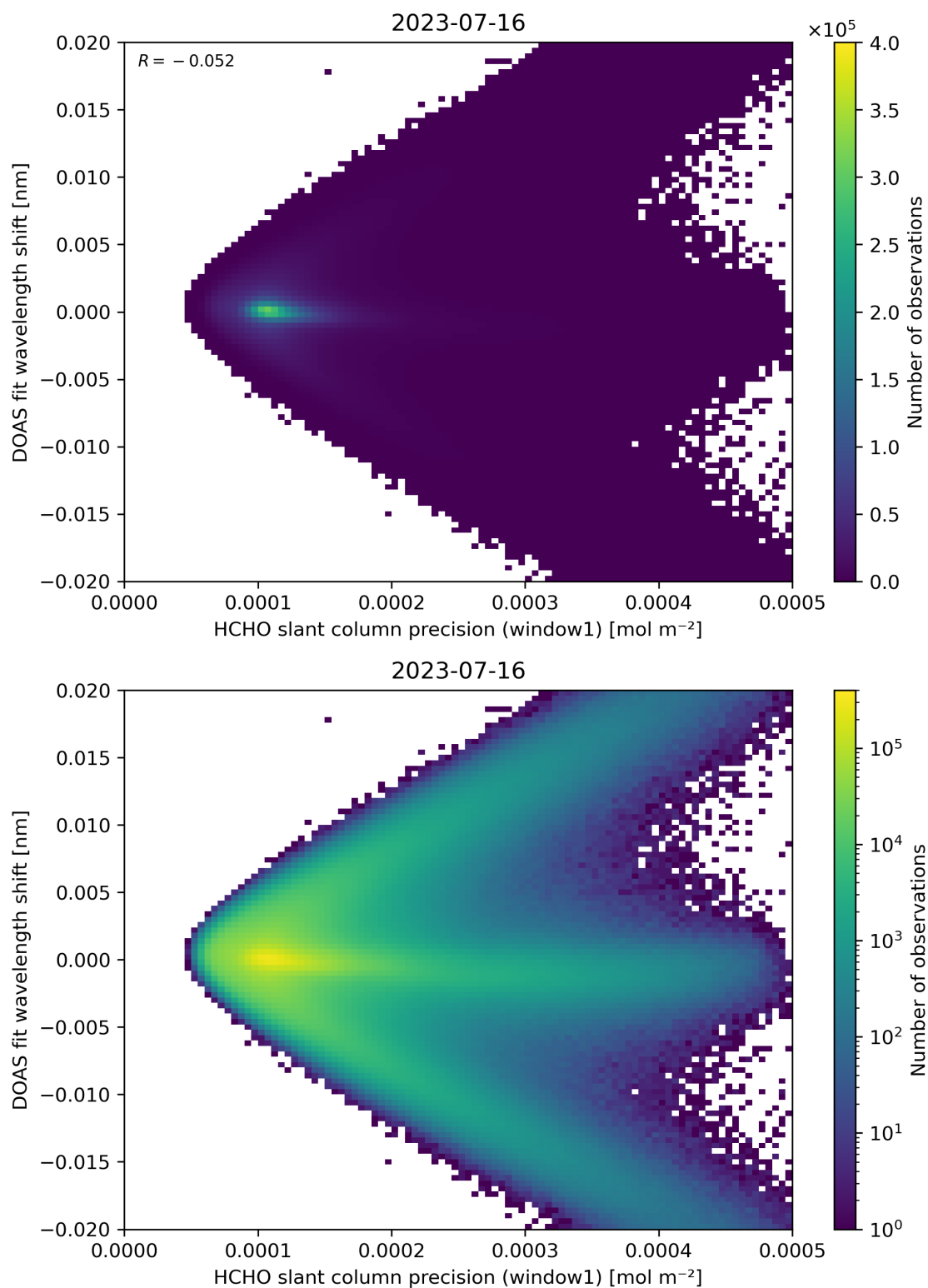
Figure 89: Scatter density plot of “HCHO slant column precision (window1)” against “DOAS fit wavelength shift” for 2023-07-15 to 2023-07-17.
