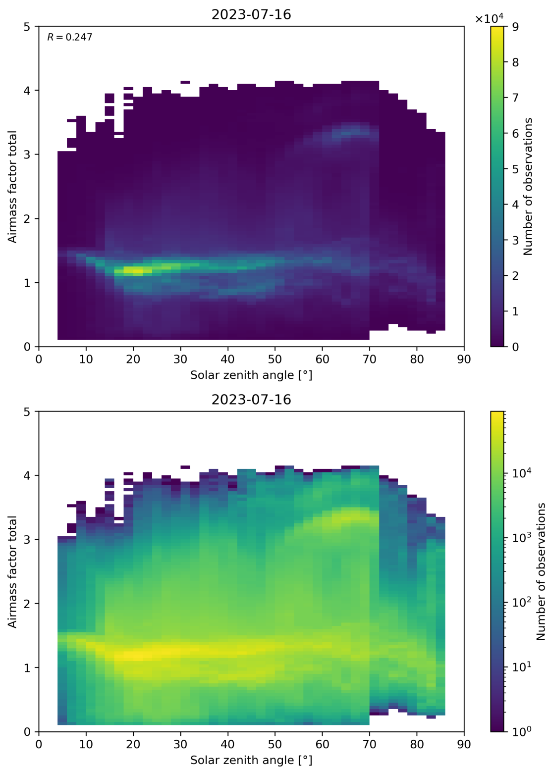
Figure 175: Scatter density plot of “Solar zenith angle” against “Airmass factor total” for 2023-07-15 to 2023-07-17.
