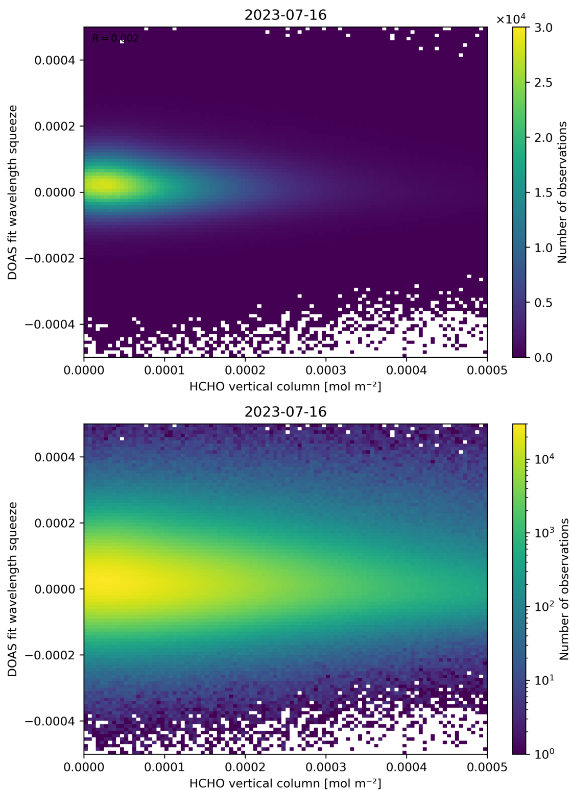
Figure 125: Scatter density plot of “HCHO vertical column” against “DOAS fit wavelength squeeze” for 2023-07-15 to 2023-07-17.
