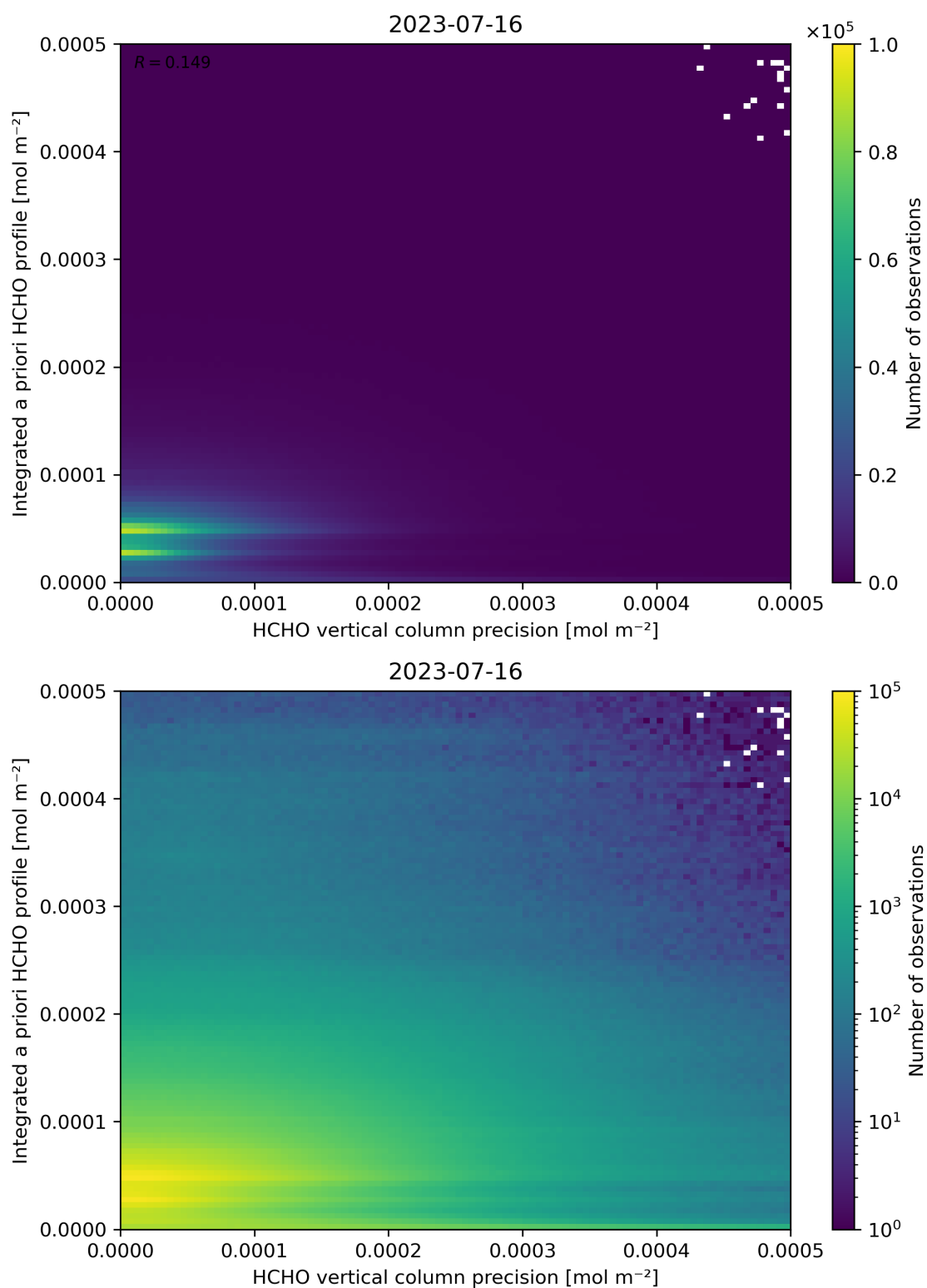
Figure 147: Scatter density plot of “HCHO vertical column precision” against “Integrated a priori HCHO profile” for 2023-07-15 to 2023-07-17.
