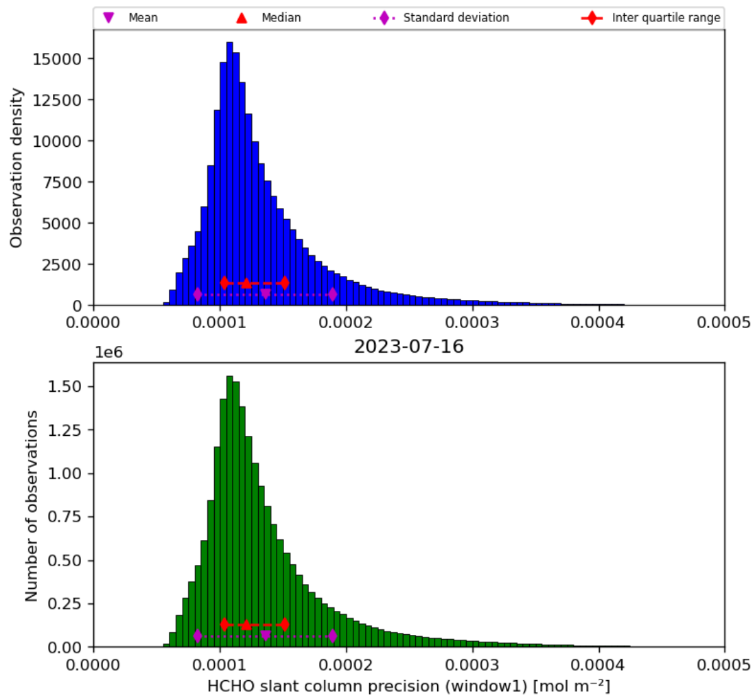
Figure 39: Histogram of “HCHO slant column precision (window1)” for 2023-07-15 to 2023-07-17
