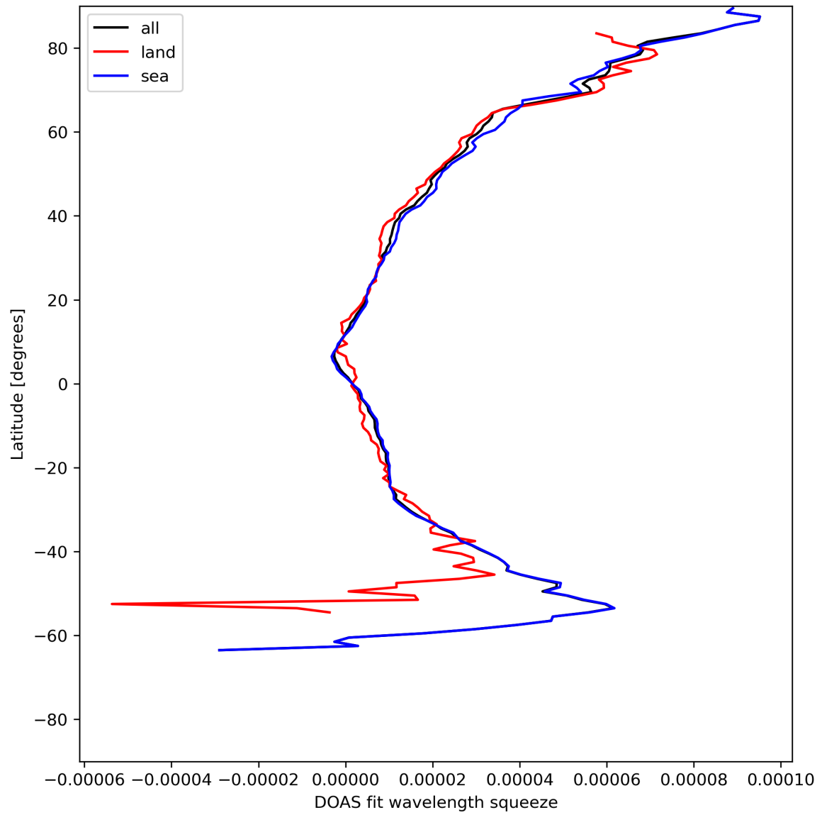
Figure 31: Zonal average of “DOAS fit wavelength squeeze” for 2023-07-15 to 2023-07-17.
