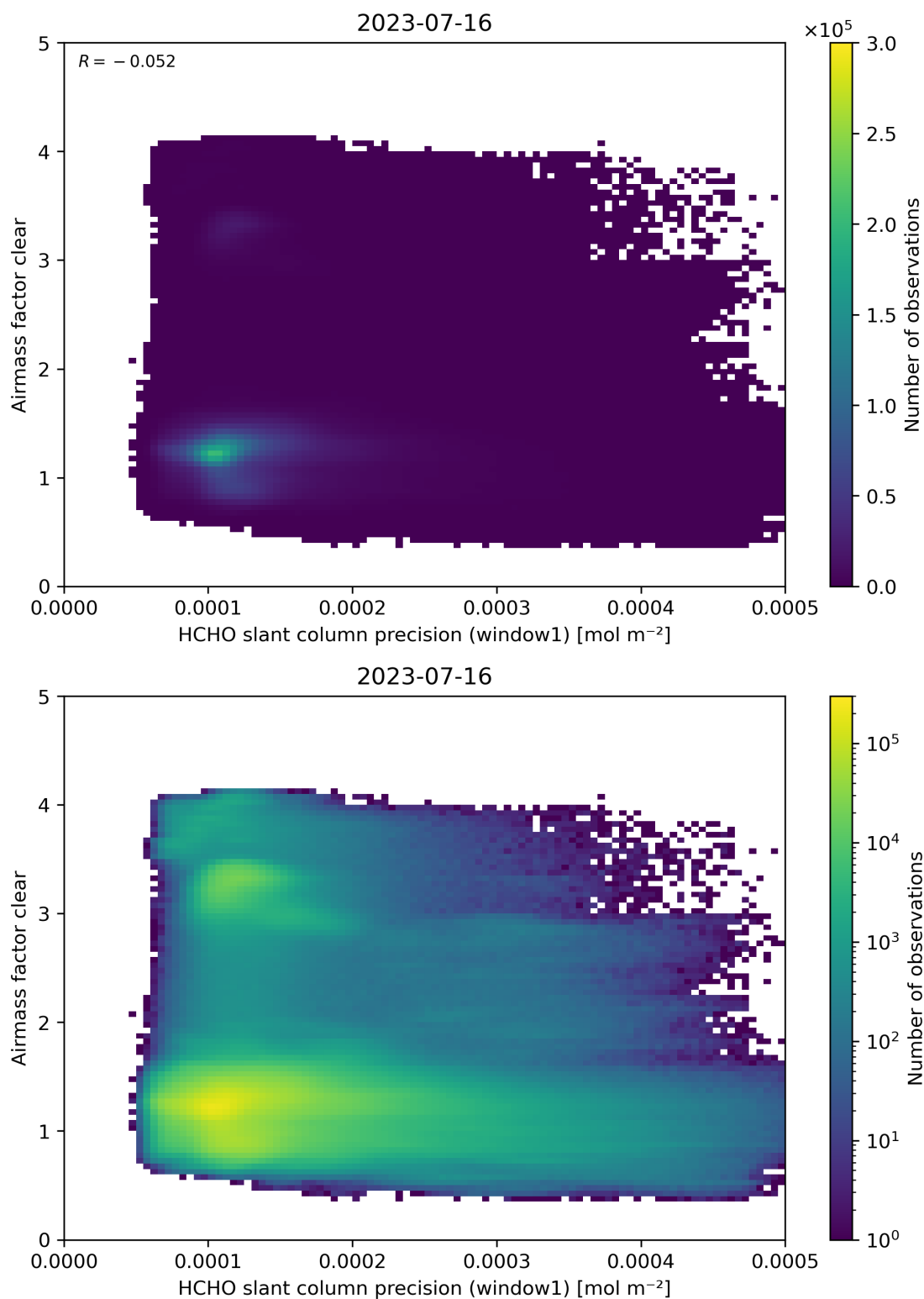
Figure 91: Scatter density plot of “HCHO slant column precision (window1)” against “Airmass factor clear” for 2023-07-15 to 2023-07-17.
