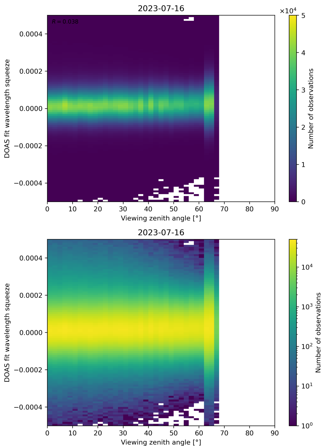
Figure 184: Scatter density plot of “Viewing zenith angle” against “DOAS fit wavelength squeeze” for 2023-07-15 to 2023-07-17.
