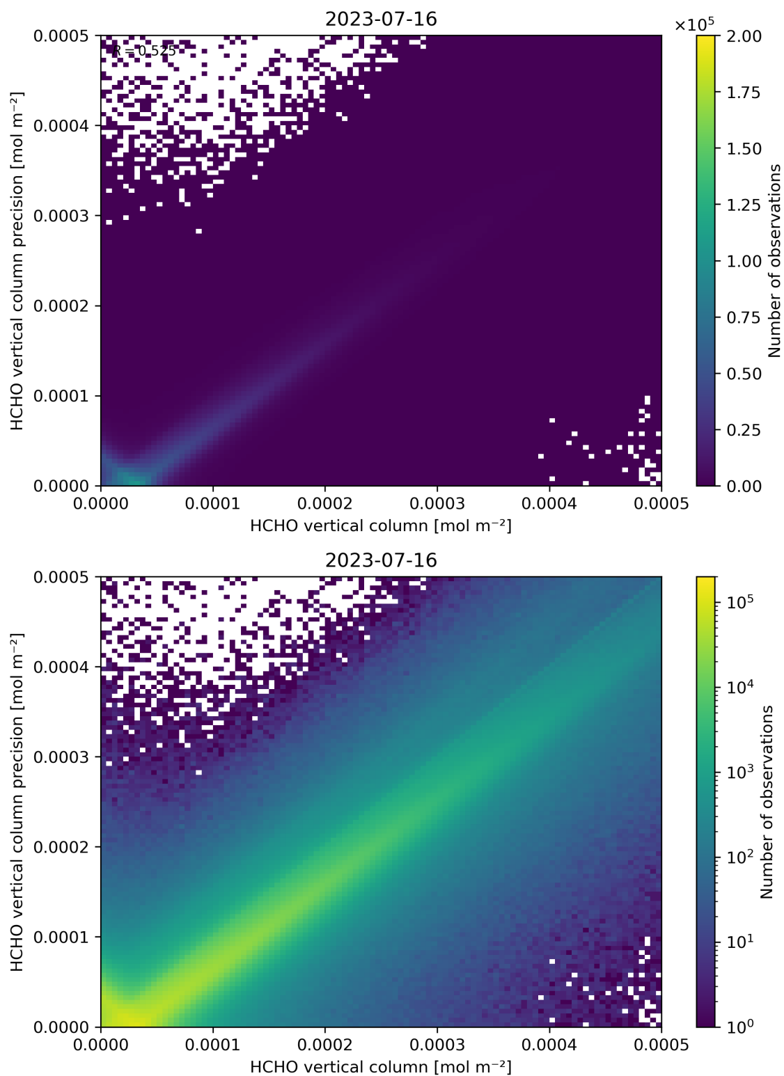
Figure 134: Scatter density plot of “HCHO vertical column” against “HCHO vertical column precision” for 2023-07-15 to 2023-07-17.
