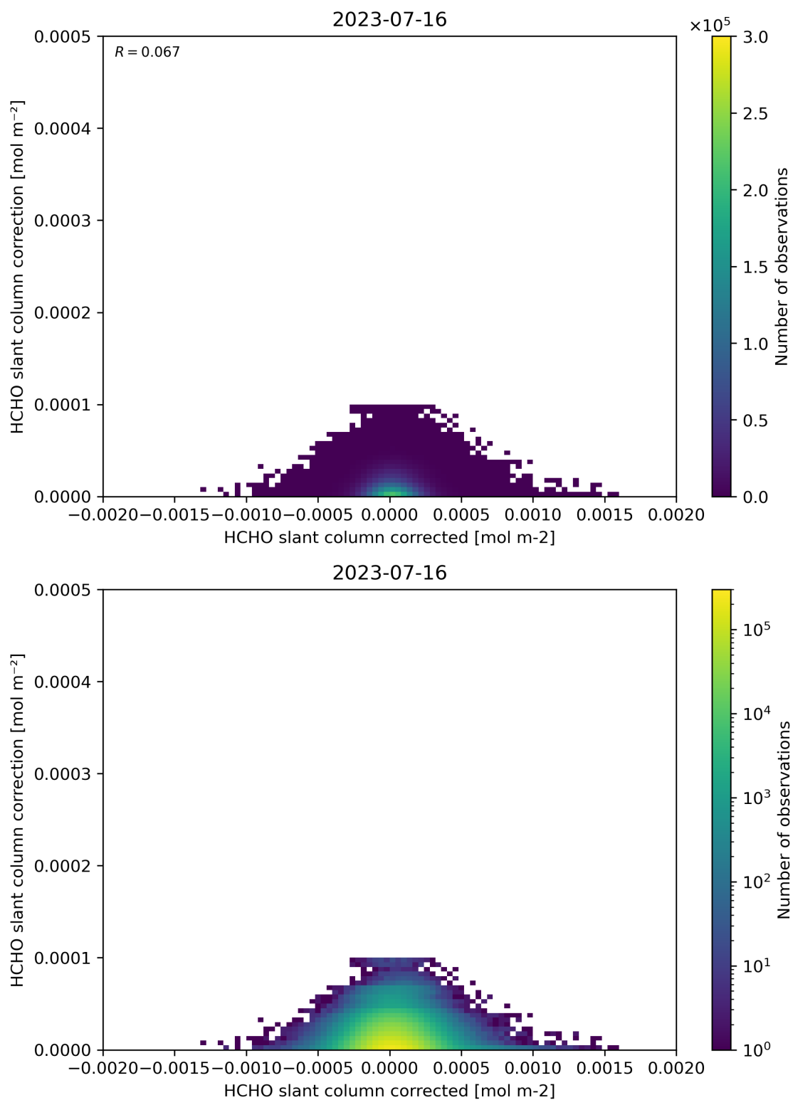
Figure 77: Scatter density plot of “HCHO slant column corrected” against “HCHO slant column correction” for 2023-07-15 to 2023-07-17.
