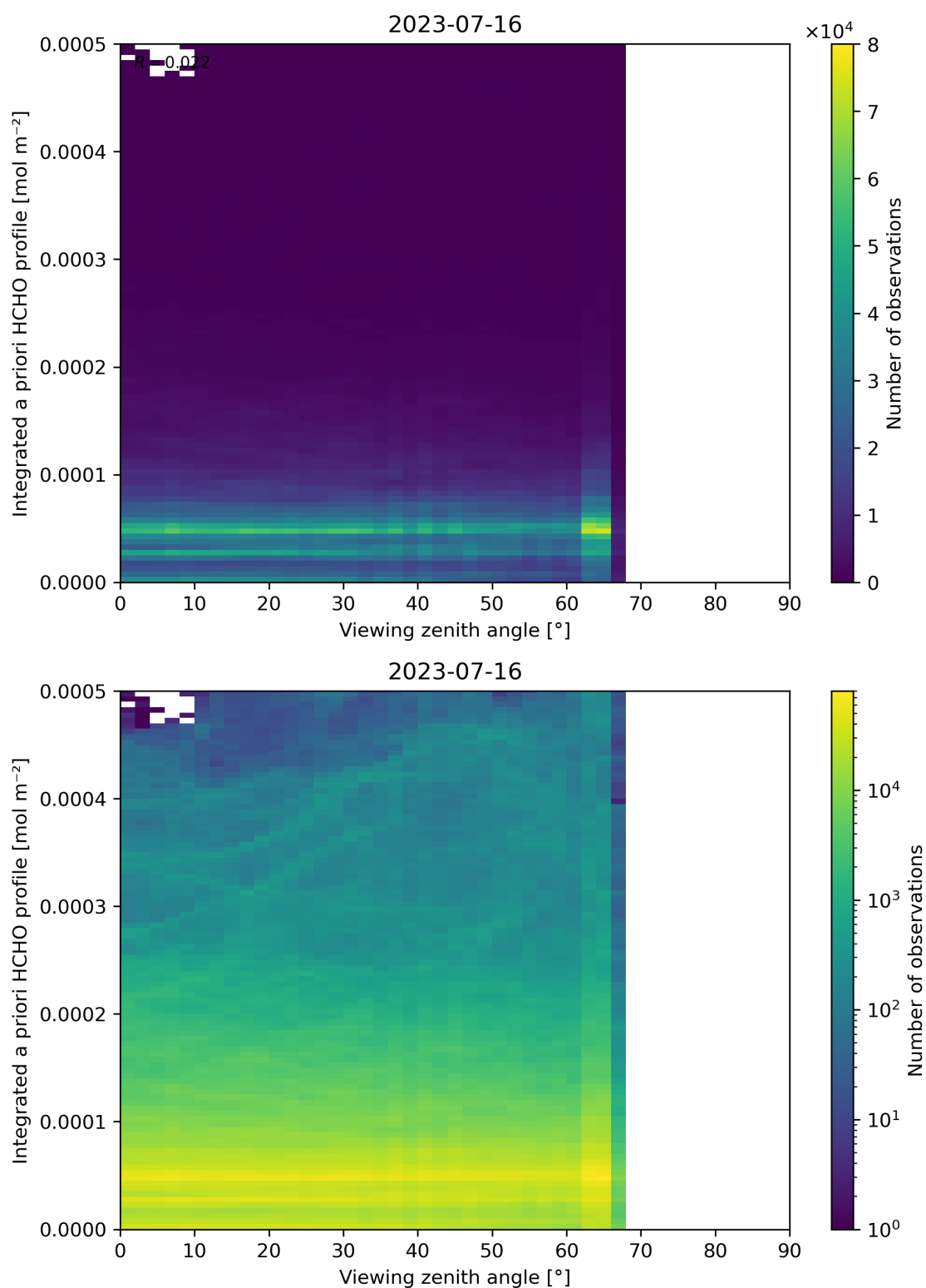
Figure 195: Scatter density plot of “Viewing zenith angle” against “Integrated a priori HCHO profile” for 2023-07-15 to 2023-07-17.
