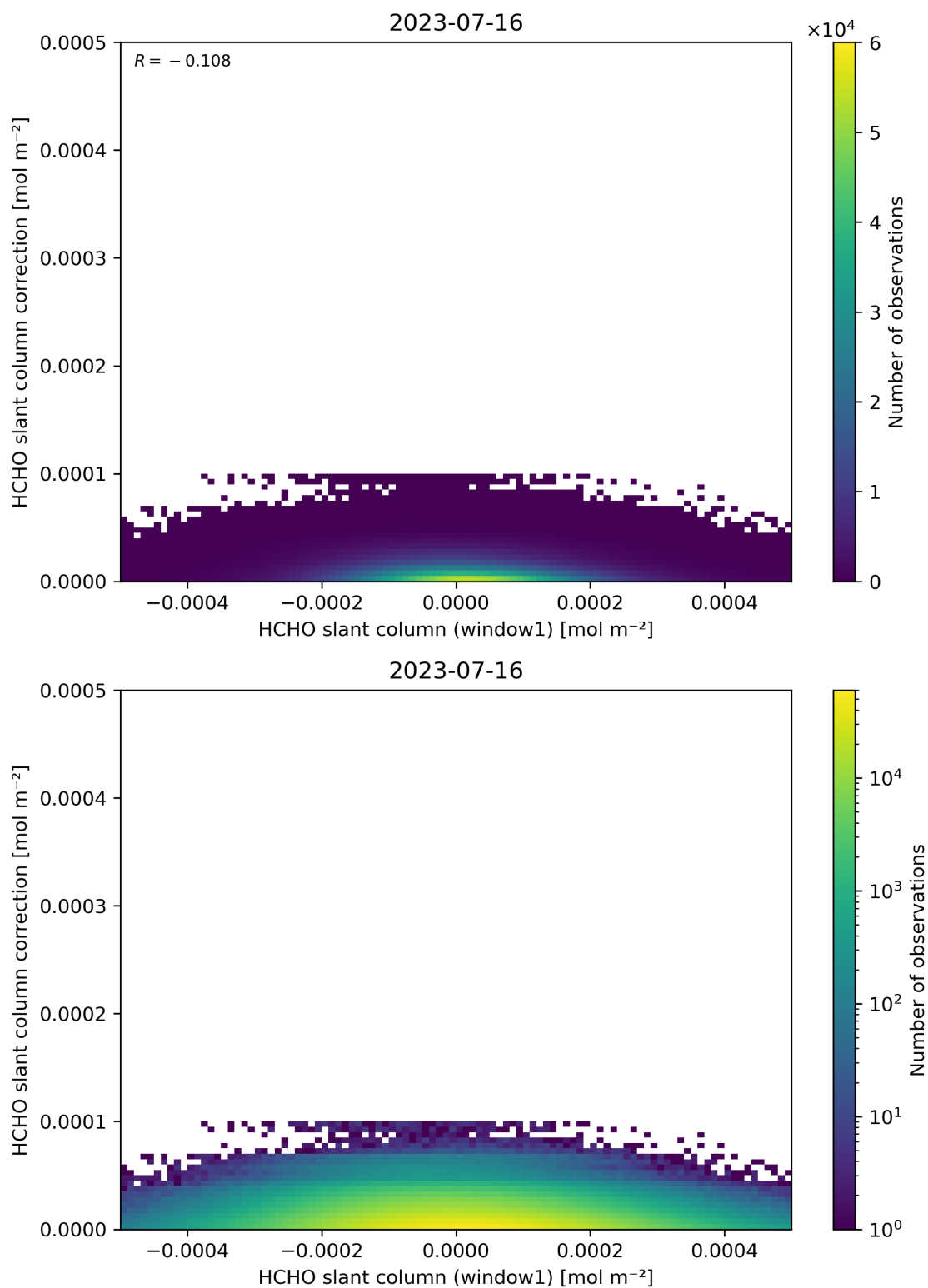
Figure 83: Scatter density plot of “HCHO slant column (window1)” against “HCHO slant column correction” for 2023-07-15 to 2023-07-17.
