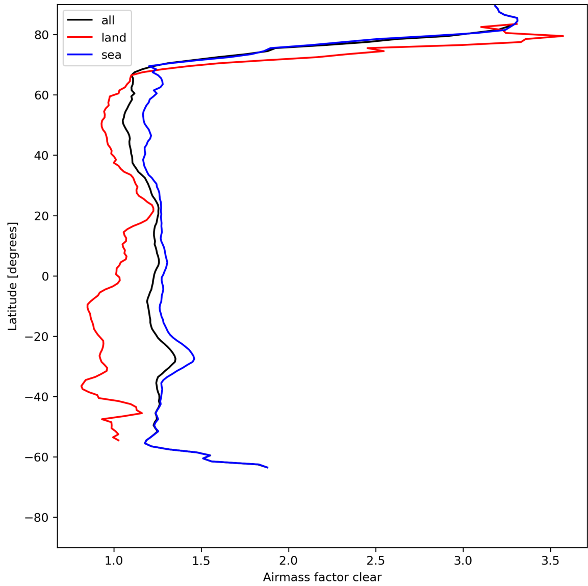
Figure 28: Zonal average of “Airmass factor clear” for 2023-07-17 to 2023-07-19.
