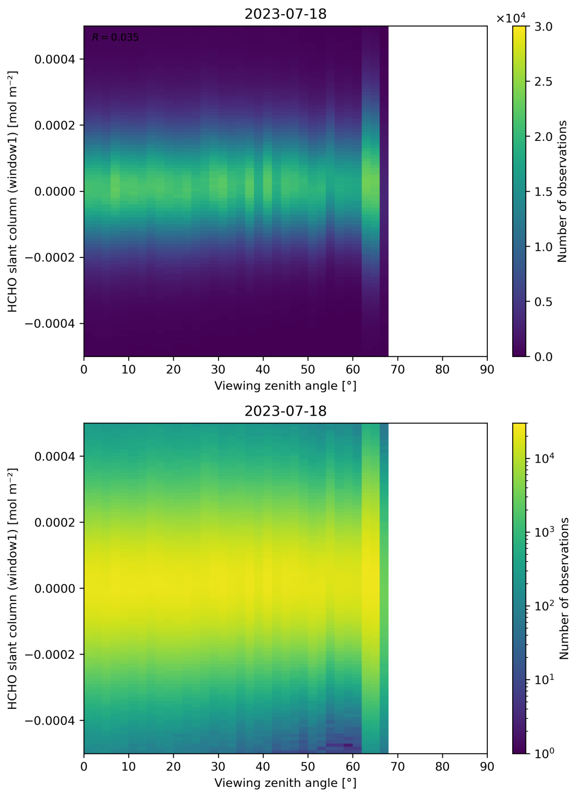
Figure 188: Scatter density plot of “Viewing zenith angle” against “HCHO slant column (window1)” for 2023-07-17 to 2023-07-19.
