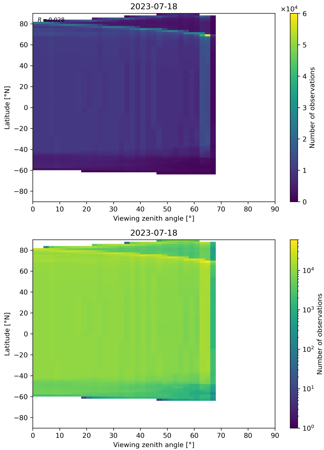
Figure 196: Scatter density plot of “Viewing zenith angle” against “Latitude” for 2023-07-17 to 2023-07-19.
