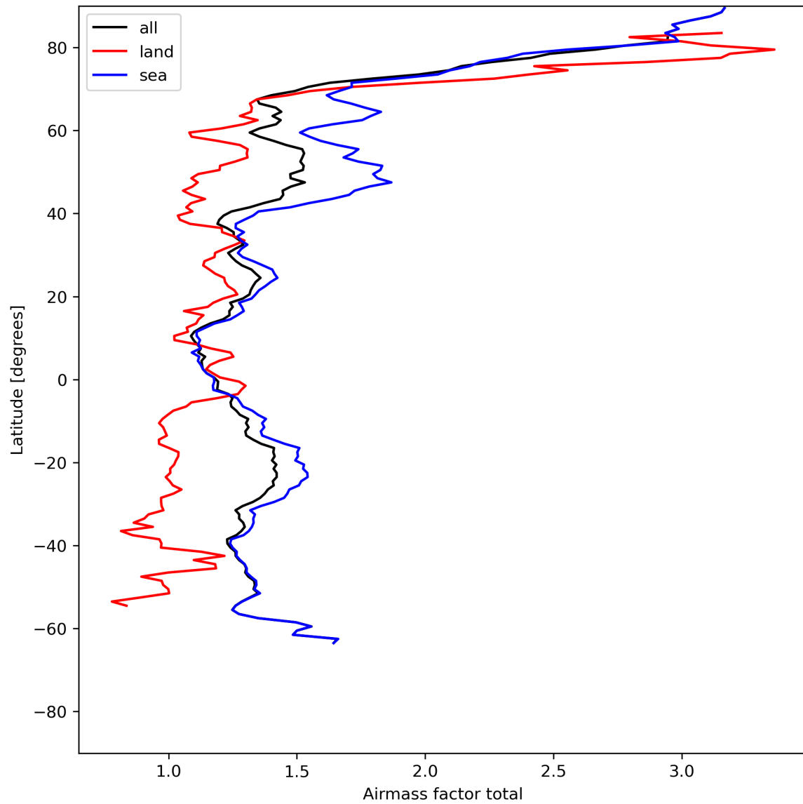
Figure 26: Zonal average of “Airmass factor total” for 2023-07-17 to 2023-07-19.
