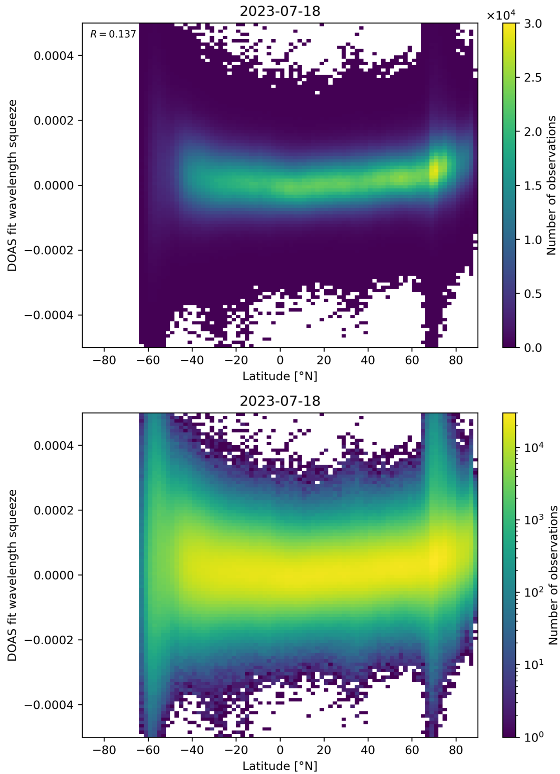
Figure 155: Scatter density plot of “Latitude” against “DOAS fit wavelength squeeze” for 2023-07-17 to 2023-07-19.
