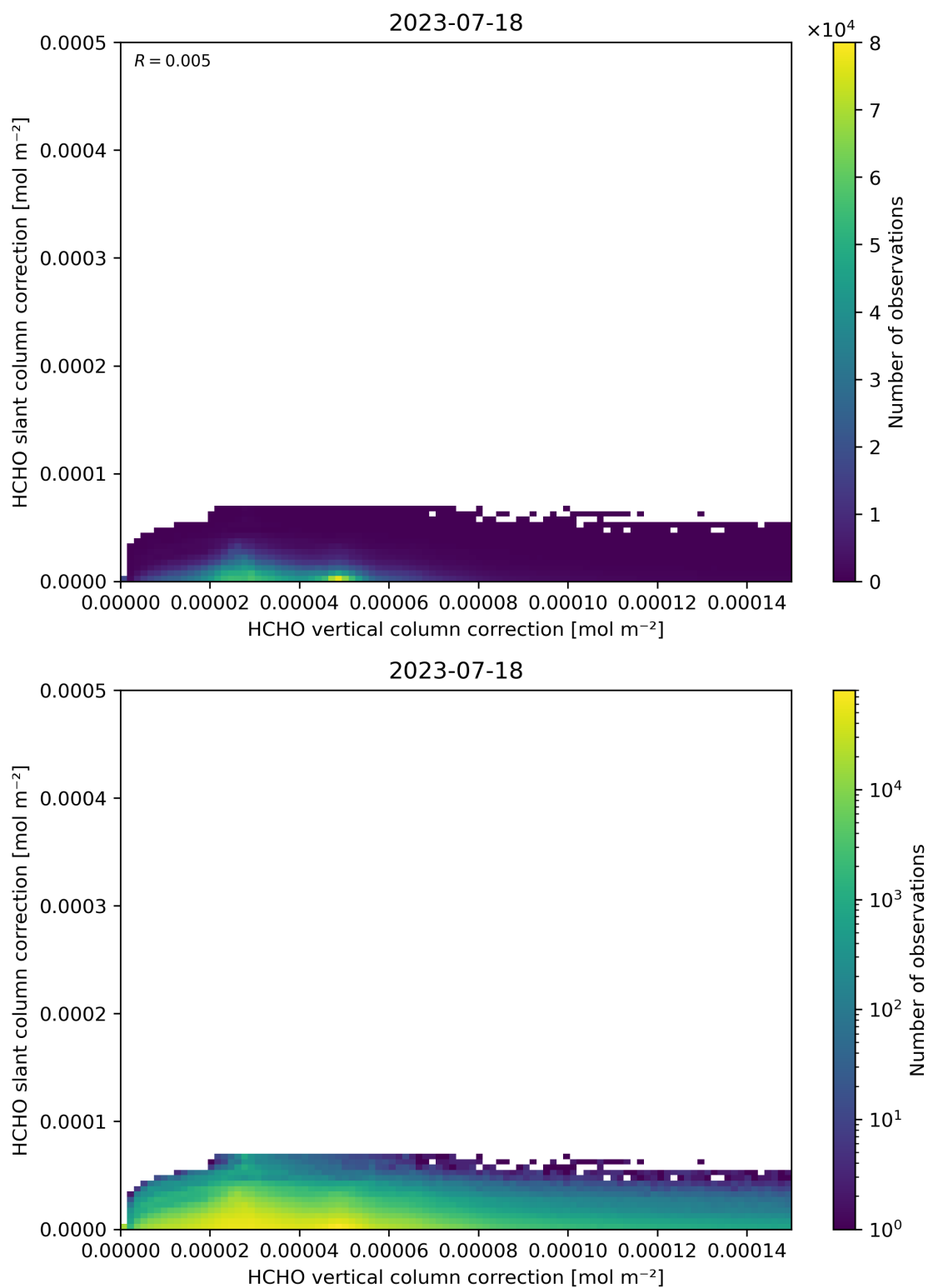
Figure 117: Scatter density plot of “HCHO vertical column correction” against “HCHO slant column correction” for 2023-07-17 to 2023-07-19.
