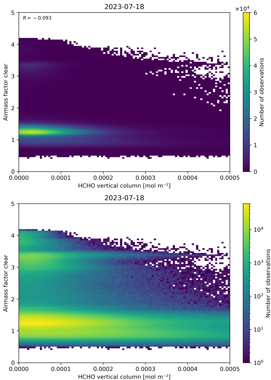
Figure 126: Scatter density plot of “HCHO vertical column” against “Airmass factor clear” for 2023-07-17 to 2023-07-19.
