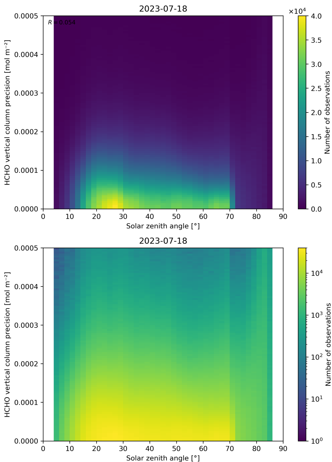
Figure 179: Scatter density plot of “Solar zenith angle” against “HCHO vertical column precision” for 2023-07-17 to 2023-07-19.
