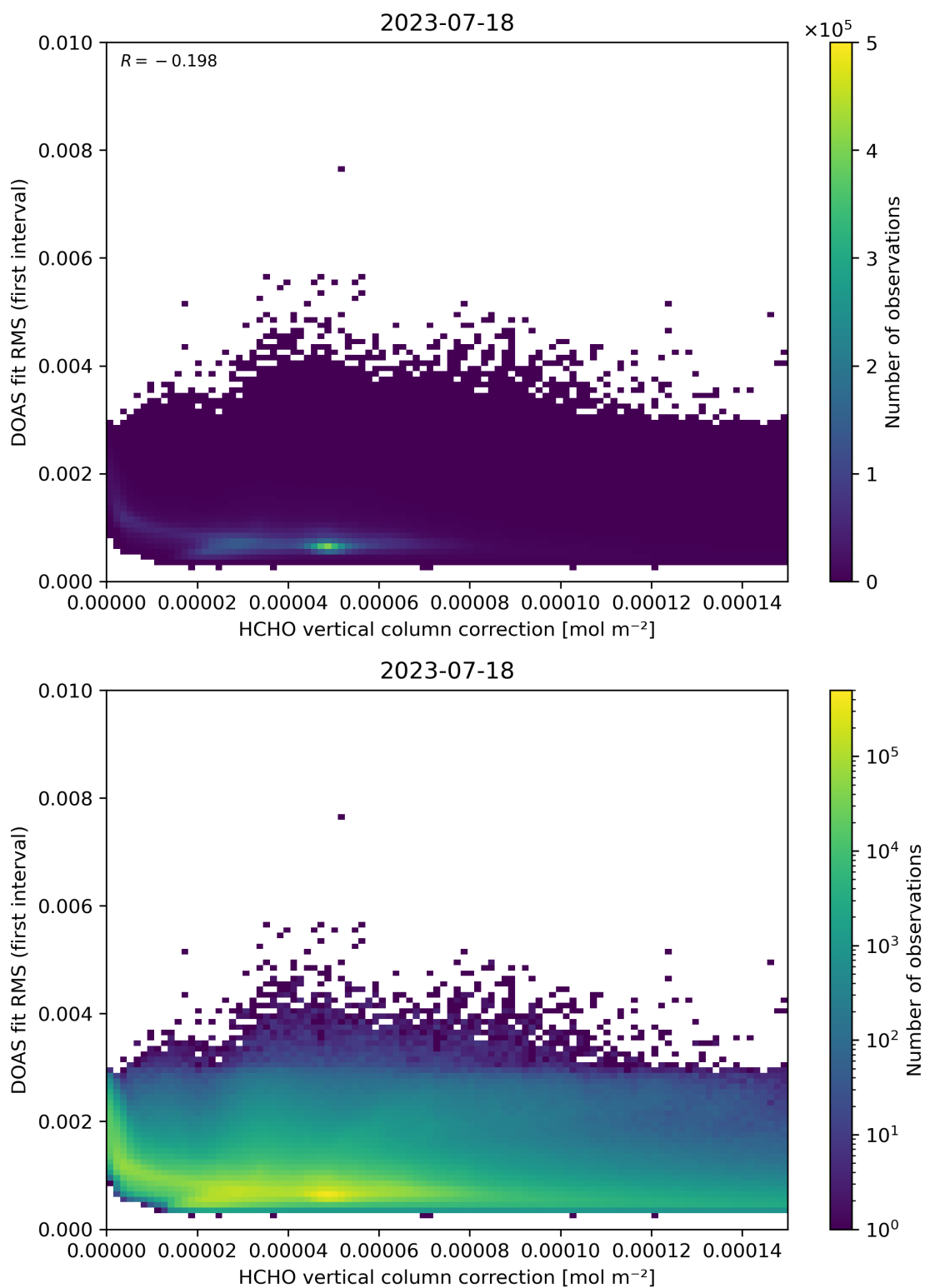
Figure 112: Scatter density plot of “HCHO vertical column correction” against “DOAS fit RMS (first interval)” for 2023-07-17 to 2023-07-19.
