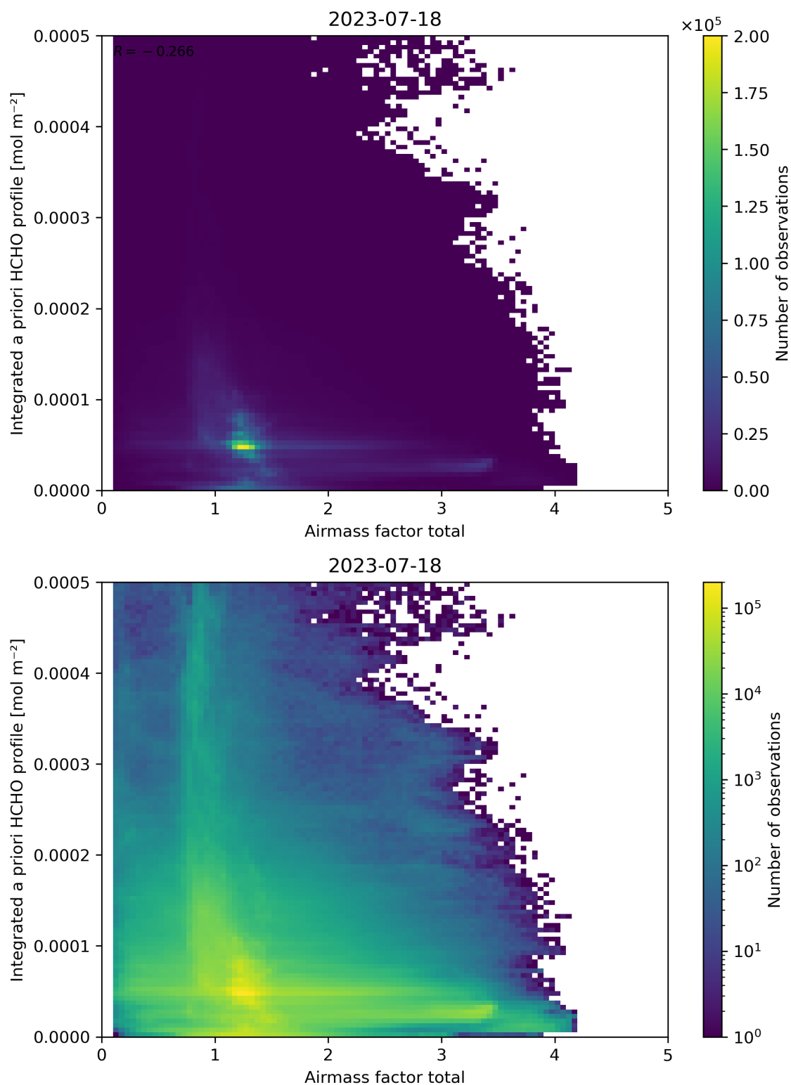
Figure 104: Scatter density plot of “Air mass factor total” against “Integrated a priori HCHO profile” for 2023-07-17 to 2023-07-19.
