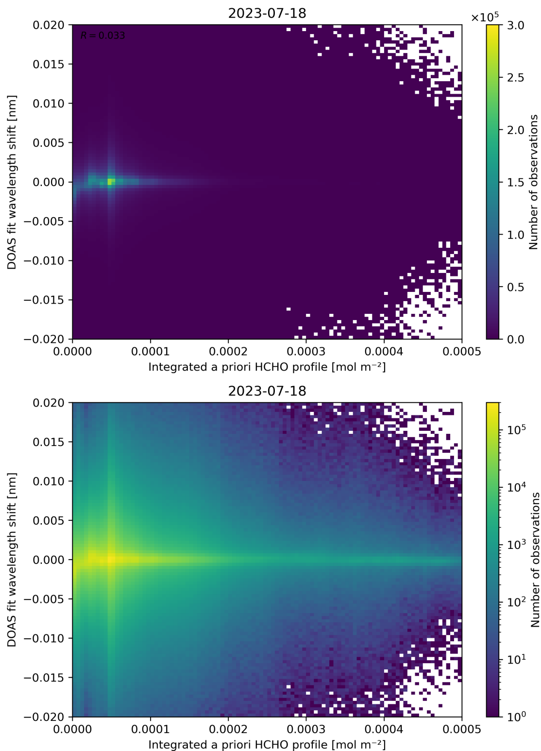
Figure 149: Scatter density plot of “Integrated a priori HCHO profile” against “DOAS fit wavelength shift” for 2023-07-17 to 2023-07-19.
