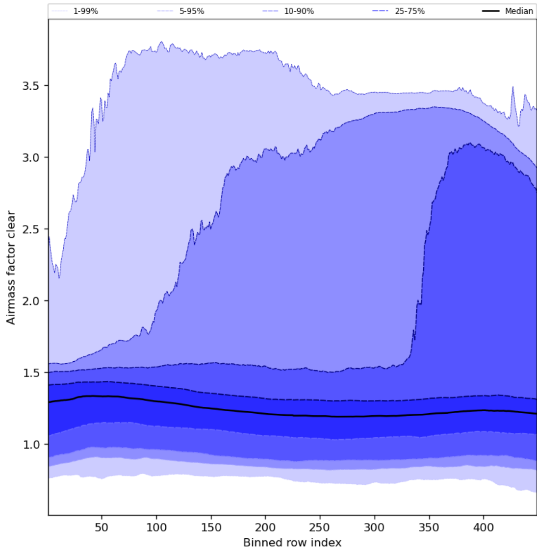
Figure 56: Along track statistics of “Airmass factor clear” for 2023-07-17 to 2023-07-19
