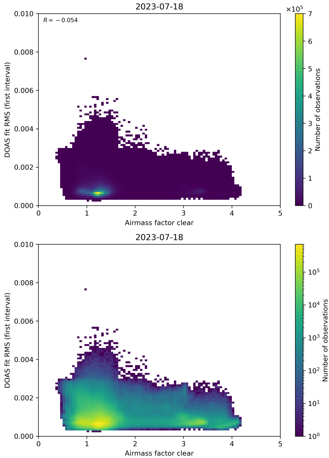
Figure 71: Scatter density plot of “Airmass factor clear” against “DOAS fit RMS (first interval)” for 2023-07-17 to 2023-07-19.
