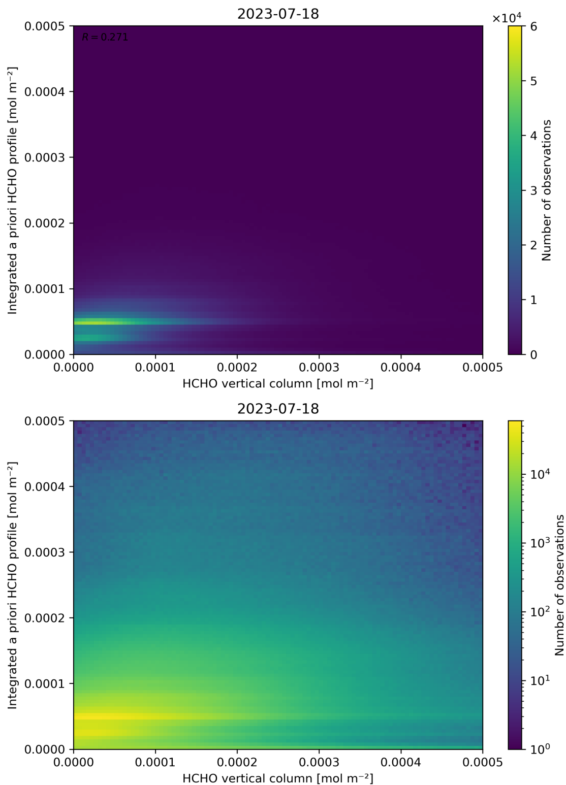
Figure 135: Scatter density plot of “HCHO vertical column” against “Integrated a priori HCHO profile” for 2023-07-17 to 2023-07-19.
