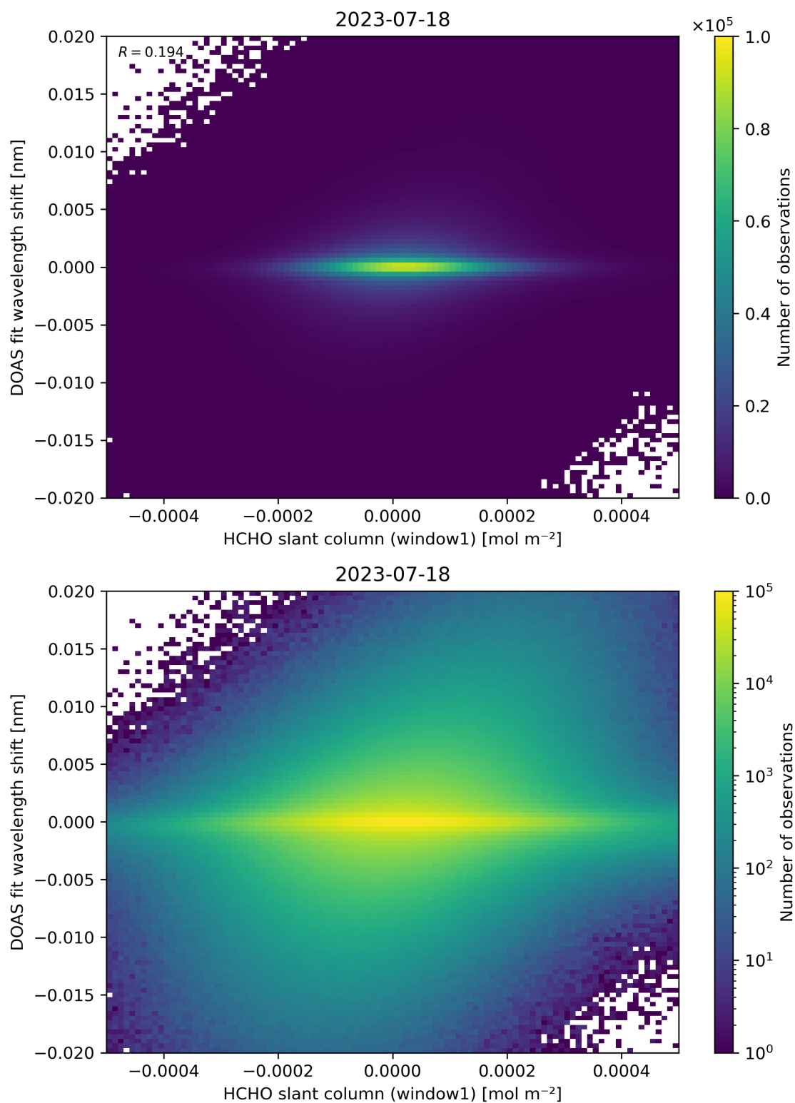
Figure 79: Scatter density plot of “HCHO slant column (window1)” against “DOAS fit wavelength shift” for 2023-07-17 to 2023-07-19.
