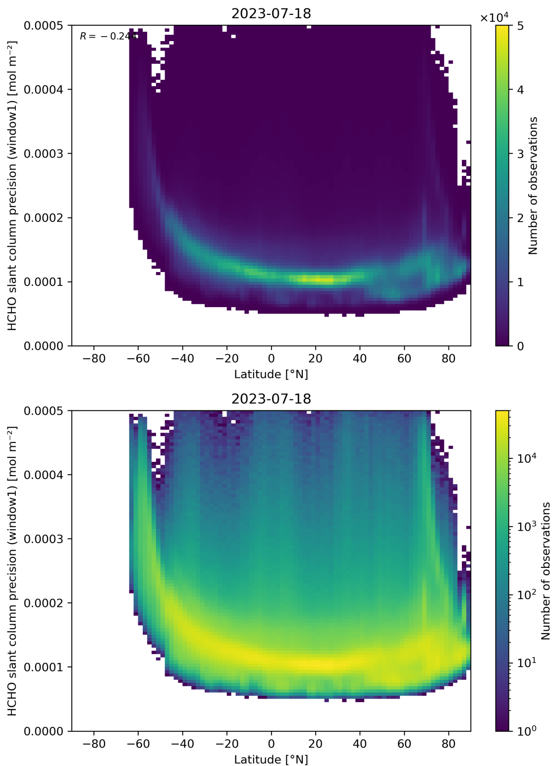
Figure 160: Scatter density plot of “Latitude” against “HCHO slant column precision (window1)” for 2023-07-17 to 2023-07-19.
