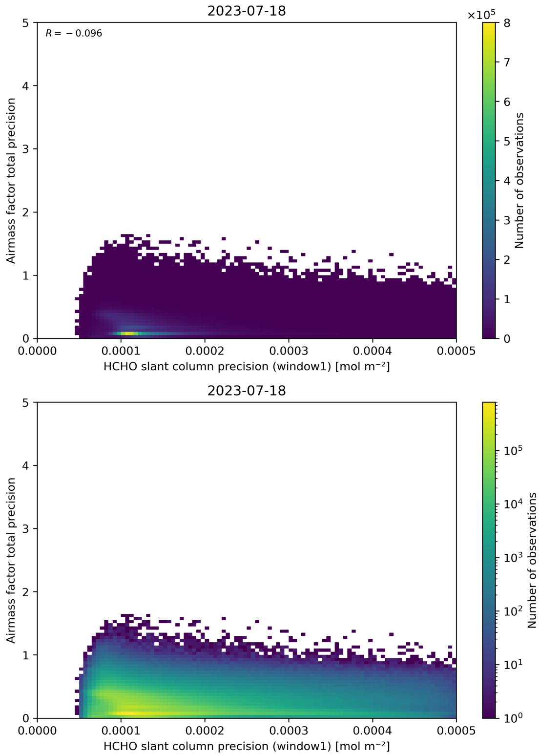
Figure 95: Scatter density plot of “HCHO slant column precision (window1)” against “Airmass factor total precision” for 2023-07-17 to 2023-07-19.
