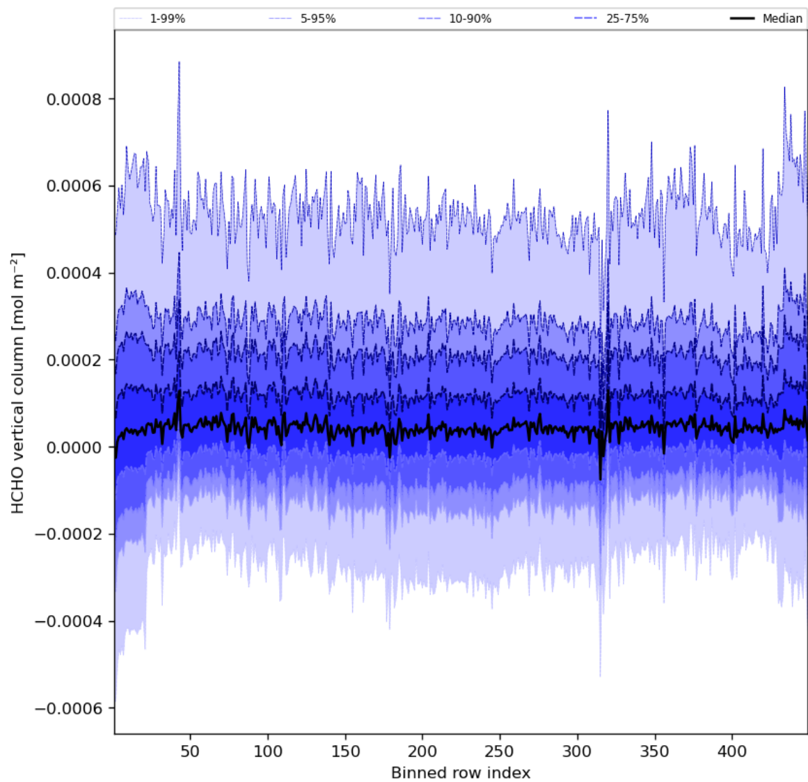
Figure 49: Along track statistics of “HCHO vertical column” for 2023-07-17 to 2023-07-19
