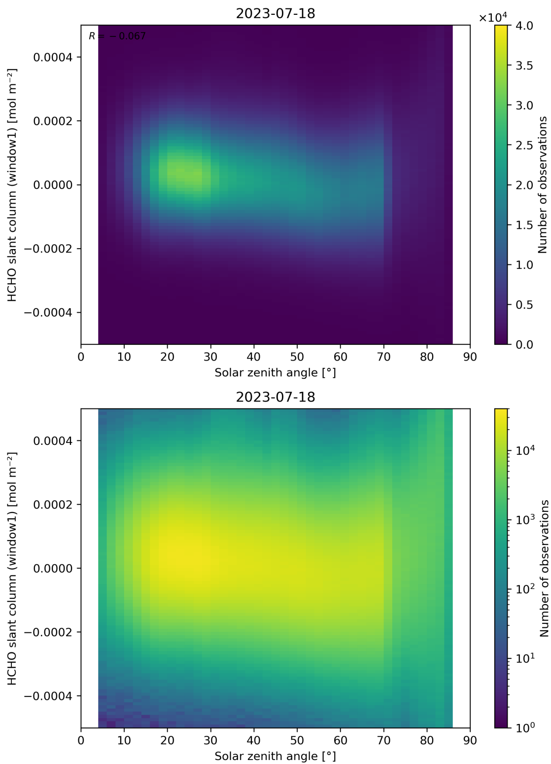
Figure 173: Scatter density plot of “Solar zenith angle” against “HCHO slant column (window1)” for 2023-07-17 to 2023-07-19.
