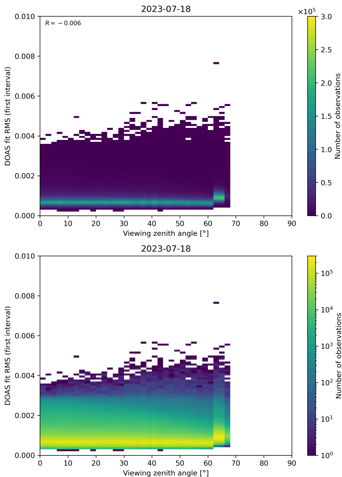
Figure 182: Scatter density plot of “Viewing zenith angle” against “DOAS fit RMS (first interval)” for 2023-07-17 to 2023-07-19.
