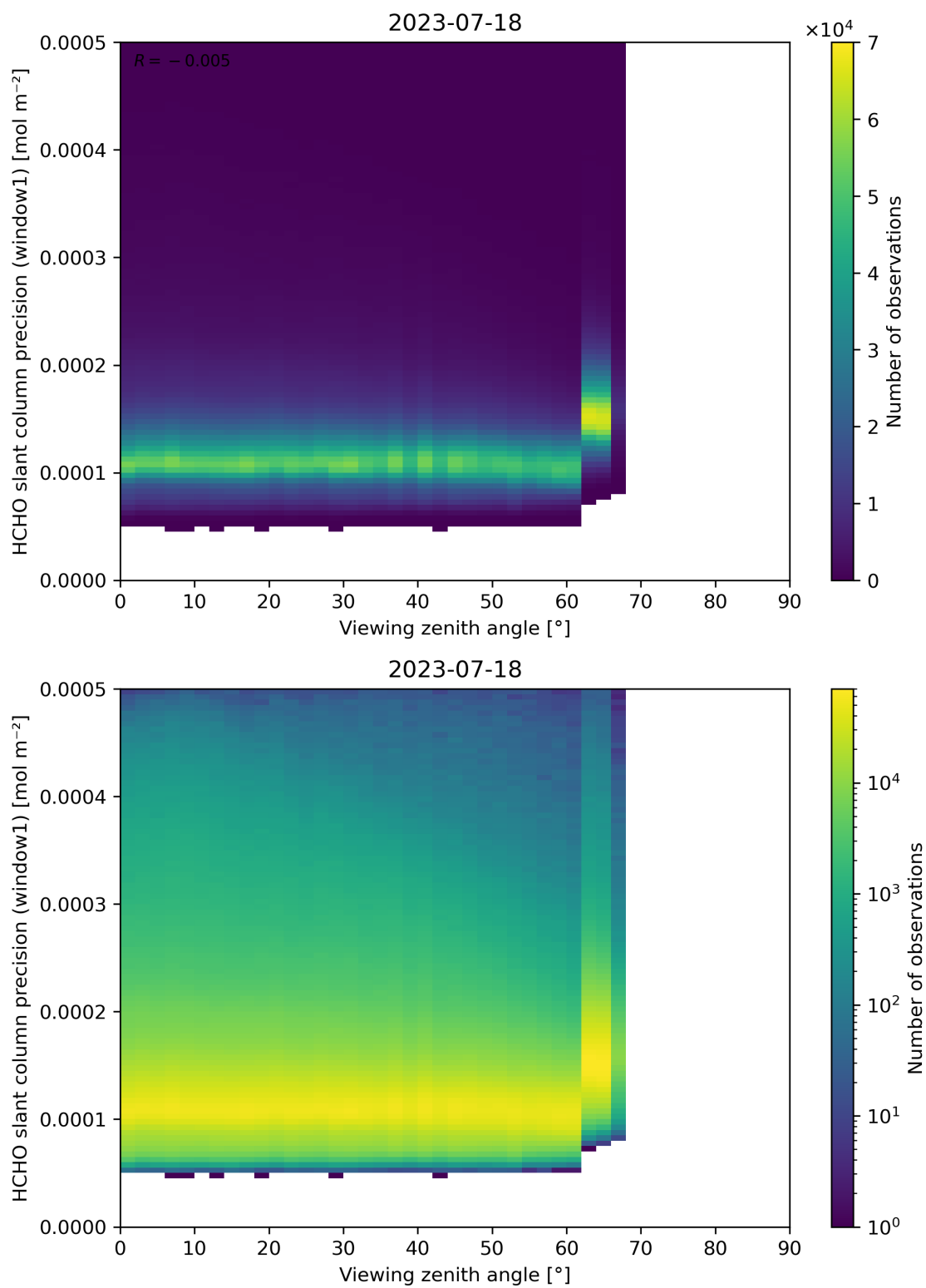
Figure 189: Scatter density plot of “Viewing zenith angle” against “HCHO slant column precision (window1)” for 2023-07-17 to 2023-07-19.
