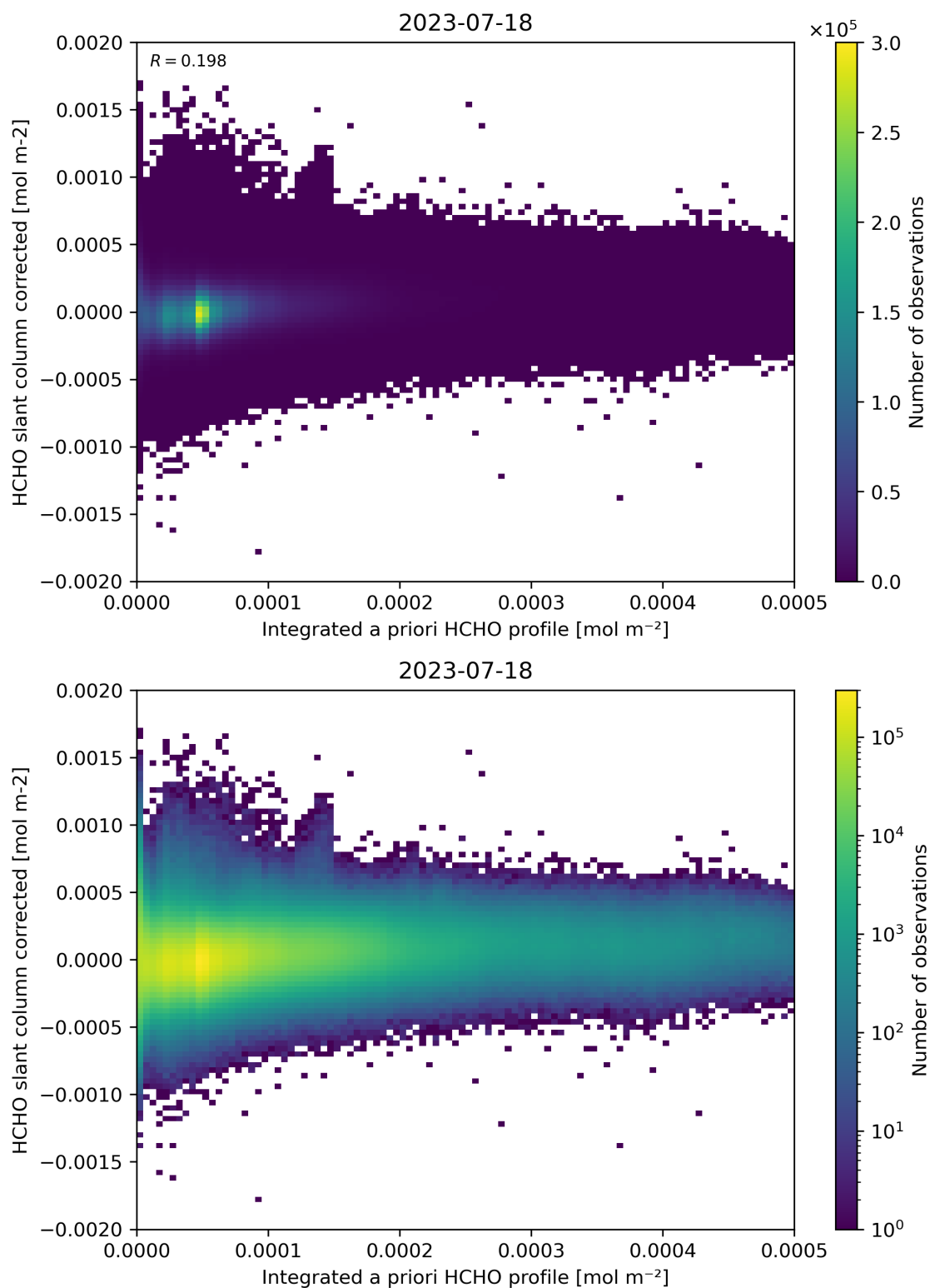
Figure 151: Scatter density plot of “Integrated a priori HCHO profile” against “HCHO slant column corrected” for 2023-07-17 to 2023-07-19.
