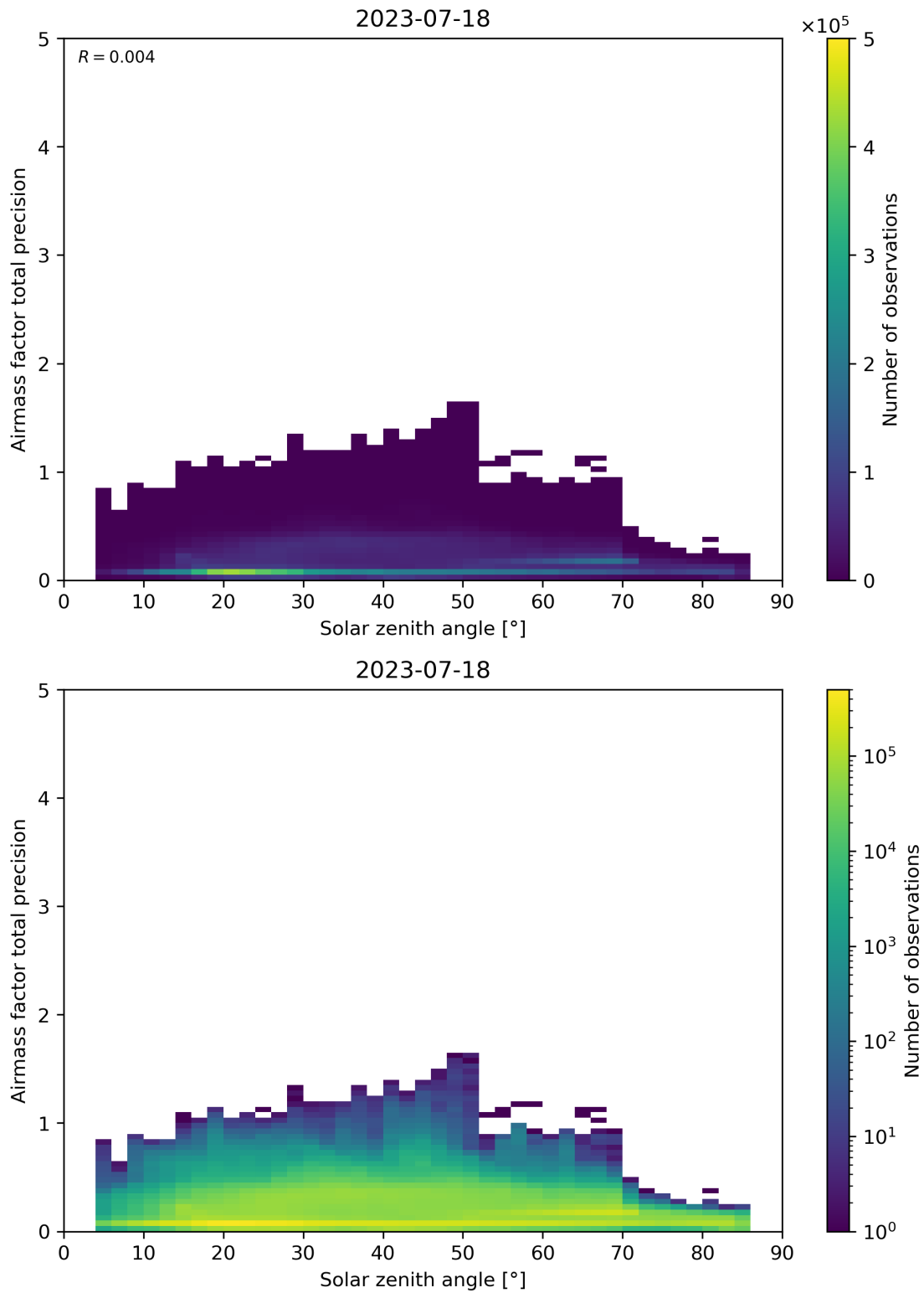
Figure 176: Scatter density plot of “Solar zenith angle” against “Airmass factor total precision” for 2023-07-17 to 2023-07-19.
