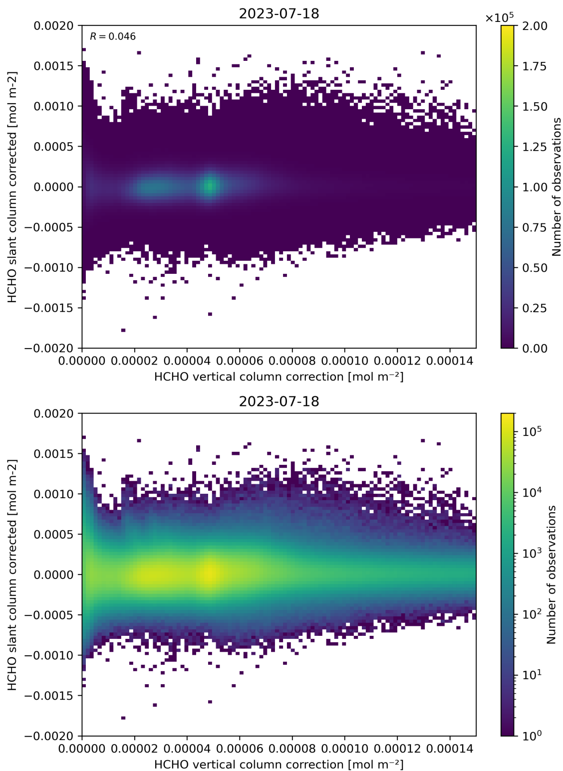
Figure 116: Scatter density plot of “HCHO vertical column correction” against “HCHO slant column corrected” for 2023-07-17 to 2023-07-19.
