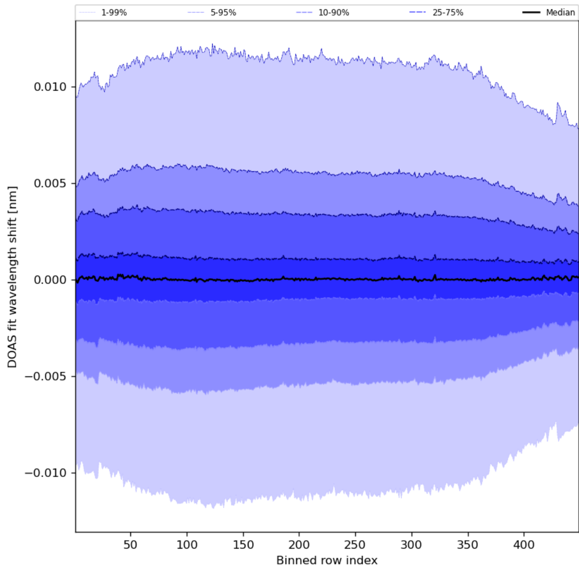
Figure 58: Along track statistics of “DOAS fit wavelength shift” for 2023-07-17 to 2023-07-19
