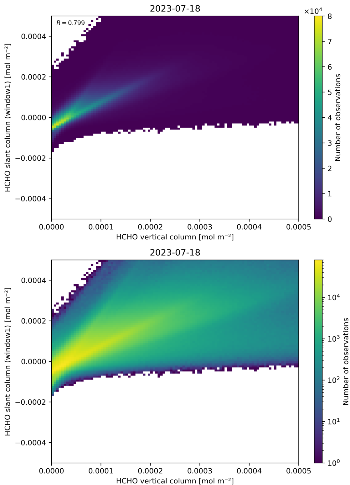
Figure 129: Scatter density plot of “HCHO vertical column” against “HCHO slant column (window1)” for 2023-07-17 to 2023-07-19.
