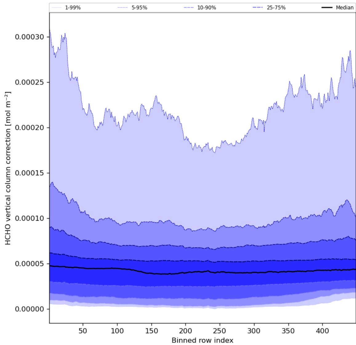
Figure 51: Along track statistics of “HCHO vertical column correction” for 2023-07-17 to 2023-07-19
