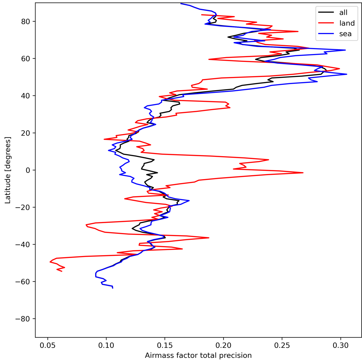
Figure 27: Zonal average of “Airmass factor total precision” for 2023-07-17 to 2023-07-19.
