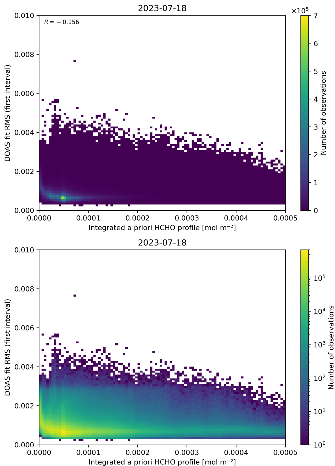
Figure 148: Scatter density plot of “Integrated a priori HCHO profile” against “DOAS fit RMS (first interval)” for 2023-07-17 to 2023-07-19.
