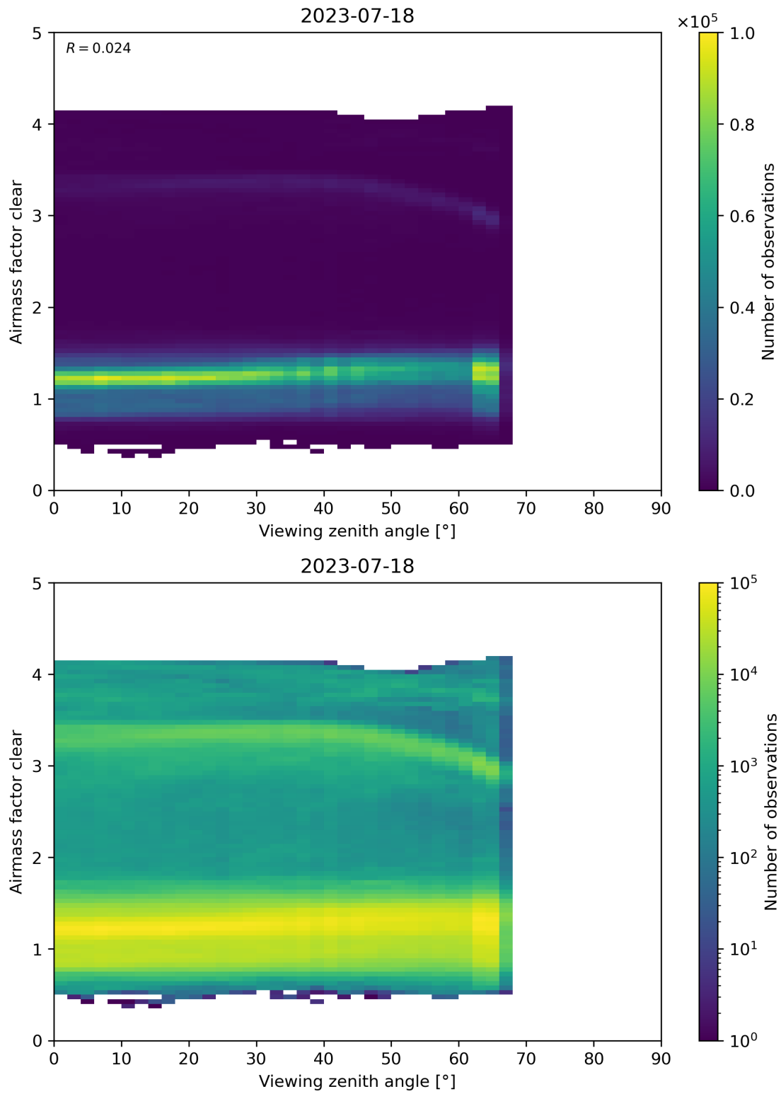
Figure 185: Scatter density plot of “Viewing zenith angle” against “Airmass factor clear” for 2023-07-17 to 2023-07-19.
