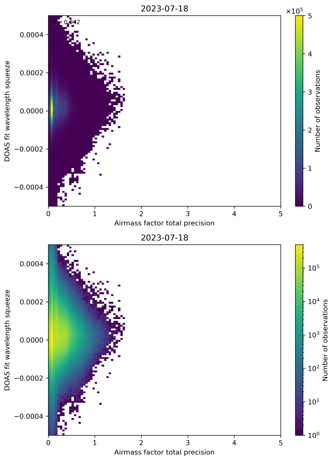
Figure 107: Scatter density plot of “Airmass factor total precision” against “DOAS fit wavelength squeeze” for 2023-07-17 to 2023-07-19.
