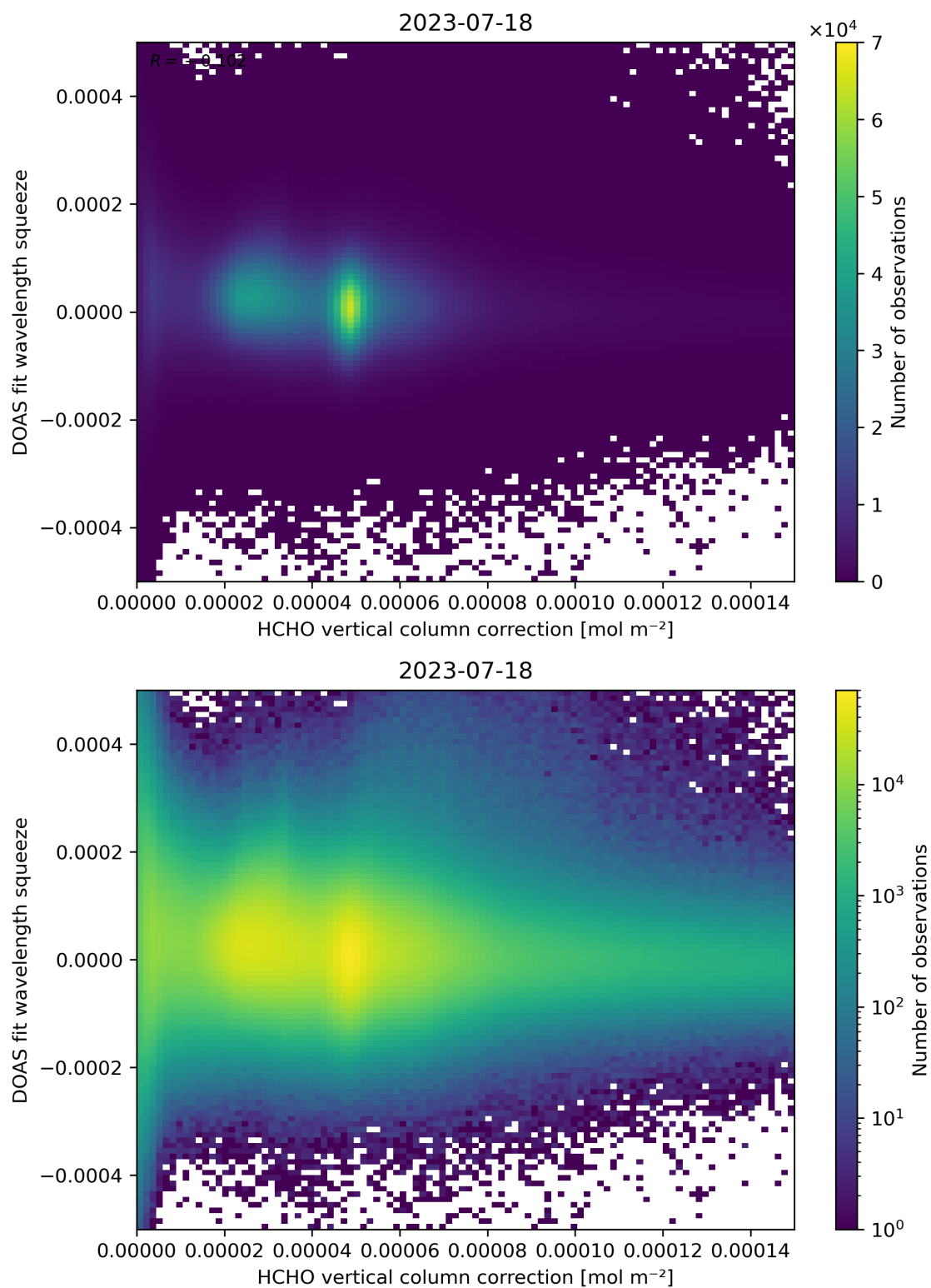
Figure 114: Scatter density plot of “HCHO vertical column correction” against “DOAS fit wavelength squeeze” for 2023-07-17 to 2023-07-19.
