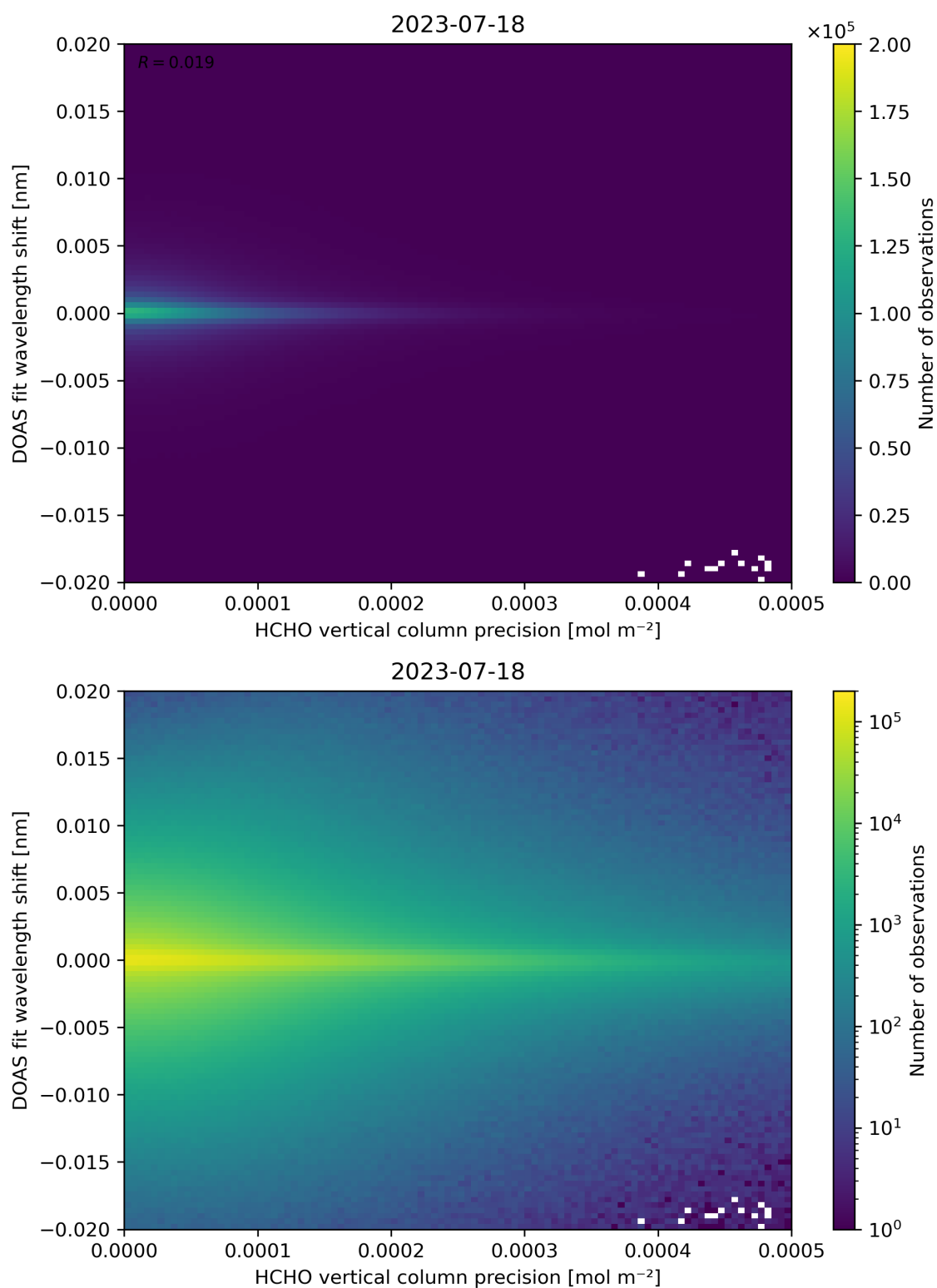
Figure 137: Scatter density plot of “HCHO vertical column precision” against “DOAS fit wavelength shift” for 2023-07-17 to 2023-07-19.
