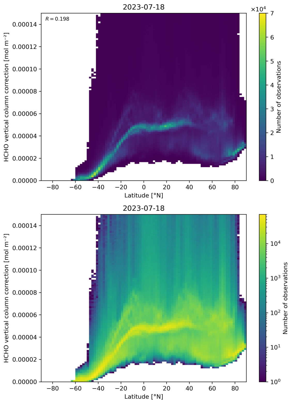
Figure 164: Scatter density plot of “Latitude” against “HCHO vertical column correction” for 2023-07-17 to 2023-07-19.
