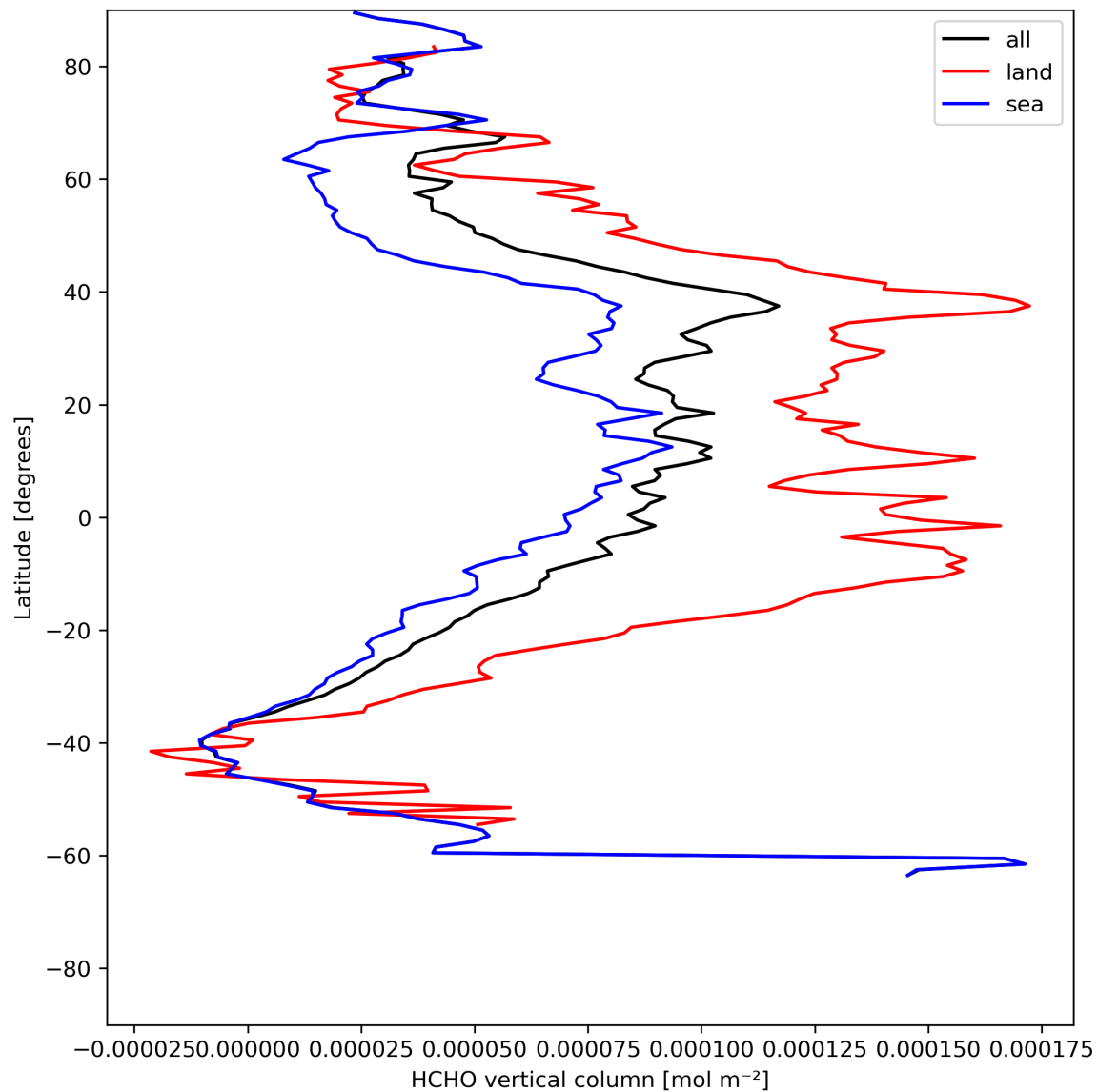
Figure 21: Zonal average of “HCHO vertical column” for 2023-07-17 to 2023-07-19.
