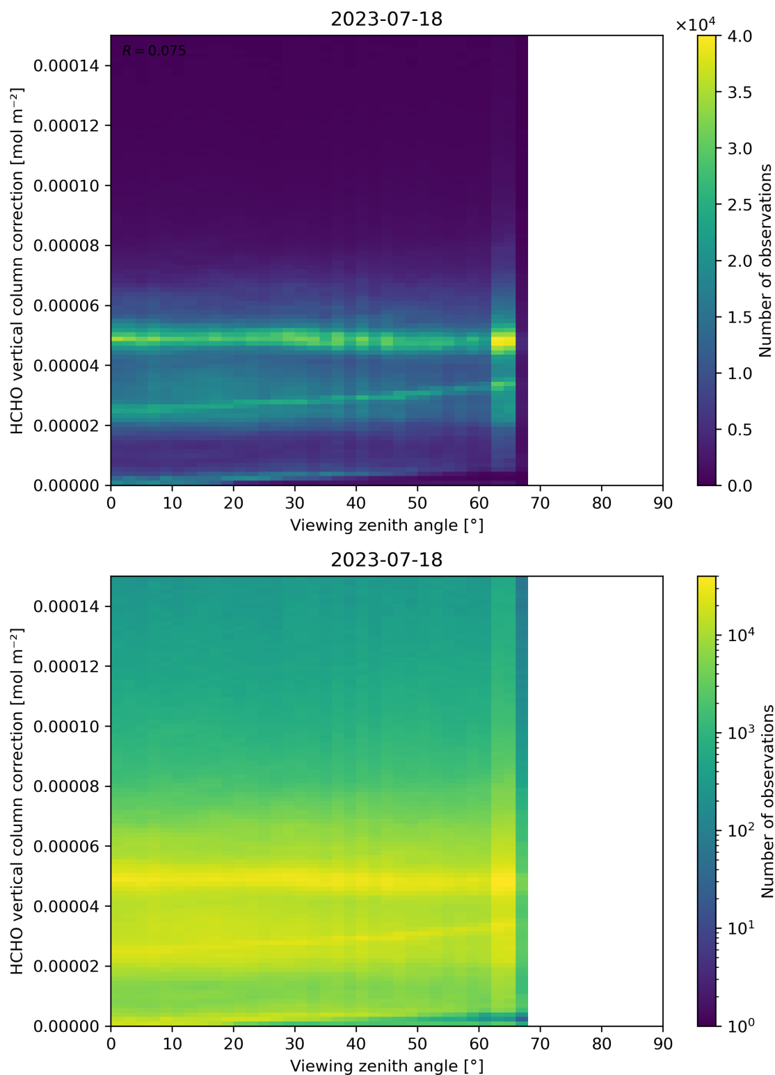
Figure 193: Scatter density plot of “Viewing zenith angle” against “HCHO vertical column correction” for 2023-07-17 to 2023-07-19.
