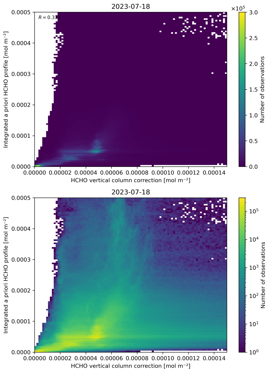
Figure 122: Scatter density plot of “HCHO vertical column correction” against “Integrated a priori HCHO profile” for 2023-07-17 to 2023-07-19.
