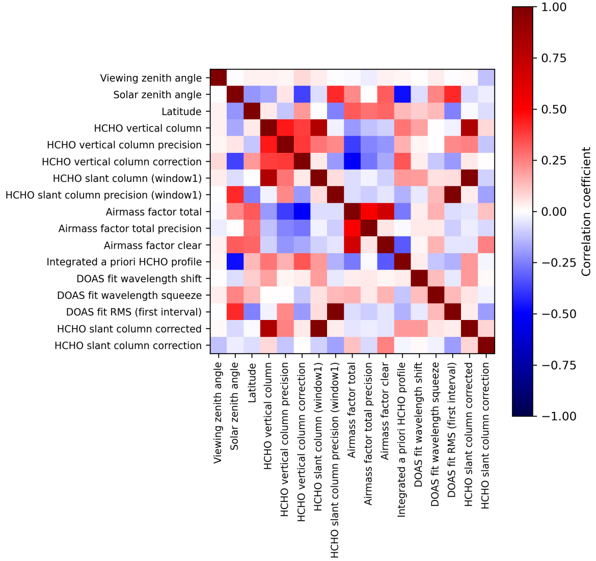
Figure 2: Map of correlation matrix for 2023-07-17 to 2023-07-19.
