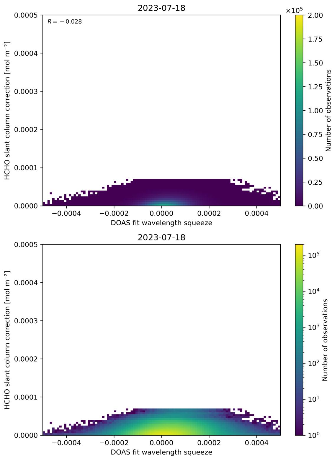
Figure 70: Scatter density plot of “DOAS fit wavelength squeeze” against “HCHO slant column correction” for 2023-07-17 to 2023-07-19.
