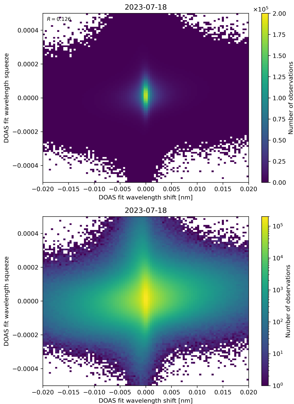
Figure 65: Scatter density plot of “DOAS fit wavelength shift” against “DOAS fit wavelength squeeze” for 2023-07-17 to 2023-07-19.
