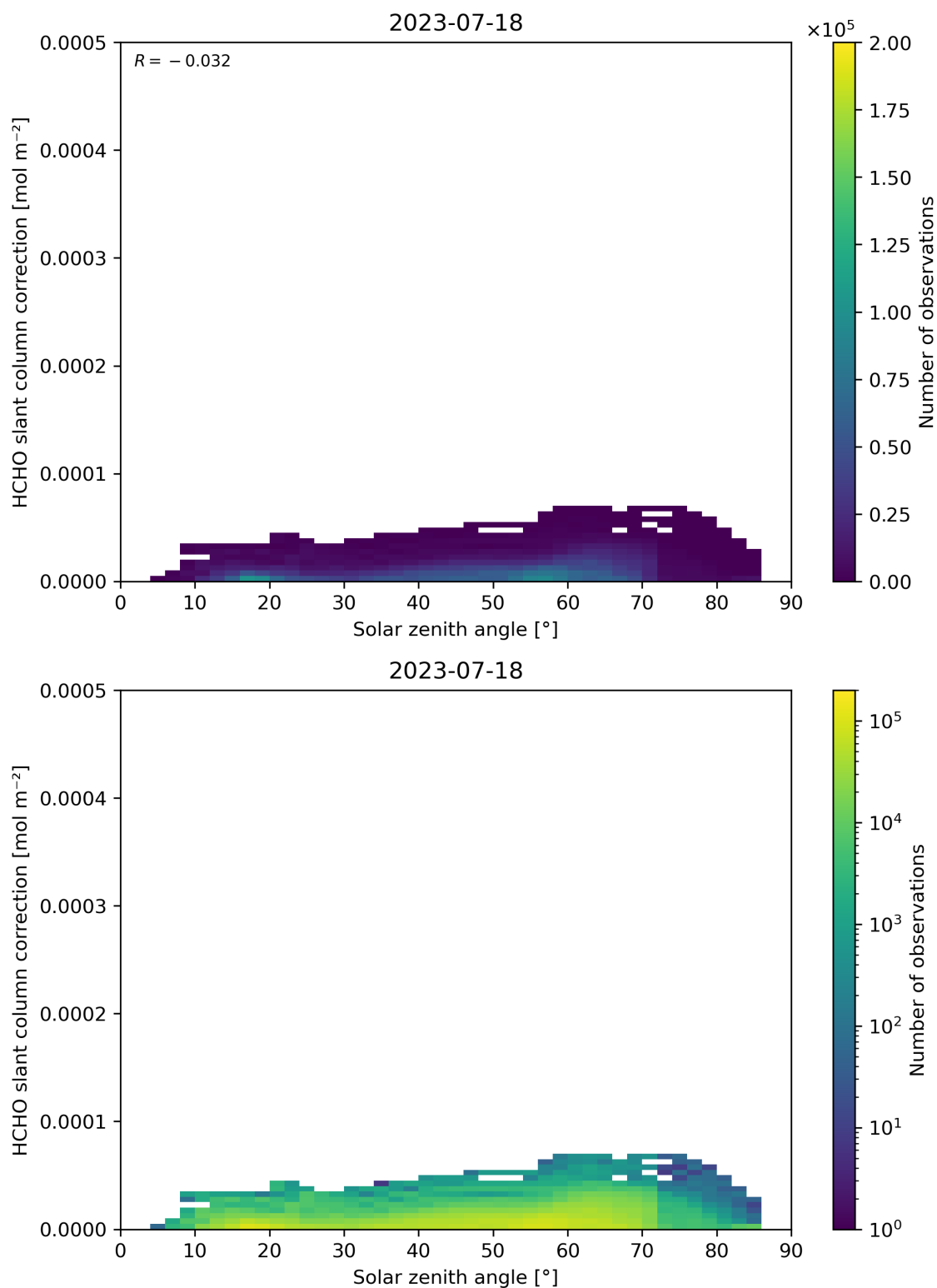
Figure 172: Scatter density plot of “Solar zenith angle” against “HCHO slant column correction” for 2023-07-17 to 2023-07-19.
