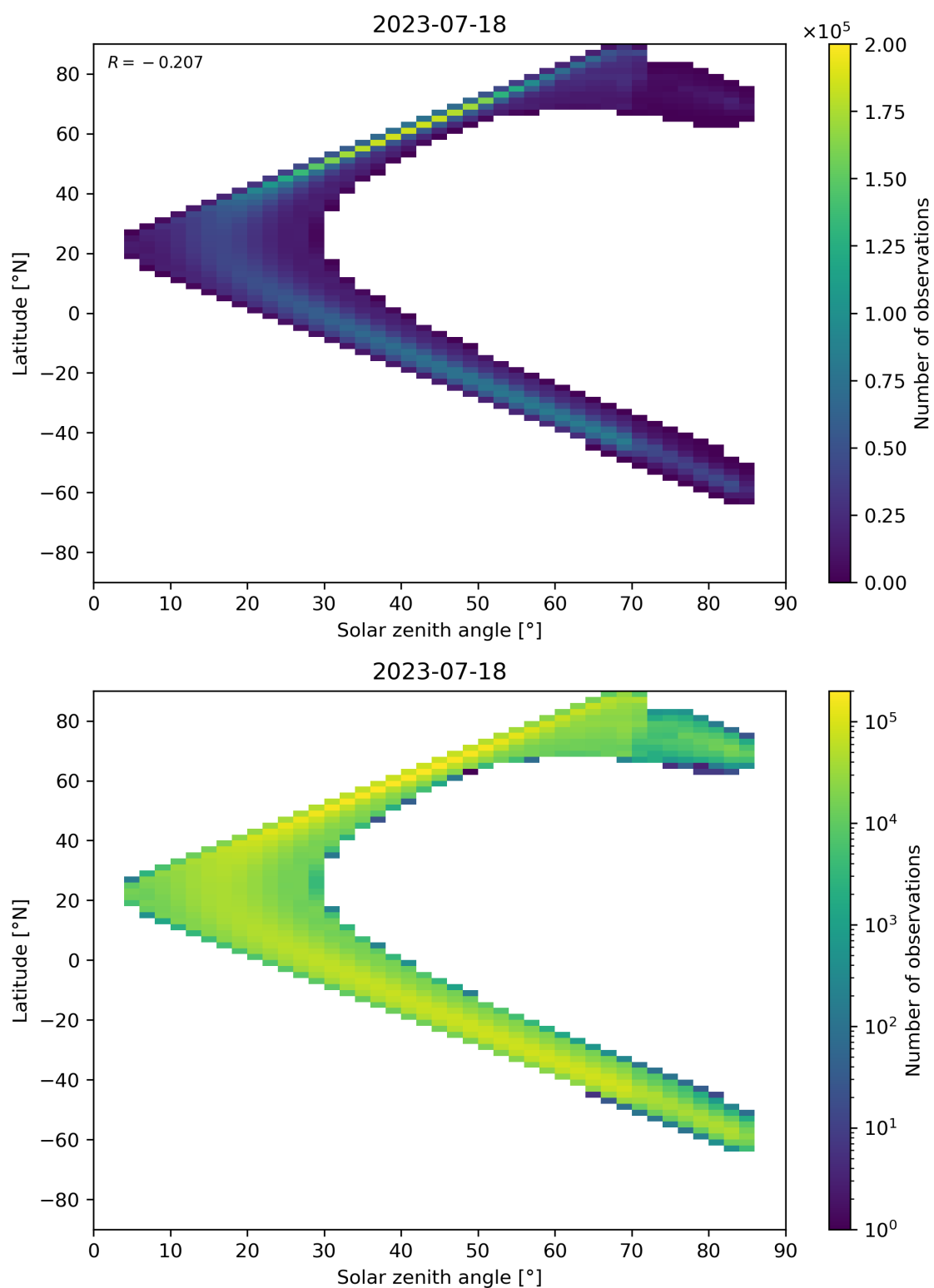
Figure 181: Scatter density plot of “Solar zenith angle” against “Latitude” for 2023-07-17 to 2023-07-19.
