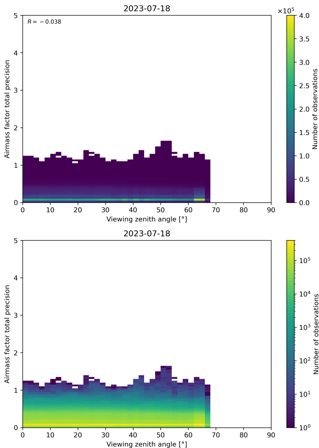
Figure 191: Scatter density plot of “Viewing zenith angle” against “Airmass factor total precision” for 2023-07-17 to 2023-07-19.
