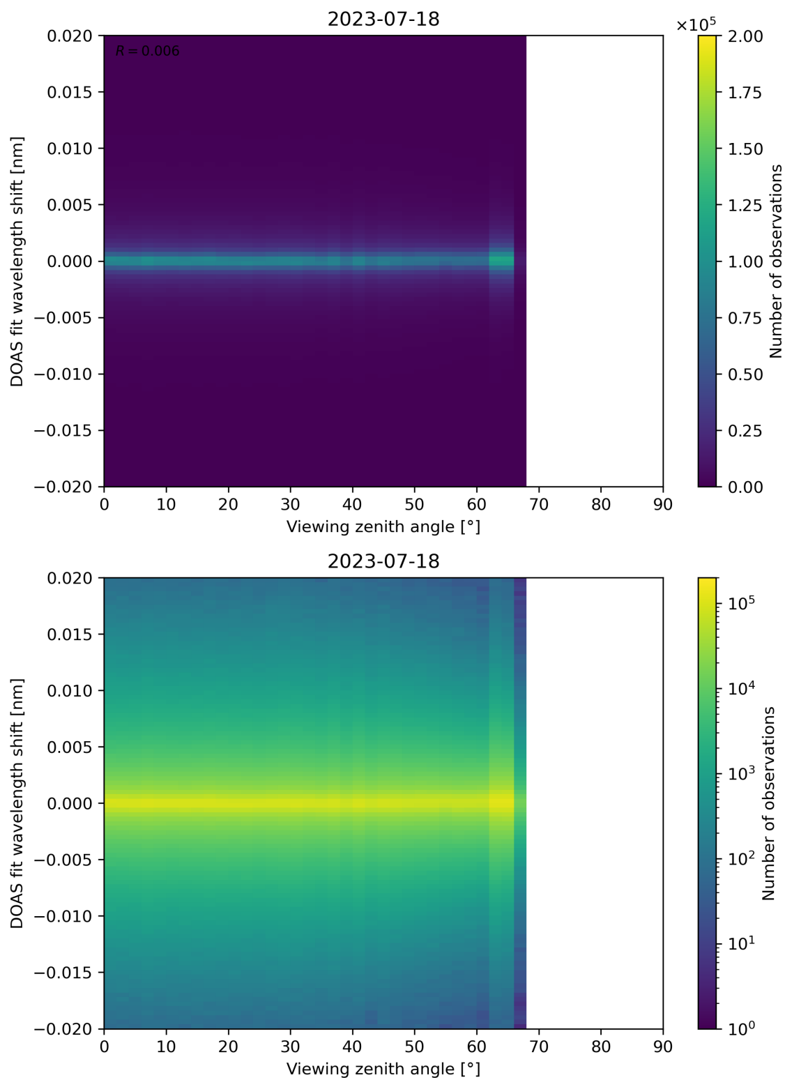
Figure 183: Scatter density plot of “Viewing zenith angle” against “DOAS fit wavelength shift” for 2023-07-17 to 2023-07-19.
