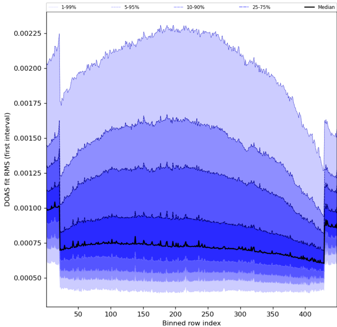
Figure 60: Along track statistics of “DOAS fit RMS (first interval)” for 2023-07-17 to 2023-07-19
