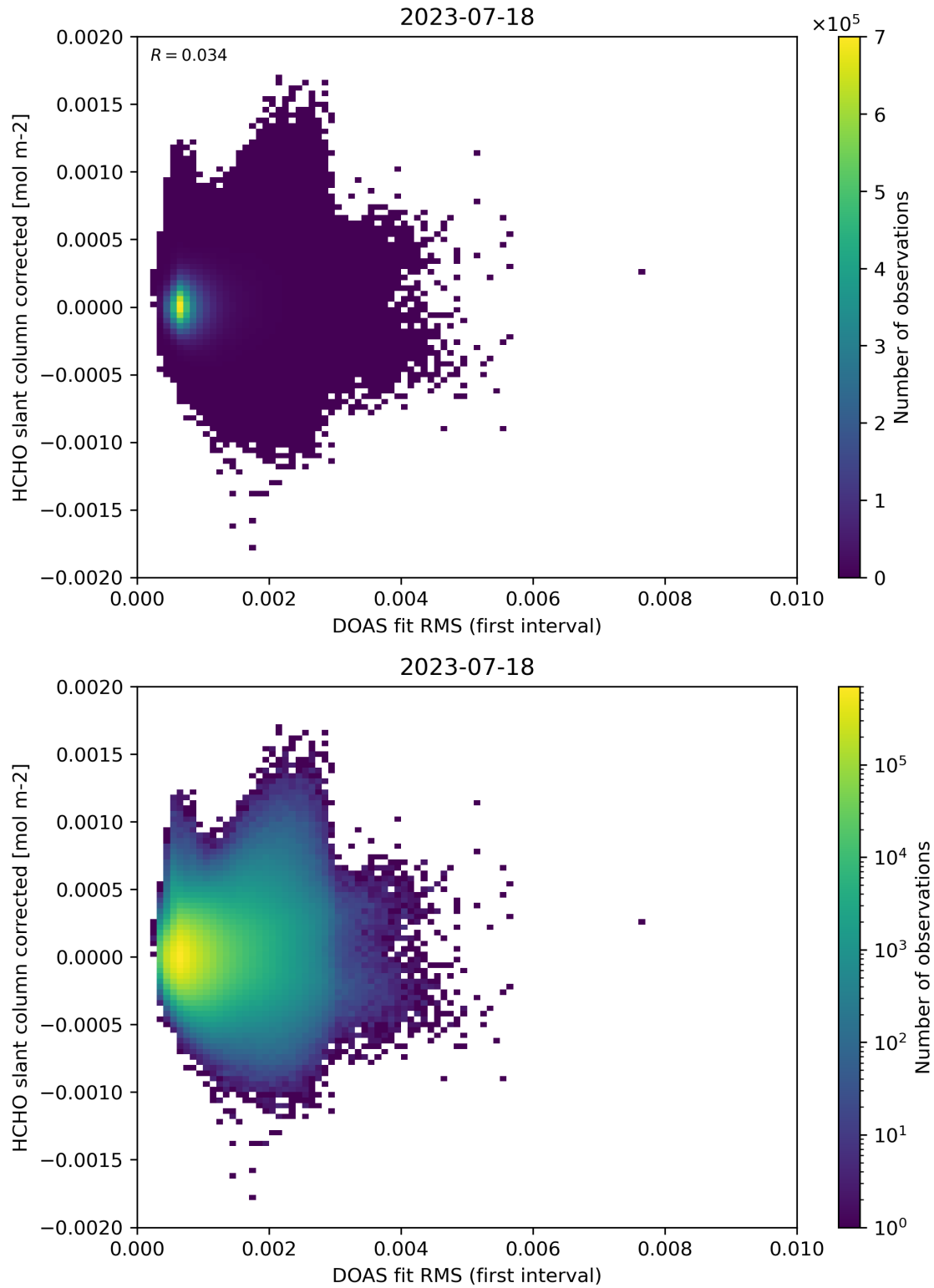
Figure 62: Scatter density plot of “DOAS fit RMS (first interval)” against “HCHO slant column corrected” for 2023-07-17 to 2023-07-19.
