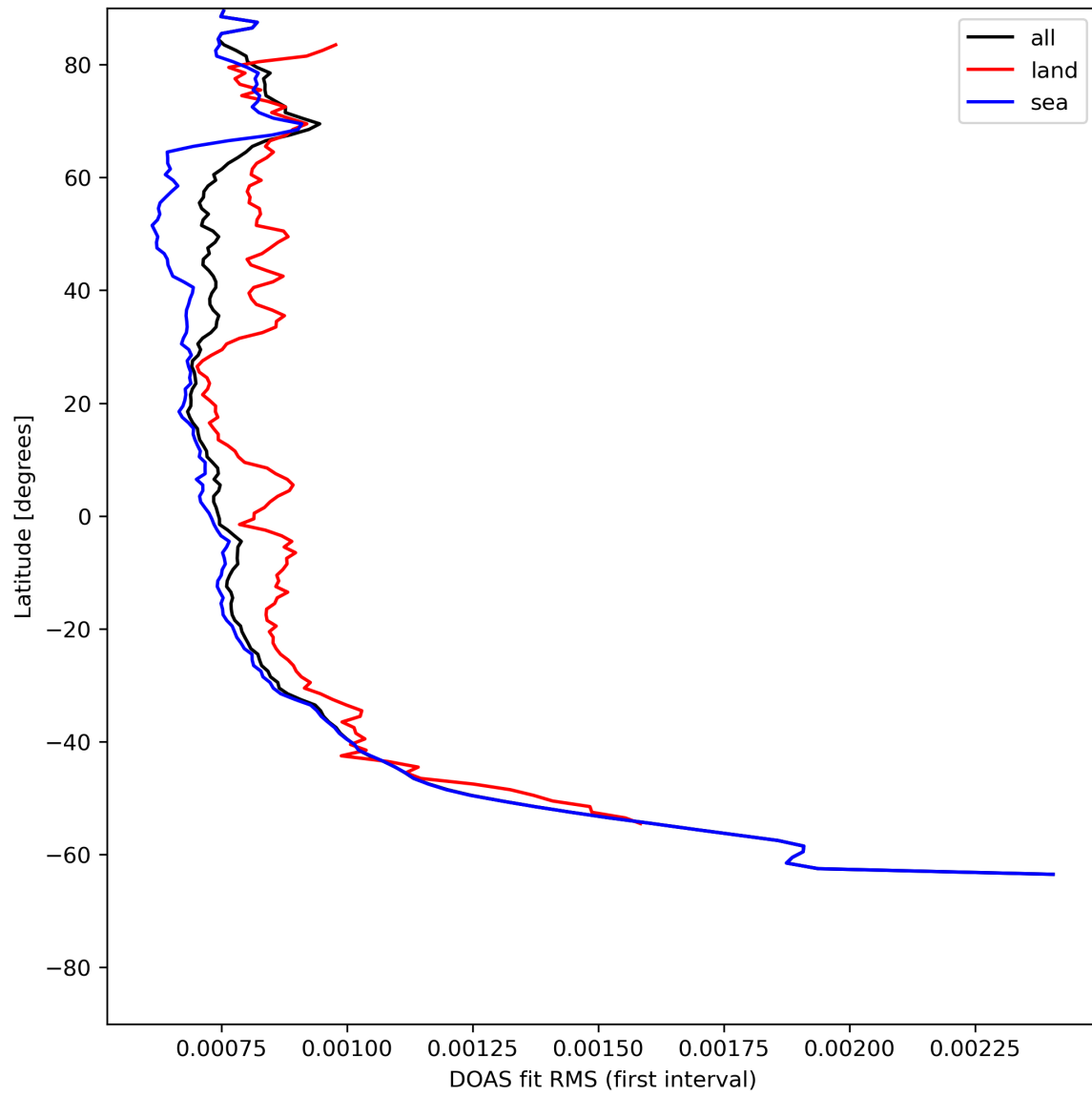
Figure 32: Zonal average of “DOAS fit RMS (first interval)” for 2023-07-17 to 2023-07-19.
