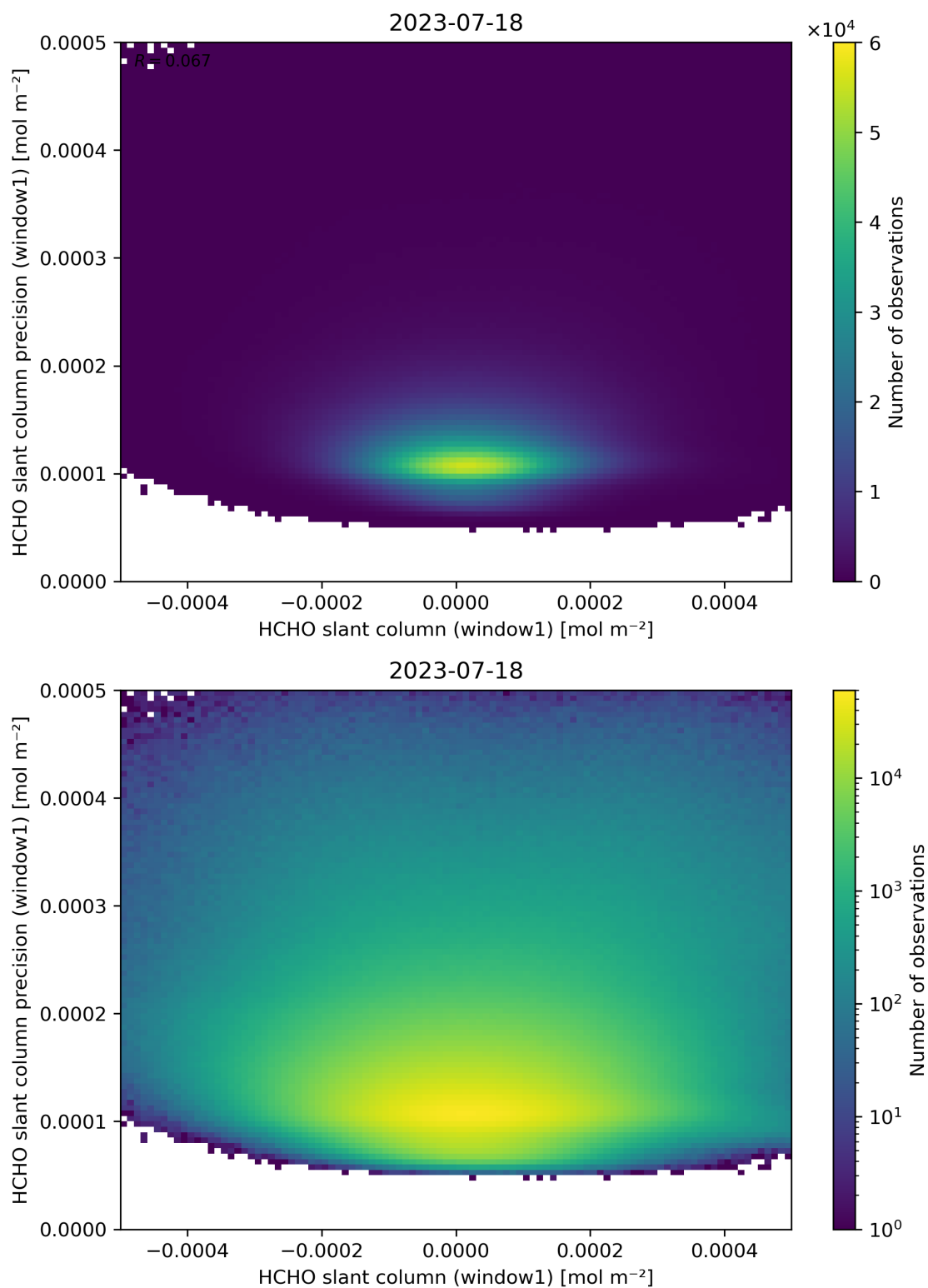
Figure 84: Scatter density plot of “HCHO slant column (window1)” against “HCHO slant column precision (window1)” for 2023-07-17 to 2023-07-19.
