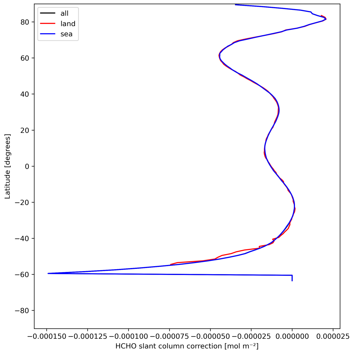
Figure 33: Zonal average of “HCHO slant column correction” for 2023-07-17 to 2023-07-19.
