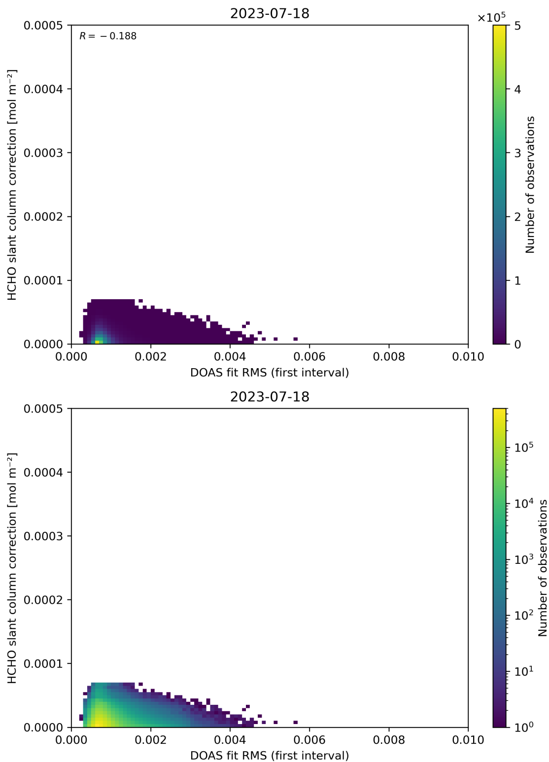
Figure 63: Scatter density plot of “DOAS fit RMS (first interval)” against “HCHO slant column correction” for 2023-07-17 to 2023-07-19.
