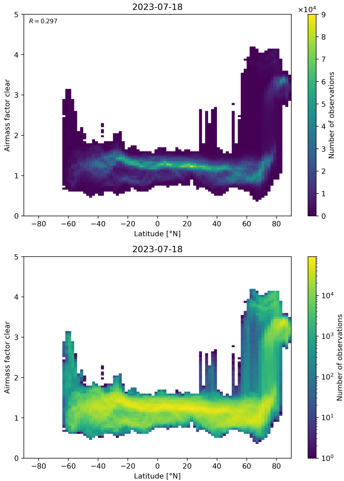
Figure 156: Scatter density plot of “Latitude” against “Airmass factor clear” for 2023-07-17 to 2023-07-19.
