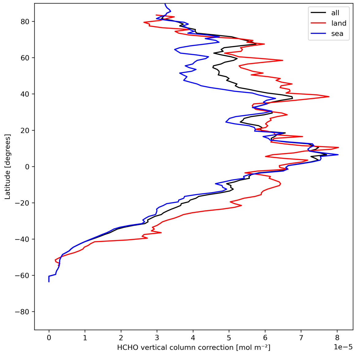
Figure 23: Zonal average of “HCHO vertical column correction” for 2023-07-17 to 2023-07-19.
