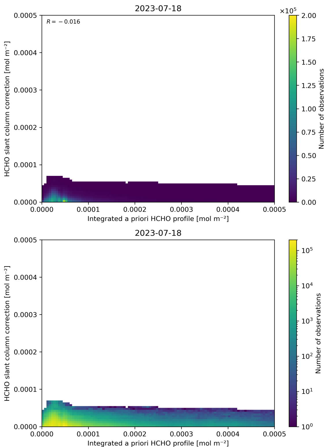
Figure 152: Scatter density plot of “Integrated a priori HCHO profile” against “HCHO slant column correction” for 2023-07-17 to 2023-07-19.
