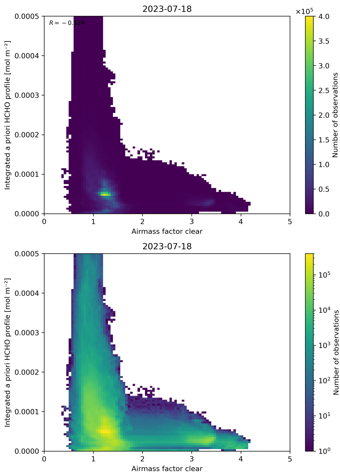
Figure 76: Scatter density plot of “Airmass factor clear” against “Integrated a priori HCHO profile” for 2023-07-17 to 2023-07-19.
