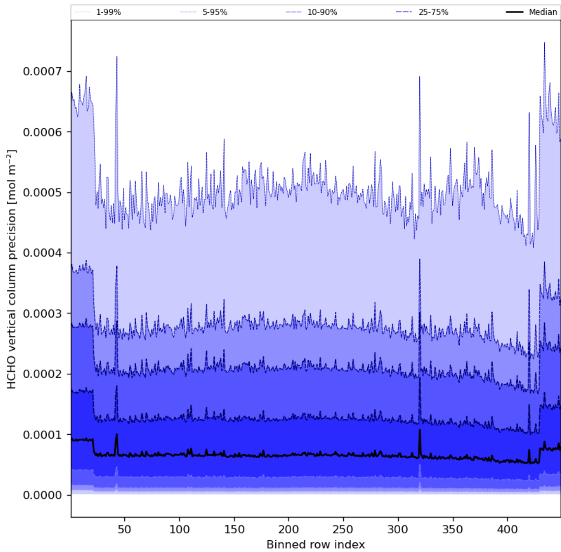
Figure 50: Along track statistics of “HCHO vertical column precision” for 2023-07-17 to 2023-07-19
