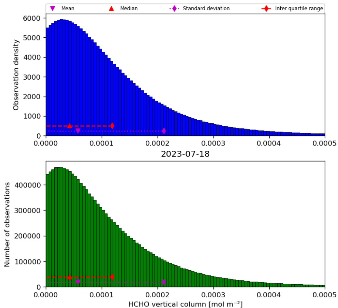
Figure 35: Histogram of “HCHO vertical column” for 2023-07-17 to 2023-07-19
