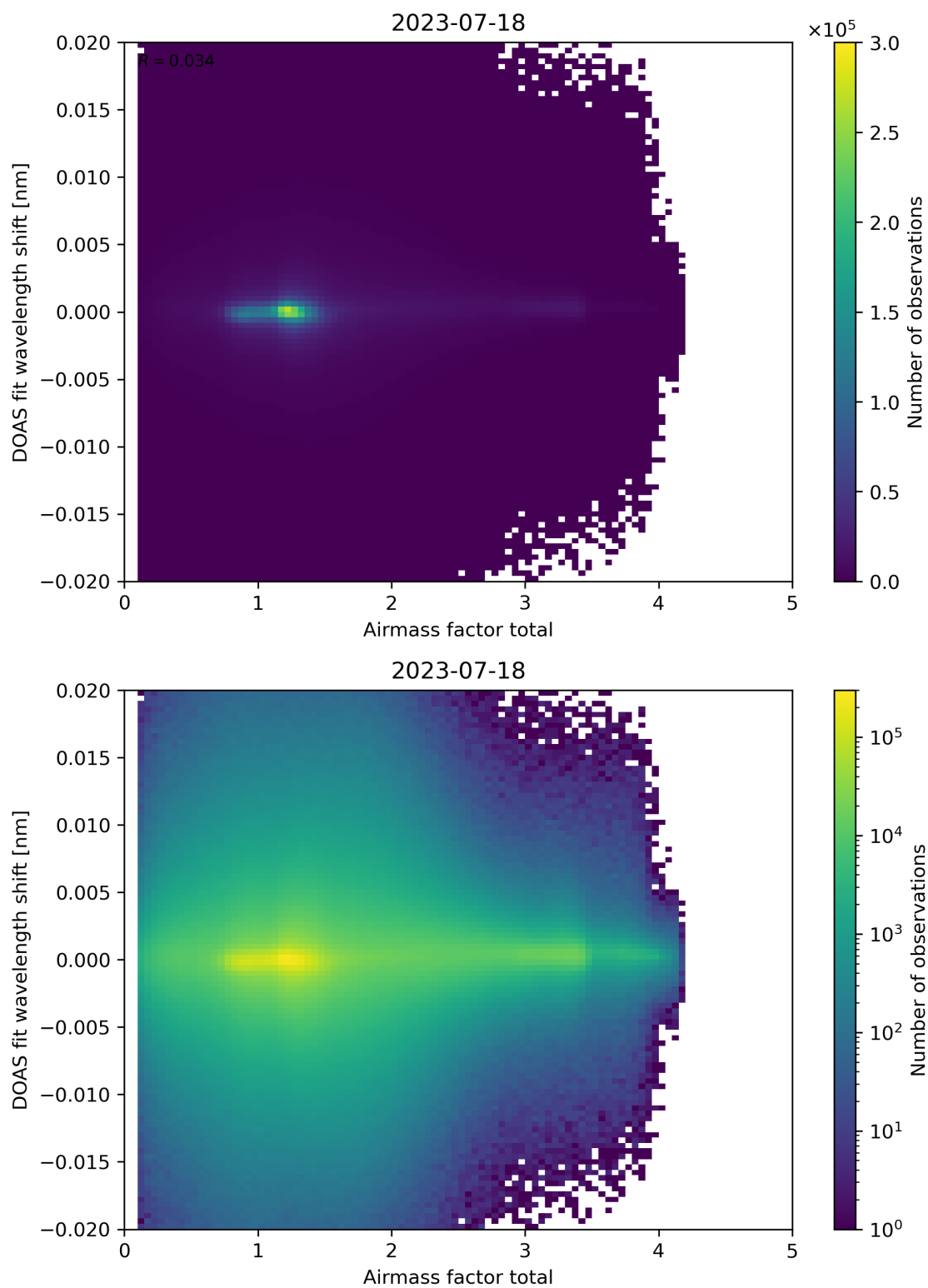
Figure 98: Scatter density plot of “Airmass factor total” against “DOAS fit wavelength shift” for 2023-07-17 to 2023-07-19.
