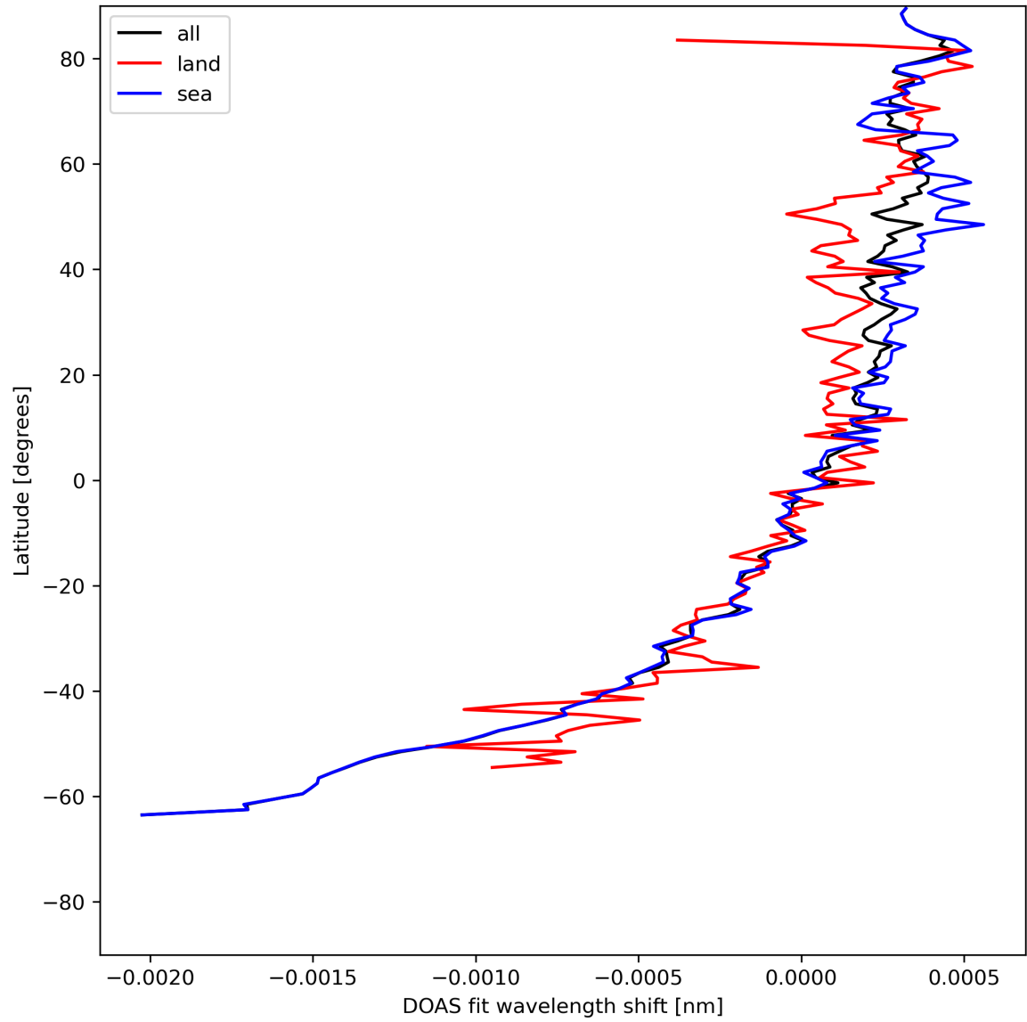
Figure 30: Zonal average of “DOAS fit wavelength shift” for 2023-07-17 to 2023-07-19.
