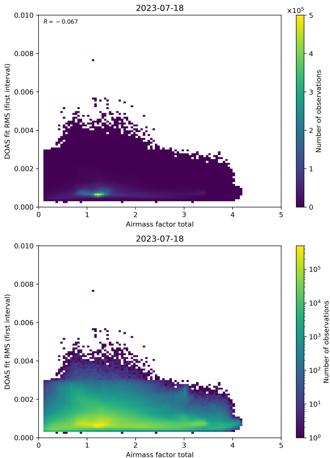
Figure 97: Scatter density plot of “Airmass factor total” against “DOAS fit RMS (first interval)” for 2023-07-17 to 2023-07-19.
