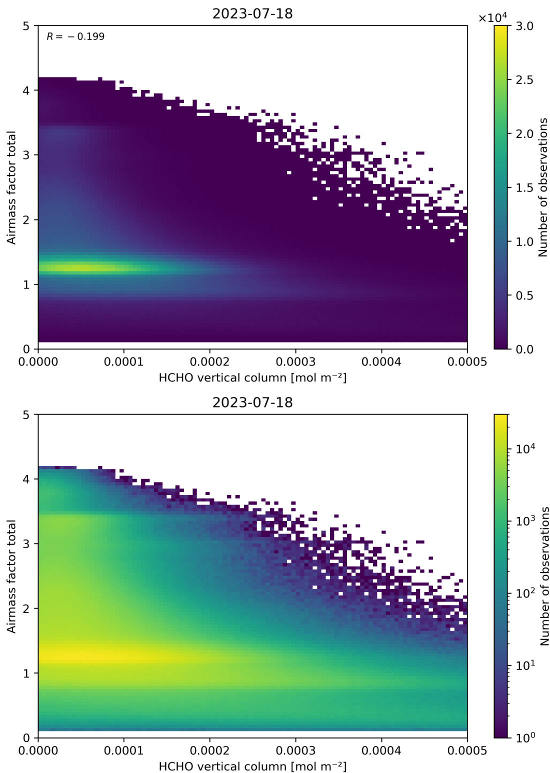
Figure 131: Scatter density plot of “HCHO vertical column” against “Airmass factor total” for 2023-07-17 to 2023-07-19.
