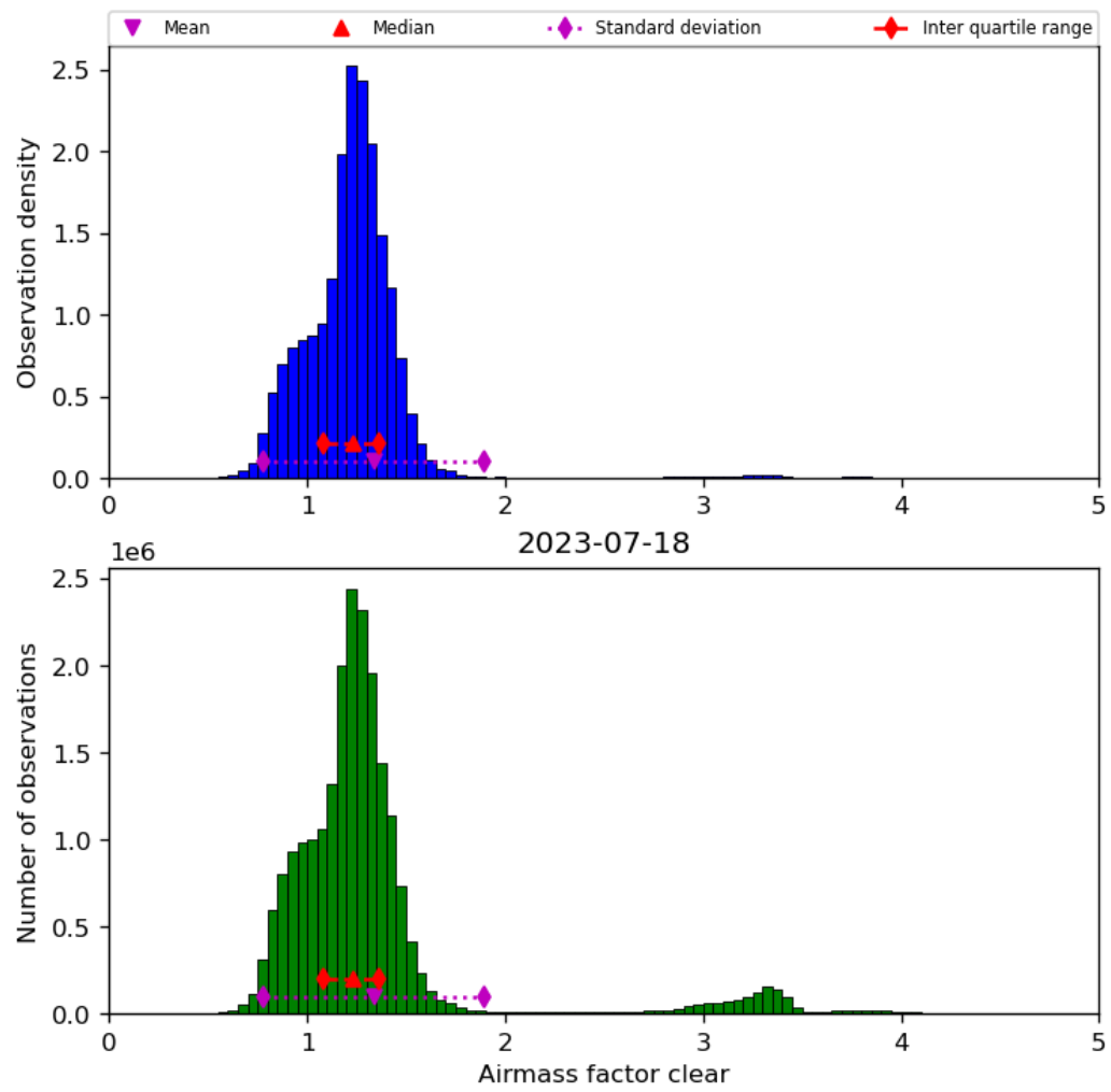
Figure 42: Histogram of “Airmass factor clear” for 2023-07-17 to 2023-07-19
