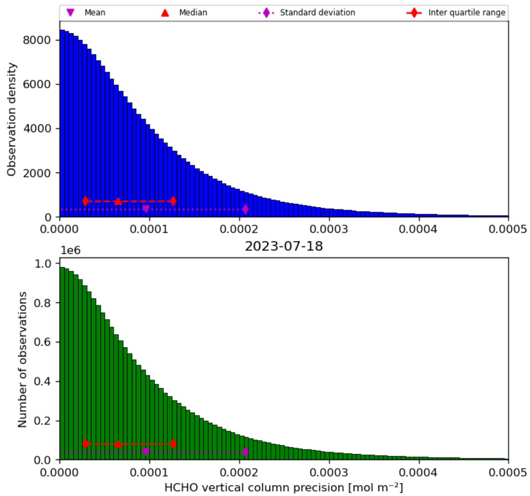
Figure 36: Histogram of “HCHO vertical column precision” for 2023-07-17 to 2023-07-19
