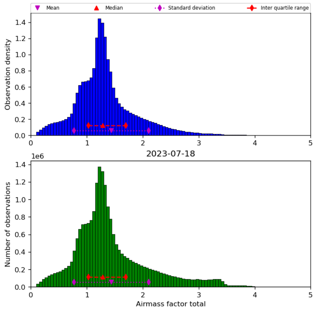
Figure 40: Histogram of “Airmass factor total” for 2023-07-17 to 2023-07-19
