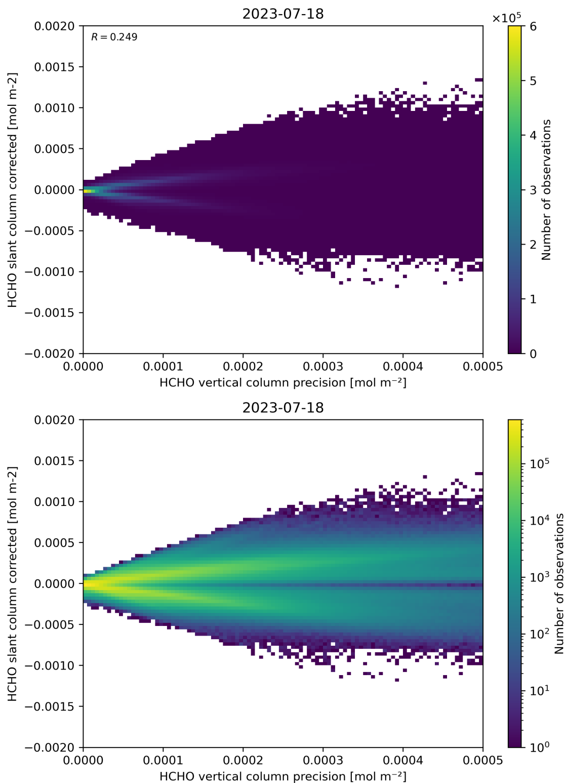
Figure 140: Scatter density plot of “HCHO vertical column precision” against “HCHO slant column corrected” for 2023-07-17 to 2023-07-19.
