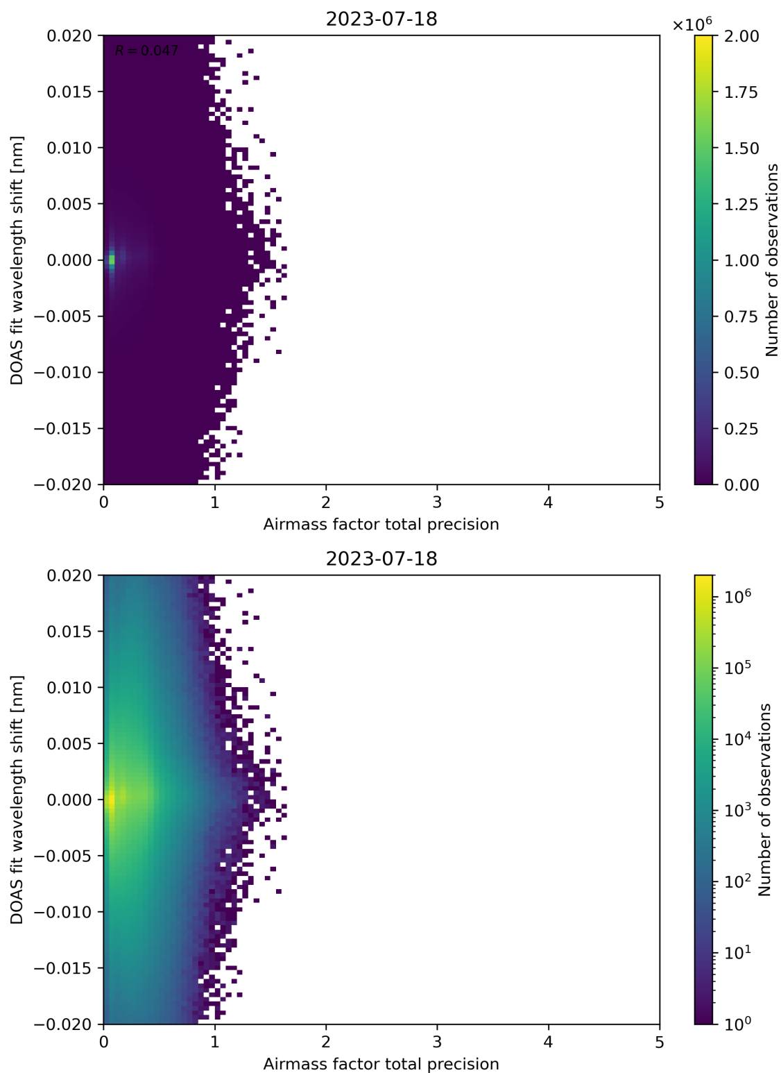
Figure 106: Scatter density plot of “Airmass factor total precision” against “DOAS fit wavelength shift” for 2023-07-17 to 2023-07-19.
