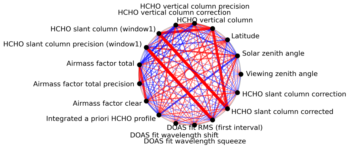
Figure 1: Map of correlation graph for 2023-07-17 to 2023-07-19.
