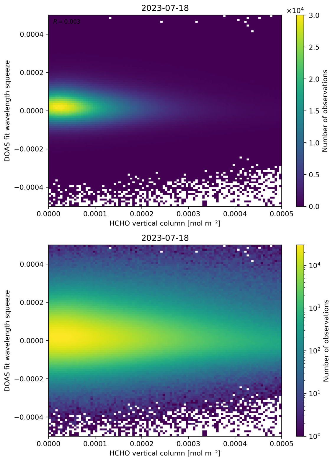
Figure 125: Scatter density plot of “HCHO vertical column” against “DOAS fit wavelength squeeze” for 2023-07-17 to 2023-07-19.
