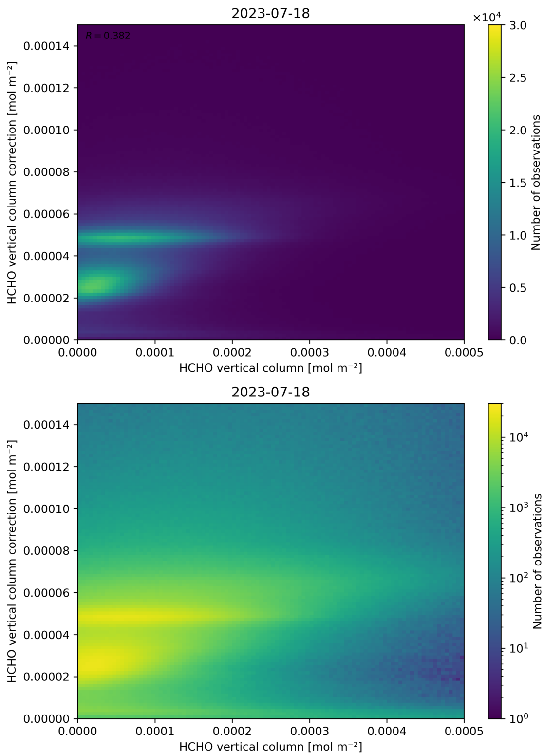
Figure 133: Scatter density plot of “HCHO vertical column” against “HCHO vertical column correction” for 2023-07-17 to 2023-07-19.
