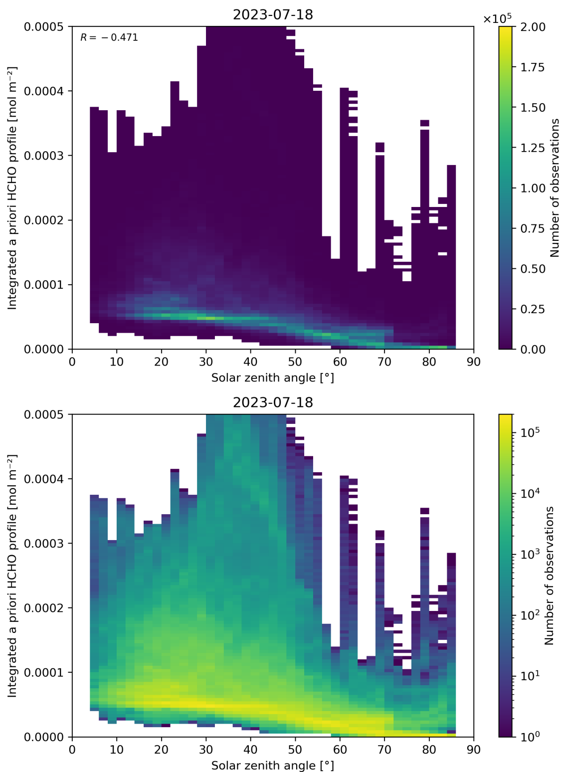
Figure 180: Scatter density plot of “Solar zenith angle” against “Integrated a priori HCHO profile” for 2023-07-17 to 2023-07-19.
