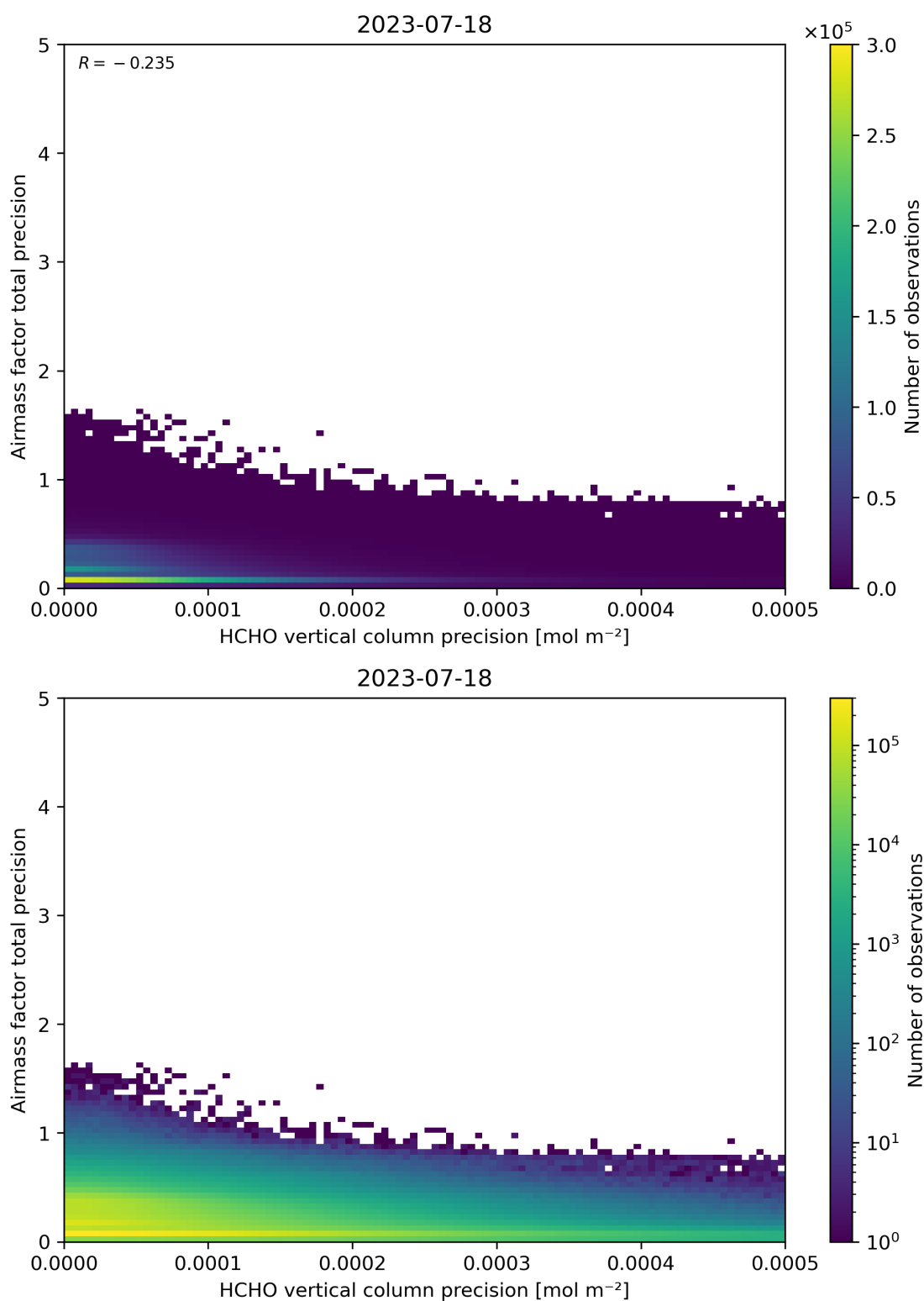
Figure 145: Scatter density plot of “HCHO vertical column precision” against “Airmass factor total precision” for 2023-07-17 to 2023-07-19.
