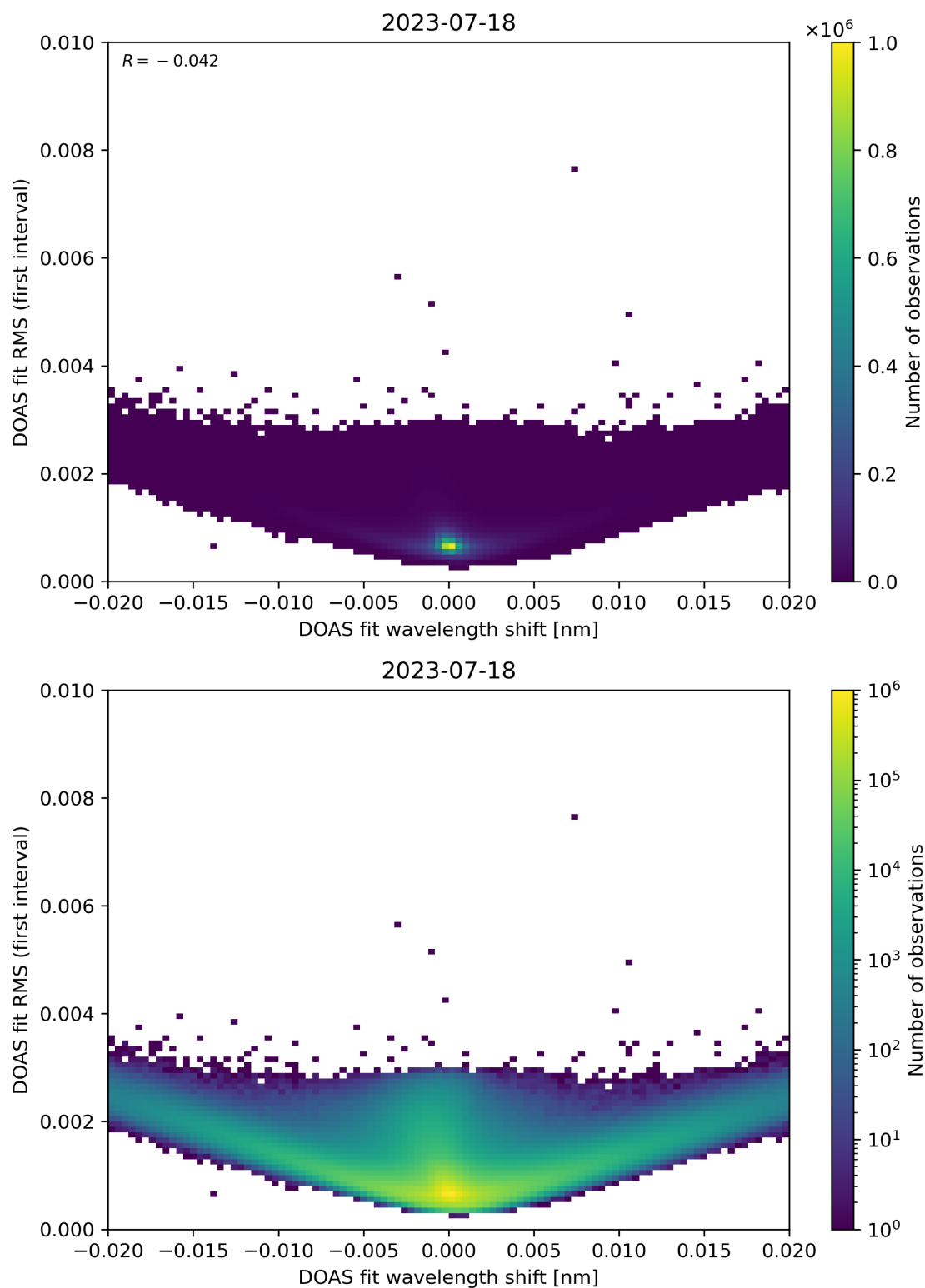
Figure 64: Scatter density plot of “DOAS fit wavelength shift” against “DOAS fit RMS (first interval)” for 2023-07-17 to 2023-07-19.
