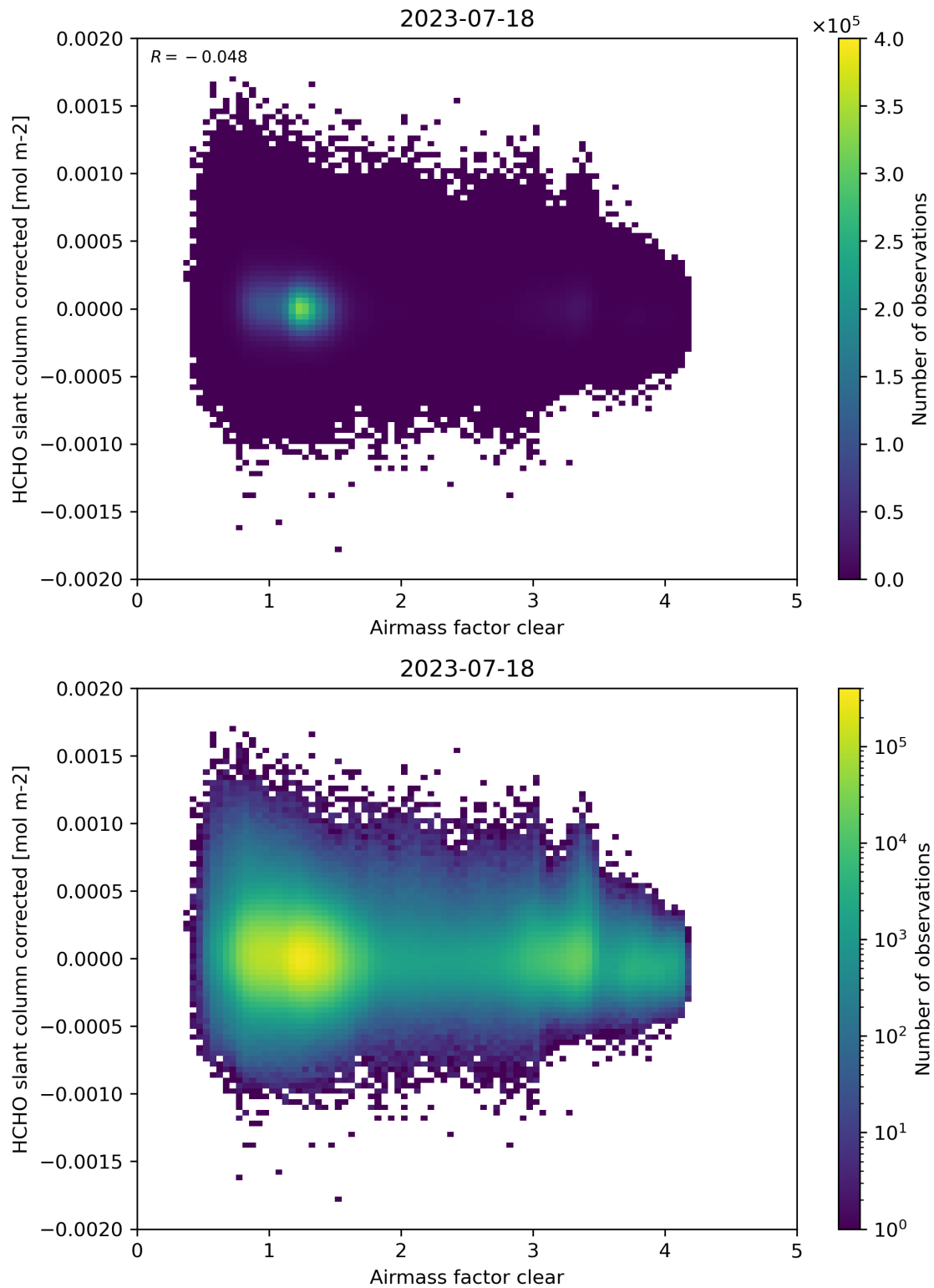
Figure 74: Scatter density plot of “Airmass factor clear” against “HCHO slant column corrected” for 2023-07-17 to 2023-07-19.
