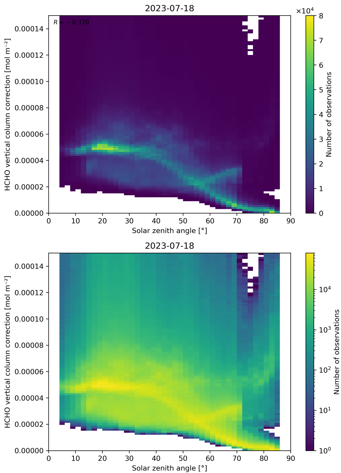
Figure 178: Scatter density plot of “Solar zenith angle” against “HCHO vertical column correction” for 2023-07-17 to 2023-07-19.
