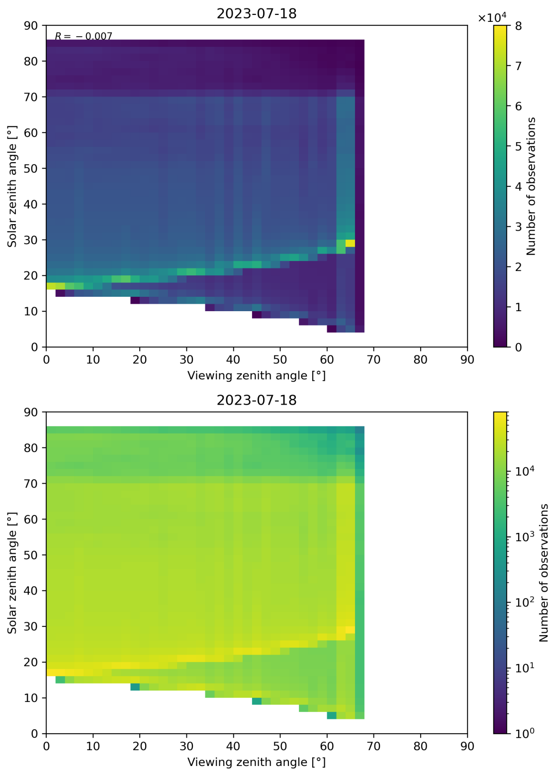
Figure 197: Scatter density plot of “Viewing zenith angle” against “Solar zenith angle” for 2023-07-17 to 2023-07-19.
