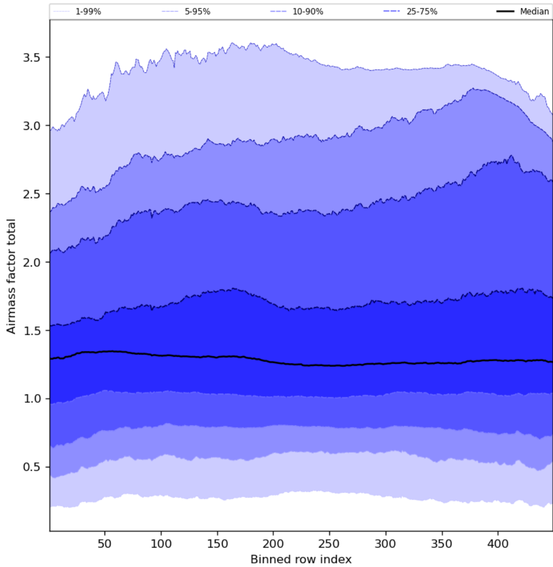
Figure 54: Along track statistics of “Airmass factor total” for 2023-07-17 to 2023-07-19
