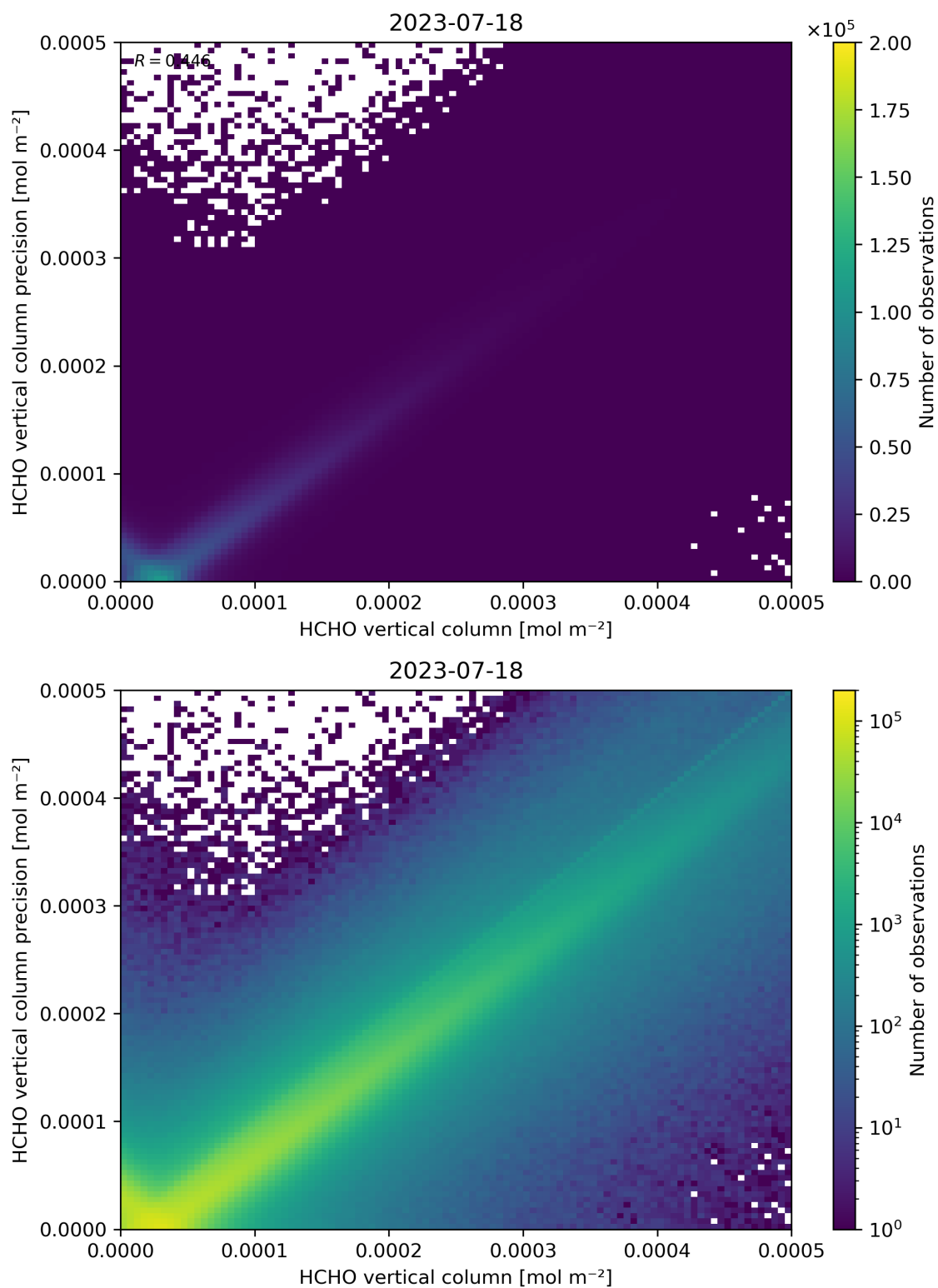
Figure 134: Scatter density plot of “HCHO vertical column” against “HCHO vertical column precision” for 2023-07-17 to 2023-07-19.
