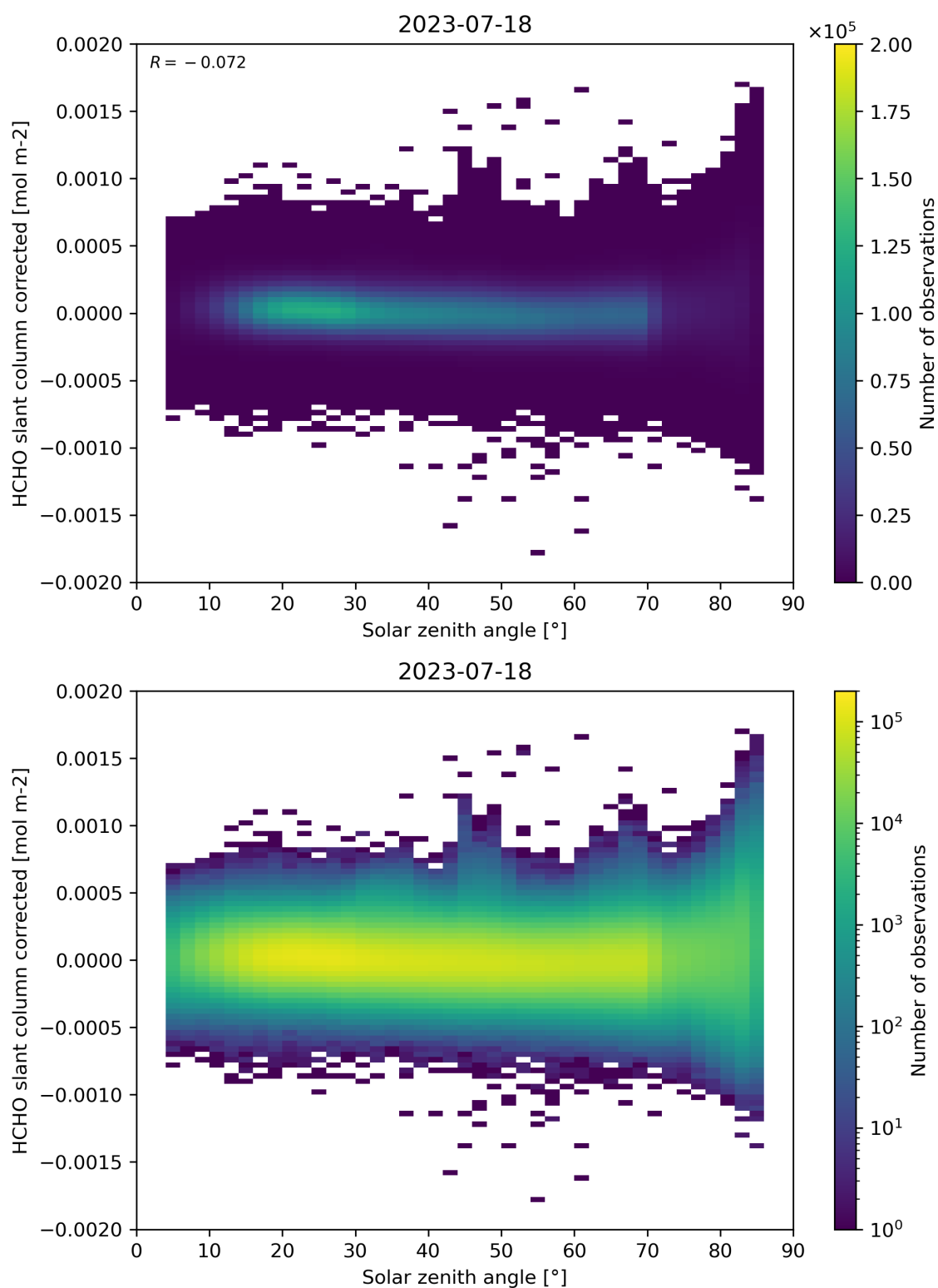
Figure 171: Scatter density plot of “Solar zenith angle” against “HCHO slant column corrected” for 2023-07-17 to 2023-07-19.
