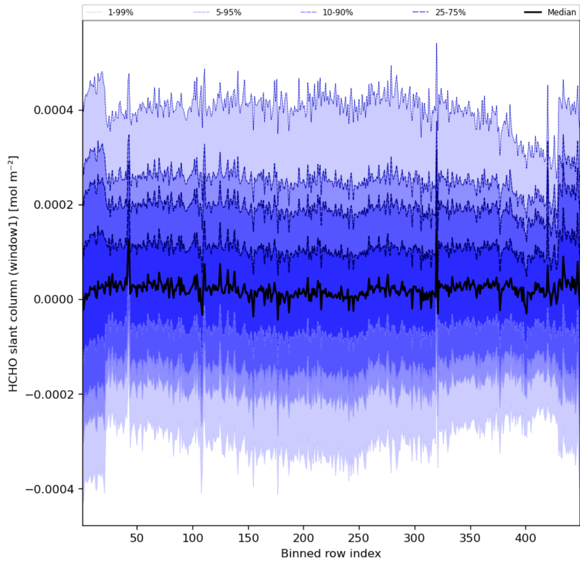
Figure 52: Along track statistics of “HCHO slant column (window1)” for 2023-07-17 to 2023-07-19
