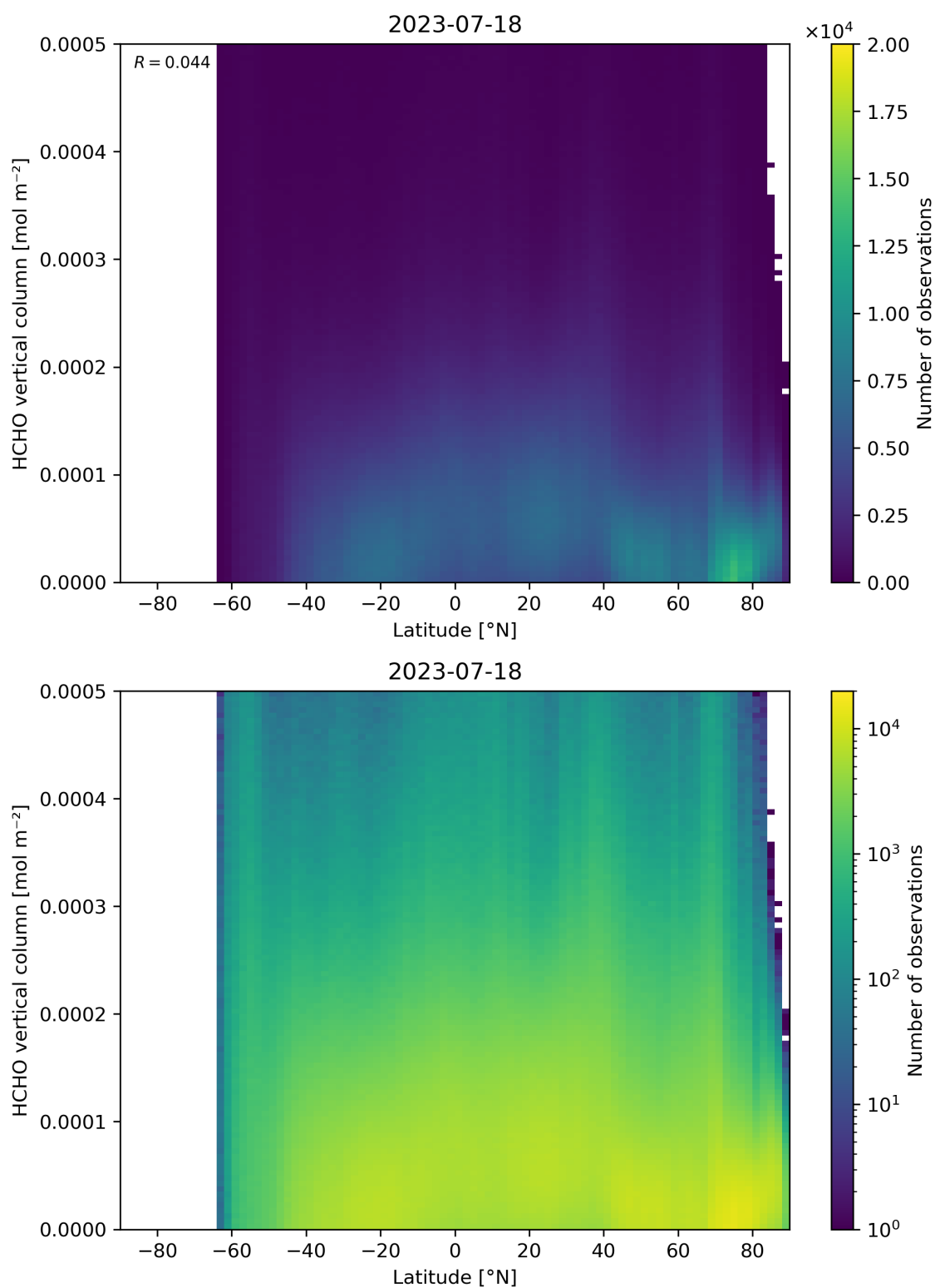
Figure 163: Scatter density plot of “Latitude” against “HCHO vertical column” for 2023-07-17 to 2023-07-19.
