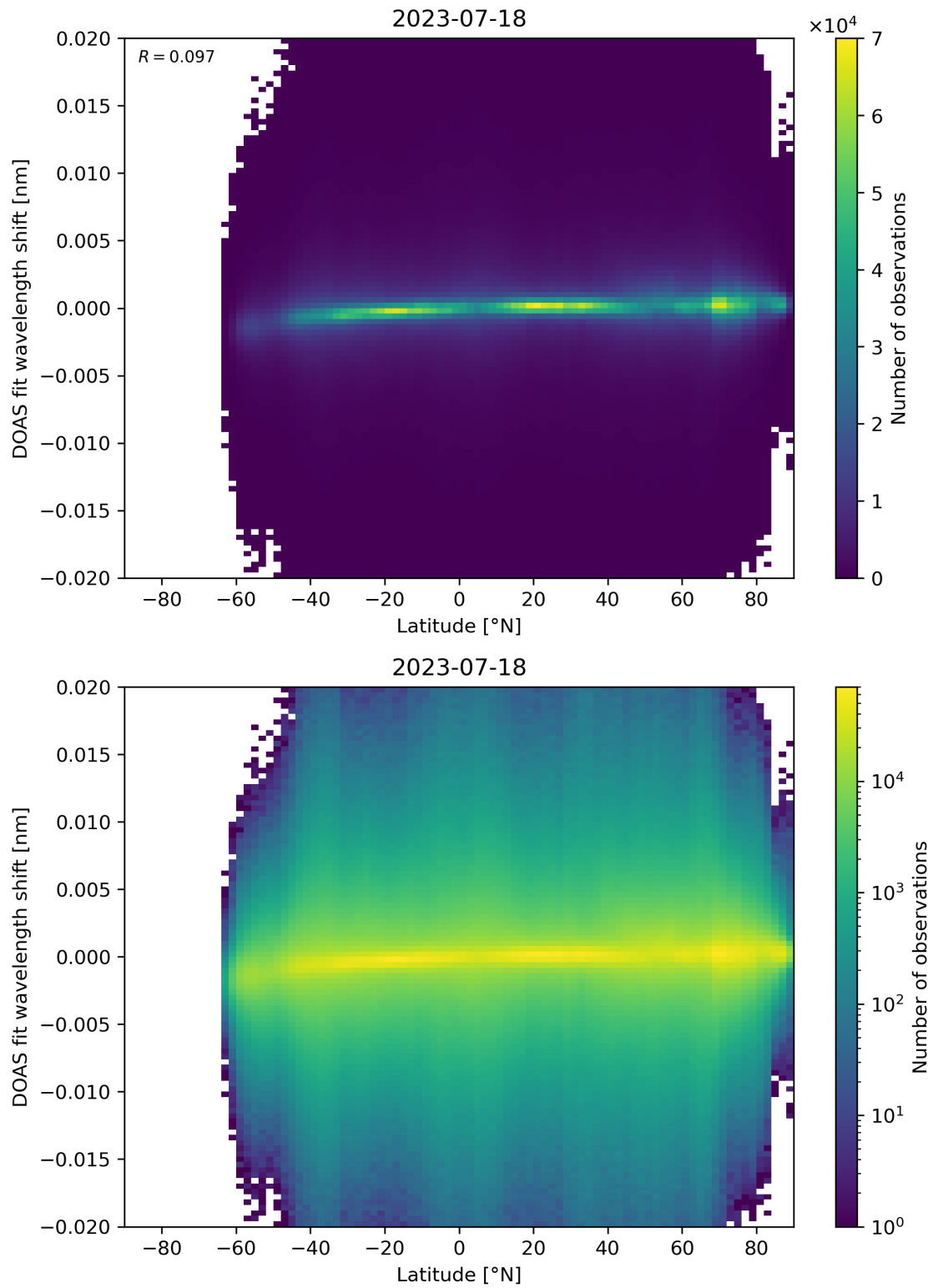
Figure 154: Scatter density plot of “Latitude” against “DOAS fit wavelength shift” for 2023-07-17 to 2023-07-19.
