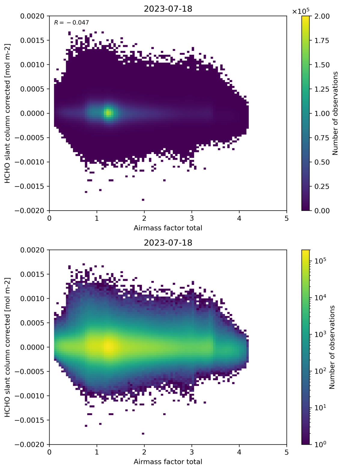
Figure 101: Scatter density plot of “Airmass factor total” against “HCHO slant column corrected” for 2023-07-17 to 2023-07-19.
