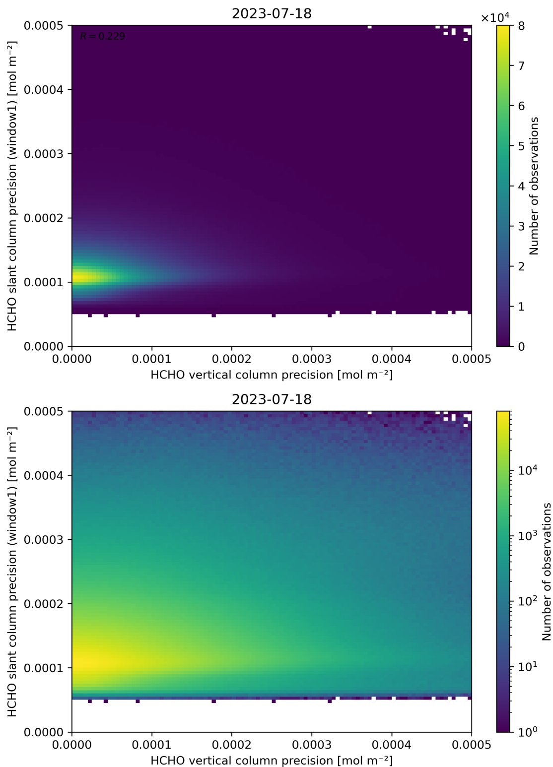
Figure 143: Scatter density plot of “HCHO vertical column precision” against “HCHO slant column precision (window1)” for 2023-07-17 to 2023-07-19.
