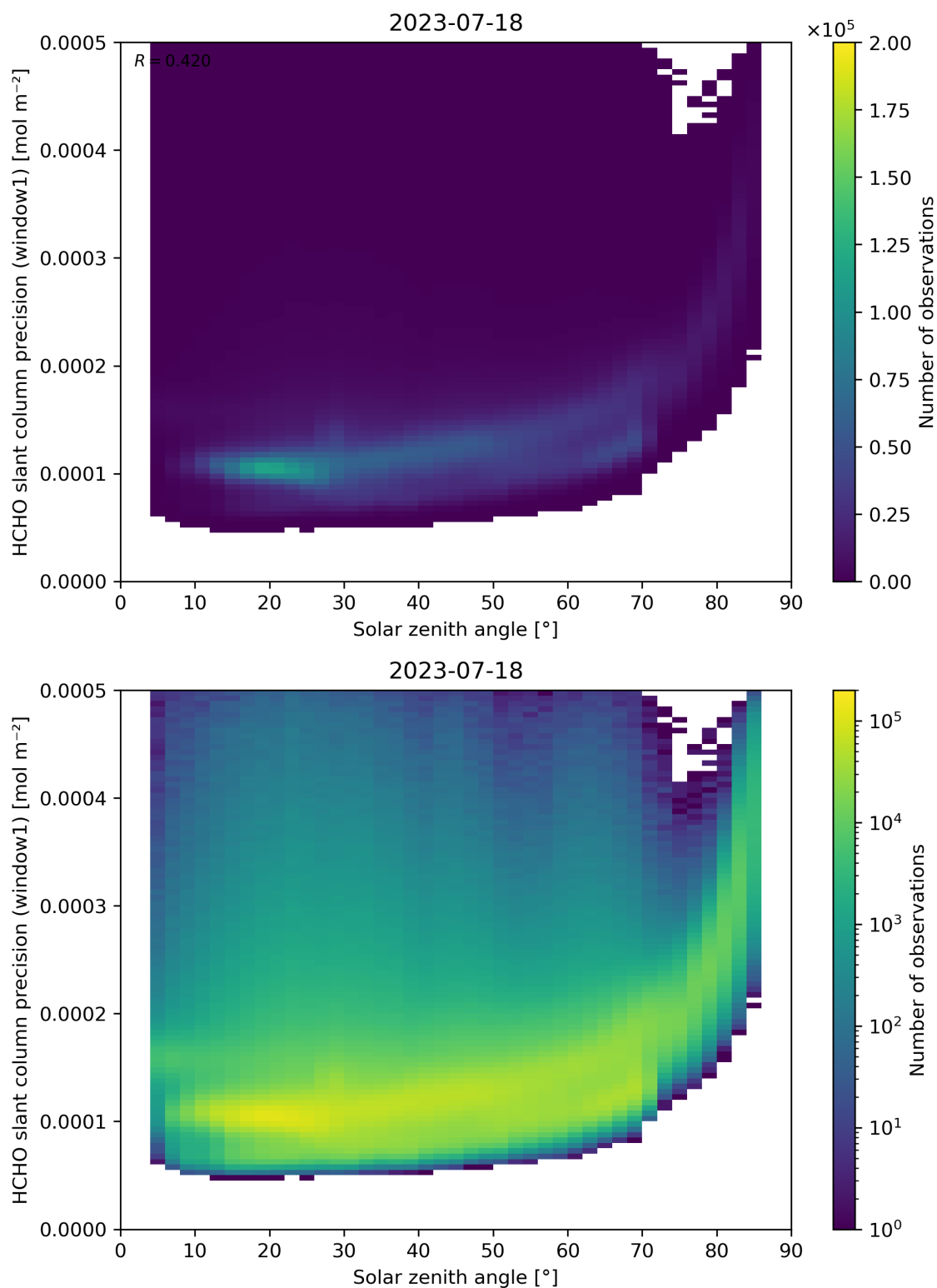
Figure 174: Scatter density plot of “Solar zenith angle” against “HCHO slant column precision (window1)” for 2023-07-17 to 2023-07-19.
