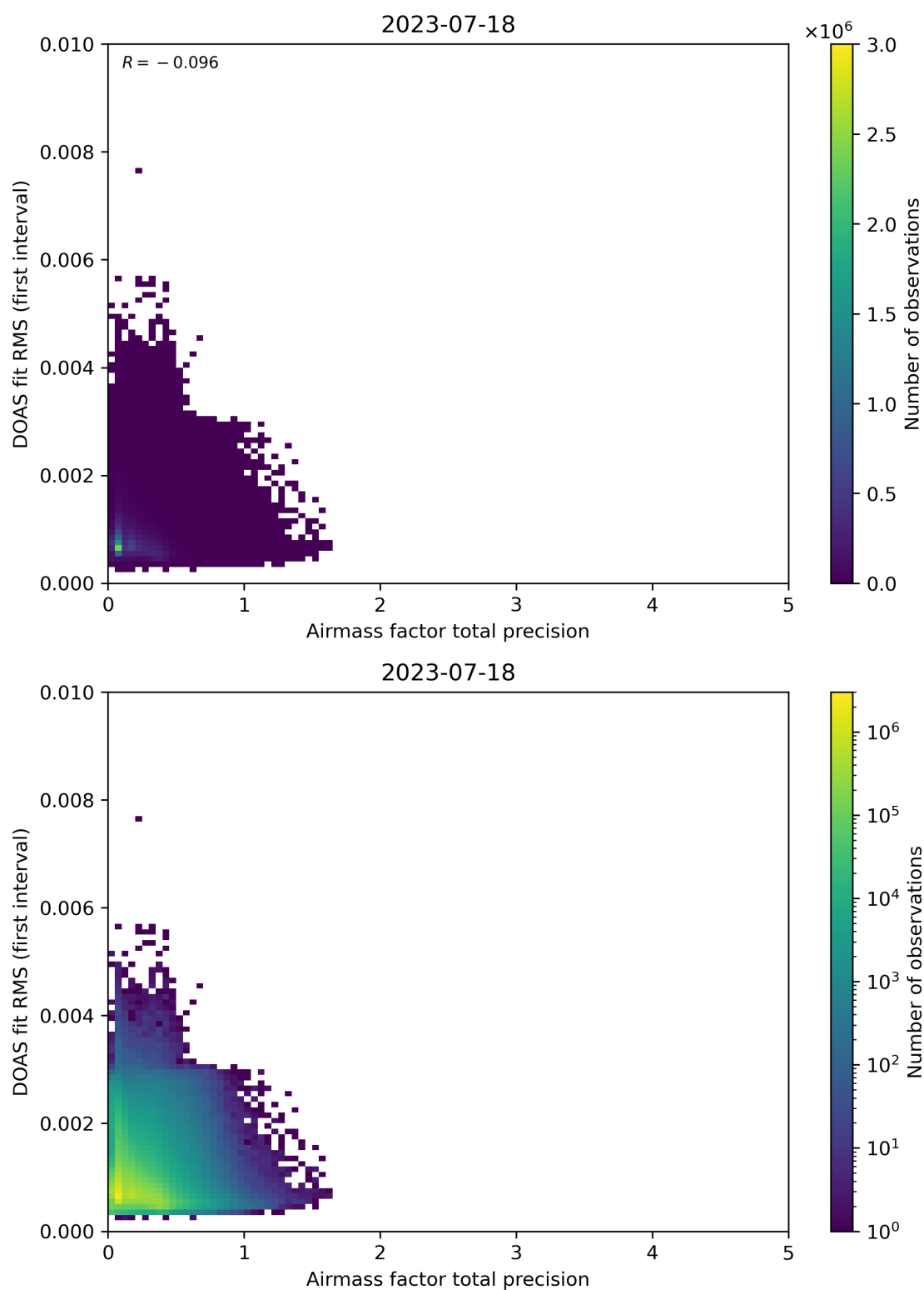
Figure 105: Scatter density plot of “Airmass factor total precision” against “DOAS fit RMS (first interval)” for 2023-07-17 to 2023-07-19.
