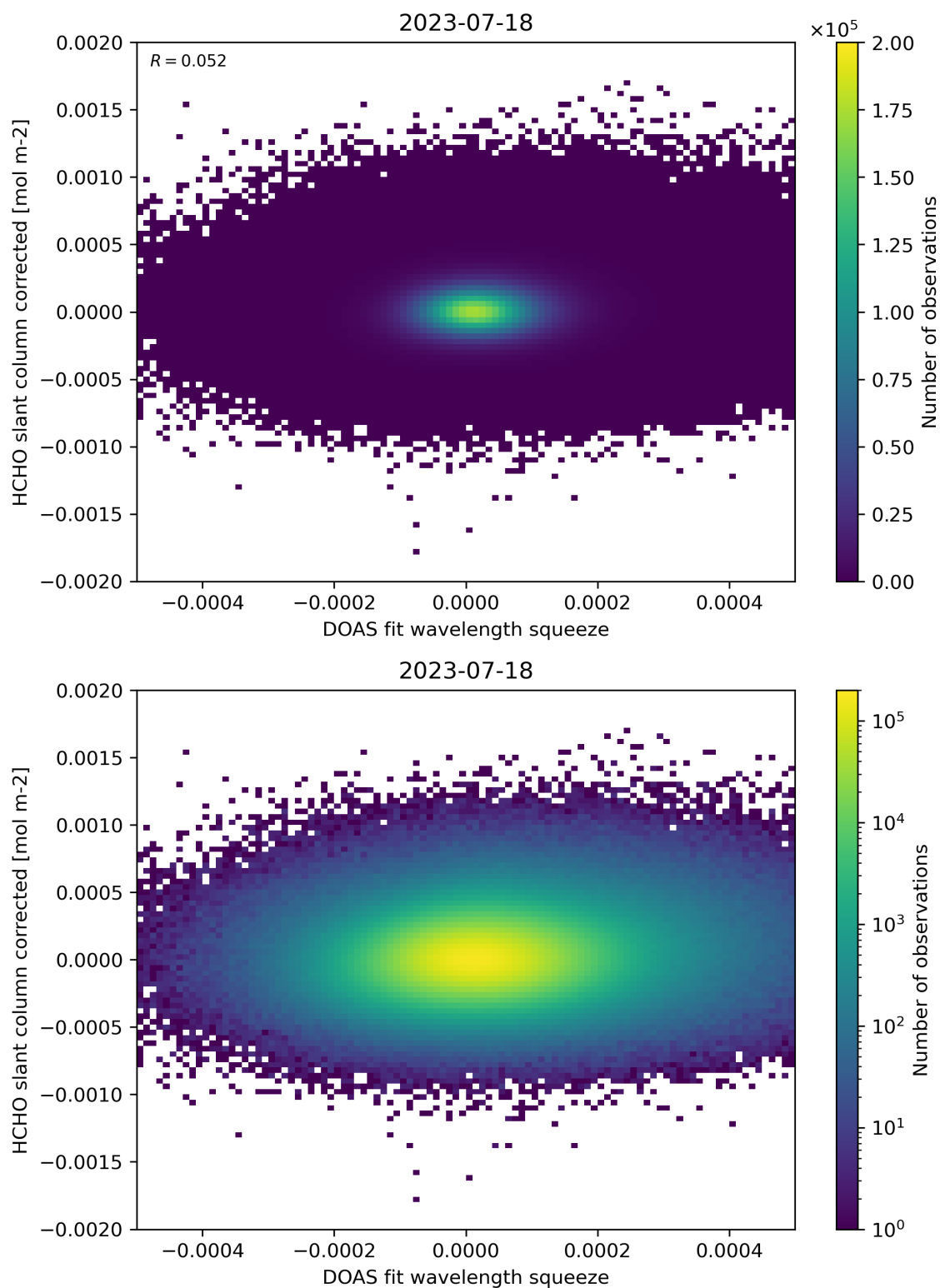
Figure 69: Scatter density plot of “DOAS fit wavelength squeeze” against “HCHO slant column corrected” for 2023-07-17 to 2023-07-19.
