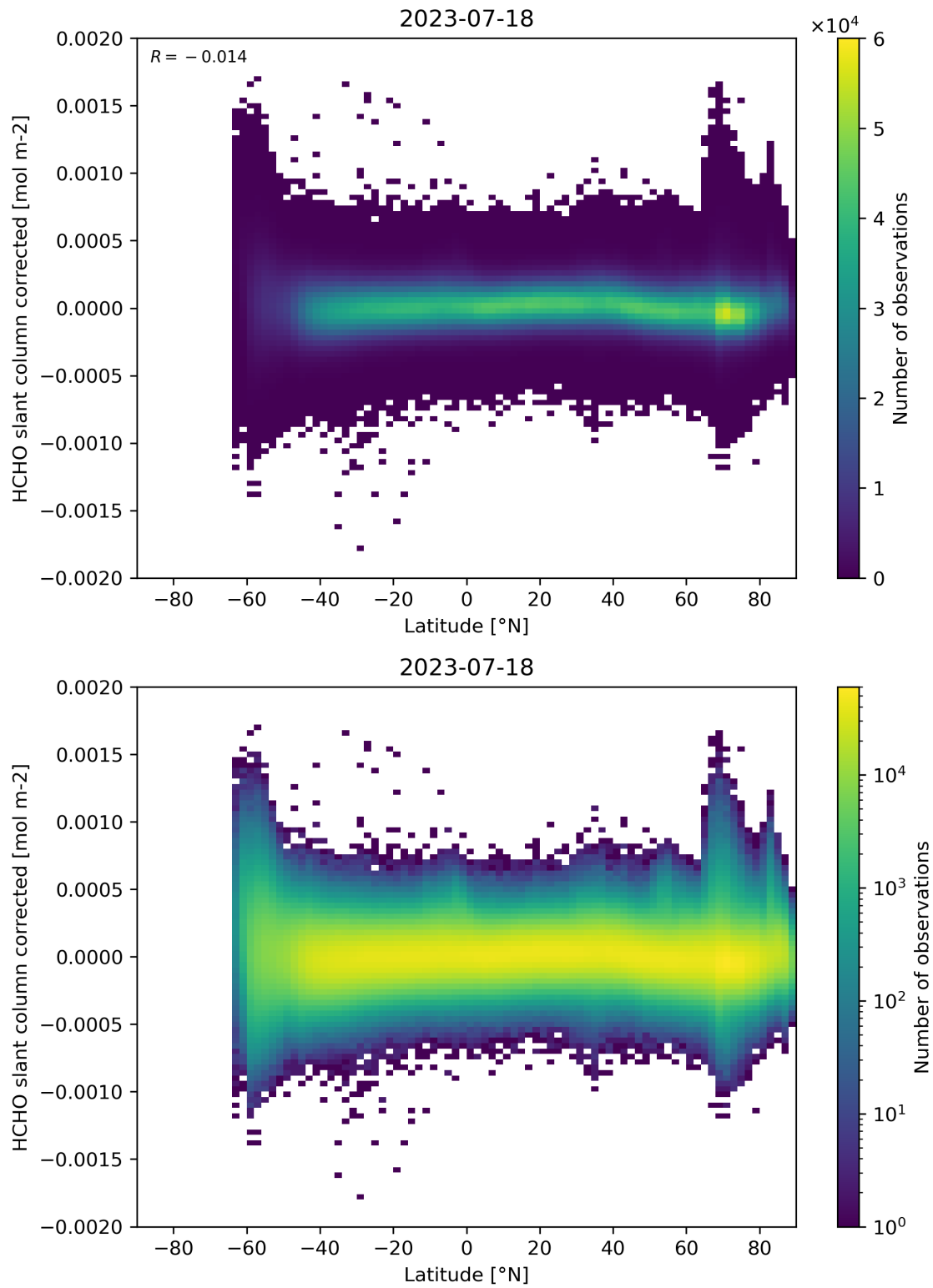
Figure 157: Scatter density plot of “Latitude” against “HCHO slant column corrected” for 2023-07-17 to 2023-07-19.
