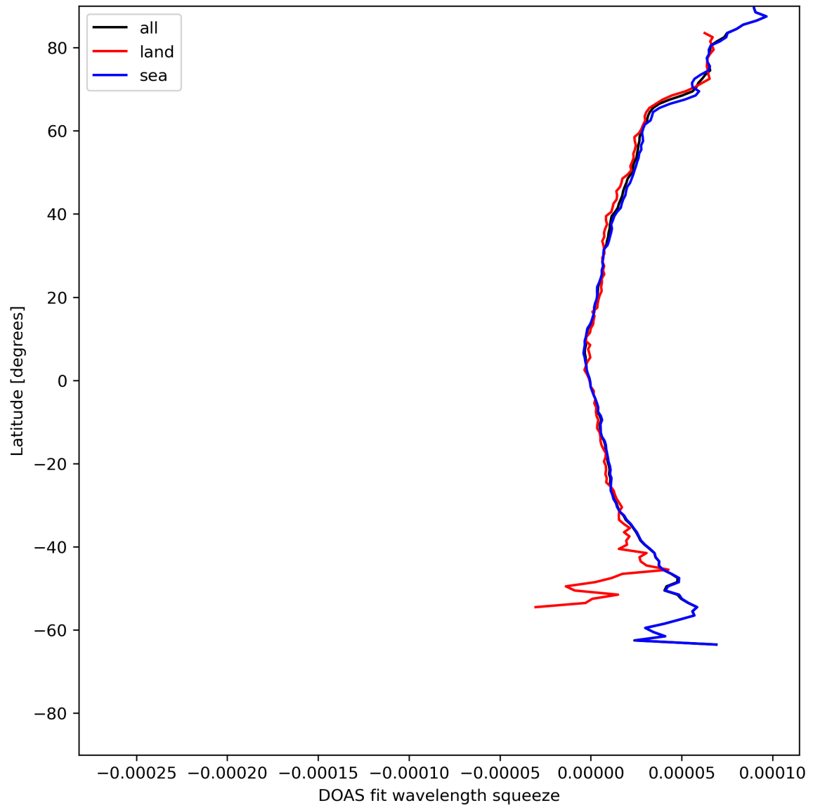
Figure 31: Zonal average of “DOAS fit wavelength squeeze” for 2023-07-17 to 2023-07-19.
