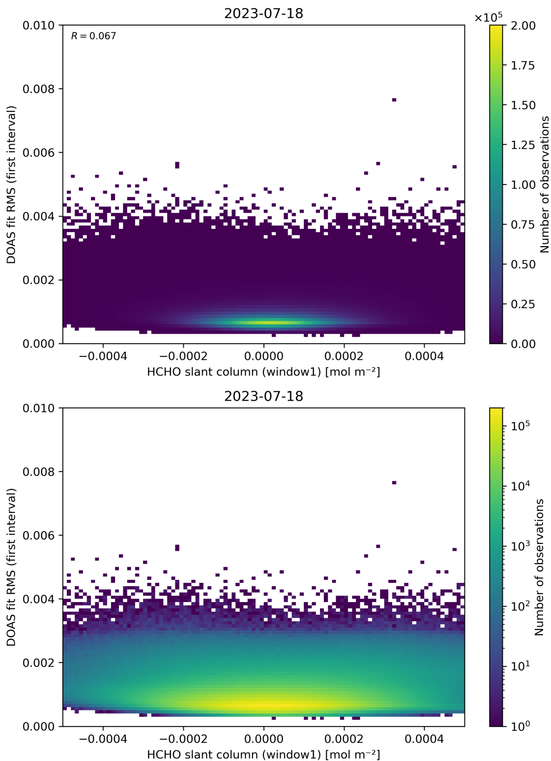
Figure 78: Scatter density plot of “HCHO slant column (window1)” against “DOAS fit RMS (first interval)” for 2023-07-17 to 2023-07-19.
