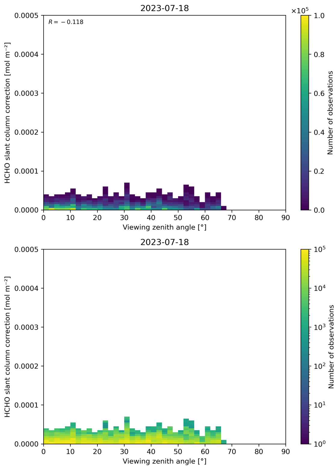
Figure 187: Scatter density plot of “Viewing zenith angle” against “HCHO slant column correction” for 2023-07-17 to 2023-07-19.
