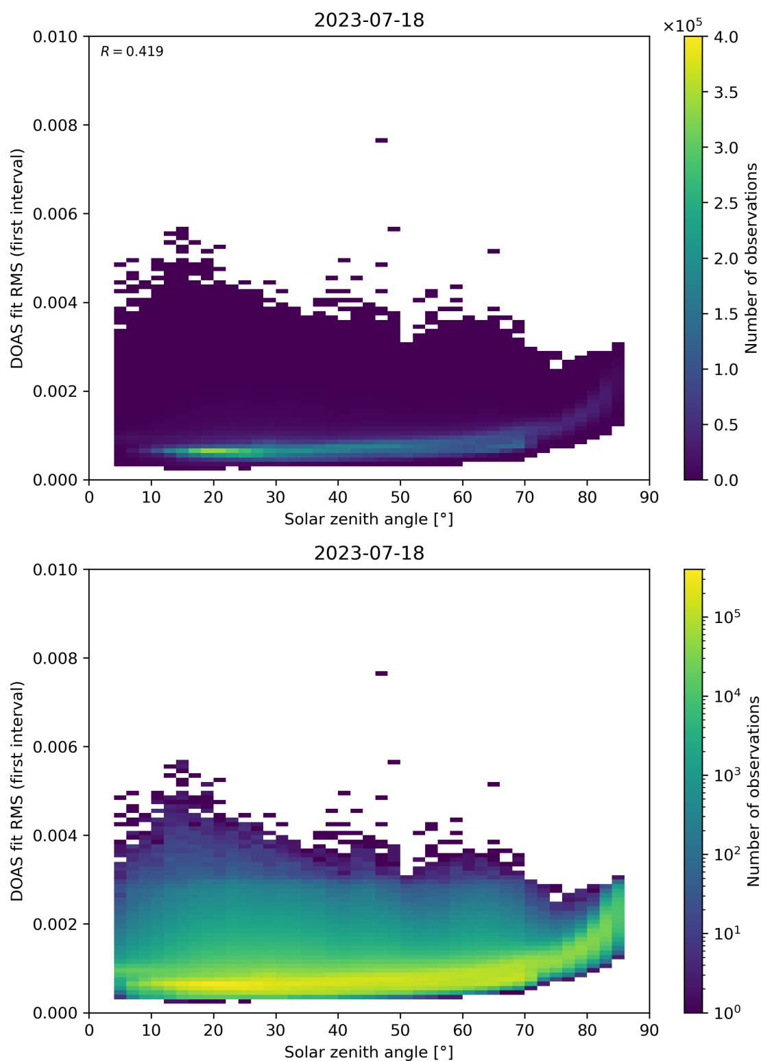
Figure 167: Scatter density plot of “Solar zenith angle” against “DOAS fit RMS (first interval)” for 2023-07-17 to 2023-07-19.
