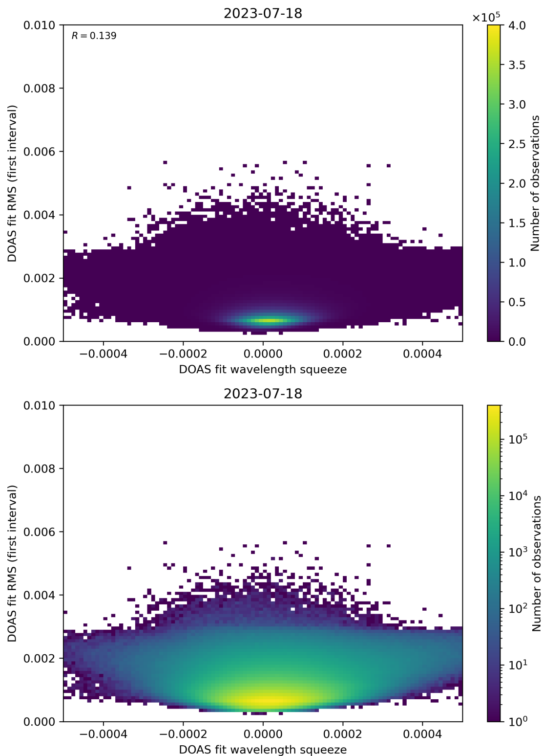
Figure 68: Scatter density plot of “DOAS fit wavelength squeeze” against “DOAS fit RMS (first interval)” for 2023-07-17 to 2023-07-19.
