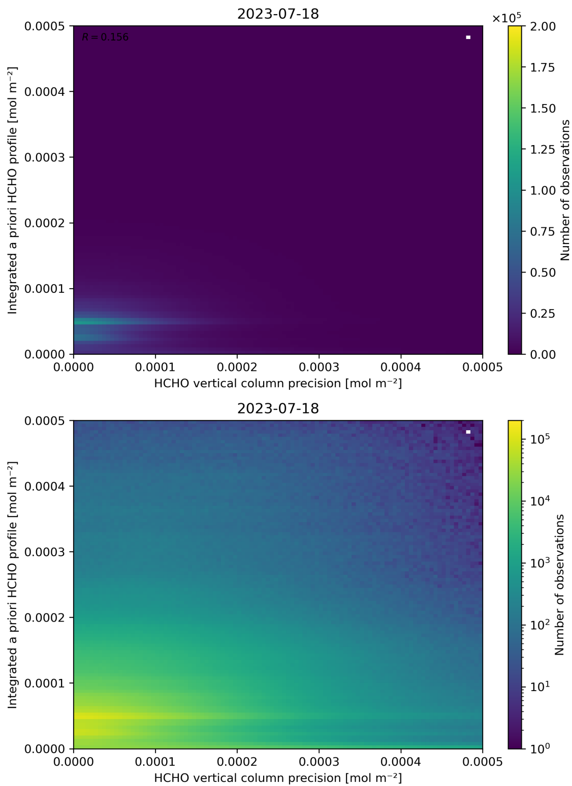
Figure 147: Scatter density plot of “HCHO vertical column precision” against “Integrated a priori HCHO profile” for 2023-07-17 to 2023-07-19.
