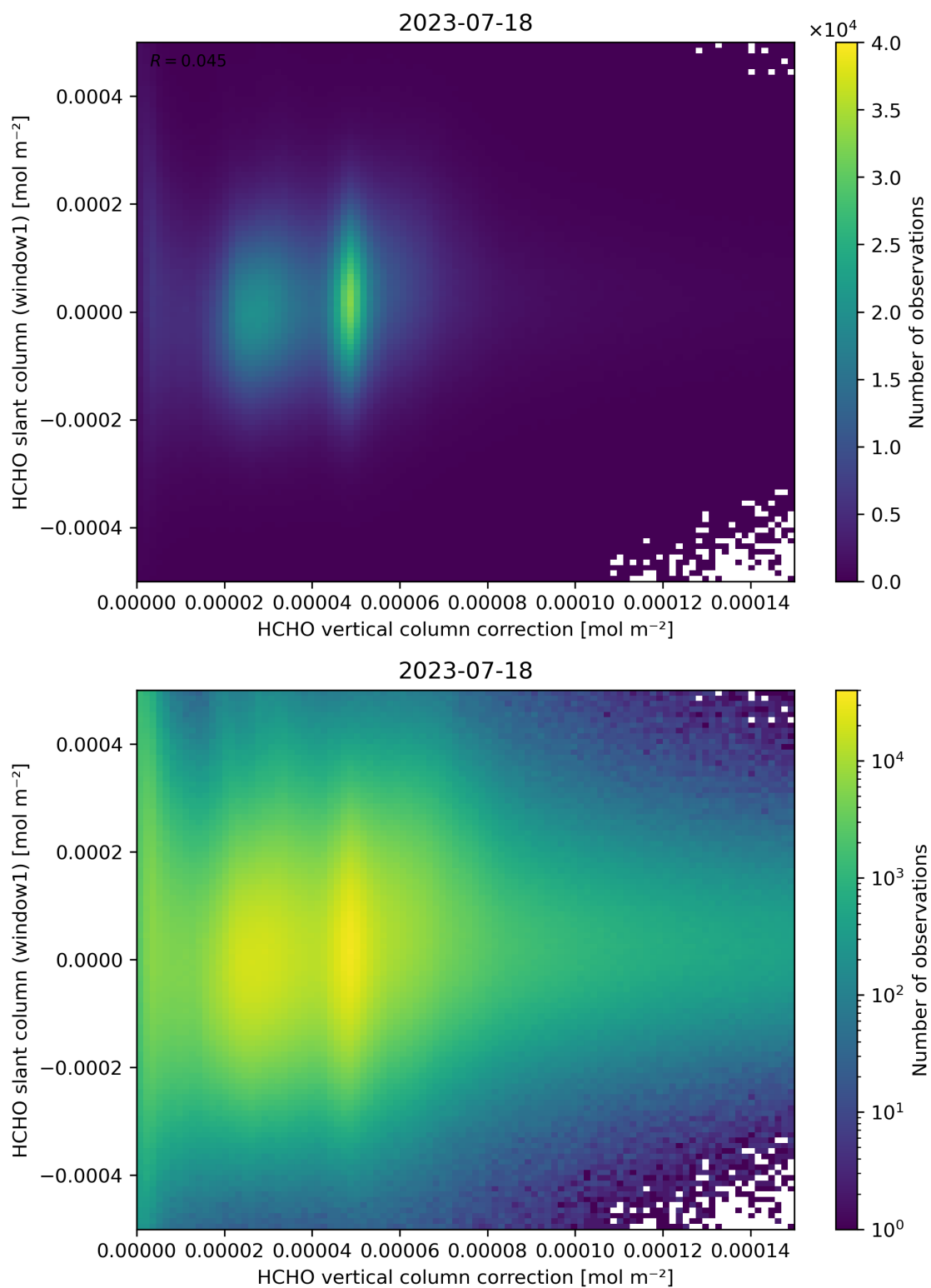
Figure 118: Scatter density plot of “HCHO vertical column correction” against “HCHO slant column (window1)” for 2023-07-17 to 2023-07-19.
