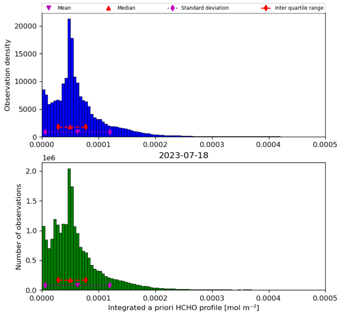
Figure 43: Histogram of “Integrated a priori HCHO profile” for 2023-07-17 to 2023-07-19
