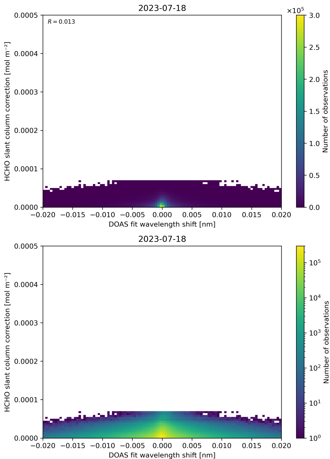
Figure 67: Scatter density plot of “DOAS fit wavelength shift” against “HCHO slant column correction” for 2023-07-17 to 2023-07-19.
