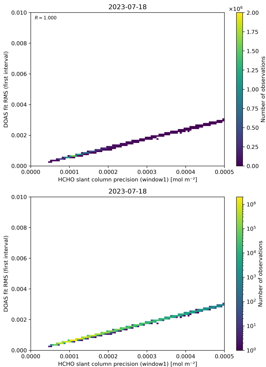
Figure 88: Scatter density plot of “HCHO slant column precision (window1)” against “DOAS fit RMS (first interval)” for 2023-07-17 to 2023-07-19.
