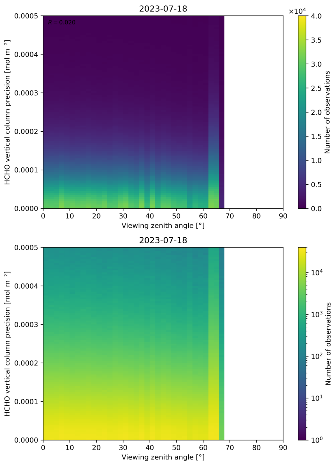
Figure 194: Scatter density plot of “Viewing zenith angle” against “HCHO vertical column precision” for 2023-07-17 to 2023-07-19.
