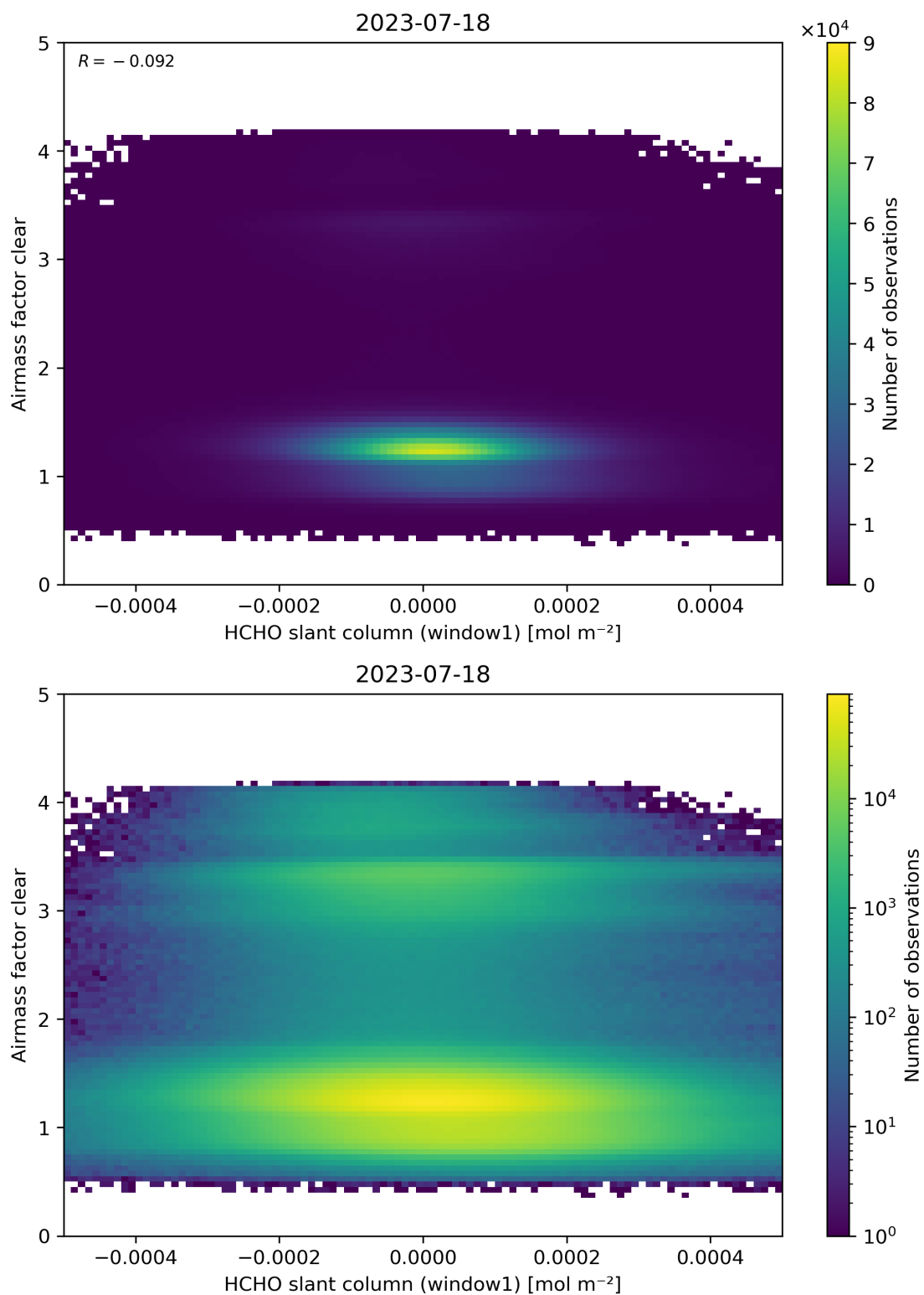
Figure 81: Scatter density plot of “HCHO slant column (window1)” against “Airmass factor clear” for 2023-07-17 to 2023-07-19.
