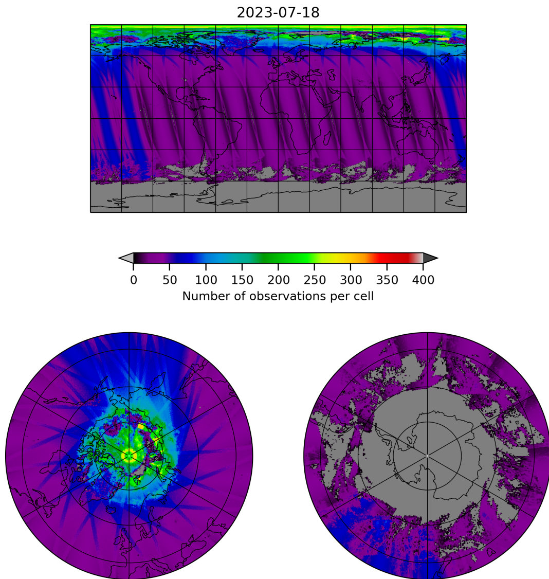
Figure 19: Map of the number of observations for 2023-07-17 to 2023-07-19
