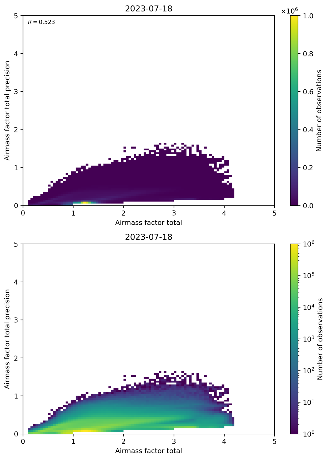
Figure 103: Scatter density plot of “Airmass factor total” against “Airmass factor total precision” for 2023-07-17 to 2023-07-19.
