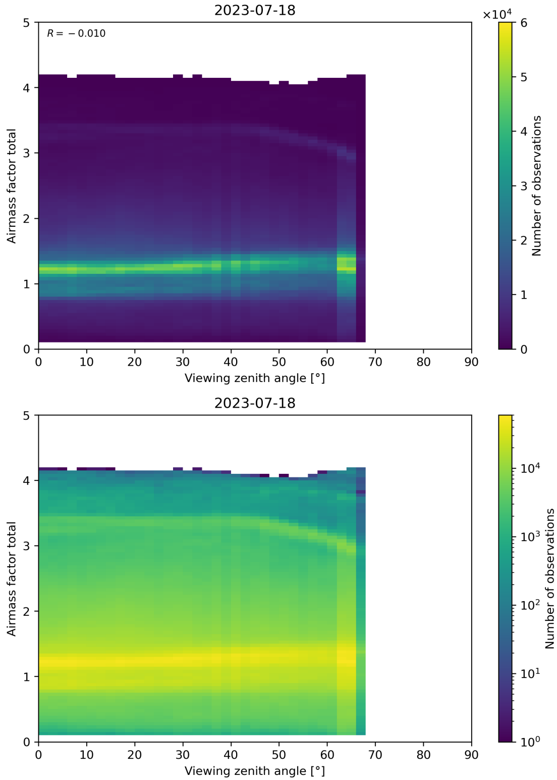
Figure 190: Scatter density plot of “Viewing zenith angle” against “Airmass factor total” for 2023-07-17 to 2023-07-19.
