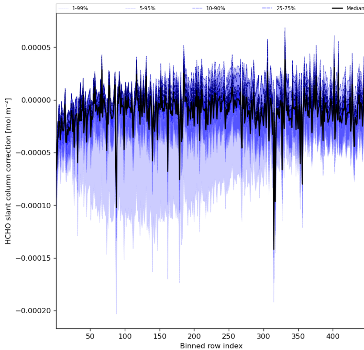
Figure 61: Along track statistics of “HCHO slant column correction” for 2023-07-17 to 2023-07-19
