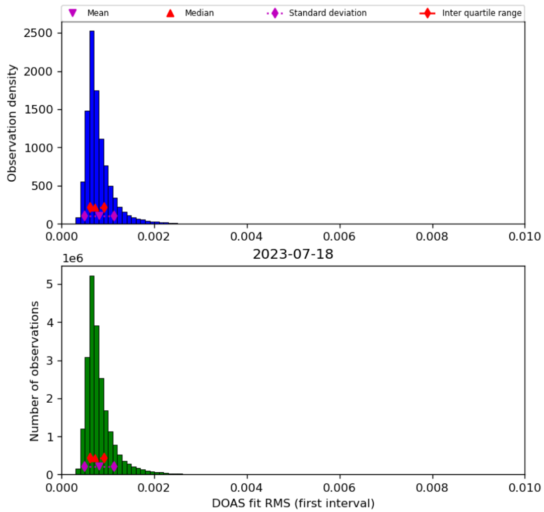
Figure 46: Histogram of “DOAS fit RMS (first interval)” for 2023-07-17 to 2023-07-19
