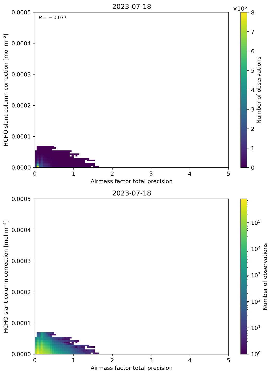
Figure 110: Scatter density plot of “Airmass factor total precision” against “HCHO slant column correction” for 2023-07-17 to 2023-07-19.
