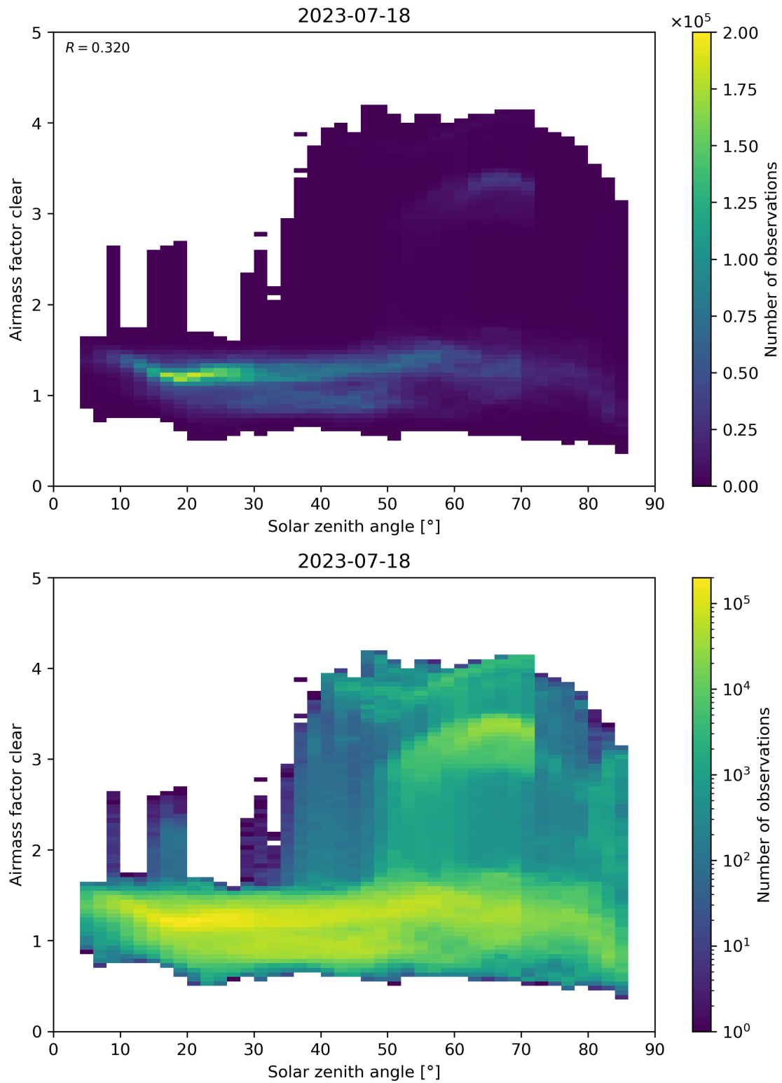
Figure 170: Scatter density plot of “Solar zenith angle” against “Airmass factor clear” for 2023-07-17 to 2023-07-19.
