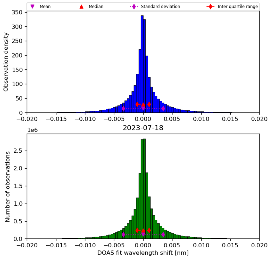
Figure 44: Histogram of “DOAS fit wavelength shift” for 2023-07-17 to 2023-07-19
