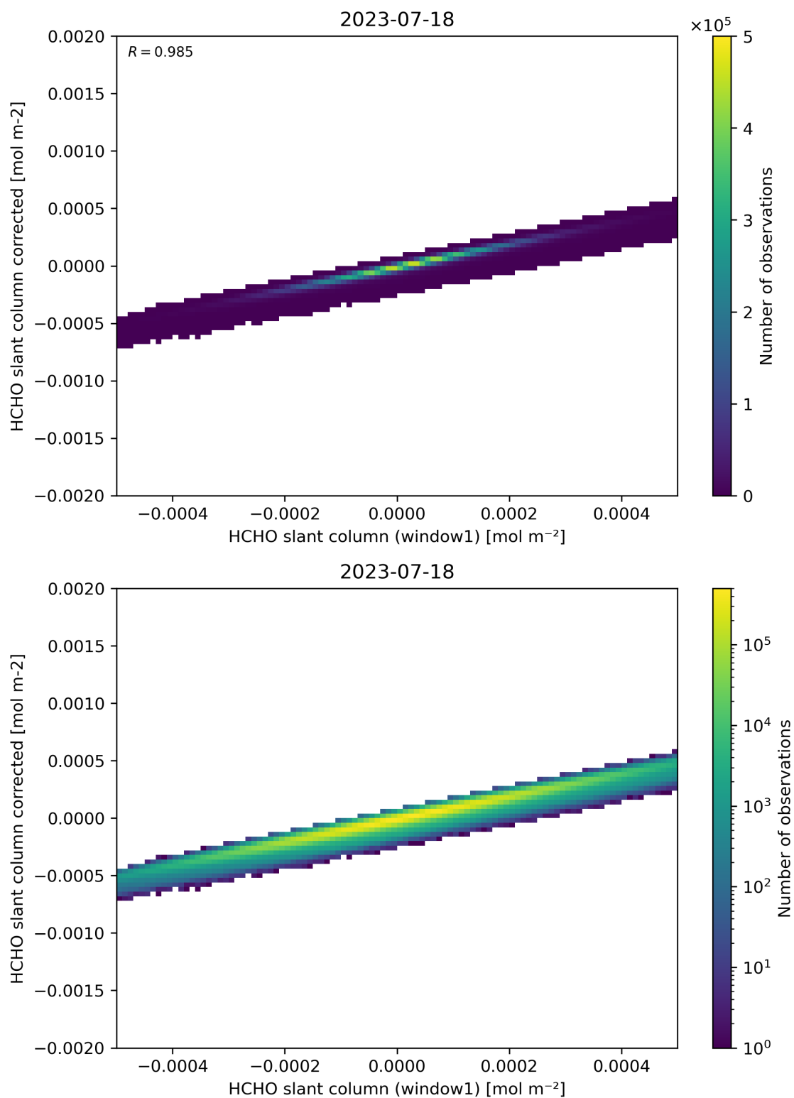
Figure 82: Scatter density plot of “HCHO slant column (window1)” against “HCHO slant column corrected” for 2023-07-17 to 2023-07-19.
