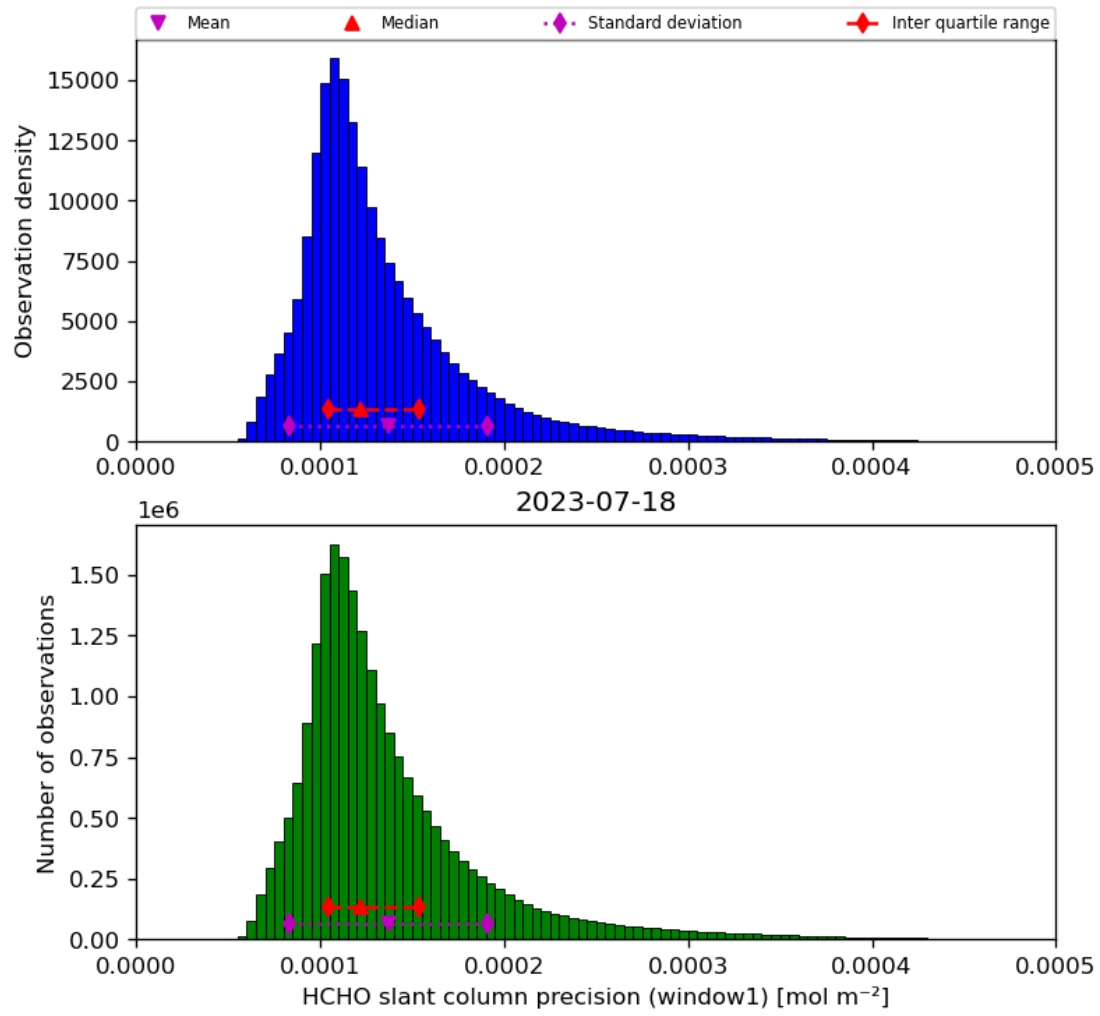
Figure 39: Histogram of “HCHO slant column precision (window1)” for 2023-07-17 to 2023-07-19
