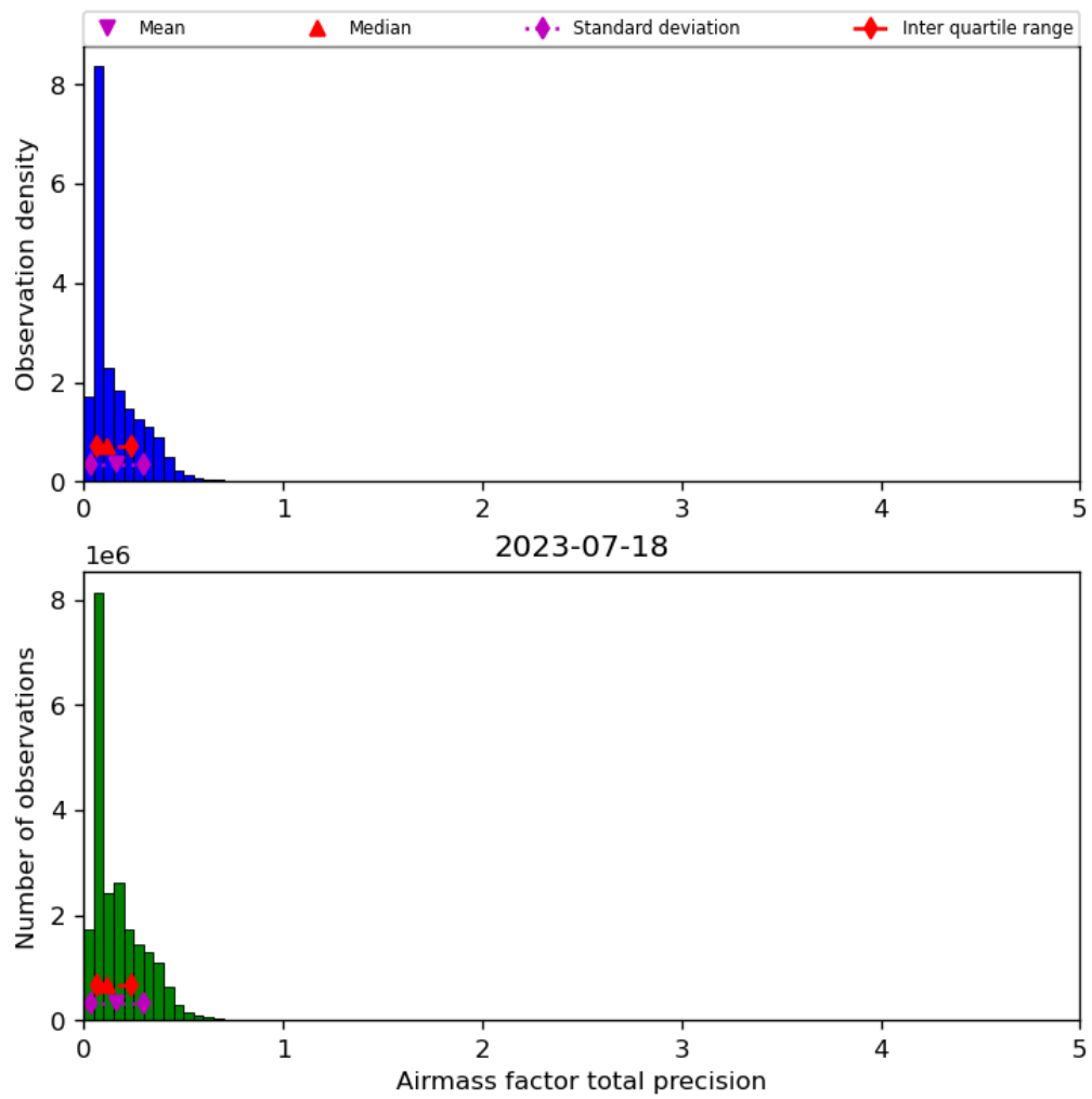
Figure 41: Histogram of “Airmass factor total precision” for 2023-07-17 to 2023-07-19
