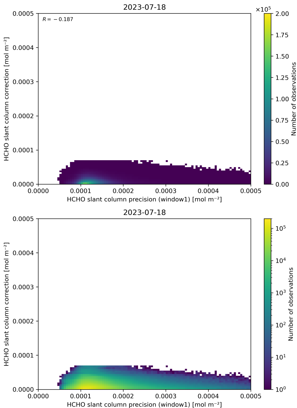
Figure 93: Scatter density plot of “HCHO slant column precision (window1)” against “HCHO slant column correction” for 2023-07-17 to 2023-07-19.
