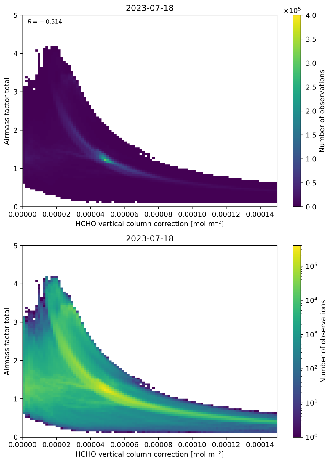
Figure 120: Scatter density plot of “HCHO vertical column correction” against “Airmass factor total” for 2023-07-17 to 2023-07-19.
