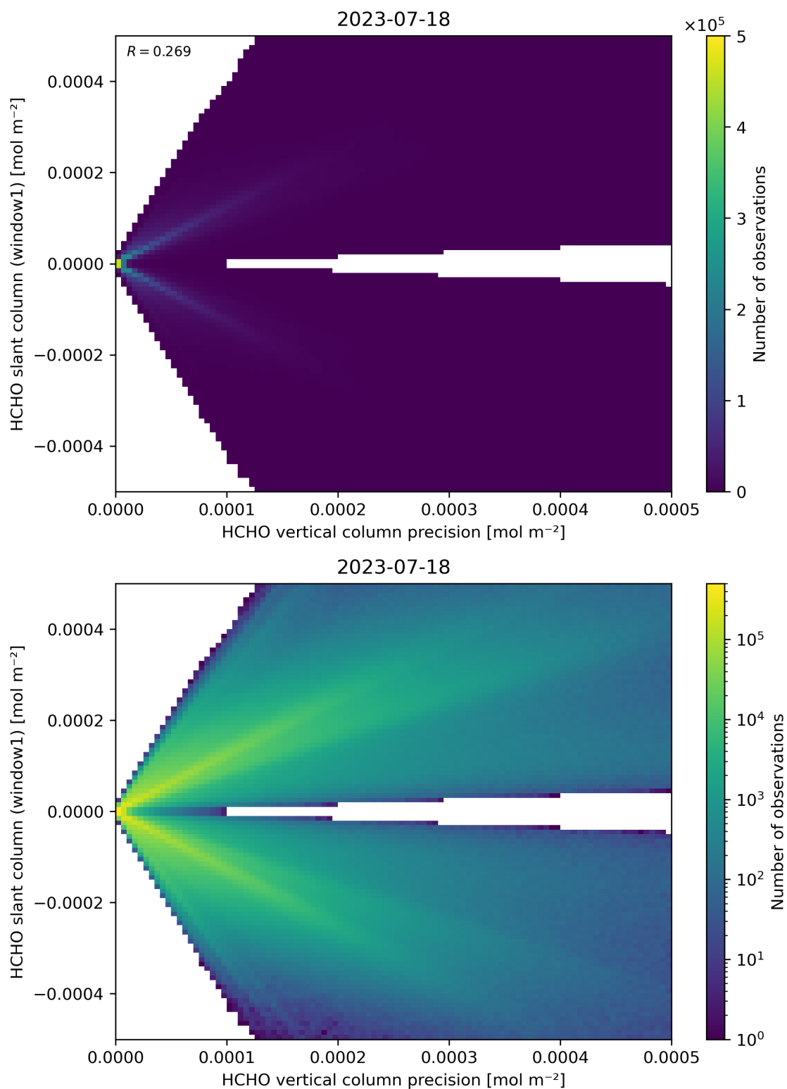
Figure 142: Scatter density plot of “HCHO vertical column precision” against “HCHO slant column (window1)” for 2023-07-17 to 2023-07-19.
