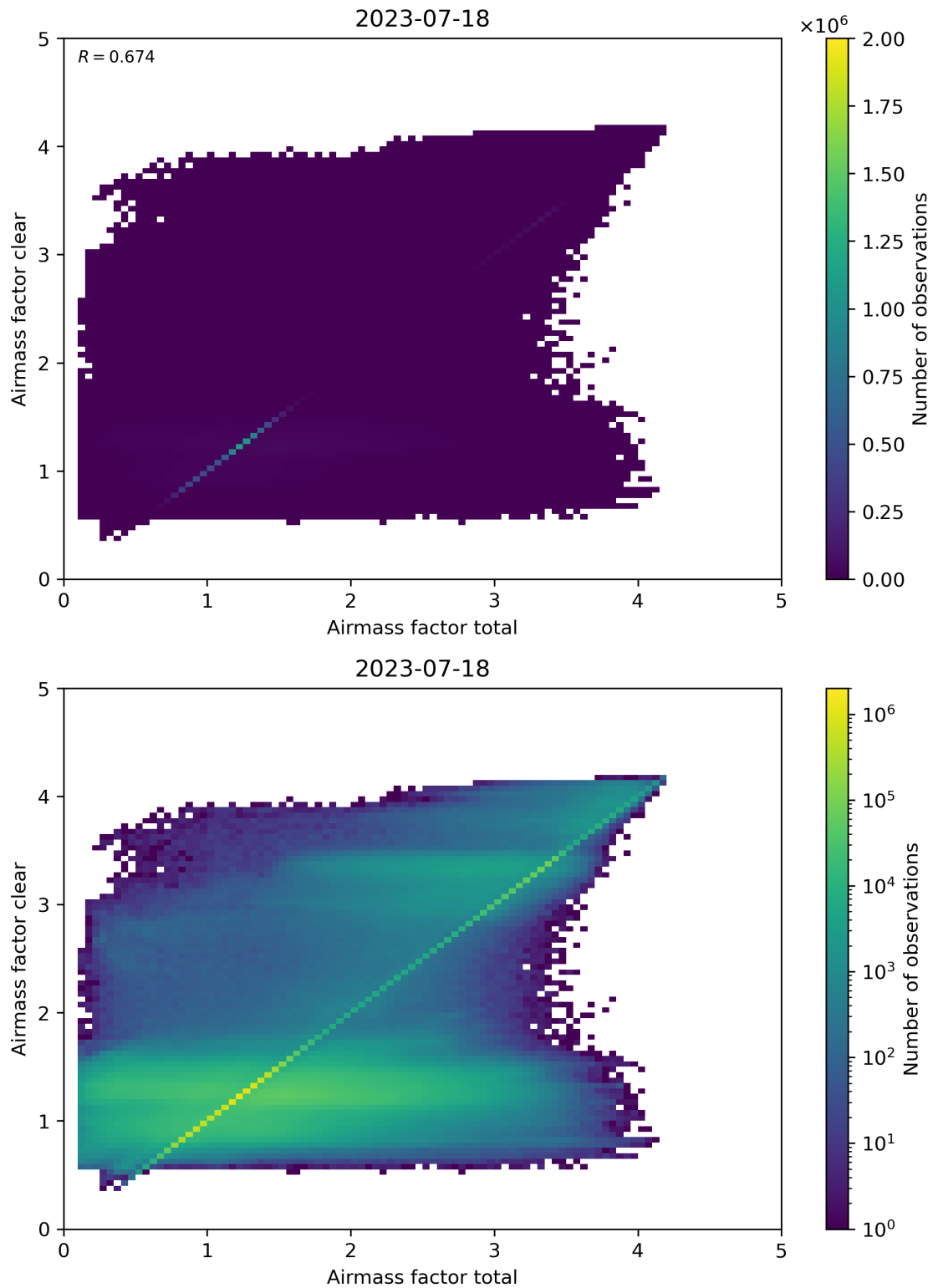
Figure 100: Scatter density plot of “Airmass factor total” against “Airmass factor clear” for 2023-07-17 to 2023-07-19.
