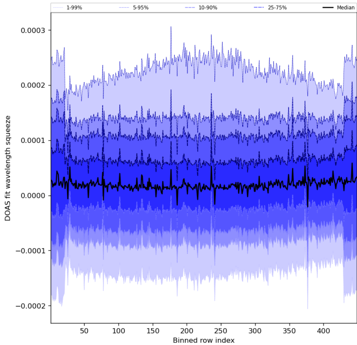
Figure 59: Along track statistics of “DOAS fit wavelength squeeze” for 2023-07-17 to 2023-07-19
