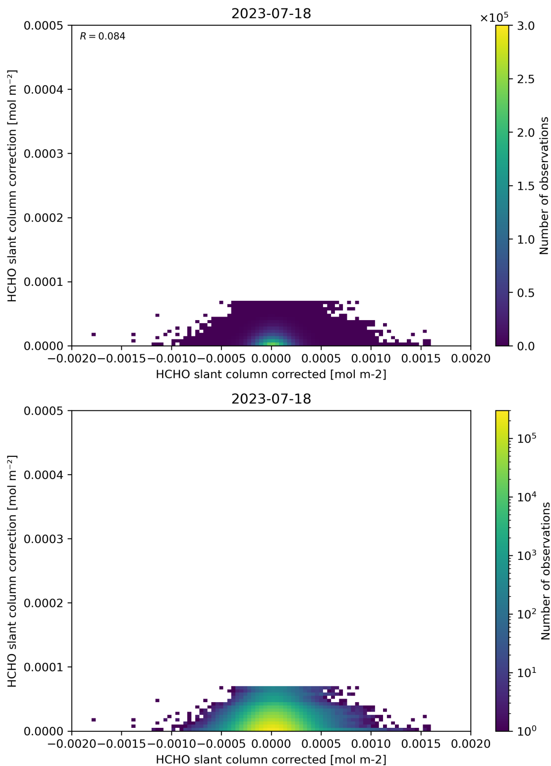
Figure 77: Scatter density plot of “HCHO slant column corrected” against “HCHO slant column correction” for 2023-07-17 to 2023-07-19.
