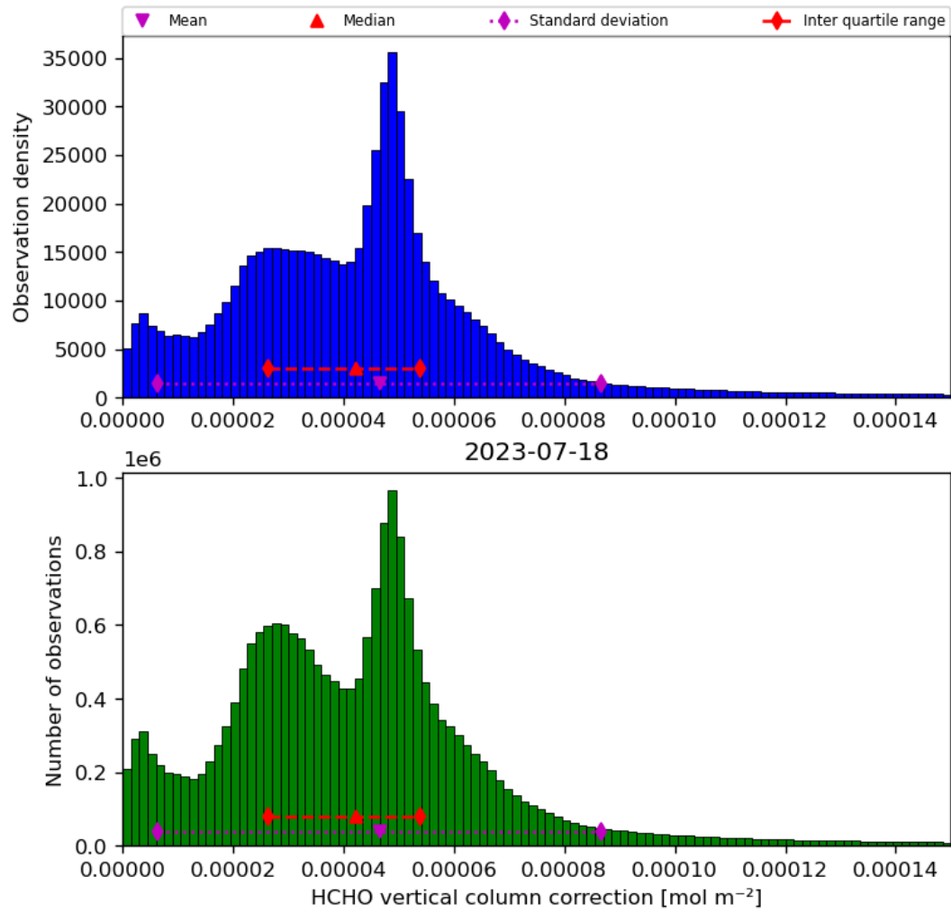
Figure 37: Histogram of “HCHO vertical column correction” for 2023-07-17 to 2023-07-19
