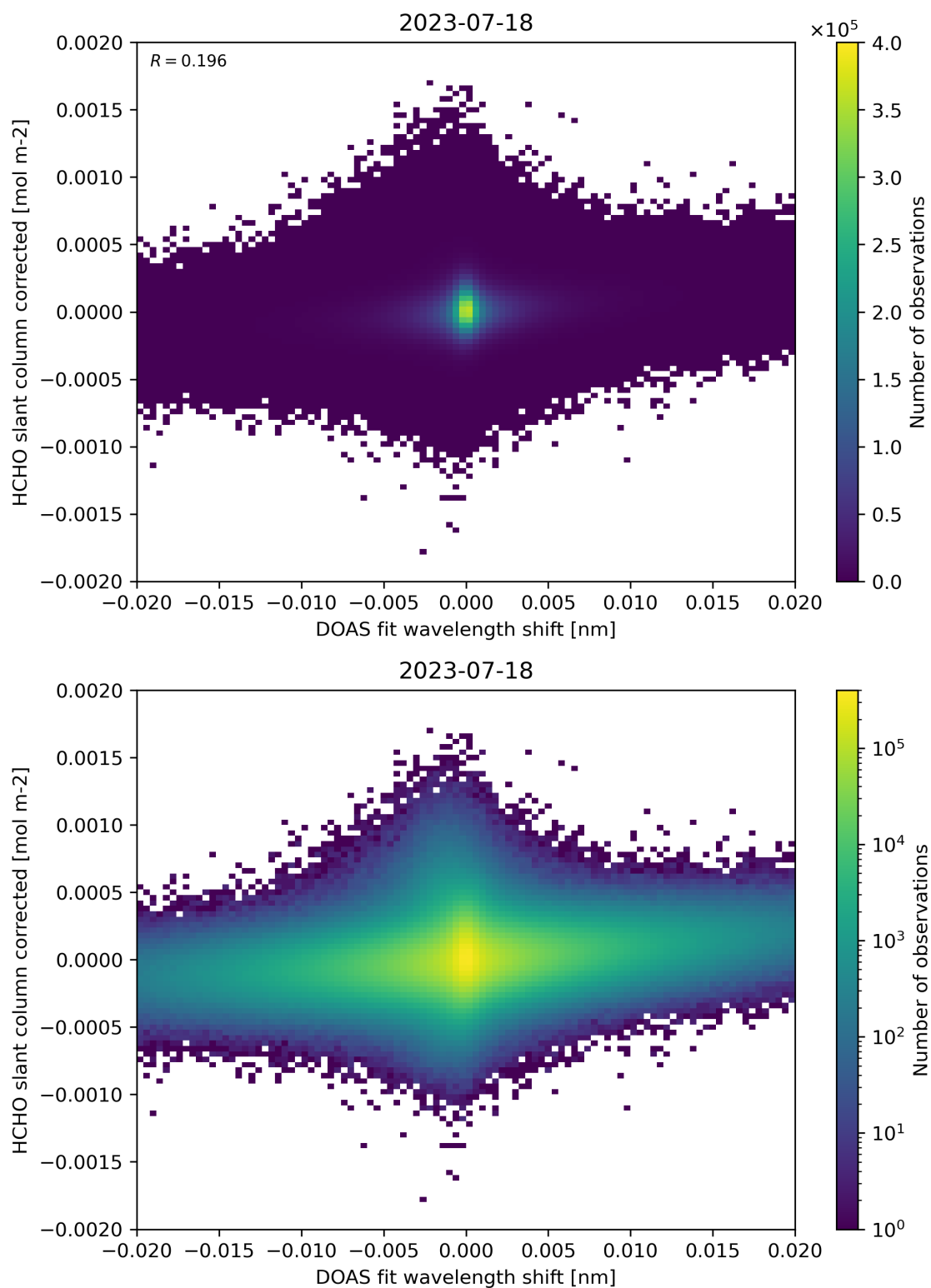
Figure 66: Scatter density plot of “DOAS fit wavelength shift” against “HCHO slant column corrected” for 2023-07-17 to 2023-07-19.
