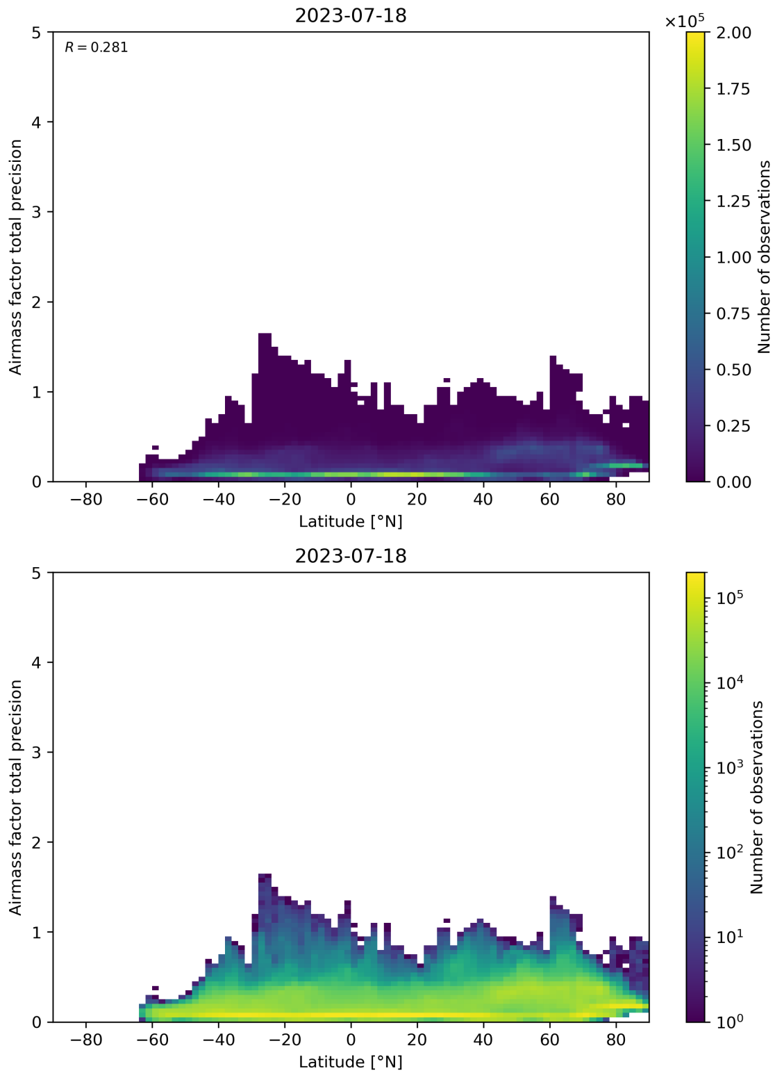
Figure 162: Scatter density plot of “Latitude” against “Airmass factor total precision” for 2023-07-17 to 2023-07-19.
