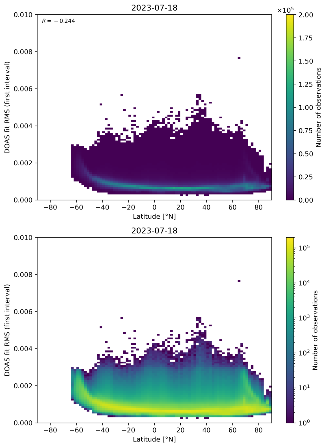
Figure 153: Scatter density plot of “Latitude” against “DOAS fit RMS (first interval)” for 2023-07-17 to 2023-07-19.
