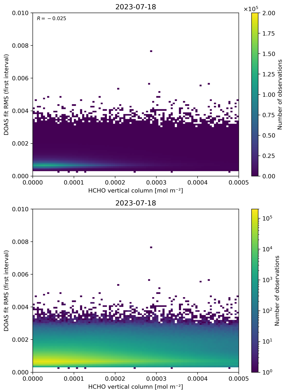
Figure 123: Scatter density plot of “HCHO vertical column” against “DOAS fit RMS (first interval)” for 2023-07-17 to 2023-07-19.
