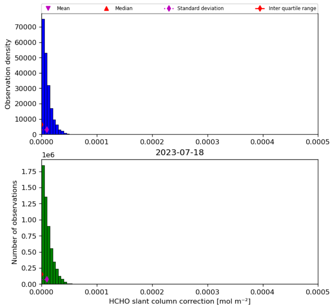
Figure 47: Histogram of “HCHO slant column correction” for 2023-07-17 to 2023-07-19
