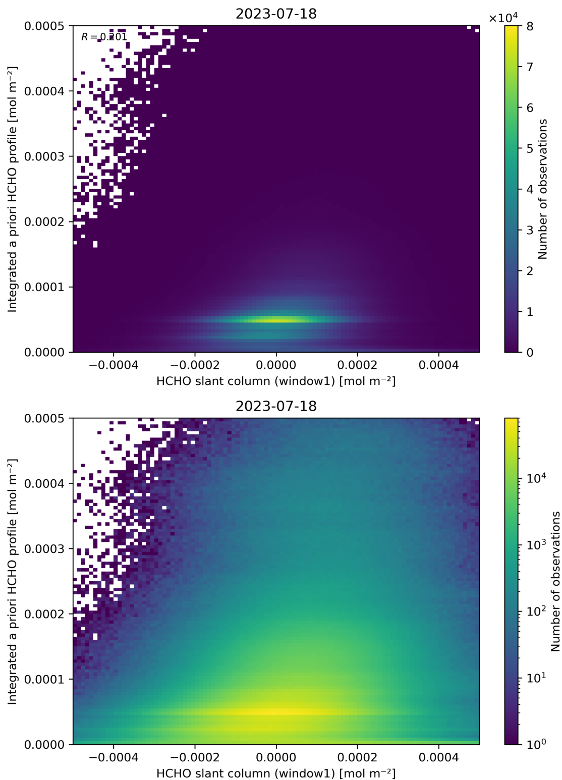
Figure 87: Scatter density plot of “HCHO slant column (window1)” against “Integrated a priori HCHO profile” for 2023-07-17 to 2023-07-19.
