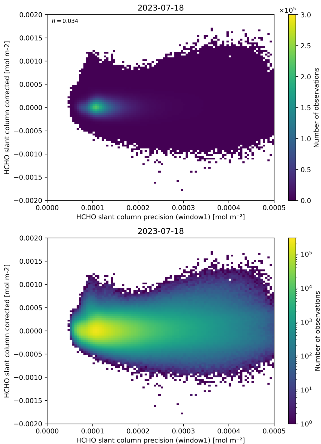
Figure 92: Scatter density plot of “HCHO slant column precision (window1)” against “HCHO slant column corrected” for 2023-07-17 to 2023-07-19.
