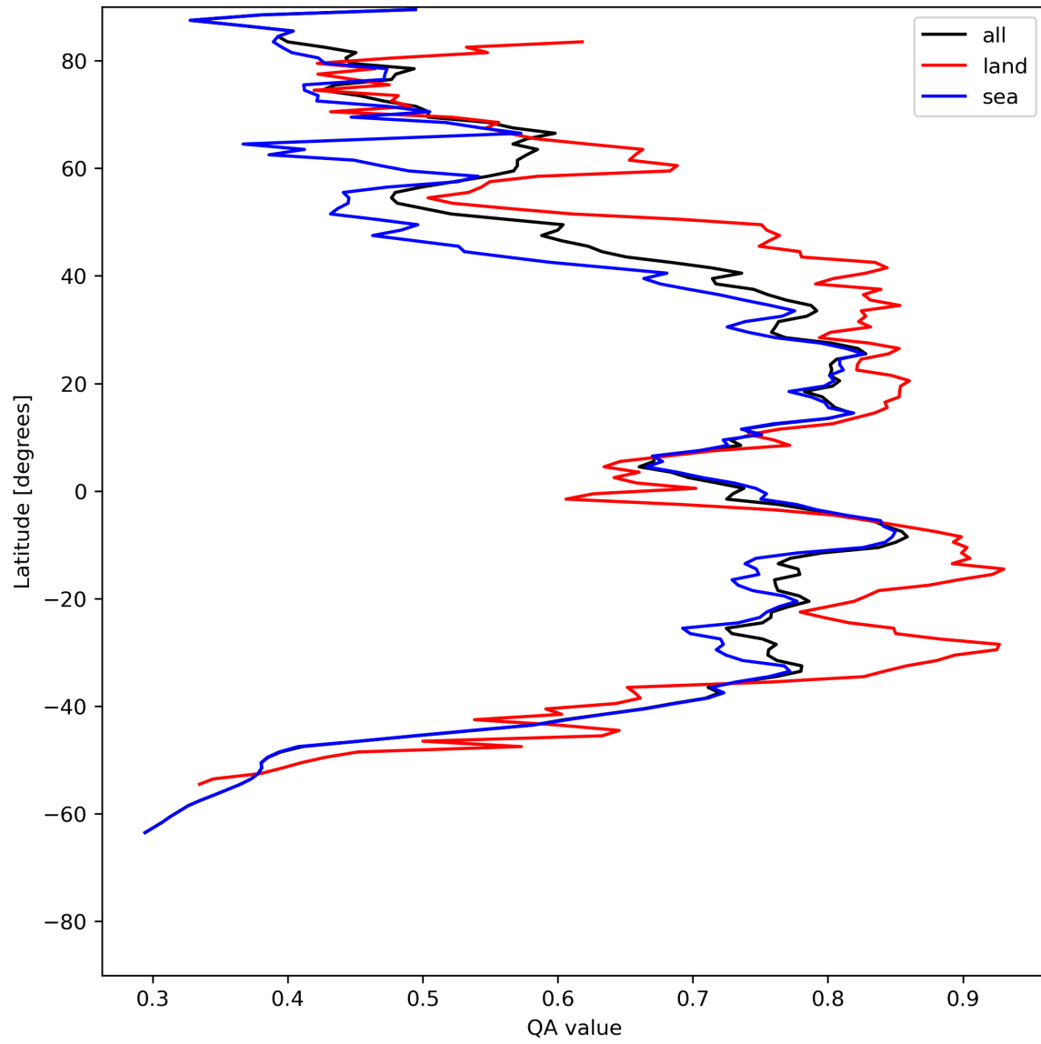
Figure 20: Zonal average of “QA value” for 2023-07-17 to 2023-07-19.
