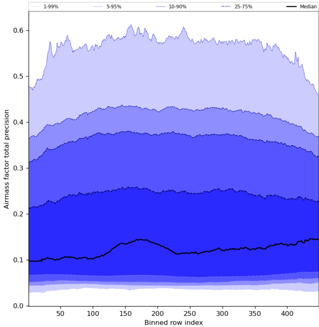
Figure 55: Along track statistics of “Airmass factor total precision” for 2023-07-17 to 2023-07-19
