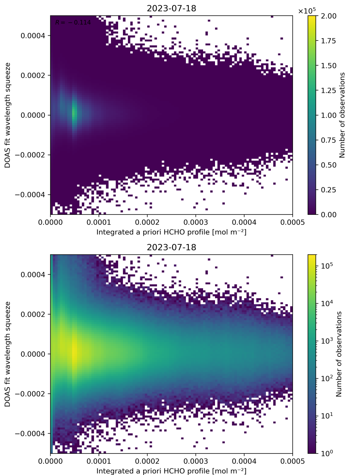
Figure 150: Scatter density plot of “Integrated a priori HCHO profile” against “DOAS fit wavelength squeeze” for 2023-07-17 to 2023-07-19.
