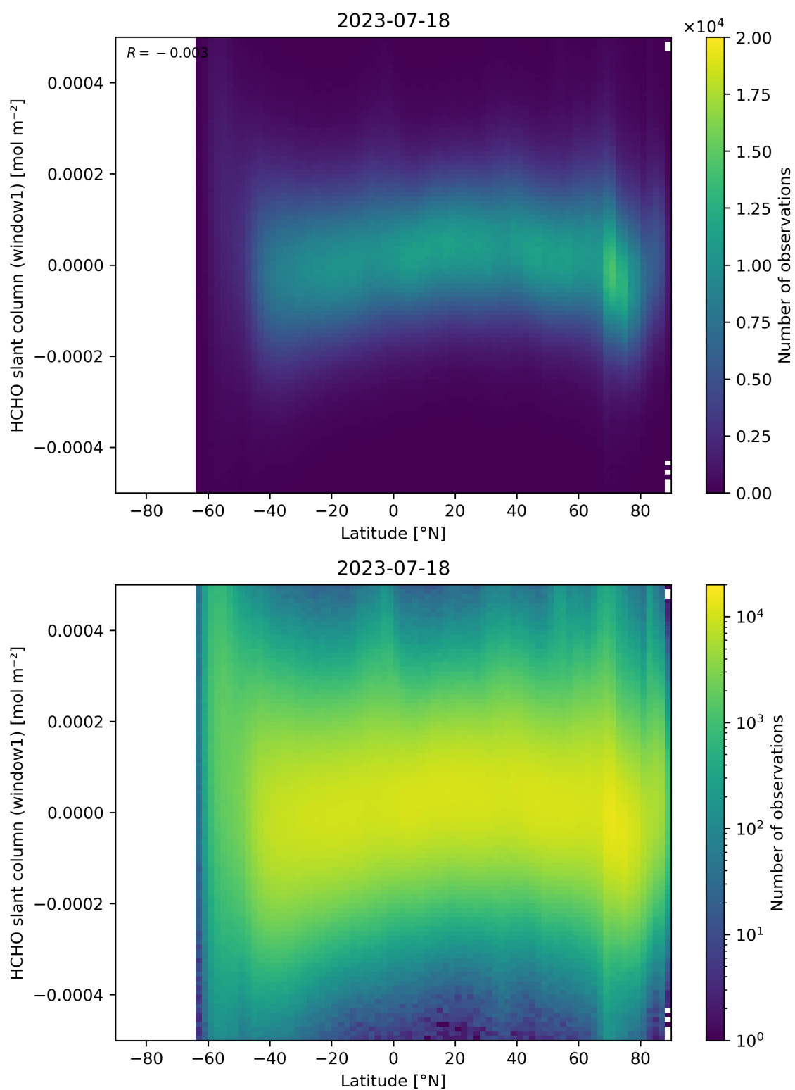
Figure 159: Scatter density plot of “Latitude” against “HCHO slant column (window1)” for 2023-07-17 to 2023-07-19.
