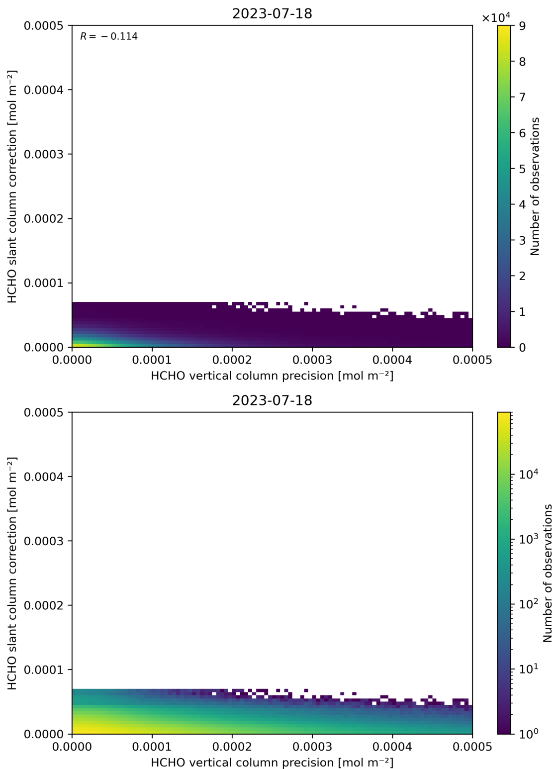
Figure 141: Scatter density plot of “HCHO vertical column precision” against “HCHO slant column correction” for 2023-07-17 to 2023-07-19.
