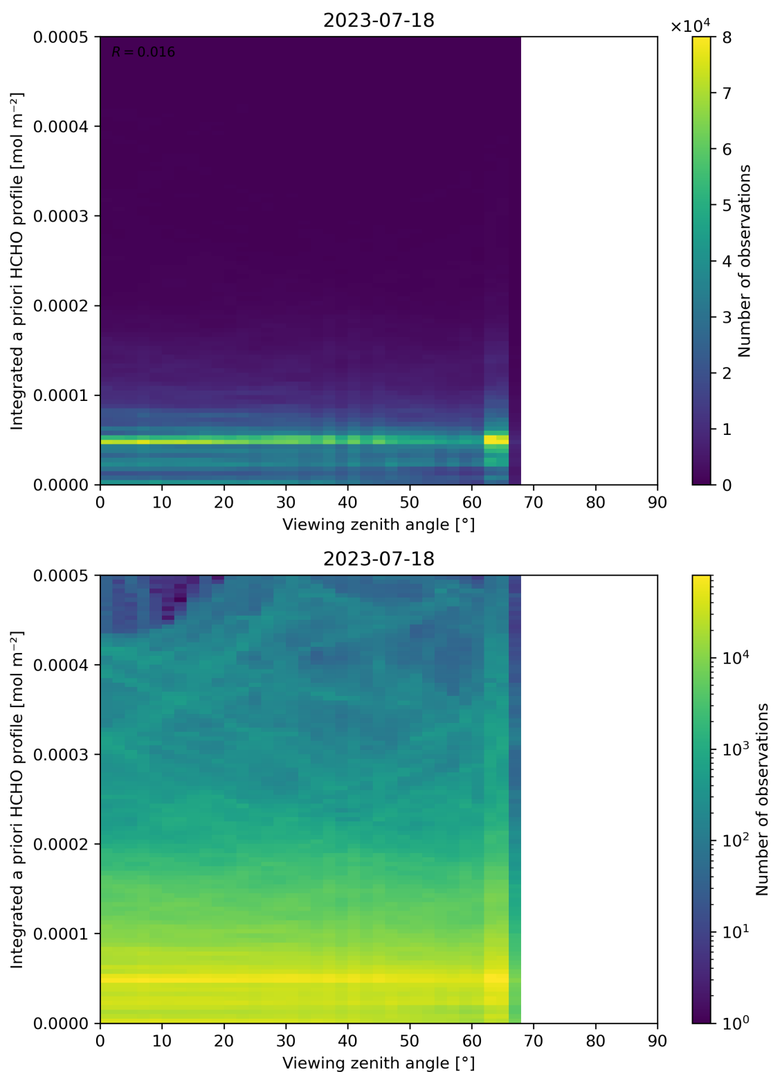
Figure 195: Scatter density plot of “Viewing zenith angle” against “Integrated a priori HCHO profile” for 2023-07-17 to 2023-07-19.
