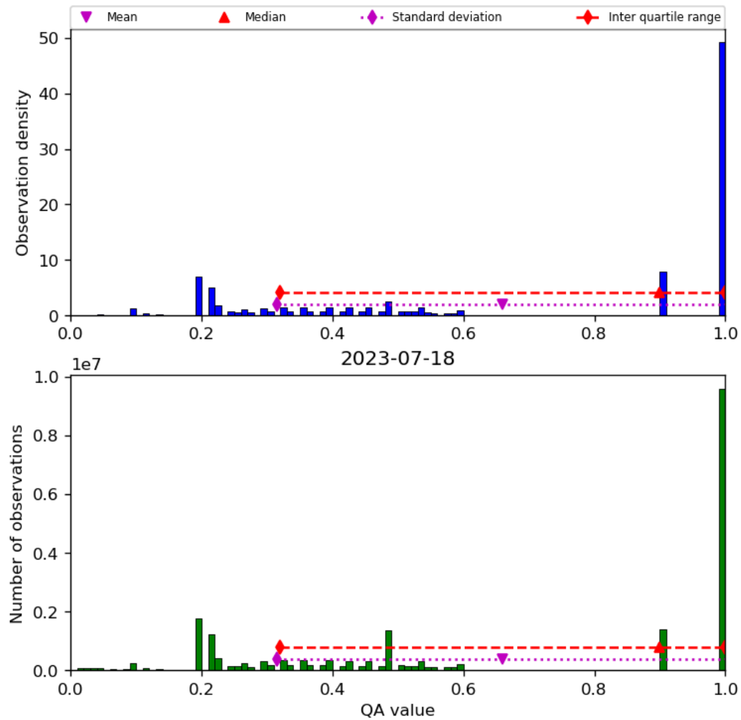
Figure 34: Histogram of “QA value” for 2023-07-17 to 2023-07-19
