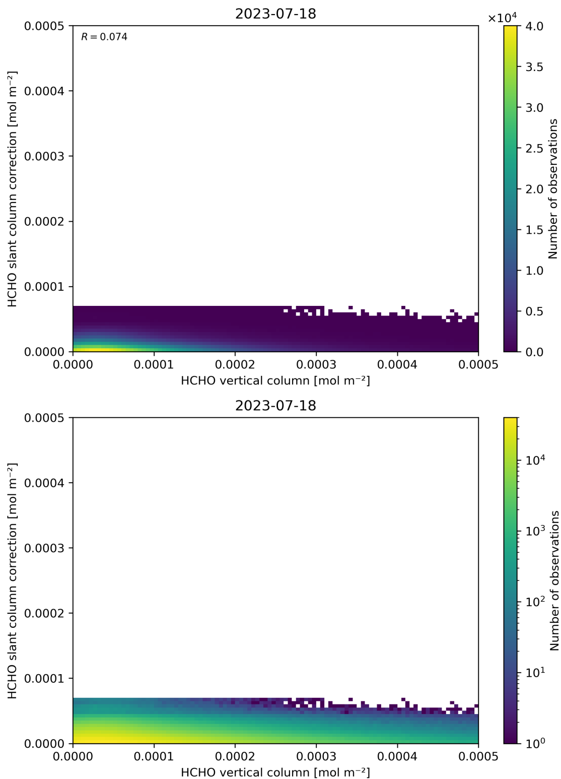
Figure 128: Scatter density plot of “HCHO vertical column” against “HCHO slant column correction” for 2023-07-17 to 2023-07-19.
