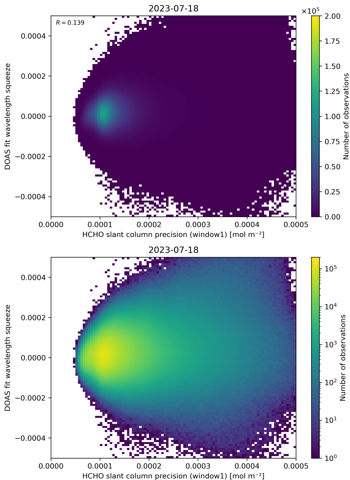
Figure 90: Scatter density plot of “HCHO slant column precision (window1)” against “DOAS fit wavelength squeeze” for 2023-07-17 to 2023-07-19.
