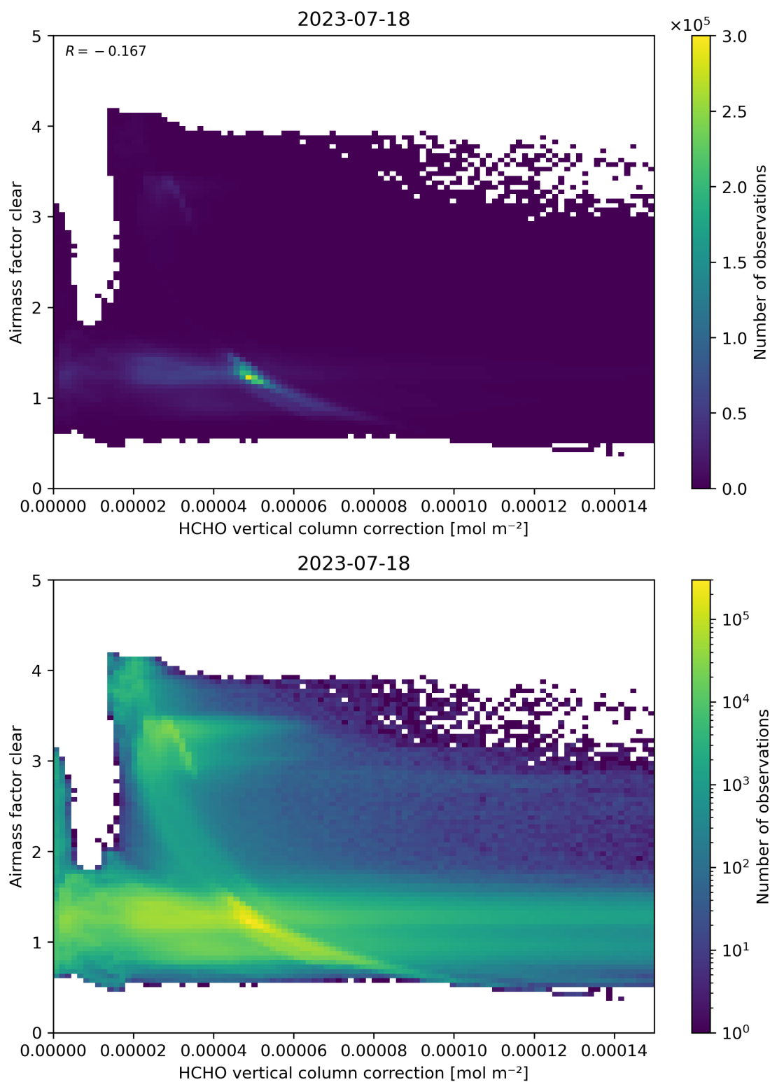
Figure 115: Scatter density plot of “HCHO vertical column correction” against “Airmass factor clear” for 2023-07-17 to 2023-07-19.
