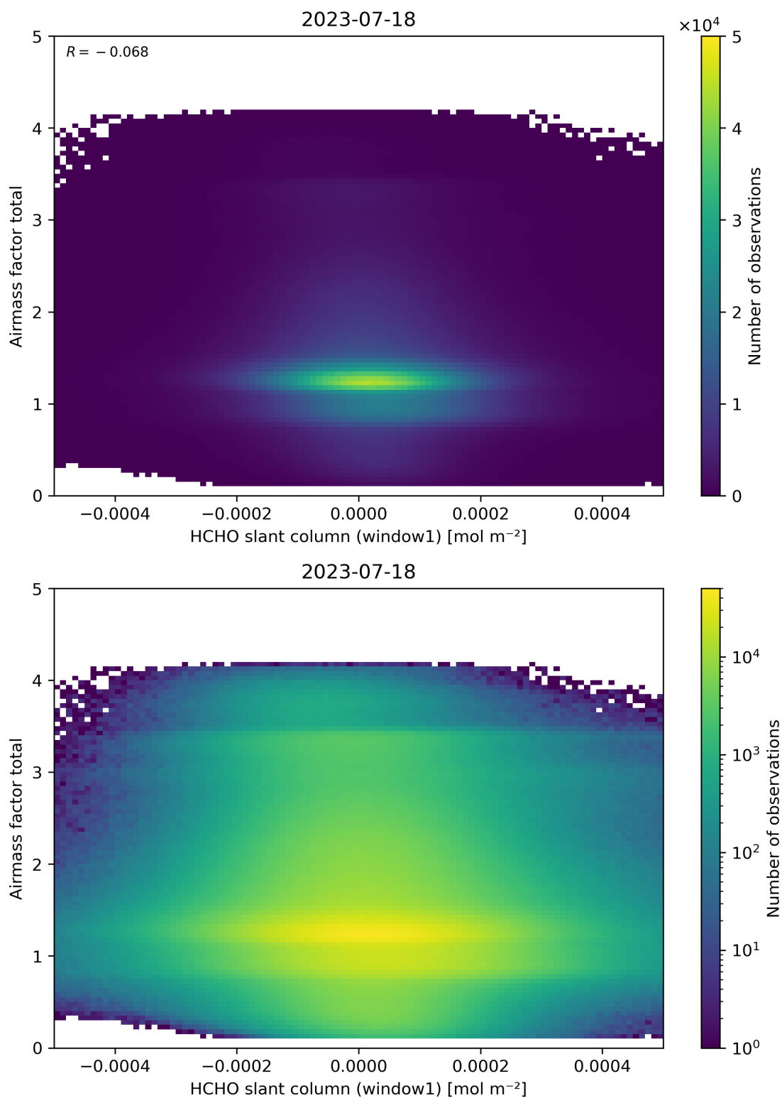
Figure 85: Scatter density plot of “HCHO slant column (window1)” against “Airmass factor total” for 2023-07-17 to 2023-07-19.
