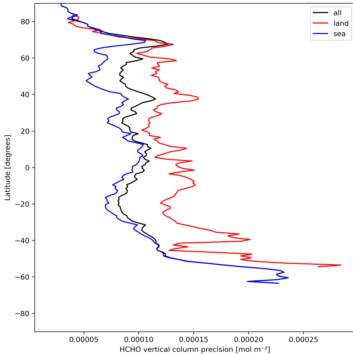
Figure 22: Zonal average of “HCHO vertical column precision” for 2023-07-17 to 2023-07-19.
