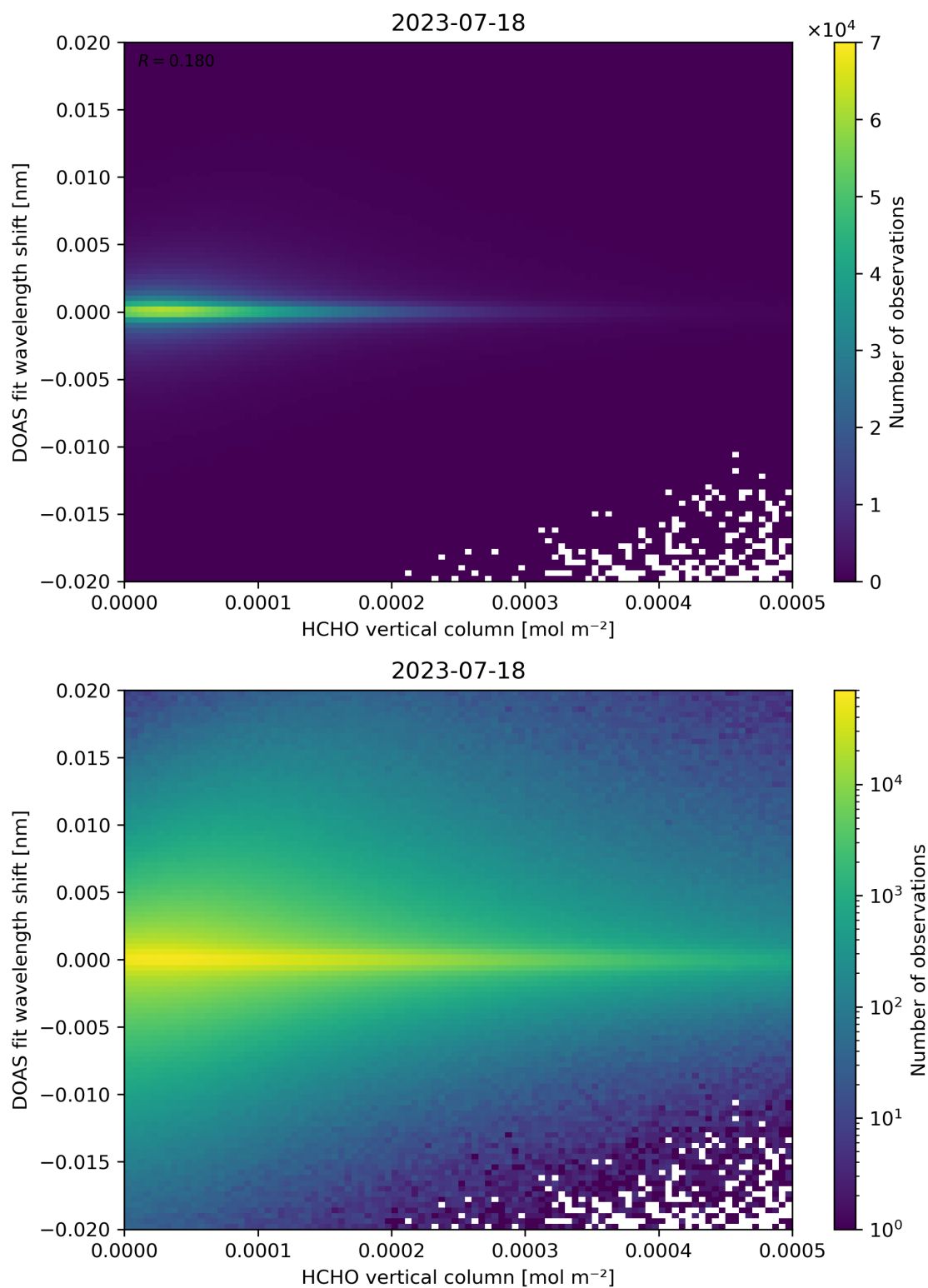
Figure 124: Scatter density plot of “HCHO vertical column” against “DOAS fit wavelength shift” for 2023-07-17 to 2023-07-19.
