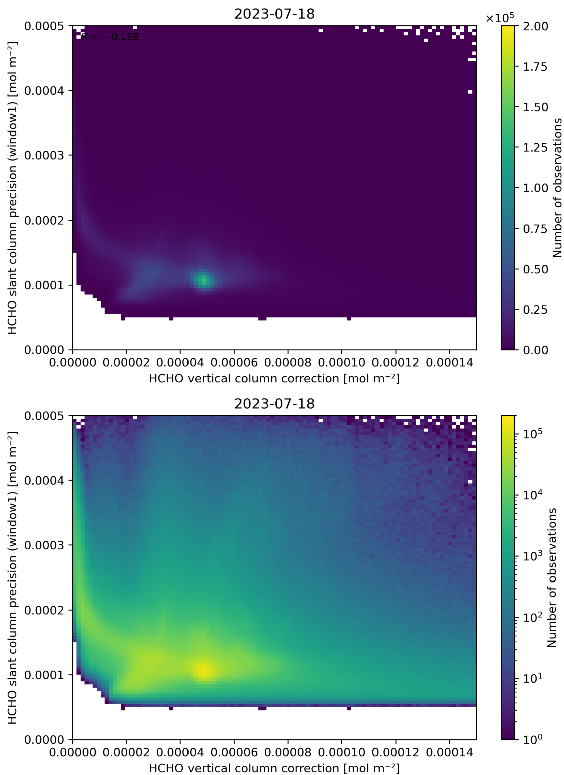
Figure 119: Scatter density plot of “HCHO vertical column correction” against “HCHO slant column precision (window1)” for 2023-07-17 to 2023-07-19.
