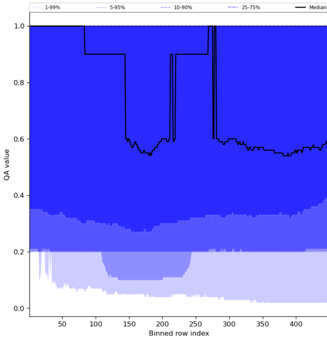
Figure 48: Along track statistics of “QA value” for 2023-07-17 to 2023-07-19
