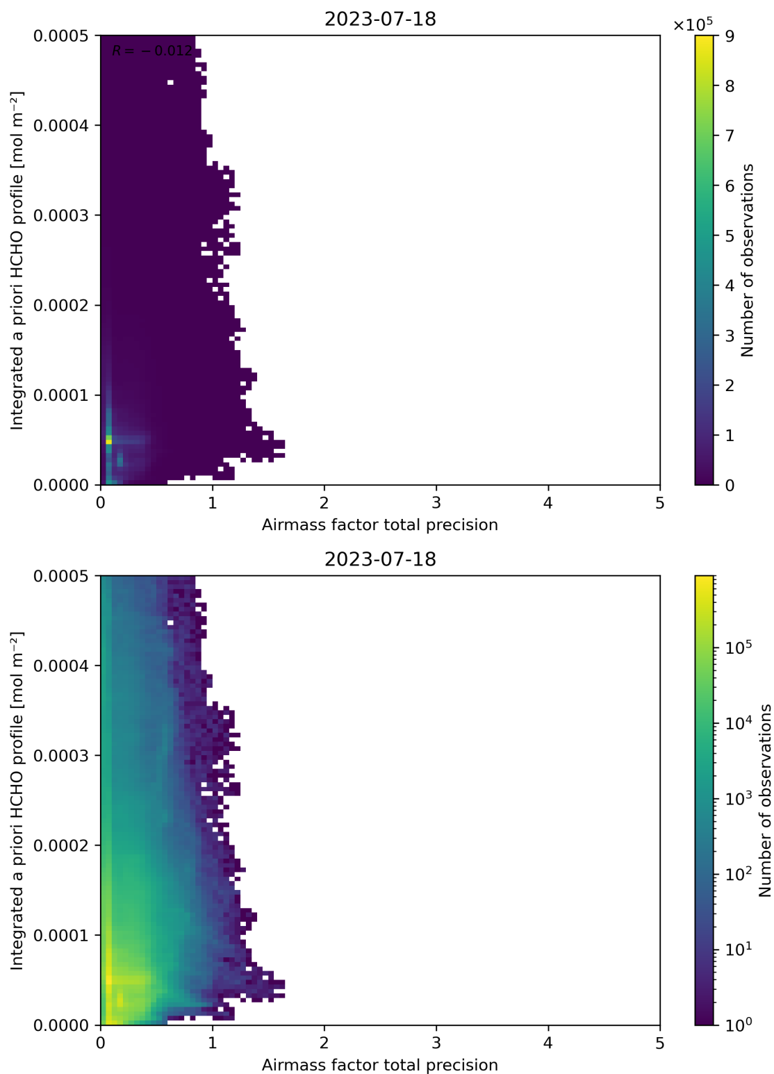
Figure 111: Scatter density plot of “Airmass factor total precision” against “Integrated a priori HCHO profile” for 2023-07-17 to 2023-07-19.
