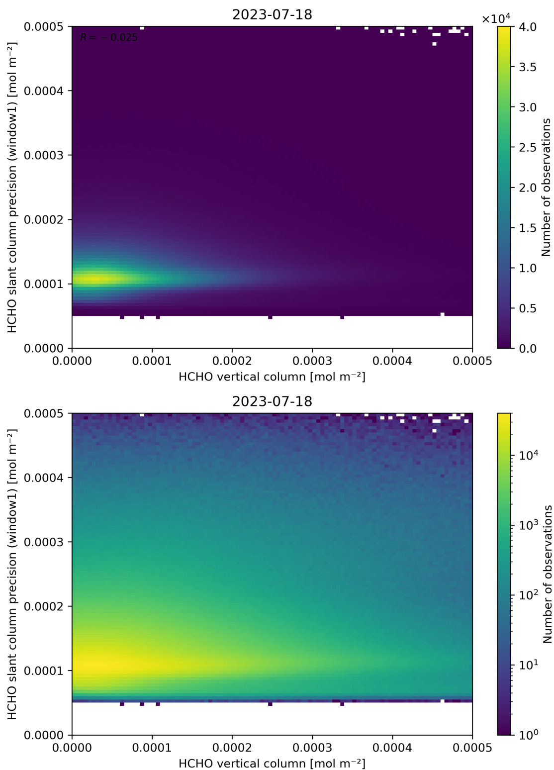
Figure 130: Scatter density plot of “HCHO vertical column” against “HCHO slant column precision (window1)” for 2023-07-17 to 2023-07-19.
