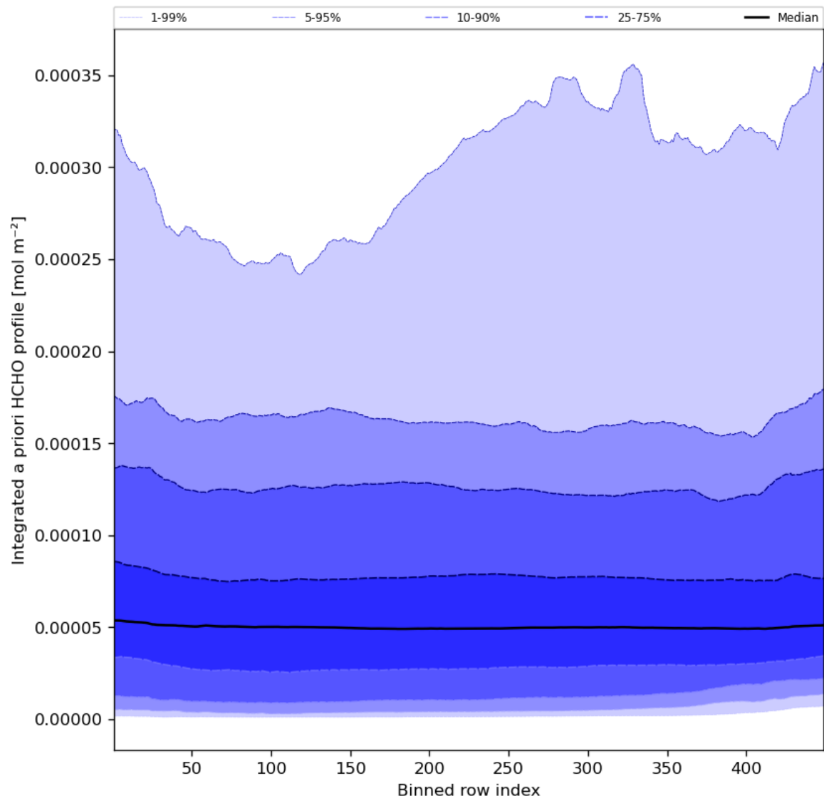
Figure 57: Along track statistics of “Integrated a priori HCHO profile” for 2023-07-17 to 2023-07-19
