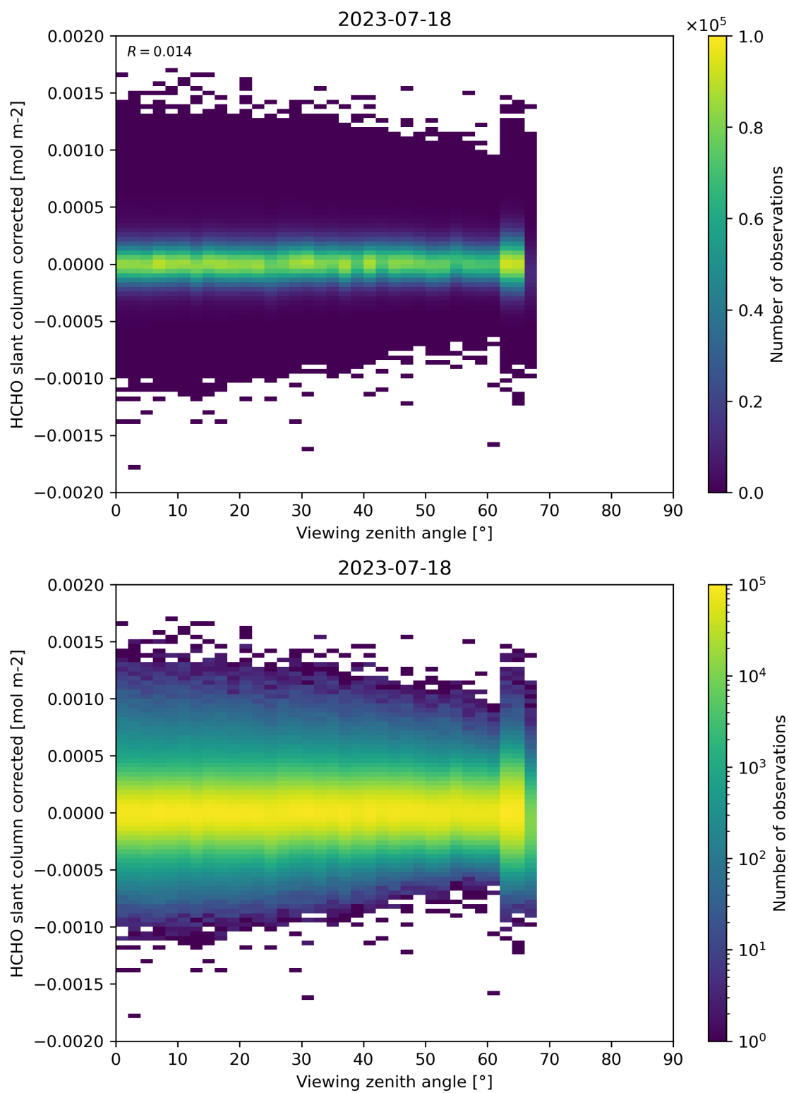
Figure 186: Scatter density plot of “Viewing zenith angle” against “HCHO slant column corrected” for 2023-07-17 to 2023-07-19.
