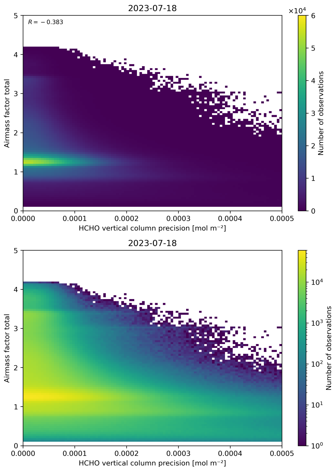
Figure 144: Scatter density plot of “HCHO vertical column precision” against “Airmass factor total” for 2023-07-17 to 2023-07-19.
