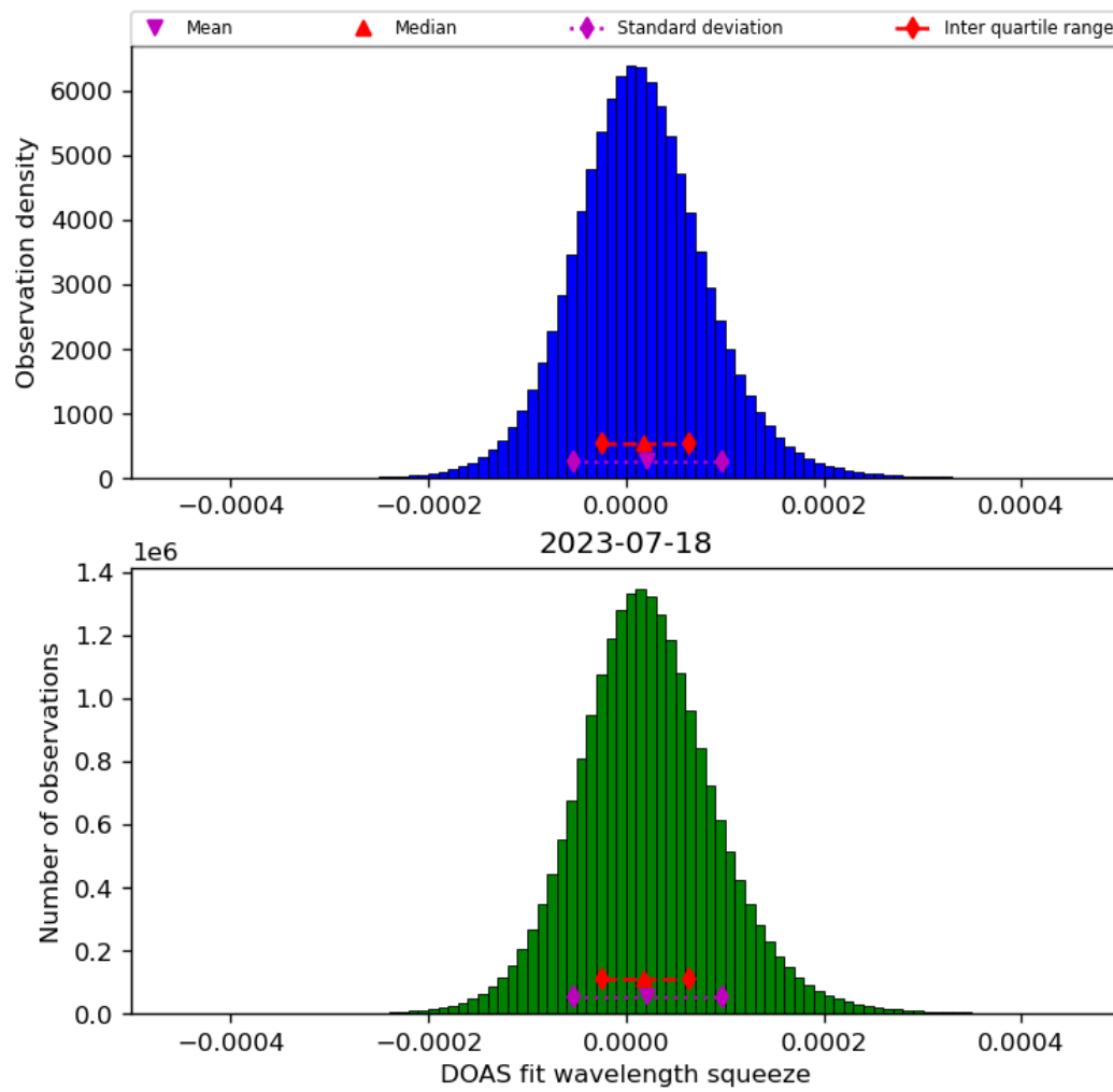
Figure 45: Histogram of “DOAS fit wavelength squeeze” for 2023-07-17 to 2023-07-19
