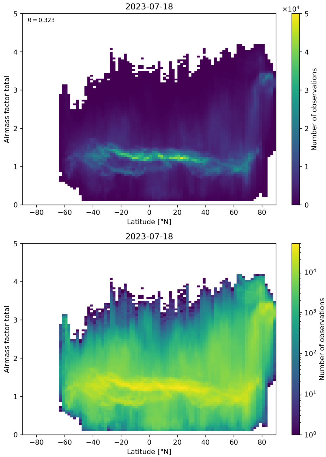
Figure 161: Scatter density plot of “Latitude” against “Airmass factor total” for 2023-07-17 to 2023-07-19.
