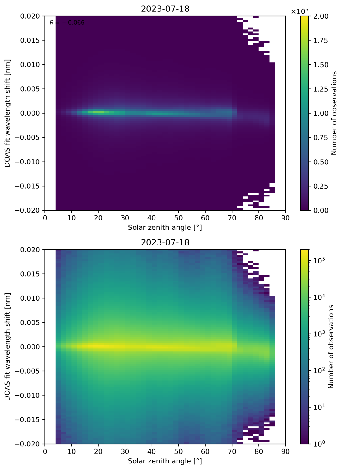
Figure 168: Scatter density plot of “Solar zenith angle” against “DOAS fit wavelength shift” for 2023-07-17 to 2023-07-19.
