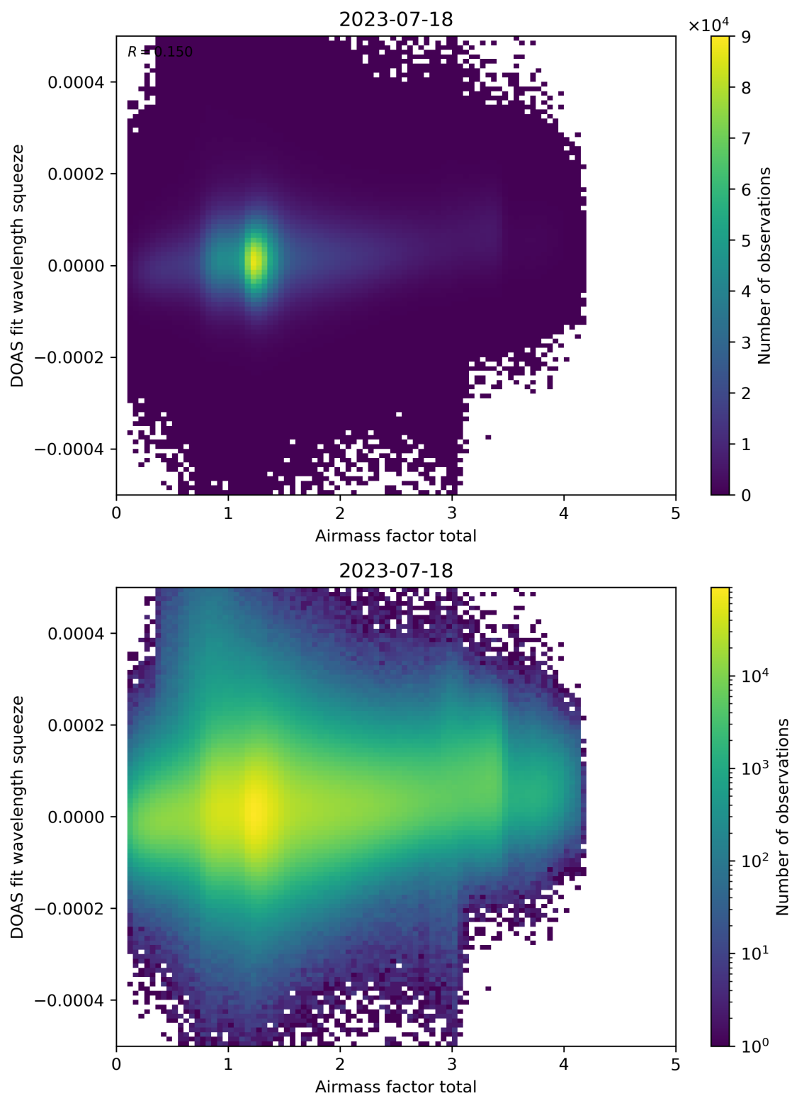
Figure 99: Scatter density plot of “Airmass factor total” against “DOAS fit wavelength squeeze” for 2023-07-17 to 2023-07-19.
