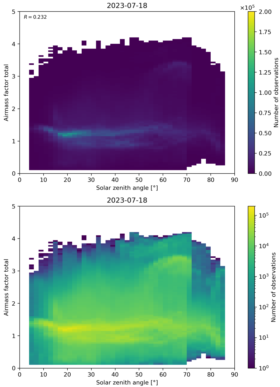
Figure 175: Scatter density plot of “Solar zenith angle” against “Airmass factor total” for 2023-07-17 to 2023-07-19.
