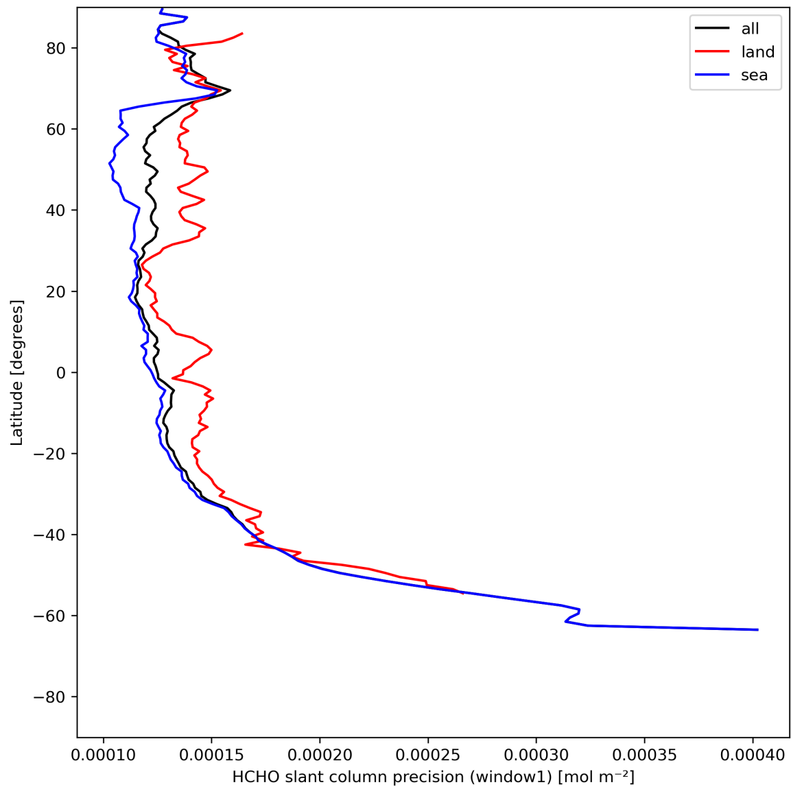
Figure 25: Zonal average of “HCHO slant column precision (window1)” for 2023-07-17 to 2023-07-19.
