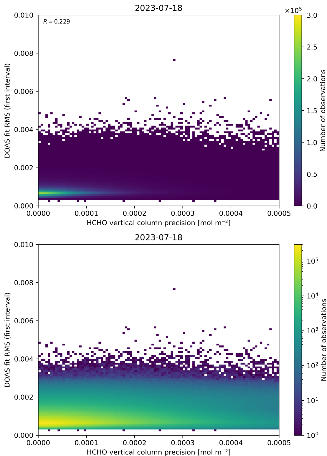
Figure 136: Scatter density plot of “HCHO vertical column precision” against “DOAS fit RMS (first interval)” for 2023-07-17 to 2023-07-19.
