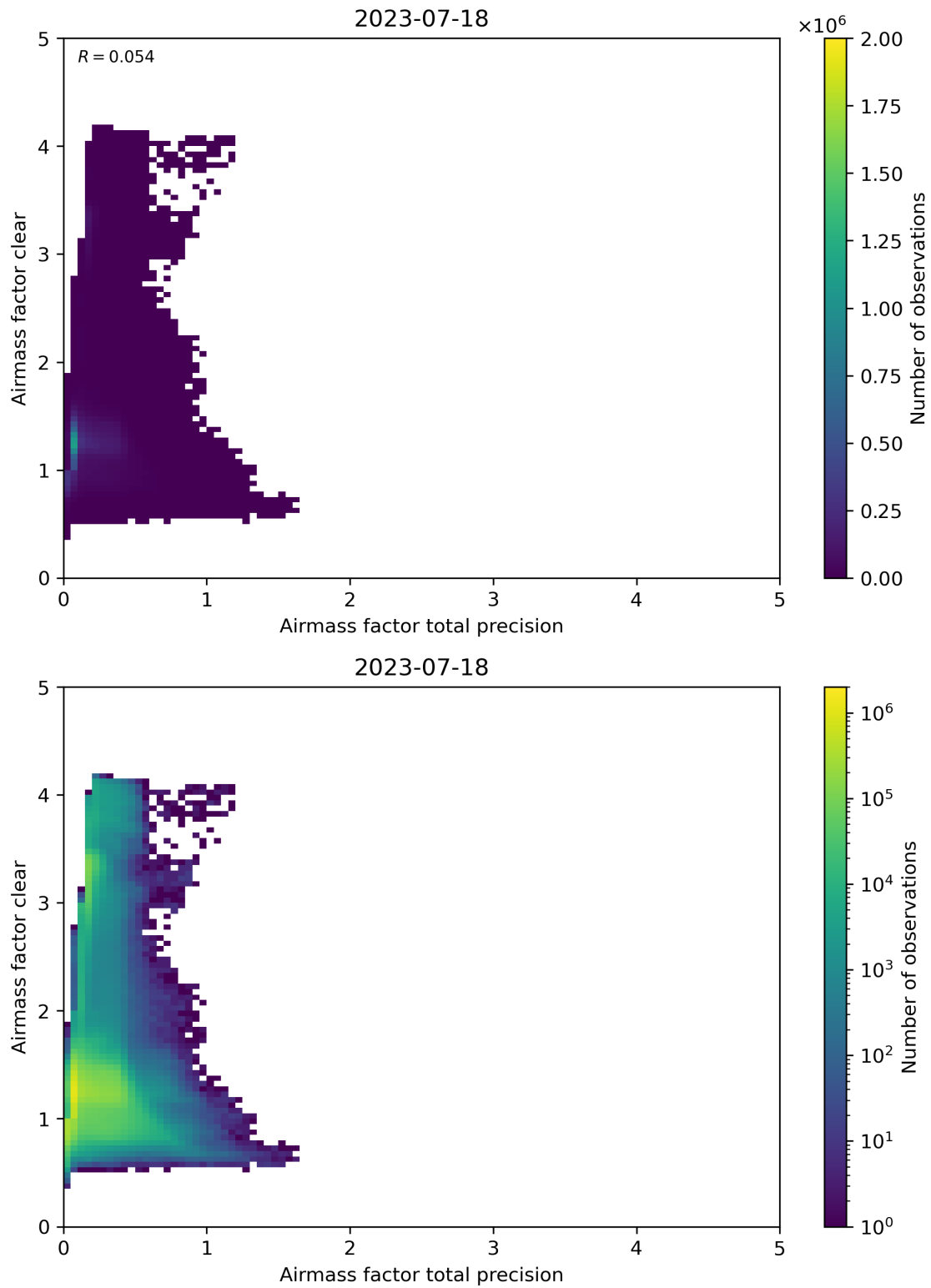
Figure 108: Scatter density plot of “Airmass factor total precision” against “Airmass factor clear” for 2023-07-17 to 2023-07-19.
