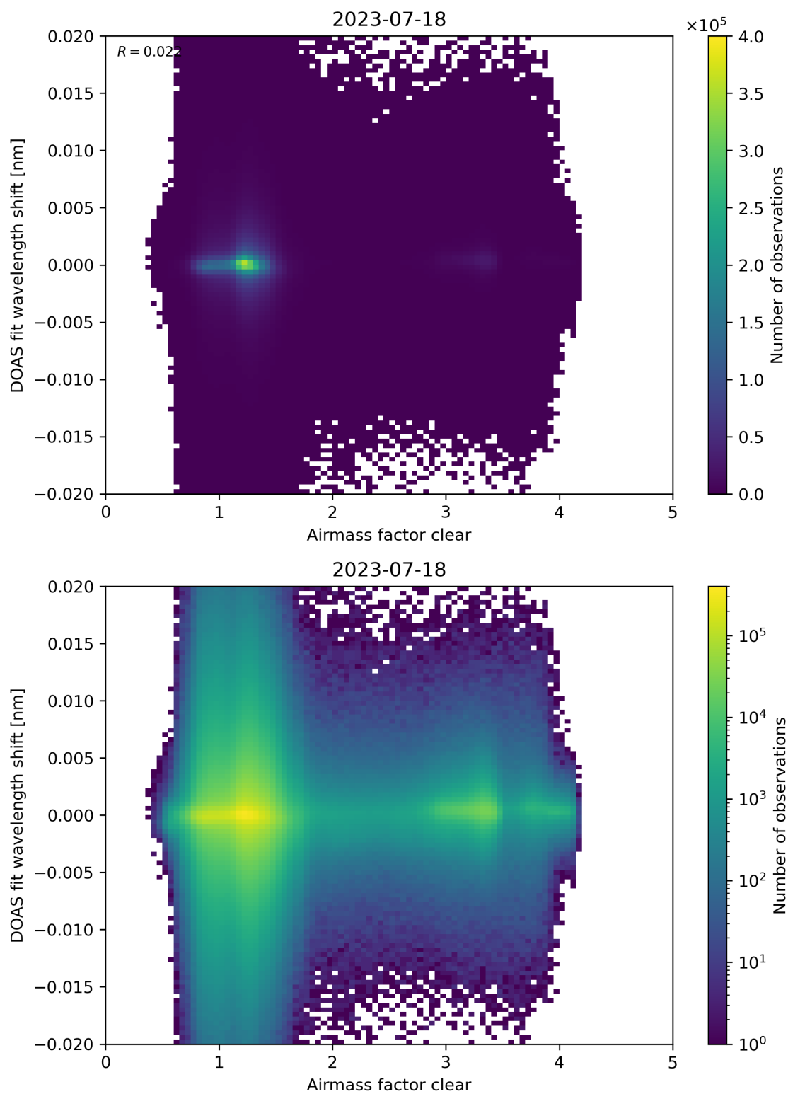
Figure 72: Scatter density plot of “Airmass factor clear” against “DOAS fit wavelength shift” for 2023-07-17 to 2023-07-19.
