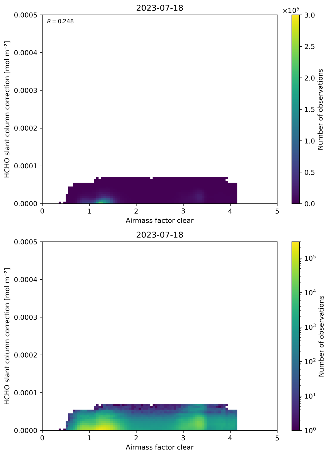
Figure 75: Scatter density plot of “Airmass factor clear” against “HCHO slant column correction” for 2023-07-17 to 2023-07-19.
