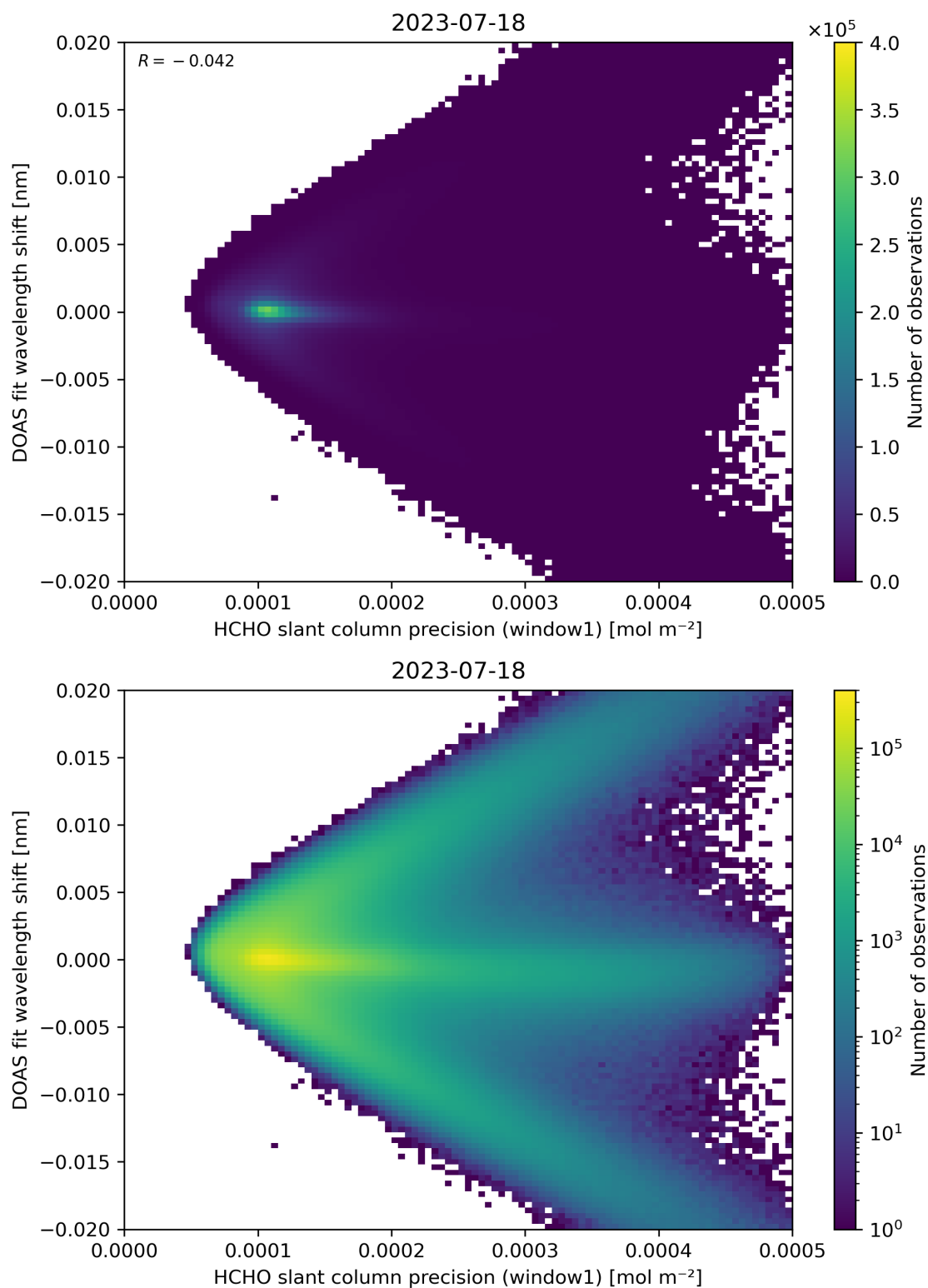
Figure 89: Scatter density plot of “HCHO slant column precision (window1)” against “DOAS fit wavelength shift” for 2023-07-17 to 2023-07-19.
