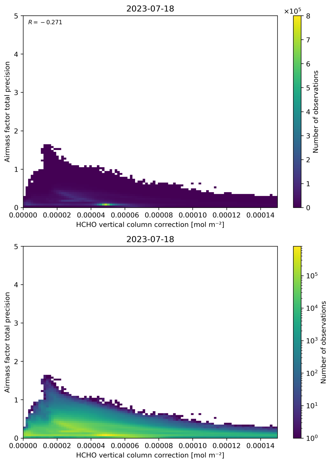
Figure 121: Scatter density plot of “HCHO vertical column correction” against “Airmass factor total precision” for 2023-07-17 to 2023-07-19.
