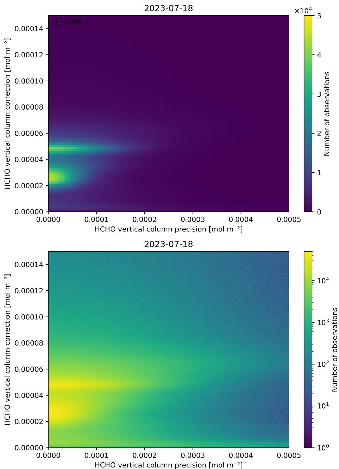
Figure 146: Scatter density plot of “HCHO vertical column precision” against “HCHO vertical column correction” for 2023-07-17 to 2023-07-19.
