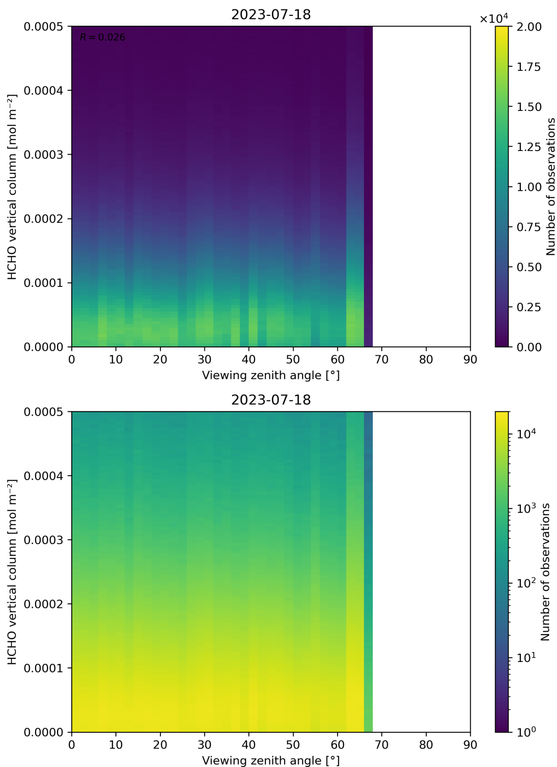
Figure 192: Scatter density plot of “Viewing zenith angle” against “HCHO vertical column” for 2023-07-17 to 2023-07-19.
