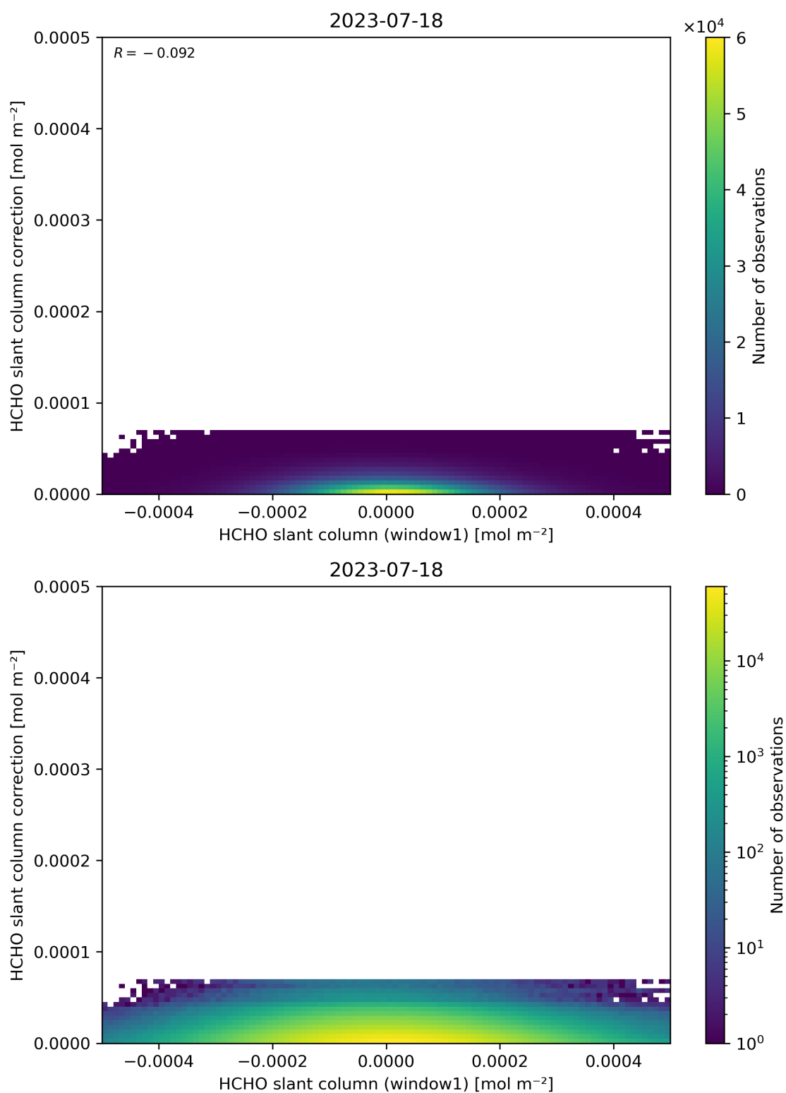
Figure 83: Scatter density plot of “HCHO slant column (window1)” against “HCHO slant column correction” for 2023-07-17 to 2023-07-19.
