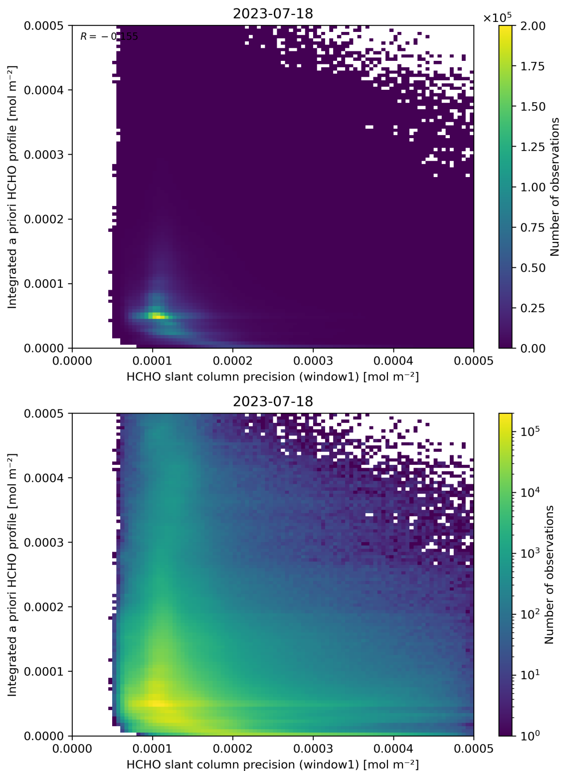
Figure 96: Scatter density plot of “HCHO slant column precision (window1)” against “Integrated a priori HCHO profile” for 2023-07-17 to 2023-07-19.
