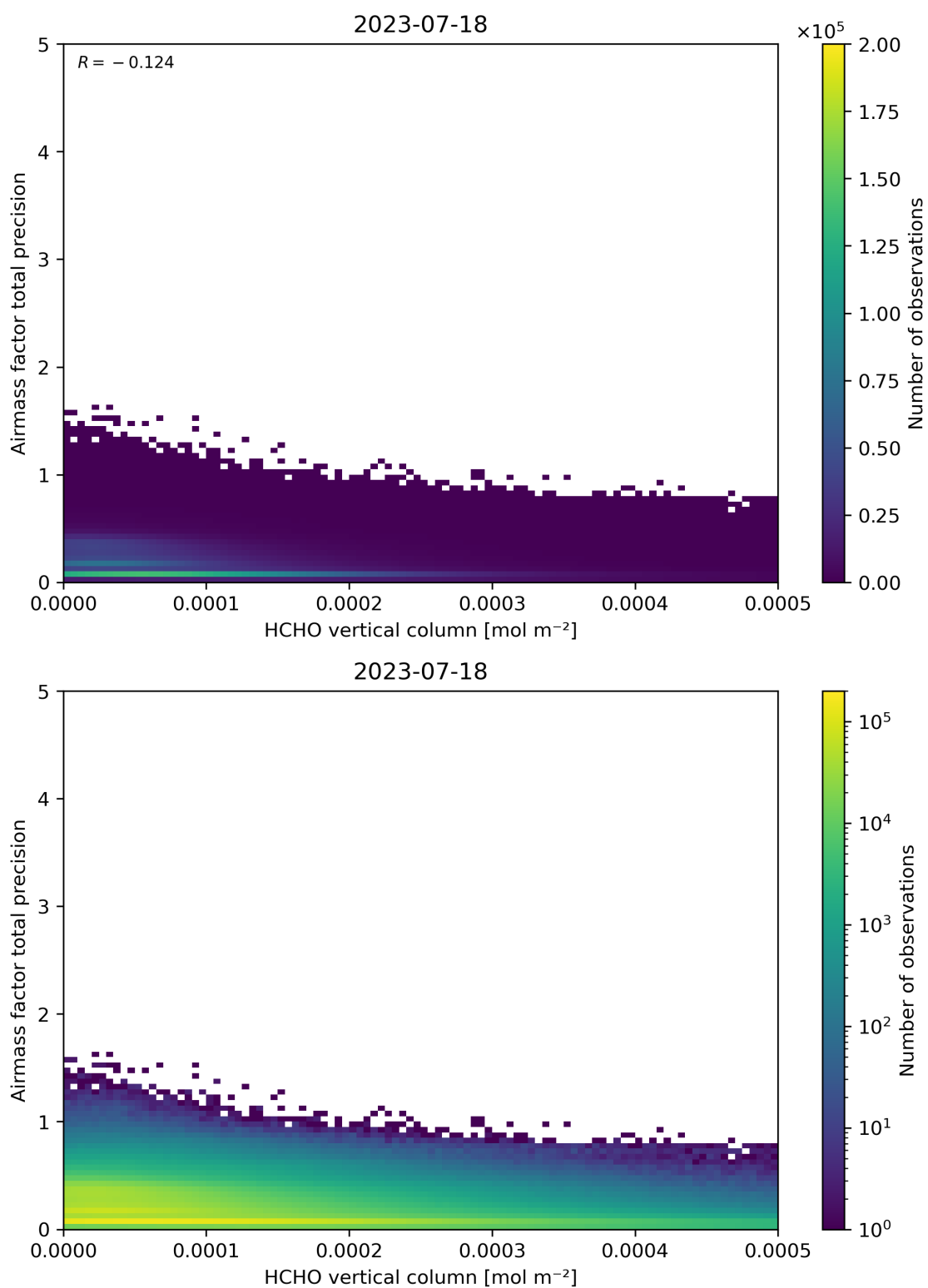
Figure 132: Scatter density plot of “HCHO vertical column” against “Airmass factor total precision” for 2023-07-17 to 2023-07-19.
