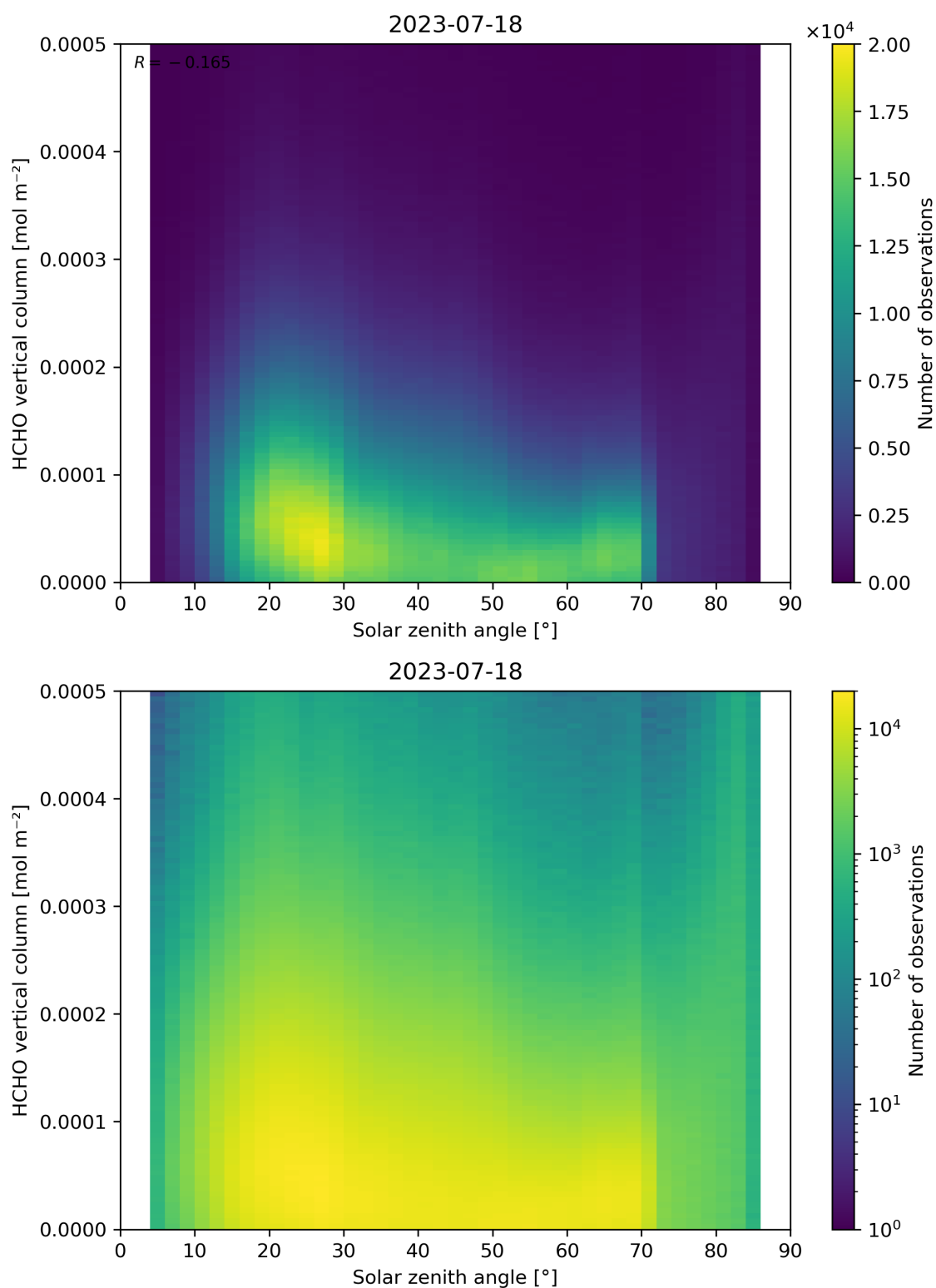
Figure 177: Scatter density plot of “Solar zenith angle” against “HCHO vertical column” for 2023-07-17 to 2023-07-19.
