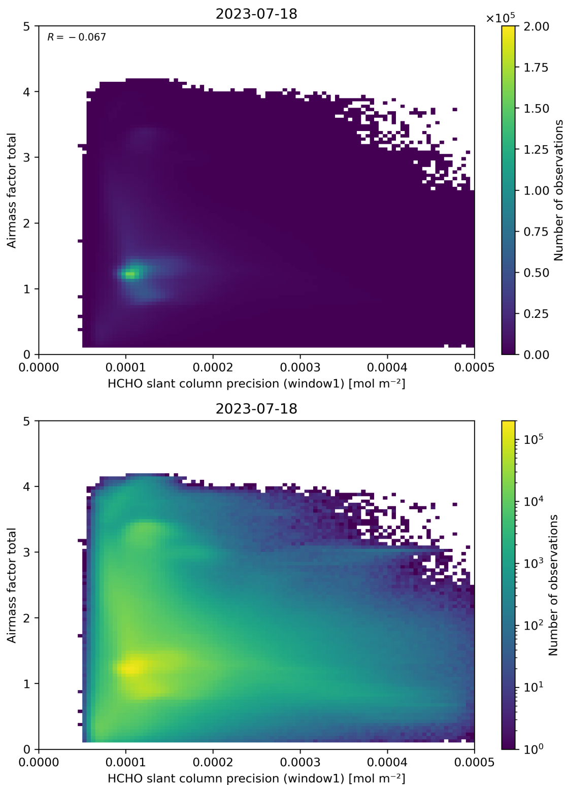
Figure 94: Scatter density plot of “HCHO slant column precision (window1)” against “Airmass factor total” for 2023-07-17 to 2023-07-19.
