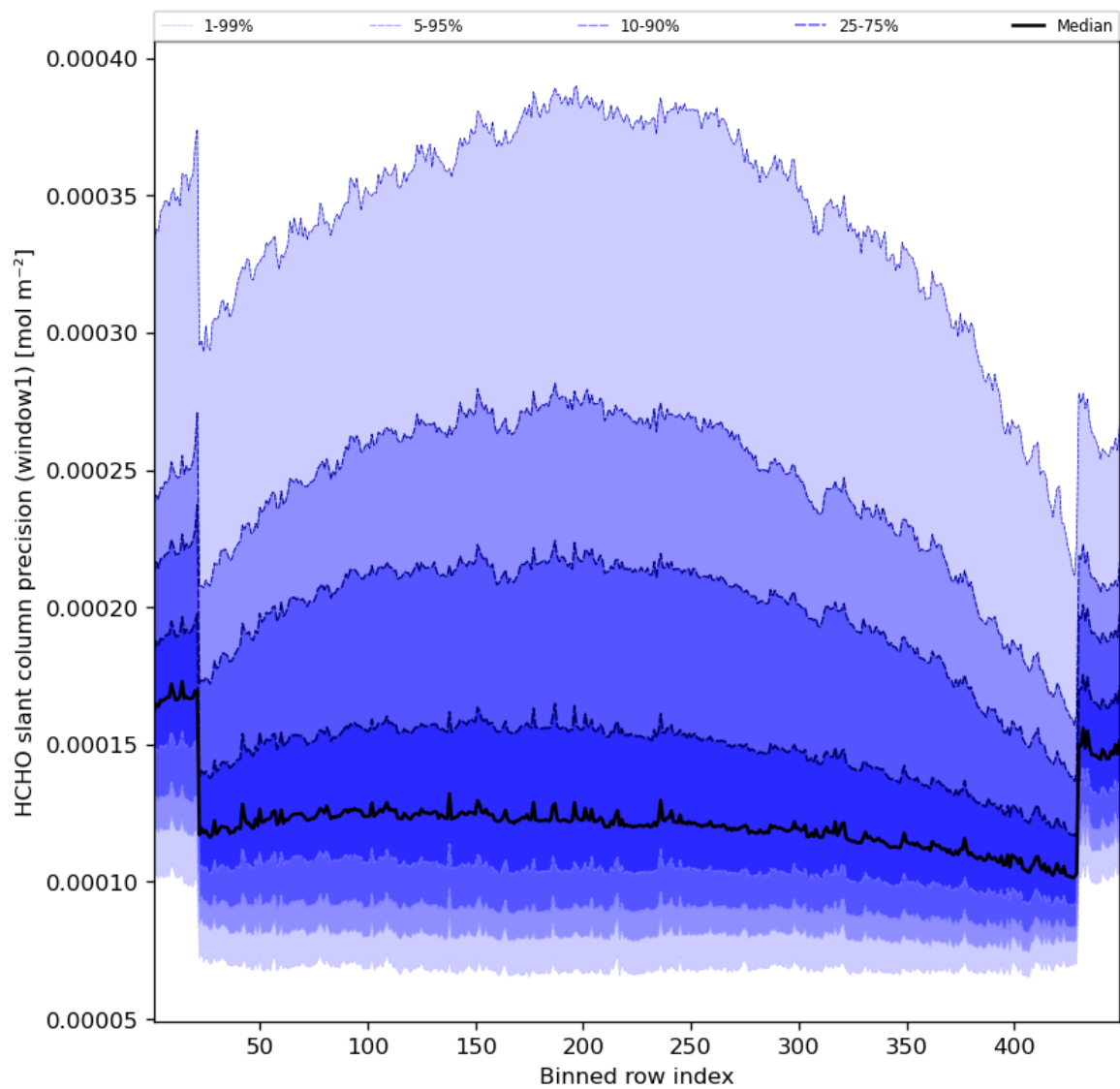
Figure 53: Along track statistics of “HCHO slant column precision (window1)” for 2023-07-17 to 2023-07-19
