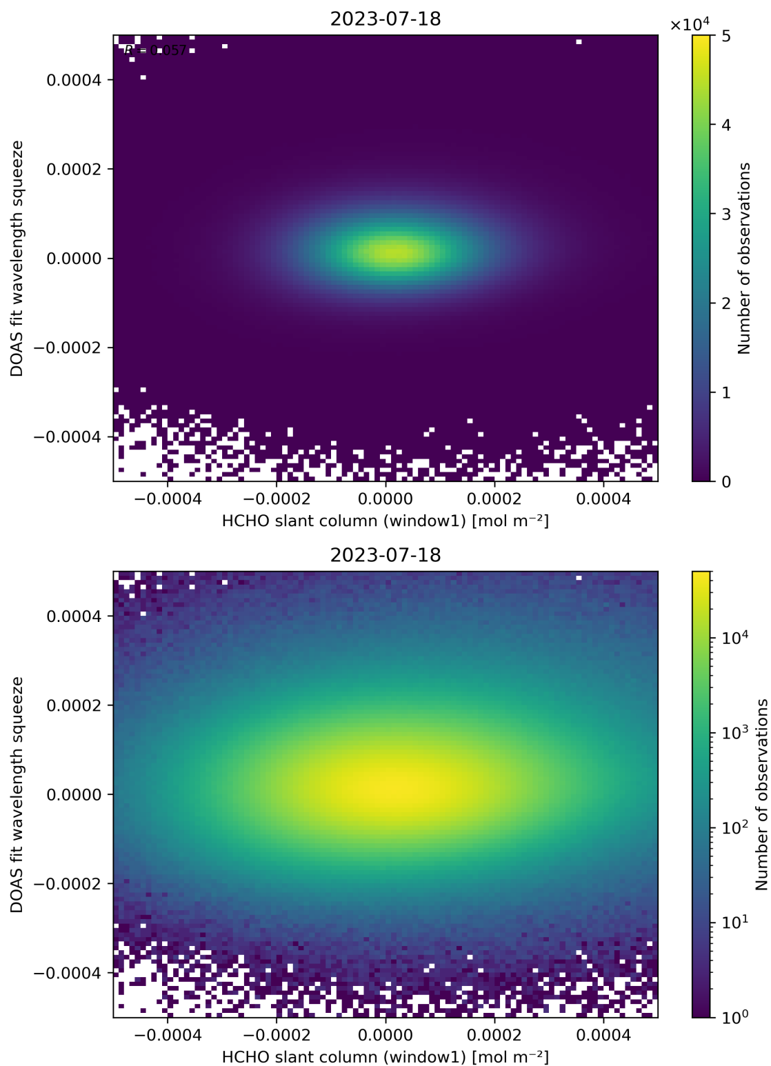
Figure 80: Scatter density plot of “HCHO slant column (window1)” against “DOAS fit wavelength squeeze” for 2023-07-17 to 2023-07-19.
