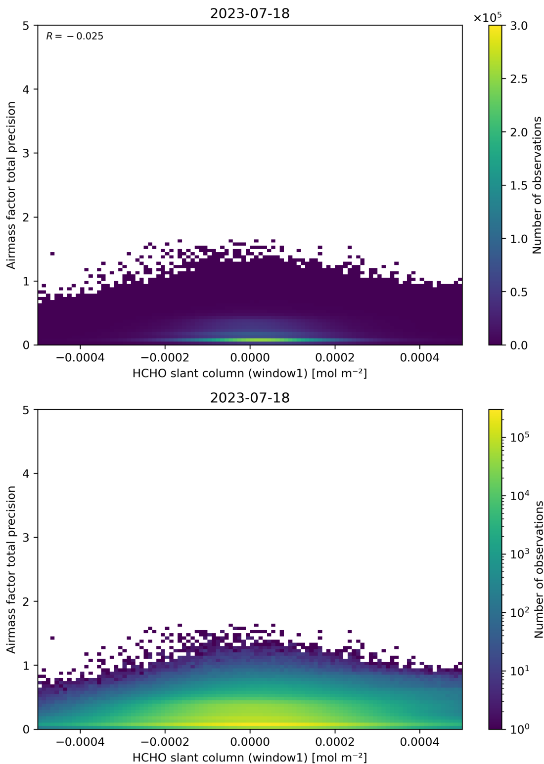
Figure 86: Scatter density plot of “HCHO slant column (window1)” against “Airmass factor total precision” for 2023-07-17 to 2023-07-19.
