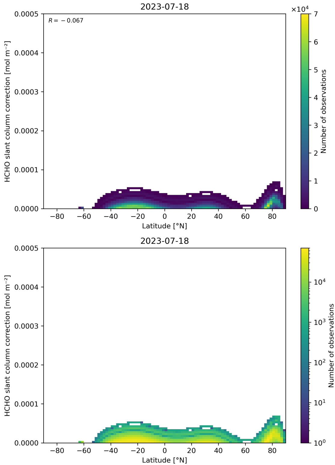
Figure 158: Scatter density plot of “Latitude” against “HCHO slant column correction” for 2023-07-17 to 2023-07-19.
