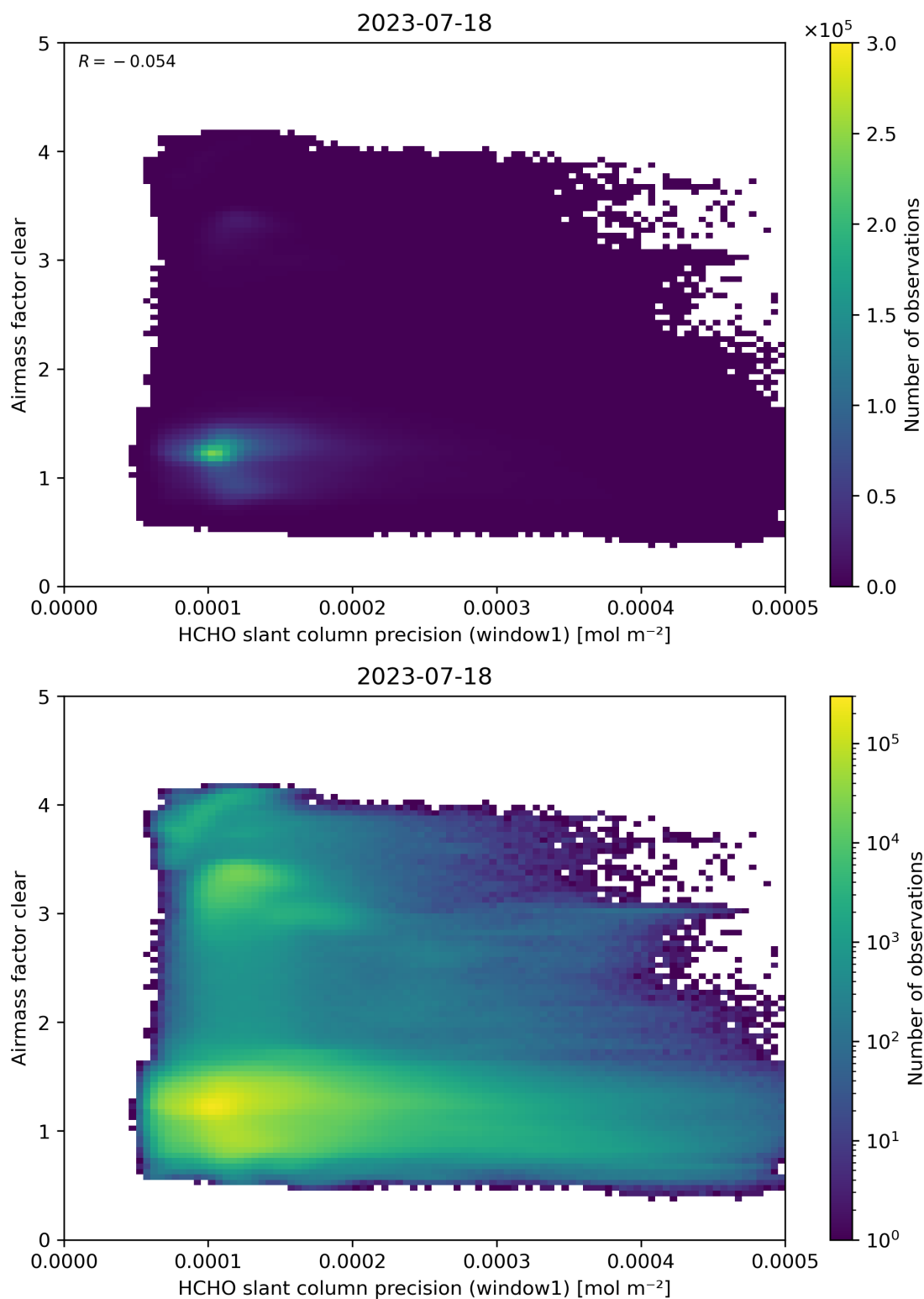
Figure 91: Scatter density plot of “HCHO slant column precision (window1)” against “Airmass factor clear” for 2023-07-17 to 2023-07-19.
