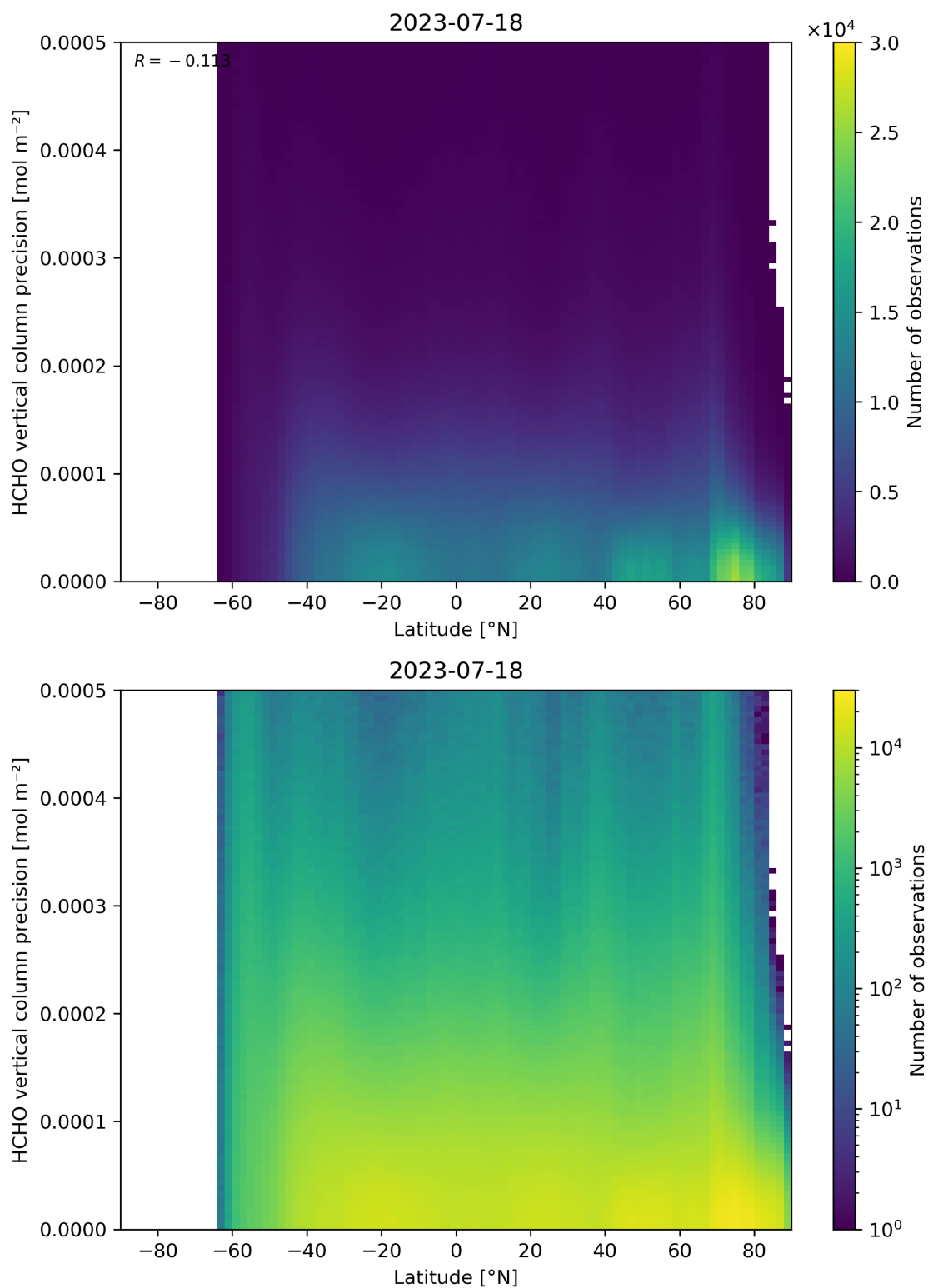
Figure 165: Scatter density plot of “Latitude” against “HCHO vertical column precision” for 2023-07-17 to 2023-07-19.
