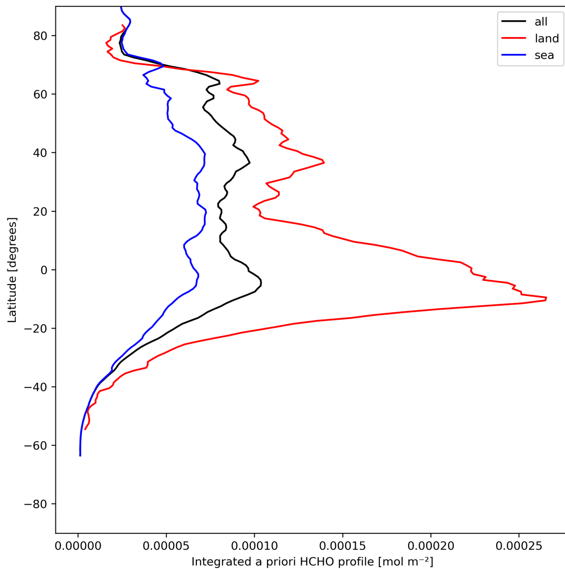
Figure 29: Zonal average of “Integrated a priori HCHO profile” for 2023-07-17 to 2023-07-19.
