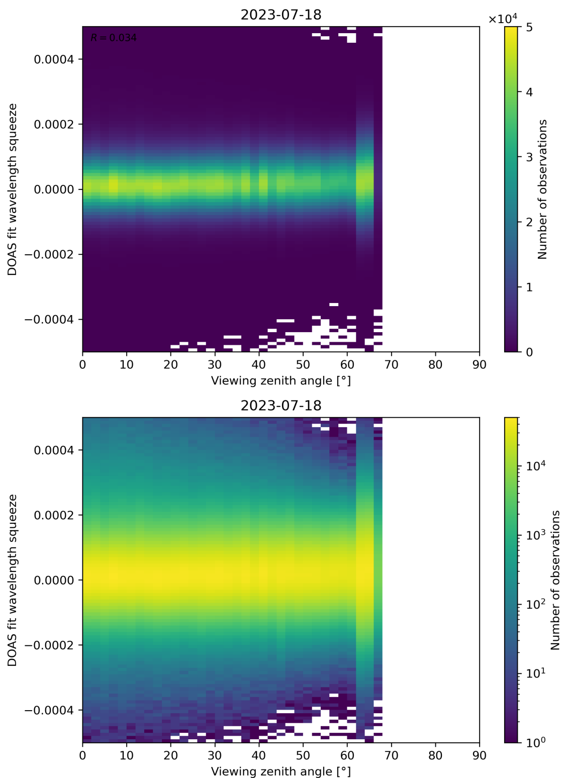
Figure 184: Scatter density plot of “Viewing zenith angle” against “DOAS fit wavelength squeeze” for 2023-07-17 to 2023-07-19.
