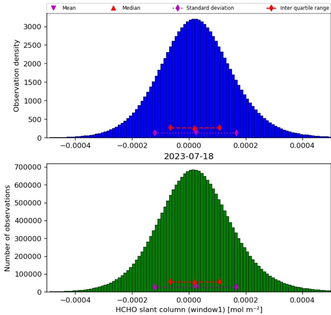
Figure 38: Histogram of “HCHO slant column (window1)” for 2023-07-17 to 2023-07-19
