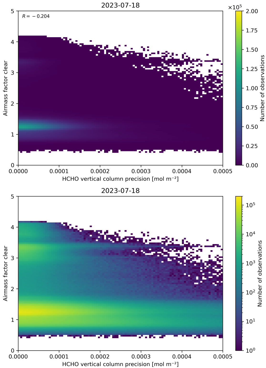
Figure 139: Scatter density plot of “HCHO vertical column precision” against “Airmass factor clear” for 2023-07-17 to 2023-07-19.
