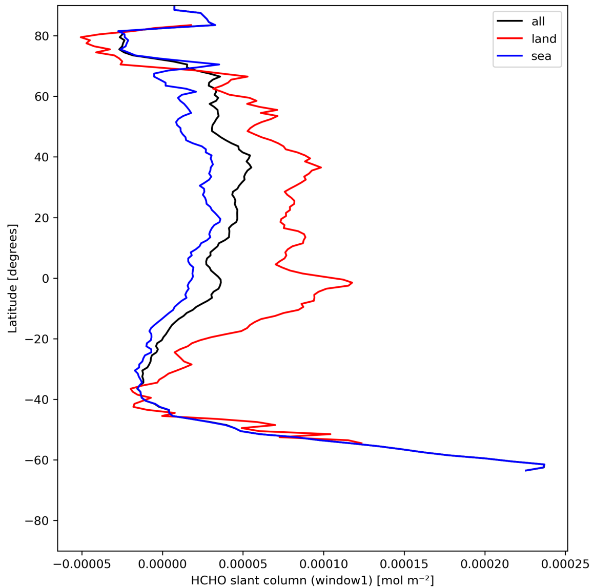
Figure 24: Zonal average of “HCHO slant column (window1)” for 2023-07-17 to 2023-07-19.
