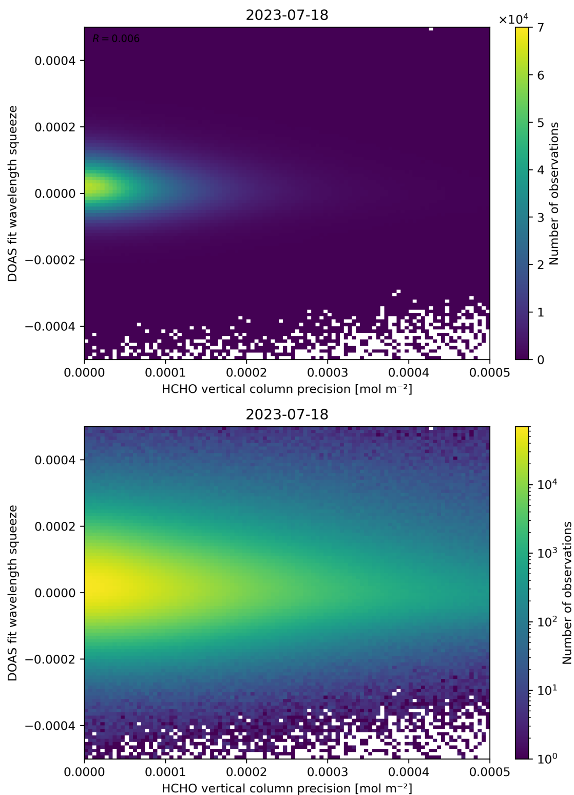
Figure 138: Scatter density plot of “HCHO vertical column precision” against “DOAS fit wavelength squeeze” for 2023-07-17 to 2023-07-19.
