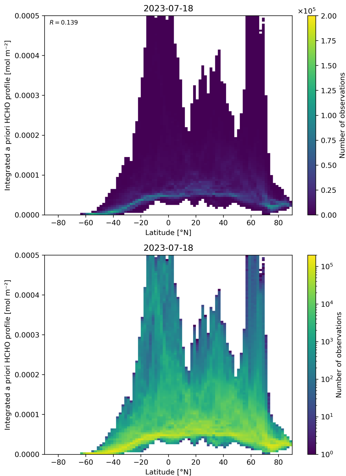
Figure 166: Scatter density plot of “Latitude” against “Integrated a priori HCHO profile” for 2023-07-17 to 2023-07-19.
