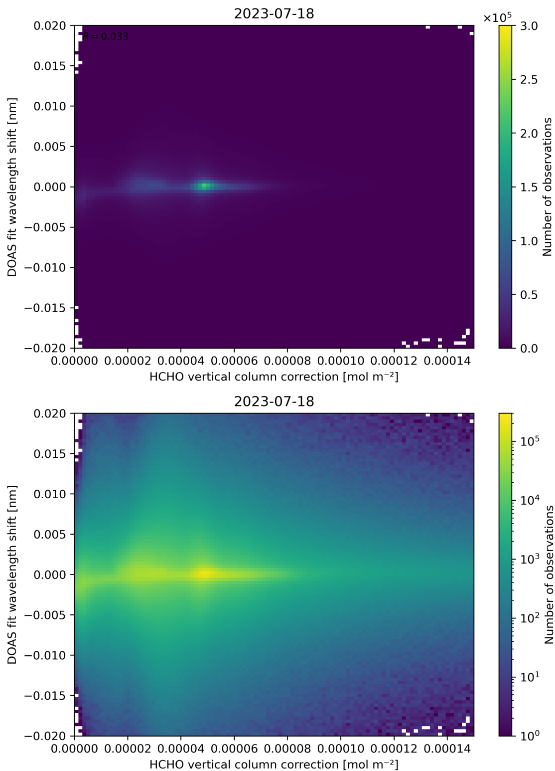
Figure 113: Scatter density plot of “HCHO vertical column correction” against “DOAS fit wavelength shift” for 2023-07-17 to 2023-07-19.
