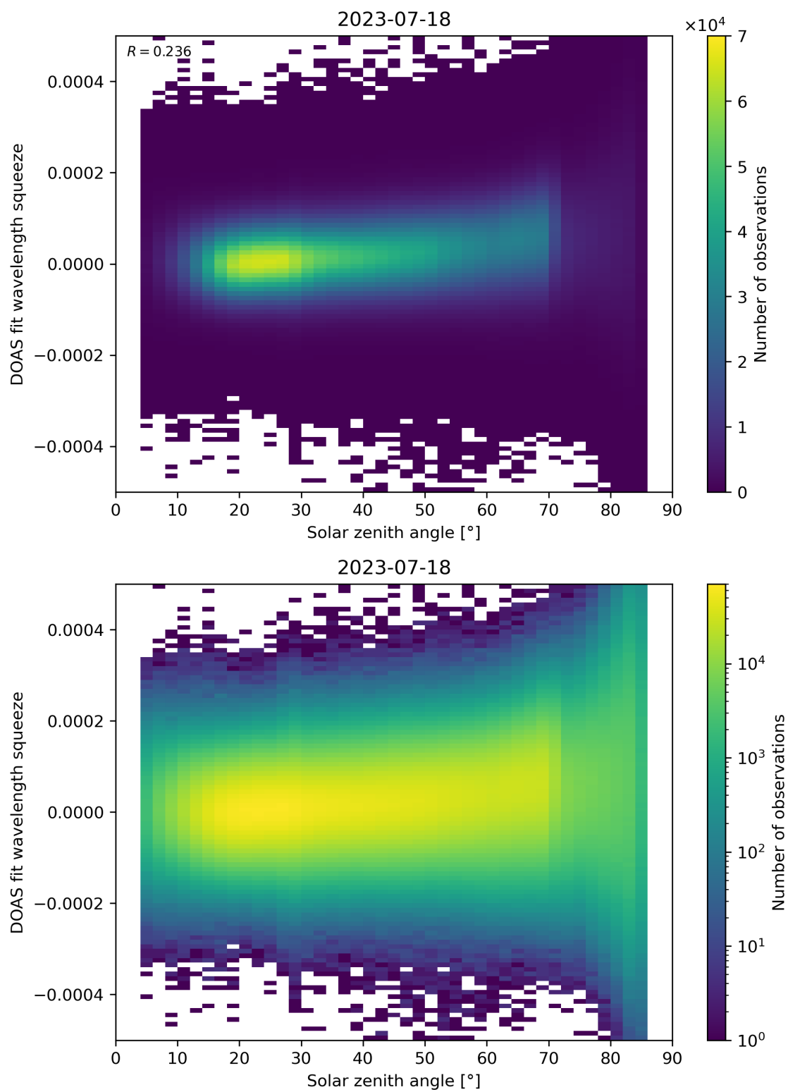
Figure 169: Scatter density plot of “Solar zenith angle” against “DOAS fit wavelength squeeze” for 2023-07-17 to 2023-07-19.
