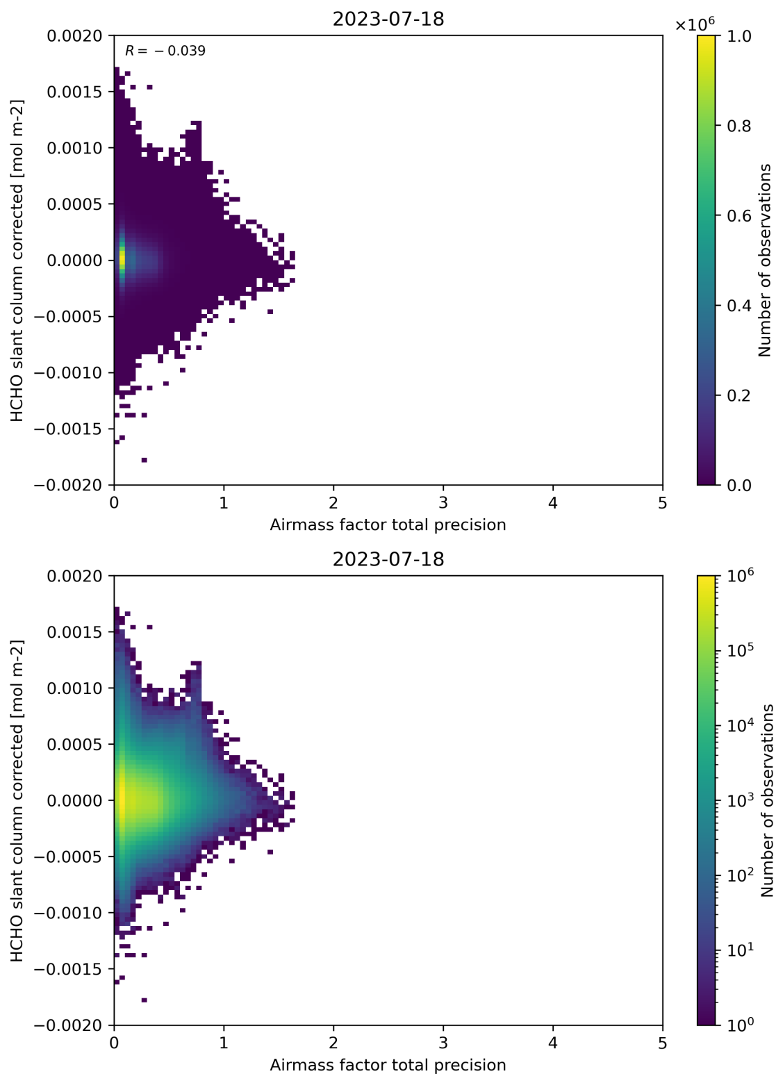
Figure 109: Scatter density plot of “Airmass factor total precision” against “HCHO slant column corrected” for 2023-07-17 to 2023-07-19.
