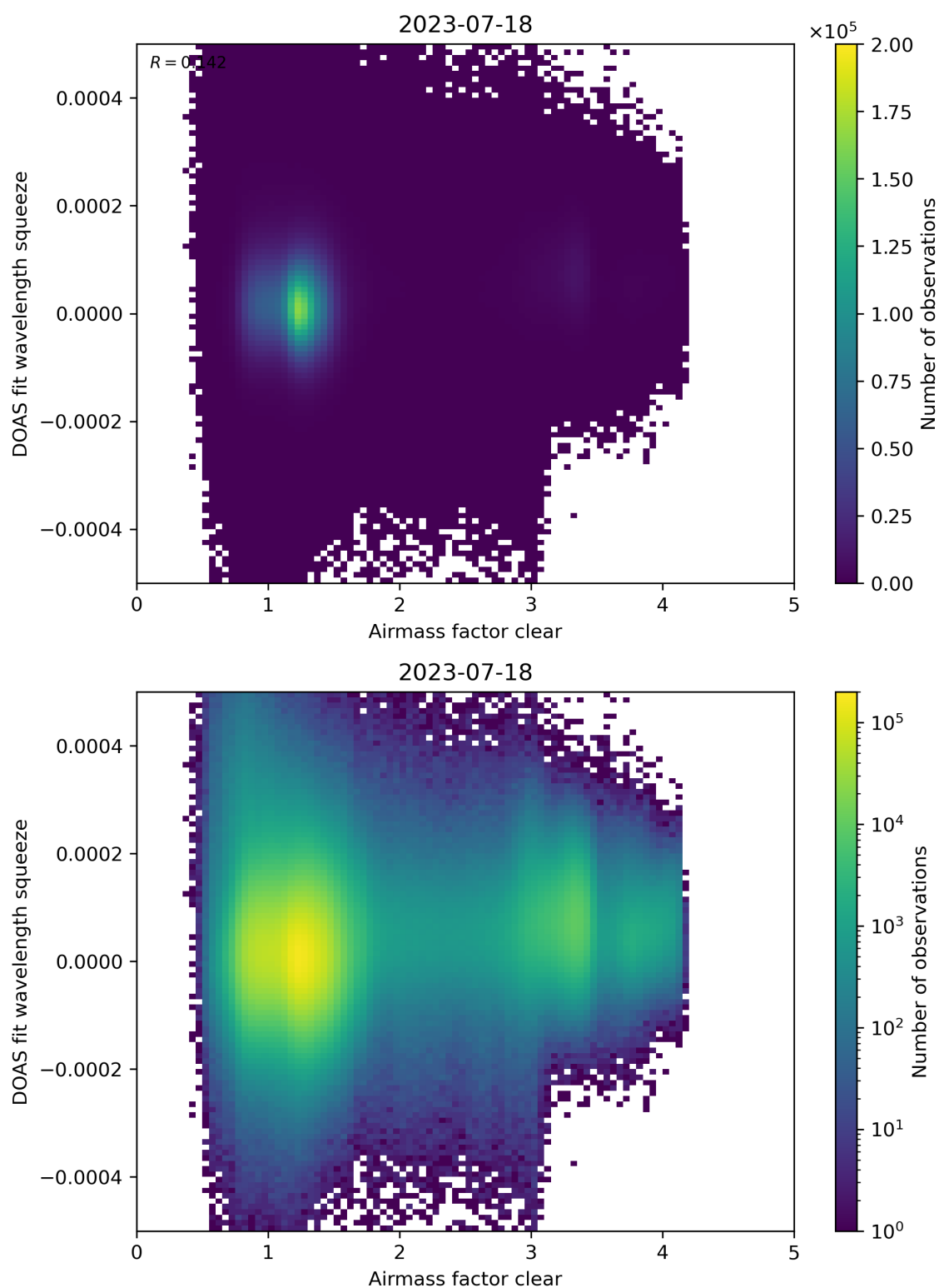
Figure 73: Scatter density plot of “Airmass factor clear” against “DOAS fit wavelength squeeze” for 2023-07-17 to 2023-07-19.
