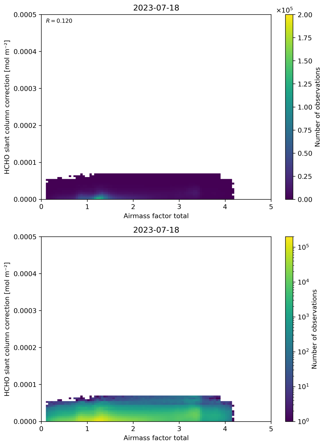
Figure 102: Scatter density plot of “Airmass factor total” against “HCHO slant column correction” for 2023-07-17 to 2023-07-19.
