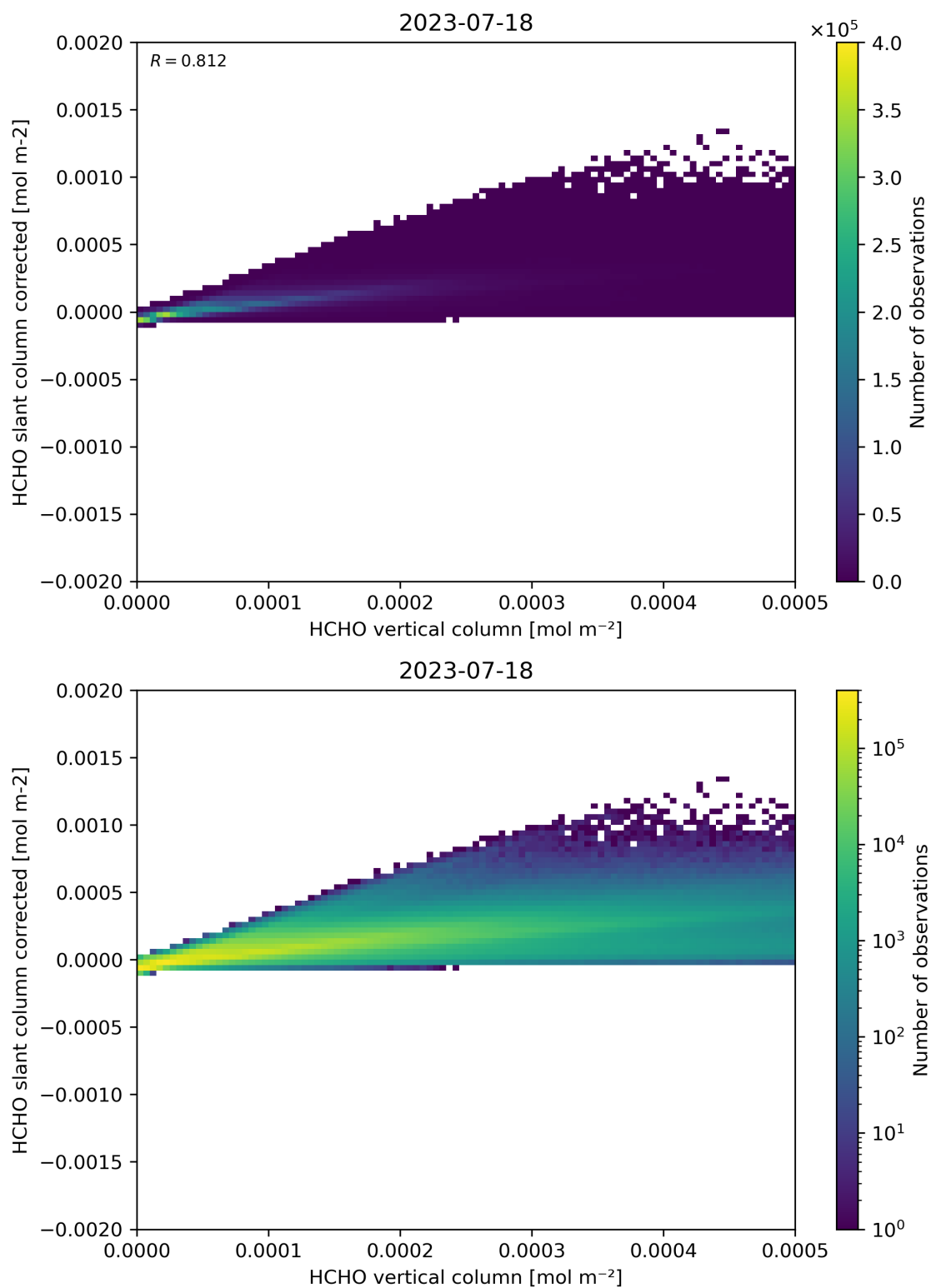
Figure 127: Scatter density plot of “HCHO vertical column” against “HCHO slant column corrected” for 2023-07-17 to 2023-07-19.
