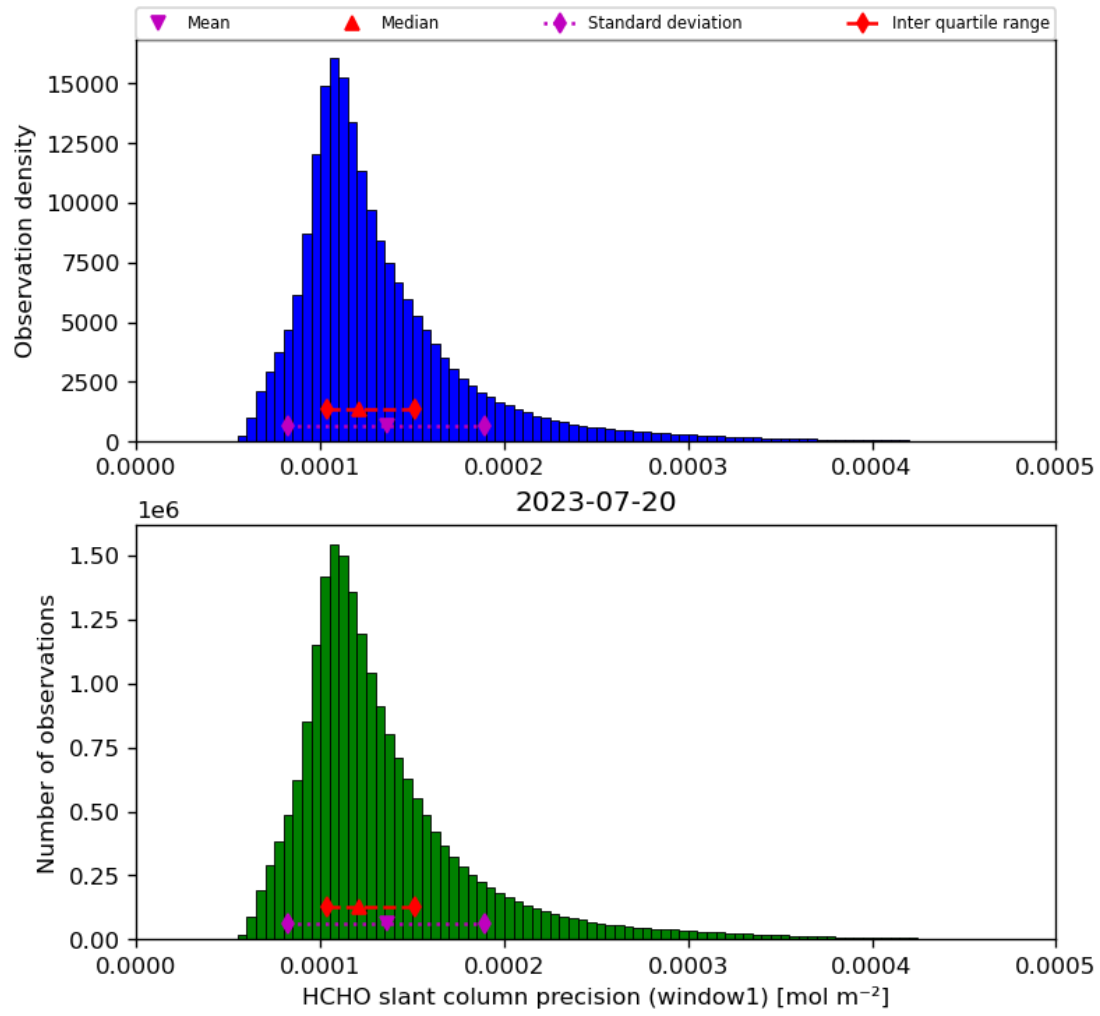
Figure 39: Histogram of “HCHO slant column precision (window1)” for 2023-07-19 to 2023-07-21
