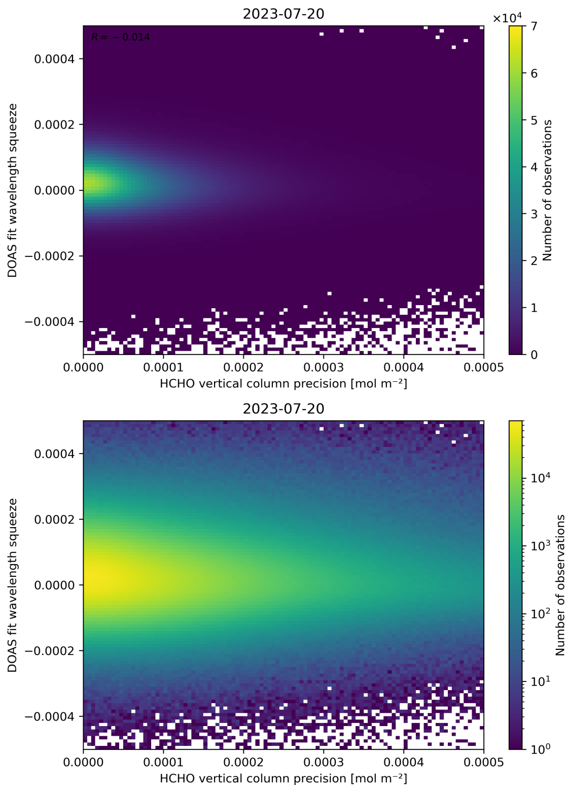
Figure 138: Scatter density plot of “HCHO vertical column precision” against “DOAS fit wavelength squeeze” for 2023-07-19 to 2023-07-21.
