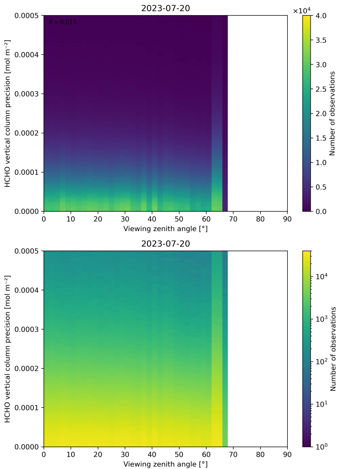
Figure 194: Scatter density plot of “Viewing zenith angle” against “HCHO vertical column precision” for 2023-07-19 to 2023-07-21.
