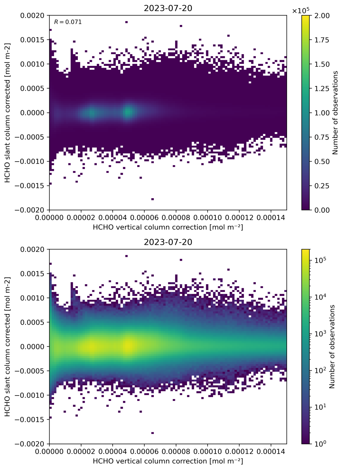
Figure 116: Scatter density plot of “HCHO vertical column correction” against “HCHO slant column corrected” for 2023-07-19 to 2023-07-21.
