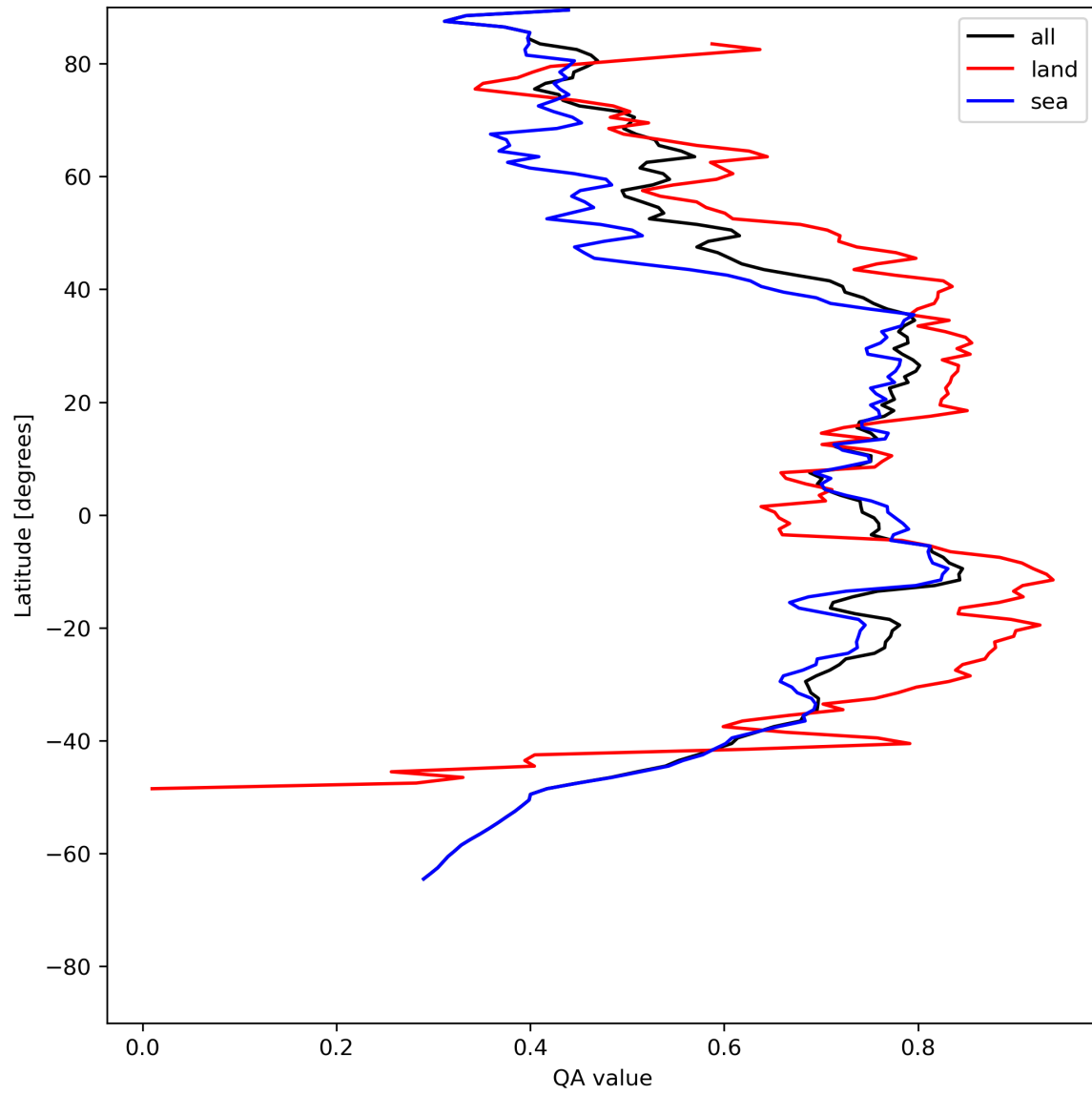
Figure 20: Zonal average of “QA value” for 2023-07-19 to 2023-07-21.
