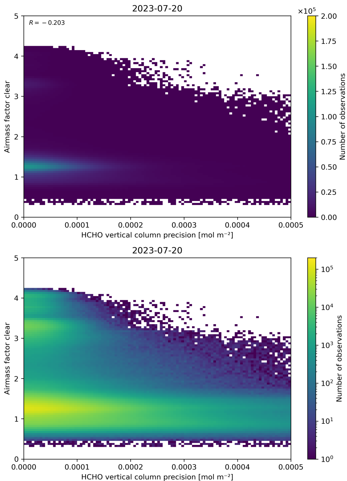
Figure 139: Scatter density plot of “HCHO vertical column precision” against “Airmass factor clear” for 2023-07-19 to 2023-07-21.
