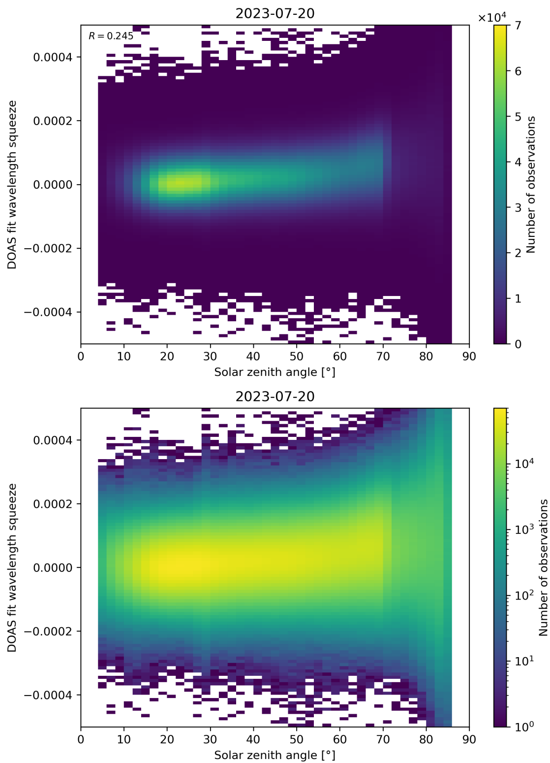
Figure 169: Scatter density plot of “Solar zenith angle” against “DOAS fit wavelength squeeze” for 2023-07-19 to 2023-07-21.
