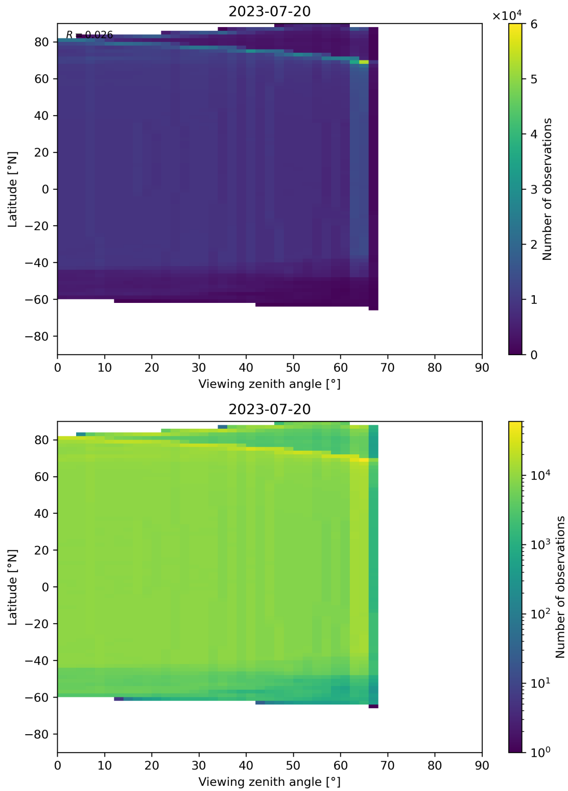
Figure 196: Scatter density plot of “Viewing zenith angle” against “Latitude” for 2023-07-19 to 2023-07-21.
