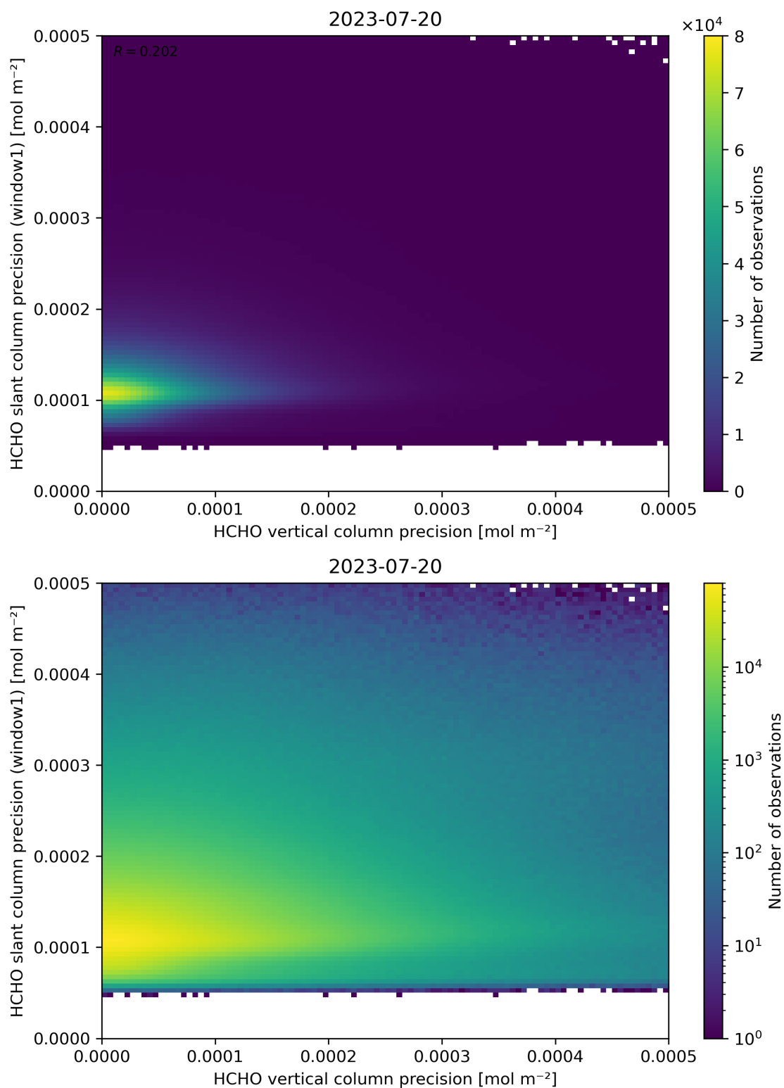
Figure 143: Scatter density plot of “HCHO vertical column precision” against “HCHO slant column precision (window1)” for 2023-07-19 to 2023-07-21.
