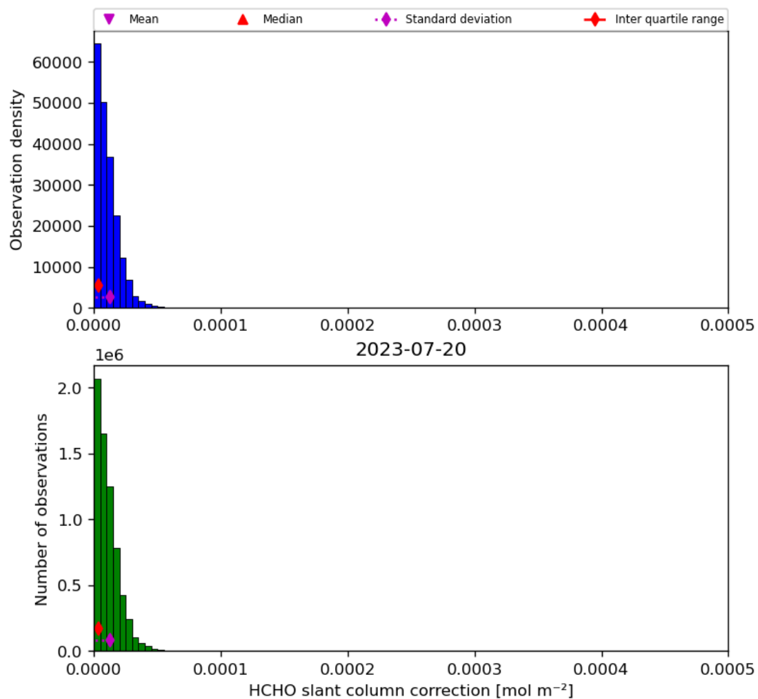
Figure 47: Histogram of “HCHO slant column correction” for 2023-07-19 to 2023-07-21
