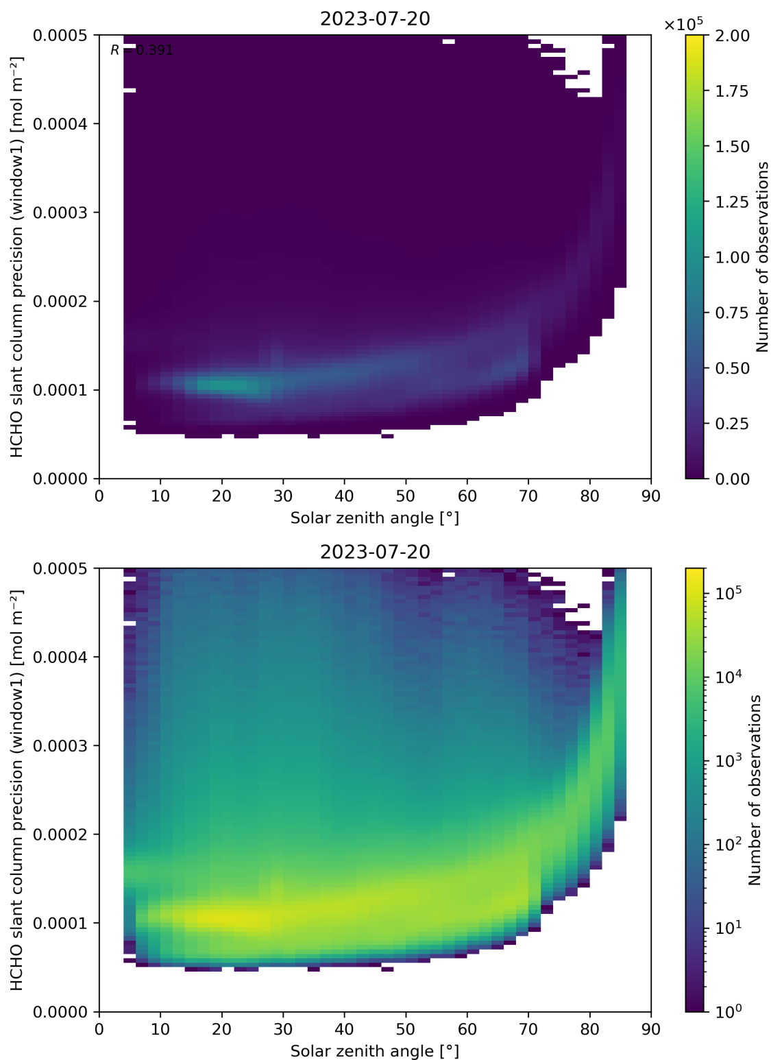
Figure 174: Scatter density plot of “Solar zenith angle” against “HCHO slant column precision (window1)” for 2023-07-19 to 2023-07-21.
