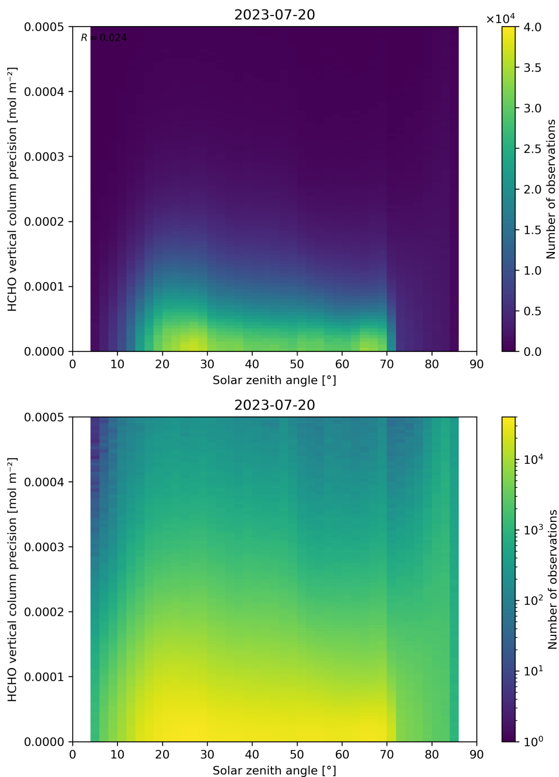
Figure 179: Scatter density plot of “Solar zenith angle” against “HCHO vertical column precision” for 2023-07-19 to 2023-07-21.
