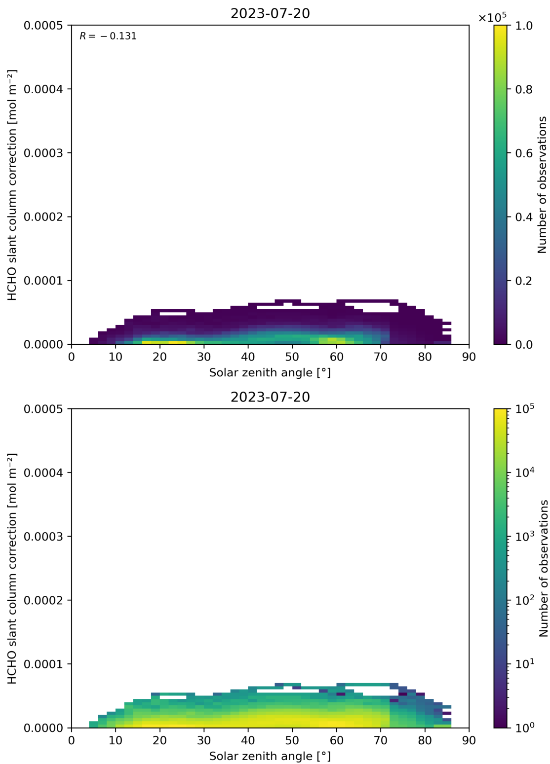
Figure 172: Scatter density plot of “Solar zenith angle” against “HCHO slant column correction” for 2023-07-19 to 2023-07-21.
