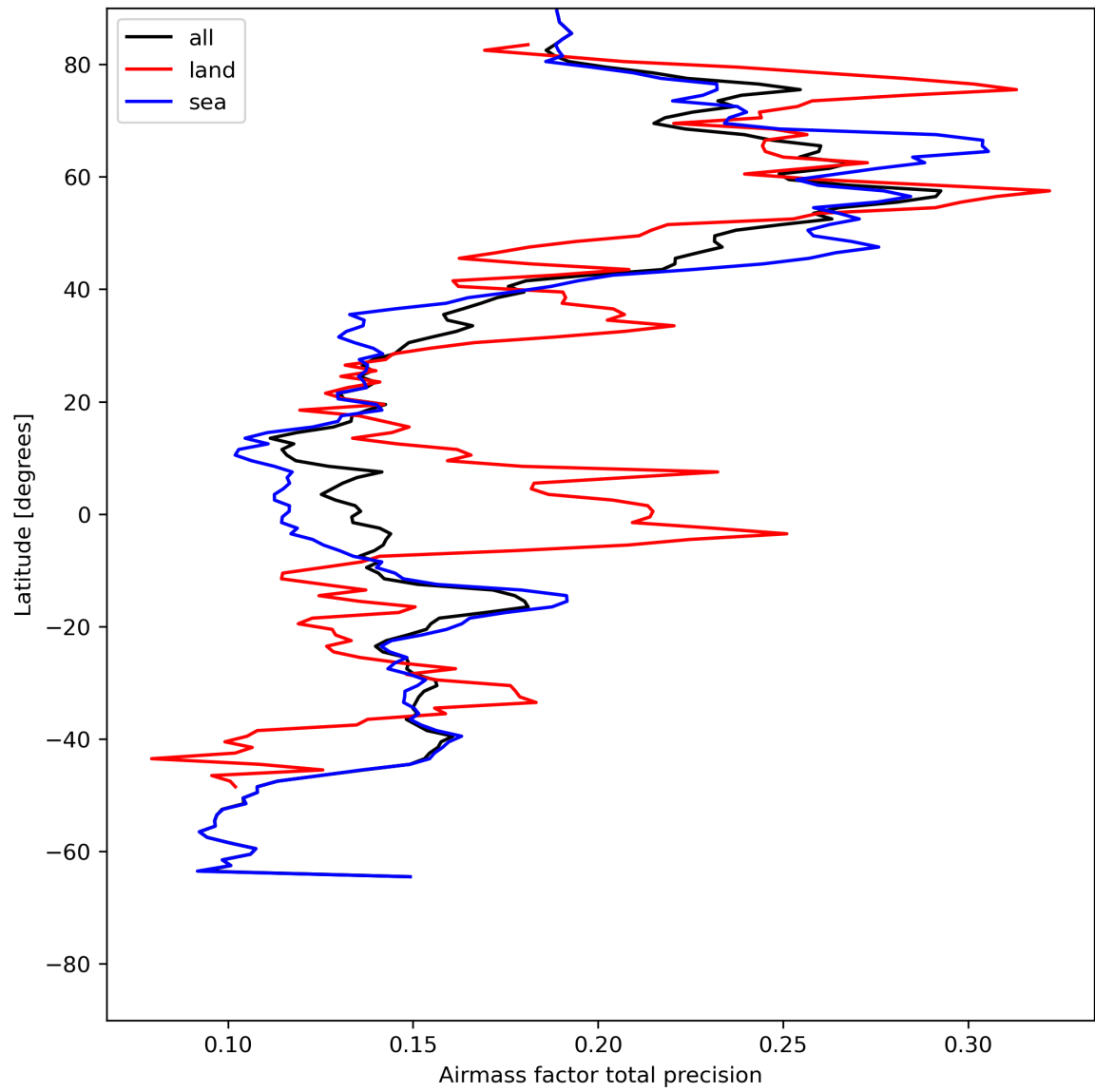
Figure 27: Zonal average of “Airmass factor total precision” for 2023-07-19 to 2023-07-21.
