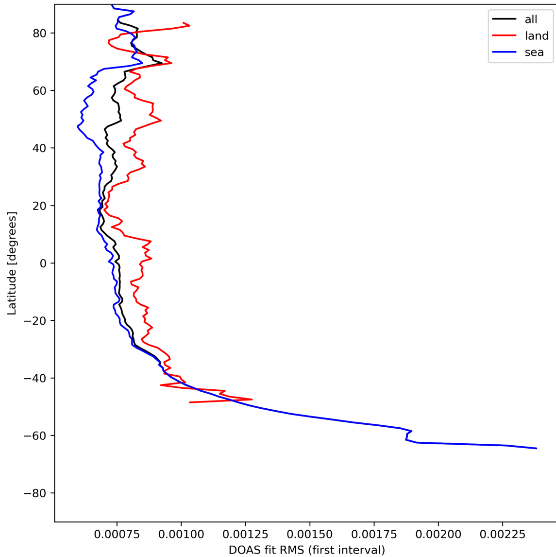
Figure 32: Zonal average of “DOAS fit RMS (first interval)” for 2023-07-19 to 2023-07-21.
