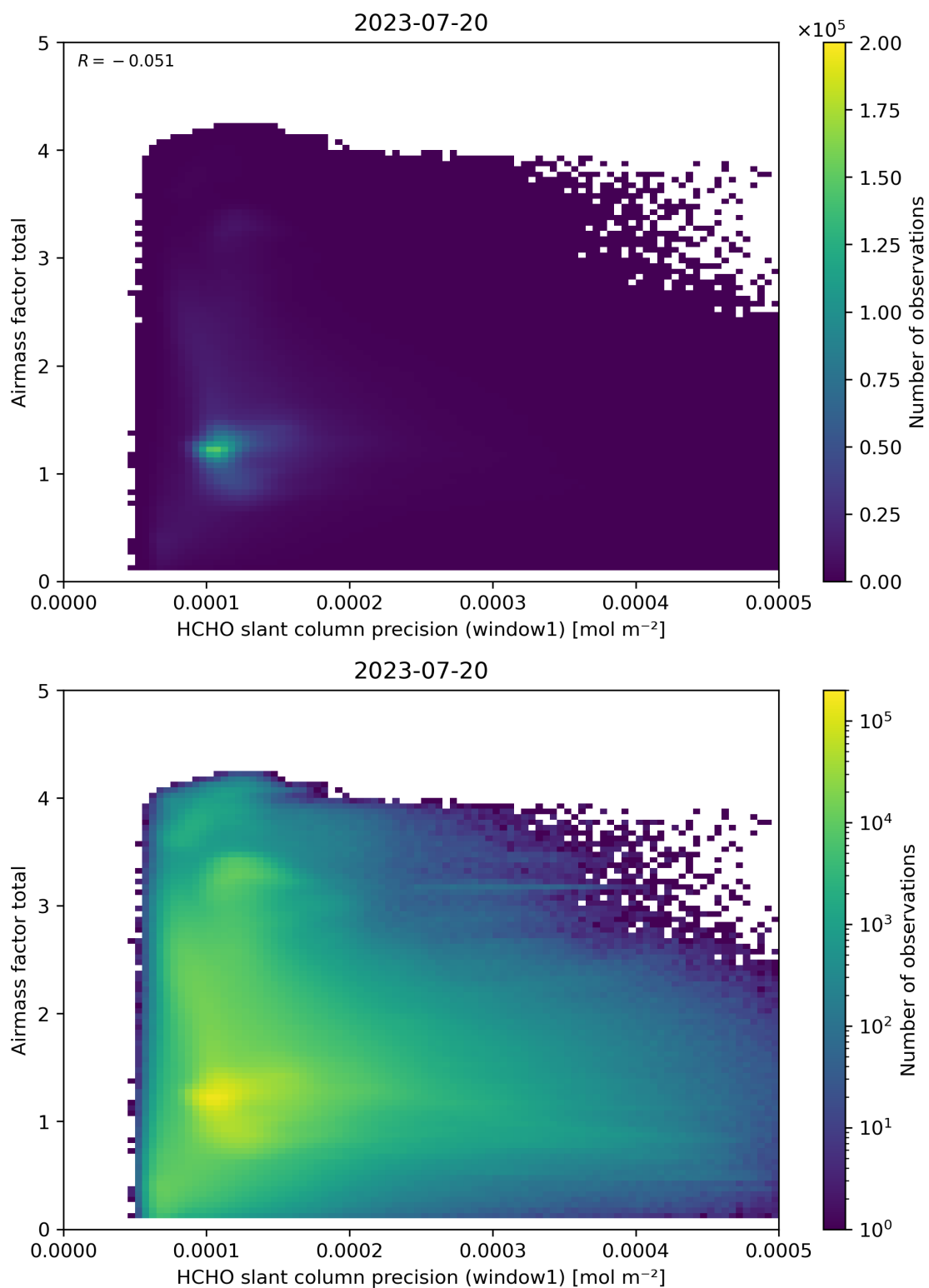
Figure 94: Scatter density plot of “HCHO slant column precision (window1)” against “Airmass factor total” for 2023-07-19 to 2023-07-21.
