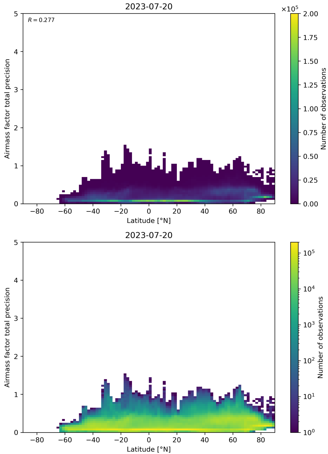
Figure 162: Scatter density plot of “Latitude” against “Airmass factor total precision” for 2023-07-19 to 2023-07-21.
