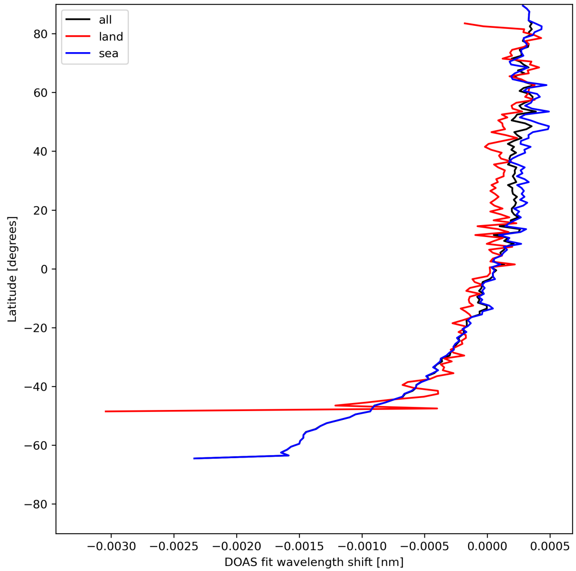
Figure 30: Zonal average of “DOAS fit wavelength shift” for 2023-07-19 to 2023-07-21.
