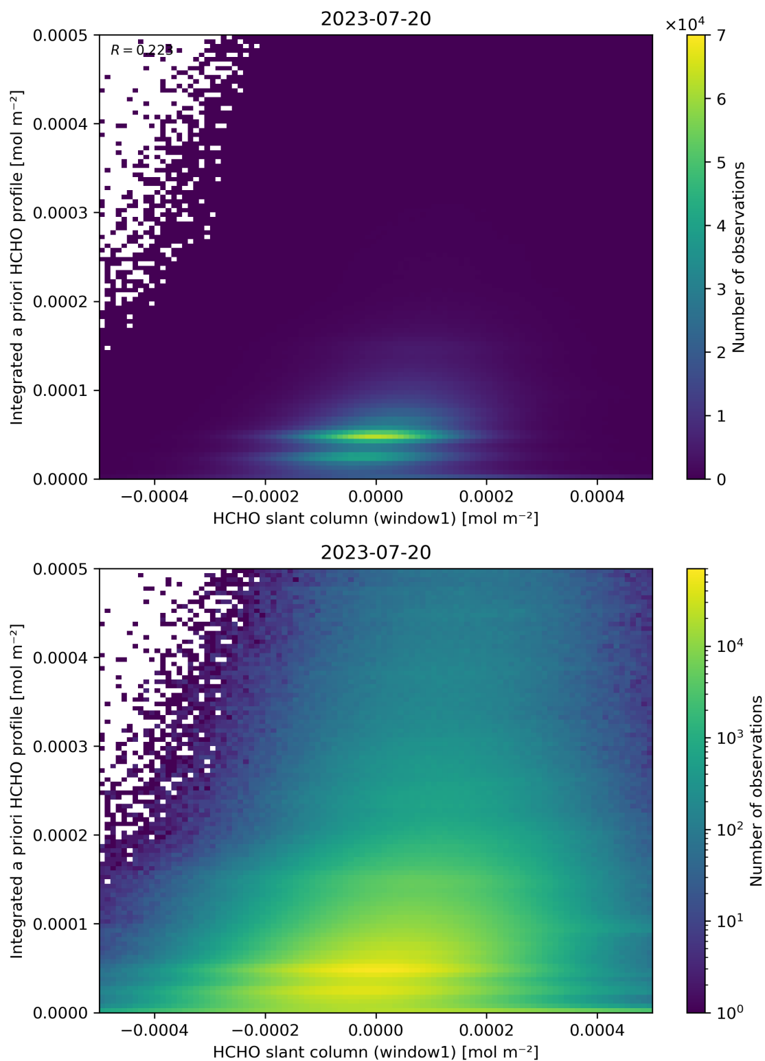
Figure 87: Scatter density plot of “HCHO slant column (window1)” against “Integrated a priori HCHO profile” for 2023-07-19 to 2023-07-21.
