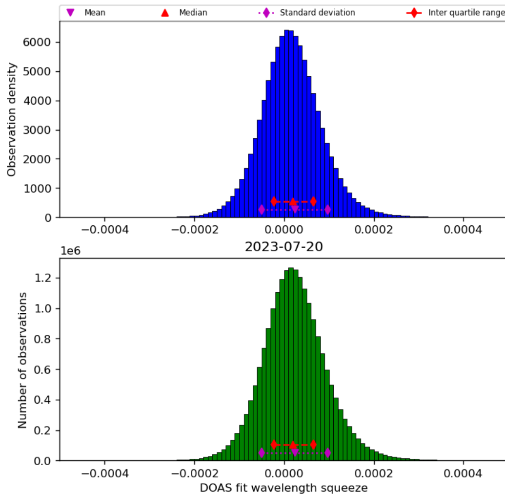
Figure 45: Histogram of “DOAS fit wavelength squeeze” for 2023-07-19 to 2023-07-21
