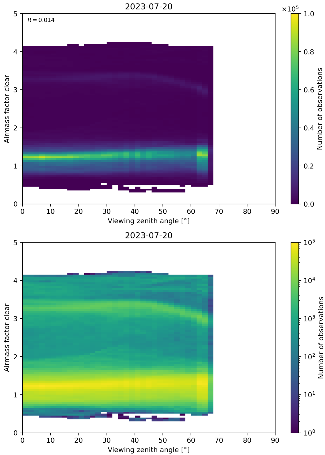
Figure 185: Scatter density plot of “Viewing zenith angle” against “Airmass factor clear” for 2023-07-19 to 2023-07-21.
