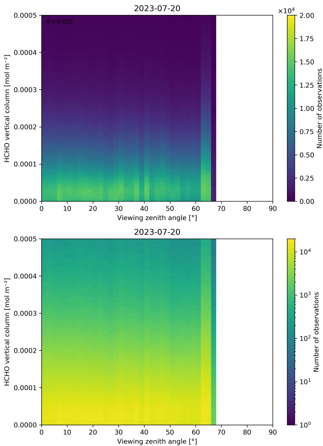
Figure 192: Scatter density plot of “Viewing zenith angle” against “HCHO vertical column” for 2023-07-19 to 2023-07-21.
