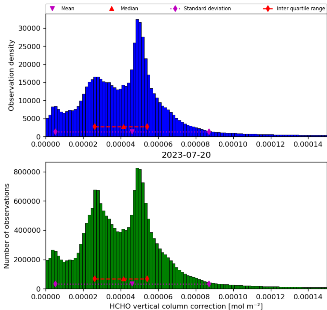
Figure 37: Histogram of “HCHO vertical column correction” for 2023-07-19 to 2023-07-21
