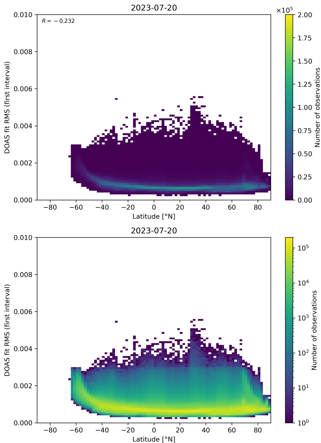
Figure 153: Scatter density plot of “Latitude” against “DOAS fit RMS (first interval)” for 2023-07-19 to 2023-07-21.
