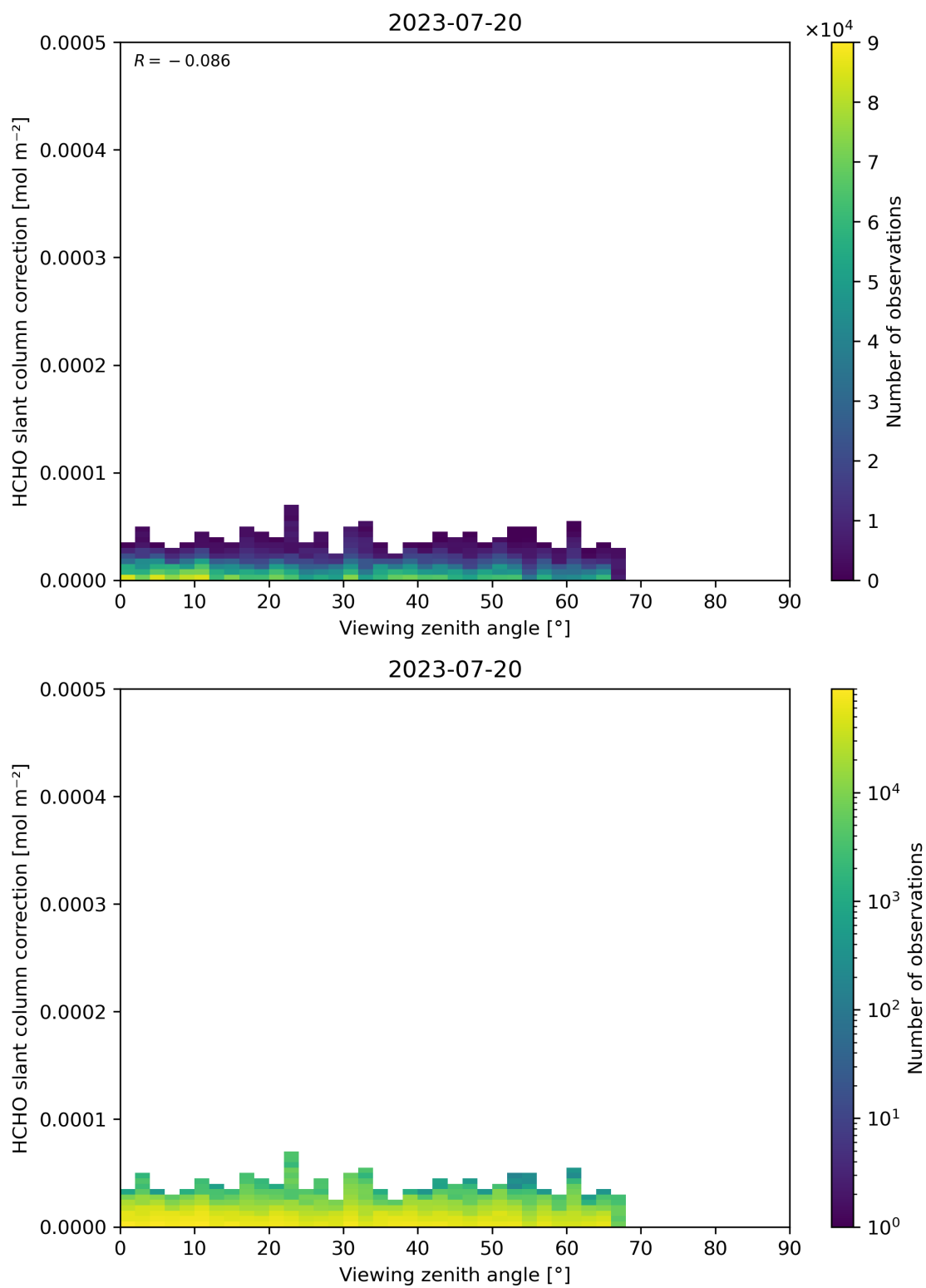
Figure 187: Scatter density plot of “Viewing zenith angle” against “HCHO slant column correction” for 2023-07-19 to 2023-07-21.
