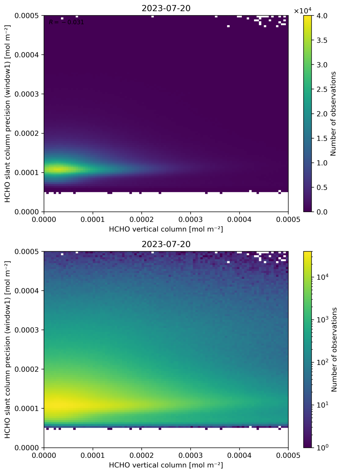
Figure 130: Scatter density plot of “HCHO vertical column” against “HCHO slant column precision (window1)” for 2023-07-19 to 2023-07-21.
