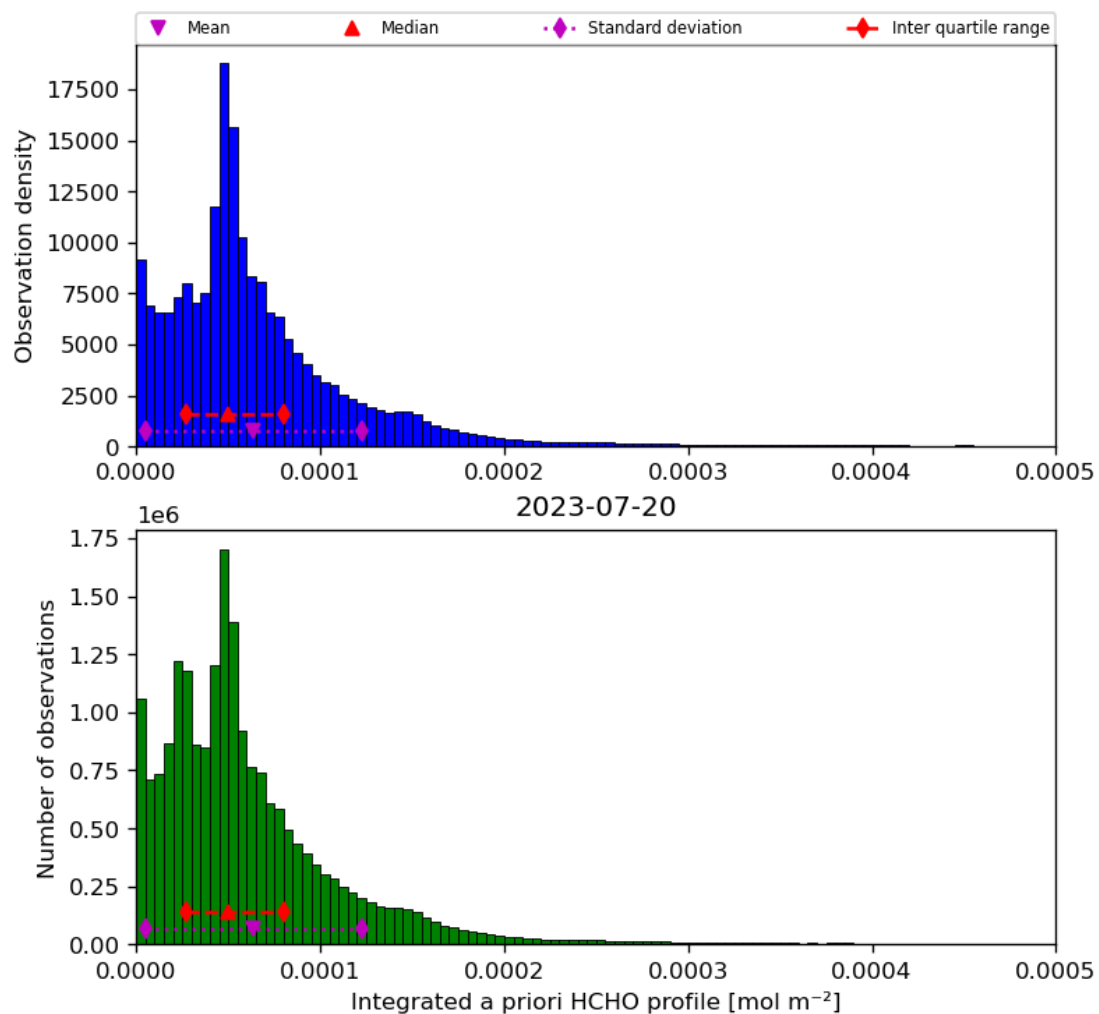
Figure 43: Histogram of “Integrated a priori HCHO profile” for 2023-07-19 to 2023-07-21
