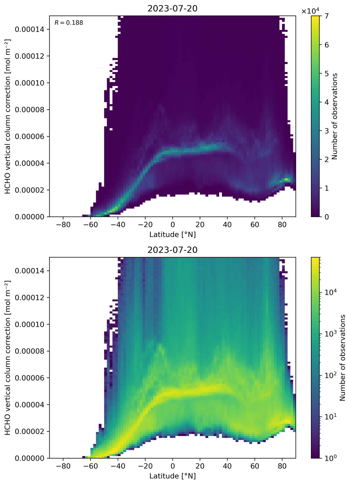
Figure 164: Scatter density plot of “Latitude” against “HCHO vertical column correction” for 2023-07-19 to 2023-07-21.
