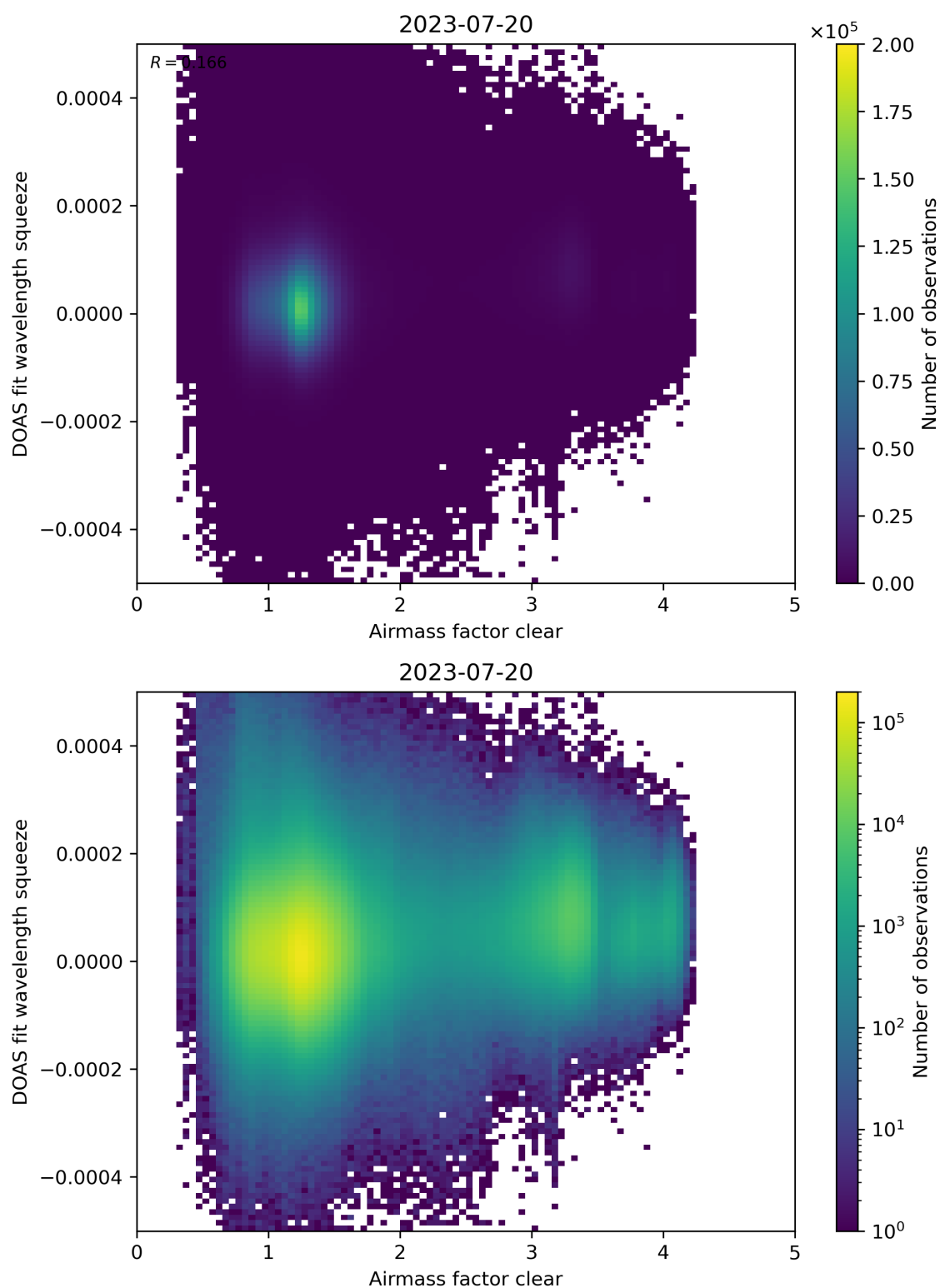
Figure 73: Scatter density plot of “Airmass factor clear” against “DOAS fit wavelength squeeze” for 2023-07-19 to 2023-07-21.
