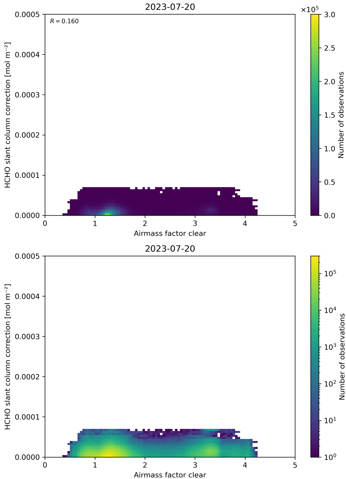
Figure 75: Scatter density plot of “Airmass factor clear” against “HCHO slant column correction” for 2023-07-19 to 2023-07-21.
