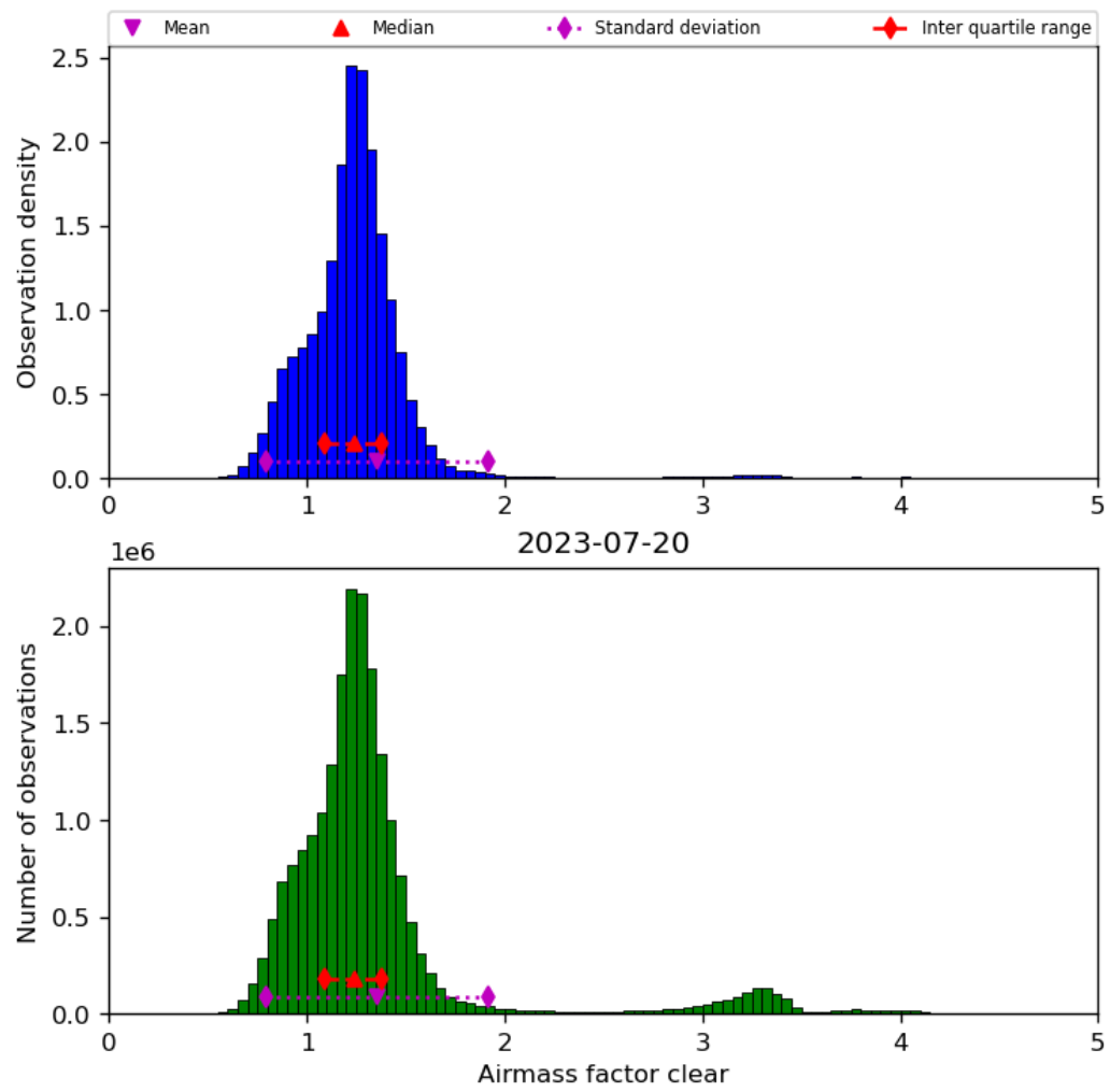
Figure 42: Histogram of “Airmass factor clear” for 2023-07-19 to 2023-07-21
