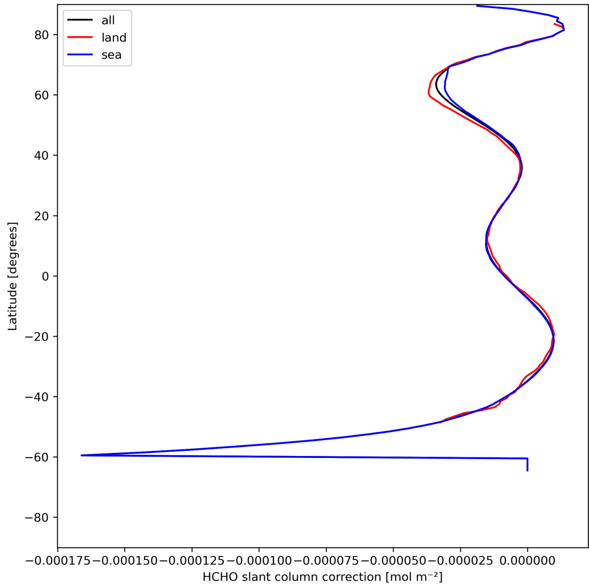
Figure 33: Zonal average of “HCHO slant column correction” for 2023-07-19 to 2023-07-21.
