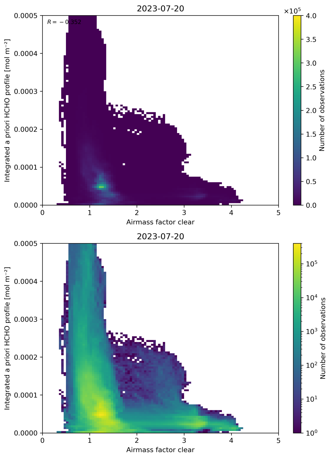
Figure 76: Scatter density plot of “Airmass factor clear” against “Integrated a priori HCHO profile” for 2023-07-19 to 2023-07-21.
