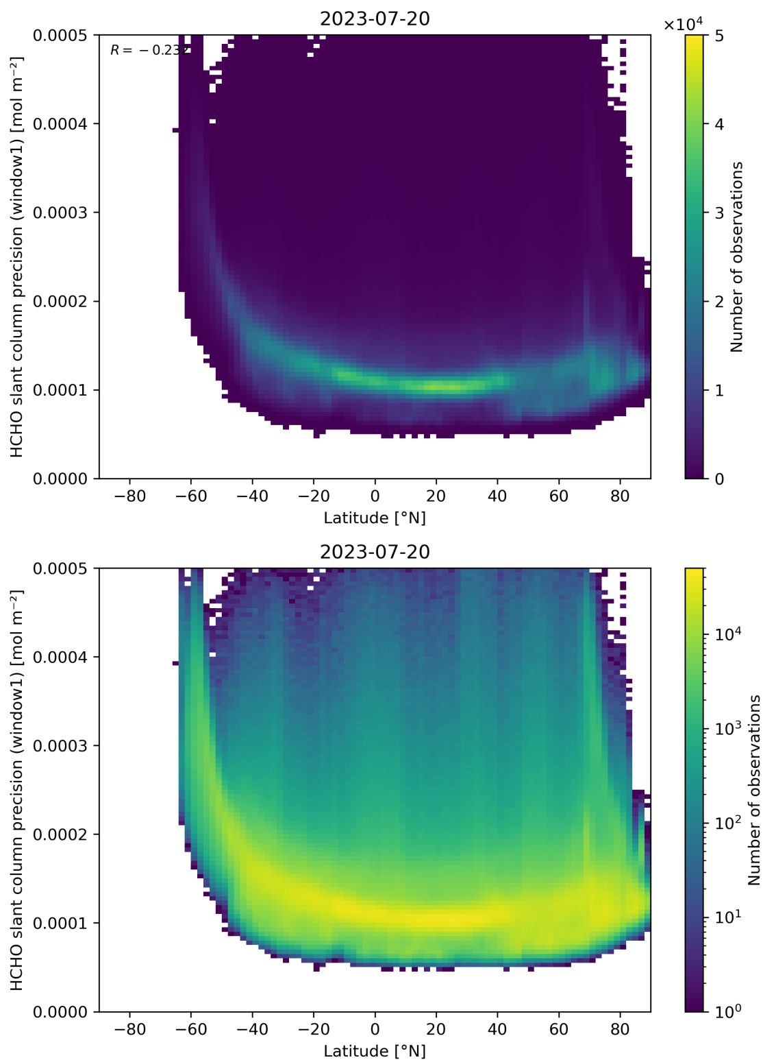
Figure 160: Scatter density plot of “Latitude” against “HCHO slant column precision (window1)” for 2023-07-19 to 2023-07-21.
