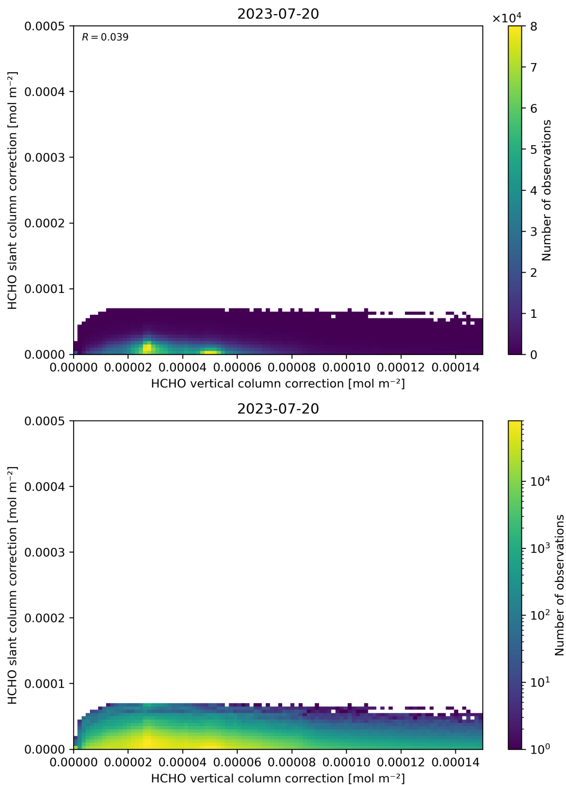
Figure 117: Scatter density plot of “HCHO vertical column correction” against “HCHO slant column correction” for 2023-07-19 to 2023-07-21.
