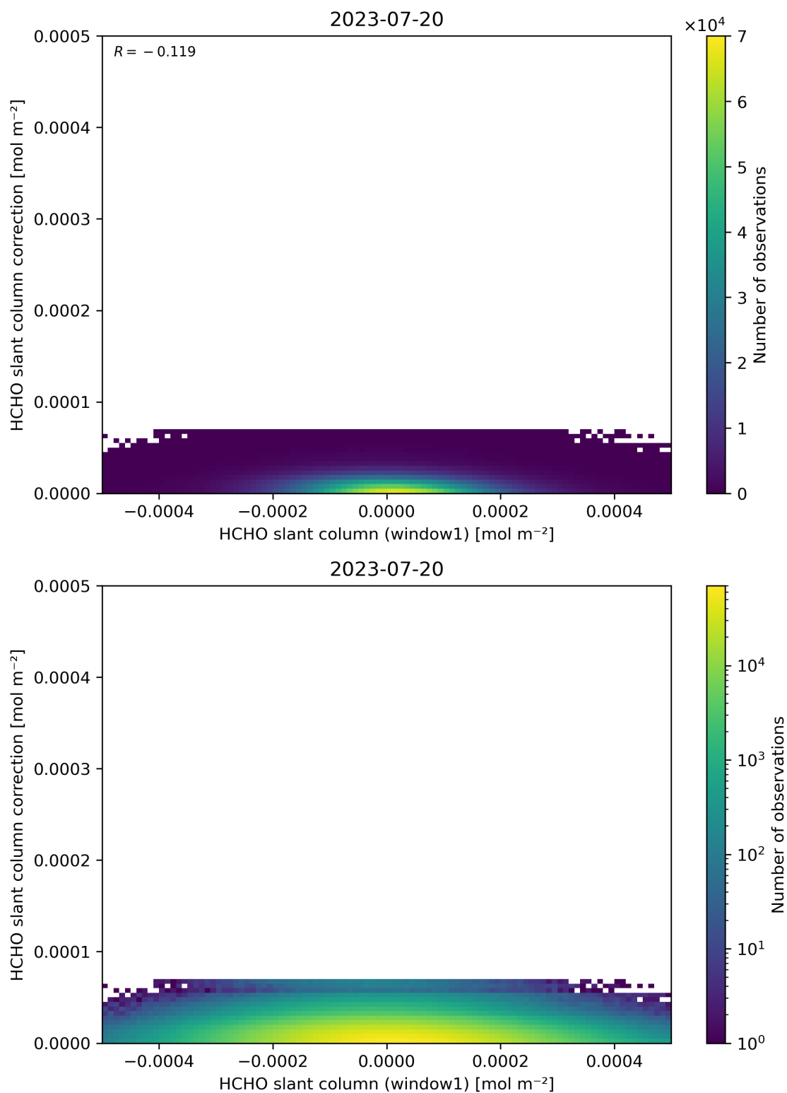
Figure 83: Scatter density plot of “HCHO slant column (window1)” against “HCHO slant column correction” for 2023-07-19 to 2023-07-21.
