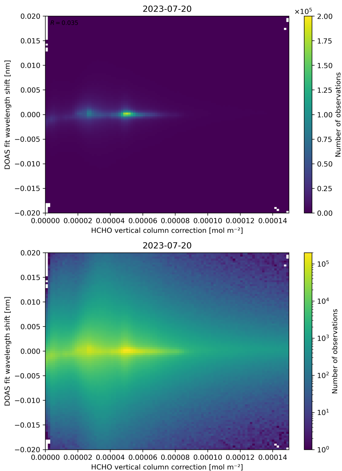
Figure 113: Scatter density plot of “HCHO vertical column correction” against “DOAS fit wavelength shift” for 2023-07-19 to 2023-07-21.
