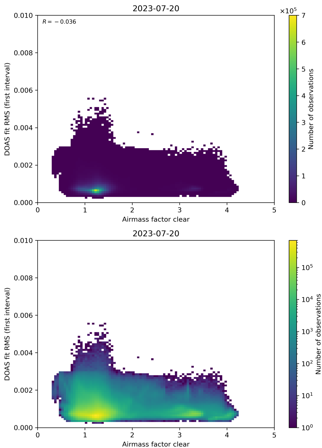
Figure 71: Scatter density plot of “Airmass factor clear” against “DOAS fit RMS (first interval)” for 2023-07-19 to 2023-07-21.
