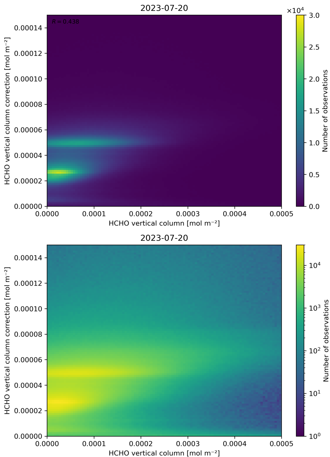
Figure 133: Scatter density plot of “HCHO vertical column” against “HCHO vertical column correction” for 2023-07-19 to 2023-07-21.
