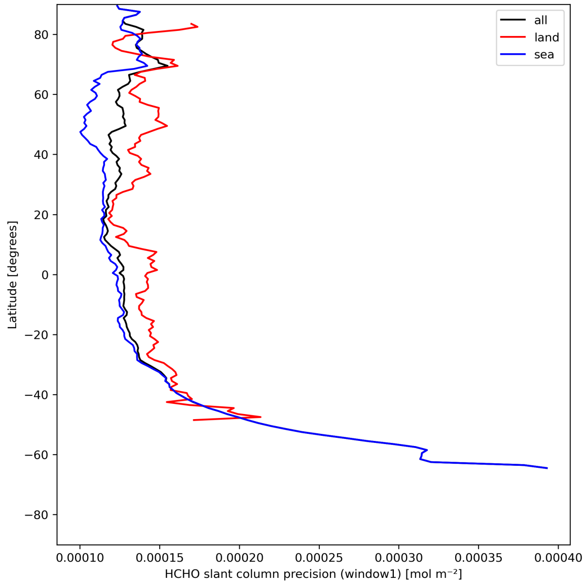
Figure 25: Zonal average of “HCHO slant column precision (window1)” for 2023-07-19 to 2023-07-21.
