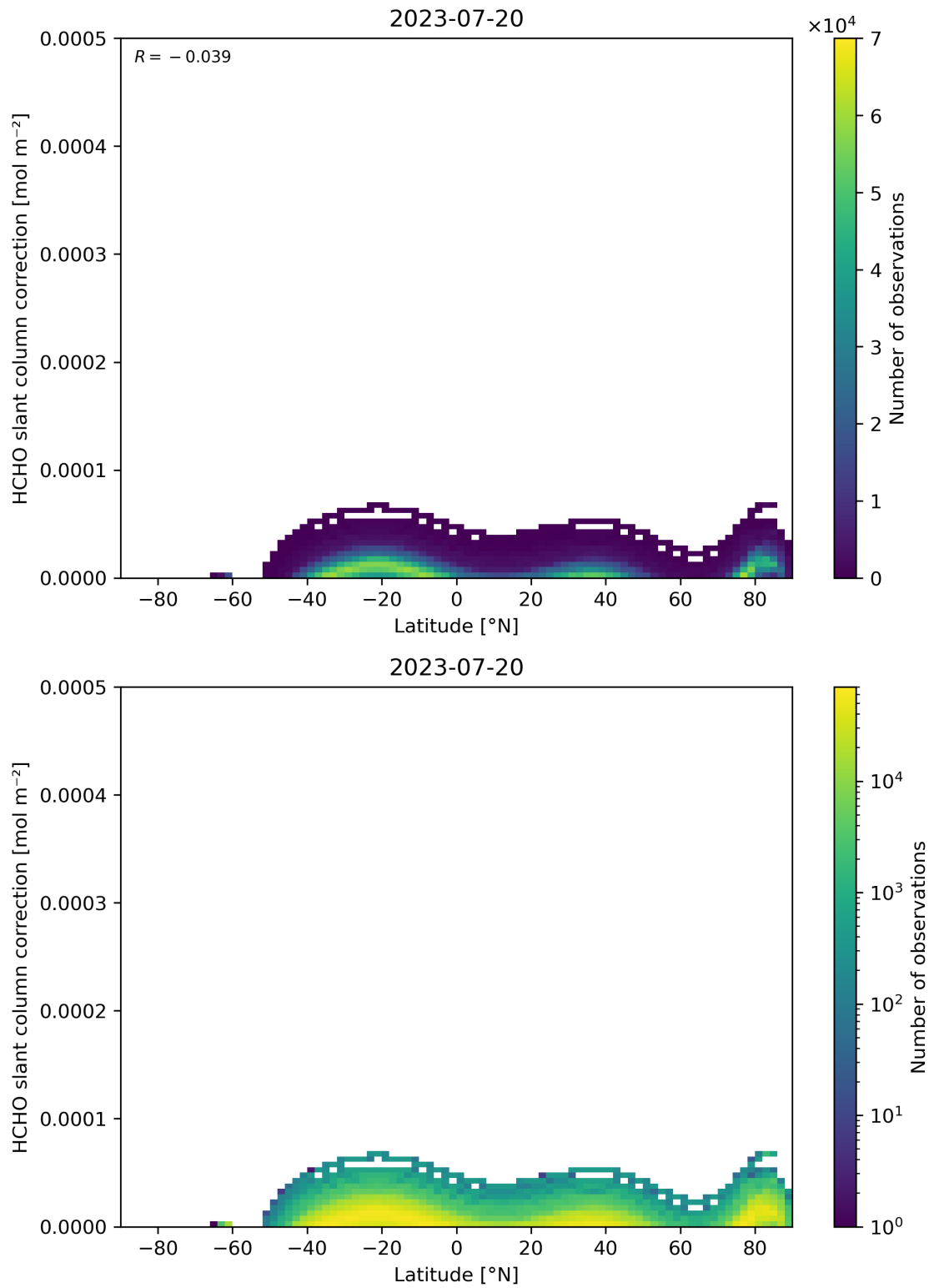
Figure 158: Scatter density plot of “Latitude” against “HCHO slant column correction” for 2023-07-19 to 2023-07-21.
