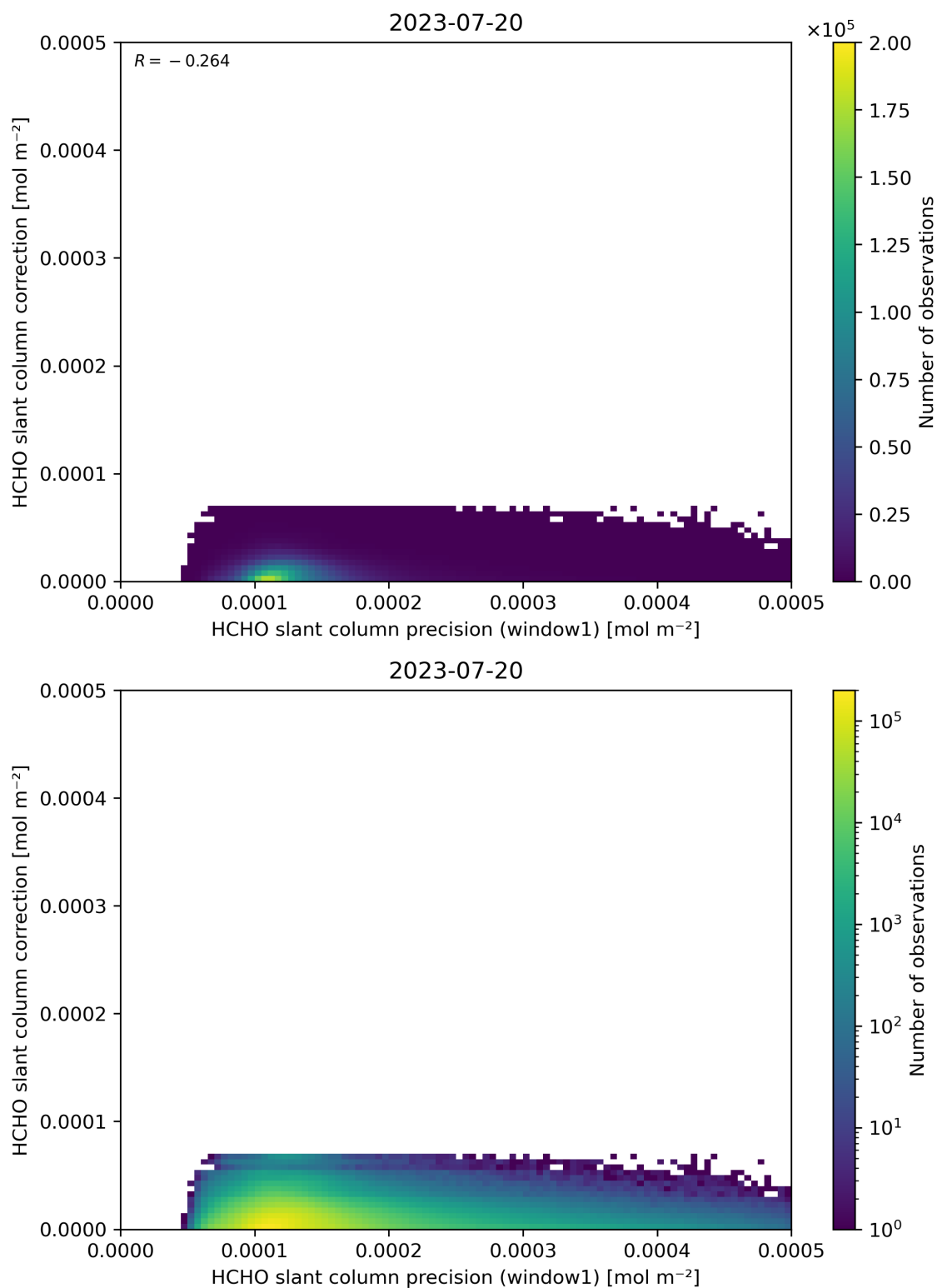
Figure 93: Scatter density plot of “HCHO slant column precision (window1)” against “HCHO slant column correction” for 2023-07-19 to 2023-07-21.
