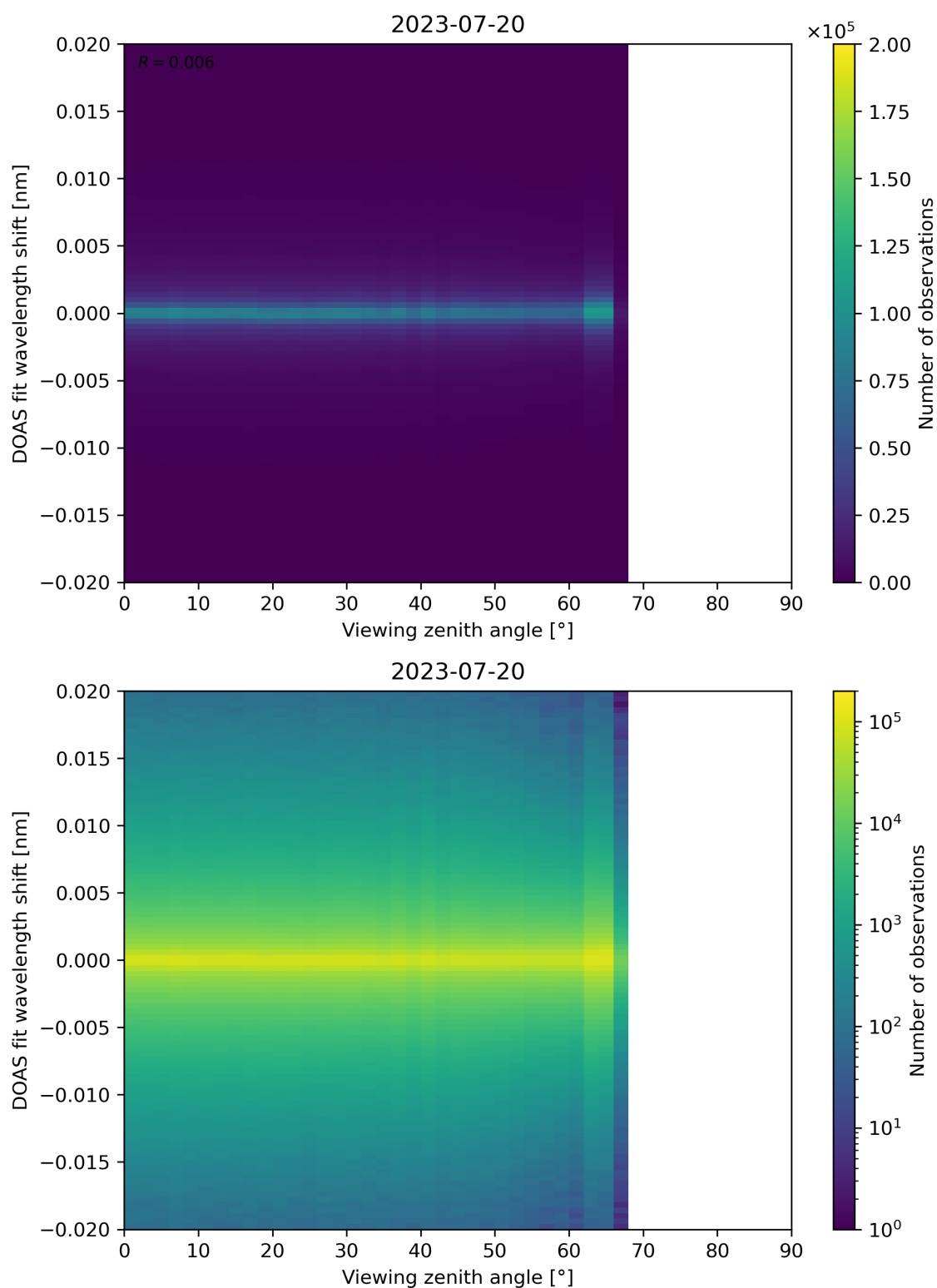
Figure 183: Scatter density plot of “Viewing zenith angle” against “DOAS fit wavelength shift” for 2023-07-19 to 2023-07-21.
