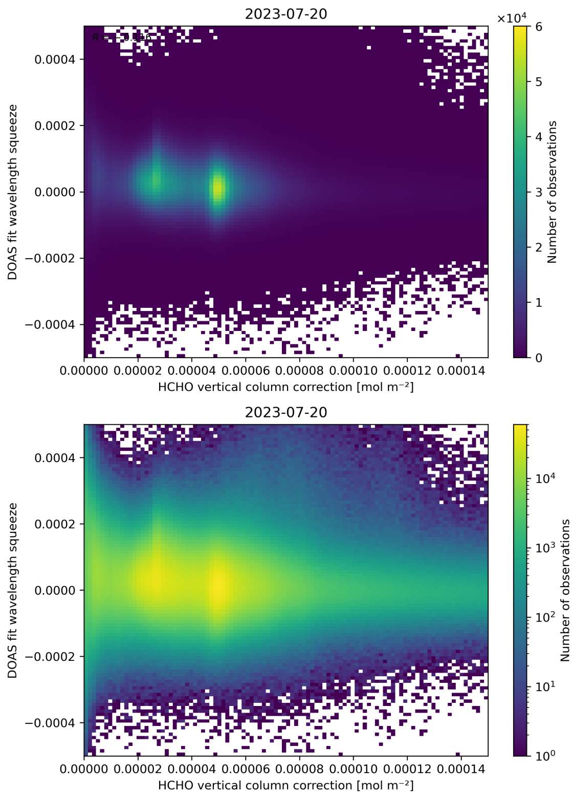
Figure 114: Scatter density plot of “HCHO vertical column correction” against “DOAS fit wavelength squeeze” for 2023-07-19 to 2023-07-21.
