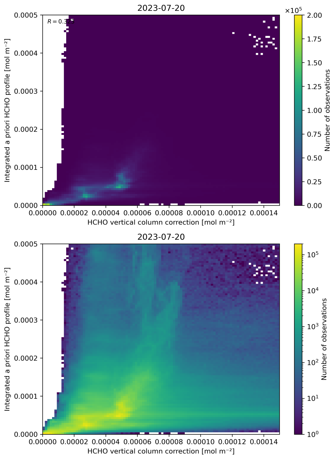
Figure 122: Scatter density plot of “HCHO vertical column correction” against “Integrated a priori HCHO profile” for 2023-07-19 to 2023-07-21.
