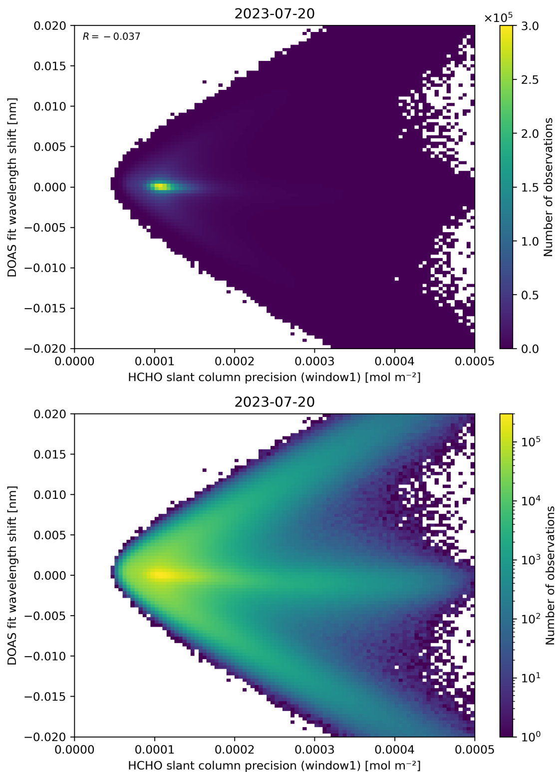
Figure 89: Scatter density plot of “HCHO slant column precision (window1)” against “DOAS fit wavelength shift” for 2023-07-19 to 2023-07-21.
