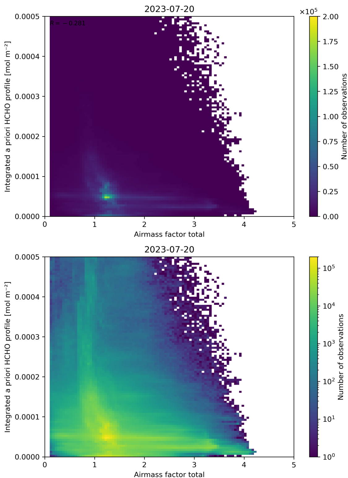
Figure 104: Scatter density plot of “Airmass factor total” against “Integrated a priori HCHO profile” for 2023-07-19 to 2023-07-21.
