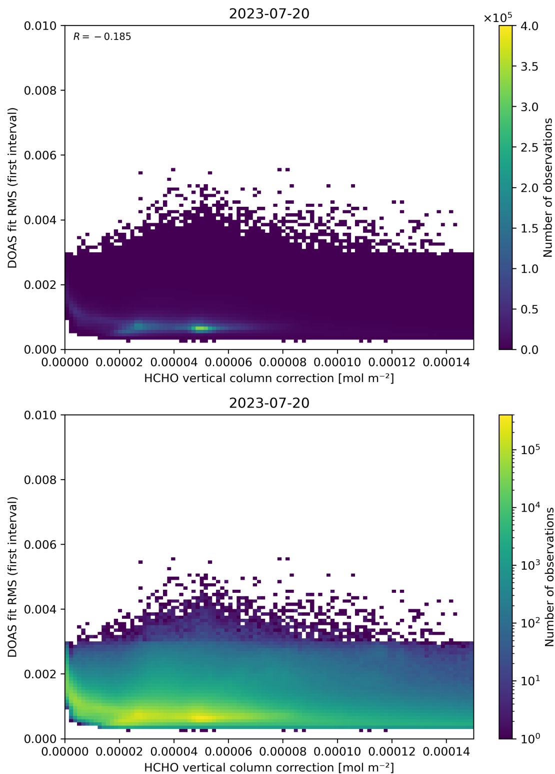
Figure 112: Scatter density plot of “HCHO vertical column correction” against “DOAS fit RMS (first interval)” for 2023-07-19 to 2023-07-21.
