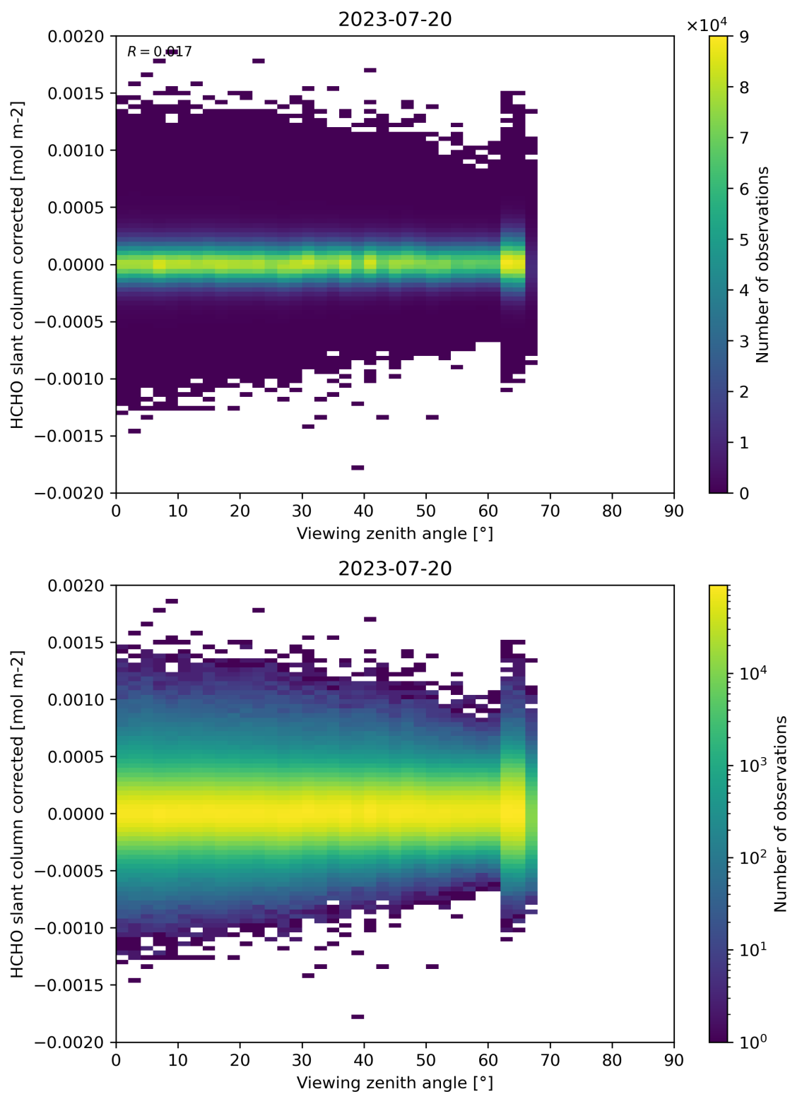
Figure 186: Scatter density plot of “Viewing zenith angle” against “HCHO slant column corrected” for 2023-07-19 to 2023-07-21.
