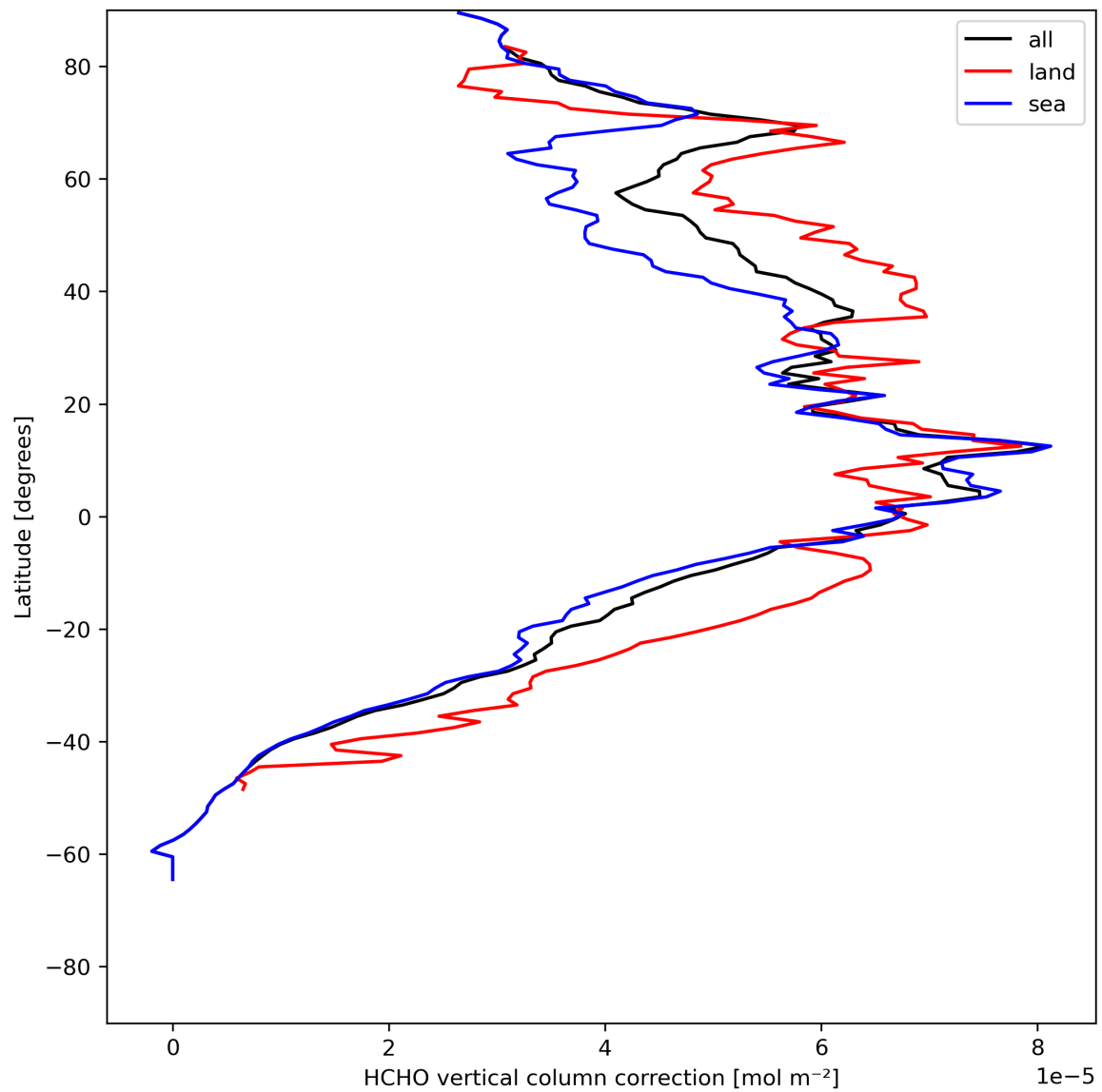
Figure 23: Zonal average of “HCHO vertical column correction” for 2023-07-19 to 2023-07-21.
