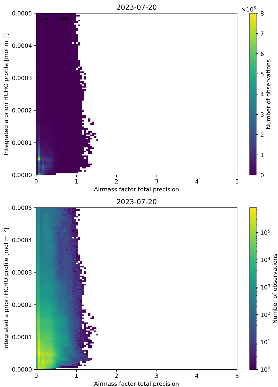
Figure 111: Scatter density plot of “Airmass factor total precision” against “Integrated a priori HCHO profile” for 2023-07-19 to 2023-07-21.
