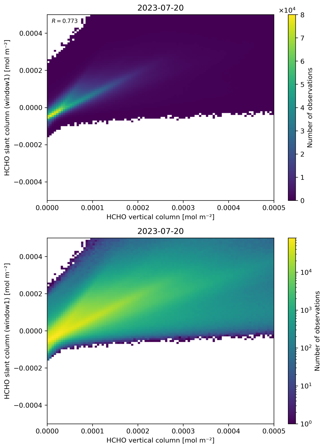
Figure 129: Scatter density plot of “HCHO vertical column” against “HCHO slant column (window1)” for 2023-07-19 to 2023-07-21.
