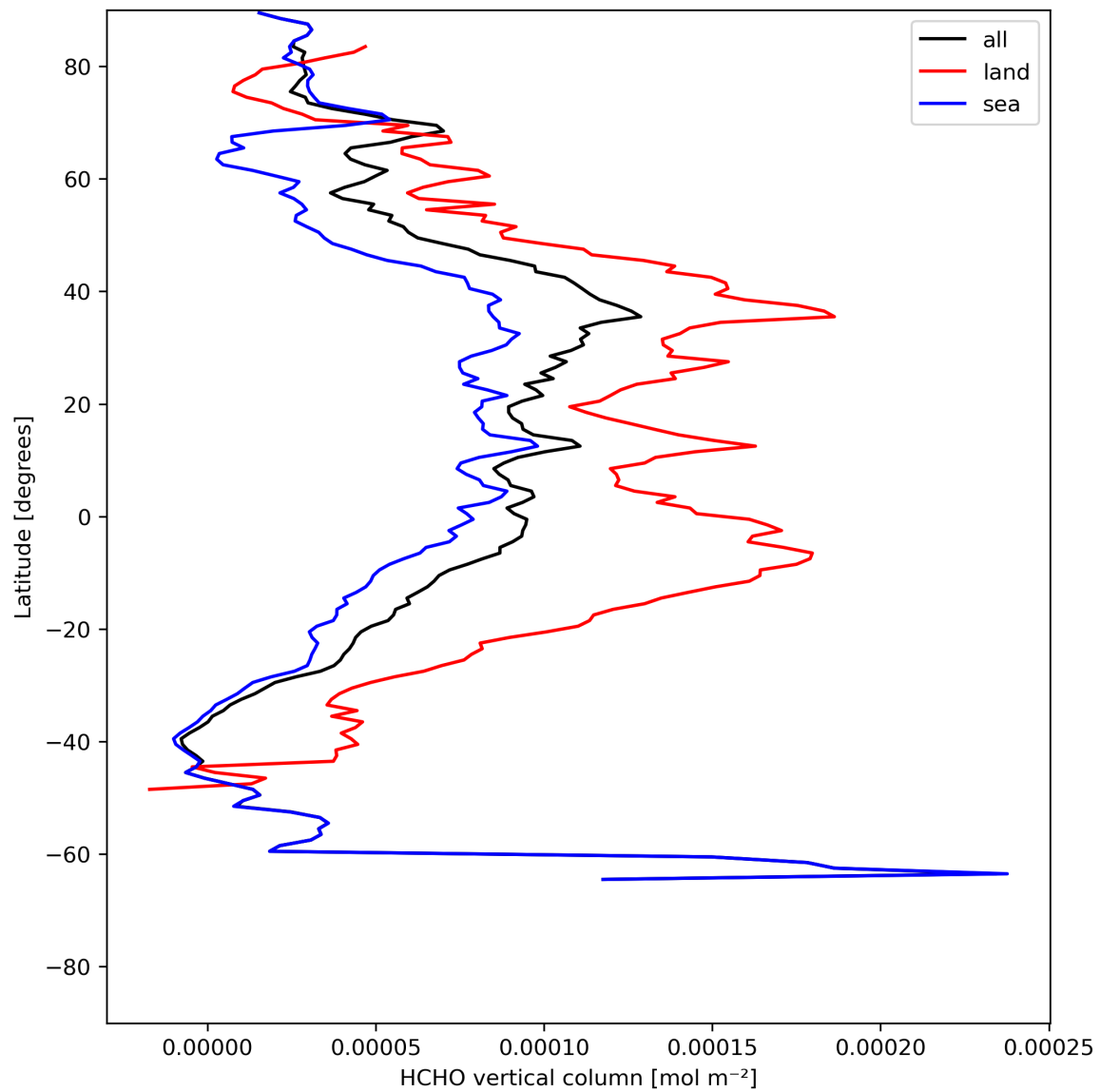
Figure 21: Zonal average of “HCHO vertical column” for 2023-07-19 to 2023-07-21.
