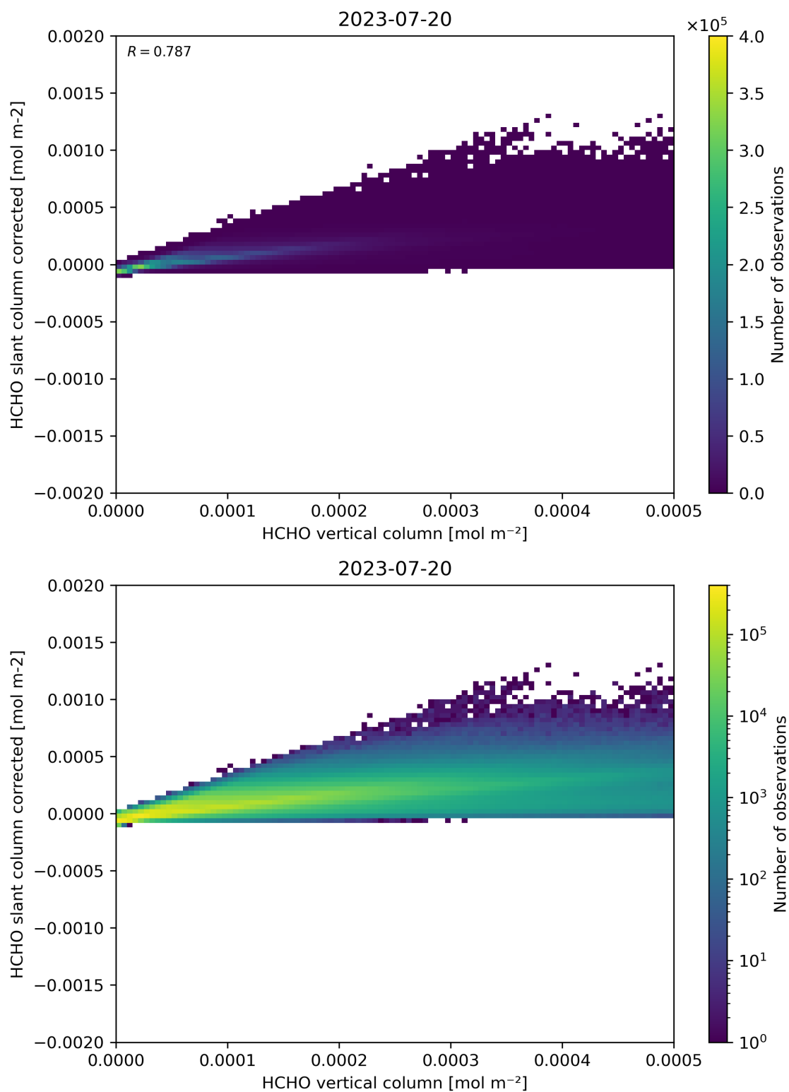
Figure 127: Scatter density plot of “HCHO vertical column” against “HCHO slant column corrected” for 2023-07-19 to 2023-07-21.
