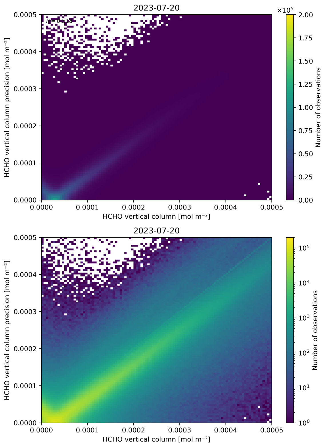
Figure 134: Scatter density plot of “HCHO vertical column” against “HCHO vertical column precision” for 2023-07-19 to 2023-07-21.
