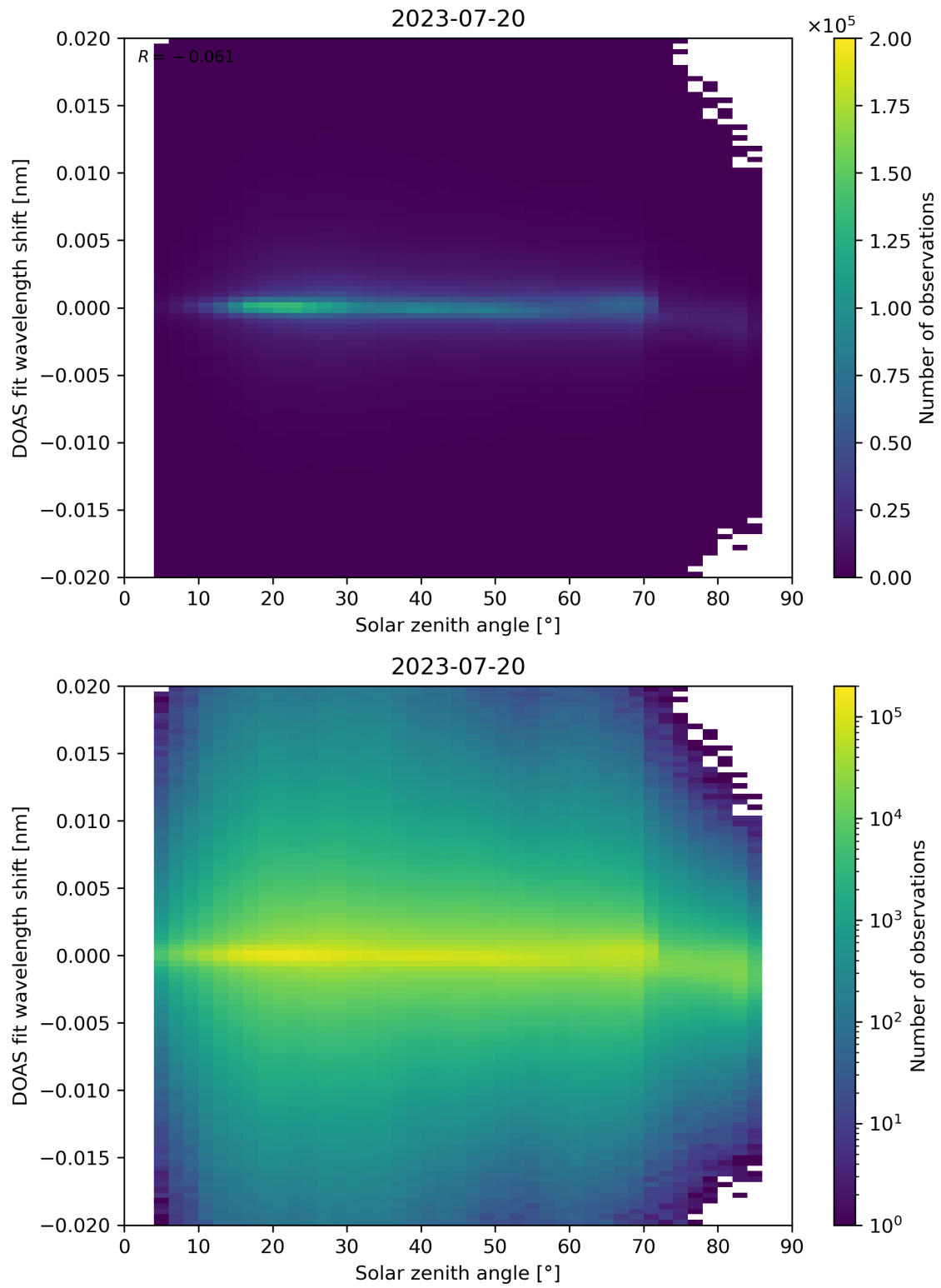
Figure 168: Scatter density plot of “Solar zenith angle” against “DOAS fit wavelength shift” for 2023-07-19 to 2023-07-21.
