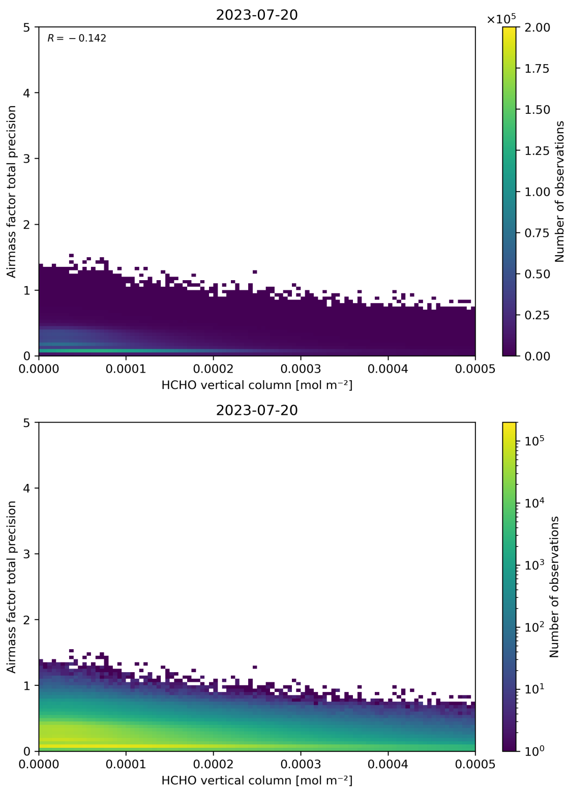
Figure 132: Scatter density plot of “HCHO vertical column” against “Airmass factor total precision” for 2023-07-19 to 2023-07-21.
