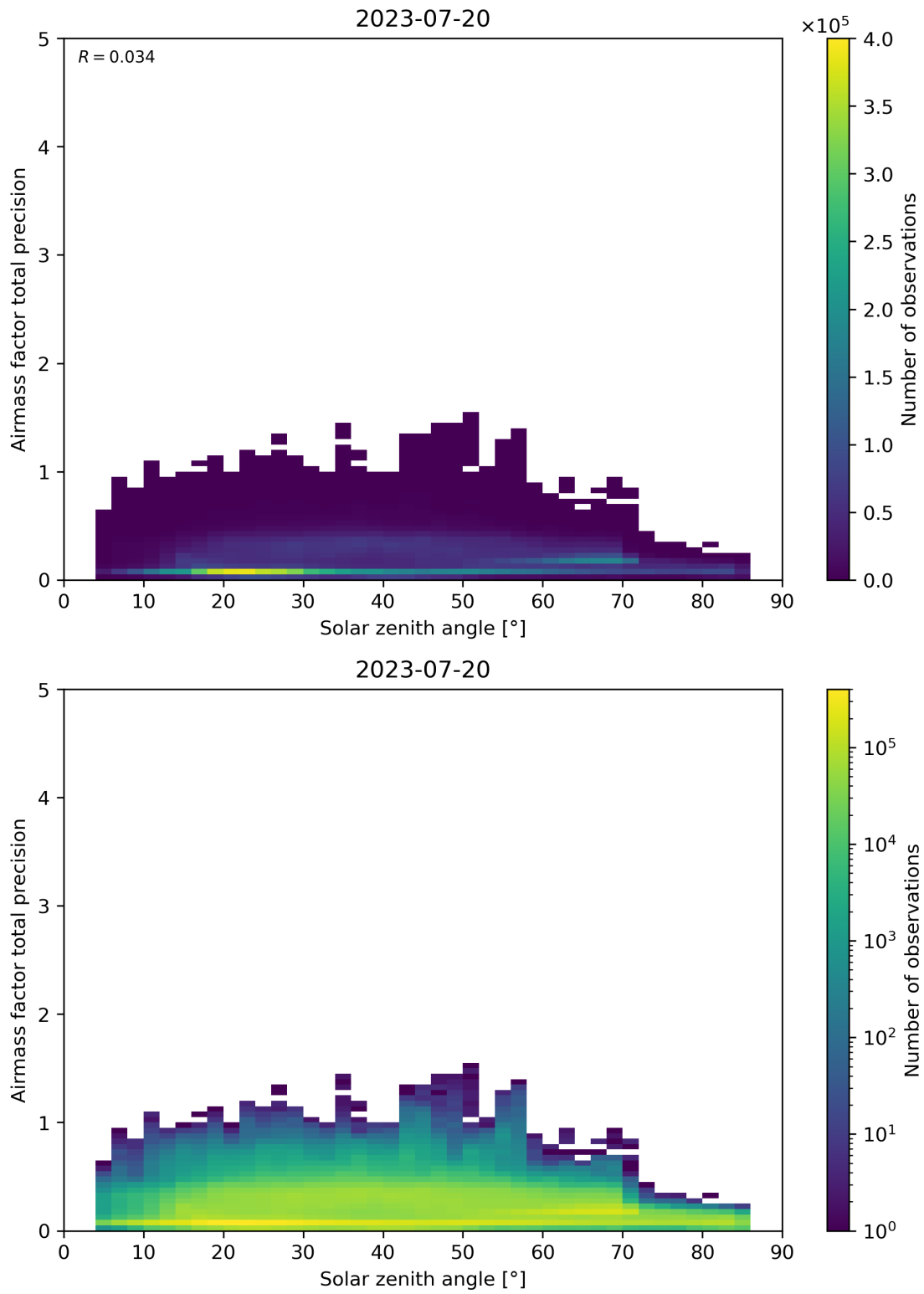
Figure 176: Scatter density plot of “Solar zenith angle” against “Airmass factor total precision” for 2023-07-19 to 2023-07-21.
