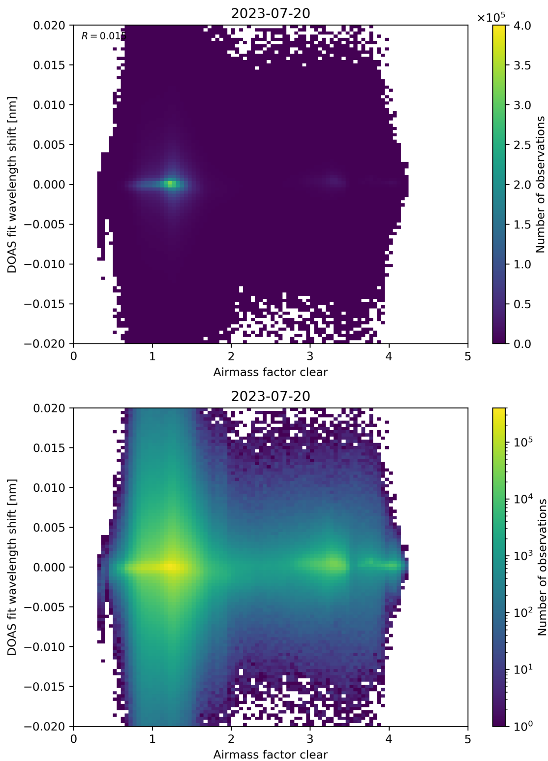
Figure 72: Scatter density plot of “Airmass factor clear” against “DOAS fit wavelength shift” for 2023-07-19 to 2023-07-21.
