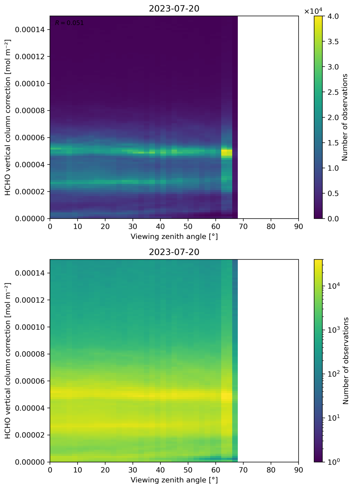
Figure 193: Scatter density plot of “Viewing zenith angle” against “HCHO vertical column correction” for 2023-07-19 to 2023-07-21.
