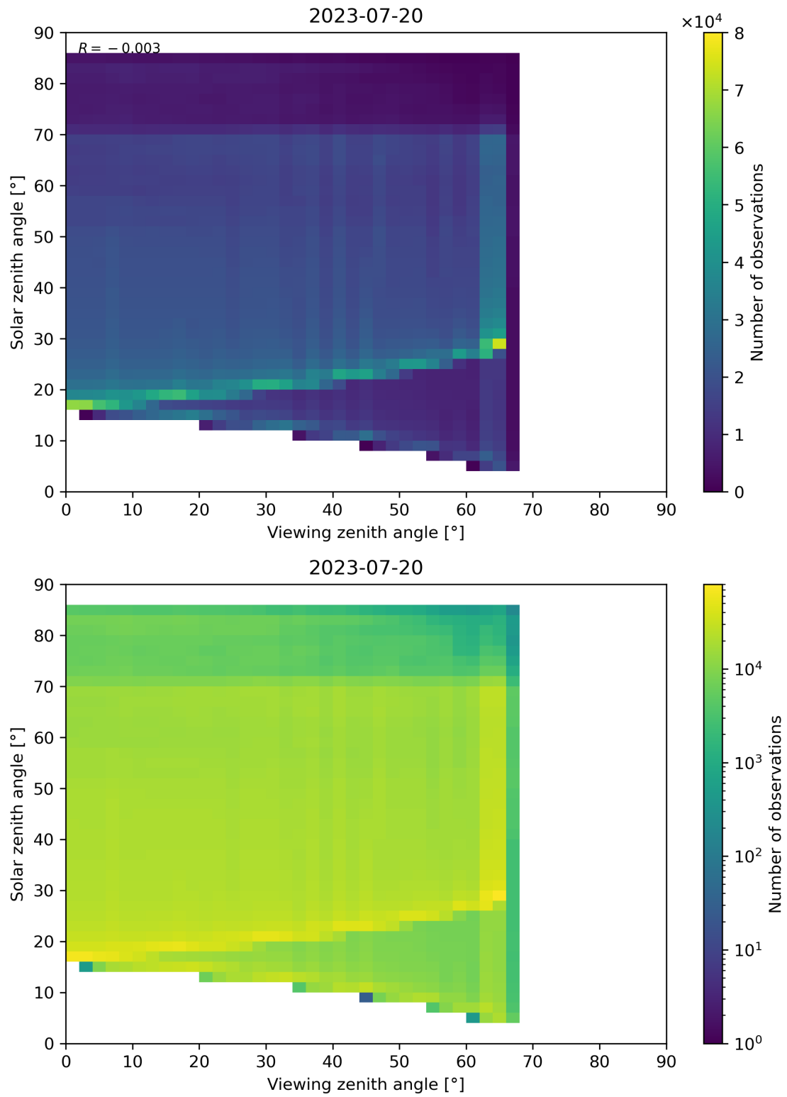
Figure 197: Scatter density plot of “Viewing zenith angle” against “Solar zenith angle” for 2023-07-19 to 2023-07-21.
