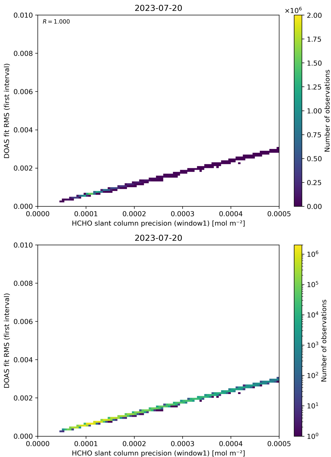
Figure 88: Scatter density plot of “HCHO slant column precision (window1)” against “DOAS fit RMS (first interval)” for 2023-07-19 to 2023-07-21.
