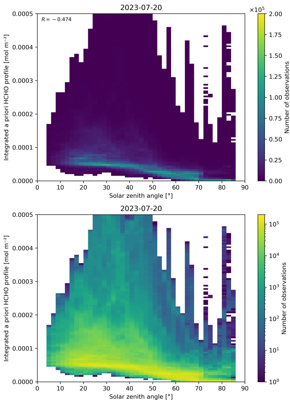
Figure 180: Scatter density plot of “Solar zenith angle” against “Integrated a priori HCHO profile” for 2023-07-19 to 2023-07-21.
