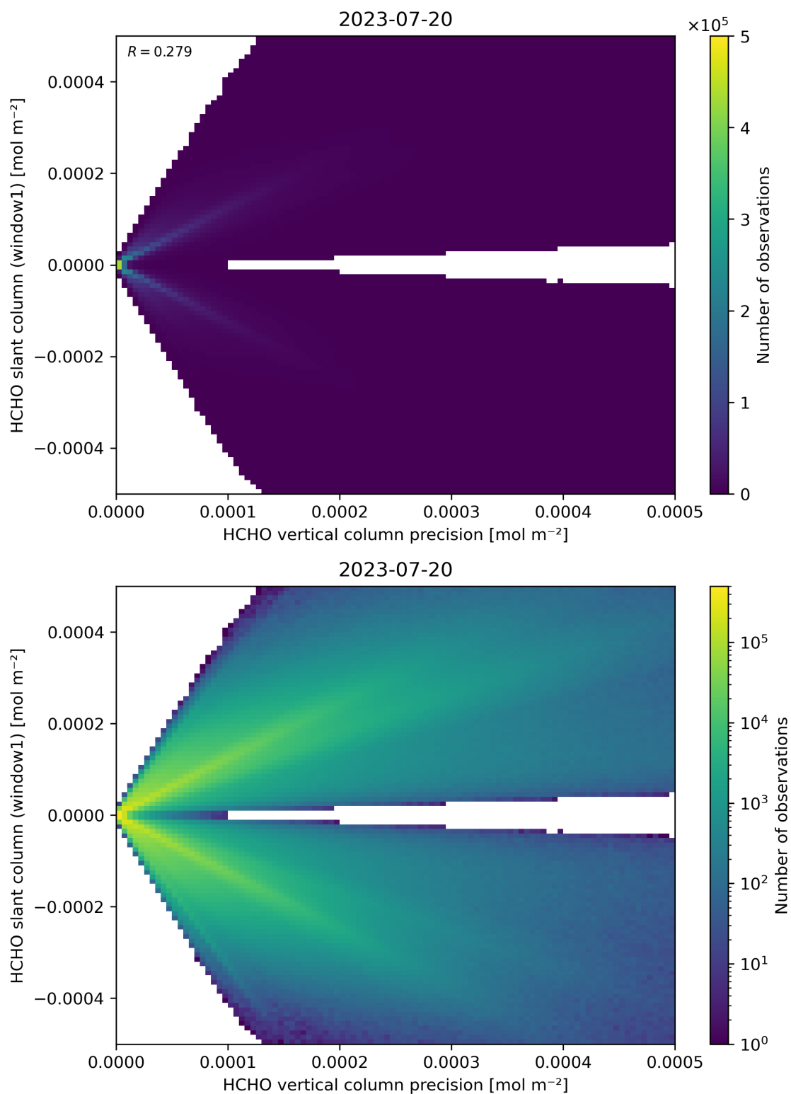
Figure 142: Scatter density plot of “HCHO vertical column precision” against “HCHO slant column (window1)” for 2023-07-19 to 2023-07-21.
