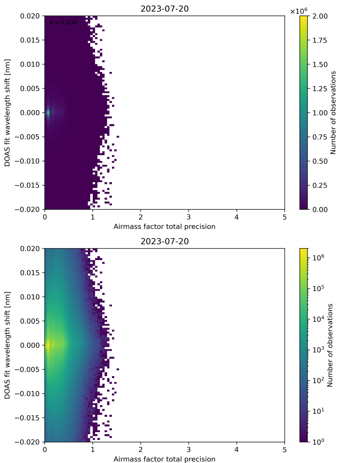
Figure 106: Scatter density plot of “Airmass factor total precision” against “DOAS fit wavelength shift” for 2023-07-19 to 2023-07-21.
