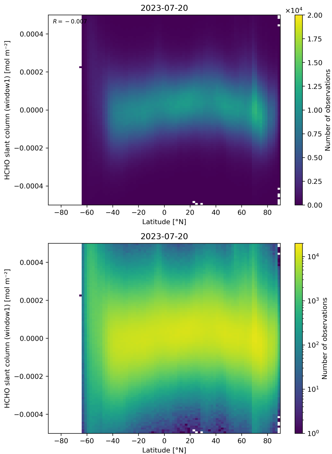
Figure 159: Scatter density plot of “Latitude” against “HCHO slant column (window1)” for 2023-07-19 to 2023-07-21.
