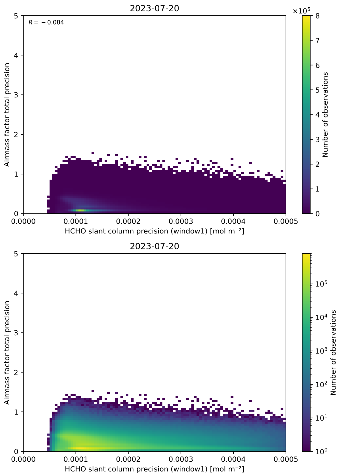
Figure 95: Scatter density plot of “HCHO slant column precision (window1)” against “Airmass factor total precision” for 2023-07-19 to 2023-07-21.
