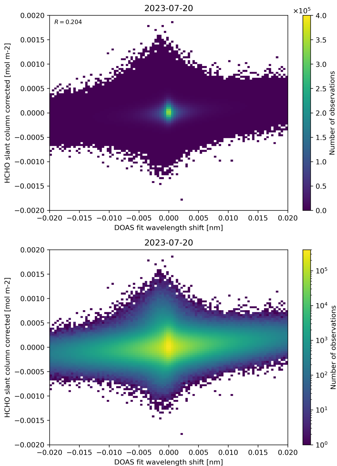
Figure 66: Scatter density plot of “DOAS fit wavelength shift” against “HCHO slant column corrected” for 2023-07-19 to 2023-07-21.
