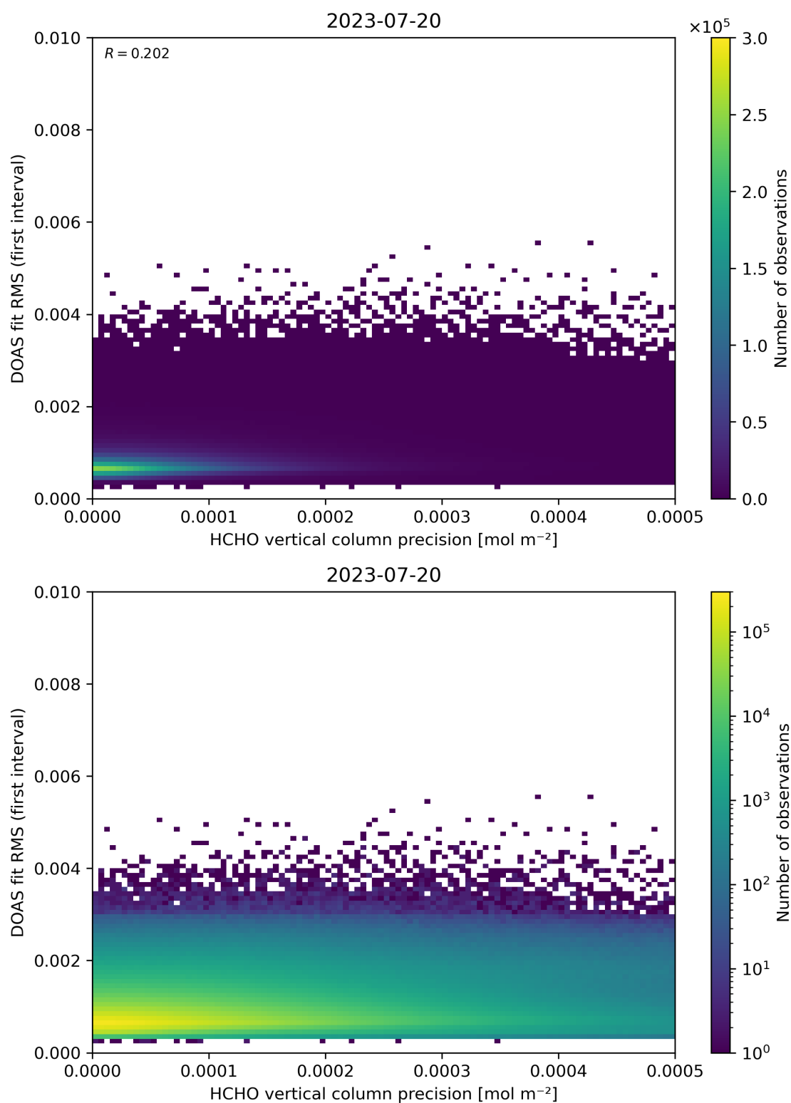
Figure 136: Scatter density plot of “HCHO vertical column precision” against “DOAS fit RMS (first interval)” for 2023-07-19 to 2023-07-21.
