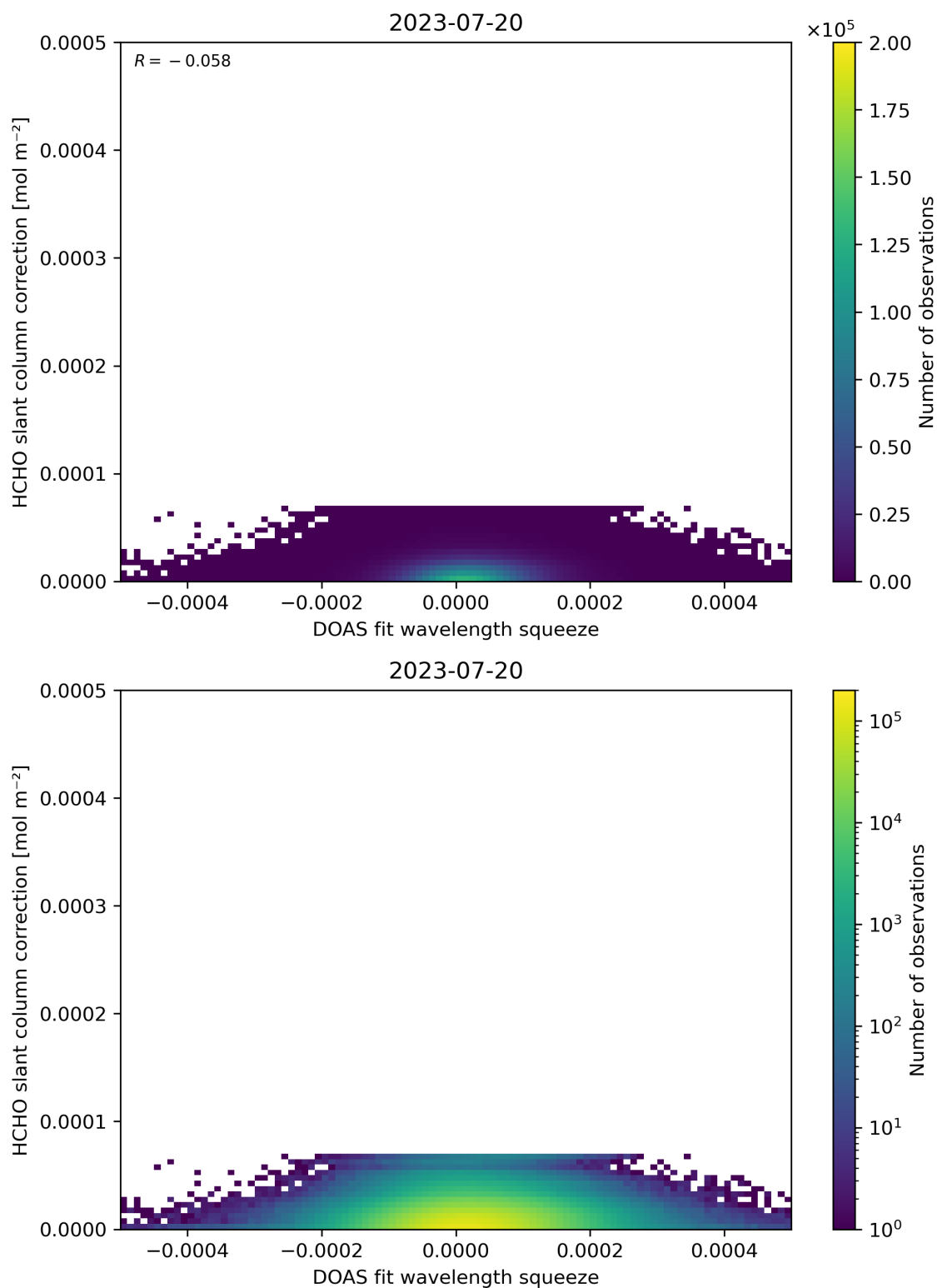
Figure 70: Scatter density plot of “DOAS fit wavelength squeeze” against “HCHO slant column correction” for 2023-07-19 to 2023-07-21.
