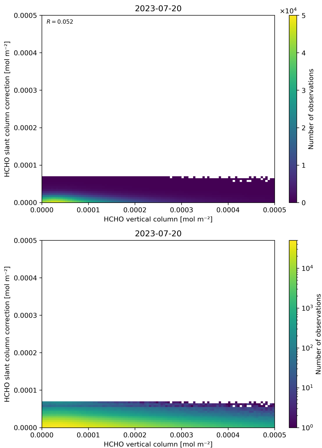
Figure 128: Scatter density plot of “HCHO vertical column” against “HCHO slant column correction” for 2023-07-19 to 2023-07-21.
