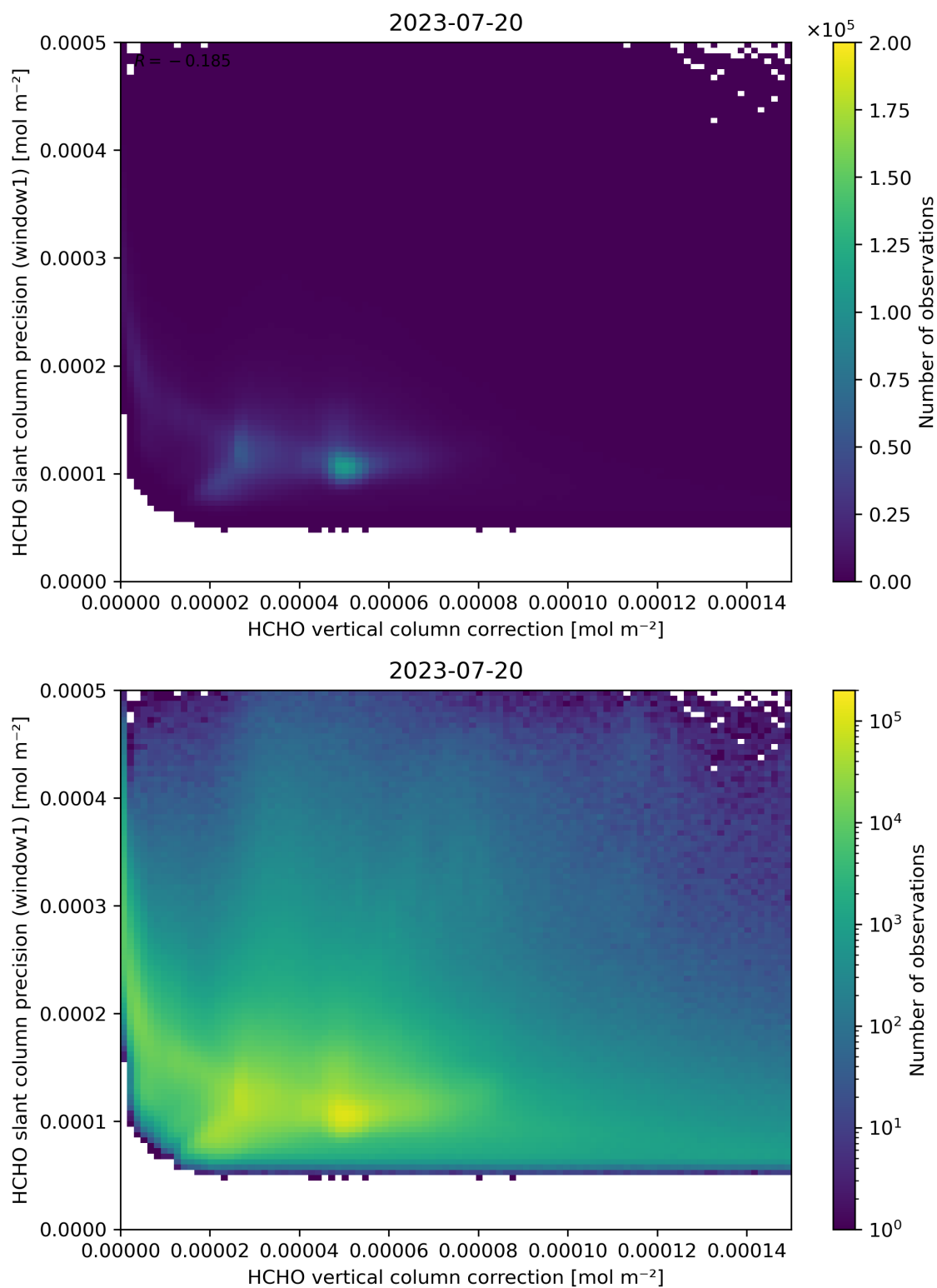
Figure 119: Scatter density plot of “HCHO vertical column correction” against “HCHO slant column precision (window1)” for 2023-07-19 to 2023-07-21.
