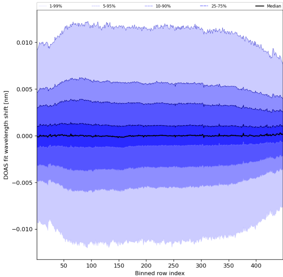
Figure 58: Along track statistics of “DOAS fit wavelength shift” for 2023-07-19 to 2023-07-21
