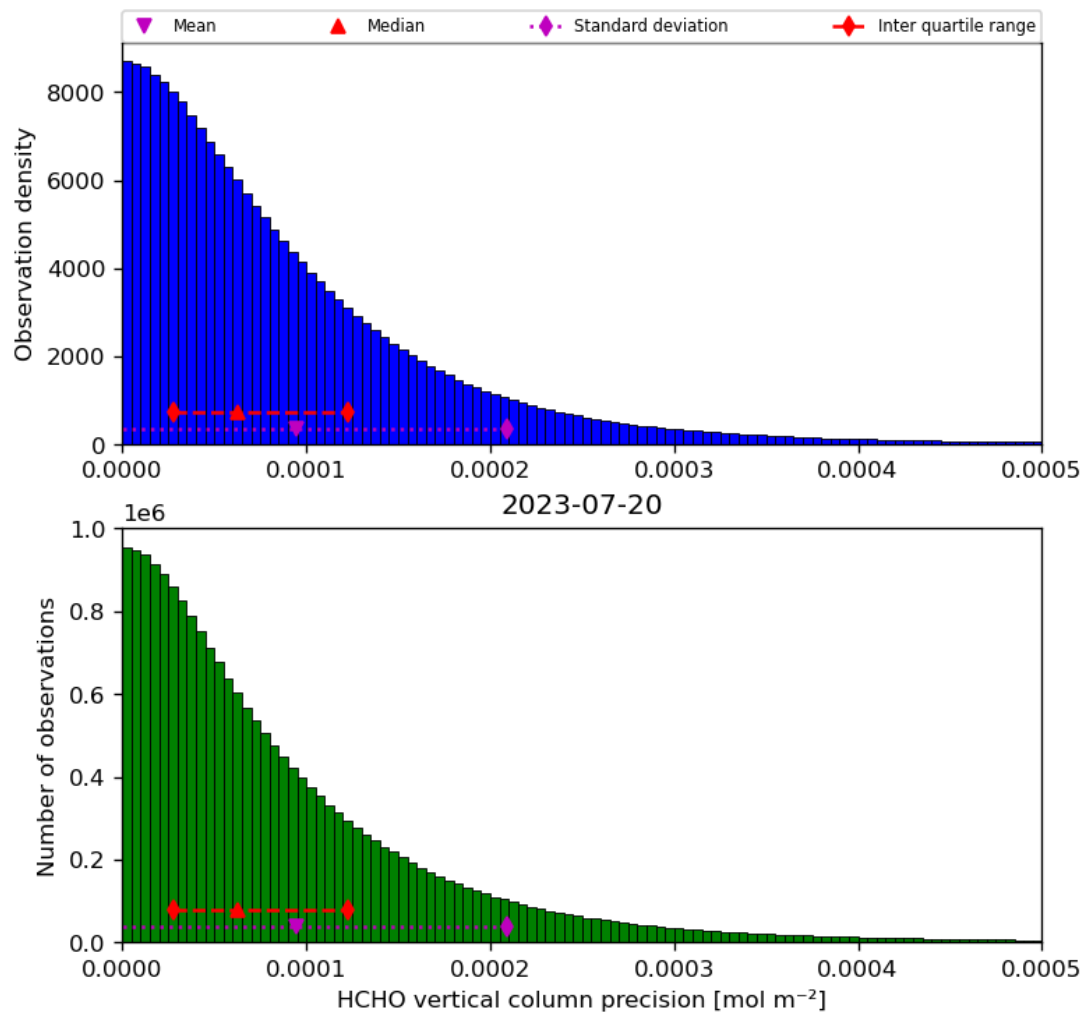
Figure 36: Histogram of “HCHO vertical column precision” for 2023-07-19 to 2023-07-21
