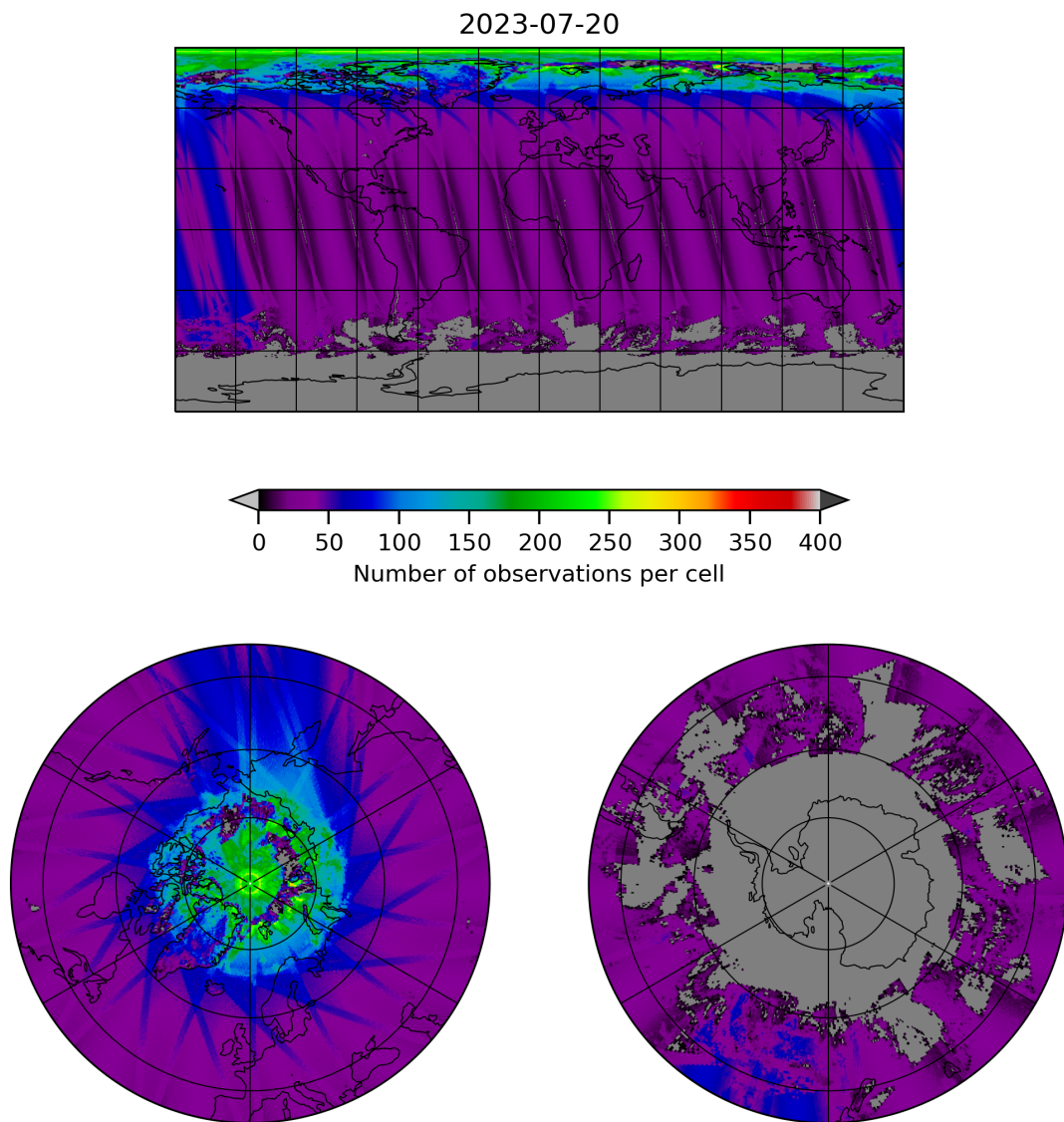
Figure 19: Map of the number of observations for 2023-07-19 to 2023-07-21
