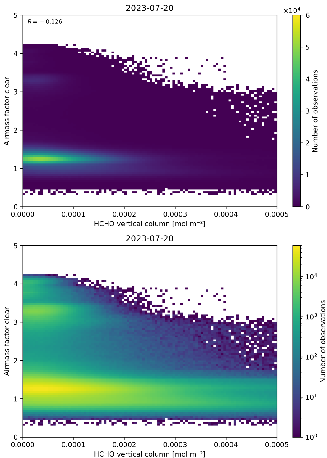
Figure 126: Scatter density plot of “HCHO vertical column” against “Airmass factor clear” for 2023-07-19 to 2023-07-21.
