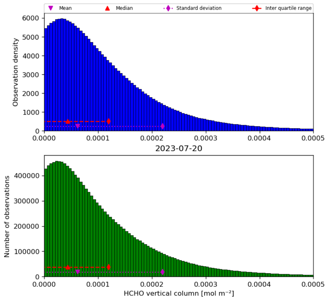
Figure 35: Histogram of “HCHO vertical column” for 2023-07-19 to 2023-07-21
