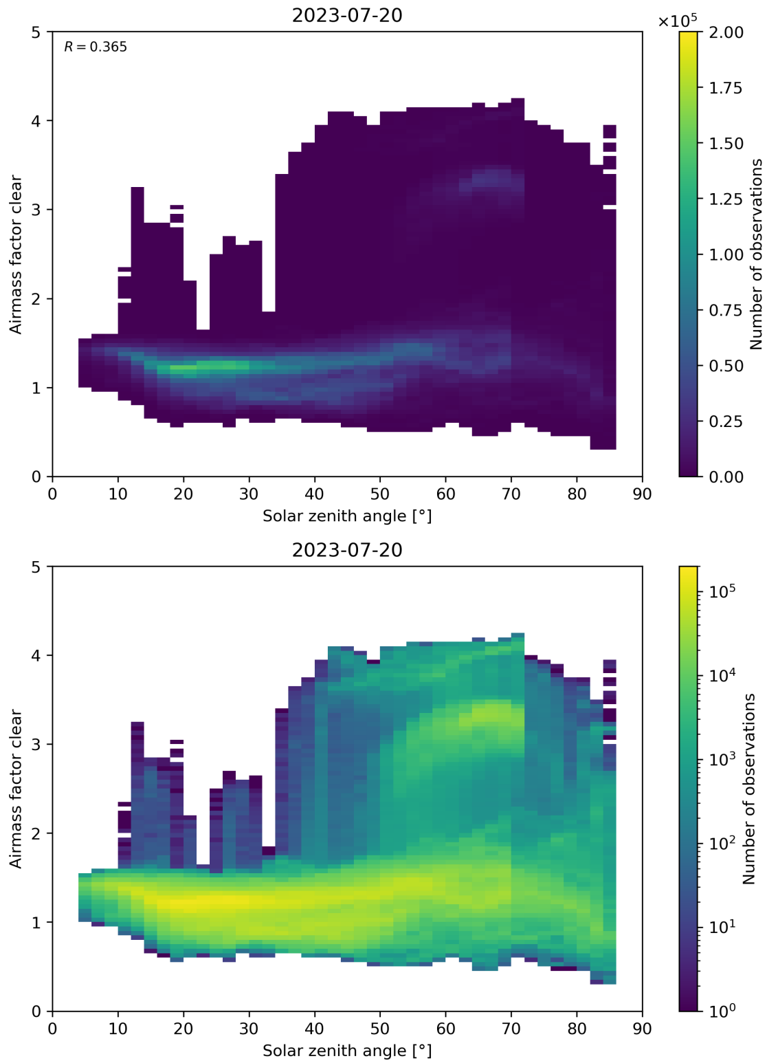
Figure 170: Scatter density plot of “Solar zenith angle” against “Airmass factor clear” for 2023-07-19 to 2023-07-21.
