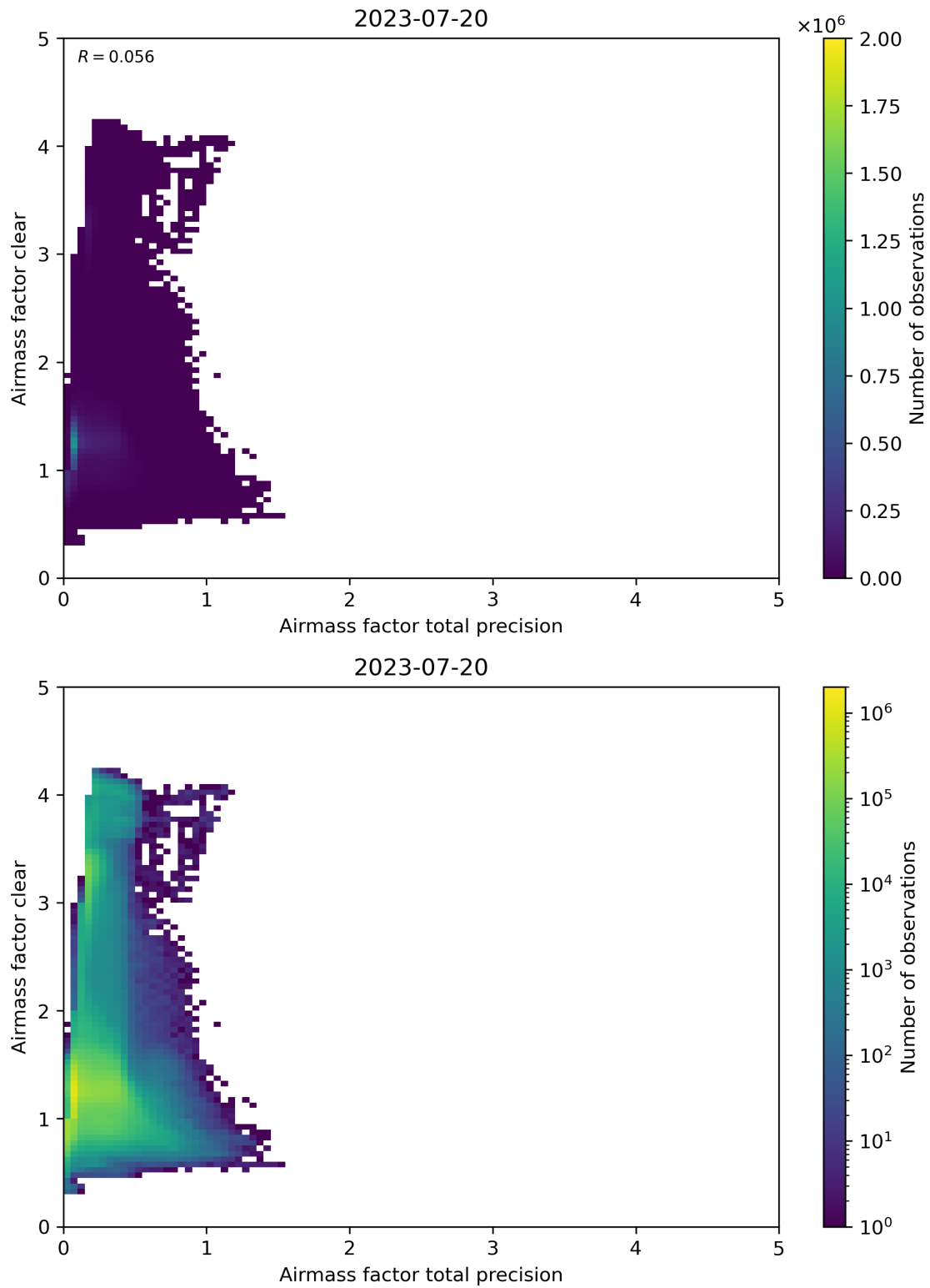
Figure 108: Scatter density plot of “Airmass factor total precision” against “Airmass factor clear” for 2023-07-19 to 2023-07-21.
