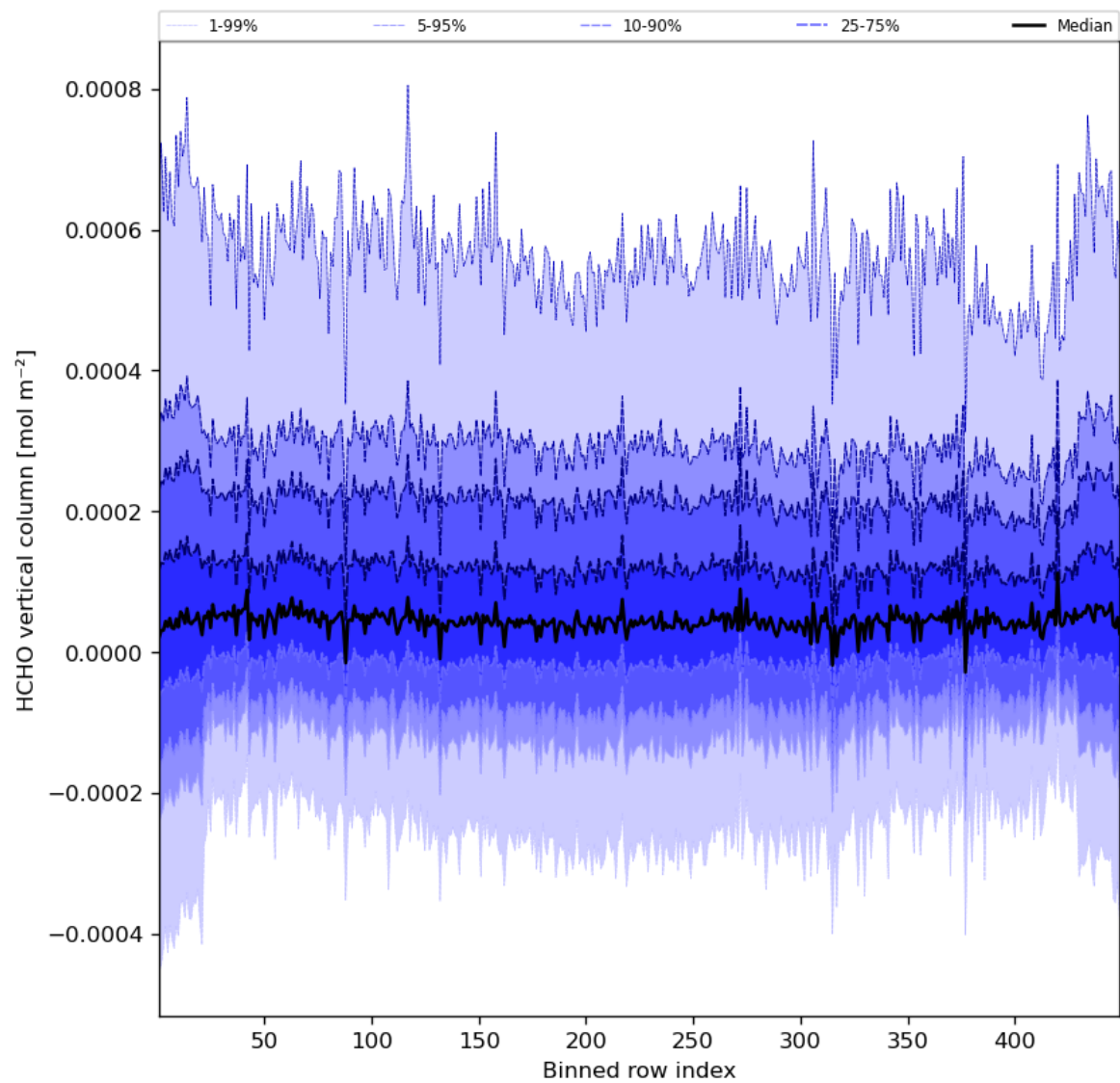
Figure 49: Along track statistics of “HCHO vertical column” for 2023-07-19 to 2023-07-21
