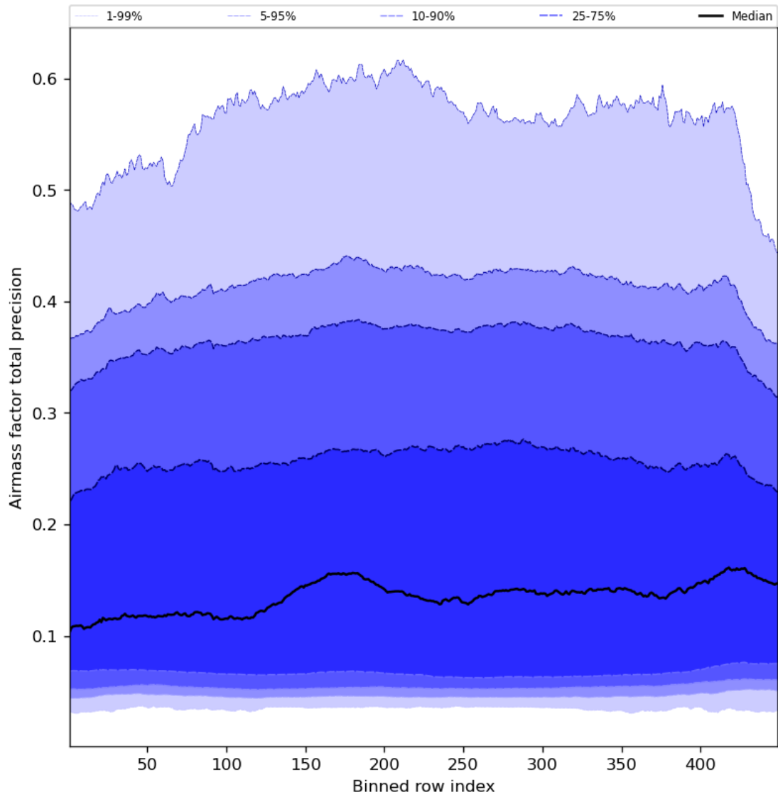
Figure 55: Along track statistics of “Airmass factor total precision” for 2023-07-19 to 2023-07-21
