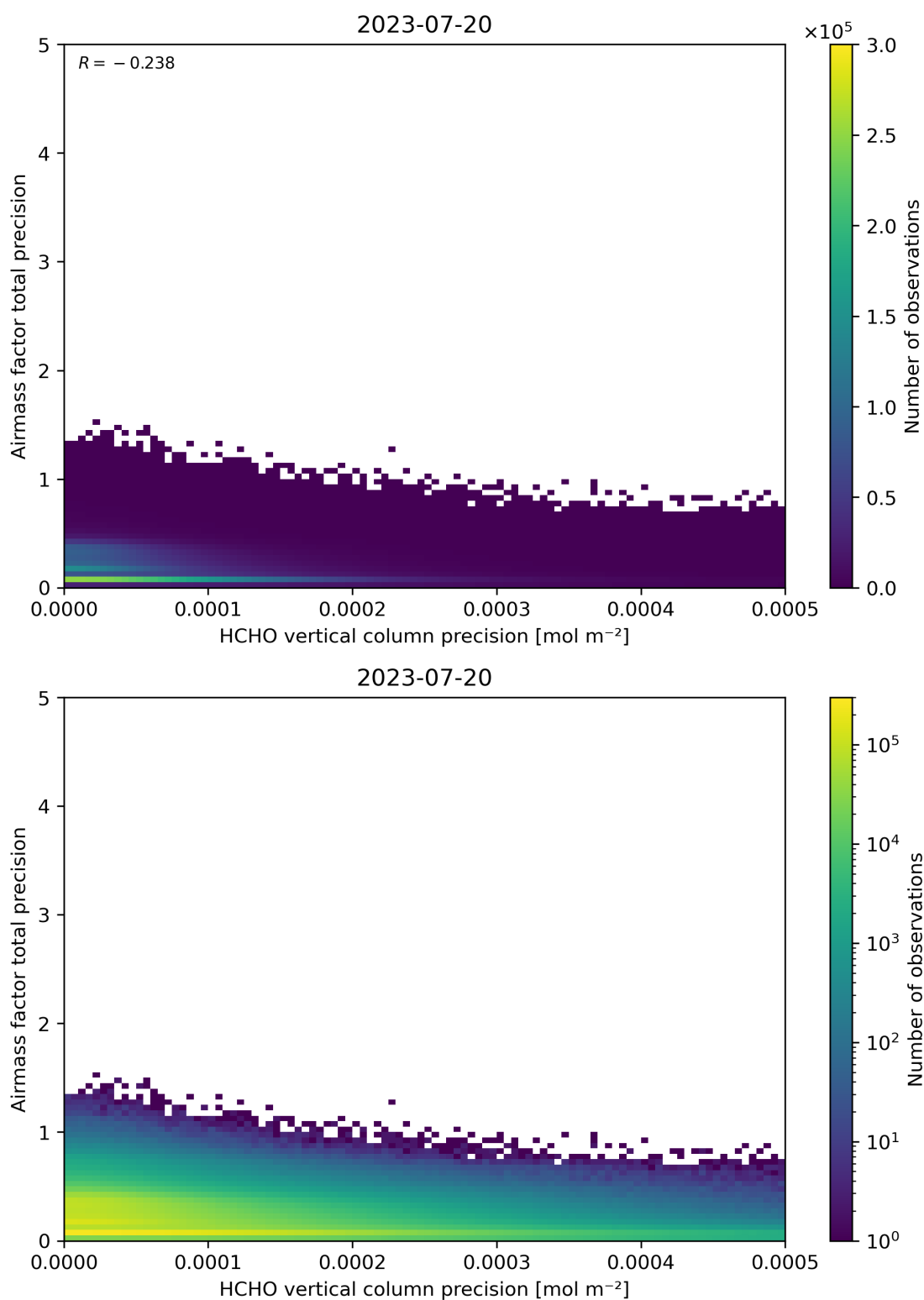
Figure 145: Scatter density plot of “HCHO vertical column precision” against “Airmass factor total precision” for 2023-07-19 to 2023-07-21.
