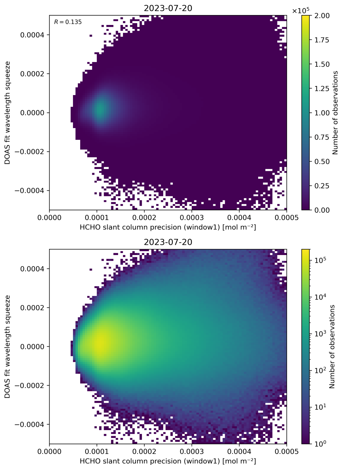
Figure 90: Scatter density plot of “HCHO slant column precision (window1)” against “DOAS fit wavelength squeeze” for 2023-07-19 to 2023-07-21.
