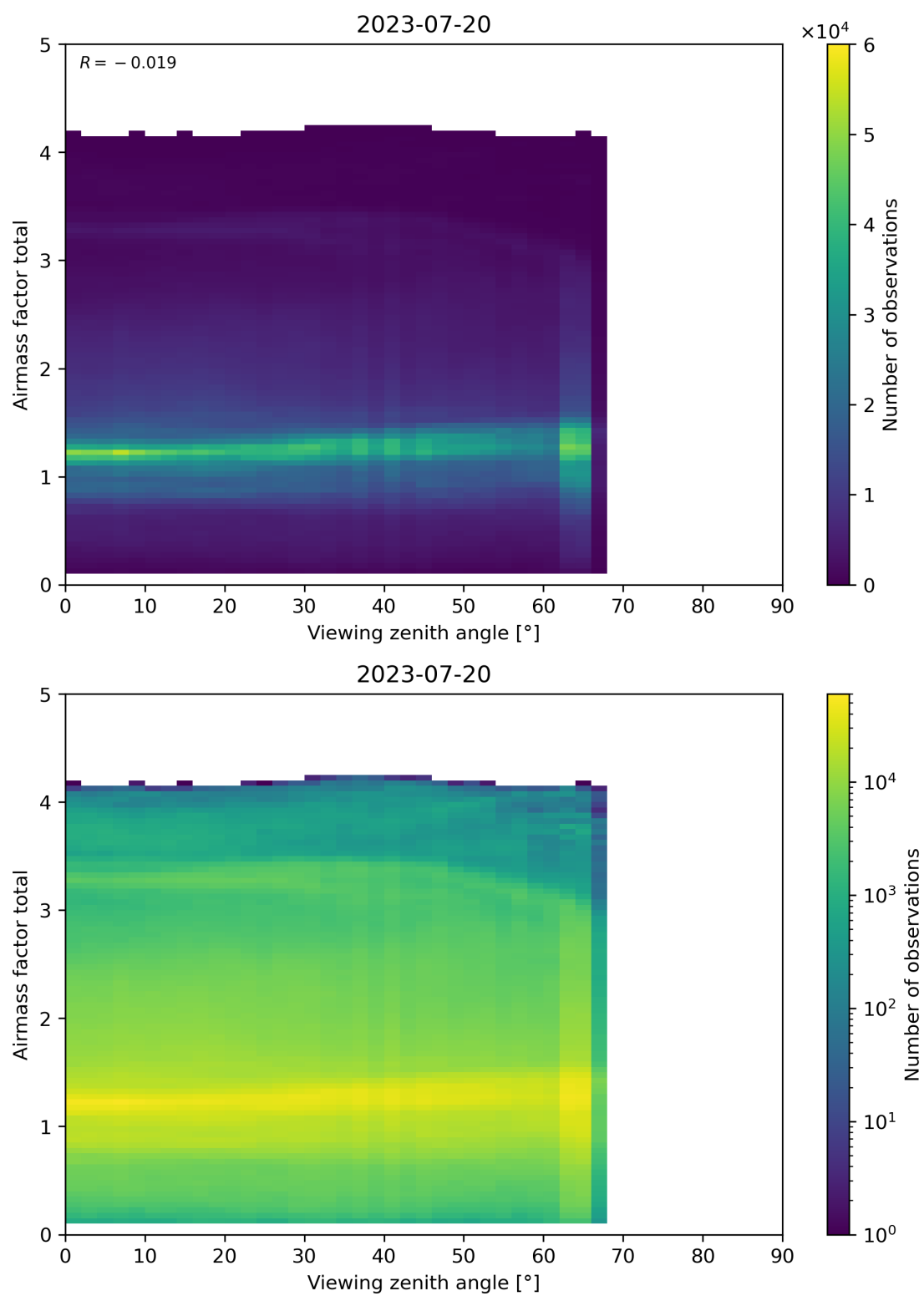
Figure 190: Scatter density plot of “Viewing zenith angle” against “Airmass factor total” for 2023-07-19 to 2023-07-21.
