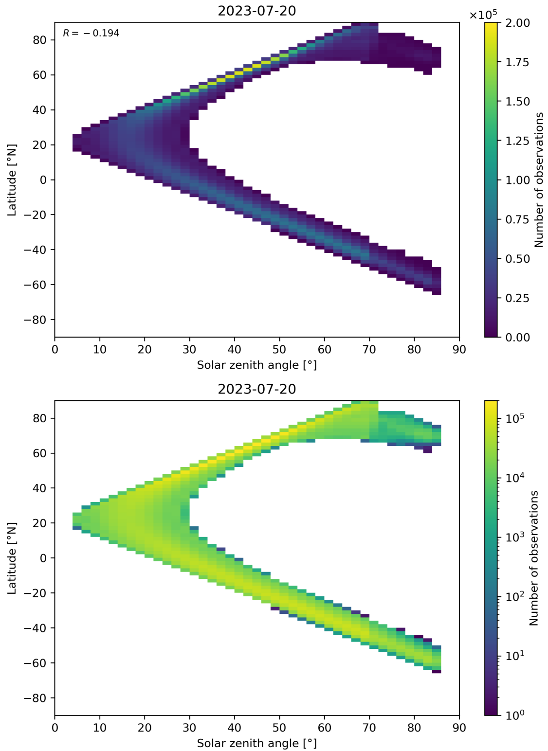
Figure 181: Scatter density plot of “Solar zenith angle” against “Latitude” for 2023-07-19 to 2023-07-21.
