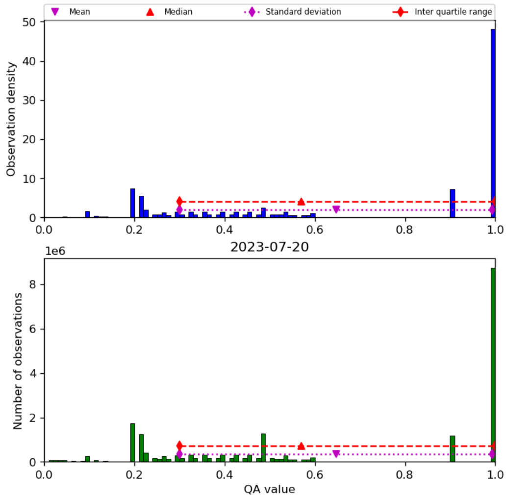
Figure 34: Histogram of “QA value” for 2023-07-19 to 2023-07-21
