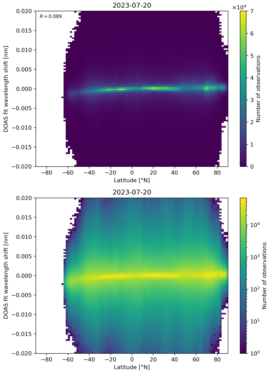
Figure 154: Scatter density plot of “Latitude” against “DOAS fit wavelength shift” for 2023-07-19 to 2023-07-21.
