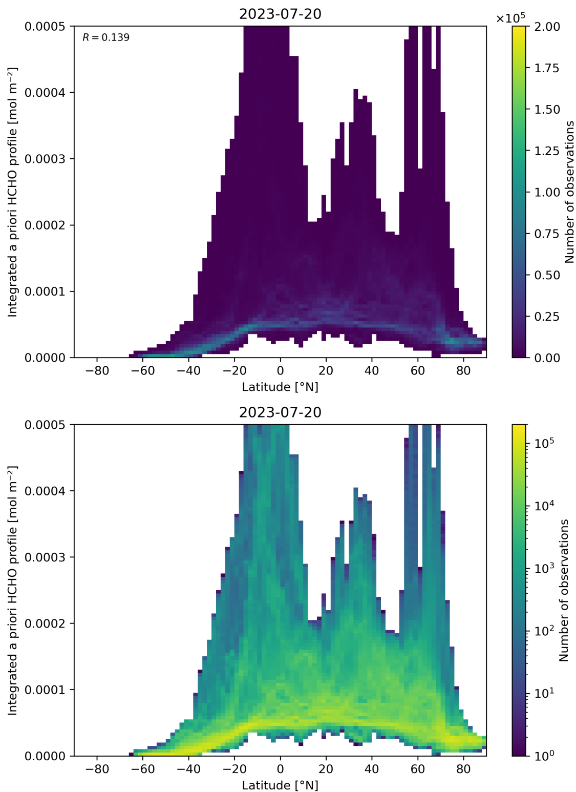
Figure 166: Scatter density plot of “Latitude” against “Integrated a priori HCHO profile” for 2023-07-19 to 2023-07-21.
