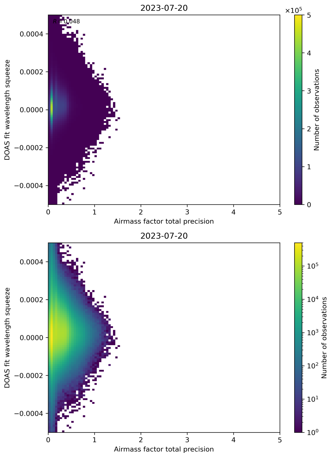
Figure 107: Scatter density plot of “Airmass factor total precision” against “DOAS fit wavelength squeeze” for 2023-07-19 to 2023-07-21.
