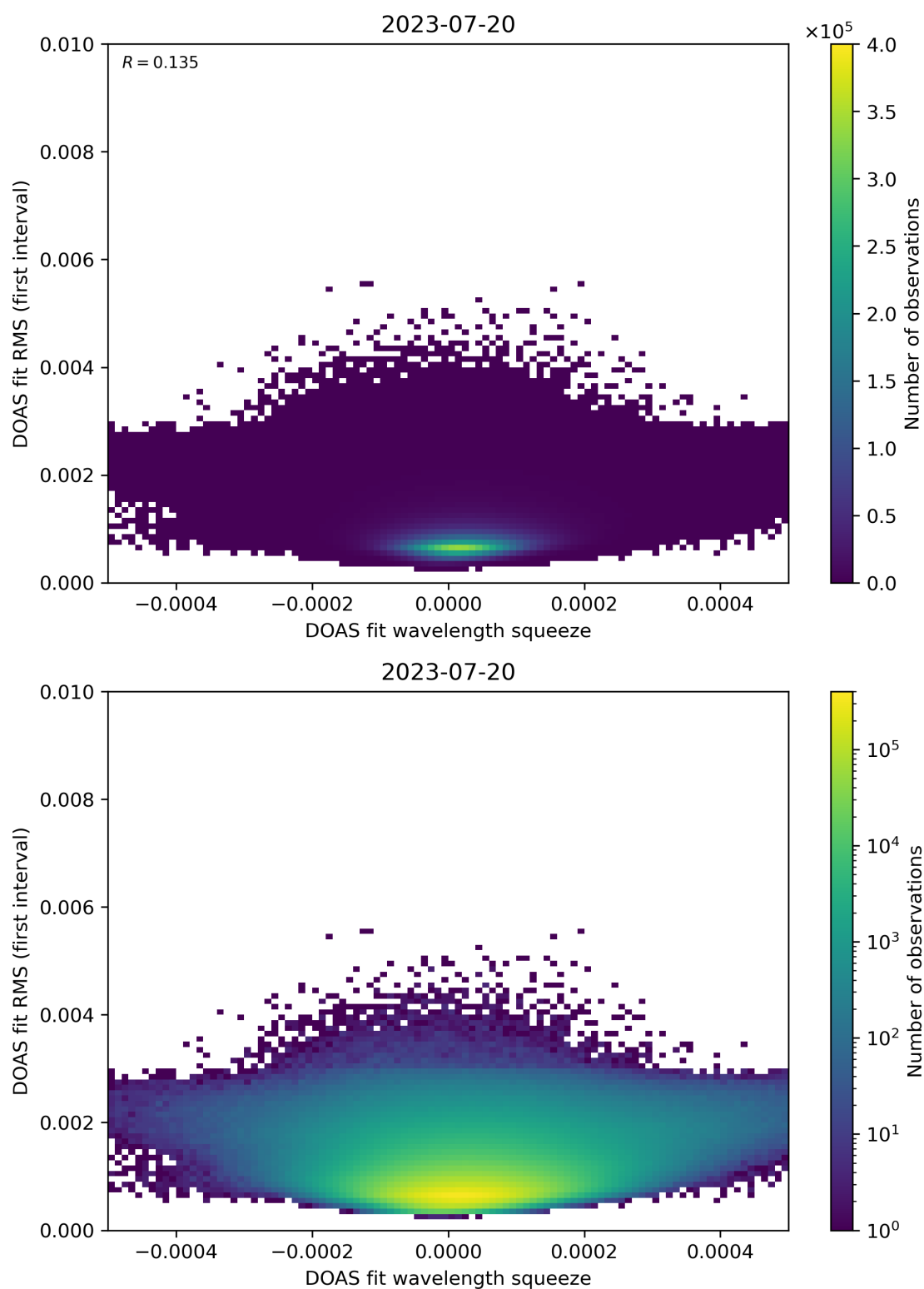
Figure 68: Scatter density plot of “DOAS fit wavelength squeeze” against “DOAS fit RMS (first interval)” for 2023-07-19 to 2023-07-21.
