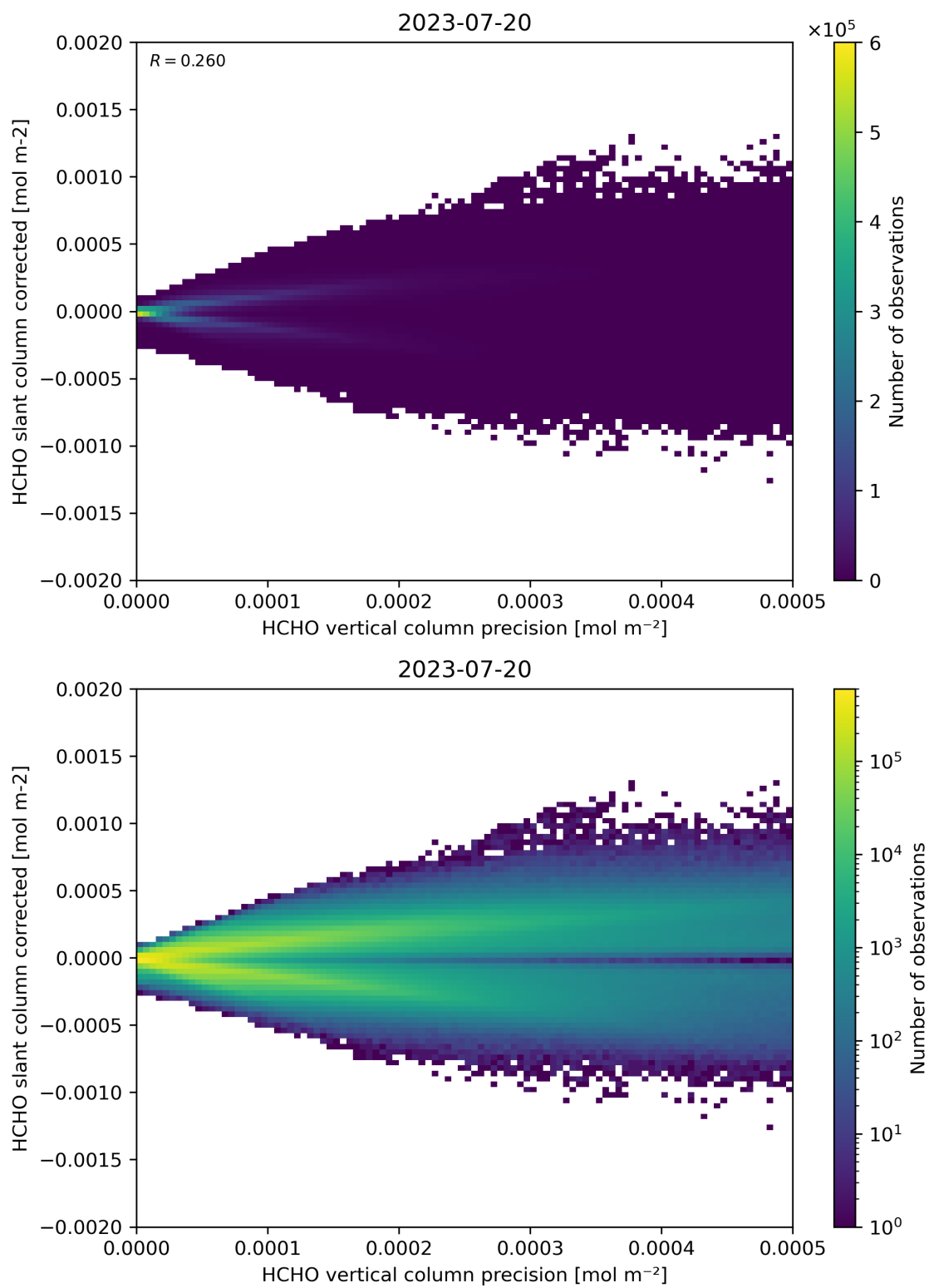
Figure 140: Scatter density plot of “HCHO vertical column precision” against “HCHO slant column corrected” for 2023-07-19 to 2023-07-21.
