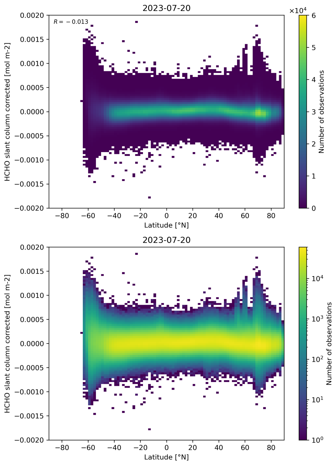
Figure 157: Scatter density plot of “Latitude” against “HCHO slant column corrected” for 2023-07-19 to 2023-07-21.
