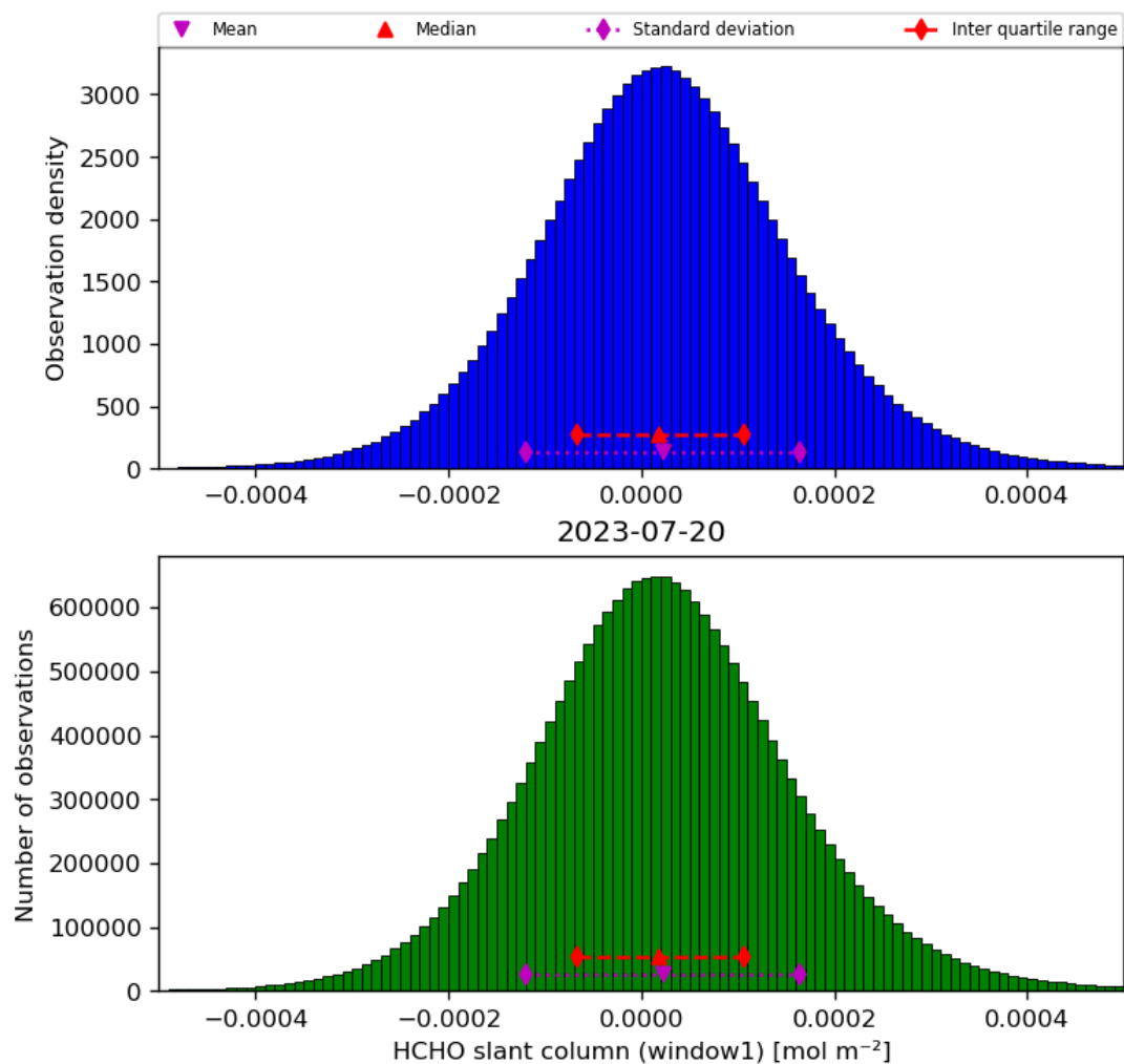
Figure 38: Histogram of “HCHO slant column (window1)” for 2023-07-19 to 2023-07-21
