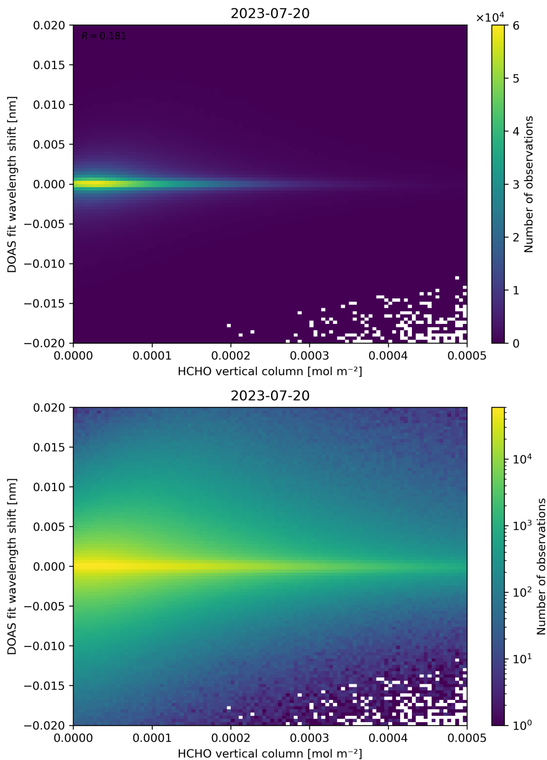
Figure 124: Scatter density plot of “HCHO vertical column” against “DOAS fit wavelength shift” for 2023-07-19 to 2023-07-21.
