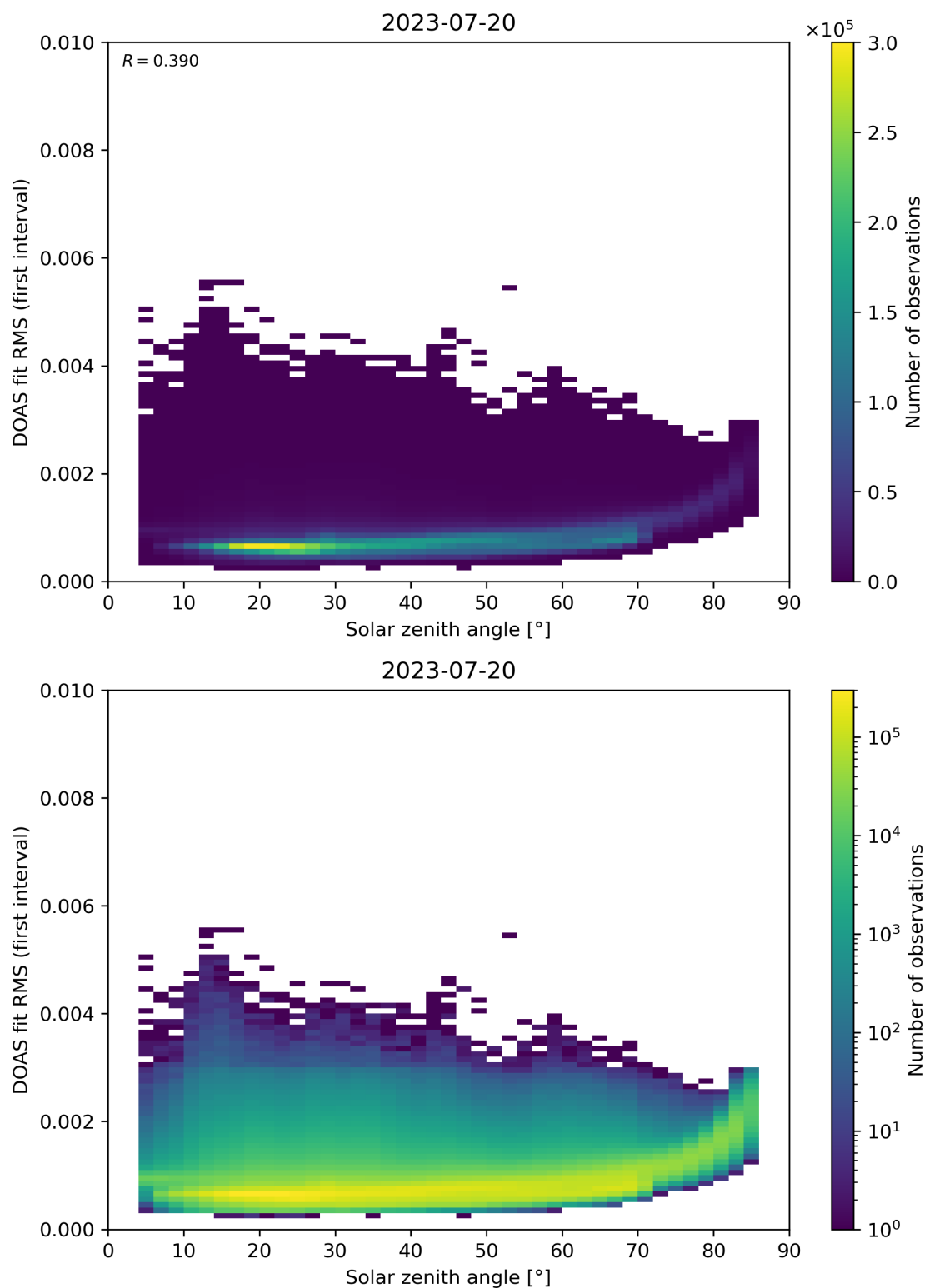
Figure 167: Scatter density plot of “Solar zenith angle” against “DOAS fit RMS (first interval)” for 2023-07-19 to 2023-07-21.
