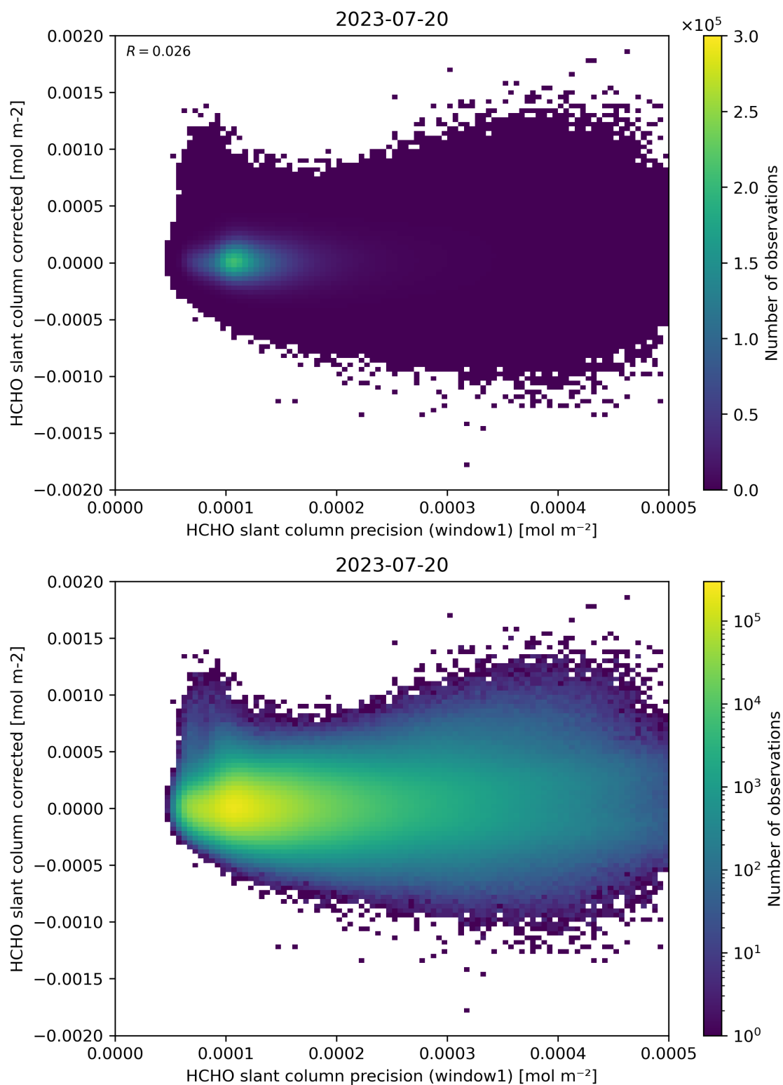
Figure 92: Scatter density plot of “HCHO slant column precision (window1)” against “HCHO slant column corrected” for 2023-07-19 to 2023-07-21.
