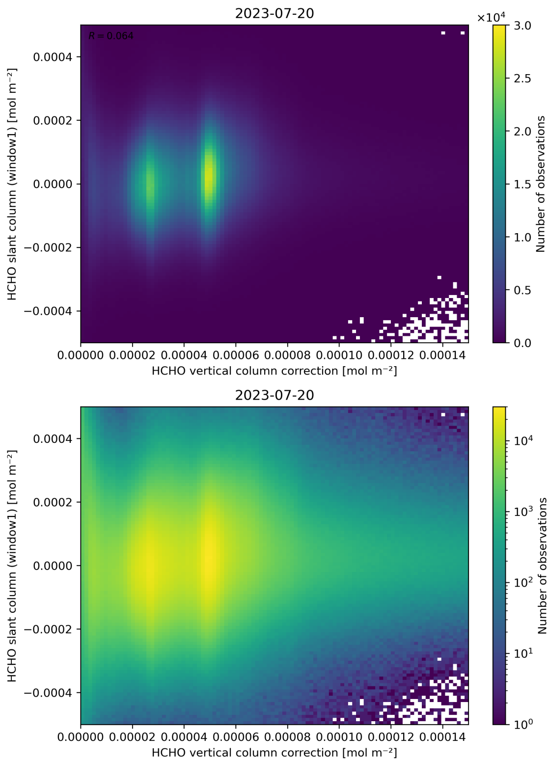
Figure 118: Scatter density plot of “HCHO vertical column correction” against “HCHO slant column (window1)” for 2023-07-19 to 2023-07-21.
