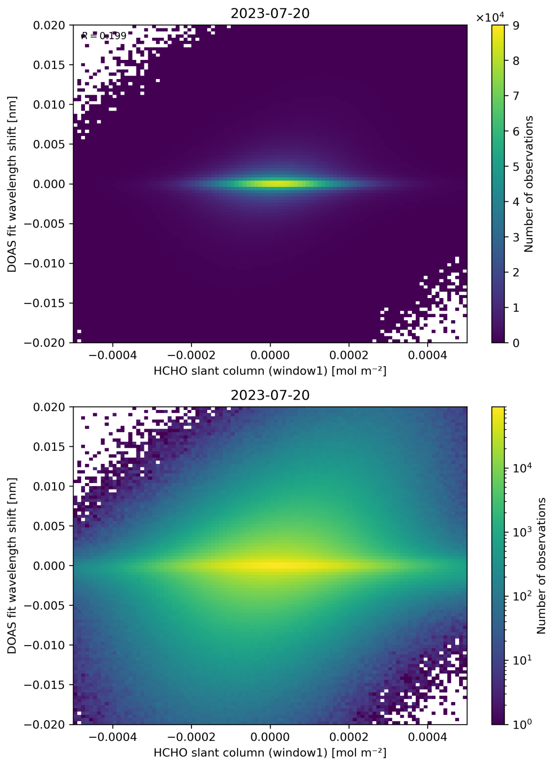
Figure 79: Scatter density plot of “HCHO slant column (window1)” against “DOAS fit wavelength shift” for 2023-07-19 to 2023-07-21.
