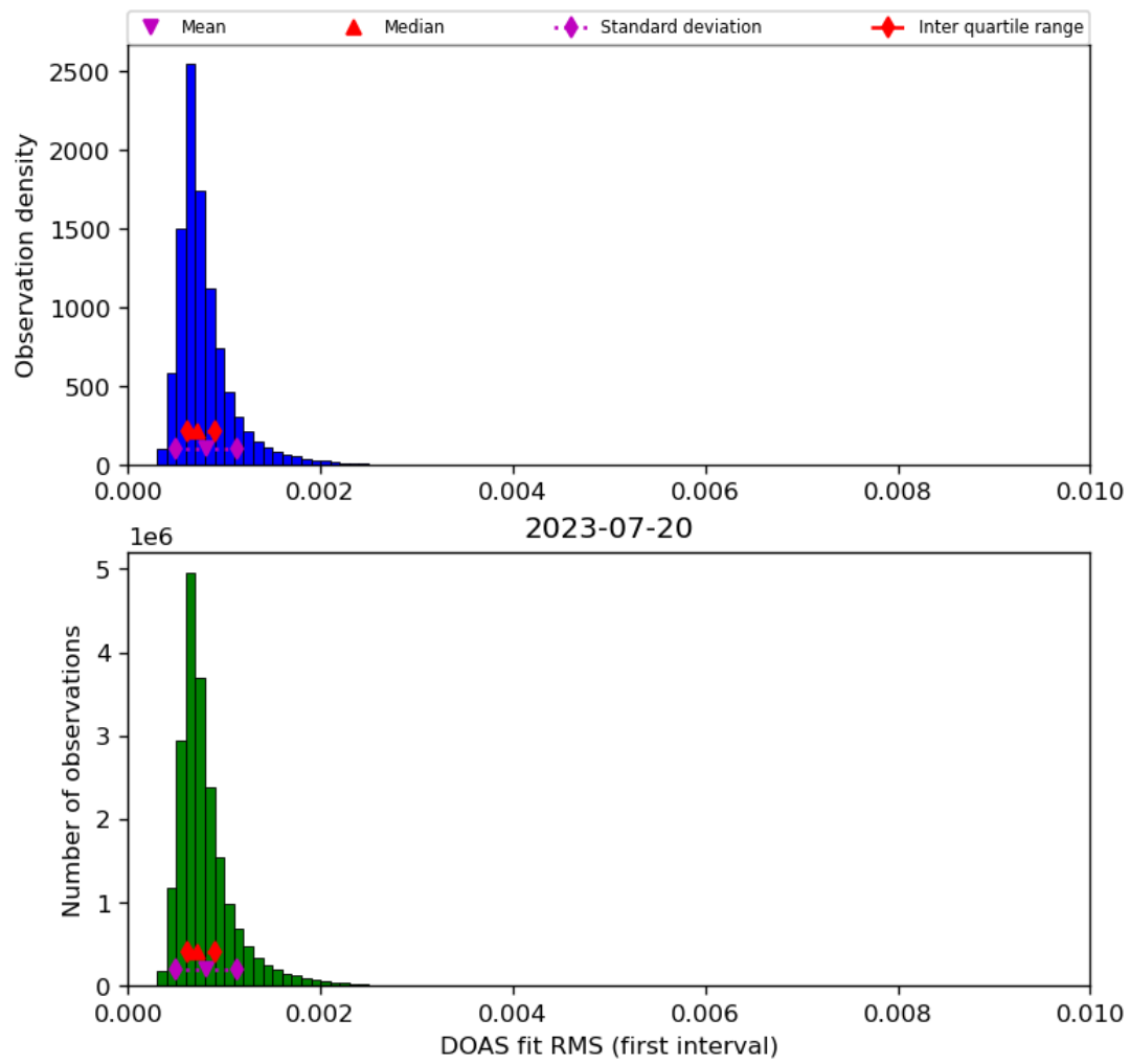
Figure 46: Histogram of “DOAS fit RMS (first interval)” for 2023-07-19 to 2023-07-21
