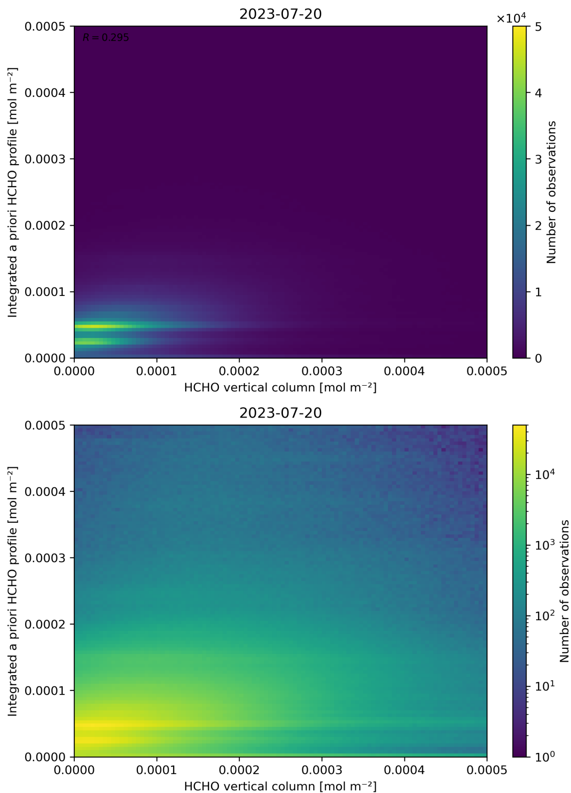
Figure 135: Scatter density plot of “HCHO vertical column” against “Integrated a priori HCHO profile” for 2023-07-19 to 2023-07-21.
