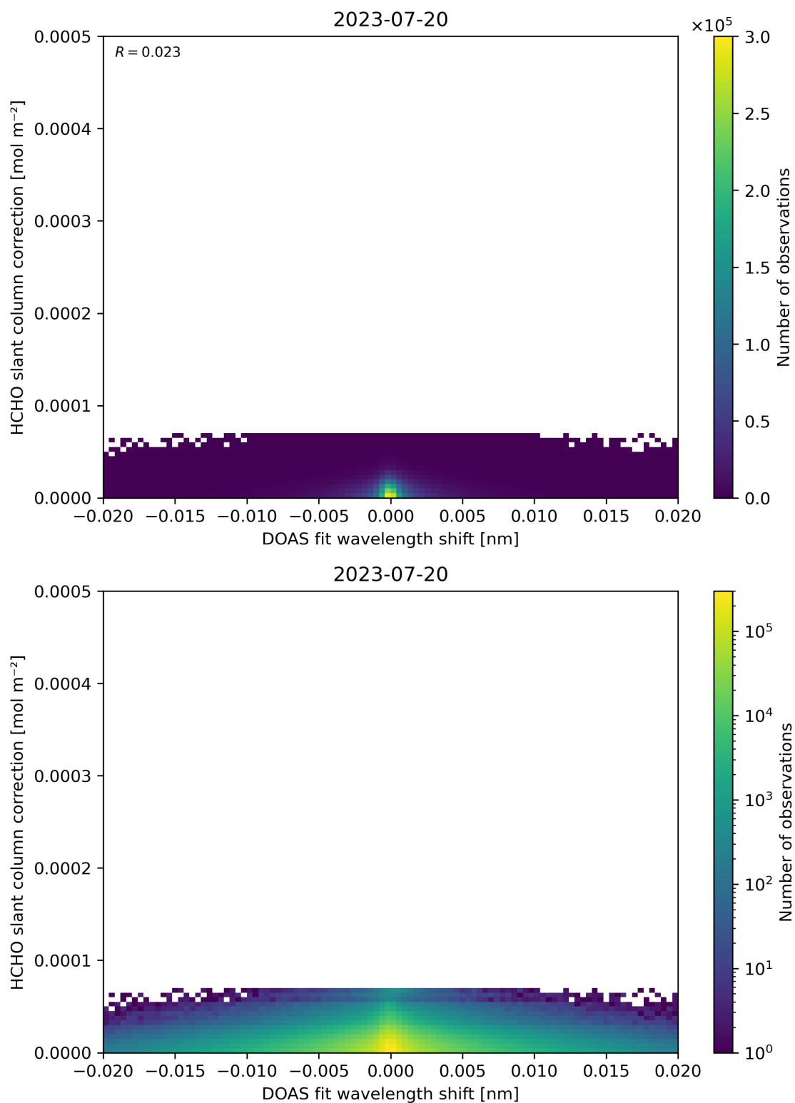
Figure 67: Scatter density plot of “DOAS fit wavelength shift” against “HCHO slant column correction” for 2023-07-19 to 2023-07-21.
