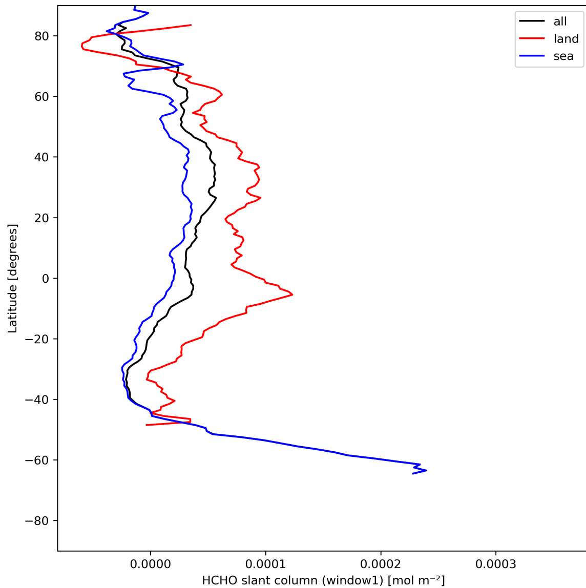
Figure 24: Zonal average of “HCHO slant column (window1)” for 2023-07-19 to 2023-07-21.
