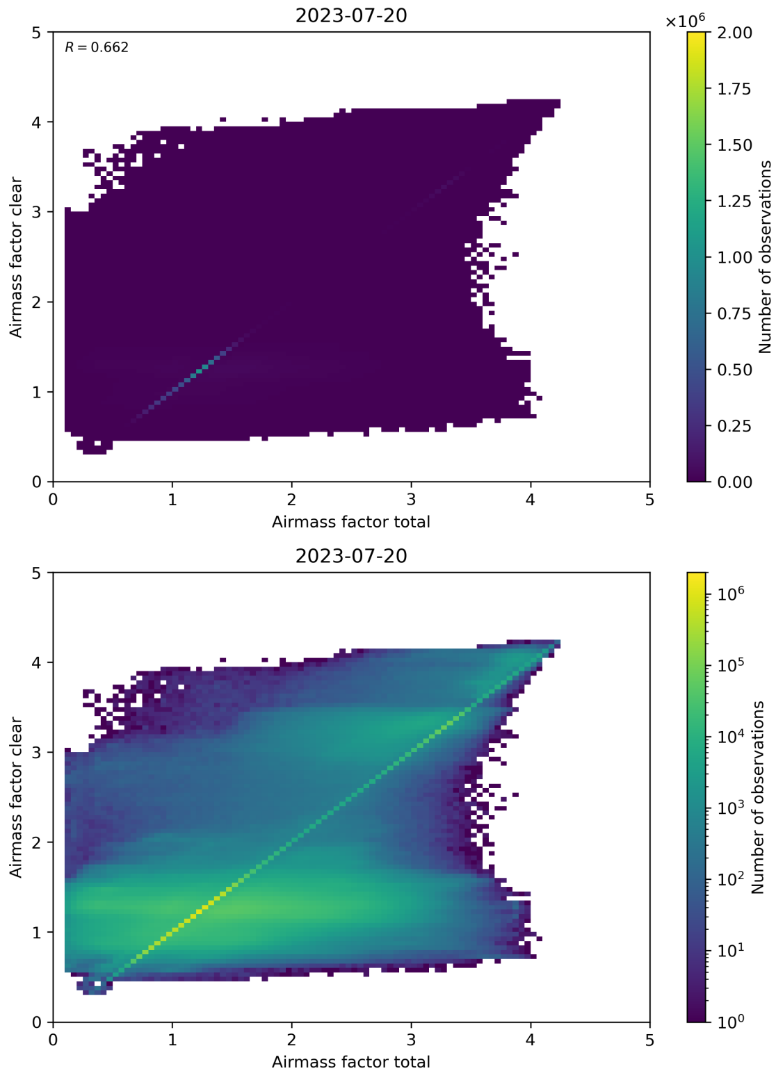
Figure 100: Scatter density plot of “Airmass factor total” against “Airmass factor clear” for 2023-07-19 to 2023-07-21.
