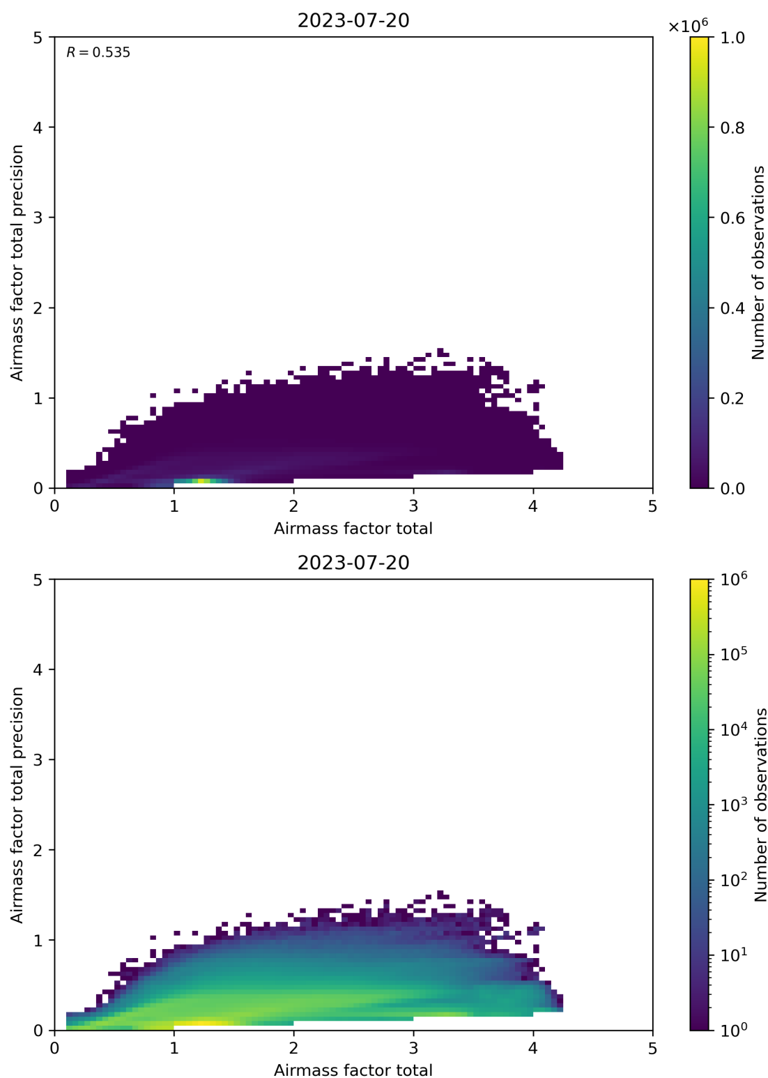
Figure 103: Scatter density plot of “Airmass factor total” against “Airmass factor total precision” for 2023-07-19 to 2023-07-21.
