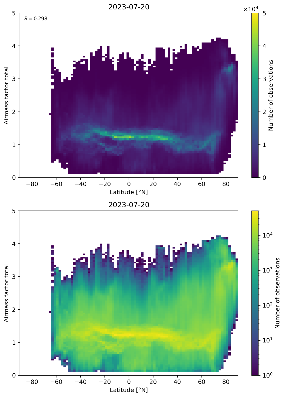
Figure 161: Scatter density plot of “Latitude” against “Airmass factor total” for 2023-07-19 to 2023-07-21.
