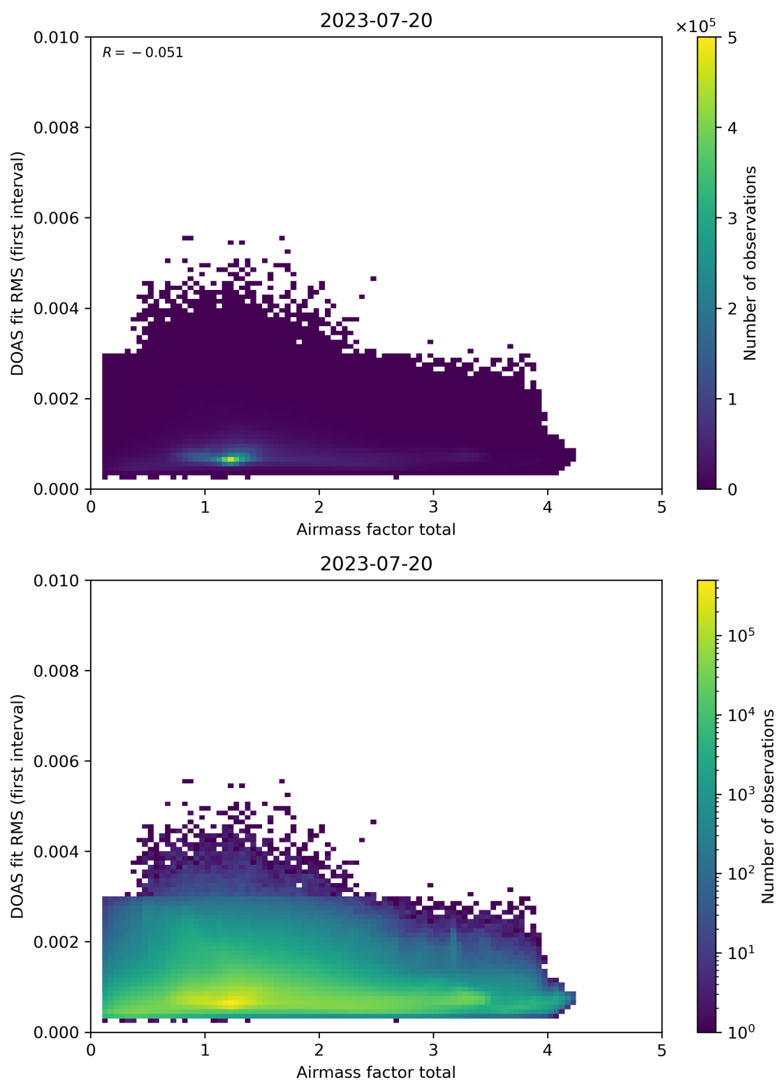
Figure 97: Scatter density plot of “Airmass factor total” against “DOAS fit RMS (first interval)” for 2023-07-19 to 2023-07-21.
