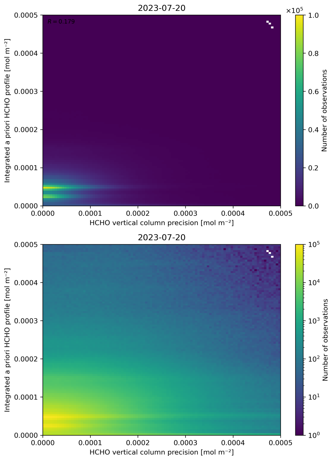
Figure 147: Scatter density plot of “HCHO vertical column precision” against “Integrated a priori HCHO profile” for 2023-07-19 to 2023-07-21.
