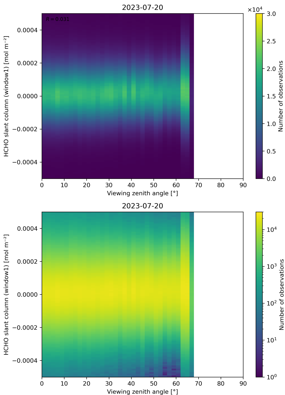
Figure 188: Scatter density plot of “Viewing zenith angle” against “HCHO slant column (window1)” for 2023-07-19 to 2023-07-21.
