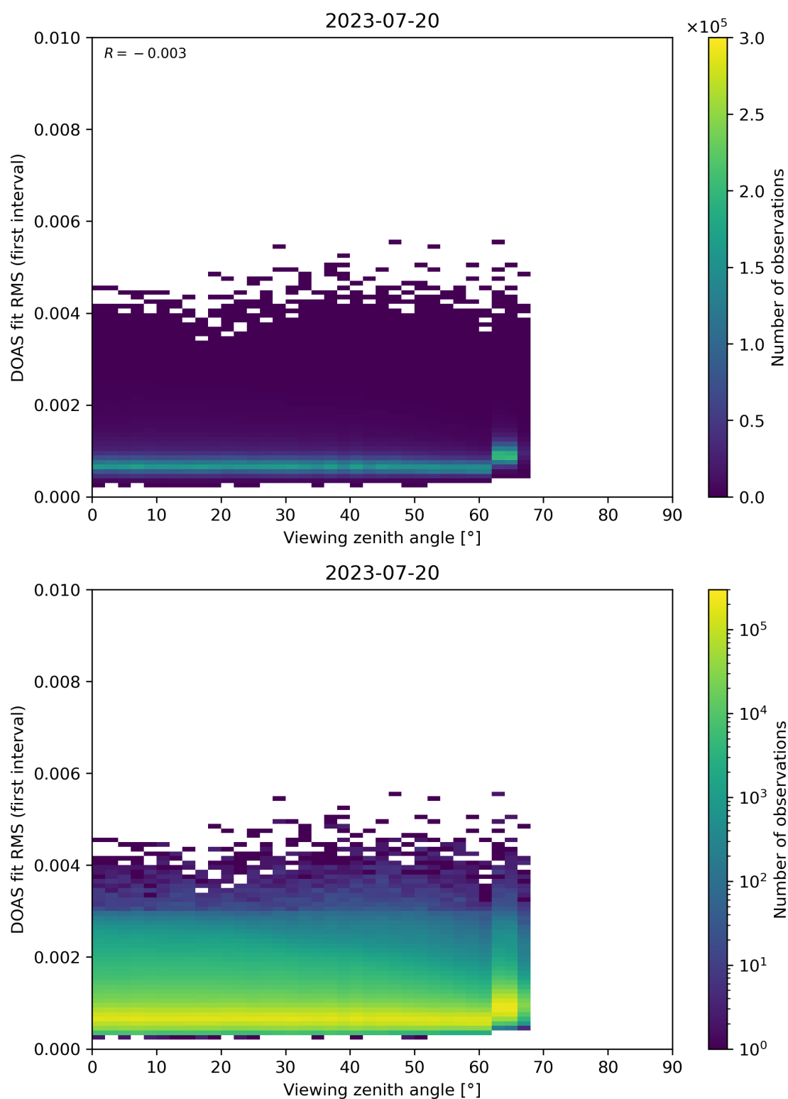
Figure 182: Scatter density plot of “Viewing zenith angle” against “DOAS fit RMS (first interval)” for 2023-07-19 to 2023-07-21.
