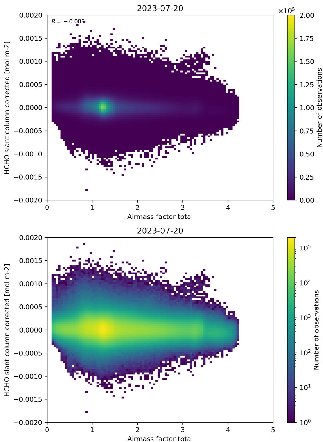
Figure 101: Scatter density plot of “Airmass factor total” against “HCHO slant column corrected” for 2023-07-19 to 2023-07-21.
