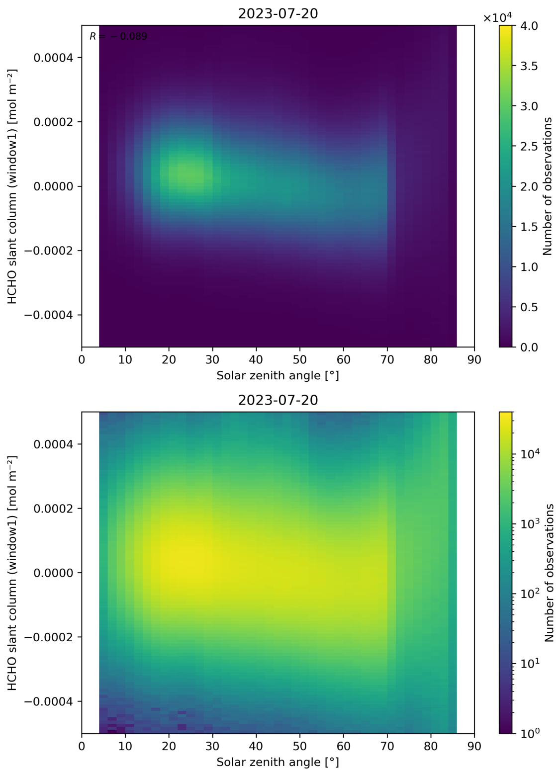
Figure 173: Scatter density plot of “Solar zenith angle” against “HCHO slant column (window1)” for 2023-07-19 to 2023-07-21.
