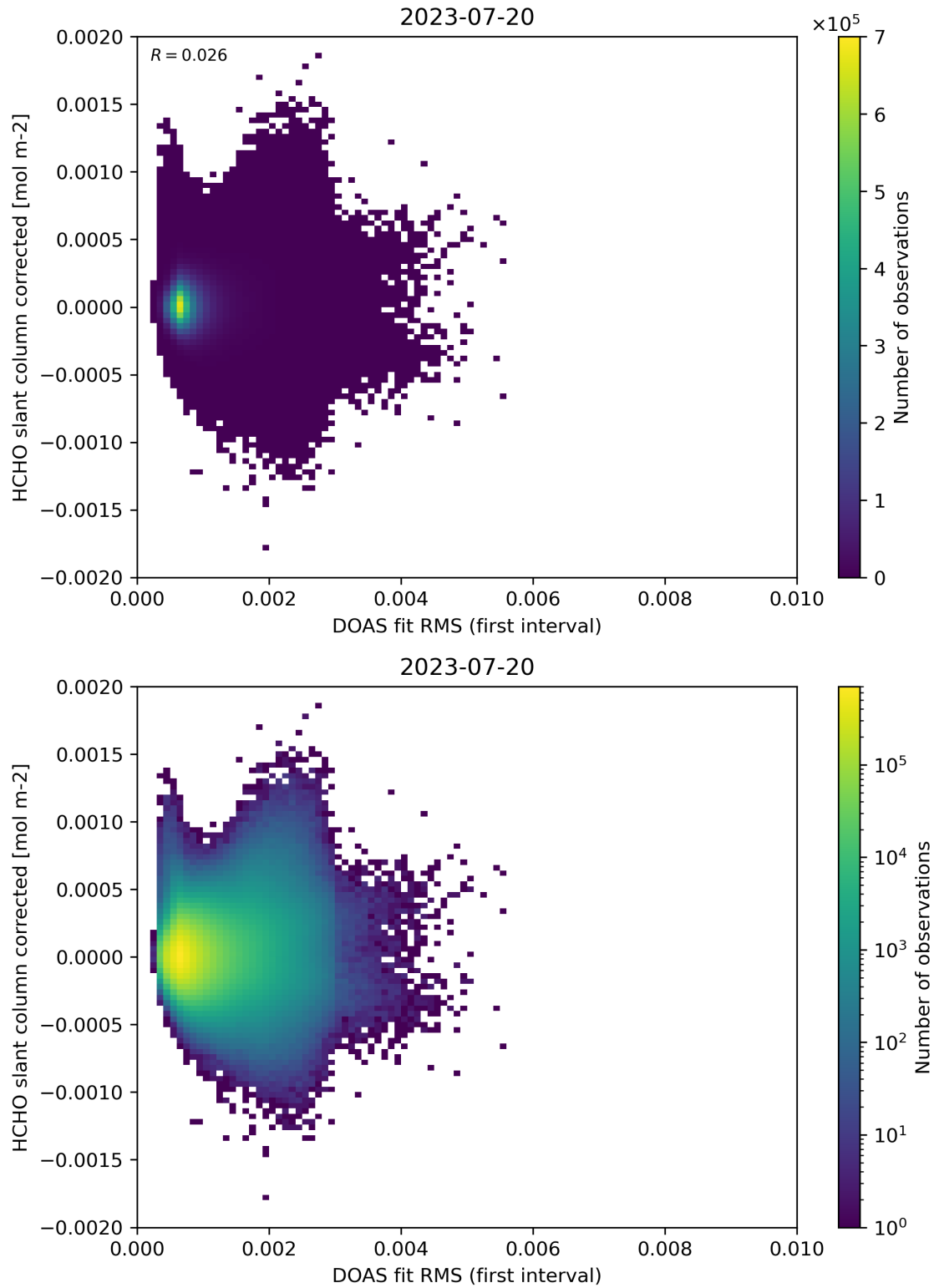
Figure 62: Scatter density plot of “DOAS fit RMS (first interval)” against “HCHO slant column corrected” for 2023-07-19 to 2023-07-21.
