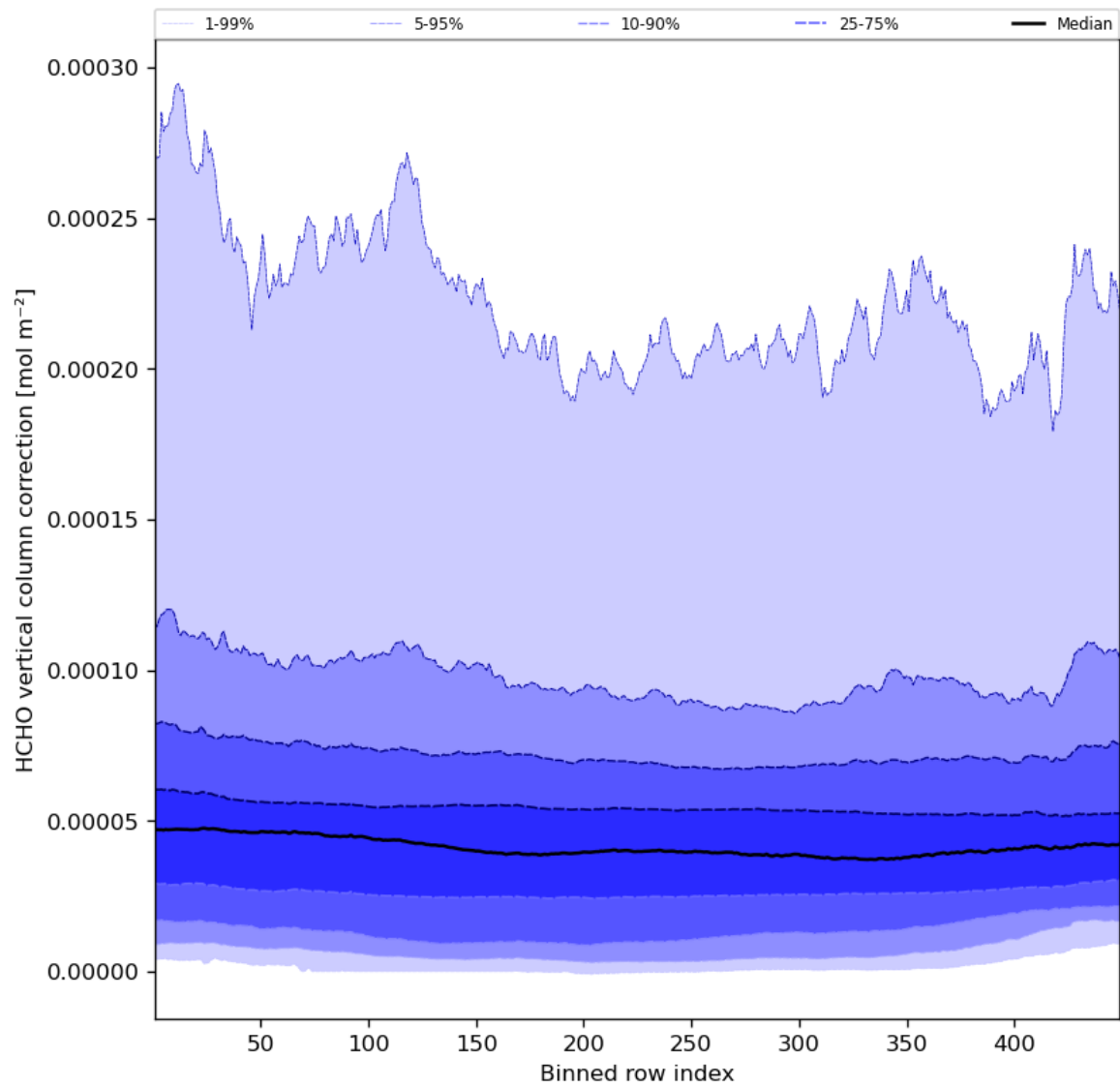
Figure 51: Along track statistics of “HCHO vertical column correction” for 2023-07-19 to 2023-07-21
