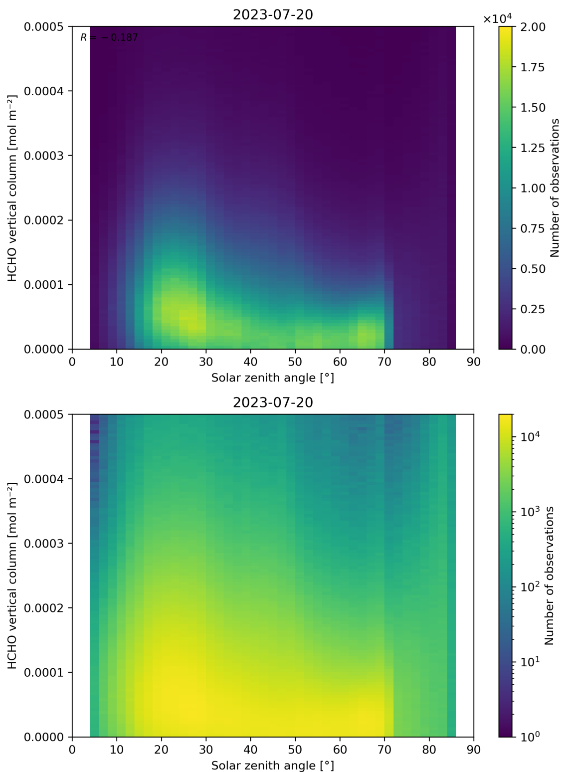
Figure 177: Scatter density plot of “Solar zenith angle” against “HCHO vertical column” for 2023-07-19 to 2023-07-21.
