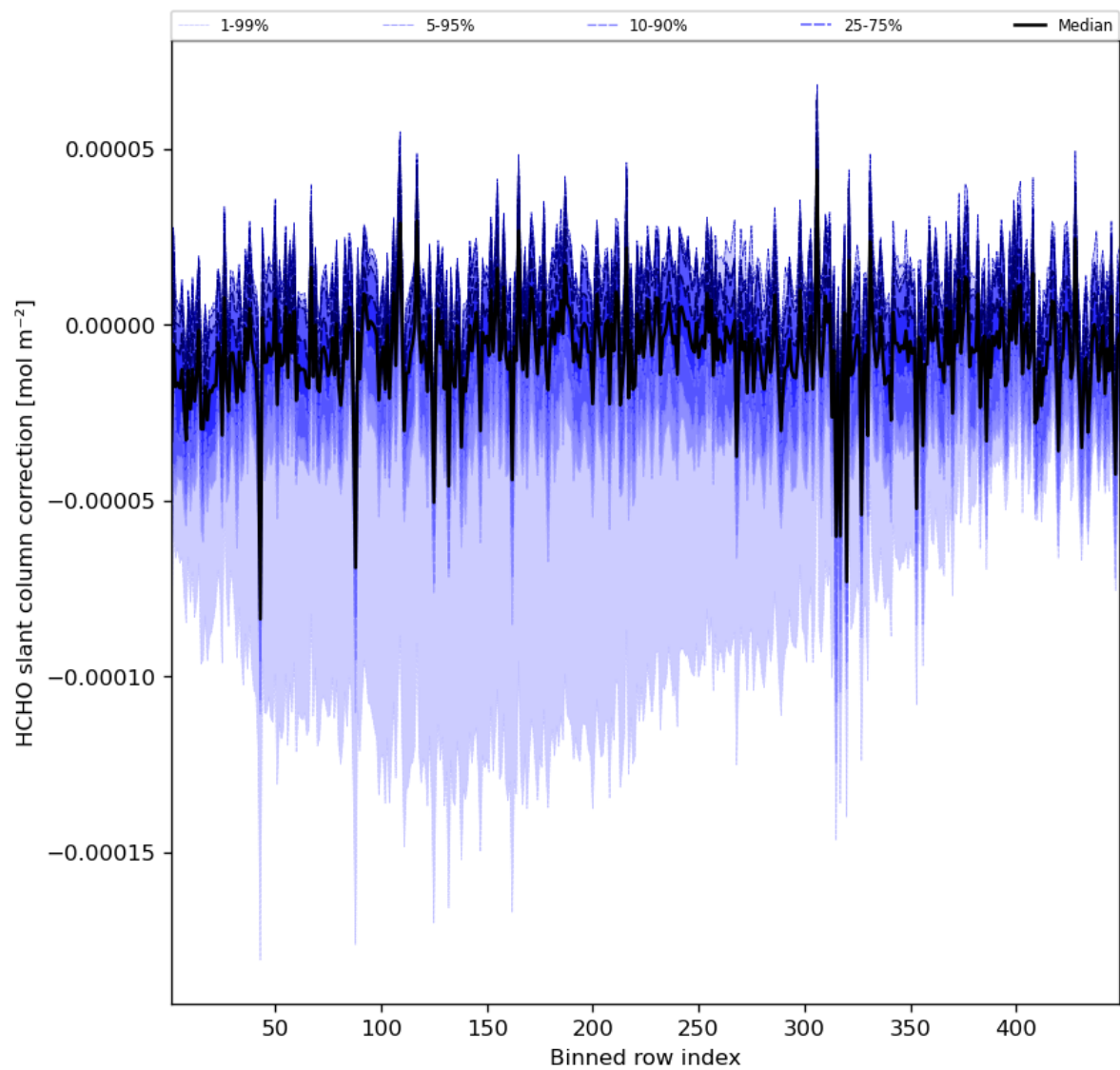
Figure 61: Along track statistics of “HCHO slant column correction” for 2023-07-19 to 2023-07-21
