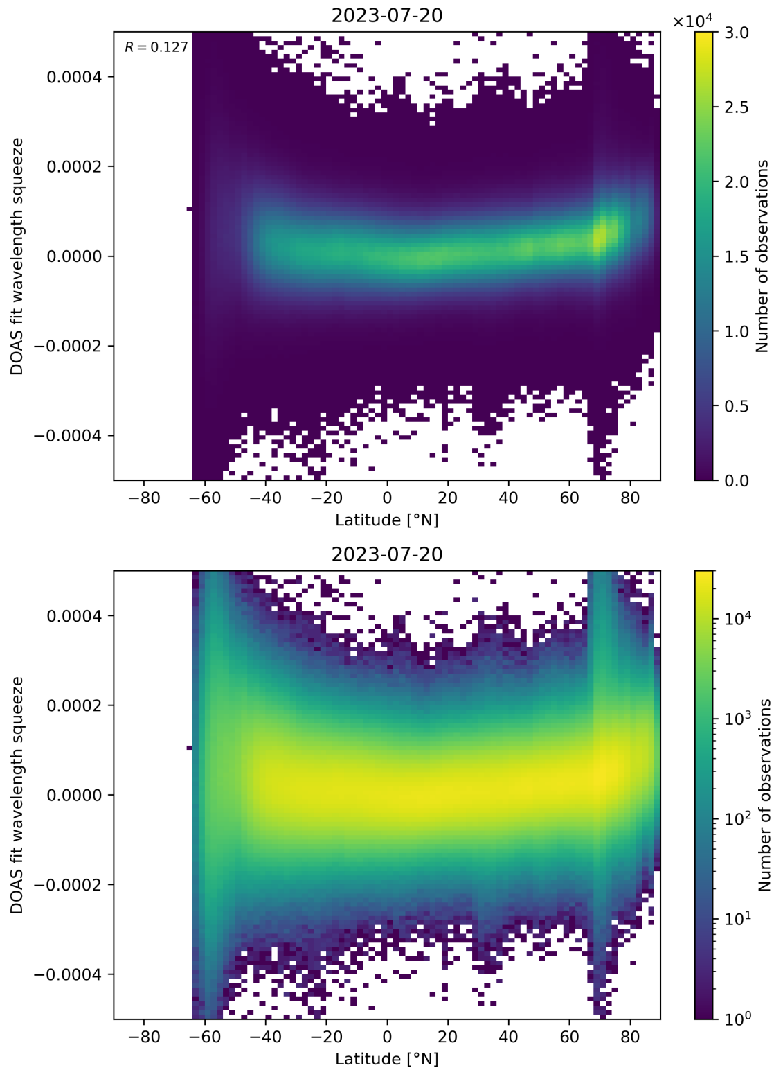
Figure 155: Scatter density plot of “Latitude” against “DOAS fit wavelength squeeze” for 2023-07-19 to 2023-07-21.
