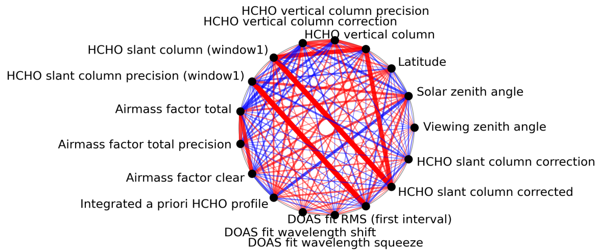
Figure 1: Map of correlation graph for 2023-07-19 to 2023-07-21.
