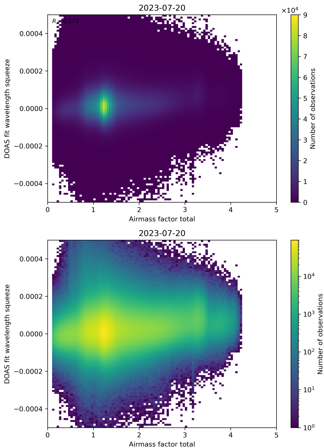
Figure 99: Scatter density plot of “Airmass factor total” against “DOAS fit wavelength squeeze” for 2023-07-19 to 2023-07-21.
