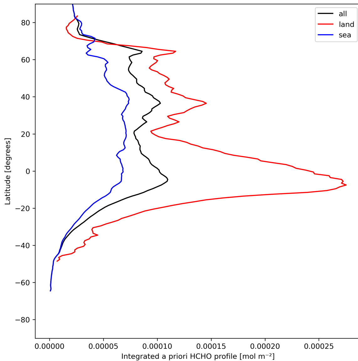
Figure 29: Zonal average of “Integrated a priori HCHO profile” for 2023-07-19 to 2023-07-21.
