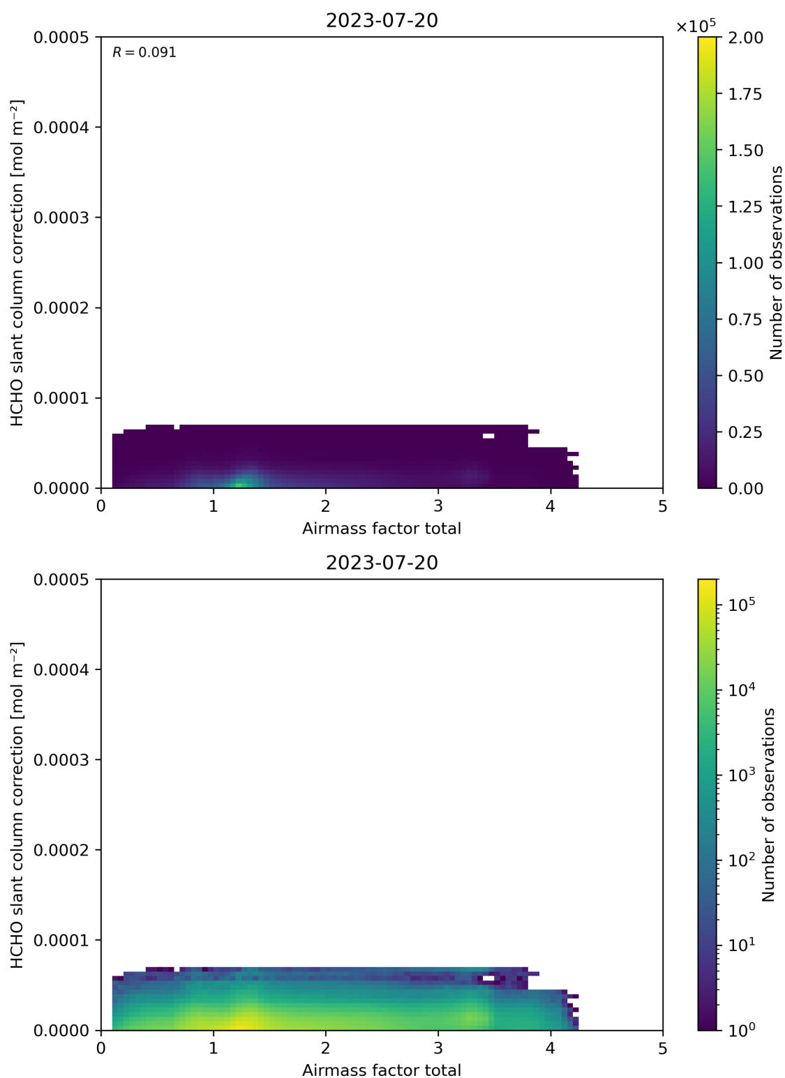
Figure 102: Scatter density plot of “Airmass factor total” against “HCHO slant column correction” for 2023-07-19 to 2023-07-21.
