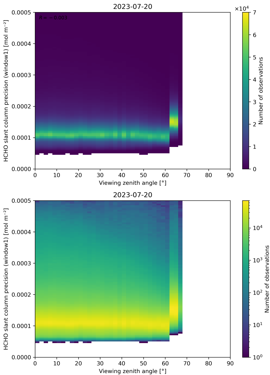
Figure 189: Scatter density plot of “Viewing zenith angle” against “HCHO slant column precision (window1)” for 2023-07-19 to 2023-07-21.
