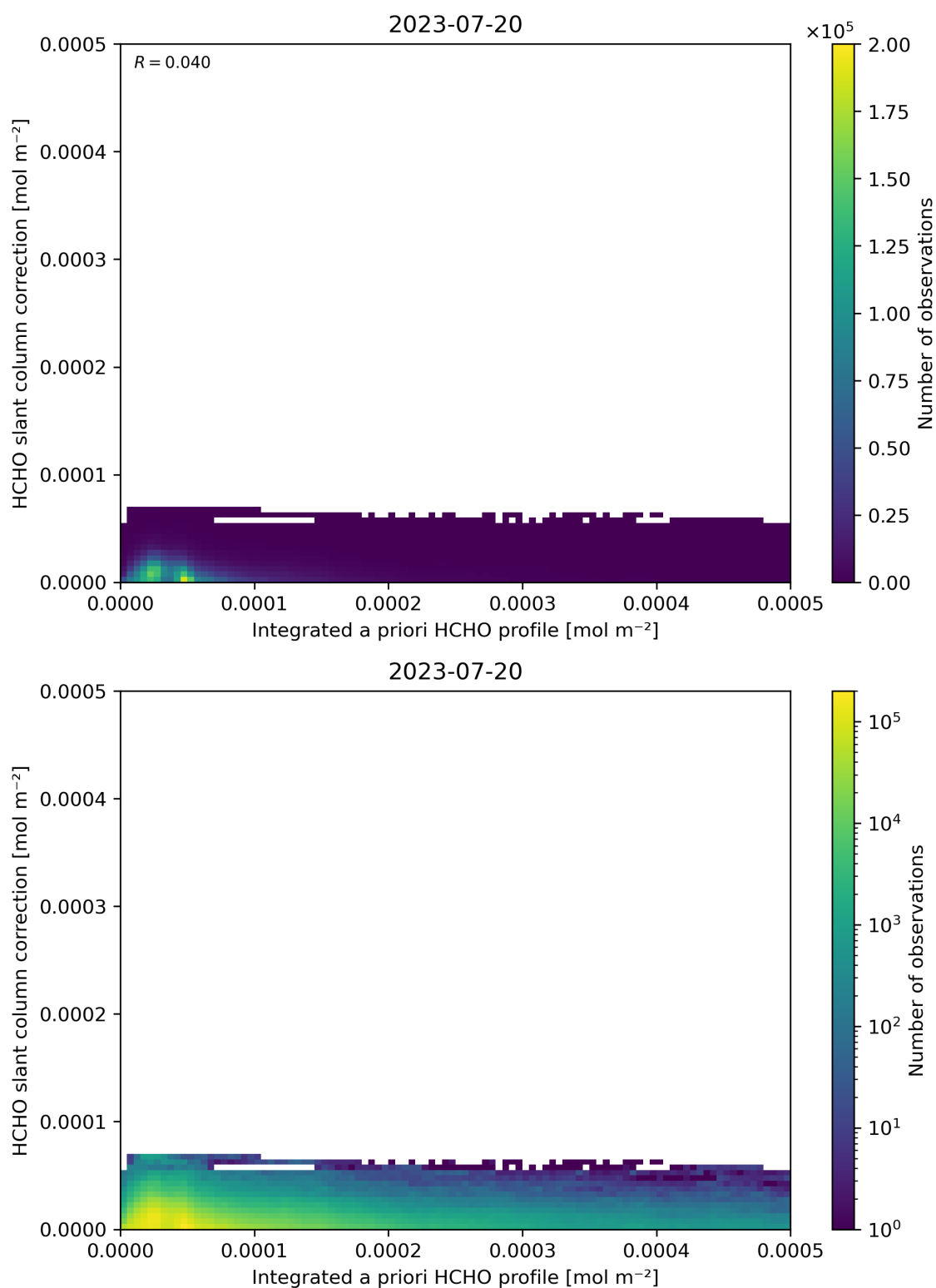
Figure 152: Scatter density plot of “Integrated a priori HCHO profile” against “HCHO slant column correction” for 2023-07-19 to 2023-07-21.
