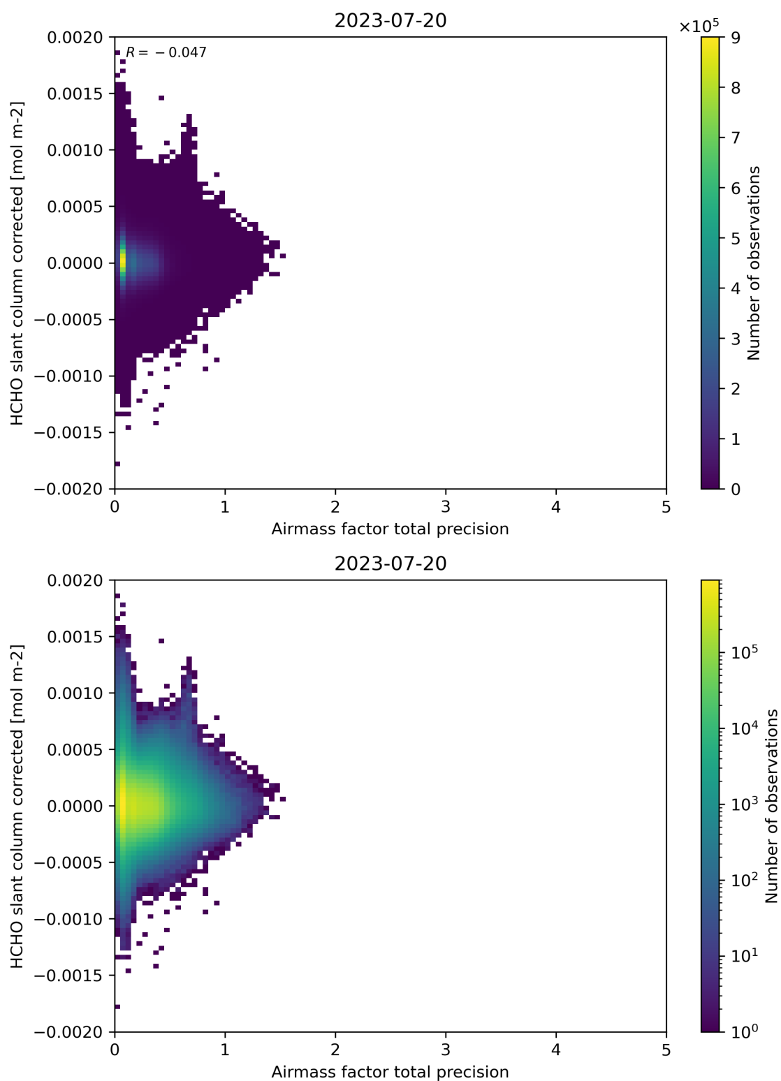
Figure 109: Scatter density plot of “Airmass factor total precision” against “HCHO slant column corrected” for 2023-07-19 to 2023-07-21.
