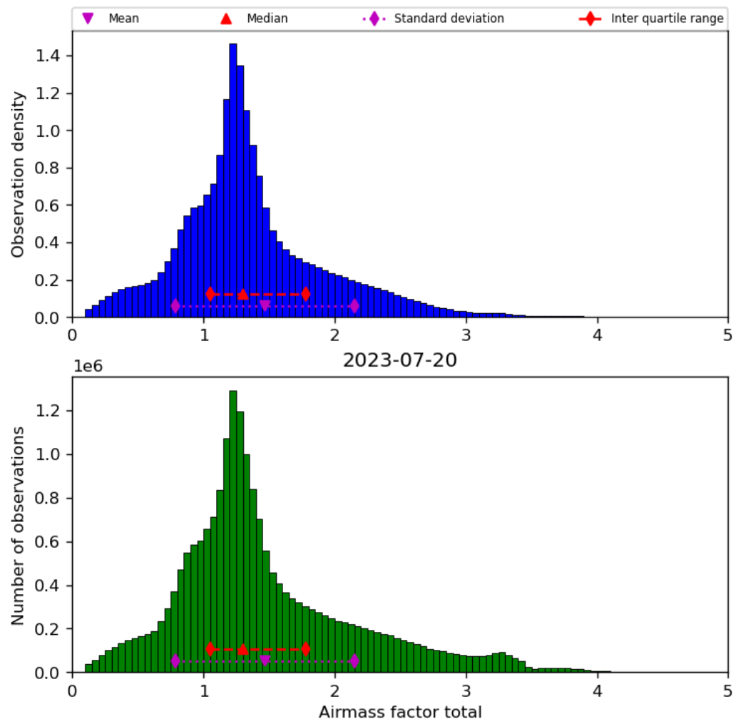
Figure 40: Histogram of “Airmass factor total” for 2023-07-19 to 2023-07-21
