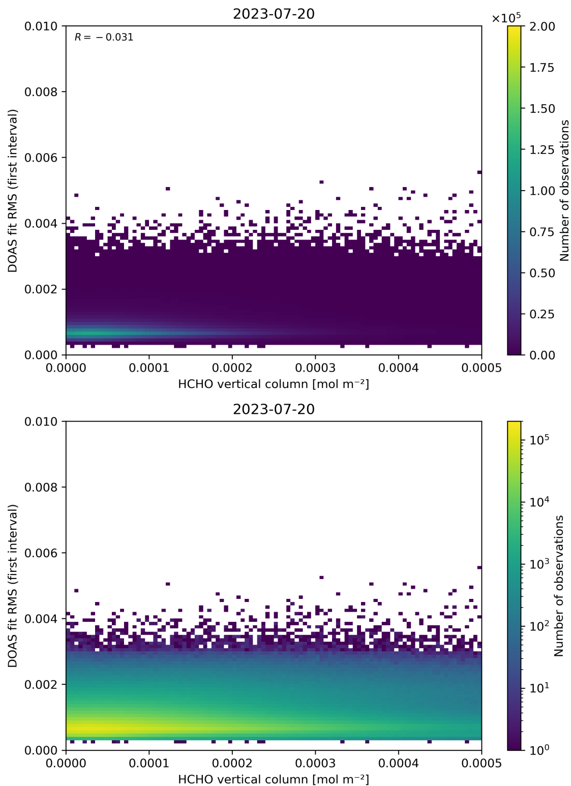
Figure 123: Scatter density plot of “HCHO vertical column” against “DOAS fit RMS (first interval)” for 2023-07-19 to 2023-07-21.
