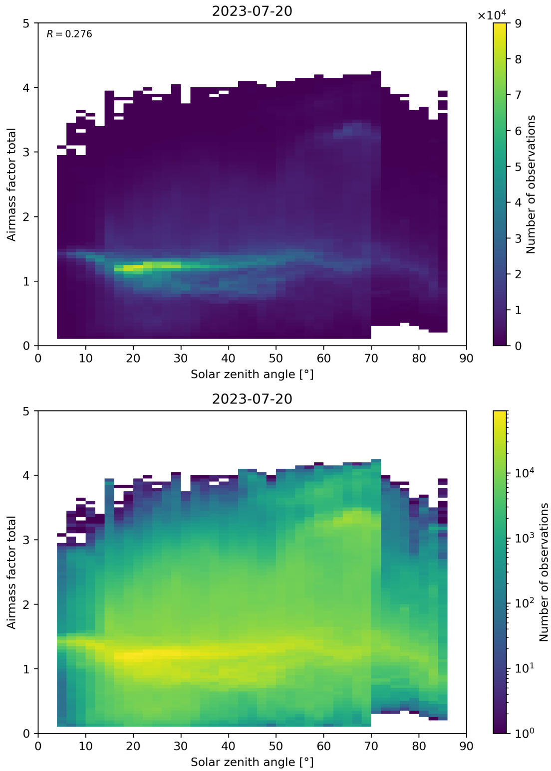
Figure 175: Scatter density plot of “Solar zenith angle” against “Airmass factor total” for 2023-07-19 to 2023-07-21.
