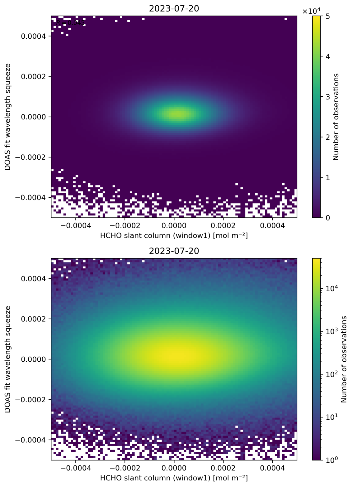
Figure 80: Scatter density plot of “HCHO slant column (window1)” against “DOAS fit wavelength squeeze” for 2023-07-19 to 2023-07-21.
