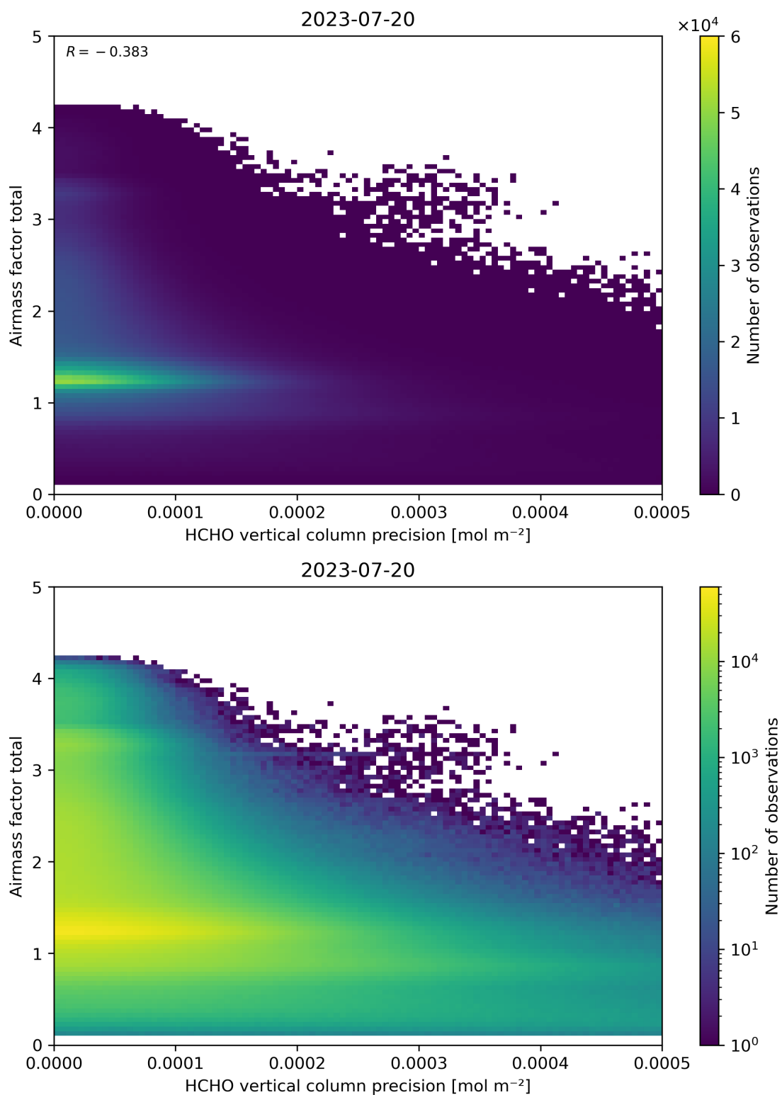
Figure 144: Scatter density plot of “HCHO vertical column precision” against “Airmass factor total” for 2023-07-19 to 2023-07-21.
