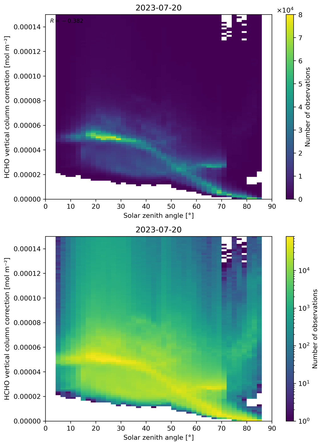
Figure 178: Scatter density plot of “Solar zenith angle” against “HCHO vertical column correction” for 2023-07-19 to 2023-07-21.
