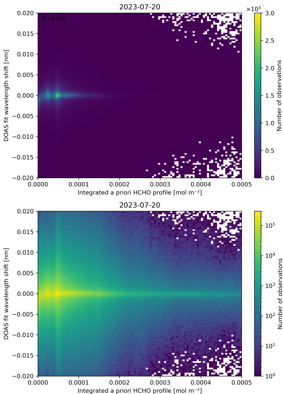
Figure 149: Scatter density plot of “Integrated a priori HCHO profile” against “DOAS fit wavelength shift” for 2023-07-19 to 2023-07-21.
