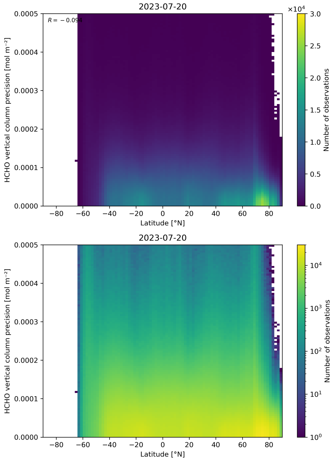
Figure 165: Scatter density plot of “Latitude” against “HCHO vertical column precision” for 2023-07-19 to 2023-07-21.
