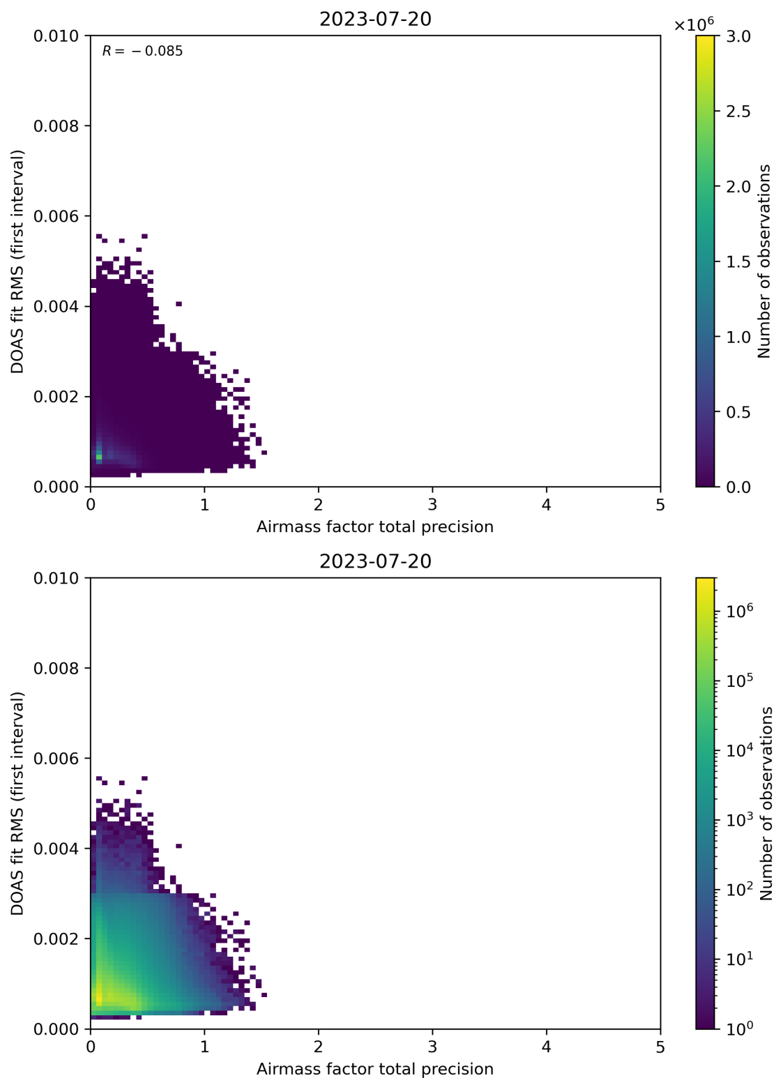
Figure 105: Scatter density plot of “Airmass factor total precision” against “DOAS fit RMS (first interval)” for 2023-07-19 to 2023-07-21.
