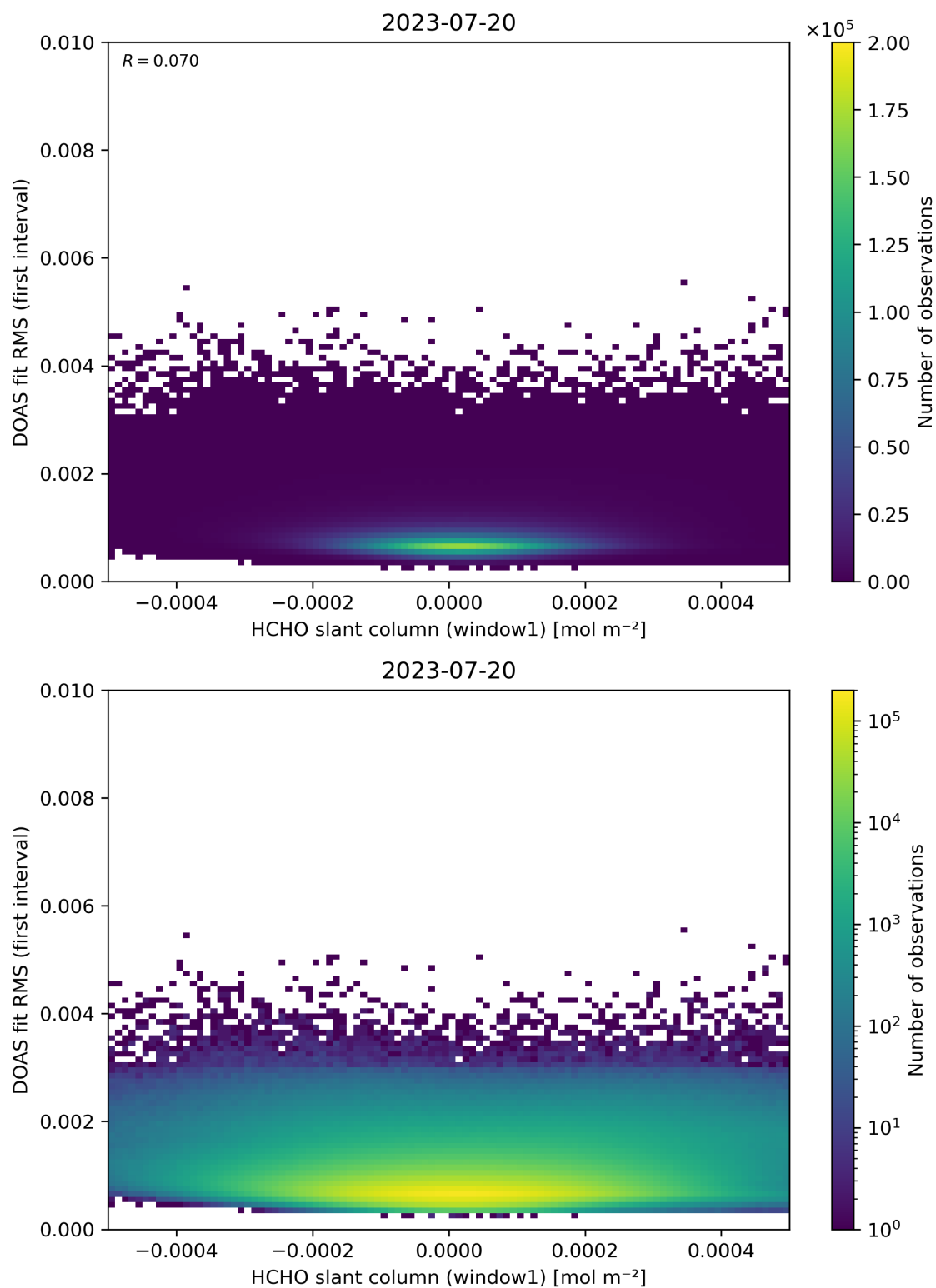
Figure 78: Scatter density plot of “HCHO slant column (window1)” against “DOAS fit RMS (first interval)” for 2023-07-19 to 2023-07-21.
