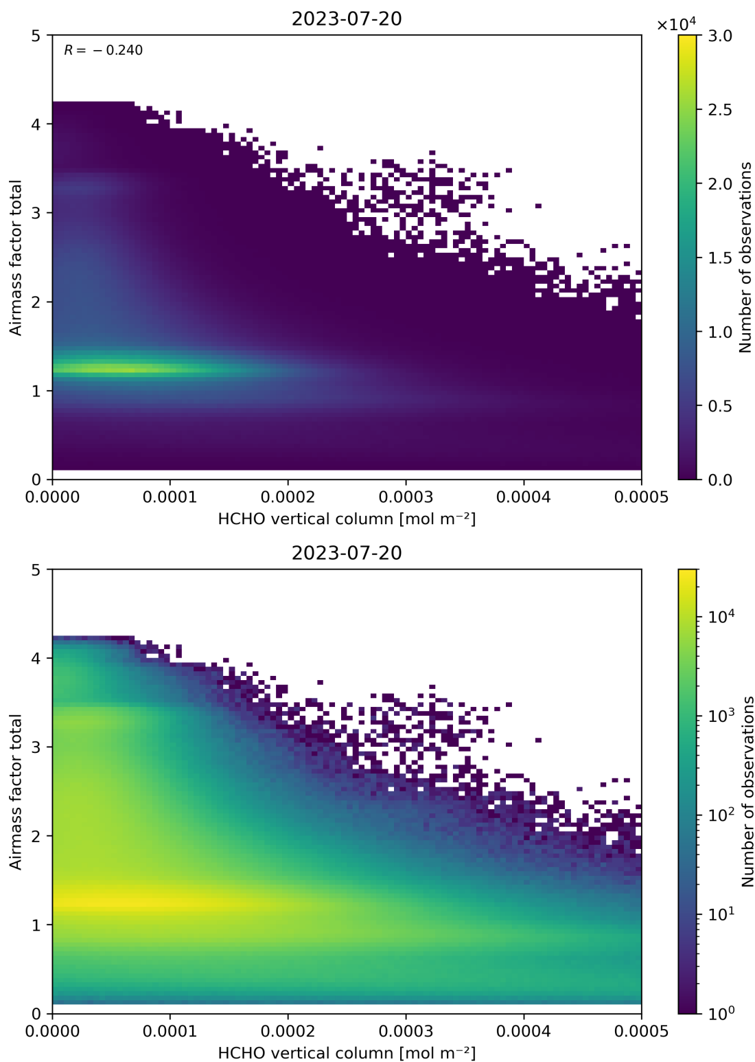
Figure 131: Scatter density plot of “HCHO vertical column” against “Airmass factor total” for 2023-07-19 to 2023-07-21.
