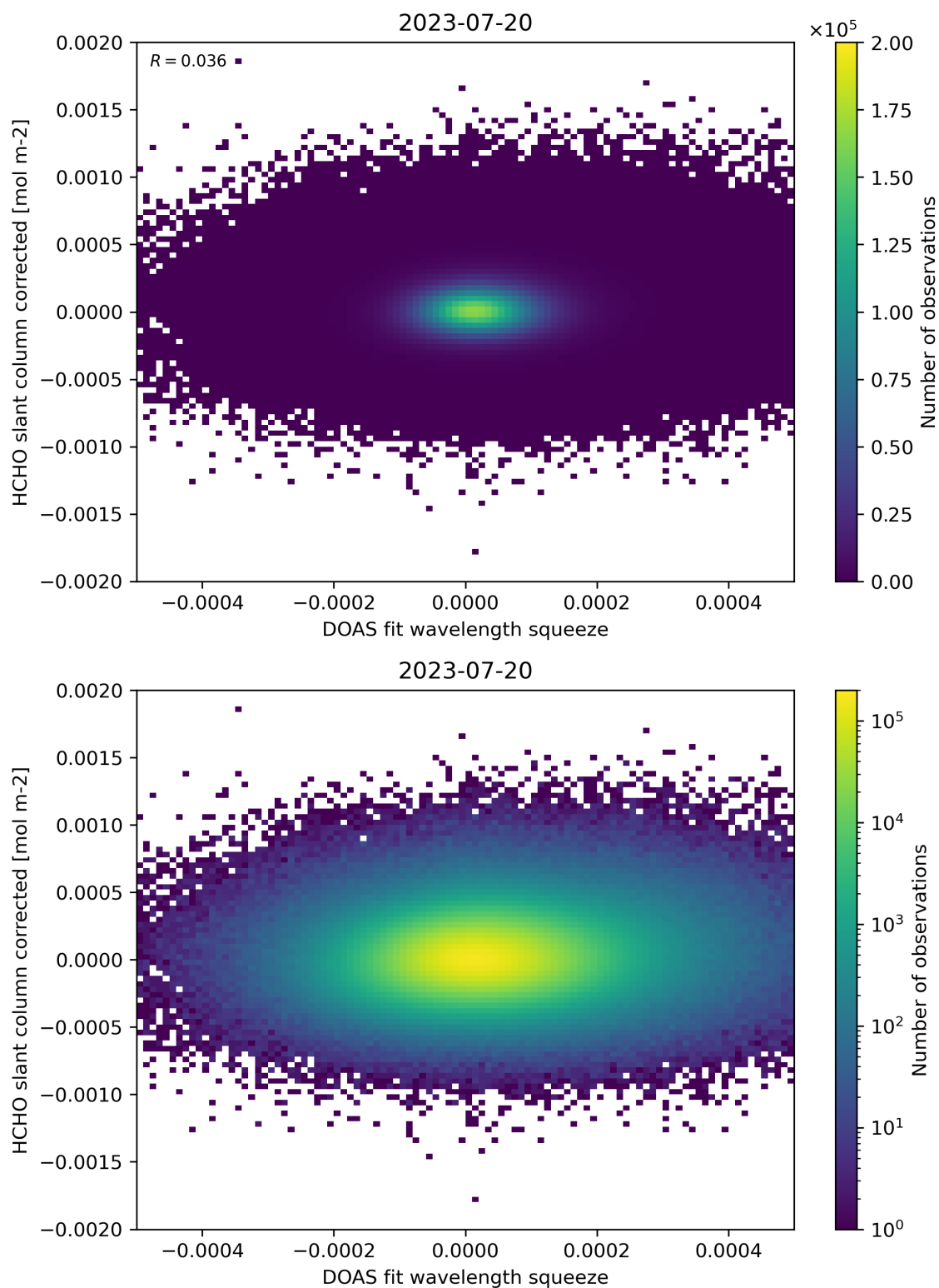
Figure 69: Scatter density plot of “DOAS fit wavelength squeeze” against “HCHO slant column corrected” for 2023-07-19 to 2023-07-21.
