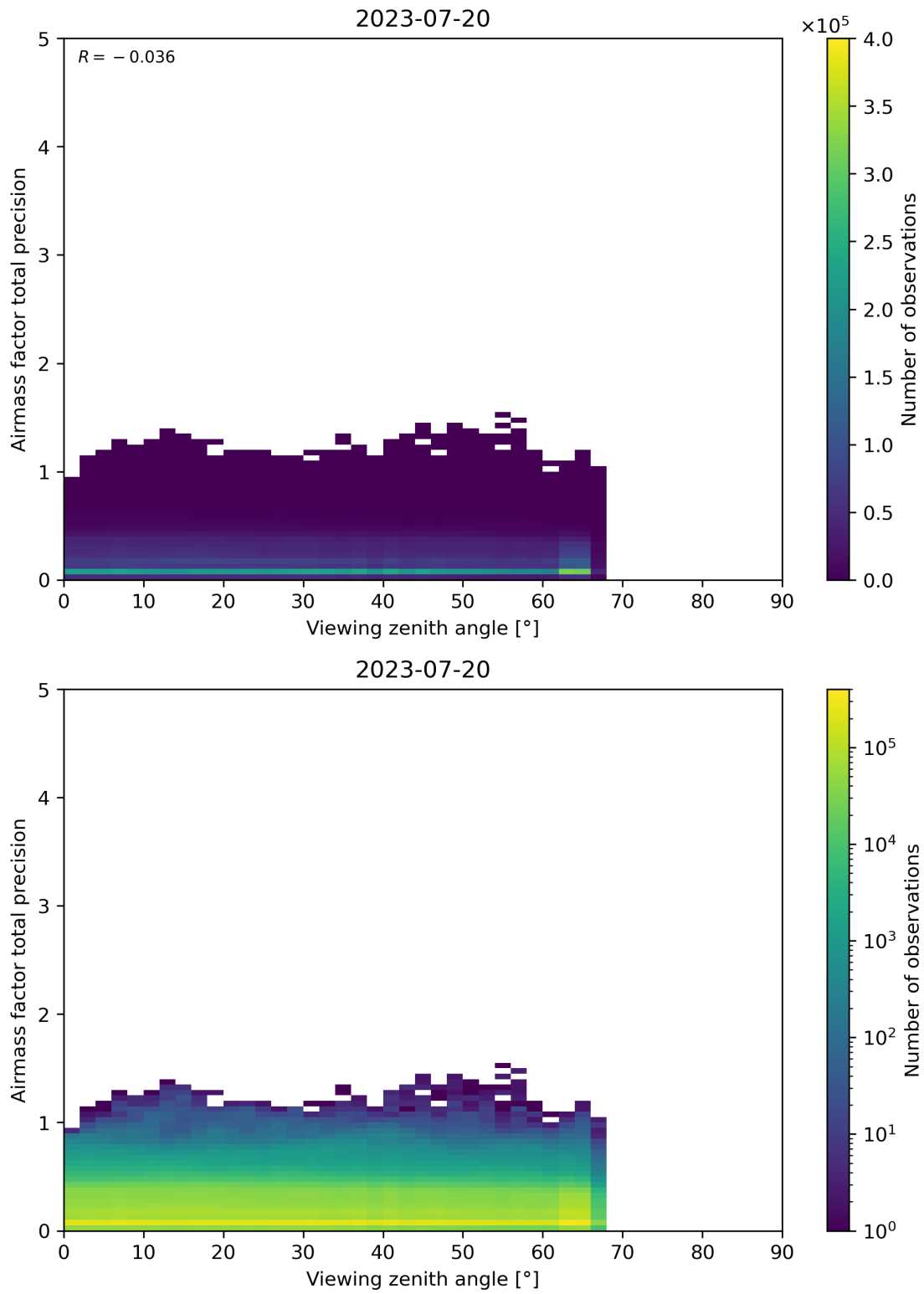
Figure 191: Scatter density plot of “Viewing zenith angle” against “Airmass factor total precision” for 2023-07-19 to 2023-07-21.
