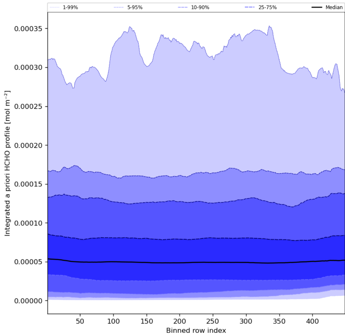
Figure 57: Along track statistics of “Integrated a priori HCHO profile” for 2023-07-19 to 2023-07-21
