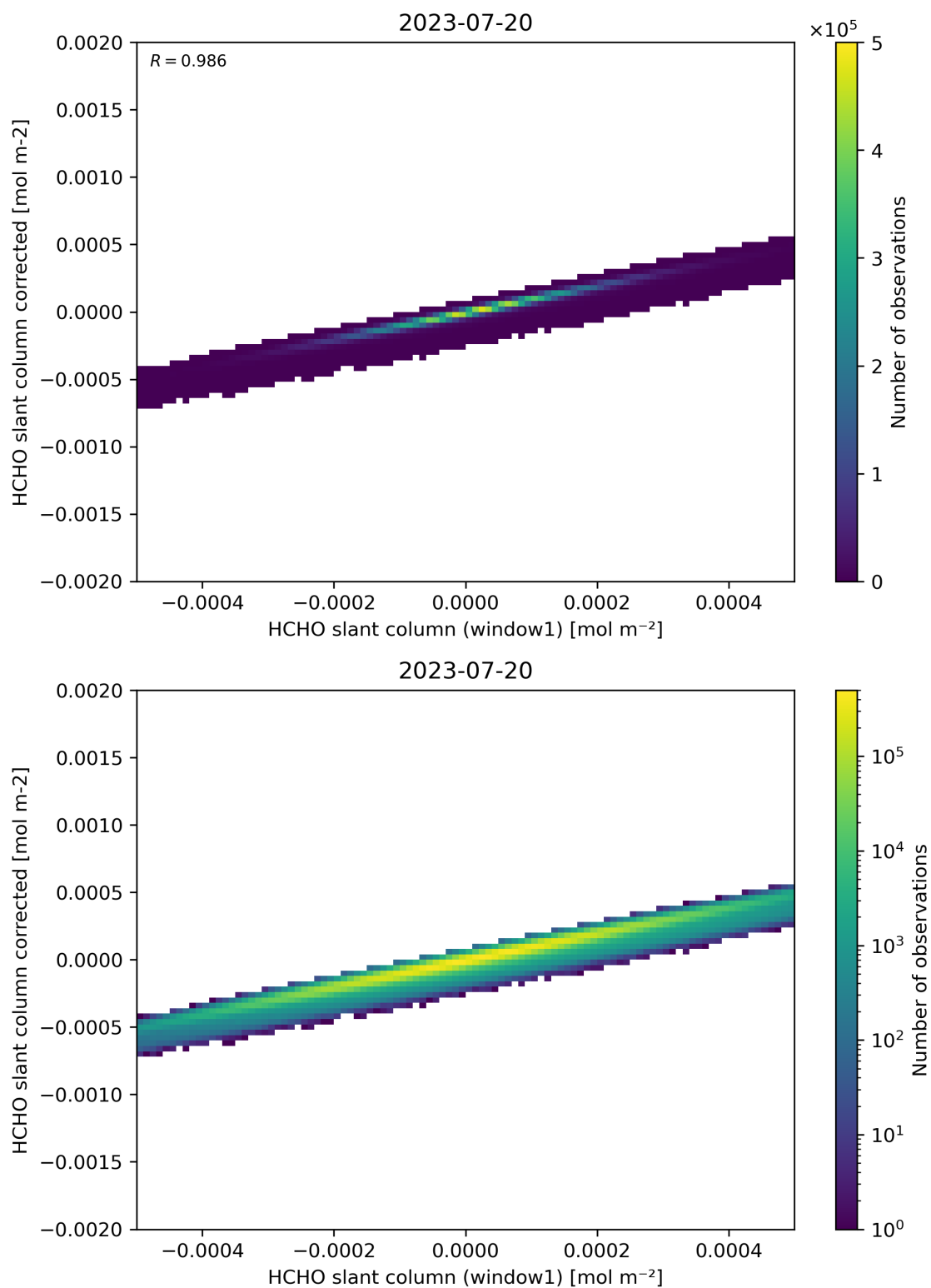
Figure 82: Scatter density plot of “HCHO slant column (window1)” against “HCHO slant column corrected” for 2023-07-19 to 2023-07-21.
