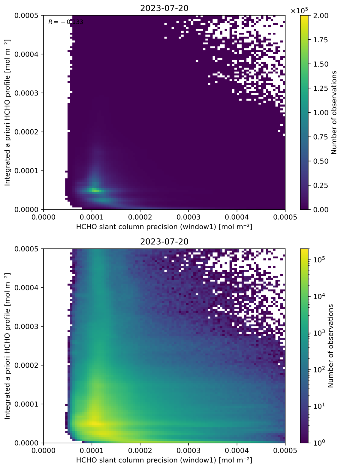
Figure 96: Scatter density plot of “HCHO slant column precision (window1)” against “Integrated a priori HCHO profile” for 2023-07-19 to 2023-07-21.
