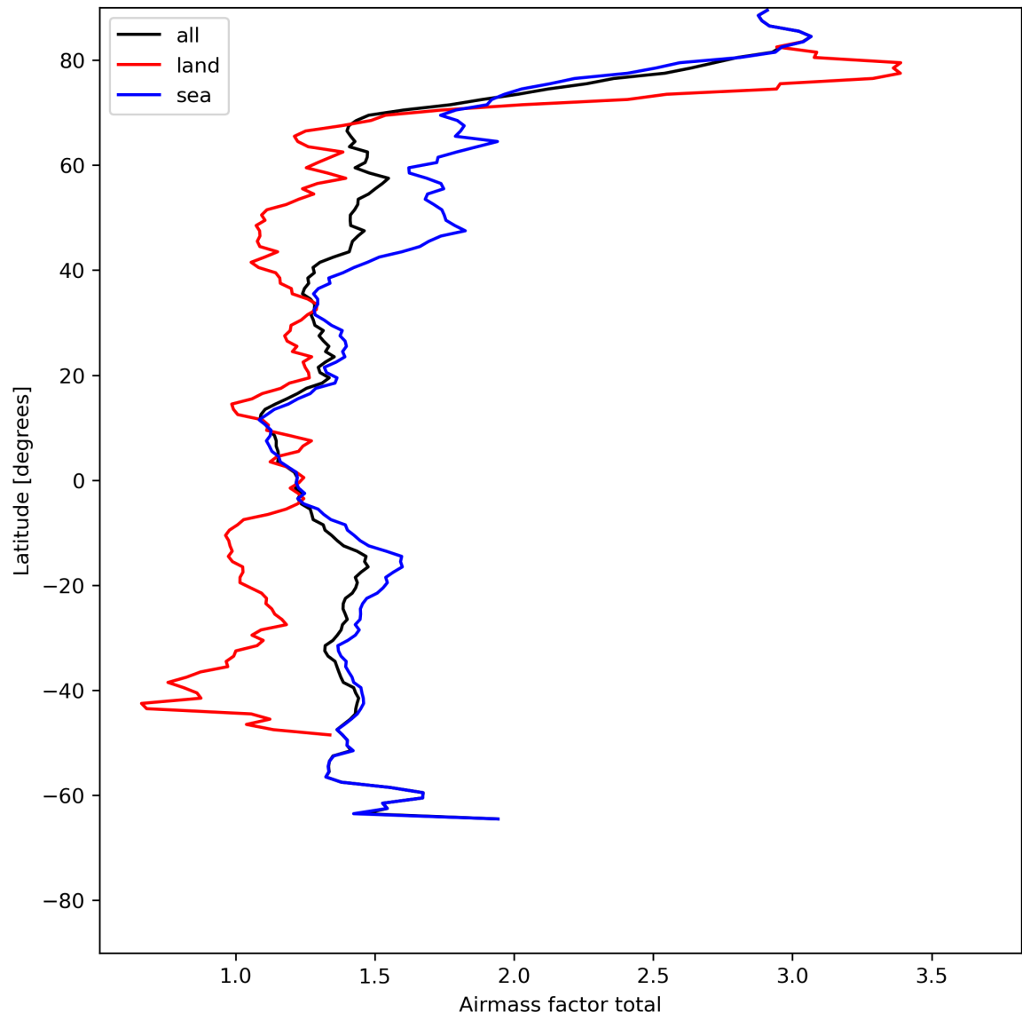
Figure 26: Zonal average of “Airmass factor total” for 2023-07-19 to 2023-07-21.
