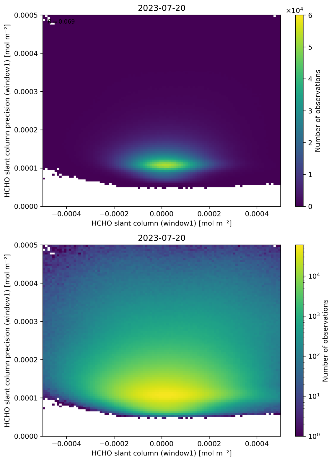
Figure 84: Scatter density plot of “HCHO slant column (window1)” against “HCHO slant column precision (window1)” for 2023-07-19 to 2023-07-21.
