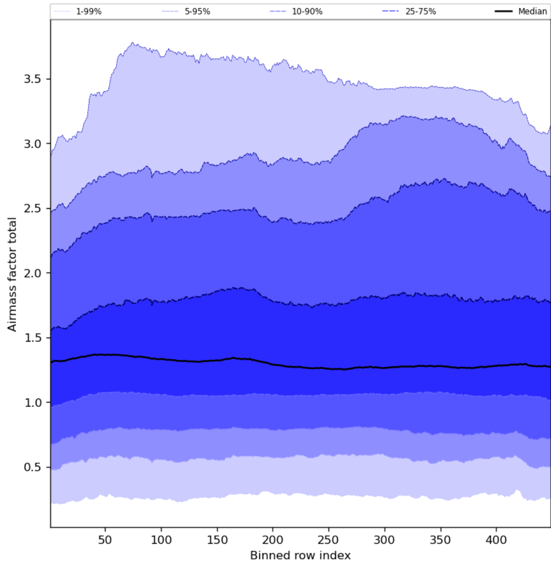
Figure 54: Along track statistics of “Airmass factor total” for 2023-07-19 to 2023-07-21
