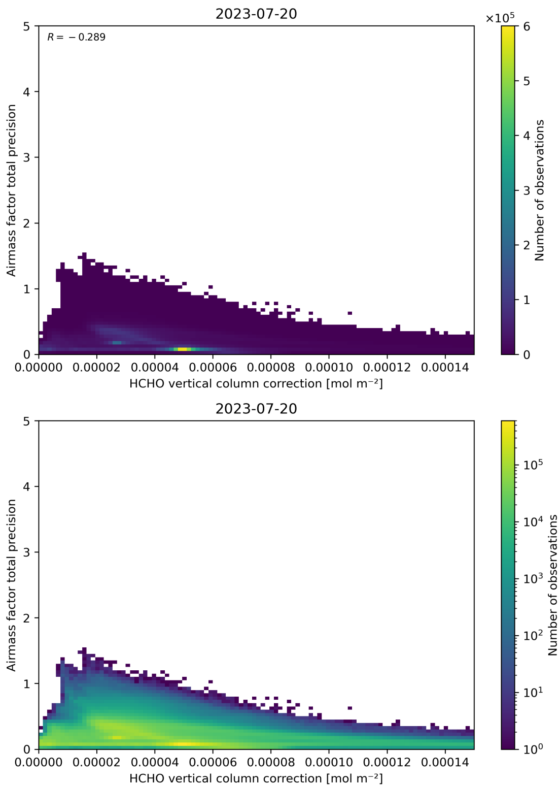
Figure 121: Scatter density plot of “HCHO vertical column correction” against “Airmass factor total precision” for 2023-07-19 to 2023-07-21.
