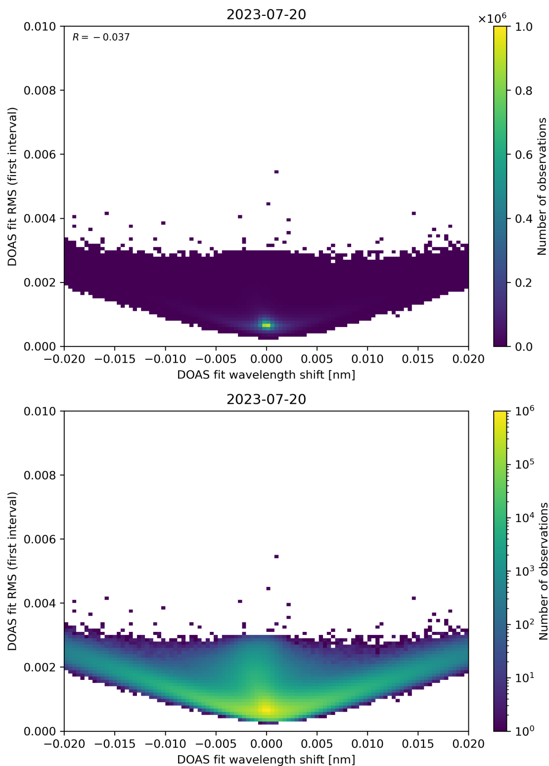
Figure 64: Scatter density plot of “DOAS fit wavelength shift” against “DOAS fit RMS (first interval)” for 2023-07-19 to 2023-07-21.
