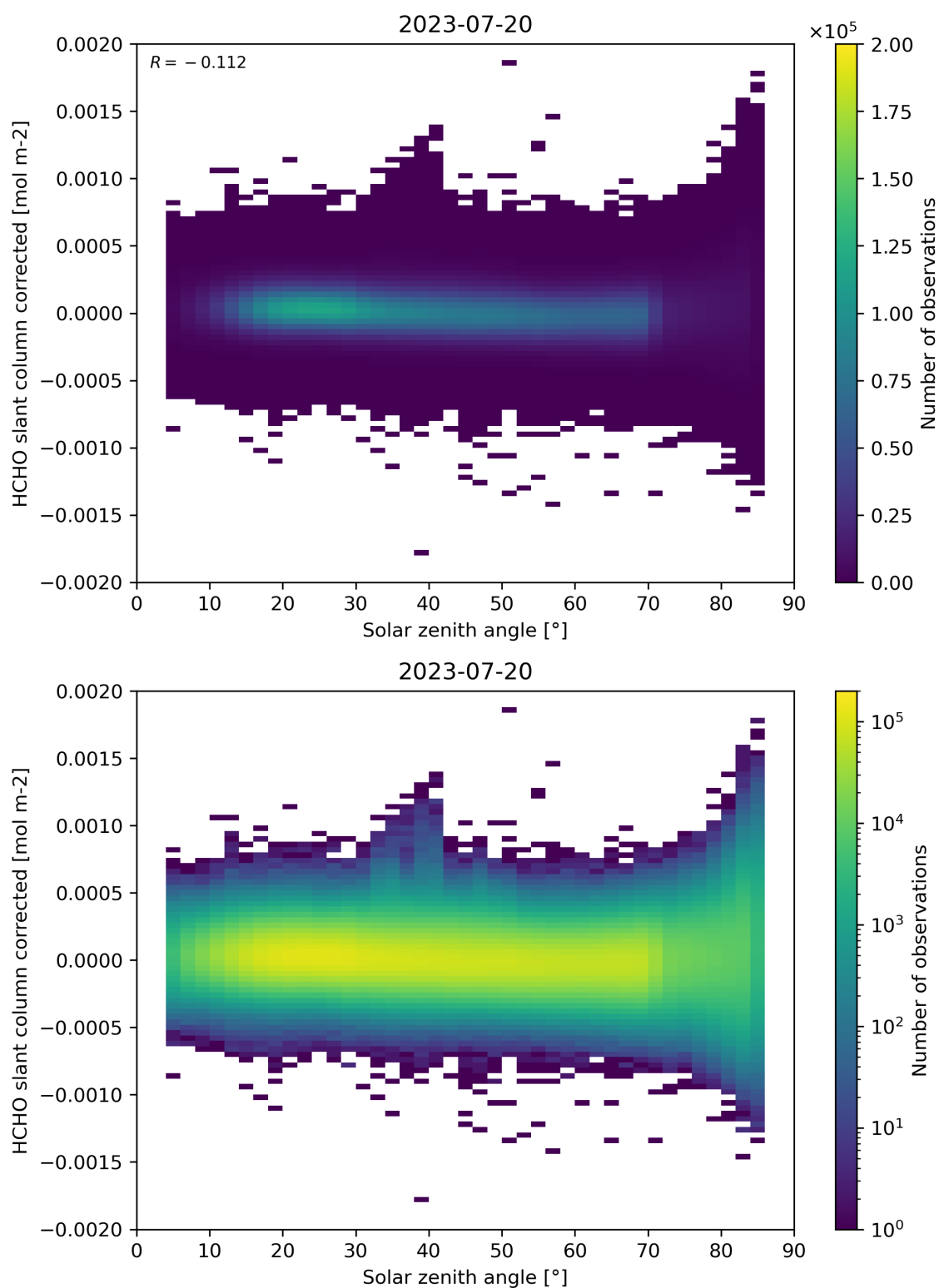
Figure 171: Scatter density plot of “Solar zenith angle” against “HCHO slant column corrected” for 2023-07-19 to 2023-07-21.
