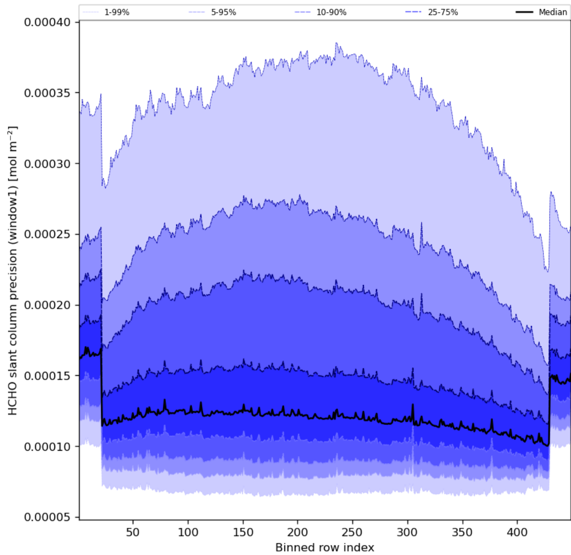
Figure 53: Along track statistics of “HCHO slant column precision (window1)” for 2023-07-19 to 2023-07-21
