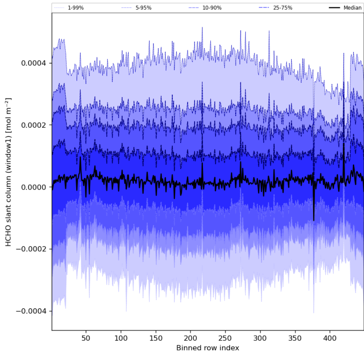
Figure 52: Along track statistics of “HCHO slant column (window1)” for 2023-07-19 to 2023-07-21
