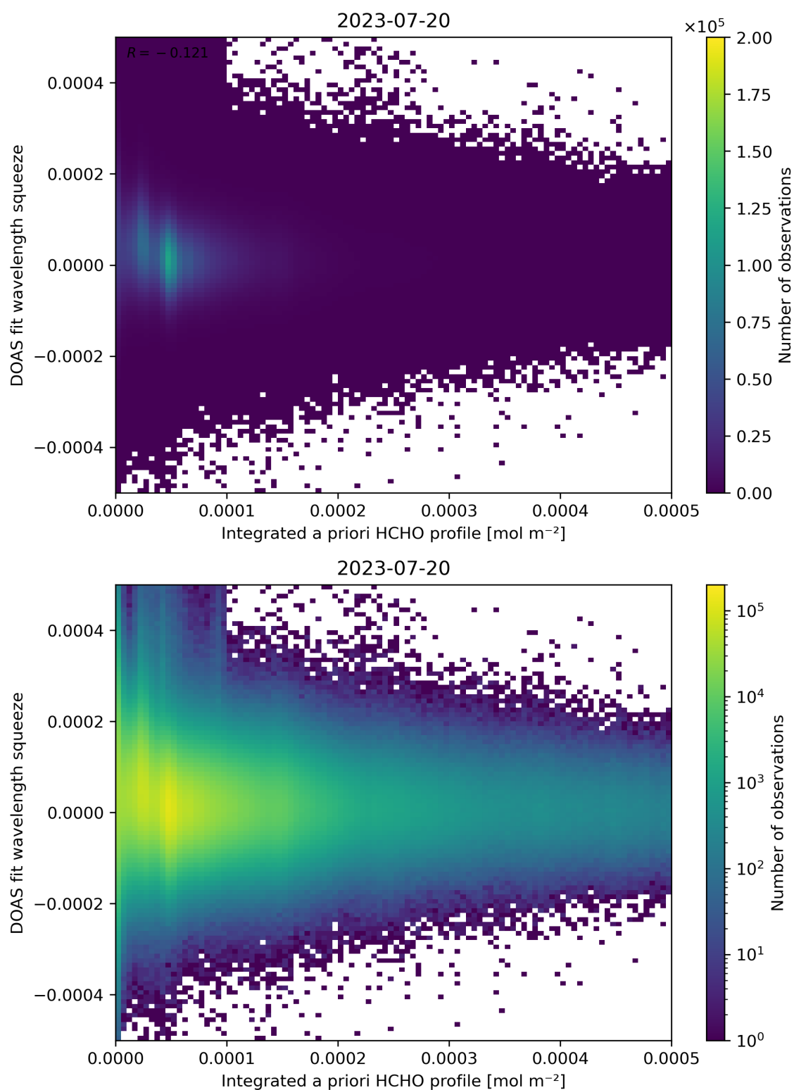
Figure 150: Scatter density plot of “Integrated a priori HCHO profile” against “DOAS fit wavelength squeeze” for 2023-07-19 to 2023-07-21.
