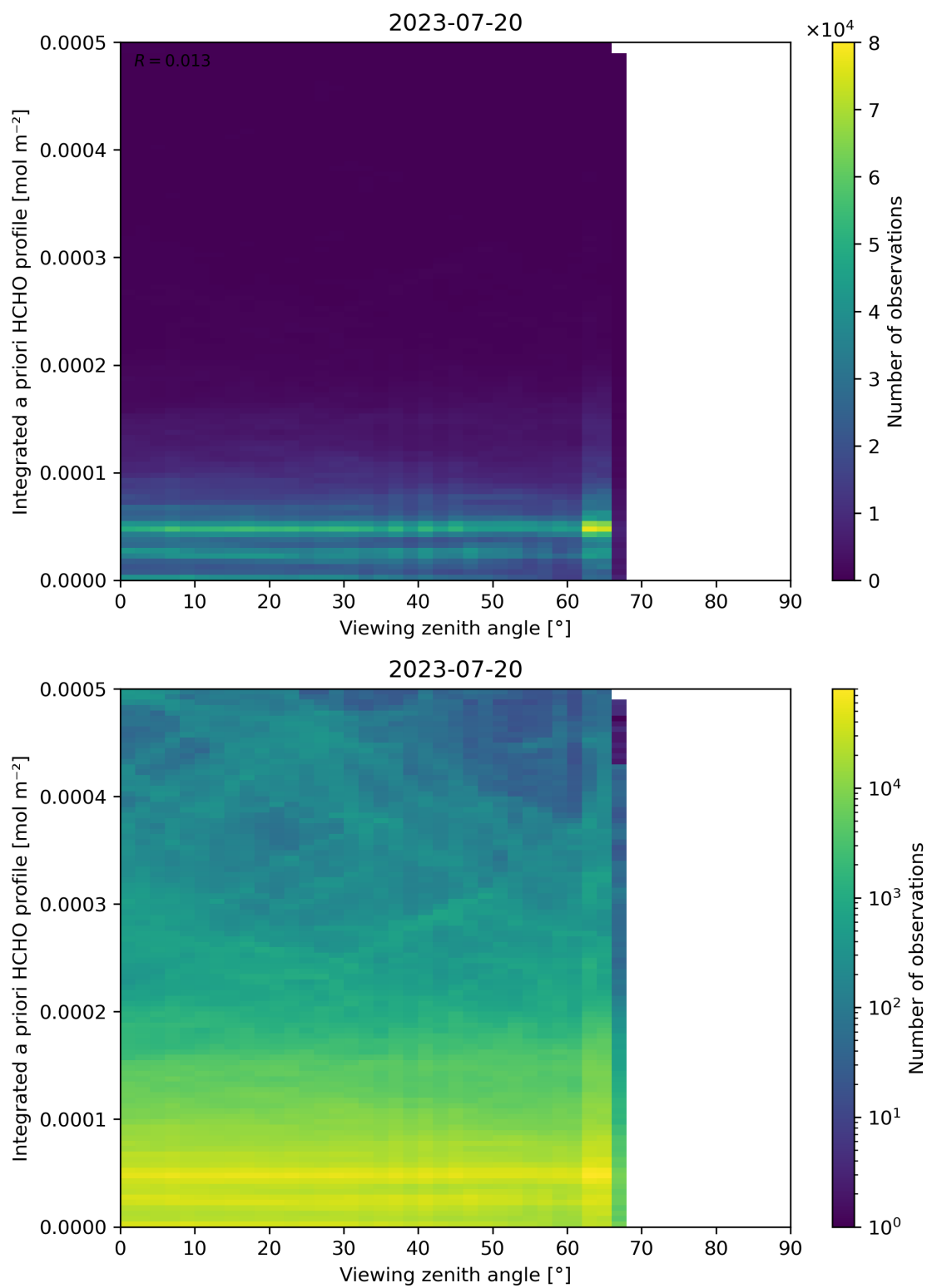
Figure 195: Scatter density plot of “Viewing zenith angle” against “Integrated a priori HCHO profile” for 2023-07-19 to 2023-07-21.
