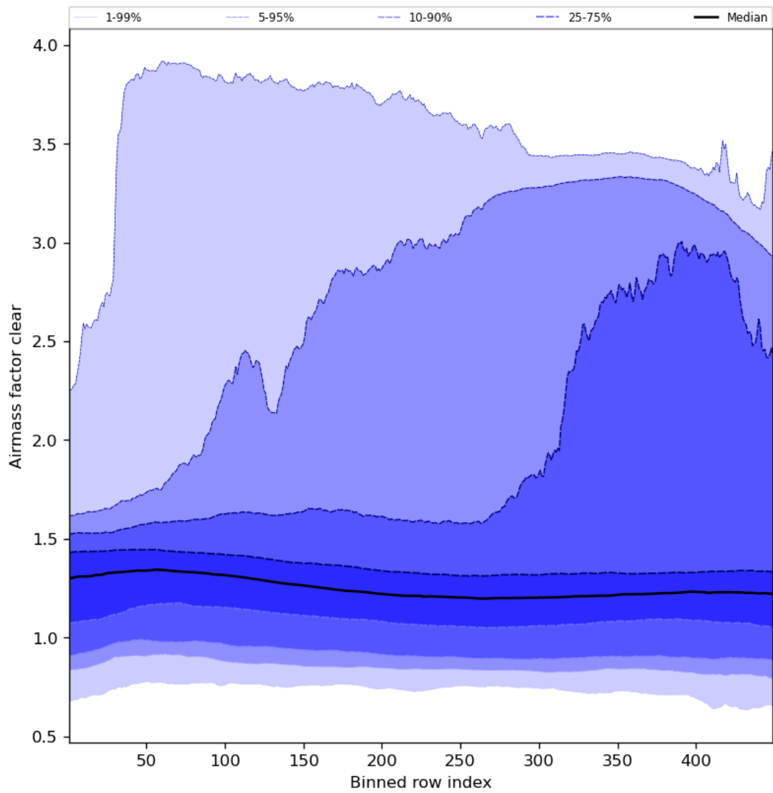
Figure 56: Along track statistics of “Airmass factor clear” for 2023-07-19 to 2023-07-21
