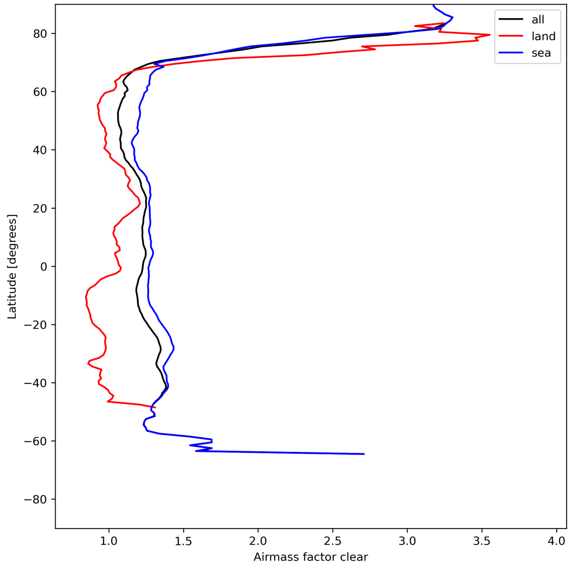
Figure 28: Zonal average of “Airmass factor clear” for 2023-07-19 to 2023-07-21.
