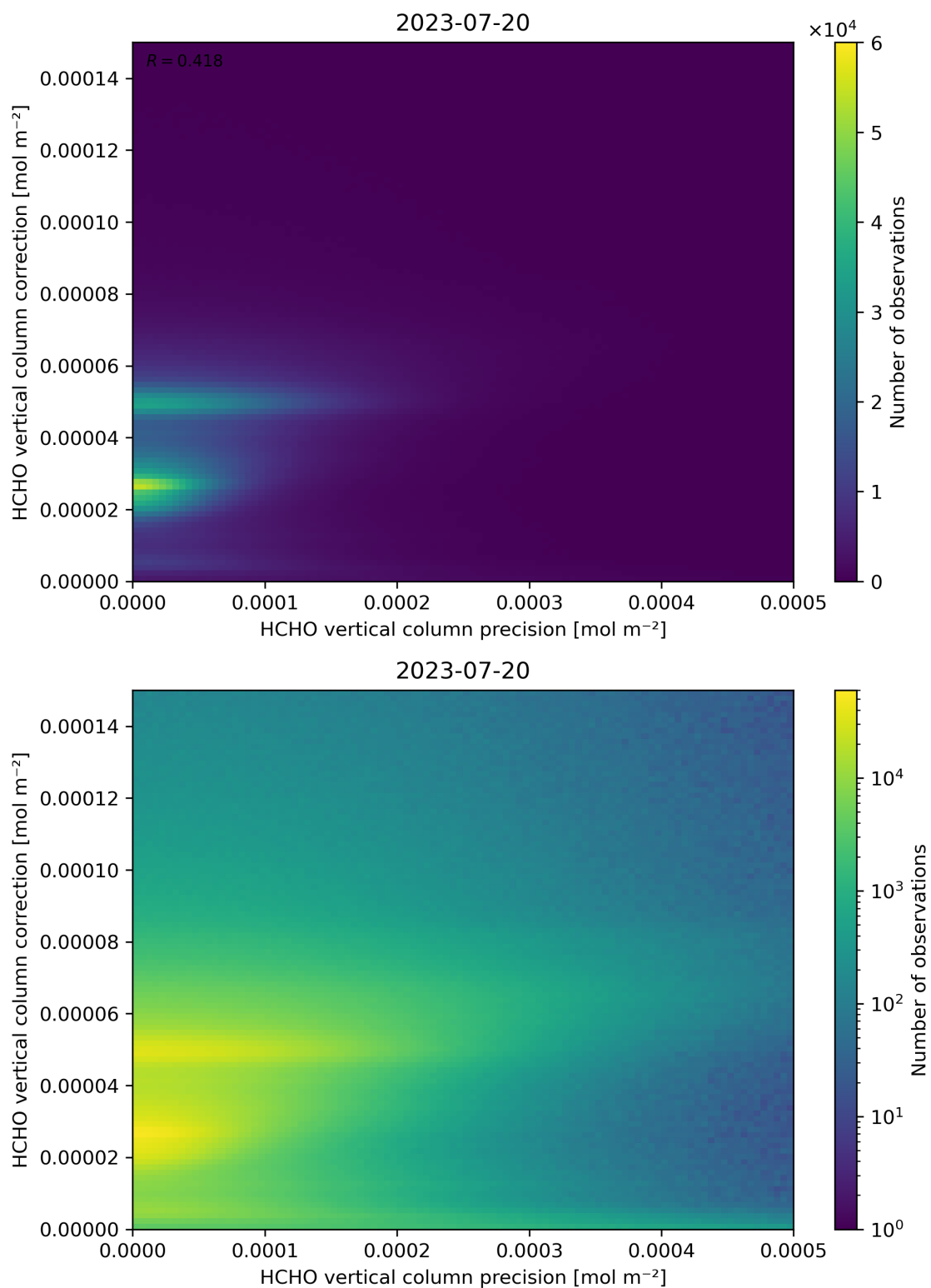
Figure 146: Scatter density plot of “HCHO vertical column precision” against “HCHO vertical column correction” for 2023-07-19 to 2023-07-21.
