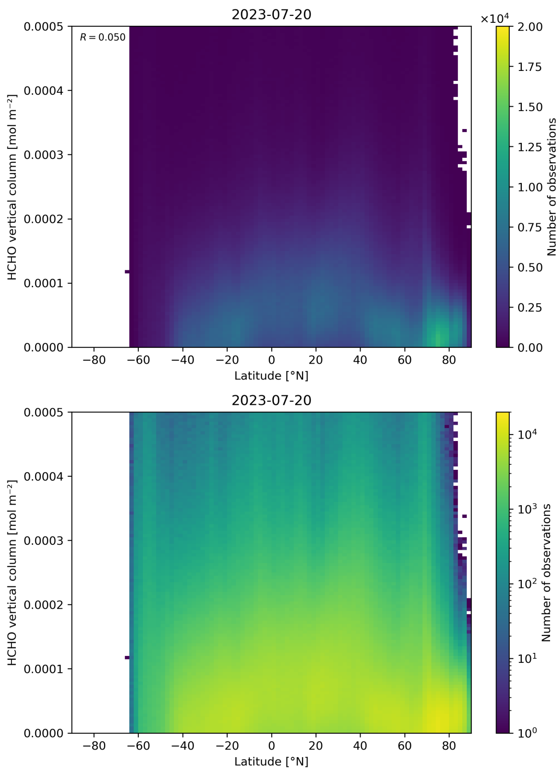
Figure 163: Scatter density plot of “Latitude” against “HCHO vertical column” for 2023-07-19 to 2023-07-21.
