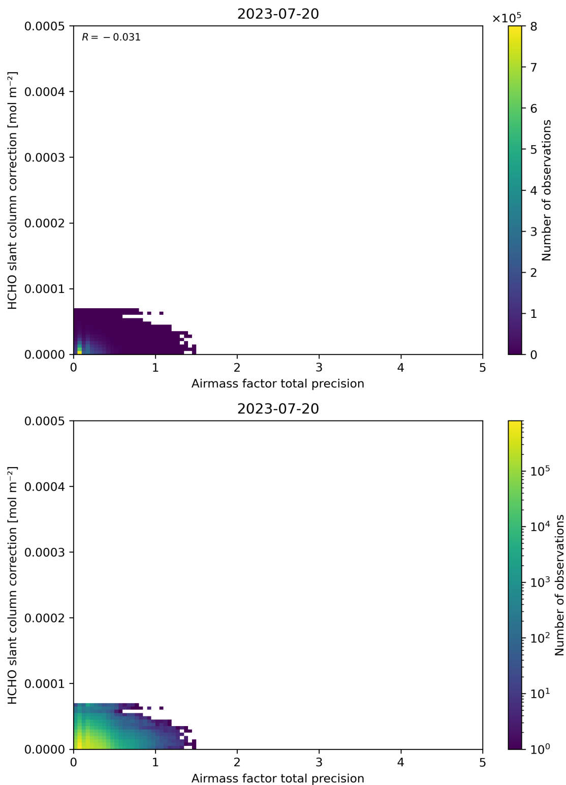
Figure 110: Scatter density plot of “Airmass factor total precision” against “HCHO slant column correction” for 2023-07-19 to 2023-07-21.
