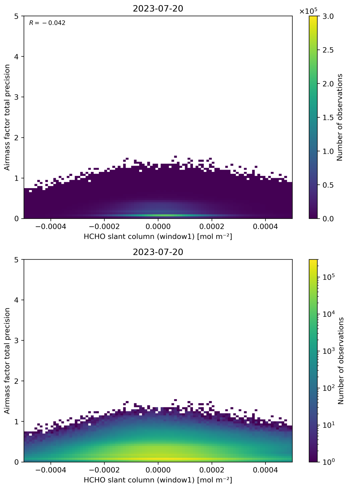
Figure 86: Scatter density plot of “HCHO slant column (window1)” against “Airmass factor total precision” for 2023-07-19 to 2023-07-21.
