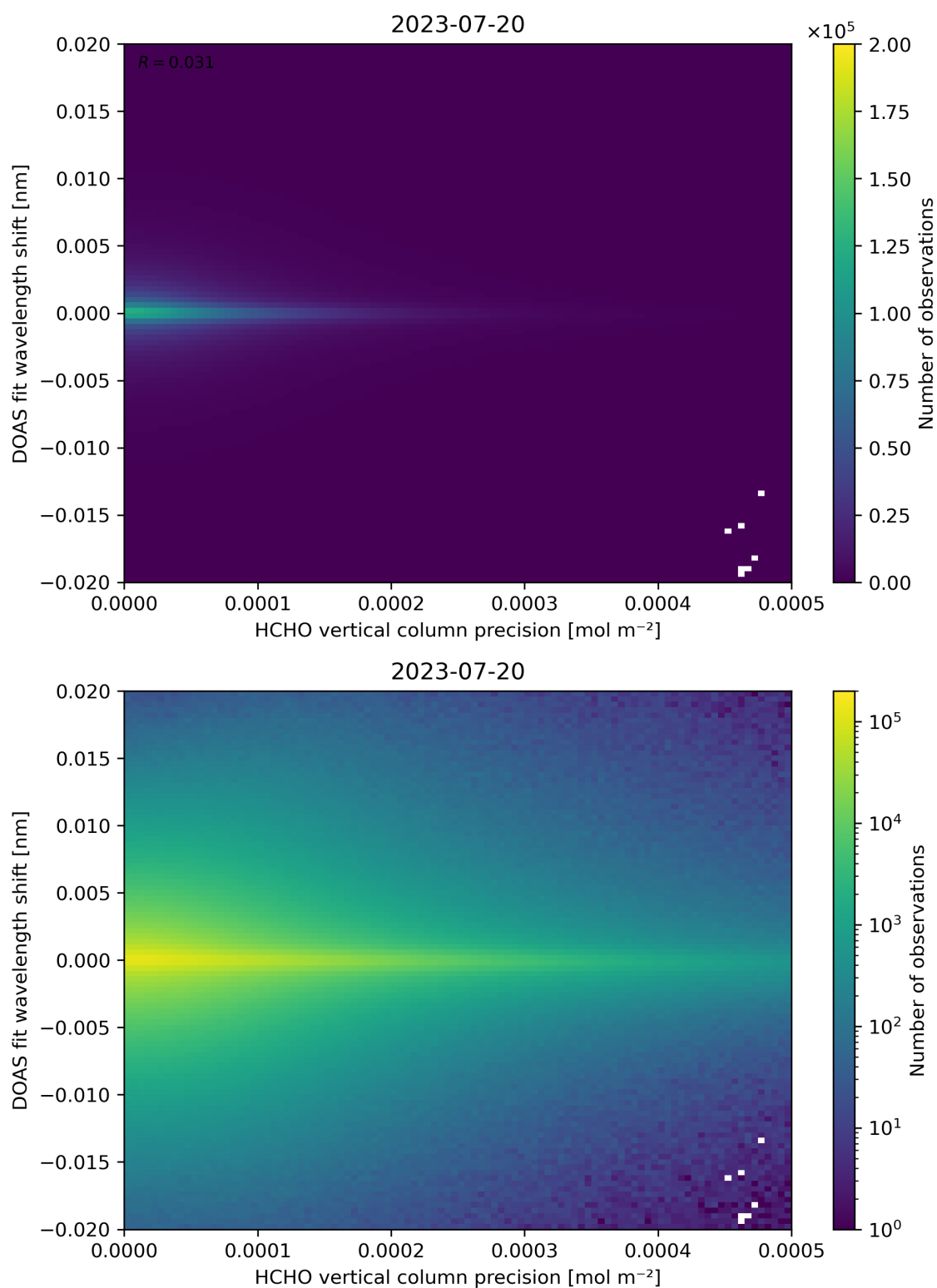
Figure 137: Scatter density plot of “HCHO vertical column precision” against “DOAS fit wavelength shift” for 2023-07-19 to 2023-07-21.
