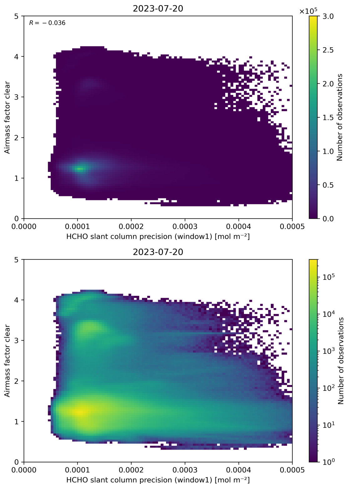
Figure 91: Scatter density plot of “HCHO slant column precision (window1)” against “Airmass factor clear” for 2023-07-19 to 2023-07-21.
