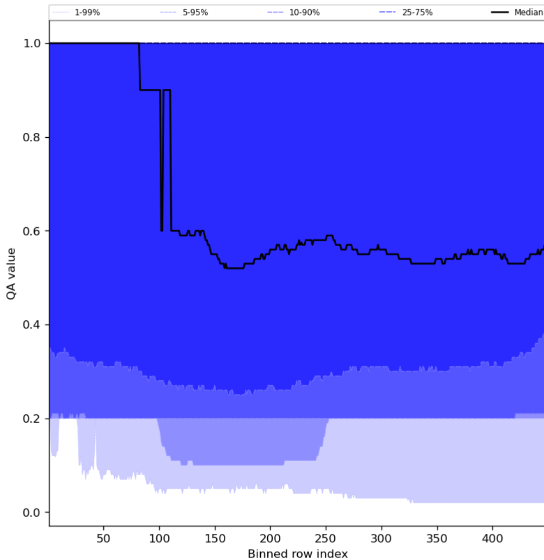
Figure 48: Along track statistics of “QA value” for 2023-07-19 to 2023-07-21
