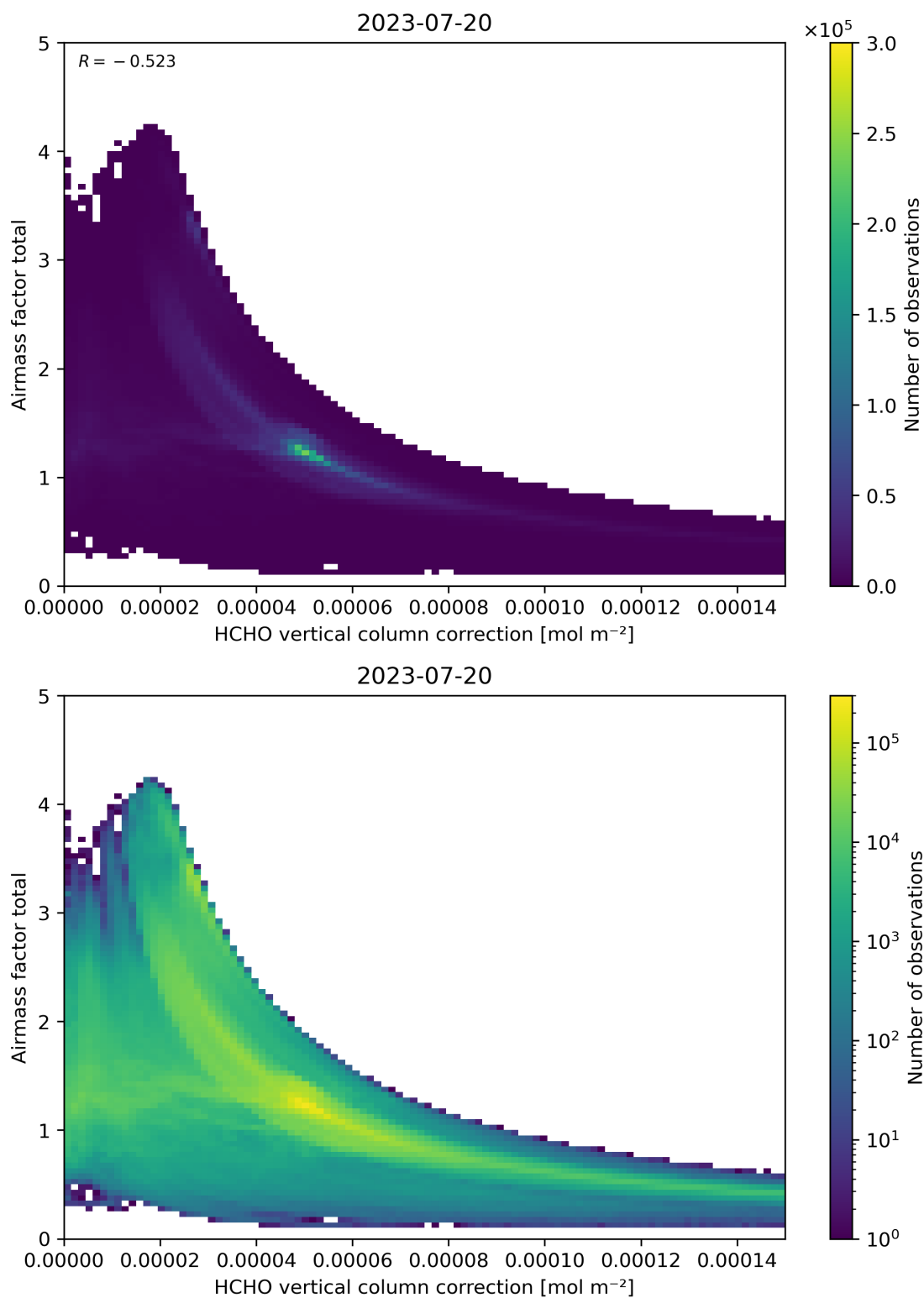
Figure 120: Scatter density plot of “HCHO vertical column correction” against “Airmass factor total” for 2023-07-19 to 2023-07-21.
