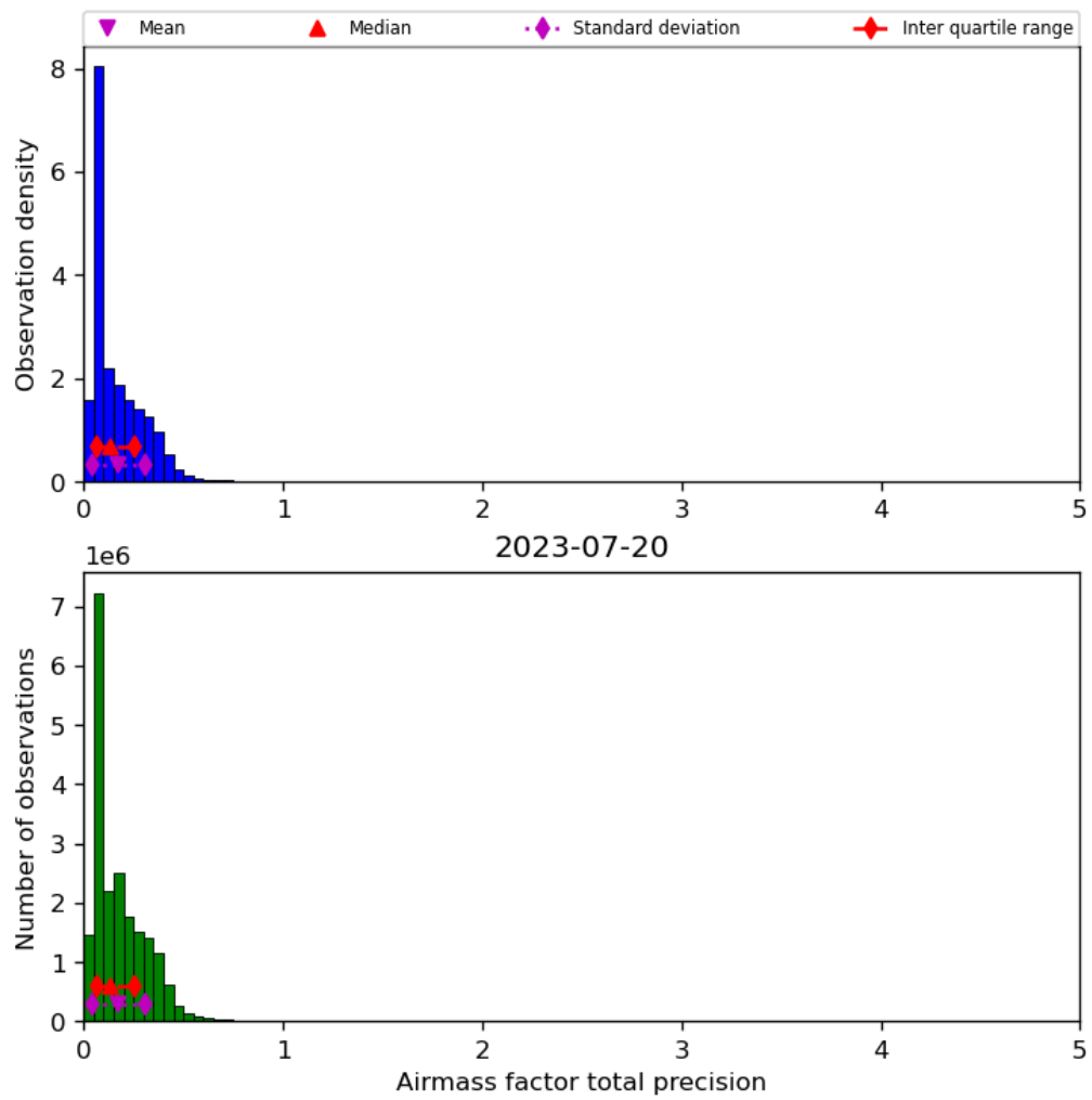
Figure 41: Histogram of “Airmass factor total precision” for 2023-07-19 to 2023-07-21
