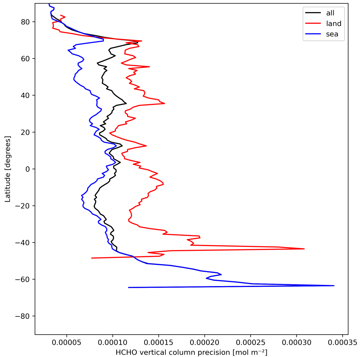
Figure 22: Zonal average of “HCHO vertical column precision” for 2023-07-19 to 2023-07-21.
