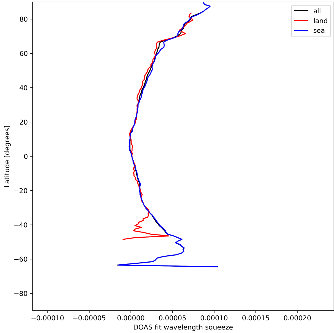
Figure 31: Zonal average of “DOAS fit wavelength squeeze” for 2023-07-19 to 2023-07-21.
