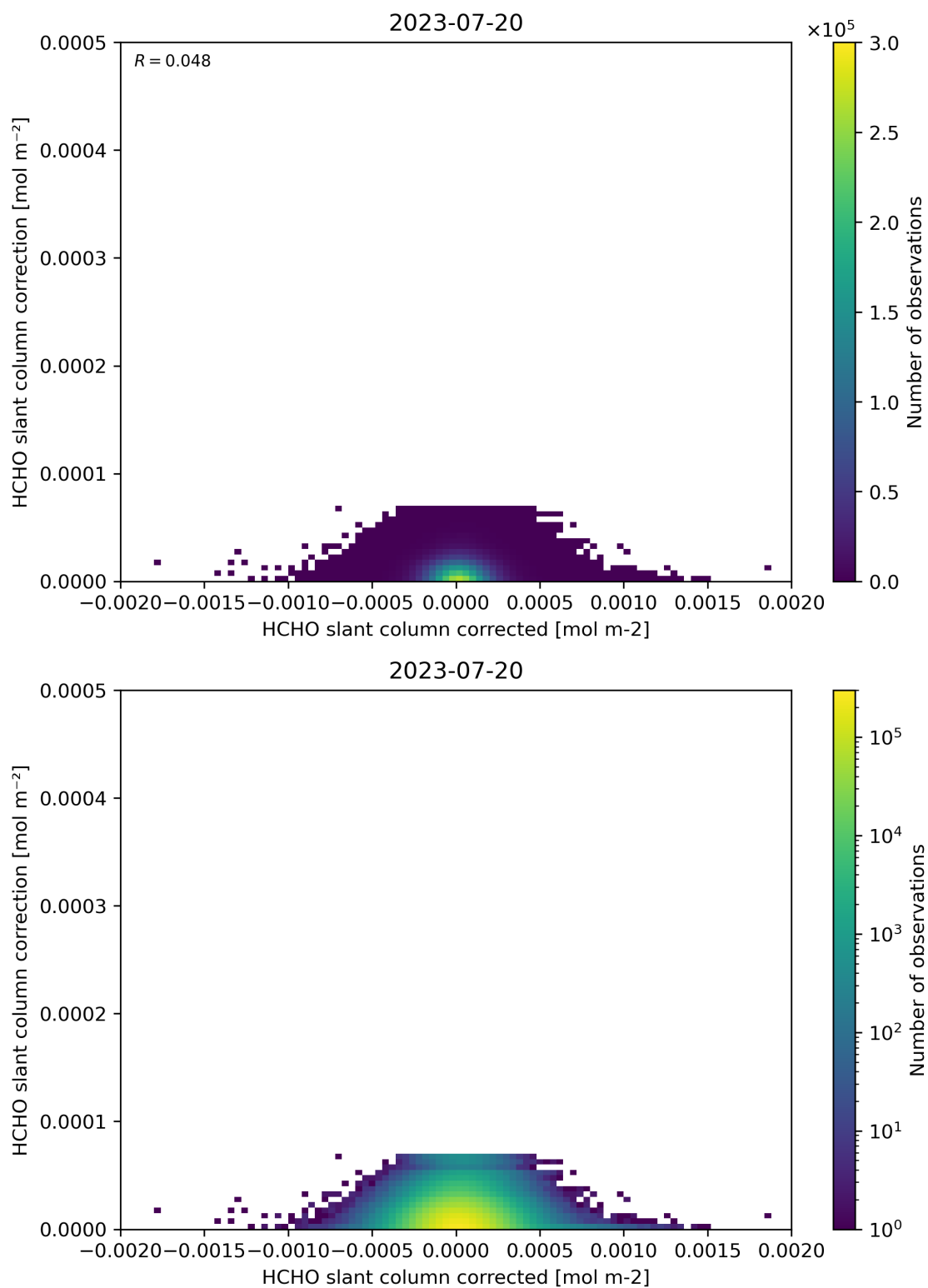
Figure 77: Scatter density plot of “HCHO slant column corrected” against “HCHO slant column correction” for 2023-07-19 to 2023-07-21.
