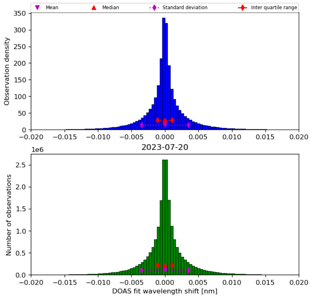
Figure 44: Histogram of “DOAS fit wavelength shift” for 2023-07-19 to 2023-07-21
