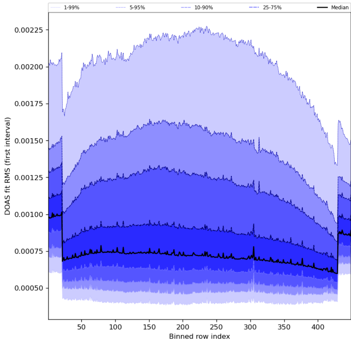
Figure 60: Along track statistics of “DOAS fit RMS (first interval)” for 2023-07-19 to 2023-07-21
