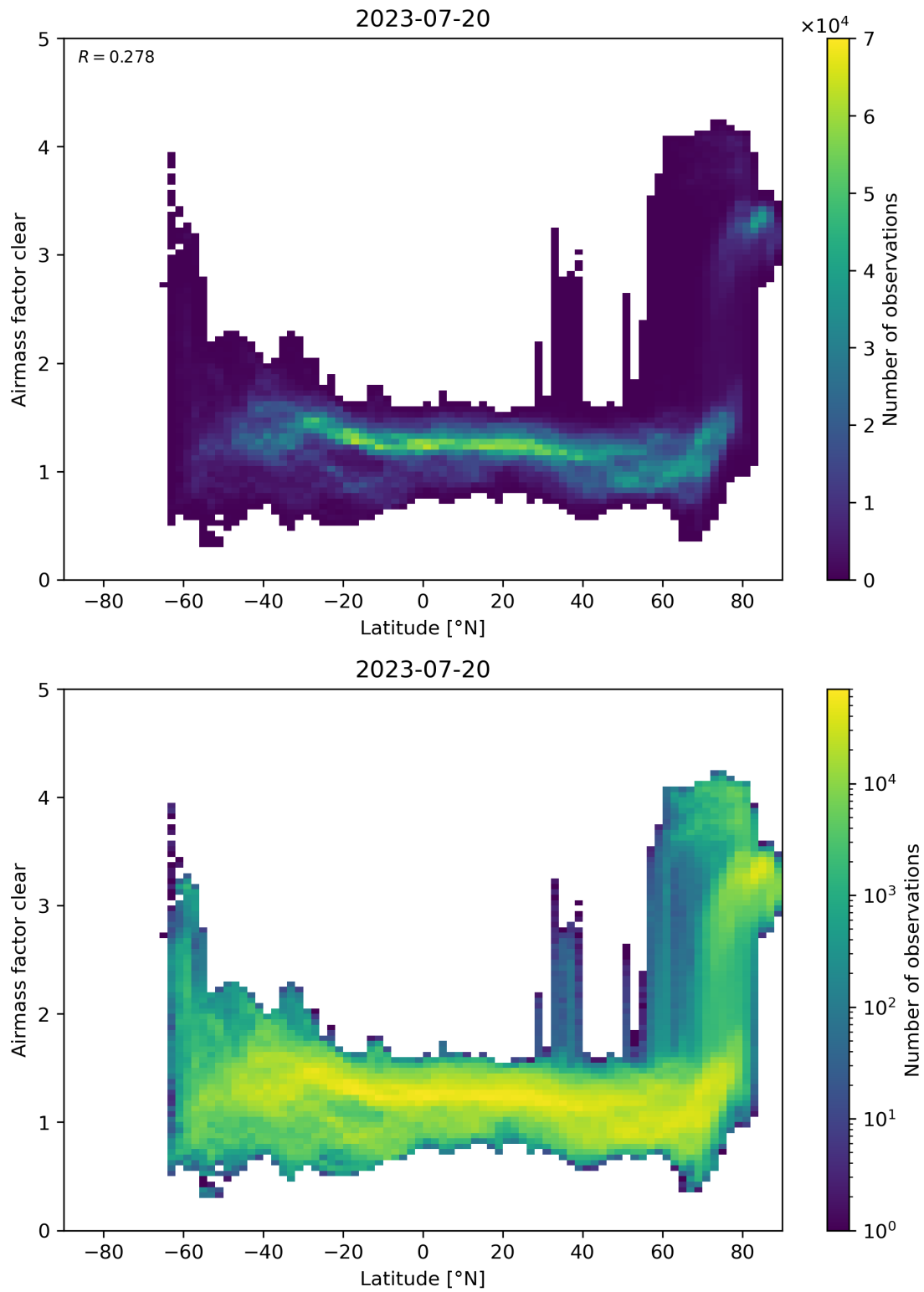
Figure 156: Scatter density plot of “Latitude” against “Airmass factor clear” for 2023-07-19 to 2023-07-21.
