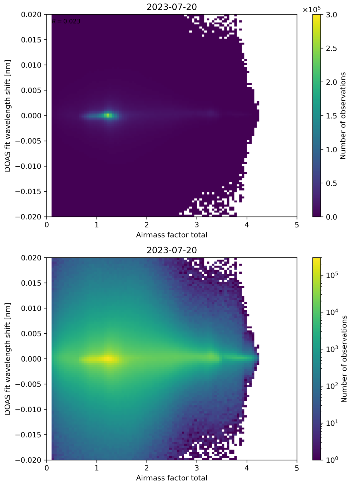
Figure 98: Scatter density plot of “Airmass factor total” against “DOAS fit wavelength shift” for 2023-07-19 to 2023-07-21.
