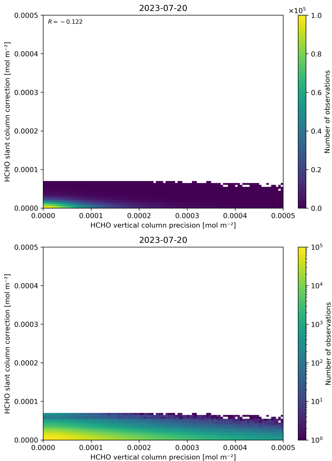
Figure 141: Scatter density plot of “HCHO vertical column precision” against “HCHO slant column correction” for 2023-07-19 to 2023-07-21.
