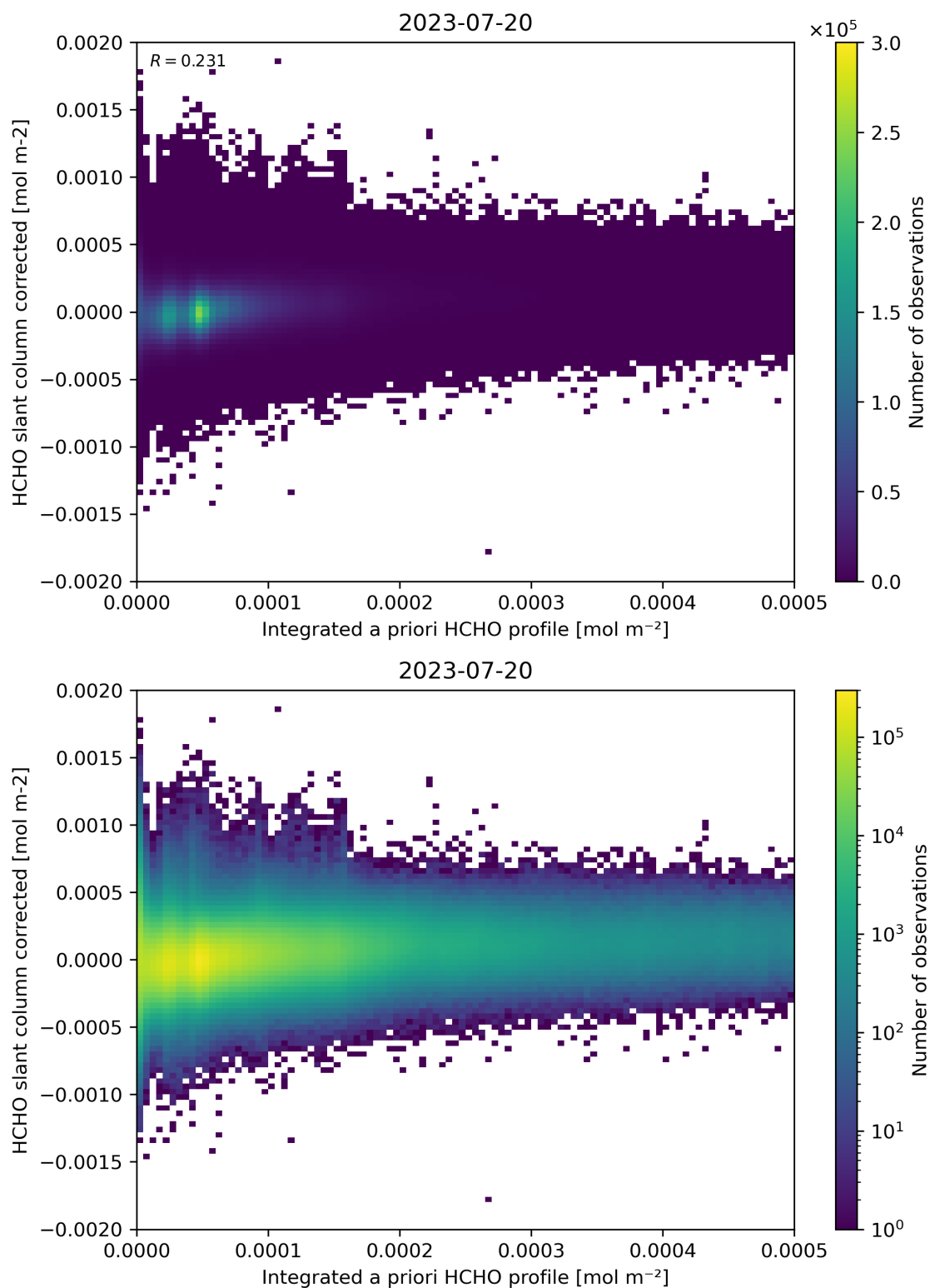
Figure 151: Scatter density plot of “Integrated a priori HCHO profile” against “HCHO slant column corrected” for 2023-07-19 to 2023-07-21.
