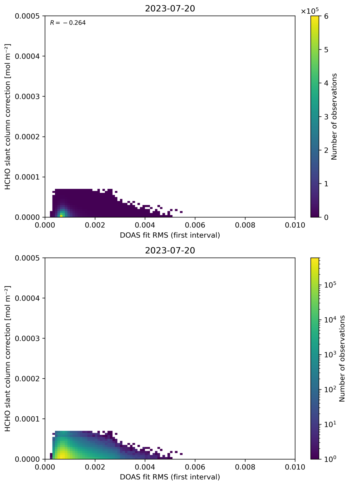
Figure 63: Scatter density plot of “DOAS fit RMS (first interval)” against “HCHO slant column correction” for 2023-07-19 to 2023-07-21.
