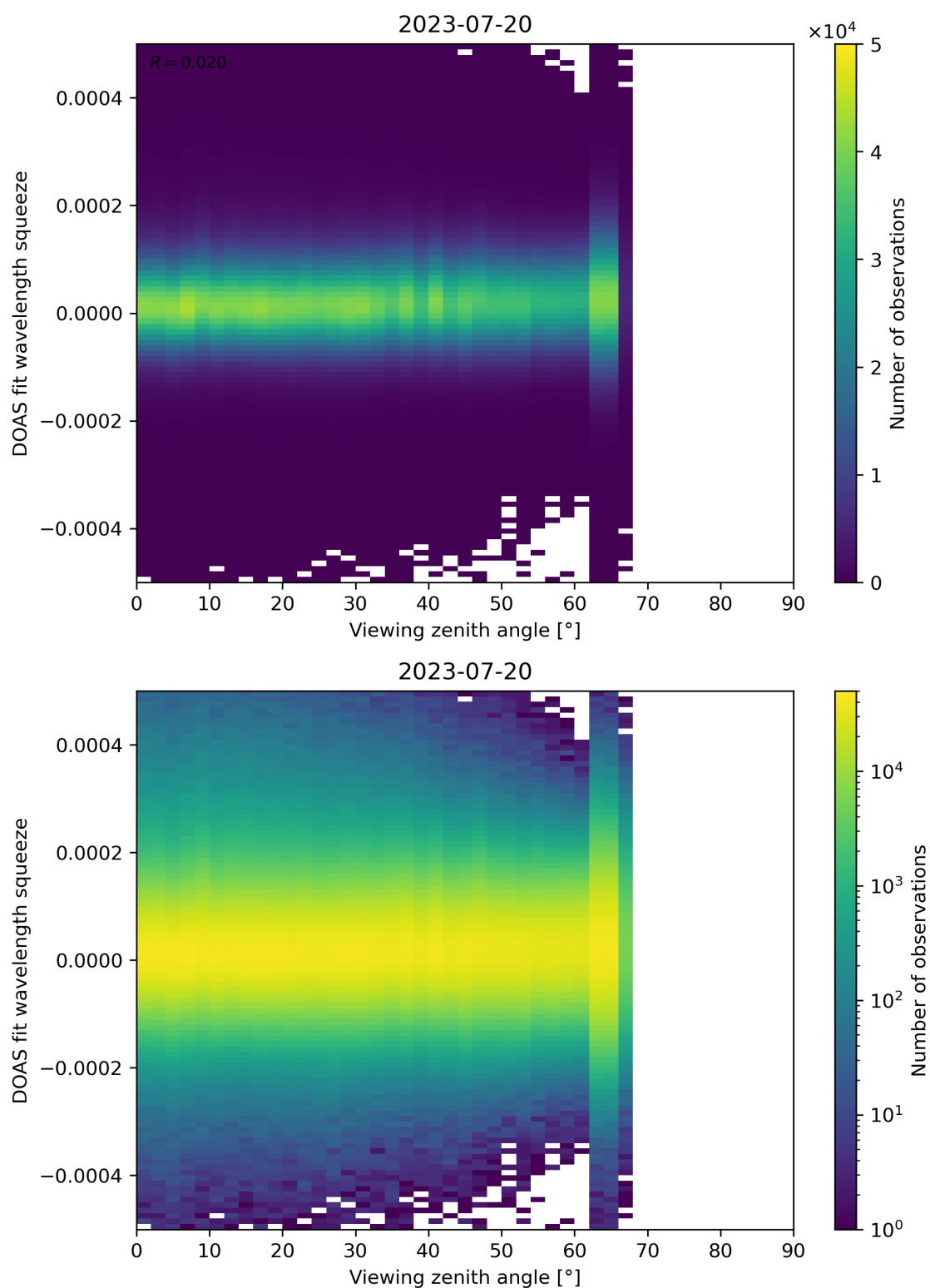
Figure 184: Scatter density plot of “Viewing zenith angle” against “DOAS fit wavelength squeeze” for 2023-07-19 to 2023-07-21.
