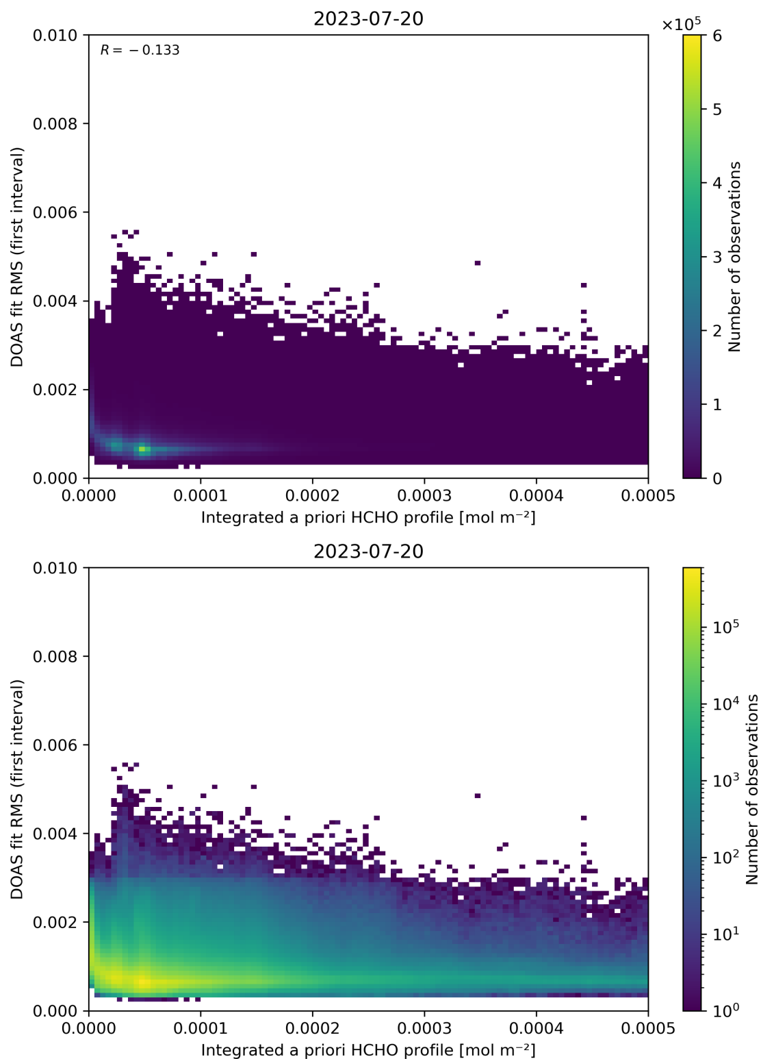
Figure 148: Scatter density plot of “Integrated a priori HCHO profile” against “DOAS fit RMS (first interval)” for 2023-07-19 to 2023-07-21.
