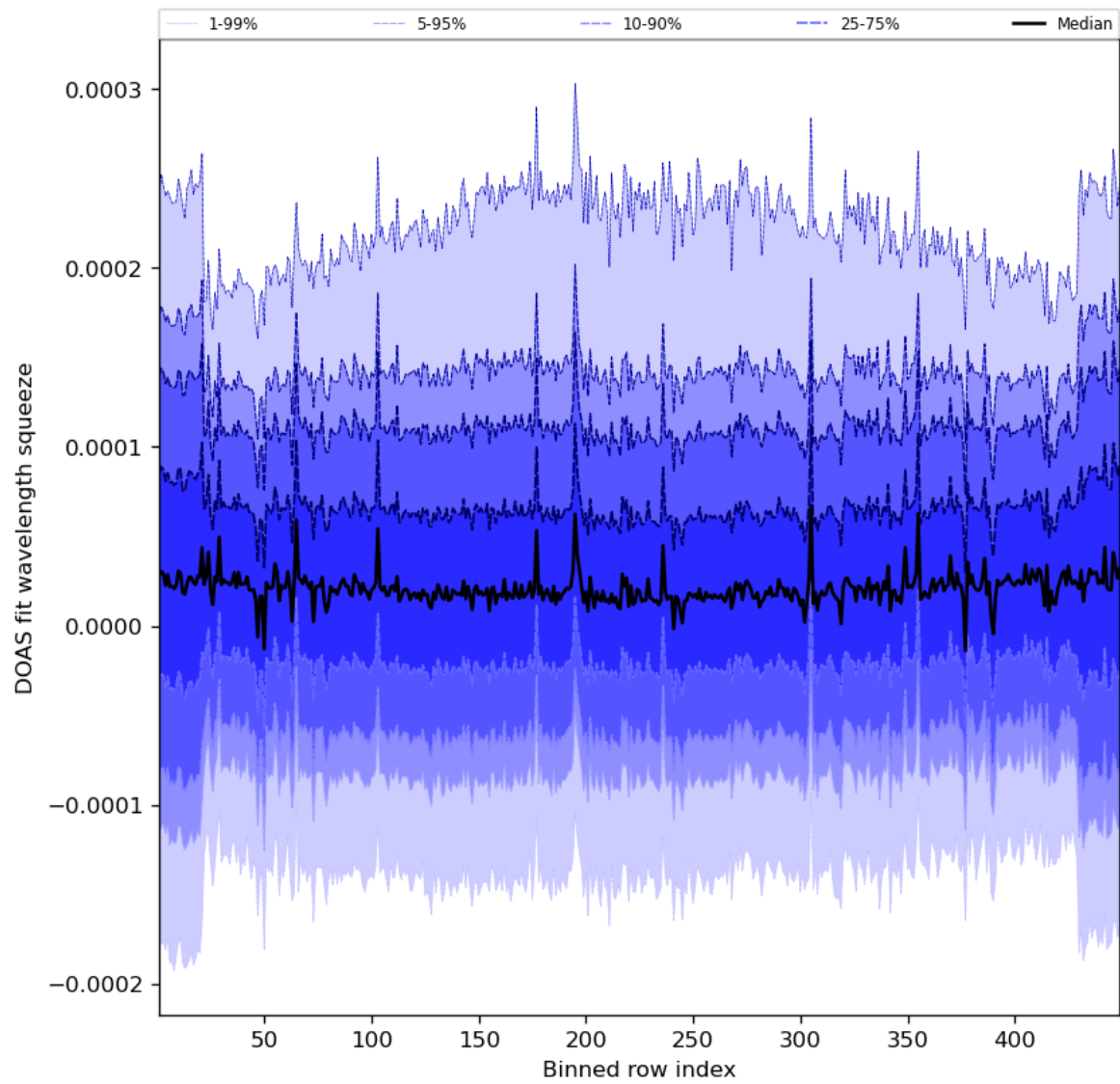
Figure 59: Along track statistics of “DOAS fit wavelength squeeze” for 2023-07-19 to 2023-07-21
