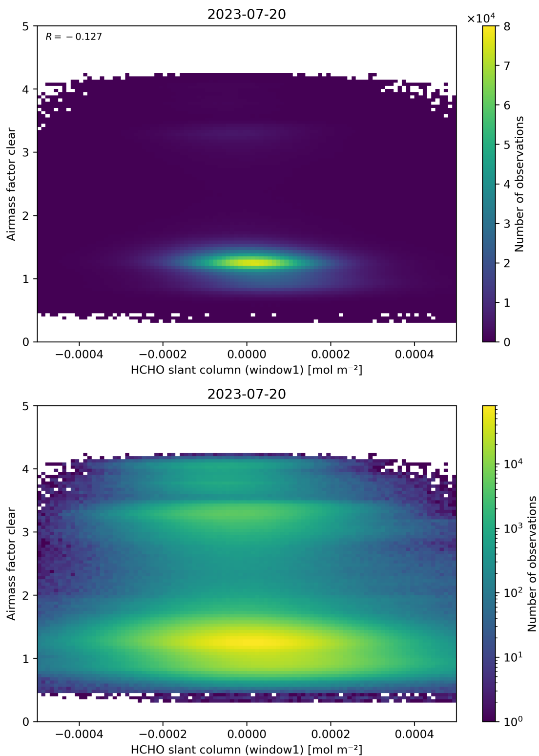
Figure 81: Scatter density plot of “HCHO slant column (window1)” against “Airmass factor clear” for 2023-07-19 to 2023-07-21.
