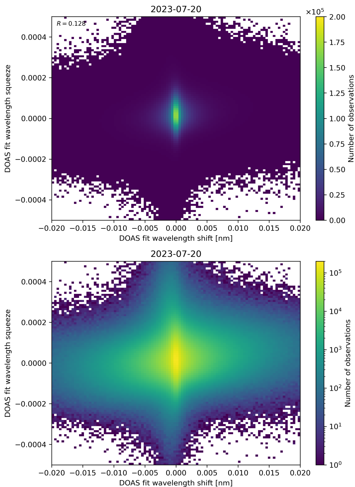
Figure 65: Scatter density plot of “DOAS fit wavelength shift” against “DOAS fit wavelength squeeze” for 2023-07-19 to 2023-07-21.
