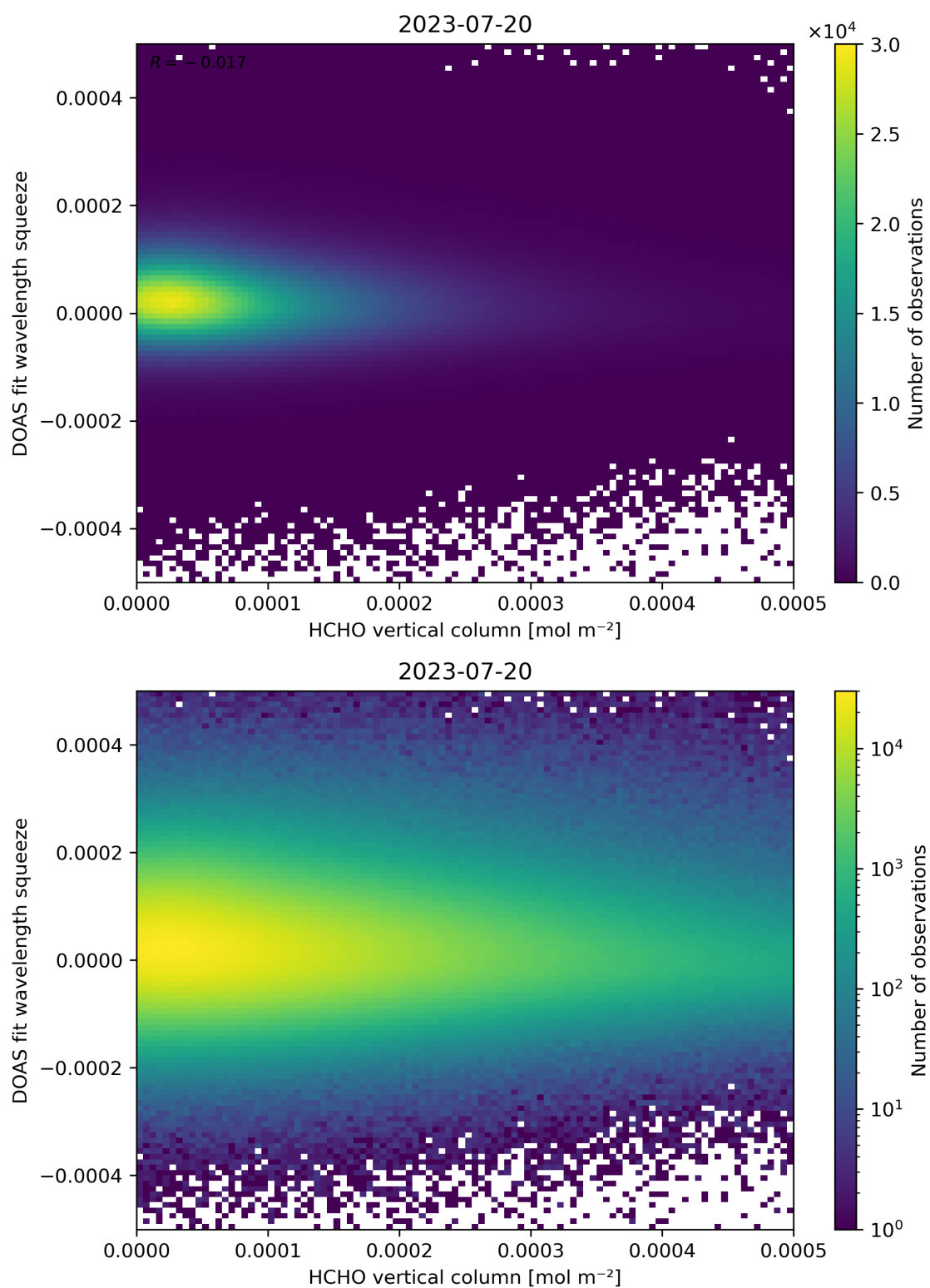
Figure 125: Scatter density plot of “HCHO vertical column” against “DOAS fit wavelength squeeze” for 2023-07-19 to 2023-07-21.
