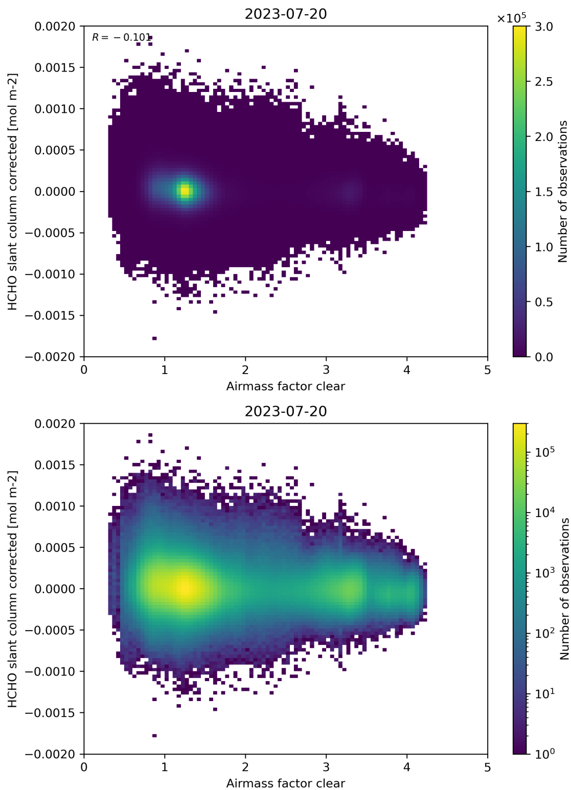
Figure 74: Scatter density plot of “Airmass factor clear” against “HCHO slant column corrected” for 2023-07-19 to 2023-07-21.
