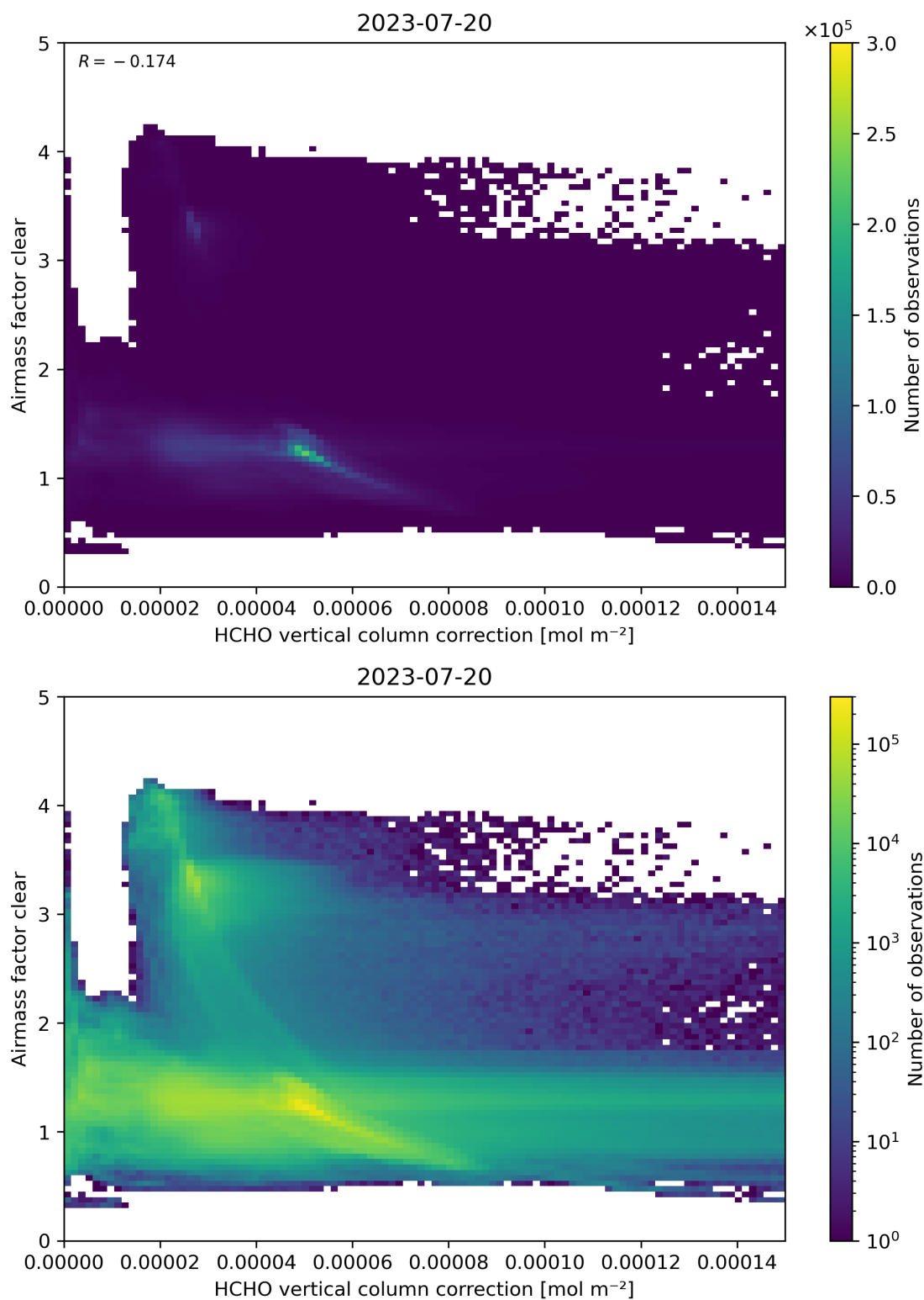
Figure 115: Scatter density plot of “HCHO vertical column correction” against “Airmass factor clear” for 2023-07-19 to 2023-07-21.
