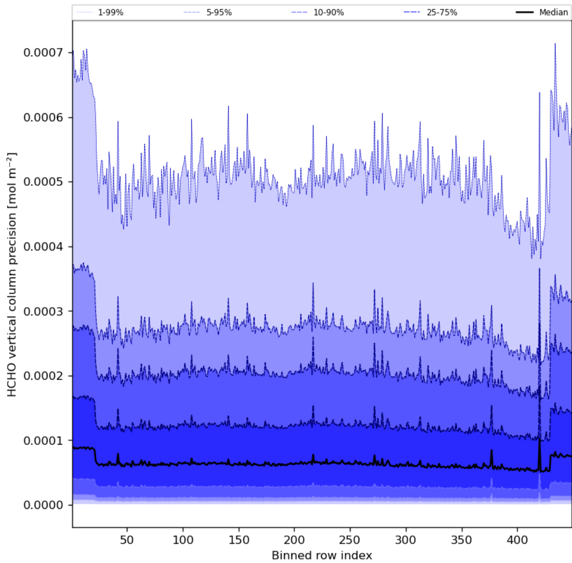
Figure 50: Along track statistics of “HCHO vertical column precision” for 2023-07-19 to 2023-07-21
