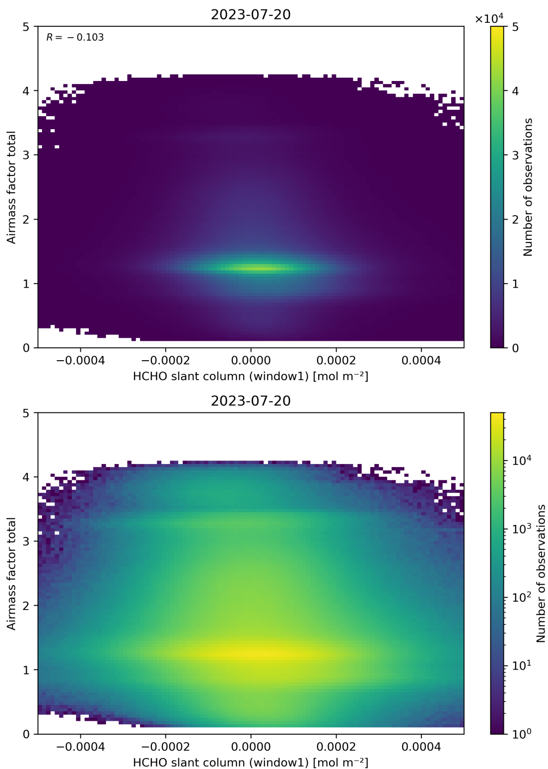
Figure 85: Scatter density plot of “HCHO slant column (window1)” against “Airmass factor total” for 2023-07-19 to 2023-07-21.
