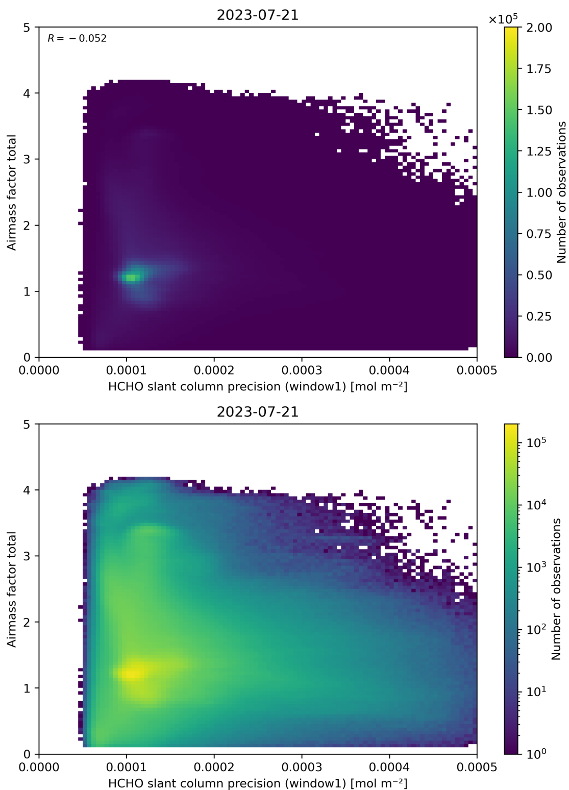
Figure 94: Scatter density plot of “HCHO slant column precision (window1)” against “Airmass factor total” for 2023-07-20 to 2023-07-22.
