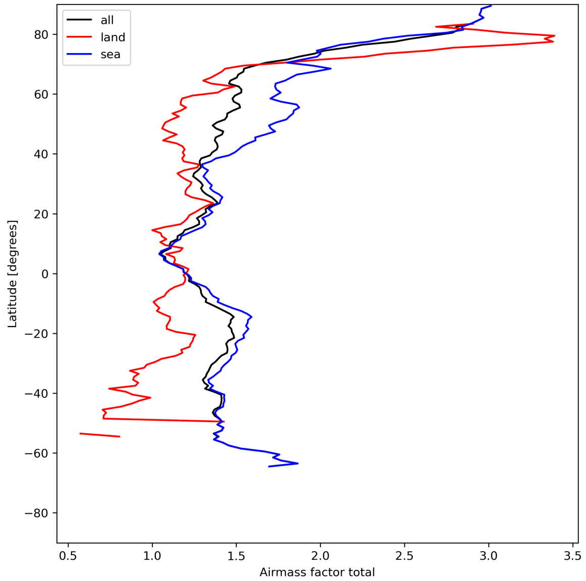
Figure 26: Zonal average of “Airmass factor total” for 2023-07-20 to 2023-07-22.
