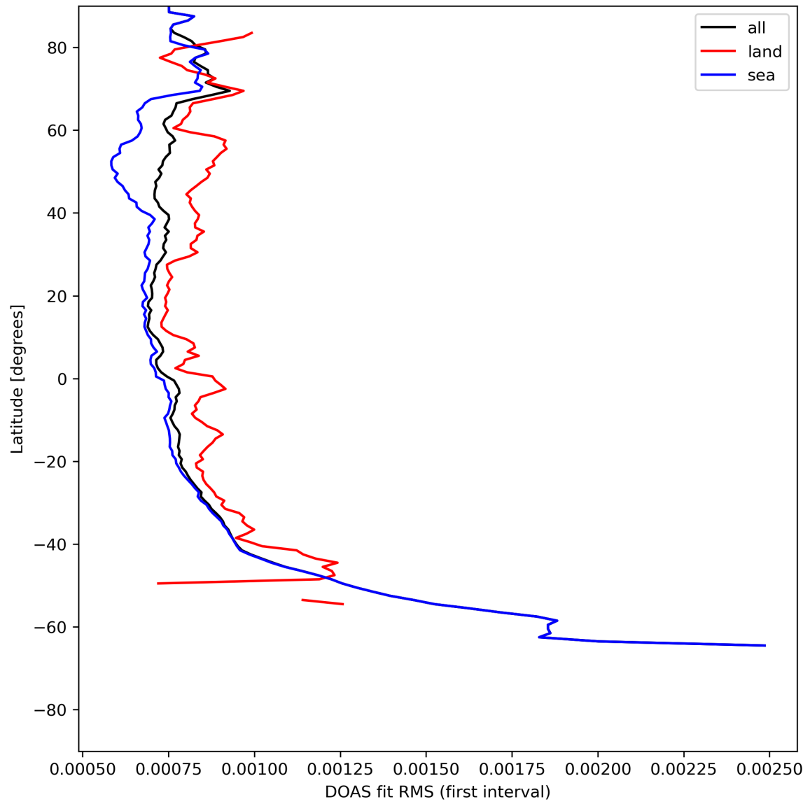
Figure 32: Zonal average of “DOAS fit RMS (first interval)” for 2023-07-20 to 2023-07-22.
