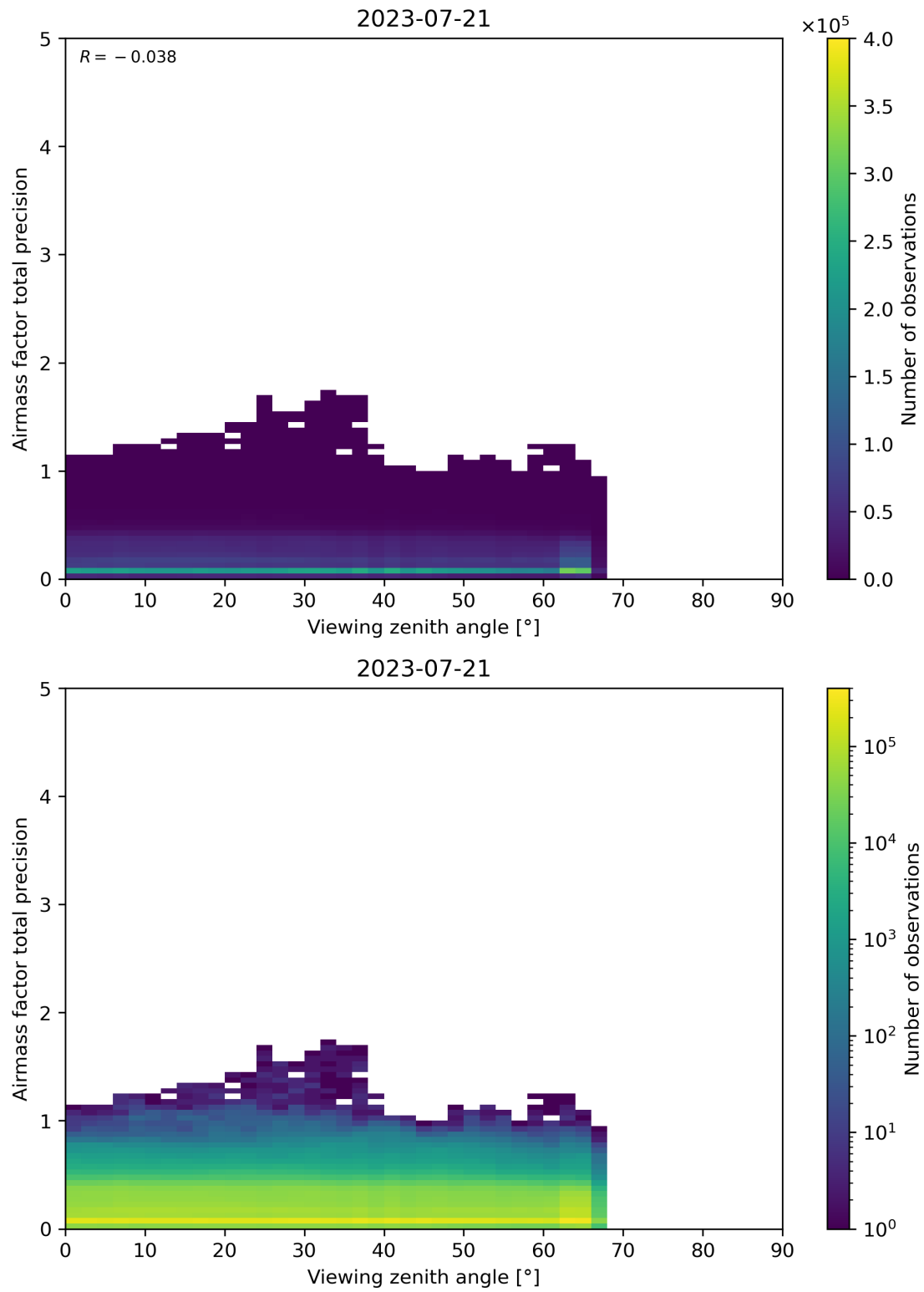
Figure 191: Scatter density plot of “Viewing zenith angle” against “Airmass factor total precision” for 2023-07-20 to 2023-07-22.
