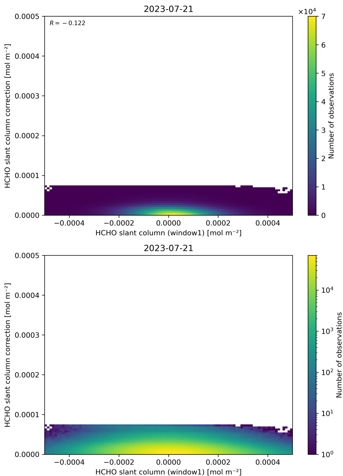
Figure 83: Scatter density plot of “HCHO slant column (window1)” against “HCHO slant column correction” for 2023-07-20 to 2023-07-22.
