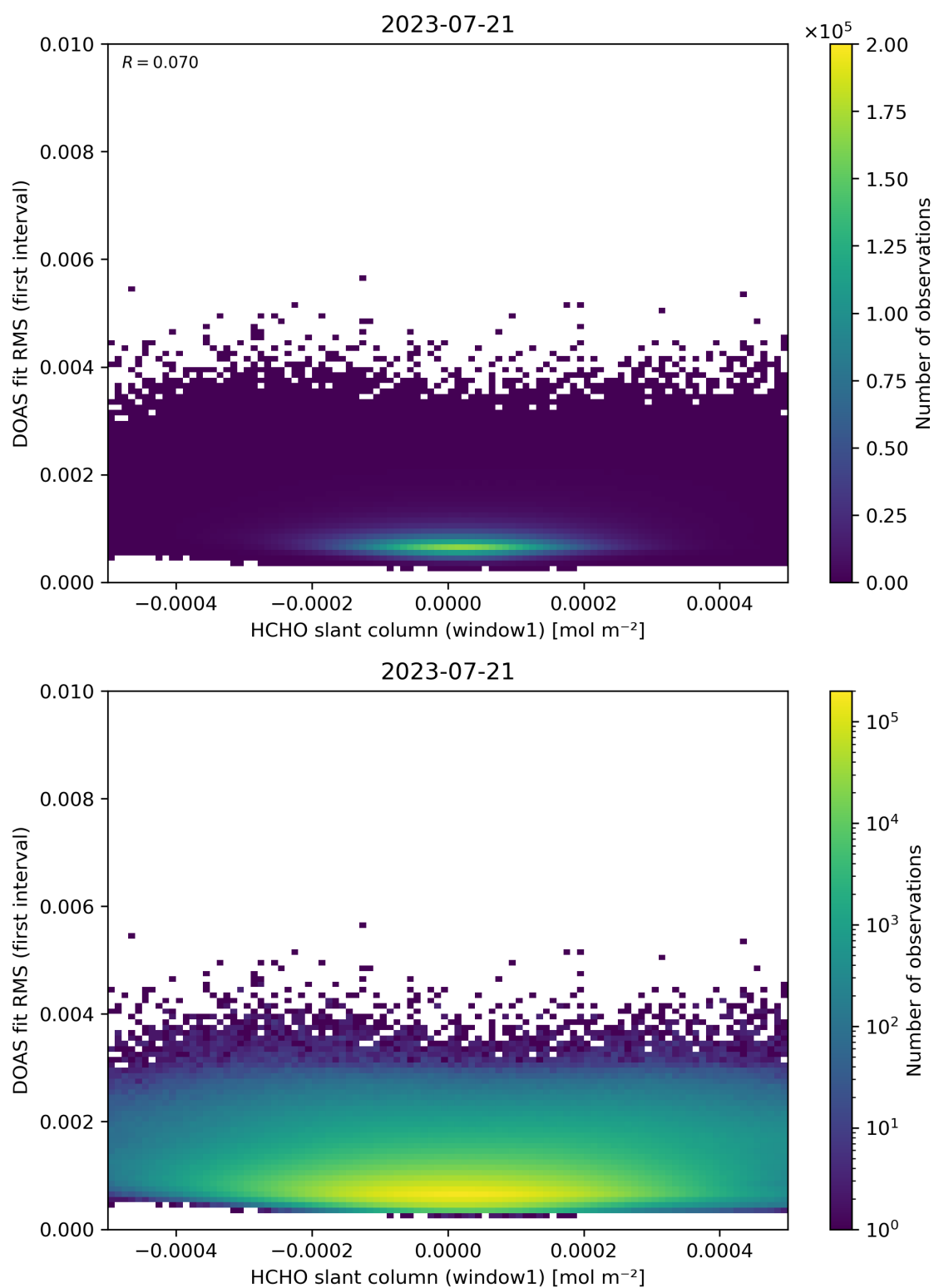
Figure 78: Scatter density plot of “HCHO slant column (window1)” against “DOAS fit RMS (first interval)” for 2023-07-20 to 2023-07-22.
