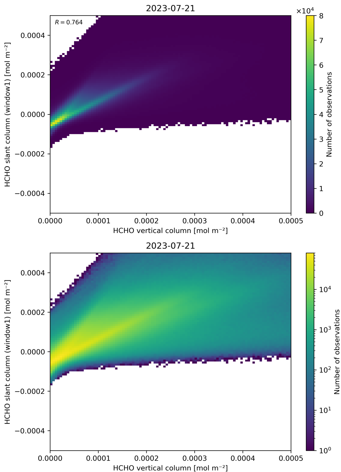
Figure 129: Scatter density plot of “HCHO vertical column” against “HCHO slant column (window1)” for 2023-07-20 to 2023-07-22.
