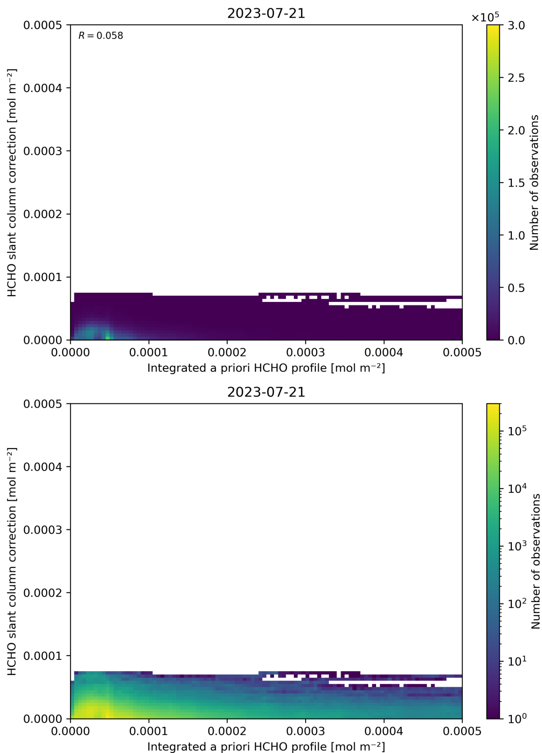
Figure 152: Scatter density plot of “Integrated a priori HCHO profile” against “HCHO slant column correction” for 2023-07-20 to 2023-07-22.
