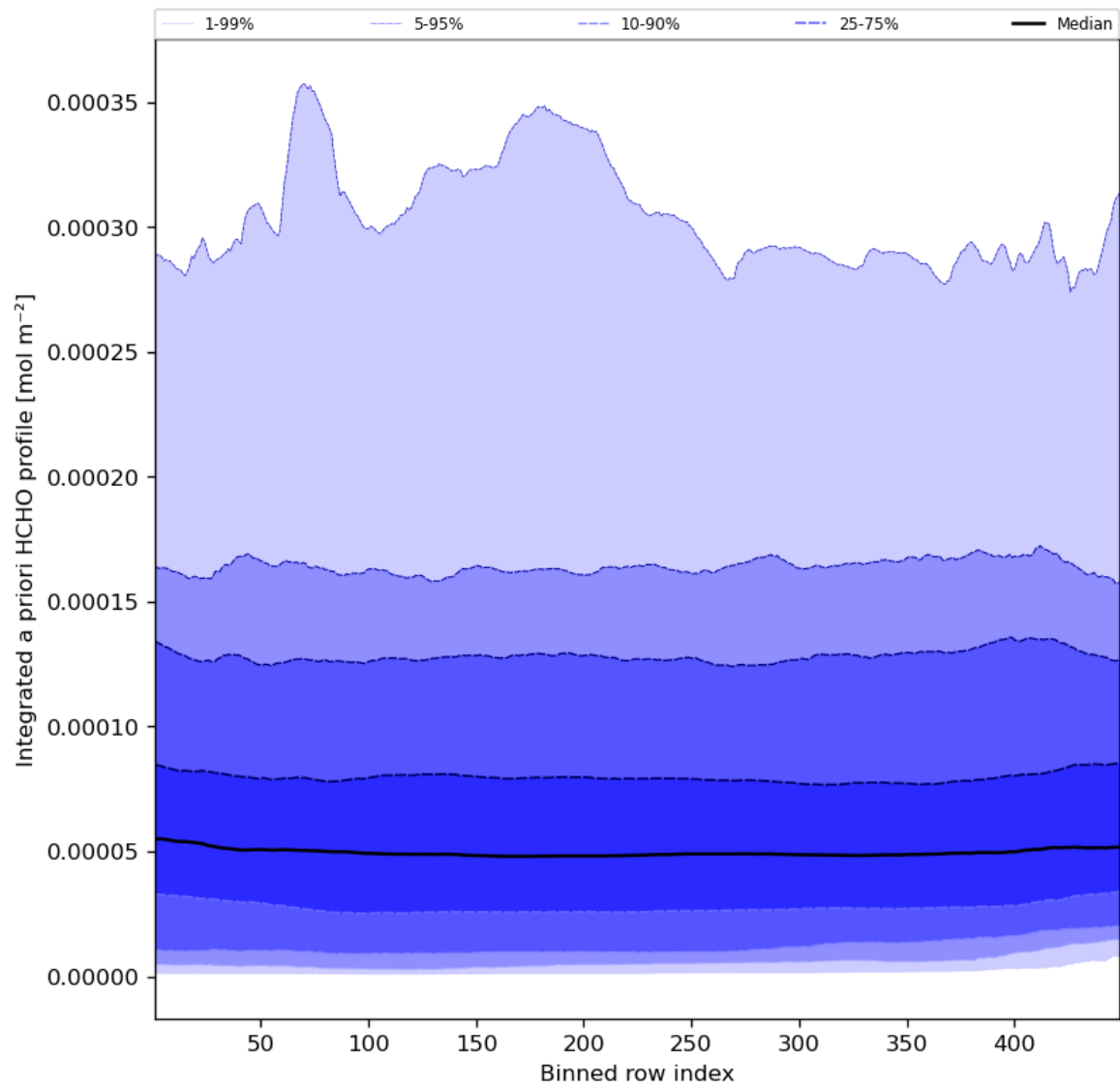
Figure 57: Along track statistics of "Integrated a priori HCHO profile" for 2023-07-20 to 2023-07-22
