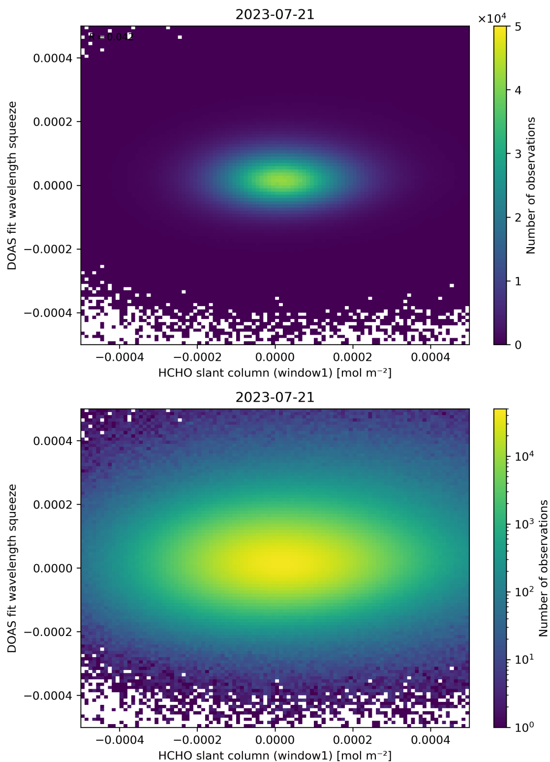
Figure 80: Scatter density plot of “HCHO slant column (window1)” against “DOAS fit wavelength squeeze” for 2023-07-20 to 2023-07-22.
