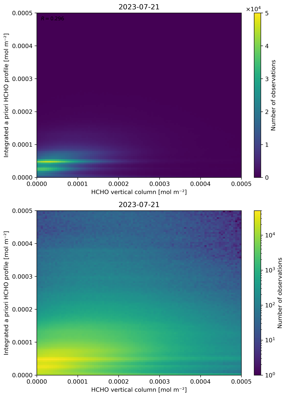
Figure 135: Scatter density plot of “HCHO vertical column” against “Integrated a priori HCHO profile” for 2023-07-20 to 2023-07-22.
