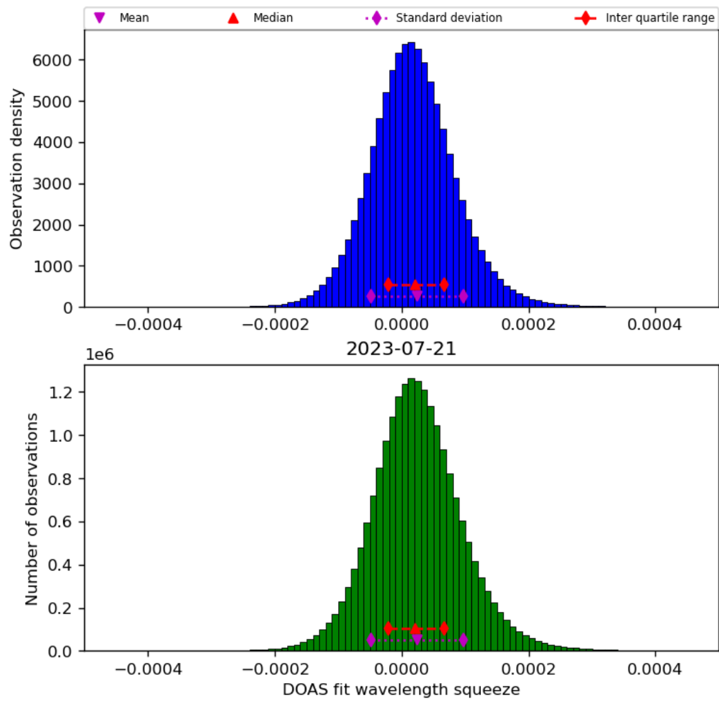
Figure 45: Histogram of “DOAS fit wavelength squeeze” for 2023-07-20 to 2023-07-22
