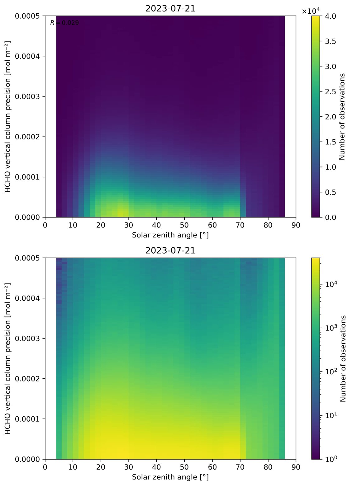
Figure 179: Scatter density plot of “Solar zenith angle” against “HCHO vertical column precision” for 2023-07-20 to 2023-07-22.
