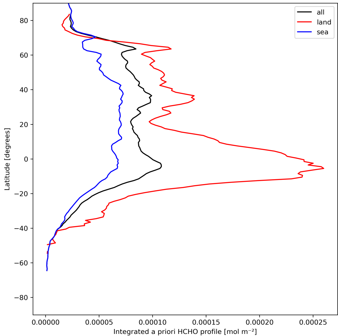
Figure 29: Zonal average of “Integrated a priori HCHO profile” for 2023-07-20 to 2023-07-22.
