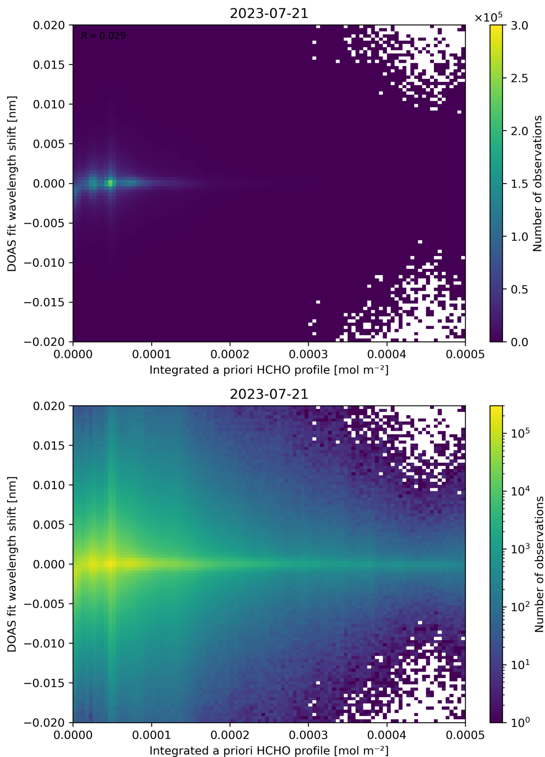
Figure 149: Scatter density plot of “Integrated a priori HCHO profile” against “DOAS fit wavelength shift” for 2023-07-20 to 2023-07-22.
