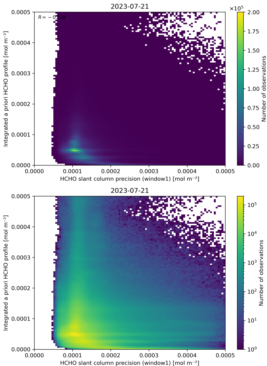
Figure 96: Scatter density plot of “HCHO slant column precision (window1)” against “Integrated a priori HCHO profile” for 2023-07-20 to 2023-07-22.
