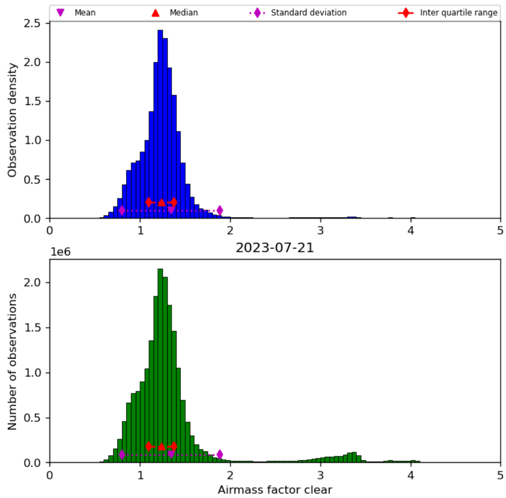
Figure 42: Histogram of “Airmass factor clear” for 2023-07-20 to 2023-07-22
