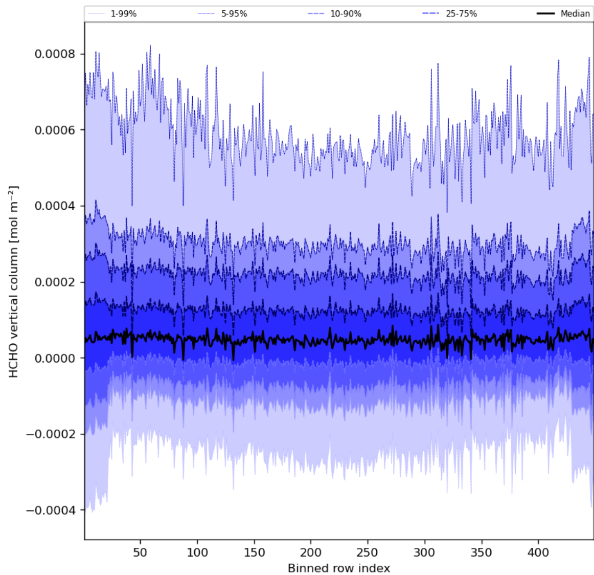
Figure 49: Along track statistics of “HCHO vertical column” for 2023-07-20 to 2023-07-22
