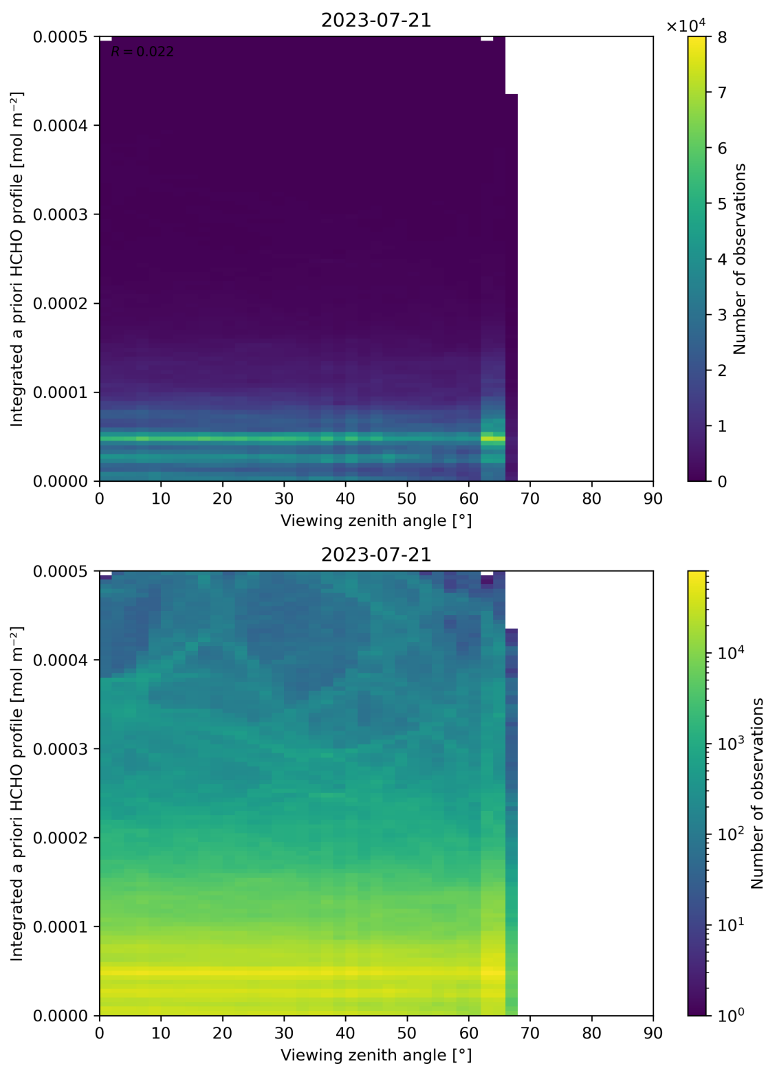
Figure 195: Scatter density plot of “Viewing zenith angle” against “Integrated a priori HCHO profile” for 2023-07-20 to 2023-07-22.
