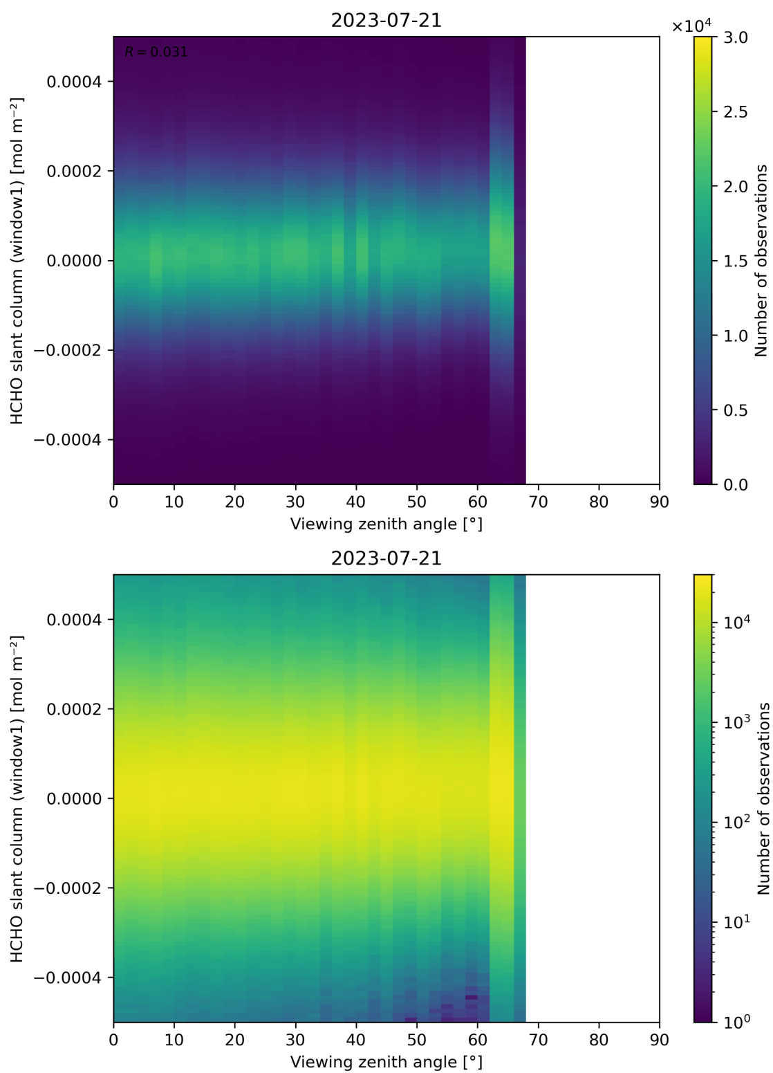
Figure 188: Scatter density plot of “Viewing zenith angle” against “HCHO slant column (window1)” for 2023-07-20 to 2023-07-22.
