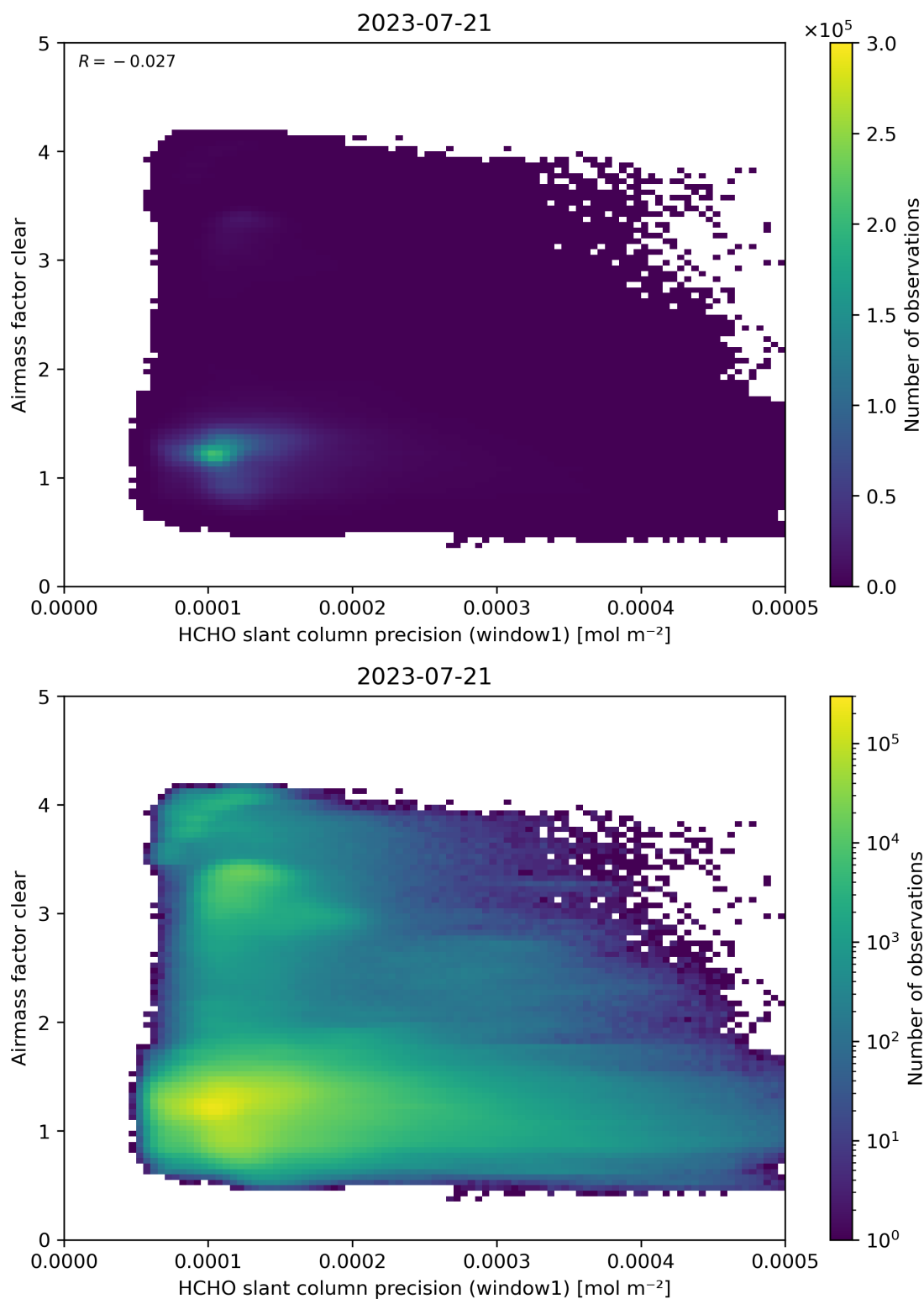
Figure 91: Scatter density plot of “HCHO slant column precision (window1)” against “Airmass factor clear” for 2023-07-20 to 2023-07-22.
