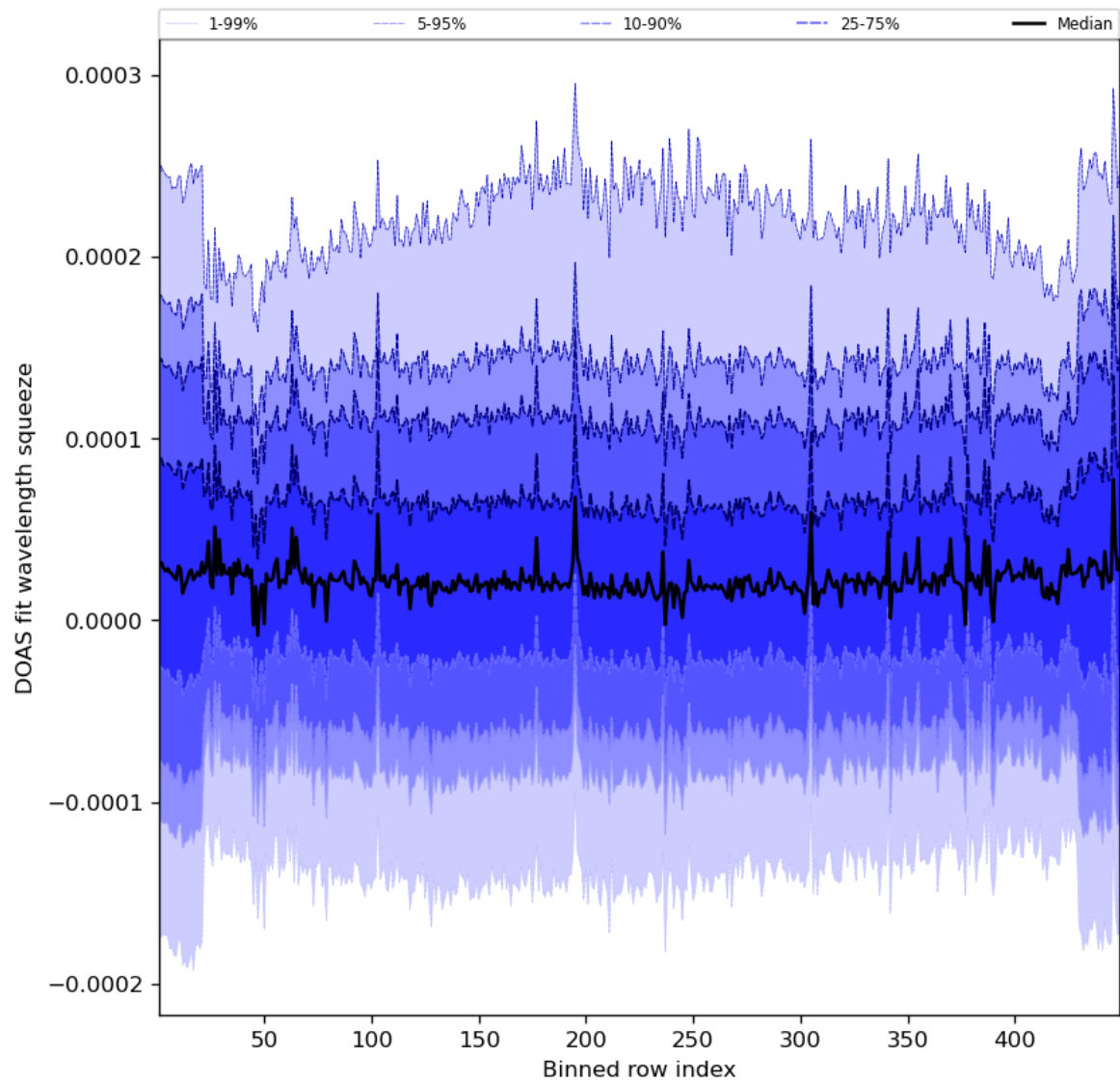
Figure 59: Along track statistics of “DOAS fit wavelength squeeze” for 2023-07-20 to 2023-07-22
