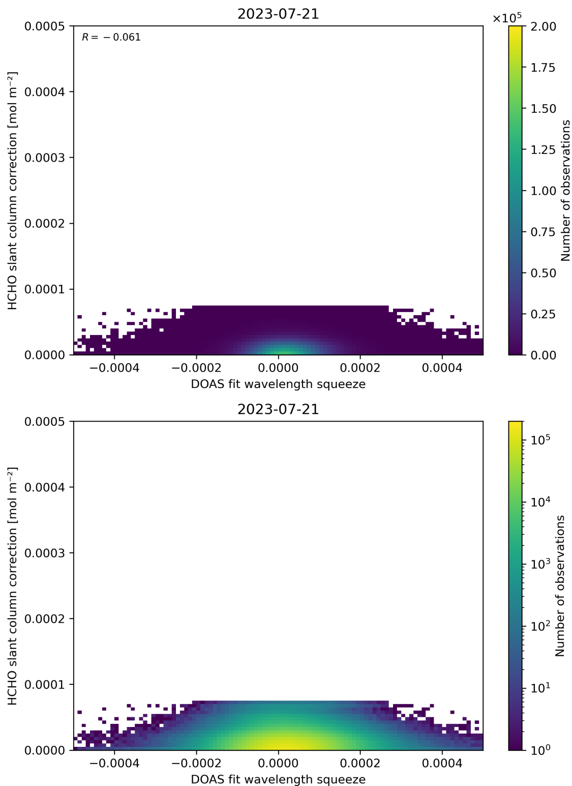
Figure 70: Scatter density plot of “DOAS fit wavelength squeeze” against “HCHO slant column correction” for 2023-07-20 to 2023-07-22.
