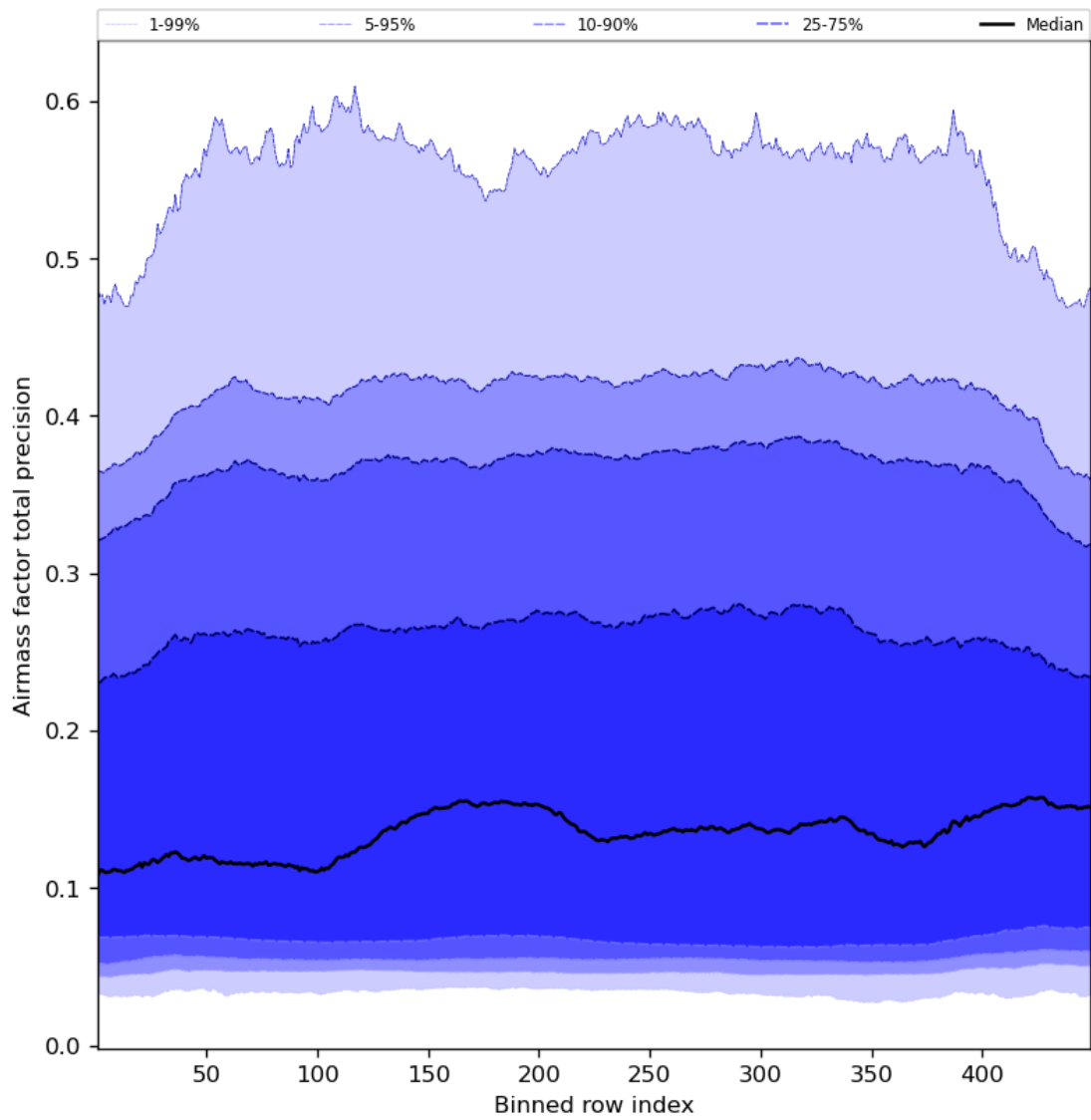
Figure 55: Along track statistics of “Airmass factor total precision” for 2023-07-20 to 2023-07-22
