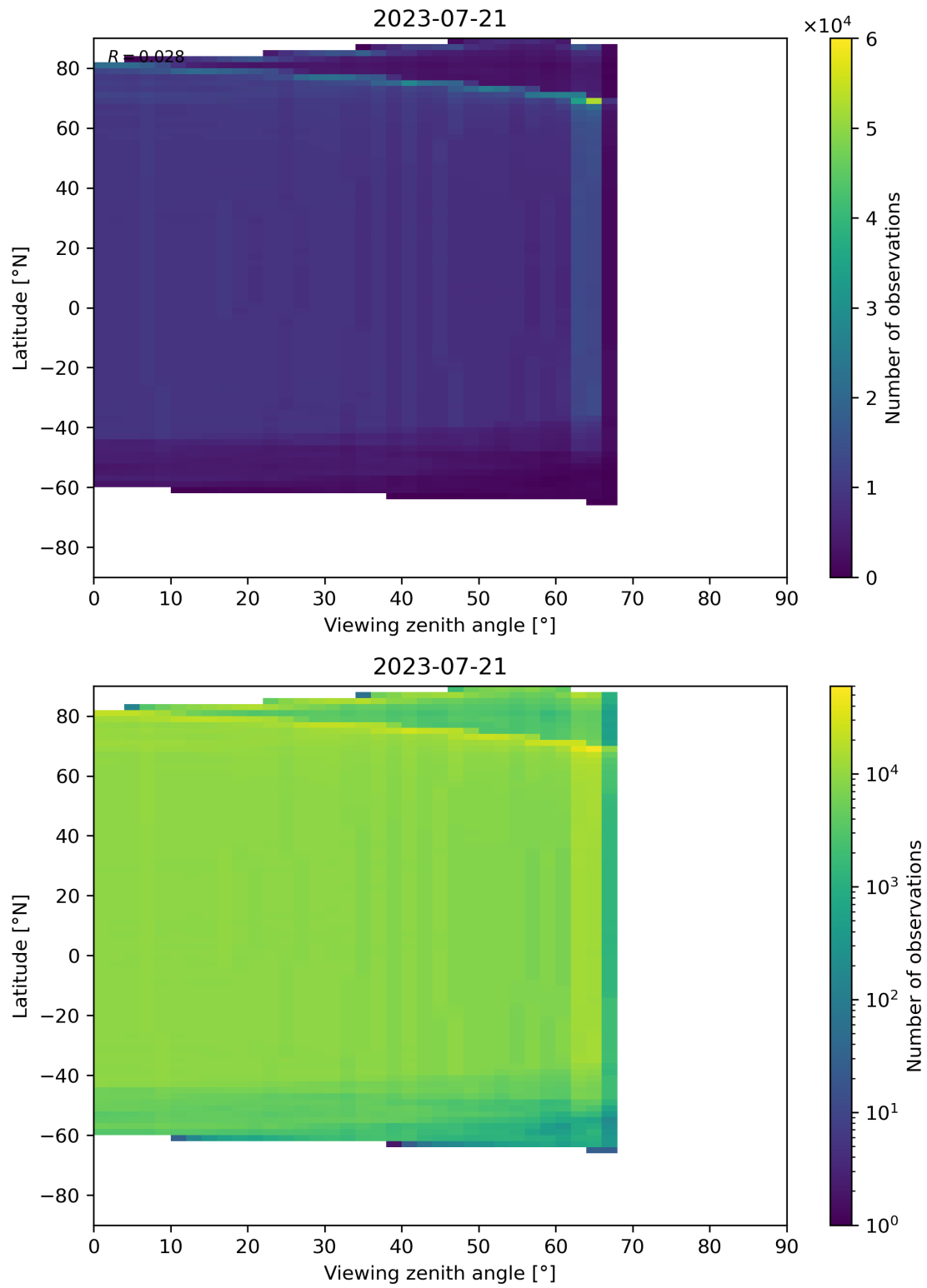
Figure 196: Scatter density plot of “Viewing zenith angle” against “Latitude” for 2023-07-20 to 2023-07-22.
