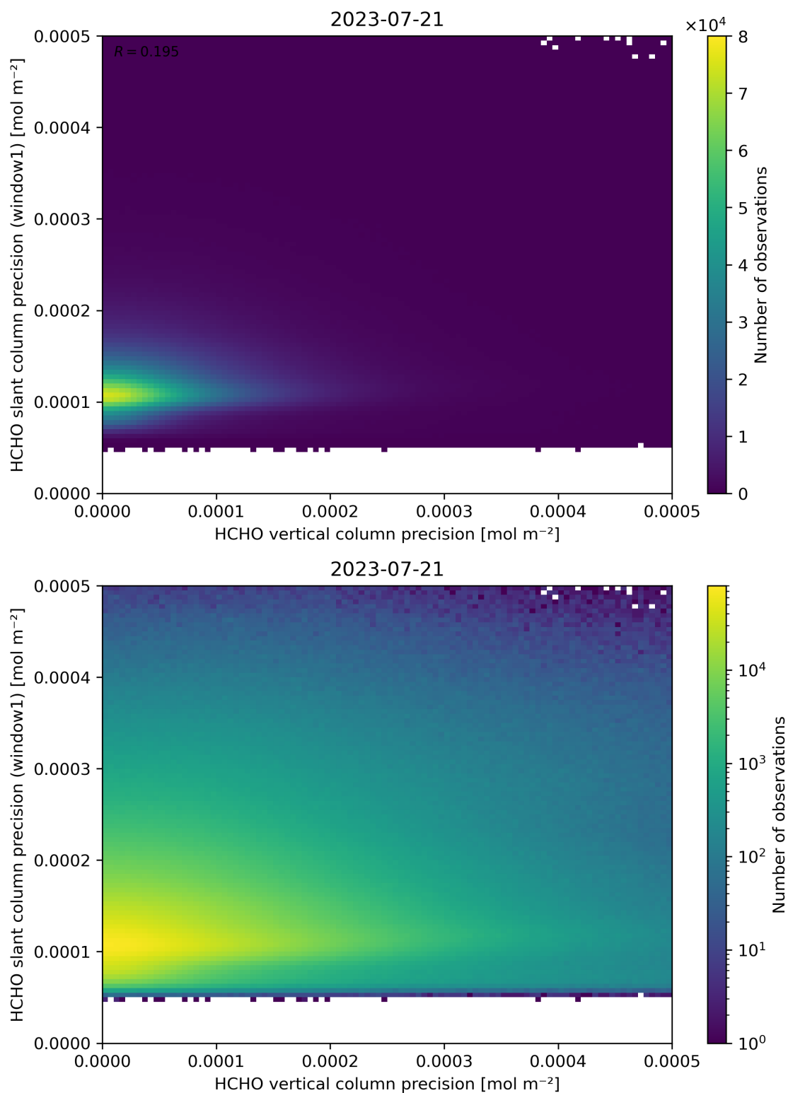
Figure 143: Scatter density plot of “HCHO vertical column precision” against “HCHO slant column precision (window1)” for 2023-07-20 to 2023-07-22.
