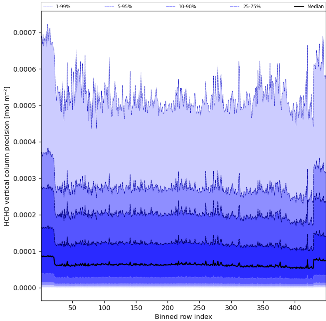
Figure 50: Along track statistics of “HCHO vertical column precision” for 2023-07-20 to 2023-07-22
