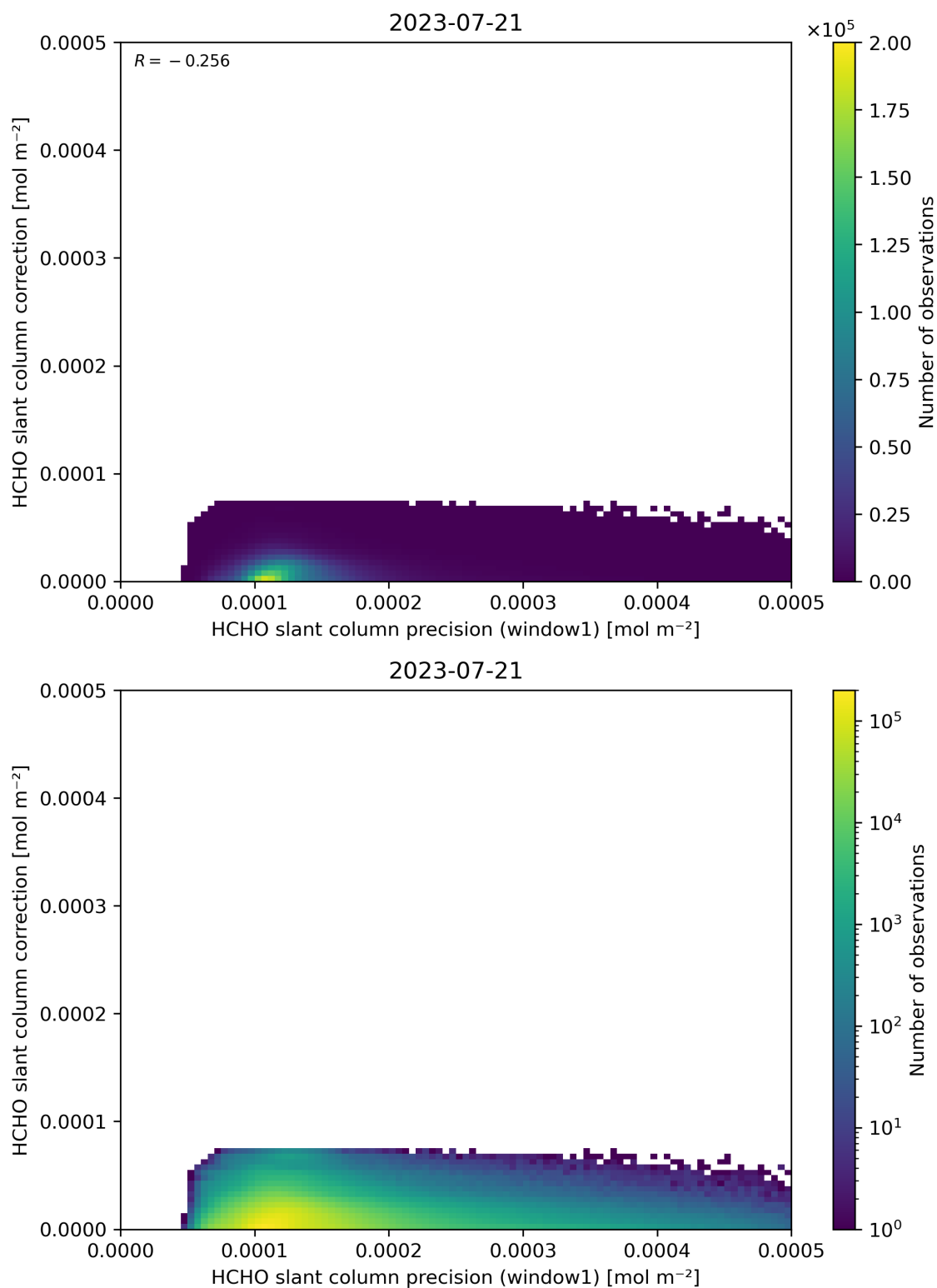
Figure 93: Scatter density plot of “HCHO slant column precision (window1)” against “HCHO slant column correction” for 2023-07-20 to 2023-07-22.
