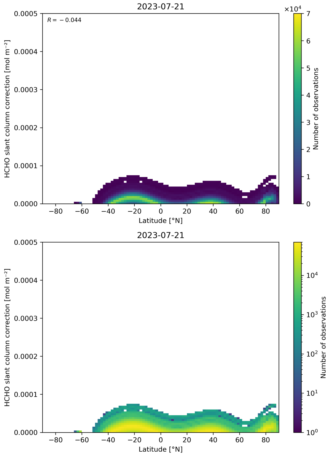
Figure 158: Scatter density plot of “Latitude” against “HCHO slant column correction” for 2023-07-20 to 2023-07-22.
