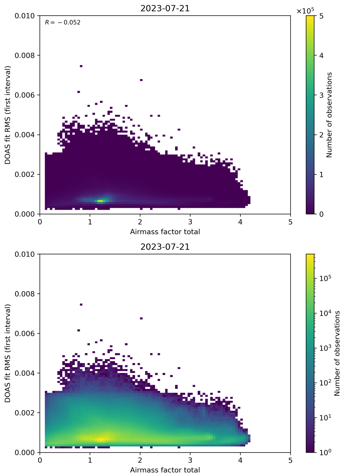
Figure 97: Scatter density plot of “Airmass factor total” against “DOAS fit RMS (first interval)” for 2023-07-20 to 2023-07-22.
