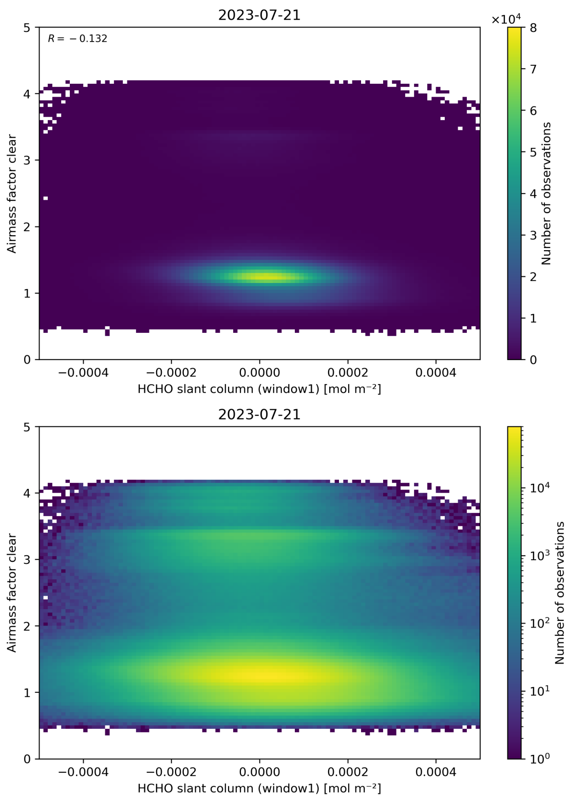
Figure 81: Scatter density plot of “HCHO slant column (window1)” against “Airmass factor clear” for 2023-07-20 to 2023-07-22.
