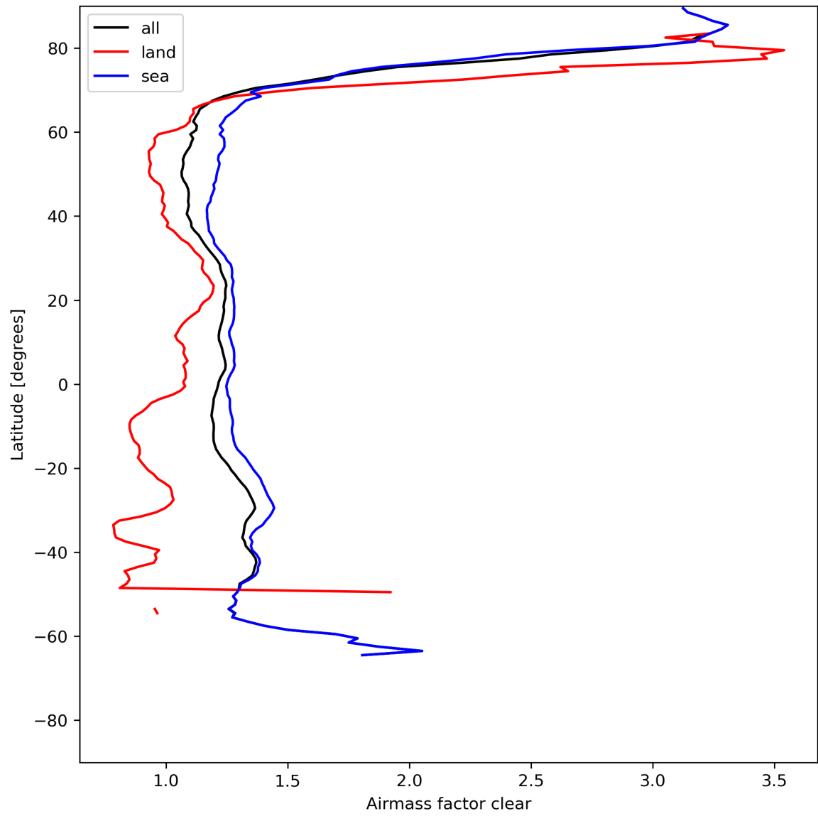
Figure 28: Zonal average of “Airmass factor clear” for 2023-07-20 to 2023-07-22.
