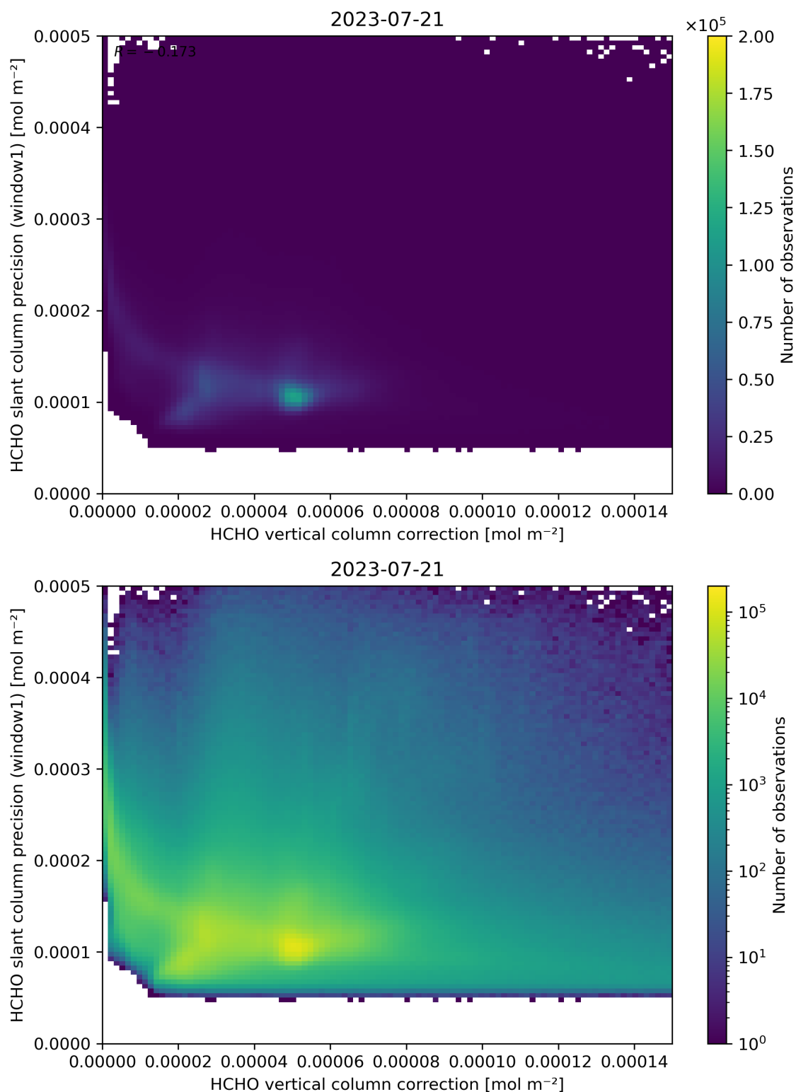
Figure 119: Scatter density plot of “HCHO vertical column correction” against “HCHO slant column precision (window1)” for 2023-07-20 to 2023-07-22.
