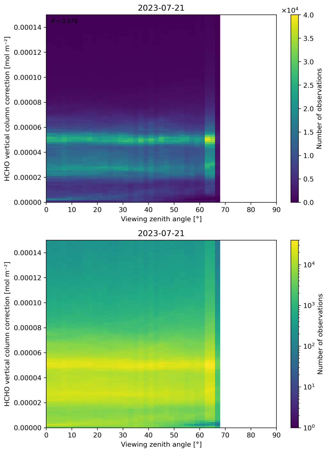
Figure 193: Scatter density plot of “Viewing zenith angle” against “HCHO vertical column correction” for 2023-07-20 to 2023-07-22.
