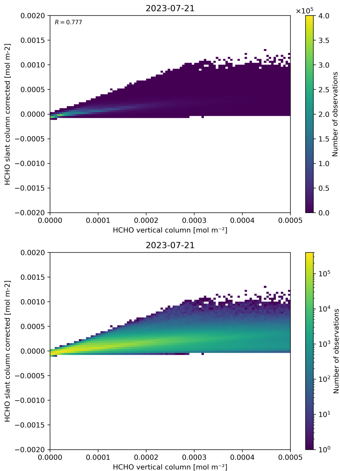
Figure 127: Scatter density plot of “HCHO vertical column” against “HCHO slant column corrected” for 2023-07-20 to 2023-07-22.
