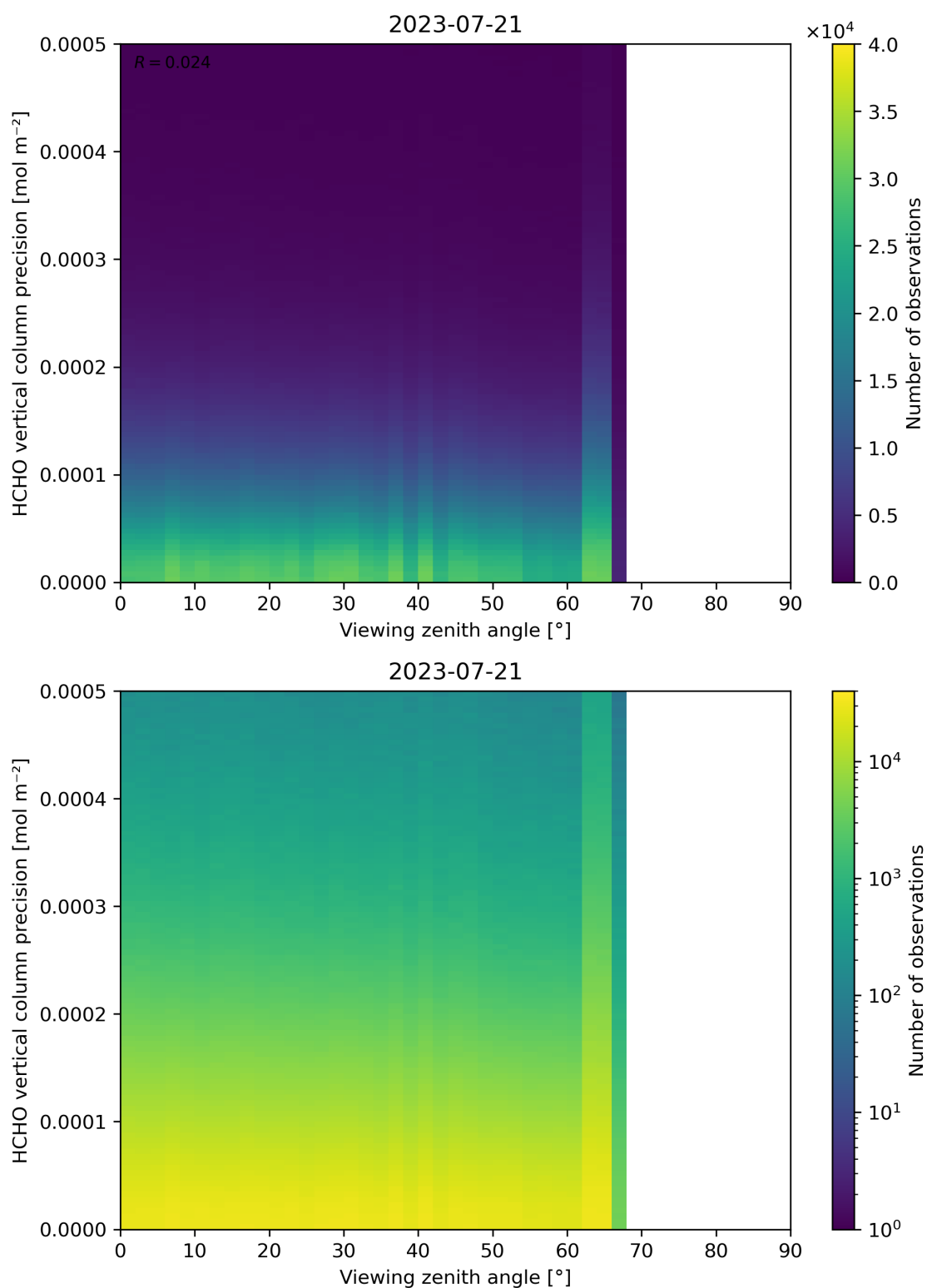
Figure 194: Scatter density plot of “Viewing zenith angle” against “HCHO vertical column precision” for 2023-07-20 to 2023-07-22.
