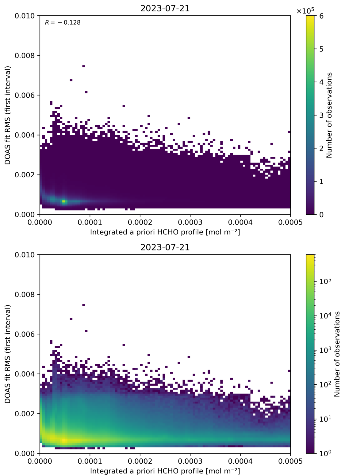
Figure 148: Scatter density plot of “Integrated a priori HCHO profile” against “DOAS fit RMS (first interval)” for 2023-07-20 to 2023-07-22.
