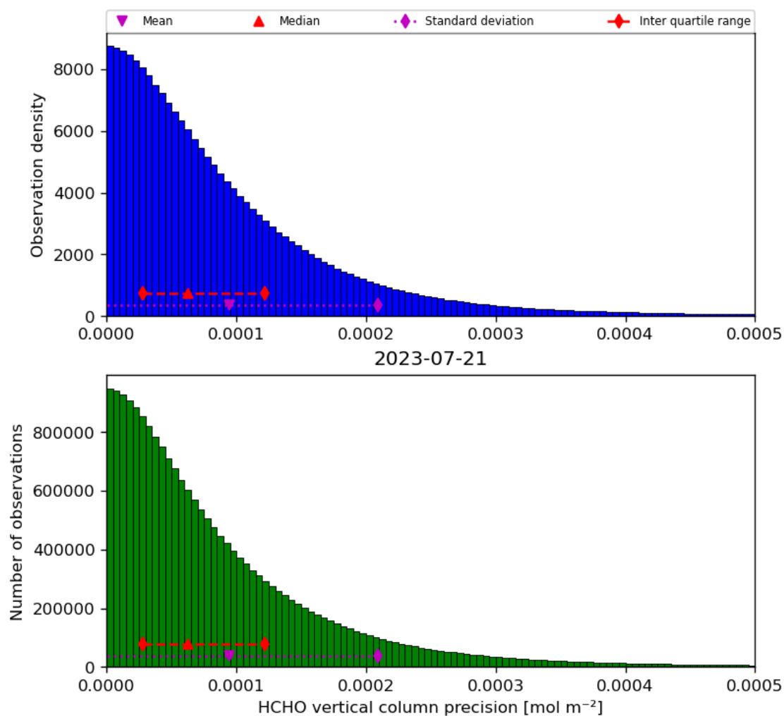
Figure 36: Histogram of “HCHO vertical column precision” for 2023-07-20 to 2023-07-22
