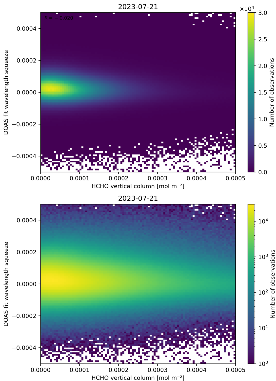
Figure 125: Scatter density plot of “HCHO vertical column” against “DOAS fit wavelength squeeze” for 2023-07-20 to 2023-07-22.
