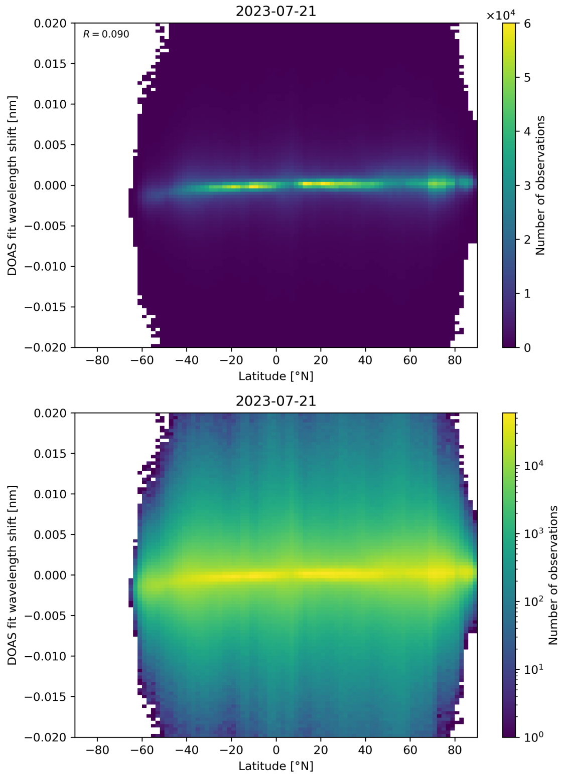
Figure 154: Scatter density plot of “Latitude” against “DOAS fit wavelength shift” for 2023-07-20 to 2023-07-22.
