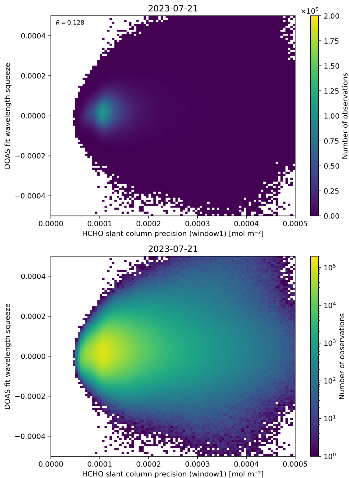
Figure 90: Scatter density plot of “HCHO slant column precision (window1)” against “DOAS fit wavelength squeeze” for 2023-07-20 to 2023-07-22.
