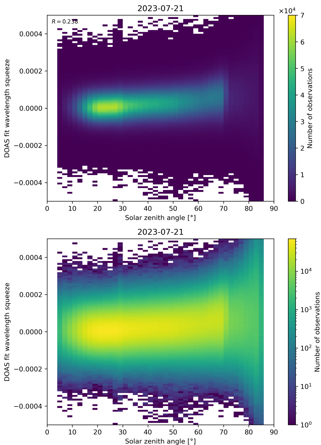
Figure 169: Scatter density plot of “Solar zenith angle” against “DOAS fit wavelength squeeze” for 2023-07-20 to 2023-07-22.
