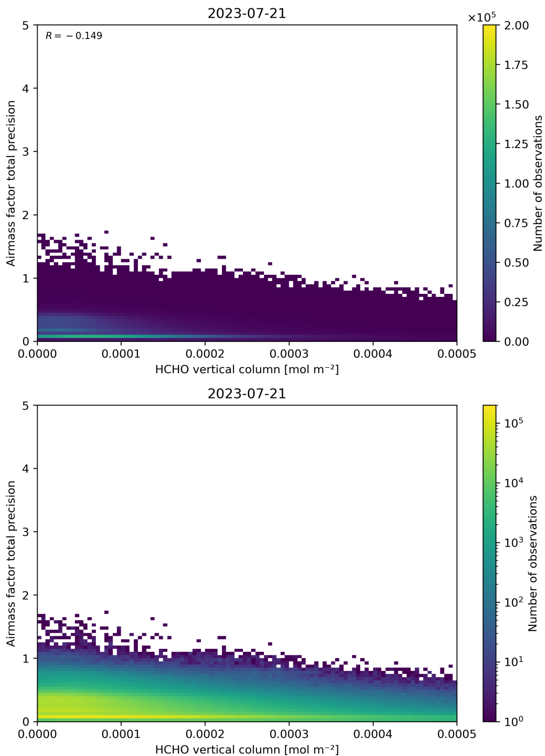
Figure 132: Scatter density plot of “HCHO vertical column” against “Airmass factor total precision” for 2023-07-20 to 2023-07-22.
