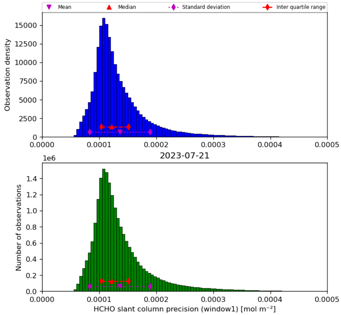
Figure 39: Histogram of “HCHO slant column precision (window1)” for 2023-07-20 to 2023-07-22
