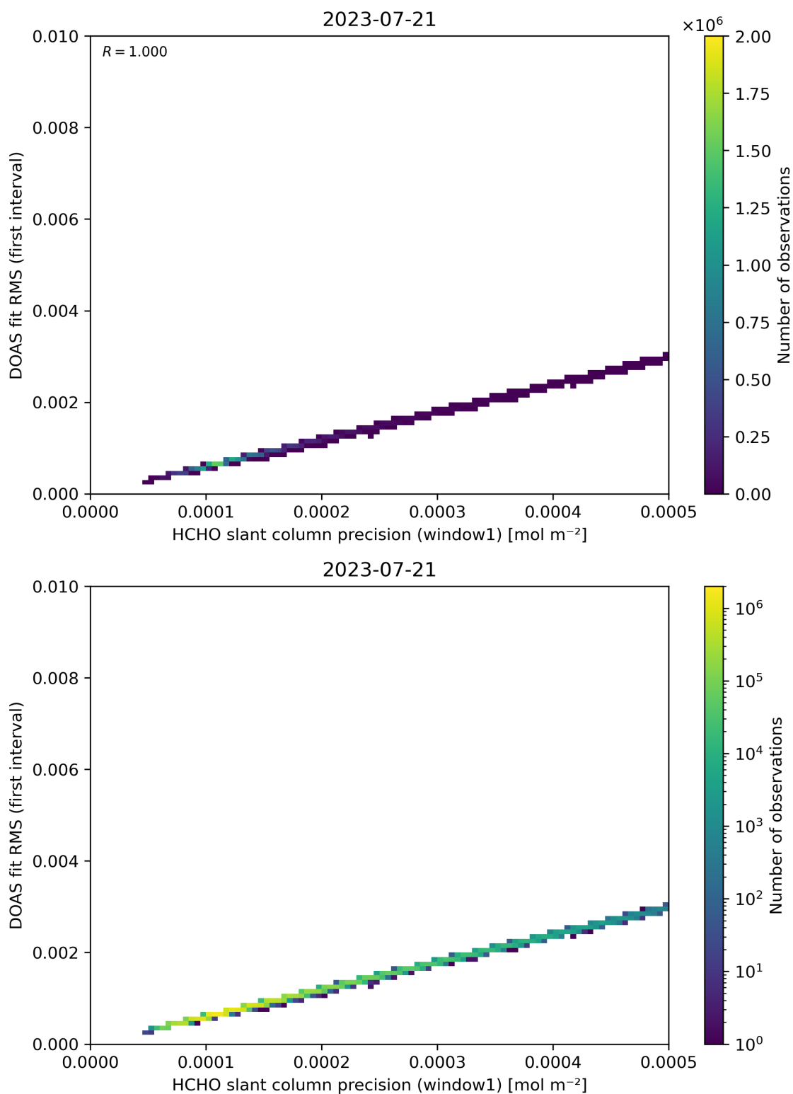
Figure 88: Scatter density plot of “HCHO slant column precision (window1)” against “DOAS fit RMS (first interval)” for 2023-07-20 to 2023-07-22.
