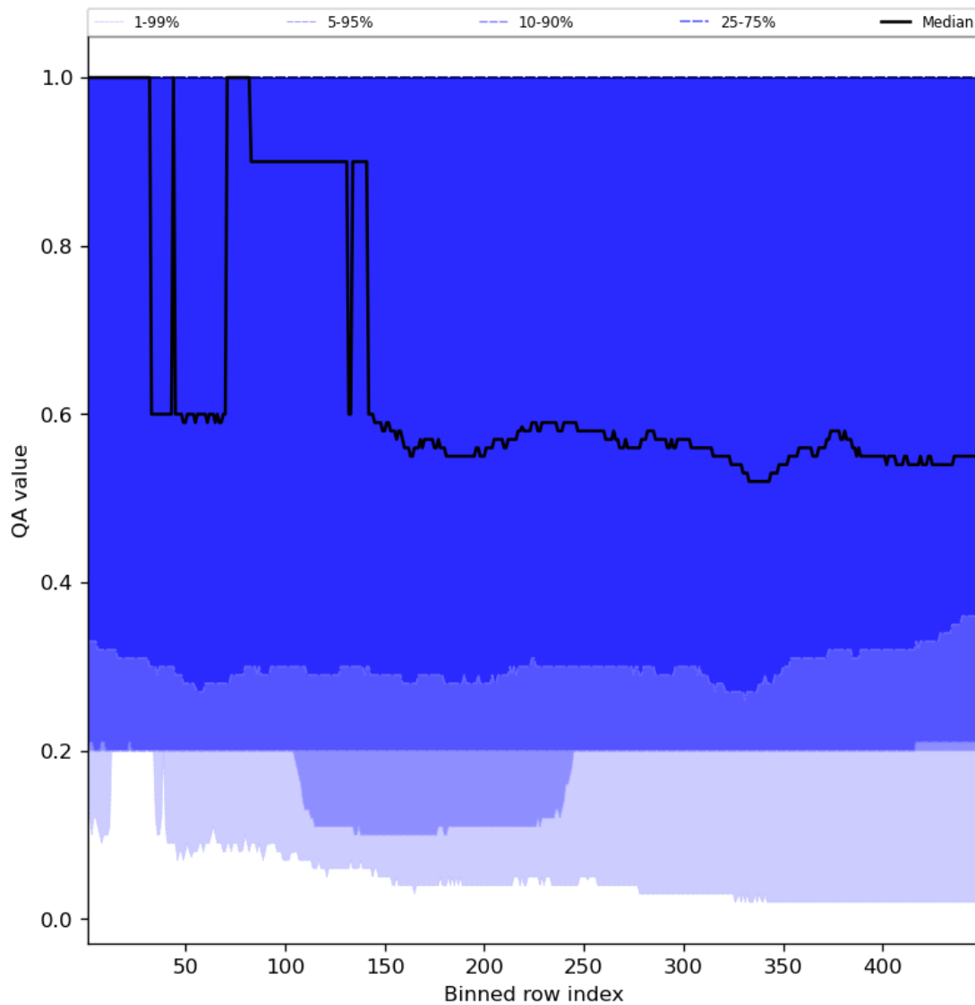
Figure 48: Along track statistics of “QA value” for 2023-07-20 to 2023-07-22
