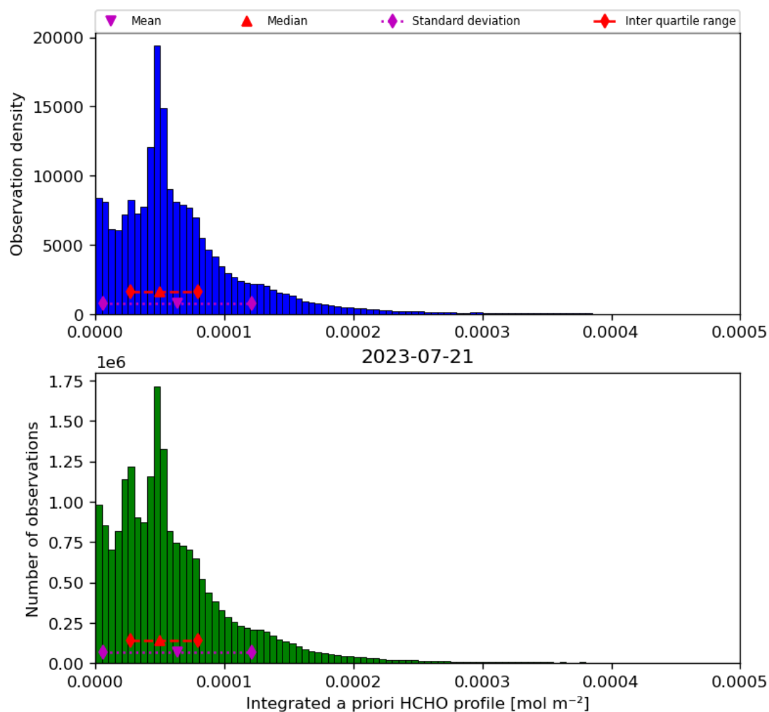
Figure 43: Histogram of “Integrated a priori HCHO profile” for 2023-07-20 to 2023-07-22
