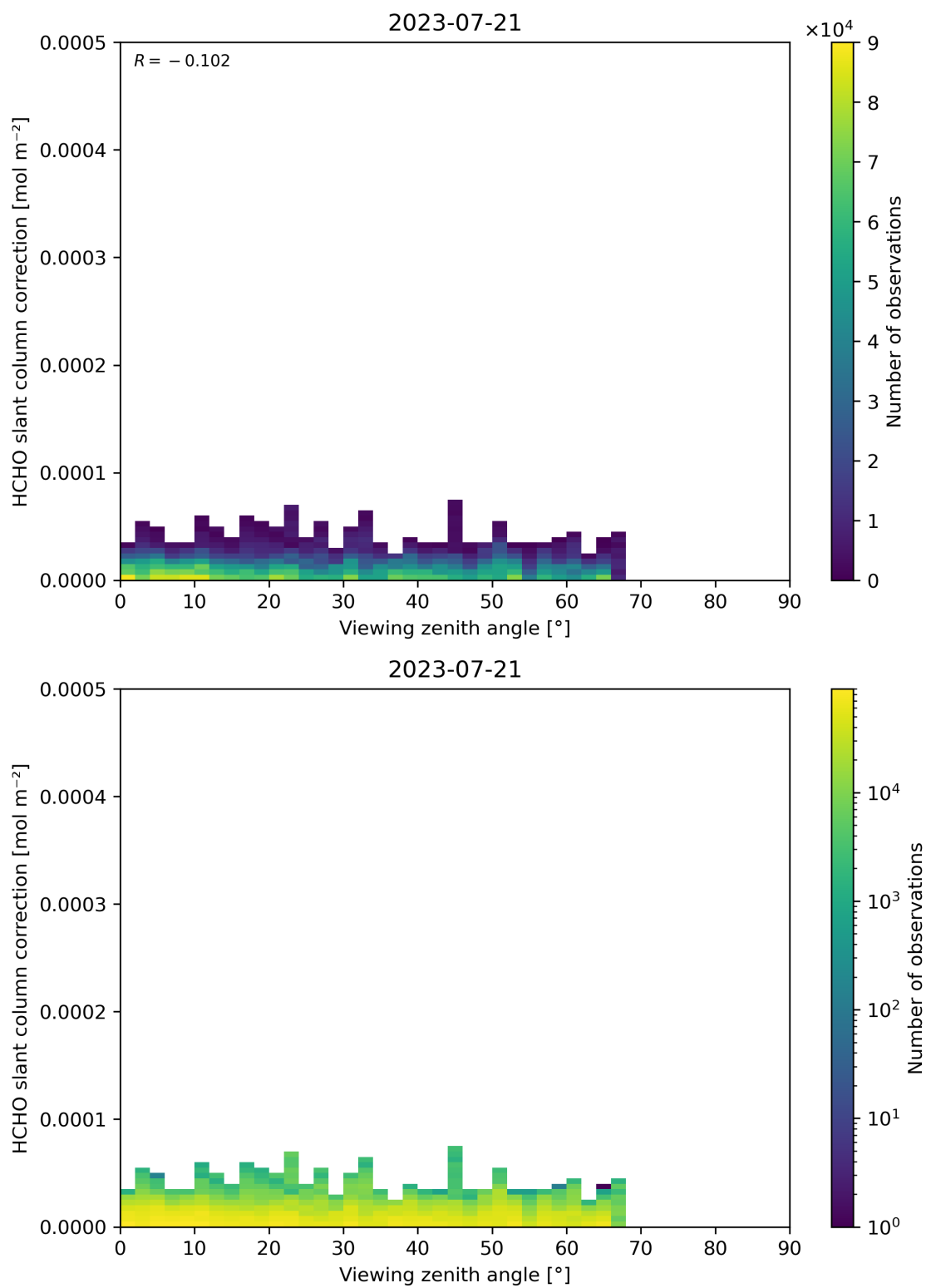
Figure 187: Scatter density plot of “Viewing zenith angle” against “HCHO slant column correction” for 2023-07-20 to 2023-07-22.
