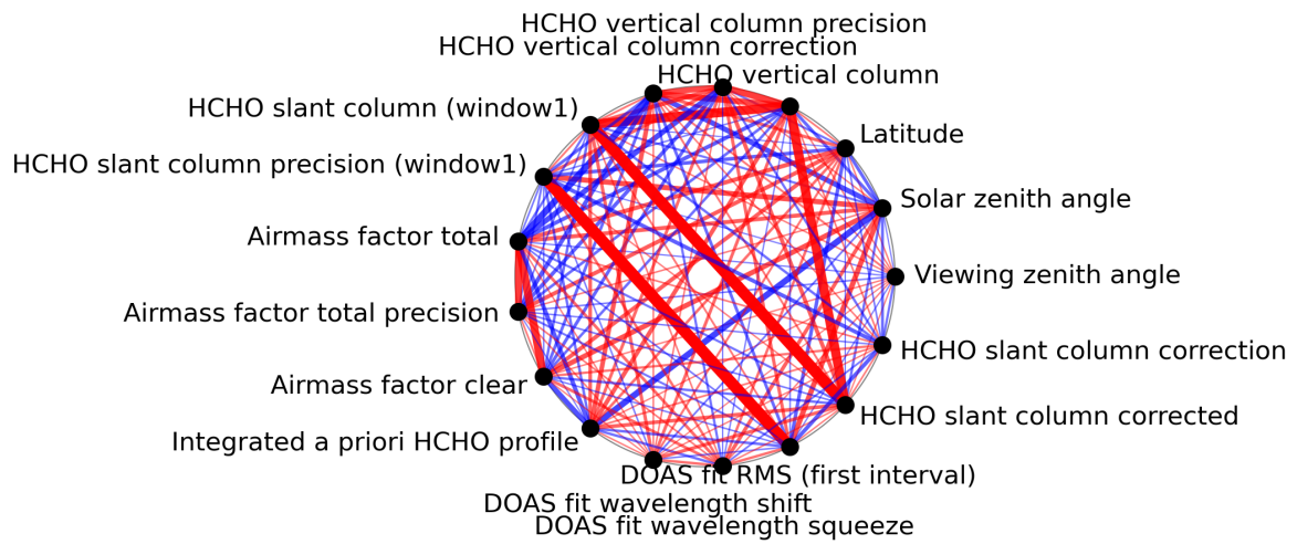
Figure 1: Map of correlation graph for 2023-07-20 to 2023-07-22.
