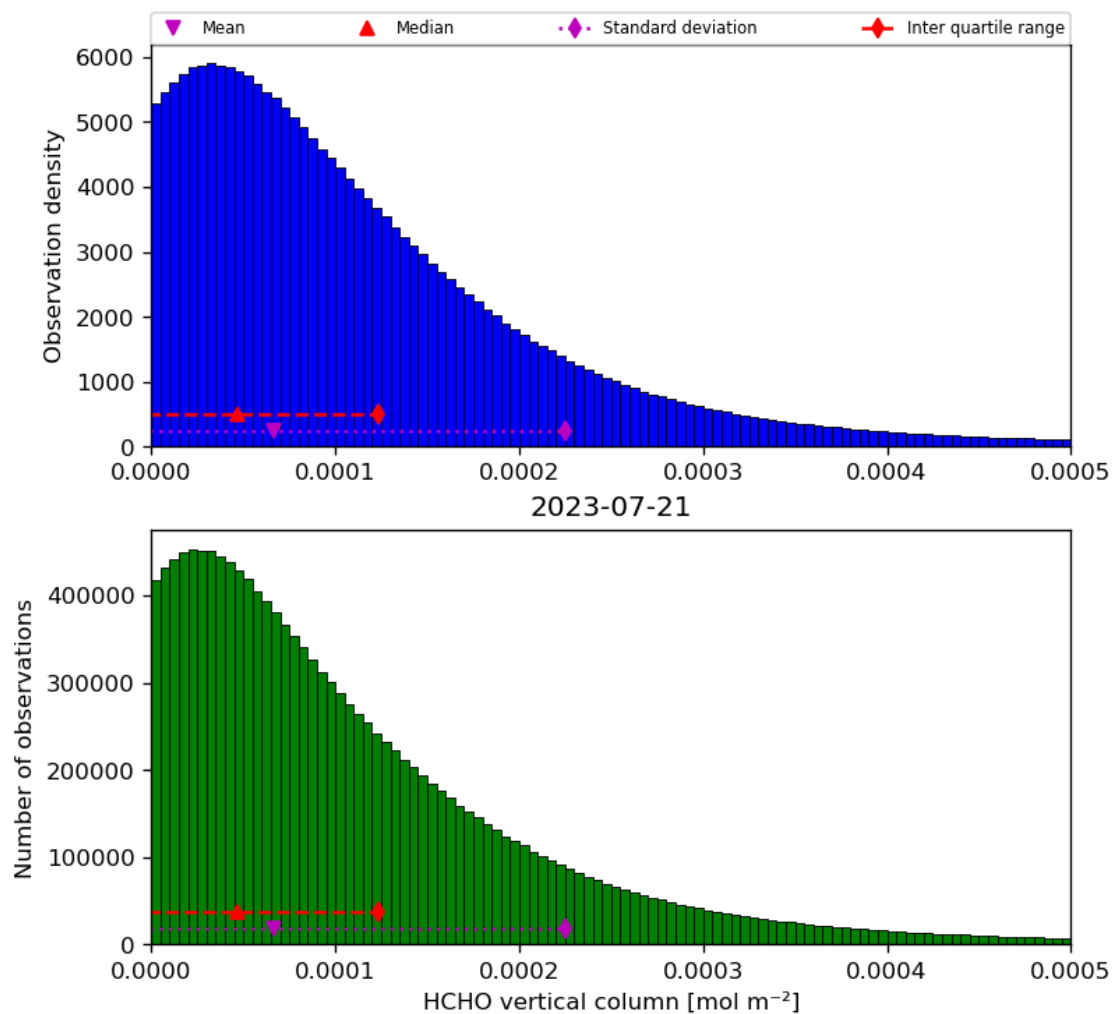
Figure 35: Histogram of “HCHO vertical column” for 2023-07-20 to 2023-07-22
