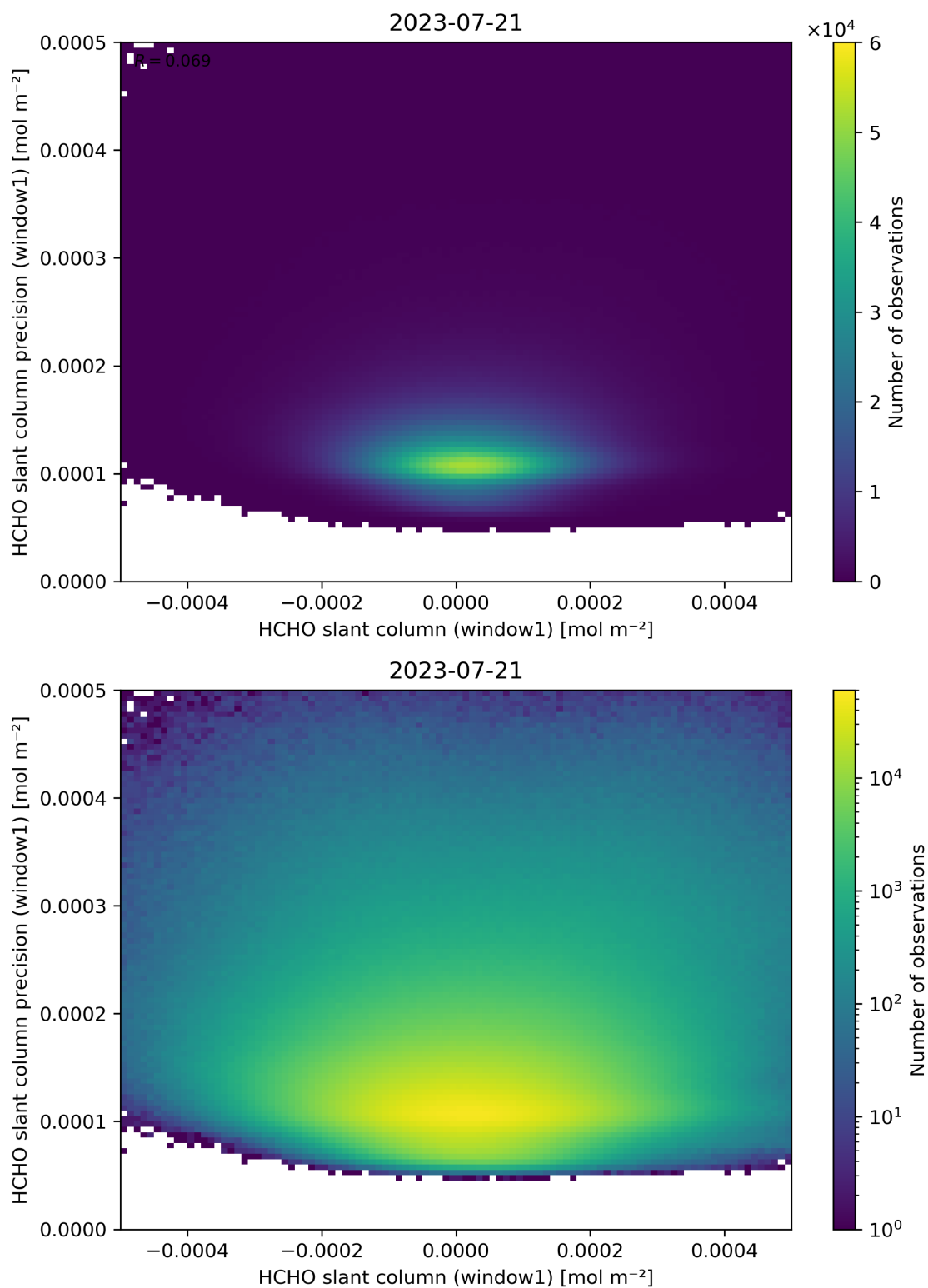
Figure 84: Scatter density plot of “HCHO slant column (window1)” against “HCHO slant column precision (window1)” for 2023-07-20 to 2023-07-22.
