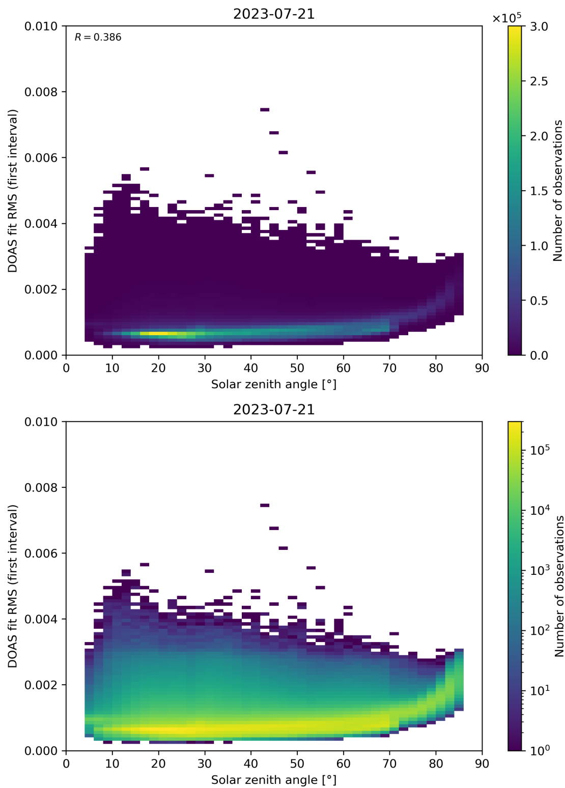
Figure 167: Scatter density plot of “Solar zenith angle” against “DOAS fit RMS (first interval)” for 2023-07-20 to 2023-07-22.
