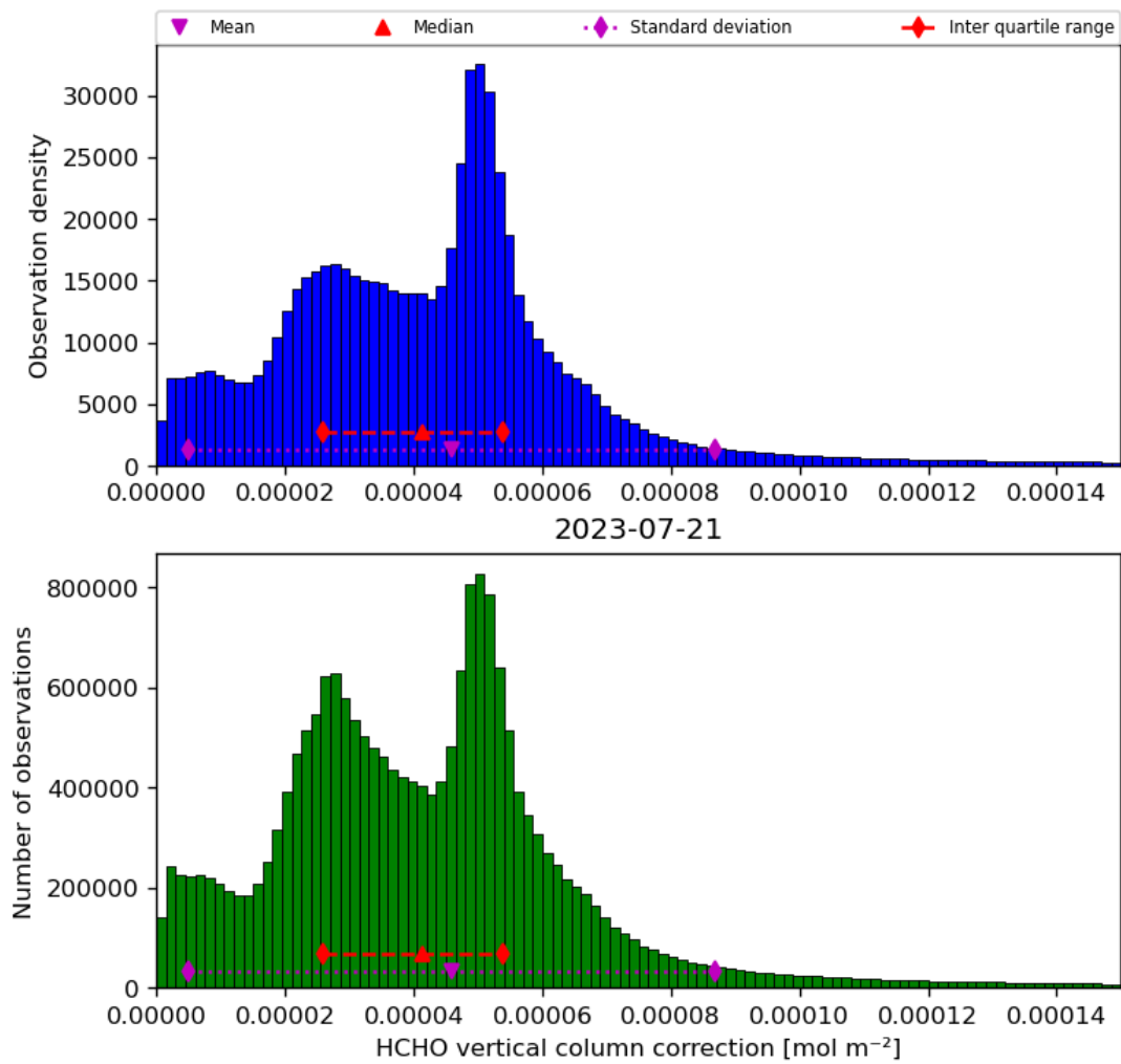
Figure 37: Histogram of “HCHO vertical column correction” for 2023-07-20 to 2023-07-22
