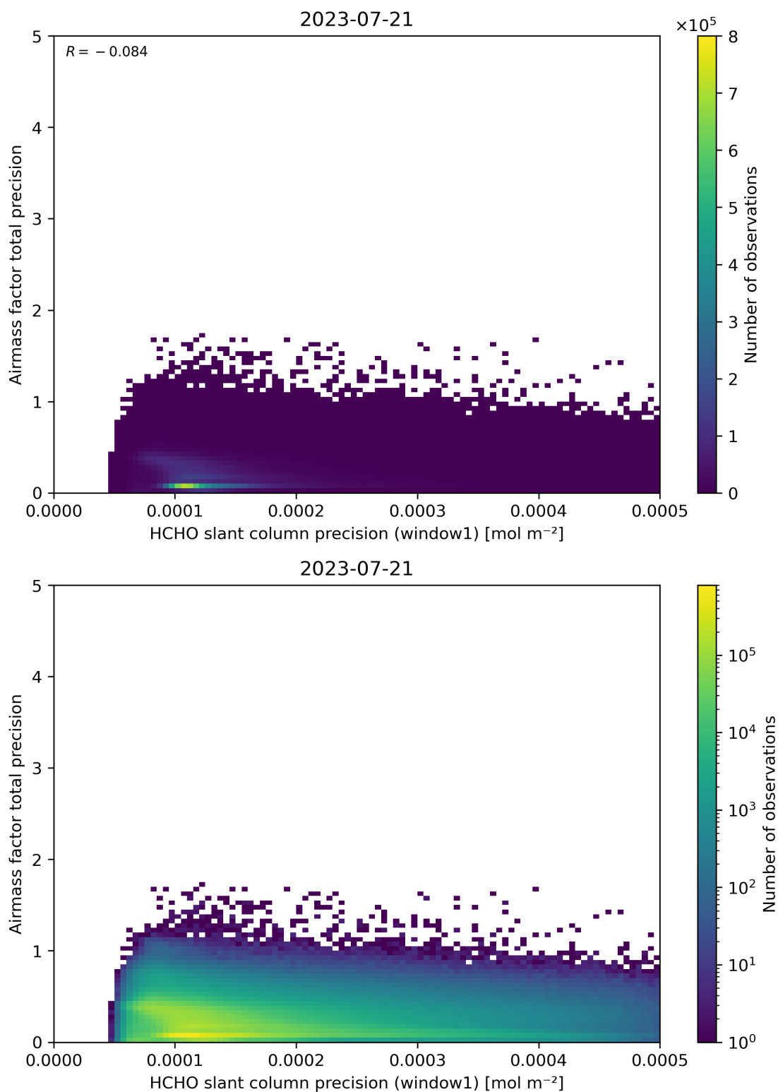
Figure 95: Scatter density plot of “HCHO slant column precision (window1)” against “Airmass factor total precision” for 2023-07-20 to 2023-07-22.
