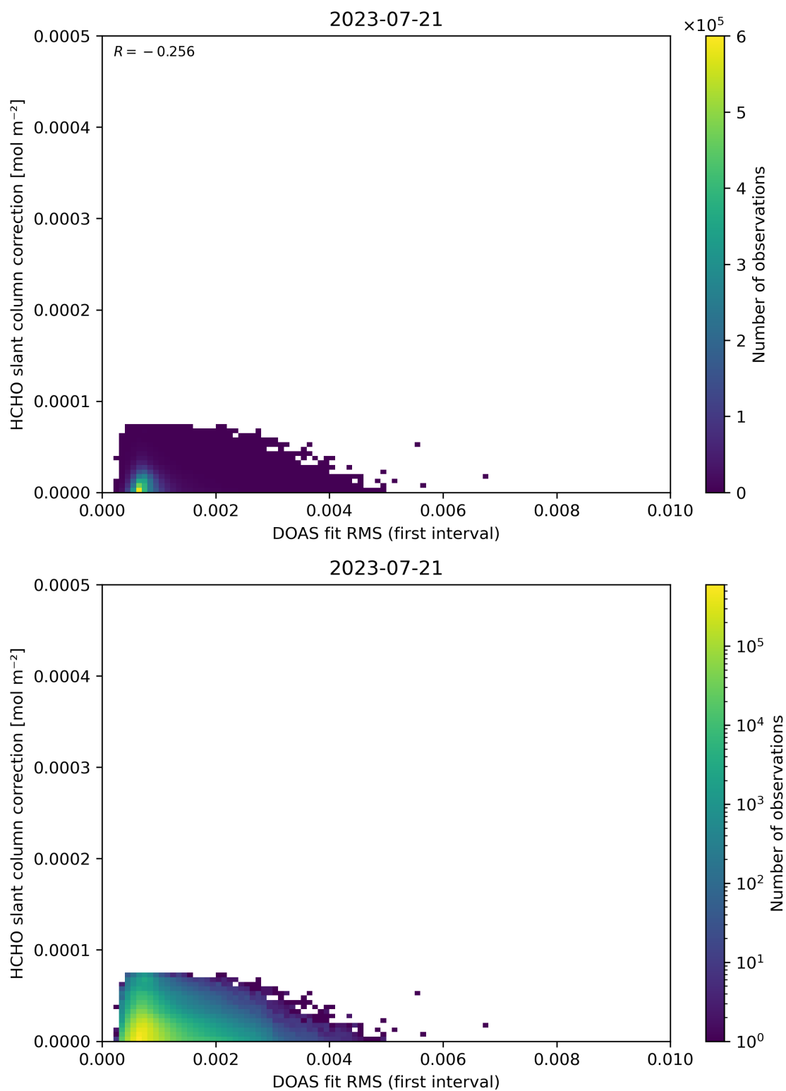
Figure 63: Scatter density plot of “DOAS fit RMS (first interval)” against “HCHO slant column correction” for 2023-07-20 to 2023-07-22.
