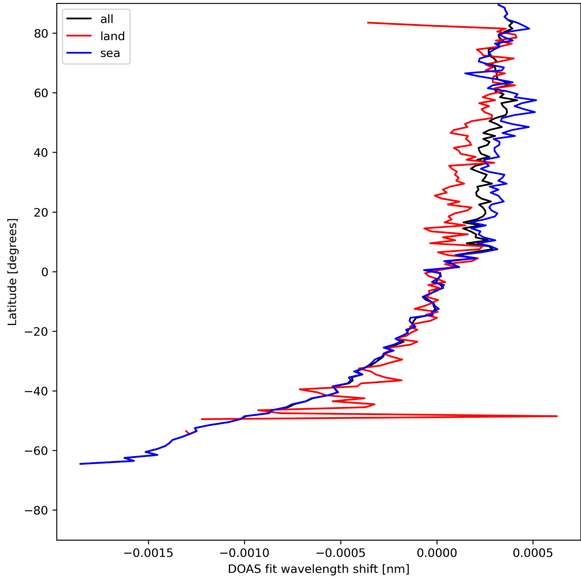
Figure 30: Zonal average of “DOAS fit wavelength shift” for 2023-07-20 to 2023-07-22.
