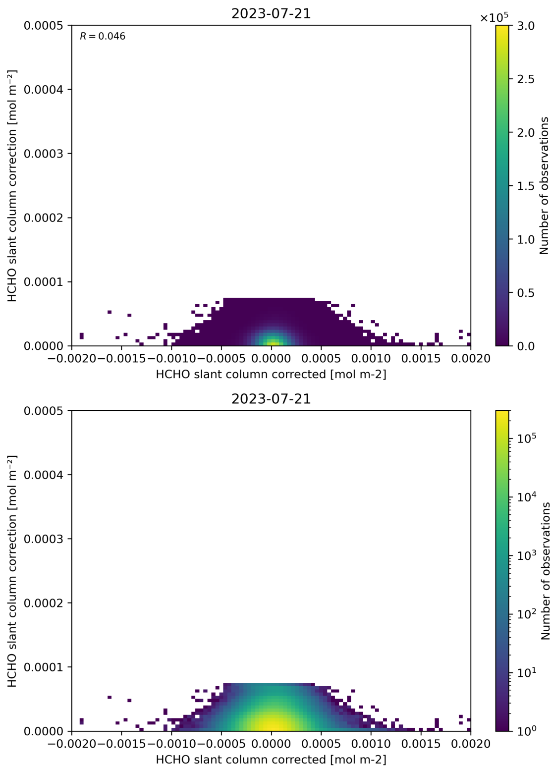
Figure 77: Scatter density plot of “HCHO slant column corrected” against “HCHO slant column correction” for 2023-07-20 to 2023-07-22.
