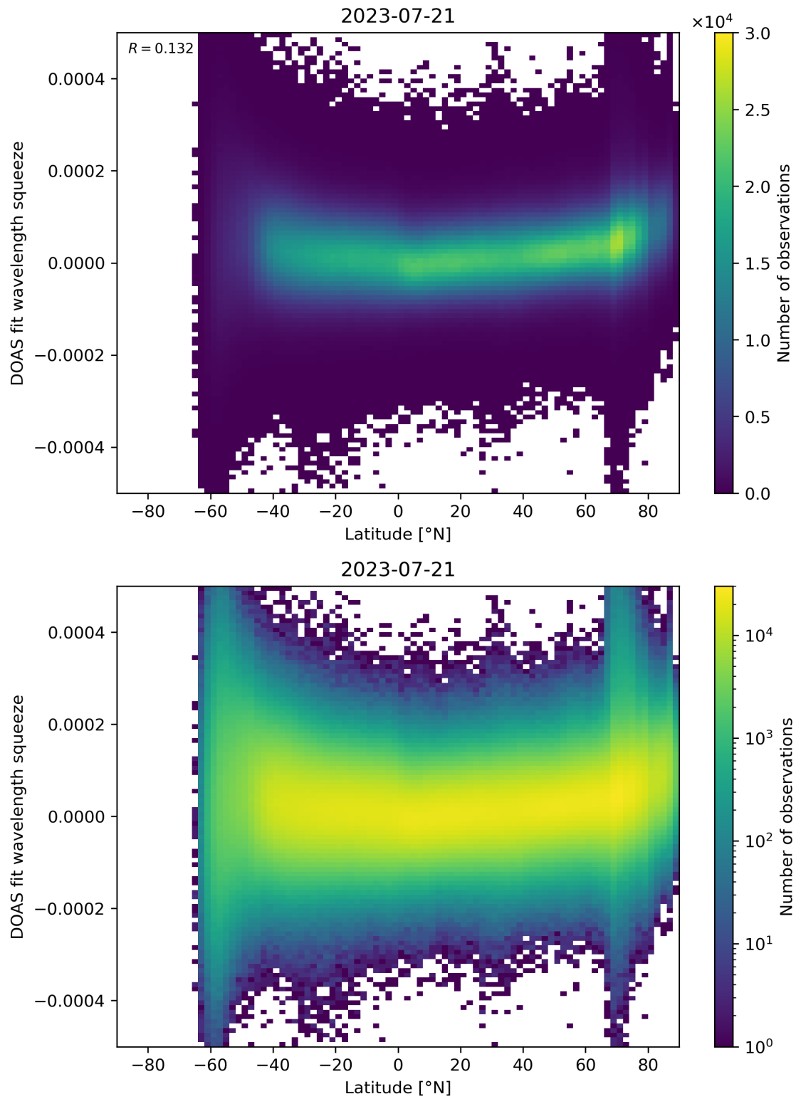
Figure 155: Scatter density plot of “Latitude” against “DOAS fit wavelength squeeze” for 2023-07-20 to 2023-07-22.
