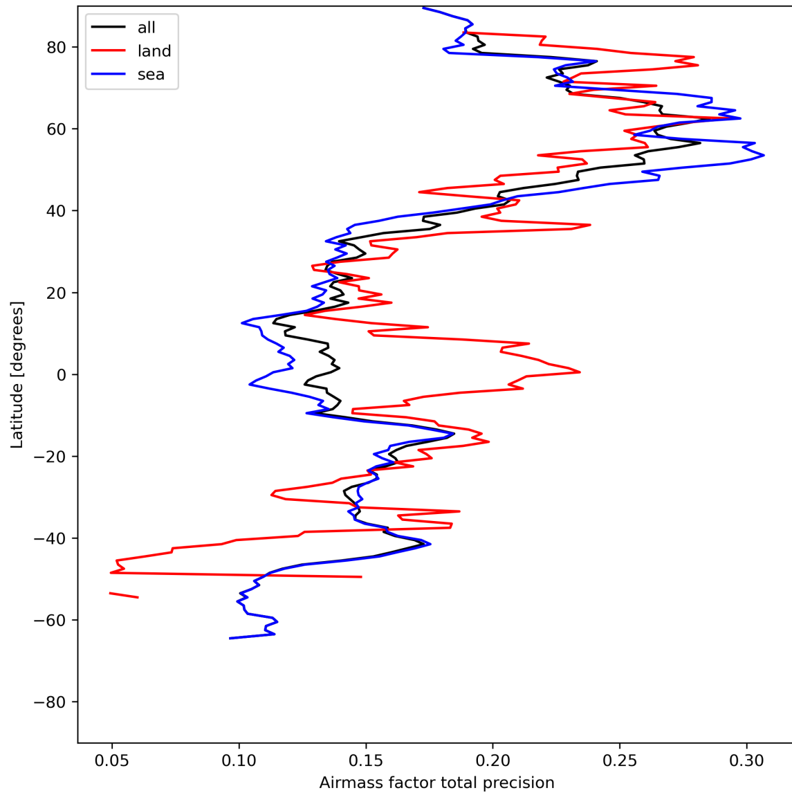
Figure 27: Zonal average of “Airmass factor total precision” for 2023-07-20 to 2023-07-22.
