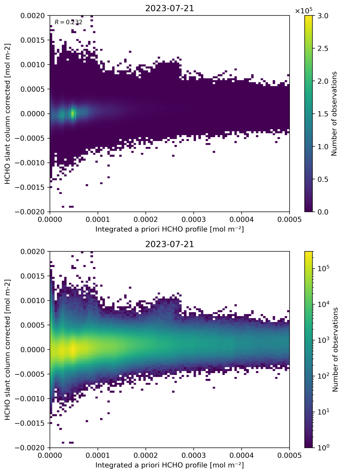
Figure 151: Scatter density plot of “Integrated a priori HCHO profile” against “HCHO slant column corrected” for 2023-07-20 to 2023-07-22.
