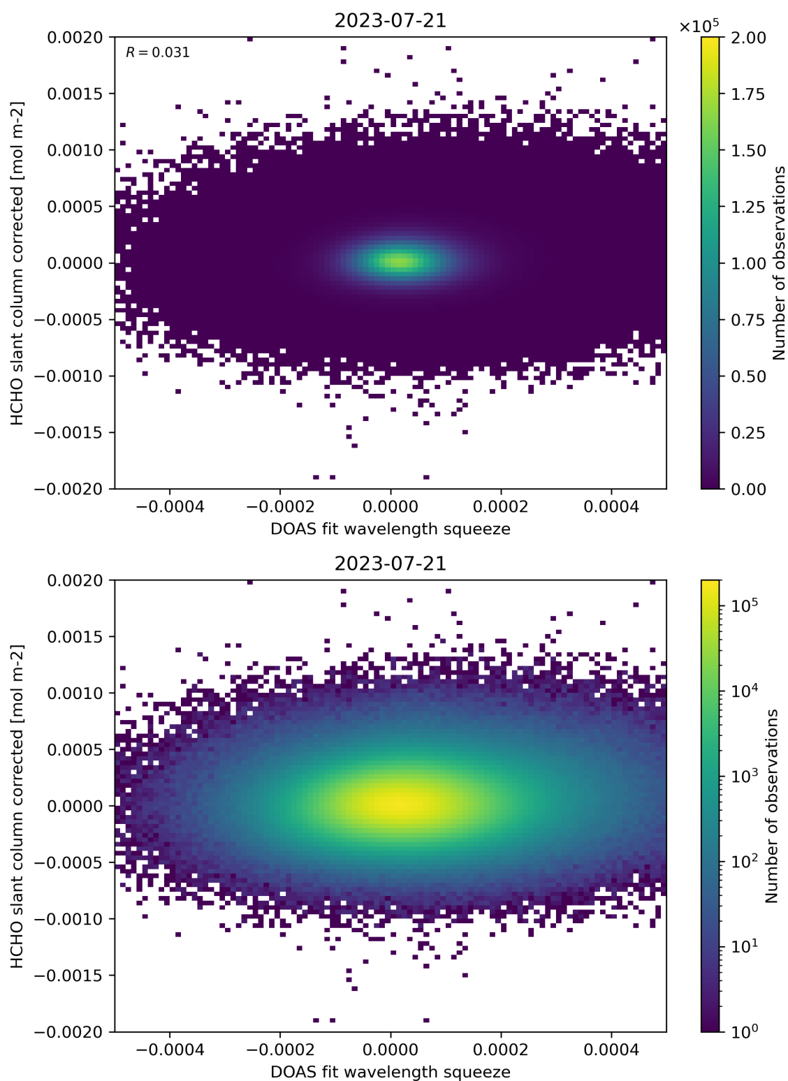
Figure 69: Scatter density plot of “DOAS fit wavelength squeeze” against “HCHO slant column corrected” for 2023-07-20 to 2023-07-22.
