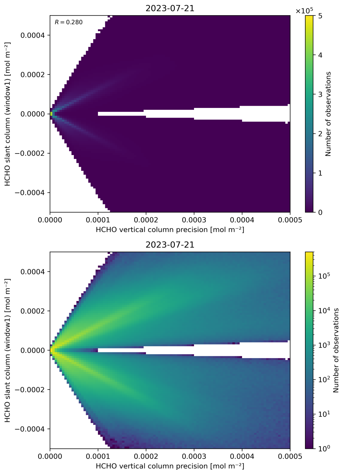
Figure 142: Scatter density plot of “HCHO vertical column precision” against “HCHO slant column (window1)” for 2023-07-20 to 2023-07-22.
