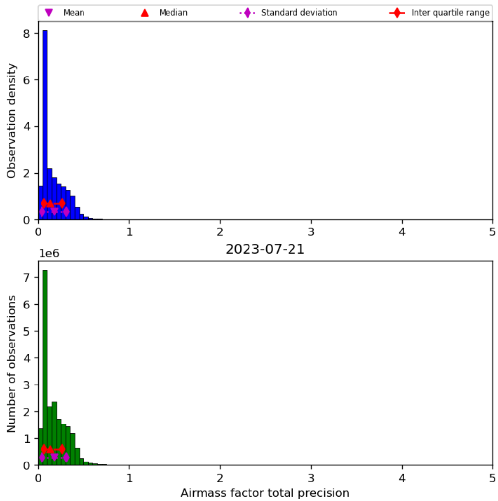
Figure 41: Histogram of “Airmass factor total precision” for 2023-07-20 to 2023-07-22
