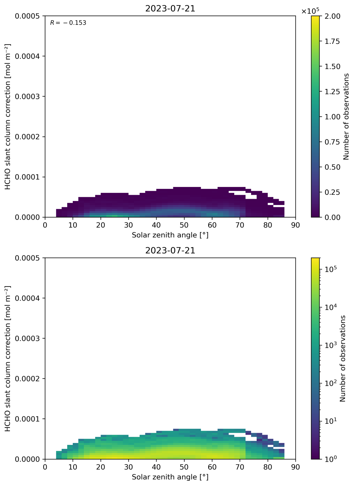
Figure 172: Scatter density plot of “Solar zenith angle” against “HCHO slant column correction” for 2023-07-20 to 2023-07-22.
