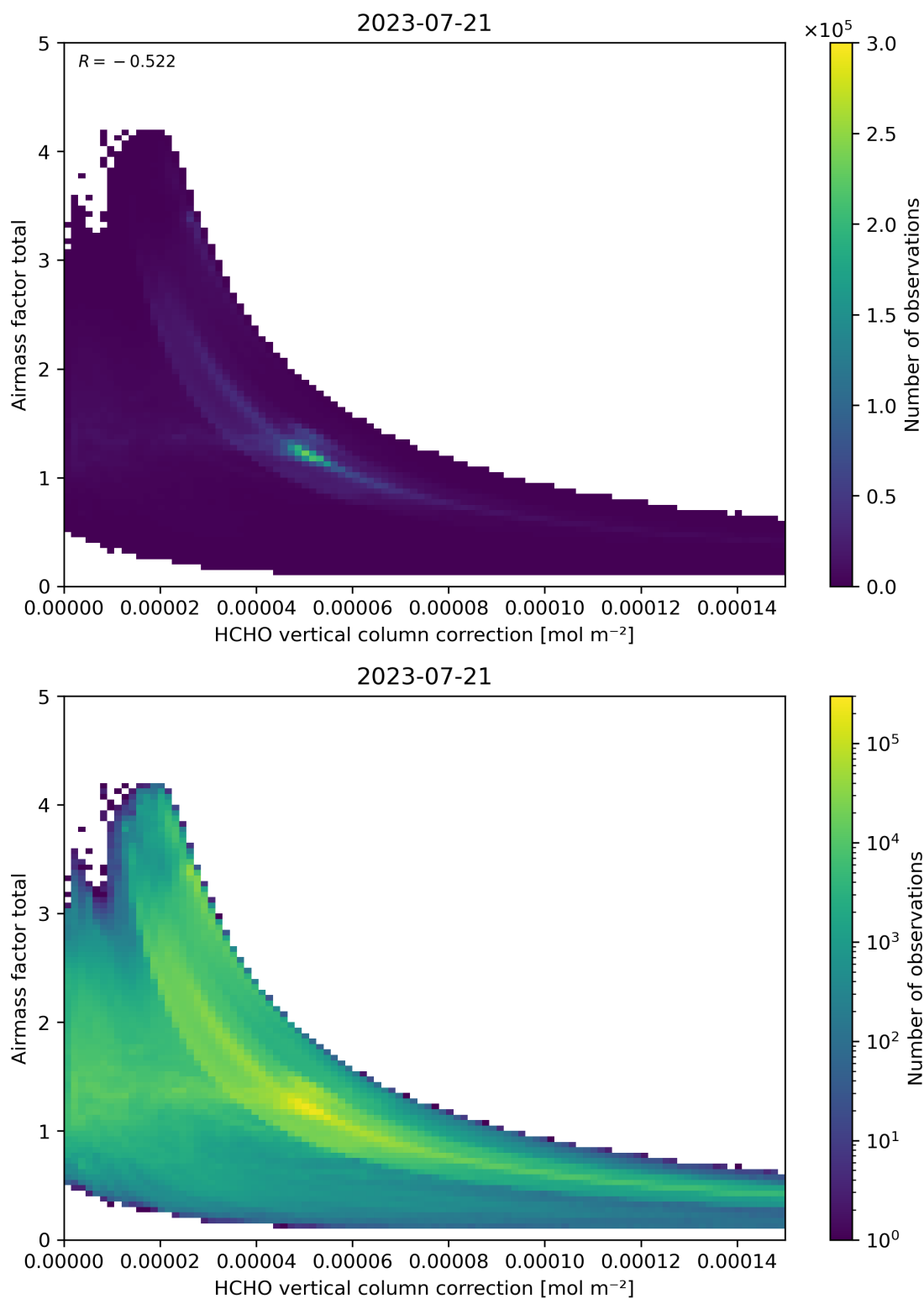
Figure 120: Scatter density plot of “HCHO vertical column correction” against “Airmass factor total” for 2023-07-20 to 2023-07-22.
