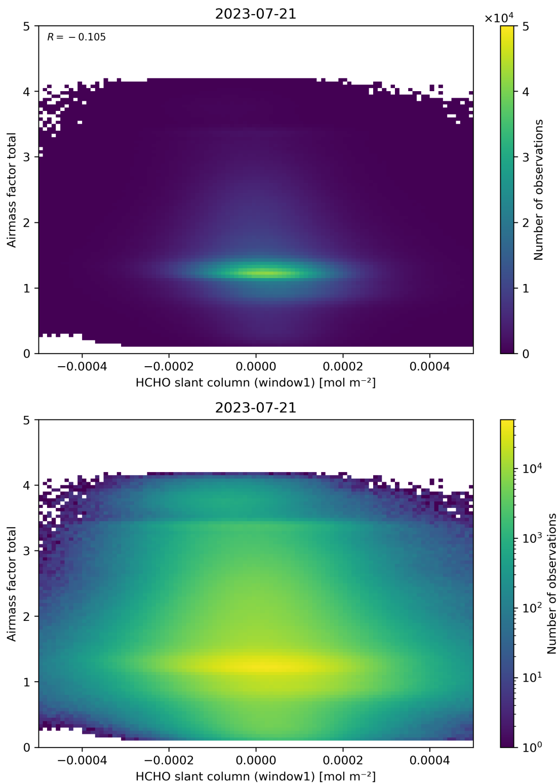
Figure 85: Scatter density plot of “HCHO slant column (window1)” against “Airmass factor total” for 2023-07-20 to 2023-07-22.
