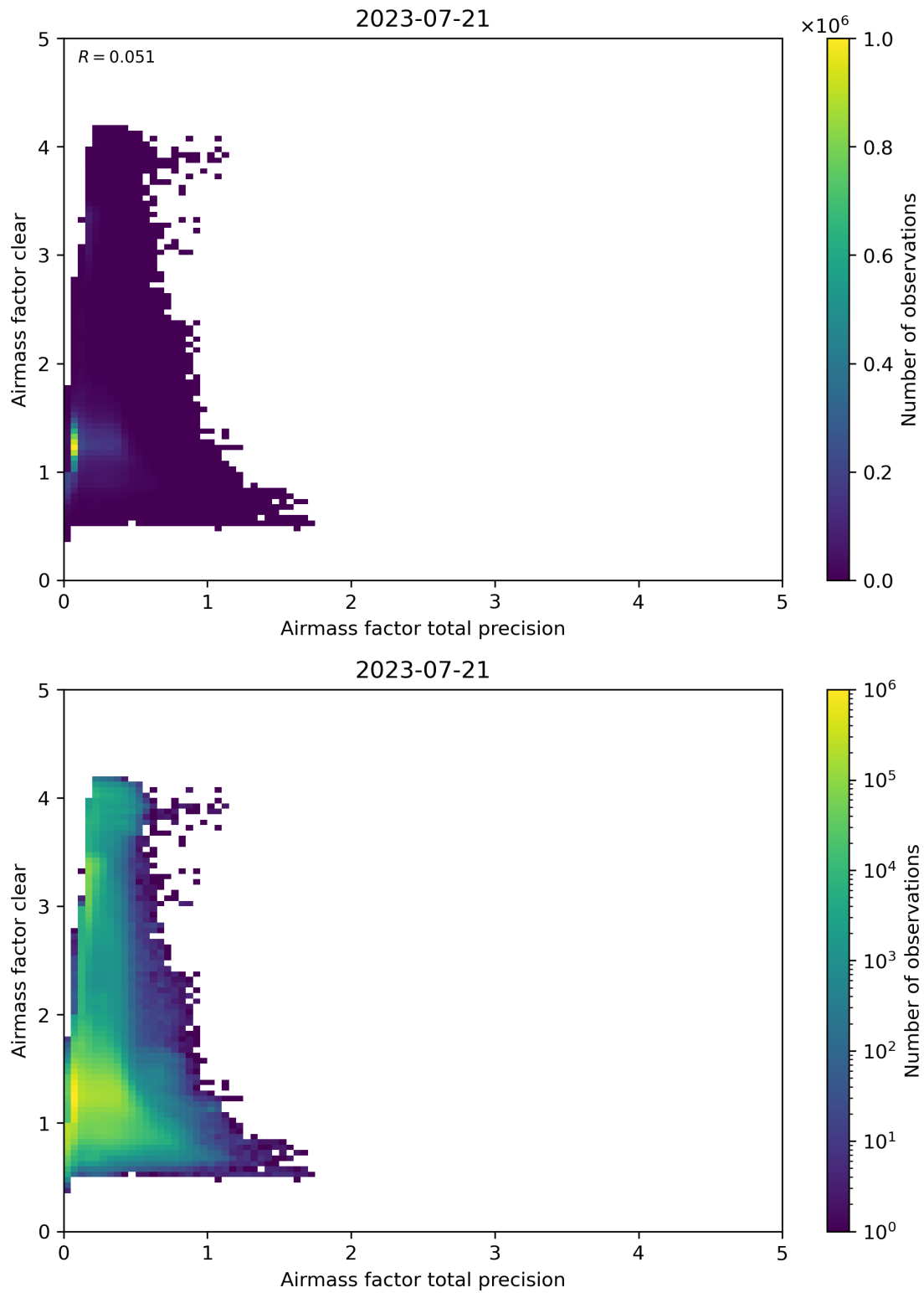
Figure 108: Scatter density plot of “Airmass factor total precision” against “Airmass factor clear” for 2023-07-20 to 2023-07-22.
