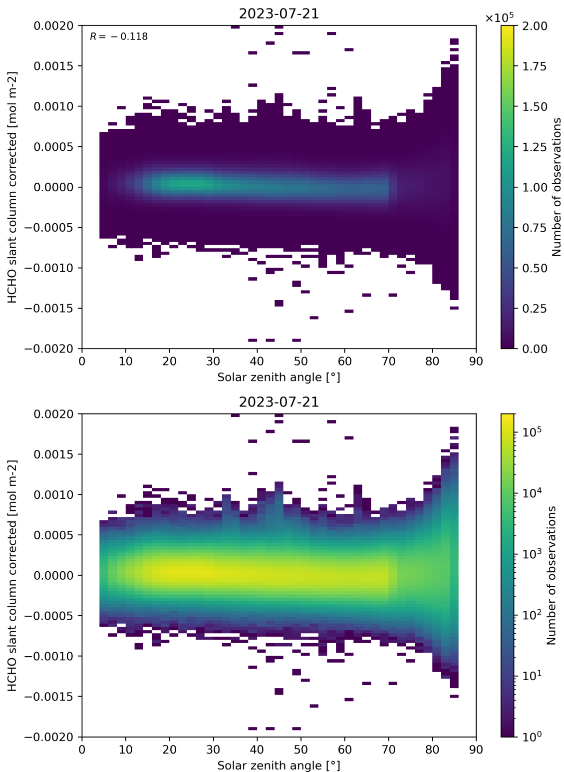
Figure 171: Scatter density plot of “Solar zenith angle” against “HCHO slant column corrected” for 2023-07-20 to 2023-07-22.
