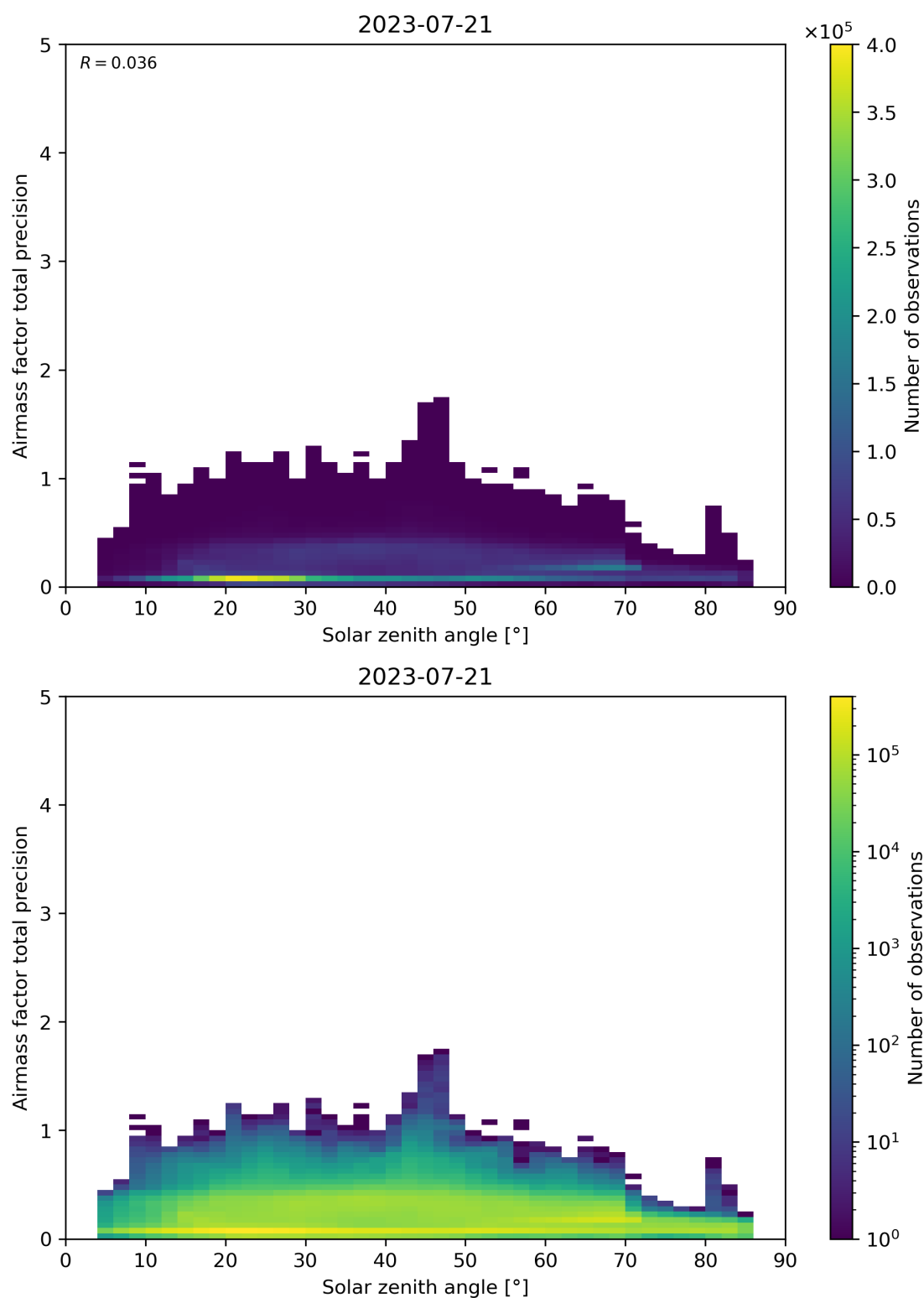
Figure 176: Scatter density plot of “Solar zenith angle” against “Airmass factor total precision” for 2023-07-20 to 2023-07-22.
