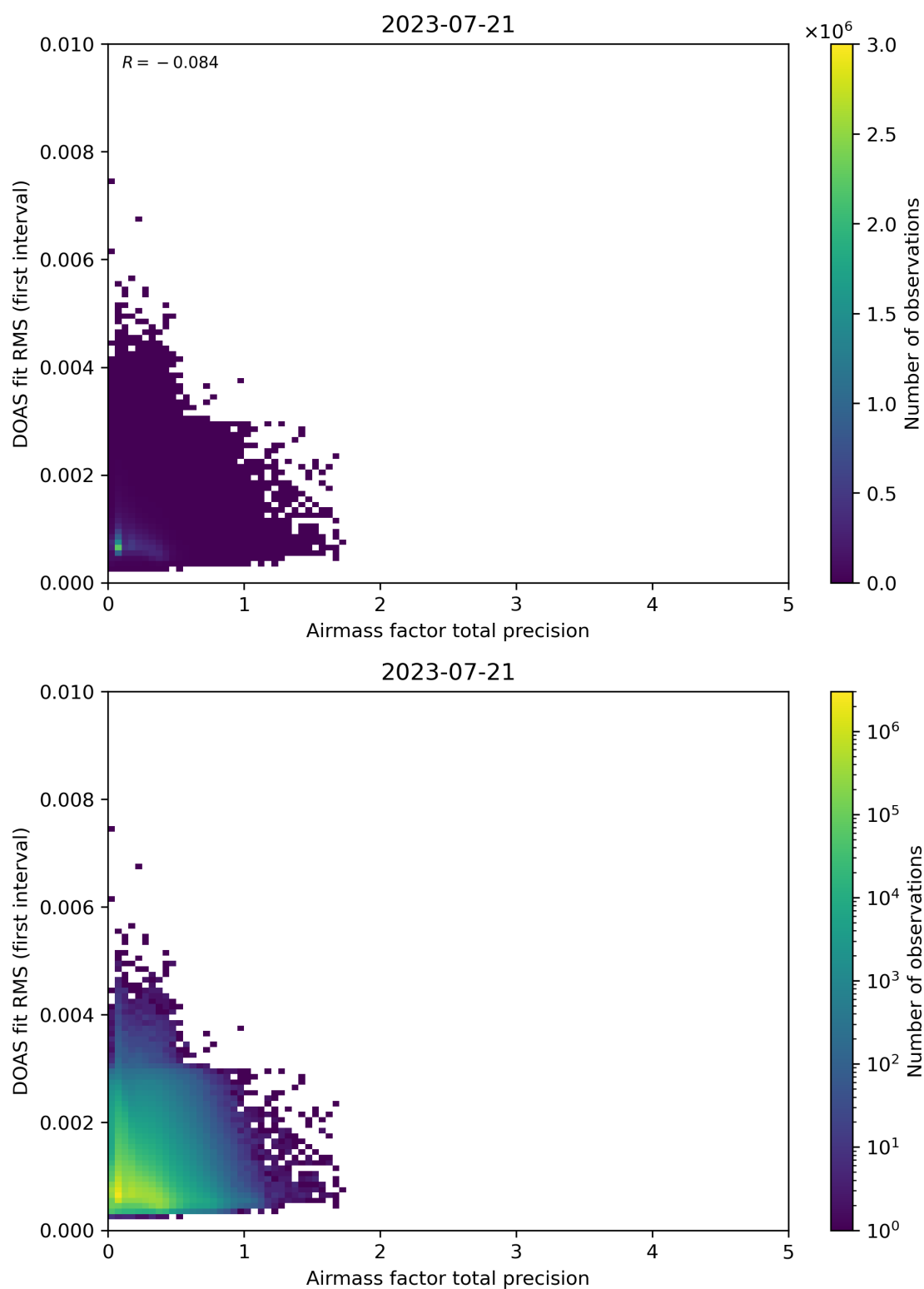
Figure 105: Scatter density plot of “Airmass factor total precision” against “DOAS fit RMS (first interval)” for 2023-07-20 to 2023-07-22.
