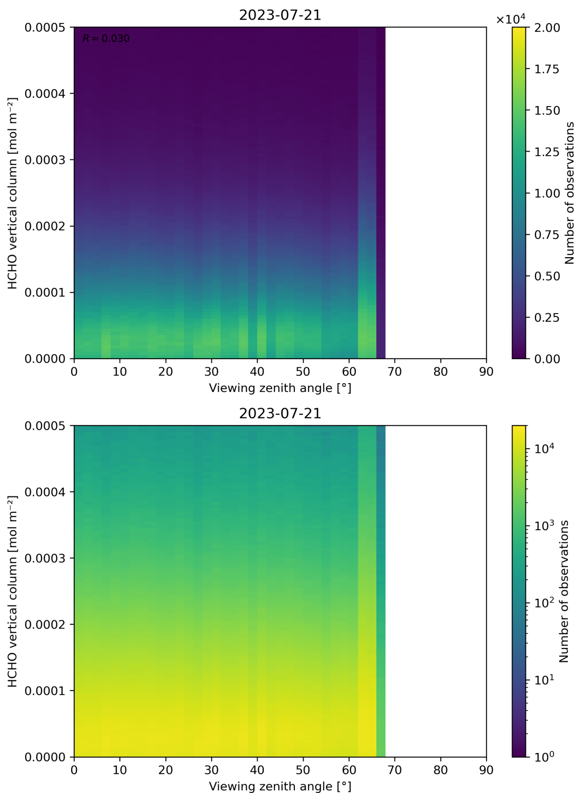
Figure 192: Scatter density plot of “Viewing zenith angle” against “HCHO vertical column” for 2023-07-20 to 2023-07-22.
