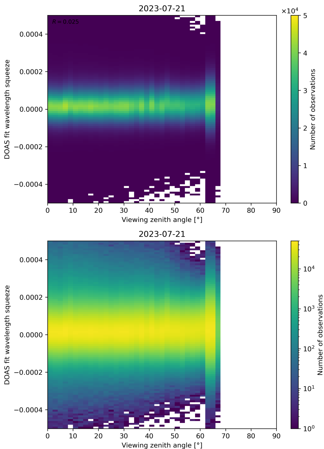
Figure 184: Scatter density plot of “Viewing zenith angle” against “DOAS fit wavelength squeeze” for 2023-07-20 to 2023-07-22.
