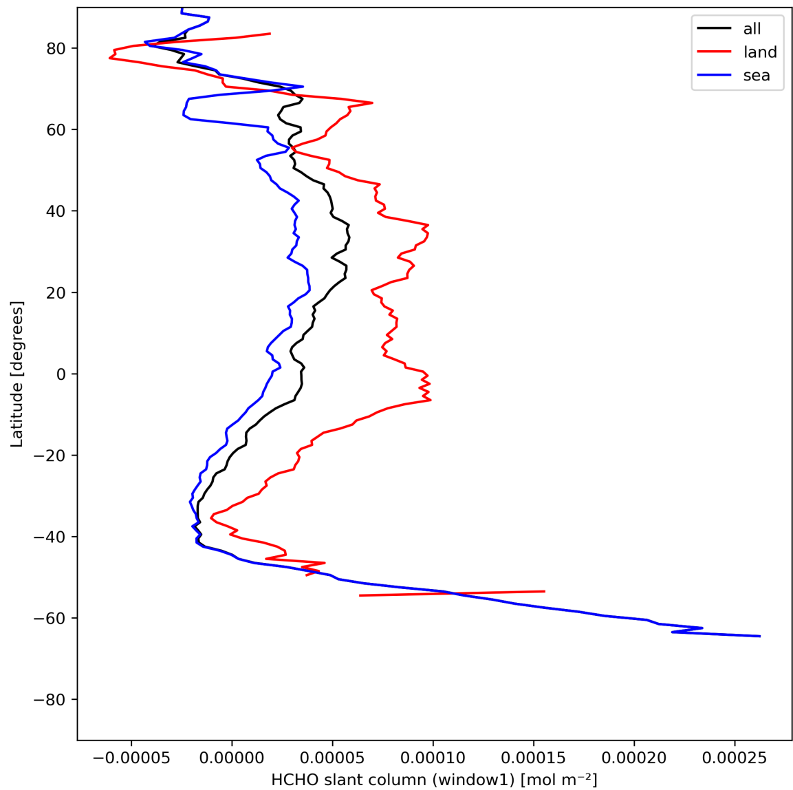
Figure 24: Zonal average of “HCHO slant column (window1)” for 2023-07-20 to 2023-07-22.
