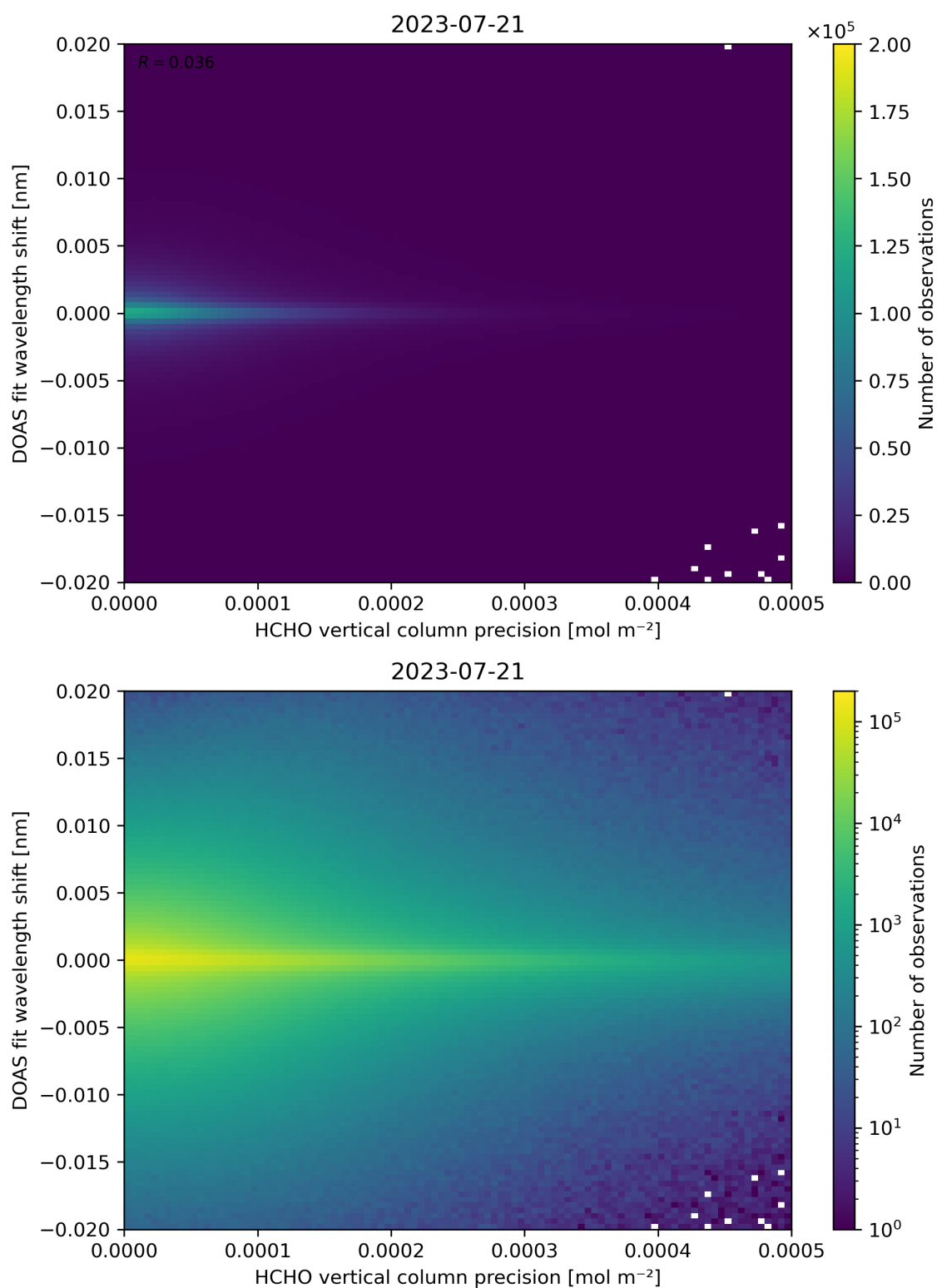
Figure 137: Scatter density plot of “HCHO vertical column precision” against “DOAS fit wavelength shift” for 2023-07-20 to 2023-07-22.
