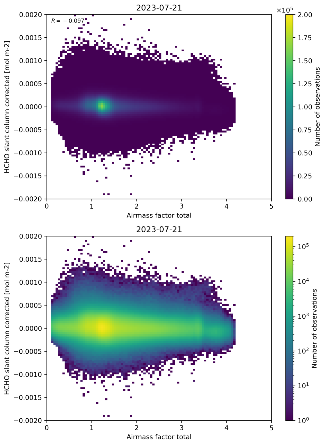
Figure 101: Scatter density plot of “Airmass factor total” against “HCHO slant column corrected” for 2023-07-20 to 2023-07-22.
