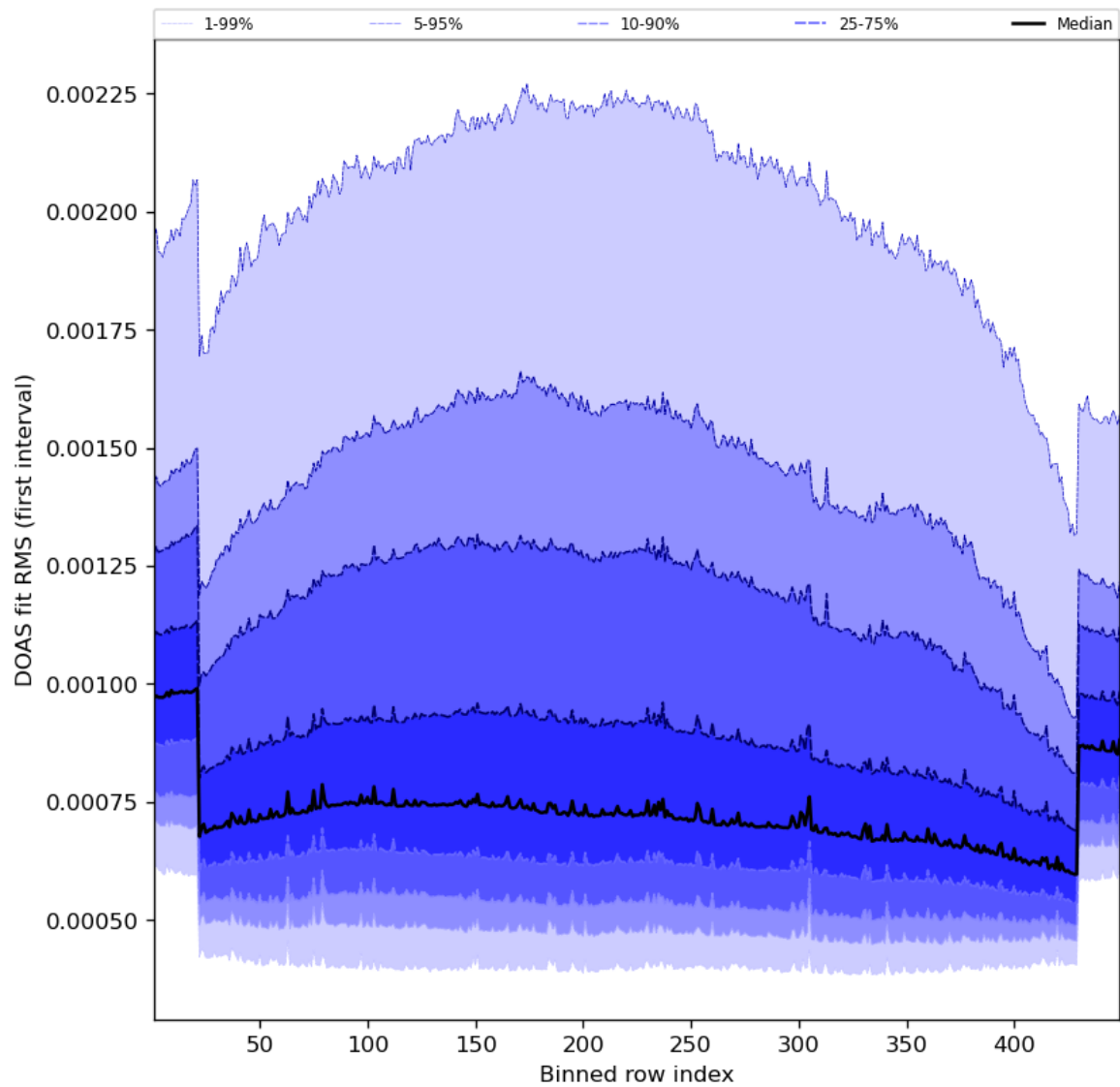
Figure 60: Along track statistics of “DOAS fit RMS (first interval)” for 2023-07-20 to 2023-07-22
