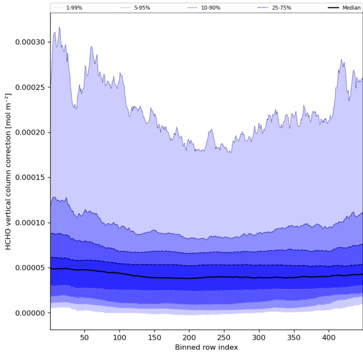
Figure 51: Along track statistics of “HCHO vertical column correction” for 2023-07-20 to 2023-07-22
