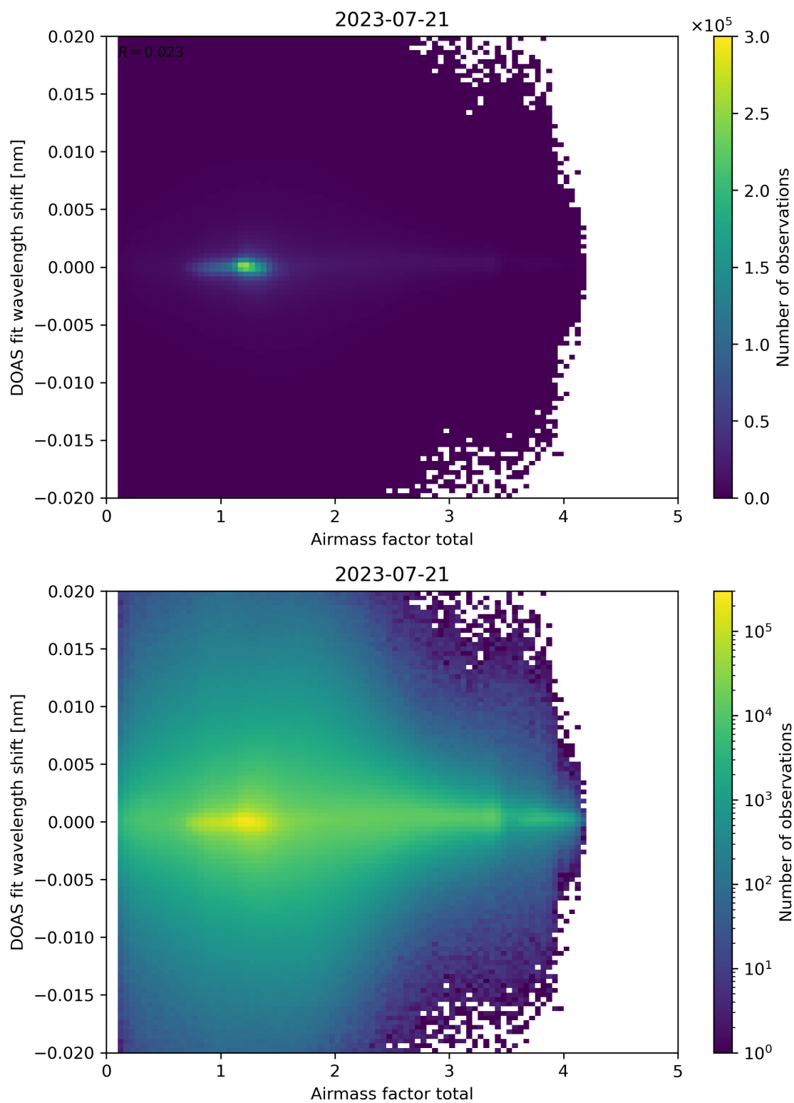
Figure 98: Scatter density plot of “Airmass factor total” against “DOAS fit wavelength shift” for 2023-07-20 to 2023-07-22.
