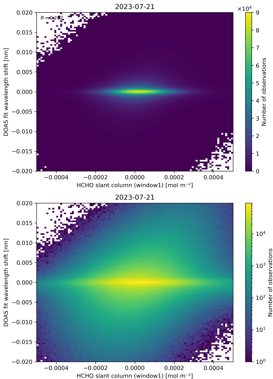
Figure 79: Scatter density plot of “HCHO slant column (window1)” against “DOAS fit wavelength shift” for 2023-07-20 to 2023-07-22.
