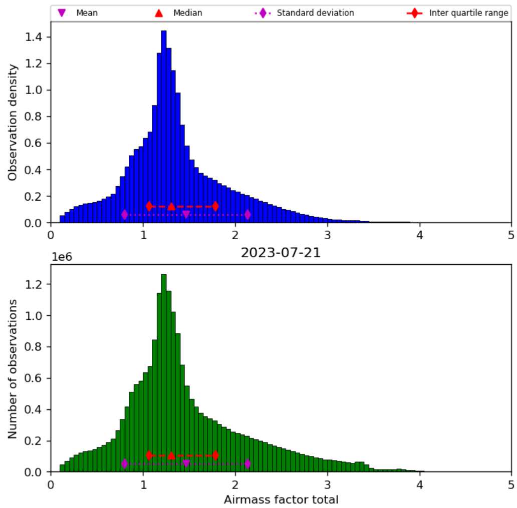
Figure 40: Histogram of “Airmass factor total” for 2023-07-20 to 2023-07-22
