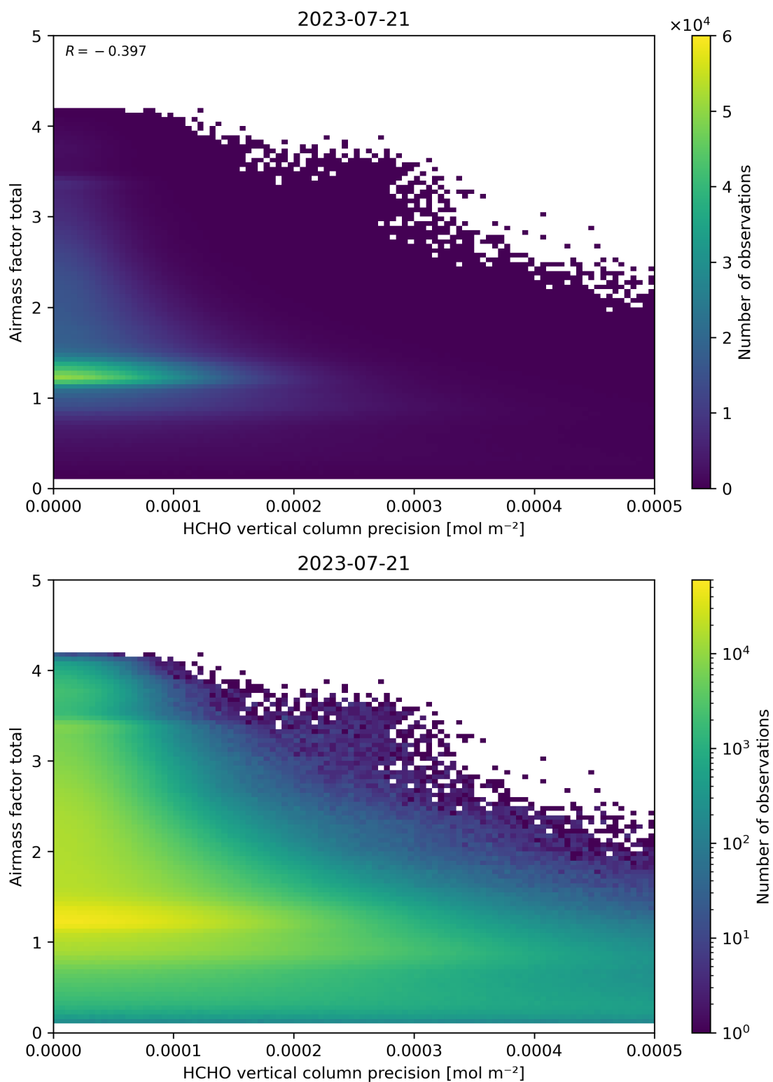
Figure 144: Scatter density plot of “HCHO vertical column precision” against “Airmass factor total” for 2023-07-20 to 2023-07-22.
