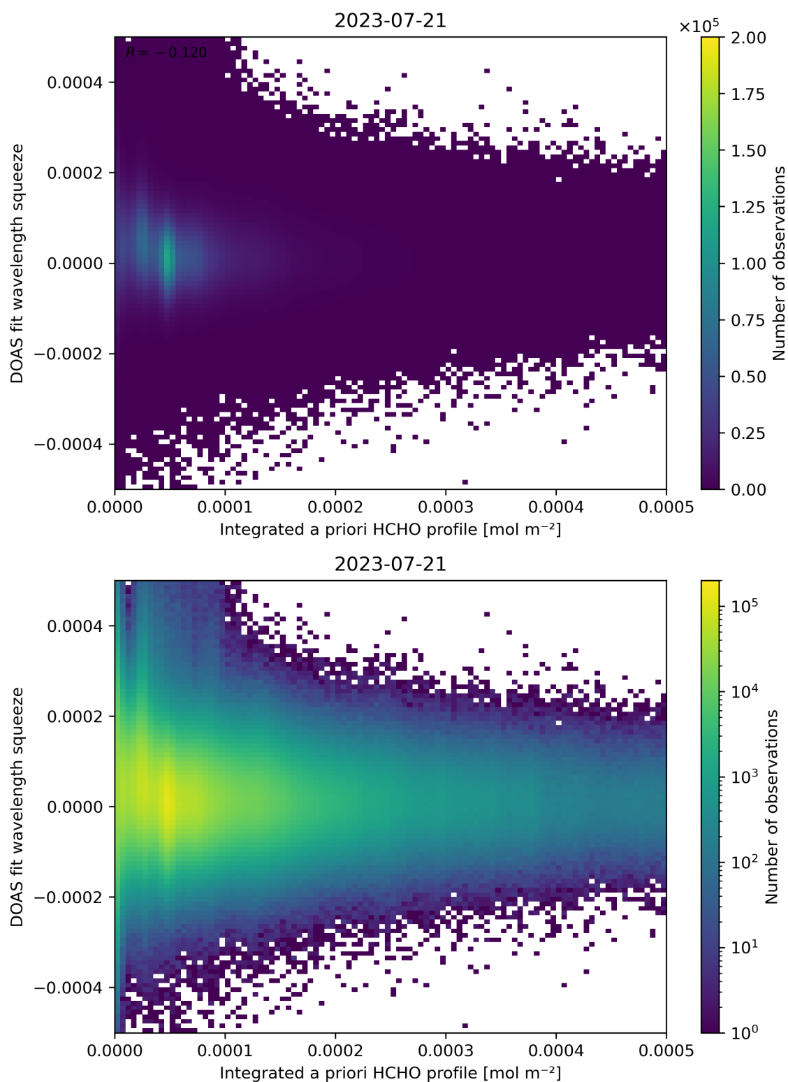
Figure 150: Scatter density plot of “Integrated a priori HCHO profile” against “DOAS fit wavelength squeeze” for 2023-07-20 to 2023-07-22.
