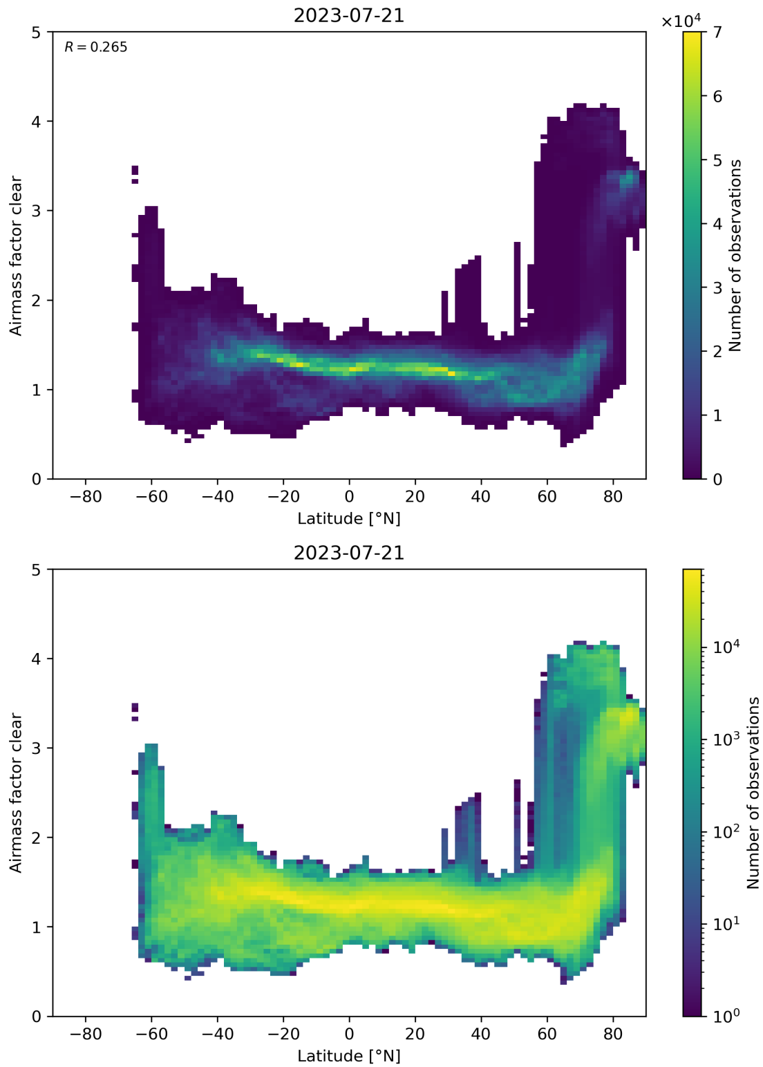
Figure 156: Scatter density plot of “Latitude” against “Airmass factor clear” for 2023-07-20 to 2023-07-22.
