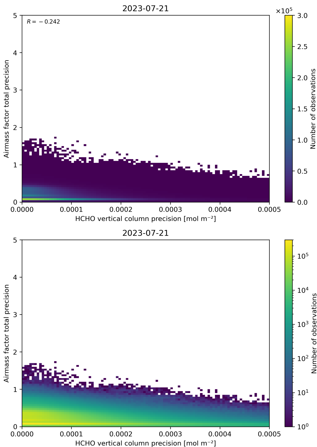
Figure 145: Scatter density plot of “HCHO vertical column precision” against “Airmass factor total precision” for 2023-07-20 to 2023-07-22.
