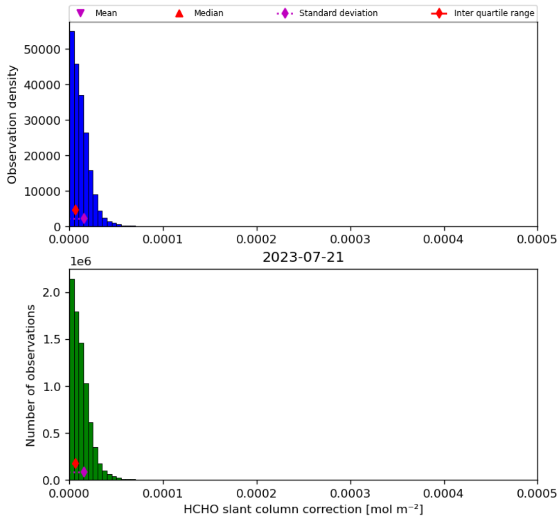
Figure 47: Histogram of “HCHO slant column correction” for 2023-07-20 to 2023-07-22
