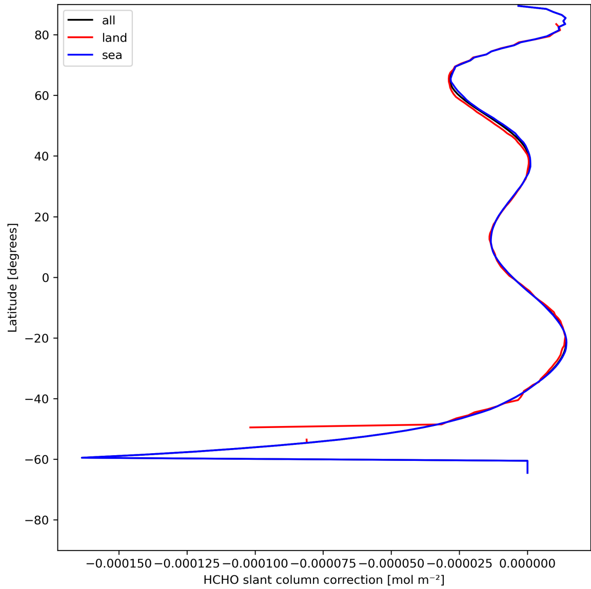
Figure 33: Zonal average of “HCHO slant column correction” for 2023-07-20 to 2023-07-22.
