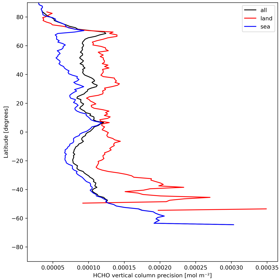
Figure 22: Zonal average of “HCHO vertical column precision” for 2023-07-20 to 2023-07-22.
