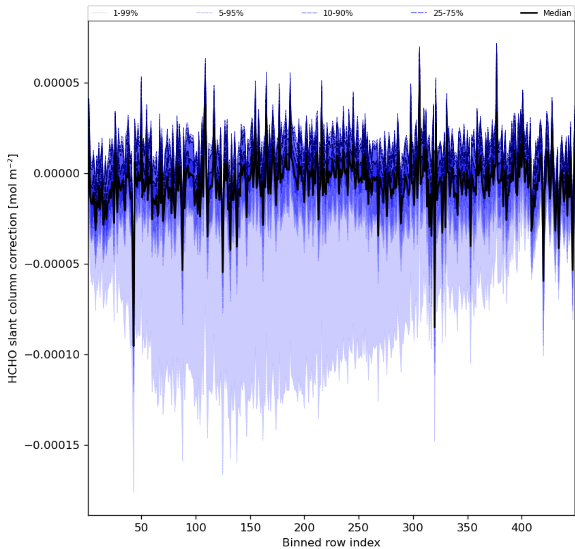
Figure 61: Along track statistics of “HCHO slant column correction” for 2023-07-20 to 2023-07-22
