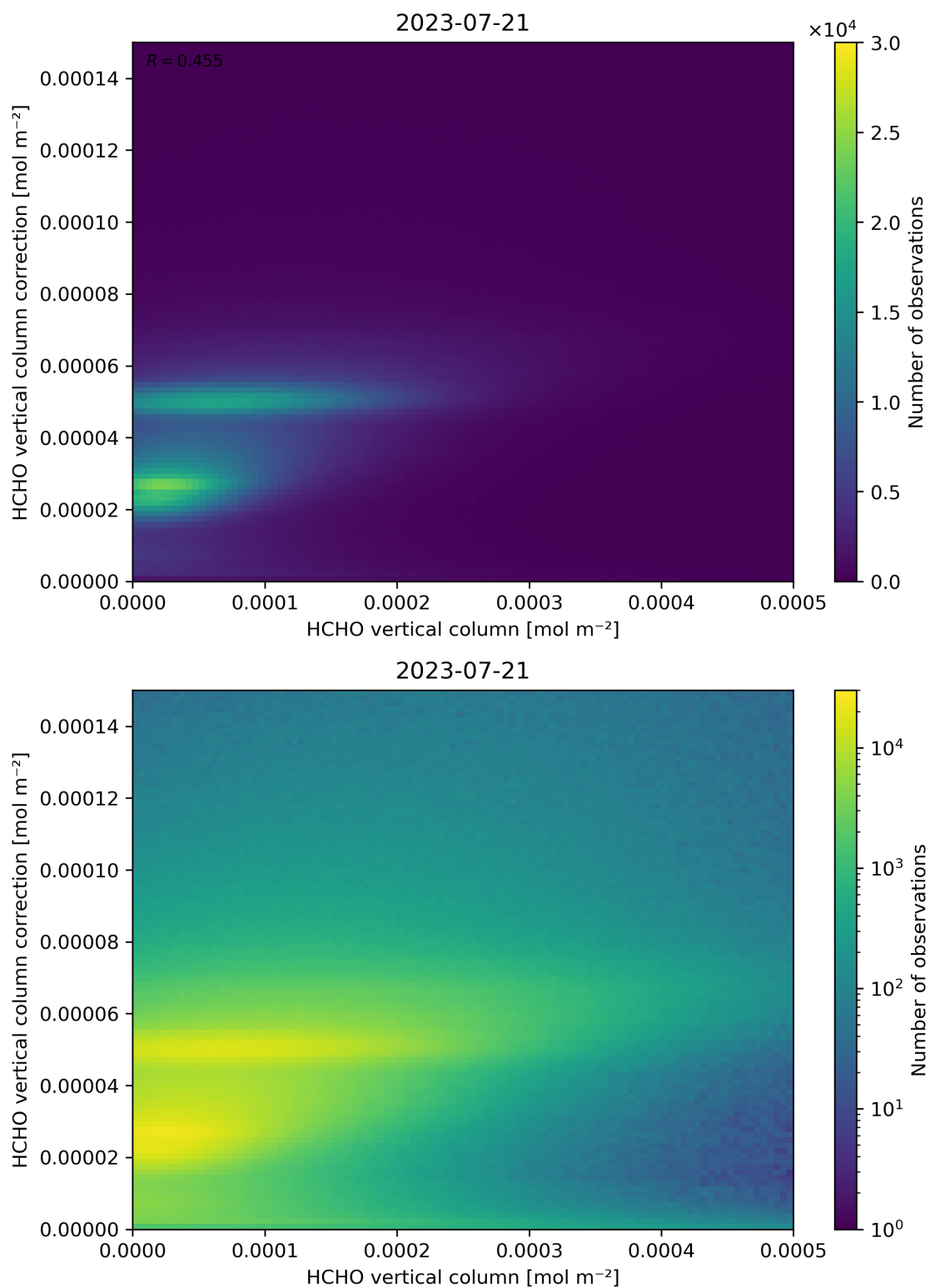
Figure 133: Scatter density plot of “HCHO vertical column” against “HCHO vertical column correction” for 2023-07-20 to 2023-07-22.
