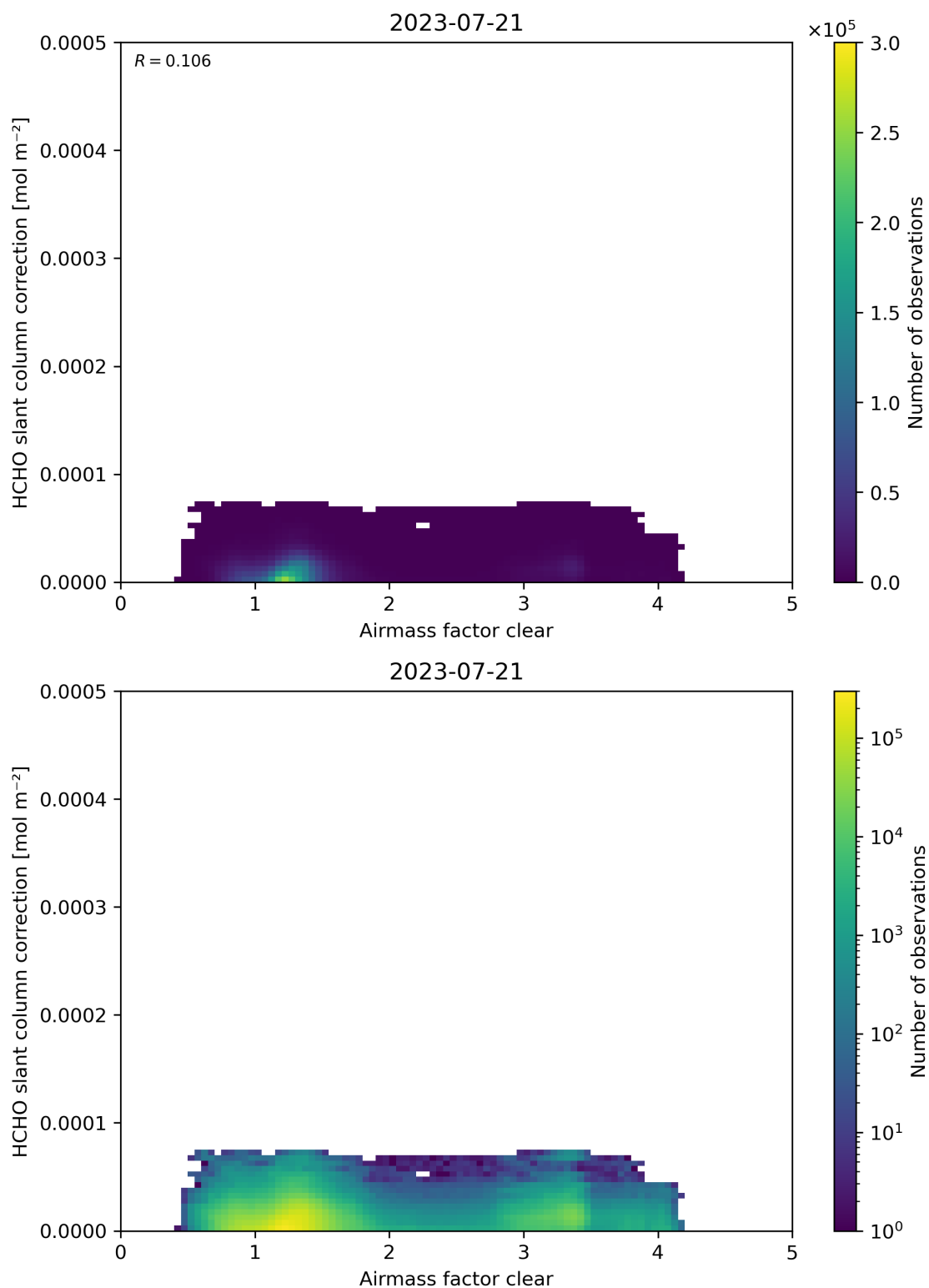
Figure 75: Scatter density plot of “Airmass factor clear” against “HCHO slant column correction” for 2023-07-20 to 2023-07-22.
