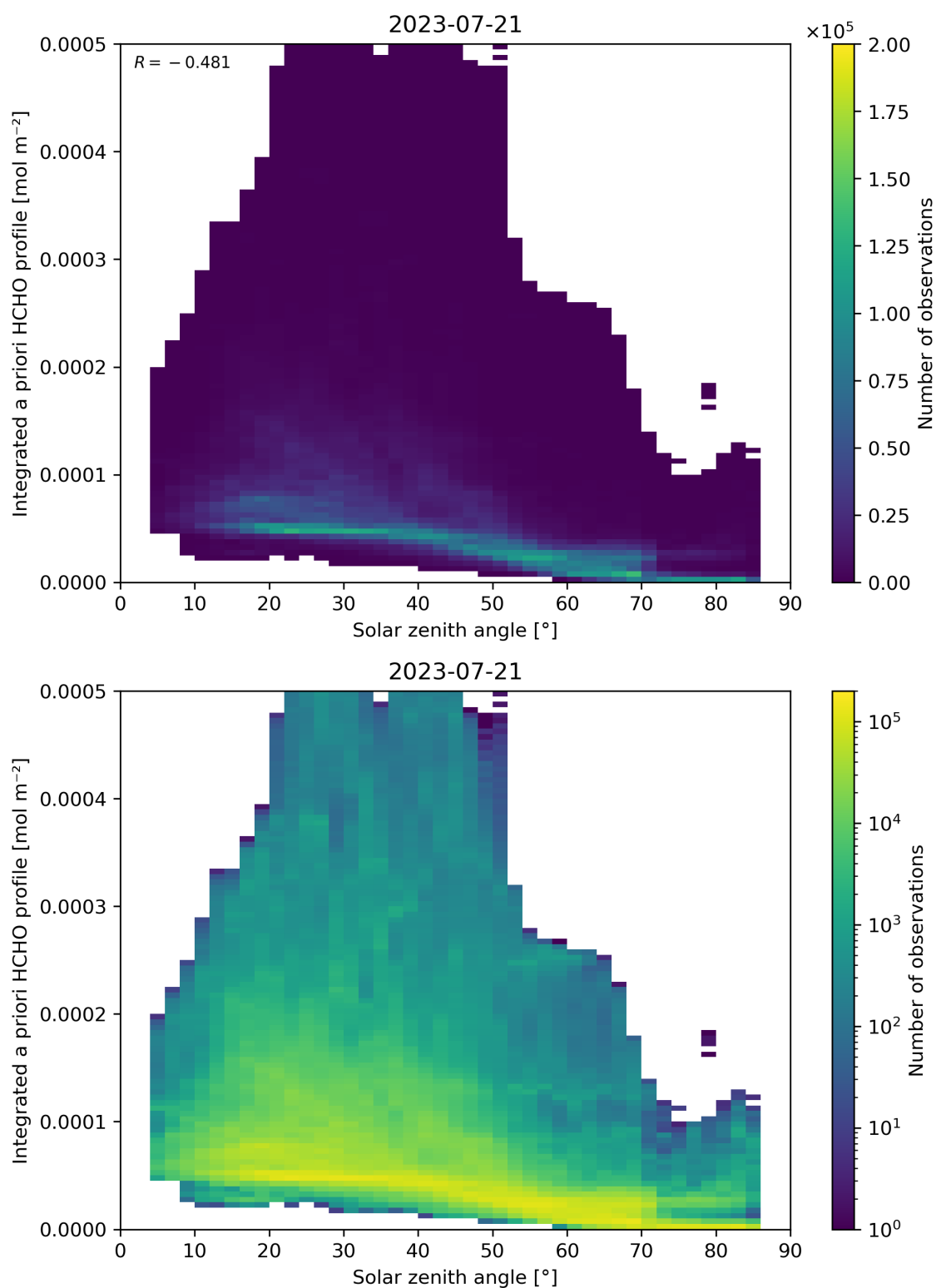
Figure 180: Scatter density plot of “Solar zenith angle” against “Integrated a priori HCHO profile” for 2023-07-20 to 2023-07-22.
