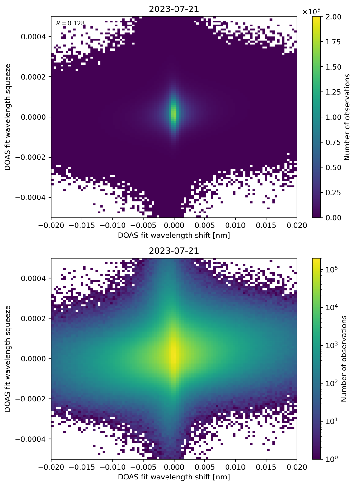
Figure 65: Scatter density plot of “DOAS fit wavelength shift” against “DOAS fit wavelength squeeze” for 2023-07-20 to 2023-07-22.
