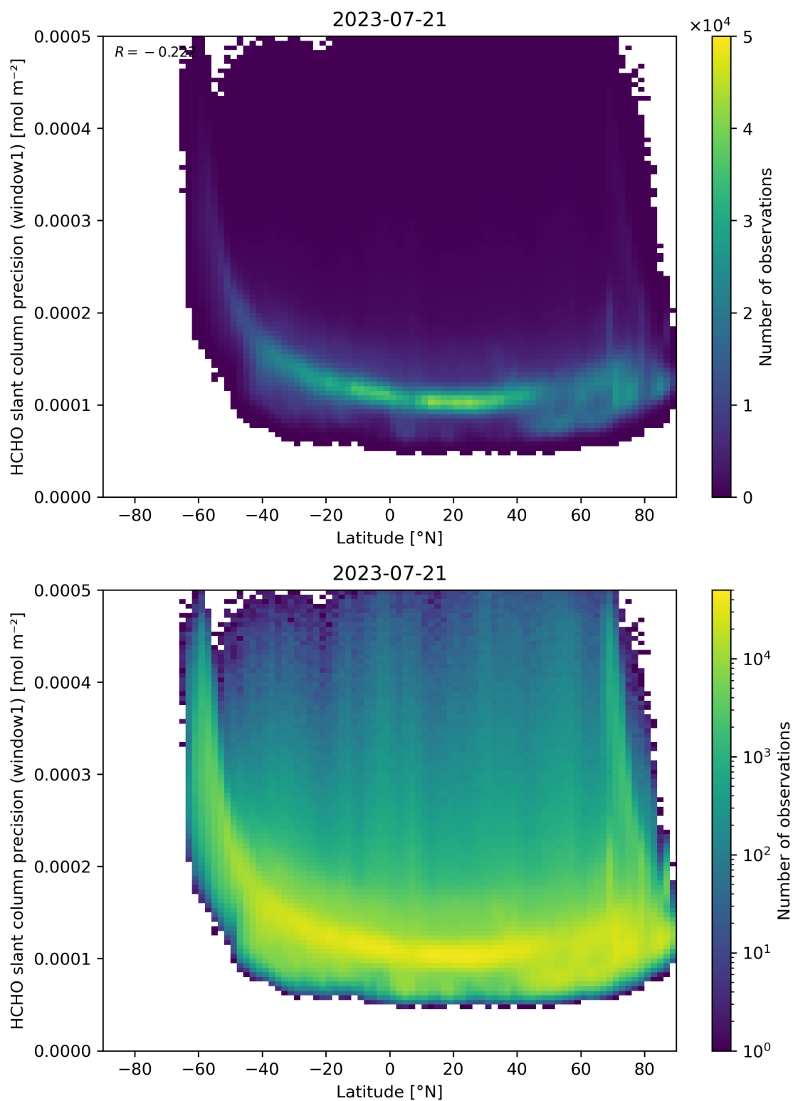
Figure 160: Scatter density plot of “Latitude” against “HCHO slant column precision (window1)” for 2023-07-20 to 2023-07-22.
