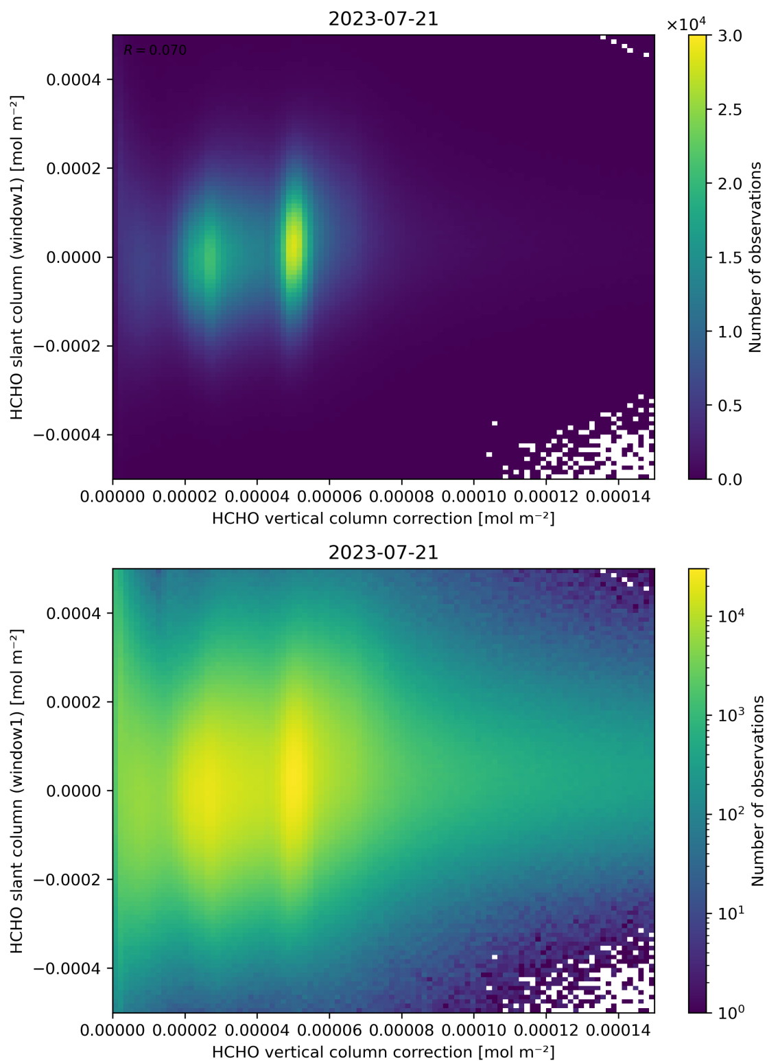
Figure 118: Scatter density plot of “HCHO vertical column correction” against “HCHO slant column (window1)” for 2023-07-20 to 2023-07-22.
