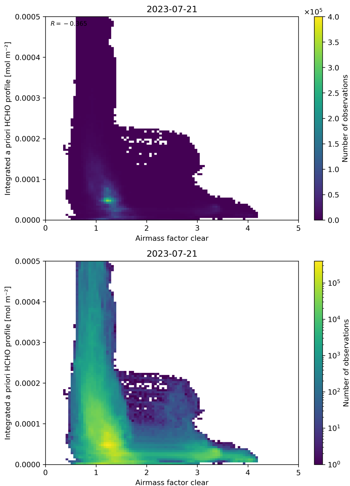
Figure 76: Scatter density plot of “Airmass factor clear” against “Integrated a priori HCHO profile” for 2023-07-20 to 2023-07-22.
