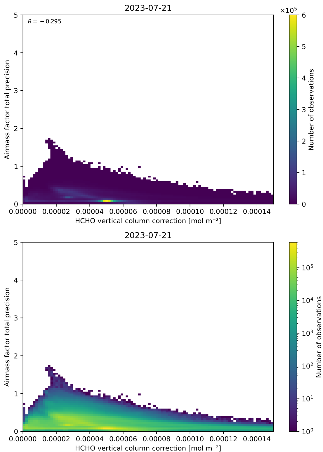
Figure 121: Scatter density plot of “HCHO vertical column correction” against “Airmass factor total precision” for 2023-07-20 to 2023-07-22.
