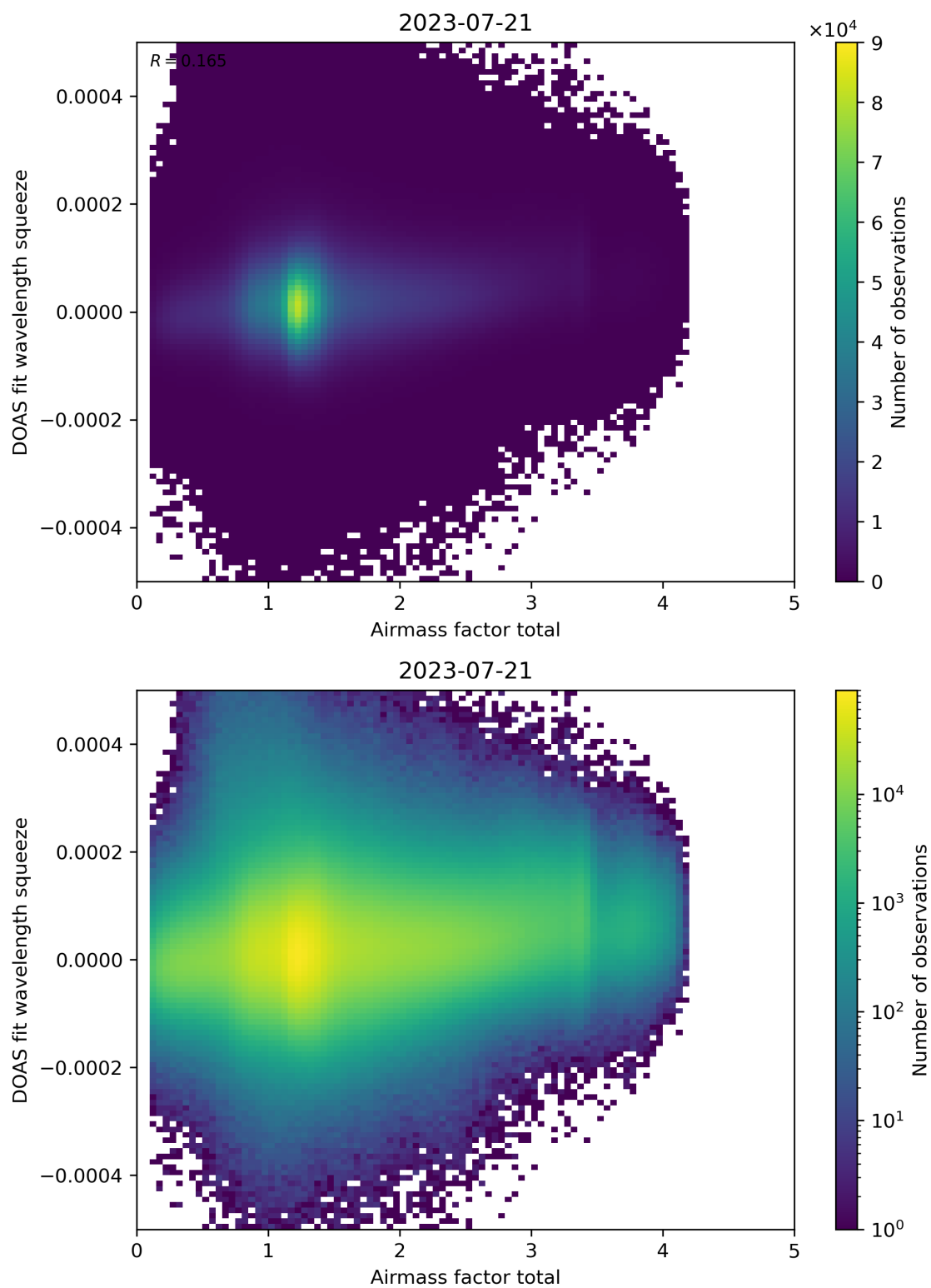
Figure 99: Scatter density plot of “Airmass factor total” against “DOAS fit wavelength squeeze” for 2023-07-20 to 2023-07-22.
