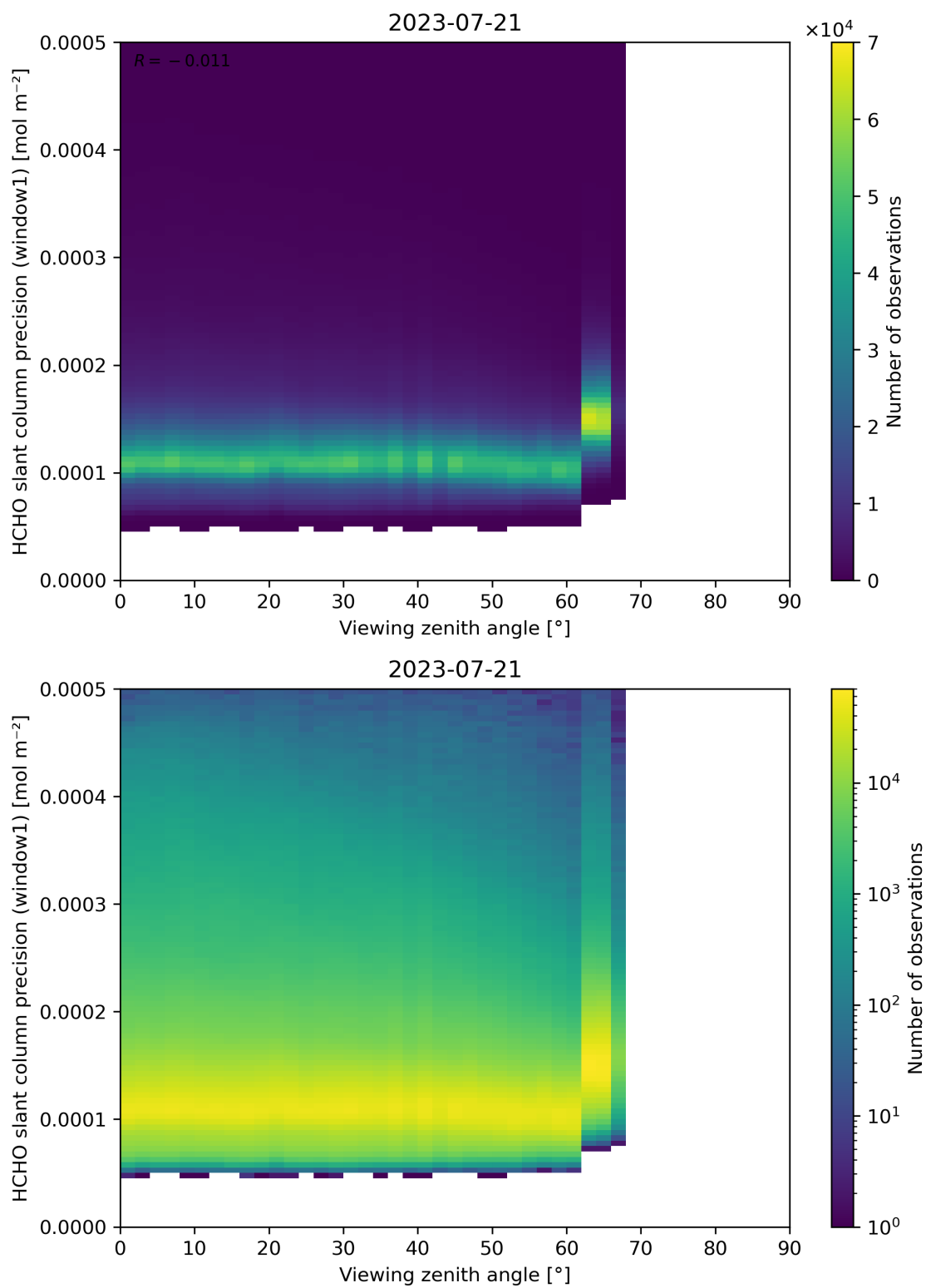
Figure 189: Scatter density plot of “Viewing zenith angle” against “HCHO slant column precision (window1)” for 2023-07-20 to 2023-07-22.
