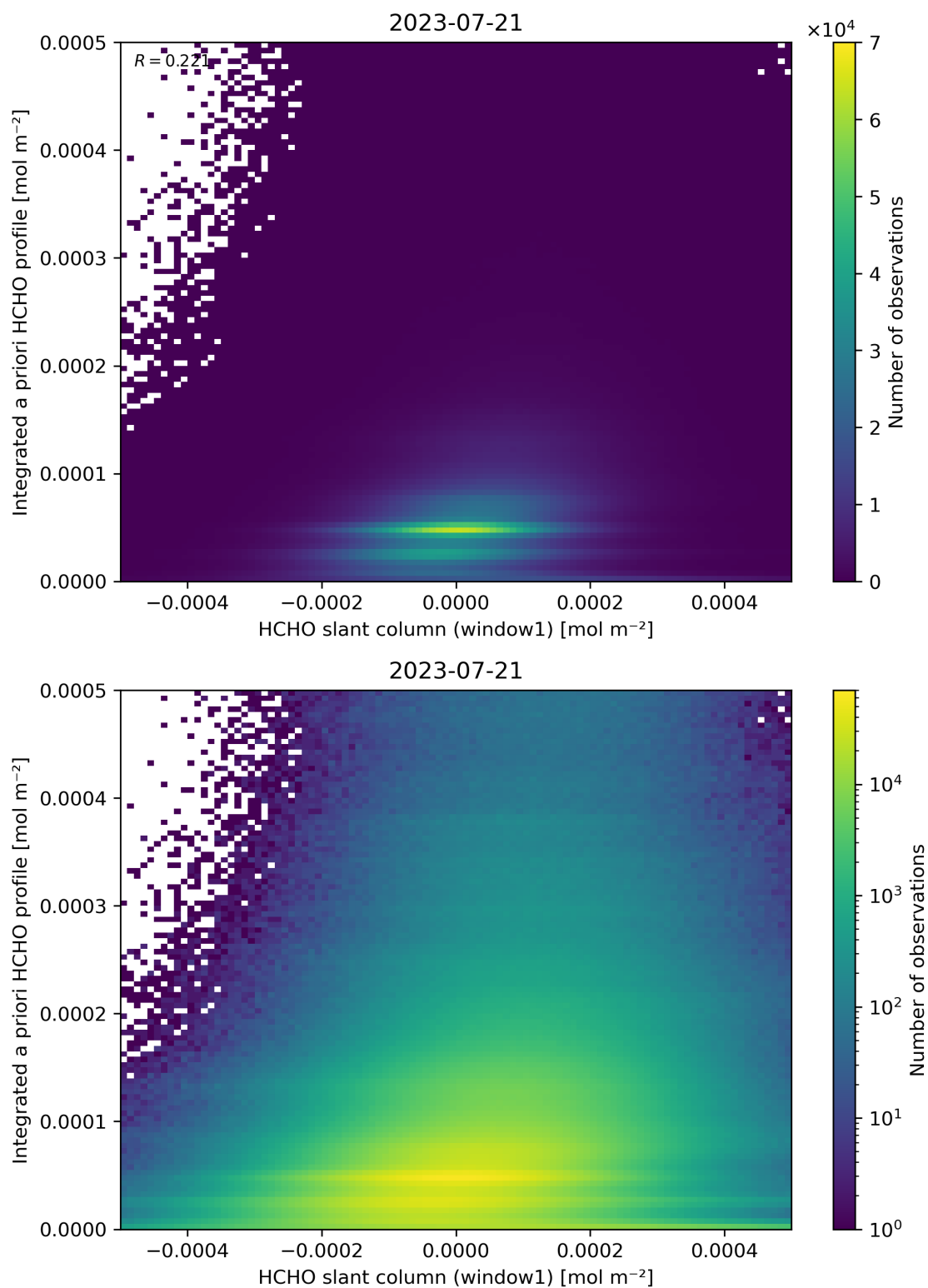
Figure 87: Scatter density plot of “HCHO slant column (window1)” against “Integrated a priori HCHO profile” for 2023-07-20 to 2023-07-22.
