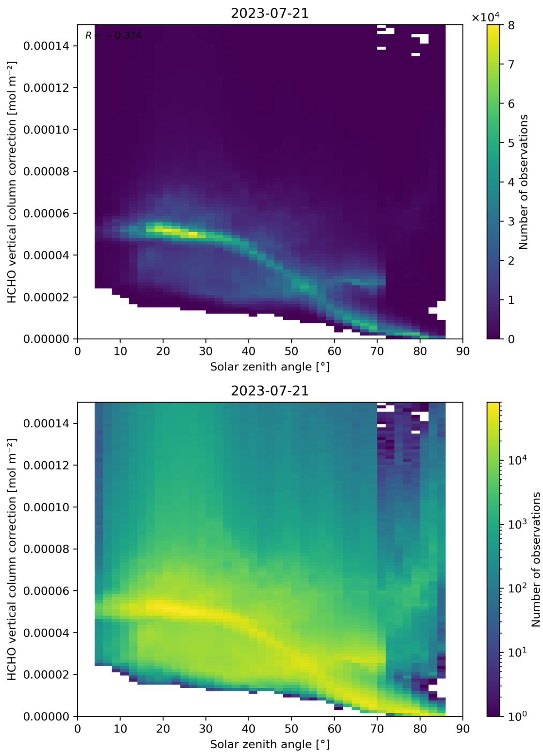
Figure 178: Scatter density plot of “Solar zenith angle” against “HCHO vertical column correction” for 2023-07-20 to 2023-07-22.
