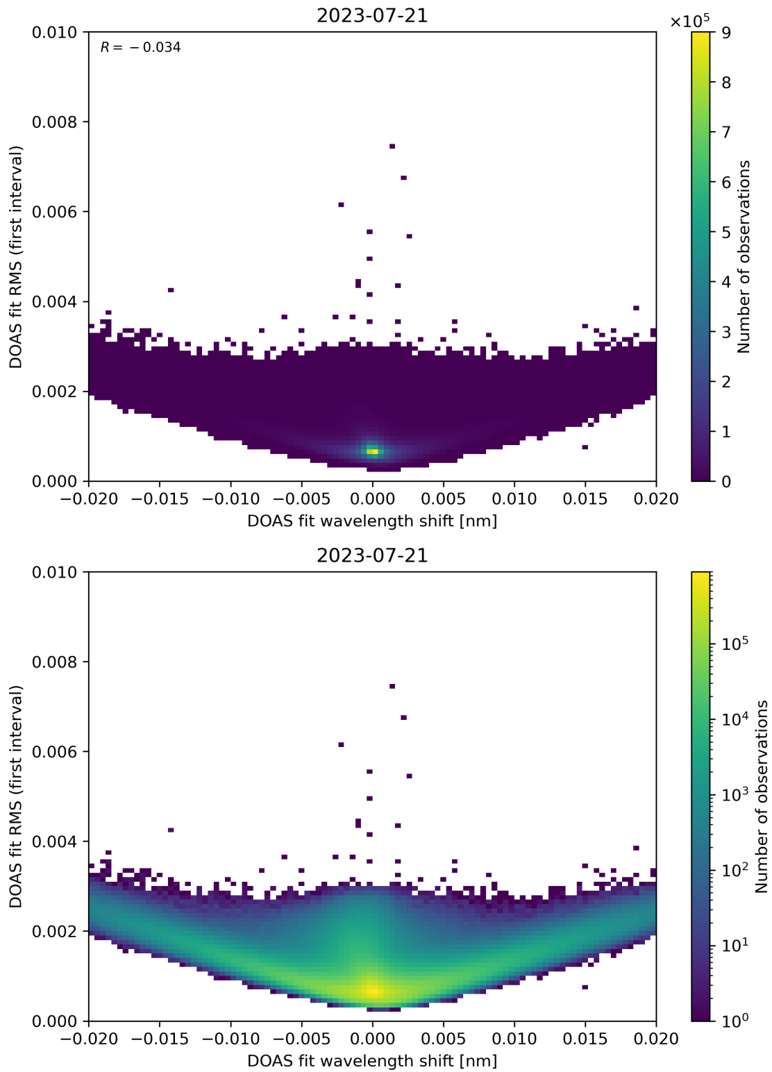
Figure 64: Scatter density plot of “DOAS fit wavelength shift” against “DOAS fit RMS (first interval)” for 2023-07-20 to 2023-07-22.
