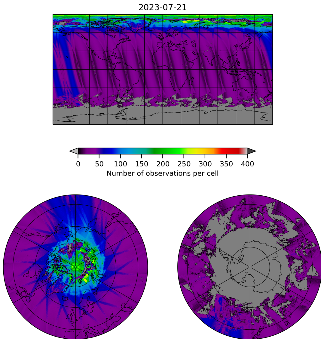
Figure 19: Map of the number of observations for 2023-07-20 to 2023-07-22
