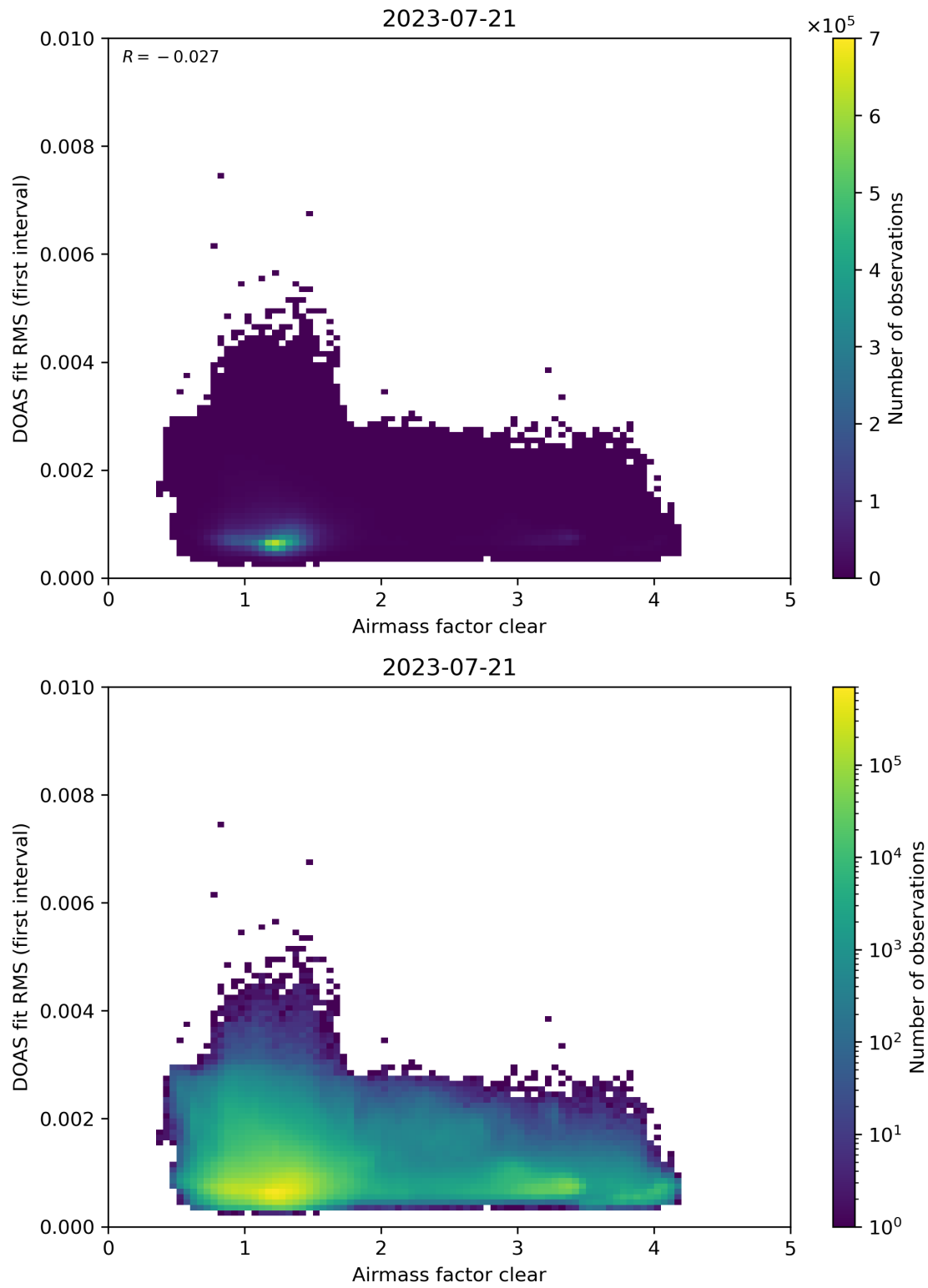
Figure 71: Scatter density plot of “Airmass factor clear” against “DOAS fit RMS (first interval)” for 2023-07-20 to 2023-07-22.
