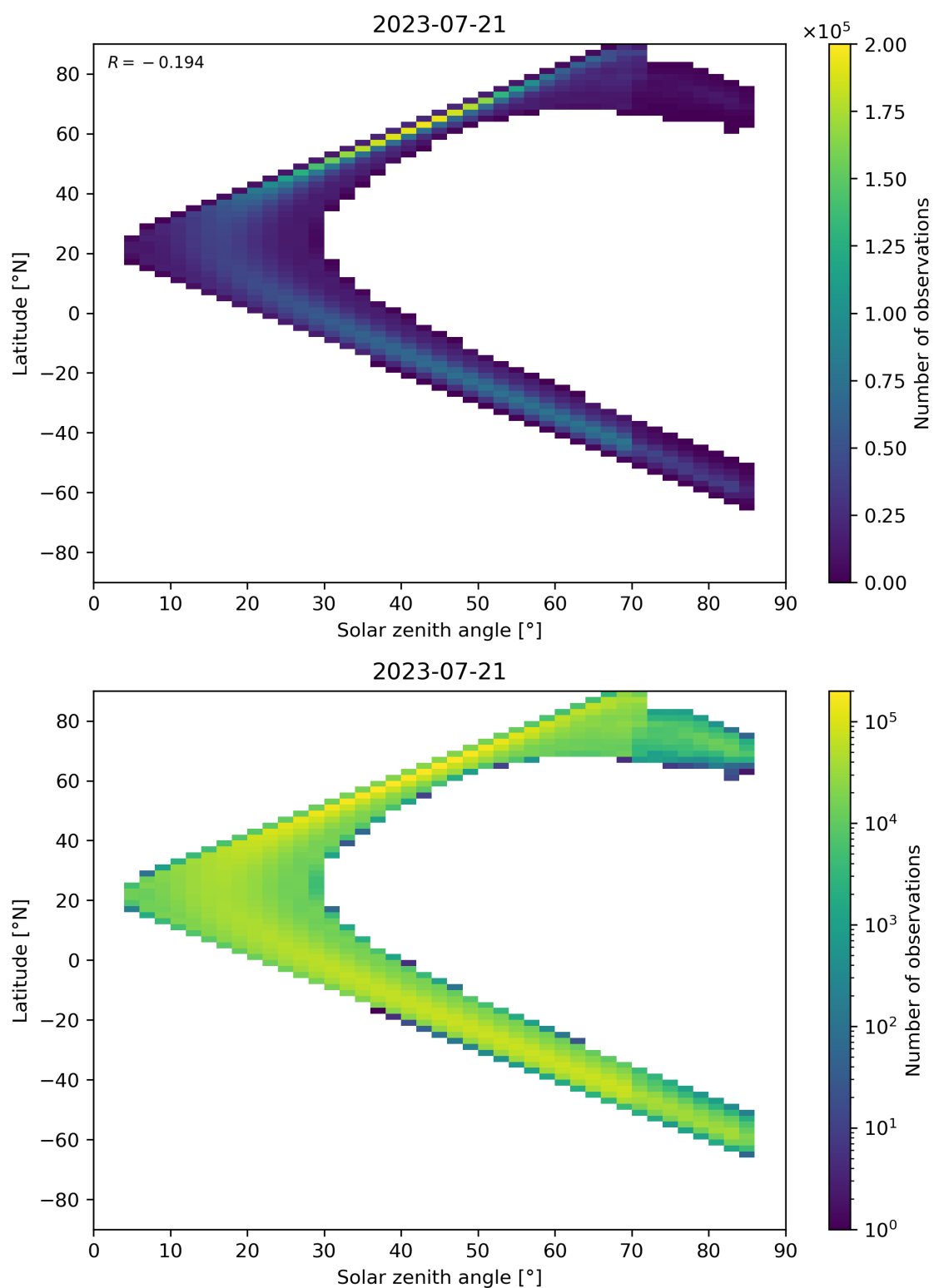
Figure 181: Scatter density plot of “Solar zenith angle” against “Latitude” for 2023-07-20 to 2023-07-22.
