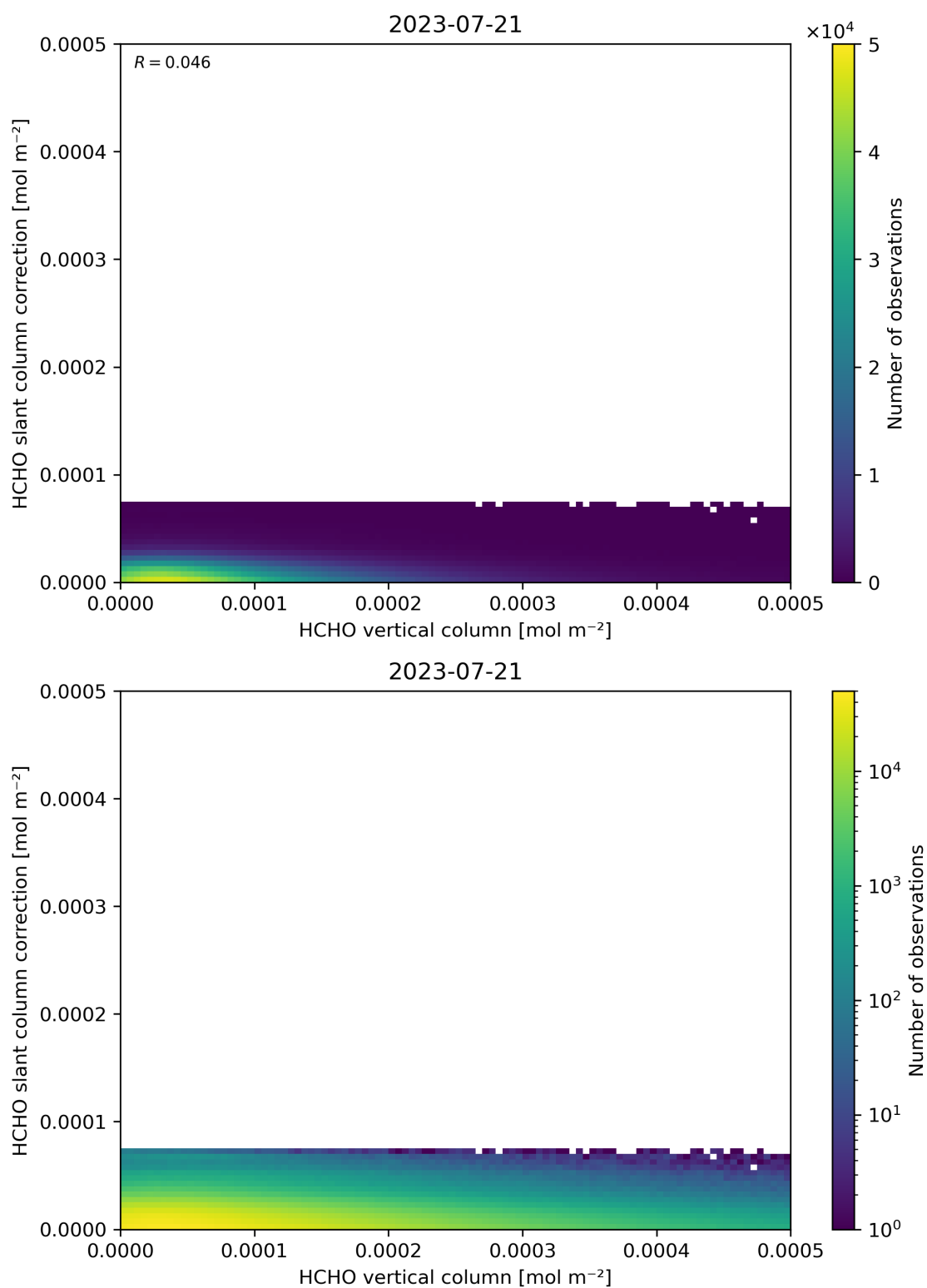
Figure 128: Scatter density plot of “HCHO vertical column” against “HCHO slant column correction” for 2023-07-20 to 2023-07-22.
