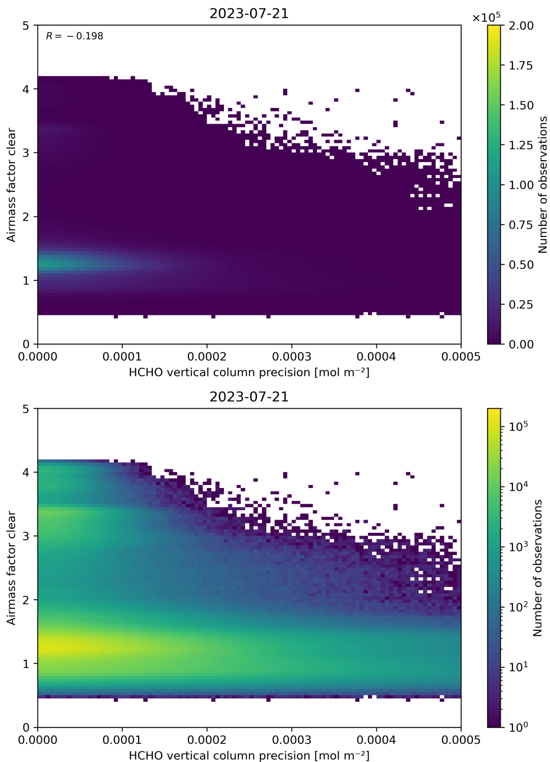
Figure 139: Scatter density plot of “HCHO vertical column precision” against “Airmass factor clear” for 2023-07-20 to 2023-07-22.
