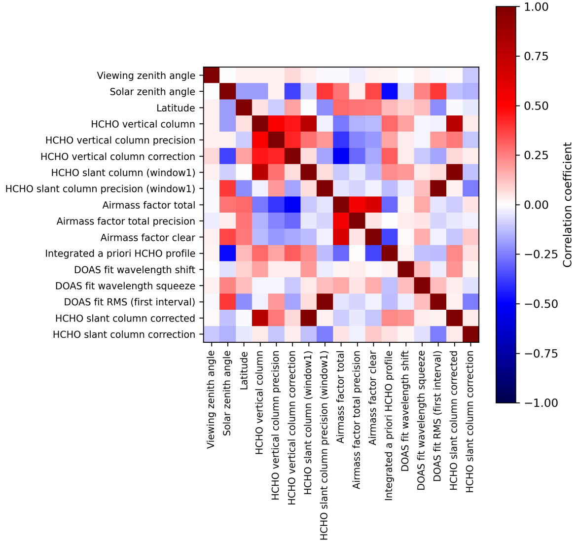
Figure 2: Map of correlation matrix for 2023-07-20 to 2023-07-22.
