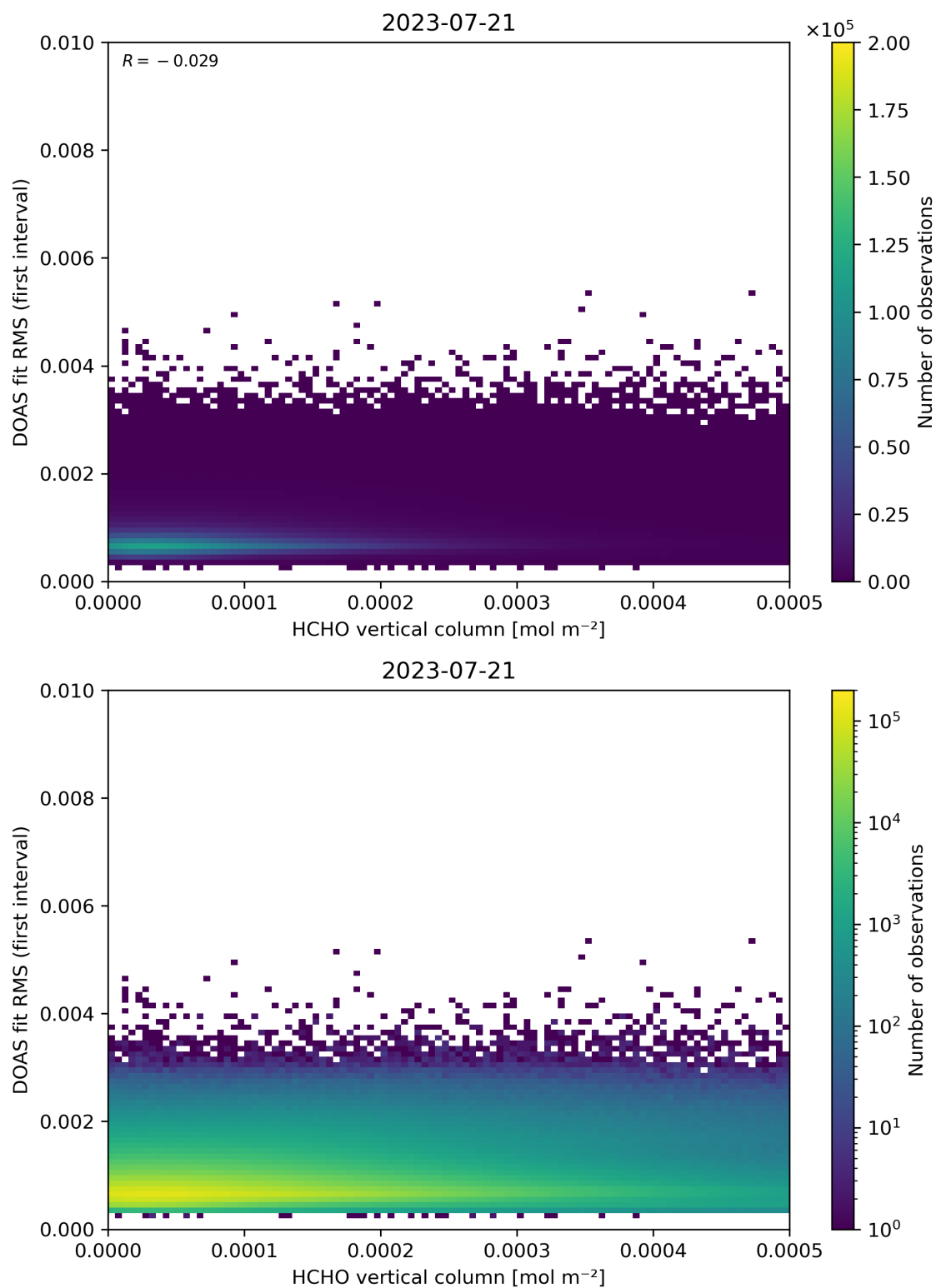
Figure 123: Scatter density plot of “HCHO vertical column” against “DOAS fit RMS (first interval)” for 2023-07-20 to 2023-07-22.
