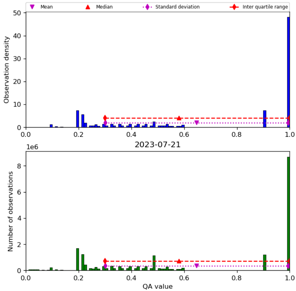
Figure 34: Histogram of “QA value” for 2023-07-20 to 2023-07-22
