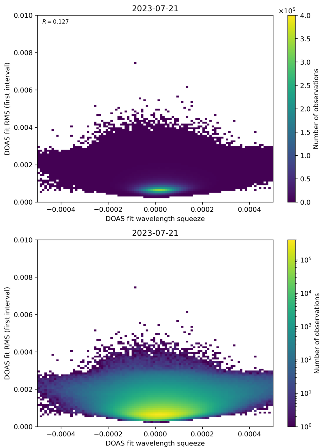
Figure 68: Scatter density plot of “DOAS fit wavelength squeeze” against “DOAS fit RMS (first interval)” for 2023-07-20 to 2023-07-22.
