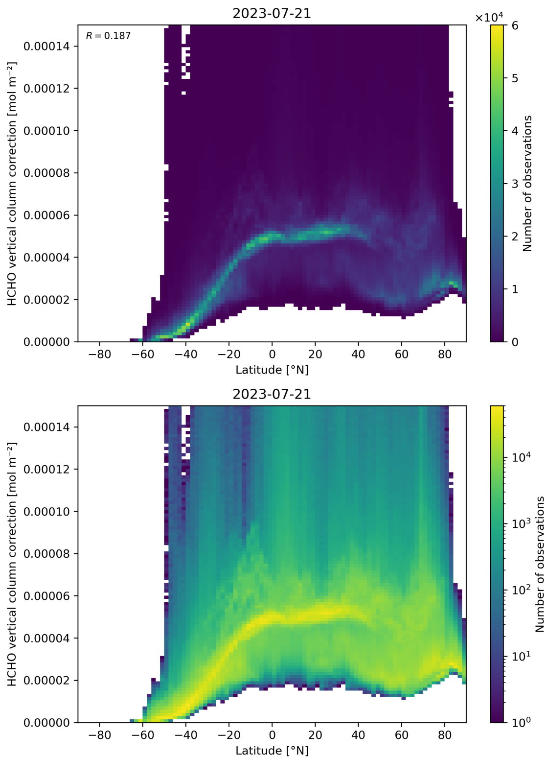
Figure 164: Scatter density plot of “Latitude” against “HCHO vertical column correction” for 2023-07-20 to 2023-07-22.
