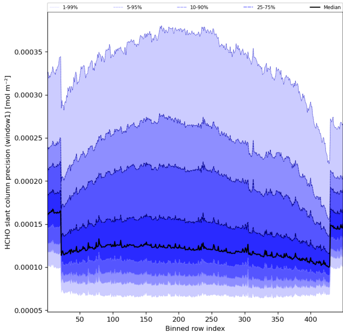
Figure 53: Along track statistics of “HCHO slant column precision (window1)” for 2023-07-20 to 2023-07-22
