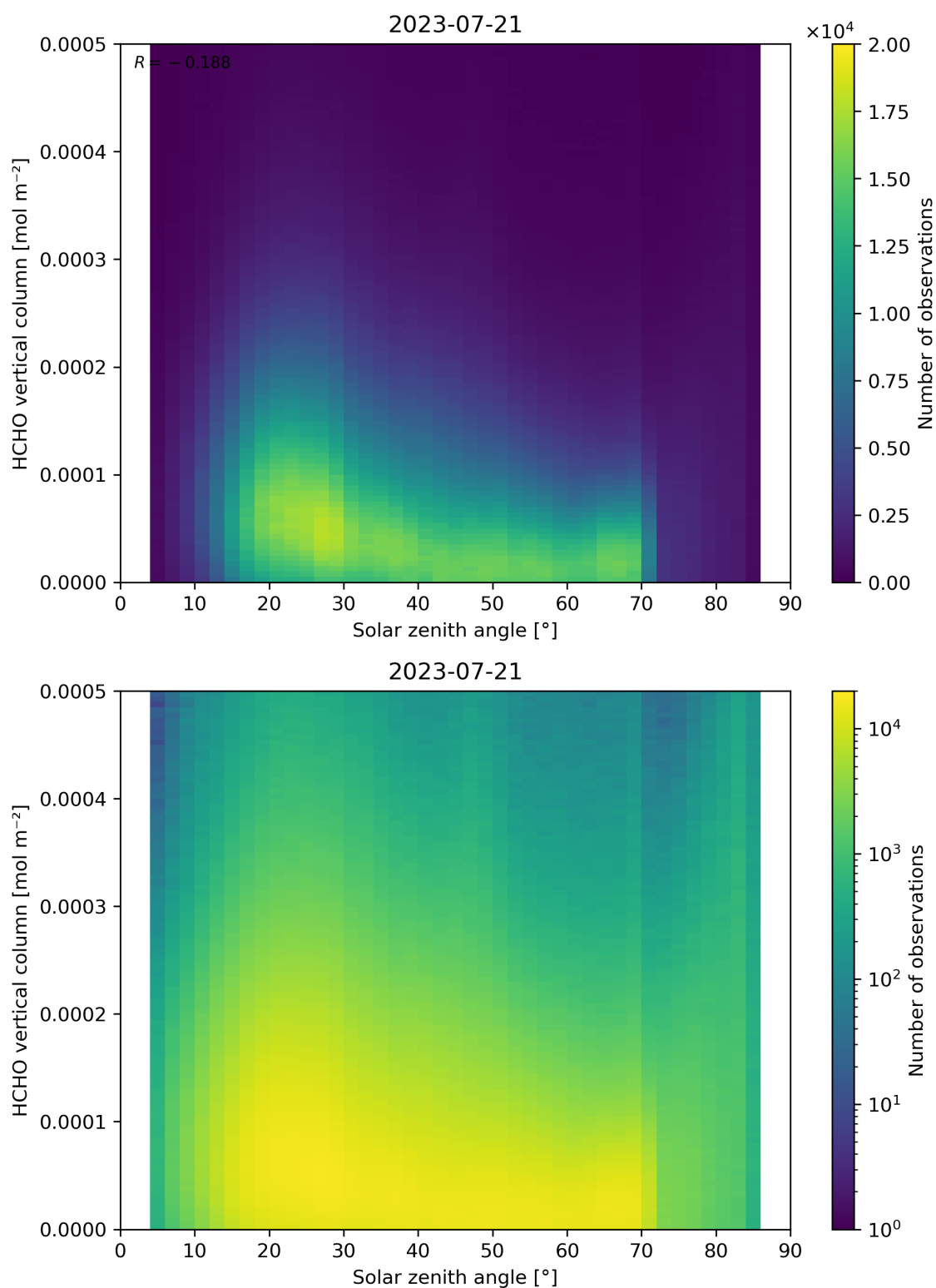
Figure 177: Scatter density plot of “Solar zenith angle” against “HCHO vertical column” for 2023-07-20 to 2023-07-22.
