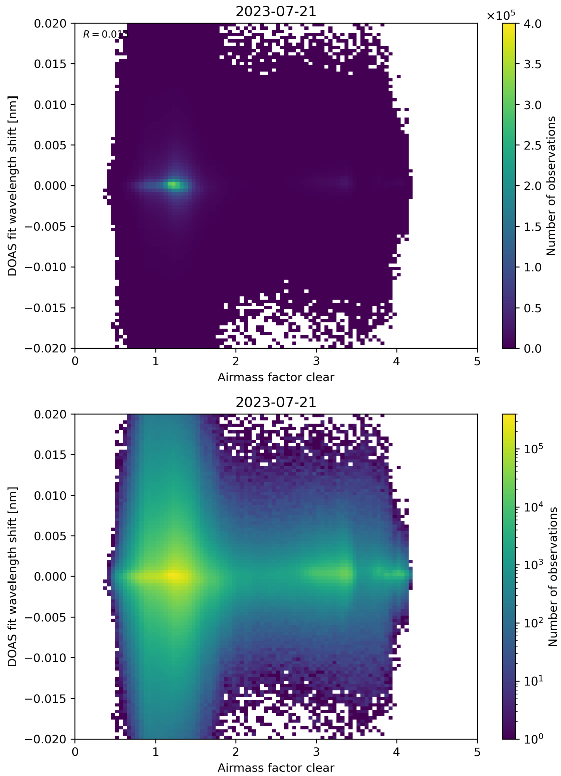
Figure 72: Scatter density plot of “Airmass factor clear” against “DOAS fit wavelength shift” for 2023-07-20 to 2023-07-22.
