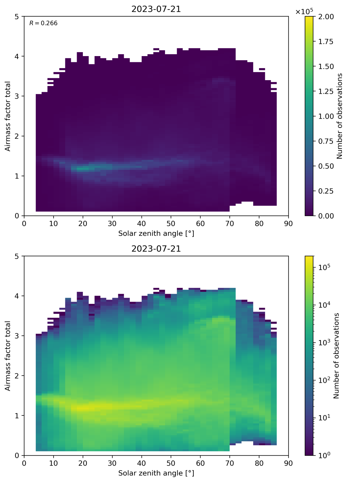
Figure 175: Scatter density plot of “Solar zenith angle” against “Airmass factor total” for 2023-07-20 to 2023-07-22.
