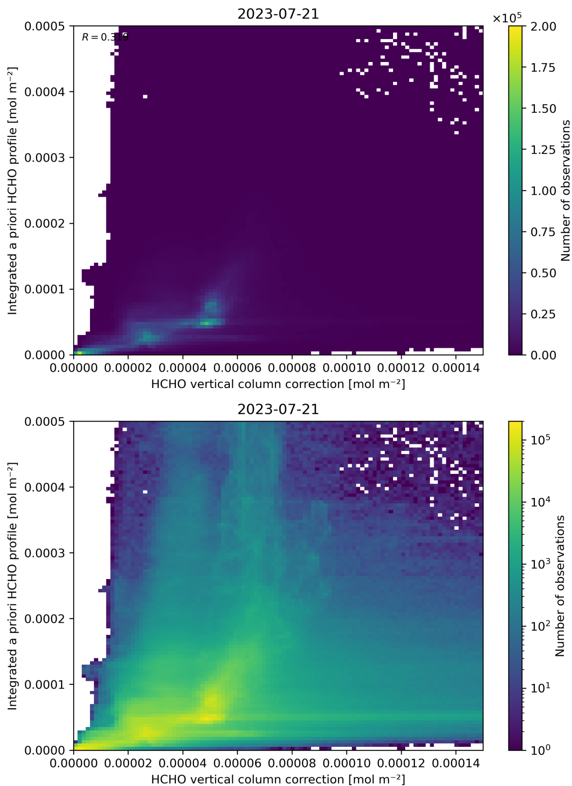
Figure 122: Scatter density plot of “HCHO vertical column correction” against “Integrated a priori HCHO profile” for 2023-07-20 to 2023-07-22.
