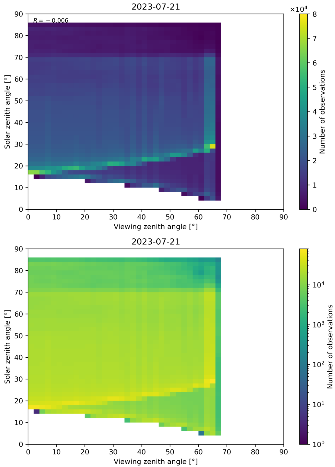
Figure 197: Scatter density plot of “Viewing zenith angle” against “Solar zenith angle” for 2023-07-20 to 2023-07-22.
