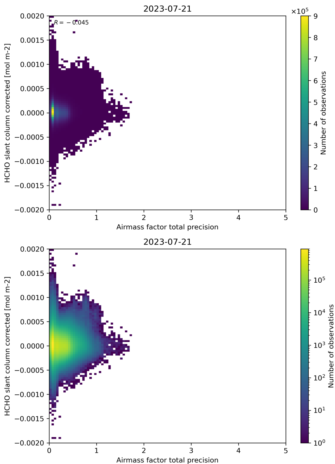
Figure 109: Scatter density plot of “Airmass factor total precision” against “HCHO slant column corrected” for 2023-07-20 to 2023-07-22.
