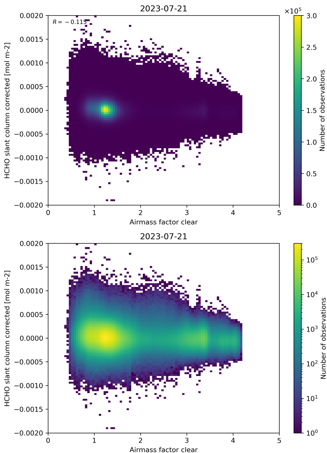
Figure 74: Scatter density plot of “Airmass factor clear” against “HCHO slant column corrected” for 2023-07-20 to 2023-07-22.
