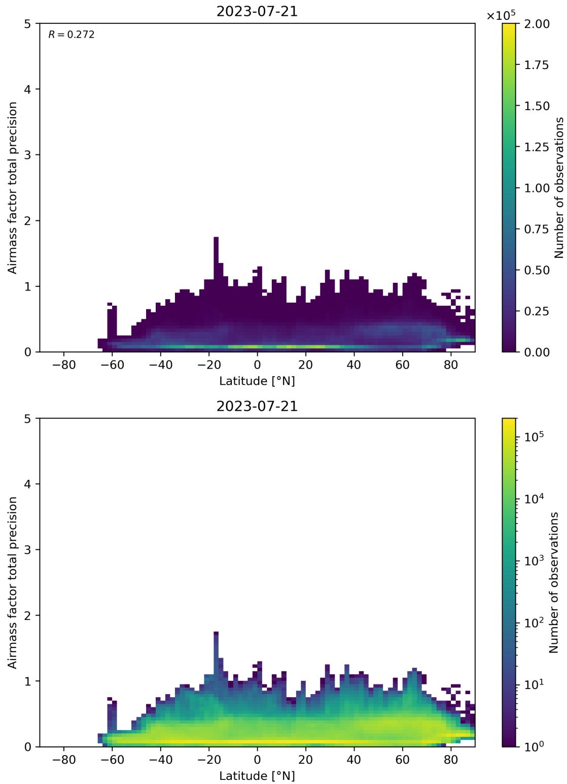
Figure 162: Scatter density plot of “Latitude” against “Airmass factor total precision” for 2023-07-20 to 2023-07-22.
