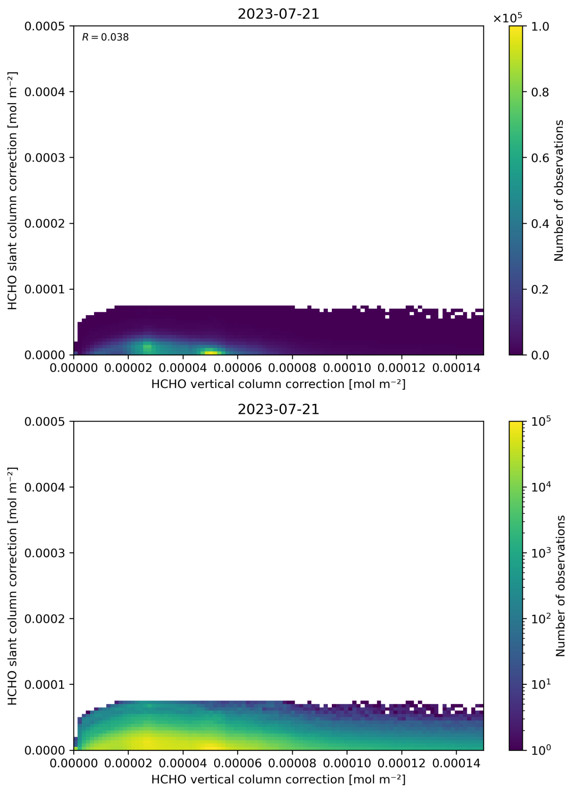
Figure 117: Scatter density plot of “HCHO vertical column correction” against “HCHO slant column correction” for 2023-07-20 to 2023-07-22.
