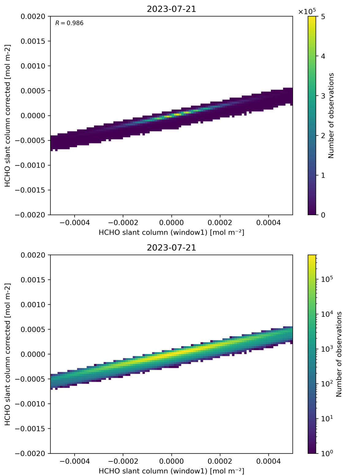
Figure 82: Scatter density plot of “HCHO slant column (window1)” against “HCHO slant column corrected” for 2023-07-20 to 2023-07-22.
