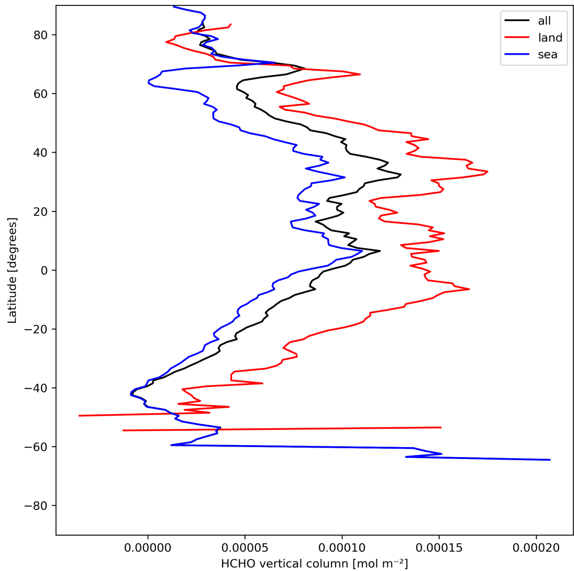
Figure 21: Zonal average of “HCHO vertical column” for 2023-07-20 to 2023-07-22.
