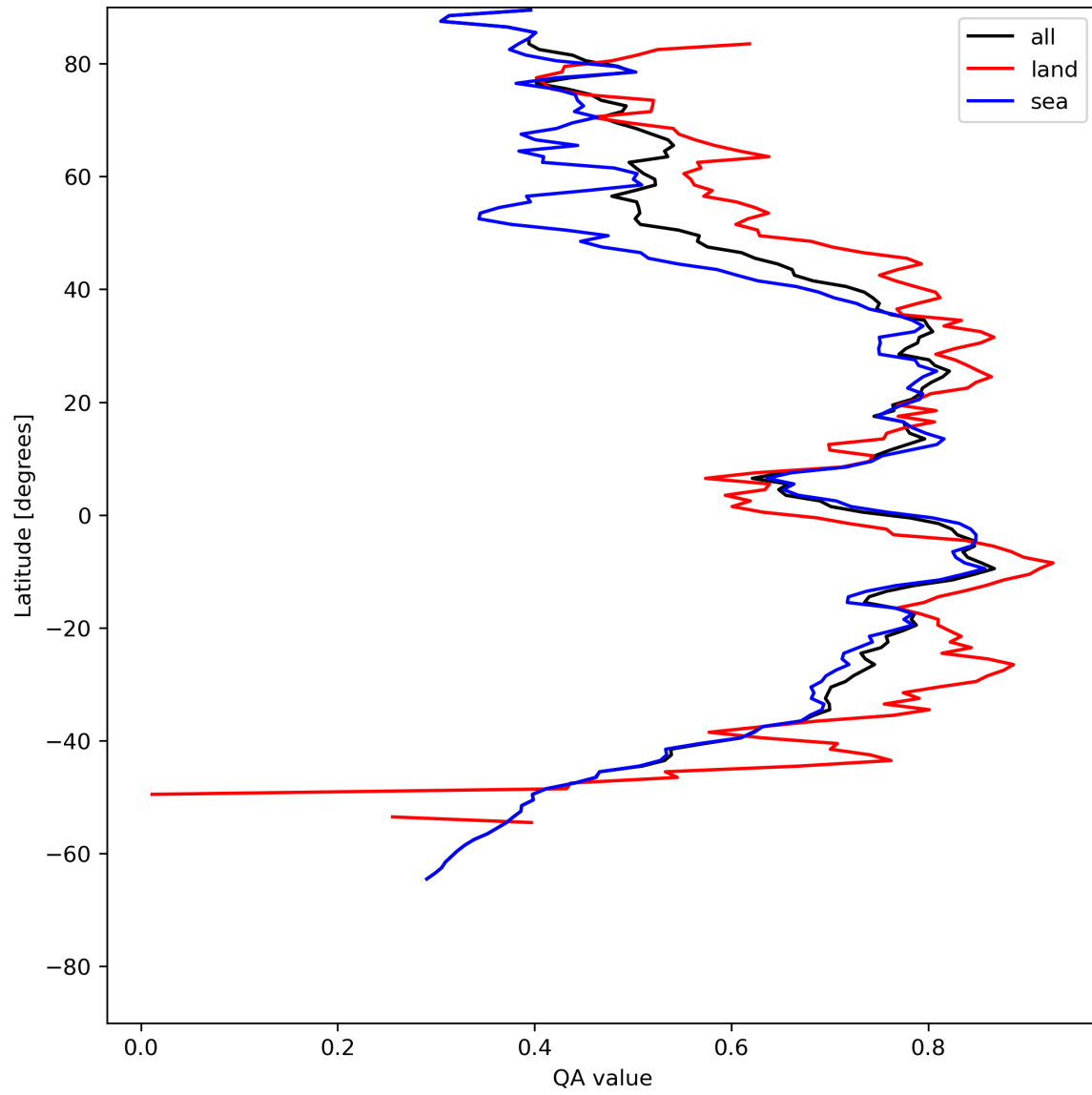
Figure 20: Zonal average of “QA value” for 2023-07-20 to 2023-07-22.
