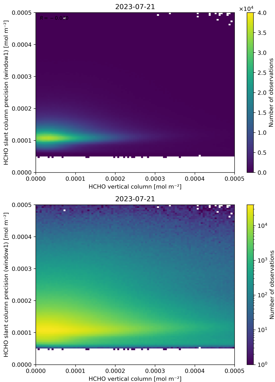
Figure 130: Scatter density plot of “HCHO vertical column” against “HCHO slant column precision (window1)” for 2023-07-20 to 2023-07-22.
