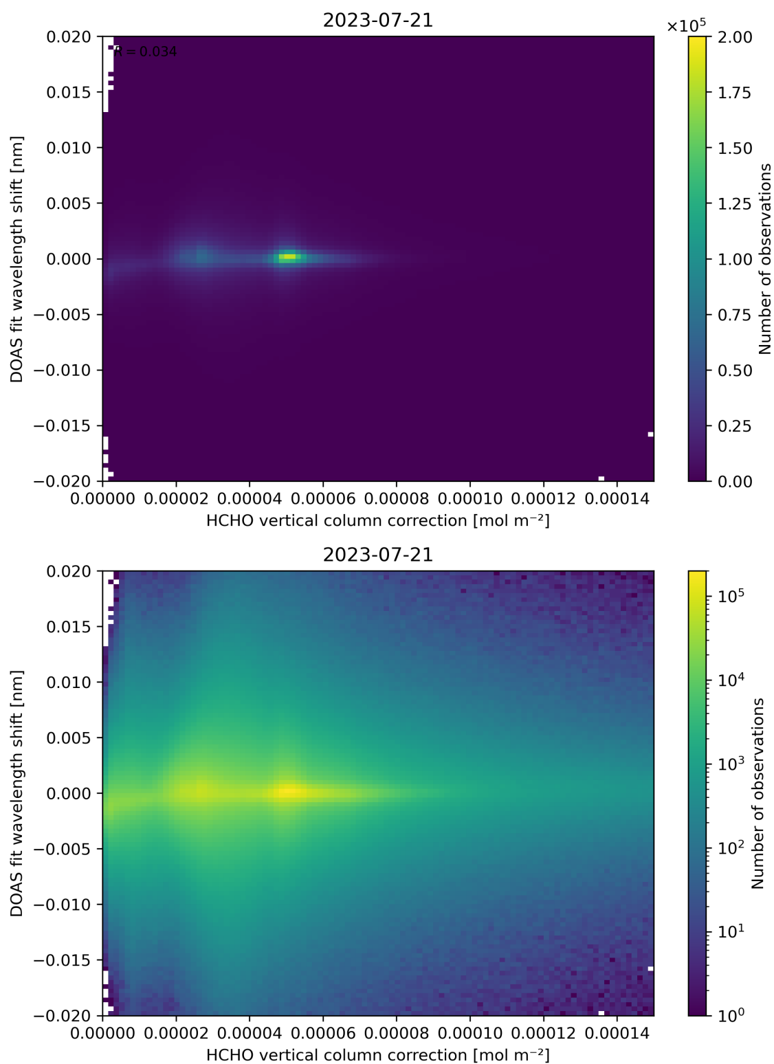
Figure 113: Scatter density plot of “HCHO vertical column correction” against “DOAS fit wavelength shift” for 2023-07-20 to 2023-07-22.
