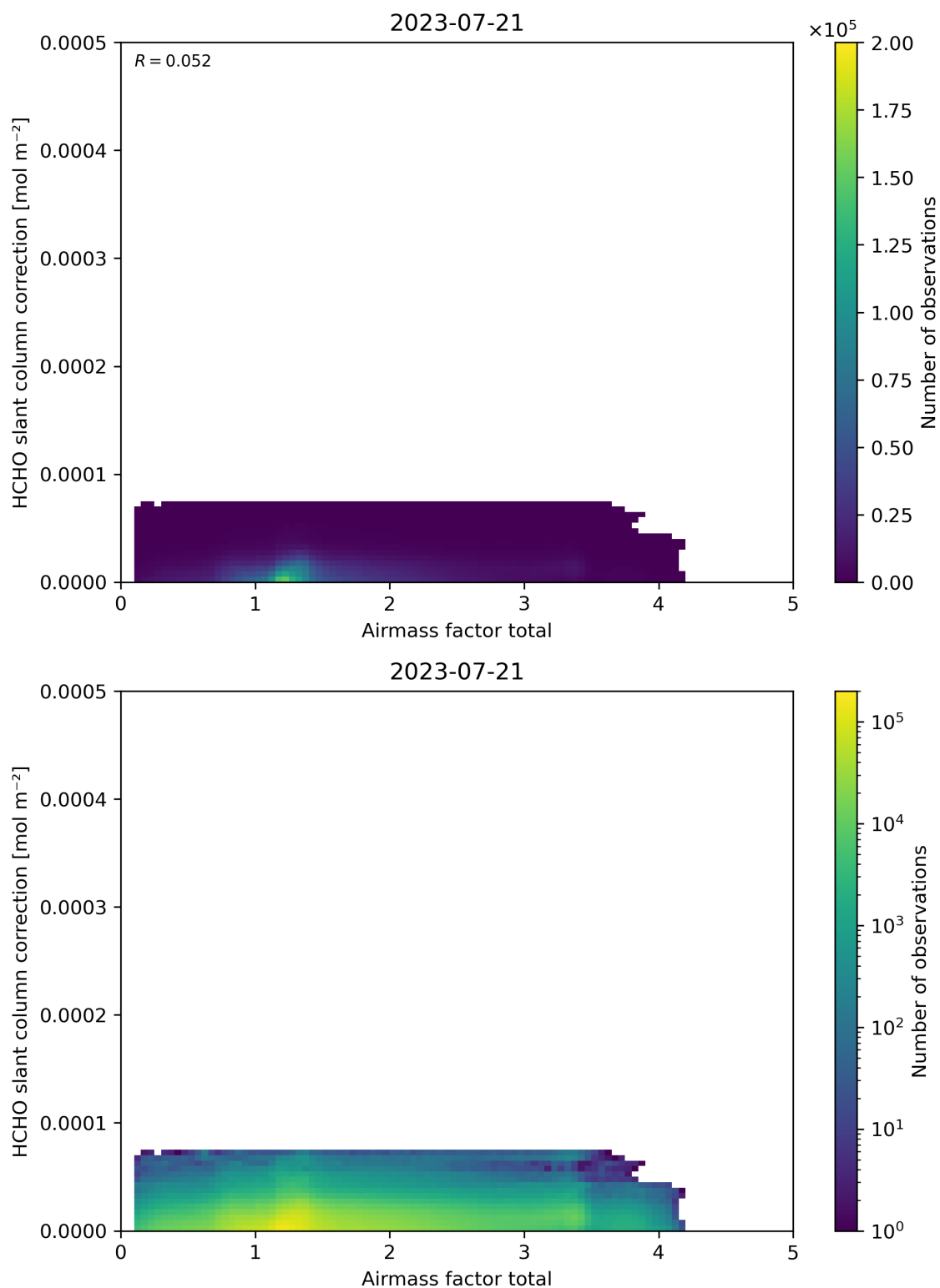
Figure 102: Scatter density plot of “Airmass factor total” against “HCHO slant column correction” for 2023-07-20 to 2023-07-22.
