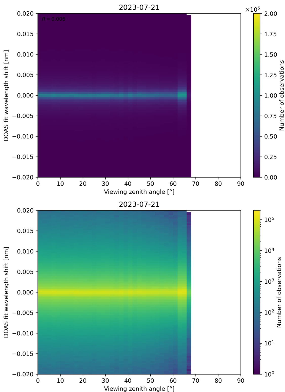
Figure 183: Scatter density plot of “Viewing zenith angle” against “DOAS fit wavelength shift” for 2023-07-20 to 2023-07-22.
