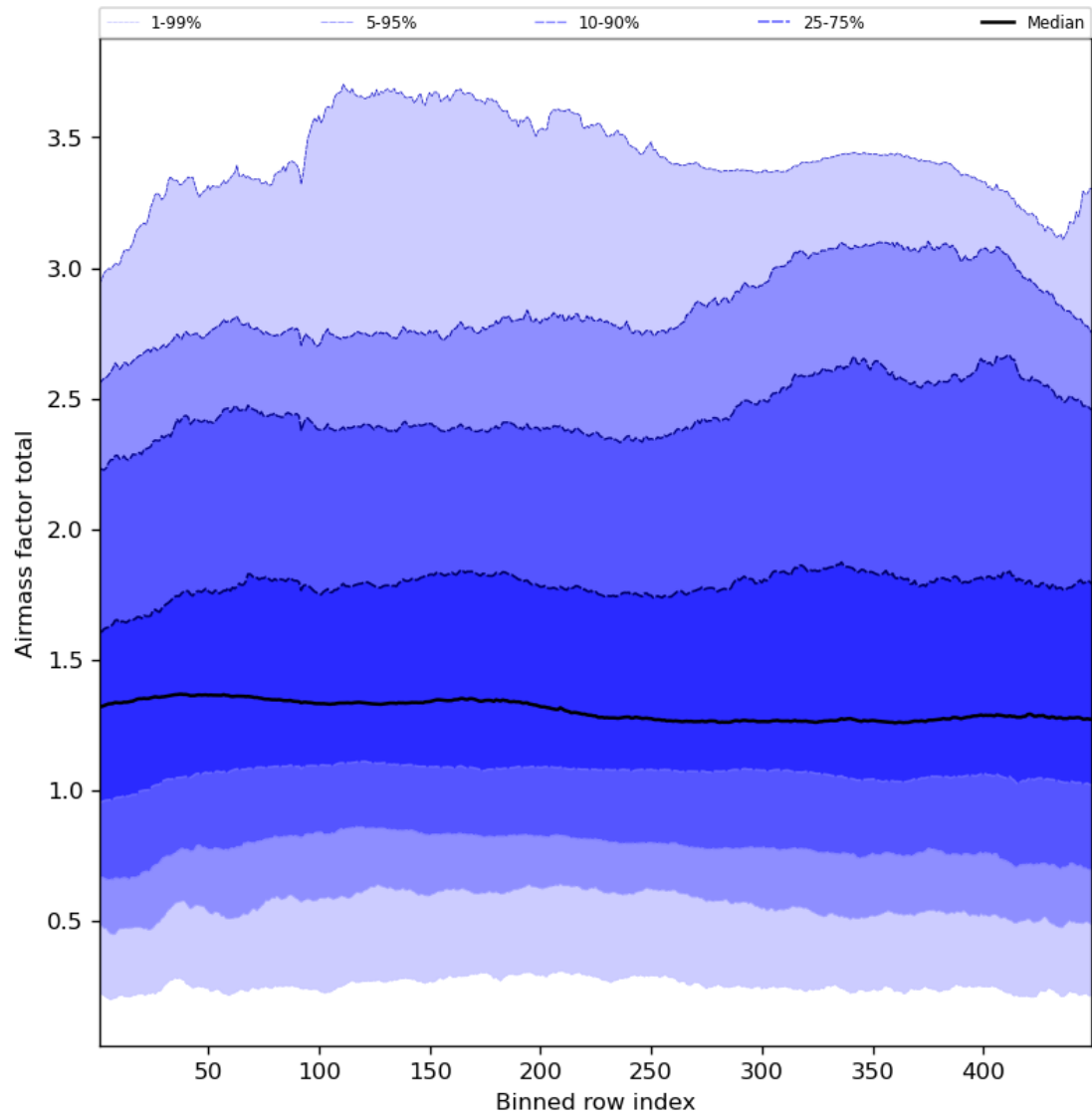
Figure 54: Along track statistics of “Airmass factor total” for 2023-07-20 to 2023-07-22
