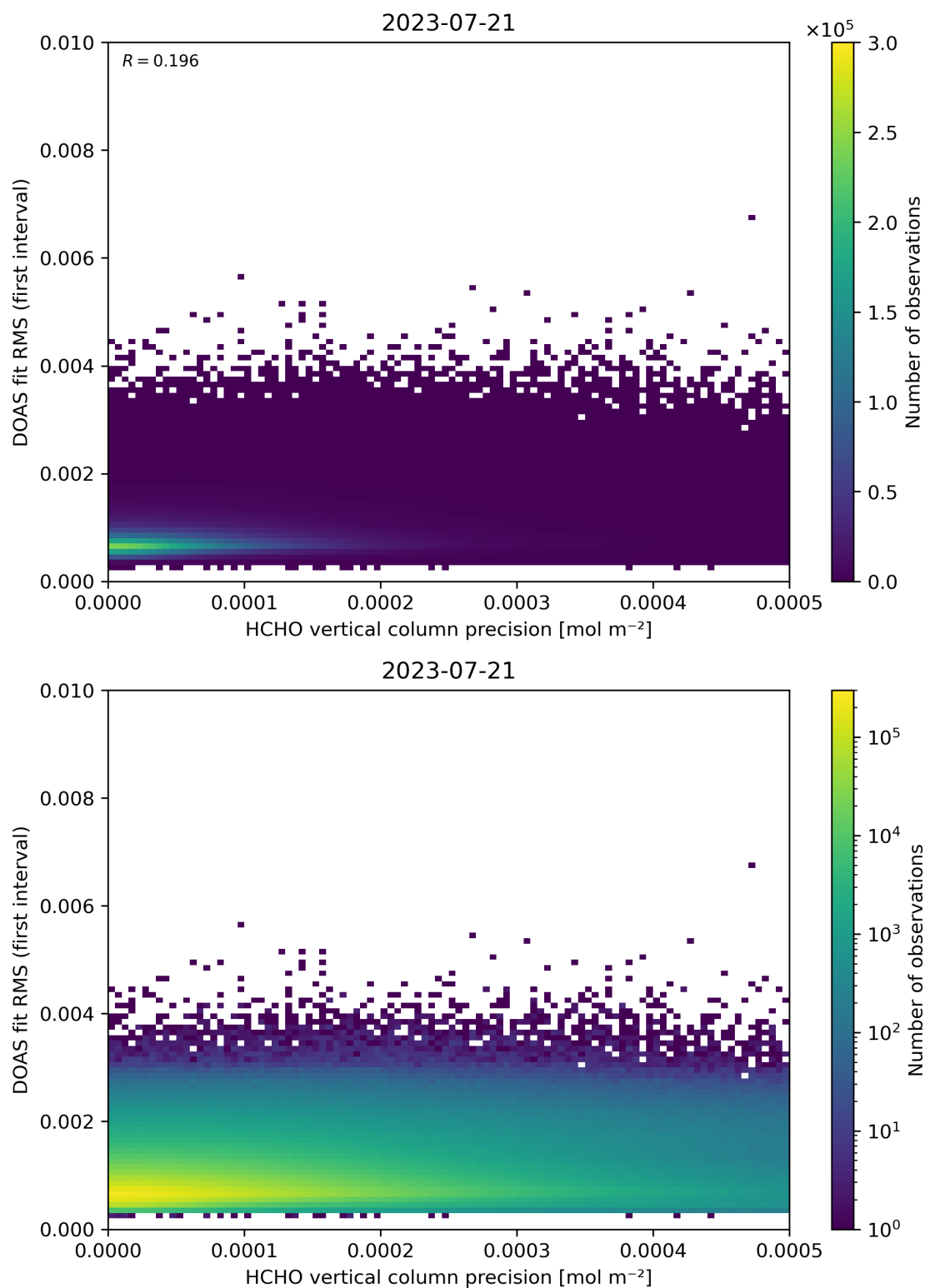
Figure 136: Scatter density plot of “HCHO vertical column precision” against “DOAS fit RMS (first interval)” for 2023-07-20 to 2023-07-22.
