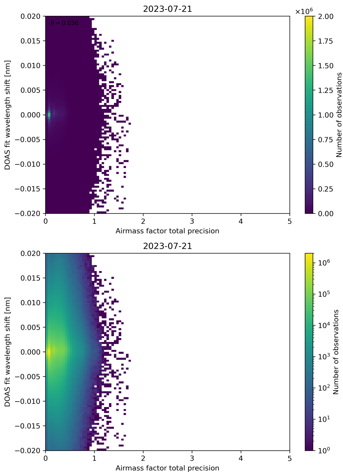
Figure 106: Scatter density plot of “Airmass factor total precision” against “DOAS fit wavelength shift” for 2023-07-20 to 2023-07-22.
