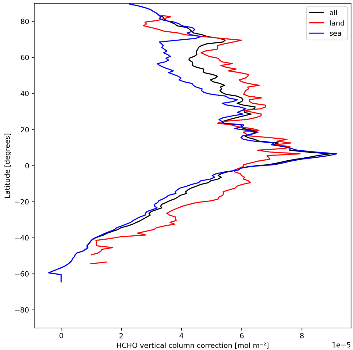
Figure 23: Zonal average of “HCHO vertical column correction” for 2023-07-20 to 2023-07-22.
