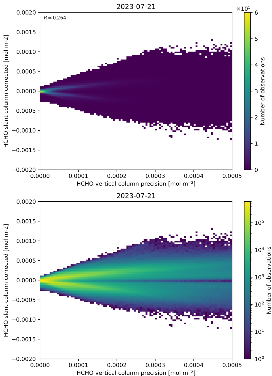
Figure 140: Scatter density plot of “HCHO vertical column precision” against “HCHO slant column corrected” for 2023-07-20 to 2023-07-22.
