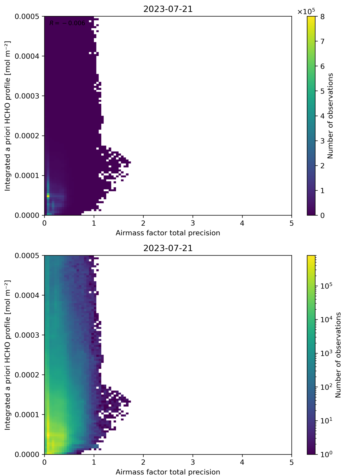
Figure 111: Scatter density plot of “Airmass factor total precision” against “Integrated a priori HCHO profile” for 2023-07-20 to 2023-07-22.
