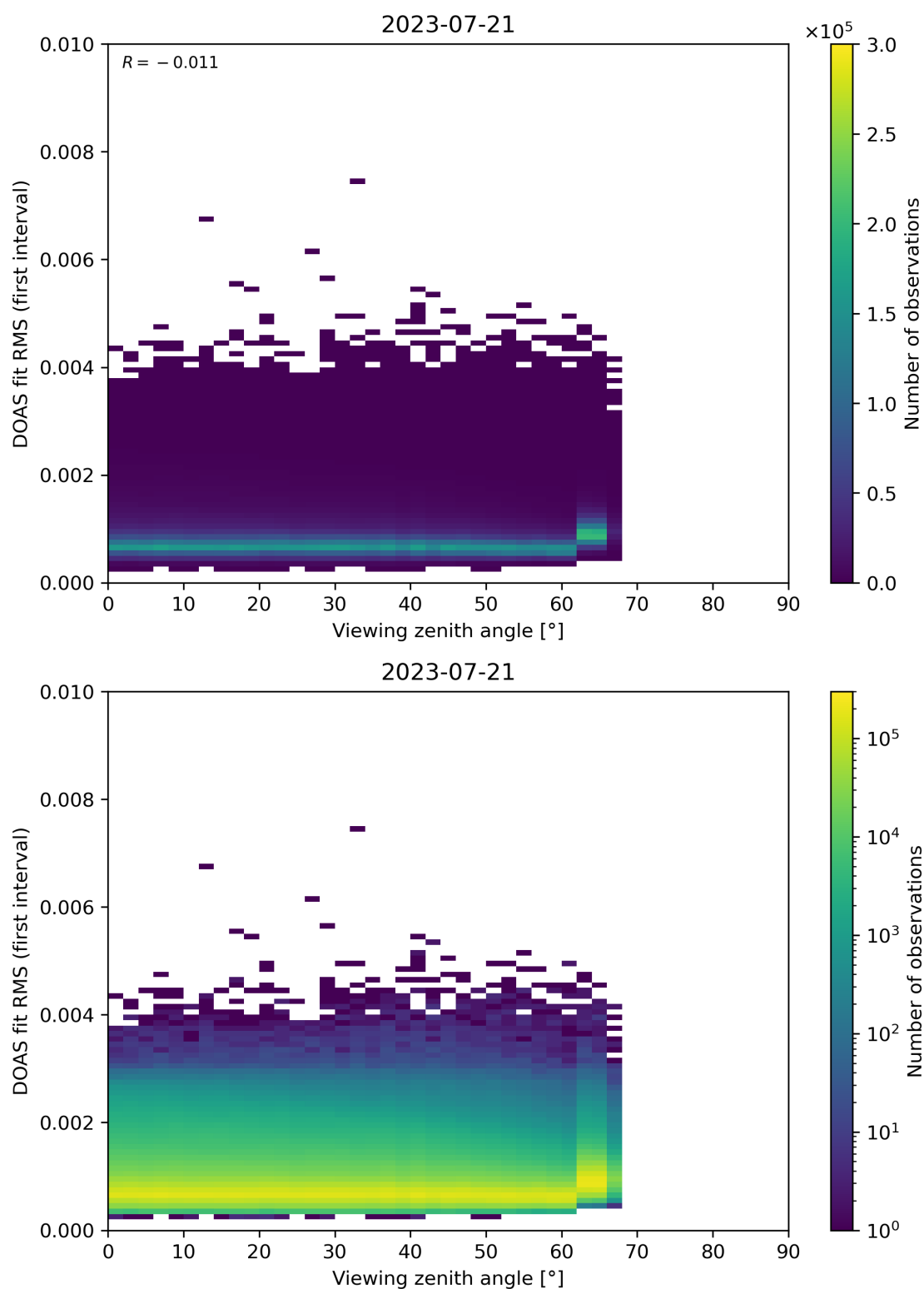
Figure 182: Scatter density plot of “Viewing zenith angle” against “DOAS fit RMS (first interval)” for 2023-07-20 to 2023-07-22.
