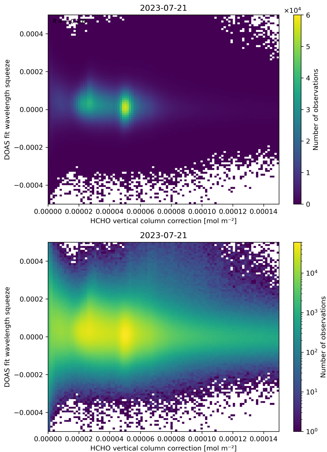
Figure 114: Scatter density plot of “HCHO vertical column correction” against “DOAS fit wavelength squeeze” for 2023-07-20 to 2023-07-22.
