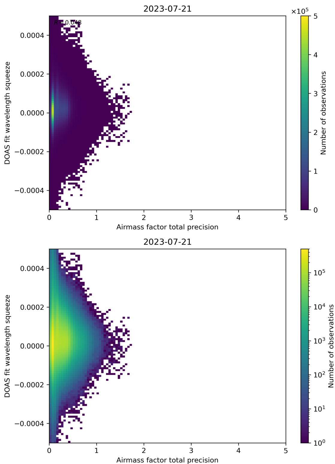
Figure 107: Scatter density plot of “Airmass factor total precision” against “DOAS fit wavelength squeeze” for 2023-07-20 to 2023-07-22.
