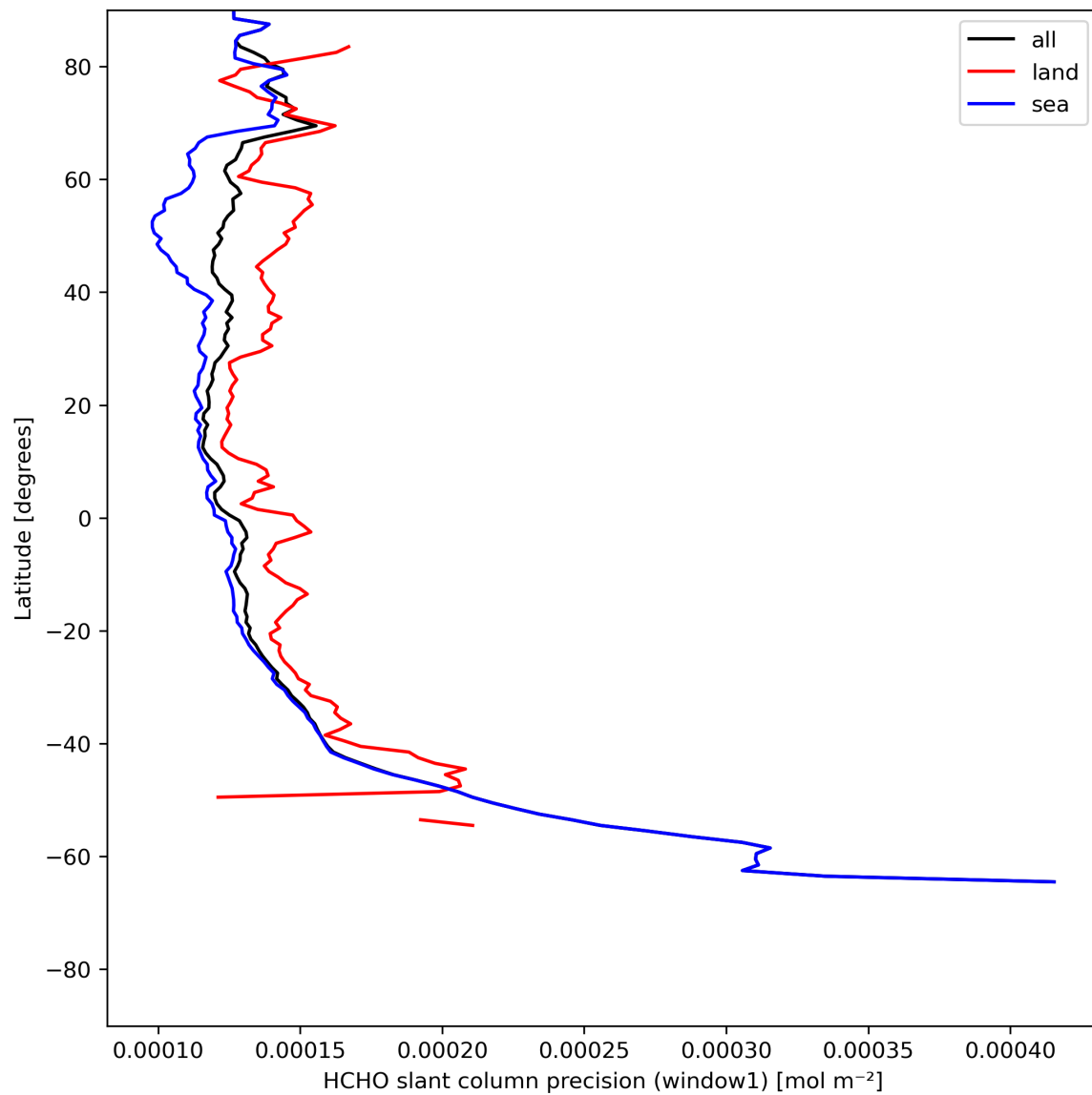
Figure 25: Zonal average of “HCHO slant column precision (window1)” for 2023-07-20 to 2023-07-22.
