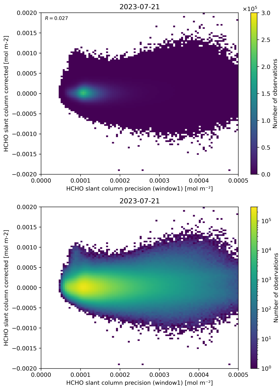
Figure 92: Scatter density plot of “HCHO slant column precision (window1)” against “HCHO slant column corrected” for 2023-07-20 to 2023-07-22.
