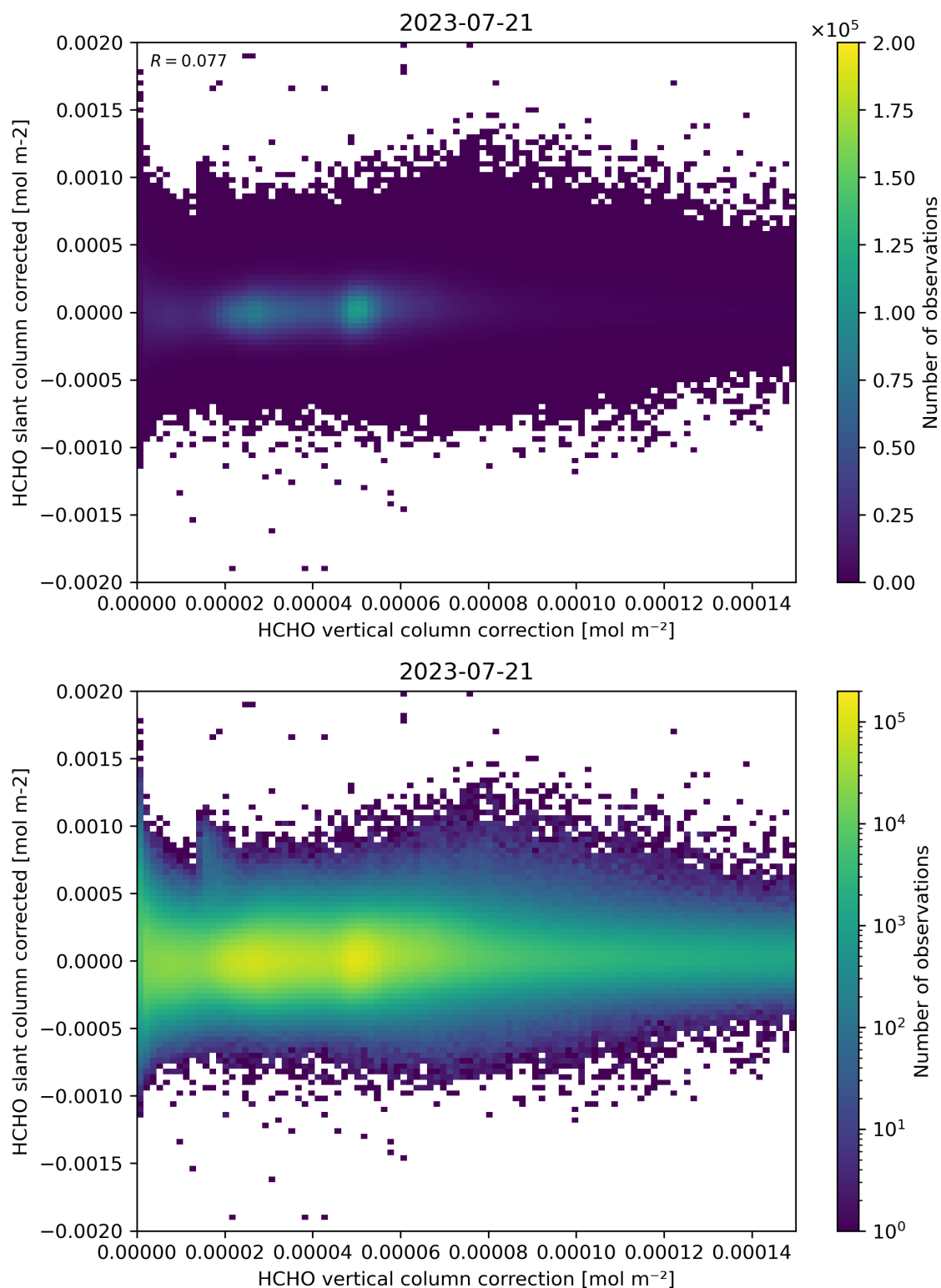
Figure 116: Scatter density plot of “HCHO vertical column correction” against “HCHO slant column corrected” for 2023-07-20 to 2023-07-22.
