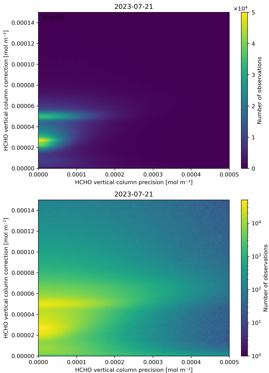
Figure 146: Scatter density plot of “HCHO vertical column precision” against “HCHO vertical column correction” for 2023-07-20 to 2023-07-22.
