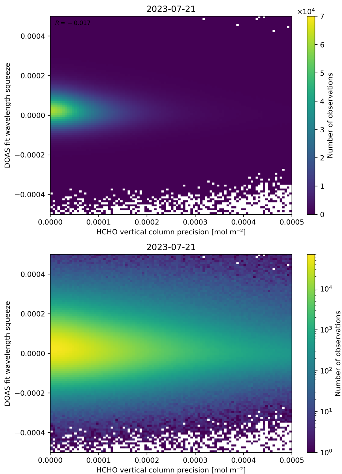
Figure 138: Scatter density plot of “HCHO vertical column precision” against “DOAS fit wavelength squeeze” for 2023-07-20 to 2023-07-22.
