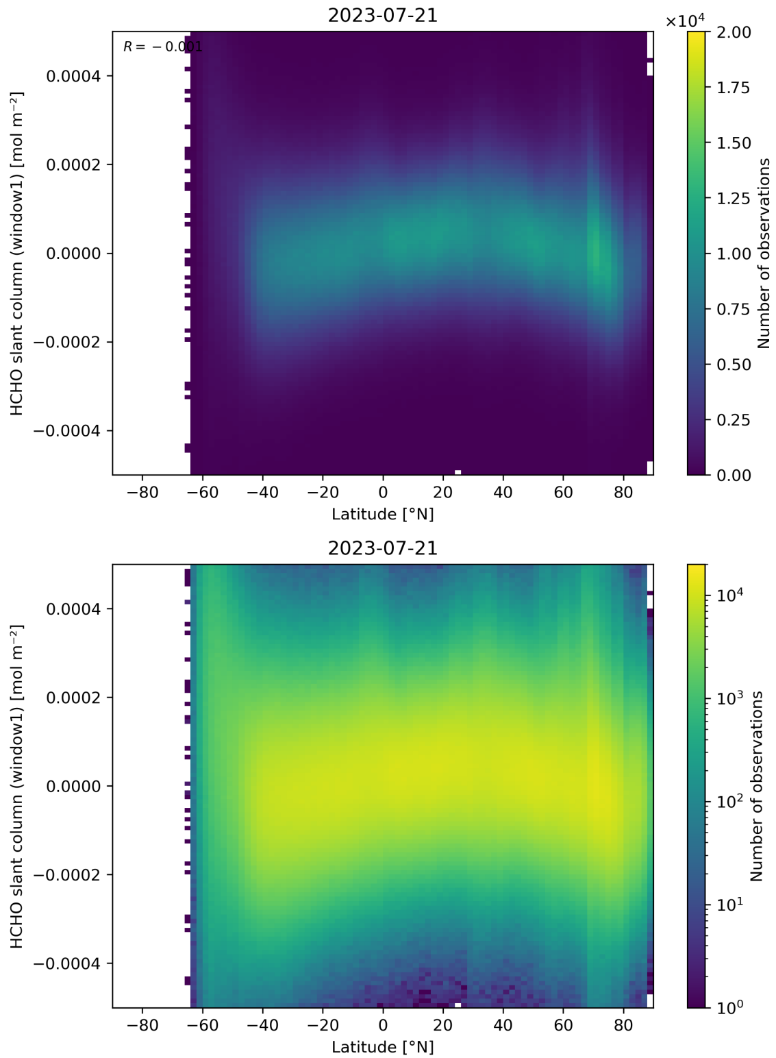
Figure 159: Scatter density plot of “Latitude” against “HCHO slant column (window1)” for 2023-07-20 to 2023-07-22.
