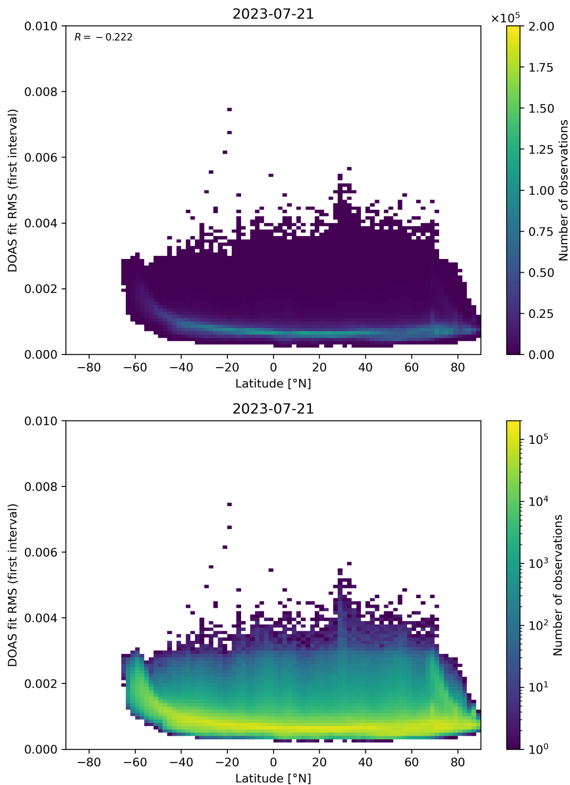
Figure 153: Scatter density plot of “Latitude” against “DOAS fit RMS (first interval)” for 2023-07-20 to 2023-07-22.
