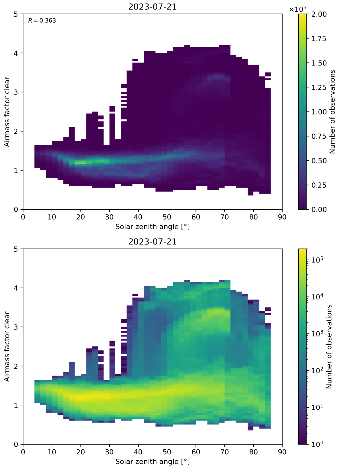
Figure 170: Scatter density plot of “Solar zenith angle” against “Airmass factor clear” for 2023-07-20 to 2023-07-22.
