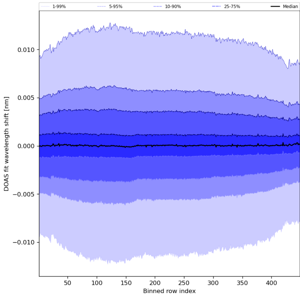
Figure 58: Along track statistics of “DOAS fit wavelength shift” for 2023-07-20 to 2023-07-22
