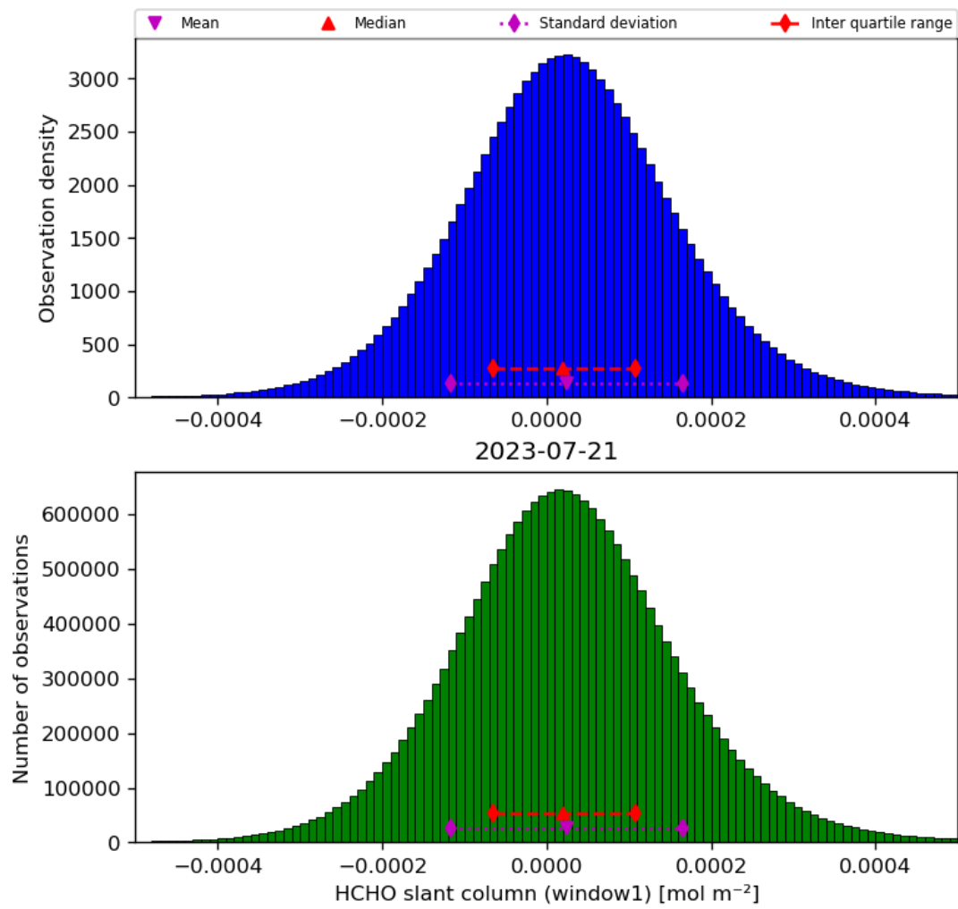
Figure 38: Histogram of “HCHO slant column (window1)” for 2023-07-20 to 2023-07-22
