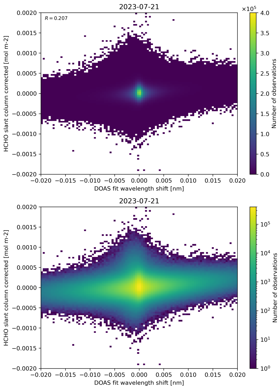
Figure 66: Scatter density plot of “DOAS fit wavelength shift” against “HCHO slant column corrected” for 2023-07-20 to 2023-07-22.
