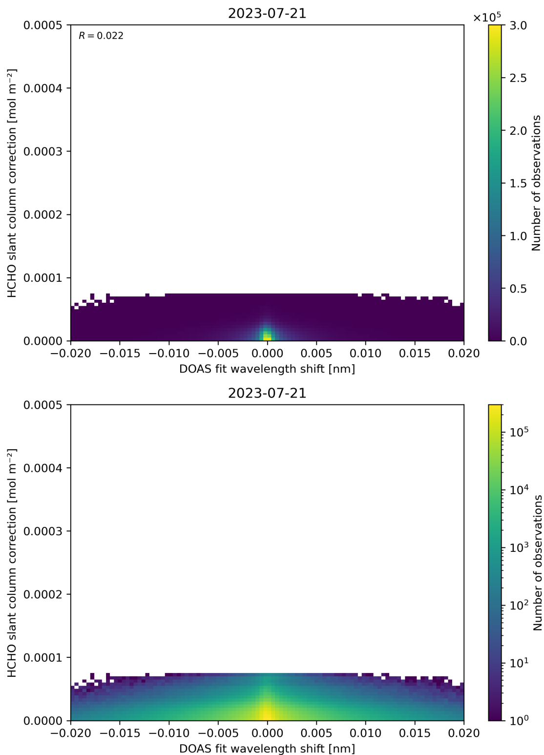
Figure 67: Scatter density plot of “DOAS fit wavelength shift” against “HCHO slant column correction” for 2023-07-20 to 2023-07-22.
