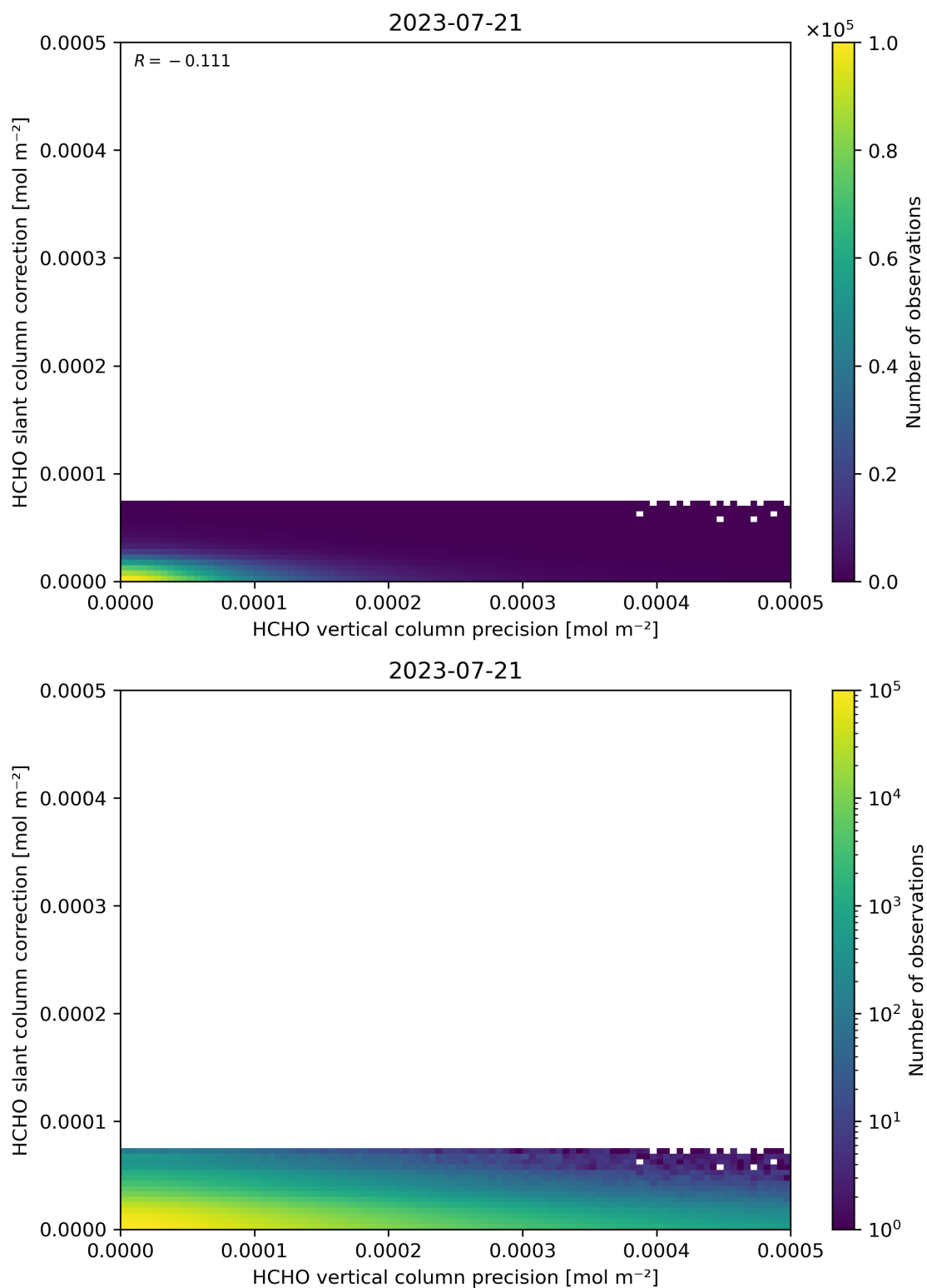
Figure 141: Scatter density plot of “HCHO vertical column precision” against “HCHO slant column correction” for 2023-07-20 to 2023-07-22.
