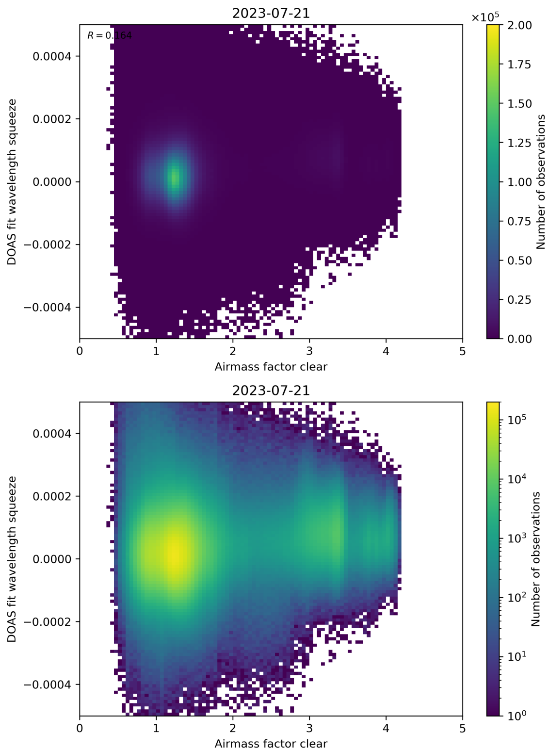
Figure 73: Scatter density plot of “Airmass factor clear” against “DOAS fit wavelength squeeze” for 2023-07-20 to 2023-07-22.
