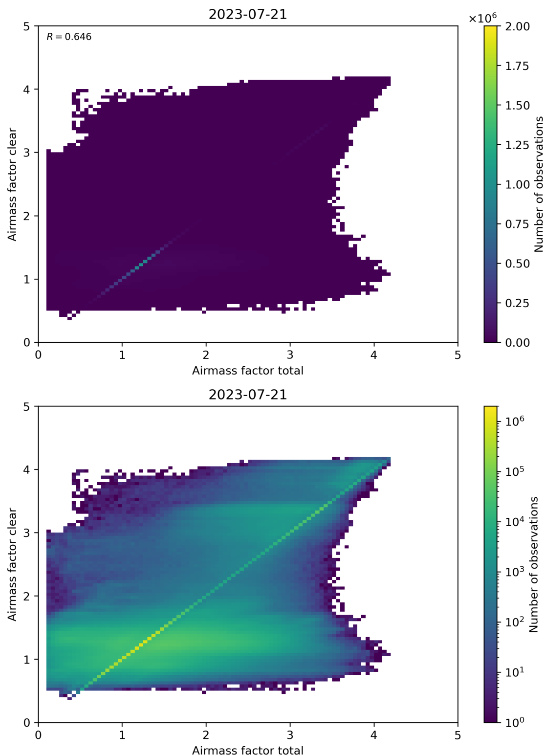
Figure 100: Scatter density plot of “Airmass factor total” against “Airmass factor clear” for 2023-07-20 to 2023-07-22.
