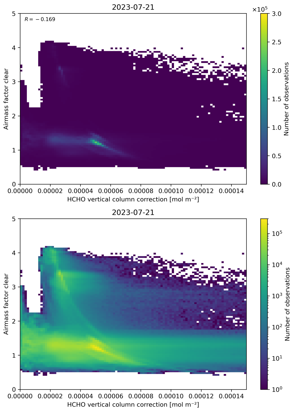
Figure 115: Scatter density plot of “HCHO vertical column correction” against “Airmass factor clear” for 2023-07-20 to 2023-07-22.
