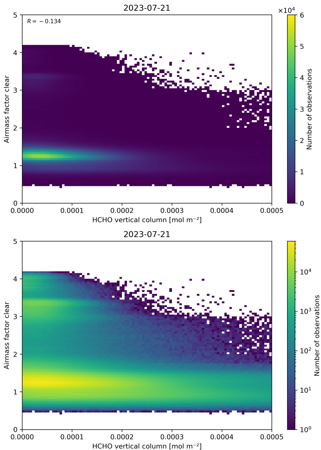
Figure 126: Scatter density plot of “HCHO vertical column” against “Airmass factor clear” for 2023-07-20 to 2023-07-22.
