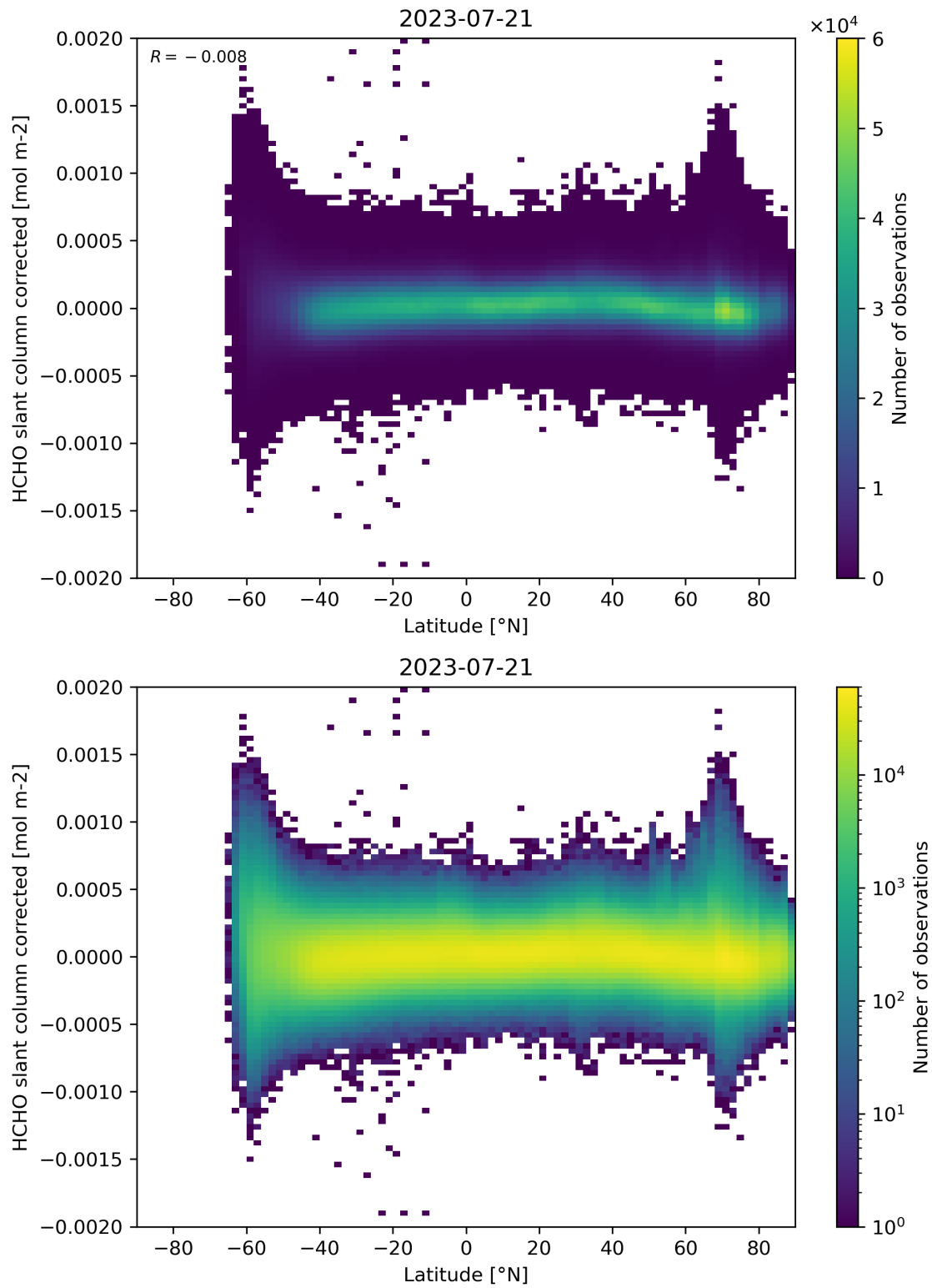
Figure 157: Scatter density plot of “Latitude” against “HCHO slant column corrected” for 2023-07-20 to 2023-07-22.
