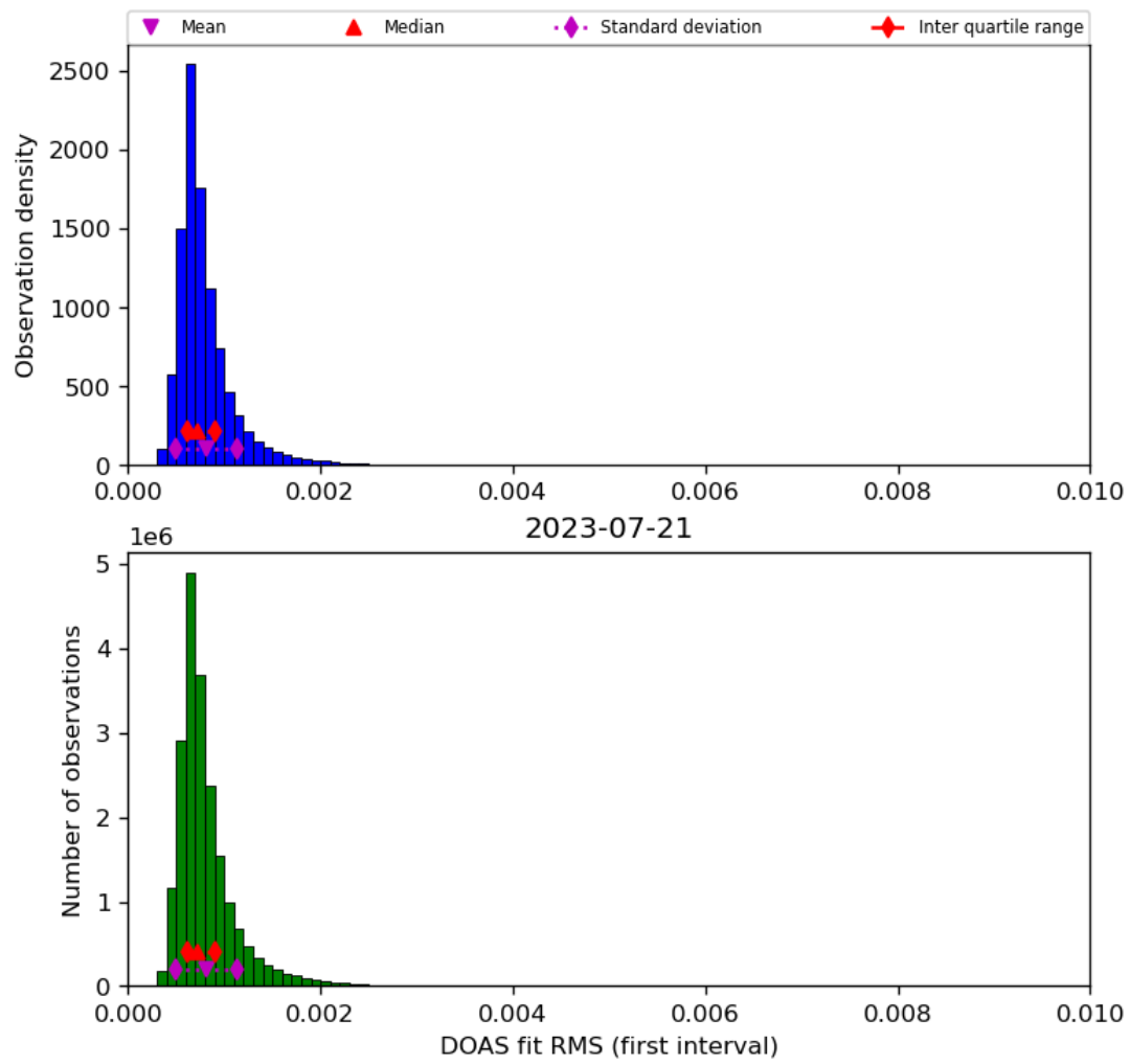
Figure 46: Histogram of “DOAS fit RMS (first interval)” for 2023-07-20 to 2023-07-22
