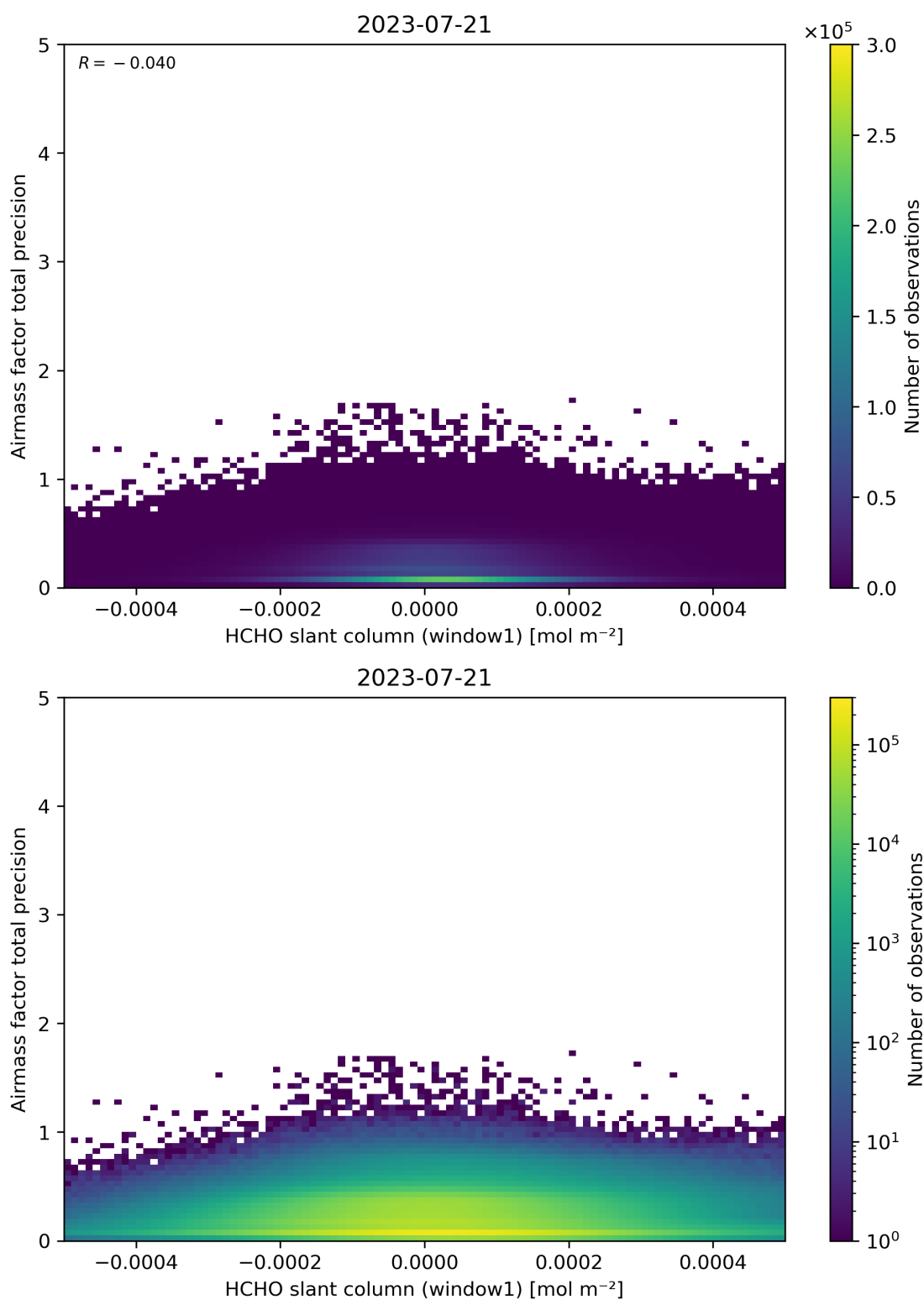
Figure 86: Scatter density plot of “HCHO slant column (window1)” against “Airmass factor total precision” for 2023-07-20 to 2023-07-22.
