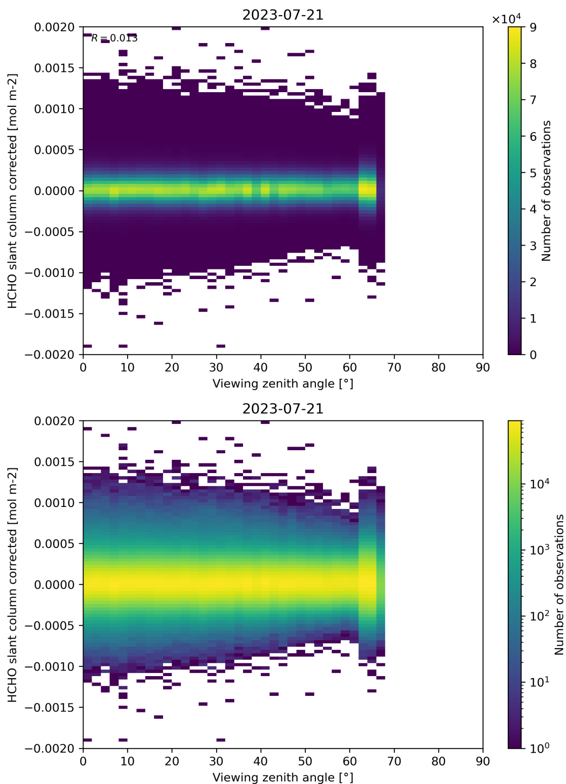
Figure 186: Scatter density plot of “Viewing zenith angle” against “HCHO slant column corrected” for 2023-07-20 to 2023-07-22.
