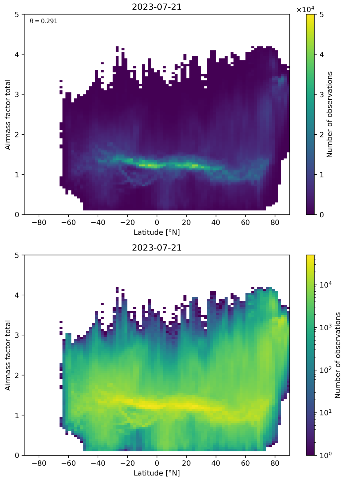
Figure 161: Scatter density plot of “Latitude” against “Airmass factor total” for 2023-07-20 to 2023-07-22.
