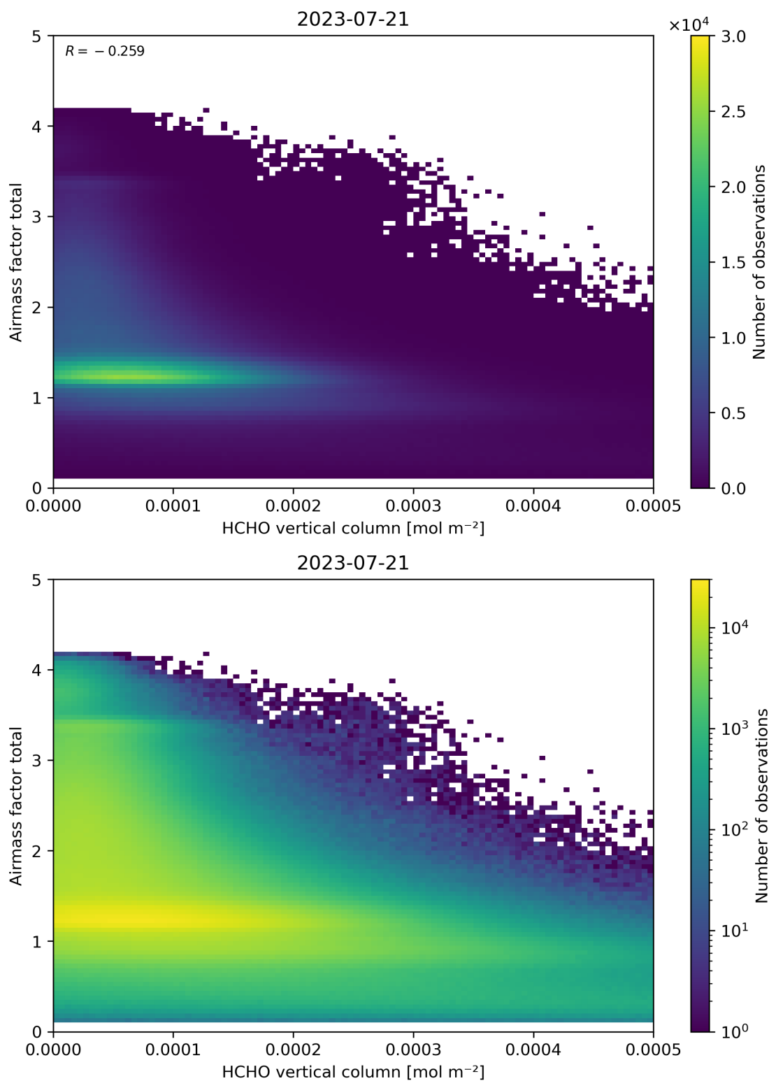
Figure 131: Scatter density plot of “HCHO vertical column” against “Airmass factor total” for 2023-07-20 to 2023-07-22.
