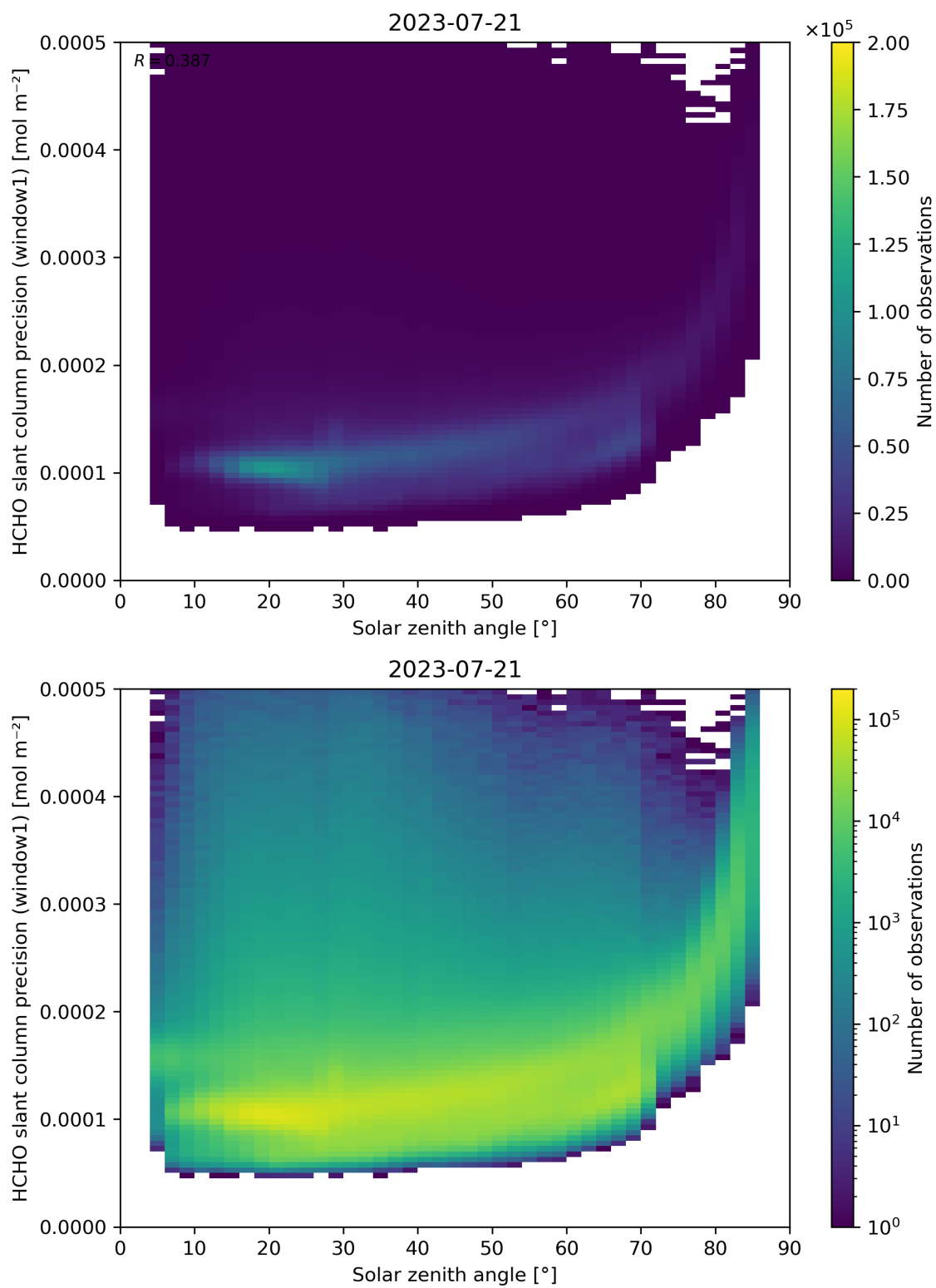
Figure 174: Scatter density plot of “Solar zenith angle” against “HCHO slant column precision (window1)” for 2023-07-20 to 2023-07-22.
