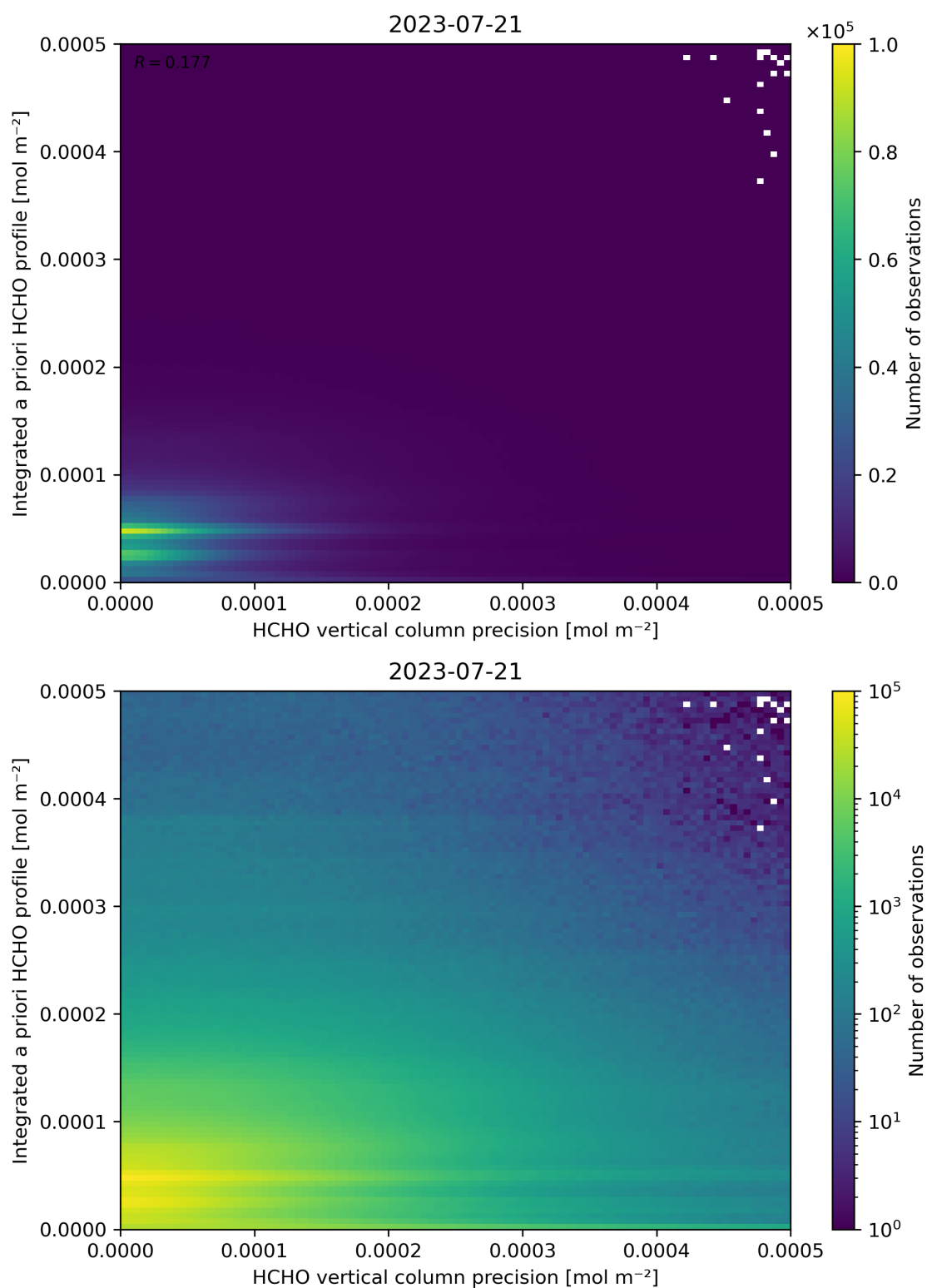
Figure 147: Scatter density plot of “HCHO vertical column precision” against “Integrated a priori HCHO profile” for 2023-07-20 to 2023-07-22.
