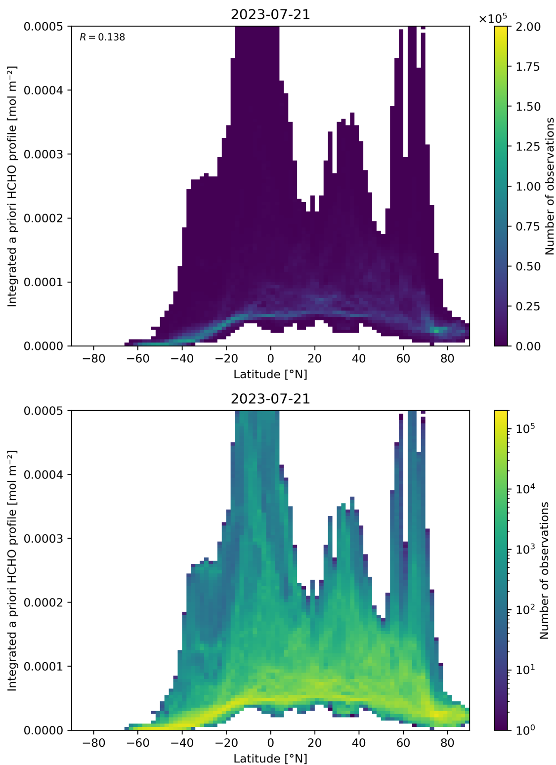
Figure 166: Scatter density plot of “Latitude” against “Integrated a priori HCHO profile” for 2023-07-20 to 2023-07-22.
