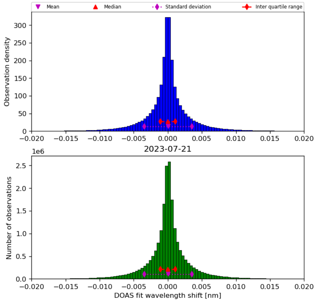
Figure 44: Histogram of “DOAS fit wavelength shift” for 2023-07-20 to 2023-07-22
