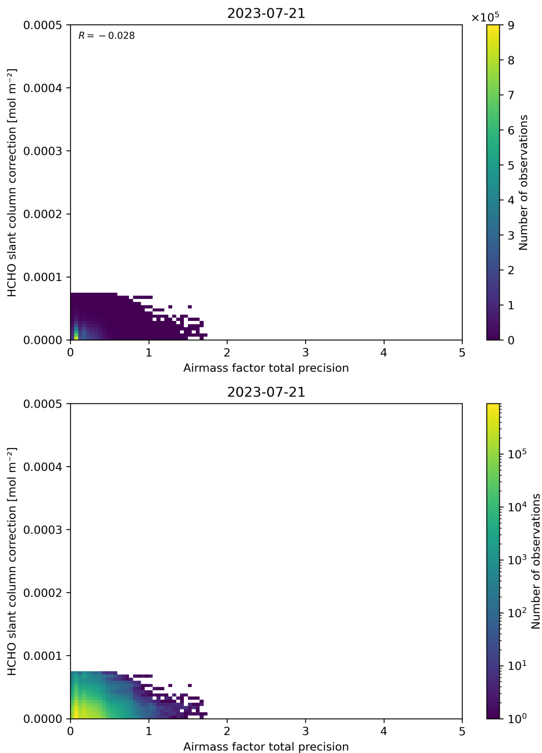
Figure 110: Scatter density plot of “Airmass factor total precision” against “HCHO slant column correction” for 2023-07-20 to 2023-07-22.
