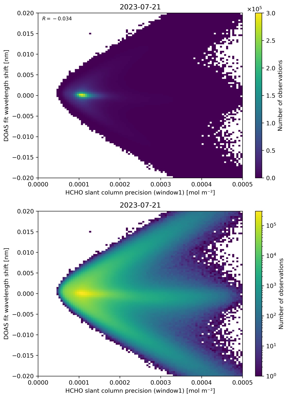
Figure 89: Scatter density plot of “HCHO slant column precision (window1)” against “DOAS fit wavelength shift” for 2023-07-20 to 2023-07-22.
