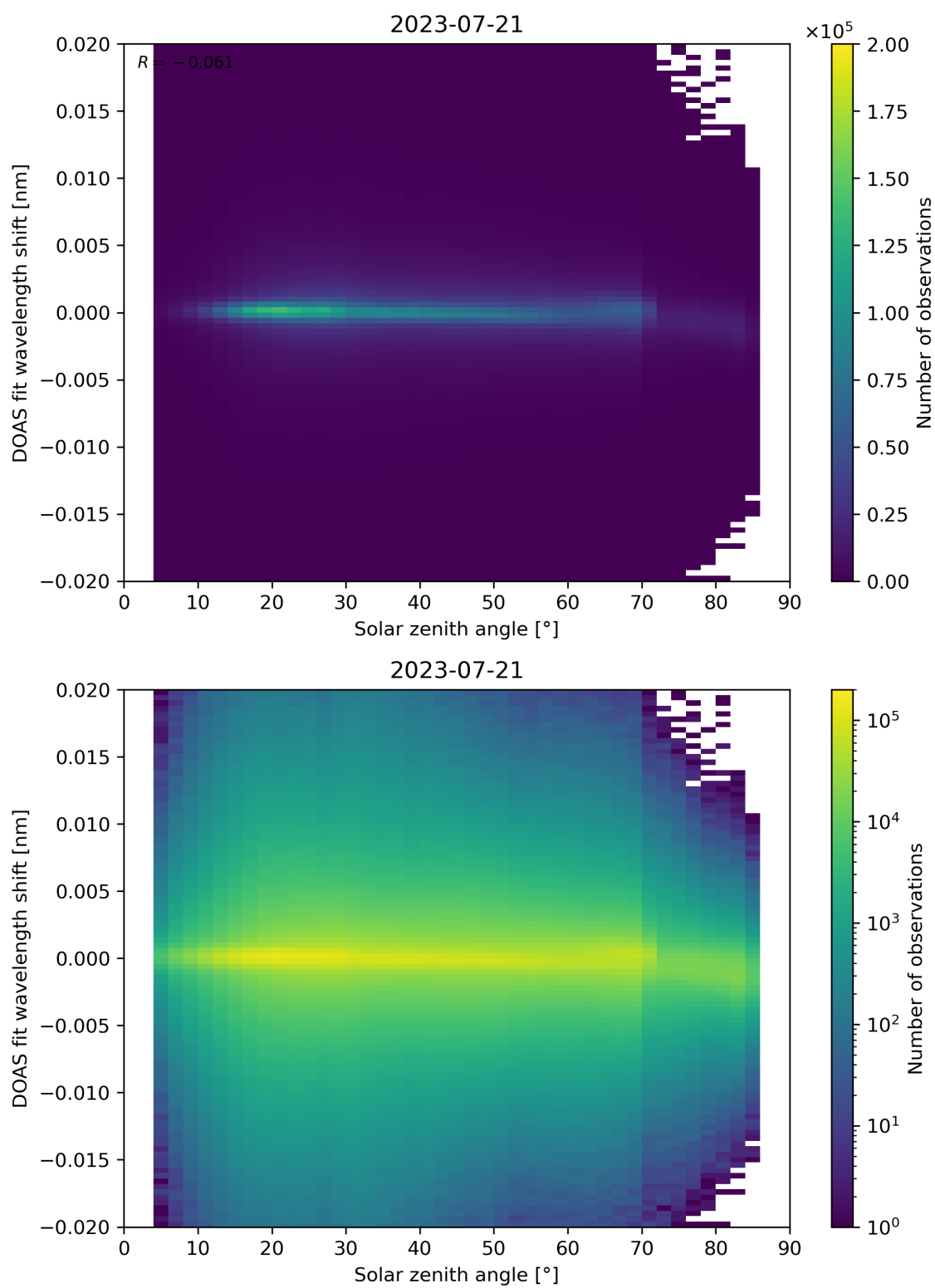
Figure 168: Scatter density plot of “Solar zenith angle” against “DOAS fit wavelength shift” for 2023-07-20 to 2023-07-22.
