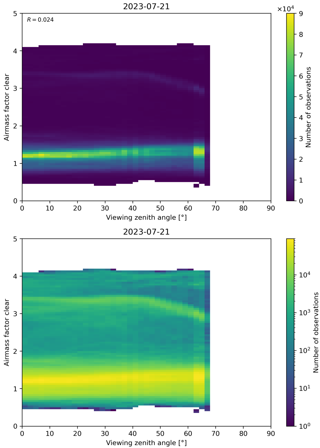
Figure 185: Scatter density plot of “Viewing zenith angle” against “Airmass factor clear” for 2023-07-20 to 2023-07-22.
