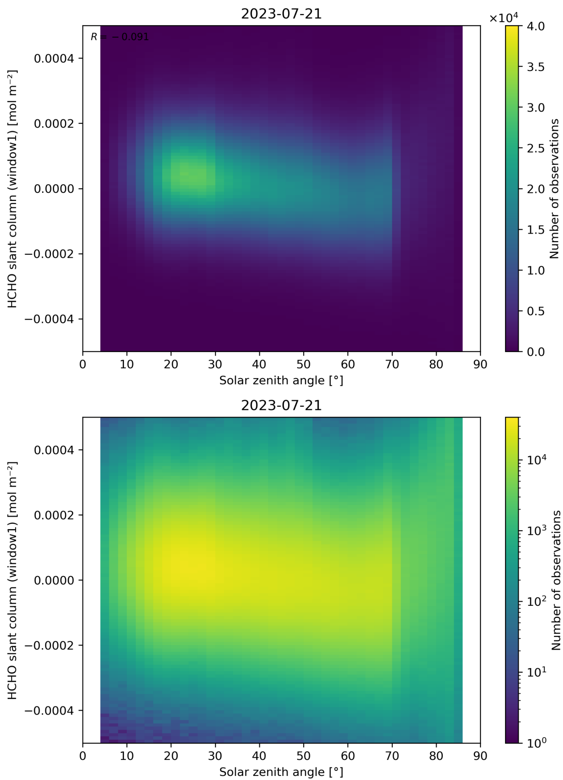
Figure 173: Scatter density plot of “Solar zenith angle” against “HCHO slant column (window1)” for 2023-07-20 to 2023-07-22.
