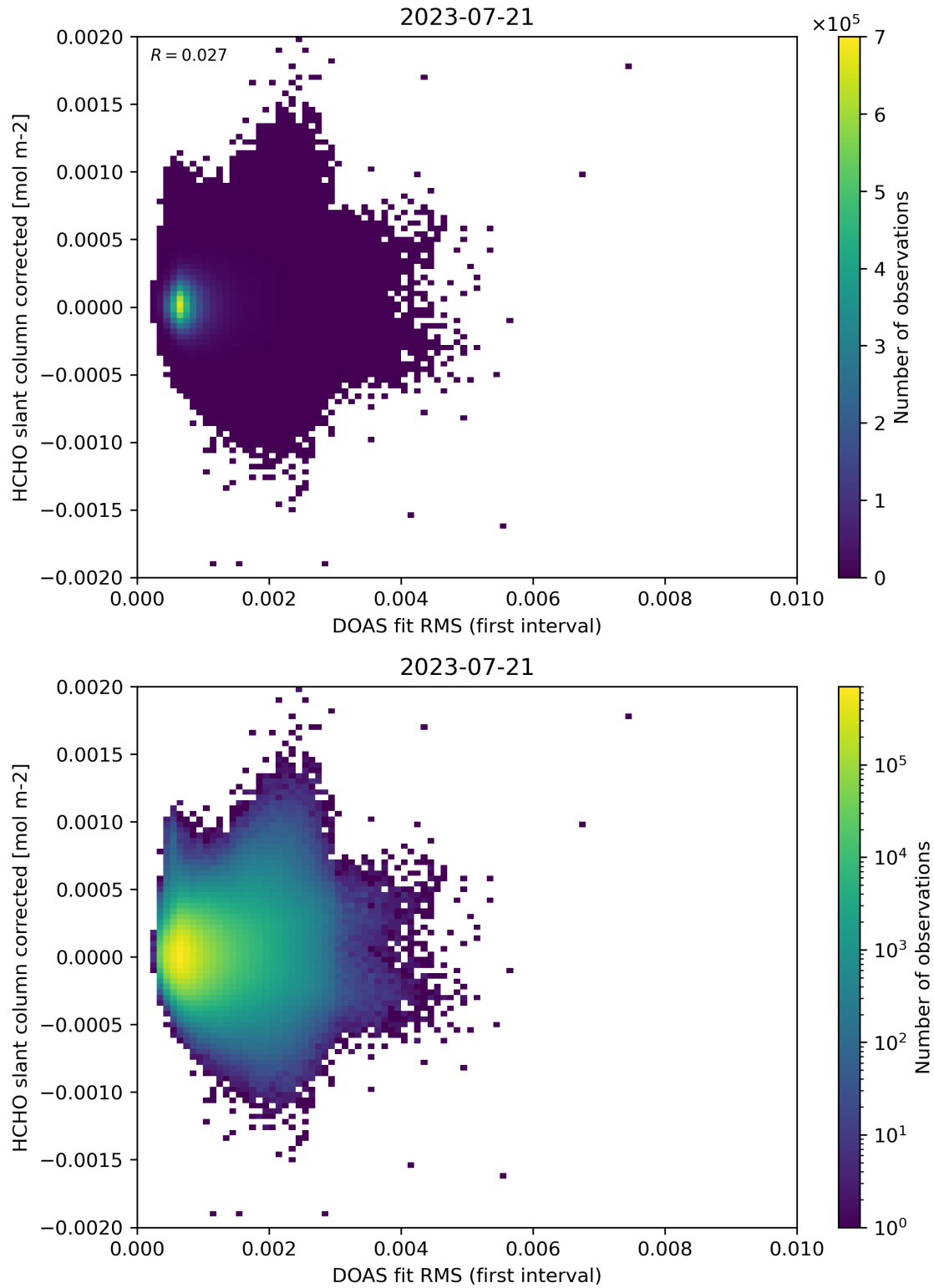
Figure 62: Scatter density plot of “DOAS fit RMS (first interval)” against “HCHO slant column corrected” for 2023-07-20 to 2023-07-22.
