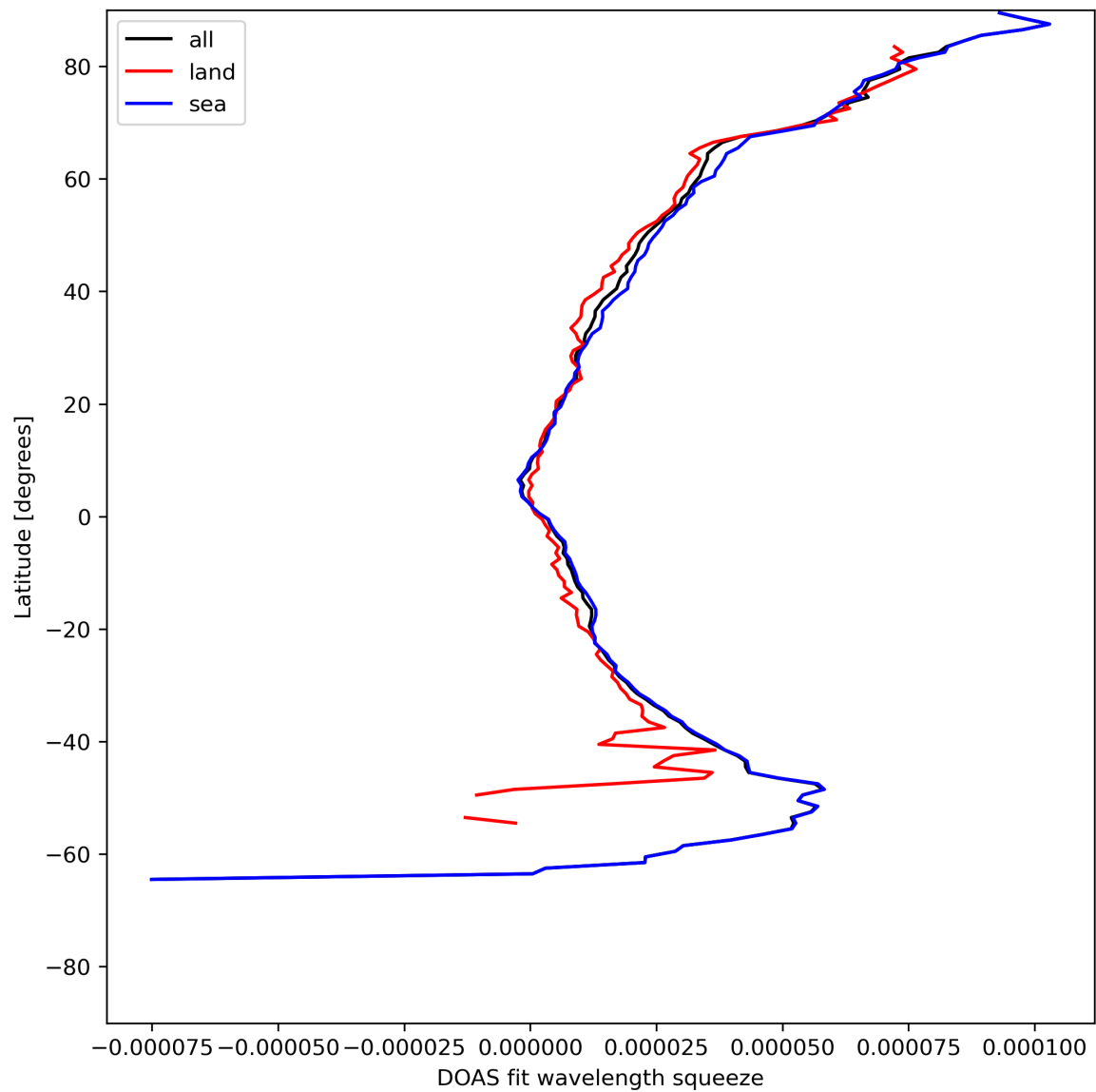
Figure 31: Zonal average of “DOAS fit wavelength squeeze” for 2023-07-20 to 2023-07-22.
