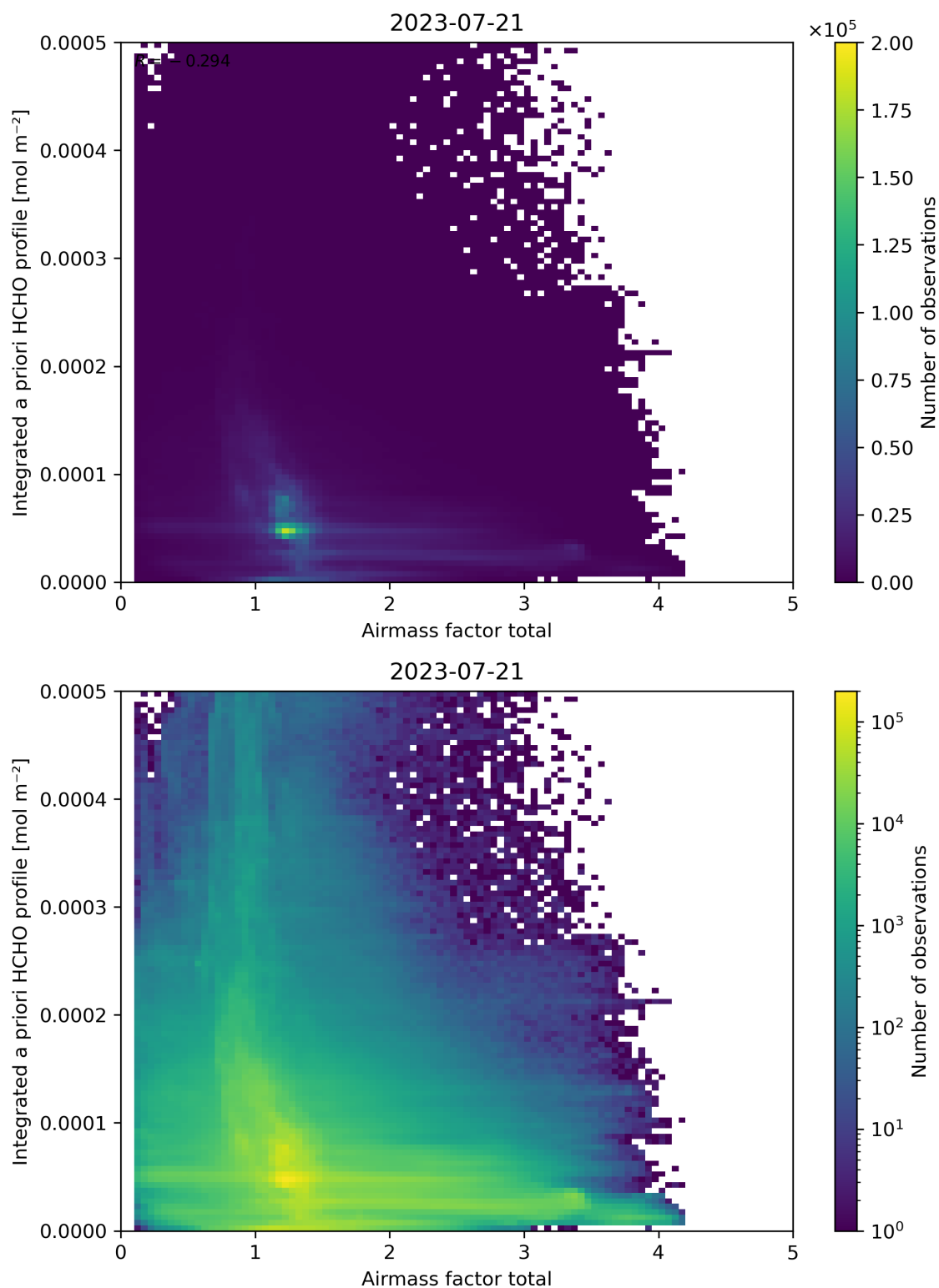
Figure 104: Scatter density plot of “Airmass factor total” against “Integrated a priori HCHO profile” for 2023-07-20 to 2023-07-22.
