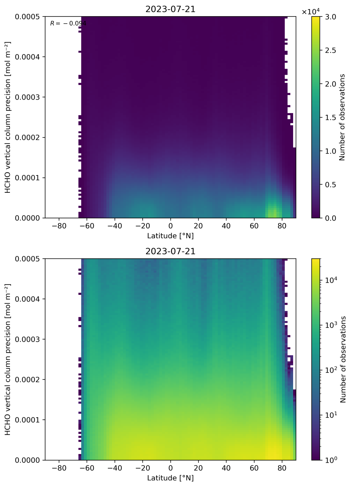
Figure 165: Scatter density plot of “Latitude” against “HCHO vertical column precision” for 2023-07-20 to 2023-07-22.
