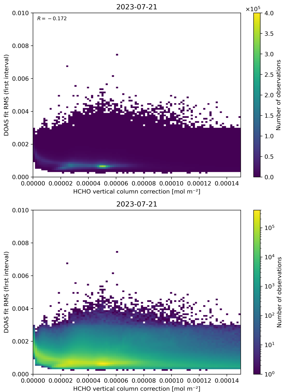
Figure 112: Scatter density plot of “HCHO vertical column correction” against “DOAS fit RMS (first interval)” for 2023-07-20 to 2023-07-22.
