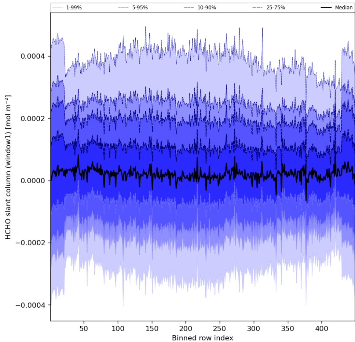
Figure 52: Along track statistics of “HCHO slant column (window1)” for 2023-07-20 to 2023-07-22
