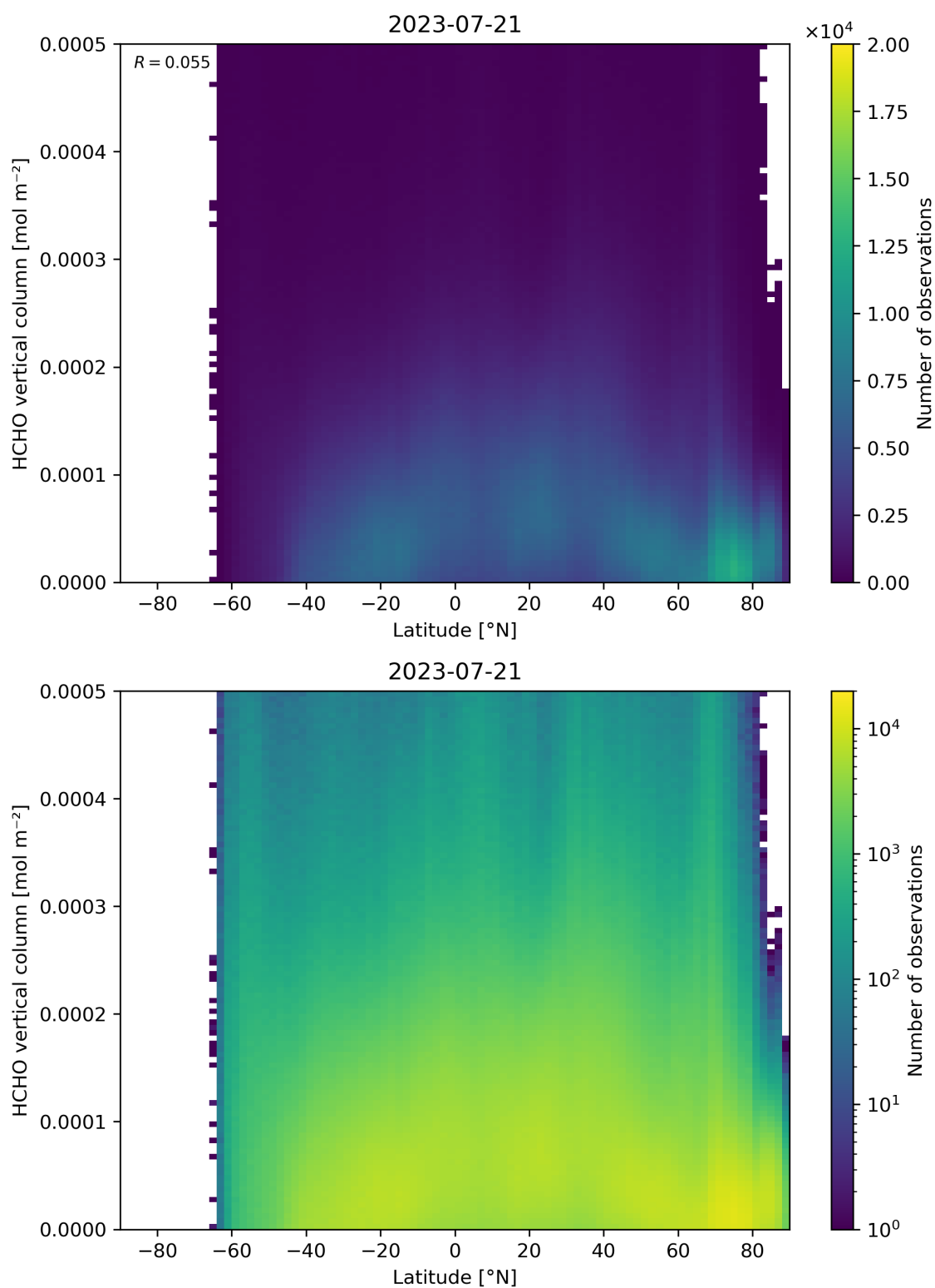
Figure 163: Scatter density plot of “Latitude” against “HCHO vertical column” for 2023-07-20 to 2023-07-22.
