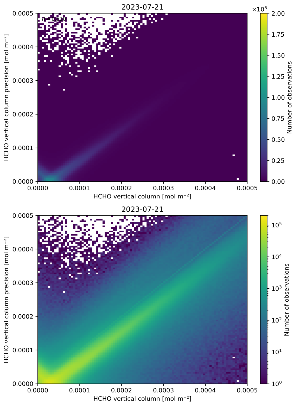
Figure 134: Scatter density plot of “HCHO vertical column” against “HCHO vertical column precision” for 2023-07-20 to 2023-07-22.
