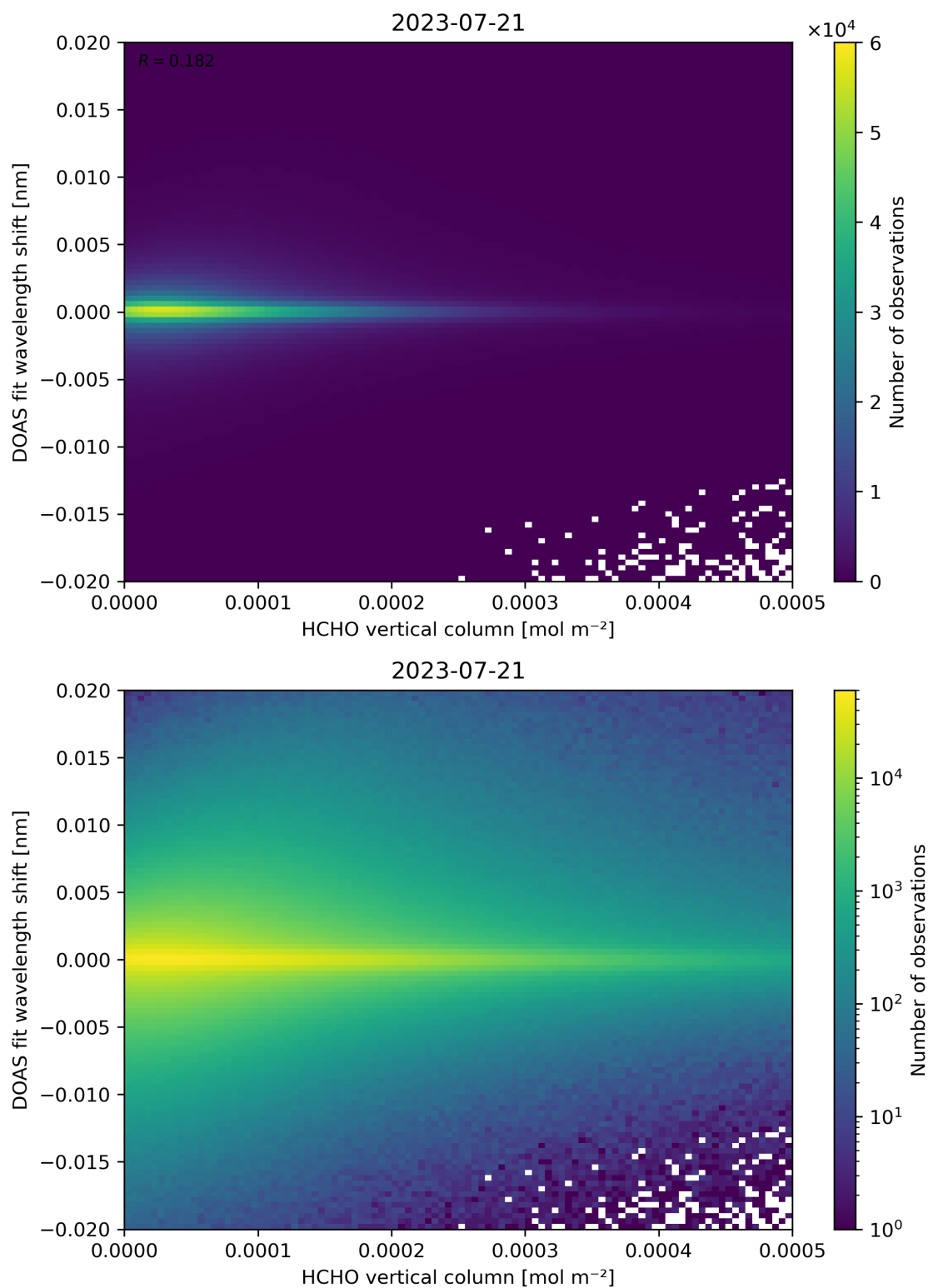
Figure 124: Scatter density plot of “HCHO vertical column” against “DOAS fit wavelength shift” for 2023-07-20 to 2023-07-22.
