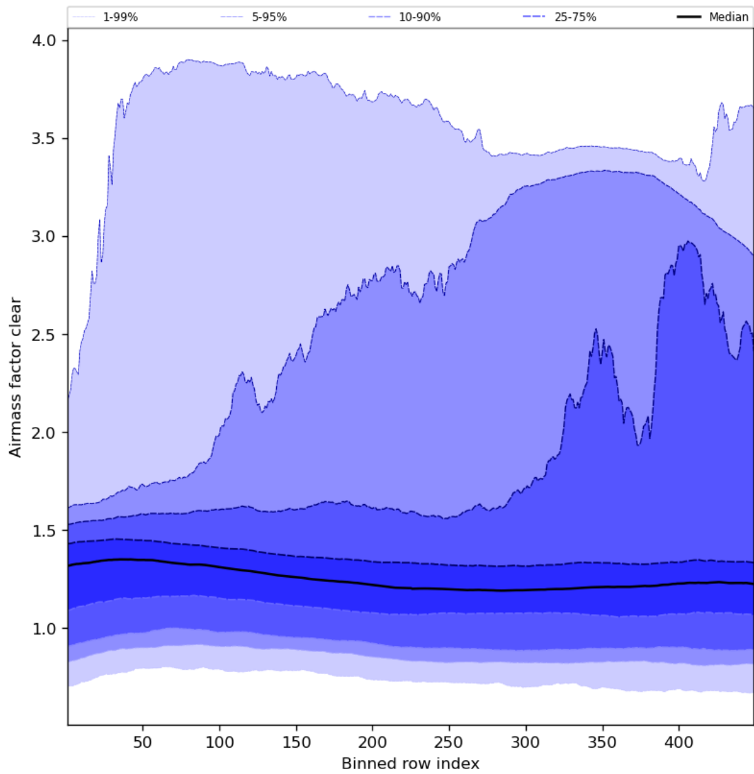
Figure 56: Along track statistics of “Airmass factor clear” for 2023-07-20 to 2023-07-22
