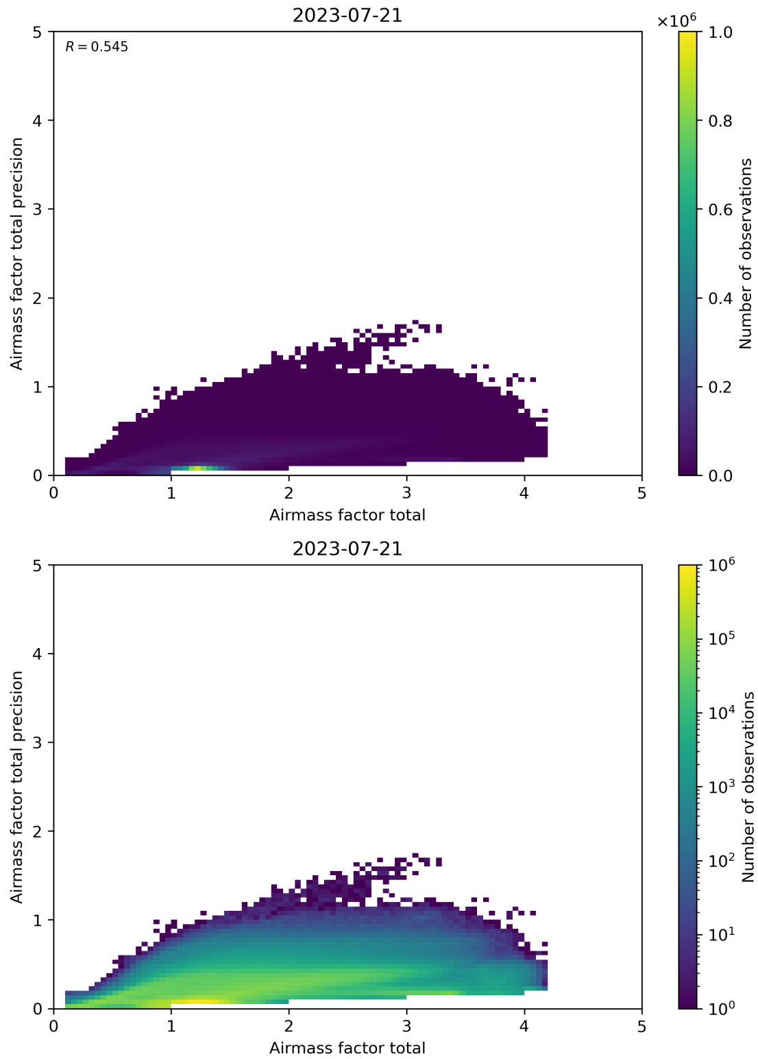
Figure 103: Scatter density plot of “Airmass factor total” against “Airmass factor total precision” for 2023-07-20 to 2023-07-22.
