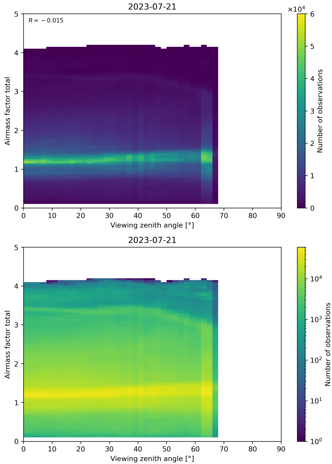
Figure 190: Scatter density plot of “Viewing zenith angle” against “Airmass factor total” for 2023-07-20 to 2023-07-22.
