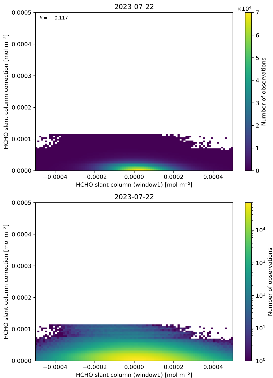
Figure 83: Scatter density plot of “HCHO slant column (window1)” against “HCHO slant column correction” for 2023-07-21 to 2023-07-23.
