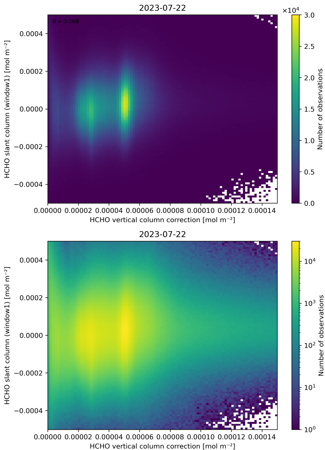
Figure 118: Scatter density plot of “HCHO vertical column correction” against “HCHO slant column (window1)” for 2023-07-21 to 2023-07-23.
