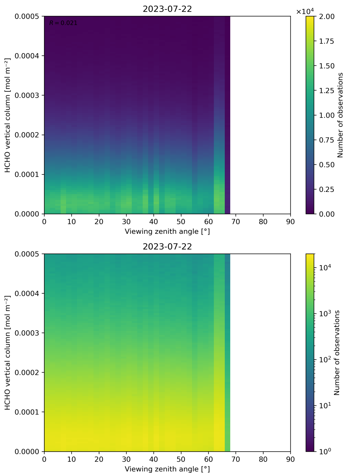
Figure 192: Scatter density plot of “Viewing zenith angle” against “HCHO vertical column” for 2023-07-21 to 2023-07-23.
