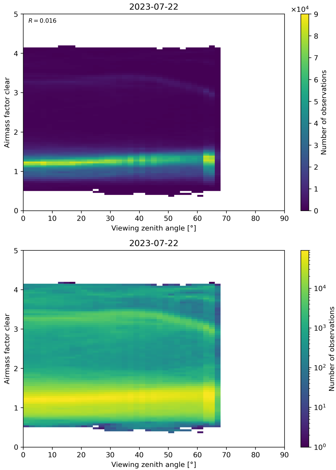
Figure 185: Scatter density plot of “Viewing zenith angle” against “Airmass factor clear” for 2023-07-21 to 2023-07-23.
