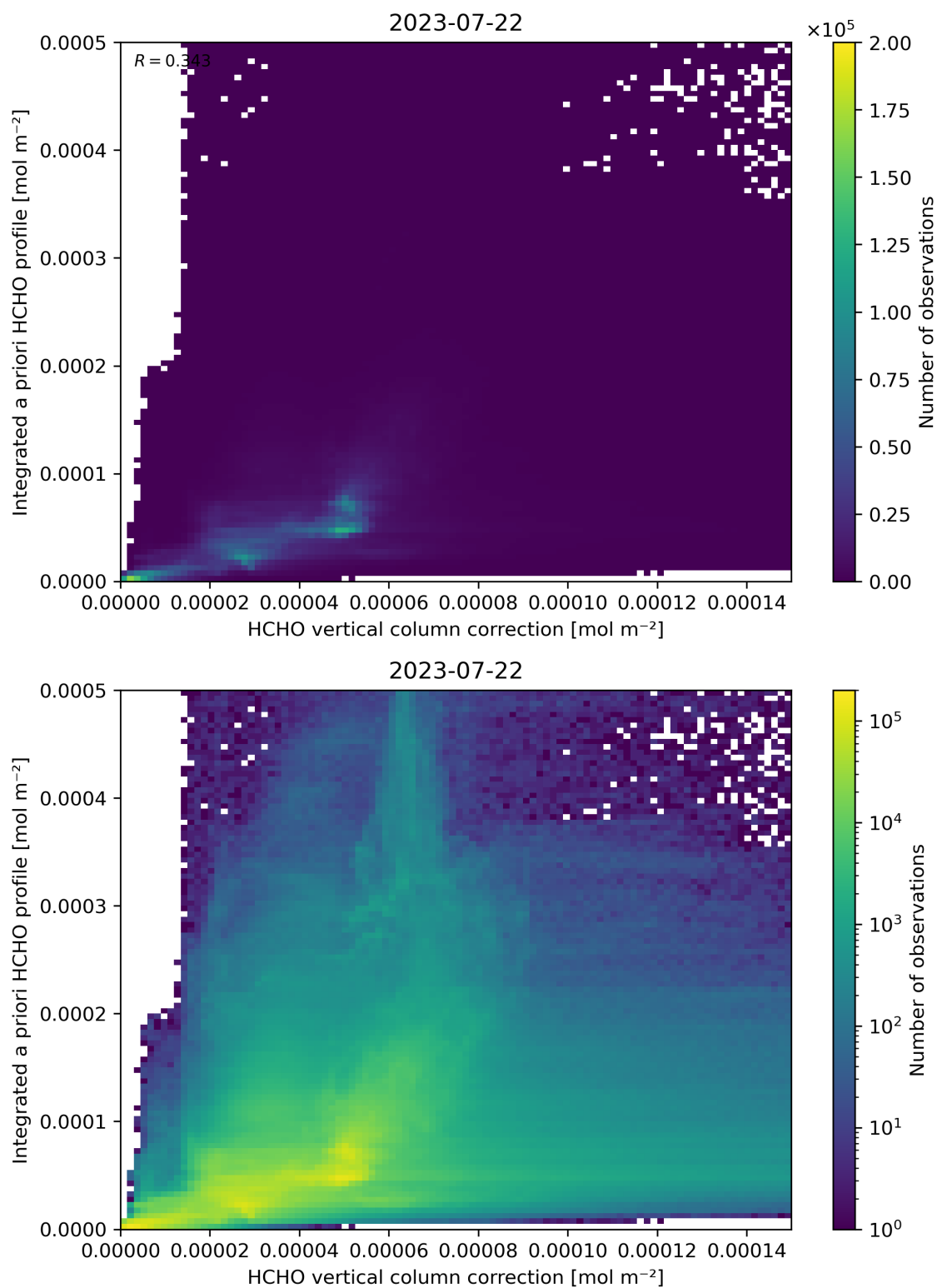
Figure 122: Scatter density plot of “HCHO vertical column correction” against “Integrated a priori HCHO profile” for 2023-07-21 to 2023-07-23.
