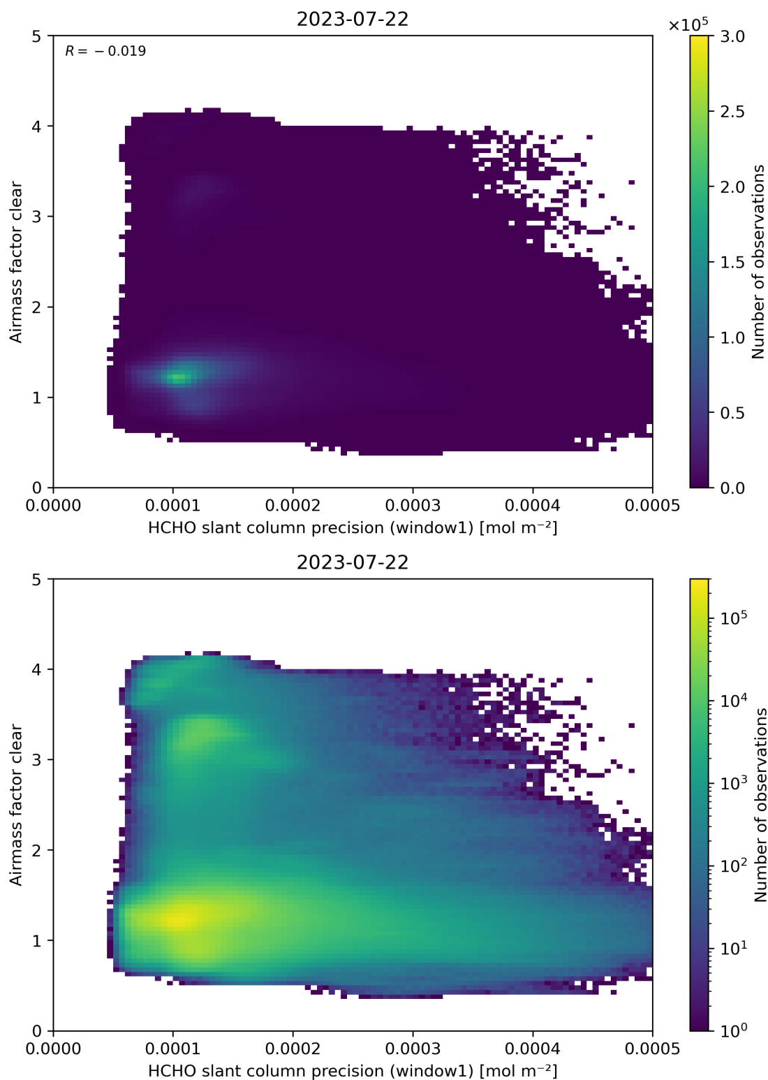
Figure 91: Scatter density plot of “HCHO slant column precision (window1)” against “Airmass factor clear” for 2023-07-21 to 2023-07-23.
