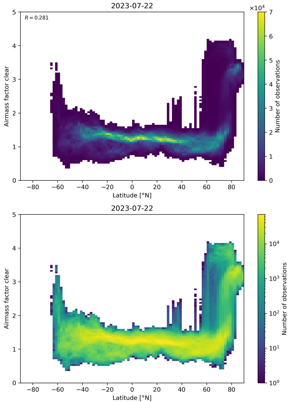
Figure 156: Scatter density plot of “Latitude” against “Airmass factor clear” for 2023-07-21 to 2023-07-23.
