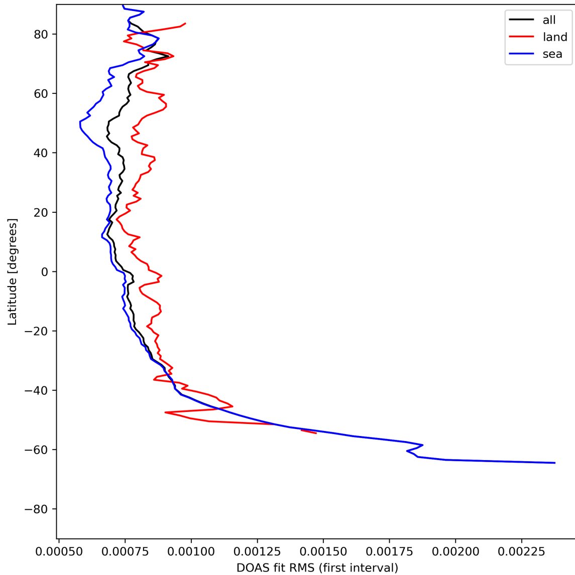
Figure 32: Zonal average of "DOAS fit RMS (first interval)" for 2023-07-21 to 2023-07-23.
