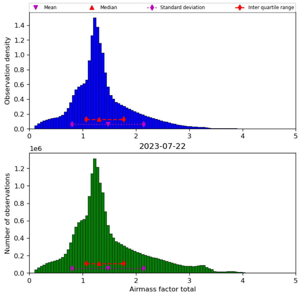
Figure 40: Histogram of “Airmass factor total” for 2023-07-21 to 2023-07-23
