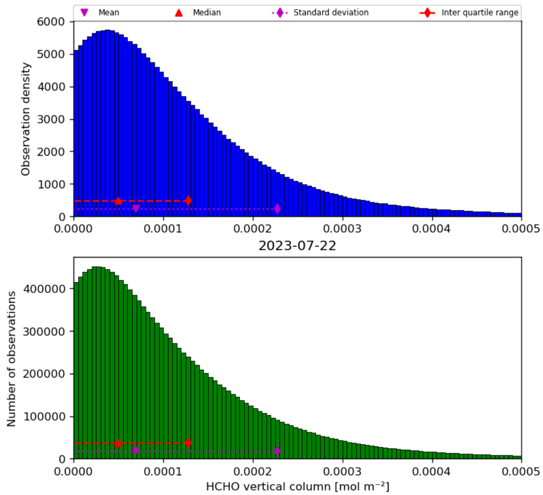
Figure 35: Histogram of “HCHO vertical column” for 2023-07-21 to 2023-07-23
