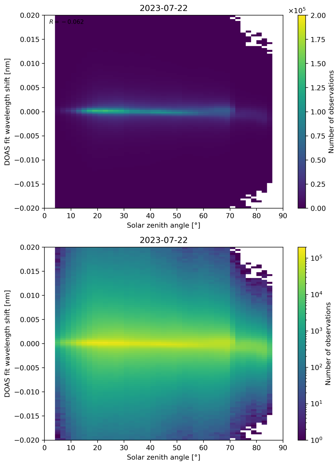
Figure 168: Scatter density plot of “Solar zenith angle” against “DOAS fit wavelength shift” for 2023-07-21 to 2023-07-23.
