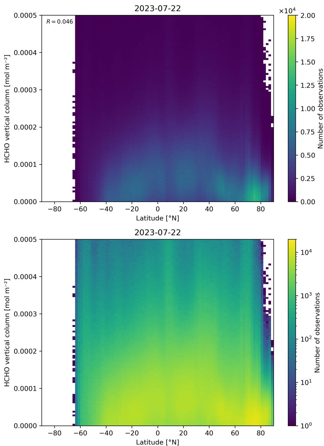
Figure 163: Scatter density plot of “Latitude” against “HCHO vertical column” for 2023-07-21 to 2023-07-23.
