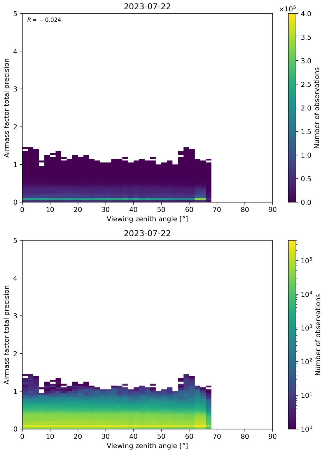
Figure 191: Scatter density plot of “Viewing zenith angle” against “Airmass factor total precision” for 2023-07-21 to 2023-07-23.
