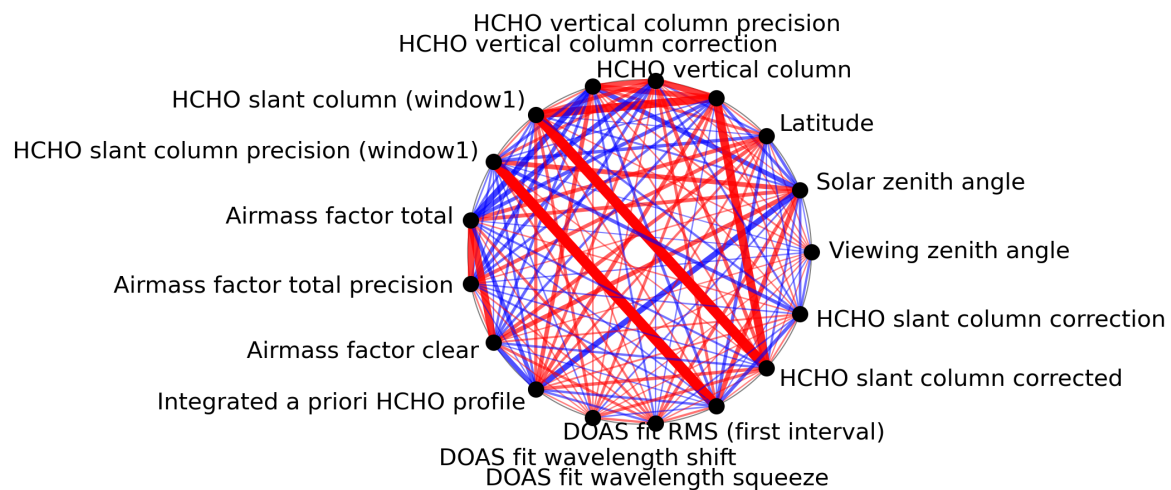
Figure 1: Map of correlation graph for 2023-07-21 to 2023-07-23.
