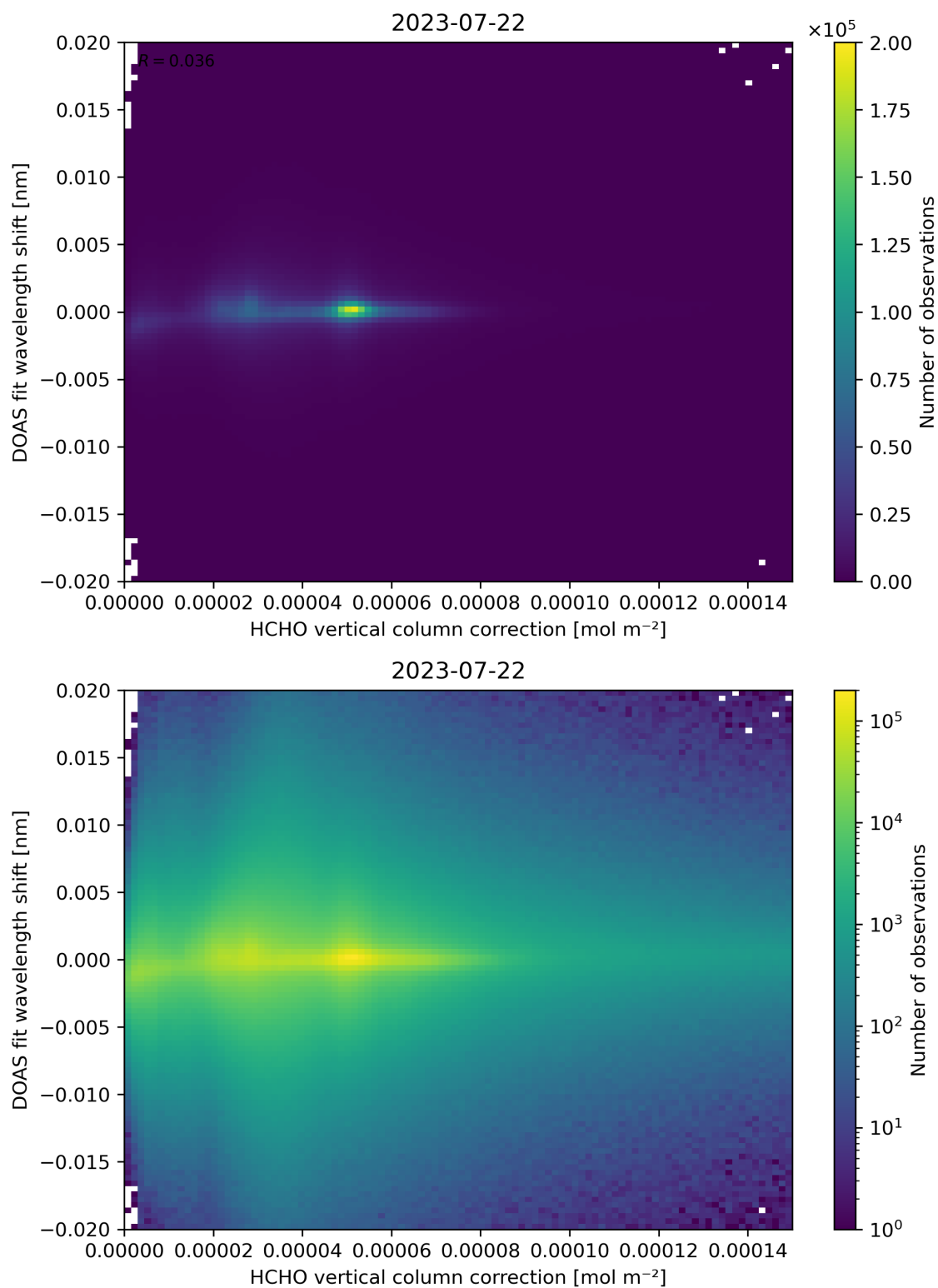
Figure 113: Scatter density plot of “HCHO vertical column correction” against “DOAS fit wavelength shift” for 2023-07-21 to 2023-07-23.
