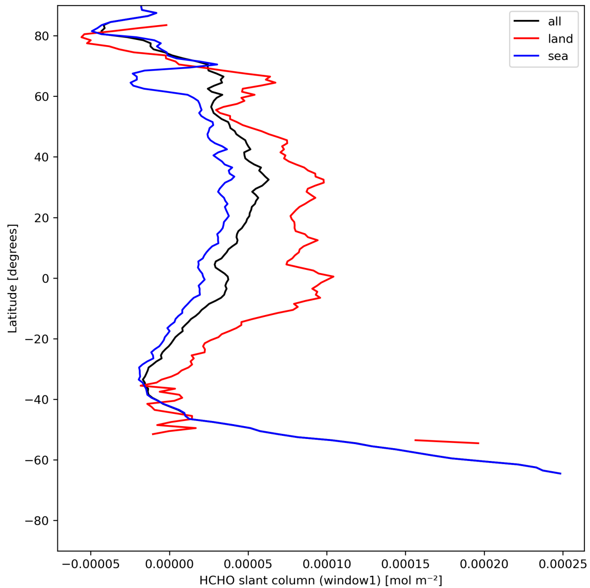
Figure 24: Zonal average of “HCHO slant column (window1)” for 2023-07-21 to 2023-07-23.
