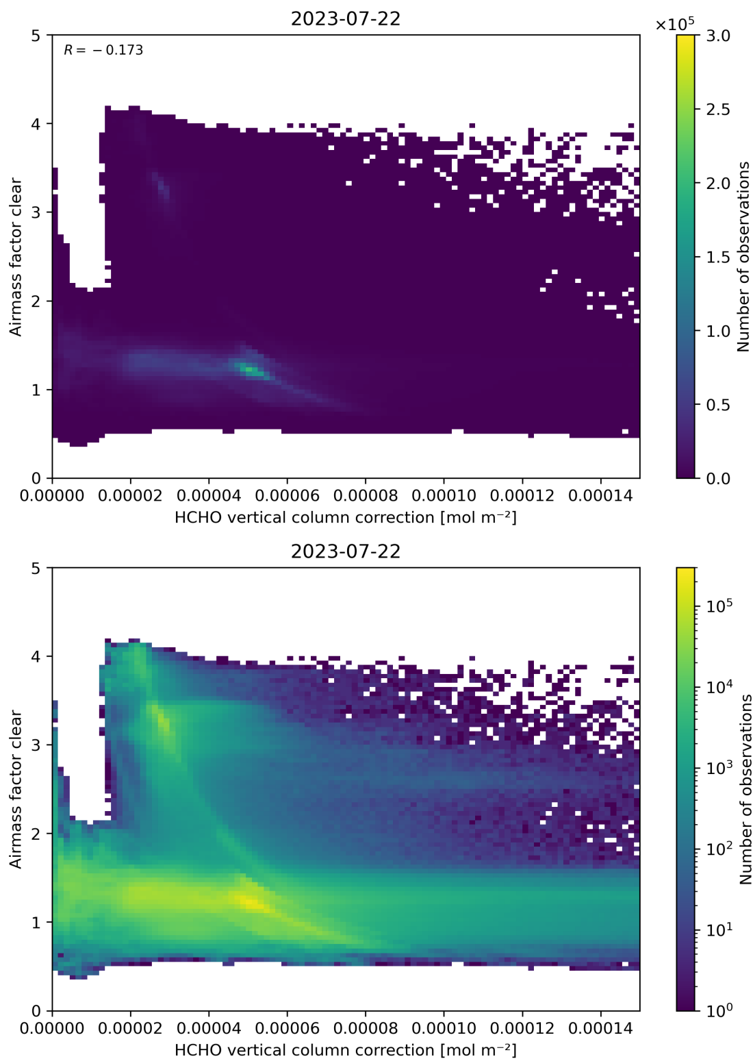
Figure 115: Scatter density plot of “HCHO vertical column correction” against “Airmass factor clear” for 2023-07-21 to 2023-07-23.
