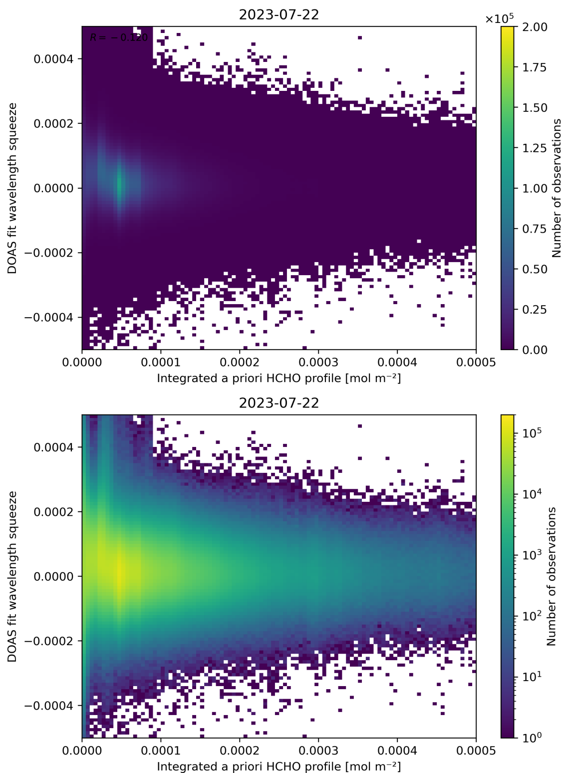
Figure 150: Scatter density plot of “Integrated a priori HCHO profile” against “DOAS fit wavelength squeeze” for 2023-07-21 to 2023-07-23.
