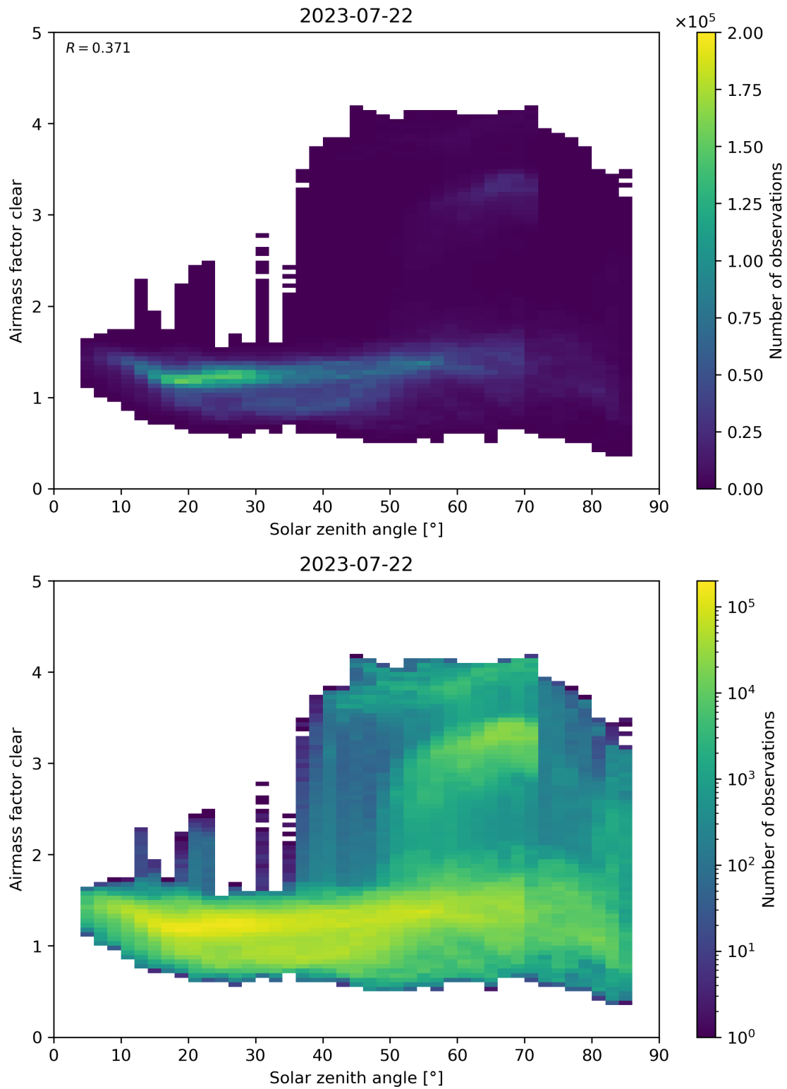
Figure 170: Scatter density plot of “Solar zenith angle” against “Airmass factor clear” for 2023-07-21 to 2023-07-23.
