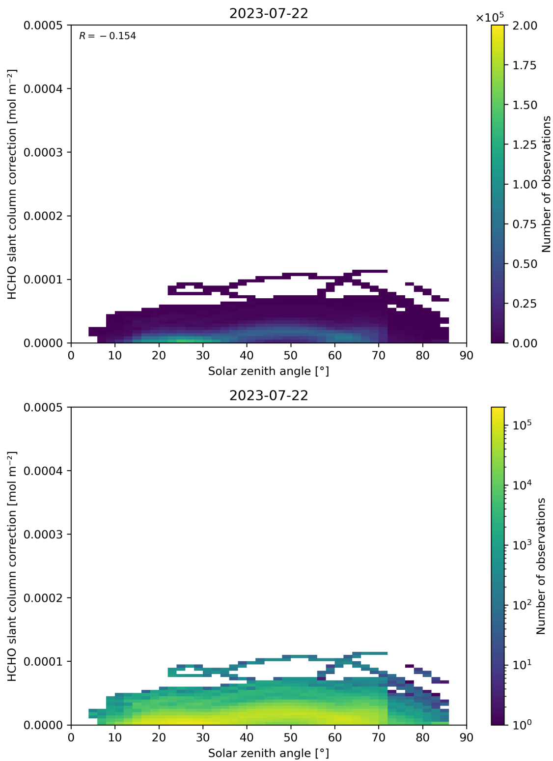
Figure 172: Scatter density plot of “Solar zenith angle” against “HCHO slant column correction” for 2023-07-21 to 2023-07-23.
