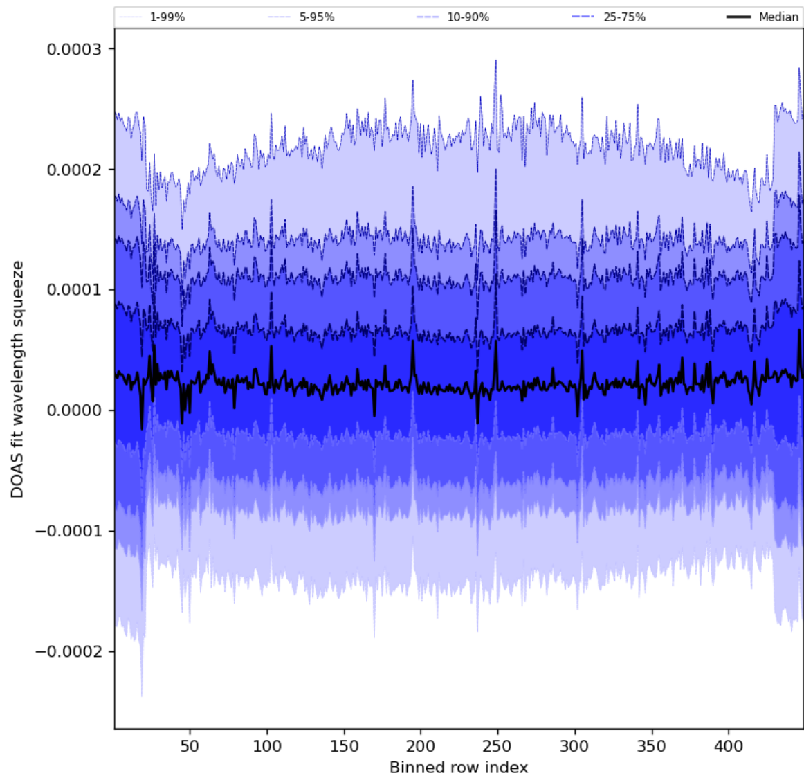
Figure 59: Along track statistics of “DOAS fit wavelength squeeze” for 2023-07-21 to 2023-07-23
