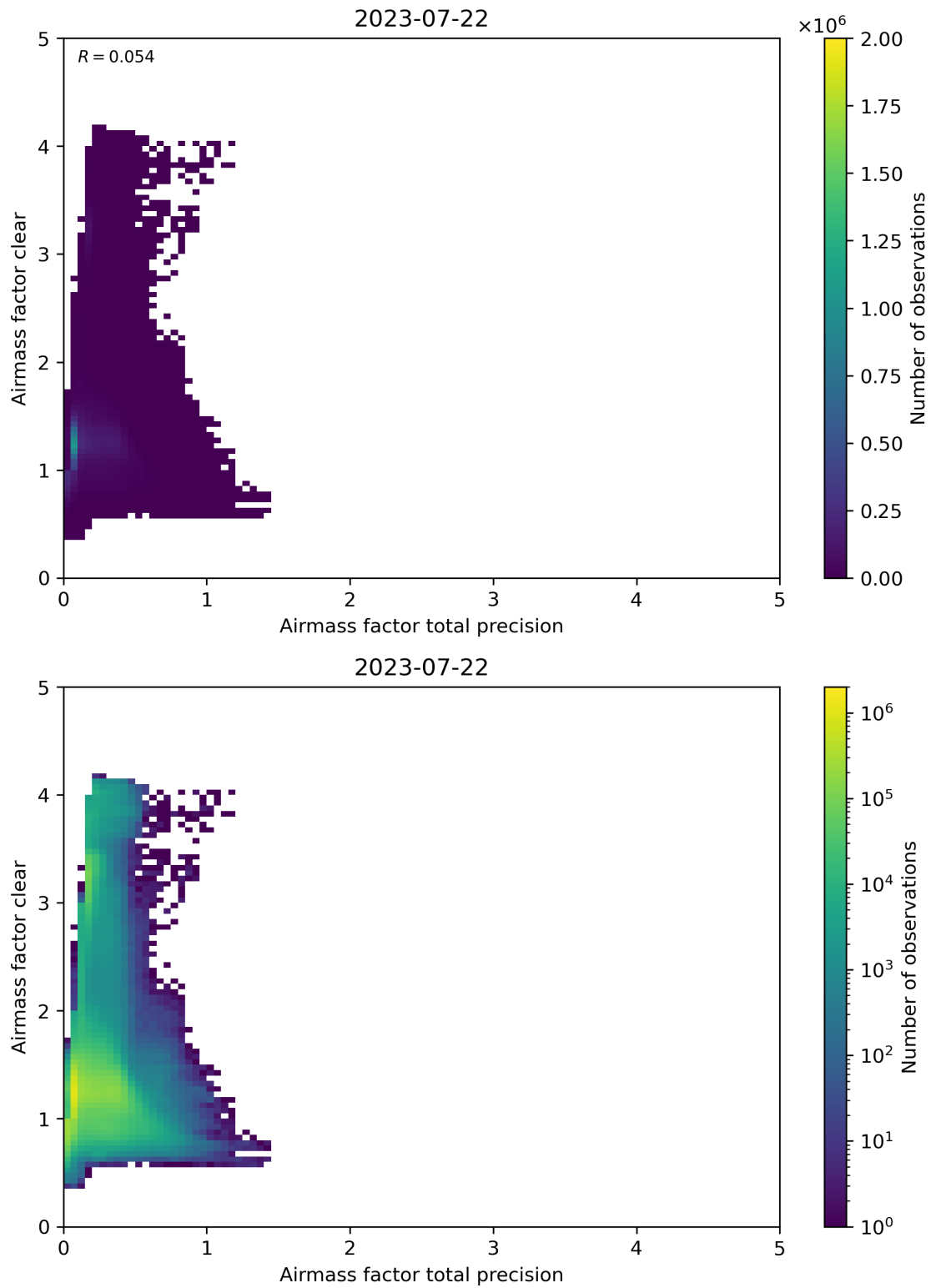
Figure 108: Scatter density plot of “Airmass factor total precision” against “Airmass factor clear” for 2023-07-21 to 2023-07-23.
