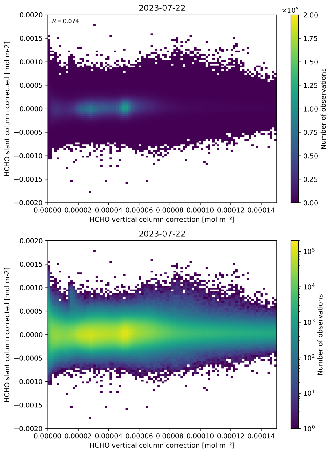
Figure 116: Scatter density plot of “HCHO vertical column correction” against “HCHO slant column corrected” for 2023-07-21 to 2023-07-23.
