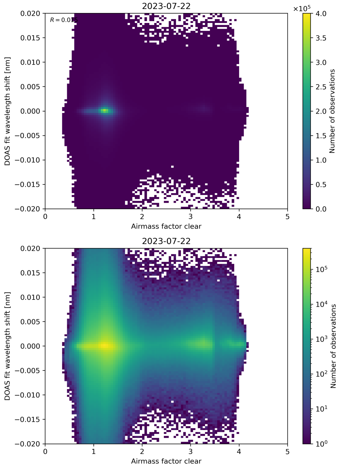
Figure 72: Scatter density plot of “Airmass factor clear” against “DOAS fit wavelength shift” for 2023-07-21 to 2023-07-23.
