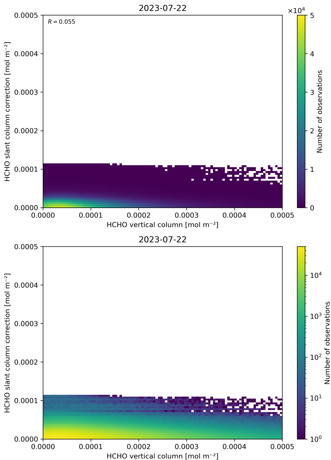
Figure 128: Scatter density plot of “HCHO vertical column” against “HCHO slant column correction” for 2023-07-21 to 2023-07-23.
