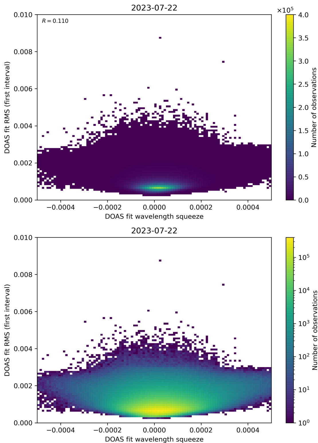
Figure 68: Scatter density plot of “DOAS fit wavelength squeeze” against “DOAS fit RMS (first interval)” for 2023-07-21 to 2023-07-23.
