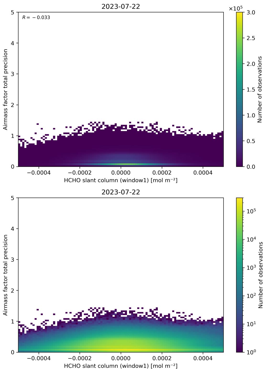
Figure 86: Scatter density plot of “HCHO slant column (window1)” against “Airmass factor total precision” for 2023-07-21 to 2023-07-23.
