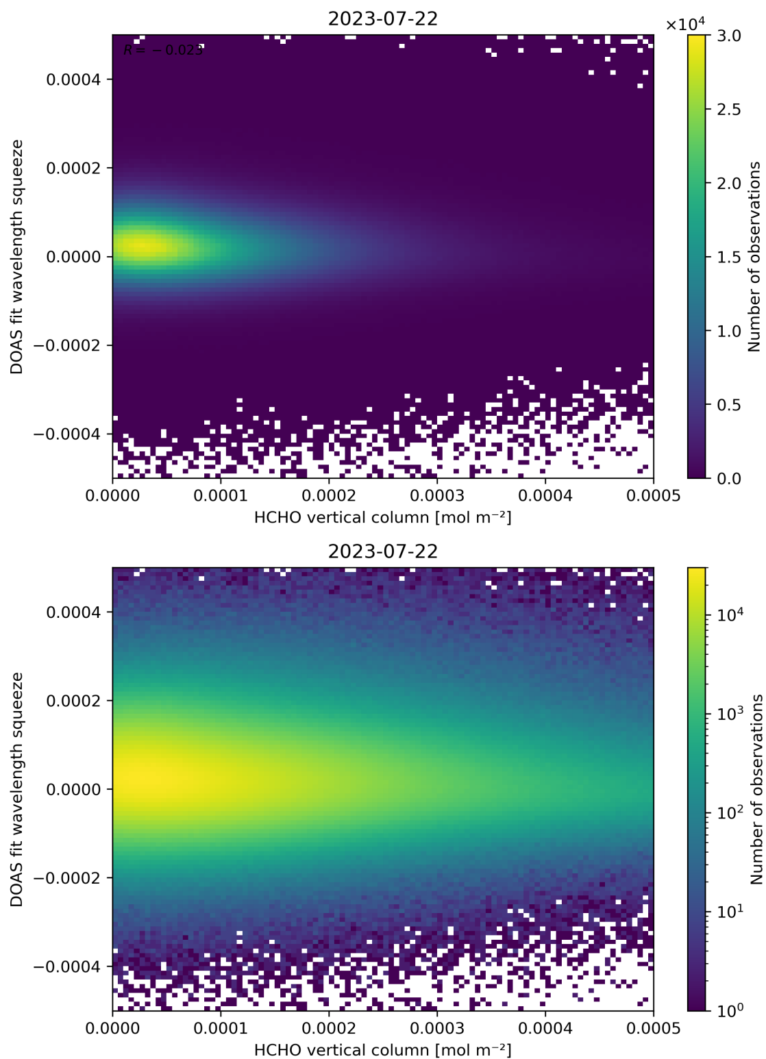
Figure 125: Scatter density plot of “HCHO vertical column” against “DOAS fit wavelength squeeze” for 2023-07-21 to 2023-07-23.
