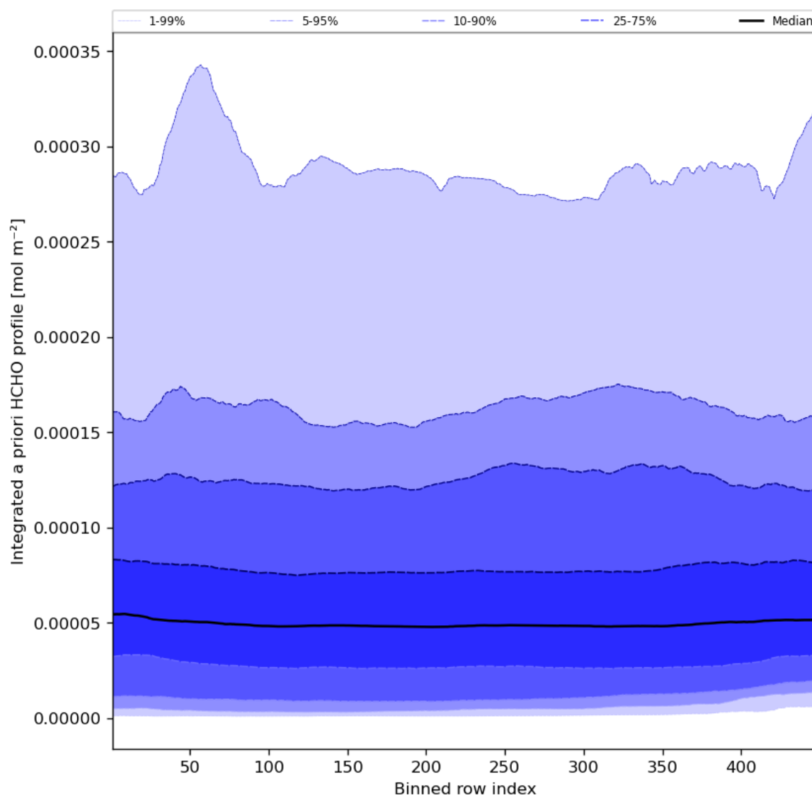
Figure 57: Along track statistics of “Integrated a priori HCHO profile” for 2023-07-21 to 2023-07-23
