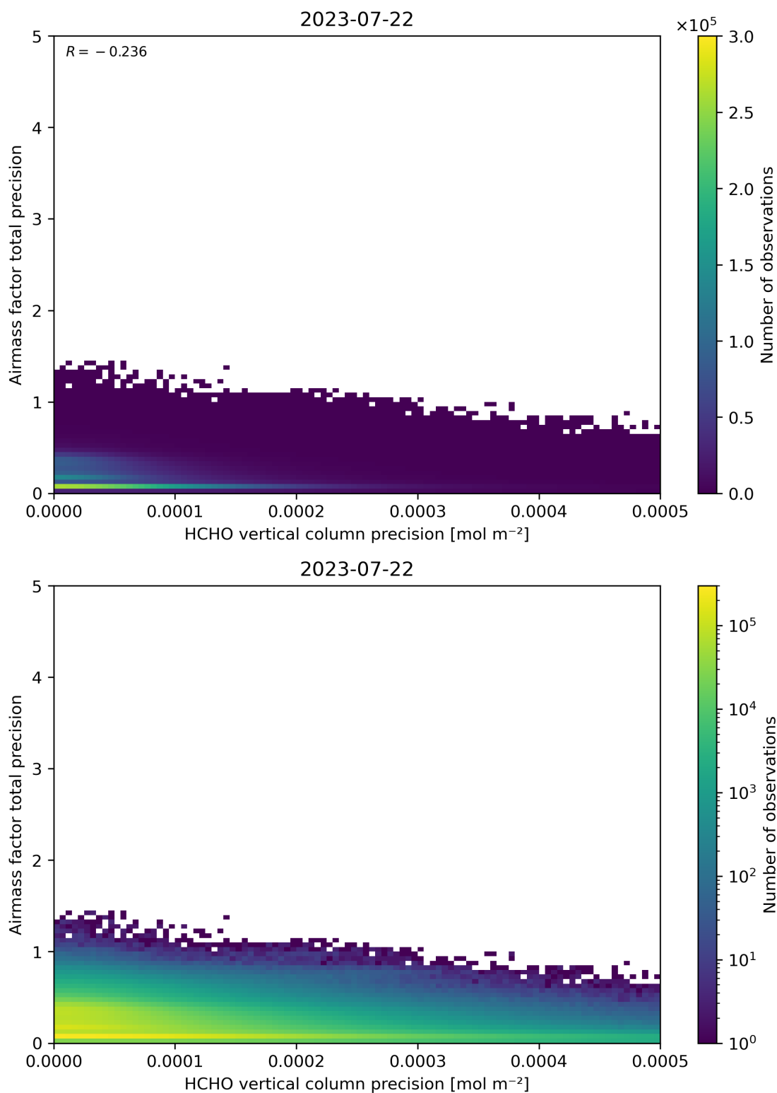
Figure 145: Scatter density plot of “HCHO vertical column precision” against “Airmass factor total precision” for 2023-07-21 to 2023-07-23.
