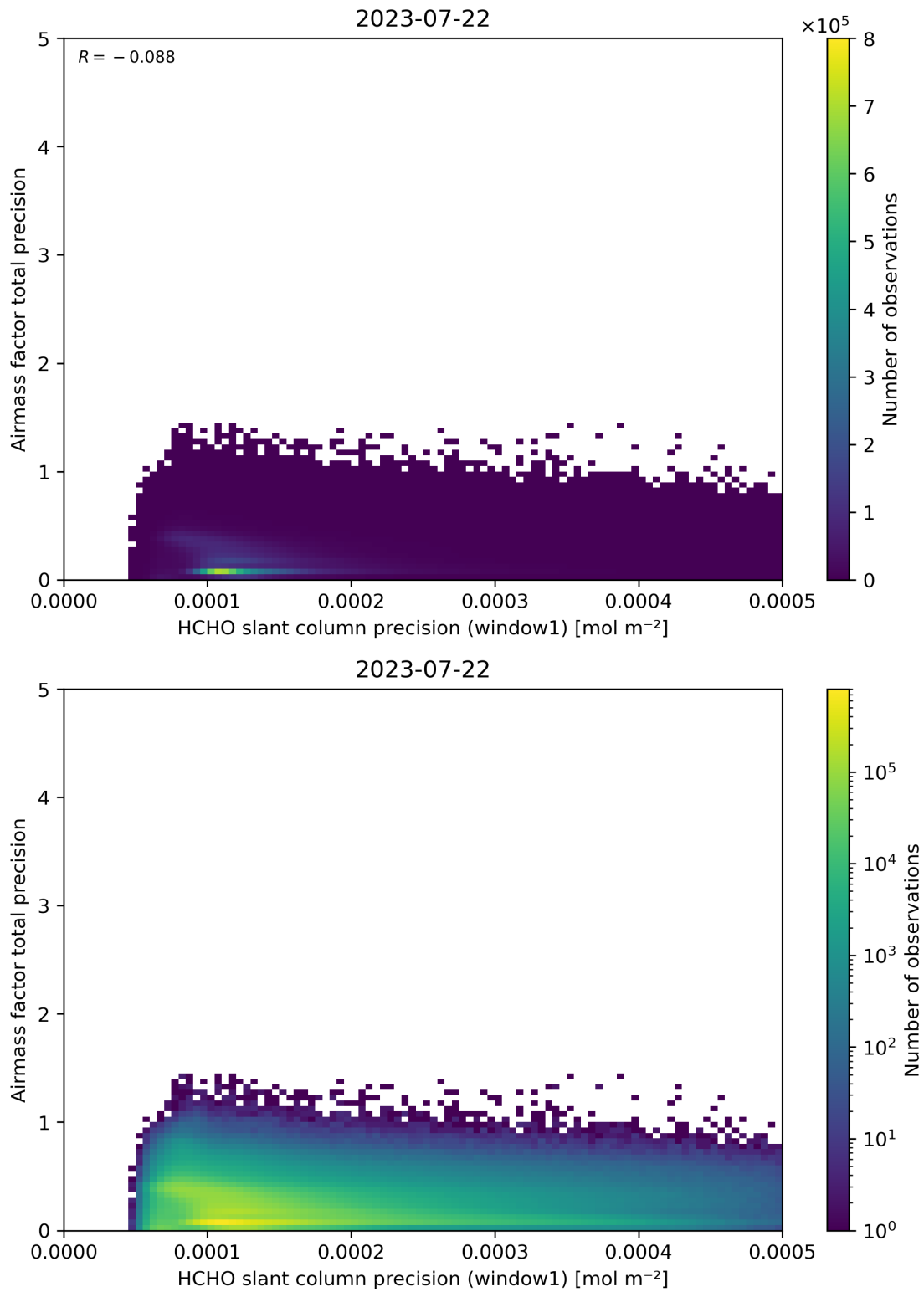
Figure 95: Scatter density plot of “HCHO slant column precision (window1)” against “Airmass factor total precision” for 2023-07-21 to 2023-07-23.
