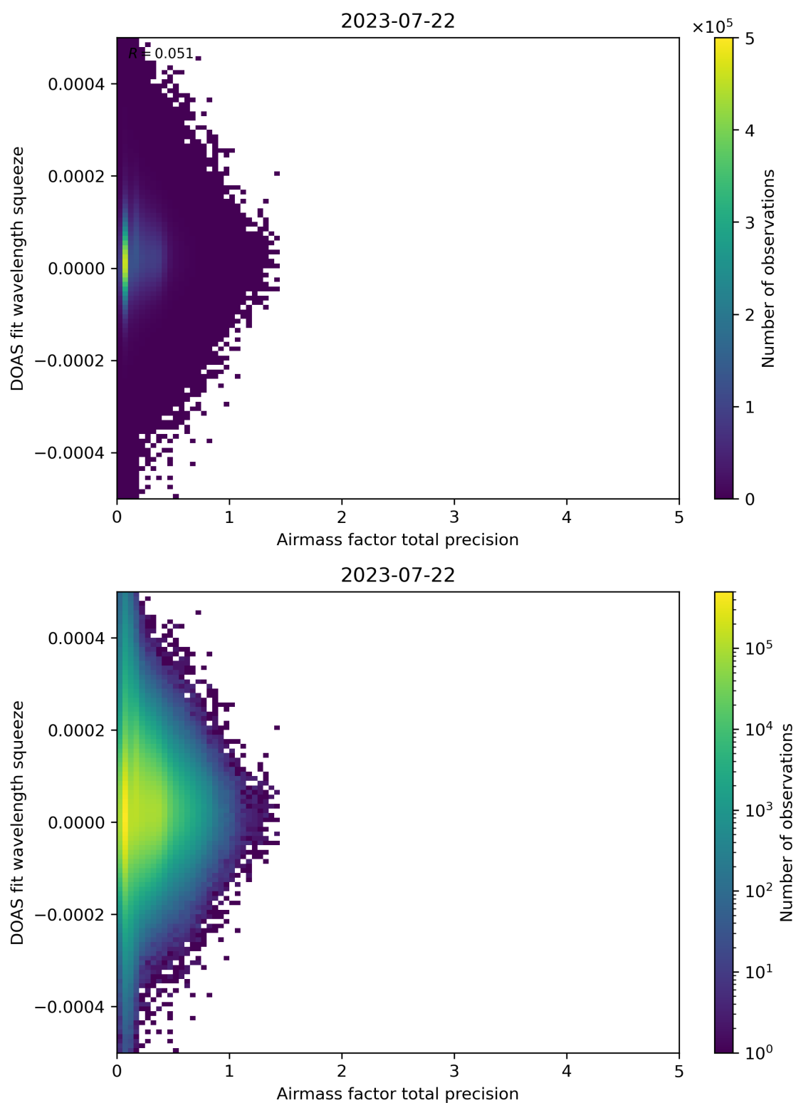
Figure 107: Scatter density plot of “Airmass factor total precision” against “DOAS fit wavelength squeeze” for 2023-07-21 to 2023-07-23.
