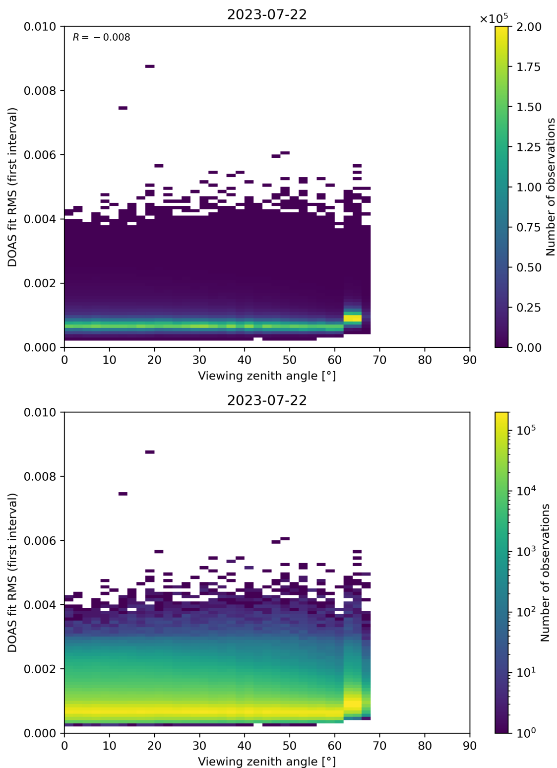
Figure 182: Scatter density plot of “Viewing zenith angle” against “DOAS fit RMS (first interval)” for 2023-07-21 to 2023-07-23.
