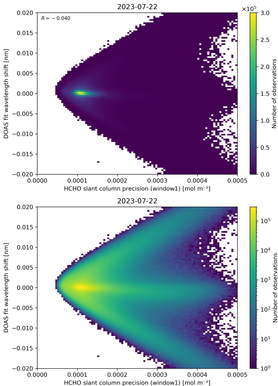
Figure 89: Scatter density plot of “HCHO slant column precision (window1)” against “DOAS fit wavelength shift” for 2023-07-21 to 2023-07-23.
