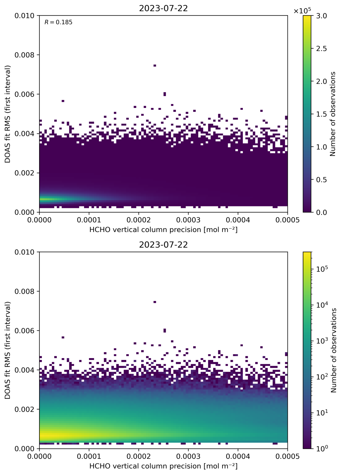
Figure 136: Scatter density plot of “HCHO vertical column precision” against “DOAS fit RMS (first interval)” for 2023-07-21 to 2023-07-23.
