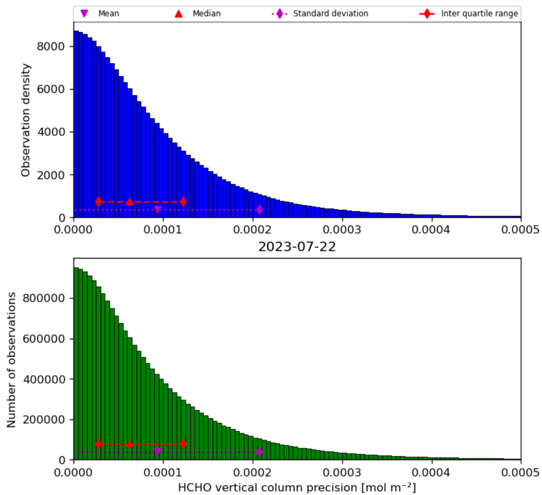
Figure 36: Histogram of “HCHO vertical column precision” for 2023-07-21 to 2023-07-23
