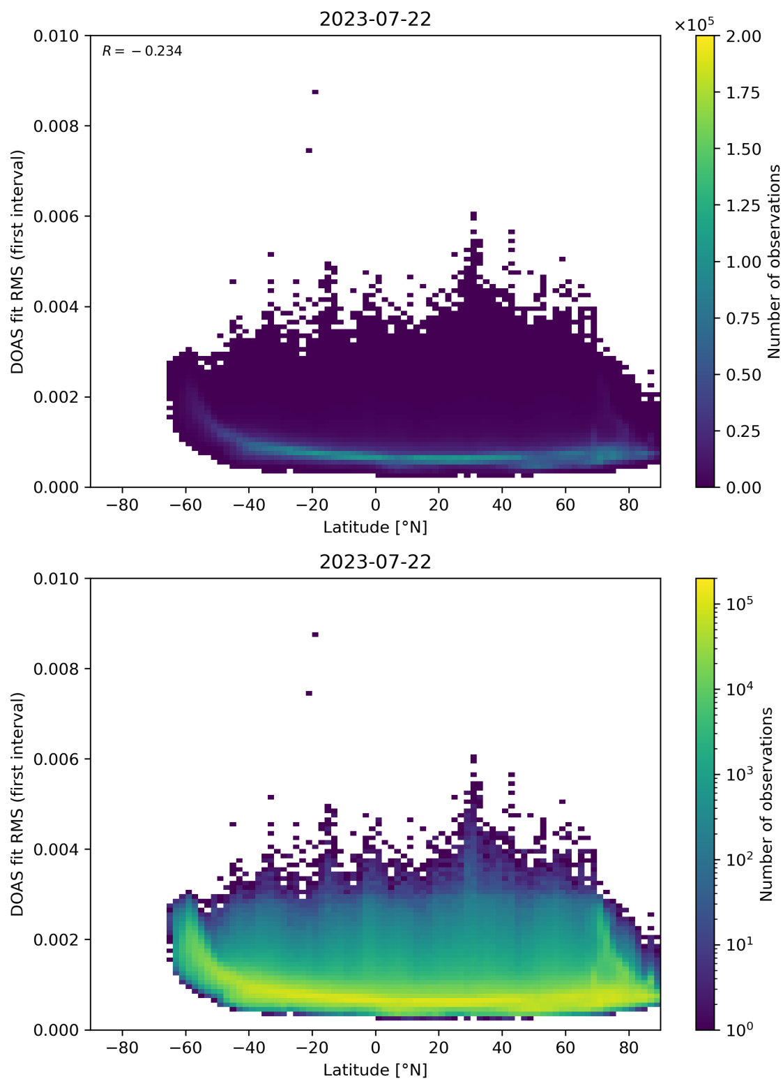
Figure 153: Scatter density plot of “Latitude” against “DOAS fit RMS (first interval)” for 2023-07-21 to 2023-07-23.
