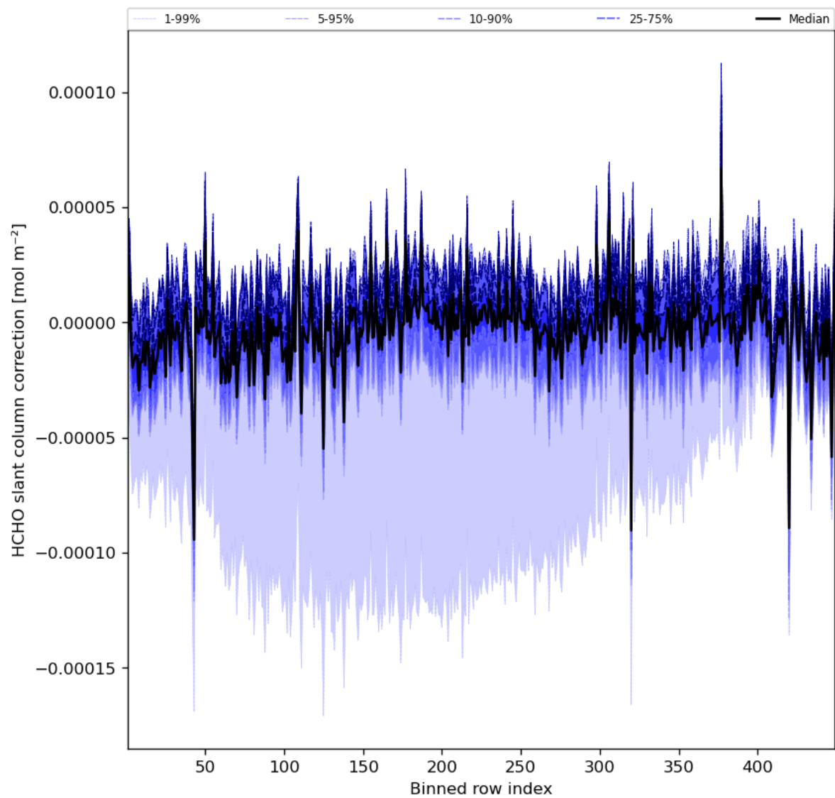
Figure 61: Along track statistics of “HCHO slant column correction” for 2023-07-21 to 2023-07-23
