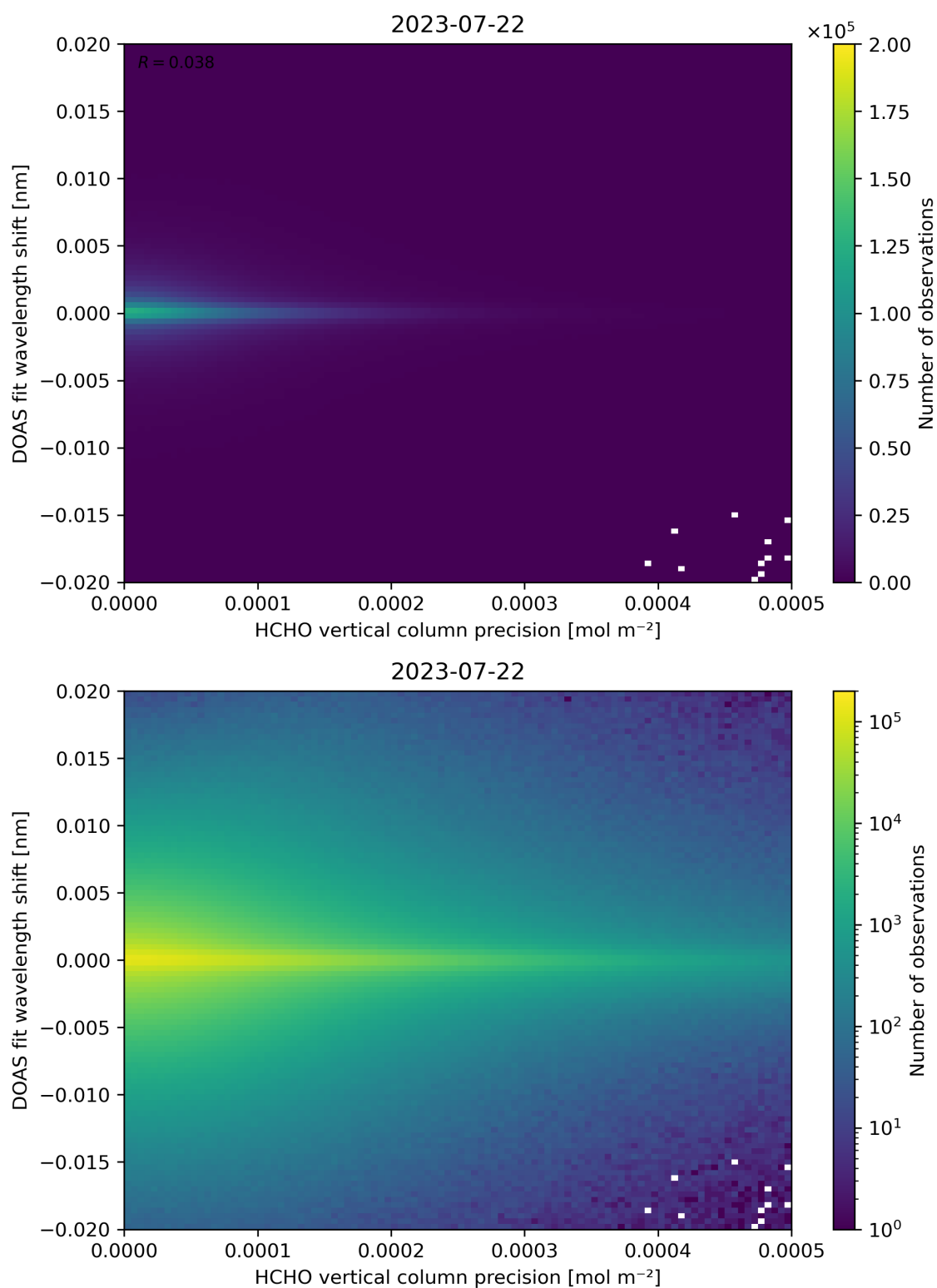
Figure 137: Scatter density plot of “HCHO vertical column precision” against “DOAS fit wavelength shift” for 2023-07-21 to 2023-07-23.
