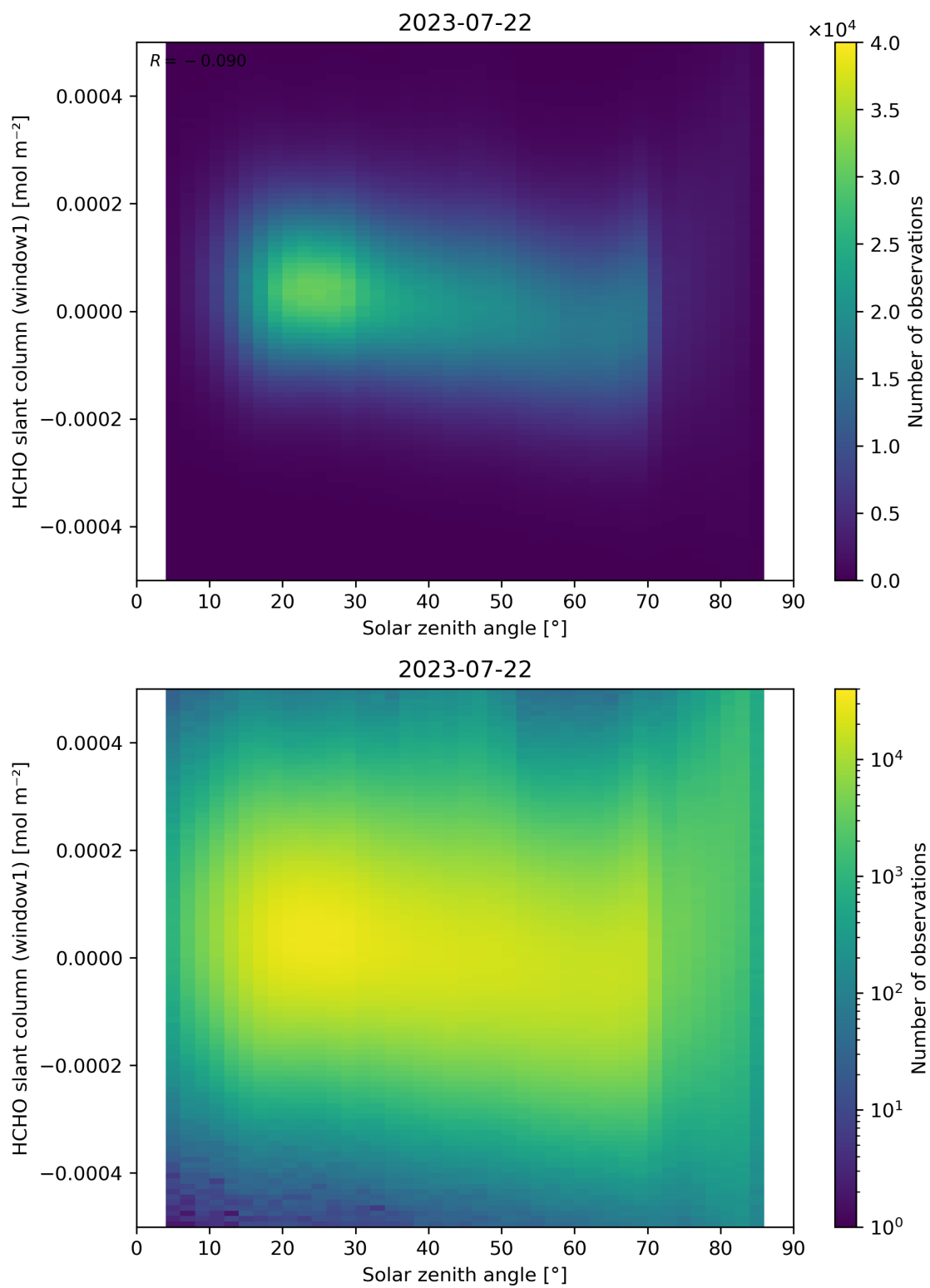
Figure 173: Scatter density plot of “Solar zenith angle” against “HCHO slant column (window1)” for 2023-07-21 to 2023-07-23.
