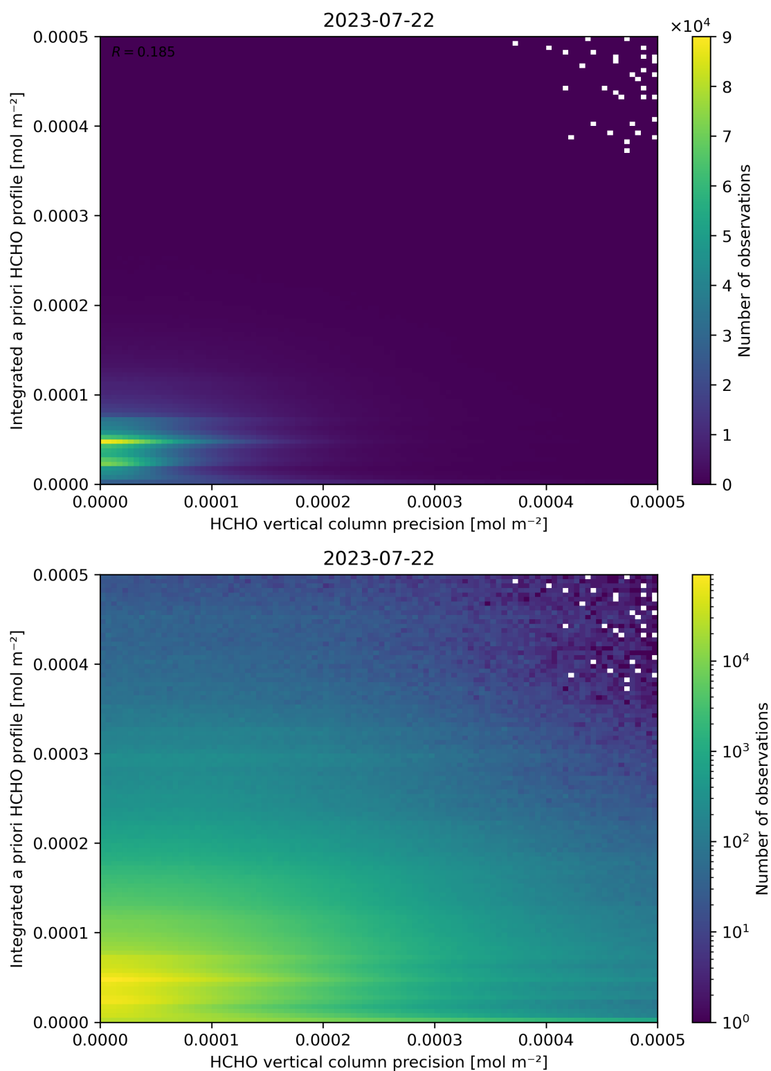
Figure 147: Scatter density plot of “HCHO vertical column precision” against “Integrated a priori HCHO profile” for 2023-07-21 to 2023-07-23.
