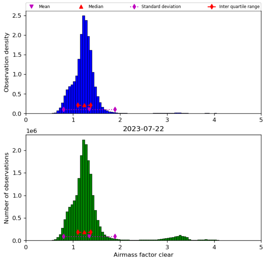
Figure 42: Histogram of “Airmass factor clear” for 2023-07-21 to 2023-07-23
