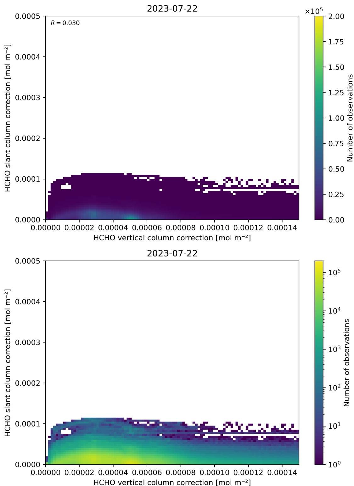
Figure 117: Scatter density plot of “HCHO vertical column correction” against “HCHO slant column correction” for 2023-07-21 to 2023-07-23.
