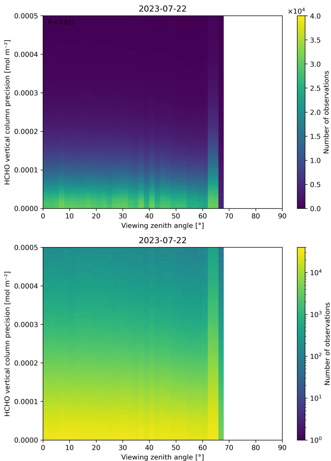
Figure 194: Scatter density plot of “Viewing zenith angle” against “HCHO vertical column precision” for 2023-07-21 to 2023-07-23.
