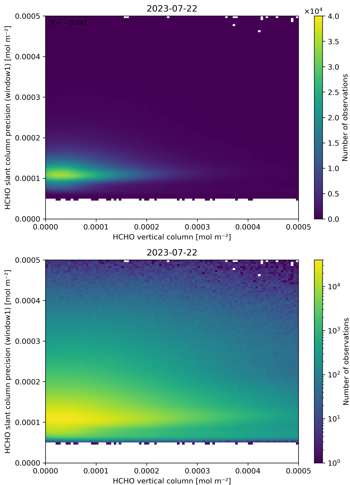
Figure 130: Scatter density plot of “HCHO vertical column” against “HCHO slant column precision (window1)” for 2023-07-21 to 2023-07-23.
