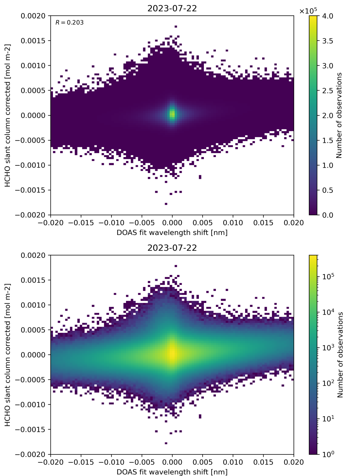
Figure 66: Scatter density plot of “DOAS fit wavelength shift” against “HCHO slant column corrected” for 2023-07-21 to 2023-07-23.
