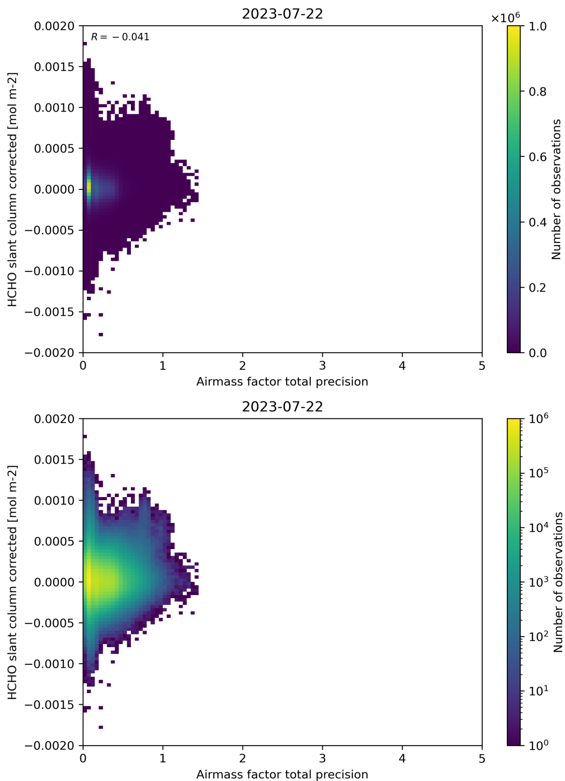
Figure 109: Scatter density plot of “Airmass factor total precision” against “HCHO slant column corrected” for 2023-07-21 to 2023-07-23.
