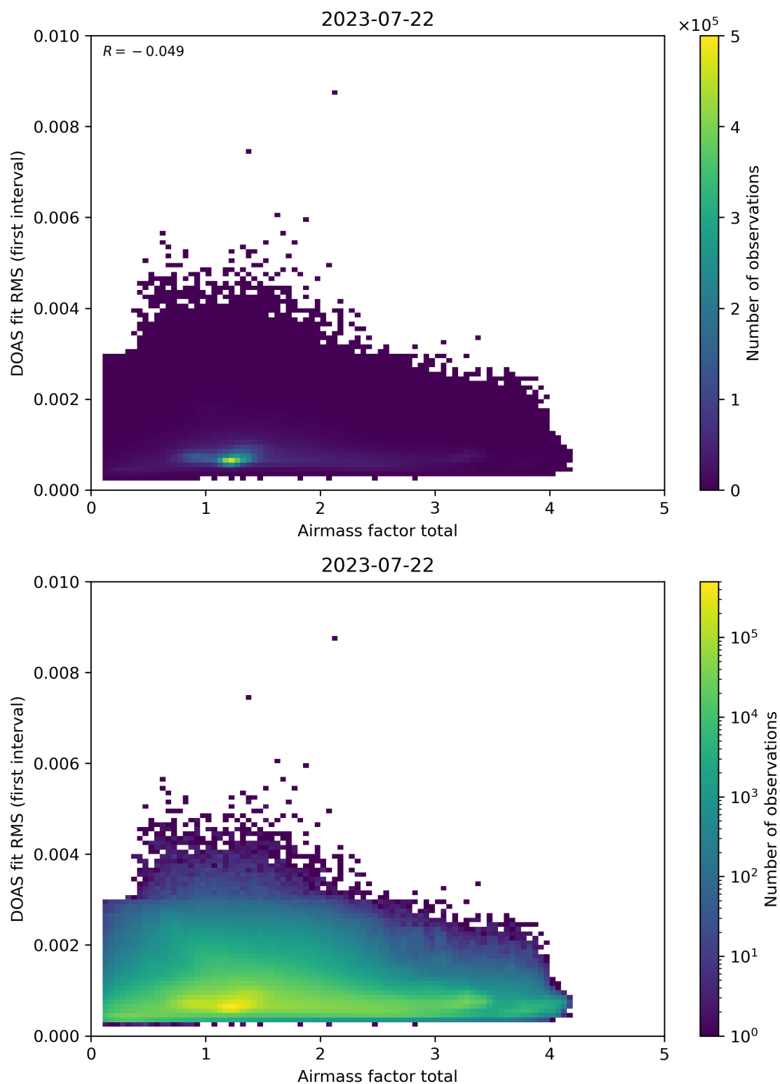
Figure 97: Scatter density plot of “Airmass factor total” against “DOAS fit RMS (first interval)” for 2023-07-21 to 2023-07-23.
