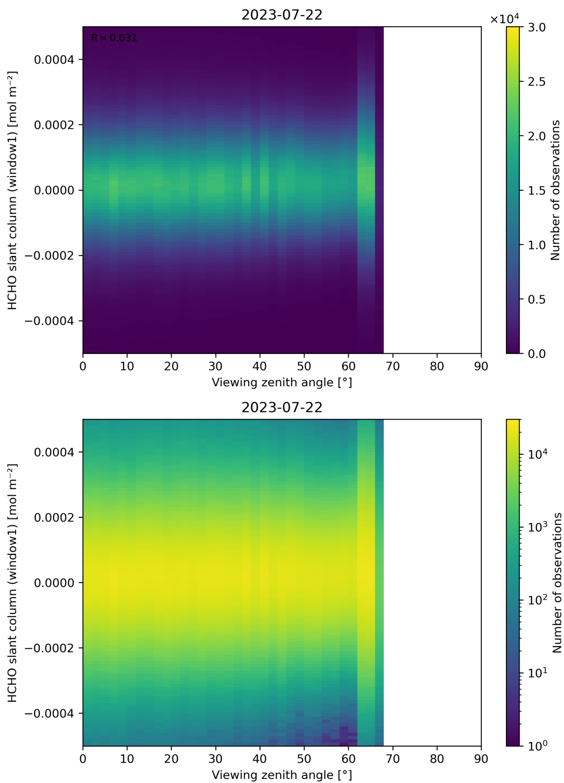
Figure 188: Scatter density plot of “Viewing zenith angle” against “HCHO slant column (window1)” for 2023-07-21 to 2023-07-23.
