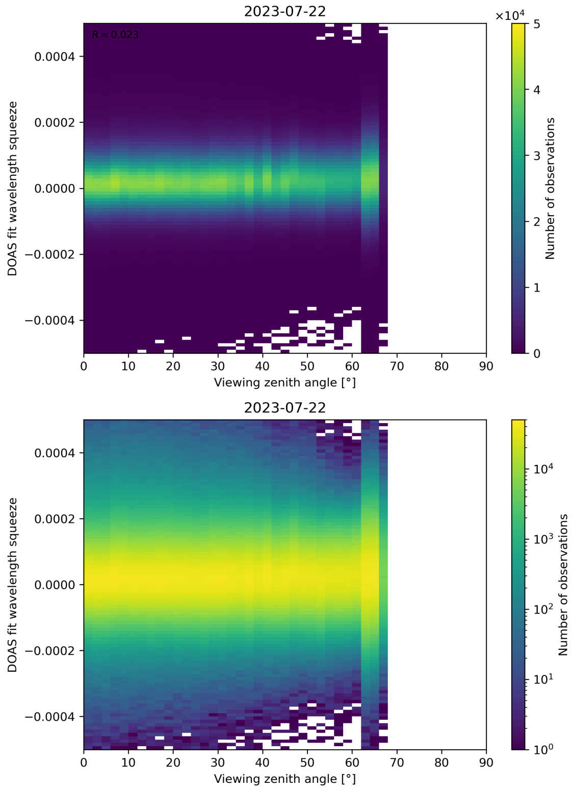
Figure 184: Scatter density plot of “Viewing zenith angle” against “DOAS fit wavelength squeeze” for 2023-07-21 to 2023-07-23.
