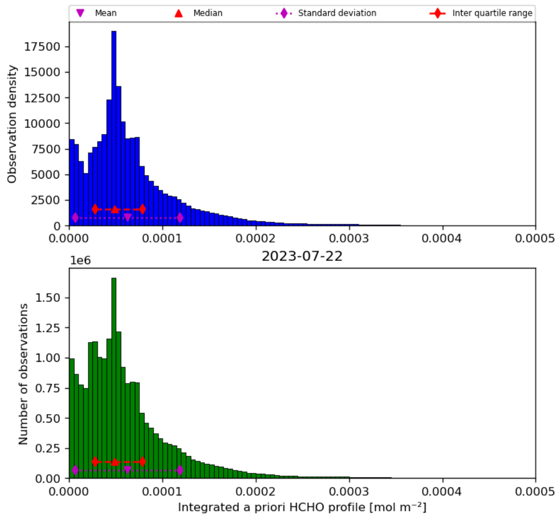
Figure 43: Histogram of “Integrated a priori HCHO profile” for 2023-07-21 to 2023-07-23
