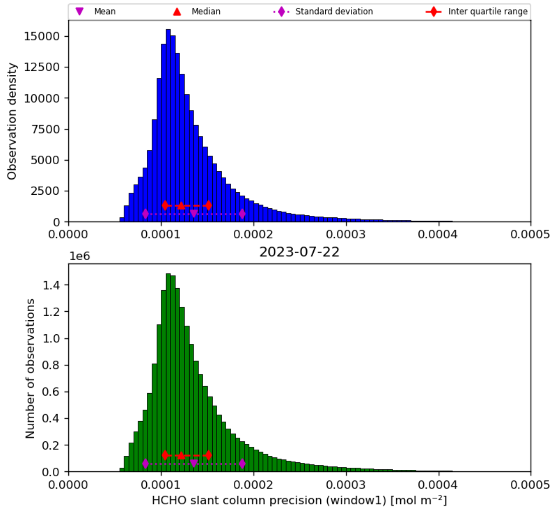
Figure 39: Histogram of “HCHO slant column precision (window1)” for 2023-07-21 to 2023-07-23
