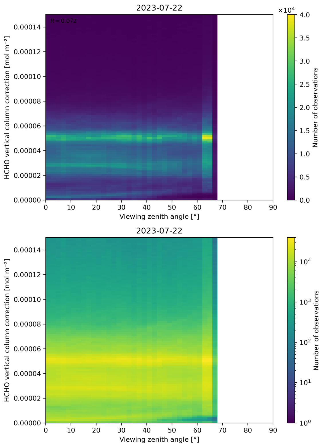
Figure 193: Scatter density plot of “Viewing zenith angle” against “HCHO vertical column correction” for 2023-07-21 to 2023-07-23.
