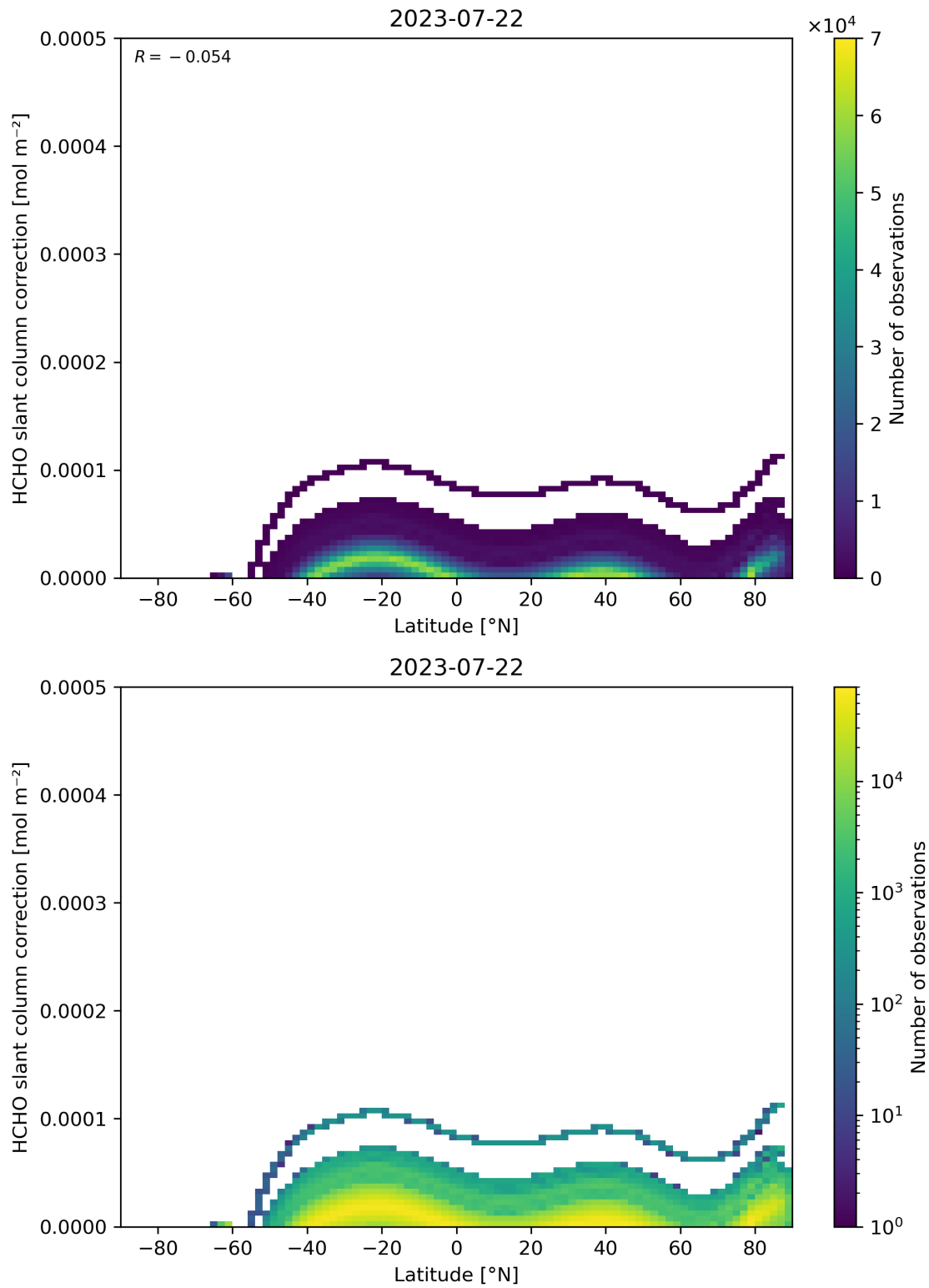
Figure 158: Scatter density plot of “Latitude” against “HCHO slant column correction” for 2023-07-21 to 2023-07-23.
