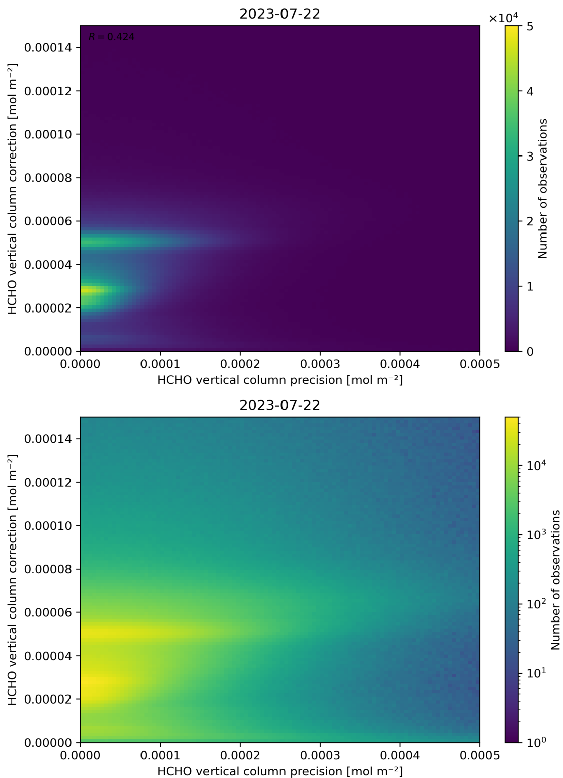
Figure 146: Scatter density plot of “HCHO vertical column precision” against “HCHO vertical column correction” for 2023-07-21 to 2023-07-23.
