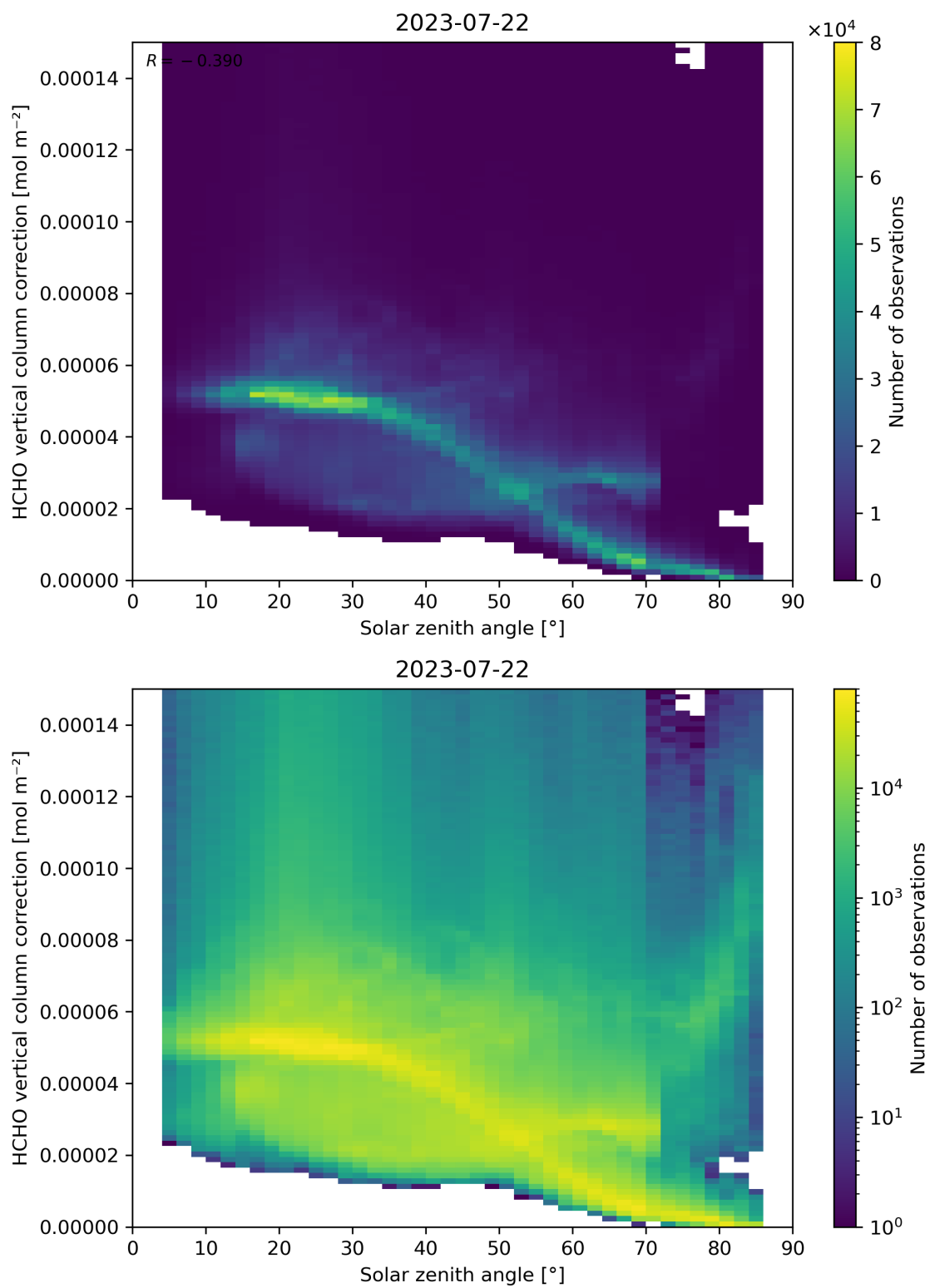
Figure 178: Scatter density plot of “Solar zenith angle” against “HCHO vertical column correction” for 2023-07-21 to 2023-07-23.
