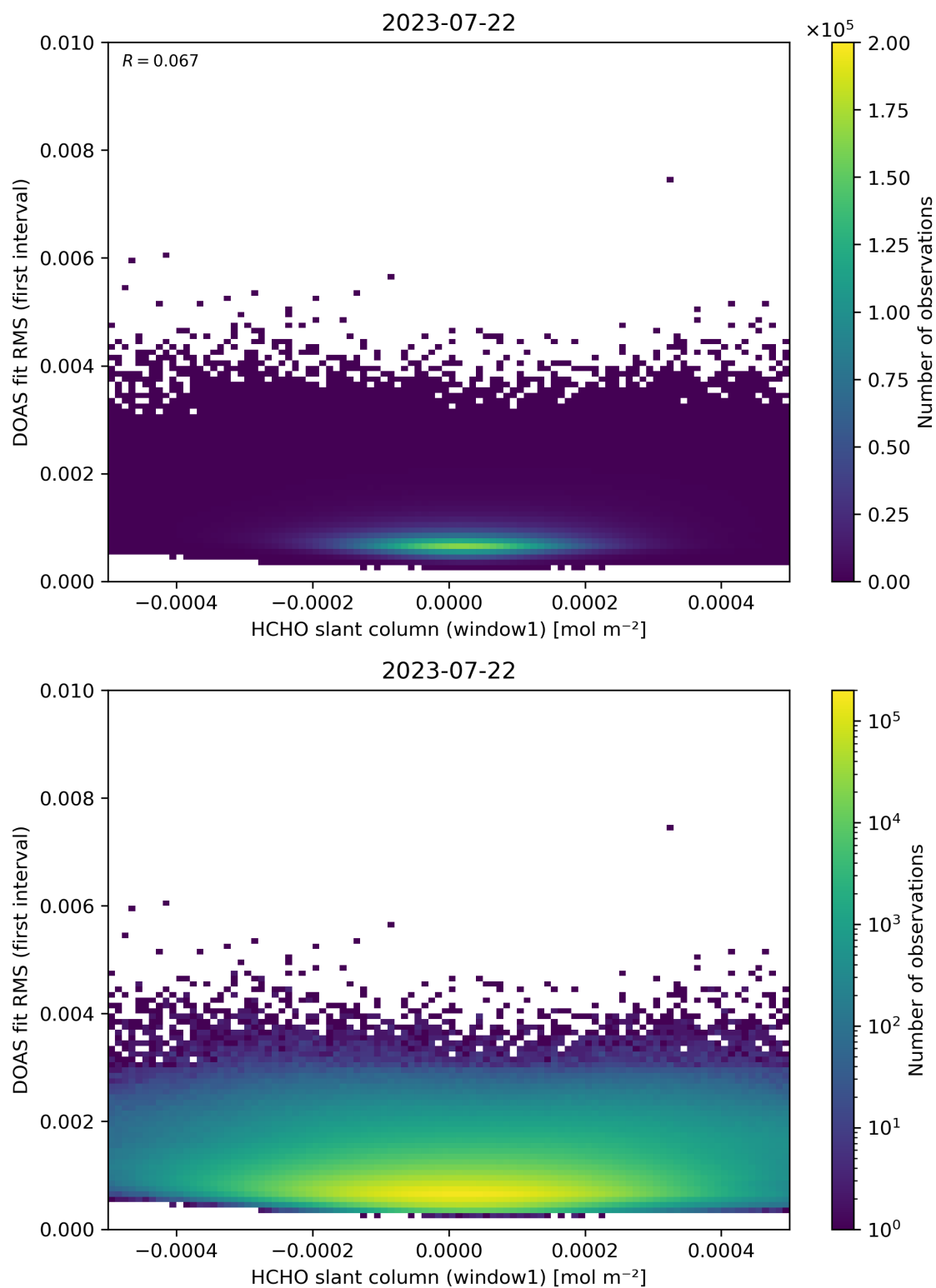
Figure 78: Scatter density plot of “HCHO slant column (window1)” against “DOAS fit RMS (first interval)” for 2023-07-21 to 2023-07-23.
