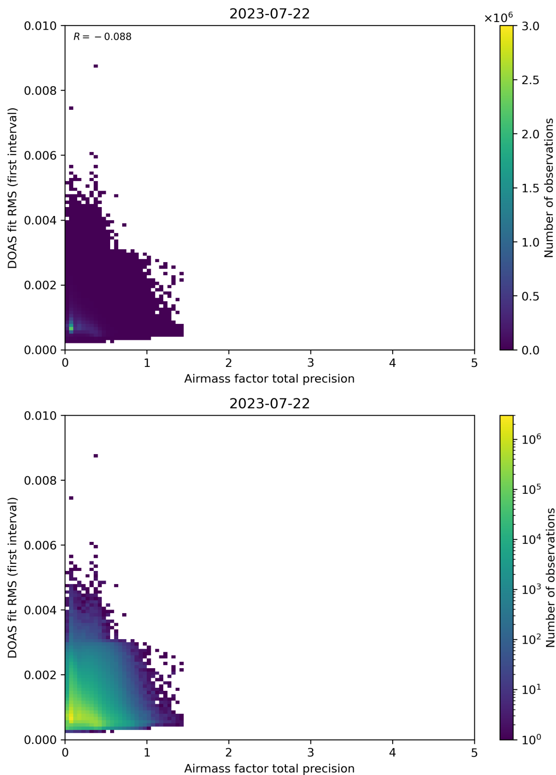
Figure 105: Scatter density plot of “Airmass factor total precision” against “DOAS fit RMS (first interval)” for 2023-07-21 to 2023-07-23.
