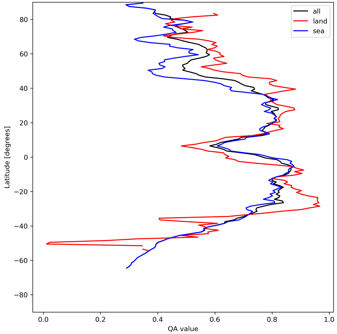
Figure 20: Zonal average of “QA value” for 2023-07-21 to 2023-07-23.
