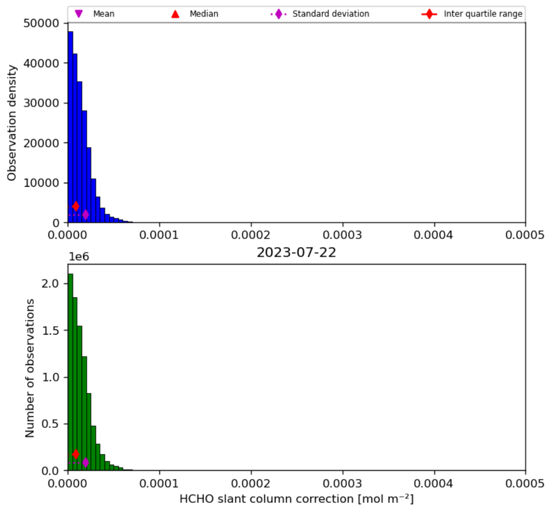
Figure 47: Histogram of “HCHO slant column correction” for 2023-07-21 to 2023-07-23
