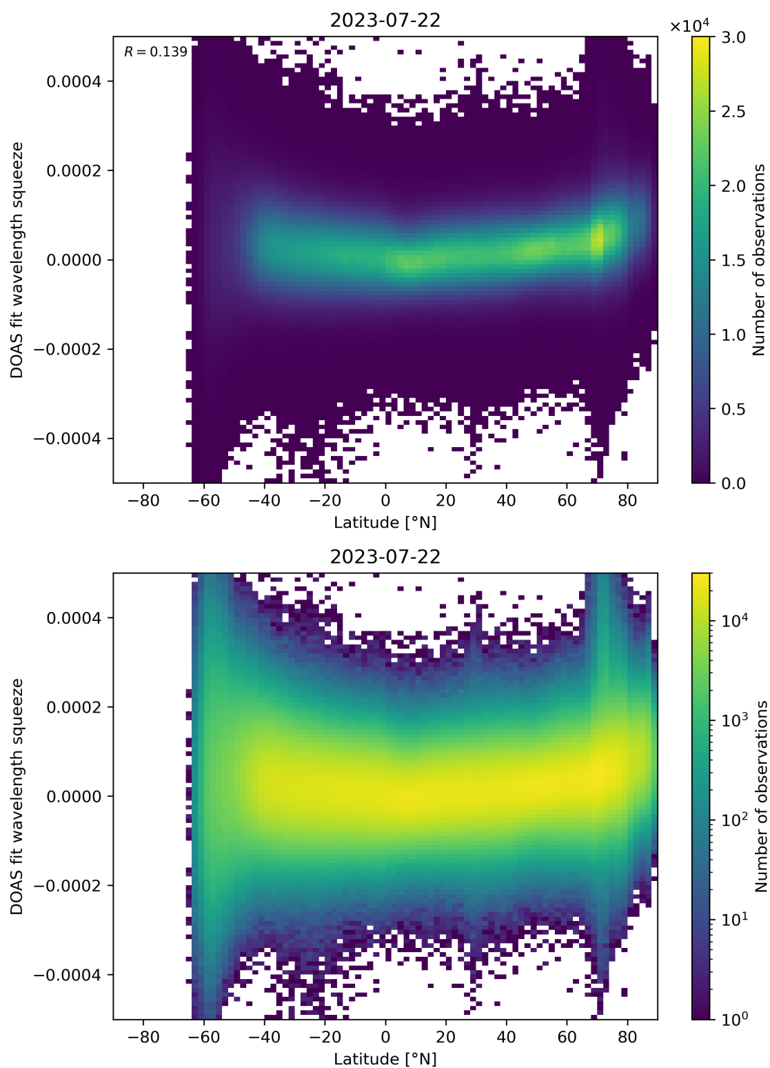
Figure 155: Scatter density plot of “Latitude” against “DOAS fit wavelength squeeze” for 2023-07-21 to 2023-07-23.
