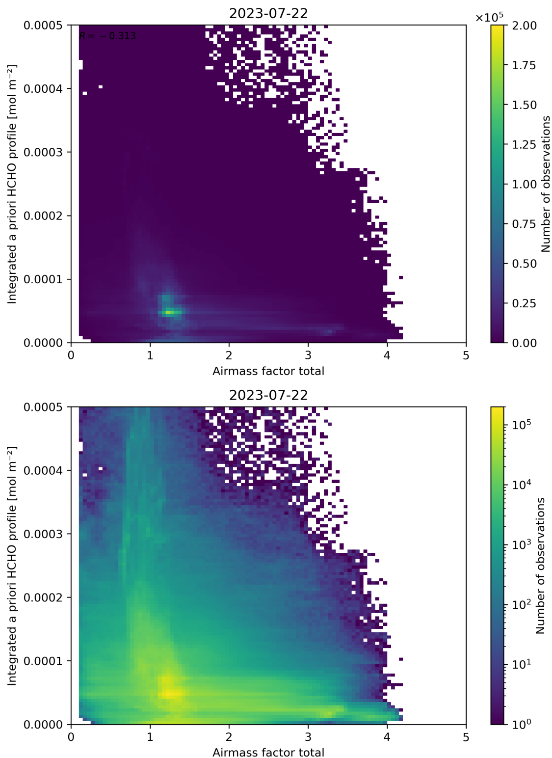
Figure 104: Scatter density plot of “Airmass factor total” against “Integrated a priori HCHO profile” for 2023-07-21 to 2023-07-23.
