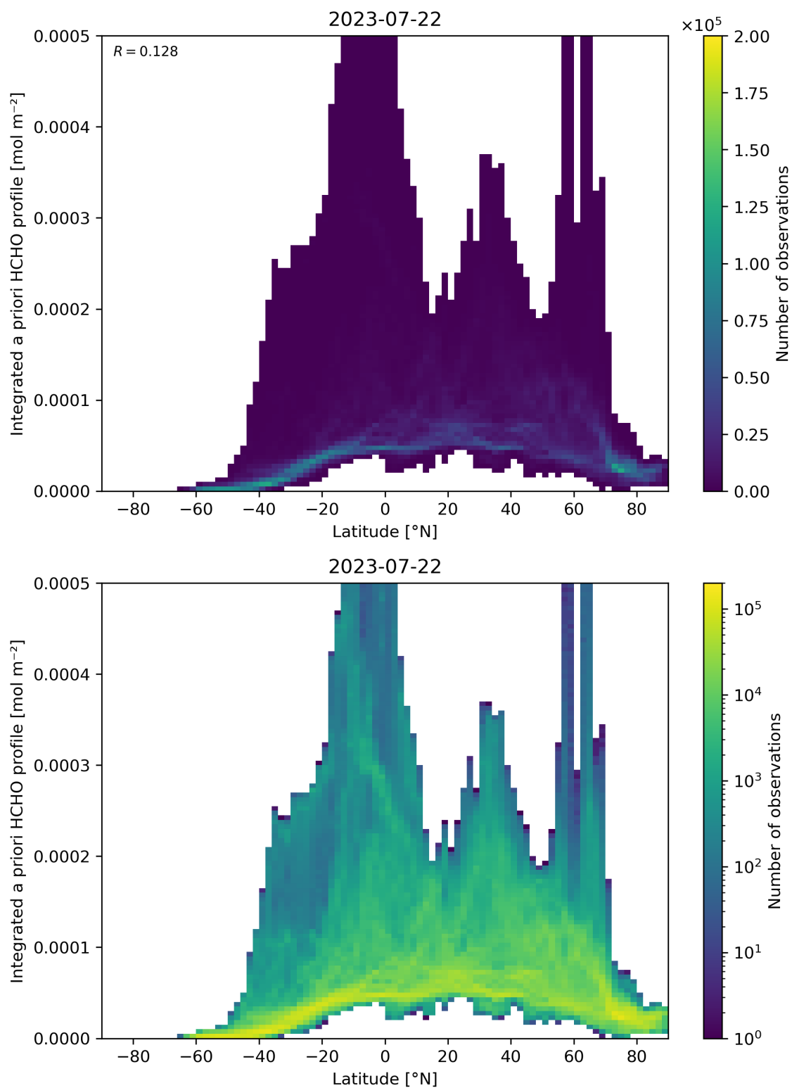
Figure 166: Scatter density plot of “Latitude” against “Integrated a priori HCHO profile” for 2023-07-21 to 2023-07-23.
