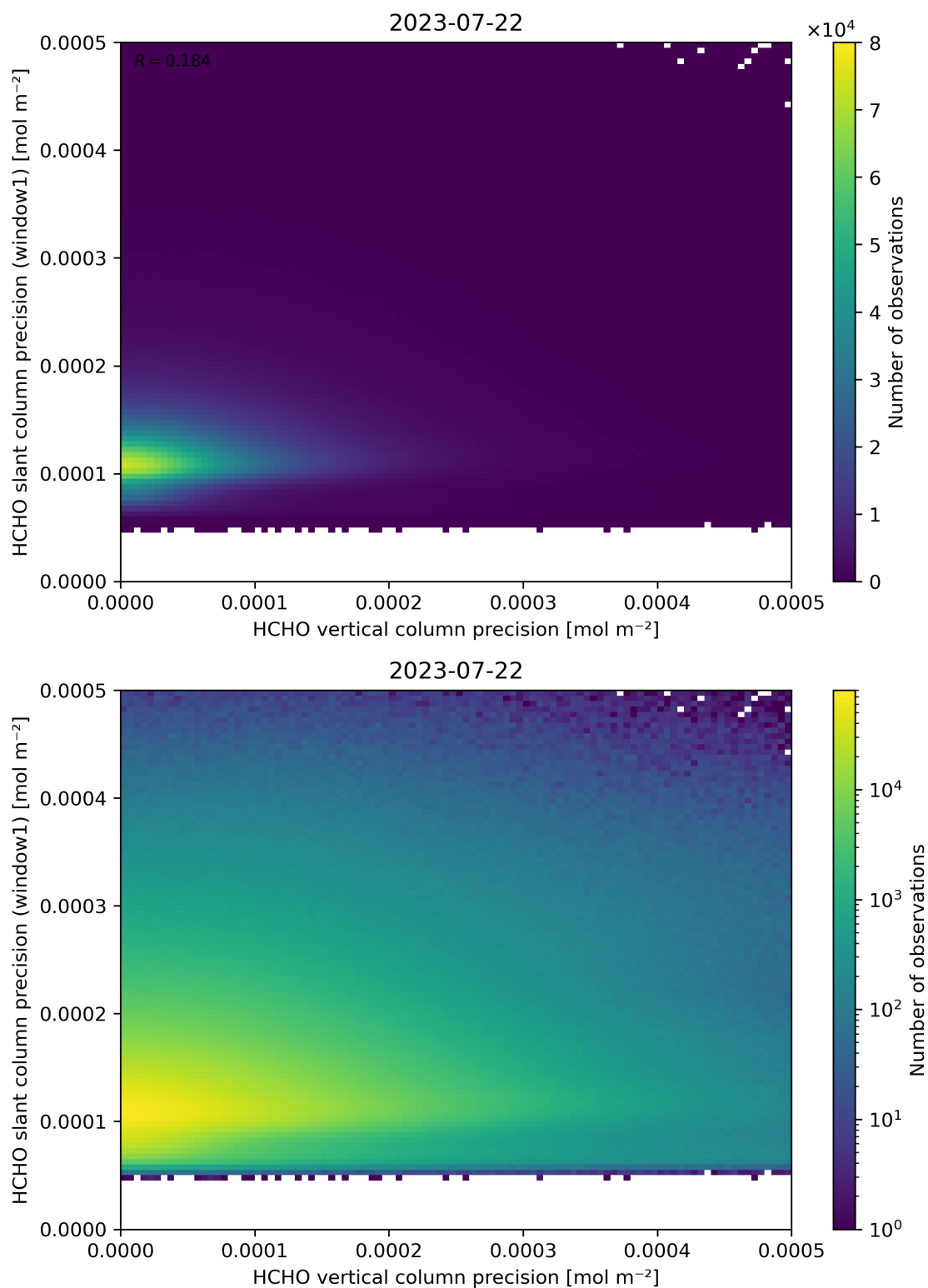
Figure 143: Scatter density plot of “HCHO vertical column precision” against “HCHO slant column precision (window1)” for 2023-07-21 to 2023-07-23.
