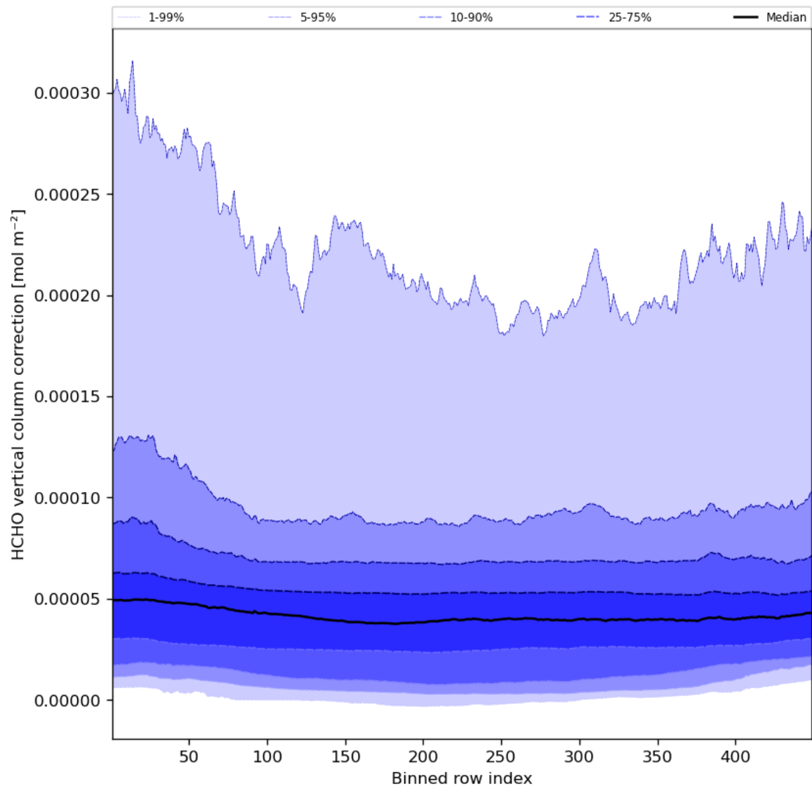
Figure 51: Along track statistics of “HCHO vertical column correction” for 2023-07-21 to 2023-07-23
