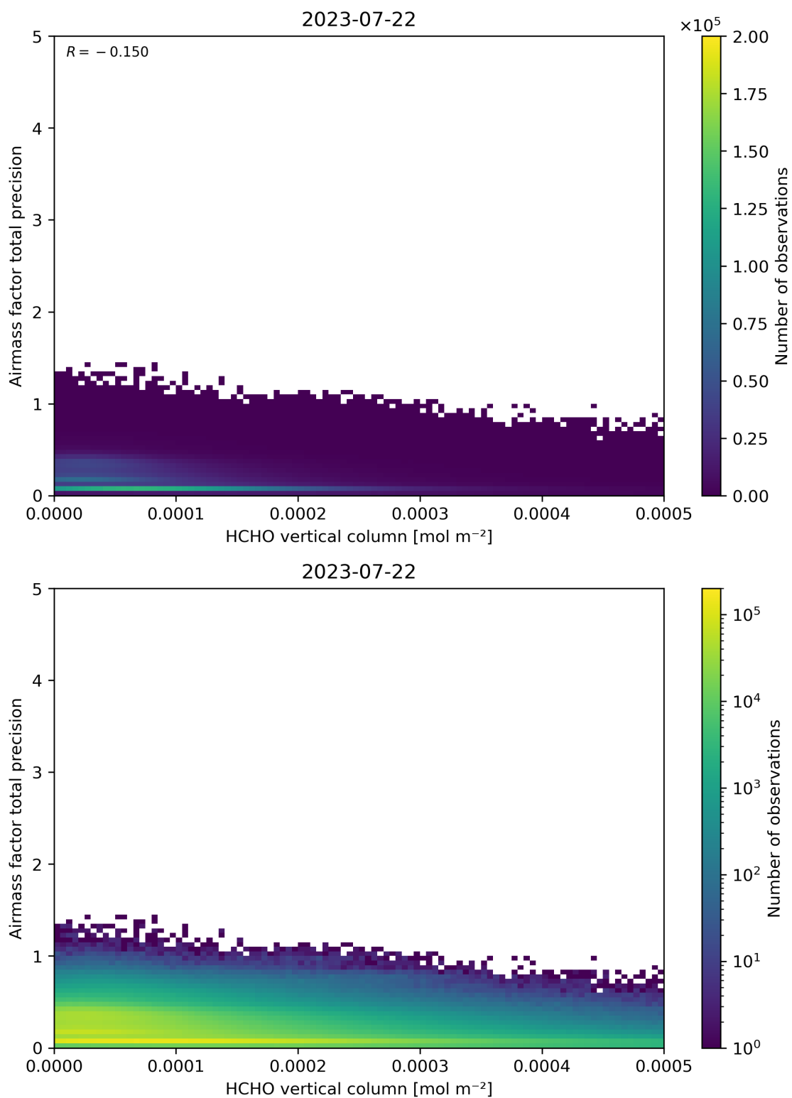
Figure 132: Scatter density plot of “HCHO vertical column” against “Airmass factor total precision” for 2023-07-21 to 2023-07-23.
