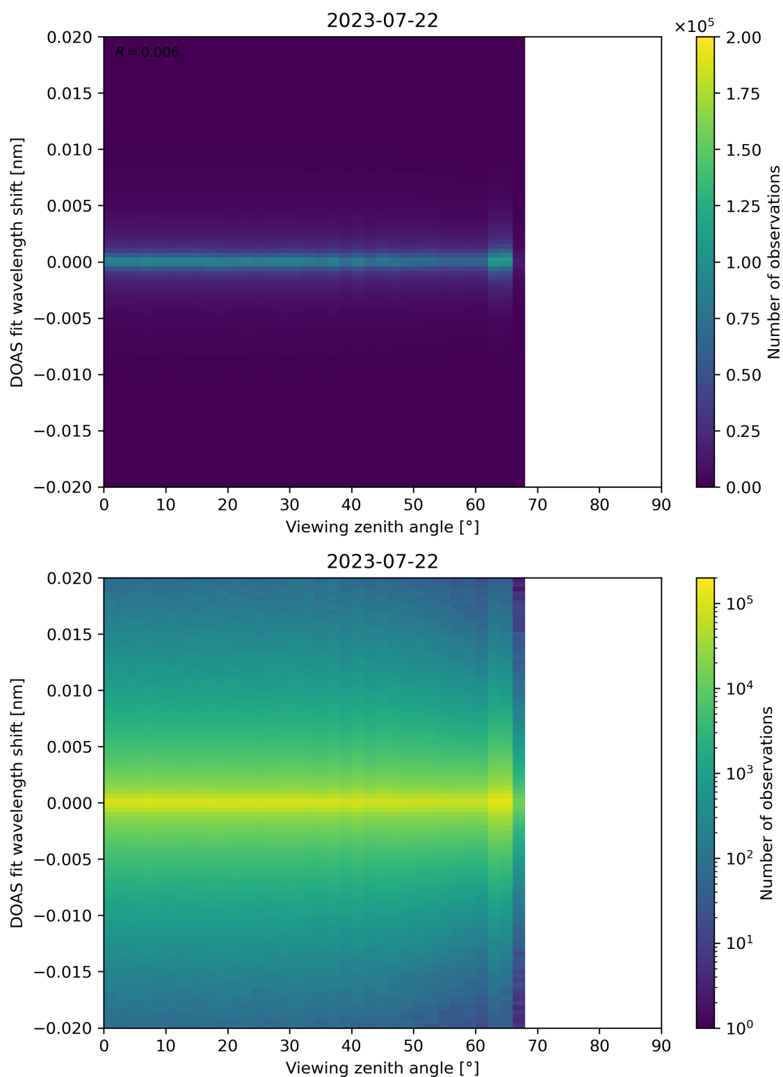
Figure 183: Scatter density plot of “Viewing zenith angle” against “DOAS fit wavelength shift” for 2023-07-21 to 2023-07-23.
