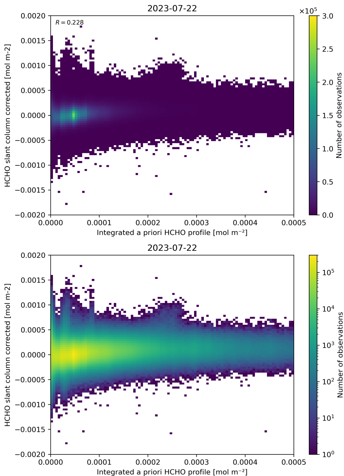
Figure 151: Scatter density plot of “Integrated a priori HCHO profile” against “HCHO slant column corrected” for 2023-07-21 to 2023-07-23.
