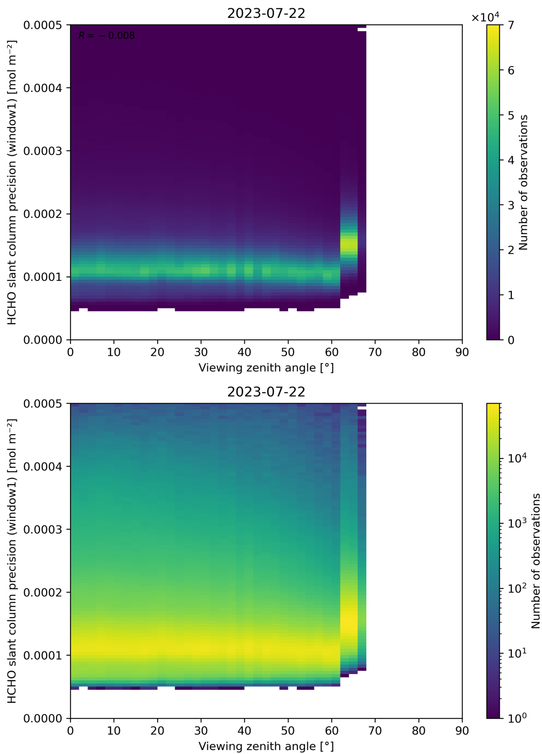
Figure 189: Scatter density plot of “Viewing zenith angle” against “HCHO slant column precision (window1)” for 2023-07-21 to 2023-07-23.
