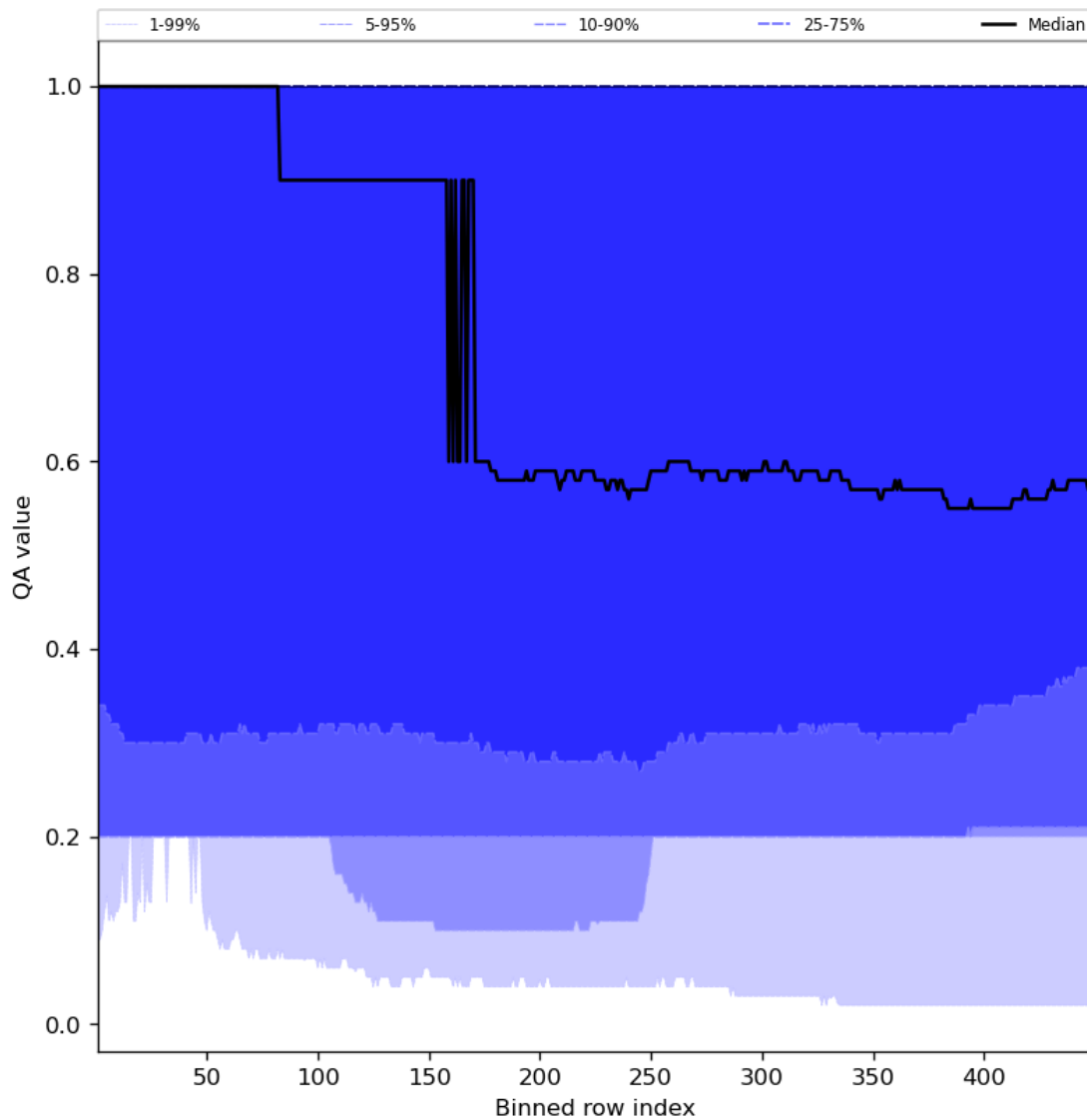
Figure 48: Along track statistics of “QA value” for 2023-07-21 to 2023-07-23
