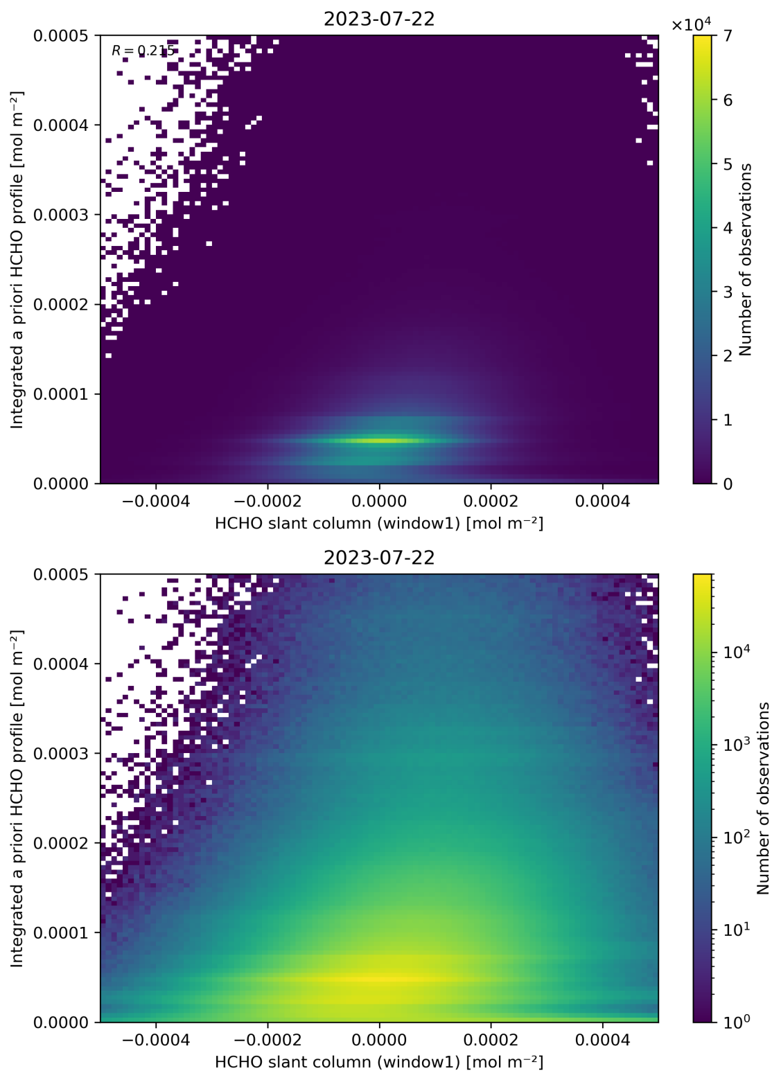
Figure 87: Scatter density plot of “HCHO slant column (window1)” against “Integrated a priori HCHO profile” for 2023-07-21 to 2023-07-23.
