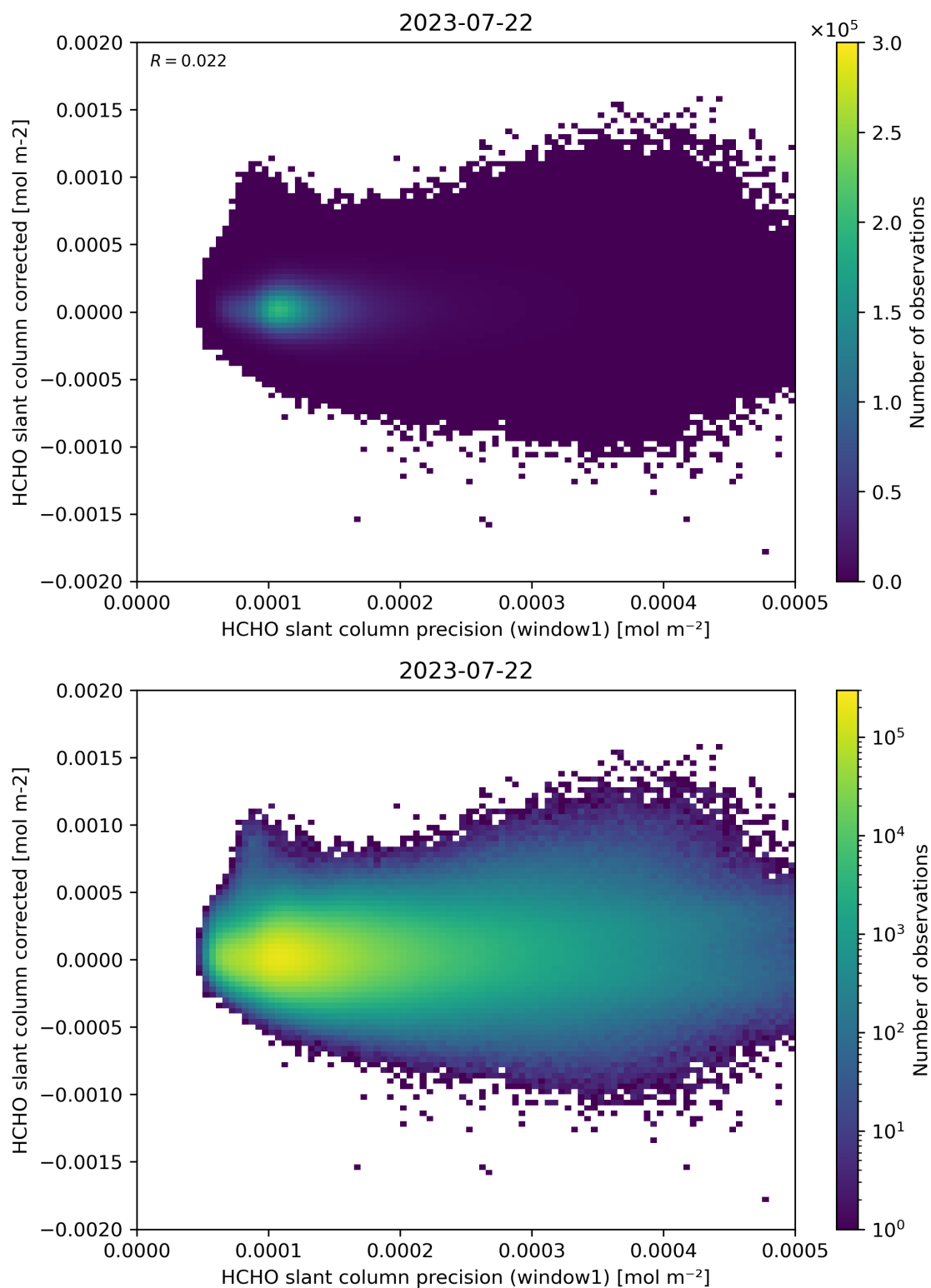
Figure 92: Scatter density plot of “HCHO slant column precision (window1)” against “HCHO slant column corrected” for 2023-07-21 to 2023-07-23.
