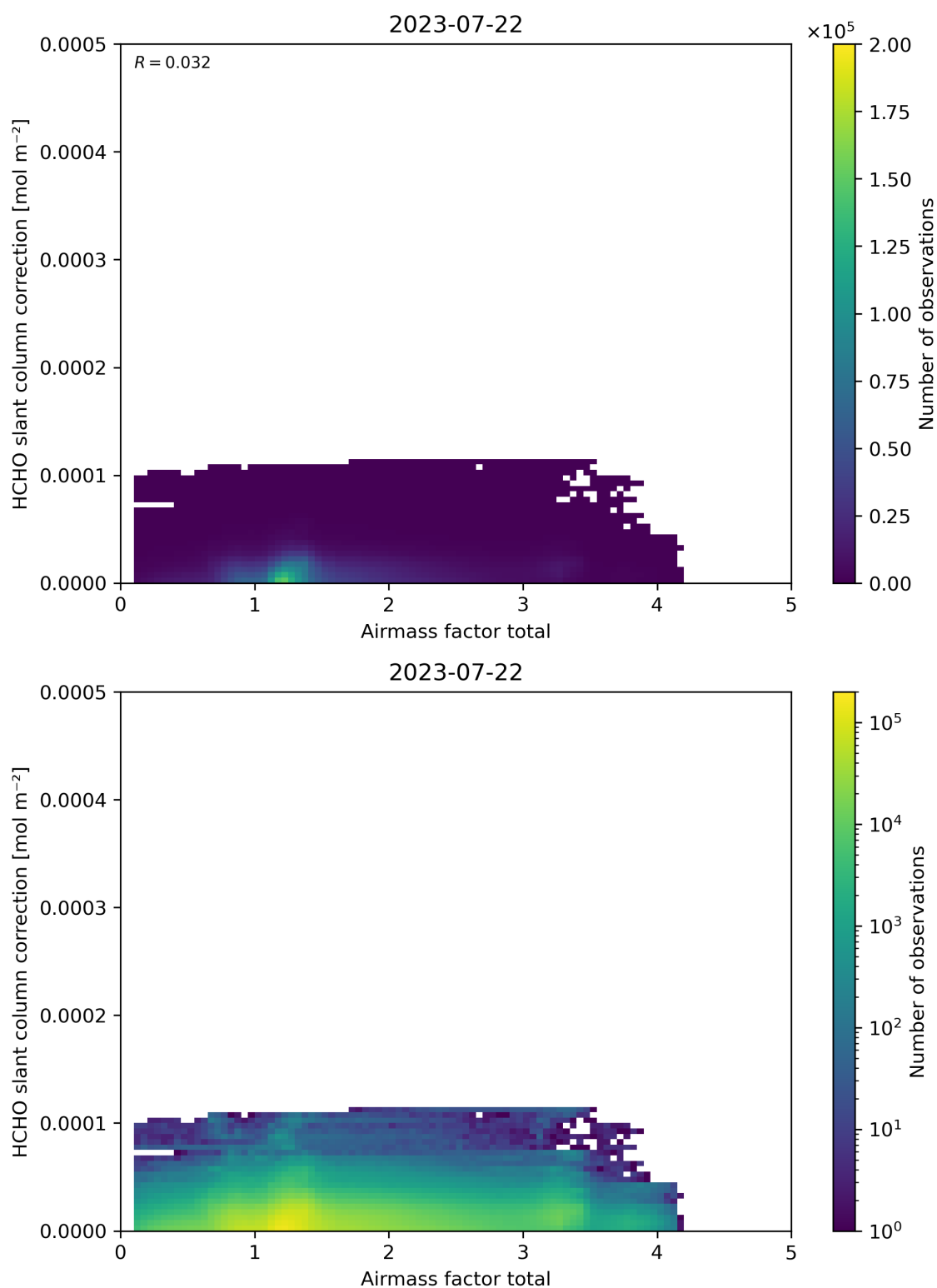
Figure 102: Scatter density plot of “Airmass factor total” against “HCHO slant column correction” for 2023-07-21 to 2023-07-23.
