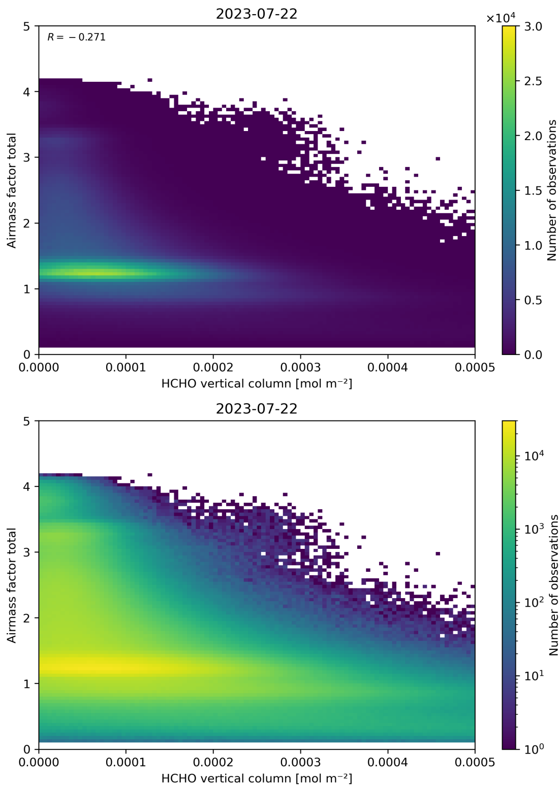
Figure 131: Scatter density plot of “HCHO vertical column” against “Airmass factor total” for 2023-07-21 to 2023-07-23.
