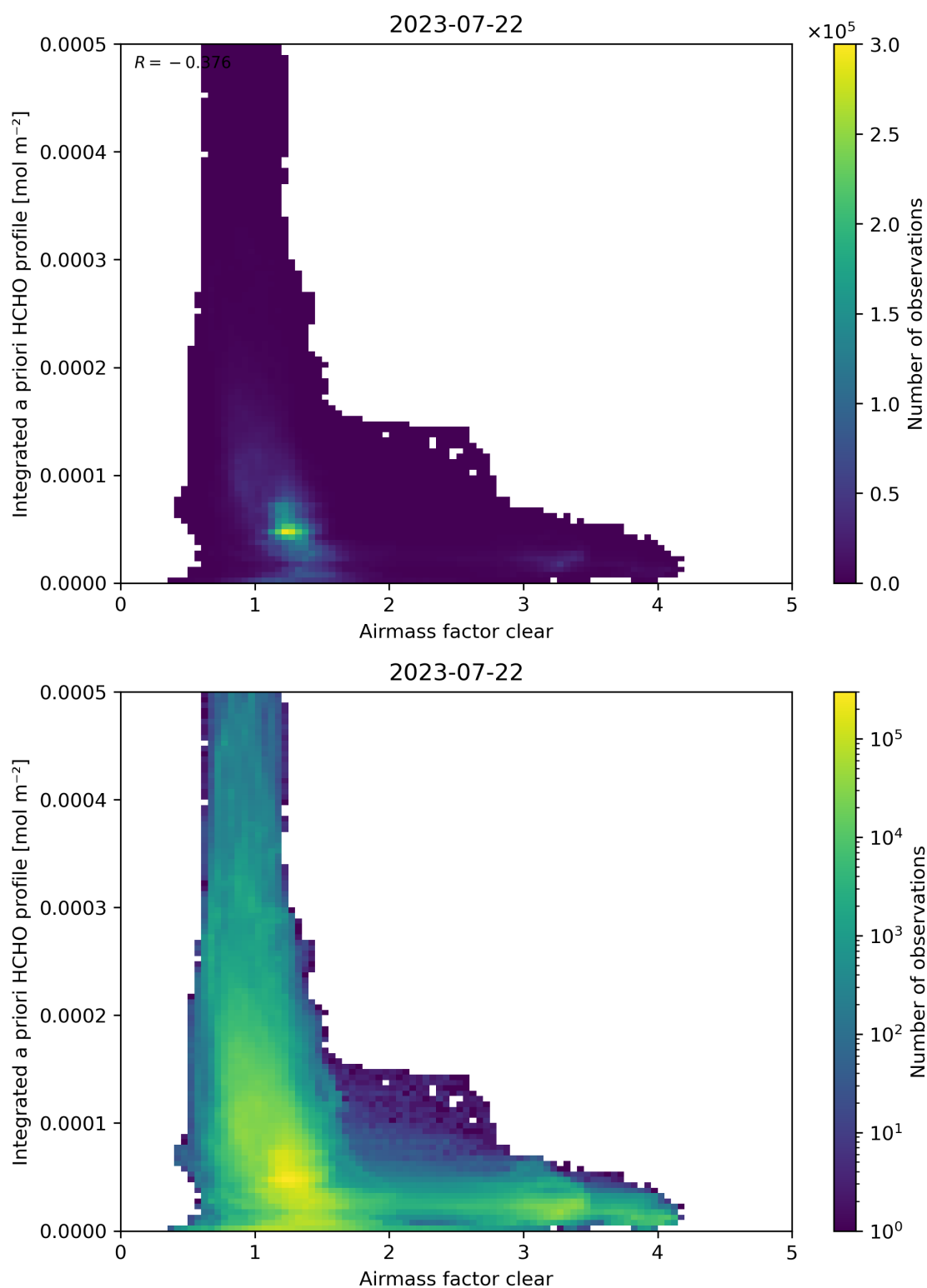
Figure 76: Scatter density plot of “Airmass factor clear” against “Integrated a priori HCHO profile” for 2023-07-21 to 2023-07-23.
