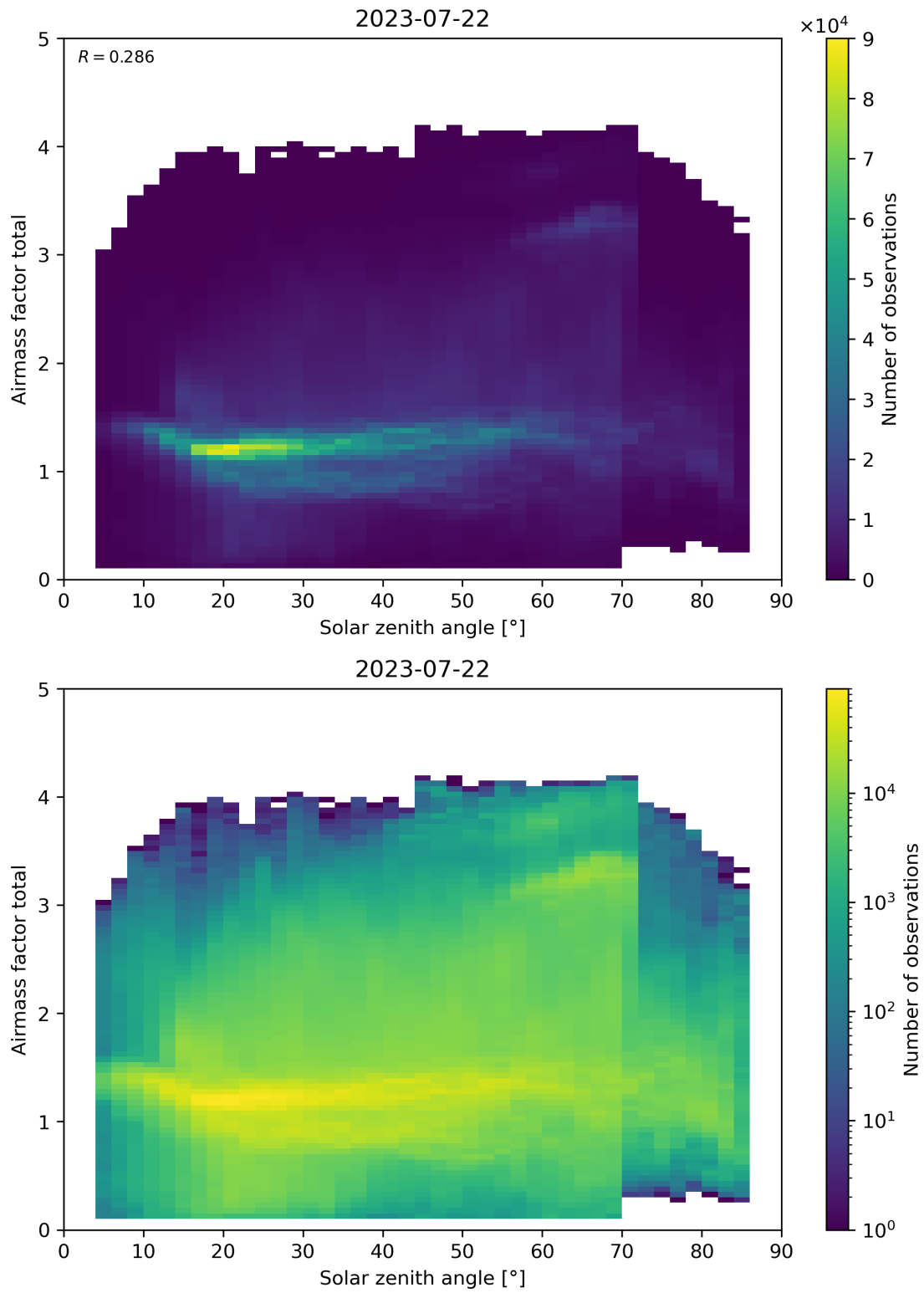
Figure 175: Scatter density plot of “Solar zenith angle” against “Airmass factor total” for 2023-07-21 to 2023-07-23.
