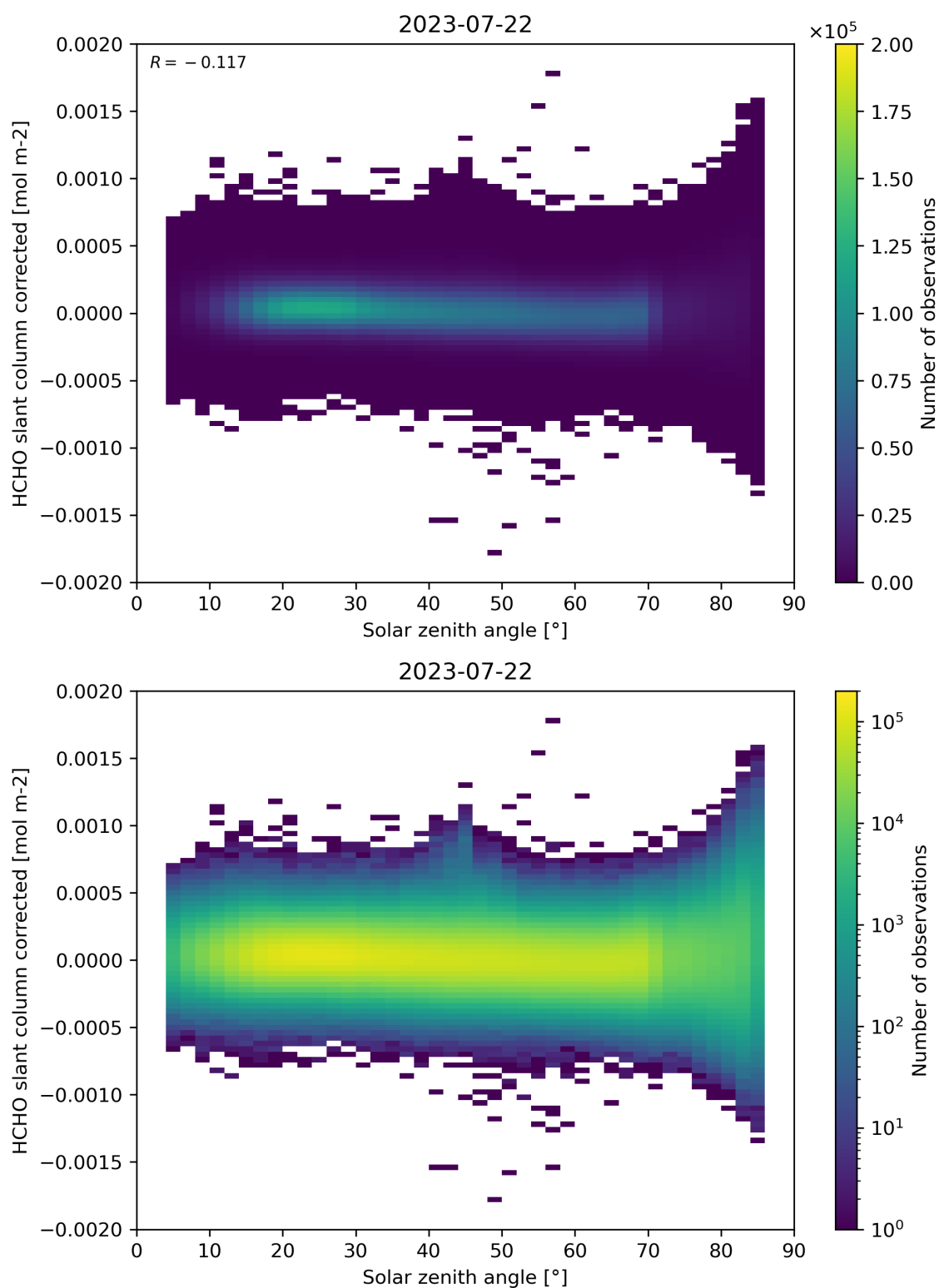
Figure 171: Scatter density plot of “Solar zenith angle” against “HCHO slant column corrected” for 2023-07-21 to 2023-07-23.
