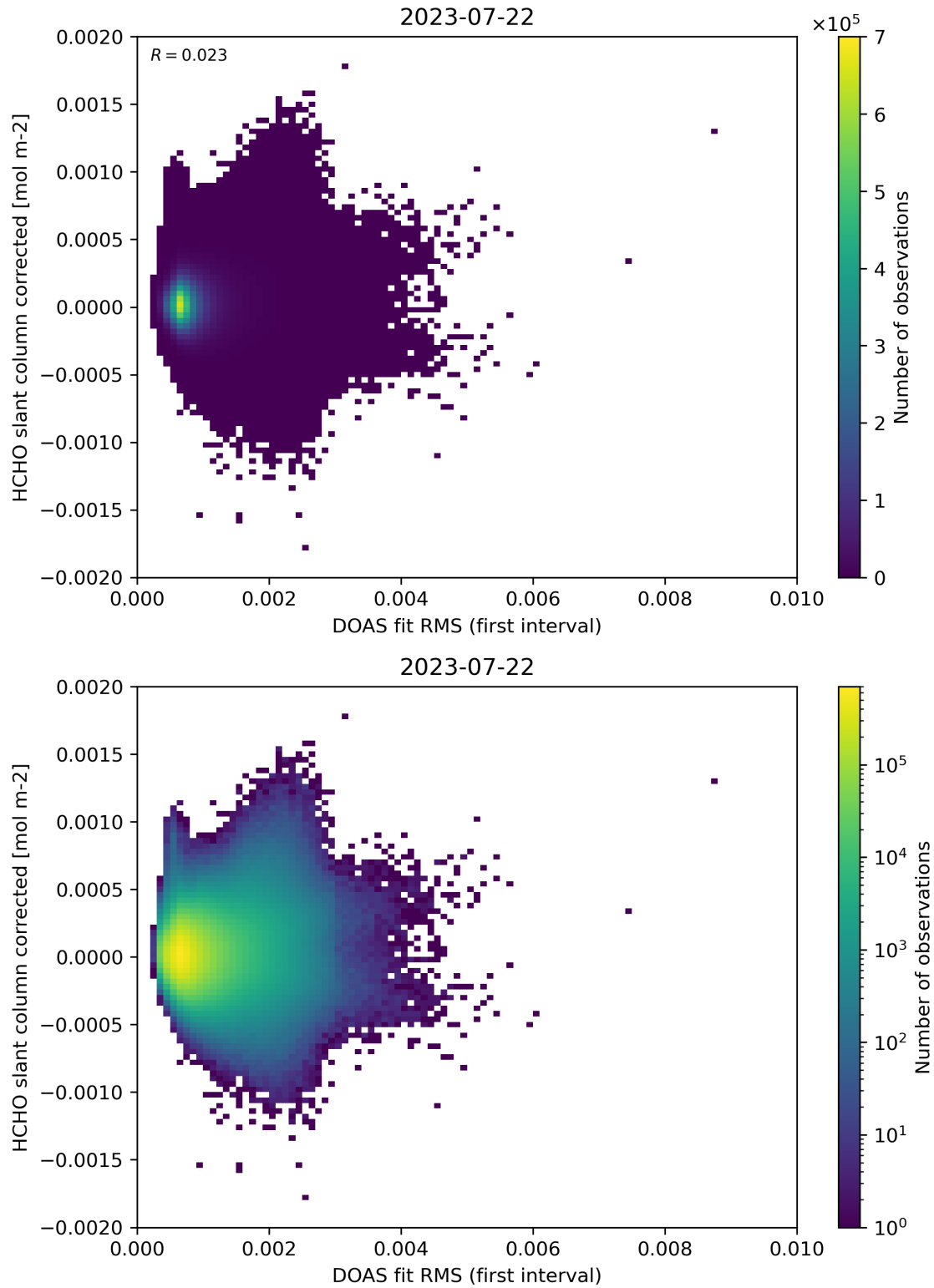
Figure 62: Scatter density plot of “DOAS fit RMS (first interval)” against “HCHO slant column corrected” for 2023-07-21 to 2023-07-23.
