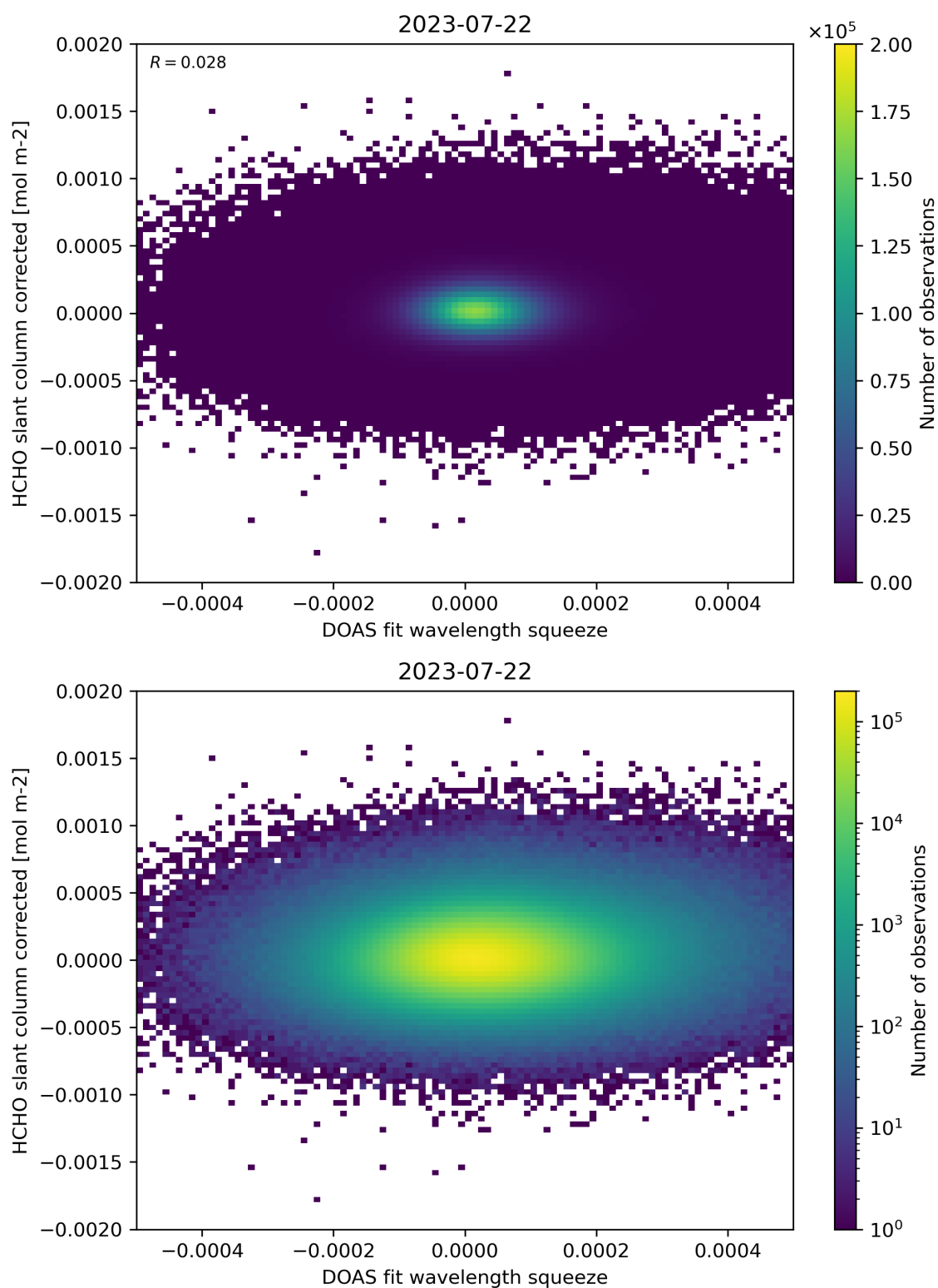
Figure 69: Scatter density plot of “DOAS fit wavelength squeeze” against “HCHO slant column corrected” for 2023-07-21 to 2023-07-23.
