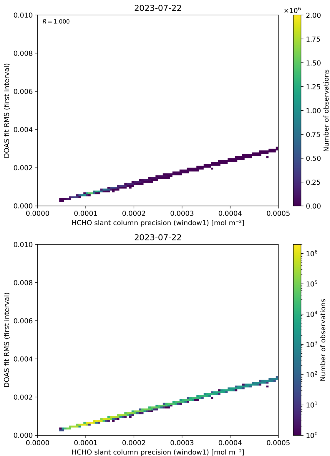
Figure 88: Scatter density plot of “HCHO slant column precision (window1)” against “DOAS fit RMS (first interval)” for 2023-07-21 to 2023-07-23.
