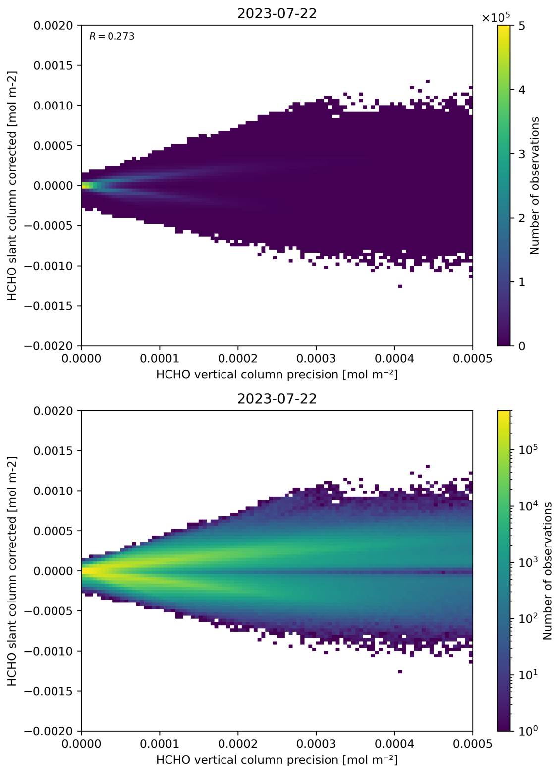
Figure 140: Scatter density plot of “HCHO vertical column precision” against “HCHO slant column corrected” for 2023-07-21 to 2023-07-23.
