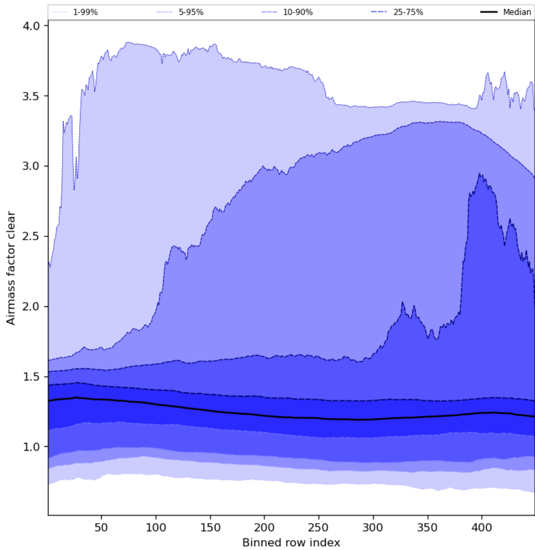
Figure 56: Along track statistics of “Airmass factor clear” for 2023-07-21 to 2023-07-23
