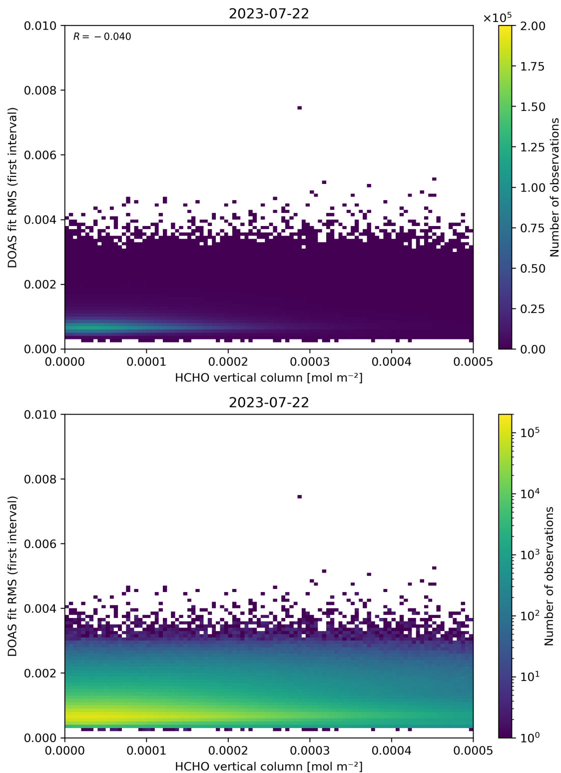
Figure 123: Scatter density plot of “HCHO vertical column” against “DOAS fit RMS (first interval)” for 2023-07-21 to 2023-07-23.
