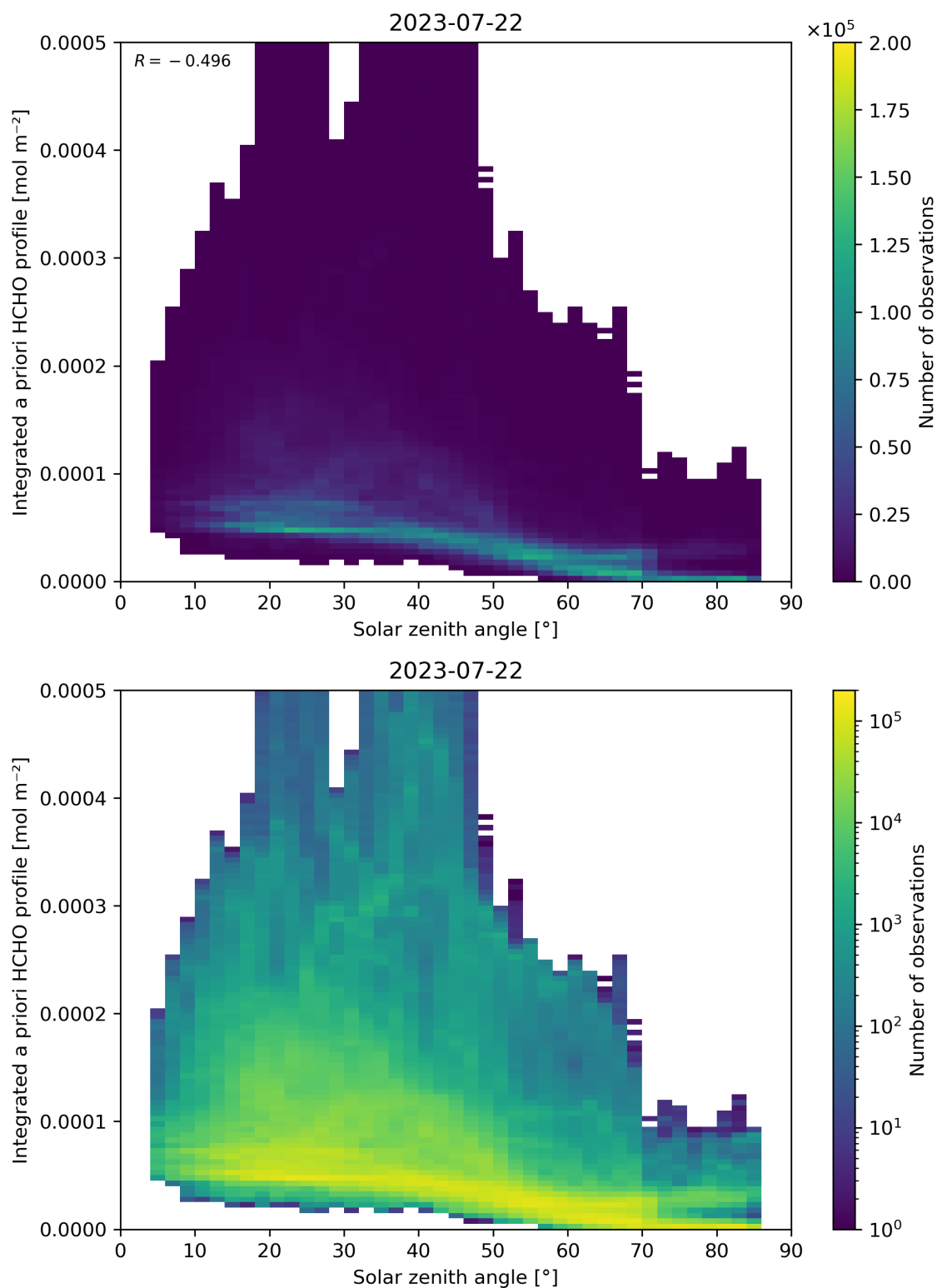
Figure 180: Scatter density plot of “Solar zenith angle” against “Integrated a priori HCHO profile” for 2023-07-21 to 2023-07-23.
