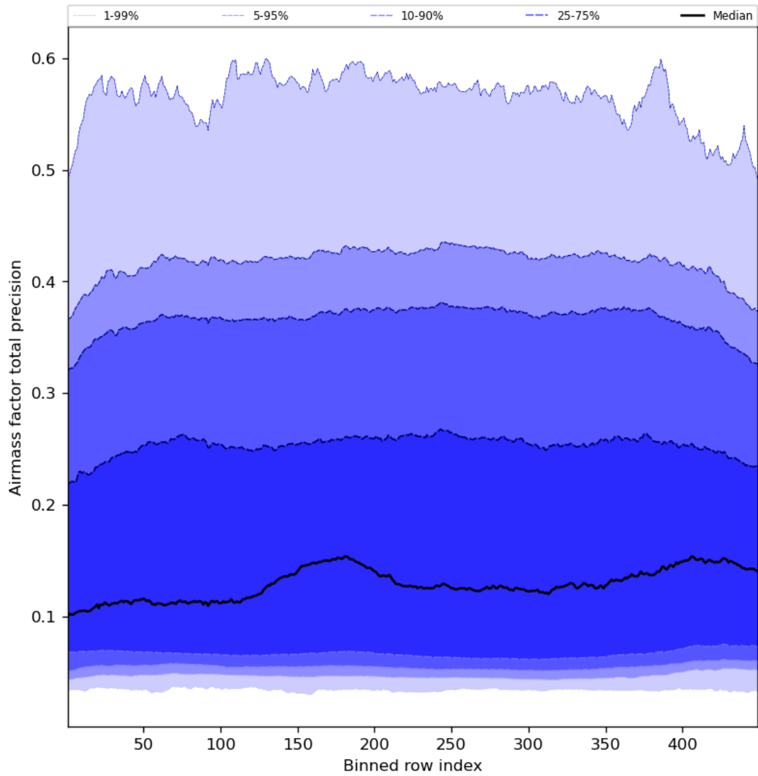
Figure 55: Along track statistics of “Airmass factor total precision” for 2023-07-21 to 2023-07-23
