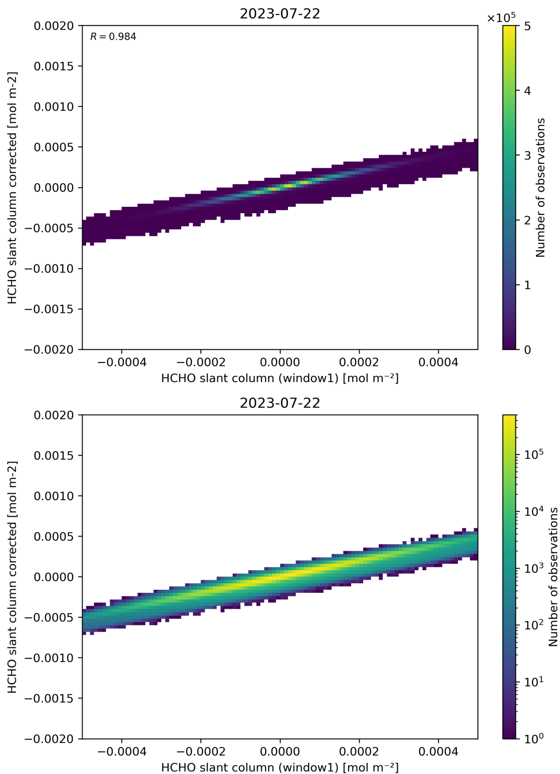
Figure 82: Scatter density plot of “HCHO slant column (window1)” against “HCHO slant column corrected” for 2023-07-21 to 2023-07-23.
