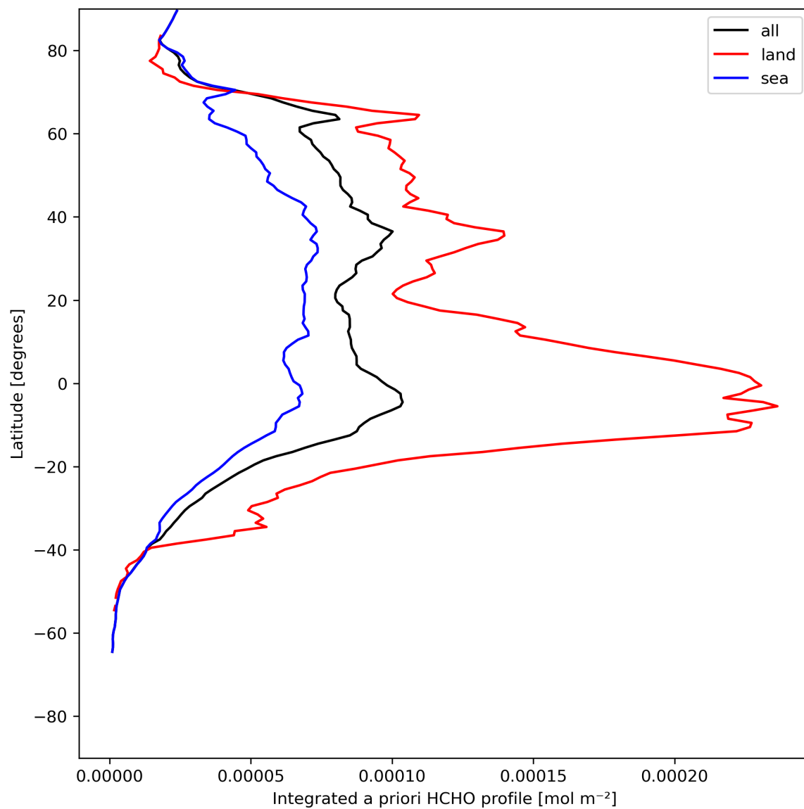
Figure 29: Zonal average of “Integrated a priori HCHO profile” for 2023-07-21 to 2023-07-23.
