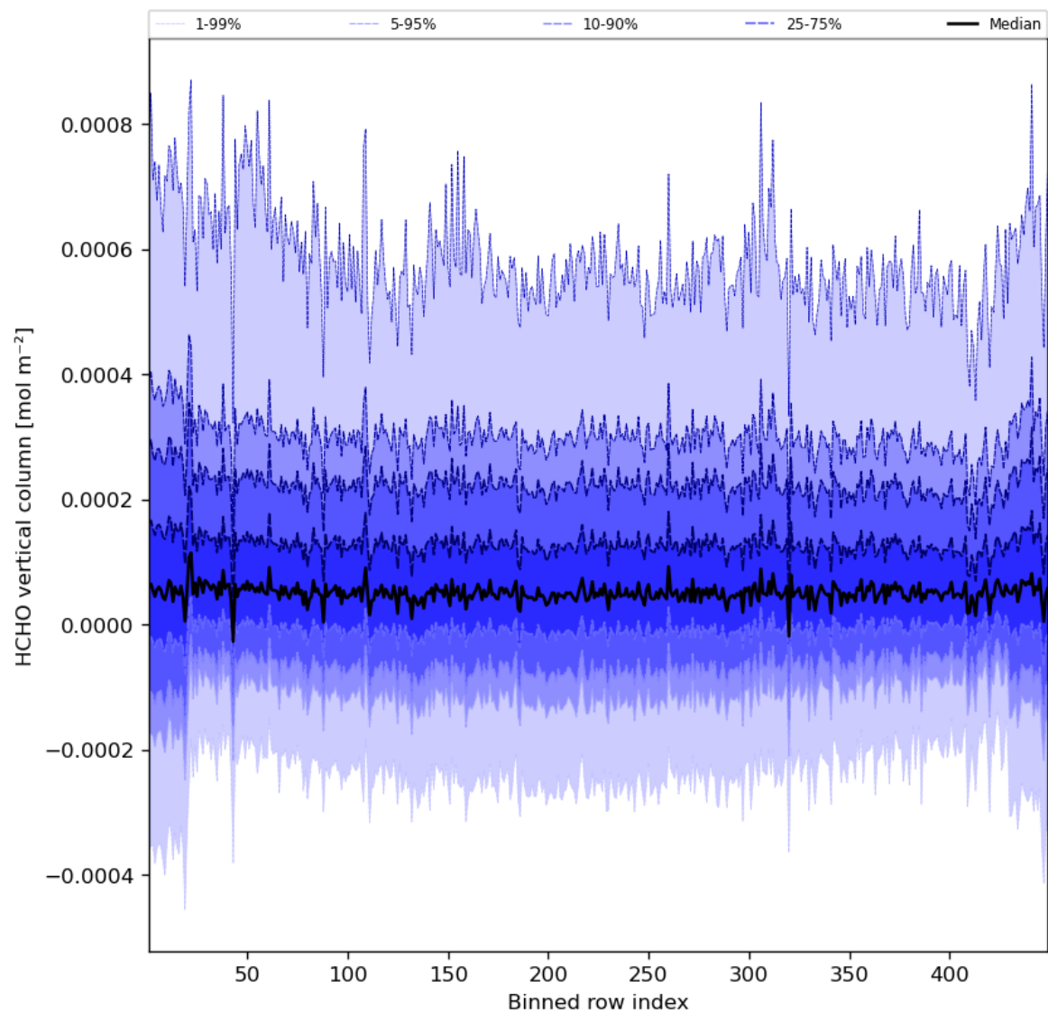
Figure 49: Along track statistics of “HCHO vertical column” for 2023-07-21 to 2023-07-23
