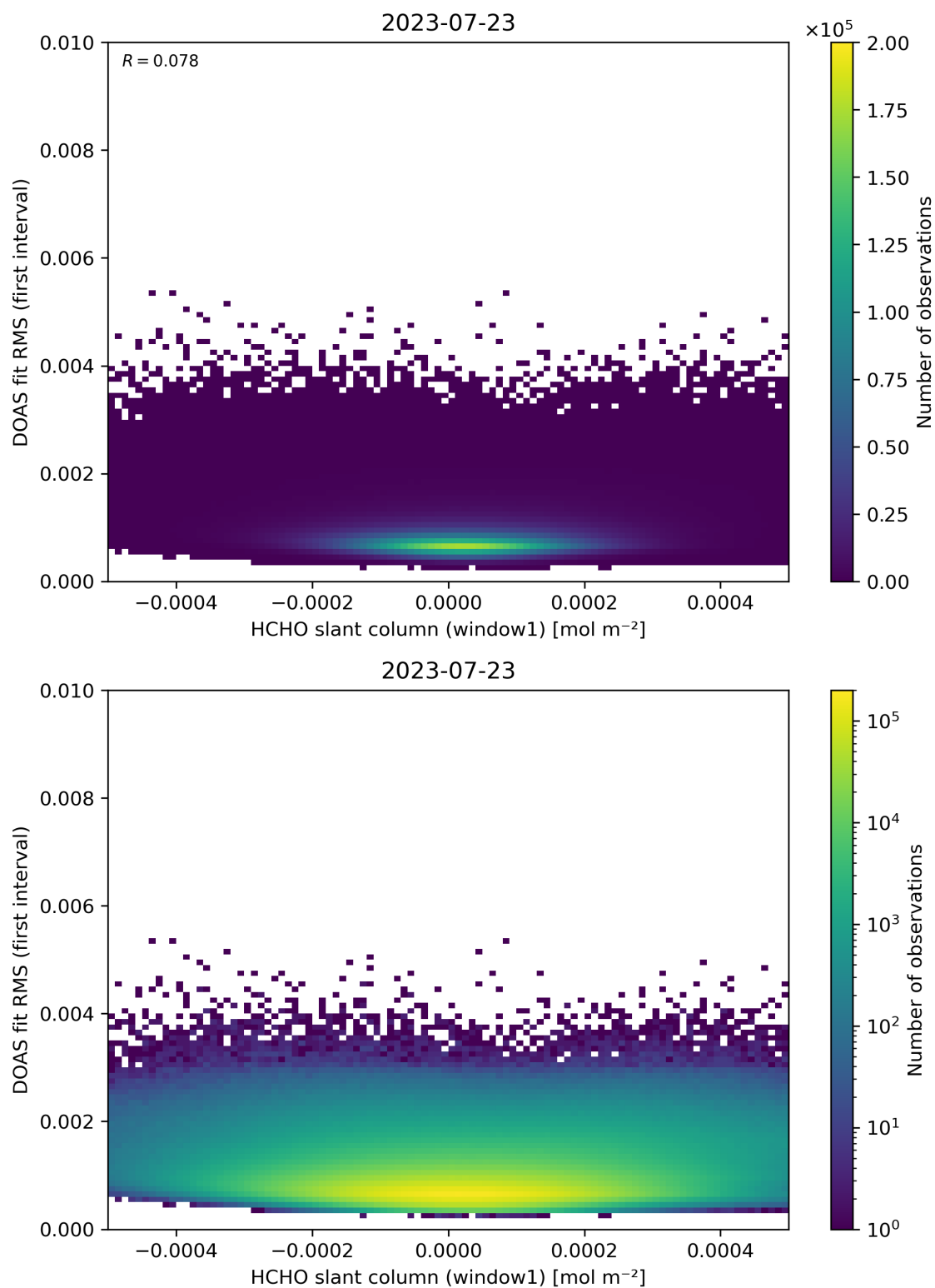
Figure 78: Scatter density plot of “HCHO slant column (window1)” against “DOAS fit RMS (first interval)” for 2023-07-22 to 2023-07-24.
