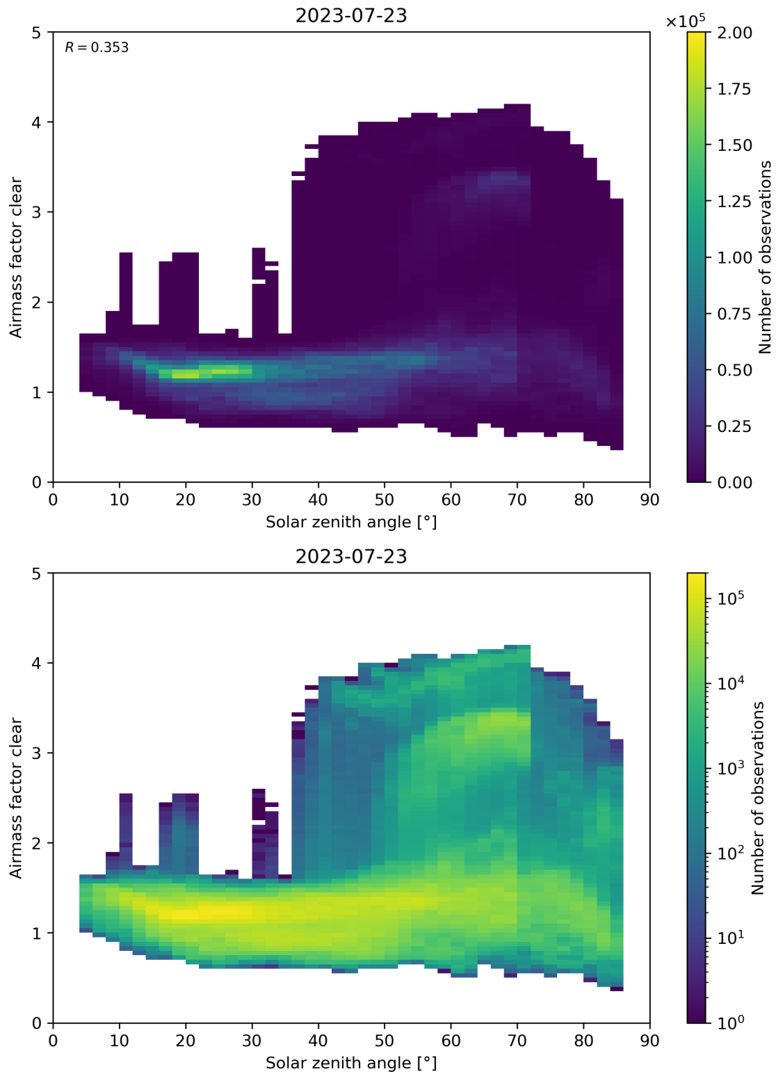
Figure 170: Scatter density plot of “Solar zenith angle” against “Airmass factor clear” for 2023-07-22 to 2023-07-24.
