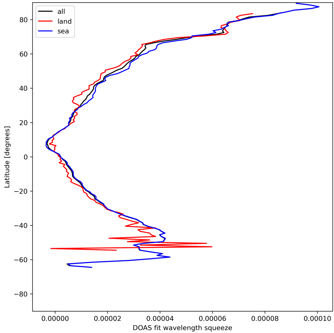
Figure 31: Zonal average of “DOAS fit wavelength squeeze” for 2023-07-22 to 2023-07-24.
