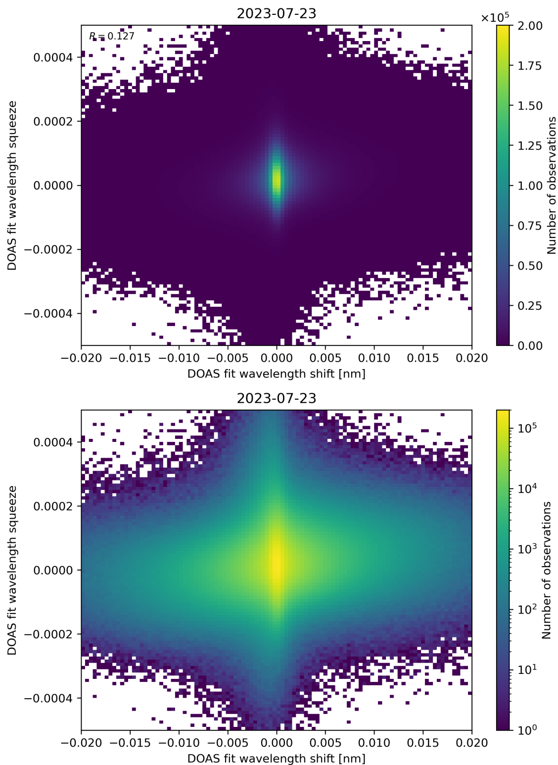
Figure 65: Scatter density plot of “DOAS fit wavelength shift” against “DOAS fit wavelength squeeze” for 2023-07-22 to 2023-07-24.
