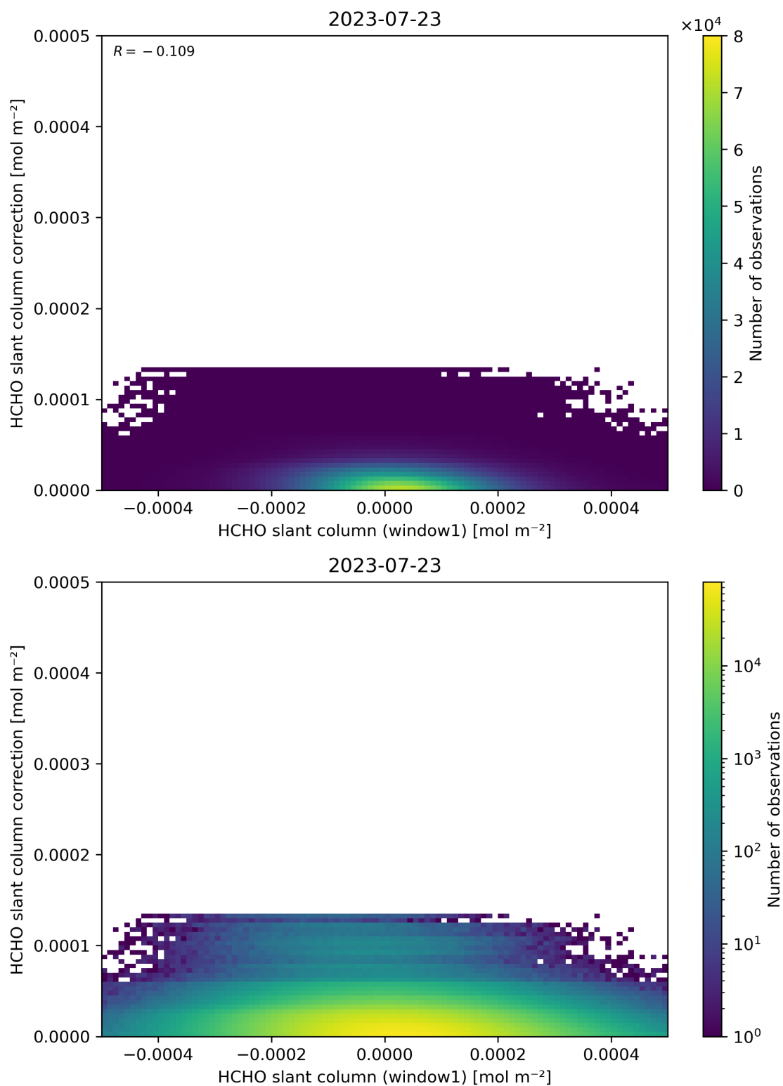
Figure 83: Scatter density plot of “HCHO slant column (window1)” against “HCHO slant column correction” for 2023-07-22 to 2023-07-24.
