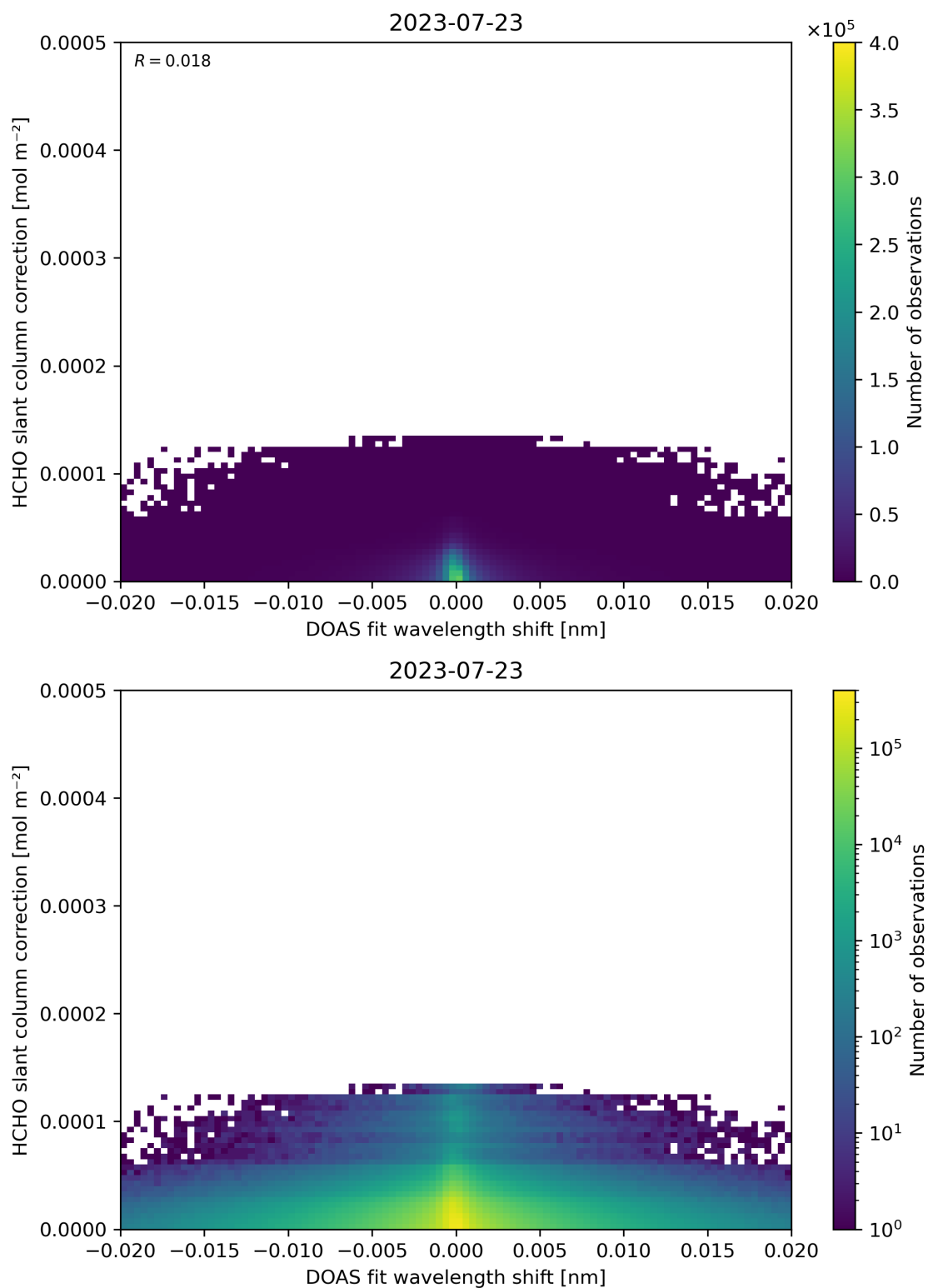
Figure 67: Scatter density plot of “DOAS fit wavelength shift” against “HCHO slant column correction” for 2023-07-22 to 2023-07-24.
