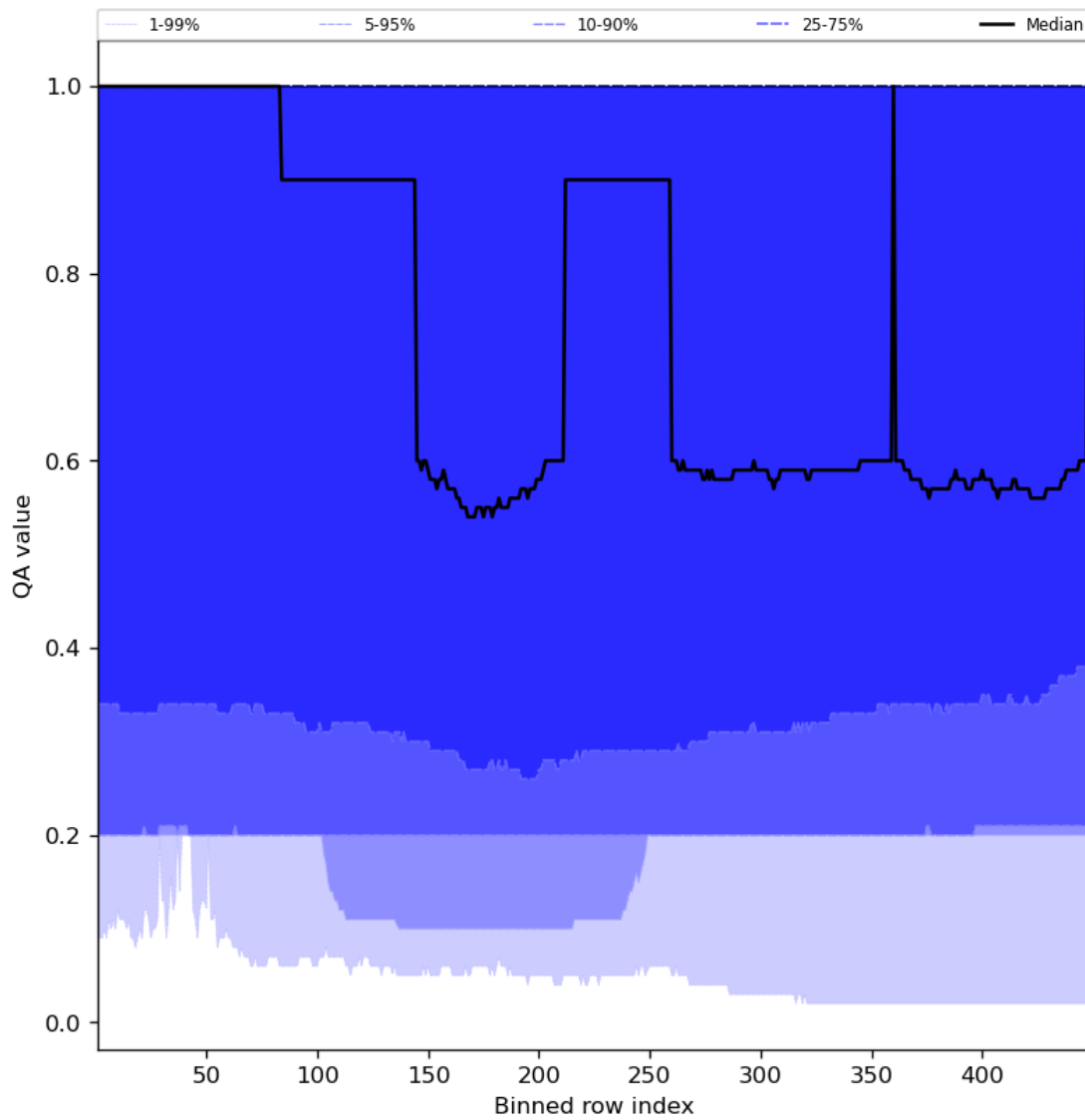
Figure 48: Along track statistics of “QA value” for 2023-07-22 to 2023-07-24
