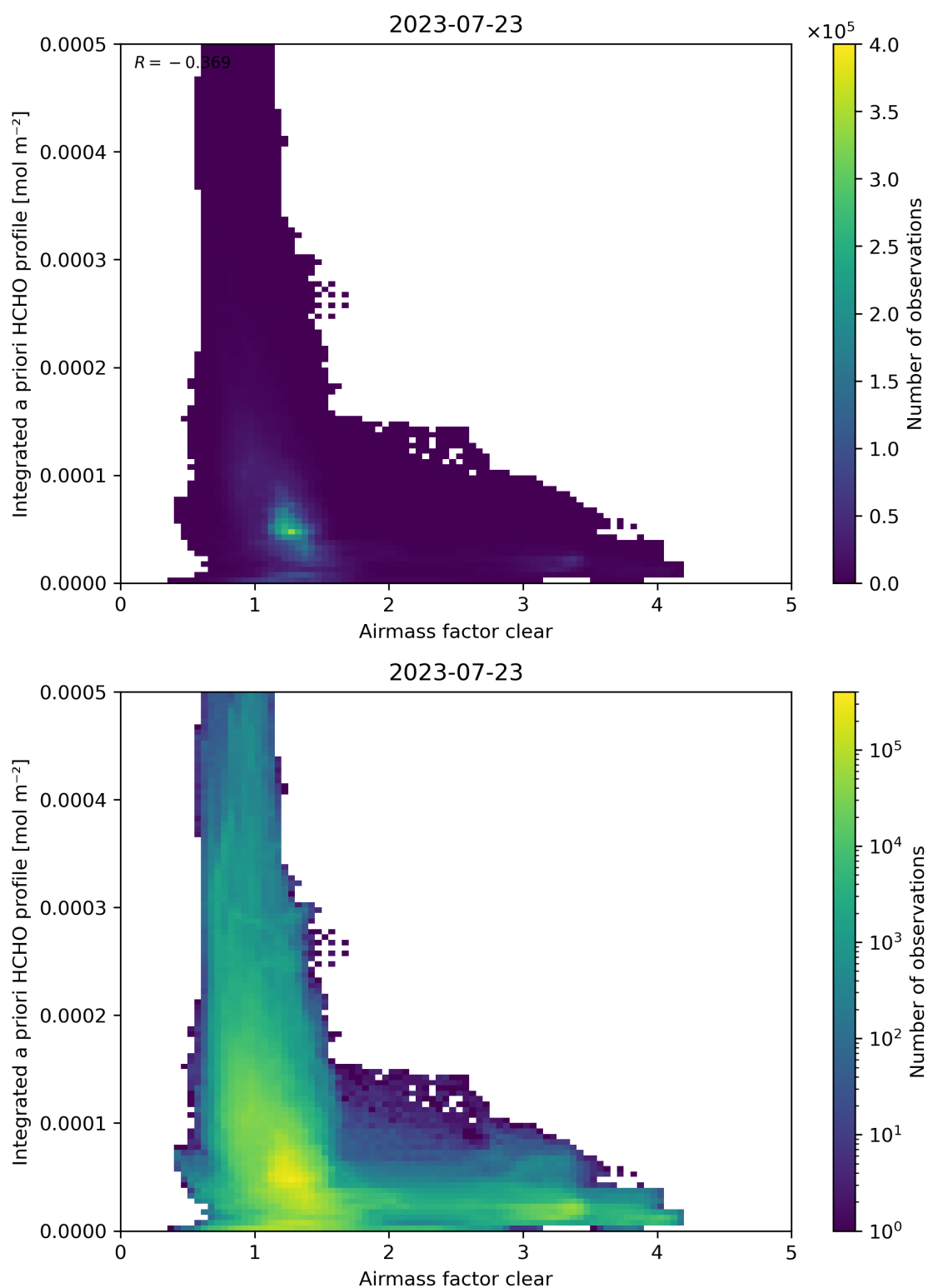
Figure 76: Scatter density plot of “Airmass factor clear” against “Integrated a priori HCHO profile” for 2023-07-22 to 2023-07-24.
