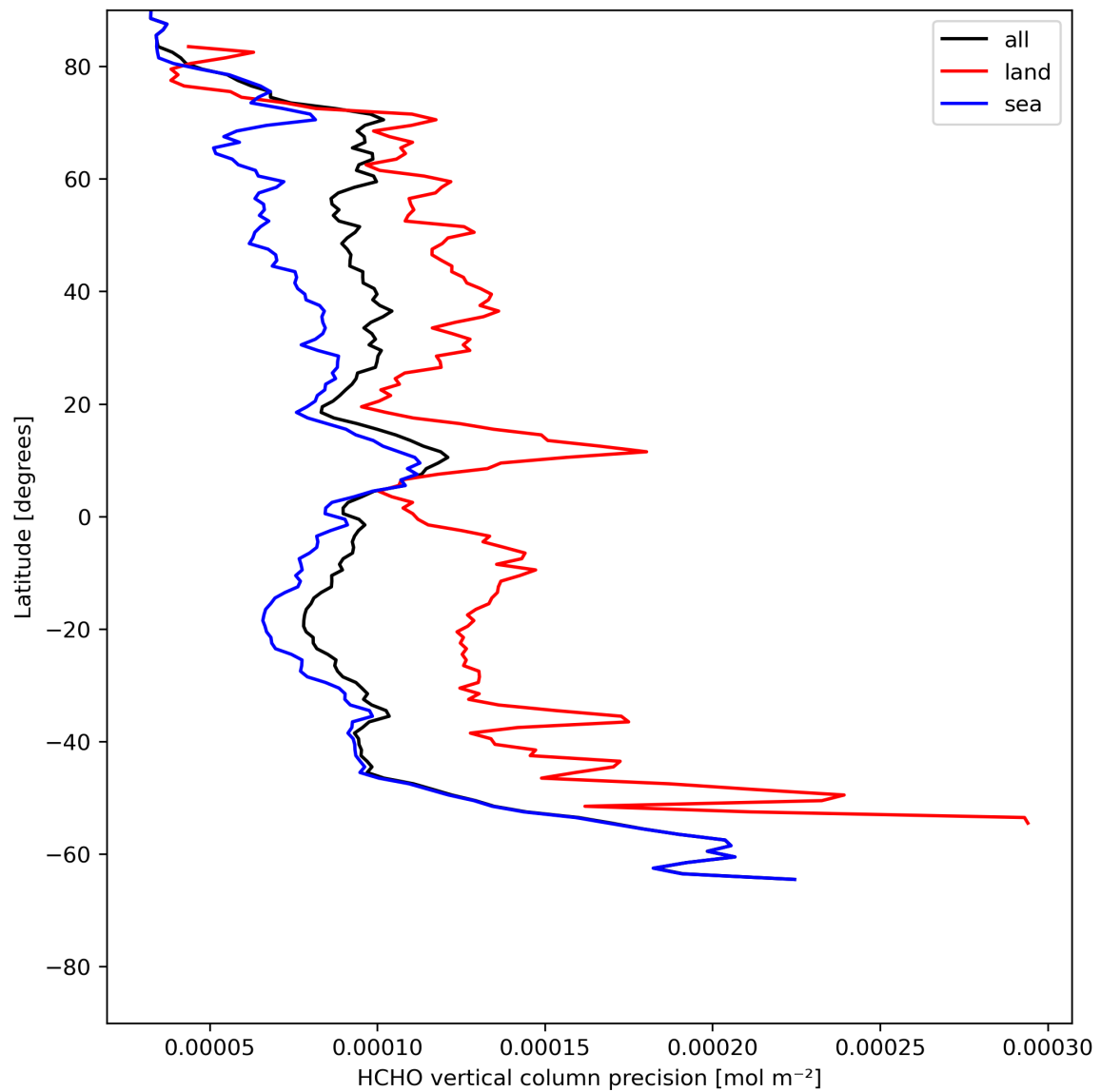
Figure 22: Zonal average of “HCHO vertical column precision” for 2023-07-22 to 2023-07-24.
