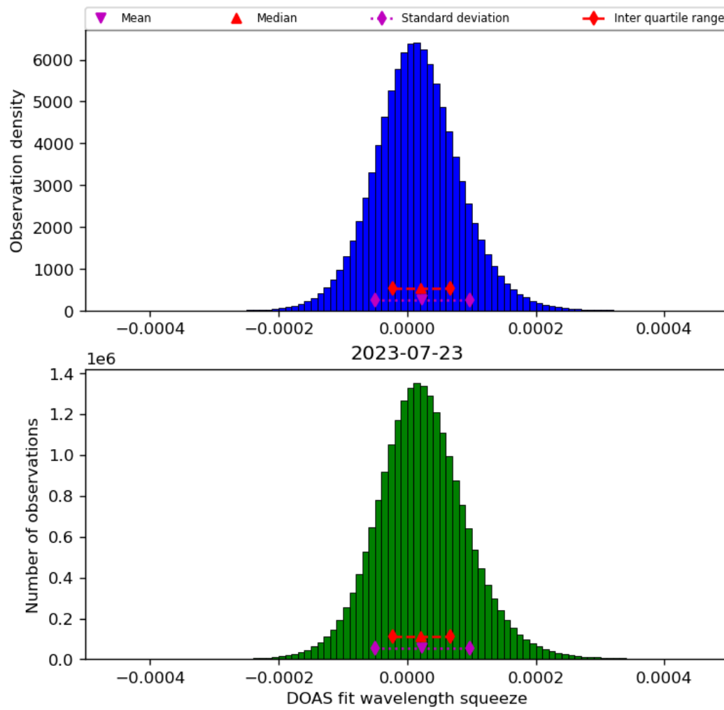
Figure 45: Histogram of “DOAS fit wavelength squeeze” for 2023-07-22 to 2023-07-24
