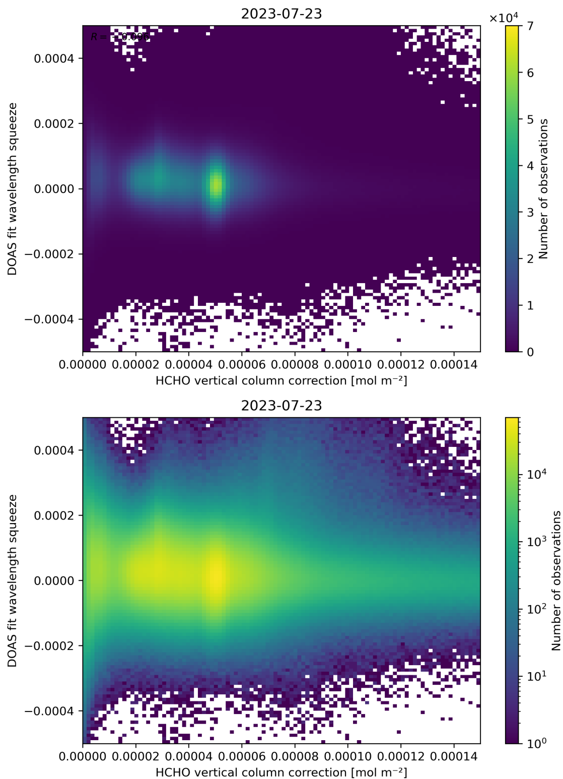
Figure 114: Scatter density plot of “HCHO vertical column correction” against “DOAS fit wavelength squeeze” for 2023-07-22 to 2023-07-24.
