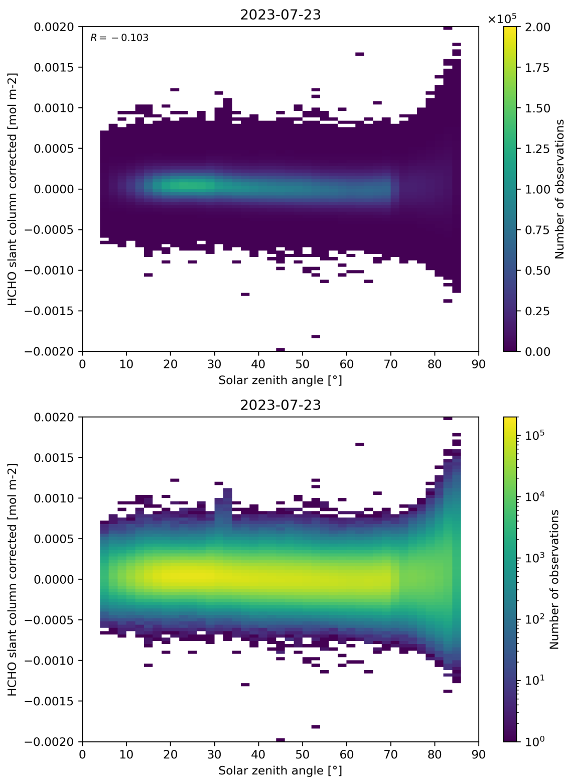
Figure 171: Scatter density plot of “Solar zenith angle” against “HCHO slant column corrected” for 2023-07-22 to 2023-07-24.
