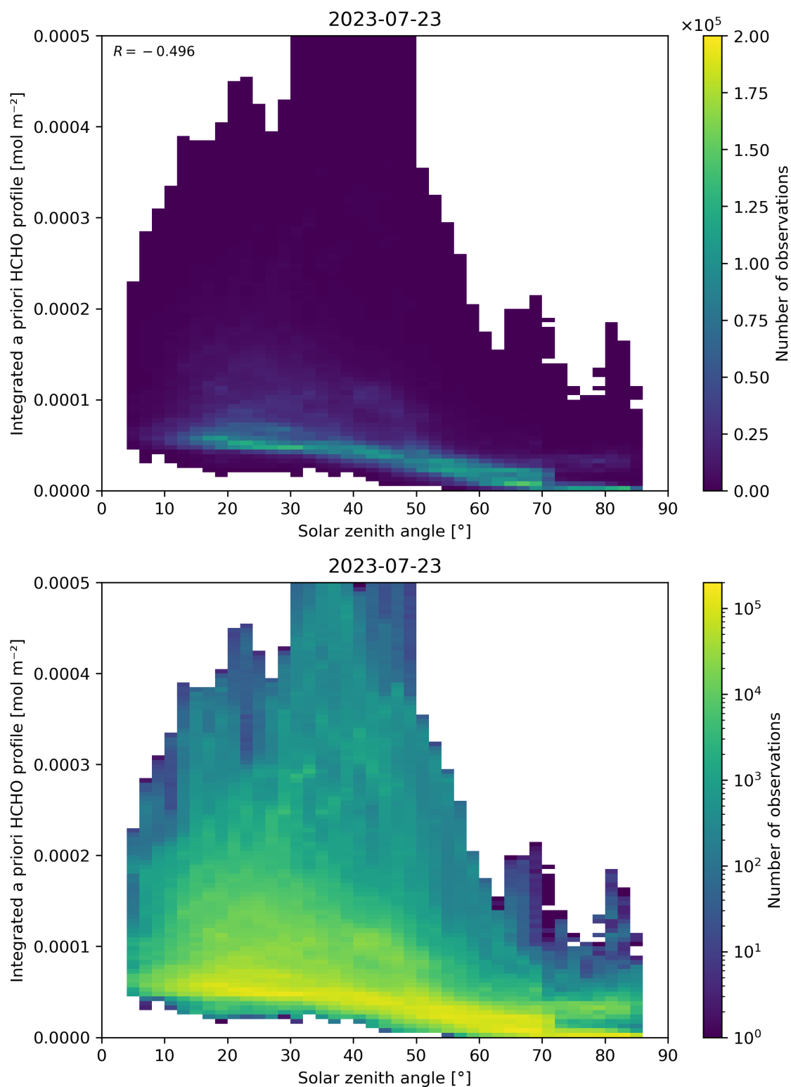
Figure 180: Scatter density plot of “Solar zenith angle” against “Integrated a priori HCHO profile” for 2023-07-22 to 2023-07-24.
