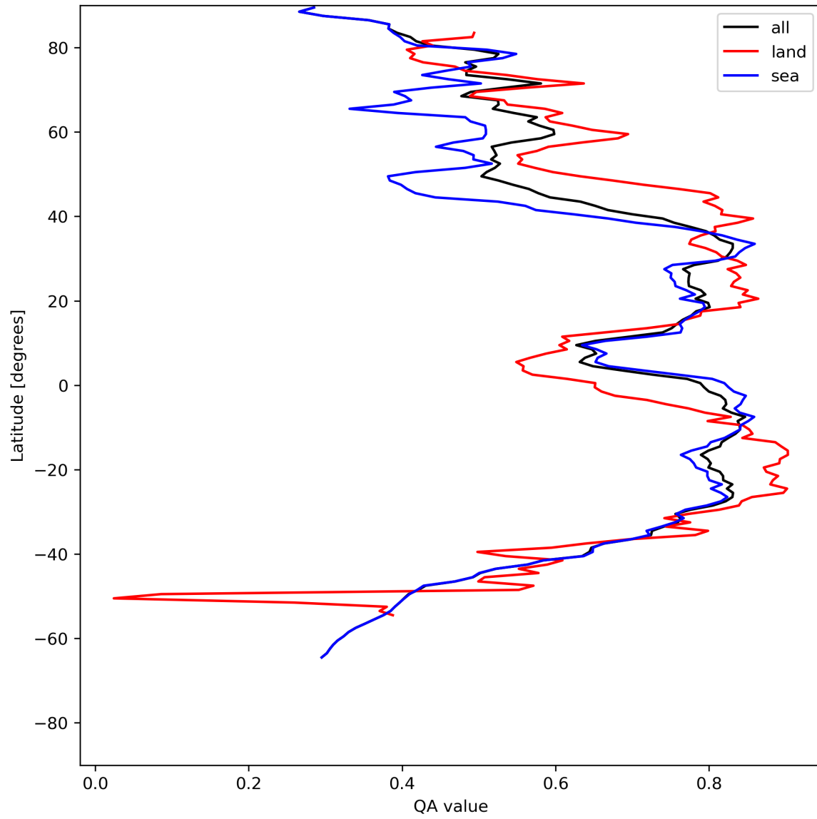
Figure 20: Zonal average of “QA value” for 2023-07-22 to 2023-07-24.
