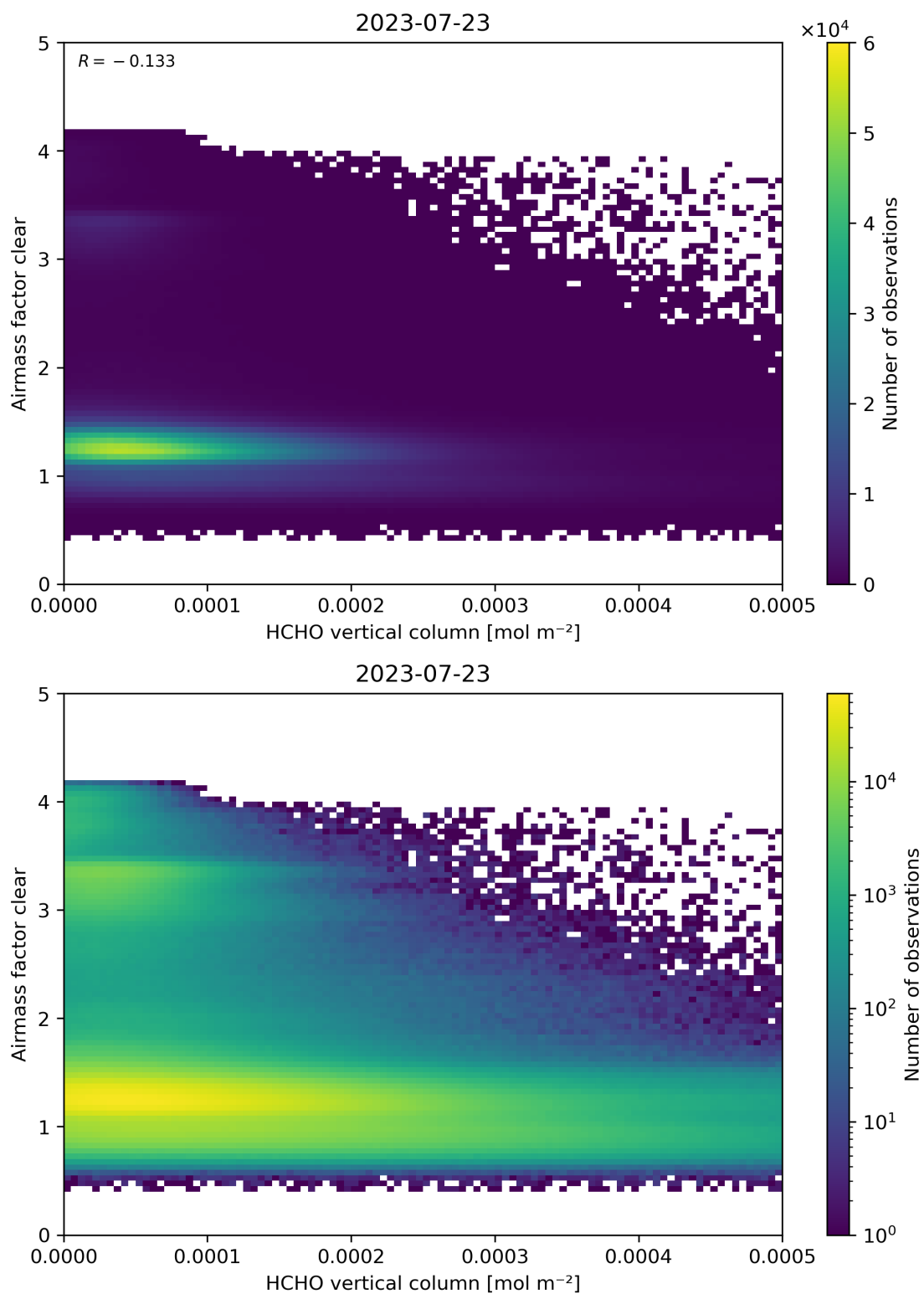
Figure 126: Scatter density plot of “HCHO vertical column” against “Airmass factor clear” for 2023-07-22 to 2023-07-24.
