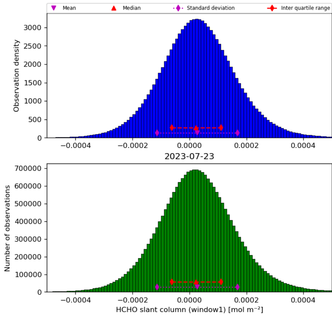
Figure 38: Histogram of “HCHO slant column (window1)” for 2023-07-22 to 2023-07-24
