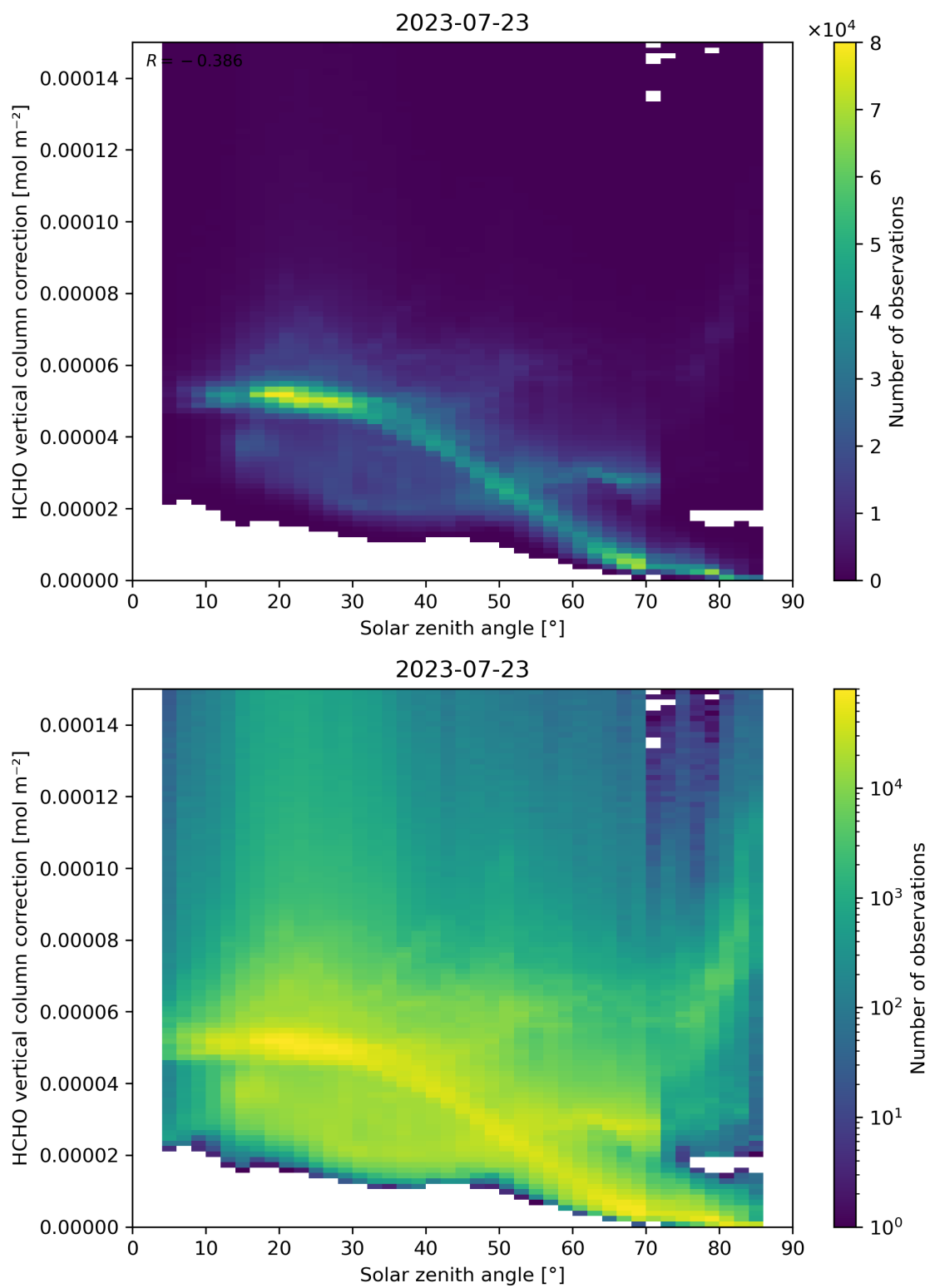
Figure 178: Scatter density plot of “Solar zenith angle” against “HCHO vertical column correction” for 2023-07-22 to 2023-07-24.
