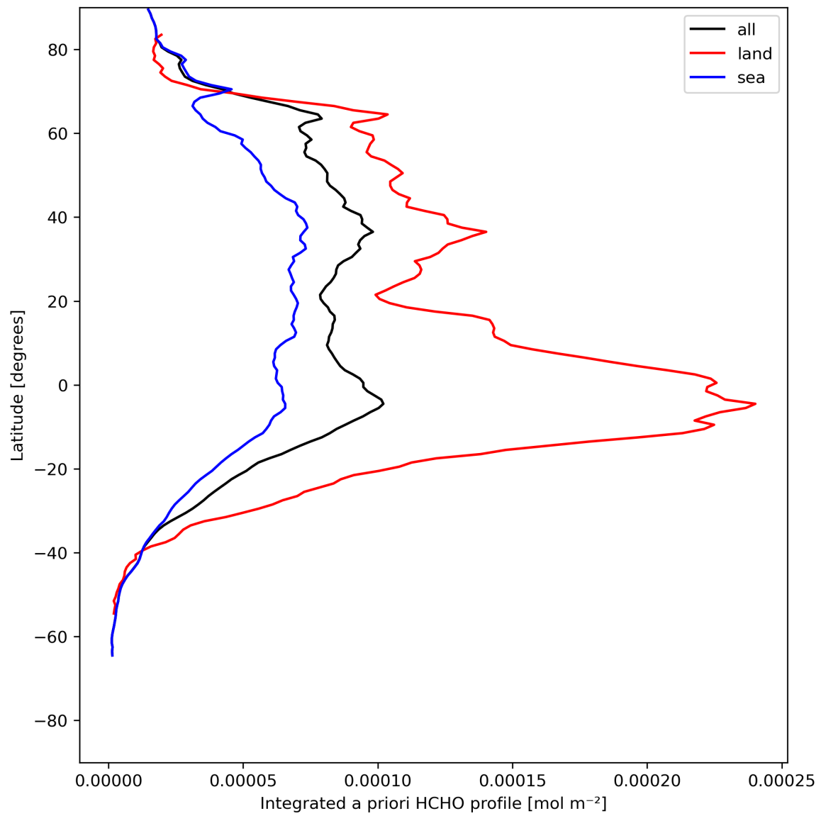
Figure 29: Zonal average of “Integrated a priori HCHO profile” for 2023-07-22 to 2023-07-24.
