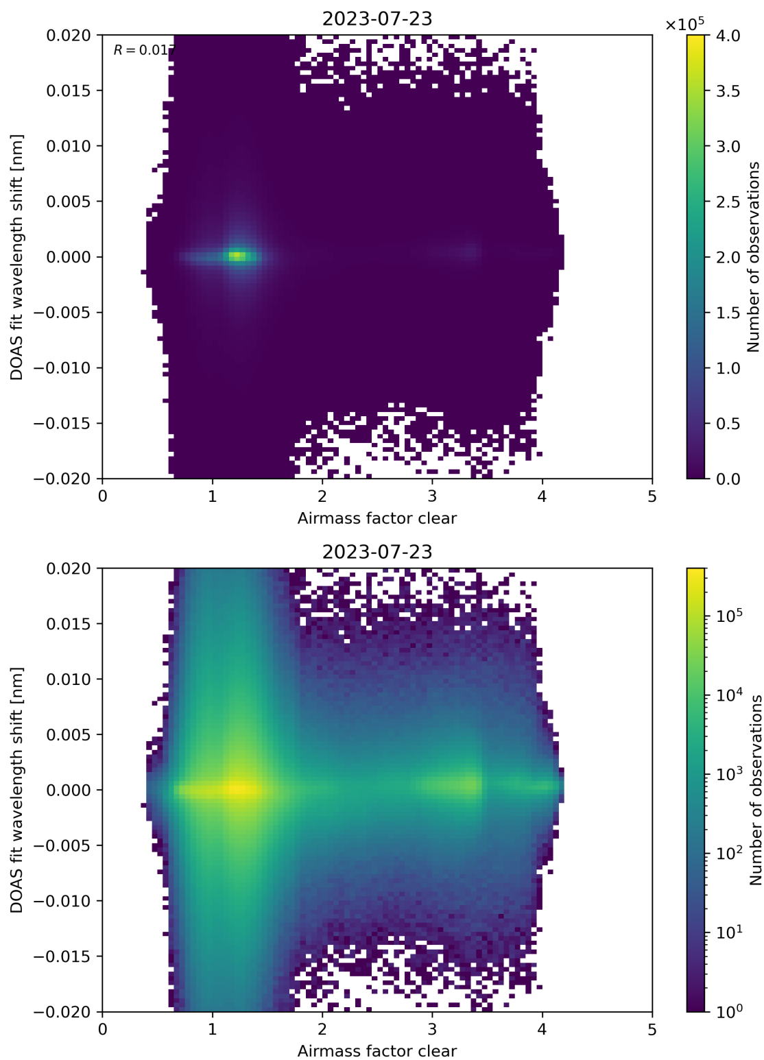
Figure 72: Scatter density plot of “Airmass factor clear” against “DOAS fit wavelength shift” for 2023-07-22 to 2023-07-24.
