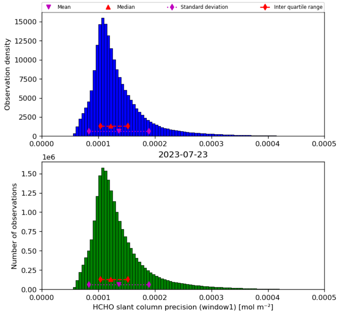
Figure 39: Histogram of “HCHO slant column precision (window1)” for 2023-07-22 to 2023-07-24
