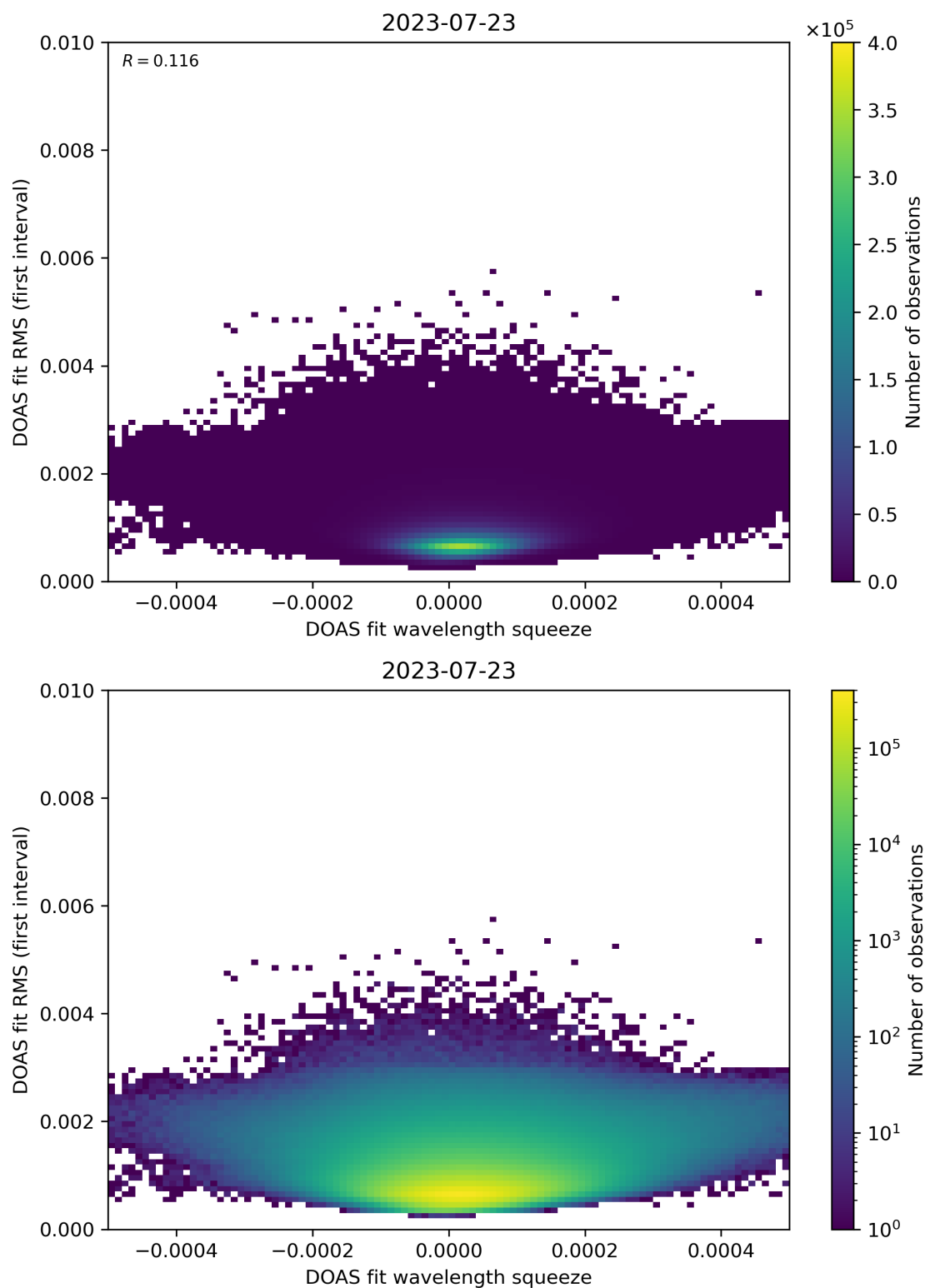
Figure 68: Scatter density plot of “DOAS fit wavelength squeeze” against “DOAS fit RMS (first interval)” for 2023-07-22 to 2023-07-24.
