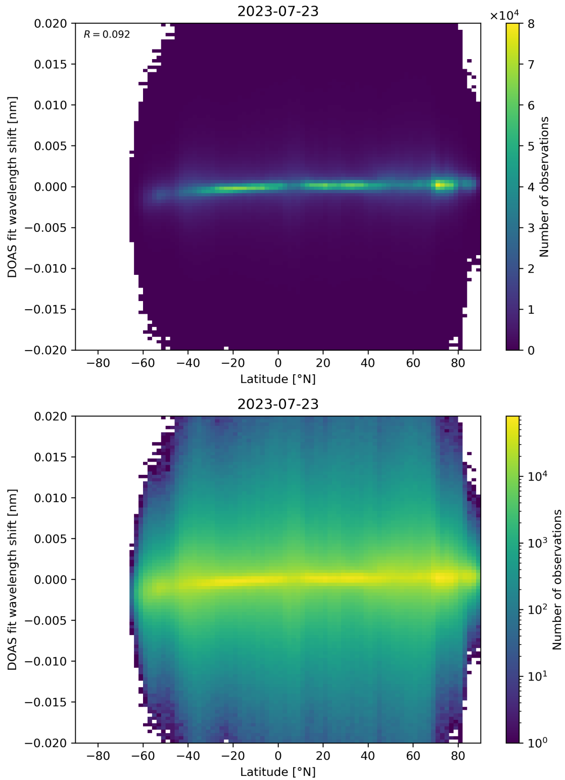
Figure 154: Scatter density plot of “Latitude” against “DOAS fit wavelength shift” for 2023-07-22 to 2023-07-24.
