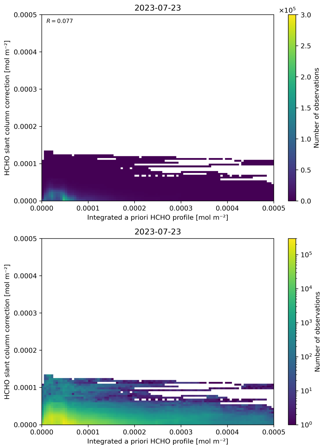
Figure 152: Scatter density plot of “Integrated a priori HCHO profile” against “HCHO slant column correction” for 2023-07-22 to 2023-07-24.
