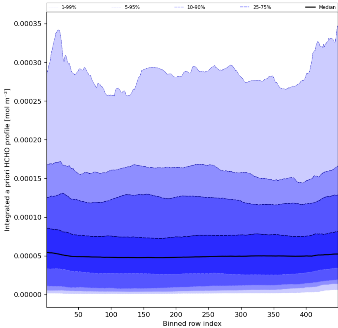
Figure 57: Along track statistics of “Integrated a priori HCHO profile” for 2023-07-22 to 2023-07-24
