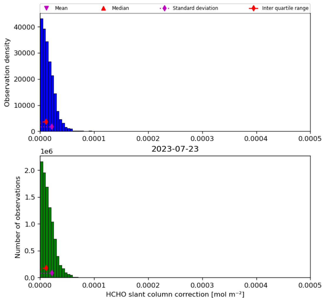
Figure 47: Histogram of “HCHO slant column correction” for 2023-07-22 to 2023-07-24
