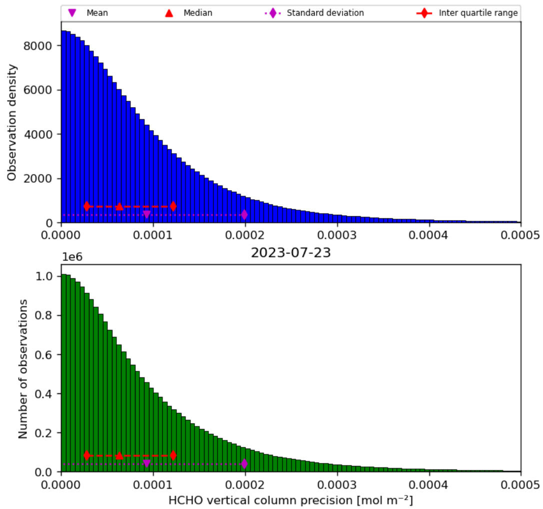
Figure 36: Histogram of “HCHO vertical column precision” for 2023-07-22 to 2023-07-24
