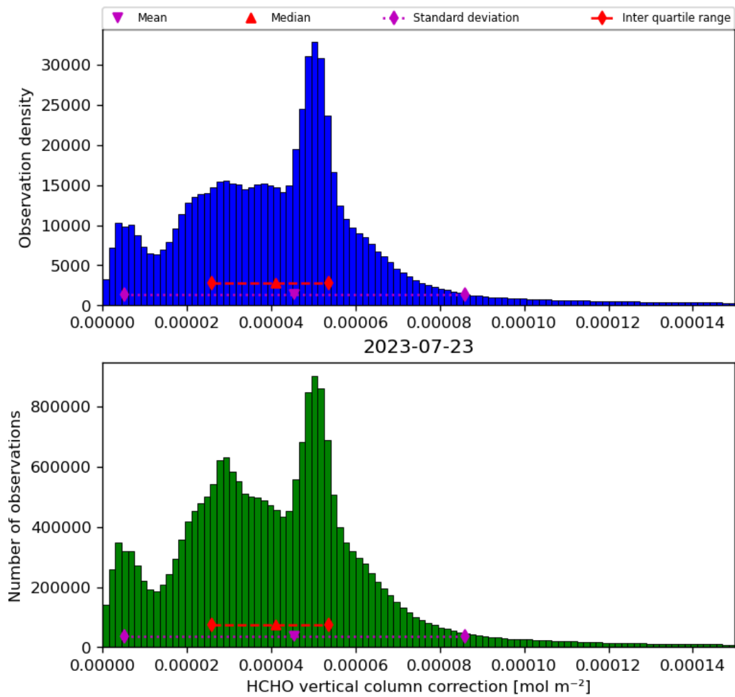
Figure 37: Histogram of “HCHO vertical column correction” for 2023-07-22 to 2023-07-24
