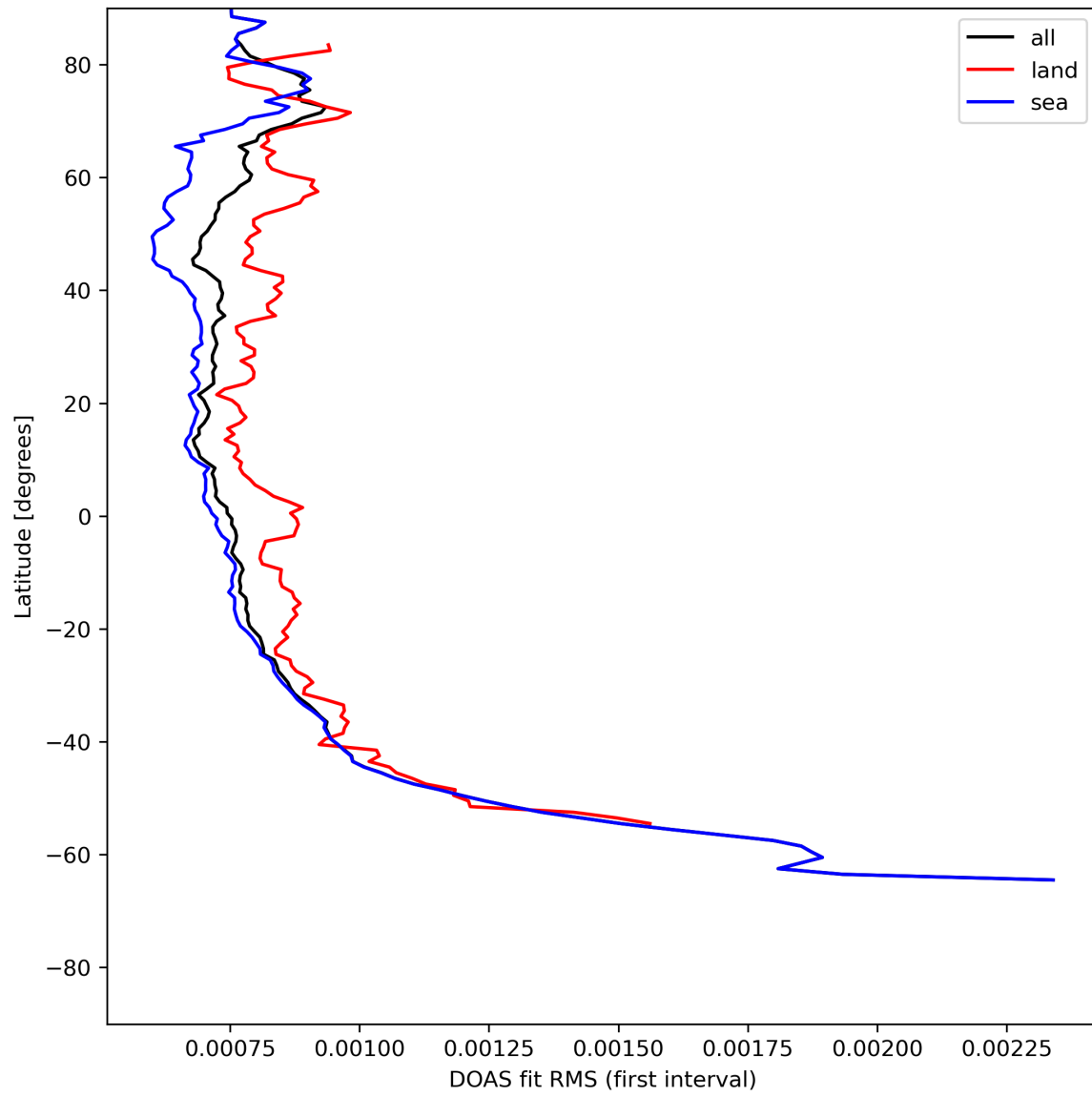
Figure 32: Zonal average of "DOAS fit RMS (first interval)" for 2023-07-22 to 2023-07-24.
