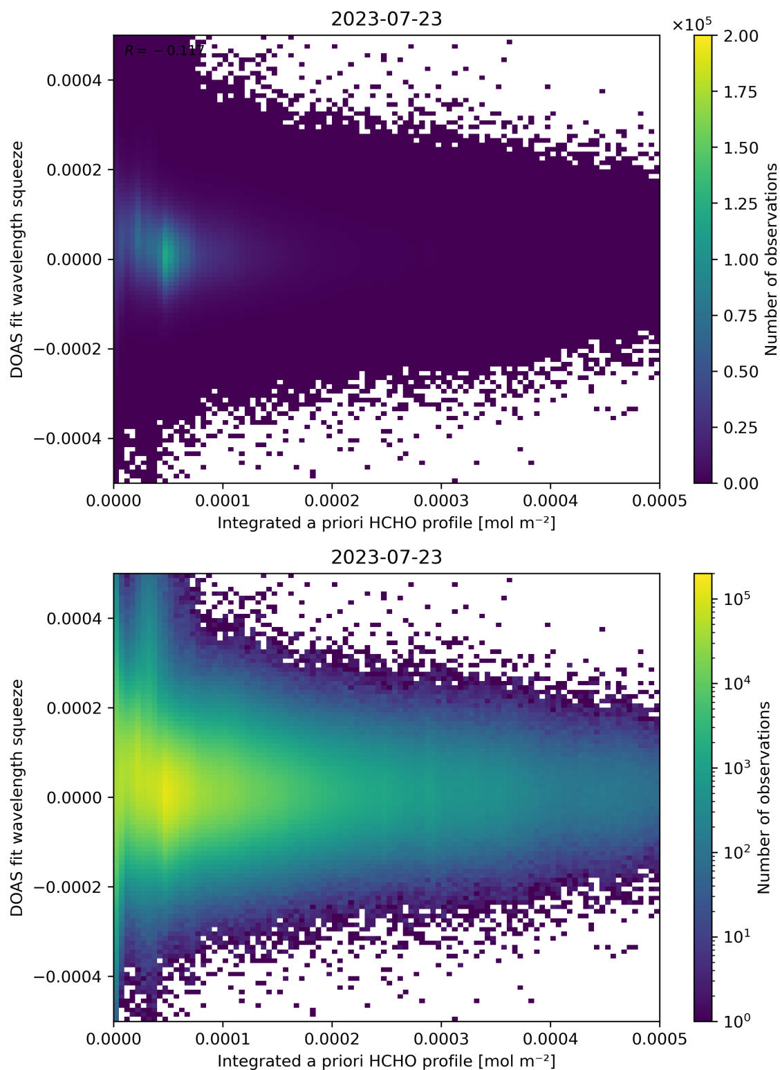
Figure 150: Scatter density plot of “Integrated a priori HCHO profile” against “DOAS fit wavelength squeeze” for 2023-07-22 to 2023-07-24.
