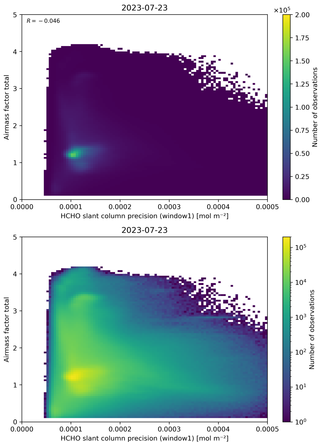
Figure 94: Scatter density plot of “HCHO slant column precision (window1)” against “Airmass factor total” for 2023-07-22 to 2023-07-24.
