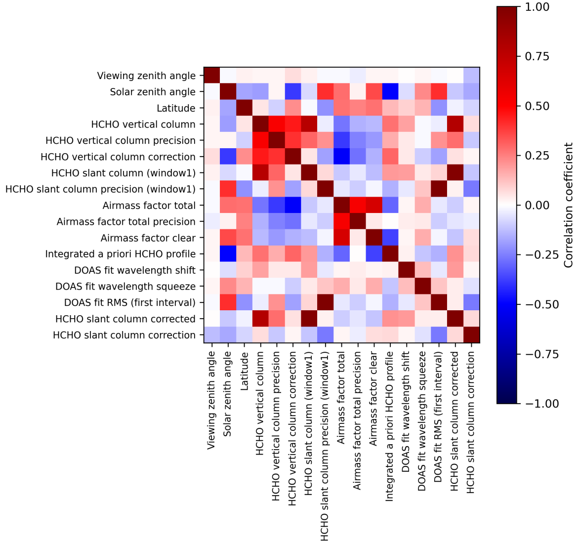
Figure 2: Map of correlation matrix for 2023-07-22 to 2023-07-24.
