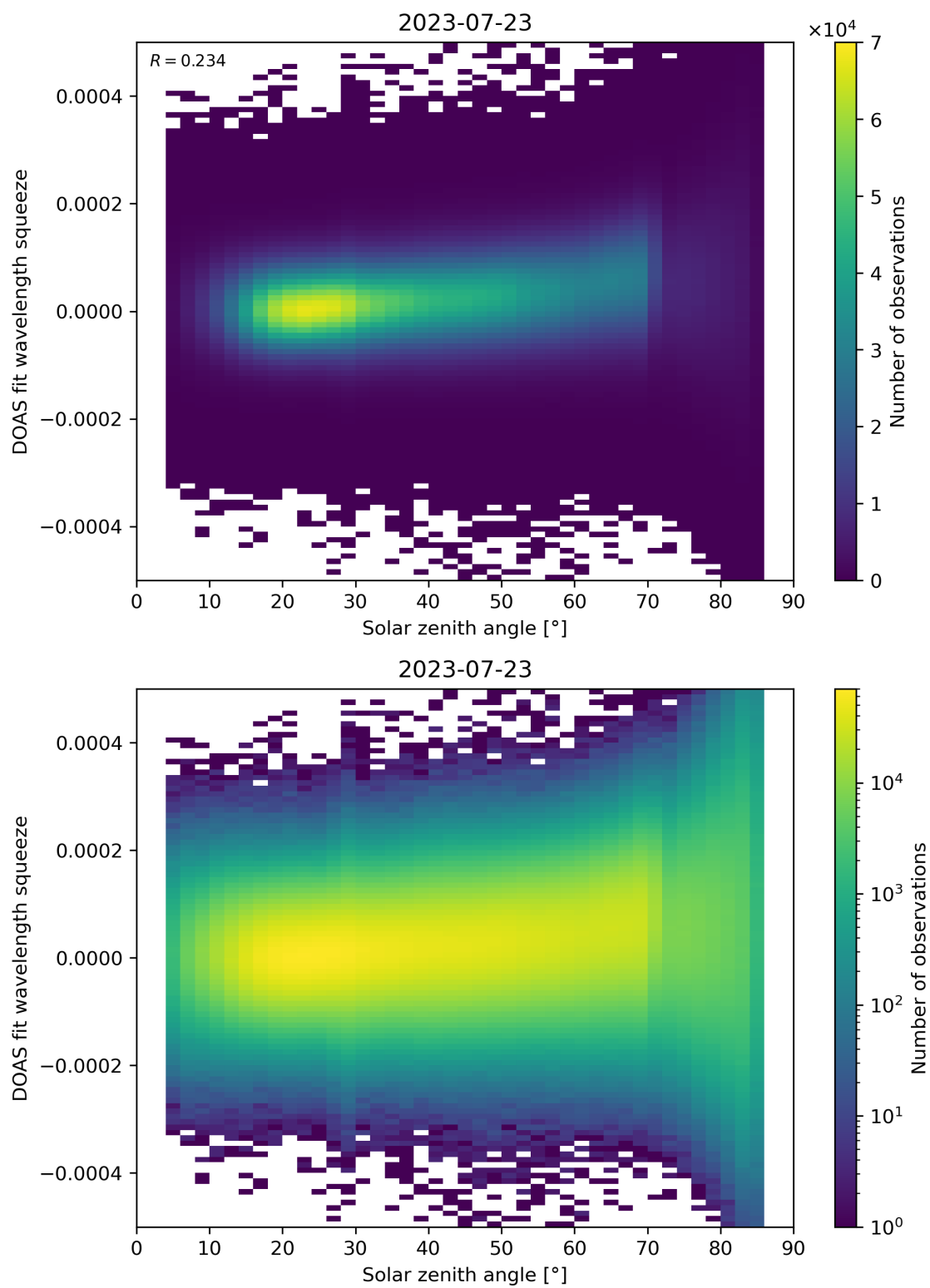
Figure 169: Scatter density plot of “Solar zenith angle” against “DOAS fit wavelength squeeze” for 2023-07-22 to 2023-07-24.
