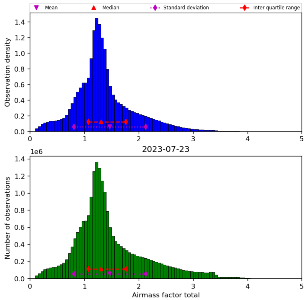
Figure 40: Histogram of “Airmass factor total” for 2023-07-22 to 2023-07-24
