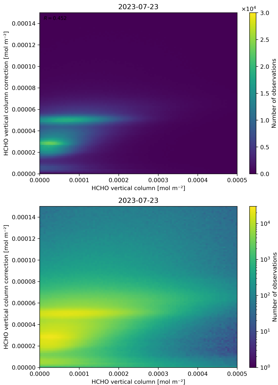
Figure 133: Scatter density plot of “HCHO vertical column” against “HCHO vertical column correction” for 2023-07-22 to 2023-07-24.
