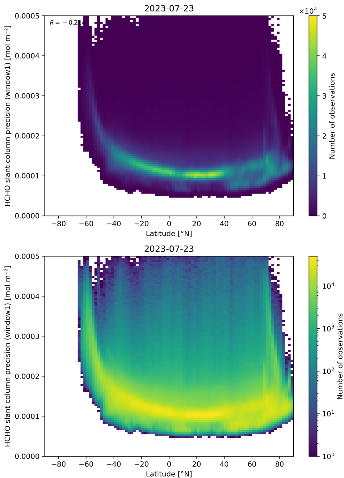
Figure 160: Scatter density plot of “Latitude” against “HCHO slant column precision (window1)” for 2023-07-22 to 2023-07-24.
