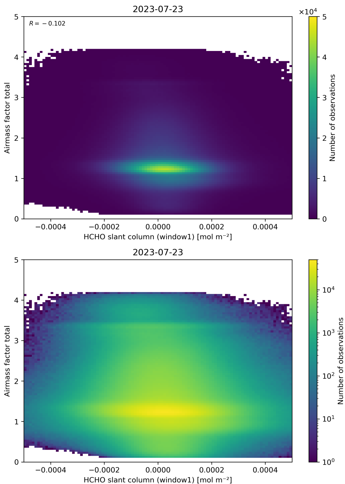
Figure 85: Scatter density plot of “HCHO slant column (window1)” against “Airmass factor total” for 2023-07-22 to 2023-07-24.
