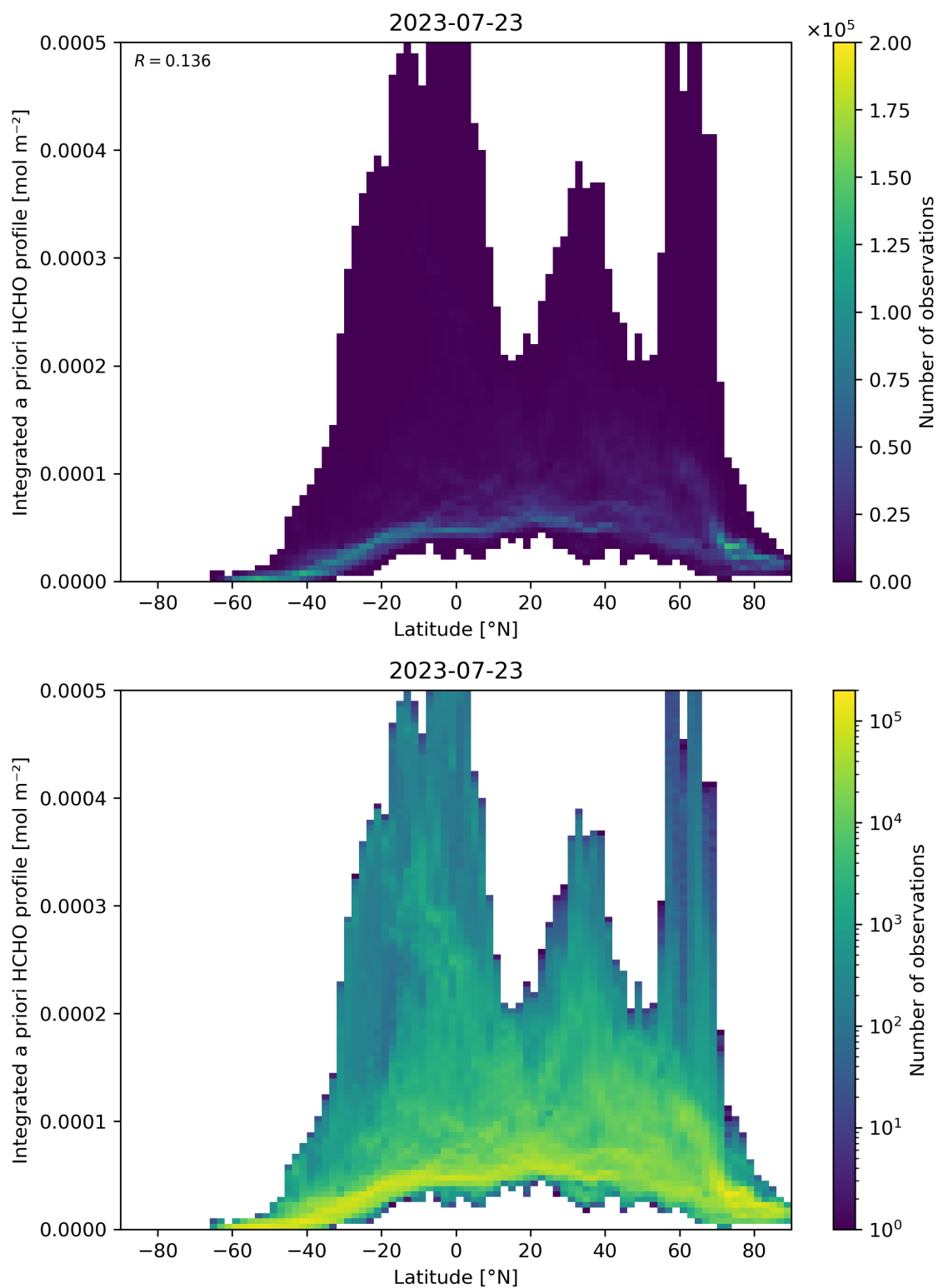
Figure 166: Scatter density plot of “Latitude” against “Integrated a priori HCHO profile” for 2023-07-22 to 2023-07-24.
