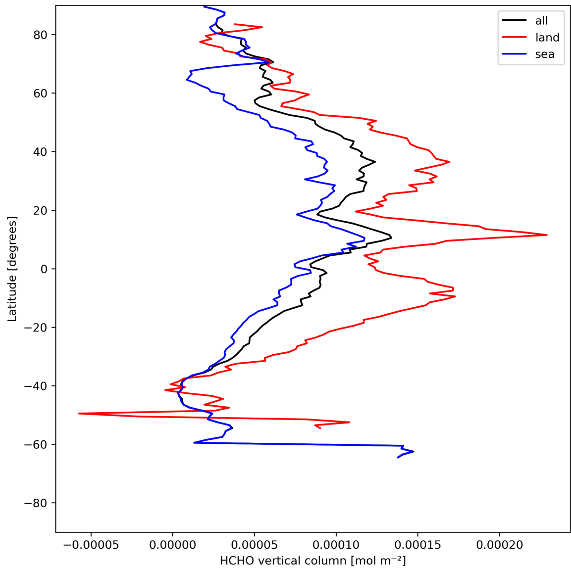
Figure 21: Zonal average of “HCHO vertical column” for 2023-07-22 to 2023-07-24.
