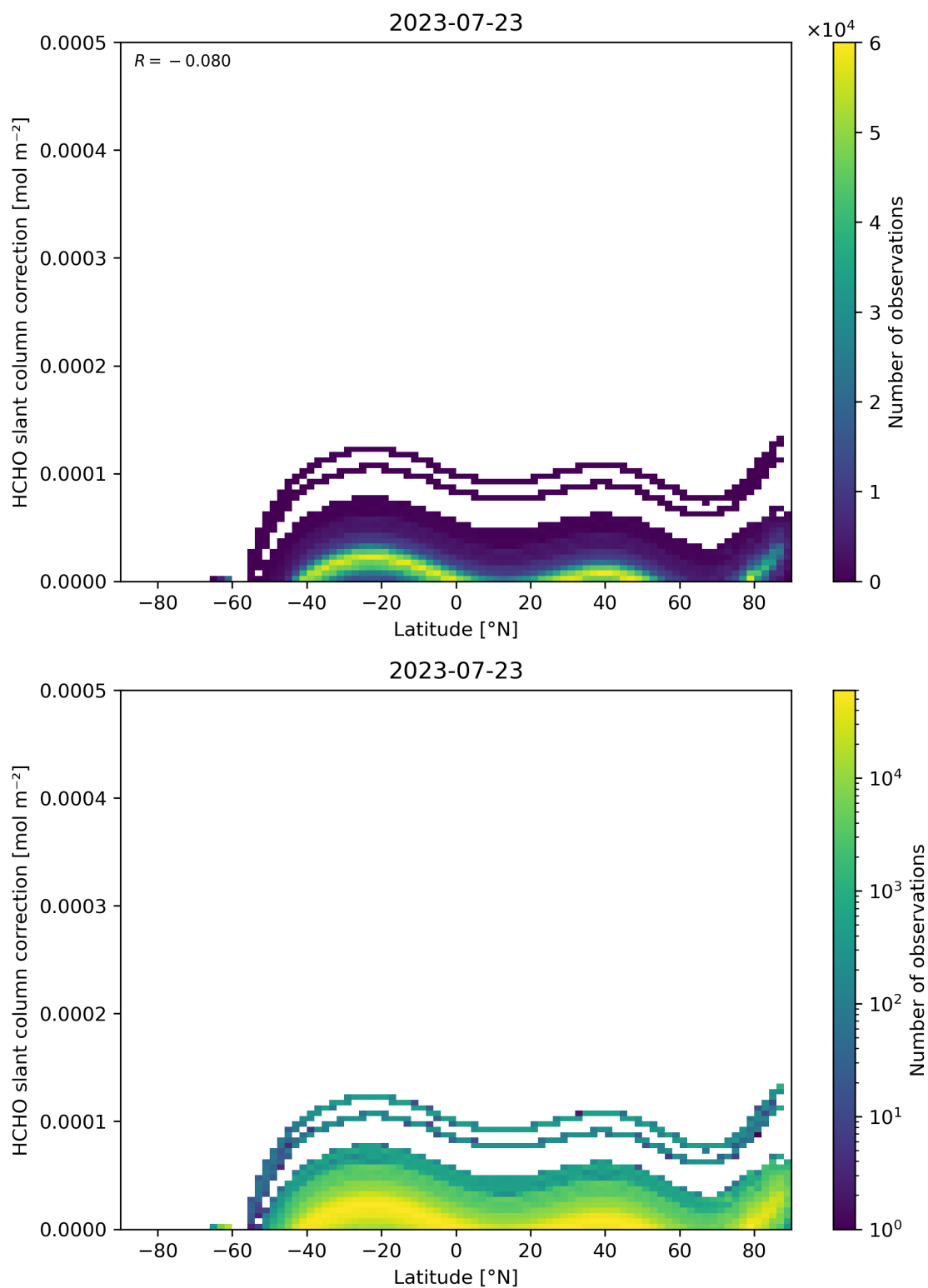
Figure 158: Scatter density plot of “Latitude” against “HCHO slant column correction” for 2023-07-22 to 2023-07-24.
