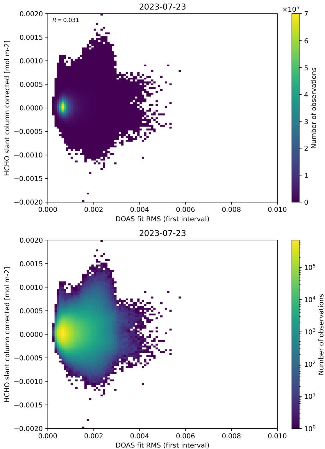
Figure 62: Scatter density plot of “DOAS fit RMS (first interval)” against “HCHO slant column corrected” for 2023-07-22 to 2023-07-24.
