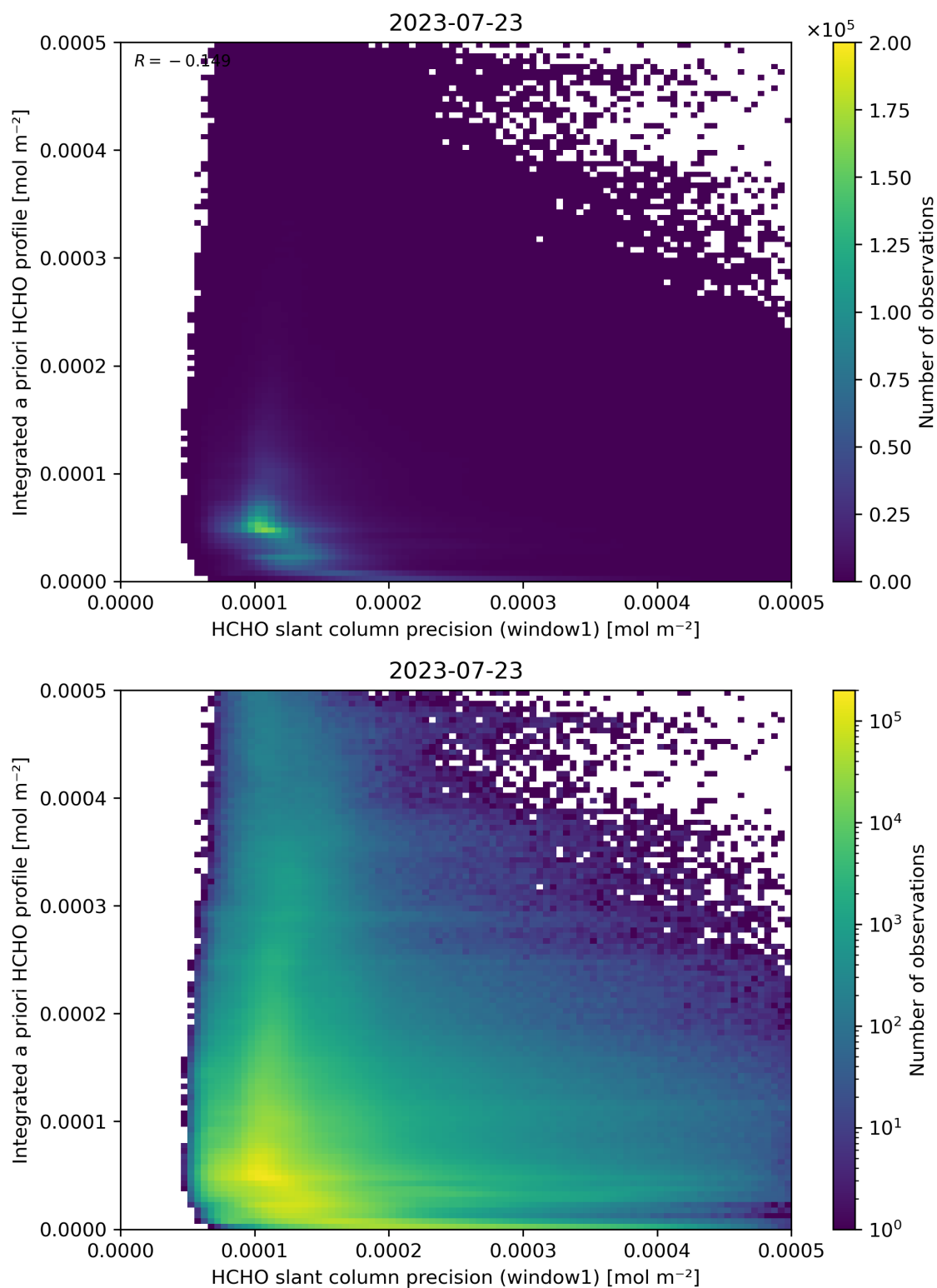
Figure 96: Scatter density plot of “HCHO slant column precision (window1)” against “Integrated a priori HCHO profile” for 2023-07-22 to 2023-07-24.
