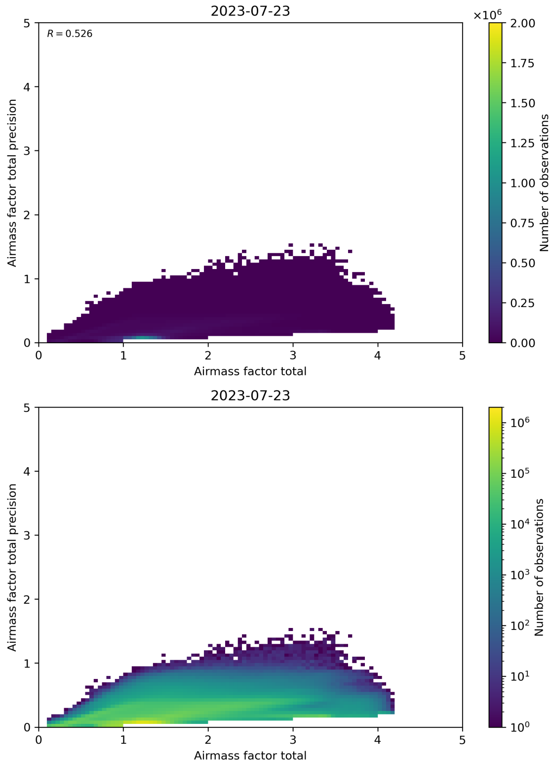
Figure 103: Scatter density plot of “Airmass factor total” against “Airmass factor total precision” for 2023-07-22 to 2023-07-24.
