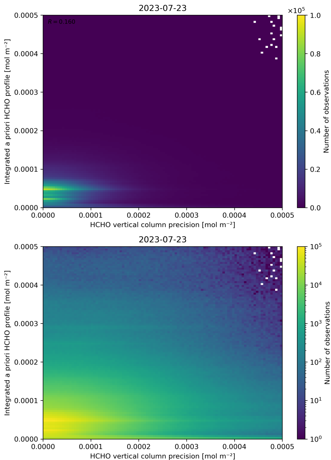
Figure 147: Scatter density plot of “HCHO vertical column precision” against “Integrated a priori HCHO profile” for 2023-07-22 to 2023-07-24.
