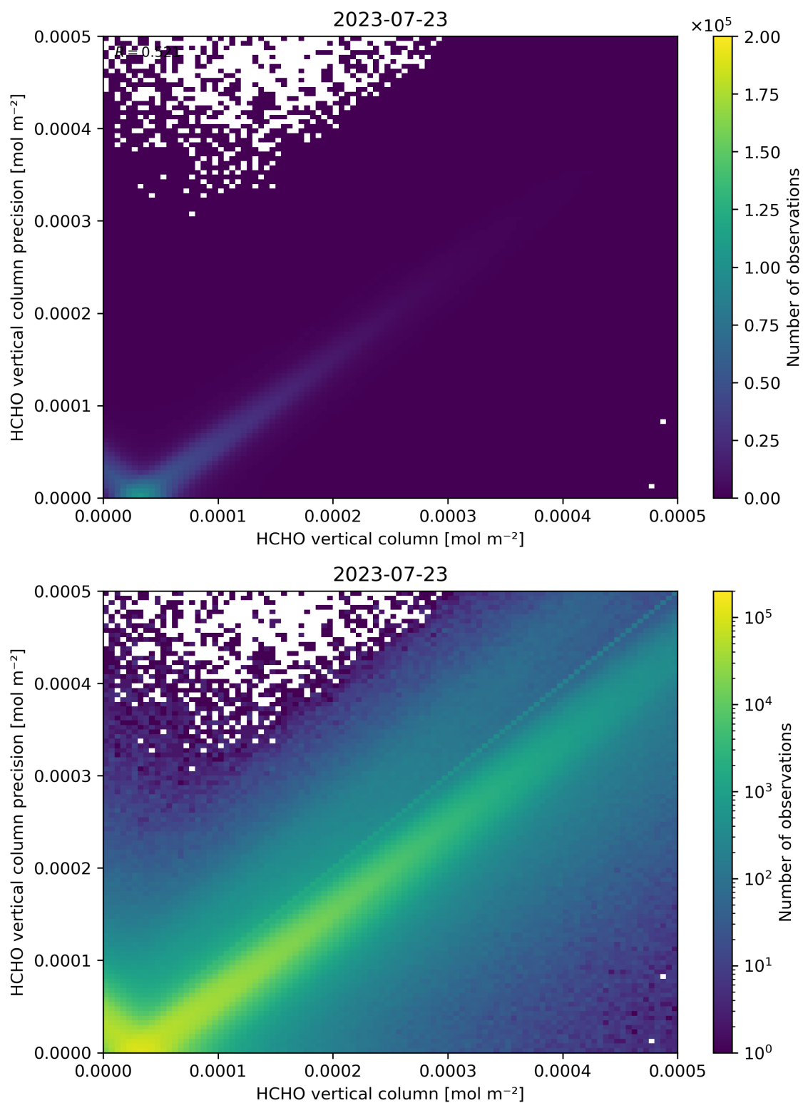
Figure 134: Scatter density plot of “HCHO vertical column” against “HCHO vertical column precision” for 2023-07-22 to 2023-07-24.
