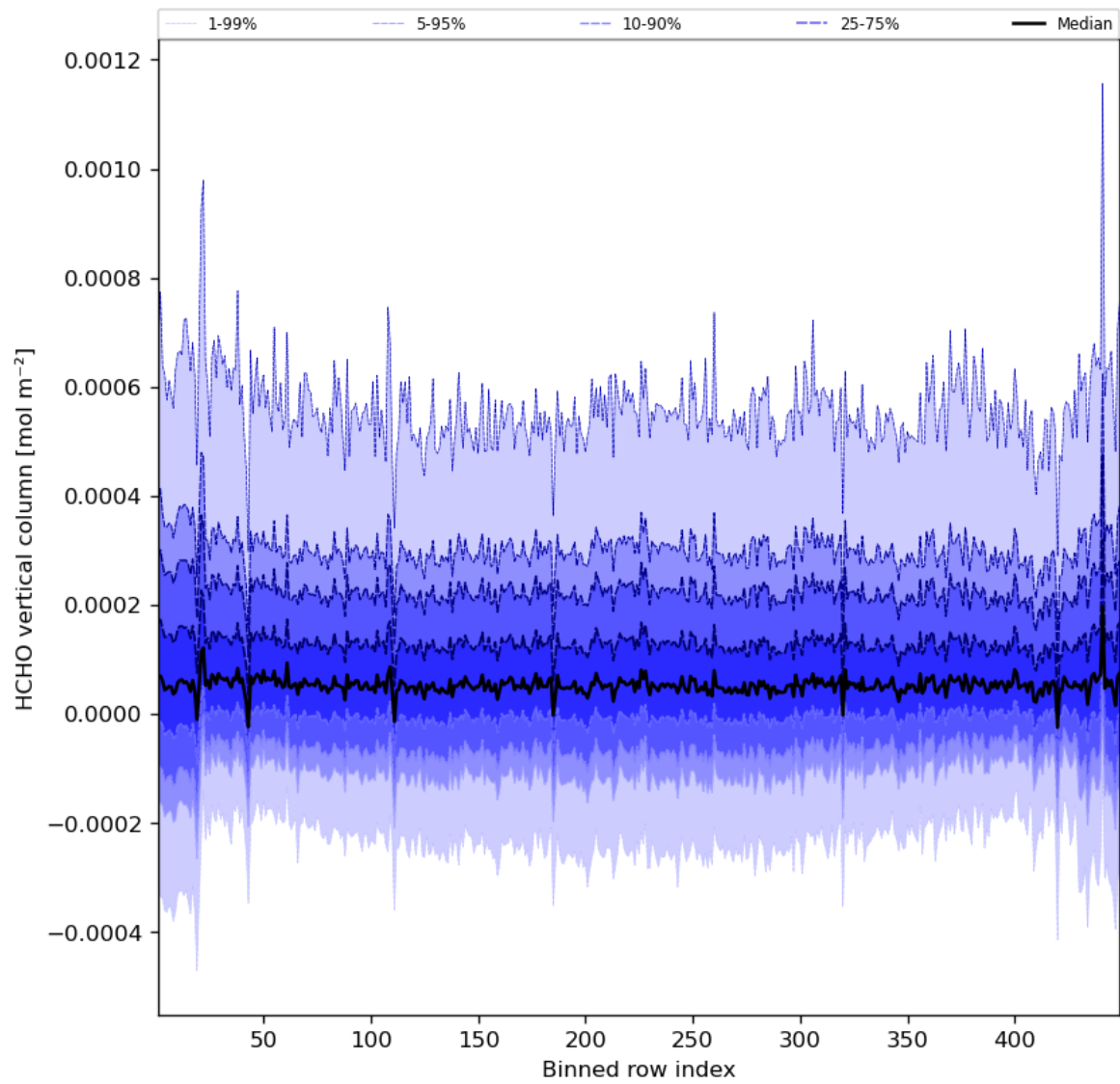
Figure 49: Along track statistics of “HCHO vertical column” for 2023-07-22 to 2023-07-24
