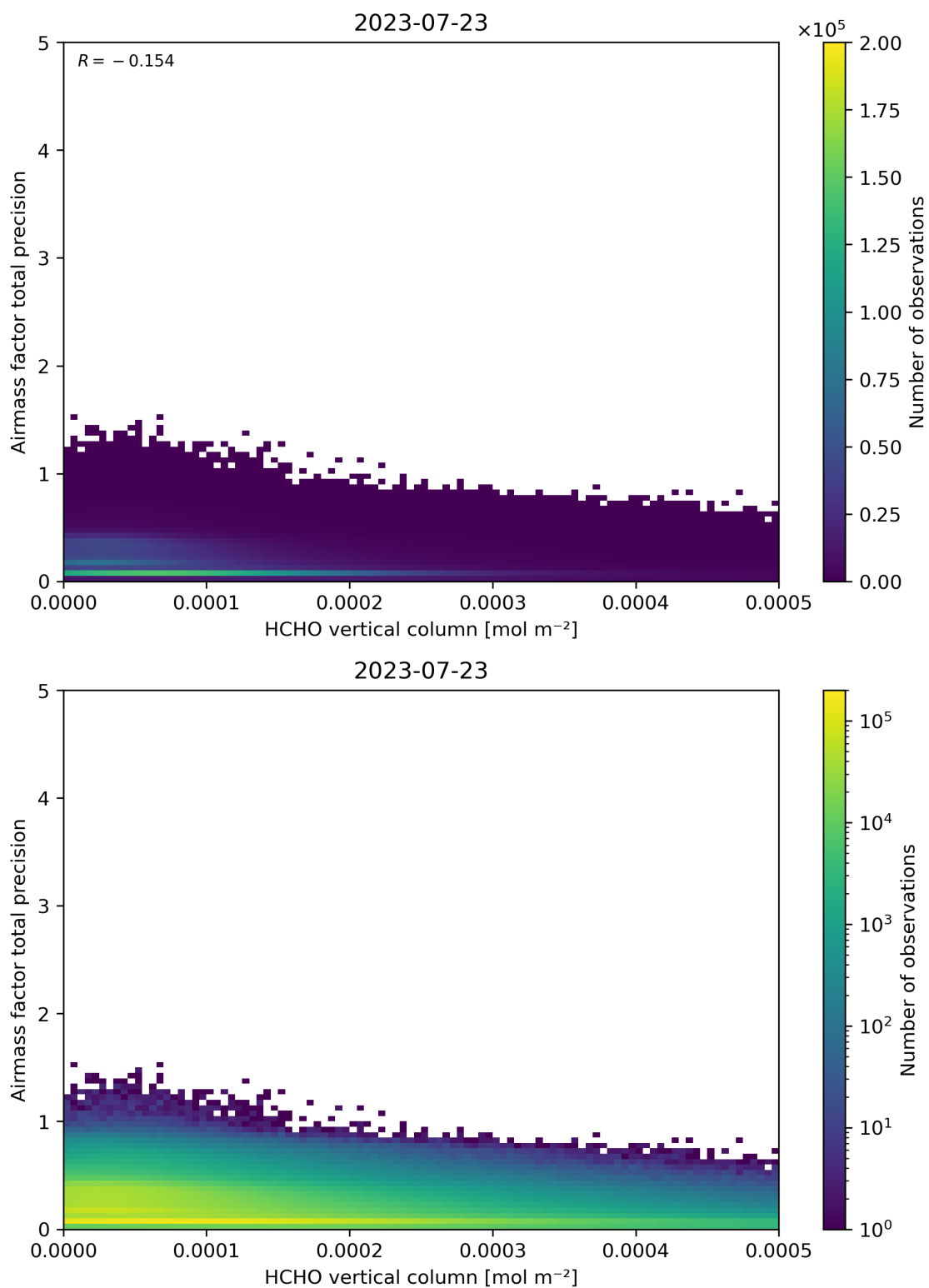
Figure 132: Scatter density plot of “HCHO vertical column” against “Airmass factor total precision” for 2023-07-22 to 2023-07-24.
