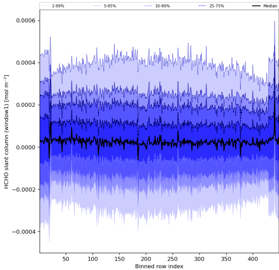
Figure 52: Along track statistics of “HCHO slant column (window1)” for 2023-07-22 to 2023-07-24
