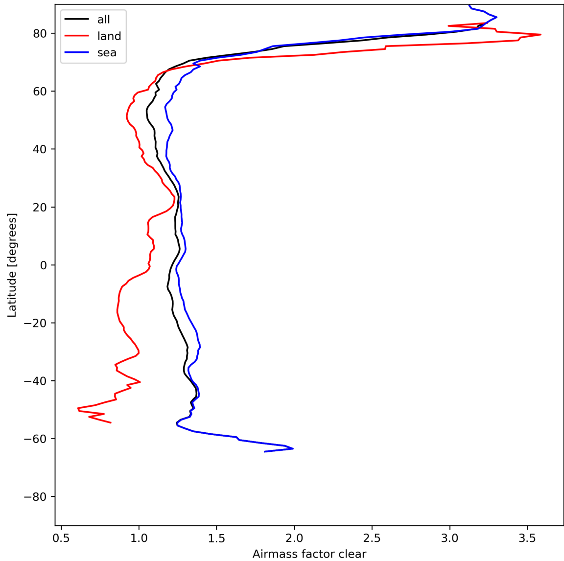
Figure 28: Zonal average of “Airmass factor clear” for 2023-07-22 to 2023-07-24.
