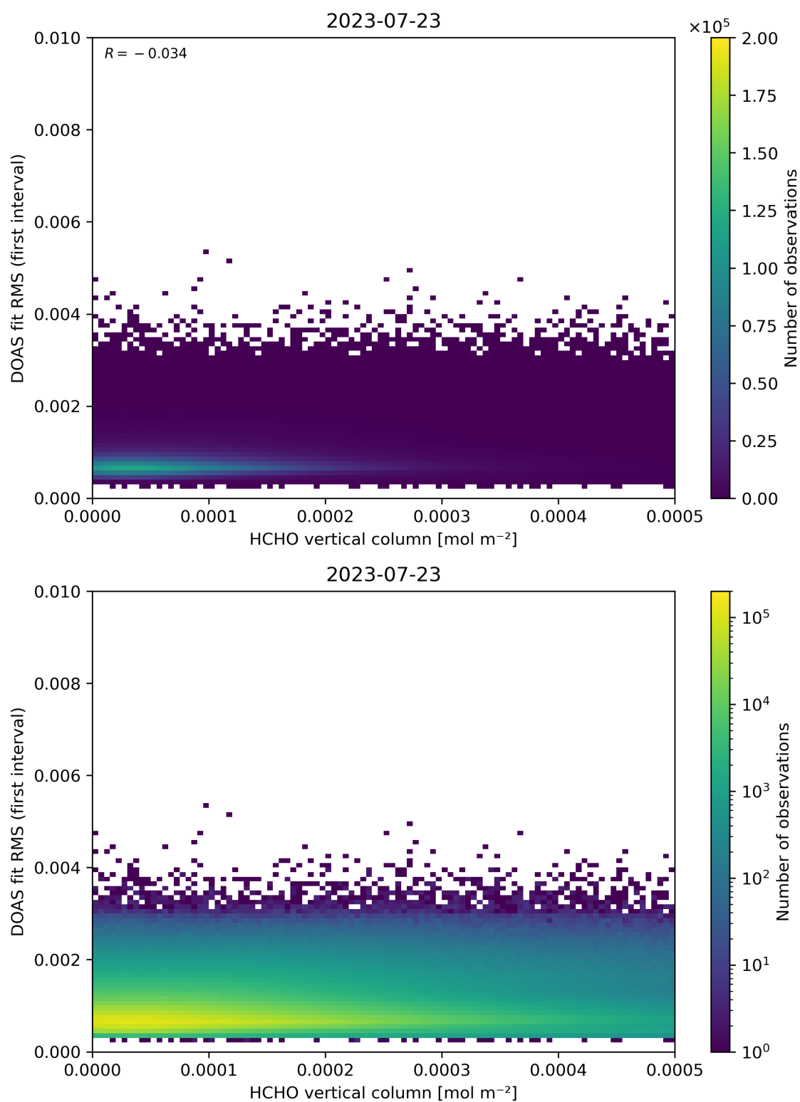
Figure 123: Scatter density plot of “HCHO vertical column” against “DOAS fit RMS (first interval)” for 2023-07-22 to 2023-07-24.
