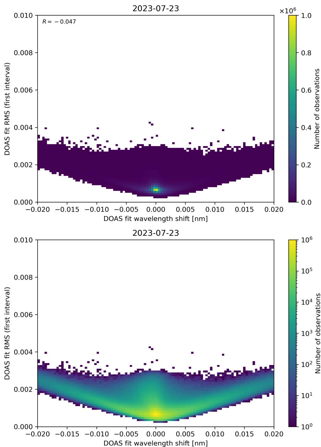
Figure 64: Scatter density plot of “DOAS fit wavelength shift” against “DOAS fit RMS (first interval)” for 2023-07-22 to 2023-07-24.
