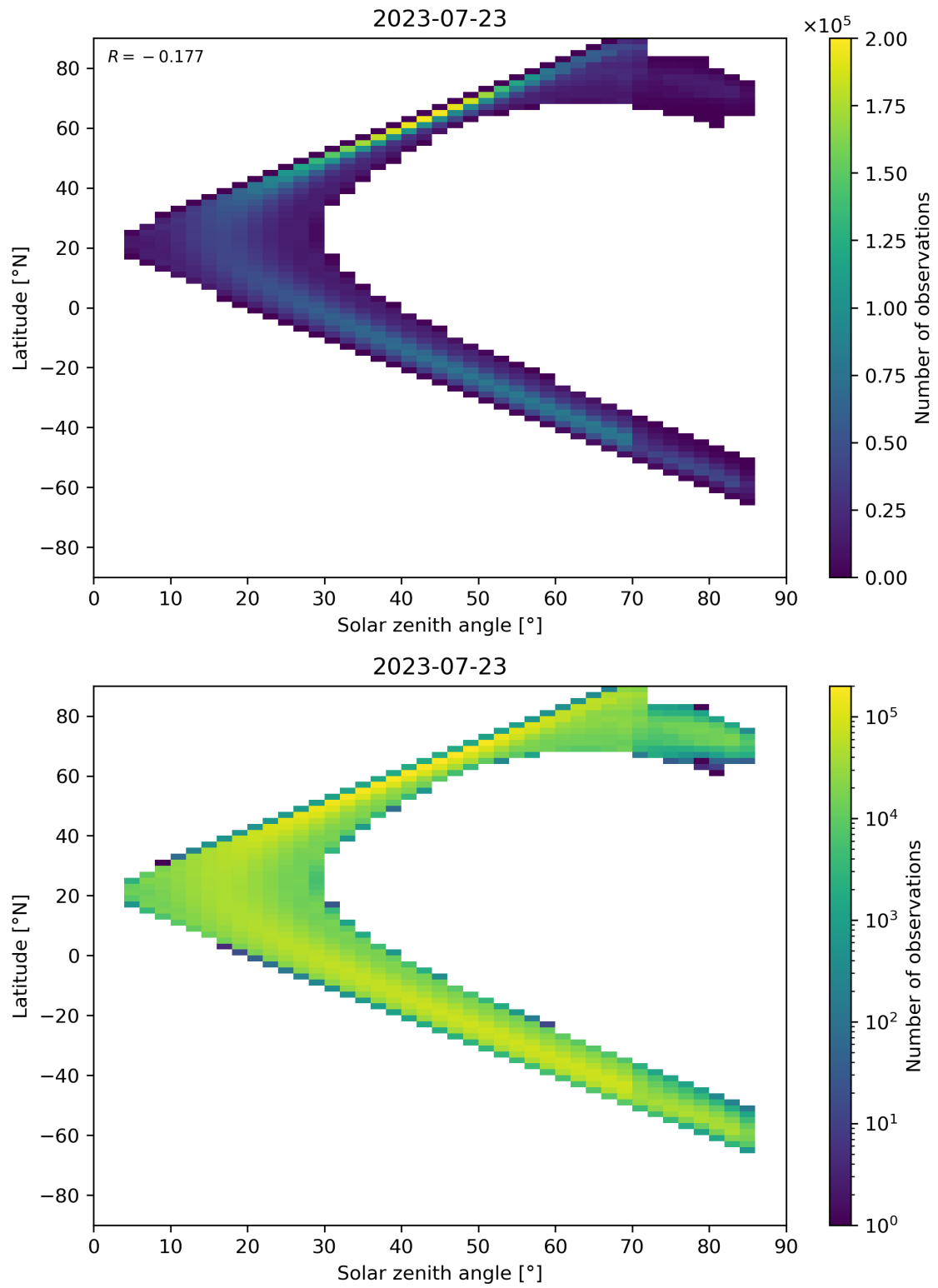
Figure 181: Scatter density plot of “Solar zenith angle” against “Latitude” for 2023-07-22 to 2023-07-24.
