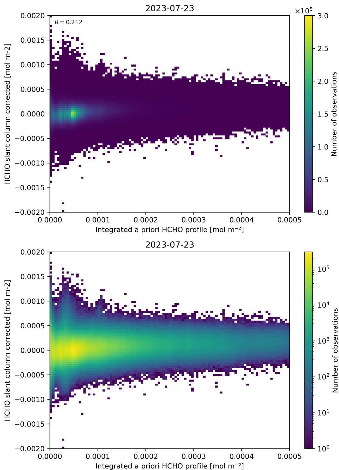
Figure 151: Scatter density plot of “Integrated a priori HCHO profile” against “HCHO slant column corrected” for 2023-07-22 to 2023-07-24.
