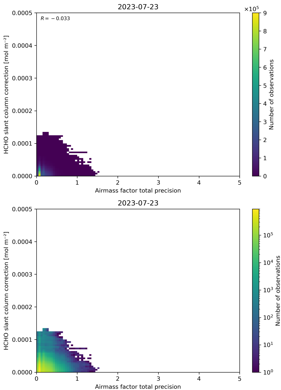
Figure 110: Scatter density plot of “Airmass factor total precision” against “HCHO slant column correction” for 2023-07-22 to 2023-07-24.
