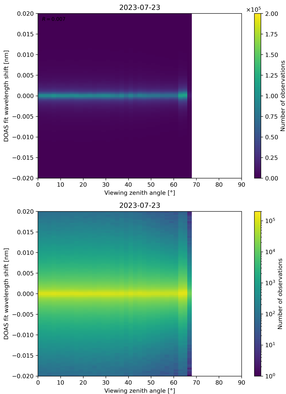
Figure 183: Scatter density plot of “Viewing zenith angle” against “DOAS fit wavelength shift” for 2023-07-22 to 2023-07-24.
