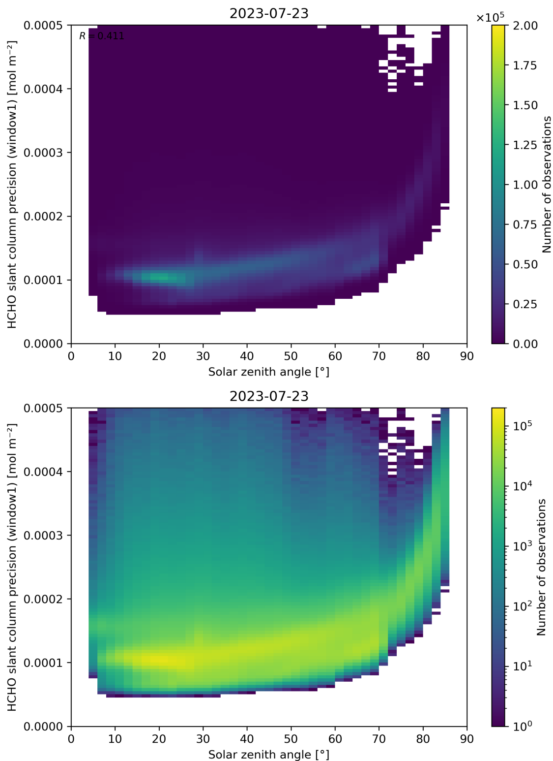
Figure 174: Scatter density plot of “Solar zenith angle” against “HCHO slant column precision (window1)” for 2023-07-22 to 2023-07-24.
