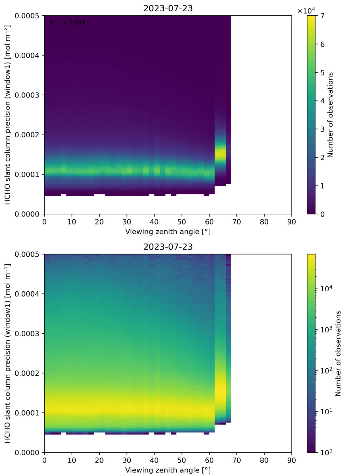
Figure 189: Scatter density plot of “Viewing zenith angle” against “HCHO slant column precision (window1)” for 2023-07-22 to 2023-07-24.
