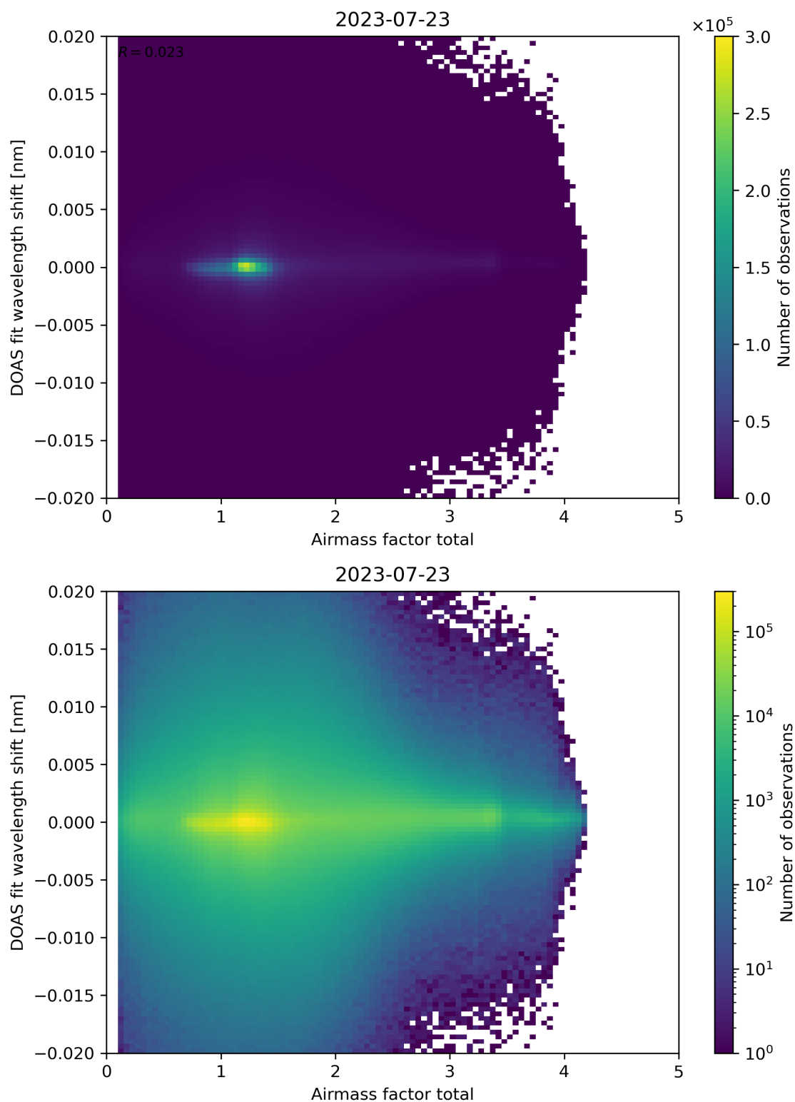
Figure 98: Scatter density plot of “Airmass factor total” against “DOAS fit wavelength shift” for 2023-07-22 to 2023-07-24.
