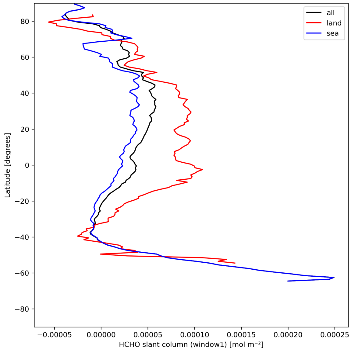
Figure 24: Zonal average of “HCHO slant column (window1)” for 2023-07-22 to 2023-07-24.
