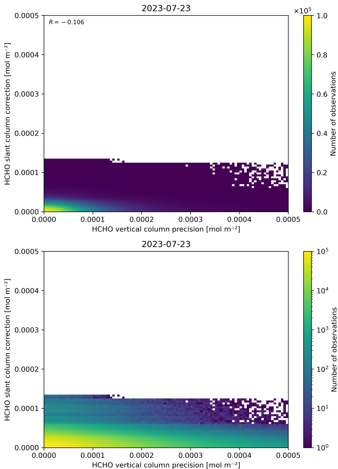
Figure 141: Scatter density plot of “HCHO vertical column precision” against “HCHO slant column correction” for 2023-07-22 to 2023-07-24.
