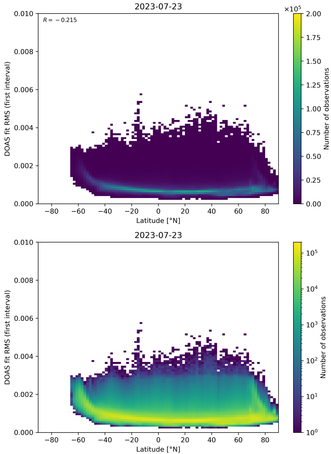
Figure 153: Scatter density plot of “Latitude” against “DOAS fit RMS (first interval)” for 2023-07-22 to 2023-07-24.
