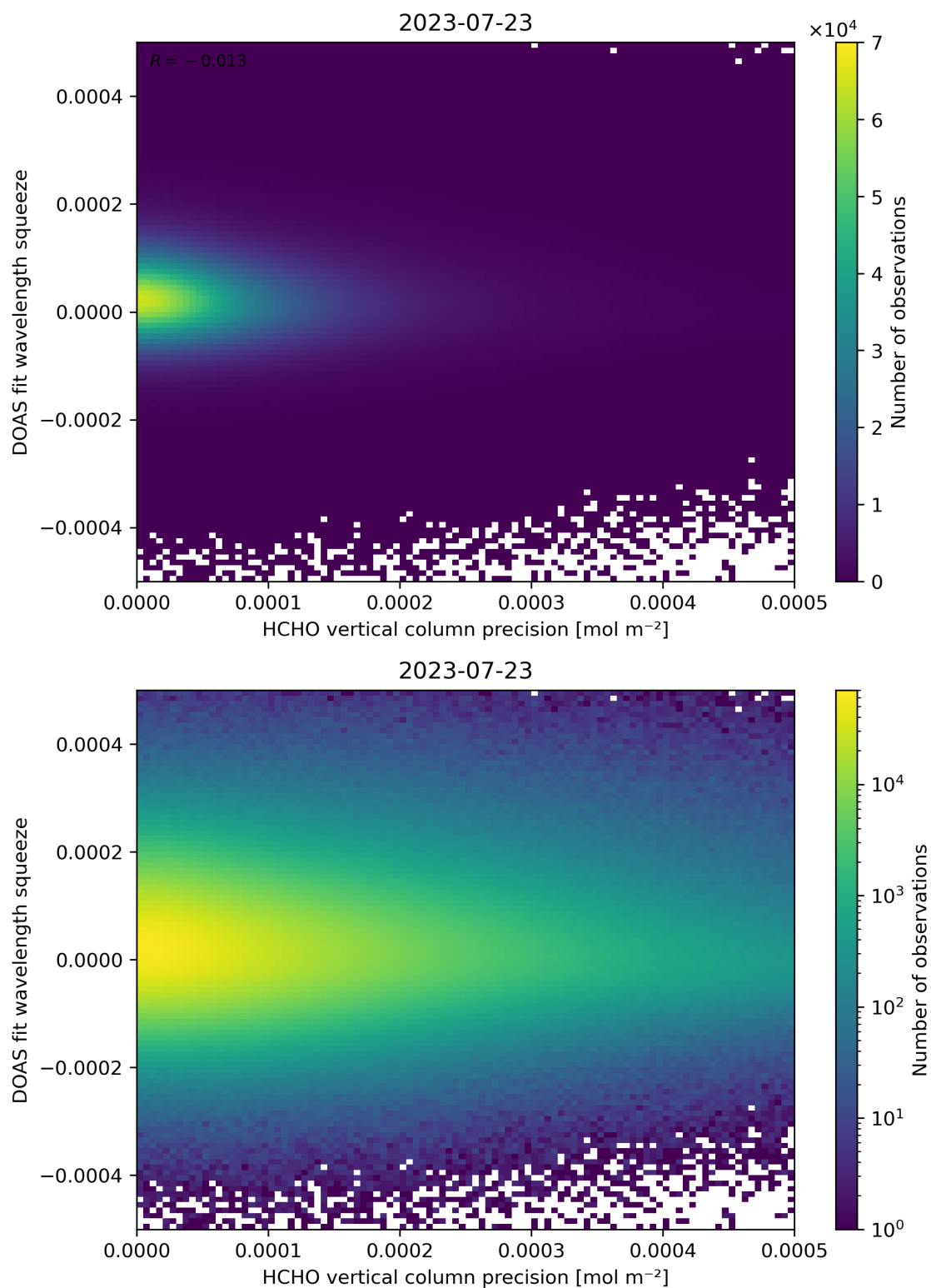
Figure 138: Scatter density plot of “HCHO vertical column precision” against “DOAS fit wavelength squeeze” for 2023-07-22 to 2023-07-24.
