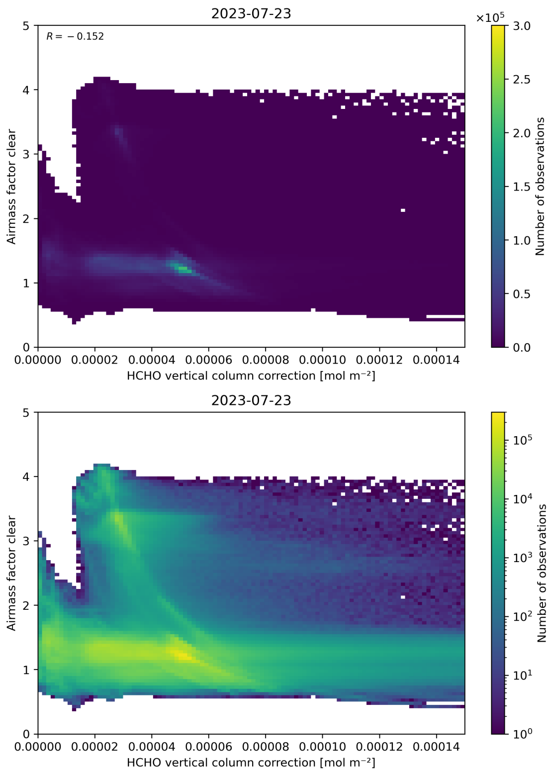
Figure 115: Scatter density plot of “HCHO vertical column correction” against “Airmass factor clear” for 2023-07-22 to 2023-07-24.
