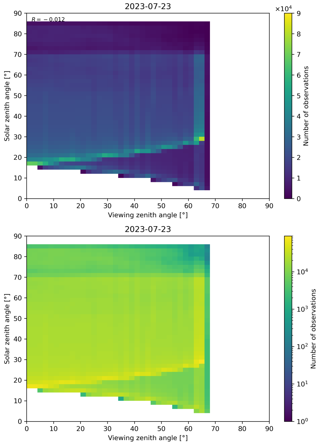
Figure 197: Scatter density plot of “Viewing zenith angle” against “Solar zenith angle” for 2023-07-22 to 2023-07-24.
