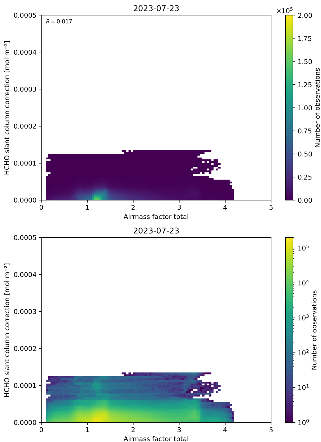
Figure 102: Scatter density plot of “Airmass factor total” against “HCHO slant column correction” for 2023-07-22 to 2023-07-24.
