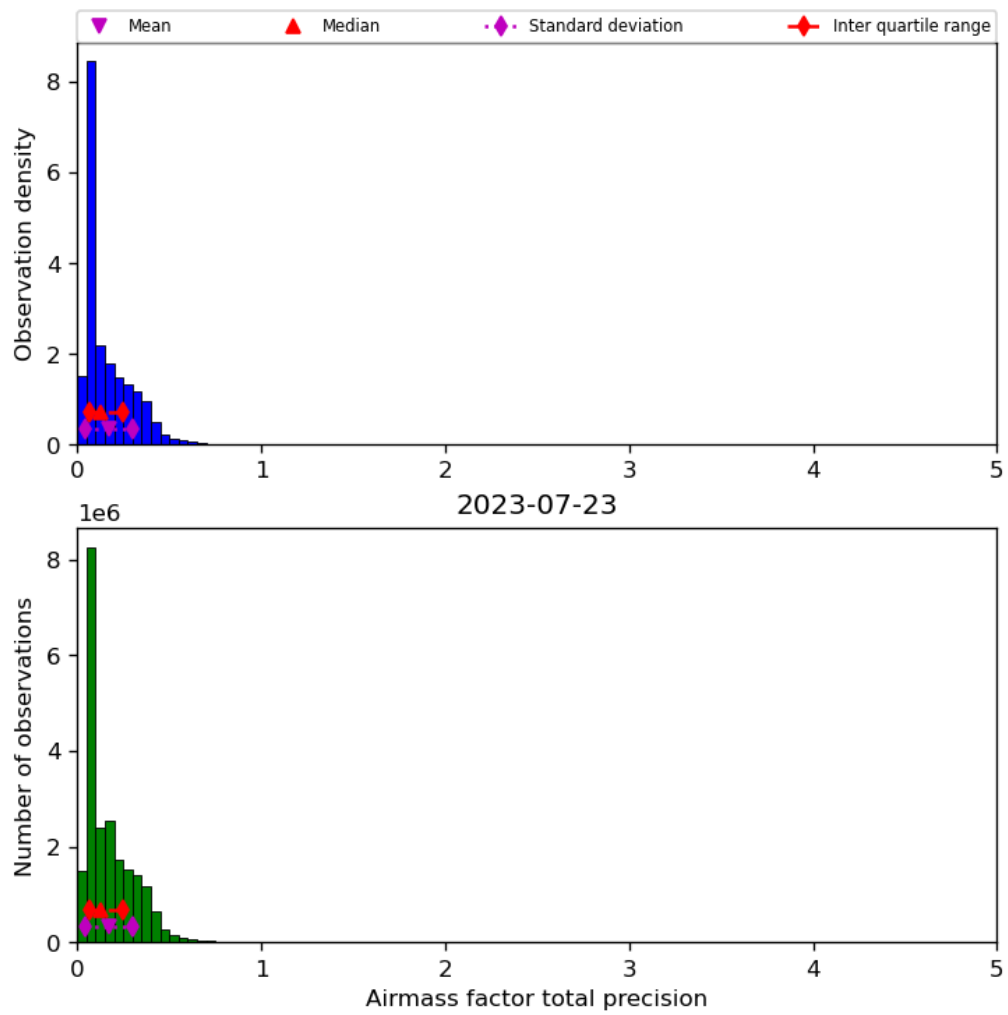
Figure 41: Histogram of "Airmass factor total precision" for 2023-07-22 to 2023-07-24
