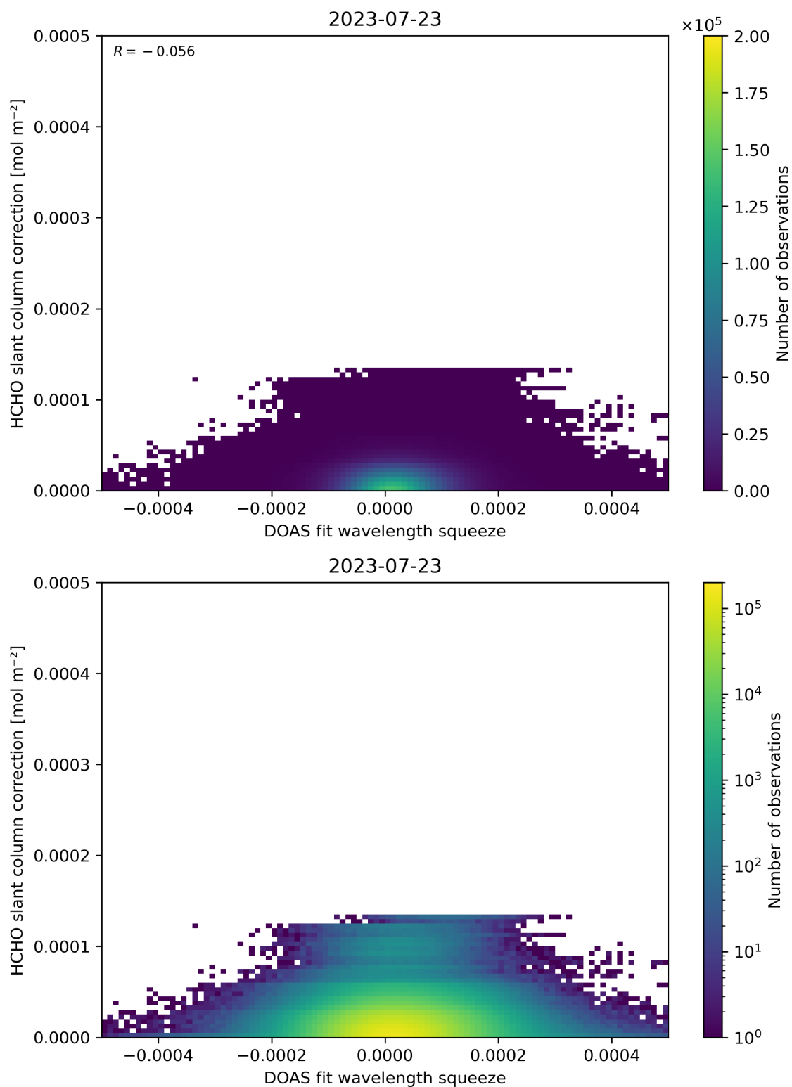
Figure 70: Scatter density plot of “DOAS fit wavelength squeeze” against “HCHO slant column correction” for 2023-07-22 to 2023-07-24.
