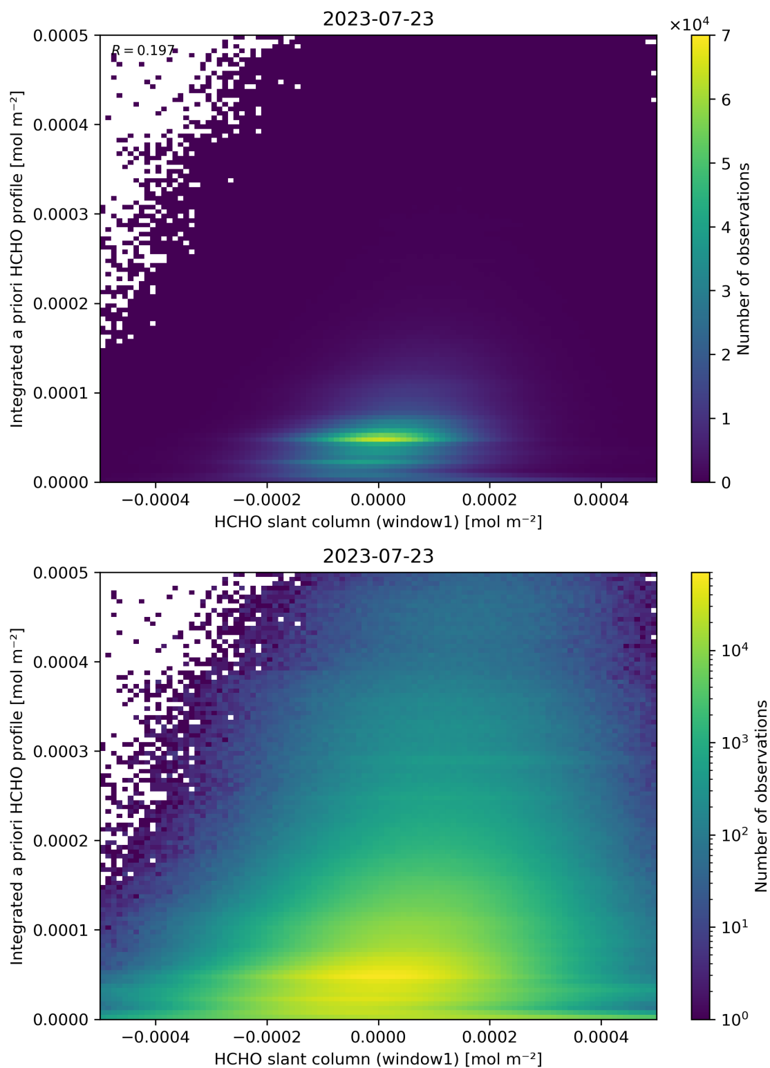
Figure 87: Scatter density plot of “HCHO slant column (window1)” against “Integrated a priori HCHO profile” for 2023-07-22 to 2023-07-24.
