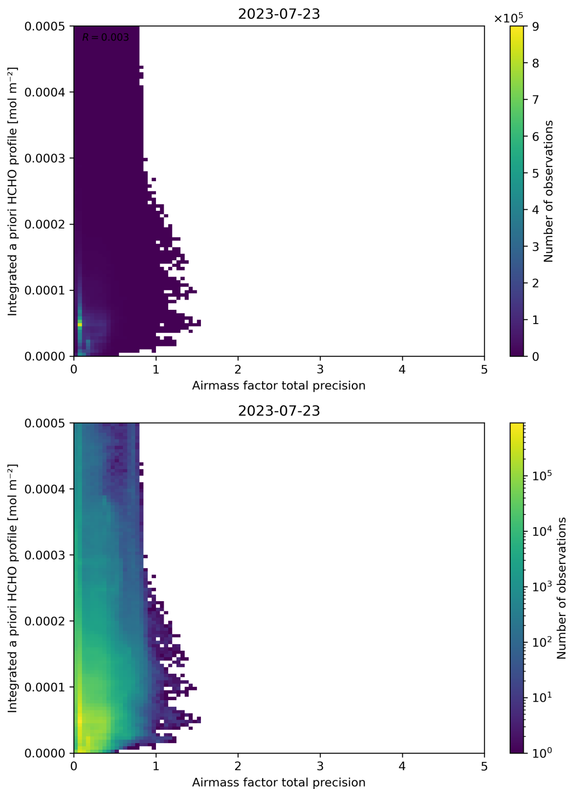
Figure 111: Scatter density plot of “Airmass factor total precision” against “Integrated a priori HCHO profile” for 2023-07-22 to 2023-07-24.
