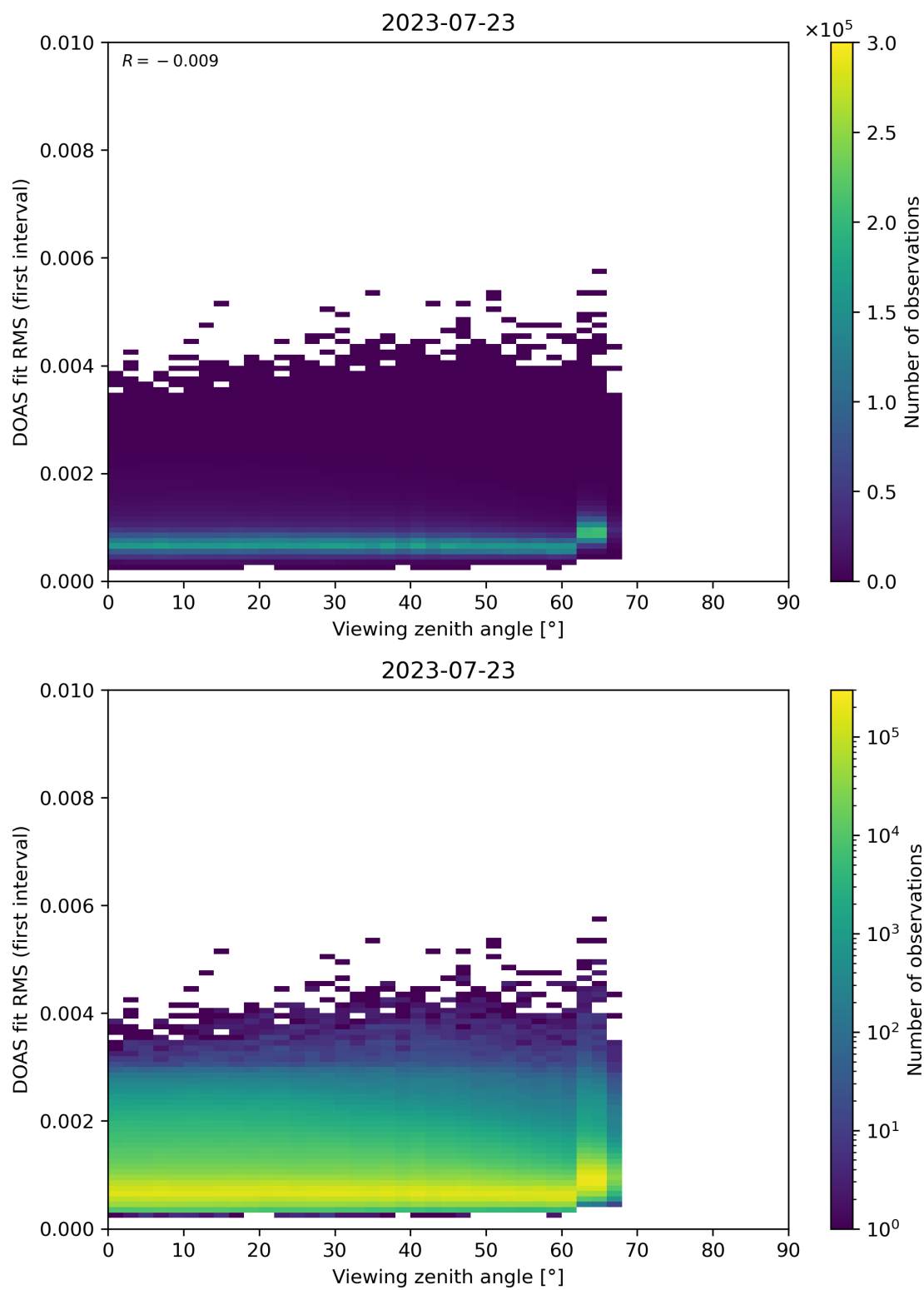
Figure 182: Scatter density plot of “Viewing zenith angle” against “DOAS fit RMS (first interval)” for 2023-07-22 to 2023-07-24.
