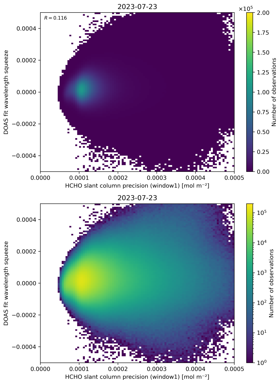
Figure 90: Scatter density plot of “HCHO slant column precision (window1)” against “DOAS fit wavelength squeeze” for 2023-07-22 to 2023-07-24.
