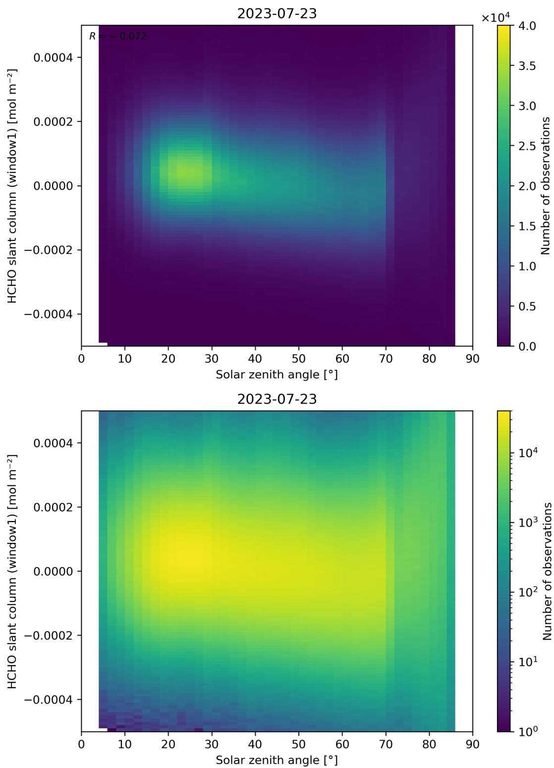
Figure 173: Scatter density plot of “Solar zenith angle” against “HCHO slant column (window1)” for 2023-07-22 to 2023-07-24.
