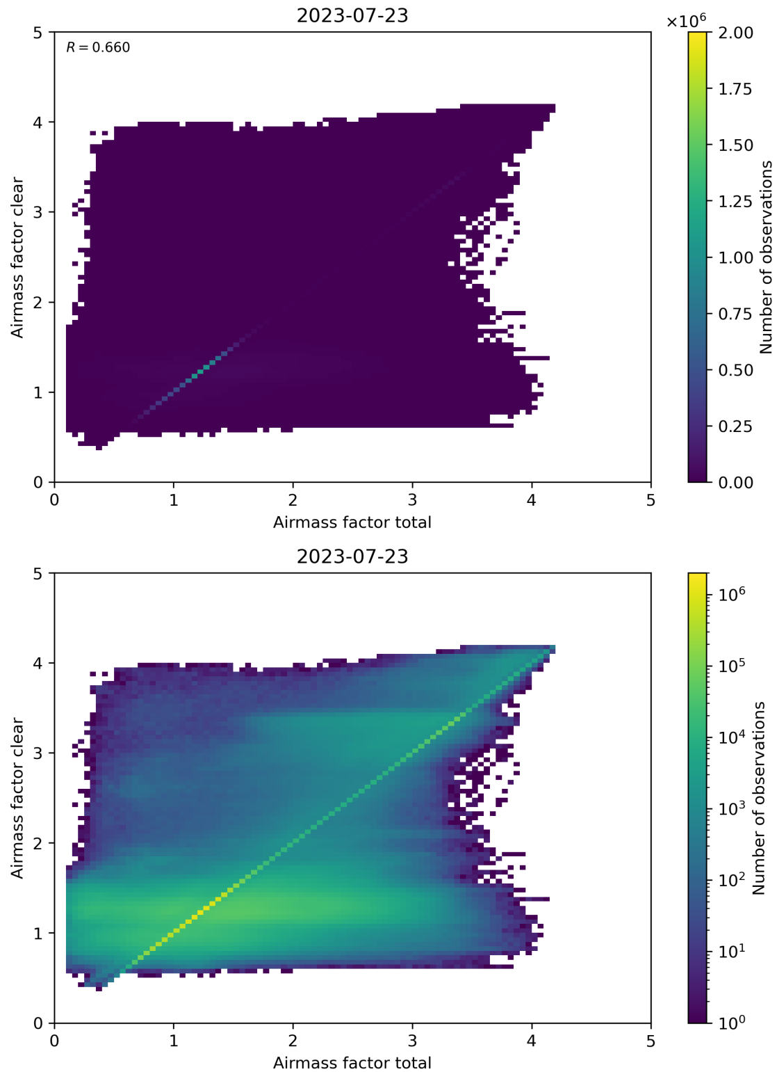
Figure 100: Scatter density plot of “Airmass factor total” against “Airmass factor clear” for 2023-07-22 to 2023-07-24.
