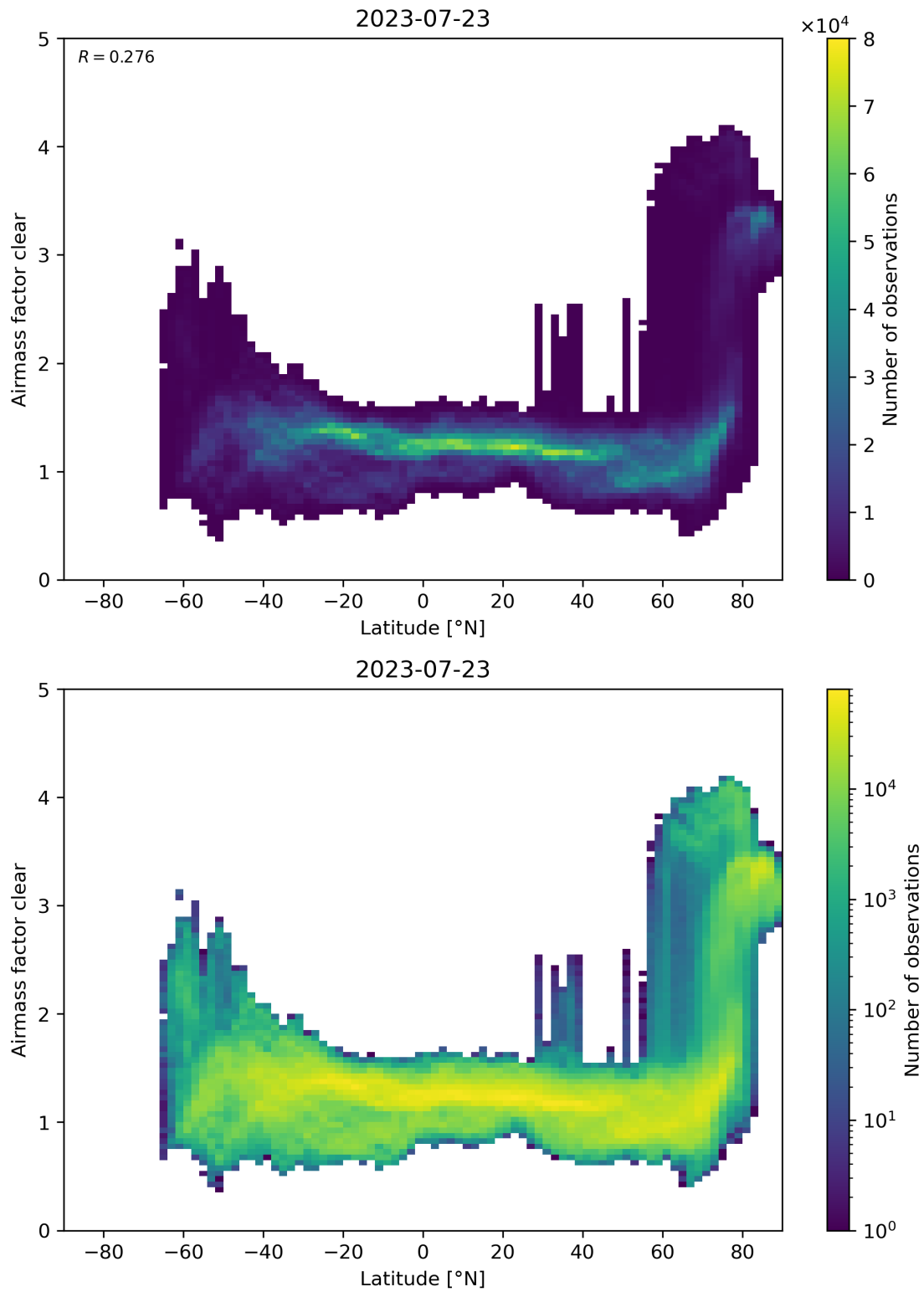
Figure 156: Scatter density plot of “Latitude” against “Airmass factor clear” for 2023-07-22 to 2023-07-24.
