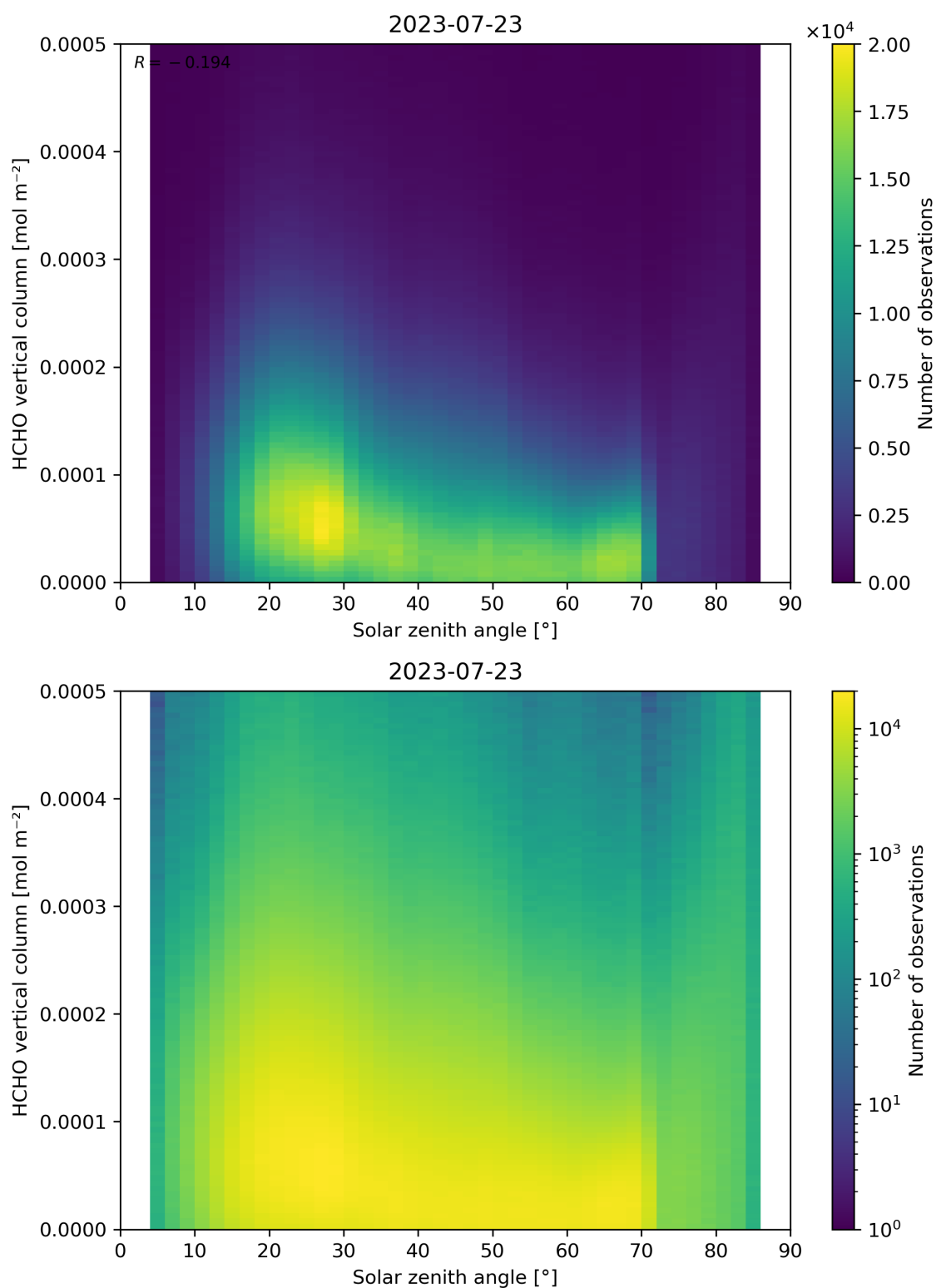
Figure 177: Scatter density plot of “Solar zenith angle” against “HCHO vertical column” for 2023-07-22 to 2023-07-24.
