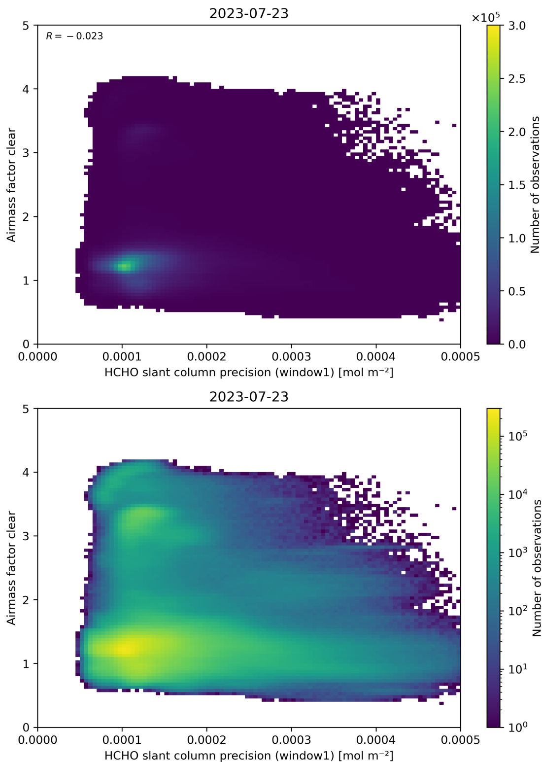
Figure 91: Scatter density plot of “HCHO slant column precision (window1)” against “Airmass factor clear” for 2023-07-22 to 2023-07-24.
