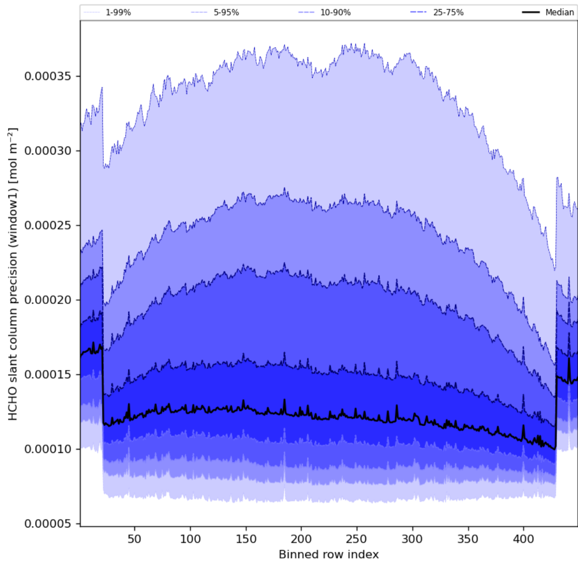
Figure 53: Along track statistics of “HCHO slant column precision (window1)” for 2023-07-22 to 2023-07-24
