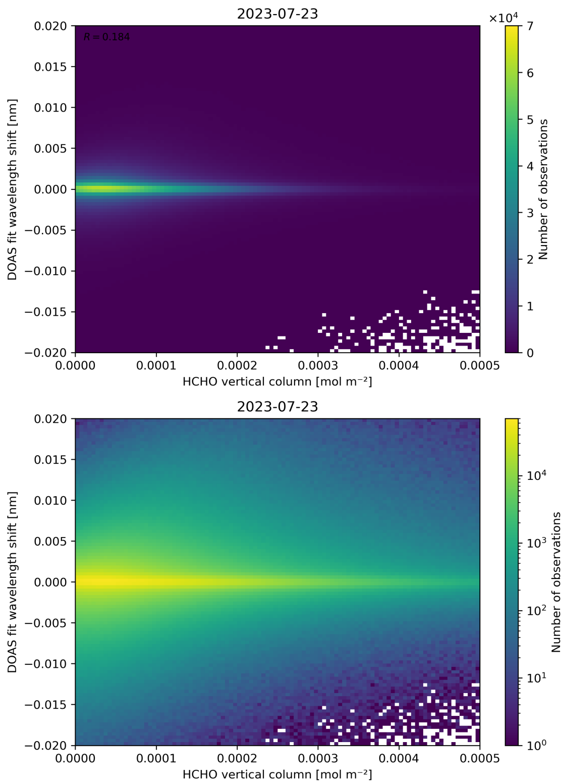
Figure 124: Scatter density plot of “HCHO vertical column” against “DOAS fit wavelength shift” for 2023-07-22 to 2023-07-24.
