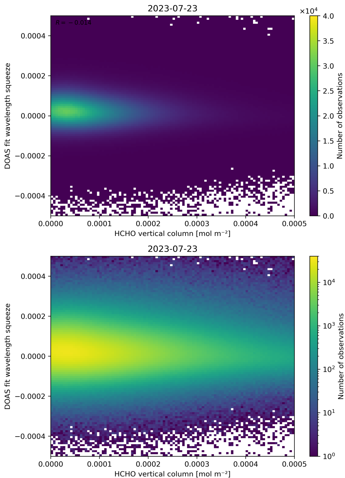
Figure 125: Scatter density plot of “HCHO vertical column” against “DOAS fit wavelength squeeze” for 2023-07-22 to 2023-07-24.
