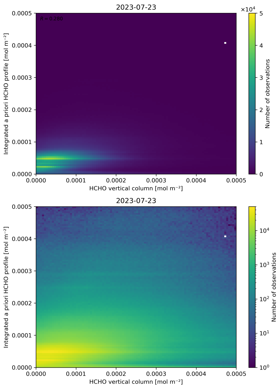
Figure 135: Scatter density plot of “HCHO vertical column” against “Integrated a priori HCHO profile” for 2023-07-22 to 2023-07-24.
