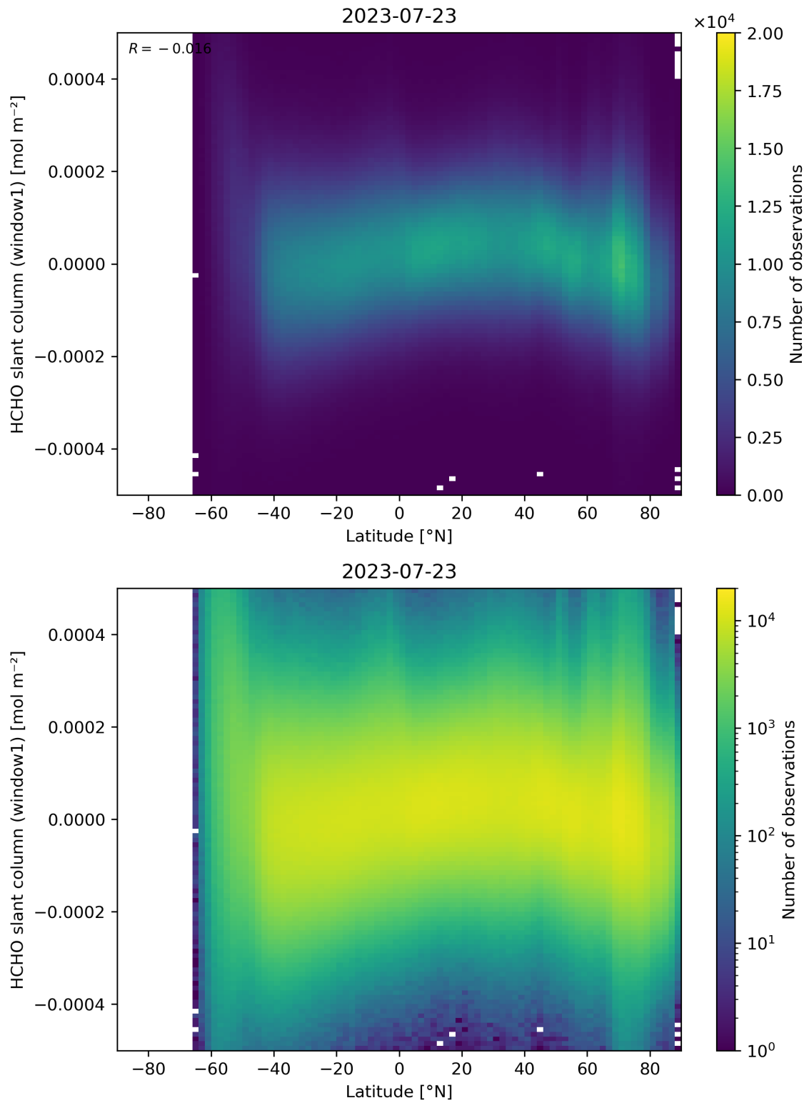
Figure 159: Scatter density plot of “Latitude” against “HCHO slant column (window1)” for 2023-07-22 to 2023-07-24.
