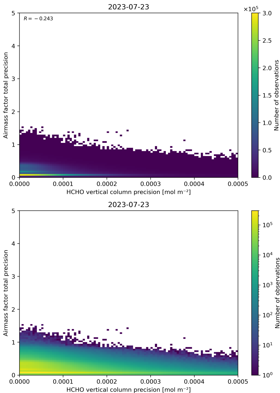
Figure 145: Scatter density plot of “HCHO vertical column precision” against “Airmass factor total precision” for 2023-07-22 to 2023-07-24.
