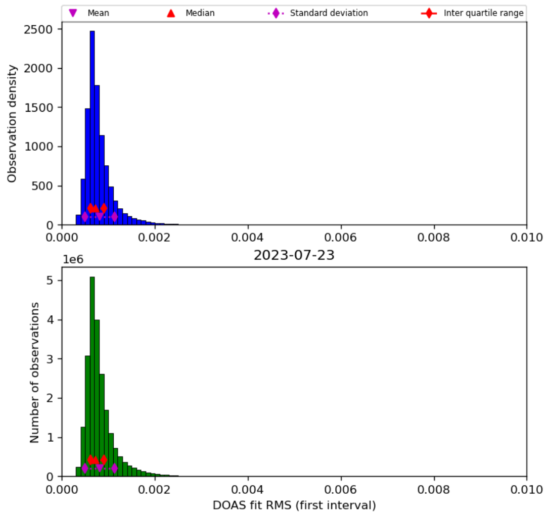
Figure 46: Histogram of “DOAS fit RMS (first interval)” for 2023-07-22 to 2023-07-24
