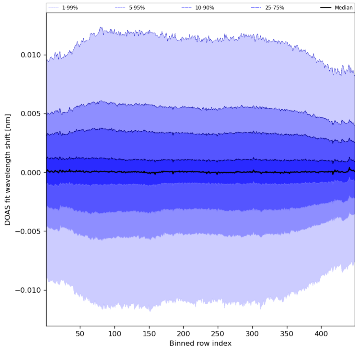
Figure 58: Along track statistics of “DOAS fit wavelength shift” for 2023-07-22 to 2023-07-24
