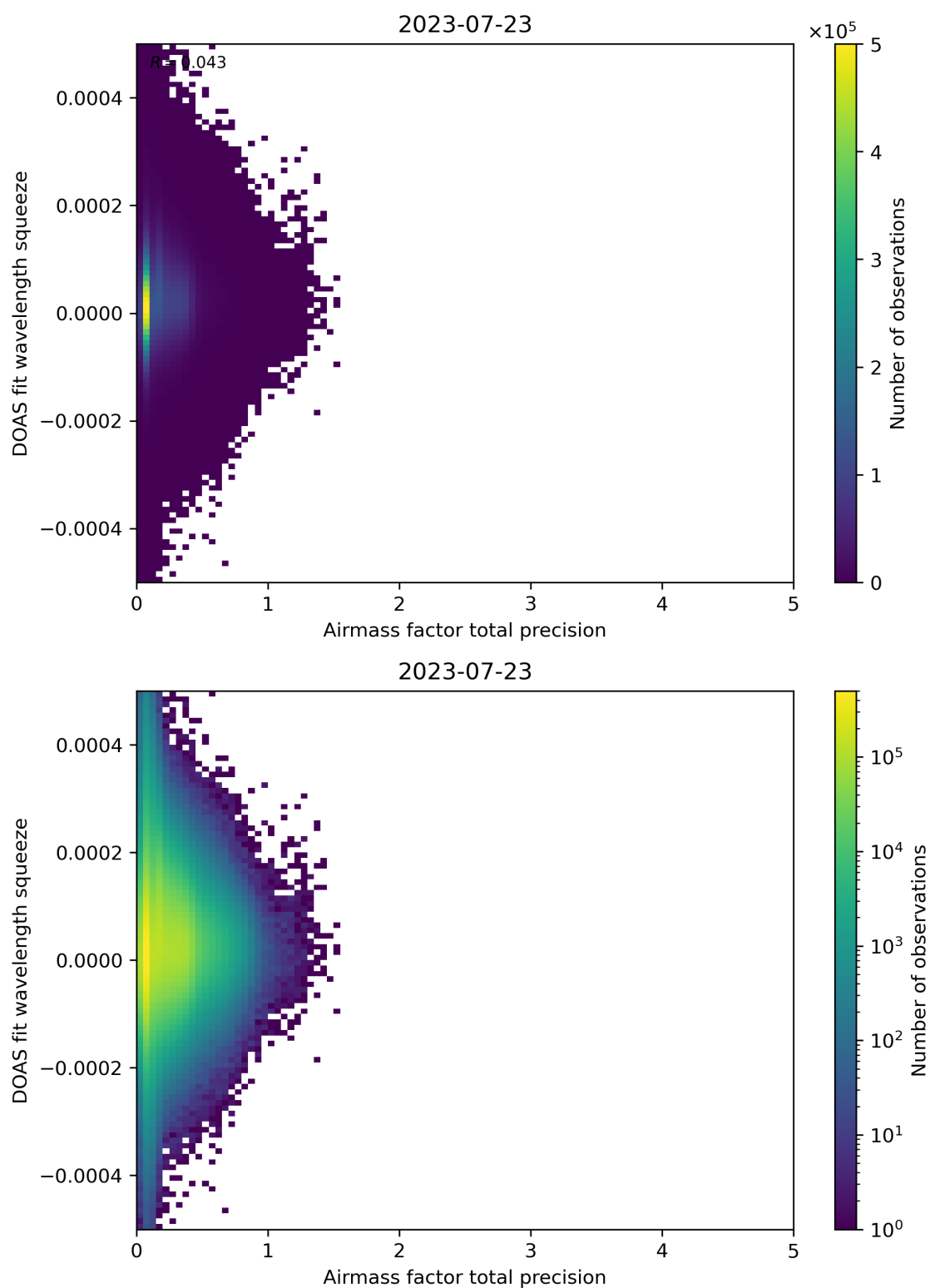
Figure 107: Scatter density plot of “Airmass factor total precision” against “DOAS fit wavelength squeeze” for 2023-07-22 to 2023-07-24.
