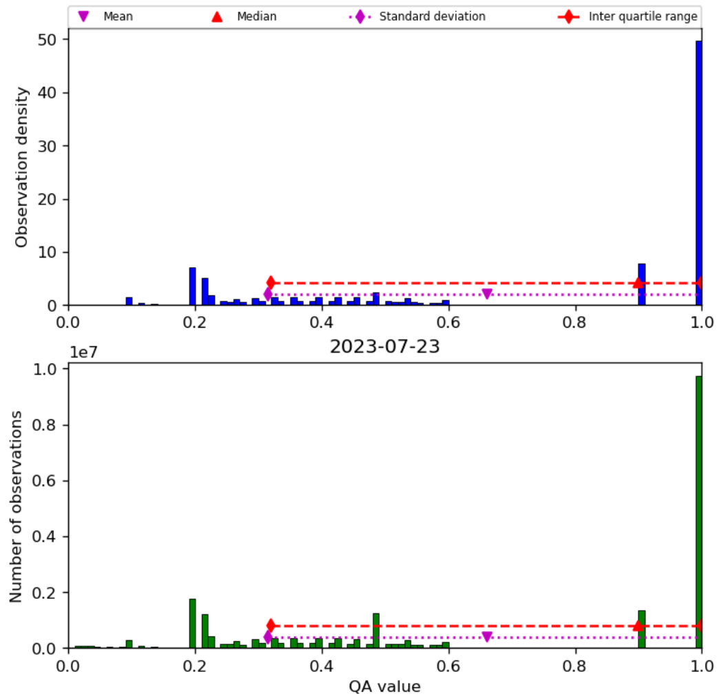
Figure 34: Histogram of “QA value” for 2023-07-22 to 2023-07-24
