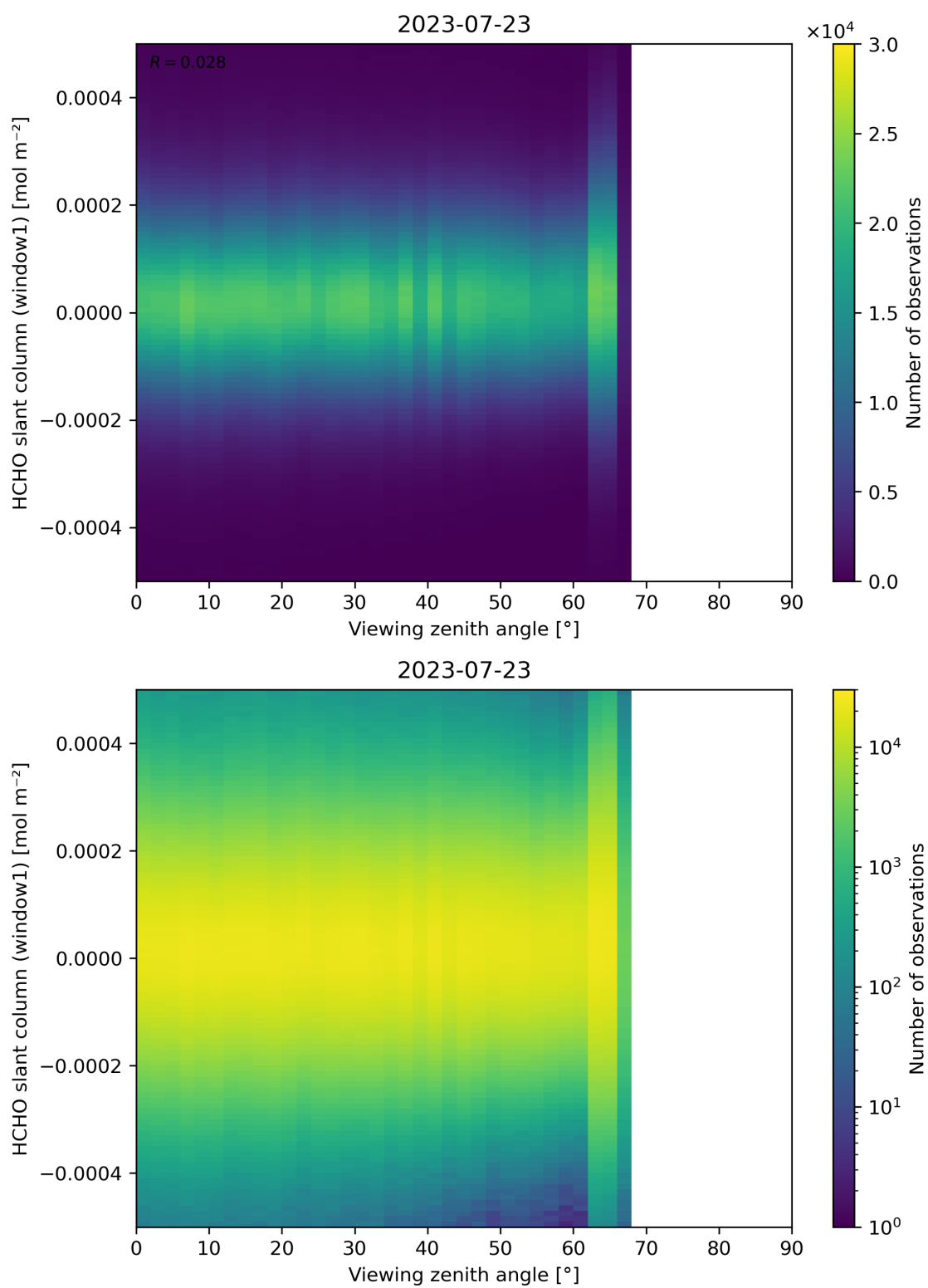
Figure 188: Scatter density plot of “Viewing zenith angle” against “HCHO slant column (window1)” for 2023-07-22 to 2023-07-24.
