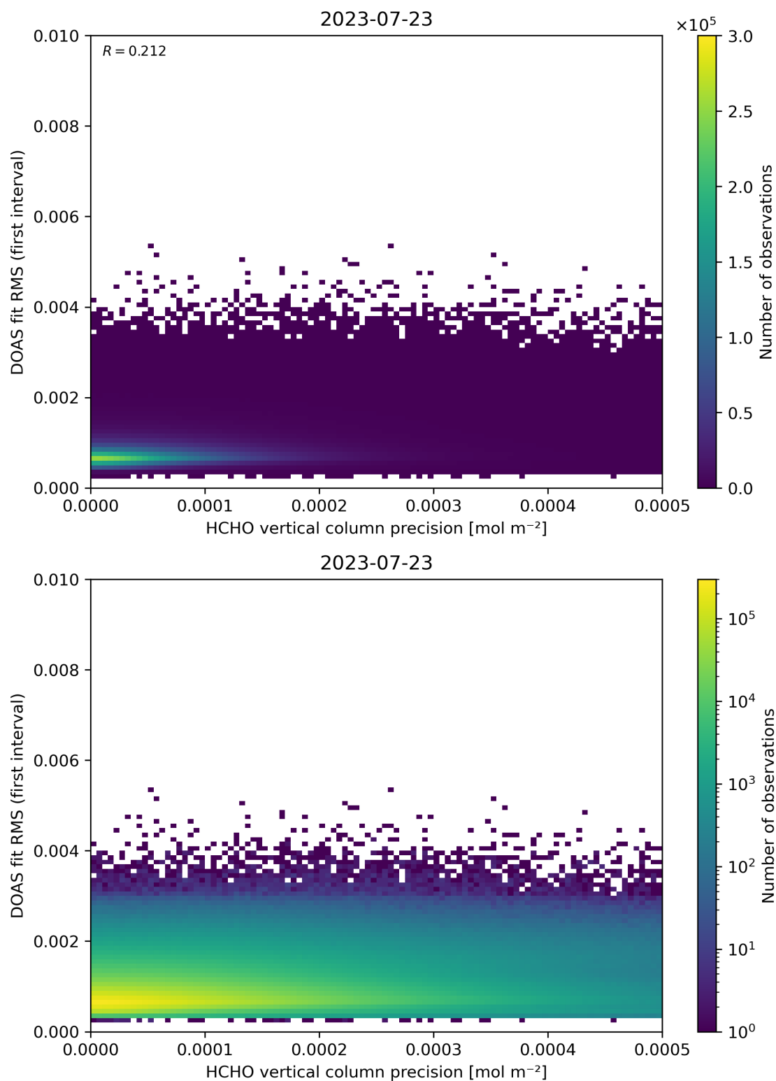
Figure 136: Scatter density plot of “HCHO vertical column precision” against “DOAS fit RMS (first interval)” for 2023-07-22 to 2023-07-24.
