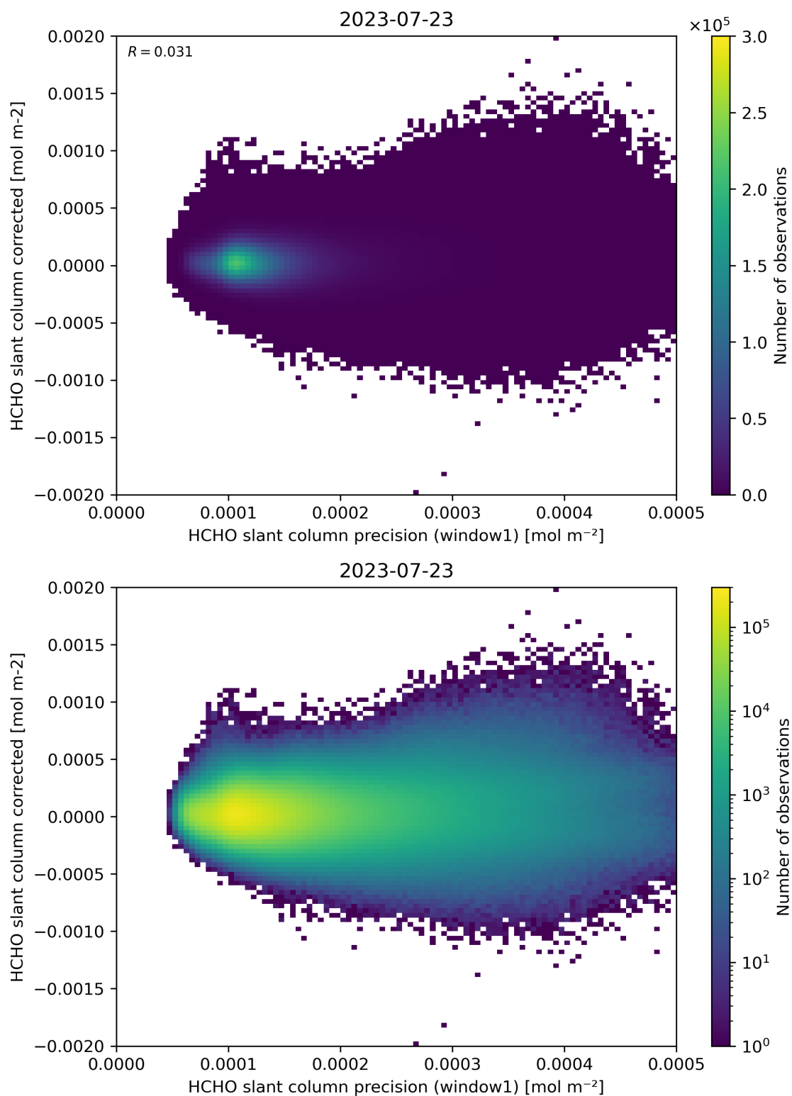
Figure 92: Scatter density plot of “HCHO slant column precision (window1)” against “HCHO slant column corrected” for 2023-07-22 to 2023-07-24.
