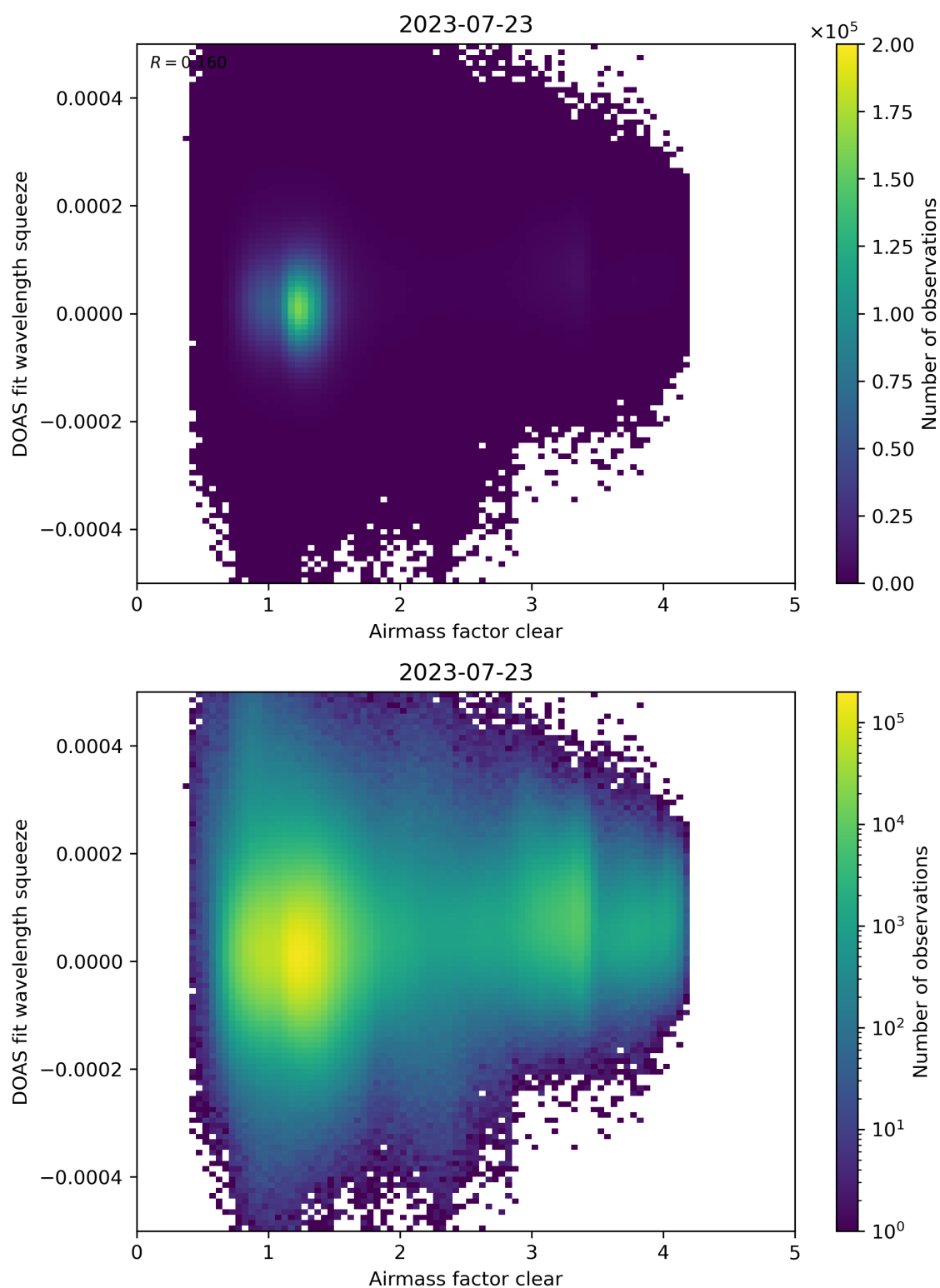
Figure 73: Scatter density plot of “Airmass factor clear” against “DOAS fit wavelength squeeze” for 2023-07-22 to 2023-07-24.
