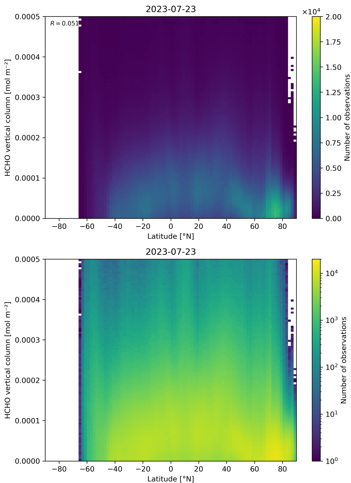
Figure 163: Scatter density plot of “Latitude” against “HCHO vertical column” for 2023-07-22 to 2023-07-24.
