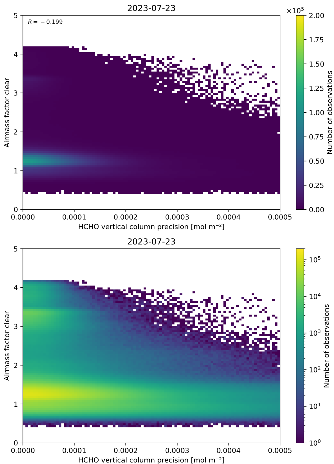
Figure 139: Scatter density plot of “HCHO vertical column precision” against “Airmass factor clear” for 2023-07-22 to 2023-07-24.
