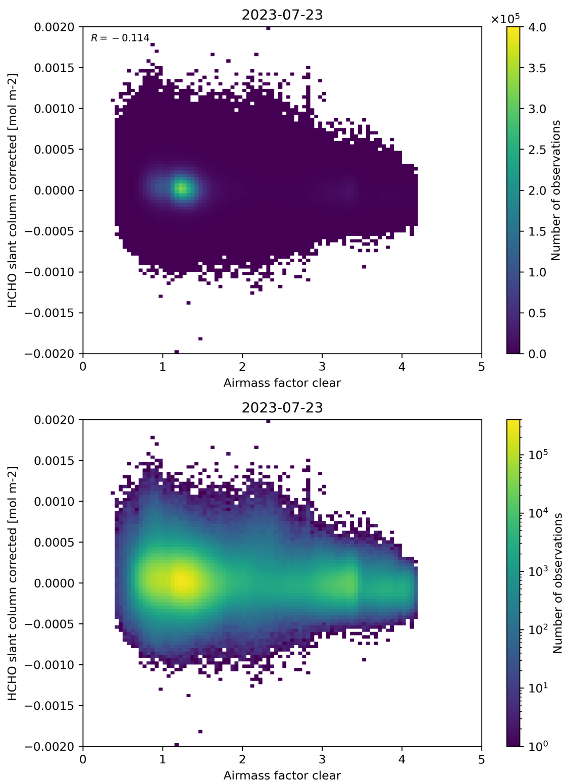
Figure 74: Scatter density plot of “Airmass factor clear” against “HCHO slant column corrected” for 2023-07-22 to 2023-07-24.
