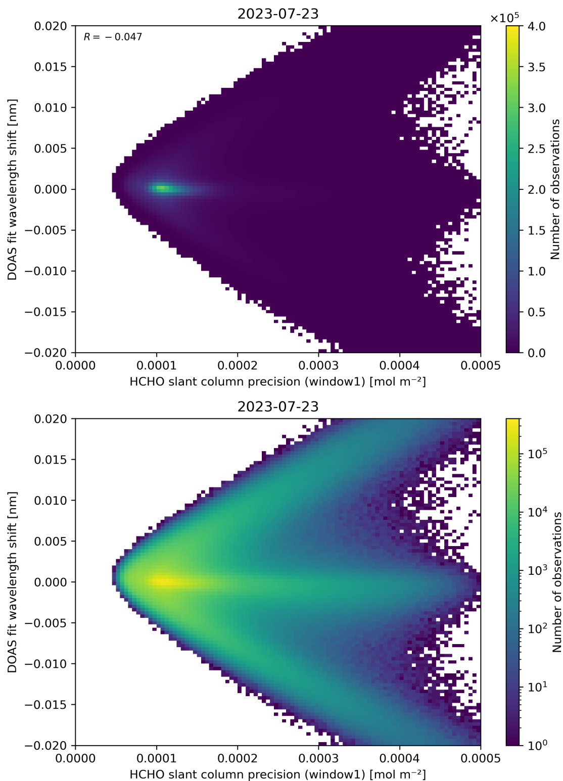
Figure 89: Scatter density plot of “HCHO slant column precision (window1)” against “DOAS fit wavelength shift” for 2023-07-22 to 2023-07-24.
