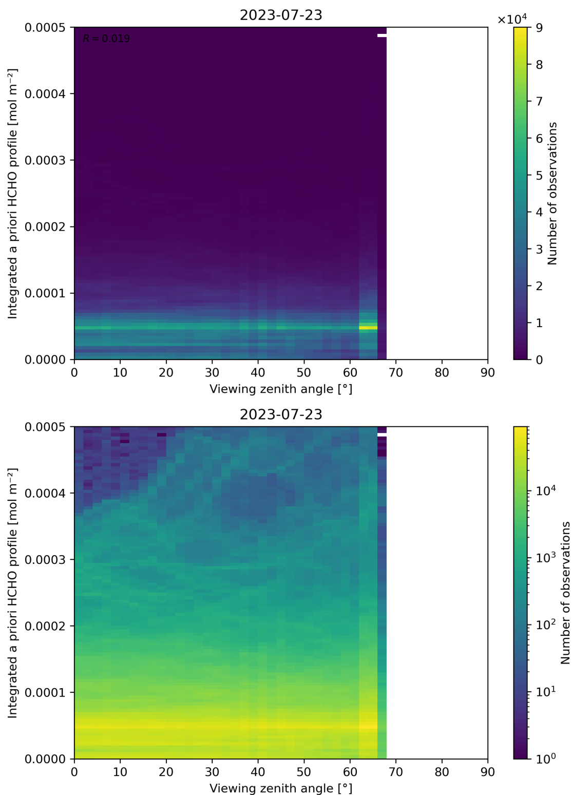
Figure 195: Scatter density plot of “Viewing zenith angle” against “Integrated a priori HCHO profile” for 2023-07-22 to 2023-07-24.
