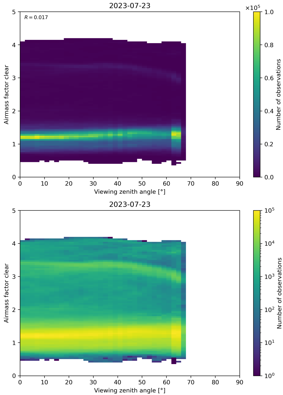
Figure 185: Scatter density plot of “Viewing zenith angle” against “Airmass factor clear” for 2023-07-22 to 2023-07-24.
