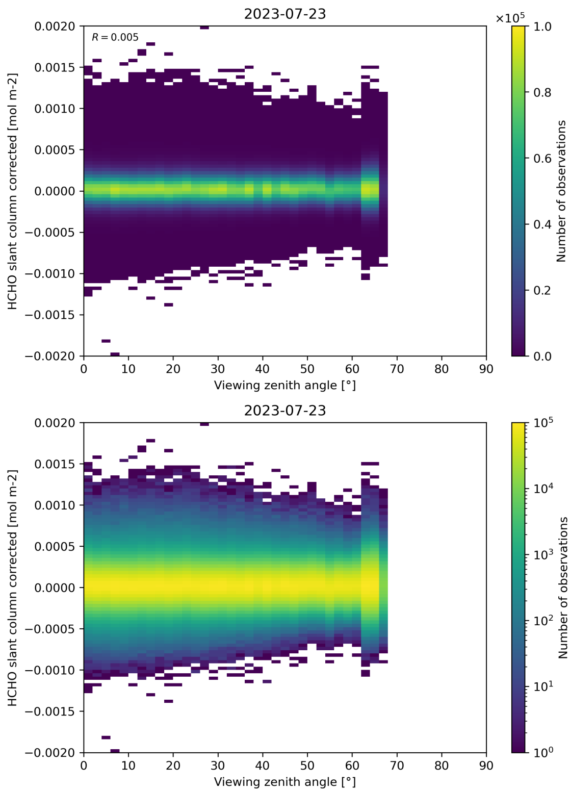
Figure 186: Scatter density plot of “Viewing zenith angle” against “HCHO slant column corrected” for 2023-07-22 to 2023-07-24.
