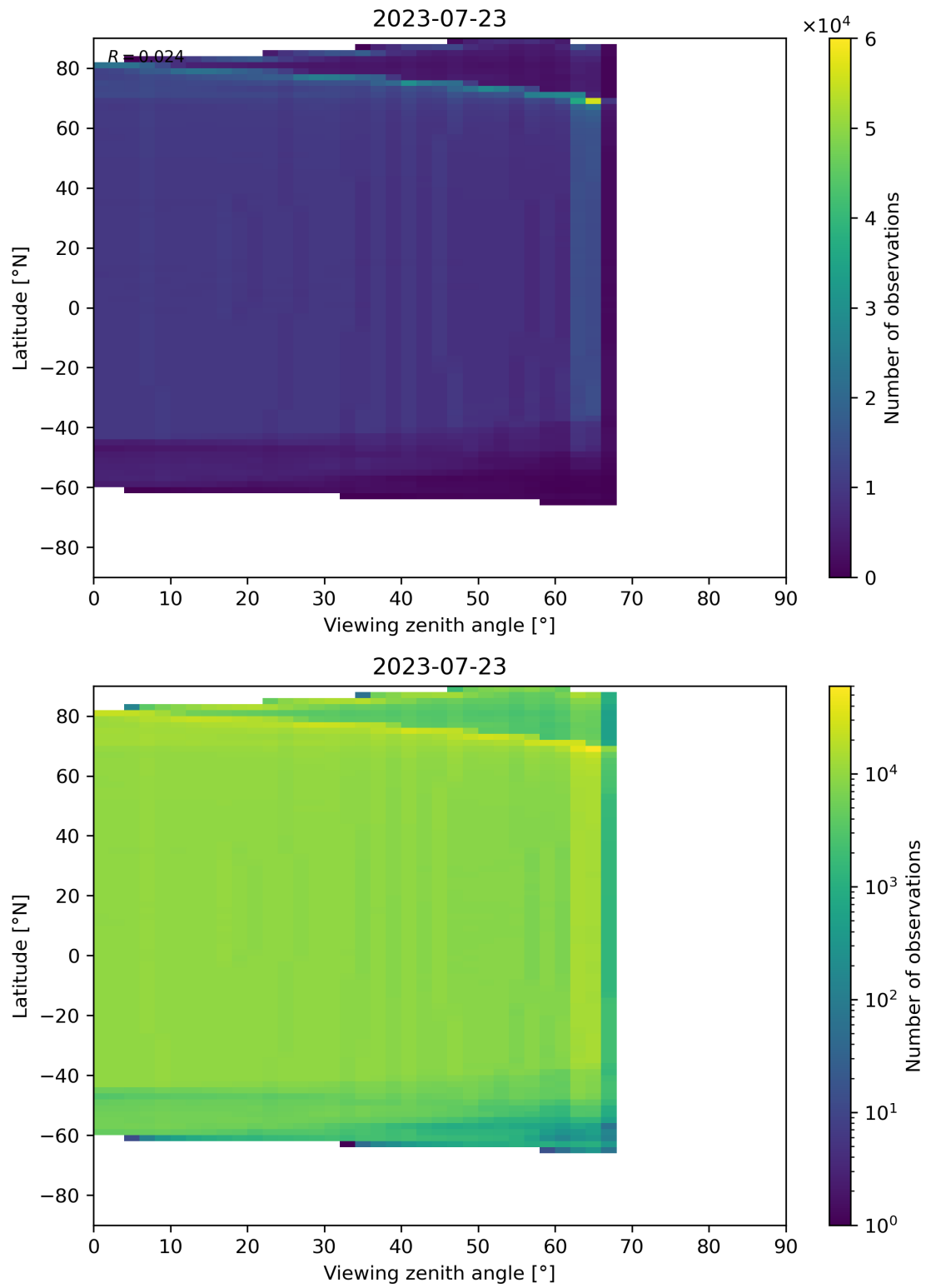
Figure 196: Scatter density plot of “Viewing zenith angle” against “Latitude” for 2023-07-22 to 2023-07-24.
