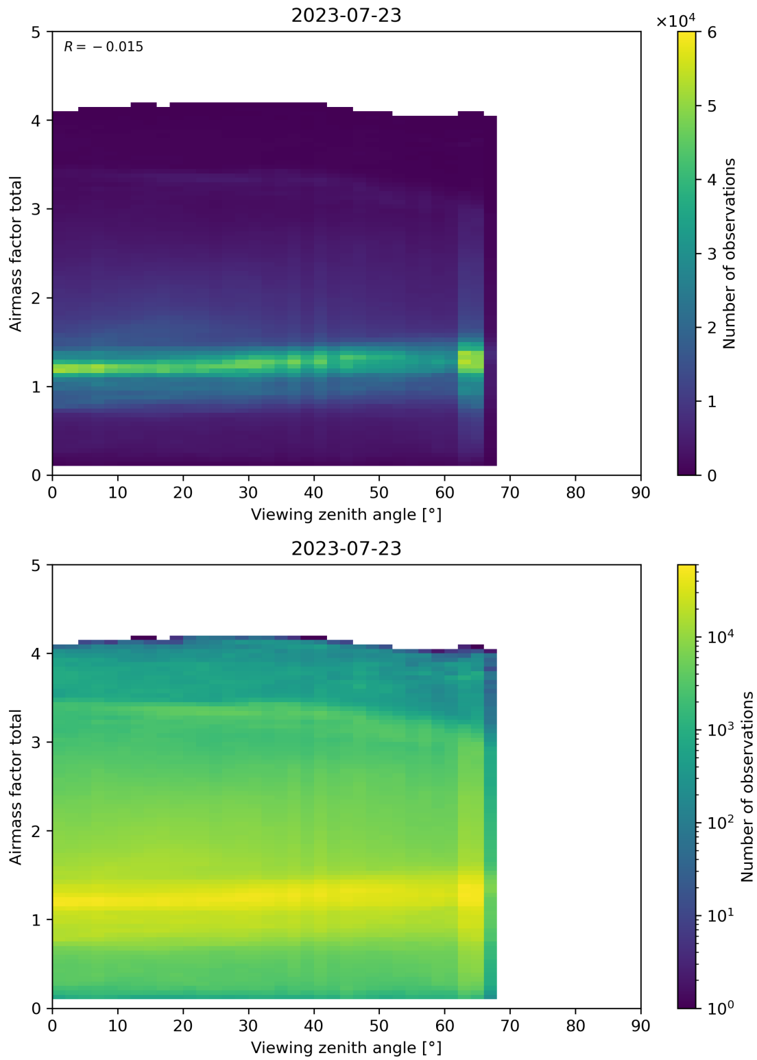
Figure 190: Scatter density plot of “Viewing zenith angle” against “Airmass factor total” for 2023-07-22 to 2023-07-24.
