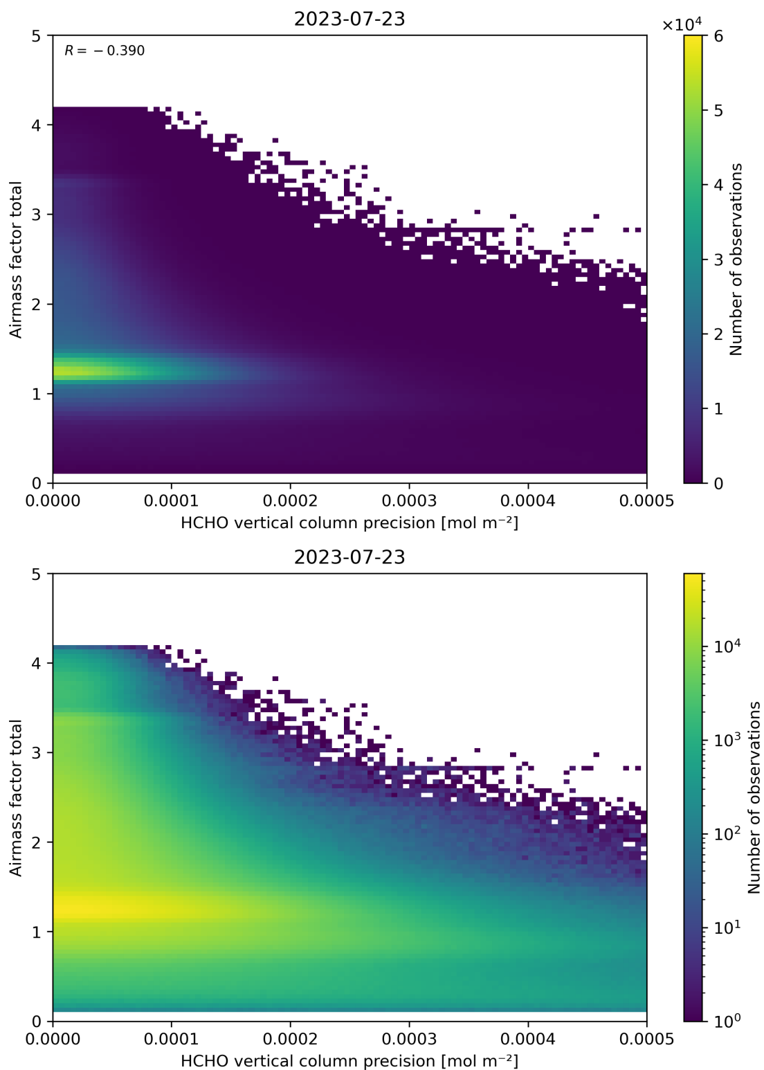
Figure 144: Scatter density plot of “HCHO vertical column precision” against “Airmass factor total” for 2023-07-22 to 2023-07-24.
