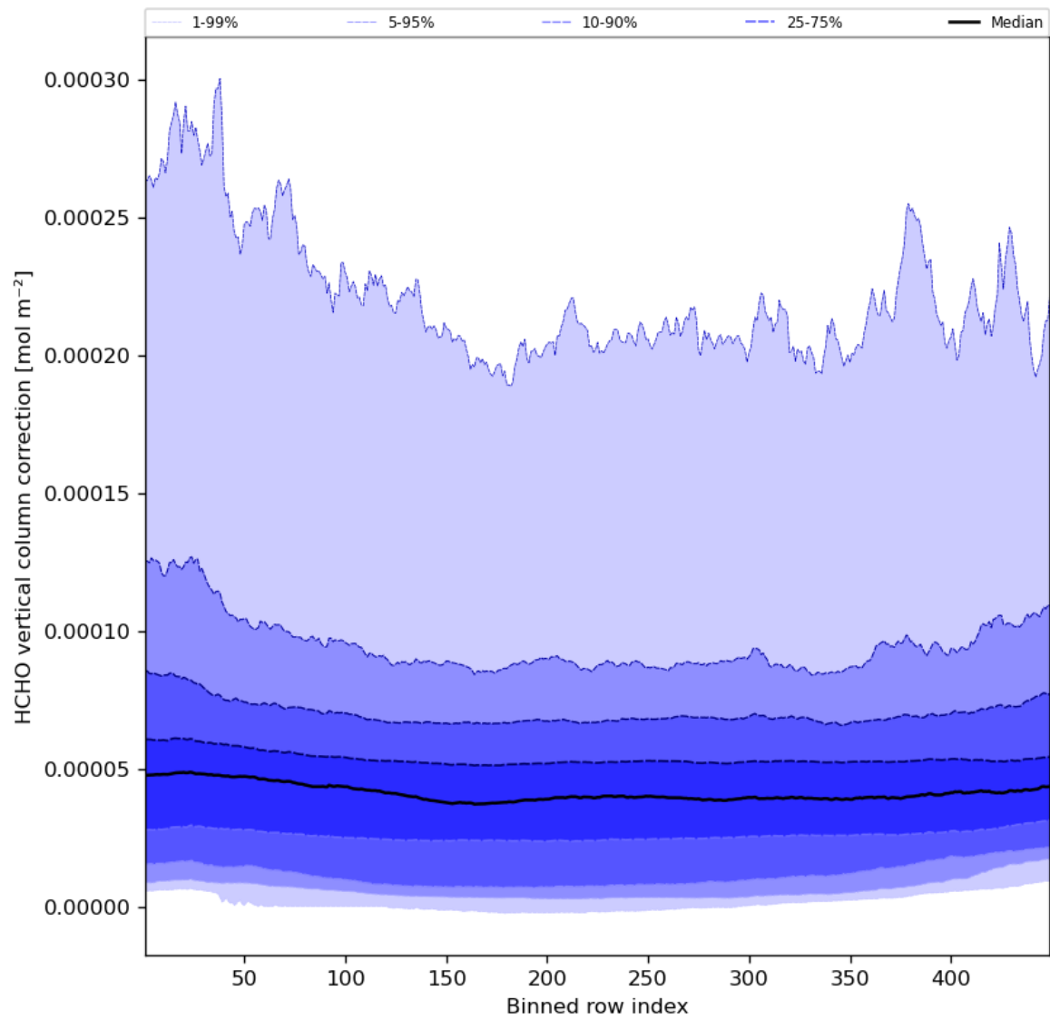
Figure 51: Along track statistics of “HCHO vertical column correction” for 2023-07-22 to 2023-07-24
