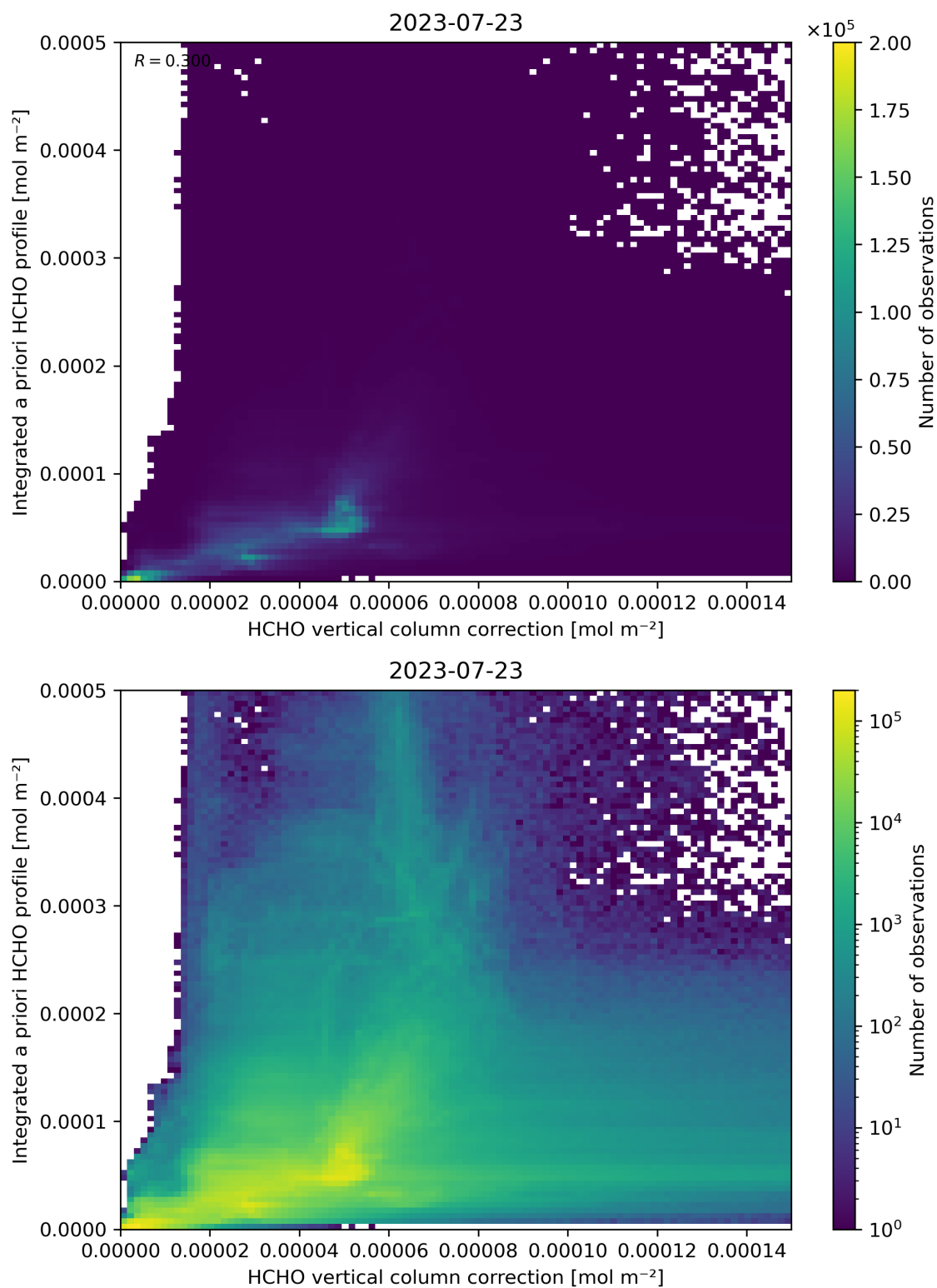
Figure 122: Scatter density plot of “HCHO vertical column correction” against “Integrated a priori HCHO profile” for 2023-07-22 to 2023-07-24.
