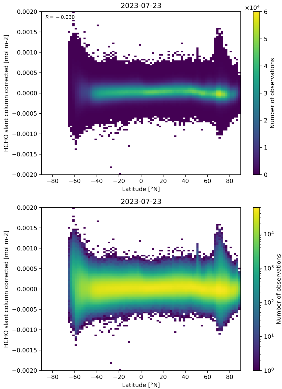
Figure 157: Scatter density plot of “Latitude” against “HCHO slant column corrected” for 2023-07-22 to 2023-07-24.
