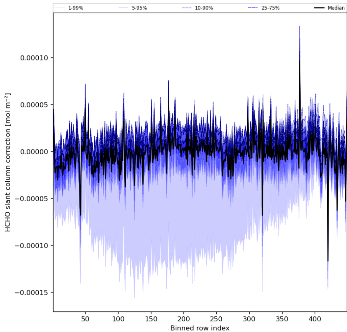
Figure 61: Along track statistics of “HCHO slant column correction” for 2023-07-22 to 2023-07-24
