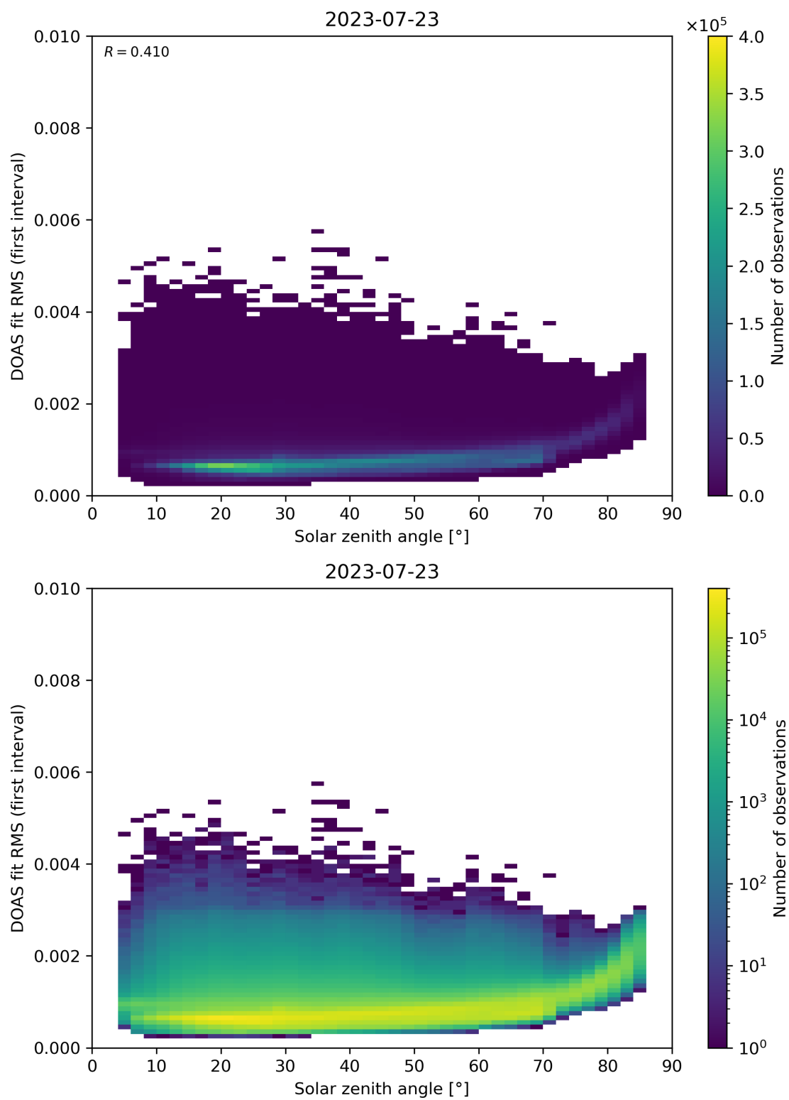
Figure 167: Scatter density plot of “Solar zenith angle” against “DOAS fit RMS (first interval)” for 2023-07-22 to 2023-07-24.
