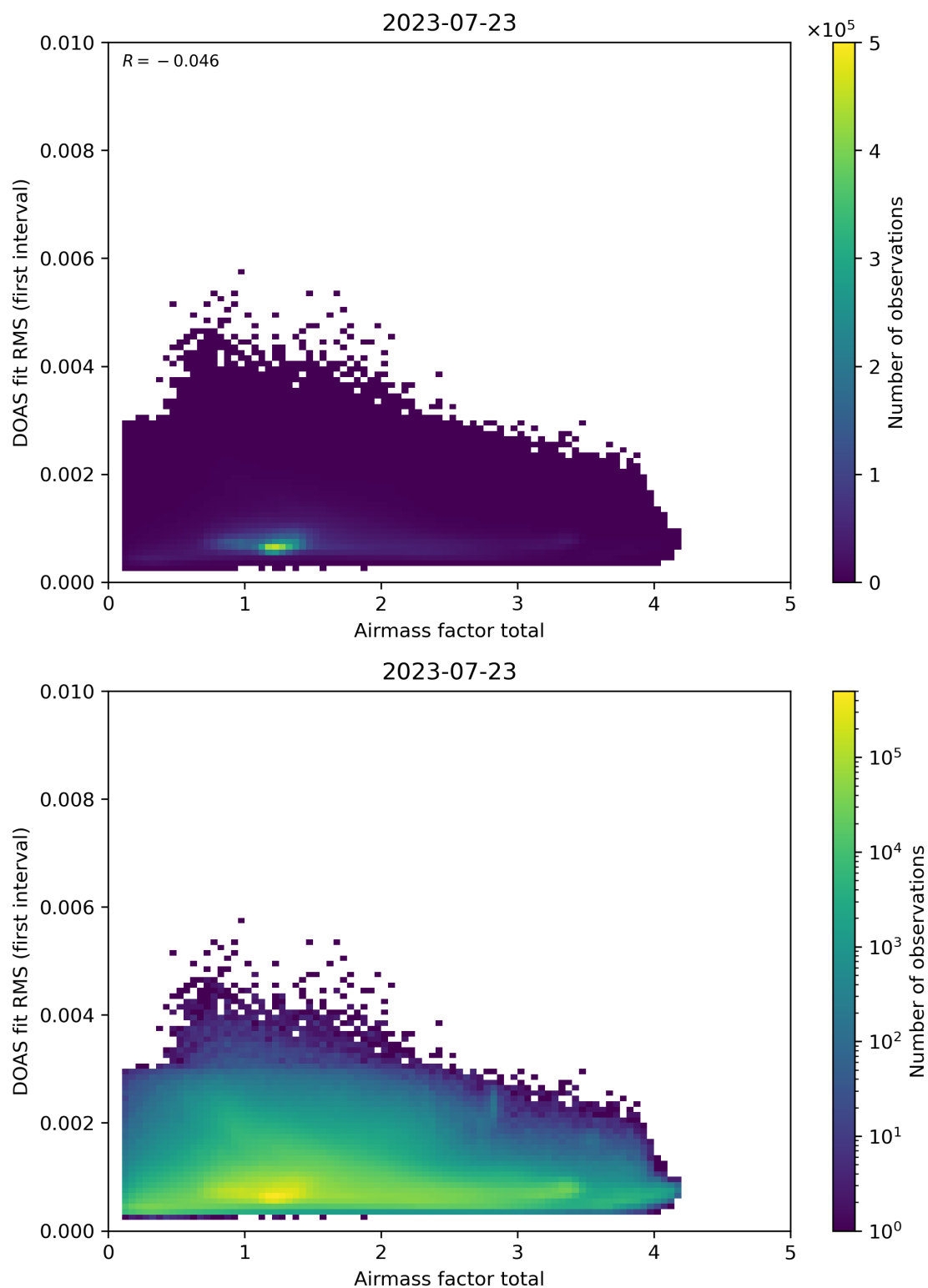
Figure 97: Scatter density plot of “Airmass factor total” against “DOAS fit RMS (first interval)” for 2023-07-22 to 2023-07-24.
