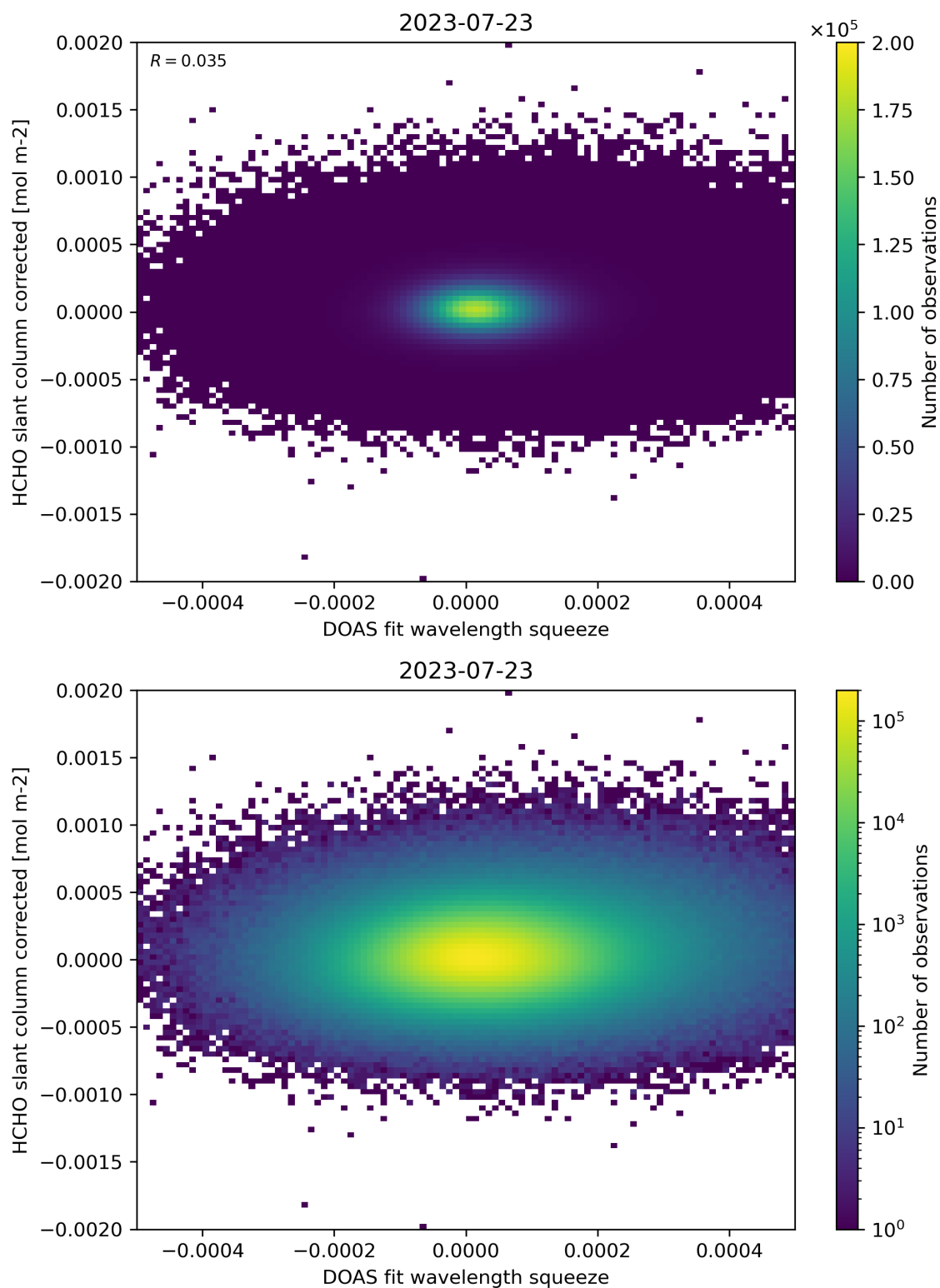
Figure 69: Scatter density plot of “DOAS fit wavelength squeeze” against “HCHO slant column corrected” for 2023-07-22 to 2023-07-24.
