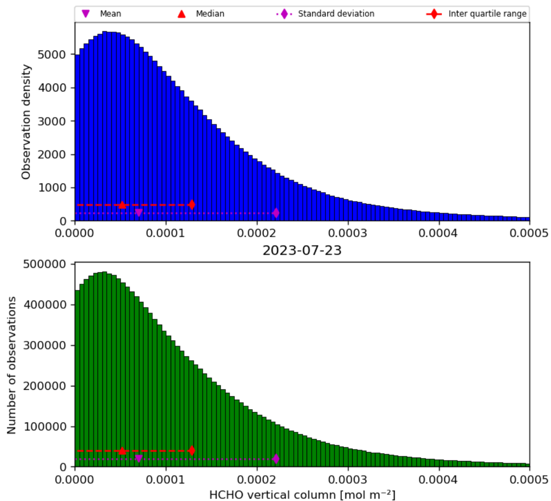
Figure 35: Histogram of “HCHO vertical column” for 2023-07-22 to 2023-07-24
