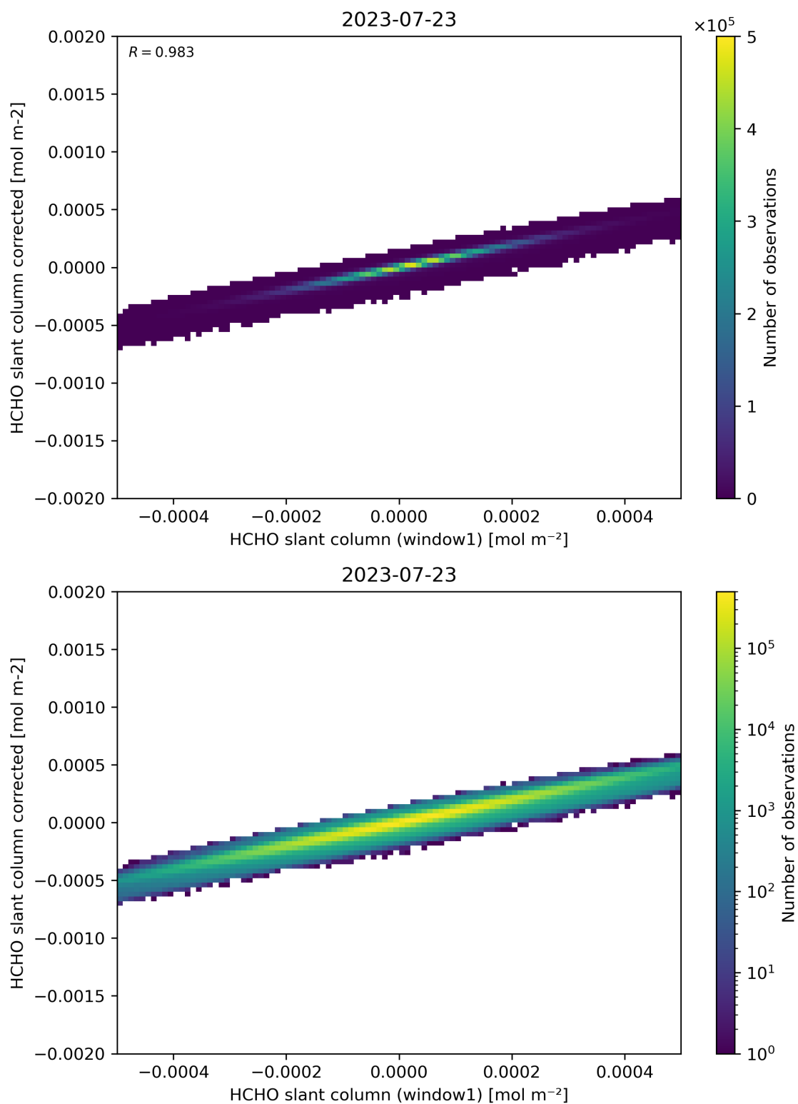
Figure 82: Scatter density plot of “HCHO slant column (window1)” against “HCHO slant column corrected” for 2023-07-22 to 2023-07-24.
