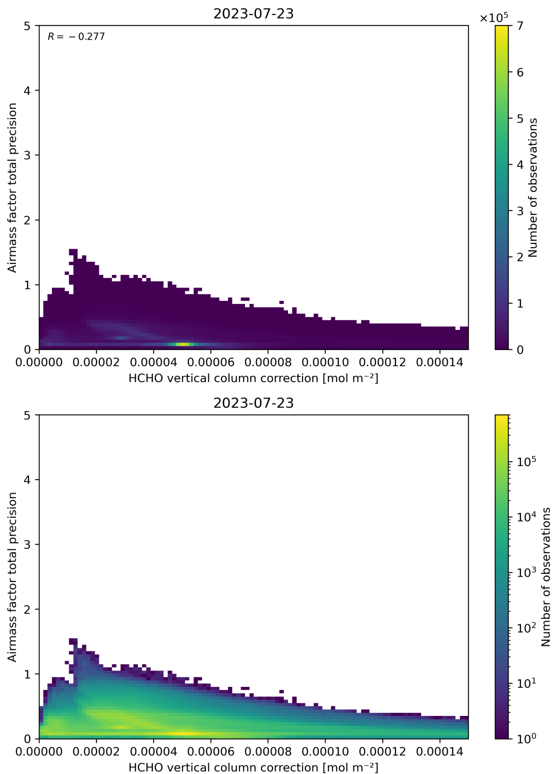
Figure 121: Scatter density plot of “HCHO vertical column correction” against “Airmass factor total precision” for 2023-07-22 to 2023-07-24.
