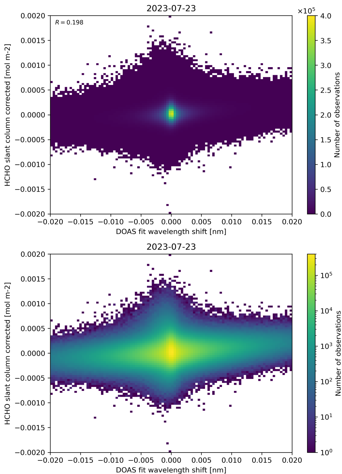
Figure 66: Scatter density plot of “DOAS fit wavelength shift” against “HCHO slant column corrected” for 2023-07-22 to 2023-07-24.
