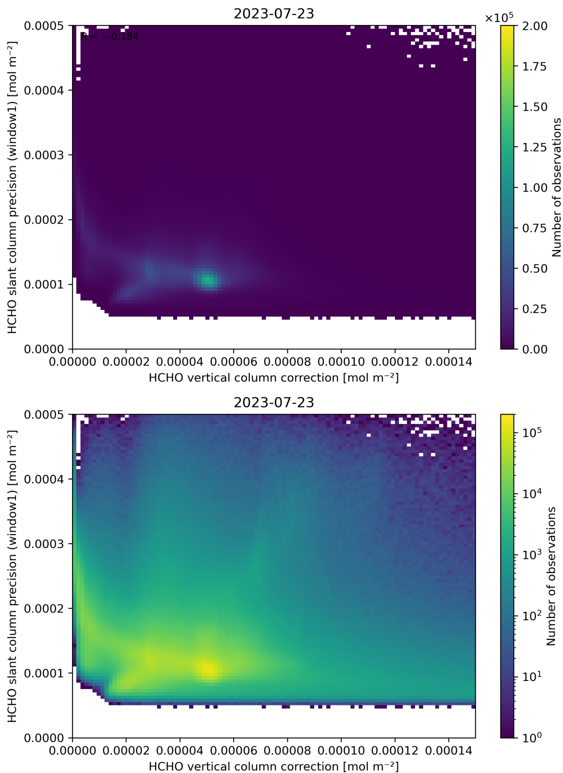
Figure 119: Scatter density plot of “HCHO vertical column correction” against “HCHO slant column precision (window1)” for 2023-07-22 to 2023-07-24.
