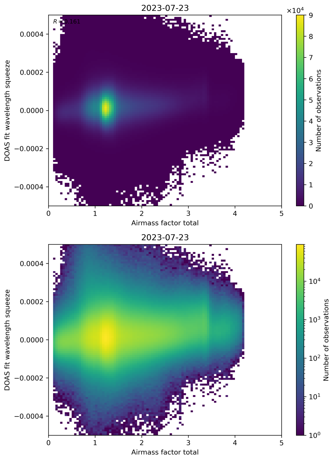
Figure 99: Scatter density plot of “Airmass factor total” against “DOAS fit wavelength squeeze” for 2023-07-22 to 2023-07-24.
