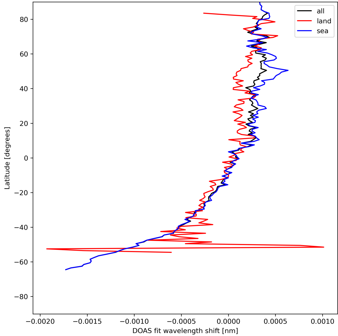
Figure 30: Zonal average of “DOAS fit wavelength shift” for 2023-07-22 to 2023-07-24.
