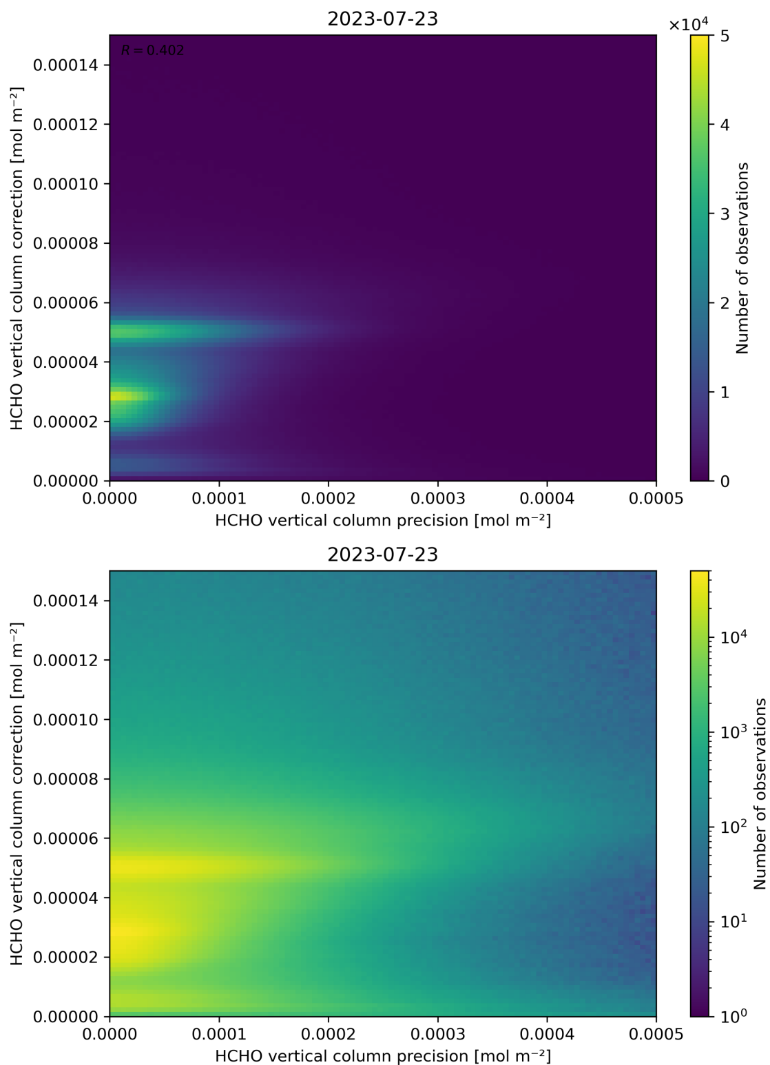
Figure 146: Scatter density plot of “HCHO vertical column precision” against “HCHO vertical column correction” for 2023-07-22 to 2023-07-24.
