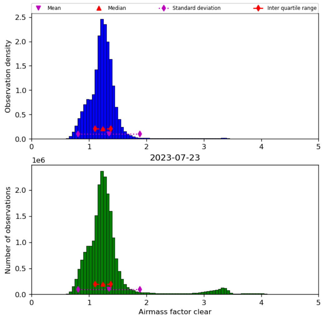
Figure 42: Histogram of “Airmass factor clear” for 2023-07-22 to 2023-07-24
