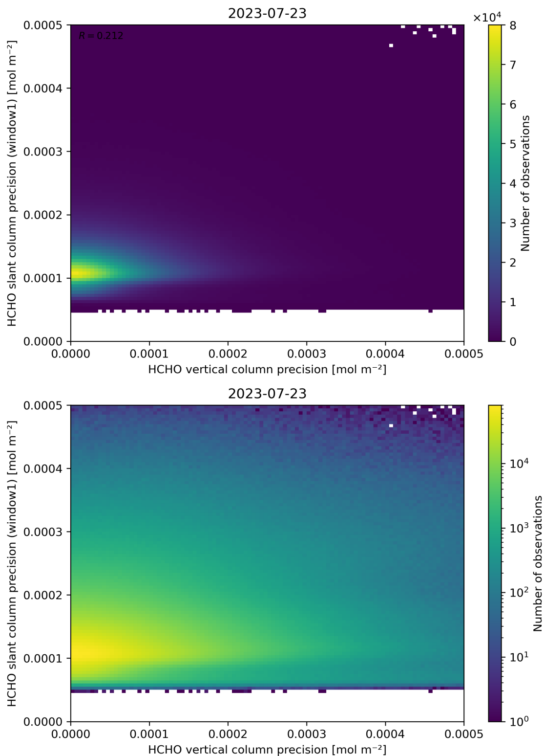
Figure 143: Scatter density plot of “HCHO vertical column precision” against “HCHO slant column precision (window1)” for 2023-07-22 to 2023-07-24.
