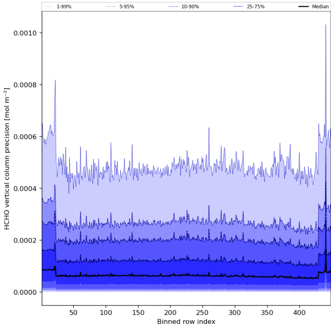
Figure 50: Along track statistics of “HCHO vertical column precision” for 2023-07-22 to 2023-07-24
