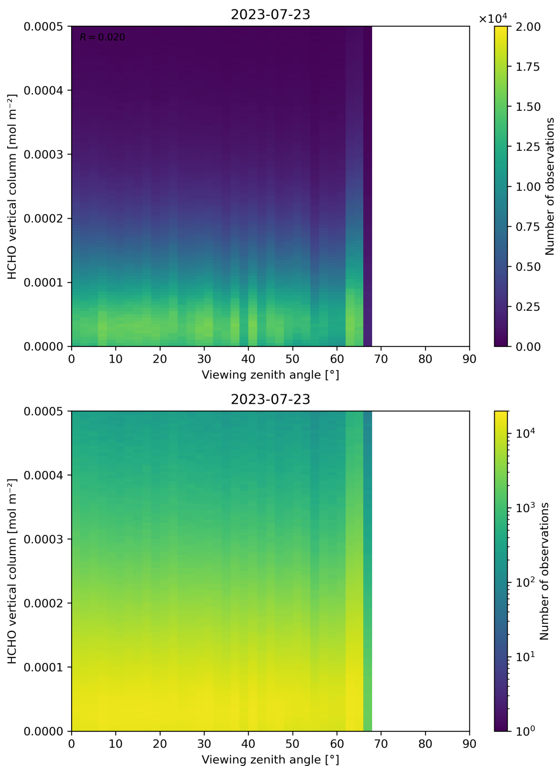
Figure 192: Scatter density plot of “Viewing zenith angle” against “HCHO vertical column” for 2023-07-22 to 2023-07-24.
