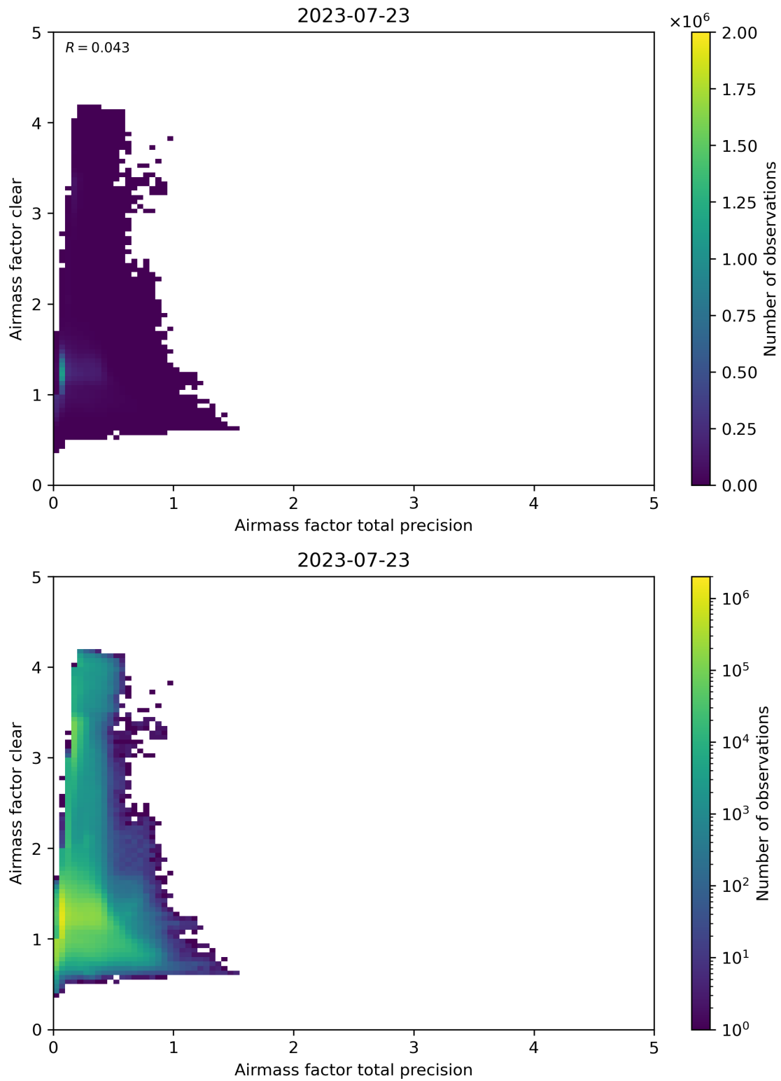
Figure 108: Scatter density plot of “Airmass factor total precision” against “Airmass factor clear” for 2023-07-22 to 2023-07-24.
