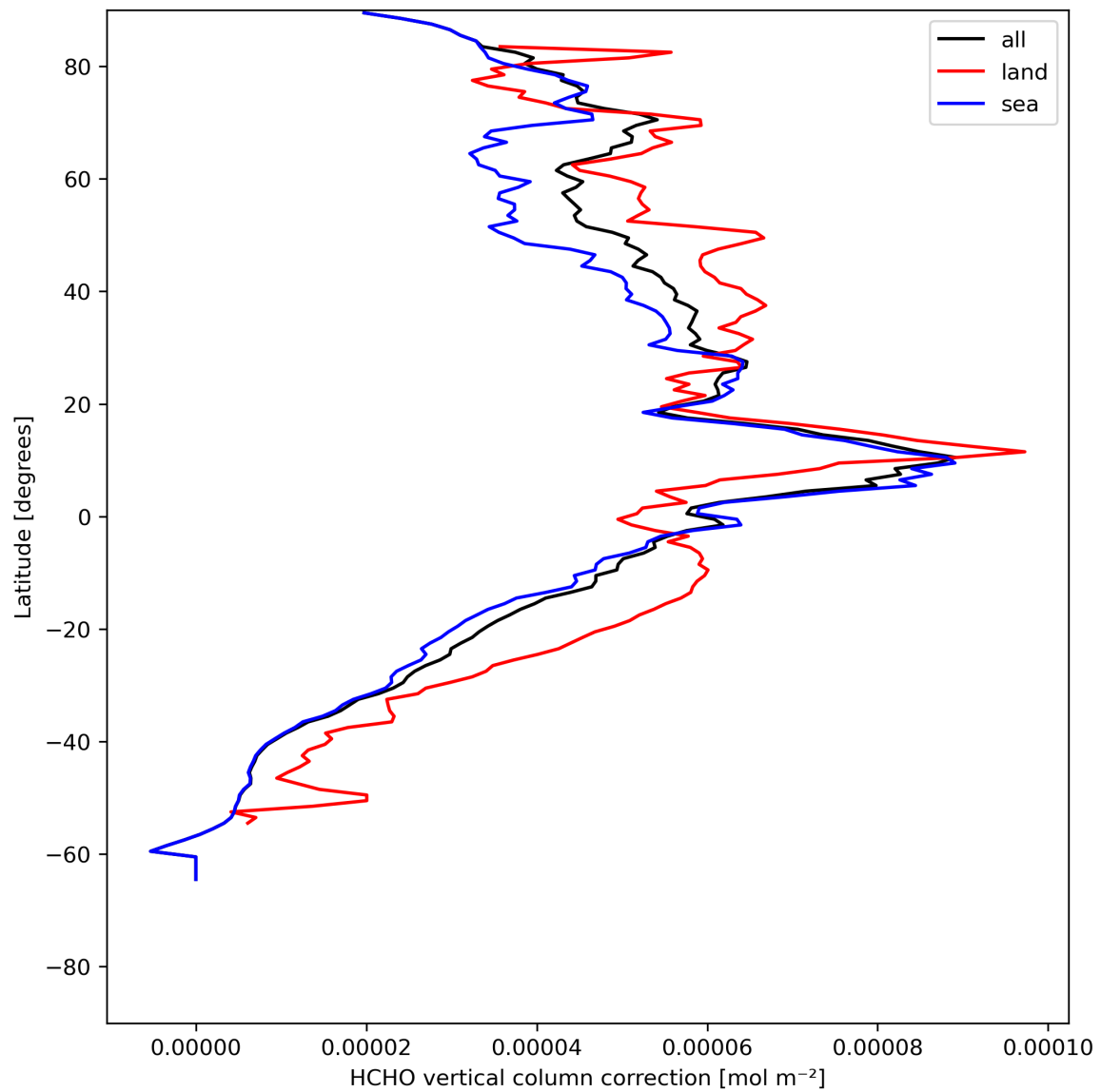
Figure 23: Zonal average of “HCHO vertical column correction” for 2023-07-22 to 2023-07-24.
