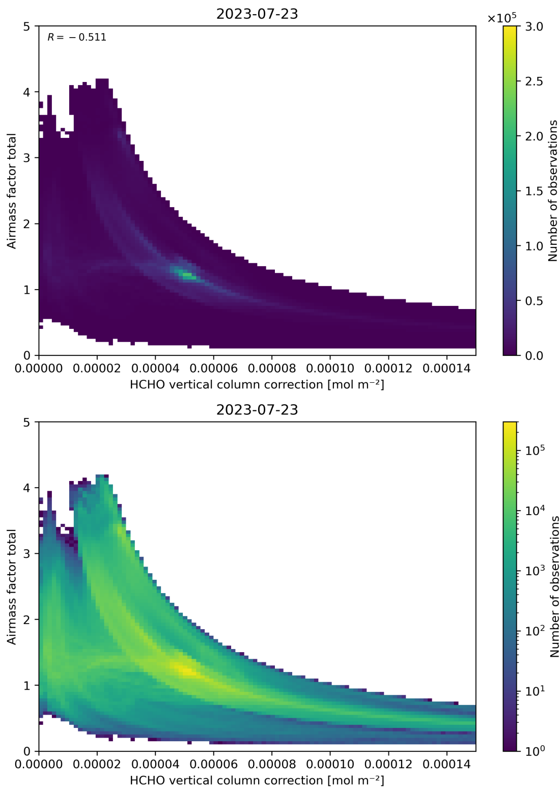
Figure 120: Scatter density plot of “HCHO vertical column correction” against “Airmass factor total” for 2023-07-22 to 2023-07-24.
