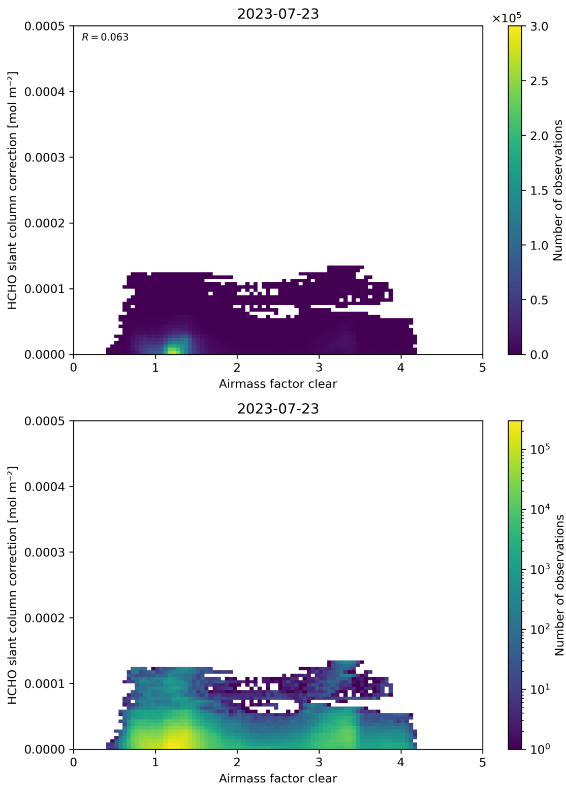
Figure 75: Scatter density plot of “Airmass factor clear” against “HCHO slant column correction” for 2023-07-22 to 2023-07-24.
