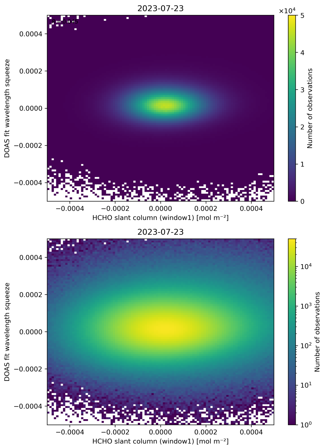
Figure 80: Scatter density plot of “HCHO slant column (window1)” against “DOAS fit wavelength squeeze” for 2023-07-22 to 2023-07-24.
