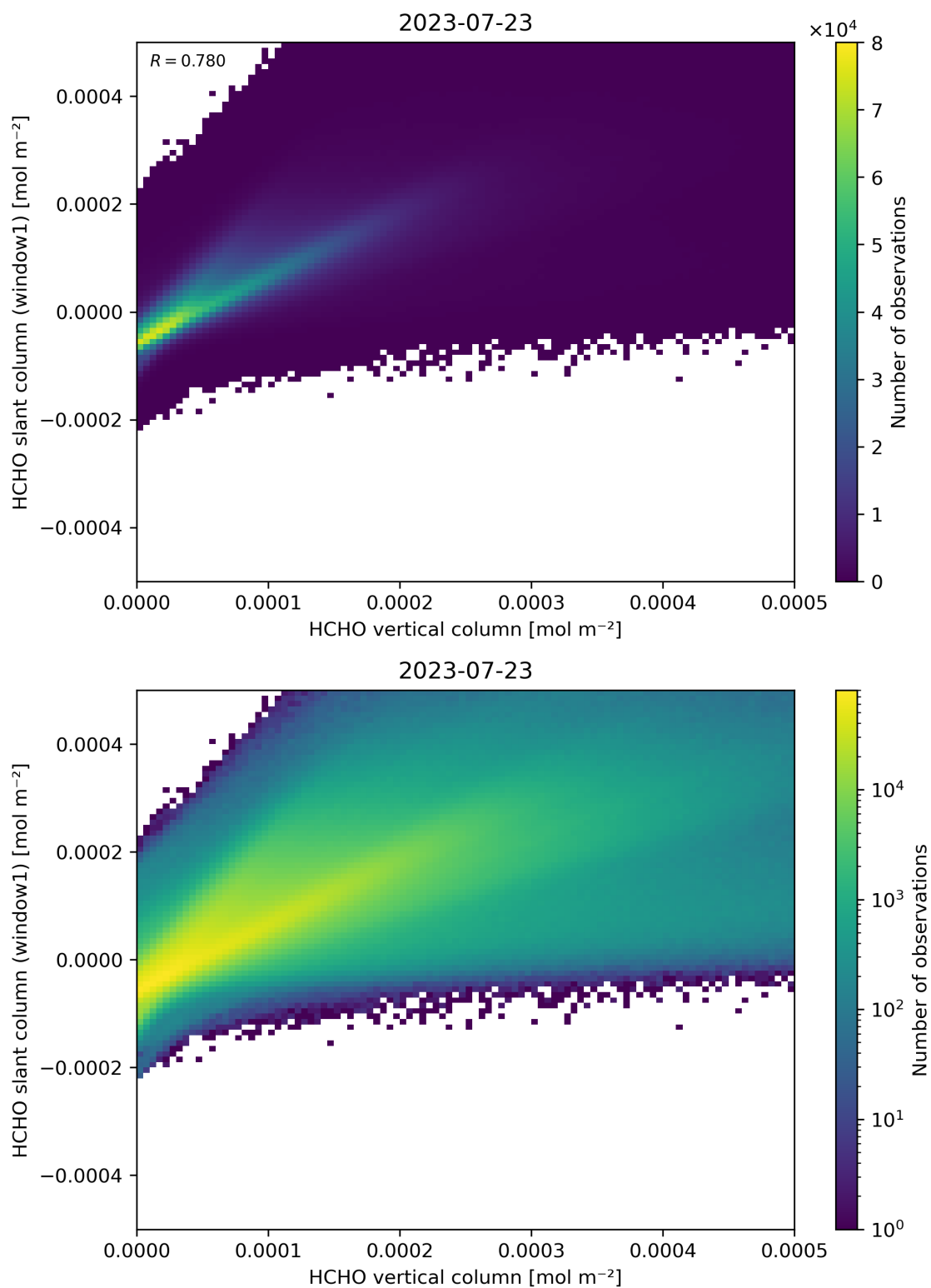
Figure 129: Scatter density plot of “HCHO vertical column” against “HCHO slant column (window1)” for 2023-07-22 to 2023-07-24.
