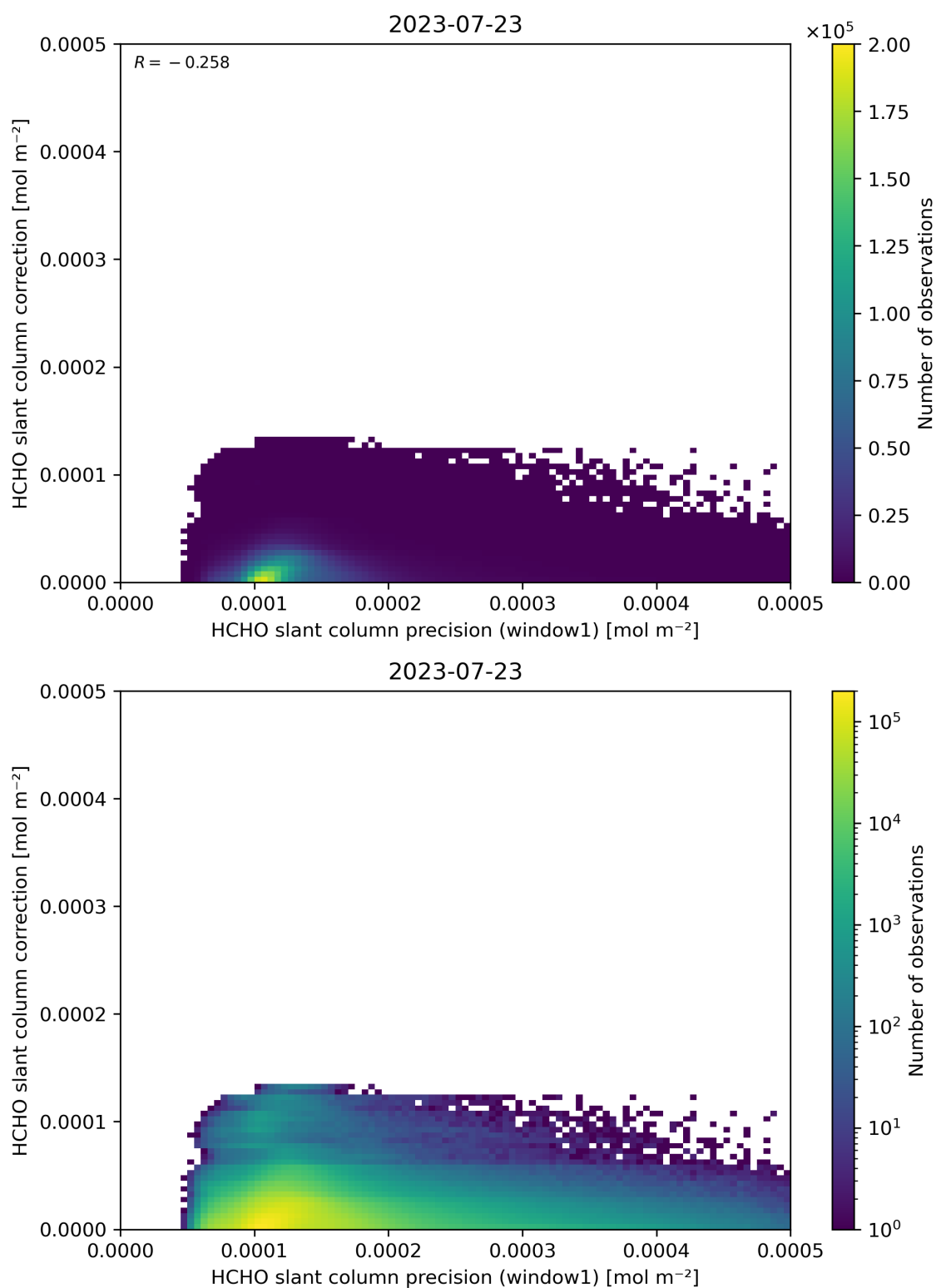
Figure 93: Scatter density plot of “HCHO slant column precision (window1)” against “HCHO slant column correction” for 2023-07-22 to 2023-07-24.
