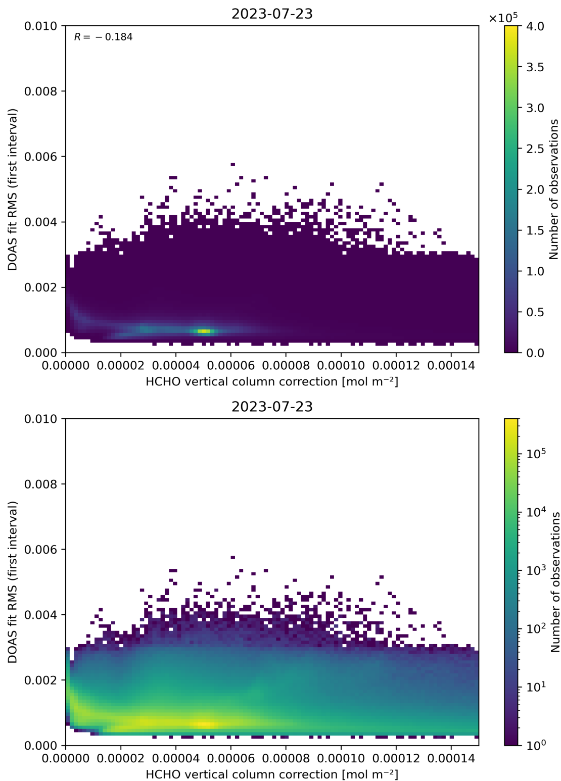
Figure 112: Scatter density plot of “HCHO vertical column correction” against “DOAS fit RMS (first interval)” for 2023-07-22 to 2023-07-24.
