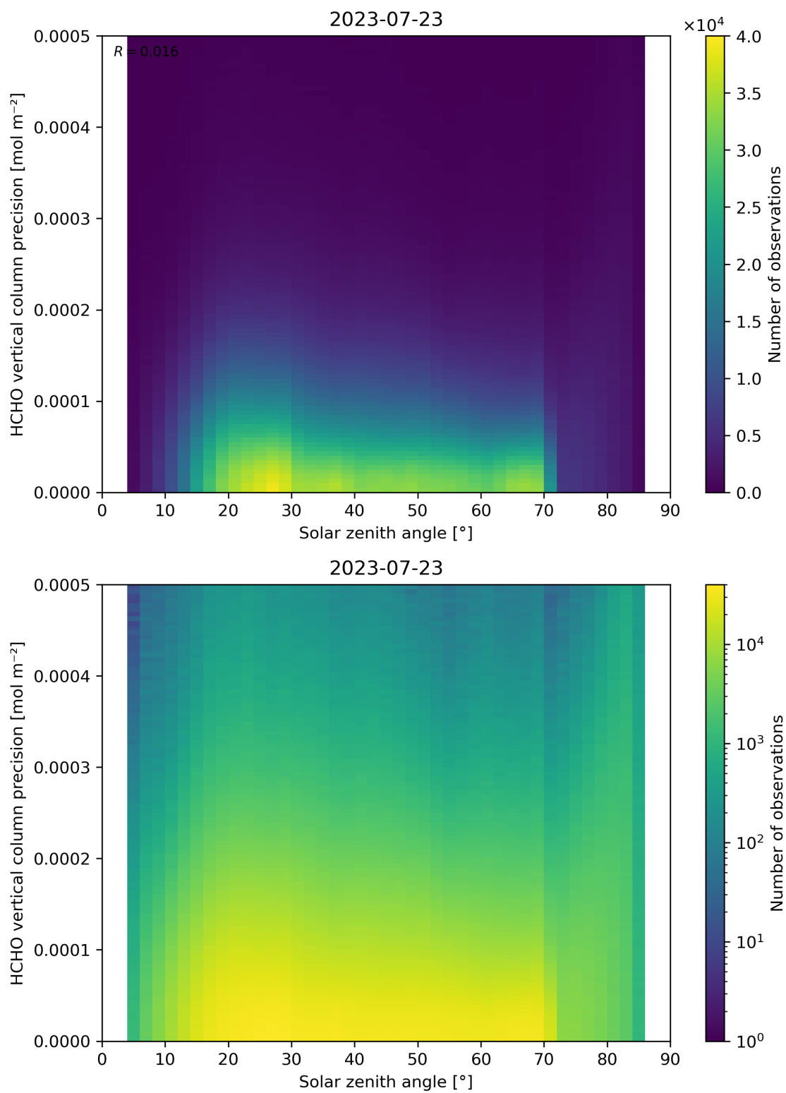
Figure 179: Scatter density plot of “Solar zenith angle” against “HCHO vertical column precision” for 2023-07-22 to 2023-07-24.
