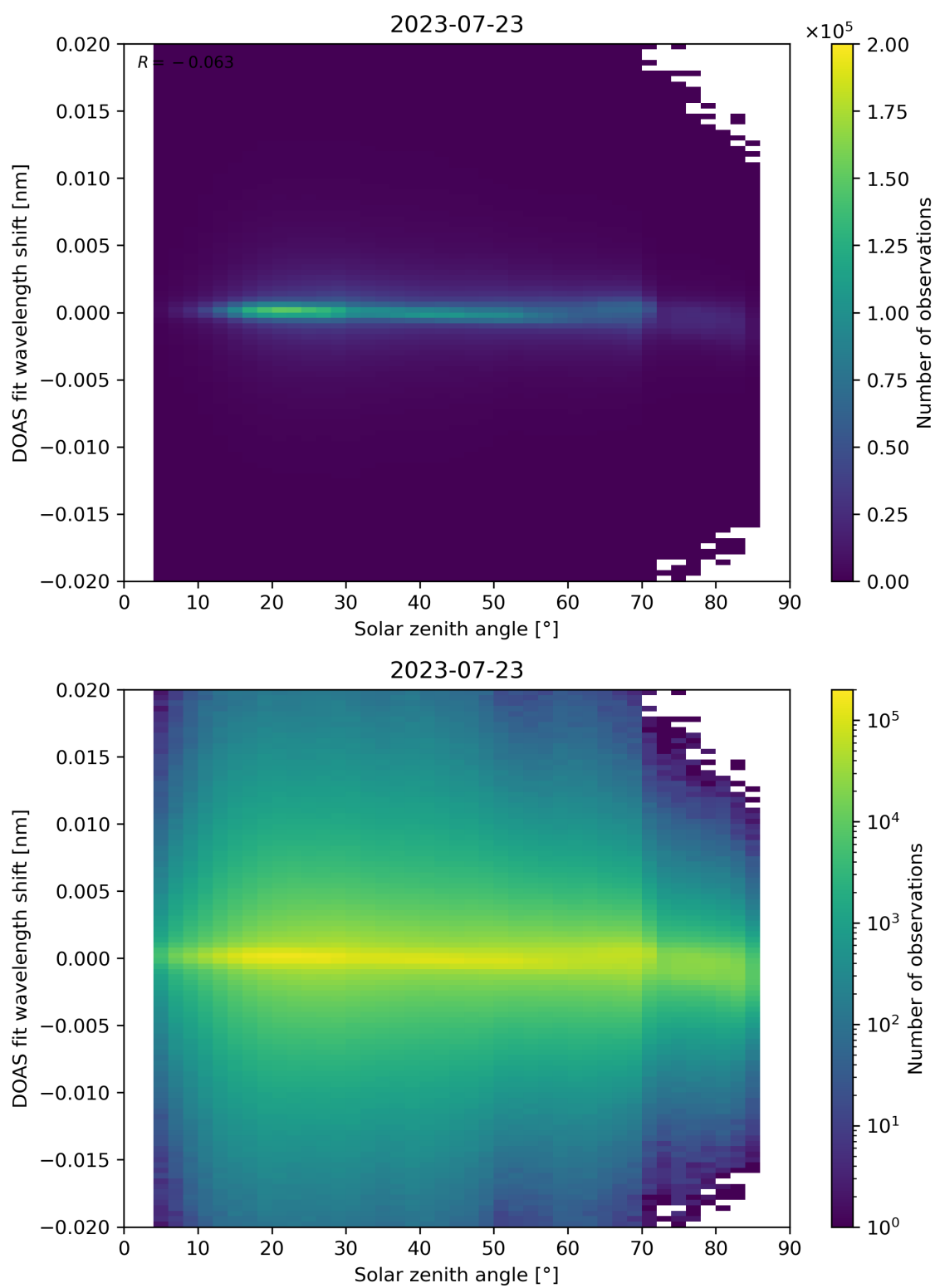
Figure 168: Scatter density plot of “Solar zenith angle” against “DOAS fit wavelength shift” for 2023-07-22 to 2023-07-24.
