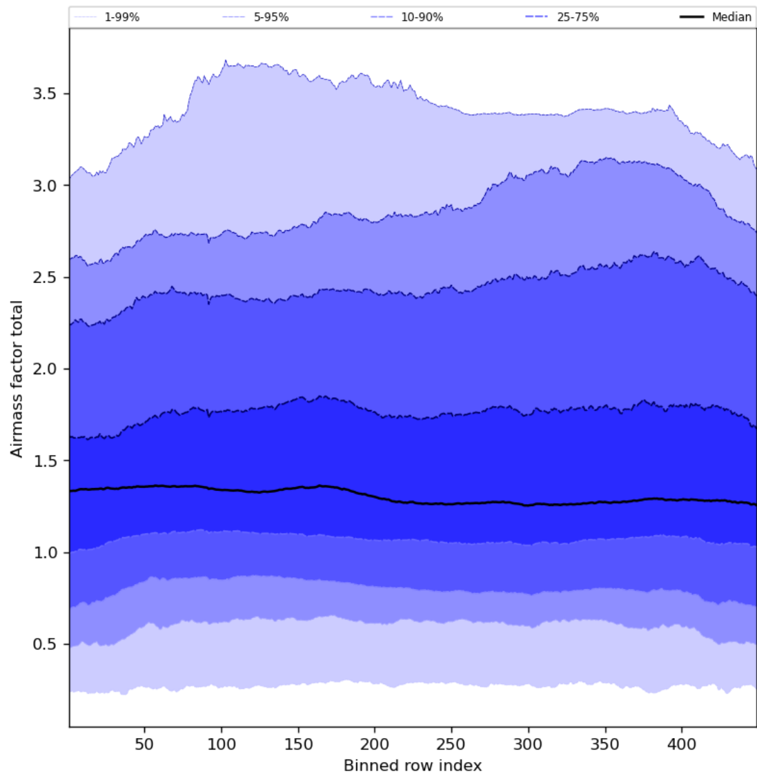
Figure 54: Along track statistics of “Airmass factor total” for 2023-07-22 to 2023-07-24
