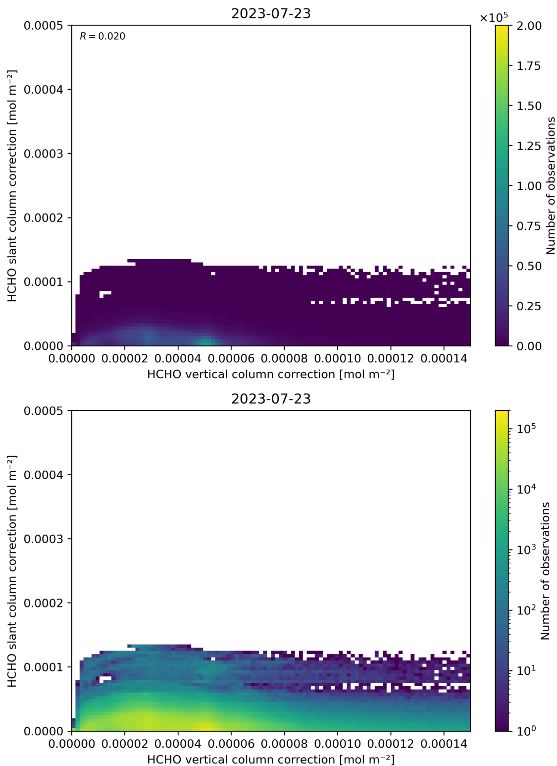
Figure 117: Scatter density plot of “HCHO vertical column correction” against “HCHO slant column correction” for 2023-07-22 to 2023-07-24.
