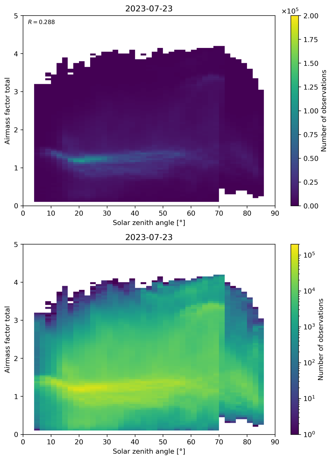
Figure 175: Scatter density plot of “Solar zenith angle” against “Airmass factor total” for 2023-07-22 to 2023-07-24.
