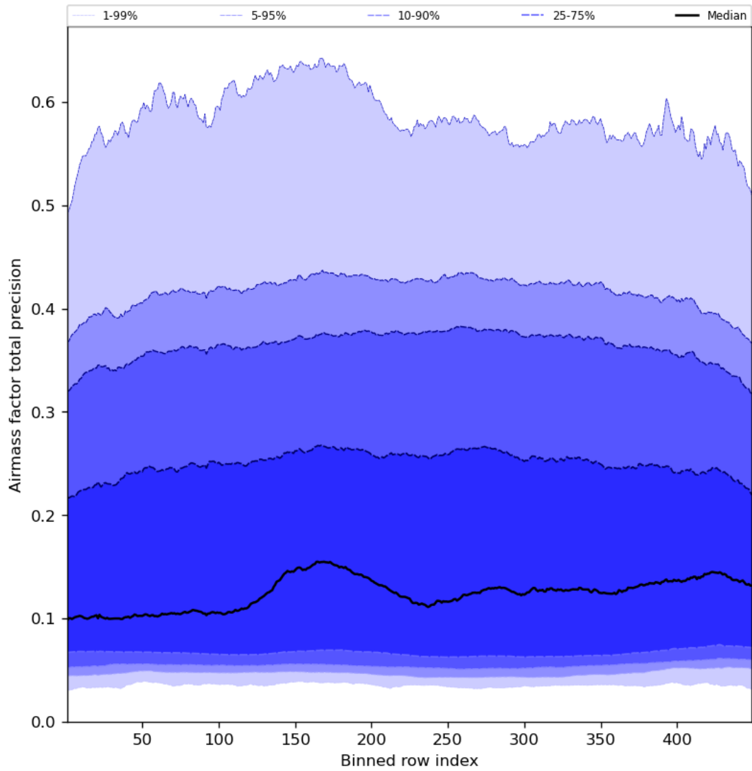
Figure 55: Along track statistics of “Airmass factor total precision” for 2023-07-22 to 2023-07-24
