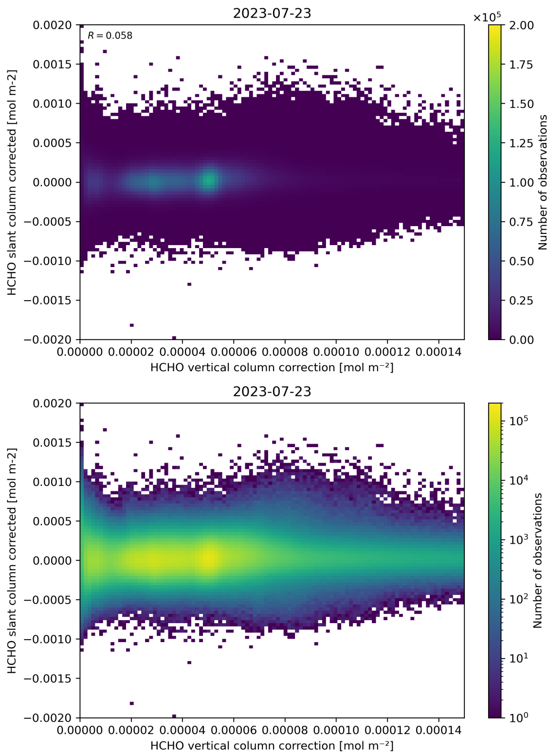
Figure 116: Scatter density plot of “HCHO vertical column correction” against “HCHO slant column corrected” for 2023-07-22 to 2023-07-24.
