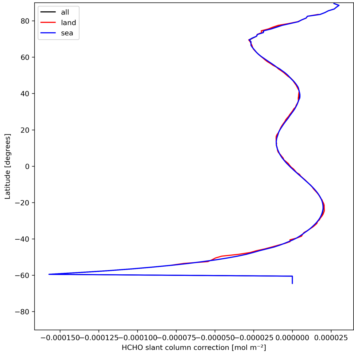
Figure 33: Zonal average of “HCHO slant column correction” for 2023-07-22 to 2023-07-24.
