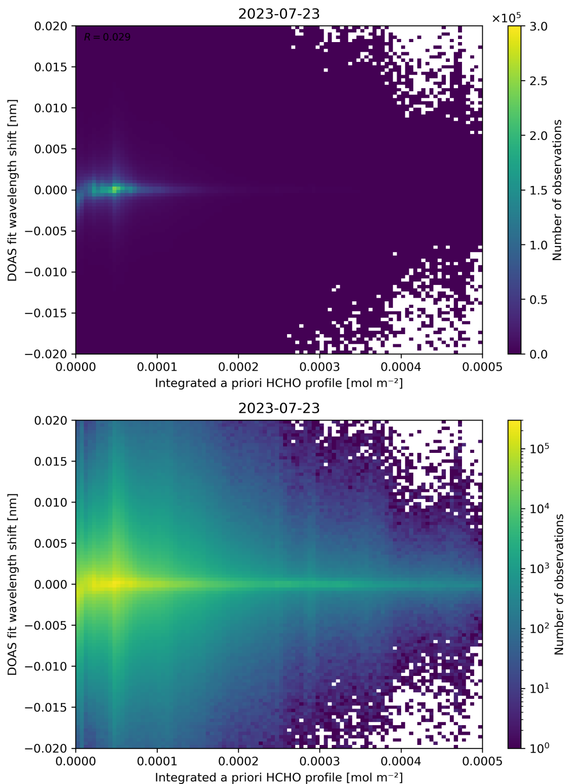
Figure 149: Scatter density plot of “Integrated a priori HCHO profile” against “DOAS fit wavelength shift” for 2023-07-22 to 2023-07-24.
