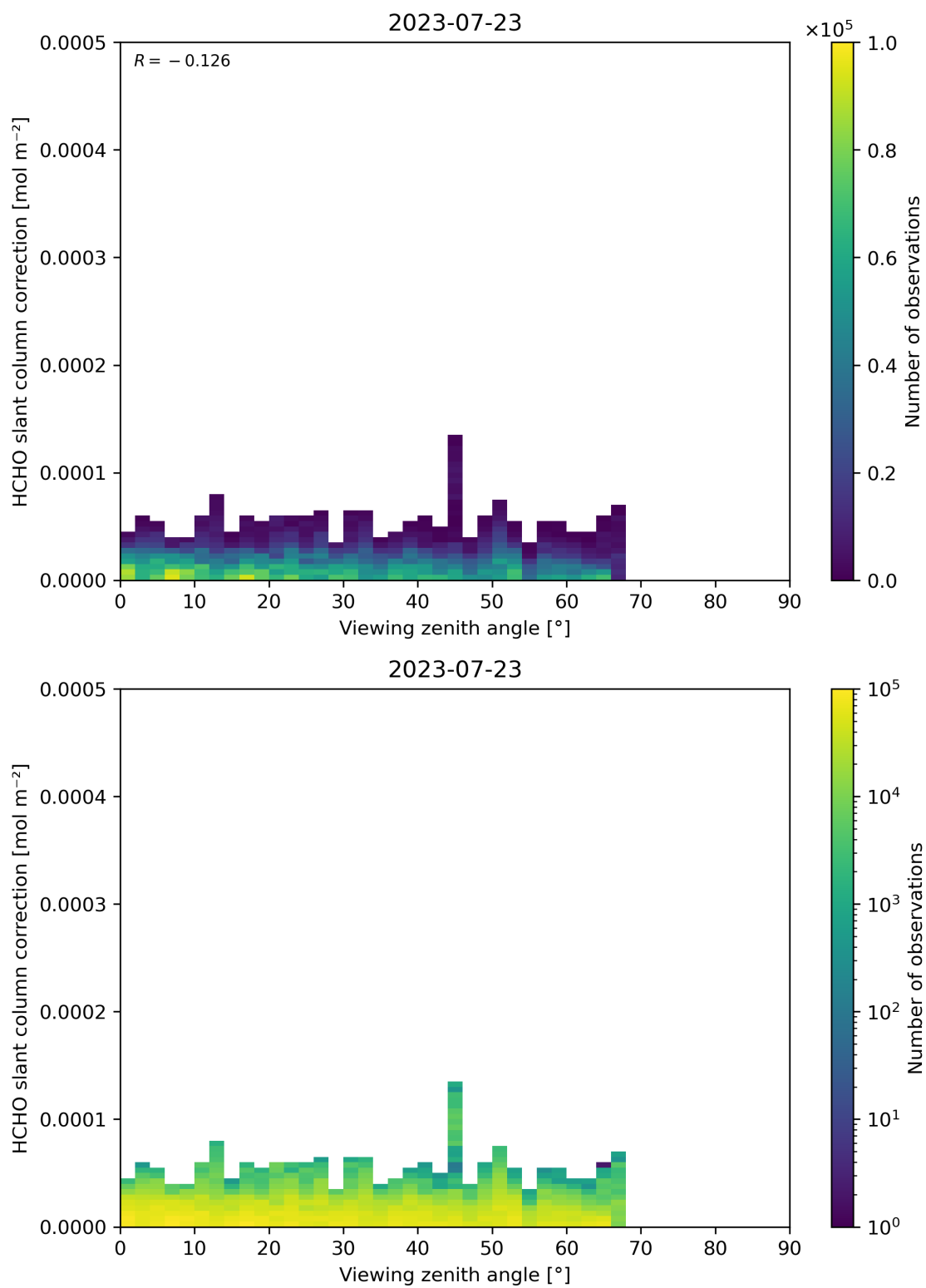
Figure 187: Scatter density plot of “Viewing zenith angle” against “HCHO slant column correction” for 2023-07-22 to 2023-07-24.
