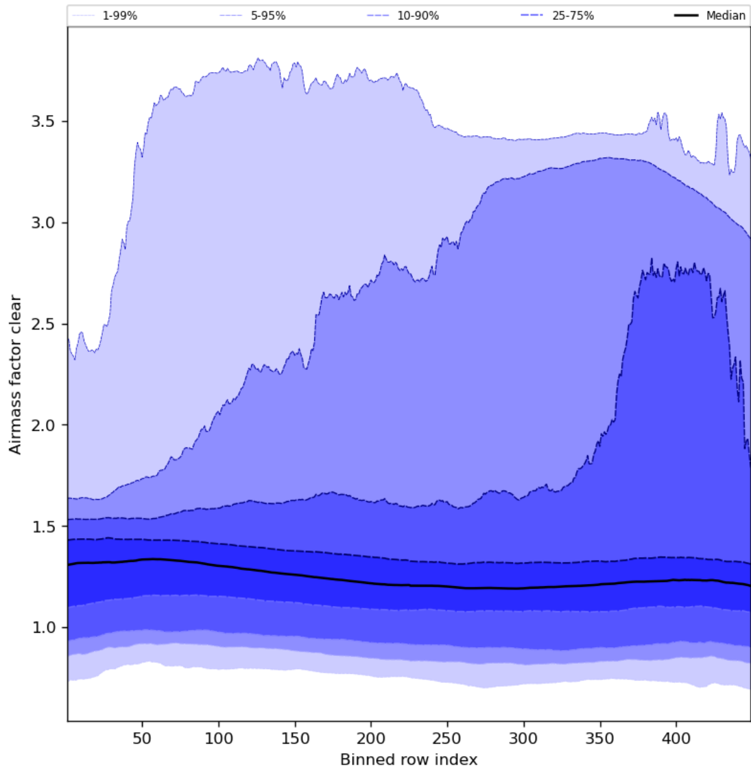
Figure 56: Along track statistics of “Airmass factor clear” for 2023-07-22 to 2023-07-24
