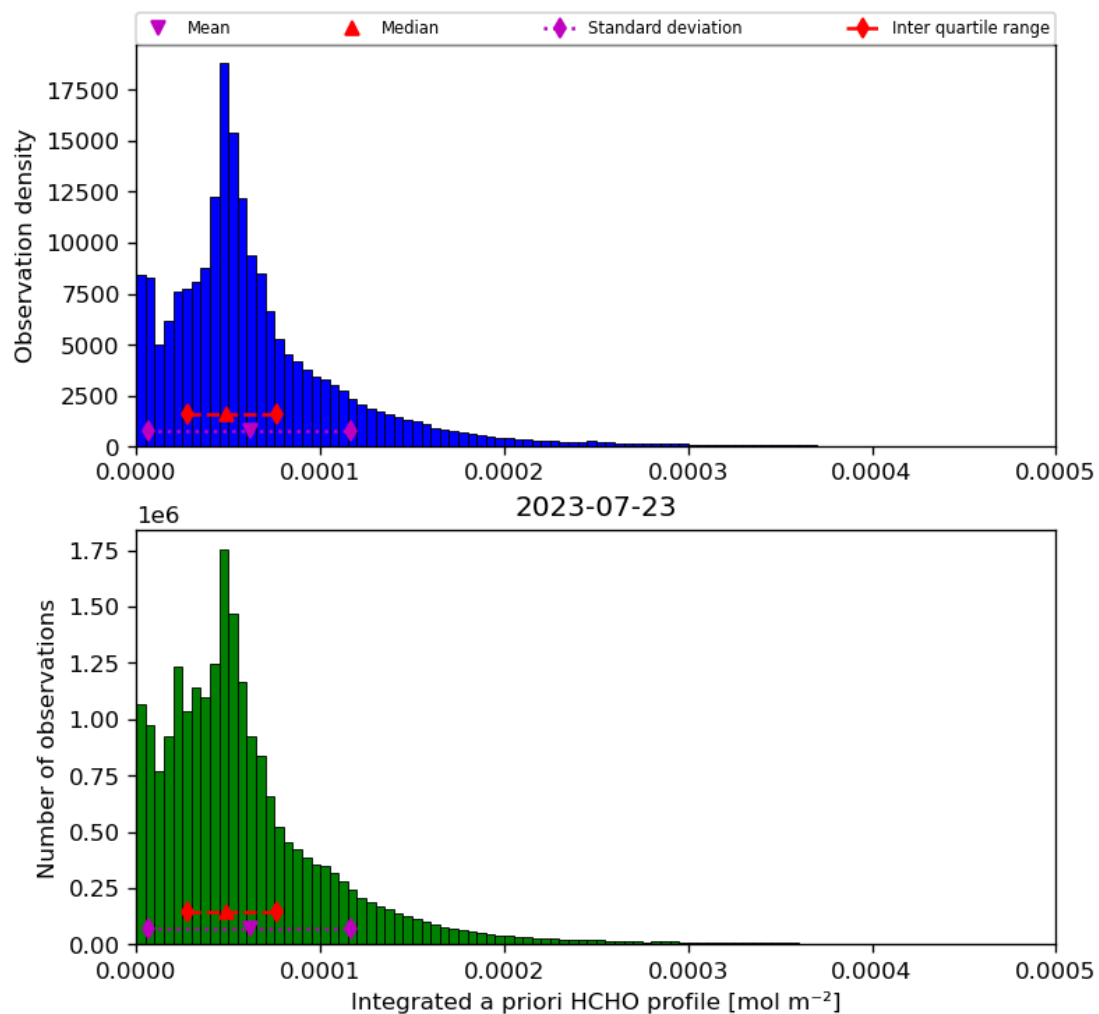
Figure 43: Histogram of “Integrated a priori HCHO profile” for 2023-07-22 to 2023-07-24
