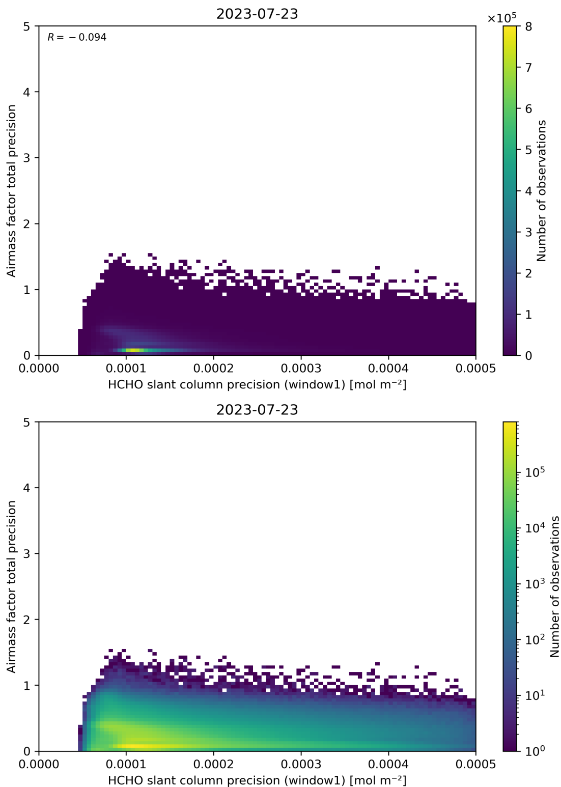
Figure 95: Scatter density plot of “HCHO slant column precision (window1)” against “Airmass factor total precision” for 2023-07-22 to 2023-07-24.
