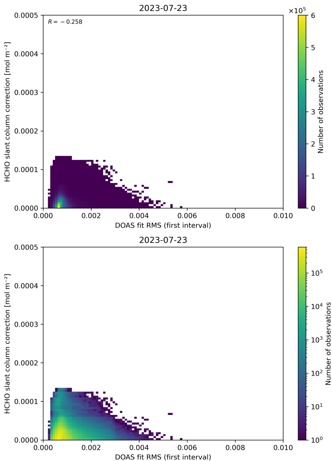
Figure 63: Scatter density plot of “DOAS fit RMS (first interval)” against “HCHO slant column correction” for 2023-07-22 to 2023-07-24.
