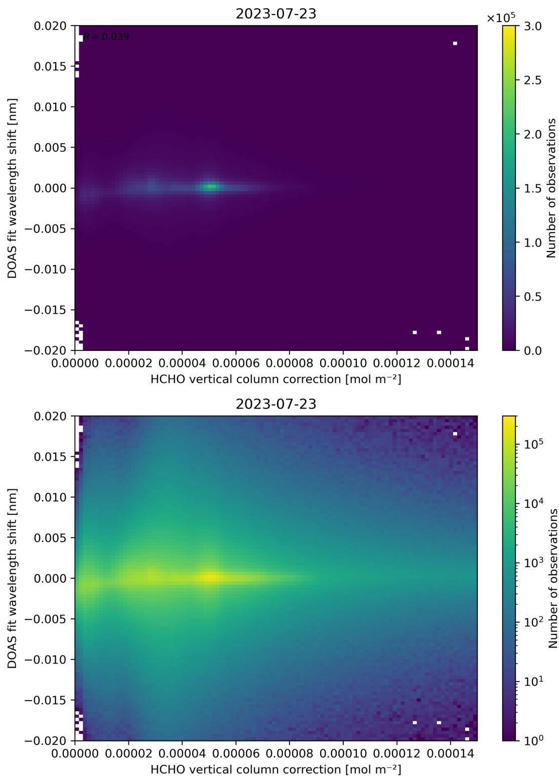
Figure 113: Scatter density plot of “HCHO vertical column correction” against “DOAS fit wavelength shift” for 2023-07-22 to 2023-07-24.
