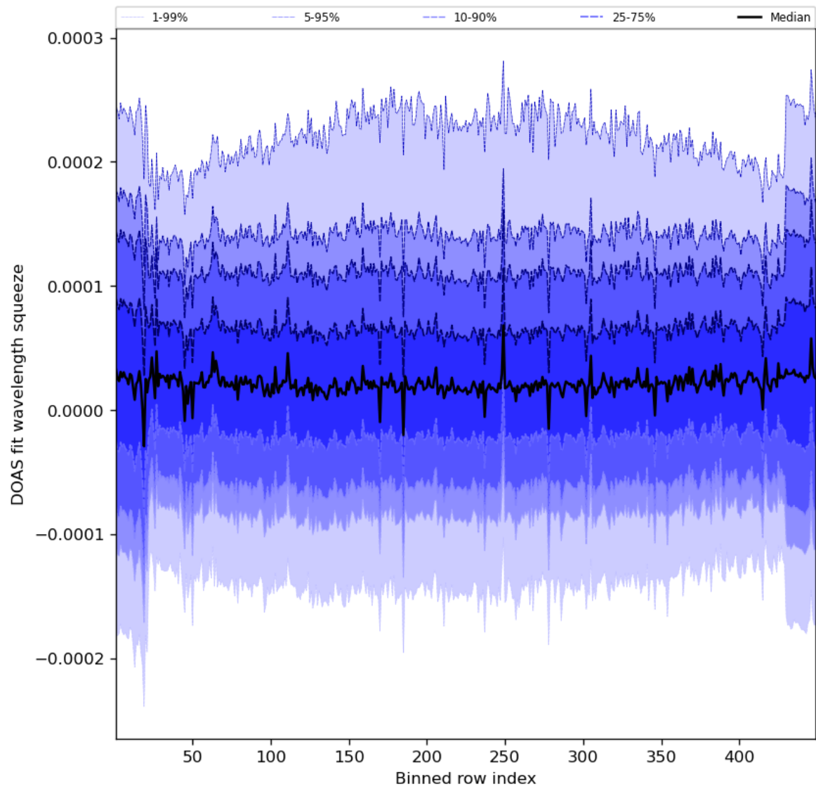
Figure 59: Along track statistics of “DOAS fit wavelength squeeze” for 2023-07-22 to 2023-07-24
