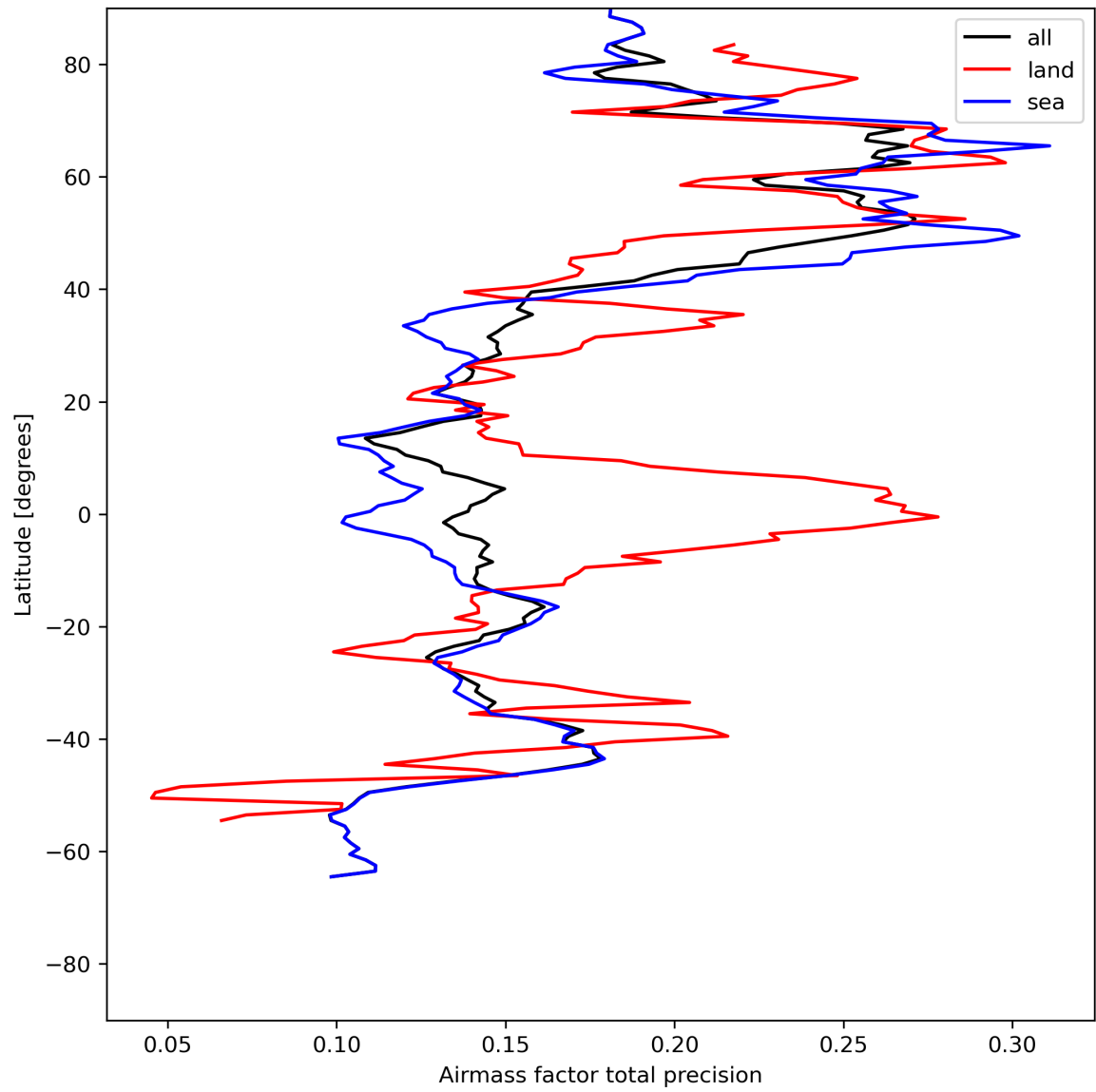
Figure 27: Zonal average of “Airmass factor total precision” for 2023-07-22 to 2023-07-24.
