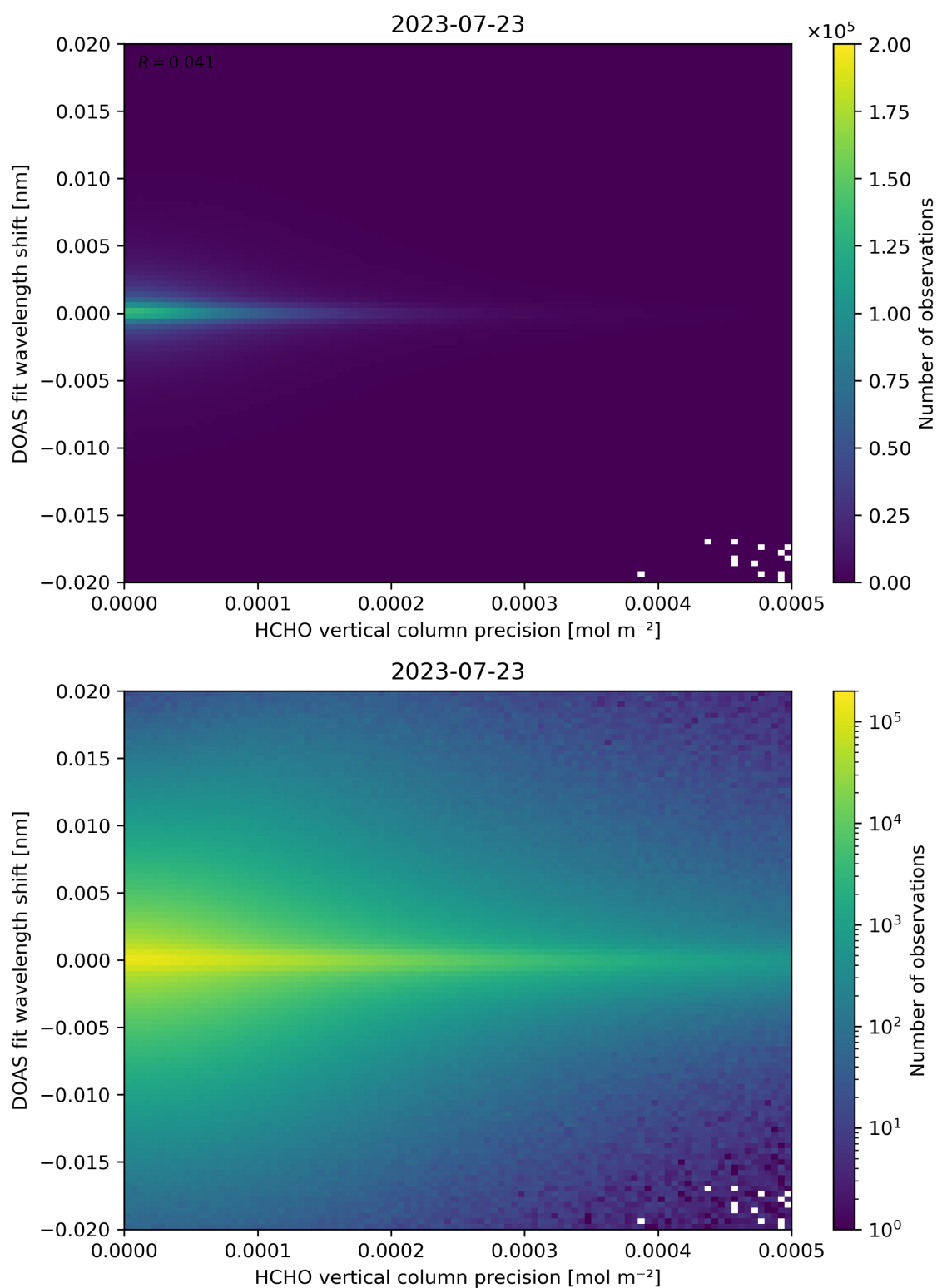
Figure 137: Scatter density plot of “HCHO vertical column precision” against “DOAS fit wavelength shift” for 2023-07-22 to 2023-07-24.
