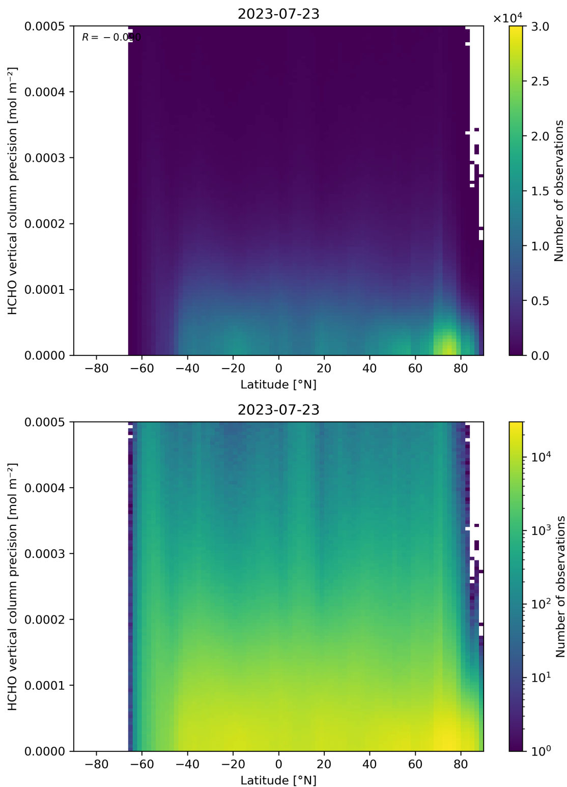
Figure 165: Scatter density plot of “Latitude” against “HCHO vertical column precision” for 2023-07-22 to 2023-07-24.
