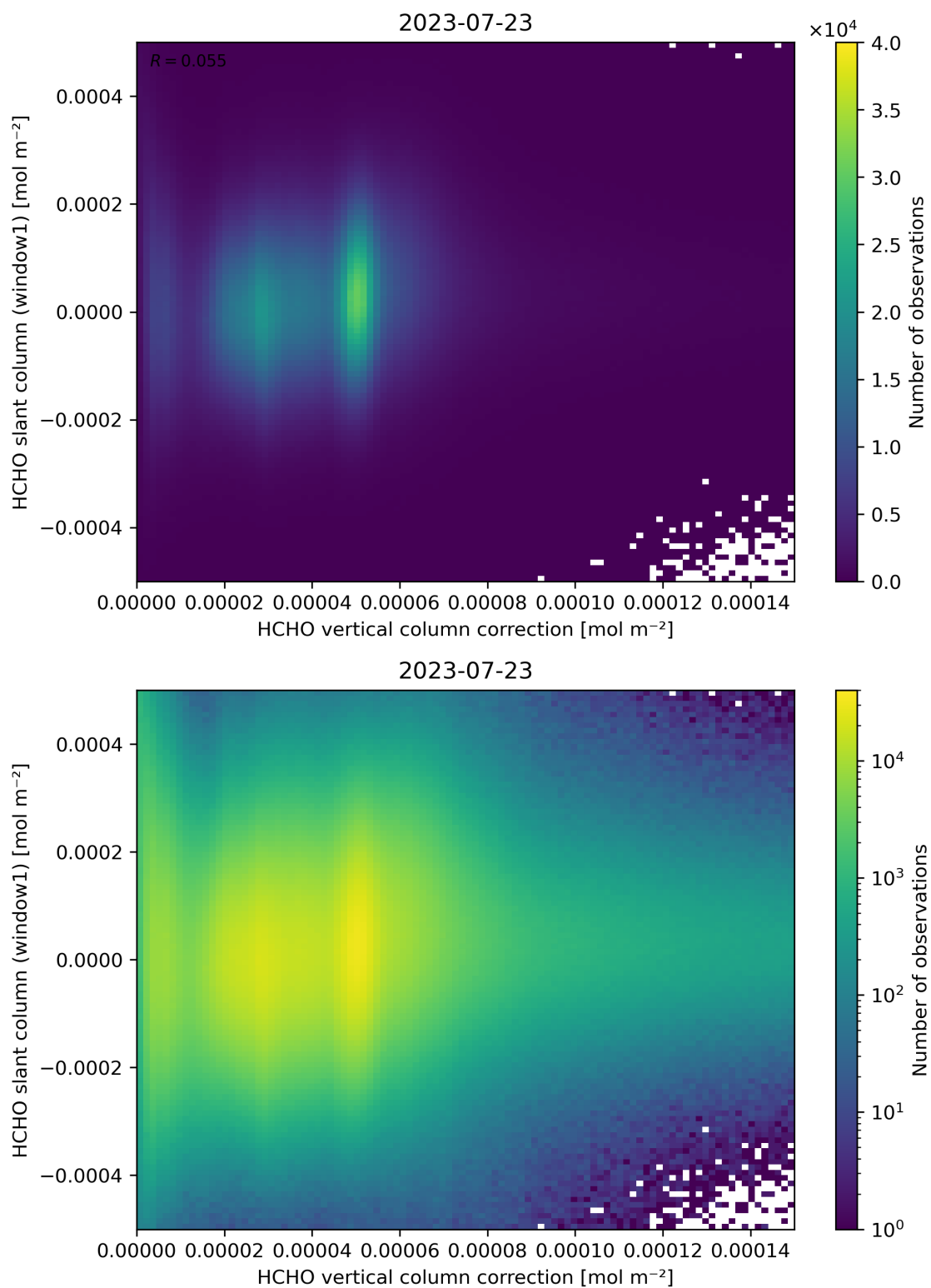
Figure 118: Scatter density plot of “HCHO vertical column correction” against “HCHO slant column (window1)” for 2023-07-22 to 2023-07-24.
