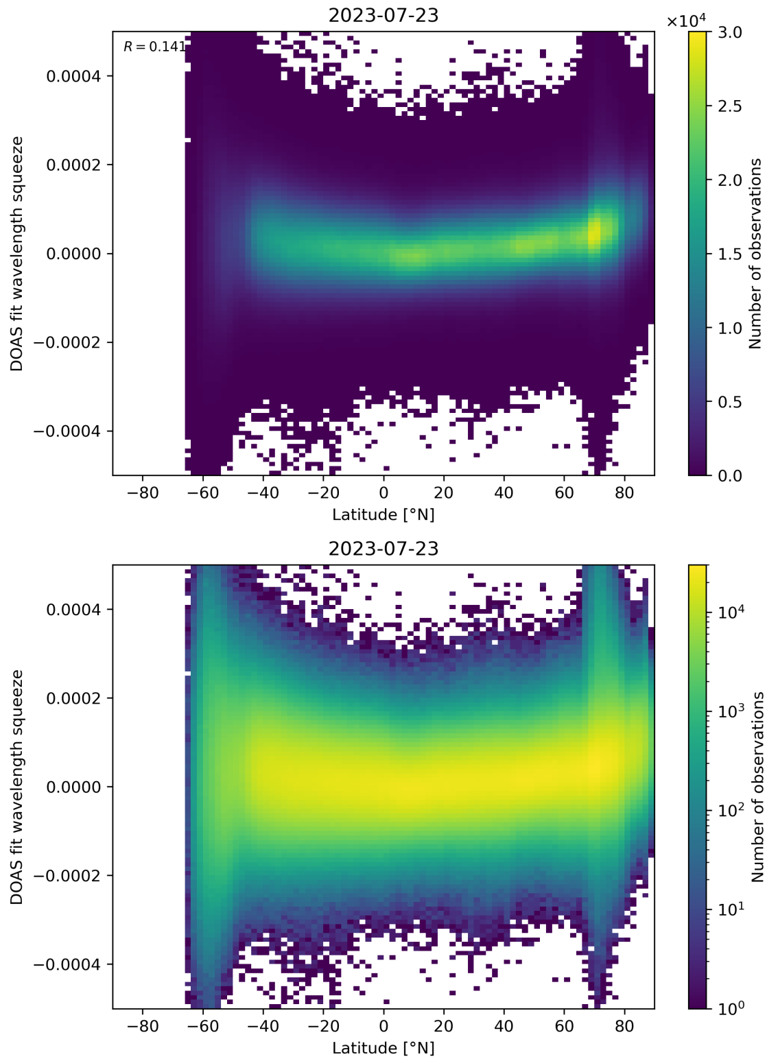
Figure 155: Scatter density plot of “Latitude” against “DOAS fit wavelength squeeze” for 2023-07-22 to 2023-07-24.
