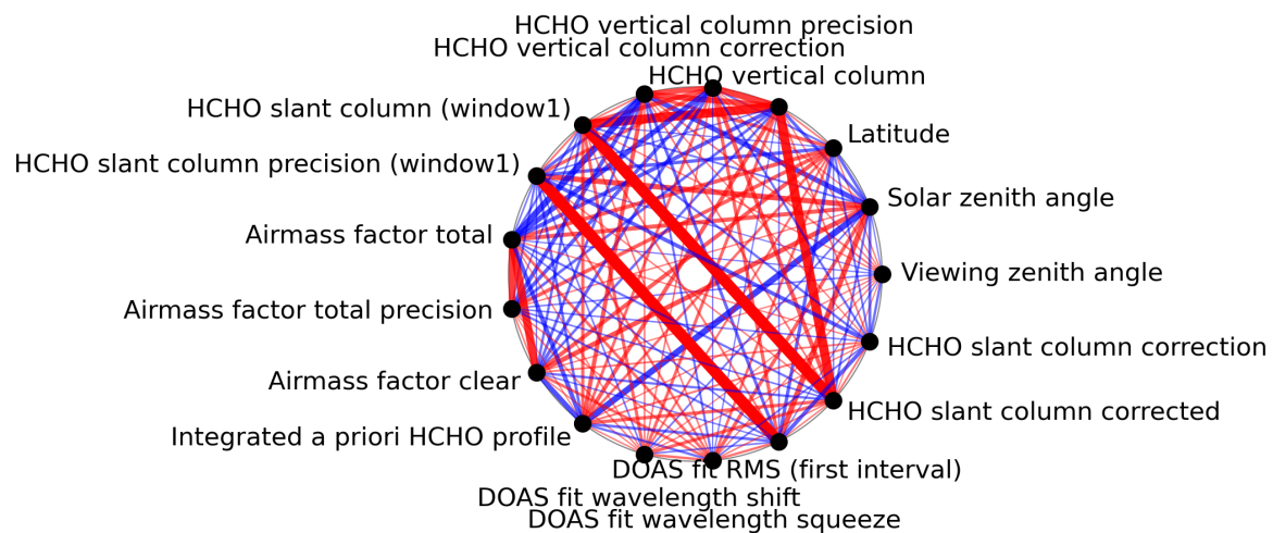
Figure 1: Map of correlation graph for 2023-07-22 to 2023-07-24.
