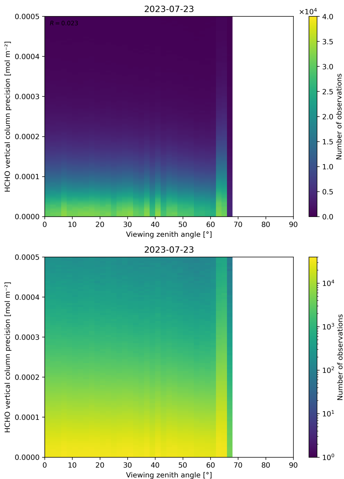
Figure 194: Scatter density plot of “Viewing zenith angle” against “HCHO vertical column precision” for 2023-07-22 to 2023-07-24.
