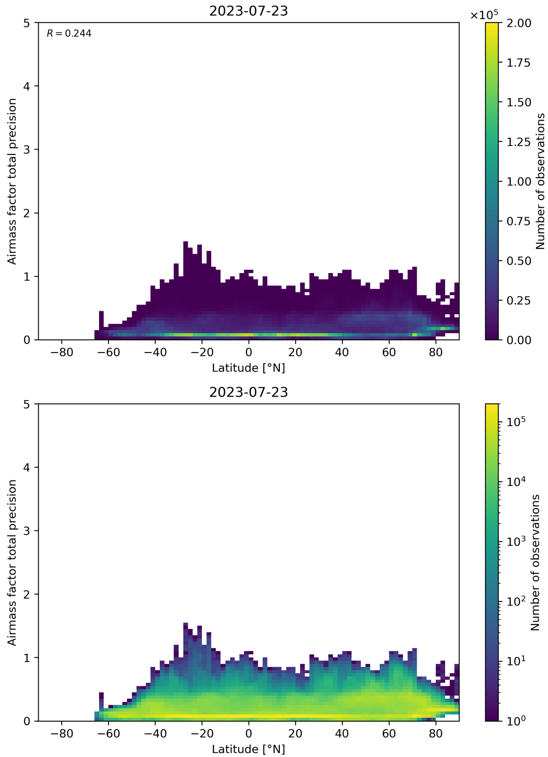
Figure 162: Scatter density plot of “Latitude” against “Airmass factor total precision” for 2023-07-22 to 2023-07-24.
