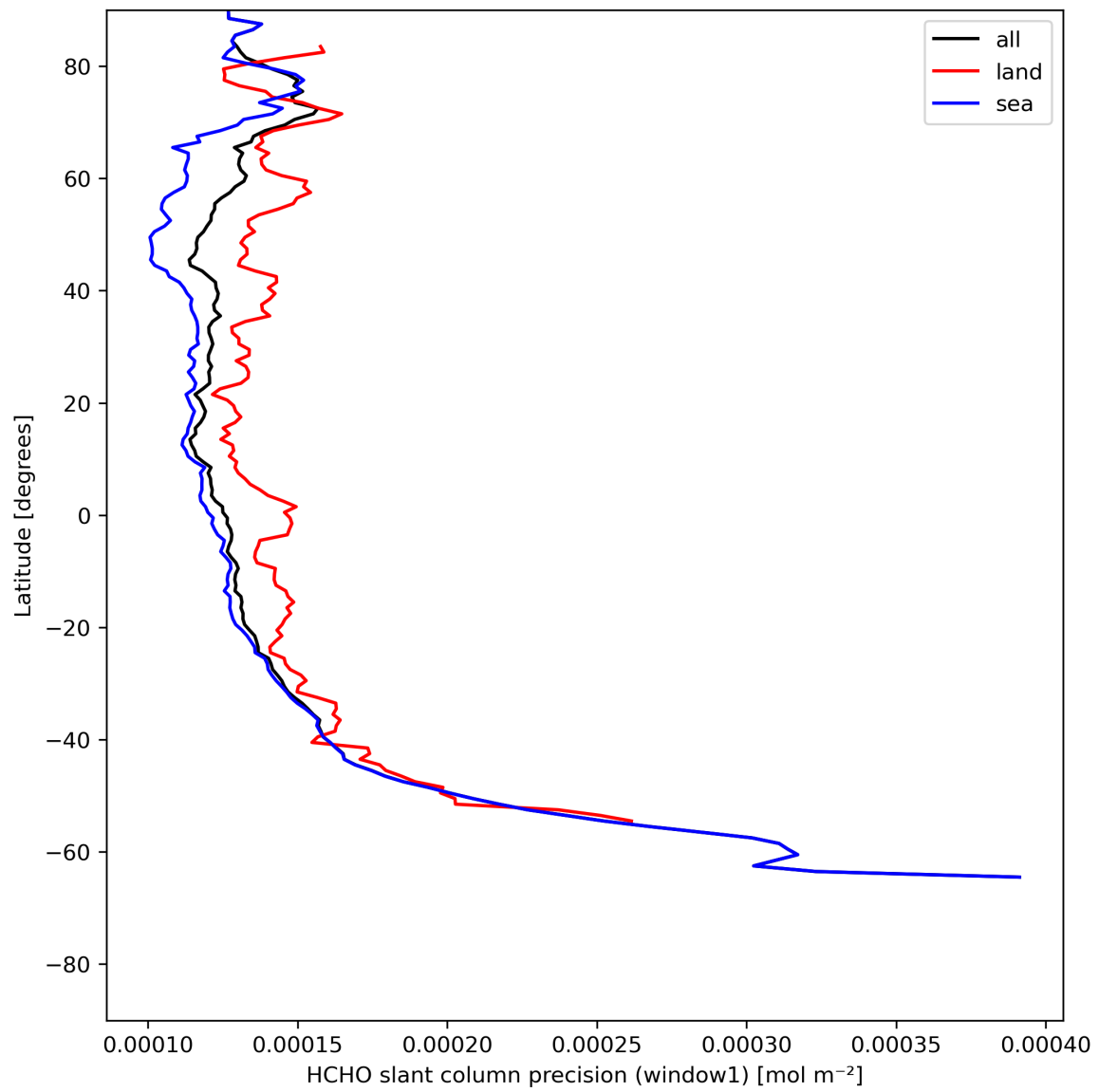
Figure 25: Zonal average of “HCHO slant column precision (window1)” for 2023-07-22 to 2023-07-24.
