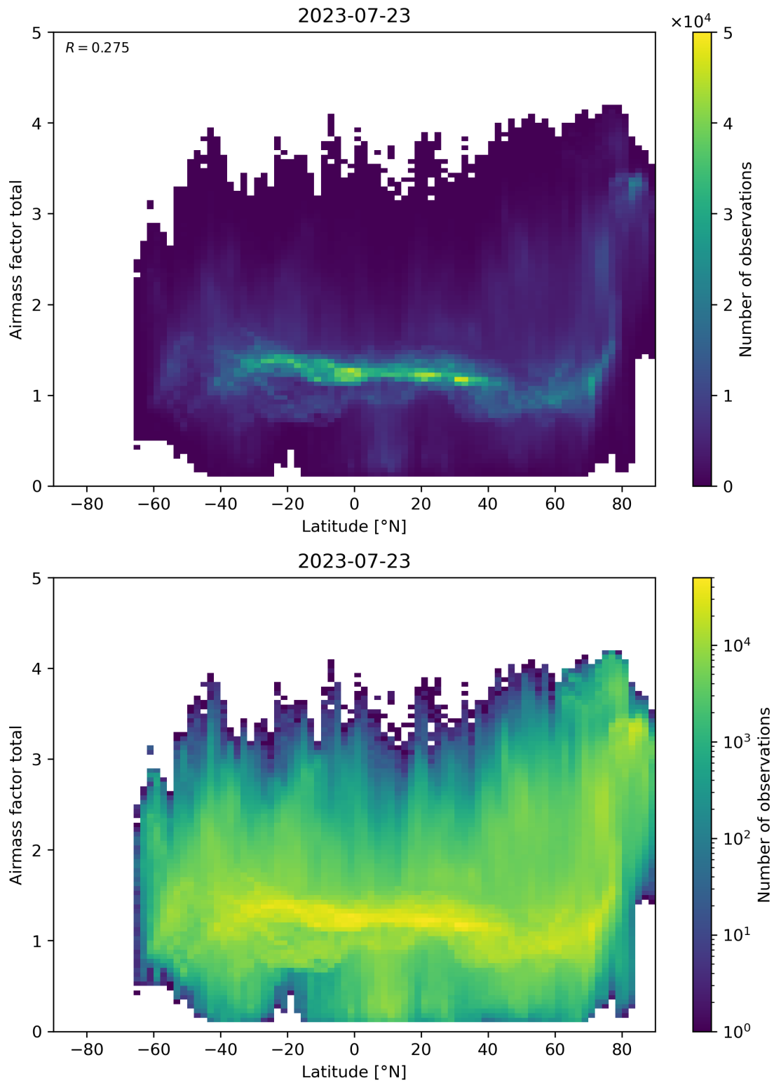
Figure 161: Scatter density plot of “Latitude” against “Airmass factor total” for 2023-07-22 to 2023-07-24.
