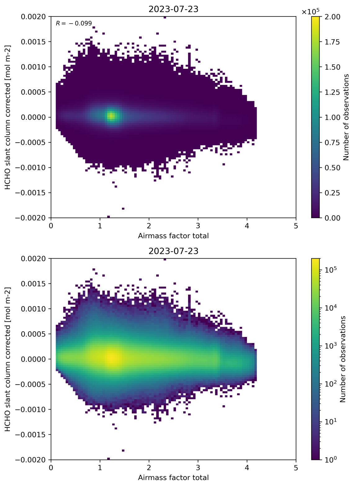
Figure 101: Scatter density plot of “Airmass factor total” against “HCHO slant column corrected” for 2023-07-22 to 2023-07-24.
