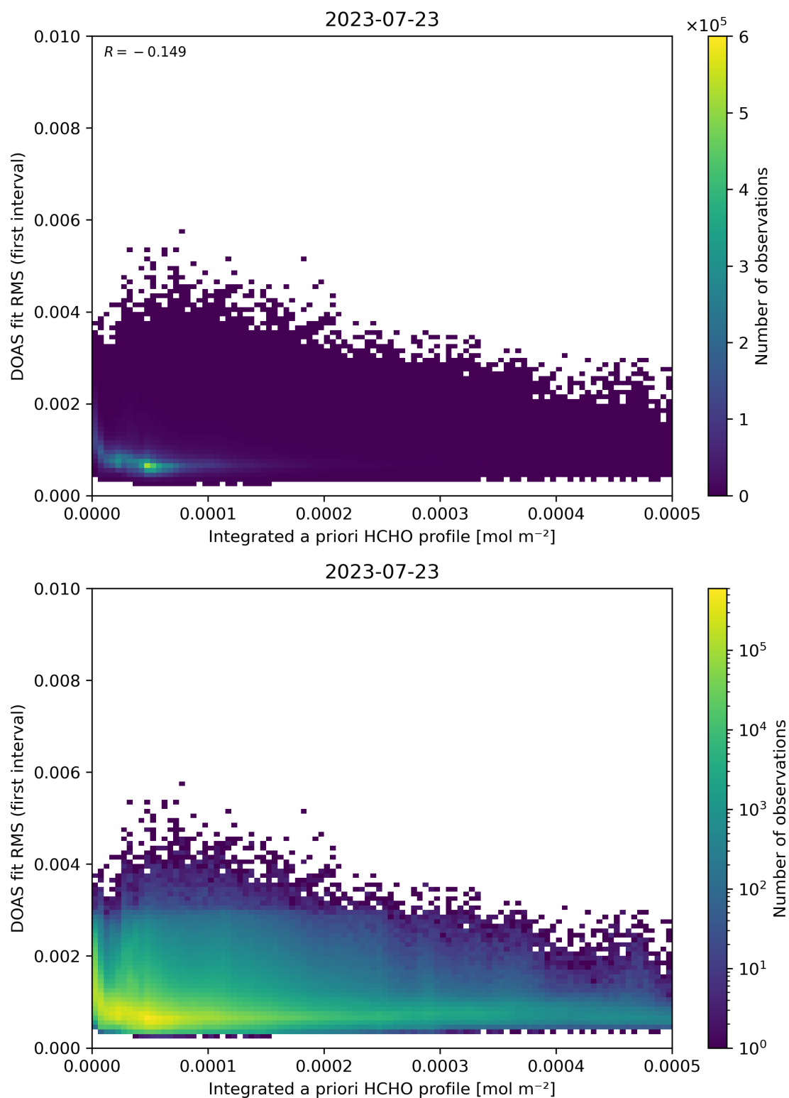
Figure 148: Scatter density plot of “Integrated a priori HCHO profile” against “DOAS fit RMS (first interval)” for 2023-07-22 to 2023-07-24.
