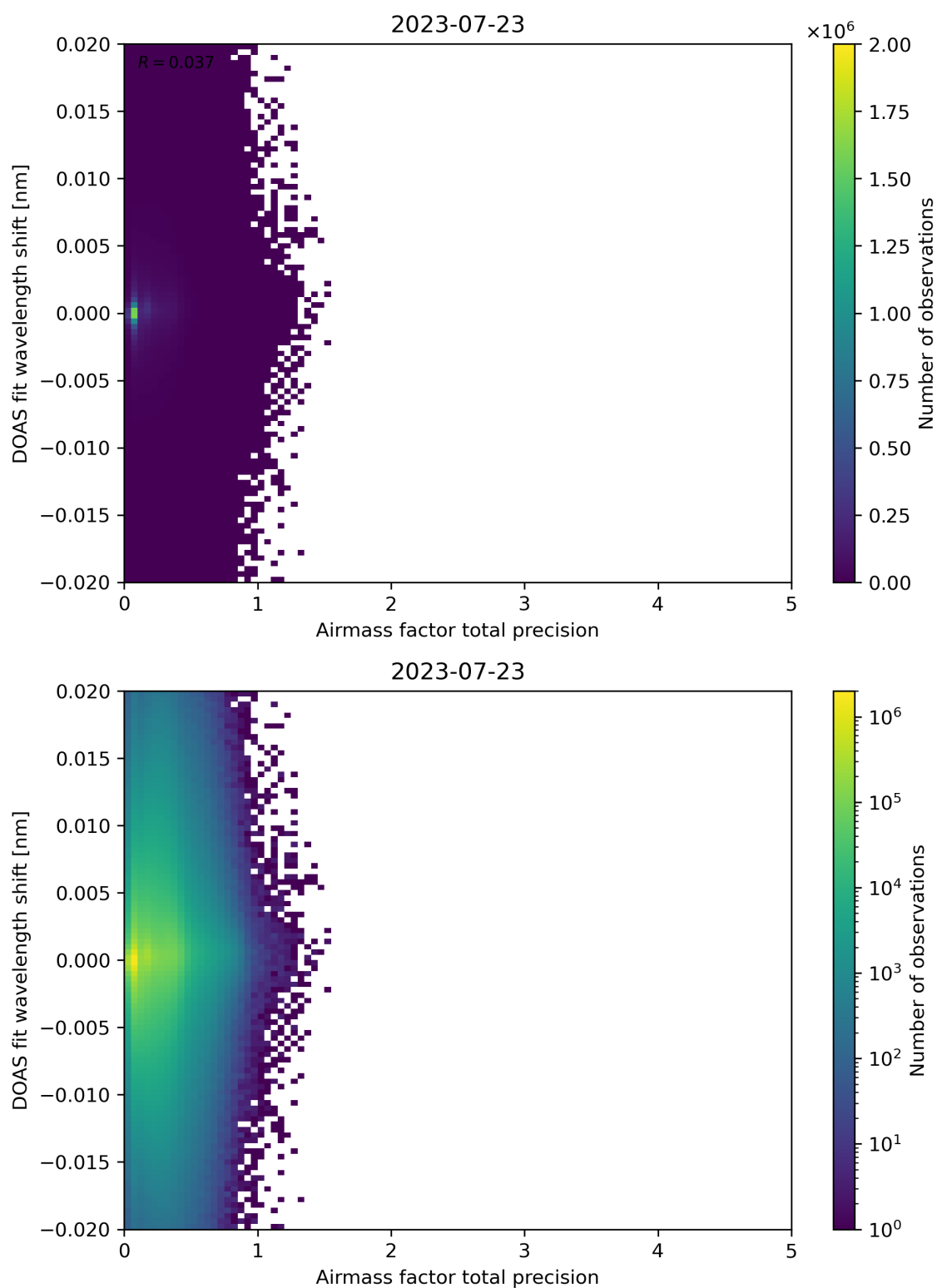
Figure 106: Scatter density plot of “Airmass factor total precision” against “DOAS fit wavelength shift” for 2023-07-22 to 2023-07-24.
