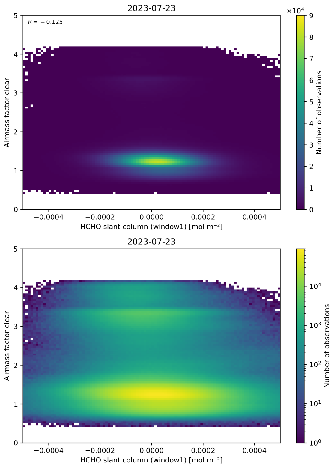
Figure 81: Scatter density plot of “HCHO slant column (window1)” against “Airmass factor clear” for 2023-07-22 to 2023-07-24.
