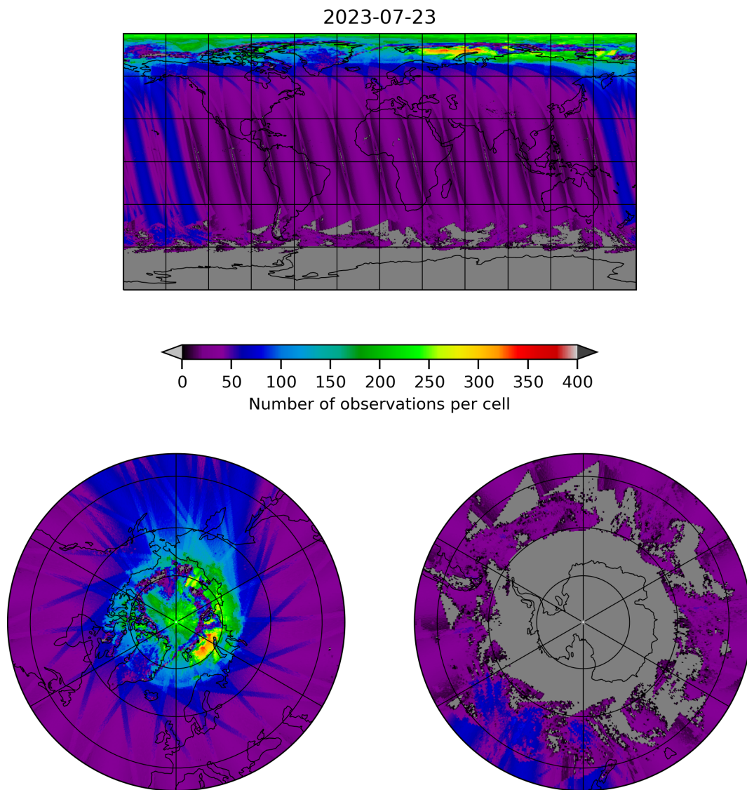
Figure 19: Map of the number of observations for 2023-07-22 to 2023-07-24
