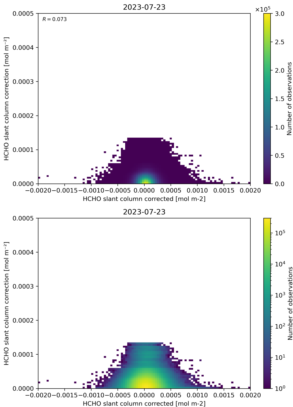
Figure 77: Scatter density plot of “HCHO slant column corrected” against “HCHO slant column correction” for 2023-07-22 to 2023-07-24.
