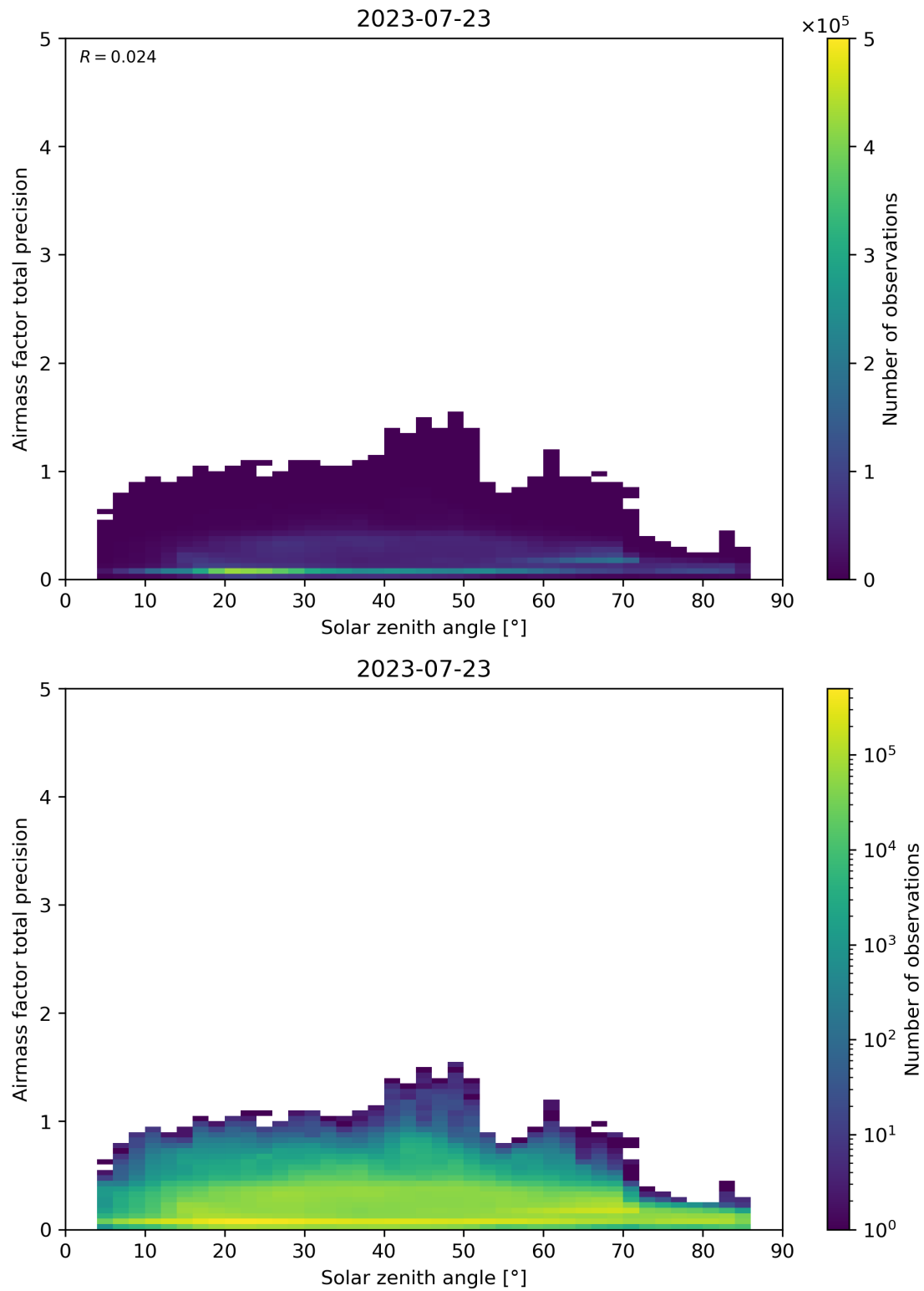
Figure 176: Scatter density plot of “Solar zenith angle” against “Airmass factor total precision” for 2023-07-22 to 2023-07-24.
