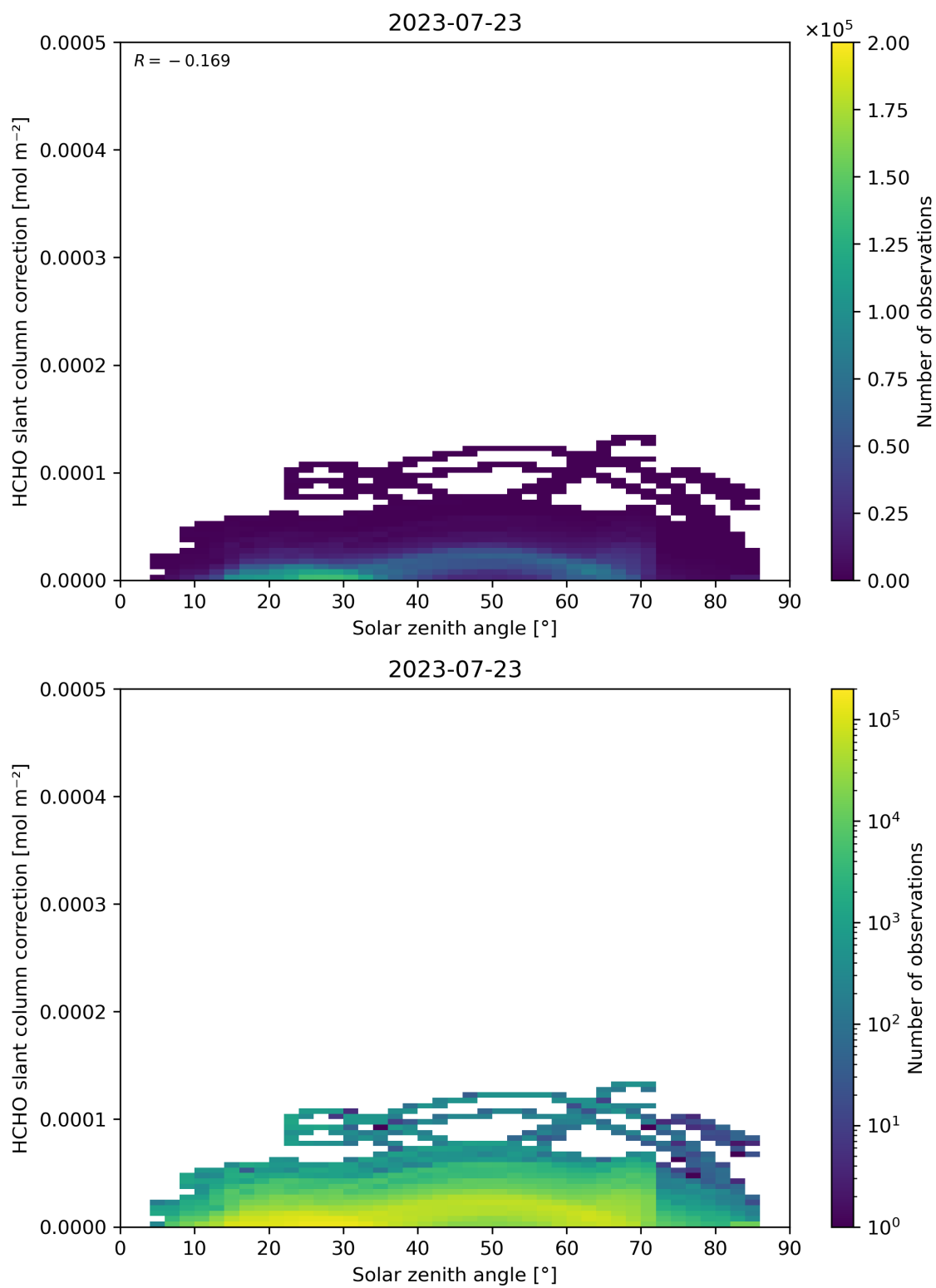
Figure 172: Scatter density plot of “Solar zenith angle” against “HCHO slant column correction” for 2023-07-22 to 2023-07-24.
