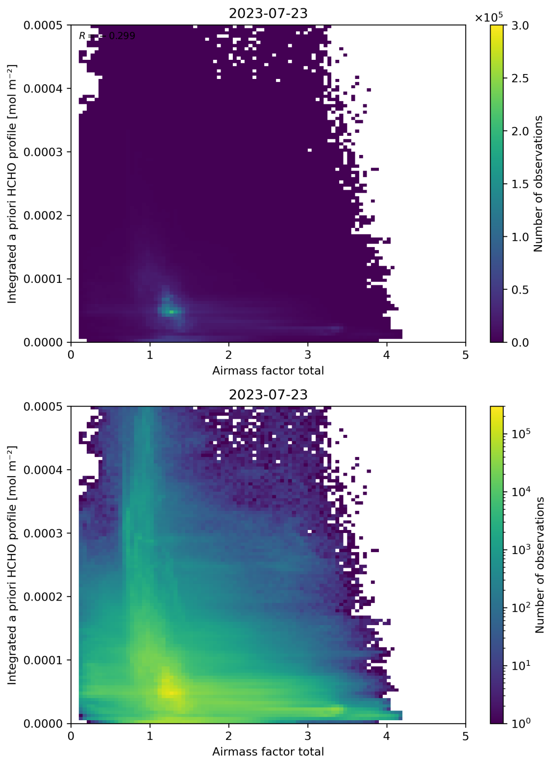
Figure 104: Scatter density plot of “Airmass factor total” against “Integrated a priori HCHO profile” for 2023-07-22 to 2023-07-24.
