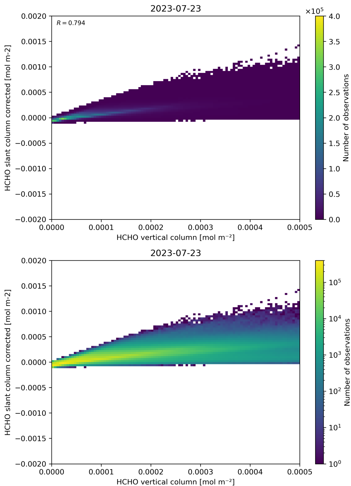
Figure 127: Scatter density plot of “HCHO vertical column” against “HCHO slant column corrected” for 2023-07-22 to 2023-07-24.
