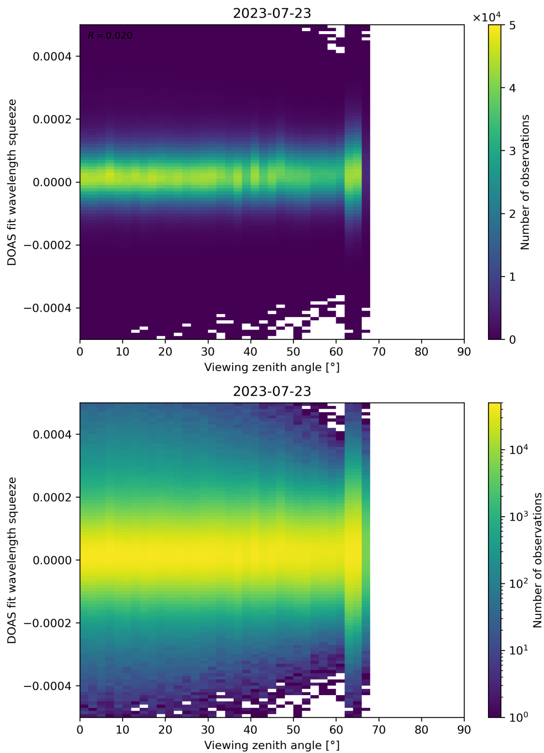
Figure 184: Scatter density plot of “Viewing zenith angle” against “DOAS fit wavelength squeeze” for 2023-07-22 to 2023-07-24.
