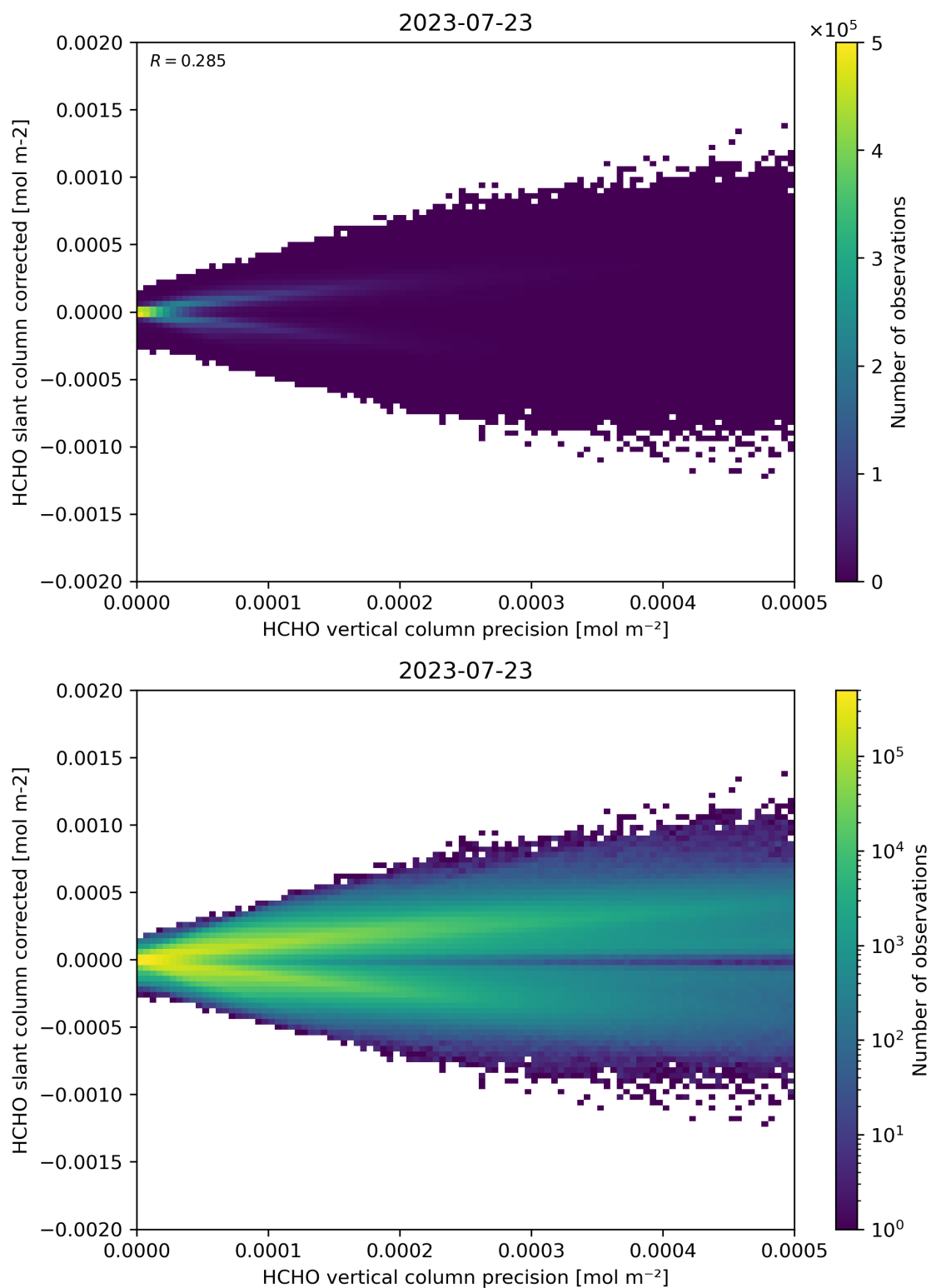
Figure 140: Scatter density plot of “HCHO vertical column precision” against “HCHO slant column corrected” for 2023-07-22 to 2023-07-24.
