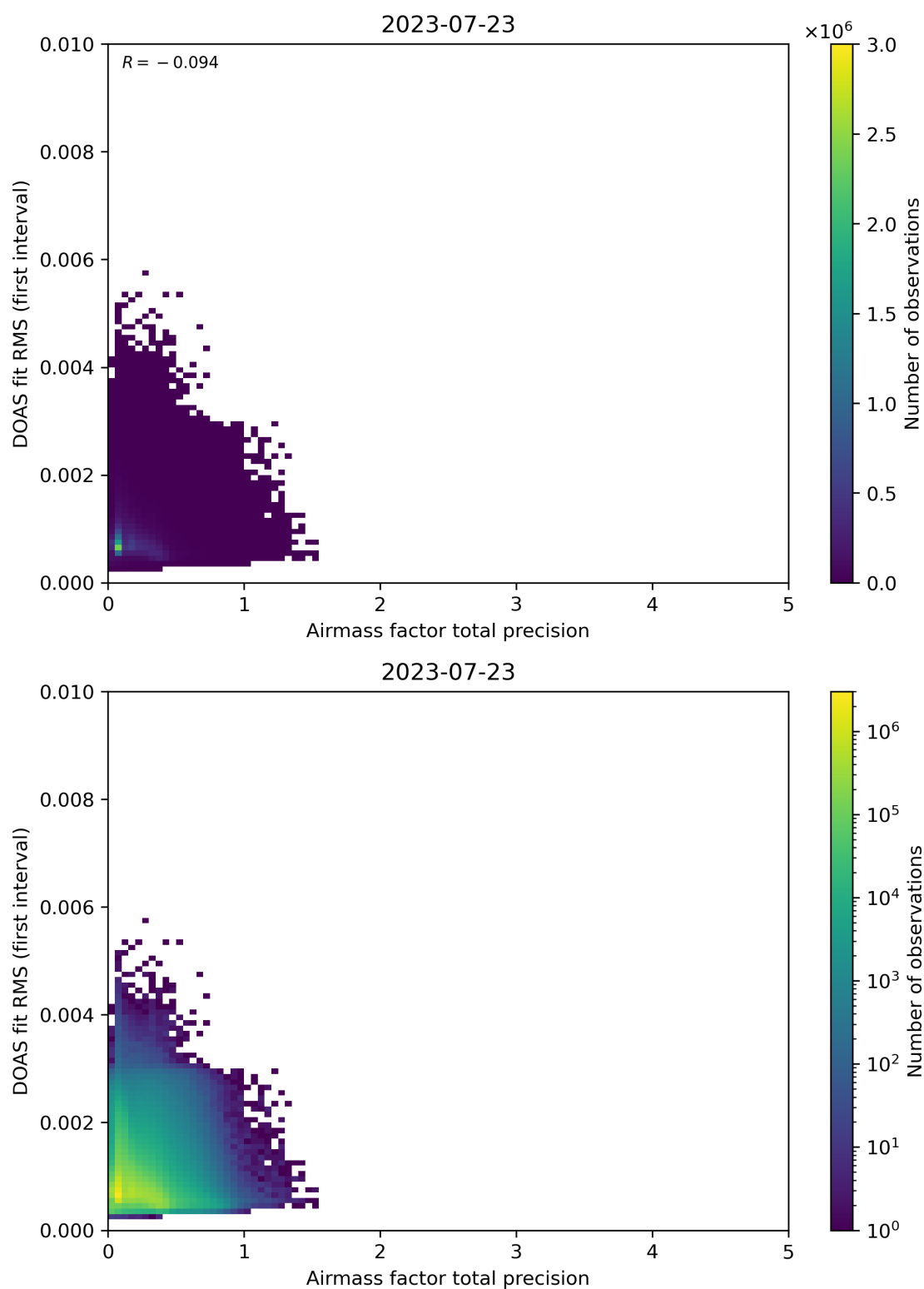
Figure 105: Scatter density plot of “Airmass factor total precision” against “DOAS fit RMS (first interval)” for 2023-07-22 to 2023-07-24.
