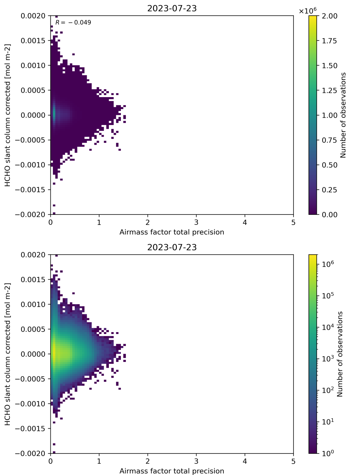
Figure 109: Scatter density plot of “Airmass factor total precision” against “HCHO slant column corrected” for 2023-07-22 to 2023-07-24.
