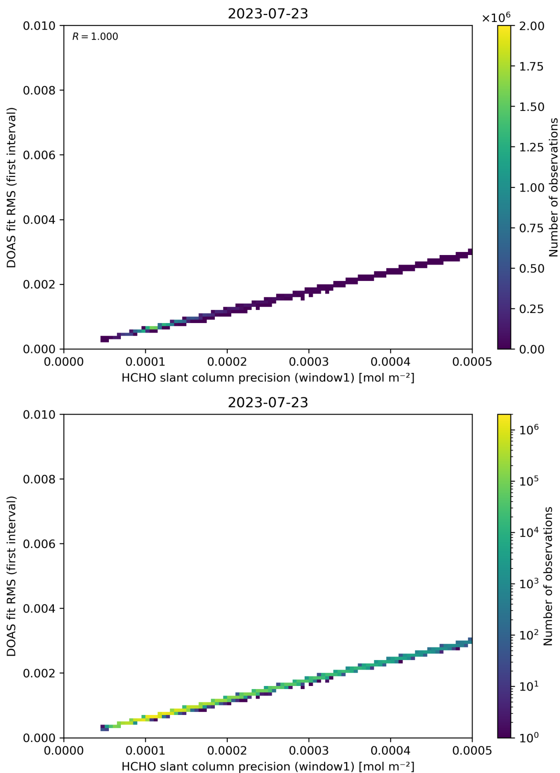
Figure 88: Scatter density plot of “HCHO slant column precision (window1)” against “DOAS fit RMS (first interval)” for 2023-07-22 to 2023-07-24.
