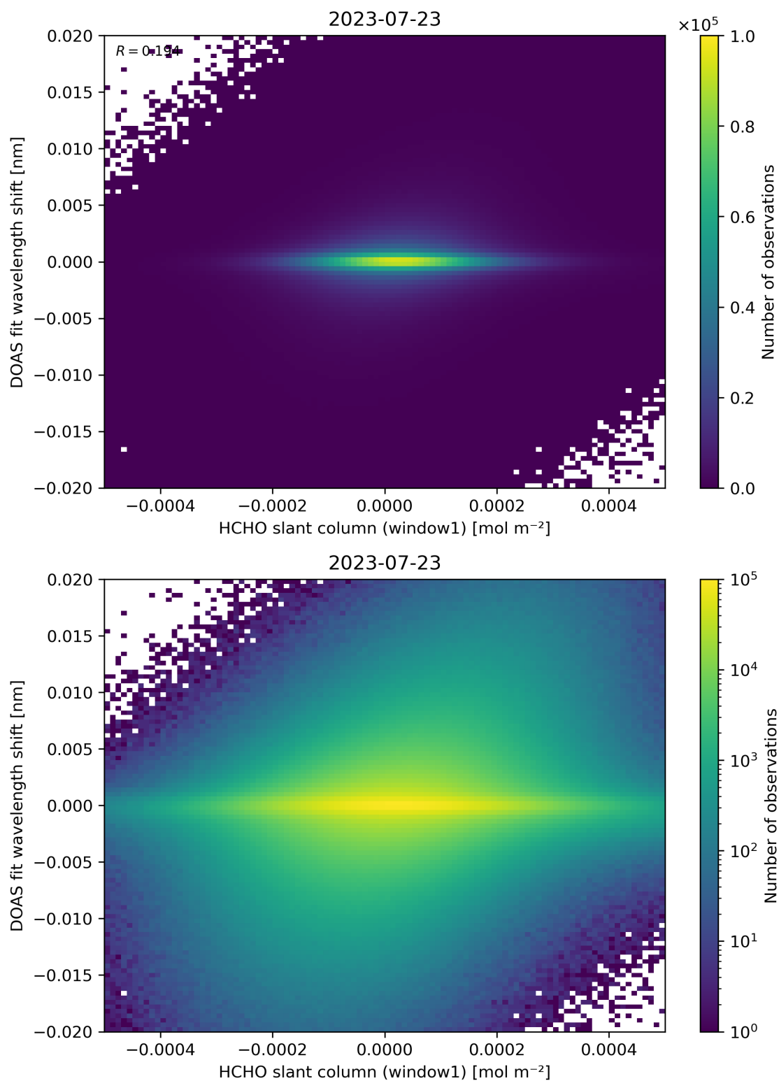
Figure 79: Scatter density plot of “HCHO slant column (window1)” against “DOAS fit wavelength shift” for 2023-07-22 to 2023-07-24.
