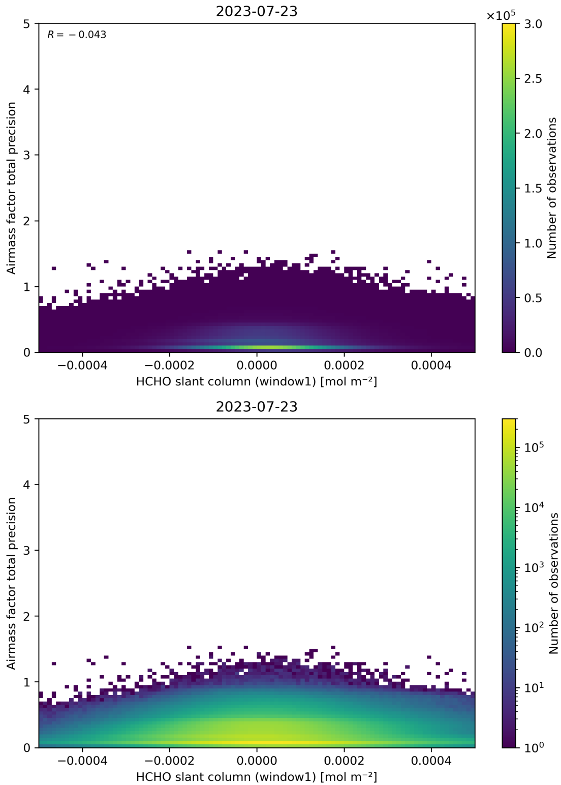
Figure 86: Scatter density plot of “HCHO slant column (window1)” against “Airmass factor total precision” for 2023-07-22 to 2023-07-24.
