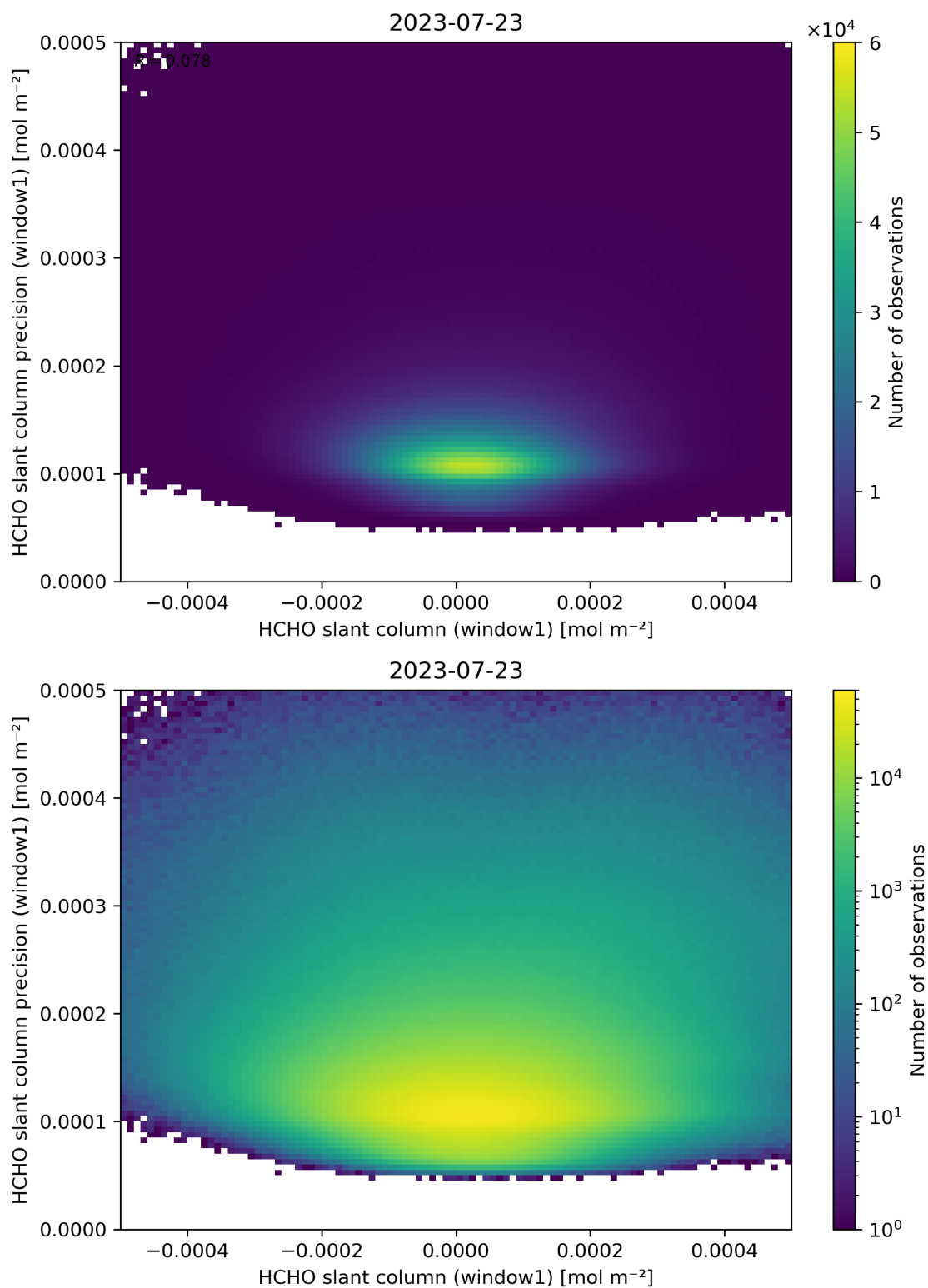
Figure 84: Scatter density plot of “HCHO slant column (window1)” against “HCHO slant column precision (window1)” for 2023-07-22 to 2023-07-24.
