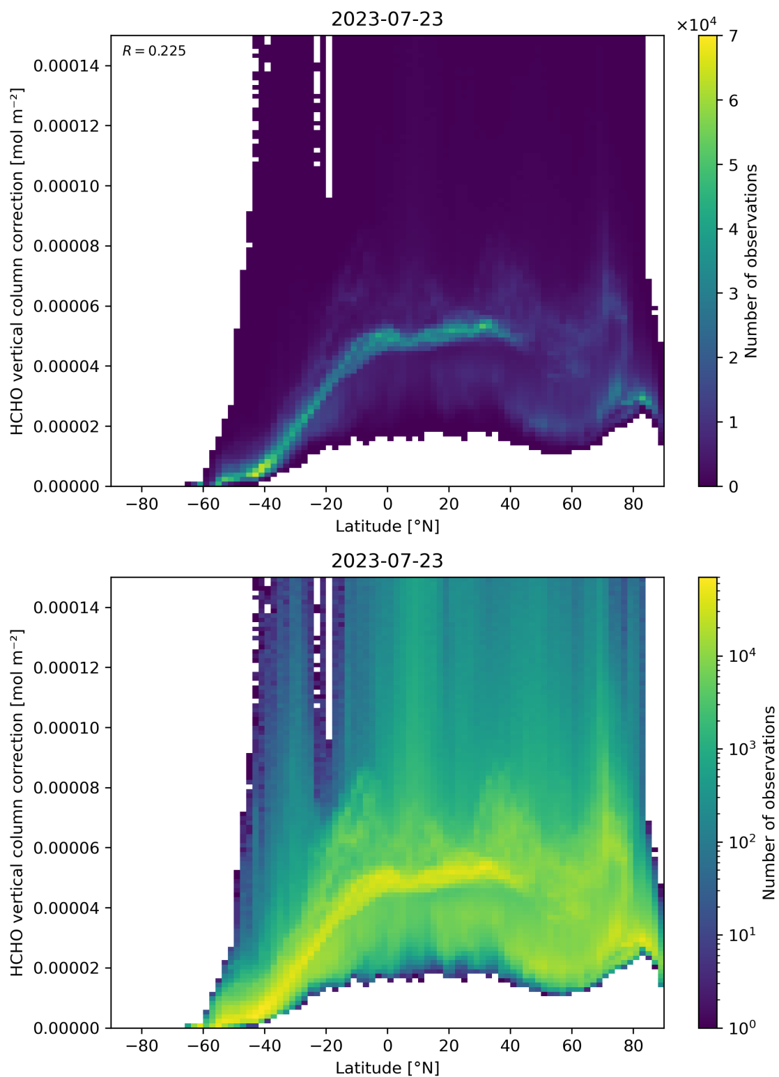
Figure 164: Scatter density plot of “Latitude” against “HCHO vertical column correction” for 2023-07-22 to 2023-07-24.
