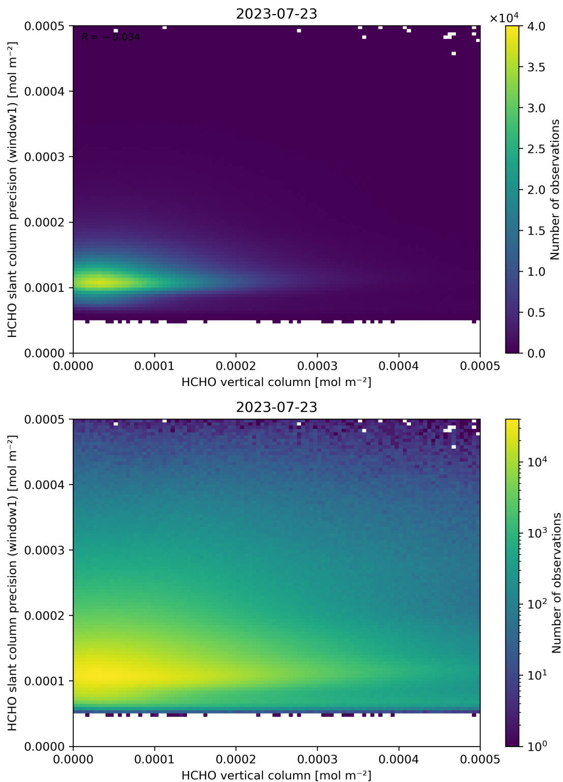
Figure 130: Scatter density plot of “HCHO vertical column” against “HCHO slant column precision (window1)” for 2023-07-22 to 2023-07-24.
