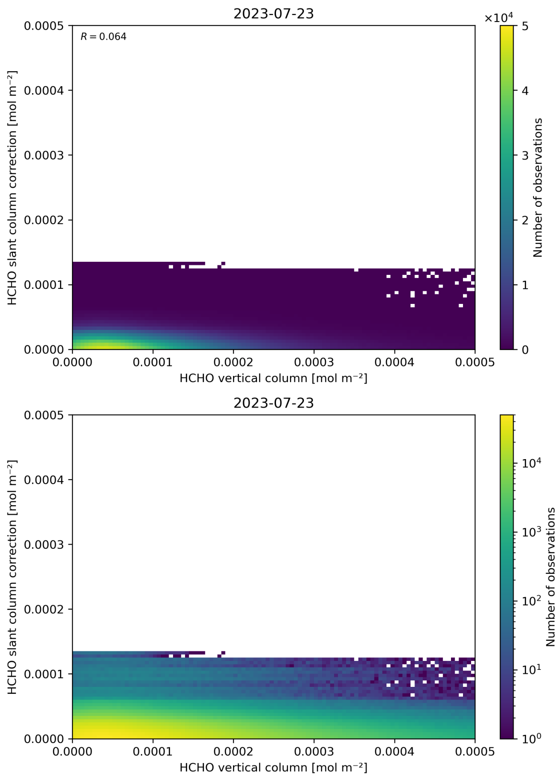
Figure 128: Scatter density plot of “HCHO vertical column” against “HCHO slant column correction” for 2023-07-22 to 2023-07-24.
