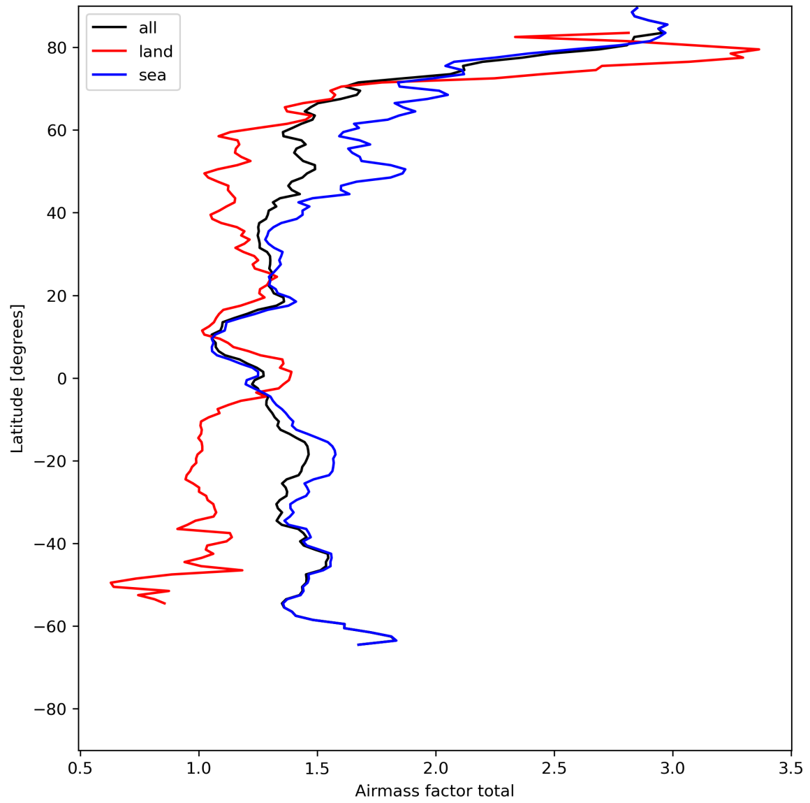
Figure 26: Zonal average of “Airmass factor total” for 2023-07-22 to 2023-07-24.
