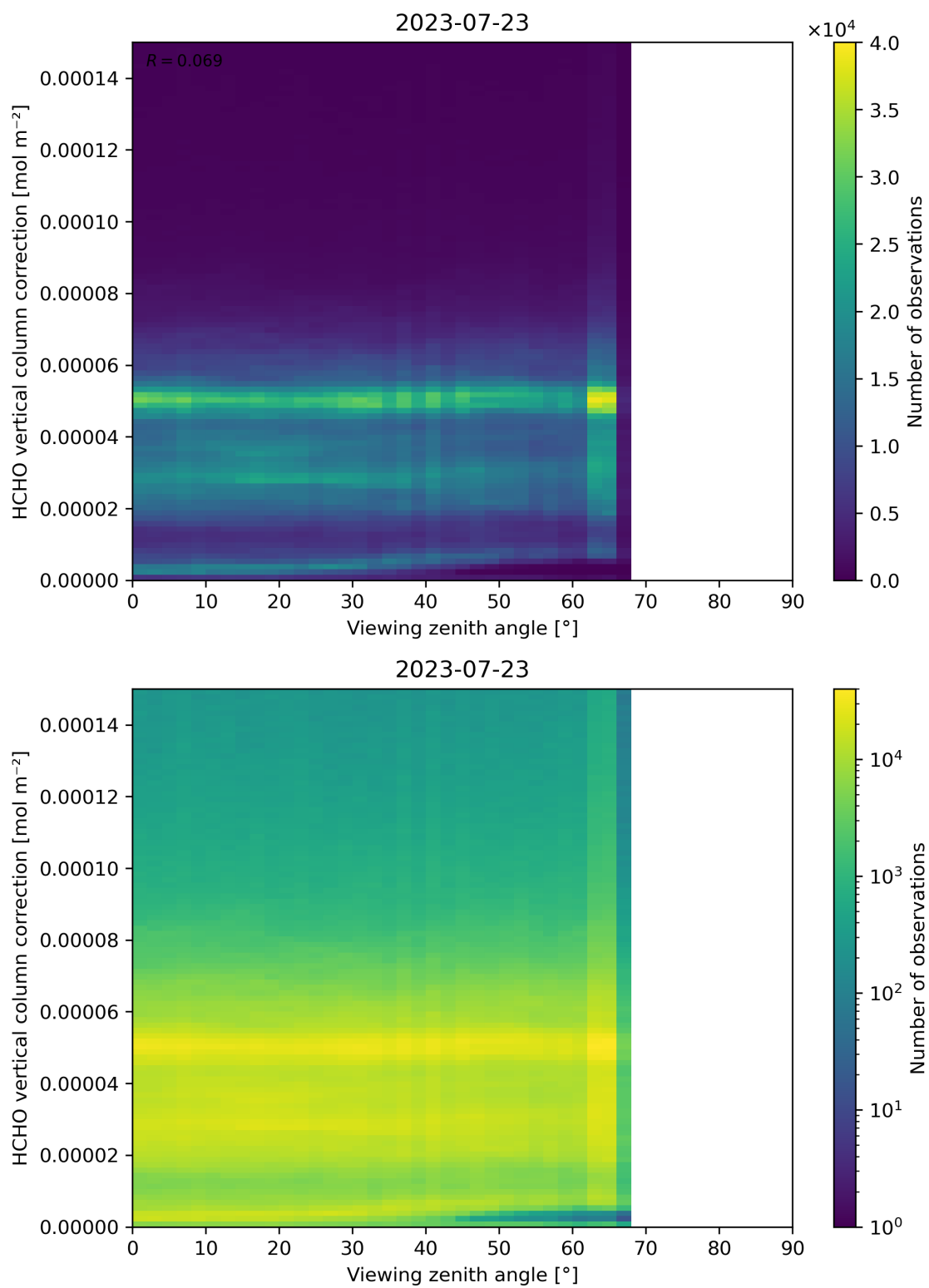
Figure 193: Scatter density plot of “Viewing zenith angle” against “HCHO vertical column correction” for 2023-07-22 to 2023-07-24.
