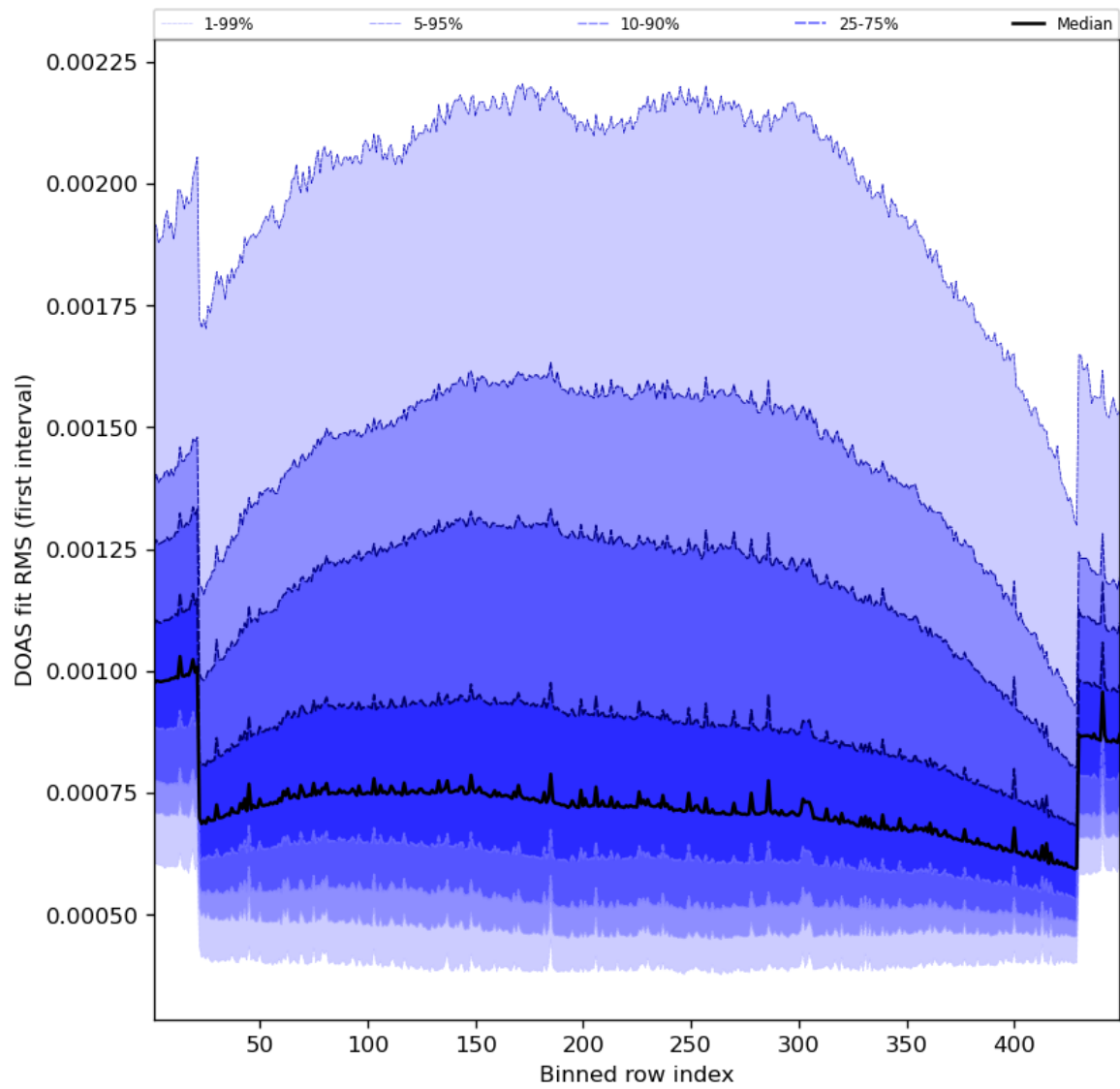
Figure 60: Along track statistics of “DOAS fit RMS (first interval)” for 2023-07-22 to 2023-07-24
