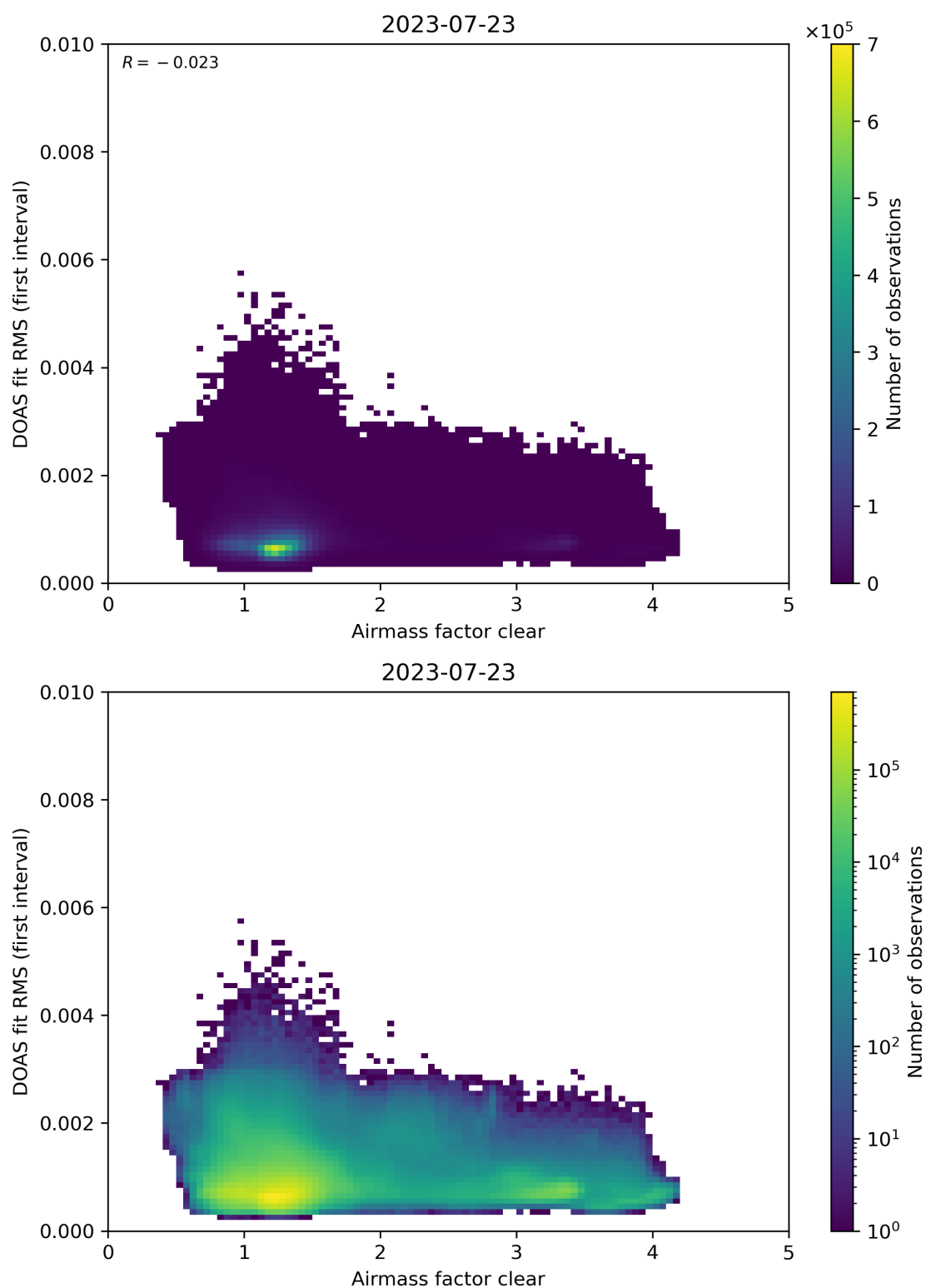
Figure 71: Scatter density plot of “Airmass factor clear” against “DOAS fit RMS (first interval)” for 2023-07-22 to 2023-07-24.
