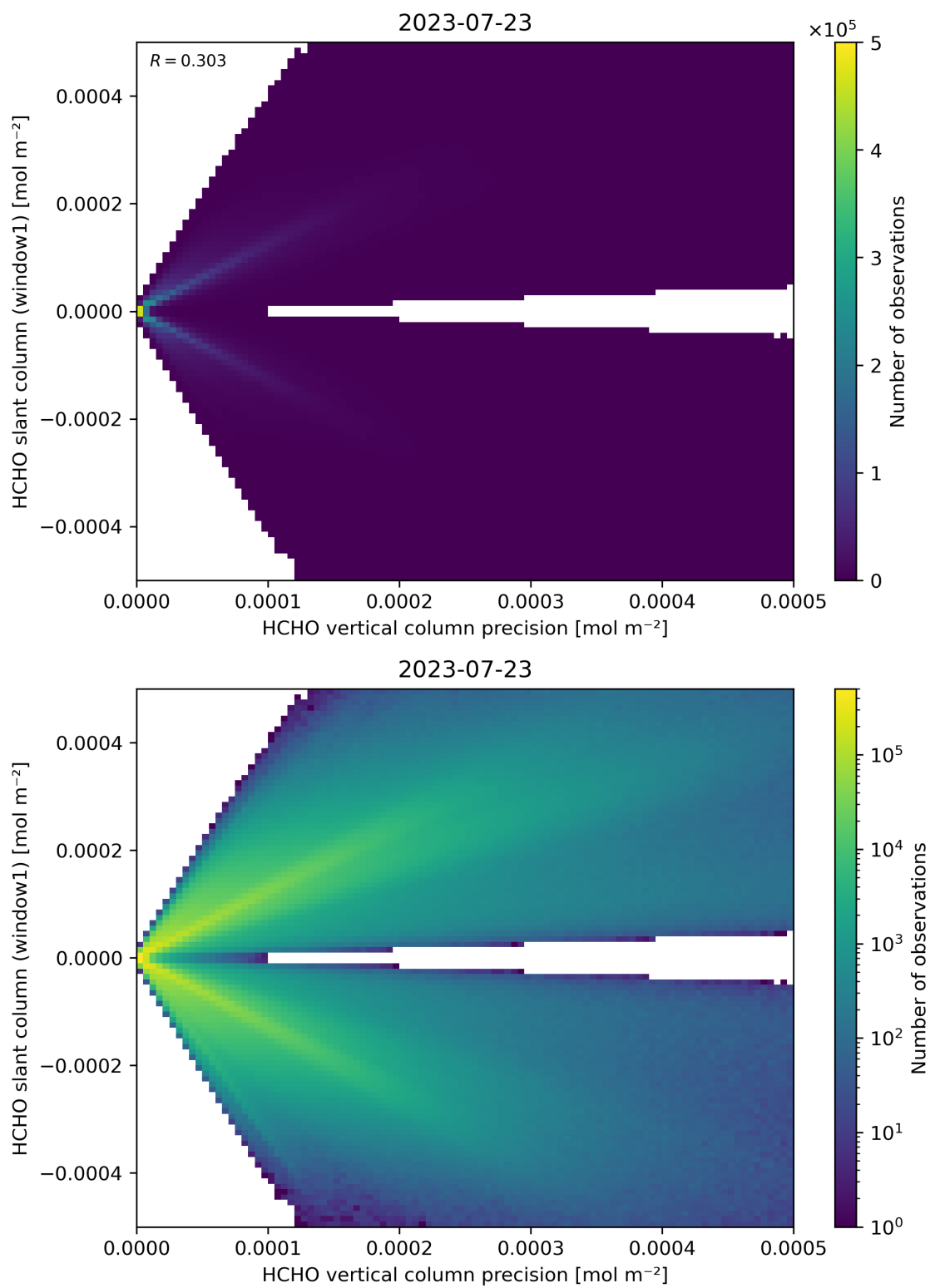
Figure 142: Scatter density plot of “HCHO vertical column precision” against “HCHO slant column (window1)” for 2023-07-22 to 2023-07-24.
