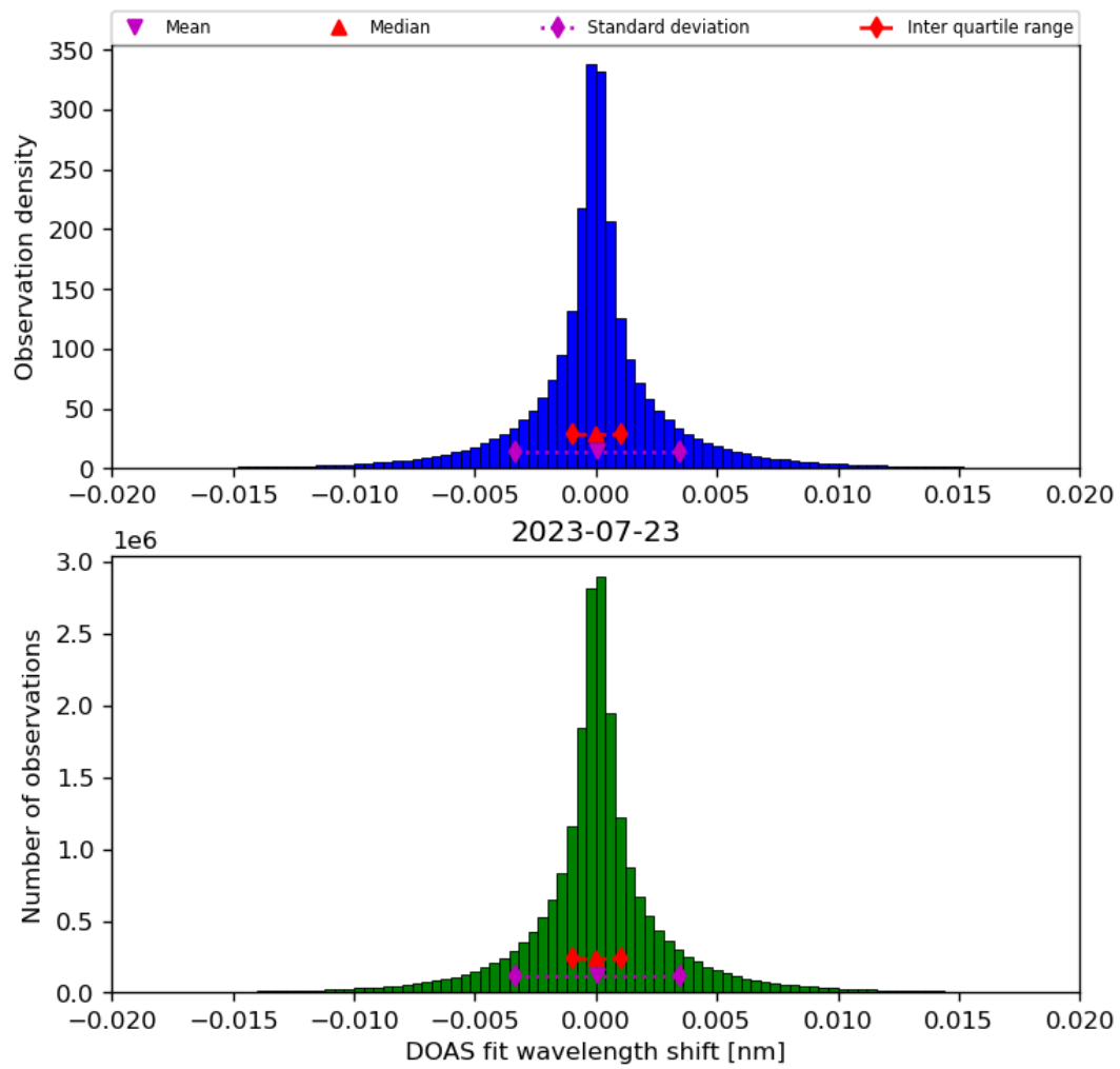
Figure 44: Histogram of “DOAS fit wavelength shift” for 2023-07-22 to 2023-07-24
