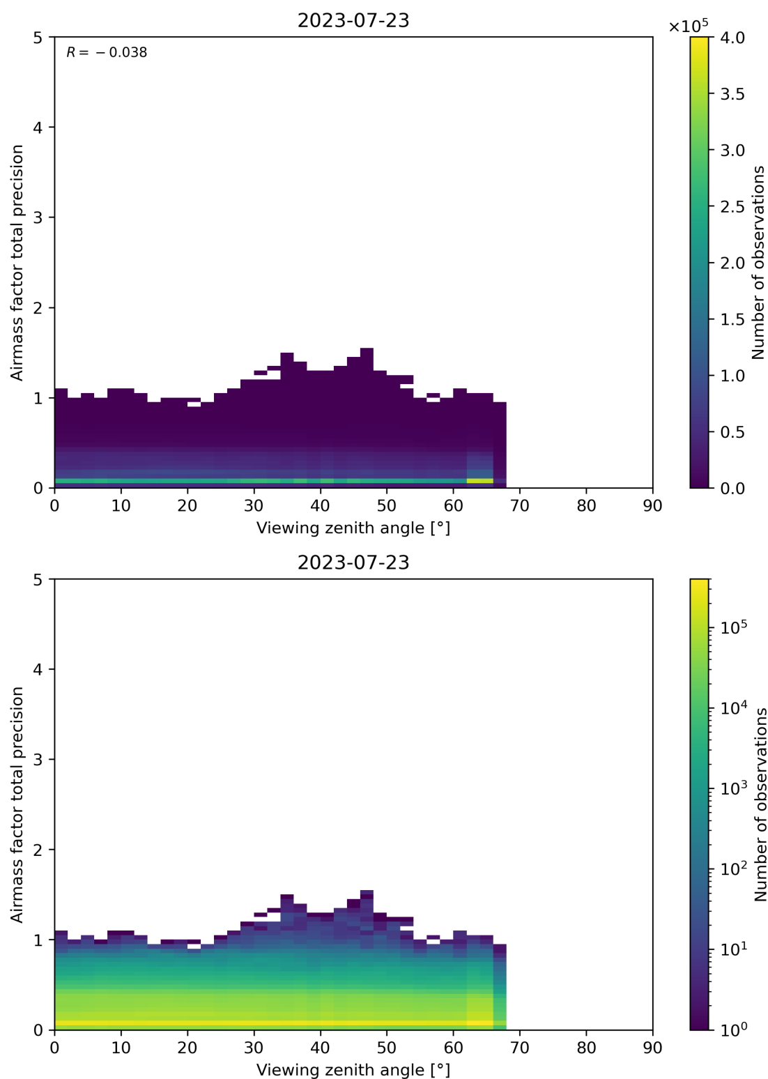
Figure 191: Scatter density plot of “Viewing zenith angle” against “Airmass factor total precision” for 2023-07-22 to 2023-07-24.
