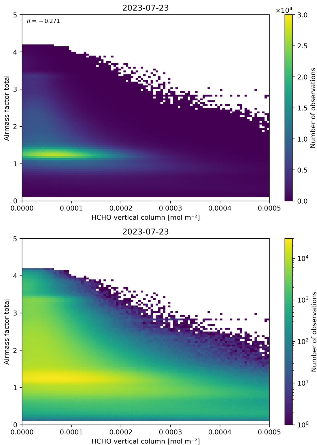
Figure 131: Scatter density plot of “HCHO vertical column” against “Airmass factor total” for 2023-07-22 to 2023-07-24.
