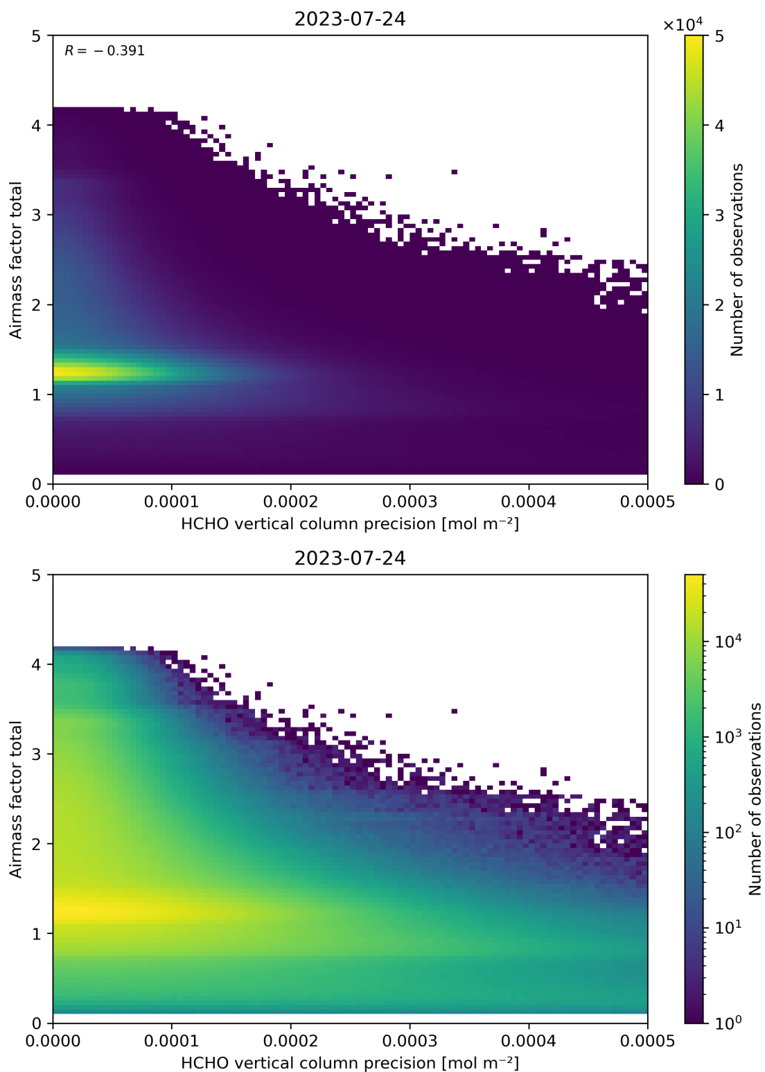
Figure 144: Scatter density plot of “HCHO vertical column precision” against “Airmass factor total” for 2023-07-24 to 2023-07-25.
