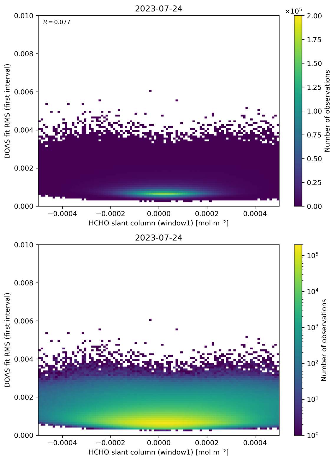
Figure 78: Scatter density plot of “HCHO slant column (window1)” against “DOAS fit RMS (first interval)” for 2023-07-24 to 2023-07-25.
