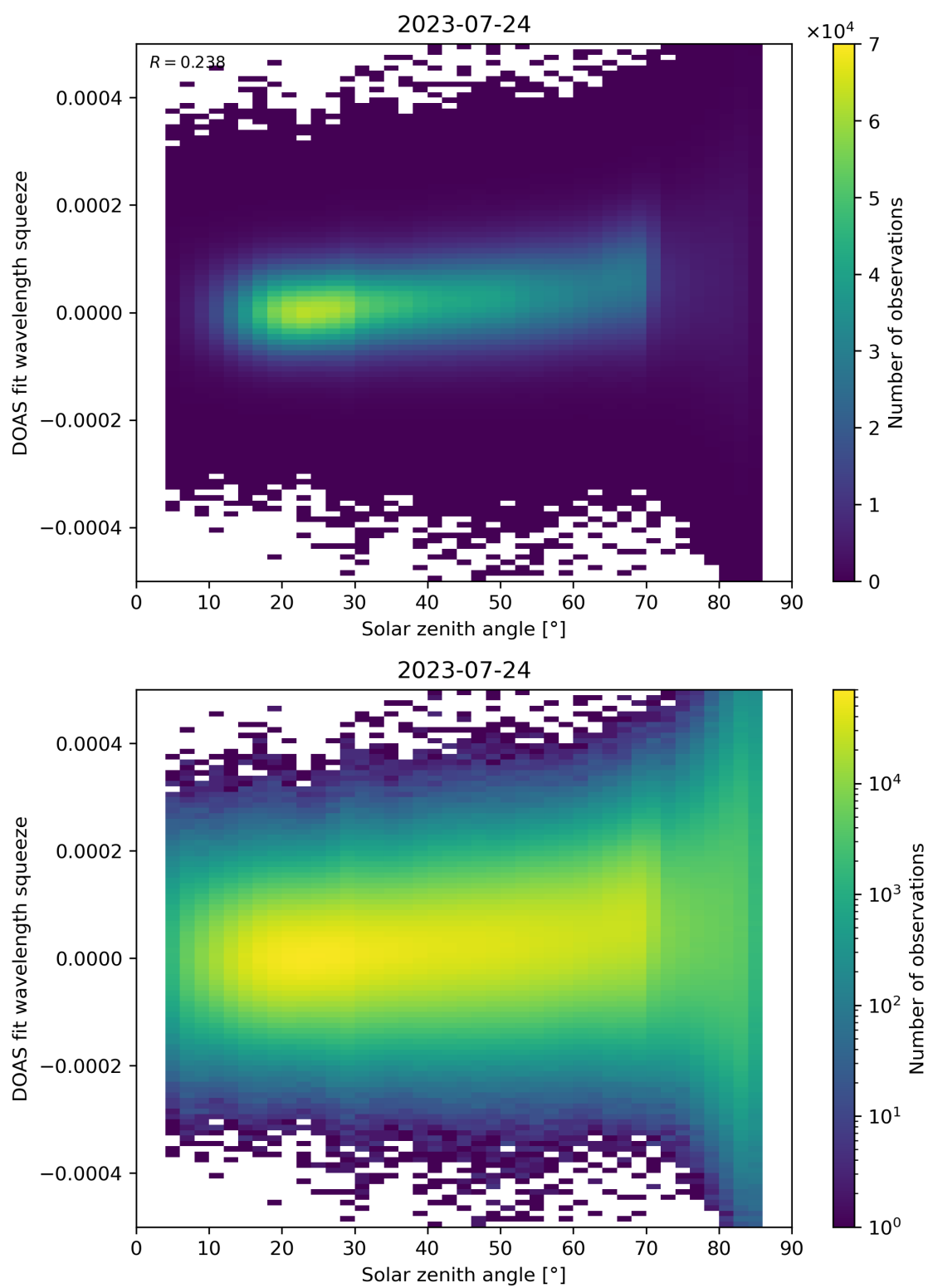
Figure 169: Scatter density plot of “Solar zenith angle” against “DOAS fit wavelength squeeze” for 2023-07-24 to 2023-07-25.
