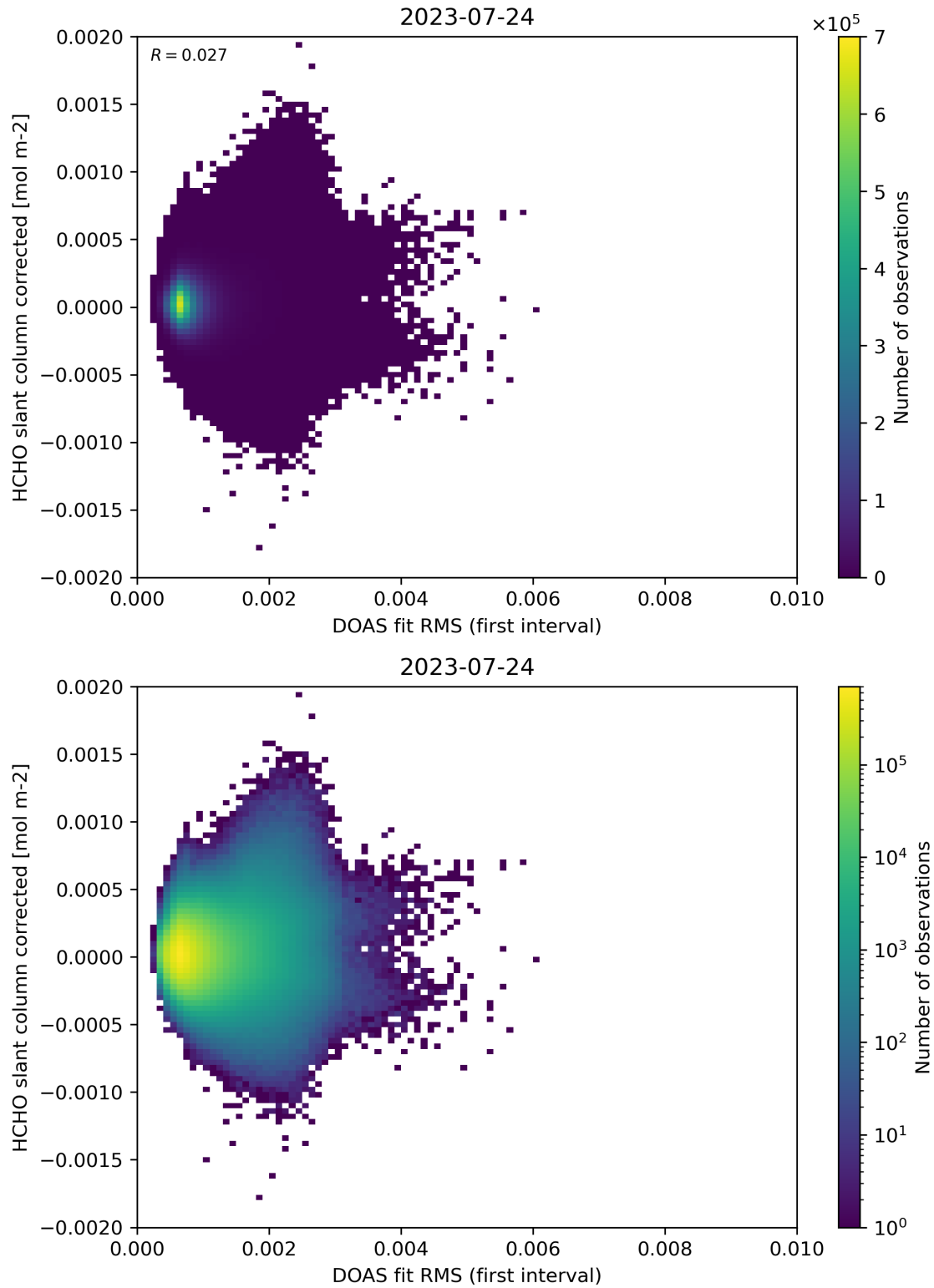
Figure 62: Scatter density plot of “DOAS fit RMS (first interval)” against “HCHO slant column corrected” for 2023-07-24 to 2023-07-25.
