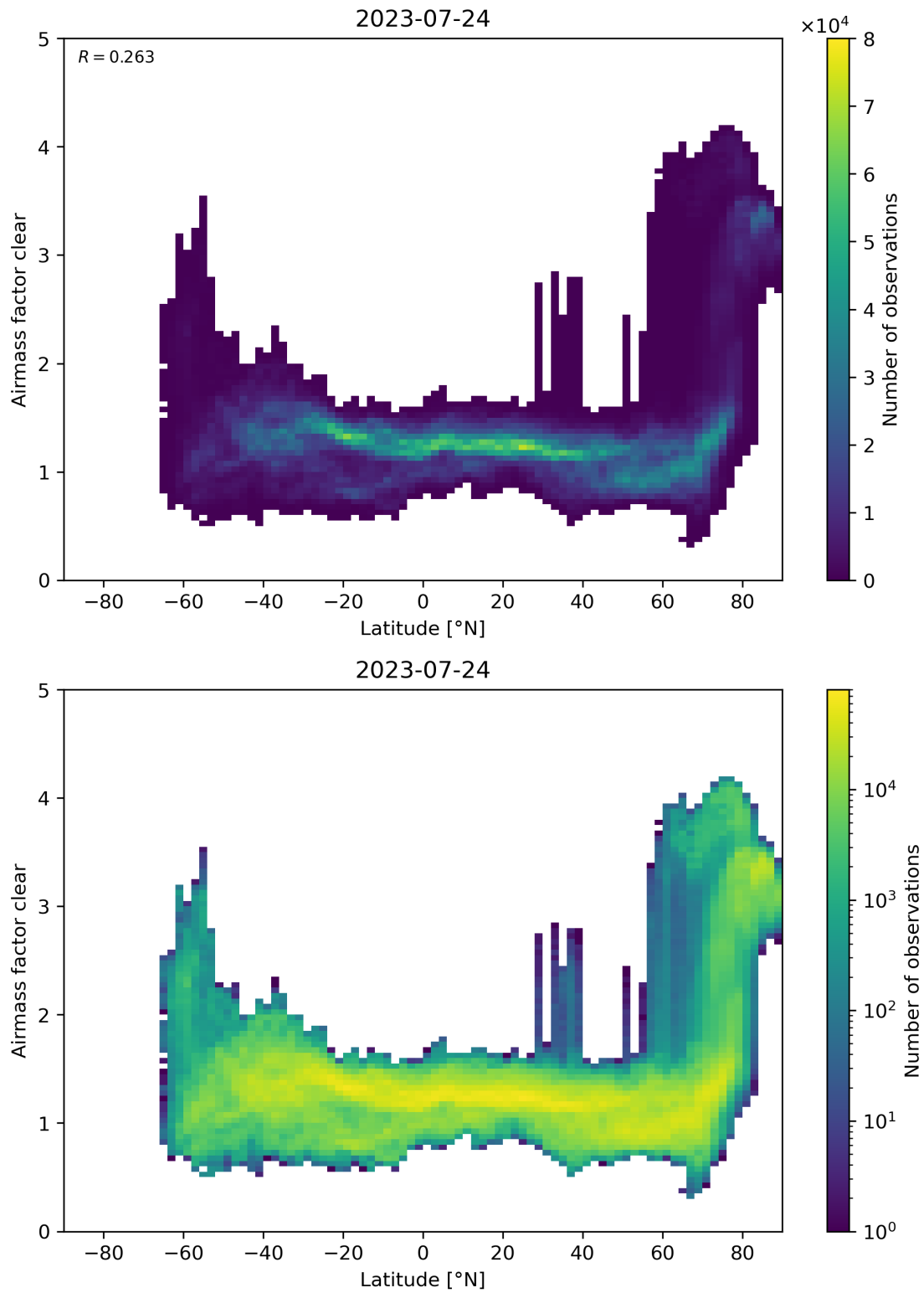
Figure 156: Scatter density plot of “Latitude” against “Airmass factor clear” for 2023-07-24 to 2023-07-25.
