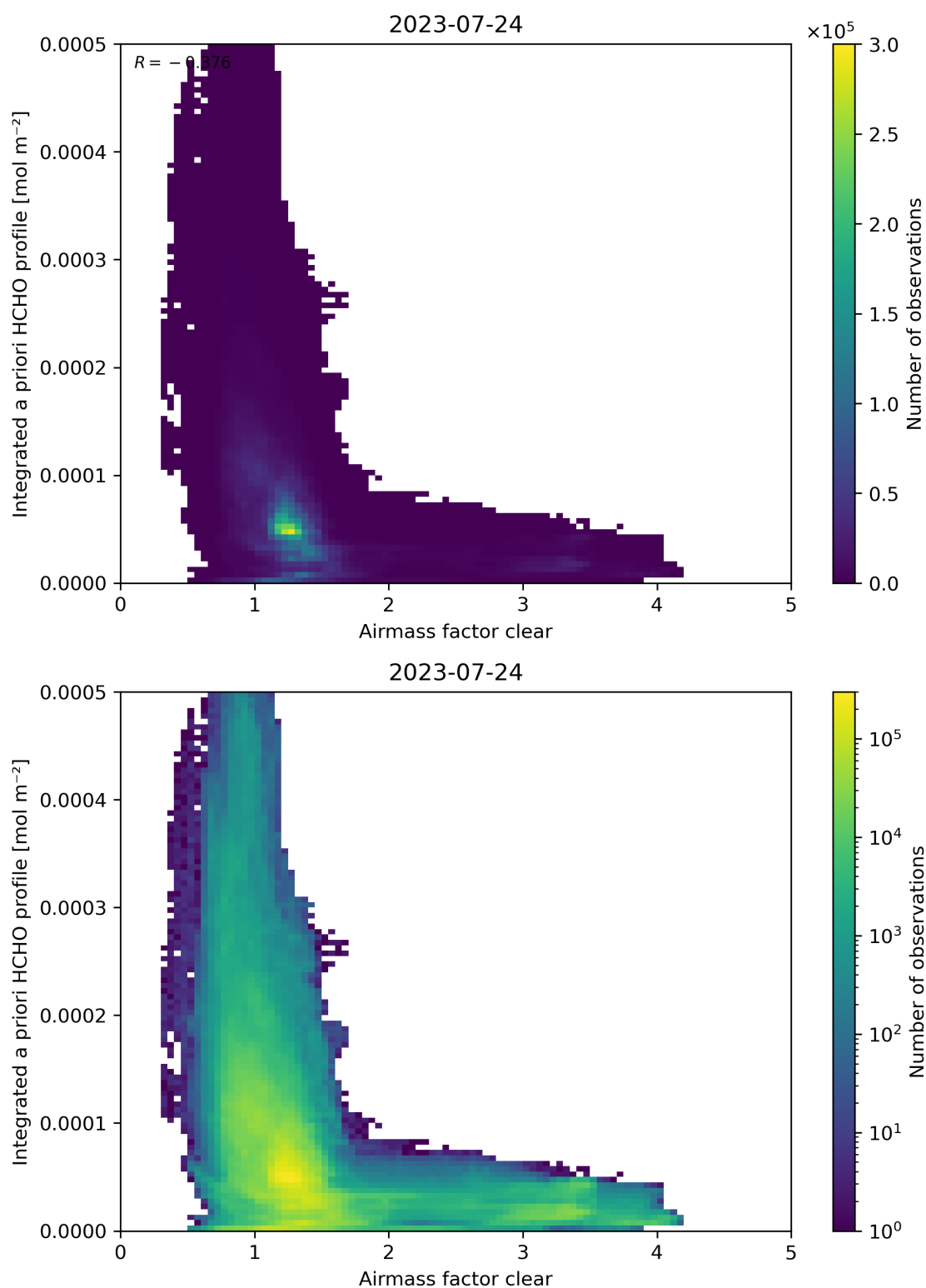
Figure 76: Scatter density plot of “Airmass factor clear” against “Integrated a priori HCHO profile” for 2023-07-24 to 2023-07-25.
