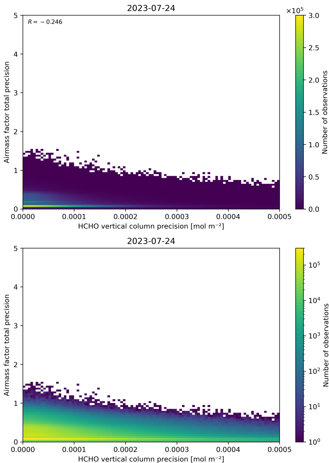
Figure 145: Scatter density plot of “HCHO vertical column precision” against “Airmass factor total precision” for 2023-07-24 to 2023-07-25.
