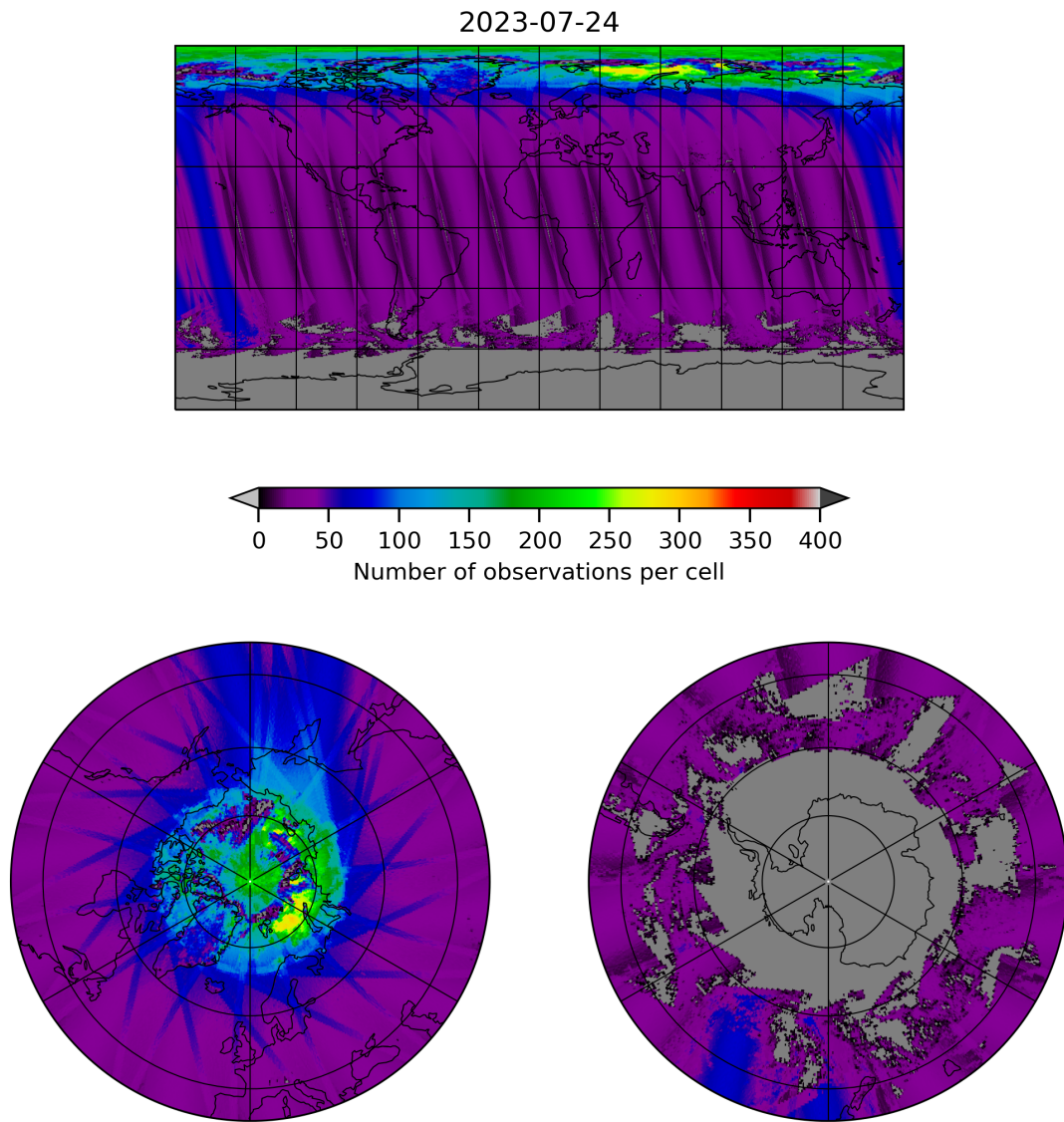
Figure 19: Map of the number of observations for 2023-07-24 to 2023-07-25
