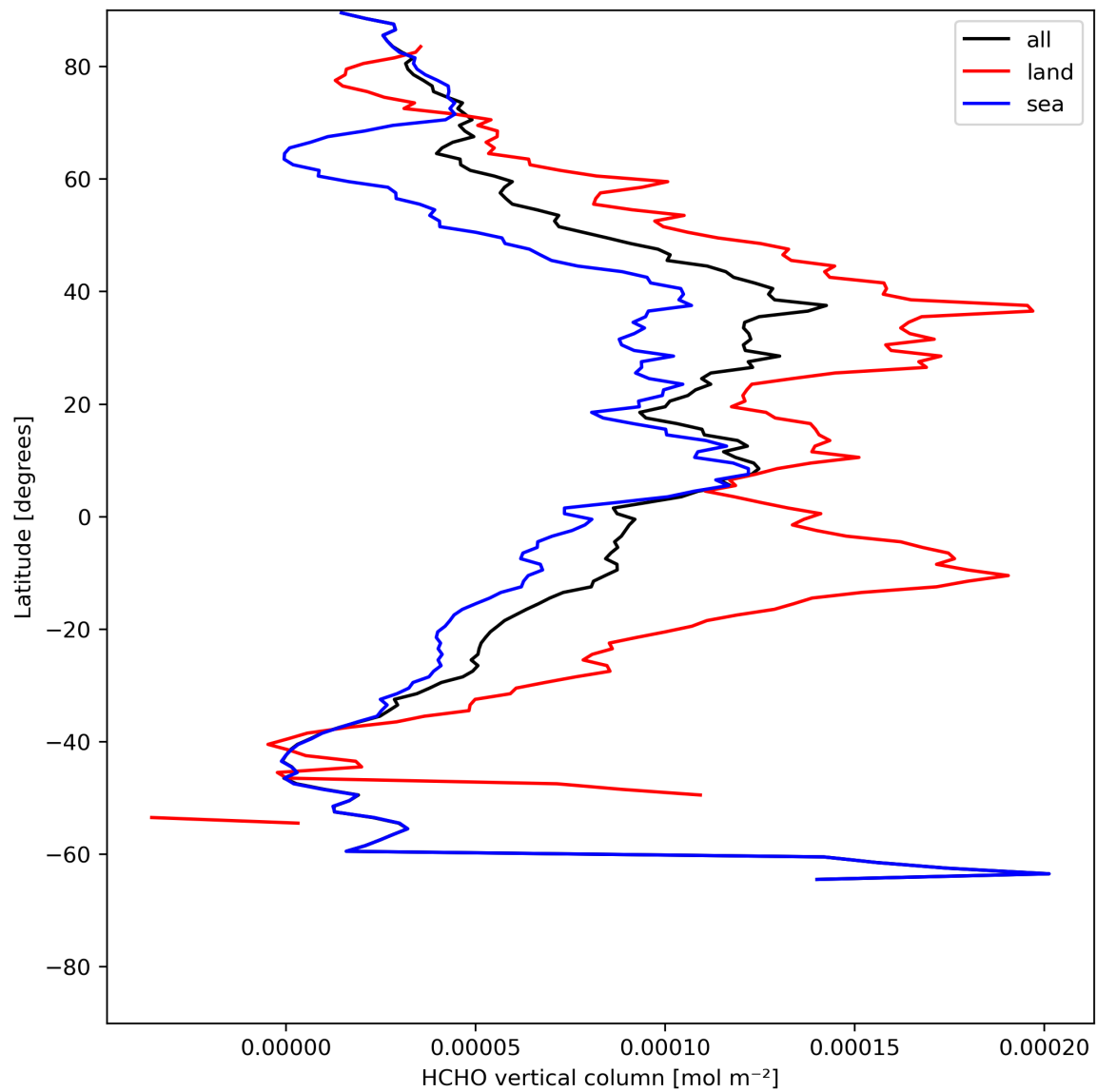
Figure 21: Zonal average of “HCHO vertical column” for 2023-07-24 to 2023-07-25.
