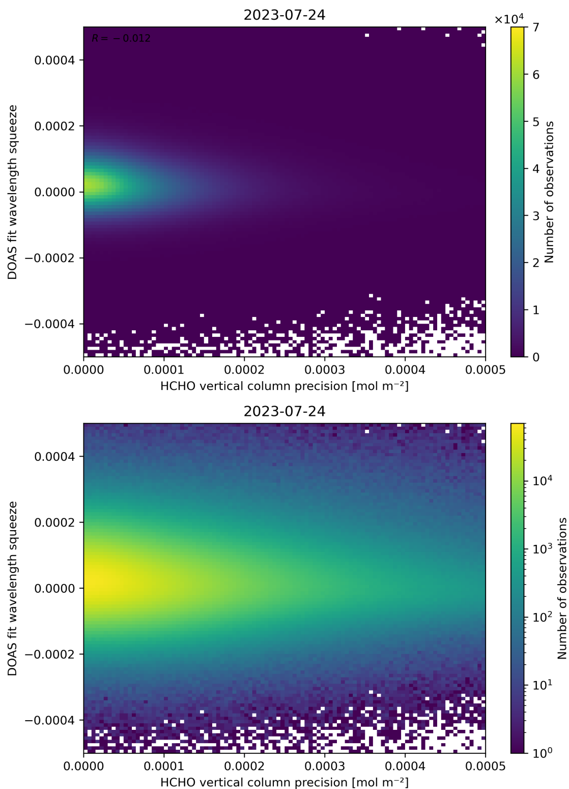
Figure 138: Scatter density plot of “HCHO vertical column precision” against “DOAS fit wavelength squeeze” for 2023-07-24 to 2023-07-25.
