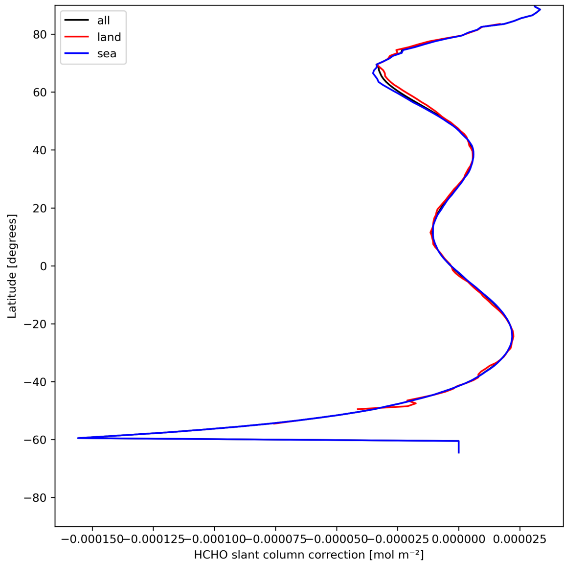
Figure 33: Zonal average of “HCHO slant column correction” for 2023-07-24 to 2023-07-25.
