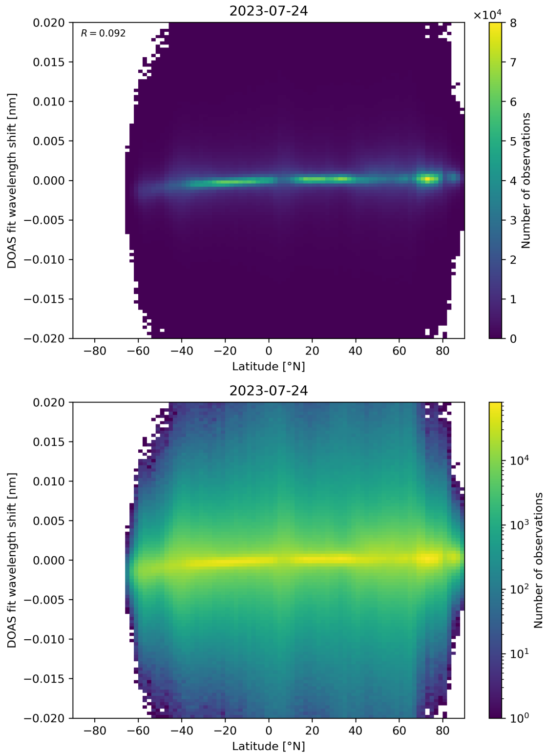
Figure 154: Scatter density plot of “Latitude” against “DOAS fit wavelength shift” for 2023-07-24 to 2023-07-25.
