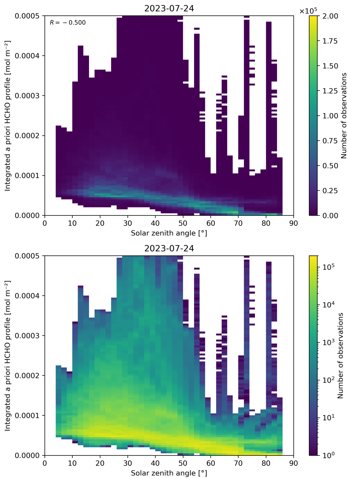
Figure 180: Scatter density plot of “Solar zenith angle” against “Integrated a priori HCHO profile” for 2023-07-24 to 2023-07-25.
