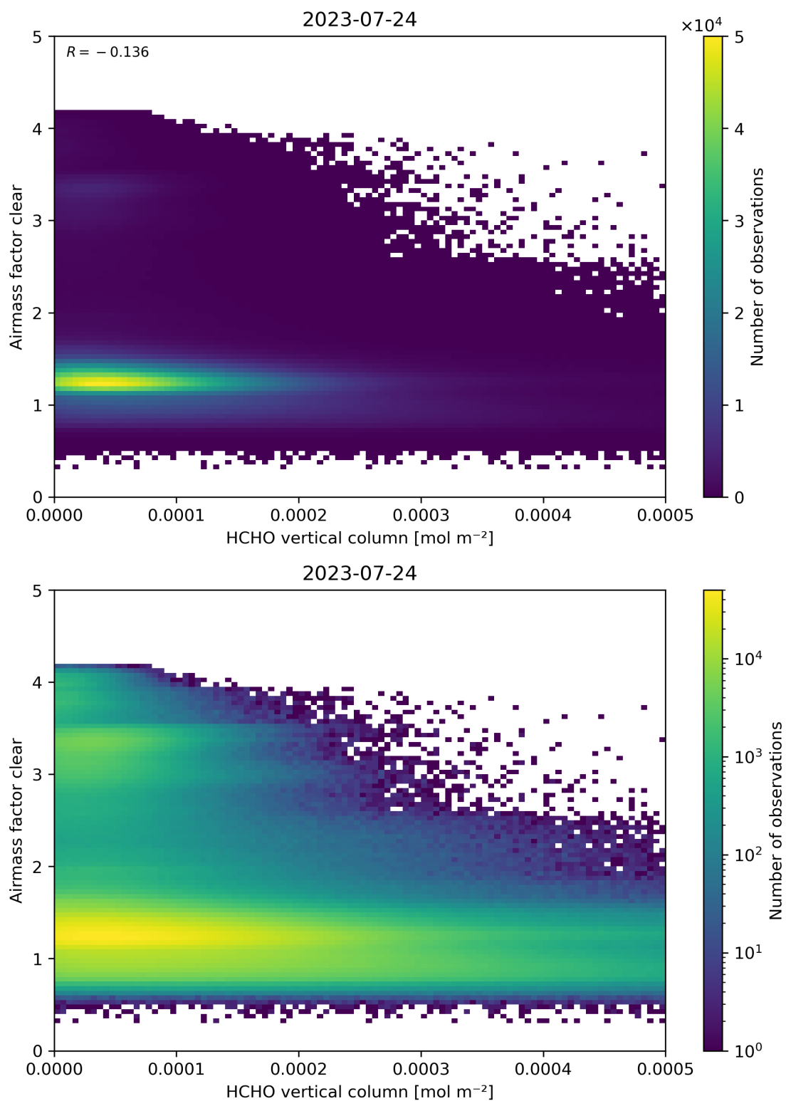
Figure 126: Scatter density plot of “HCHO vertical column” against “Airmass factor clear” for 2023-07-24 to 2023-07-25.
