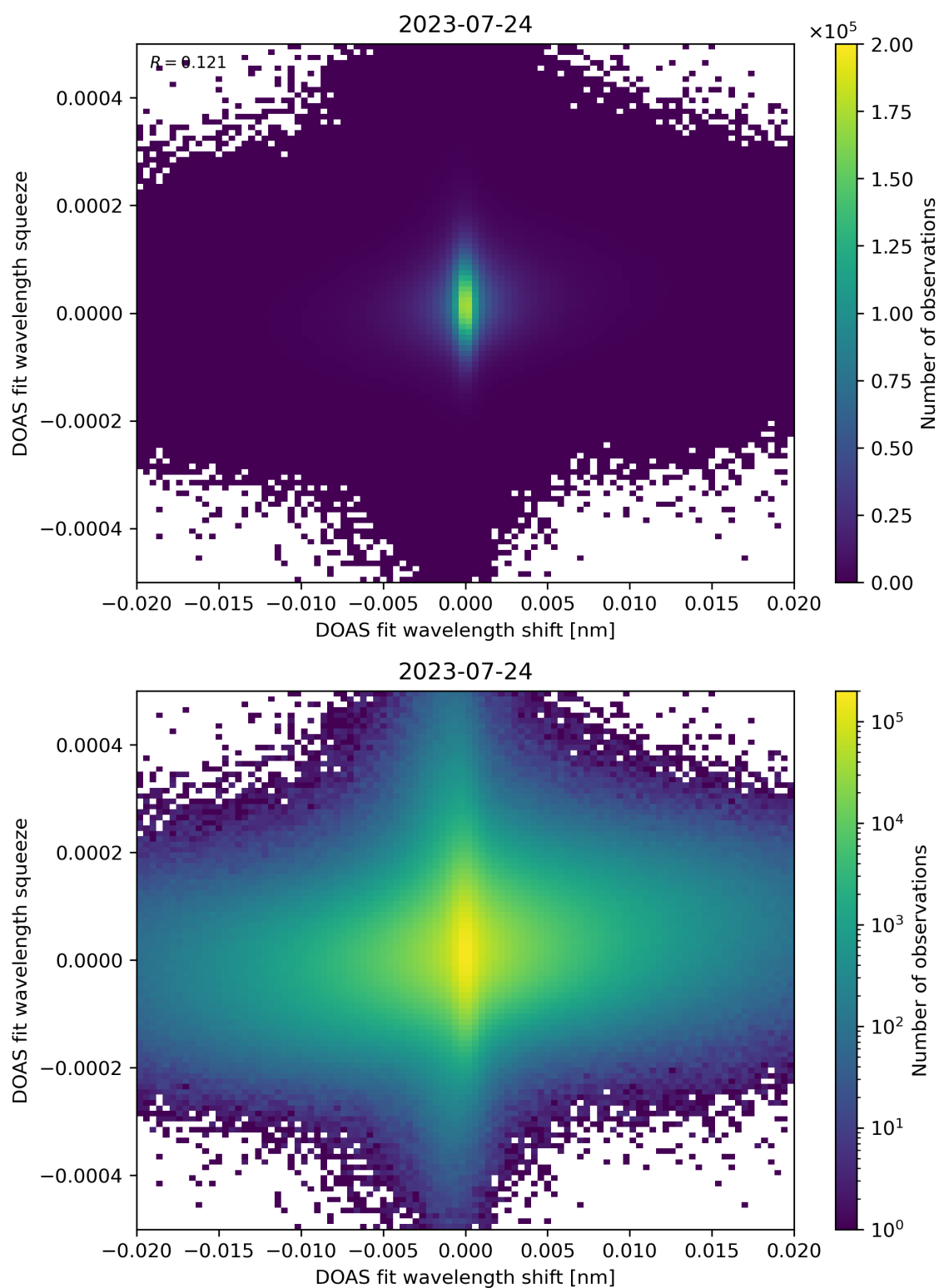
Figure 65: Scatter density plot of “DOAS fit wavelength shift” against “DOAS fit wavelength squeeze” for 2023-07-24 to 2023-07-25.
