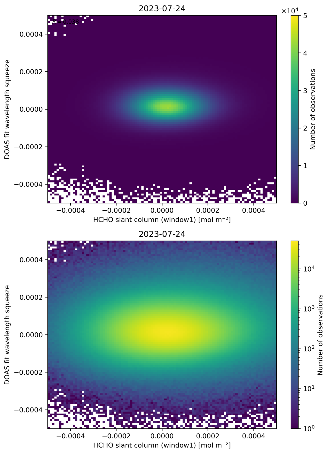
Figure 80: Scatter density plot of “HCHO slant column (window1)” against “DOAS fit wavelength squeeze” for 2023-07-24 to 2023-07-25.
