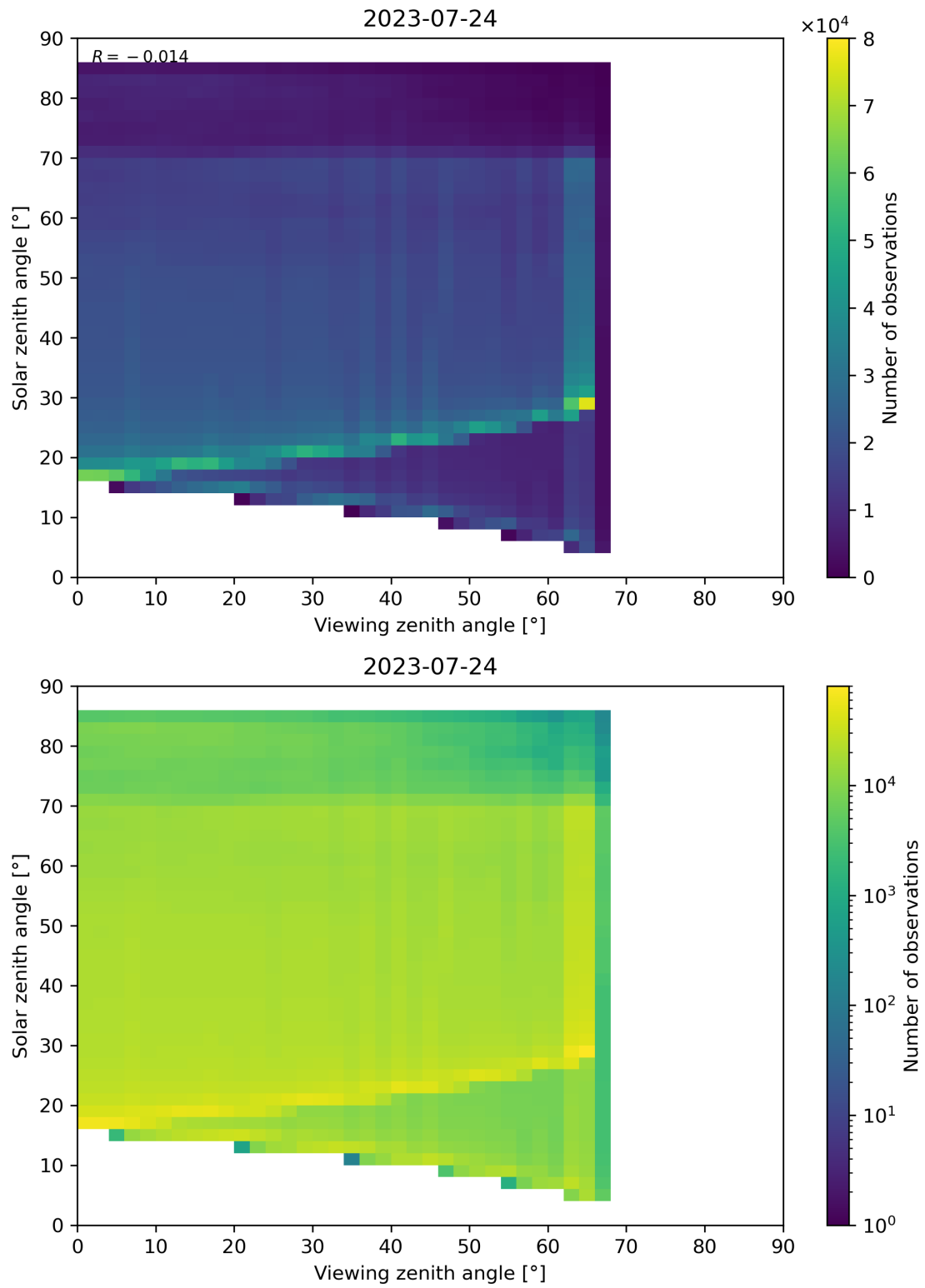
Figure 197: Scatter density plot of “Viewing zenith angle” against “Solar zenith angle” for 2023-07-24 to 2023-07-25.
