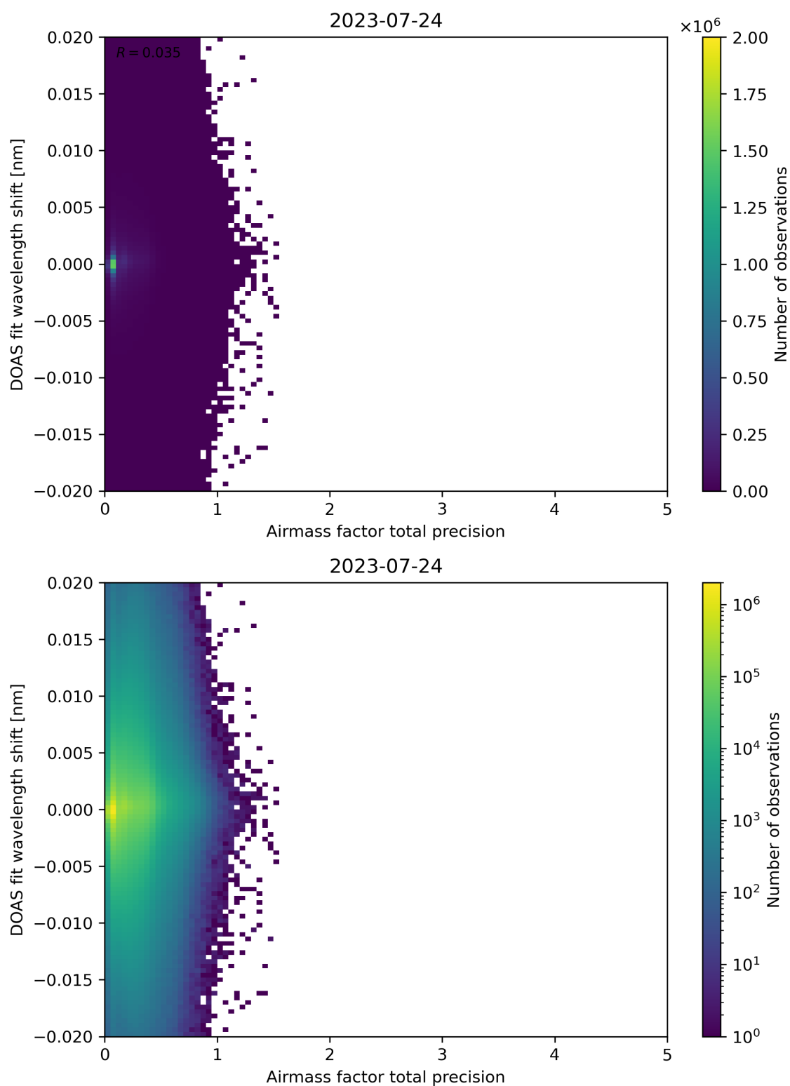
Figure 106: Scatter density plot of “Airmass factor total precision” against “DOAS fit wavelength shift” for 2023-07-24 to 2023-07-25.
