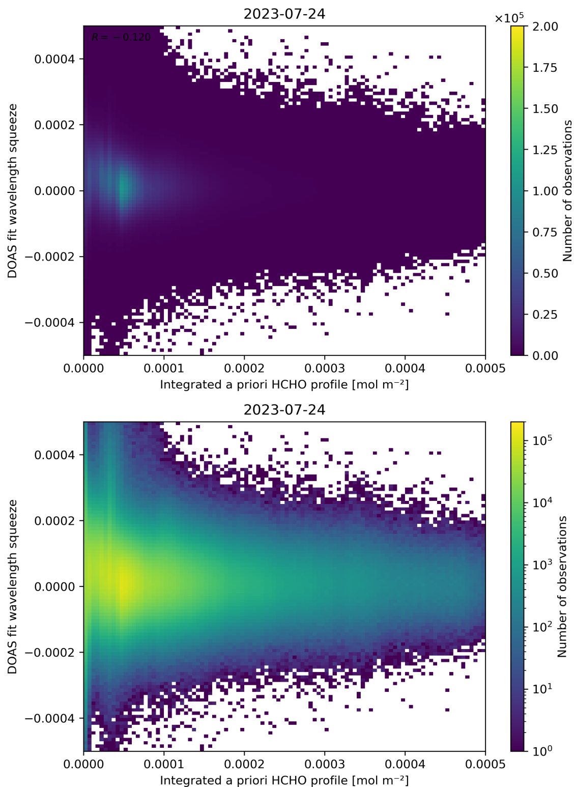
Figure 150: Scatter density plot of “Integrated a priori HCHO profile” against “DOAS fit wavelength squeeze” for 2023-07-24 to 2023-07-25.
