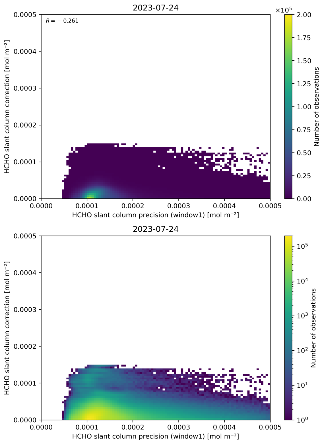
Figure 93: Scatter density plot of “HCHO slant column precision (window1)” against “HCHO slant column correction” for 2023-07-24 to 2023-07-25.
