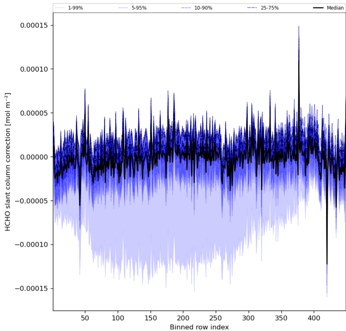
Figure 61: Along track statistics of “HCHO slant column correction” for 2023-07-24 to 2023-07-25
