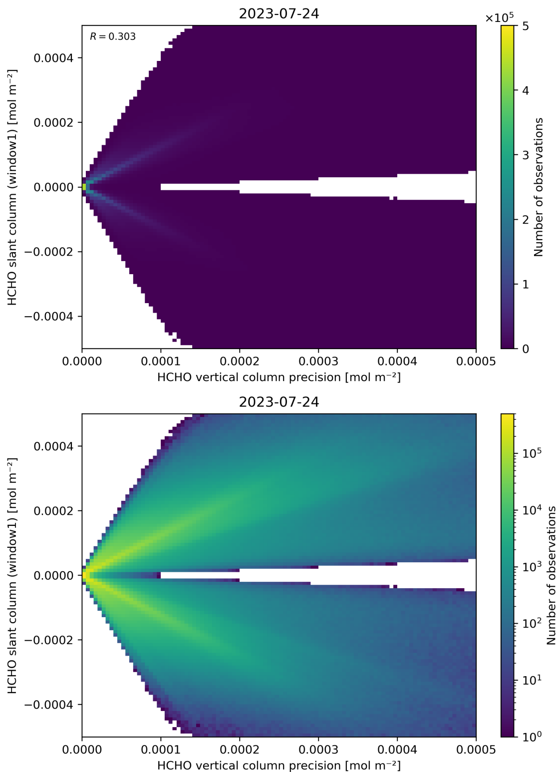
Figure 142: Scatter density plot of “HCHO vertical column precision” against “HCHO slant column (window1)” for 2023-07-24 to 2023-07-25.
