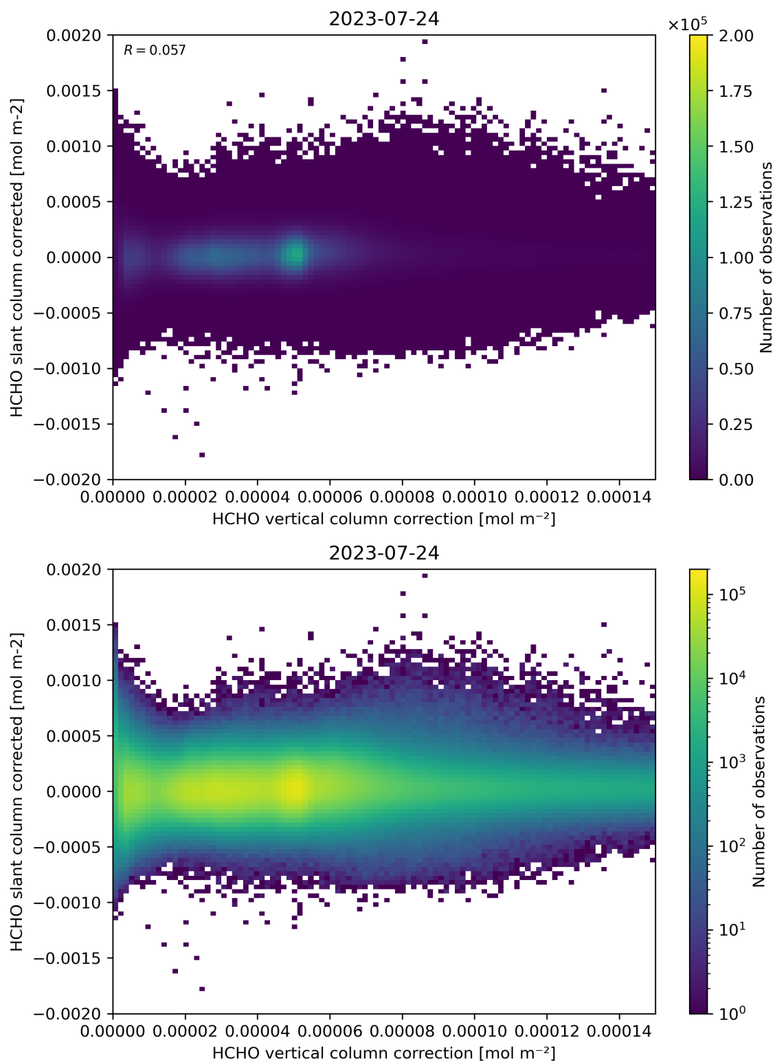
Figure 116: Scatter density plot of “HCHO vertical column correction” against “HCHO slant column corrected” for 2023-07-24 to 2023-07-25.
