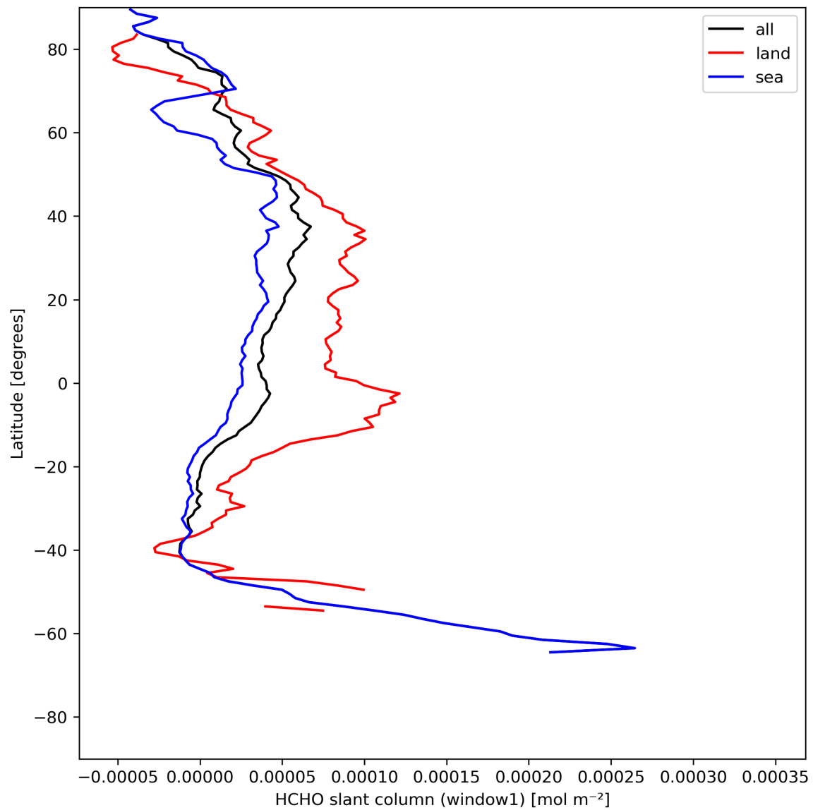
Figure 24: Zonal average of “HCHO slant column (window1)” for 2023-07-24 to 2023-07-25.
