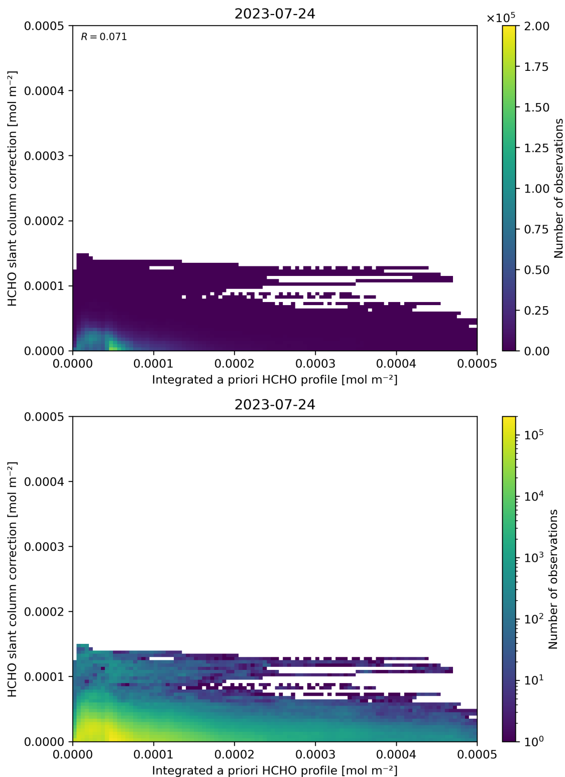
Figure 152: Scatter density plot of “Integrated a priori HCHO profile” against “HCHO slant column correction” for 2023-07-24 to 2023-07-25.
