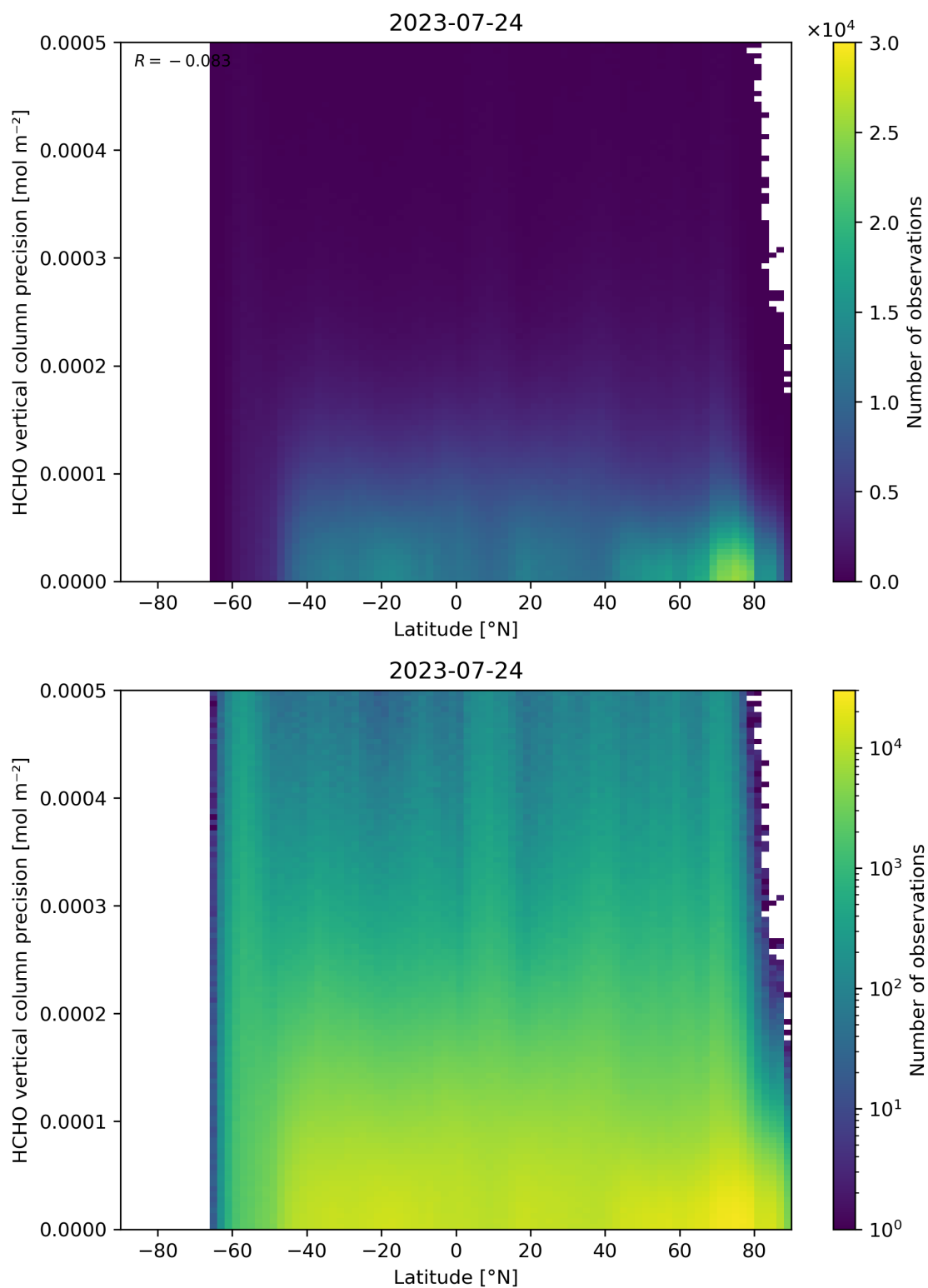
Figure 165: Scatter density plot of “Latitude” against “HCHO vertical column precision” for 2023-07-24 to 2023-07-25.
