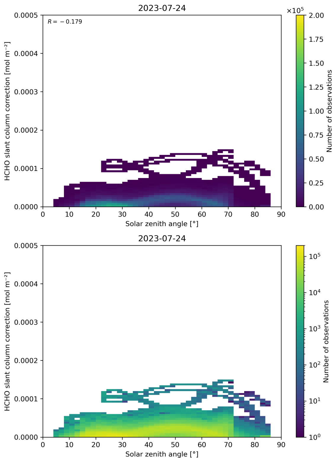
Figure 172: Scatter density plot of “Solar zenith angle” against “HCHO slant column correction” for 2023-07-24 to 2023-07-25.
