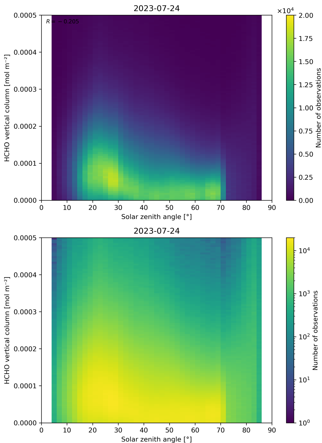
Figure 177: Scatter density plot of “Solar zenith angle” against “HCHO vertical column” for 2023-07-24 to 2023-07-25.
