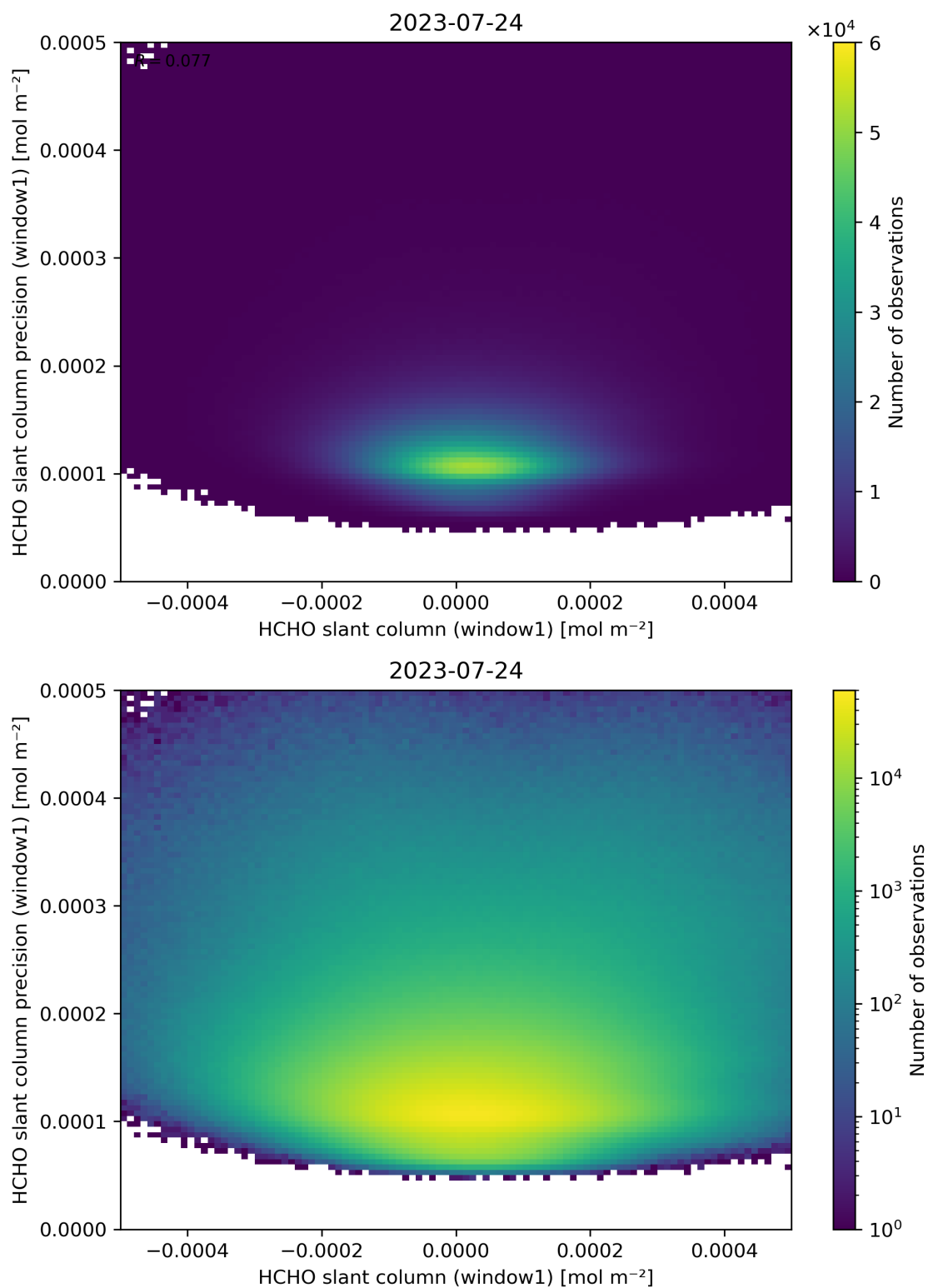
Figure 84: Scatter density plot of “HCHO slant column (window1)” against “HCHO slant column precision (window1)” for 2023-07-24 to 2023-07-25.
