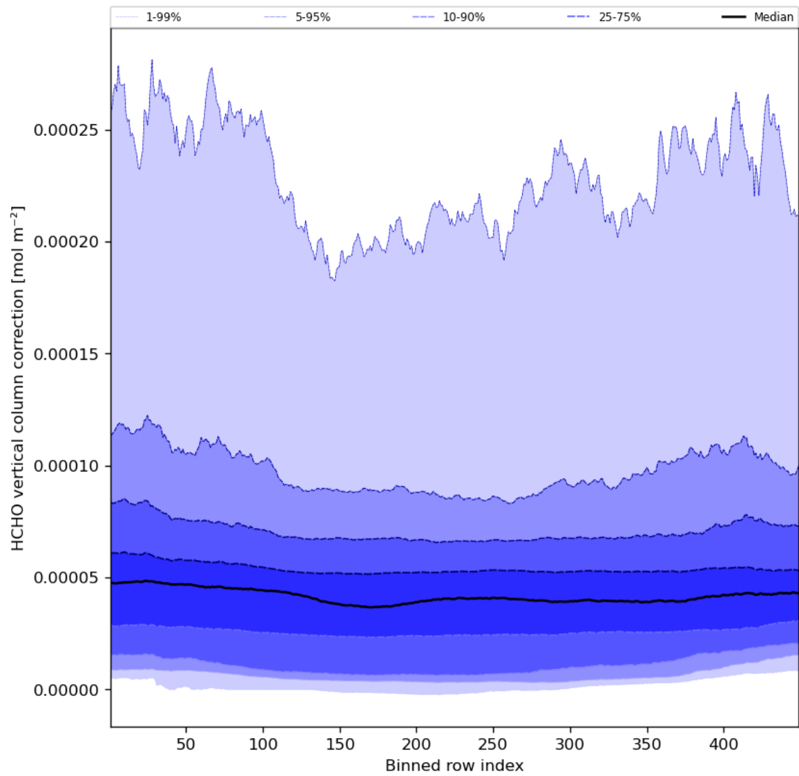
Figure 51: Along track statistics of “HCHO vertical column correction” for 2023-07-24 to 2023-07-25
