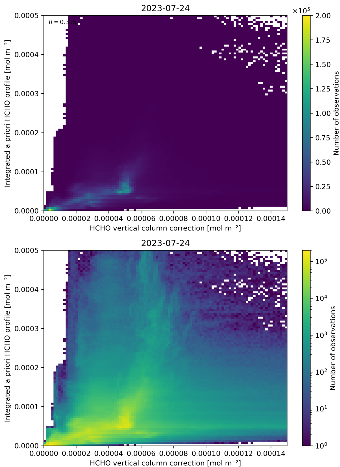
Figure 122: Scatter density plot of “HCHO vertical column correction” against “Integrated a priori HCHO profile” for 2023-07-24 to 2023-07-25.
