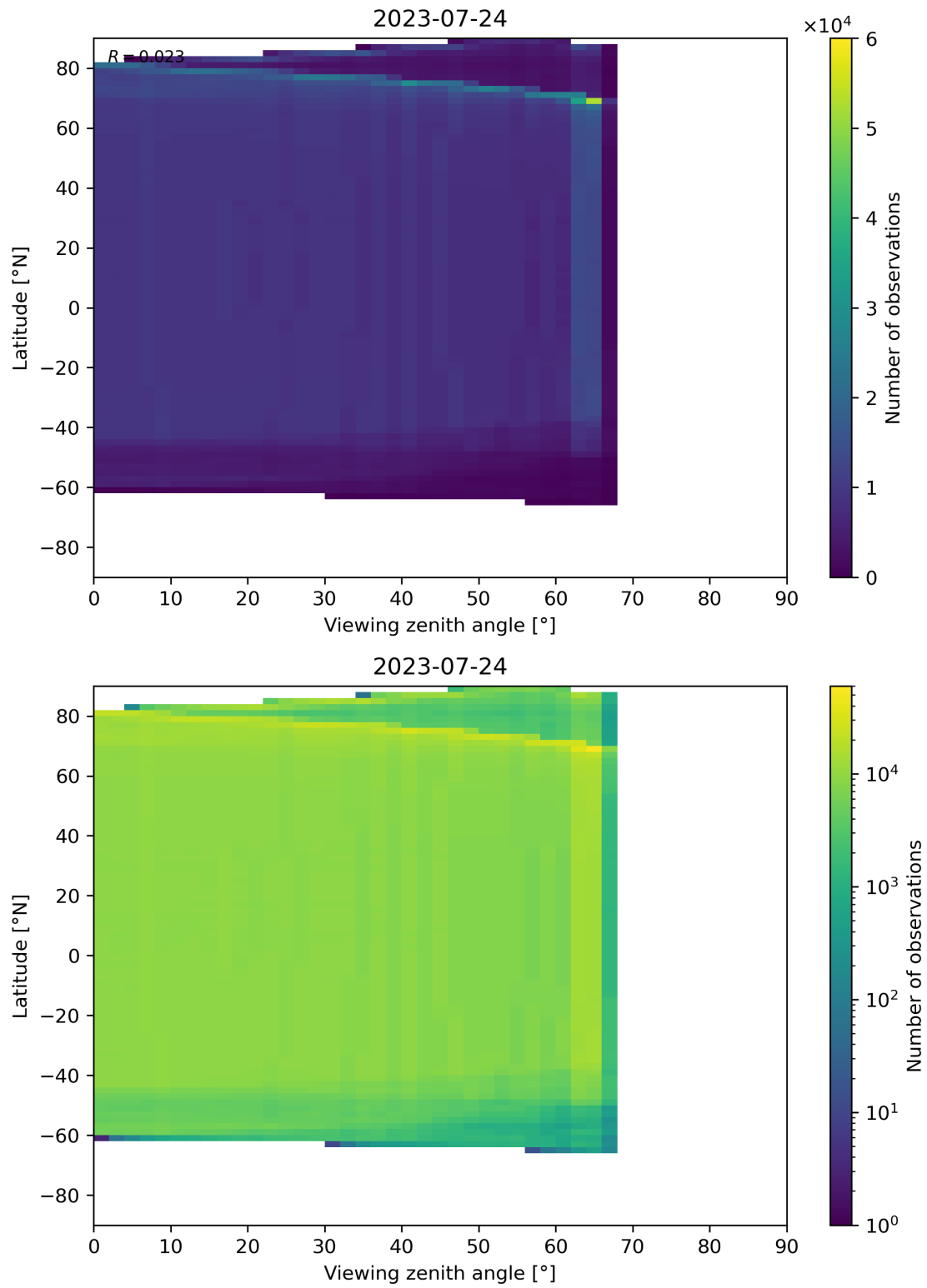
Figure 196: Scatter density plot of “Viewing zenith angle” against “Latitude” for 2023-07-24 to 2023-07-25.
