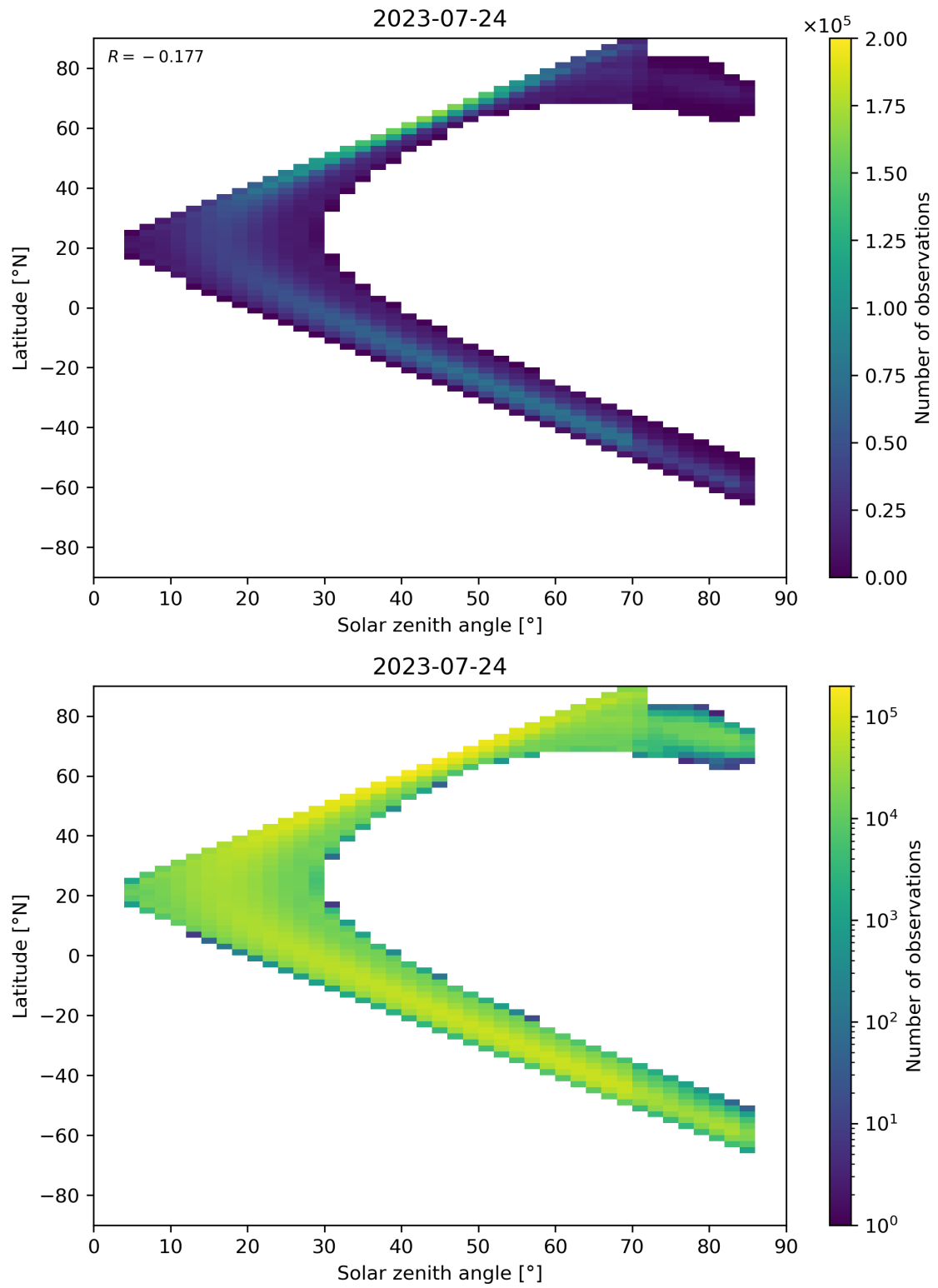
Figure 181: Scatter density plot of “Solar zenith angle” against “Latitude” for 2023-07-24 to 2023-07-25.
