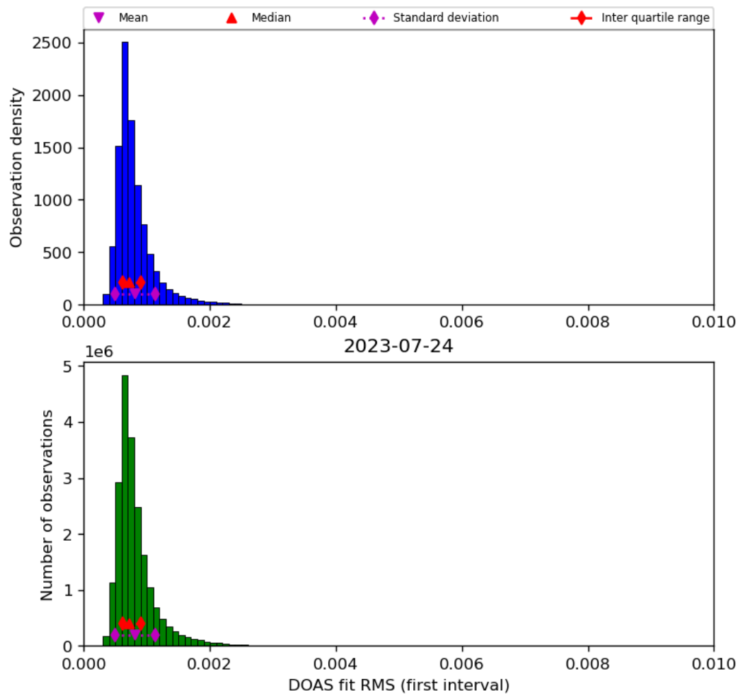
Figure 46: Histogram of “DOAS fit RMS (first interval)” for 2023-07-24 to 2023-07-25
