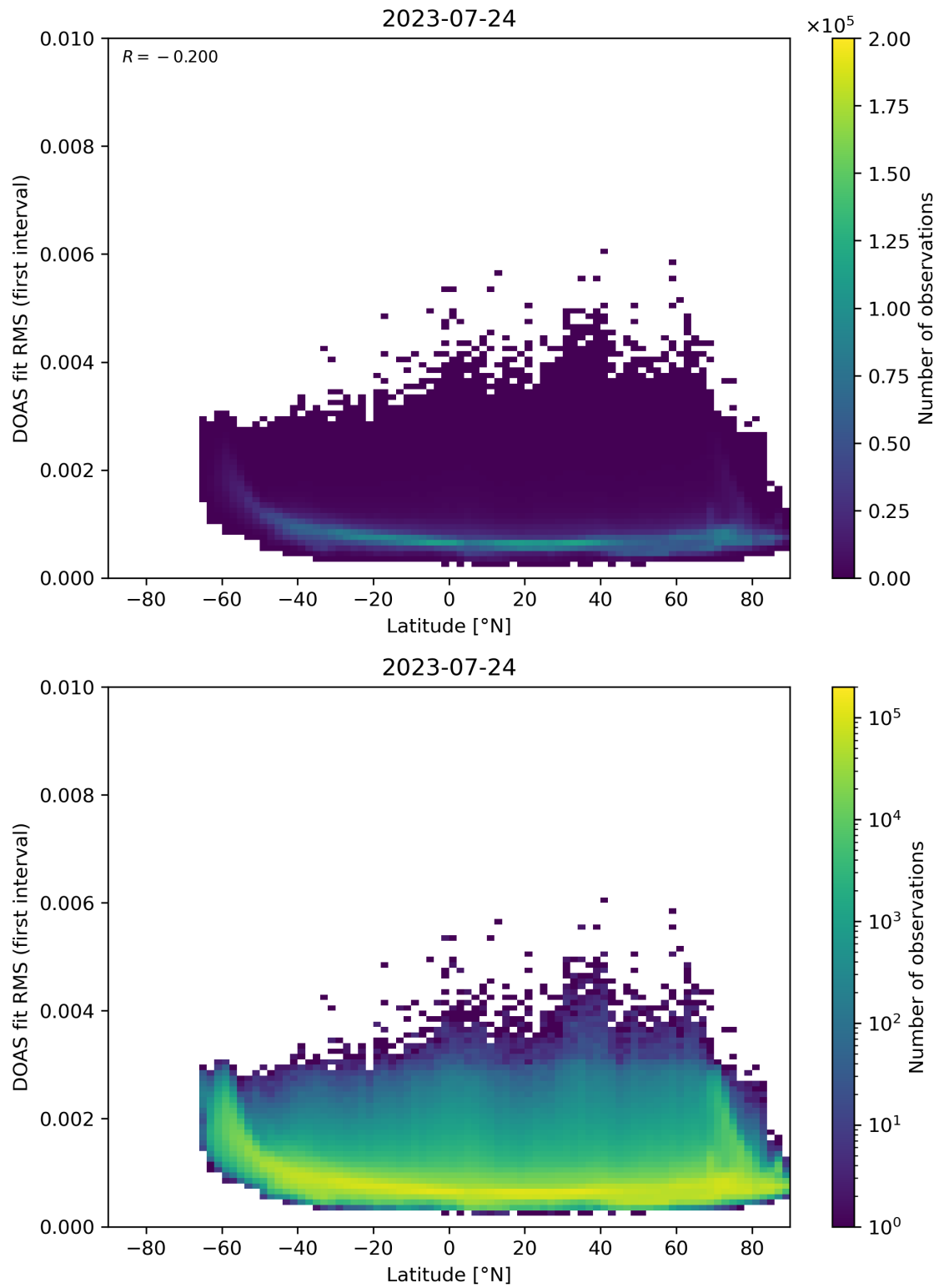
Figure 153: Scatter density plot of “Latitude” against “DOAS fit RMS (first interval)” for 2023-07-24 to 2023-07-25.
