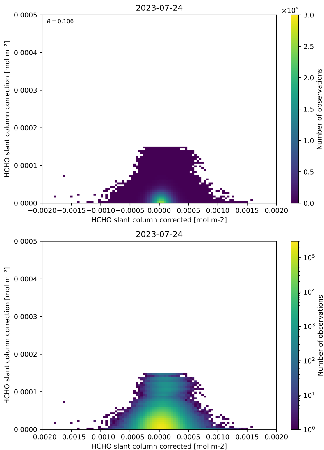
Figure 77: Scatter density plot of “HCHO slant column corrected” against “HCHO slant column correction” for 2023-07-24 to 2023-07-25.
