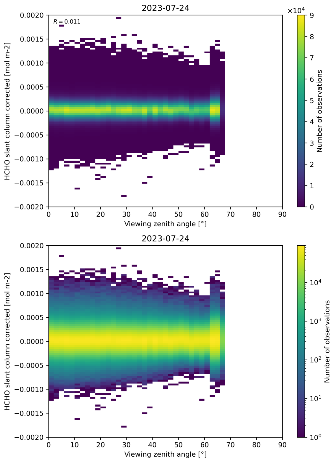
Figure 186: Scatter density plot of “Viewing zenith angle” against “HCHO slant column corrected” for 2023-07-24 to 2023-07-25.
