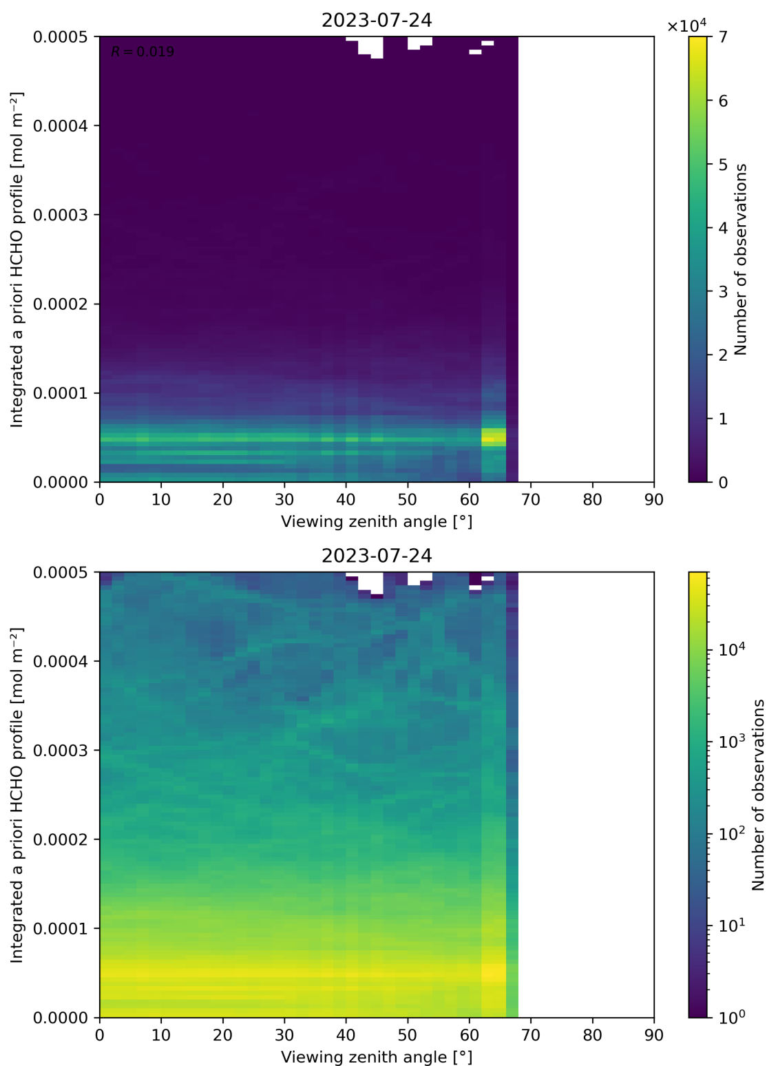
Figure 195: Scatter density plot of “Viewing zenith angle” against “Integrated a priori HCHO profile” for 2023-07-24 to 2023-07-25.
