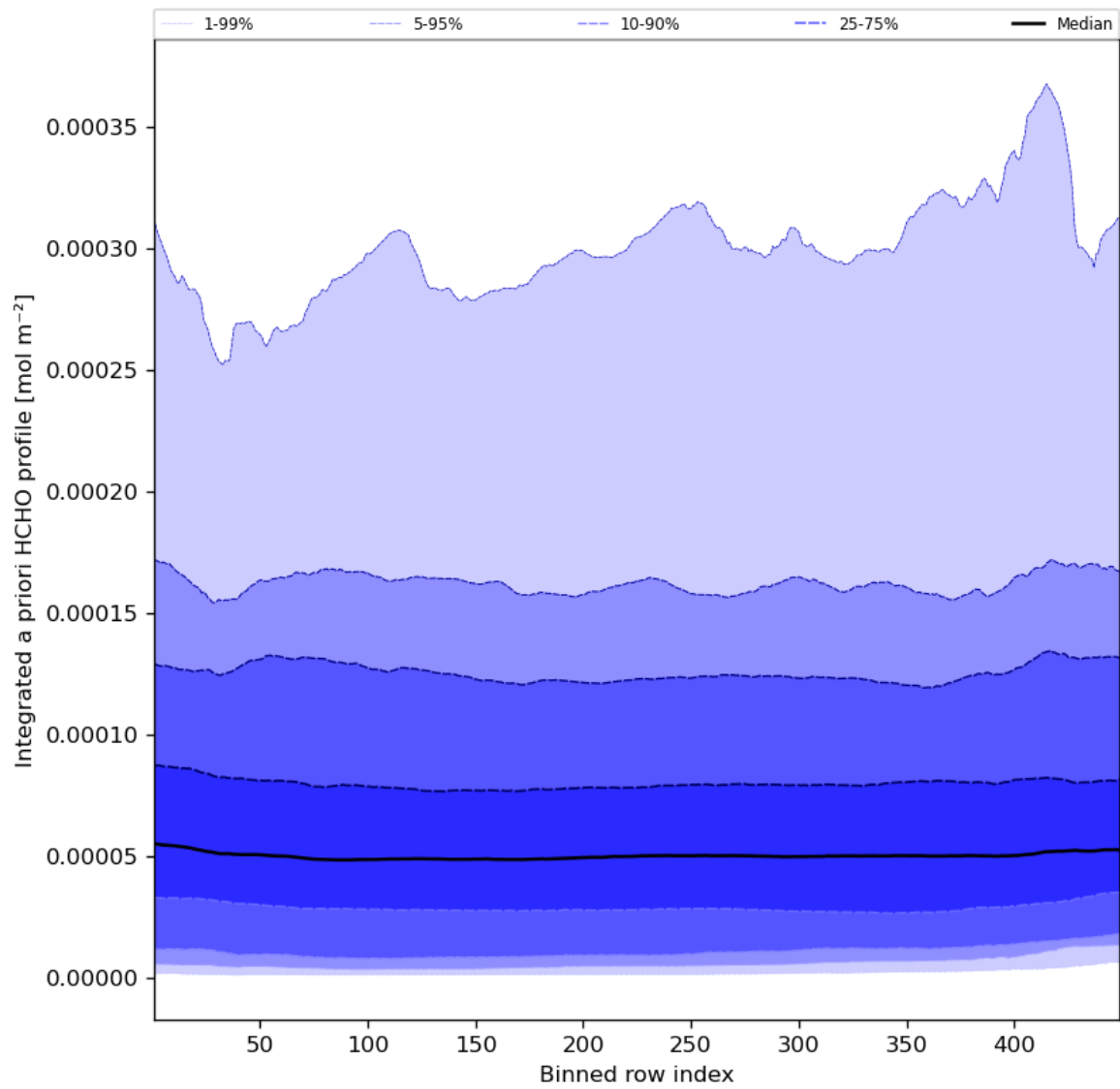
Figure 57: Along track statistics of “Integrated a priori HCHO profile” for 2023-07-24 to 2023-07-25
