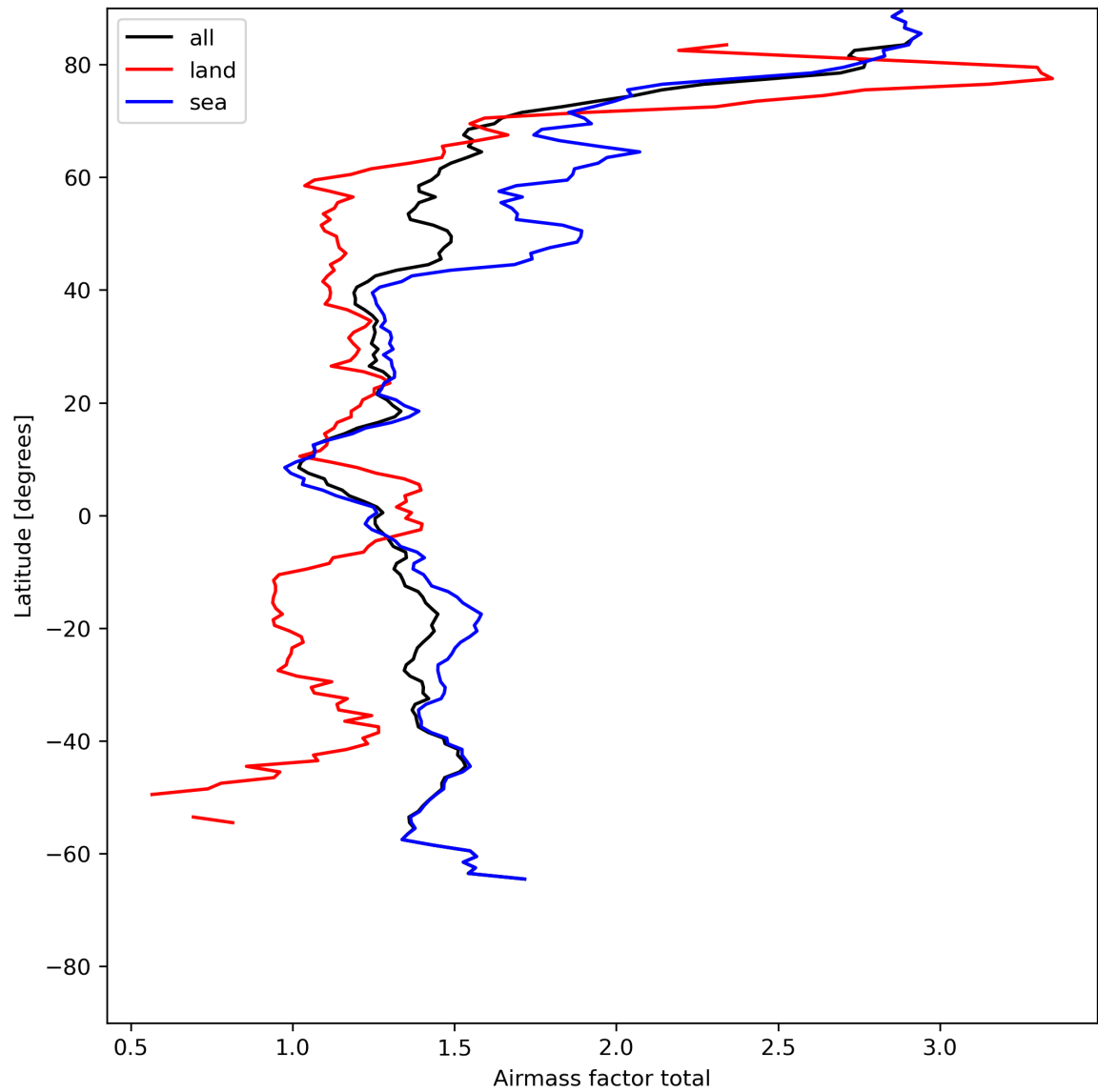
Figure 26: Zonal average of “Airmass factor total” for 2023-07-24 to 2023-07-25.
