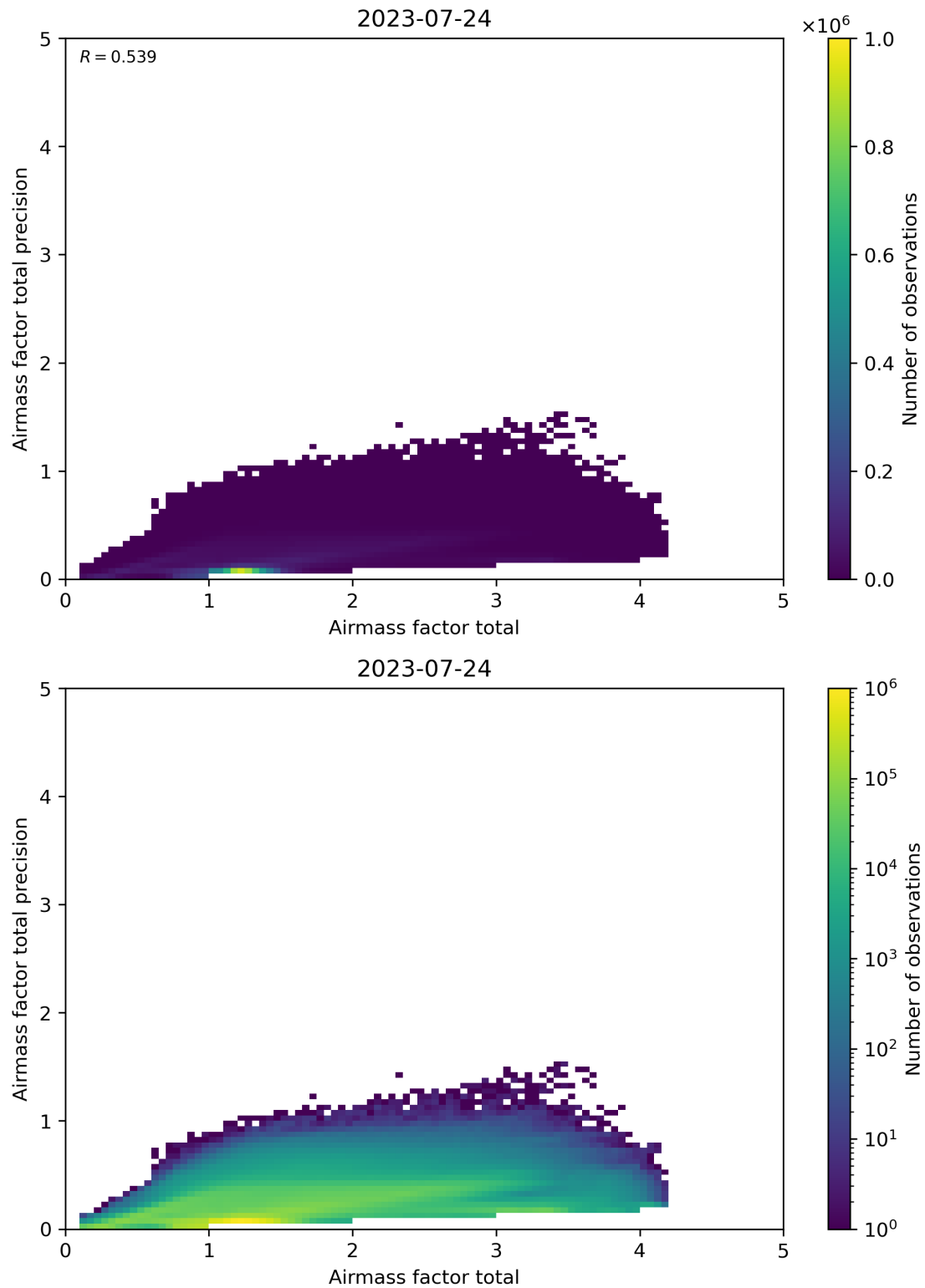
Figure 103: Scatter density plot of “Airmass factor total” against “Airmass factor total precision” for 2023-07-24 to 2023-07-25.
