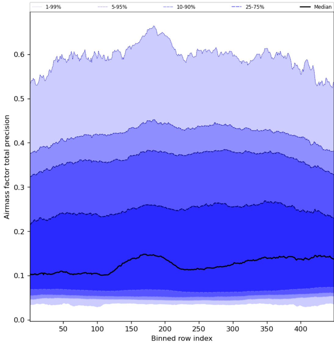
Figure 55: Along track statistics of “Airmass factor total precision” for 2023-07-24 to 2023-07-25
