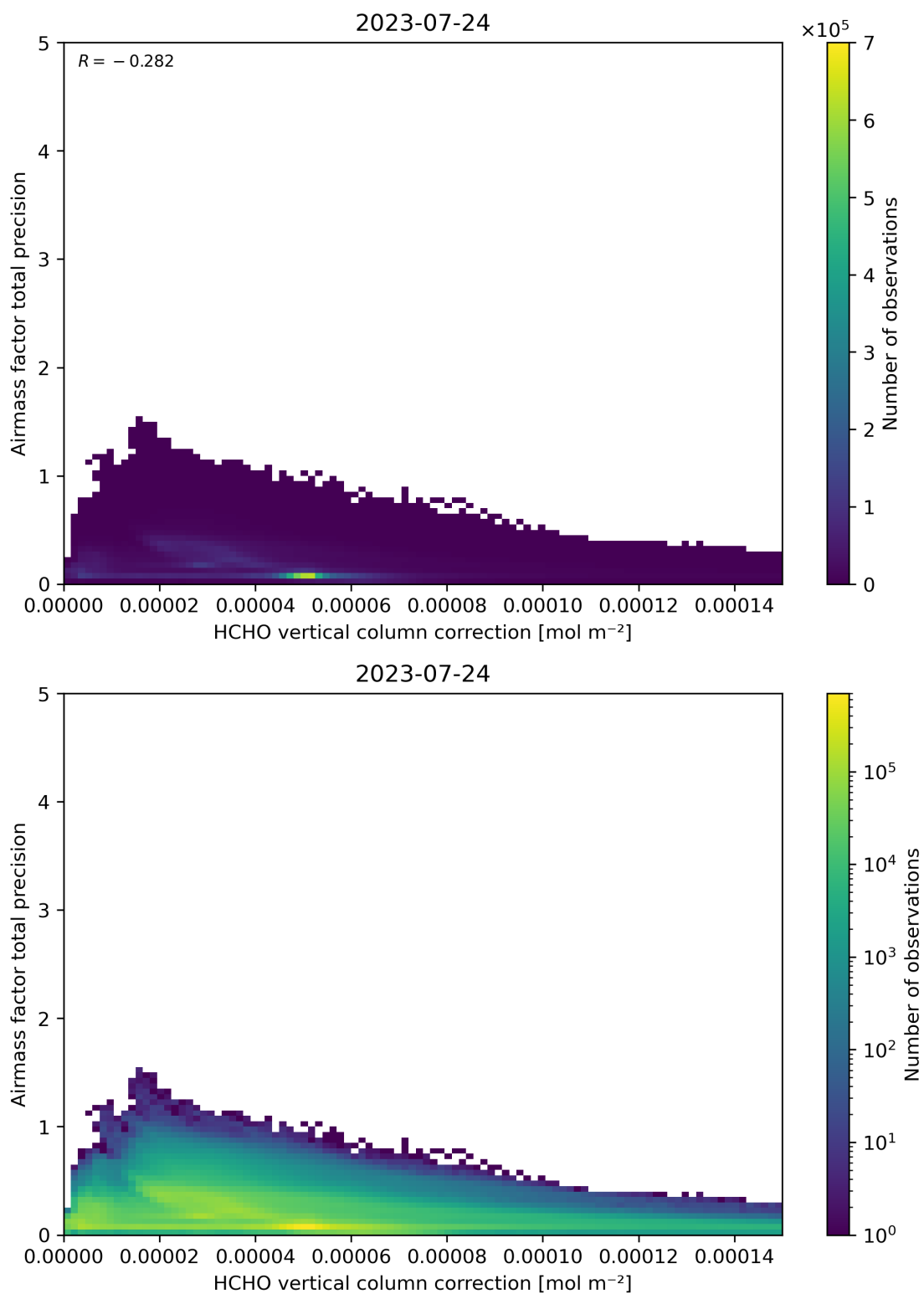
Figure 121: Scatter density plot of “HCHO vertical column correction” against “Airmass factor total precision” for 2023-07-24 to 2023-07-25.
