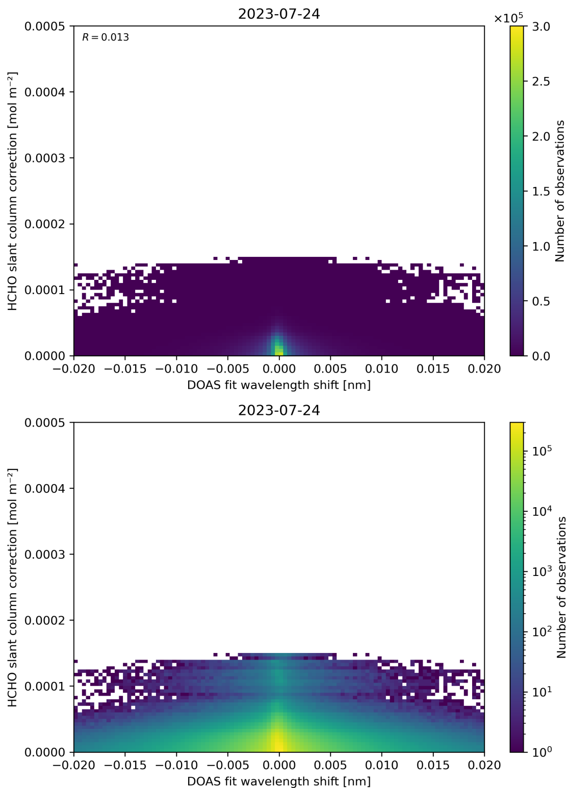
Figure 67: Scatter density plot of “DOAS fit wavelength shift” against “HCHO slant column correction” for 2023-07-24 to 2023-07-25.
