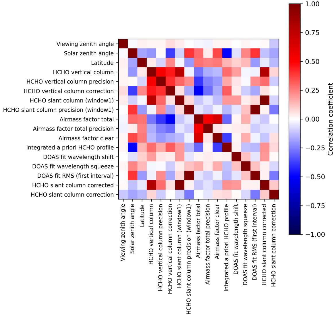
Figure 2: Map of correlation matrix for 2023-07-24 to 2023-07-25.
