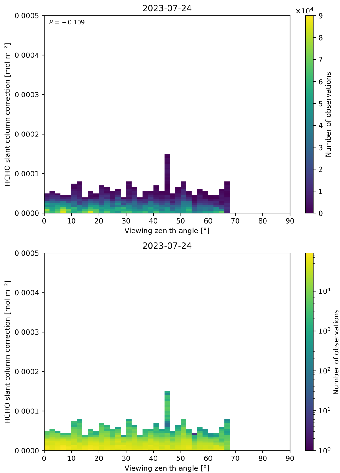
Figure 187: Scatter density plot of “Viewing zenith angle” against “HCHO slant column correction” for 2023-07-24 to 2023-07-25.
