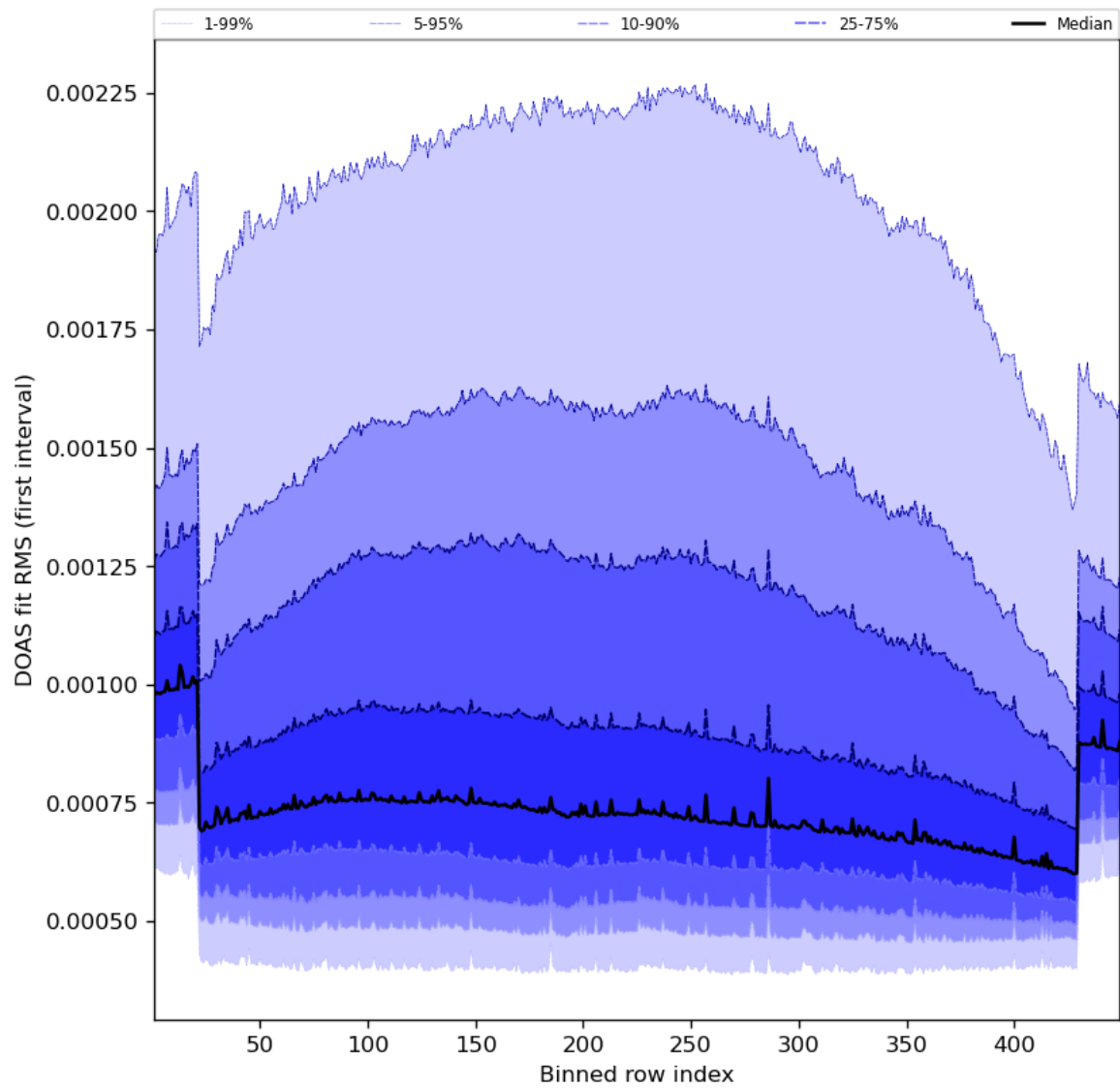
Figure 60: Along track statistics of “DOAS fit RMS (first interval)” for 2023-07-24 to 2023-07-25
