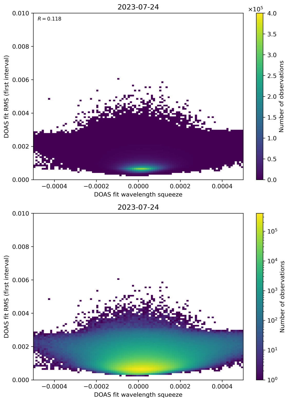
Figure 68: Scatter density plot of “DOAS fit wavelength squeeze” against “DOAS fit RMS (first interval)” for 2023-07-24 to 2023-07-25.
