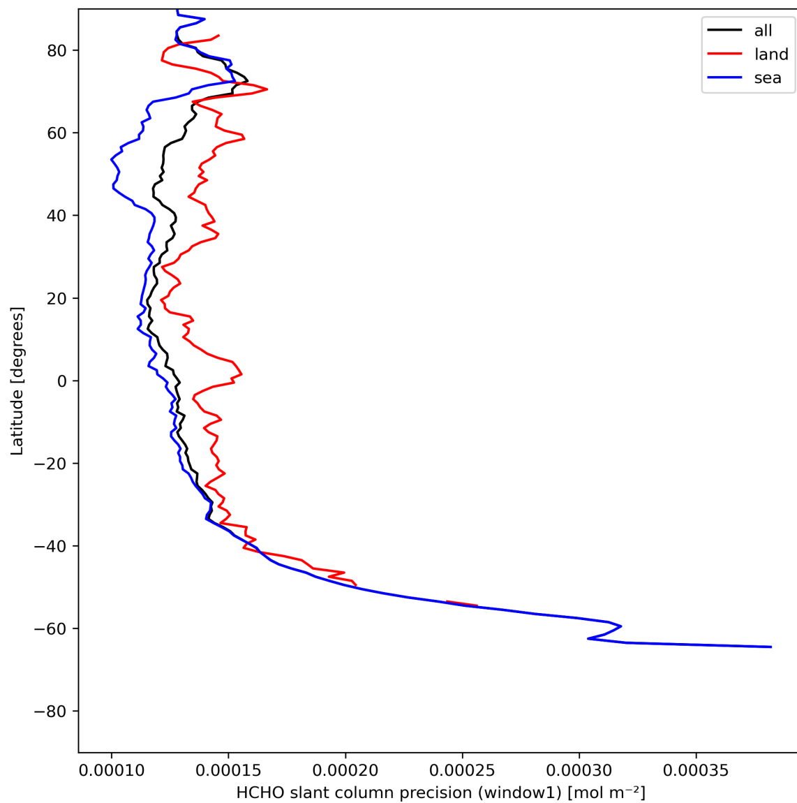
Figure 25: Zonal average of “HCHO slant column precision (window1)” for 2023-07-24 to 2023-07-25.
