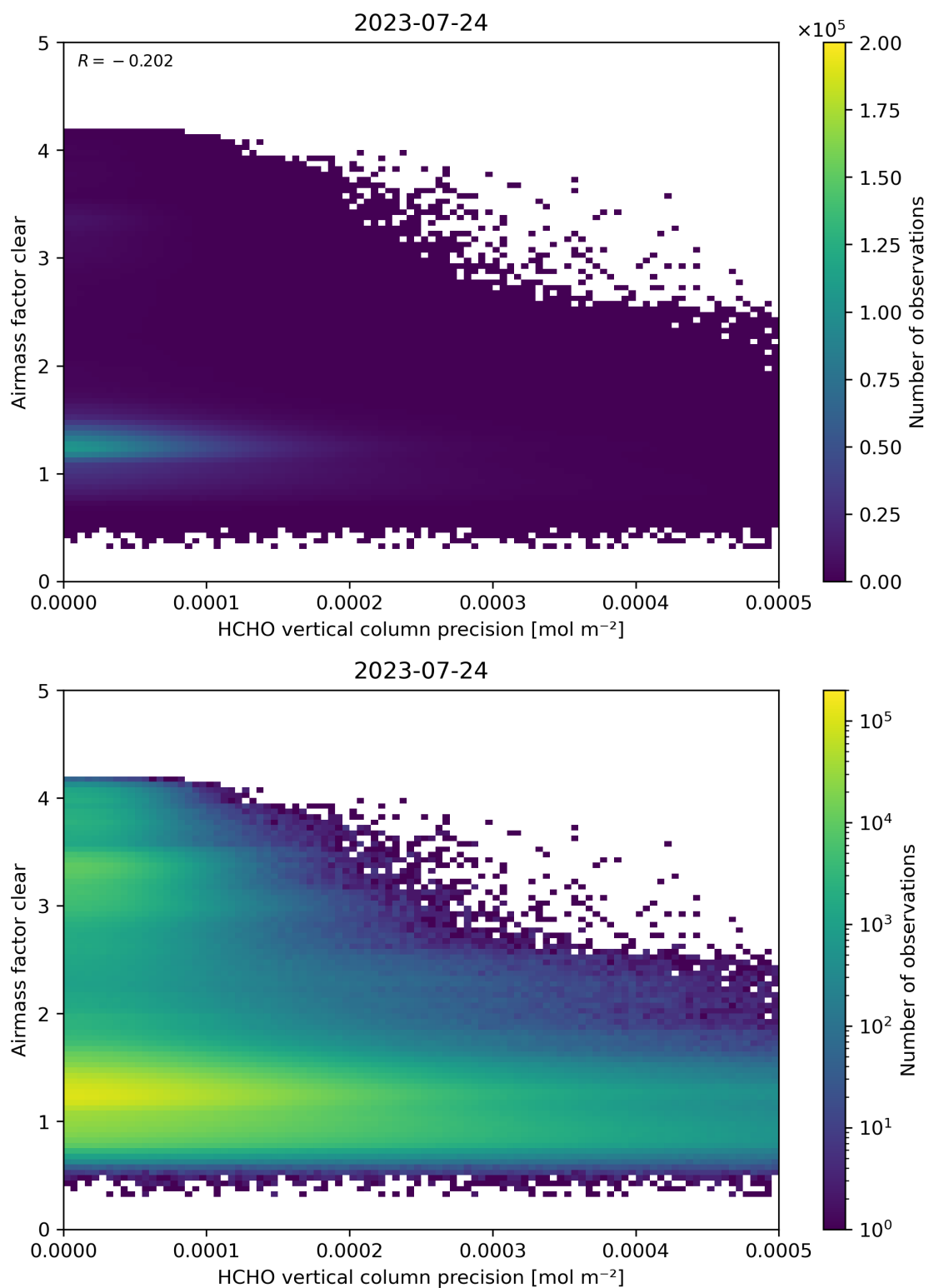
Figure 139: Scatter density plot of “HCHO vertical column precision” against “Airmass factor clear” for 2023-07-24 to 2023-07-25.
