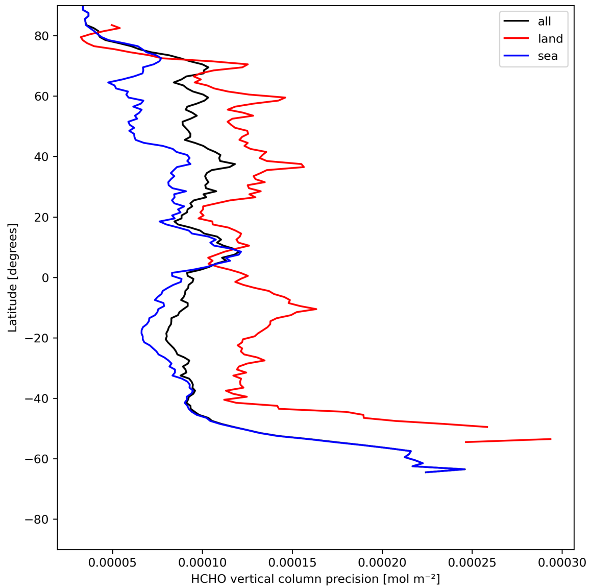
Figure 22: Zonal average of “HCHO vertical column precision” for 2023-07-24 to 2023-07-25.
