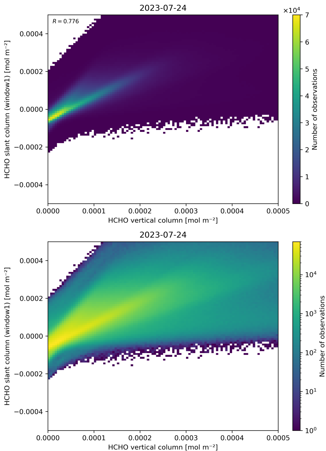
Figure 129: Scatter density plot of “HCHO vertical column” against “HCHO slant column (window1)” for 2023-07-24 to 2023-07-25.
