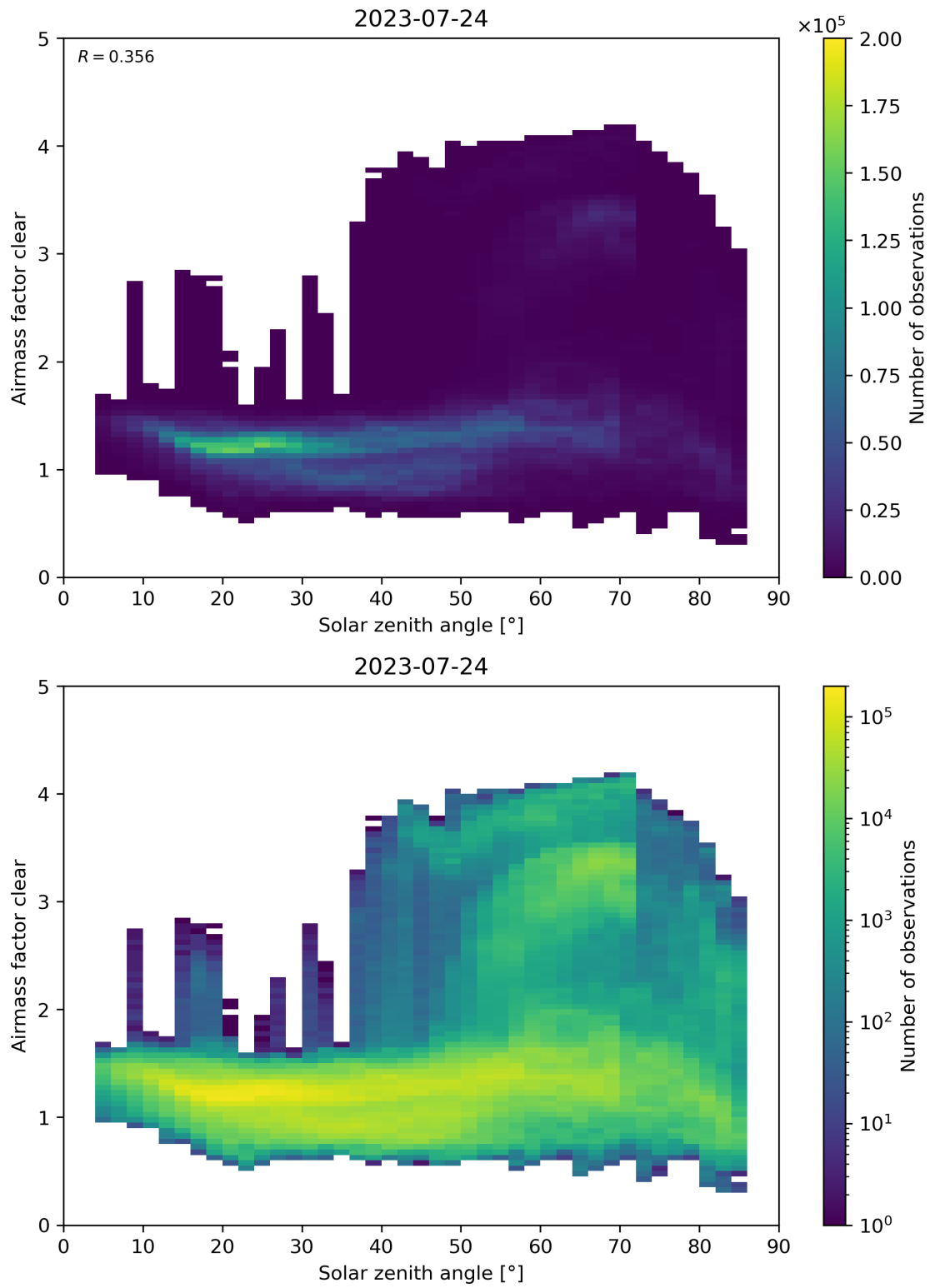
Figure 170: Scatter density plot of “Solar zenith angle” against “Airmass factor clear” for 2023-07-24 to 2023-07-25.
