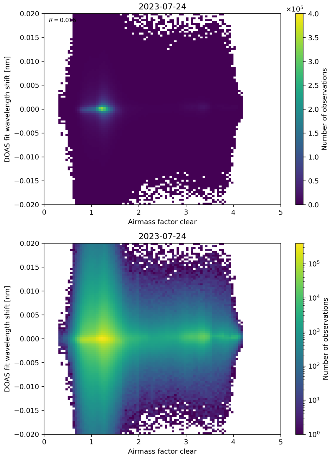
Figure 72: Scatter density plot of “Airmass factor clear” against “DOAS fit wavelength shift” for 2023-07-24 to 2023-07-25.
