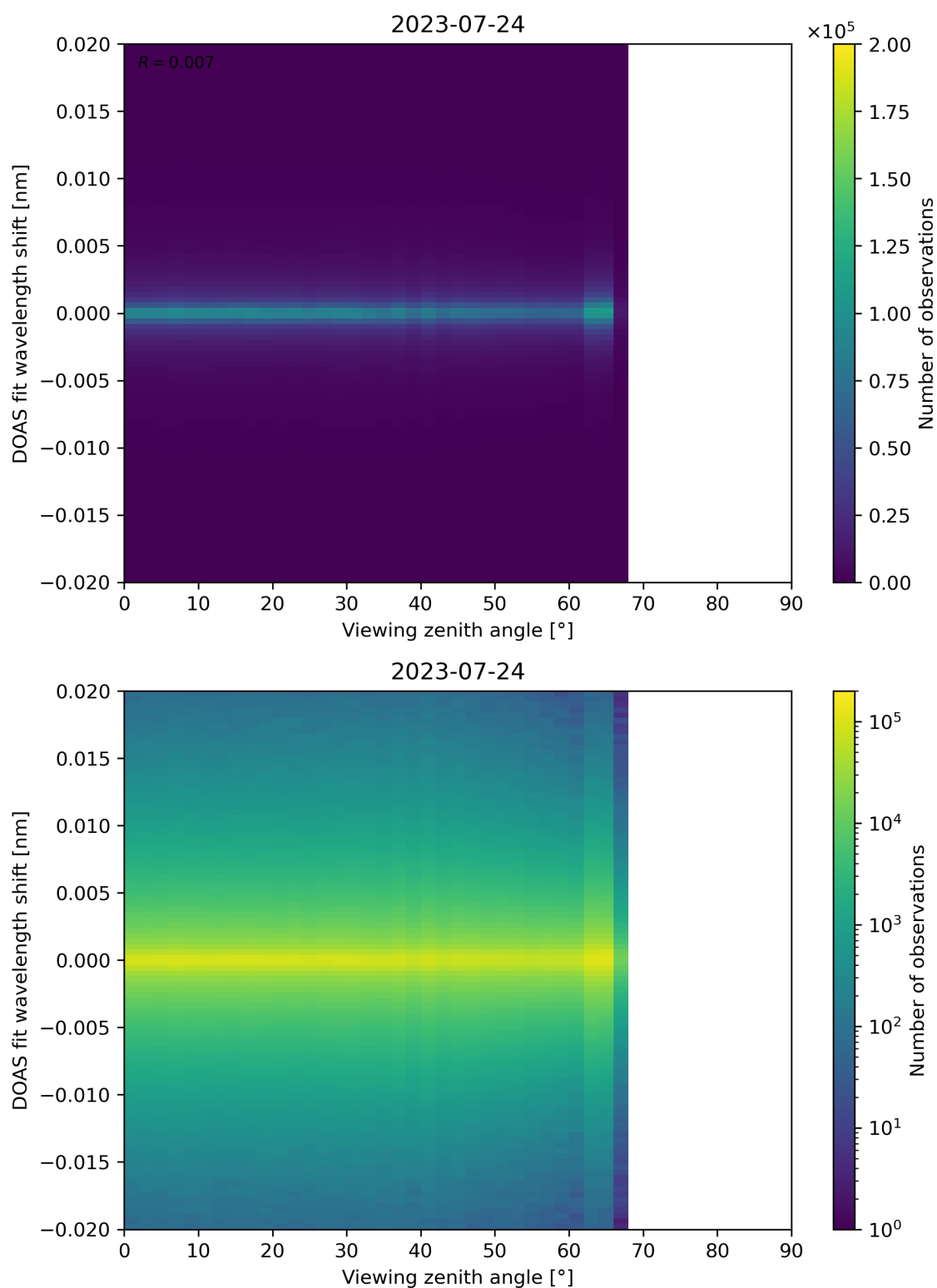
Figure 183: Scatter density plot of “Viewing zenith angle” against “DOAS fit wavelength shift” for 2023-07-24 to 2023-07-25.
