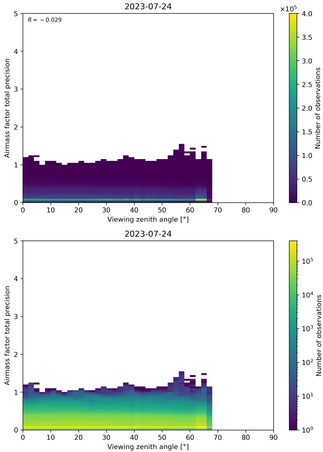
Figure 191: Scatter density plot of “Viewing zenith angle” against “Airmass factor total precision” for 2023-07-24 to 2023-07-25.
