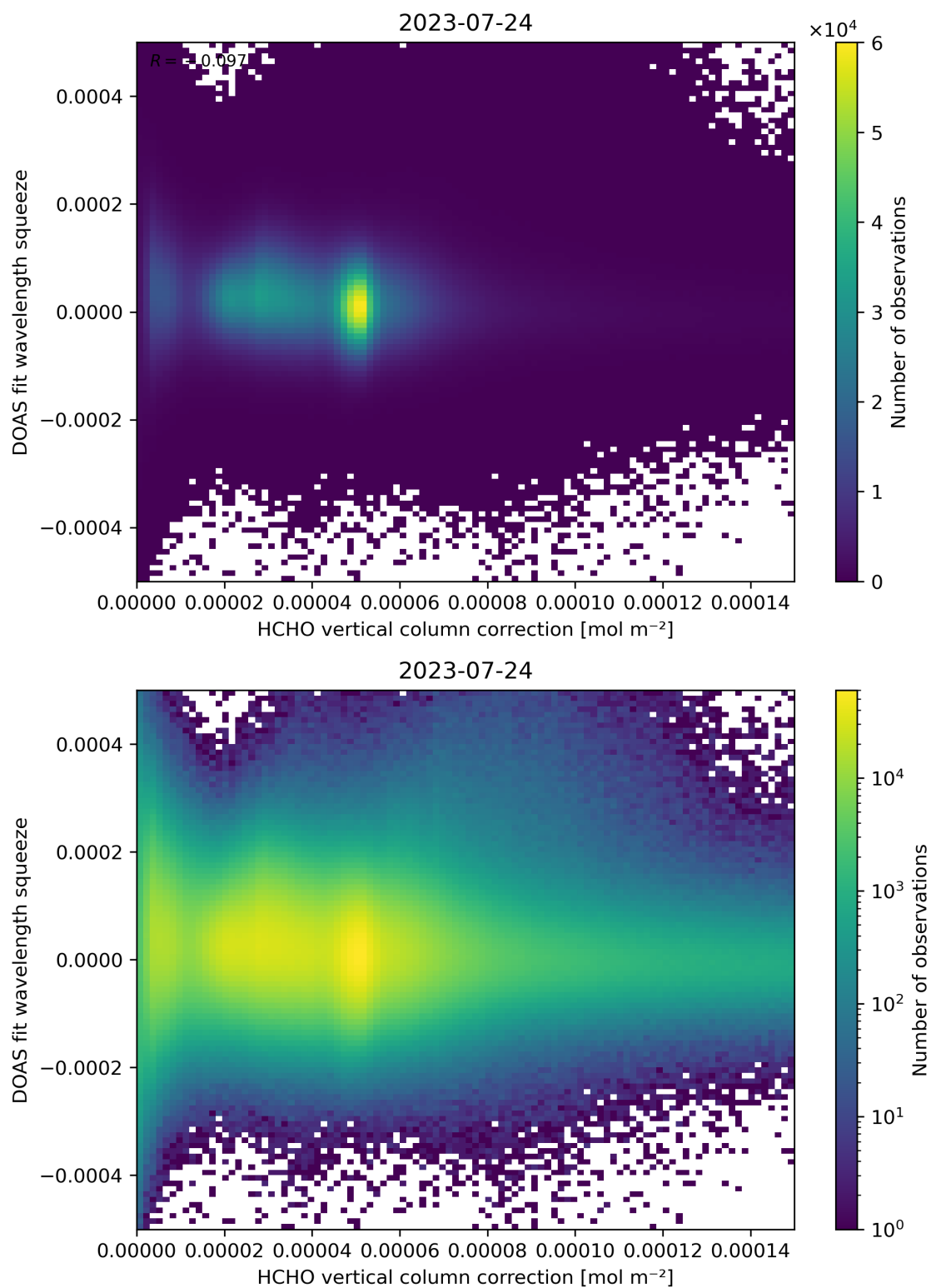
Figure 114: Scatter density plot of “HCHO vertical column correction” against “DOAS fit wavelength squeeze” for 2023-07-24 to 2023-07-25.
