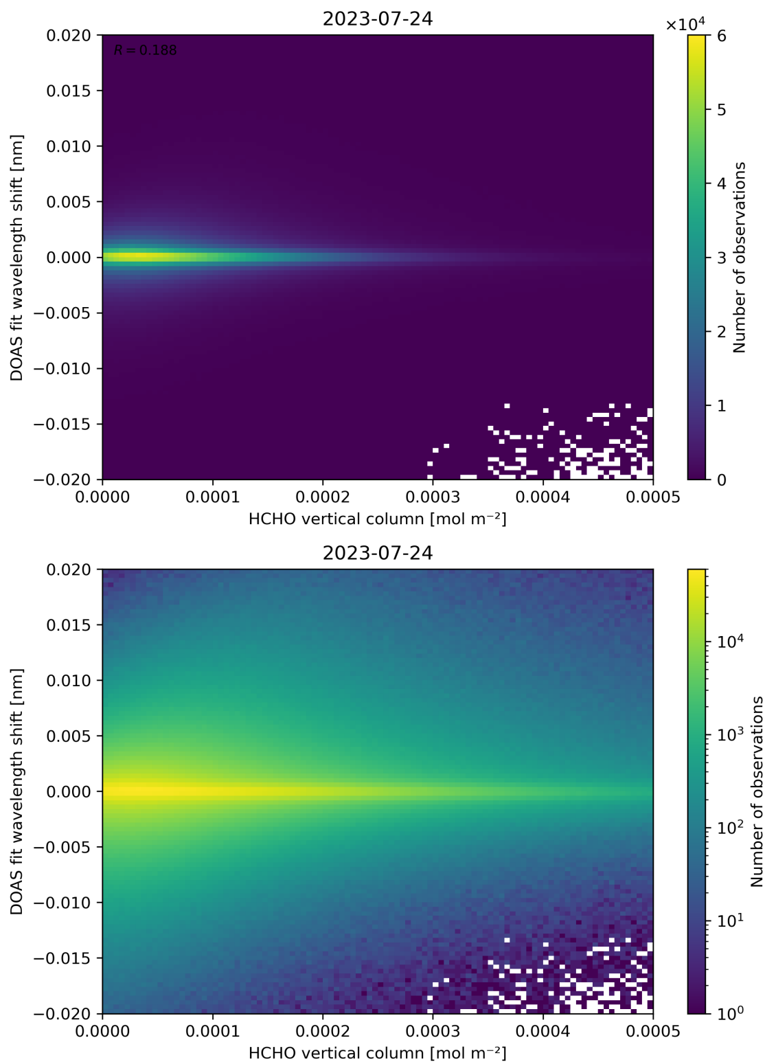
Figure 124: Scatter density plot of “HCHO vertical column” against “DOAS fit wavelength shift” for 2023-07-24 to 2023-07-25.
