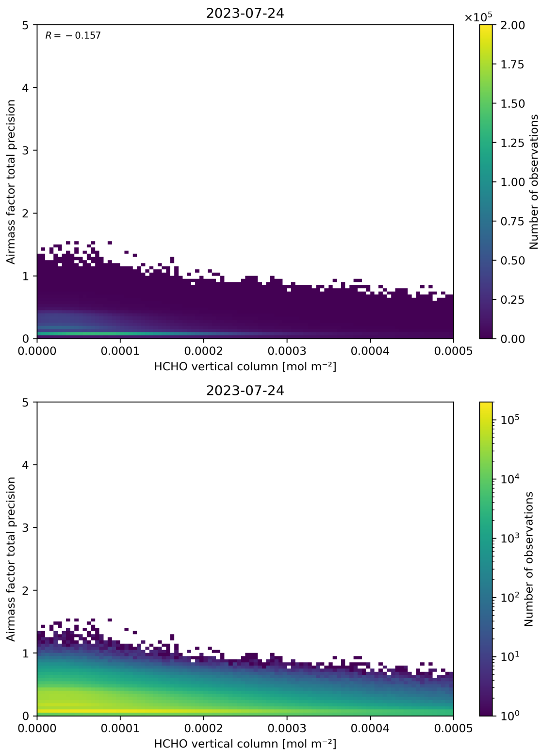
Figure 132: Scatter density plot of “HCHO vertical column” against “Airmass factor total precision” for 2023-07-24 to 2023-07-25.
