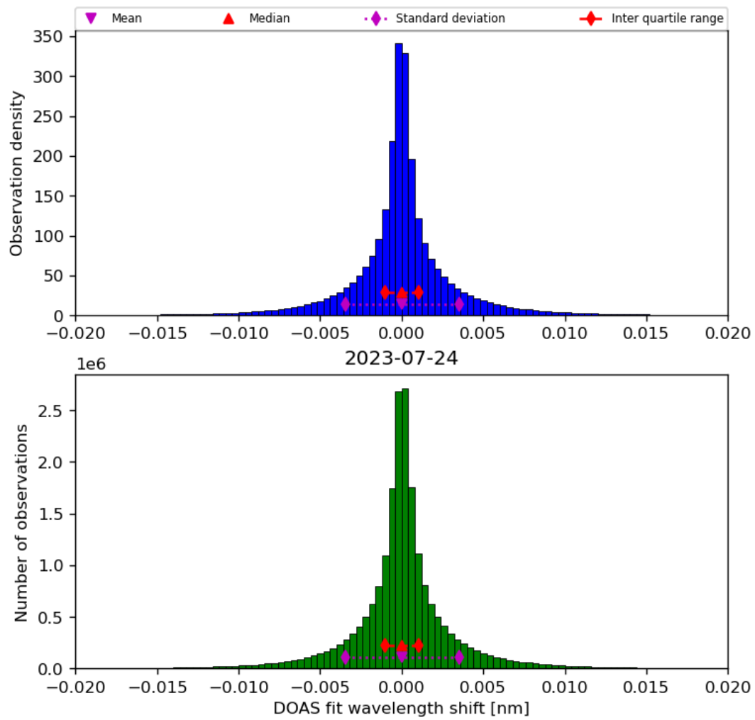
Figure 44: Histogram of “DOAS fit wavelength shift” for 2023-07-24 to 2023-07-25
