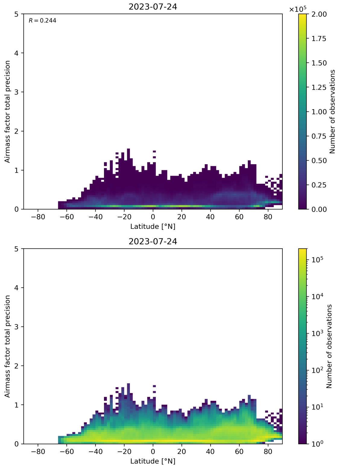
Figure 162: Scatter density plot of “Latitude” against “Airmass factor total precision” for 2023-07-24 to 2023-07-25.
