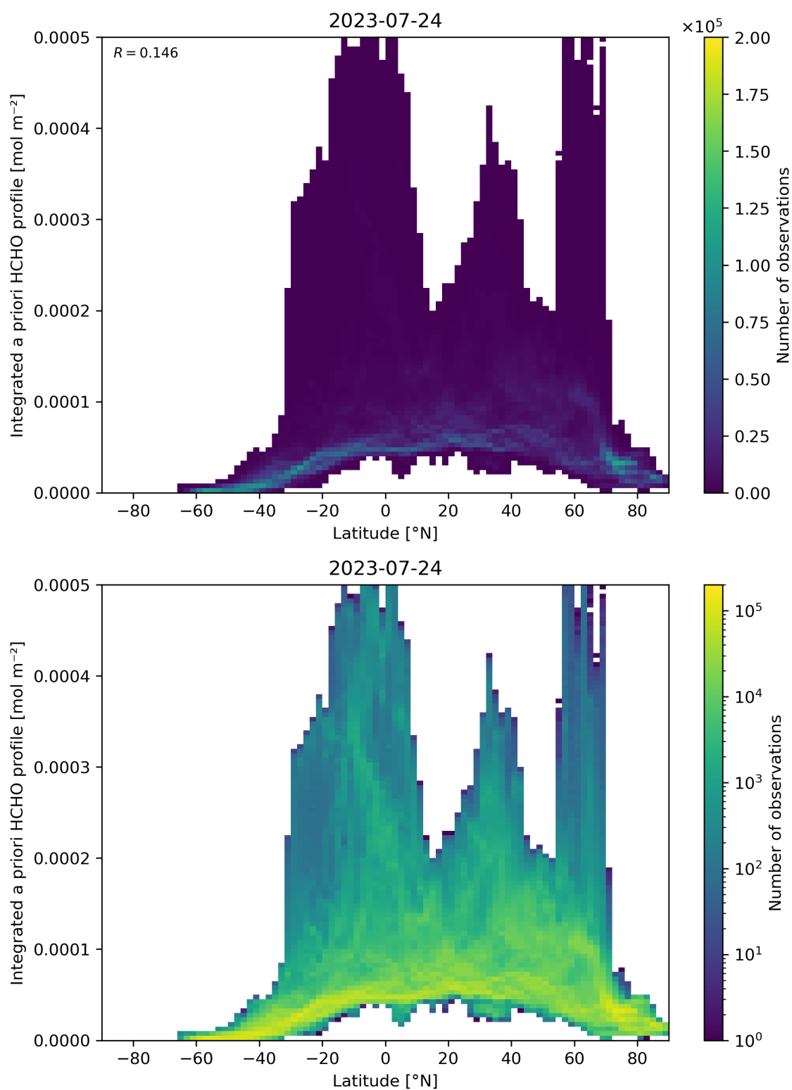
Figure 166: Scatter density plot of “Latitude” against “Integrated a priori HCHO profile” for 2023-07-24 to 2023-07-25.
