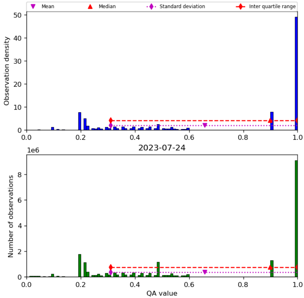
Figure 34: Histogram of “QA value” for 2023-07-24 to 2023-07-25
