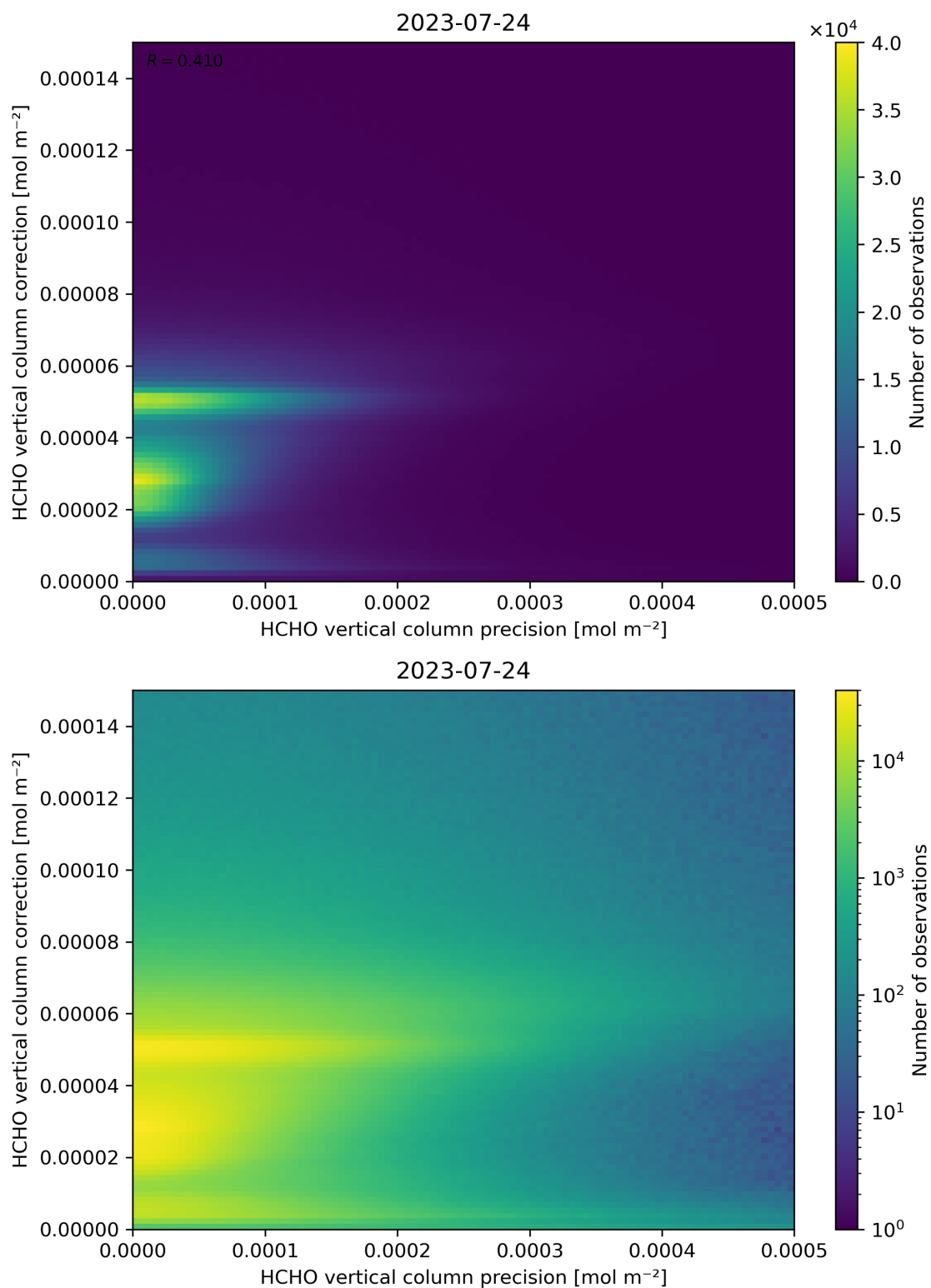
Figure 146: Scatter density plot of “HCHO vertical column precision” against “HCHO vertical column correction” for 2023-07-24 to 2023-07-25.
