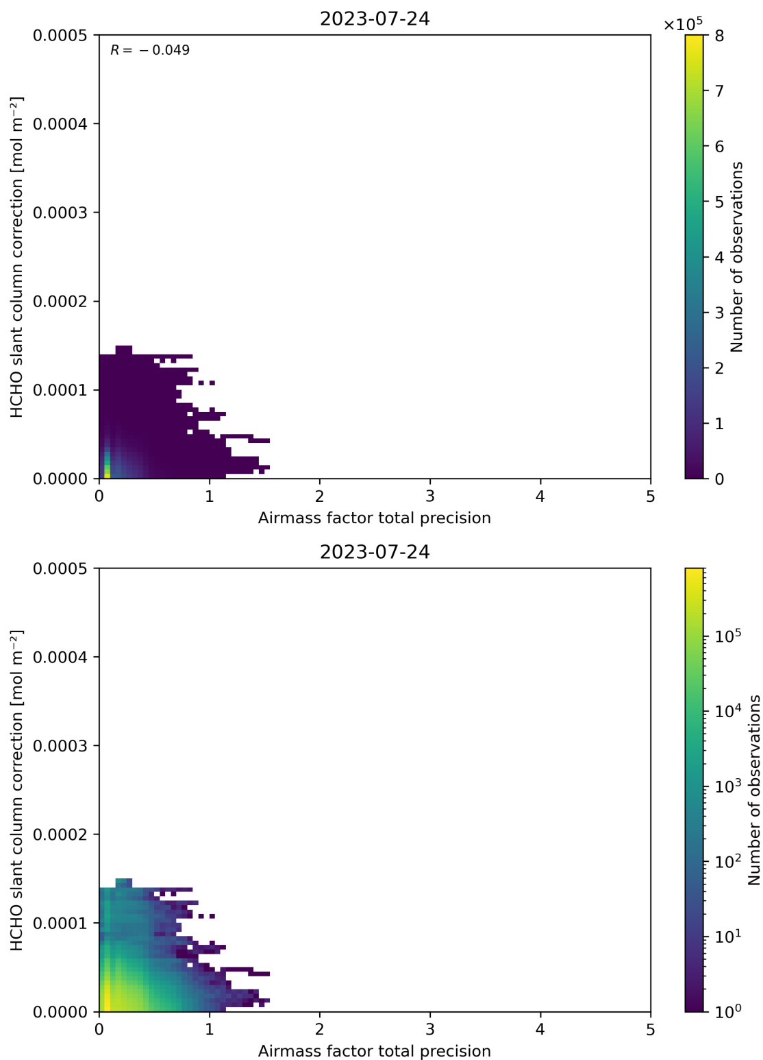
Figure 110: Scatter density plot of “Airmass factor total precision” against “HCHO slant column correction” for 2023-07-24 to 2023-07-25.
