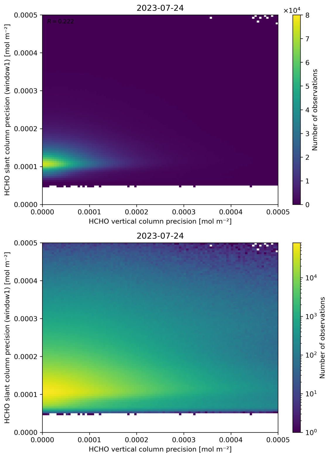
Figure 143: Scatter density plot of “HCHO vertical column precision” against “HCHO slant column precision (window1)” for 2023-07-24 to 2023-07-25.
