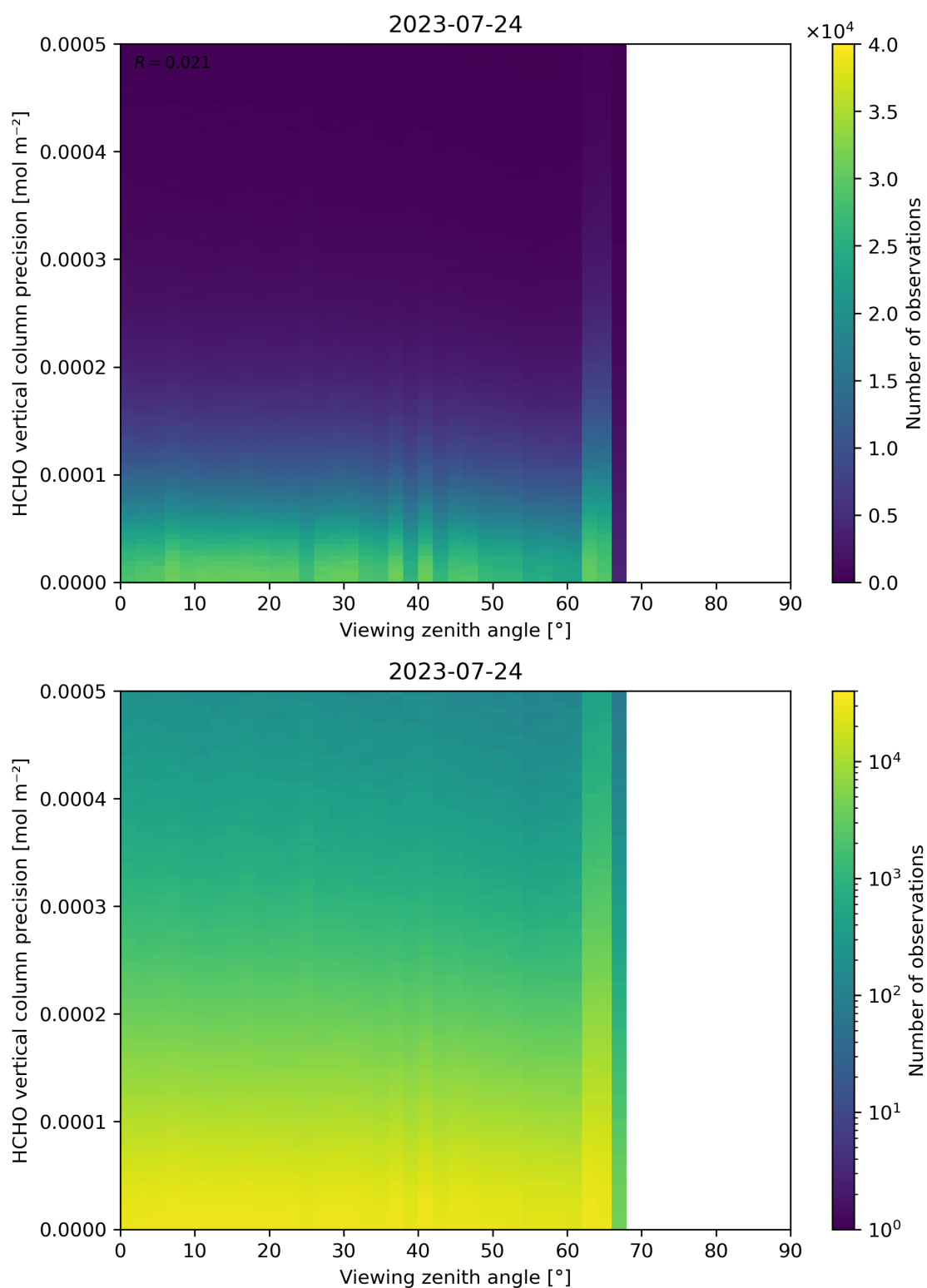
Figure 194: Scatter density plot of “Viewing zenith angle” against “HCHO vertical column precision” for 2023-07-24 to 2023-07-25.
