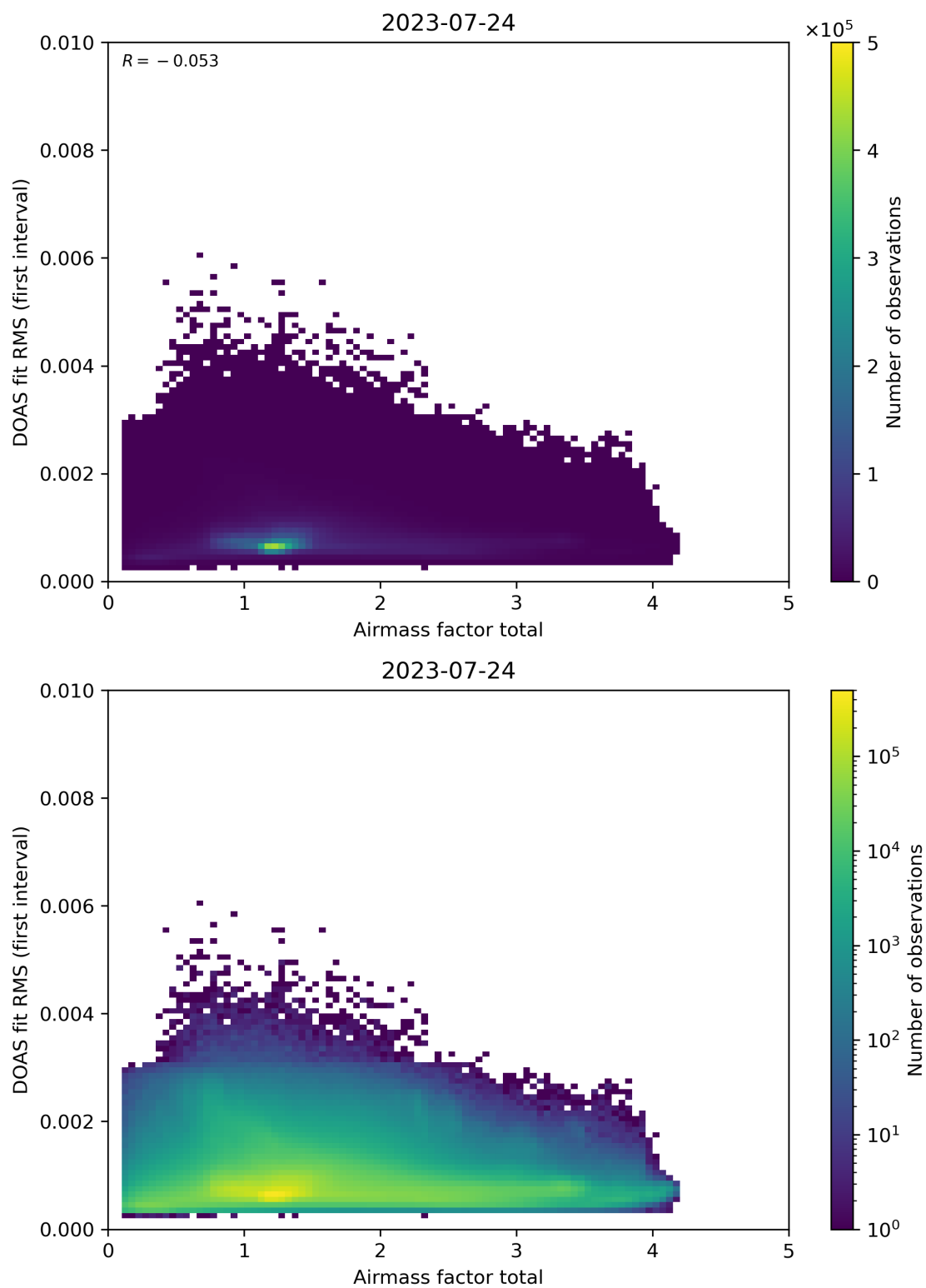
Figure 97: Scatter density plot of “Airmass factor total” against “DOAS fit RMS (first interval)” for 2023-07-24 to 2023-07-25.
