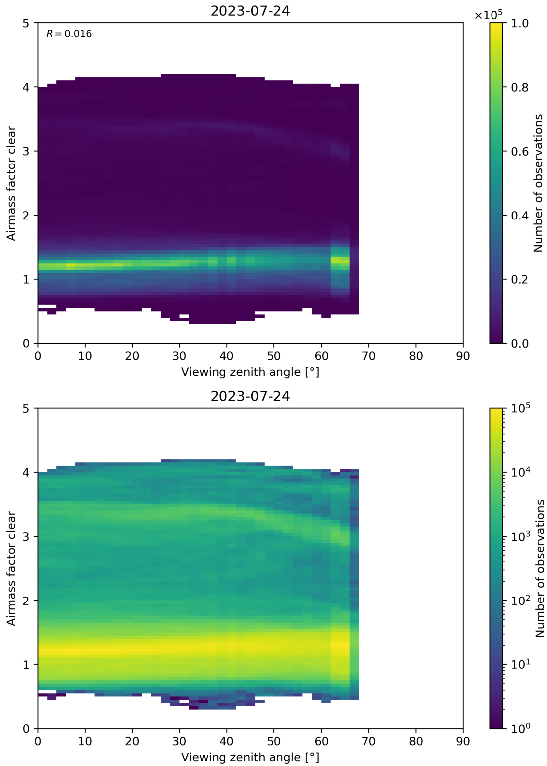
Figure 185: Scatter density plot of “Viewing zenith angle” against “Airmass factor clear” for 2023-07-24 to 2023-07-25.
