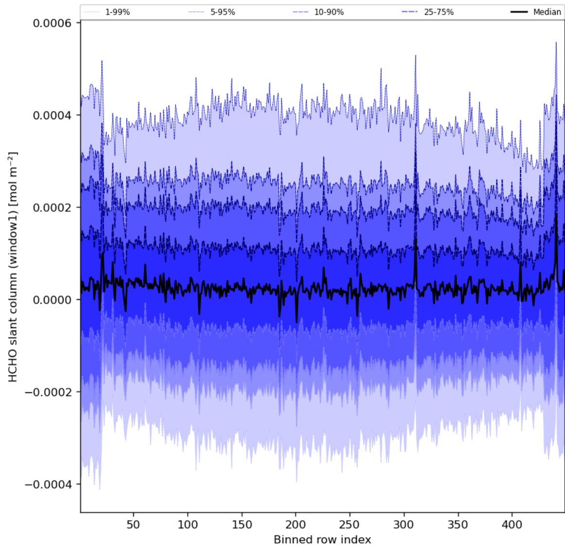
Figure 52: Along track statistics of “HCHO slant column (window1)” for 2023-07-24 to 2023-07-25
