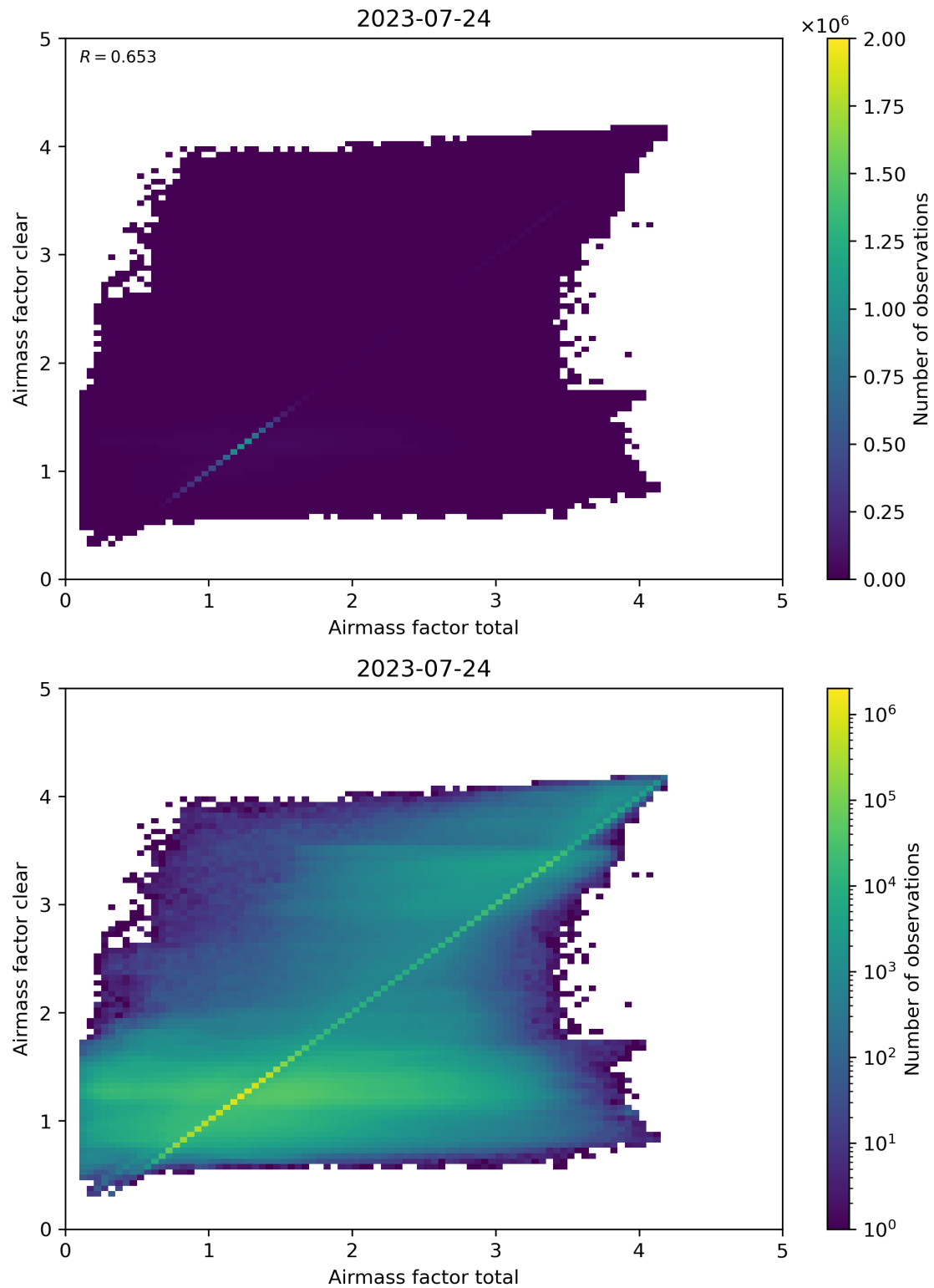
Figure 100: Scatter density plot of “Airmass factor total” against “Airmass factor clear” for 2023-07-24 to 2023-07-25.
