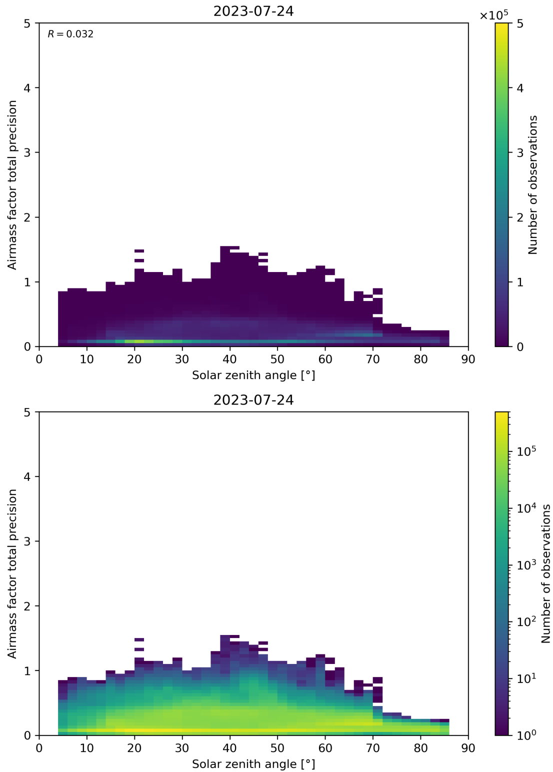
Figure 176: Scatter density plot of “Solar zenith angle” against “Airmass factor total precision” for 2023-07-24 to 2023-07-25.
