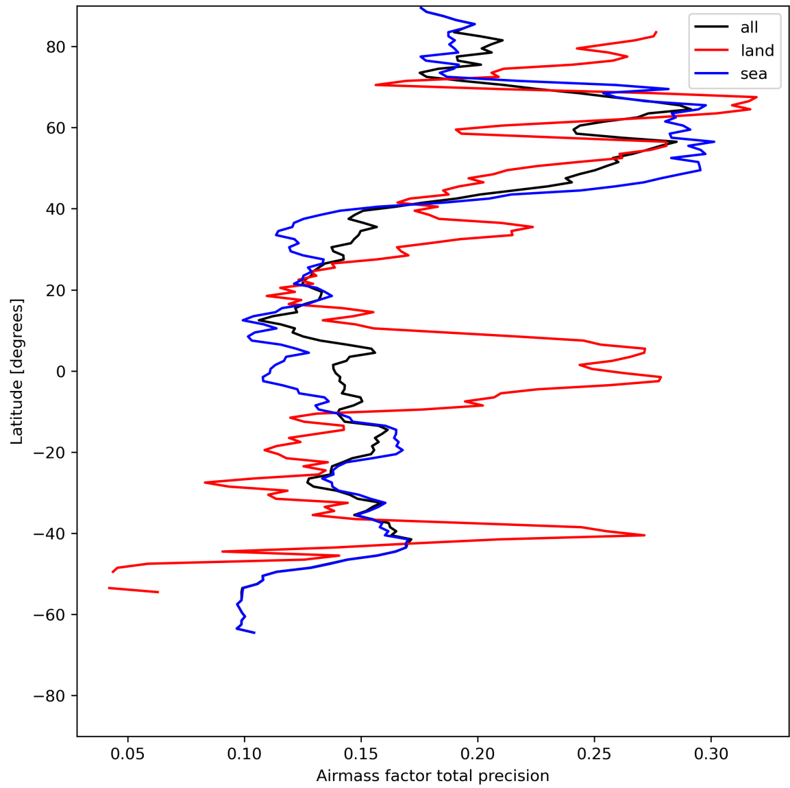
Figure 27: Zonal average of “Airmass factor total precision” for 2023-07-24 to 2023-07-25.
