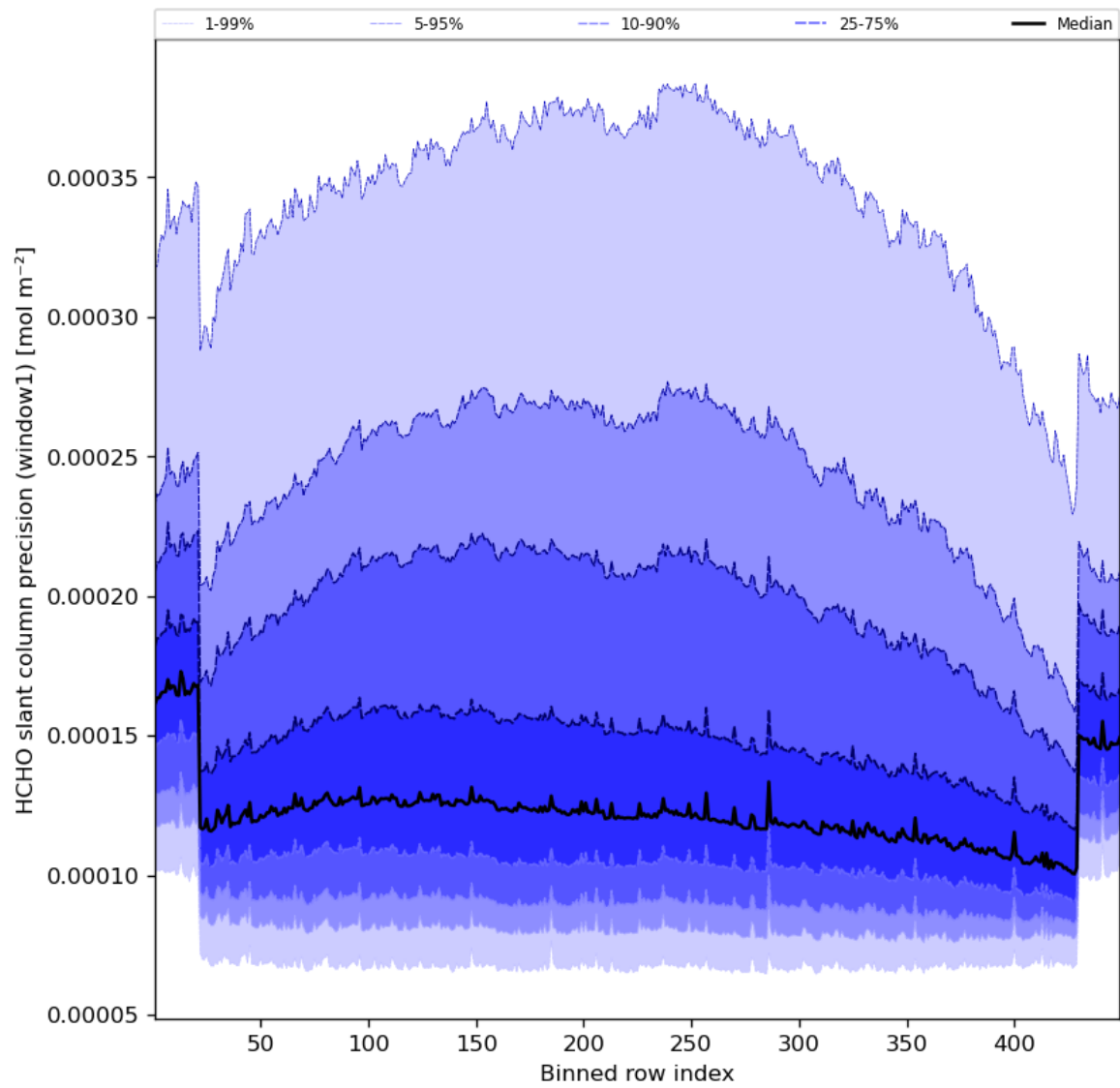
Figure 53: Along track statistics of “HCHO slant column precision (window1)” for 2023-07-24 to 2023-07-25
