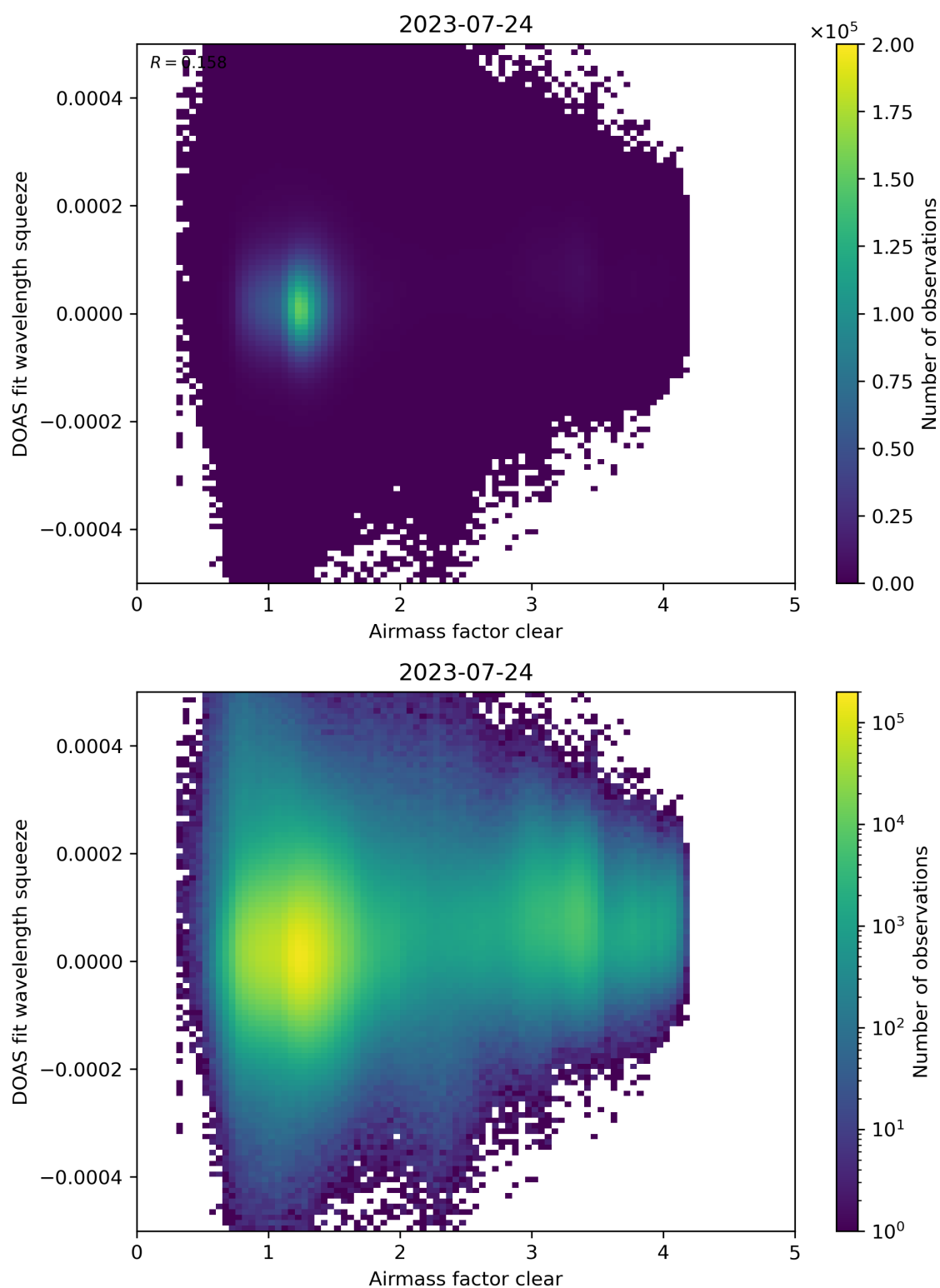
Figure 73: Scatter density plot of “Airmass factor clear” against “DOAS fit wavelength squeeze” for 2023-07-24 to 2023-07-25.
