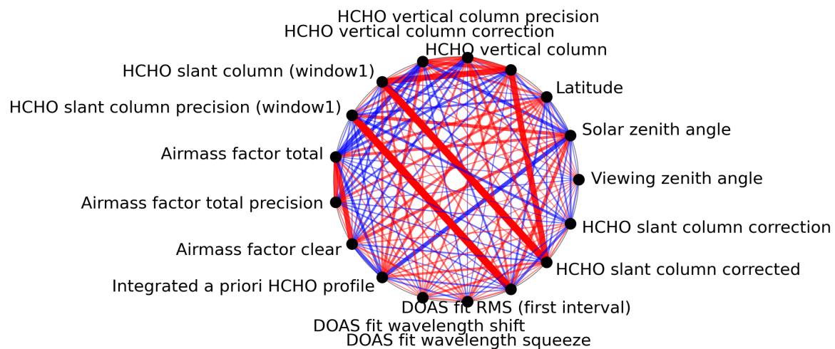
Figure 1: Map of correlation graph for 2023-07-24 to 2023-07-25.
