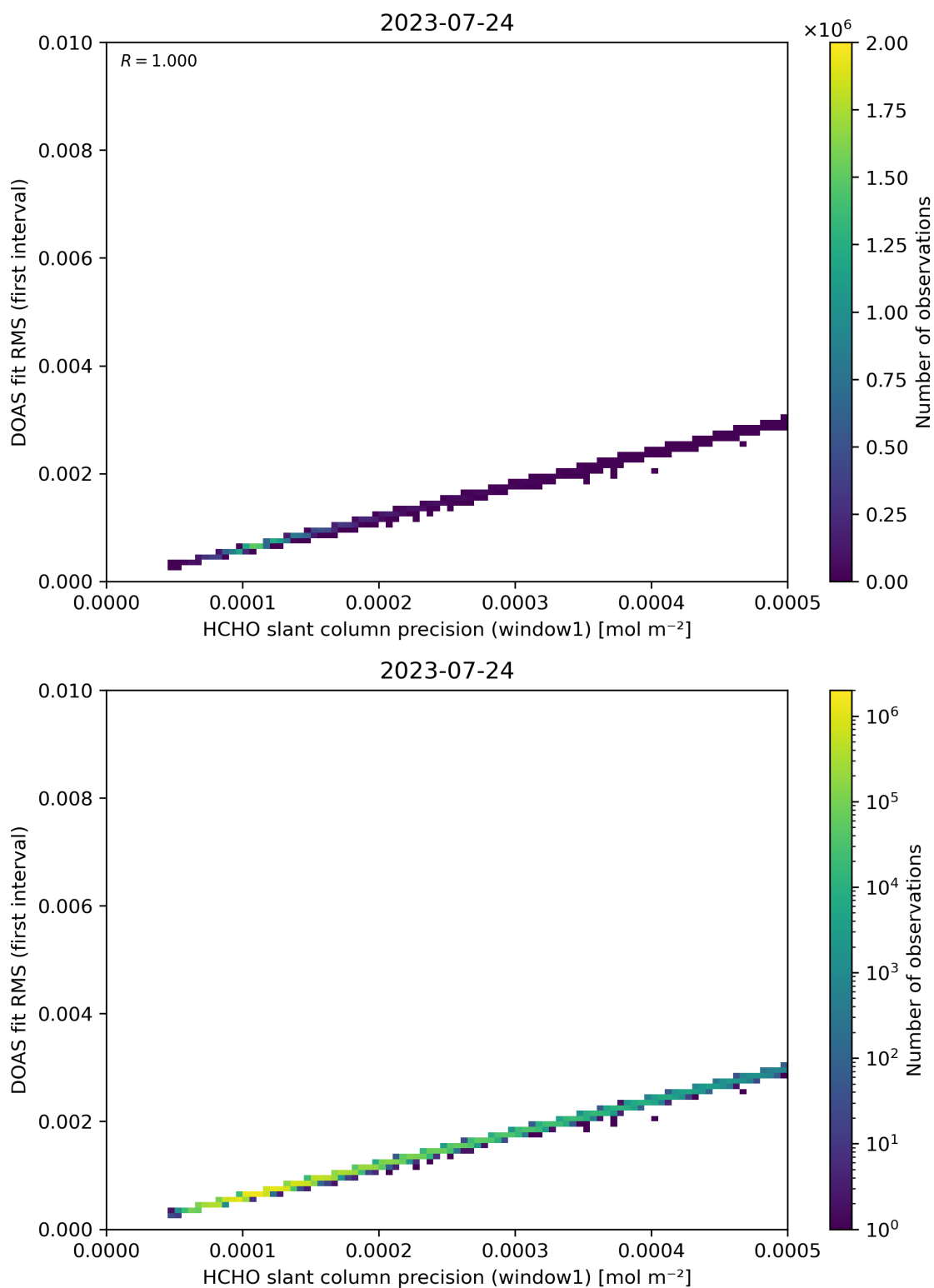
Figure 88: Scatter density plot of “HCHO slant column precision (window1)” against “DOAS fit RMS (first interval)” for 2023-07-24 to 2023-07-25.
