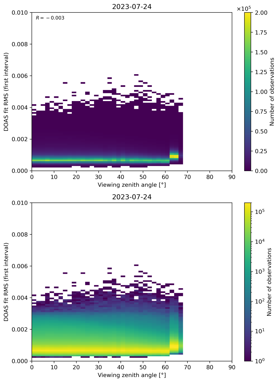
Figure 182: Scatter density plot of “Viewing zenith angle” against “DOAS fit RMS (first interval)” for 2023-07-24 to 2023-07-25.
