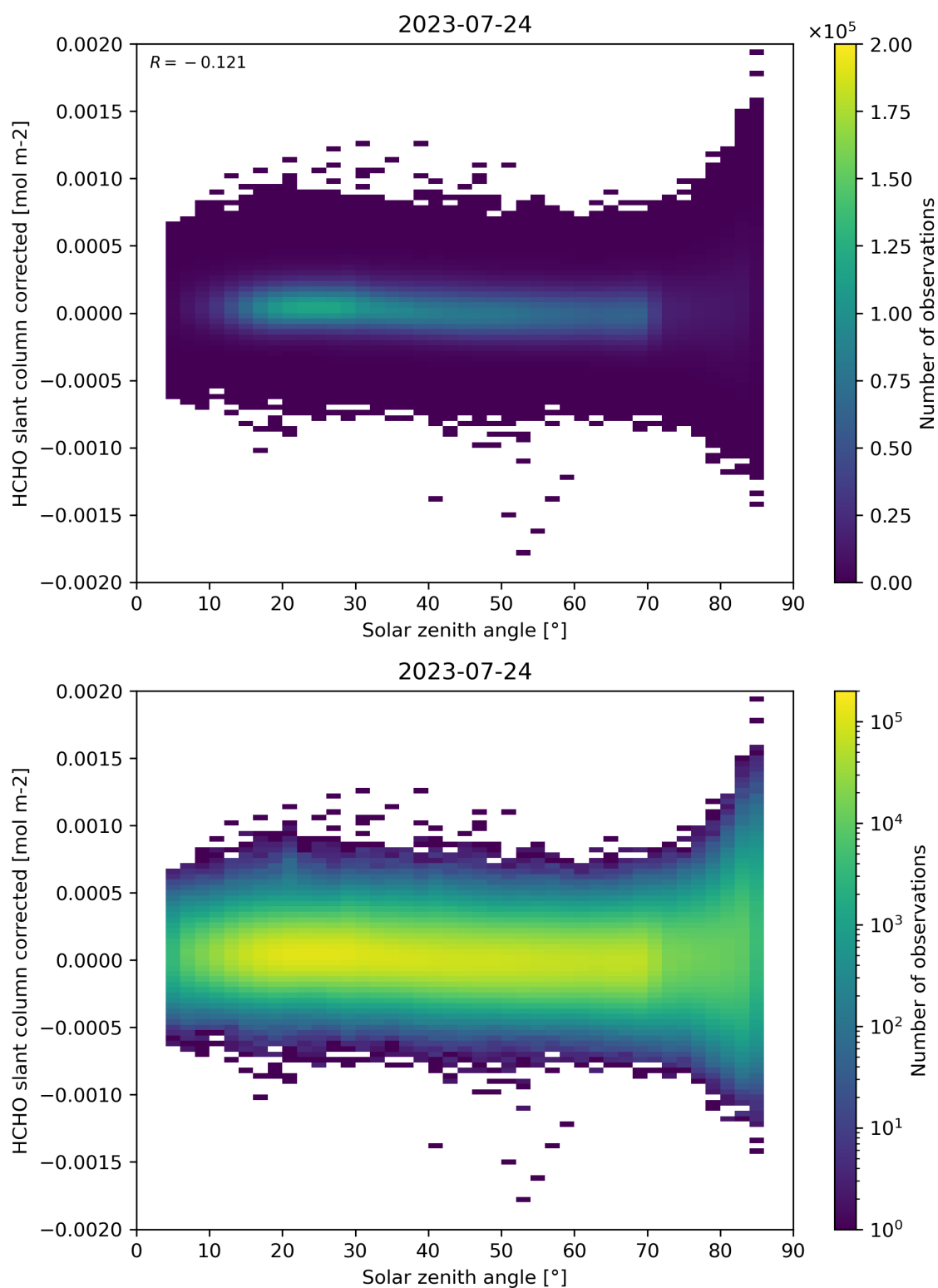
Figure 171: Scatter density plot of “Solar zenith angle” against “HCHO slant column corrected” for 2023-07-24 to 2023-07-25.
