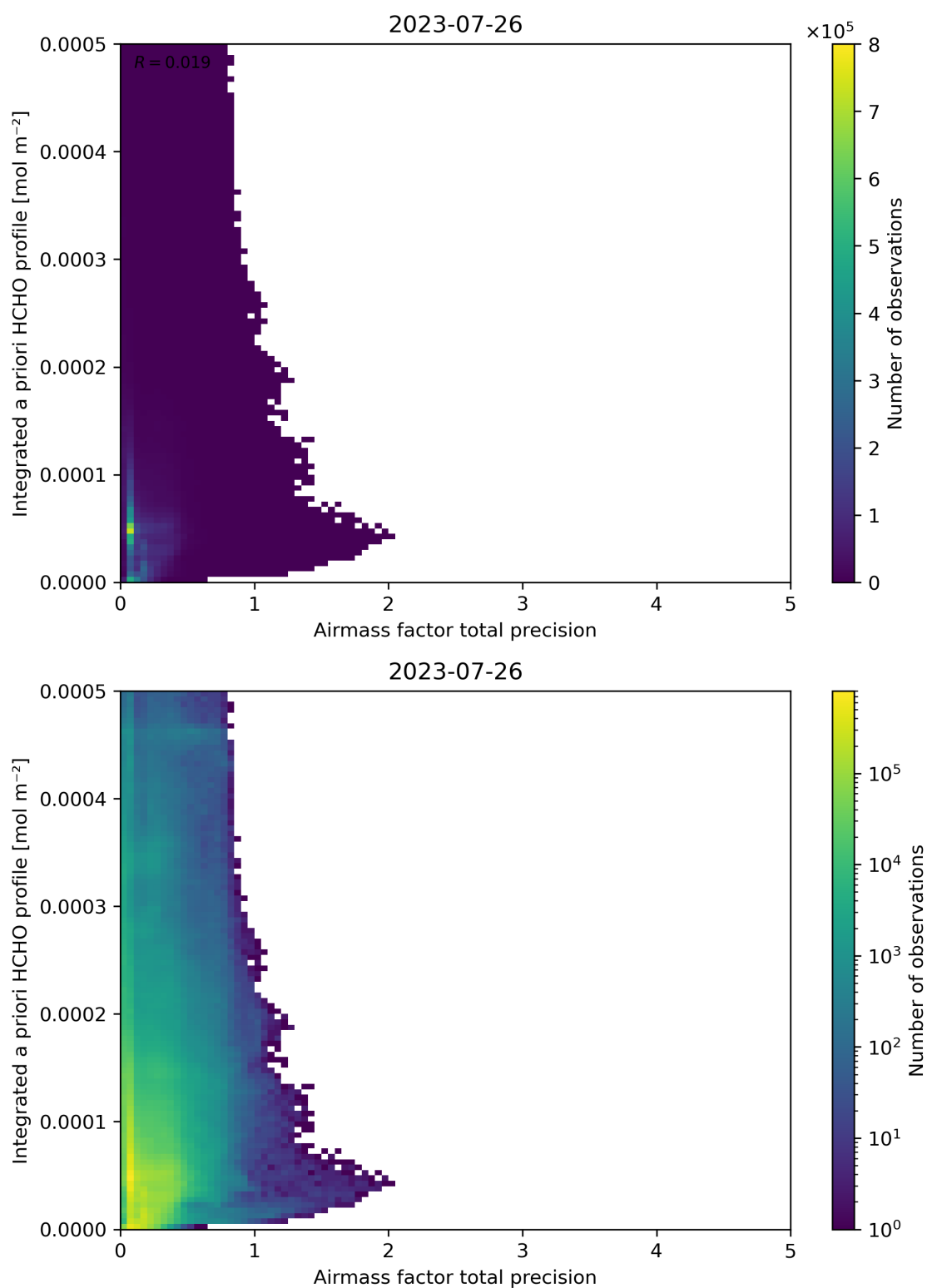
Figure 111: Scatter density plot of “Airmass factor total precision” against “Integrated a priori HCHO profile” for 2023-07-25 to 2023-07-27.
