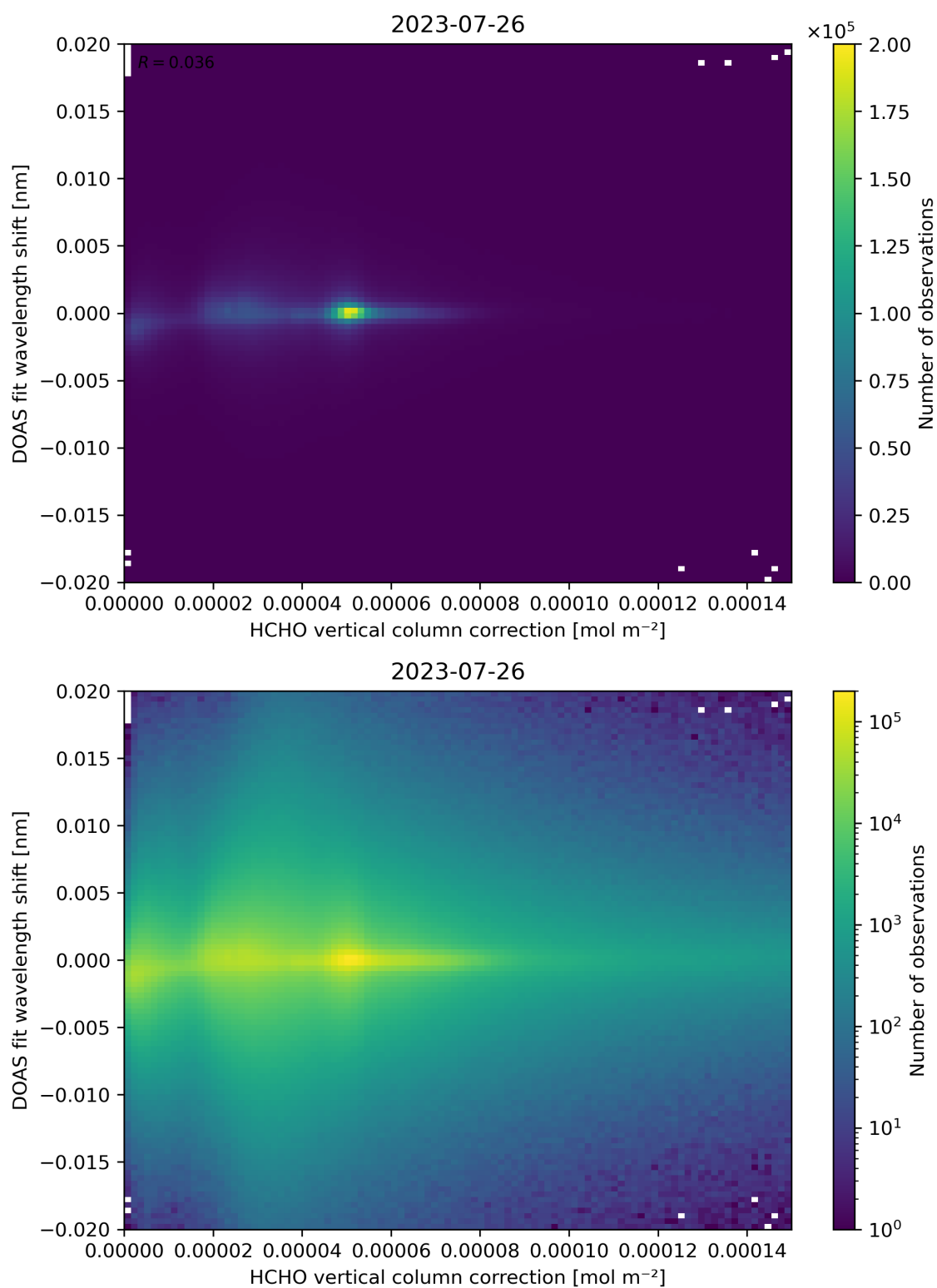
Figure 113: Scatter density plot of “HCHO vertical column correction” against “DOAS fit wavelength shift” for 2023-07-25 to 2023-07-27.
