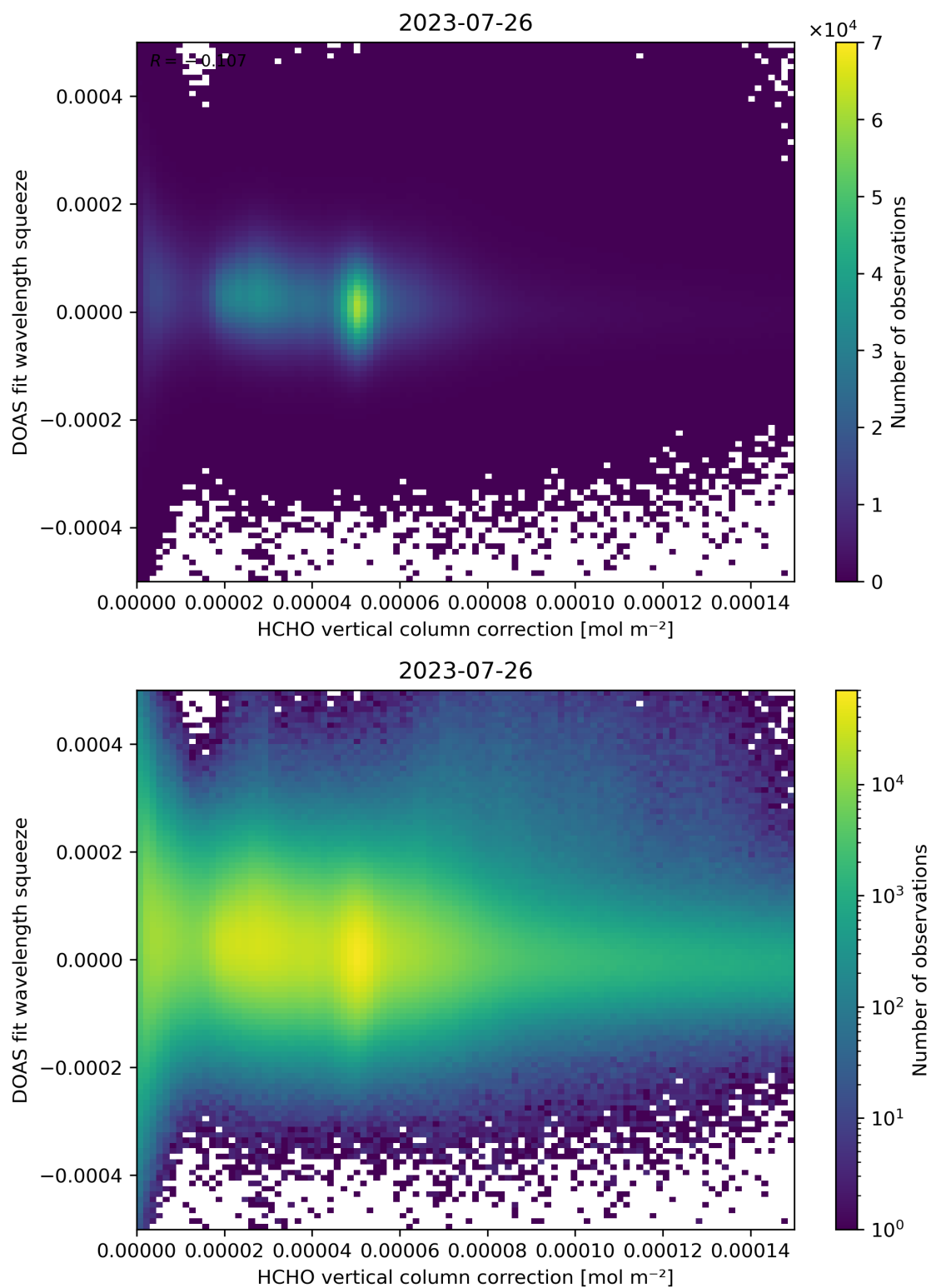
Figure 114: Scatter density plot of “HCHO vertical column correction” against “DOAS fit wavelength squeeze” for 2023-07-25 to 2023-07-27.
