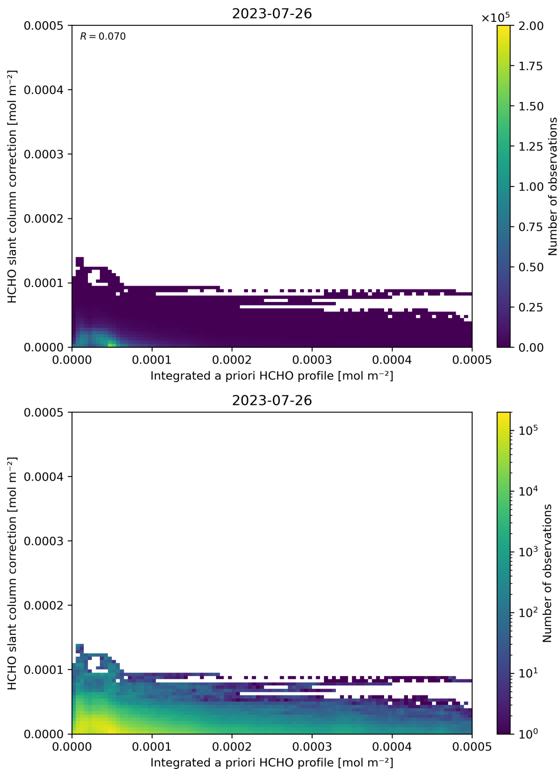
Figure 152: Scatter density plot of “Integrated a priori HCHO profile” against “HCHO slant column correction” for 2023-07-25 to 2023-07-27.
