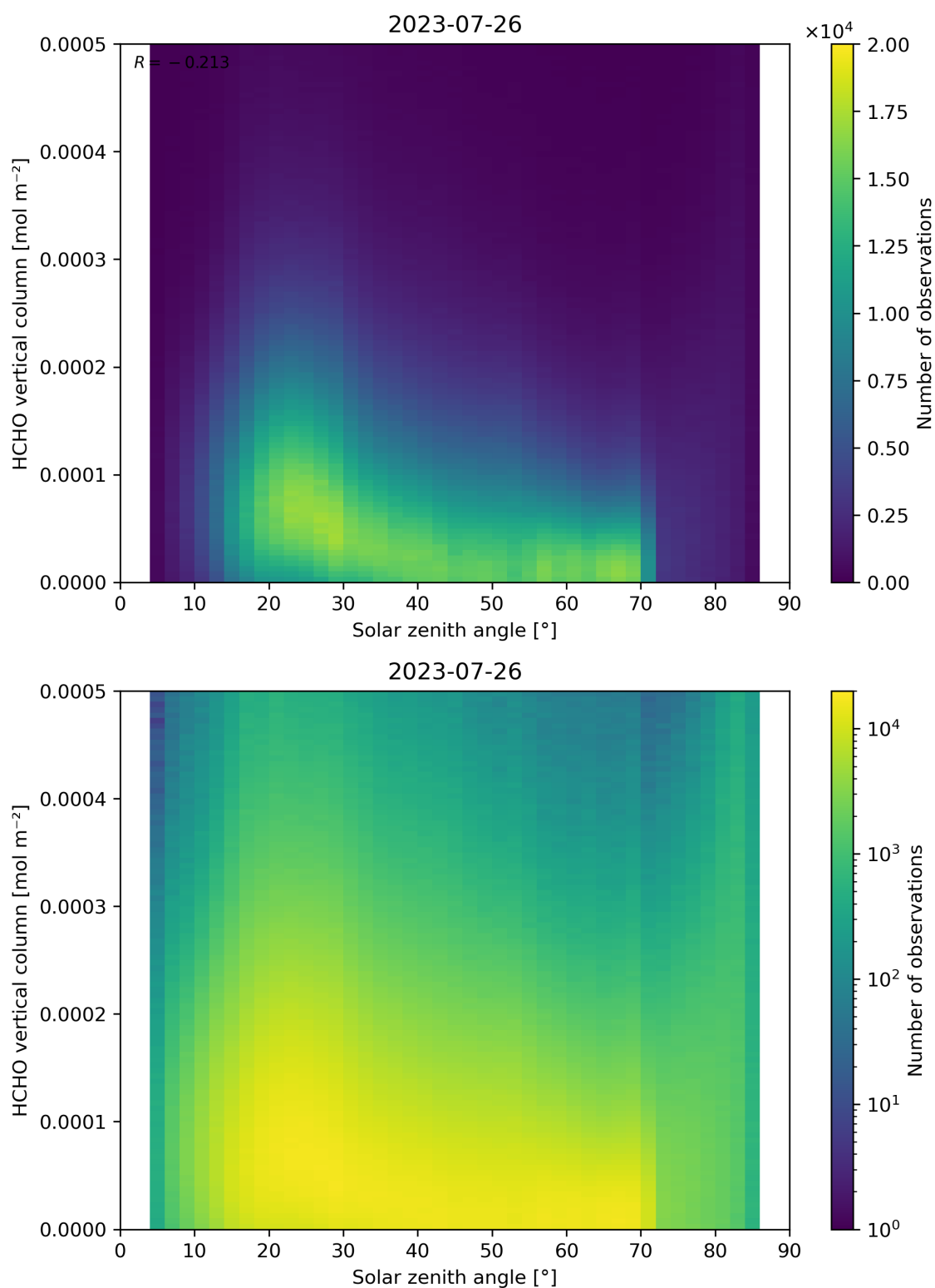
Figure 177: Scatter density plot of “Solar zenith angle” against “HCHO vertical column” for 2023-07-25 to 2023-07-27.
