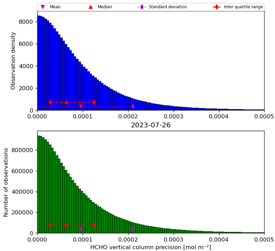
Figure 36: Histogram of “HCHO vertical column precision” for 2023-07-25 to 2023-07-27
