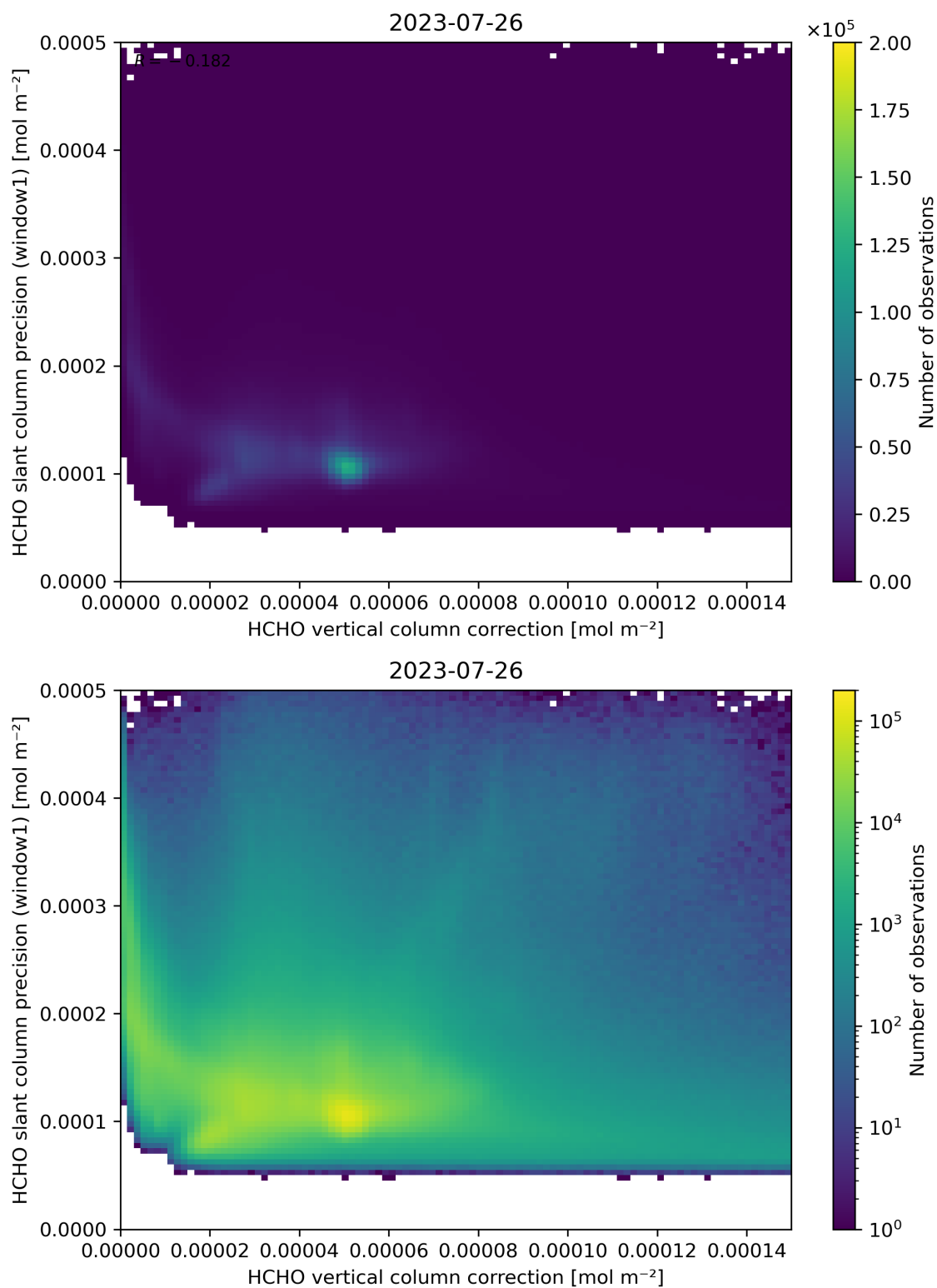
Figure 119: Scatter density plot of “HCHO vertical column correction” against “HCHO slant column precision (window1)” for 2023-07-25 to 2023-07-27.
