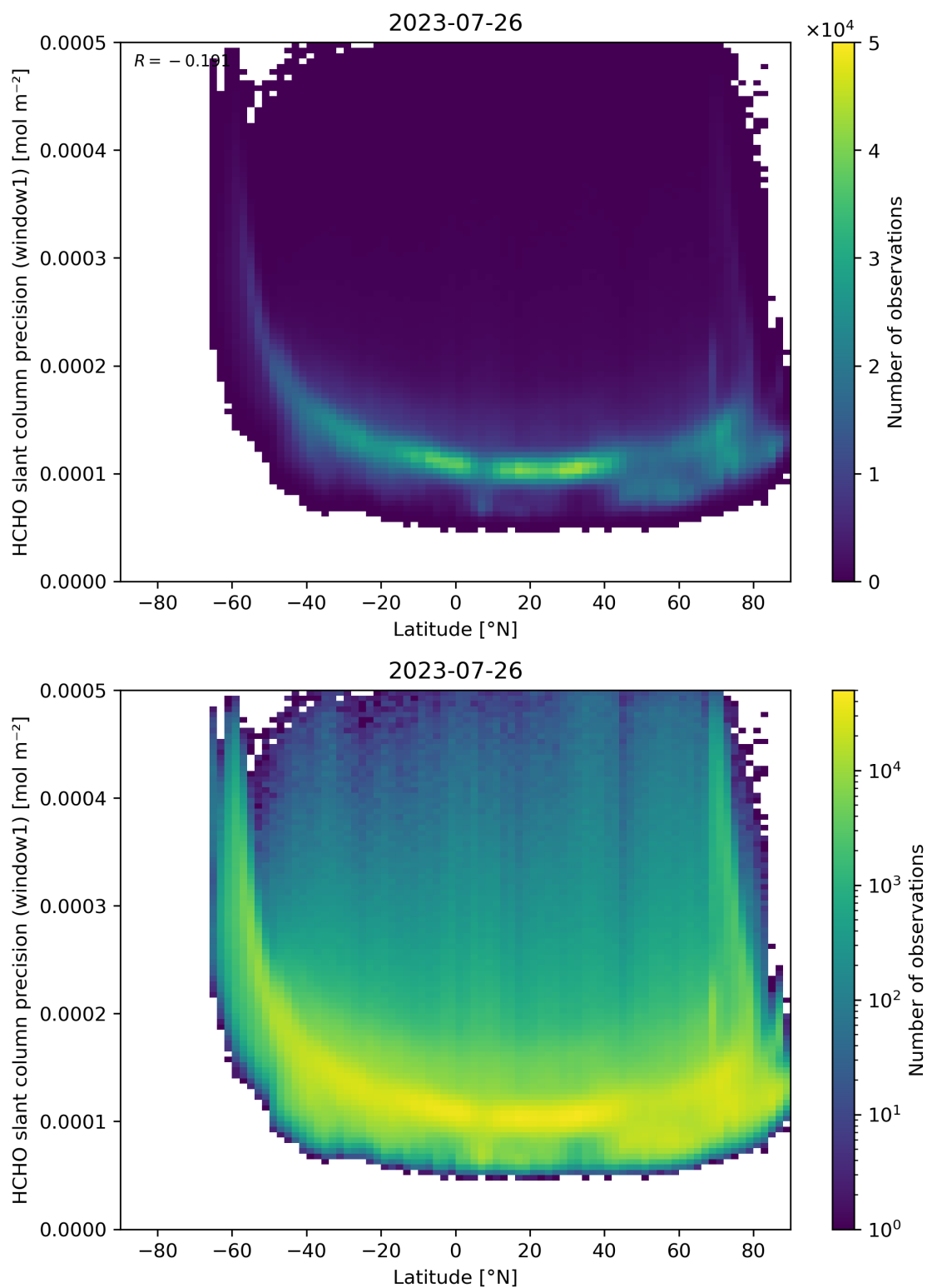
Figure 160: Scatter density plot of “Latitude” against “HCHO slant column precision (window1)” for 2023-07-25 to 2023-07-27.
