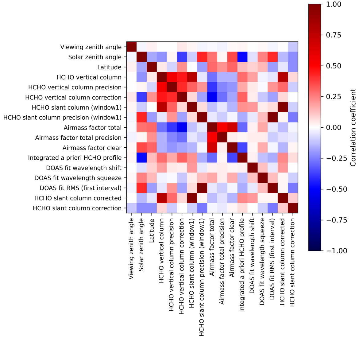
Figure 2: Map of correlation matrix for 2023-07-25 to 2023-07-27.
