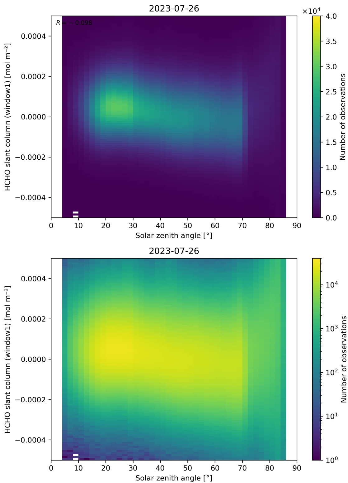
Figure 173: Scatter density plot of “Solar zenith angle” against “HCHO slant column (window1)” for 2023-07-25 to 2023-07-27.
