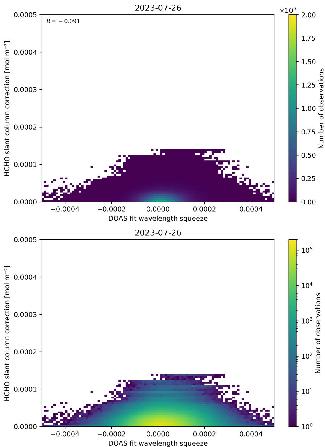
Figure 70: Scatter density plot of “DOAS fit wavelength squeeze” against “HCHO slant column correction” for 2023-07-25 to 2023-07-27.
