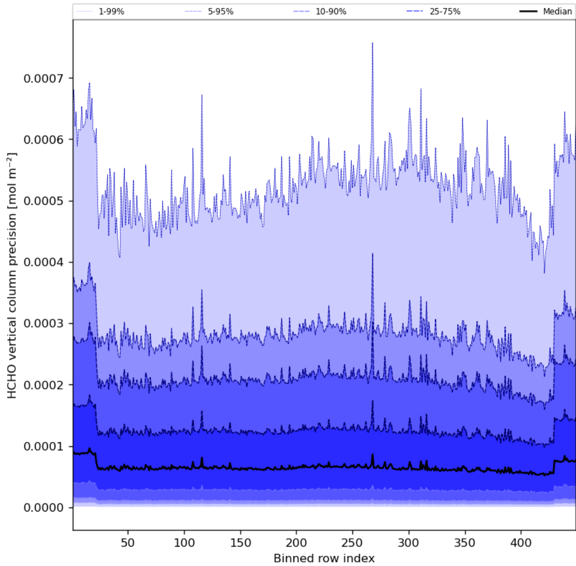
Figure 50: Along track statistics of “HCHO vertical column precision” for 2023-07-25 to 2023-07-27
