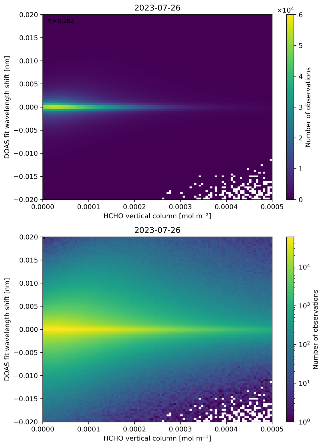
Figure 124: Scatter density plot of “HCHO vertical column” against “DOAS fit wavelength shift” for 2023-07-25 to 2023-07-27.
