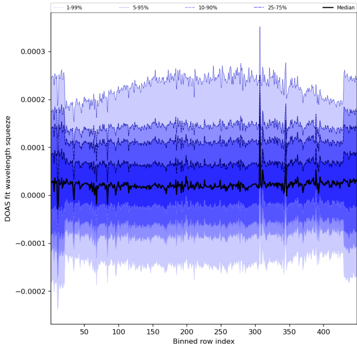
Figure 59: Along track statistics of “DOAS fit wavelength squeeze” for 2023-07-25 to 2023-07-27
