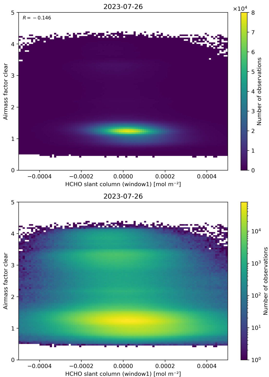
Figure 81: Scatter density plot of “HCHO slant column (window1)” against “Airmass factor clear” for 2023-07-25 to 2023-07-27.
