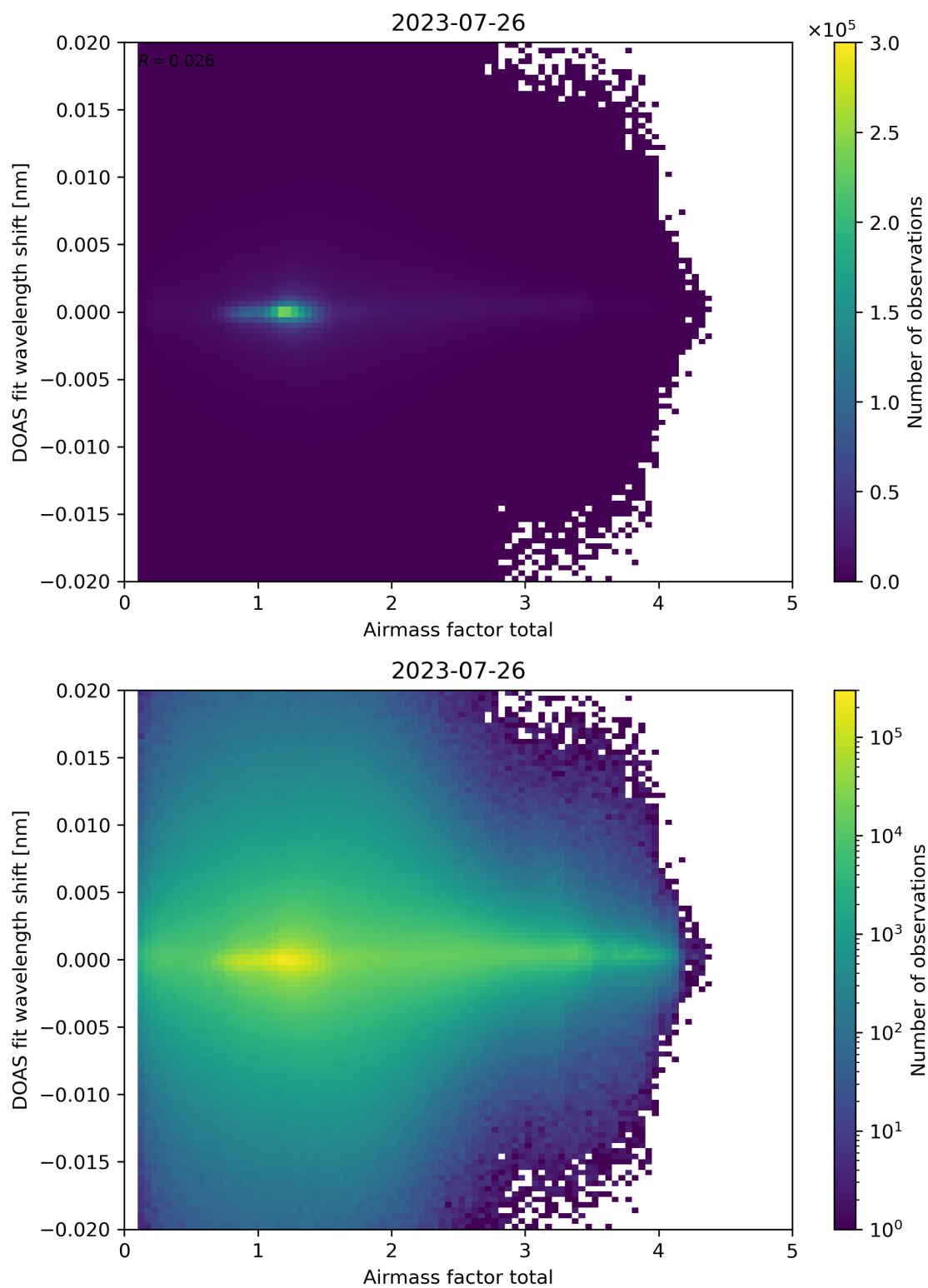
Figure 98: Scatter density plot of “Airmass factor total” against “DOAS fit wavelength shift” for 2023-07-25 to 2023-07-27.
