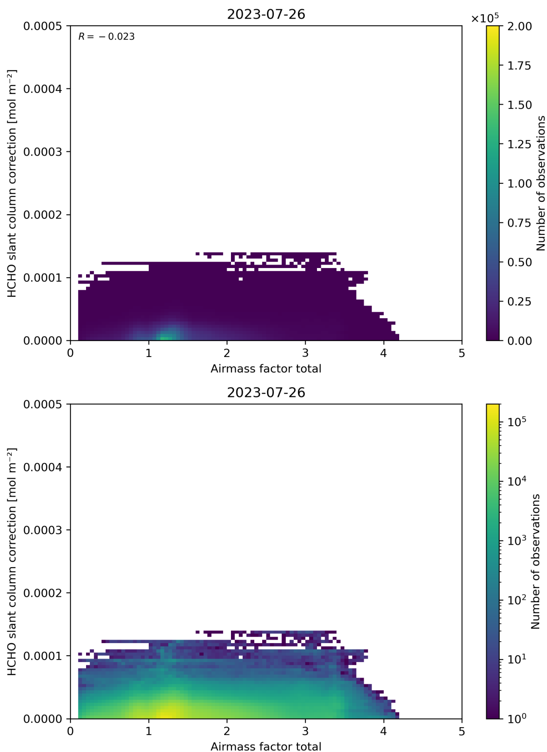
Figure 102: Scatter density plot of “Airmass factor total” against “HCHO slant column correction” for 2023-07-25 to 2023-07-27.
