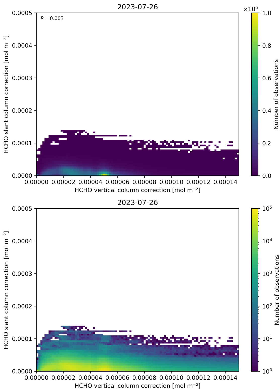
Figure 117: Scatter density plot of “HCHO vertical column correction” against “HCHO slant column correction” for 2023-07-25 to 2023-07-27.
