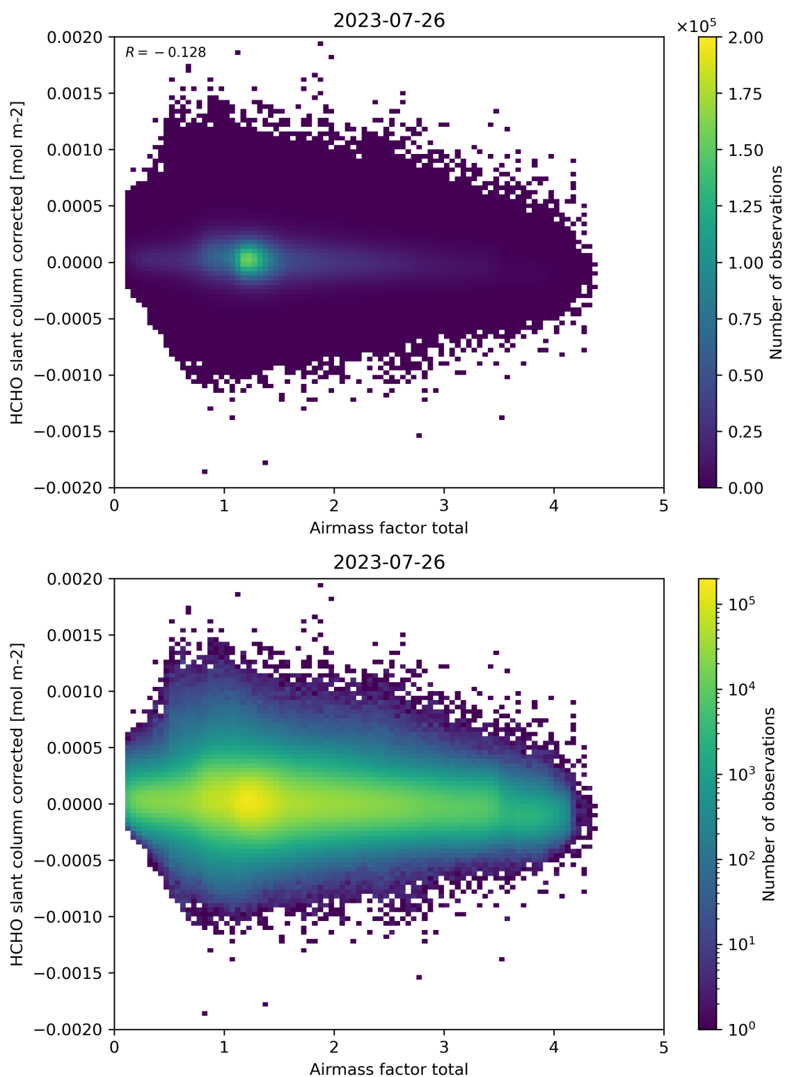
Figure 101: Scatter density plot of “Airmass factor total” against “HCHO slant column corrected” for 2023-07-25 to 2023-07-27.
