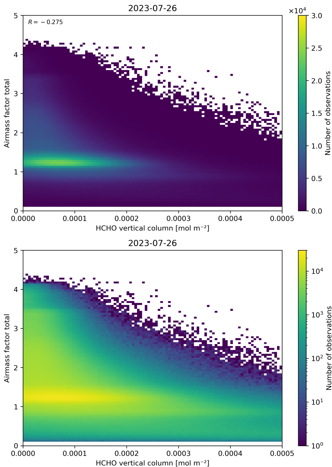
Figure 131: Scatter density plot of “HCHO vertical column” against “Airmass factor total” for 2023-07-25 to 2023-07-27.
