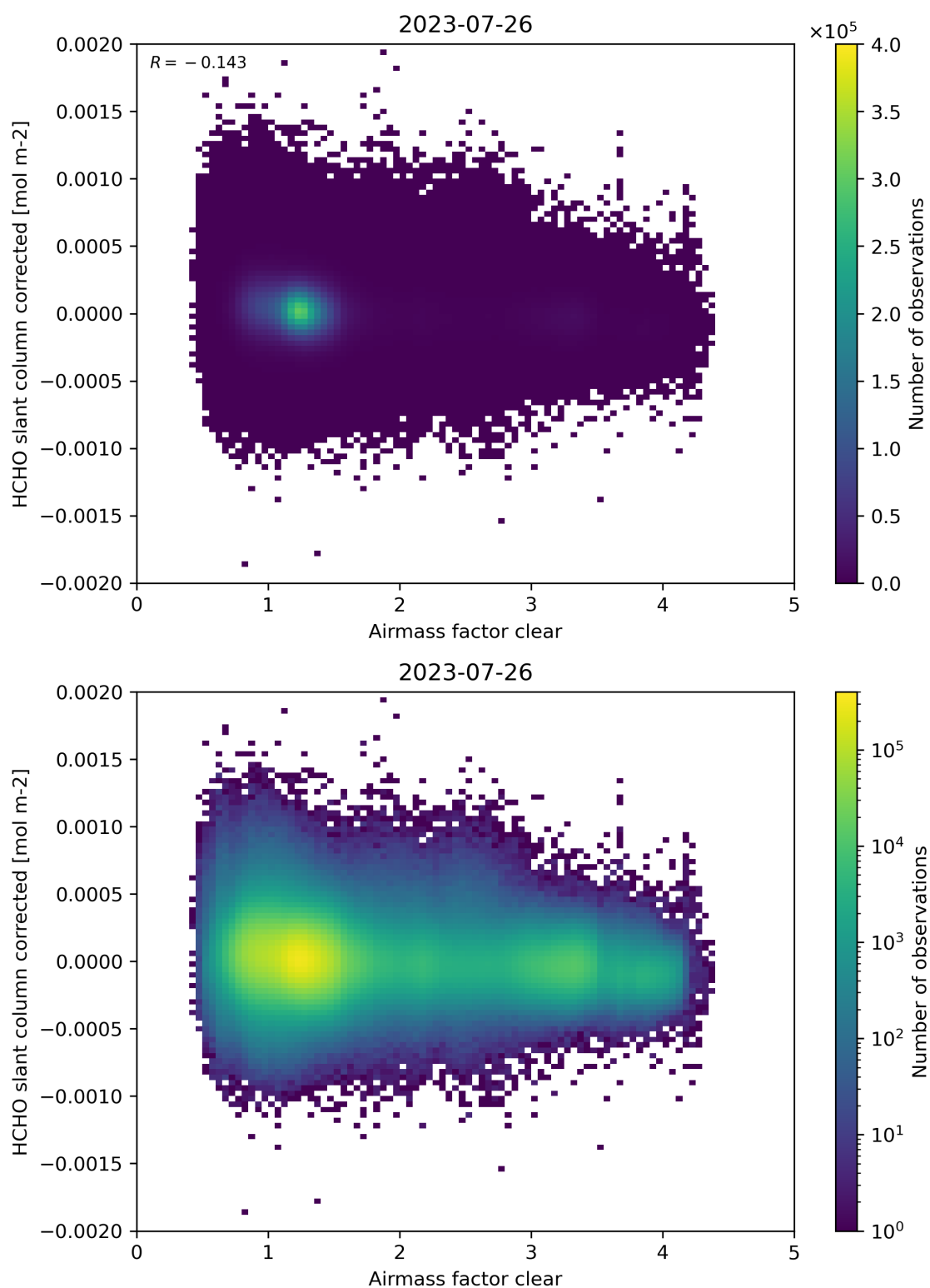
Figure 74: Scatter density plot of “Airmass factor clear” against “HCHO slant column corrected” for 2023-07-25 to 2023-07-27.
