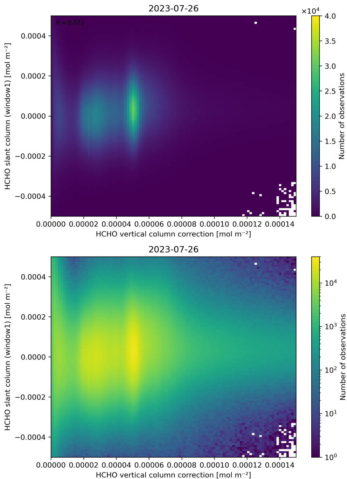
Figure 118: Scatter density plot of “HCHO vertical column correction” against “HCHO slant column (window1)” for 2023-07-25 to 2023-07-27.
