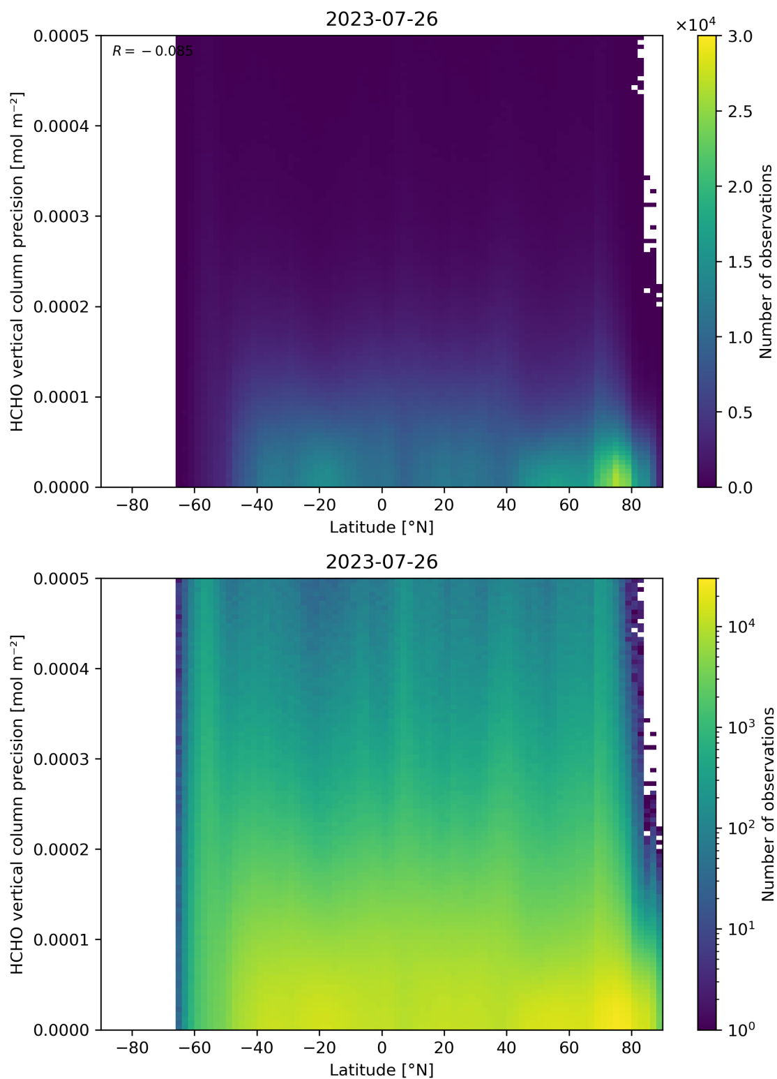
Figure 165: Scatter density plot of “Latitude” against “HCHO vertical column precision” for 2023-07-25 to 2023-07-27.
