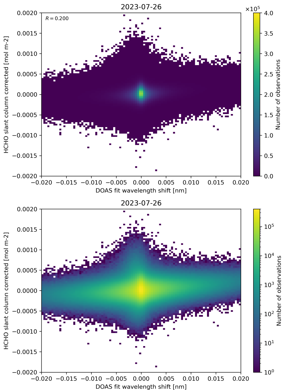
Figure 66: Scatter density plot of “DOAS fit wavelength shift” against “HCHO slant column corrected” for 2023-07-25 to 2023-07-27.
