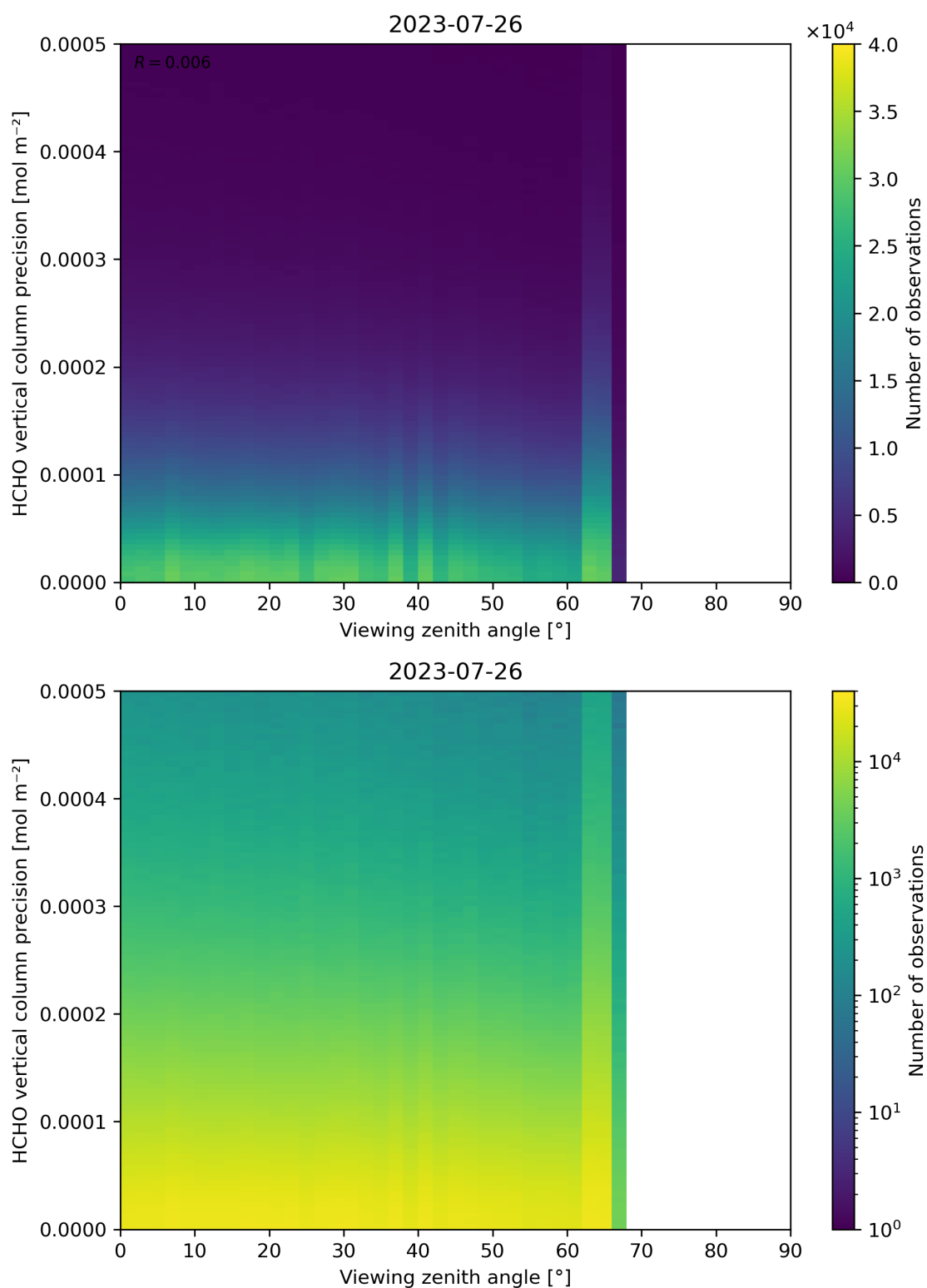
Figure 194: Scatter density plot of “Viewing zenith angle” against “HCHO vertical column precision” for 2023-07-25 to 2023-07-27.
