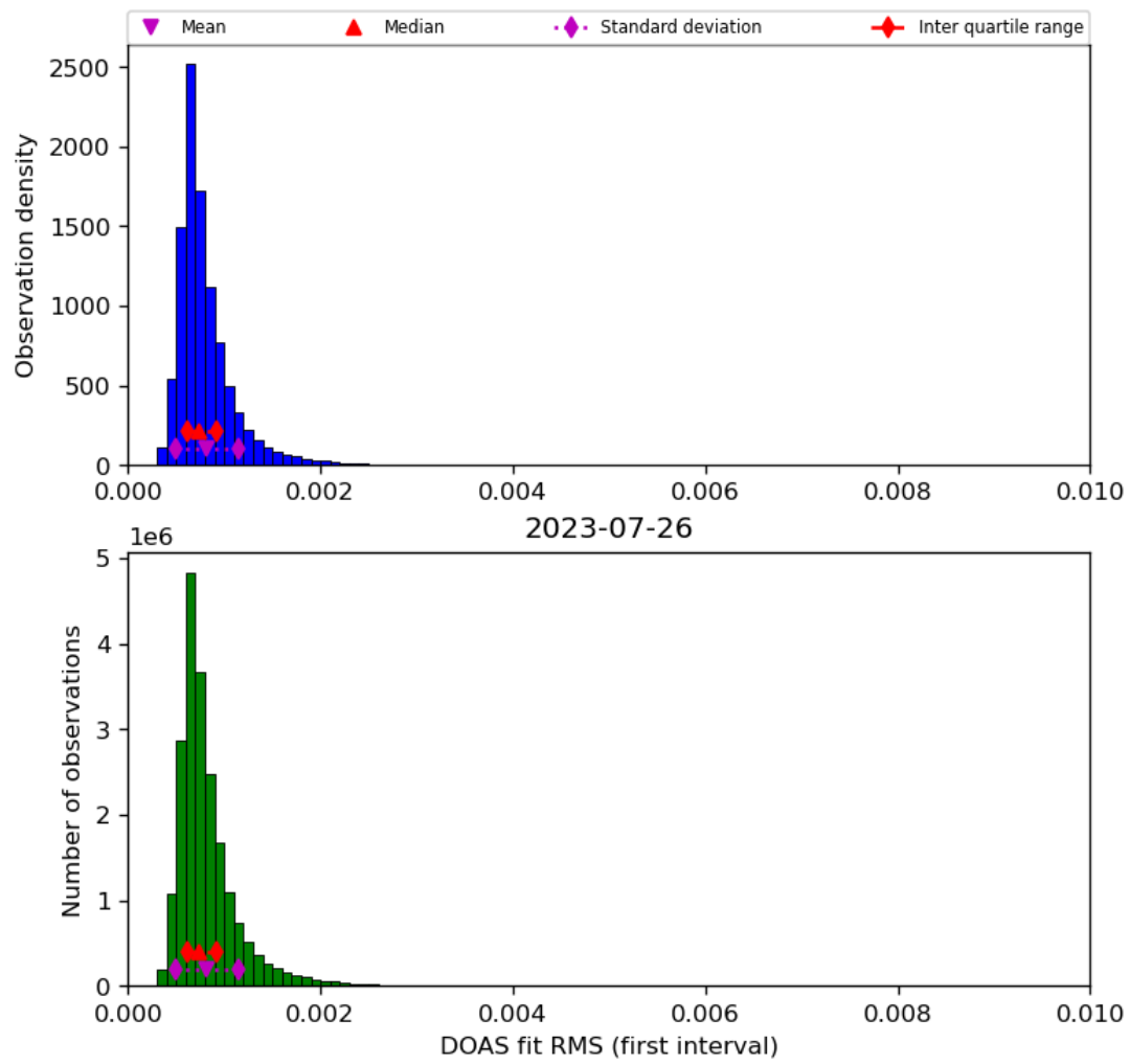
Figure 46: Histogram of “DOAS fit RMS (first interval)” for 2023-07-25 to 2023-07-27
