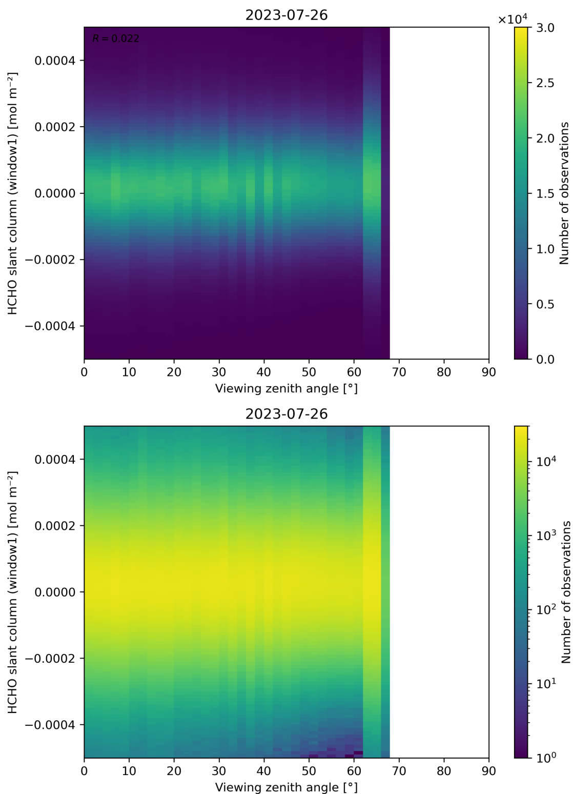
Figure 188: Scatter density plot of “Viewing zenith angle” against “HCHO slant column (window1)” for 2023-07-25 to 2023-07-27.
