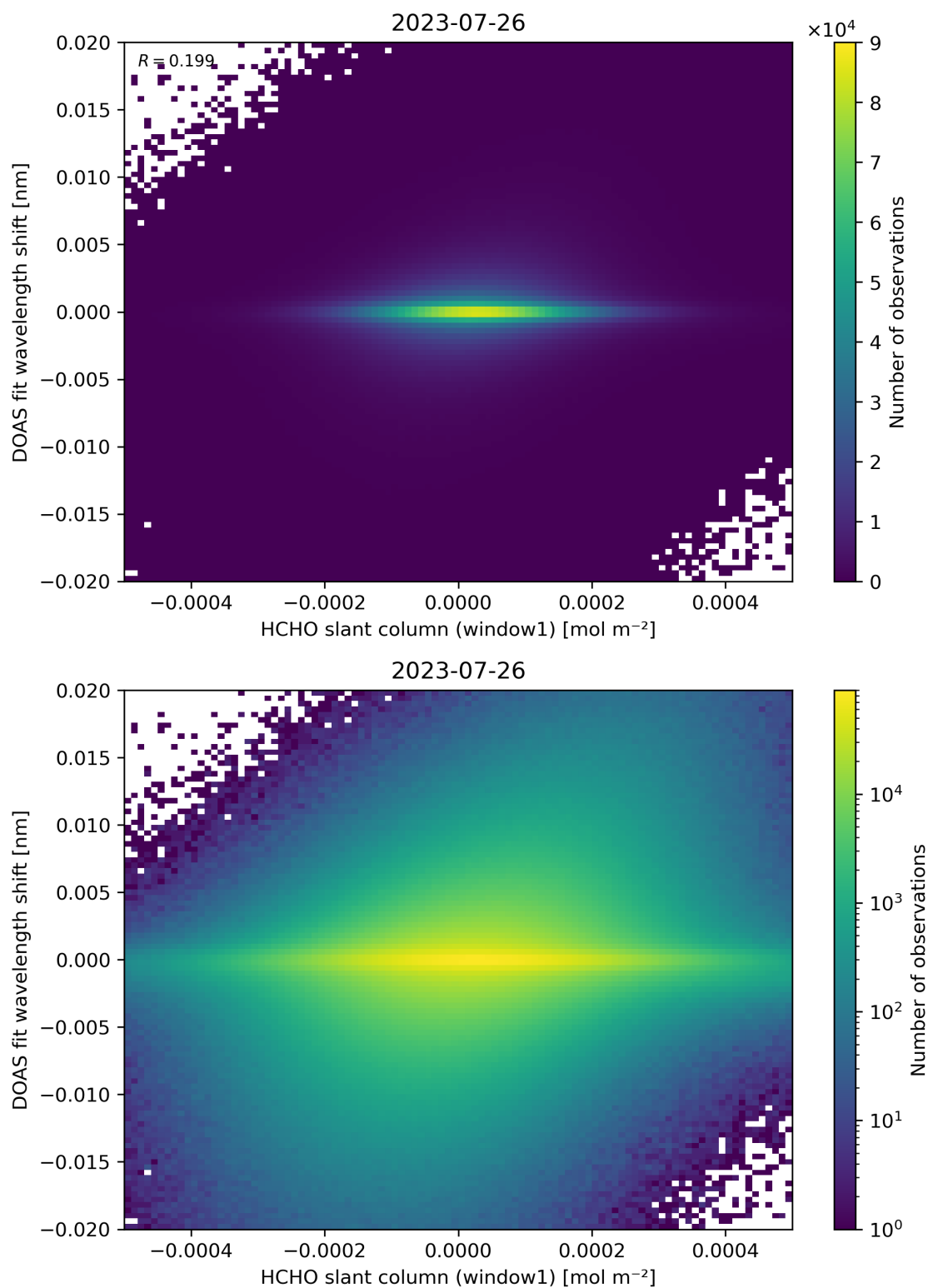
Figure 79: Scatter density plot of “HCHO slant column (window1)” against “DOAS fit wavelength shift” for 2023-07-25 to 2023-07-27.
