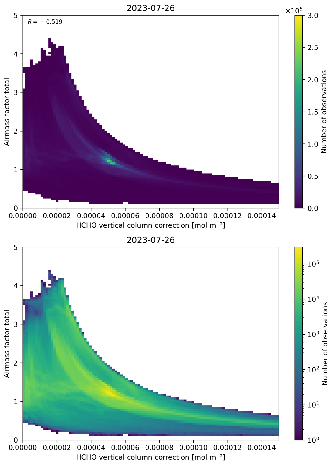
Figure 120: Scatter density plot of “HCHO vertical column correction” against “Airmass factor total” for 2023-07-25 to 2023-07-27.
