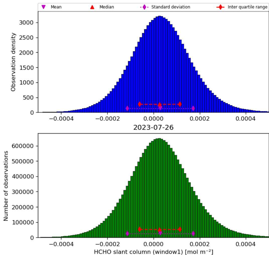
Figure 38: Histogram of “HCHO slant column (window1)” for 2023-07-25 to 2023-07-27
