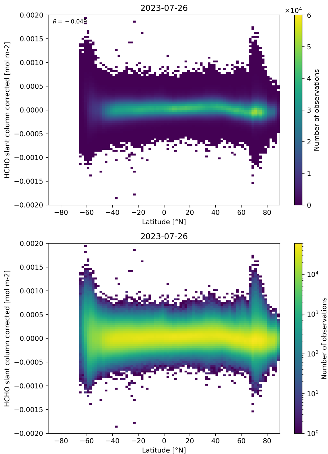
Figure 157: Scatter density plot of “Latitude” against “HCHO slant column corrected” for 2023-07-25 to 2023-07-27.
