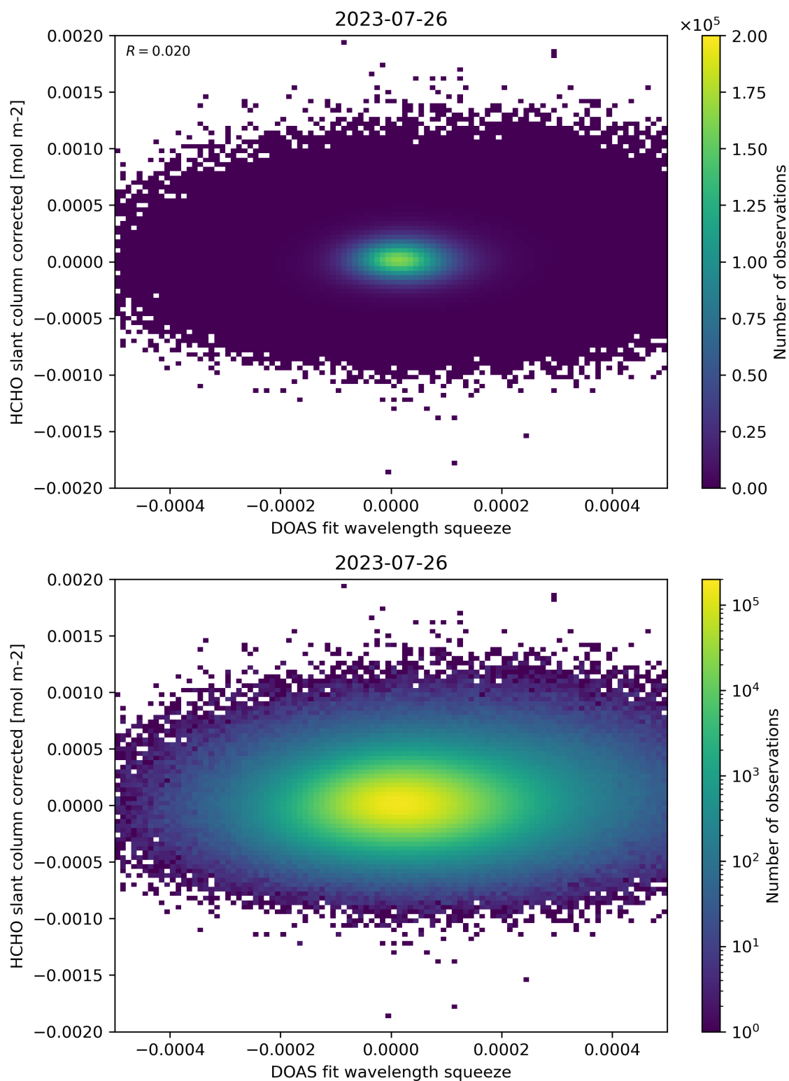
Figure 69: Scatter density plot of “DOAS fit wavelength squeeze” against “HCHO slant column corrected” for 2023-07-25 to 2023-07-27.
