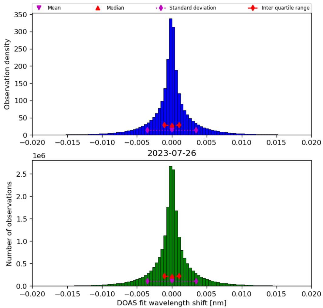
Figure 44: Histogram of “DOAS fit wavelength shift” for 2023-07-25 to 2023-07-27
