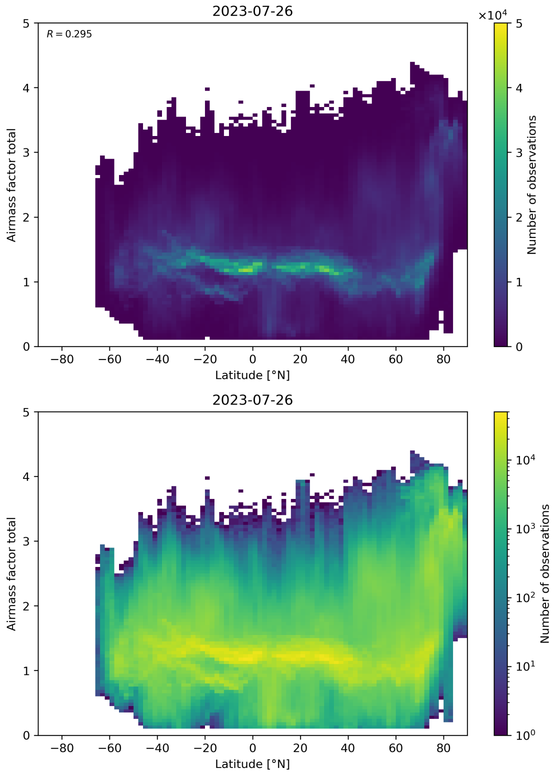
Figure 161: Scatter density plot of “Latitude” against “Airmass factor total” for 2023-07-25 to 2023-07-27.
