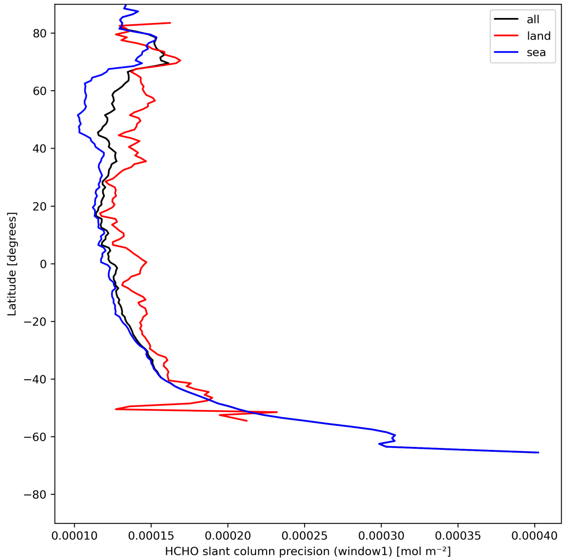
Figure 25: Zonal average of “HCHO slant column precision (window1)” for 2023-07-25 to 2023-07-27.
