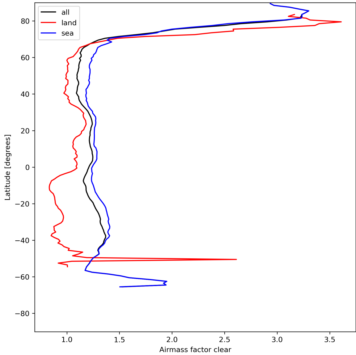
Figure 28: Zonal average of “Airmass factor clear” for 2023-07-25 to 2023-07-27.
