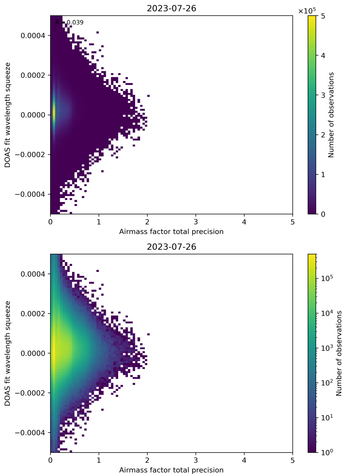
Figure 107: Scatter density plot of “Airmass factor total precision” against “DOAS fit wavelength squeeze” for 2023-07-25 to 2023-07-27.
