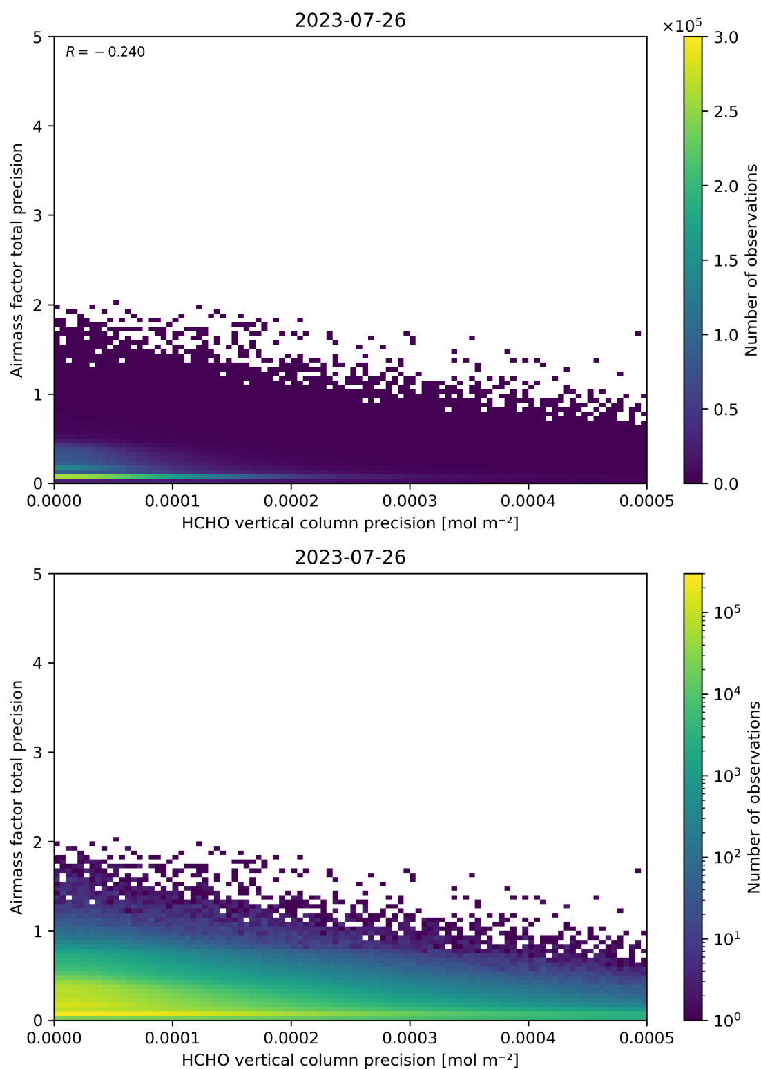
Figure 145: Scatter density plot of “HCHO vertical column precision” against “Airmass factor total precision” for 2023-07-25 to 2023-07-27.
