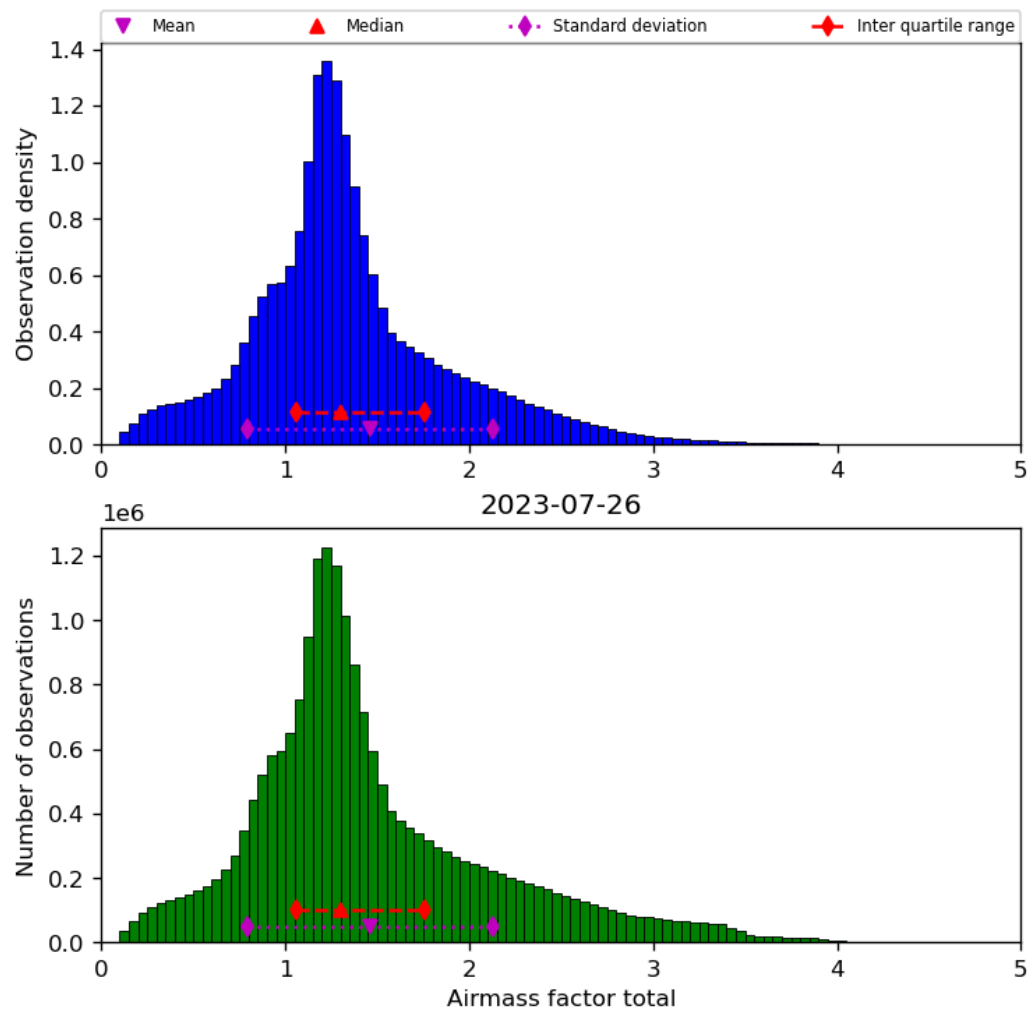
Figure 40: Histogram of “Airmass factor total” for 2023-07-25 to 2023-07-27
