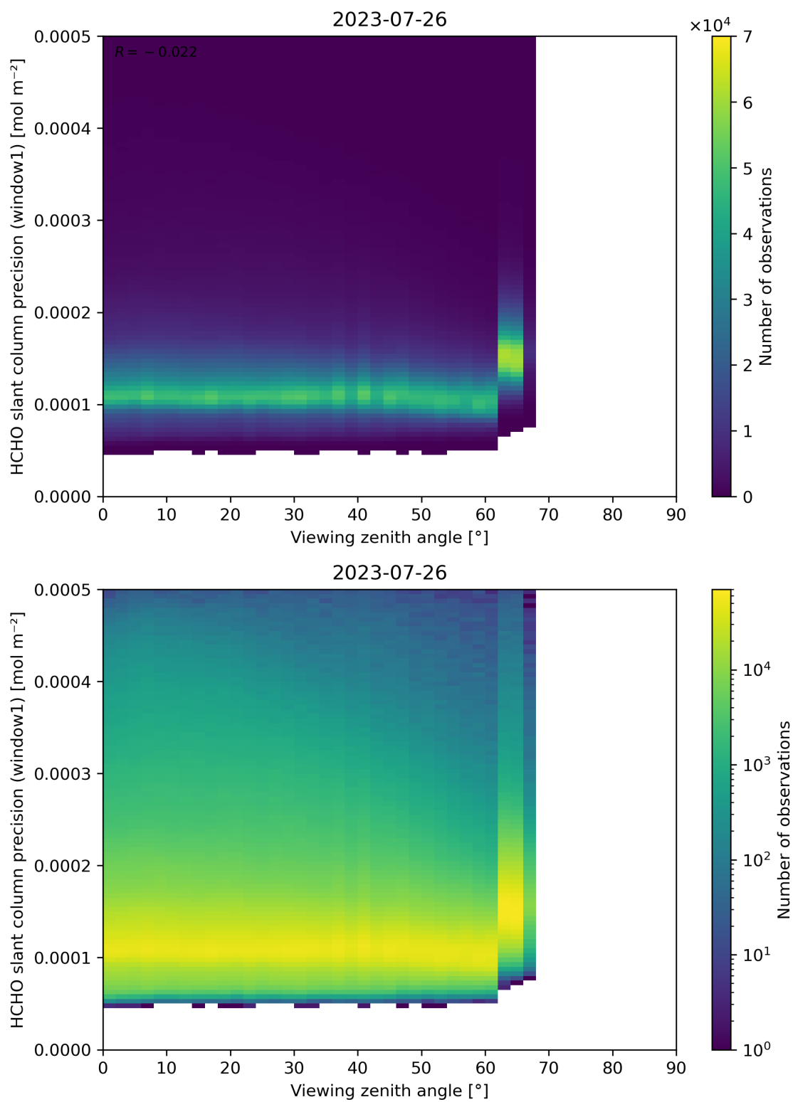
Figure 189: Scatter density plot of “Viewing zenith angle” against “HCHO slant column precision (window1)” for 2023-07-25 to 2023-07-27.
