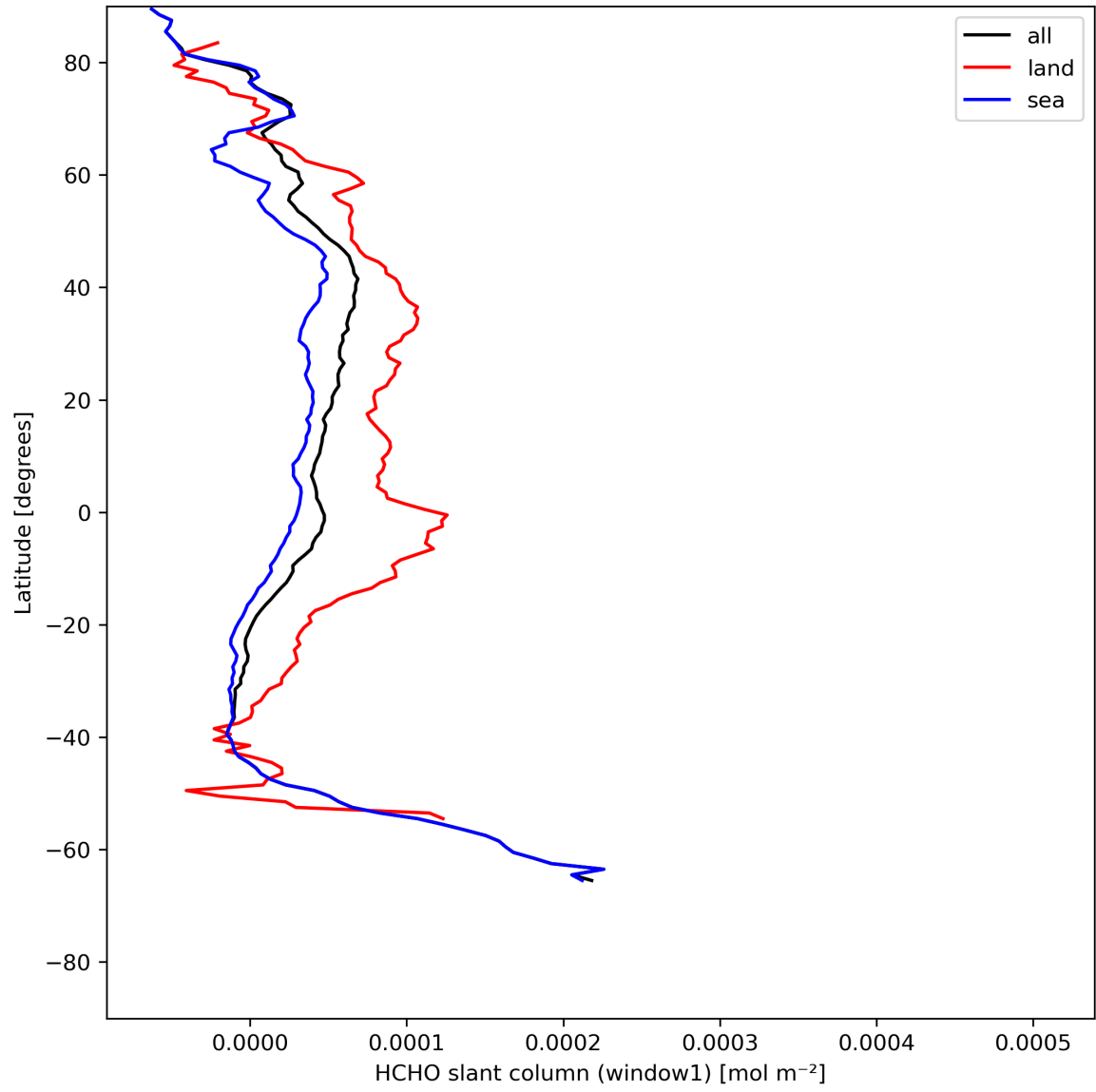
Figure 24: Zonal average of “HCHO slant column (window1)” for 2023-07-25 to 2023-07-27.
