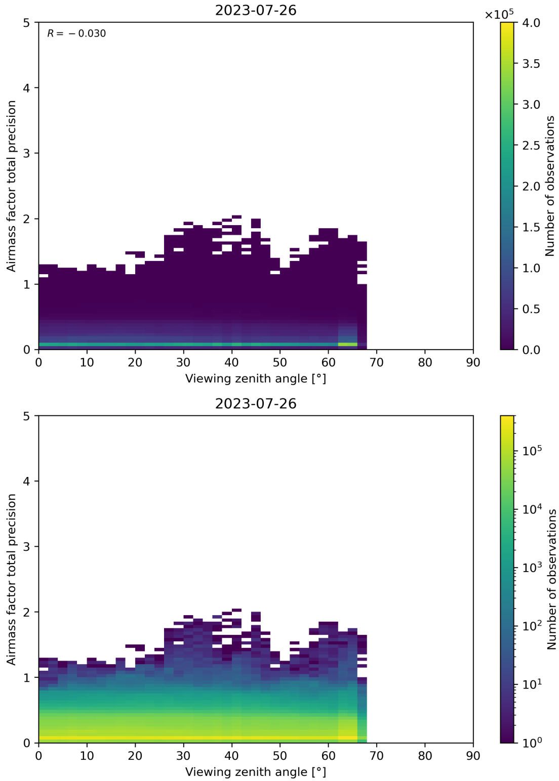
Figure 191: Scatter density plot of “Viewing zenith angle” against “Airmass factor total precision” for 2023-07-25 to 2023-07-27.
