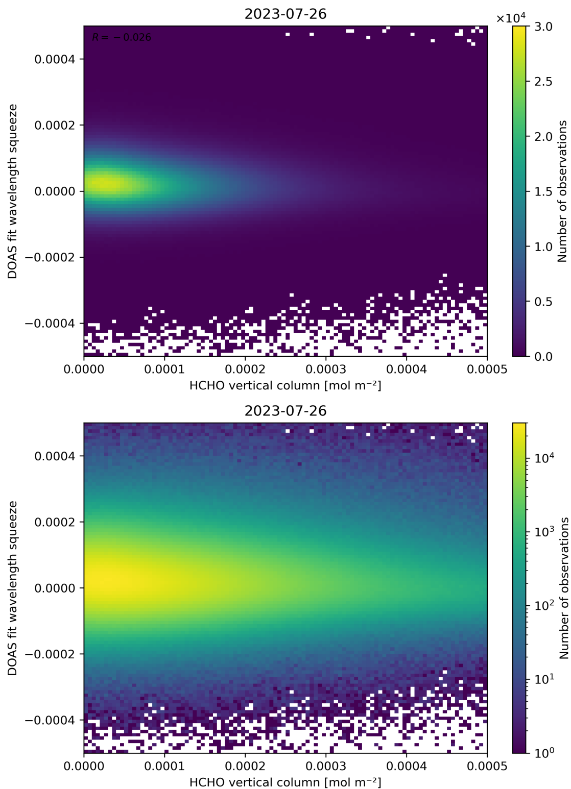
Figure 125: Scatter density plot of “HCHO vertical column” against “DOAS fit wavelength squeeze” for 2023-07-25 to 2023-07-27.
