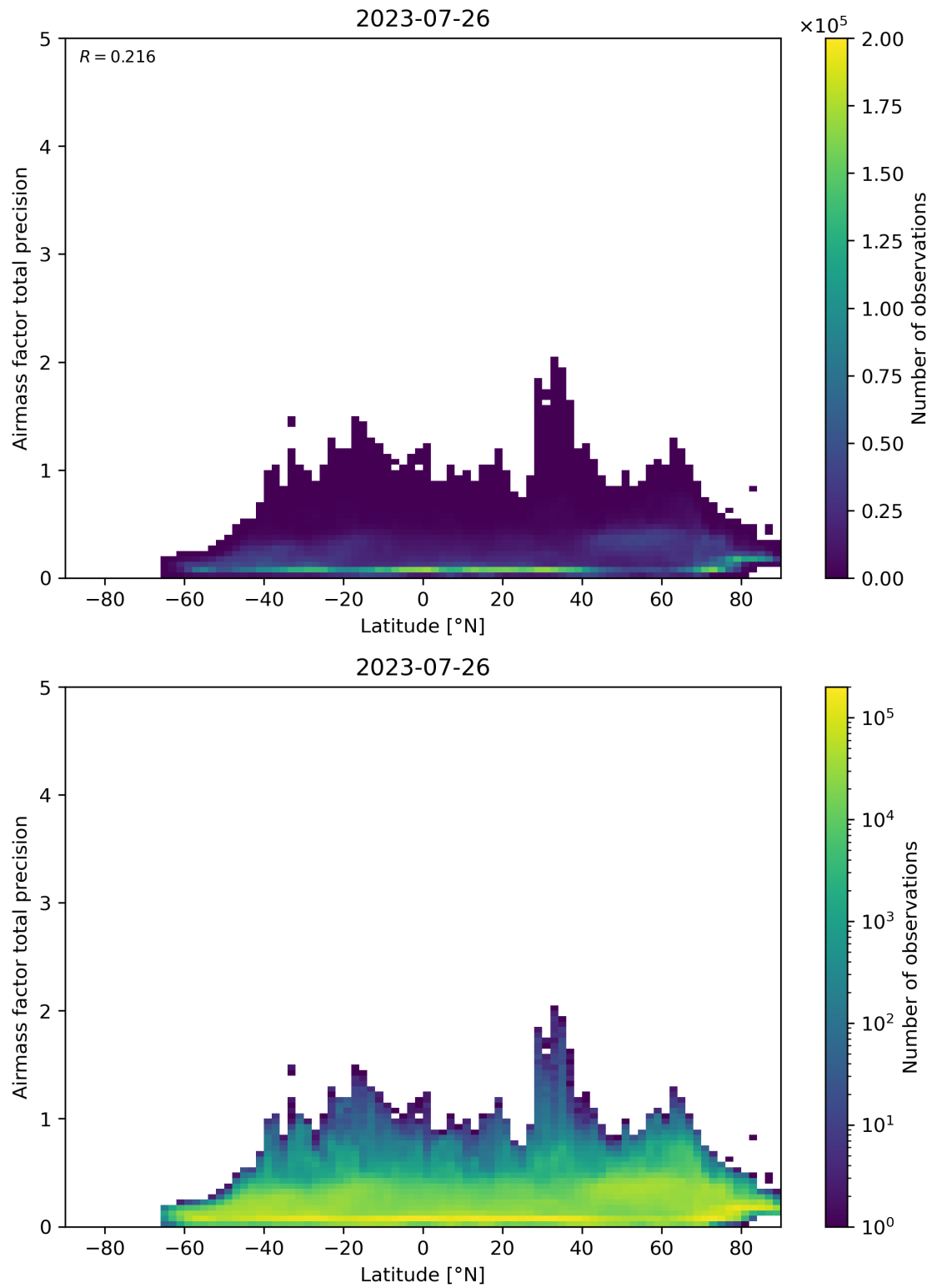
Figure 162: Scatter density plot of “Latitude” against “Airmass factor total precision” for 2023-07-25 to 2023-07-27.
