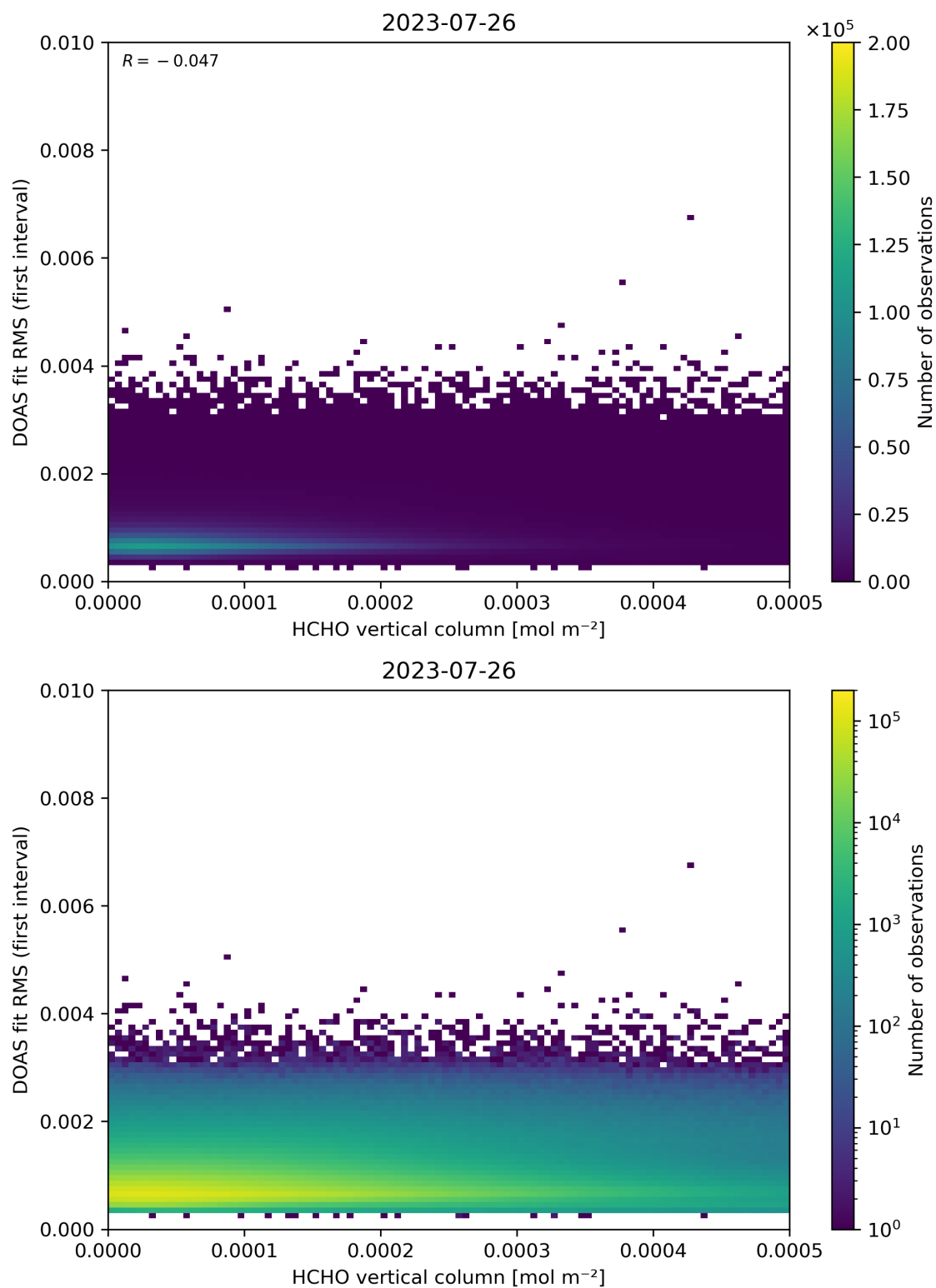
Figure 123: Scatter density plot of “HCHO vertical column” against “DOAS fit RMS (first interval)” for 2023-07-25 to 2023-07-27.
