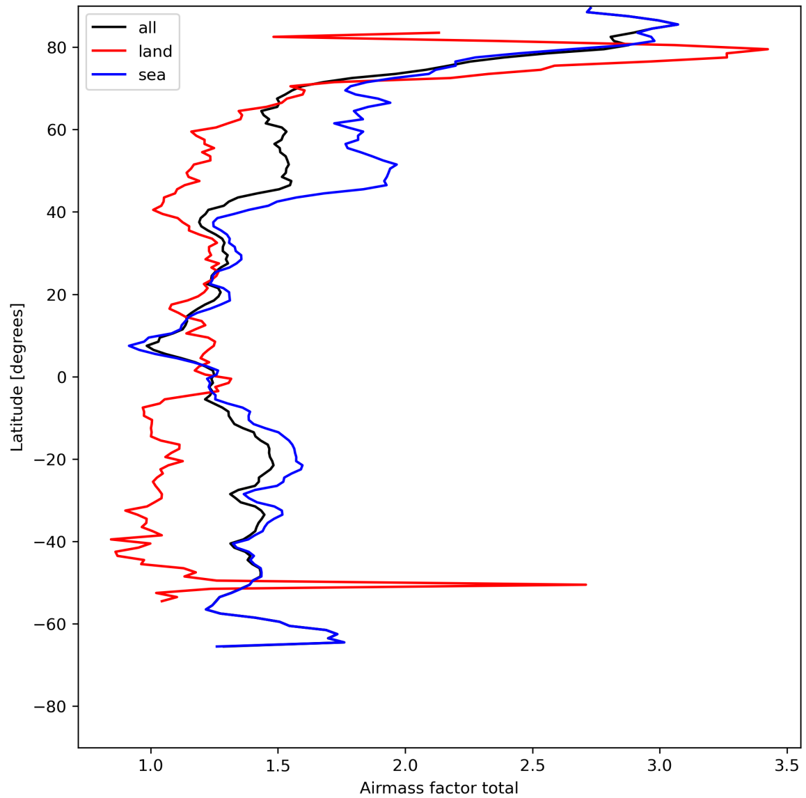
Figure 26: Zonal average of “Airmass factor total” for 2023-07-25 to 2023-07-27.
