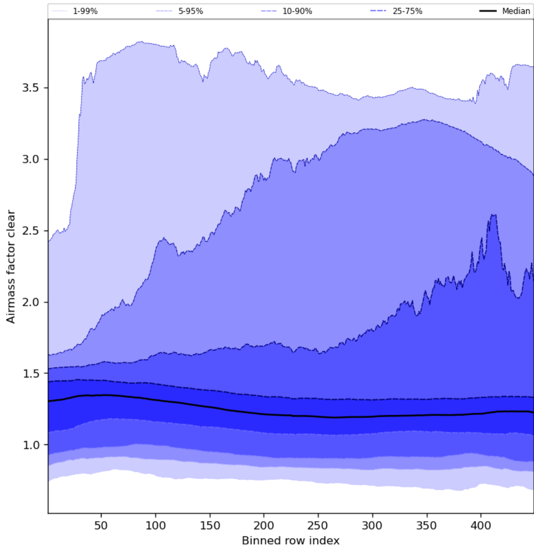
Figure 56: Along track statistics of “Airmass factor clear” for 2023-07-25 to 2023-07-27
