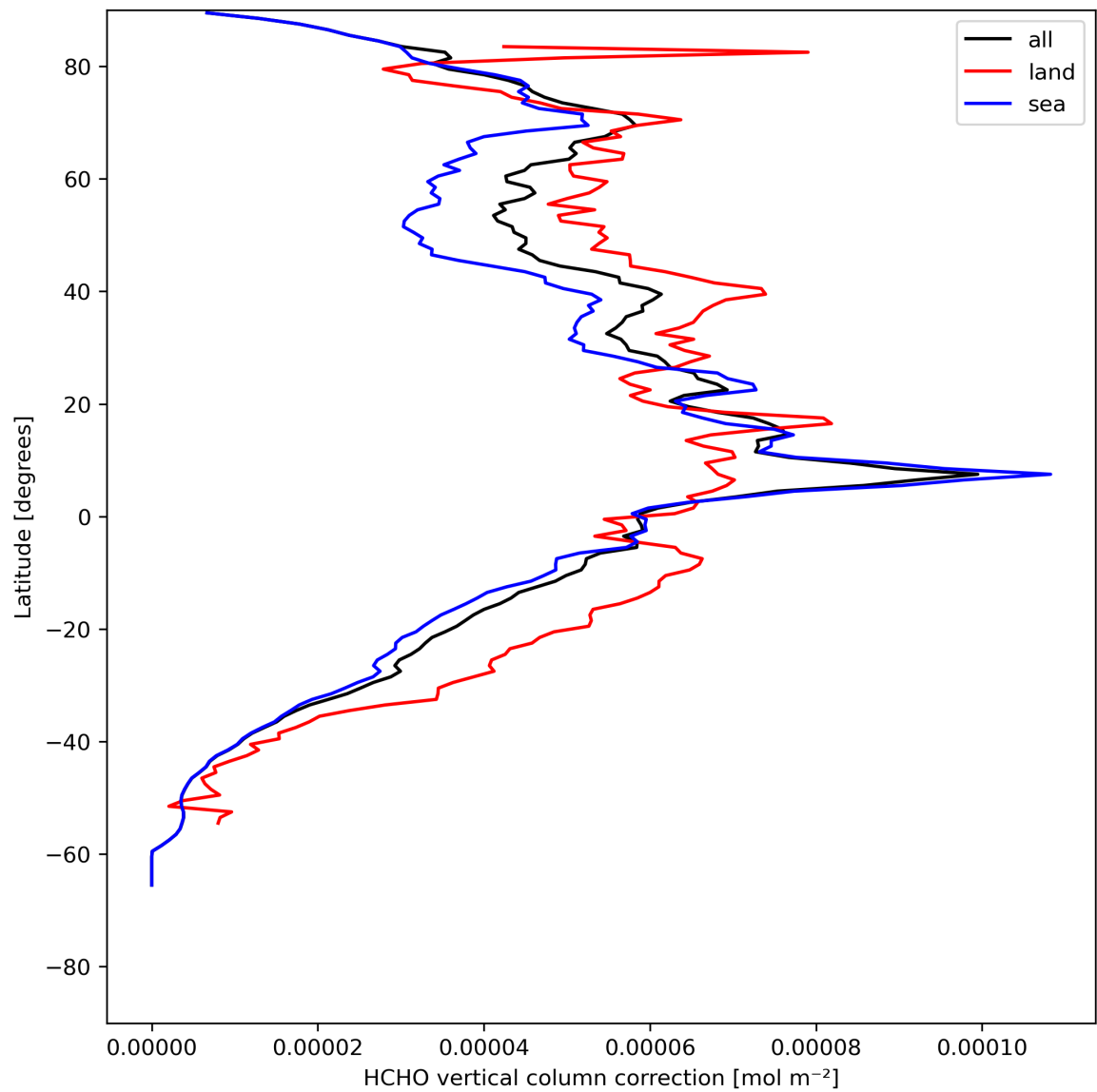
Figure 23: Zonal average of “HCHO vertical column correction” for 2023-07-25 to 2023-07-27.
