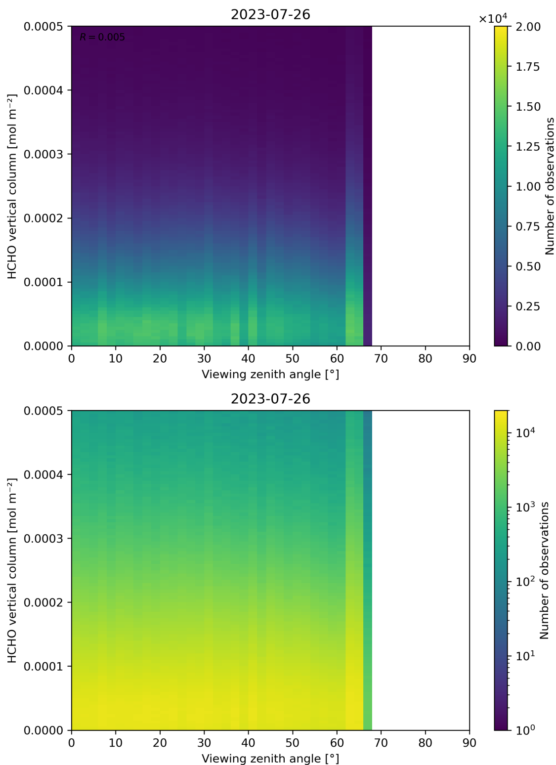
Figure 192: Scatter density plot of “Viewing zenith angle” against “HCHO vertical column” for 2023-07-25 to 2023-07-27.
