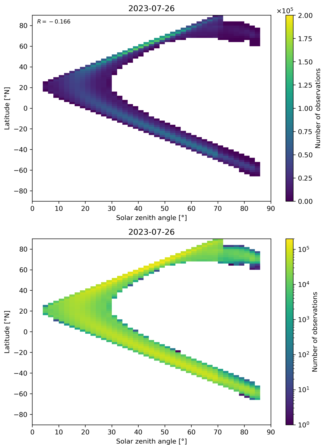
Figure 181: Scatter density plot of “Solar zenith angle” against “Latitude” for 2023-07-25 to 2023-07-27.
