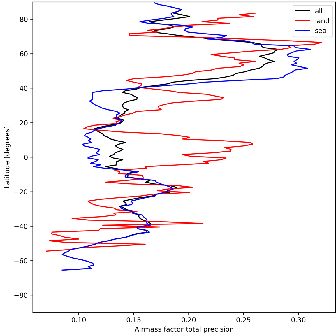
Figure 27: Zonal average of “Airmass factor total precision” for 2023-07-25 to 2023-07-27.
