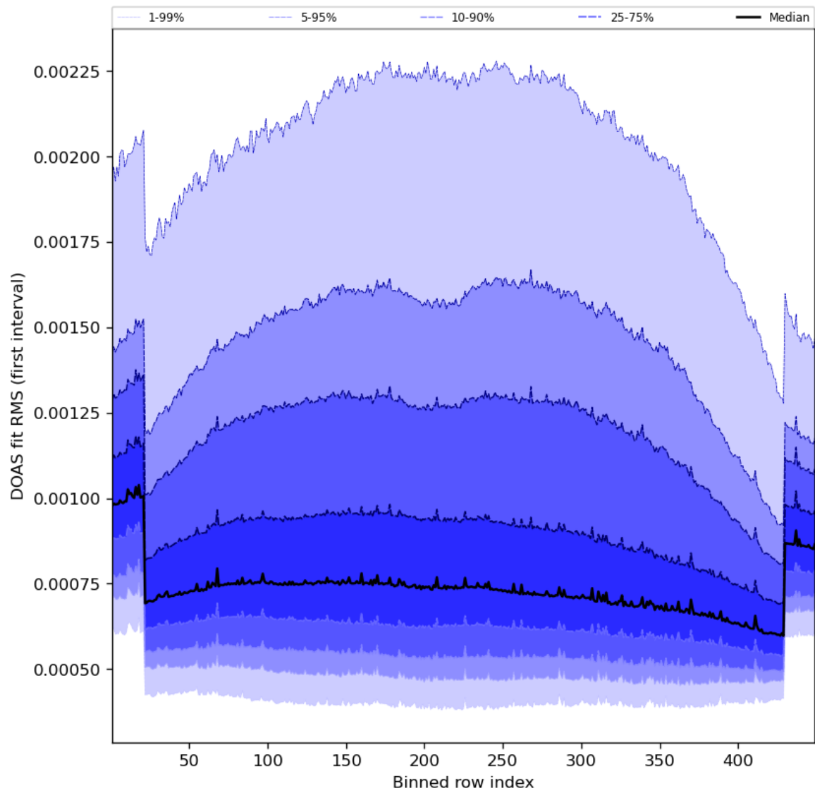
Figure 60: Along track statistics of “DOAS fit RMS (first interval)” for 2023-07-25 to 2023-07-27
