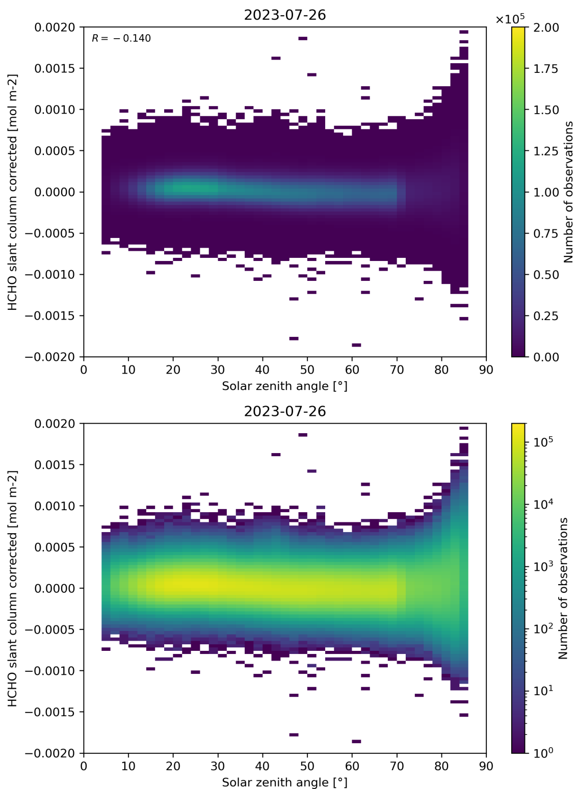
Figure 171: Scatter density plot of “Solar zenith angle” against “HCHO slant column corrected” for 2023-07-25 to 2023-07-27.
