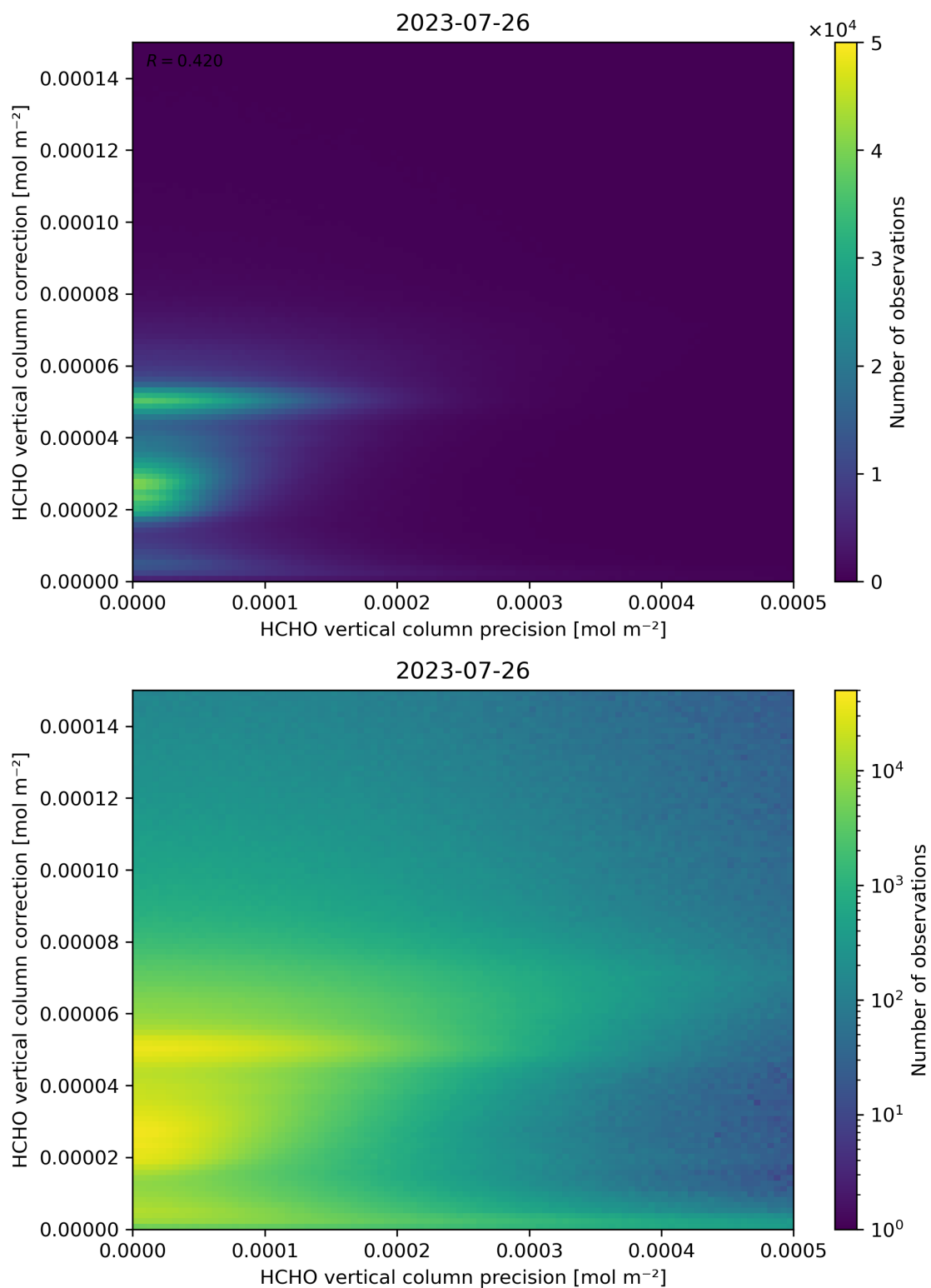
Figure 146: Scatter density plot of “HCHO vertical column precision” against “HCHO vertical column correction” for 2023-07-25 to 2023-07-27.
