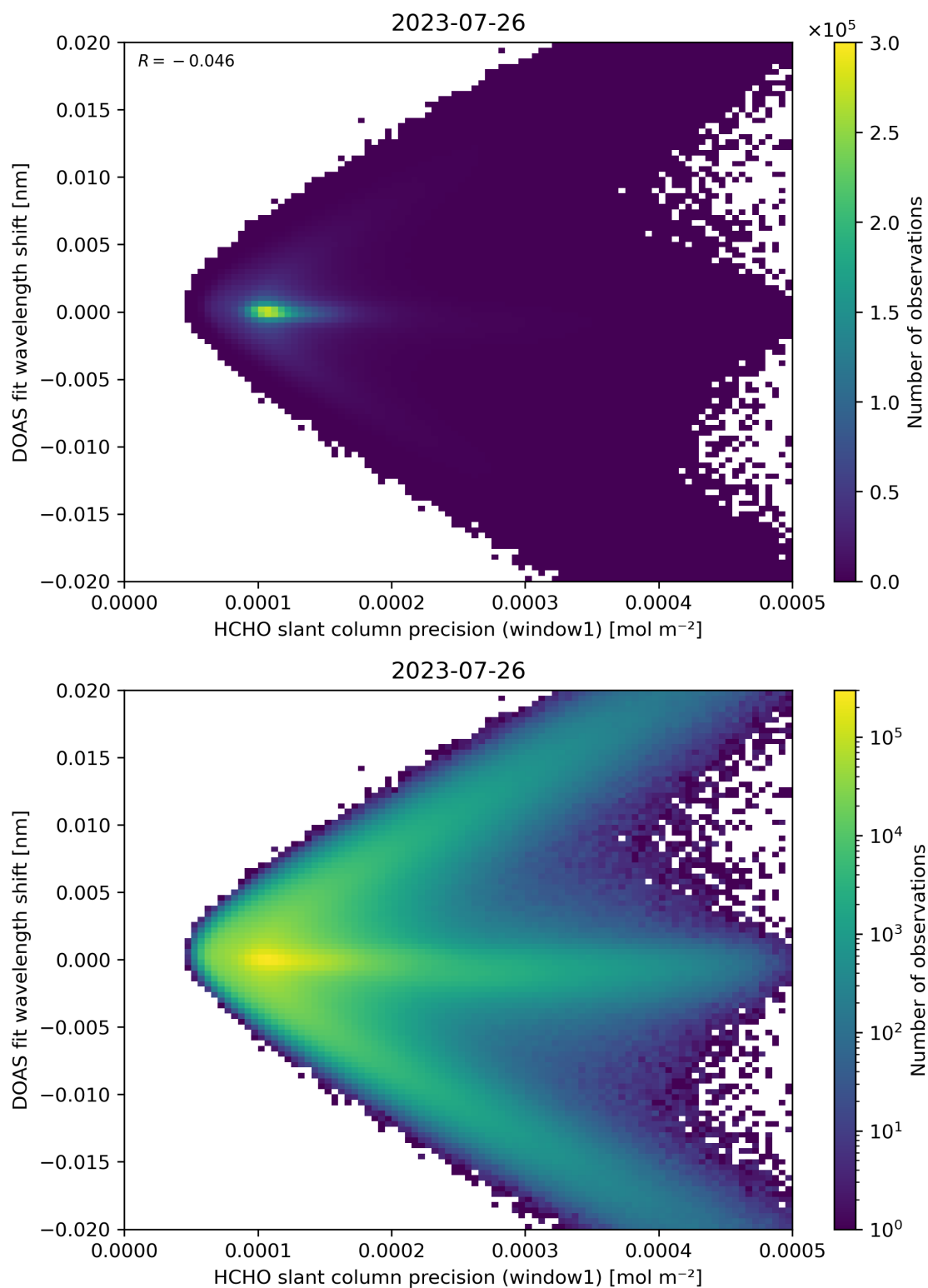
Figure 89: Scatter density plot of “HCHO slant column precision (window1)” against “DOAS fit wavelength shift” for 2023-07-25 to 2023-07-27.
