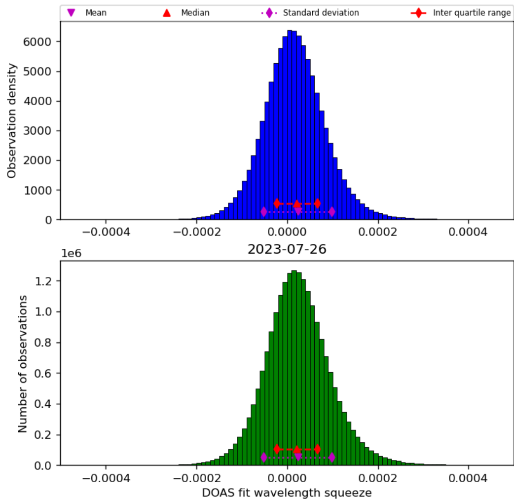
Figure 45: Histogram of “DOAS fit wavelength squeeze” for 2023-07-25 to 2023-07-27
