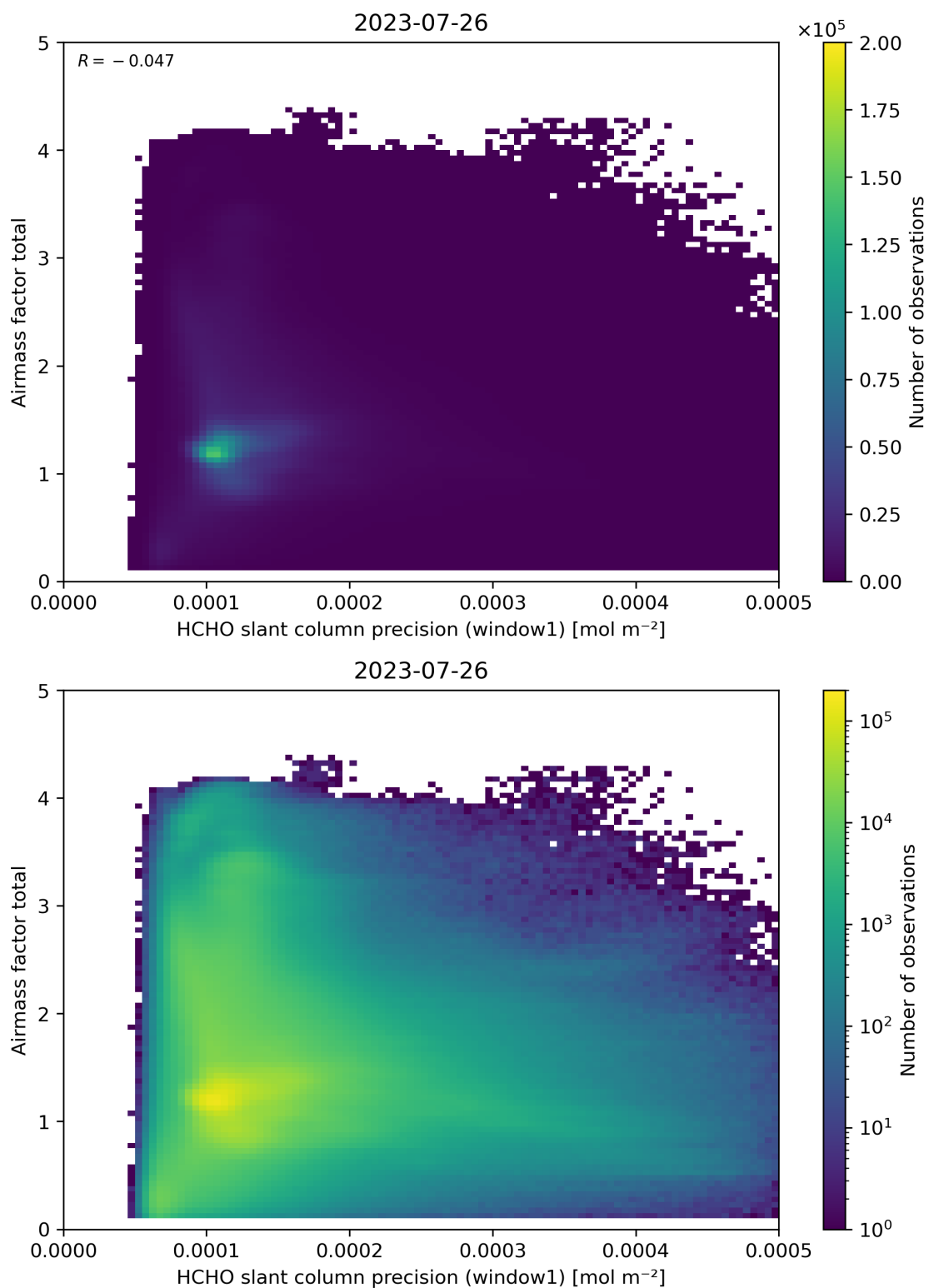
Figure 94: Scatter density plot of “HCHO slant column precision (window1)” against “Airmass factor total” for 2023-07-25 to 2023-07-27.
