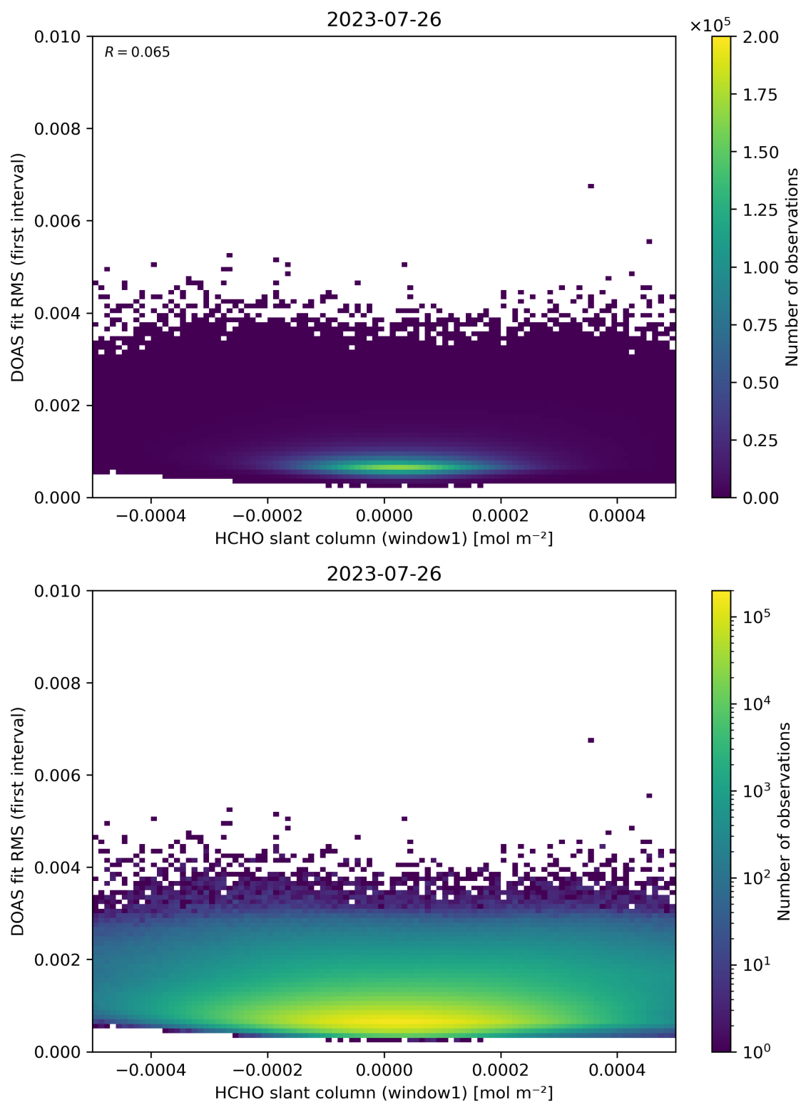
Figure 78: Scatter density plot of “HCHO slant column (window1)” against “DOAS fit RMS (first interval)” for 2023-07-25 to 2023-07-27.
