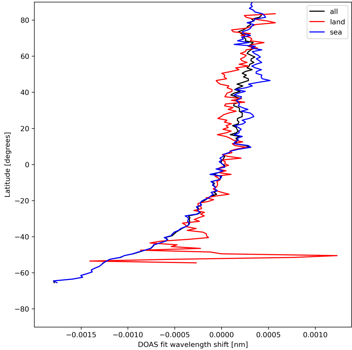
Figure 30: Zonal average of “DOAS fit wavelength shift” for 2023-07-25 to 2023-07-27.
