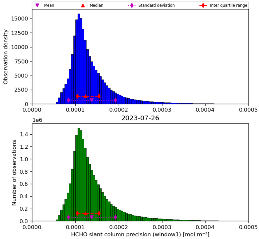
Figure 39: Histogram of “HCHO slant column precision (window1)” for 2023-07-25 to 2023-07-27
