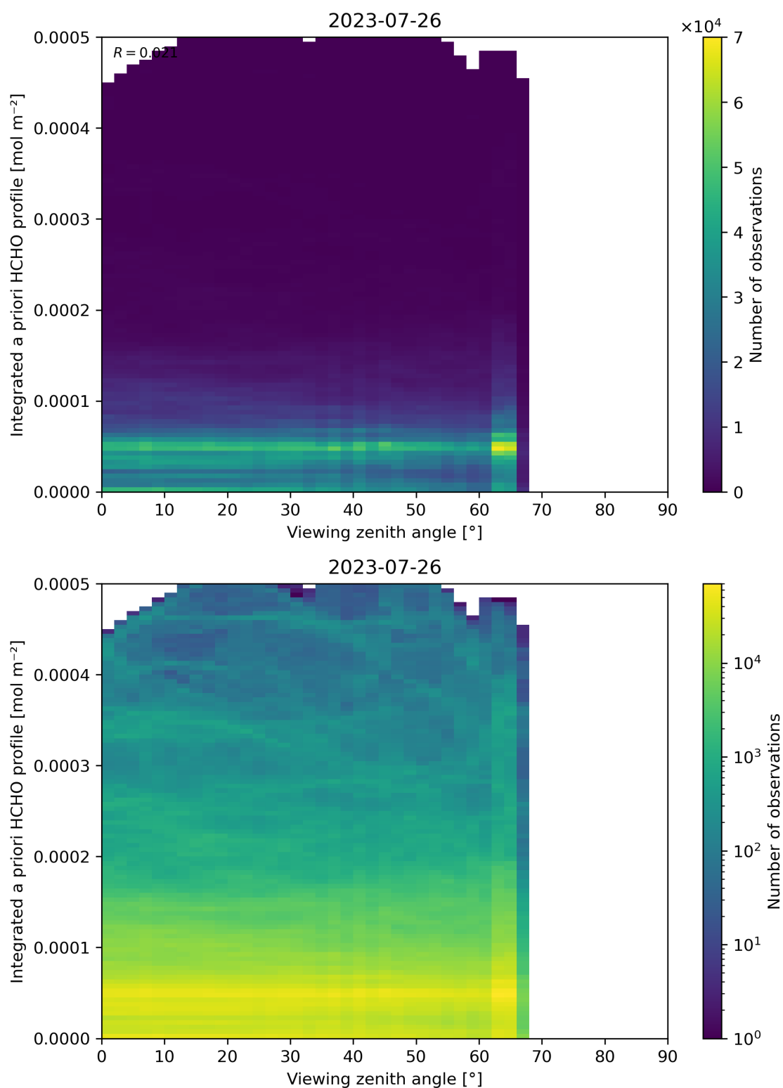
Figure 195: Scatter density plot of “Viewing zenith angle” against “Integrated a priori HCHO profile” for 2023-07-25 to 2023-07-27.
