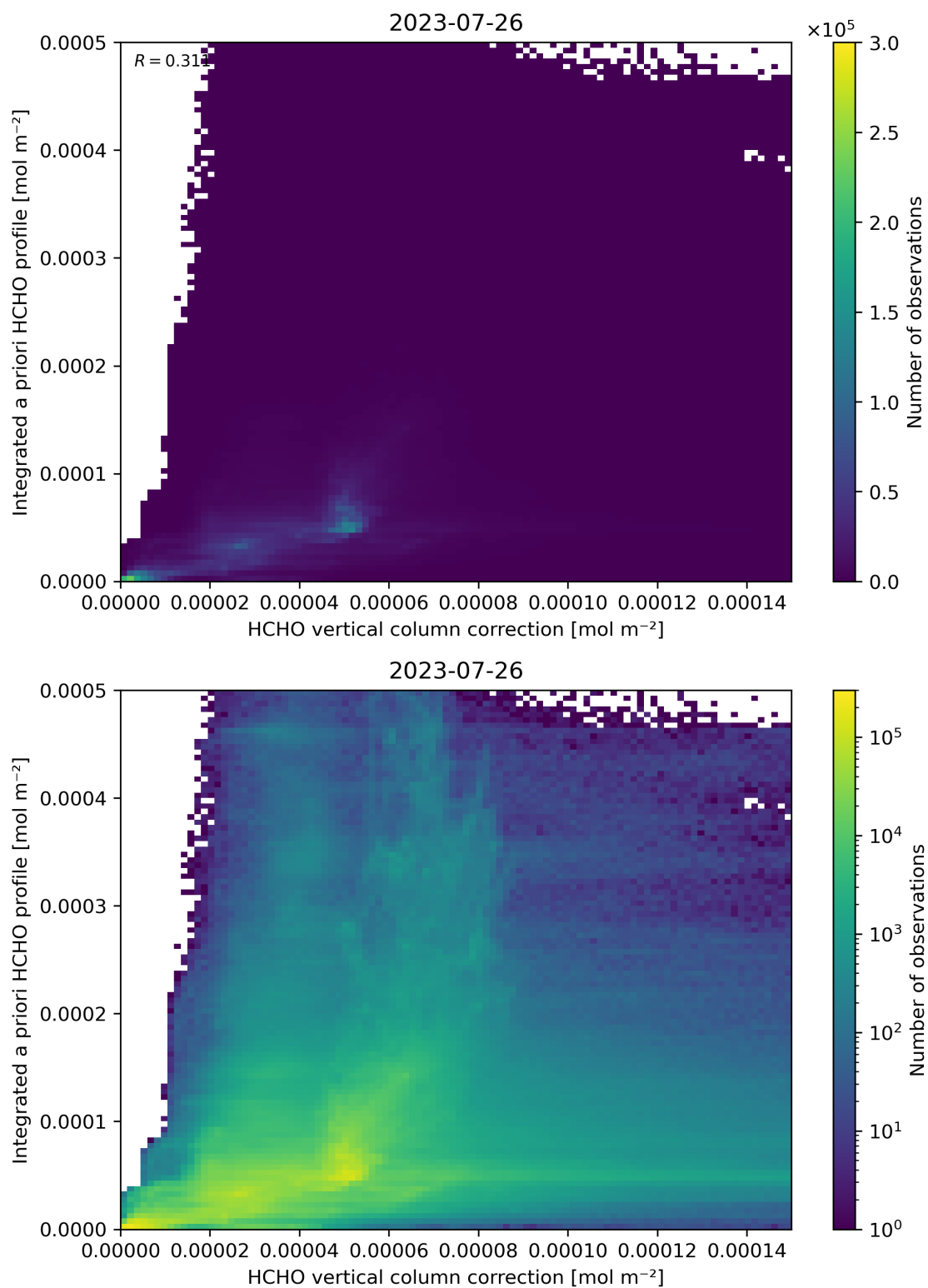
Figure 122: Scatter density plot of “HCHO vertical column correction” against “Integrated a priori HCHO profile” for 2023-07-25 to 2023-07-27.
