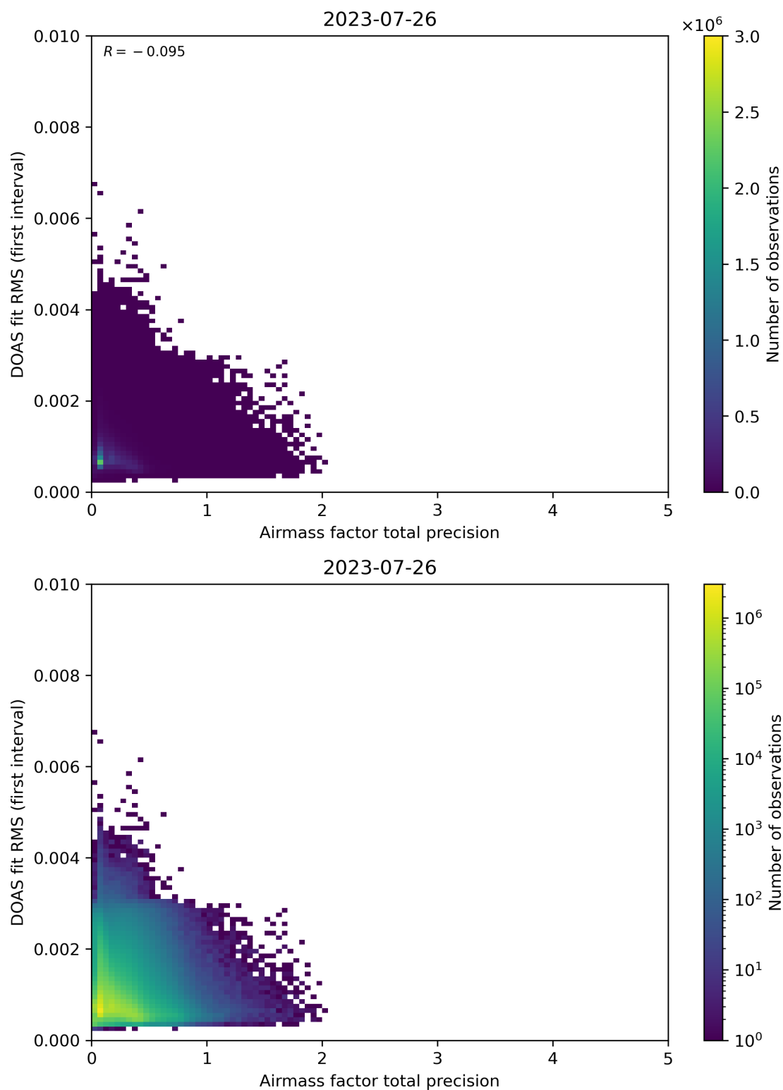
Figure 105: Scatter density plot of “Airmass factor total precision” against “DOAS fit RMS (first interval)” for 2023-07-25 to 2023-07-27.
