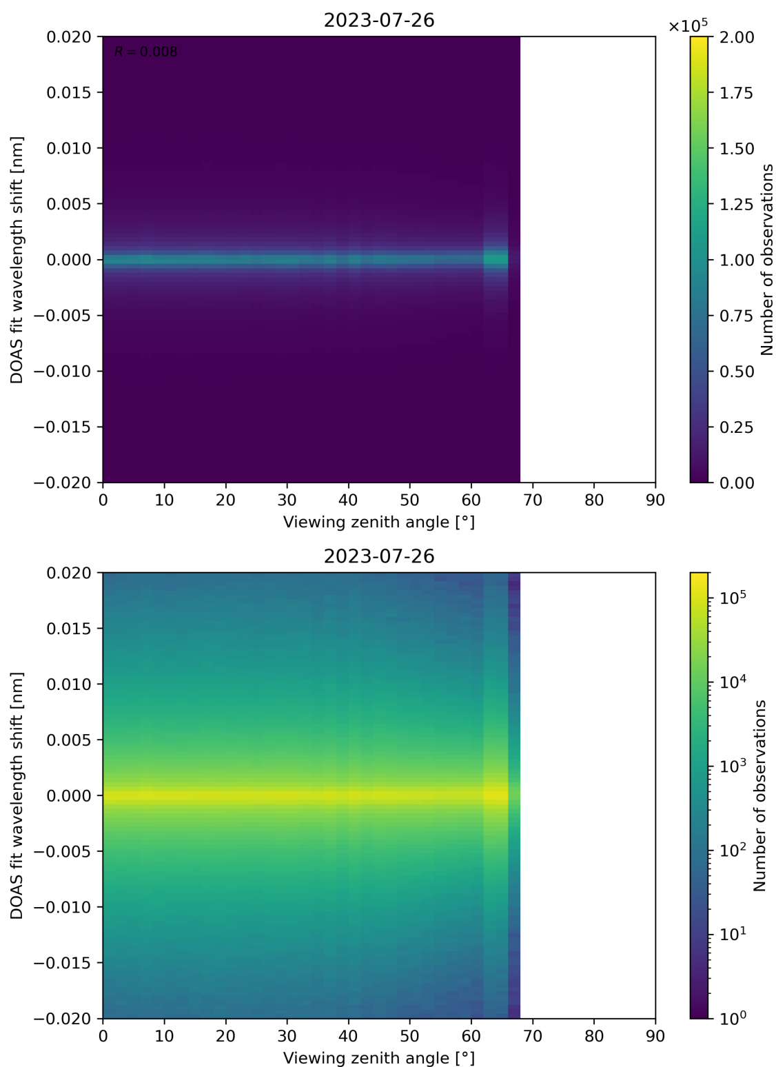
Figure 183: Scatter density plot of “Viewing zenith angle” against “DOAS fit wavelength shift” for 2023-07-25 to 2023-07-27.
