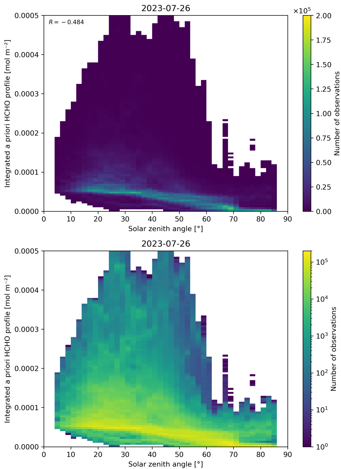
Figure 180: Scatter density plot of “Solar zenith angle” against “Integrated a priori HCHO profile” for 2023-07-25 to 2023-07-27.
