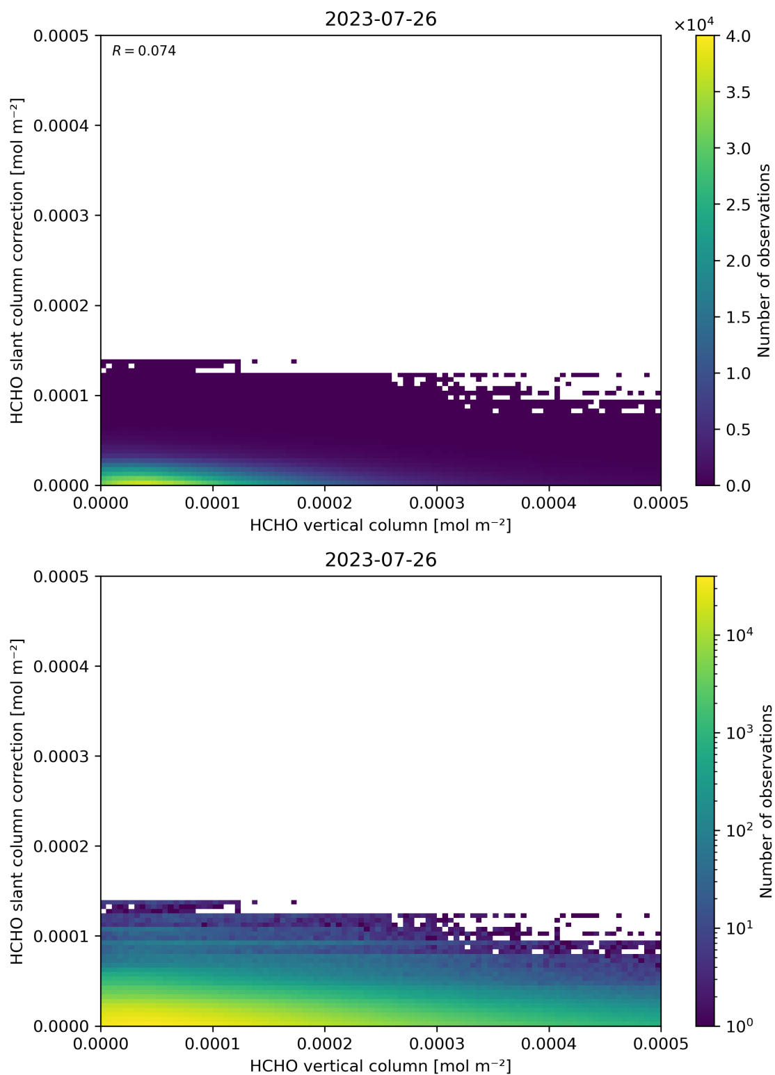
Figure 128: Scatter density plot of “HCHO vertical column” against “HCHO slant column correction” for 2023-07-25 to 2023-07-27.
