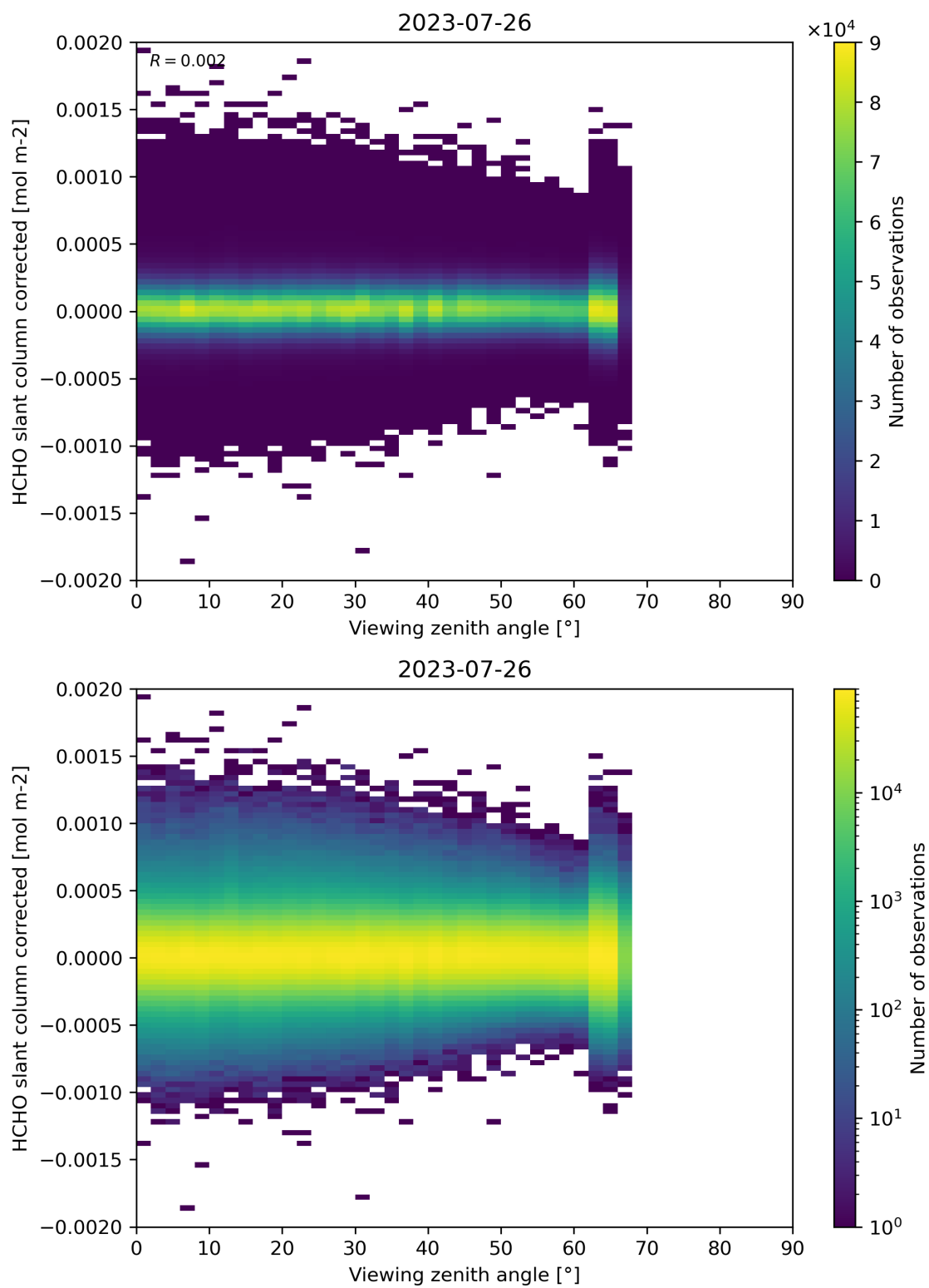
Figure 186: Scatter density plot of “Viewing zenith angle” against “HCHO slant column corrected” for 2023-07-25 to 2023-07-27.
