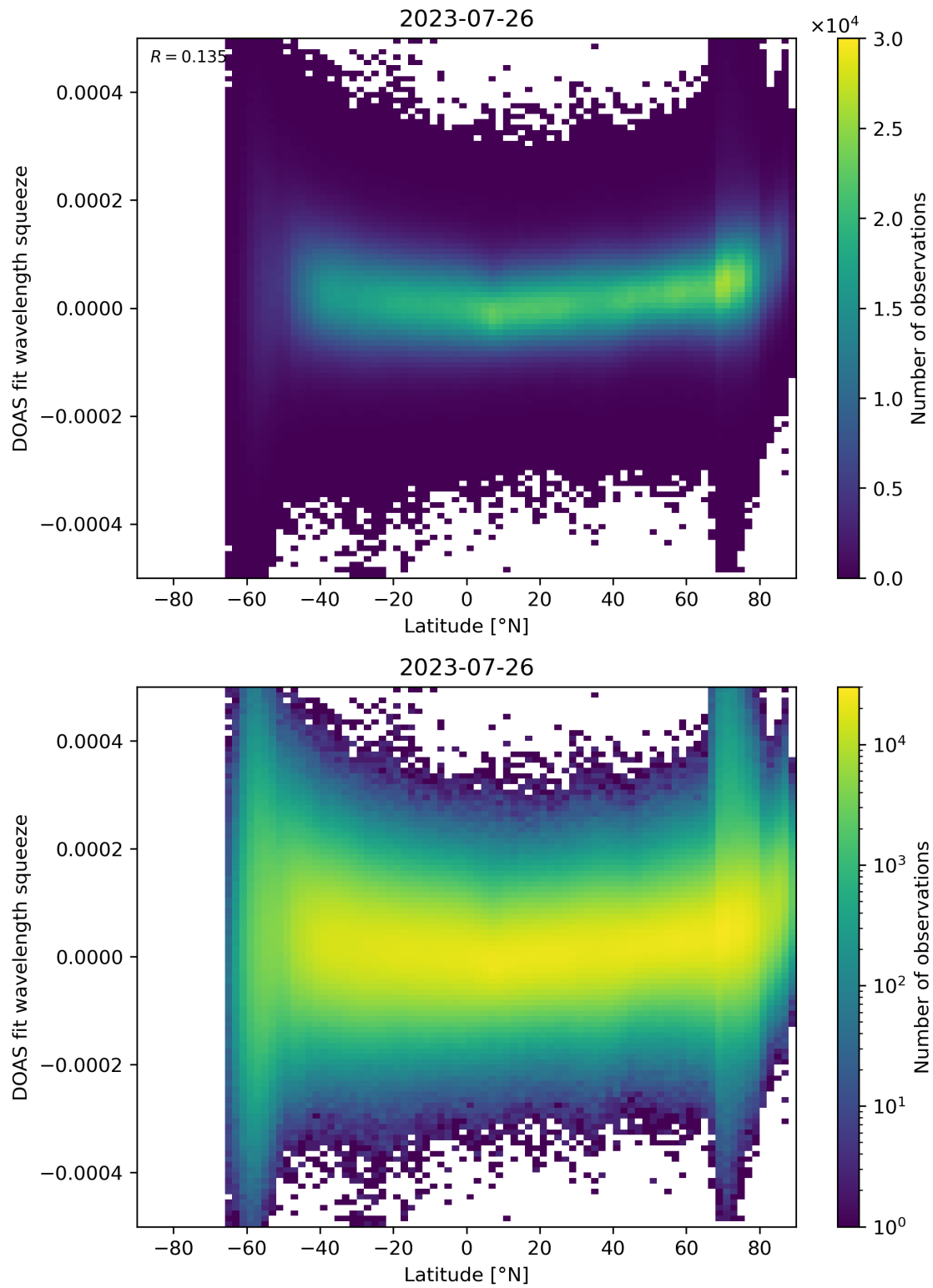
Figure 155: Scatter density plot of “Latitude” against “DOAS fit wavelength squeeze” for 2023-07-25 to 2023-07-27.
