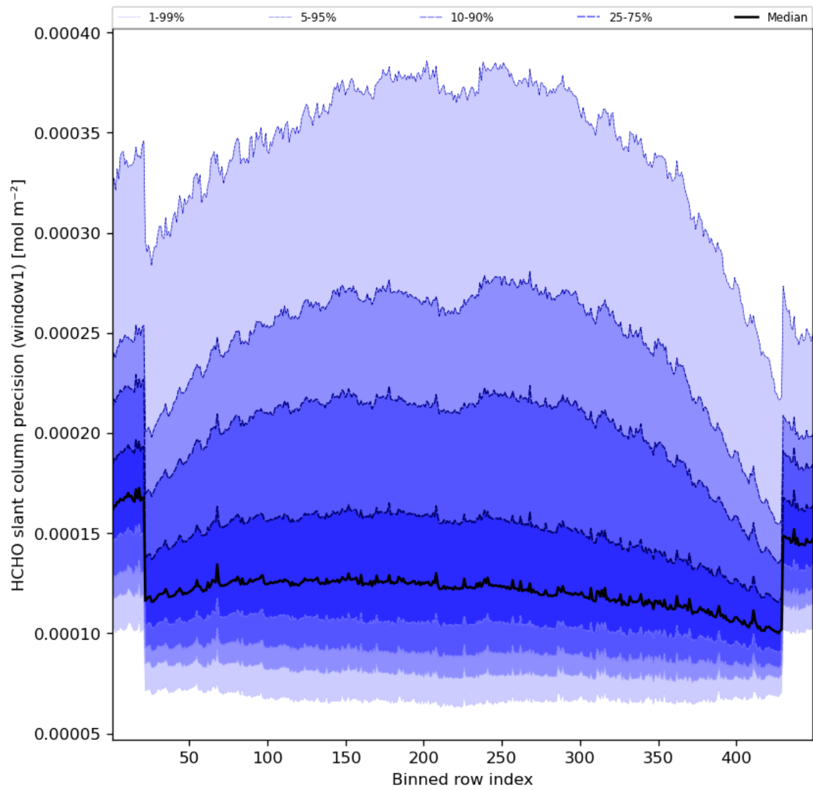
Figure 53: Along track statistics of “HCHO slant column precision (window1)” for 2023-07-25 to 2023-07-27
