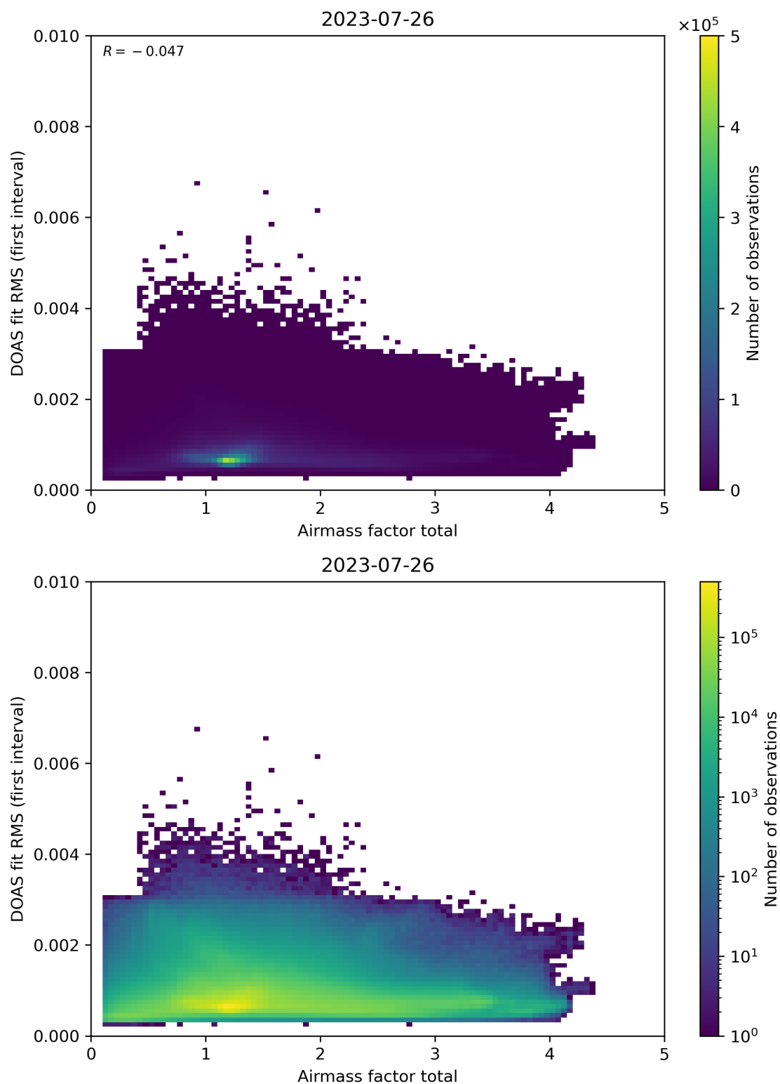
Figure 97: Scatter density plot of “Airmass factor total” against “DOAS fit RMS (first interval)” for 2023-07-25 to 2023-07-27.
