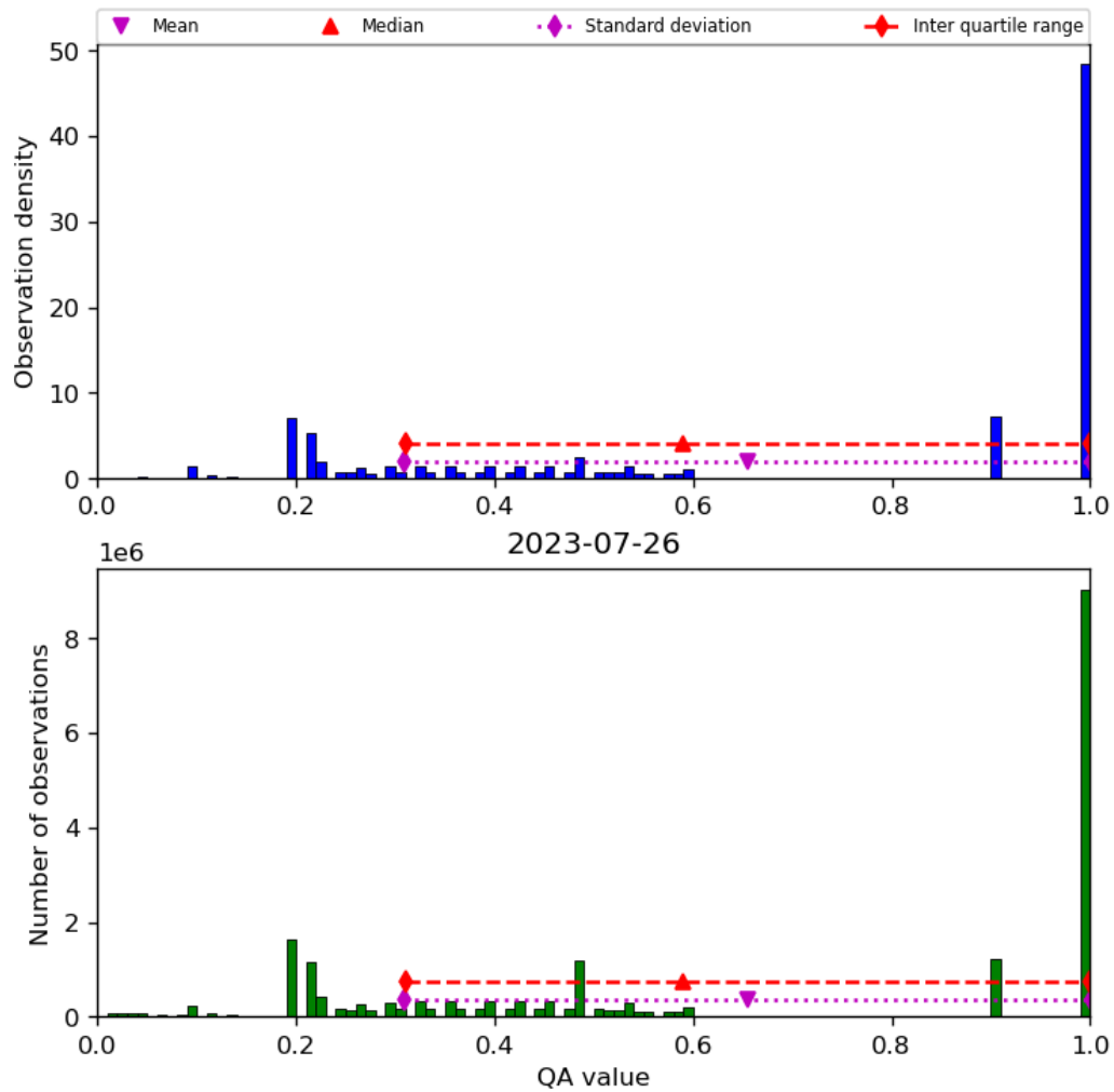
Figure 34: Histogram of “QA value” for 2023-07-25 to 2023-07-27
