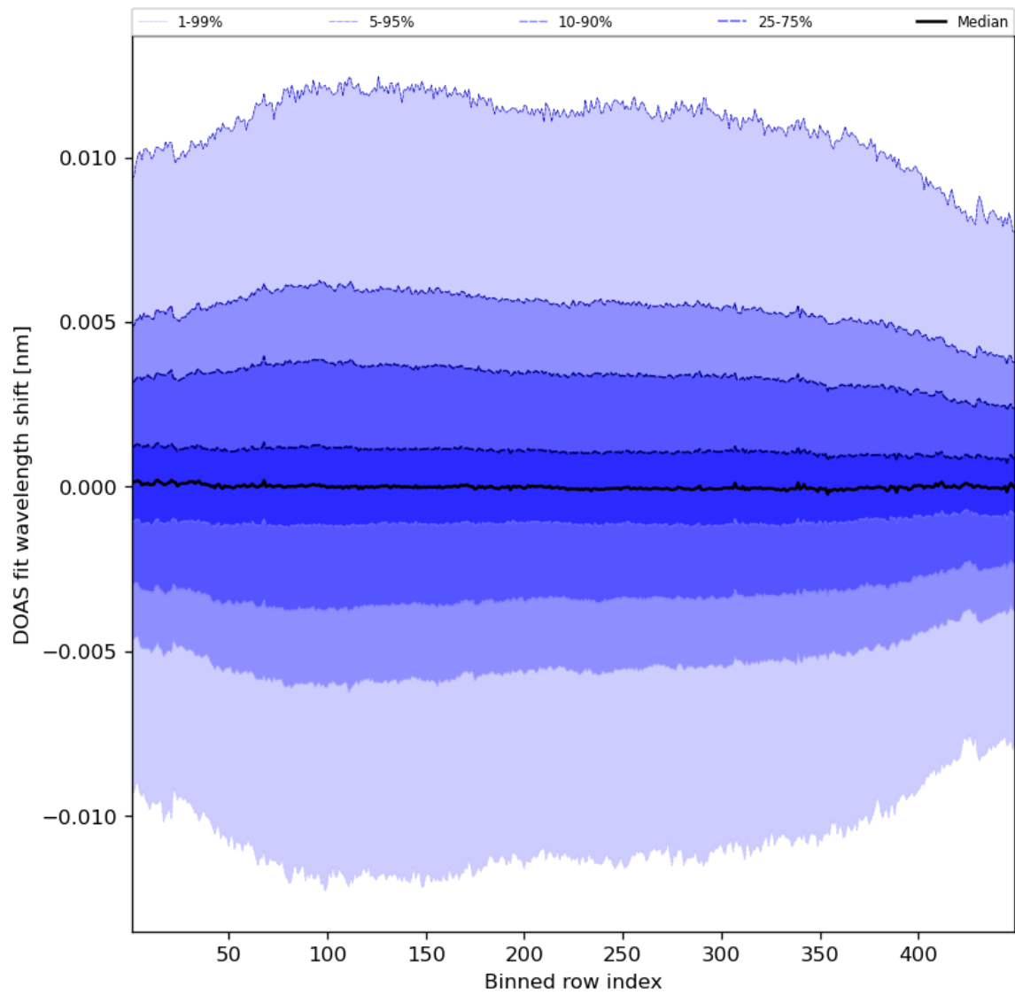
Figure 58: Along track statistics of “DOAS fit wavelength shift” for 2023-07-25 to 2023-07-27
