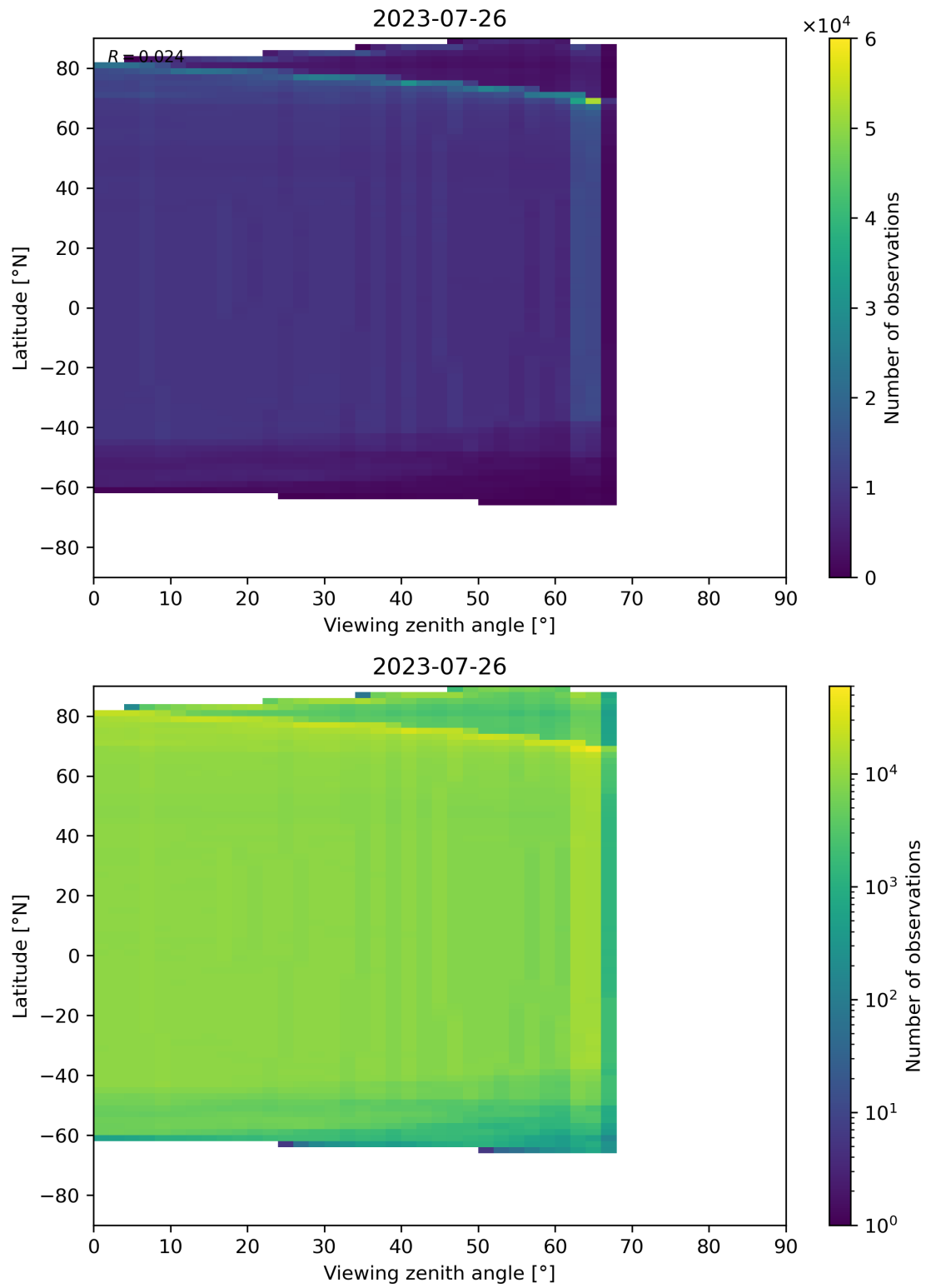
Figure 196: Scatter density plot of “Viewing zenith angle” against “Latitude” for 2023-07-25 to 2023-07-27.
