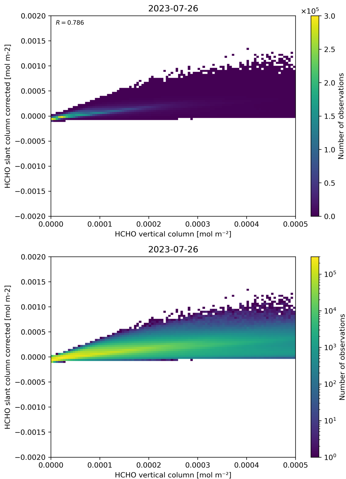
Figure 127: Scatter density plot of “HCHO vertical column” against “HCHO slant column corrected” for 2023-07-25 to 2023-07-27.
