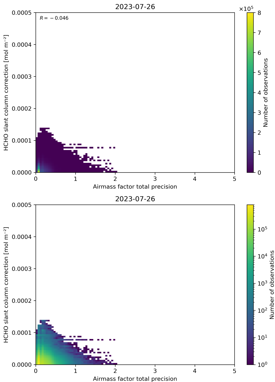
Figure 110: Scatter density plot of “Airmass factor total precision” against “HCHO slant column correction” for 2023-07-25 to 2023-07-27.
