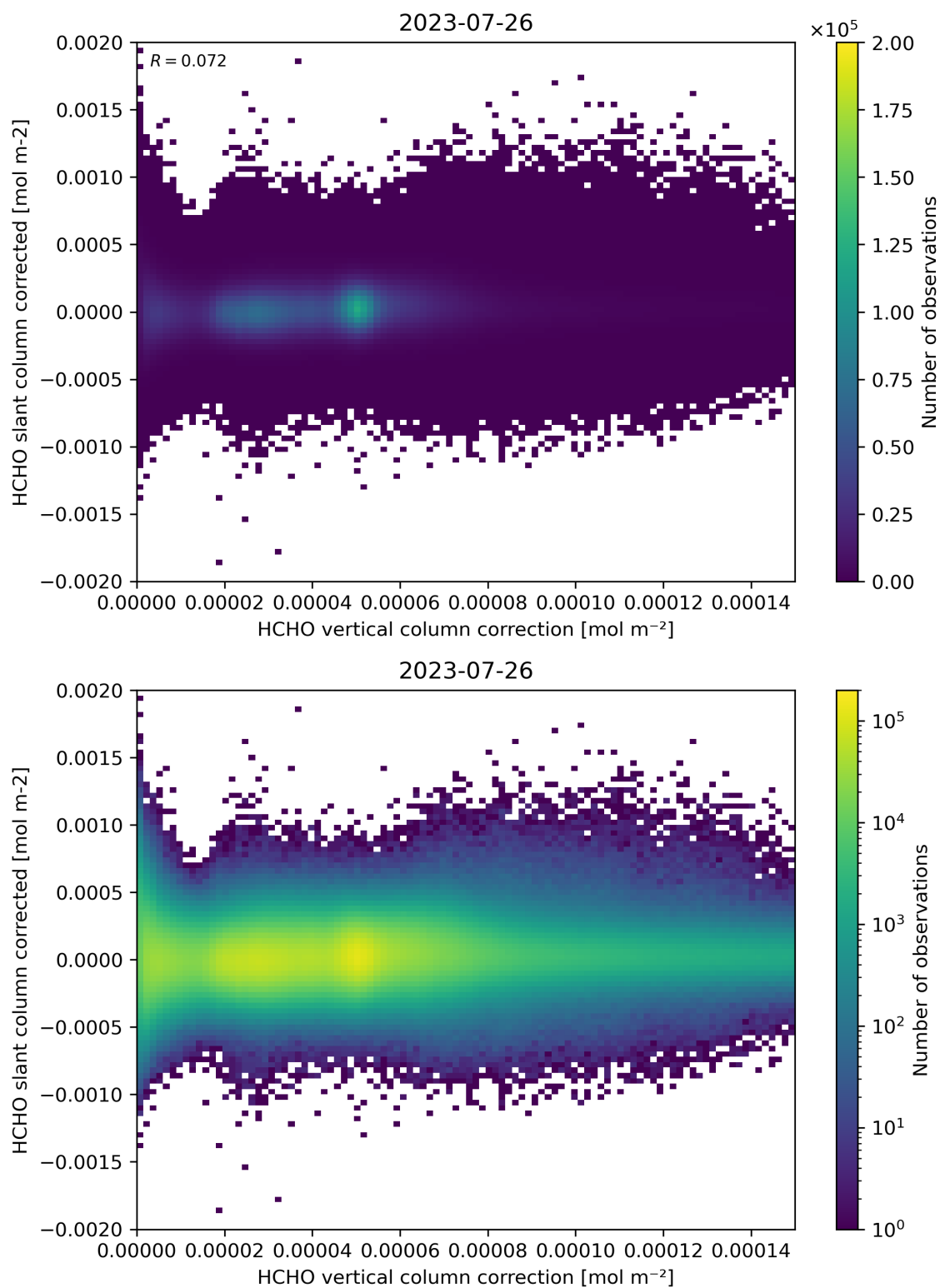
Figure 116: Scatter density plot of “HCHO vertical column correction” against “HCHO slant column corrected” for 2023-07-25 to 2023-07-27.
