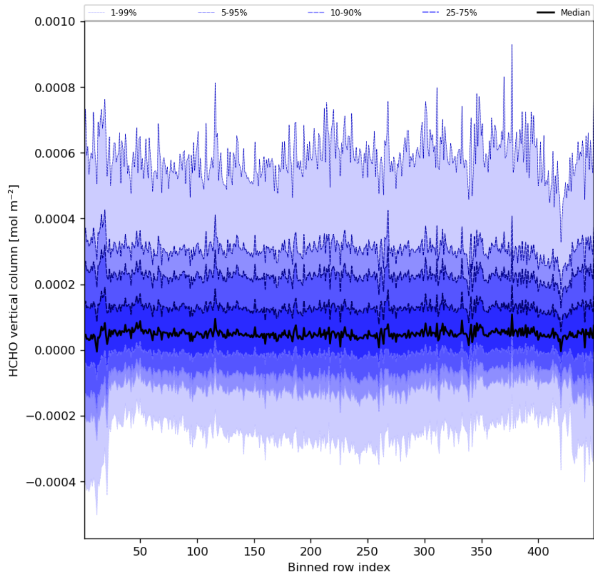
Figure 49: Along track statistics of “HCHO vertical column” for 2023-07-25 to 2023-07-27
