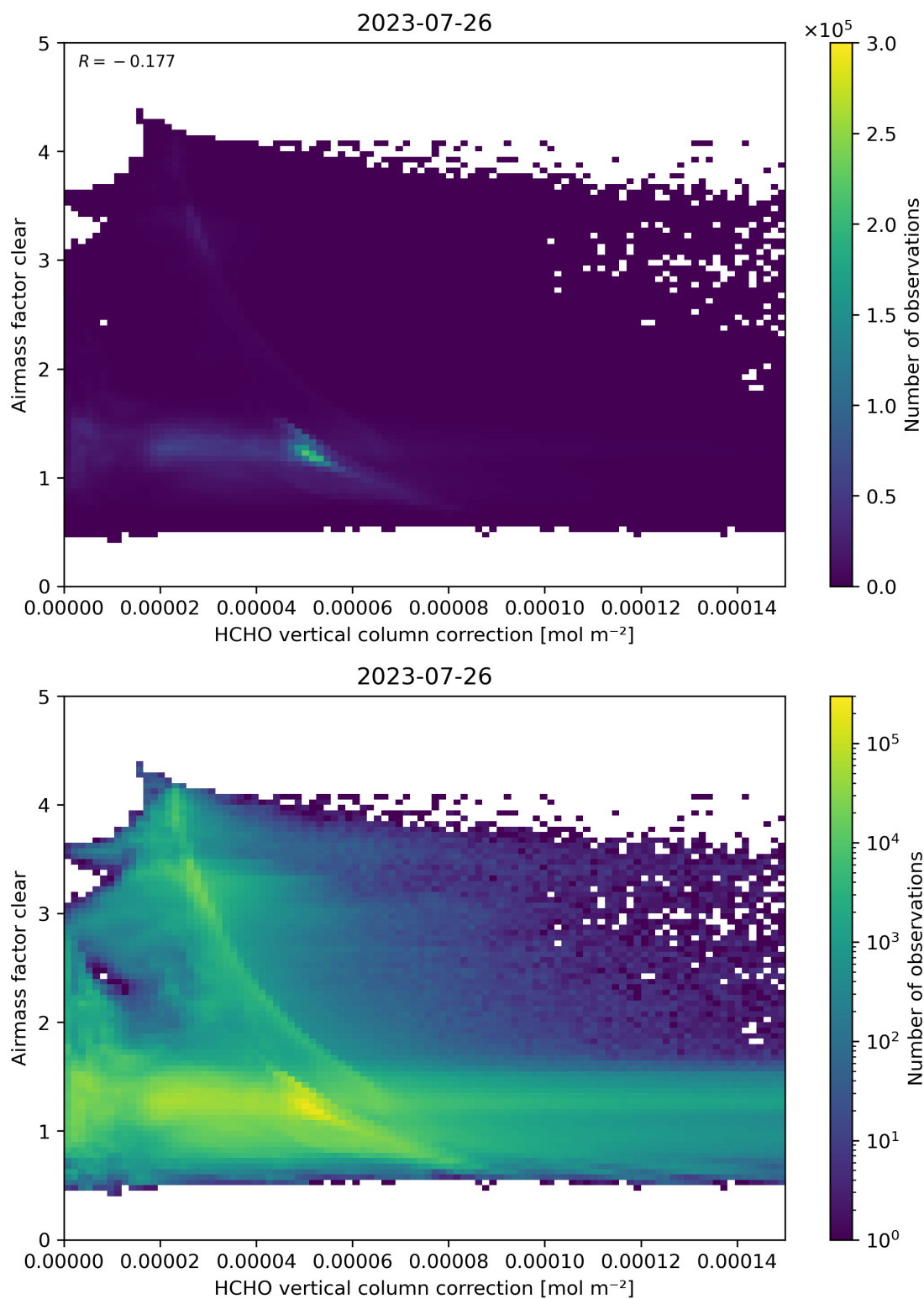
Figure 115: Scatter density plot of “HCHO vertical column correction” against “Airmass factor clear” for 2023-07-25 to 2023-07-27.
