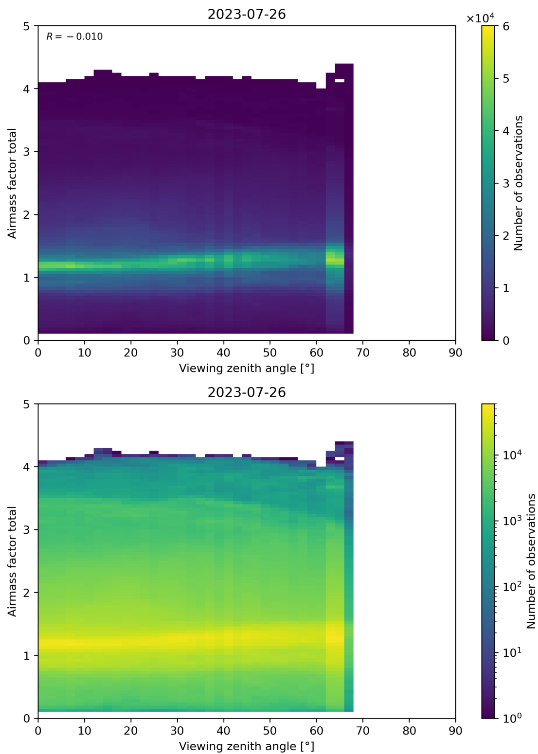
Figure 190: Scatter density plot of “Viewing zenith angle” against “Airmass factor total” for 2023-07-25 to 2023-07-27.
