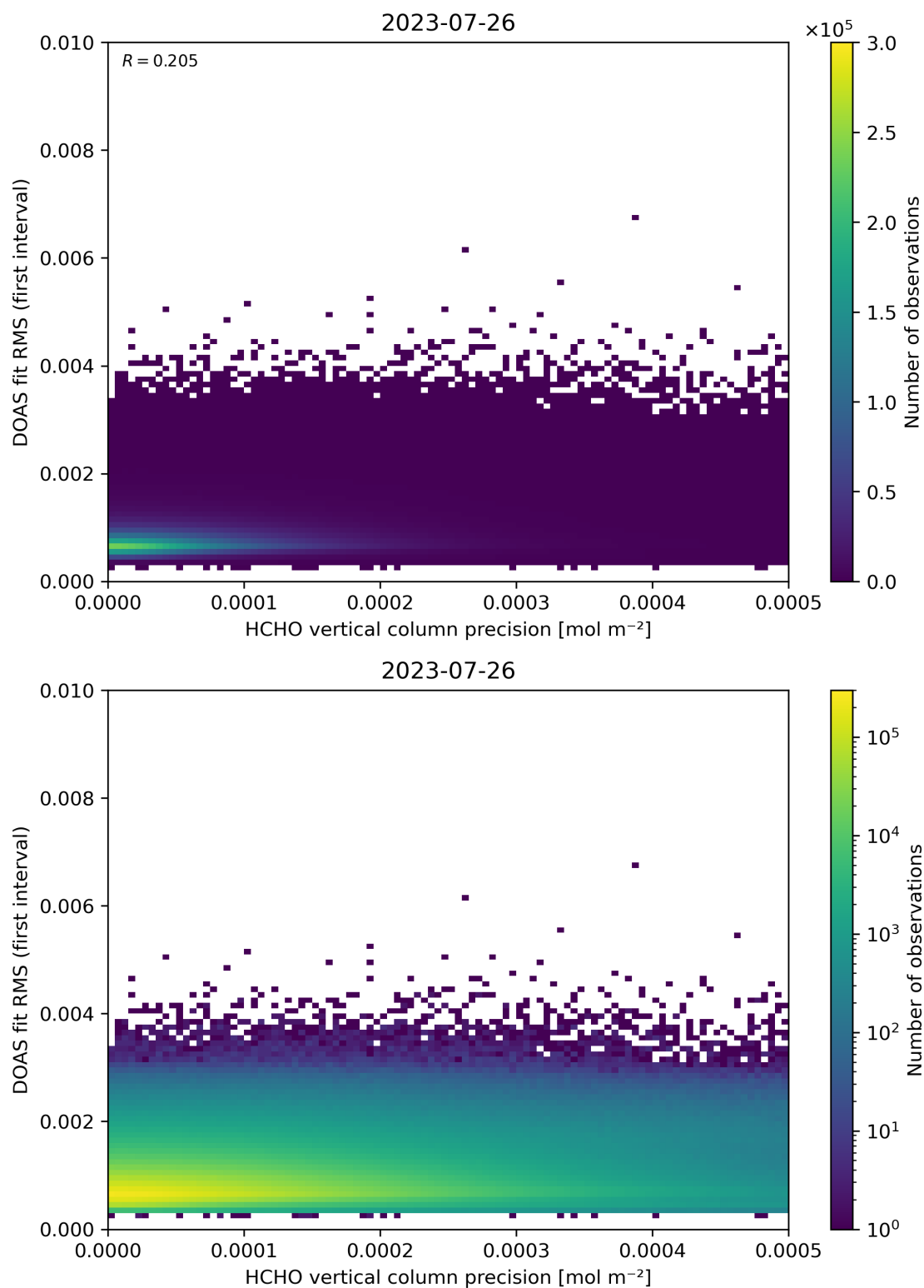
Figure 136: Scatter density plot of “HCHO vertical column precision” against “DOAS fit RMS (first interval)” for 2023-07-25 to 2023-07-27.
