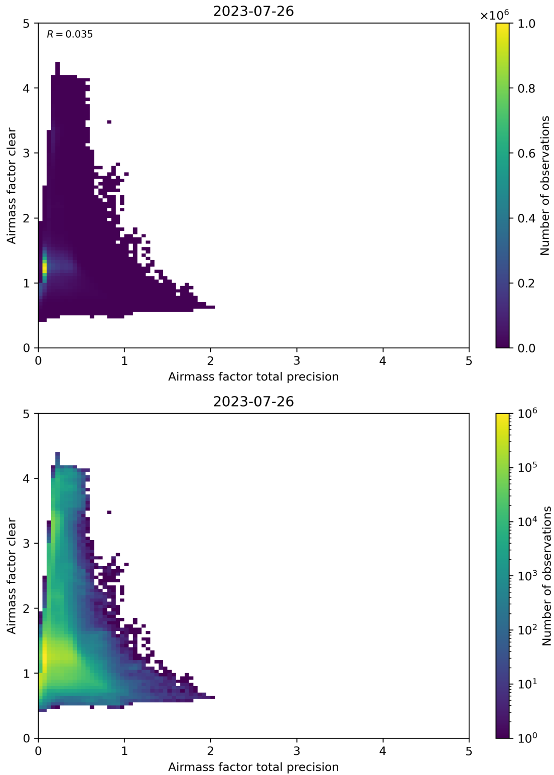
Figure 108: Scatter density plot of “Airmass factor total precision” against “Airmass factor clear” for 2023-07-25 to 2023-07-27.
