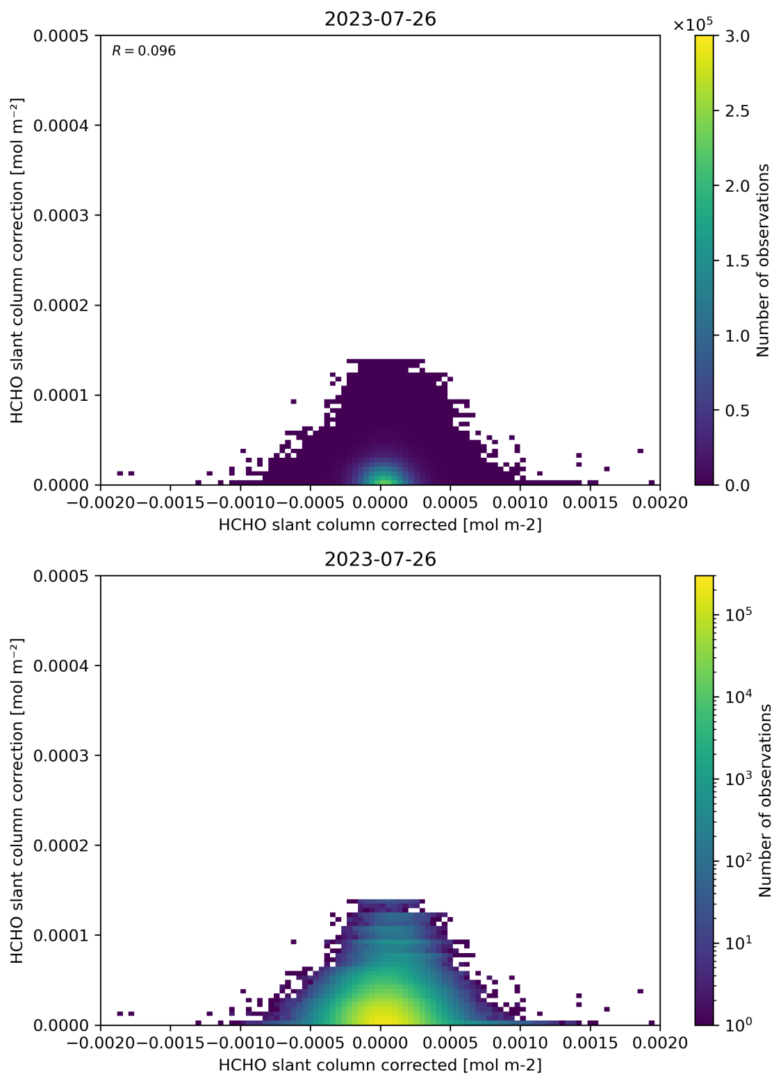
Figure 77: Scatter density plot of “HCHO slant column corrected” against “HCHO slant column correction” for 2023-07-25 to 2023-07-27.
