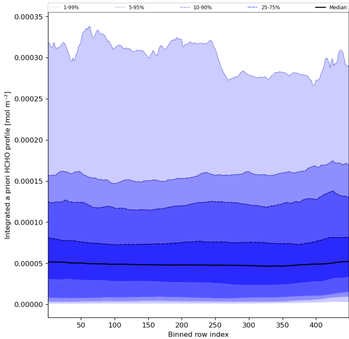
Figure 57: Along track statistics of “Integrated a priori HCHO profile” for 2023-07-25 to 2023-07-27
