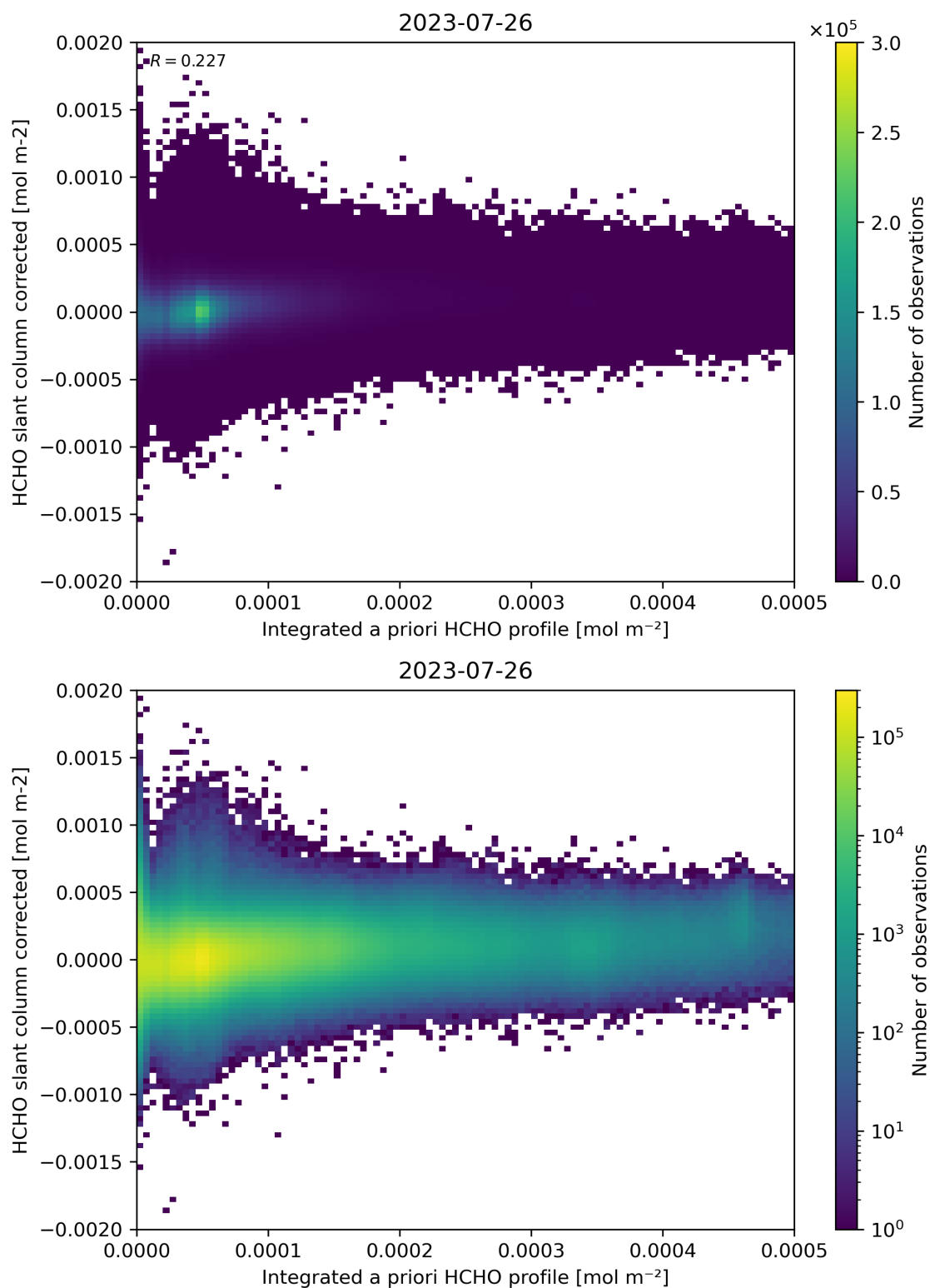
Figure 151: Scatter density plot of “Integrated a priori HCHO profile” against “HCHO slant column corrected” for 2023-07-25 to 2023-07-27.
