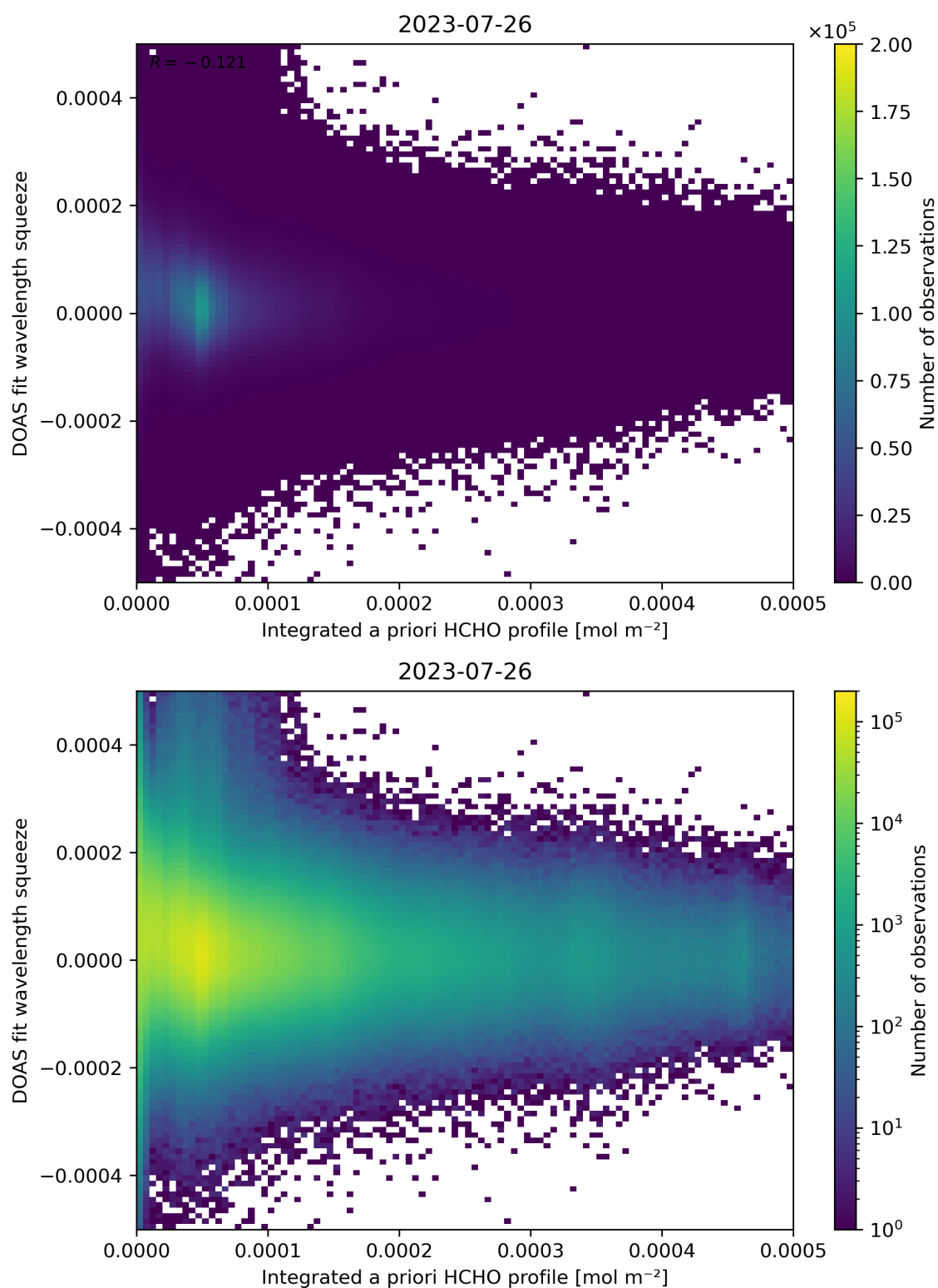
Figure 150: Scatter density plot of “Integrated a priori HCHO profile” against “DOAS fit wavelength squeeze” for 2023-07-25 to 2023-07-27.
