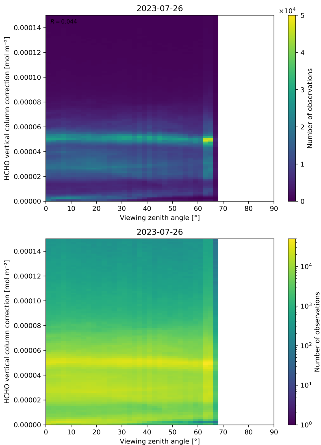
Figure 193: Scatter density plot of “Viewing zenith angle” against “HCHO vertical column correction” for 2023-07-25 to 2023-07-27.
