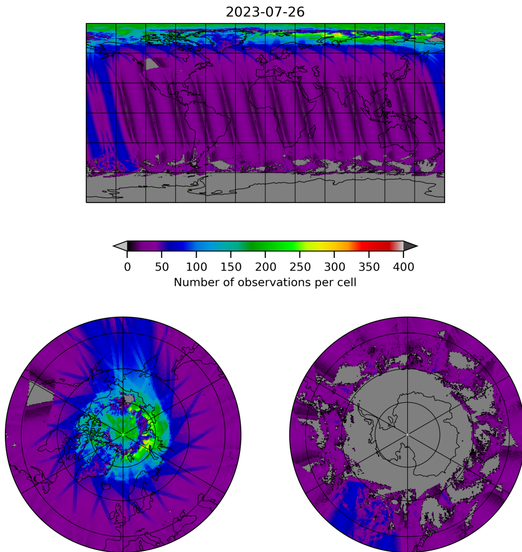
Figure 19: Map of the number of observations for 2023-07-25 to 2023-07-27
