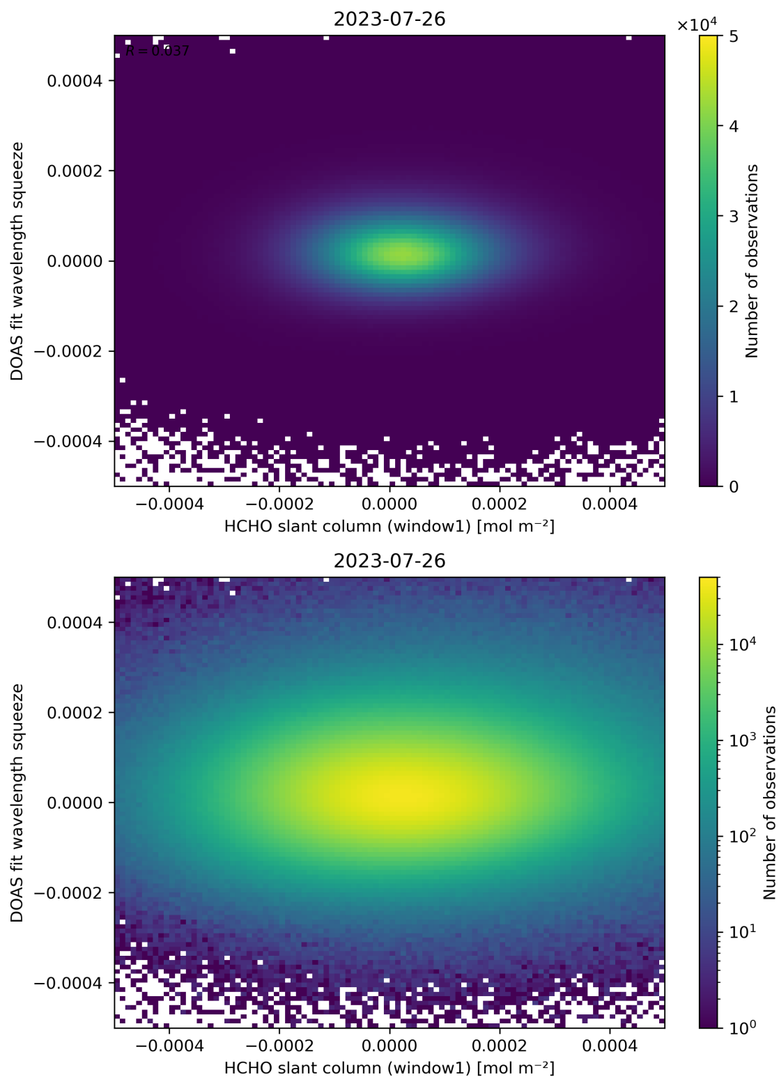
Figure 80: Scatter density plot of “HCHO slant column (window1)” against “DOAS fit wavelength squeeze” for 2023-07-25 to 2023-07-27.
