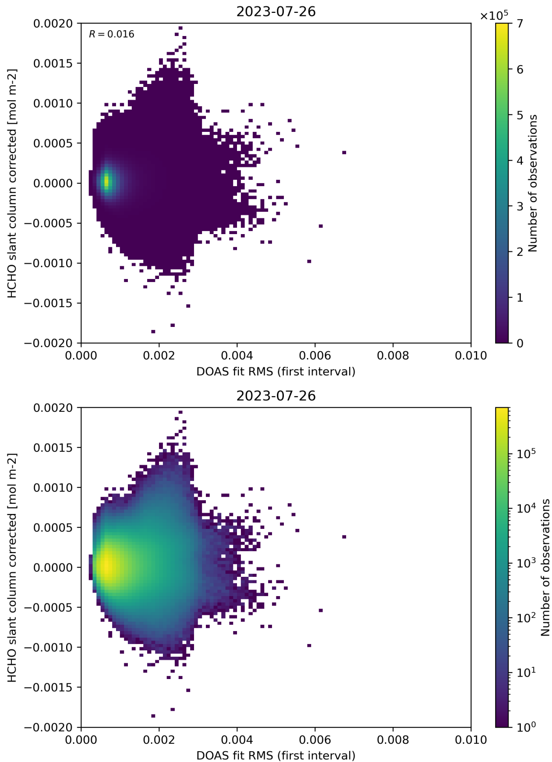
Figure 62: Scatter density plot of “DOAS fit RMS (first interval)” against “HCHO slant column corrected” for 2023-07-25 to 2023-07-27.
