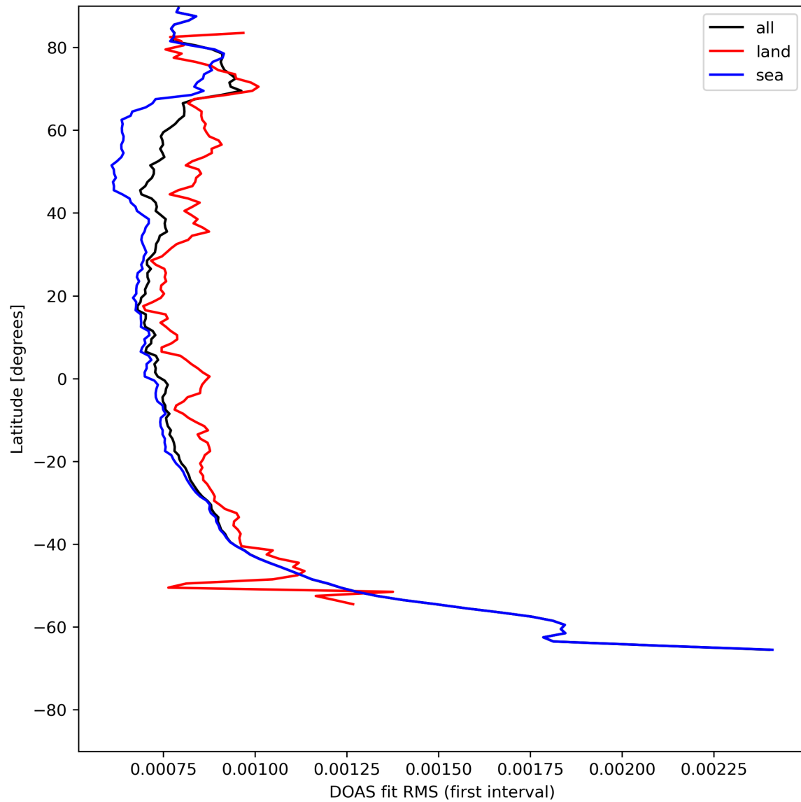
Figure 32: Zonal average of “DOAS fit RMS (first interval)” for 2023-07-25 to 2023-07-27.
