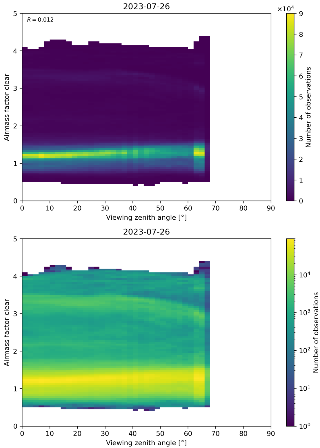
Figure 185: Scatter density plot of “Viewing zenith angle” against “Airmass factor clear” for 2023-07-25 to 2023-07-27.
