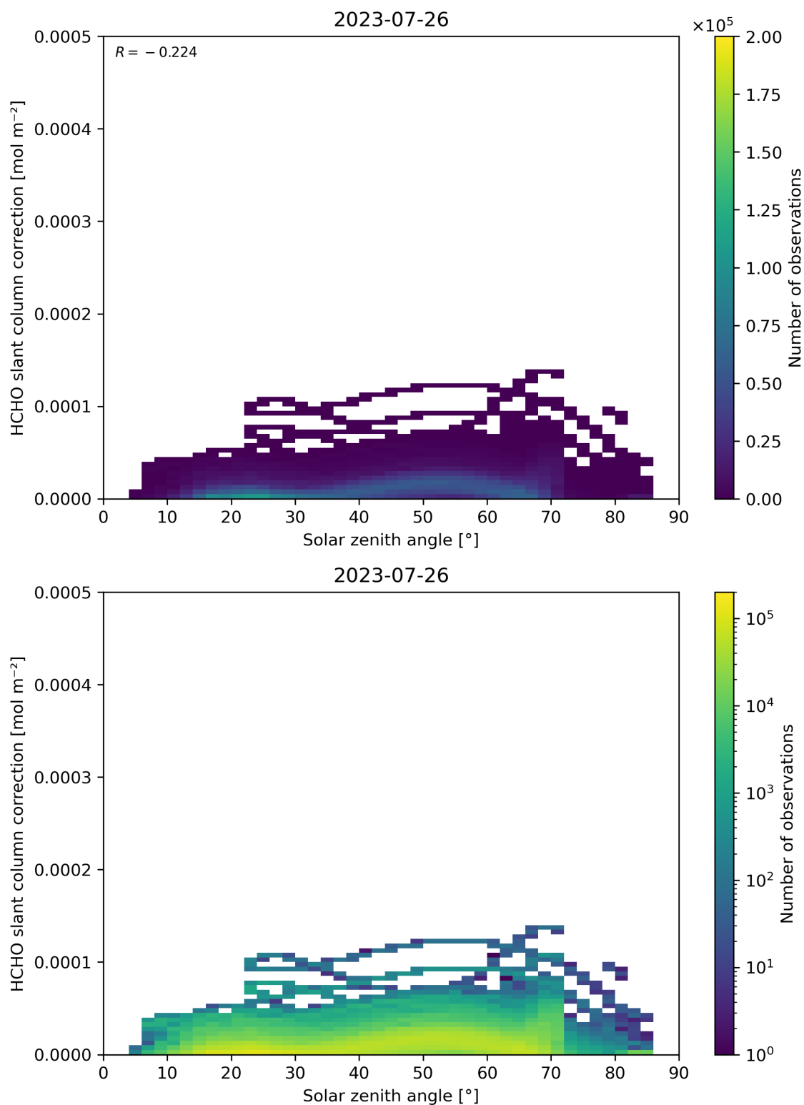
Figure 172: Scatter density plot of “Solar zenith angle” against “HCHO slant column correction” for 2023-07-25 to 2023-07-27.
