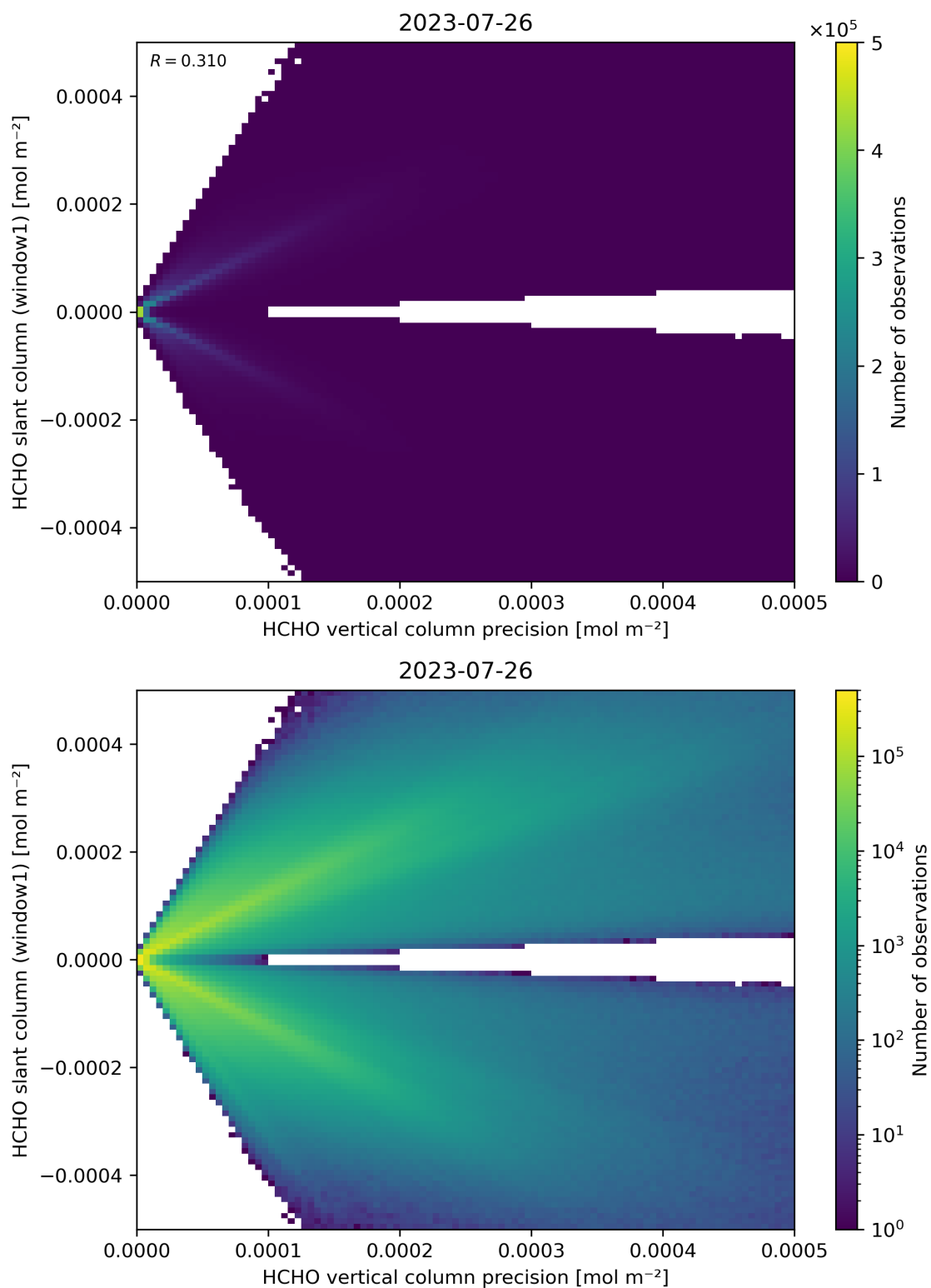
Figure 142: Scatter density plot of “HCHO vertical column precision” against “HCHO slant column (window1)” for 2023-07-25 to 2023-07-27.
