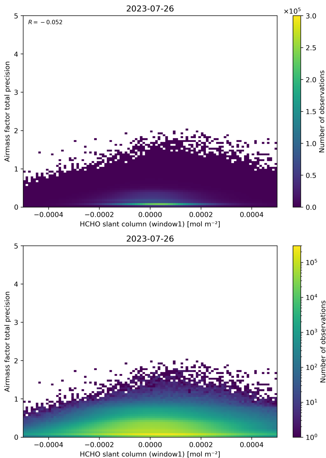
Figure 86: Scatter density plot of “HCHO slant column (window1)” against “Airmass factor total precision” for 2023-07-25 to 2023-07-27.
