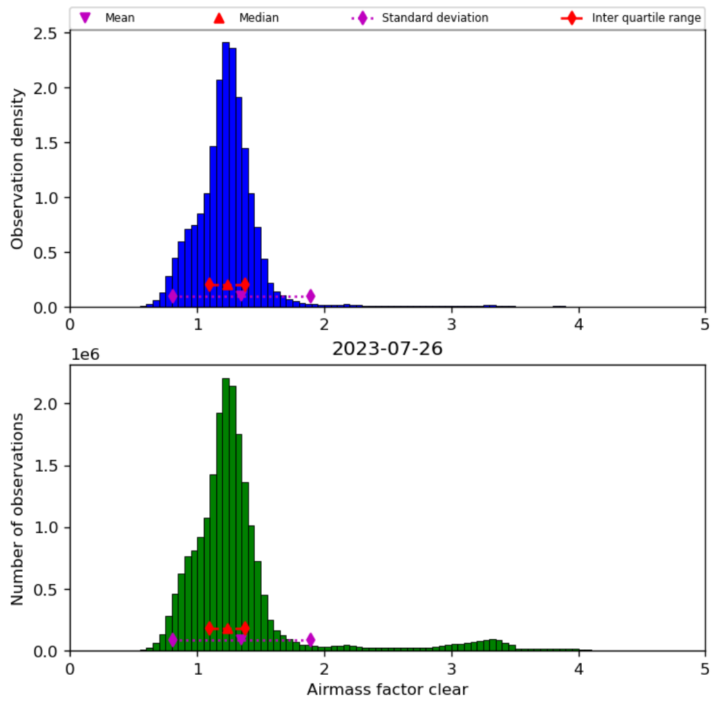
Figure 42: Histogram of “Airmass factor clear” for 2023-07-25 to 2023-07-27
