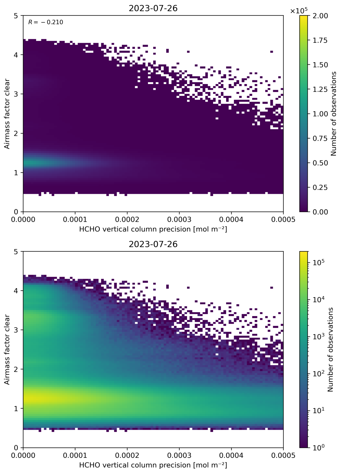
Figure 139: Scatter density plot of “HCHO vertical column precision” against “Airmass factor clear” for 2023-07-25 to 2023-07-27.
