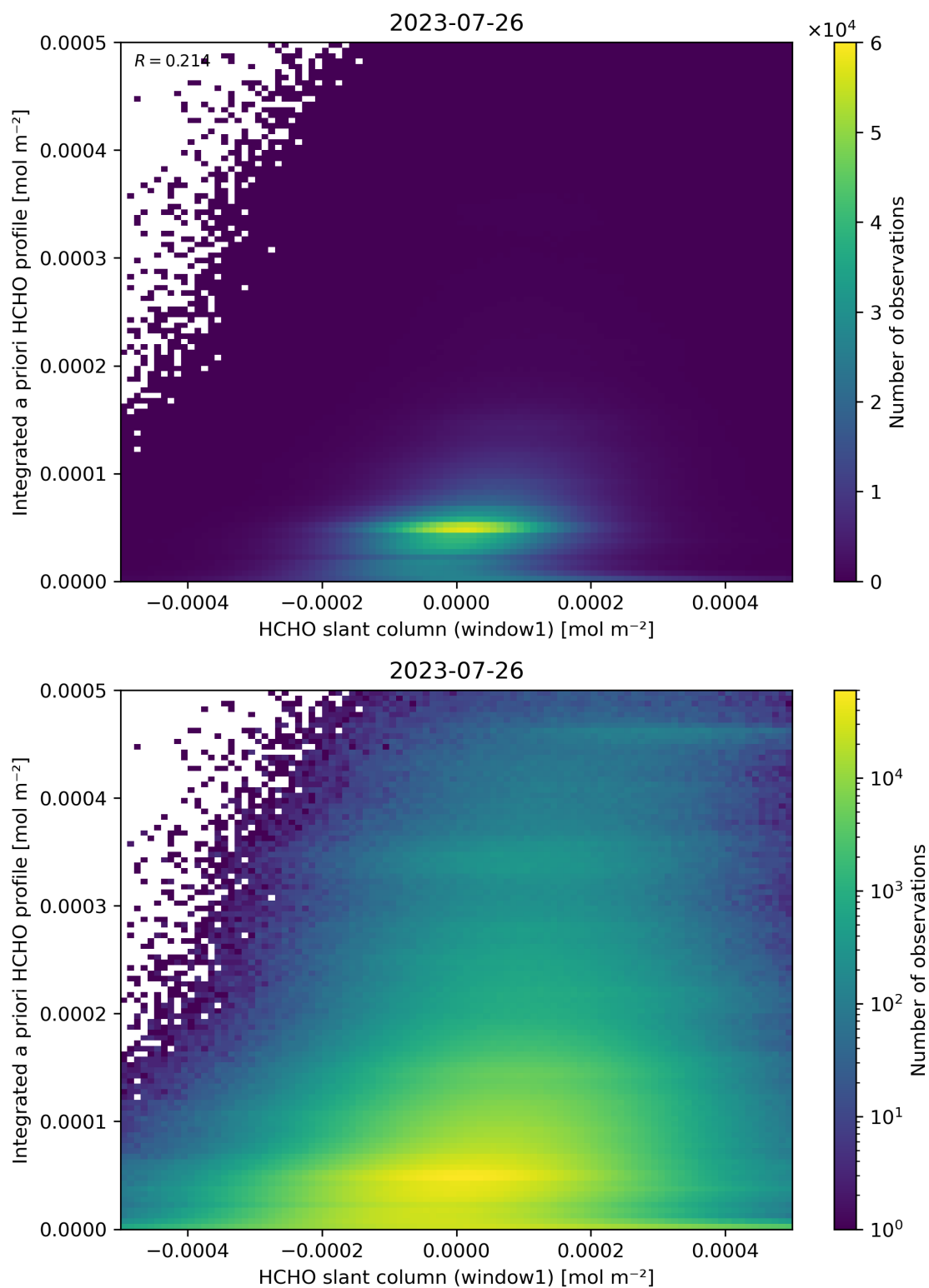
Figure 87: Scatter density plot of “HCHO slant column (window1)” against “Integrated a priori HCHO profile” for 2023-07-25 to 2023-07-27.
