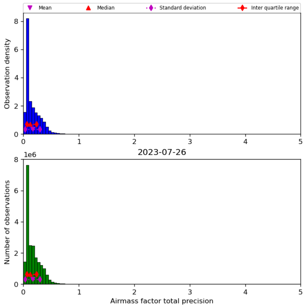
Figure 41: Histogram of "Airmass factor total precision" for 2023-07-25 to 2023-07-27
