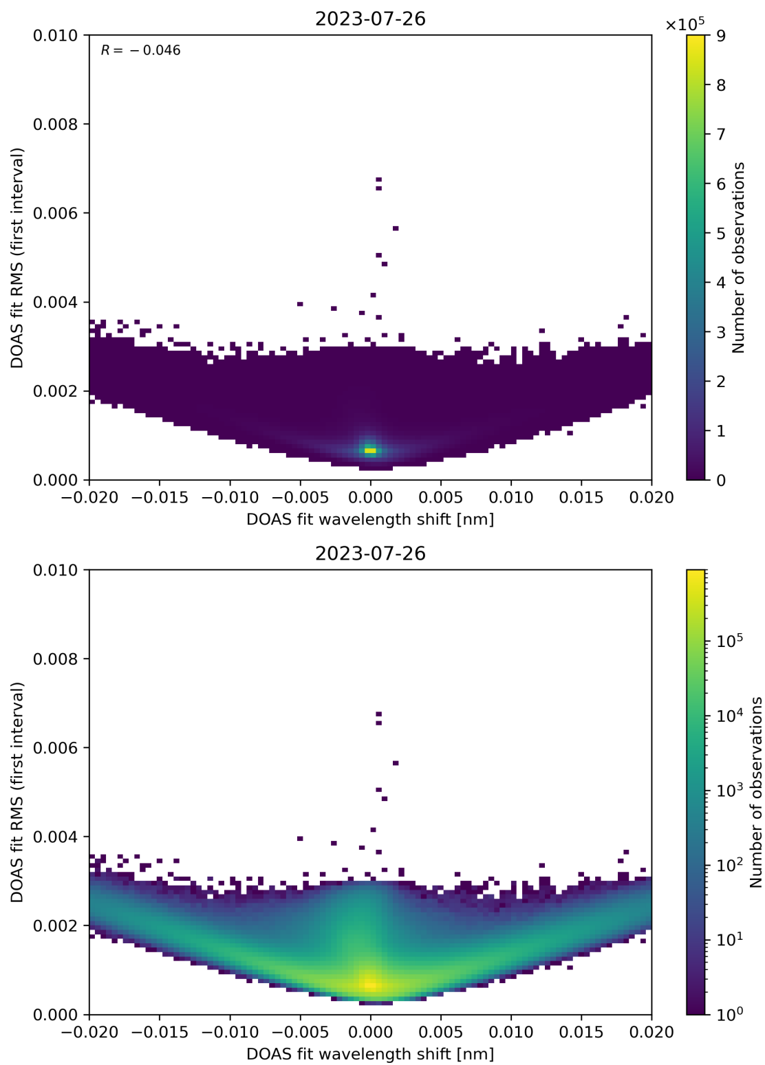
Figure 64: Scatter density plot of “DOAS fit wavelength shift” against “DOAS fit RMS (first interval)” for 2023-07-25 to 2023-07-27.
