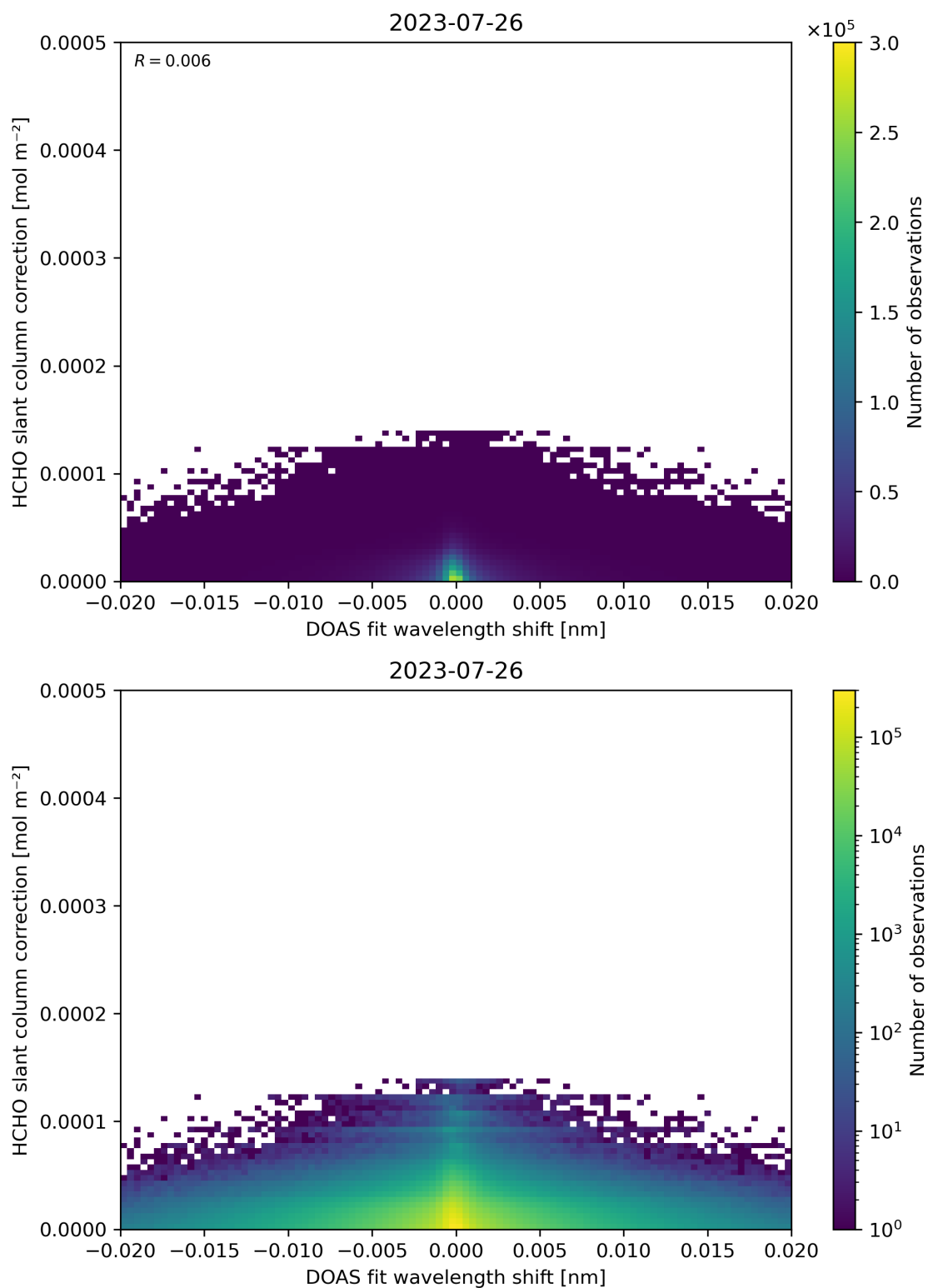
Figure 67: Scatter density plot of “DOAS fit wavelength shift” against “HCHO slant column correction” for 2023-07-25 to 2023-07-27.
