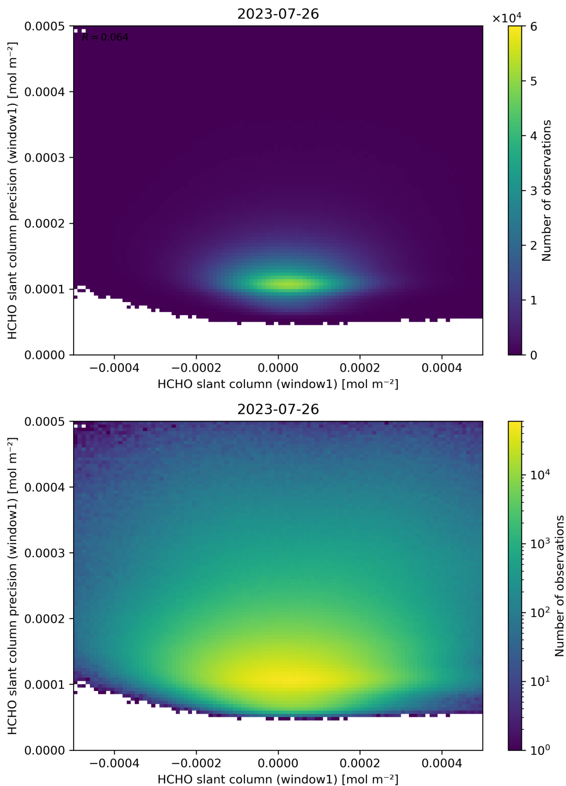
Figure 84: Scatter density plot of “HCHO slant column (window1)” against “HCHO slant column precision (window1)” for 2023-07-25 to 2023-07-27.
