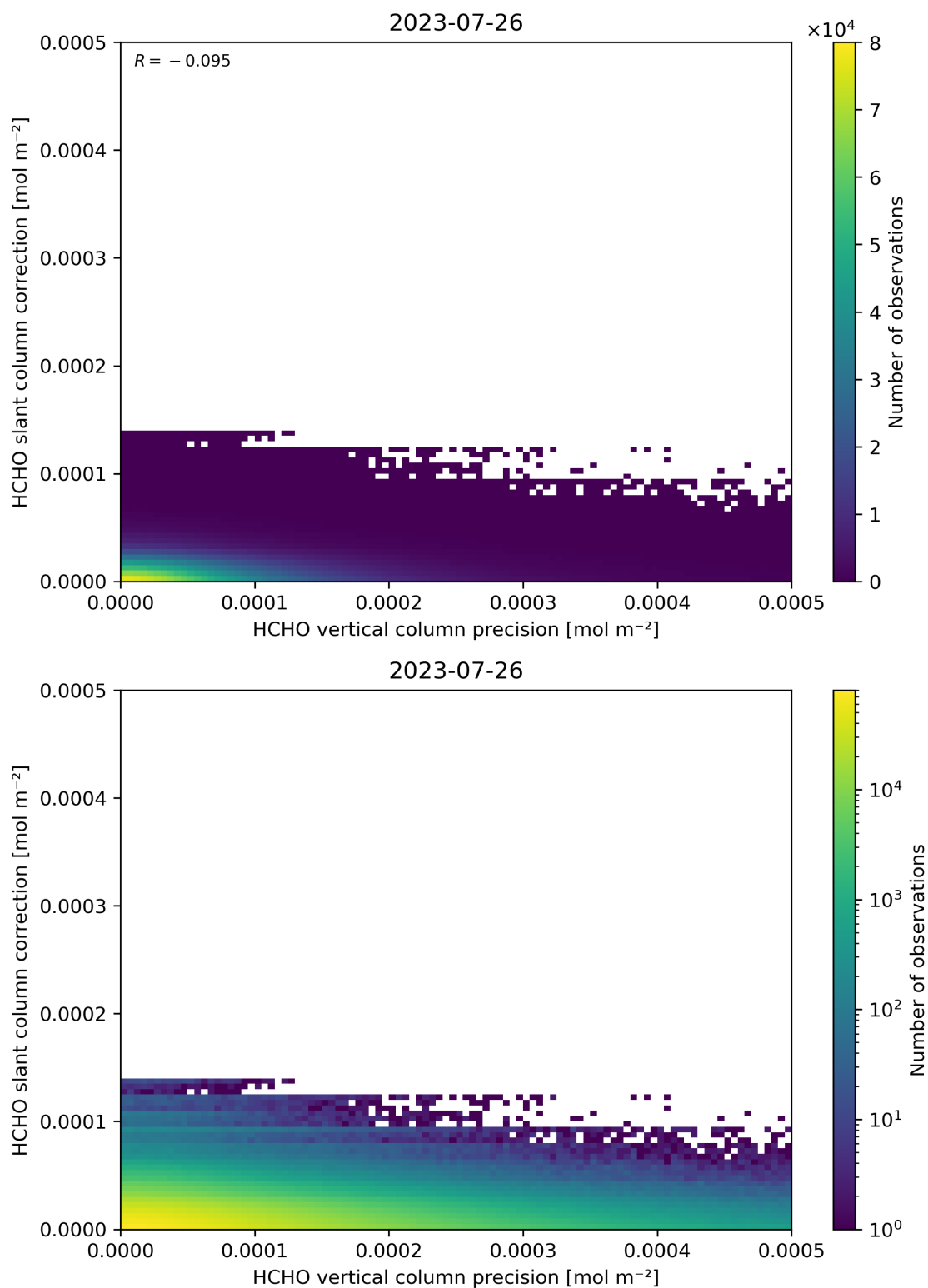
Figure 141: Scatter density plot of “HCHO vertical column precision” against “HCHO slant column correction” for 2023-07-25 to 2023-07-27.
