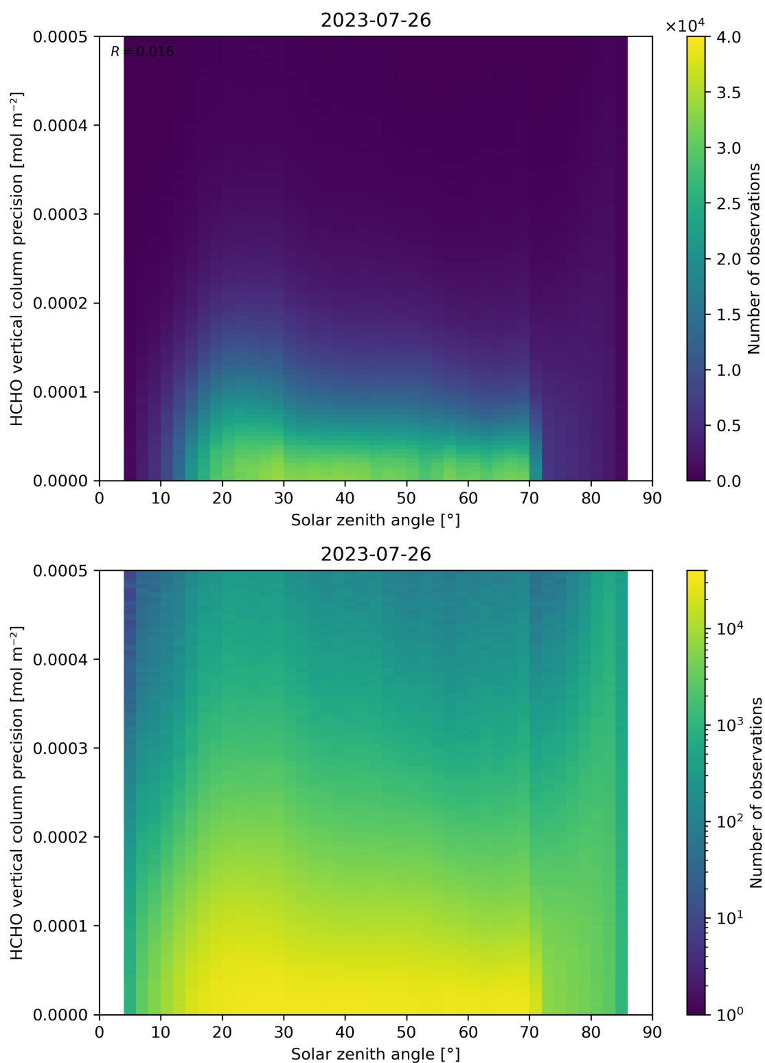
Figure 179: Scatter density plot of “Solar zenith angle” against “HCHO vertical column precision” for 2023-07-25 to 2023-07-27.
