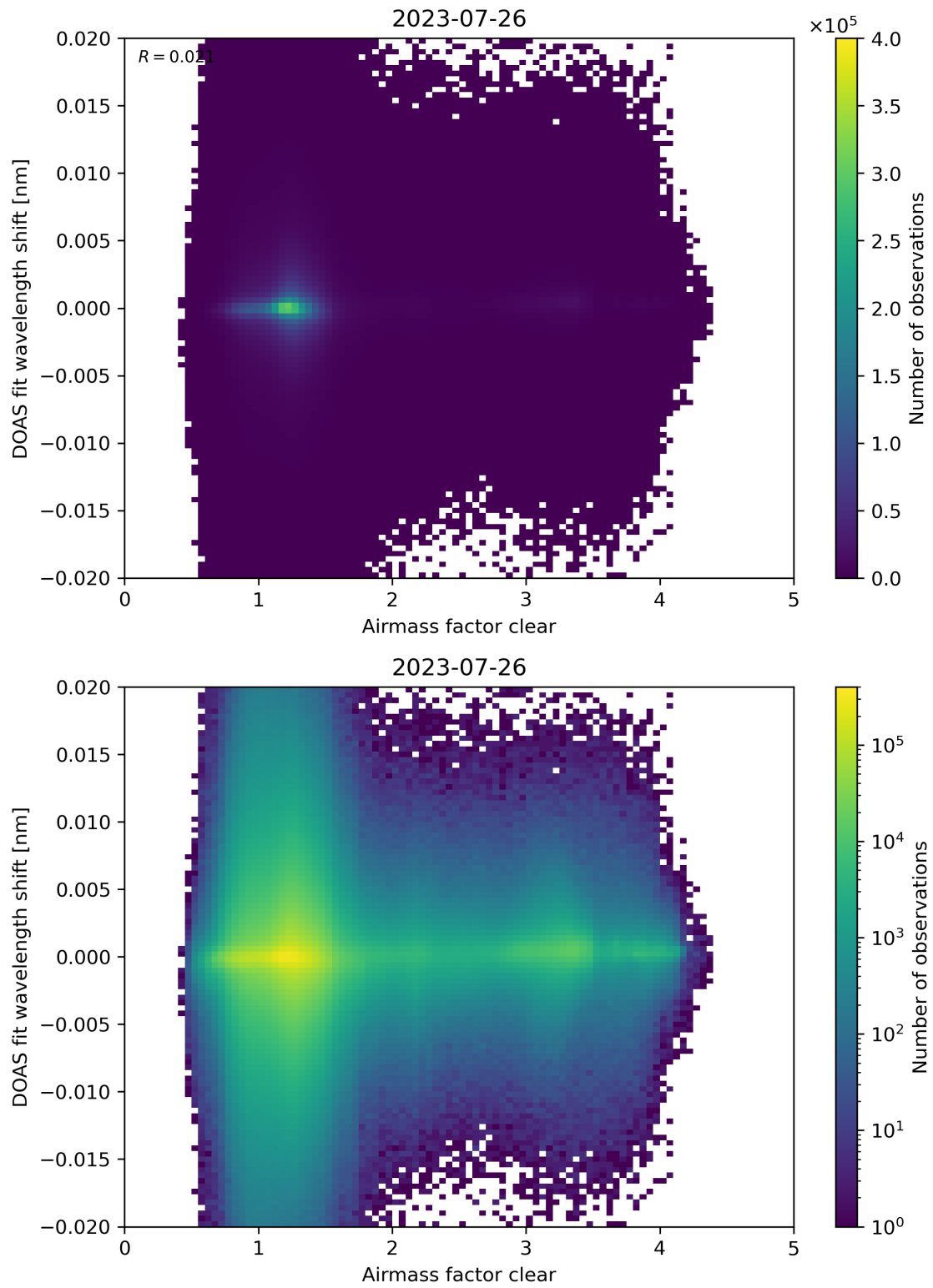
Figure 72: Scatter density plot of “Airmass factor clear” against “DOAS fit wavelength shift” for 2023-07-25 to 2023-07-27.
