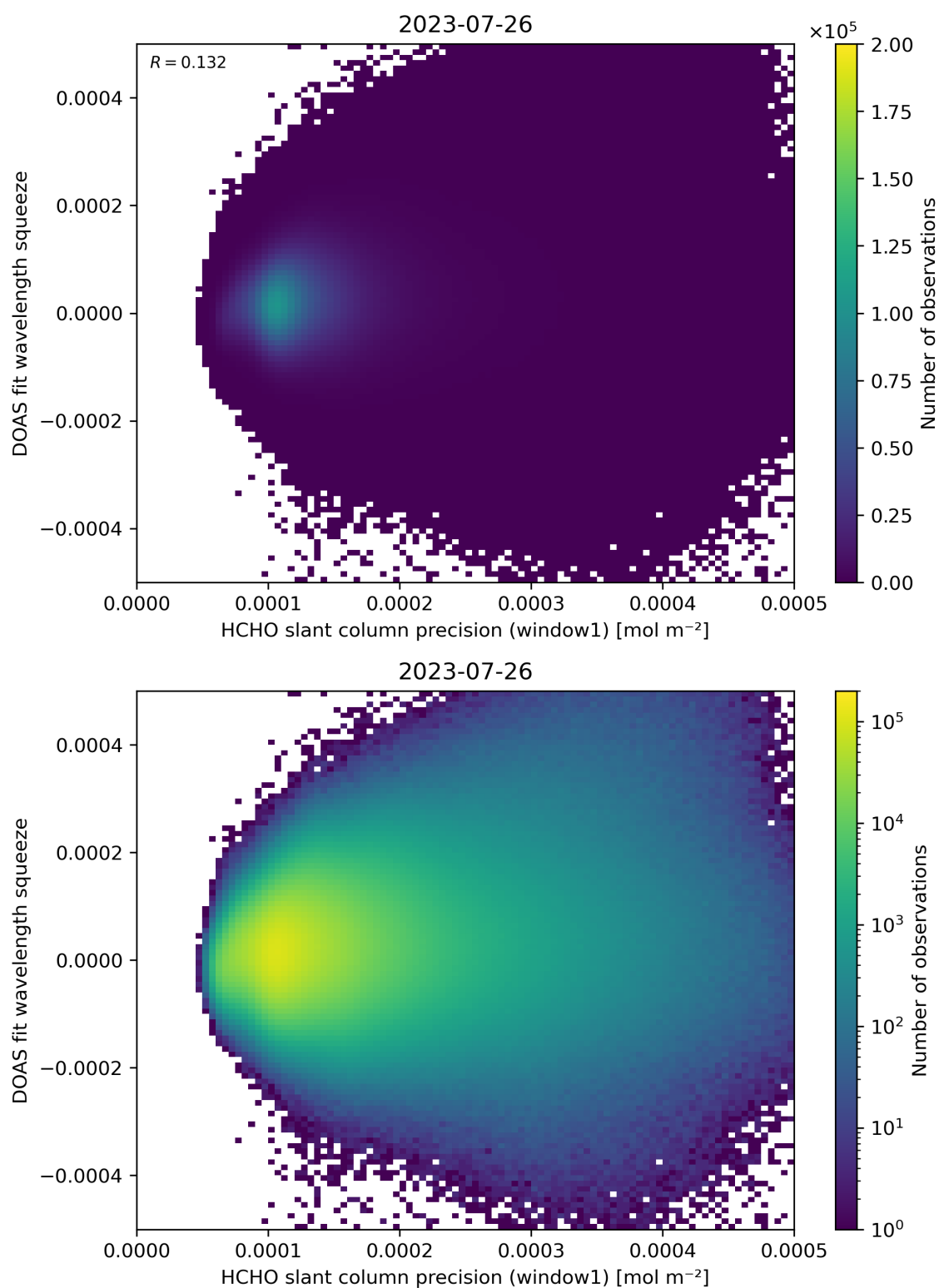
Figure 90: Scatter density plot of “HCHO slant column precision (window1)” against “DOAS fit wavelength squeeze” for 2023-07-25 to 2023-07-27.
