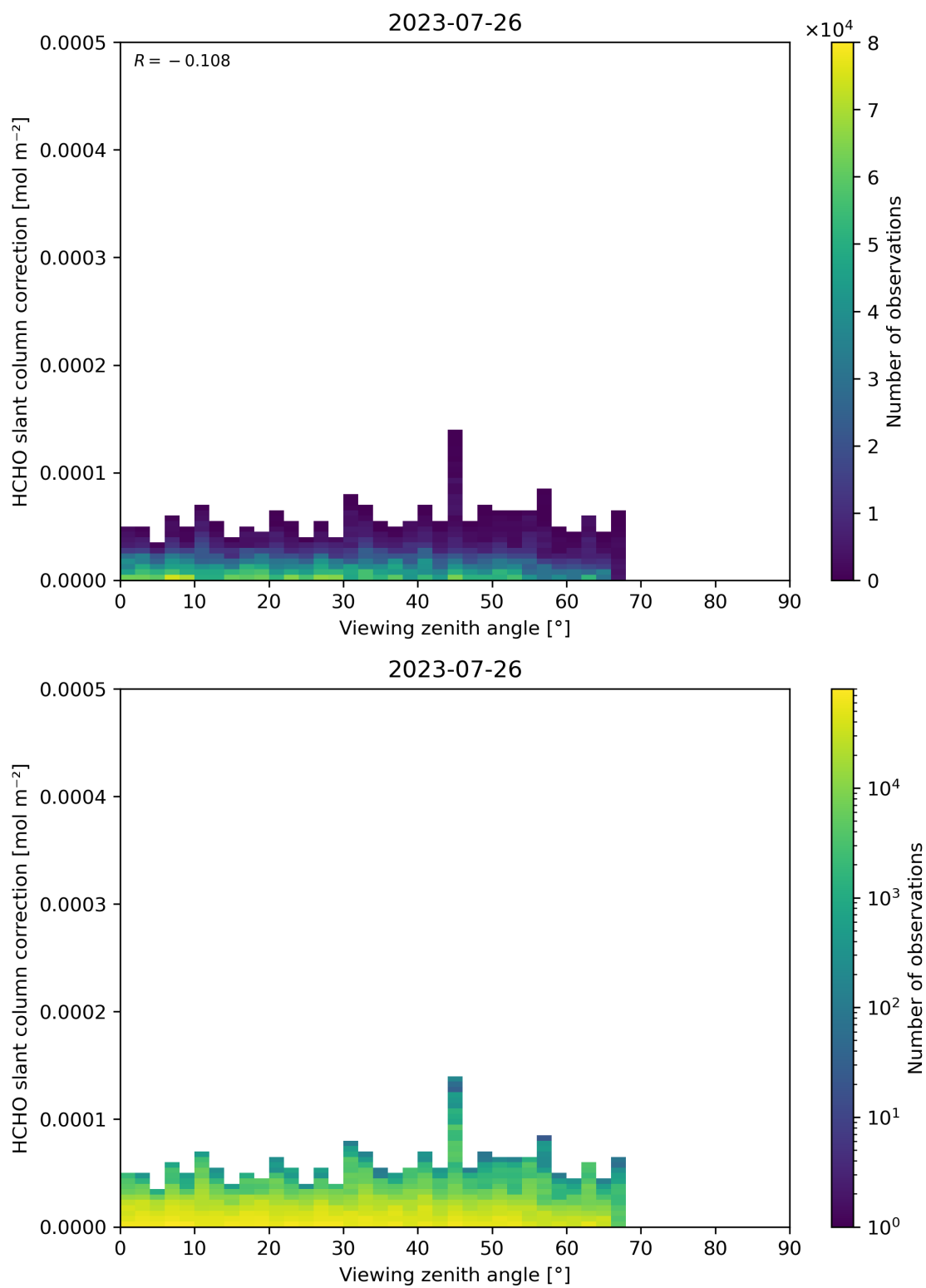
Figure 187: Scatter density plot of “Viewing zenith angle” against “HCHO slant column correction” for 2023-07-25 to 2023-07-27.
