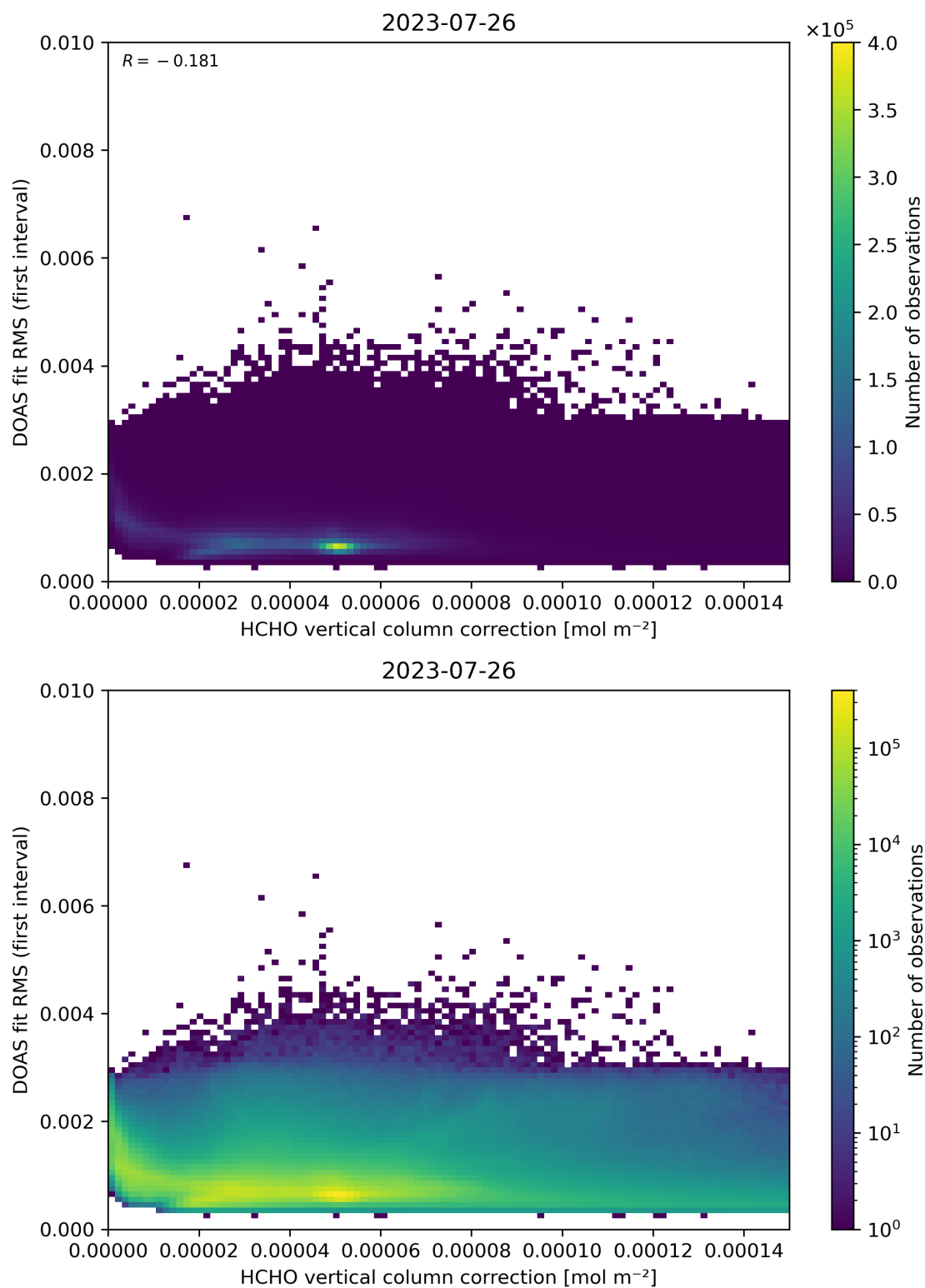
Figure 112: Scatter density plot of “HCHO vertical column correction” against “DOAS fit RMS (first interval)” for 2023-07-25 to 2023-07-27.
