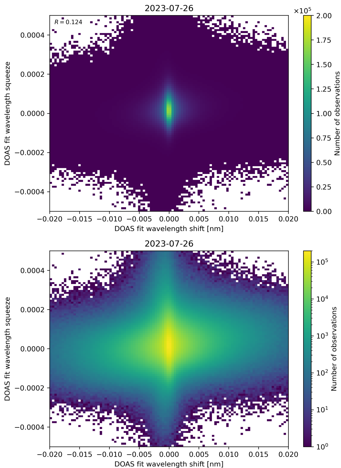
Figure 65: Scatter density plot of “DOAS fit wavelength shift” against “DOAS fit wavelength squeeze” for 2023-07-25 to 2023-07-27.
