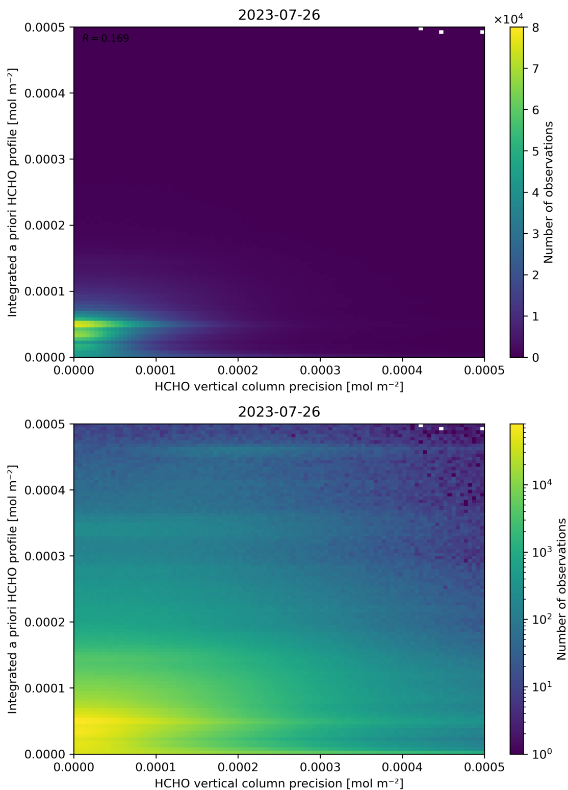
Figure 147: Scatter density plot of “HCHO vertical column precision” against “Integrated a priori HCHO profile” for 2023-07-25 to 2023-07-27.
