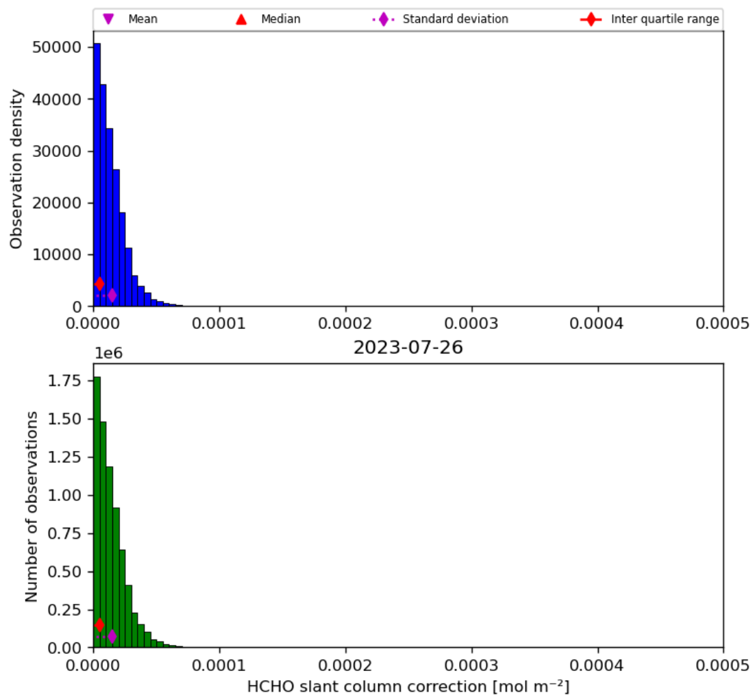
Figure 47: Histogram of “HCHO slant column correction” for 2023-07-25 to 2023-07-27
