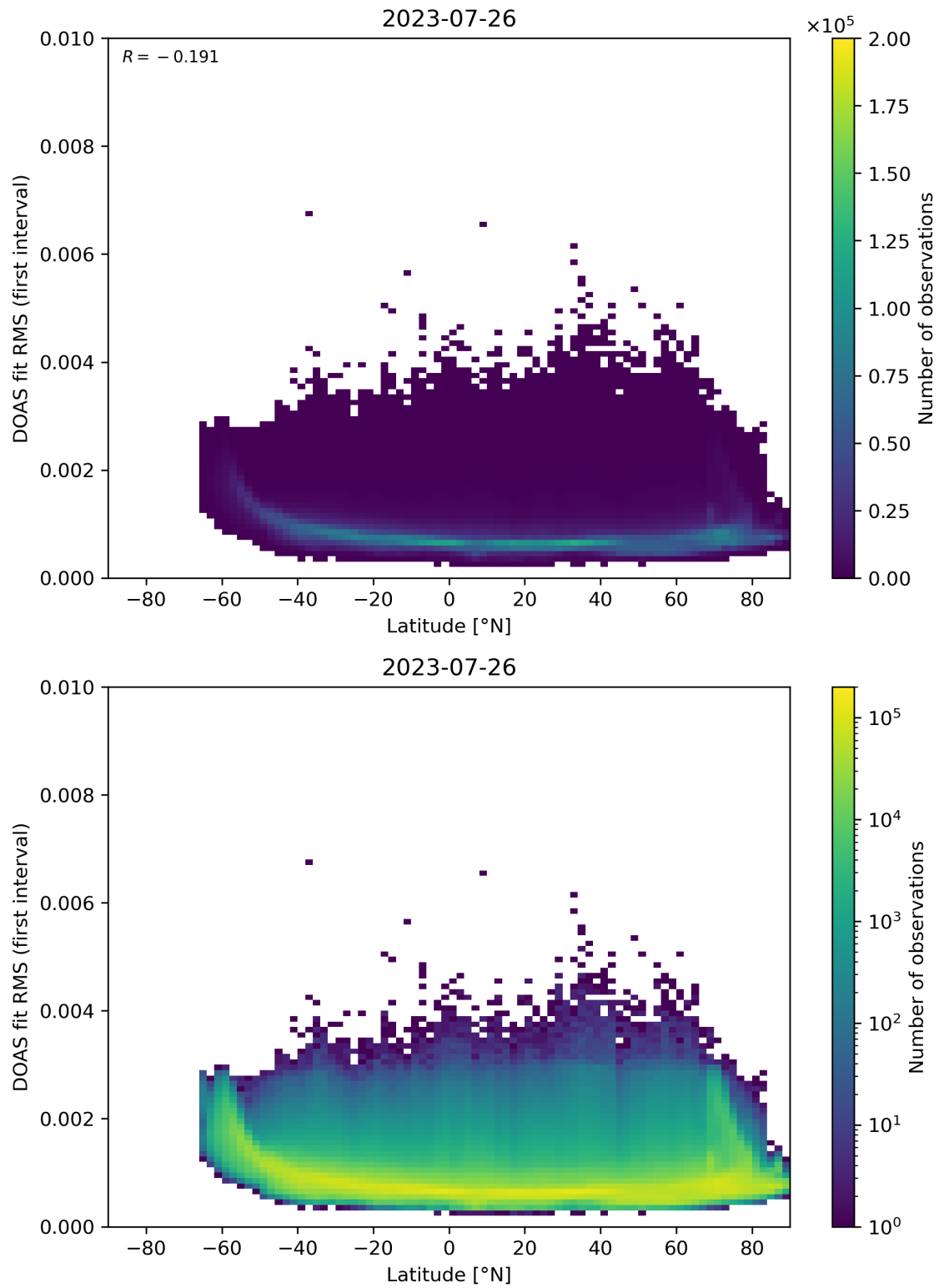
Figure 153: Scatter density plot of “Latitude” against “DOAS fit RMS (first interval)” for 2023-07-25 to 2023-07-27.
