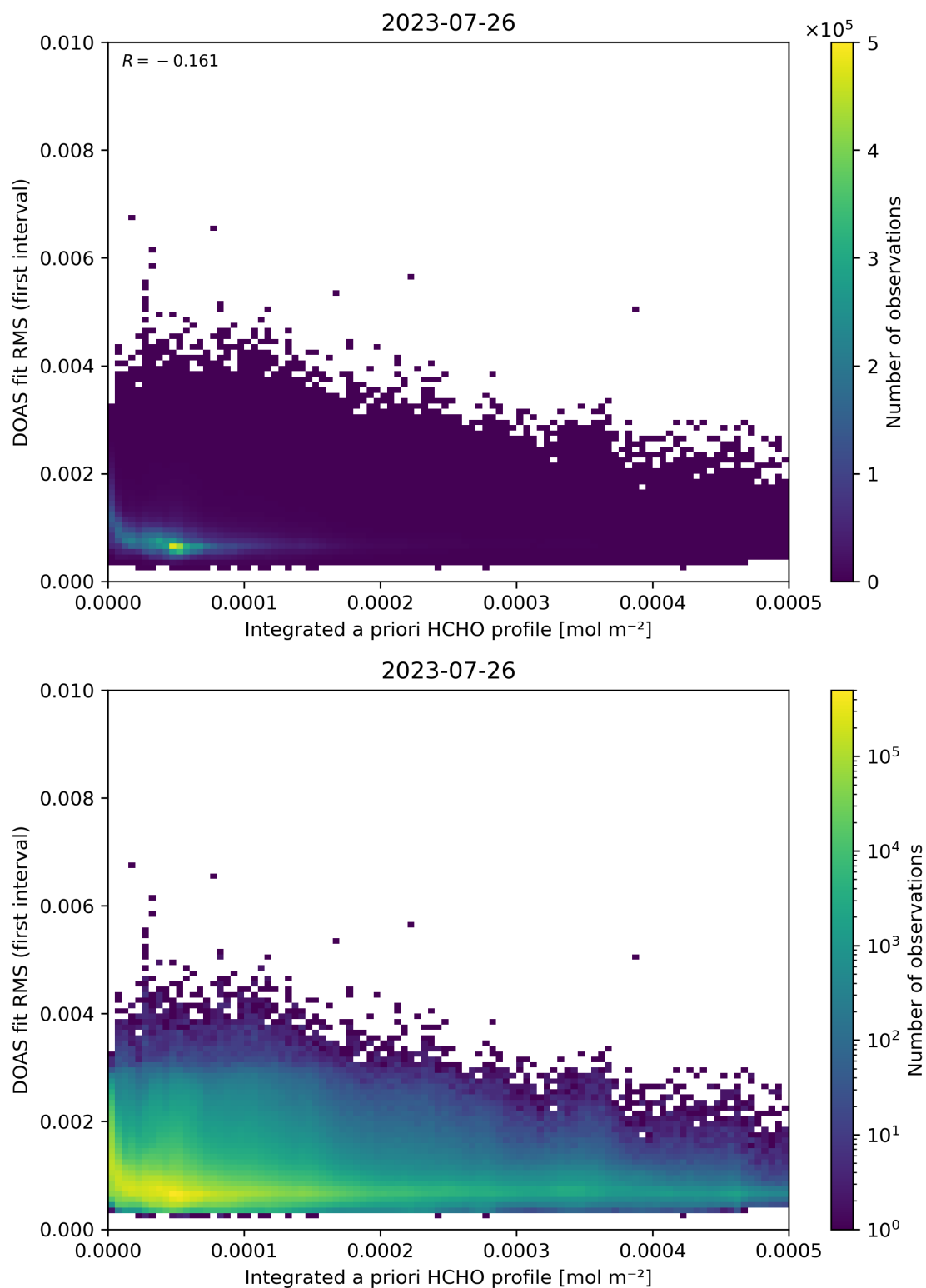
Figure 148: Scatter density plot of “Integrated a priori HCHO profile” against “DOAS fit RMS (first interval)” for 2023-07-25 to 2023-07-27.
