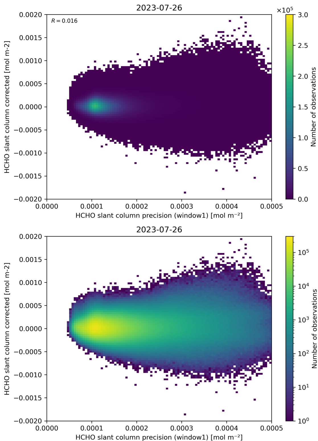
Figure 92: Scatter density plot of “HCHO slant column precision (window1)” against “HCHO slant column corrected” for 2023-07-25 to 2023-07-27.
