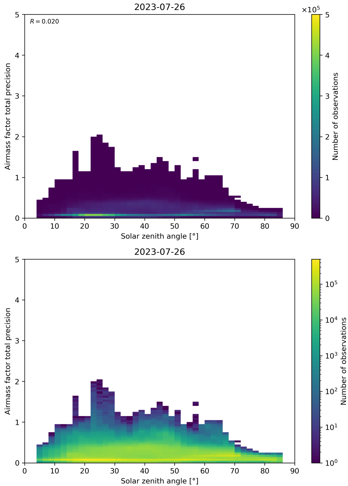
Figure 176: Scatter density plot of “Solar zenith angle” against “Airmass factor total precision” for 2023-07-25 to 2023-07-27.
