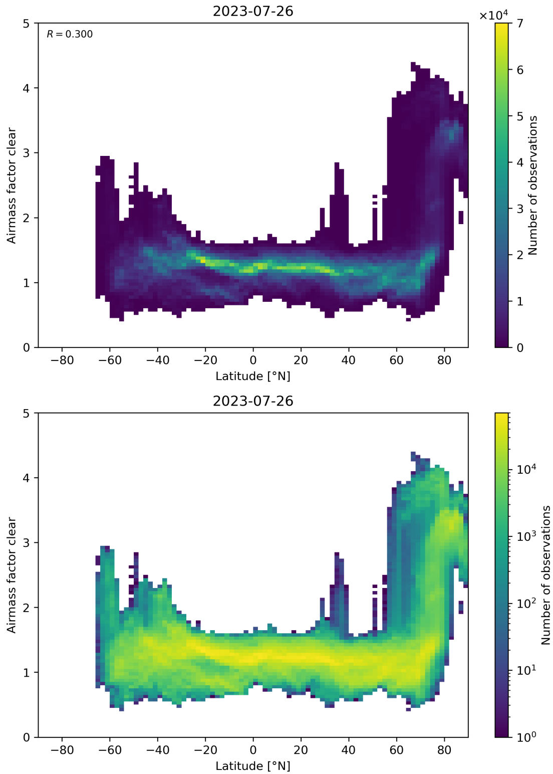
Figure 156: Scatter density plot of “Latitude” against “Airmass factor clear” for 2023-07-25 to 2023-07-27.
