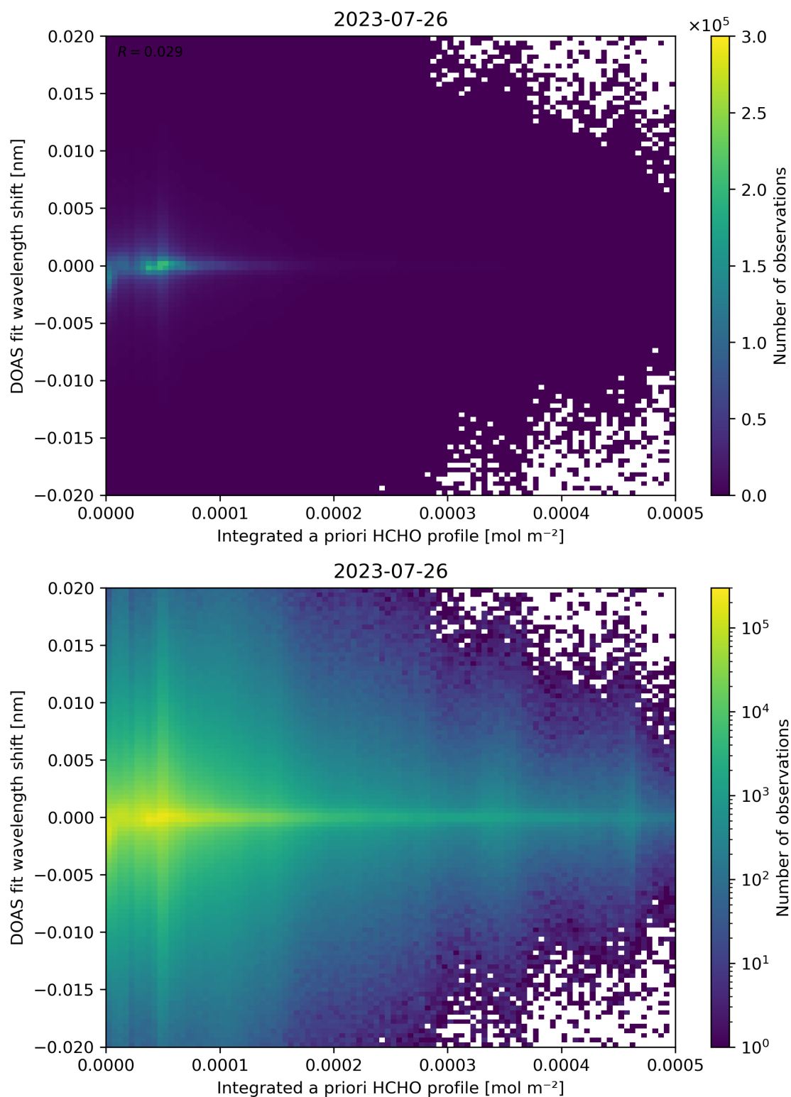
Figure 149: Scatter density plot of “Integrated a priori HCHO profile” against “DOAS fit wavelength shift” for 2023-07-25 to 2023-07-27.
