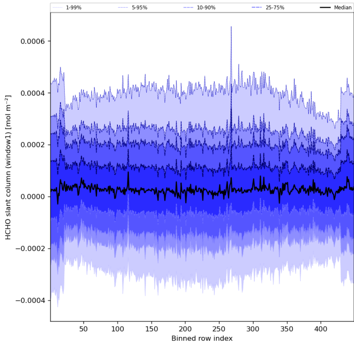
Figure 52: Along track statistics of “HCHO slant column (window1)” for 2023-07-25 to 2023-07-27
