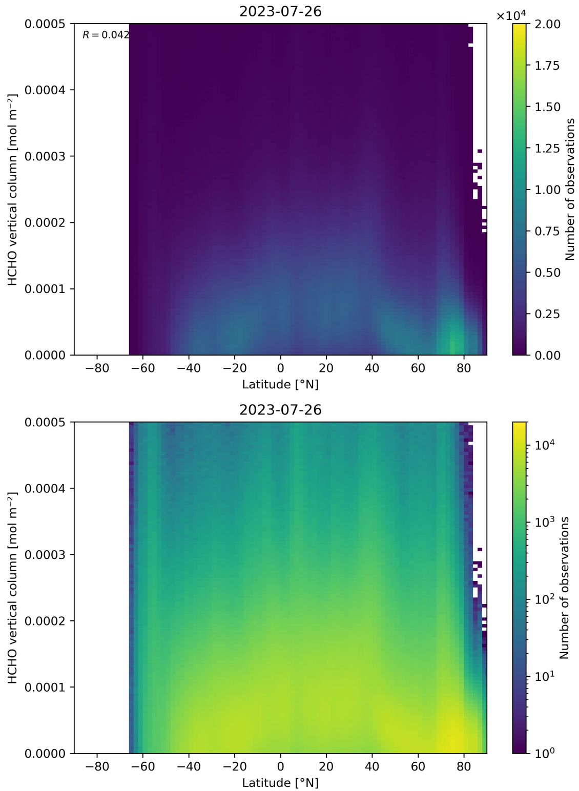
Figure 163: Scatter density plot of “Latitude” against “HCHO vertical column” for 2023-07-25 to 2023-07-27.
