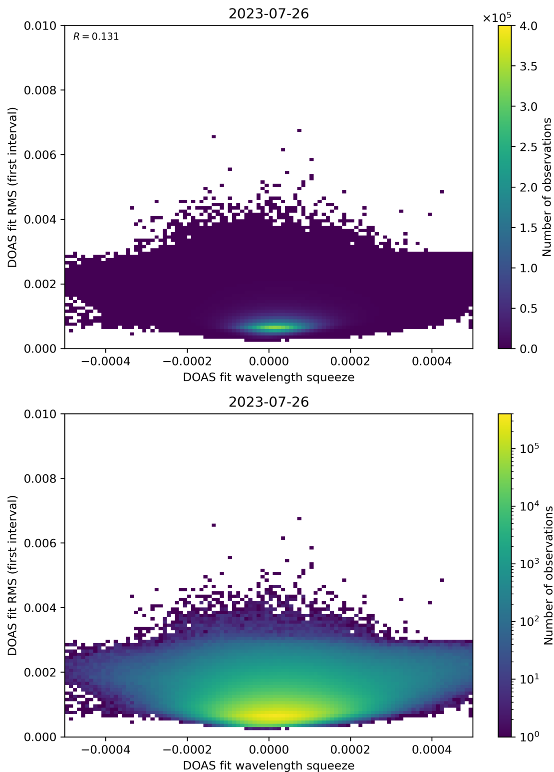
Figure 68: Scatter density plot of “DOAS fit wavelength squeeze” against “DOAS fit RMS (first interval)” for 2023-07-25 to 2023-07-27.
