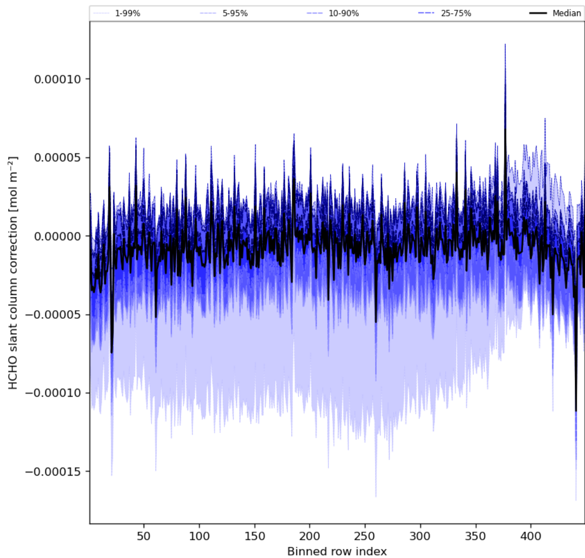
Figure 61: Along track statistics of “HCHO slant column correction” for 2023-07-25 to 2023-07-27
