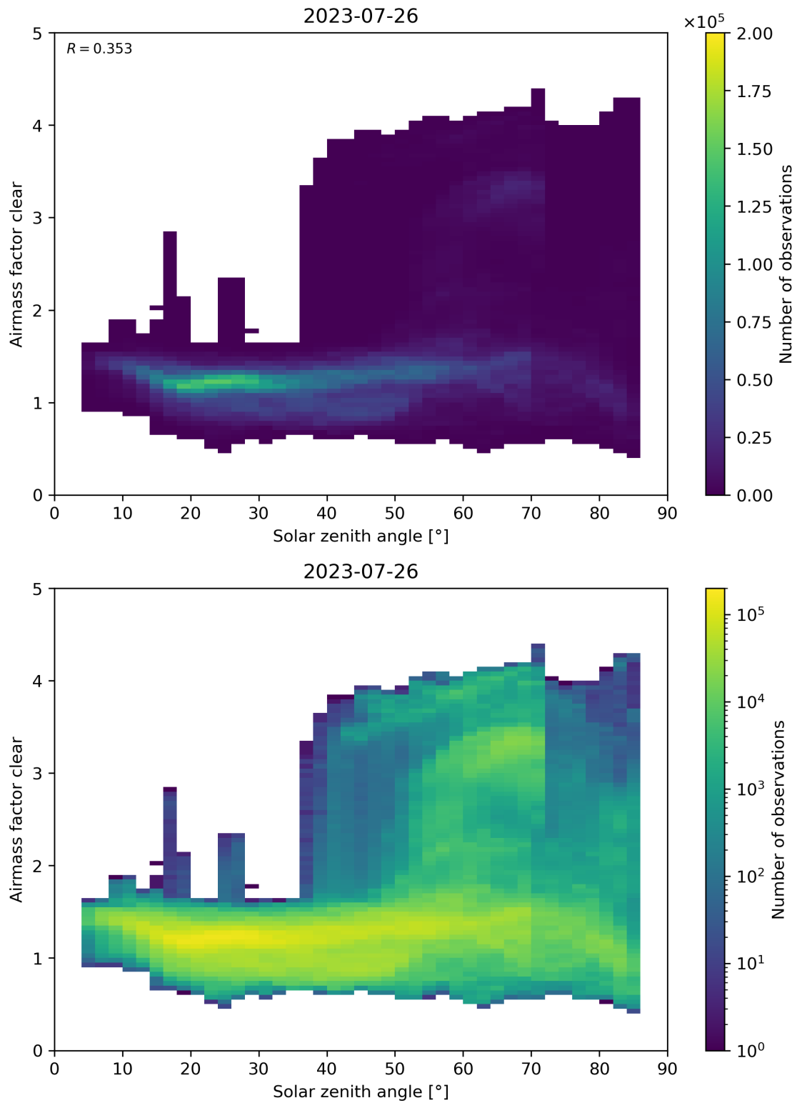
Figure 170: Scatter density plot of “Solar zenith angle” against “Airmass factor clear” for 2023-07-25 to 2023-07-27.
