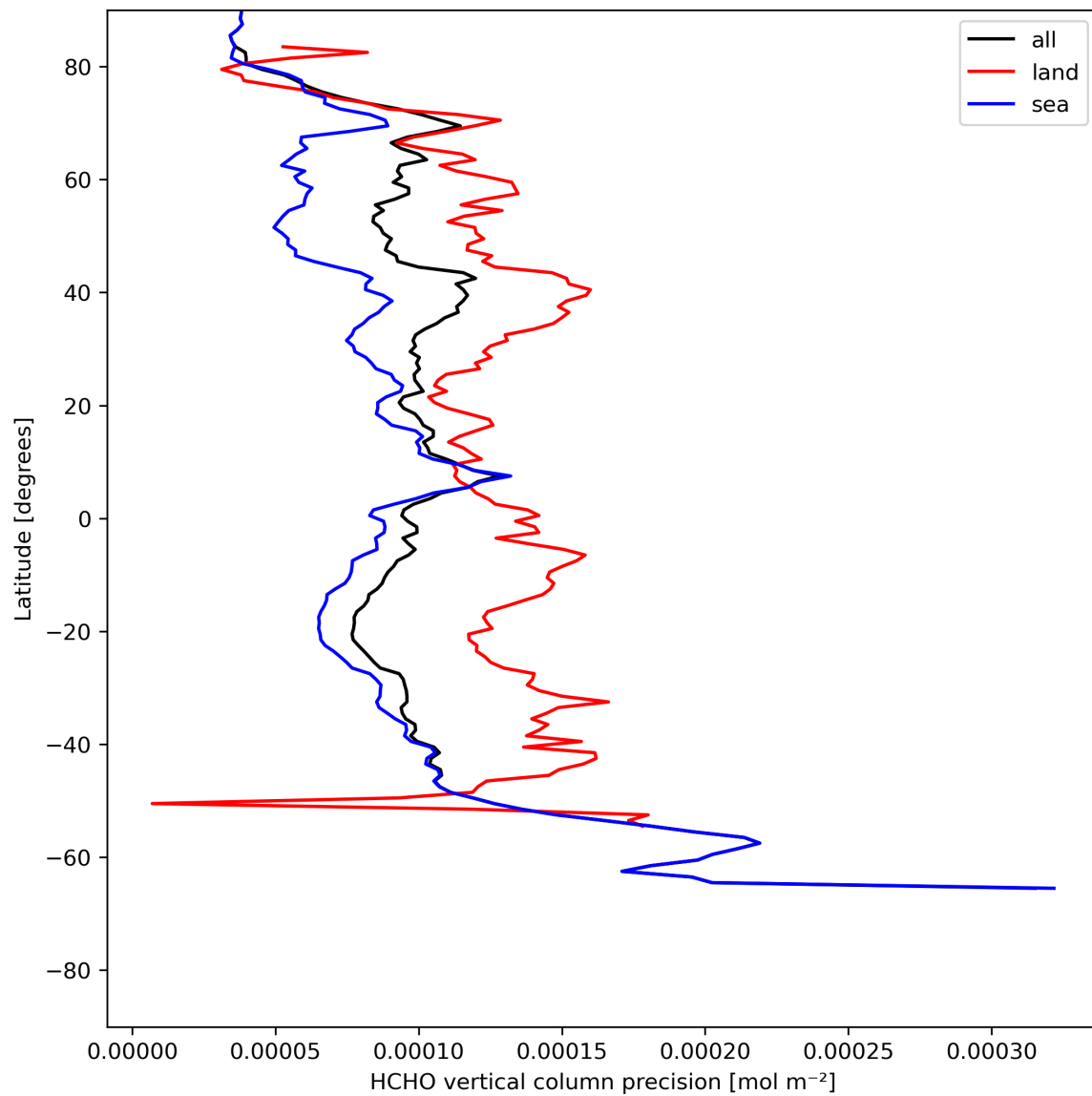
Figure 22: Zonal average of “HCHO vertical column precision” for 2023-07-25 to 2023-07-27.
