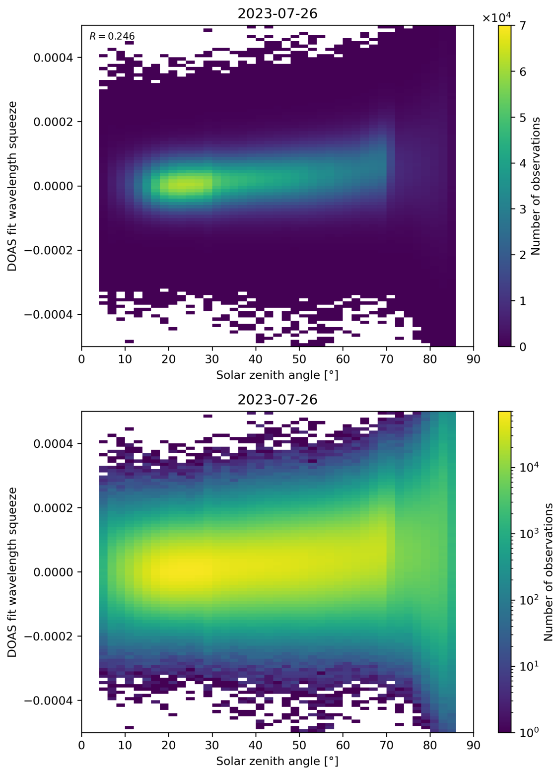
Figure 169: Scatter density plot of “Solar zenith angle” against “DOAS fit wavelength squeeze” for 2023-07-25 to 2023-07-27.
