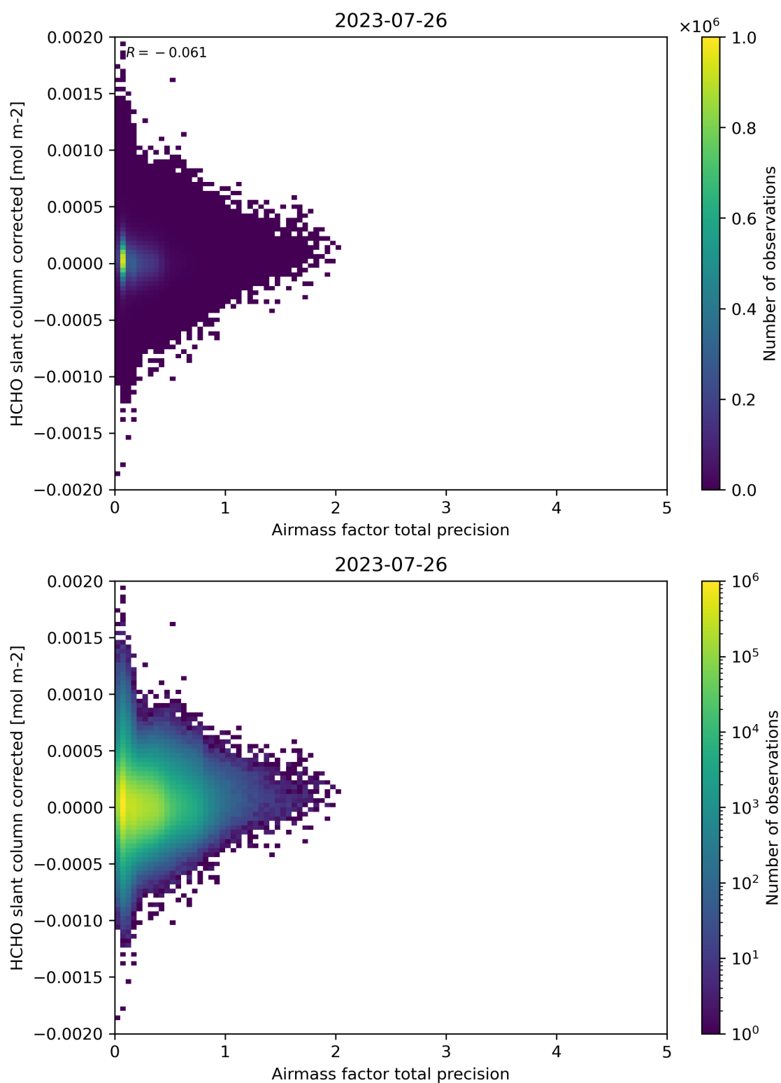
Figure 109: Scatter density plot of “Airmass factor total precision” against “HCHO slant column corrected” for 2023-07-25 to 2023-07-27.
