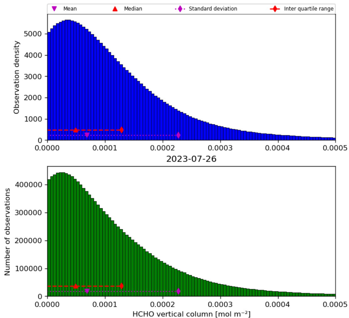
Figure 35: Histogram of “HCHO vertical column” for 2023-07-25 to 2023-07-27
