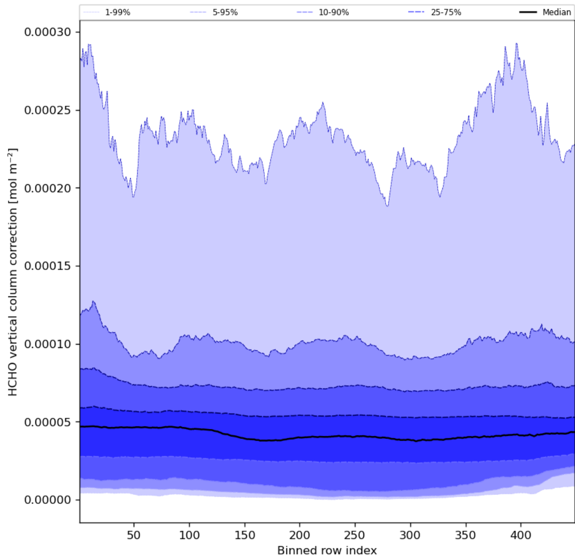
Figure 51: Along track statistics of “HCHO vertical column correction” for 2023-07-25 to 2023-07-27
