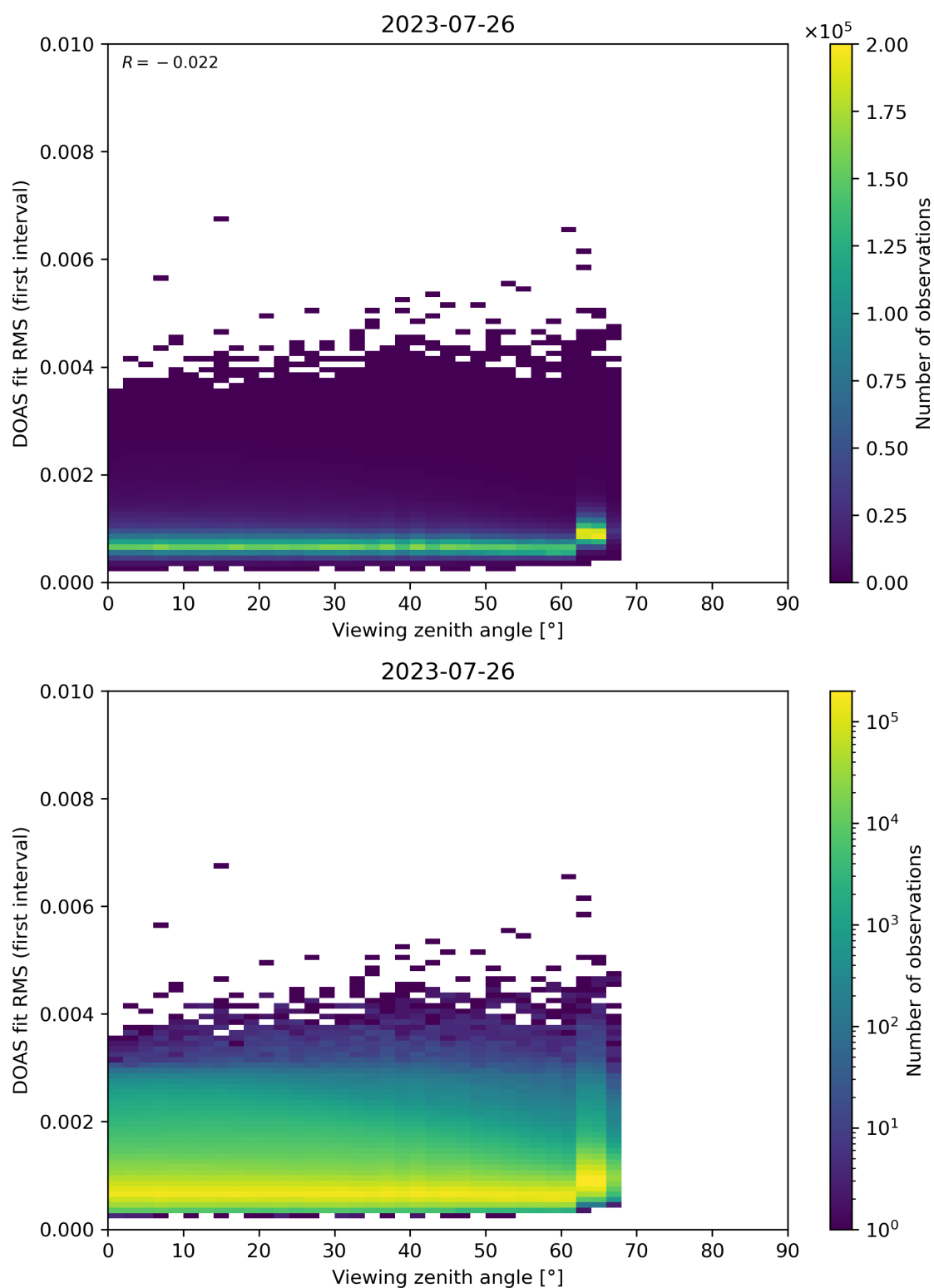
Figure 182: Scatter density plot of “Viewing zenith angle” against “DOAS fit RMS (first interval)” for 2023-07-25 to 2023-07-27.
