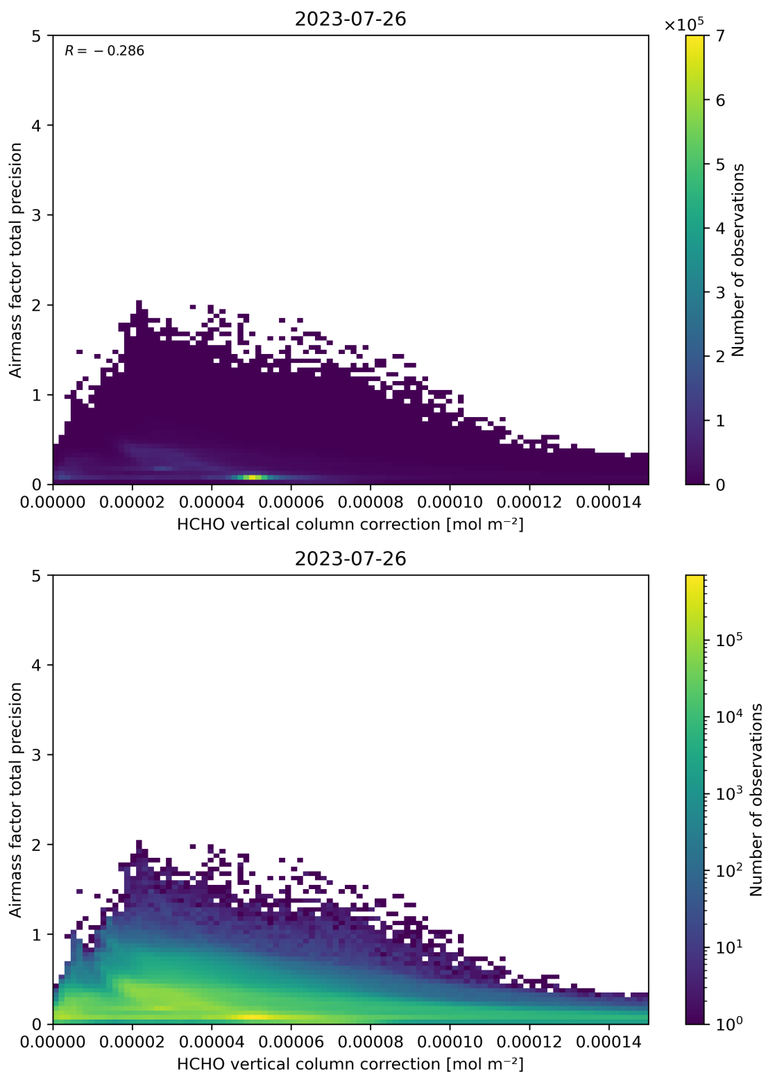
Figure 121: Scatter density plot of “HCHO vertical column correction” against “Airmass factor total precision” for 2023-07-25 to 2023-07-27.
