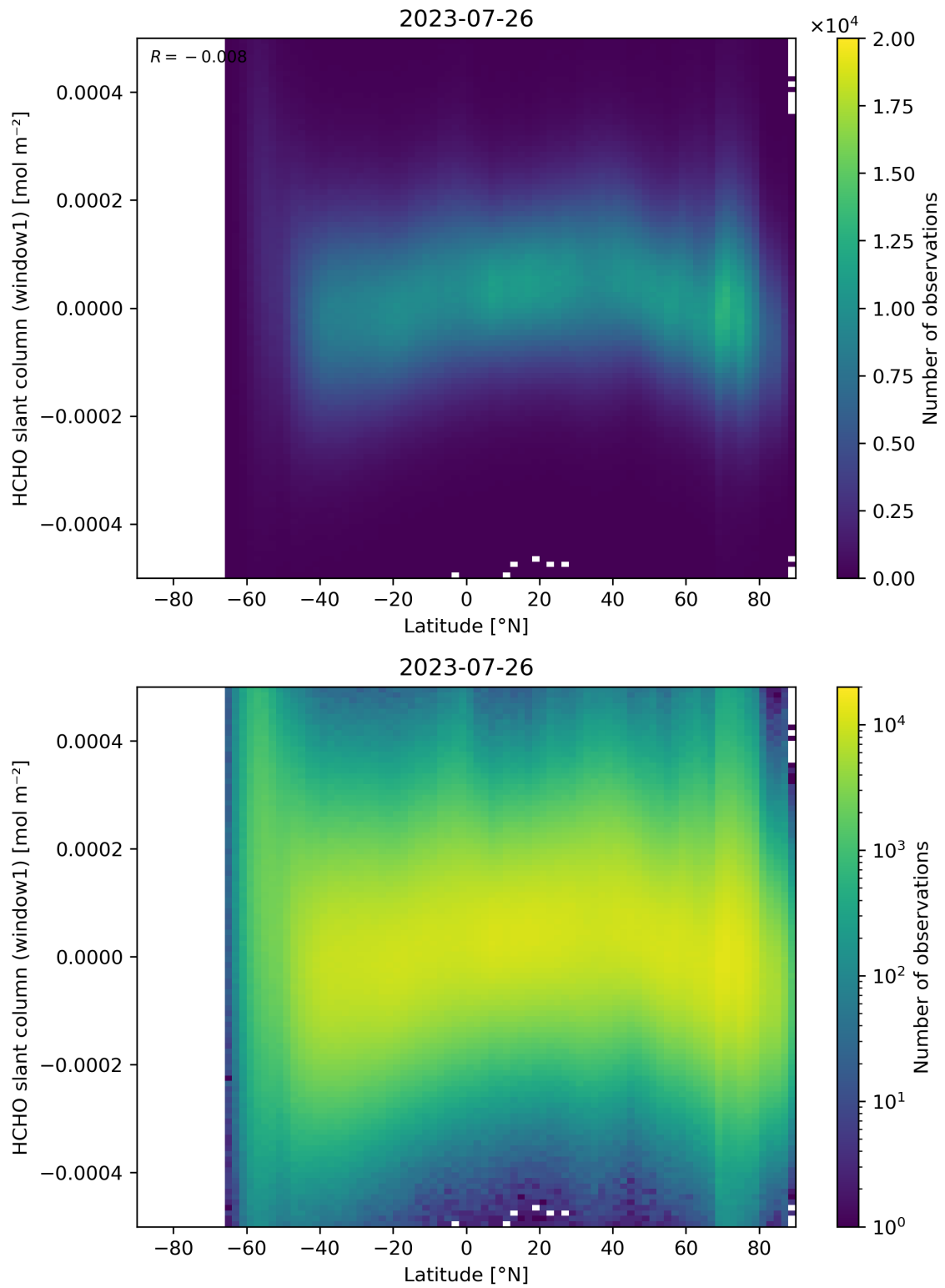
Figure 159: Scatter density plot of “Latitude” against “HCHO slant column (window1)” for 2023-07-25 to 2023-07-27.
