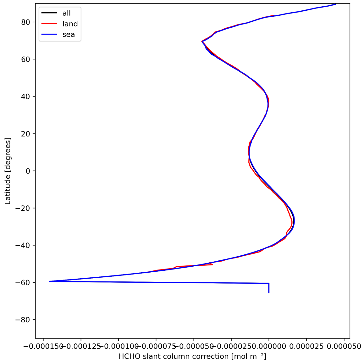
Figure 33: Zonal average of “HCHO slant column correction” for 2023-07-25 to 2023-07-27.
