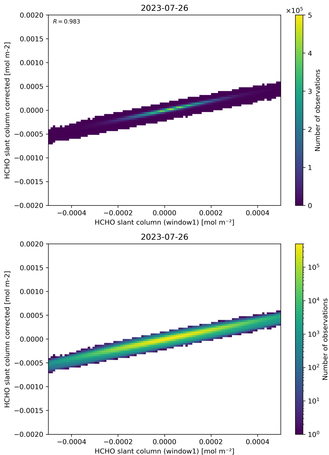
Figure 82: Scatter density plot of “HCHO slant column (window1)” against “HCHO slant column corrected” for 2023-07-25 to 2023-07-27.
