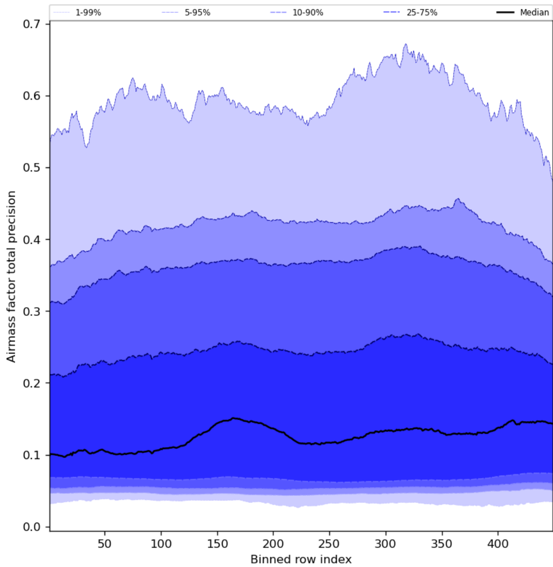
Figure 55: Along track statistics of “Airmass factor total precision” for 2023-07-25 to 2023-07-27
