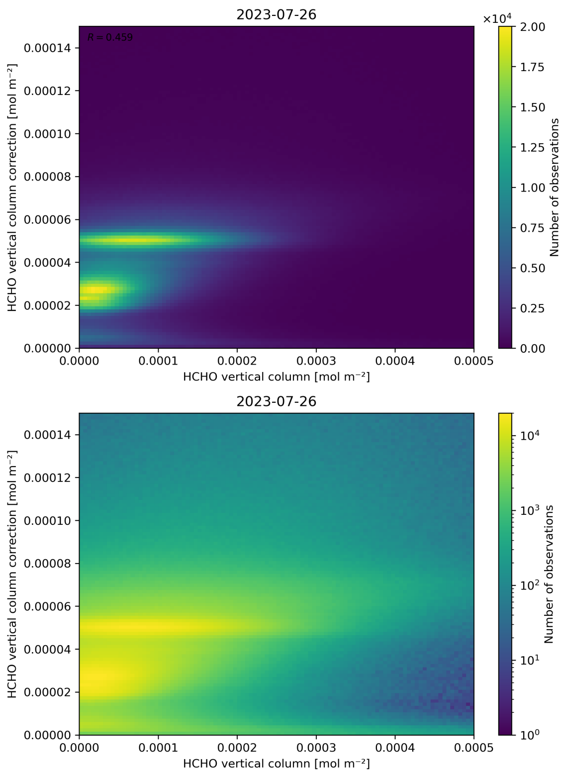
Figure 133: Scatter density plot of “HCHO vertical column” against “HCHO vertical column correction” for 2023-07-25 to 2023-07-27.
