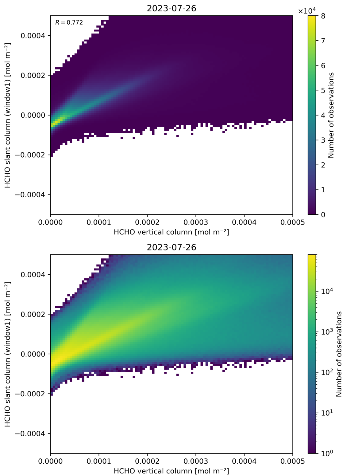
Figure 129: Scatter density plot of “HCHO vertical column” against “HCHO slant column (window1)” for 2023-07-25 to 2023-07-27.
