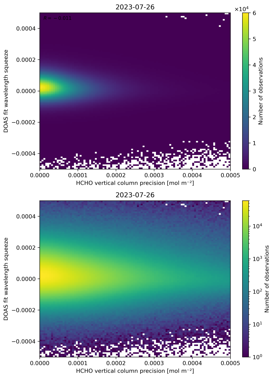
Figure 138: Scatter density plot of “HCHO vertical column precision” against “DOAS fit wavelength squeeze” for 2023-07-25 to 2023-07-27.
