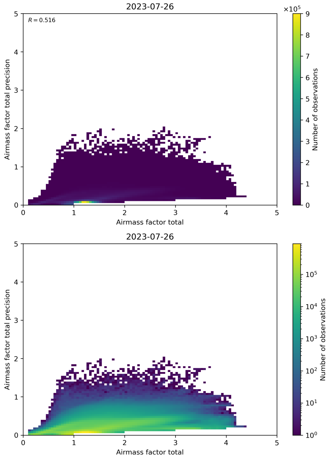
Figure 103: Scatter density plot of “Airmass factor total” against “Airmass factor total precision” for 2023-07-25 to 2023-07-27.
