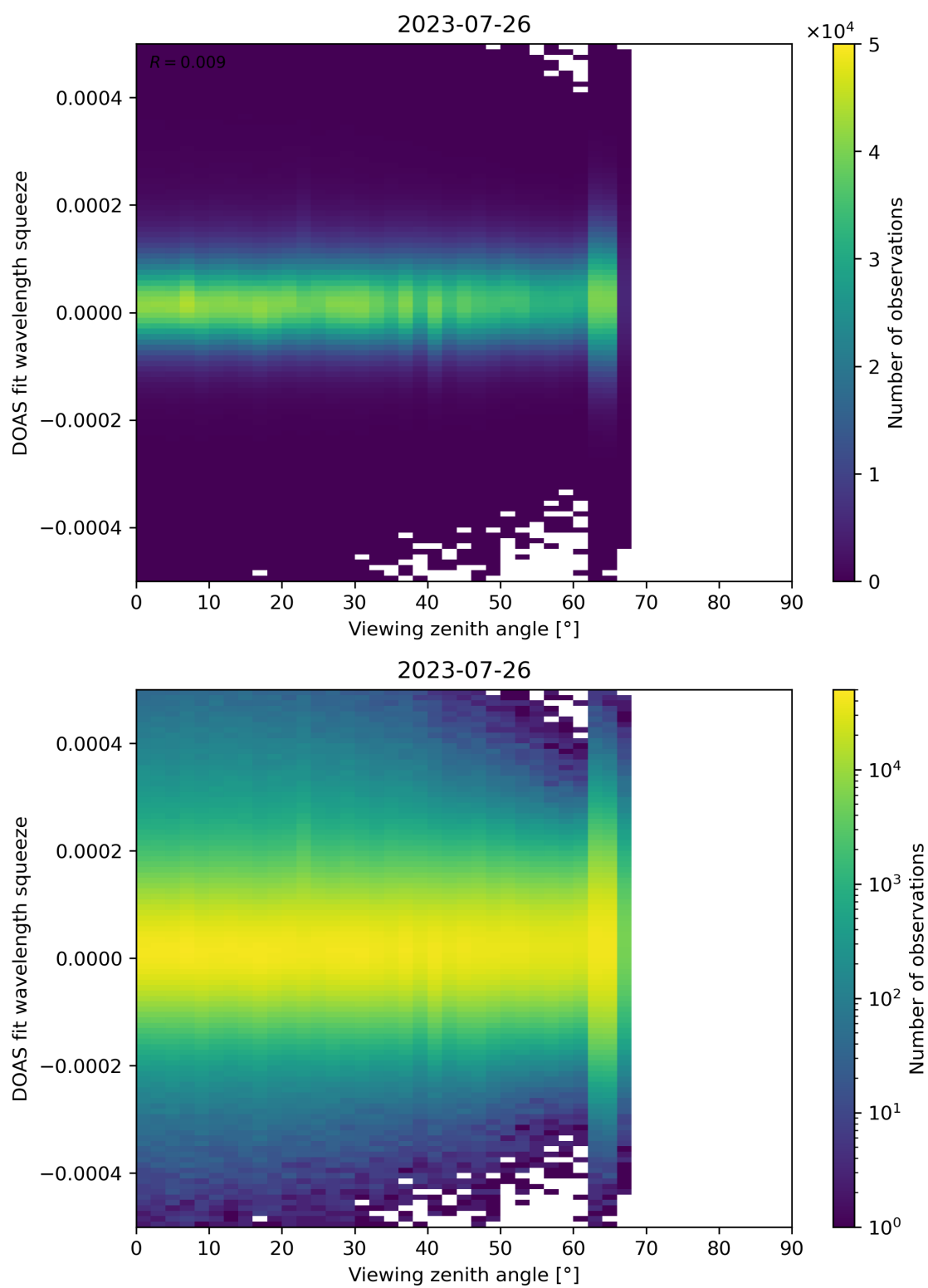
Figure 184: Scatter density plot of “Viewing zenith angle” against “DOAS fit wavelength squeeze” for 2023-07-25 to 2023-07-27.
