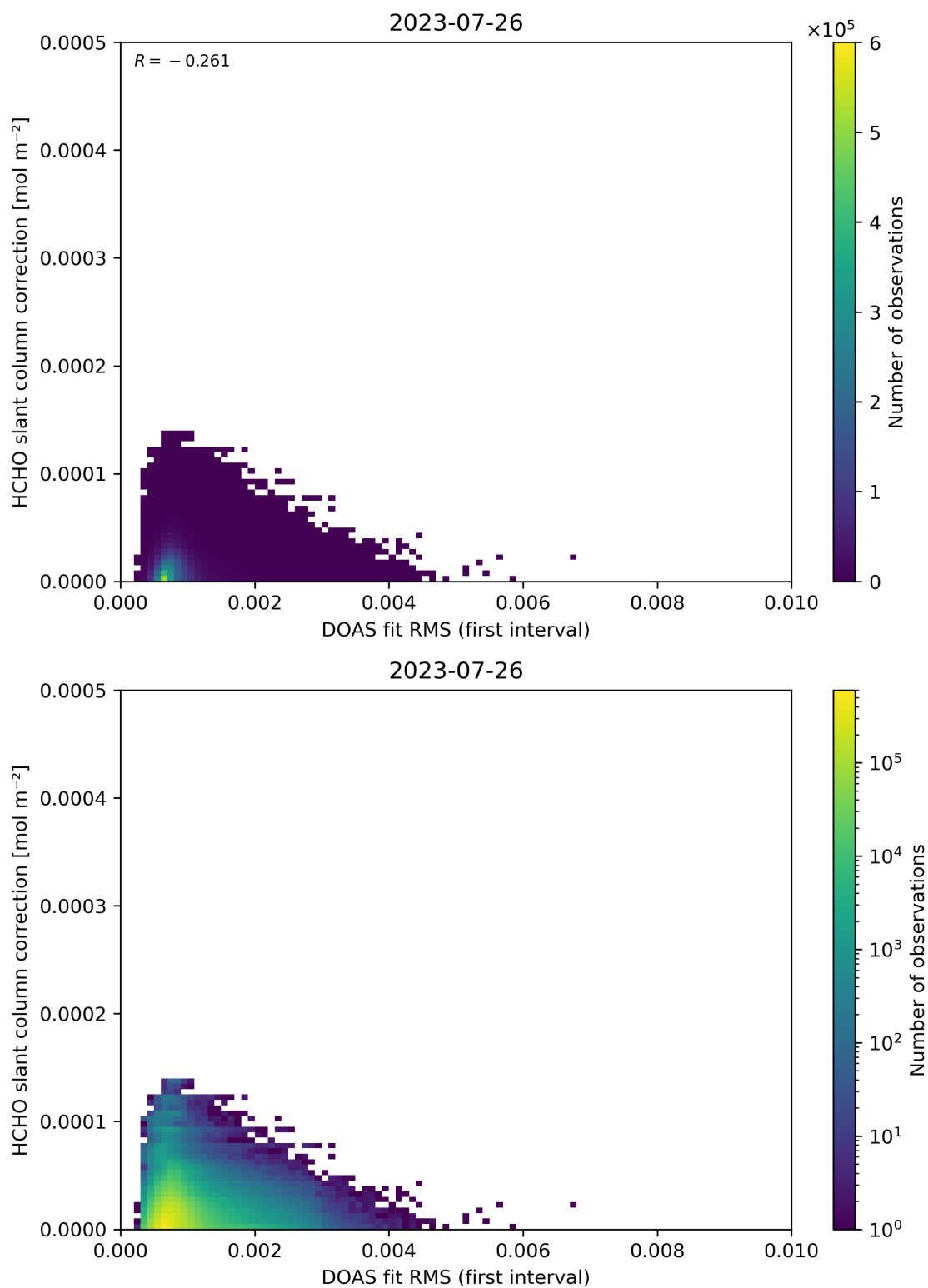
Figure 63: Scatter density plot of “DOAS fit RMS (first interval)” against “HCHO slant column correction” for 2023-07-25 to 2023-07-27.
