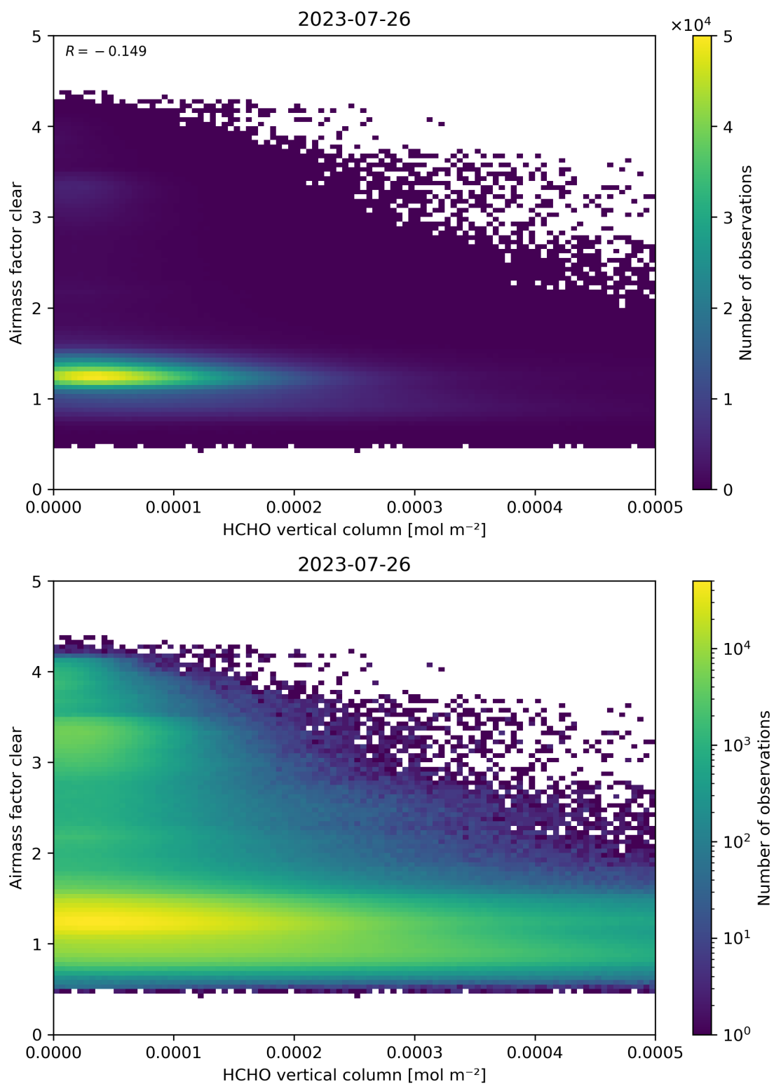
Figure 126: Scatter density plot of “HCHO vertical column” against “Airmass factor clear” for 2023-07-25 to 2023-07-27.
