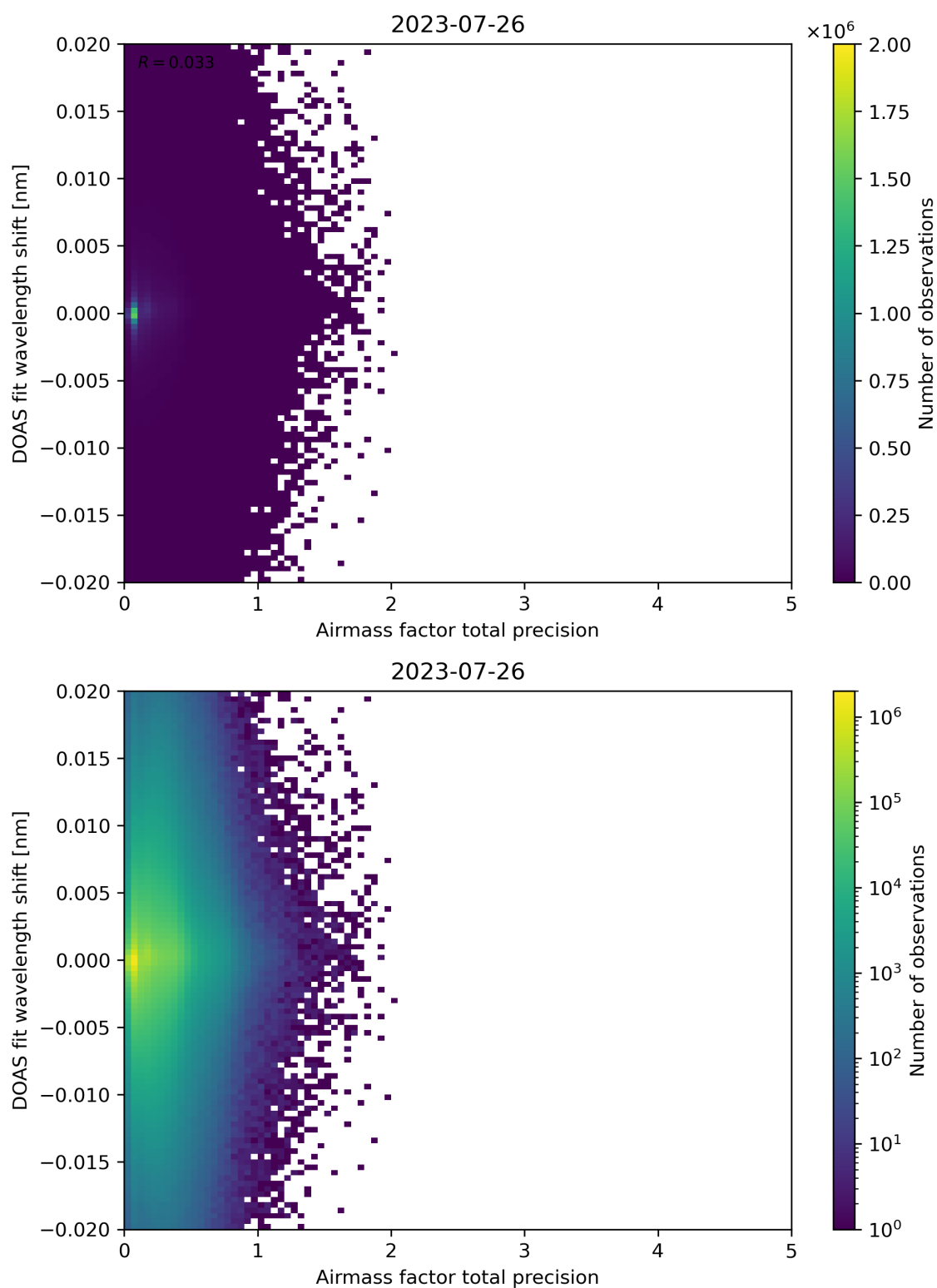
Figure 106: Scatter density plot of “Airmass factor total precision” against “DOAS fit wavelength shift” for 2023-07-25 to 2023-07-27.
