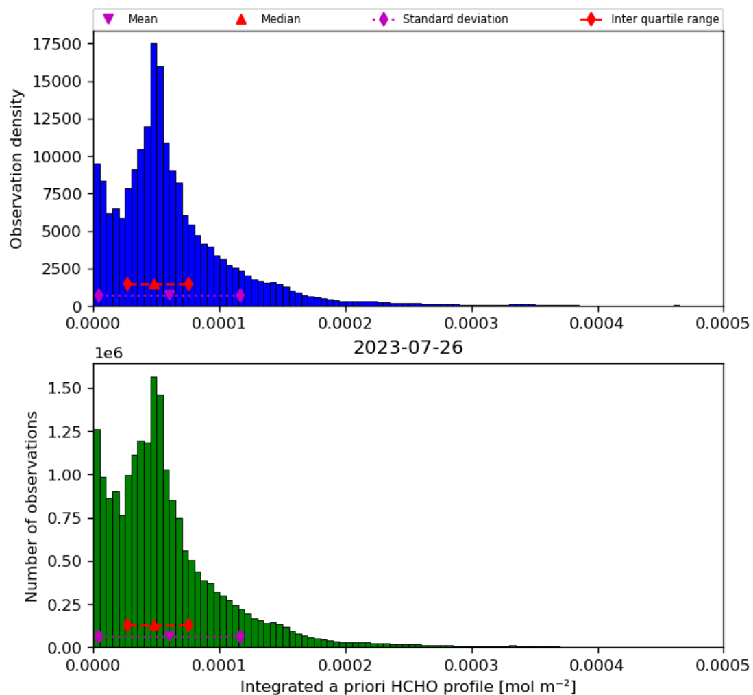
Figure 43: Histogram of “Integrated a priori HCHO profile” for 2023-07-25 to 2023-07-27
