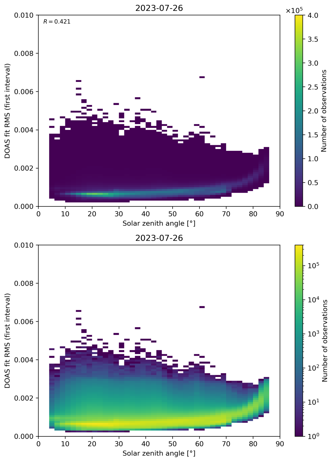
Figure 167: Scatter density plot of “Solar zenith angle” against “DOAS fit RMS (first interval)” for 2023-07-25 to 2023-07-27.
