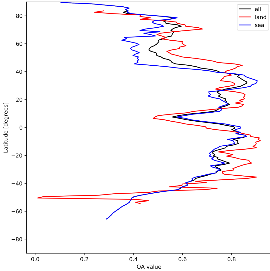
Figure 20: Zonal average of “QA value” for 2023-07-25 to 2023-07-27.
