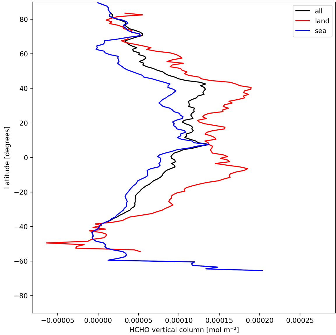
Figure 21: Zonal average of “HCHO vertical column” for 2023-07-25 to 2023-07-27.
