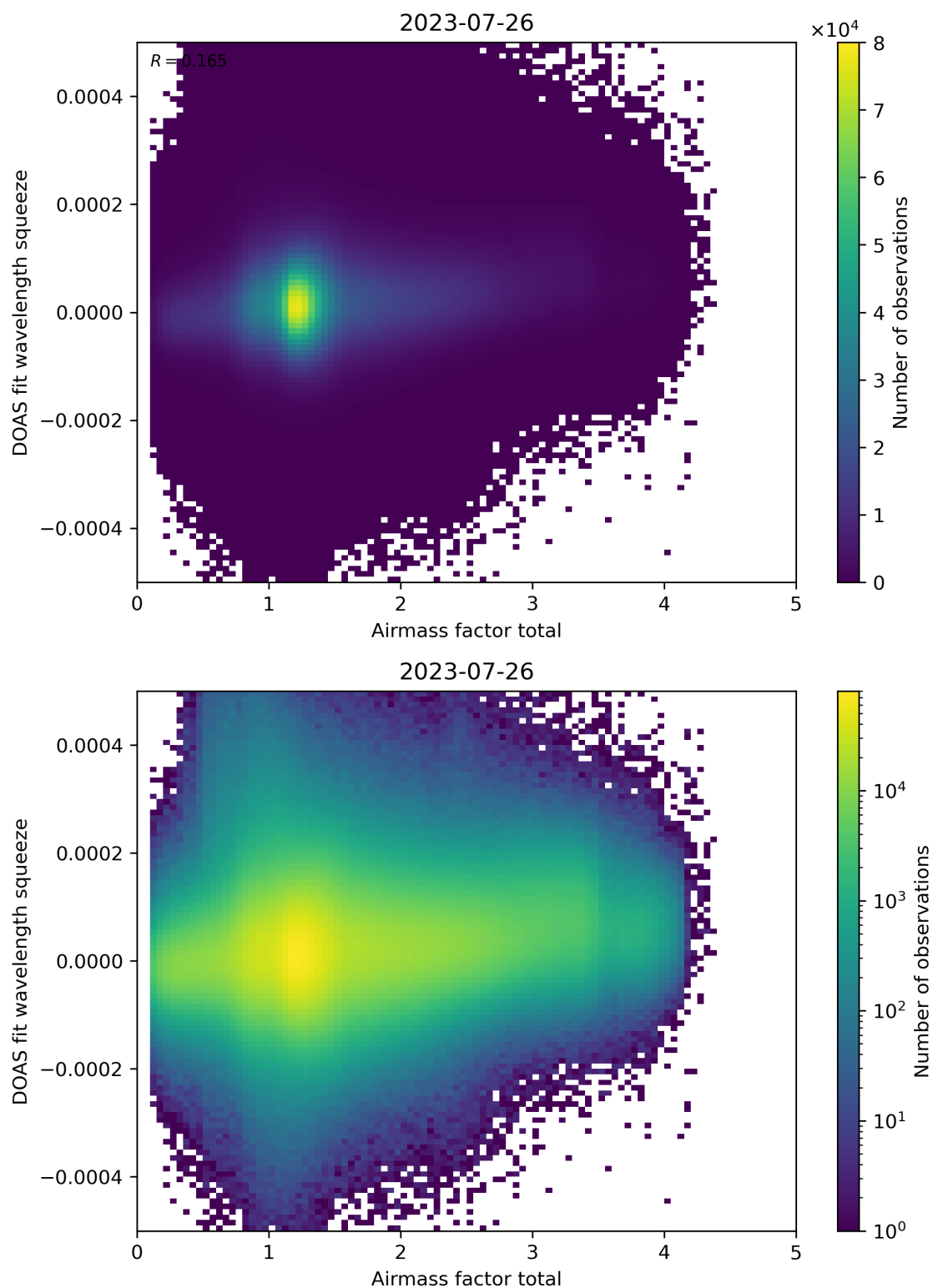
Figure 99: Scatter density plot of “Airmass factor total” against “DOAS fit wavelength squeeze” for 2023-07-25 to 2023-07-27.
