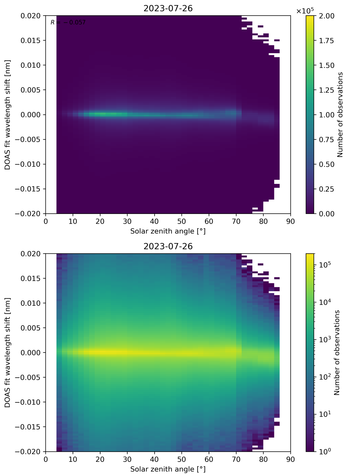
Figure 168: Scatter density plot of “Solar zenith angle” against “DOAS fit wavelength shift” for 2023-07-25 to 2023-07-27.
