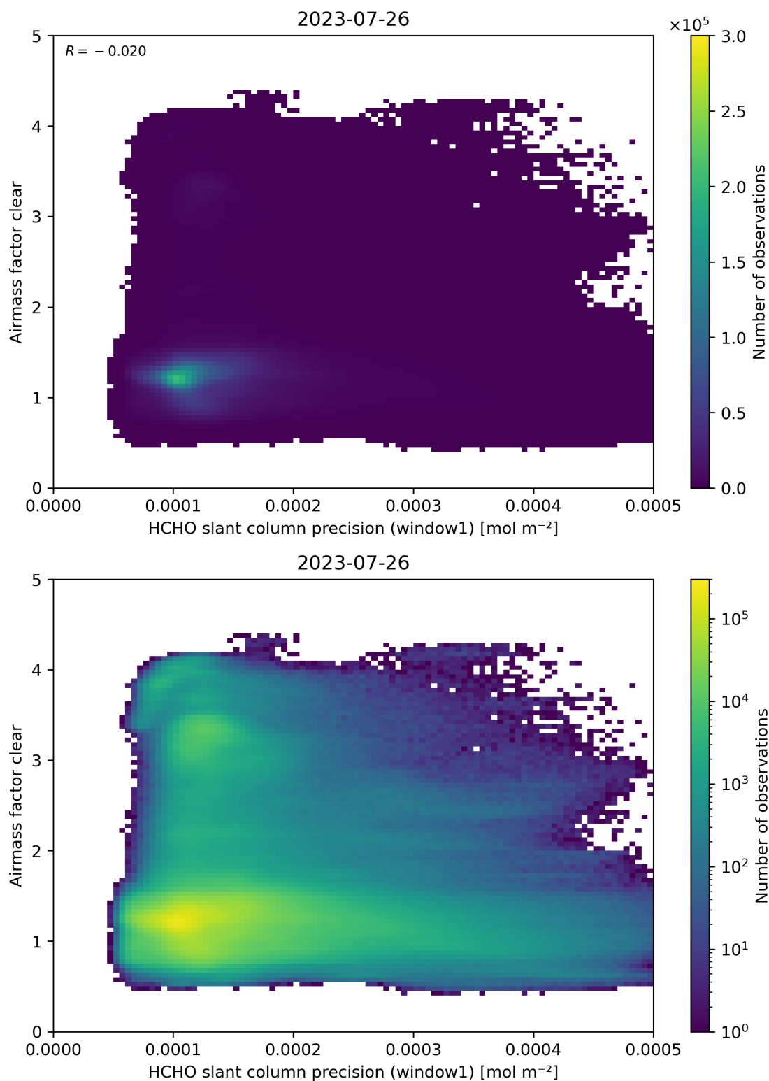
Figure 91: Scatter density plot of “HCHO slant column precision (window1)” against “Airmass factor clear” for 2023-07-25 to 2023-07-27.
