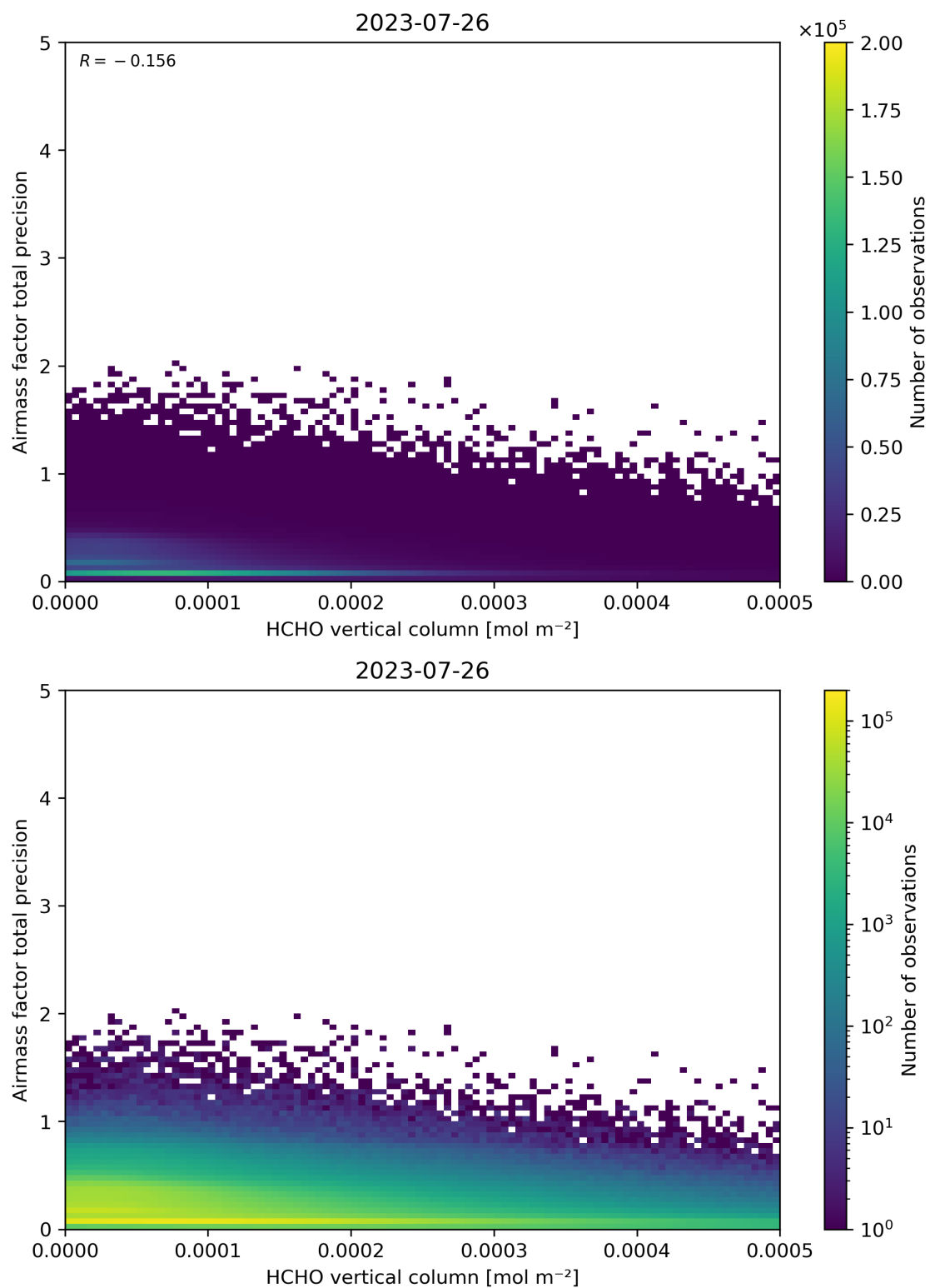
Figure 132: Scatter density plot of “HCHO vertical column” against “Airmass factor total precision” for 2023-07-25 to 2023-07-27.
