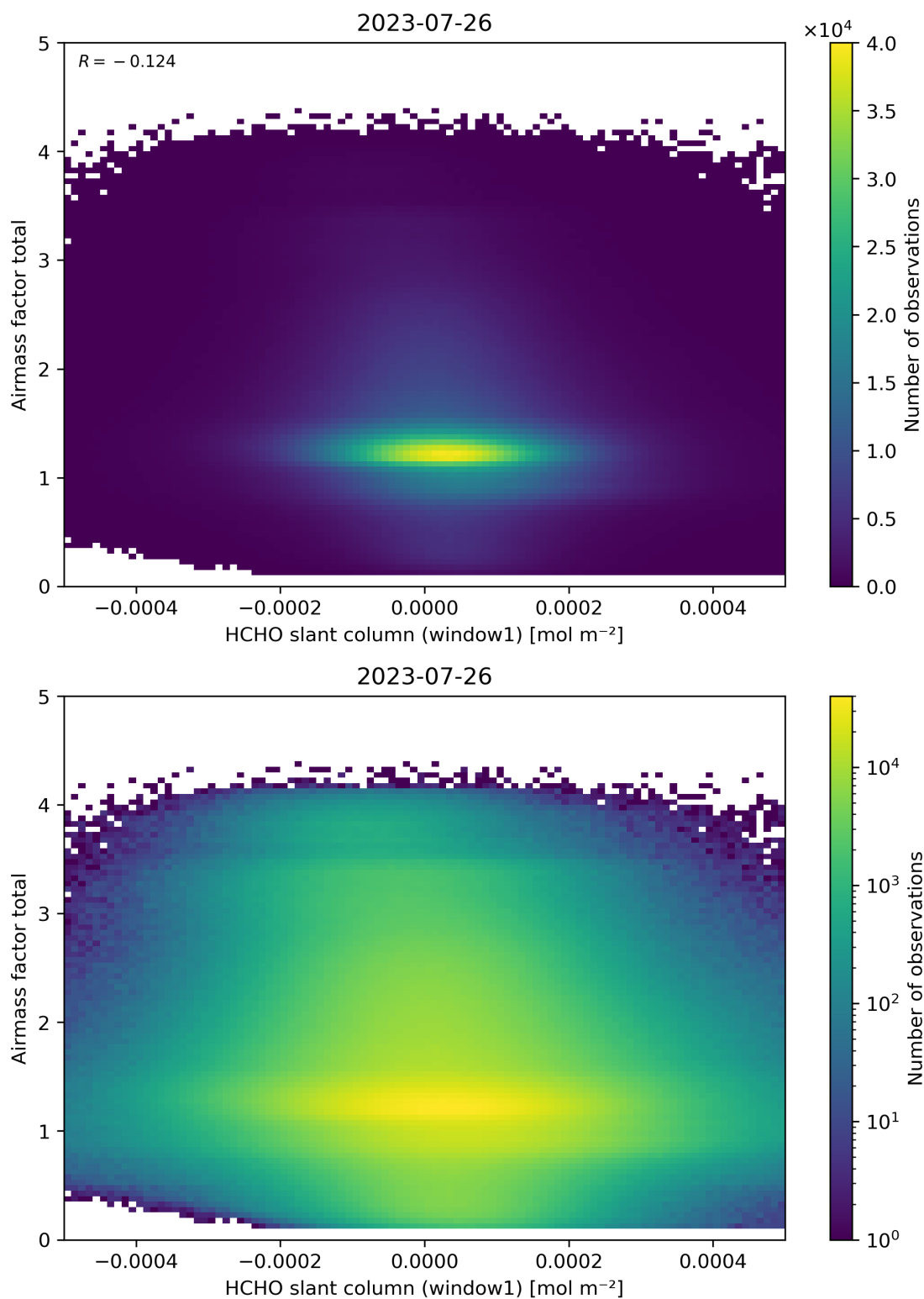
Figure 85: Scatter density plot of “HCHO slant column (window1)” against “Airmass factor total” for 2023-07-25 to 2023-07-27.
