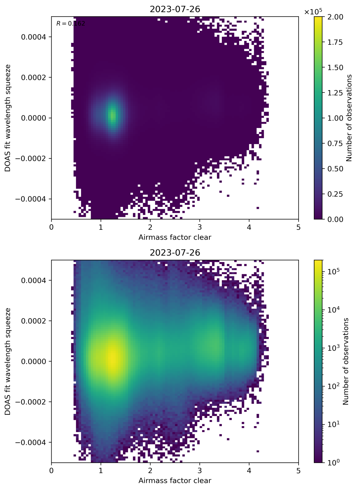
Figure 73: Scatter density plot of “Airmass factor clear” against “DOAS fit wavelength squeeze” for 2023-07-25 to 2023-07-27.
