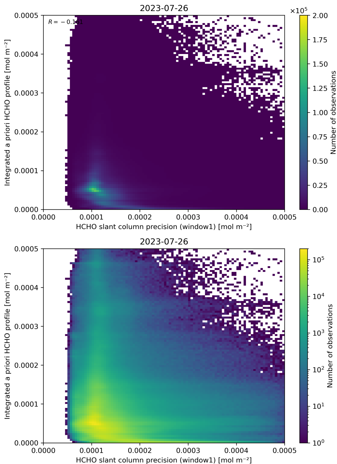
Figure 96: Scatter density plot of “HCHO slant column precision (window1)” against “Integrated a priori HCHO profile” for 2023-07-25 to 2023-07-27.
