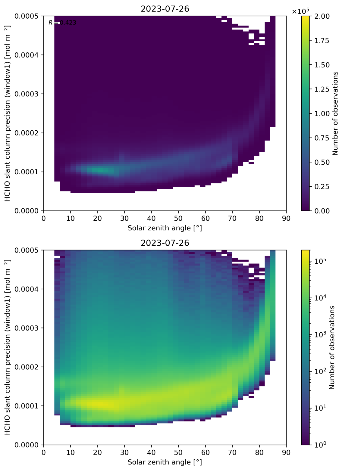
Figure 174: Scatter density plot of “Solar zenith angle” against “HCHO slant column precision (window1)” for 2023-07-25 to 2023-07-27.
