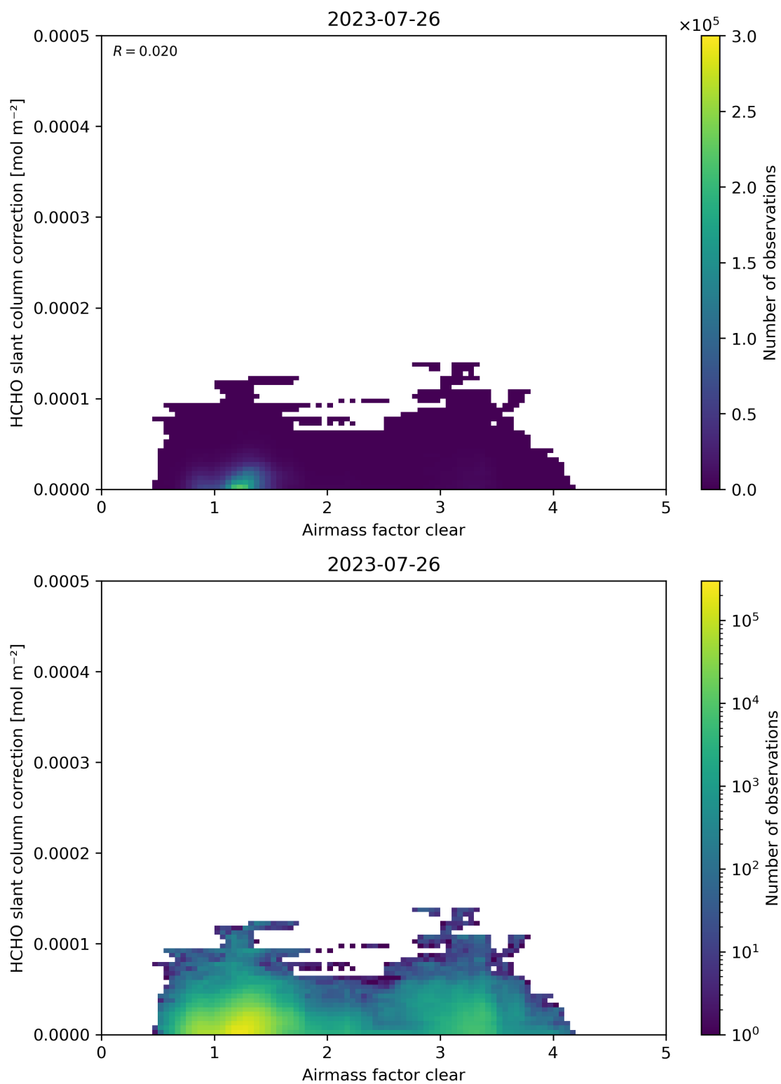
Figure 75: Scatter density plot of “Airmass factor clear” against “HCHO slant column correction” for 2023-07-25 to 2023-07-27.
