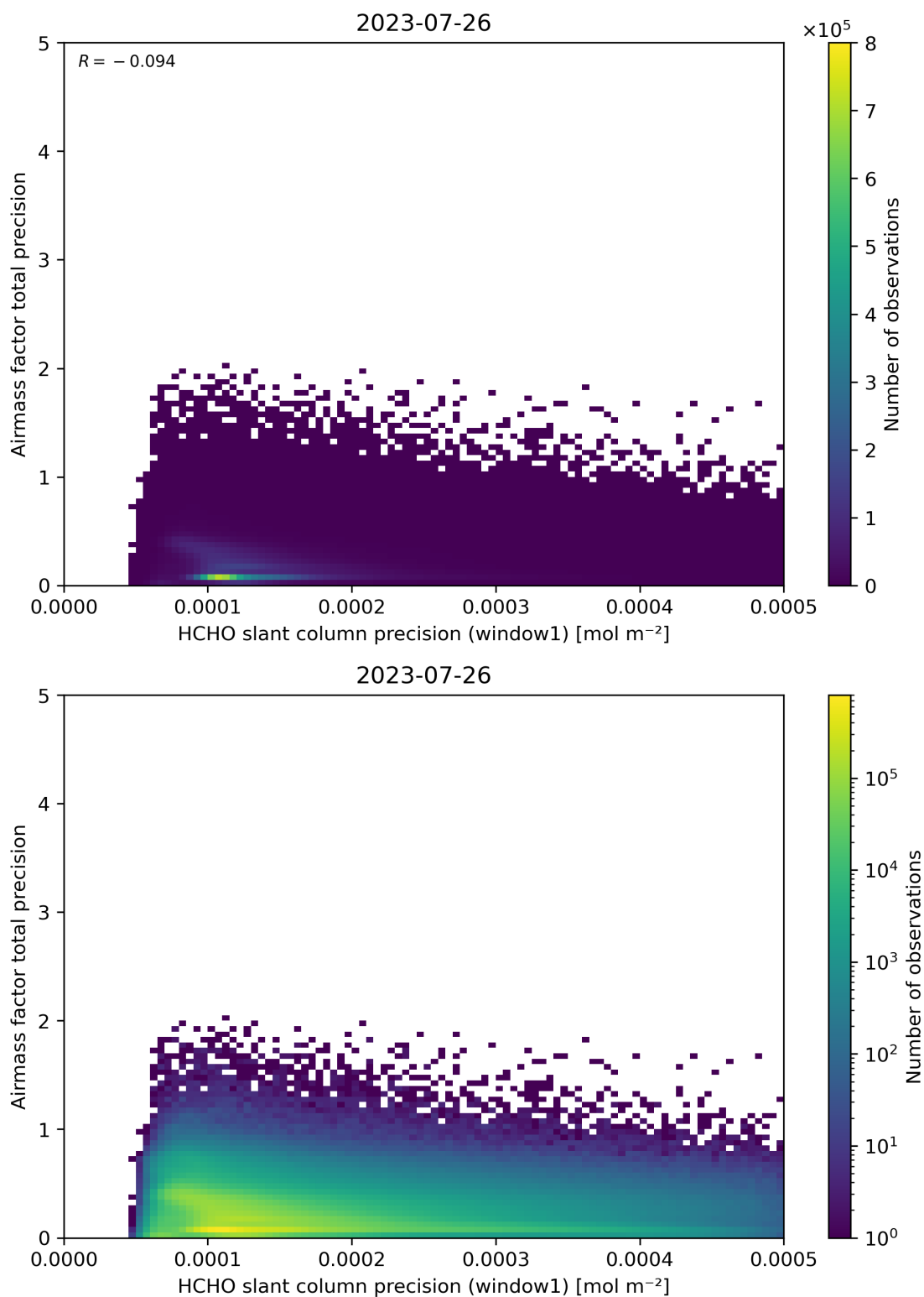
Figure 95: Scatter density plot of “HCHO slant column precision (window1)” against “Airmass factor total precision” for 2023-07-25 to 2023-07-27.
