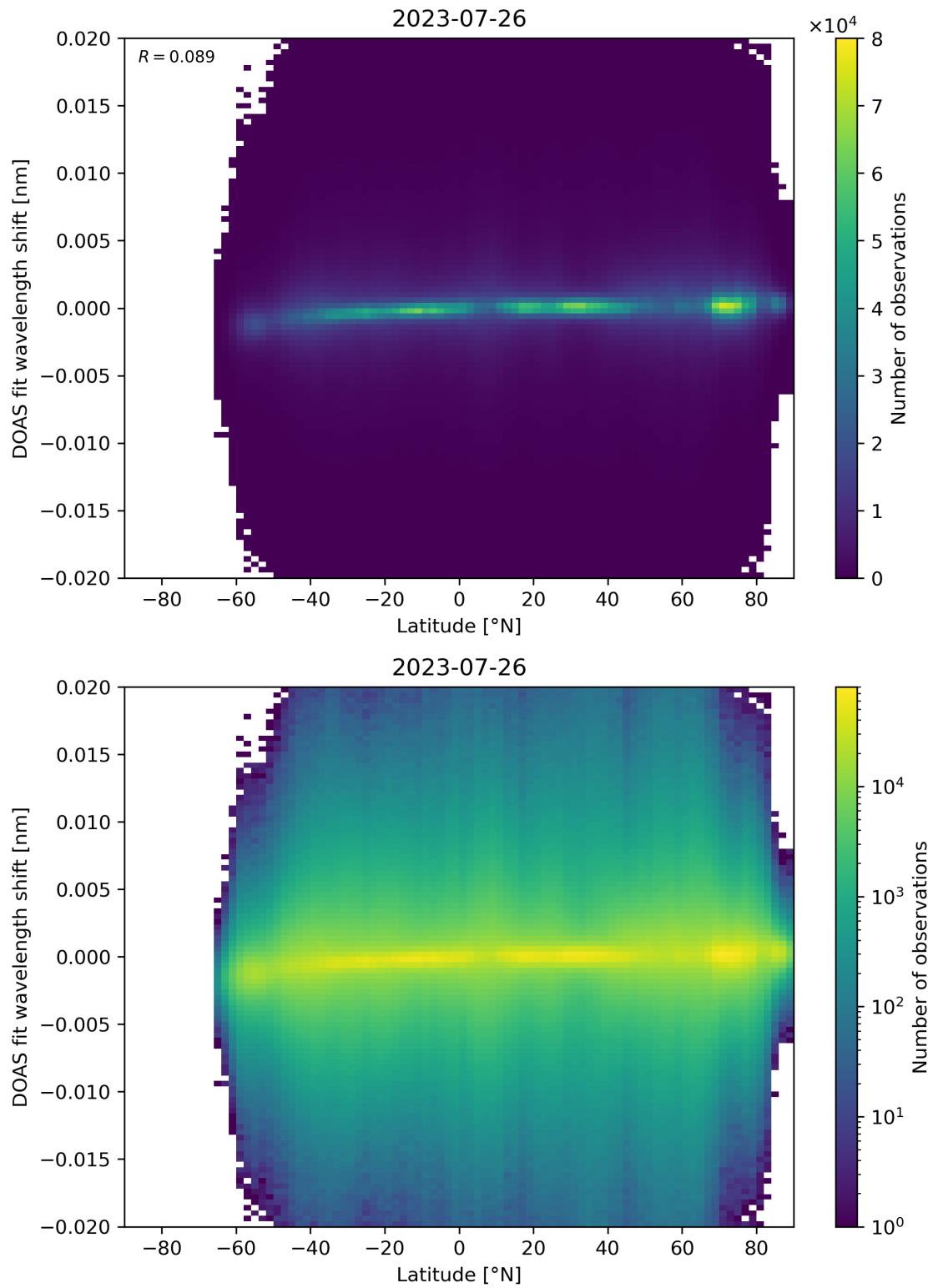
Figure 154: Scatter density plot of “Latitude” against “DOAS fit wavelength shift” for 2023-07-25 to 2023-07-27.
