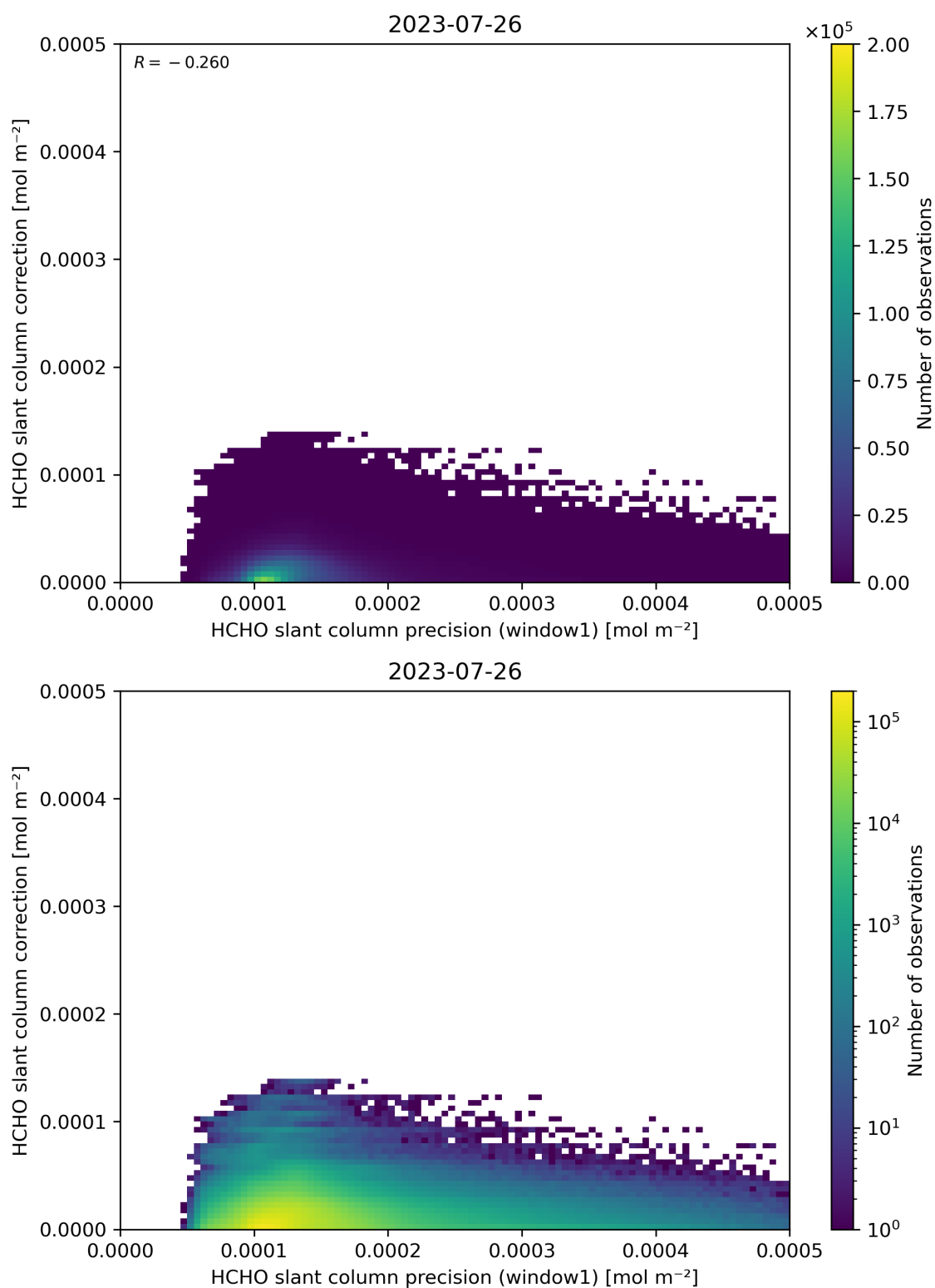
Figure 93: Scatter density plot of “HCHO slant column precision (window1)” against “HCHO slant column correction” for 2023-07-25 to 2023-07-27.
