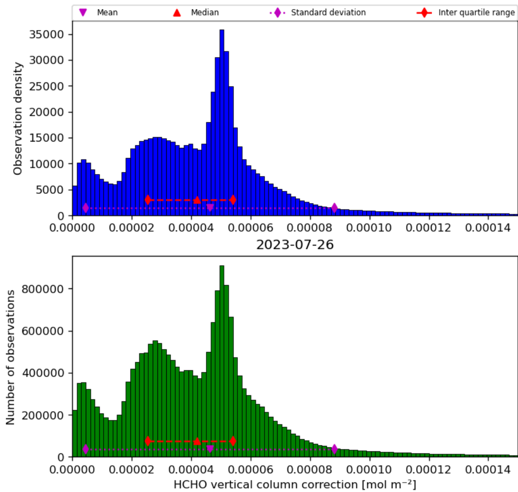
Figure 37: Histogram of “HCHO vertical column correction” for 2023-07-25 to 2023-07-27
