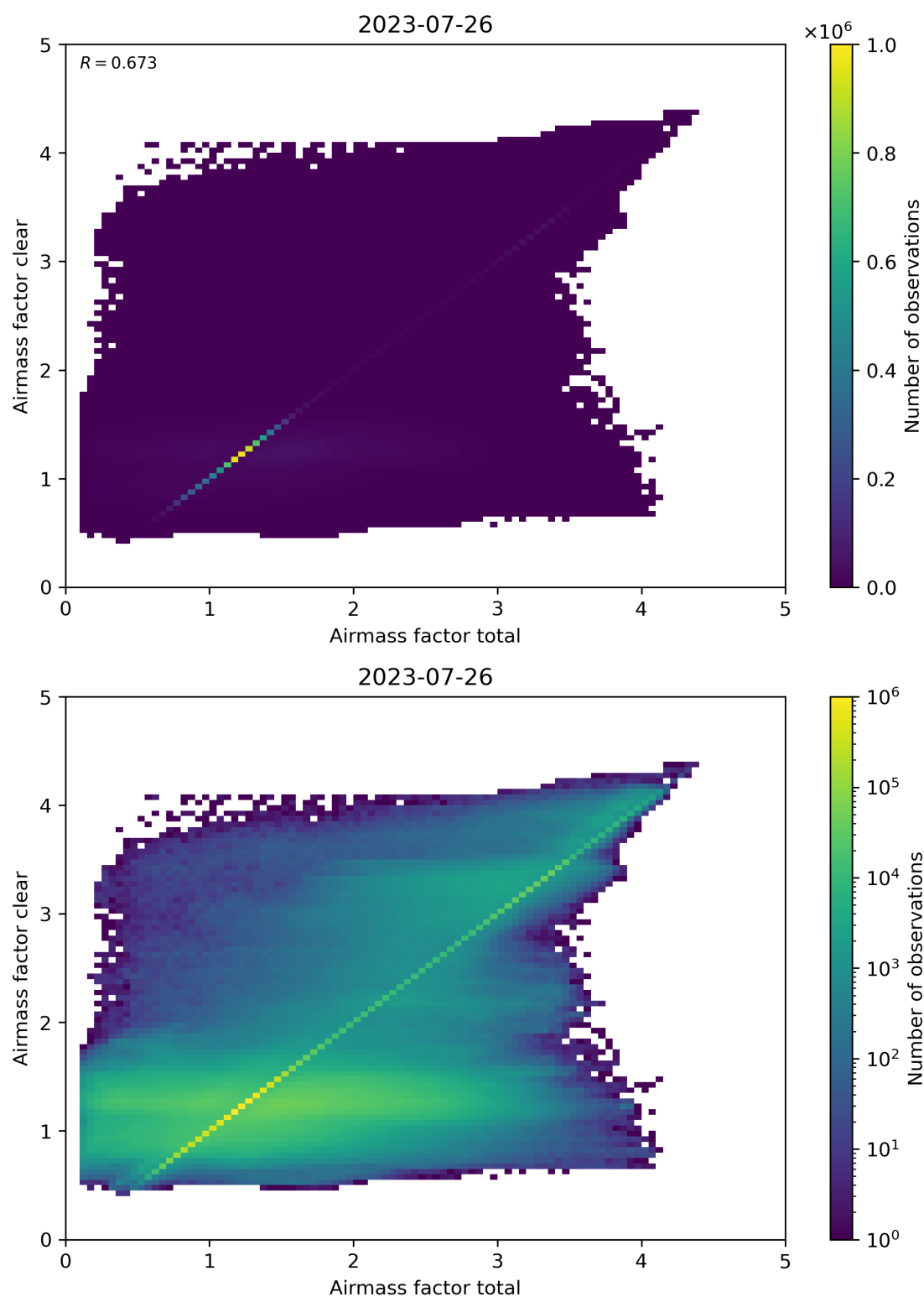
Figure 100: Scatter density plot of “Airmass factor total” against “Airmass factor clear” for 2023-07-25 to 2023-07-27.
