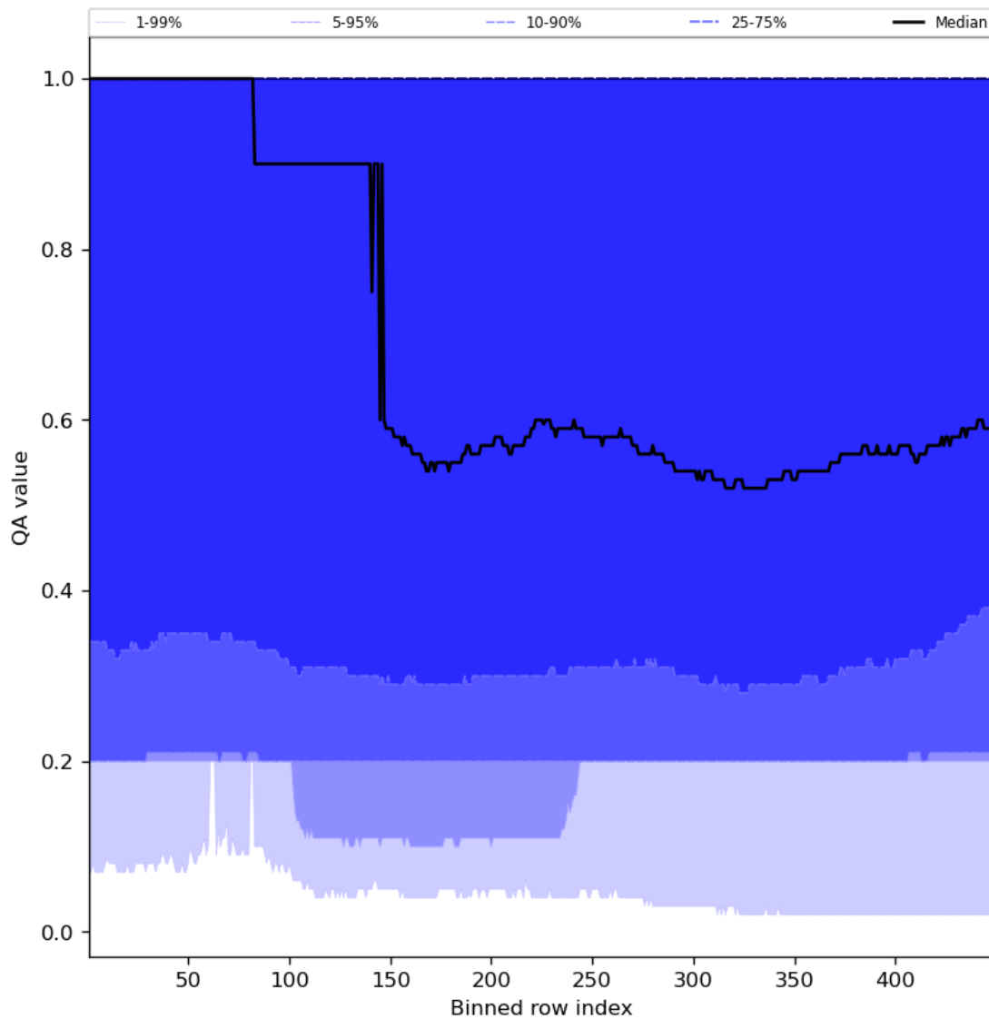
Figure 48: Along track statistics of “QA value” for 2023-07-25 to 2023-07-27
