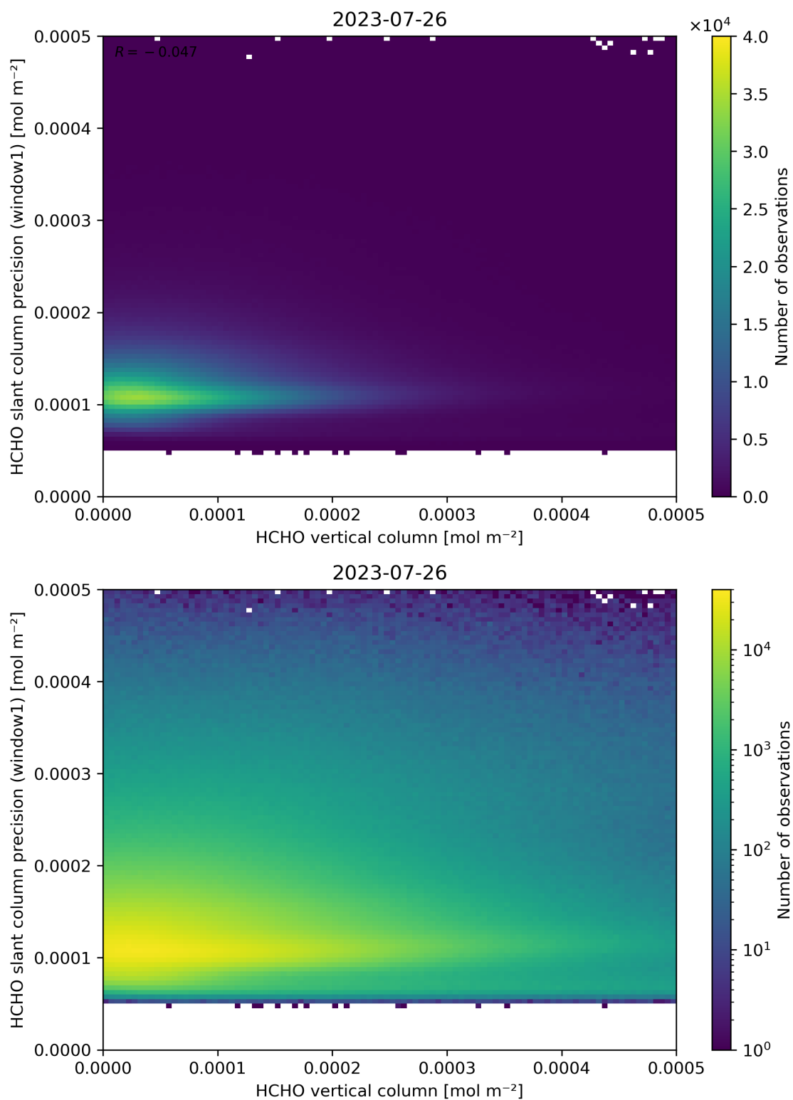
Figure 130: Scatter density plot of “HCHO vertical column” against “HCHO slant column precision (window1)” for 2023-07-25 to 2023-07-27.
