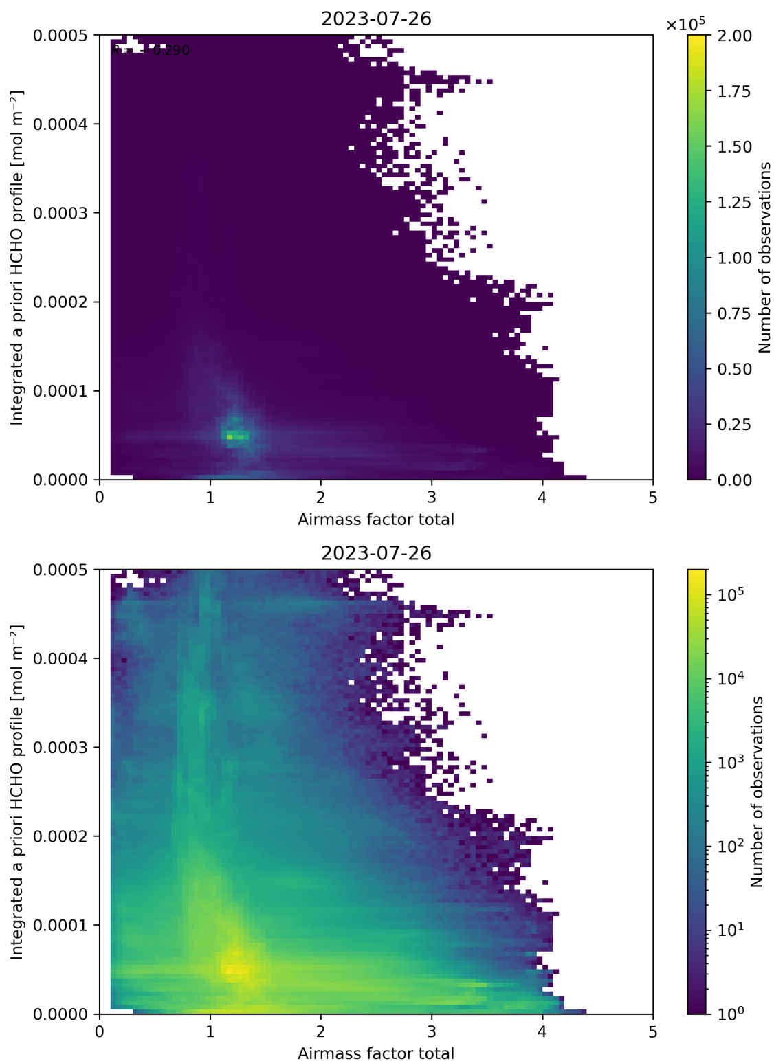
Figure 104: Scatter density plot of “Airmass factor total” against “Integrated a priori HCHO profile” for 2023-07-25 to 2023-07-27.
