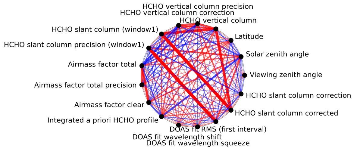
Figure 1: Map of correlation graph for 2023-07-25 to 2023-07-27.
