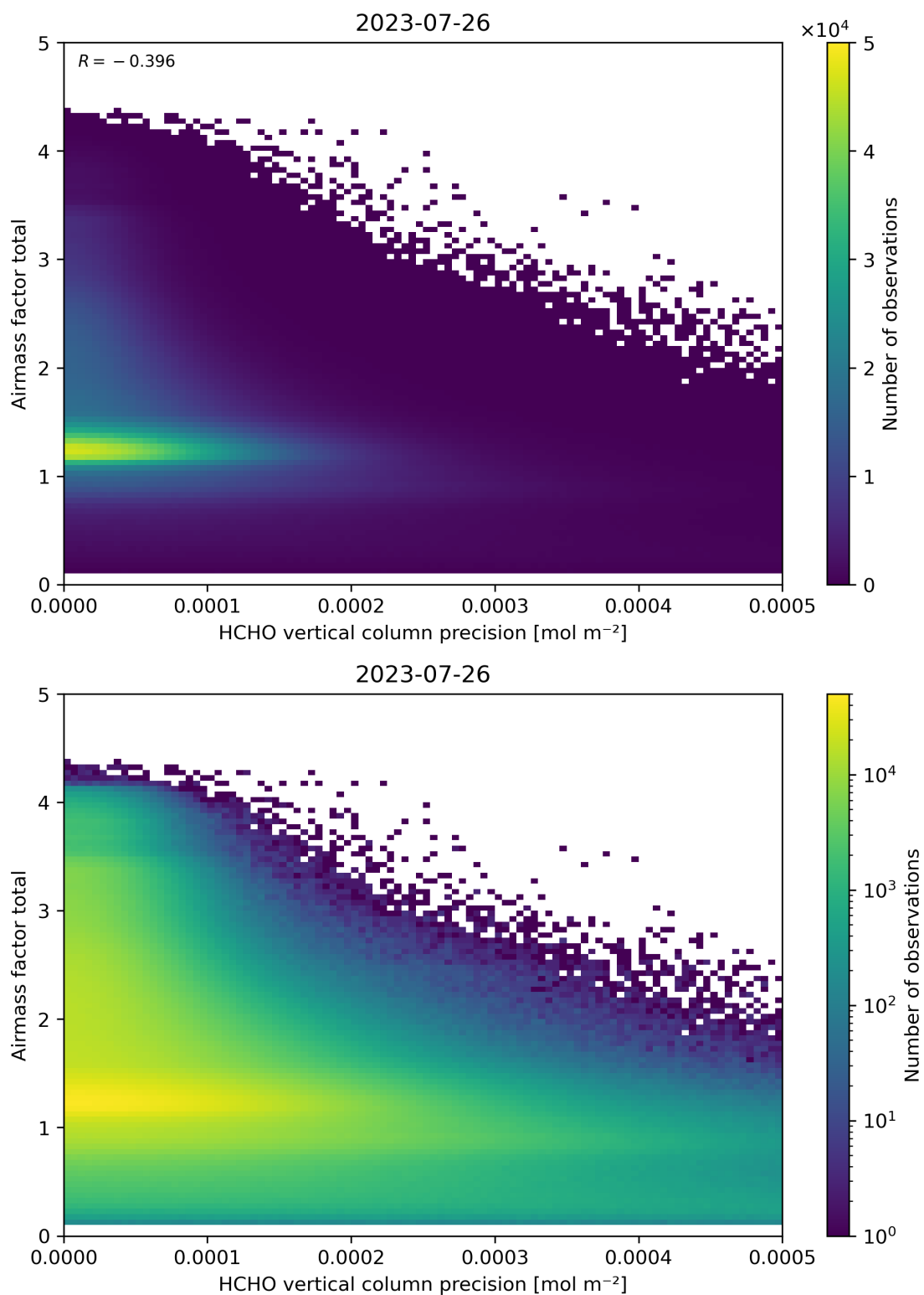
Figure 144: Scatter density plot of “HCHO vertical column precision” against “Airmass factor total” for 2023-07-25 to 2023-07-27.
