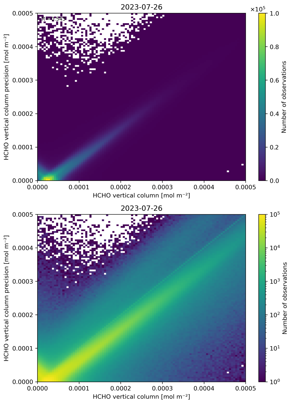
Figure 134: Scatter density plot of “HCHO vertical column” against “HCHO vertical column precision” for 2023-07-25 to 2023-07-27.
