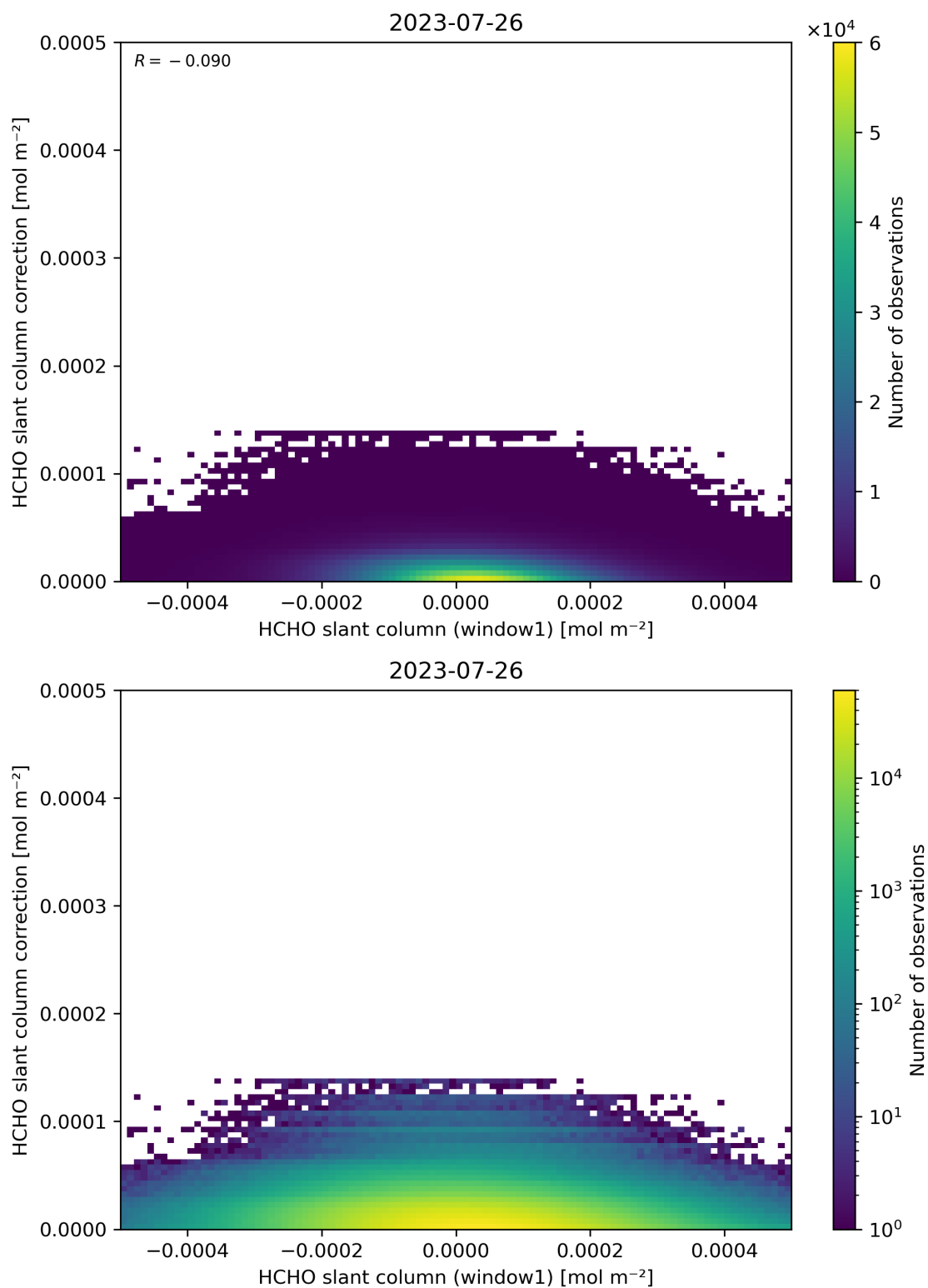
Figure 83: Scatter density plot of “HCHO slant column (window1)” against “HCHO slant column correction” for 2023-07-25 to 2023-07-27.
