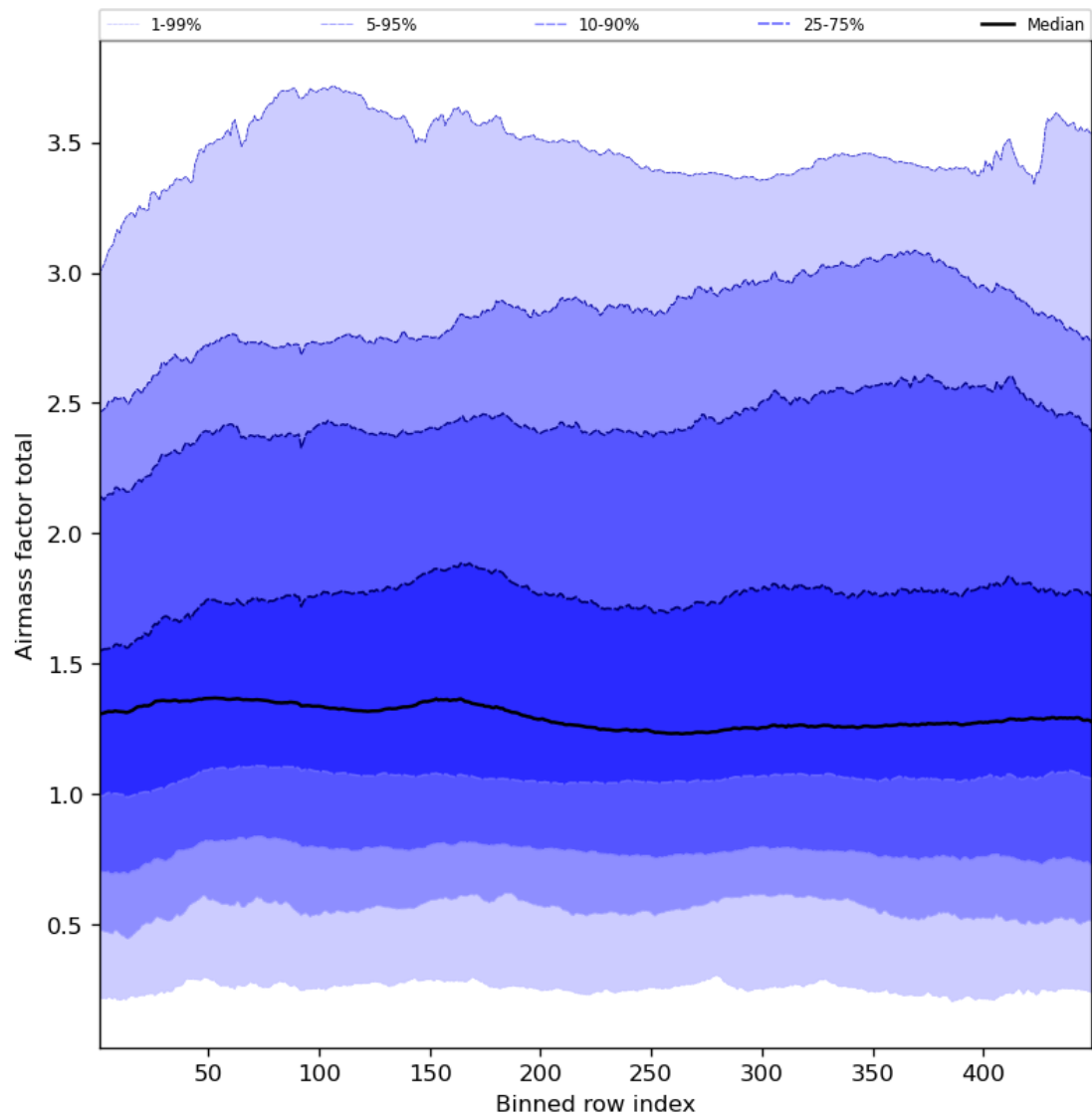
Figure 54: Along track statistics of “Airmass factor total” for 2023-07-25 to 2023-07-27
