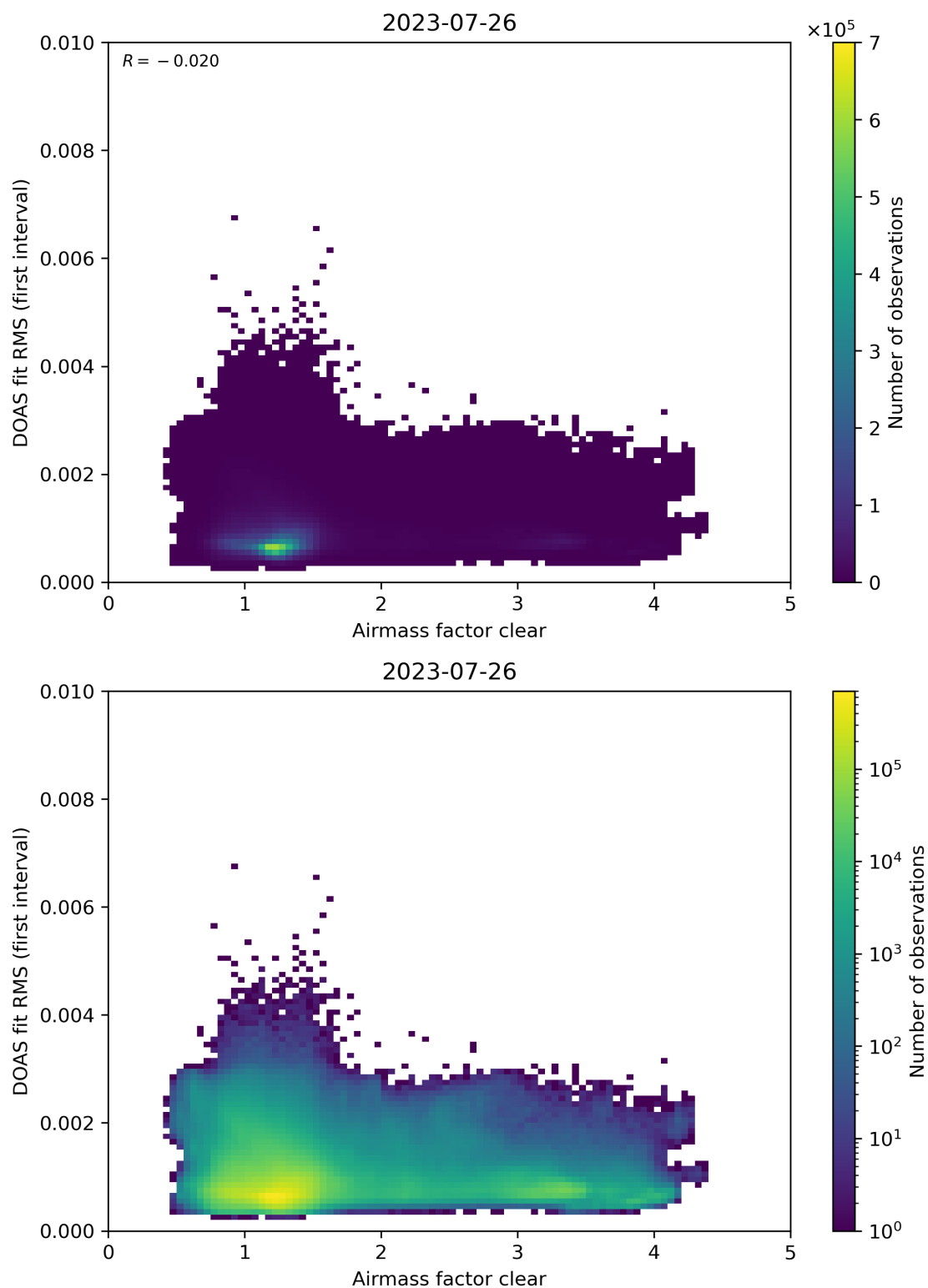
Figure 71: Scatter density plot of “Airmass factor clear” against “DOAS fit RMS (first interval)” for 2023-07-25 to 2023-07-27.
