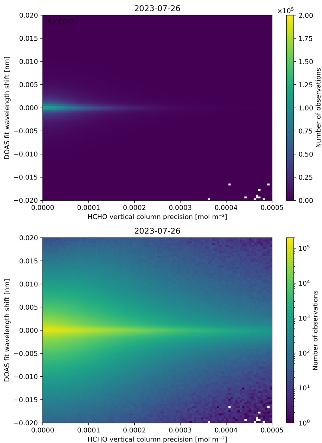
Figure 137: Scatter density plot of “HCHO vertical column precision” against “DOAS fit wavelength shift” for 2023-07-25 to 2023-07-27.
