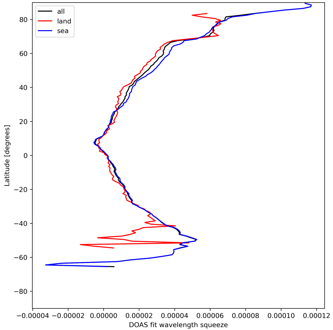
Figure 31: Zonal average of “DOAS fit wavelength squeeze” for 2023-07-25 to 2023-07-27.
