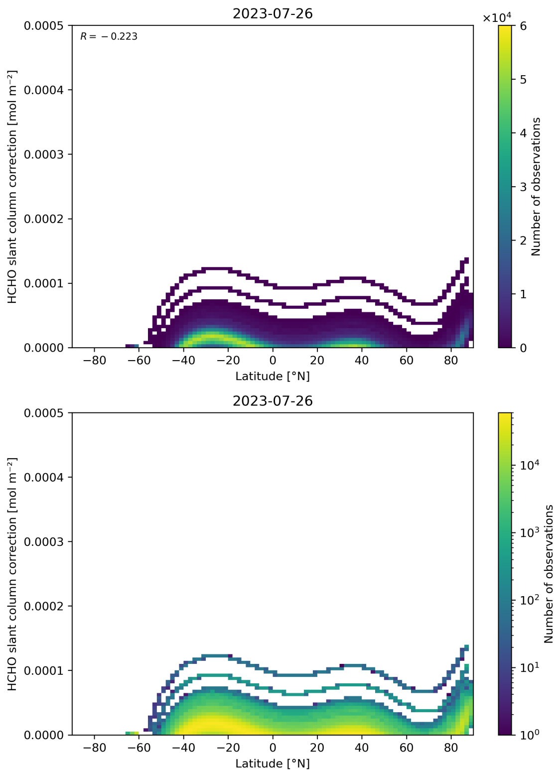
Figure 158: Scatter density plot of “Latitude” against “HCHO slant column correction” for 2023-07-25 to 2023-07-27.
