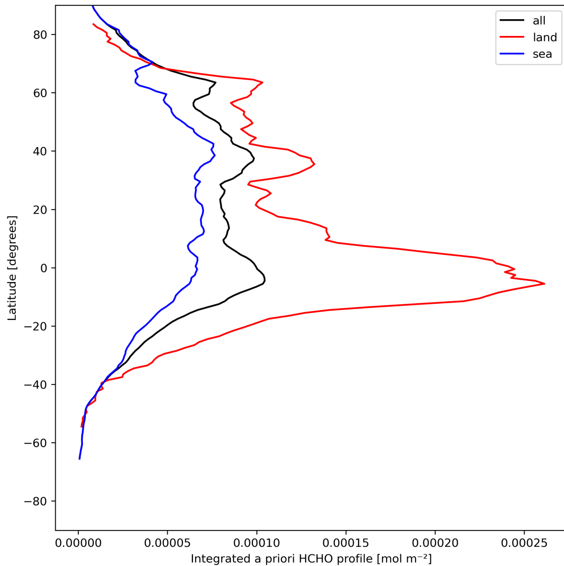
Figure 29: Zonal average of “Integrated a priori HCHO profile” for 2023-07-25 to 2023-07-27.
