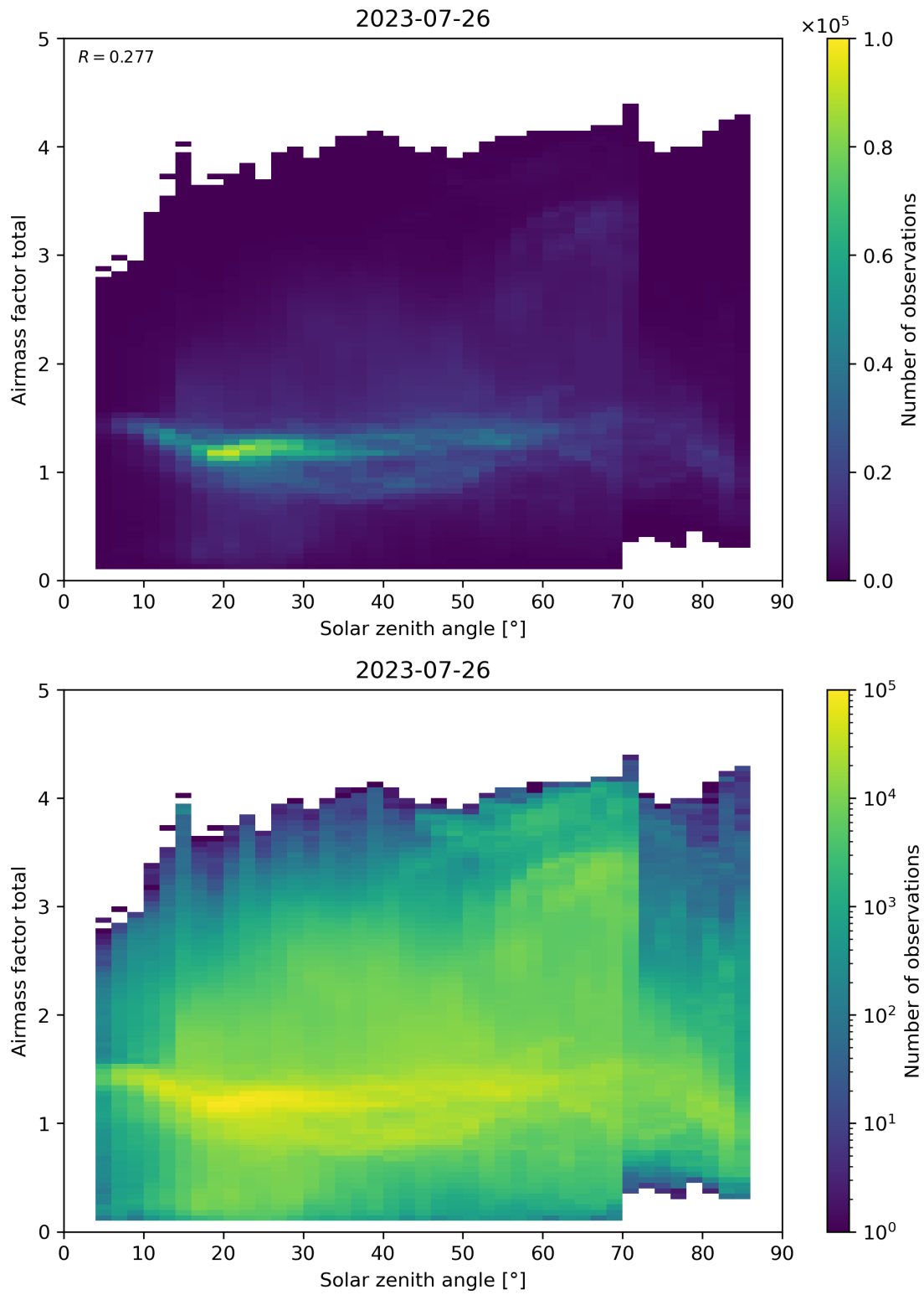
Figure 175: Scatter density plot of “Solar zenith angle” against “Airmass factor total” for 2023-07-25 to 2023-07-27.
