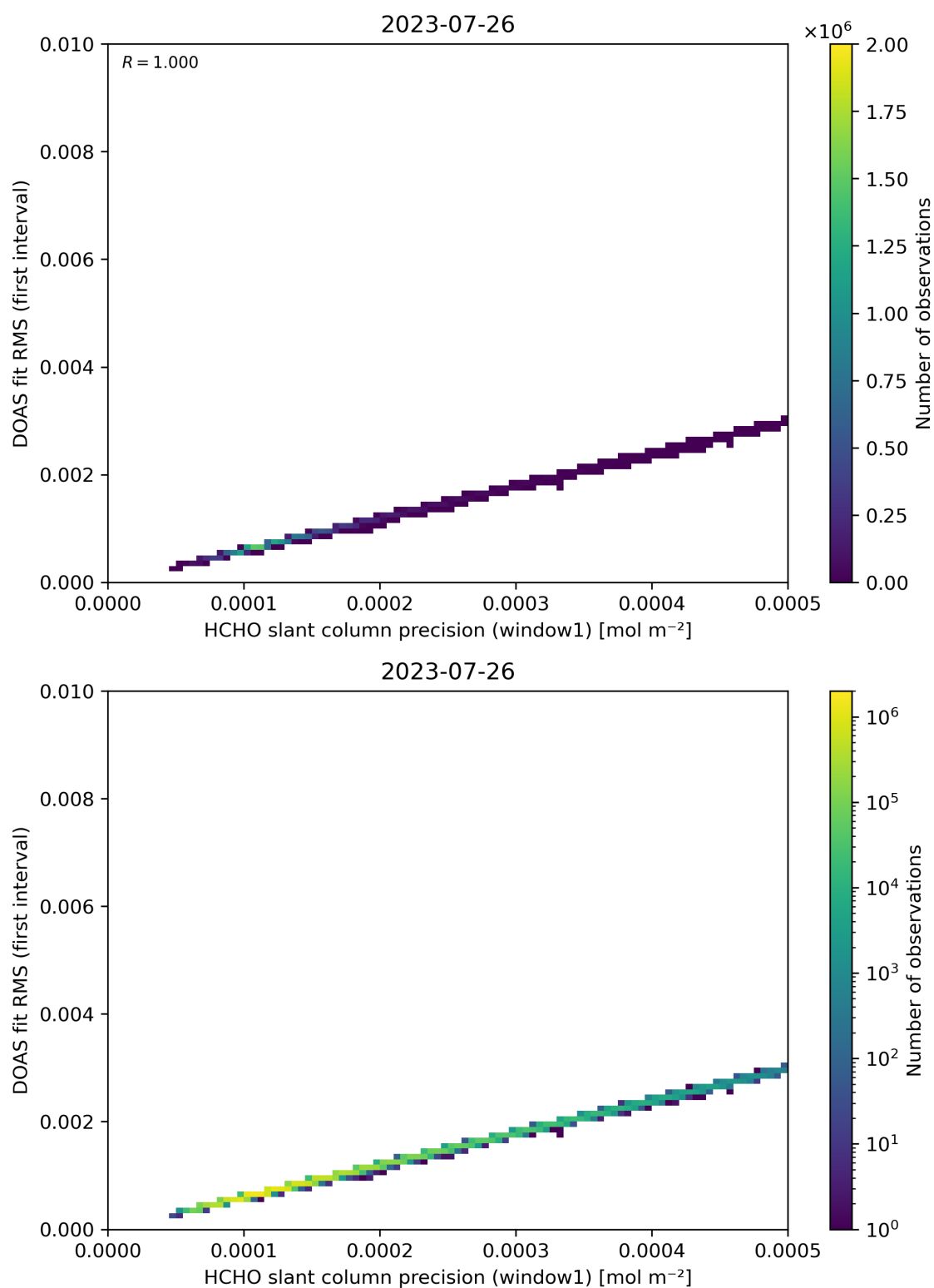
Figure 88: Scatter density plot of “HCHO slant column precision (window1)” against “DOAS fit RMS (first interval)” for 2023-07-25 to 2023-07-27.
