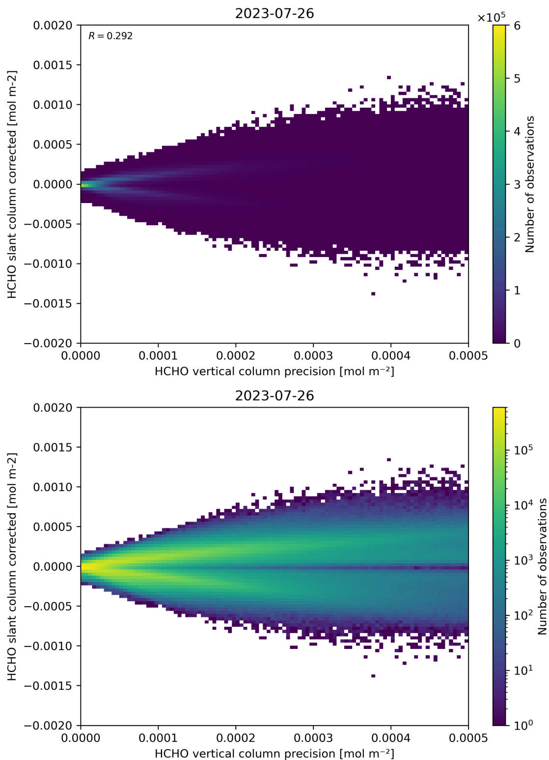
Figure 140: Scatter density plot of “HCHO vertical column precision” against “HCHO slant column corrected” for 2023-07-25 to 2023-07-27.
