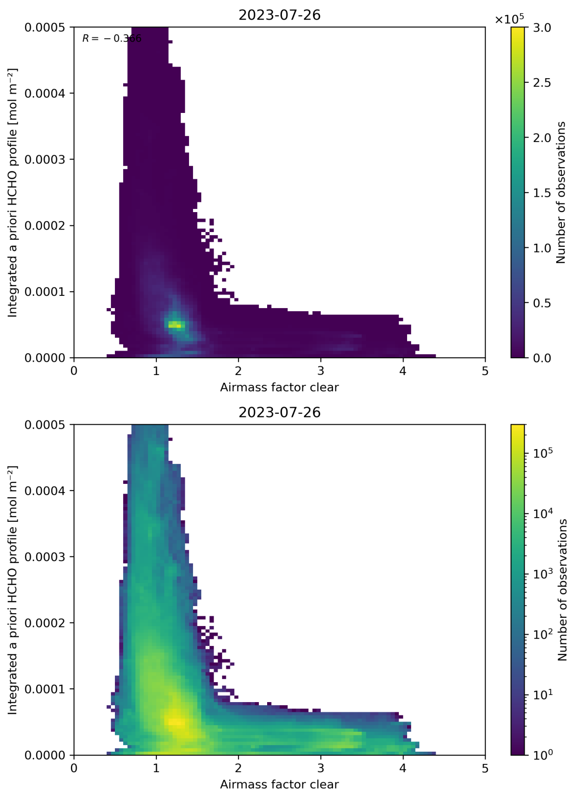
Figure 76: Scatter density plot of “Airmass factor clear” against “Integrated a priori HCHO profile” for 2023-07-25 to 2023-07-27.
