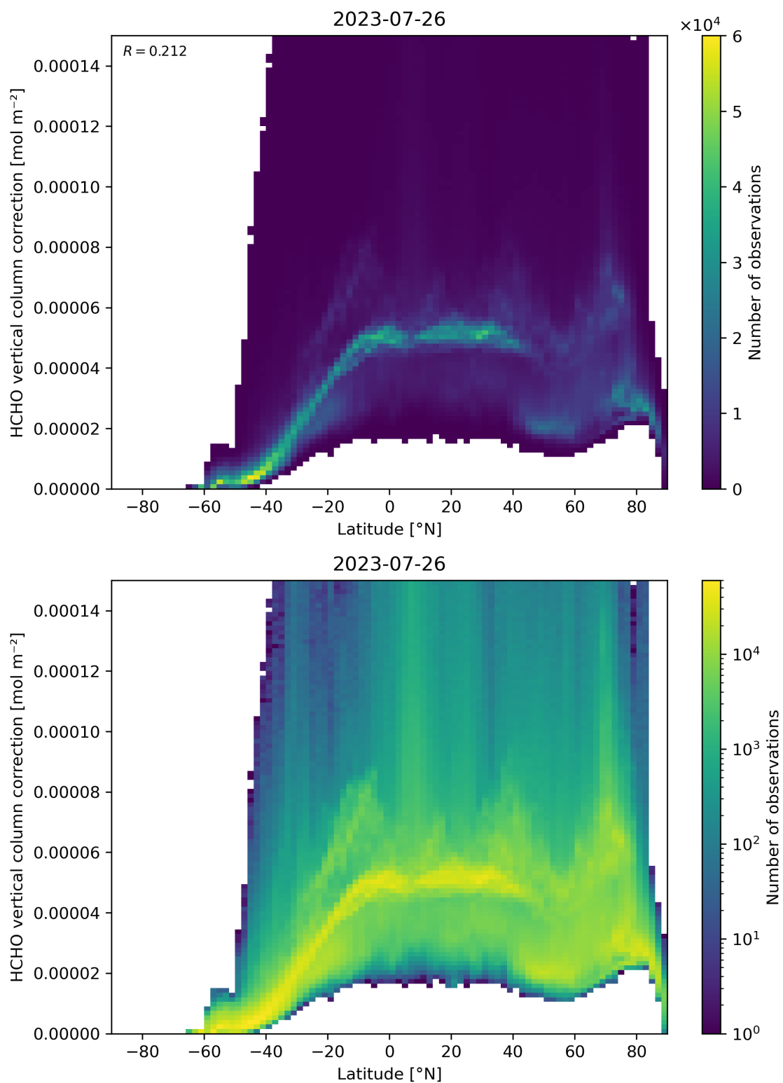
Figure 164: Scatter density plot of “Latitude” against “HCHO vertical column correction” for 2023-07-25 to 2023-07-27.
