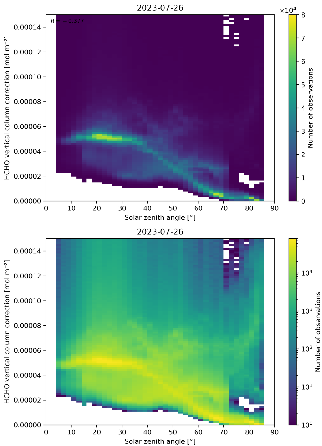
Figure 178: Scatter density plot of “Solar zenith angle” against “HCHO vertical column correction” for 2023-07-25 to 2023-07-27.
