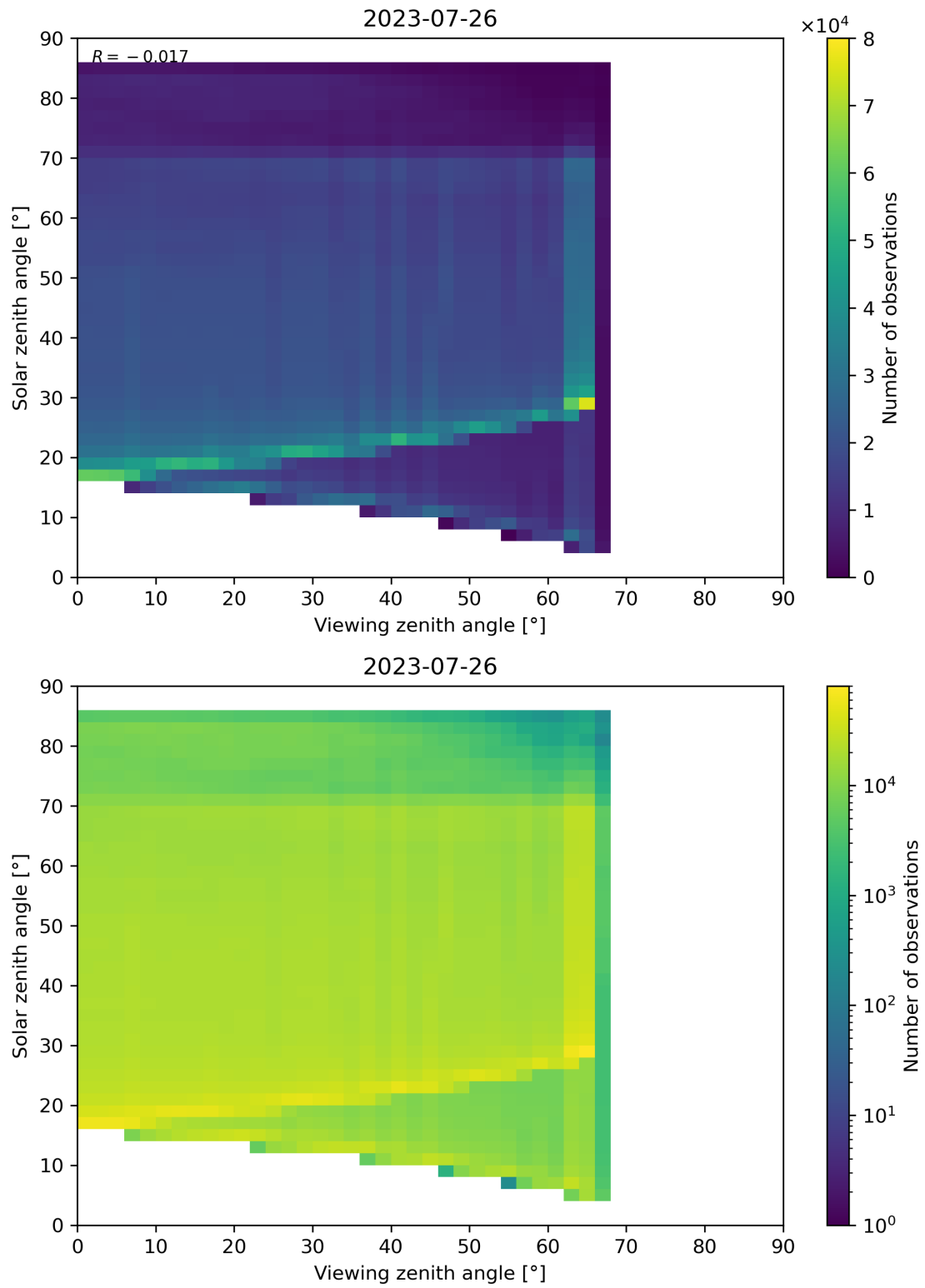
Figure 197: Scatter density plot of “Viewing zenith angle” against “Solar zenith angle” for 2023-07-25 to 2023-07-27.
