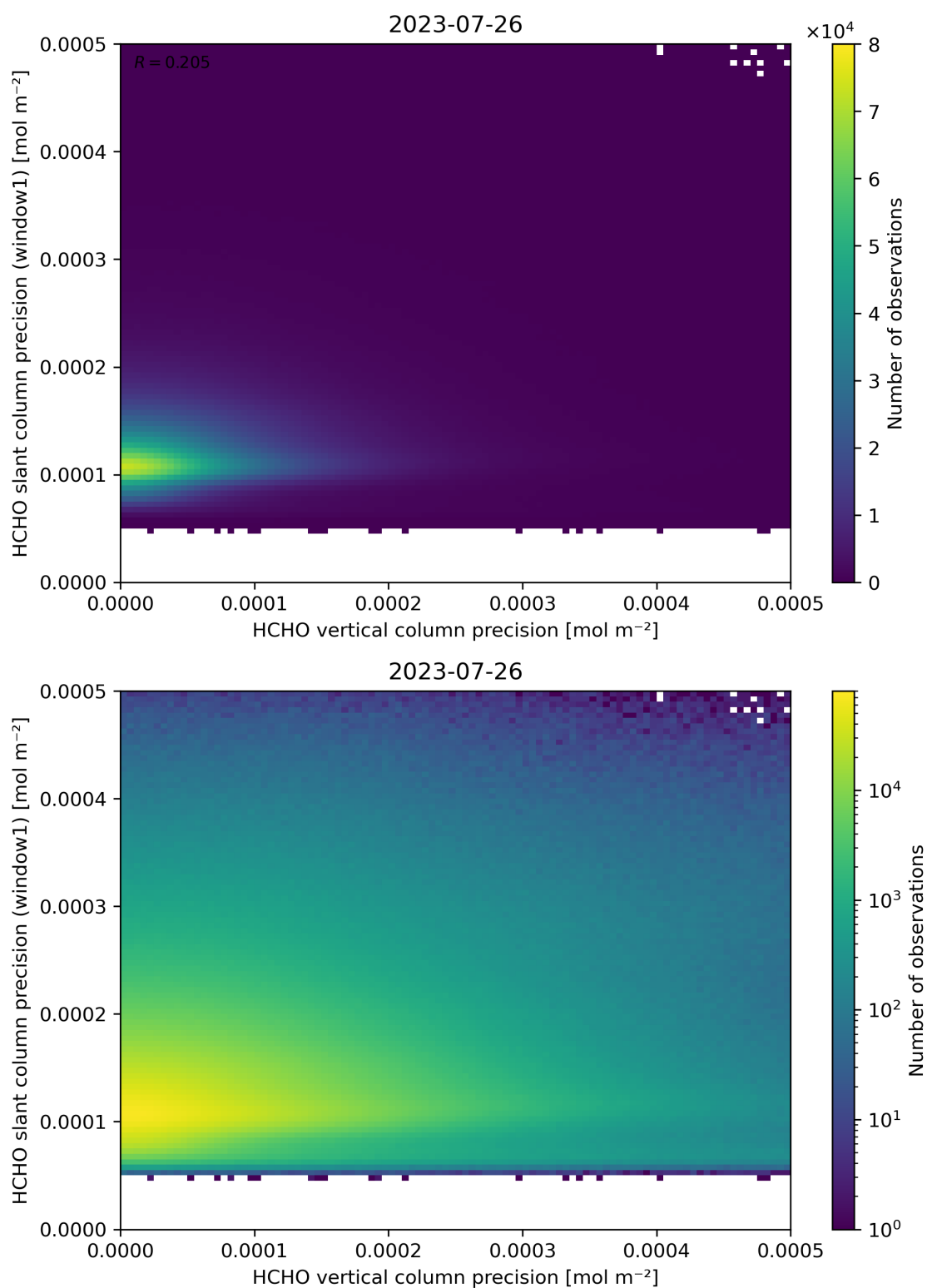
Figure 143: Scatter density plot of “HCHO vertical column precision” against “HCHO slant column precision (window1)” for 2023-07-25 to 2023-07-27.
