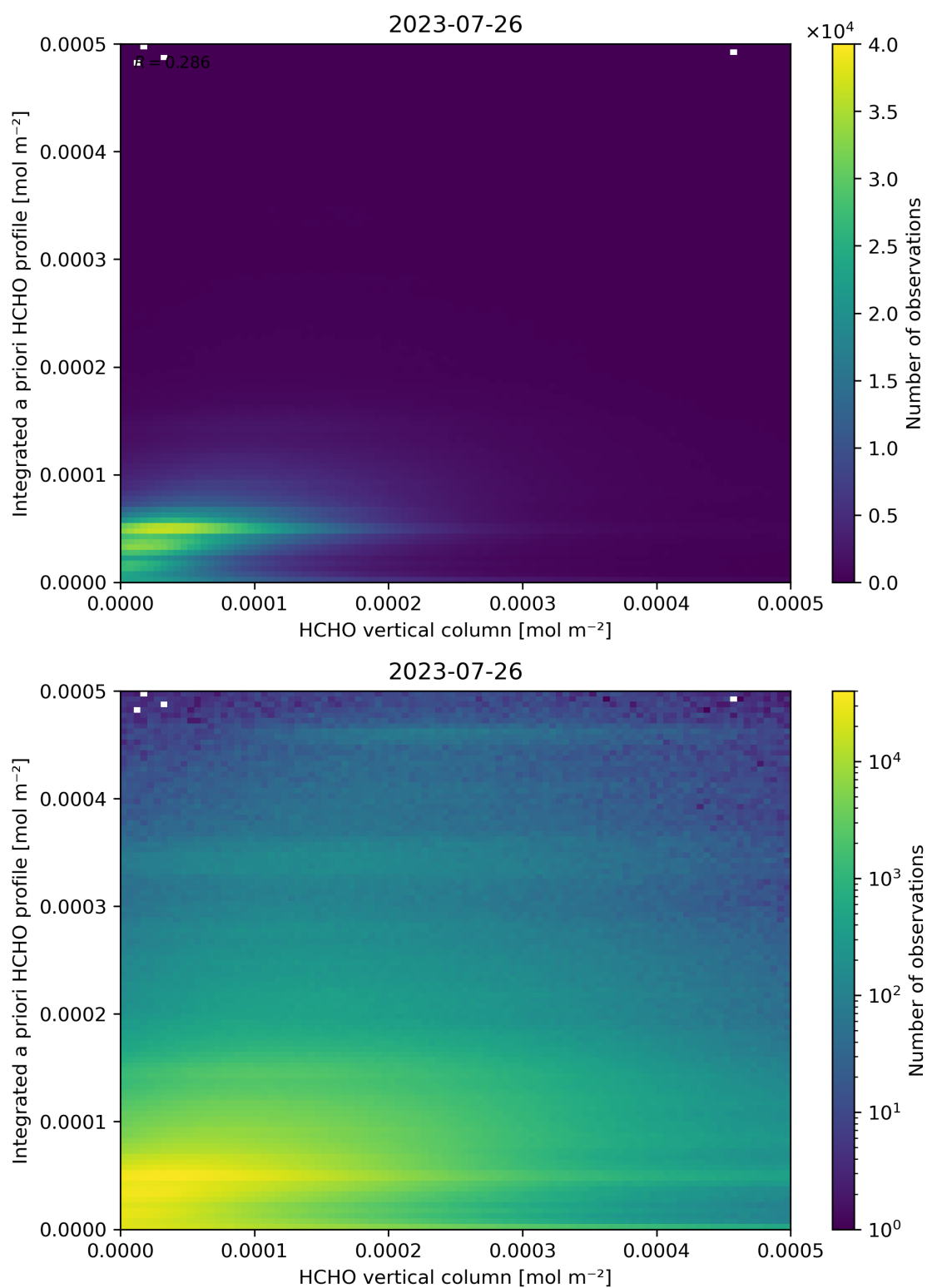
Figure 135: Scatter density plot of “HCHO vertical column” against “Integrated a priori HCHO profile” for 2023-07-25 to 2023-07-27.
