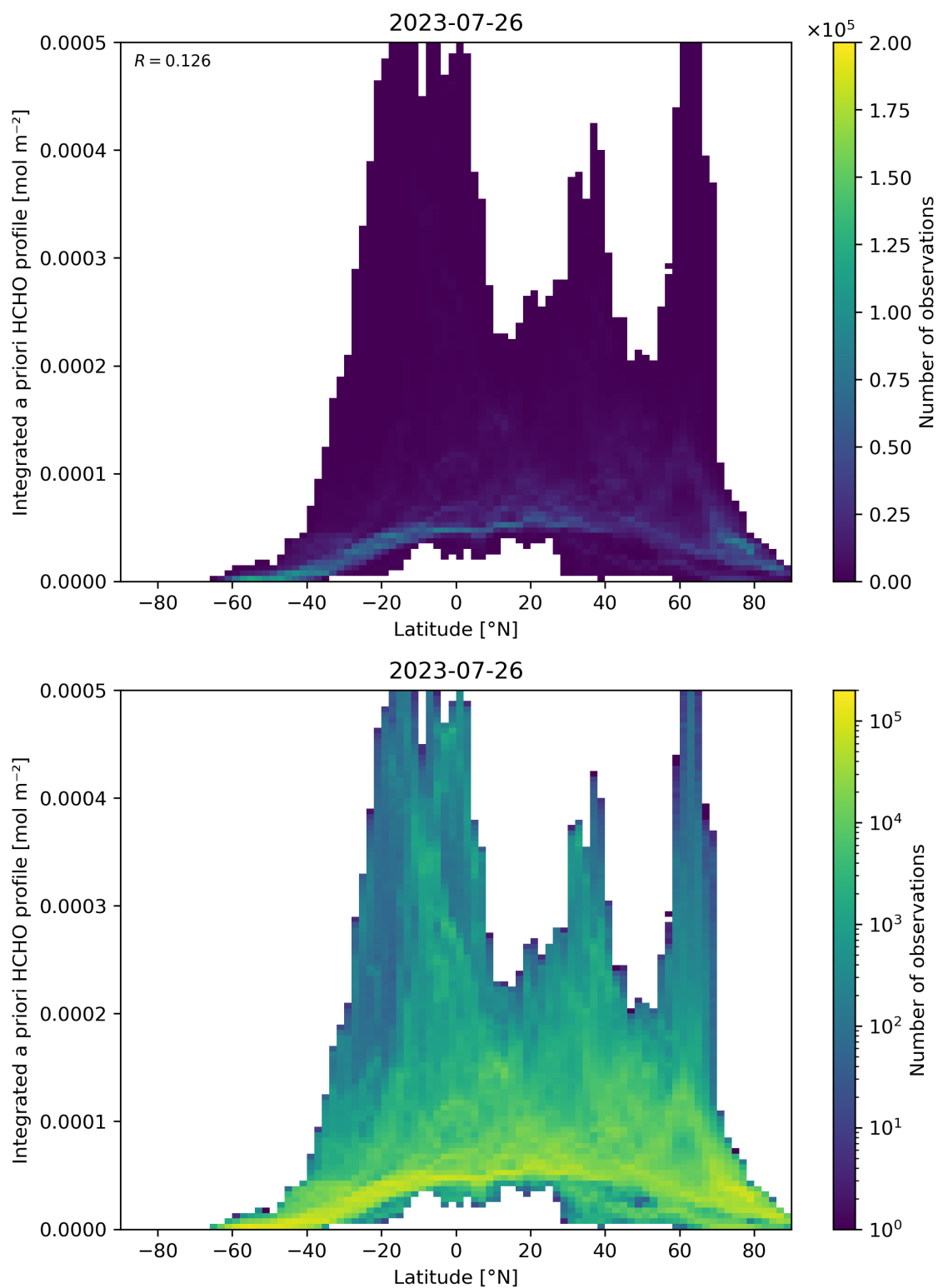
Figure 166: Scatter density plot of “Latitude” against “Integrated a priori HCHO profile” for 2023-07-25 to 2023-07-27.
