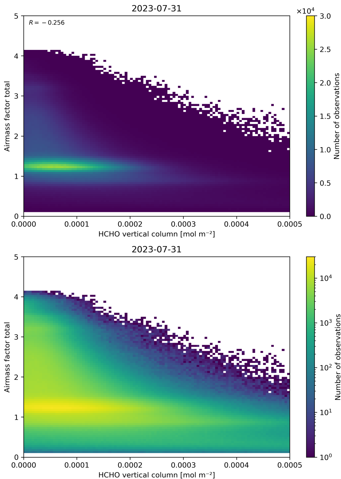
Figure 131: Scatter density plot of “HCHO vertical column” against “Airmass factor total” for 2023-07-30 to 2023-08-01.
