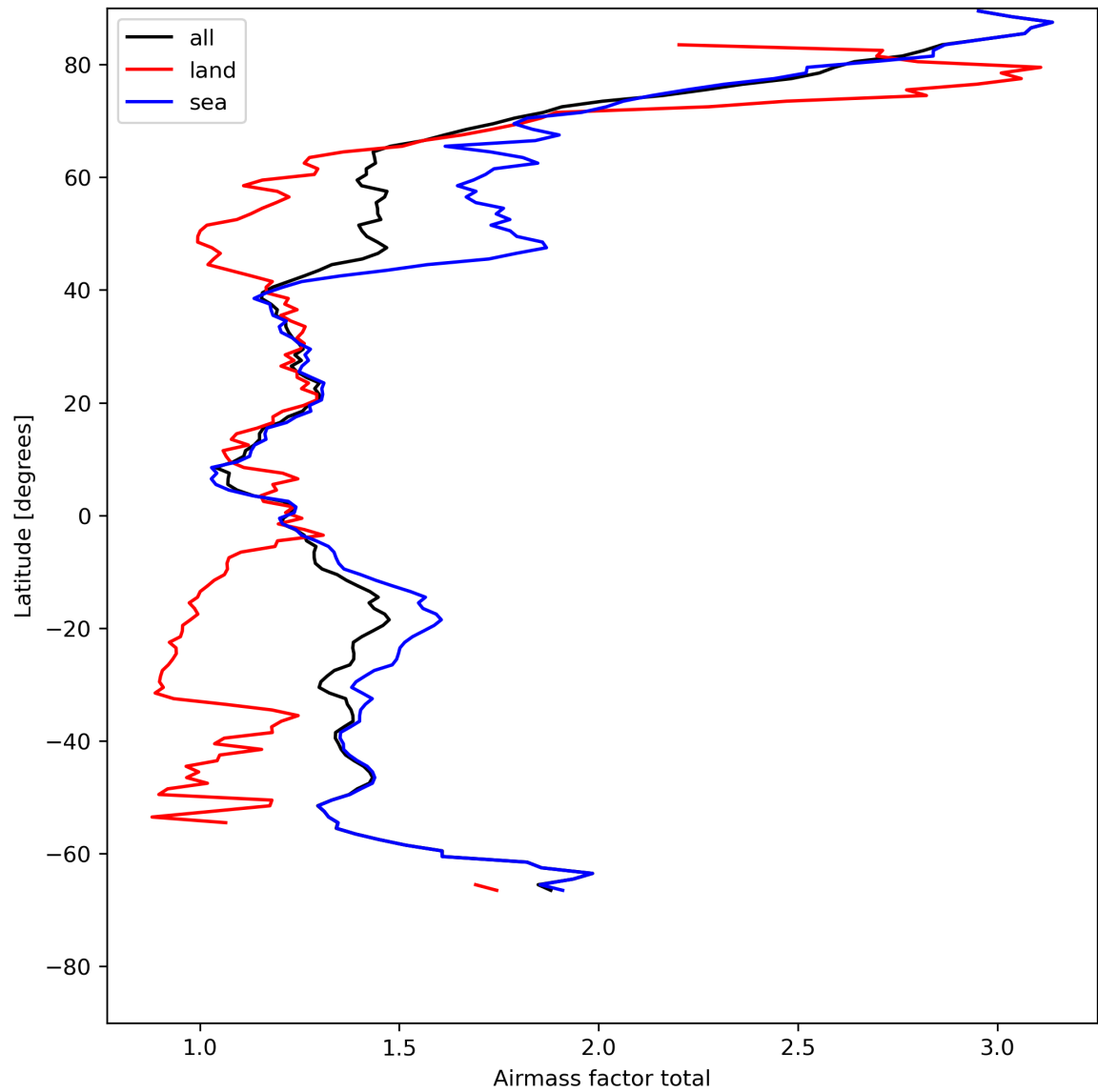
Figure 26: Zonal average of “Airmass factor total” for 2023-07-30 to 2023-08-01.
