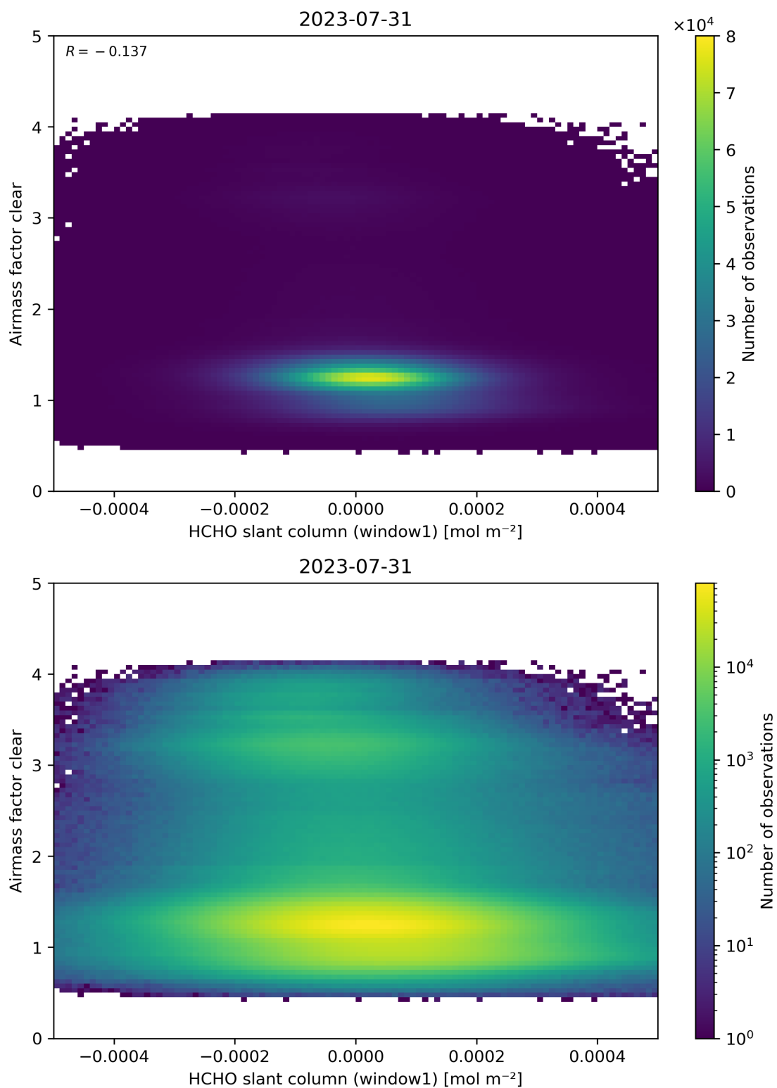
Figure 81: Scatter density plot of “HCHO slant column (window1)” against “Airmass factor clear” for 2023-07-30 to 2023-08-01.
