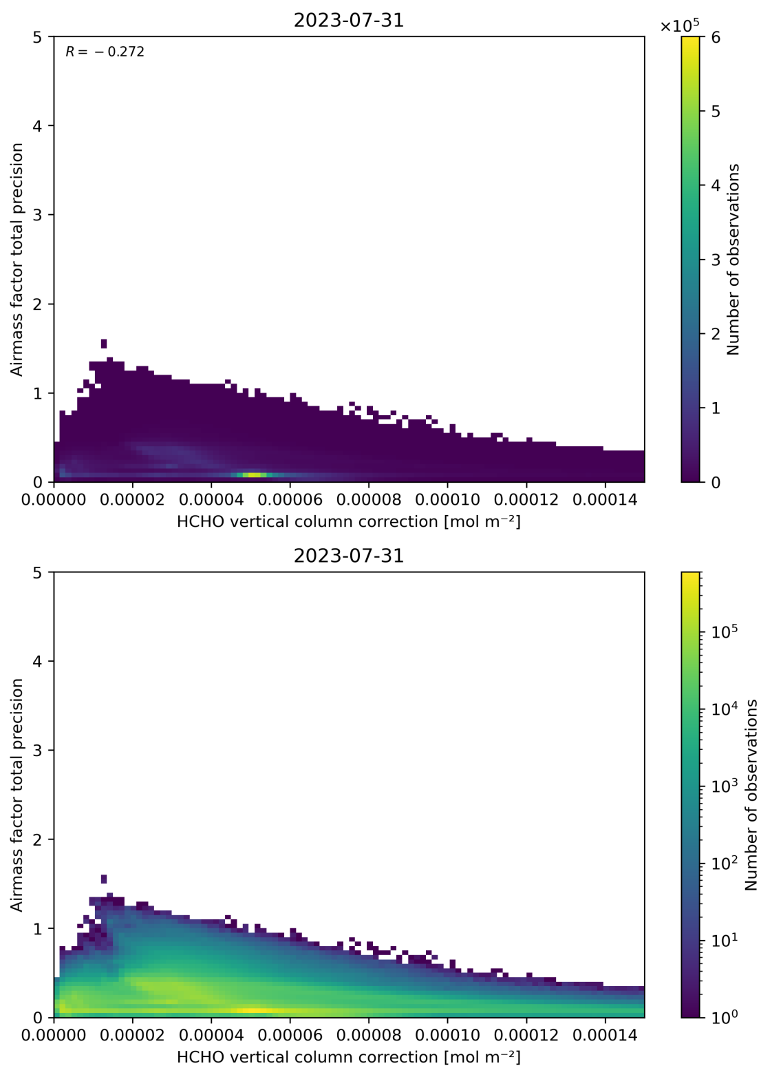
Figure 121: Scatter density plot of “HCHO vertical column correction” against “Airmass factor total precision” for 2023-07-30 to 2023-08-01.
