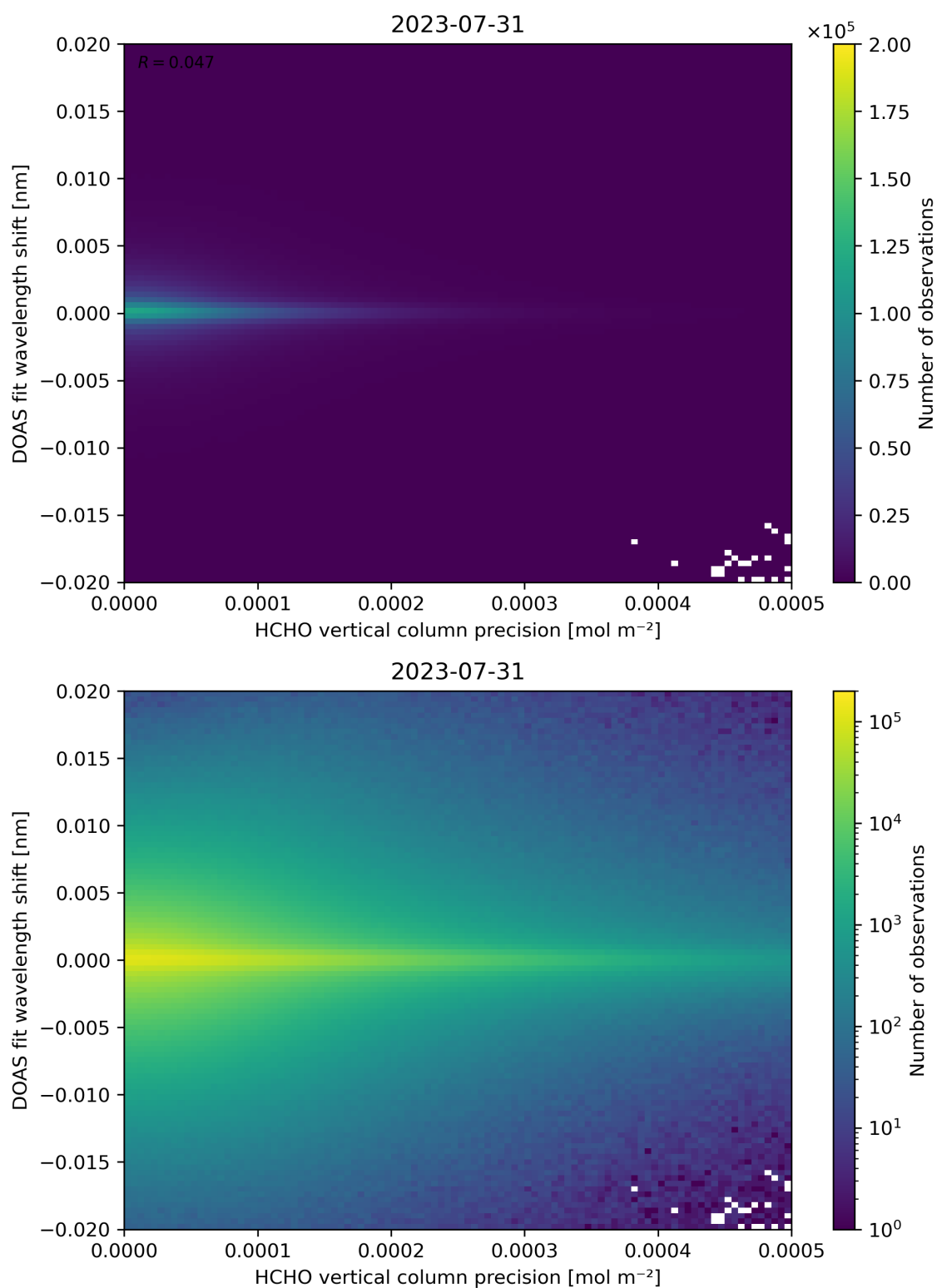
Figure 137: Scatter density plot of “HCHO vertical column precision” against “DOAS fit wavelength shift” for 2023-07-30 to 2023-08-01.
