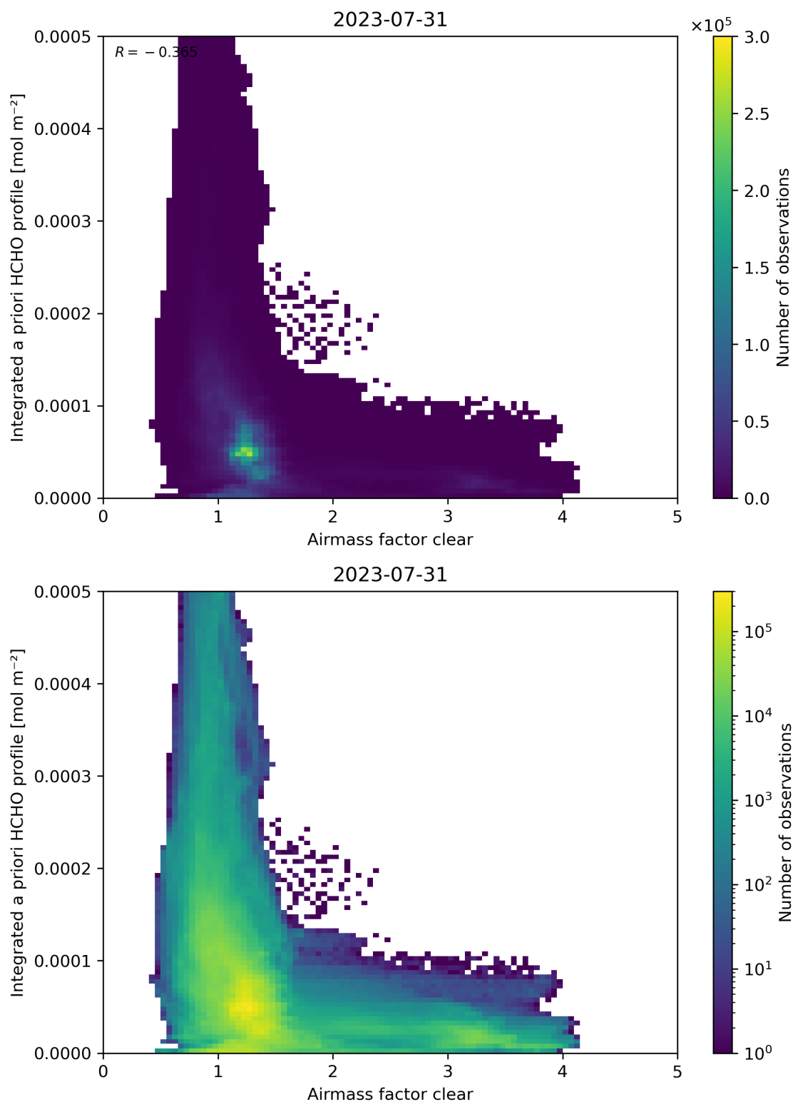
Figure 76: Scatter density plot of “Airmass factor clear” against “Integrated a priori HCHO profile” for 2023-07-30 to 2023-08-01.
