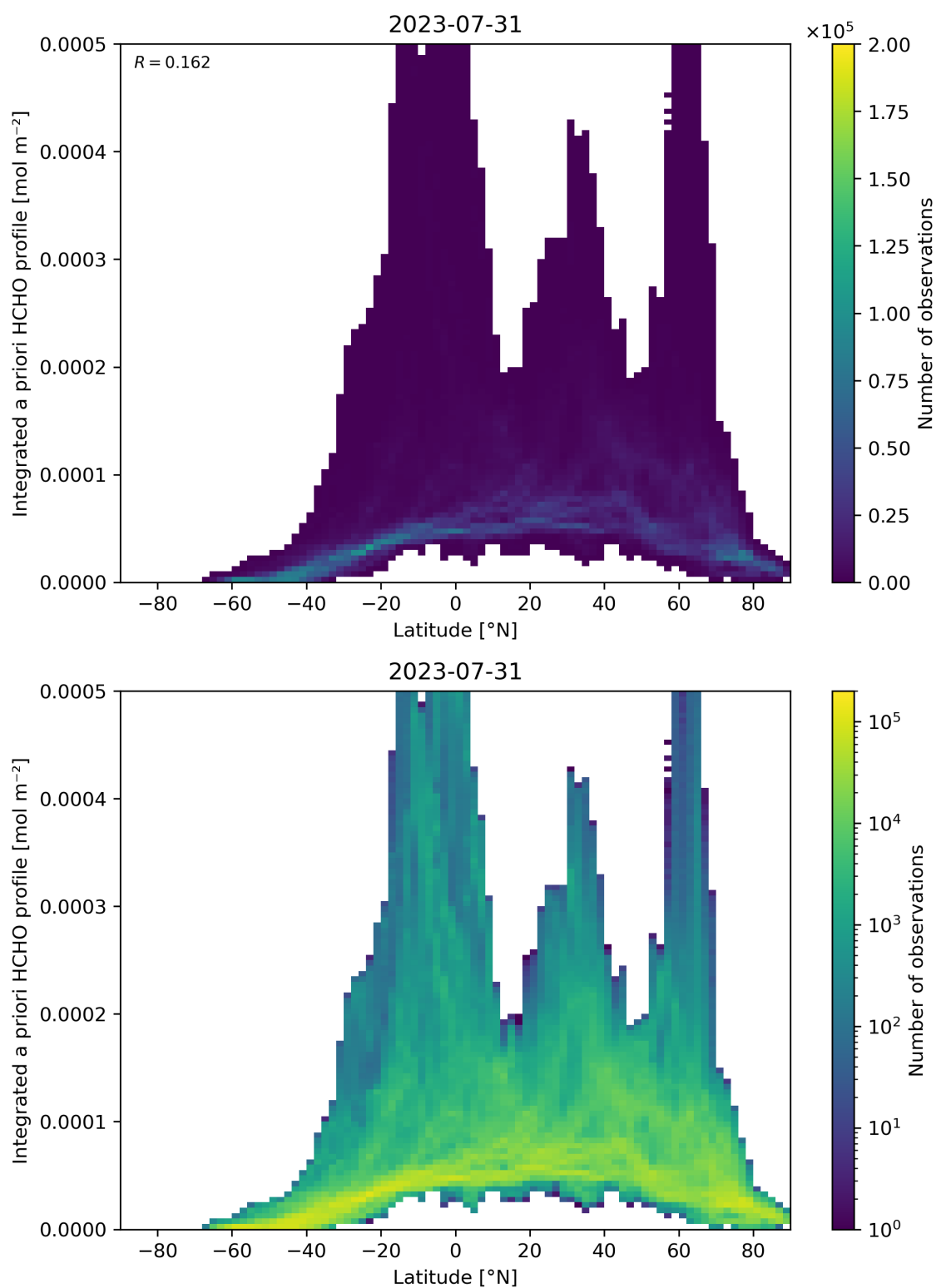
Figure 166: Scatter density plot of “Latitude” against “Integrated a priori HCHO profile” for 2023-07-30 to 2023-08-01.
