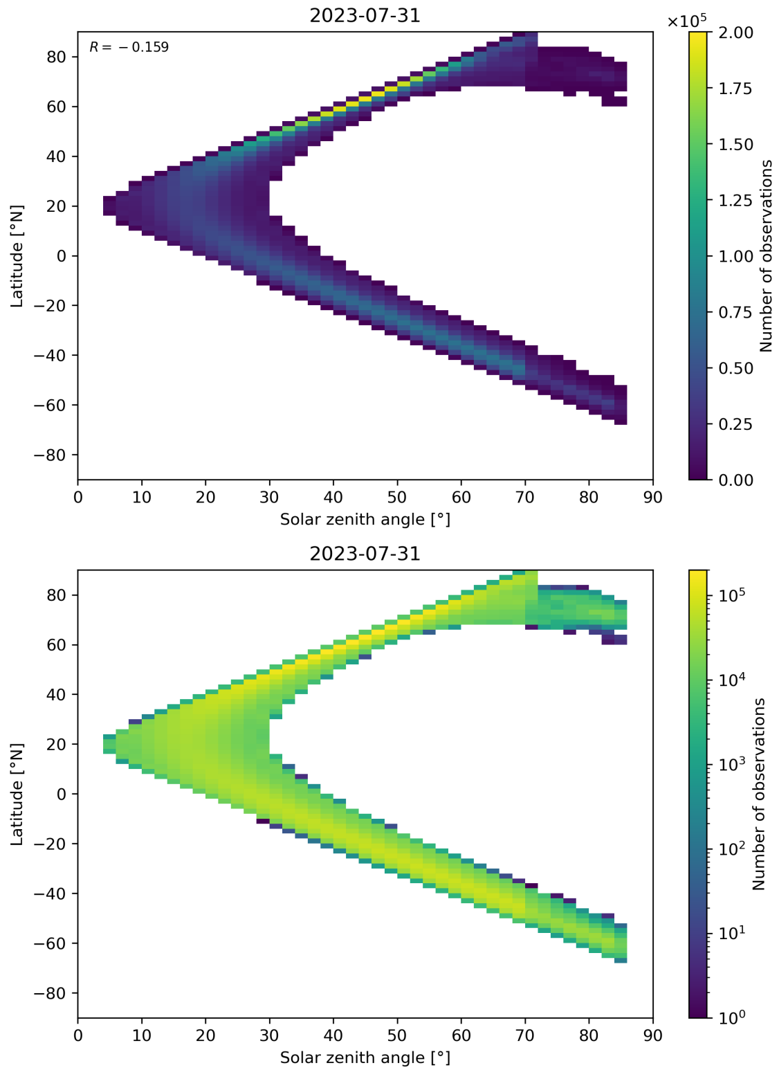
Figure 181: Scatter density plot of “Solar zenith angle” against “Latitude” for 2023-07-30 to 2023-08-01.
