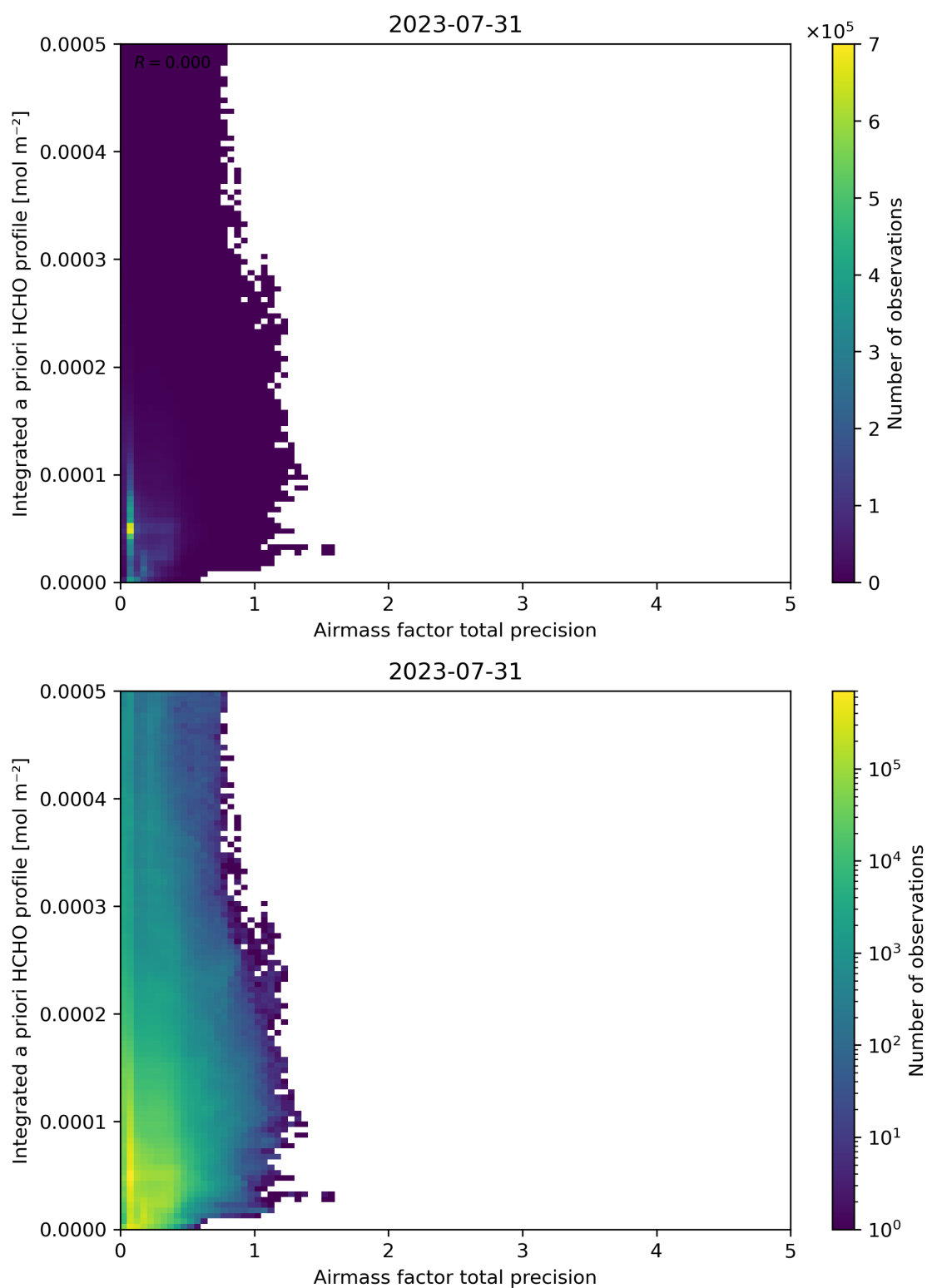
Figure 111: Scatter density plot of “Airmass factor total precision” against “Integrated a priori HCHO profile” for 2023-07-30 to 2023-08-01.
