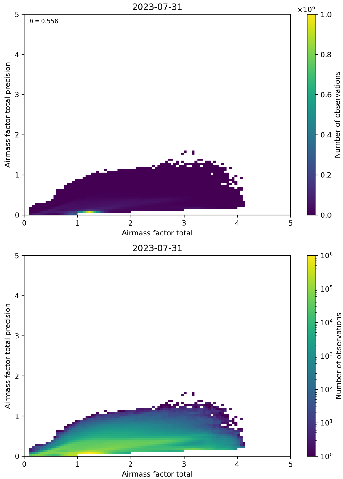
Figure 103: Scatter density plot of “Airmass factor total” against “Airmass factor total precision” for 2023-07-30 to 2023-08-01.
