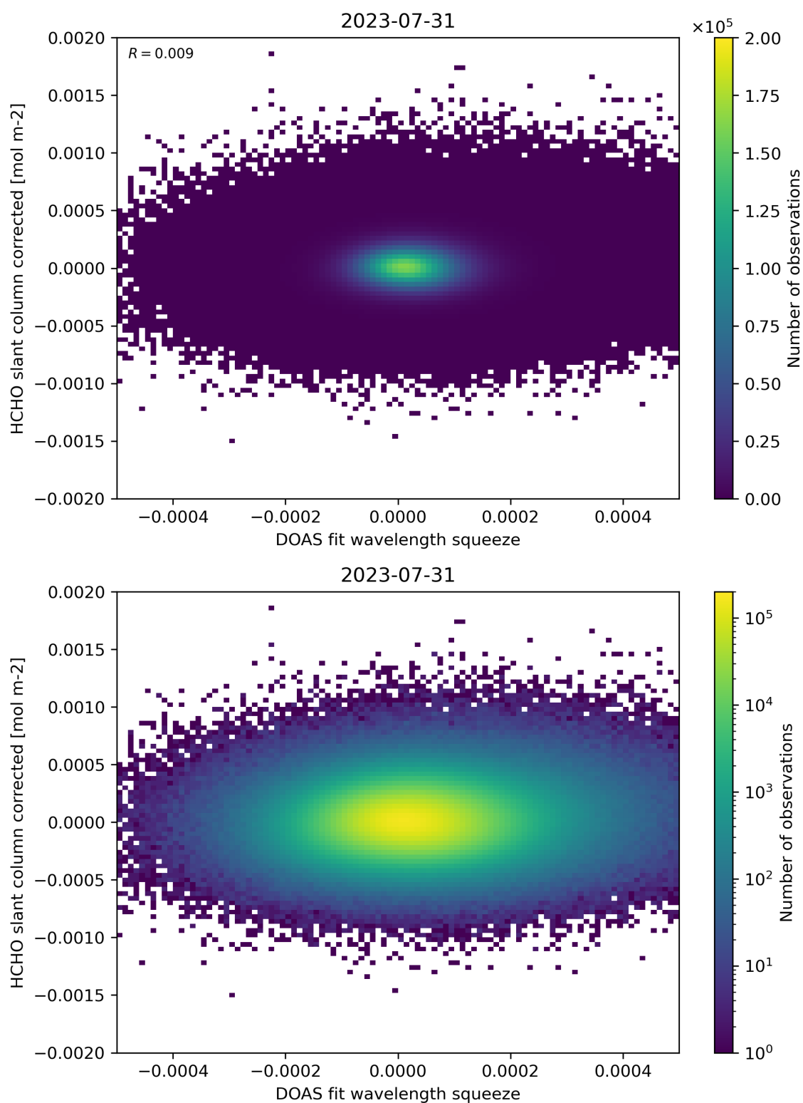
Figure 69: Scatter density plot of “DOAS fit wavelength squeeze” against “HCHO slant column corrected” for 2023-07-30 to 2023-08-01.
