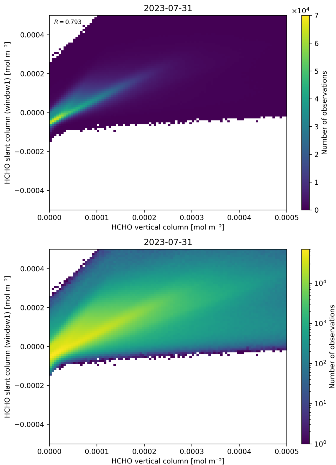
Figure 129: Scatter density plot of “HCHO vertical column” against “HCHO slant column (window1)” for 2023-07-30 to 2023-08-01.
