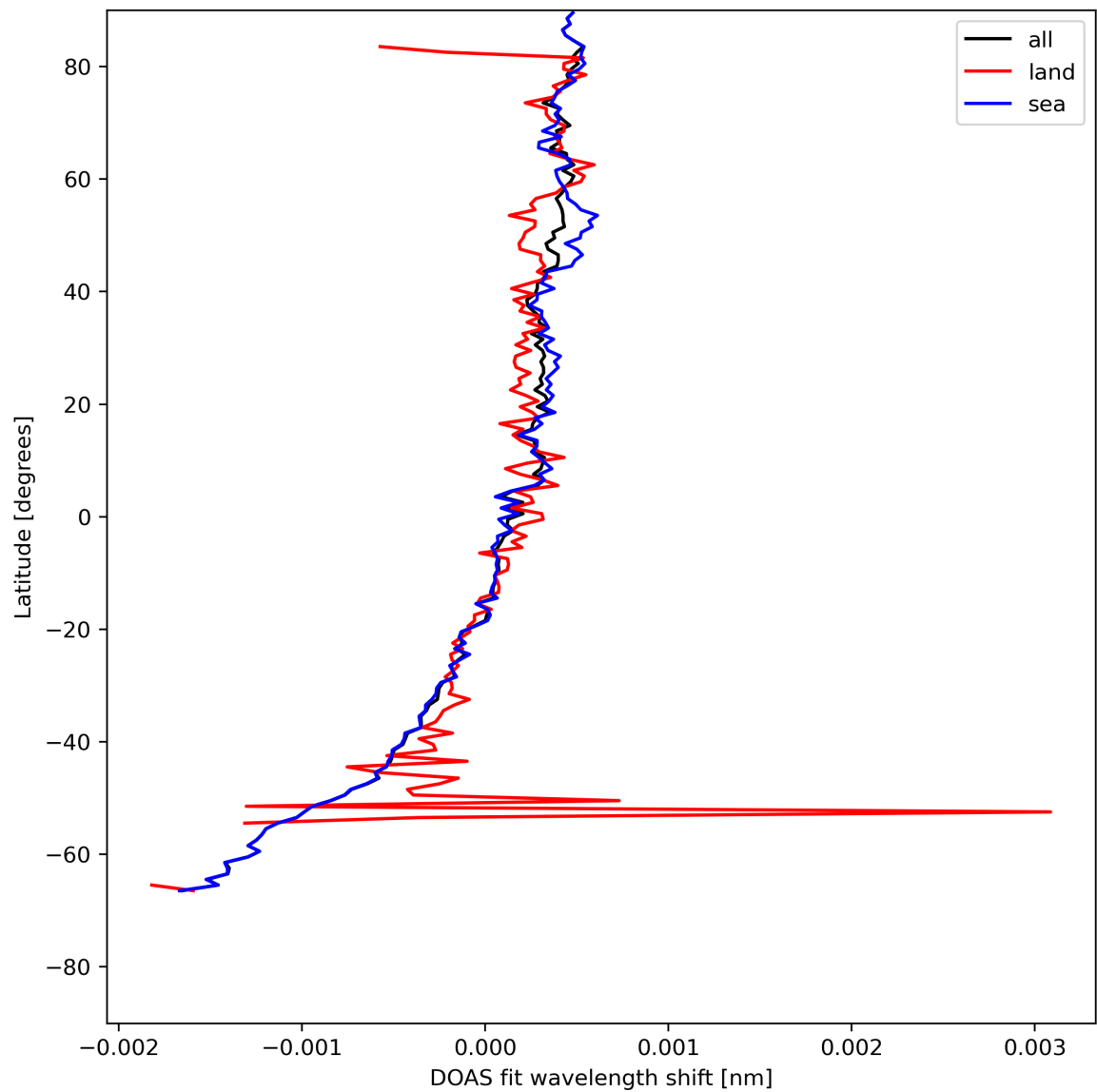
Figure 30: Zonal average of "DOAS fit wavelength shift" for 2023-07-30 to 2023-08-01.
