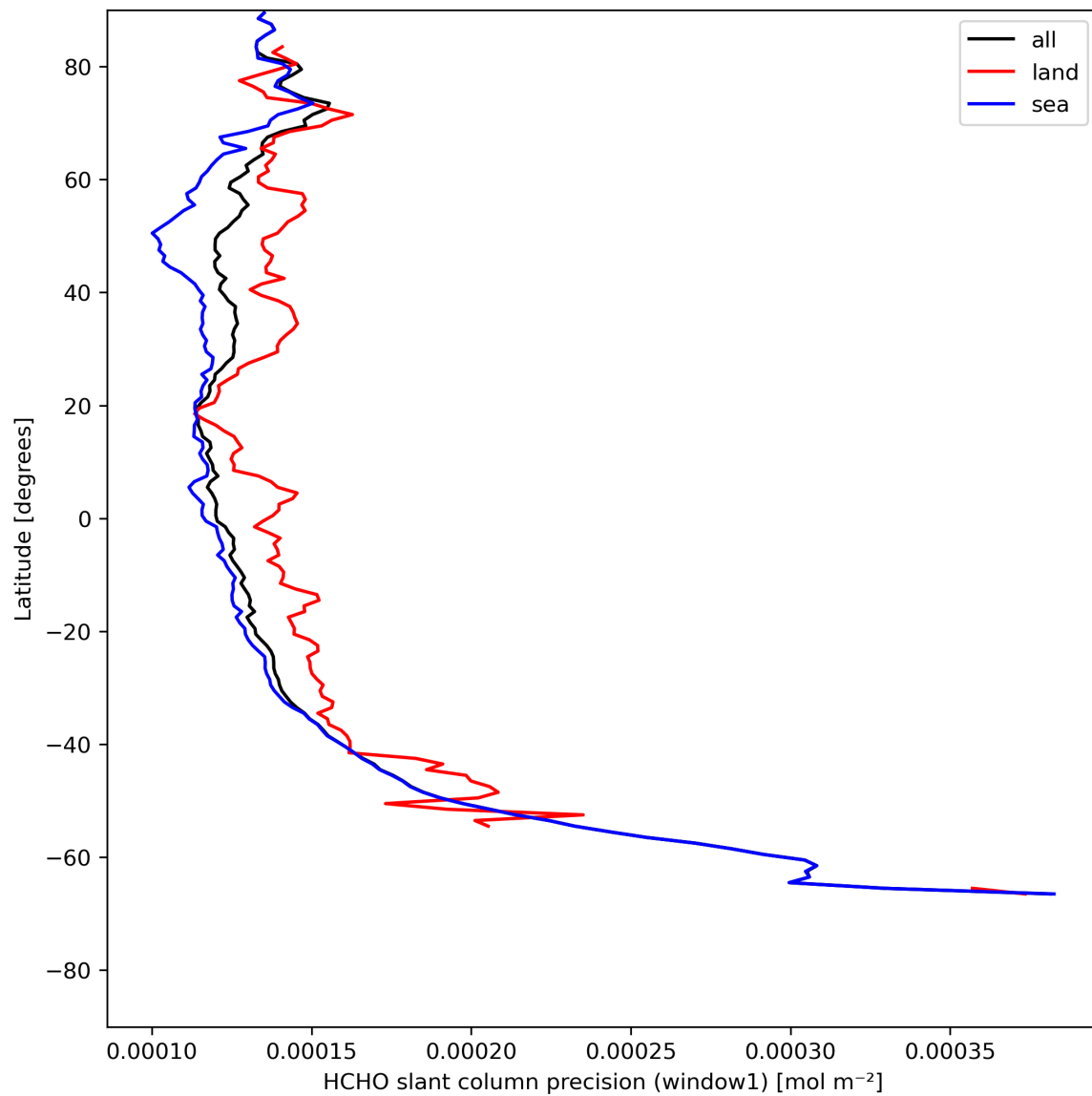
Figure 25: Zonal average of “HCHO slant column precision (window1)” for 2023-07-30 to 2023-08-01.
