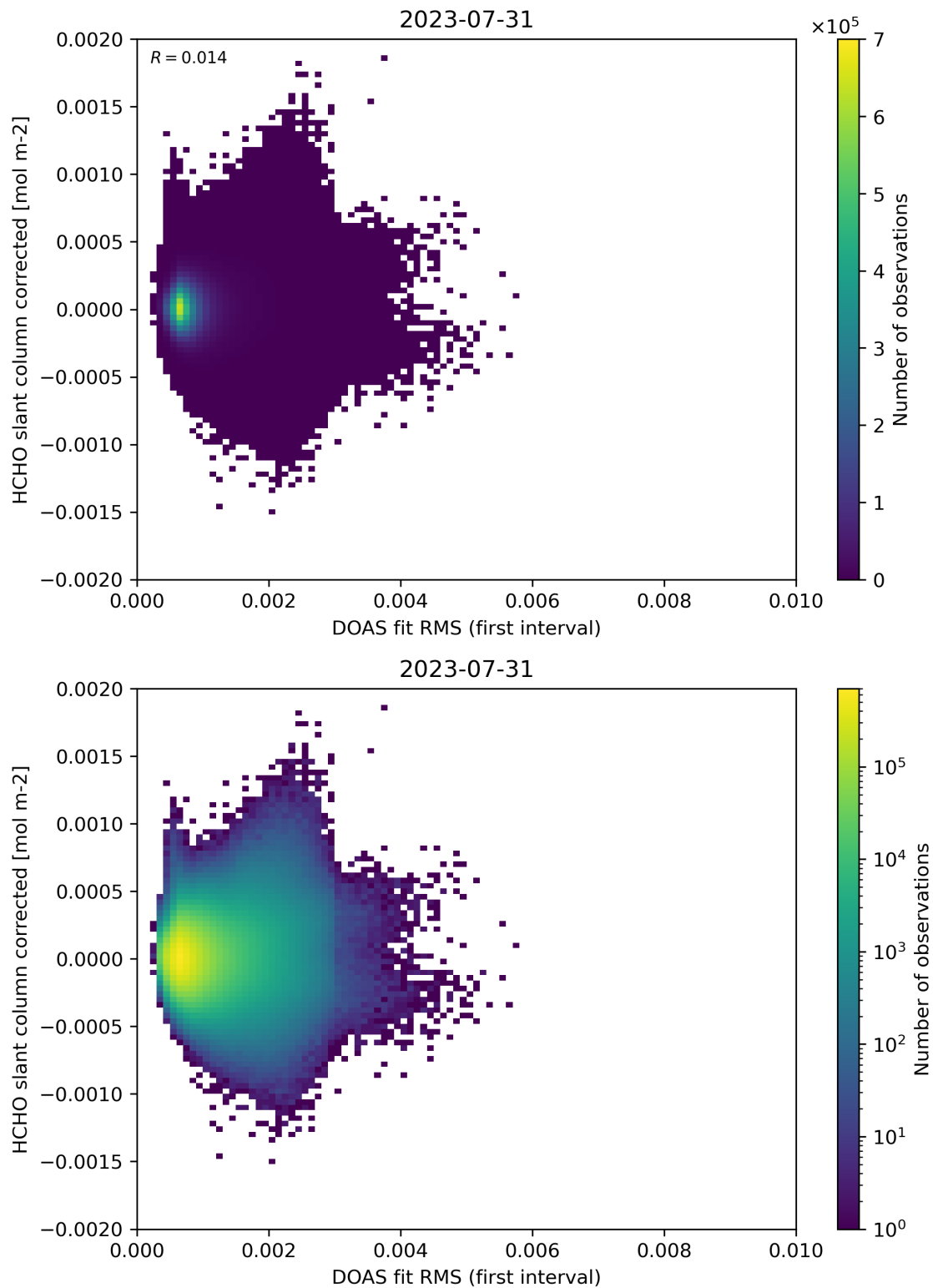
Figure 62: Scatter density plot of “DOAS fit RMS (first interval)” against “HCHO slant column corrected” for 2023-07-30 to 2023-08-01.
