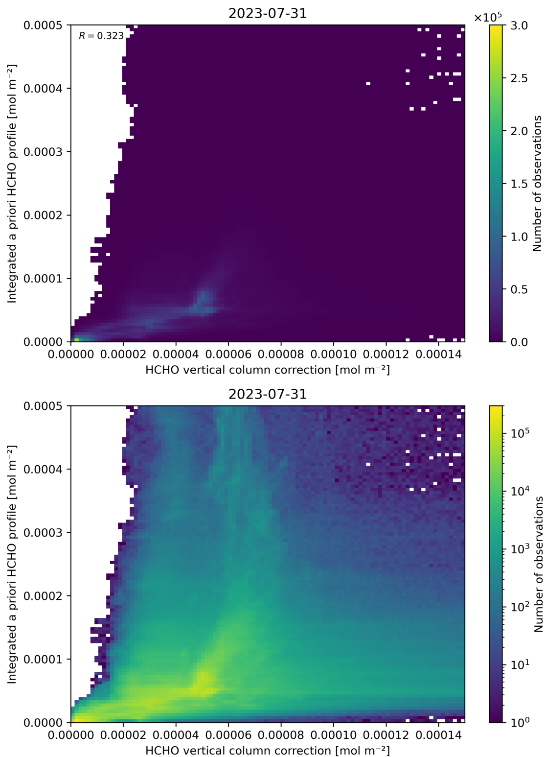
Figure 122: Scatter density plot of “HCHO vertical column correction” against “Integrated a priori HCHO profile” for 2023-07-30 to 2023-08-01.
