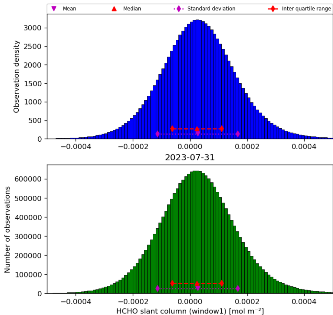
Figure 38: Histogram of “HCHO slant column (window1)” for 2023-07-30 to 2023-08-01
