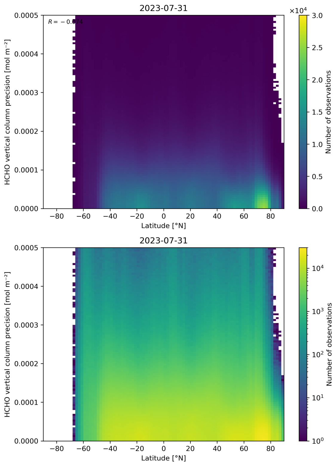
Figure 165: Scatter density plot of “Latitude” against “HCHO vertical column precision” for 2023-07-30 to 2023-08-01.
