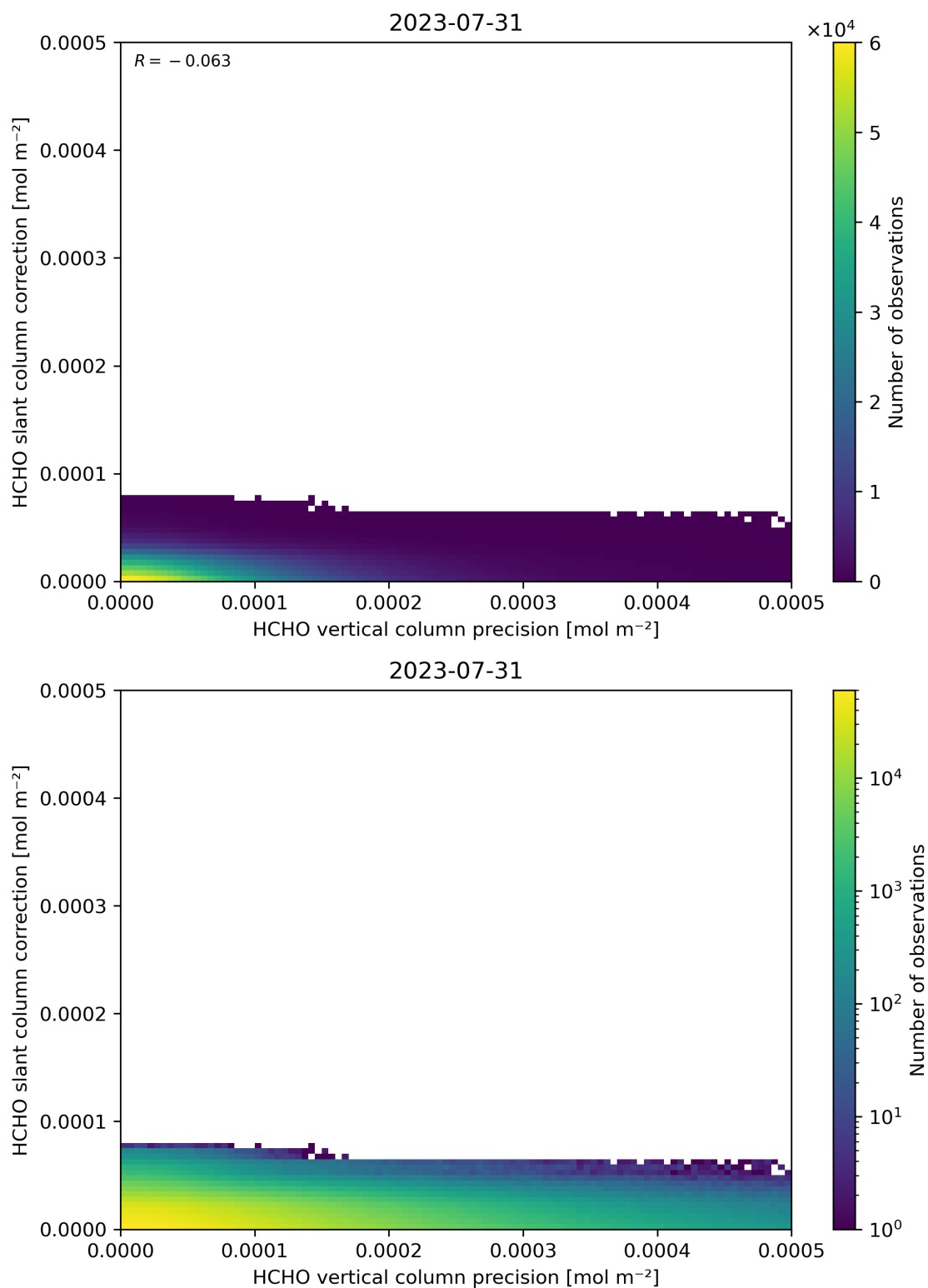
Figure 141: Scatter density plot of “HCHO vertical column precision” against “HCHO slant column correction” for 2023-07-30 to 2023-08-01.
