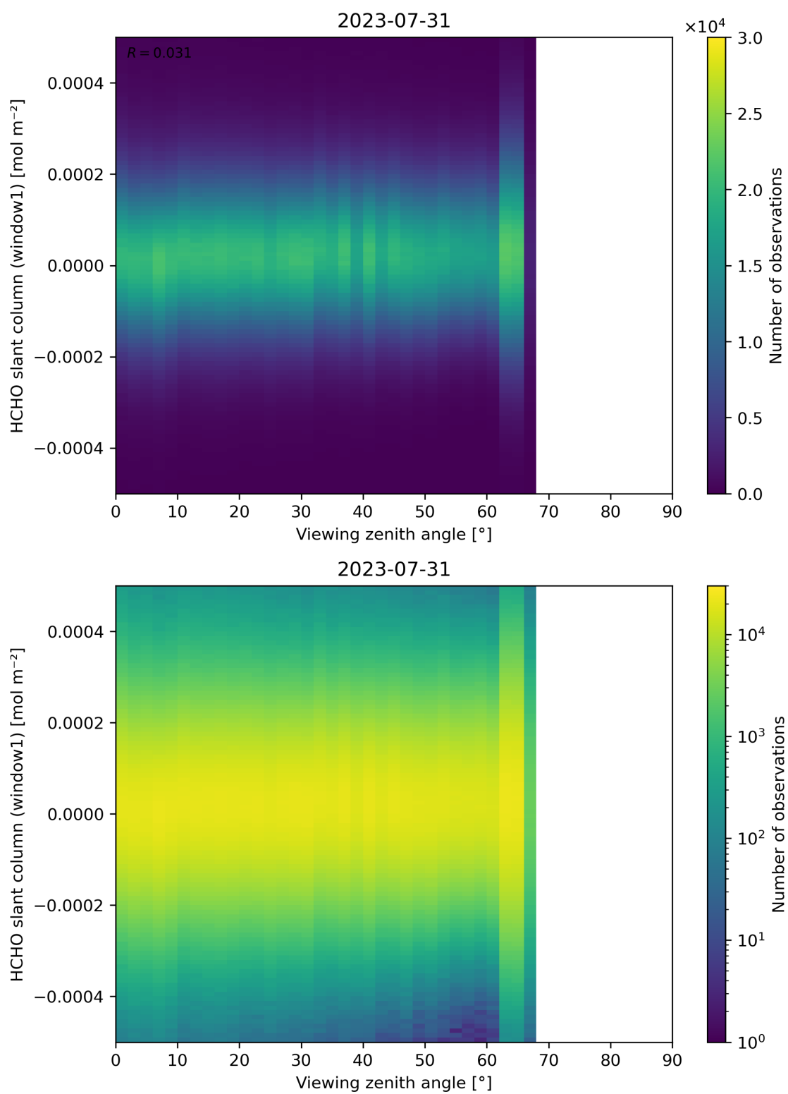
Figure 188: Scatter density plot of “Viewing zenith angle” against “HCHO slant column (window1)” for 2023-07-30 to 2023-08-01.
