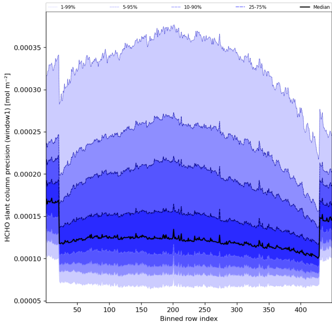
Figure 53: Along track statistics of “HCHO slant column precision (window1)” for 2023-07-30 to 2023-08-01
