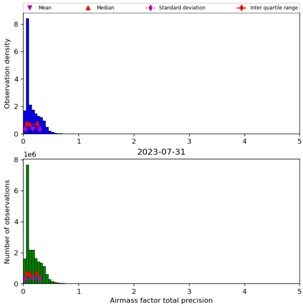
Figure 41: Histogram of “Airmass factor total precision” for 2023-07-30 to 2023-08-01
