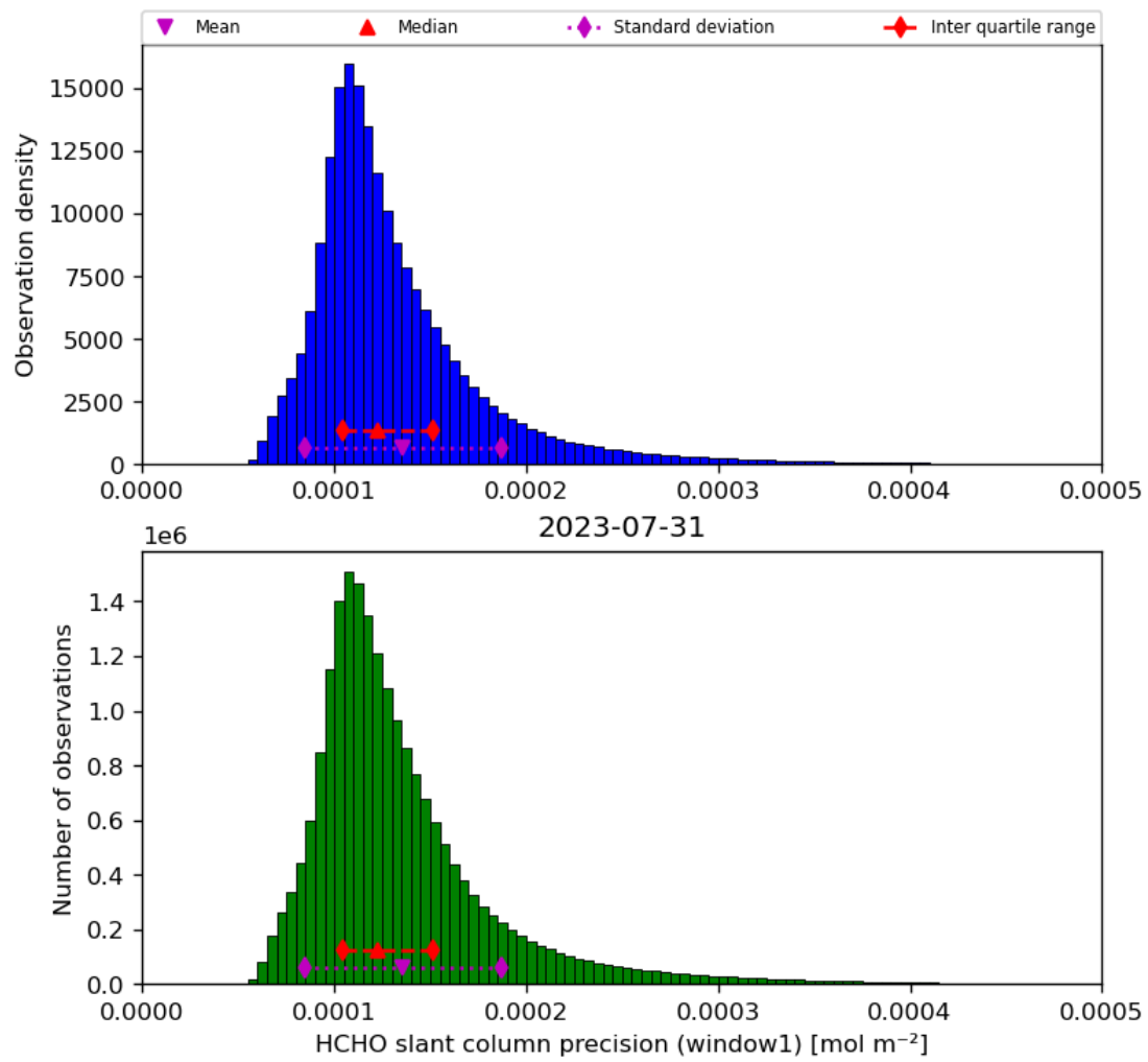
Figure 39: Histogram of “HCHO slant column precision (window1)” for 2023-07-30 to 2023-08-01
