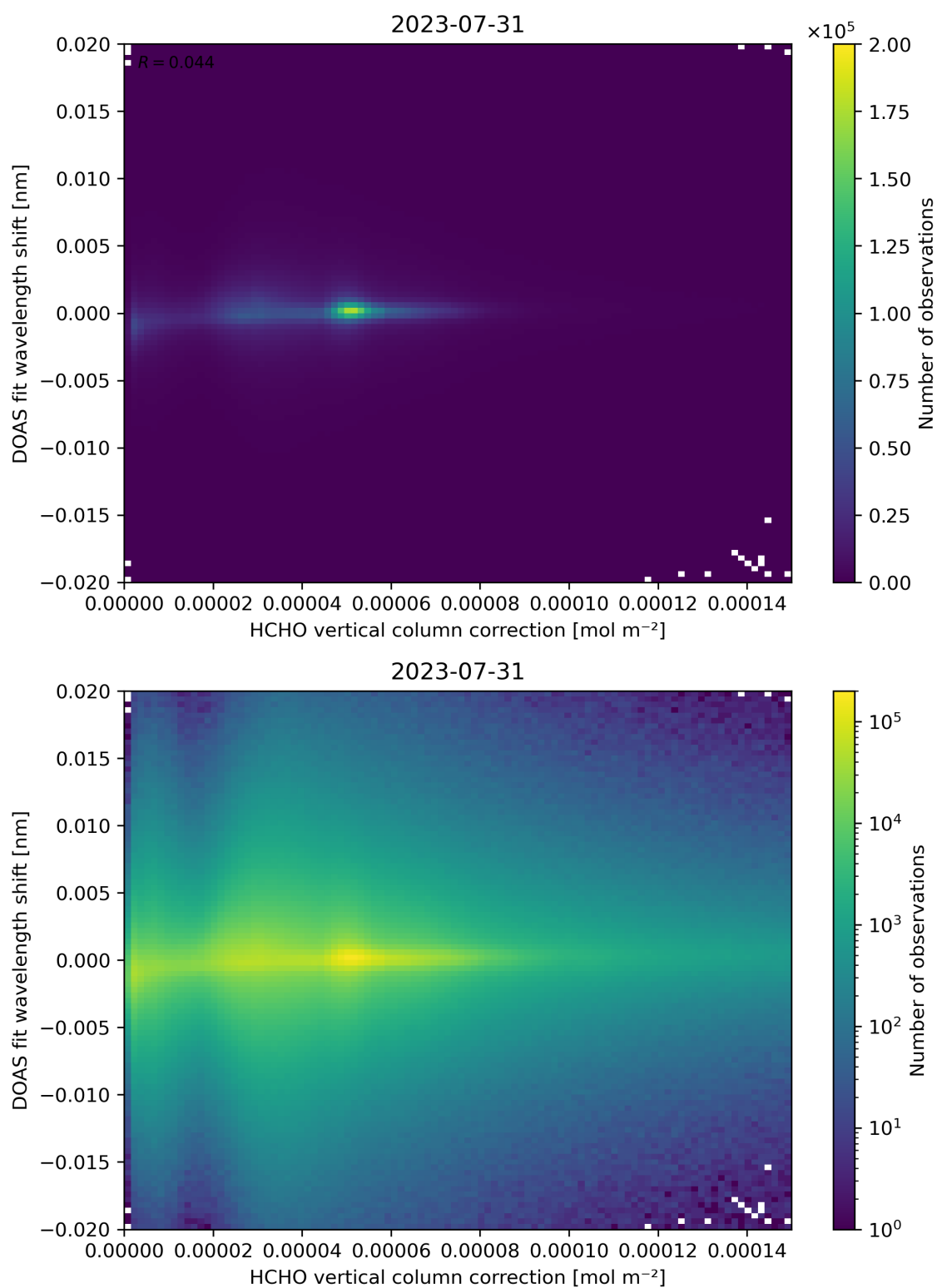
Figure 113: Scatter density plot of “HCHO vertical column correction” against “DOAS fit wavelength shift” for 2023-07-30 to 2023-08-01.
