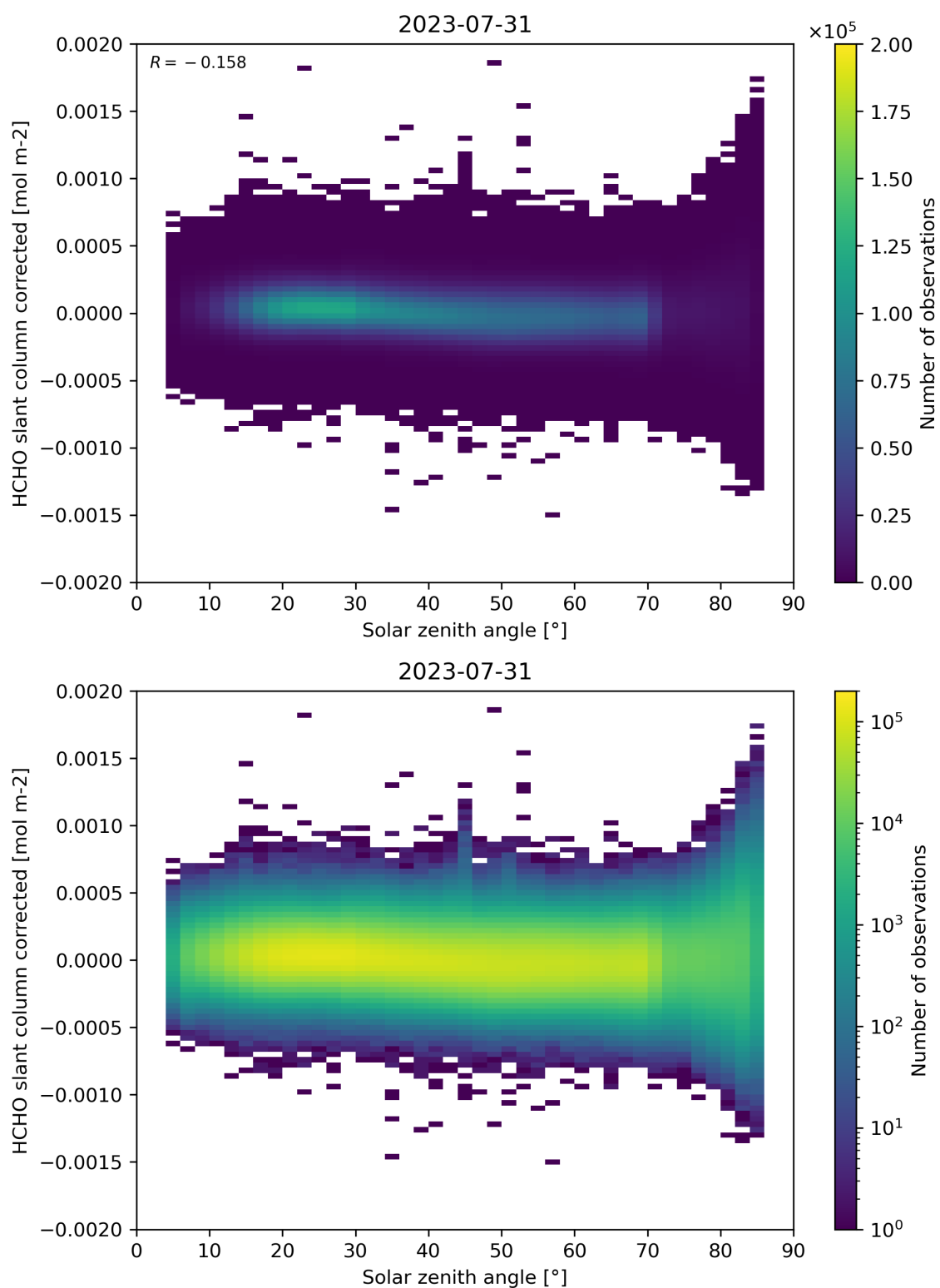
Figure 171: Scatter density plot of “Solar zenith angle” against “HCHO slant column corrected” for 2023-07-30 to 2023-08-01.
