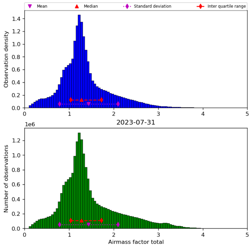
Figure 40: Histogram of “Airmass factor total” for 2023-07-30 to 2023-08-01
