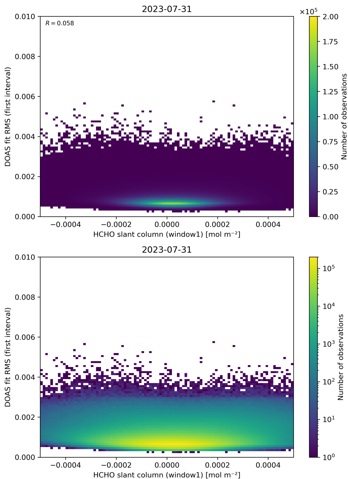
Figure 78: Scatter density plot of “HCHO slant column (window1)” against “DOAS fit RMS (first interval)” for 2023-07-30 to 2023-08-01.
