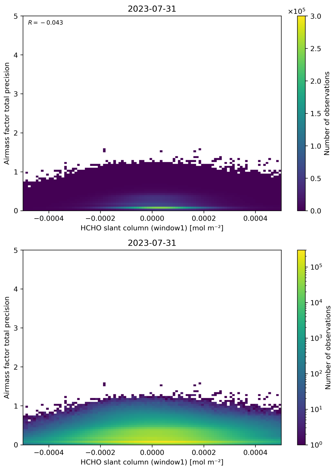
Figure 86: Scatter density plot of “HCHO slant column (window1)” against “Airmass factor total precision” for 2023-07-30 to 2023-08-01.
