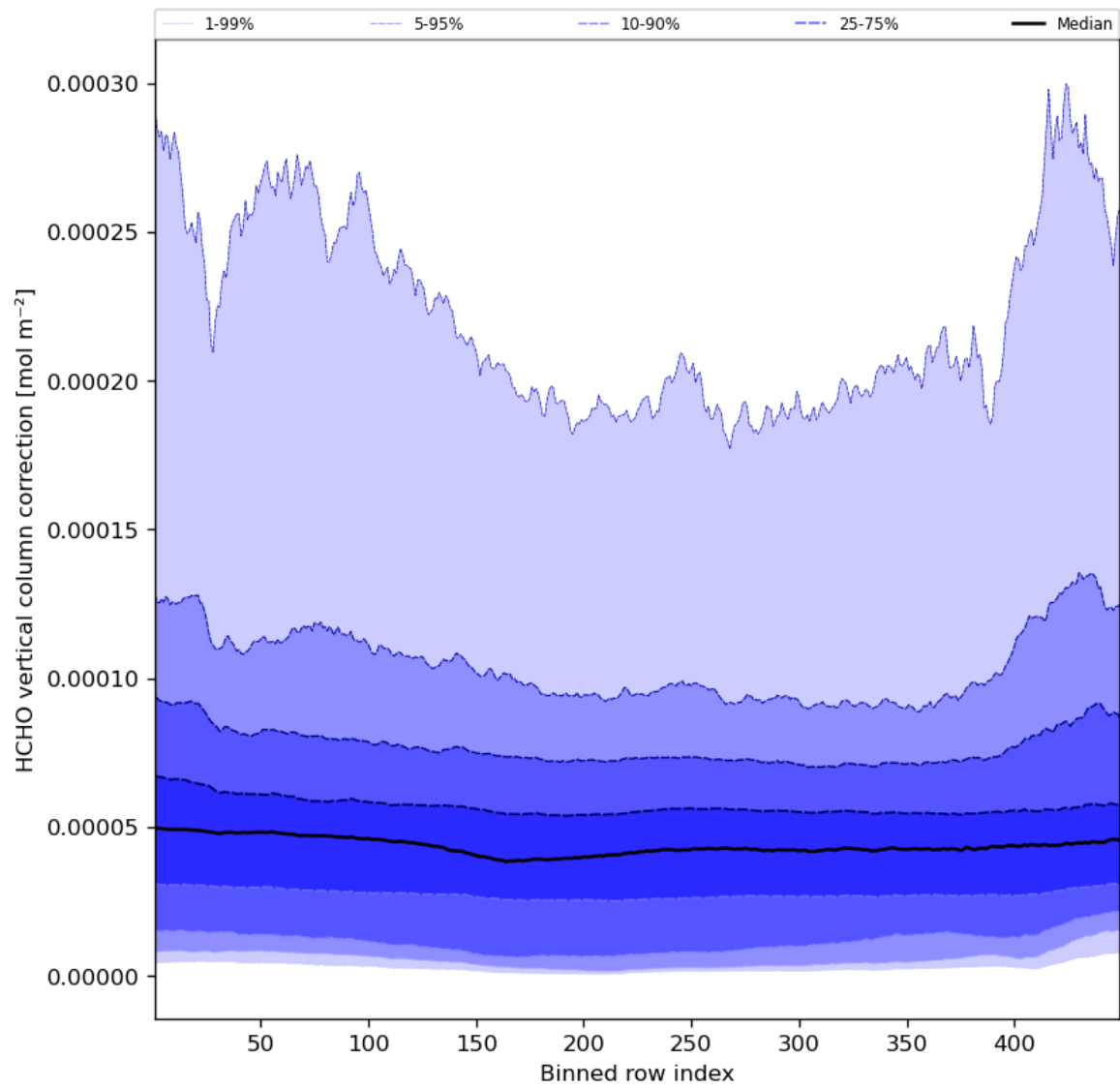
Figure 51: Along track statistics of “HCHO vertical column correction” for 2023-07-30 to 2023-08-01
