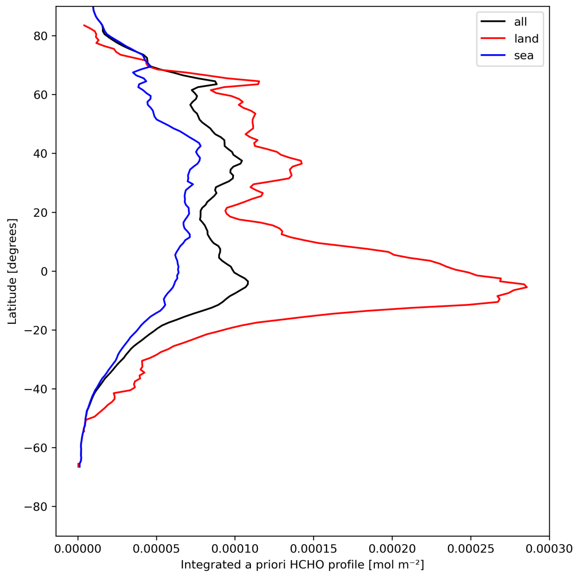
Figure 29: Zonal average of “Integrated a priori HCHO profile” for 2023-07-30 to 2023-08-01.
