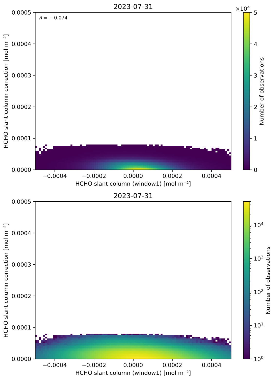
Figure 83: Scatter density plot of “HCHO slant column (window1)” against “HCHO slant column correction” for 2023-07-30 to 2023-08-01.
