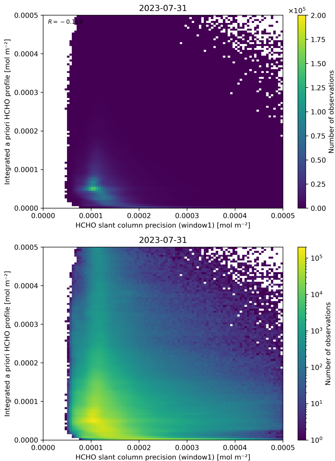
Figure 96: Scatter density plot of “HCHO slant column precision (window1)” against “Integrated a priori HCHO profile” for 2023-07-30 to 2023-08-01.
