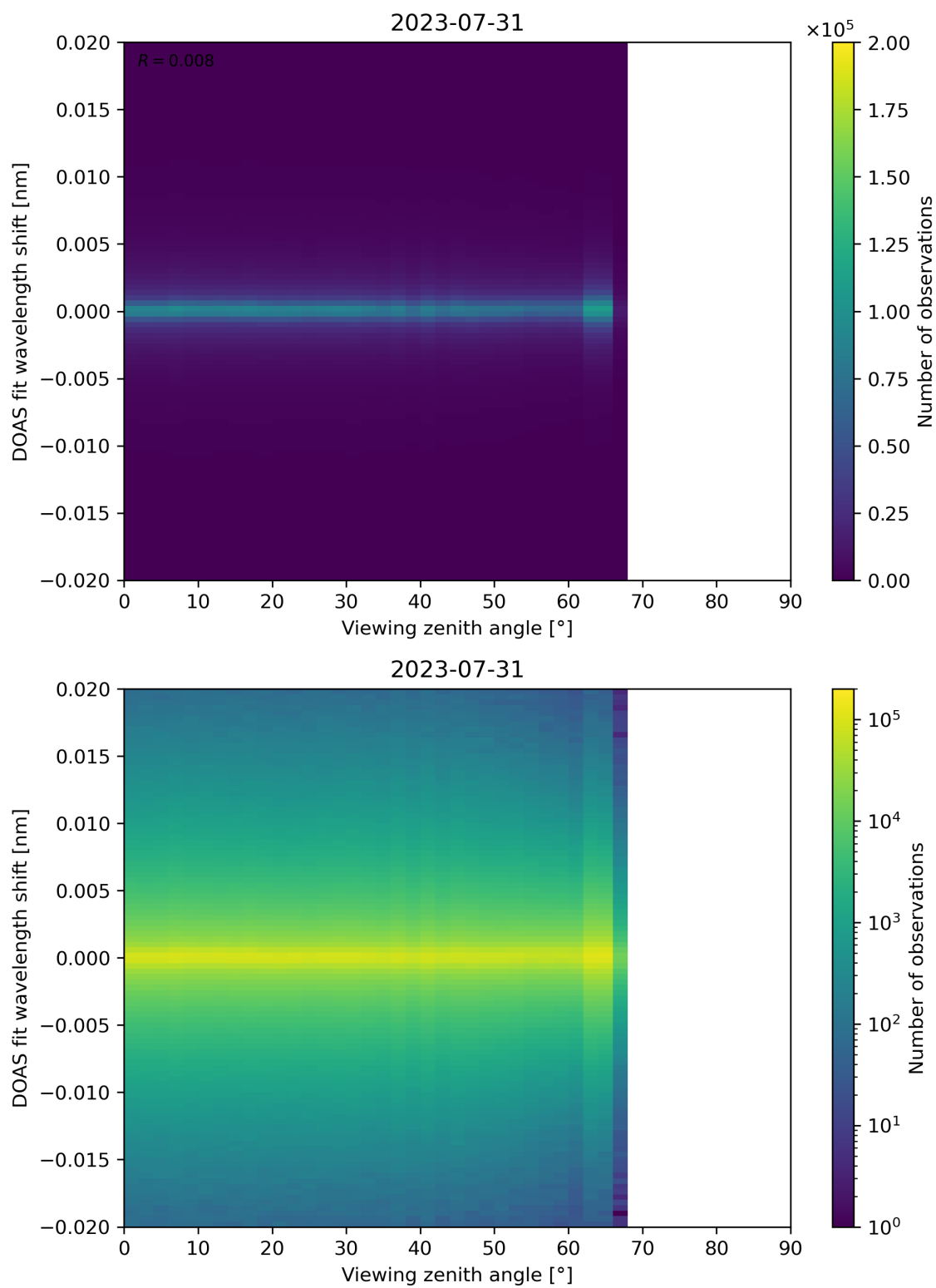
Figure 183: Scatter density plot of “Viewing zenith angle” against “DOAS fit wavelength shift” for 2023-07-30 to 2023-08-01.
