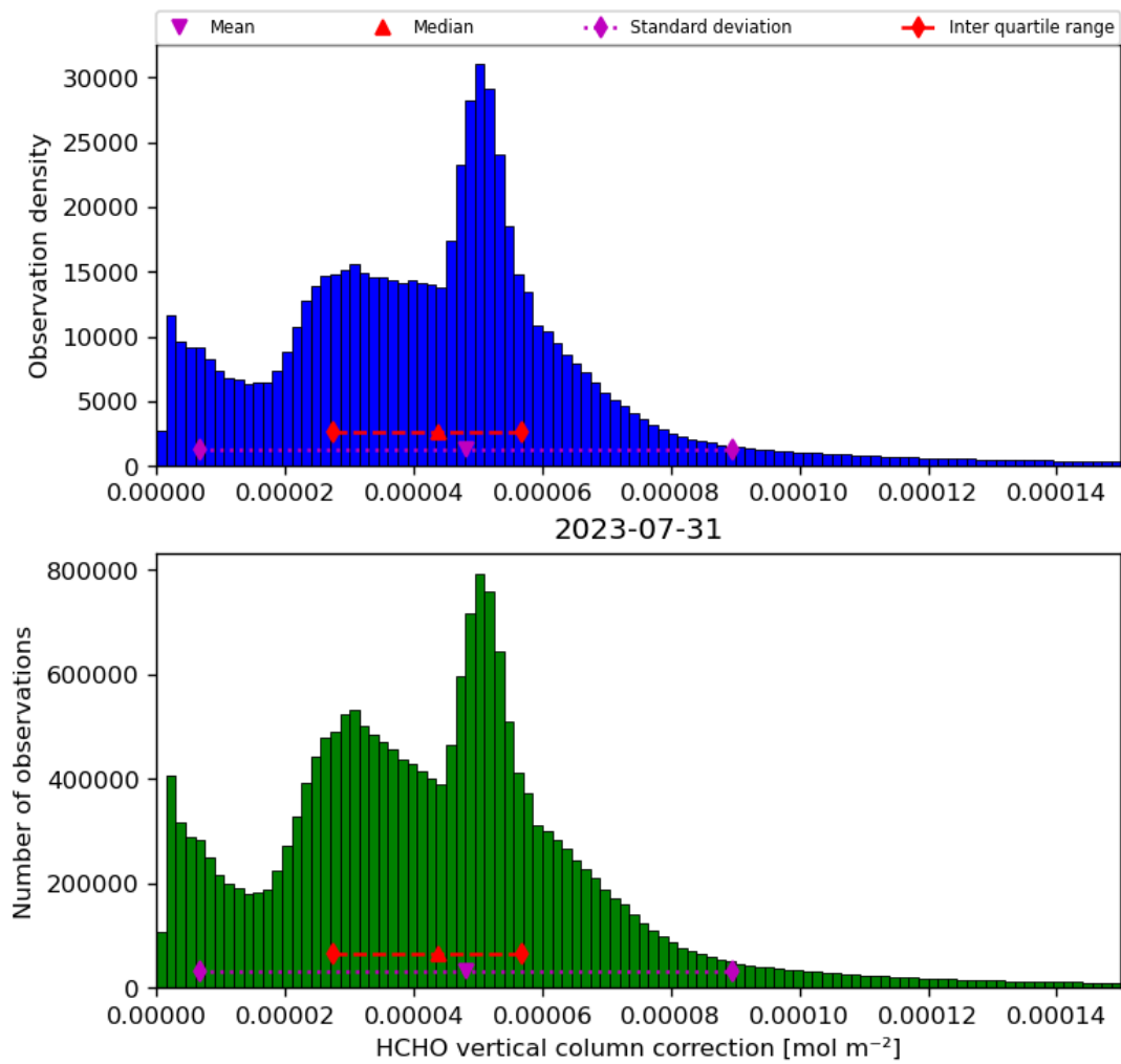
Figure 37: Histogram of “HCHO vertical column correction” for 2023-07-30 to 2023-08-01
