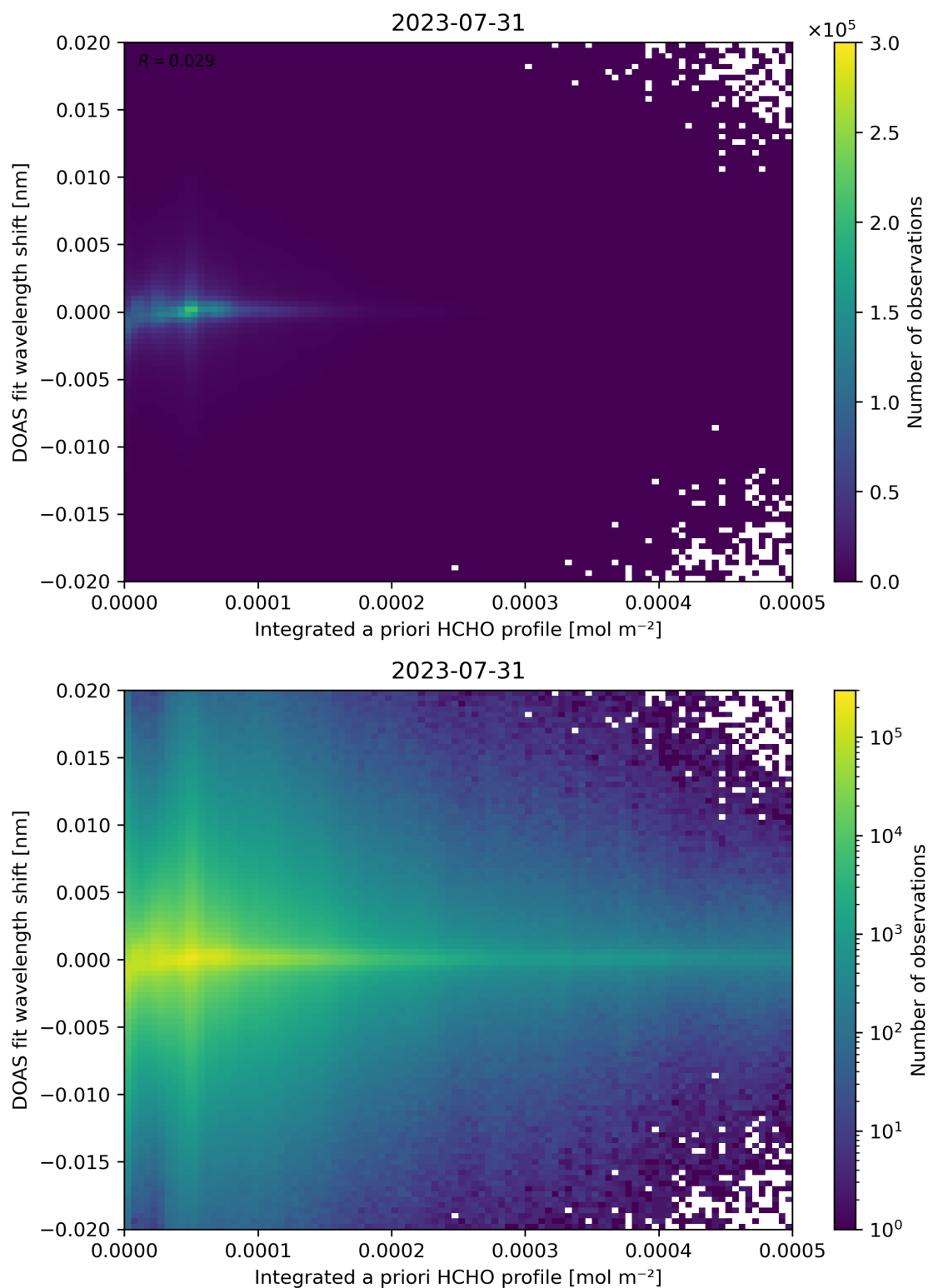
Figure 149: Scatter density plot of “Integrated a priori HCHO profile” against “DOAS fit wavelength shift” for 2023-07-30 to 2023-08-01.
