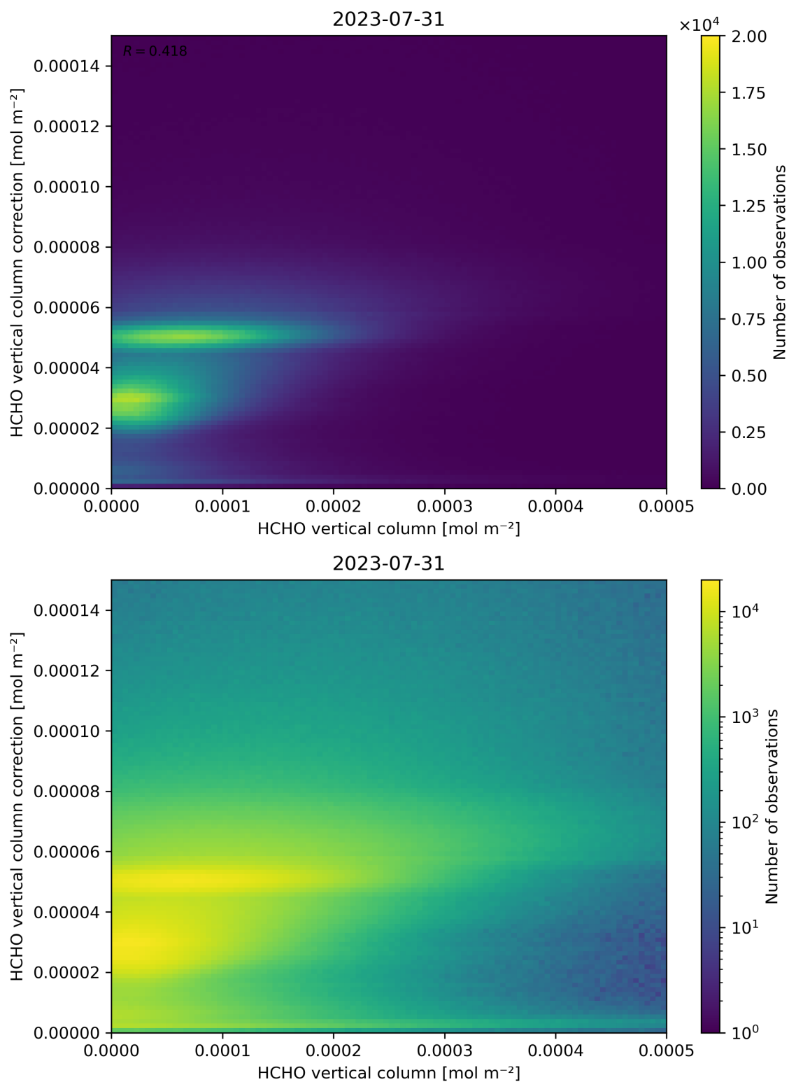
Figure 133: Scatter density plot of “HCHO vertical column” against “HCHO vertical column correction” for 2023-07-30 to 2023-08-01.
