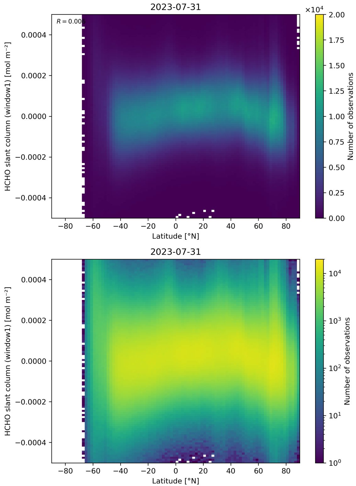
Figure 159: Scatter density plot of “Latitude” against “HCHO slant column (window1)” for 2023-07-30 to 2023-08-01.
