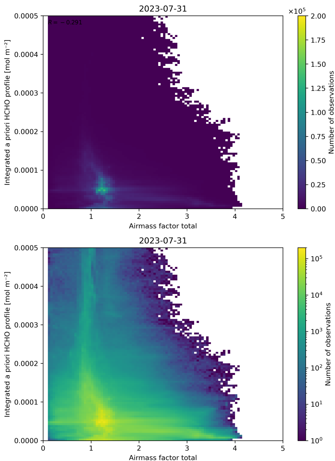
Figure 104: Scatter density plot of “Air mass factor total” against “Integrated a priori HCHO profile” for 2023-07-30 to 2023-08-01.
