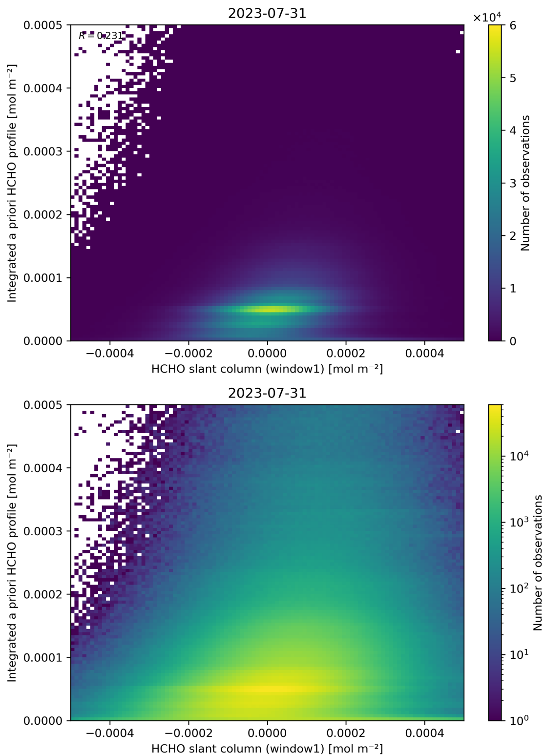
Figure 87: Scatter density plot of “HCHO slant column (window1)” against “Integrated a priori HCHO profile” for 2023-07-30 to 2023-08-01.
