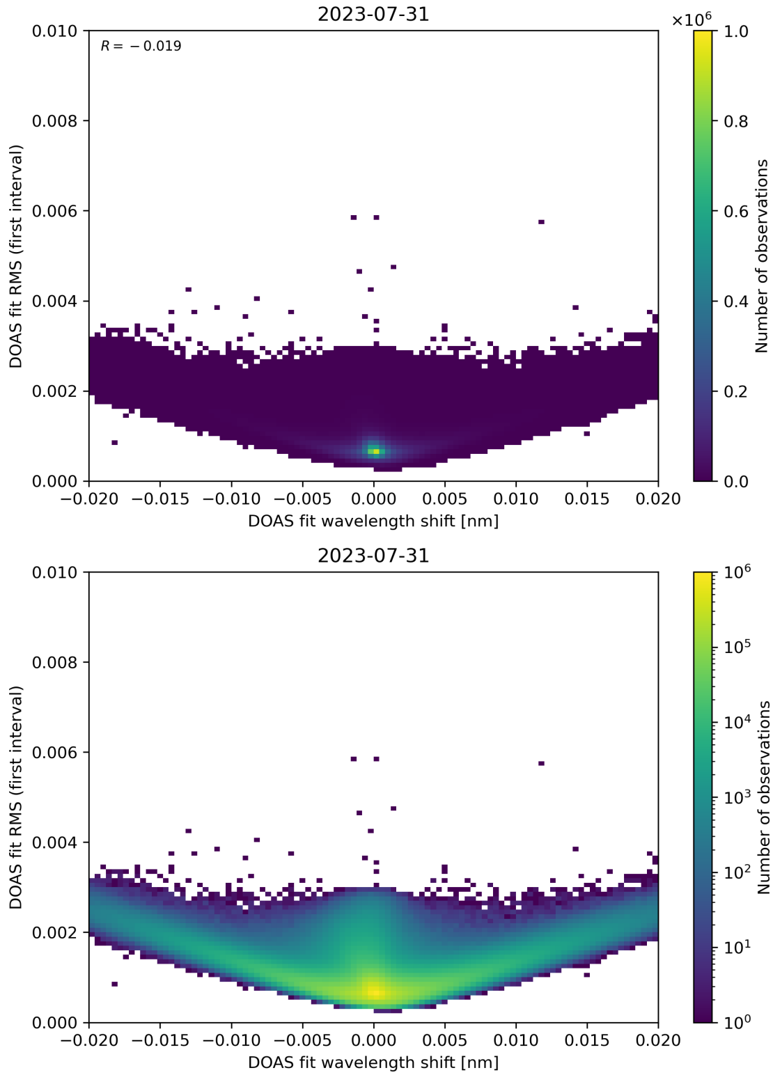
Figure 64: Scatter density plot of “DOAS fit wavelength shift” against “DOAS fit RMS (first interval)” for 2023-07-30 to 2023-08-01.
