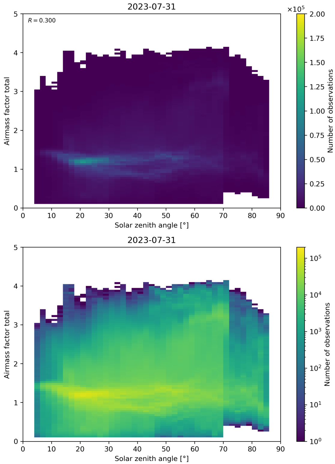
Figure 175: Scatter density plot of “Solar zenith angle” against “Airmass factor total” for 2023-07-30 to 2023-08-01.
