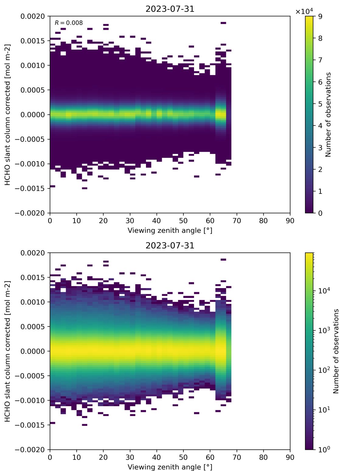
Figure 186: Scatter density plot of “Viewing zenith angle” against “HCHO slant column corrected” for 2023-07-30 to 2023-08-01.
