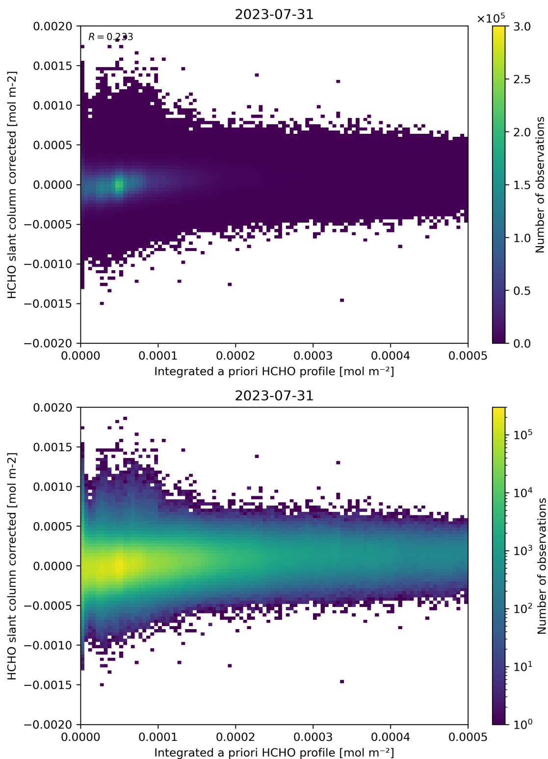
Figure 151: Scatter density plot of “Integrated a priori HCHO profile” against “HCHO slant column corrected” for 2023-07-30 to 2023-08-01.
