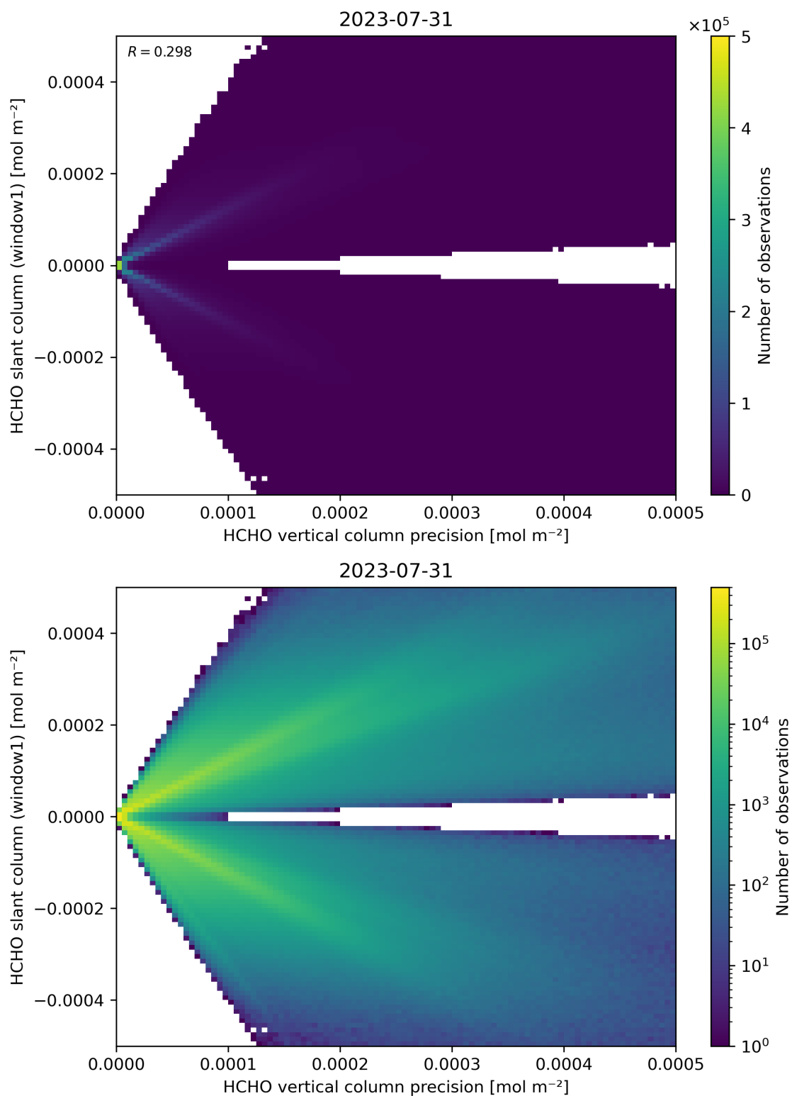
Figure 142: Scatter density plot of “HCHO vertical column precision” against “HCHO slant column (window1)” for 2023-07-30 to 2023-08-01.
