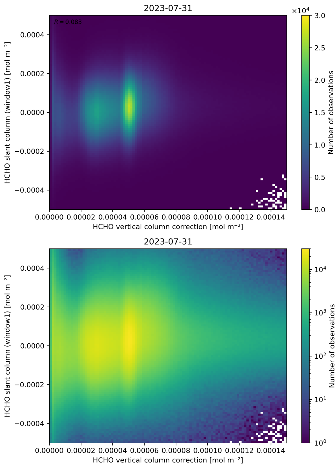
Figure 118: Scatter density plot of “HCHO vertical column correction” against “HCHO slant column (window1)” for 2023-07-30 to 2023-08-01.
