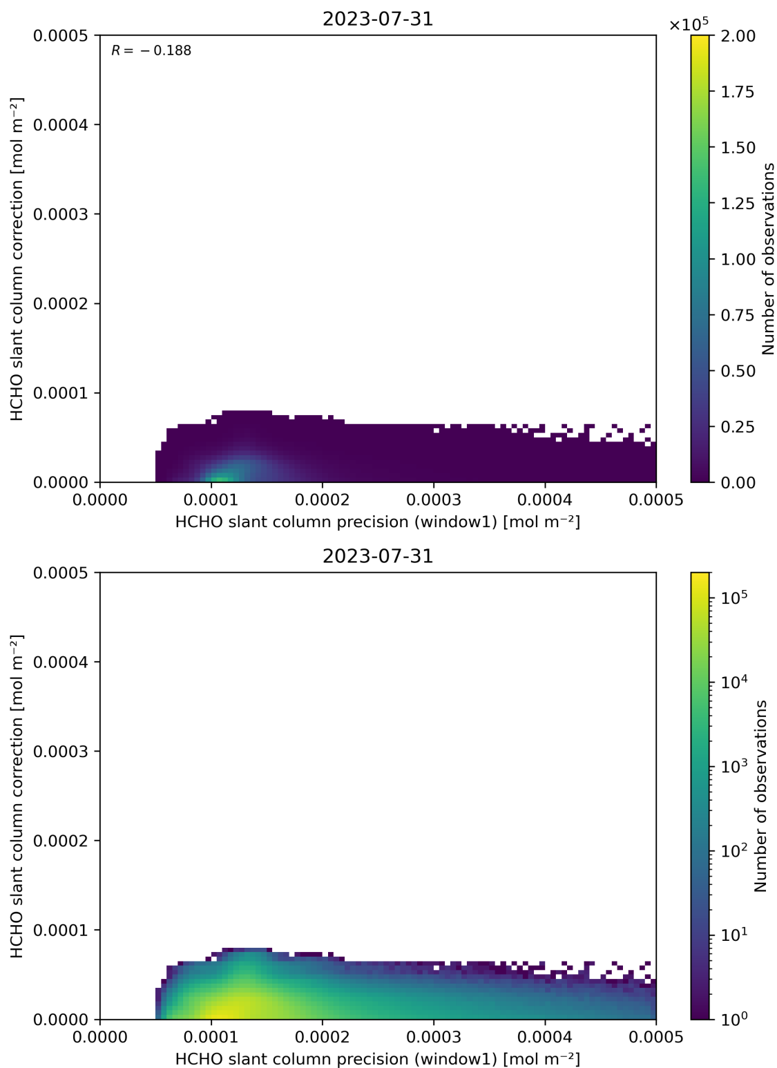
Figure 93: Scatter density plot of “HCHO slant column precision (window1)” against “HCHO slant column correction” for 2023-07-30 to 2023-08-01.
