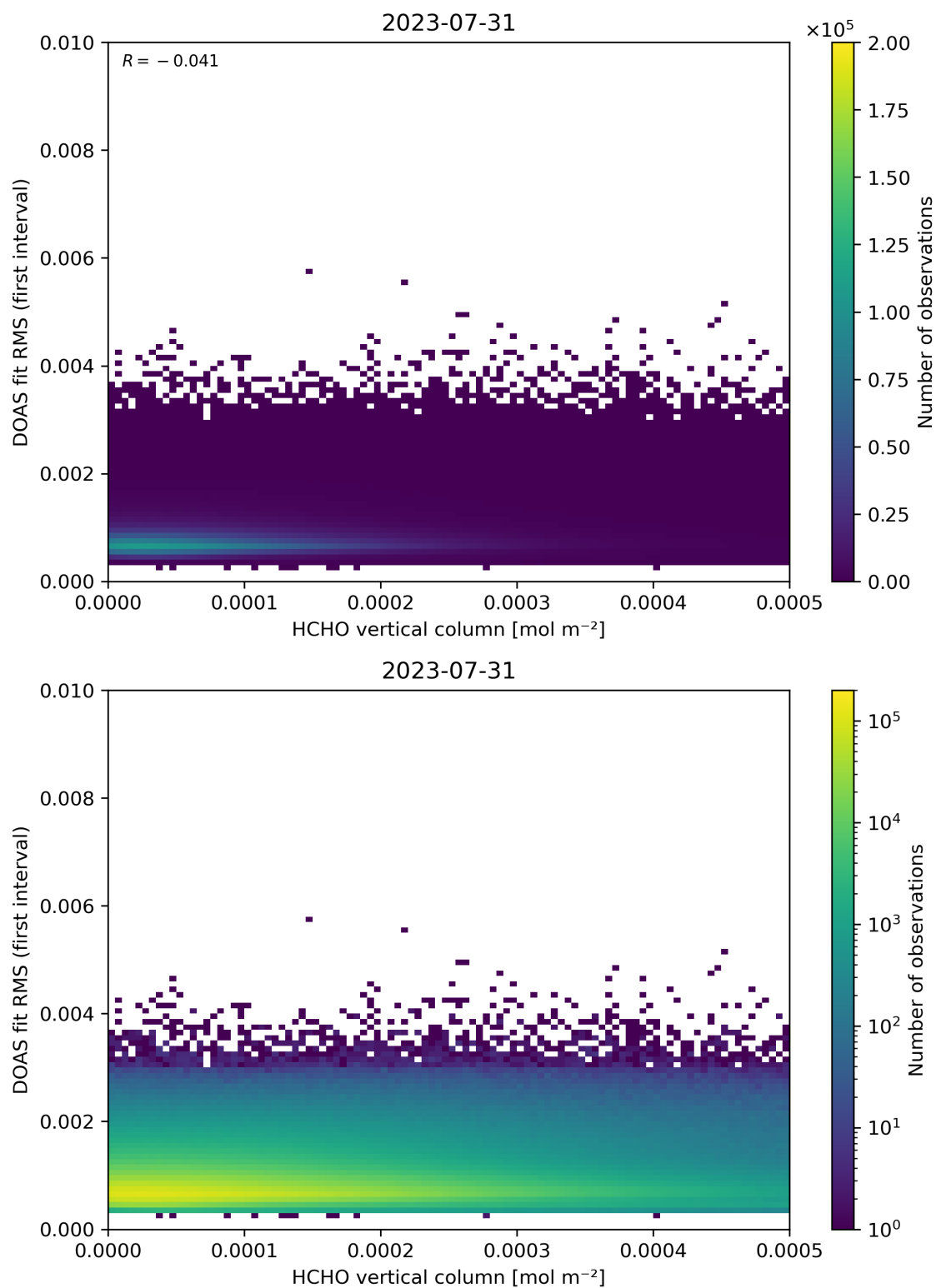
Figure 123: Scatter density plot of “HCHO vertical column” against “DOAS fit RMS (first interval)” for 2023-07-30 to 2023-08-01.
