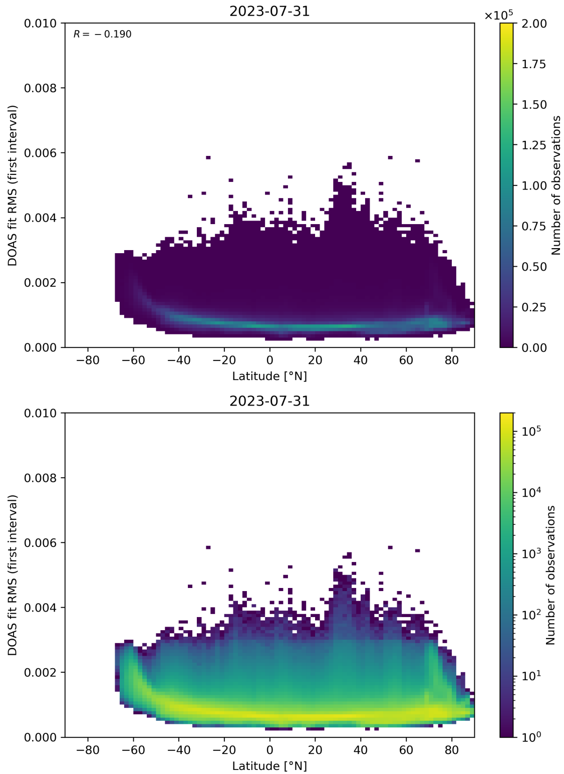
Figure 153: Scatter density plot of “Latitude” against “DOAS fit RMS (first interval)” for 2023-07-30 to 2023-08-01.
