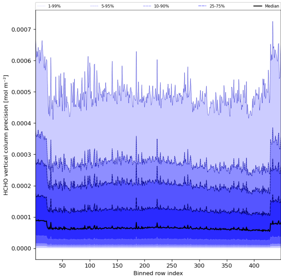
Figure 50: Along track statistics of “HCHO vertical column precision” for 2023-07-30 to 2023-08-01
