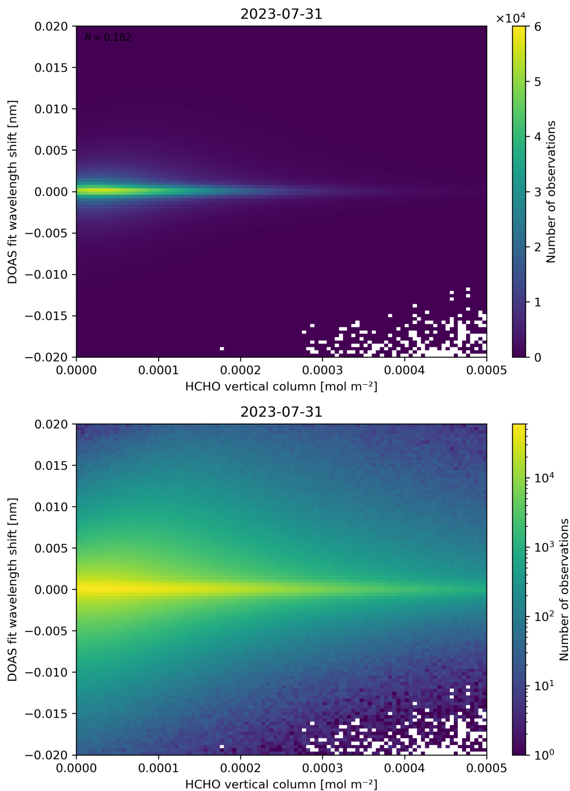
Figure 124: Scatter density plot of “HCHO vertical column” against “DOAS fit wavelength shift” for 2023-07-30 to 2023-08-01.
