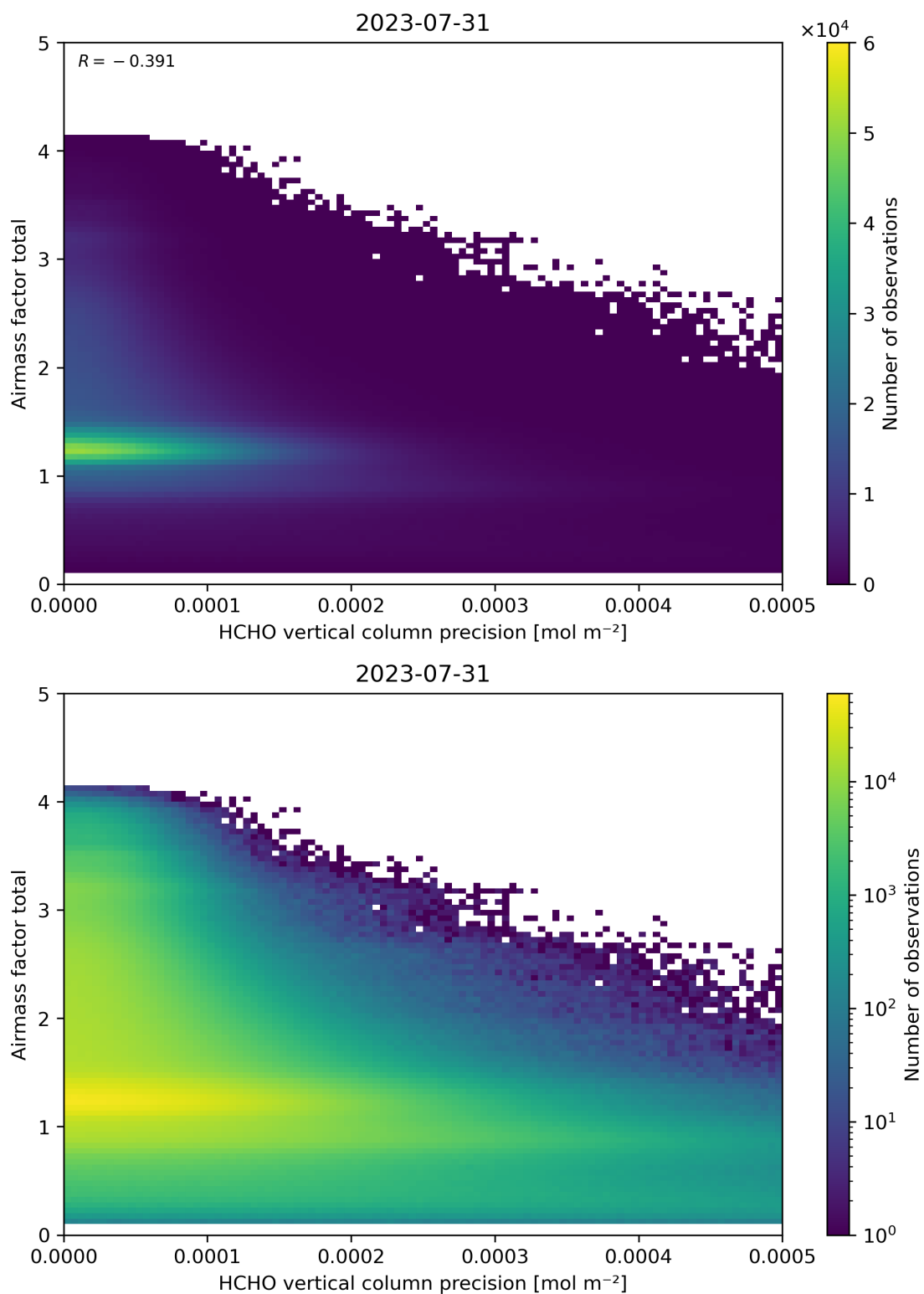
Figure 144: Scatter density plot of “HCHO vertical column precision” against “Airmass factor total” for 2023-07-30 to 2023-08-01.
