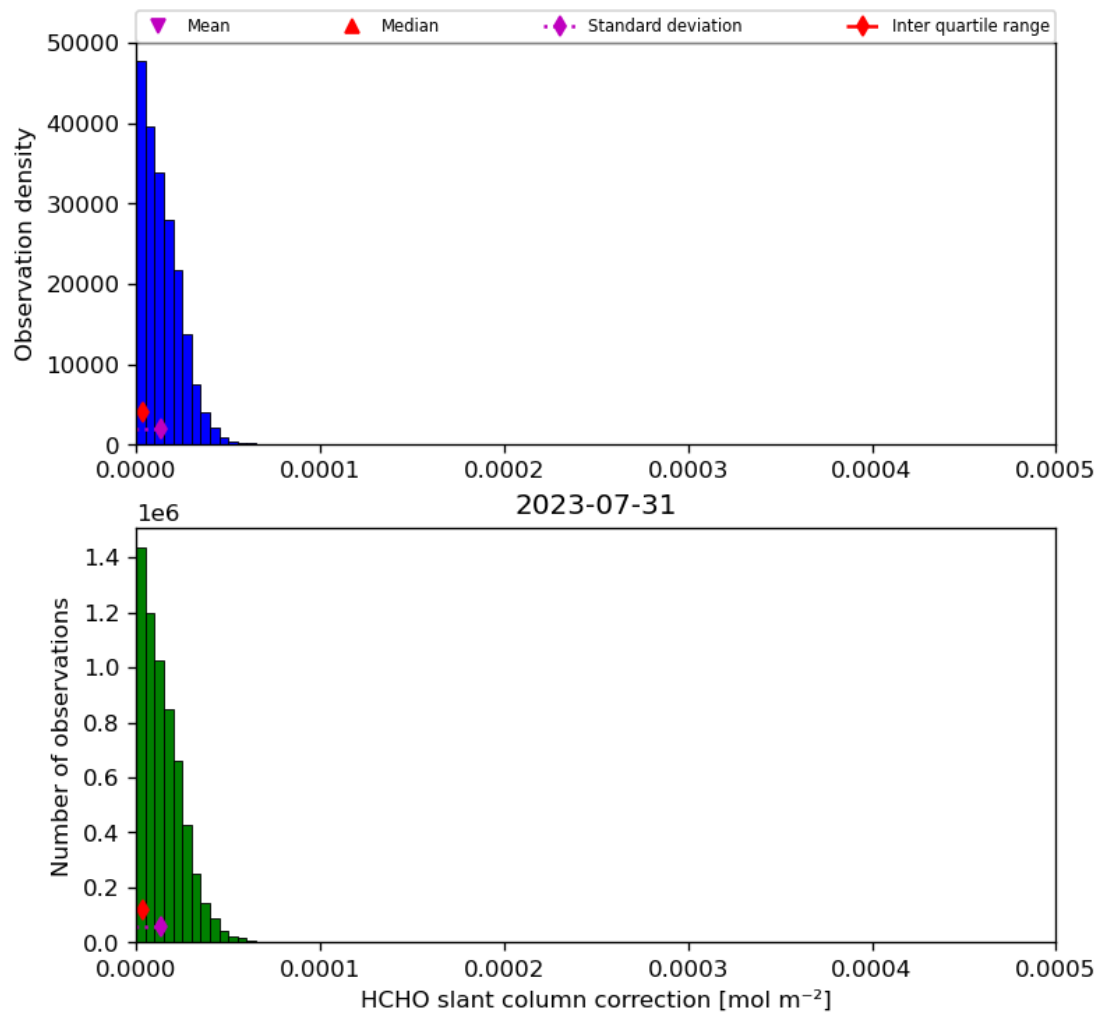
Figure 47: Histogram of “HCHO slant column correction” for 2023-07-30 to 2023-08-01
