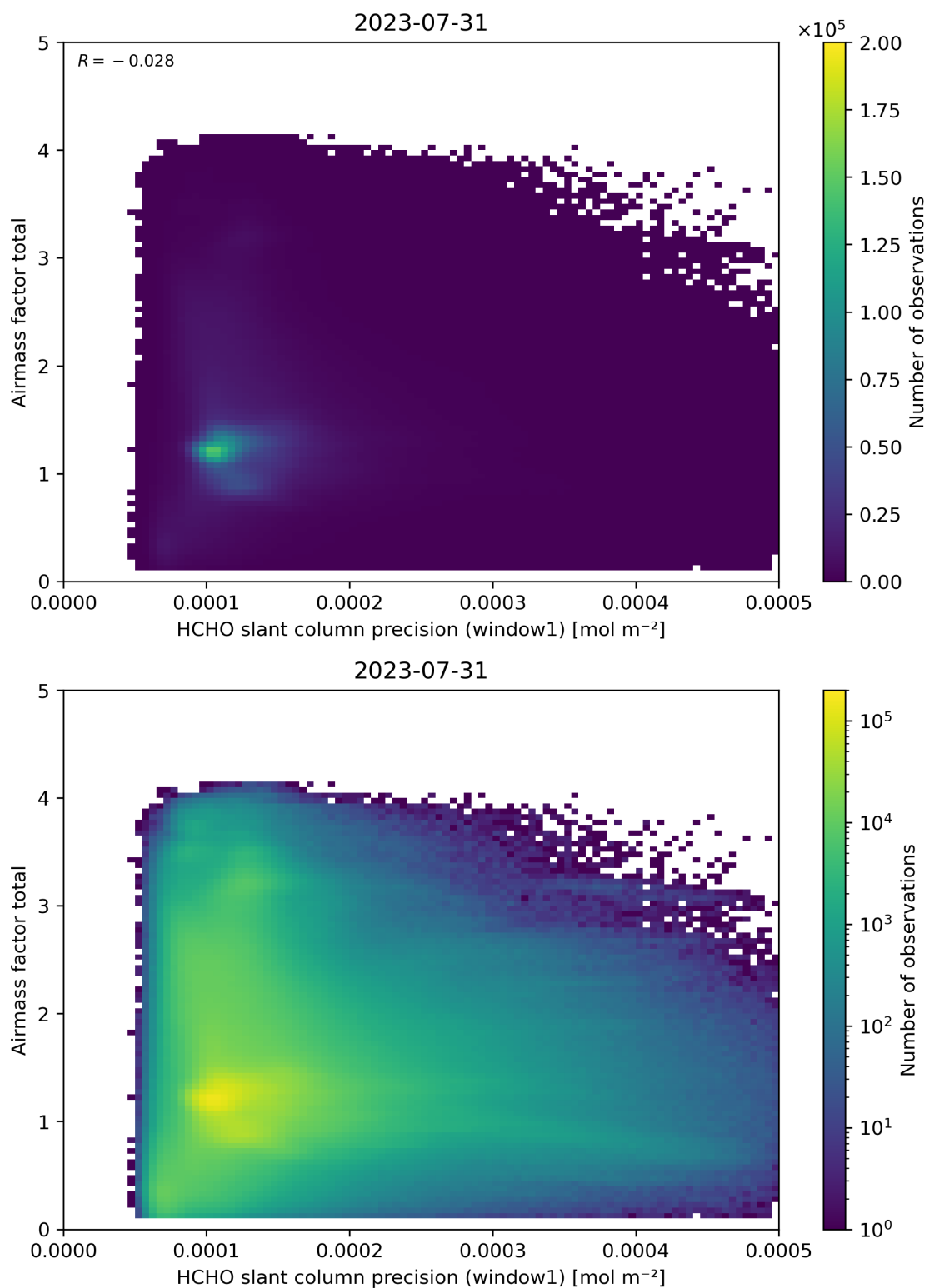
Figure 94: Scatter density plot of “HCHO slant column precision (window1)” against “Airmass factor total” for 2023-07-30 to 2023-08-01.
