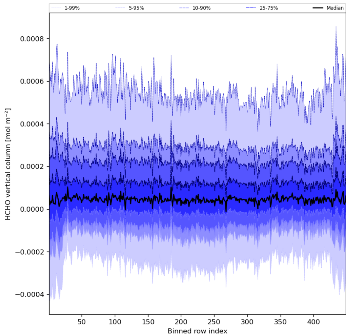
Figure 49: Along track statistics of “HCHO vertical column” for 2023-07-30 to 2023-08-01
