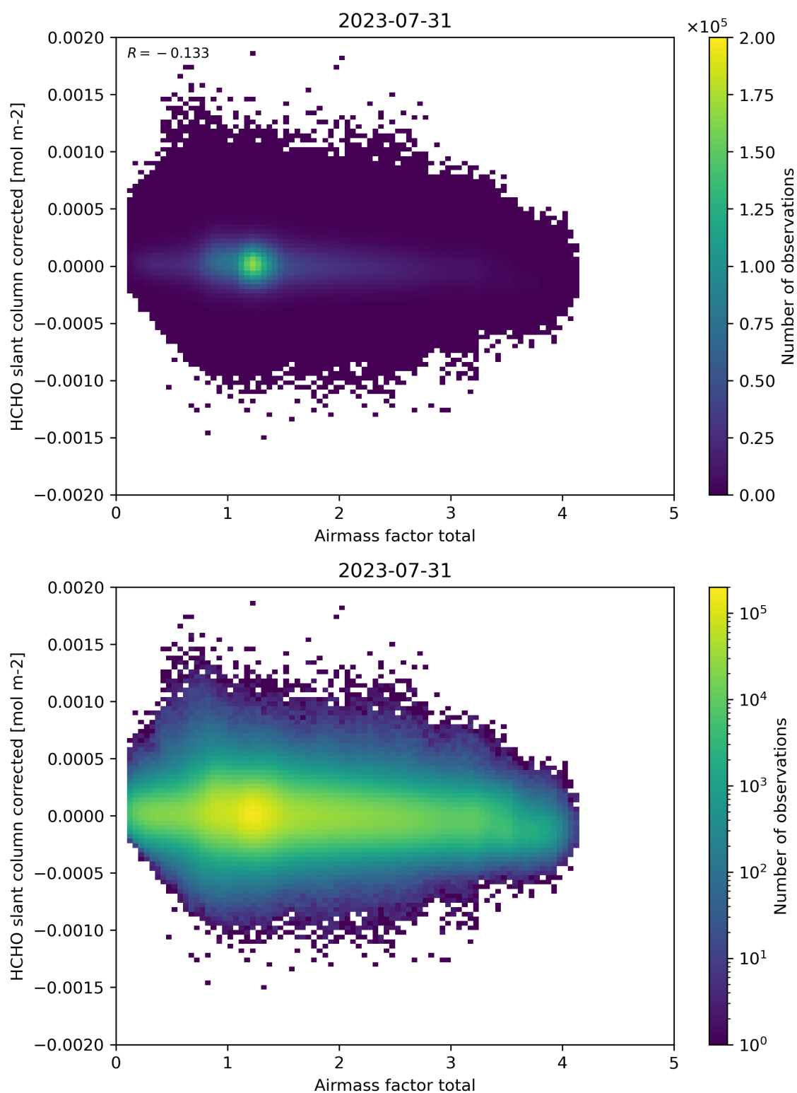
Figure 101: Scatter density plot of “Airmass factor total” against “HCHO slant column corrected” for 2023-07-30 to 2023-08-01.
