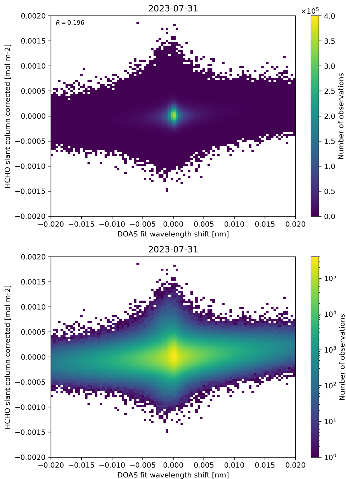
Figure 66: Scatter density plot of “DOAS fit wavelength shift” against “HCHO slant column corrected” for 2023-07-30 to 2023-08-01.
