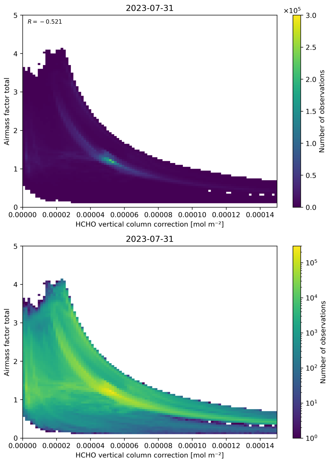
Figure 120: Scatter density plot of “HCHO vertical column correction” against “Airmass factor total” for 2023-07-30 to 2023-08-01.
