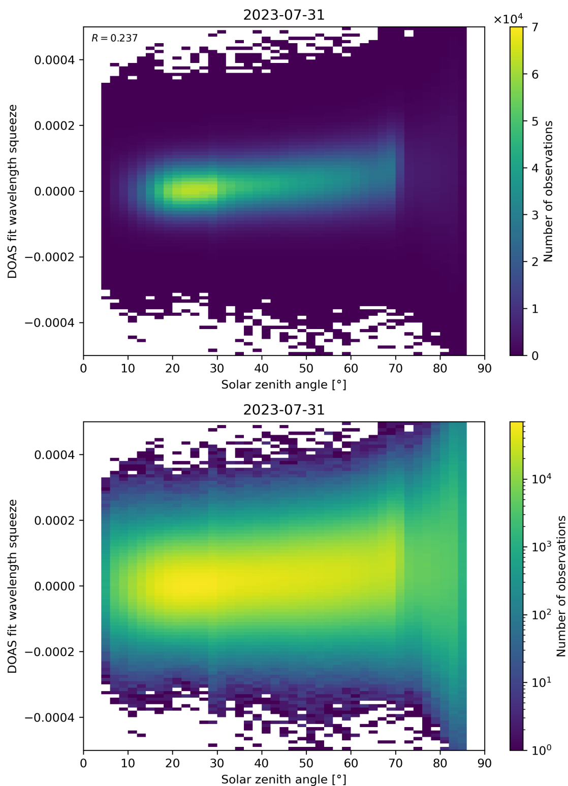
Figure 169: Scatter density plot of “Solar zenith angle” against “DOAS fit wavelength squeeze” for 2023-07-30 to 2023-08-01.
