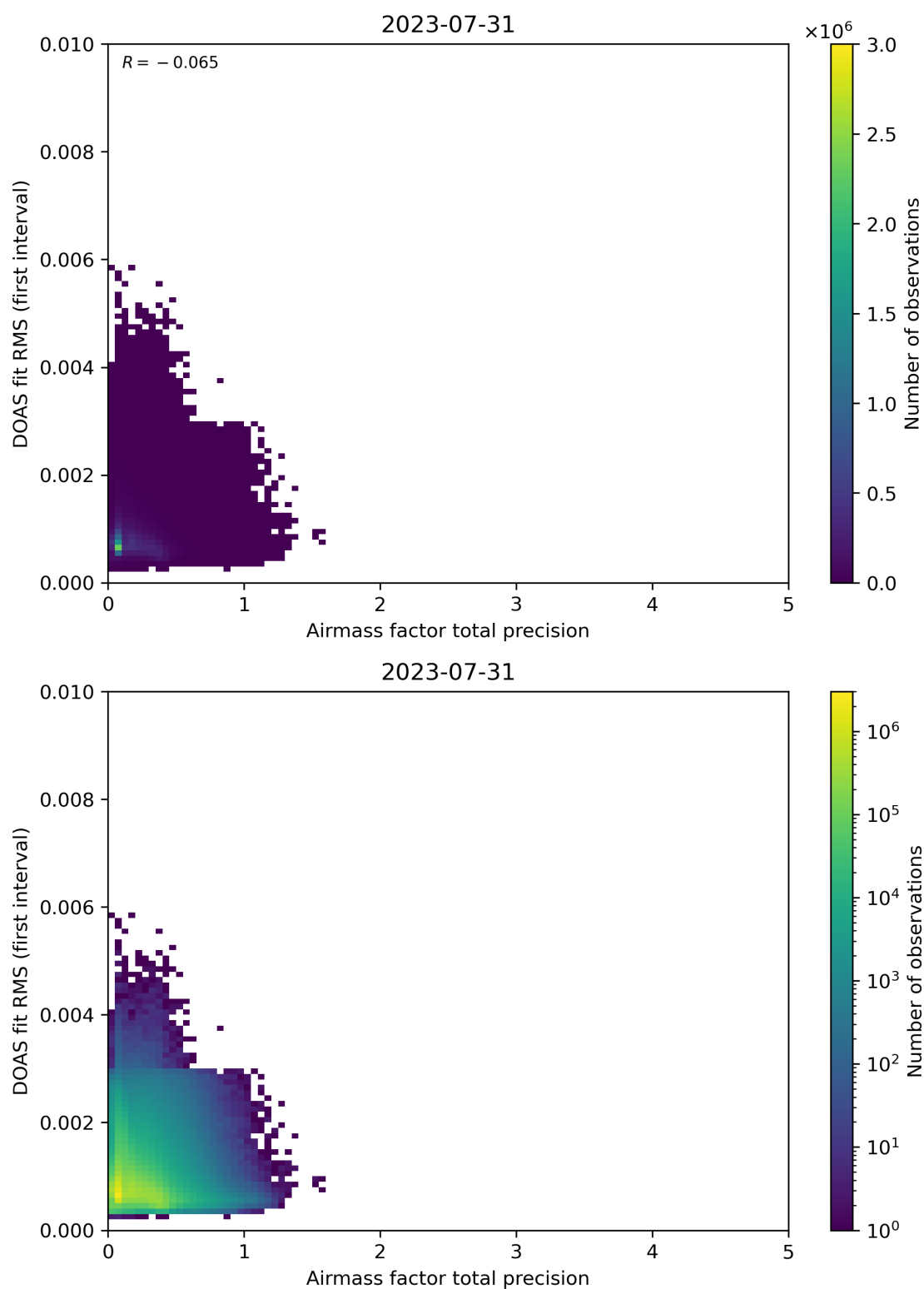
Figure 105: Scatter density plot of “Airmass factor total precision” against “DOAS fit RMS (first interval)” for 2023-07-30 to 2023-08-01.
