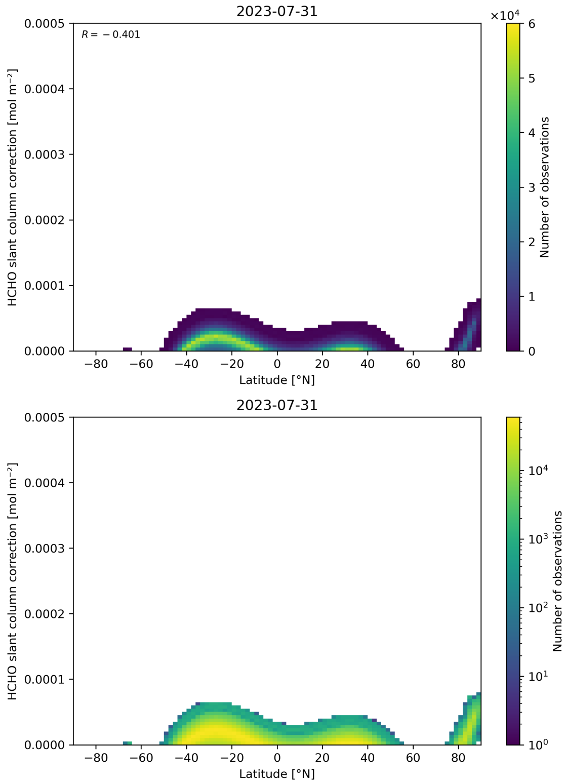
Figure 158: Scatter density plot of “Latitude” against “HCHO slant column correction” for 2023-07-30 to 2023-08-01.
