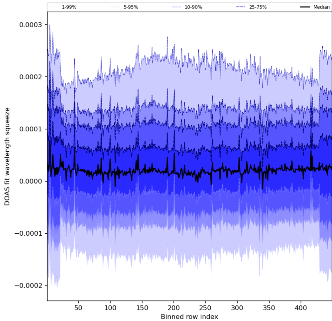
Figure 59: Along track statistics of “DOAS fit wavelength squeeze” for 2023-07-30 to 2023-08-01
