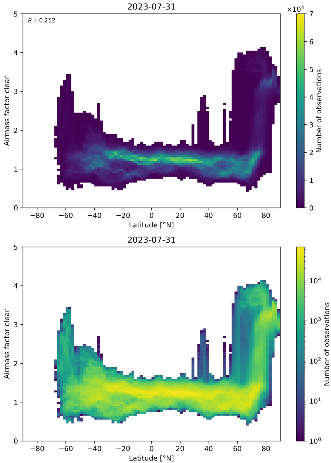
Figure 156: Scatter density plot of “Latitude” against “Airmass factor clear” for 2023-07-30 to 2023-08-01.
