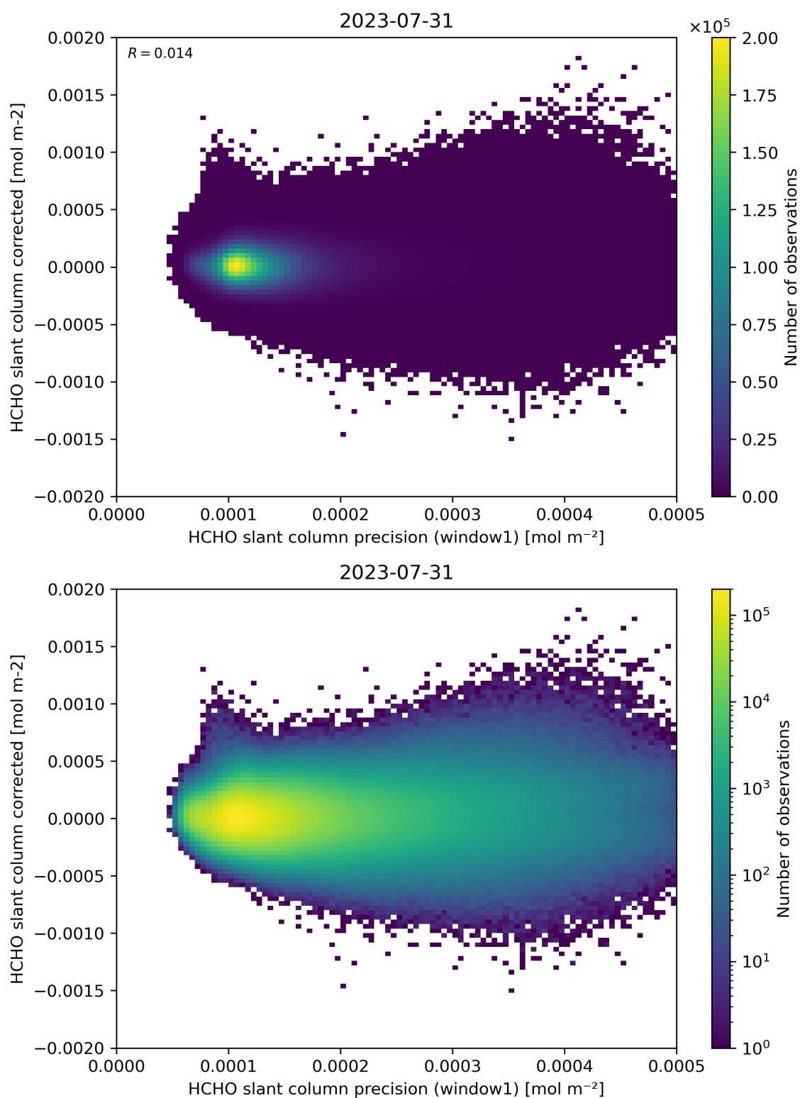
Figure 92: Scatter density plot of “HCHO slant column precision (window1)” against “HCHO slant column corrected” for 2023-07-30 to 2023-08-01.
