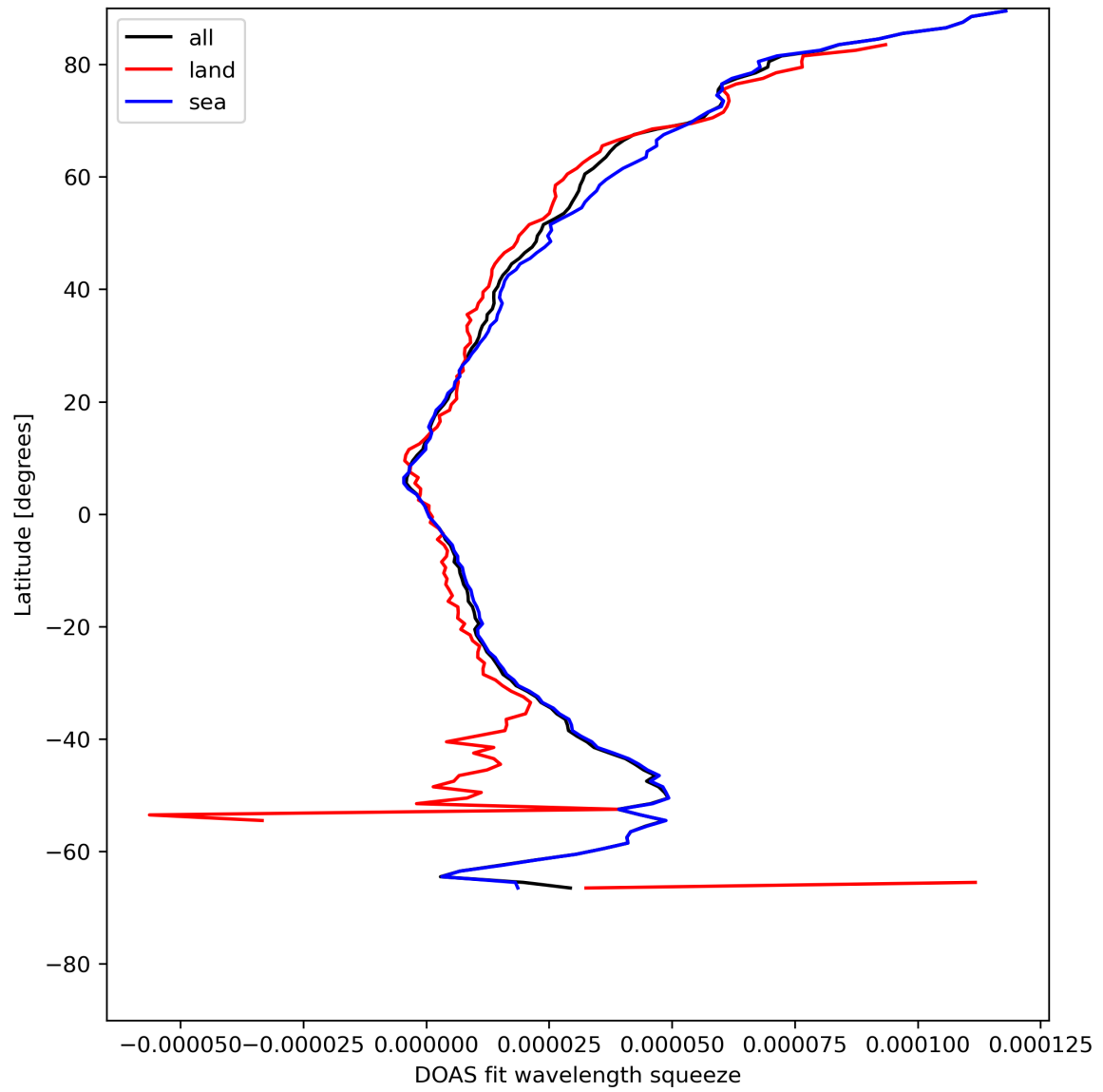
Figure 31: Zonal average of “DOAS fit wavelength squeeze” for 2023-07-30 to 2023-08-01.
