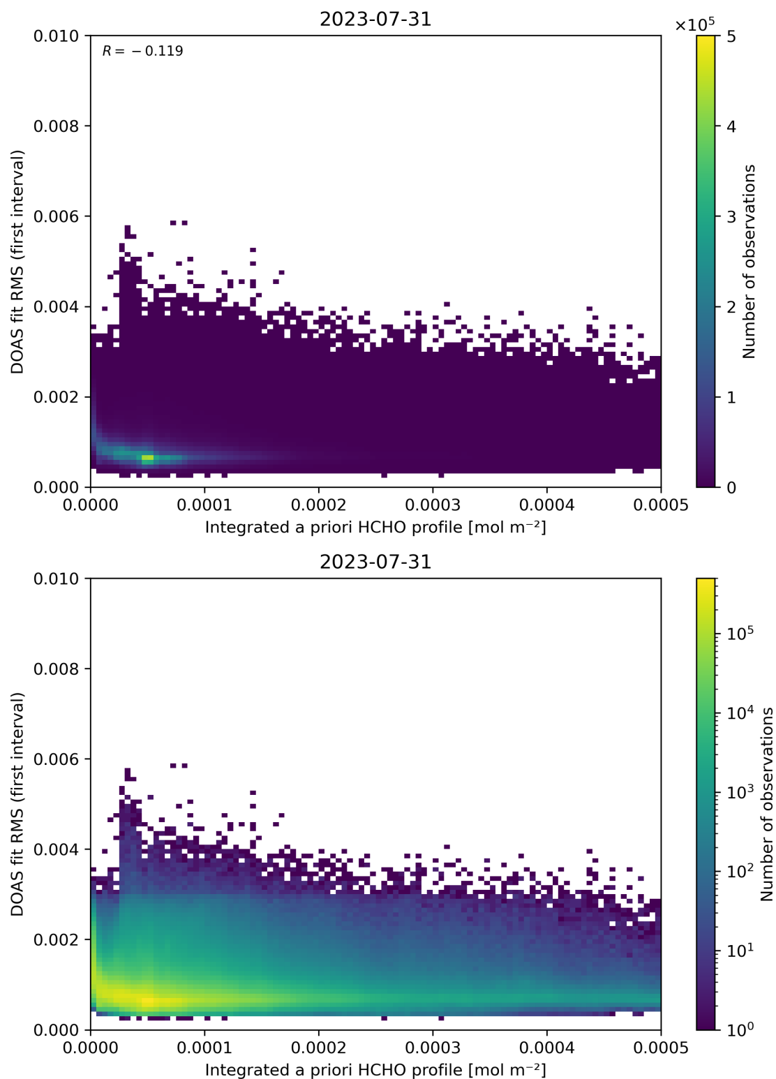
Figure 148: Scatter density plot of “Integrated a priori HCHO profile” against “DOAS fit RMS (first interval)” for 2023-07-30 to 2023-08-01.
