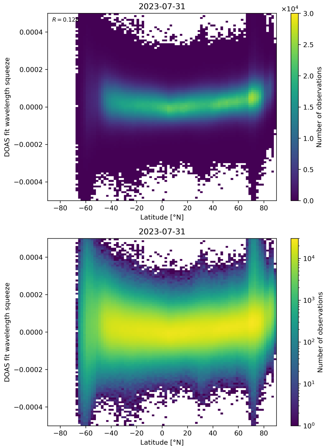
Figure 155: Scatter density plot of “Latitude” against “DOAS fit wavelength squeeze” for 2023-07-30 to 2023-08-01.
