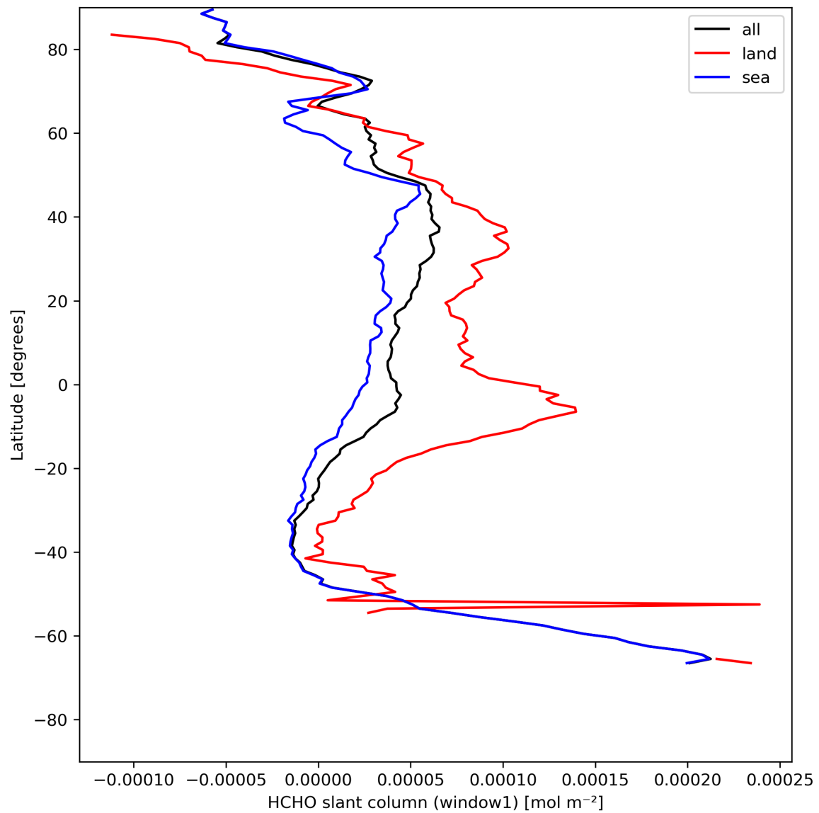
Figure 24: Zonal average of "HCHO slant column (window1)" for 2023-07-30 to 2023-08-01.
