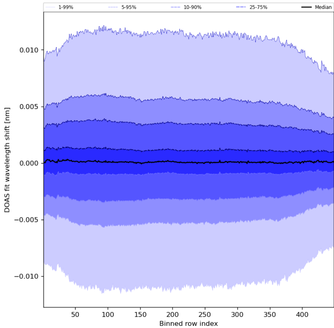
Figure 58: Along track statistics of “DOAS fit wavelength shift” for 2023-07-30 to 2023-08-01
