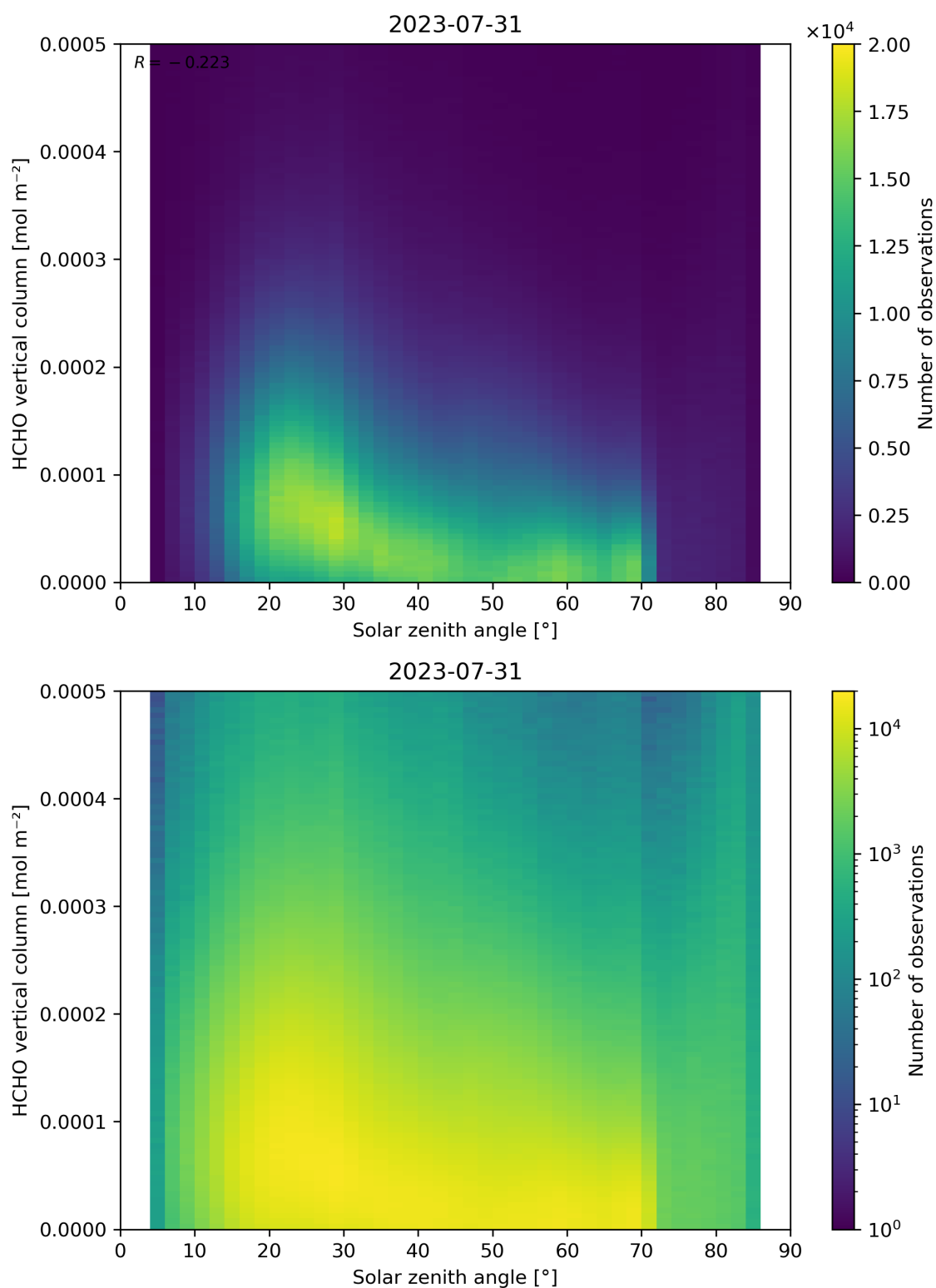
Figure 177: Scatter density plot of “Solar zenith angle” against “HCHO vertical column” for 2023-07-30 to 2023-08-01.
