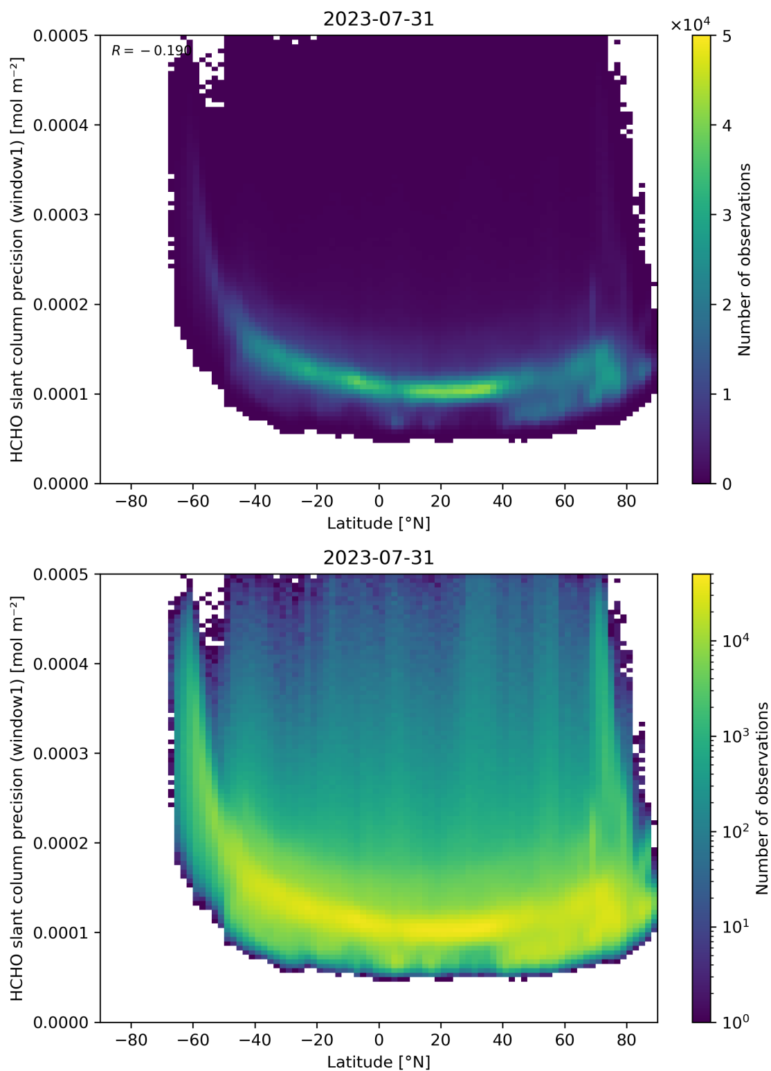
Figure 160: Scatter density plot of “Latitude” against “HCHO slant column precision (window1)” for 2023-07-30 to 2023-08-01.
