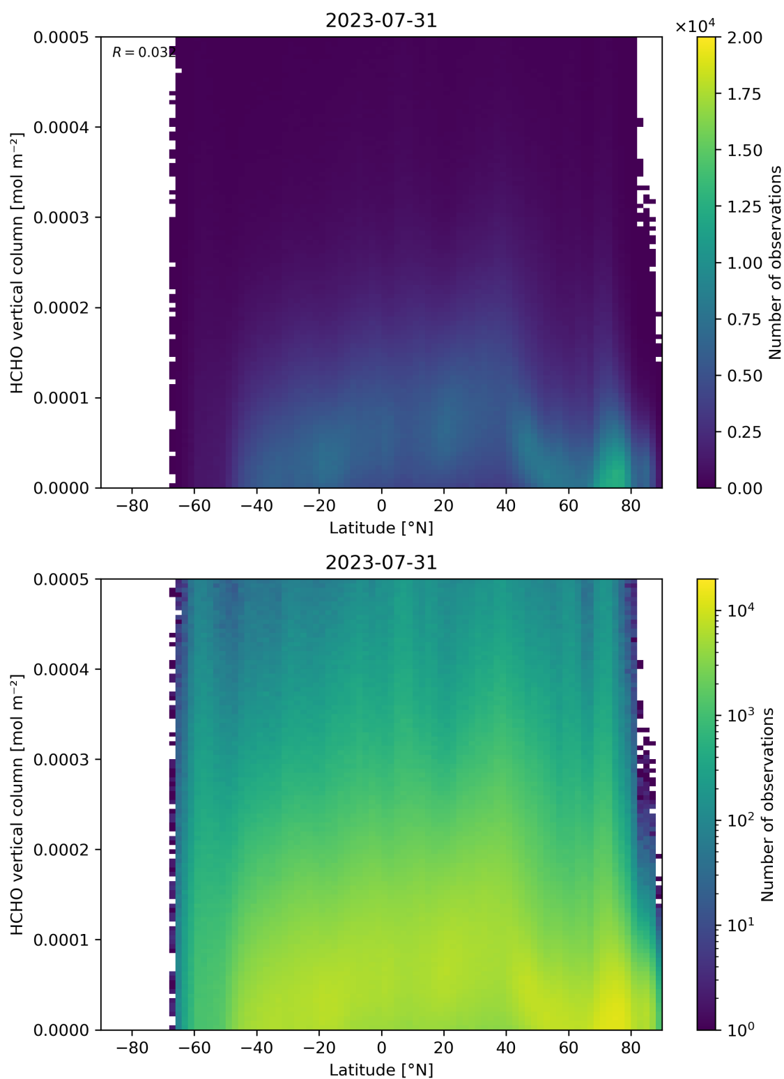
Figure 163: Scatter density plot of “Latitude” against “HCHO vertical column” for 2023-07-30 to 2023-08-01.
