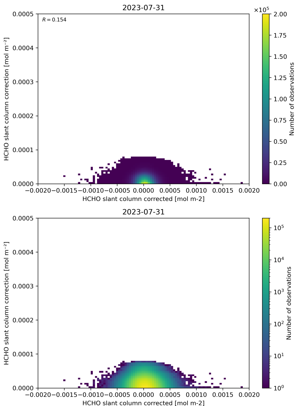
Figure 77: Scatter density plot of “HCHO slant column corrected” against “HCHO slant column correction” for 2023-07-30 to 2023-08-01.
