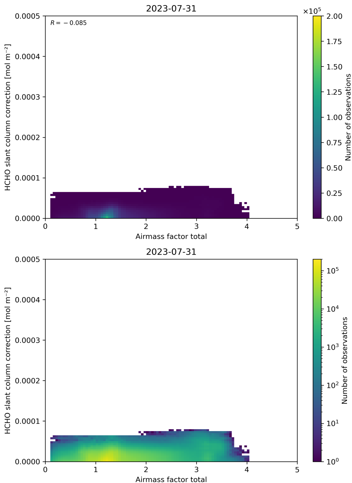
Figure 102: Scatter density plot of “Airmass factor total” against “HCHO slant column correction” for 2023-07-30 to 2023-08-01.
