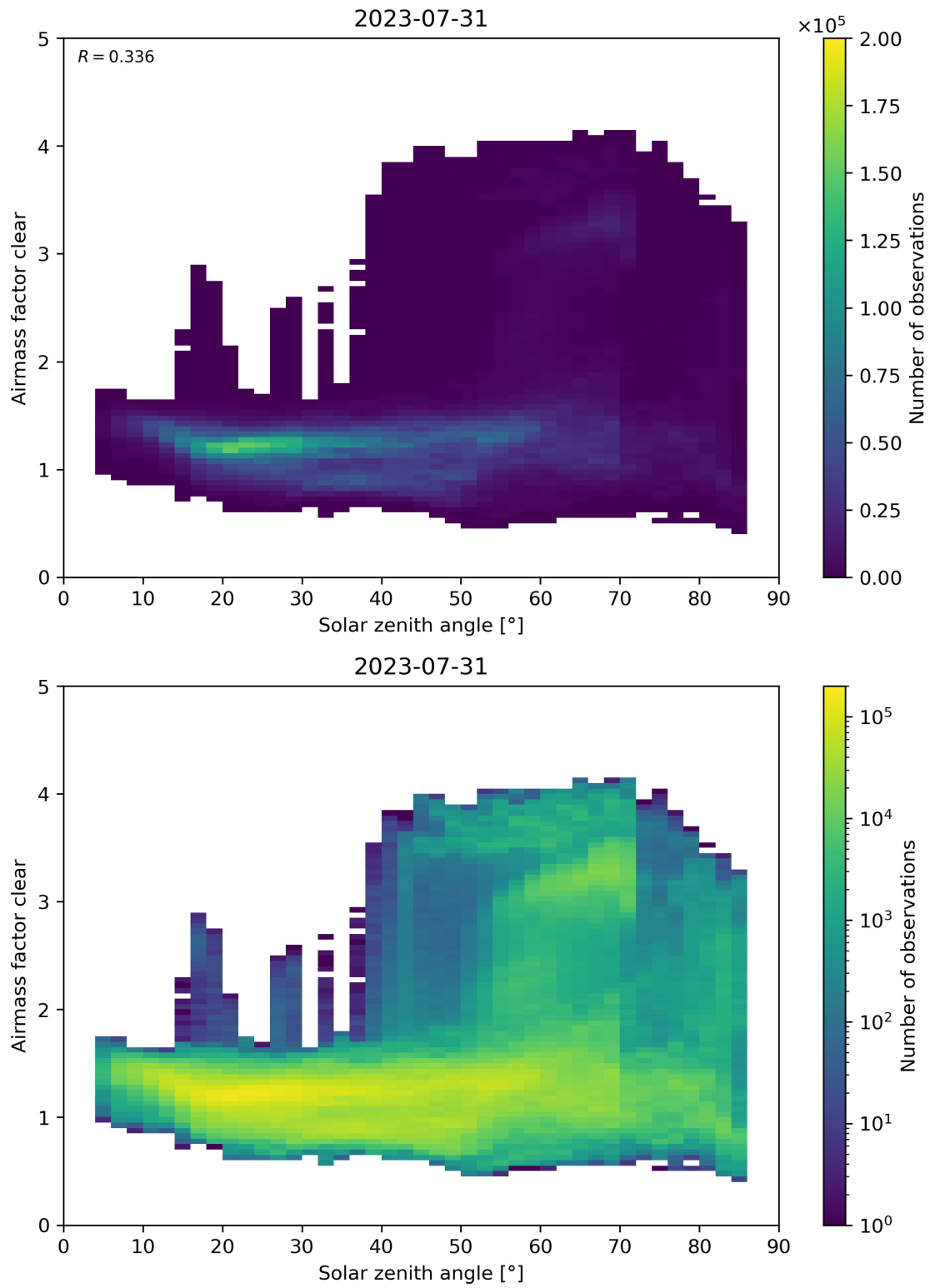
Figure 170: Scatter density plot of “Solar zenith angle” against “Airmass factor clear” for 2023-07-30 to 2023-08-01.
