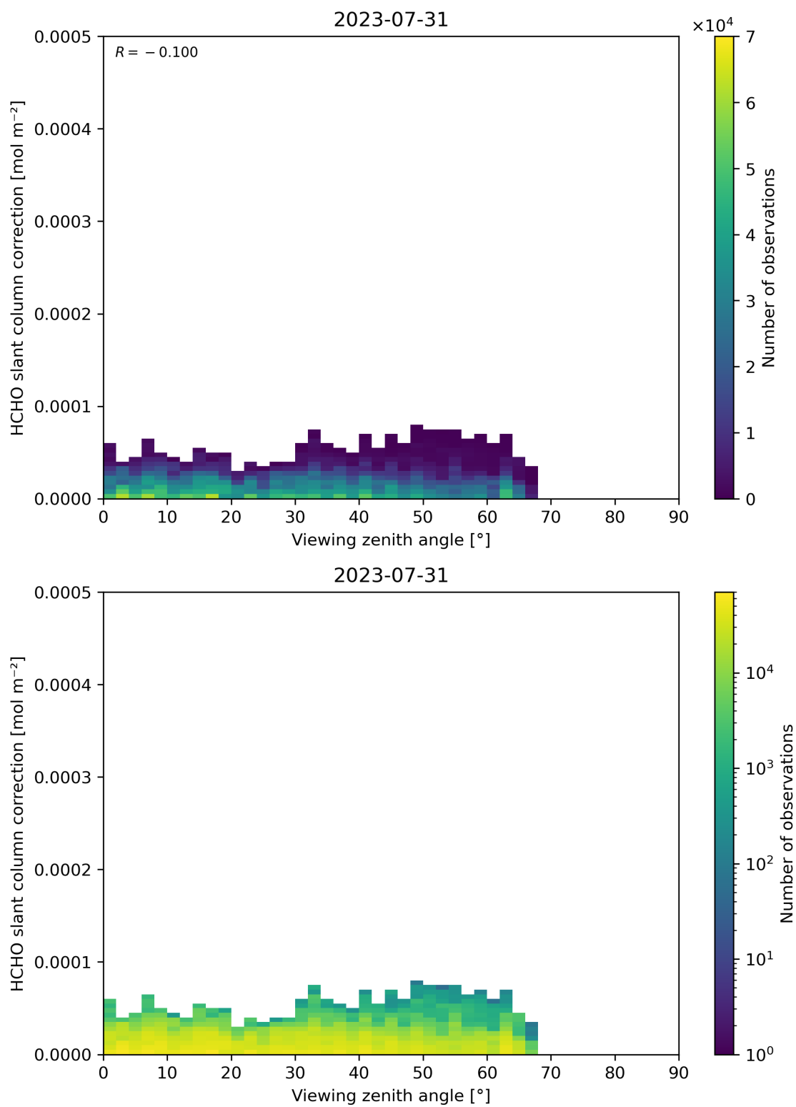
Figure 187: Scatter density plot of “Viewing zenith angle” against “HCHO slant column correction” for 2023-07-30 to 2023-08-01.
