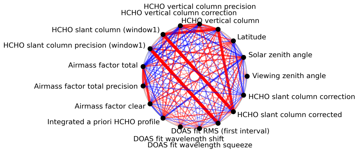
Figure 1: Map of correlation graph for 2023-07-30 to 2023-08-01.
