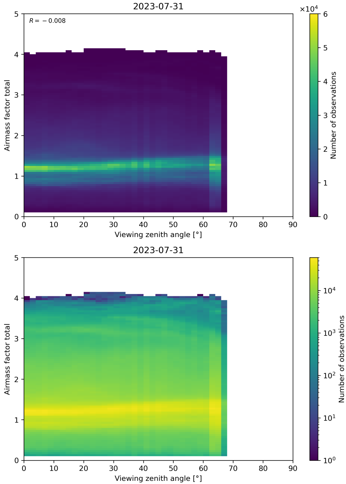
Figure 190: Scatter density plot of “Viewing zenith angle” against “Airmass factor total” for 2023-07-30 to 2023-08-01.
