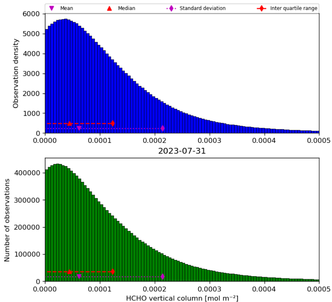
Figure 35: Histogram of “HCHO vertical column” for 2023-07-30 to 2023-08-01
