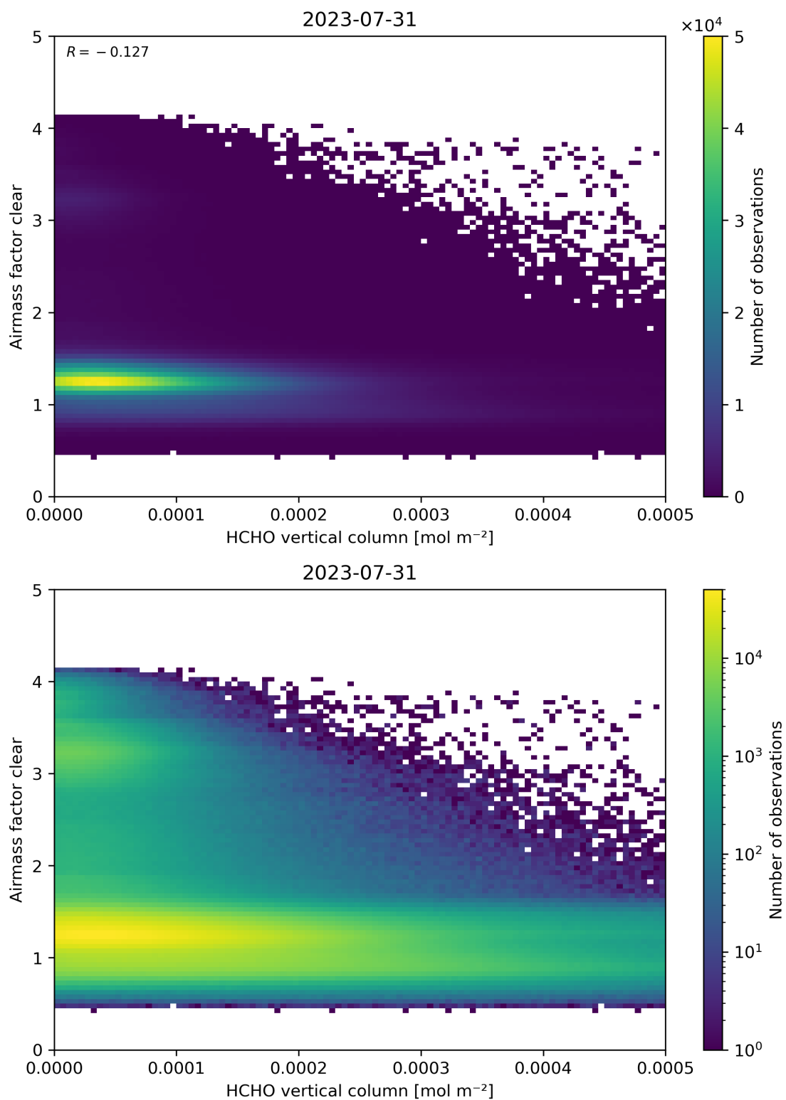
Figure 126: Scatter density plot of “HCHO vertical column” against “Airmass factor clear” for 2023-07-30 to 2023-08-01.
