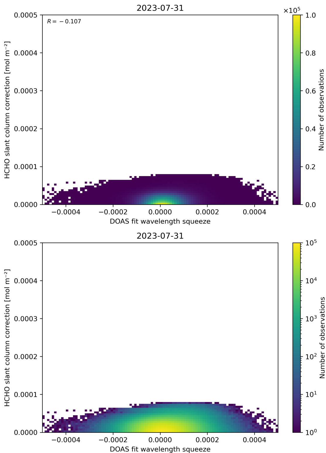
Figure 70: Scatter density plot of “DOAS fit wavelength squeeze” against “HCHO slant column correction” for 2023-07-30 to 2023-08-01.
