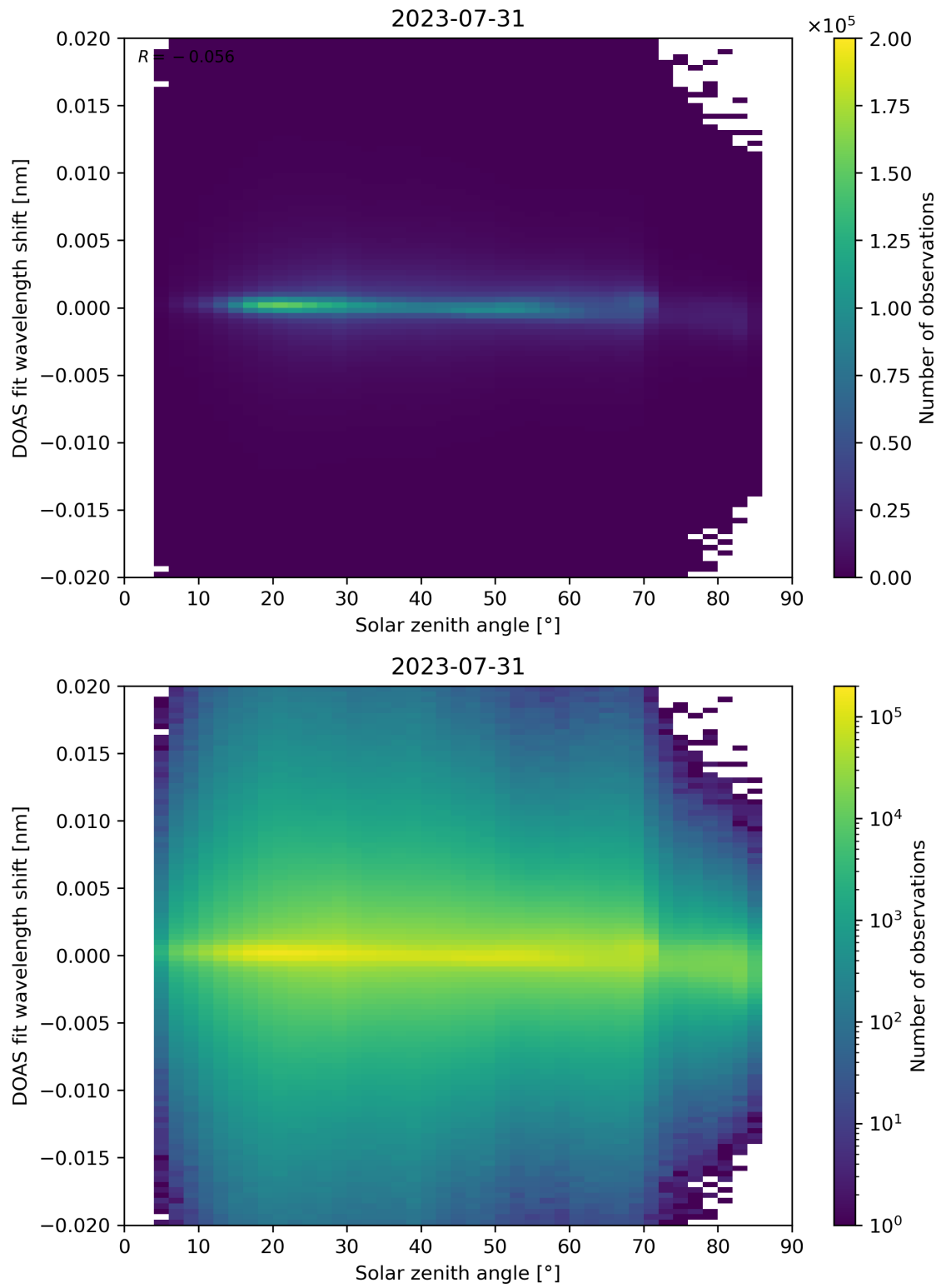
Figure 168: Scatter density plot of “Solar zenith angle” against “DOAS fit wavelength shift” for 2023-07-30 to 2023-08-01.
