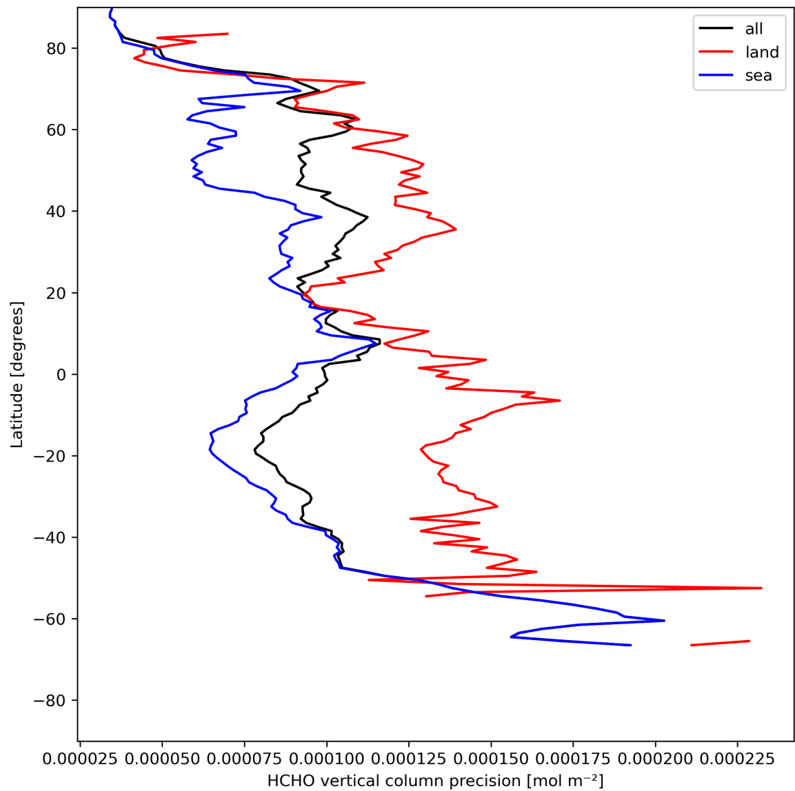
Figure 22: Zonal average of “HCHO vertical column precision” for 2023-07-30 to 2023-08-01.
