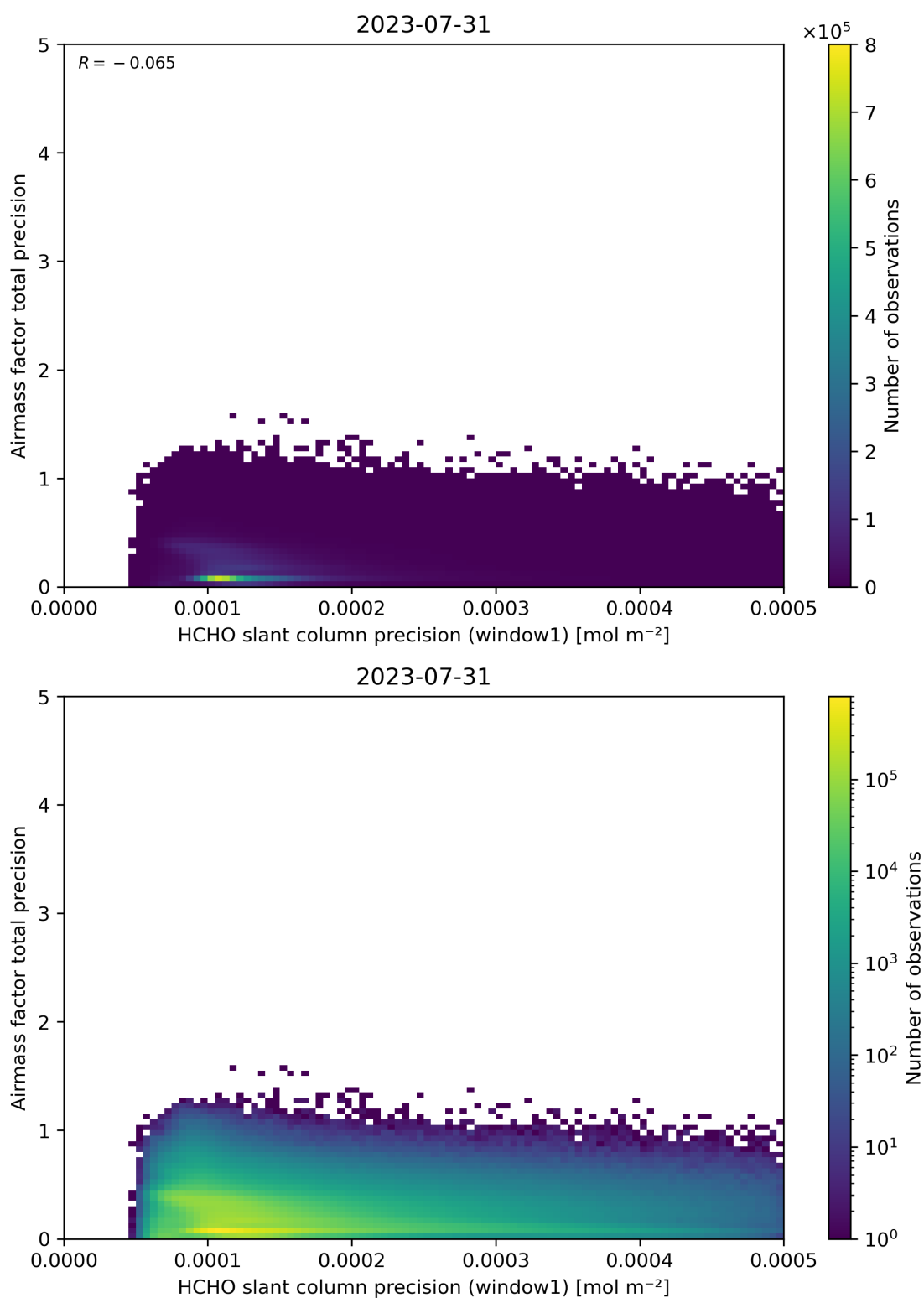
Figure 95: Scatter density plot of “HCHO slant column precision (window1)” against “Airmass factor total precision” for 2023-07-30 to 2023-08-01.
