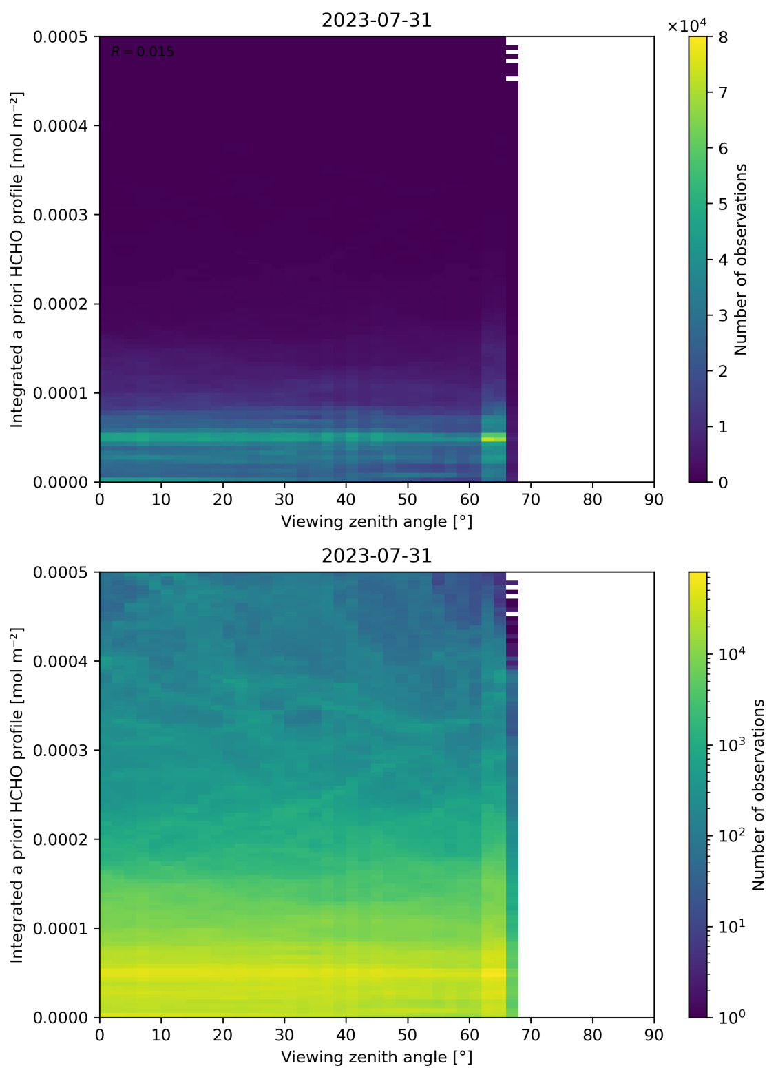
Figure 195: Scatter density plot of “Viewing zenith angle” against “Integrated a priori HCHO profile” for 2023-07-30 to 2023-08-01.
