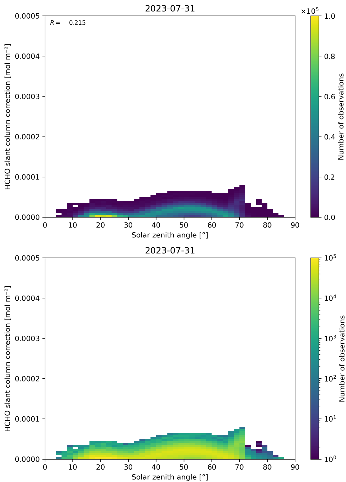
Figure 172: Scatter density plot of “Solar zenith angle” against “HCHO slant column correction” for 2023-07-30 to 2023-08-01.
