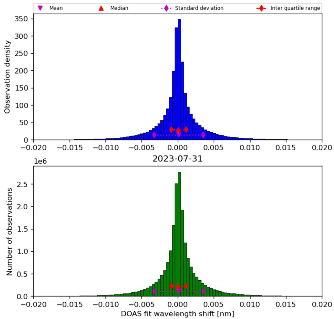
Figure 44: Histogram of “DOAS fit wavelength shift” for 2023-07-30 to 2023-08-01
