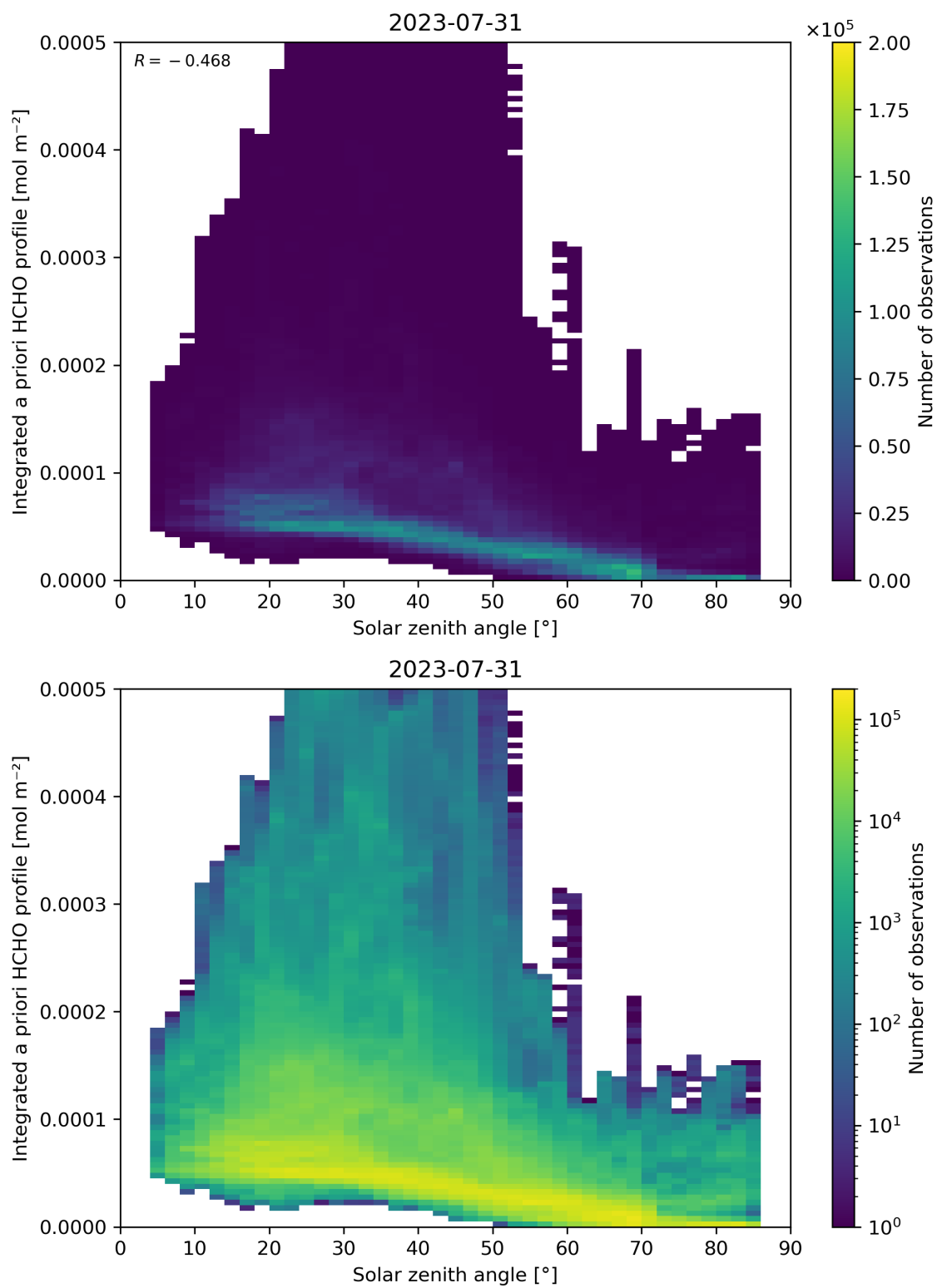
Figure 180: Scatter density plot of “Solar zenith angle” against “Integrated a priori HCHO profile” for 2023-07-30 to 2023-08-01.
