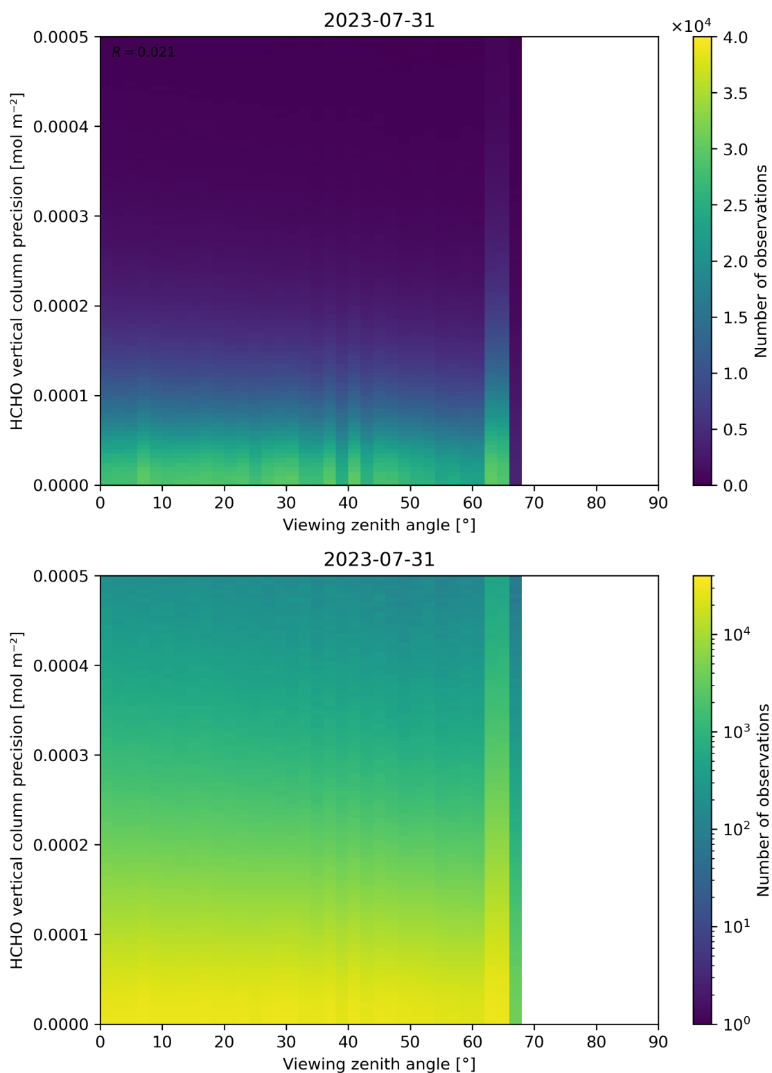
Figure 194: Scatter density plot of “Viewing zenith angle” against “HCHO vertical column precision” for 2023-07-30 to 2023-08-01.
