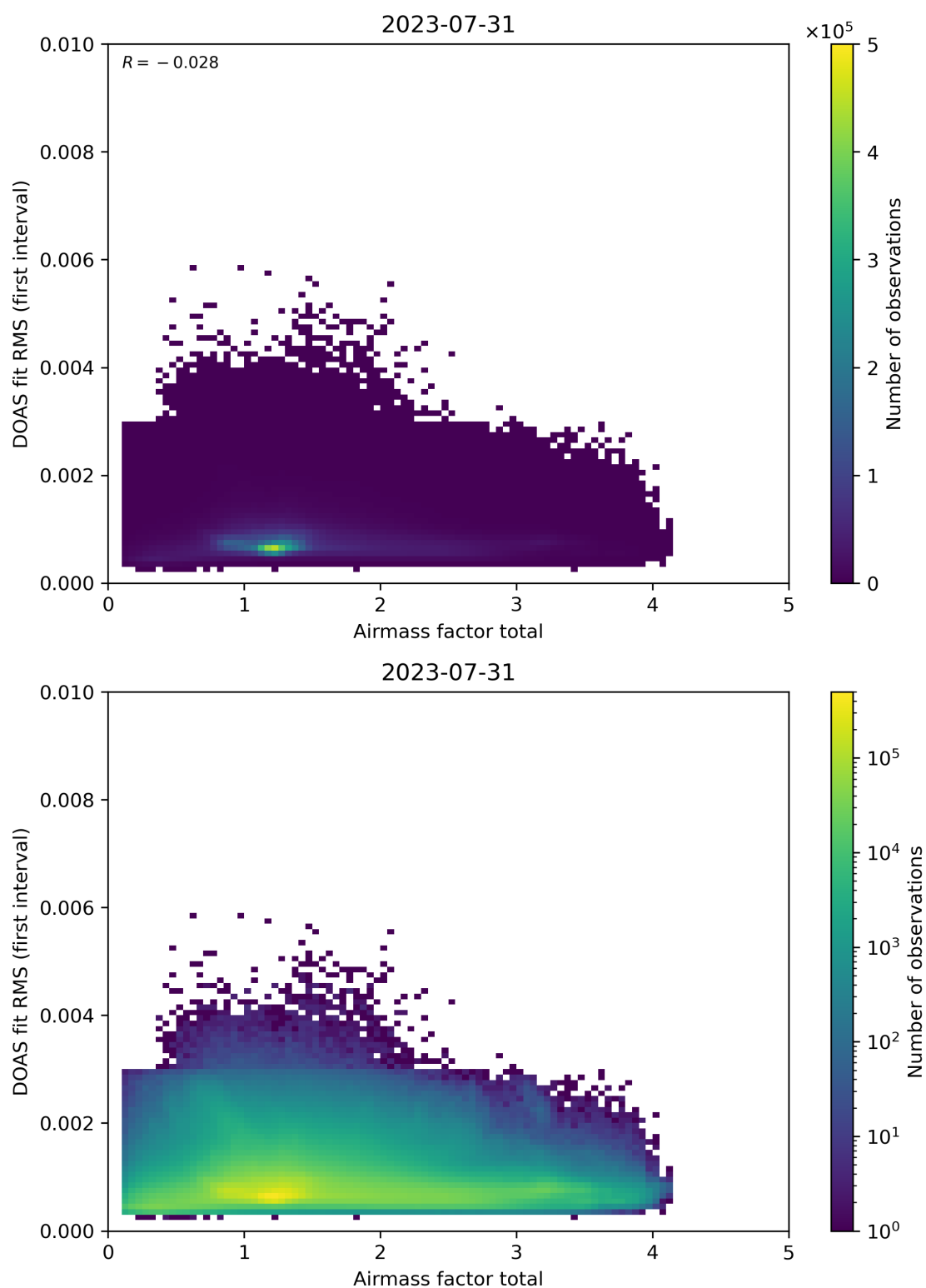
Figure 97: Scatter density plot of “Airmass factor total” against “DOAS fit RMS (first interval)” for 2023-07-30 to 2023-08-01.
