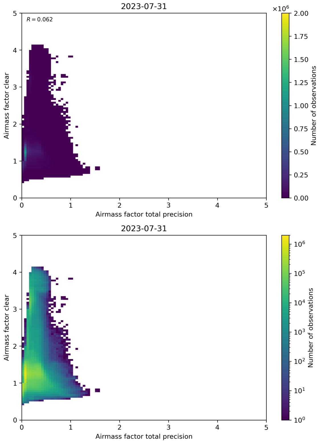
Figure 108: Scatter density plot of “Airmass factor total precision” against “Airmass factor clear” for 2023-07-30 to 2023-08-01.
