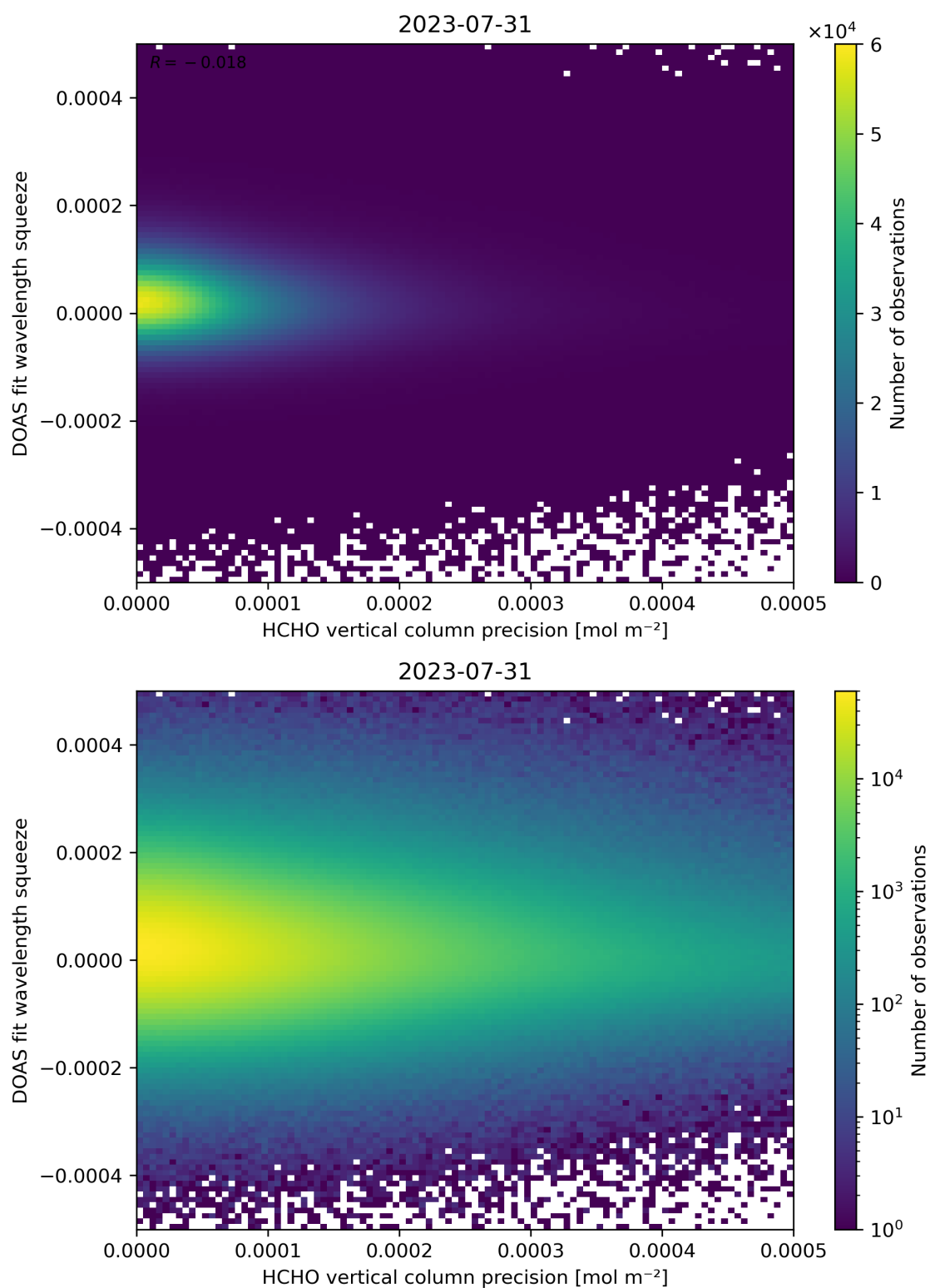
Figure 138: Scatter density plot of “HCHO vertical column precision” against “DOAS fit wavelength squeeze” for 2023-07-30 to 2023-08-01.
