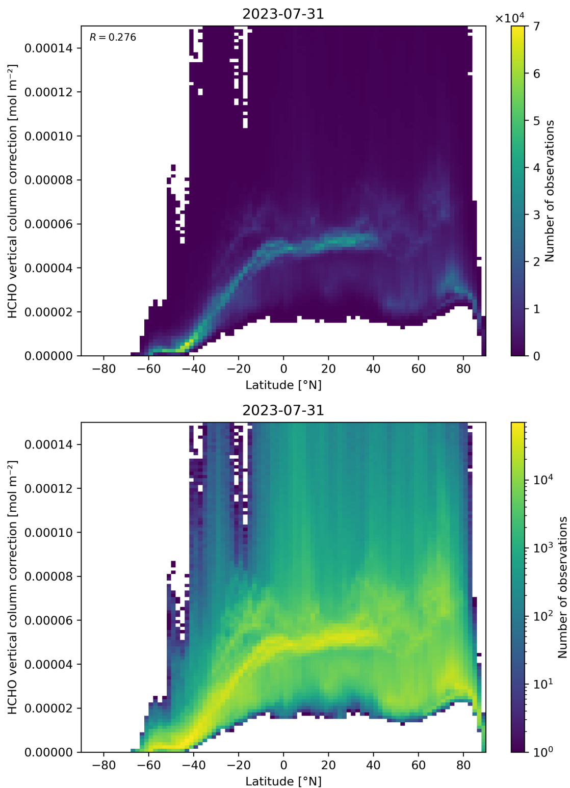
Figure 164: Scatter density plot of “Latitude” against “HCHO vertical column correction” for 2023-07-30 to 2023-08-01.
