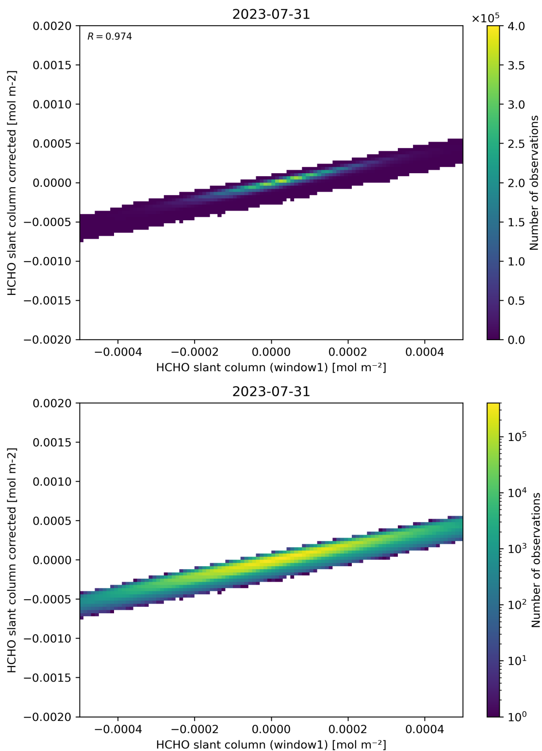
Figure 82: Scatter density plot of “HCHO slant column (window1)” against “HCHO slant column corrected” for 2023-07-30 to 2023-08-01.
