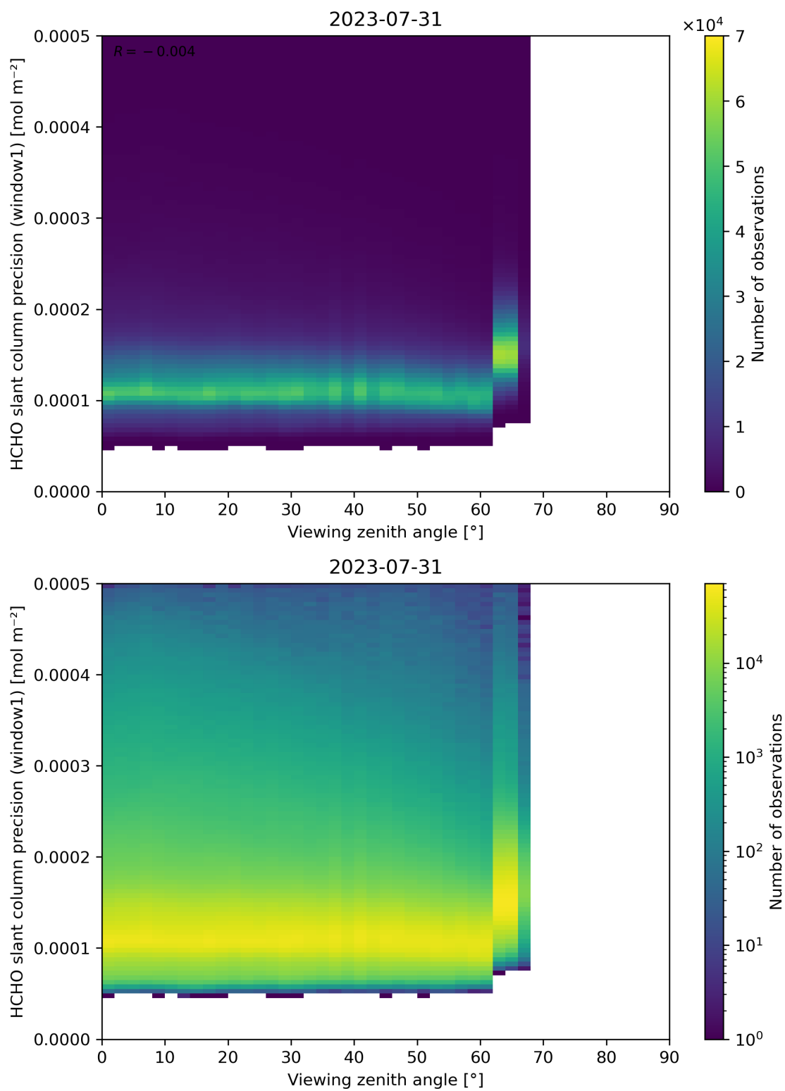
Figure 189: Scatter density plot of “Viewing zenith angle” against “HCHO slant column precision (window1)” for 2023-07-30 to 2023-08-01.
