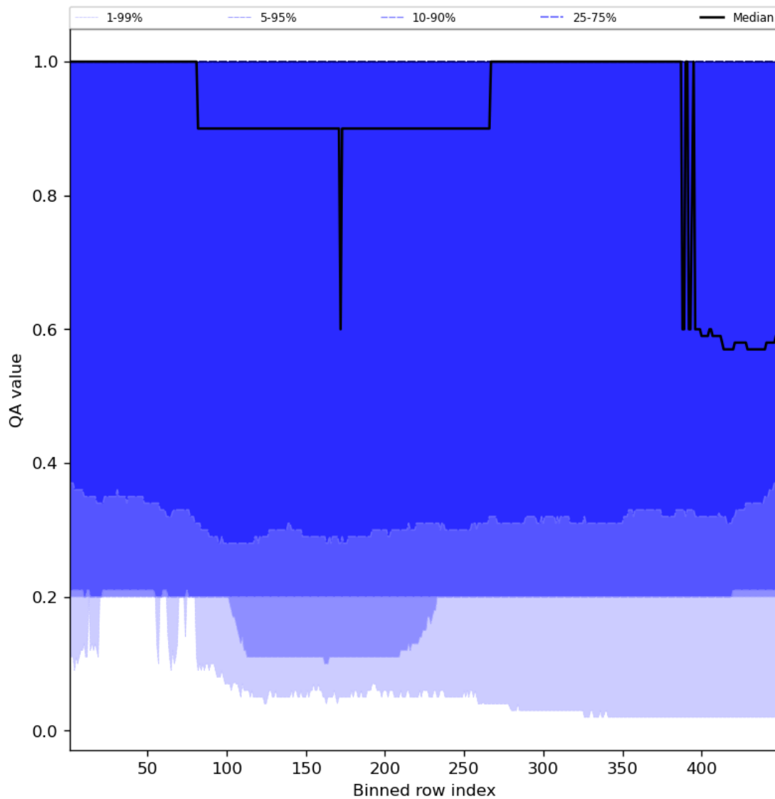
Figure 48: Along track statistics of “QA value” for 2023-07-30 to 2023-08-01
