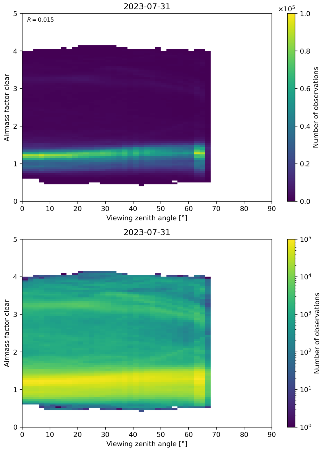
Figure 185: Scatter density plot of “Viewing zenith angle” against “Airmass factor clear” for 2023-07-30 to 2023-08-01.
