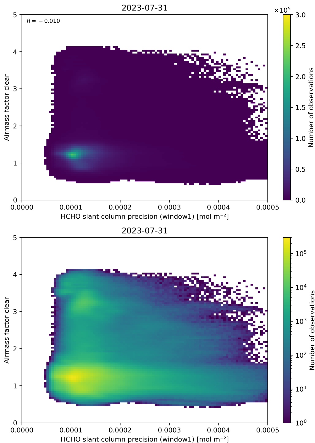
Figure 91: Scatter density plot of “HCHO slant column precision (window1)” against “Airmass factor clear” for 2023-07-30 to 2023-08-01.
