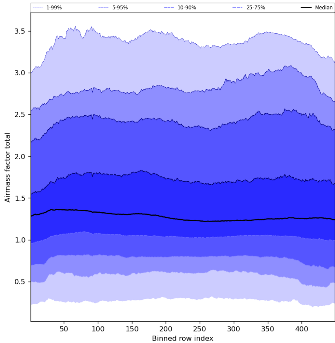
Figure 54: Along track statistics of “Airmass factor total” for 2023-07-30 to 2023-08-01
