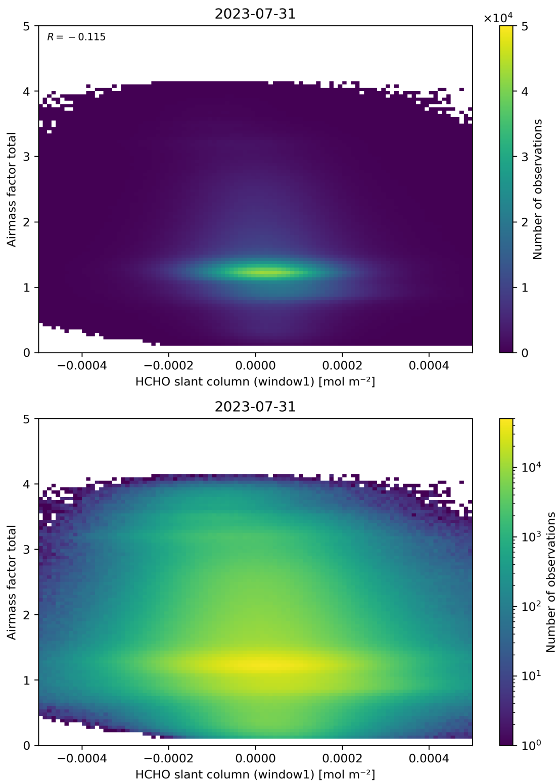
Figure 85: Scatter density plot of “HCHO slant column (window1)” against “Airmass factor total” for 2023-07-30 to 2023-08-01.
