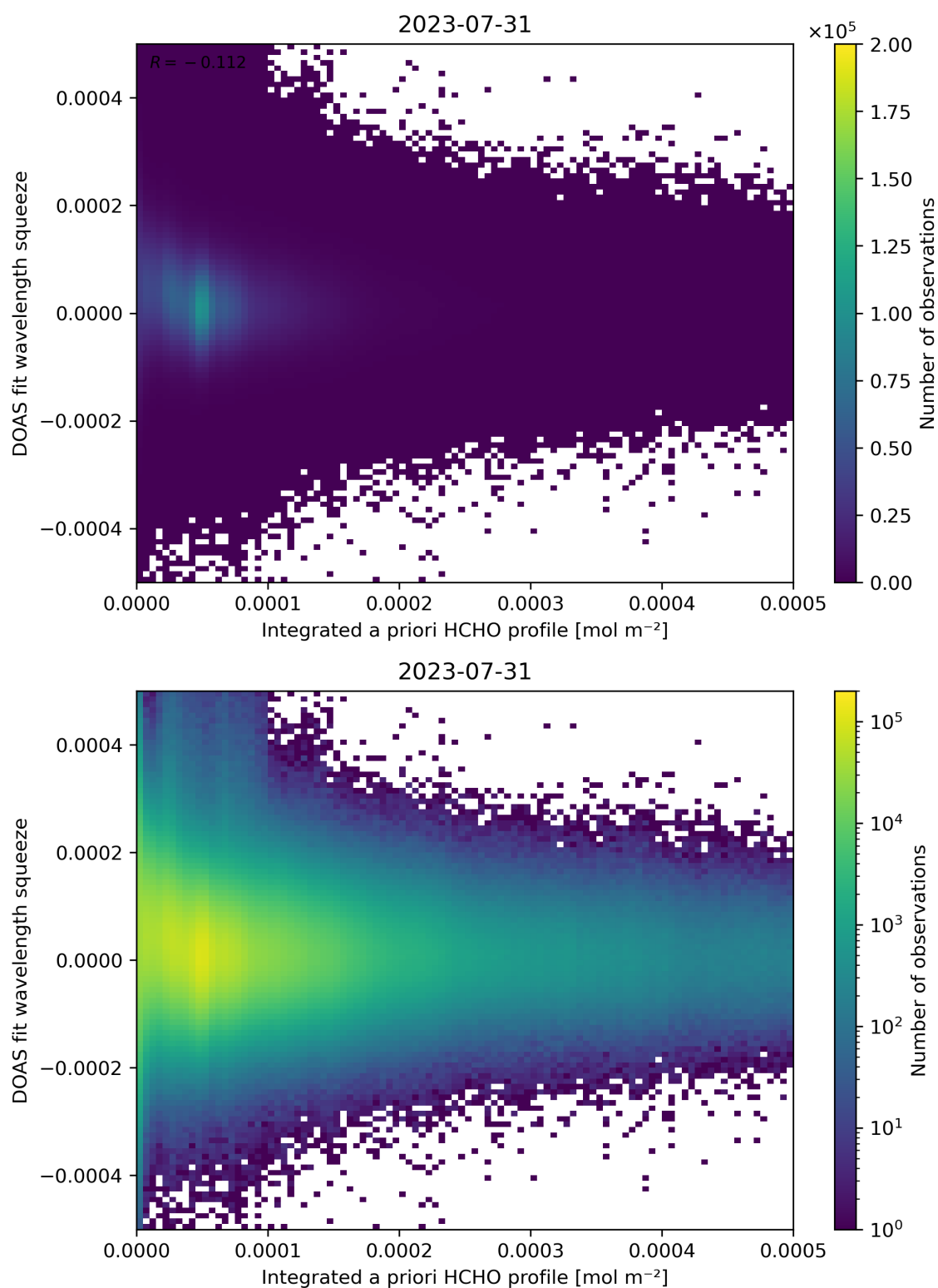
Figure 150: Scatter density plot of “Integrated a priori HCHO profile” against “DOAS fit wavelength squeeze” for 2023-07-30 to 2023-08-01.
