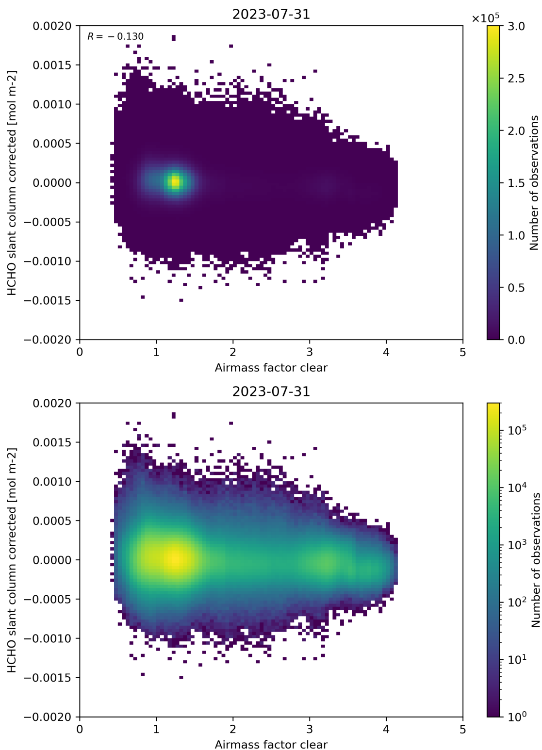
Figure 74: Scatter density plot of “Airmass factor clear” against “HCHO slant column corrected” for 2023-07-30 to 2023-08-01.
