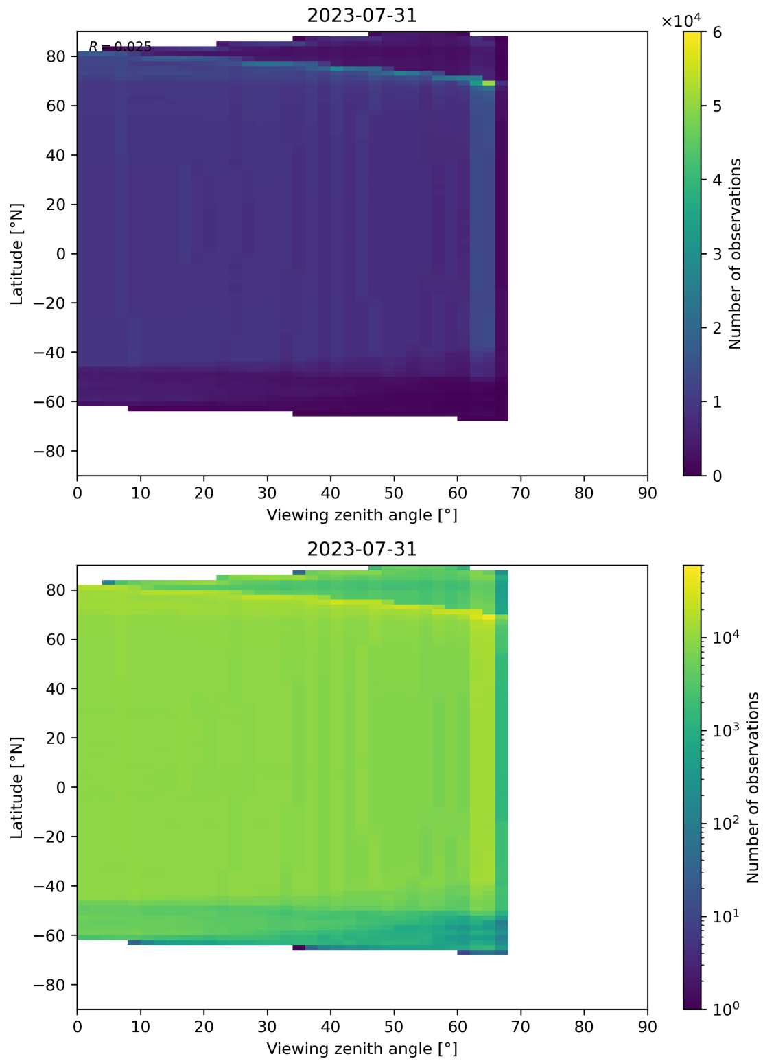
Figure 196: Scatter density plot of “Viewing zenith angle” against “Latitude” for 2023-07-30 to 2023-08-01.
