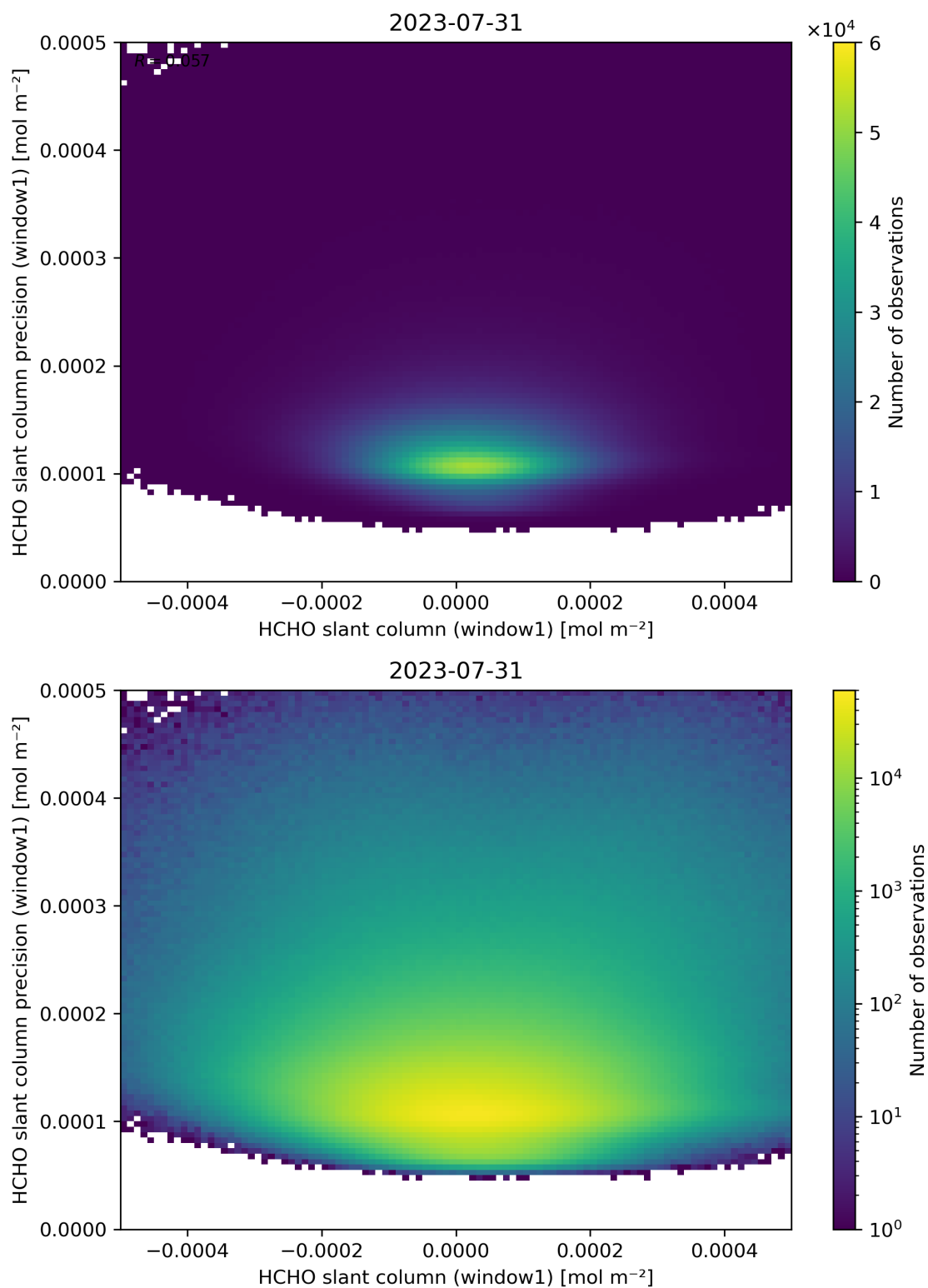
Figure 84: Scatter density plot of “HCHO slant column (window1)” against “HCHO slant column precision (window1)” for 2023-07-30 to 2023-08-01.
