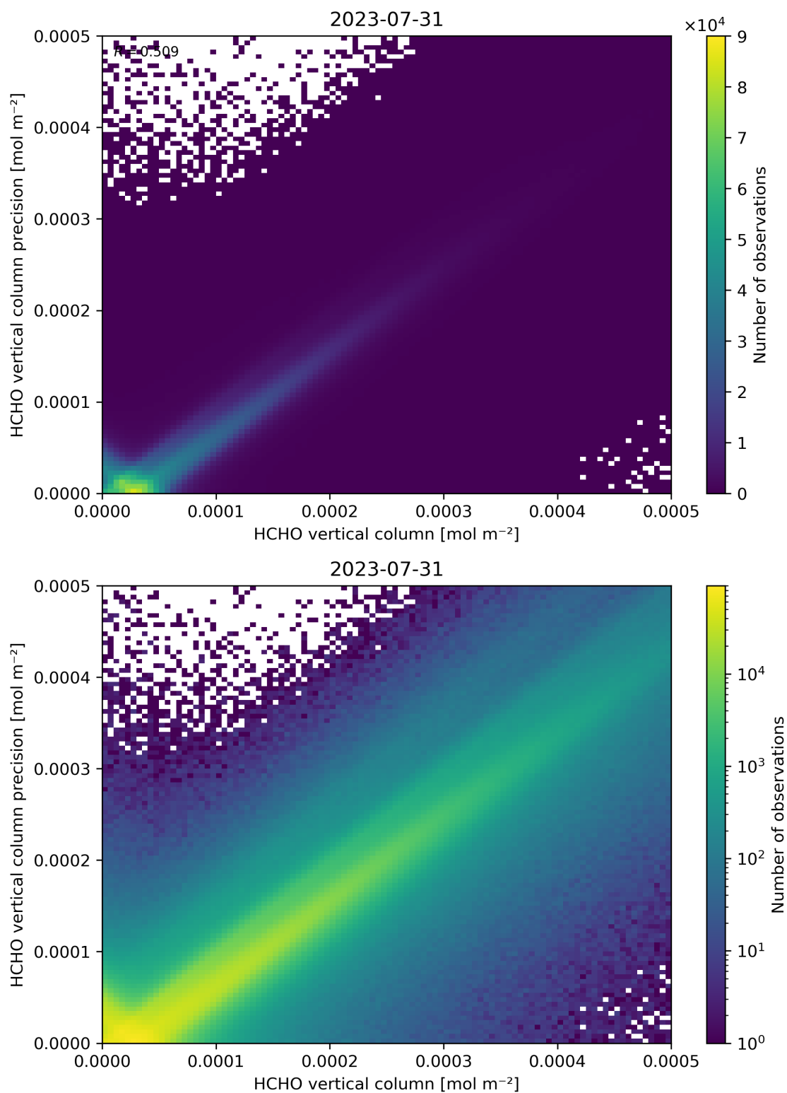
Figure 134: Scatter density plot of “HCHO vertical column” against “HCHO vertical column precision” for 2023-07-30 to 2023-08-01.
