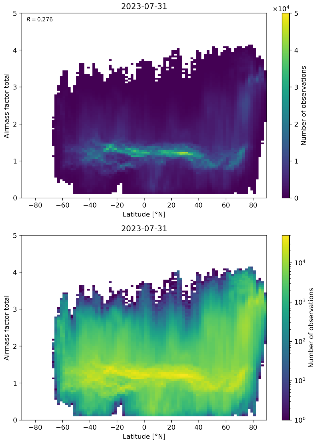
Figure 161: Scatter density plot of “Latitude” against “Airmass factor total” for 2023-07-30 to 2023-08-01.
