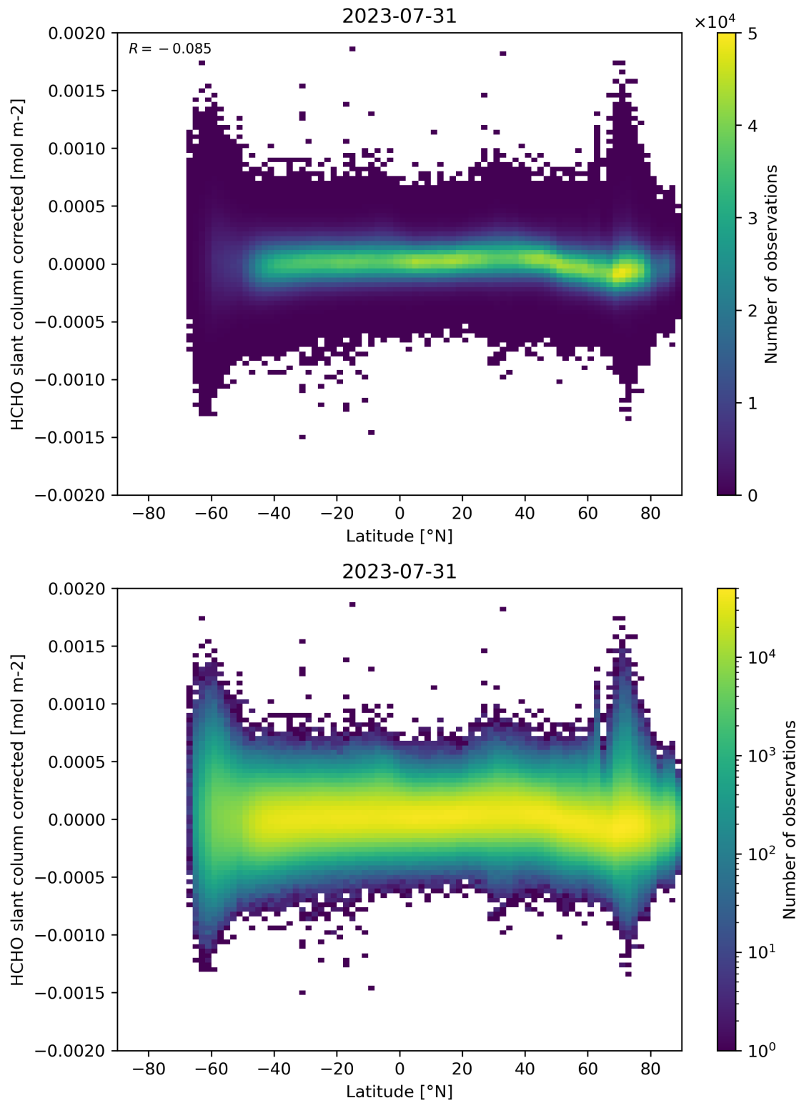
Figure 157: Scatter density plot of “Latitude” against “HCHO slant column corrected” for 2023-07-30 to 2023-08-01.
