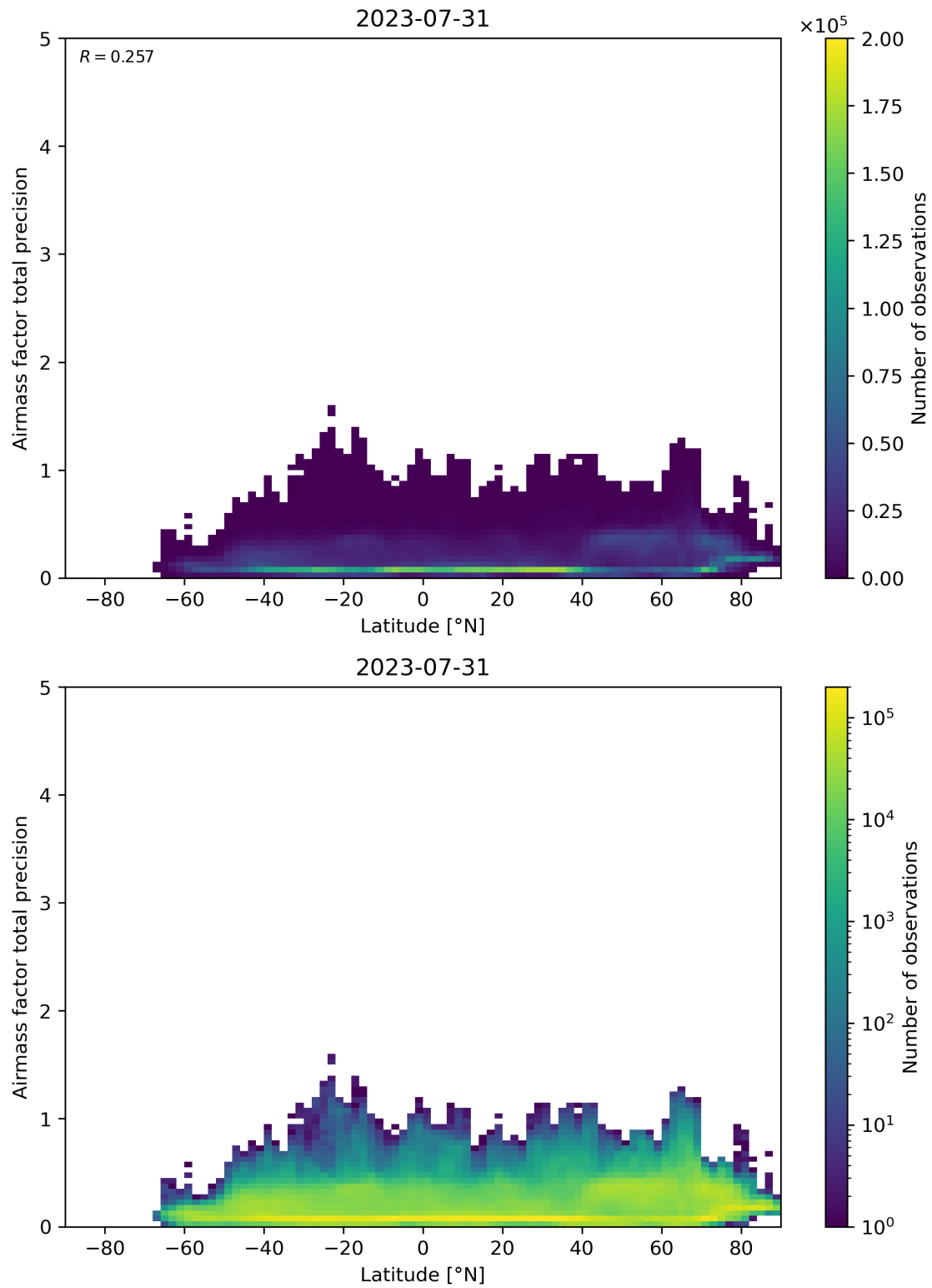
Figure 162: Scatter density plot of “Latitude” against “Airmass factor total precision” for 2023-07-30 to 2023-08-01.
