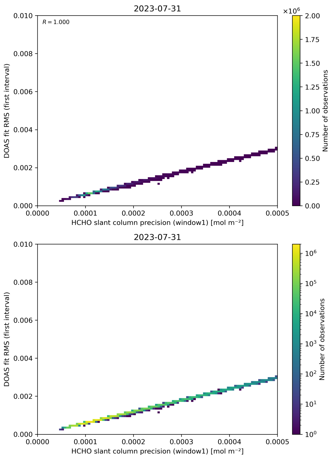
Figure 88: Scatter density plot of “HCHO slant column precision (window1)” against “DOAS fit RMS (first interval)” for 2023-07-30 to 2023-08-01.
