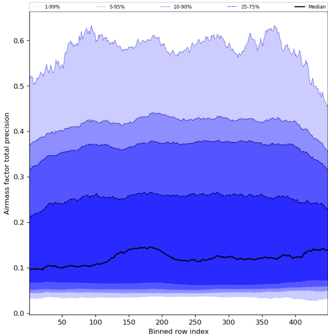
Figure 55: Along track statistics of “Airmass factor total precision” for 2023-07-30 to 2023-08-01
