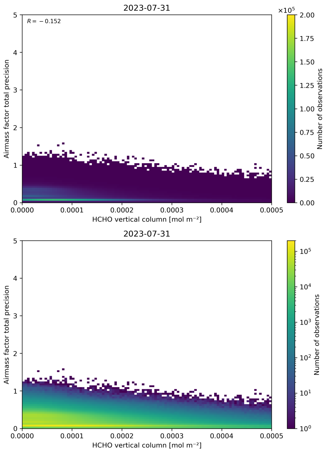
Figure 132: Scatter density plot of “HCHO vertical column” against “Airmass factor total precision” for 2023-07-30 to 2023-08-01.
