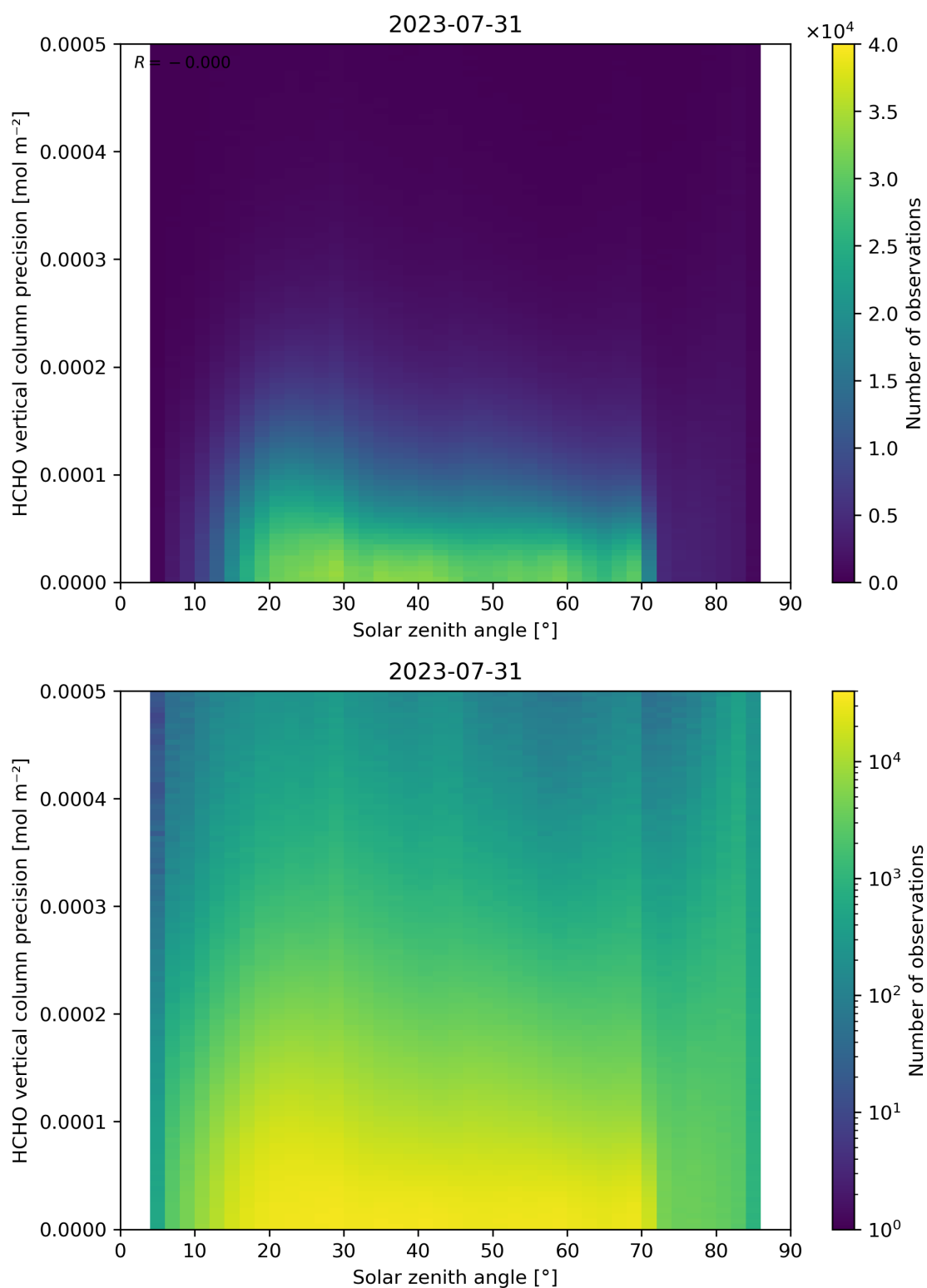
Figure 179: Scatter density plot of “Solar zenith angle” against “HCHO vertical column precision” for 2023-07-30 to 2023-08-01.
