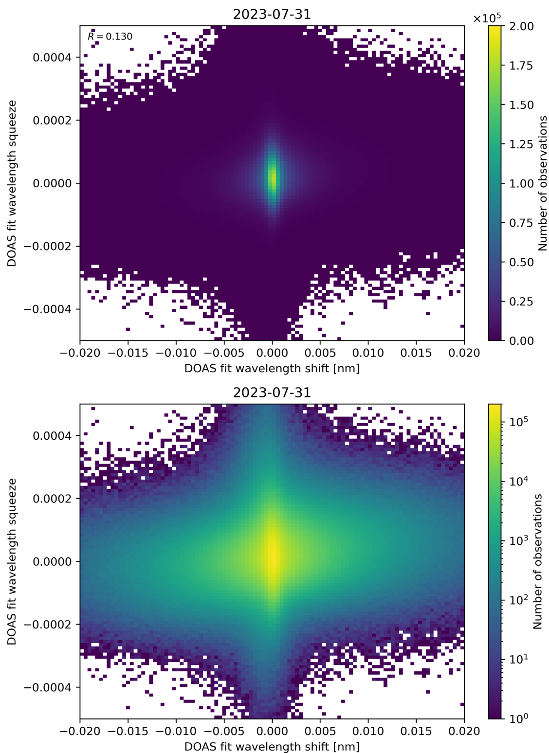
Figure 65: Scatter density plot of “DOAS fit wavelength shift” against “DOAS fit wavelength squeeze” for 2023-07-30 to 2023-08-01.
