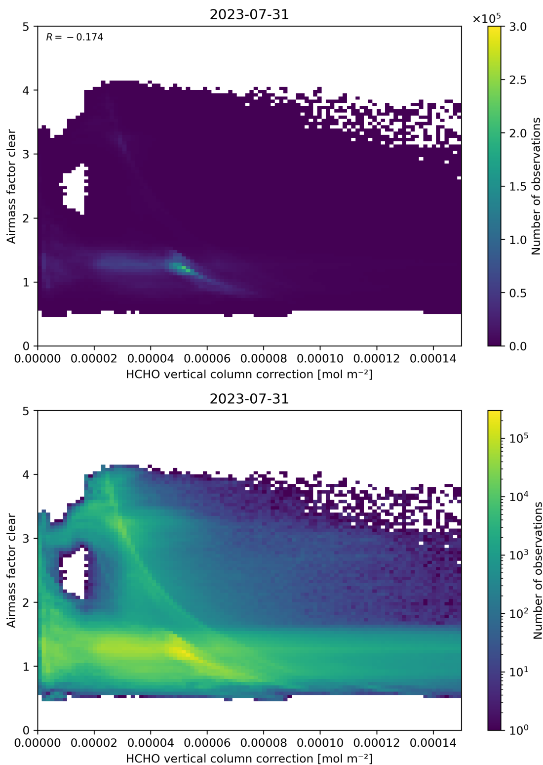
Figure 115: Scatter density plot of “HCHO vertical column correction” against “Airmass factor clear” for 2023-07-30 to 2023-08-01.
