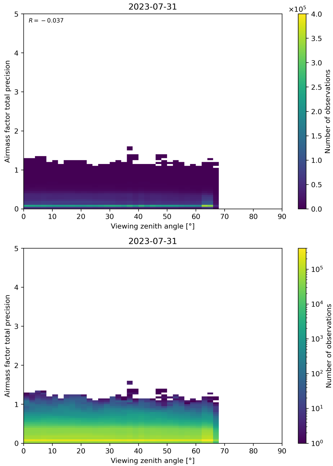
Figure 191: Scatter density plot of “Viewing zenith angle” against “Airmass factor total precision” for 2023-07-30 to 2023-08-01.
