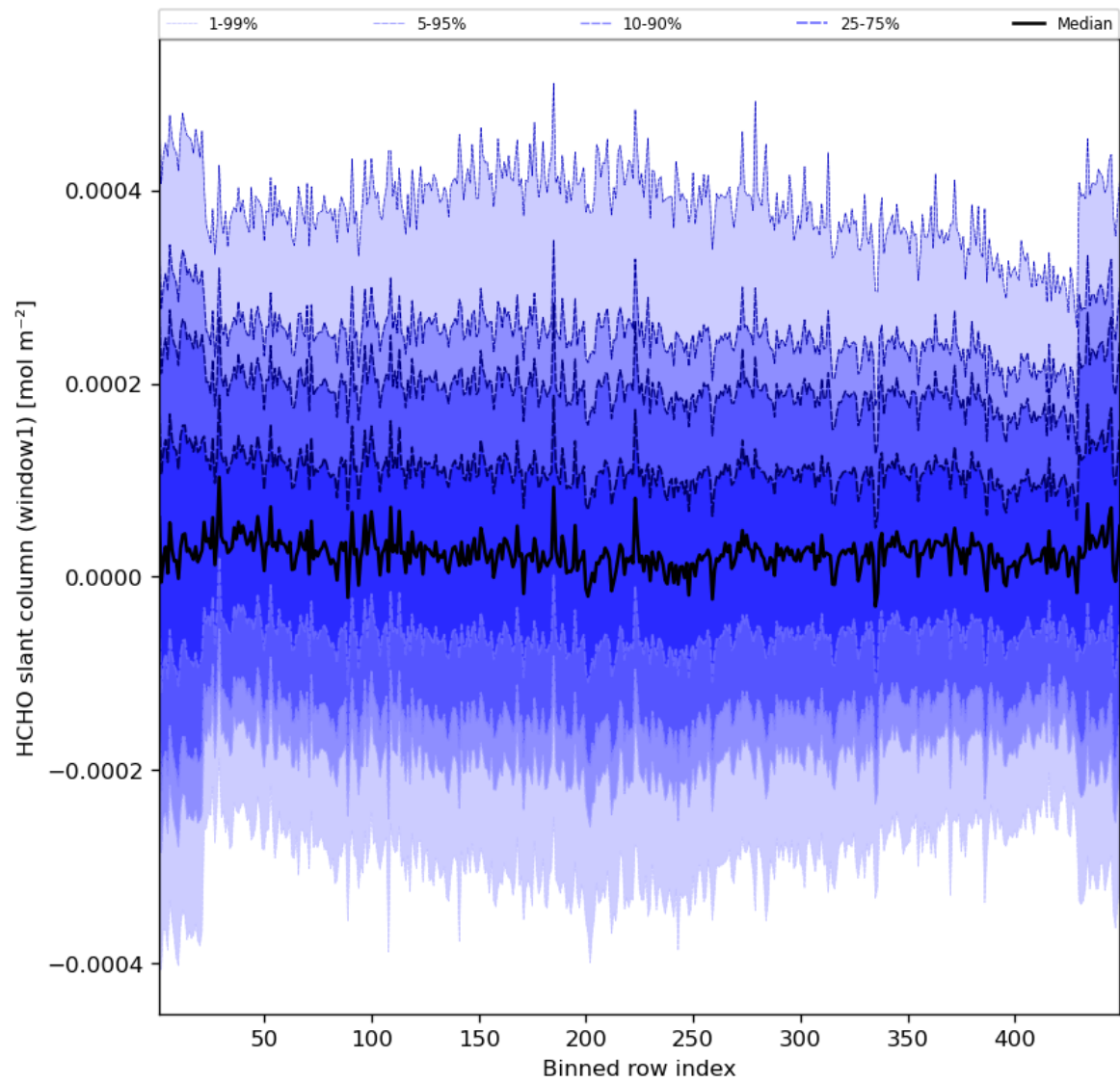
Figure 52: Along track statistics of “HCHO slant column (window1)” for 2023-07-30 to 2023-08-01
