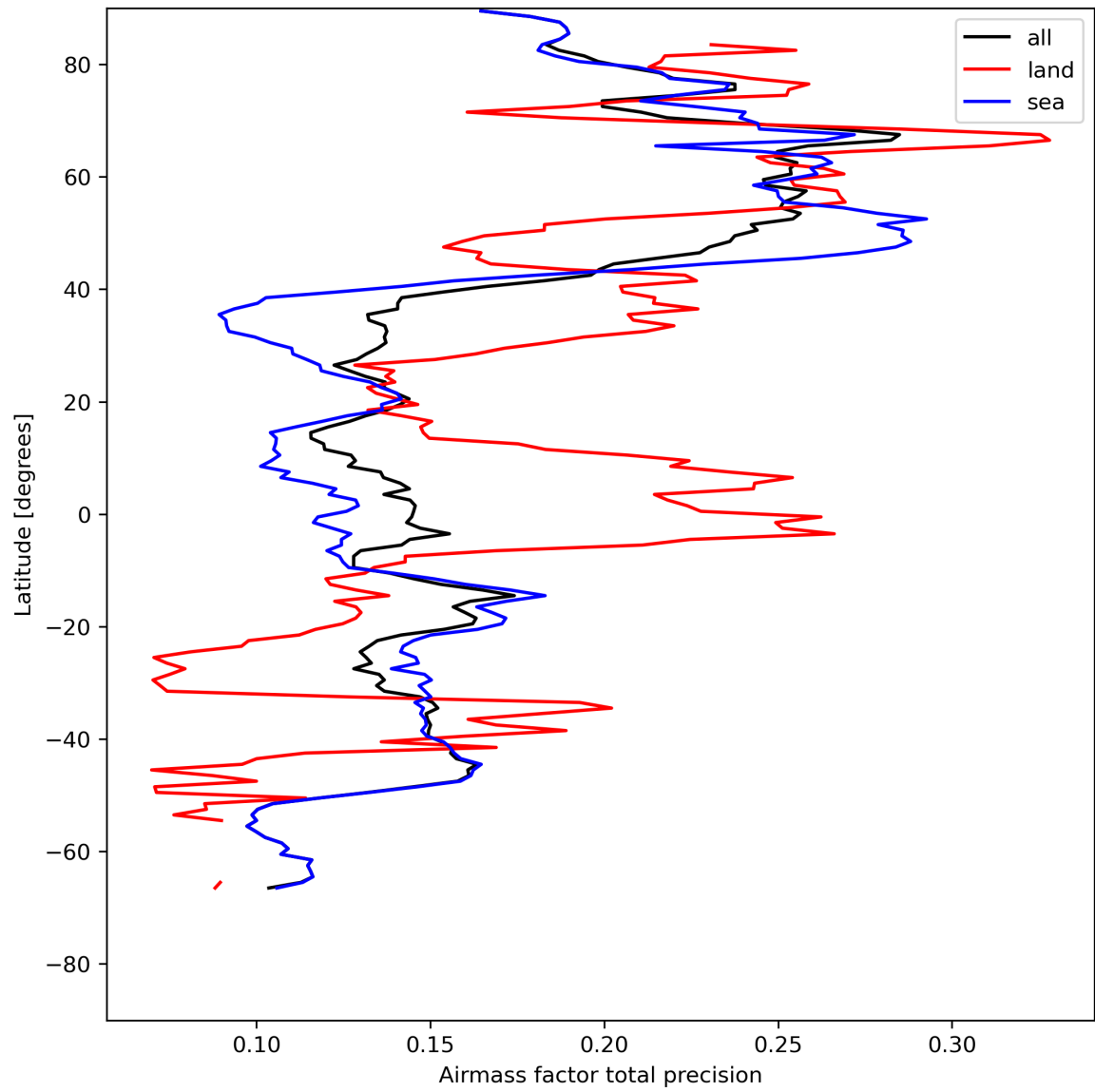
Figure 27: Zonal average of “Airmass factor total precision” for 2023-07-30 to 2023-08-01.
