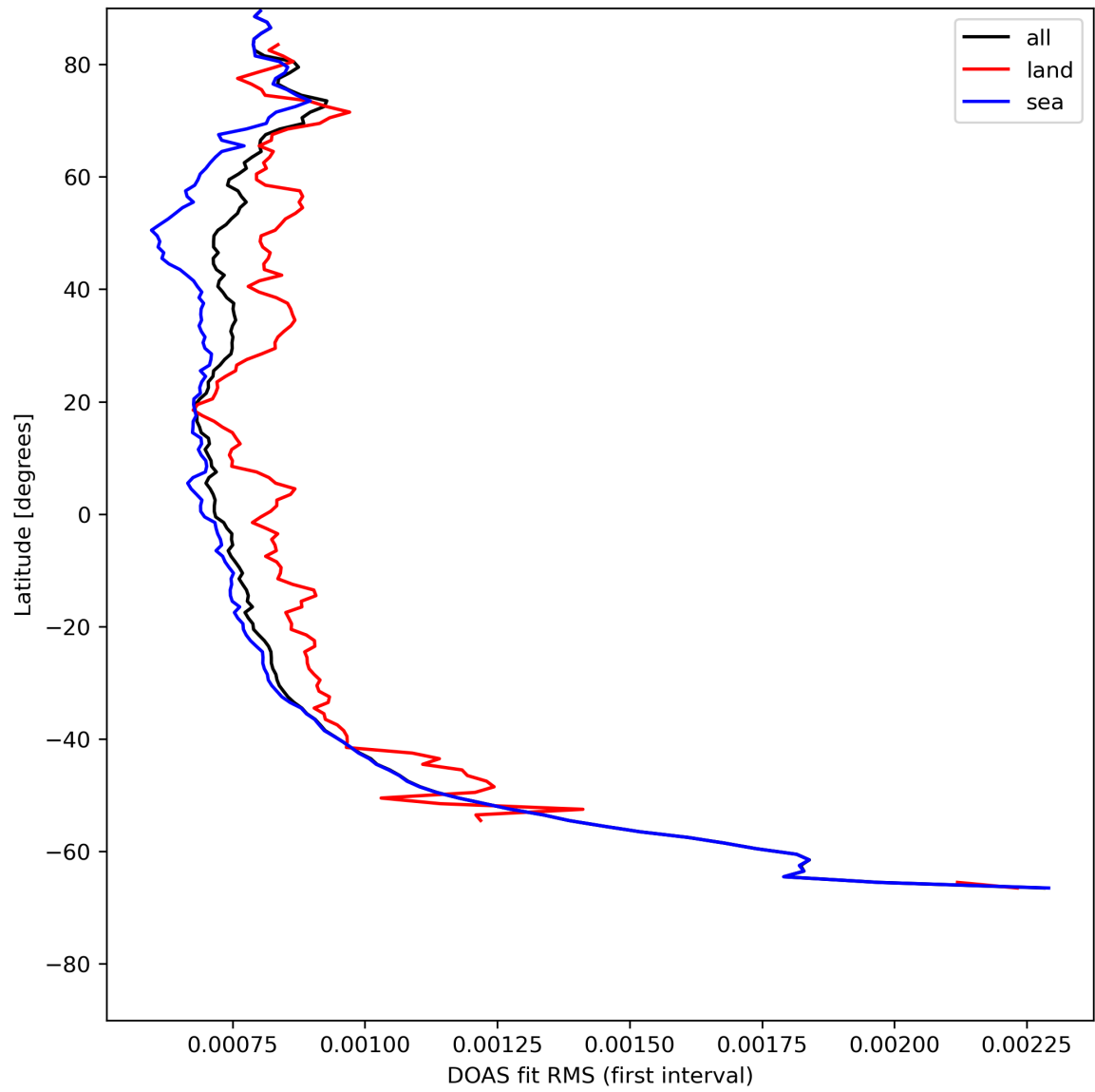
Figure 32: Zonal average of “DOAS fit RMS (first interval)” for 2023-07-30 to 2023-08-01.
