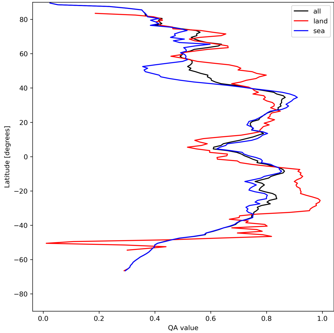
Figure 20: Zonal average of “QA value” for 2023-07-30 to 2023-08-01.
