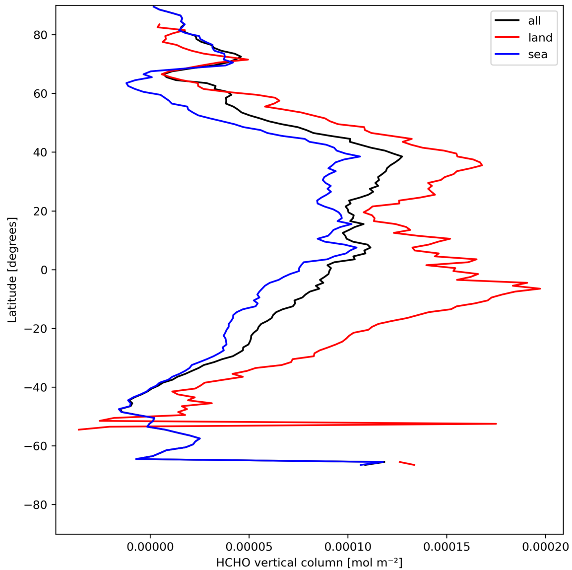
Figure 21: Zonal average of “HCHO vertical column” for 2023-07-30 to 2023-08-01.
