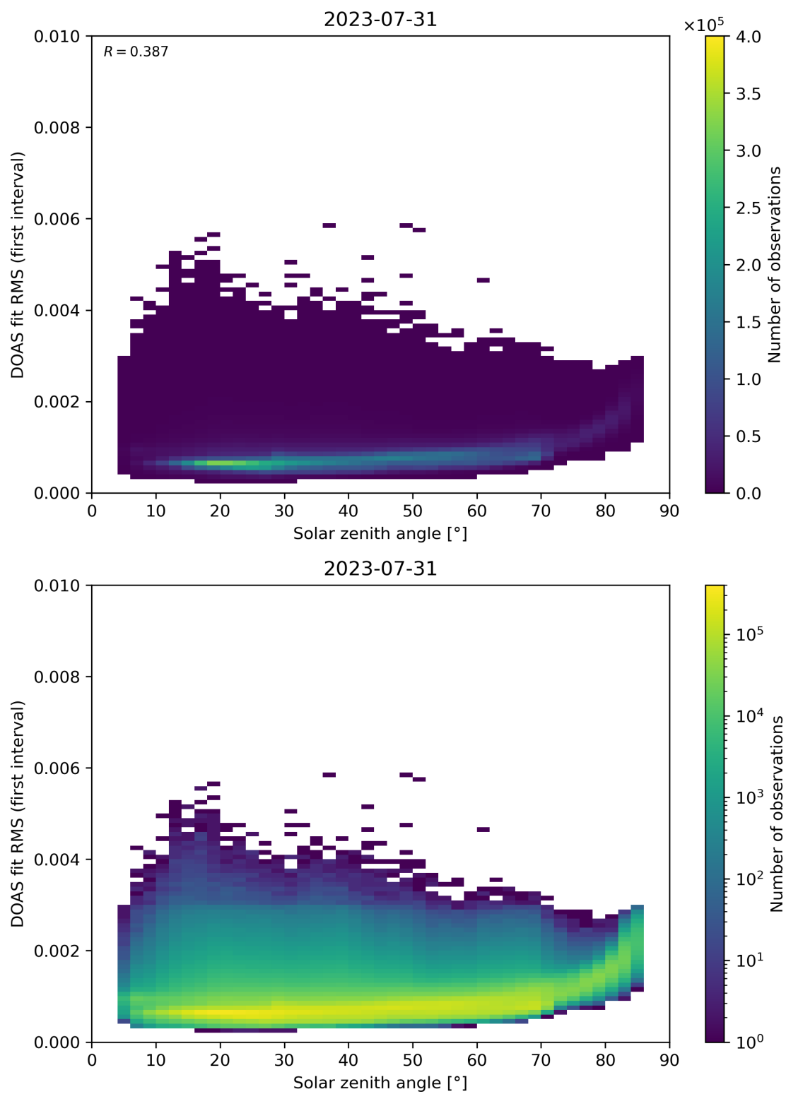
Figure 167: Scatter density plot of “Solar zenith angle” against “DOAS fit RMS (first interval)” for 2023-07-30 to 2023-08-01.
