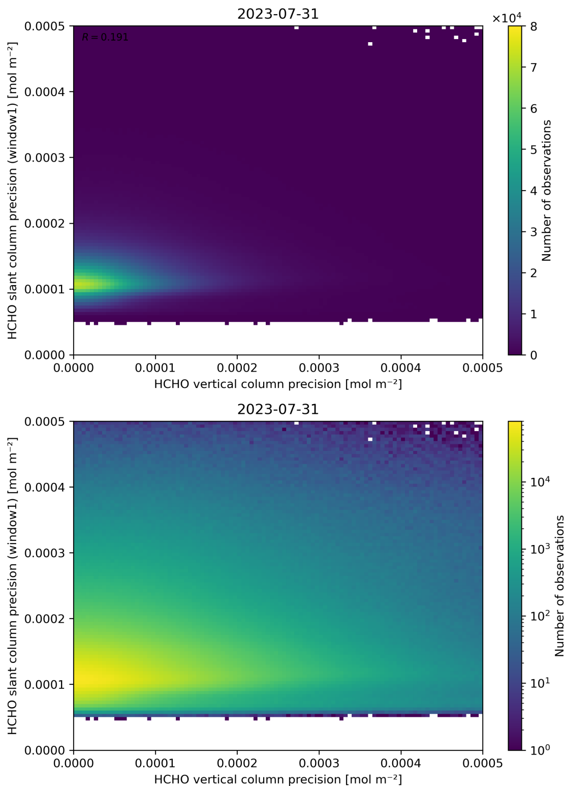
Figure 143: Scatter density plot of “HCHO vertical column precision” against “HCHO slant column precision (window1)” for 2023-07-30 to 2023-08-01.
