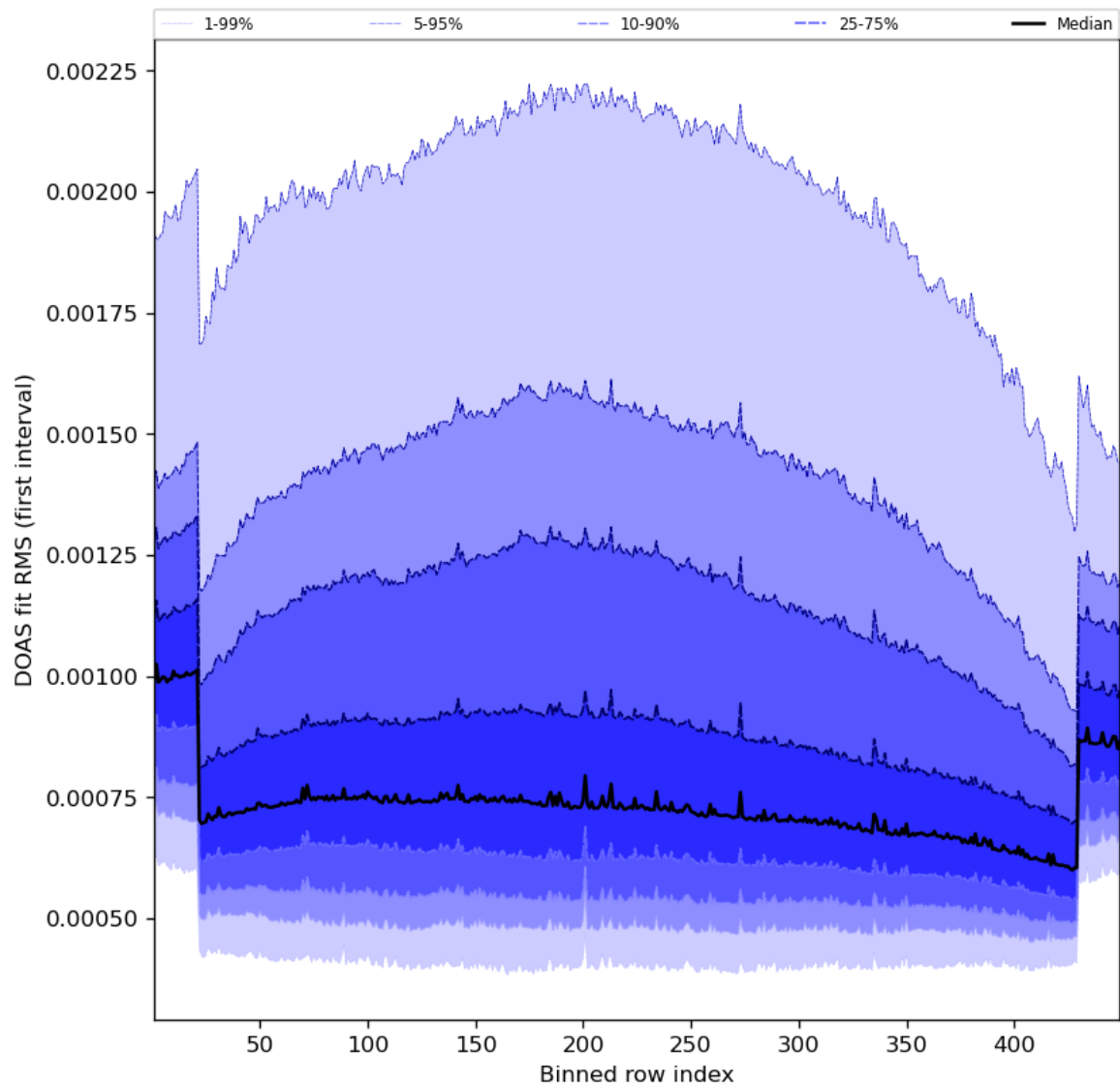
Figure 60: Along track statistics of “DOAS fit RMS (first interval)” for 2023-07-30 to 2023-08-01
