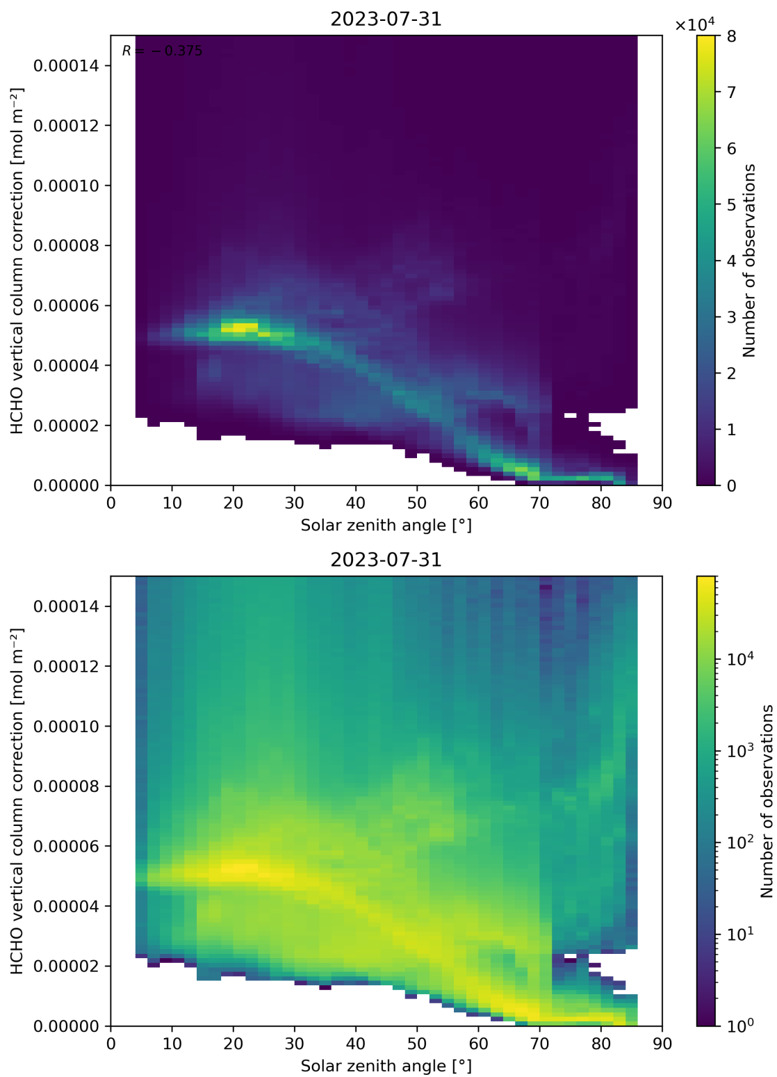
Figure 178: Scatter density plot of “Solar zenith angle” against “HCHO vertical column correction” for 2023-07-30 to 2023-08-01.
