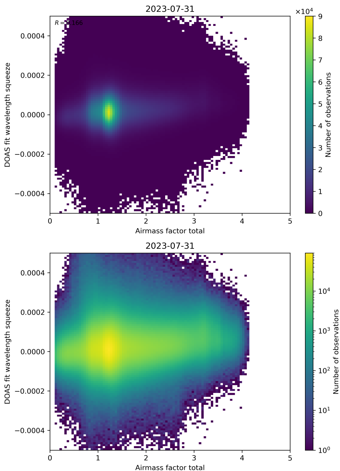
Figure 99: Scatter density plot of “Airmass factor total” against “DOAS fit wavelength squeeze” for 2023-07-30 to 2023-08-01.
