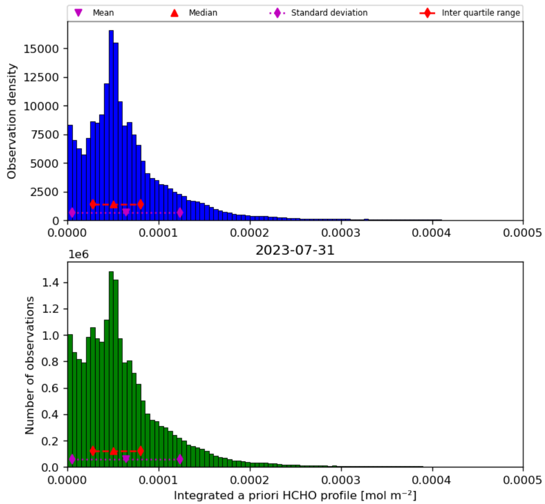
Figure 43: Histogram of “Integrated a priori HCHO profile” for 2023-07-30 to 2023-08-01
