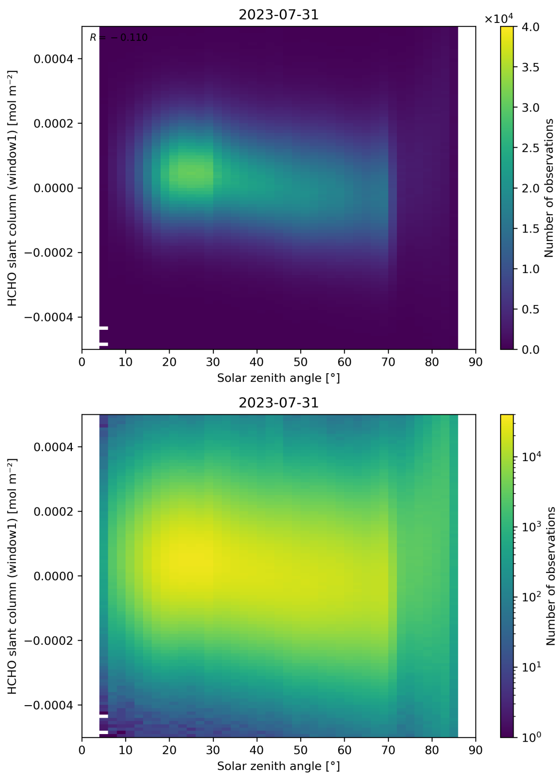
Figure 173: Scatter density plot of “Solar zenith angle” against “HCHO slant column (window1)” for 2023-07-30 to 2023-08-01.
