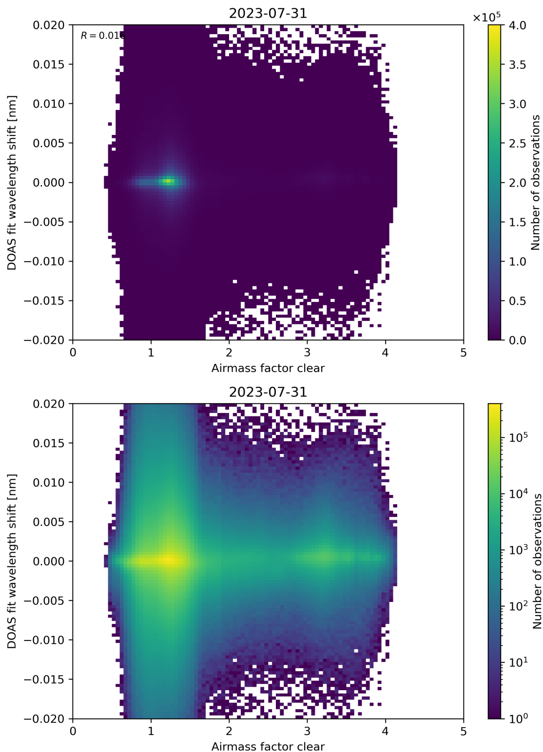
Figure 72: Scatter density plot of “Airmass factor clear” against “DOAS fit wavelength shift” for 2023-07-30 to 2023-08-01.
