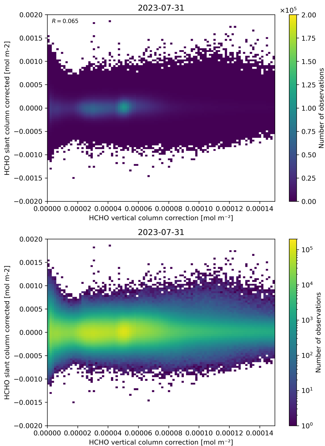
Figure 116: Scatter density plot of “HCHO vertical column correction” against “HCHO slant column corrected” for 2023-07-30 to 2023-08-01.
