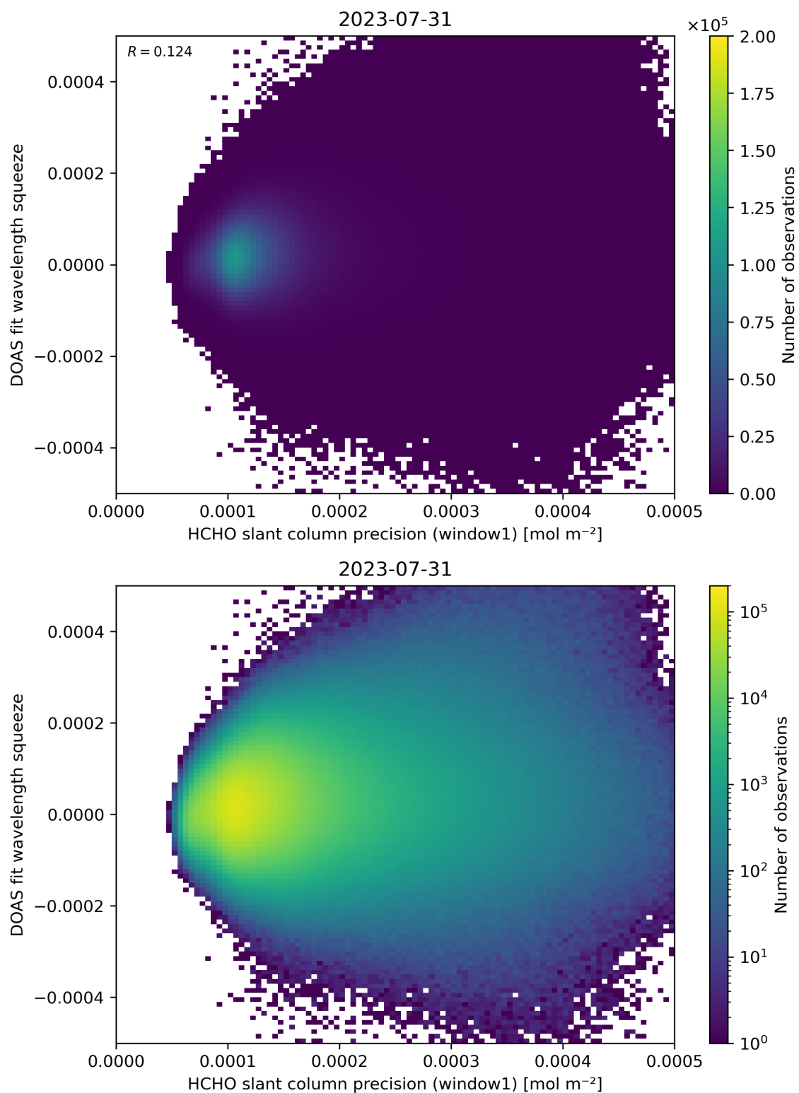
Figure 90: Scatter density plot of “HCHO slant column precision (window1)” against “DOAS fit wavelength squeeze” for 2023-07-30 to 2023-08-01.
