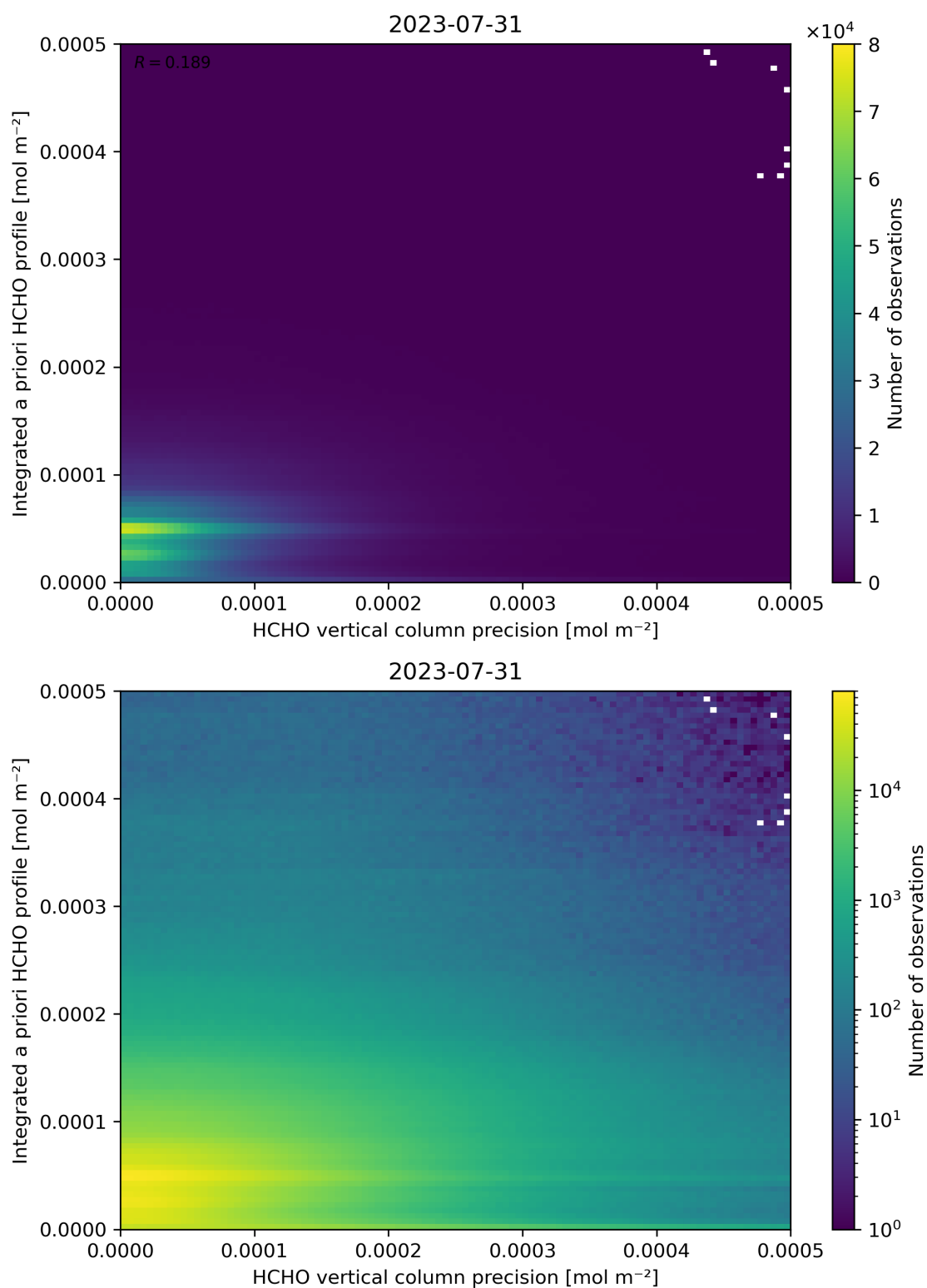
Figure 147: Scatter density plot of “HCHO vertical column precision” against “Integrated a priori HCHO profile” for 2023-07-30 to 2023-08-01.
