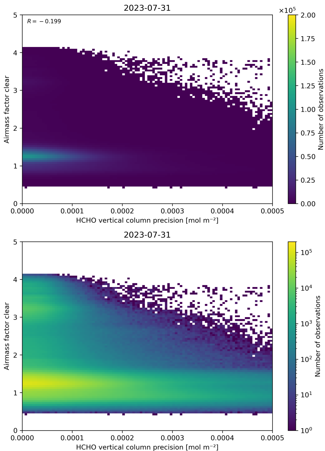
Figure 139: Scatter density plot of “HCHO vertical column precision” against “Airmass factor clear” for 2023-07-30 to 2023-08-01.
