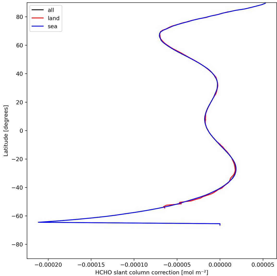
Figure 33: Zonal average of “HCHO slant column correction” for 2023-07-30 to 2023-08-01.
