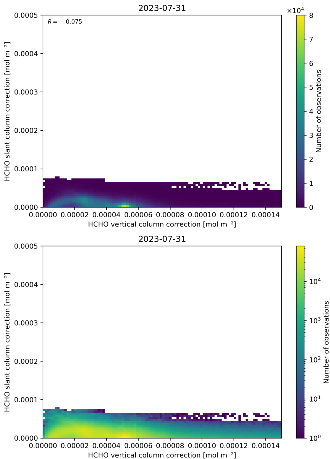
Figure 117: Scatter density plot of “HCHO vertical column correction” against “HCHO slant column correction” for 2023-07-30 to 2023-08-01.
