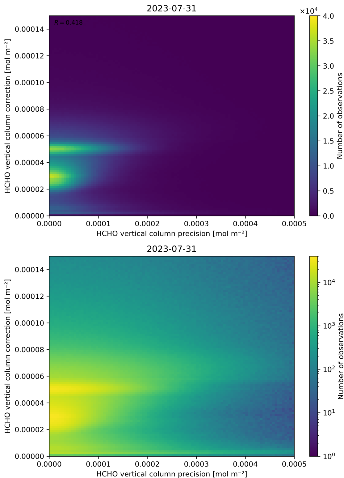
Figure 146: Scatter density plot of “HCHO vertical column precision” against “HCHO vertical column correction” for 2023-07-30 to 2023-08-01.
