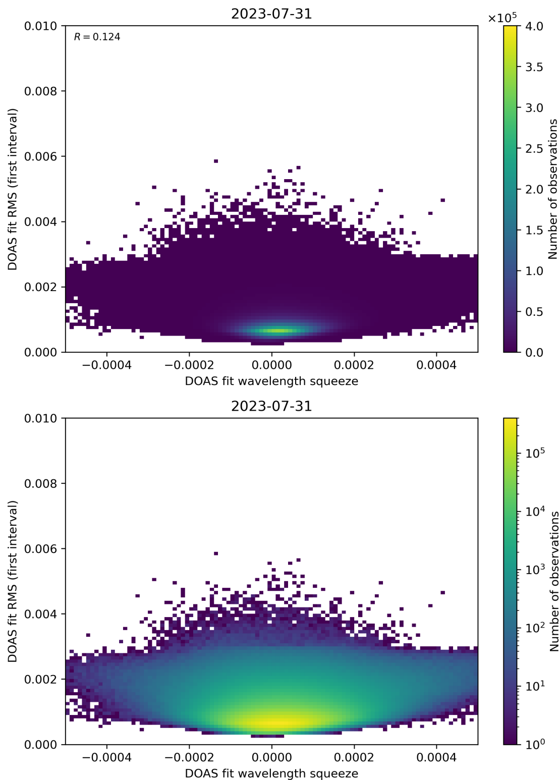
Figure 68: Scatter density plot of “DOAS fit wavelength squeeze” against “DOAS fit RMS (first interval)” for 2023-07-30 to 2023-08-01.
