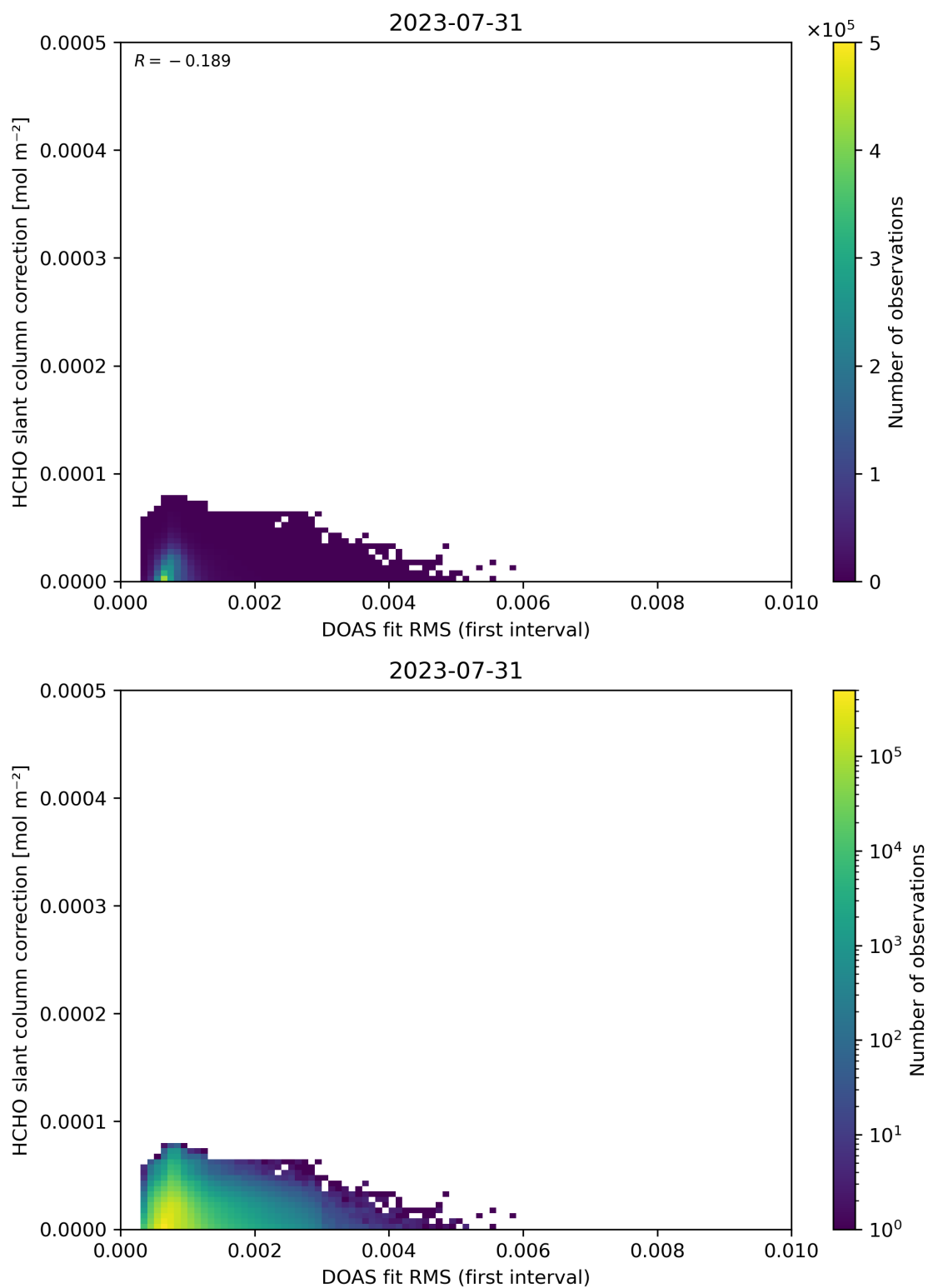
Figure 63: Scatter density plot of “DOAS fit RMS (first interval)” against “HCHO slant column correction” for 2023-07-30 to 2023-08-01.
