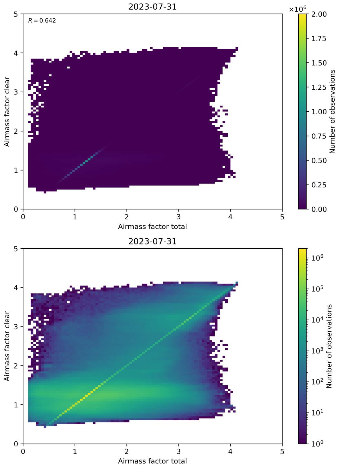
Figure 100: Scatter density plot of “Airmass factor total” against “Airmass factor clear” for 2023-07-30 to 2023-08-01.
