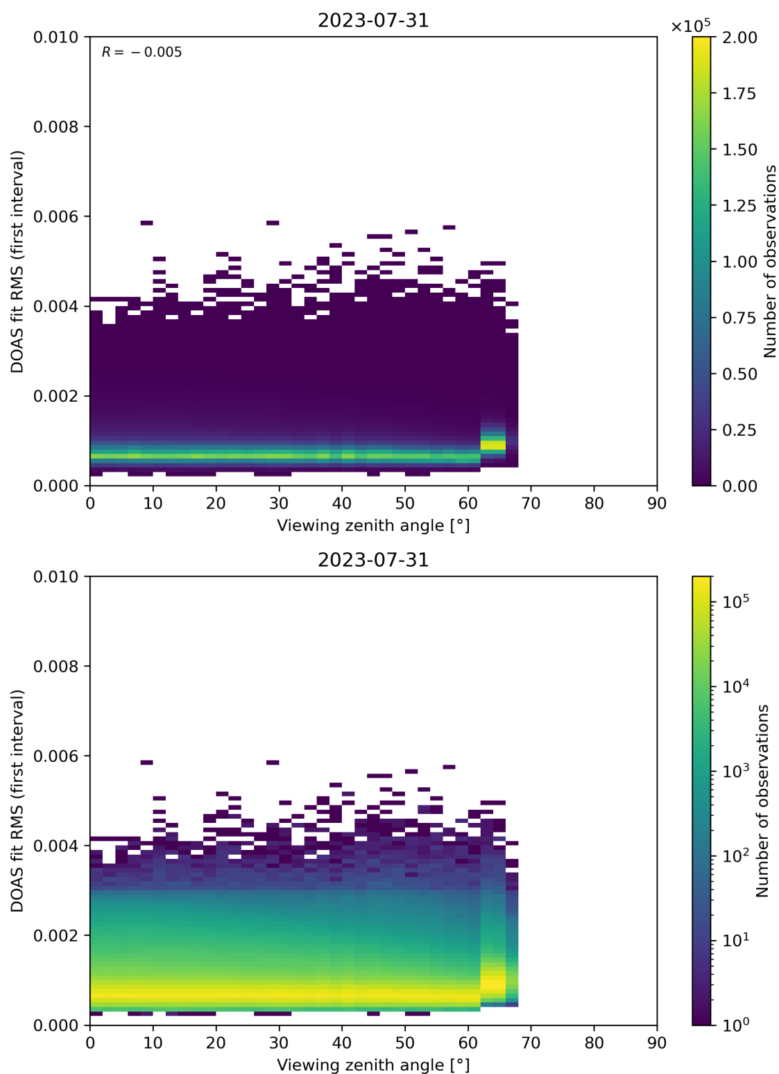
Figure 182: Scatter density plot of “Viewing zenith angle” against “DOAS fit RMS (first interval)” for 2023-07-30 to 2023-08-01.
