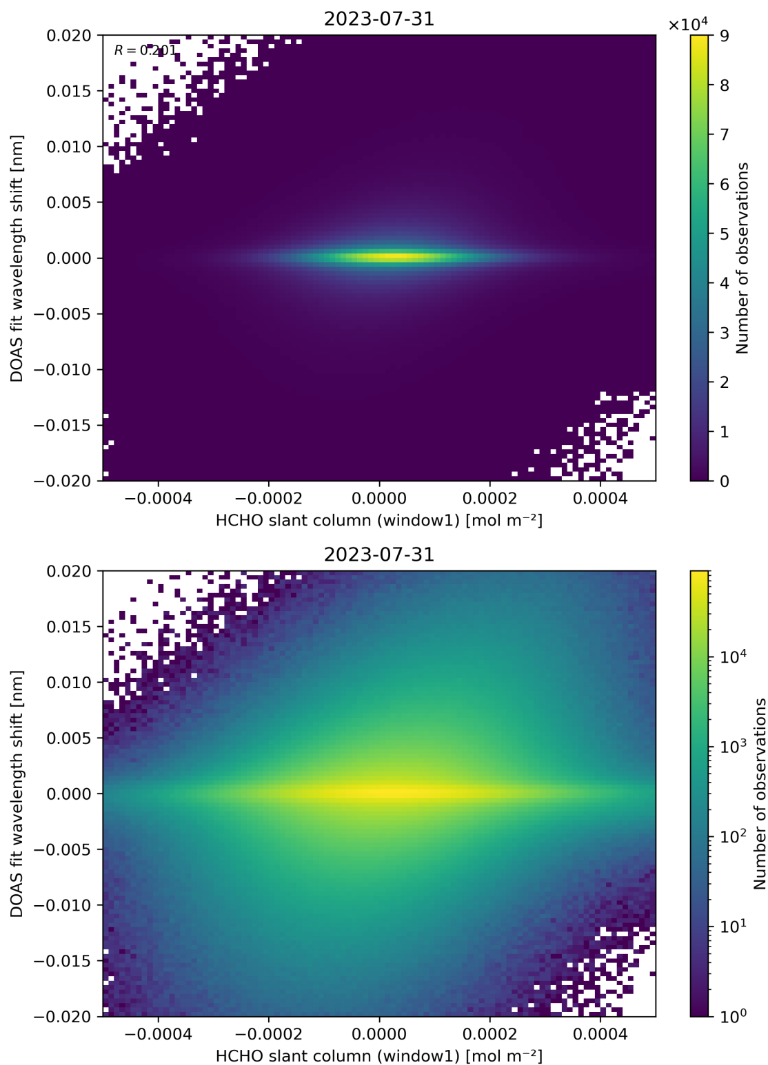
Figure 79: Scatter density plot of “HCHO slant column (window1)” against “DOAS fit wavelength shift” for 2023-07-30 to 2023-08-01.
