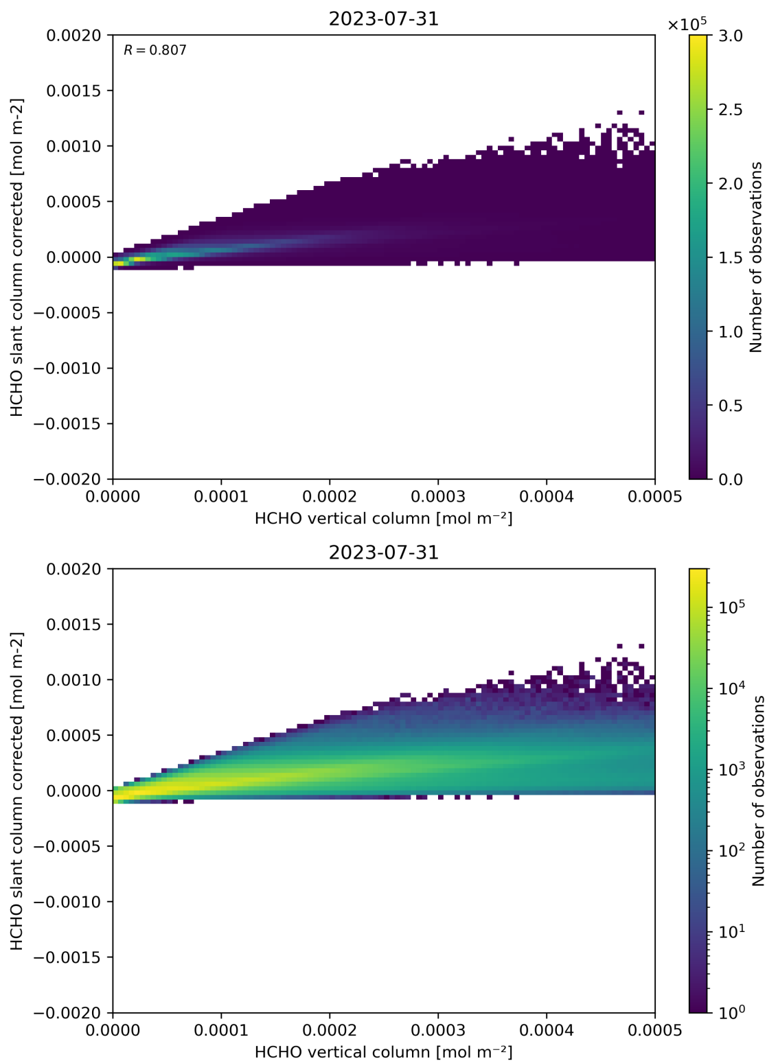
Figure 127: Scatter density plot of “HCHO vertical column” against “HCHO slant column corrected” for 2023-07-30 to 2023-08-01.
