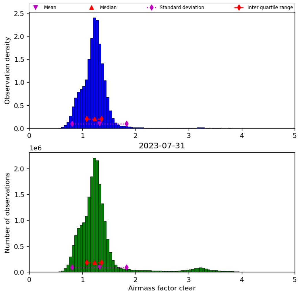
Figure 42: Histogram of “Airmass factor clear” for 2023-07-30 to 2023-08-01
