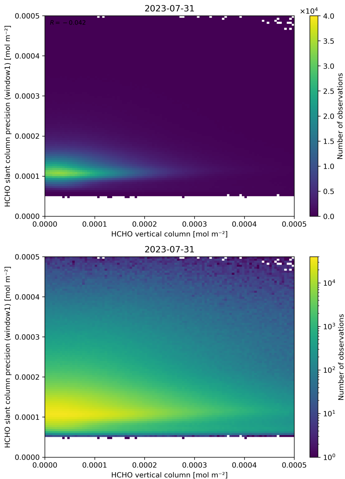
Figure 130: Scatter density plot of “HCHO vertical column” against “HCHO slant column precision (window1)” for 2023-07-30 to 2023-08-01.
