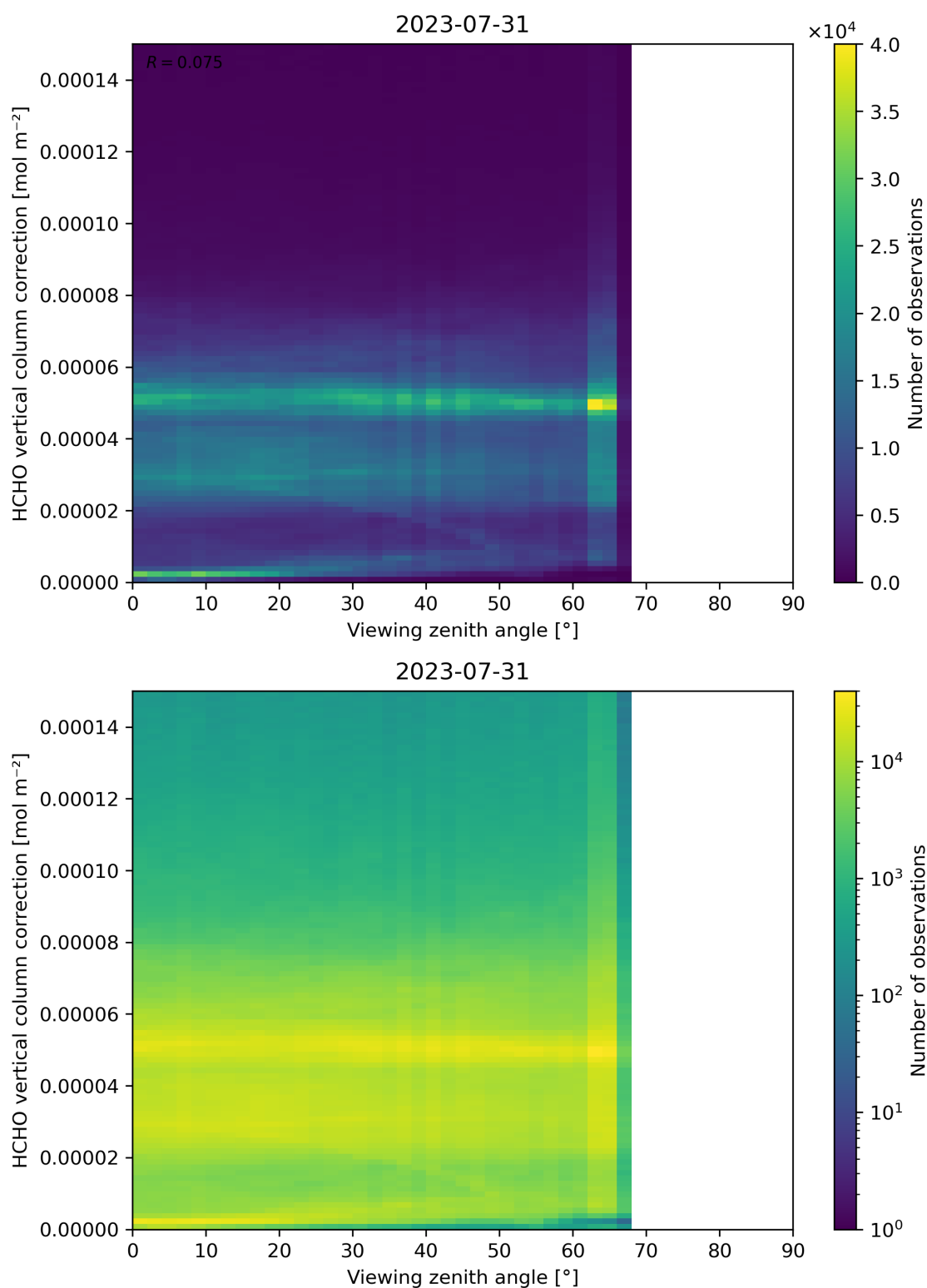
Figure 193: Scatter density plot of “Viewing zenith angle” against “HCHO vertical column correction” for 2023-07-30 to 2023-08-01.
