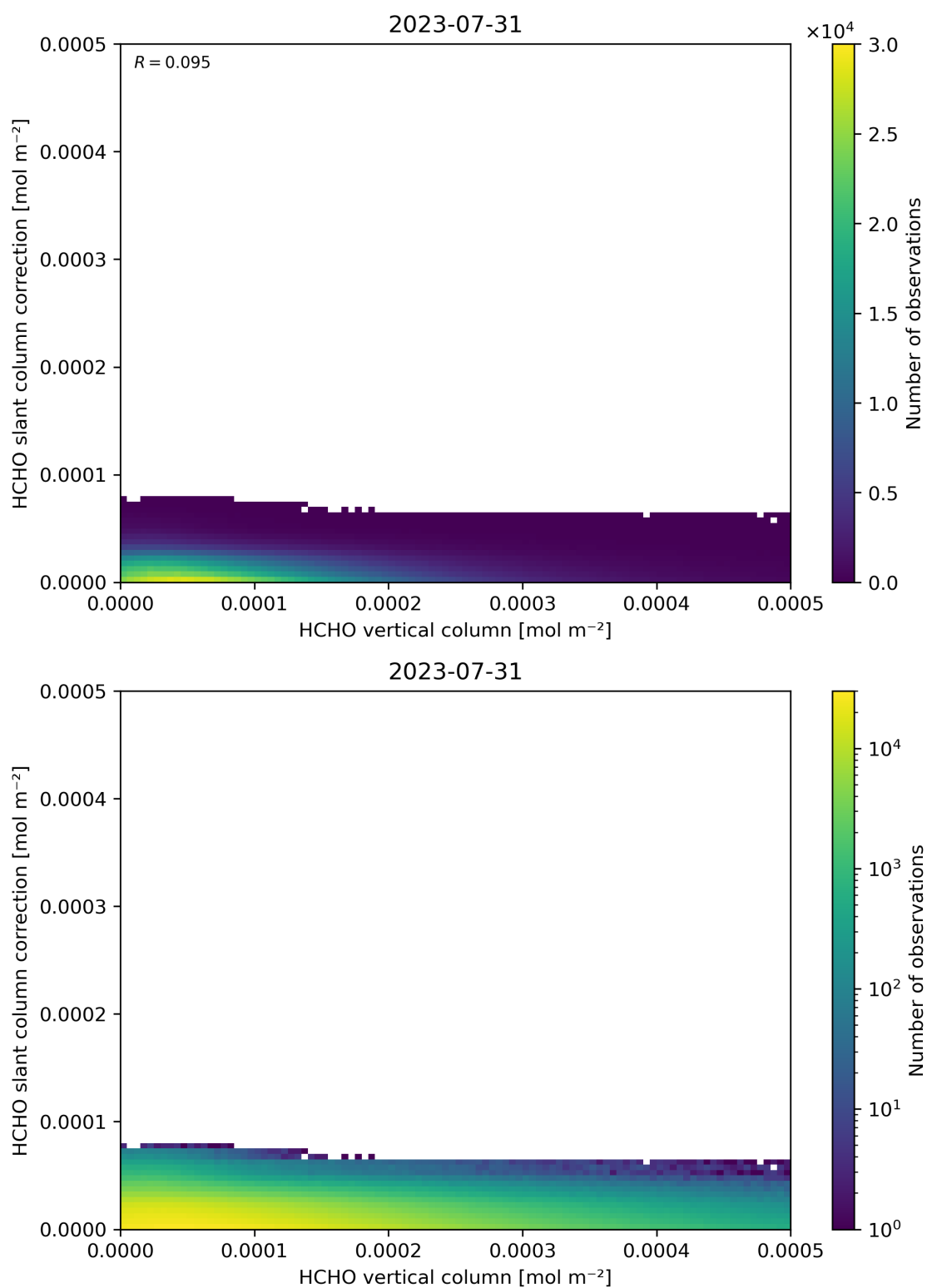
Figure 128: Scatter density plot of “HCHO vertical column” against “HCHO slant column correction” for 2023-07-30 to 2023-08-01.
