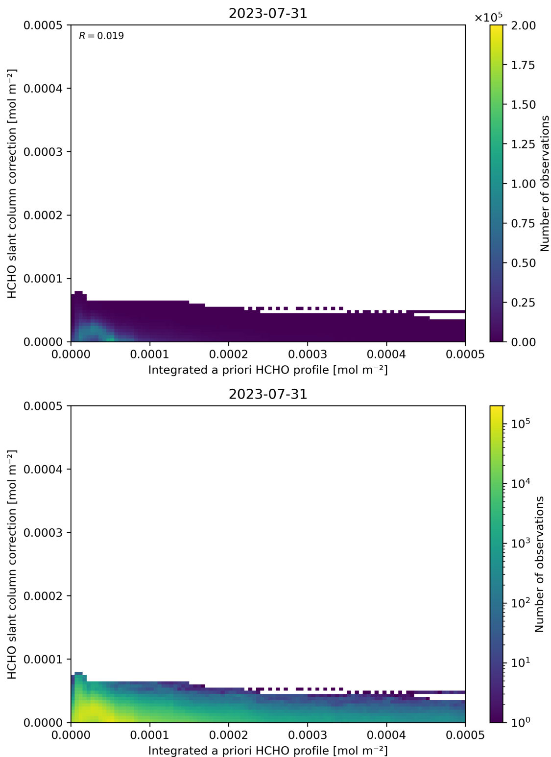
Figure 152: Scatter density plot of “Integrated a priori HCHO profile” against “HCHO slant column correction” for 2023-07-30 to 2023-08-01.
