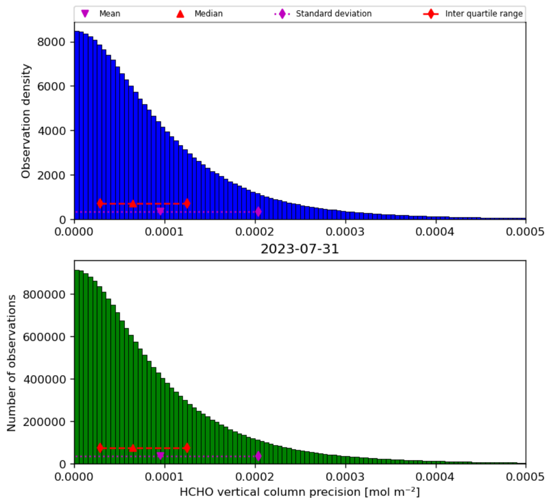
Figure 36: Histogram of “HCHO vertical column precision” for 2023-07-30 to 2023-08-01
