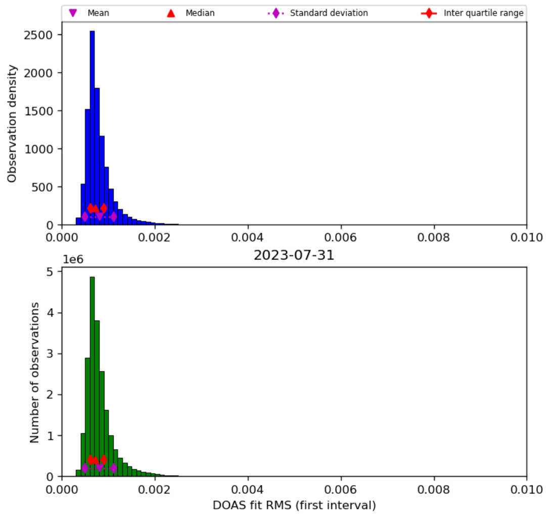
Figure 46: Histogram of “DOAS fit RMS (first interval)” for 2023-07-30 to 2023-08-01
