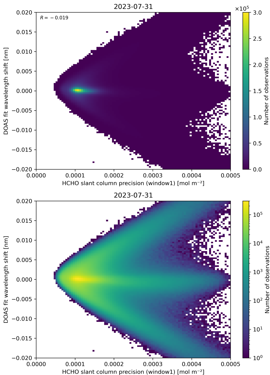
Figure 89: Scatter density plot of “HCHO slant column precision (window1)” against “DOAS fit wavelength shift” for 2023-07-30 to 2023-08-01.
