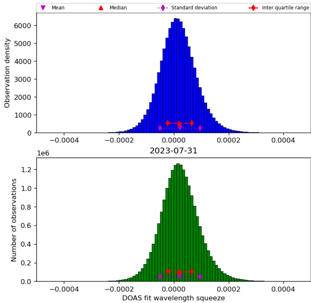
Figure 45: Histogram of “DOAS fit wavelength squeeze” for 2023-07-30 to 2023-08-01
