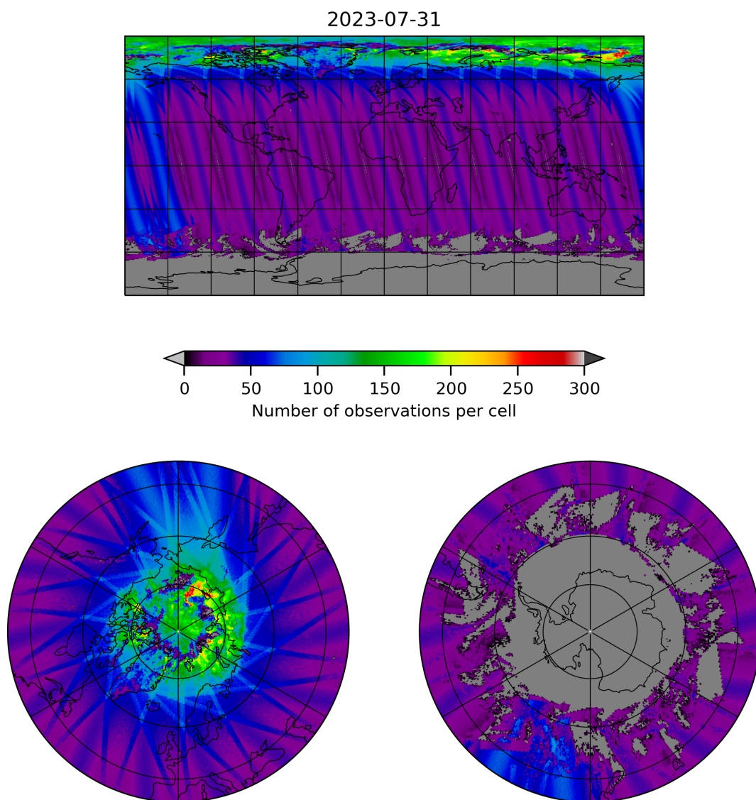
Figure 19: Map of the number of observations for 2023-07-30 to 2023-08-01
