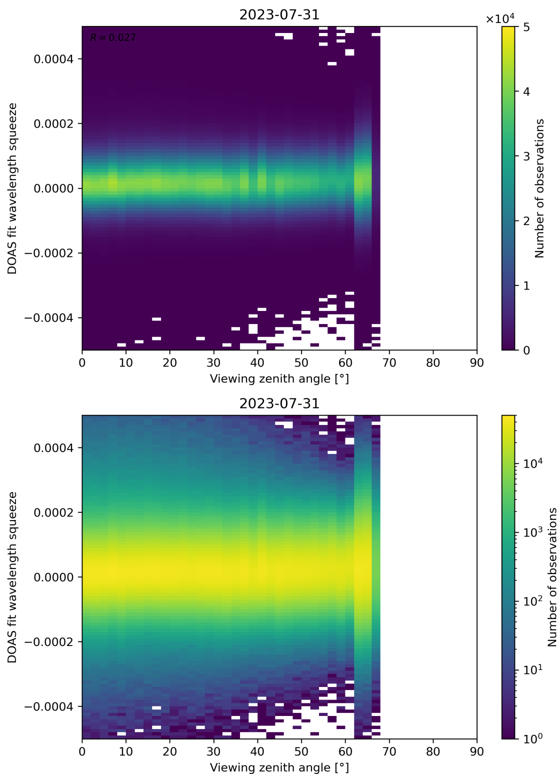
Figure 184: Scatter density plot of “Viewing zenith angle” against “DOAS fit wavelength squeeze” for 2023-07-30 to 2023-08-01.
