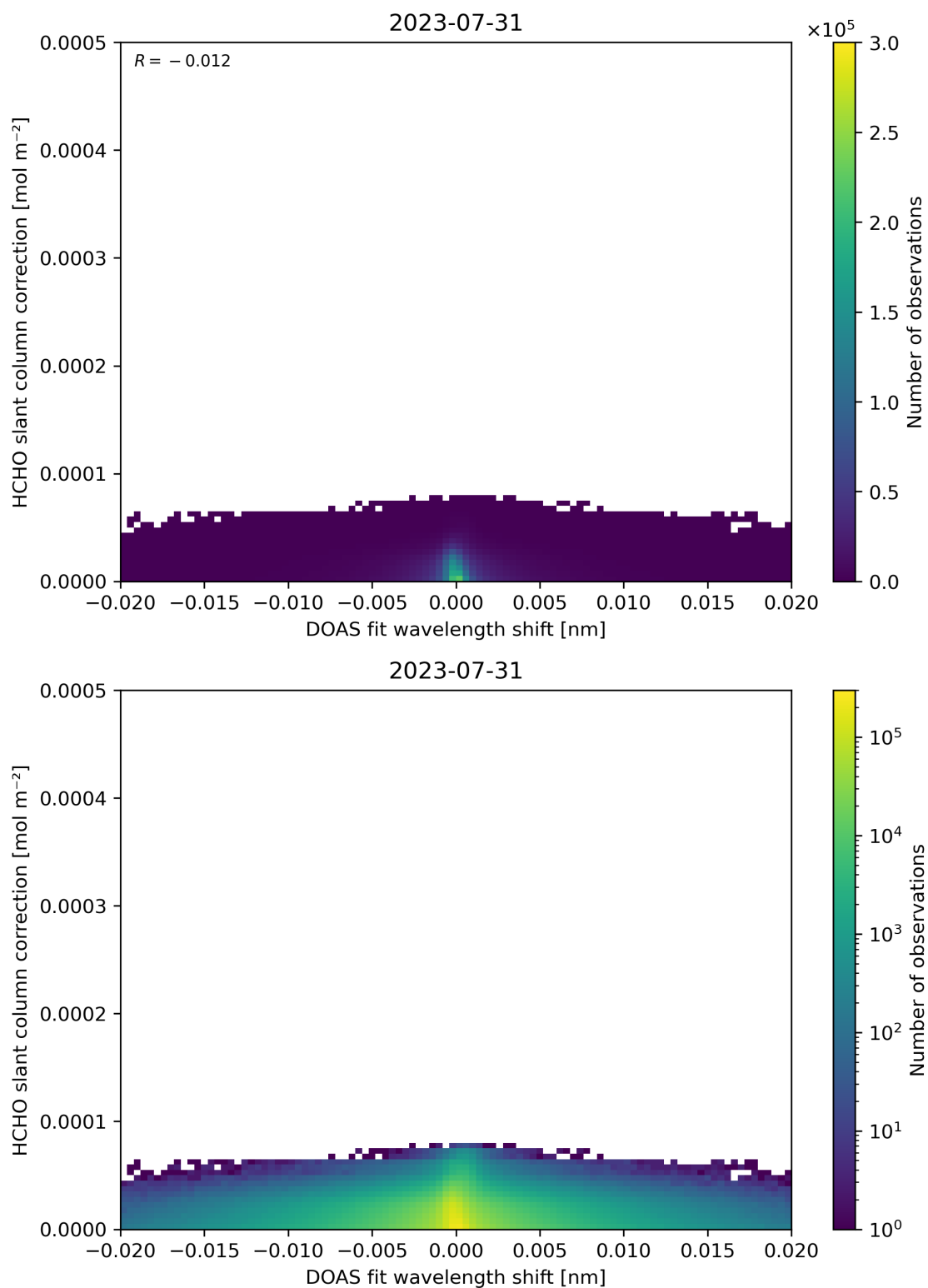
Figure 67: Scatter density plot of “DOAS fit wavelength shift” against “HCHO slant column correction” for 2023-07-30 to 2023-08-01.
