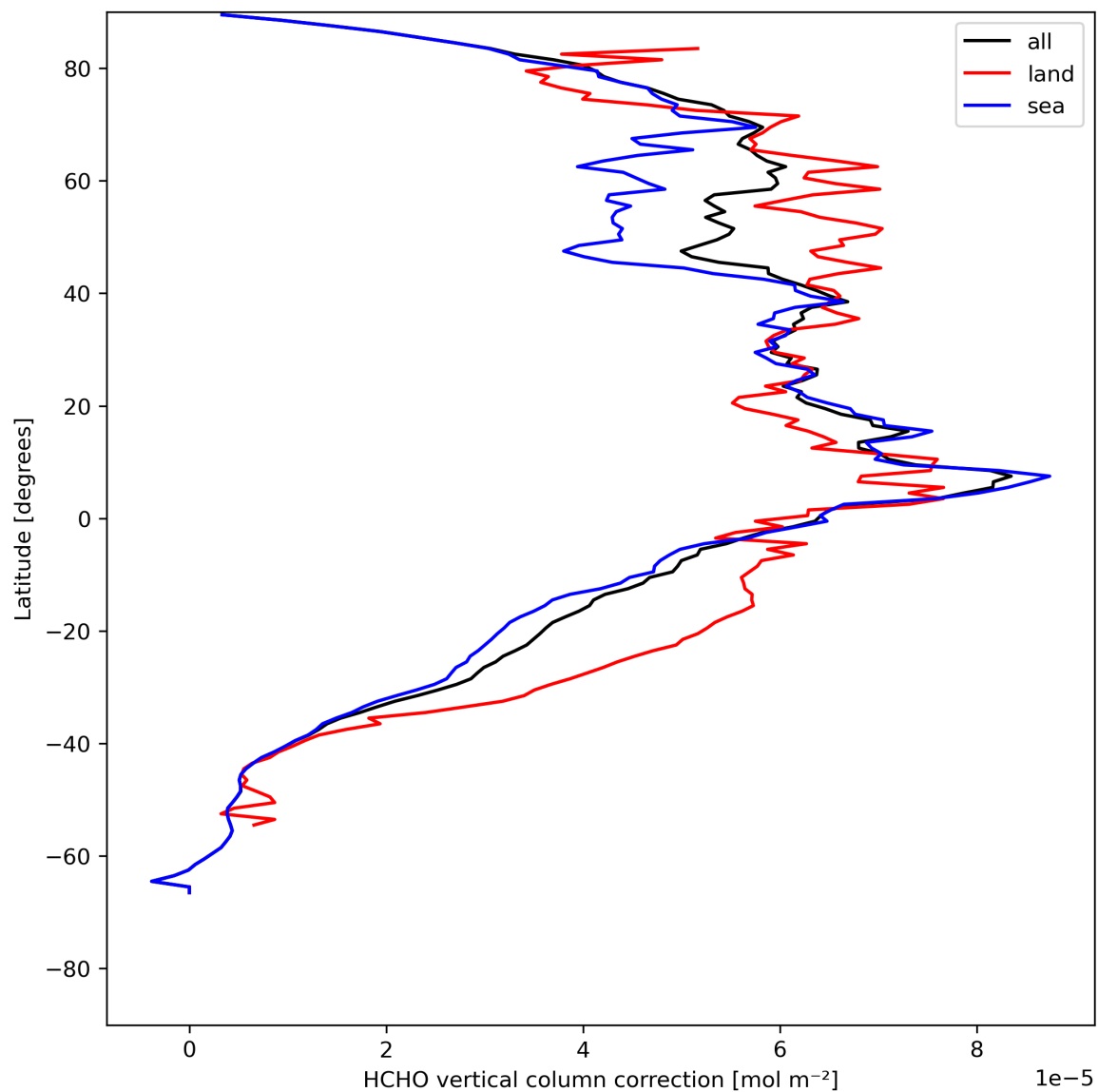
Figure 23: Zonal average of “HCHO vertical column correction” for 2023-07-30 to 2023-08-01.
