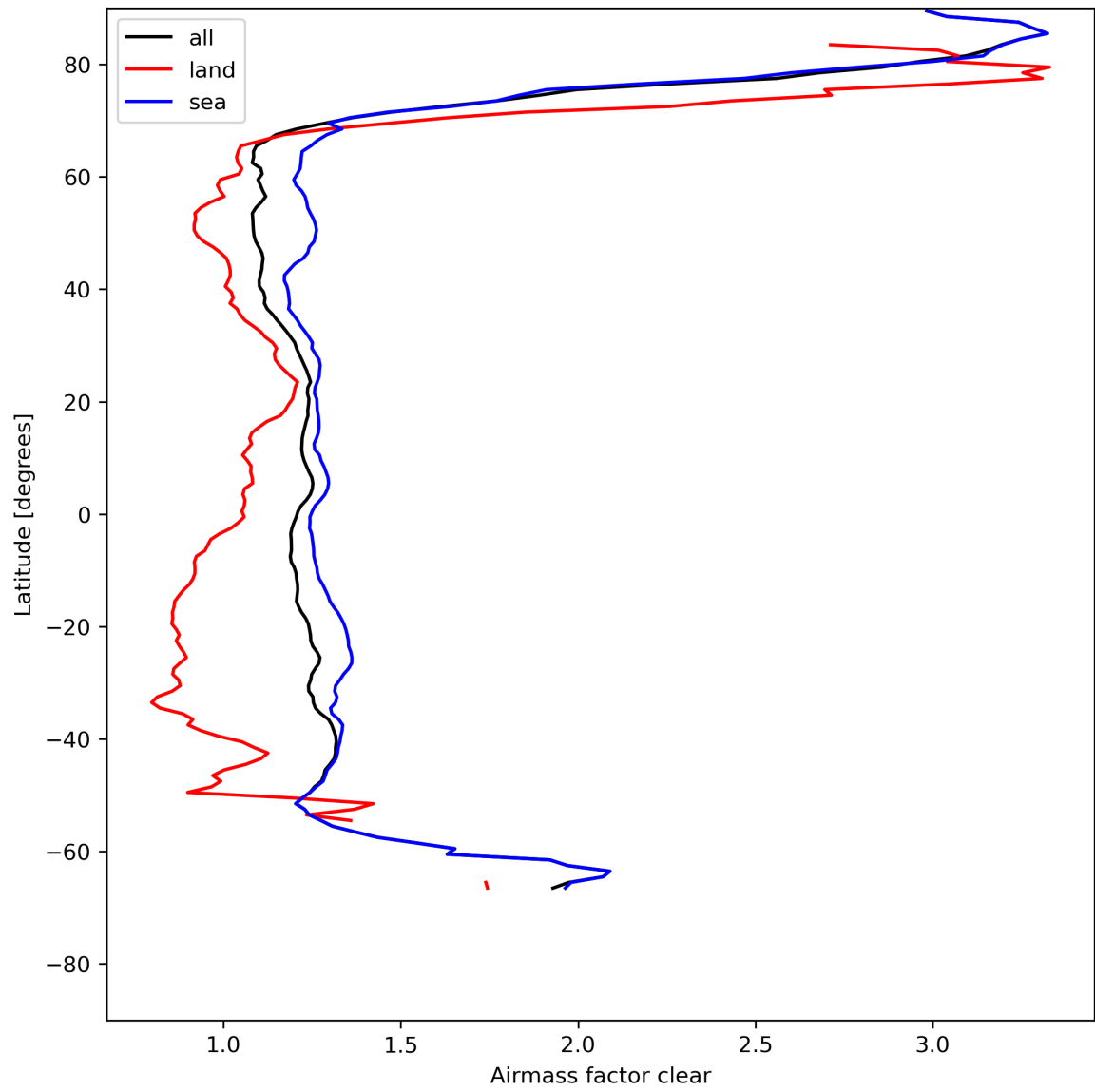
Figure 28: Zonal average of “Airmass factor clear” for 2023-07-30 to 2023-08-01.
