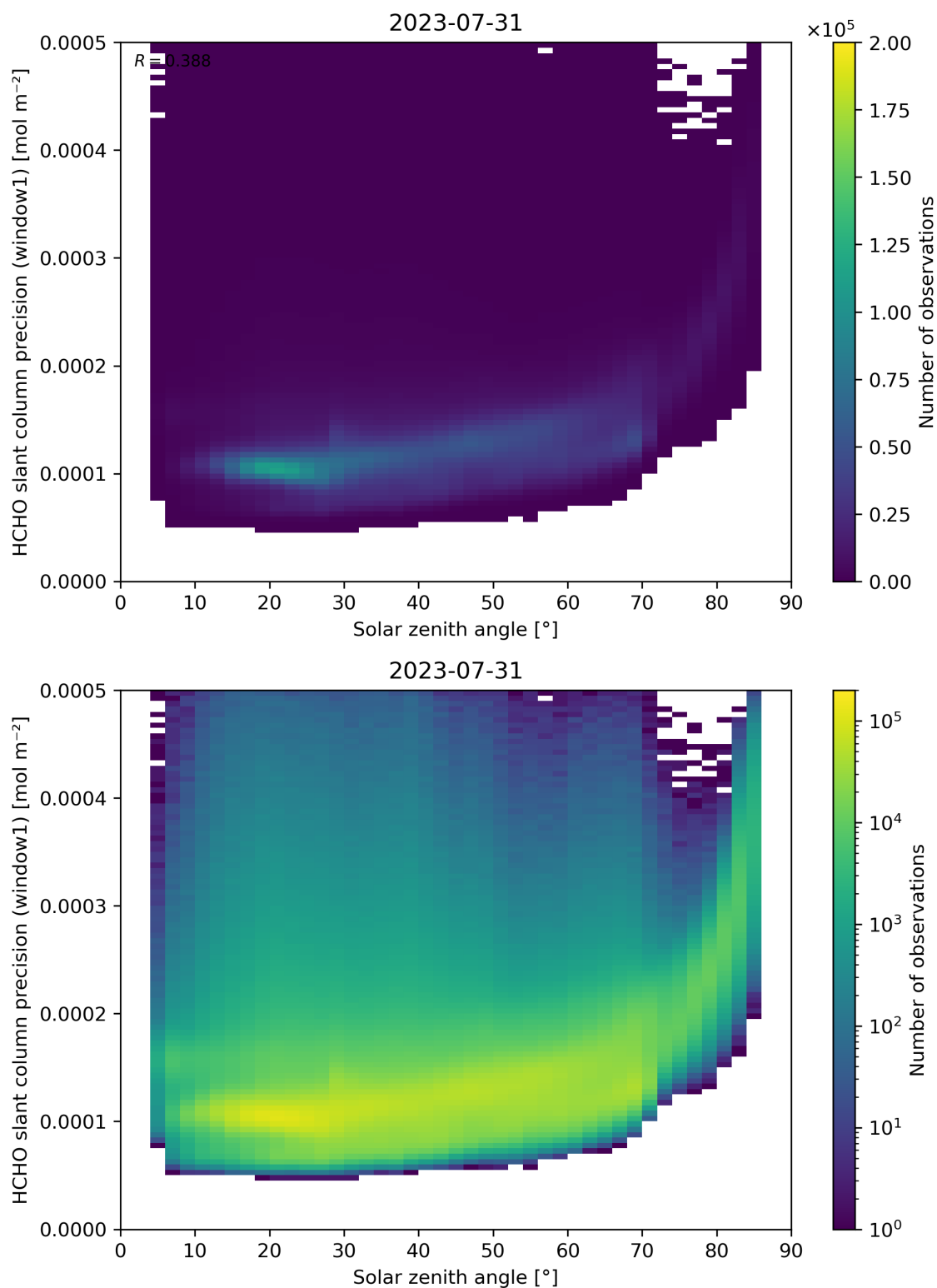
Figure 174: Scatter density plot of “Solar zenith angle” against “HCHO slant column precision (window1)” for 2023-07-30 to 2023-08-01.
