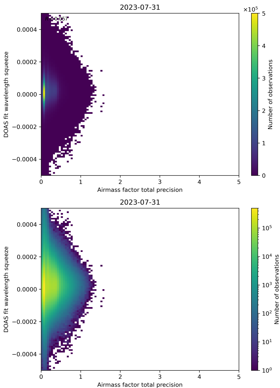
Figure 107: Scatter density plot of “Airmass factor total precision” against “DOAS fit wavelength squeeze” for 2023-07-30 to 2023-08-01.
