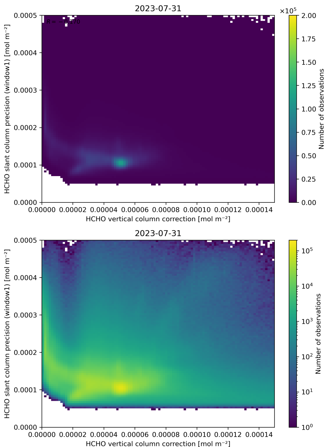
Figure 119: Scatter density plot of “HCHO vertical column correction” against “HCHO slant column precision (window1)” for 2023-07-30 to 2023-08-01.
