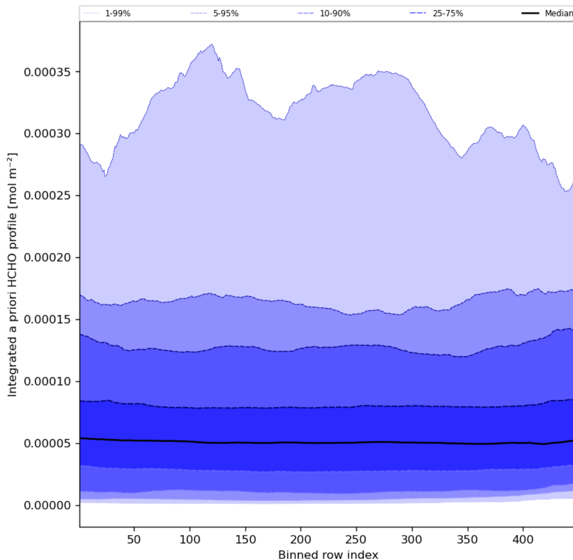
Figure 57: Along track statistics of “Integrated a priori HCHO profile” for 2023-07-30 to 2023-08-01
