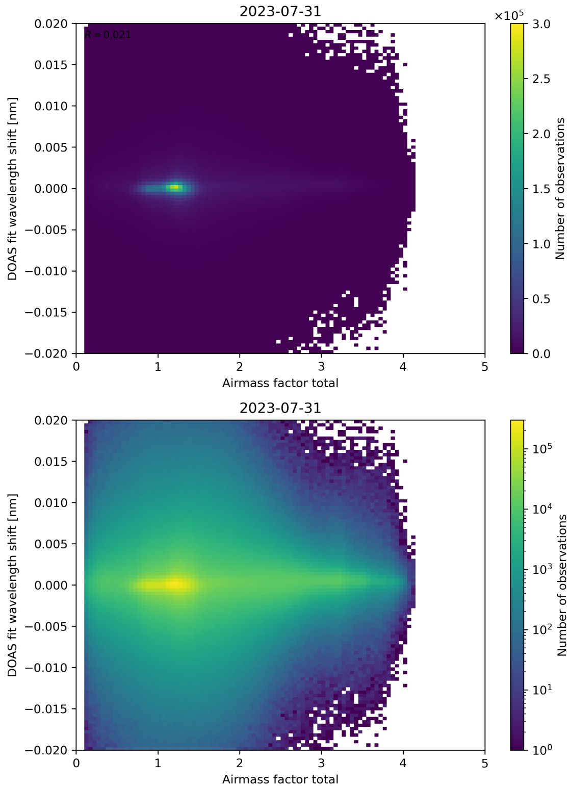
Figure 98: Scatter density plot of “Airmass factor total” against “DOAS fit wavelength shift” for 2023-07-30 to 2023-08-01.
