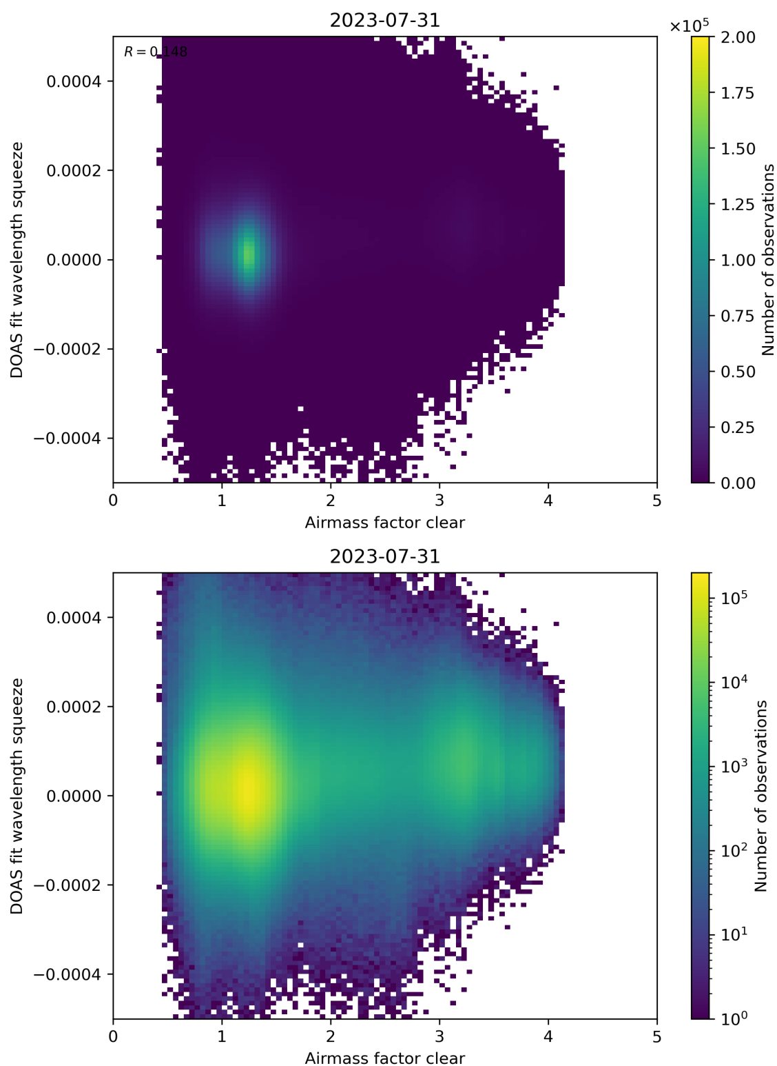
Figure 73: Scatter density plot of “Airmass factor clear” against “DOAS fit wavelength squeeze” for 2023-07-30 to 2023-08-01.
