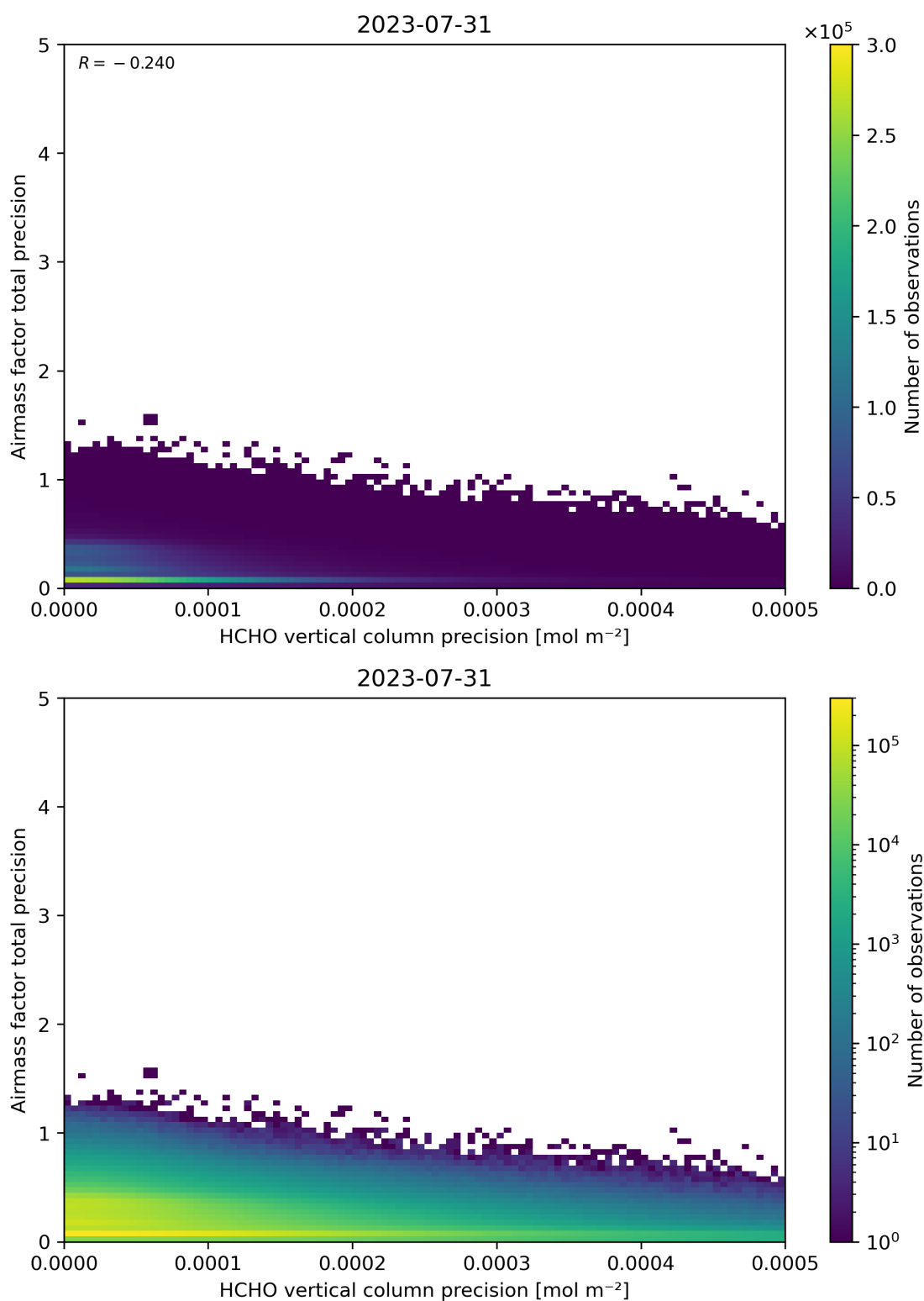
Figure 145: Scatter density plot of “HCHO vertical column precision” against “Airmass factor total precision” for 2023-07-30 to 2023-08-01.
