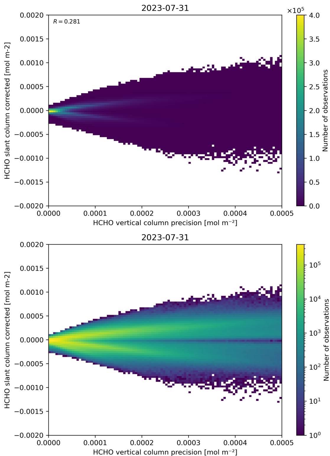
Figure 140: Scatter density plot of “HCHO vertical column precision” against “HCHO slant column corrected” for 2023-07-30 to 2023-08-01.
