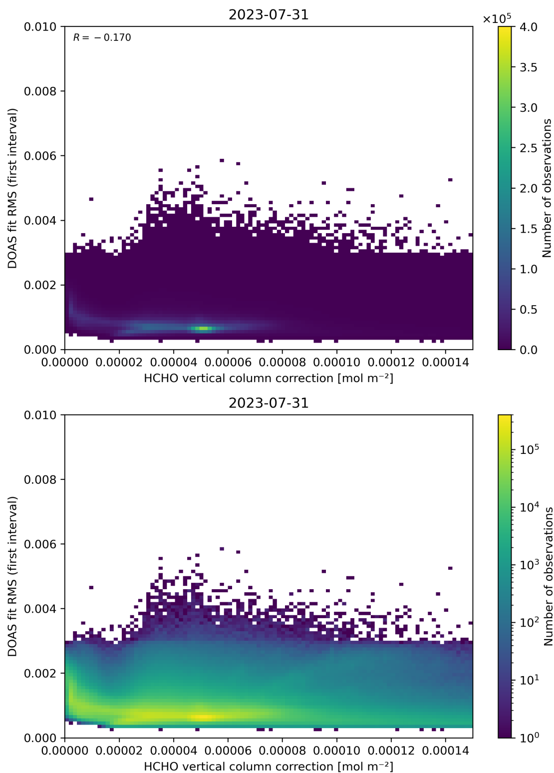
Figure 112: Scatter density plot of “HCHO vertical column correction” against “DOAS fit RMS (first interval)” for 2023-07-30 to 2023-08-01.
