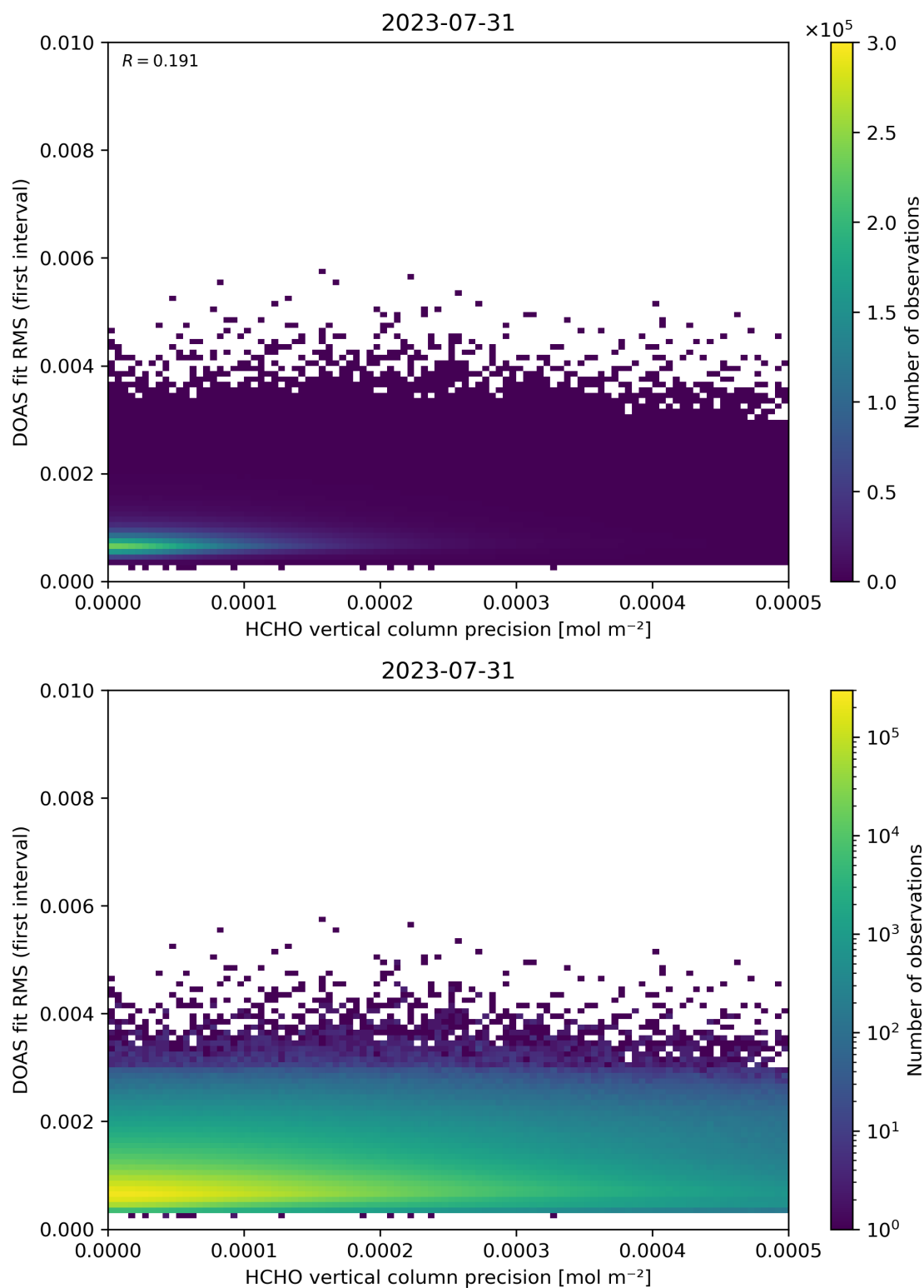
Figure 136: Scatter density plot of “HCHO vertical column precision” against “DOAS fit RMS (first interval)” for 2023-07-30 to 2023-08-01.
