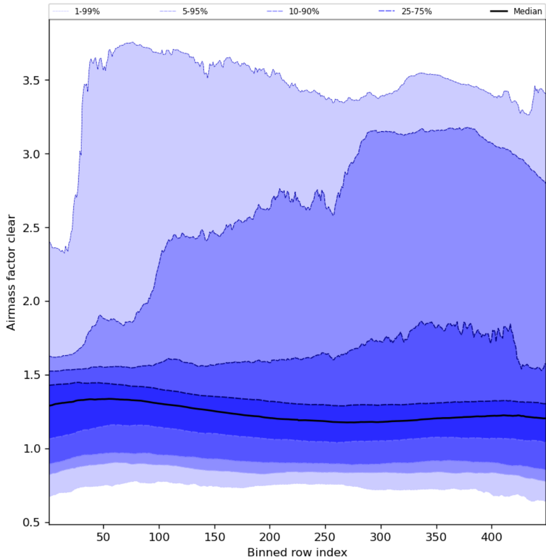
Figure 56: Along track statistics of “Airmass factor clear” for 2023-07-30 to 2023-08-01
