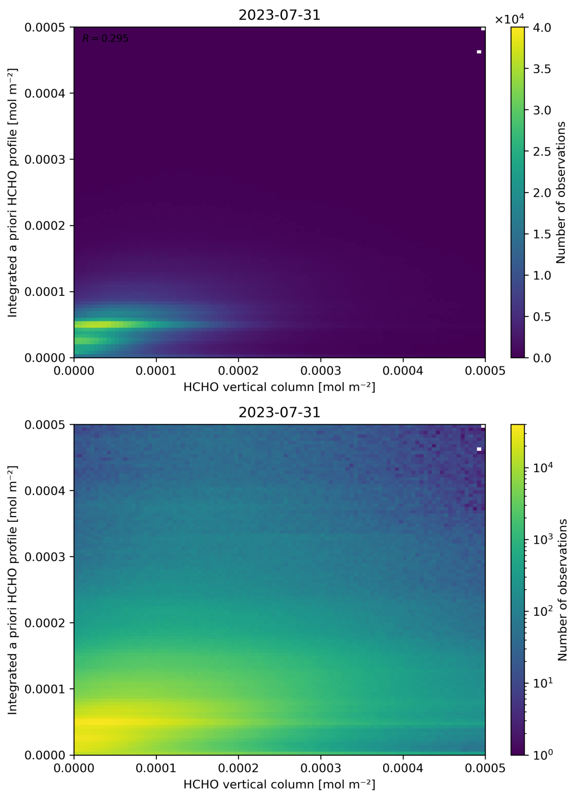
Figure 135: Scatter density plot of “HCHO vertical column” against “Integrated a priori HCHO profile” for 2023-07-30 to 2023-08-01.
