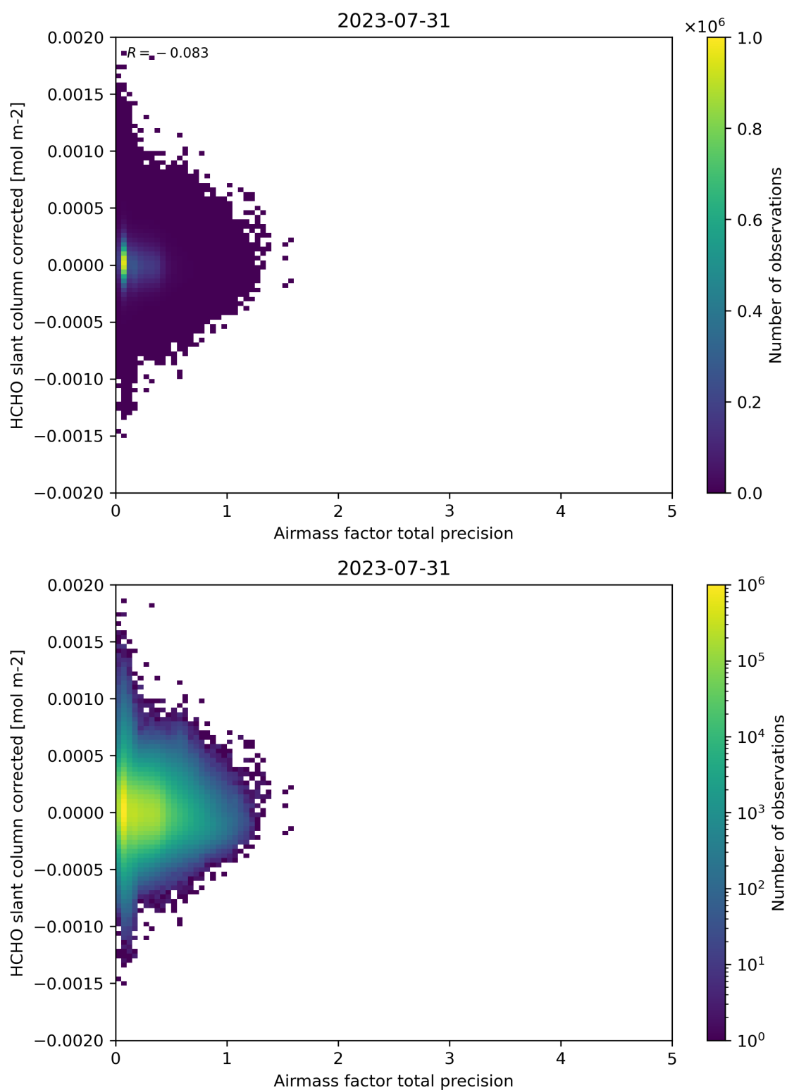
Figure 109: Scatter density plot of “Airmass factor total precision” against “HCHO slant column corrected” for 2023-07-30 to 2023-08-01.
