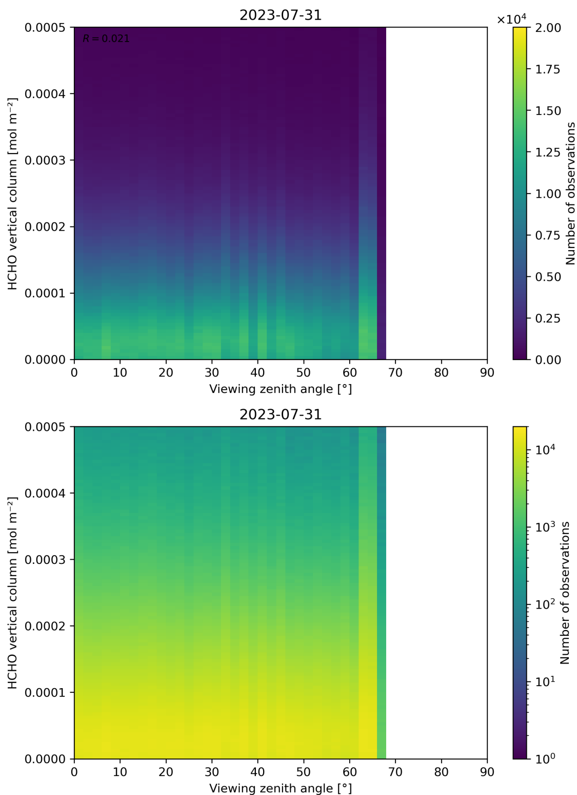
Figure 192: Scatter density plot of “Viewing zenith angle” against “HCHO vertical column” for 2023-07-30 to 2023-08-01.
