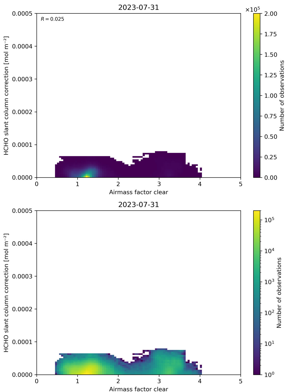
Figure 75: Scatter density plot of “Air mass factor clear” against “HCHO slant column correction” for 2023-07-30 to 2023-08-01.
