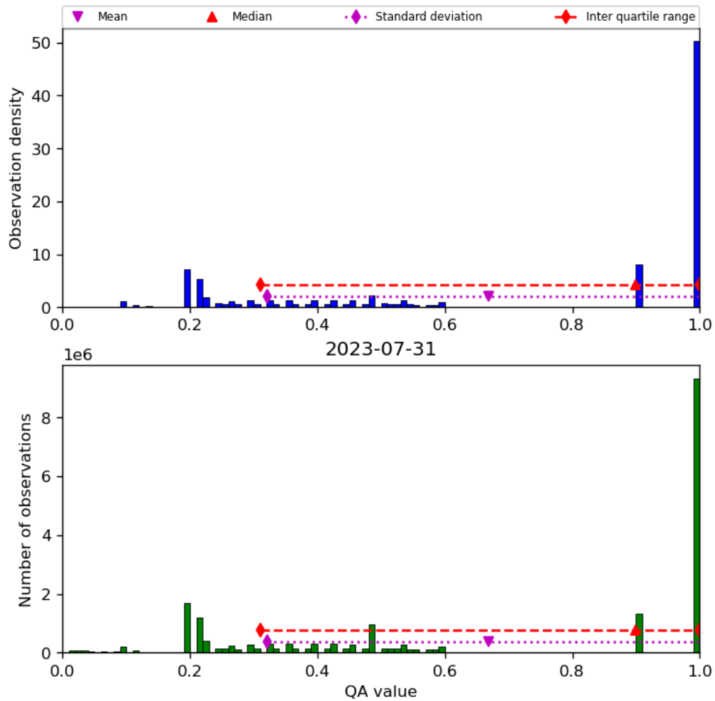
Figure 34: Histogram of “QA value” for 2023-07-30 to 2023-08-01
