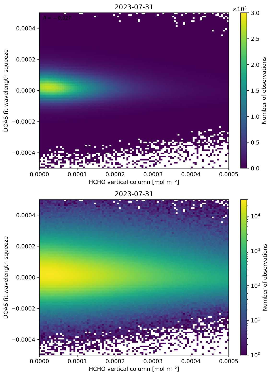
Figure 125: Scatter density plot of “HCHO vertical column” against “DOAS fit wavelength squeeze” for 2023-07-30 to 2023-08-01.
