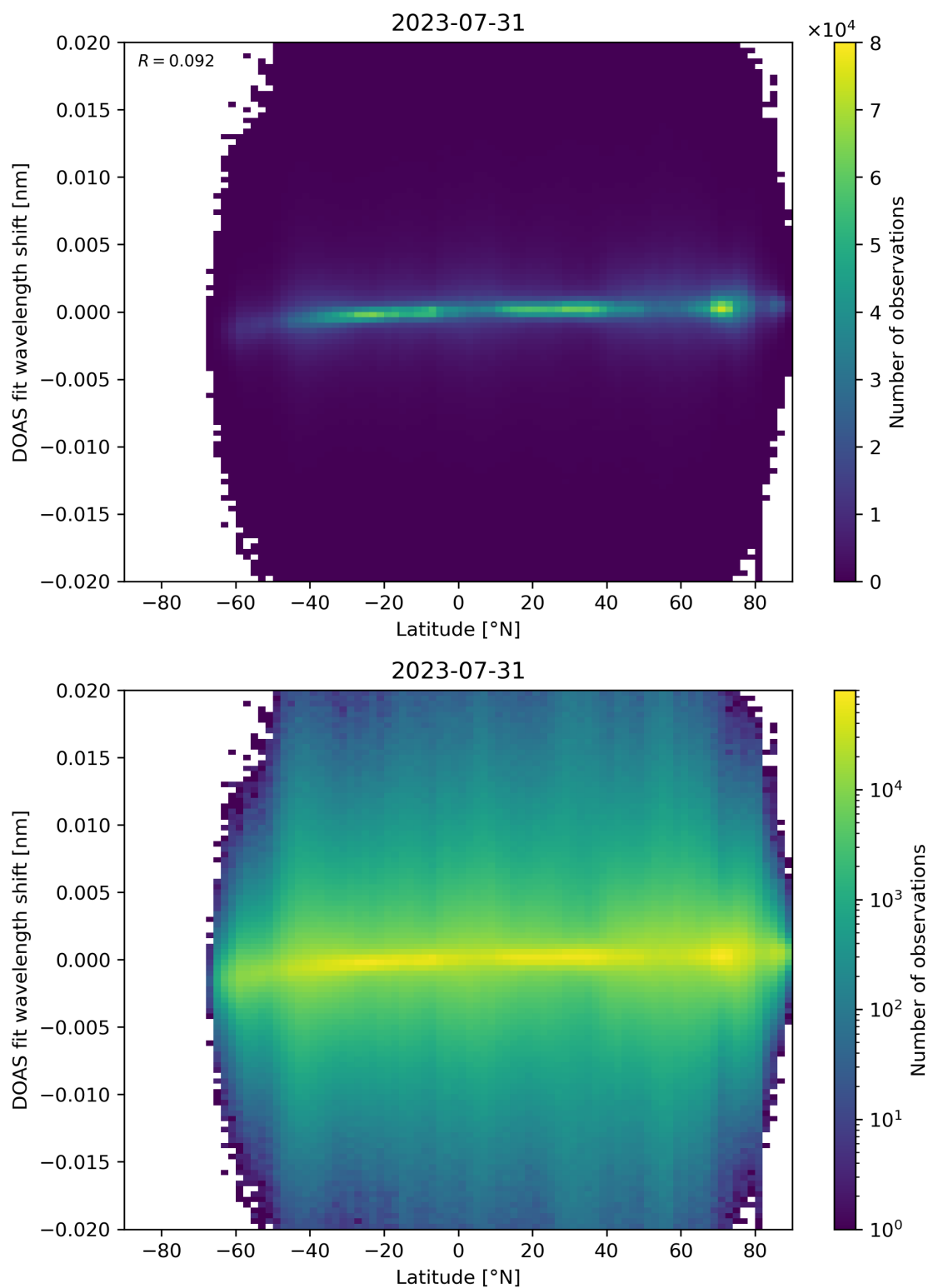
Figure 154: Scatter density plot of “Latitude” against “DOAS fit wavelength shift” for 2023-07-30 to 2023-08-01.
