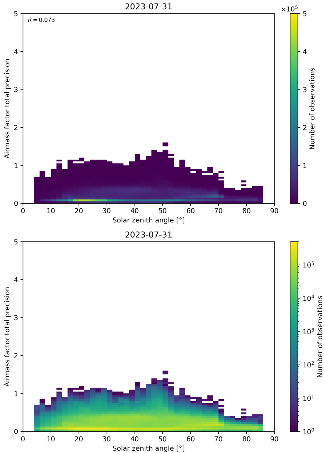
Figure 176: Scatter density plot of “Solar zenith angle” against “Airmass factor total precision” for 2023-07-30 to 2023-08-01.
