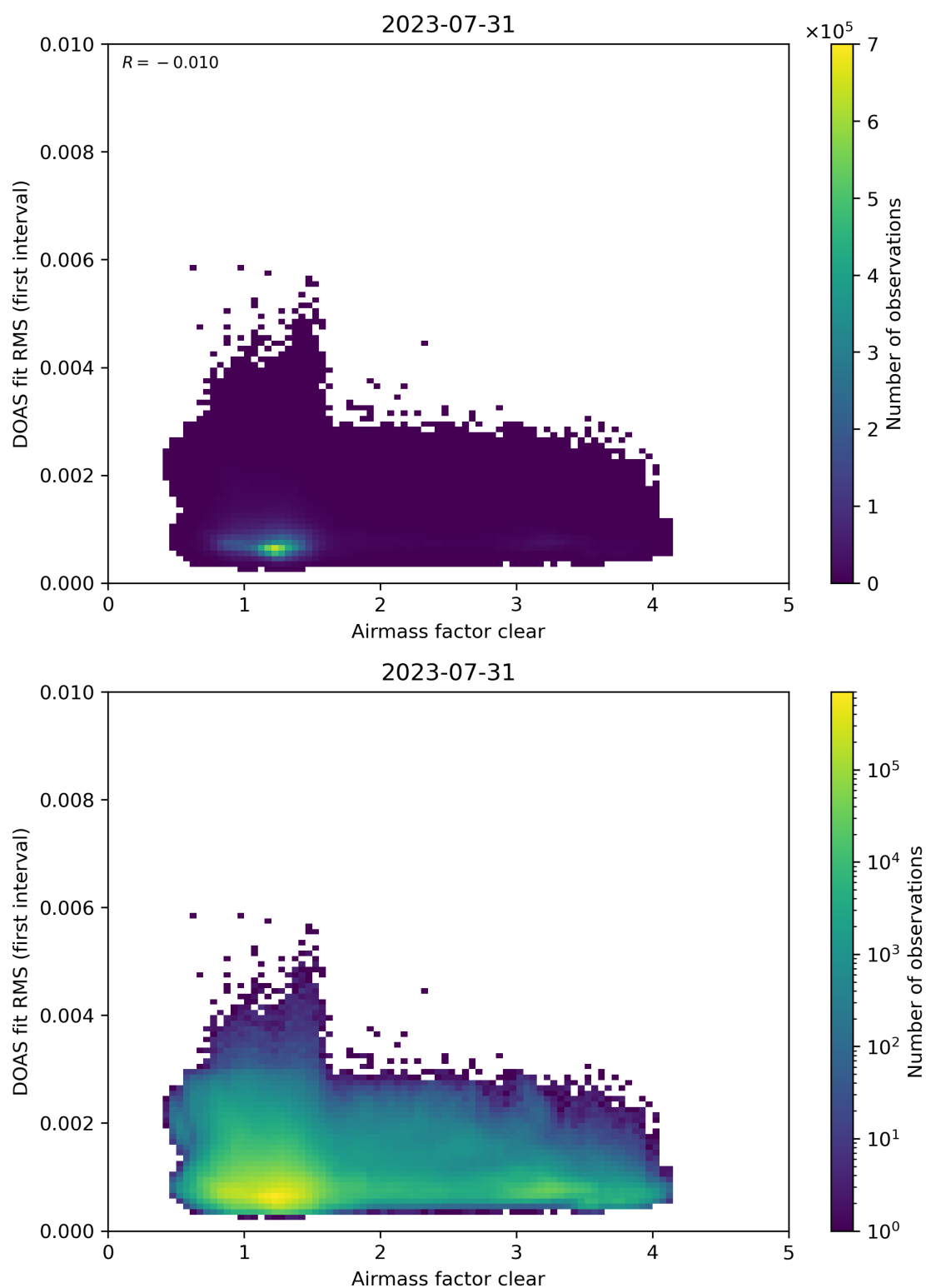
Figure 71: Scatter density plot of “Airmass factor clear” against “DOAS fit RMS (first interval)” for 2023-07-30 to 2023-08-01.
