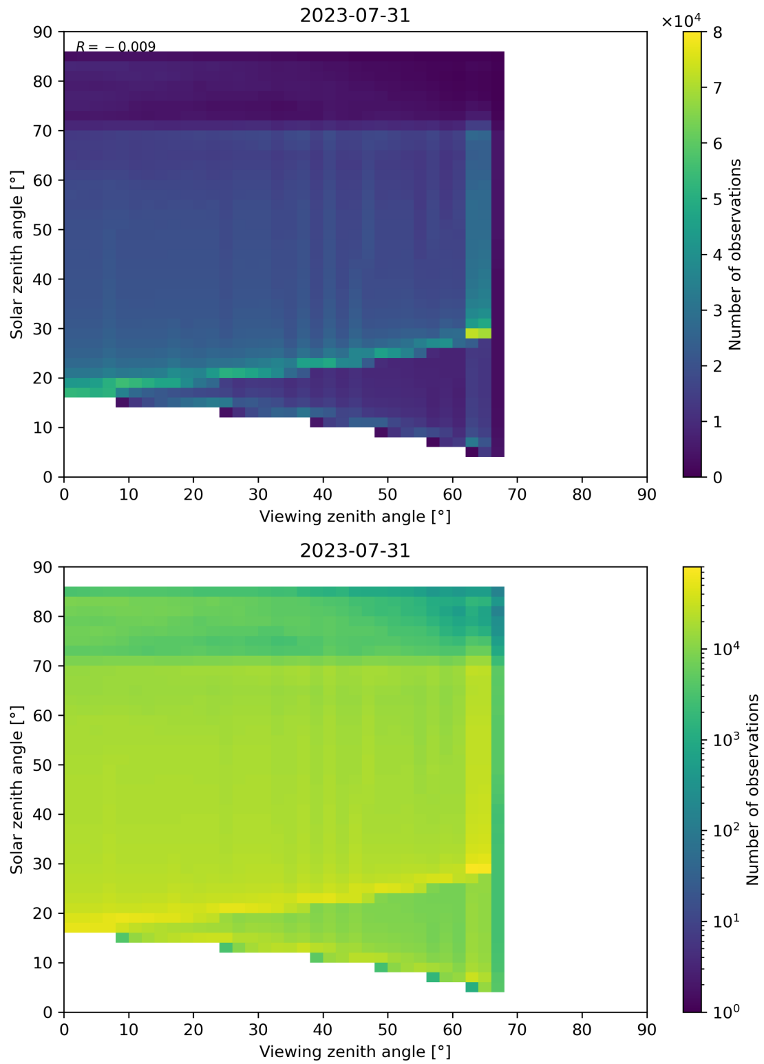
Figure 197: Scatter density plot of “Viewing zenith angle” against “Solar zenith angle” for 2023-07-30 to 2023-08-01.
