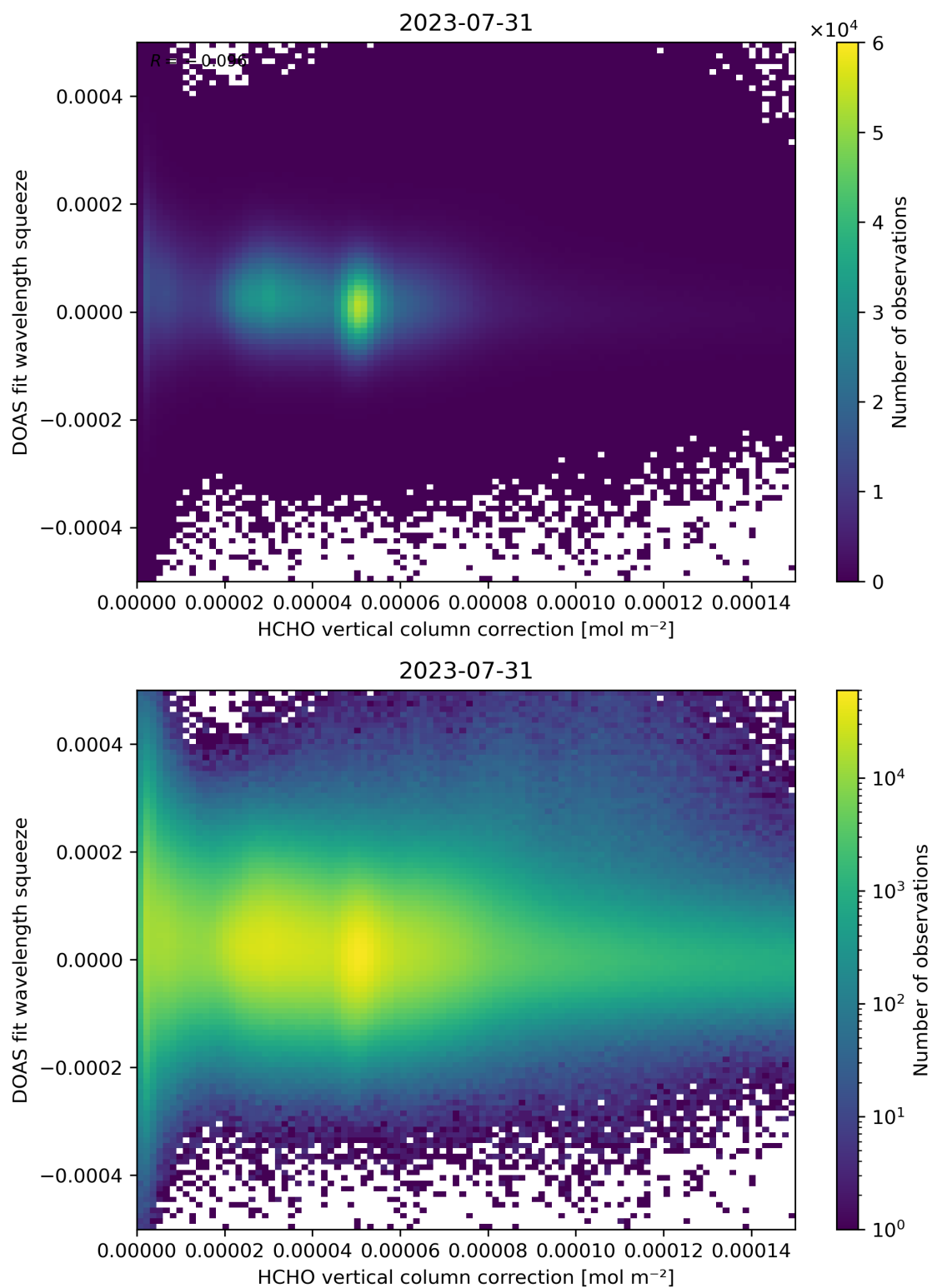
Figure 114: Scatter density plot of “HCHO vertical column correction” against “DOAS fit wavelength squeeze” for 2023-07-30 to 2023-08-01.
