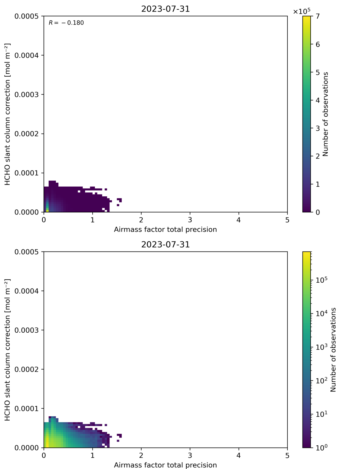
Figure 110: Scatter density plot of “Airmass factor total precision” against “HCHO slant column correction” for 2023-07-30 to 2023-08-01.
