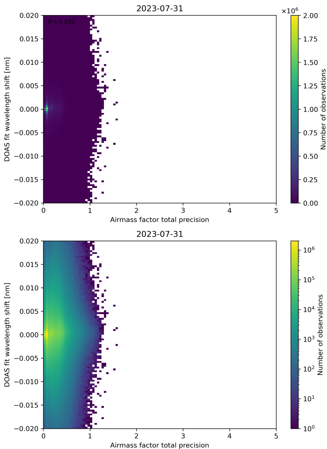
Figure 106: Scatter density plot of “Airmass factor total precision” against “DOAS fit wavelength shift” for 2023-07-30 to 2023-08-01.
