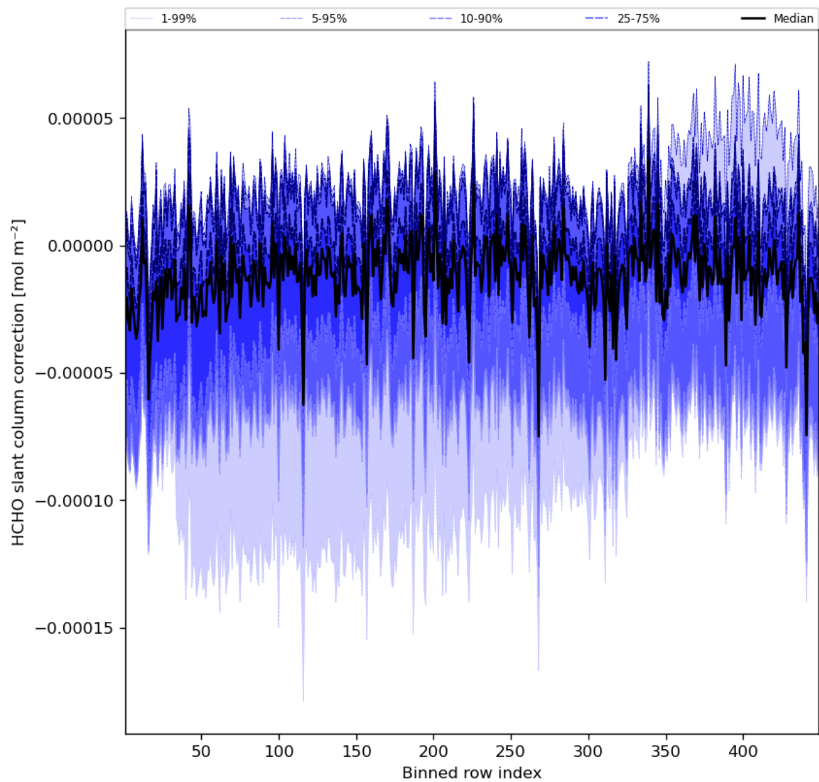
Figure 61: Along track statistics of “HCHO slant column correction” for 2023-07-30 to 2023-08-01
