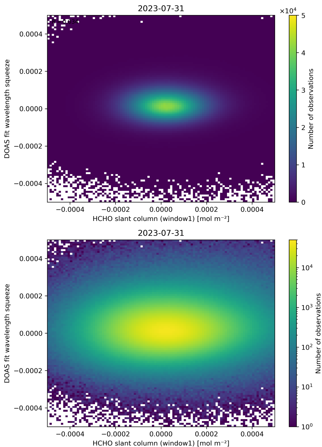
Figure 80: Scatter density plot of “HCHO slant column (window1)” against “DOAS fit wavelength squeeze” for 2023-07-30 to 2023-08-01.
