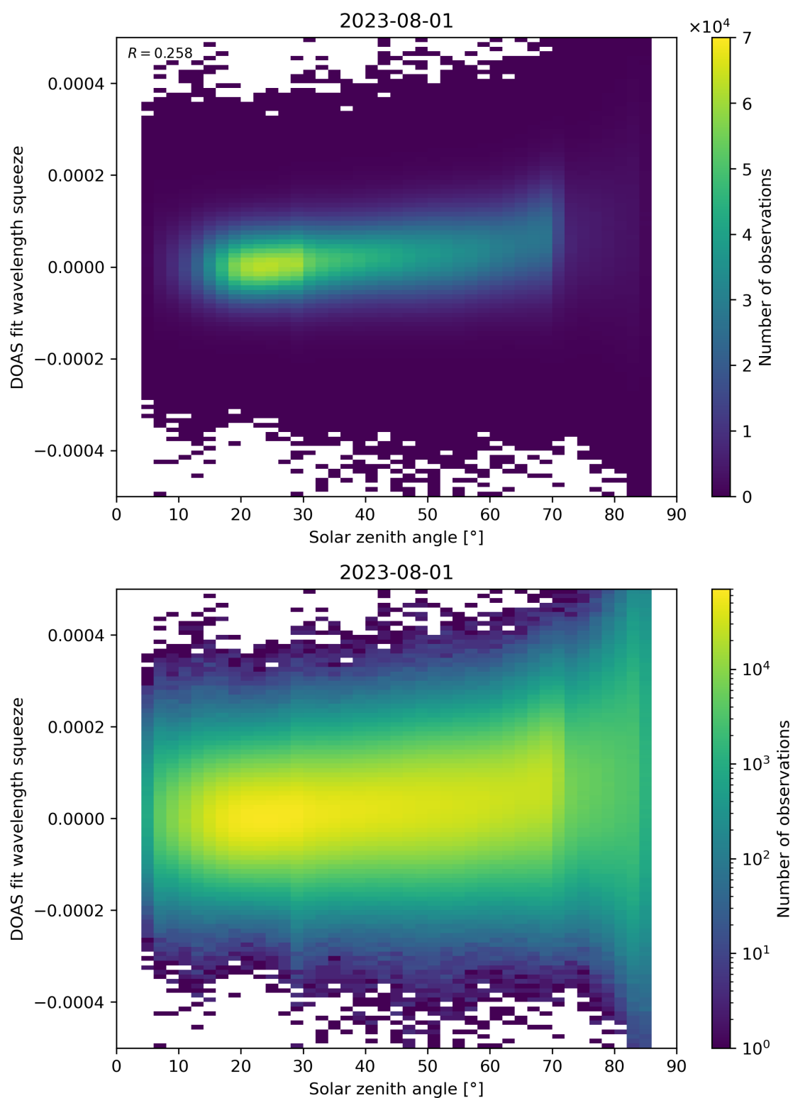
Figure 169: Scatter density plot of “Solar zenith angle” against “DOAS fit wavelength squeeze” for 2023-07-31 to 2023-08-02.
