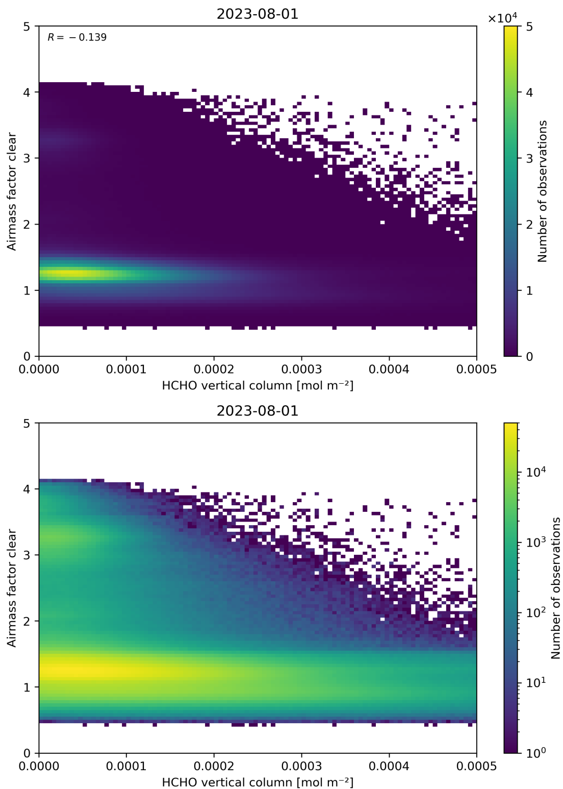
Figure 126: Scatter density plot of “HCHO vertical column” against “Airmass factor clear” for 2023-07-31 to 2023-08-02.
