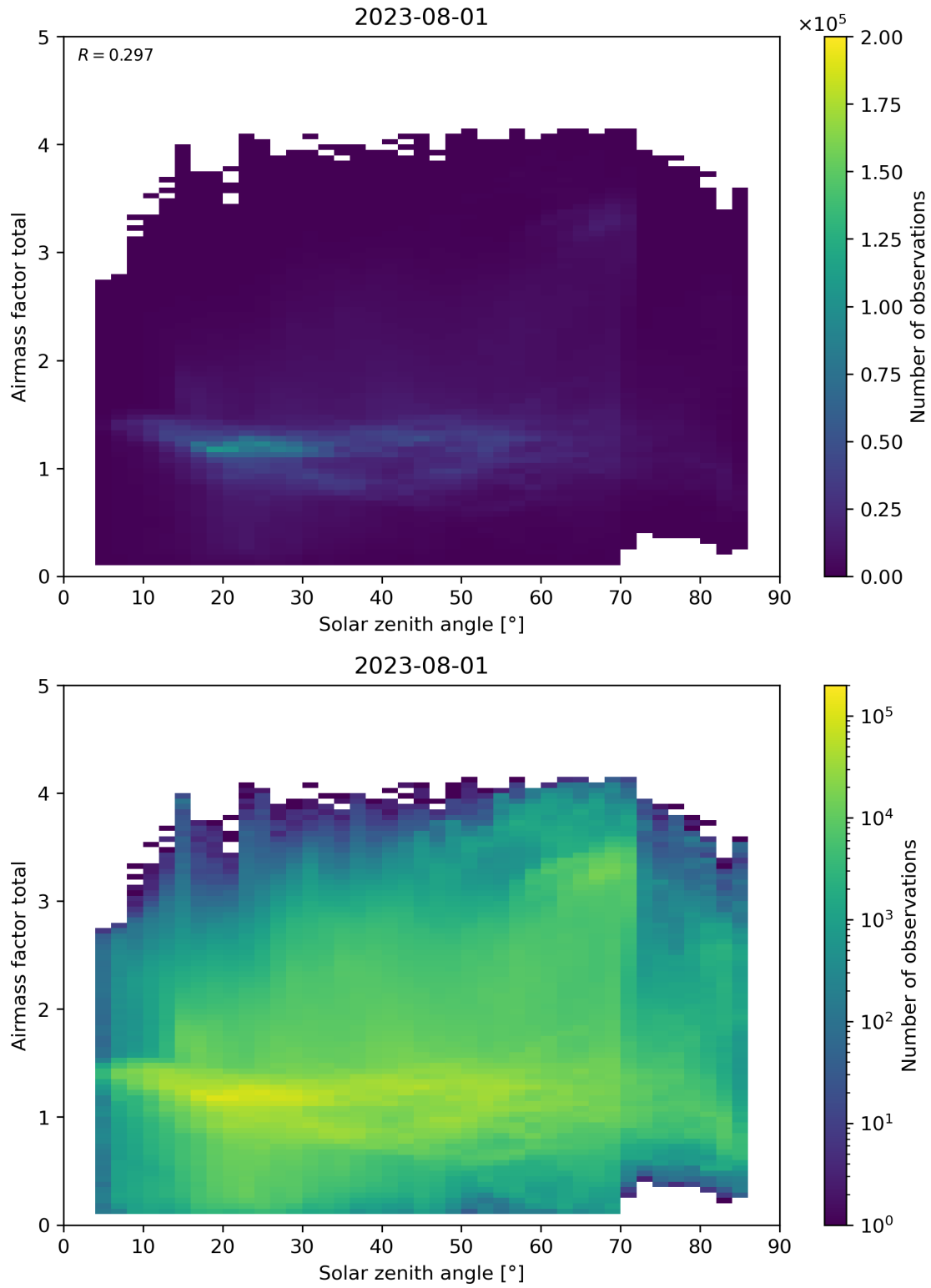
Figure 175: Scatter density plot of “Solar zenith angle” against “Airmass factor total” for 2023-07-31 to 2023-08-02.
