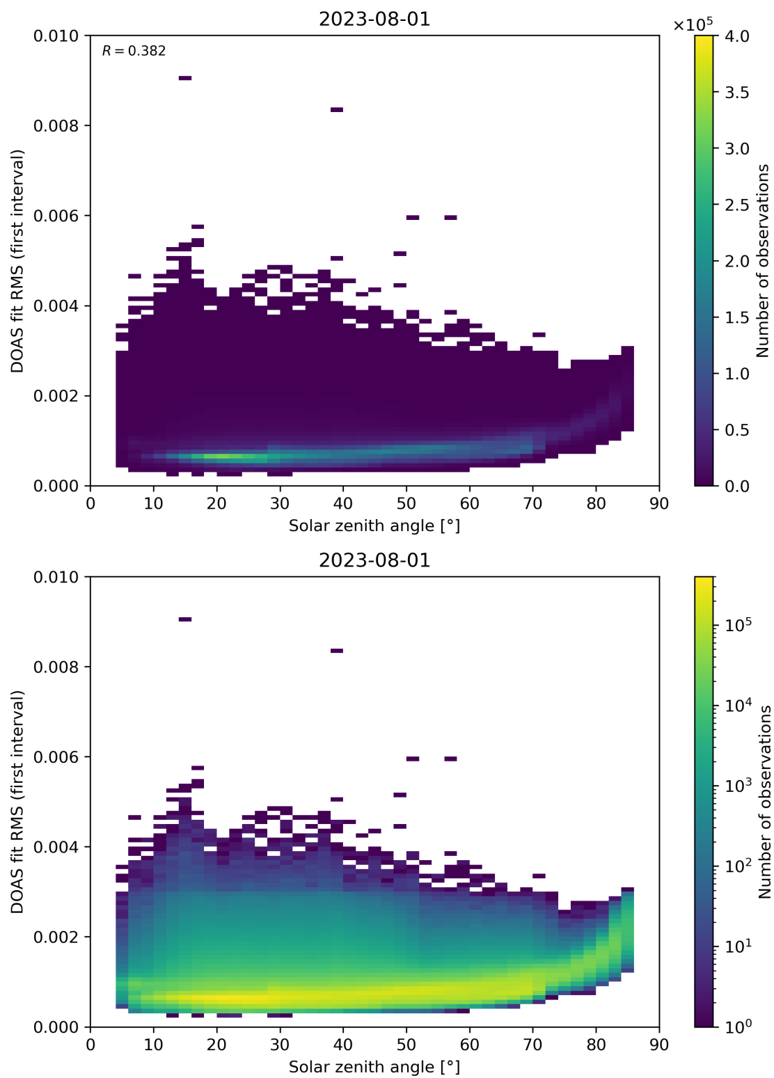
Figure 167: Scatter density plot of “Solar zenith angle” against “DOAS fit RMS (first interval)” for 2023-07-31 to 2023-08-02.
