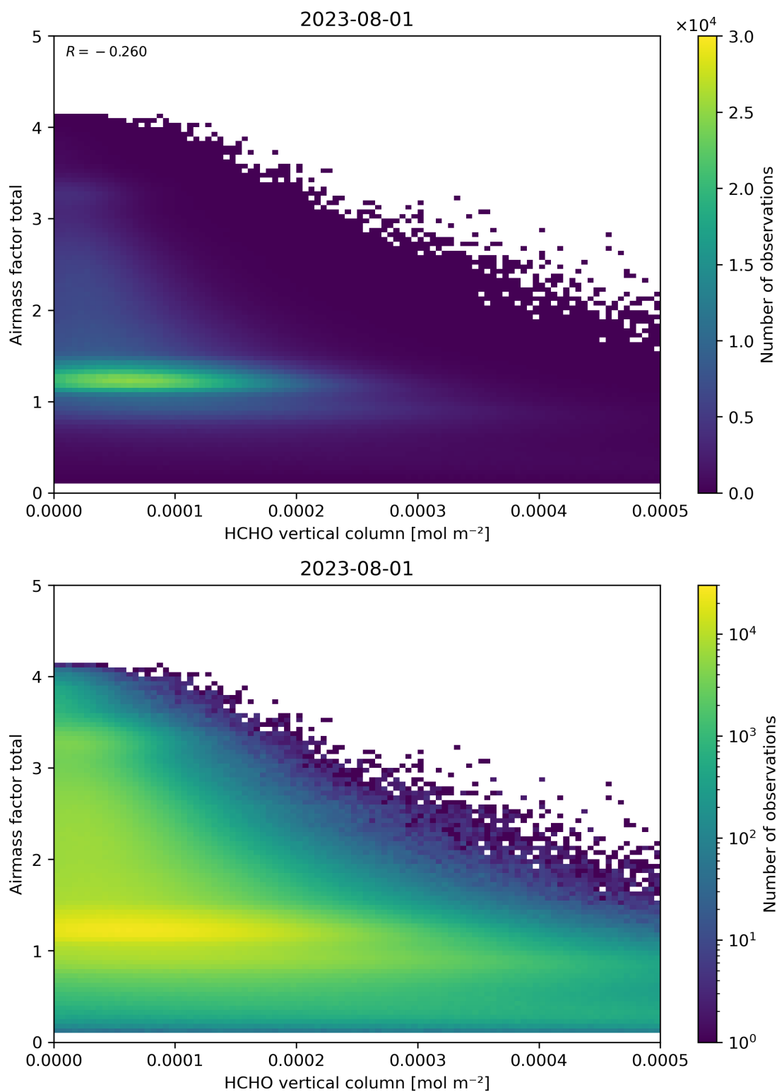
Figure 131: Scatter density plot of “HCHO vertical column” against “Airmass factor total” for 2023-07-31 to 2023-08-02.
