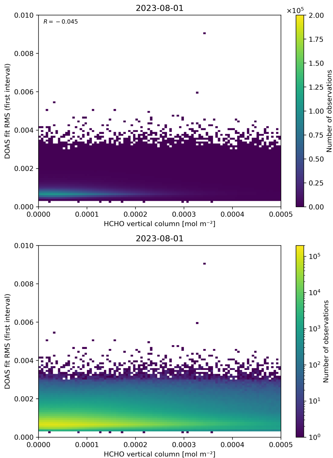
Figure 123: Scatter density plot of “HCHO vertical column” against “DOAS fit RMS (first interval)” for 2023-07-31 to 2023-08-02.
