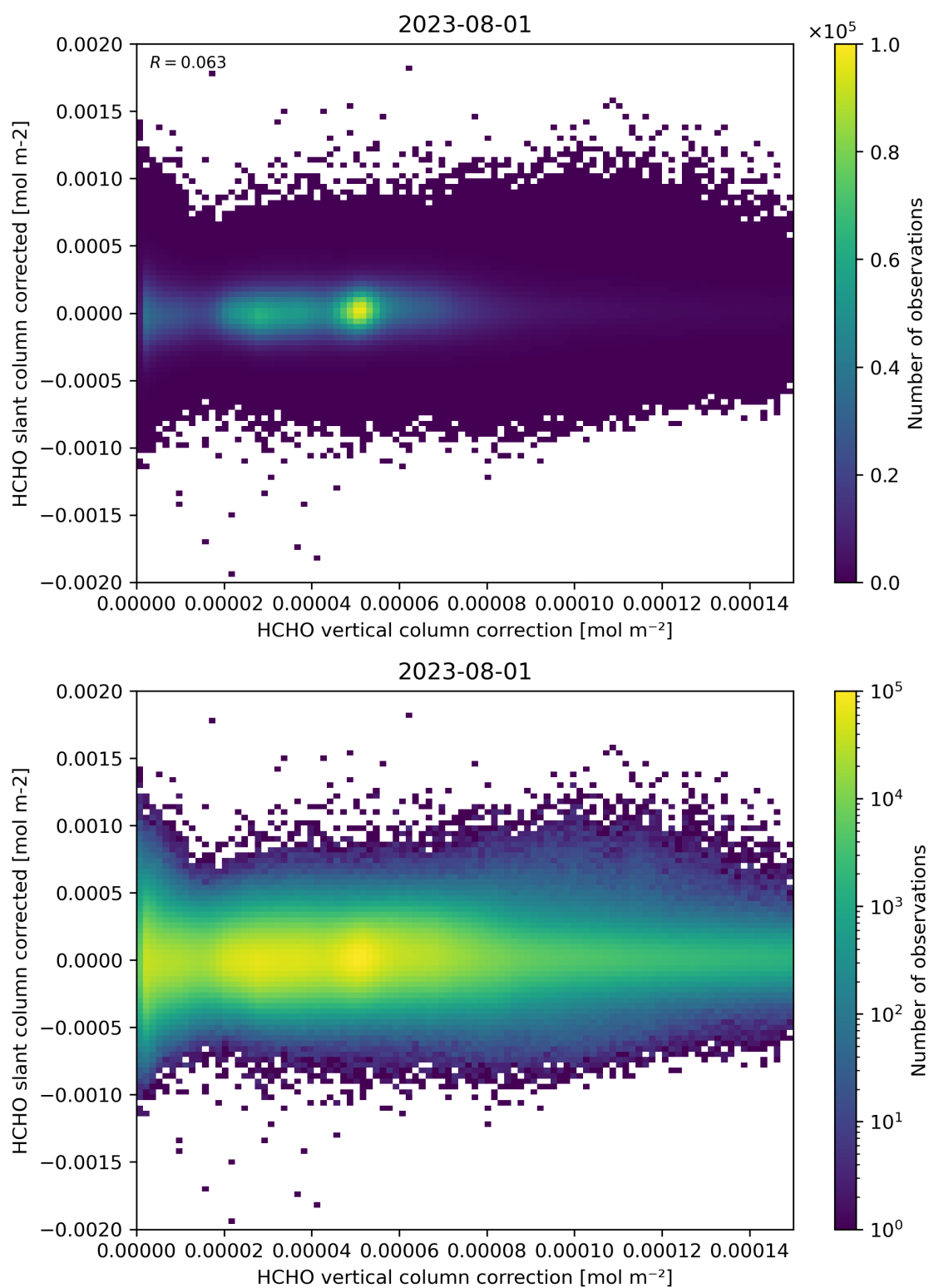
Figure 116: Scatter density plot of “HCHO vertical column correction” against “HCHO slant column corrected” for 2023-07-31 to 2023-08-02.
