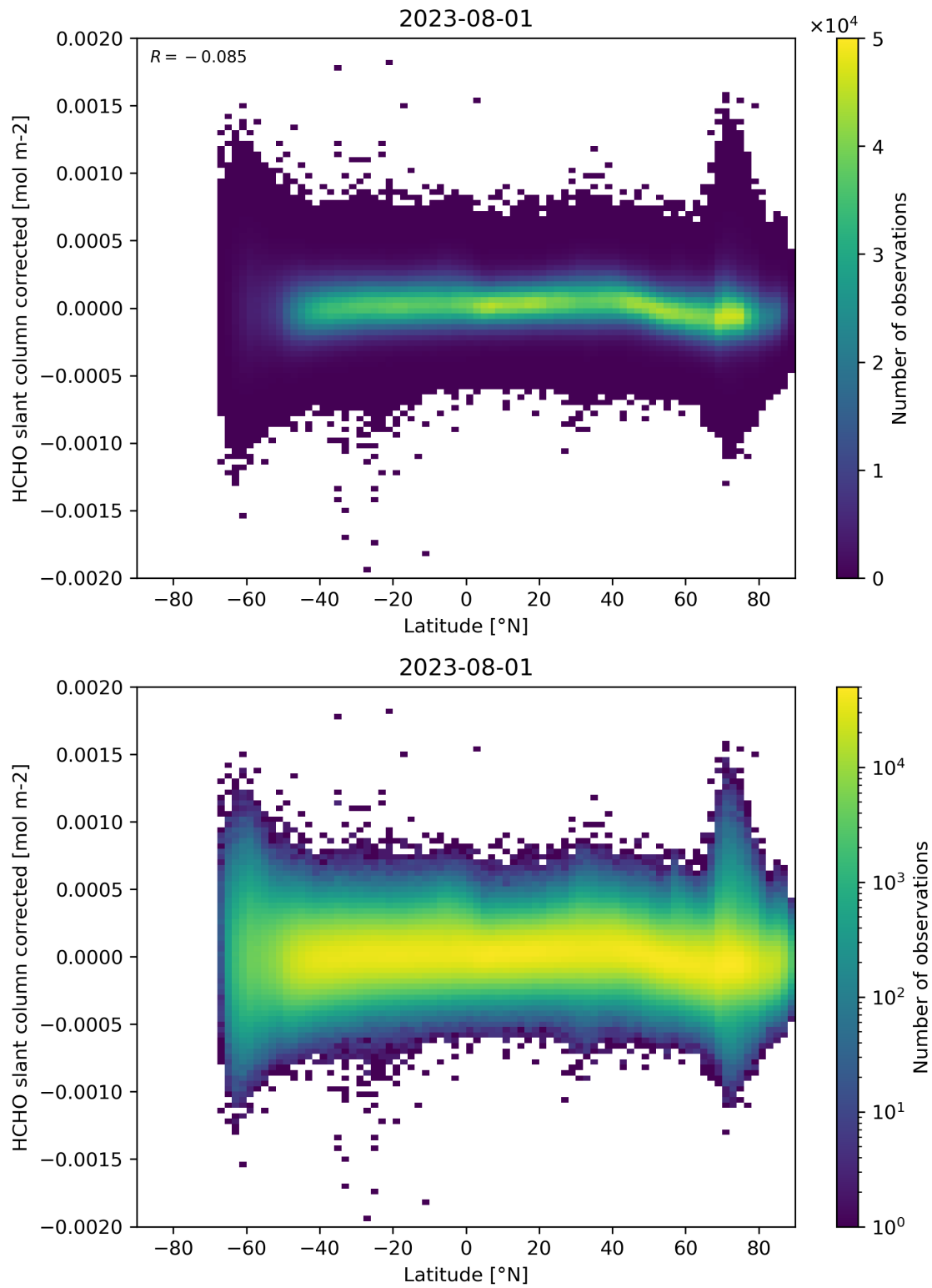
Figure 157: Scatter density plot of “Latitude” against “HCHO slant column corrected” for 2023-07-31 to 2023-08-02.
