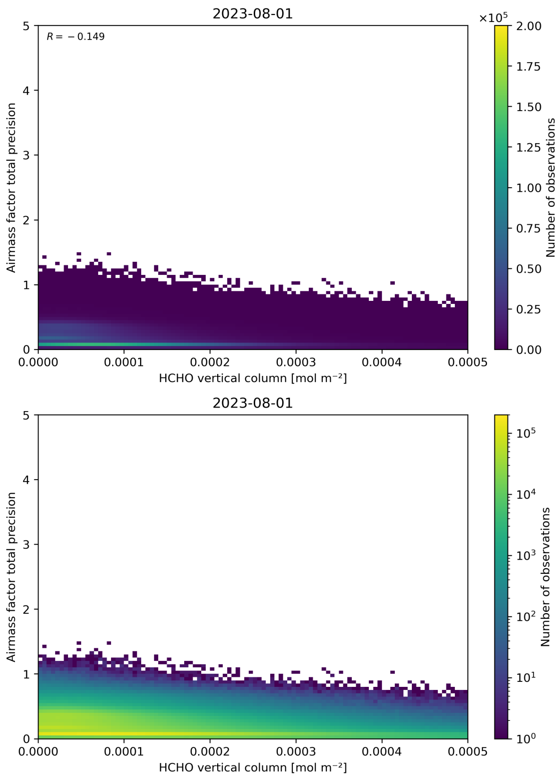
Figure 132: Scatter density plot of “HCHO vertical column” against “Airmass factor total precision” for 2023-07-31 to 2023-08-02.
