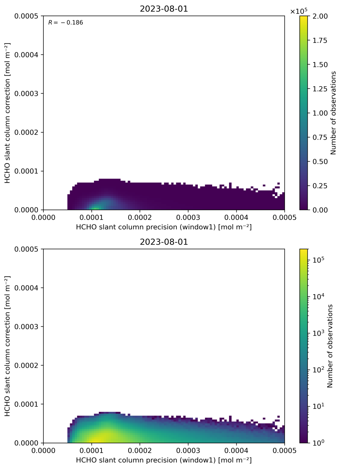
Figure 93: Scatter density plot of “HCHO slant column precision (window1)” against “HCHO slant column correction” for 2023-07-31 to 2023-08-02.
