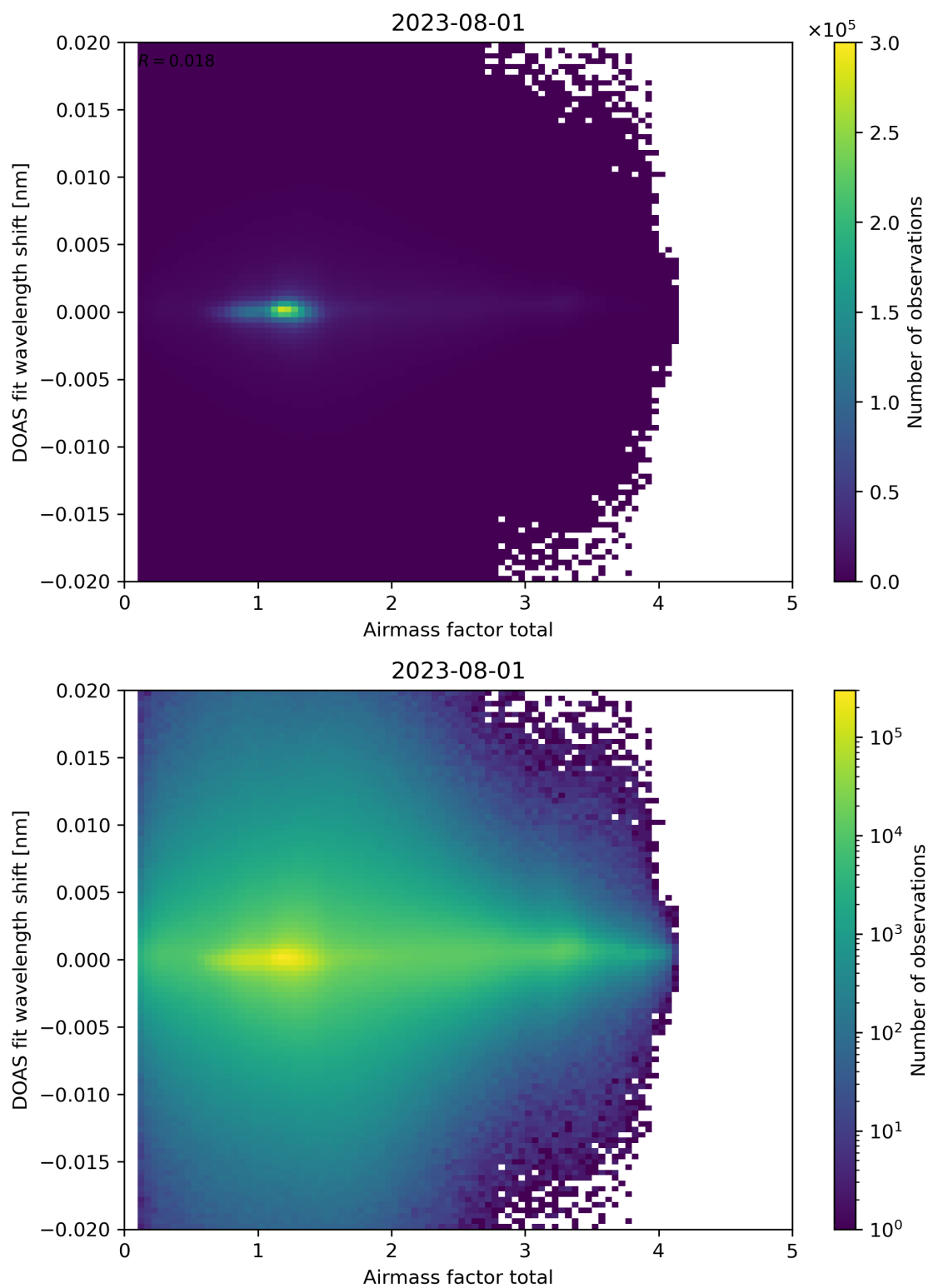
Figure 98: Scatter density plot of “Airmass factor total” against “DOAS fit wavelength shift” for 2023-07-31 to 2023-08-02.
