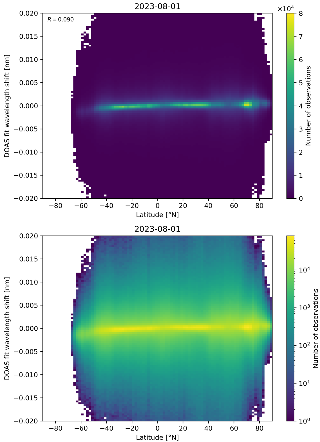
Figure 154: Scatter density plot of “Latitude” against “DOAS fit wavelength shift” for 2023-07-31 to 2023-08-02.
