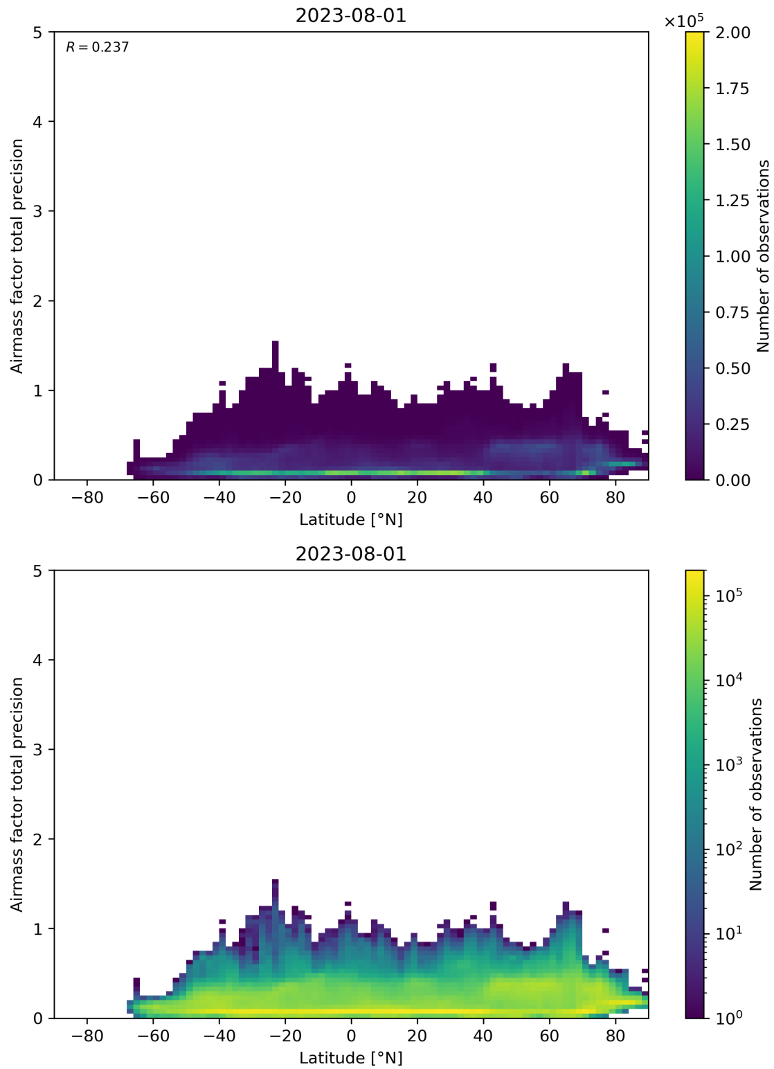
Figure 162: Scatter density plot of “Latitude” against “Airmass factor total precision” for 2023-07-31 to 2023-08-02.
