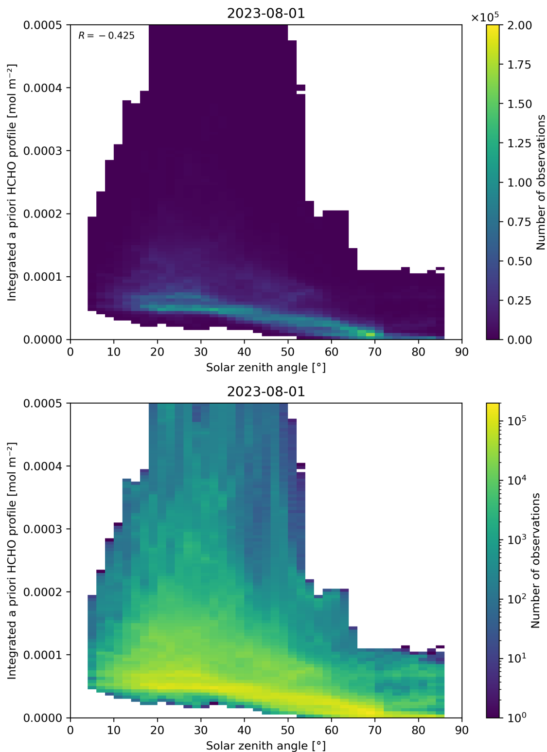
Figure 180: Scatter density plot of “Solar zenith angle” against “Integrated a priori HCHO profile” for 2023-07-31 to 2023-08-02.
