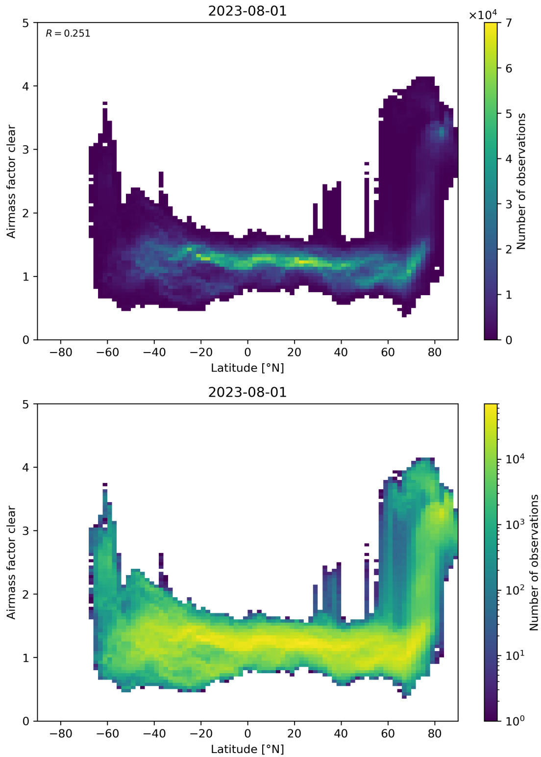
Figure 156: Scatter density plot of “Latitude” against “Airmass factor clear” for 2023-07-31 to 2023-08-02.
