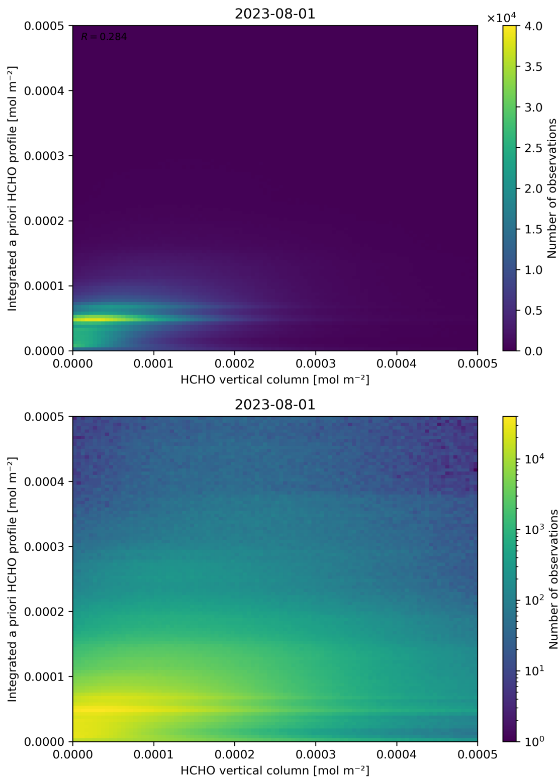
Figure 135: Scatter density plot of “HCHO vertical column” against “Integrated a priori HCHO profile” for 2023-07-31 to 2023-08-02.
