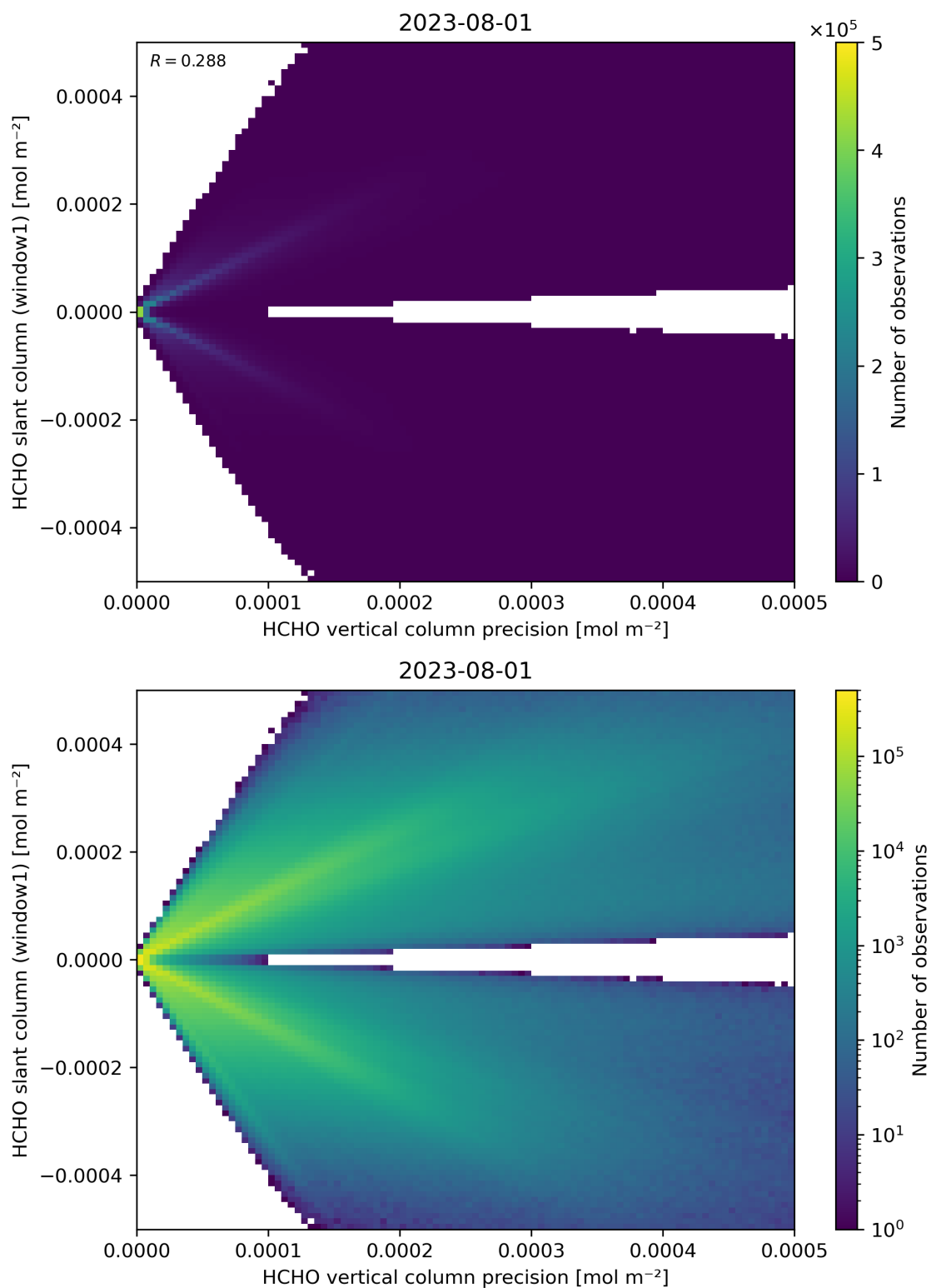
Figure 142: Scatter density plot of “HCHO vertical column precision” against “HCHO slant column (window1)” for 2023-07-31 to 2023-08-02.
