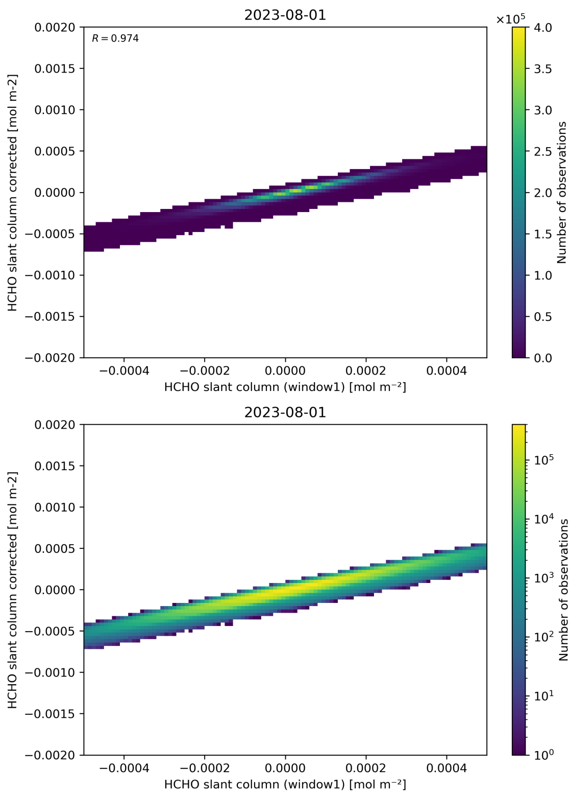
Figure 82: Scatter density plot of “HCHO slant column (window1)” against “HCHO slant column corrected” for 2023-07-31 to 2023-08-02.
