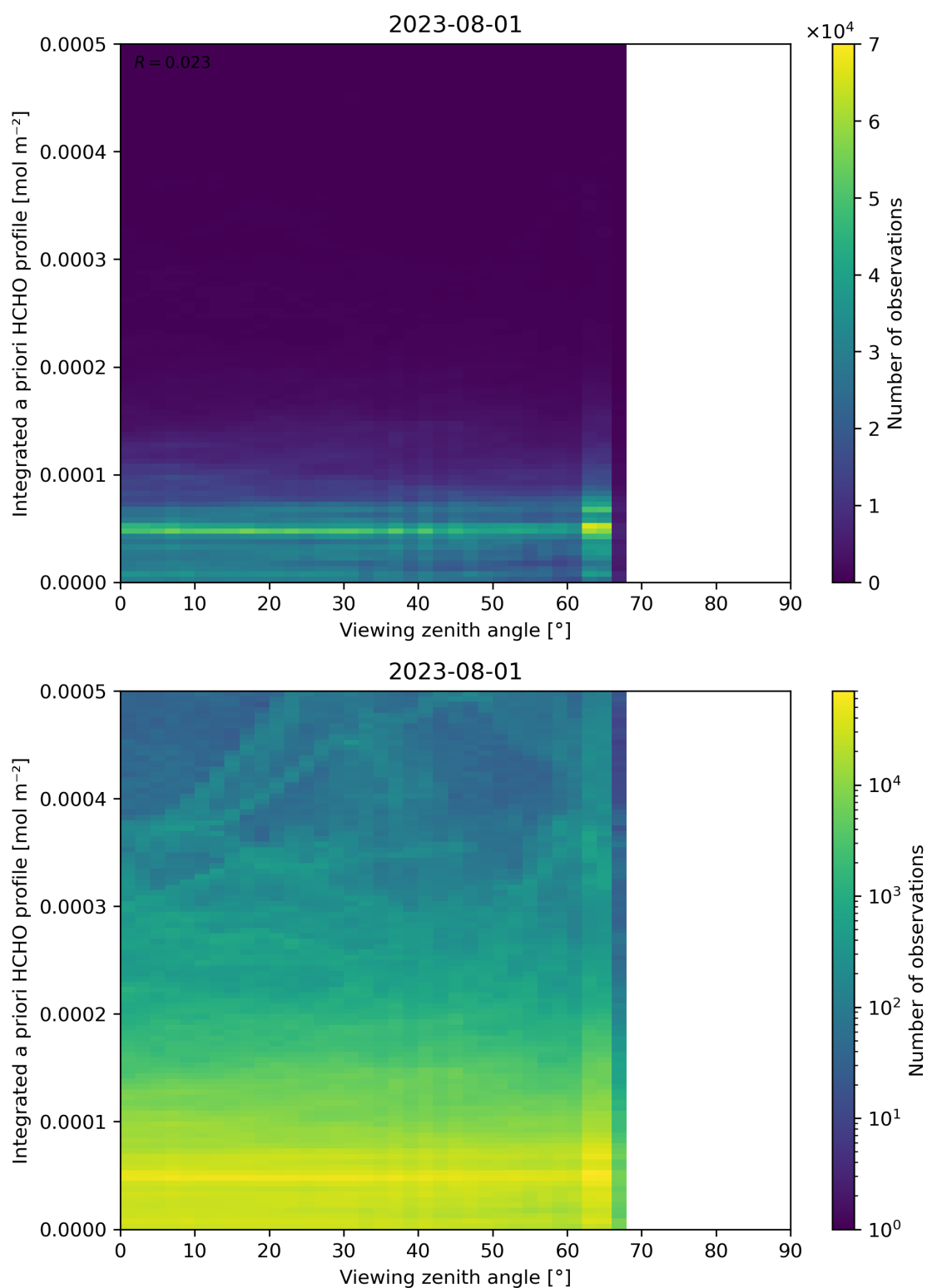
Figure 195: Scatter density plot of “Viewing zenith angle” against “Integrated a priori HCHO profile” for 2023-07-31 to 2023-08-02.
