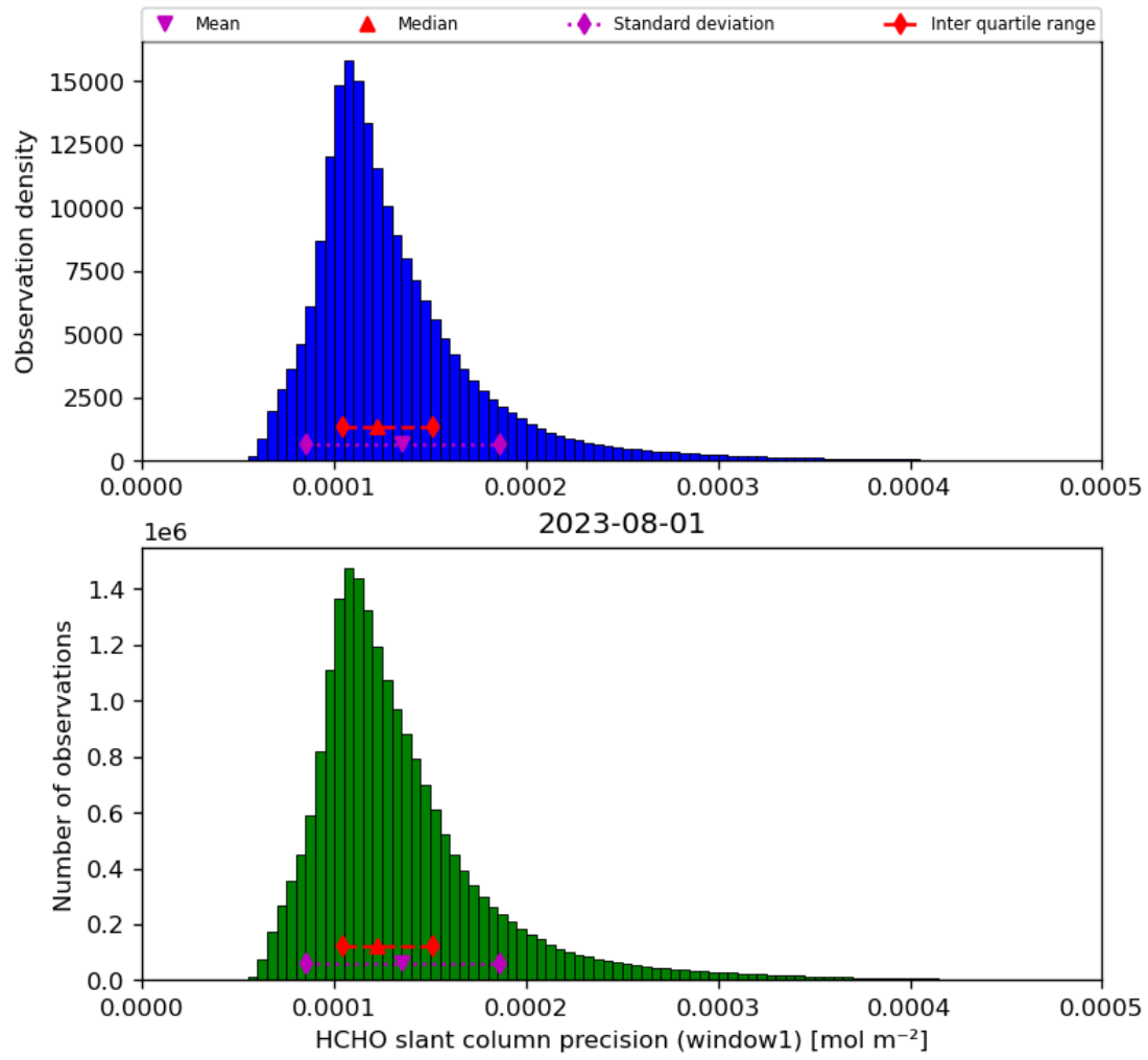
Figure 39: Histogram of “HCHO slant column precision (window1)” for 2023-07-31 to 2023-08-02
