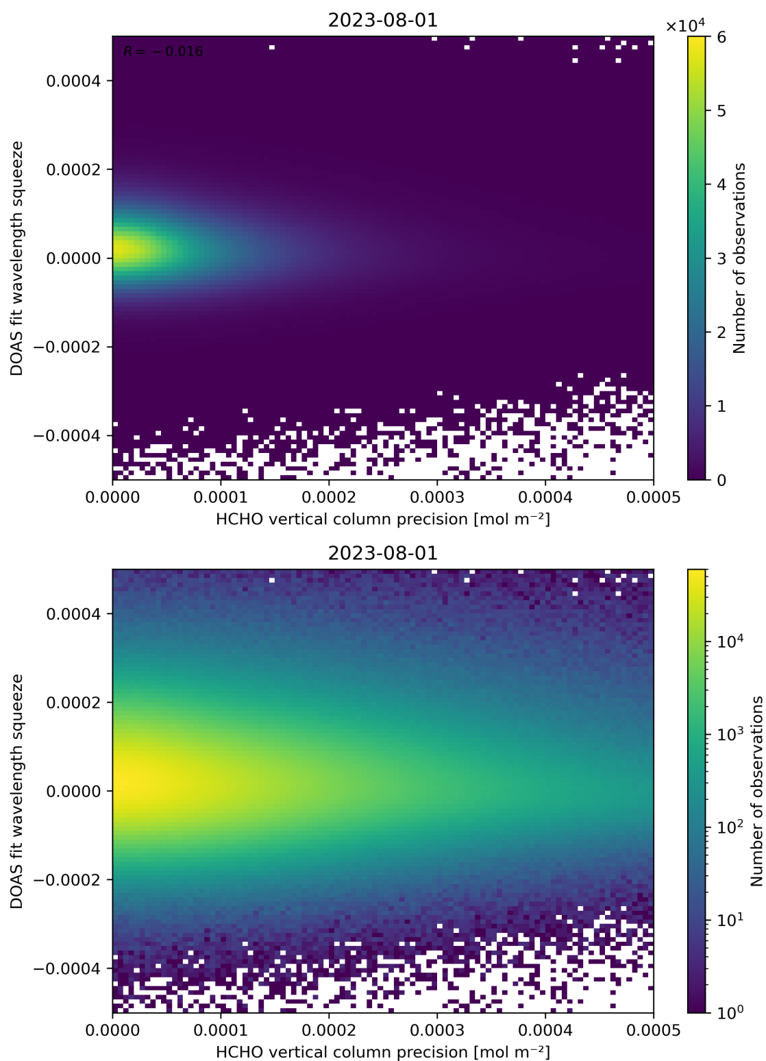
Figure 138: Scatter density plot of “HCHO vertical column precision” against “DOAS fit wavelength squeeze” for 2023-07-31 to 2023-08-02.
