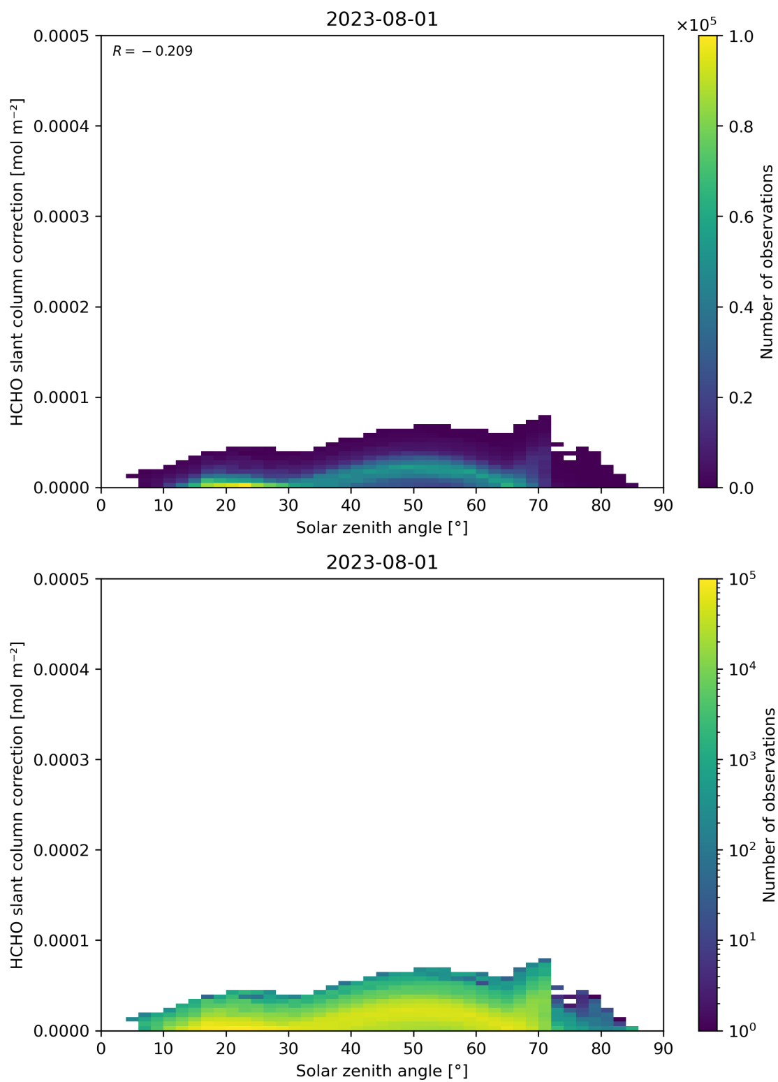
Figure 172: Scatter density plot of “Solar zenith angle” against “HCHO slant column correction” for 2023-07-31 to 2023-08-02.
