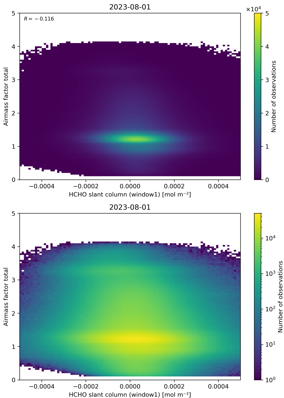
Figure 85: Scatter density plot of “HCHO slant column (window1)” against “Airmass factor total” for 2023-07-31 to 2023-08-02.
