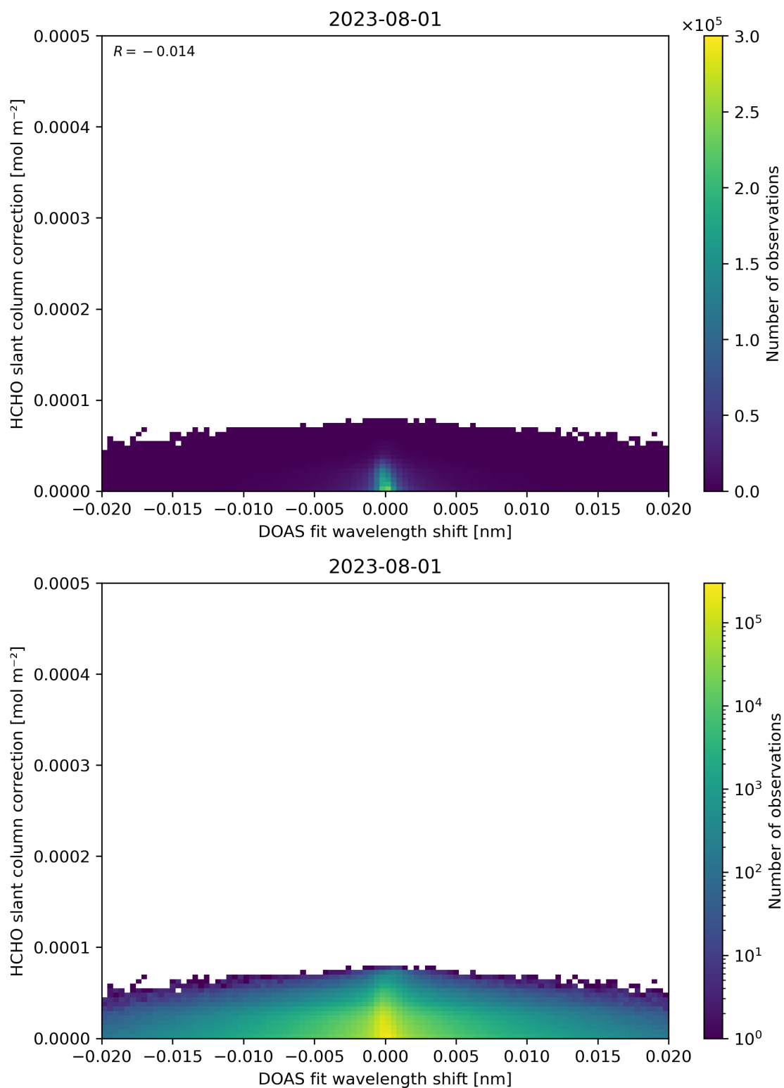
Figure 67: Scatter density plot of “DOAS fit wavelength shift” against “HCHO slant column correction” for 2023-07-31 to 2023-08-02.
