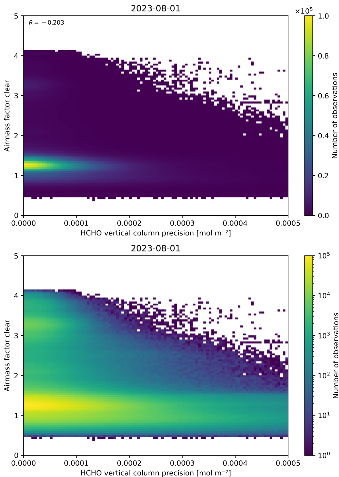
Figure 139: Scatter density plot of “HCHO vertical column precision” against “Airmass factor clear” for 2023-07-31 to 2023-08-02.
