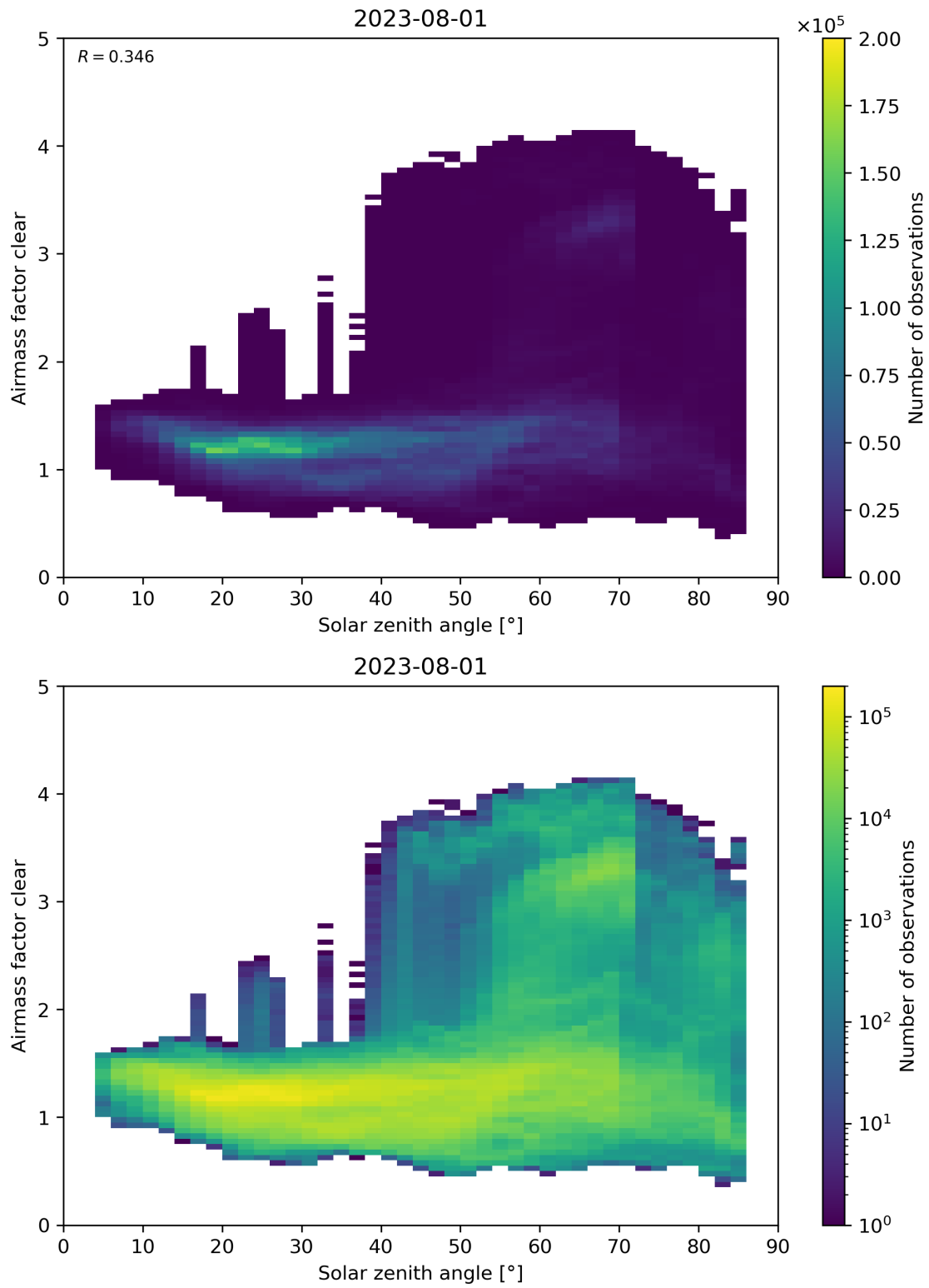
Figure 170: Scatter density plot of “Solar zenith angle” against “Airmass factor clear” for 2023-07-31 to 2023-08-02.
