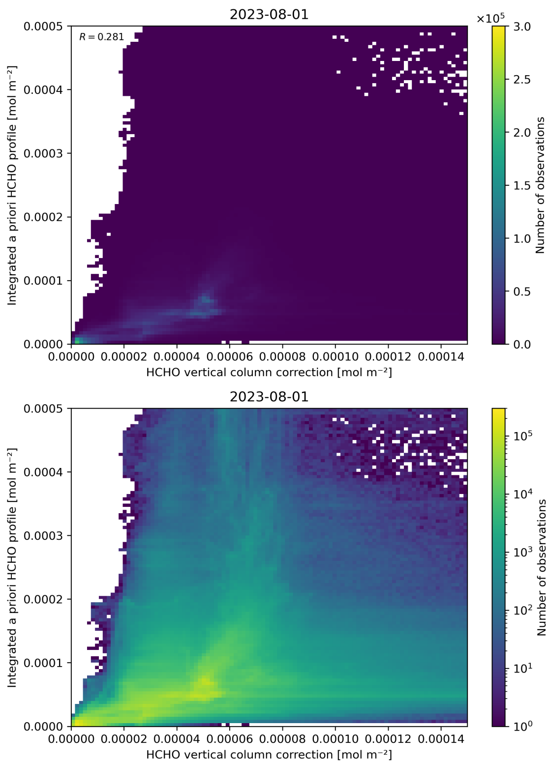
Figure 122: Scatter density plot of “HCHO vertical column correction” against “Integrated a priori HCHO profile” for 2023-07-31 to 2023-08-02.
