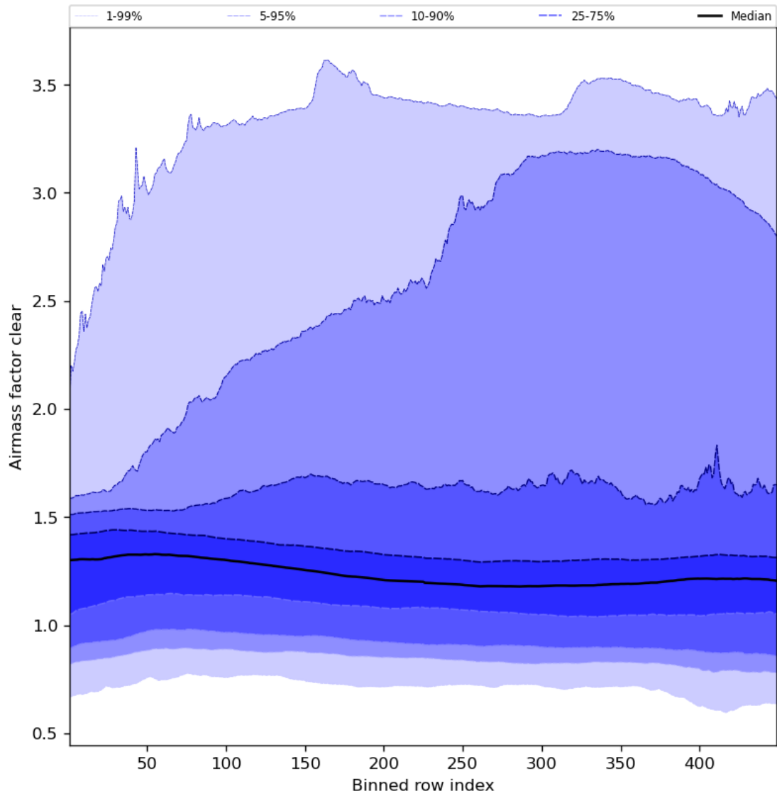
Figure 56: Along track statistics of “Airmass factor clear” for 2023-07-31 to 2023-08-02
