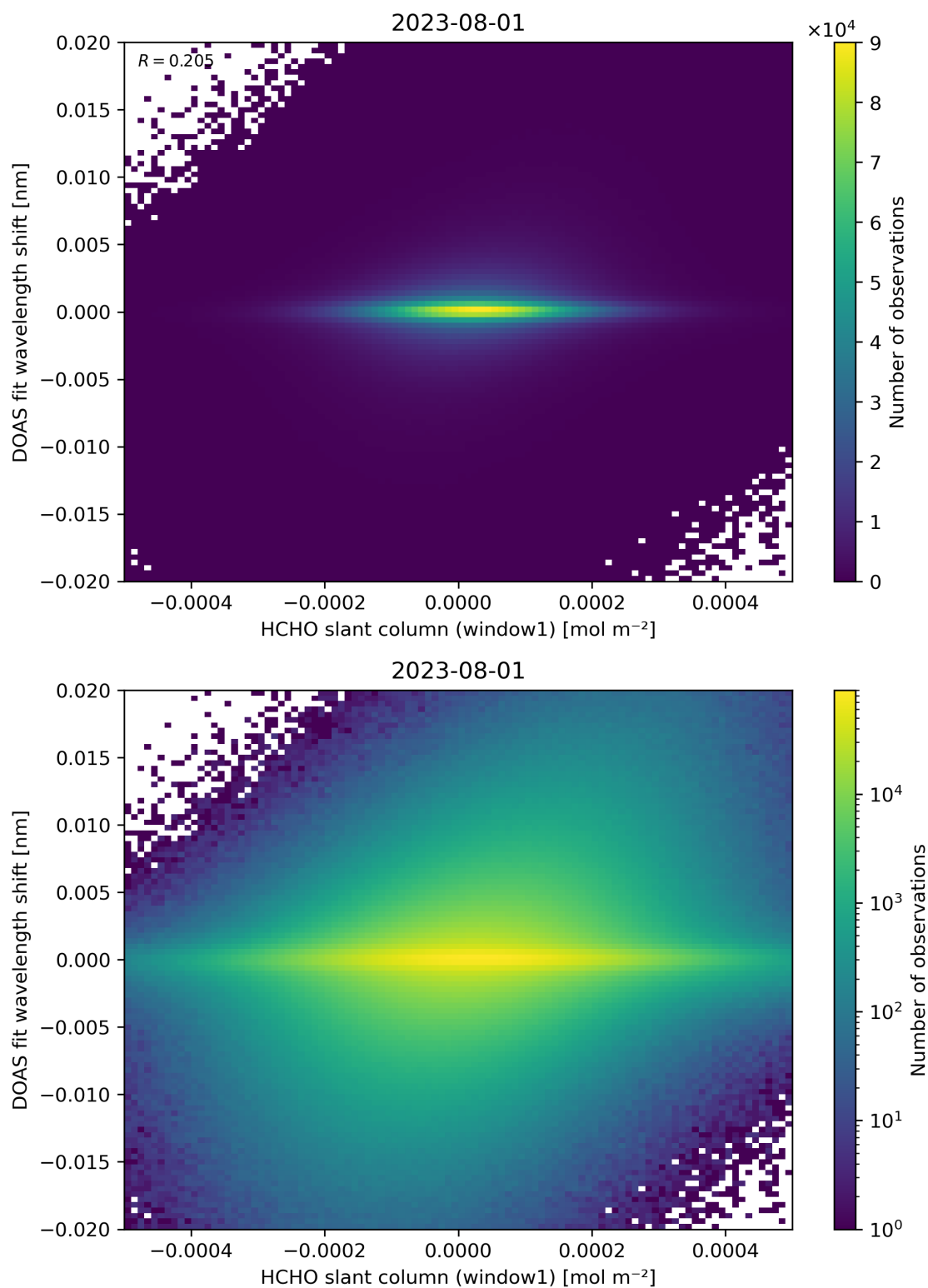
Figure 79: Scatter density plot of “HCHO slant column (window1)” against “DOAS fit wavelength shift” for 2023-07-31 to 2023-08-02.
