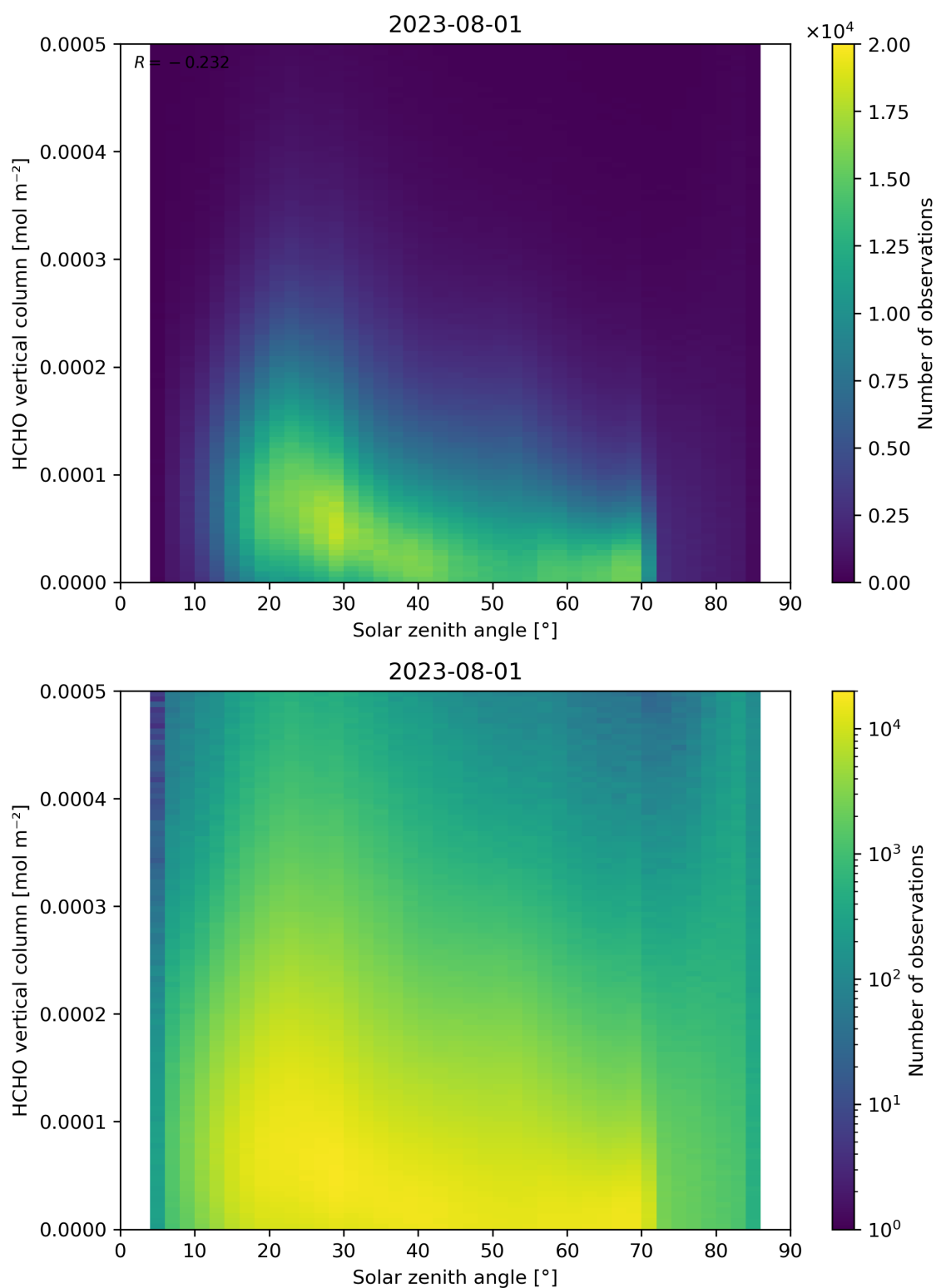
Figure 177: Scatter density plot of “Solar zenith angle” against “HCHO vertical column” for 2023-07-31 to 2023-08-02.
