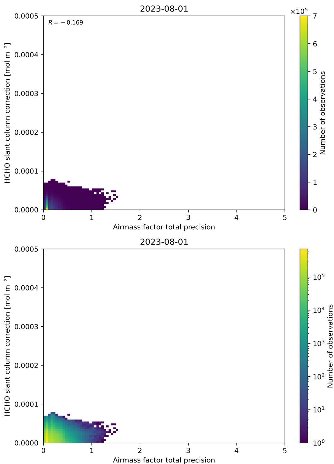
Figure 110: Scatter density plot of “Airmass factor total precision” against “HCHO slant column correction” for 2023-07-31 to 2023-08-02.
