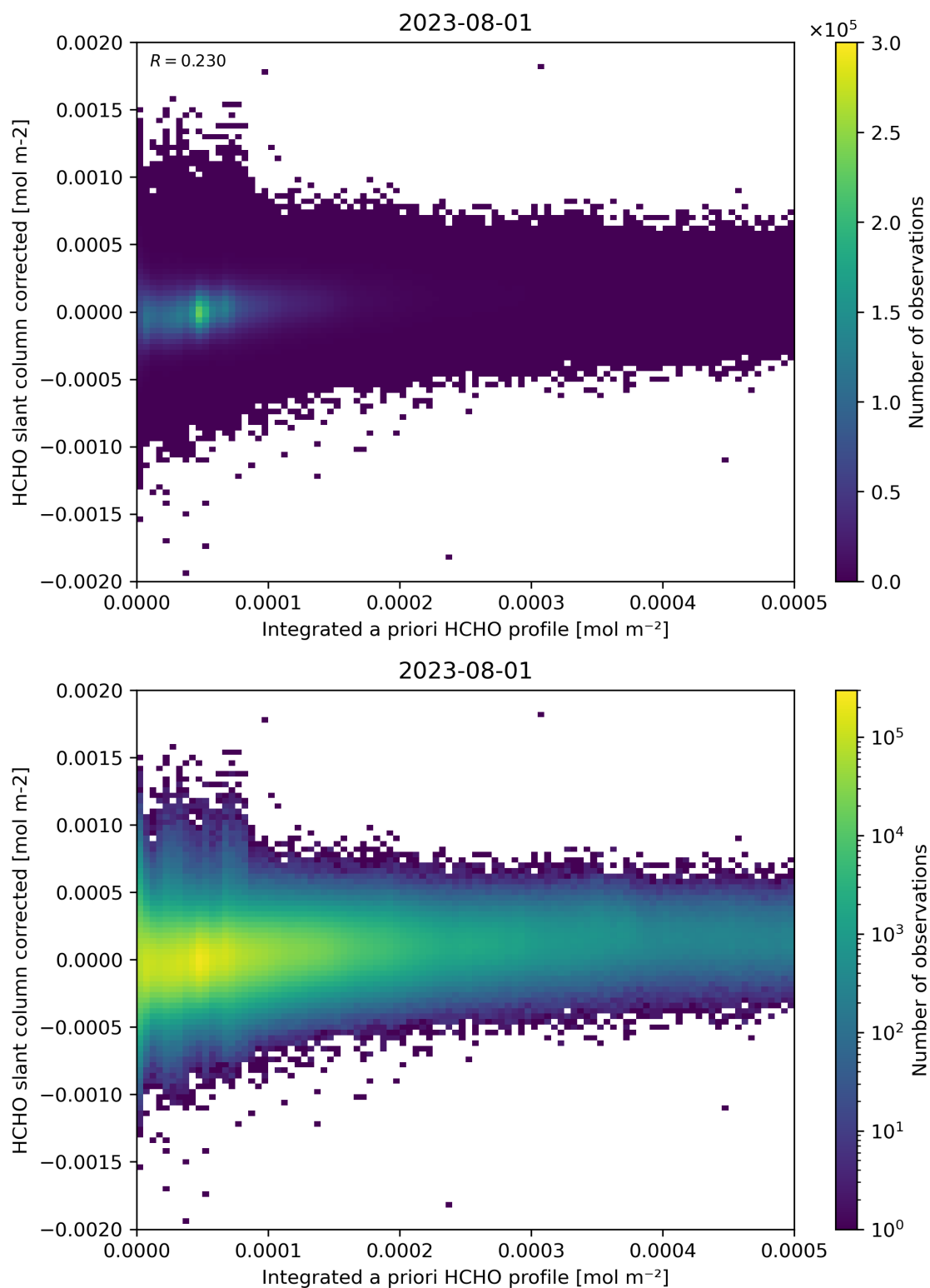
Figure 151: Scatter density plot of “Integrated a priori HCHO profile” against “HCHO slant column corrected” for 2023-07-31 to 2023-08-02.
