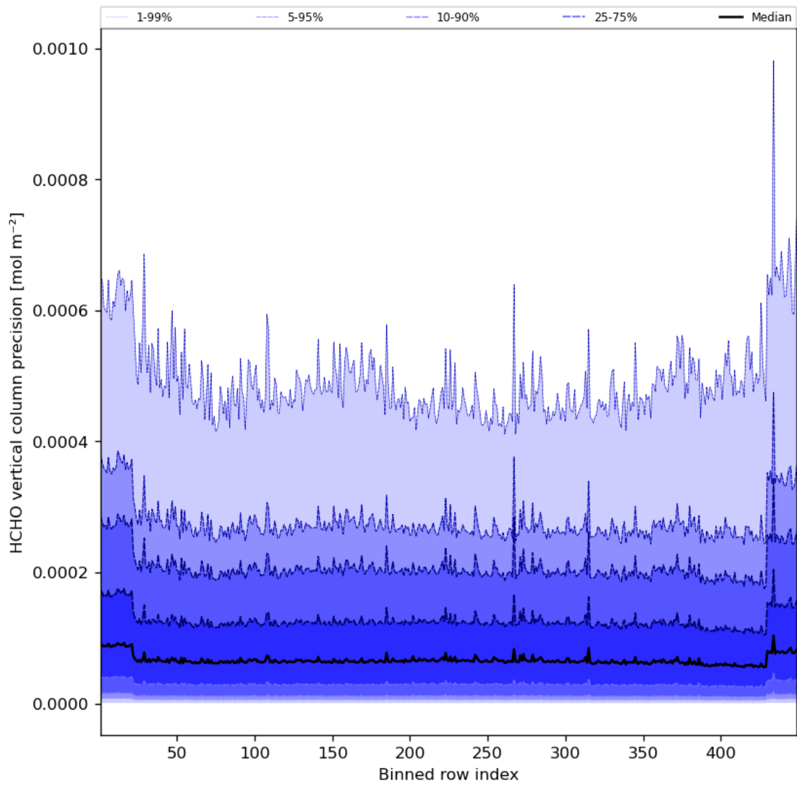
Figure 50: Along track statistics of “HCHO vertical column precision” for 2023-07-31 to 2023-08-02
