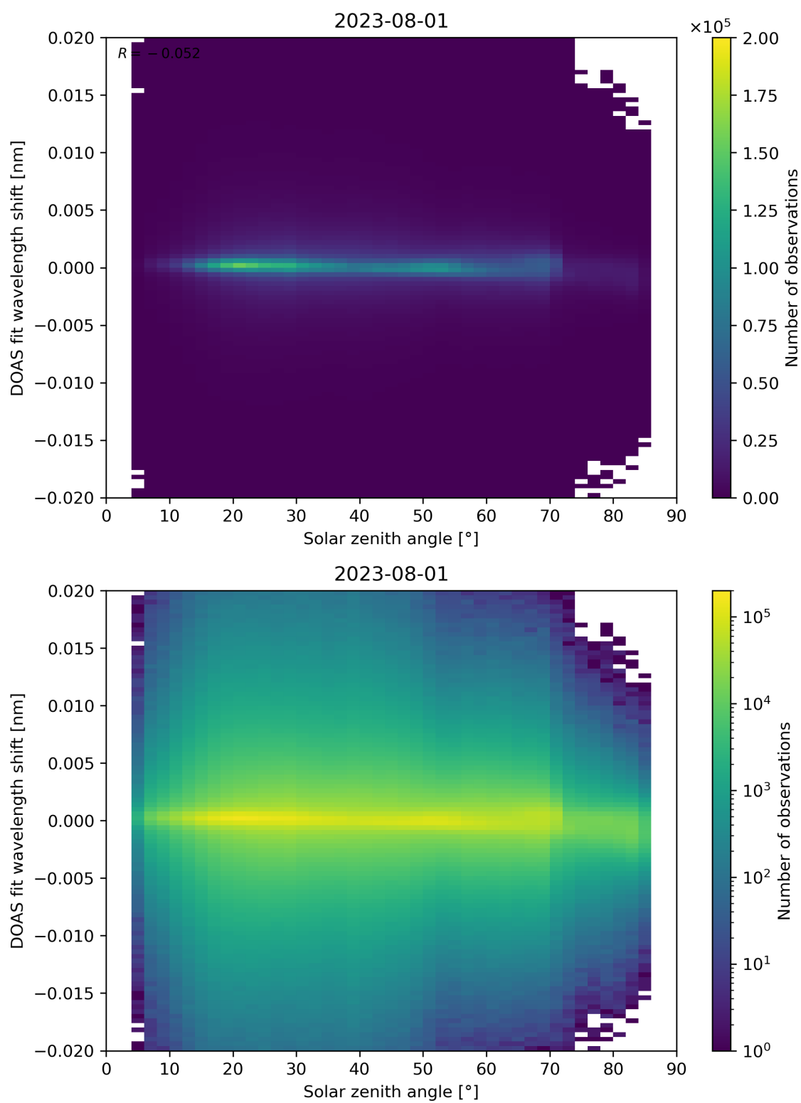
Figure 168: Scatter density plot of “Solar zenith angle” against “DOAS fit wavelength shift” for 2023-07-31 to 2023-08-02.
