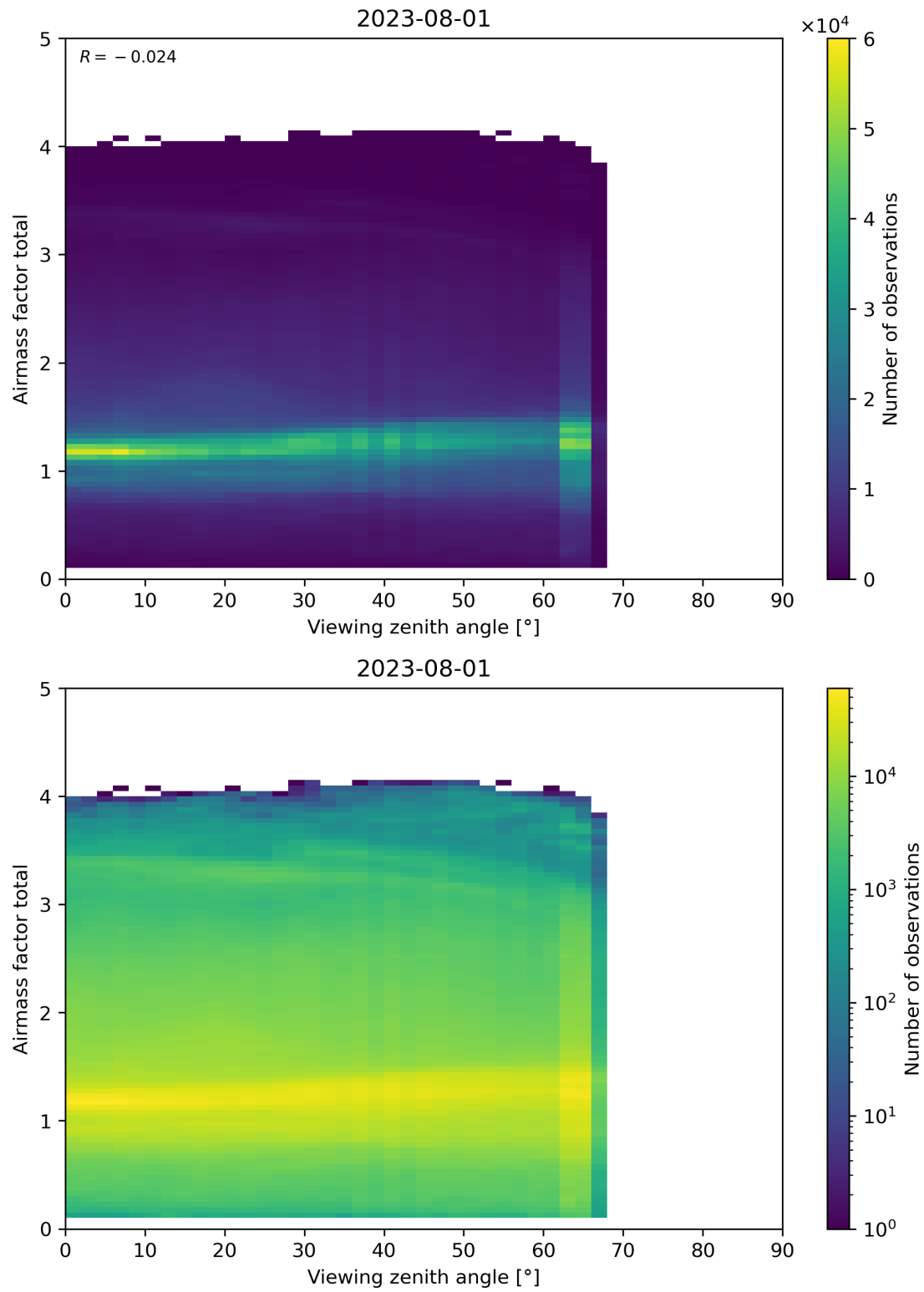
Figure 190: Scatter density plot of “Viewing zenith angle” against “Airmass factor total” for 2023-07-31 to 2023-08-02.
