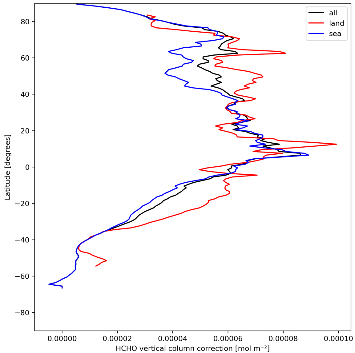
Figure 23: Zonal average of “HCHO vertical column correction” for 2023-07-31 to 2023-08-02.
