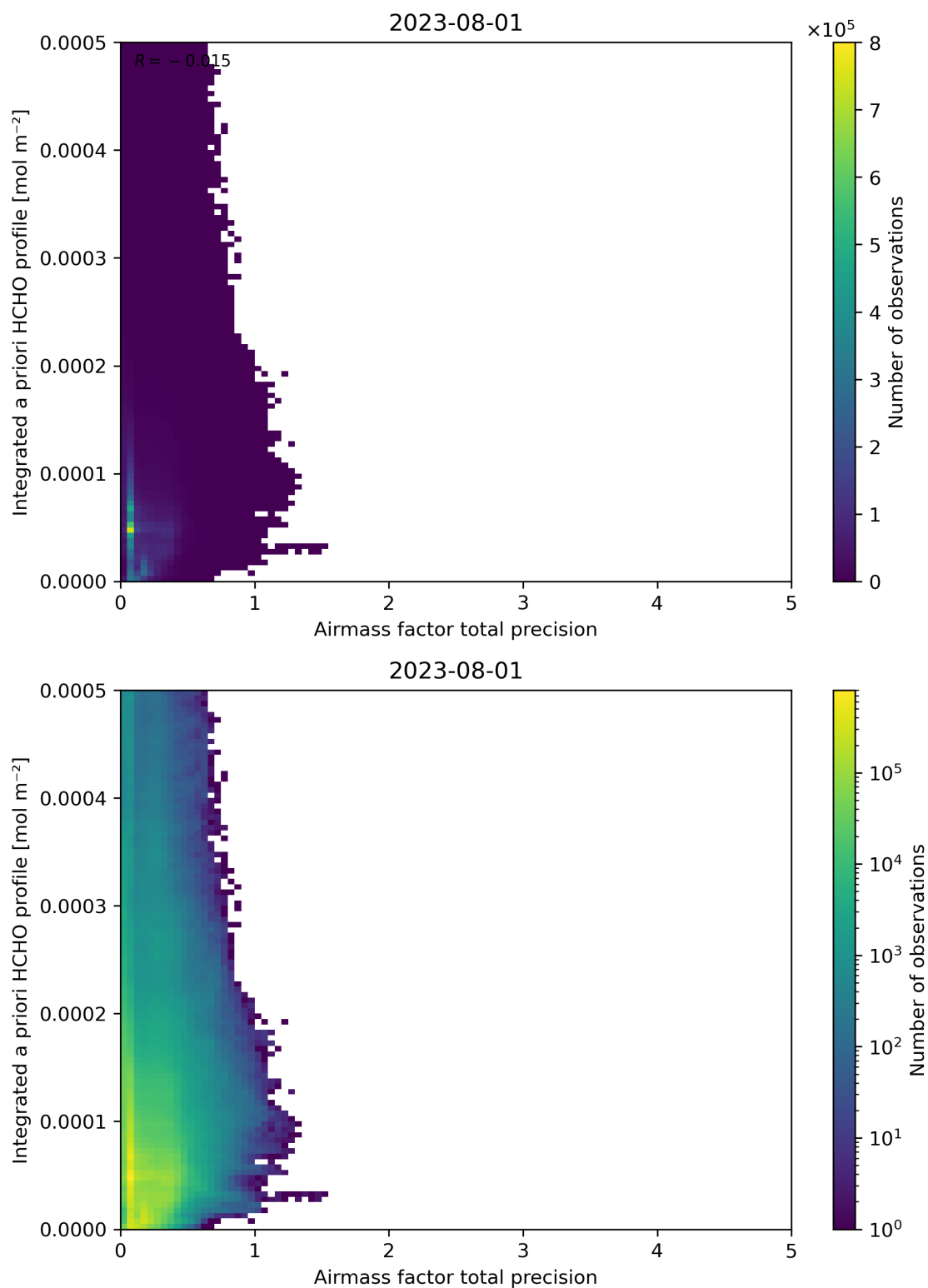
Figure 111: Scatter density plot of “Airmass factor total precision” against “Integrated a priori HCHO profile” for 2023-07-31 to 2023-08-02.
