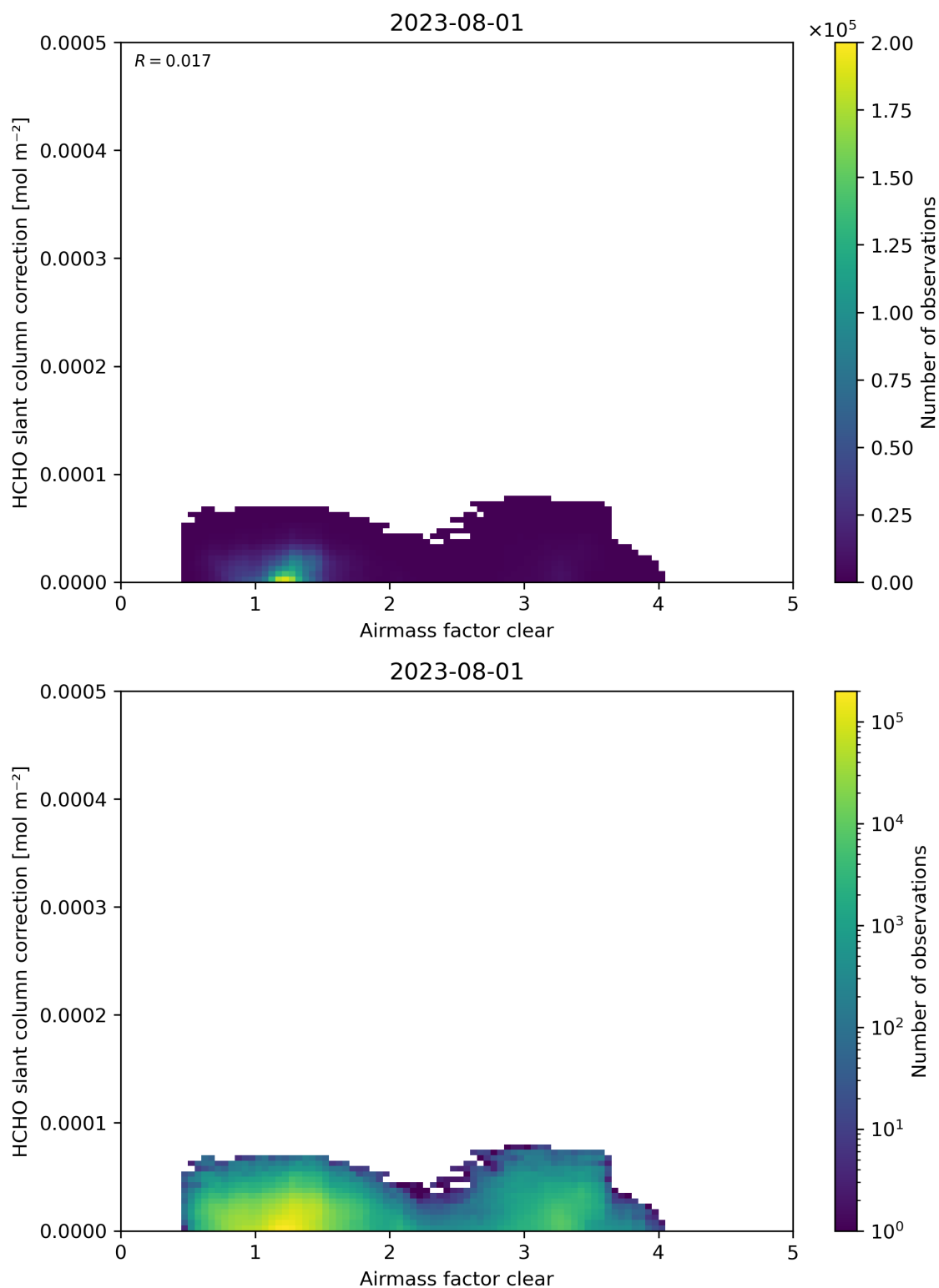
Figure 75: Scatter density plot of “Airmass factor clear” against “HCHO slant column correction” for 2023-07-31 to 2023-08-02.
