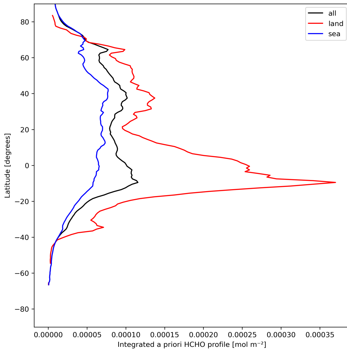
Figure 29: Zonal average of “Integrated a priori HCHO profile” for 2023-07-31 to 2023-08-02.
