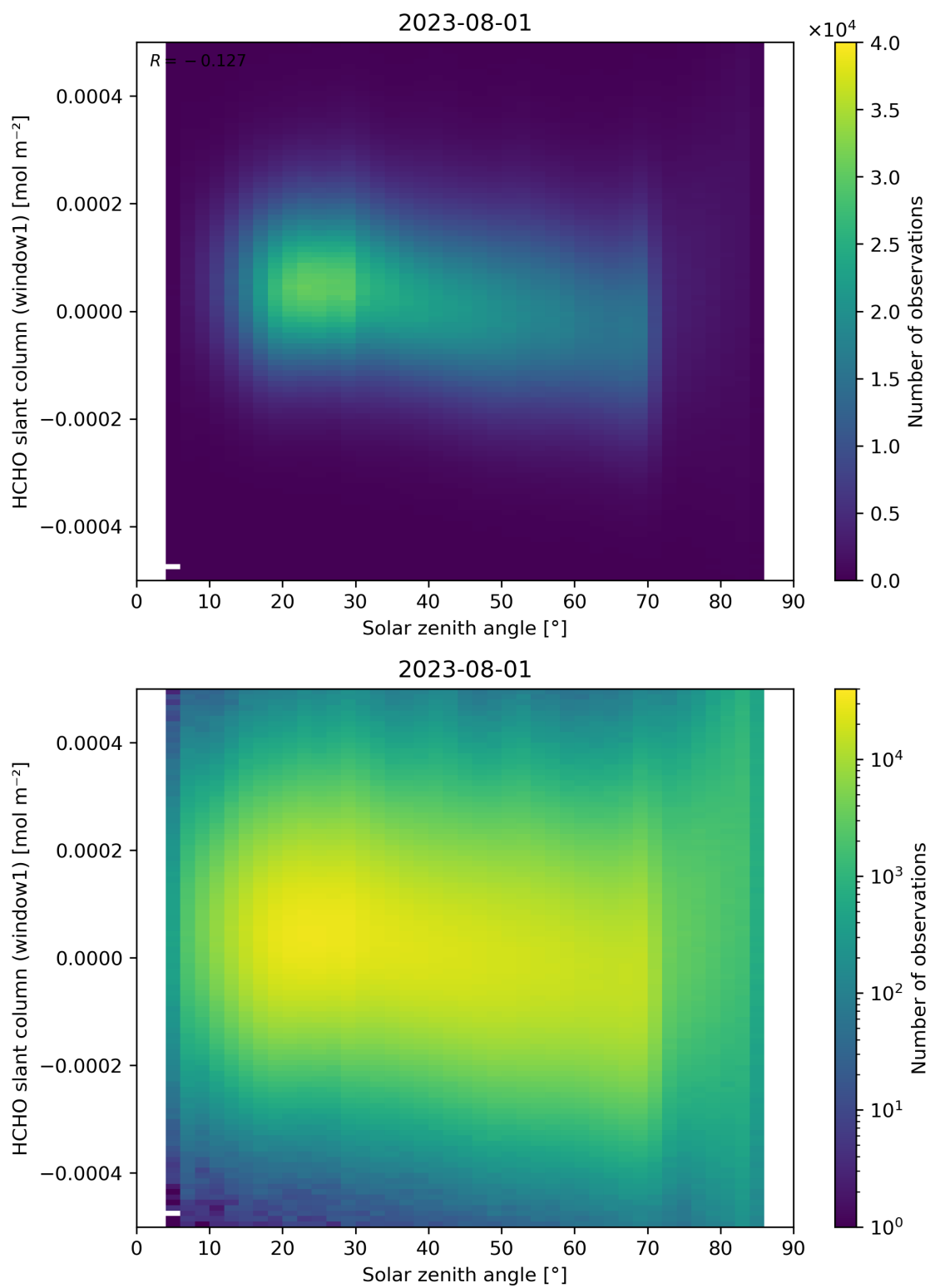
Figure 173: Scatter density plot of “Solar zenith angle” against “HCHO slant column (window1)” for 2023-07-31 to 2023-08-02.
