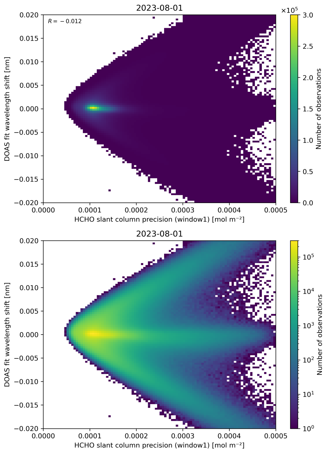
Figure 89: Scatter density plot of “HCHO slant column precision (window1)” against “DOAS fit wavelength shift” for 2023-07-31 to 2023-08-02.
