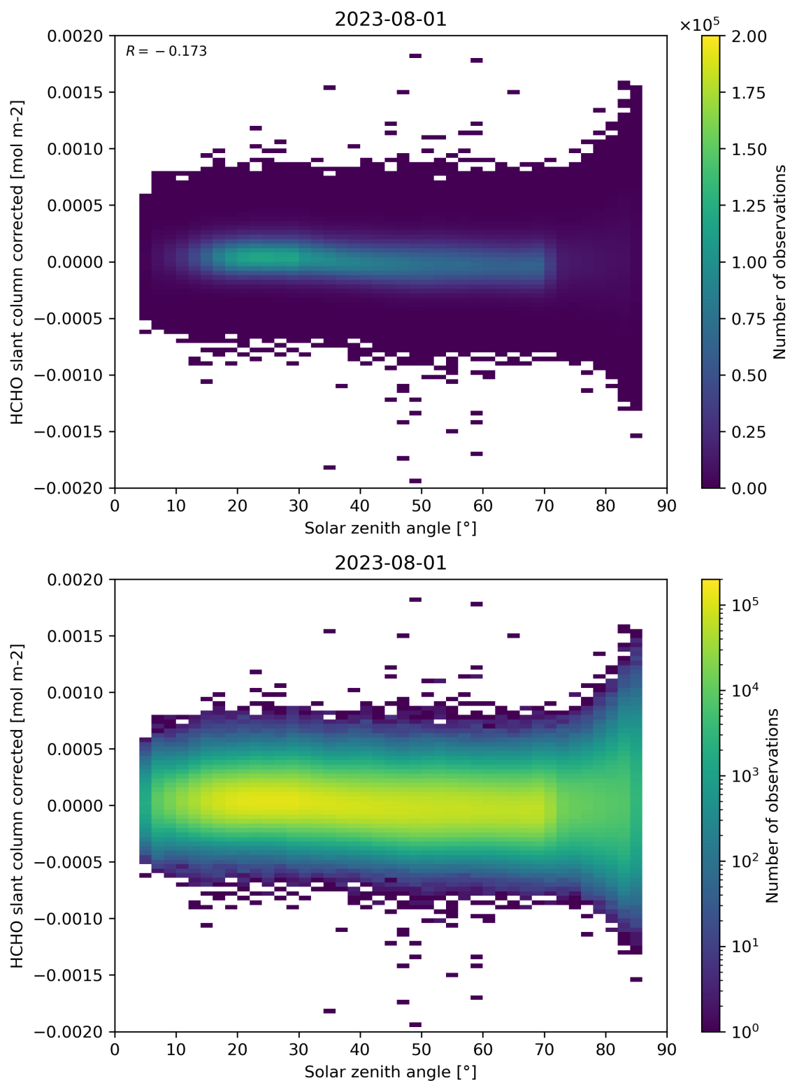
Figure 171: Scatter density plot of “Solar zenith angle” against “HCHO slant column corrected” for 2023-07-31 to 2023-08-02.
