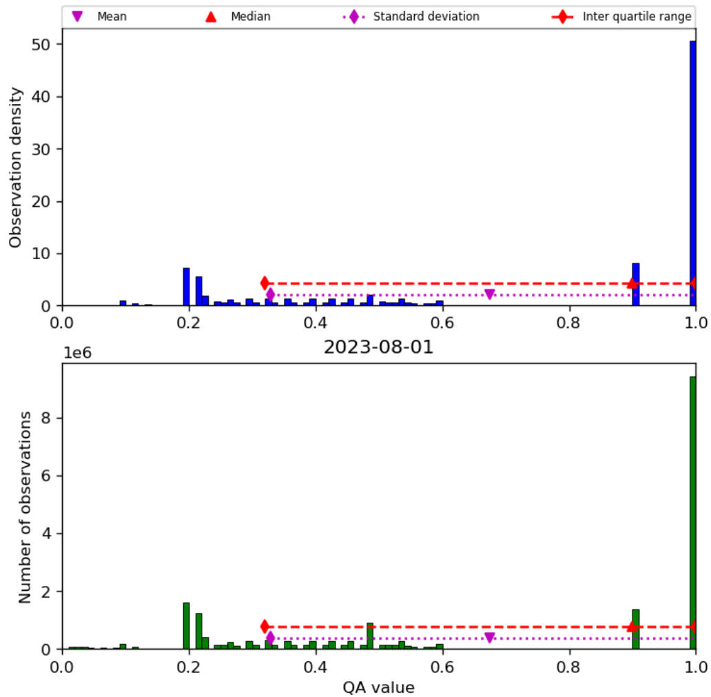
Figure 34: Histogram of “QA value” for 2023-07-31 to 2023-08-02
