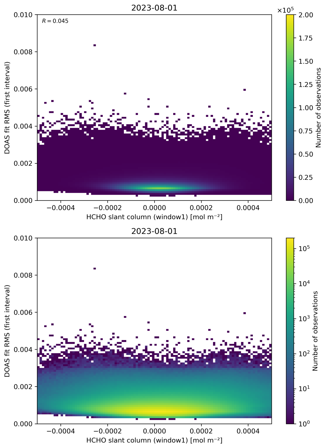
Figure 78: Scatter density plot of “HCHO slant column (window1)” against “DOAS fit RMS (first interval)” for 2023-07-31 to 2023-08-02.
