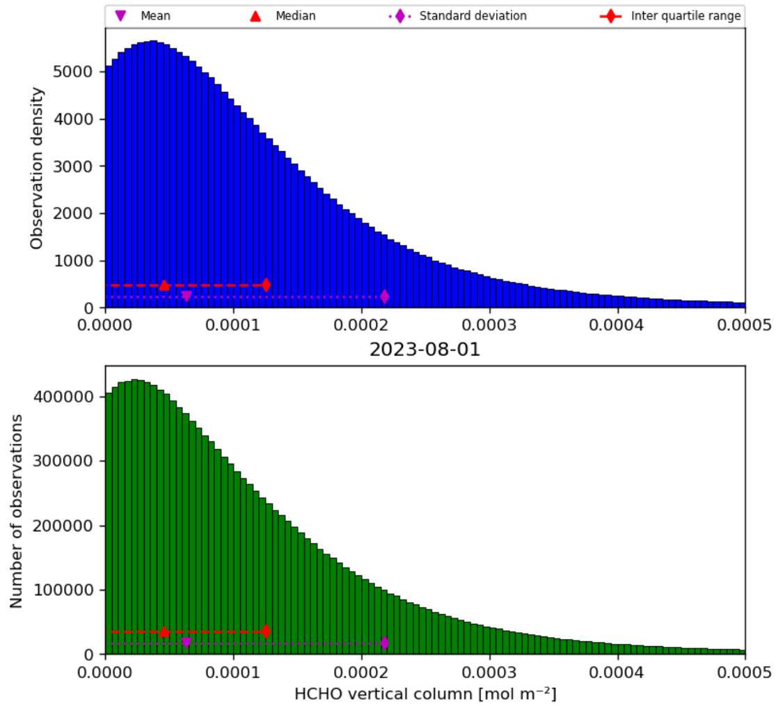
Figure 35: Histogram of “HCHO vertical column” for 2023-07-31 to 2023-08-02
