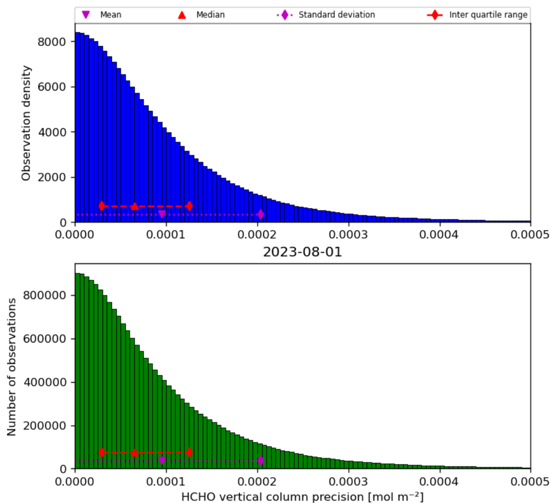
Figure 36: Histogram of “HCHO vertical column precision” for 2023-07-31 to 2023-08-02
