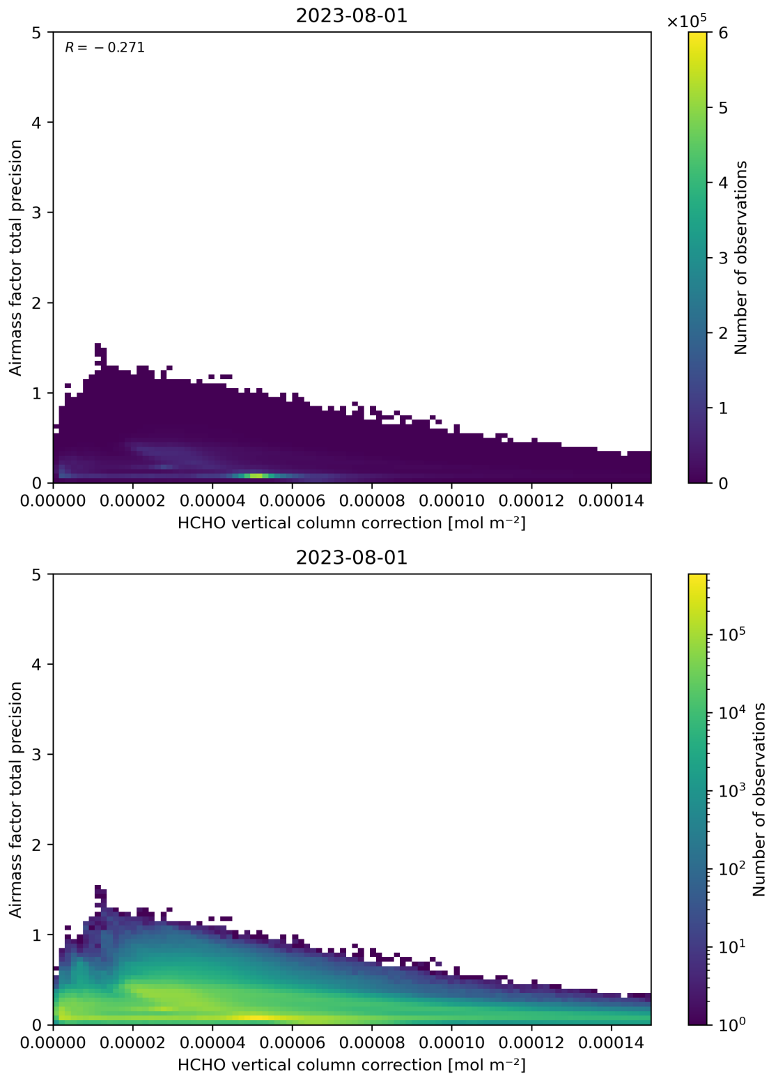
Figure 121: Scatter density plot of “HCHO vertical column correction” against “Airmass factor total precision” for 2023-07-31 to 2023-08-02.
