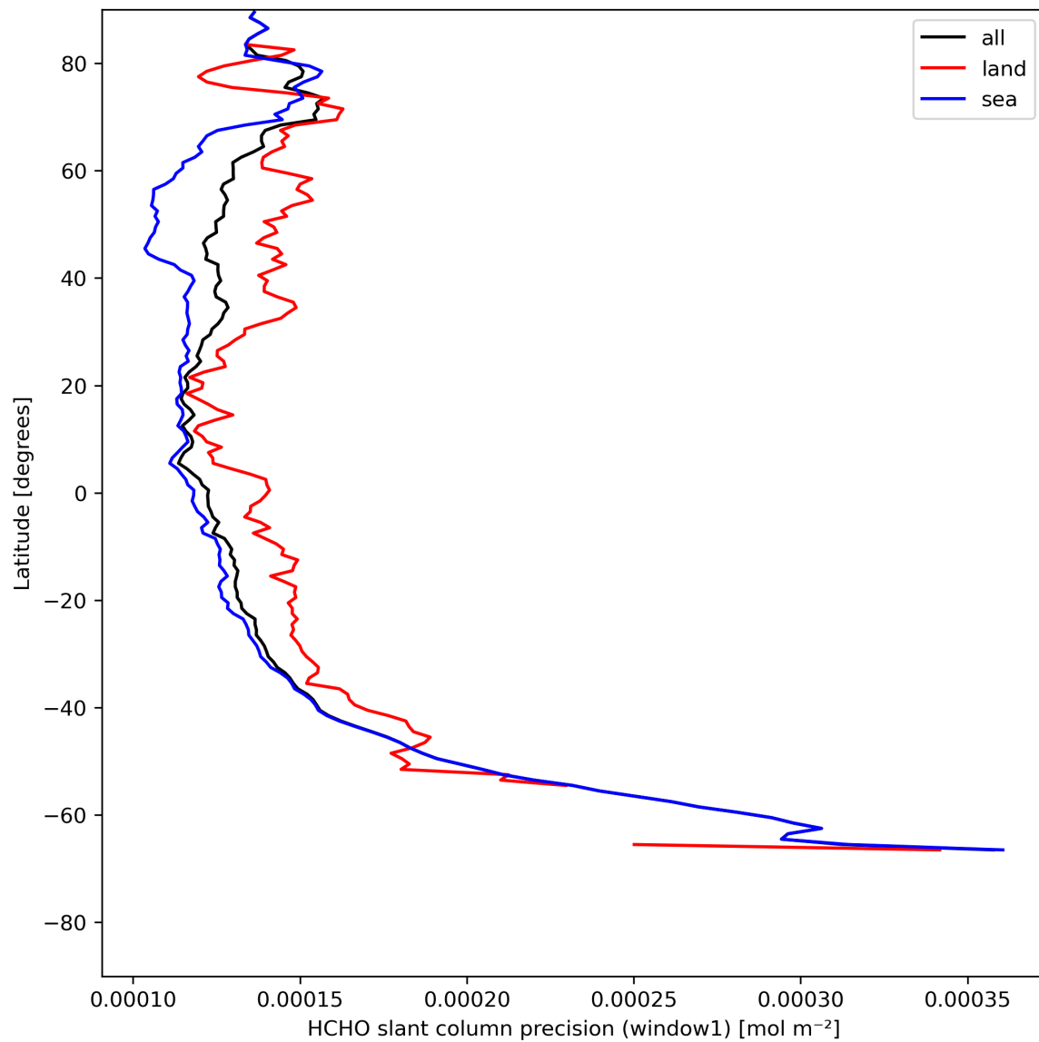
Figure 25: Zonal average of “HCHO slant column precision (window1)” for 2023-07-31 to 2023-08-02.
