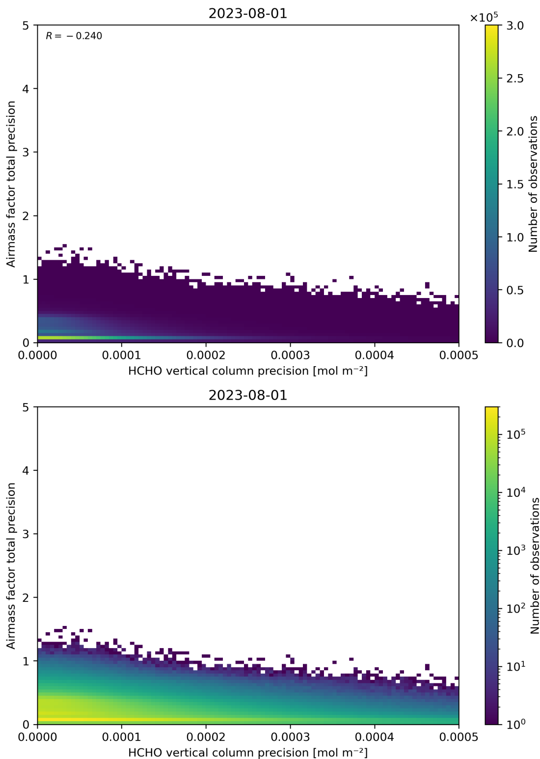
Figure 145: Scatter density plot of “HCHO vertical column precision” against “Airmass factor total precision” for 2023-07-31 to 2023-08-02.
