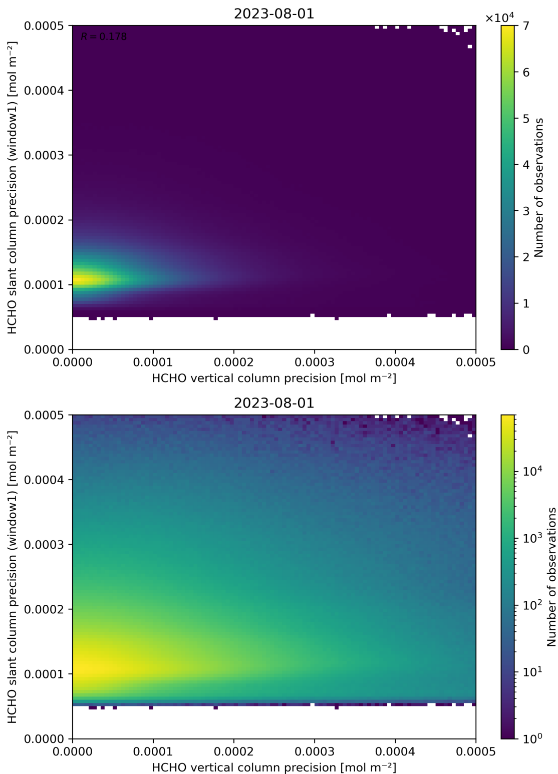
Figure 143: Scatter density plot of “HCHO vertical column precision” against “HCHO slant column precision (window1)” for 2023-07-31 to 2023-08-02.
