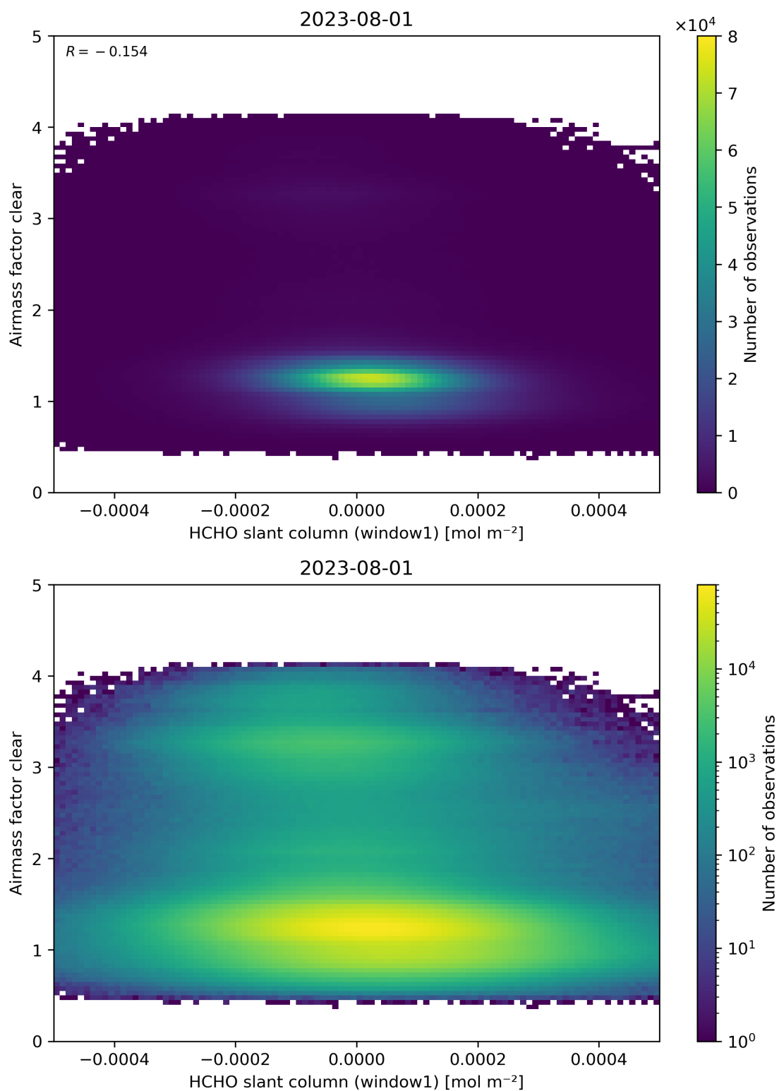
Figure 81: Scatter density plot of “HCHO slant column (window1)” against “Airmass factor clear” for 2023-07-31 to 2023-08-02.
