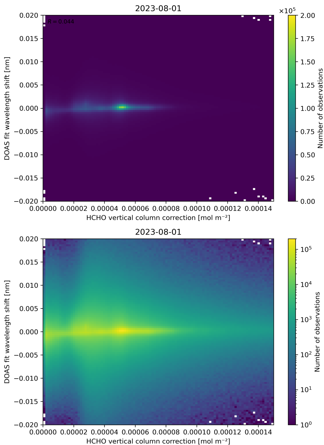
Figure 113: Scatter density plot of “HCHO vertical column correction” against “DOAS fit wavelength shift” for 2023-07-31 to 2023-08-02.
