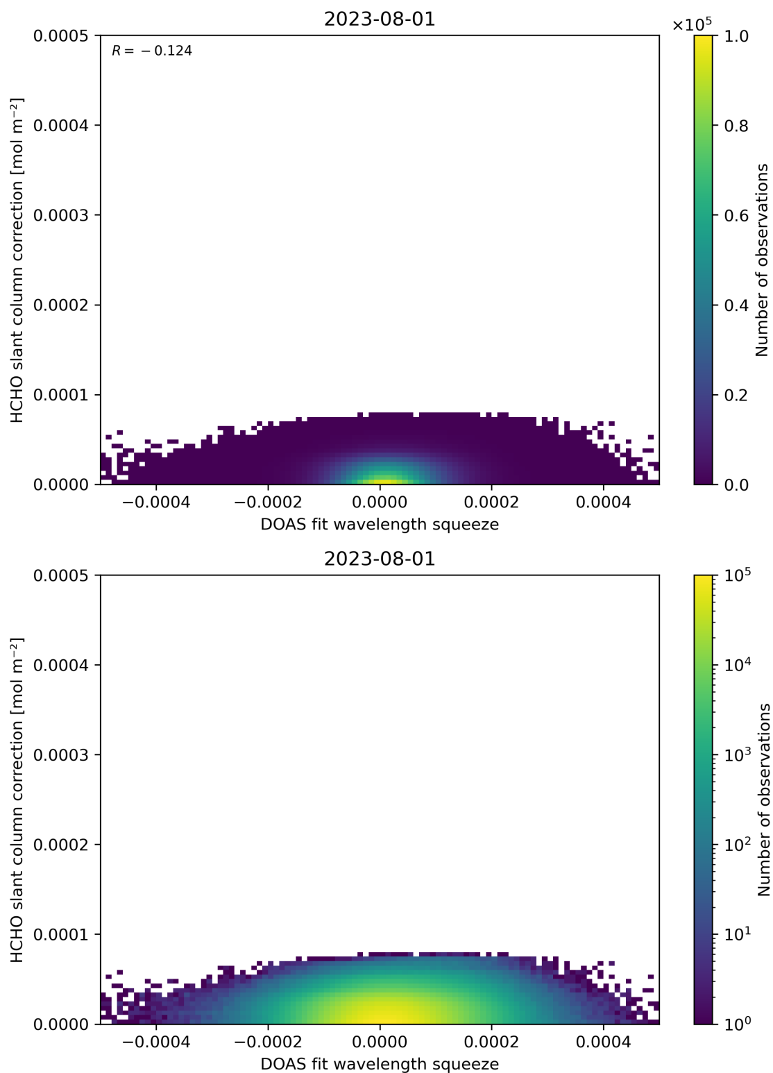
Figure 70: Scatter density plot of “DOAS fit wavelength squeeze” against “HCHO slant column correction” for 2023-07-31 to 2023-08-02.
