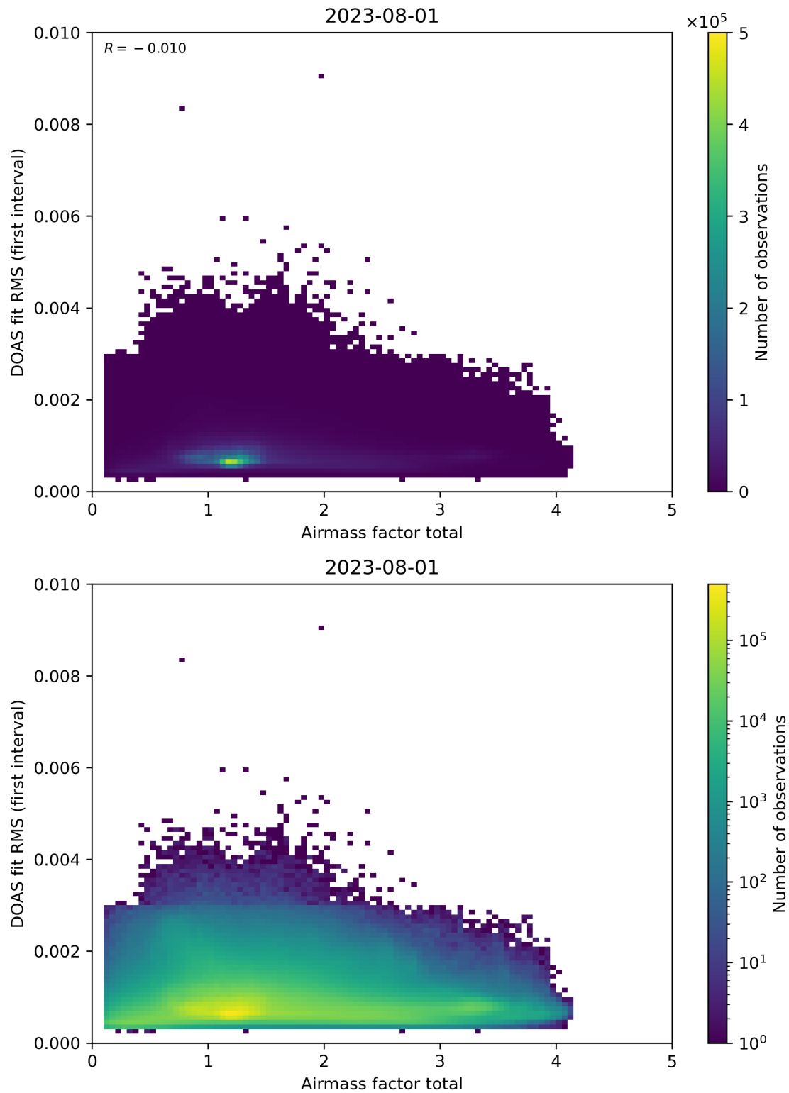
Figure 97: Scatter density plot of “Airmass factor total” against “DOAS fit RMS (first interval)” for 2023-07-31 to 2023-08-02.
