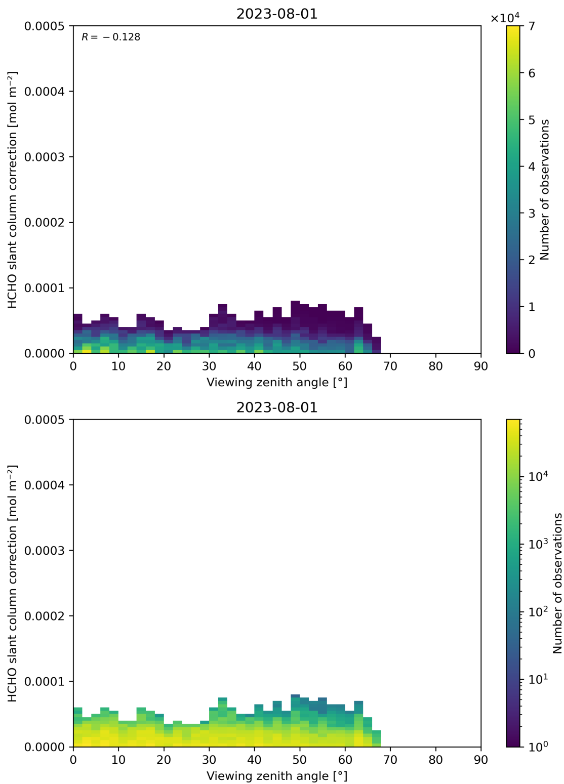
Figure 187: Scatter density plot of “Viewing zenith angle” against “HCHO slant column correction” for 2023-07-31 to 2023-08-02.
