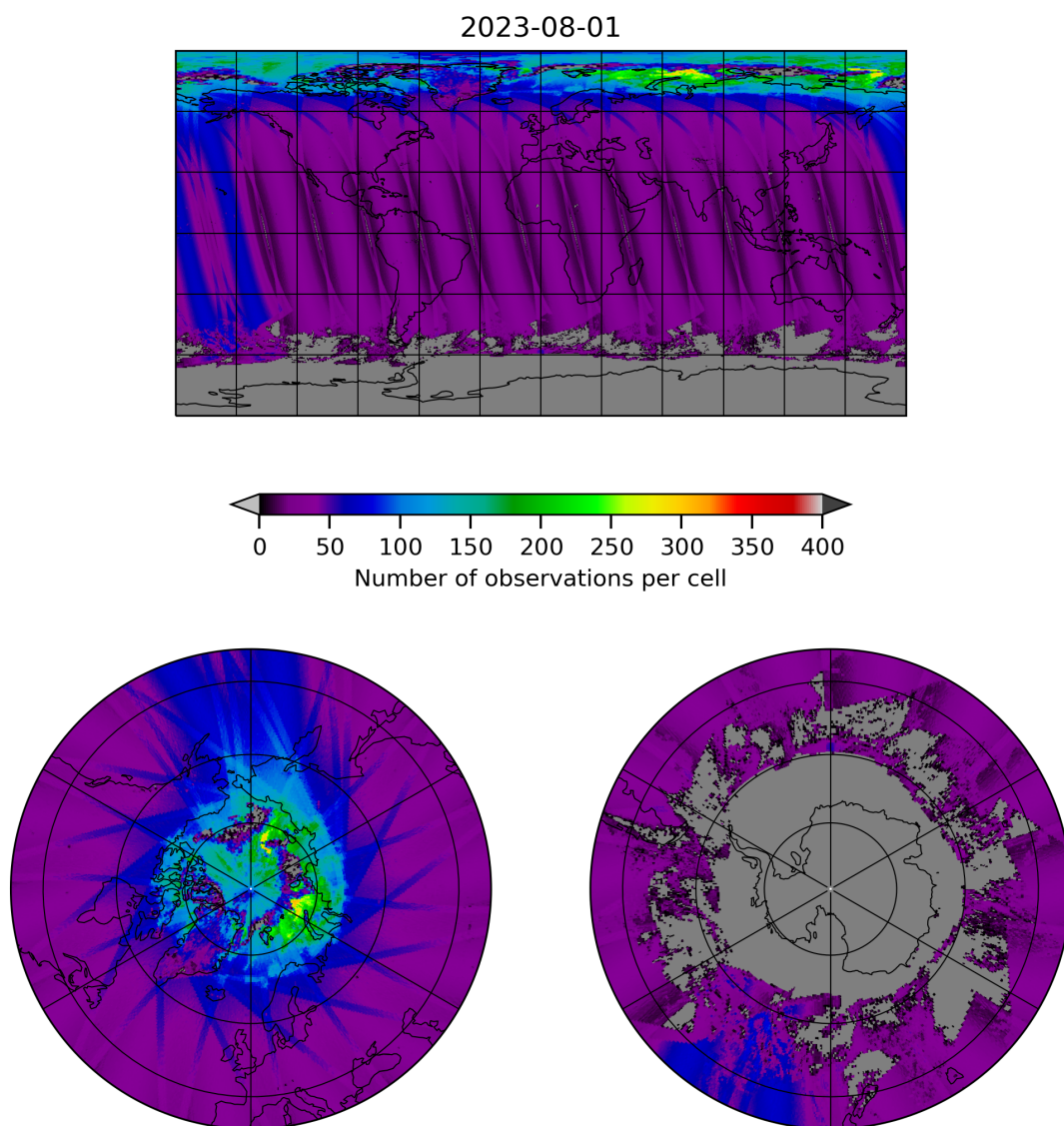
Figure 19: Map of the number of observations for 2023-07-31 to 2023-08-02
