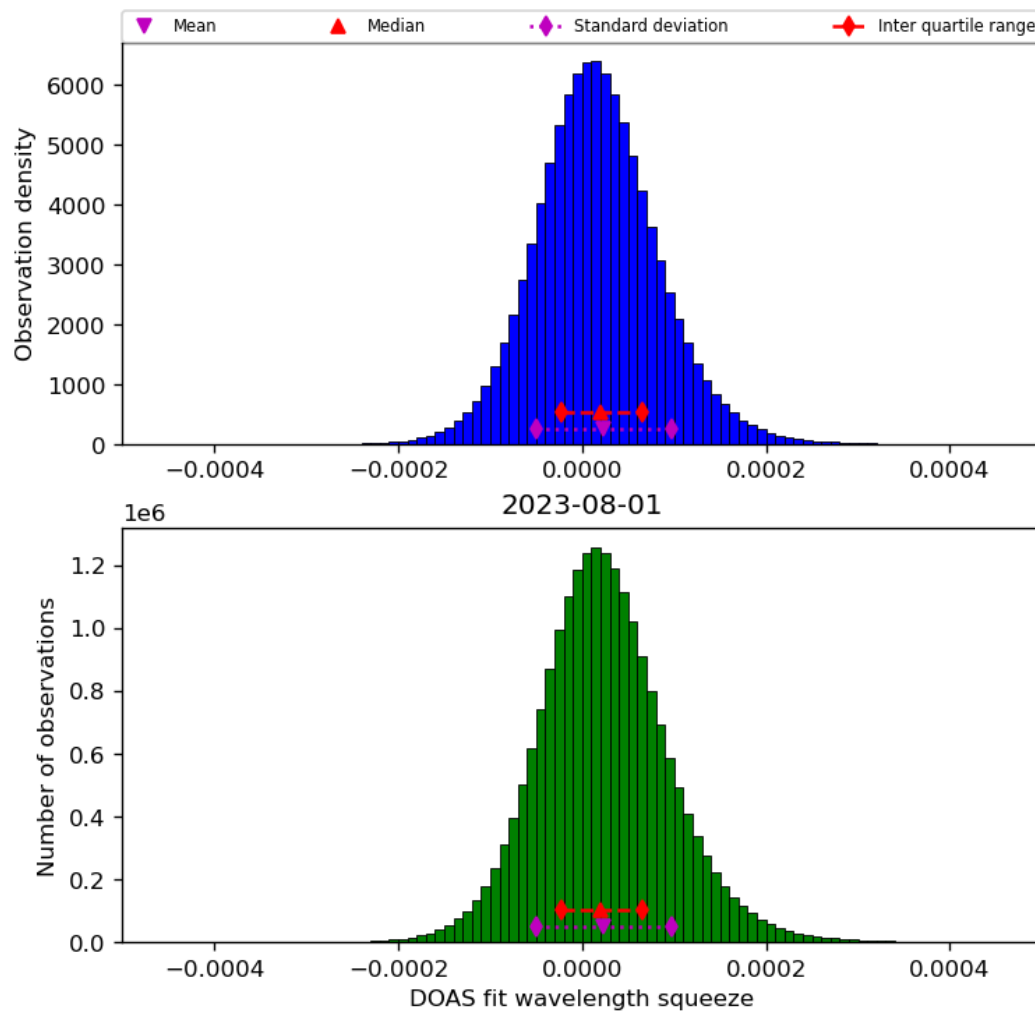
Figure 45: Histogram of “DOAS fit wavelength squeeze” for 2023-07-31 to 2023-08-02
