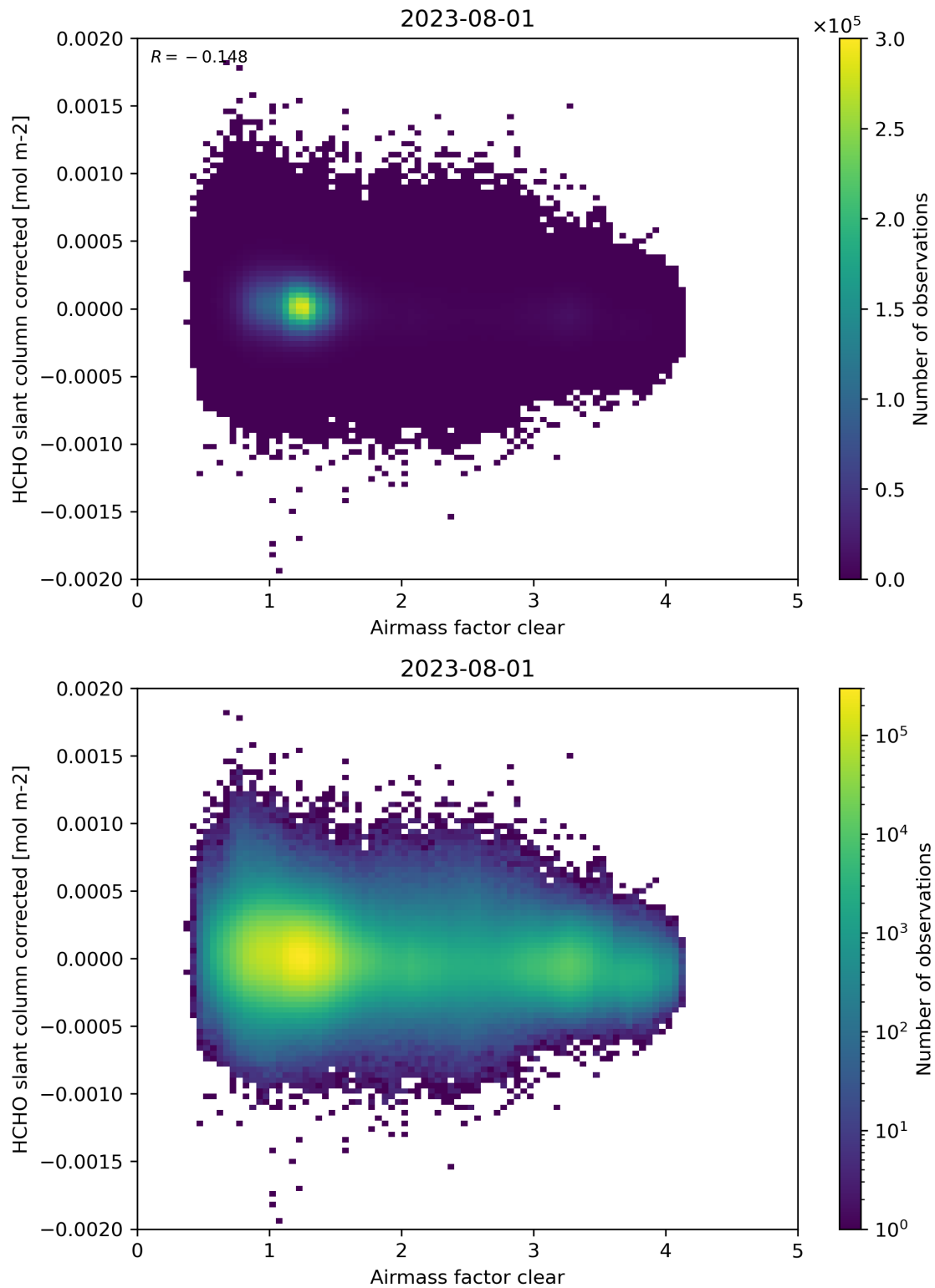
Figure 74: Scatter density plot of “Airmass factor clear” against “HCHO slant column corrected” for 2023-07-31 to 2023-08-02.
