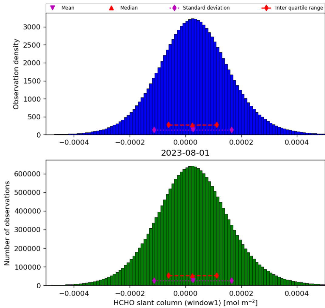
Figure 38: Histogram of “HCHO slant column (window1)” for 2023-07-31 to 2023-08-02
