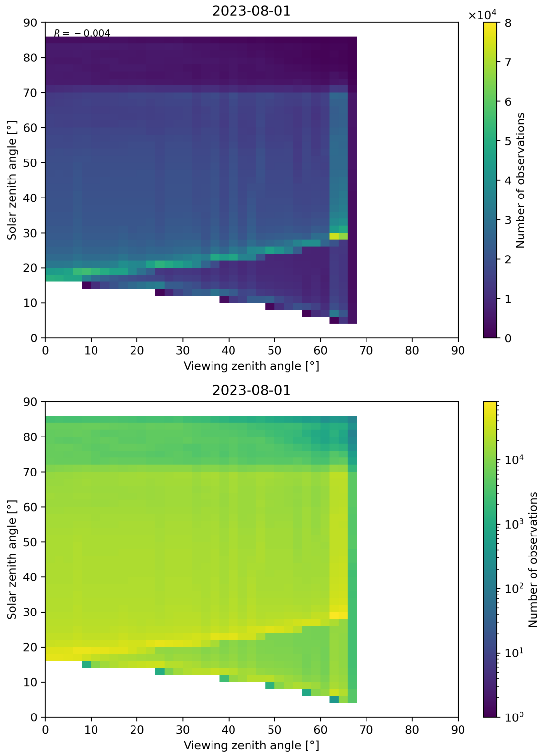
Figure 197: Scatter density plot of “Viewing zenith angle” against “Solar zenith angle” for 2023-07-31 to 2023-08-02.
