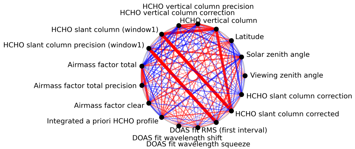
Figure 1: Map of correlation graph for 2023-07-31 to 2023-08-02.
