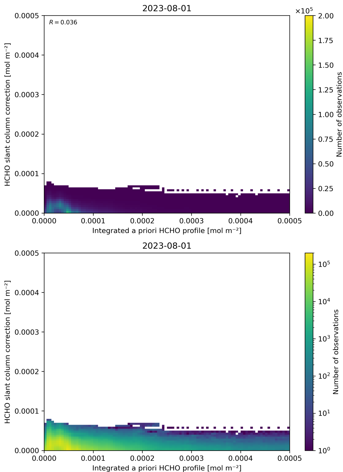
Figure 152: Scatter density plot of “Integrated a priori HCHO profile” against “HCHO slant column correction” for 2023-07-31 to 2023-08-02.
