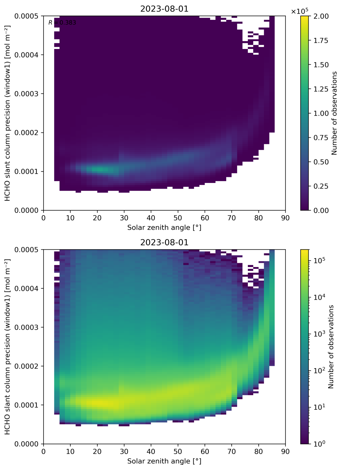
Figure 174: Scatter density plot of “Solar zenith angle” against “HCHO slant column precision (window1)” for 2023-07-31 to 2023-08-02.
