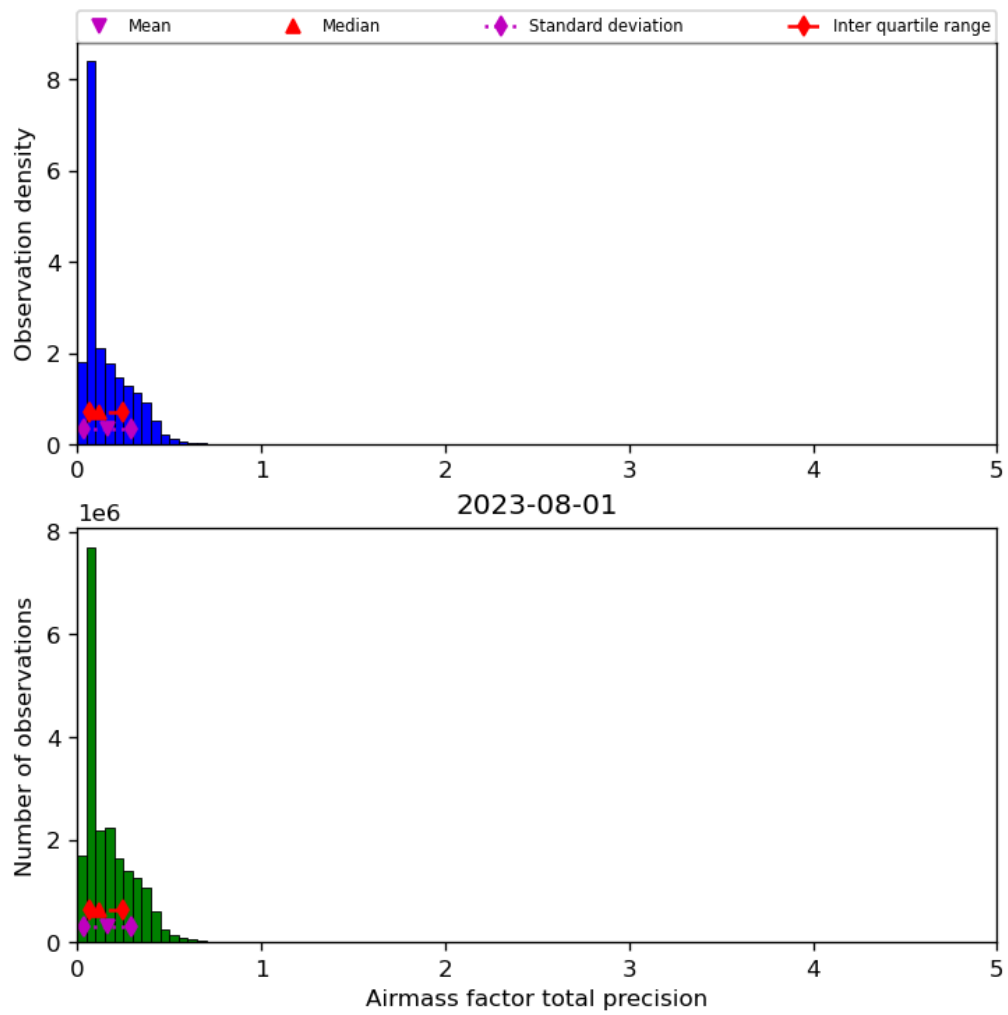
Figure 41: Histogram of “Airmass factor total precision” for 2023-07-31 to 2023-08-02
