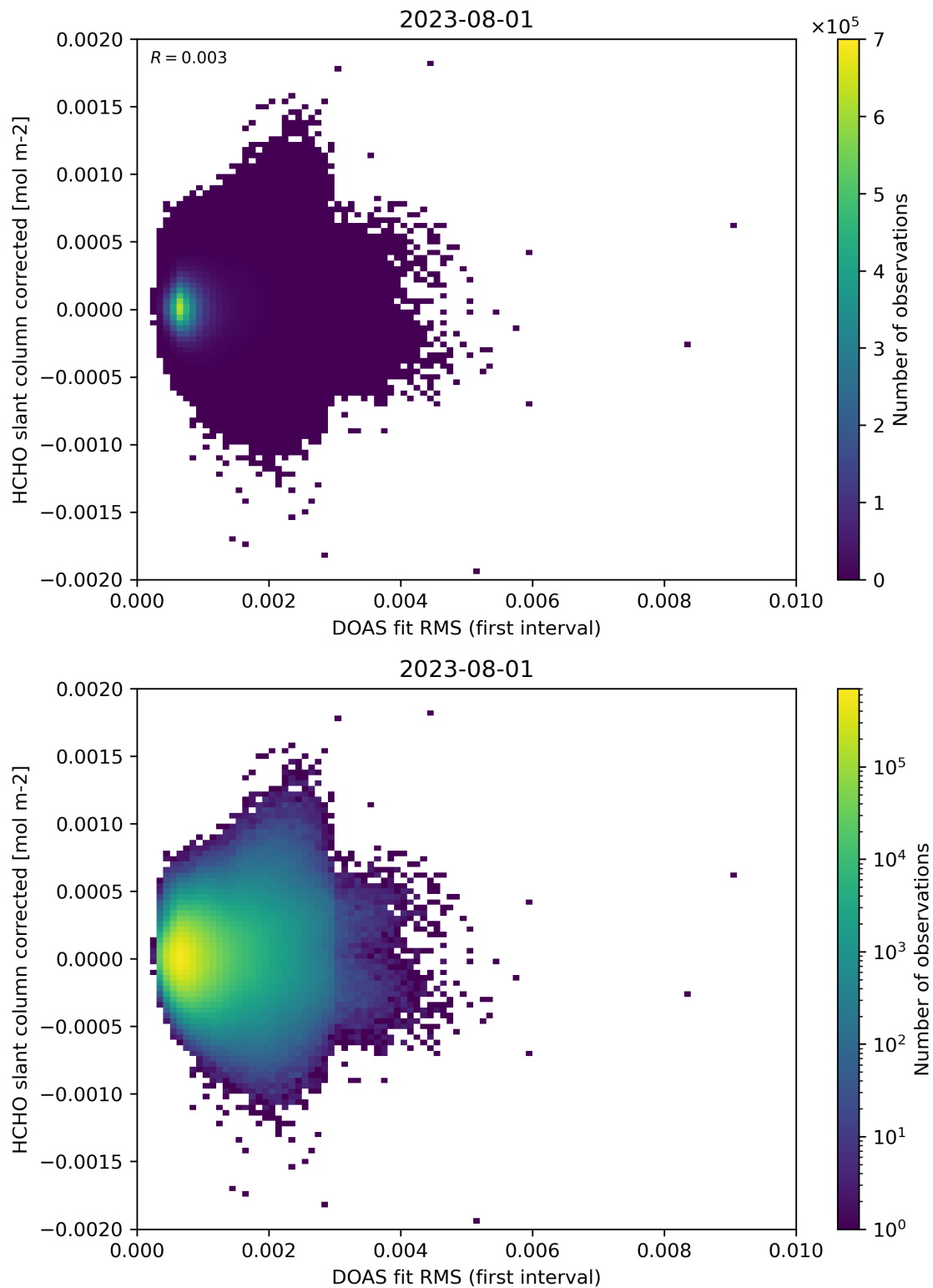
Figure 62: Scatter density plot of “DOAS fit RMS (first interval)” against “HCHO slant column corrected” for 2023-07-31 to 2023-08-02.
