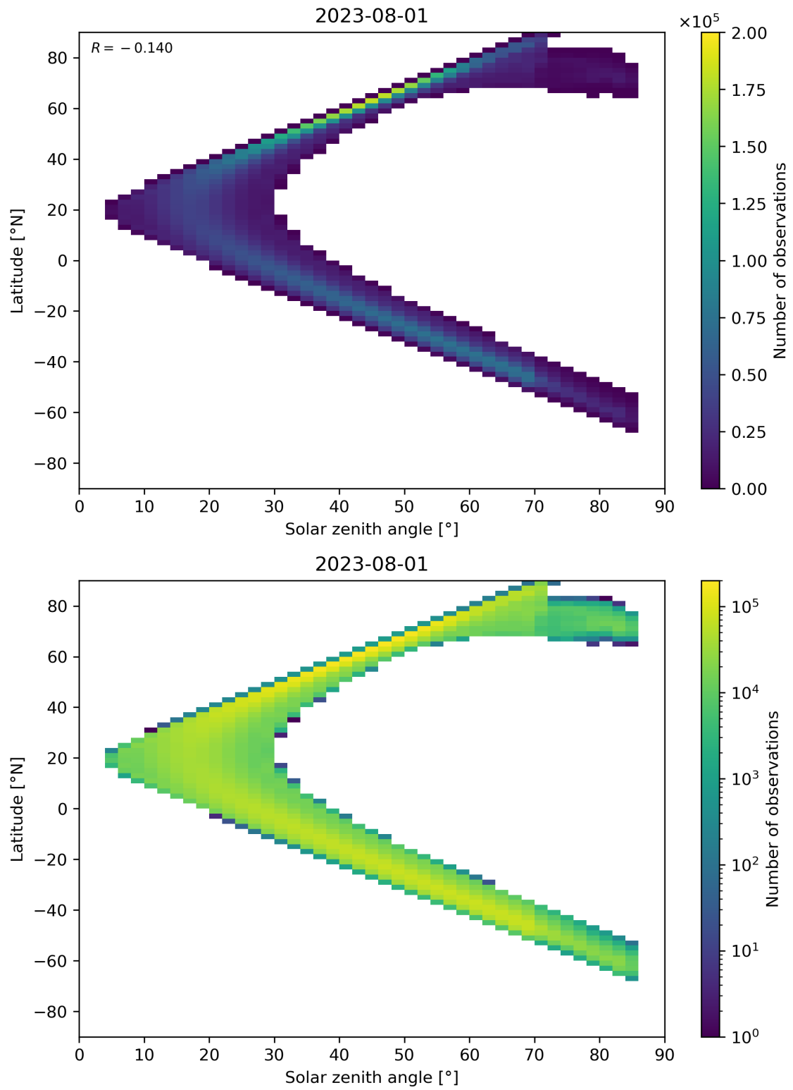
Figure 181: Scatter density plot of “Solar zenith angle” against “Latitude” for 2023-07-31 to 2023-08-02.
