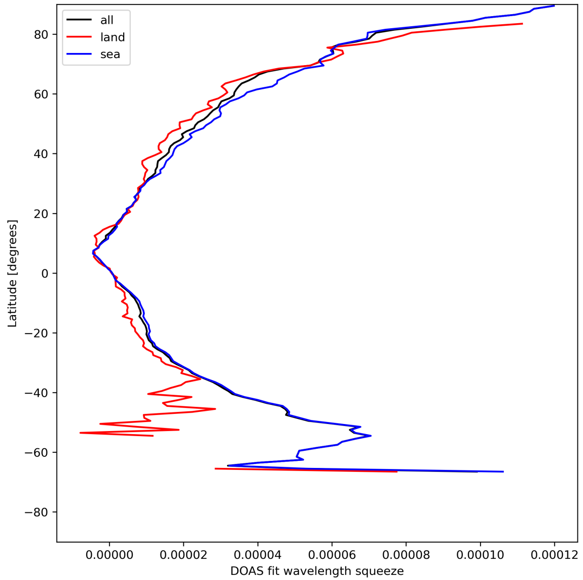
Figure 31: Zonal average of “DOAS fit wavelength squeeze” for 2023-07-31 to 2023-08-02.
