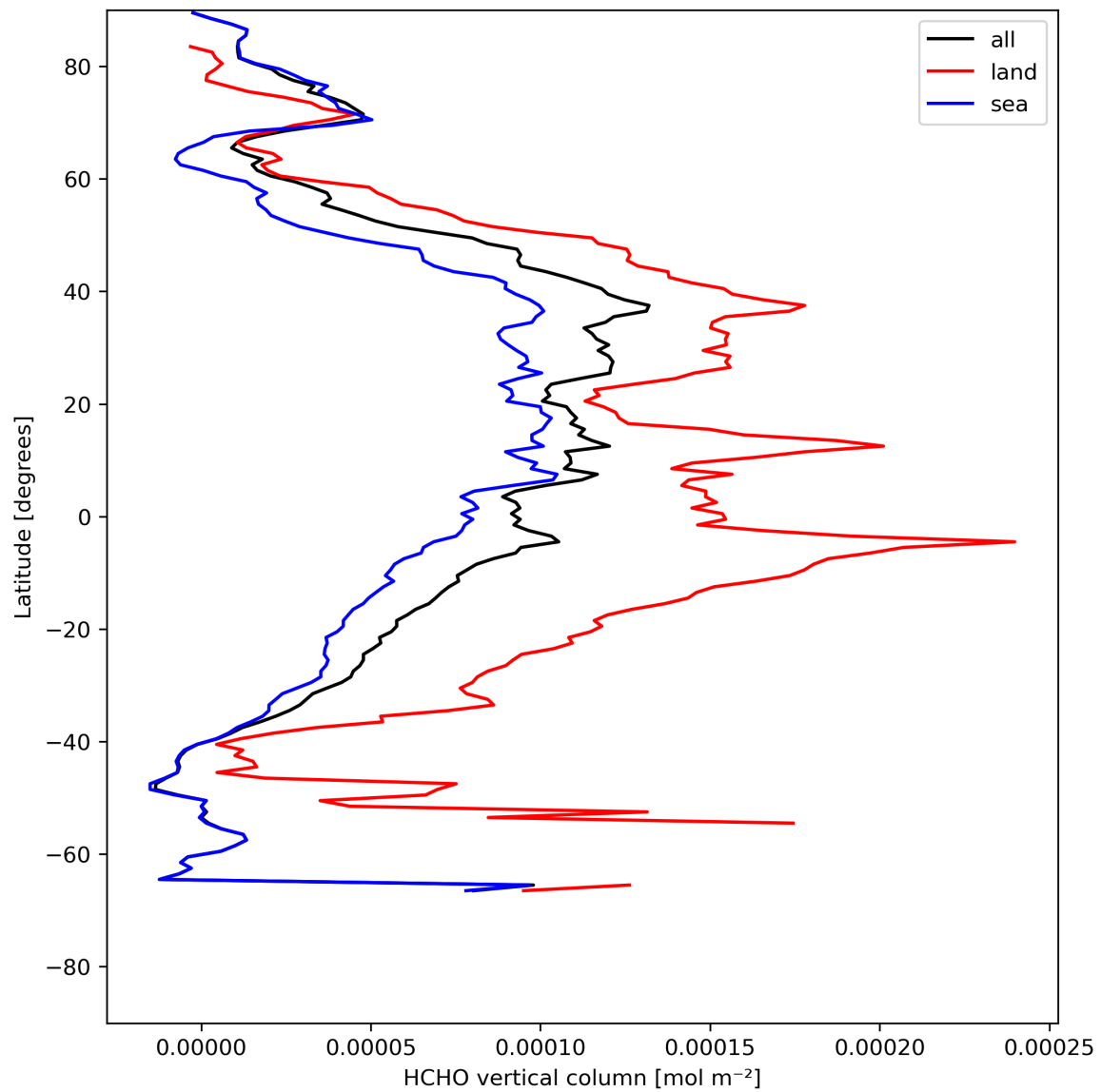
Figure 21: Zonal average of “HCHO vertical column” for 2023-07-31 to 2023-08-02.
