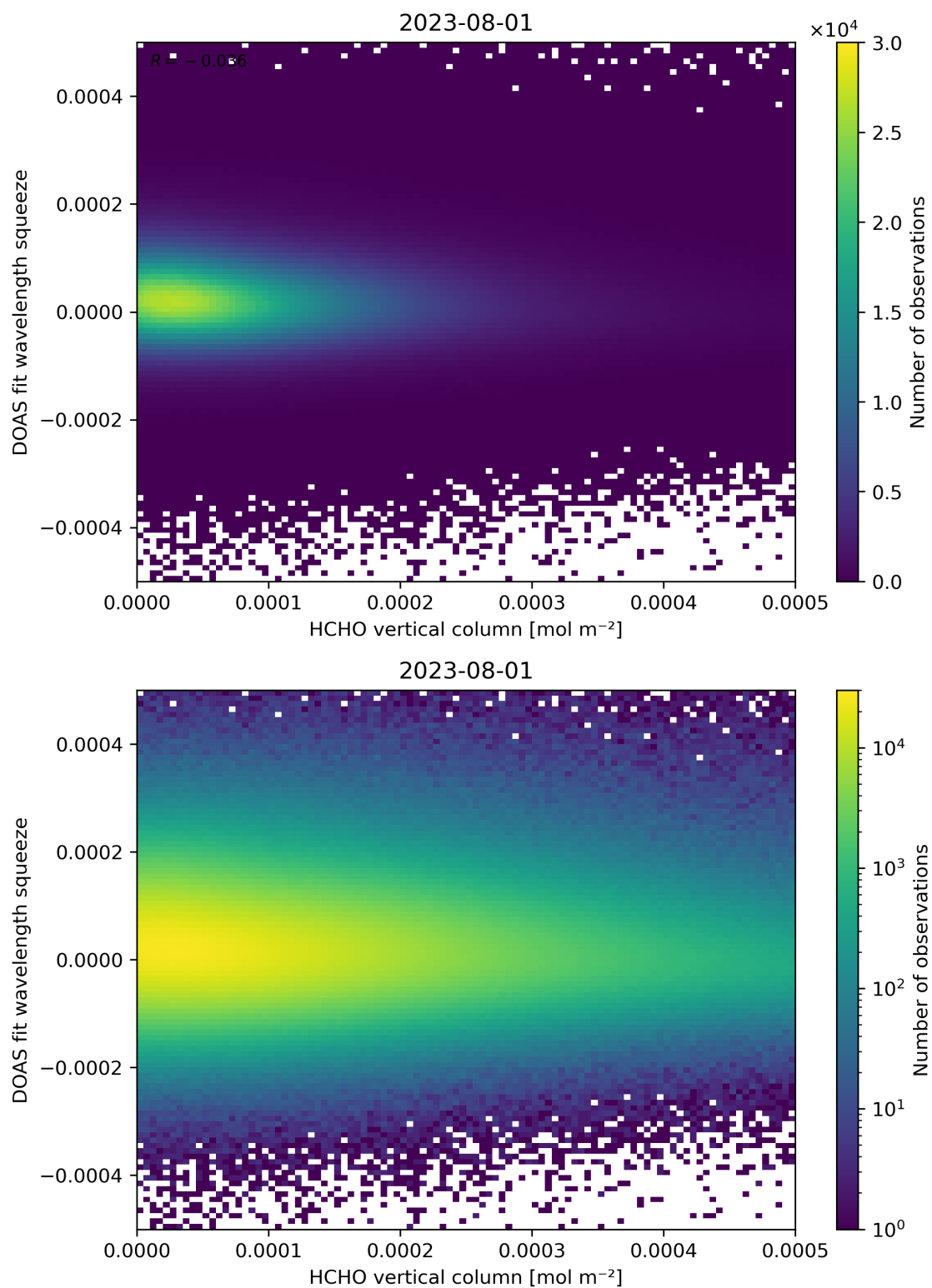
Figure 125: Scatter density plot of “HCHO vertical column” against “DOAS fit wavelength squeeze” for 2023-07-31 to 2023-08-02.
