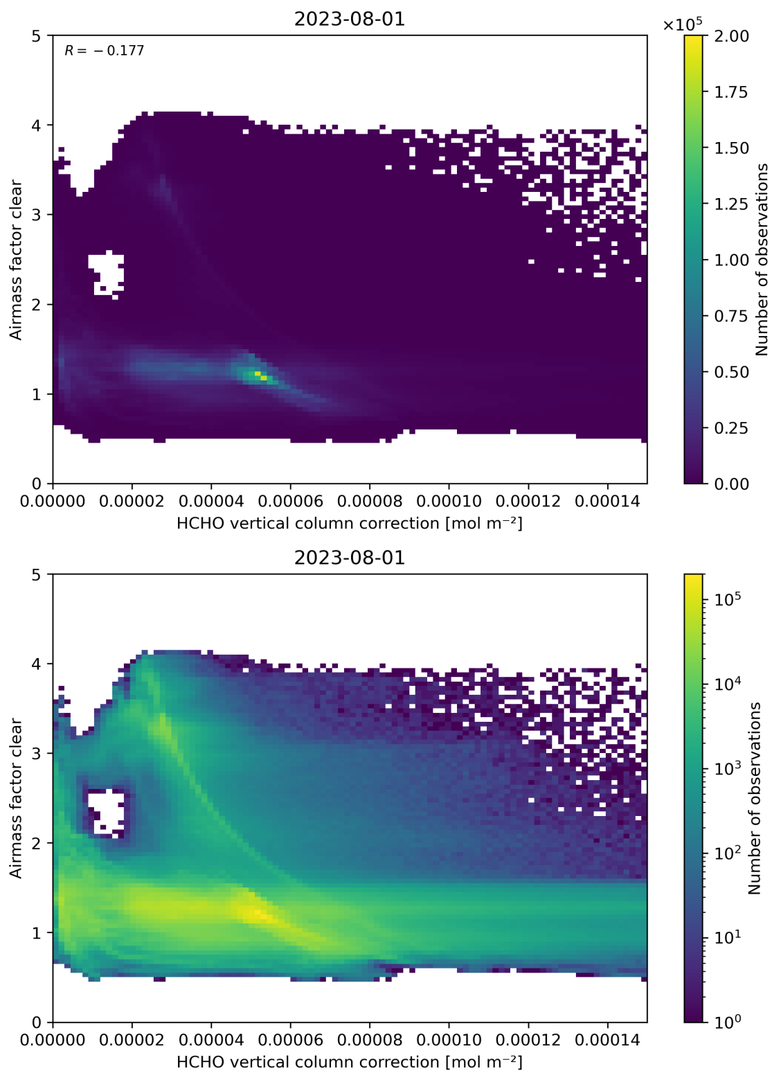
Figure 115: Scatter density plot of “HCHO vertical column correction” against “Airmass factor clear” for 2023-07-31 to 2023-08-02.
