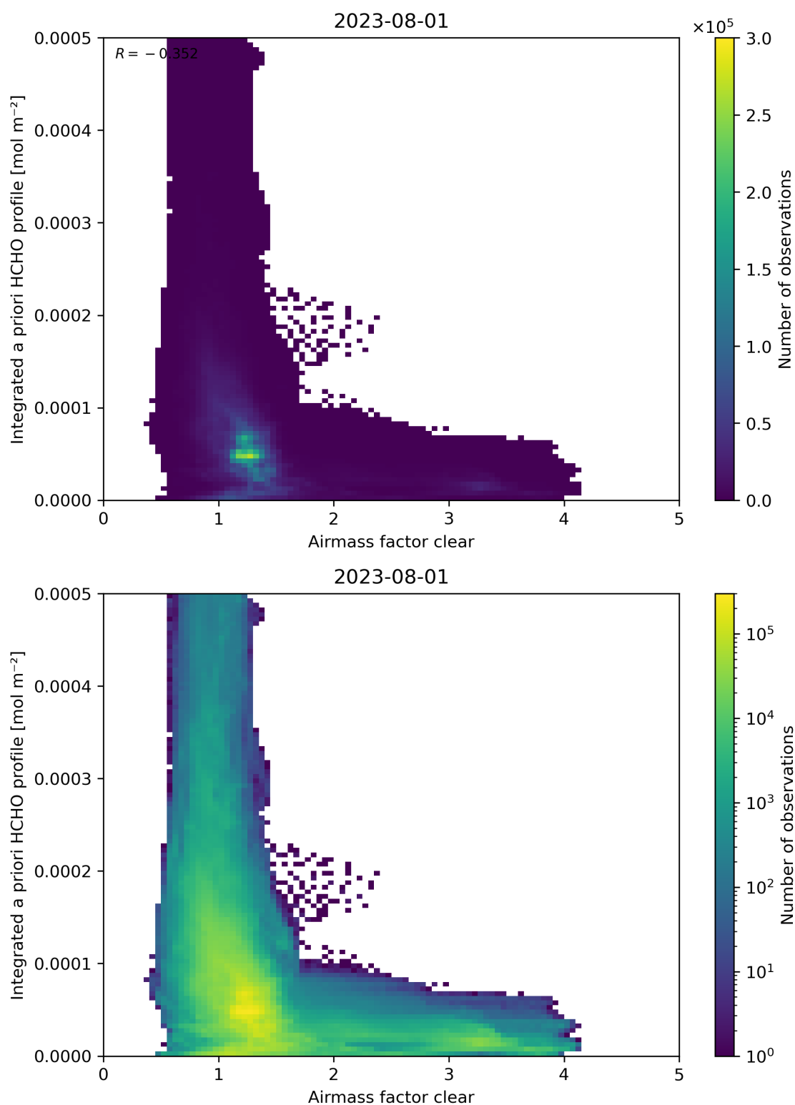
Figure 76: Scatter density plot of “Airmass factor clear” against “Integrated a priori HCHO profile” for 2023-07-31 to 2023-08-02.
