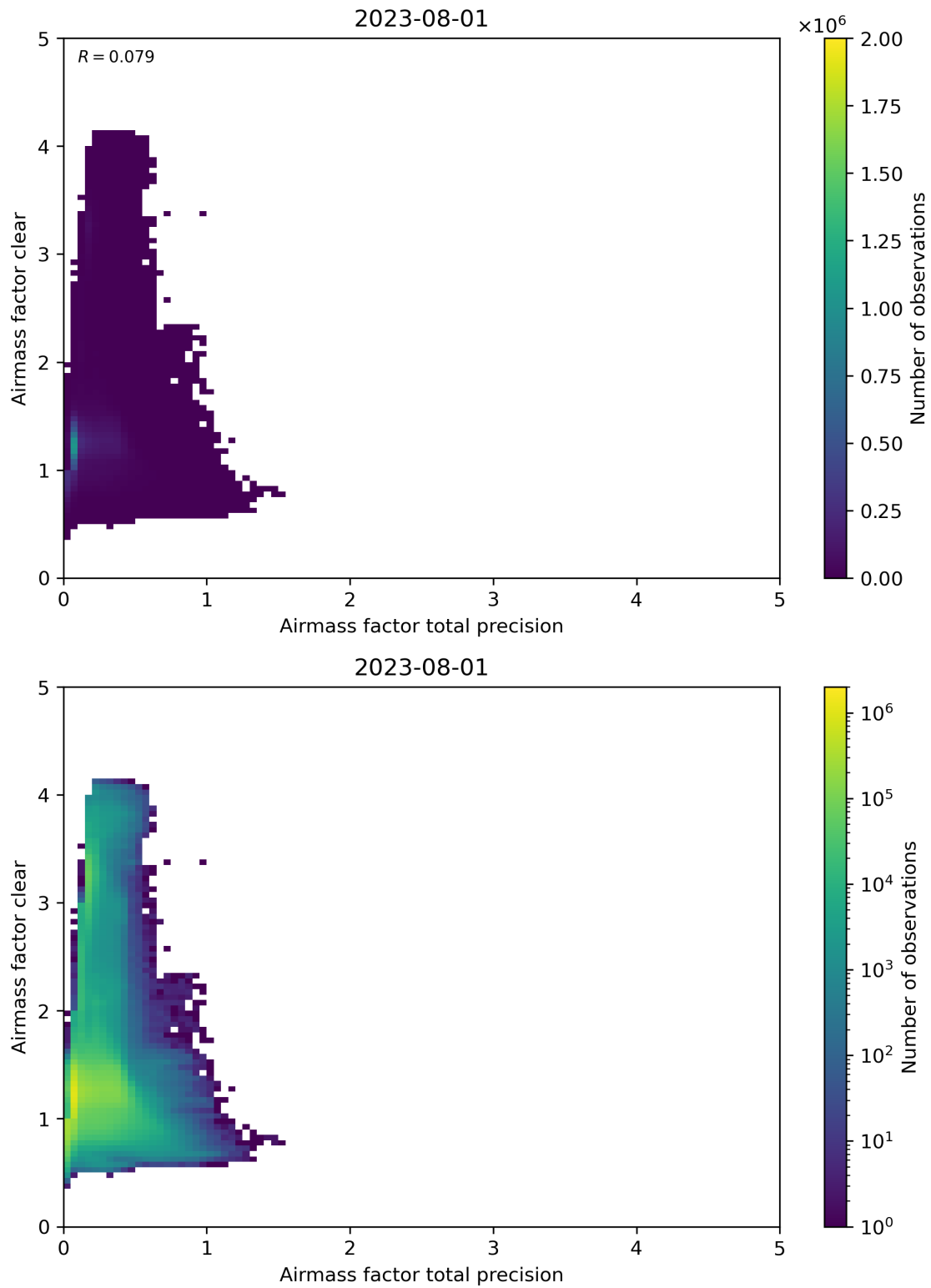
Figure 108: Scatter density plot of “Airmass factor total precision” against “Airmass factor clear” for 2023-07-31 to 2023-08-02.
