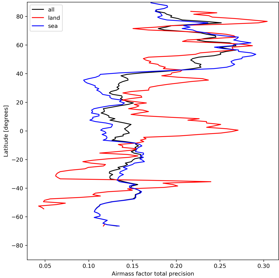
Figure 27: Zonal average of “Airmass factor total precision” for 2023-07-31 to 2023-08-02.
