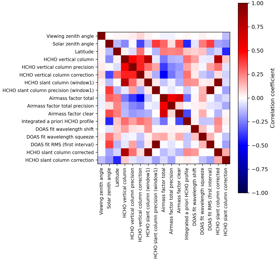
Figure 2: Map of correlation matrix for 2023-07-31 to 2023-08-02.
