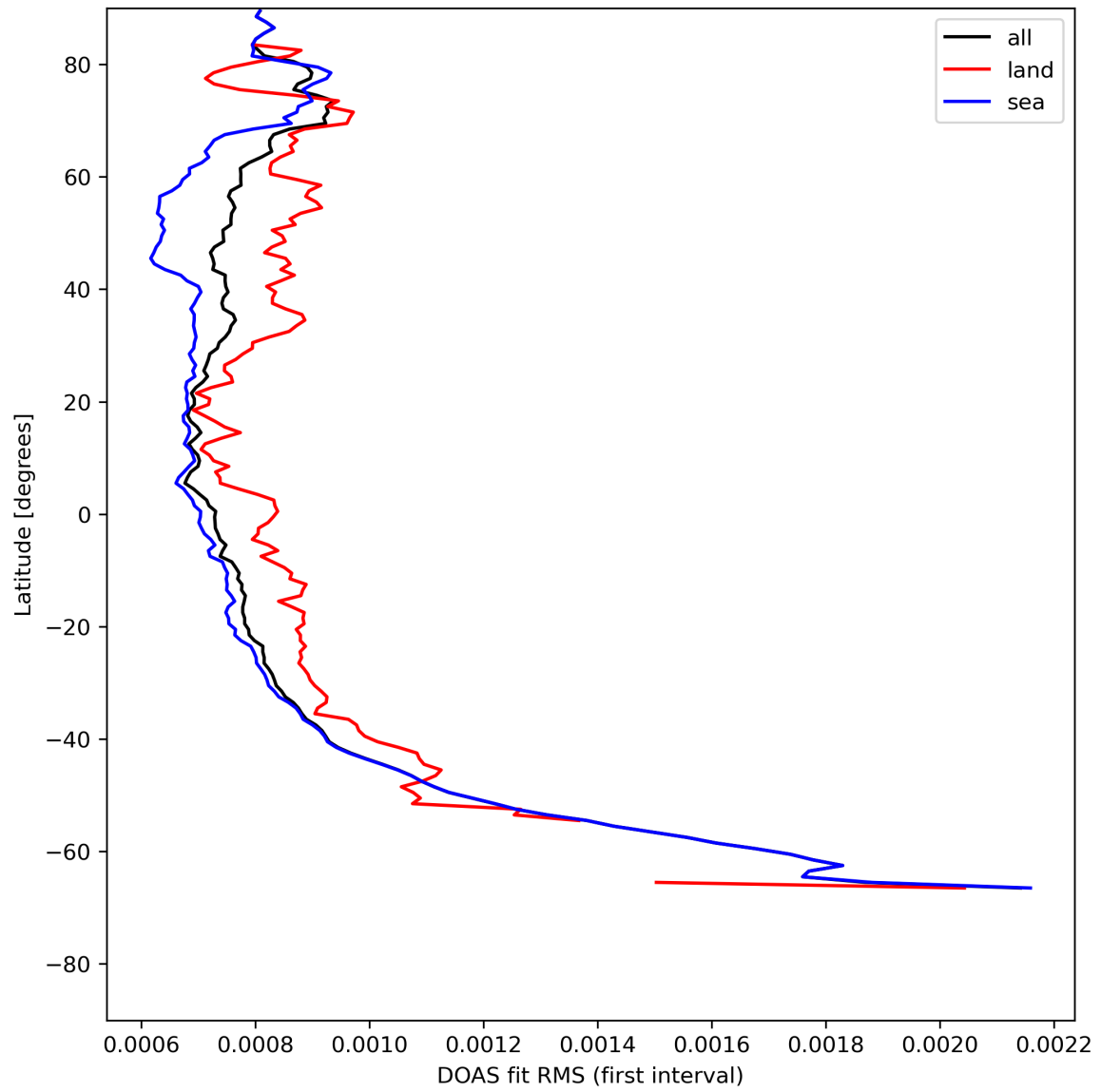
Figure 32: Zonal average of “DOAS fit RMS (first interval)” for 2023-07-31 to 2023-08-02.
