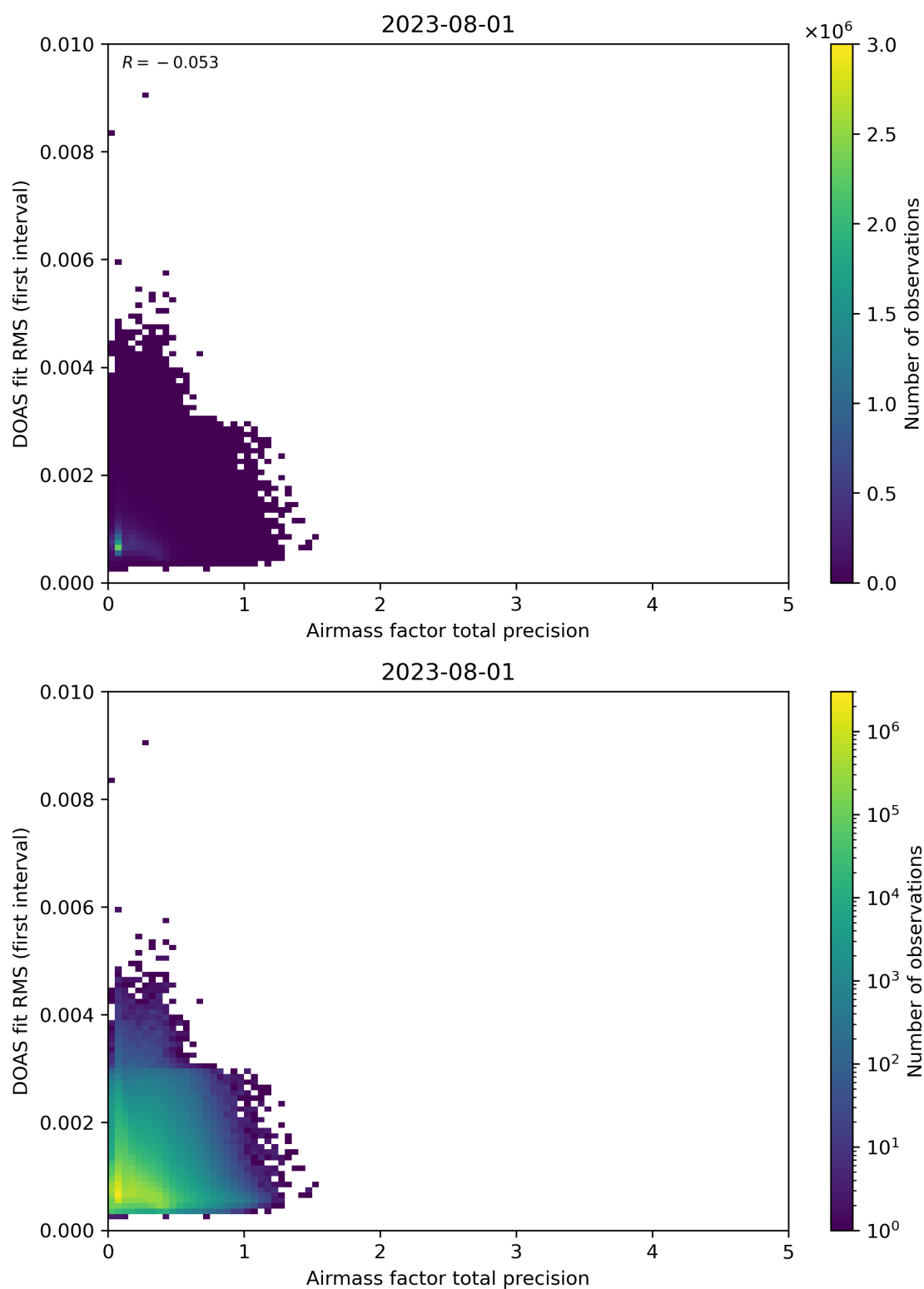
Figure 105: Scatter density plot of “Airmass factor total precision” against “DOAS fit RMS (first interval)” for 2023-07-31 to 2023-08-02.
