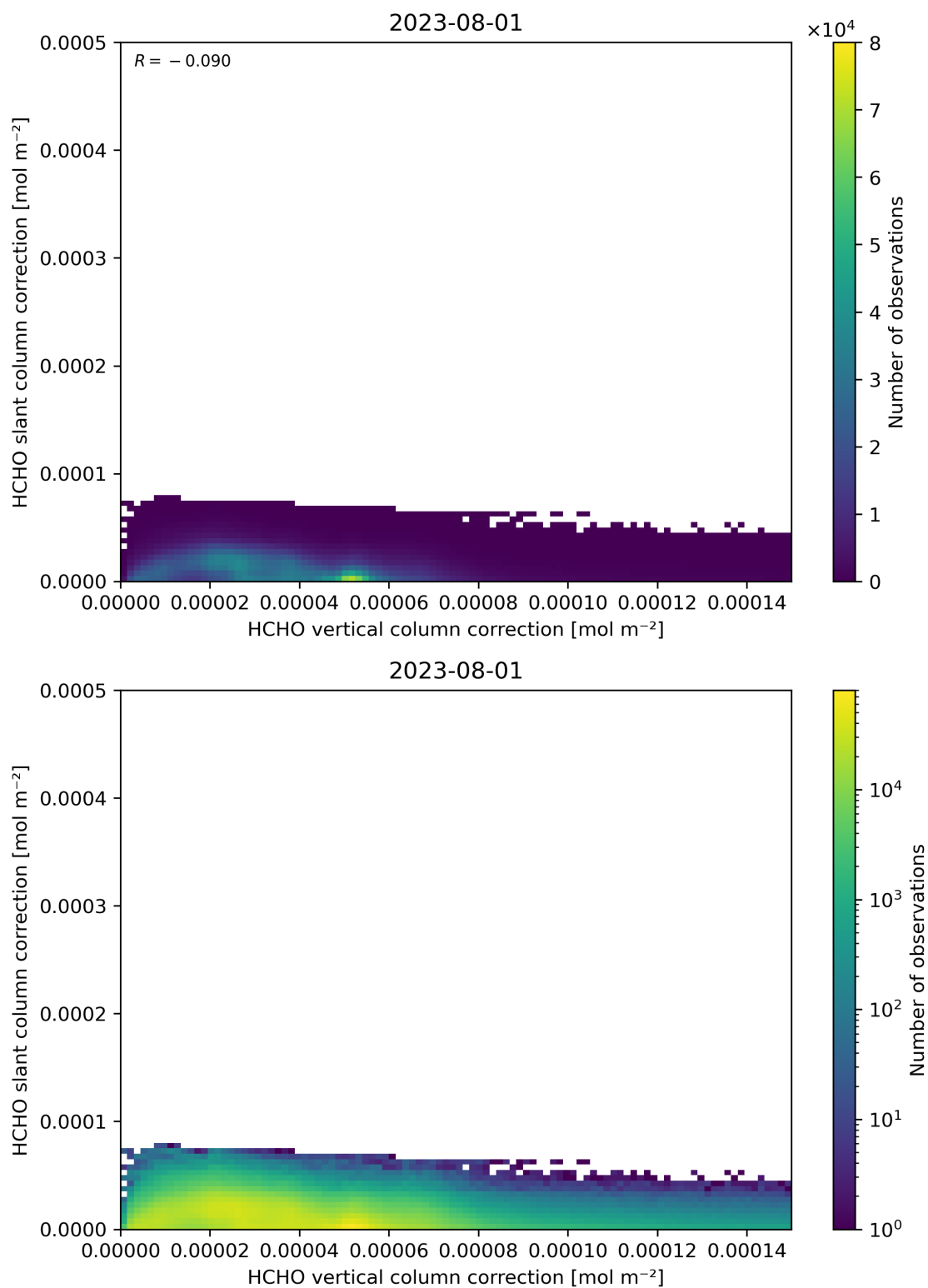
Figure 117: Scatter density plot of “HCHO vertical column correction” against “HCHO slant column correction” for 2023-07-31 to 2023-08-02.
