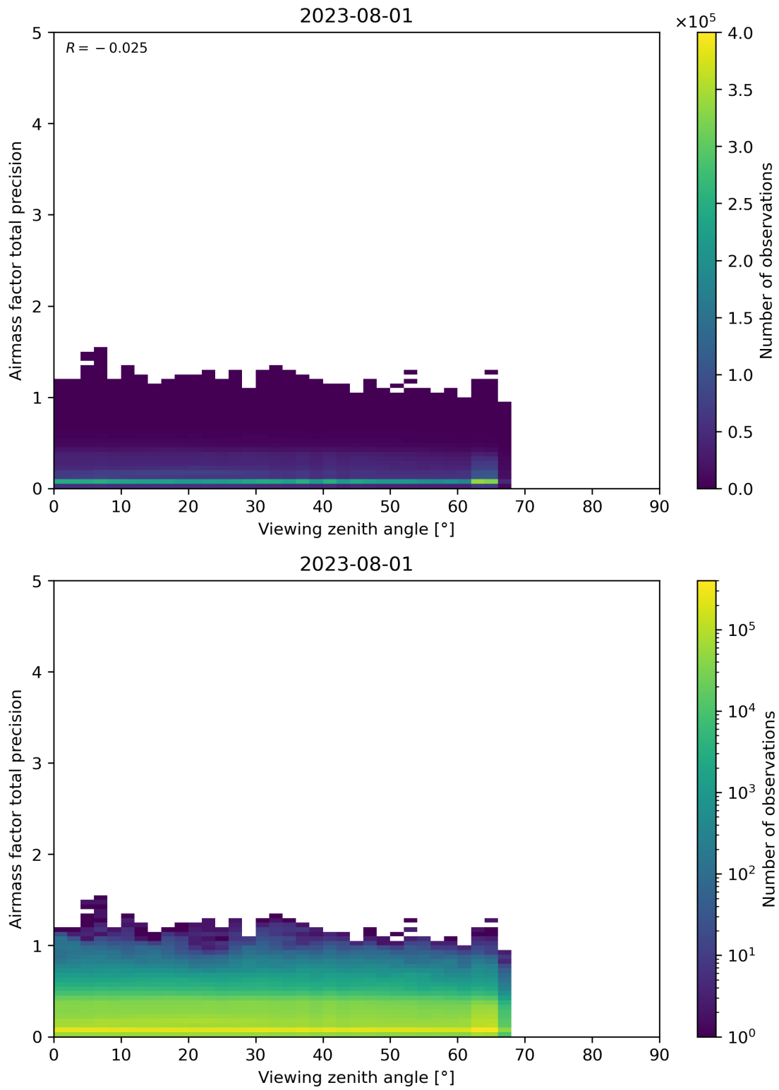
Figure 191: Scatter density plot of “Viewing zenith angle” against “Airmass factor total precision” for 2023-07-31 to 2023-08-02.
