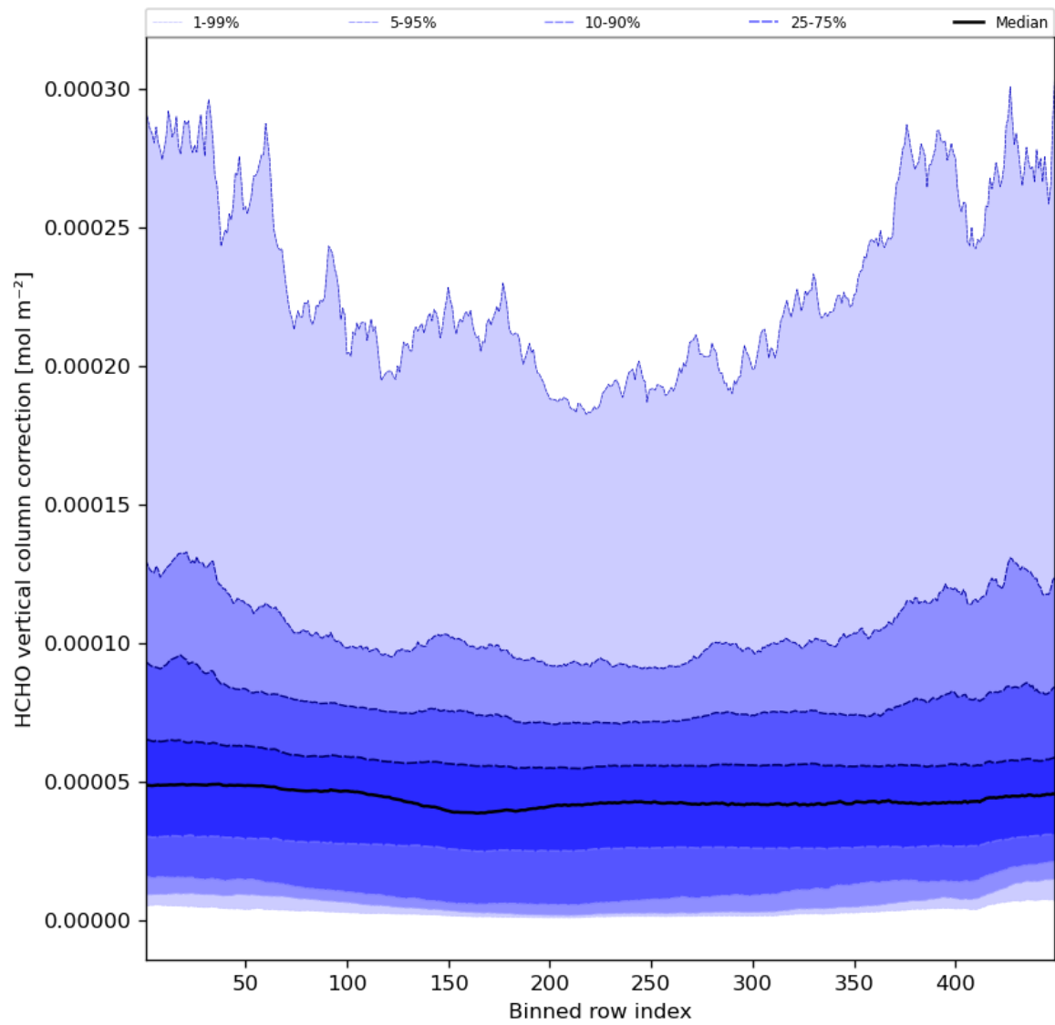
Figure 51: Along track statistics of “HCHO vertical column correction” for 2023-07-31 to 2023-08-02
