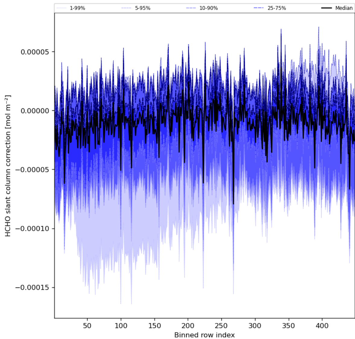
Figure 61: Along track statistics of “HCHO slant column correction” for 2023-07-31 to 2023-08-02
