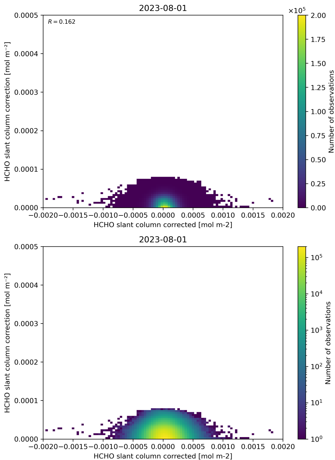
Figure 77: Scatter density plot of “HCHO slant column corrected” against “HCHO slant column correction” for 2023-07-31 to 2023-08-02.
