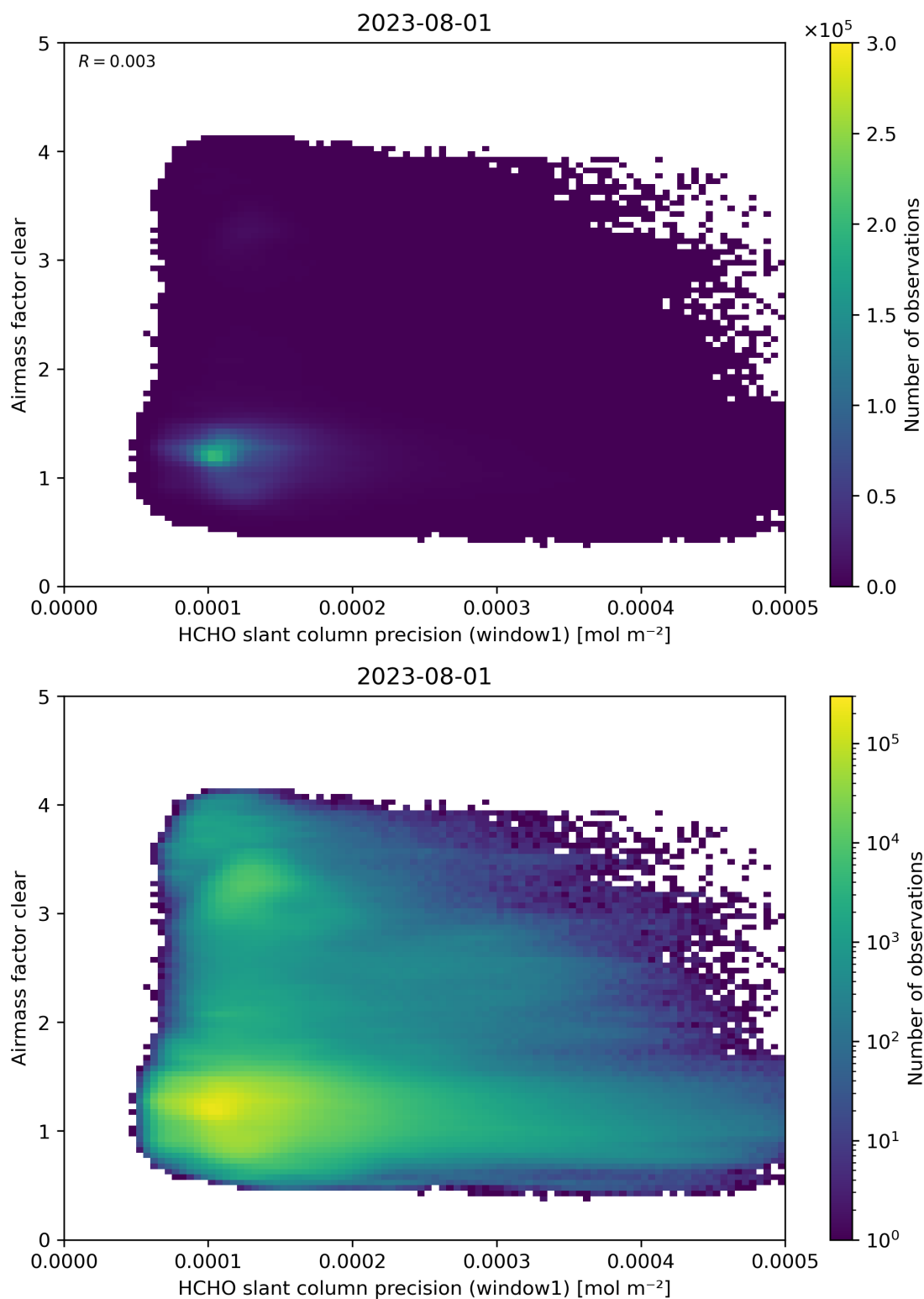
Figure 91: Scatter density plot of “HCHO slant column precision (window1)” against “Airmass factor clear” for 2023-07-31 to 2023-08-02.
