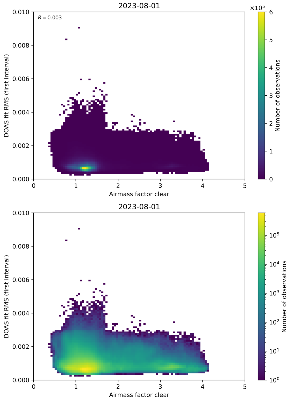
Figure 71: Scatter density plot of “Airmass factor clear” against “DOAS fit RMS (first interval)” for 2023-07-31 to 2023-08-02.
