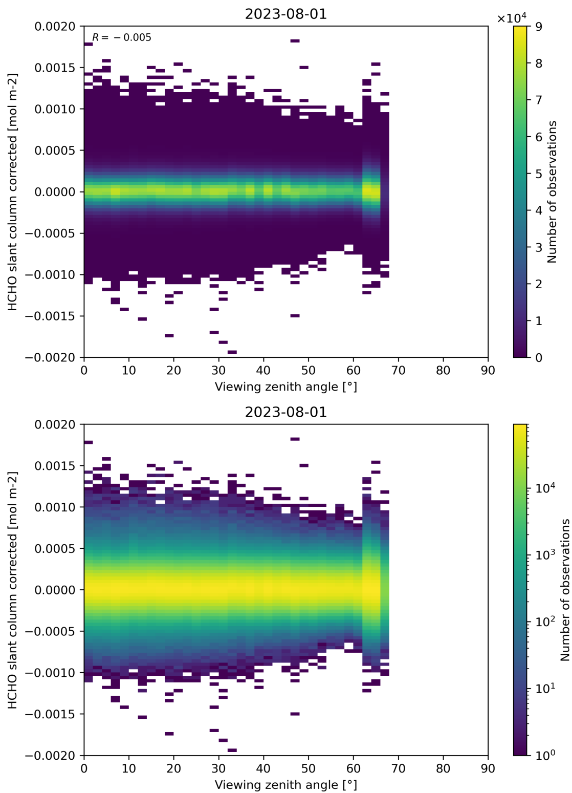
Figure 186: Scatter density plot of “Viewing zenith angle” against “HCHO slant column corrected” for 2023-07-31 to 2023-08-02.
