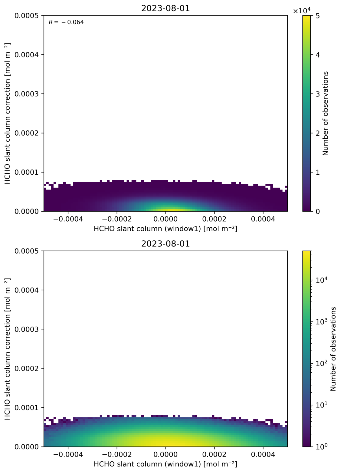
Figure 83: Scatter density plot of “HCHO slant column (window1)” against “HCHO slant column correction” for 2023-07-31 to 2023-08-02.
