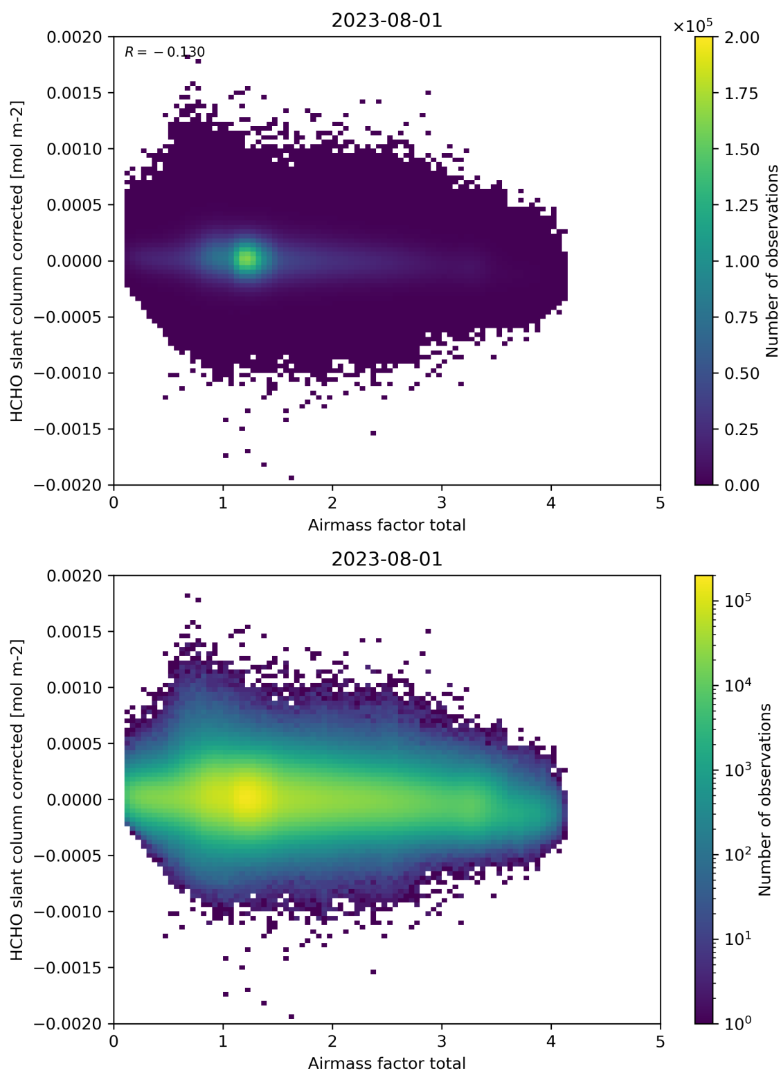
Figure 101: Scatter density plot of “Airmass factor total” against “HCHO slant column corrected” for 2023-07-31 to 2023-08-02.
