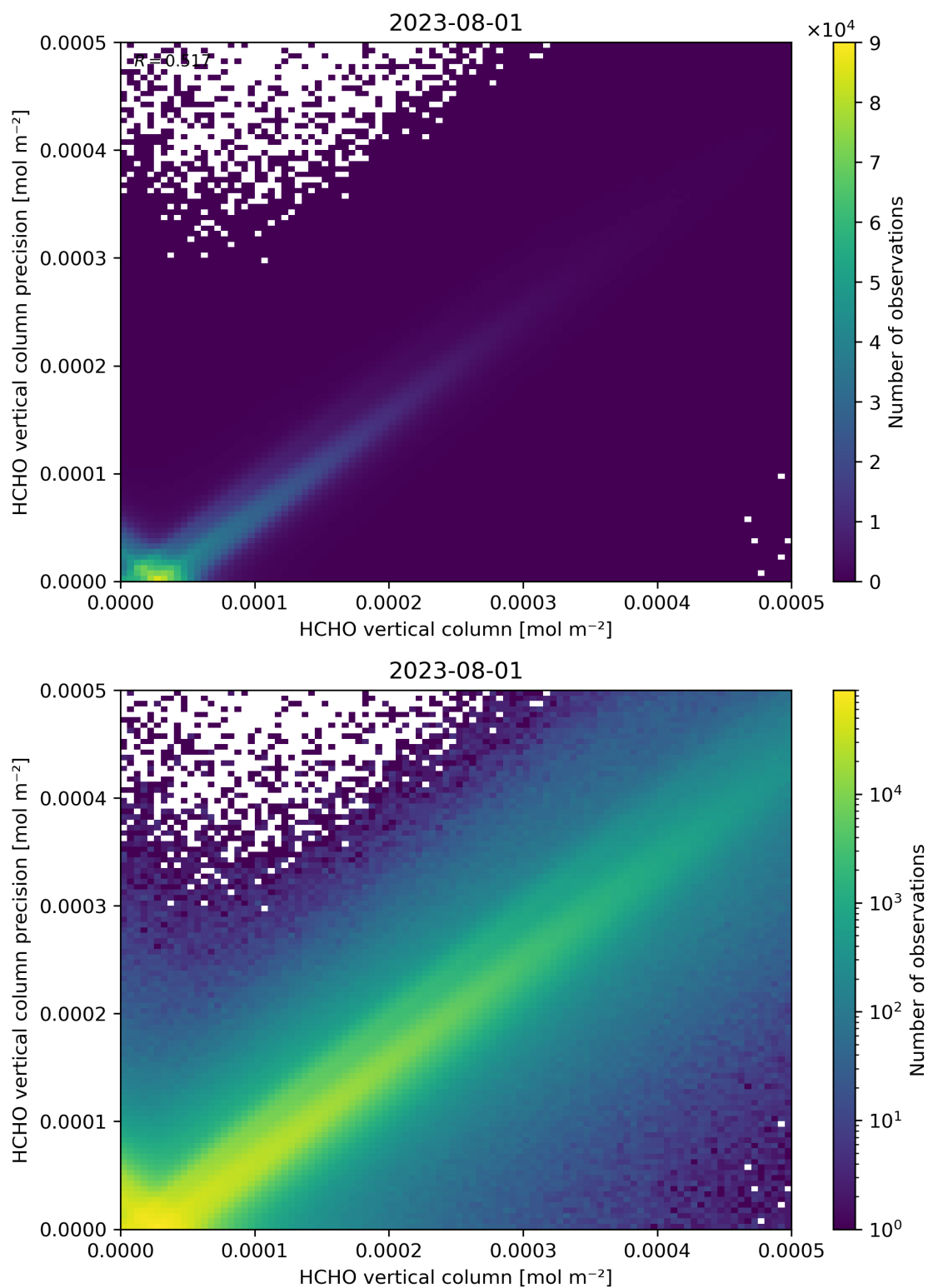
Figure 134: Scatter density plot of “HCHO vertical column” against “HCHO vertical column precision” for 2023-07-31 to 2023-08-02.
