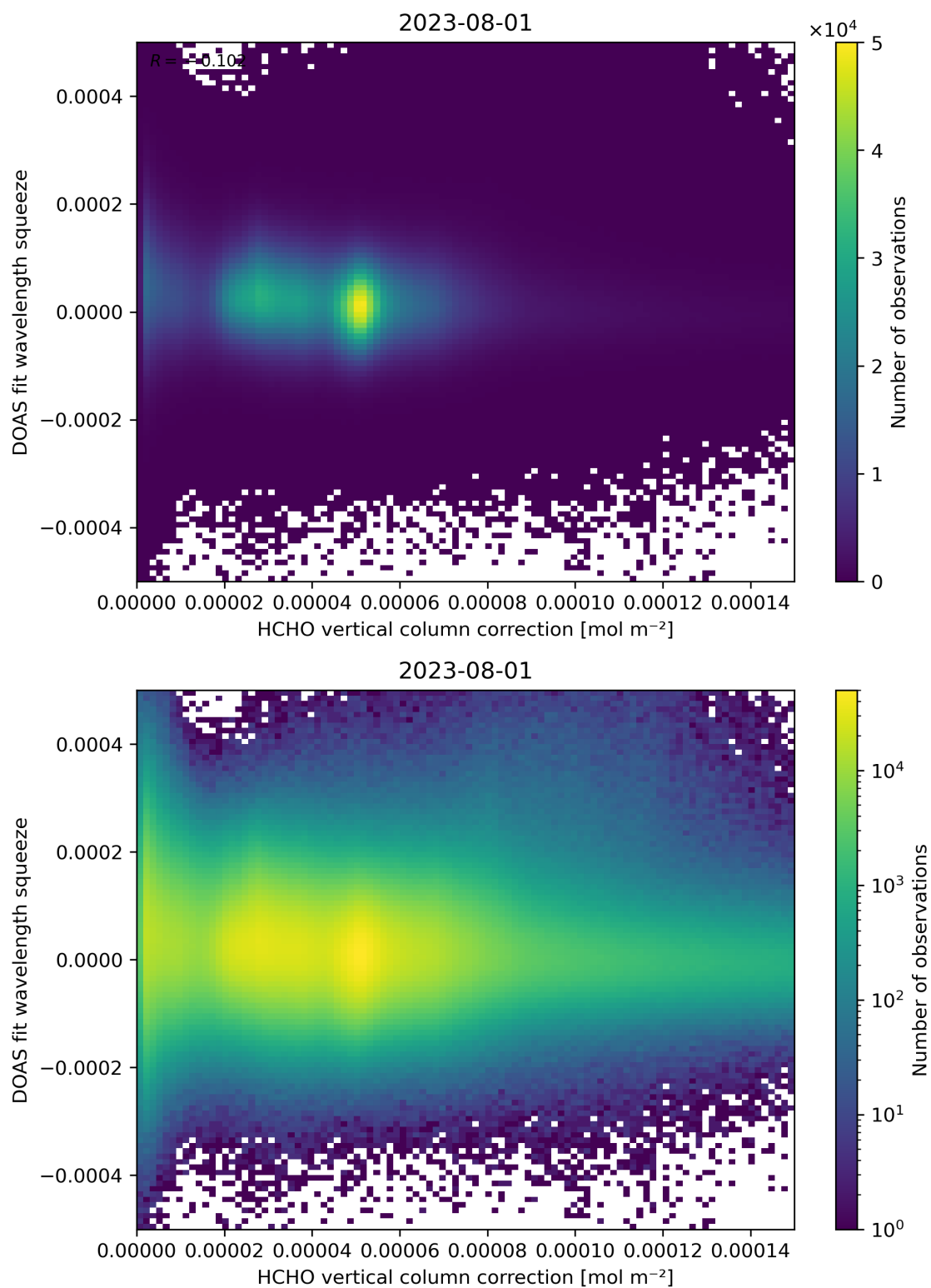
Figure 114: Scatter density plot of “HCHO vertical column correction” against “DOAS fit wavelength squeeze” for 2023-07-31 to 2023-08-02.
