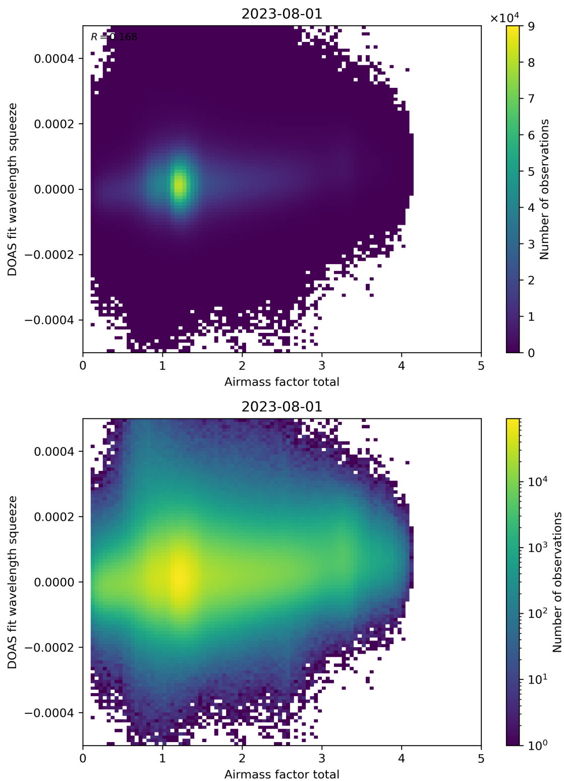
Figure 99: Scatter density plot of “Airmass factor total” against “DOAS fit wavelength squeeze” for 2023-07-31 to 2023-08-02.
