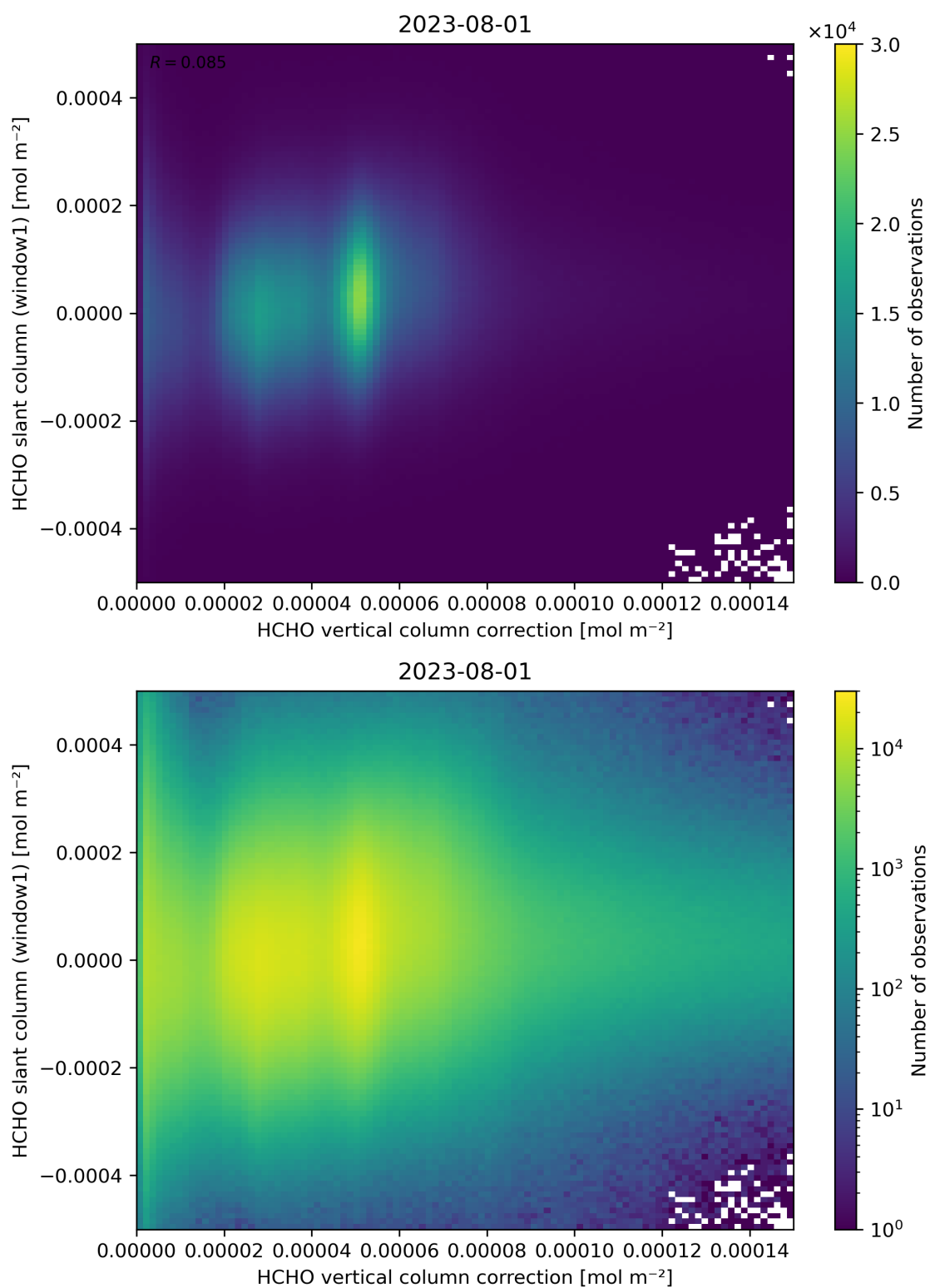
Figure 118: Scatter density plot of “HCHO vertical column correction” against “HCHO slant column (window1)” for 2023-07-31 to 2023-08-02.
