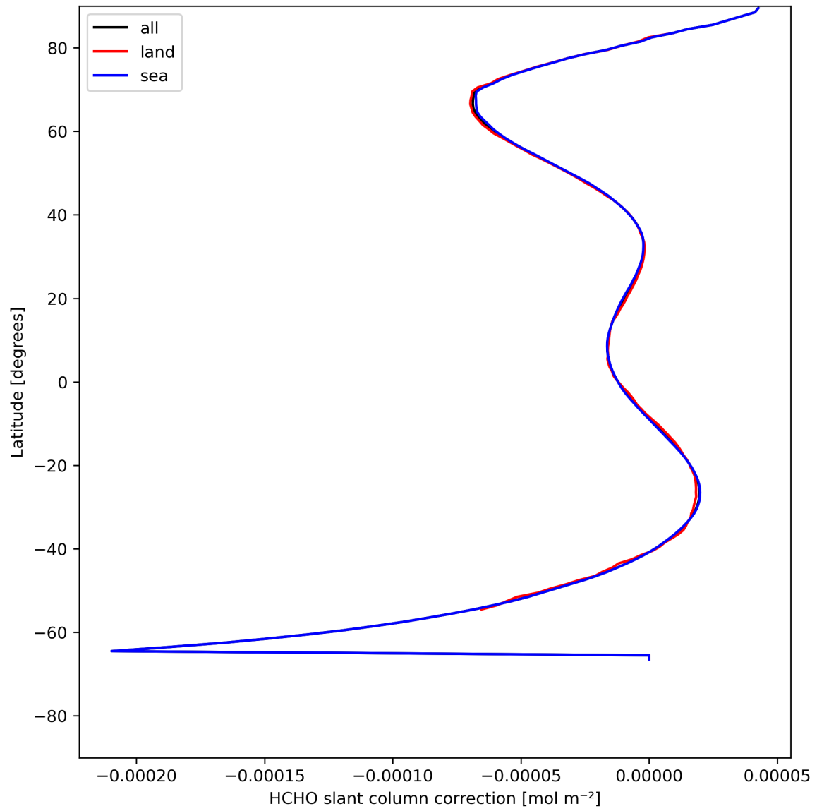
Figure 33: Zonal average of “HCHO slant column correction” for 2023-07-31 to 2023-08-02.
