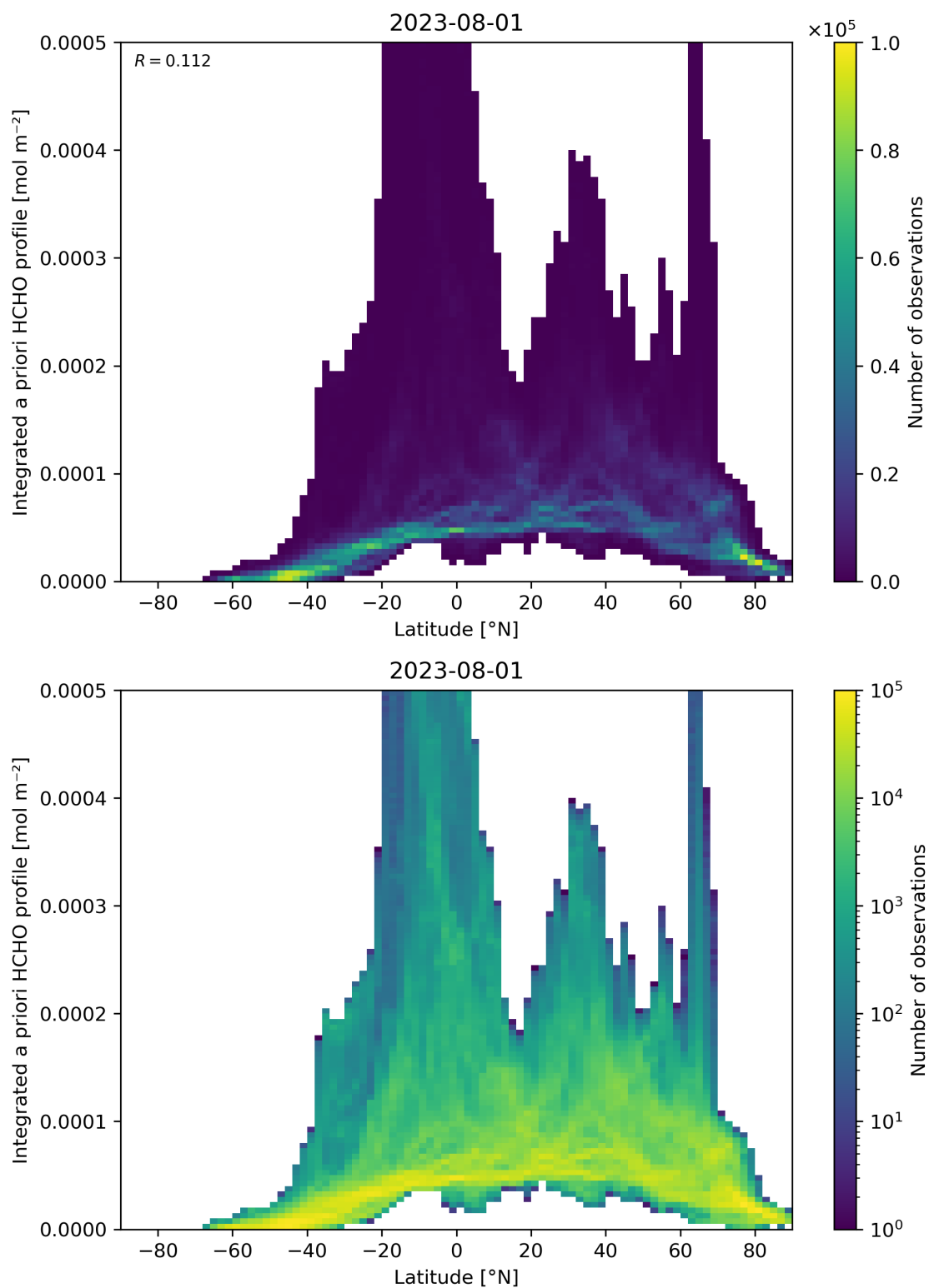
Figure 166: Scatter density plot of “Latitude” against “Integrated a priori HCHO profile” for 2023-07-31 to 2023-08-02.
