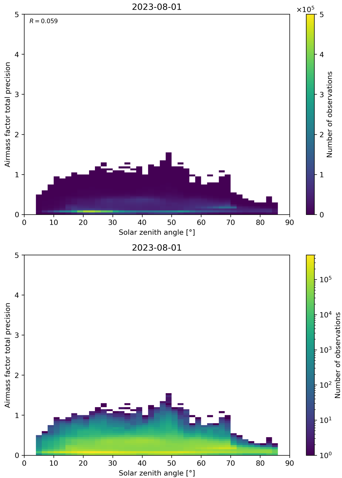
Figure 176: Scatter density plot of “Solar zenith angle” against “Airmass factor total precision” for 2023-07-31 to 2023-08-02.
