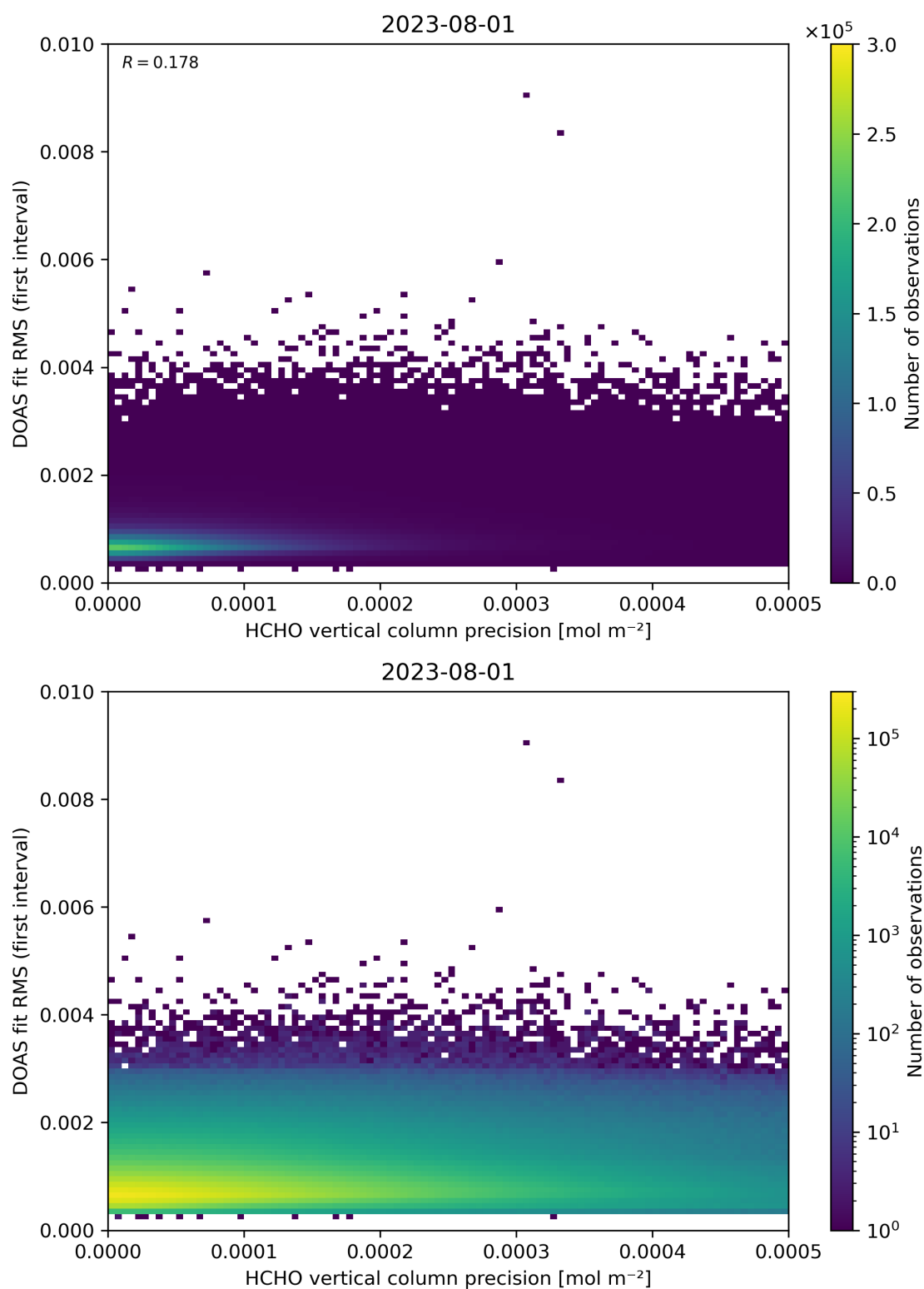
Figure 136: Scatter density plot of “HCHO vertical column precision” against “DOAS fit RMS (first interval)” for 2023-07-31 to 2023-08-02.
