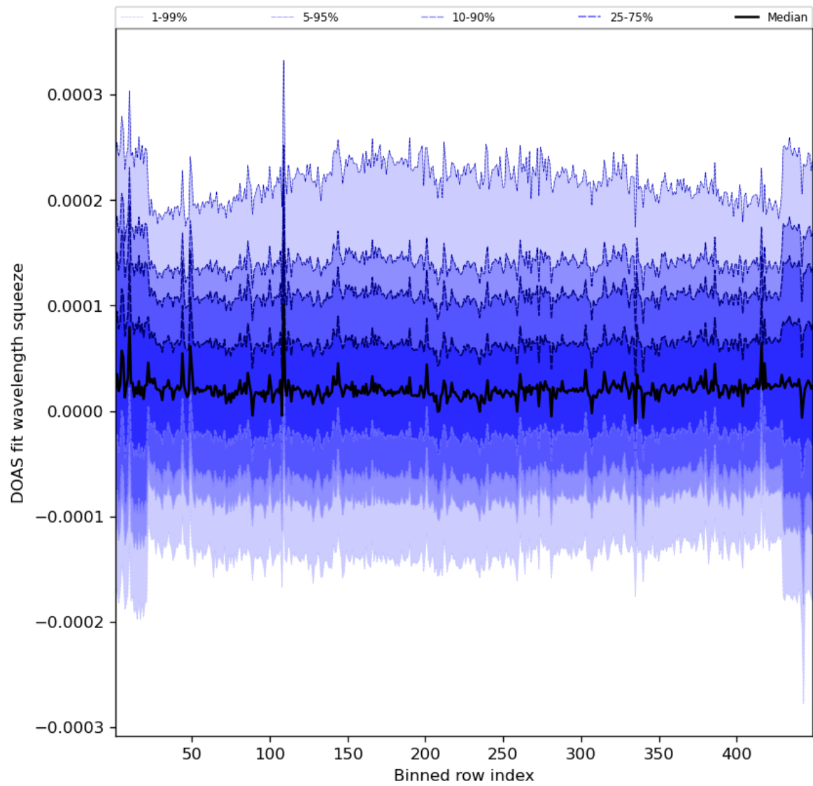
Figure 59: Along track statistics of “DOAS fit wavelength squeeze” for 2023-07-31 to 2023-08-02
