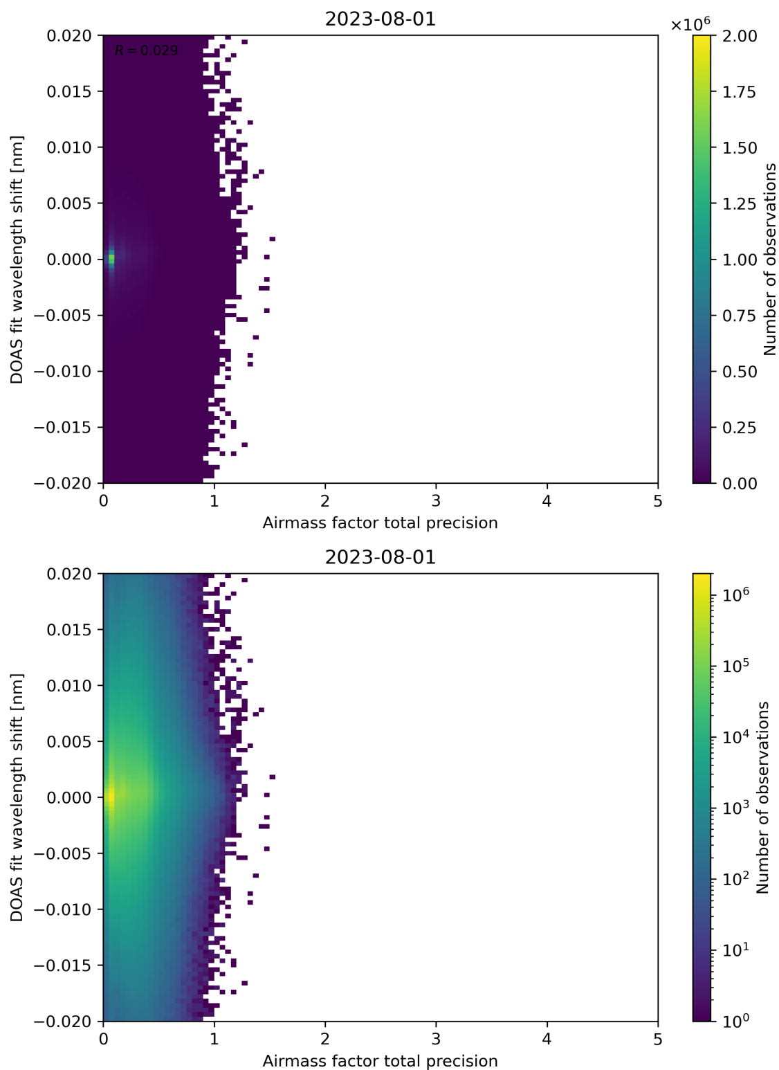
Figure 106: Scatter density plot of “Airmass factor total precision” against “DOAS fit wavelength shift” for 2023-07-31 to 2023-08-02.
