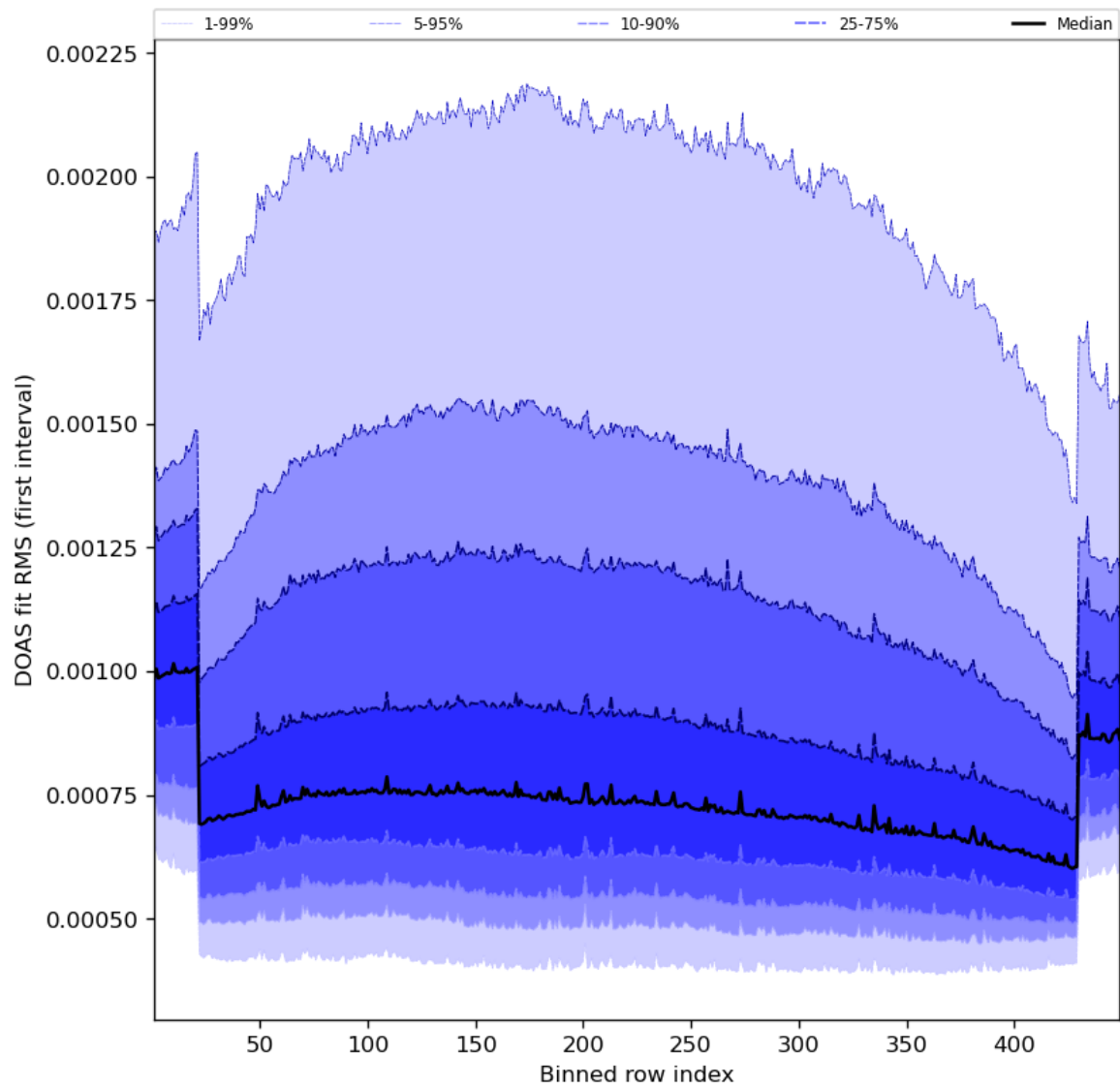
Figure 60: Along track statistics of “DOAS fit RMS (first interval)” for 2023-07-31 to 2023-08-02
