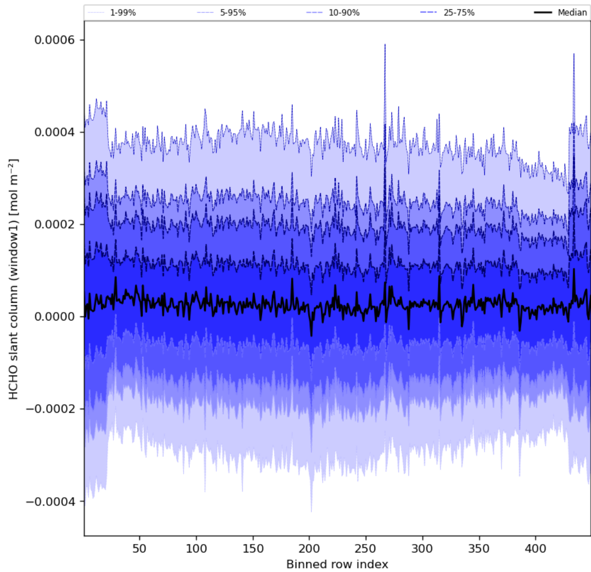
Figure 52: Along track statistics of “HCHO slant column (window1)” for 2023-07-31 to 2023-08-02
