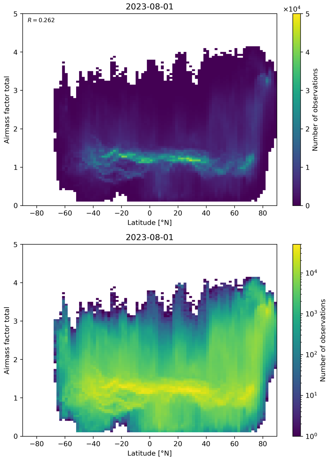
Figure 161: Scatter density plot of “Latitude” against “Airmass factor total” for 2023-07-31 to 2023-08-02.
