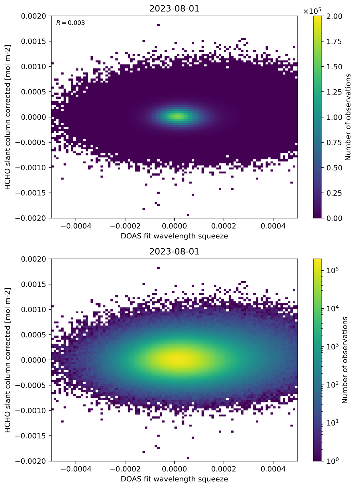
Figure 69: Scatter density plot of “DOAS fit wavelength squeeze” against “HCHO slant column corrected” for 2023-07-31 to 2023-08-02.
