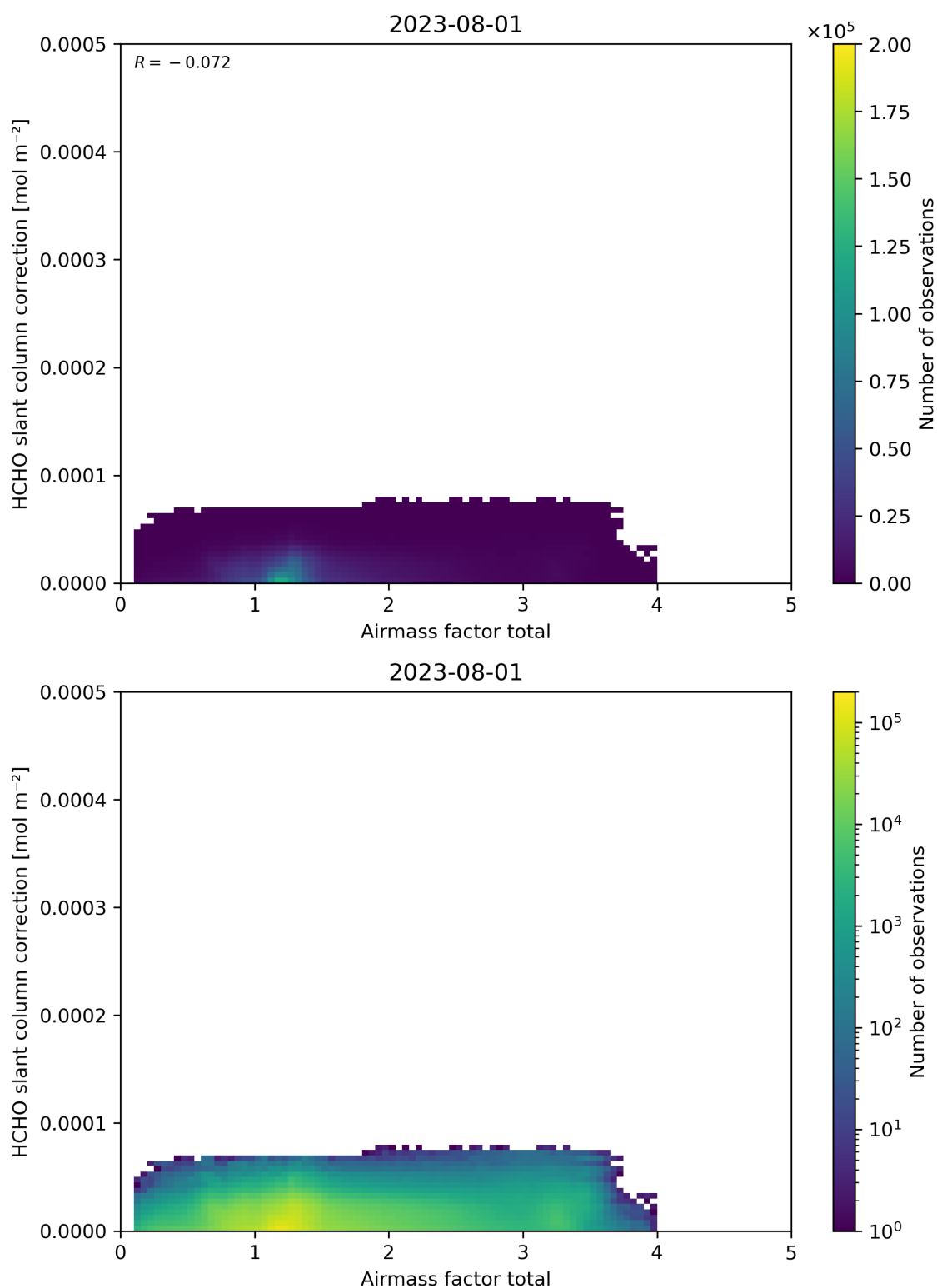
Figure 102: Scatter density plot of “Airmass factor total” against “HCHO slant column correction” for 2023-07-31 to 2023-08-02.
