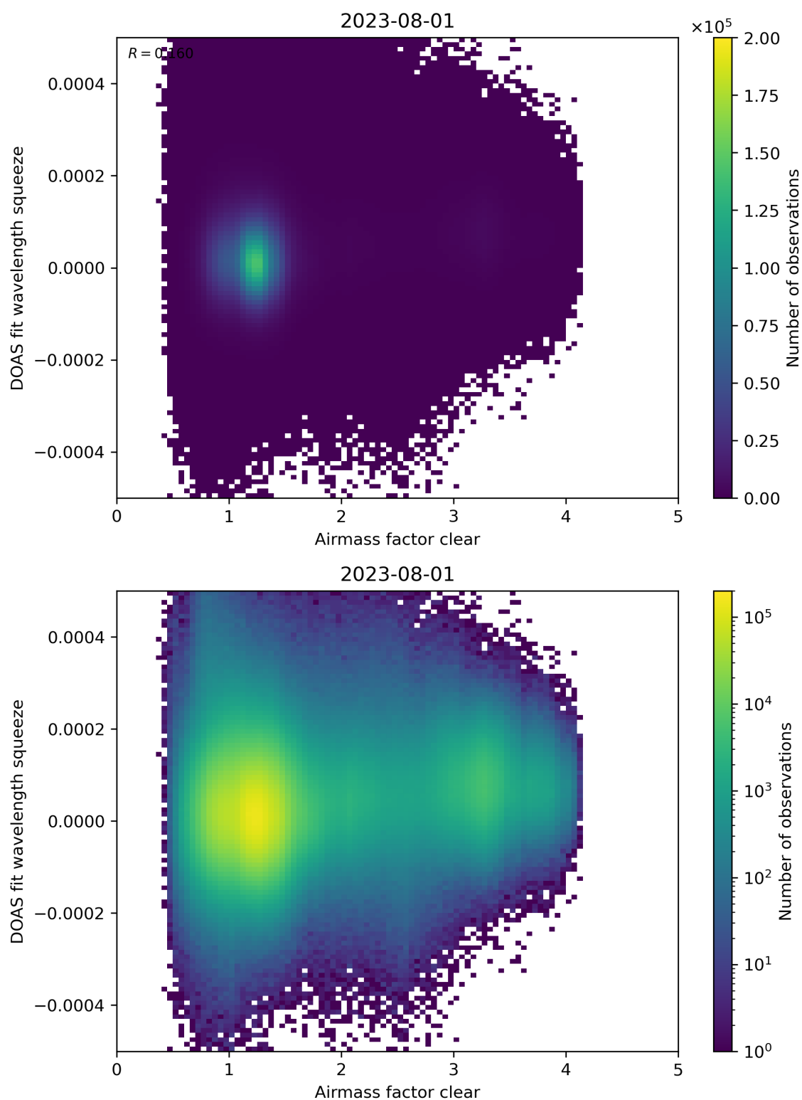
Figure 73: Scatter density plot of “Airmass factor clear” against “DOAS fit wavelength squeeze” for 2023-07-31 to 2023-08-02.
