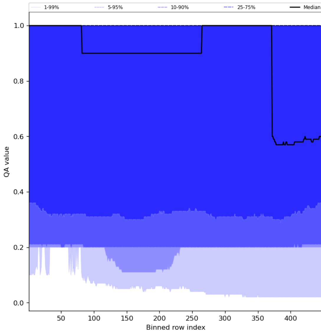
Figure 48: Along track statistics of “QA value” for 2023-07-31 to 2023-08-02
