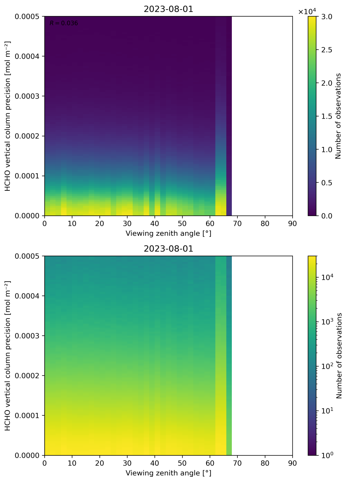
Figure 194: Scatter density plot of “Viewing zenith angle” against “HCHO vertical column precision” for 2023-07-31 to 2023-08-02.
