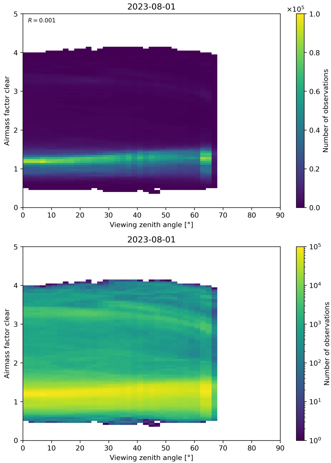
Figure 185: Scatter density plot of “Viewing zenith angle” against “Airmass factor clear” for 2023-07-31 to 2023-08-02.
