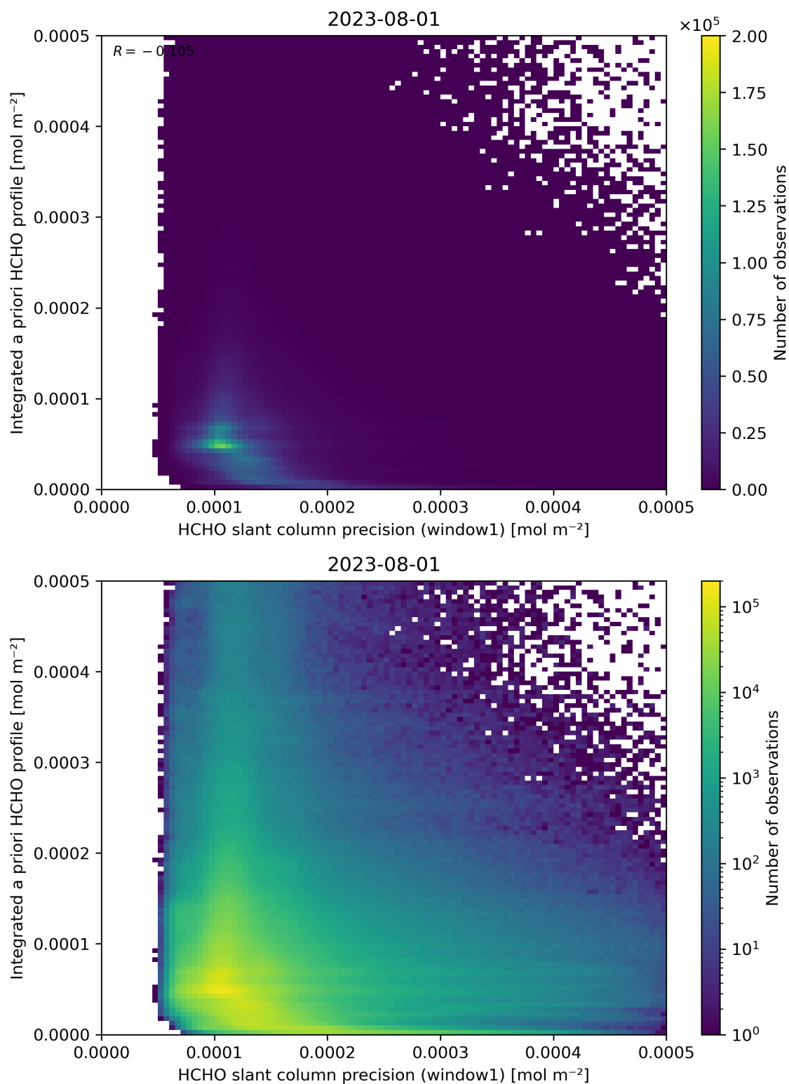
Figure 96: Scatter density plot of “HCHO slant column precision (window1)” against “Integrated a priori HCHO profile” for 2023-07-31 to 2023-08-02.
