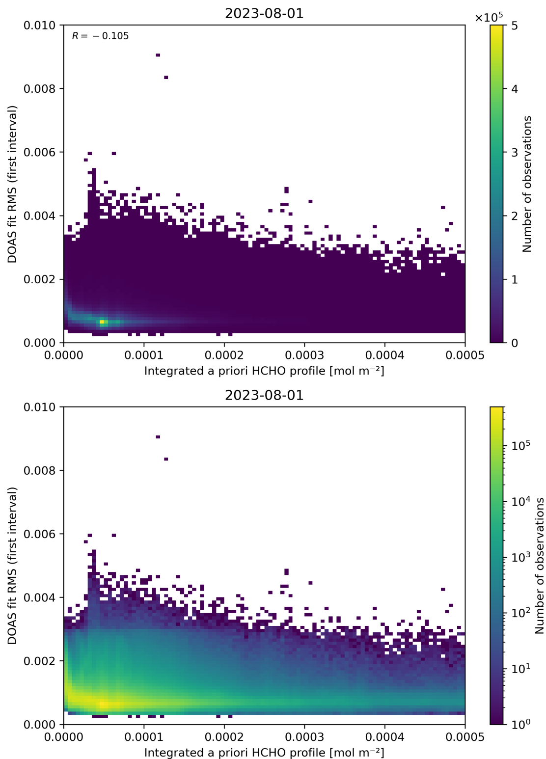
Figure 148: Scatter density plot of “Integrated a priori HCHO profile” against “DOAS fit RMS (first interval)” for 2023-07-31 to 2023-08-02.
