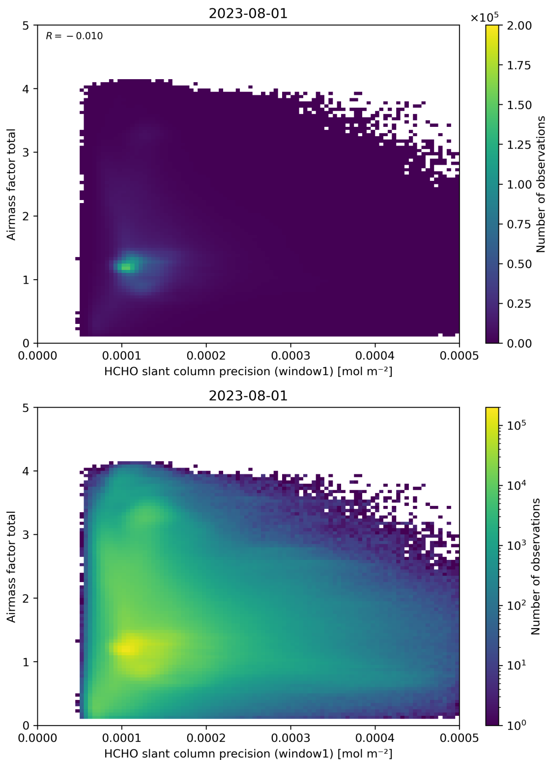
Figure 94: Scatter density plot of “HCHO slant column precision (window1)” against “Airmass factor total” for 2023-07-31 to 2023-08-02.
