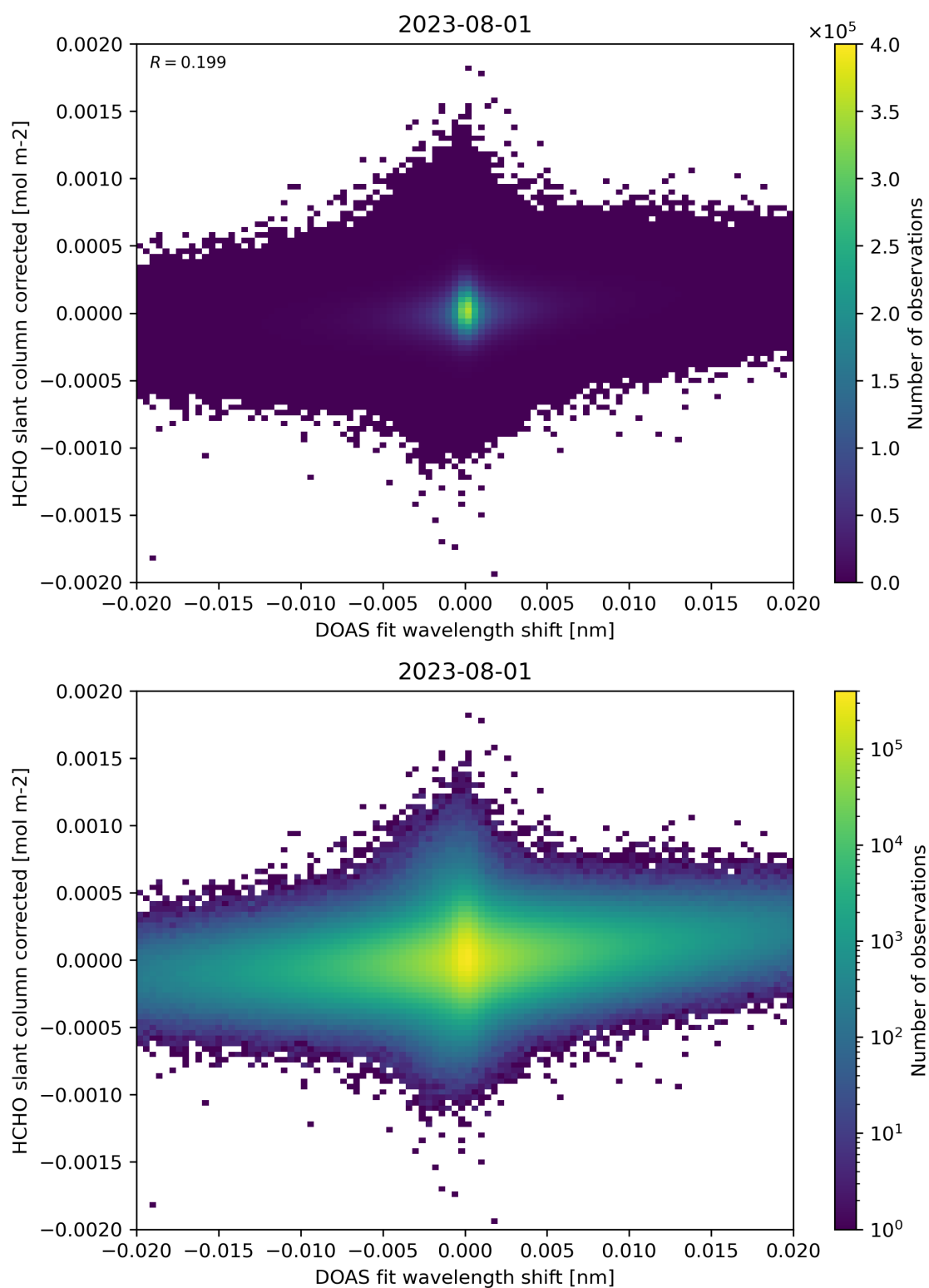
Figure 66: Scatter density plot of “DOAS fit wavelength shift” against “HCHO slant column corrected” for 2023-07-31 to 2023-08-02.
