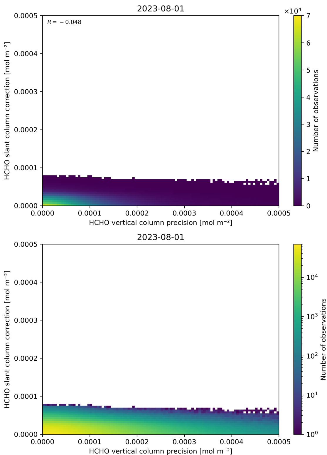
Figure 141: Scatter density plot of “HCHO vertical column precision” against “HCHO slant column correction” for 2023-07-31 to 2023-08-02.
