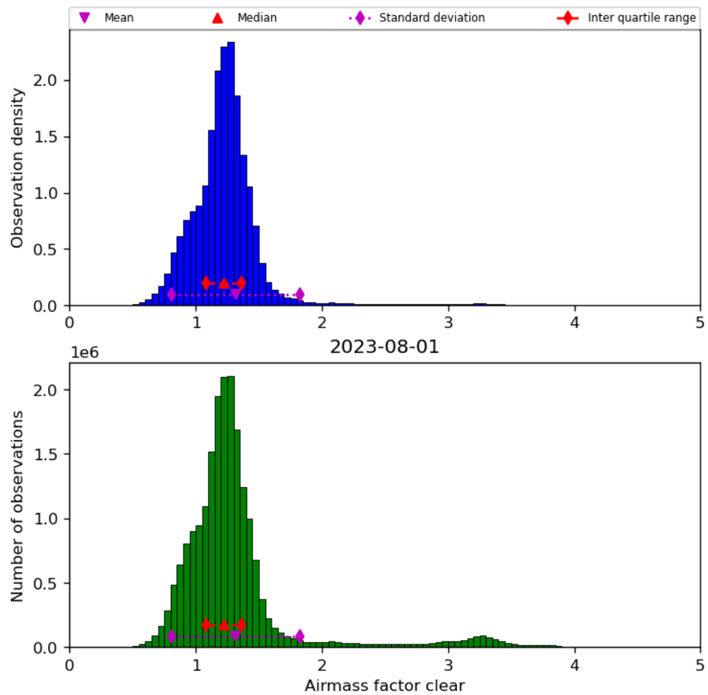
Figure 42: Histogram of “Airmass factor clear” for 2023-07-31 to 2023-08-02
