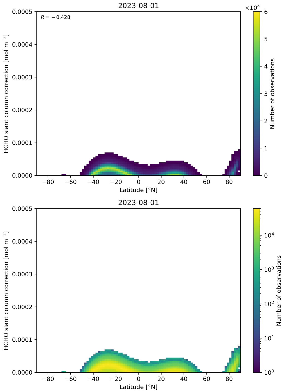
Figure 158: Scatter density plot of “Latitude” against “HCHO slant column correction” for 2023-07-31 to 2023-08-02.
