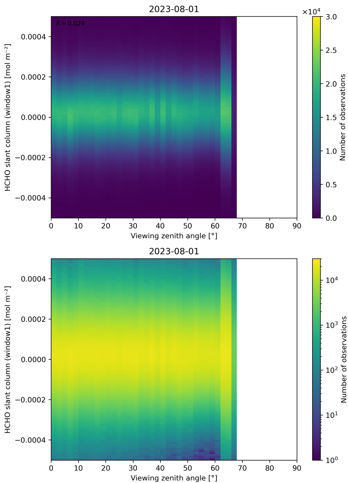
Figure 188: Scatter density plot of “Viewing zenith angle” against “HCHO slant column (window1)” for 2023-07-31 to 2023-08-02.
