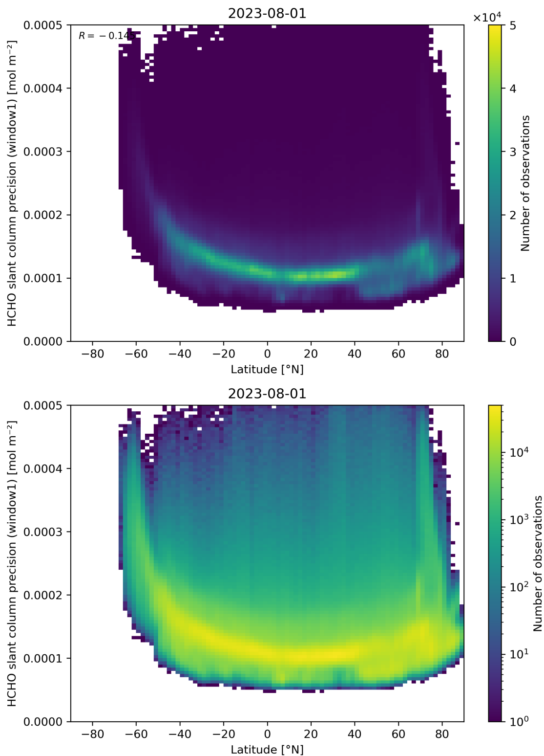
Figure 160: Scatter density plot of “Latitude” against “HCHO slant column precision (window1)” for 2023-07-31 to 2023-08-02.
