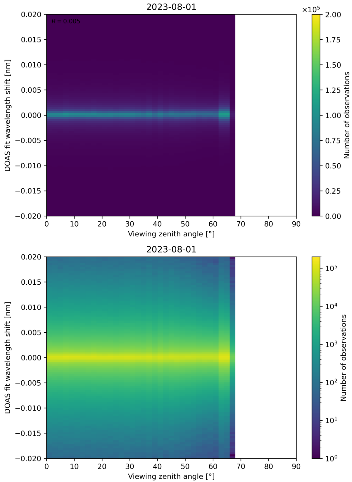
Figure 183: Scatter density plot of “Viewing zenith angle” against “DOAS fit wavelength shift” for 2023-07-31 to 2023-08-02.
