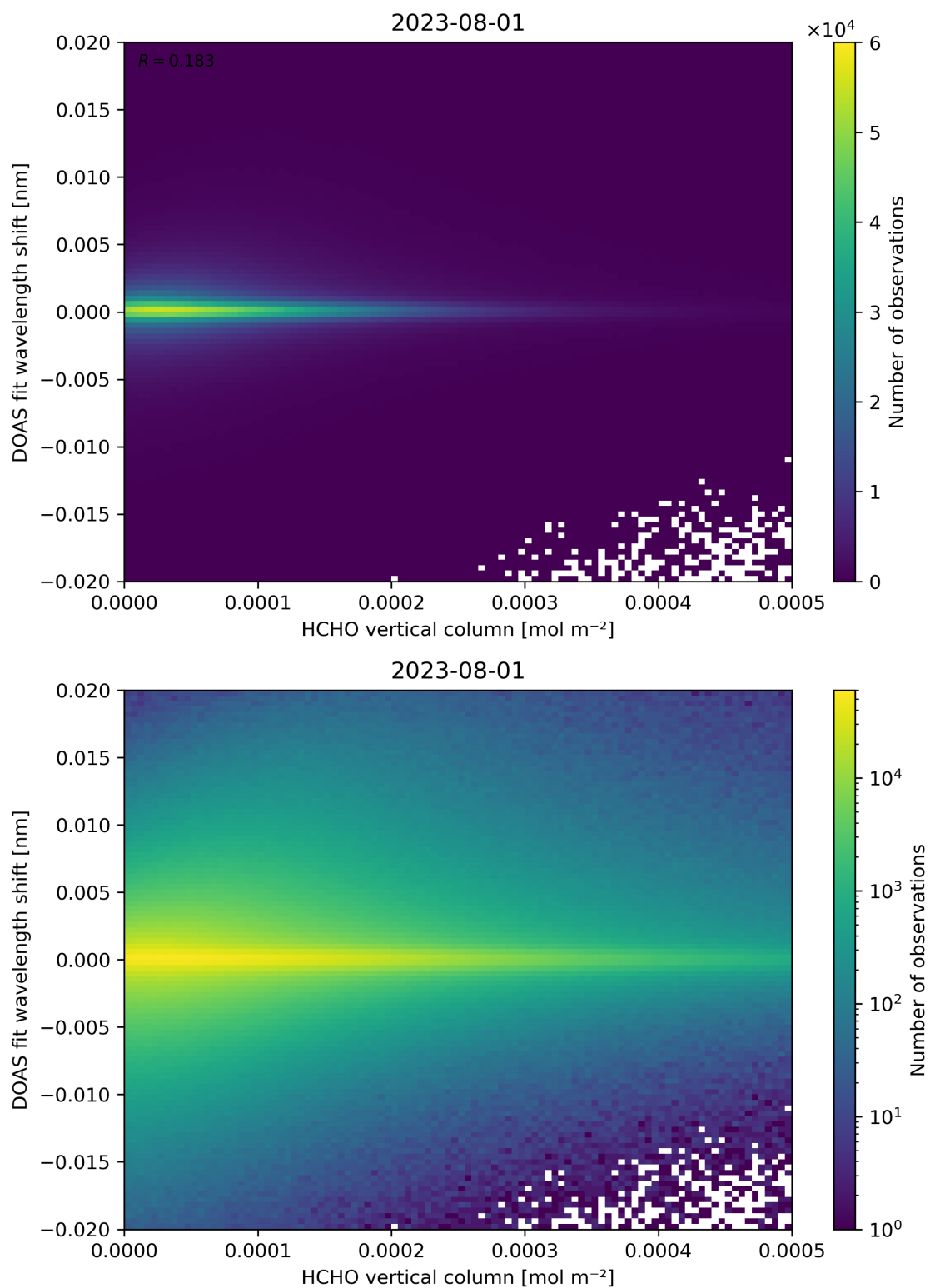
Figure 124: Scatter density plot of “HCHO vertical column” against “DOAS fit wavelength shift” for 2023-07-31 to 2023-08-02.
