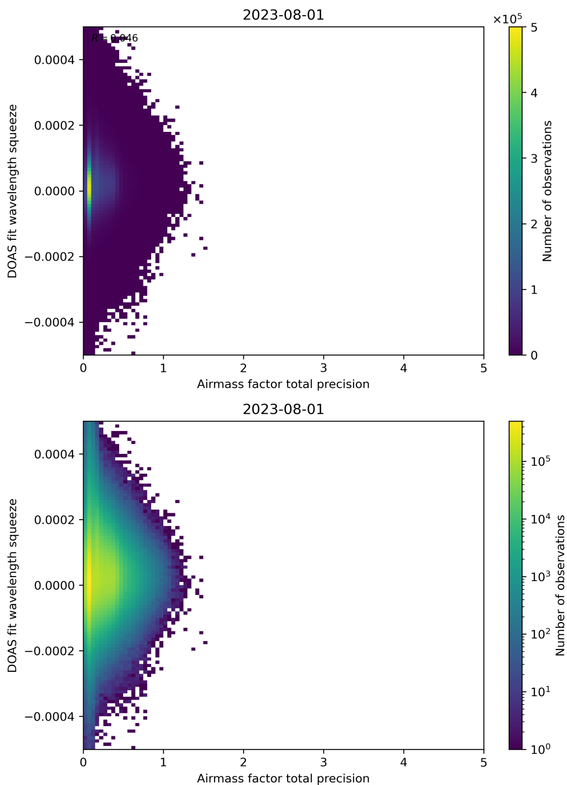
Figure 107: Scatter density plot of “Airmass factor total precision” against “DOAS fit wavelength squeeze” for 2023-07-31 to 2023-08-02.
