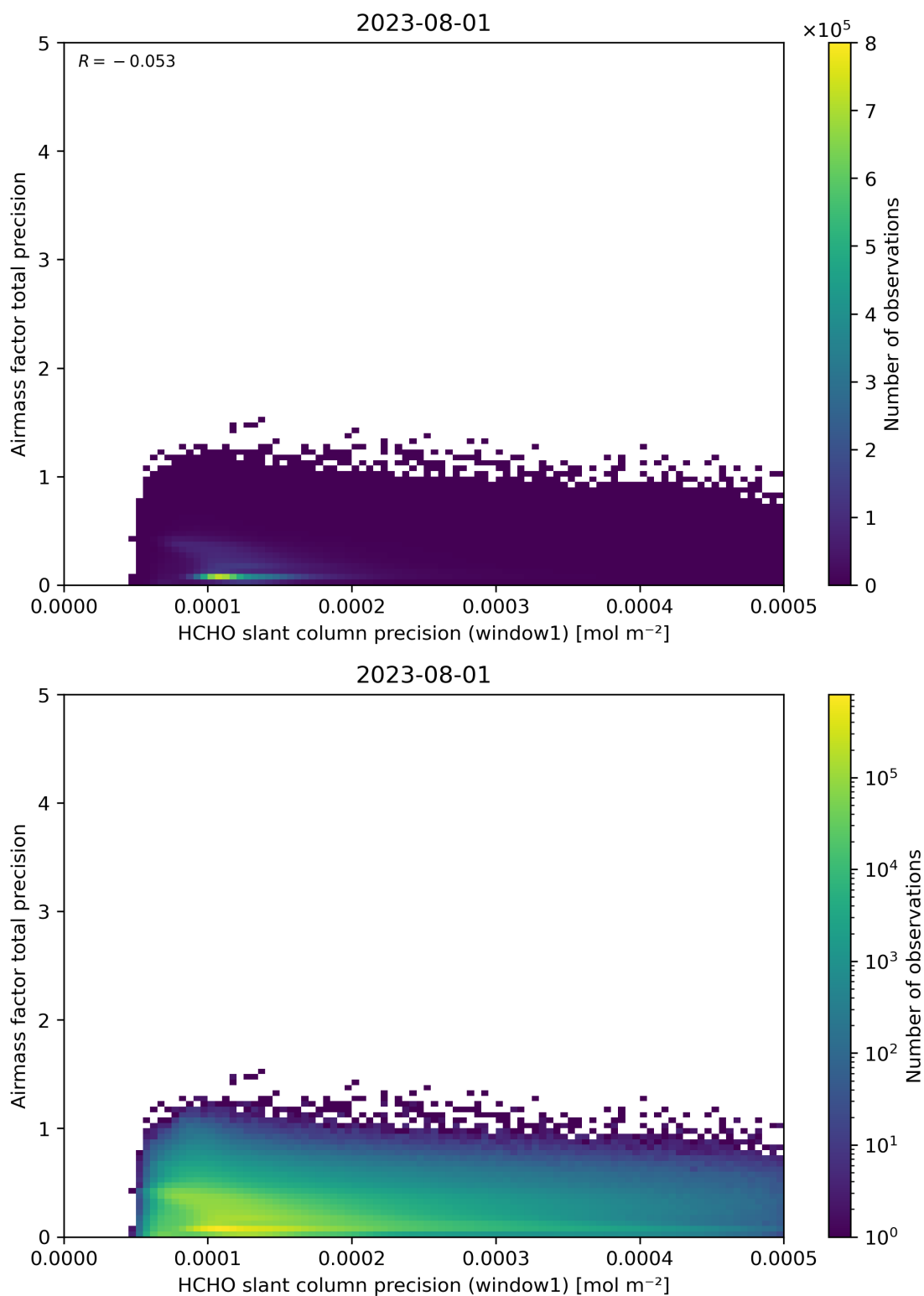
Figure 95: Scatter density plot of “HCHO slant column precision (window1)” against “Airmass factor total precision” for 2023-07-31 to 2023-08-02.
