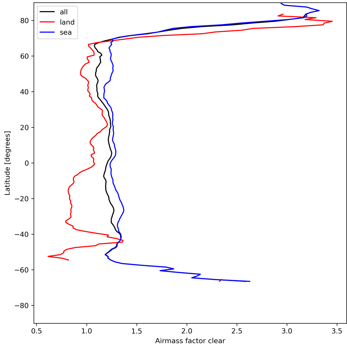
Figure 28: Zonal average of “Airmass factor clear” for 2023-07-31 to 2023-08-02.
