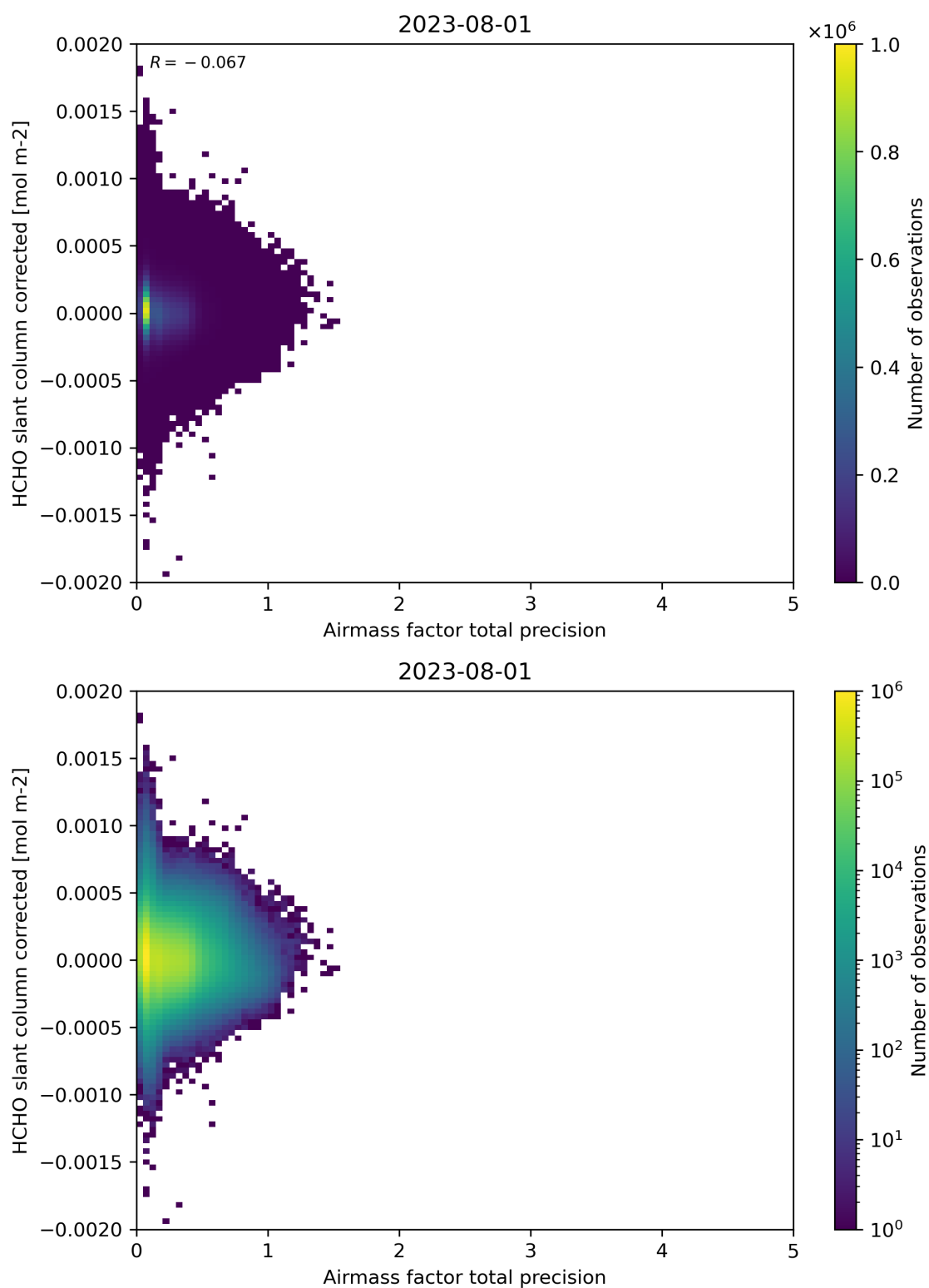
Figure 109: Scatter density plot of “Airmass factor total precision” against “HCHO slant column corrected” for 2023-07-31 to 2023-08-02.
