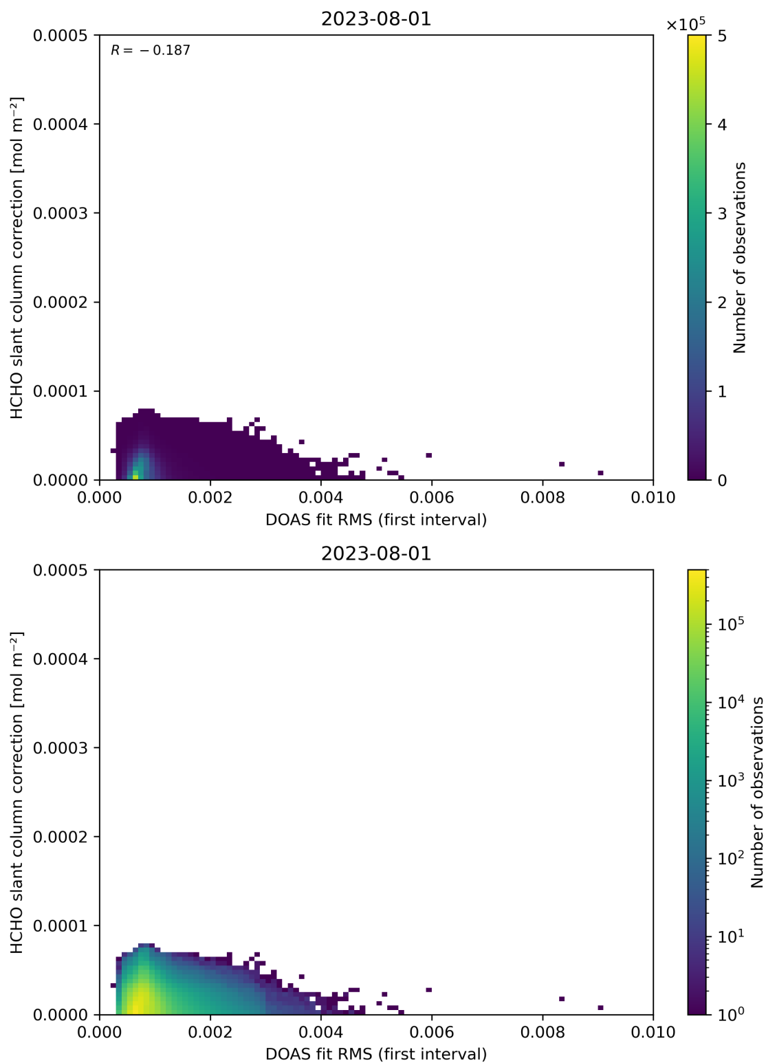
Figure 63: Scatter density plot of “DOAS fit RMS (first interval)” against “HCHO slant column correction” for 2023-07-31 to 2023-08-02.
