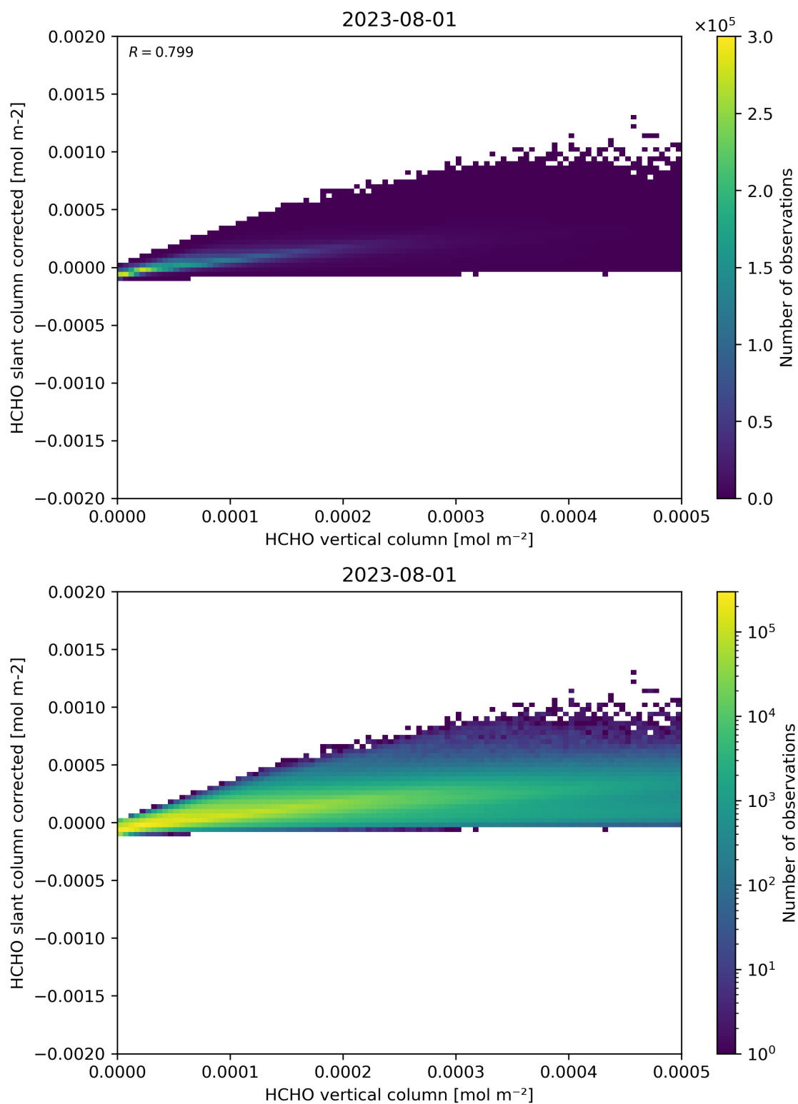
Figure 127: Scatter density plot of “HCHO vertical column” against “HCHO slant column corrected” for 2023-07-31 to 2023-08-02.
