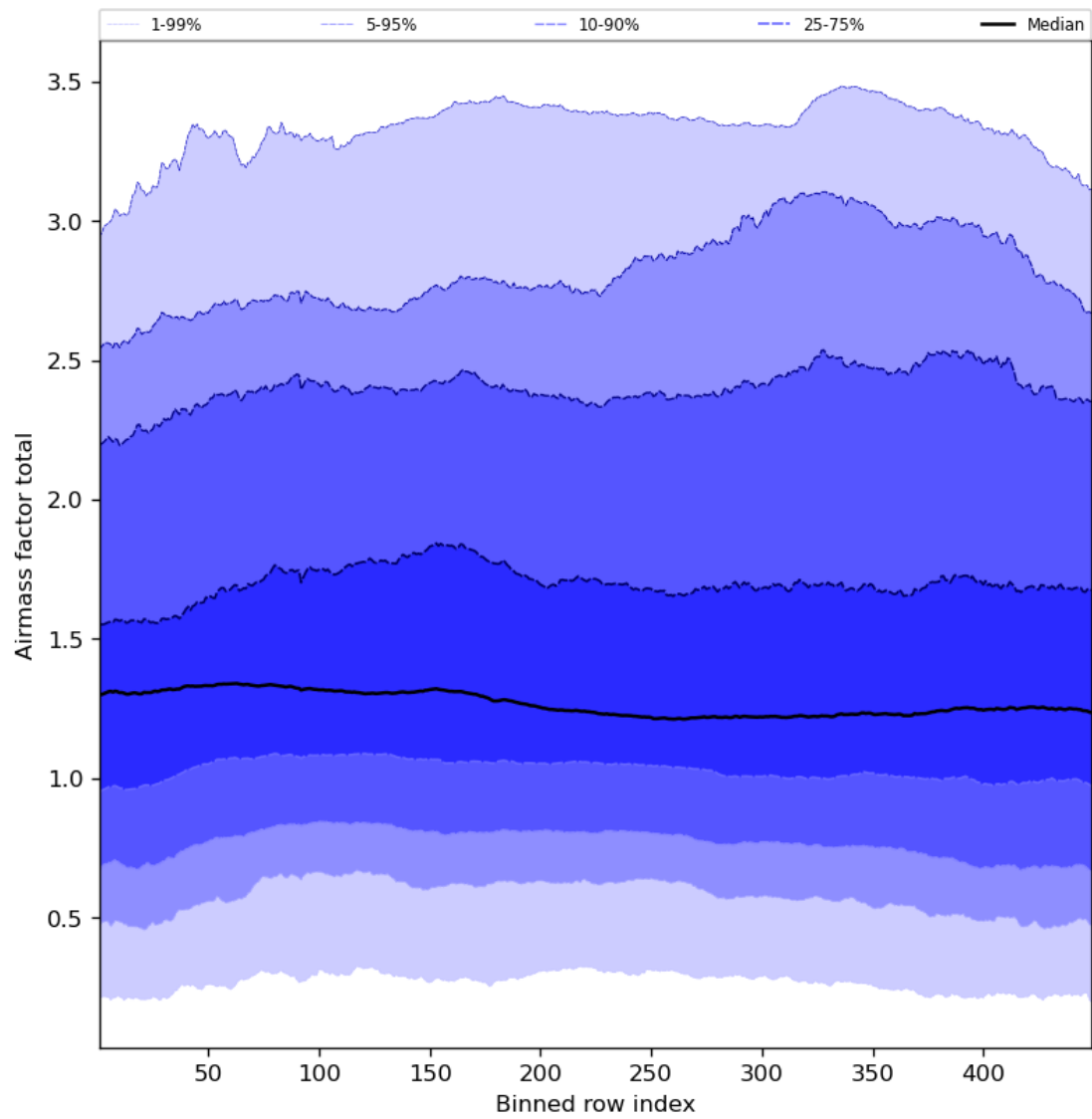
Figure 54: Along track statistics of “Airmass factor total” for 2023-07-31 to 2023-08-02
