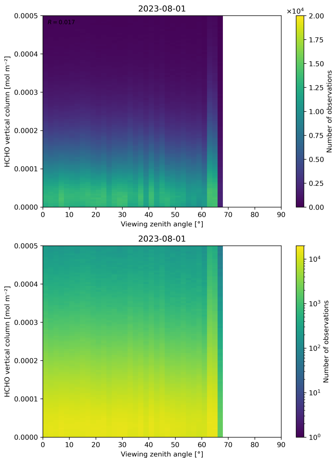
Figure 192: Scatter density plot of “Viewing zenith angle” against “HCHO vertical column” for 2023-07-31 to 2023-08-02.
