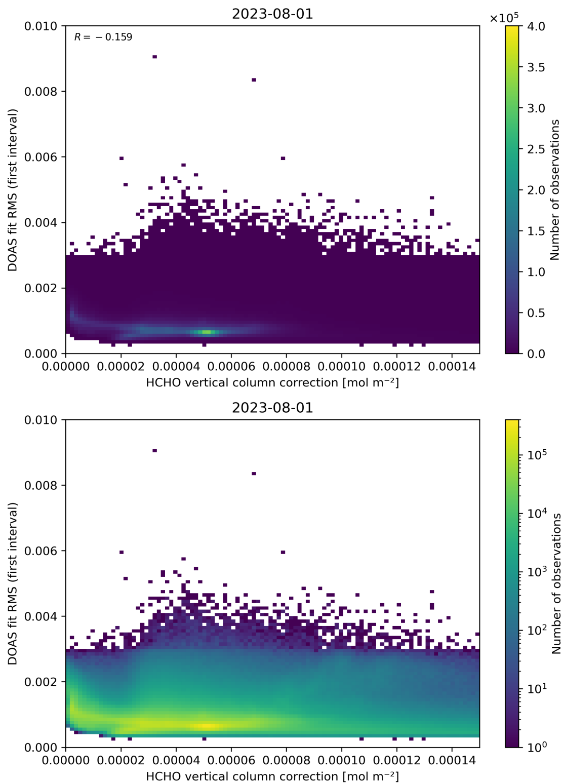
Figure 112: Scatter density plot of “HCHO vertical column correction” against “DOAS fit RMS (first interval)” for 2023-07-31 to 2023-08-02.
