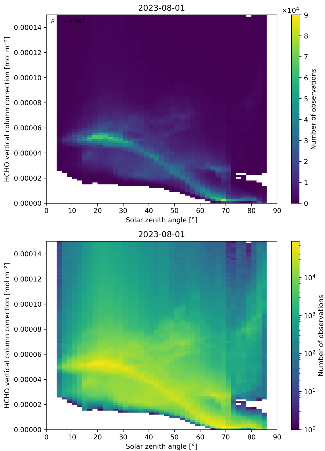
Figure 178: Scatter density plot of “Solar zenith angle” against “HCHO vertical column correction” for 2023-07-31 to 2023-08-02.
