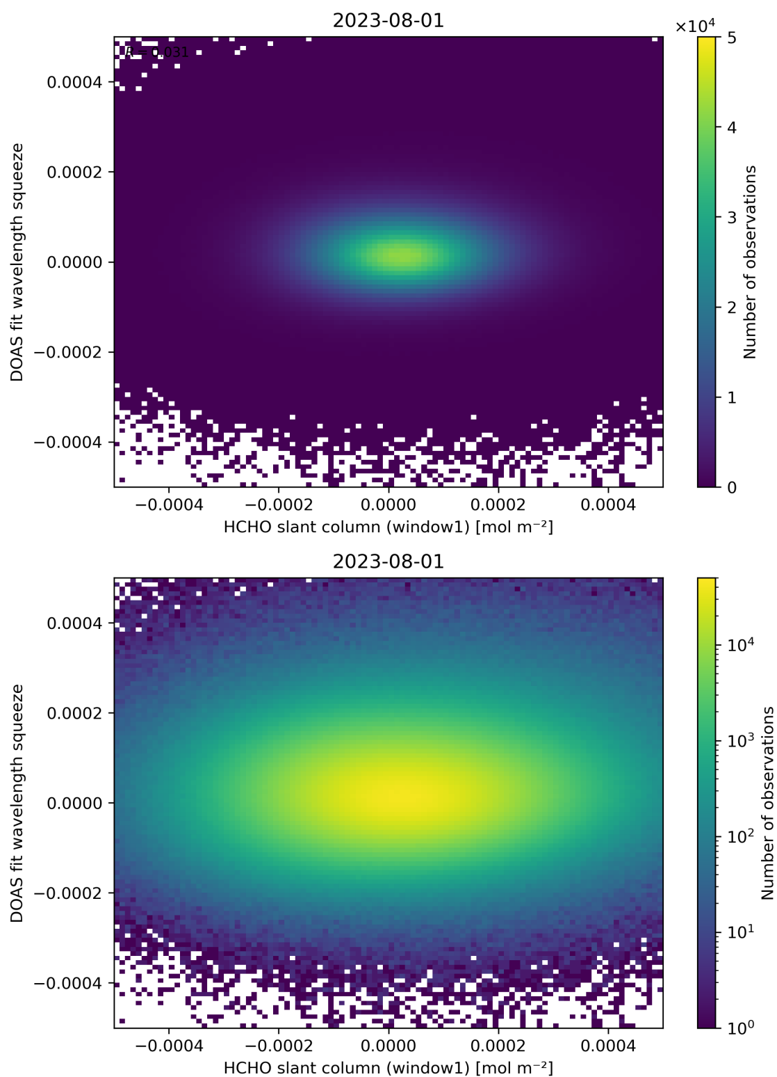
Figure 80: Scatter density plot of “HCHO slant column (window1)” against “DOAS fit wavelength squeeze” for 2023-07-31 to 2023-08-02.
