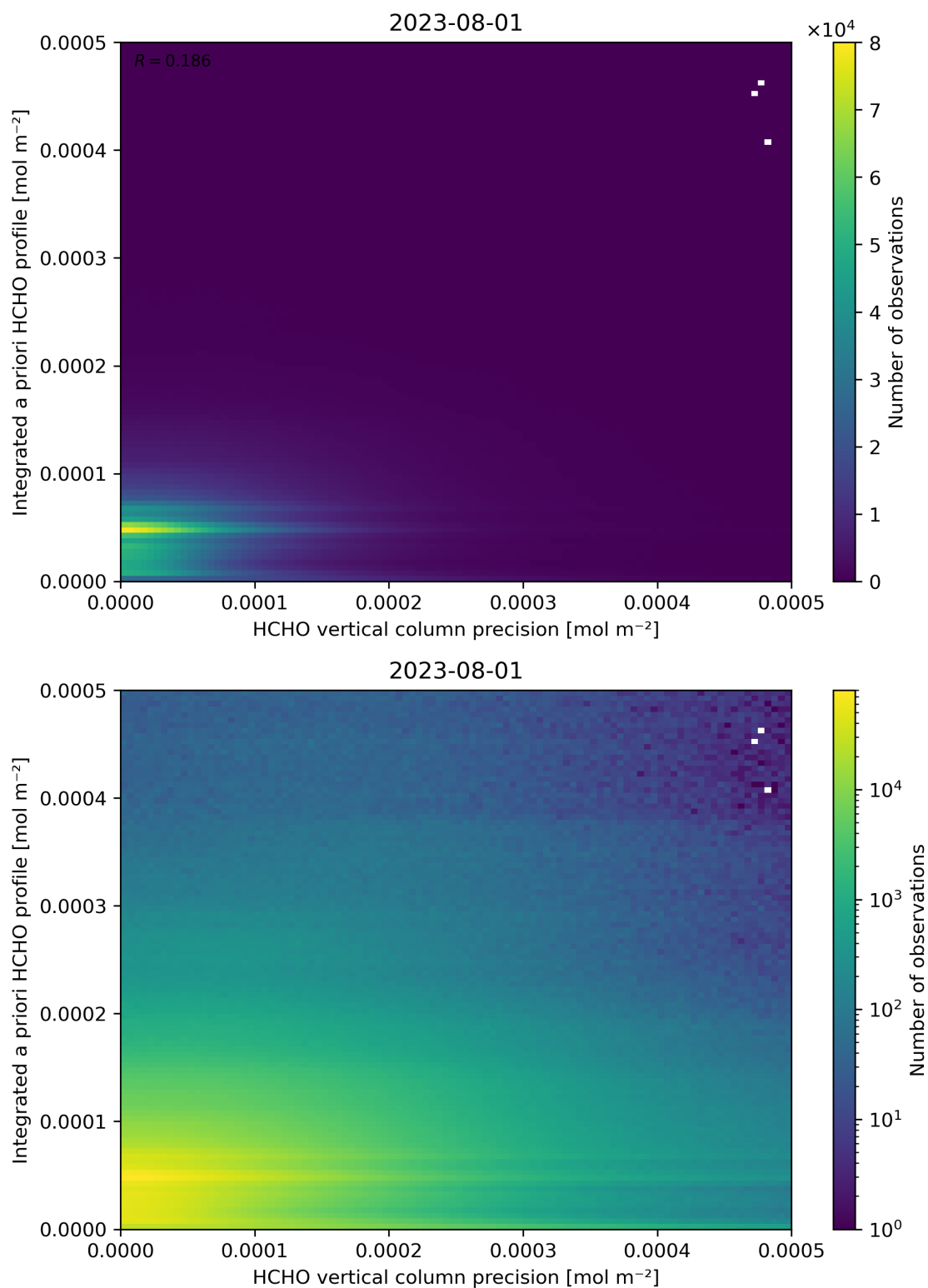
Figure 147: Scatter density plot of “HCHO vertical column precision” against “Integrated a priori HCHO profile” for 2023-07-31 to 2023-08-02.
