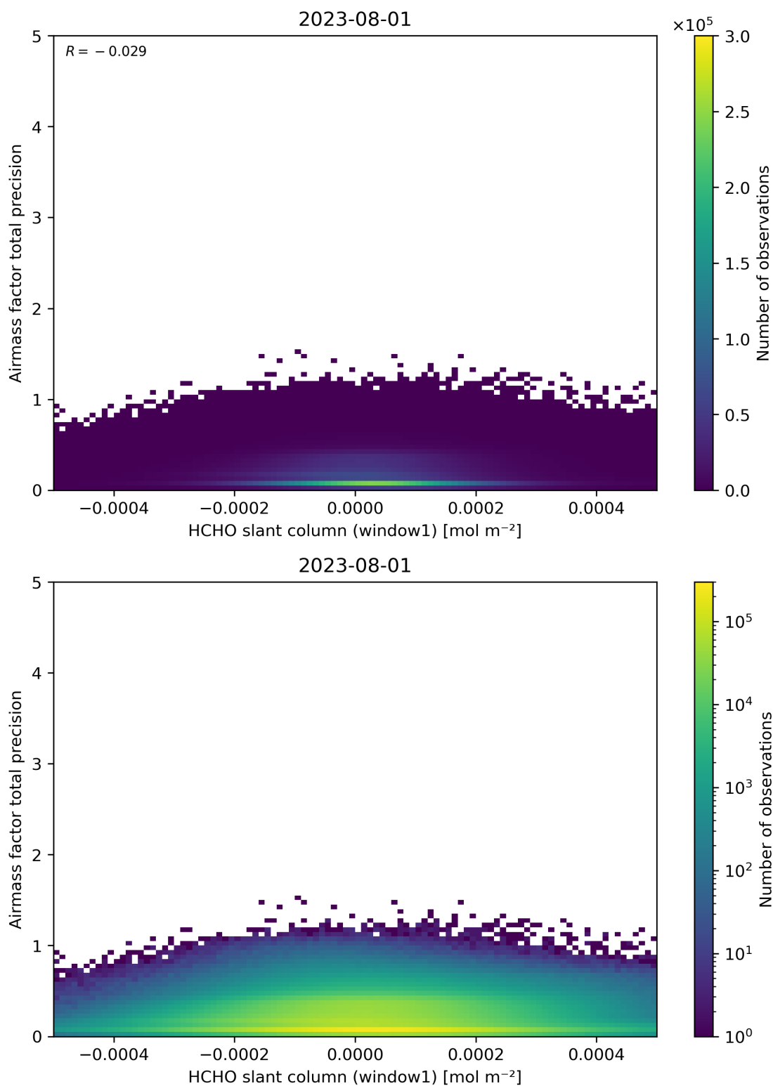
Figure 86: Scatter density plot of “HCHO slant column (window1)” against “Airmass factor total precision” for 2023-07-31 to 2023-08-02.
