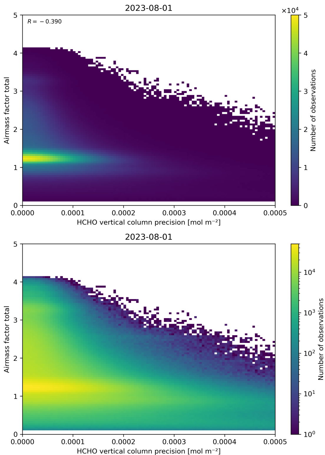
Figure 144: Scatter density plot of “HCHO vertical column precision” against “Airmass factor total” for 2023-07-31 to 2023-08-02.
