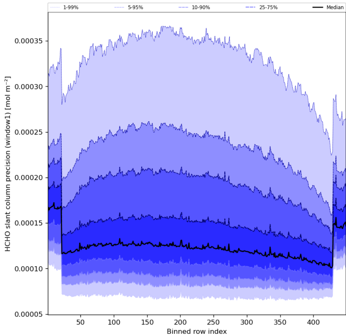
Figure 53: Along track statistics of “HCHO slant column precision (window1)” for 2023-07-31 to 2023-08-02
