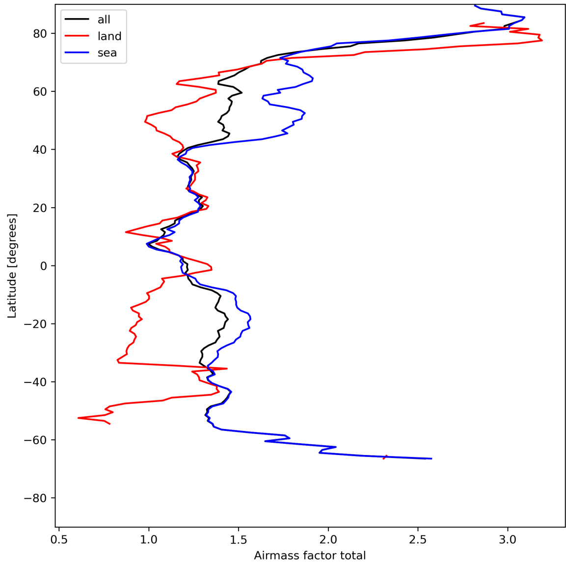
Figure 26: Zonal average of “Airmass factor total” for 2023-07-31 to 2023-08-02.
