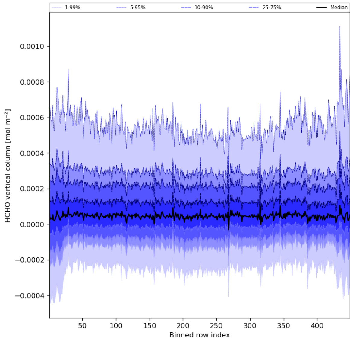
Figure 49: Along track statistics of “HCHO vertical column” for 2023-07-31 to 2023-08-02
