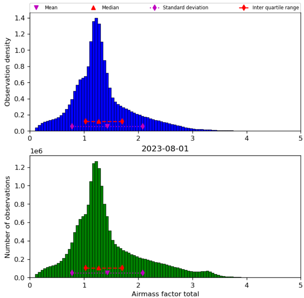
Figure 40: Histogram of “Airmass factor total” for 2023-07-31 to 2023-08-02
