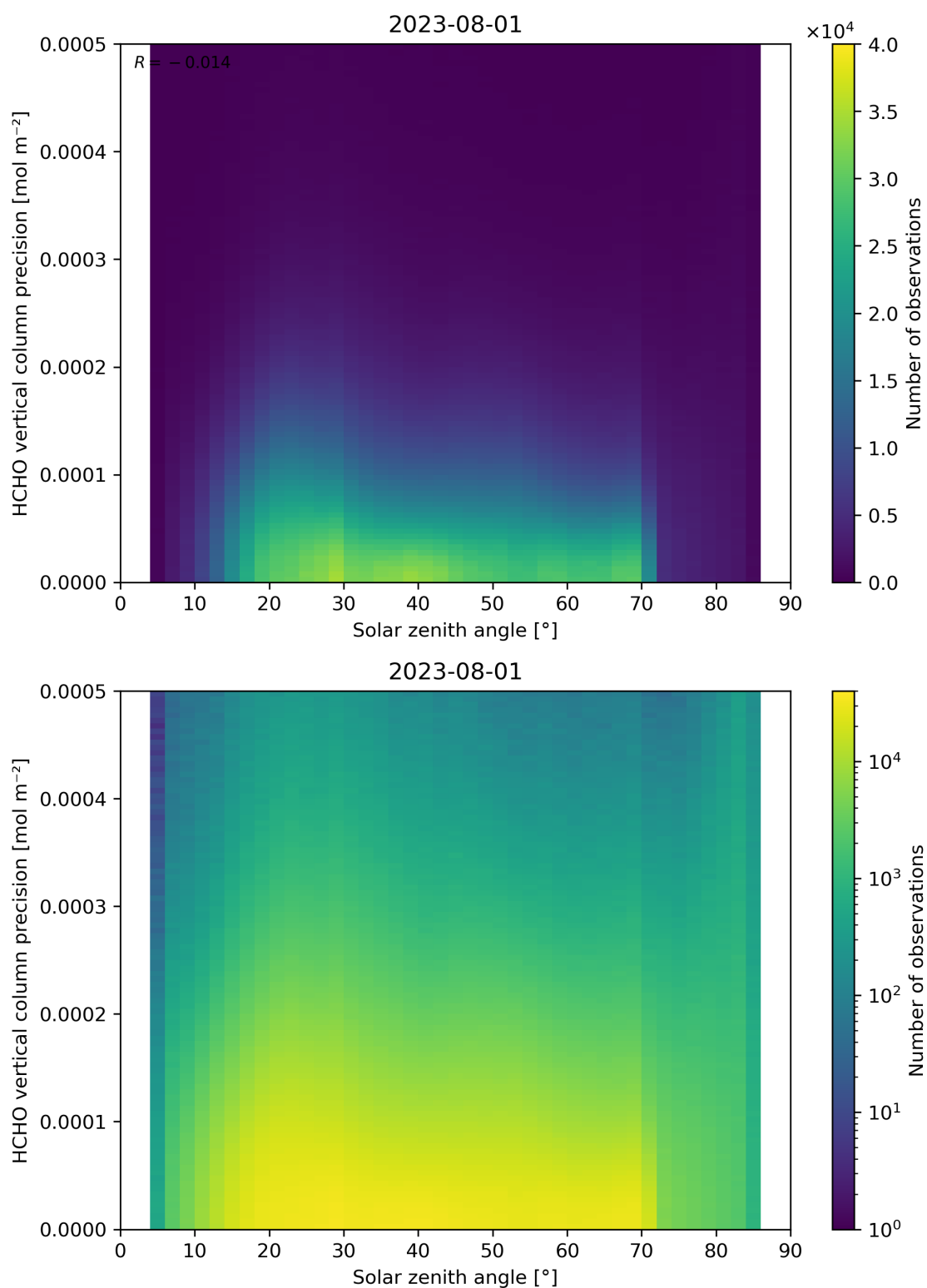
Figure 179: Scatter density plot of “Solar zenith angle” against “HCHO vertical column precision” for 2023-07-31 to 2023-08-02.
