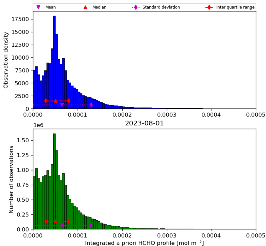
Figure 43: Histogram of “Integrated a priori HCHO profile” for 2023-07-31 to 2023-08-02
