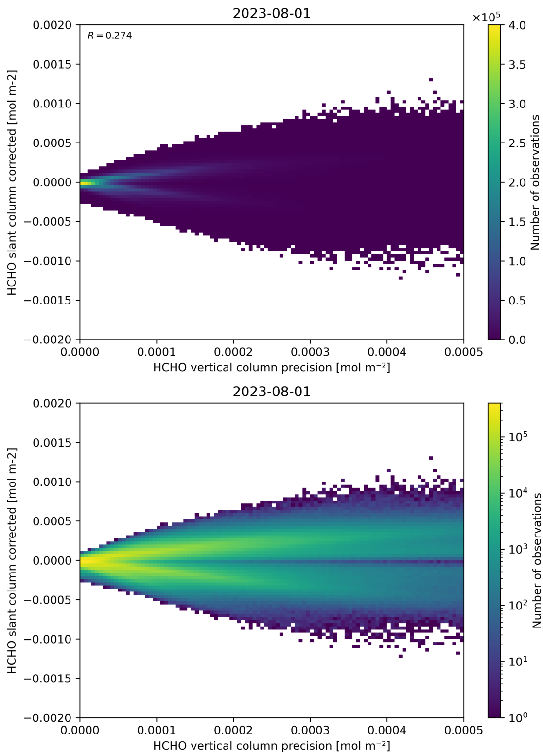
Figure 140: Scatter density plot of “HCHO vertical column precision” against “HCHO slant column corrected” for 2023-07-31 to 2023-08-02.
