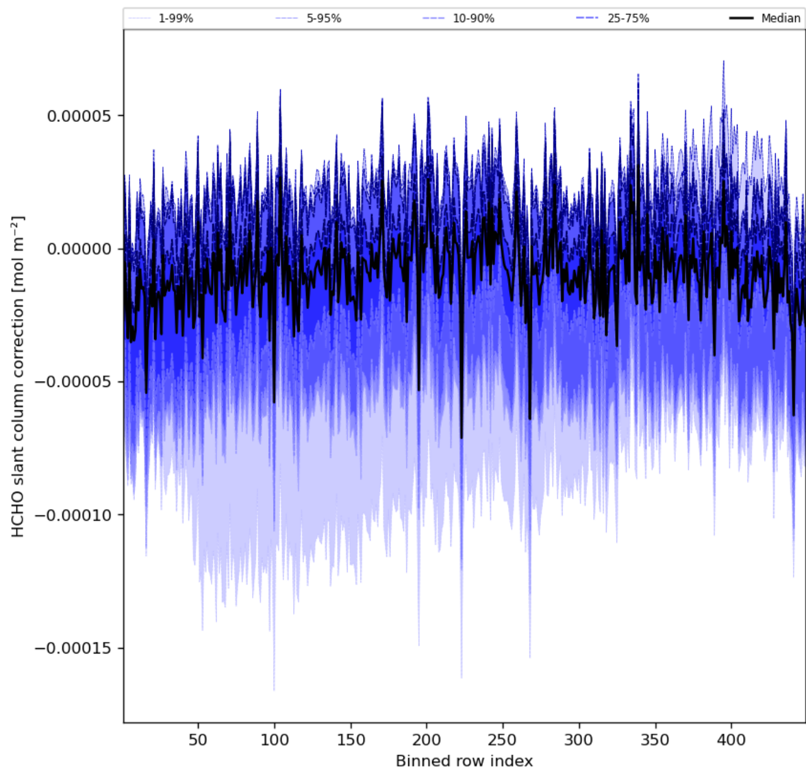
Figure 61: Along track statistics of “HCHO slant column correction” for 2023-08-01 to 2023-08-03
