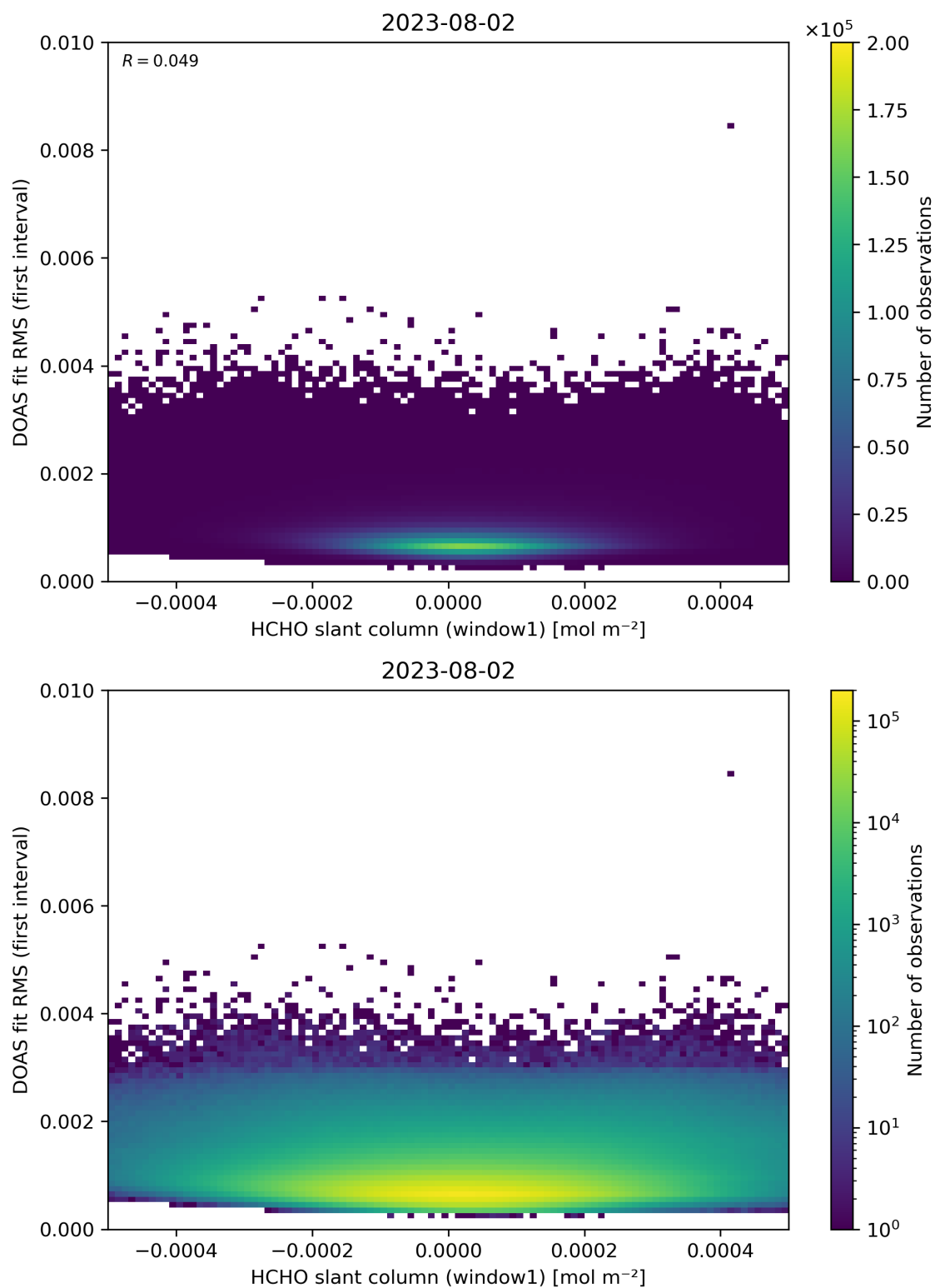
Figure 78: Scatter density plot of “HCHO slant column (window1)” against “DOAS fit RMS (first interval)” for 2023-08-01 to 2023-08-03.
