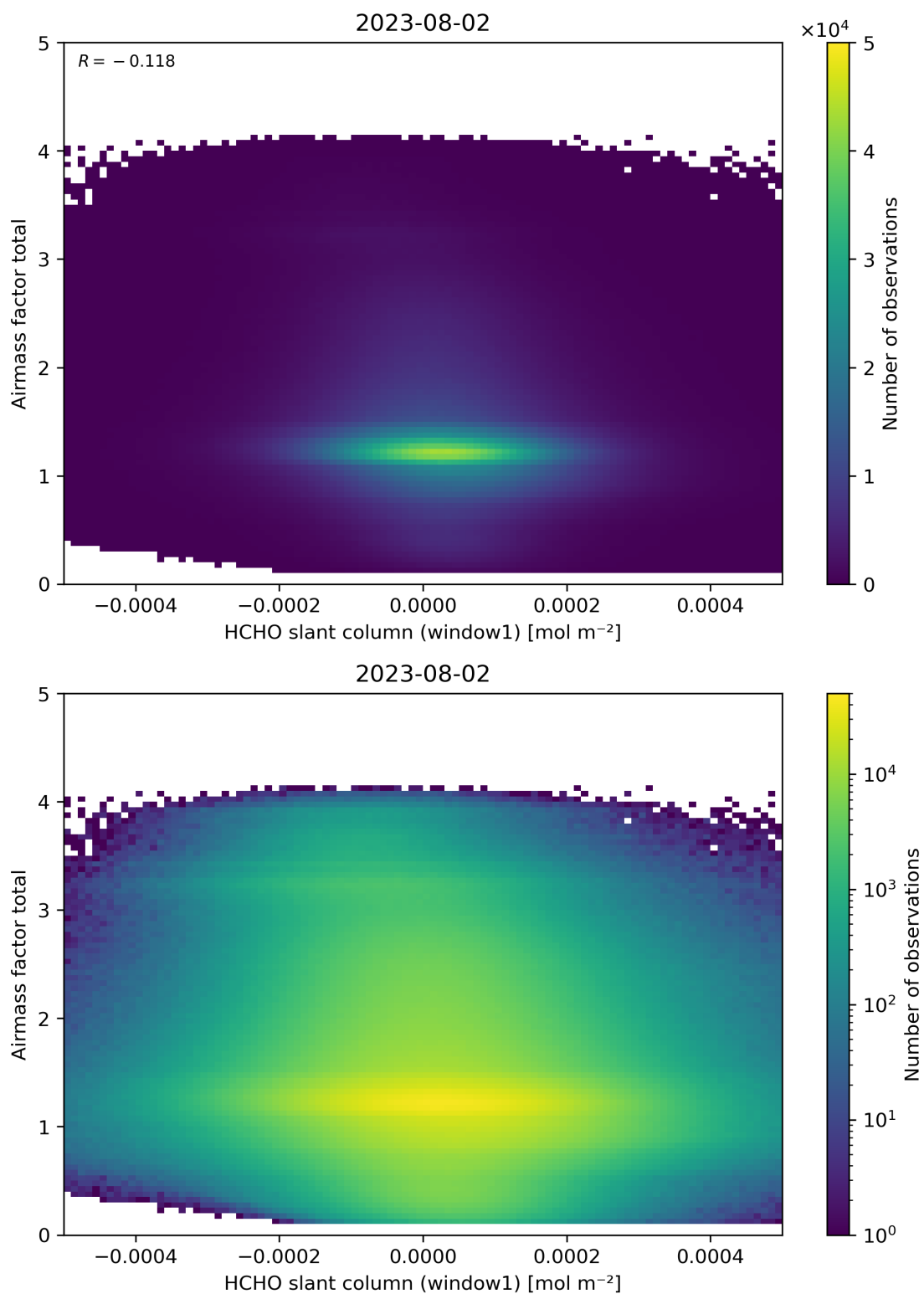
Figure 85: Scatter density plot of “HCHO slant column (window1)” against “Airmass factor total” for 2023-08-01 to 2023-08-03.
