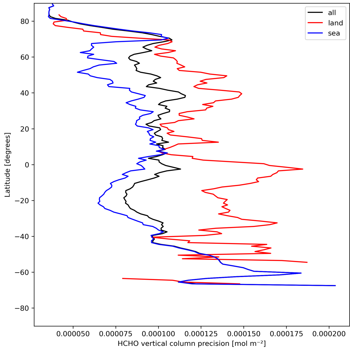
Figure 22: Zonal average of “HCHO vertical column precision” for 2023-08-01 to 2023-08-03.
