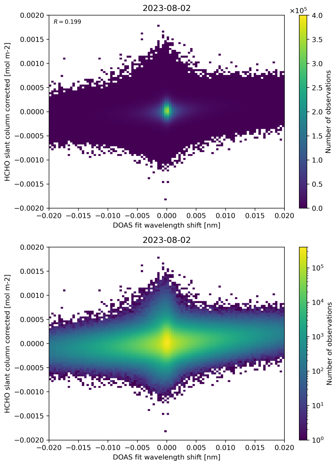
Figure 66: Scatter density plot of “DOAS fit wavelength shift” against “HCHO slant column corrected” for 2023-08-01 to 2023-08-03.
