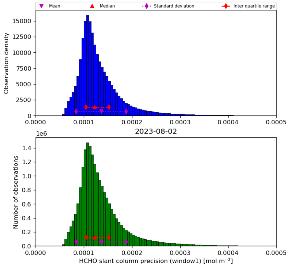
Figure 39: Histogram of “HCHO slant column precision (window1)” for 2023-08-01 to 2023-08-03
