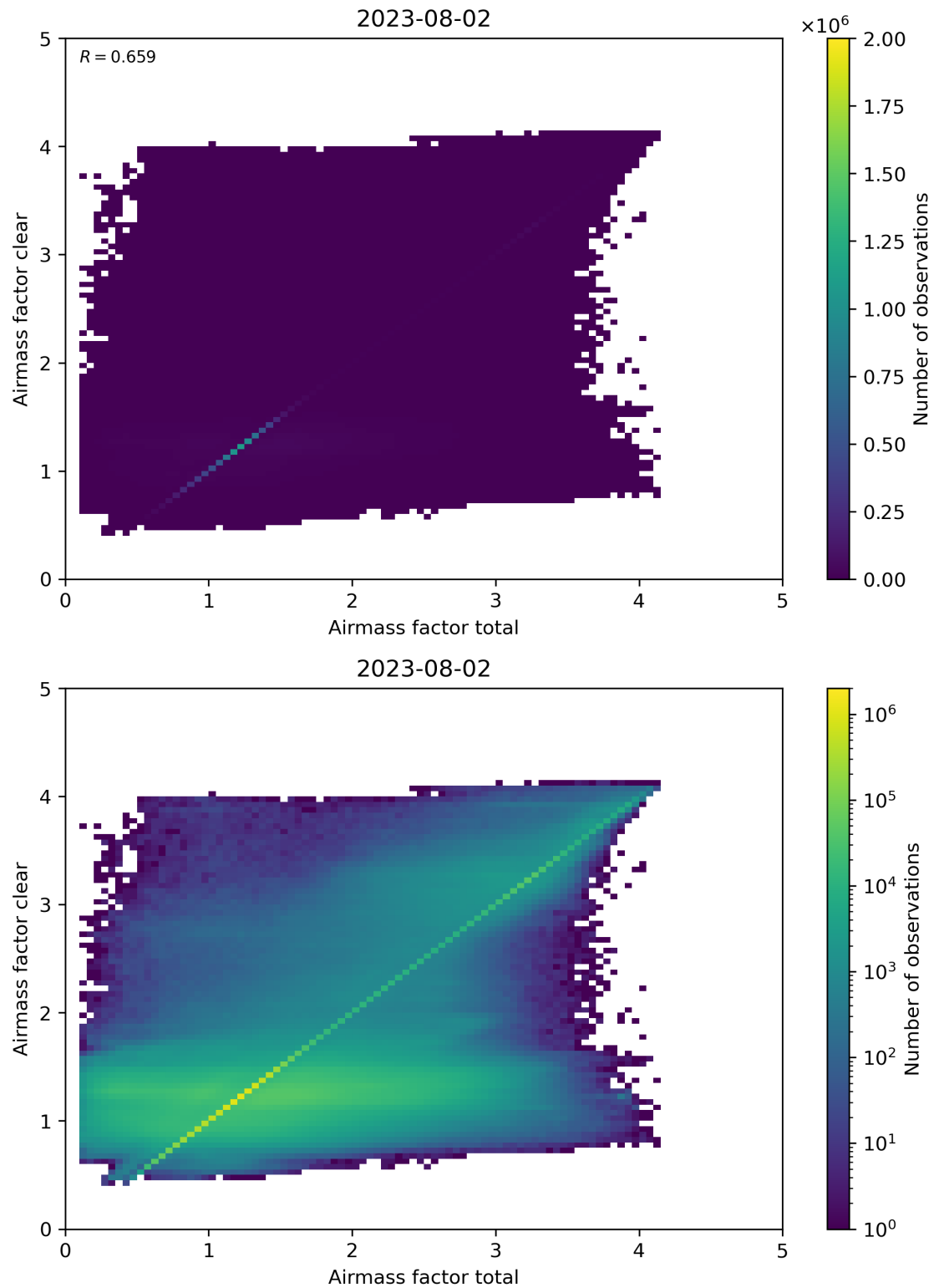
Figure 100: Scatter density plot of “Airmass factor total” against “Airmass factor clear” for 2023-08-01 to 2023-08-03.
