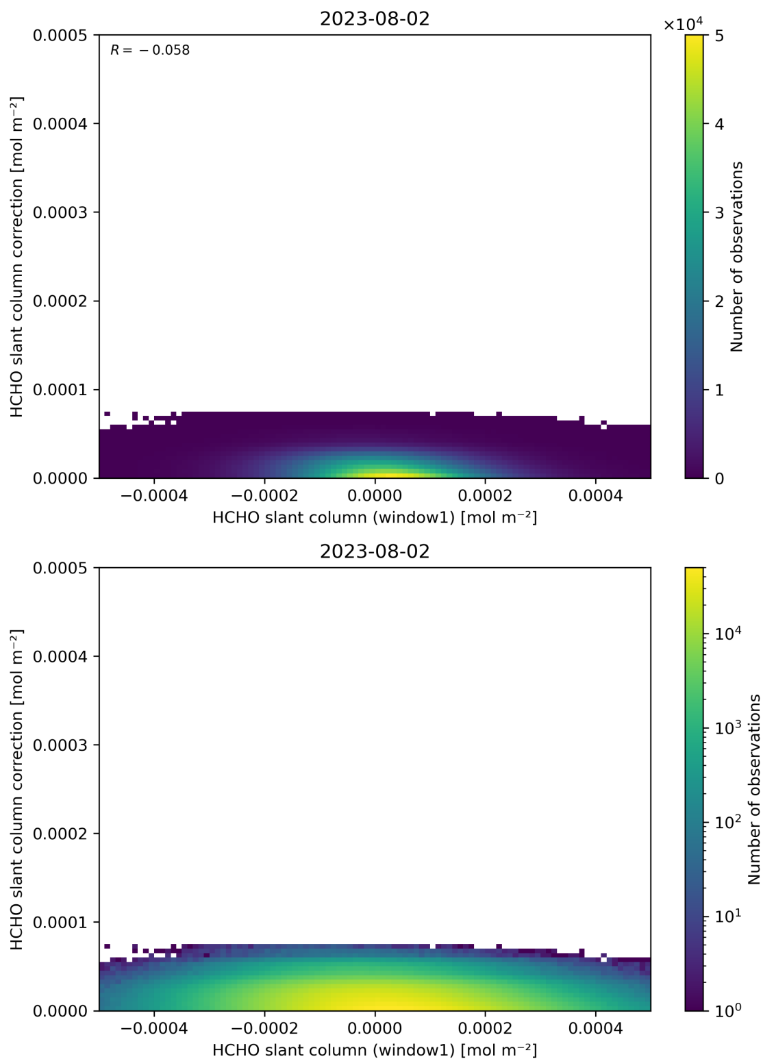
Figure 83: Scatter density plot of “HCHO slant column (window1)” against “HCHO slant column correction” for 2023-08-01 to 2023-08-03.
