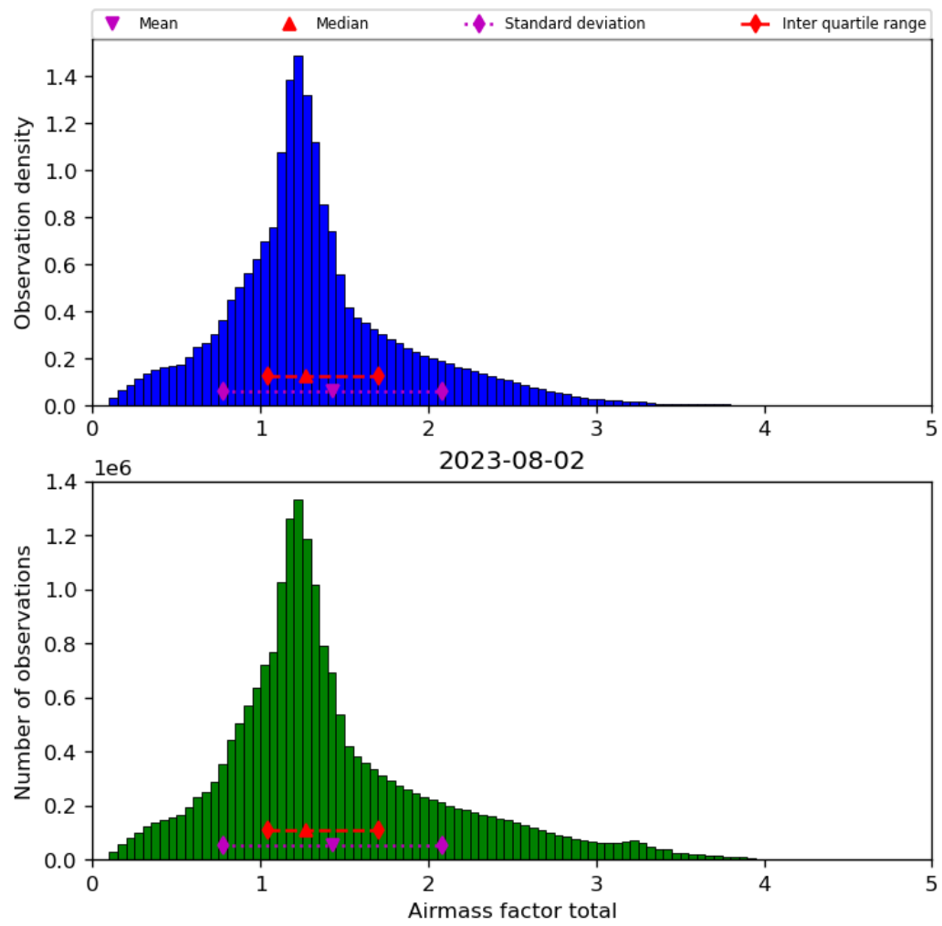
Figure 40: Histogram of “Airmass factor total” for 2023-08-01 to 2023-08-03
