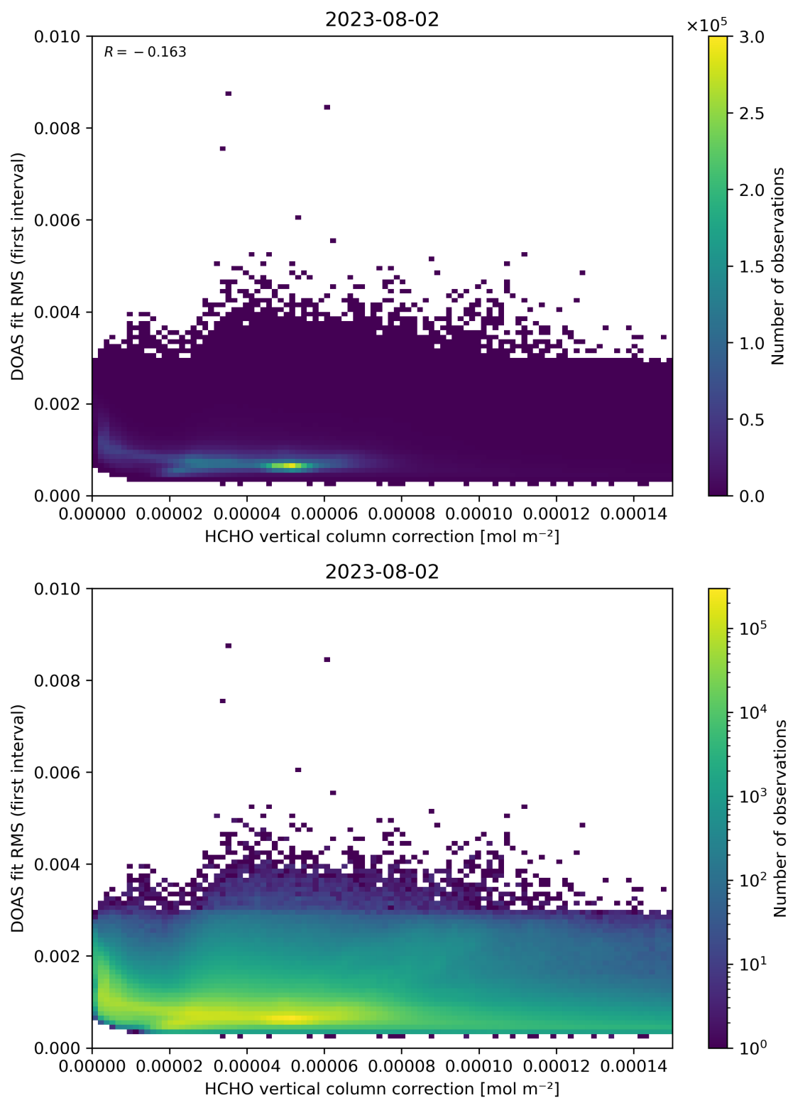
Figure 112: Scatter density plot of “HCHO vertical column correction” against “DOAS fit RMS (first interval)” for 2023-08-01 to 2023-08-03.
