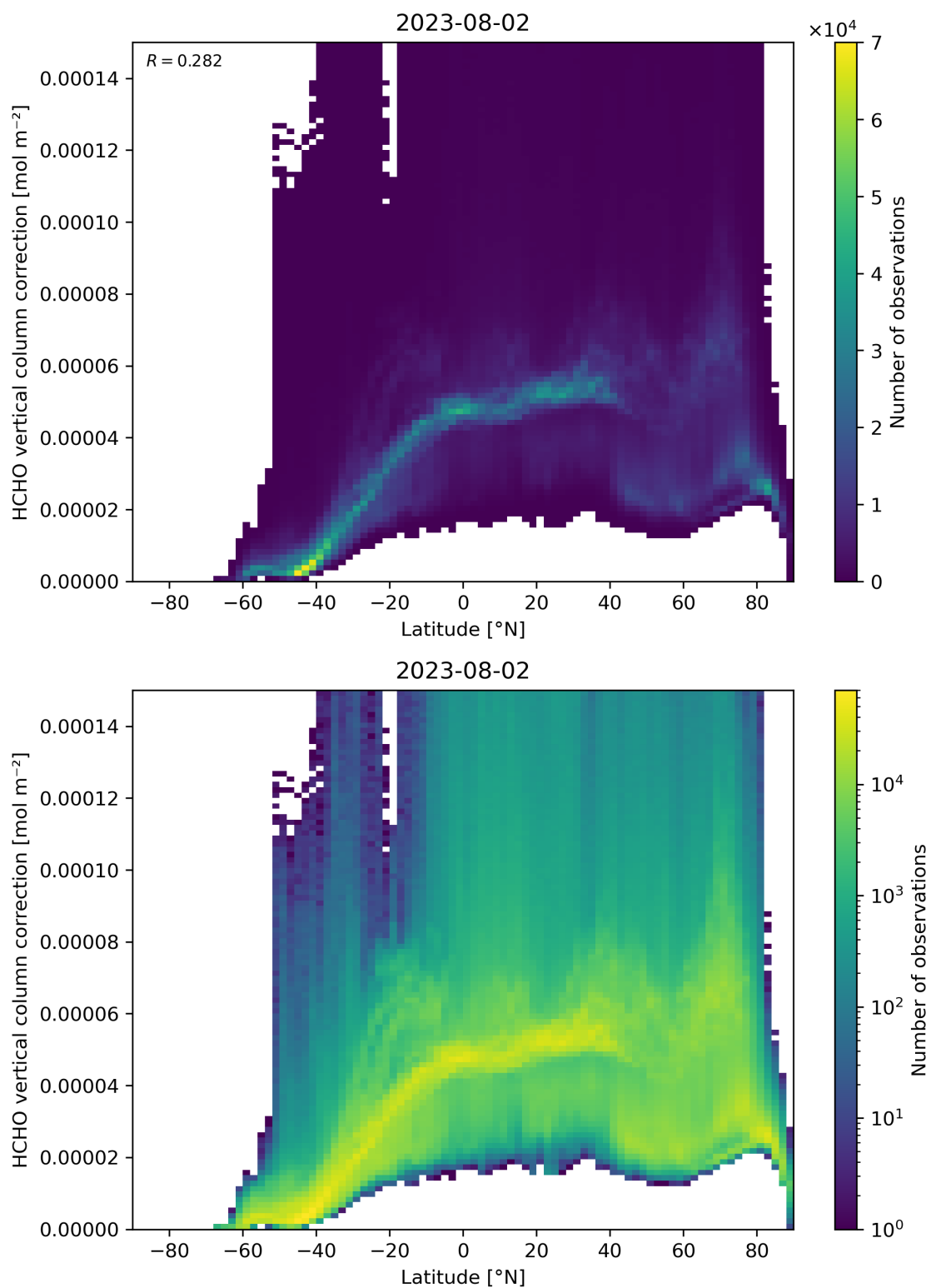
Figure 164: Scatter density plot of “Latitude” against “HCHO vertical column correction” for 2023-08-01 to 2023-08-03.
