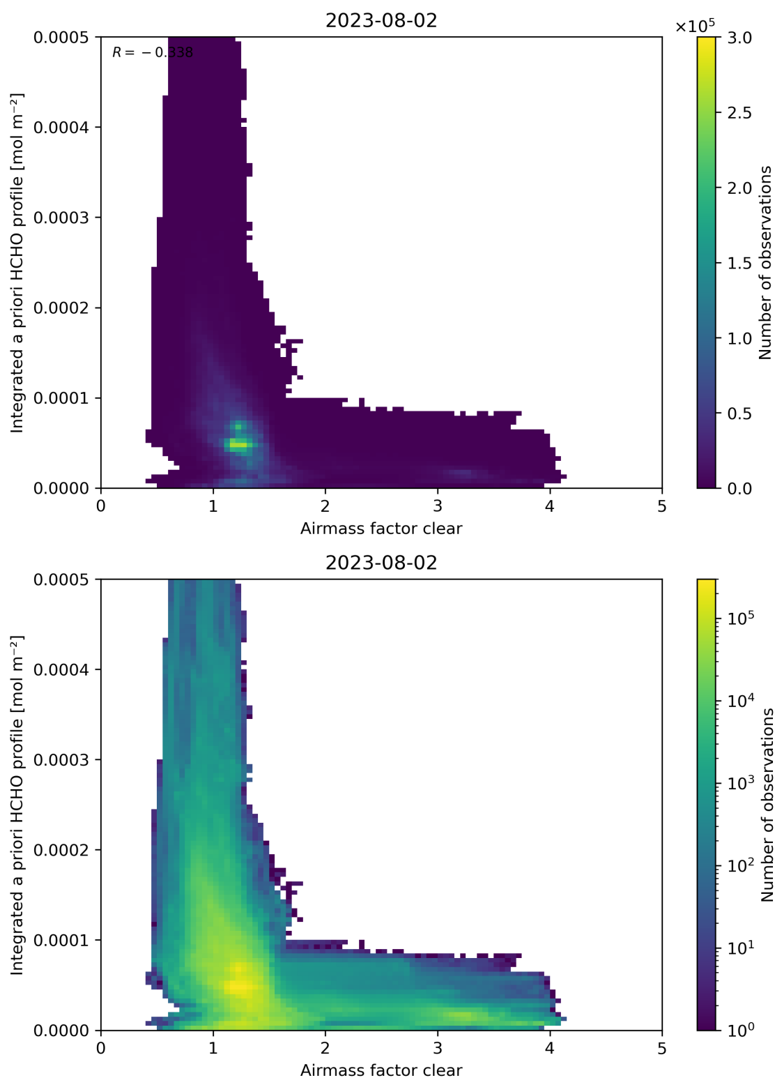
Figure 76: Scatter density plot of “Airmass factor clear” against “Integrated a priori HCHO profile” for 2023-08-01 to 2023-08-03.
