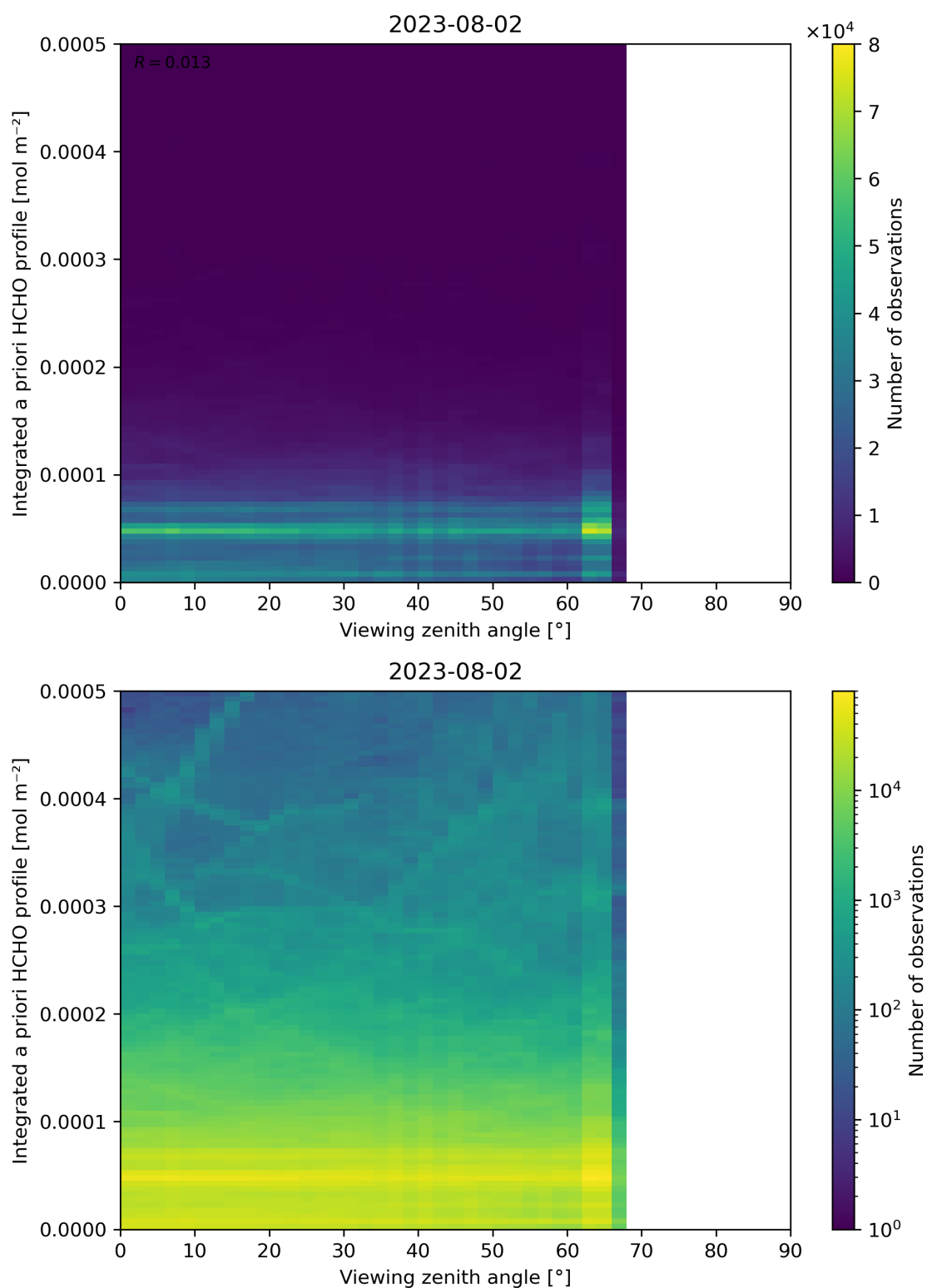
Figure 195: Scatter density plot of “Viewing zenith angle” against “Integrated a priori HCHO profile” for 2023-08-01 to 2023-08-03.
