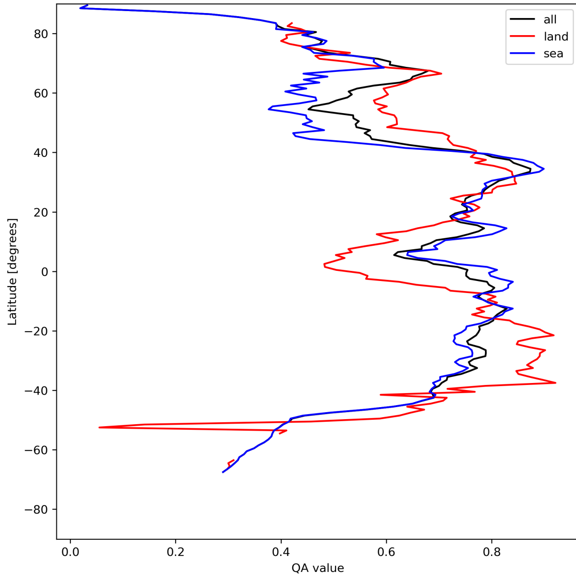
Figure 20: Zonal average of “QA value” for 2023-08-01 to 2023-08-03.
