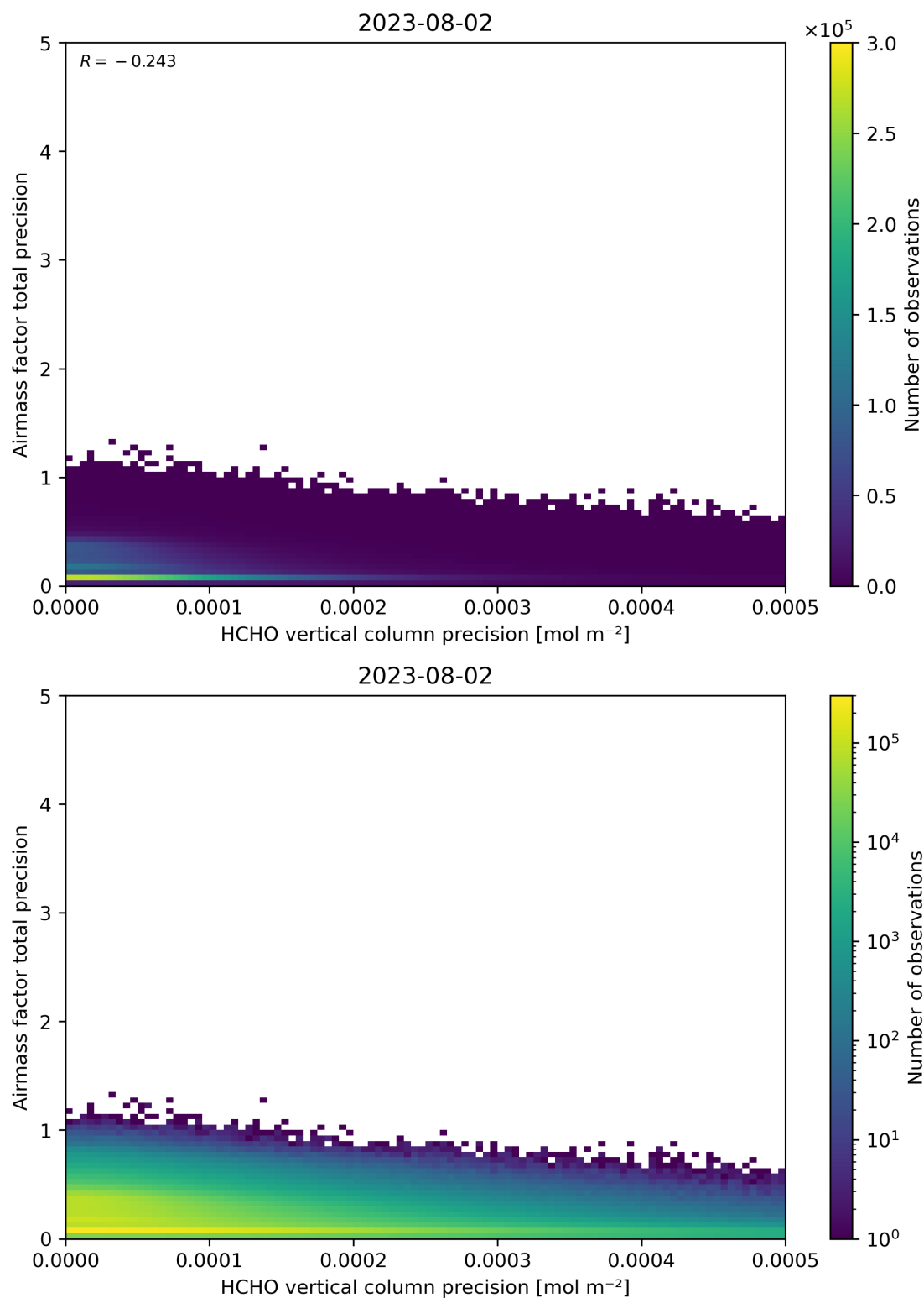
Figure 145: Scatter density plot of “HCHO vertical column precision” against “Airmass factor total precision” for 2023-08-01 to 2023-08-03.
