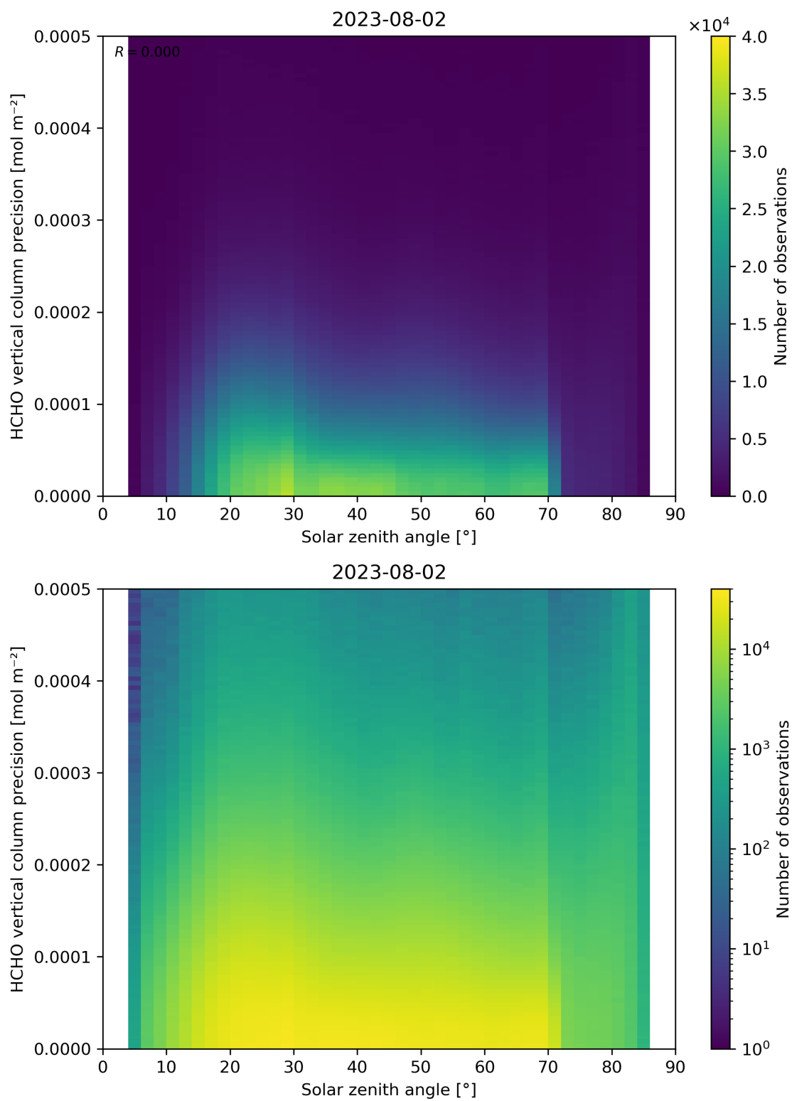
Figure 179: Scatter density plot of “Solar zenith angle” against “HCHO vertical column precision” for 2023-08-01 to 2023-08-03.
