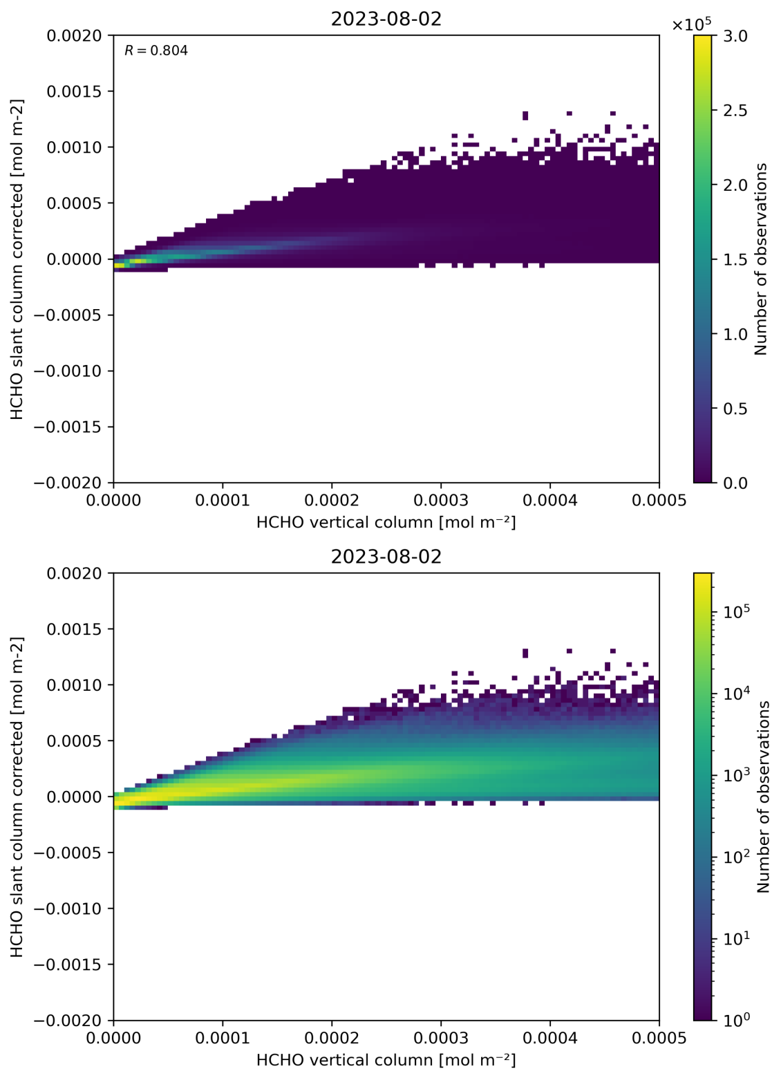
Figure 127: Scatter density plot of “HCHO vertical column” against “HCHO slant column corrected” for 2023-08-01 to 2023-08-03.
