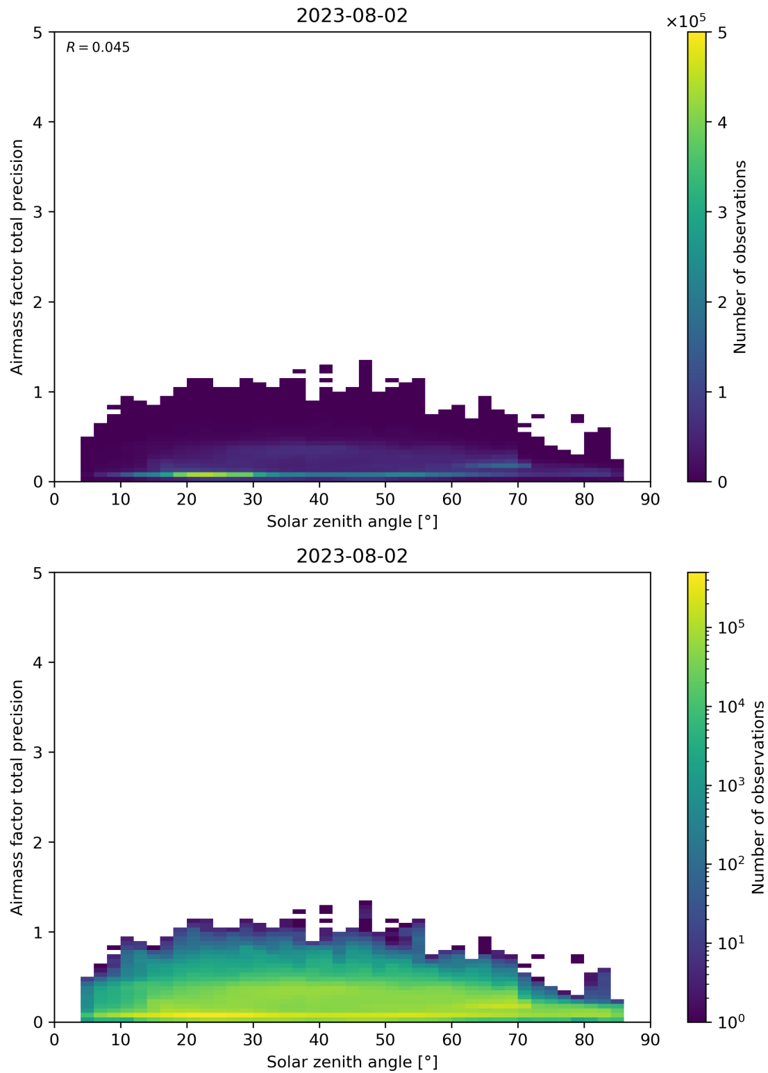
Figure 176: Scatter density plot of “Solar zenith angle” against “Airmass factor total precision” for 2023-08-01 to 2023-08-03.
