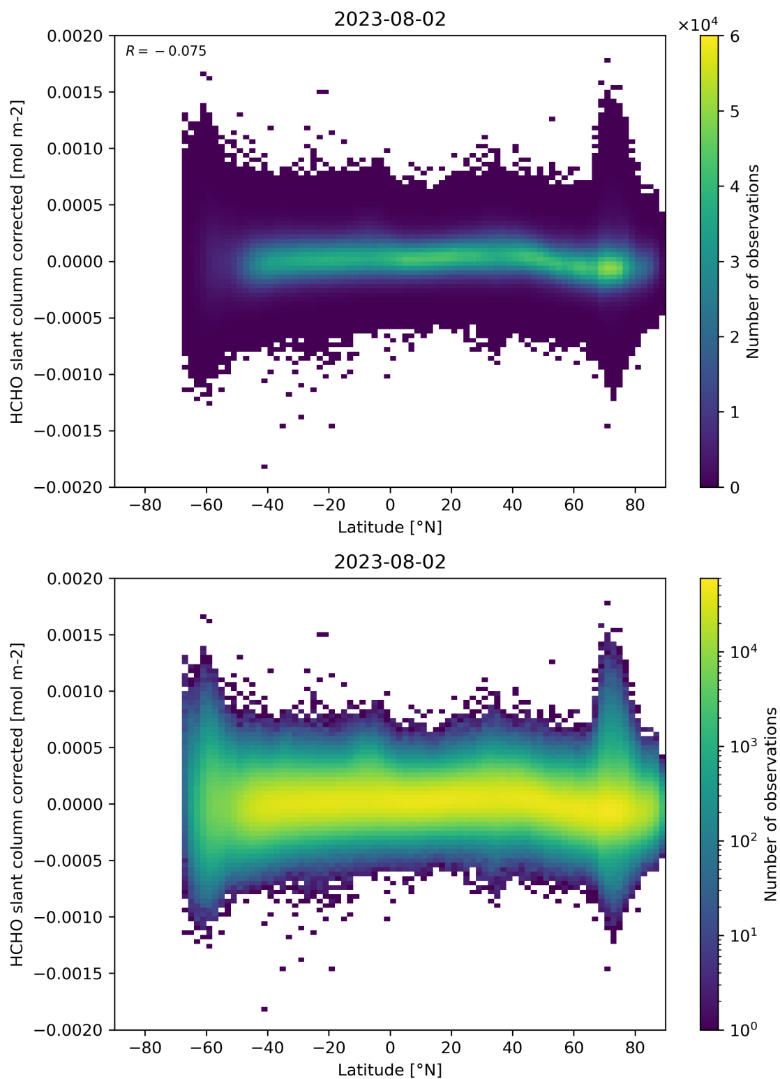
Figure 157: Scatter density plot of “Latitude” against “HCHO slant column corrected” for 2023-08-01 to 2023-08-03.
