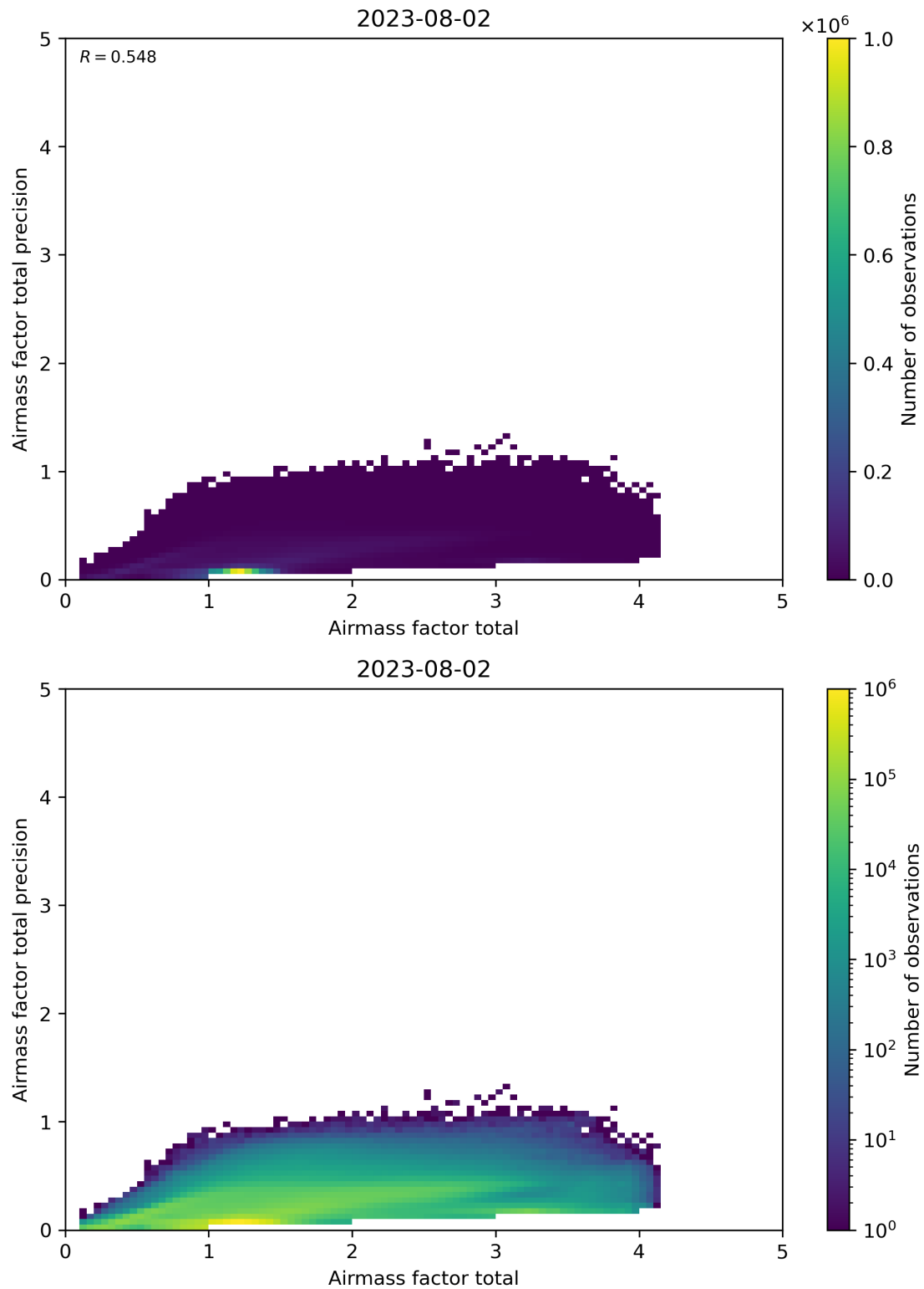
Figure 103: Scatter density plot of “Airmass factor total” against “Airmass factor total precision” for 2023-08-01 to 2023-08-03.
