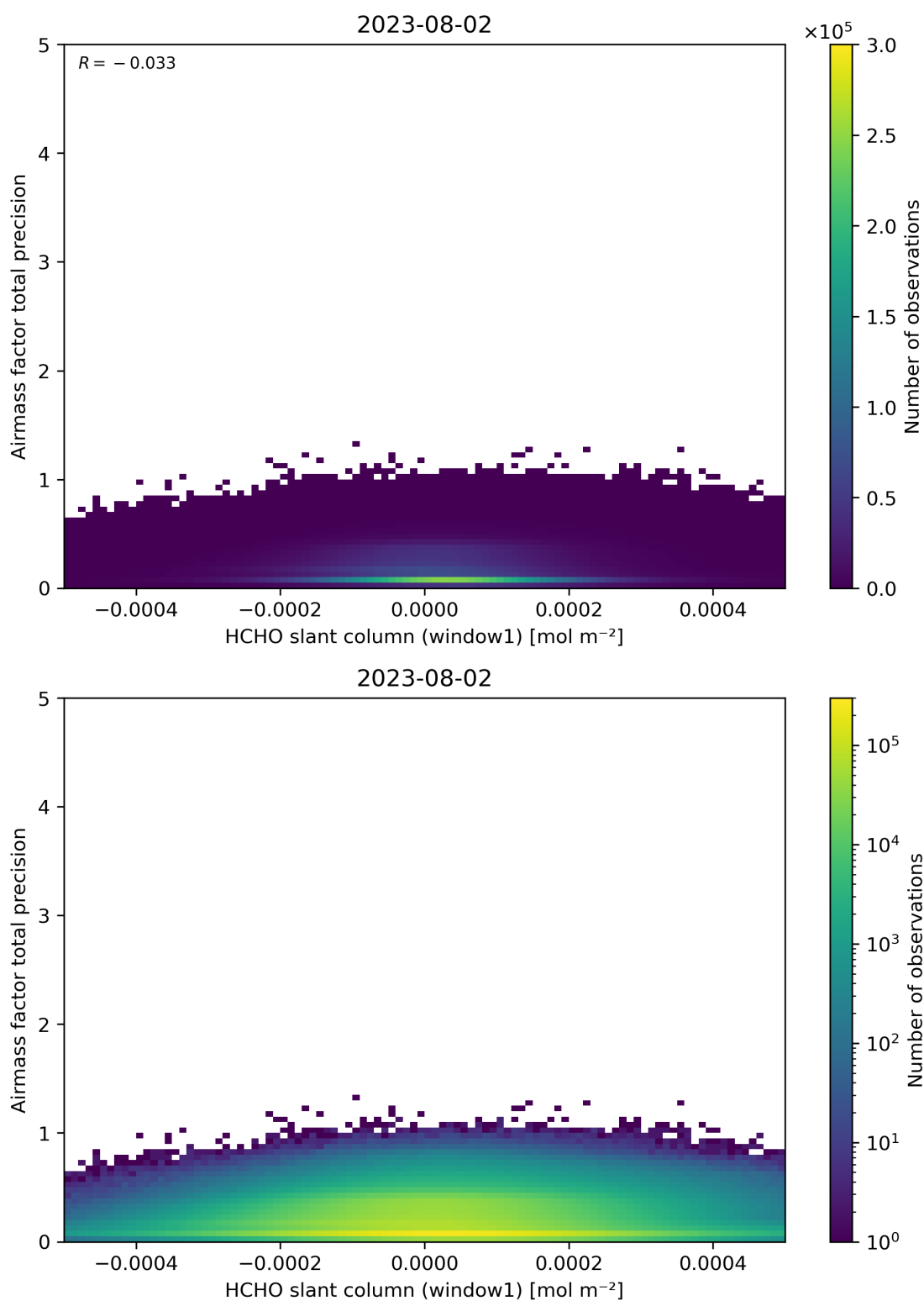
Figure 86: Scatter density plot of “HCHO slant column (window1)” against “Airmass factor total precision” for 2023-08-01 to 2023-08-03.
