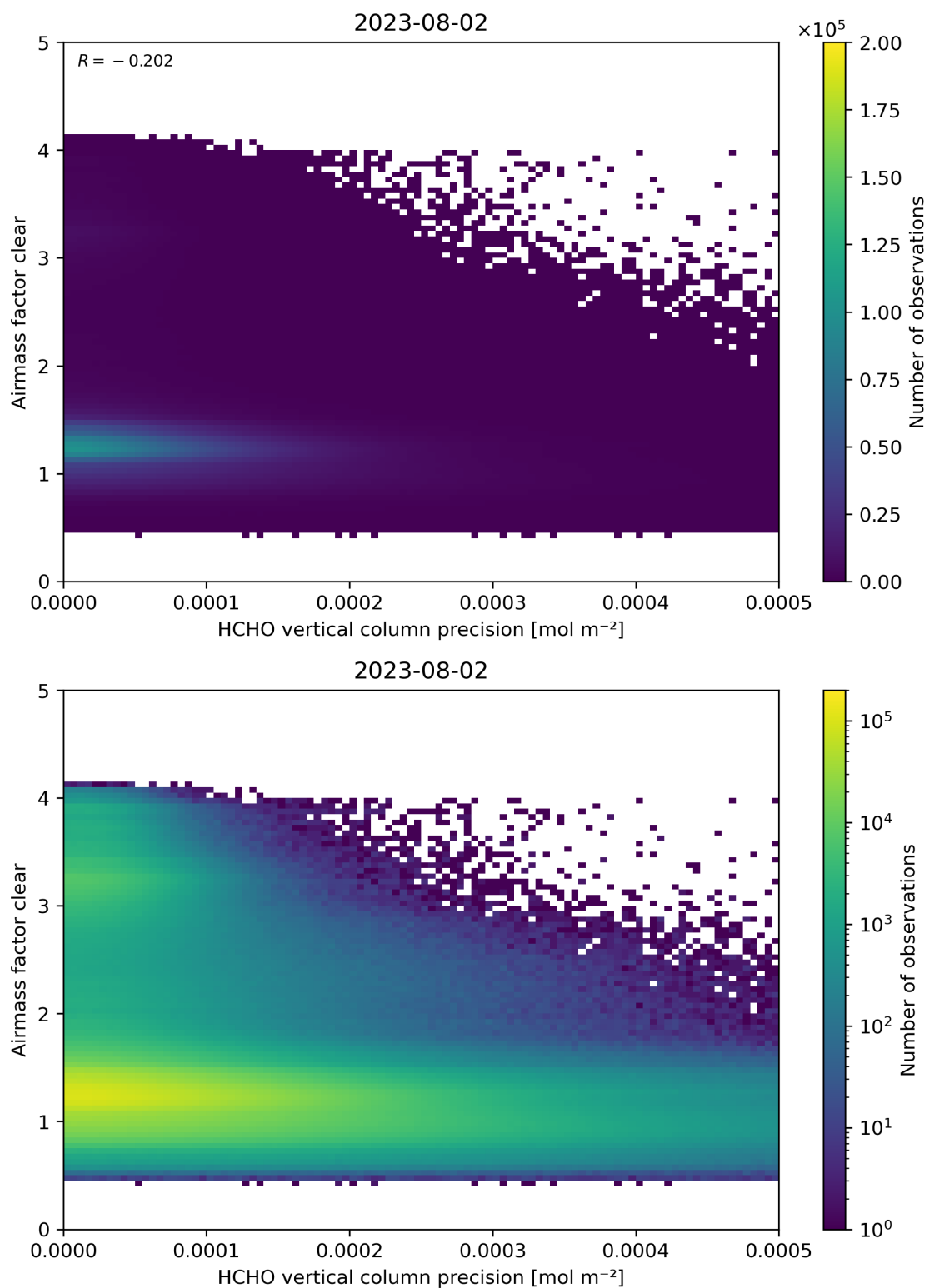
Figure 139: Scatter density plot of “HCHO vertical column precision” against “Airmass factor clear” for 2023-08-01 to 2023-08-03.
