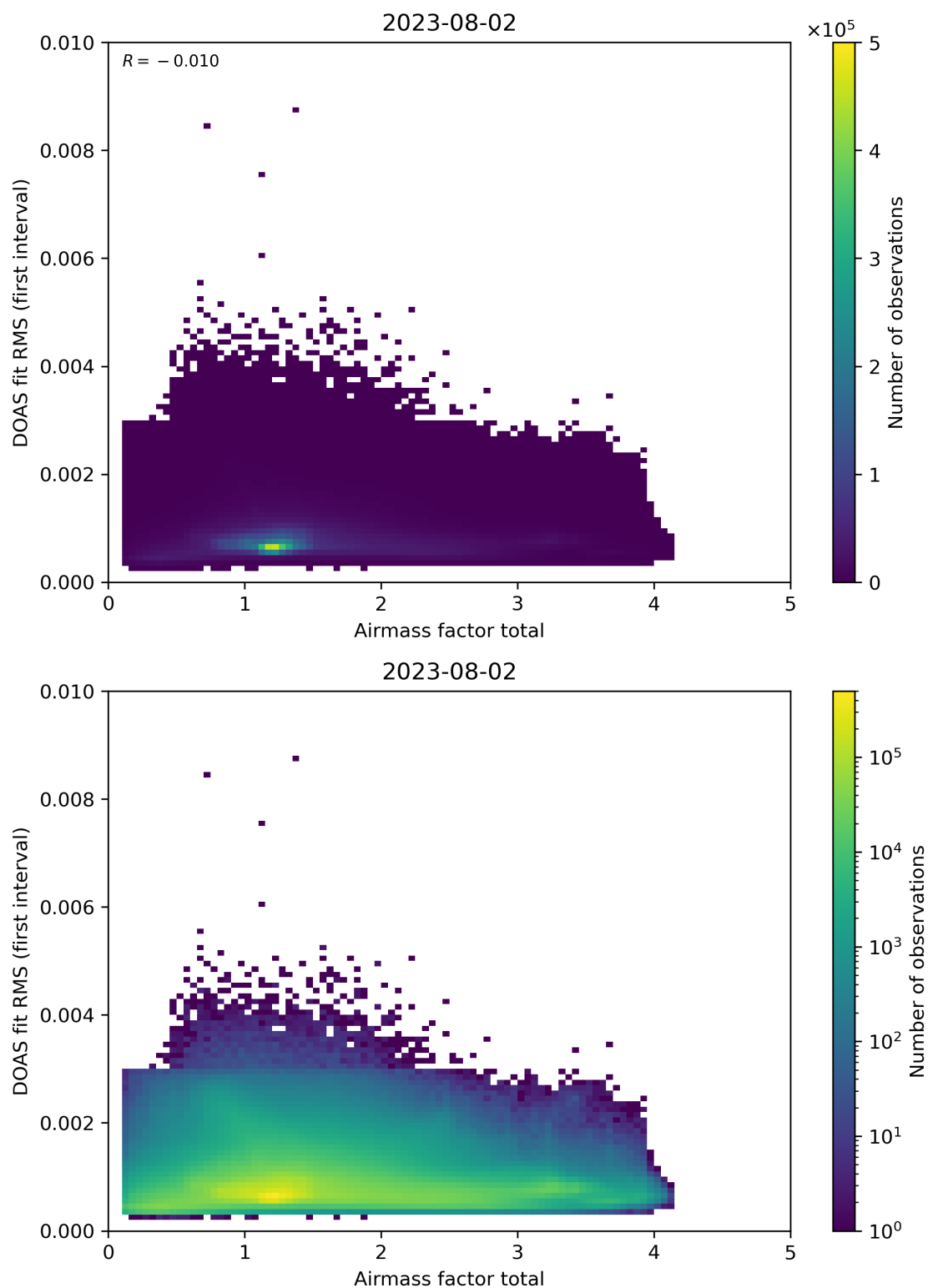
Figure 97: Scatter density plot of “Airmass factor total” against “DOAS fit RMS (first interval)” for 2023-08-01 to 2023-08-03.
