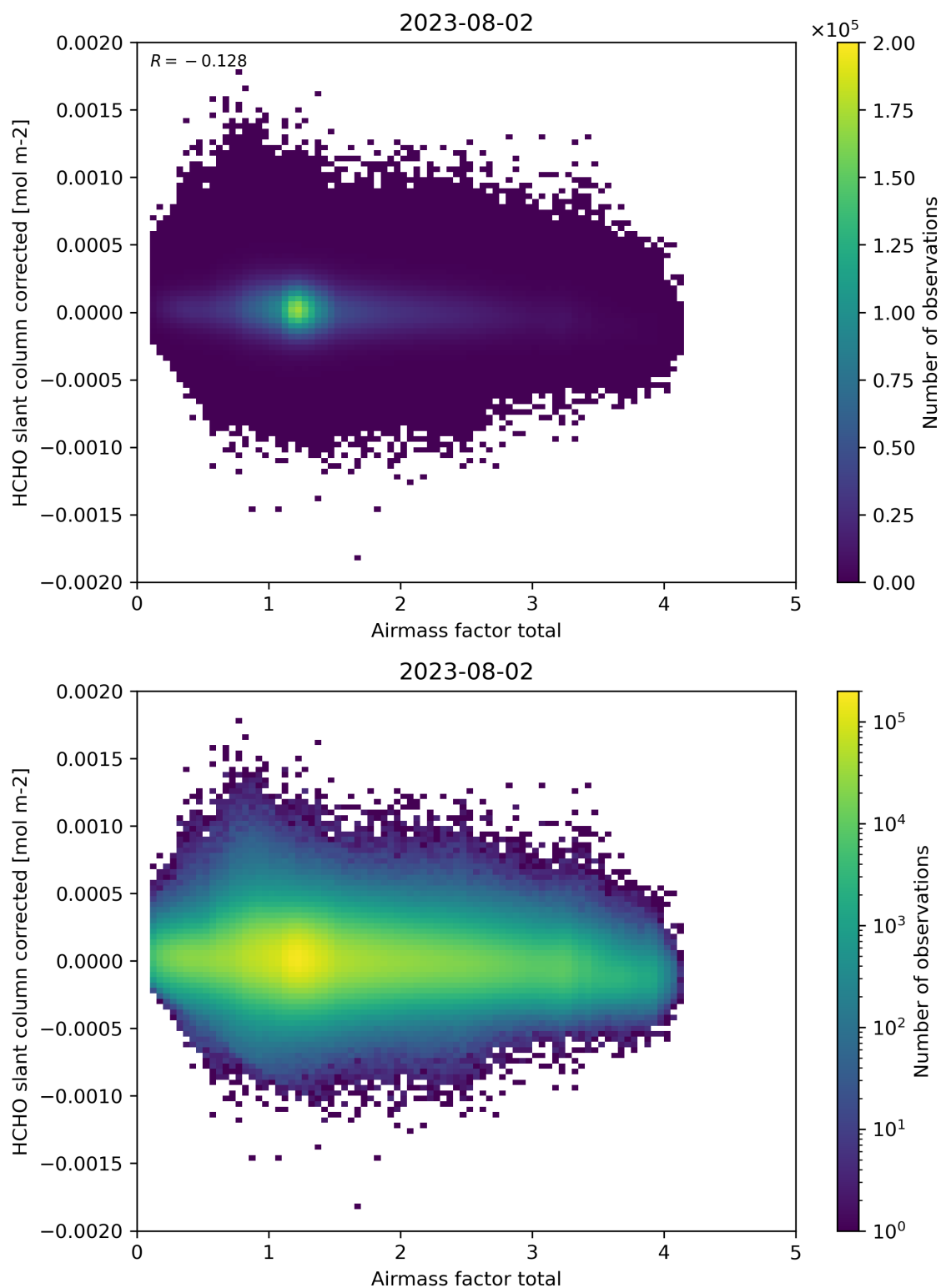
Figure 101: Scatter density plot of “Airmass factor total” against “HCHO slant column corrected” for 2023-08-01 to 2023-08-03.
