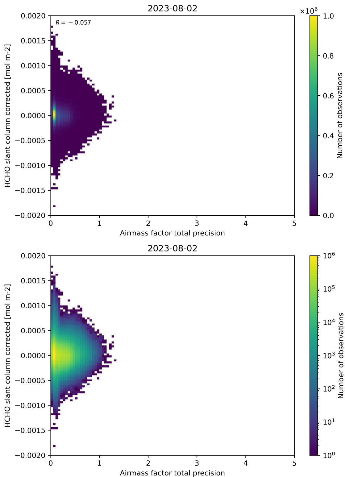
Figure 109: Scatter density plot of “Airmass factor total precision” against “HCHO slant column corrected” for 2023-08-01 to 2023-08-03.
