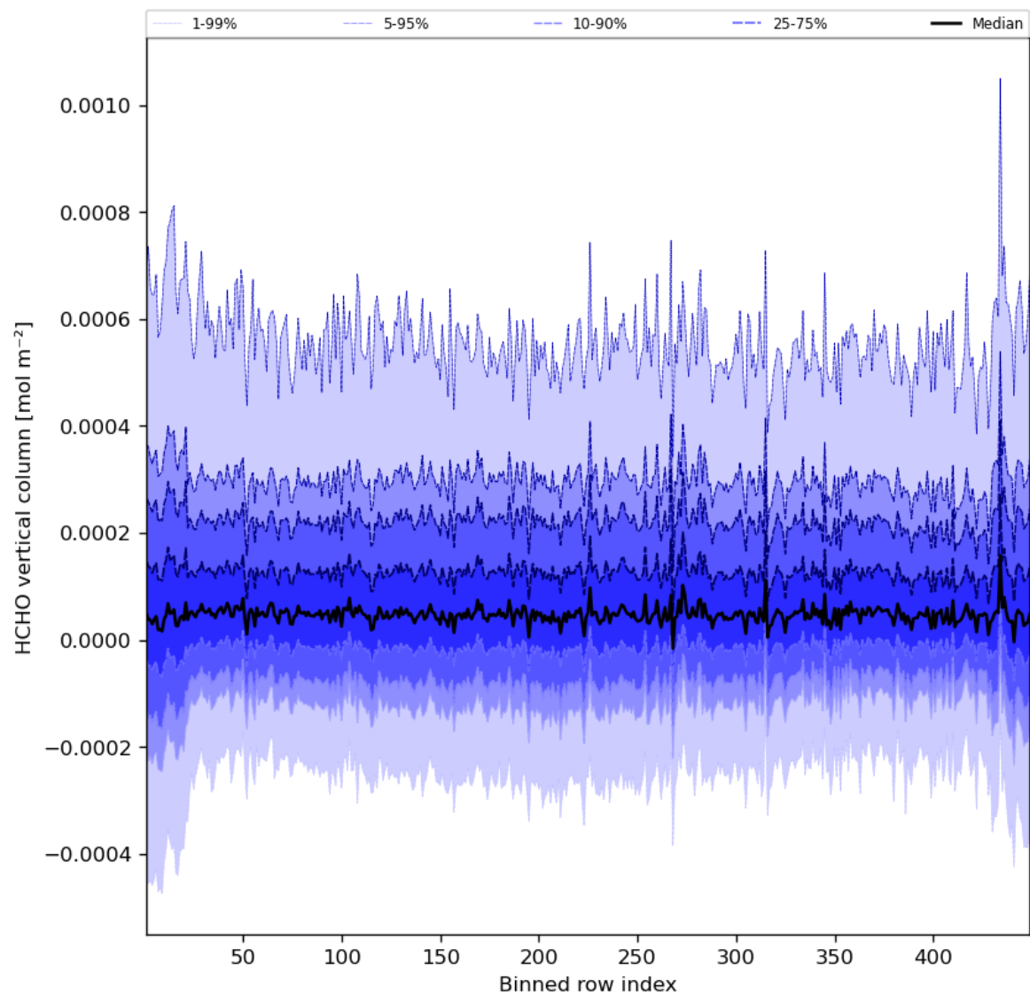
Figure 49: Along track statistics of “HCHO vertical column” for 2023-08-01 to 2023-08-03
