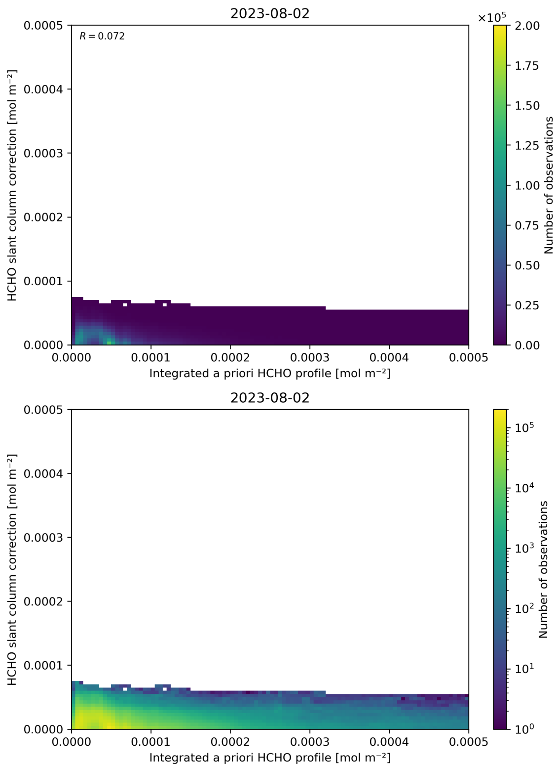
Figure 152: Scatter density plot of “Integrated a priori HCHO profile” against “HCHO slant column correction” for 2023-08-01 to 2023-08-03.
