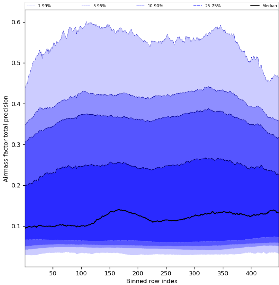
Figure 55: Along track statistics of “Airmass factor total precision” for 2023-08-01 to 2023-08-03
