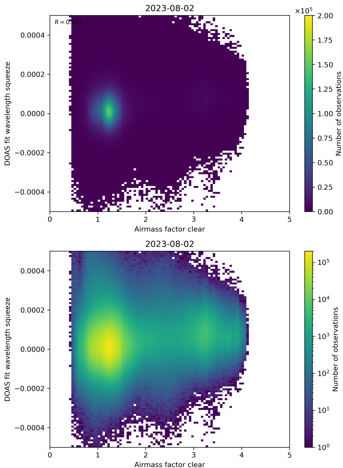
Figure 73: Scatter density plot of “Airmass factor clear” against “DOAS fit wavelength squeeze” for 2023-08-01 to 2023-08-03.
