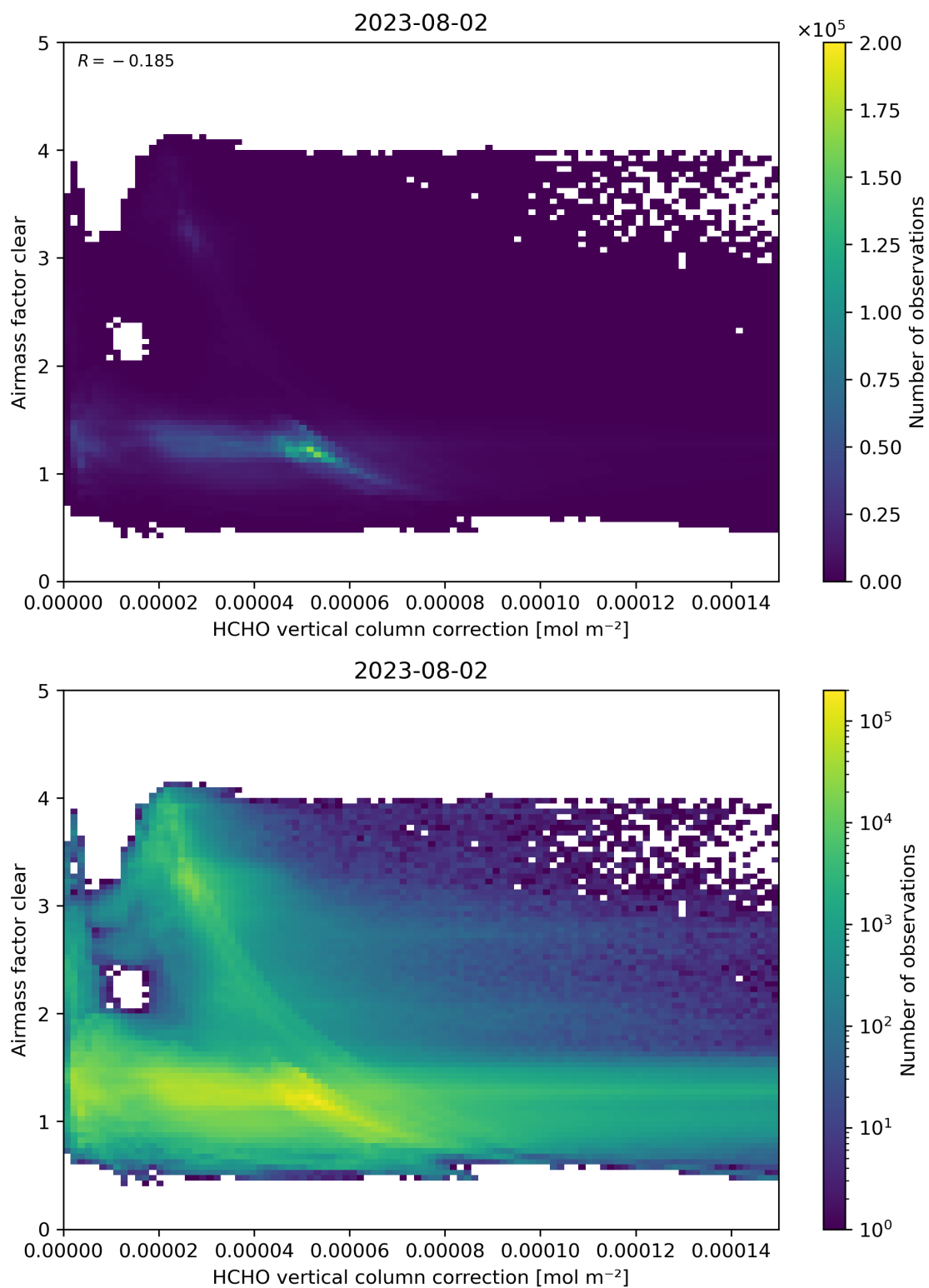
Figure 115: Scatter density plot of “HCHO vertical column correction” against “Airmass factor clear” for 2023-08-01 to 2023-08-03.
