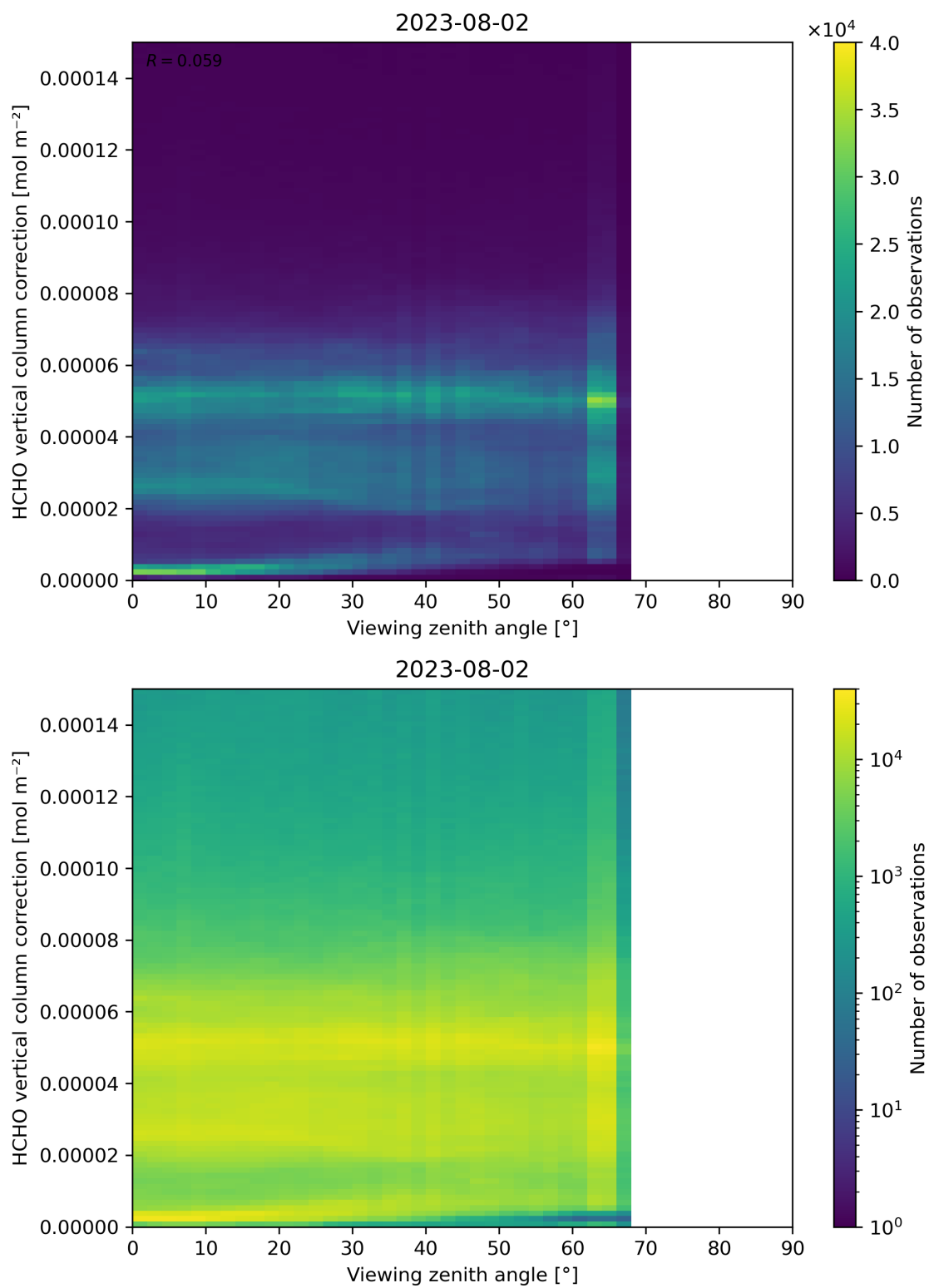
Figure 193: Scatter density plot of “Viewing zenith angle” against “HCHO vertical column correction” for 2023-08-01 to 2023-08-03.
