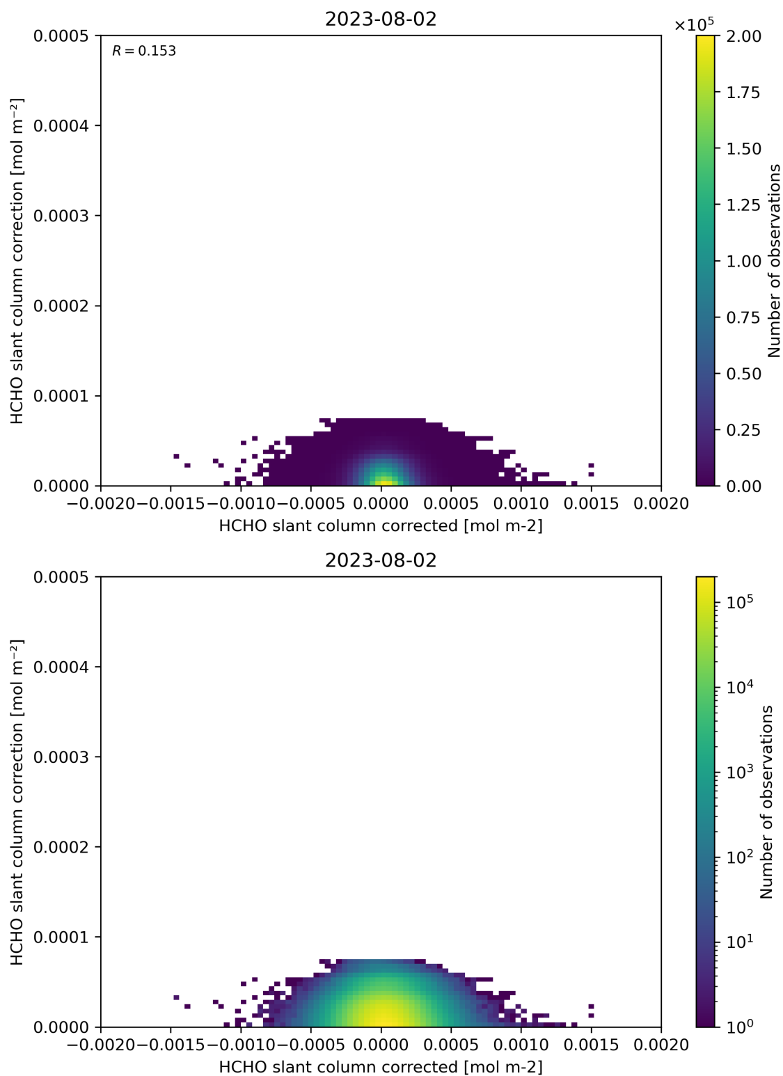
Figure 77: Scatter density plot of “HCHO slant column corrected” against “HCHO slant column correction” for 2023-08-01 to 2023-08-03.
