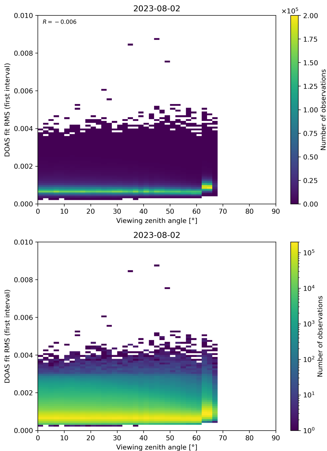
Figure 182: Scatter density plot of “Viewing zenith angle” against “DOAS fit RMS (first interval)” for 2023-08-01 to 2023-08-03.
