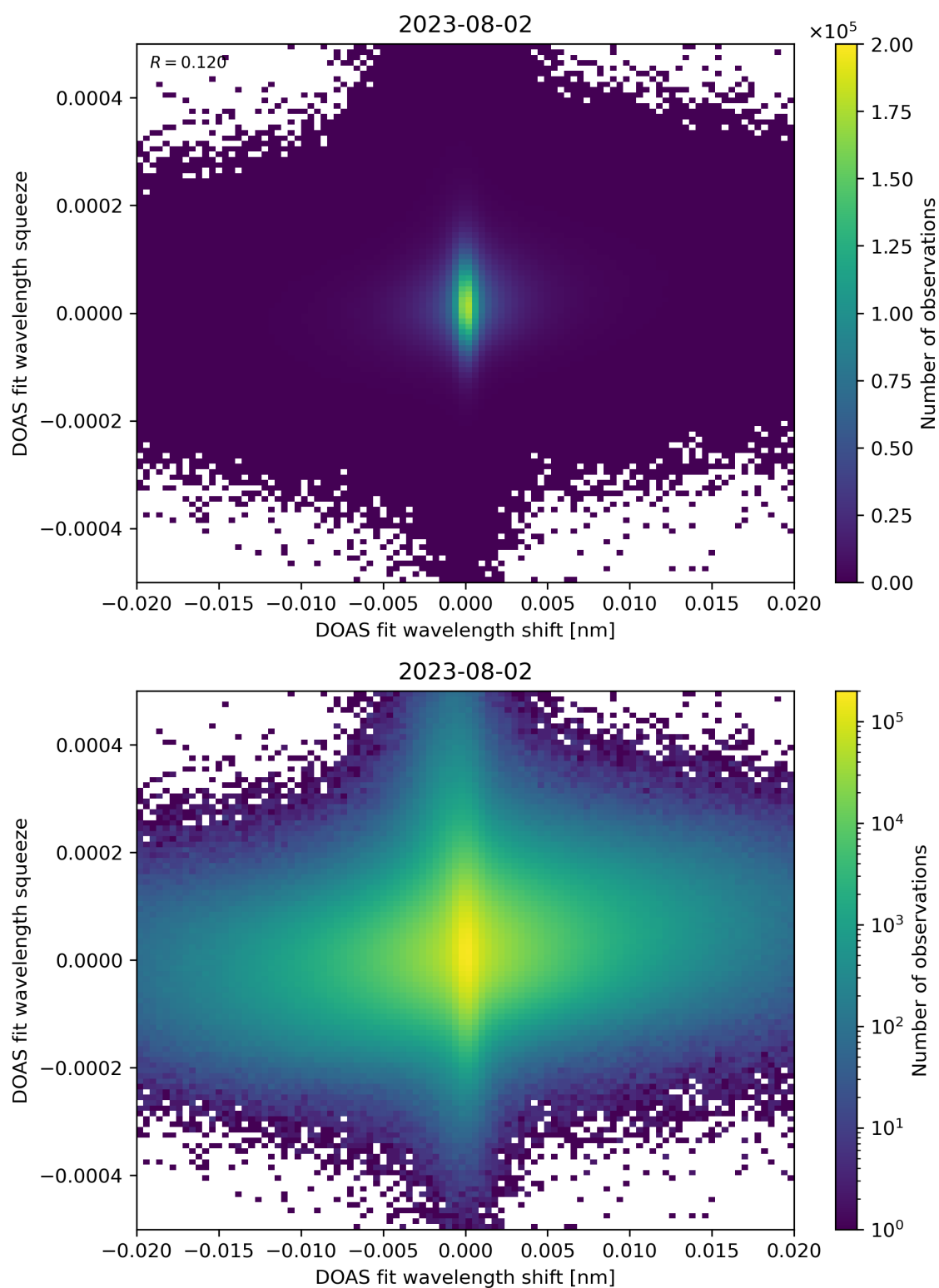
Figure 65: Scatter density plot of “DOAS fit wavelength shift” against “DOAS fit wavelength squeeze” for 2023-08-01 to 2023-08-03.
