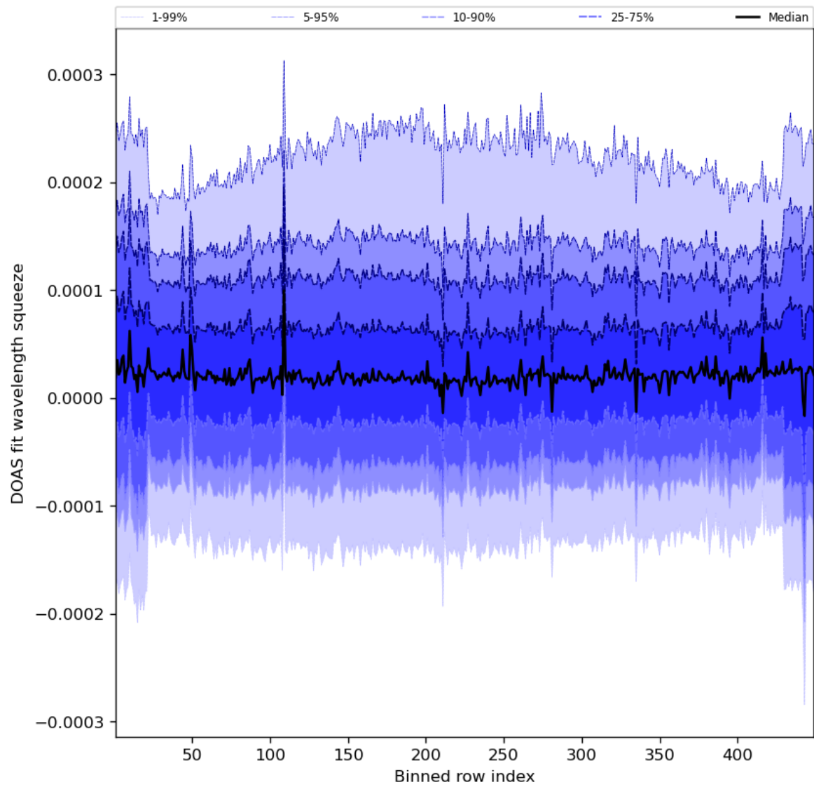
Figure 59: Along track statistics of “DOAS fit wavelength squeeze” for 2023-08-01 to 2023-08-03
