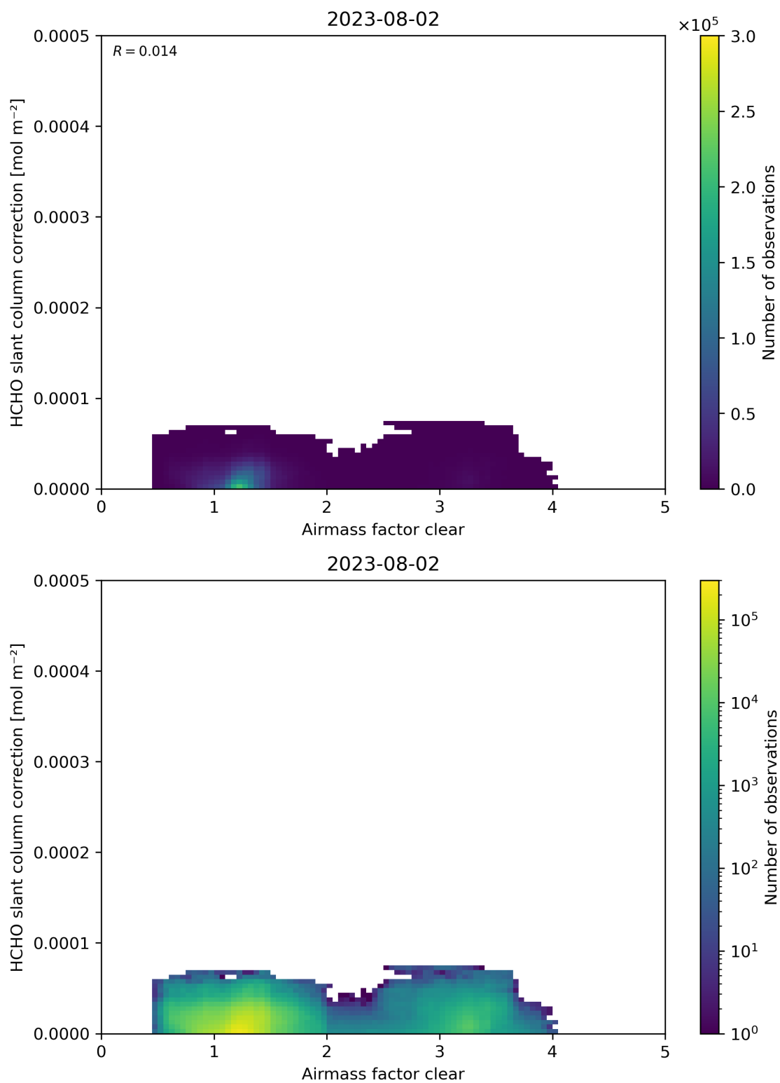
Figure 75: Scatter density plot of “Airmass factor clear” against “HCHO slant column correction” for 2023-08-01 to 2023-08-03.
