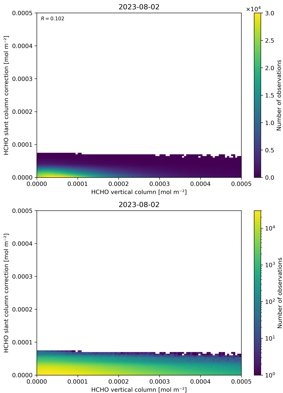
Figure 128: Scatter density plot of “HCHO vertical column” against “HCHO slant column correction” for 2023-08-01 to 2023-08-03.
