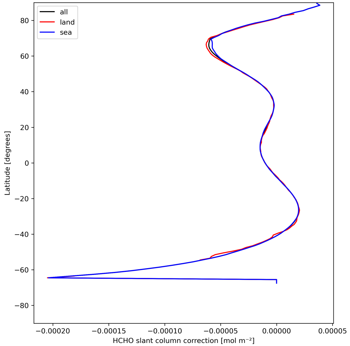
Figure 33: Zonal average of “HCHO slant column correction” for 2023-08-01 to 2023-08-03.
