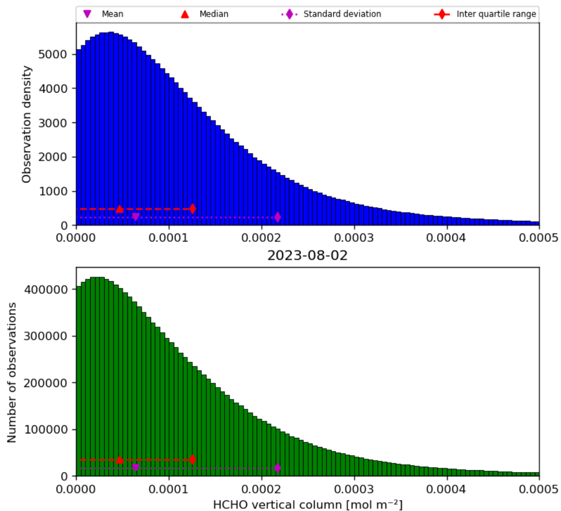
Figure 35: Histogram of “HCHO vertical column” for 2023-08-01 to 2023-08-03
