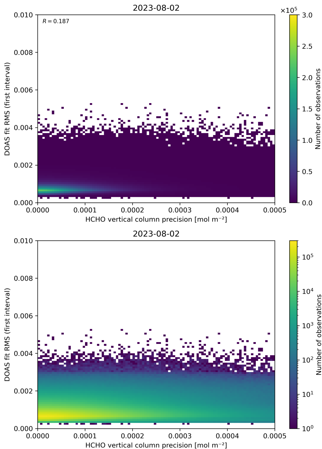
Figure 136: Scatter density plot of “HCHO vertical column precision” against “DOAS fit RMS (first interval)” for 2023-08-01 to 2023-08-03.
