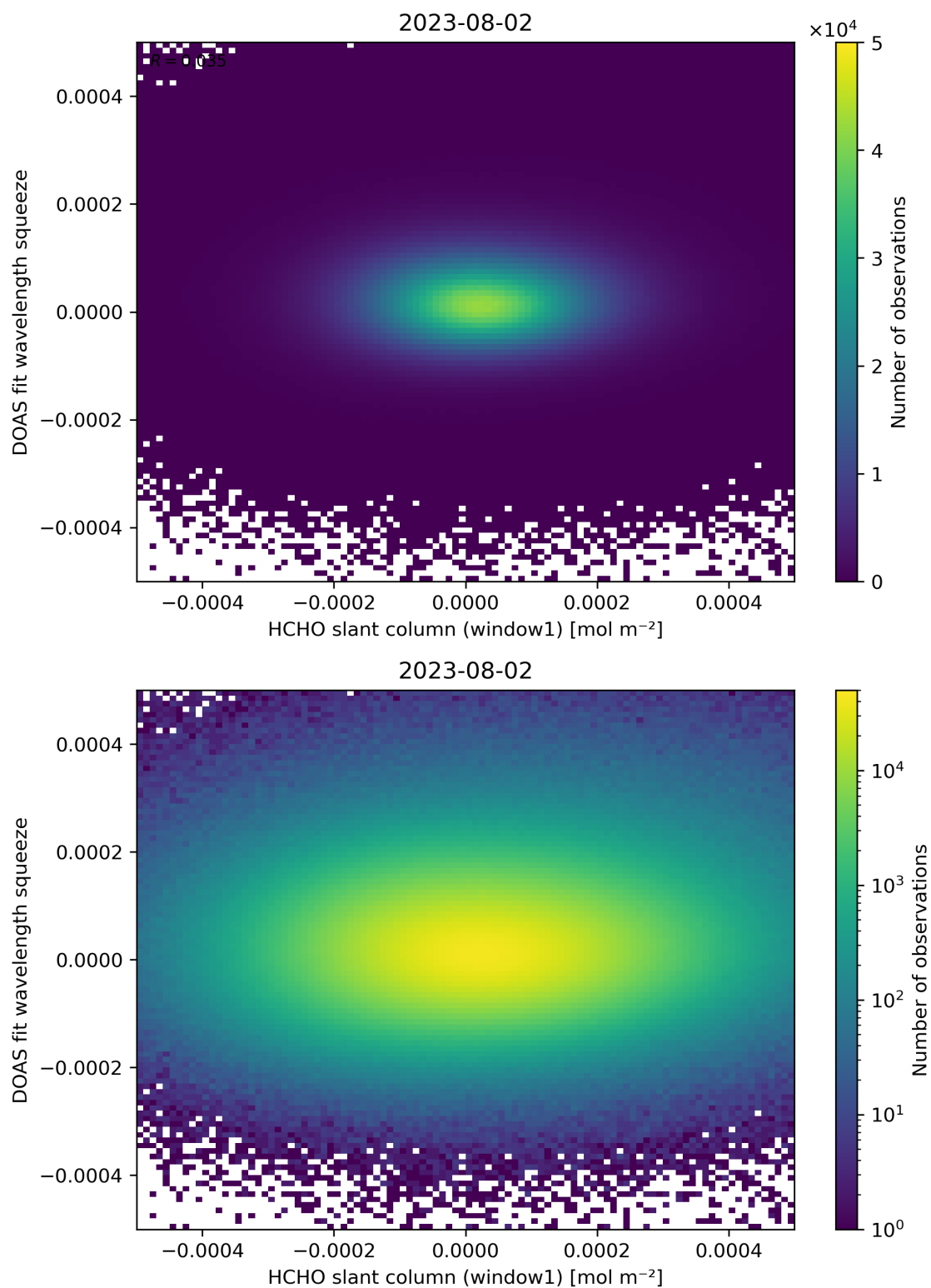
Figure 80: Scatter density plot of “HCHO slant column (window1)” against “DOAS fit wavelength squeeze” for 2023-08-01 to 2023-08-03.
