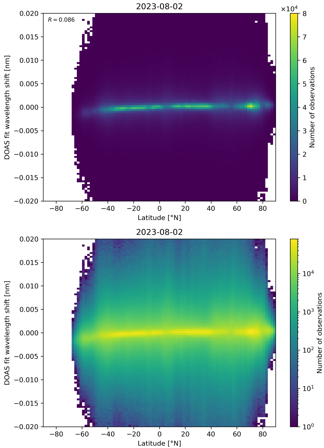
Figure 154: Scatter density plot of “Latitude” against “DOAS fit wavelength shift” for 2023-08-01 to 2023-08-03.
