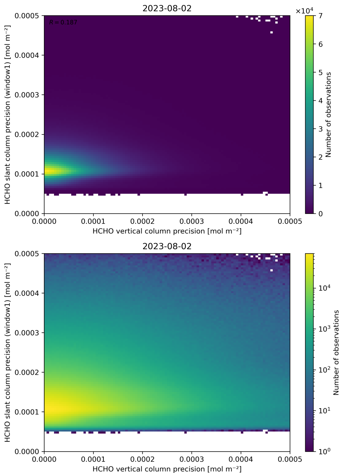
Figure 143: Scatter density plot of “HCHO vertical column precision” against “HCHO slant column precision (window1)” for 2023-08-01 to 2023-08-03.
