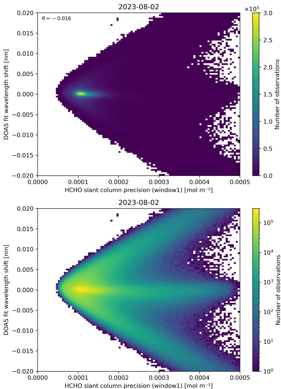
Figure 89: Scatter density plot of “HCHO slant column precision (window1)” against “DOAS fit wavelength shift” for 2023-08-01 to 2023-08-03.
