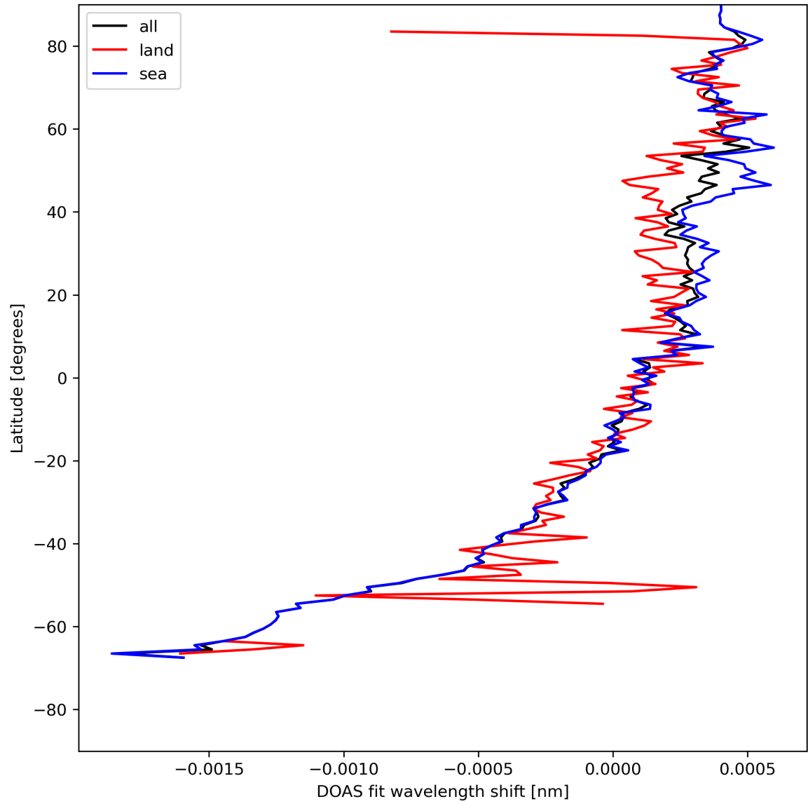
Figure 30: Zonal average of “DOAS fit wavelength shift” for 2023-08-01 to 2023-08-03.
