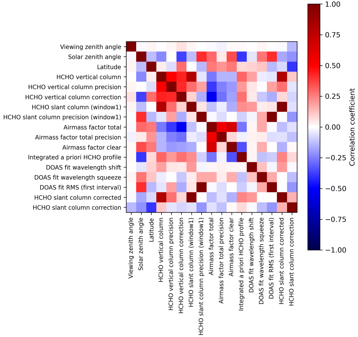
Figure 2: Map of correlation matrix for 2023-08-01 to 2023-08-03.
