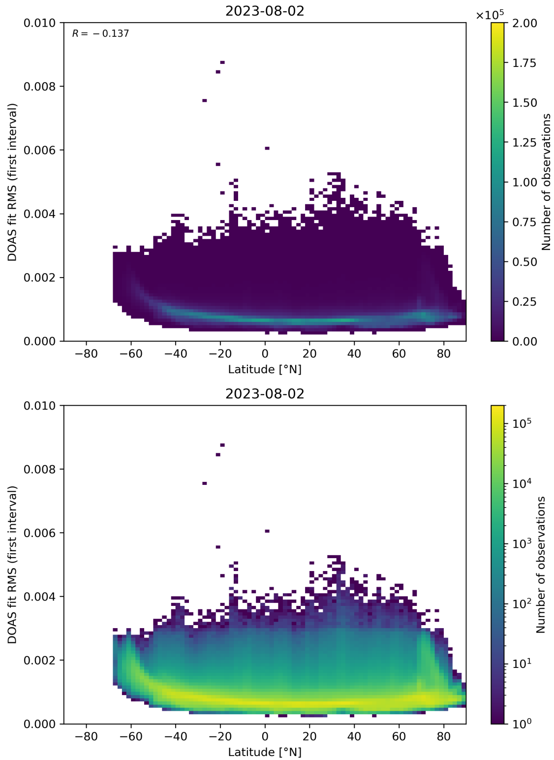
Figure 153: Scatter density plot of “Latitude” against “DOAS fit RMS (first interval)” for 2023-08-01 to 2023-08-03.
