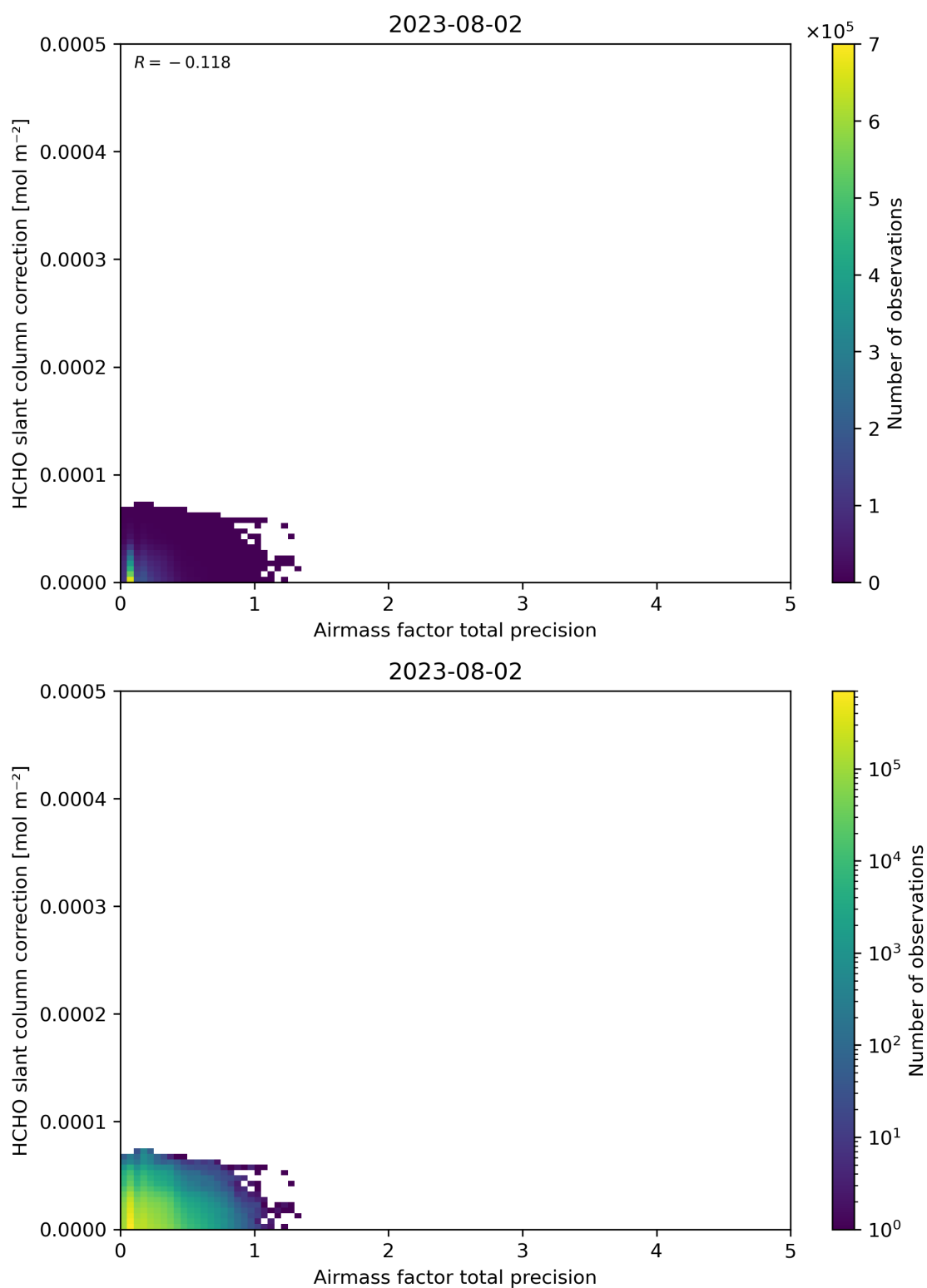
Figure 110: Scatter density plot of “Airmass factor total precision” against “HCHO slant column correction” for 2023-08-01 to 2023-08-03.
