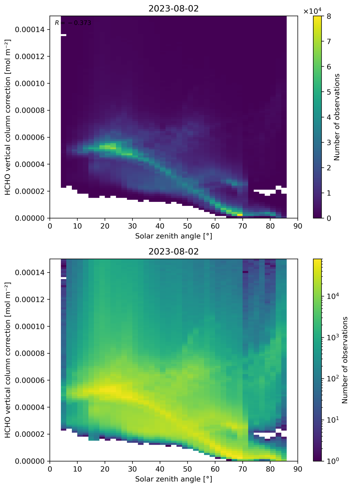
Figure 178: Scatter density plot of “Solar zenith angle” against “HCHO vertical column correction” for 2023-08-01 to 2023-08-03.
