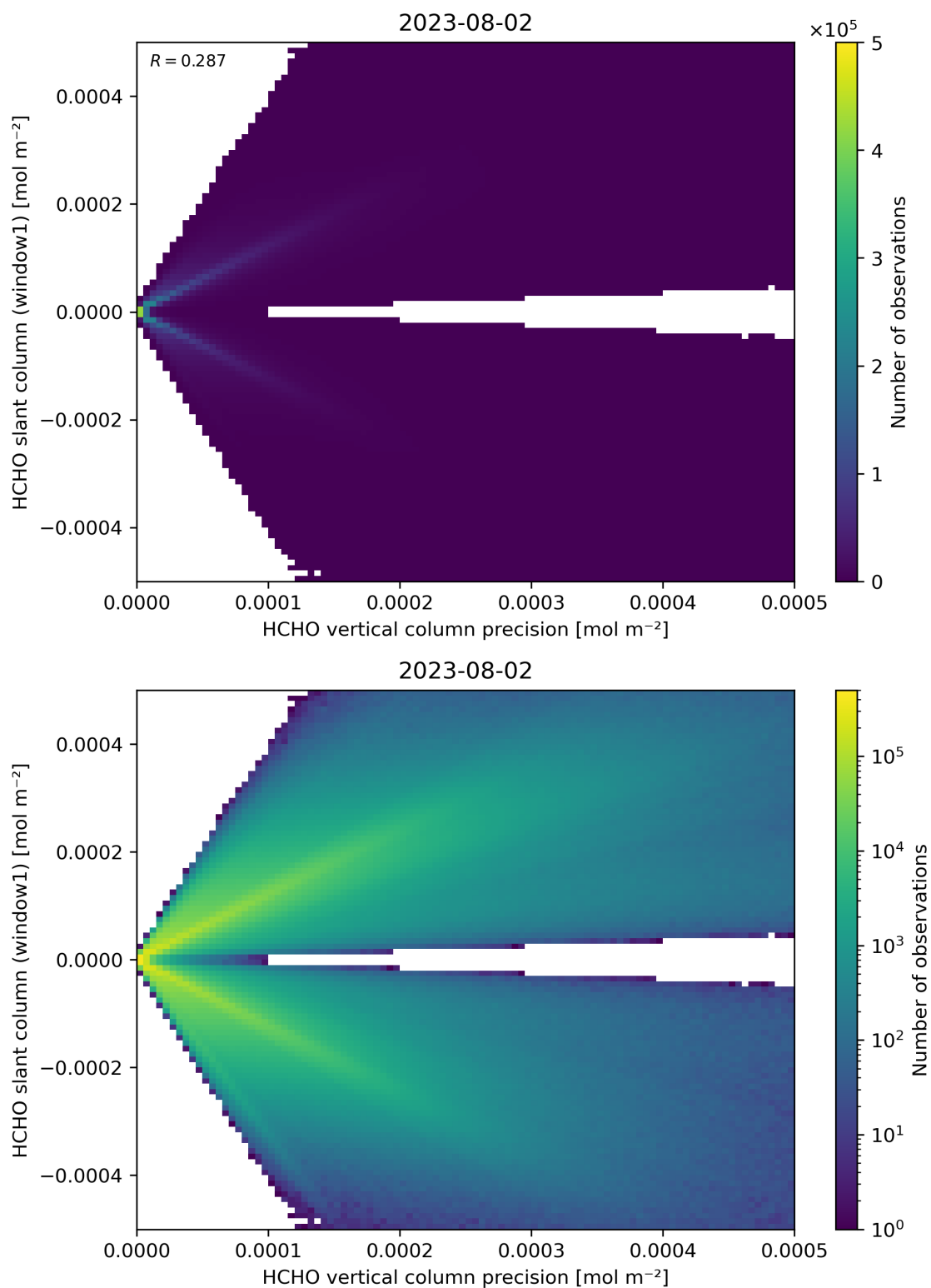
Figure 142: Scatter density plot of “HCHO vertical column precision” against “HCHO slant column (window1)” for 2023-08-01 to 2023-08-03.
