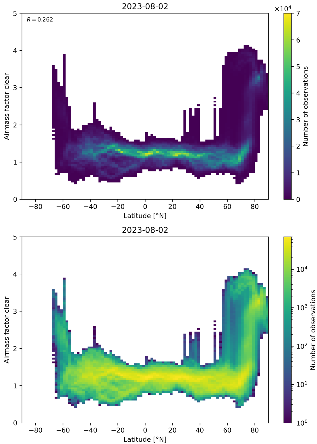
Figure 156: Scatter density plot of “Latitude” against “Airmass factor clear” for 2023-08-01 to 2023-08-03.
