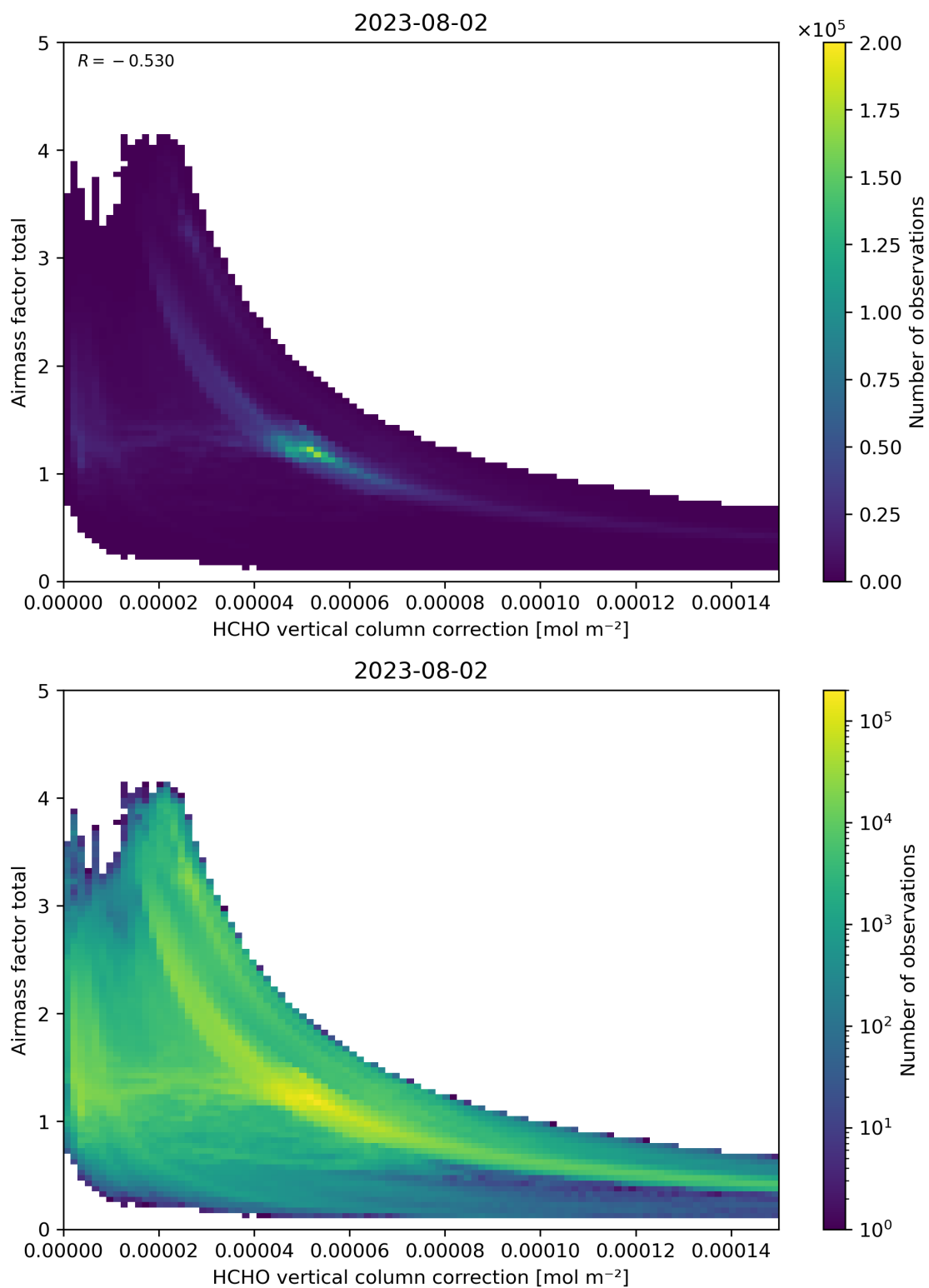
Figure 120: Scatter density plot of “HCHO vertical column correction” against “Airmass factor total” for 2023-08-01 to 2023-08-03.
