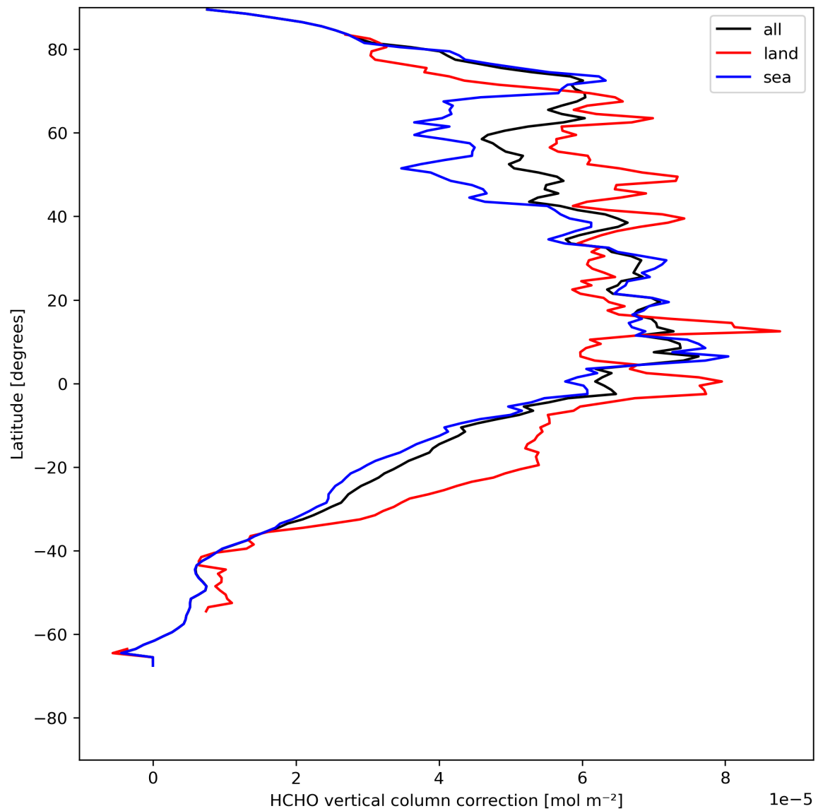
Figure 23: Zonal average of “HCHO vertical column correction” for 2023-08-01 to 2023-08-03.
