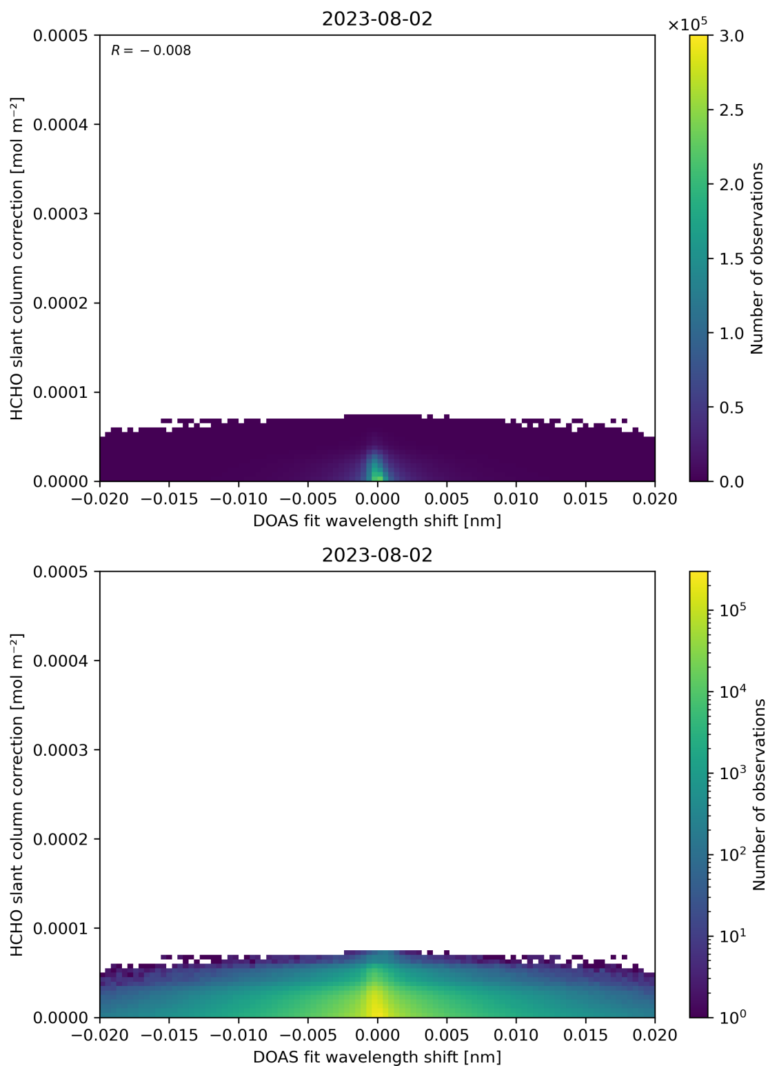
Figure 67: Scatter density plot of “DOAS fit wavelength shift” against “HCHO slant column correction” for 2023-08-01 to 2023-08-03.
