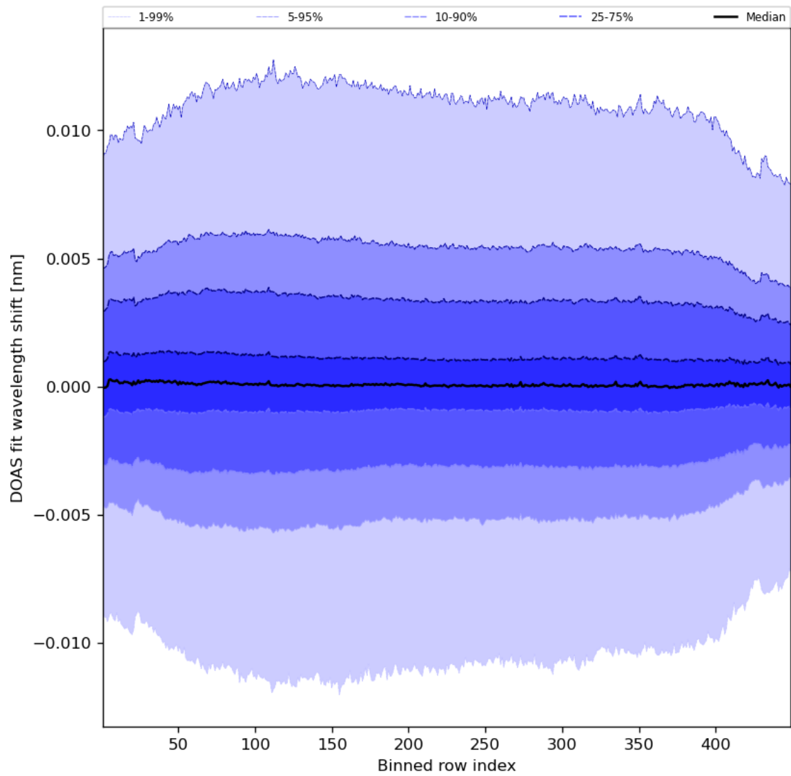
Figure 58: Along track statistics of “DOAS fit wavelength shift” for 2023-08-01 to 2023-08-03
