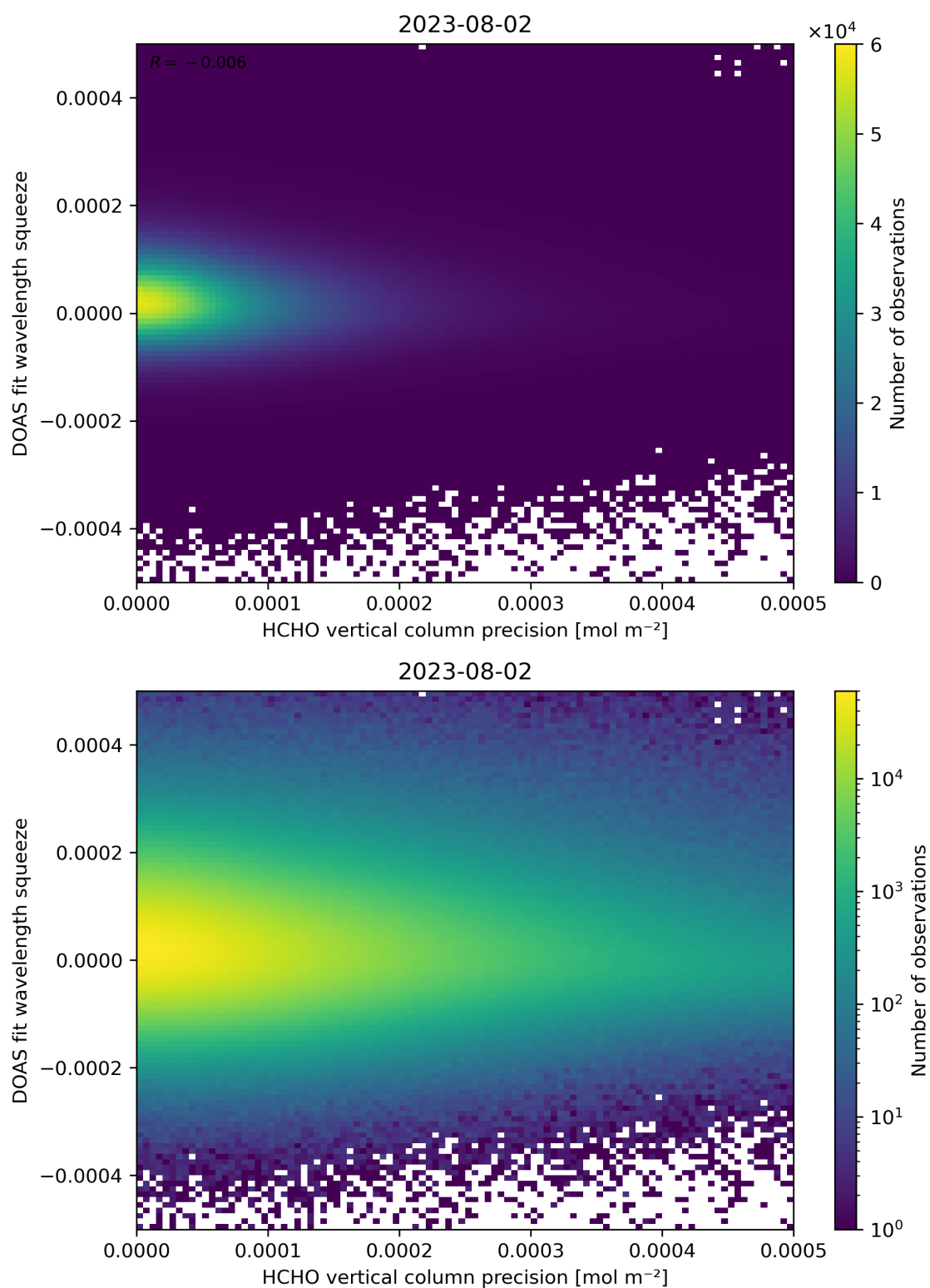
Figure 138: Scatter density plot of “HCHO vertical column precision” against “DOAS fit wavelength squeeze” for 2023-08-01 to 2023-08-03.
