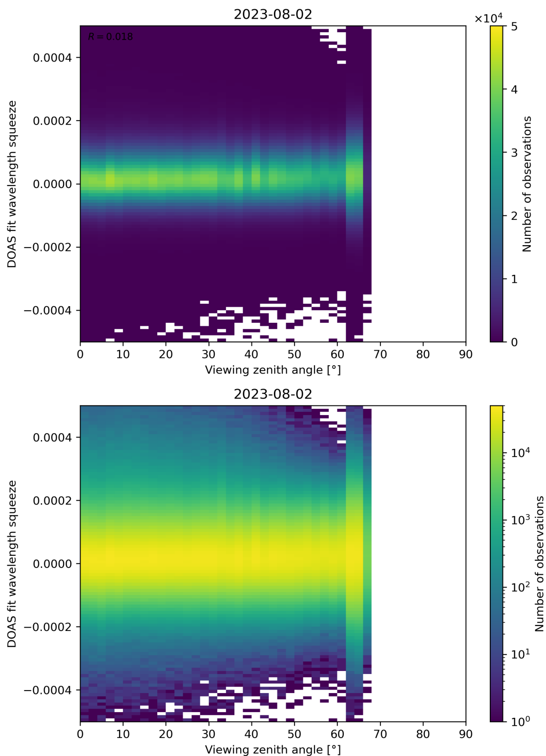
Figure 184: Scatter density plot of “Viewing zenith angle” against “DOAS fit wavelength squeeze” for 2023-08-01 to 2023-08-03.
