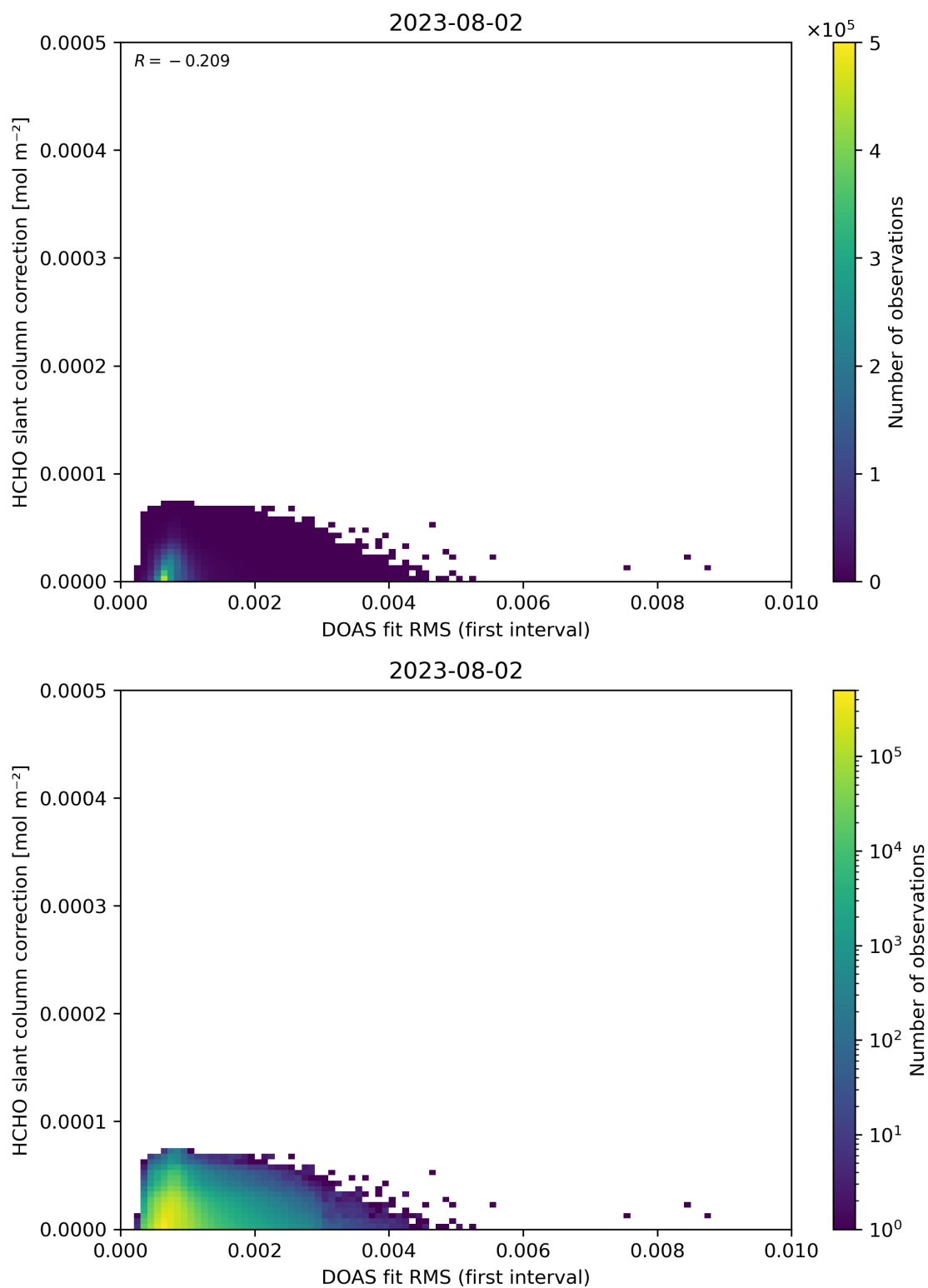
Figure 63: Scatter density plot of “DOAS fit RMS (first interval)” against “HCHO slant column correction” for 2023-08-01 to 2023-08-03.
