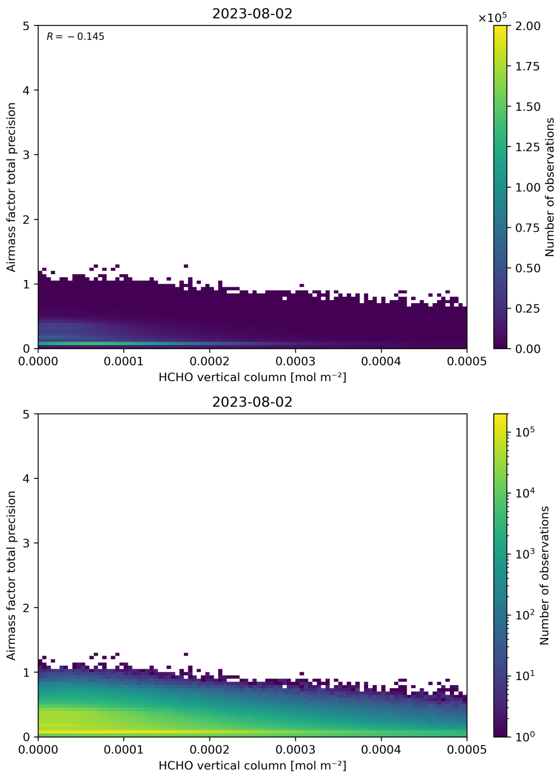
Figure 132: Scatter density plot of “HCHO vertical column” against “Airmass factor total precision” for 2023-08-01 to 2023-08-03.
