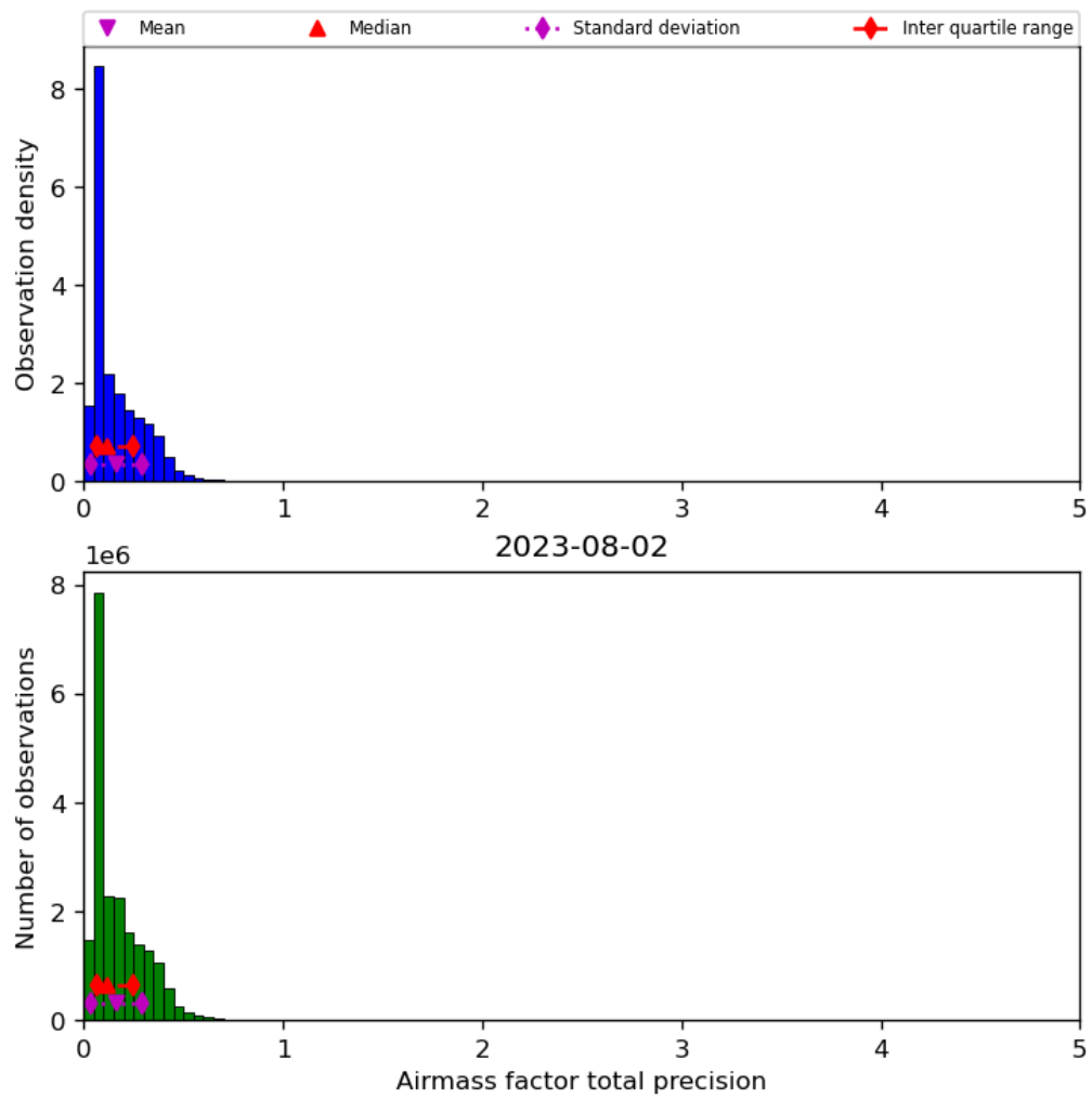
Figure 41: Histogram of “Airmass factor total precision” for 2023-08-01 to 2023-08-03
