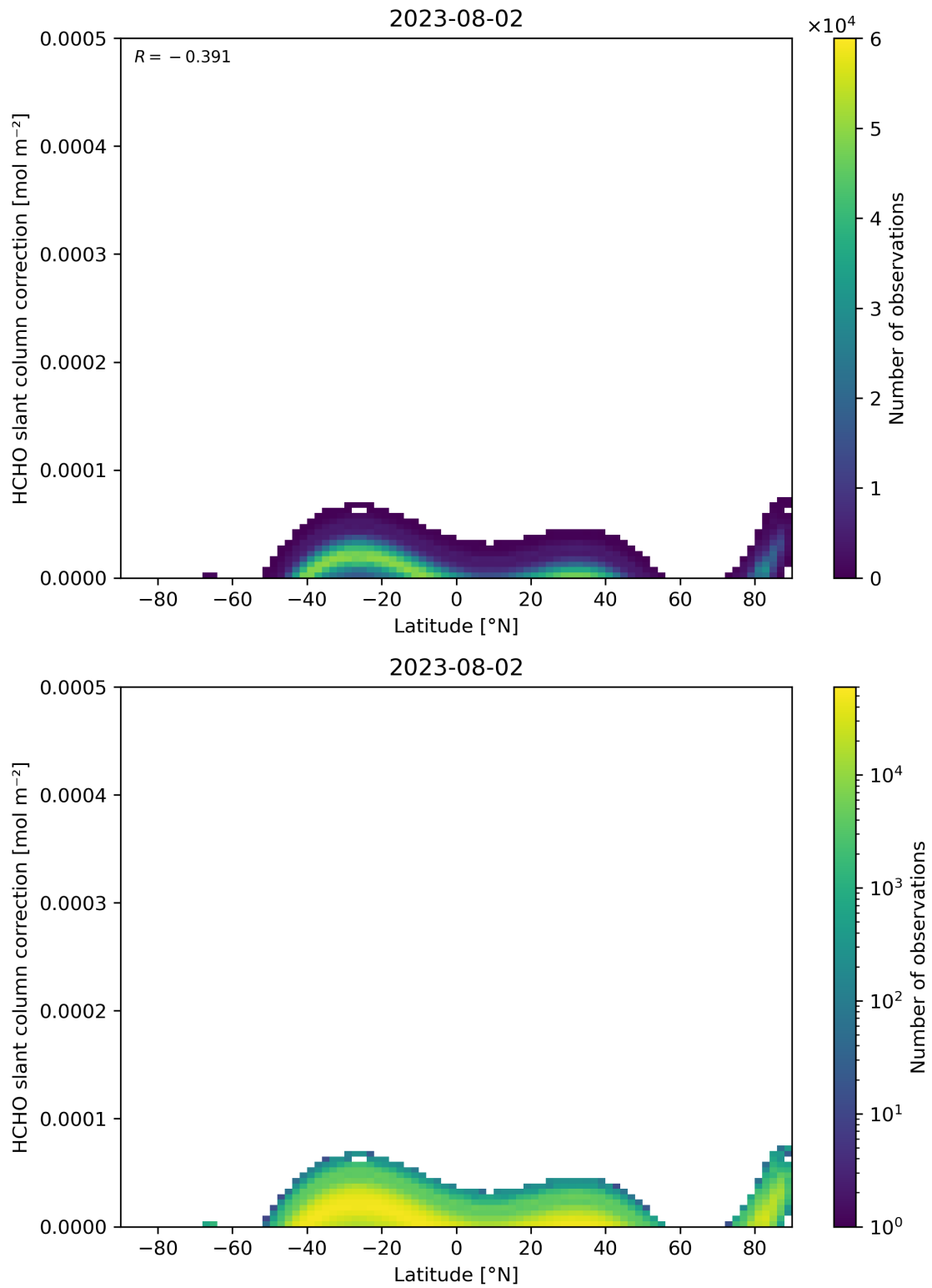
Figure 158: Scatter density plot of “Latitude” against “HCHO slant column correction” for 2023-08-01 to 2023-08-03.
