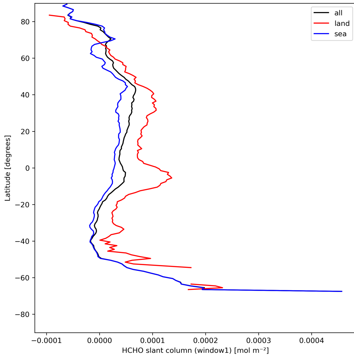
Figure 24: Zonal average of “HCHO slant column (window1)” for 2023-08-01 to 2023-08-03.
