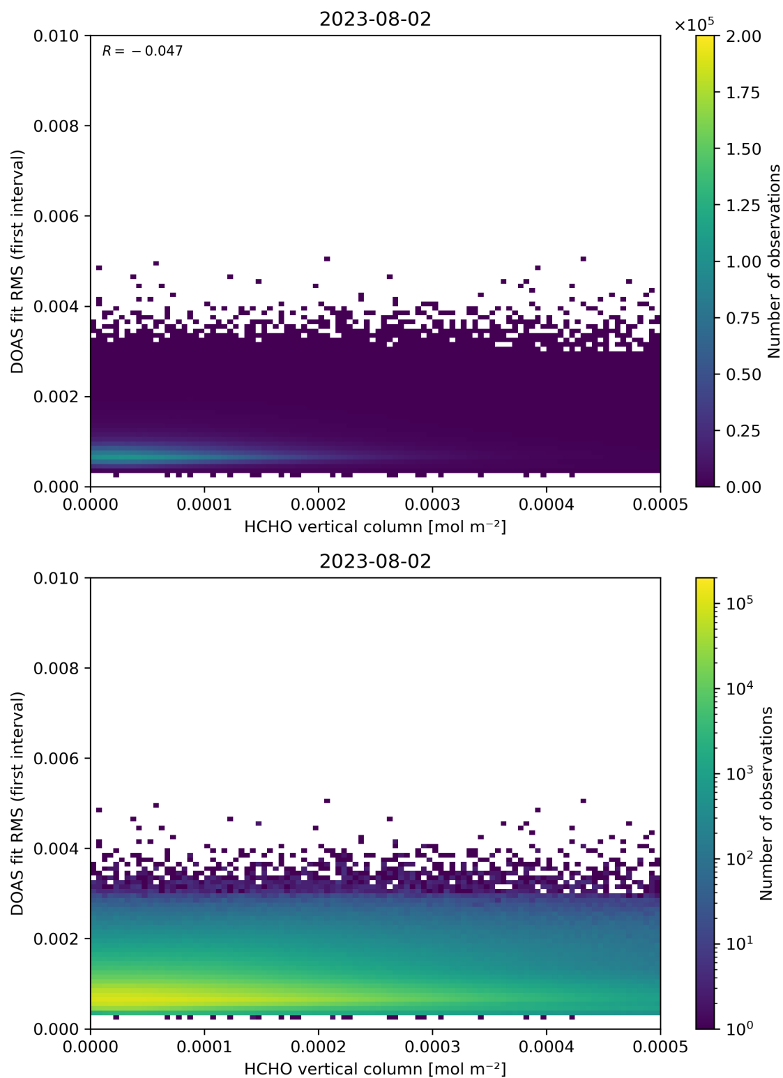
Figure 123: Scatter density plot of “HCHO vertical column” against “DOAS fit RMS (first interval)” for 2023-08-01 to 2023-08-03.
