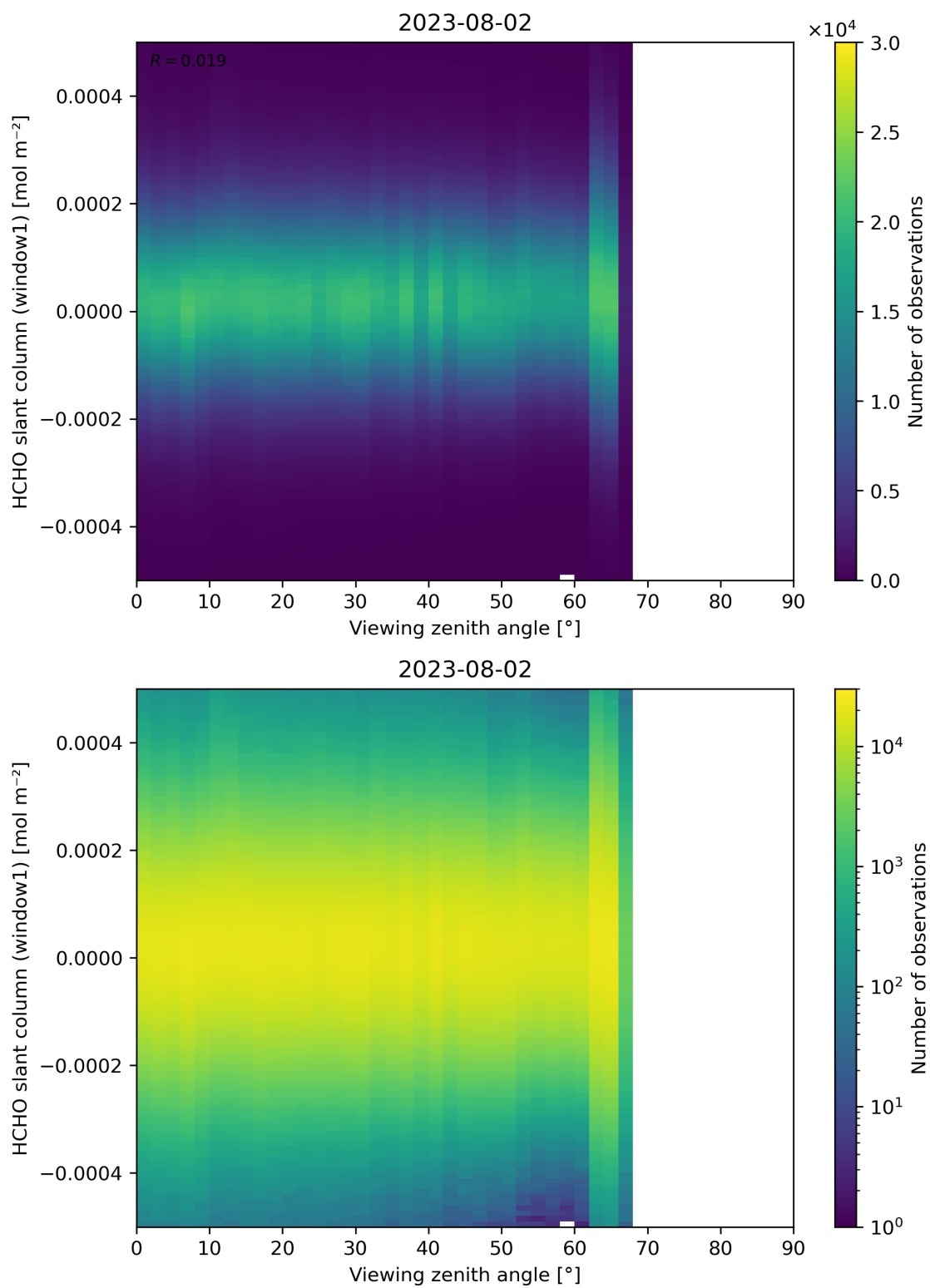
Figure 188: Scatter density plot of “Viewing zenith angle” against “HCHO slant column (window1)” for 2023-08-01 to 2023-08-03.
