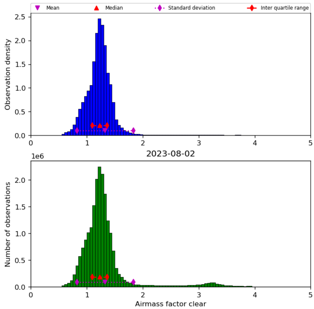
Figure 42: Histogram of “Airmass factor clear” for 2023-08-01 to 2023-08-03
