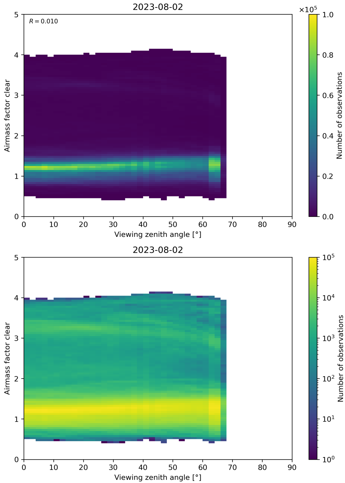
Figure 185: Scatter density plot of “Viewing zenith angle” against “Airmass factor clear” for 2023-08-01 to 2023-08-03.
