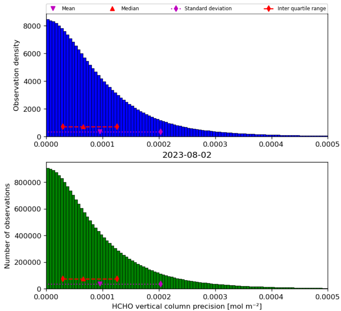
Figure 36: Histogram of “HCHO vertical column precision” for 2023-08-01 to 2023-08-03
