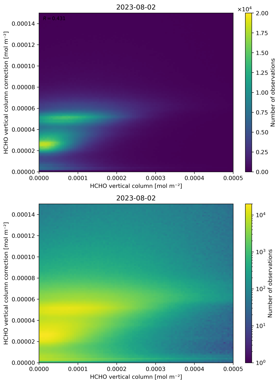
Figure 133: Scatter density plot of “HCHO vertical column” against “HCHO vertical column correction” for 2023-08-01 to 2023-08-03.
