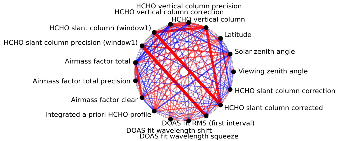
Figure 1: Map of correlation graph for 2023-08-01 to 2023-08-03.
