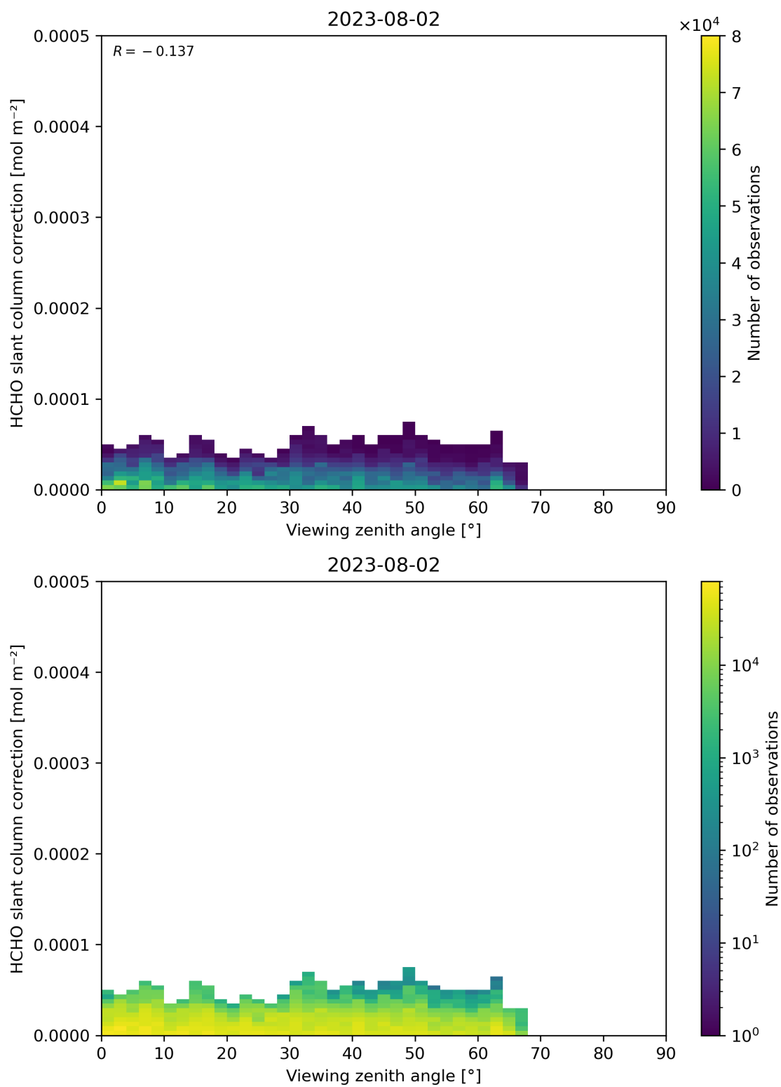
Figure 187: Scatter density plot of “Viewing zenith angle” against “HCHO slant column correction” for 2023-08-01 to 2023-08-03.
