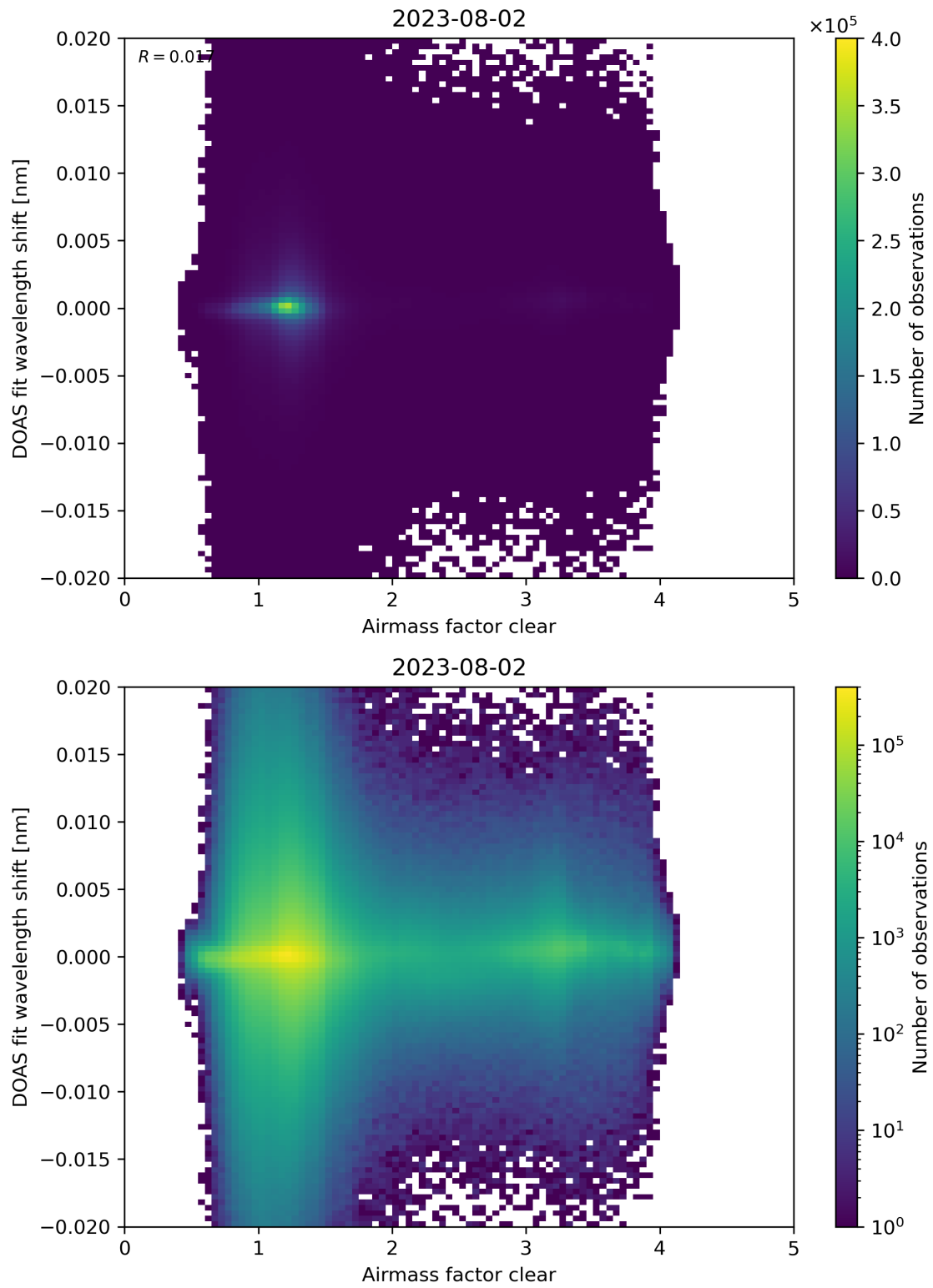
Figure 72: Scatter density plot of “Airmass factor clear” against “DOAS fit wavelength shift” for 2023-08-01 to 2023-08-03.
