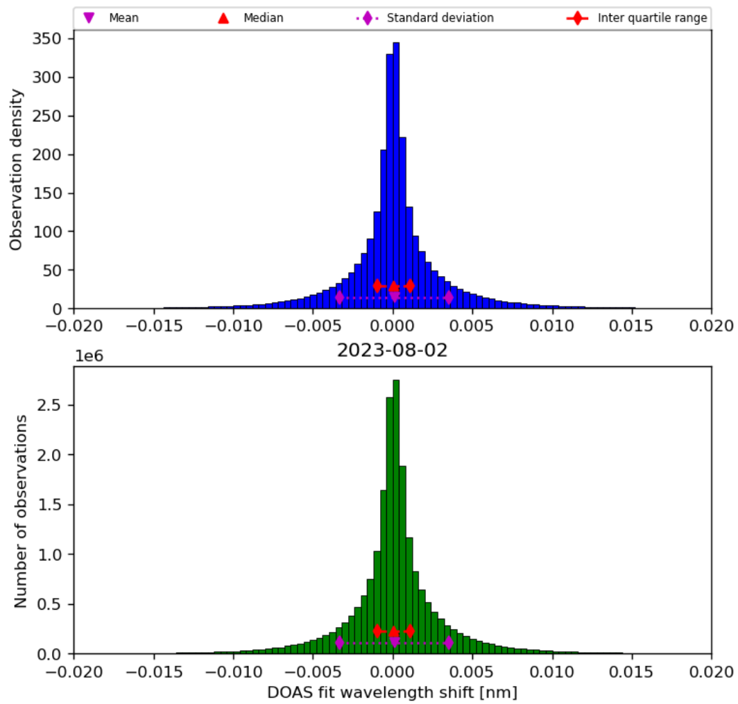
Figure 44: Histogram of “DOAS fit wavelength shift” for 2023-08-01 to 2023-08-03
