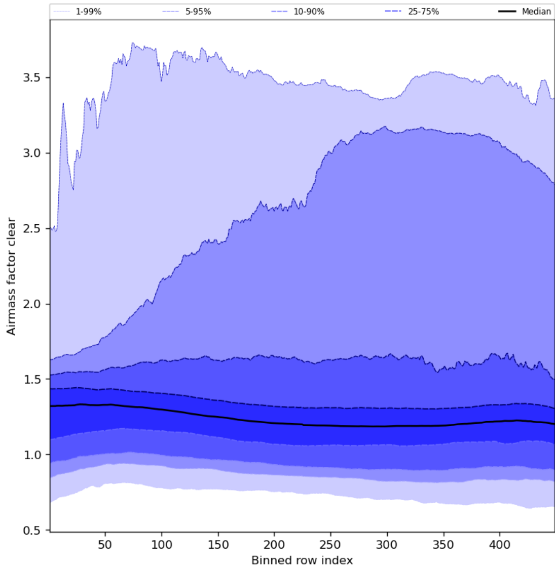
Figure 56: Along track statistics of “Airmass factor clear” for 2023-08-01 to 2023-08-03
