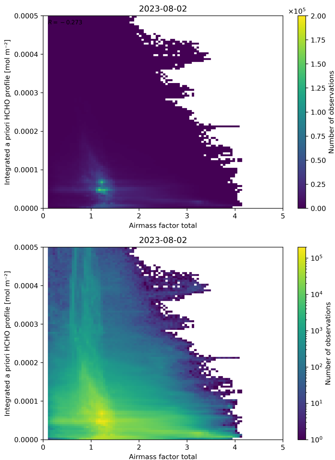
Figure 104: Scatter density plot of “Airmass factor total” against “Integrated a priori HCHO profile” for 2023-08-01 to 2023-08-03.
