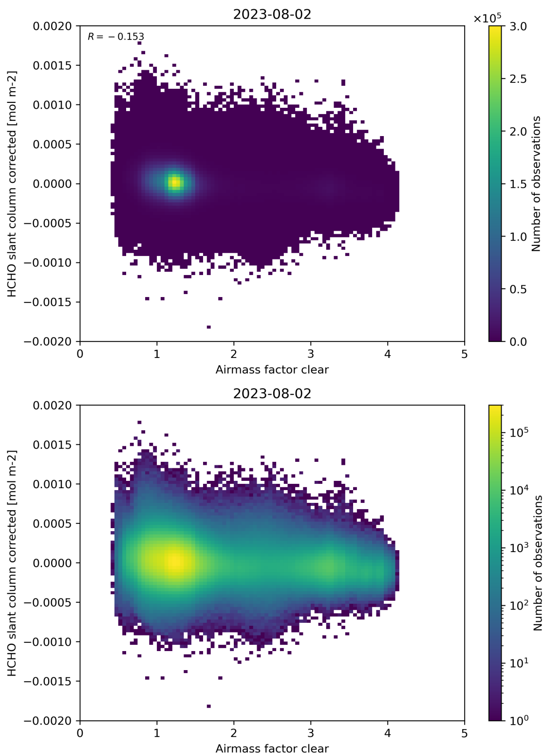
Figure 74: Scatter density plot of “Airmass factor clear” against “HCHO slant column corrected” for 2023-08-01 to 2023-08-03.
