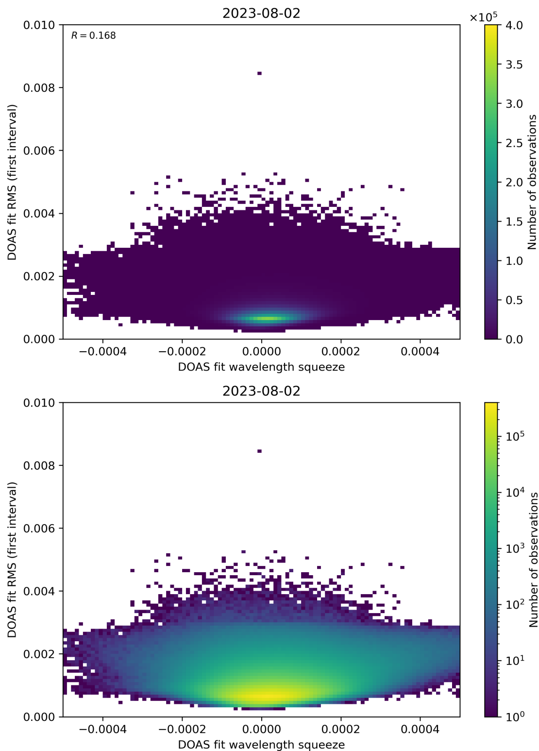
Figure 68: Scatter density plot of “DOAS fit wavelength squeeze” against “DOAS fit RMS (first interval)” for 2023-08-01 to 2023-08-03.
