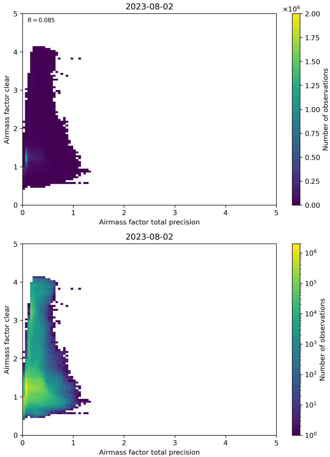
Figure 108: Scatter density plot of “Airmass factor total precision” against “Airmass factor clear” for 2023-08-01 to 2023-08-03.
