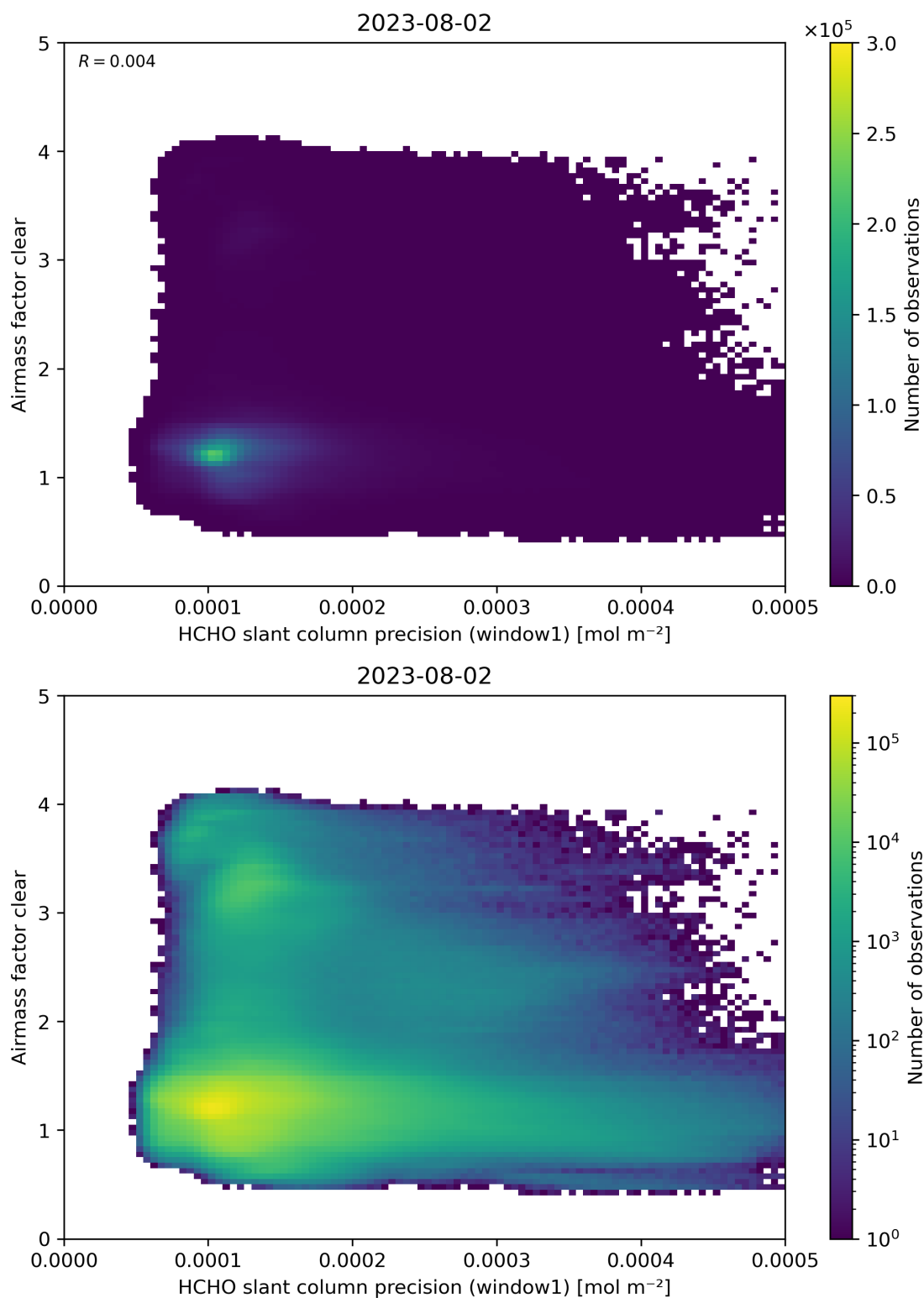
Figure 91: Scatter density plot of “HCHO slant column precision (window1)” against “Airmass factor clear” for 2023-08-01 to 2023-08-03.
