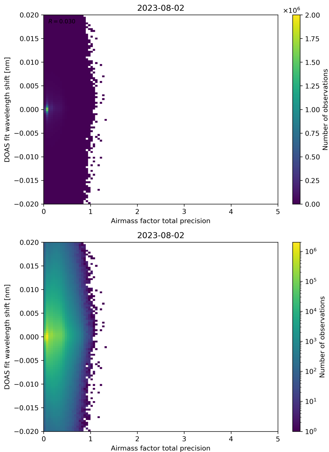
Figure 106: Scatter density plot of “Airmass factor total precision” against “DOAS fit wavelength shift” for 2023-08-01 to 2023-08-03.
