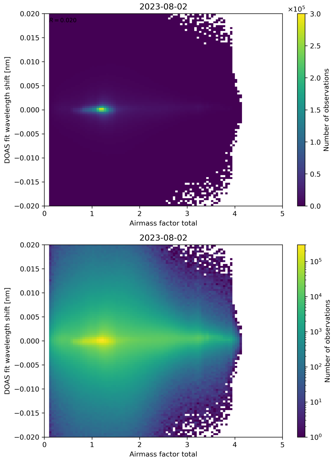
Figure 98: Scatter density plot of “Airmass factor total” against “DOAS fit wavelength shift” for 2023-08-01 to 2023-08-03.
