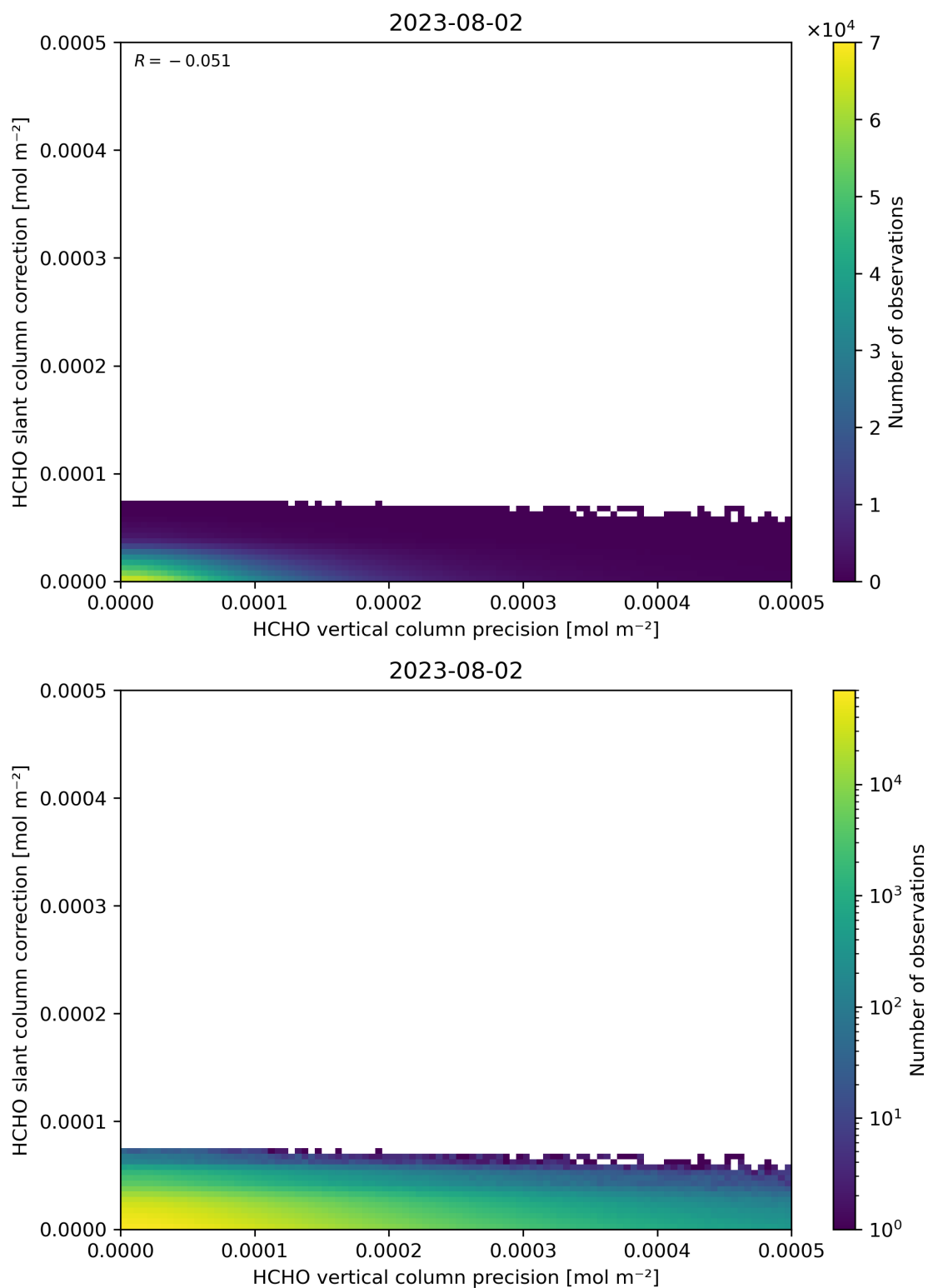
Figure 141: Scatter density plot of “HCHO vertical column precision” against “HCHO slant column correction” for 2023-08-01 to 2023-08-03.
