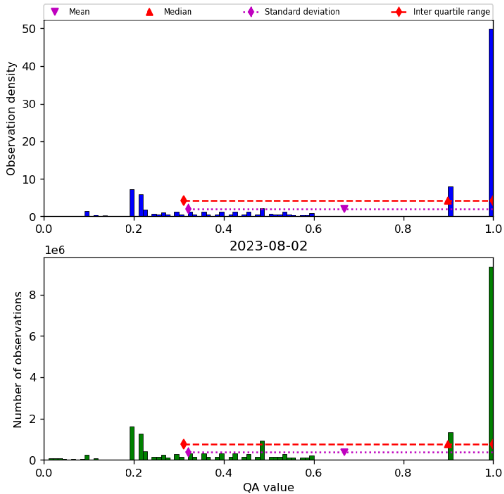
Figure 34: Histogram of “QA value” for 2023-08-01 to 2023-08-03
