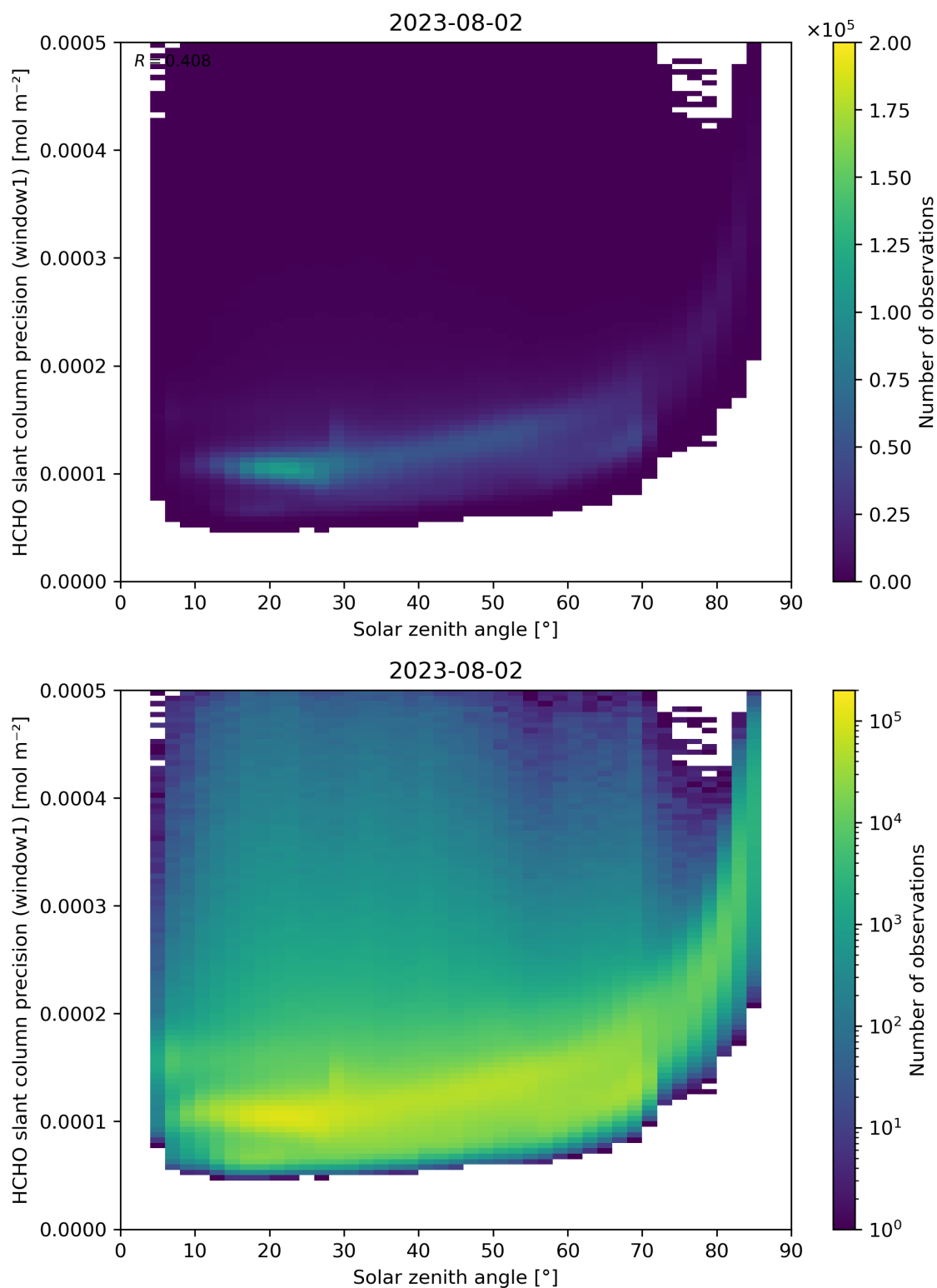
Figure 174: Scatter density plot of “Solar zenith angle” against “HCHO slant column precision (window1)” for 2023-08-01 to 2023-08-03.
