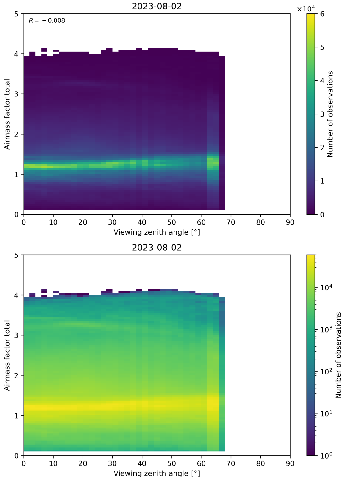
Figure 190: Scatter density plot of “Viewing zenith angle” against “Airmass factor total” for 2023-08-01 to 2023-08-03.
