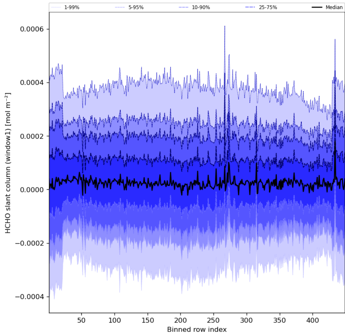
Figure 52: Along track statistics of “HCHO slant column (window1)” for 2023-08-01 to 2023-08-03
