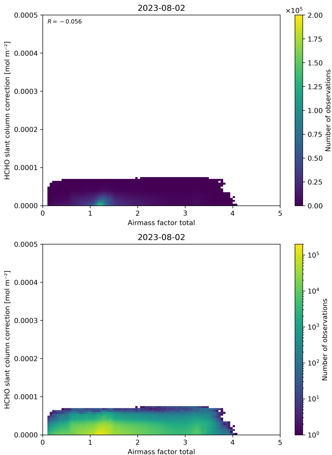
Figure 102: Scatter density plot of “Airmass factor total” against “HCHO slant column correction” for 2023-08-01 to 2023-08-03.
