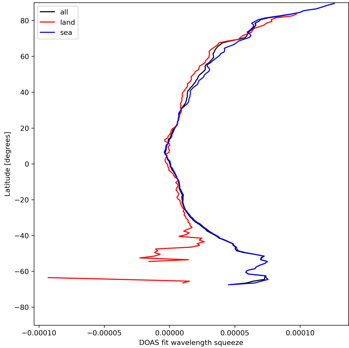
Figure 31: Zonal average of “DOAS fit wavelength squeeze” for 2023-08-01 to 2023-08-03.
