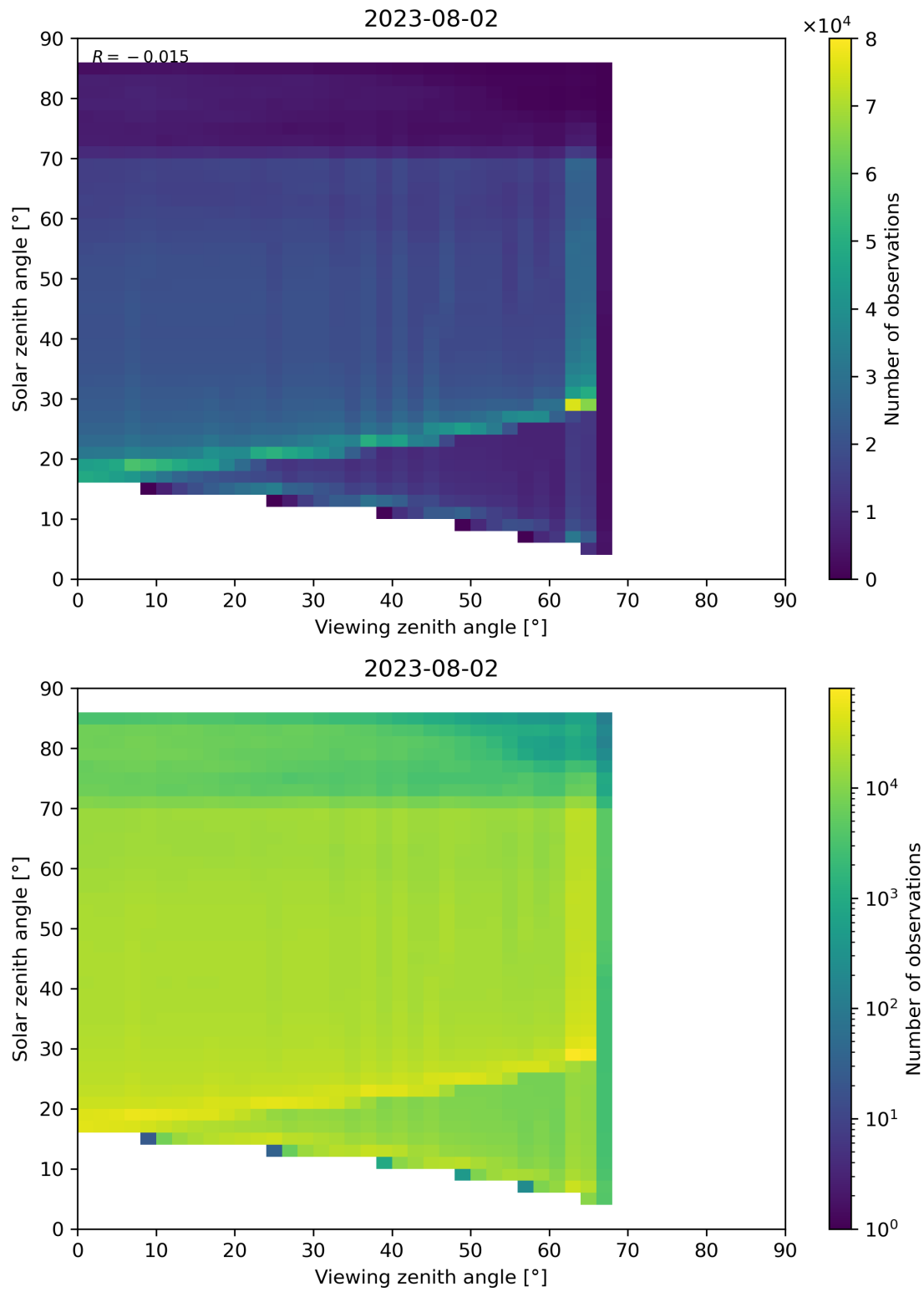
Figure 197: Scatter density plot of “Viewing zenith angle” against “Solar zenith angle” for 2023-08-01 to 2023-08-03.
