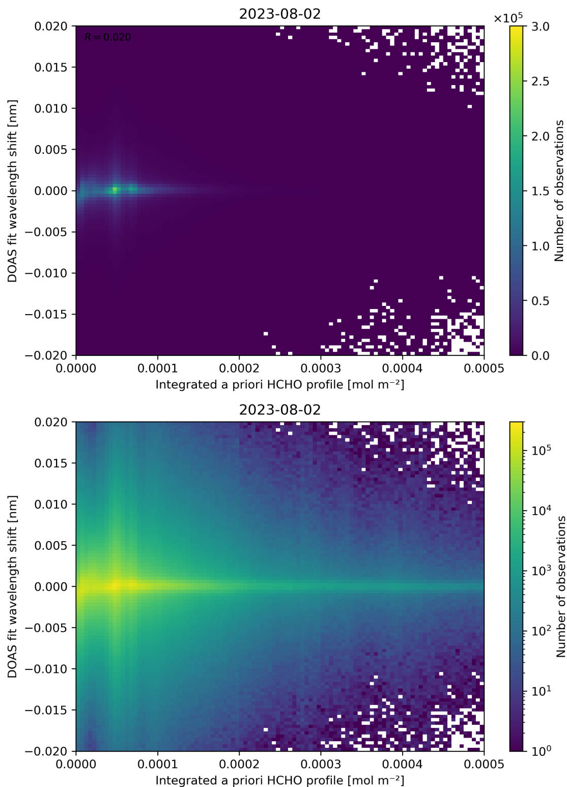
Figure 149: Scatter density plot of “Integrated a priori HCHO profile” against “DOAS fit wavelength shift” for 2023-08-01 to 2023-08-03.
