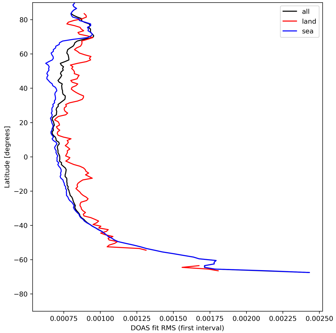
Figure 32: Zonal average of "DOAS fit RMS (first interval)" for 2023-08-01 to 2023-08-03.
