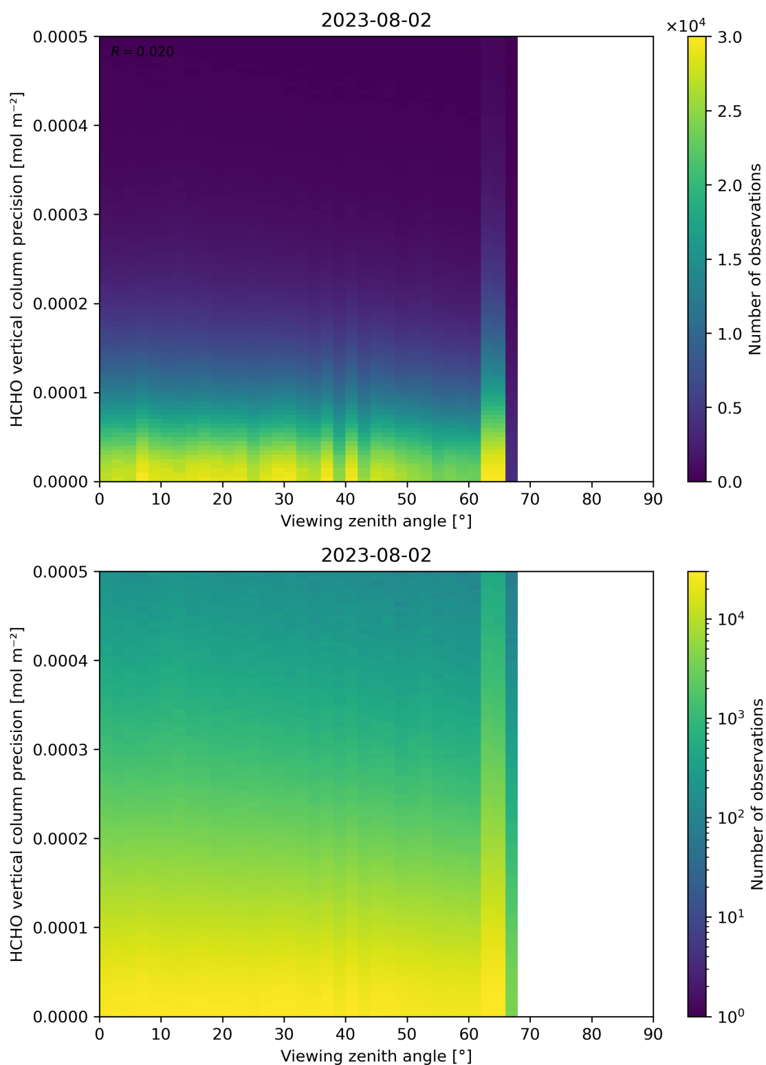
Figure 194: Scatter density plot of “Viewing zenith angle” against “HCHO vertical column precision” for 2023-08-01 to 2023-08-03.
