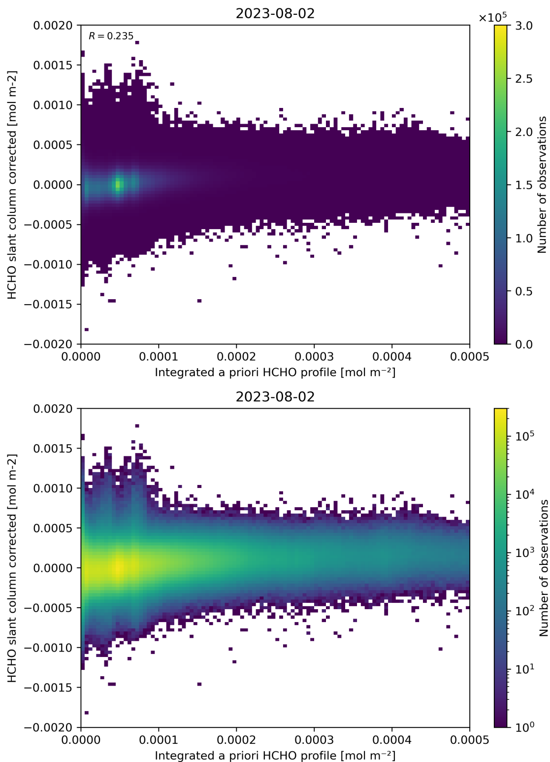
Figure 151: Scatter density plot of “Integrated a priori HCHO profile” against “HCHO slant column corrected” for 2023-08-01 to 2023-08-03.
