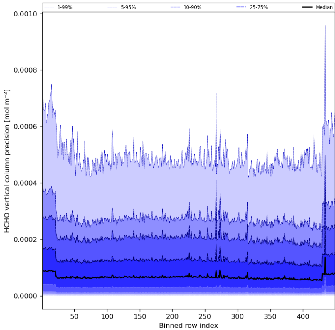
Figure 50: Along track statistics of “HCHO vertical column precision” for 2023-08-01 to 2023-08-03
