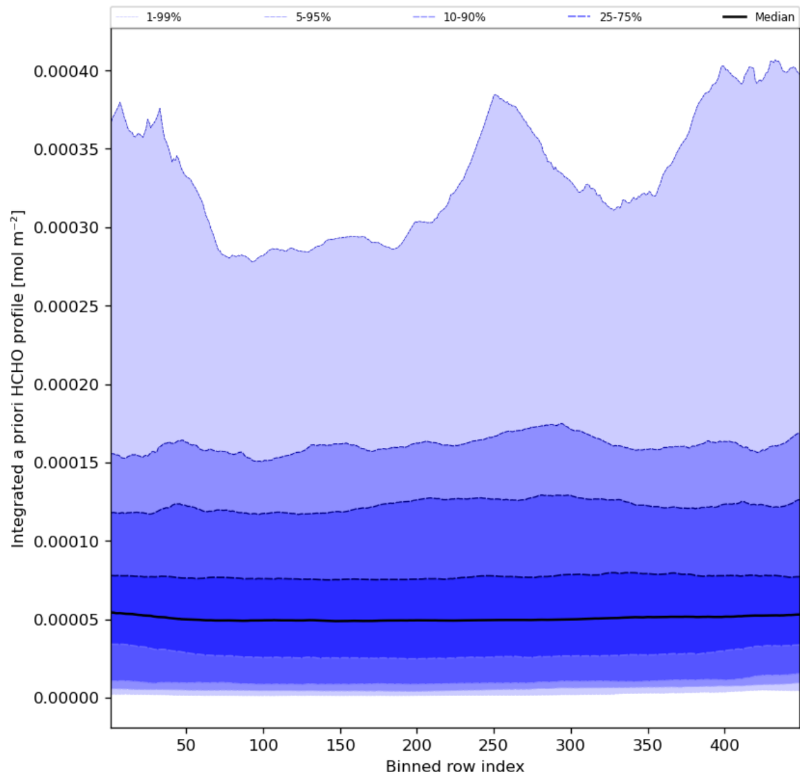
Figure 57: Along track statistics of “Integrated a priori HCHO profile” for 2023-08-01 to 2023-08-03
