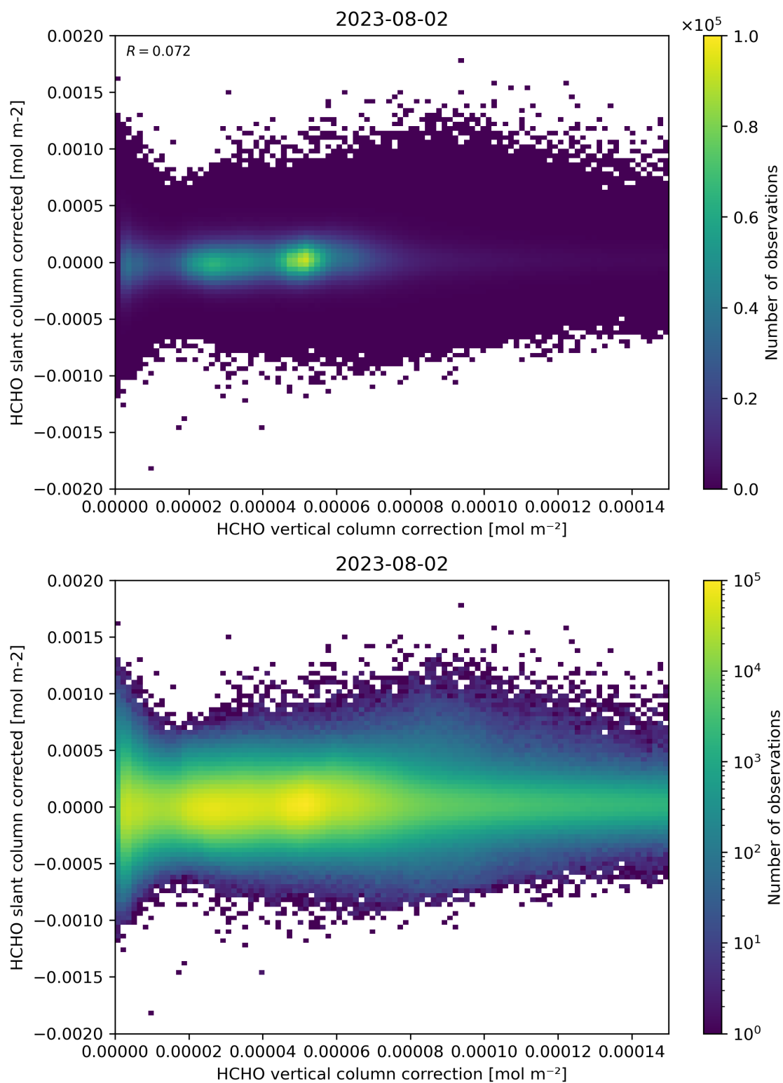
Figure 116: Scatter density plot of “HCHO vertical column correction” against “HCHO slant column corrected” for 2023-08-01 to 2023-08-03.
