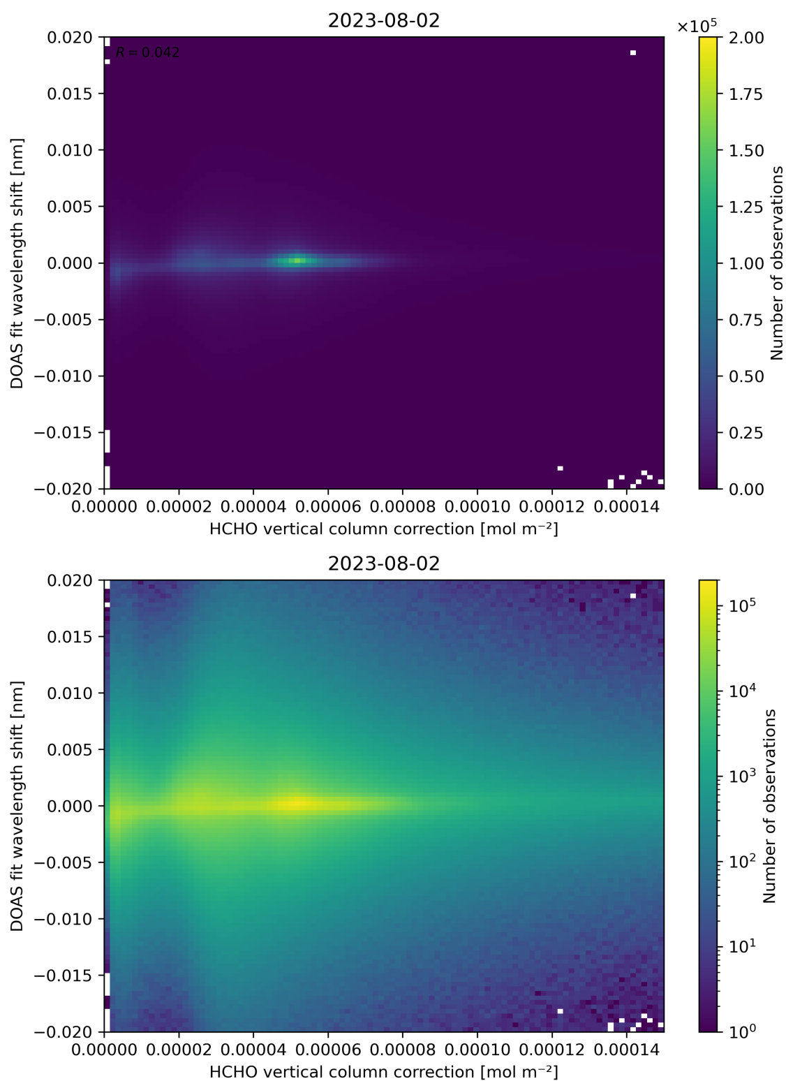
Figure 113: Scatter density plot of “HCHO vertical column correction” against “DOAS fit wavelength shift” for 2023-08-01 to 2023-08-03.
