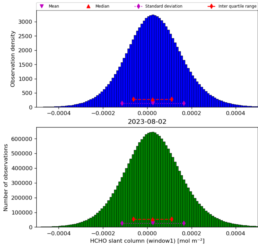
Figure 38: Histogram of “HCHO slant column (window1)” for 2023-08-01 to 2023-08-03
