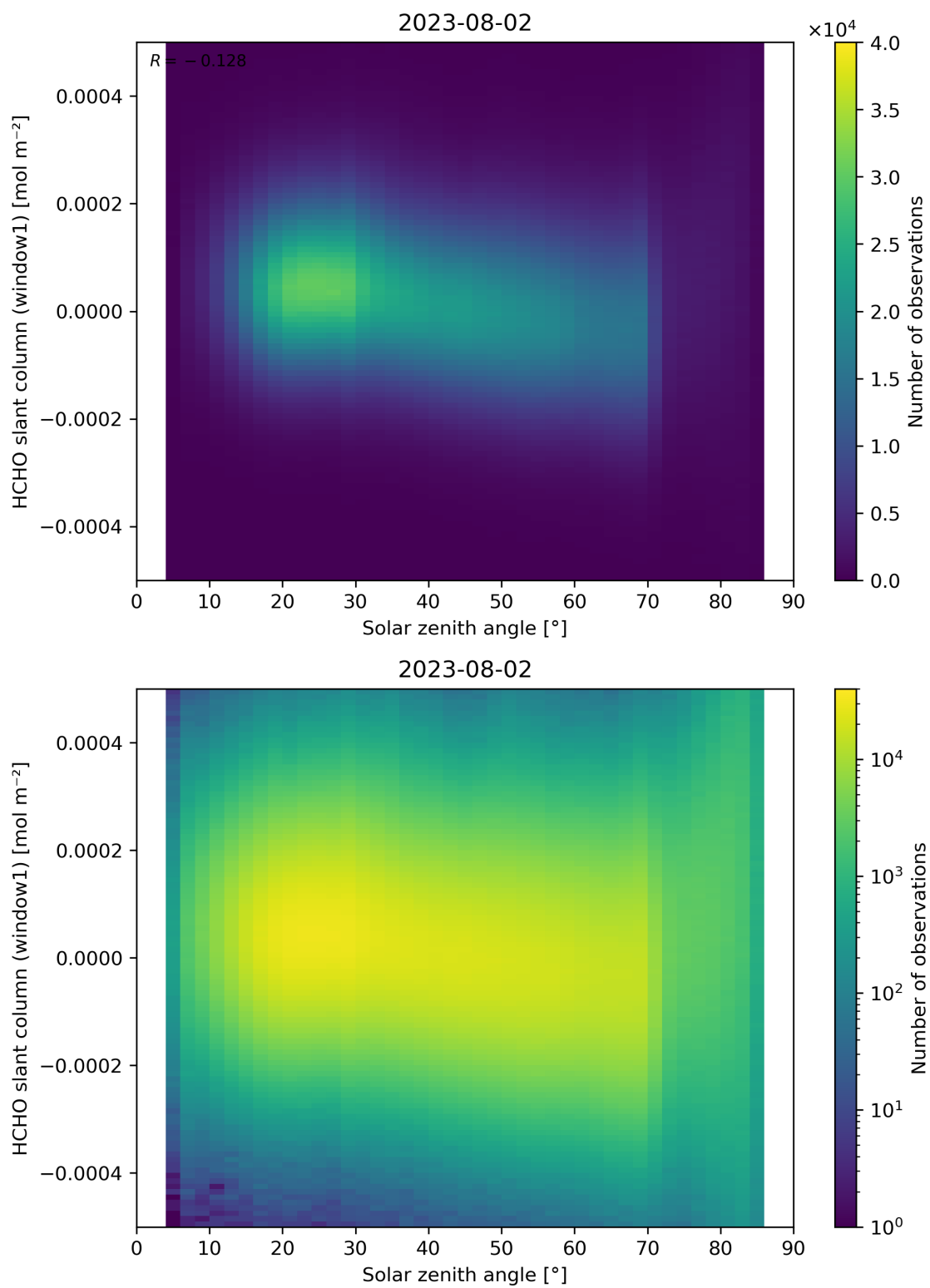
Figure 173: Scatter density plot of “Solar zenith angle” against “HCHO slant column (window1)” for 2023-08-01 to 2023-08-03.
