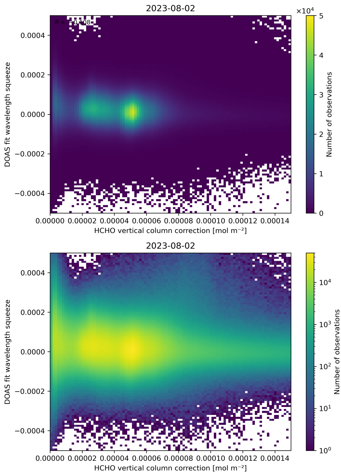
Figure 114: Scatter density plot of “HCHO vertical column correction” against “DOAS fit wavelength squeeze” for 2023-08-01 to 2023-08-03.
