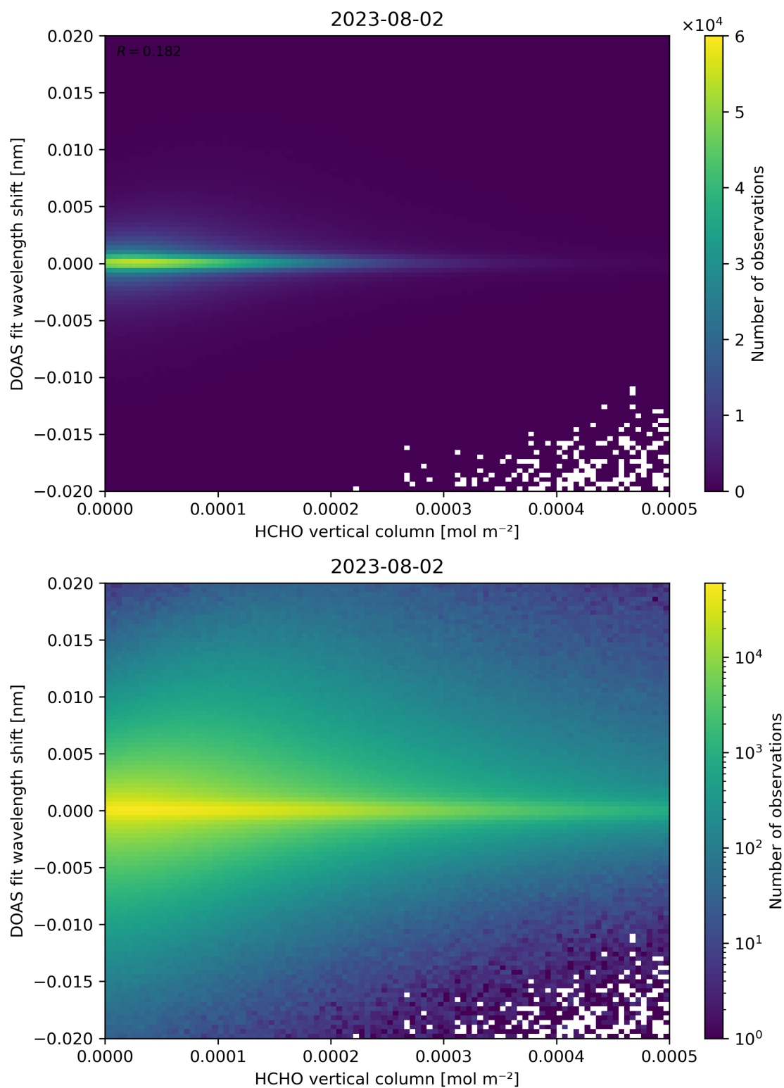
Figure 124: Scatter density plot of “HCHO vertical column” against “DOAS fit wavelength shift” for 2023-08-01 to 2023-08-03.
