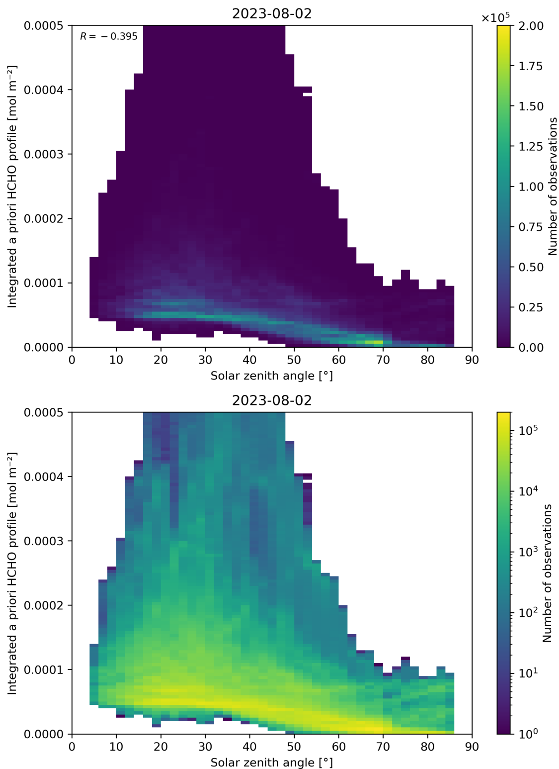
Figure 180: Scatter density plot of “Solar zenith angle” against “Integrated a priori HCHO profile” for 2023-08-01 to 2023-08-03.
