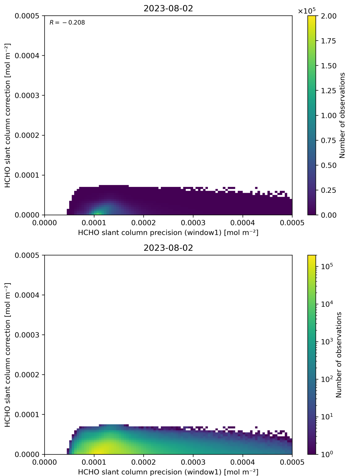
Figure 93: Scatter density plot of “HCHO slant column precision (window1)” against “HCHO slant column correction” for 2023-08-01 to 2023-08-03.
