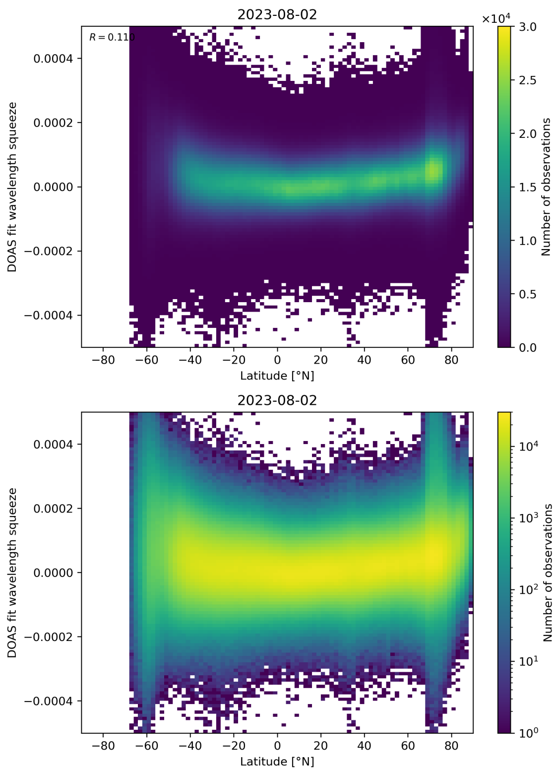
Figure 155: Scatter density plot of “Latitude” against “DOAS fit wavelength squeeze” for 2023-08-01 to 2023-08-03.
