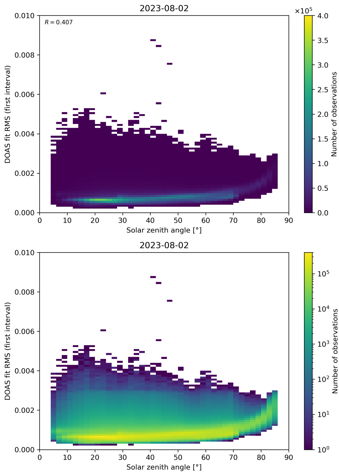
Figure 167: Scatter density plot of “Solar zenith angle” against “DOAS fit RMS (first interval)” for 2023-08-01 to 2023-08-03.
