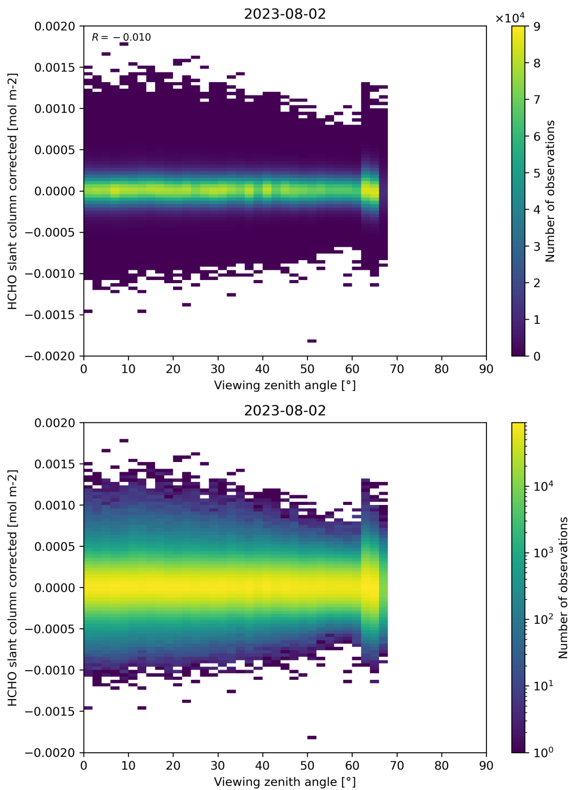
Figure 186: Scatter density plot of “Viewing zenith angle” against “HCHO slant column corrected” for 2023-08-01 to 2023-08-03.
