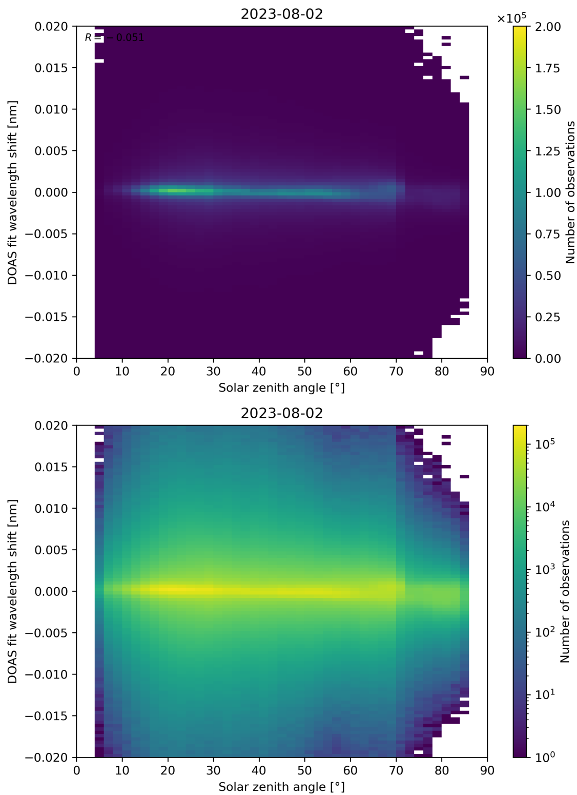
Figure 168: Scatter density plot of “Solar zenith angle” against “DOAS fit wavelength shift” for 2023-08-01 to 2023-08-03.
