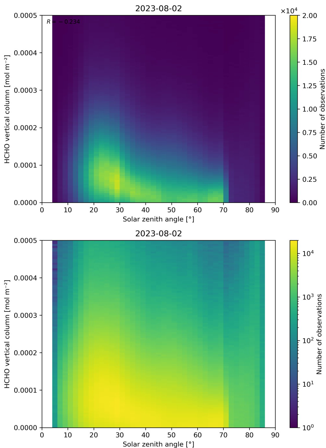
Figure 177: Scatter density plot of “Solar zenith angle” against “HCHO vertical column” for 2023-08-01 to 2023-08-03.
