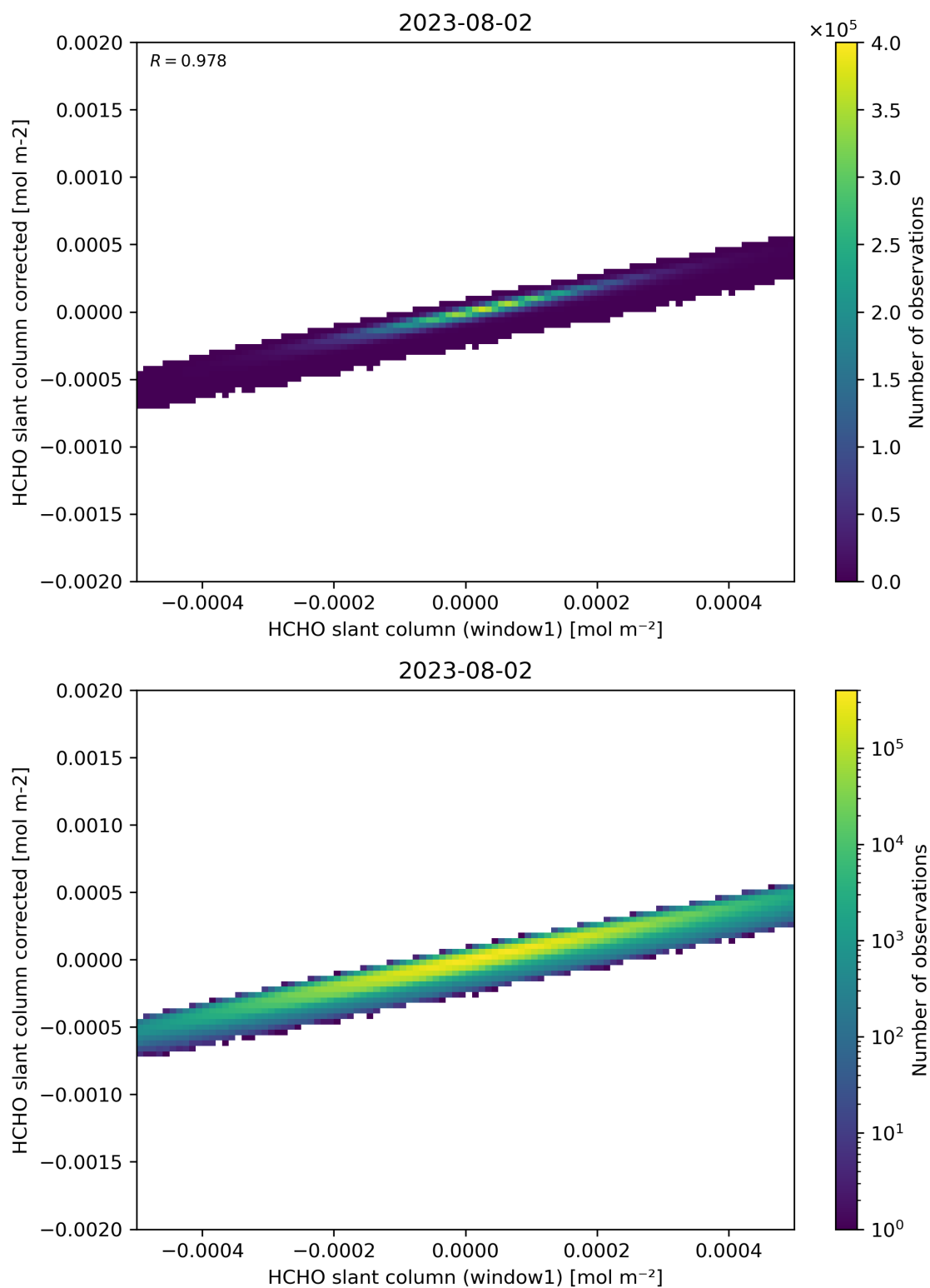
Figure 82: Scatter density plot of “HCHO slant column (window1)” against “HCHO slant column corrected” for 2023-08-01 to 2023-08-03.
