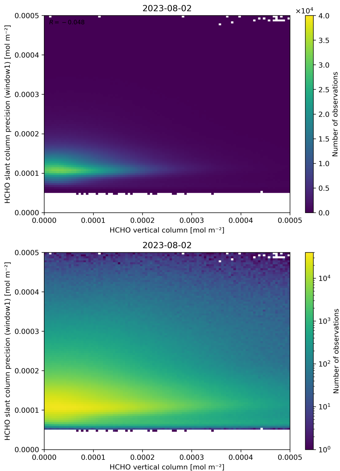
Figure 130: Scatter density plot of “HCHO vertical column” against “HCHO slant column precision (window1)” for 2023-08-01 to 2023-08-03.
