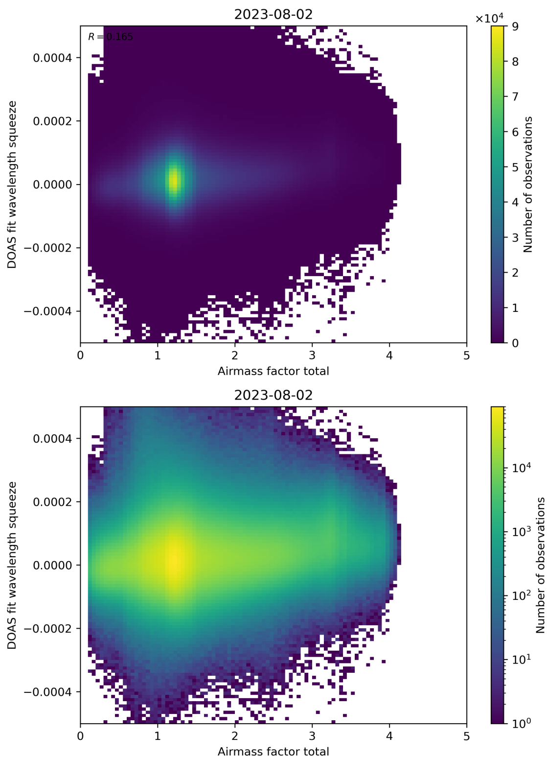
Figure 99: Scatter density plot of “Airmass factor total” against “DOAS fit wavelength squeeze” for 2023-08-01 to 2023-08-03.
