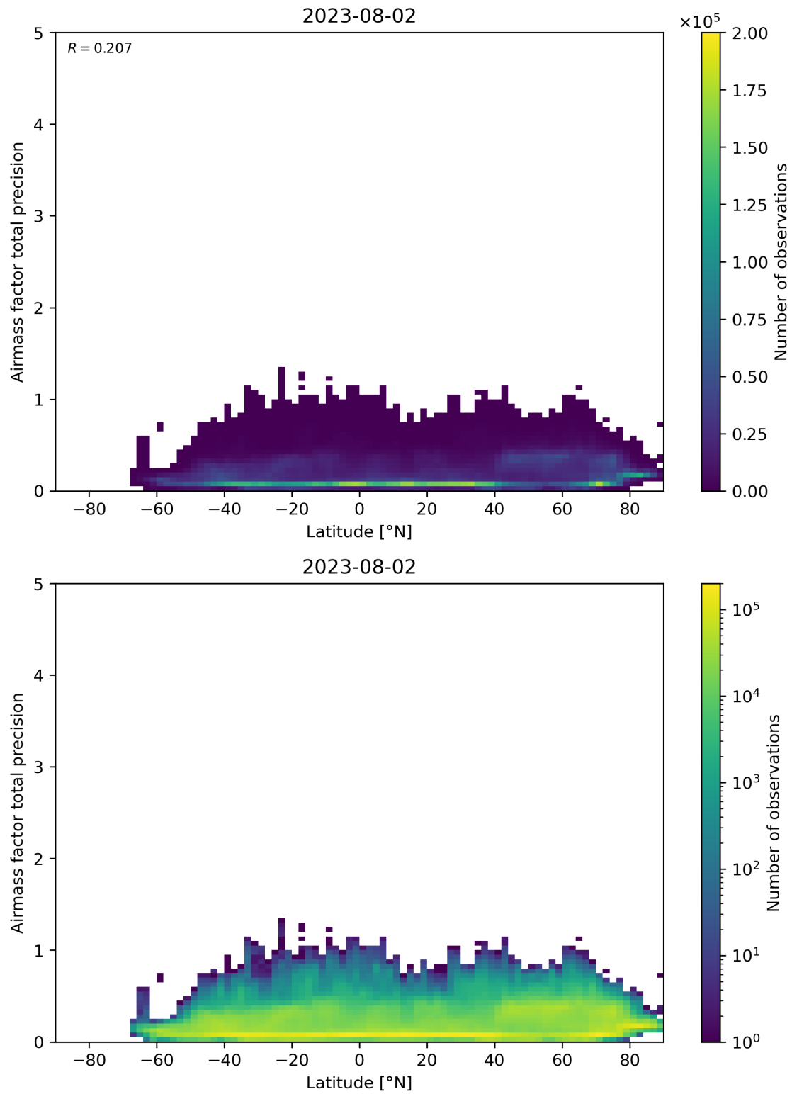
Figure 162: Scatter density plot of “Latitude” against “Airmass factor total precision” for 2023-08-01 to 2023-08-03.
