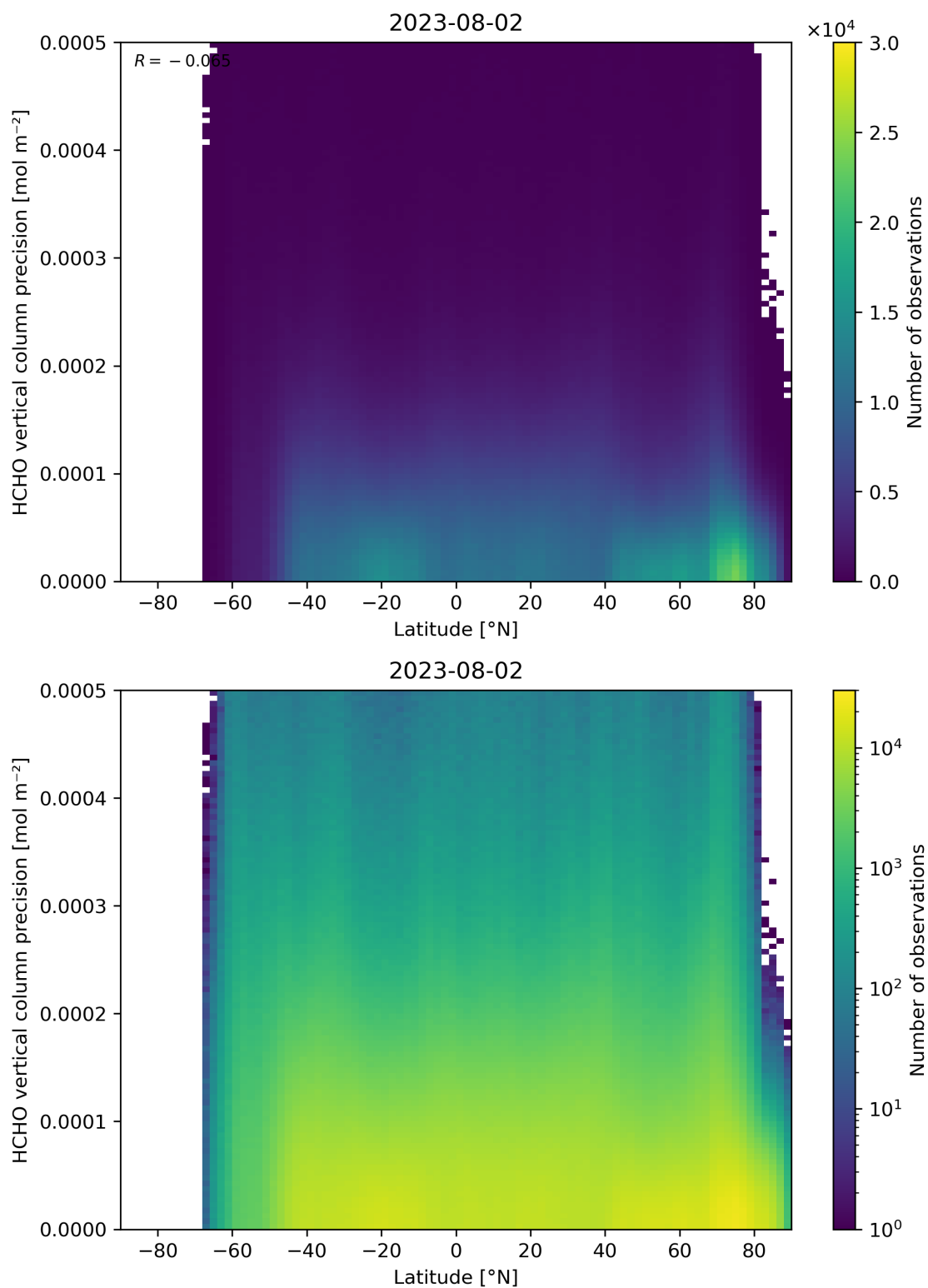
Figure 165: Scatter density plot of “Latitude” against “HCHO vertical column precision” for 2023-08-01 to 2023-08-03.
