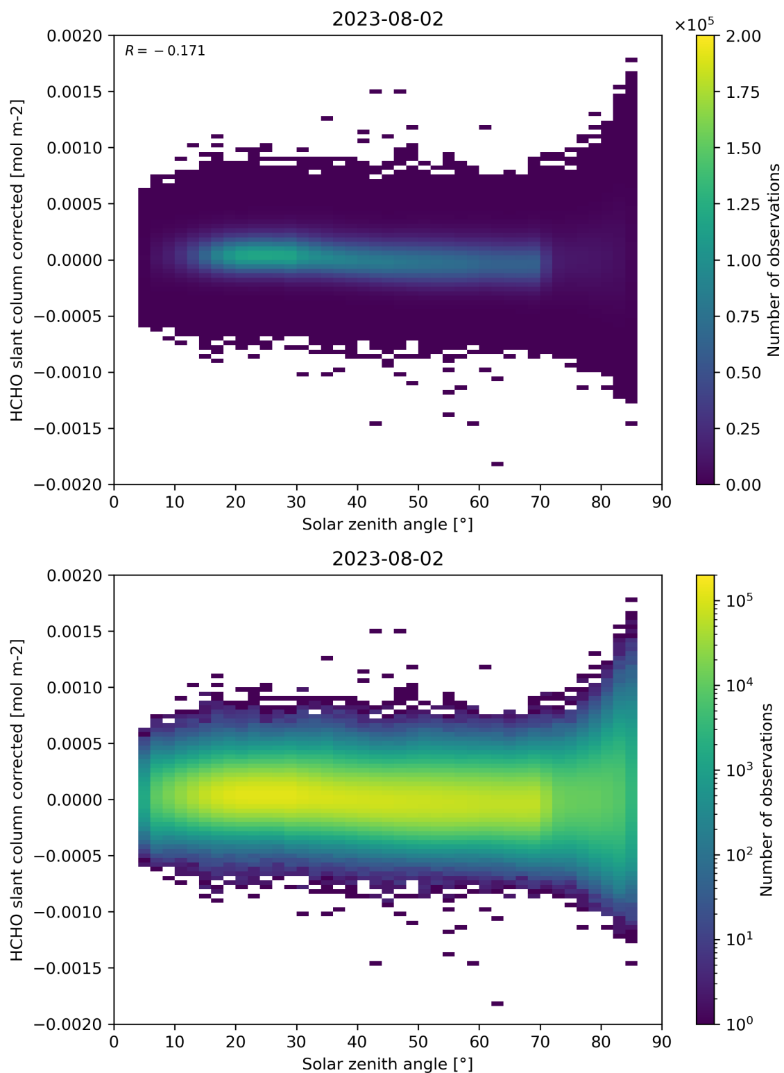
Figure 171: Scatter density plot of “Solar zenith angle” against “HCHO slant column corrected” for 2023-08-01 to 2023-08-03.
