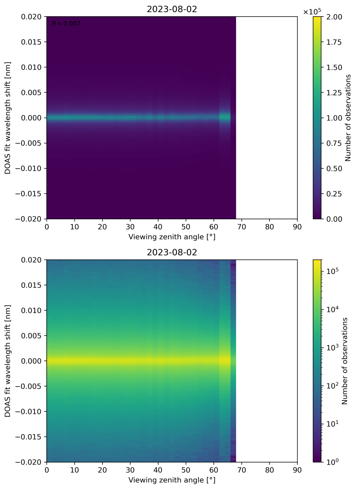
Figure 183: Scatter density plot of “Viewing zenith angle” against “DOAS fit wavelength shift” for 2023-08-01 to 2023-08-03.
