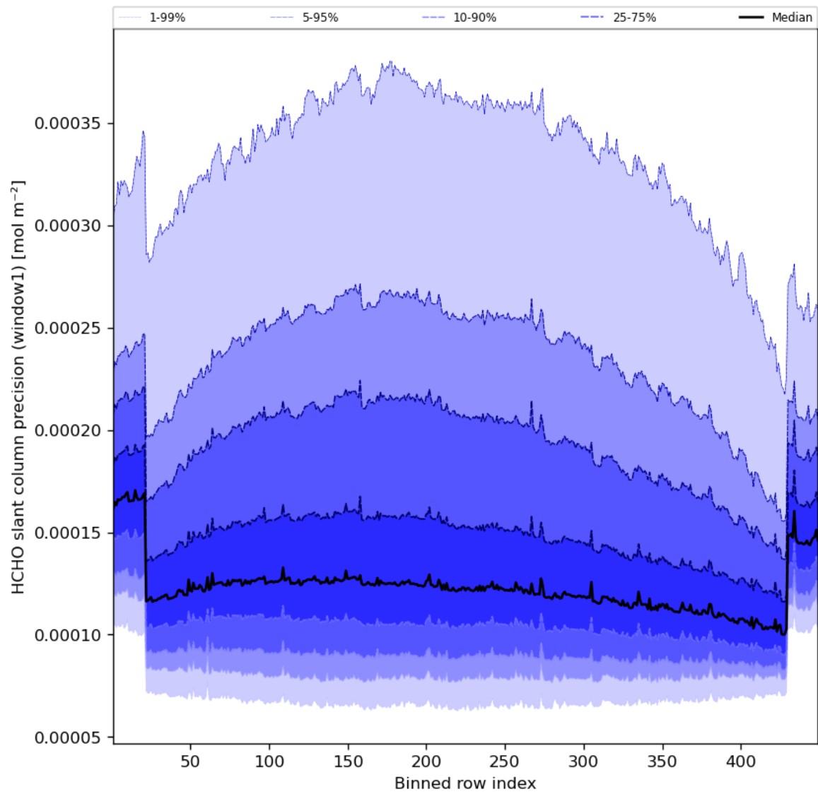
Figure 53: Along track statistics of “HCHO slant column precision (window1)” for 2023-08-01 to 2023-08-03
