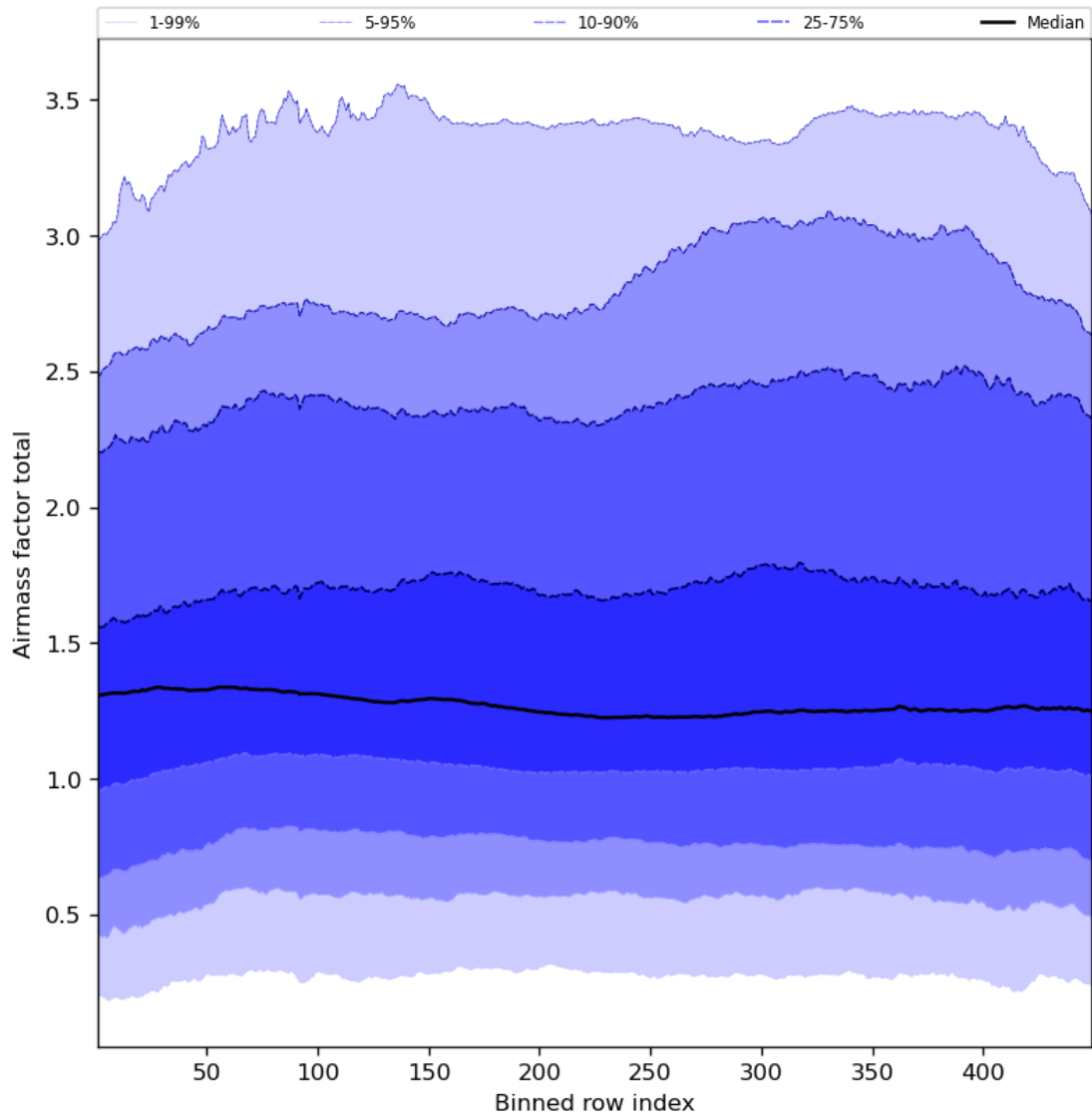
Figure 54: Along track statistics of “Airmass factor total” for 2023-08-01 to 2023-08-03
