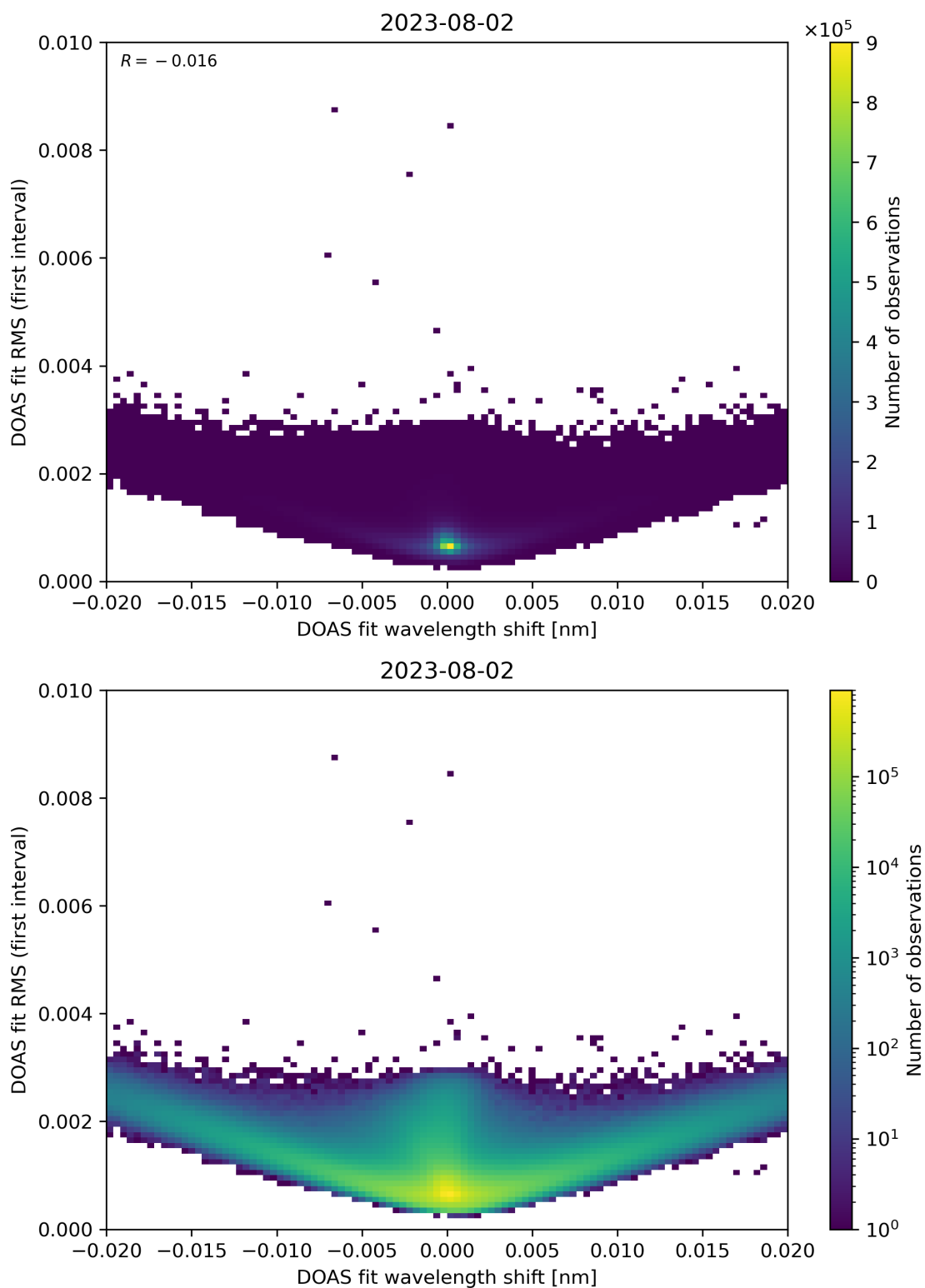
Figure 64: Scatter density plot of “DOAS fit wavelength shift” against “DOAS fit RMS (first interval)” for 2023-08-01 to 2023-08-03.
