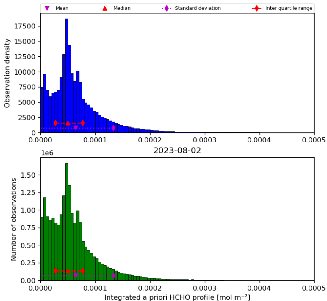
Figure 43: Histogram of “Integrated a priori HCHO profile” for 2023-08-01 to 2023-08-03
