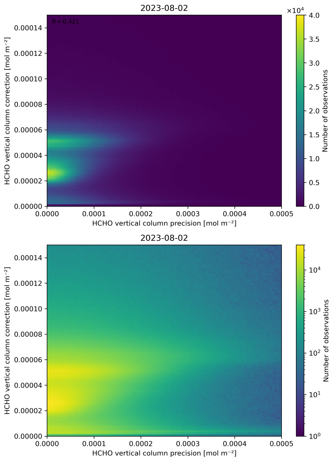
Figure 146: Scatter density plot of “HCHO vertical column precision” against “HCHO vertical column correction” for 2023-08-01 to 2023-08-03.
