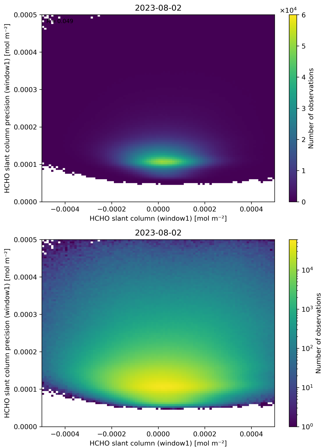
Figure 84: Scatter density plot of “HCHO slant column (window1)” against “HCHO slant column precision (window1)” for 2023-08-01 to 2023-08-03.
