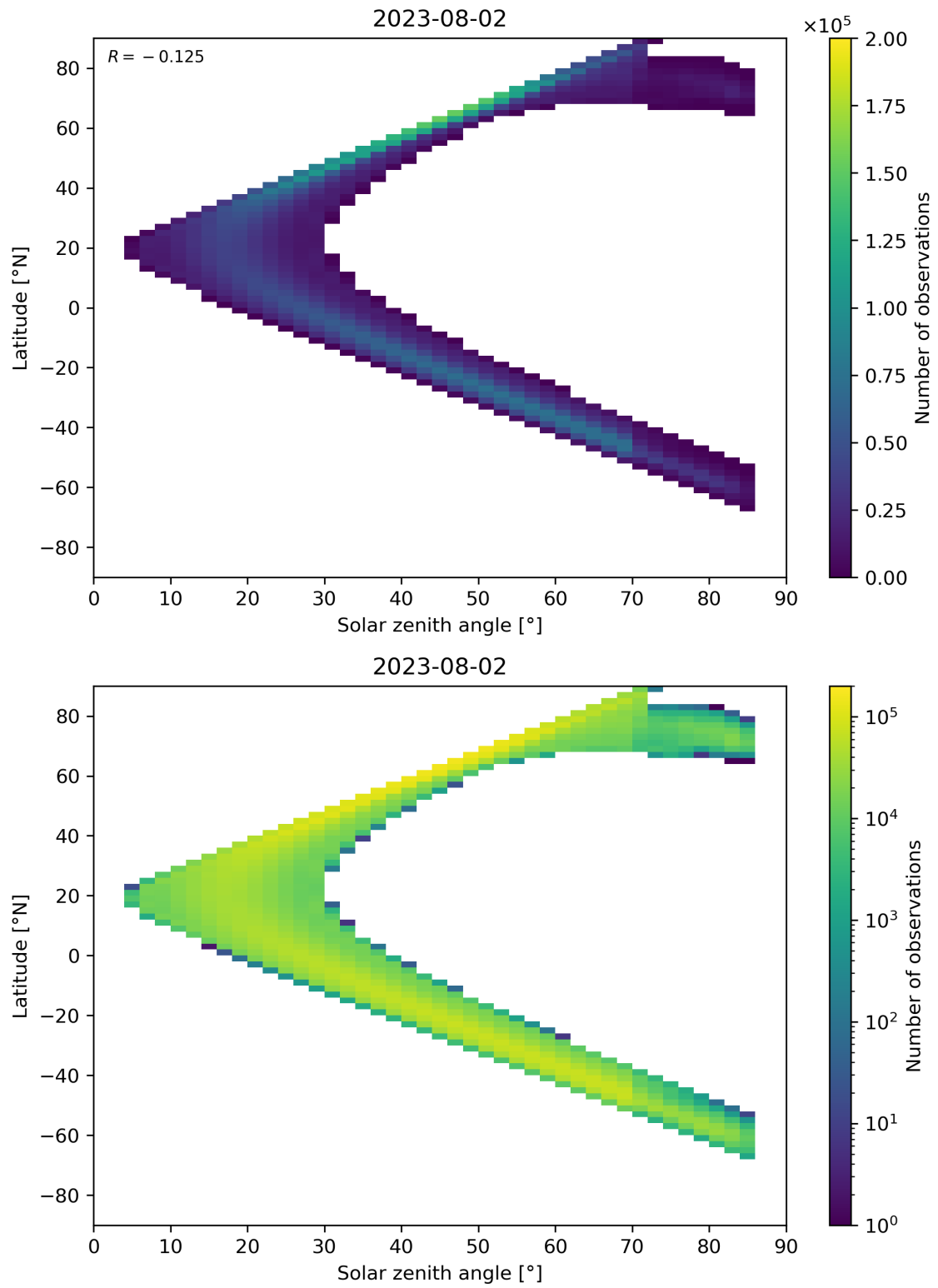
Figure 181: Scatter density plot of “Solar zenith angle” against “Latitude” for 2023-08-01 to 2023-08-03.
