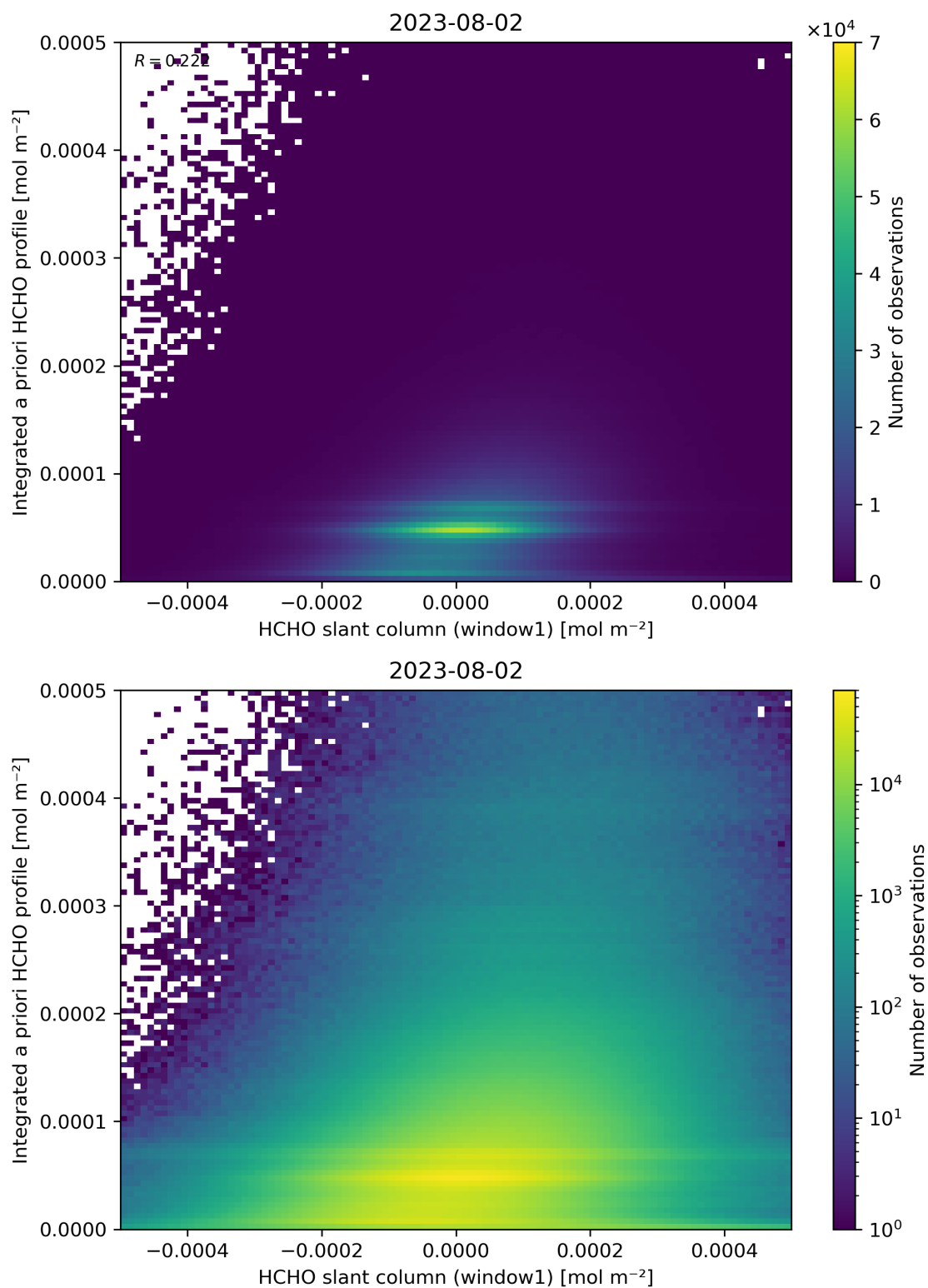
Figure 87: Scatter density plot of “HCHO slant column (window1)” against “Integrated a priori HCHO profile” for 2023-08-01 to 2023-08-03.
