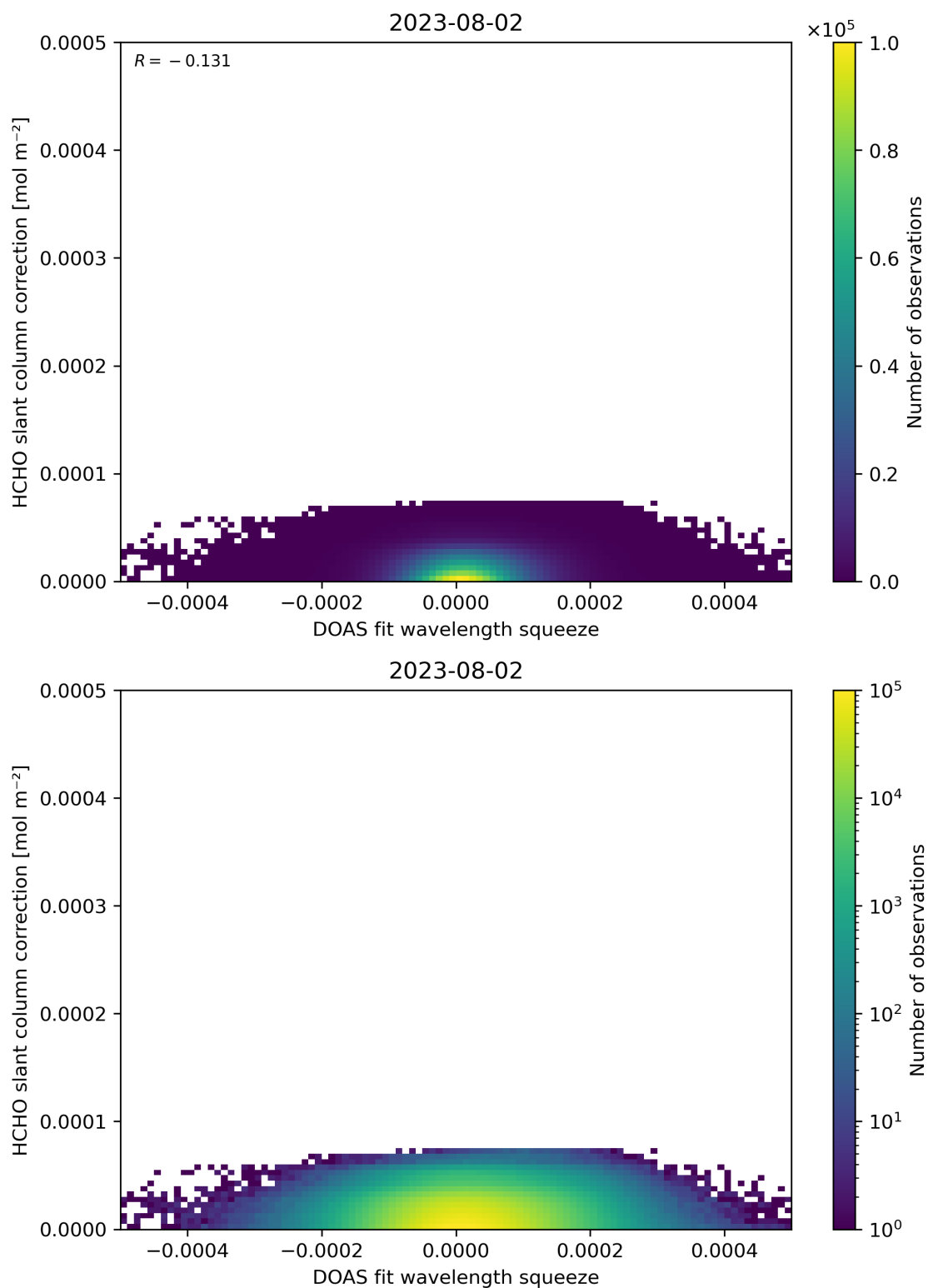
Figure 70: Scatter density plot of “DOAS fit wavelength squeeze” against “HCHO slant column correction” for 2023-08-01 to 2023-08-03.
