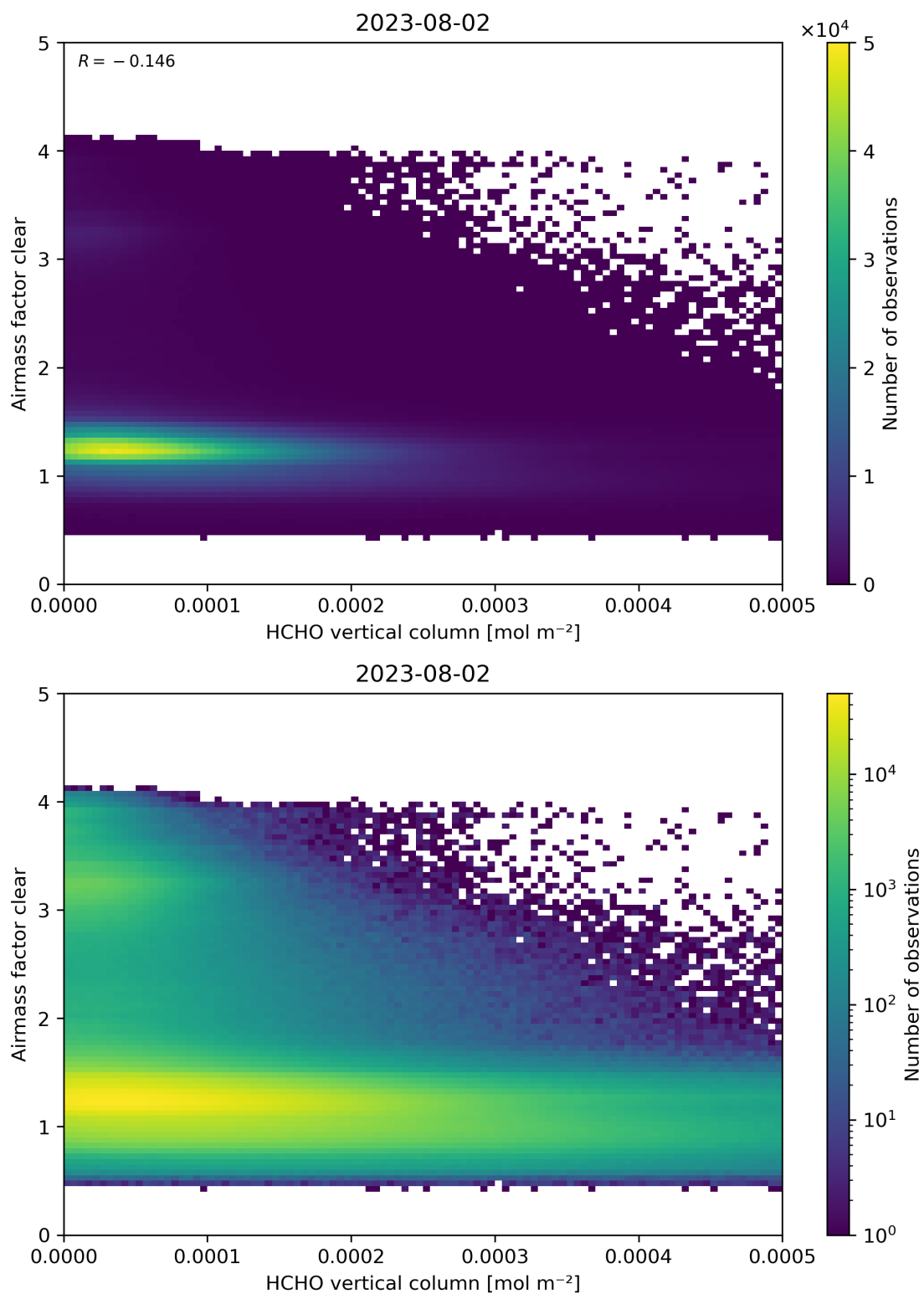
Figure 126: Scatter density plot of “HCHO vertical column” against “Airmass factor clear” for 2023-08-01 to 2023-08-03.
