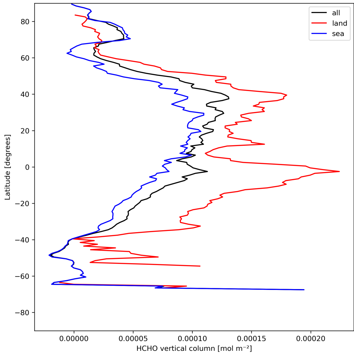
Figure 21: Zonal average of “HCHO vertical column” for 2023-08-01 to 2023-08-03.
