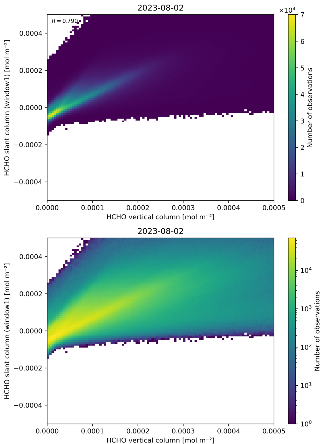
Figure 129: Scatter density plot of “HCHO vertical column” against “HCHO slant column (window1)” for 2023-08-01 to 2023-08-03.
