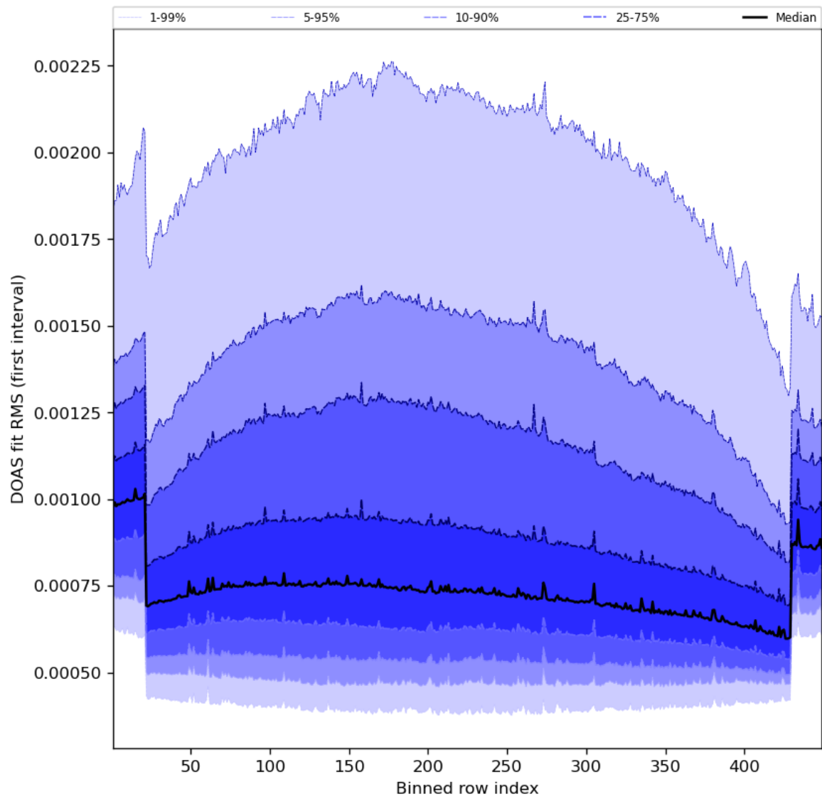
Figure 60: Along track statistics of “DOAS fit RMS (first interval)” for 2023-08-01 to 2023-08-03
