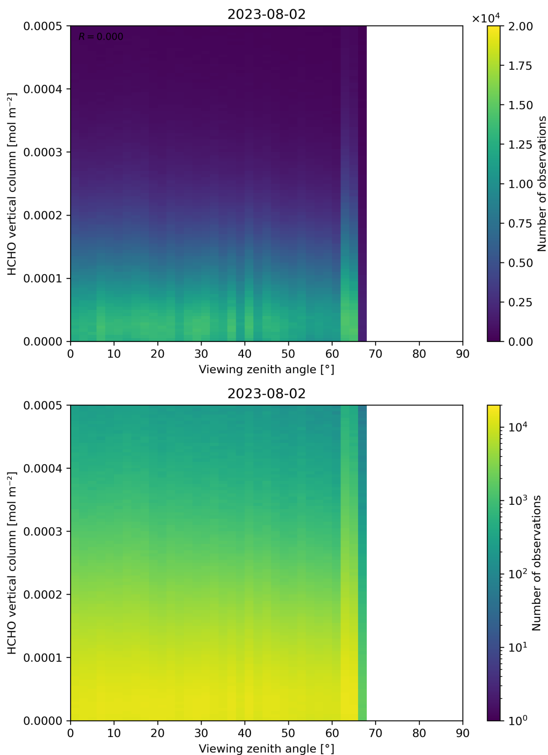
Figure 192: Scatter density plot of “Viewing zenith angle” against “HCHO vertical column” for 2023-08-01 to 2023-08-03.
