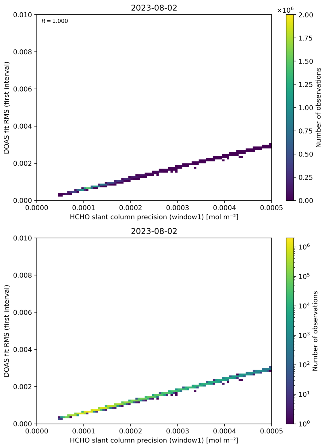
Figure 88: Scatter density plot of “HCHO slant column precision (window1)” against “DOAS fit RMS (first interval)” for 2023-08-01 to 2023-08-03.
