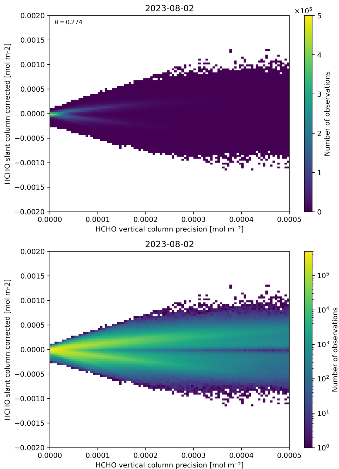
Figure 140: Scatter density plot of “HCHO vertical column precision” against “HCHO slant column corrected” for 2023-08-01 to 2023-08-03.
