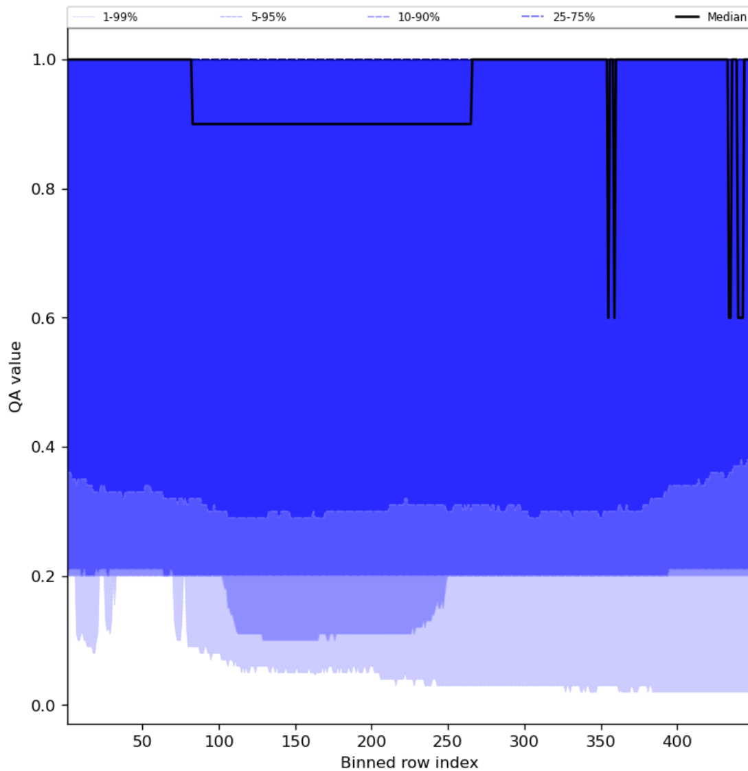
Figure 48: Along track statistics of “QA value” for 2023-08-01 to 2023-08-03
