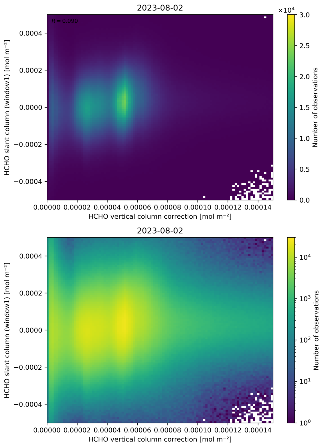
Figure 118: Scatter density plot of “HCHO vertical column correction” against “HCHO slant column (window1)” for 2023-08-01 to 2023-08-03.
