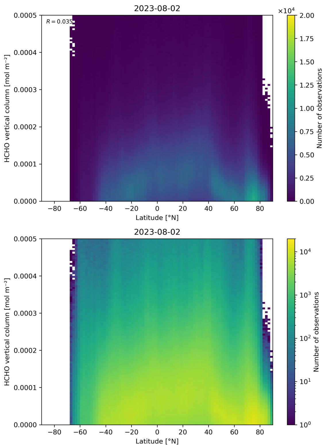
Figure 163: Scatter density plot of “Latitude” against “HCHO vertical column” for 2023-08-01 to 2023-08-03.
