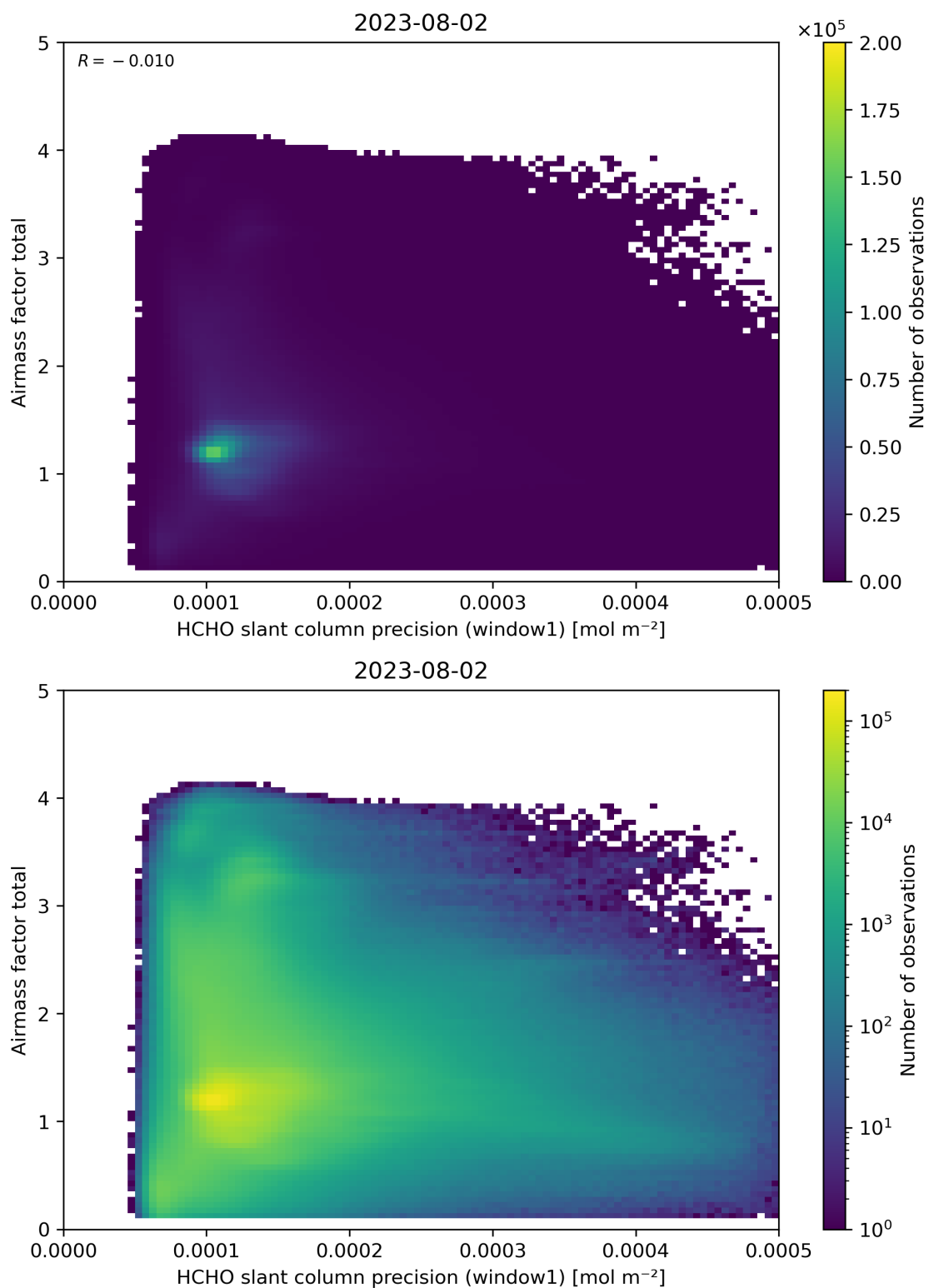
Figure 94: Scatter density plot of “HCHO slant column precision (window1)” against “Airmass factor total” for 2023-08-01 to 2023-08-03.
