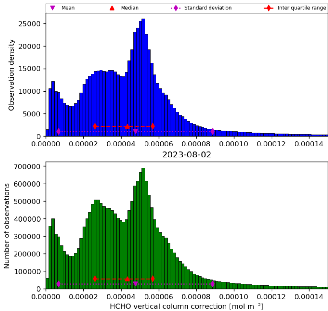
Figure 37: Histogram of “HCHO vertical column correction” for 2023-08-01 to 2023-08-03
