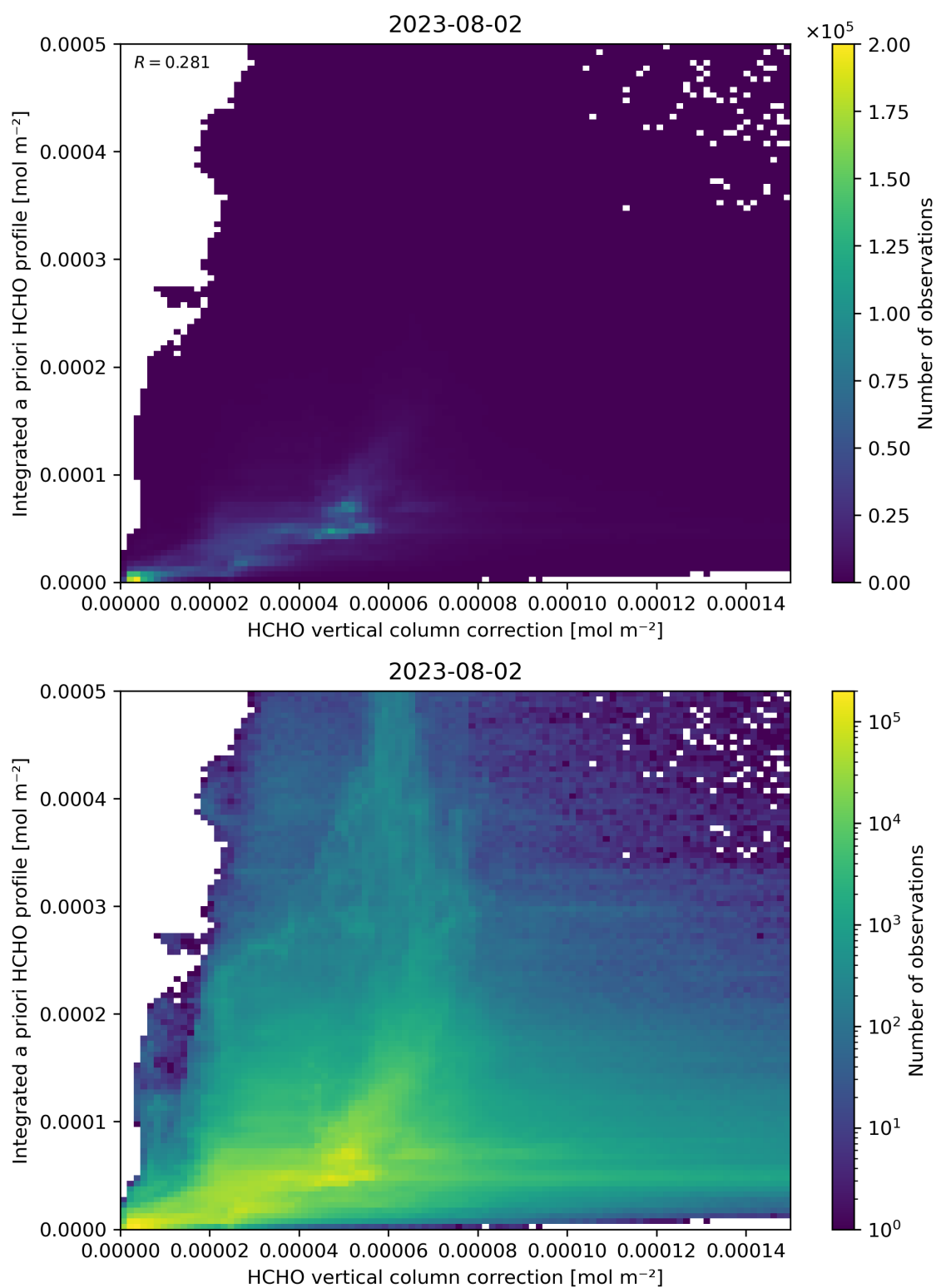
Figure 122: Scatter density plot of “HCHO vertical column correction” against “Integrated a priori HCHO profile” for 2023-08-01 to 2023-08-03.
