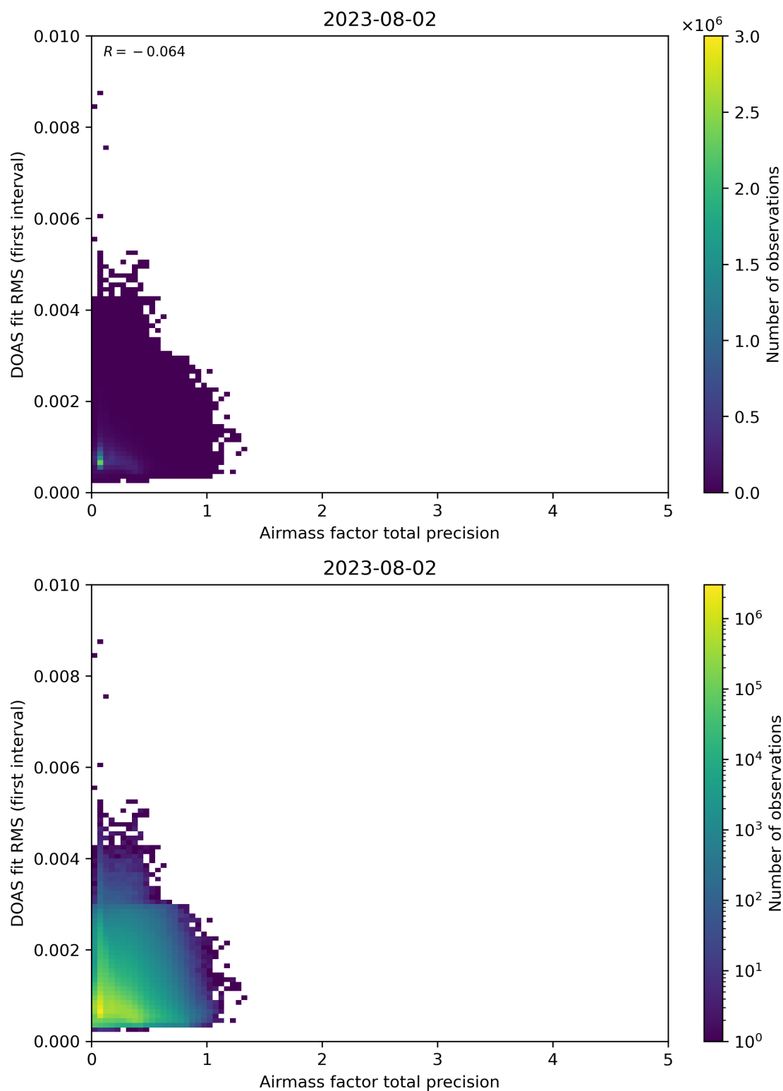
Figure 105: Scatter density plot of “Airmass factor total precision” against “DOAS fit RMS (first interval)” for 2023-08-01 to 2023-08-03.
