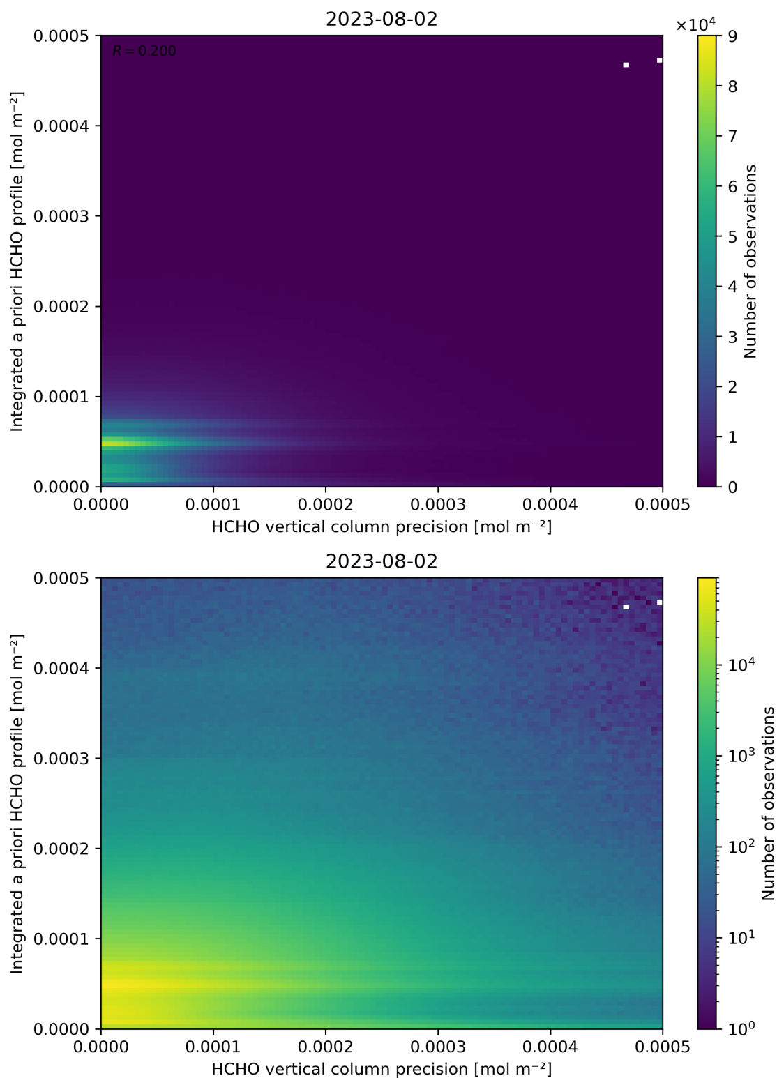
Figure 147: Scatter density plot of “HCHO vertical column precision” against “Integrated a priori HCHO profile” for 2023-08-01 to 2023-08-03.
