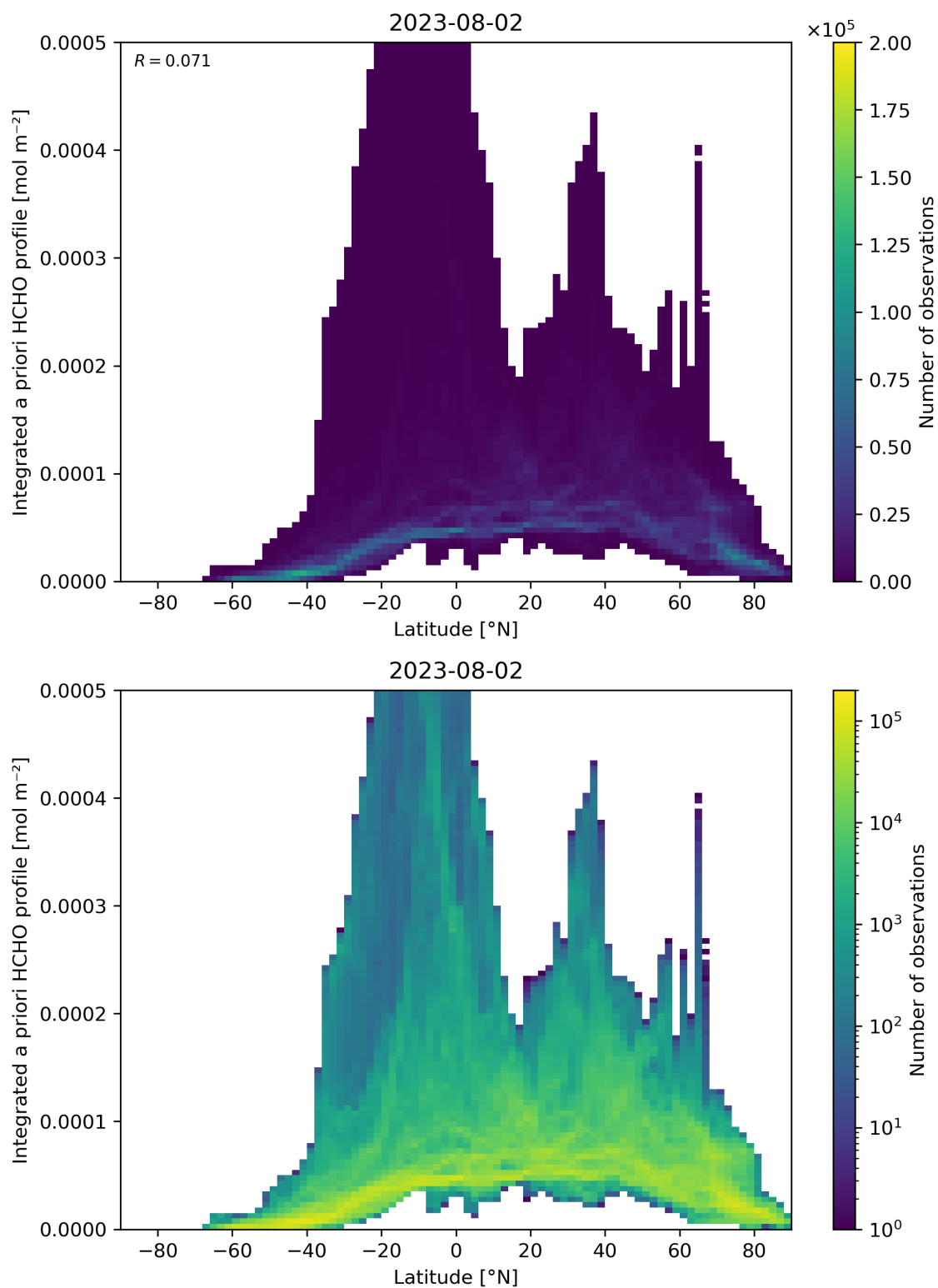
Figure 166: Scatter density plot of “Latitude” against “Integrated a priori HCHO profile” for 2023-08-01 to 2023-08-03.
