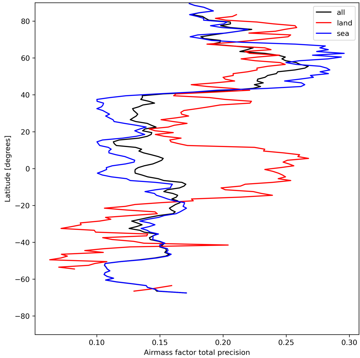
Figure 27: Zonal average of “Airmass factor total precision” for 2023-08-01 to 2023-08-03.
