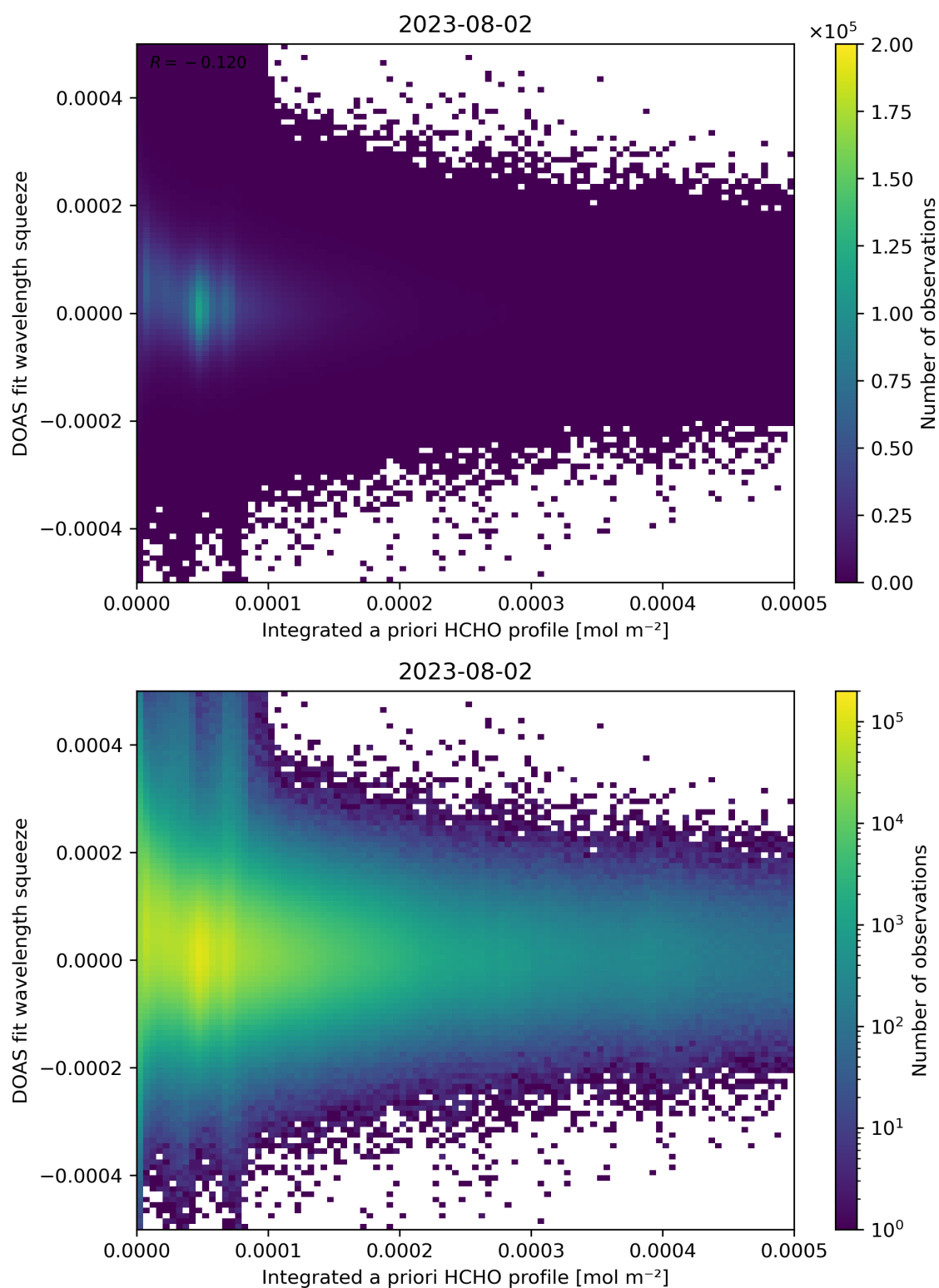
Figure 150: Scatter density plot of “Integrated a priori HCHO profile” against “DOAS fit wavelength squeeze” for 2023-08-01 to 2023-08-03.
