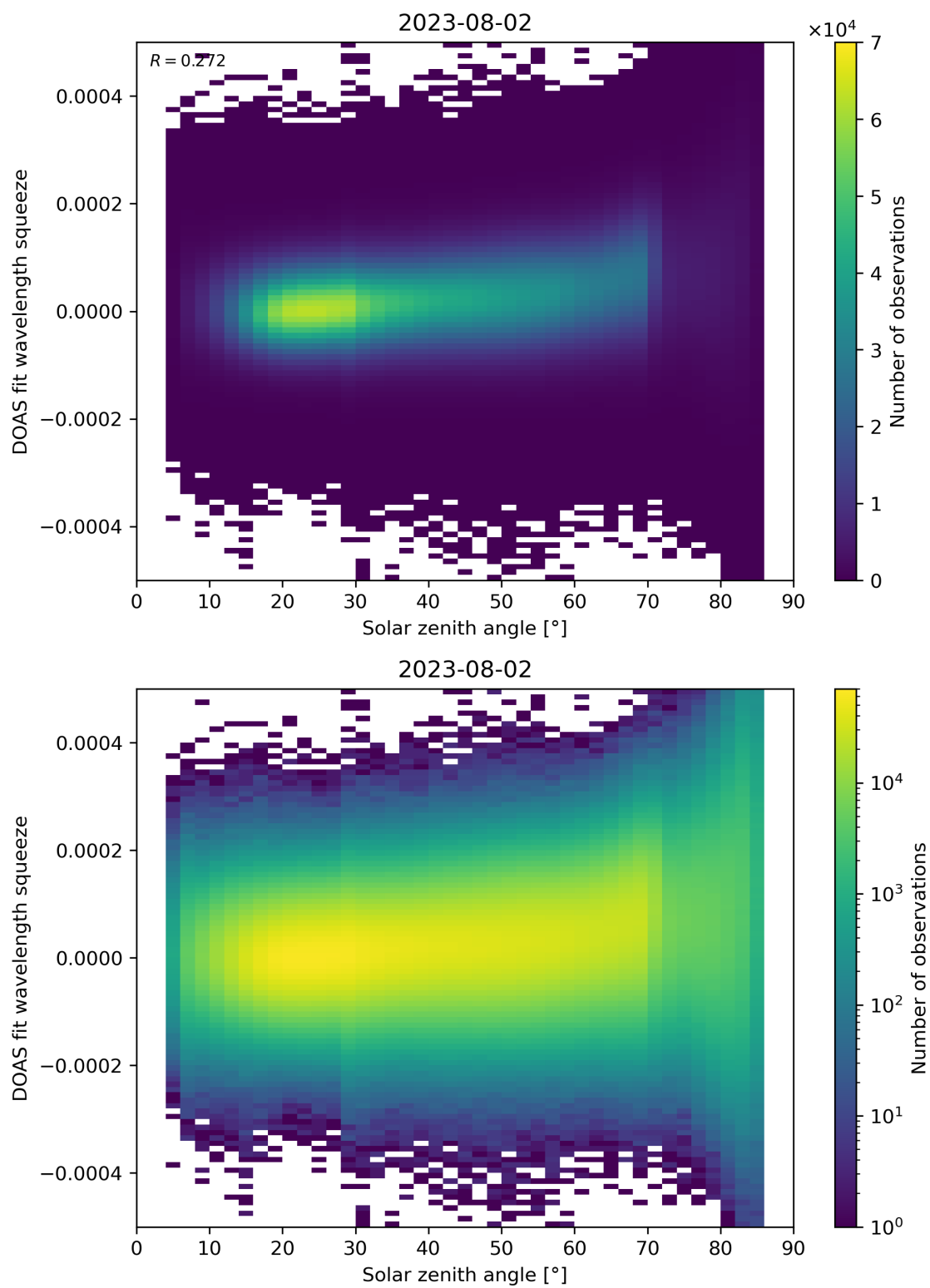
Figure 169: Scatter density plot of “Solar zenith angle” against “DOAS fit wavelength squeeze” for 2023-08-01 to 2023-08-03.
