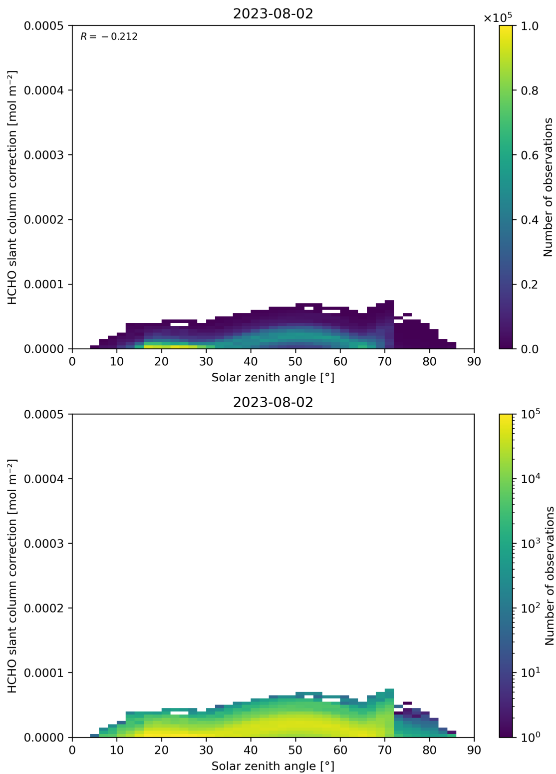
Figure 172: Scatter density plot of “Solar zenith angle” against “HCHO slant column correction” for 2023-08-01 to 2023-08-03.
