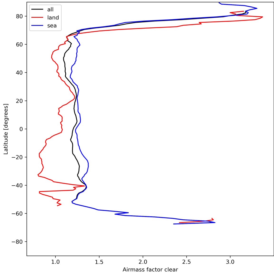
Figure 28: Zonal average of “Airmass factor clear” for 2023-08-01 to 2023-08-03.
