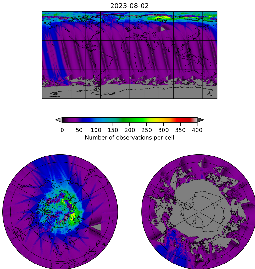
Figure 19: Map of the number of observations for 2023-08-01 to 2023-08-03
