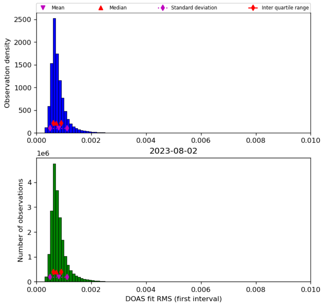
Figure 46: Histogram of “DOAS fit RMS (first interval)” for 2023-08-01 to 2023-08-03
