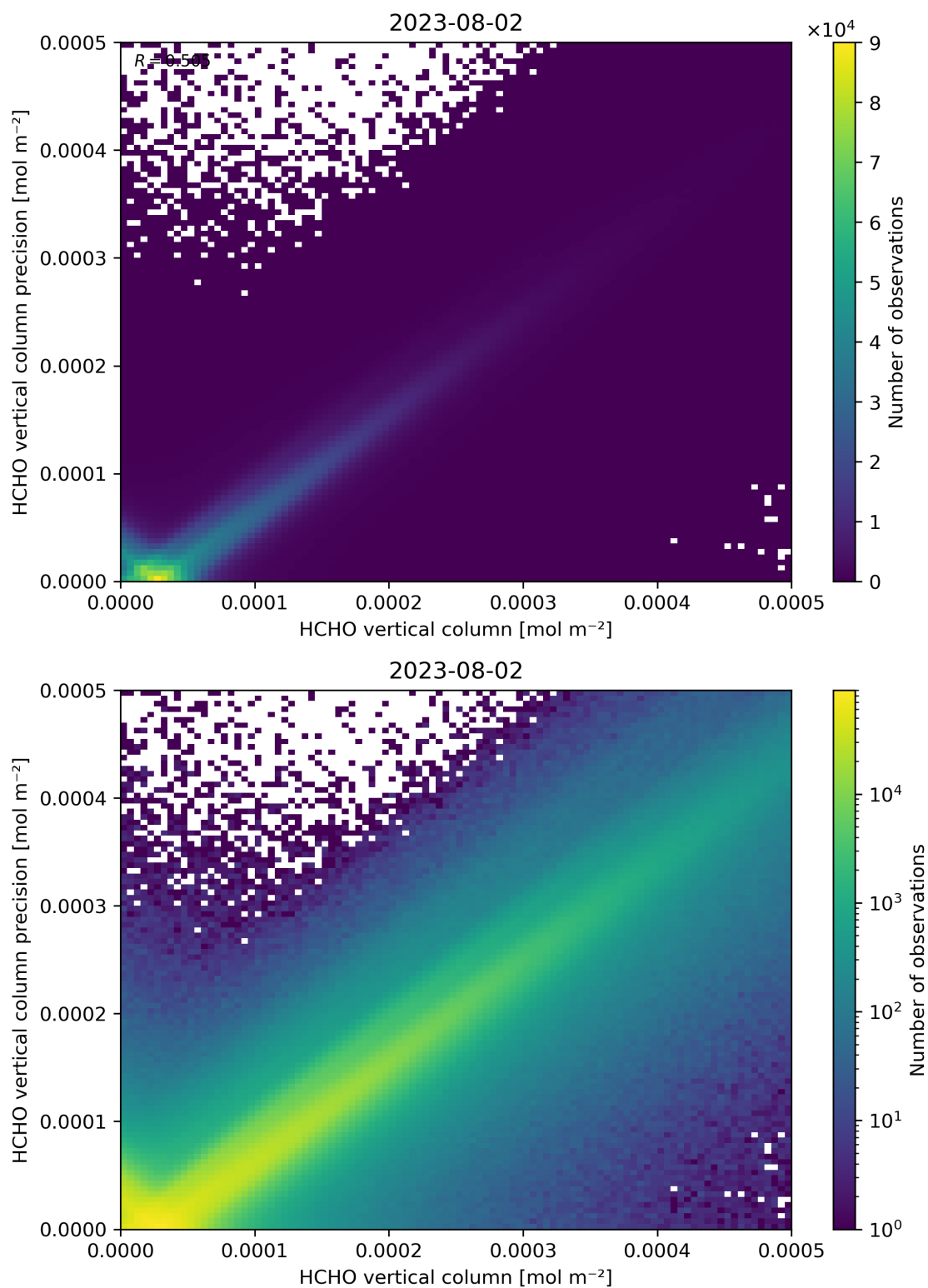
Figure 134: Scatter density plot of “HCHO vertical column” against “HCHO vertical column precision” for 2023-08-01 to 2023-08-03.
