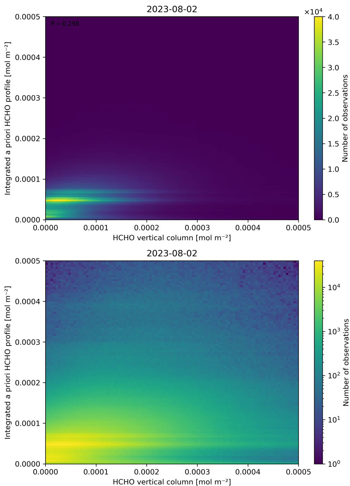
Figure 135: Scatter density plot of “HCHO vertical column” against “Integrated a priori HCHO profile” for 2023-08-01 to 2023-08-03.
