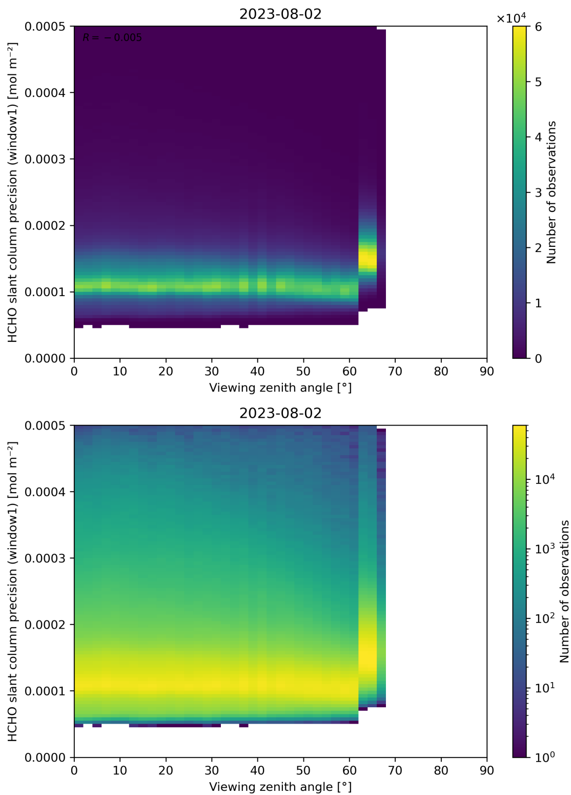
Figure 189: Scatter density plot of “Viewing zenith angle” against “HCHO slant column precision (window1)” for 2023-08-01 to 2023-08-03.
