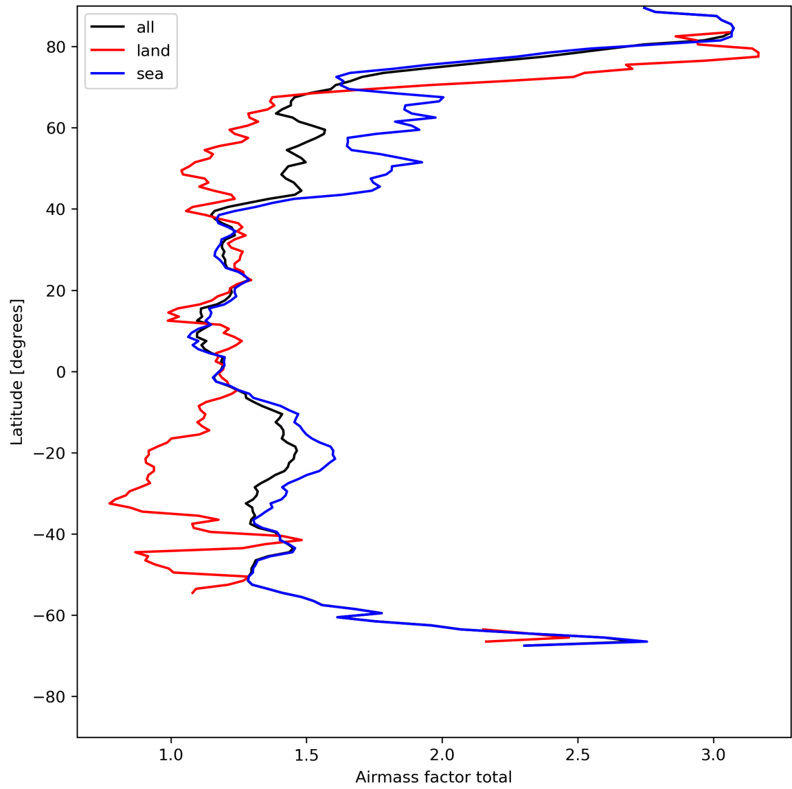
Figure 26: Zonal average of “Airmass factor total” for 2023-08-01 to 2023-08-03.
