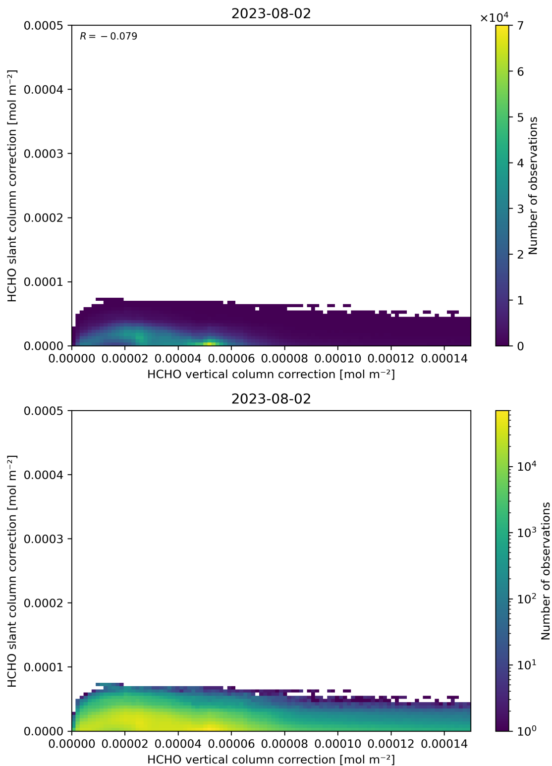
Figure 117: Scatter density plot of “HCHO vertical column correction” against “HCHO slant column correction” for 2023-08-01 to 2023-08-03.
