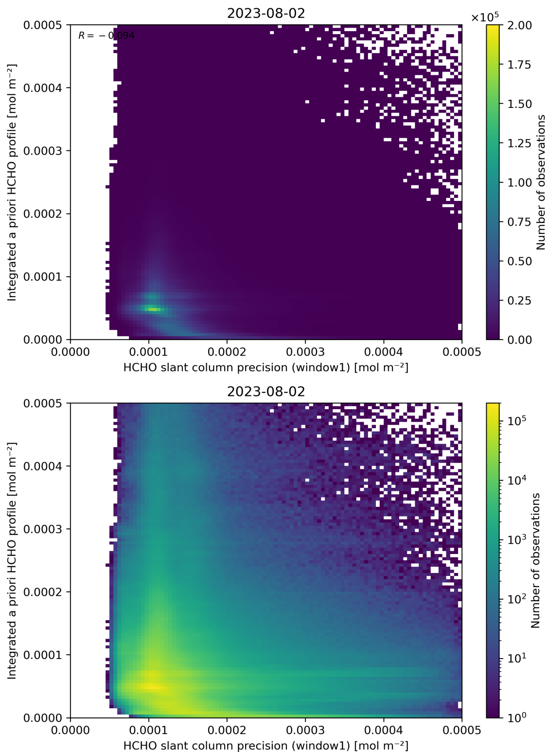
Figure 96: Scatter density plot of “HCHO slant column precision (window1)” against “Integrated a priori HCHO profile” for 2023-08-01 to 2023-08-03.
