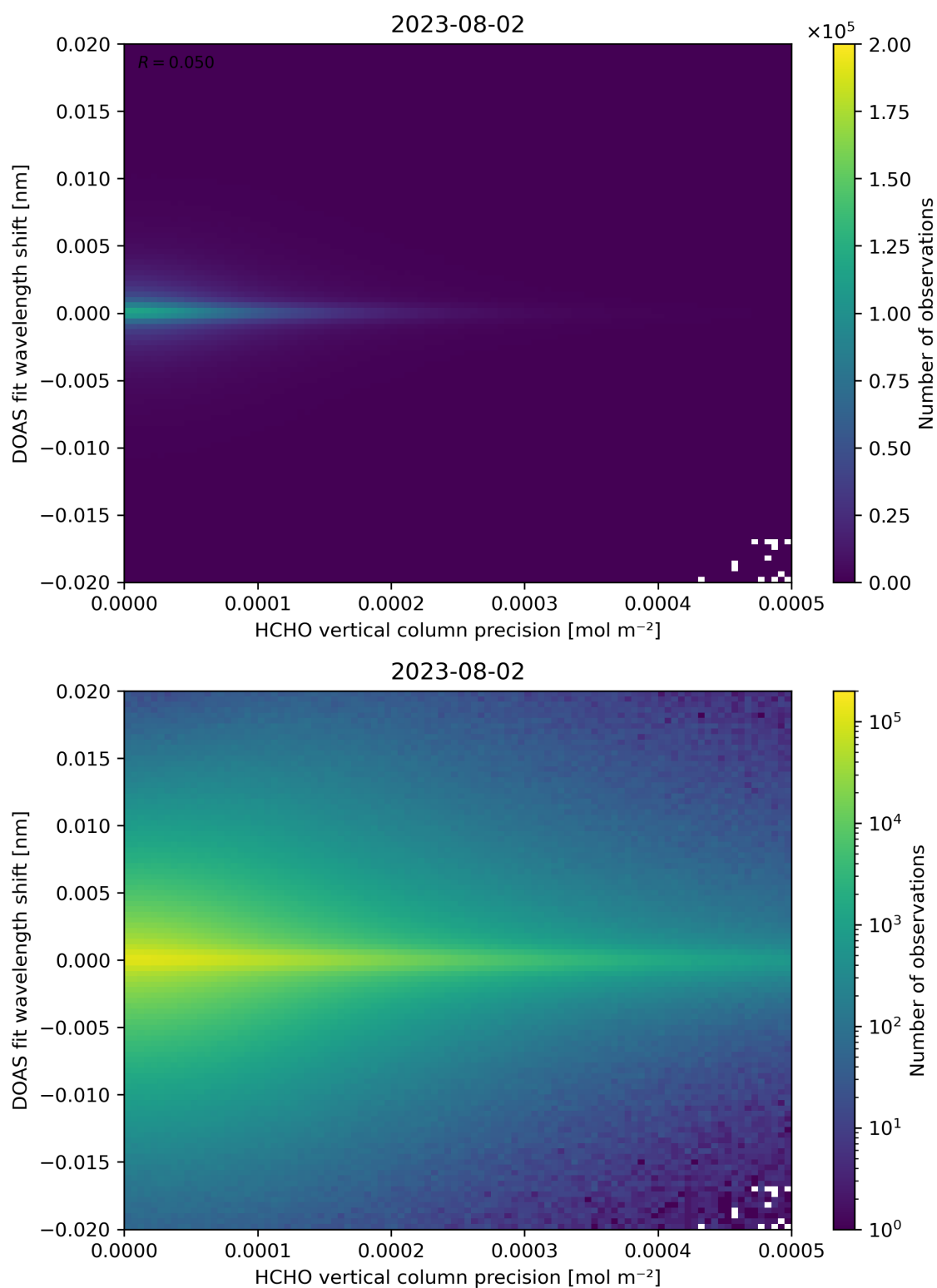
Figure 137: Scatter density plot of “HCHO vertical column precision” against “DOAS fit wavelength shift” for 2023-08-01 to 2023-08-03.
