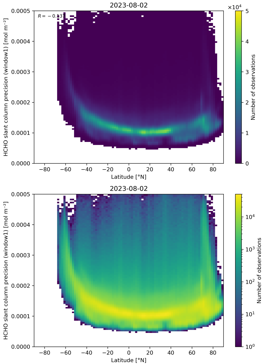
Figure 160: Scatter density plot of “Latitude” against “HCHO slant column precision (window1)” for 2023-08-01 to 2023-08-03.
