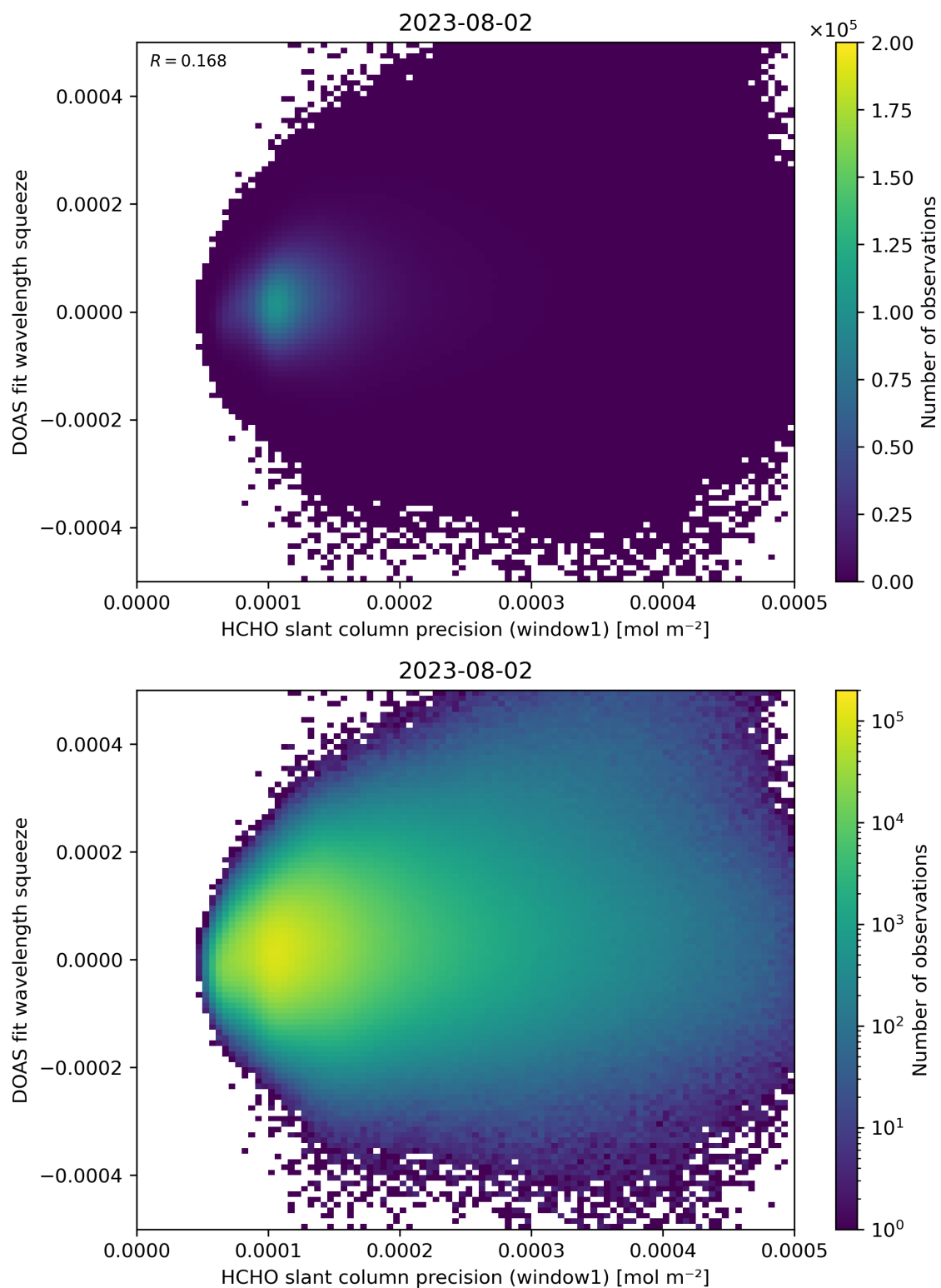
Figure 90: Scatter density plot of “HCHO slant column precision (window1)” against “DOAS fit wavelength squeeze” for 2023-08-01 to 2023-08-03.
