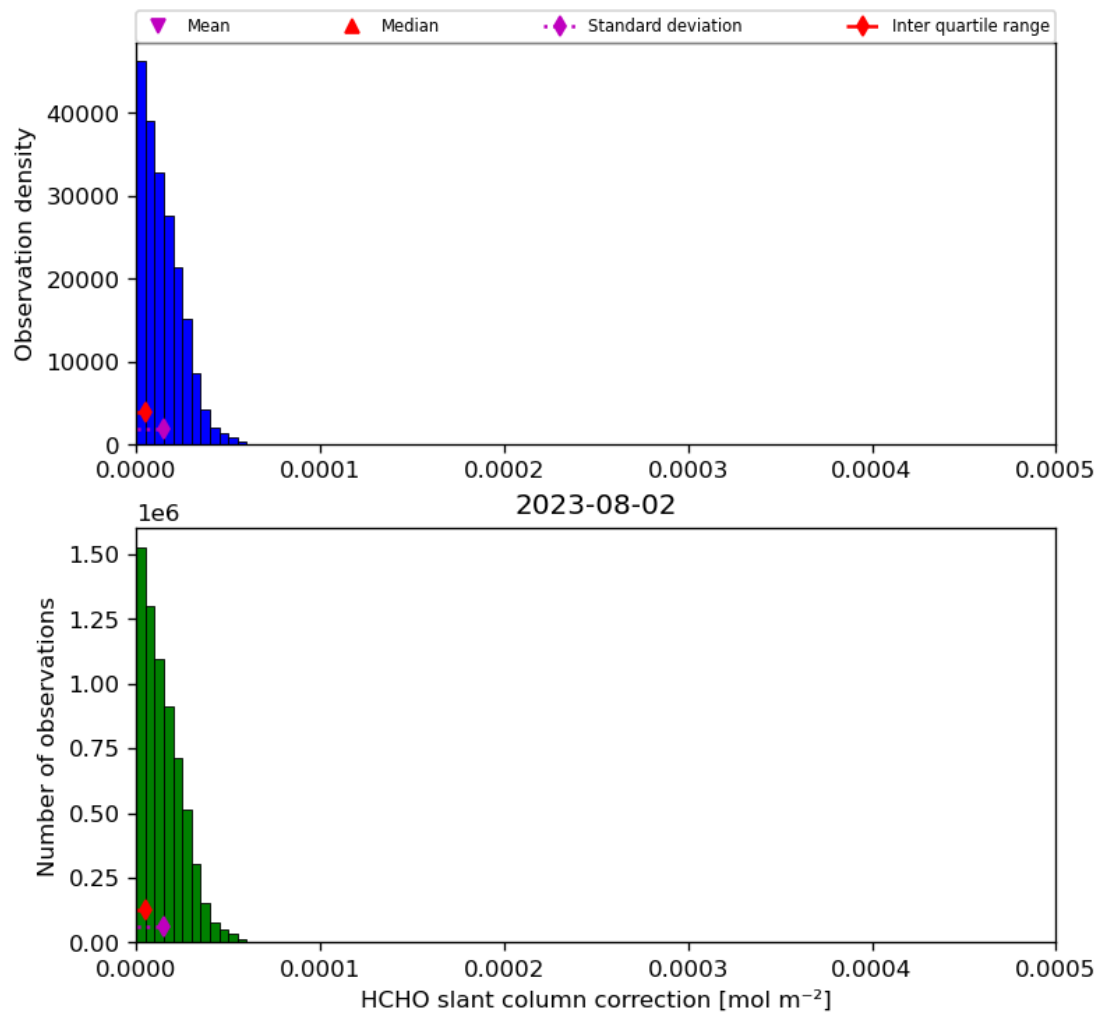
Figure 47: Histogram of “HCHO slant column correction” for 2023-08-01 to 2023-08-03
