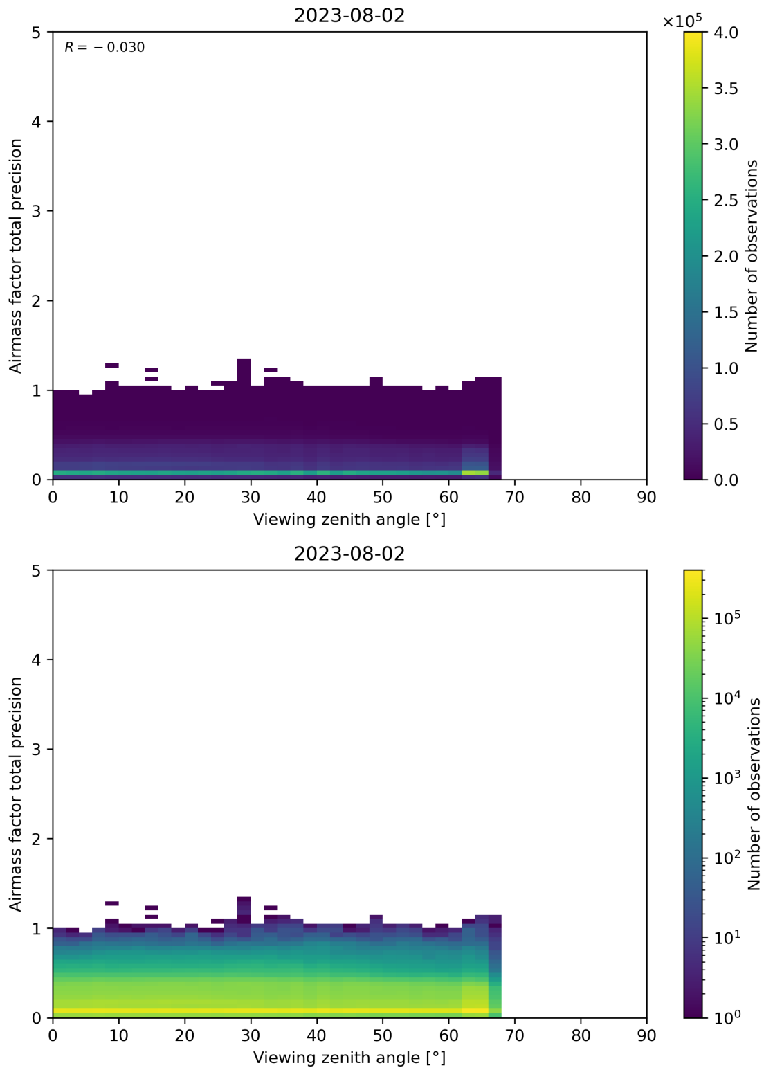
Figure 191: Scatter density plot of “Viewing zenith angle” against “Airmass factor total precision” for 2023-08-01 to 2023-08-03.
