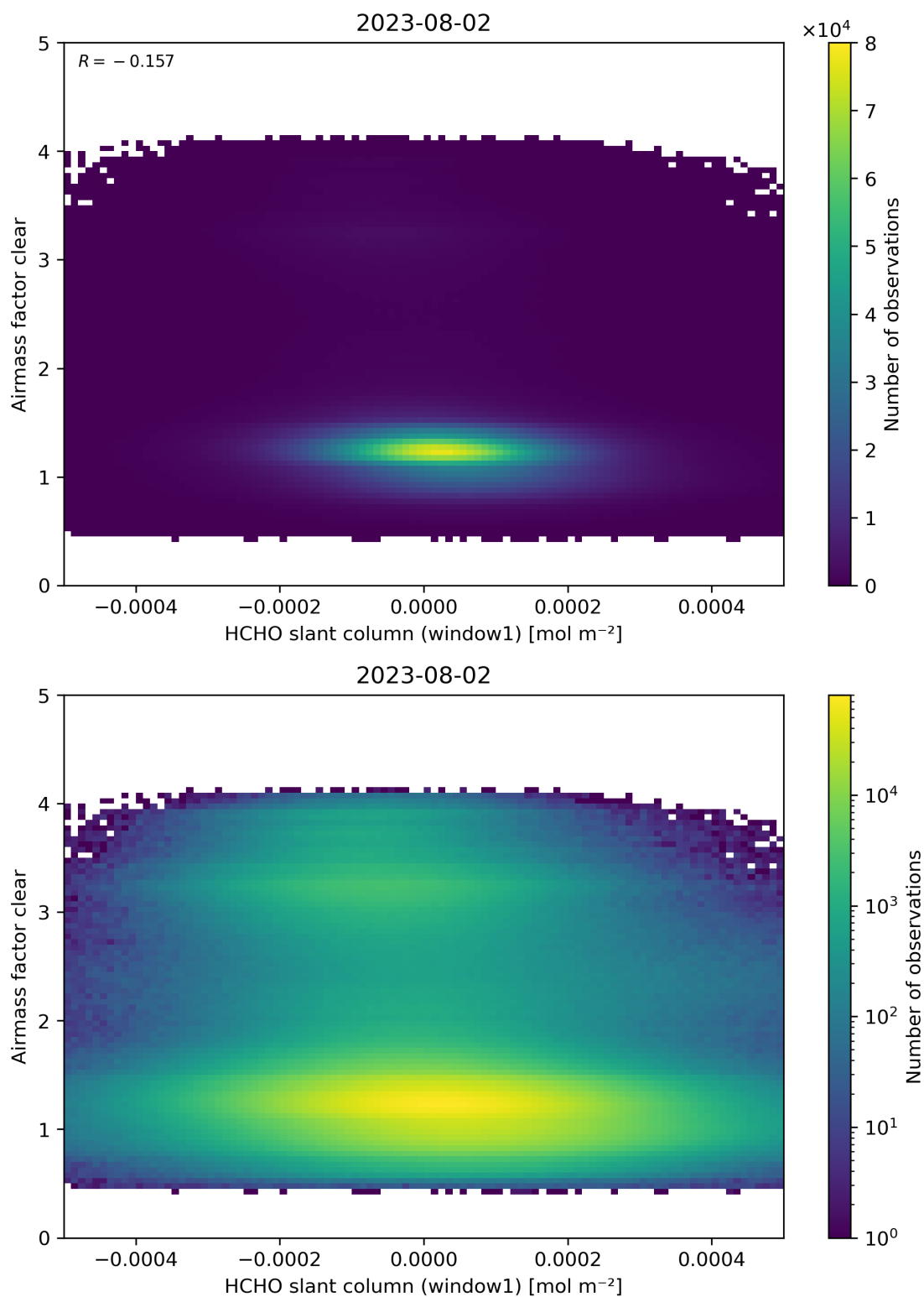
Figure 81: Scatter density plot of “HCHO slant column (window1)” against “Airmass factor clear” for 2023-08-01 to 2023-08-03.
