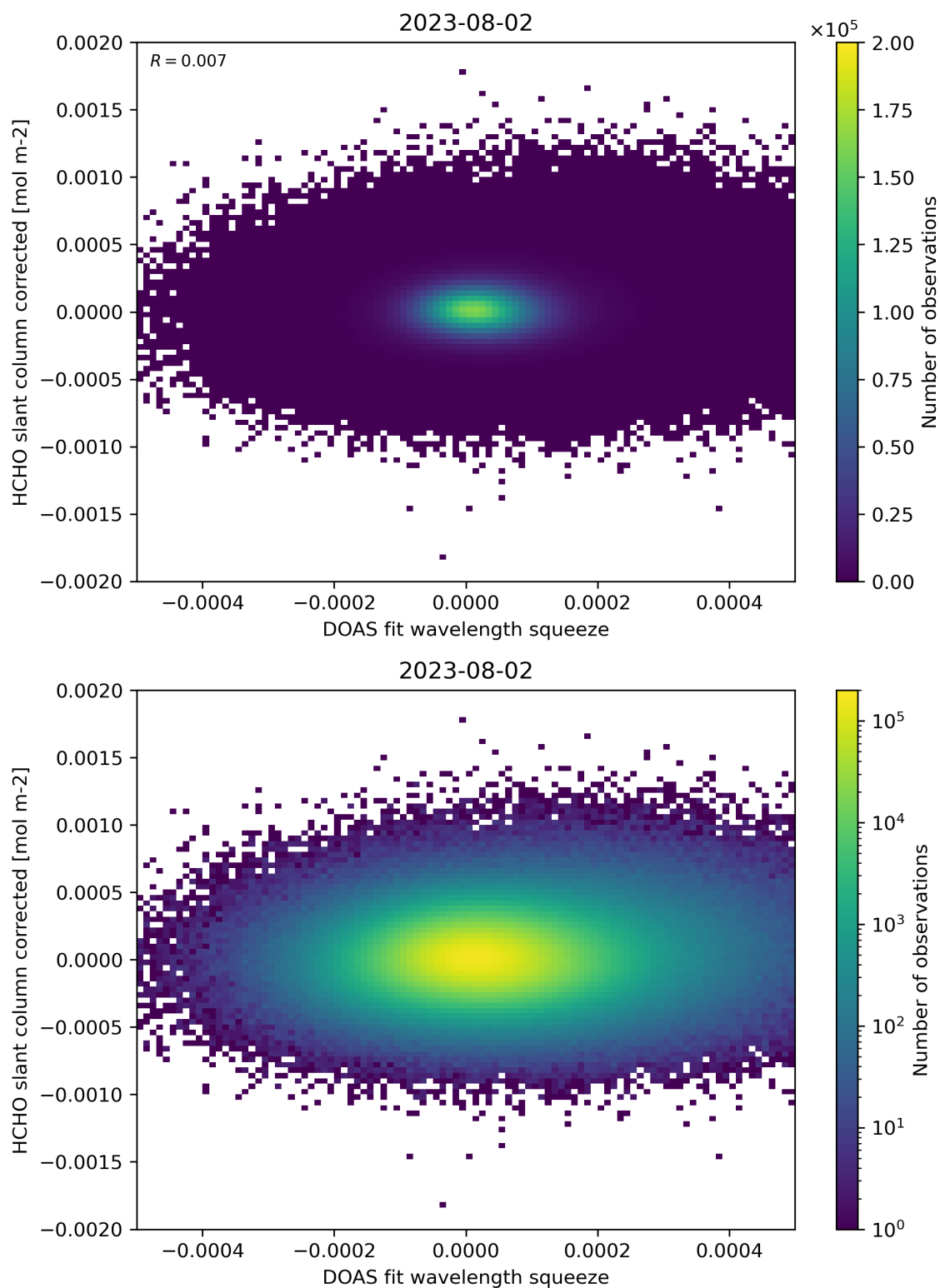
Figure 69: Scatter density plot of “DOAS fit wavelength squeeze” against “HCHO slant column corrected” for 2023-08-01 to 2023-08-03.
