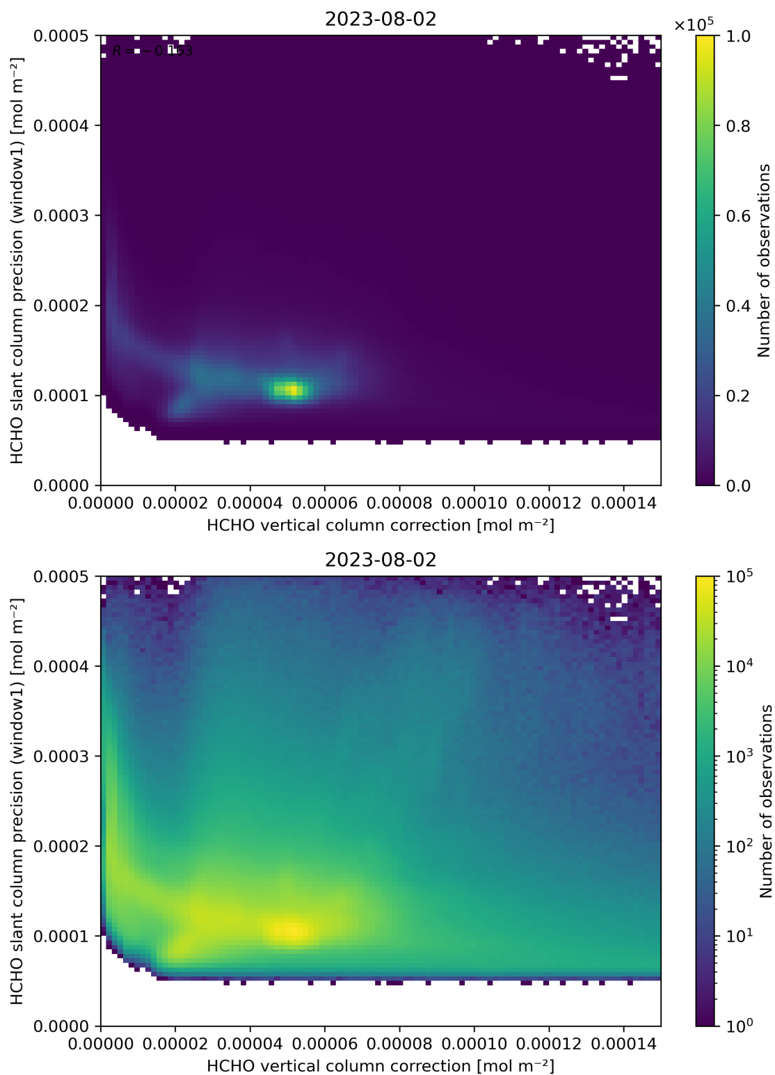
Figure 119: Scatter density plot of “HCHO vertical column correction” against “HCHO slant column precision (window1)” for 2023-08-01 to 2023-08-03.
