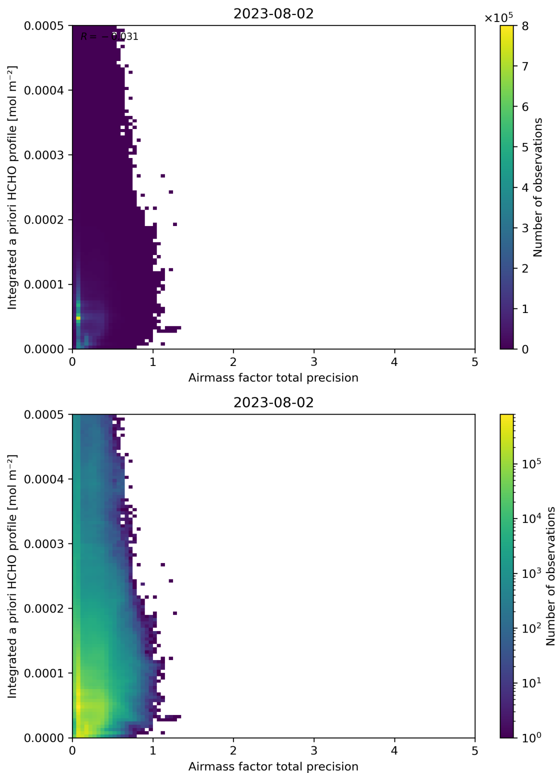
Figure 111: Scatter density plot of “Airmass factor total precision” against “Integrated a priori HCHO profile” for 2023-08-01 to 2023-08-03.
