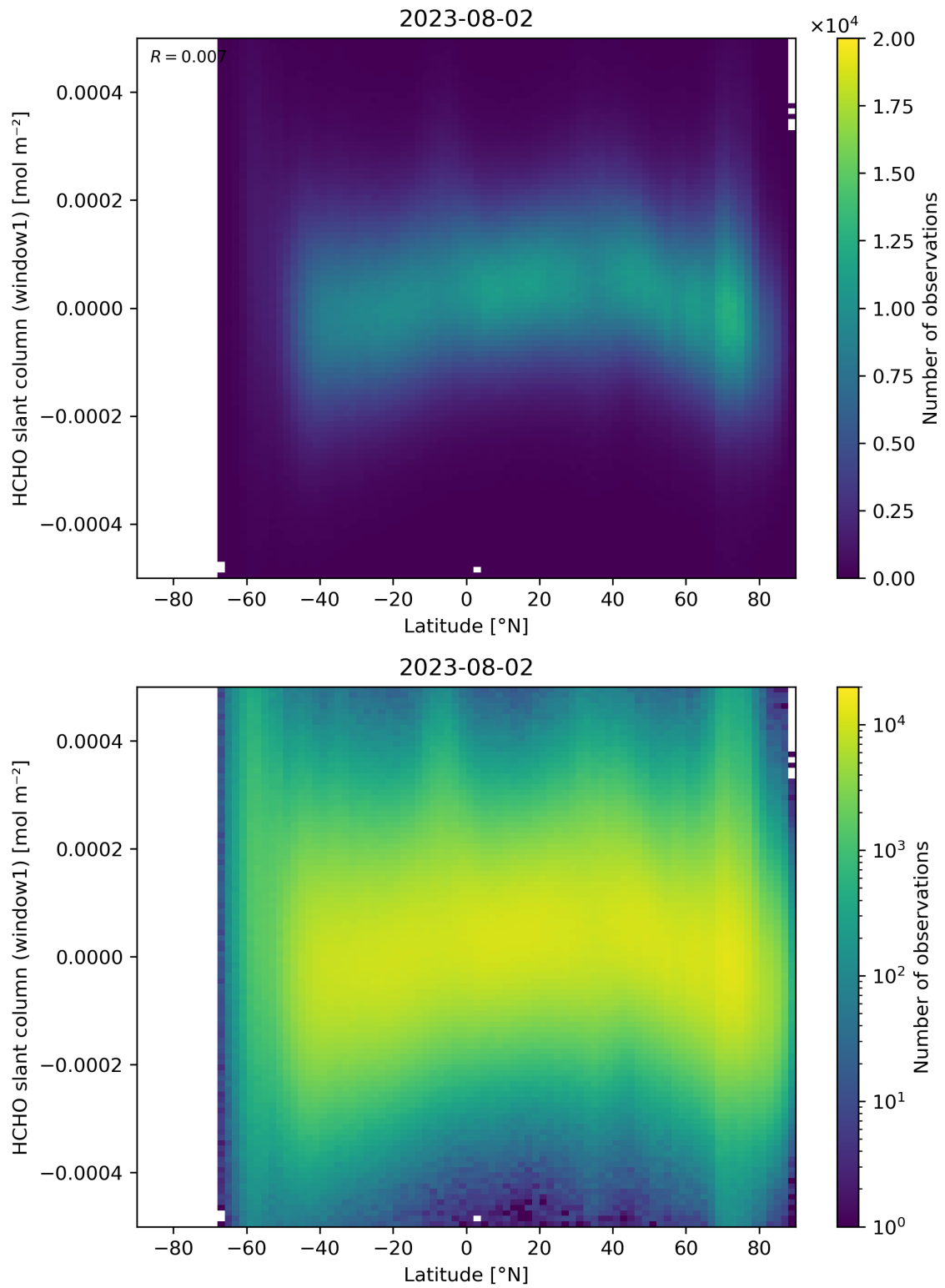
Figure 159: Scatter density plot of “Latitude” against “HCHO slant column (window1)” for 2023-08-01 to 2023-08-03.
