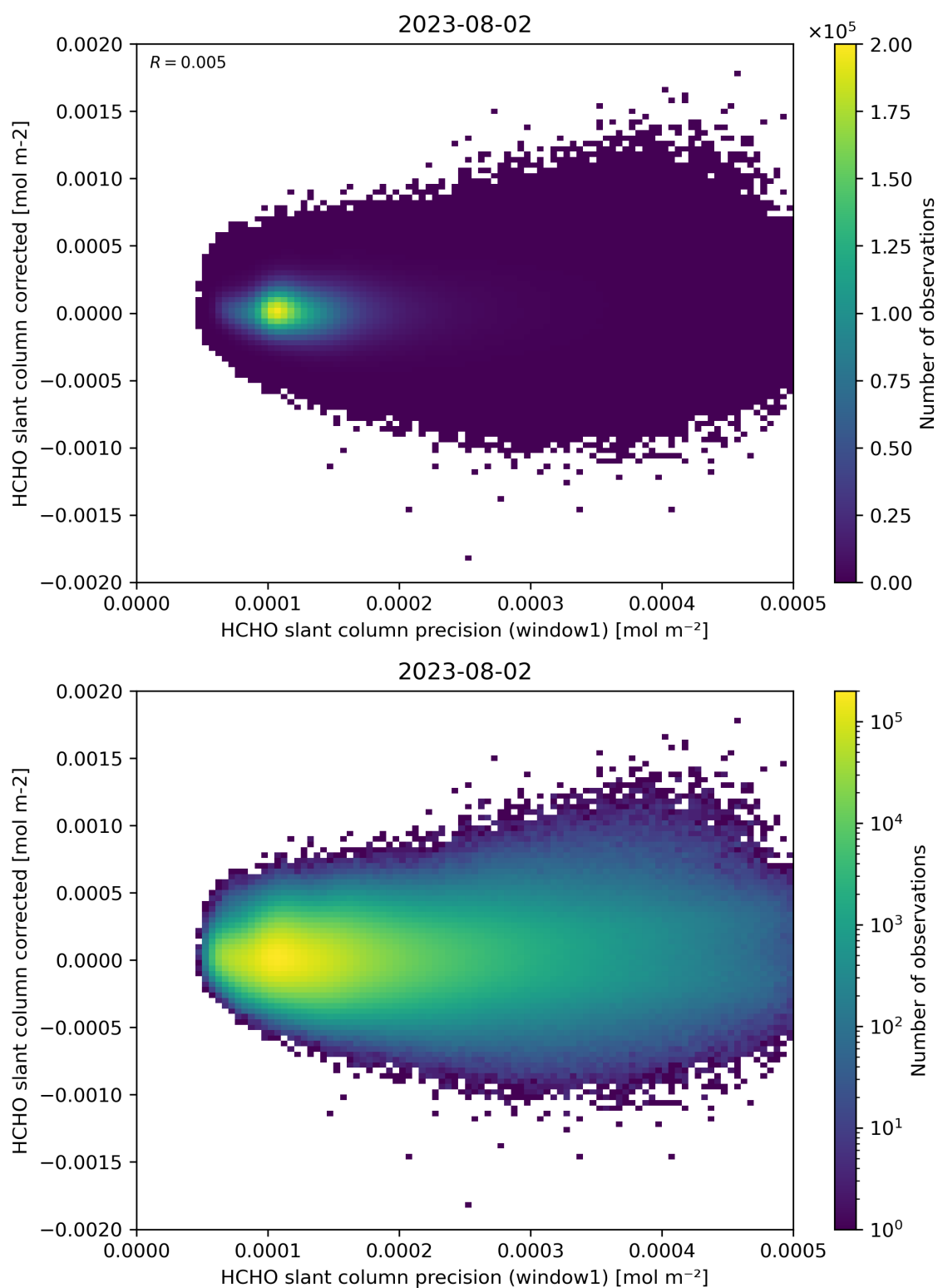
Figure 92: Scatter density plot of “HCHO slant column precision (window1)” against “HCHO slant column corrected” for 2023-08-01 to 2023-08-03.
