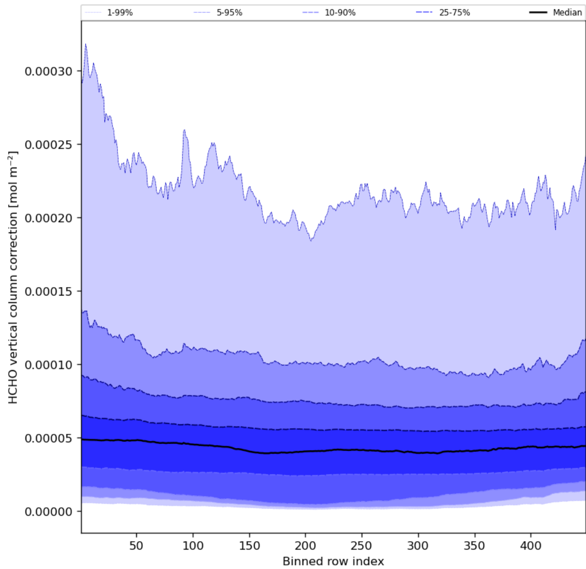
Figure 51: Along track statistics of “HCHO vertical column correction” for 2023-08-01 to 2023-08-03
