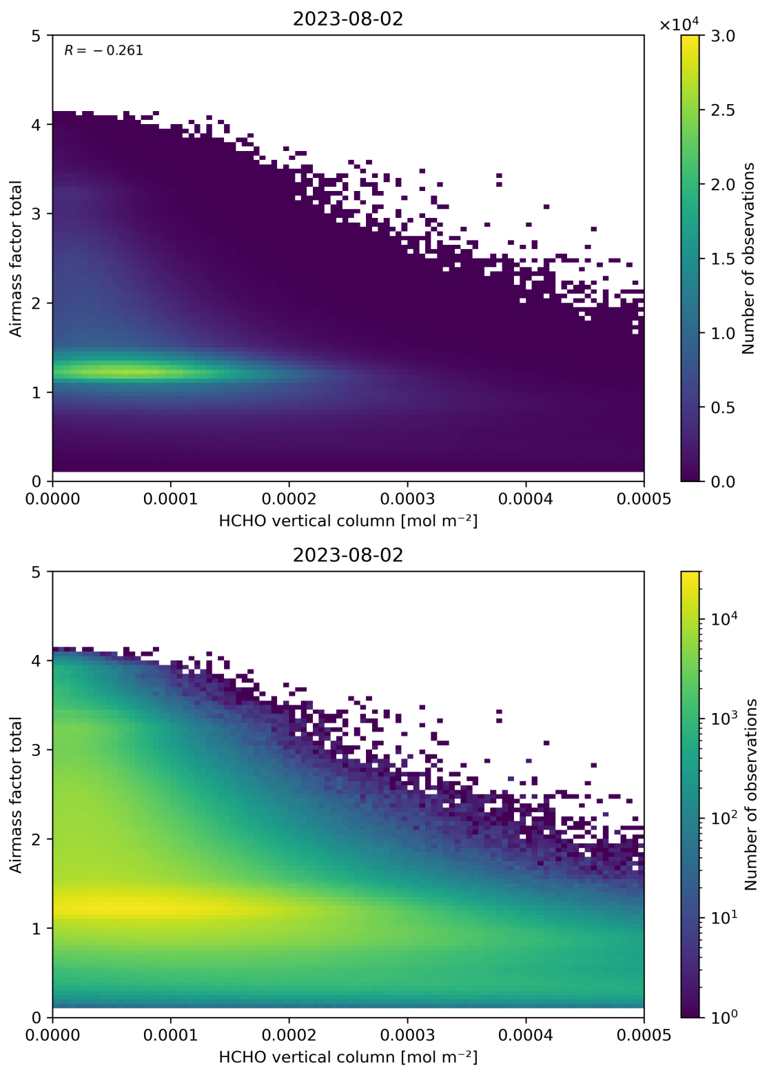
Figure 131: Scatter density plot of “HCHO vertical column” against “Airmass factor total” for 2023-08-01 to 2023-08-03.
