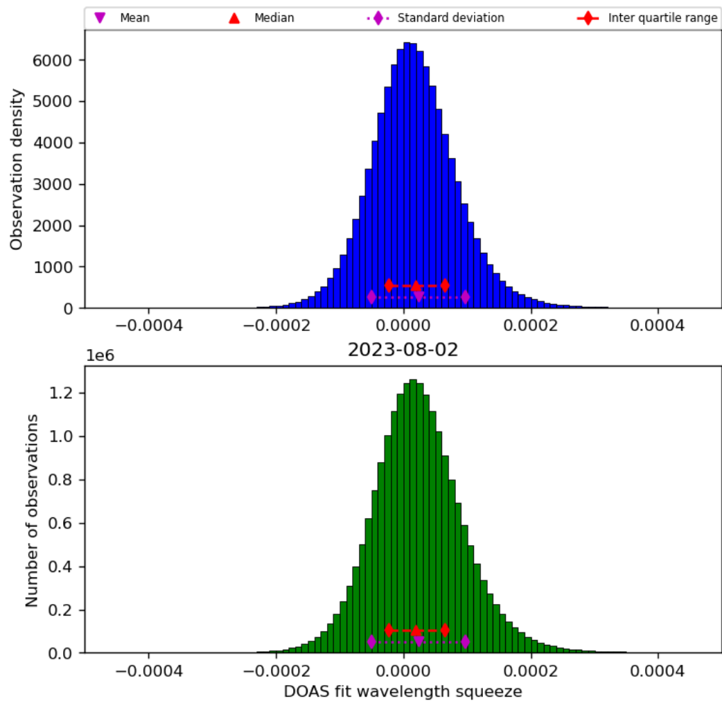
Figure 45: Histogram of “DOAS fit wavelength squeeze” for 2023-08-01 to 2023-08-03
