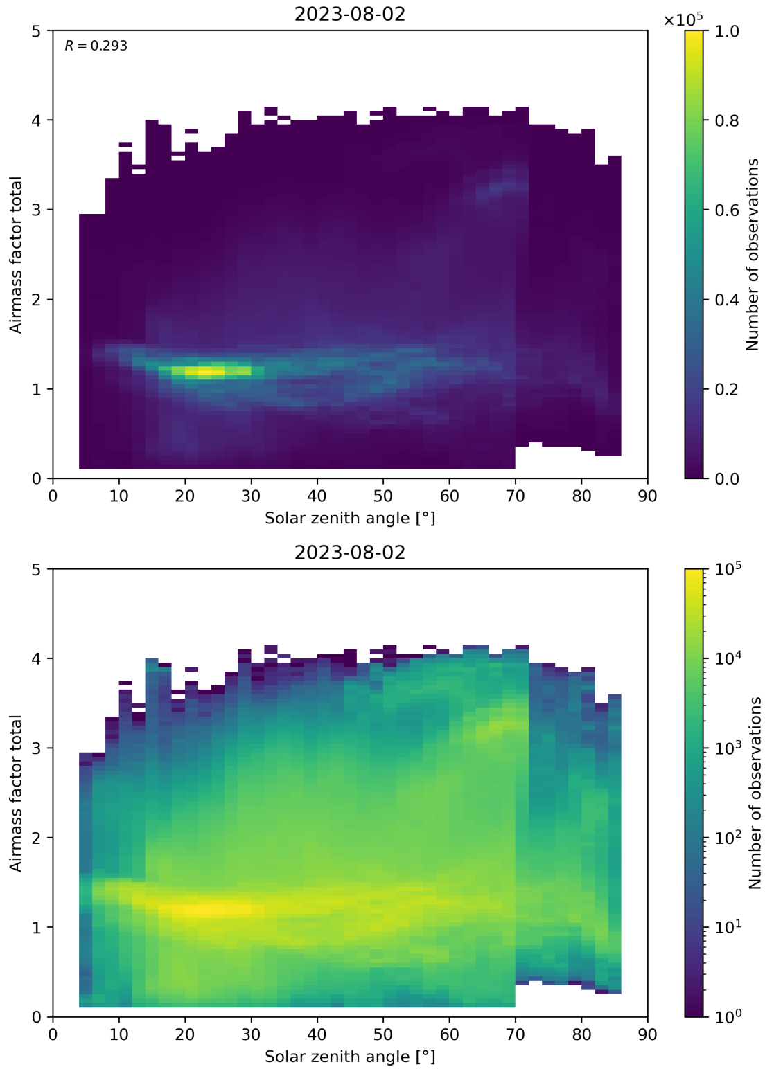
Figure 175: Scatter density plot of “Solar zenith angle” against “Airmass factor total” for 2023-08-01 to 2023-08-03.
