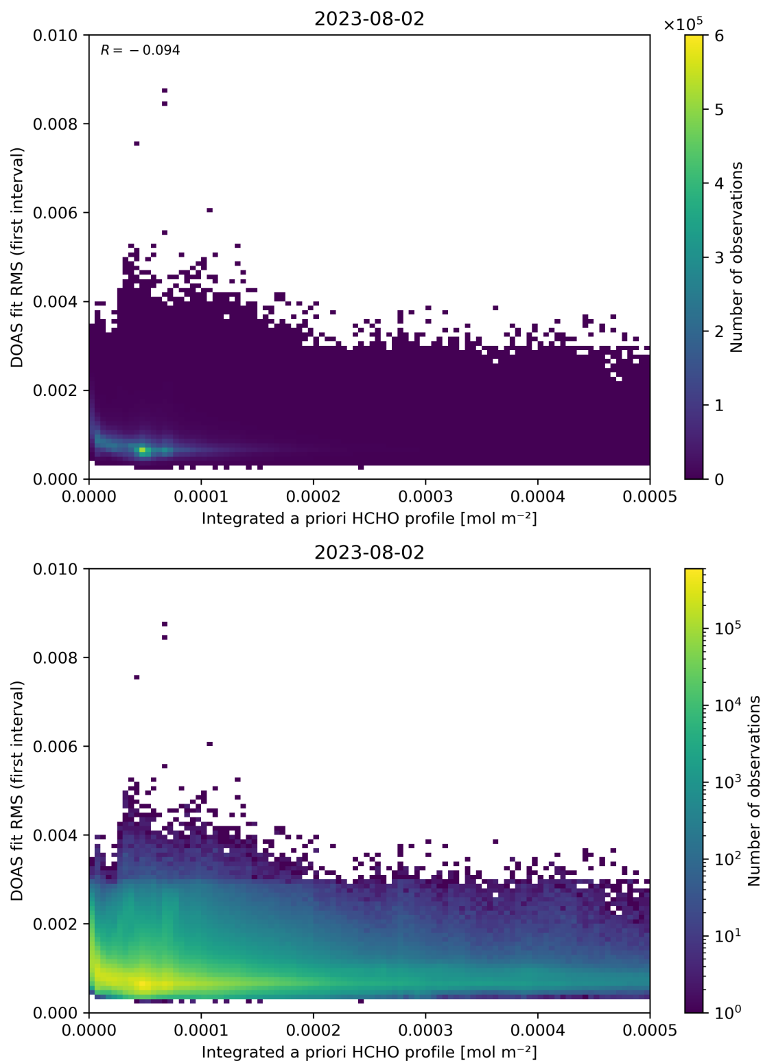
Figure 148: Scatter density plot of “Integrated a priori HCHO profile” against “DOAS fit RMS (first interval)” for 2023-08-01 to 2023-08-03.
