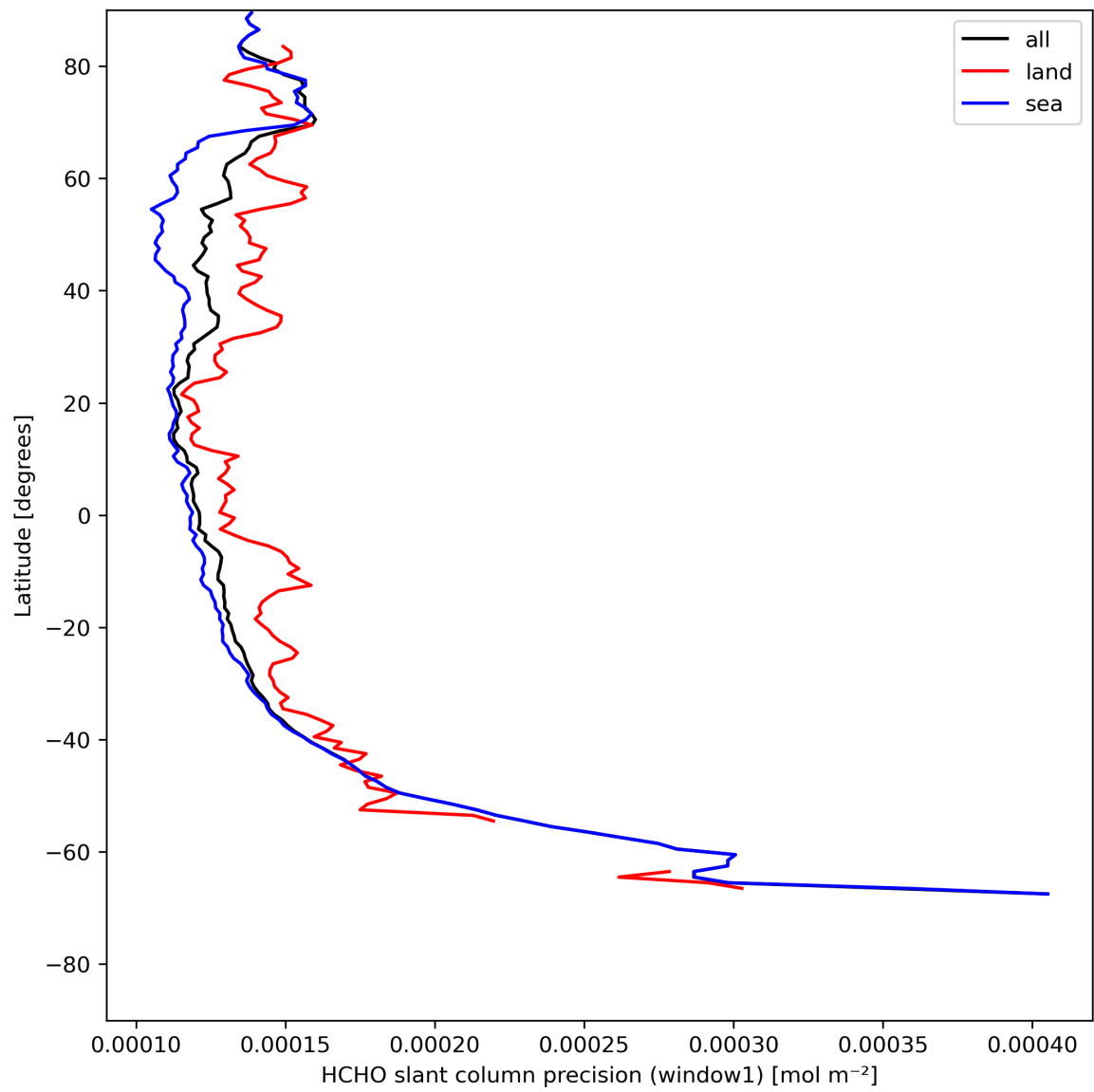
Figure 25: Zonal average of “HCHO slant column precision (window1)” for 2023-08-01 to 2023-08-03.
