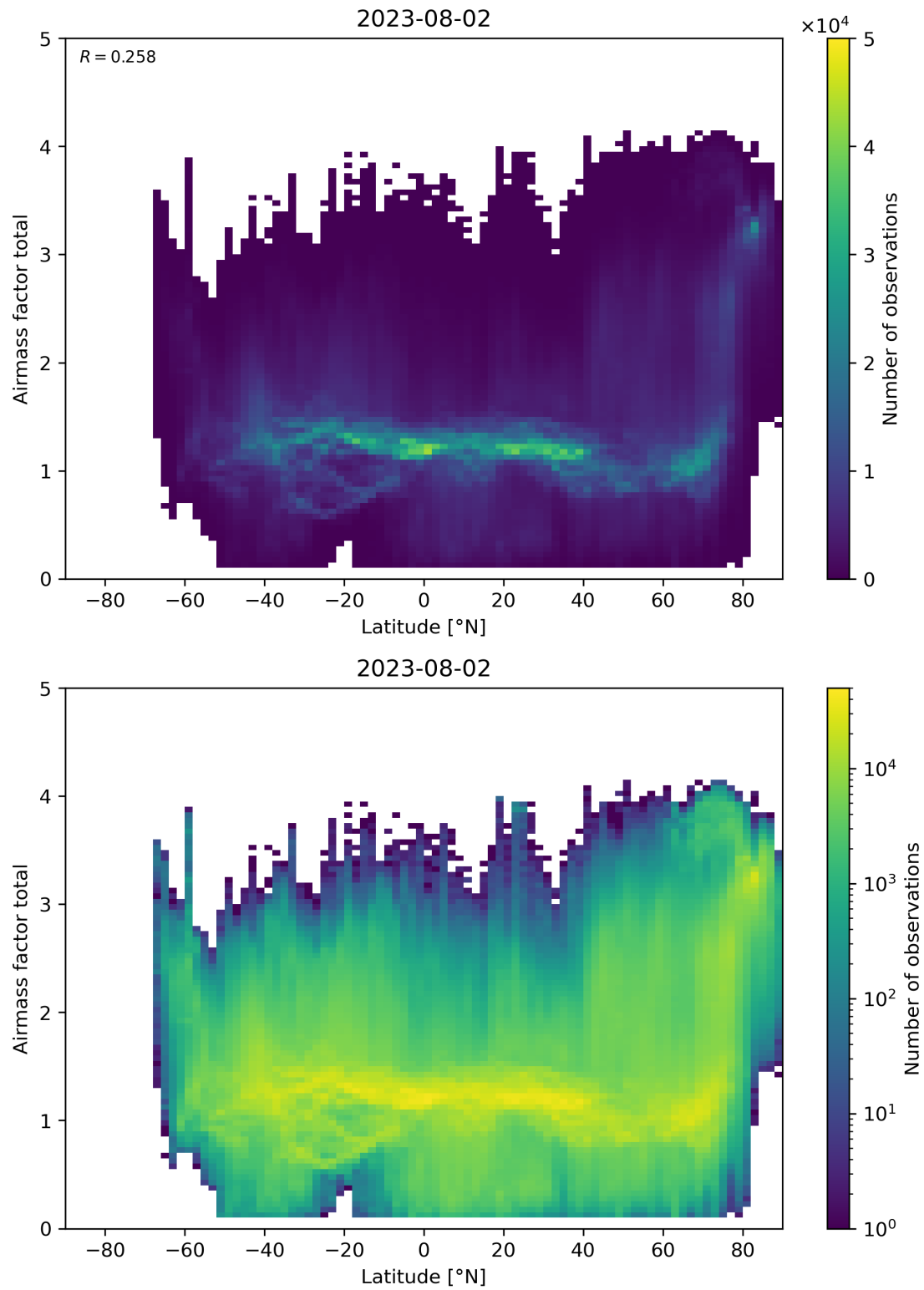
Figure 161: Scatter density plot of “Latitude” against “Airmass factor total” for 2023-08-01 to 2023-08-03.
