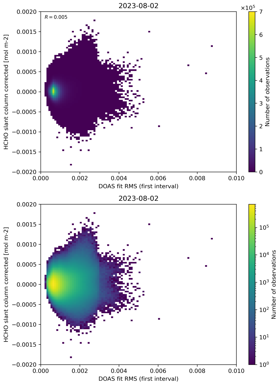
Figure 62: Scatter density plot of “DOAS fit RMS (first interval)” against “HCHO slant column corrected” for 2023-08-01 to 2023-08-03.
