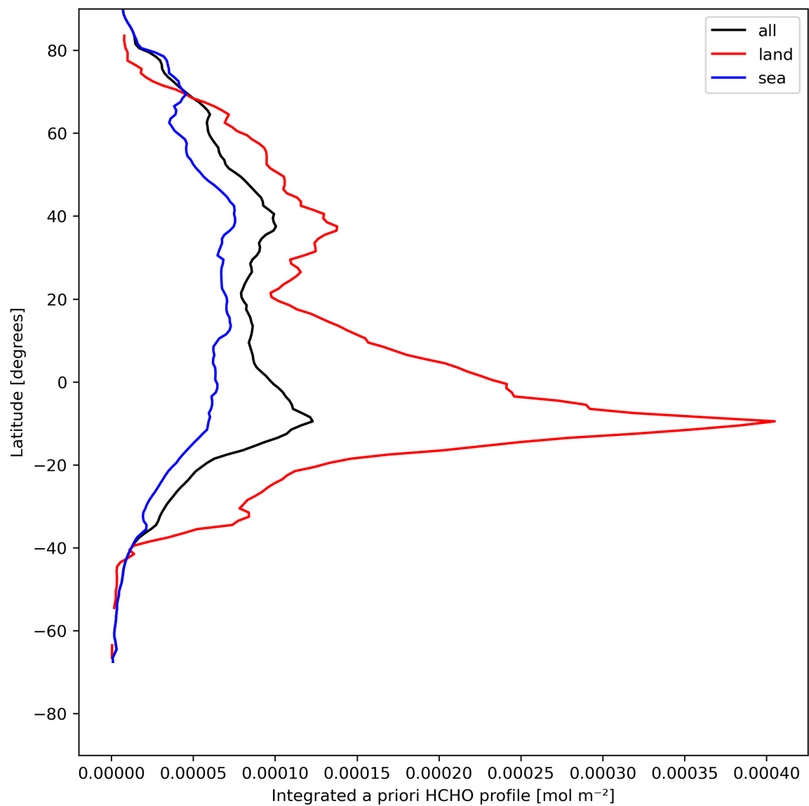
Figure 29: Zonal average of “Integrated a priori HCHO profile” for 2023-08-01 to 2023-08-03.
