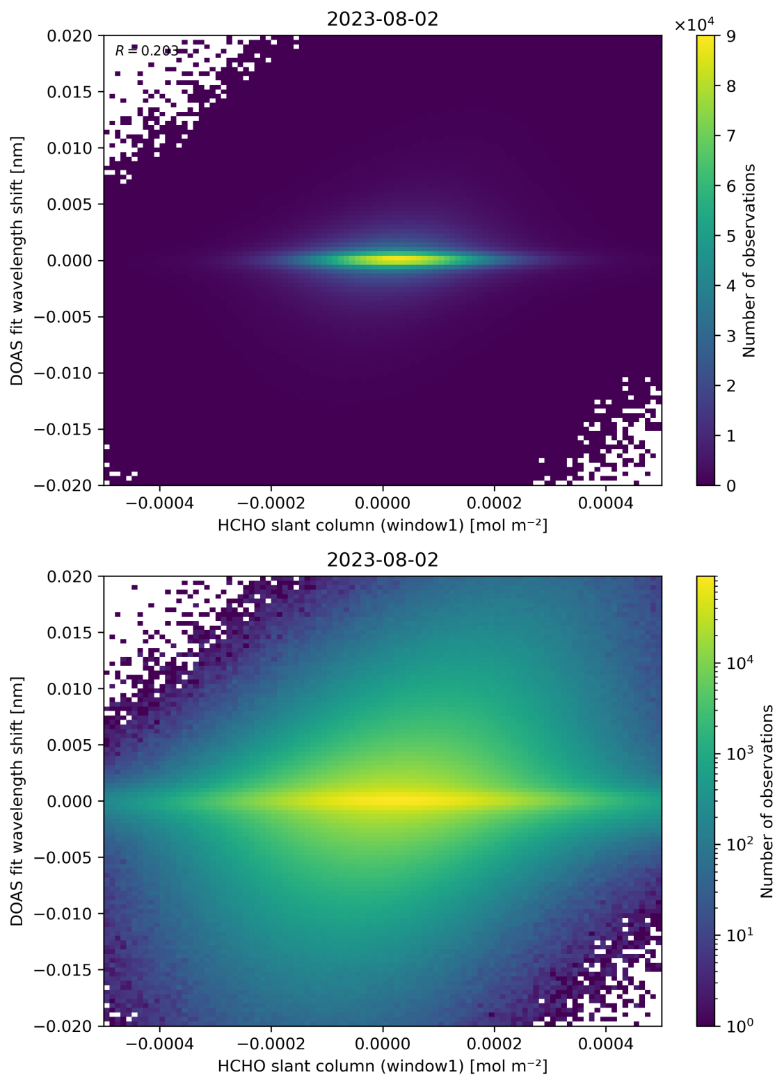
Figure 79: Scatter density plot of “HCHO slant column (window1)” against “DOAS fit wavelength shift” for 2023-08-01 to 2023-08-03.
