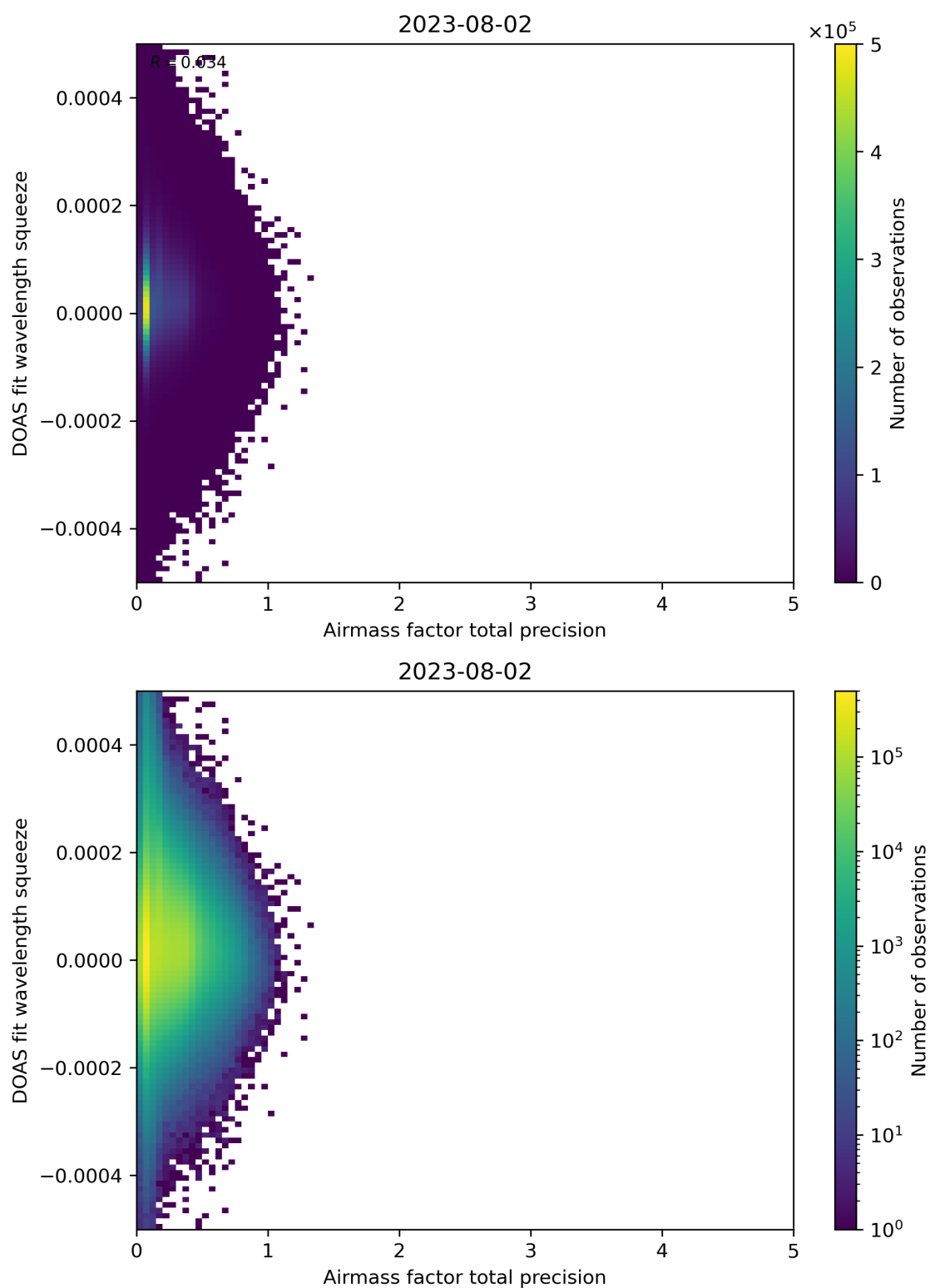
Figure 107: Scatter density plot of “Airmass factor total precision” against “DOAS fit wavelength squeeze” for 2023-08-01 to 2023-08-03.
