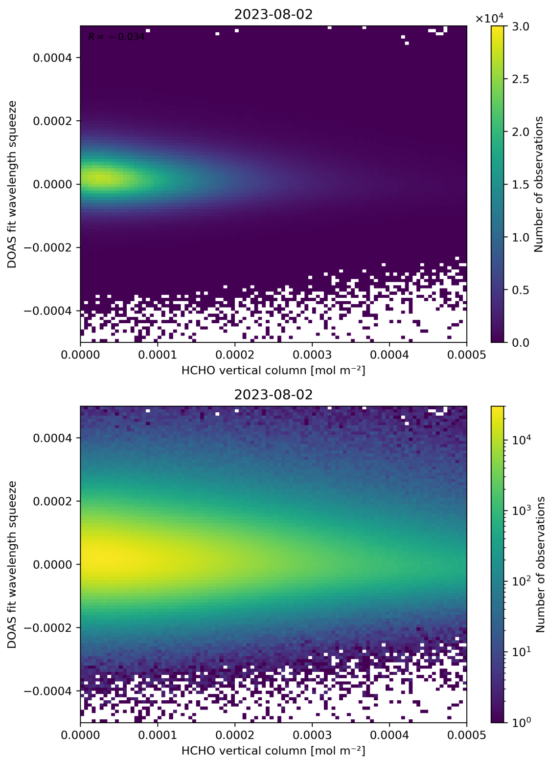
Figure 125: Scatter density plot of “HCHO vertical column” against “DOAS fit wavelength squeeze” for 2023-08-01 to 2023-08-03.
