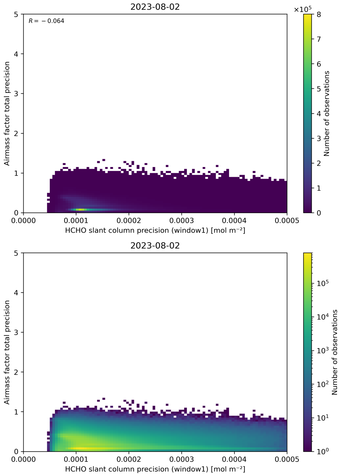
Figure 95: Scatter density plot of “HCHO slant column precision (window1)” against “Airmass factor total precision” for 2023-08-01 to 2023-08-03.
