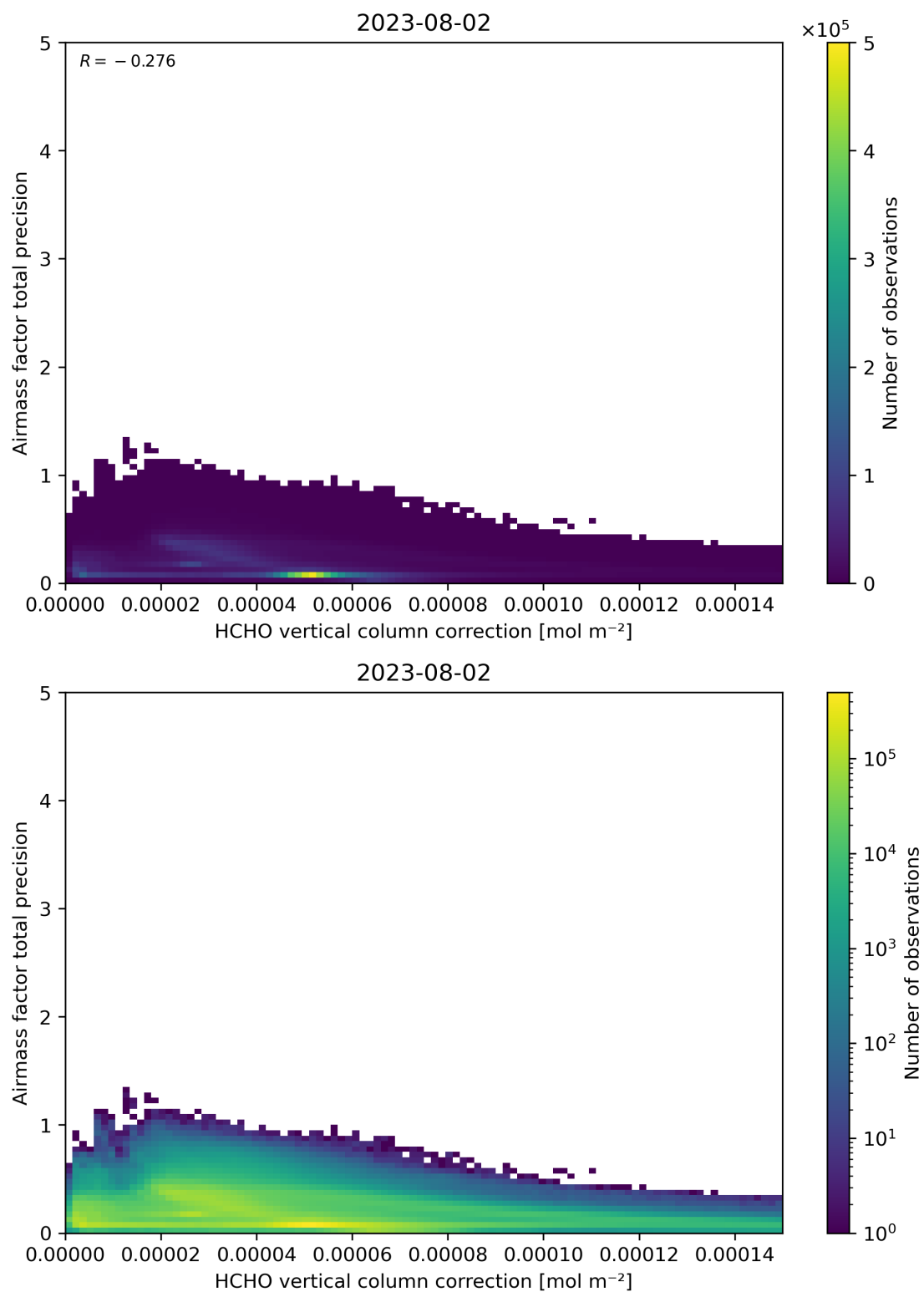
Figure 121: Scatter density plot of “HCHO vertical column correction” against “Airmass factor total precision” for 2023-08-01 to 2023-08-03.
