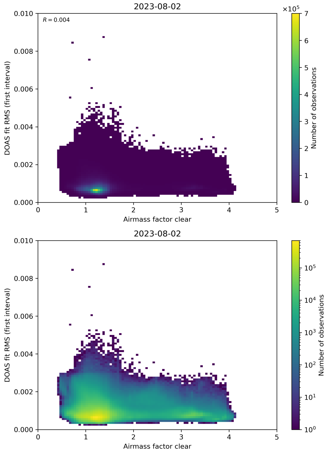
Figure 71: Scatter density plot of “Airmass factor clear” against “DOAS fit RMS (first interval)” for 2023-08-01 to 2023-08-03.
