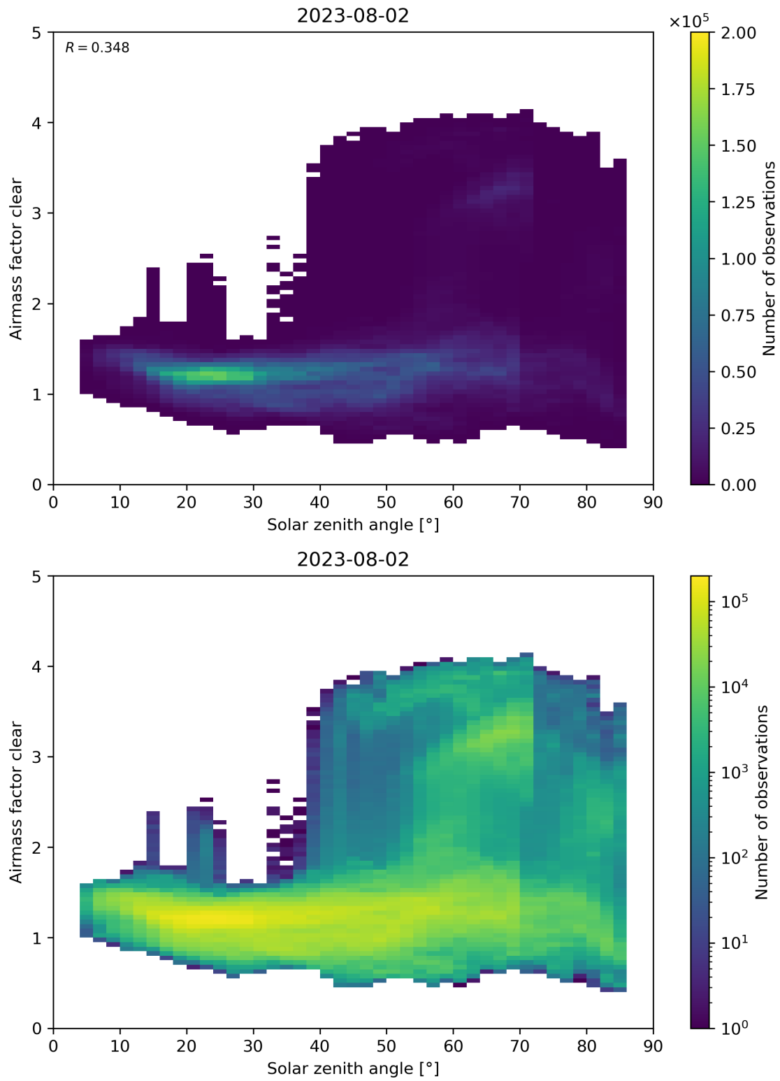
Figure 170: Scatter density plot of “Solar zenith angle” against “Airmass factor clear” for 2023-08-01 to 2023-08-03.
