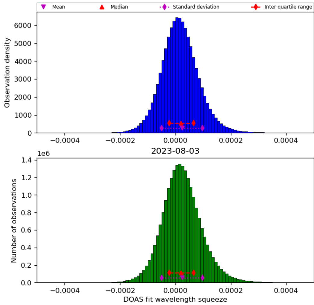
Figure 45: Histogram of “DOAS fit wavelength squeeze” for 2023-08-02 to 2023-08-04
