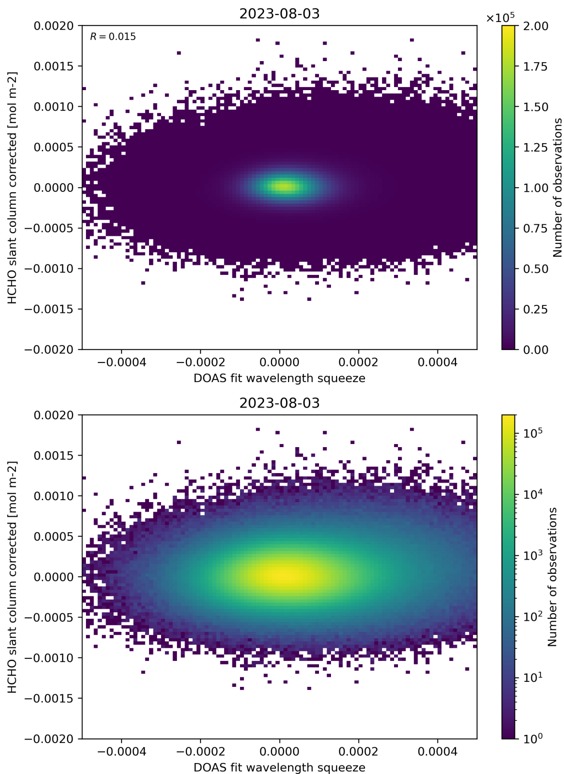
Figure 69: Scatter density plot of “DOAS fit wavelength squeeze” against “HCHO slant column corrected” for 2023-08-02 to 2023-08-04.
