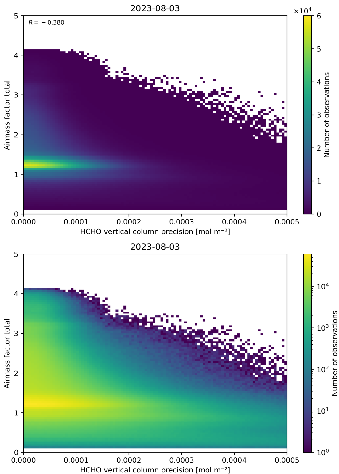
Figure 144: Scatter density plot of “HCHO vertical column precision” against “Airmass factor total” for 2023-08-02 to 2023-08-04.
