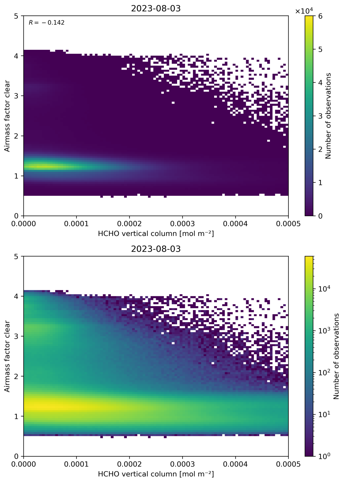
Figure 126: Scatter density plot of “HCHO vertical column” against “Airmass factor clear” for 2023-08-02 to 2023-08-04.
