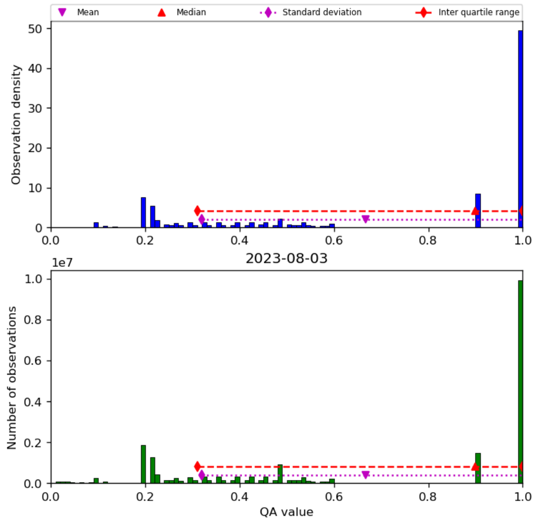
Figure 34: Histogram of “QA value” for 2023-08-02 to 2023-08-04
