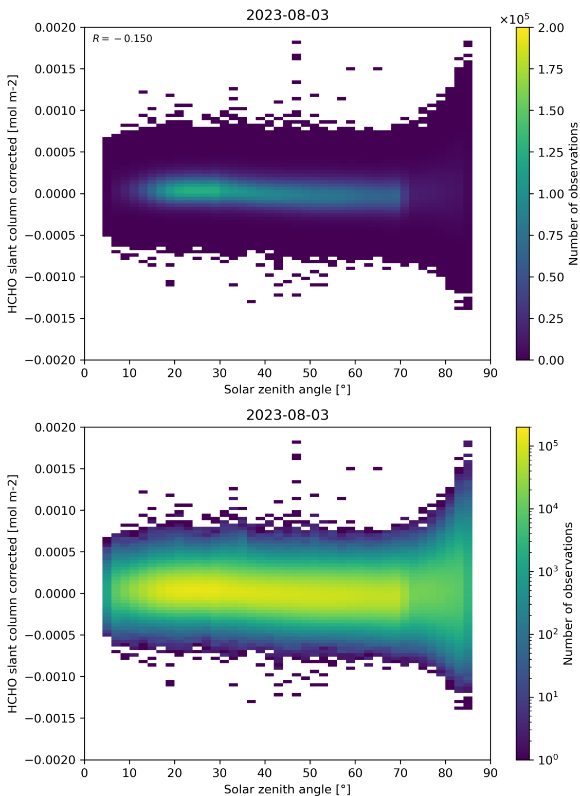
Figure 171: Scatter density plot of “Solar zenith angle” against “HCHO slant column corrected” for 2023-08-02 to 2023-08-04.
