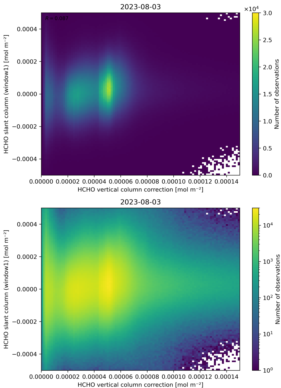
Figure 118: Scatter density plot of “HCHO vertical column correction” against “HCHO slant column (window1)” for 2023-08-02 to 2023-08-04.
