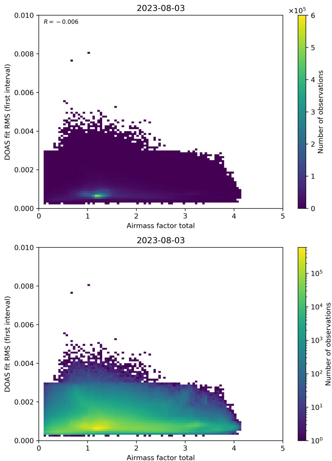
Figure 97: Scatter density plot of “Airmass factor total” against “DOAS fit RMS (first interval)” for 2023-08-02 to 2023-08-04.
