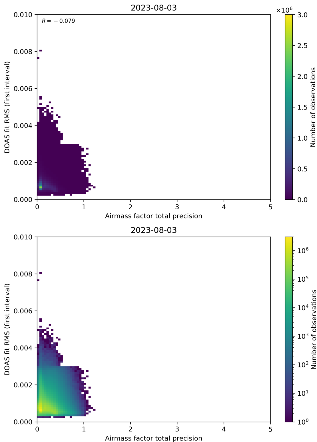
Figure 105: Scatter density plot of “Airmass factor total precision” against “DOAS fit RMS (first interval)” for 2023-08-02 to 2023-08-04.
