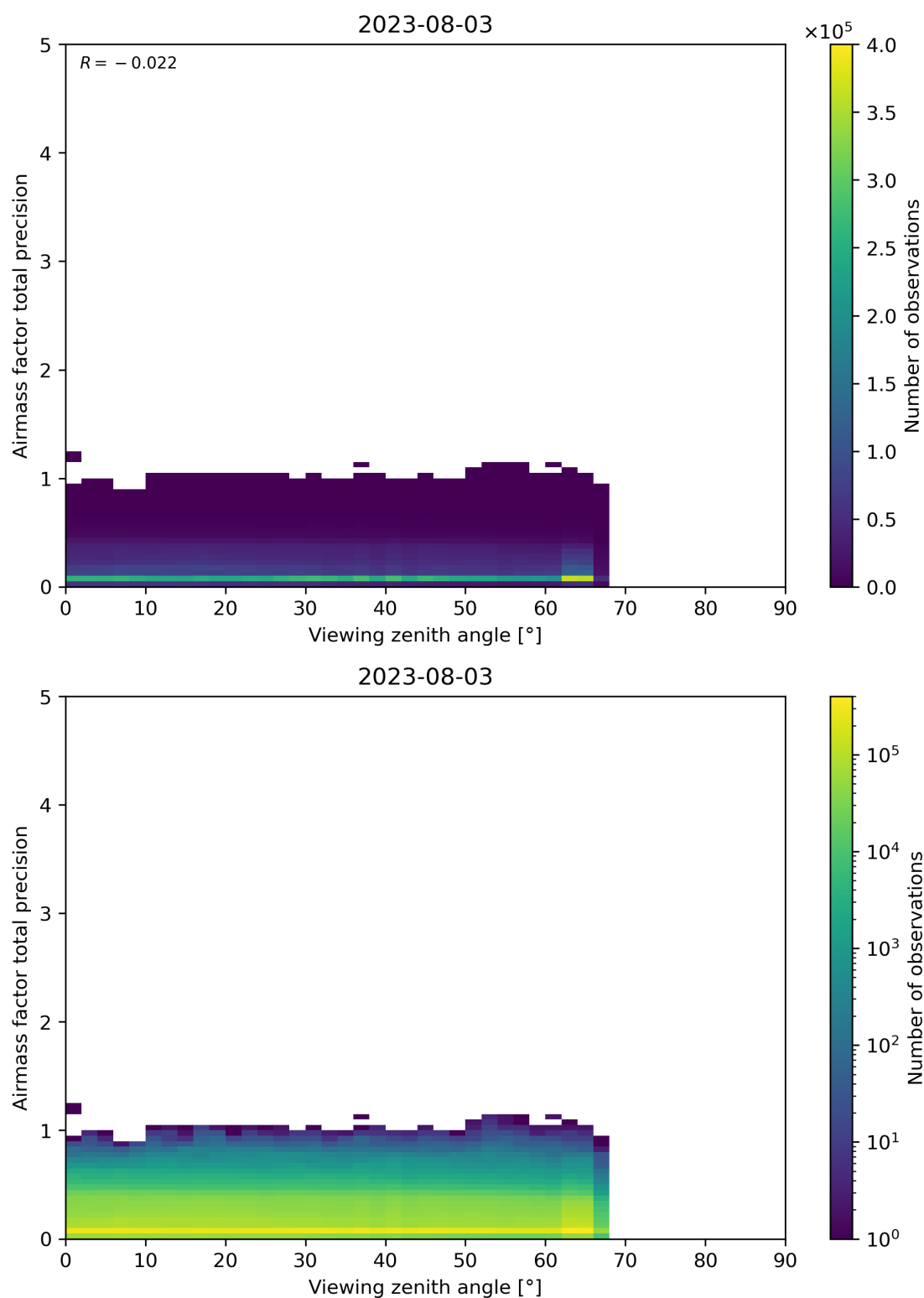
Figure 191: Scatter density plot of “Viewing zenith angle” against “Airmass factor total precision” for 2023-08-02 to 2023-08-04.
