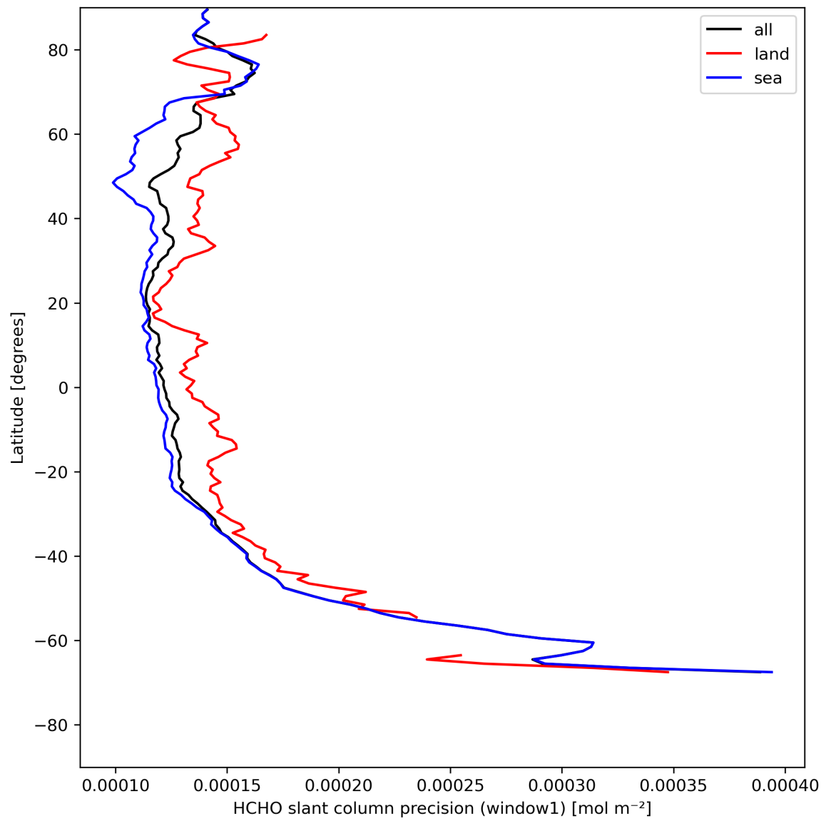
Figure 25: Zonal average of “HCHO slant column precision (window1)” for 2023-08-02 to 2023-08-04.
