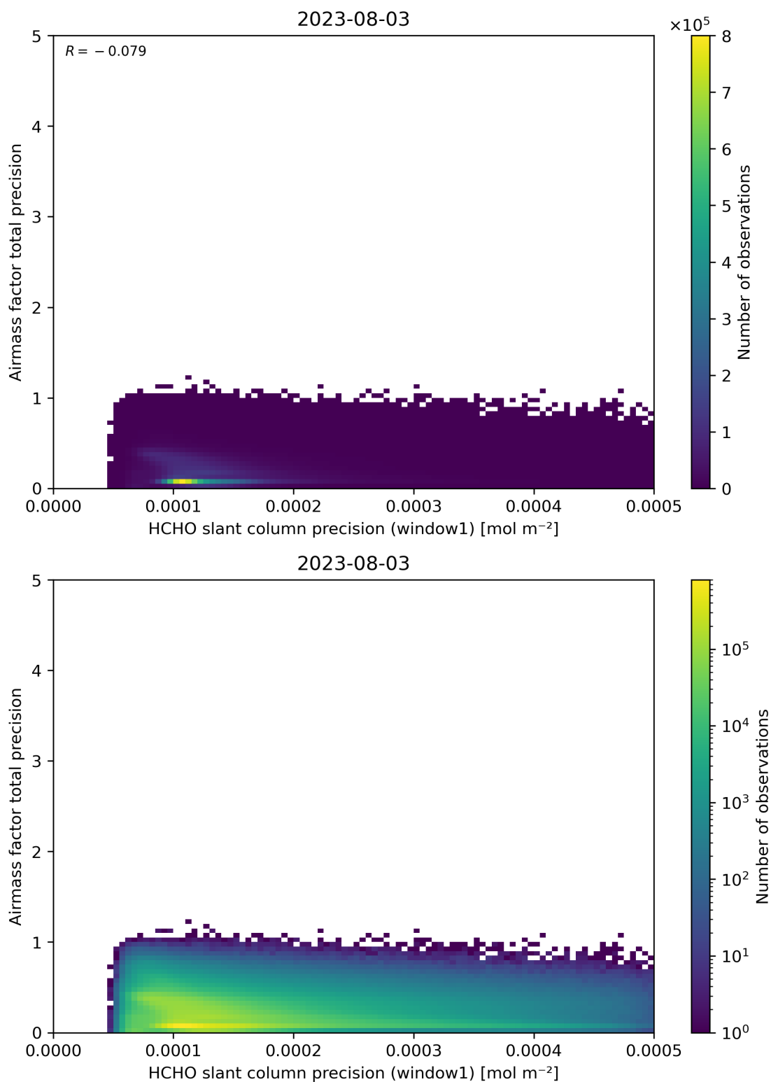
Figure 95: Scatter density plot of “HCHO slant column precision (window1)” against “Airmass factor total precision” for 2023-08-02 to 2023-08-04.
