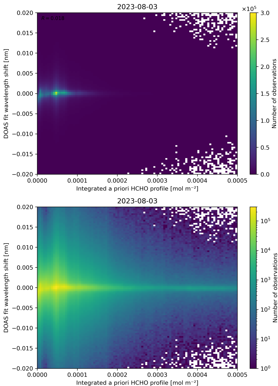
Figure 149: Scatter density plot of “Integrated a priori HCHO profile” against “DOAS fit wavelength shift” for 2023-08-02 to 2023-08-04.
