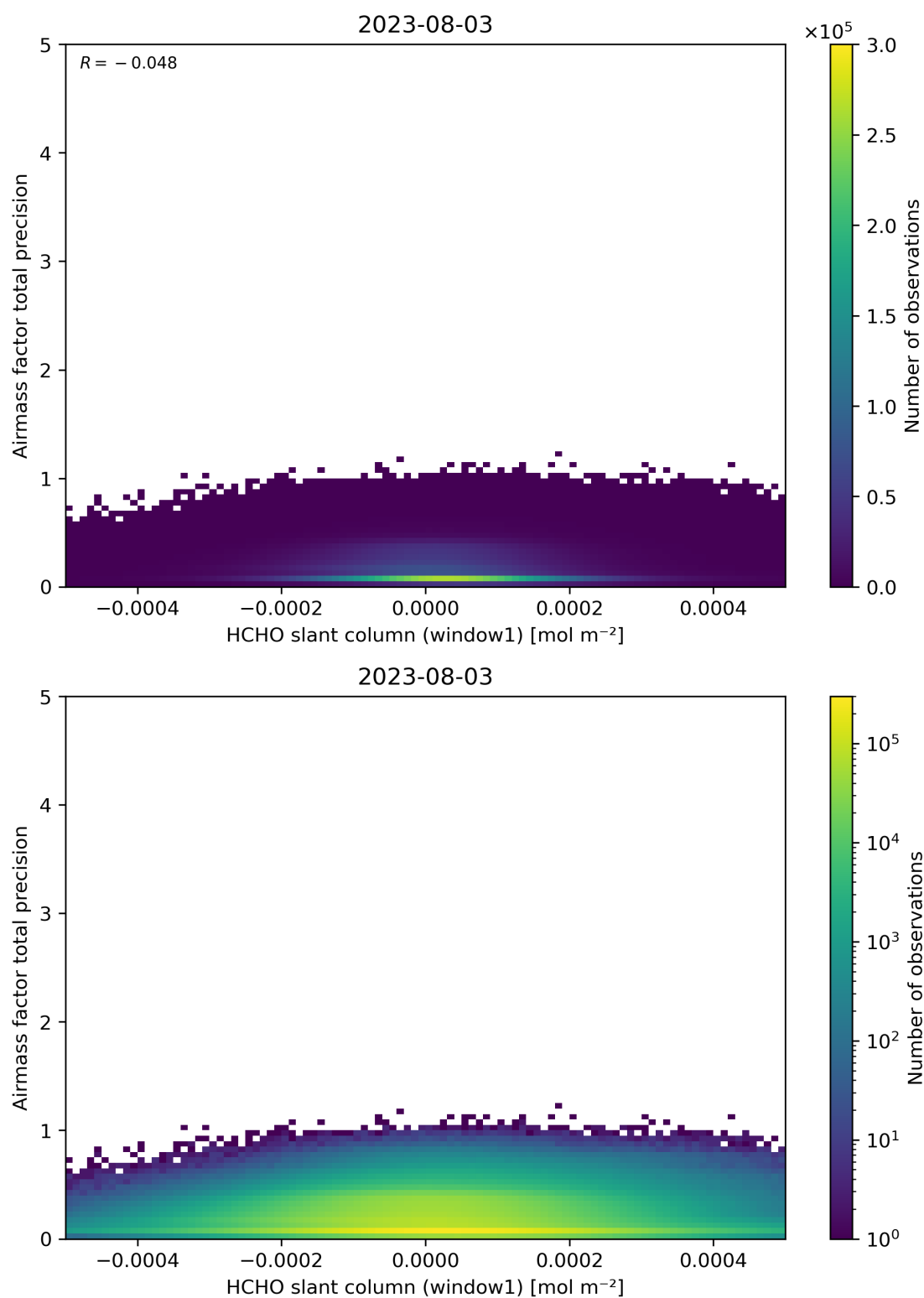
Figure 86: Scatter density plot of “HCHO slant column (window1)” against “Airmass factor total precision” for 2023-08-02 to 2023-08-04.
