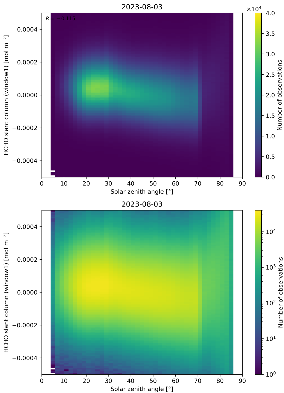
Figure 173: Scatter density plot of “Solar zenith angle” against “HCHO slant column (window1)” for 2023-08-02 to 2023-08-04.
