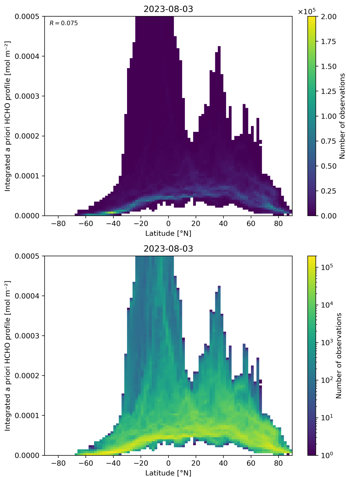
Figure 166: Scatter density plot of “Latitude” against “Integrated a priori HCHO profile” for 2023-08-02 to 2023-08-04.
