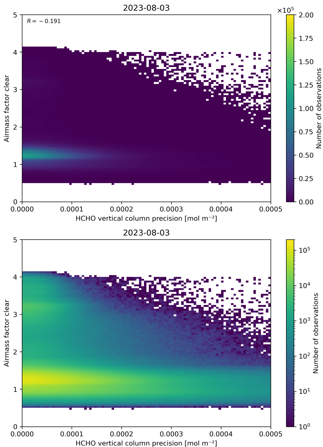
Figure 139: Scatter density plot of “HCHO vertical column precision” against “Airmass factor clear” for 2023-08-02 to 2023-08-04.
