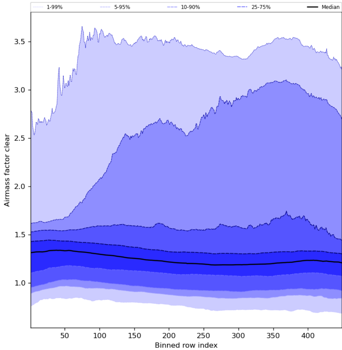
Figure 56: Along track statistics of “Airmass factor clear” for 2023-08-02 to 2023-08-04
