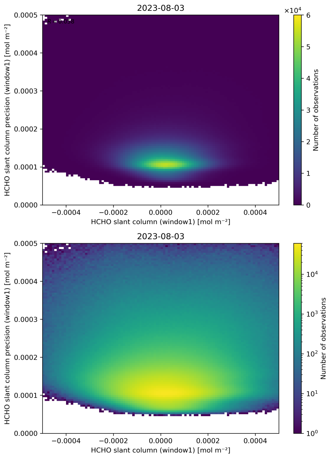
Figure 84: Scatter density plot of “HCHO slant column (window1)” against “HCHO slant column precision (window1)” for 2023-08-02 to 2023-08-04.
