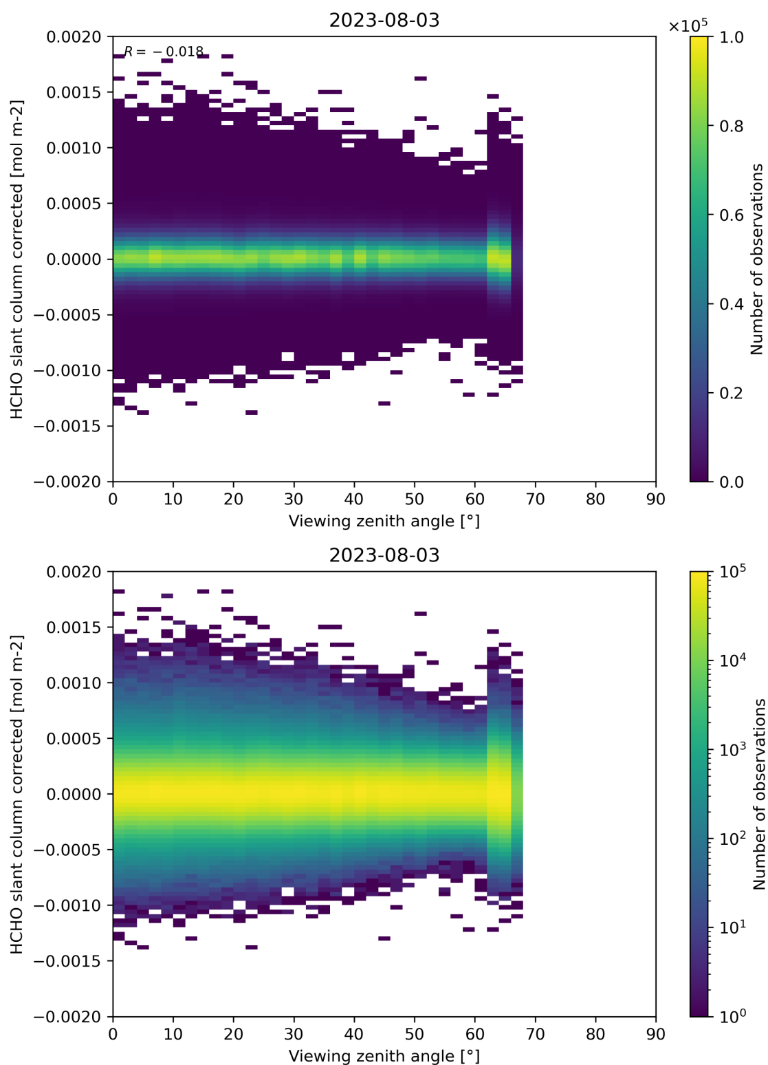
Figure 186: Scatter density plot of “Viewing zenith angle” against “HCHO slant column corrected” for 2023-08-02 to 2023-08-04.
