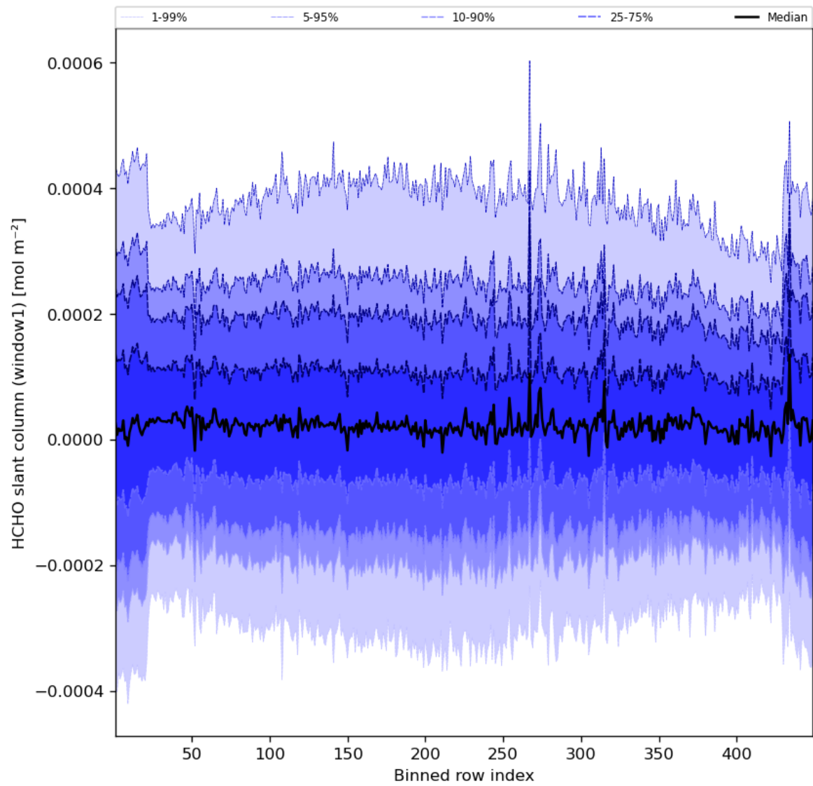
Figure 52: Along track statistics of “HCHO slant column (window1)” for 2023-08-02 to 2023-08-04
