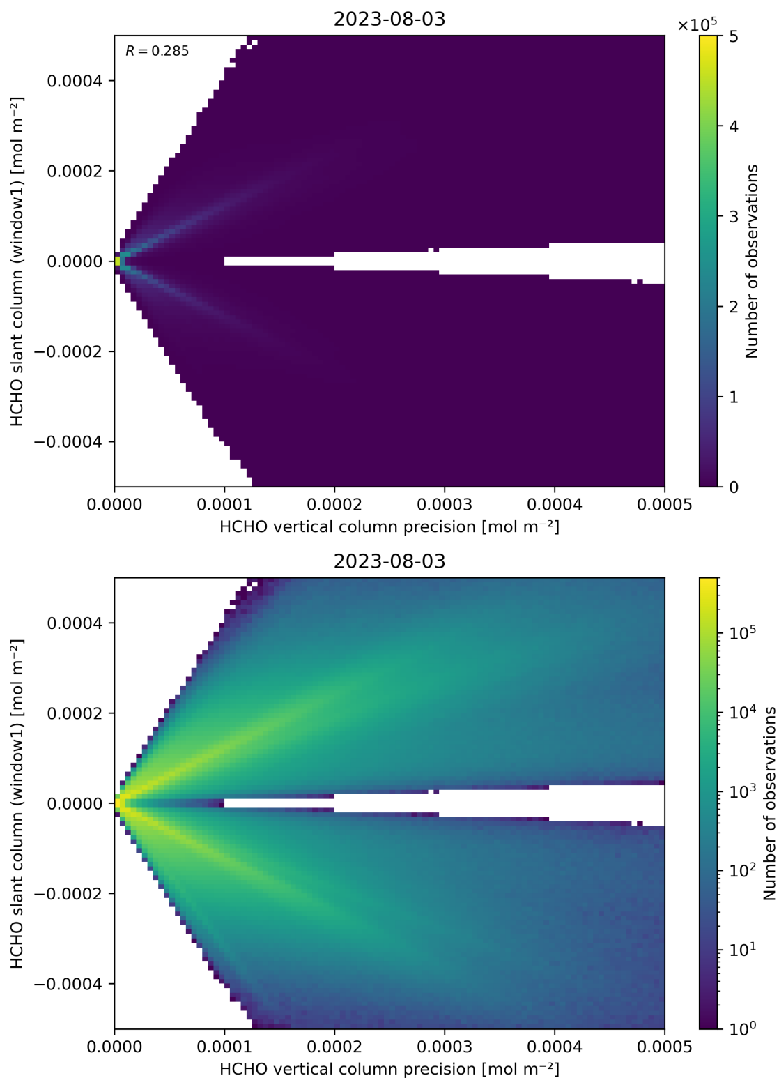
Figure 142: Scatter density plot of “HCHO vertical column precision” against “HCHO slant column (window1)” for 2023-08-02 to 2023-08-04.
