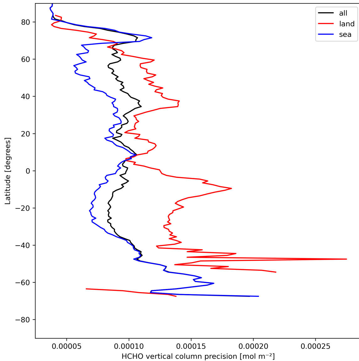
Figure 22: Zonal average of “HCHO vertical column precision” for 2023-08-02 to 2023-08-04.
