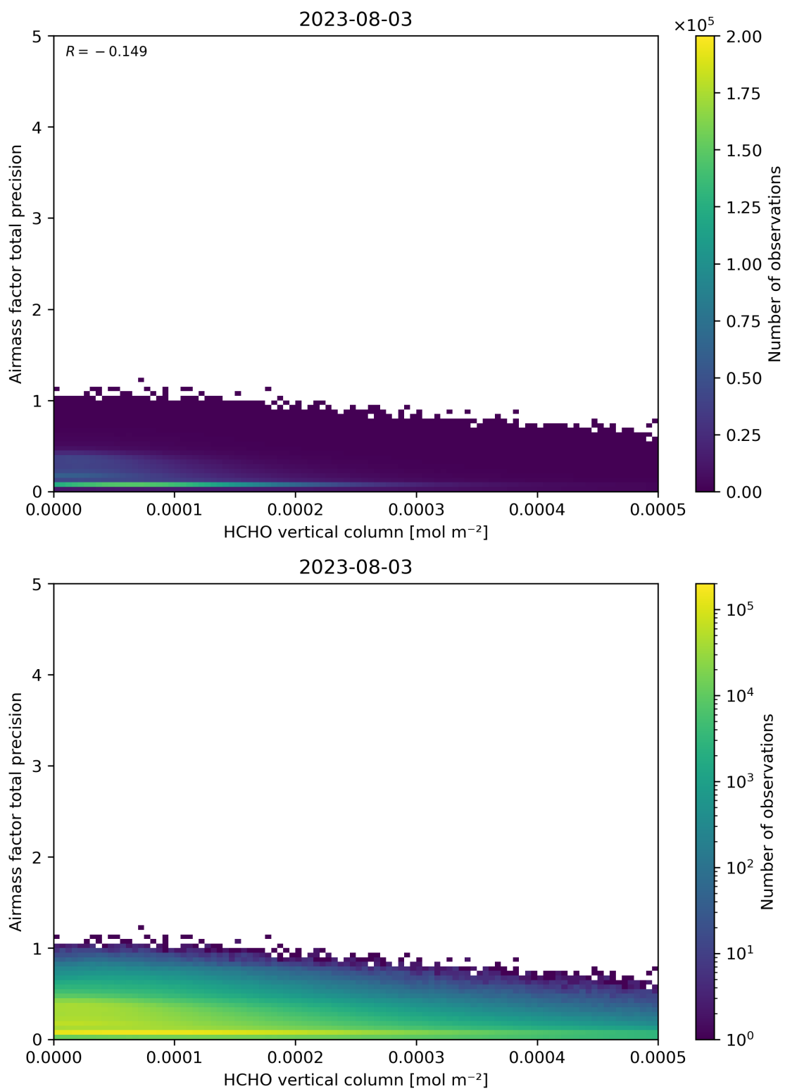
Figure 132: Scatter density plot of “HCHO vertical column” against “Airmass factor total precision” for 2023-08-02 to 2023-08-04.
