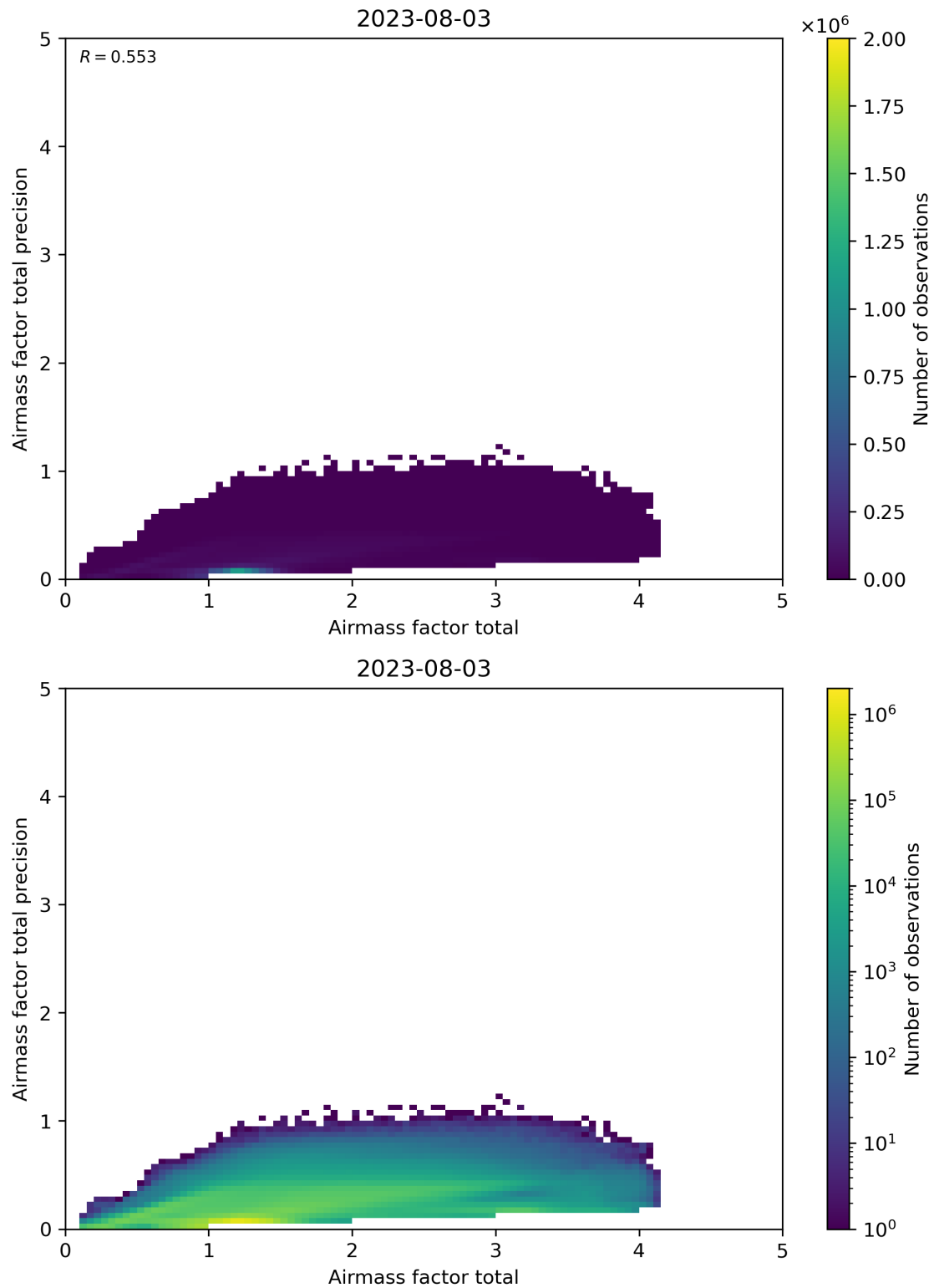
Figure 103: Scatter density plot of “Airmass factor total” against “Airmass factor total precision” for 2023-08-02 to 2023-08-04.
