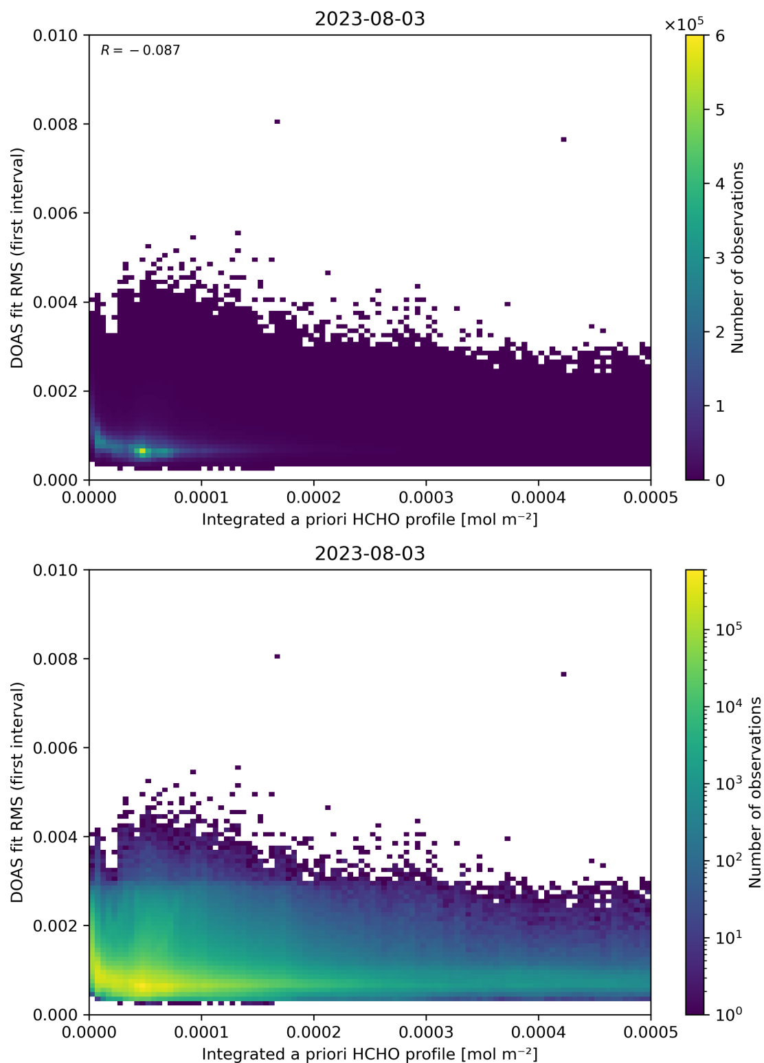
Figure 148: Scatter density plot of “Integrated a priori HCHO profile” against “DOAS fit RMS (first interval)” for 2023-08-02 to 2023-08-04.
