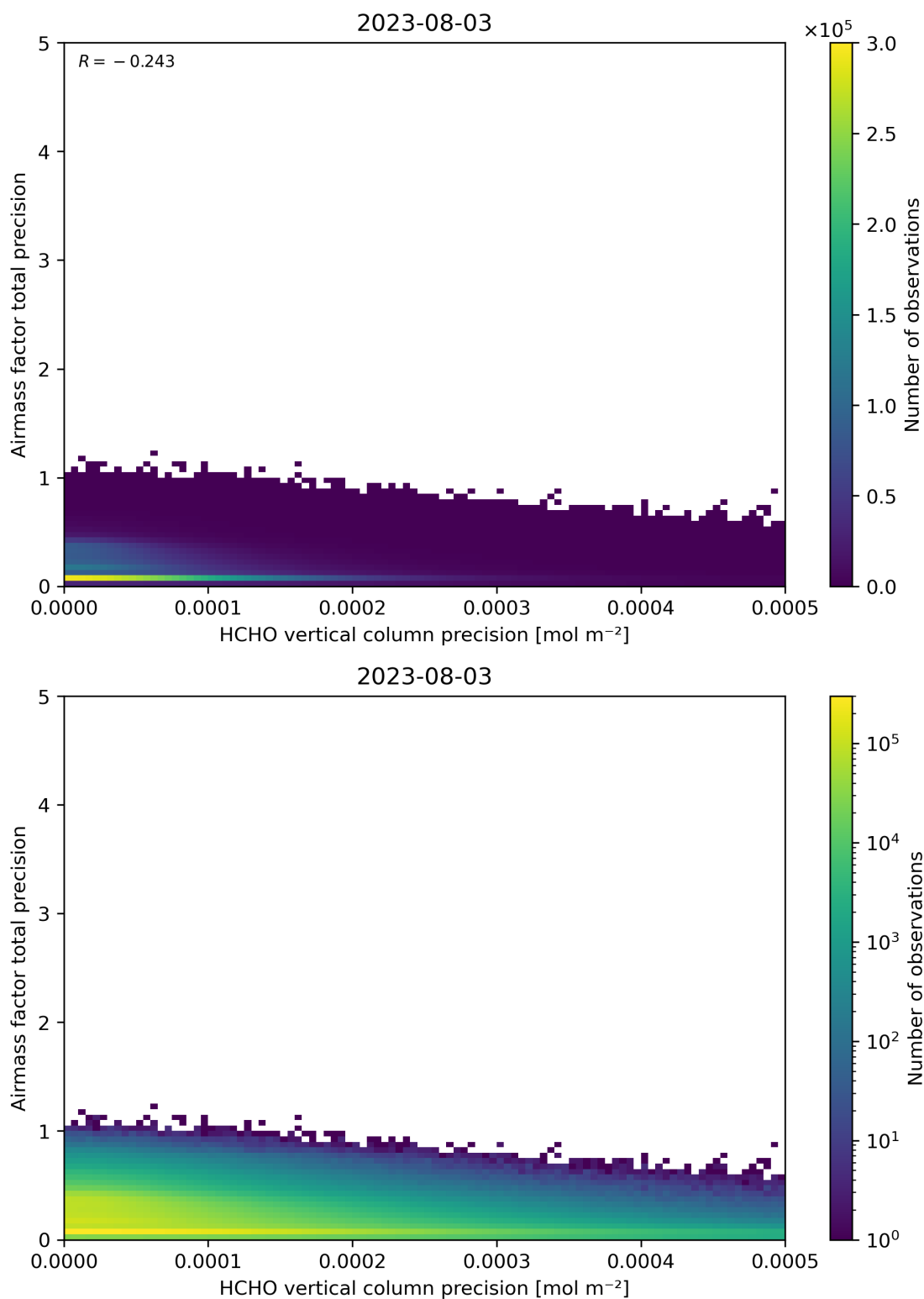
Figure 145: Scatter density plot of “HCHO vertical column precision” against “Airmass factor total precision” for 2023-08-02 to 2023-08-04.
