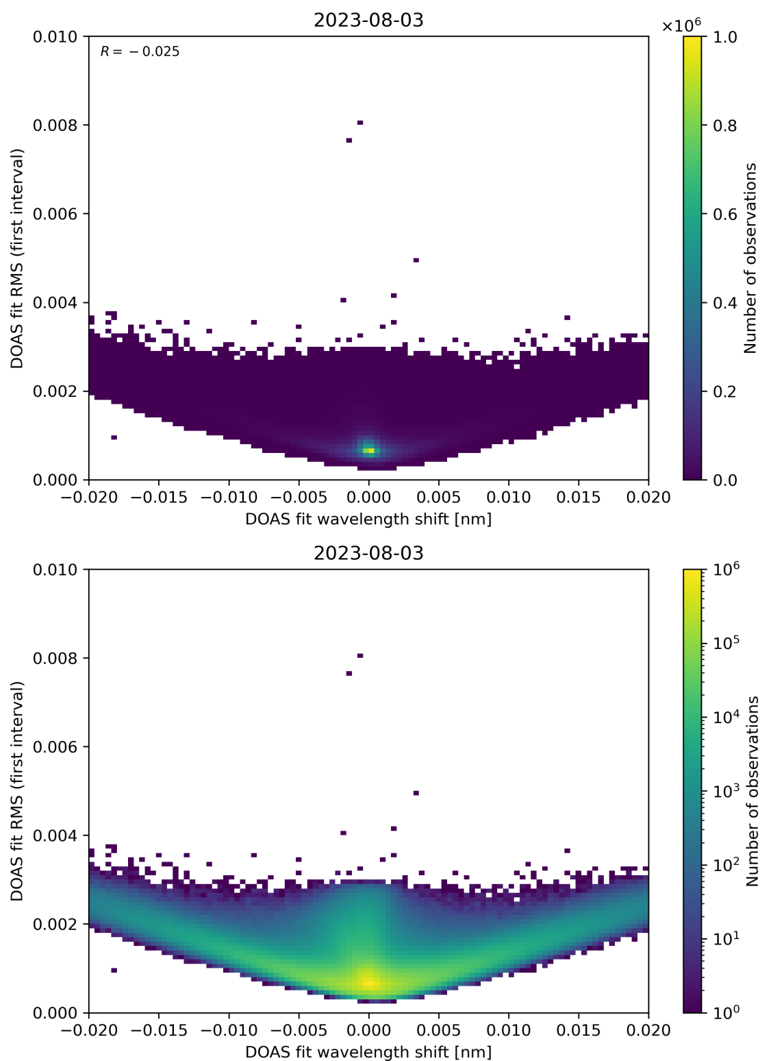
Figure 64: Scatter density plot of “DOAS fit wavelength shift” against “DOAS fit RMS (first interval)” for 2023-08-02 to 2023-08-04.
