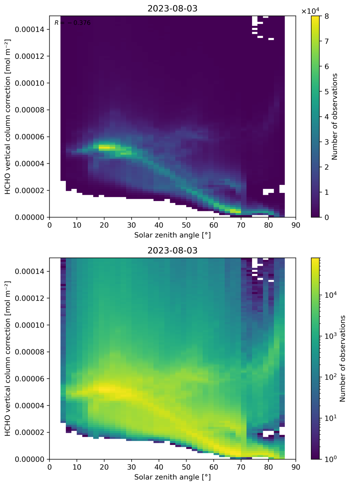
Figure 178: Scatter density plot of “Solar zenith angle” against “HCHO vertical column correction” for 2023-08-02 to 2023-08-04.
