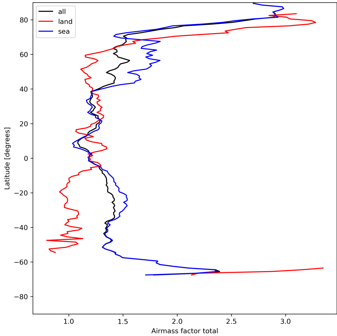
Figure 26: Zonal average of “Airmass factor total” for 2023-08-02 to 2023-08-04.
