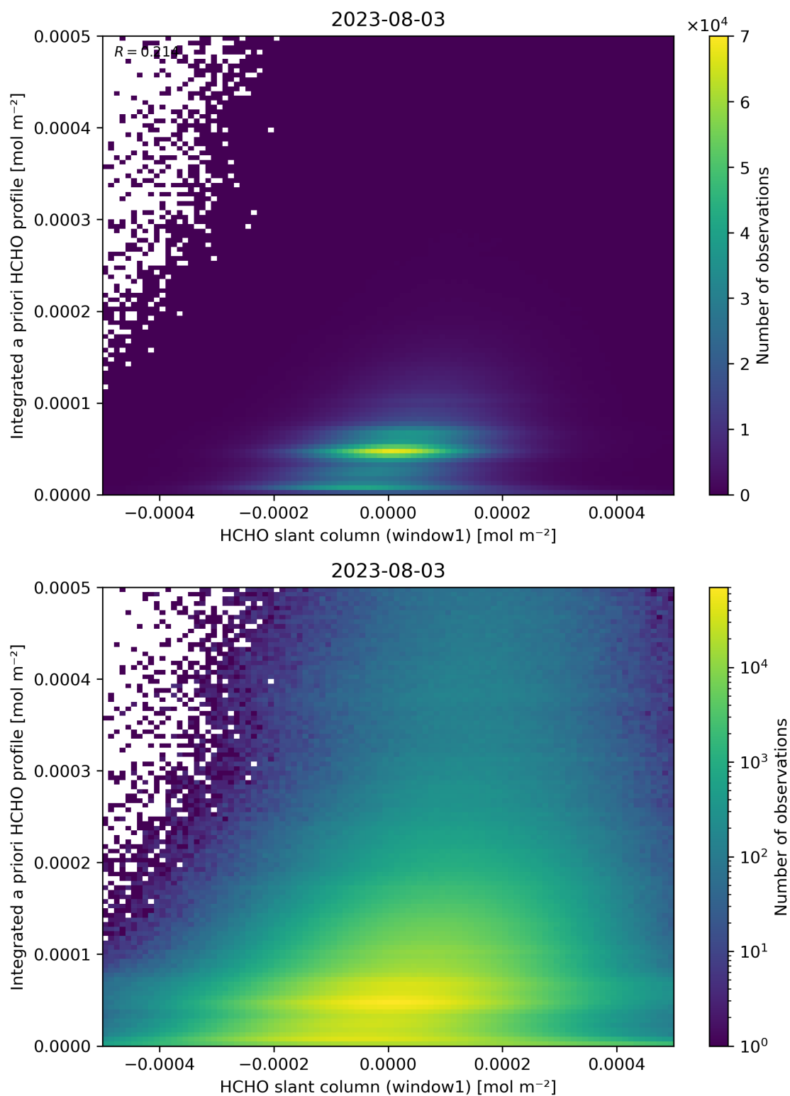
Figure 87: Scatter density plot of “HCHO slant column (window1)” against “Integrated a priori HCHO profile” for 2023-08-02 to 2023-08-04.
