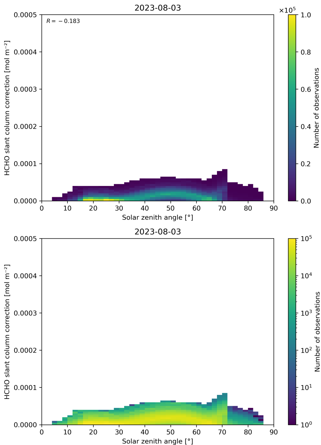
Figure 172: Scatter density plot of “Solar zenith angle” against “HCHO slant column correction” for 2023-08-02 to 2023-08-04.
