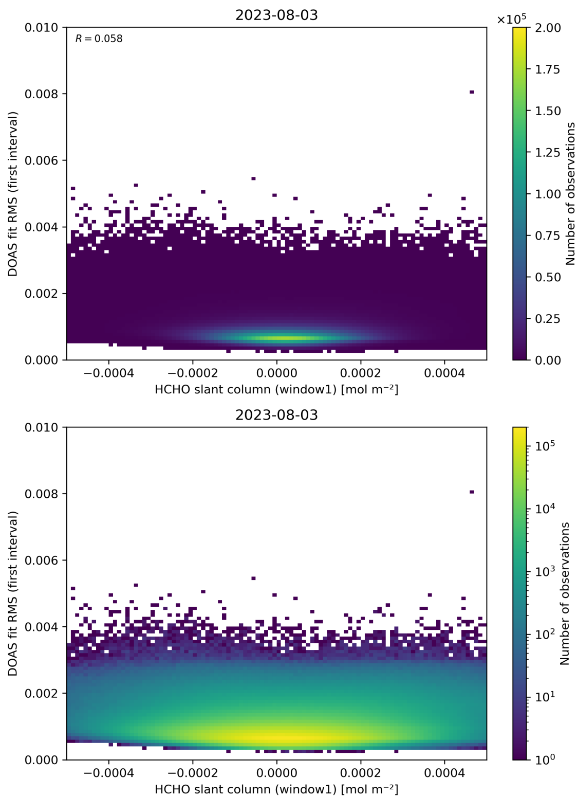
Figure 78: Scatter density plot of “HCHO slant column (window1)” against “DOAS fit RMS (first interval)” for 2023-08-02 to 2023-08-04.
