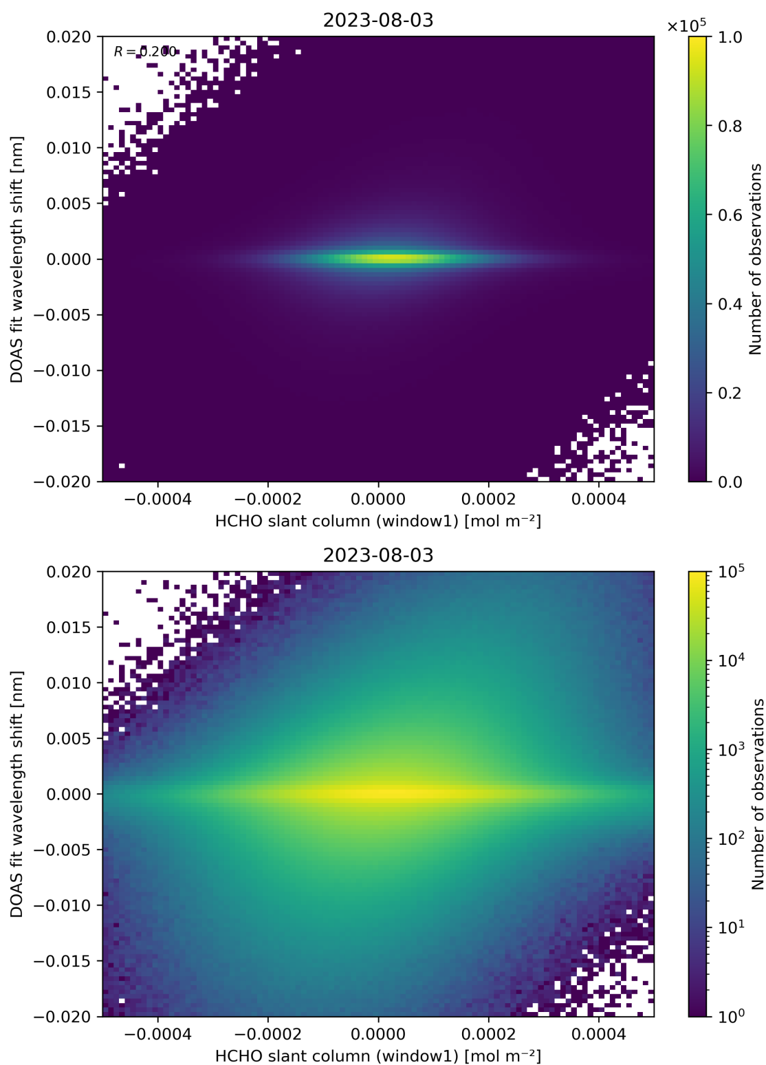
Figure 79: Scatter density plot of “HCHO slant column (window1)” against “DOAS fit wavelength shift” for 2023-08-02 to 2023-08-04.
