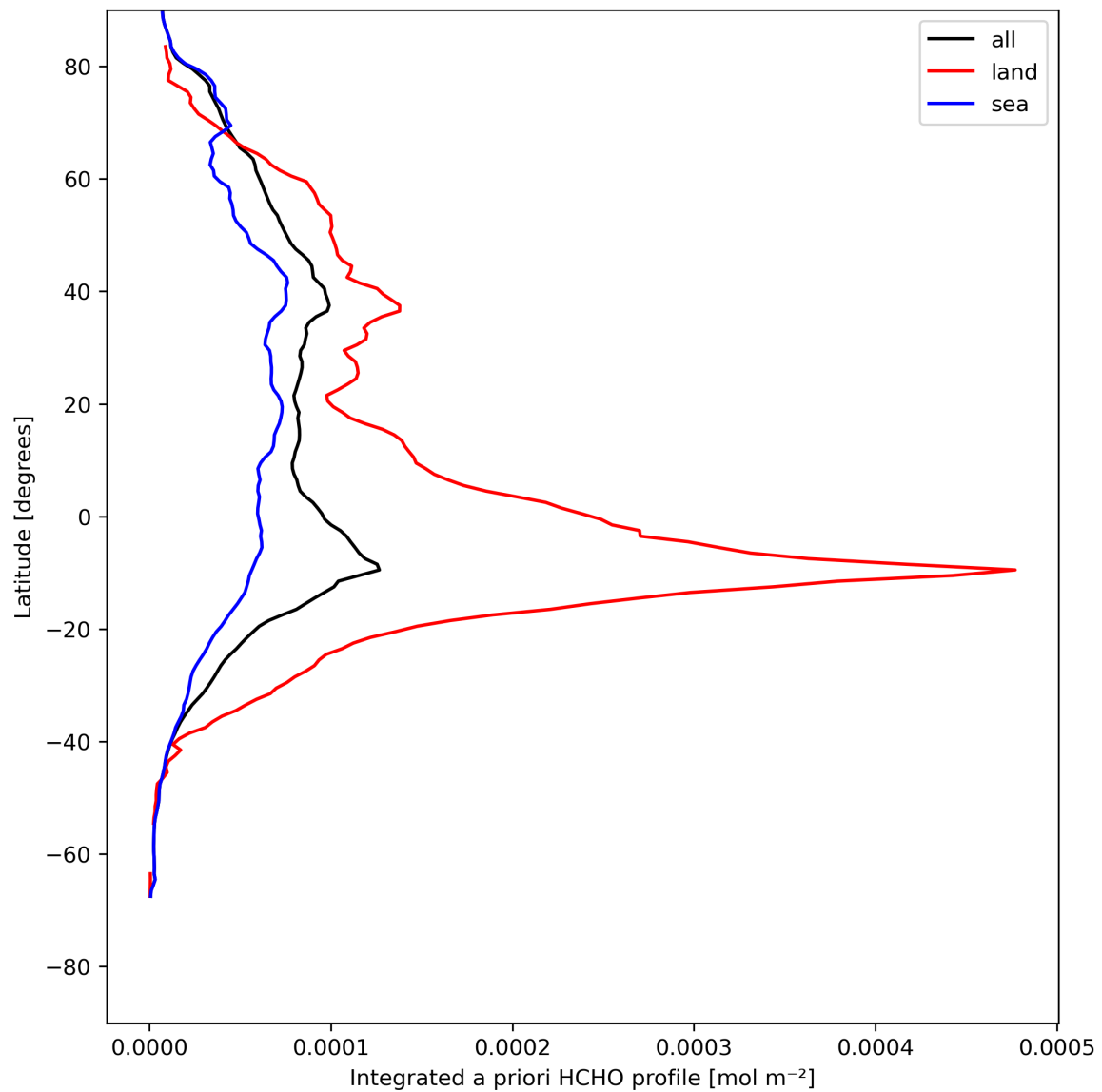
Figure 29: Zonal average of “Integrated a priori HCHO profile” for 2023-08-02 to 2023-08-04.
