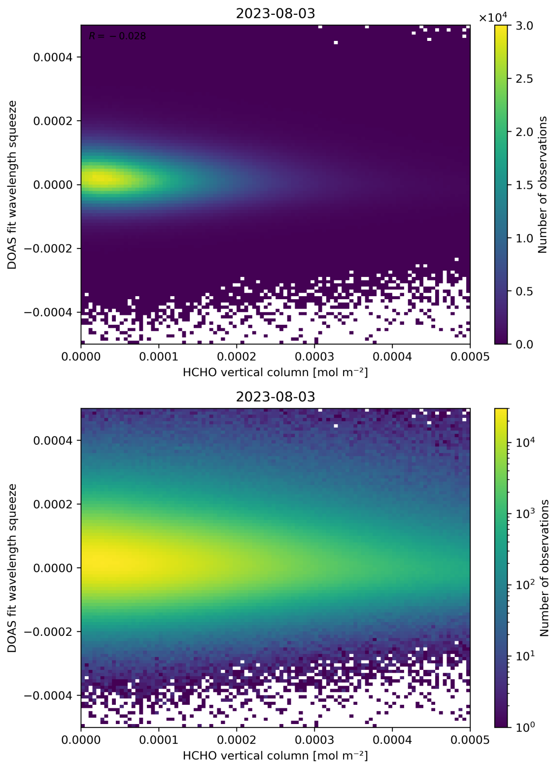
Figure 125: Scatter density plot of “HCHO vertical column” against “DOAS fit wavelength squeeze” for 2023-08-02 to 2023-08-04.
