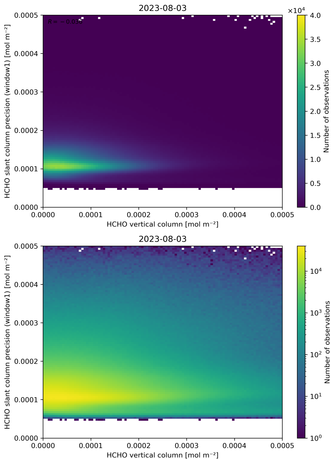
Figure 130: Scatter density plot of “HCHO vertical column” against “HCHO slant column precision (window1)” for 2023-08-02 to 2023-08-04.
