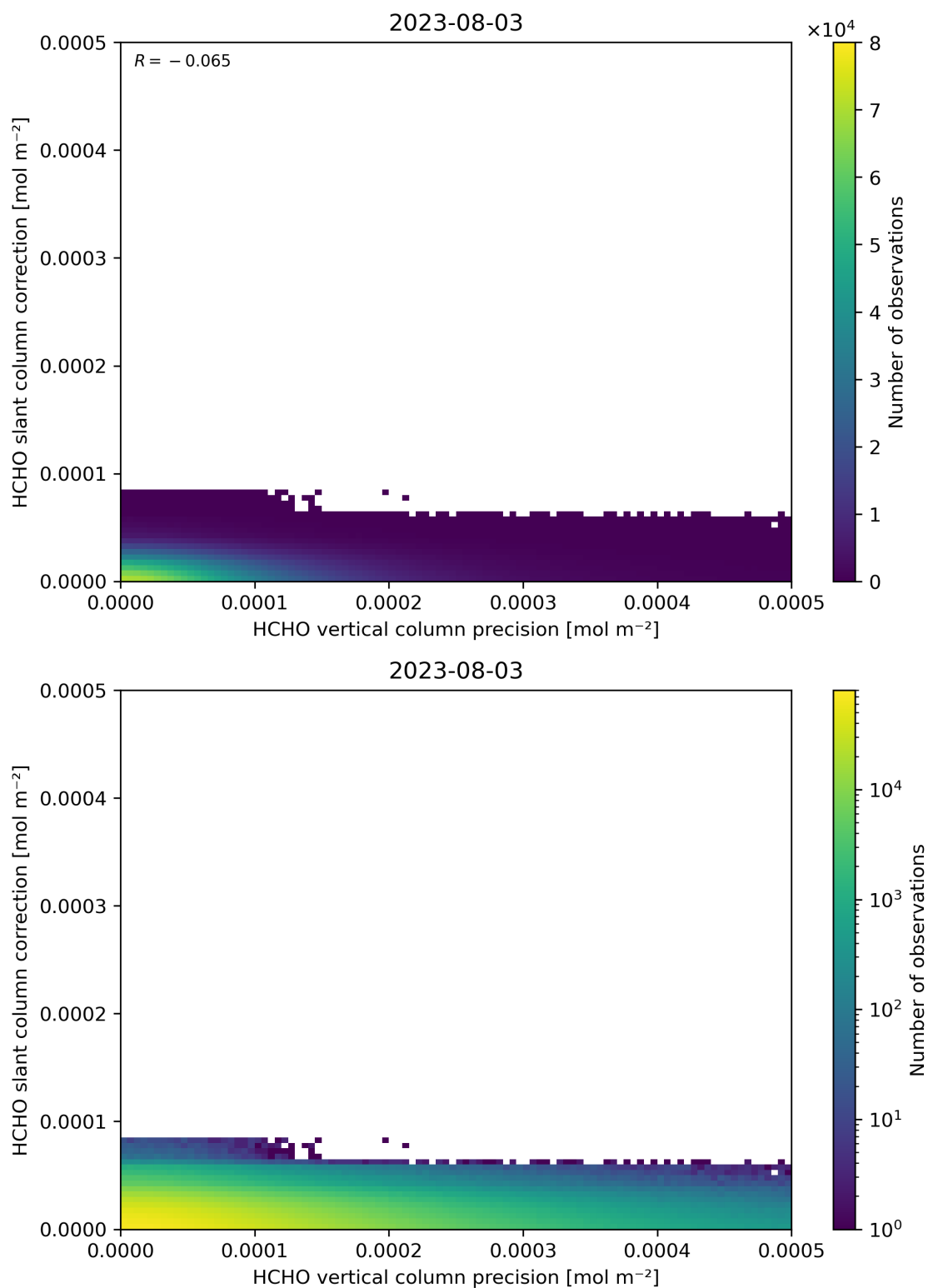
Figure 141: Scatter density plot of “HCHO vertical column precision” against “HCHO slant column correction” for 2023-08-02 to 2023-08-04.
