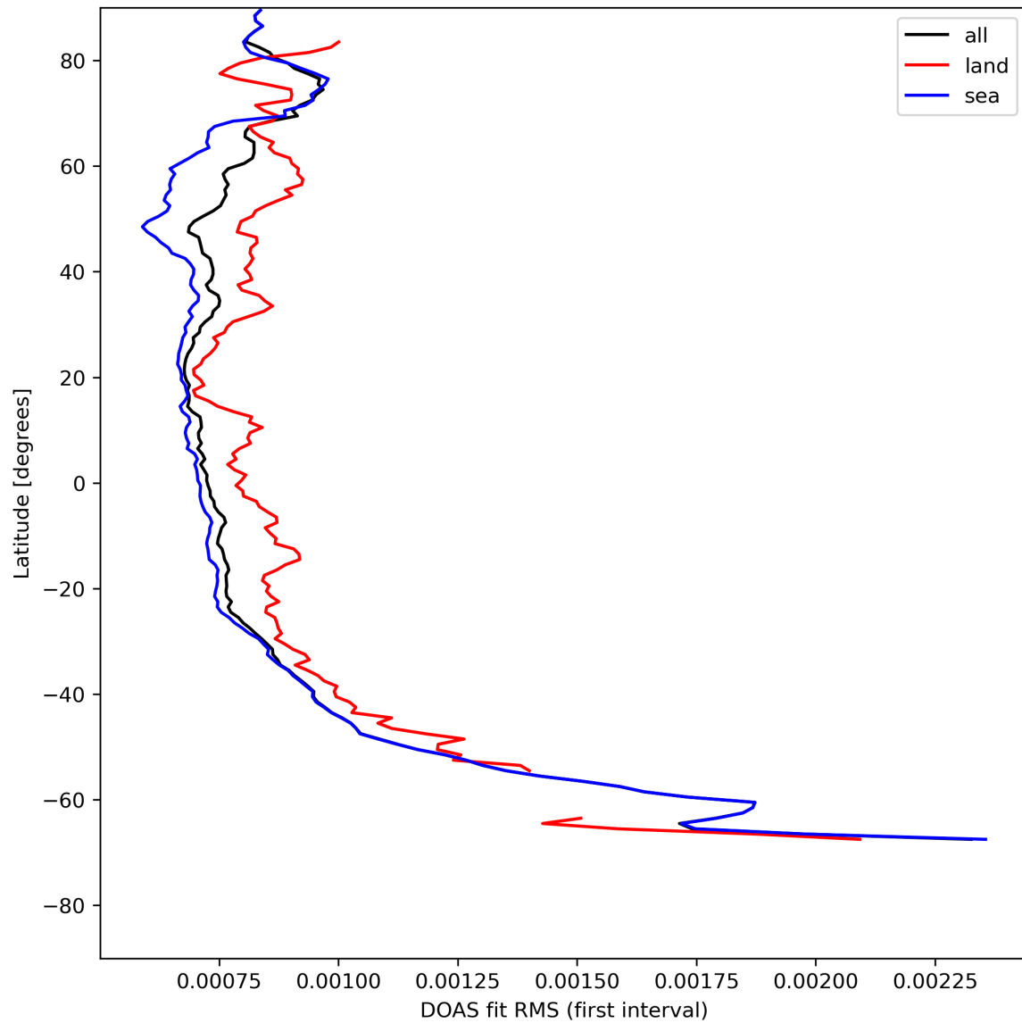
Figure 32: Zonal average of "DOAS fit RMS (first interval)" for 2023-08-02 to 2023-08-04.
