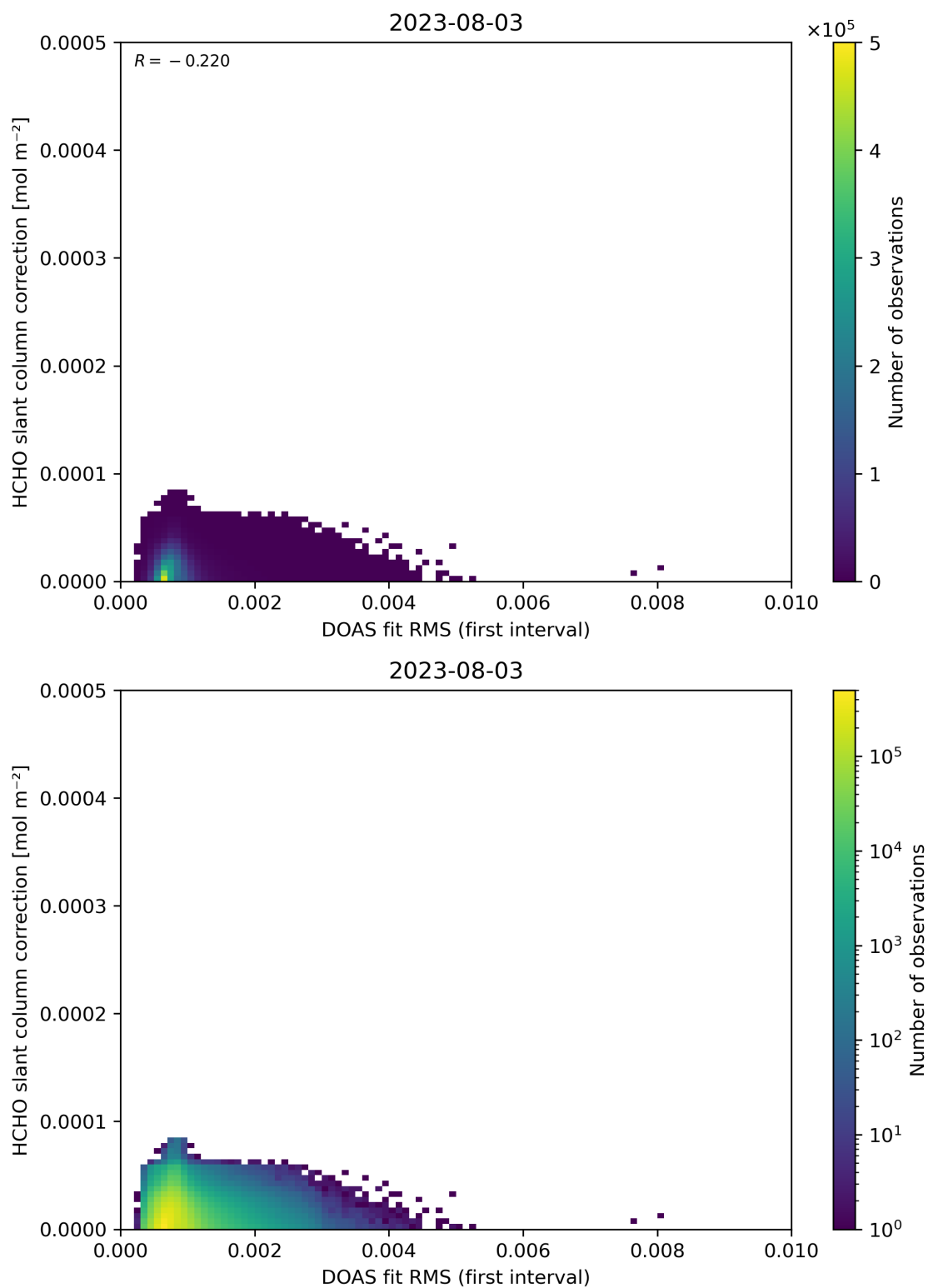
Figure 63: Scatter density plot of “DOAS fit RMS (first interval)” against “HCHO slant column correction” for 2023-08-02 to 2023-08-04.
