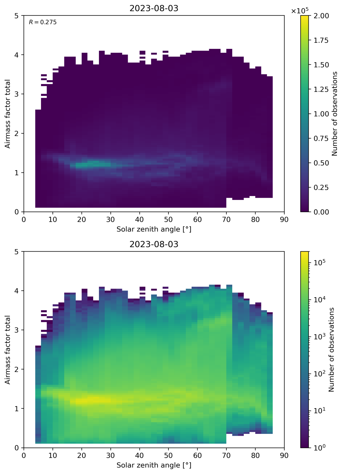
Figure 175: Scatter density plot of “Solar zenith angle” against “Airmass factor total” for 2023-08-02 to 2023-08-04.
