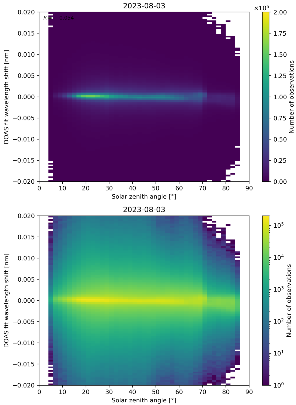
Figure 168: Scatter density plot of “Solar zenith angle” against “DOAS fit wavelength shift” for 2023-08-02 to 2023-08-04.
