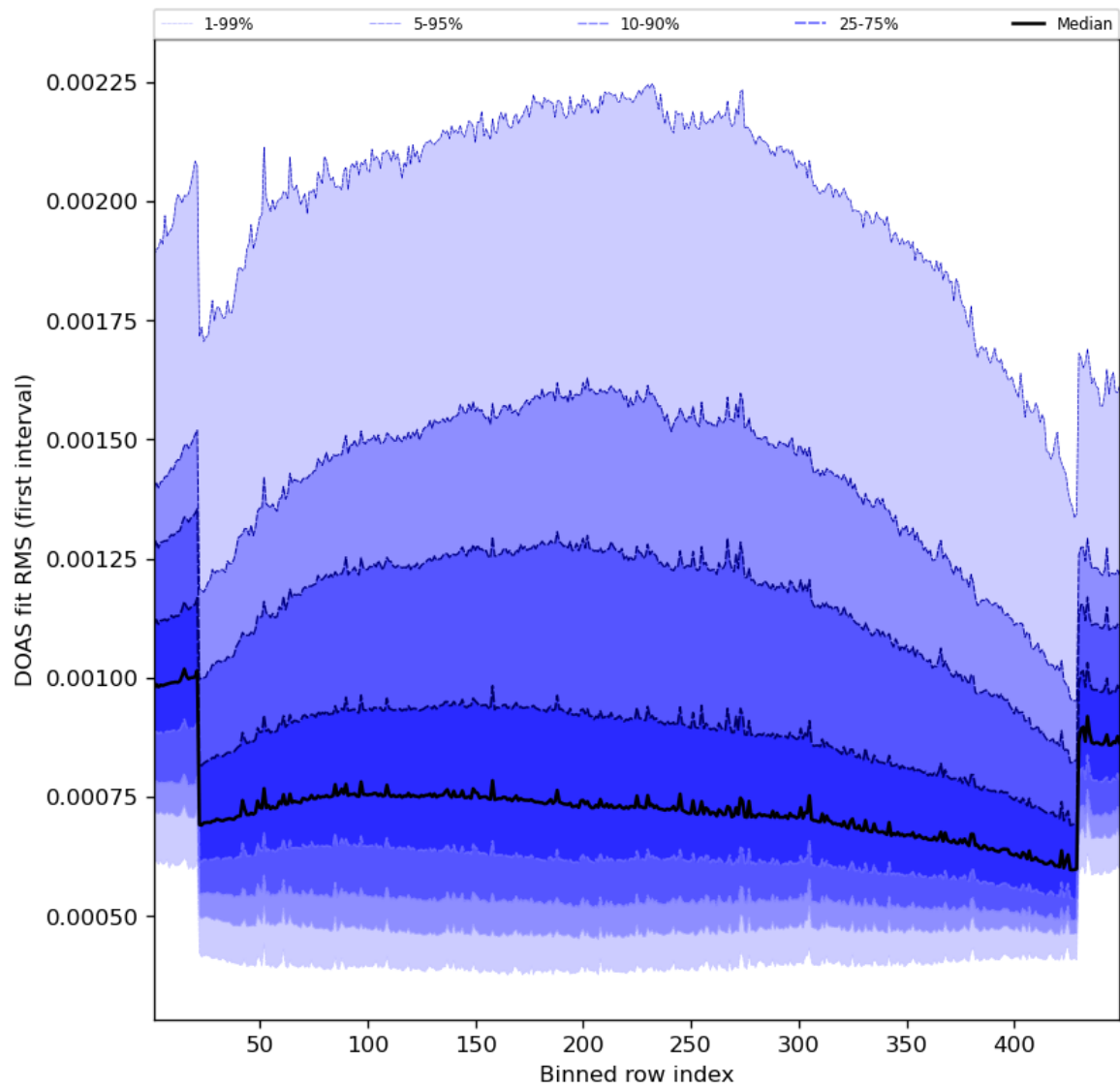
Figure 60: Along track statistics of “DOAS fit RMS (first interval)” for 2023-08-02 to 2023-08-04
