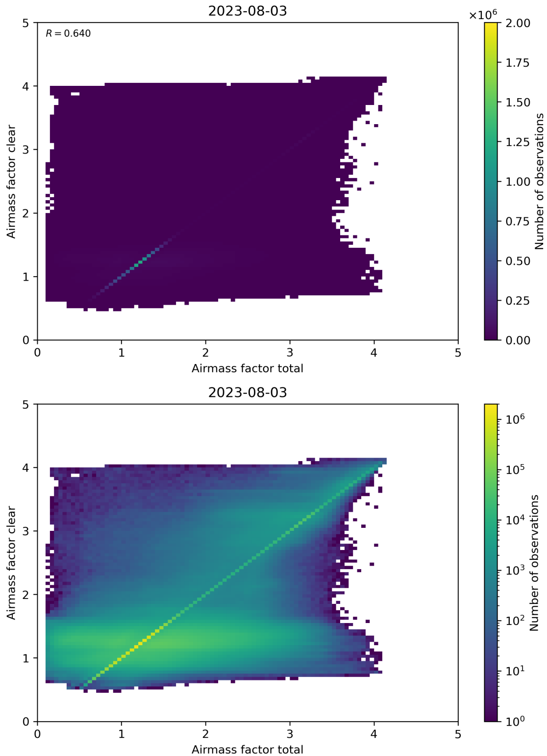
Figure 100: Scatter density plot of “Airmass factor total” against “Airmass factor clear” for 2023-08-02 to 2023-08-04.
