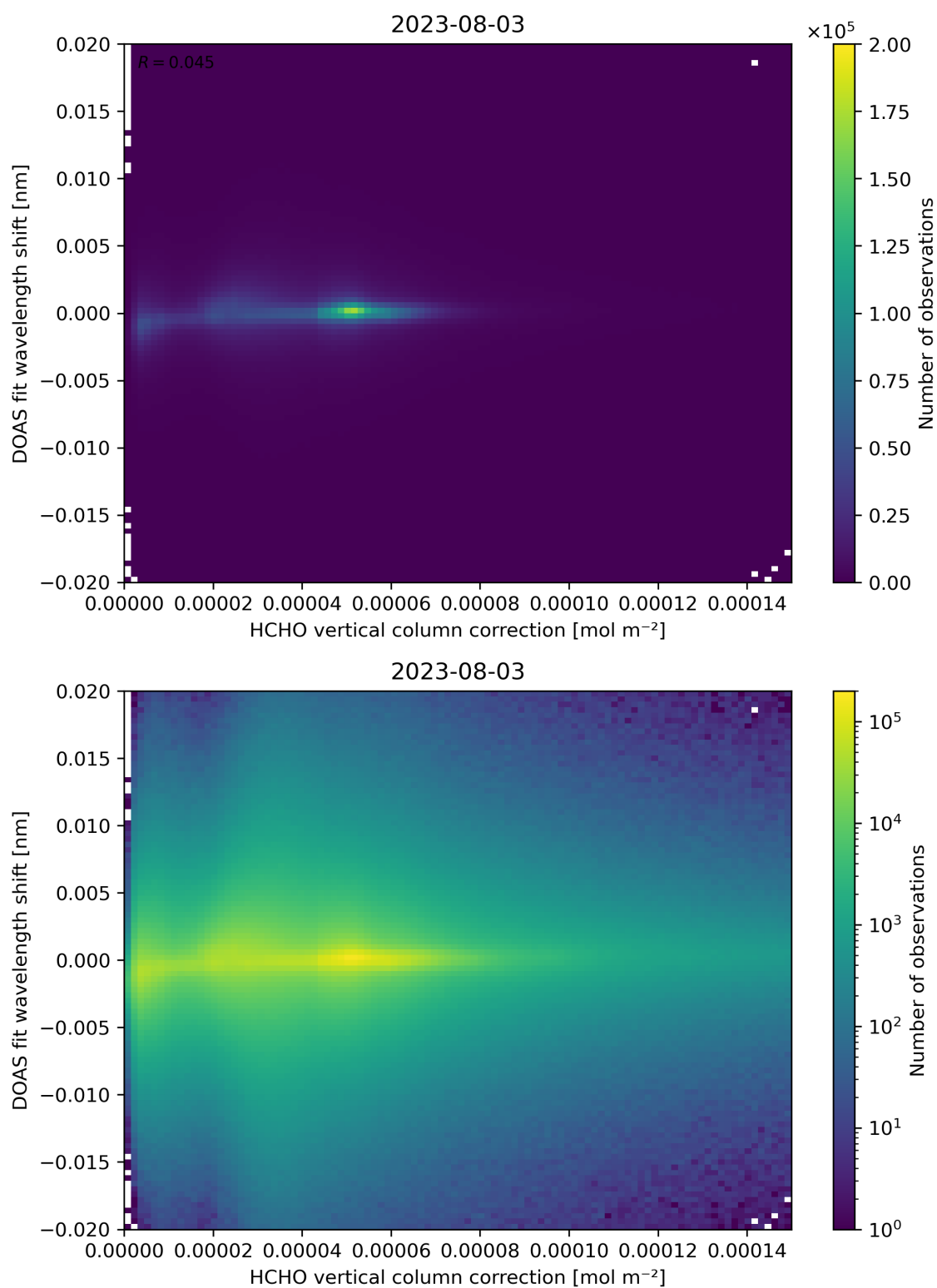
Figure 113: Scatter density plot of “HCHO vertical column correction” against “DOAS fit wavelength shift” for 2023-08-02 to 2023-08-04.
