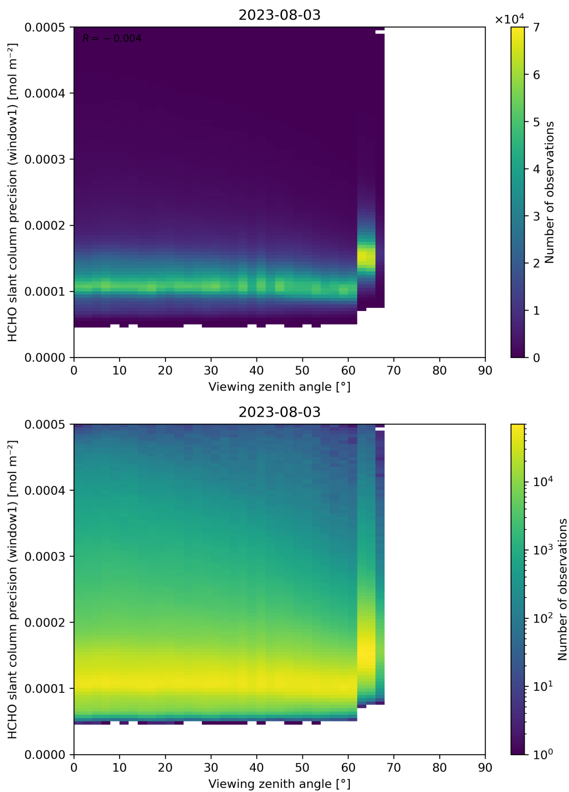
Figure 189: Scatter density plot of “Viewing zenith angle” against “HCHO slant column precision (window1)” for 2023-08-02 to 2023-08-04.
