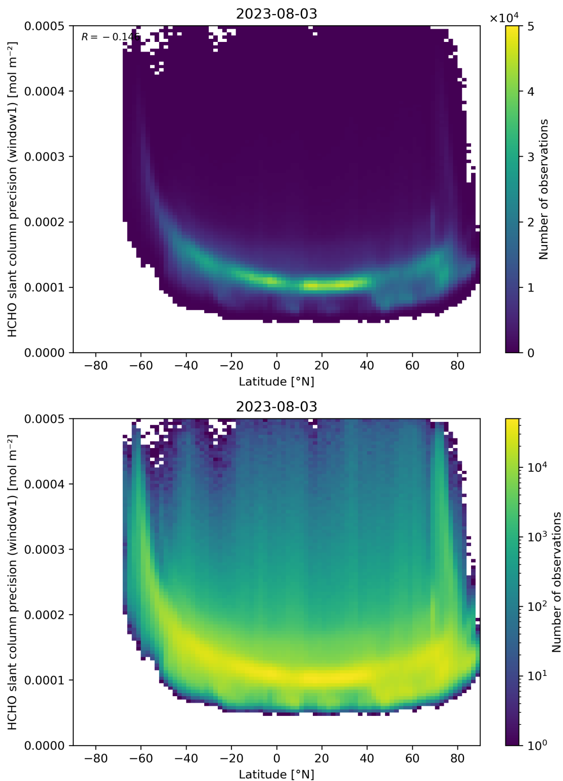
Figure 160: Scatter density plot of “Latitude” against “HCHO slant column precision (window1)” for 2023-08-02 to 2023-08-04.
