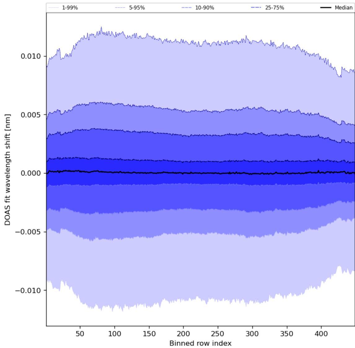
Figure 58: Along track statistics of “DOAS fit wavelength shift” for 2023-08-02 to 2023-08-04
