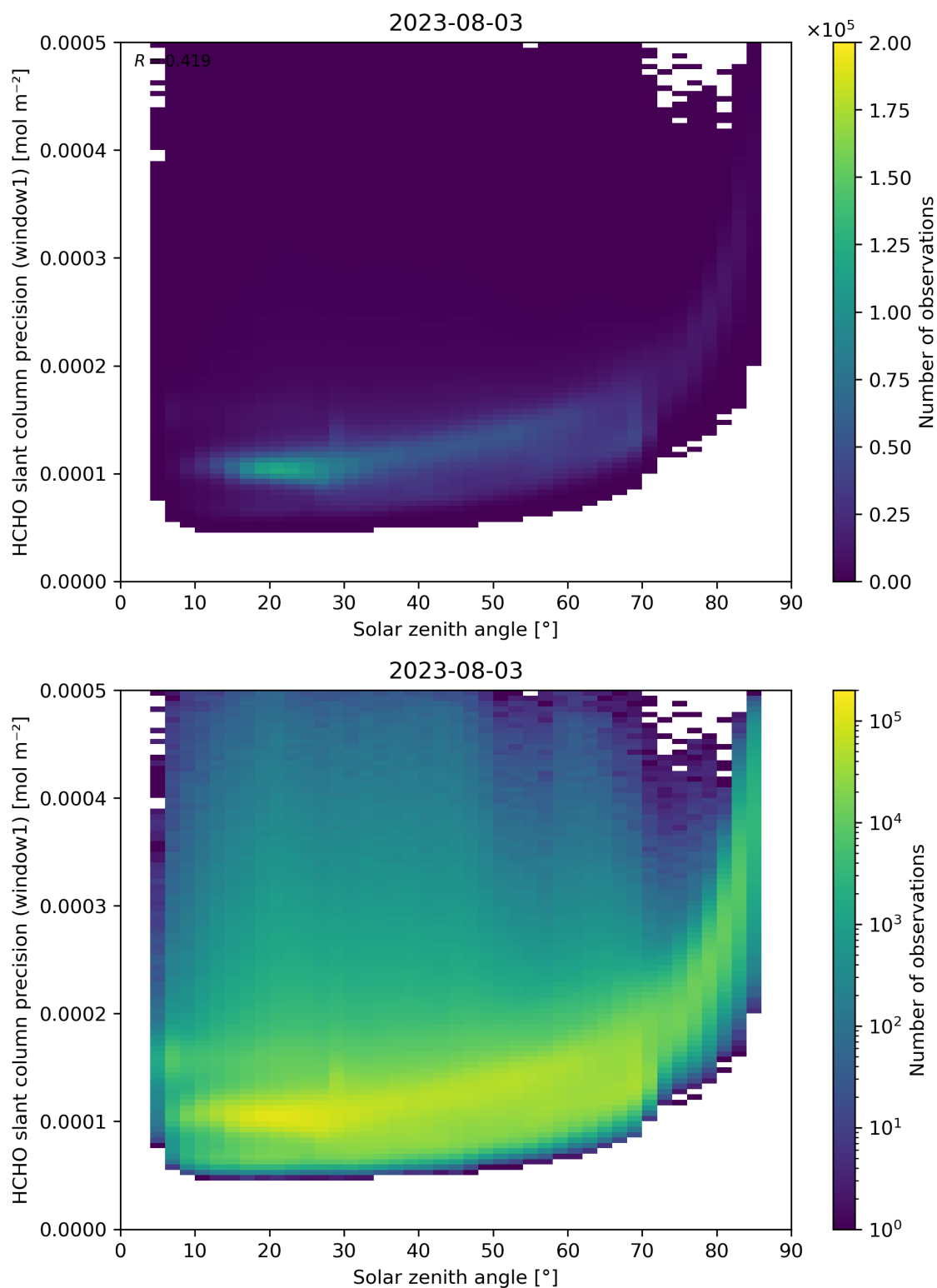
Figure 174: Scatter density plot of “Solar zenith angle” against “HCHO slant column precision (window1)” for 2023-08-02 to 2023-08-04.
