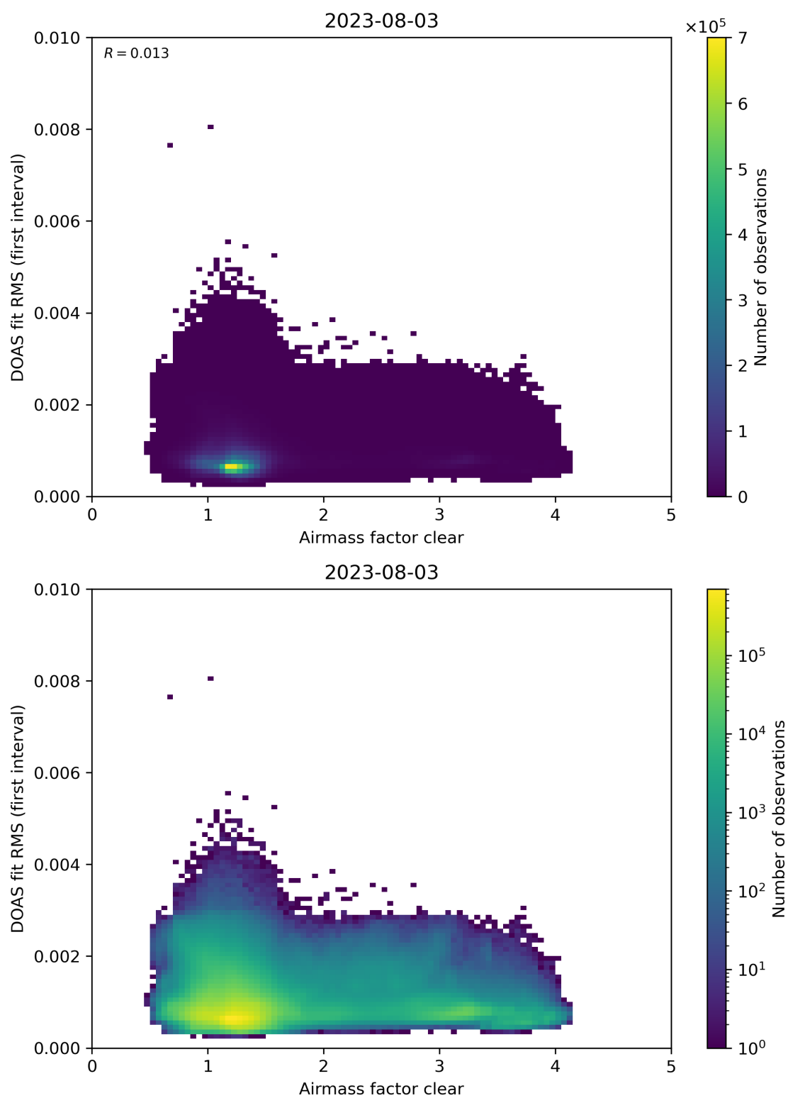
Figure 71: Scatter density plot of “Airmass factor clear” against “DOAS fit RMS (first interval)” for 2023-08-02 to 2023-08-04.
