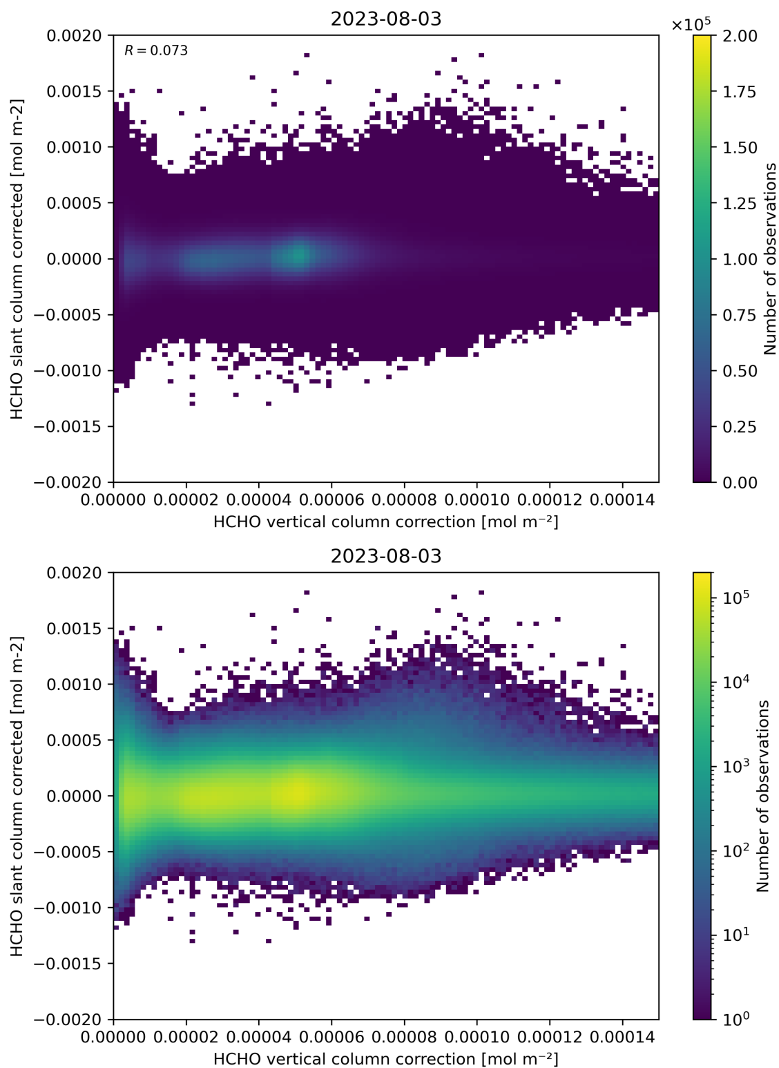
Figure 116: Scatter density plot of “HCHO vertical column correction” against “HCHO slant column corrected” for 2023-08-02 to 2023-08-04.
