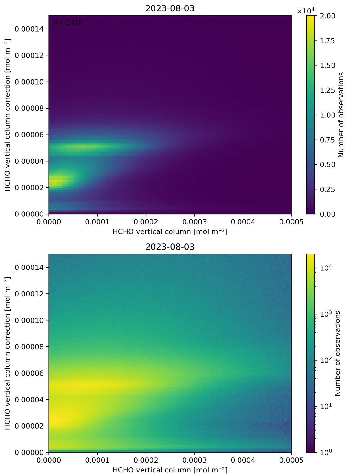
Figure 133: Scatter density plot of “HCHO vertical column” against “HCHO vertical column correction” for 2023-08-02 to 2023-08-04.
