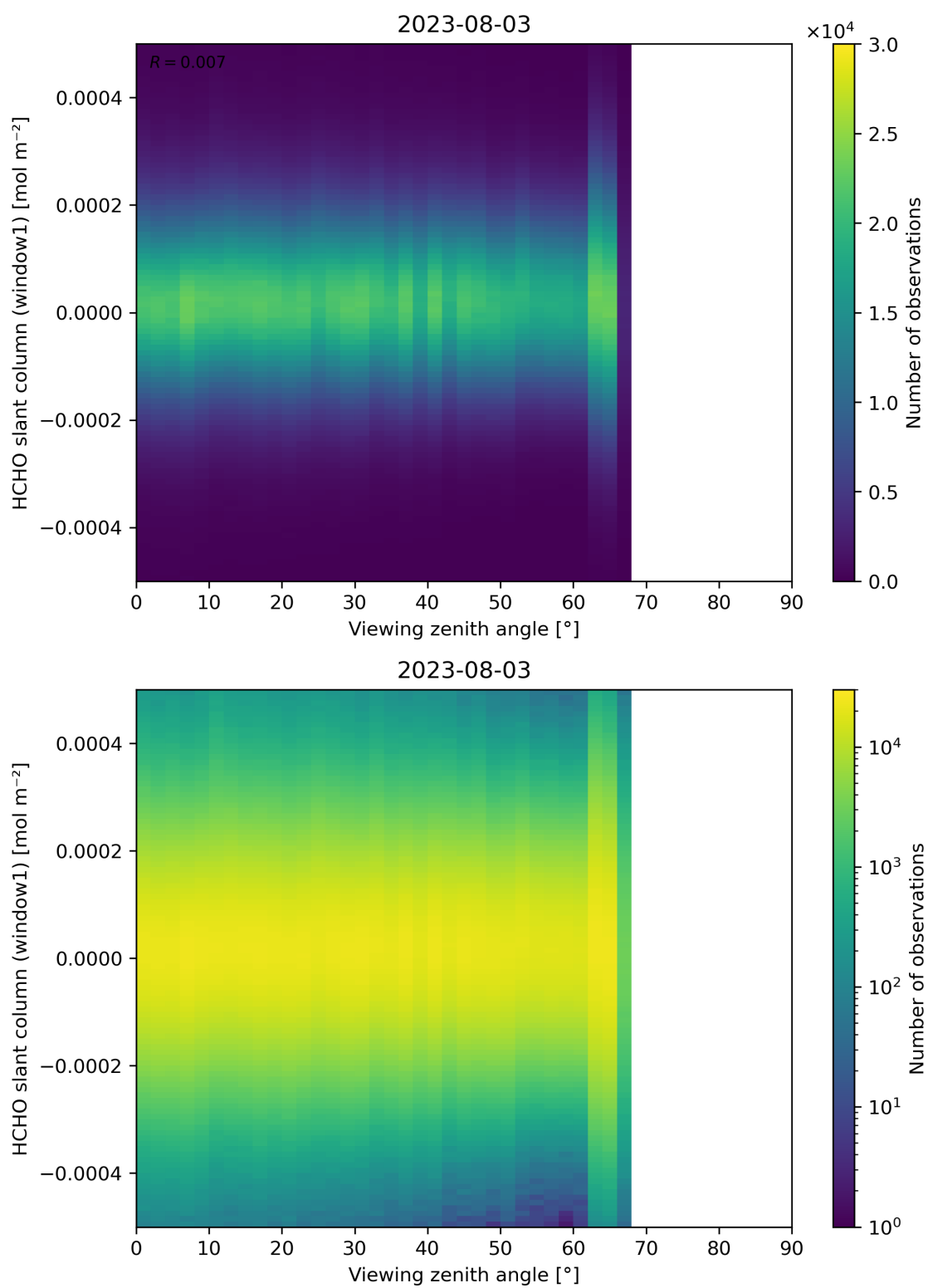
Figure 188: Scatter density plot of “Viewing zenith angle” against “HCHO slant column (window1)” for 2023-08-02 to 2023-08-04.
