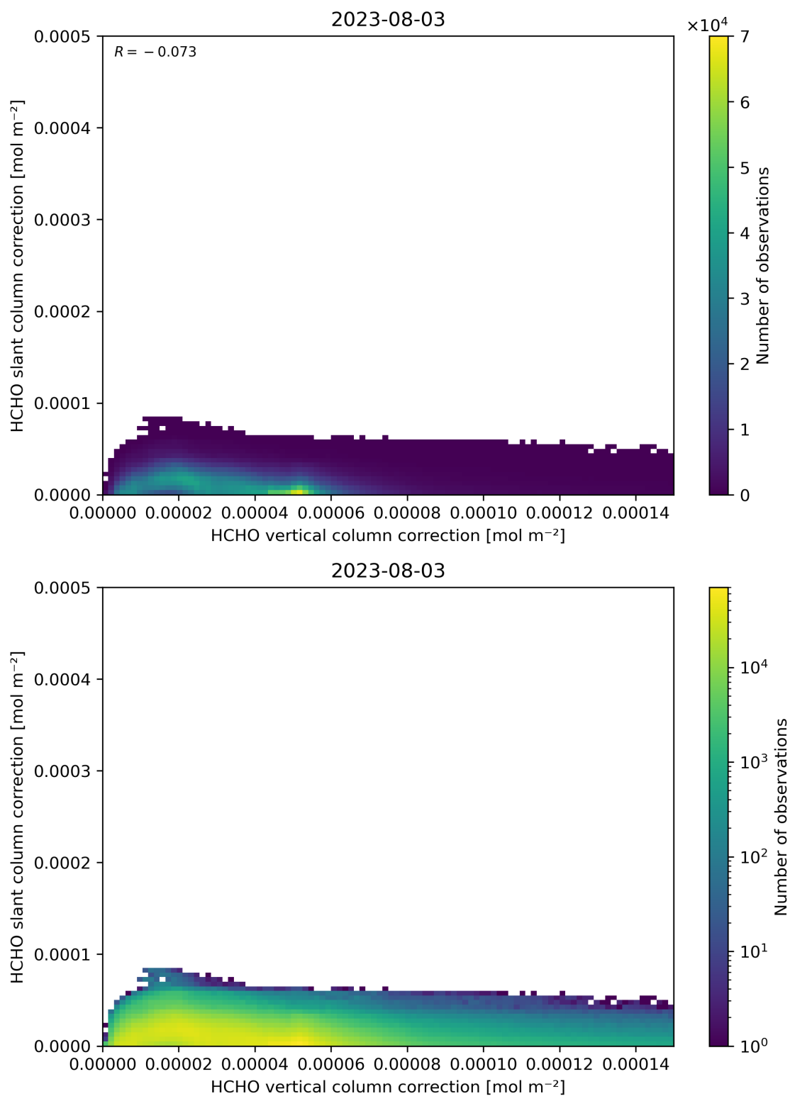
Figure 117: Scatter density plot of “HCHO vertical column correction” against “HCHO slant column correction” for 2023-08-02 to 2023-08-04.
