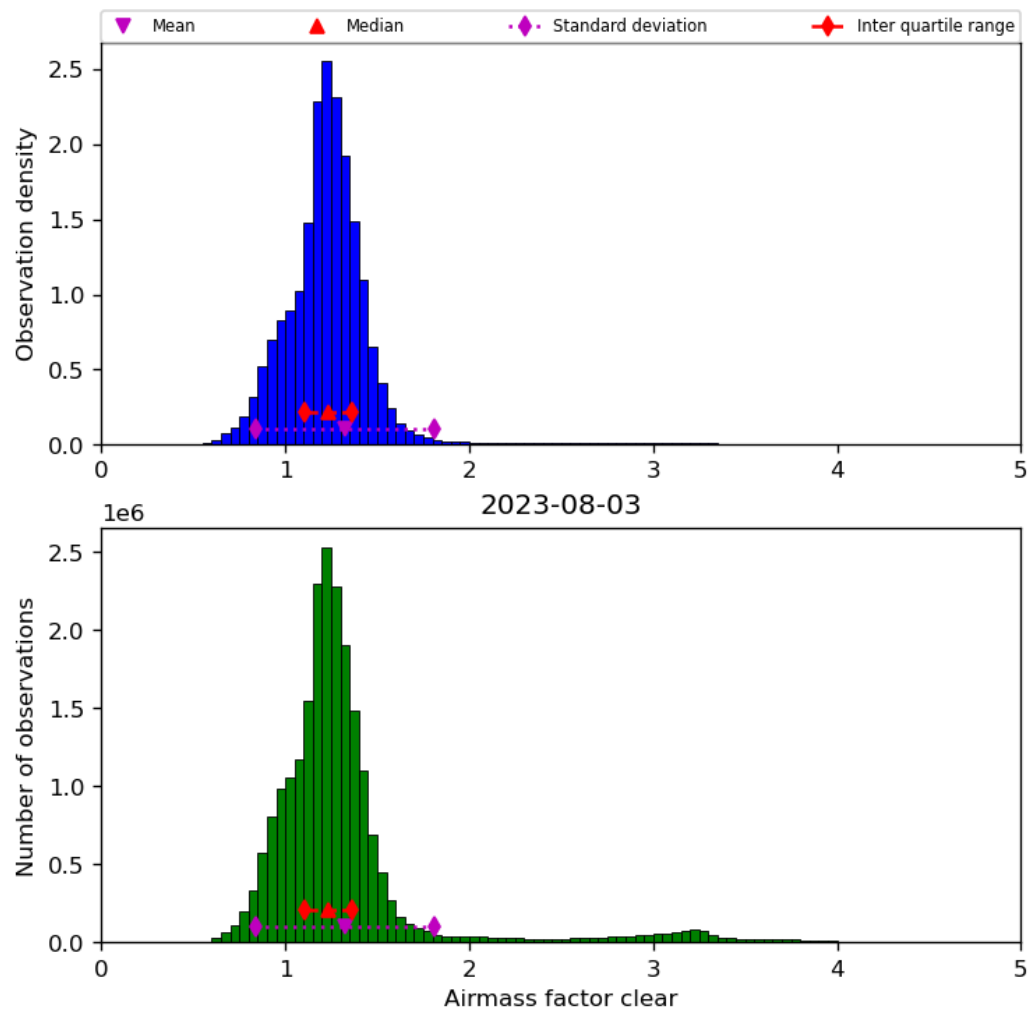
Figure 42: Histogram of “Airmass factor clear” for 2023-08-02 to 2023-08-04
