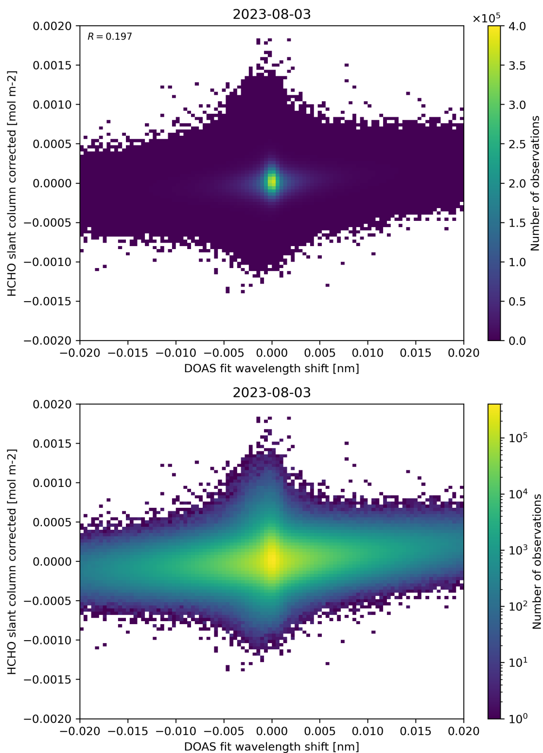
Figure 66: Scatter density plot of “DOAS fit wavelength shift” against “HCHO slant column corrected” for 2023-08-02 to 2023-08-04.
