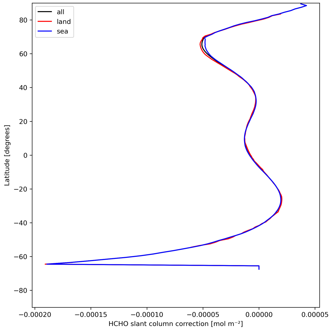
Figure 33: Zonal average of “HCHO slant column correction” for 2023-08-02 to 2023-08-04.
