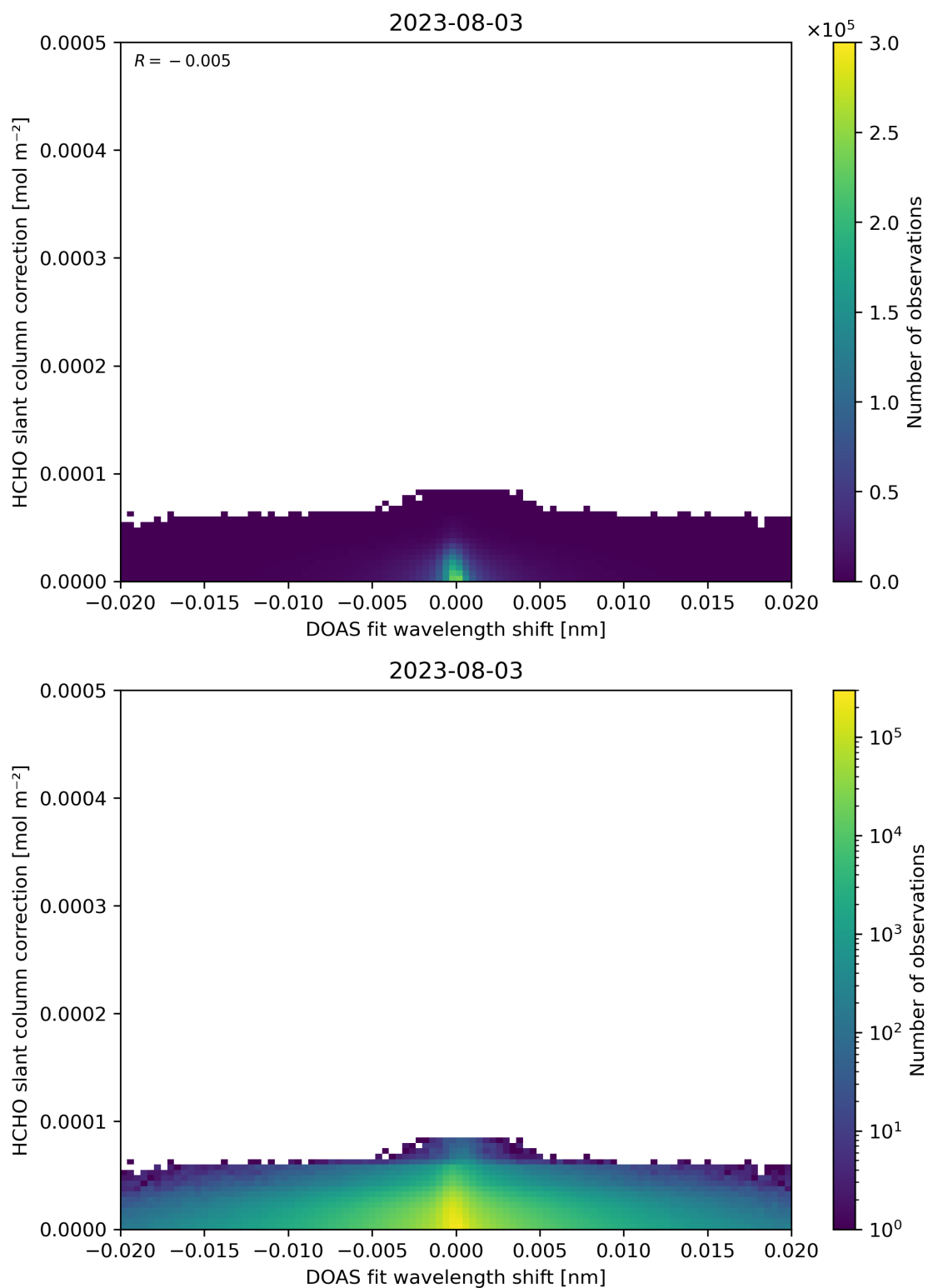
Figure 67: Scatter density plot of “DOAS fit wavelength shift” against “HCHO slant column correction” for 2023-08-02 to 2023-08-04.
