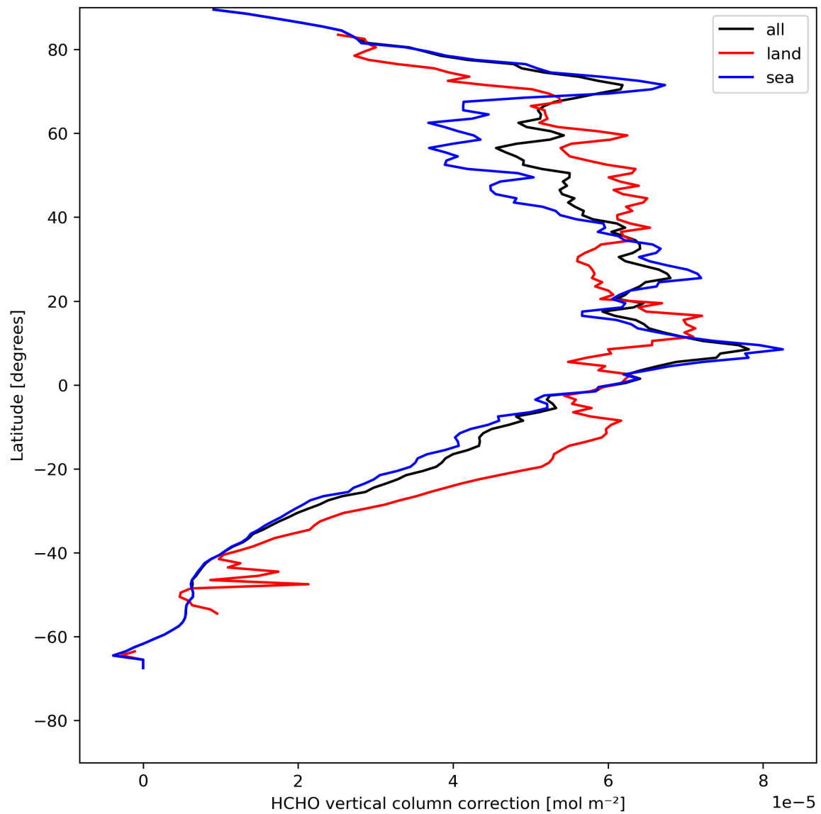
Figure 23: Zonal average of “HCHO vertical column correction” for 2023-08-02 to 2023-08-04.
