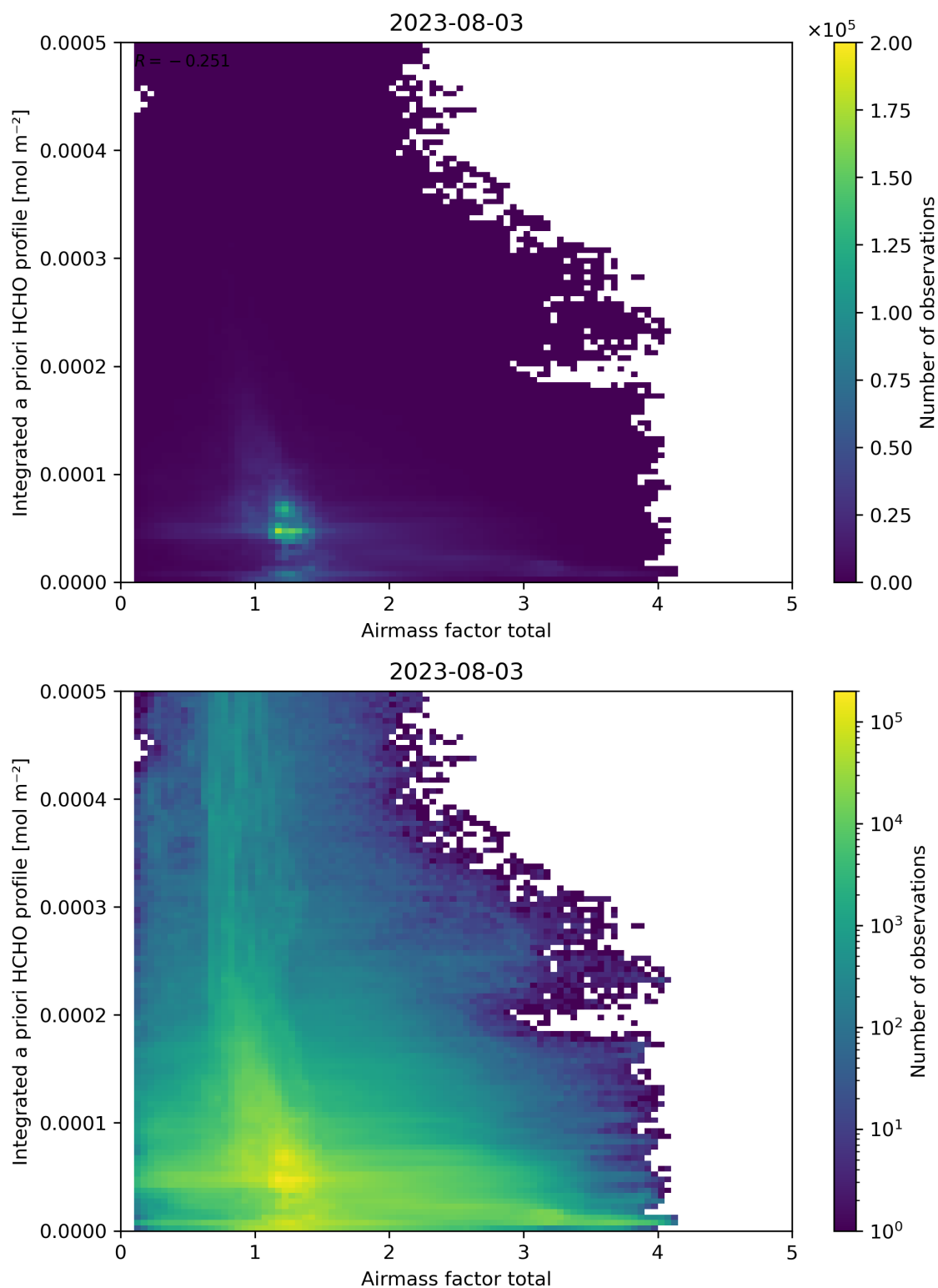
Figure 104: Scatter density plot of “Airmass factor total” against “Integrated a priori HCHO profile” for 2023-08-02 to 2023-08-04.
