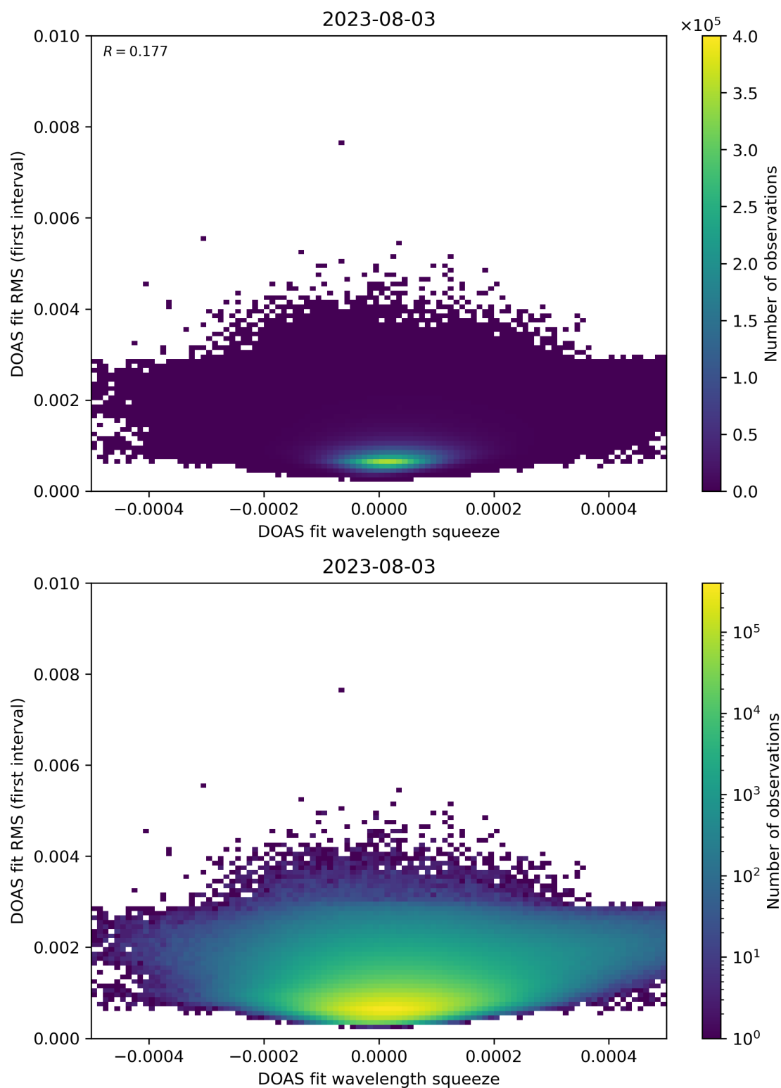
Figure 68: Scatter density plot of “DOAS fit wavelength squeeze” against “DOAS fit RMS (first interval)” for 2023-08-02 to 2023-08-04.
