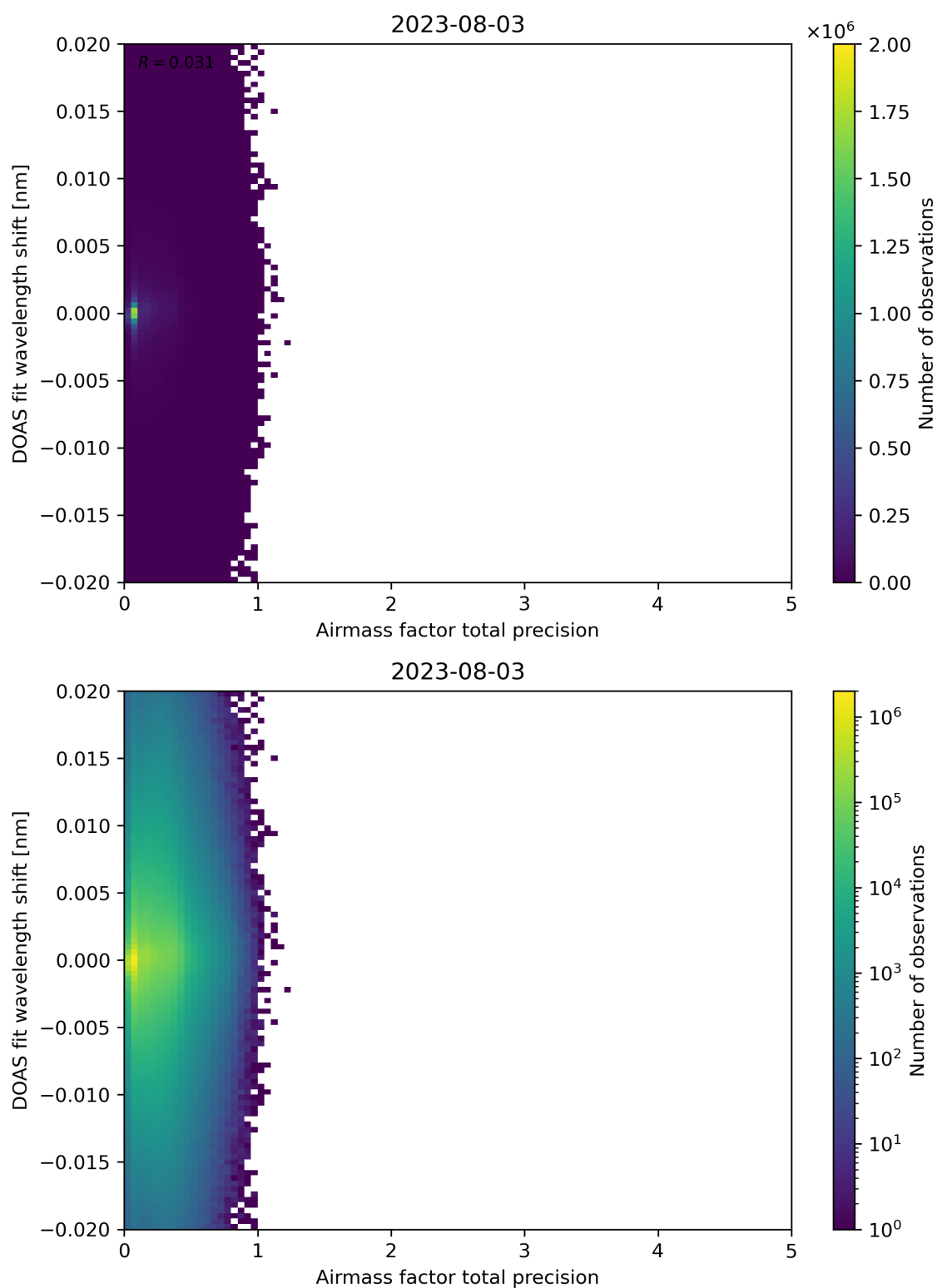
Figure 106: Scatter density plot of “Airmass factor total precision” against “DOAS fit wavelength shift” for 2023-08-02 to 2023-08-04.
