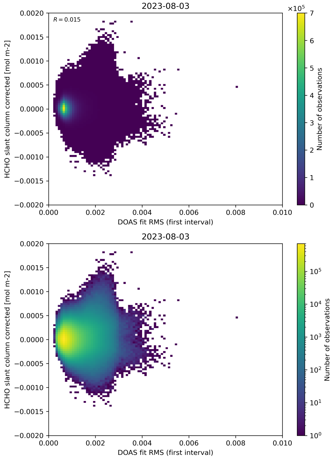
Figure 62: Scatter density plot of “DOAS fit RMS (first interval)” against “HCHO slant column corrected” for 2023-08-02 to 2023-08-04.
