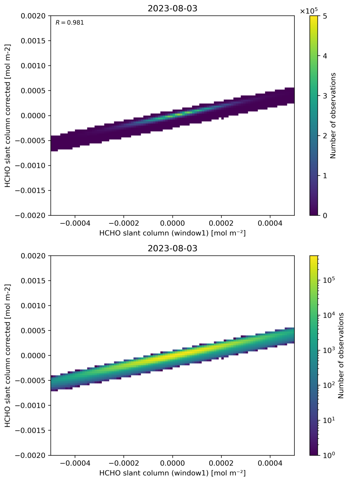
Figure 82: Scatter density plot of “HCHO slant column (window1)” against “HCHO slant column corrected” for 2023-08-02 to 2023-08-04.
