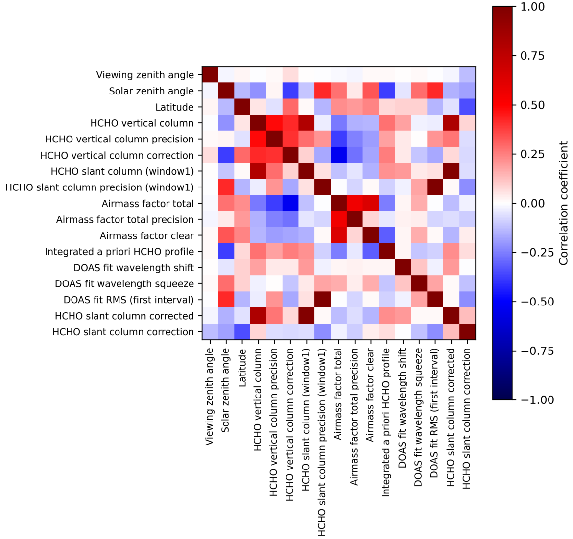
Figure 2: Map of correlation matrix for 2023-08-02 to 2023-08-04.
