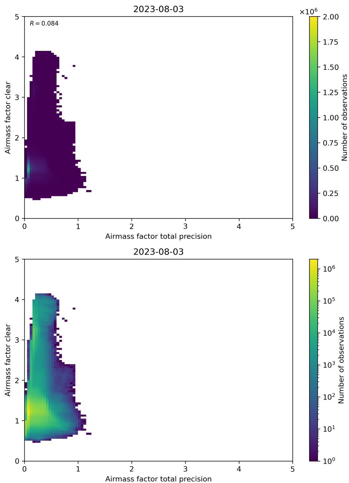
Figure 108: Scatter density plot of “Airmass factor total precision” against “Airmass factor clear” for 2023-08-02 to 2023-08-04.
