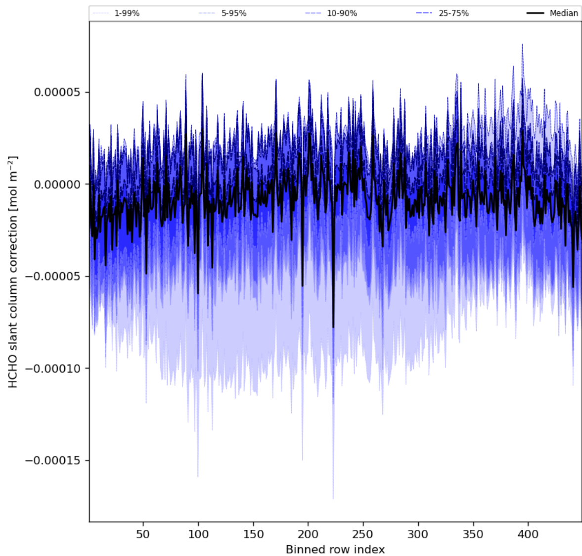
Figure 61: Along track statistics of “HCHO slant column correction” for 2023-08-02 to 2023-08-04
