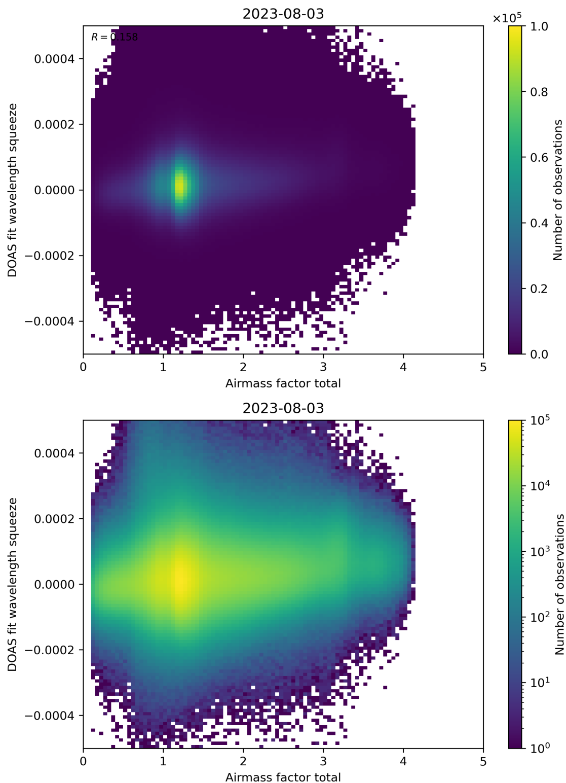
Figure 99: Scatter density plot of “Airmass factor total” against “DOAS fit wavelength squeeze” for 2023-08-02 to 2023-08-04.
