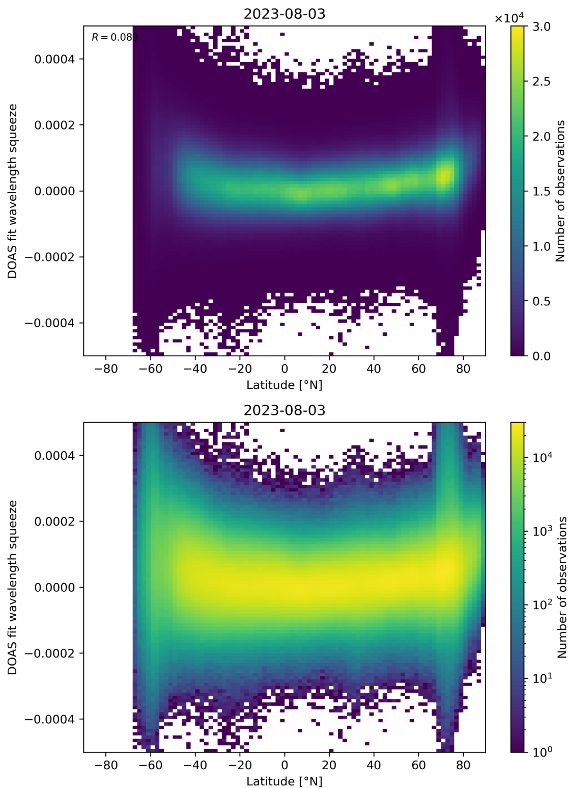
Figure 155: Scatter density plot of “Latitude” against “DOAS fit wavelength squeeze” for 2023-08-02 to 2023-08-04.
