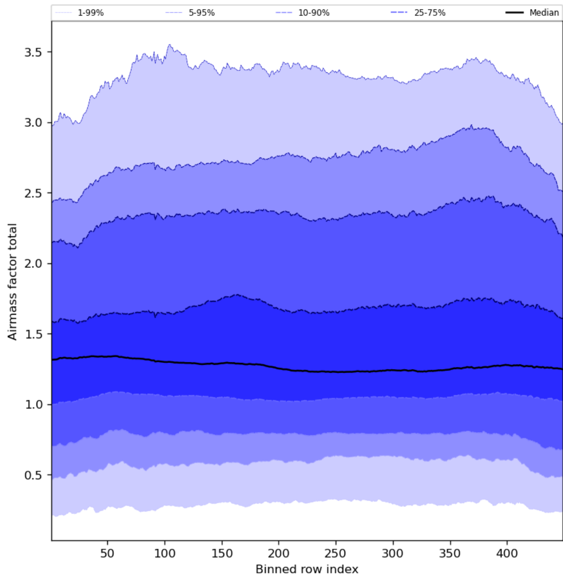
Figure 54: Along track statistics of “Airmass factor total” for 2023-08-02 to 2023-08-04
