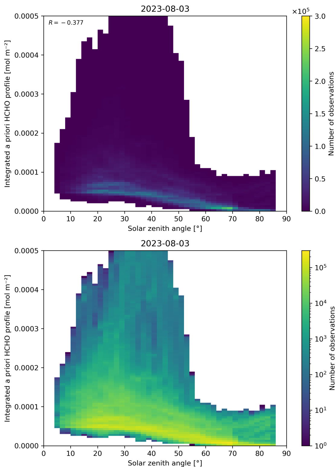
Figure 180: Scatter density plot of “Solar zenith angle” against “Integrated a priori HCHO profile” for 2023-08-02 to 2023-08-04.
