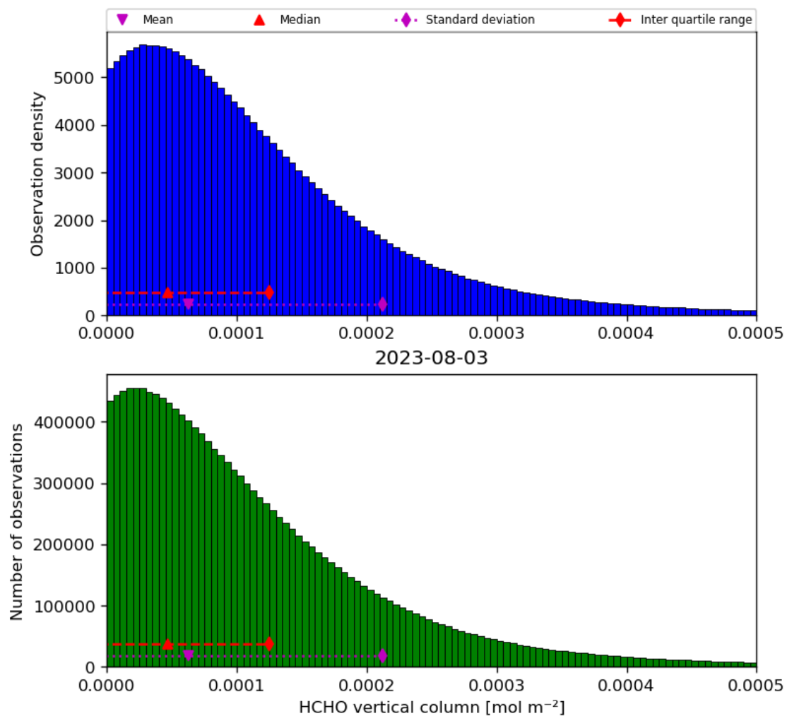
Figure 35: Histogram of “HCHO vertical column” for 2023-08-02 to 2023-08-04
