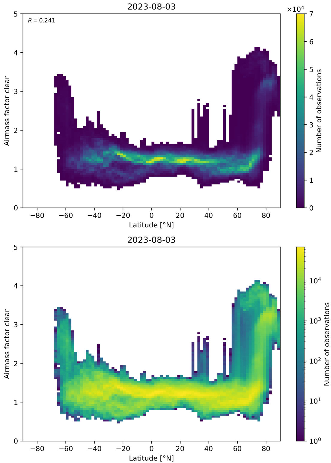
Figure 156: Scatter density plot of “Latitude” against “Airmass factor clear” for 2023-08-02 to 2023-08-04.
