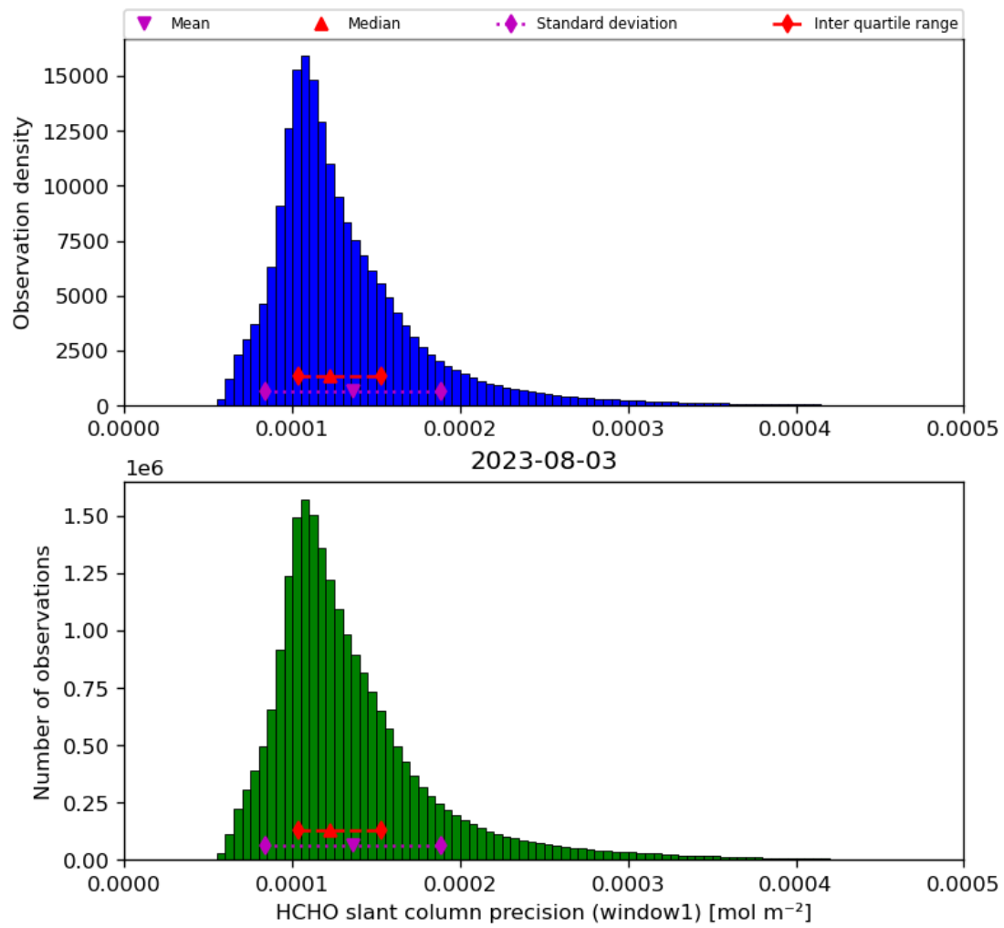
Figure 39: Histogram of “HCHO slant column precision (window1)” for 2023-08-02 to 2023-08-04
