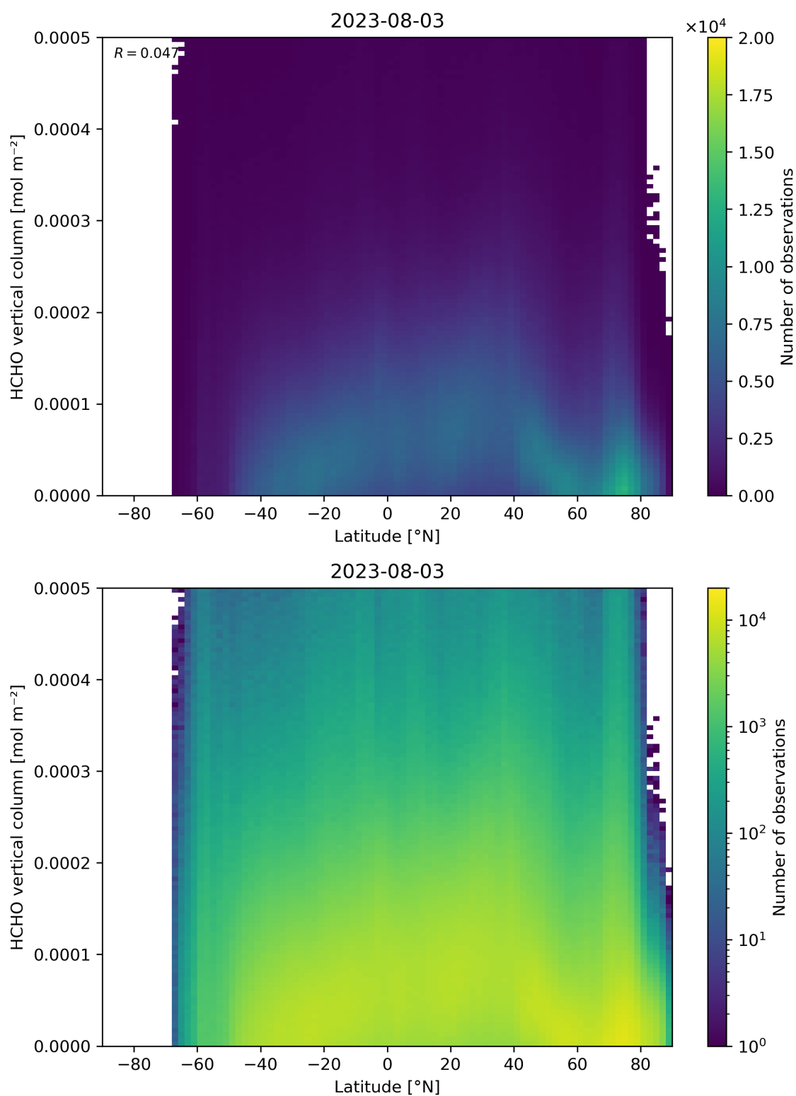
Figure 163: Scatter density plot of “Latitude” against “HCHO vertical column” for 2023-08-02 to 2023-08-04.
