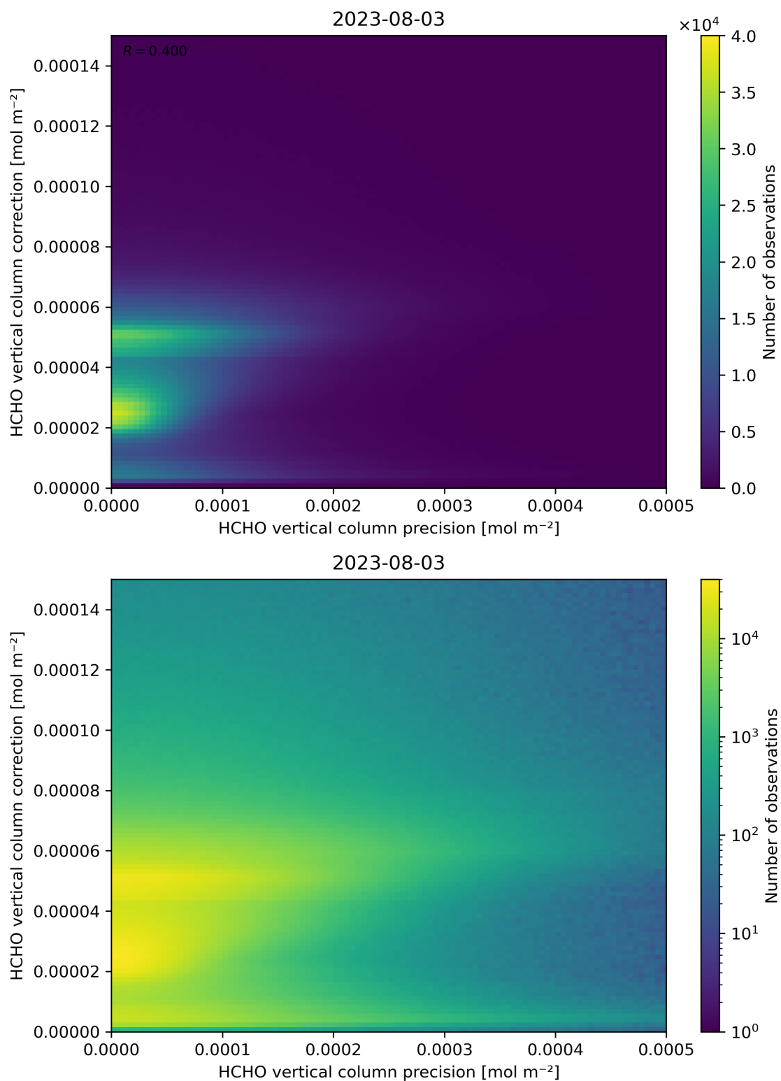
Figure 146: Scatter density plot of “HCHO vertical column precision” against “HCHO vertical column correction” for 2023-08-02 to 2023-08-04.
