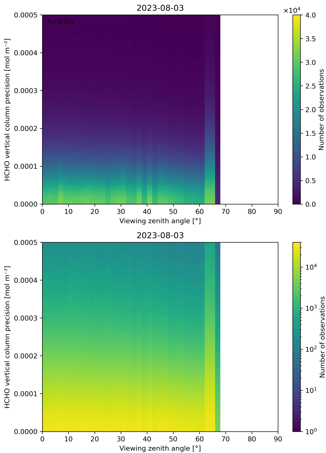
Figure 194: Scatter density plot of “Viewing zenith angle” against “HCHO vertical column precision” for 2023-08-02 to 2023-08-04.
