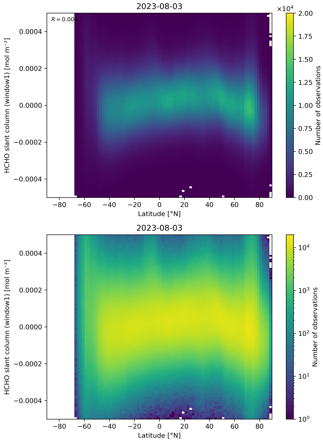
Figure 159: Scatter density plot of “Latitude” against “HCHO slant column (window1)” for 2023-08-02 to 2023-08-04.
