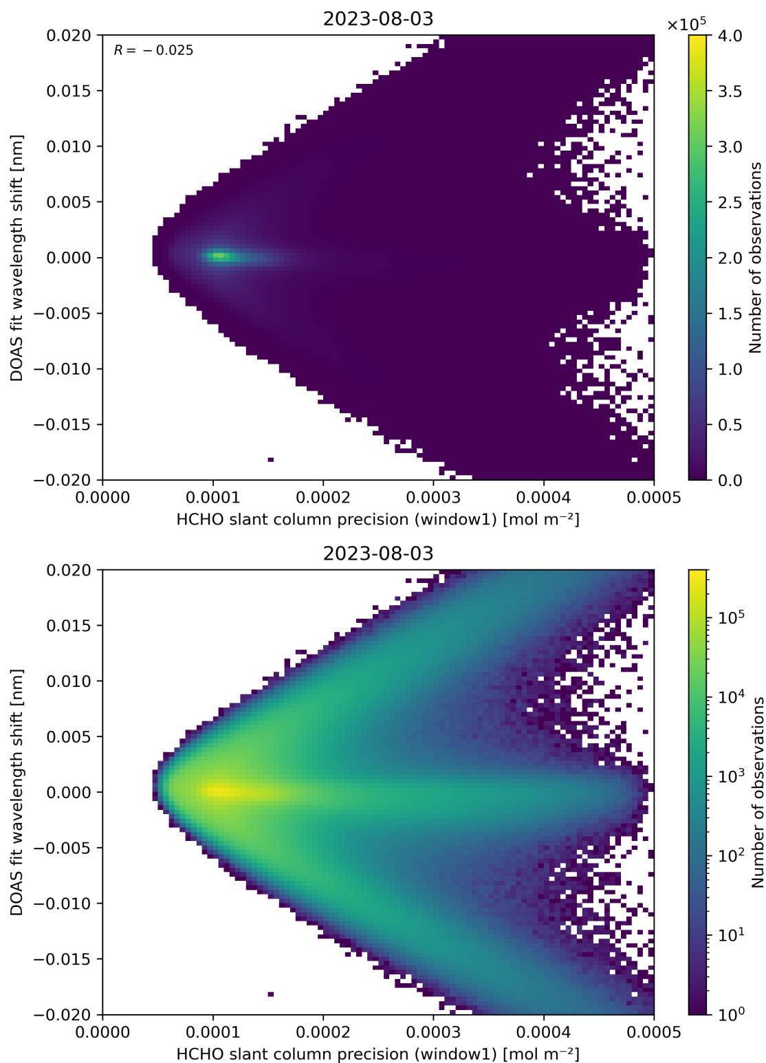
Figure 89: Scatter density plot of “HCHO slant column precision (window1)” against “DOAS fit wavelength shift” for 2023-08-02 to 2023-08-04.
