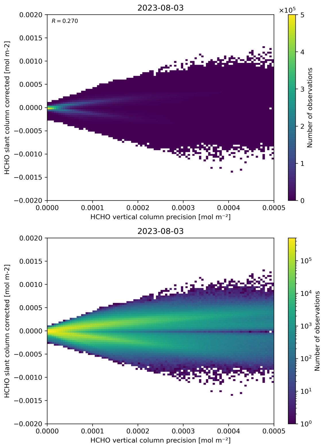
Figure 140: Scatter density plot of “HCHO vertical column precision” against “HCHO slant column corrected” for 2023-08-02 to 2023-08-04.
