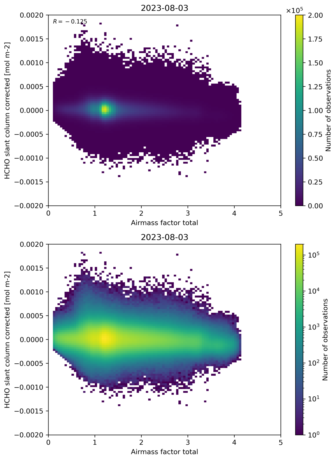
Figure 101: Scatter density plot of “Airmass factor total” against “HCHO slant column corrected” for 2023-08-02 to 2023-08-04.
