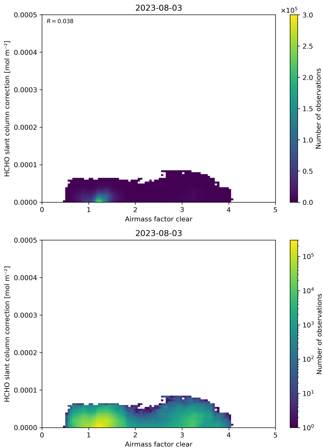
Figure 75: Scatter density plot of “Airmass factor clear” against “HCHO slant column correction” for 2023-08-02 to 2023-08-04.
