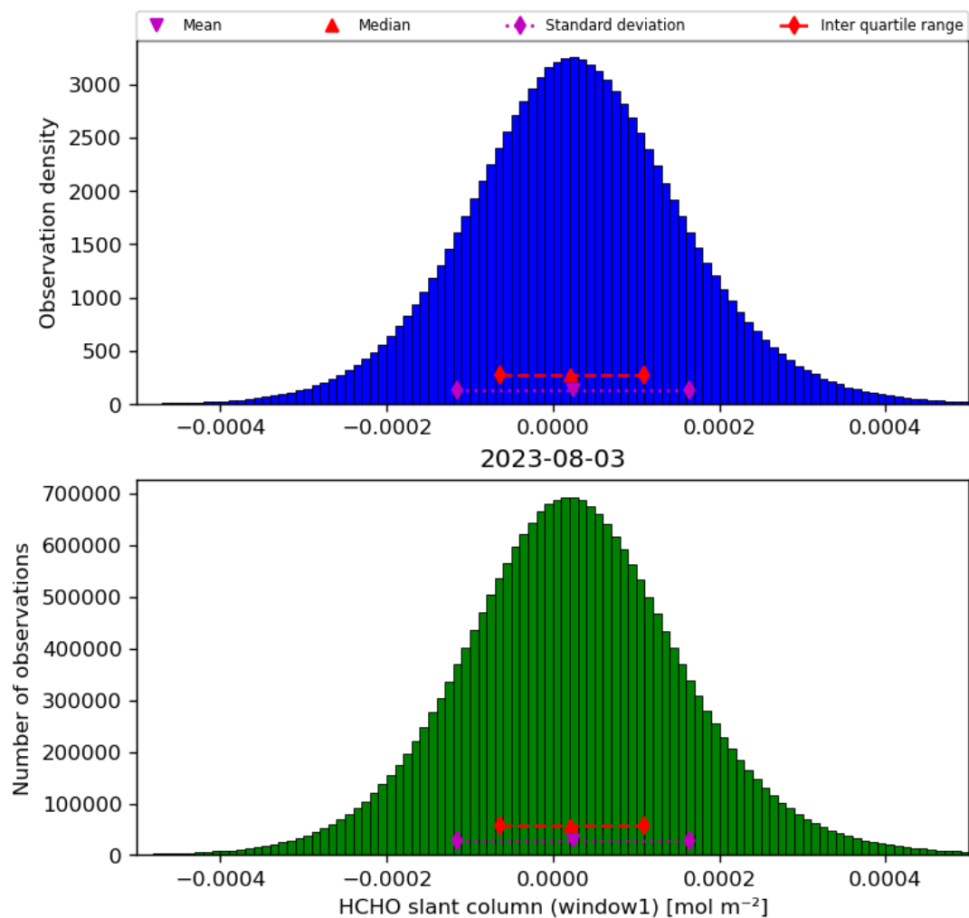
Figure 38: Histogram of “HCHO slant column (window1)” for 2023-08-02 to 2023-08-04
