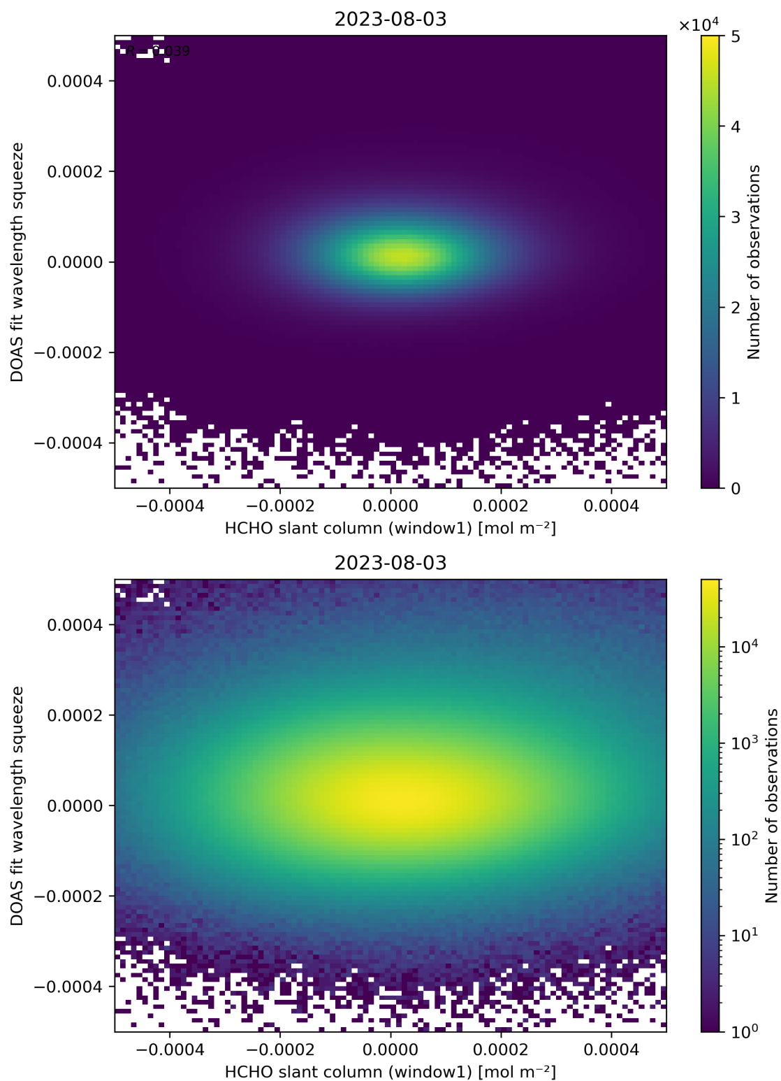
Figure 80: Scatter density plot of “HCHO slant column (window1)” against “DOAS fit wavelength squeeze” for 2023-08-02 to 2023-08-04.
