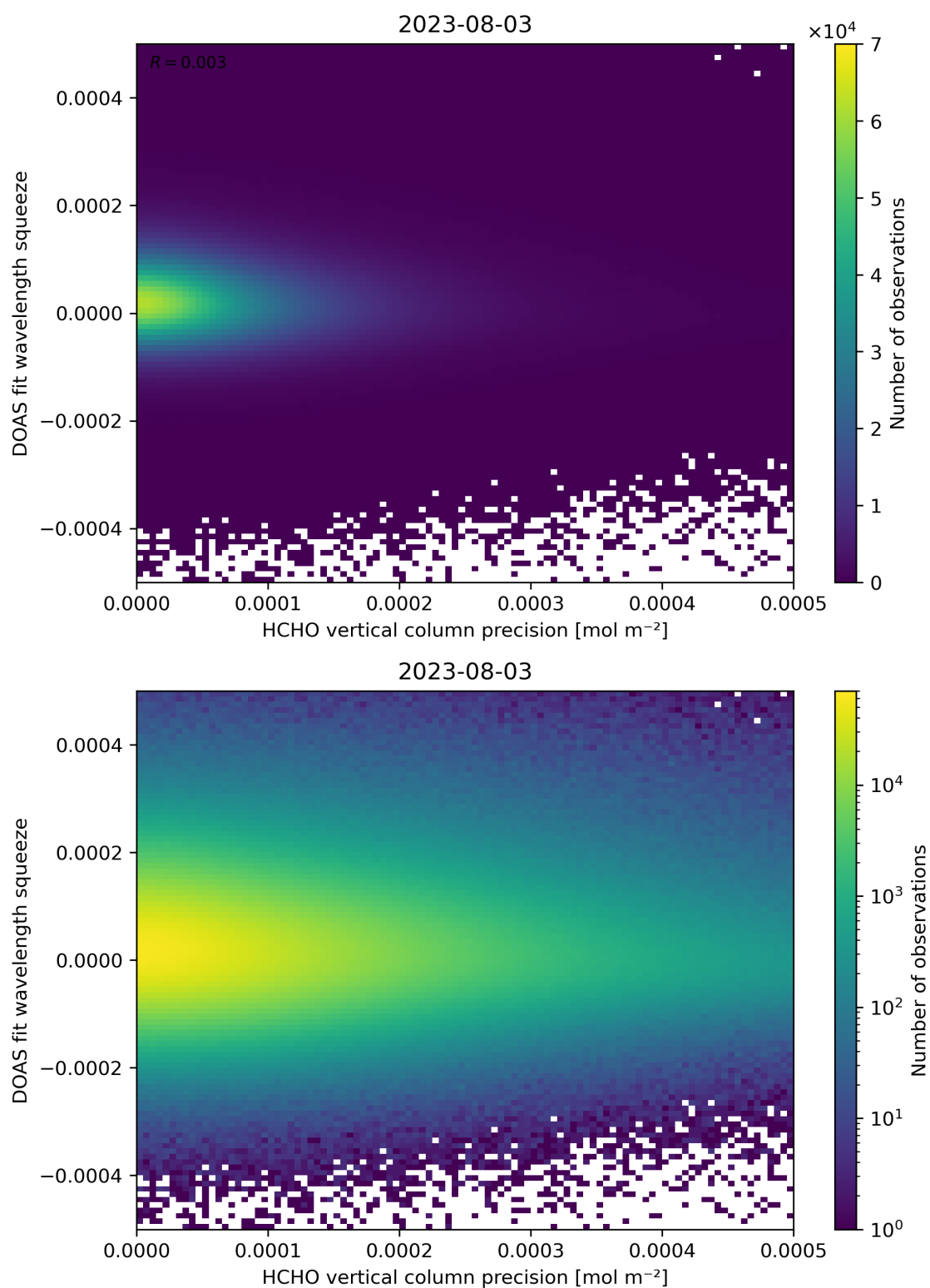
Figure 138: Scatter density plot of “HCHO vertical column precision” against “DOAS fit wavelength squeeze” for 2023-08-02 to 2023-08-04.
