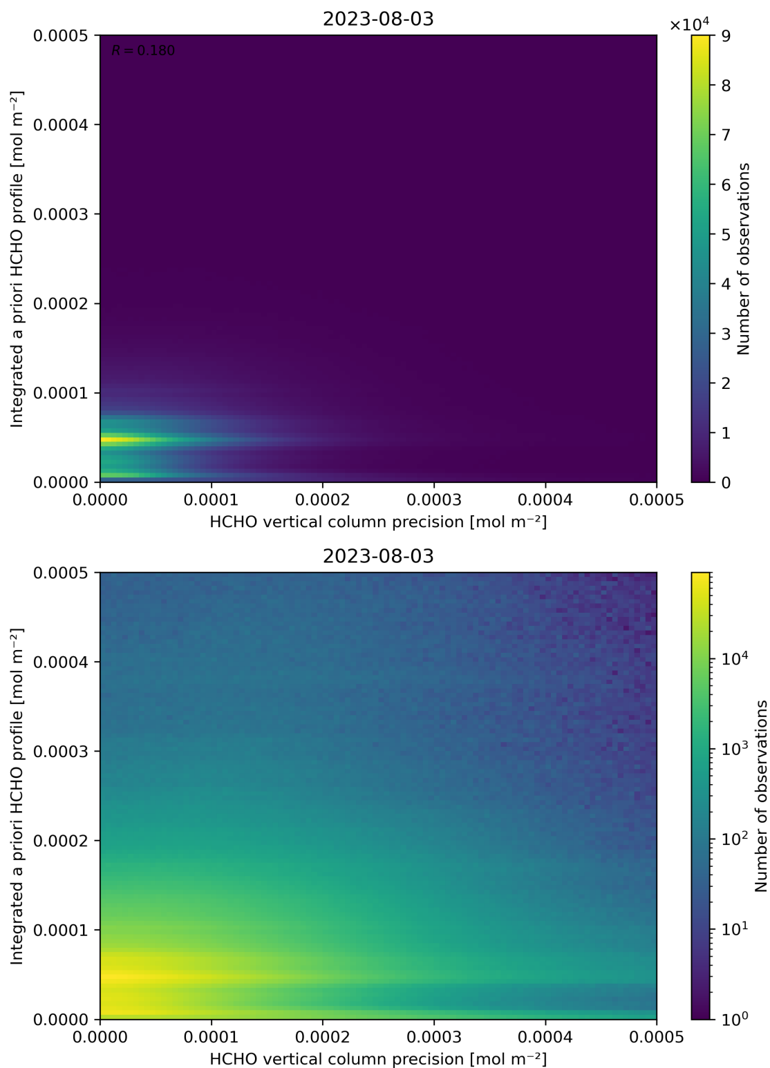
Figure 147: Scatter density plot of “HCHO vertical column precision” against “Integrated a priori HCHO profile” for 2023-08-02 to 2023-08-04.
