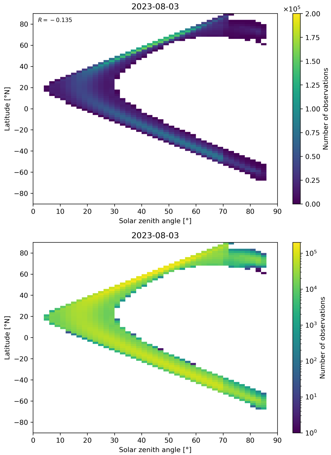
Figure 181: Scatter density plot of “Solar zenith angle” against “Latitude” for 2023-08-02 to 2023-08-04.
