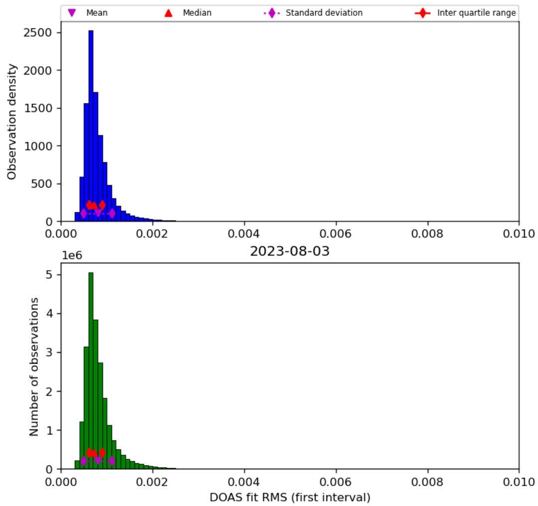
Figure 46: Histogram of “DOAS fit RMS (first interval)” for 2023-08-02 to 2023-08-04
