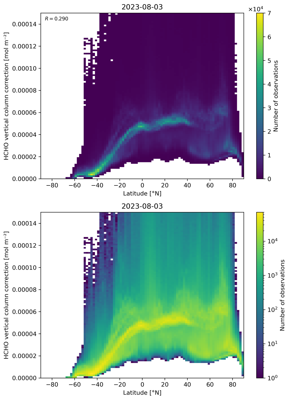
Figure 164: Scatter density plot of “Latitude” against “HCHO vertical column correction” for 2023-08-02 to 2023-08-04.
