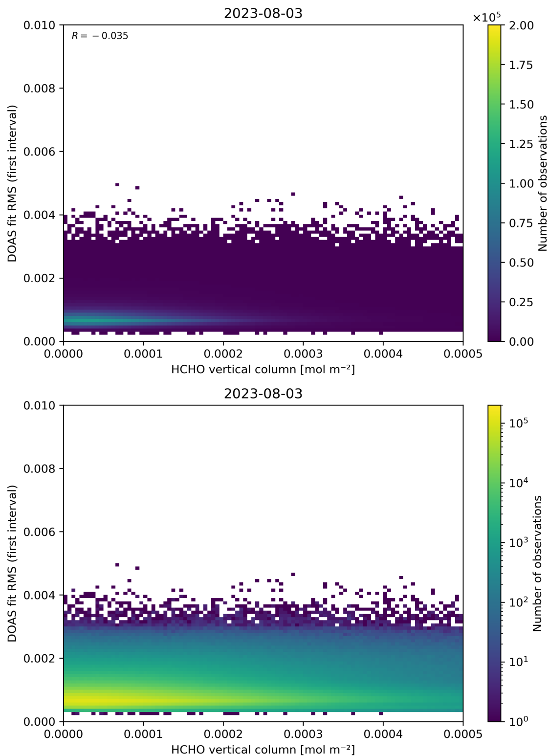
Figure 123: Scatter density plot of “HCHO vertical column” against “DOAS fit RMS (first interval)” for 2023-08-02 to 2023-08-04.
