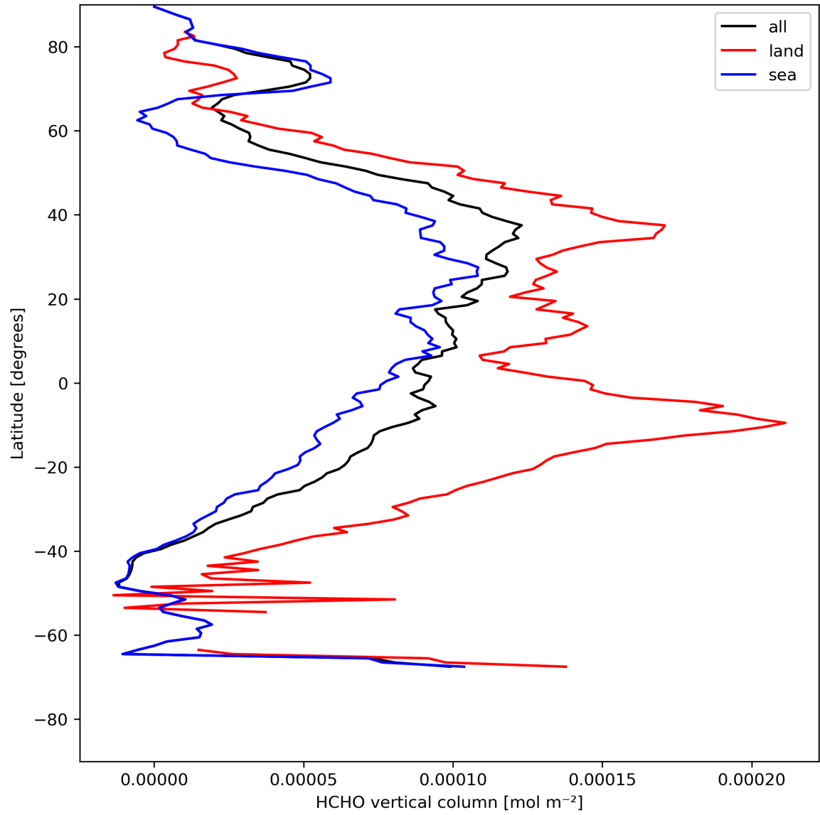
Figure 21: Zonal average of “HCHO vertical column” for 2023-08-02 to 2023-08-04.
