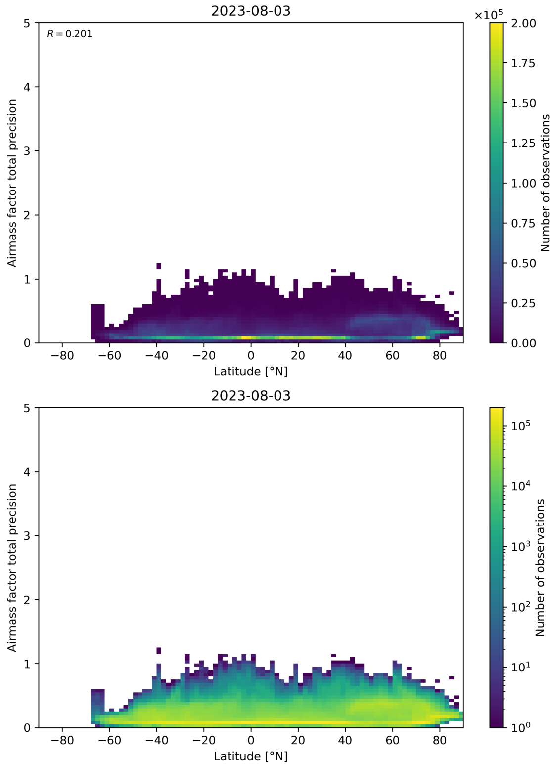
Figure 162: Scatter density plot of “Latitude” against “Airmass factor total precision” for 2023-08-02 to 2023-08-04.
