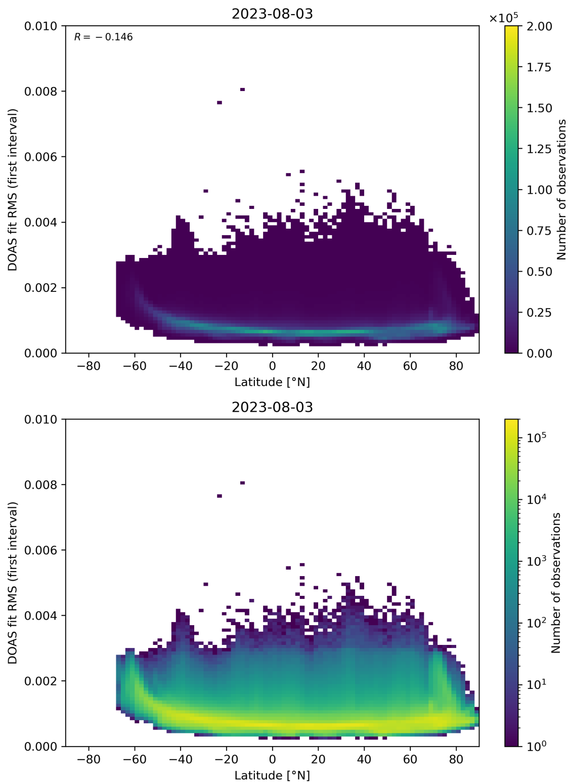
Figure 153: Scatter density plot of “Latitude” against “DOAS fit RMS (first interval)” for 2023-08-02 to 2023-08-04.
