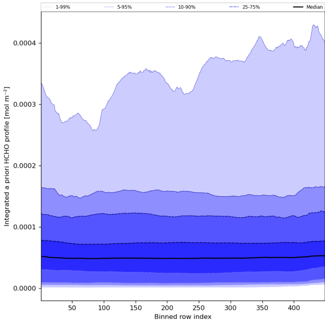
Figure 57: Along track statistics of "Integrated a priori HCHO profile" for 2023-08-02 to 2023-08-04
