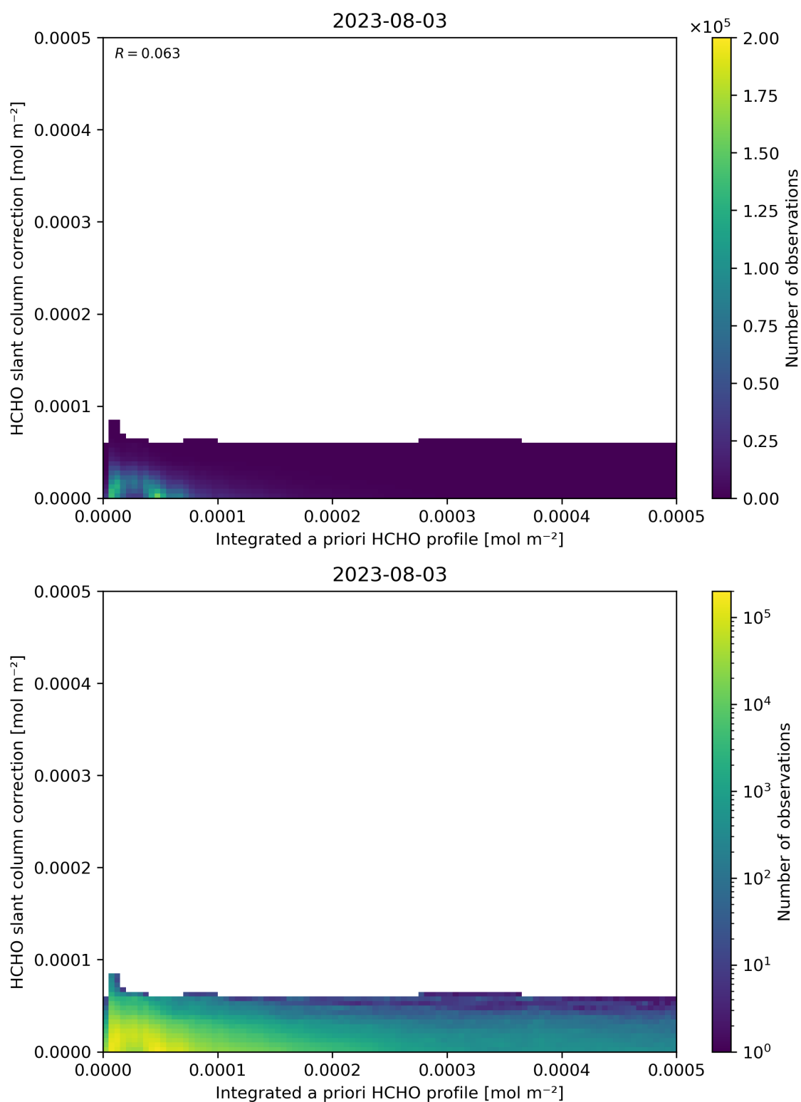
Figure 152: Scatter density plot of “Integrated a priori HCHO profile” against “HCHO slant column correction” for 2023-08-02 to 2023-08-04.
