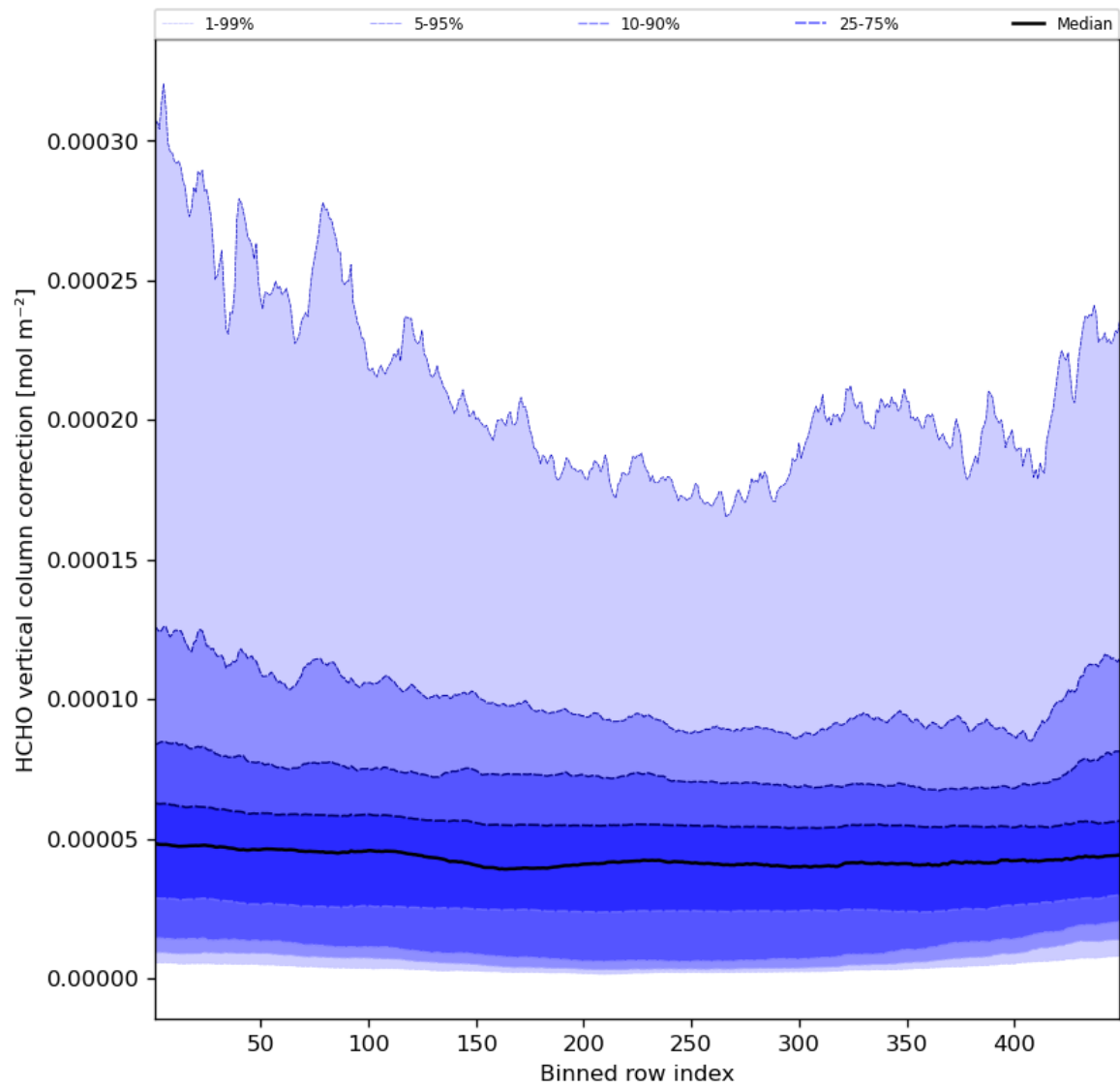
Figure 51: Along track statistics of “HCHO vertical column correction” for 2023-08-02 to 2023-08-04
