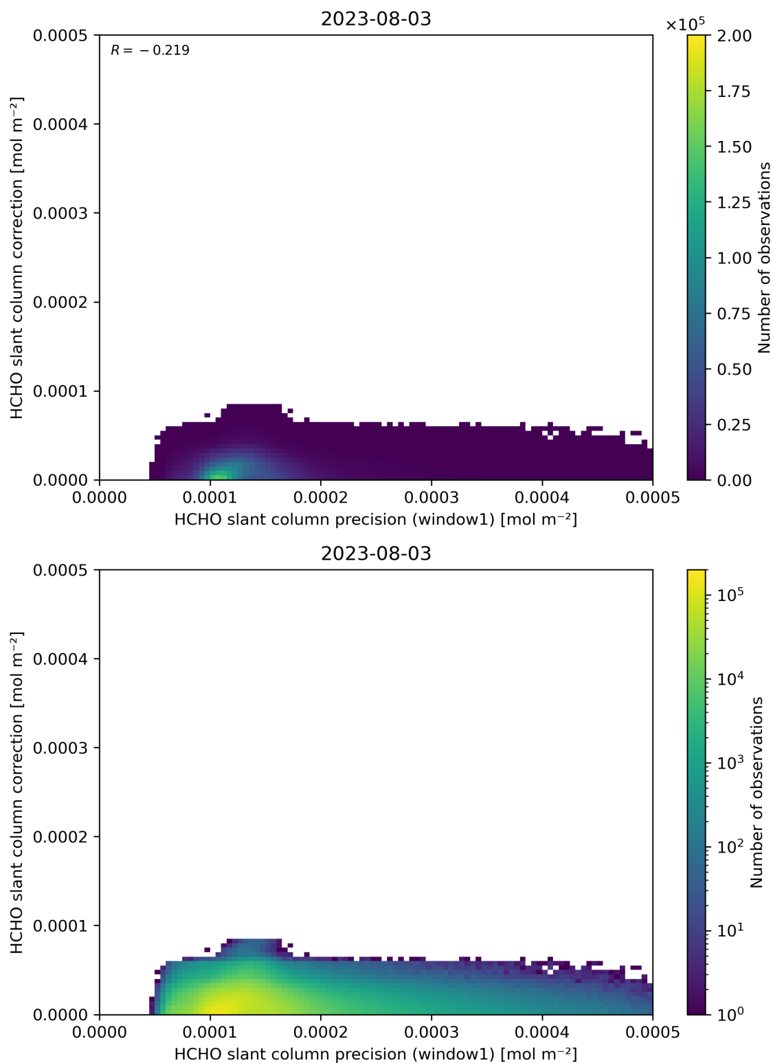
Figure 93: Scatter density plot of “HCHO slant column precision (window1)” against “HCHO slant column correction” for 2023-08-02 to 2023-08-04.
