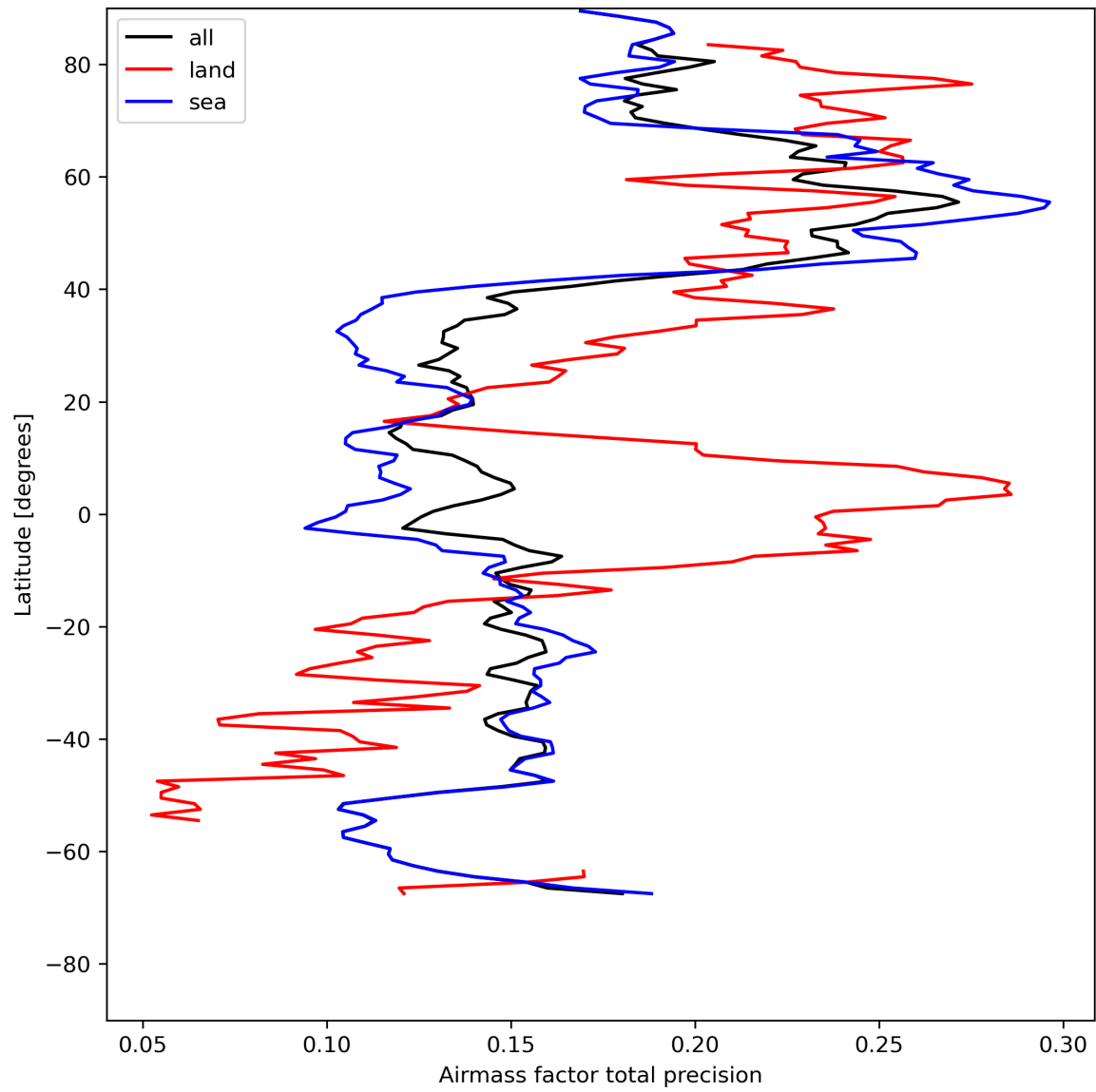
Figure 27: Zonal average of “Airmass factor total precision” for 2023-08-02 to 2023-08-04.
