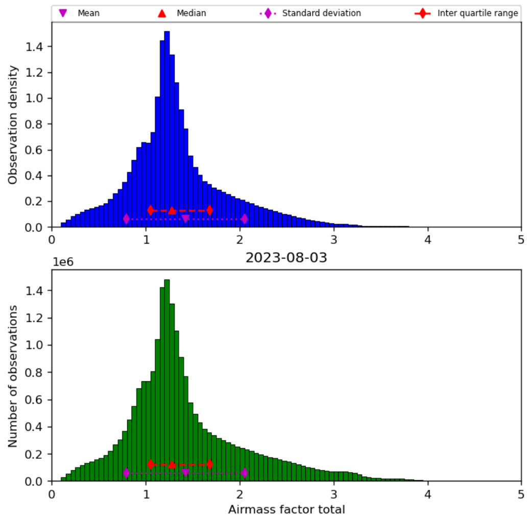
Figure 40: Histogram of “Airmass factor total” for 2023-08-02 to 2023-08-04
