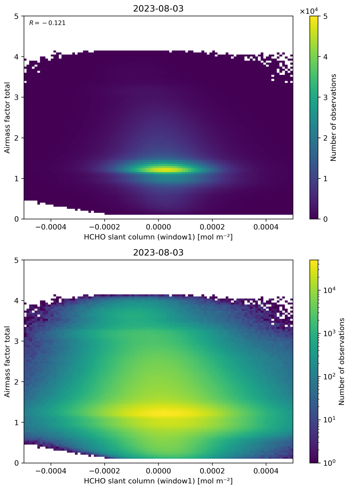
Figure 85: Scatter density plot of “HCHO slant column (window1)” against “Airmass factor total” for 2023-08-02 to 2023-08-04.
