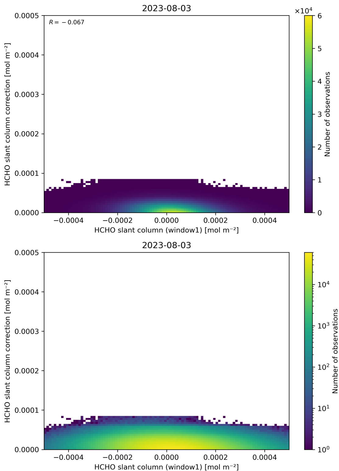
Figure 83: Scatter density plot of “HCHO slant column (window1)” against “HCHO slant column correction” for 2023-08-02 to 2023-08-04.
