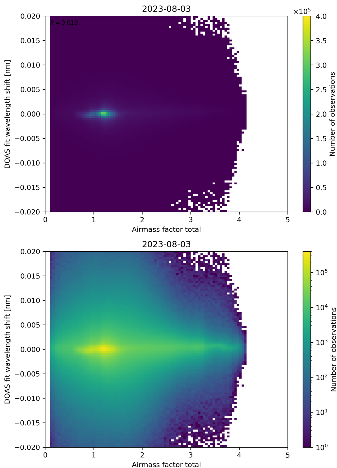
Figure 98: Scatter density plot of “Airmass factor total” against “DOAS fit wavelength shift” for 2023-08-02 to 2023-08-04.
