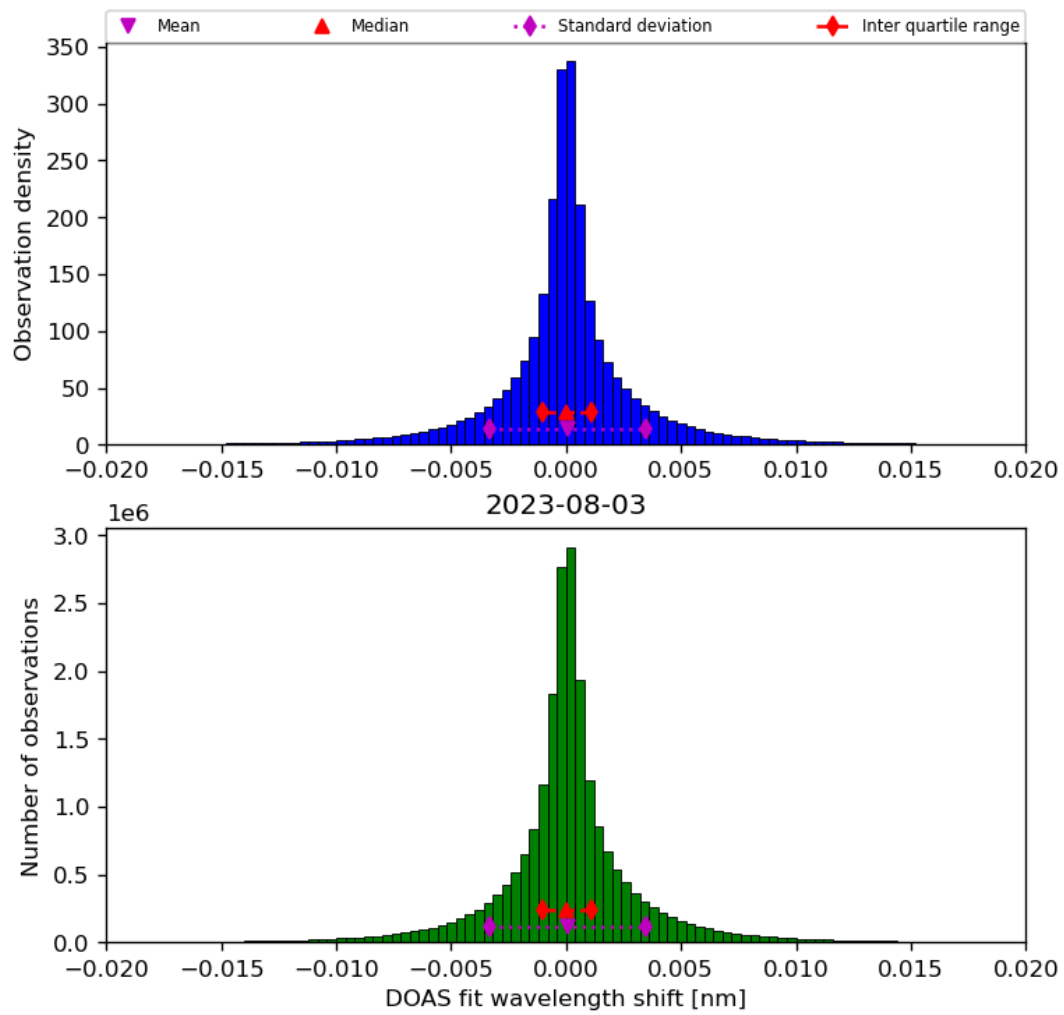
Figure 44: Histogram of “DOAS fit wavelength shift” for 2023-08-02 to 2023-08-04
