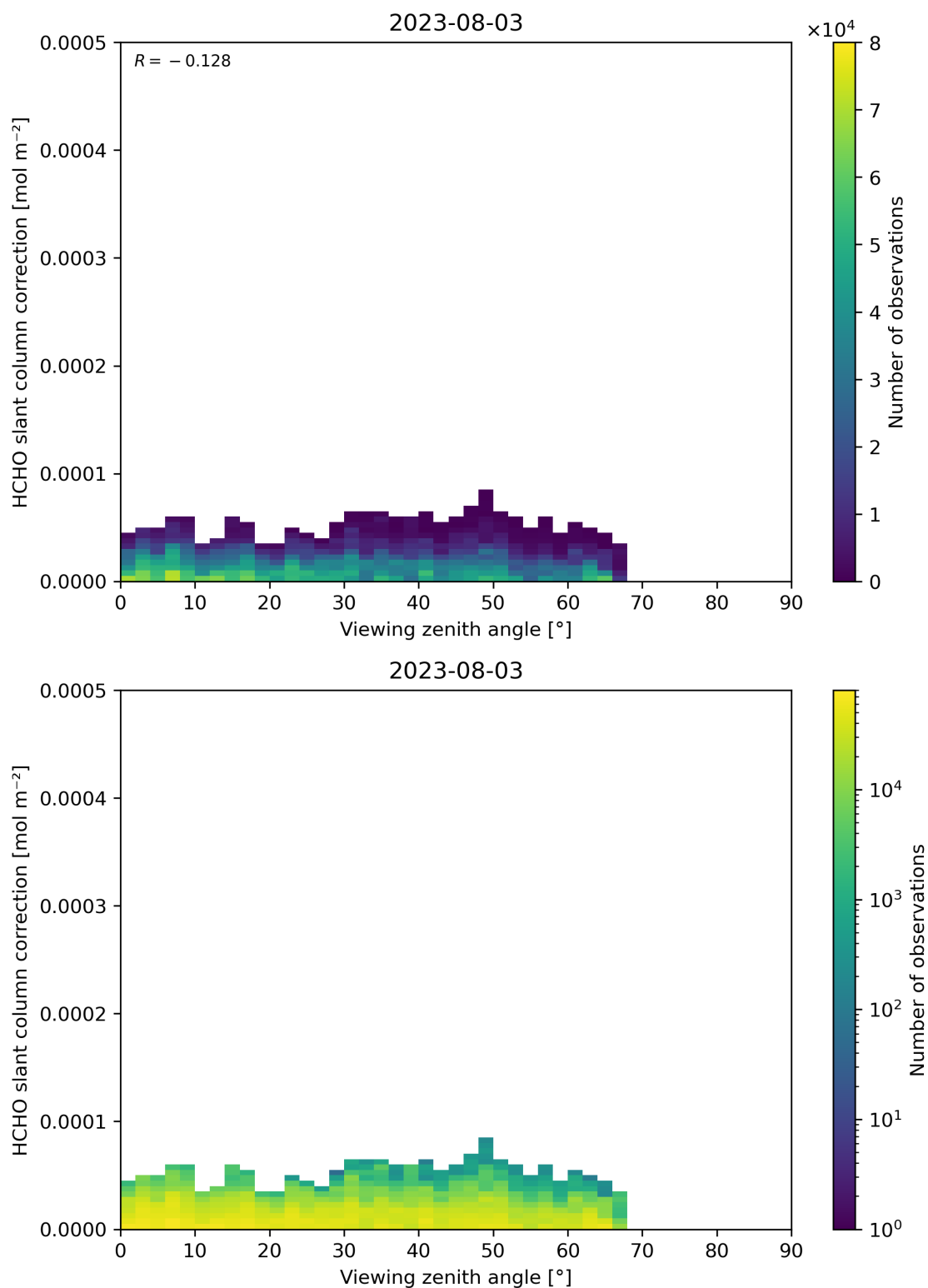
Figure 187: Scatter density plot of “Viewing zenith angle” against “HCHO slant column correction” for 2023-08-02 to 2023-08-04.
