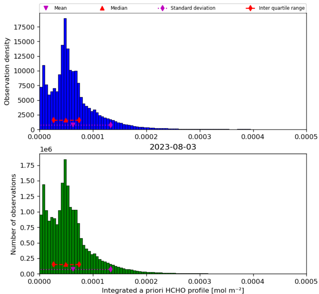
Figure 43: Histogram of “Integrated a priori HCHO profile” for 2023-08-02 to 2023-08-04
