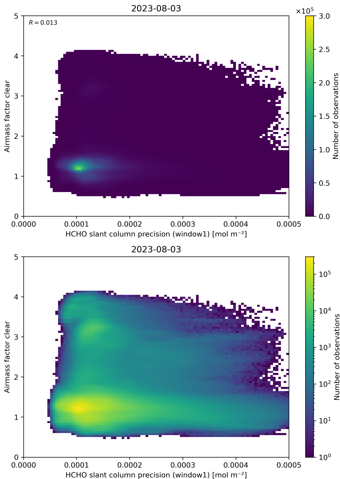
Figure 91: Scatter density plot of “HCHO slant column precision (window1)” against “Airmass factor clear” for 2023-08-02 to 2023-08-04.
