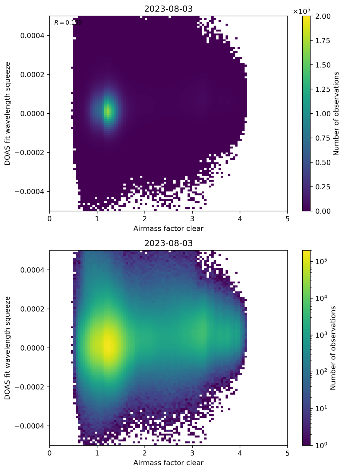
Figure 73: Scatter density plot of “Airmass factor clear” against “DOAS fit wavelength squeeze” for 2023-08-02 to 2023-08-04.
