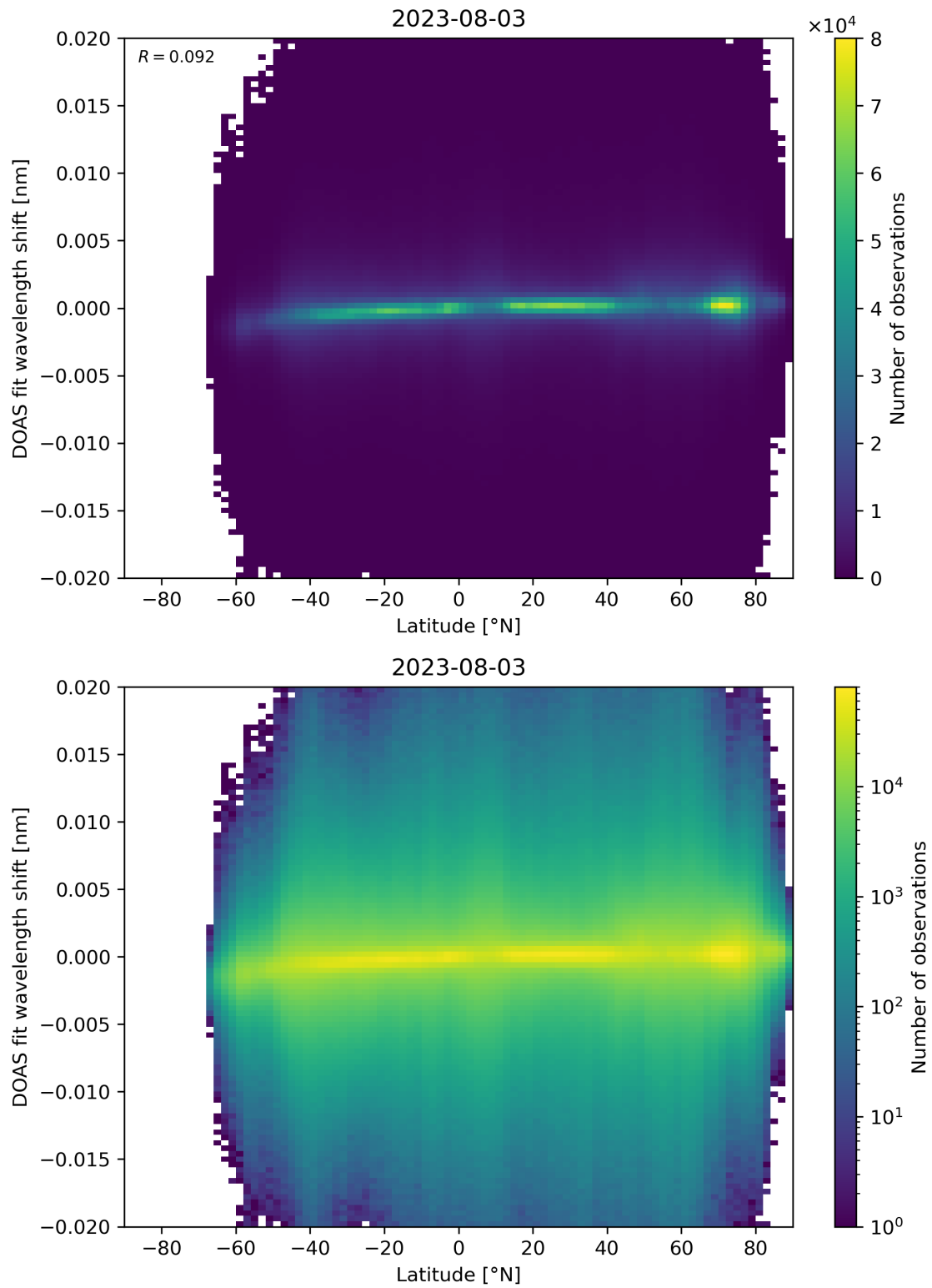
Figure 154: Scatter density plot of “Latitude” against “DOAS fit wavelength shift” for 2023-08-02 to 2023-08-04.
