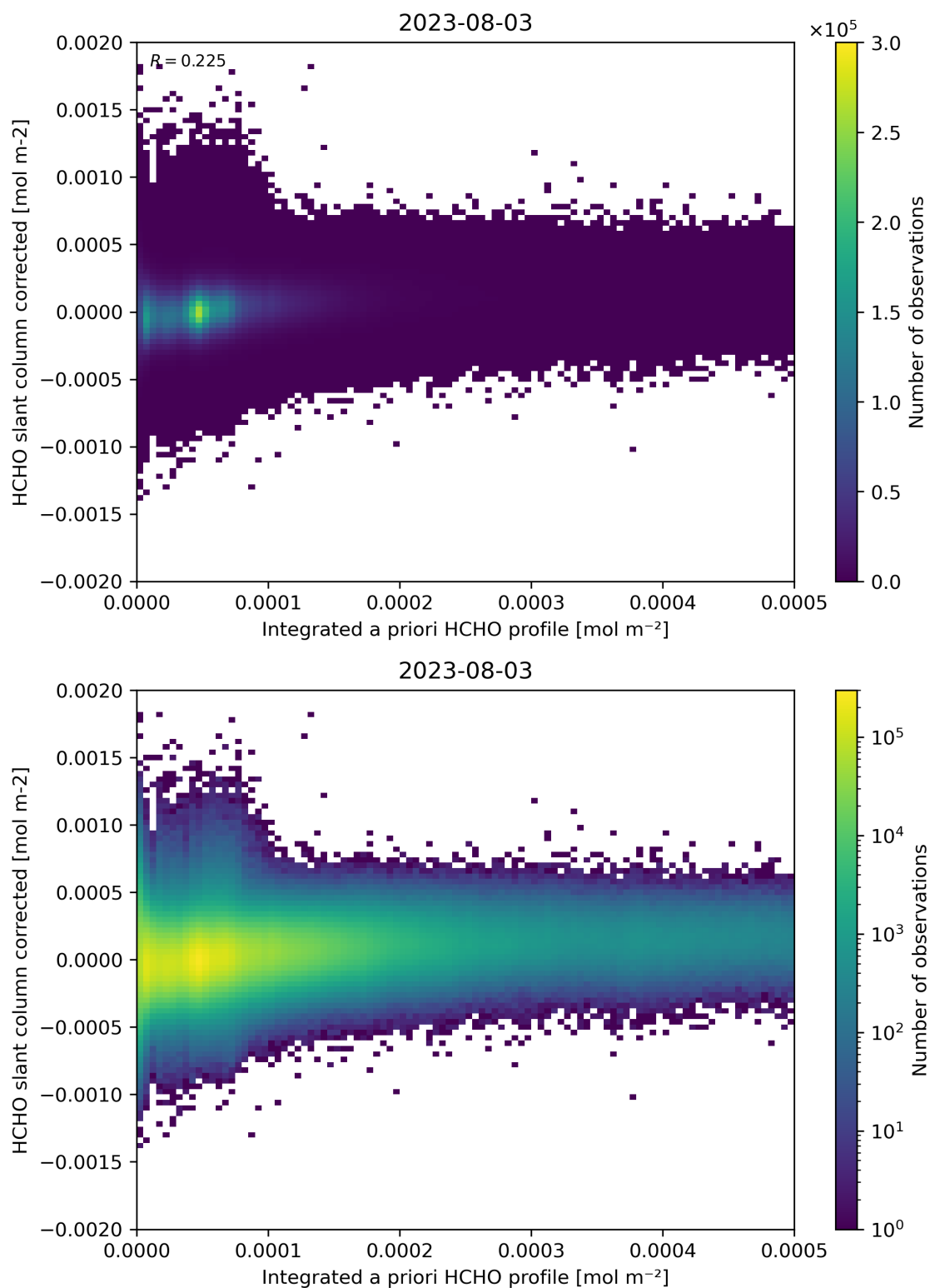
Figure 151: Scatter density plot of “Integrated a priori HCHO profile” against “HCHO slant column corrected” for 2023-08-02 to 2023-08-04.
