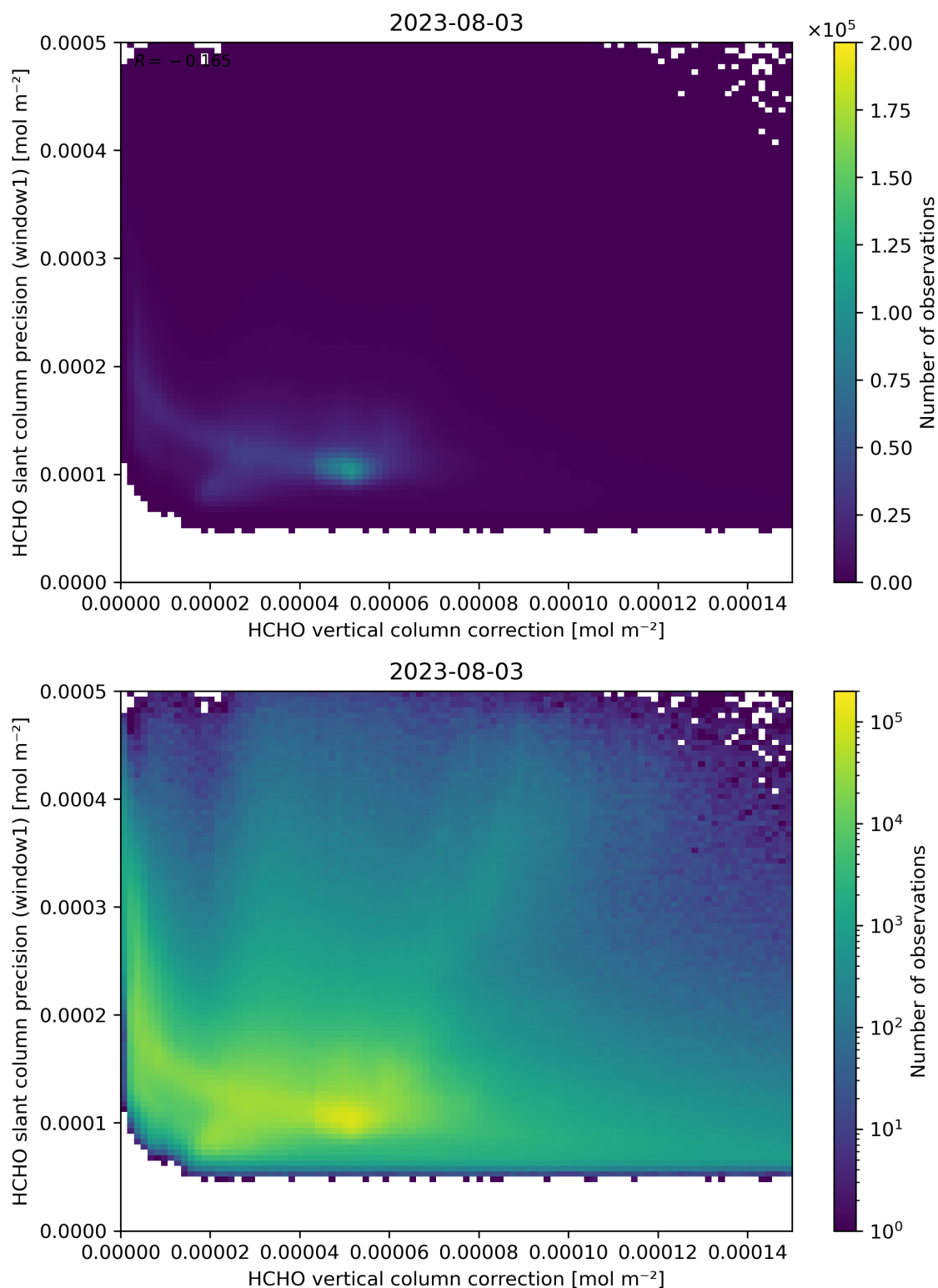
Figure 119: Scatter density plot of “HCHO vertical column correction” against “HCHO slant column precision (window1)” for 2023-08-02 to 2023-08-04.
