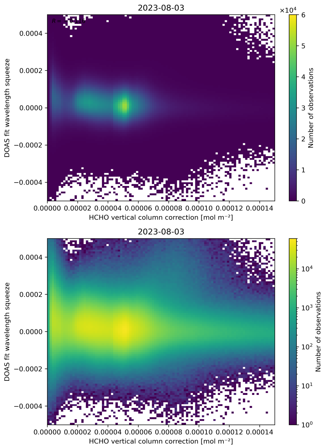
Figure 114: Scatter density plot of “HCHO vertical column correction” against “DOAS fit wavelength squeeze” for 2023-08-02 to 2023-08-04.
