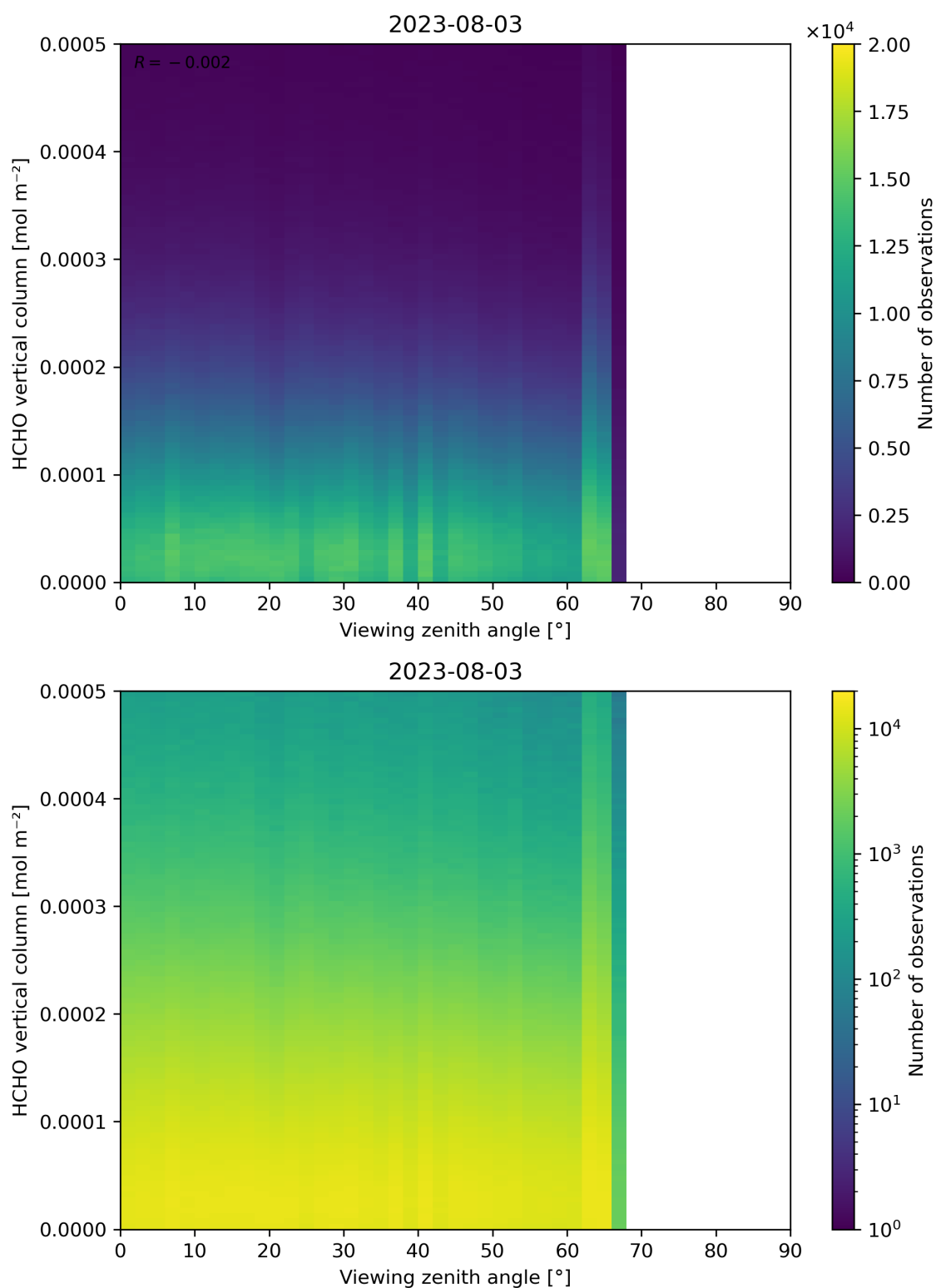
Figure 192: Scatter density plot of “Viewing zenith angle” against “HCHO vertical column” for 2023-08-02 to 2023-08-04.
