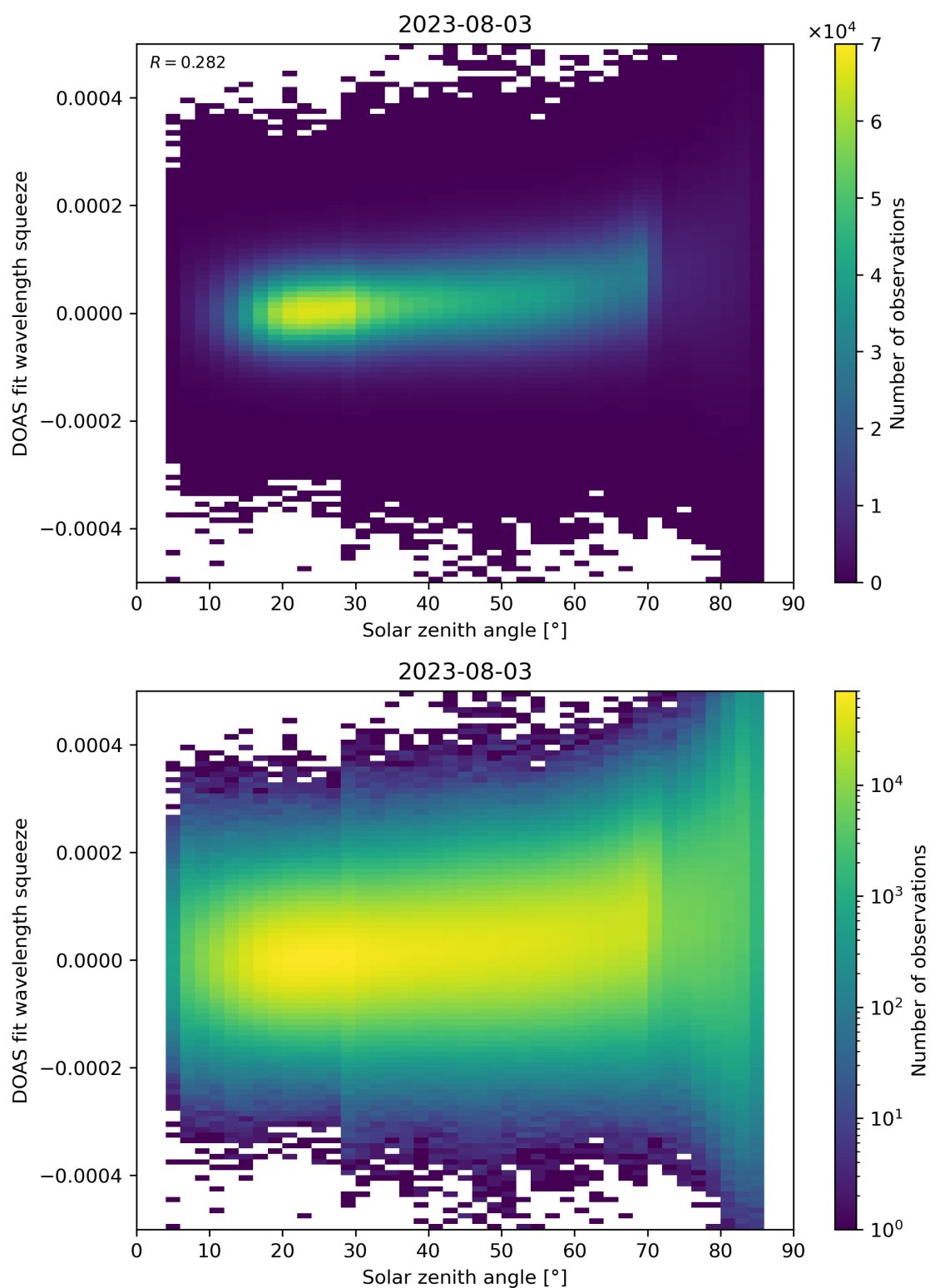
Figure 169: Scatter density plot of “Solar zenith angle” against “DOAS fit wavelength squeeze” for 2023-08-02 to 2023-08-04.
