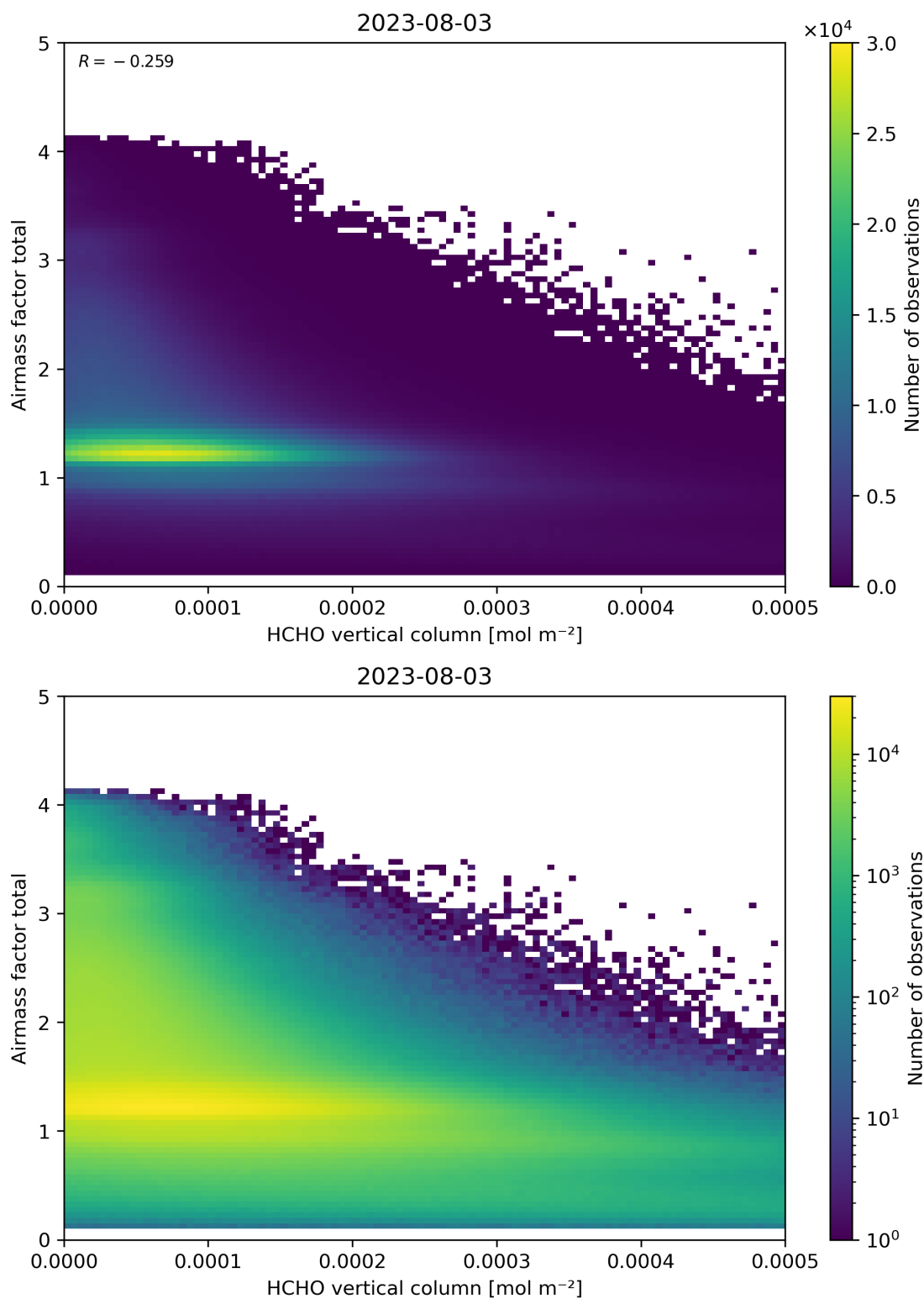
Figure 131: Scatter density plot of “HCHO vertical column” against “Airmass factor total” for 2023-08-02 to 2023-08-04.
