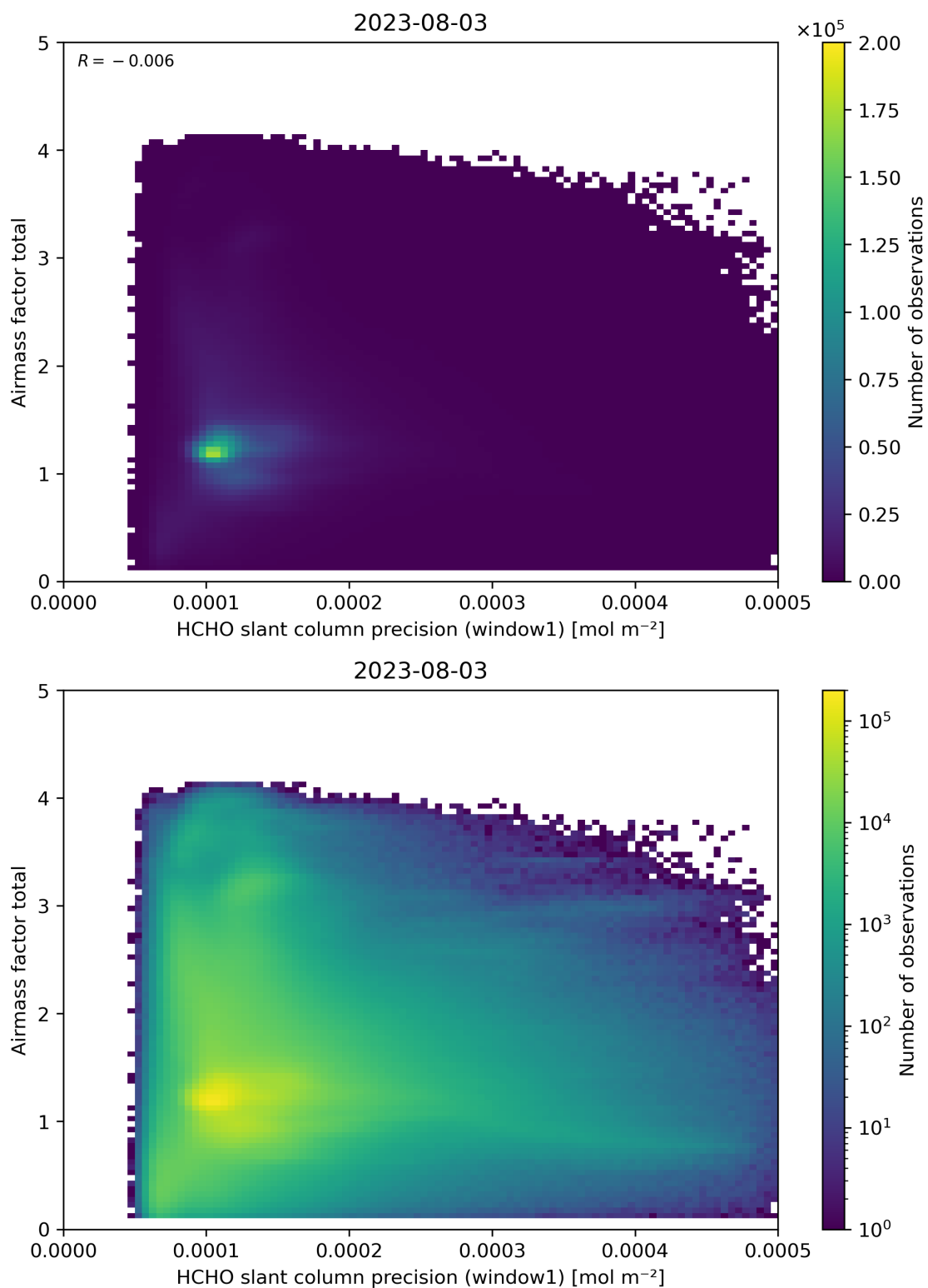
Figure 94: Scatter density plot of “HCHO slant column precision (window1)” against “Airmass factor total” for 2023-08-02 to 2023-08-04.
