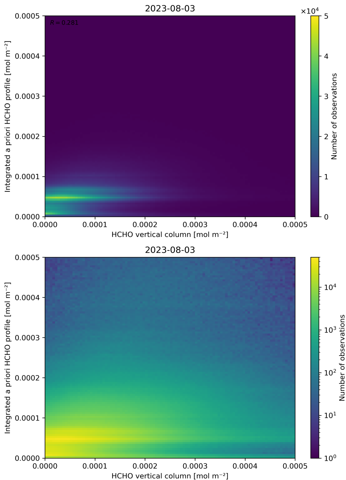
Figure 135: Scatter density plot of “HCHO vertical column” against “Integrated a priori HCHO profile” for 2023-08-02 to 2023-08-04.
