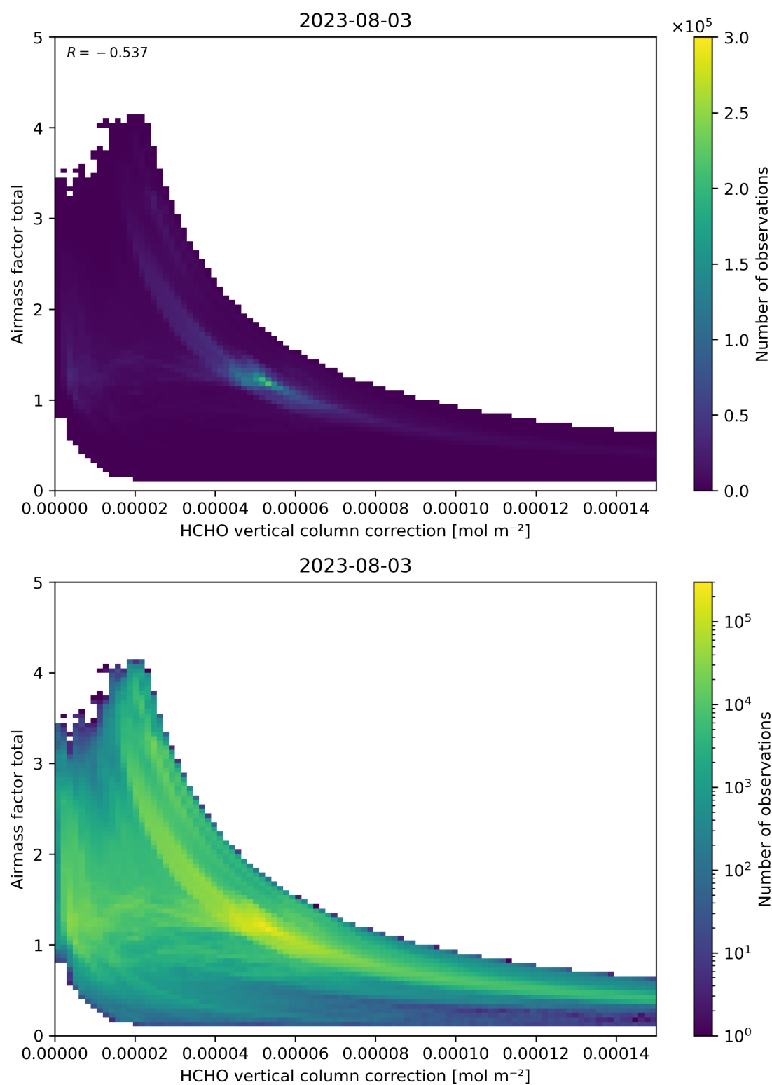
Figure 120: Scatter density plot of “HCHO vertical column correction” against “Airmass factor total” for 2023-08-02 to 2023-08-04.
