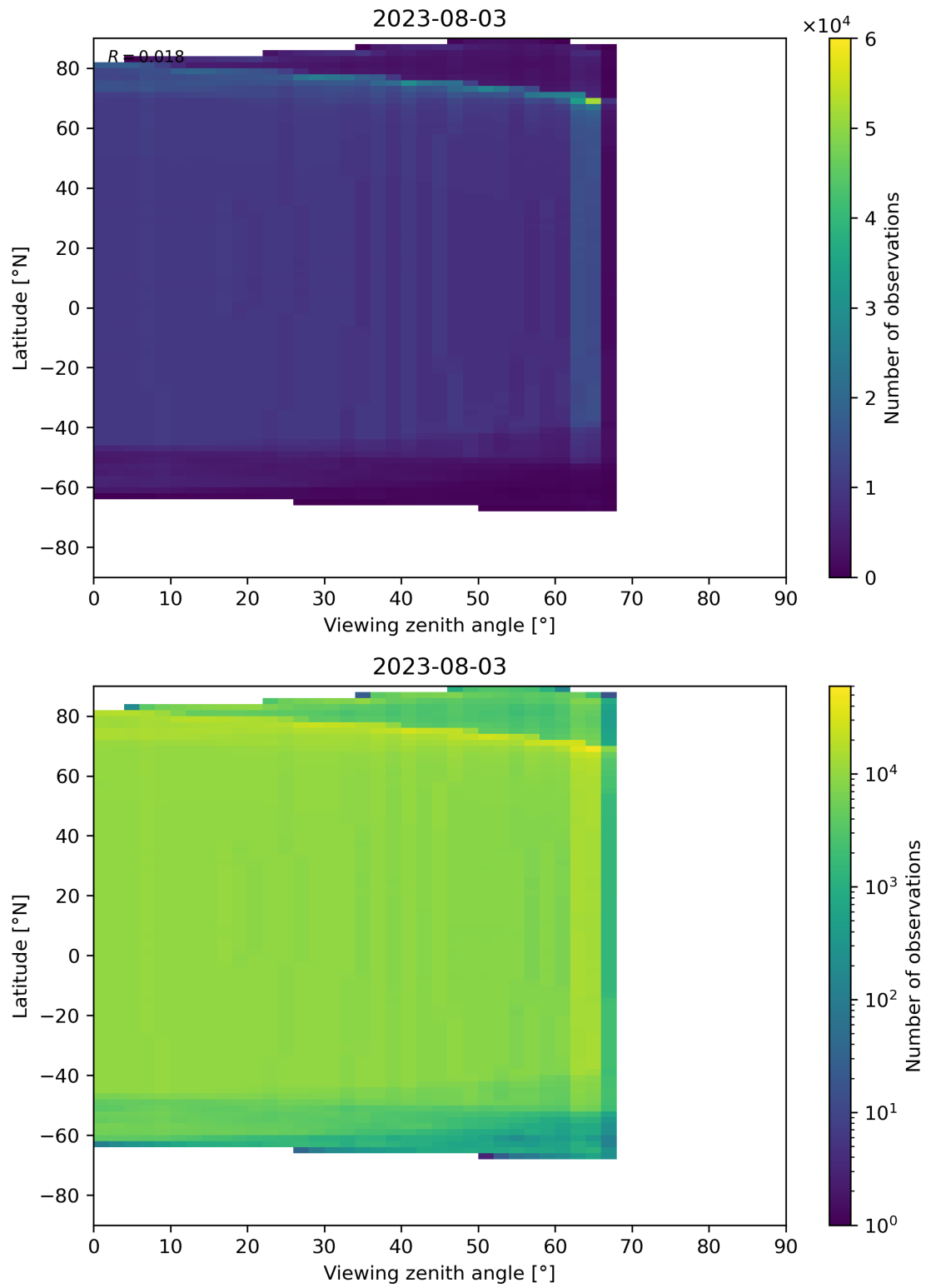
Figure 196: Scatter density plot of “Viewing zenith angle” against “Latitude” for 2023-08-02 to 2023-08-04.
