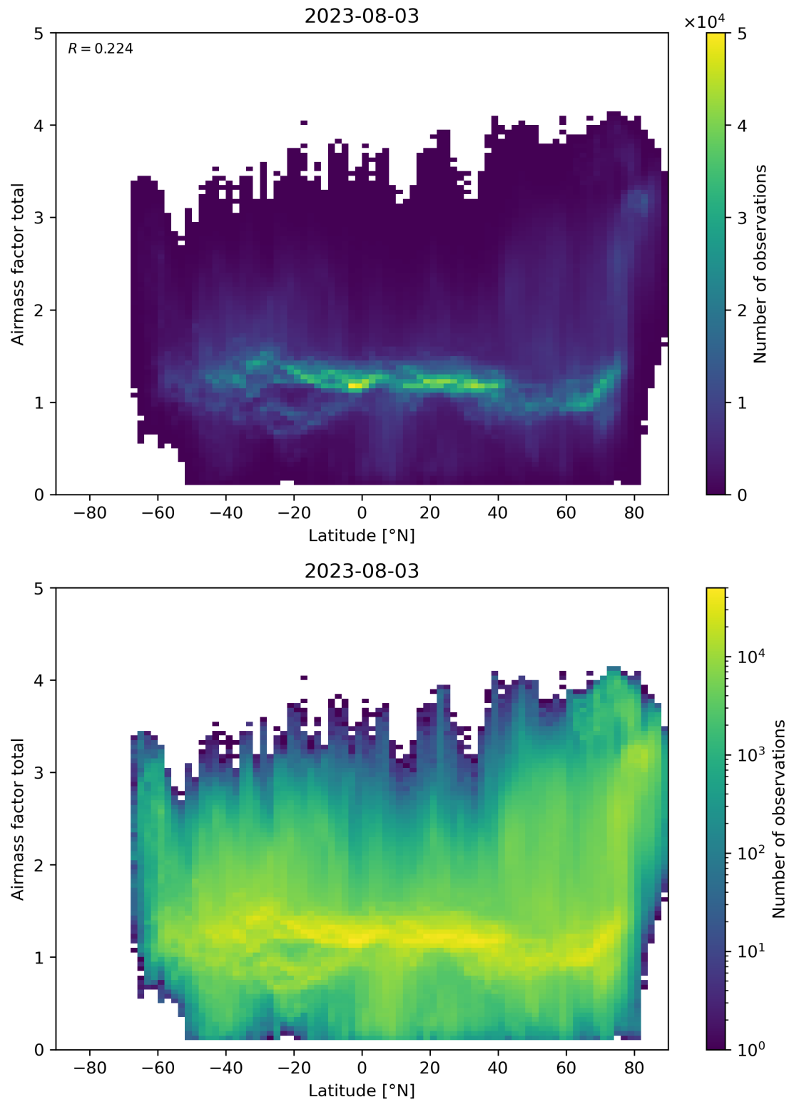
Figure 161: Scatter density plot of “Latitude” against “Airmass factor total” for 2023-08-02 to 2023-08-04.
