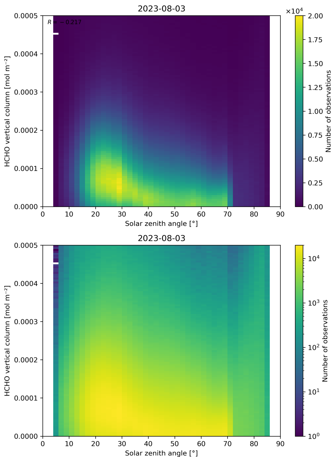
Figure 177: Scatter density plot of “Solar zenith angle” against “HCHO vertical column” for 2023-08-02 to 2023-08-04.
