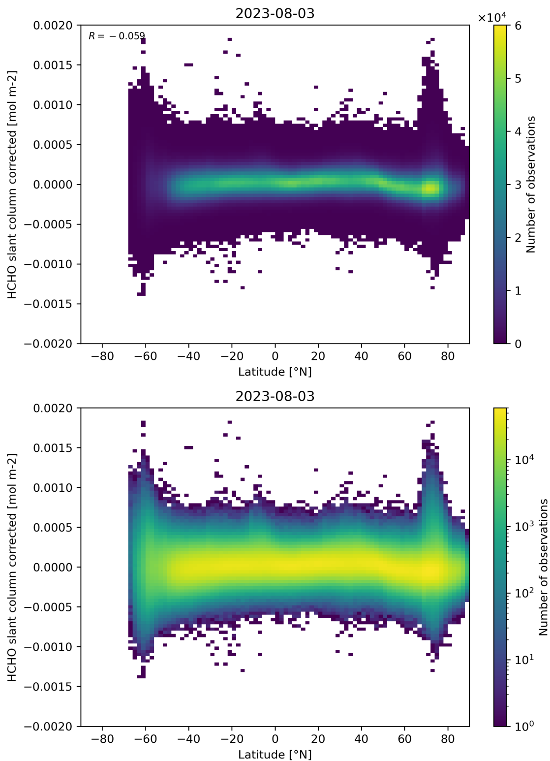
Figure 157: Scatter density plot of “Latitude” against “HCHO slant column corrected” for 2023-08-02 to 2023-08-04.
