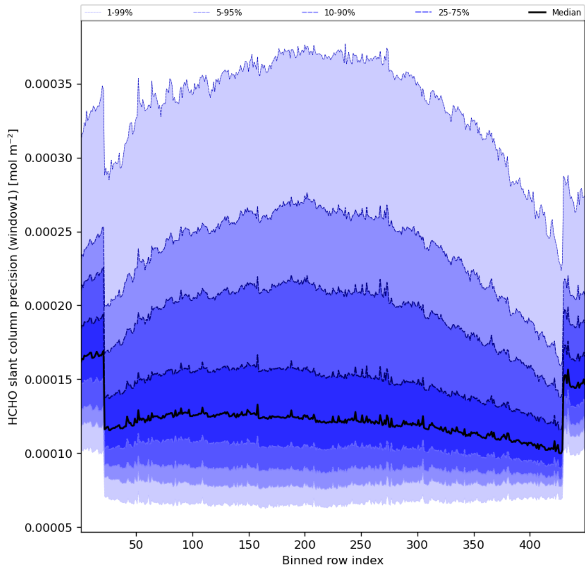
Figure 53: Along track statistics of “HCHO slant column precision (window1)” for 2023-08-02 to 2023-08-04
