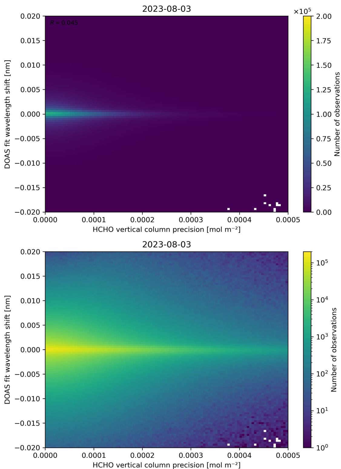
Figure 137: Scatter density plot of “HCHO vertical column precision” against “DOAS fit wavelength shift” for 2023-08-02 to 2023-08-04.
