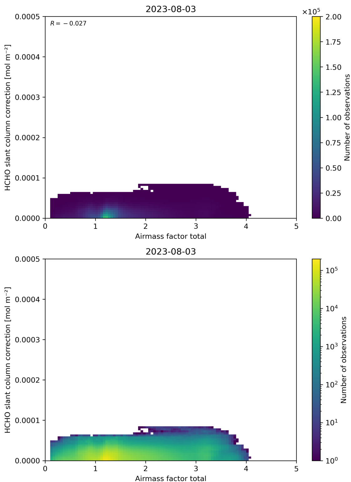
Figure 102: Scatter density plot of “Airmass factor total” against “HCHO slant column correction” for 2023-08-02 to 2023-08-04.
