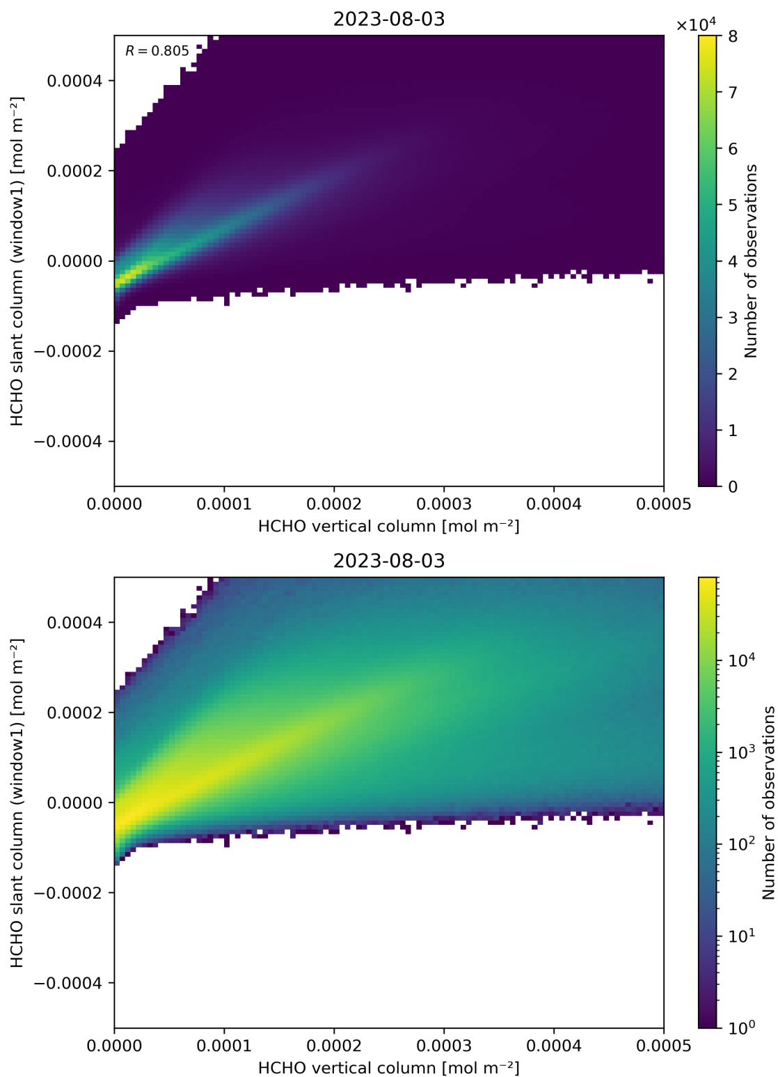
Figure 129: Scatter density plot of “HCHO vertical column” against “HCHO slant column (window1)” for 2023-08-02 to 2023-08-04.
