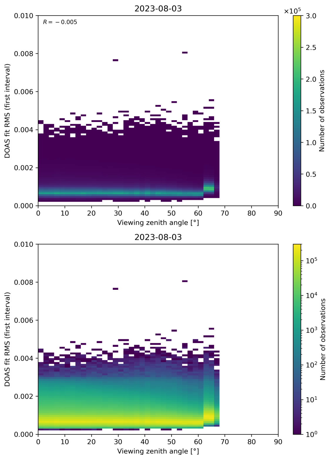
Figure 182: Scatter density plot of “Viewing zenith angle” against “DOAS fit RMS (first interval)” for 2023-08-02 to 2023-08-04.
