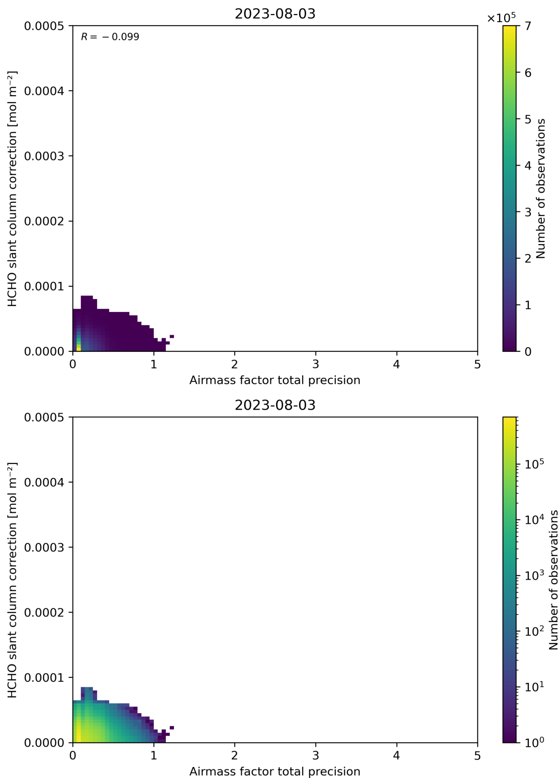
Figure 110: Scatter density plot of “Airmass factor total precision” against “HCHO slant column correction” for 2023-08-02 to 2023-08-04.
