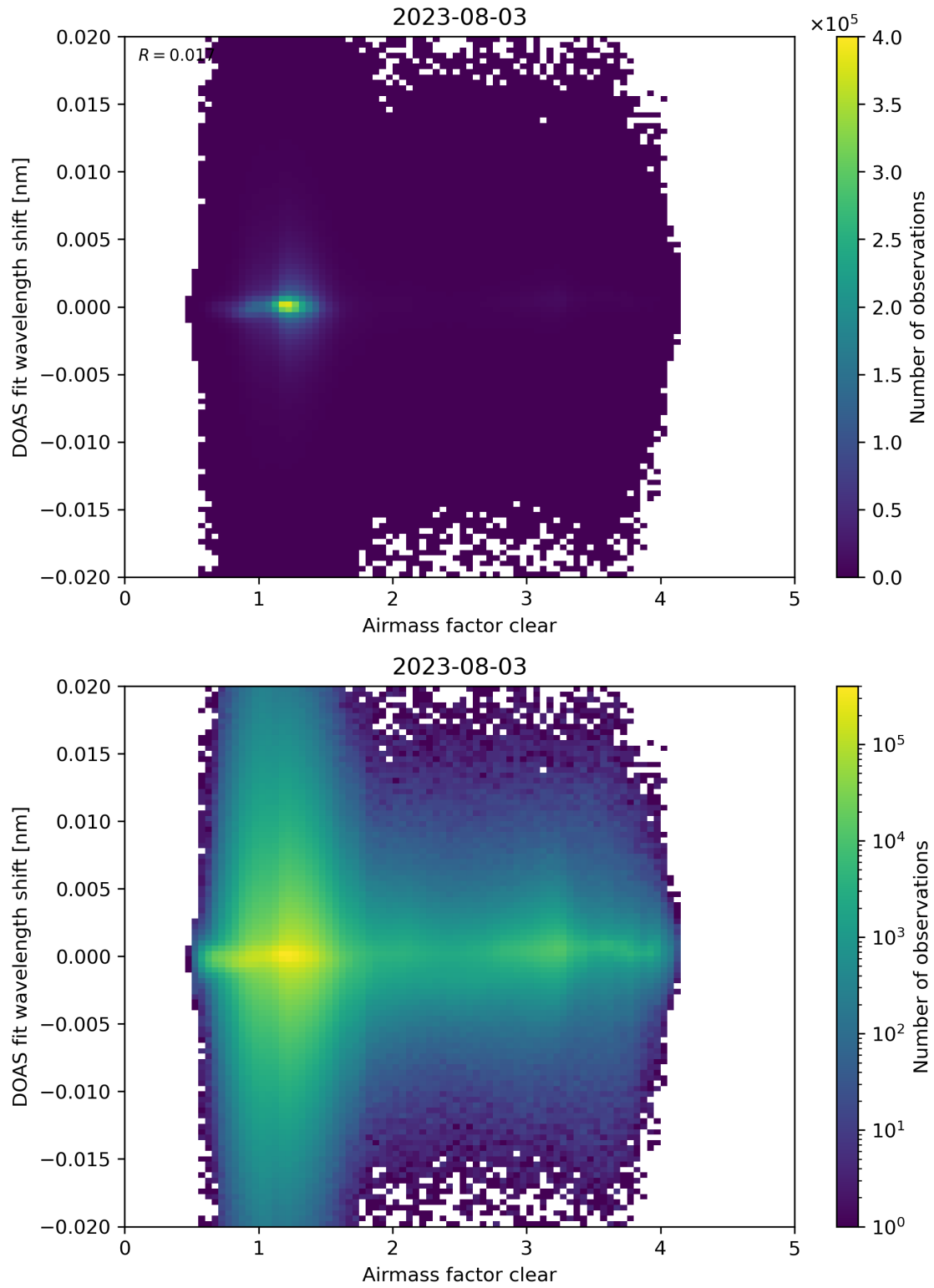
Figure 72: Scatter density plot of “Airmass factor clear” against “DOAS fit wavelength shift” for 2023-08-02 to 2023-08-04.
