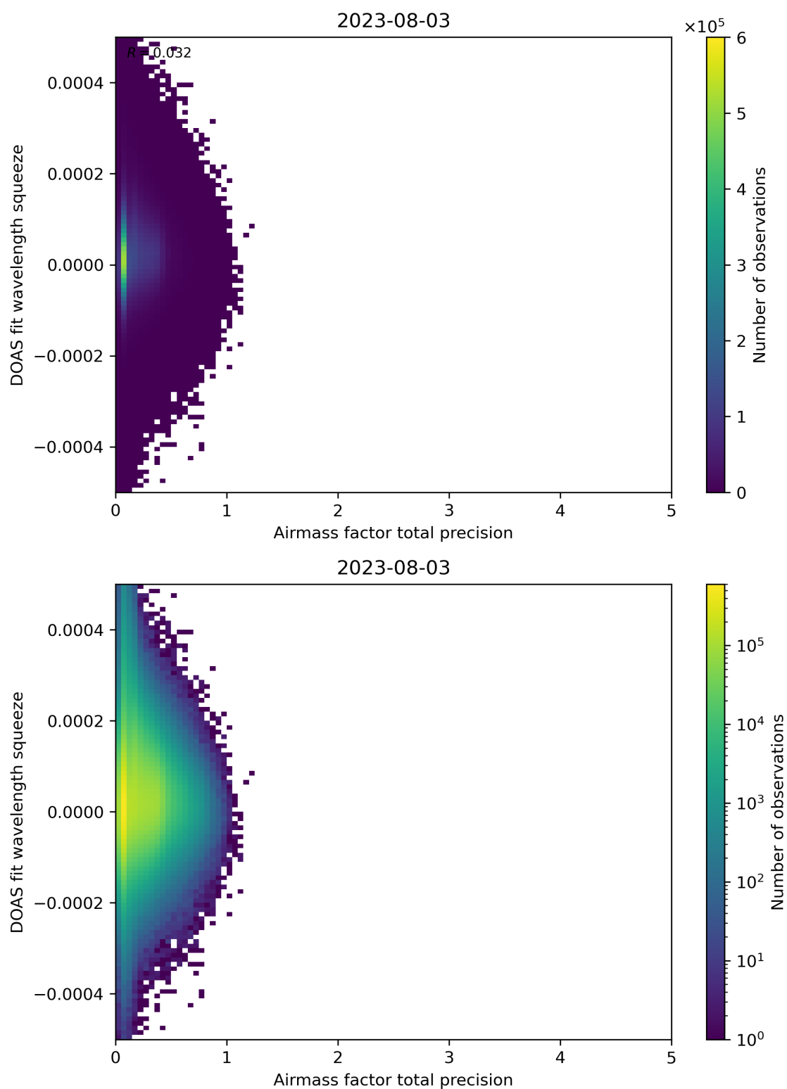
Figure 107: Scatter density plot of “Airmass factor total precision” against “DOAS fit wavelength squeeze” for 2023-08-02 to 2023-08-04.
