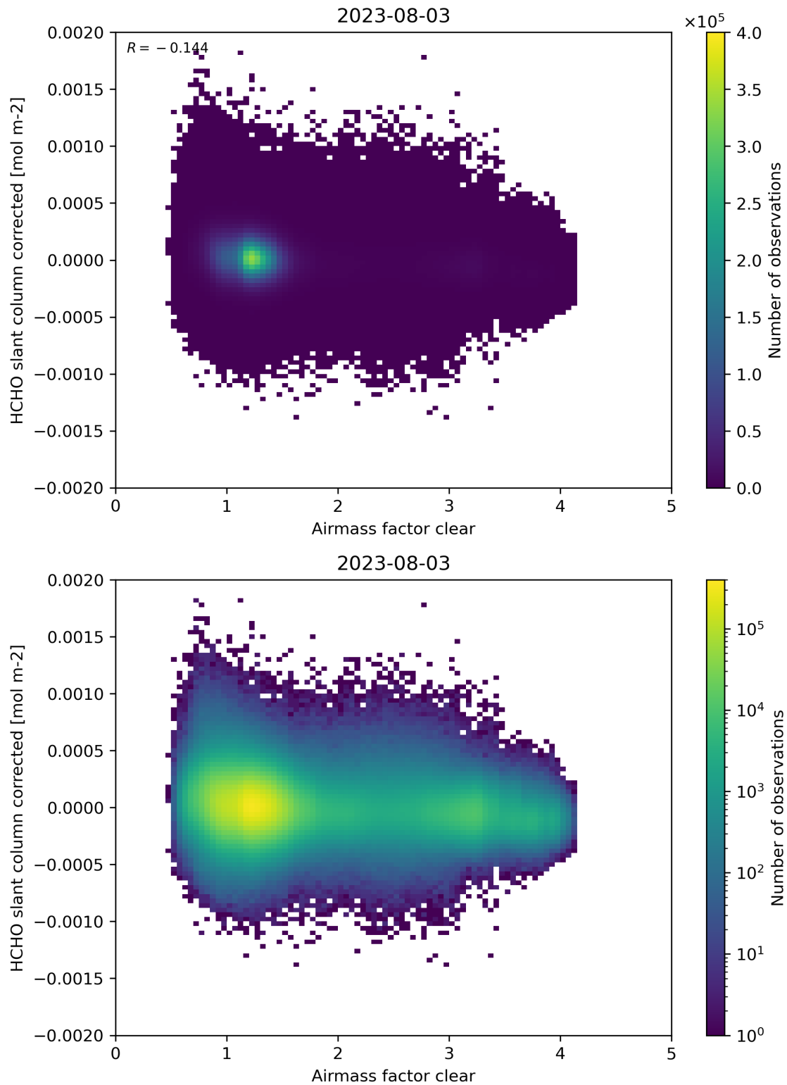
Figure 74: Scatter density plot of “Airmass factor clear” against “HCHO slant column corrected” for 2023-08-02 to 2023-08-04.
