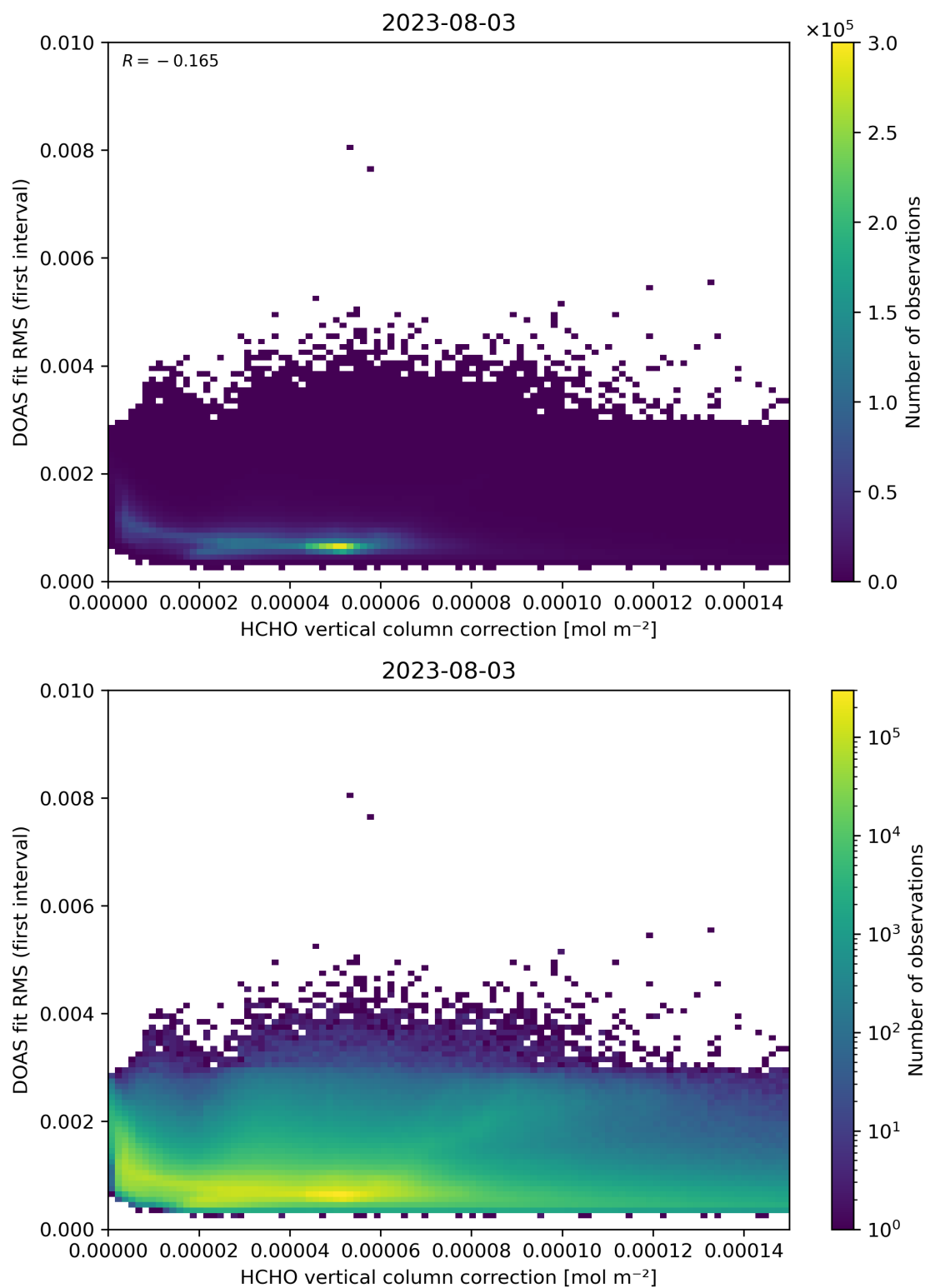
Figure 112: Scatter density plot of “HCHO vertical column correction” against “DOAS fit RMS (first interval)” for 2023-08-02 to 2023-08-04.
