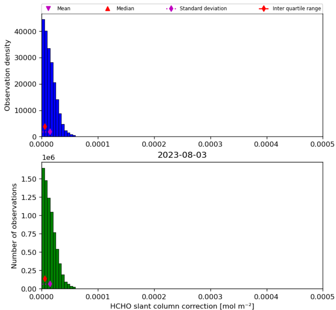
Figure 47: Histogram of “HCHO slant column correction” for 2023-08-02 to 2023-08-04
