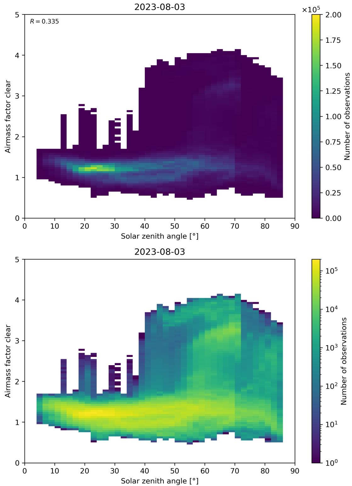
Figure 170: Scatter density plot of “Solar zenith angle” against “Airmass factor clear” for 2023-08-02 to 2023-08-04.
