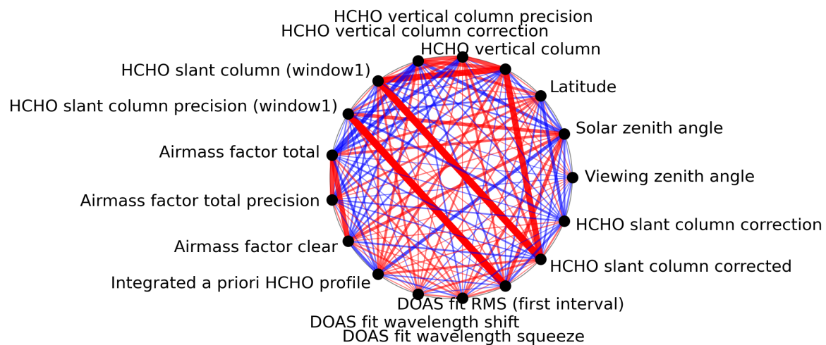
Figure 1: Map of correlation graph for 2023-08-02 to 2023-08-04.
