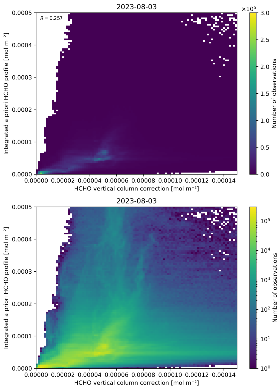
Figure 122: Scatter density plot of “HCHO vertical column correction” against “Integrated a priori HCHO profile” for 2023-08-02 to 2023-08-04.
