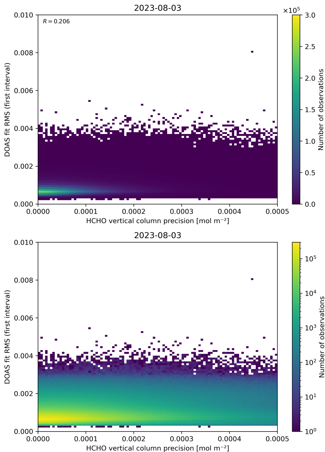
Figure 136: Scatter density plot of “HCHO vertical column precision” against “DOAS fit RMS (first interval)” for 2023-08-02 to 2023-08-04.
