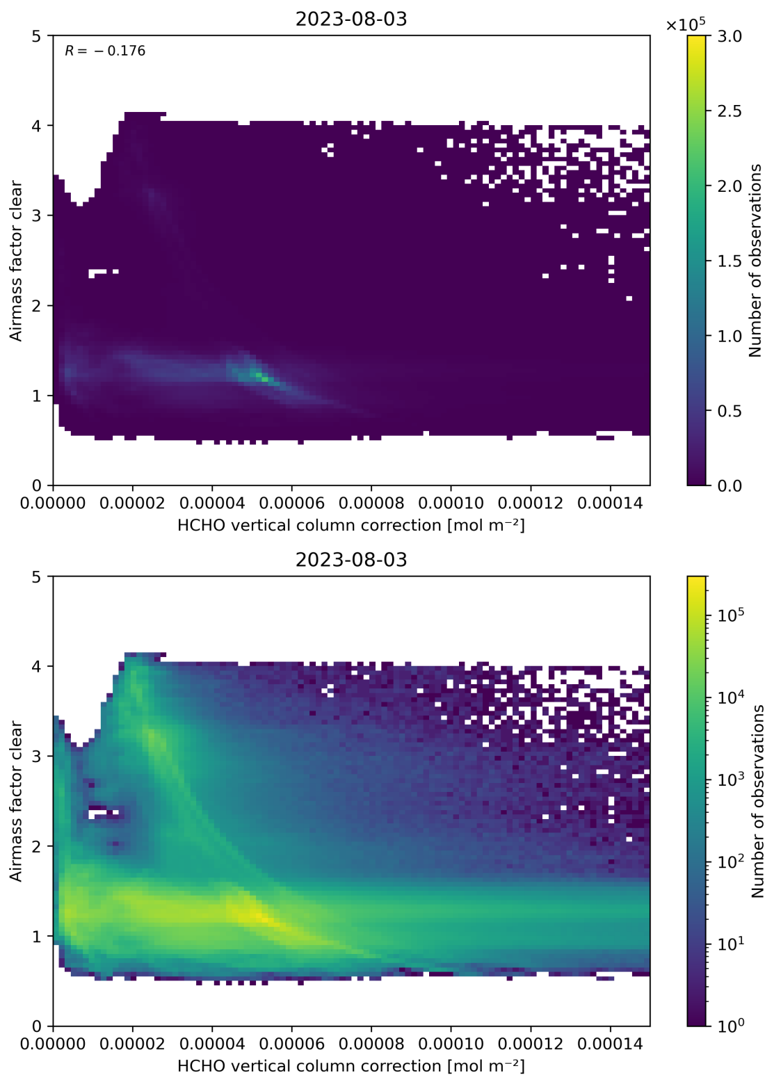
Figure 115: Scatter density plot of “HCHO vertical column correction” against “Airmass factor clear” for 2023-08-02 to 2023-08-04.
