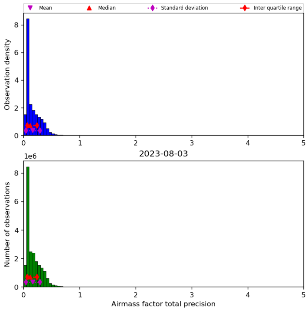
Figure 41: Histogram of “Airmass factor total precision” for 2023-08-02 to 2023-08-04
