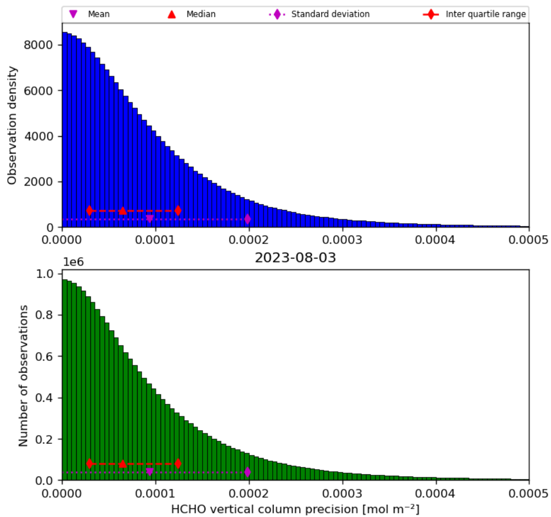
Figure 36: Histogram of “HCHO vertical column precision” for 2023-08-02 to 2023-08-04
