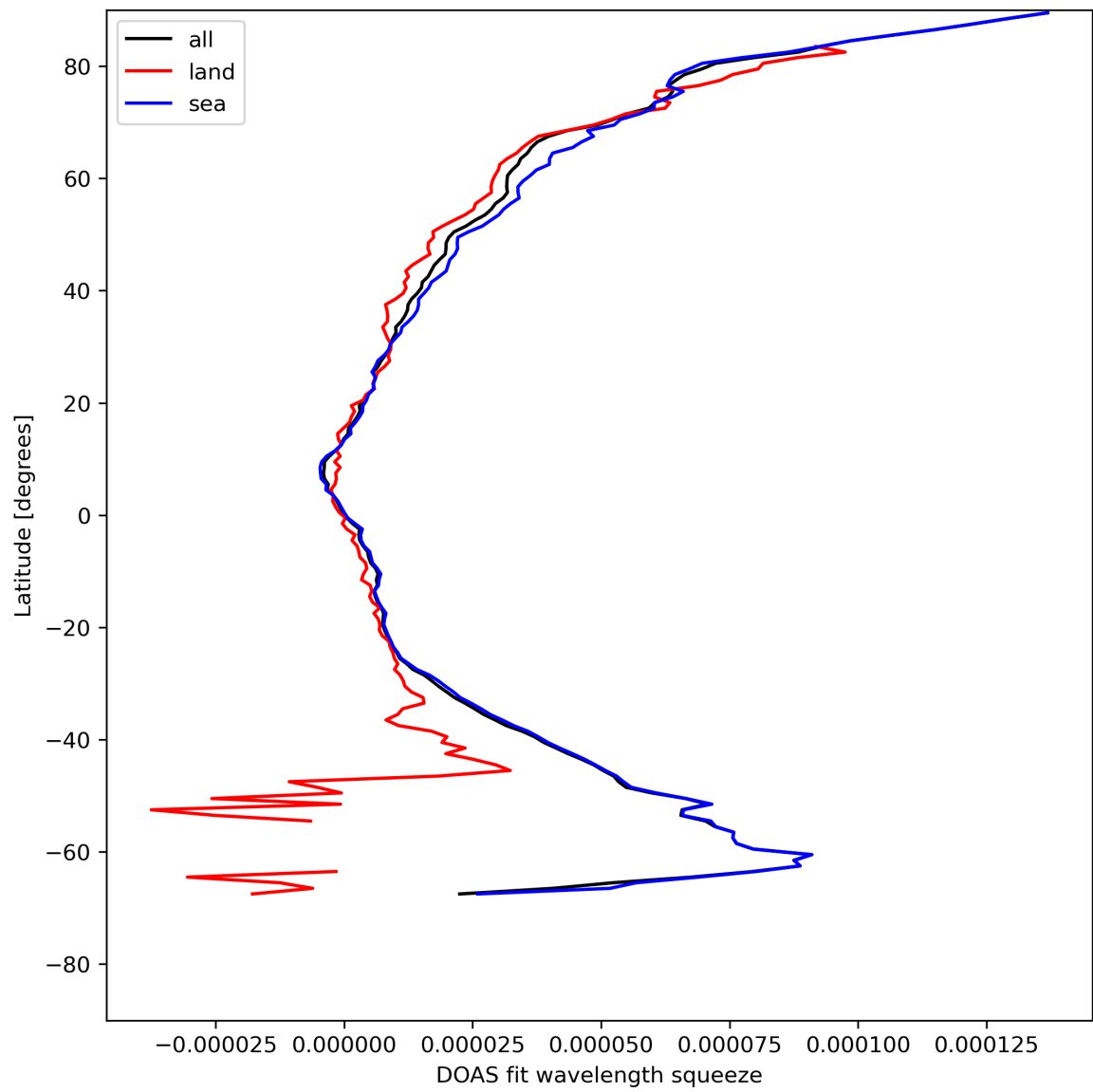
Figure 31: Zonal average of “DOAS fit wavelength squeeze” for 2023-08-02 to 2023-08-04.
