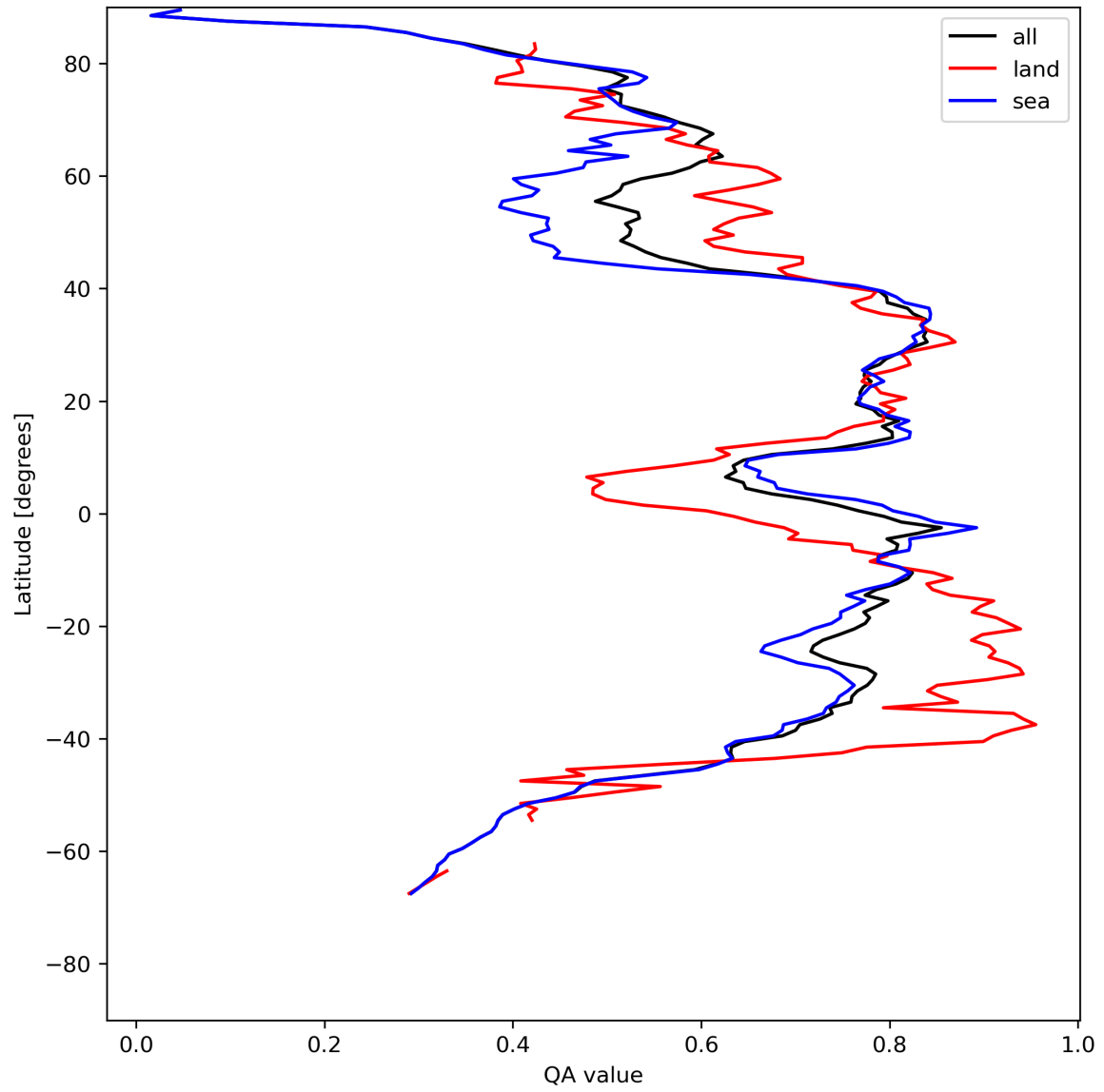
Figure 20: Zonal average of “QA value” for 2023-08-02 to 2023-08-04.
