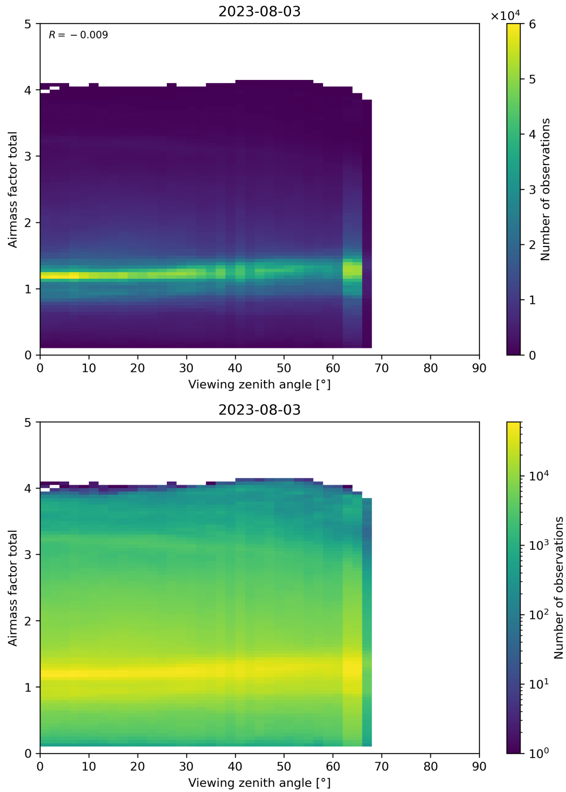
Figure 190: Scatter density plot of “Viewing zenith angle” against “Airmass factor total” for 2023-08-02 to 2023-08-04.
