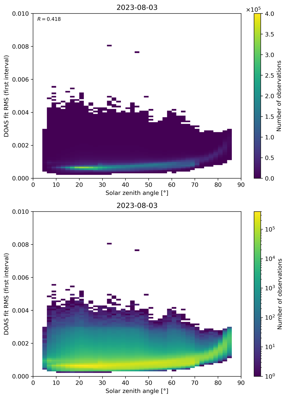
Figure 167: Scatter density plot of “Solar zenith angle” against “DOAS fit RMS (first interval)” for 2023-08-02 to 2023-08-04.
