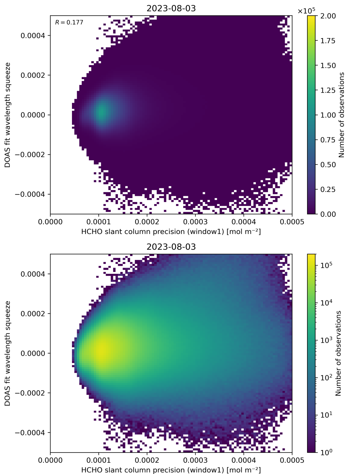
Figure 90: Scatter density plot of “HCHO slant column precision (window1)” against “DOAS fit wavelength squeeze” for 2023-08-02 to 2023-08-04.
