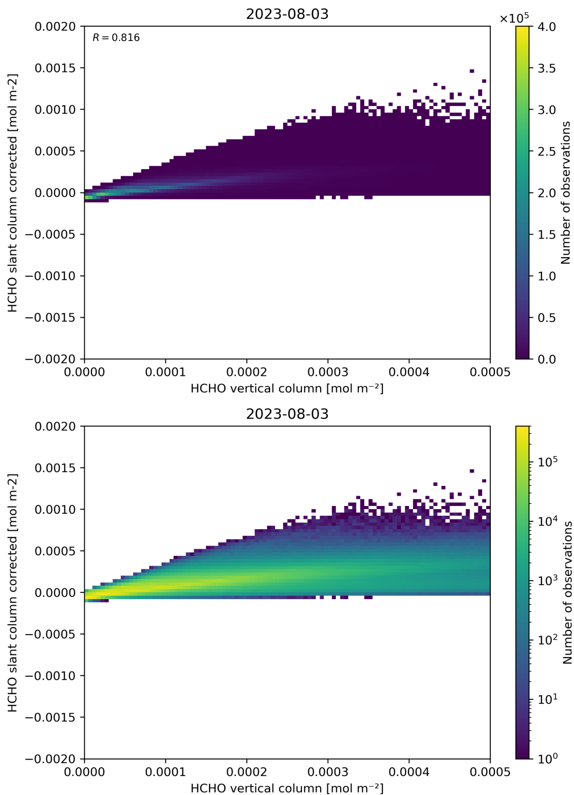
Figure 127: Scatter density plot of “HCHO vertical column” against “HCHO slant column corrected” for 2023-08-02 to 2023-08-04.
