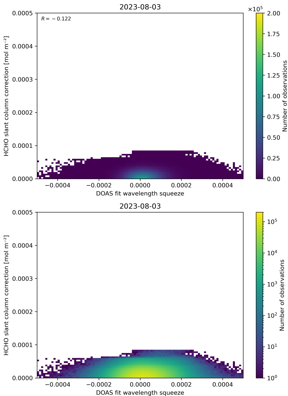
Figure 70: Scatter density plot of “DOAS fit wavelength squeeze” against “HCHO slant column correction” for 2023-08-02 to 2023-08-04.
