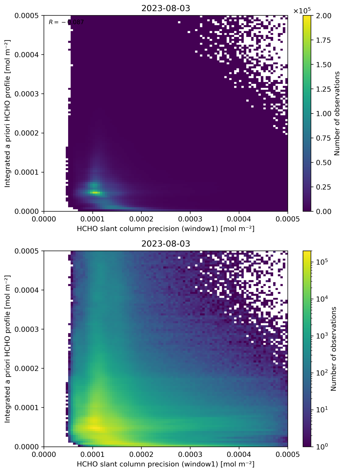
Figure 96: Scatter density plot of “HCHO slant column precision (window1)” against “Integrated a priori HCHO profile” for 2023-08-02 to 2023-08-04.
