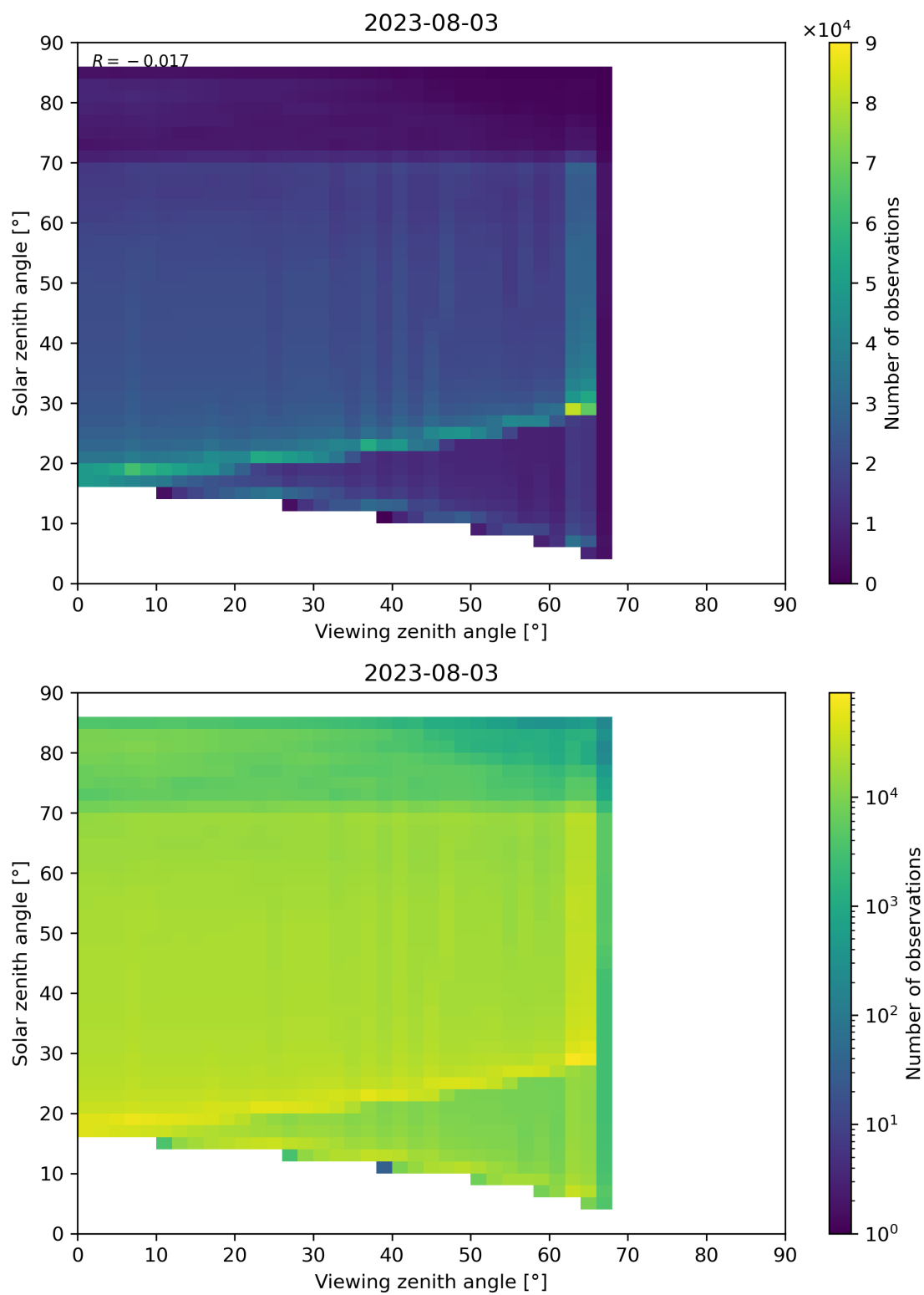
Figure 197: Scatter density plot of “Viewing zenith angle” against “Solar zenith angle” for 2023-08-02 to 2023-08-04.
