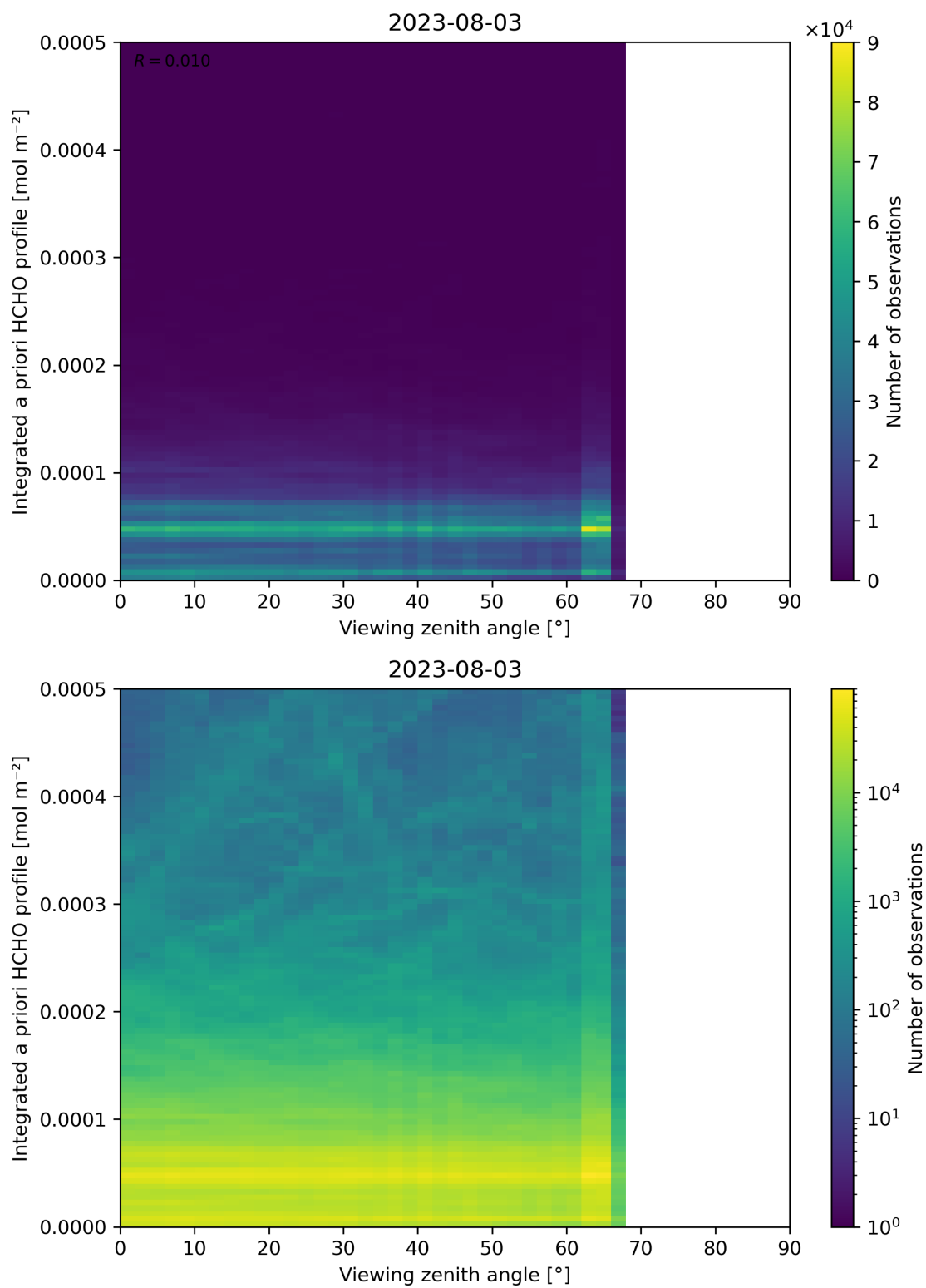
Figure 195: Scatter density plot of “Viewing zenith angle” against “Integrated a priori HCHO profile” for 2023-08-02 to 2023-08-04.
