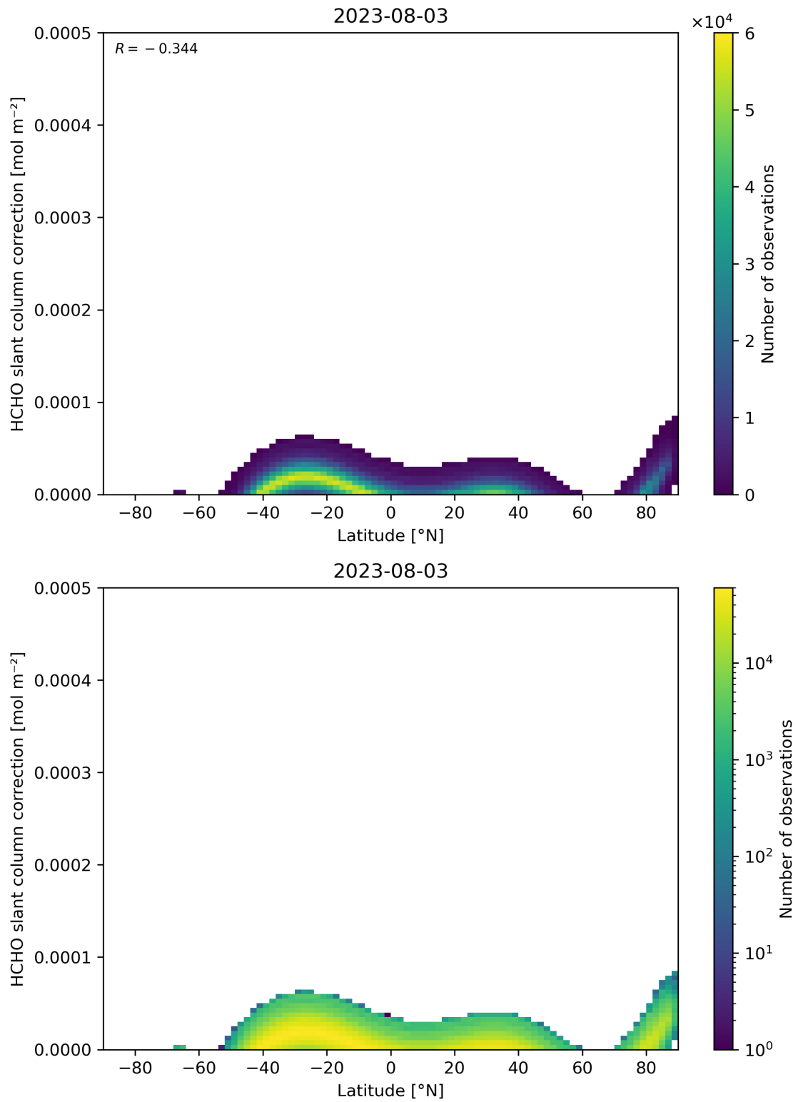
Figure 158: Scatter density plot of “Latitude” against “HCHO slant column correction” for 2023-08-02 to 2023-08-04.
