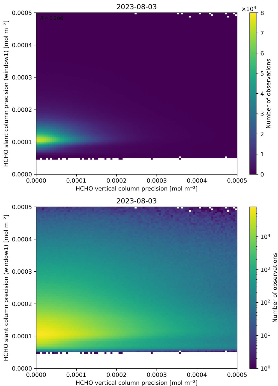
Figure 143: Scatter density plot of “HCHO vertical column precision” against “HCHO slant column precision (window1)” for 2023-08-02 to 2023-08-04.
