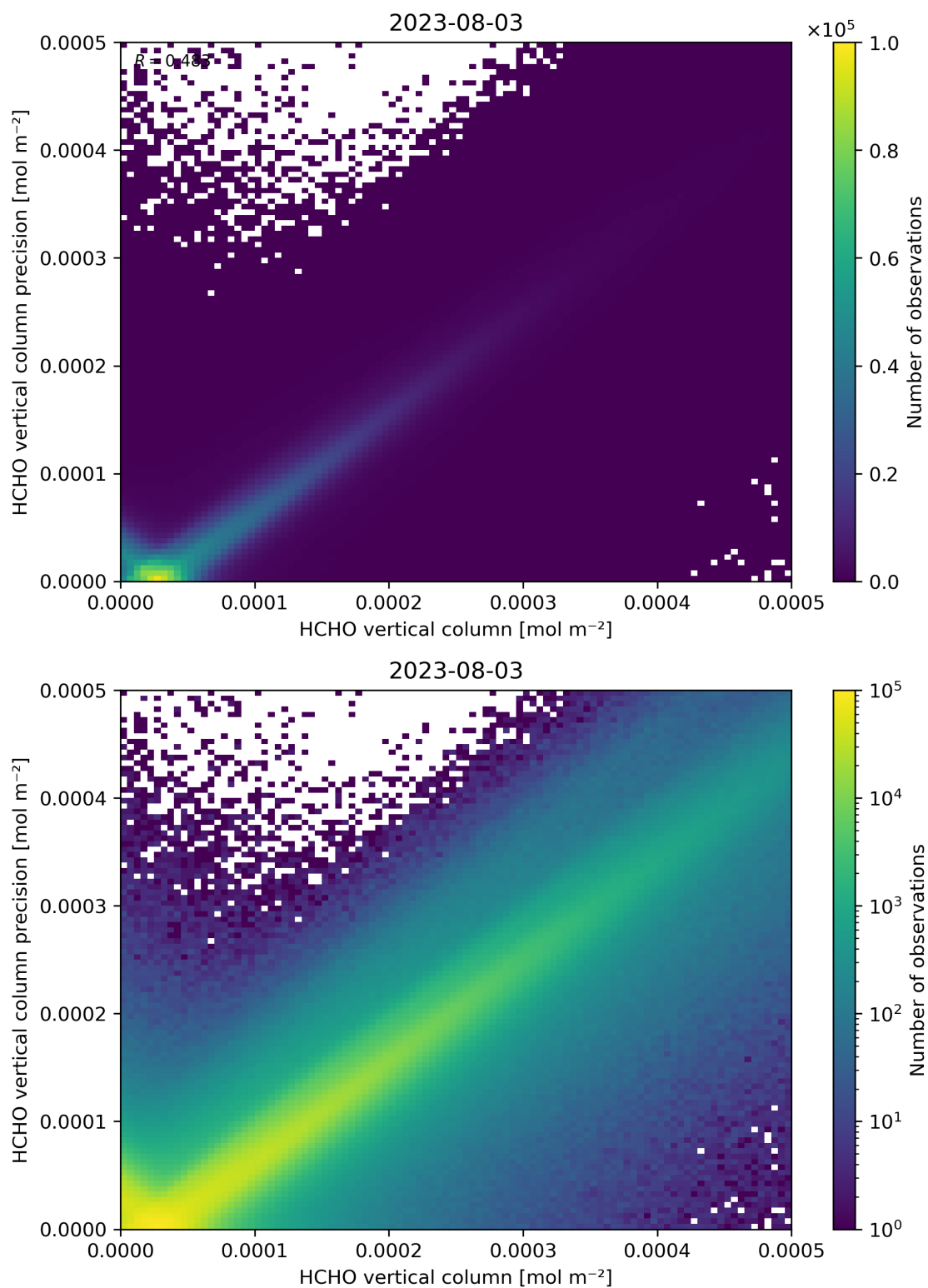
Figure 134: Scatter density plot of “HCHO vertical column” against “HCHO vertical column precision” for 2023-08-02 to 2023-08-04.
