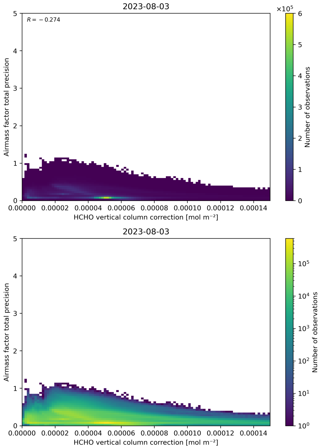
Figure 121: Scatter density plot of “HCHO vertical column correction” against “Airmass factor total precision” for 2023-08-02 to 2023-08-04.
