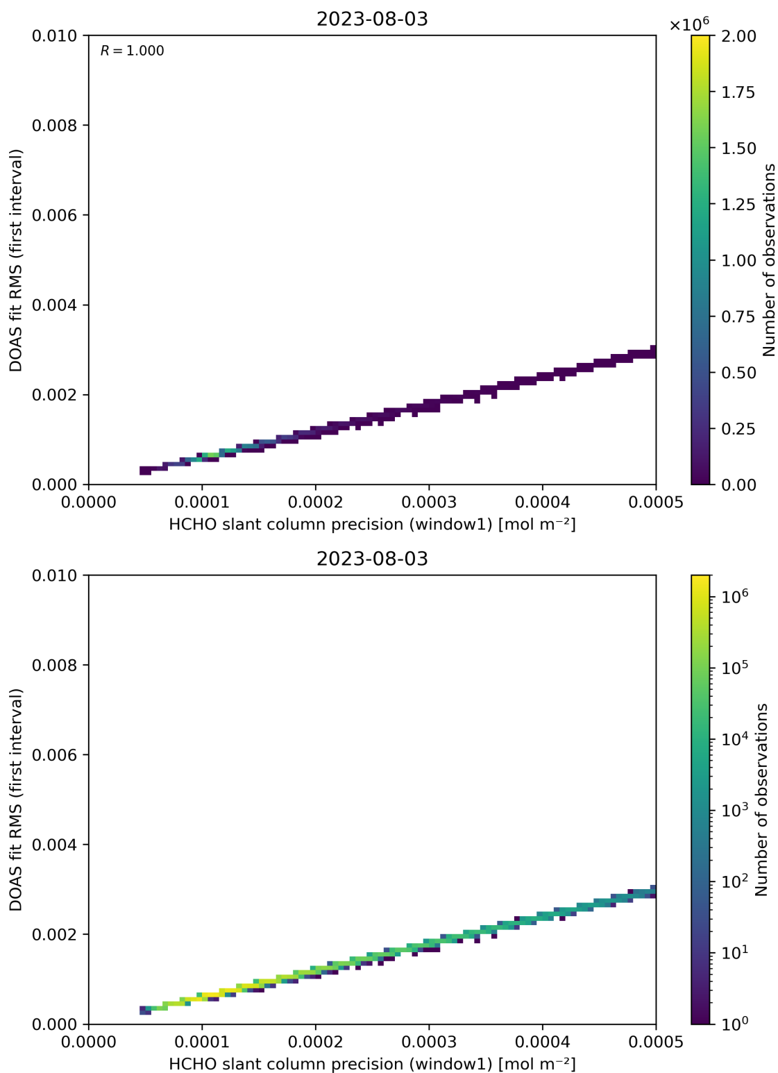
Figure 88: Scatter density plot of “HCHO slant column precision (window1)” against “DOAS fit RMS (first interval)” for 2023-08-02 to 2023-08-04.
