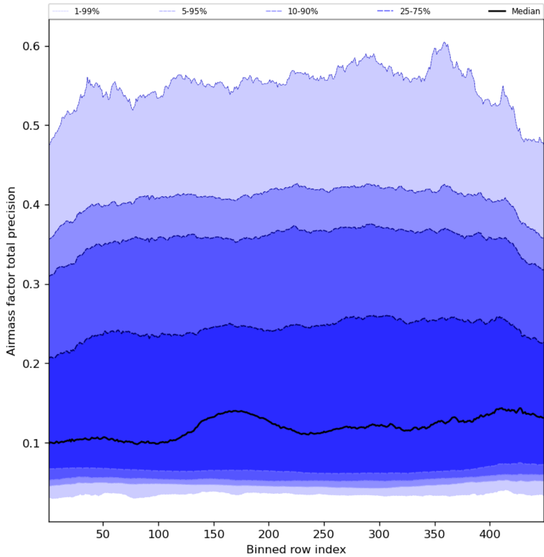
Figure 55: Along track statistics of “Airmass factor total precision” for 2023-08-02 to 2023-08-04
