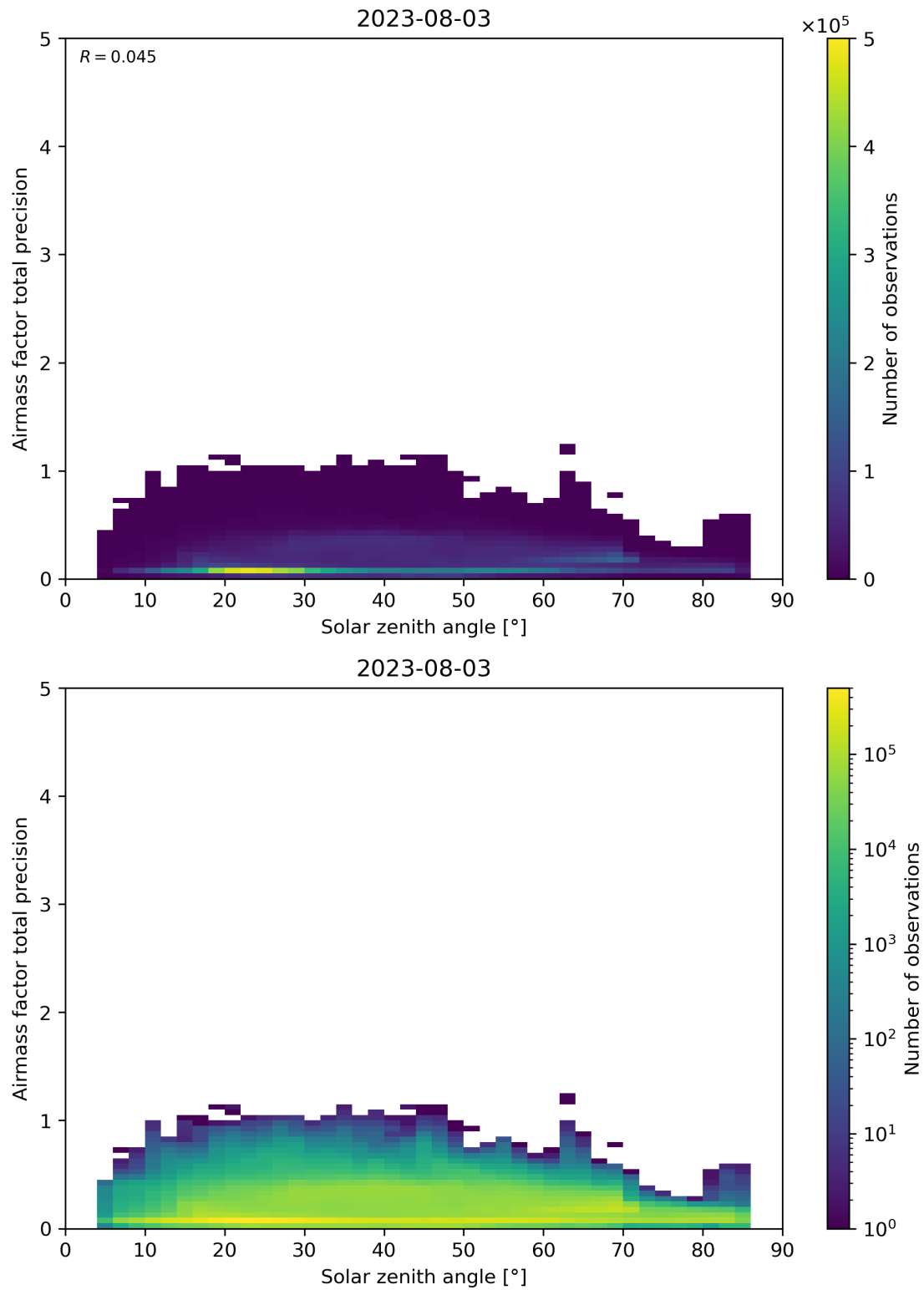
Figure 176: Scatter density plot of “Solar zenith angle” against “Airmass factor total precision” for 2023-08-02 to 2023-08-04.
