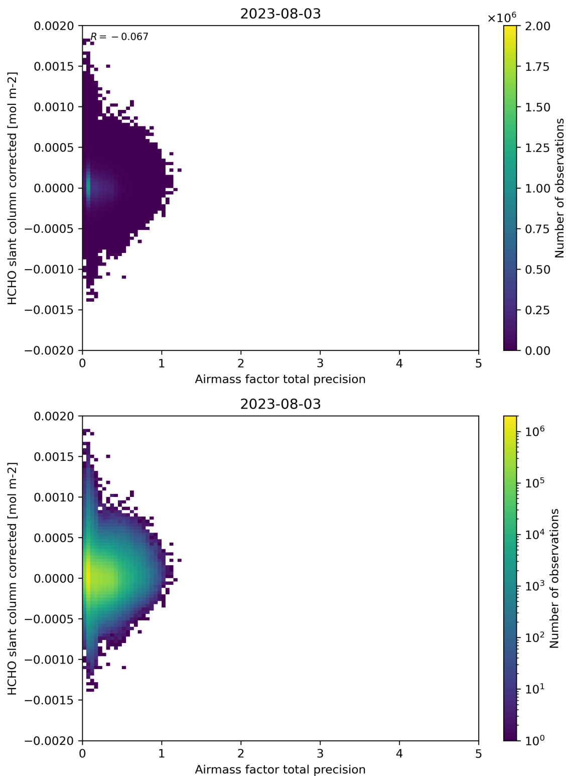
Figure 109: Scatter density plot of “Airmass factor total precision” against “HCHO slant column corrected” for 2023-08-02 to 2023-08-04.
