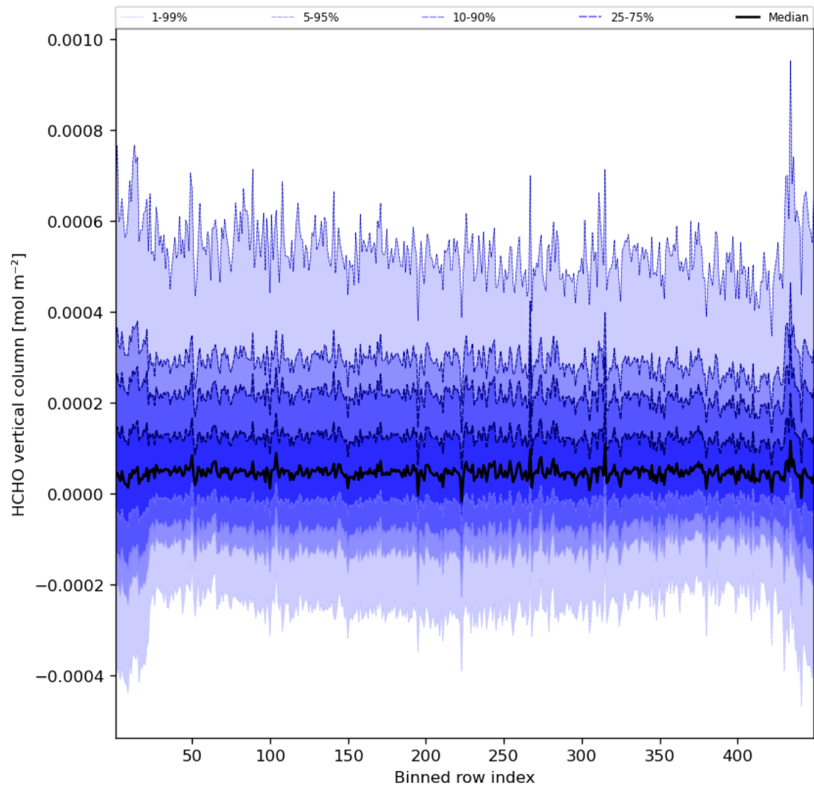
Figure 49: Along track statistics of “HCHO vertical column” for 2023-08-02 to 2023-08-04
