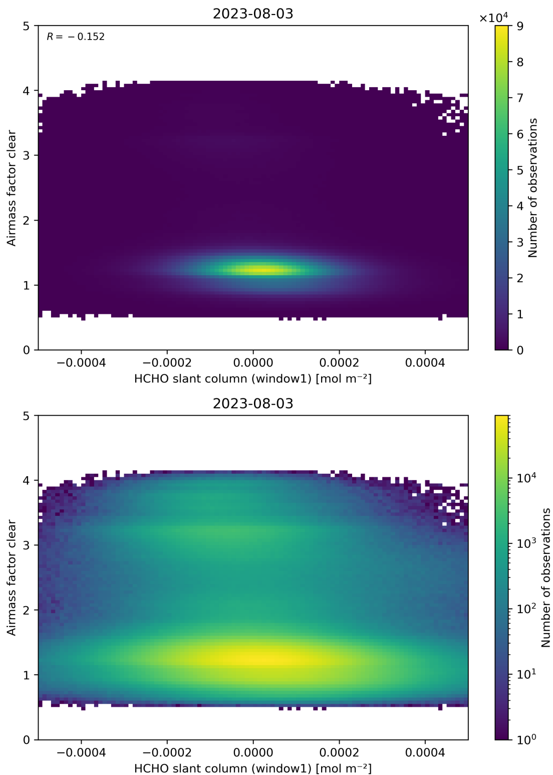
Figure 81: Scatter density plot of “HCHO slant column (window1)” against “Airmass factor clear” for 2023-08-02 to 2023-08-04.
