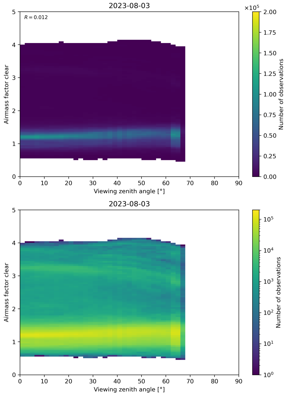
Figure 185: Scatter density plot of “Viewing zenith angle” against “Airmass factor clear” for 2023-08-02 to 2023-08-04.
