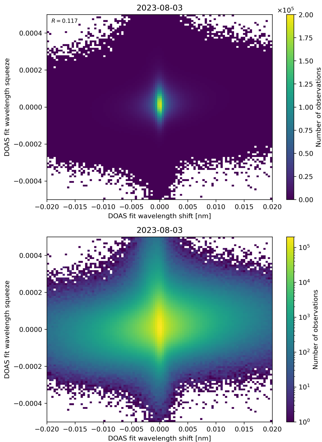
Figure 65: Scatter density plot of “DOAS fit wavelength shift” against “DOAS fit wavelength squeeze” for 2023-08-02 to 2023-08-04.
