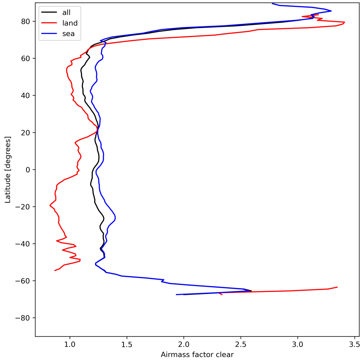
Figure 28: Zonal average of “Airmass factor clear” for 2023-08-02 to 2023-08-04.
