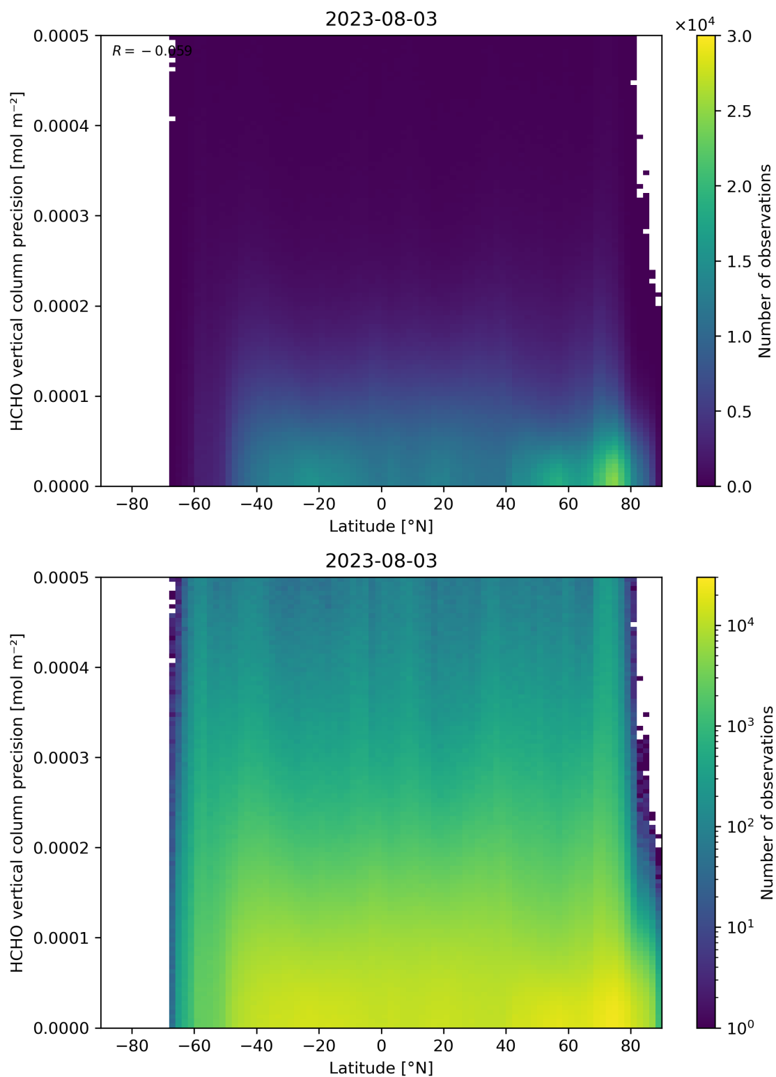
Figure 165: Scatter density plot of “Latitude” against “HCHO vertical column precision” for 2023-08-02 to 2023-08-04.
