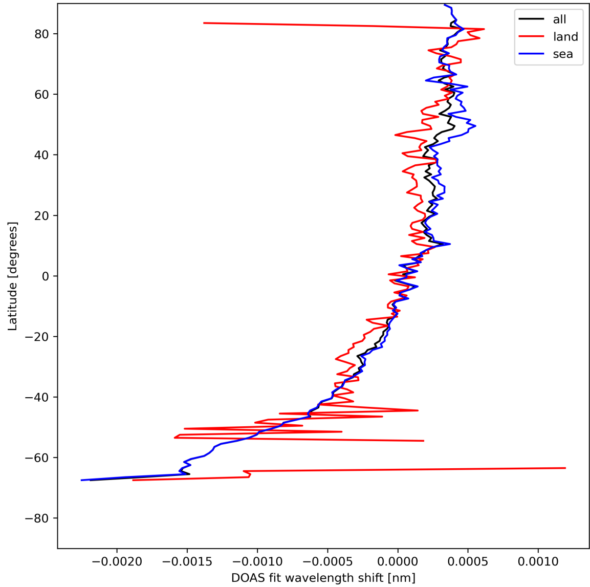
Figure 30: Zonal average of “DOAS fit wavelength shift” for 2023-08-02 to 2023-08-04.
