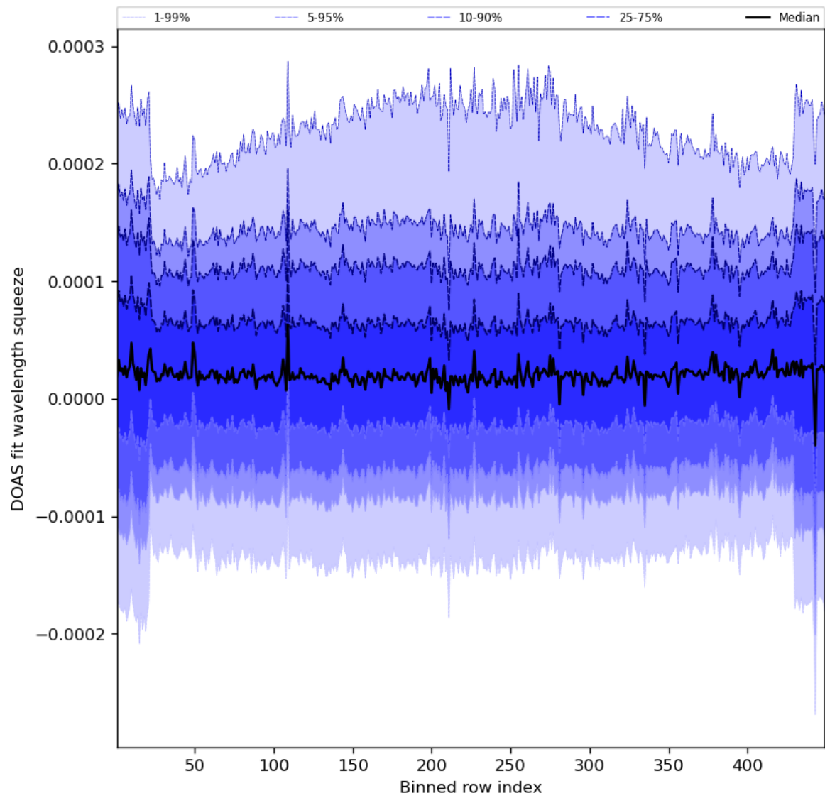
Figure 59: Along track statistics of “DOAS fit wavelength squeeze” for 2023-08-02 to 2023-08-04
