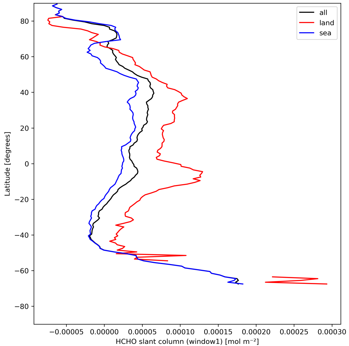
Figure 24: Zonal average of “HCHO slant column (window1)” for 2023-08-02 to 2023-08-04.
