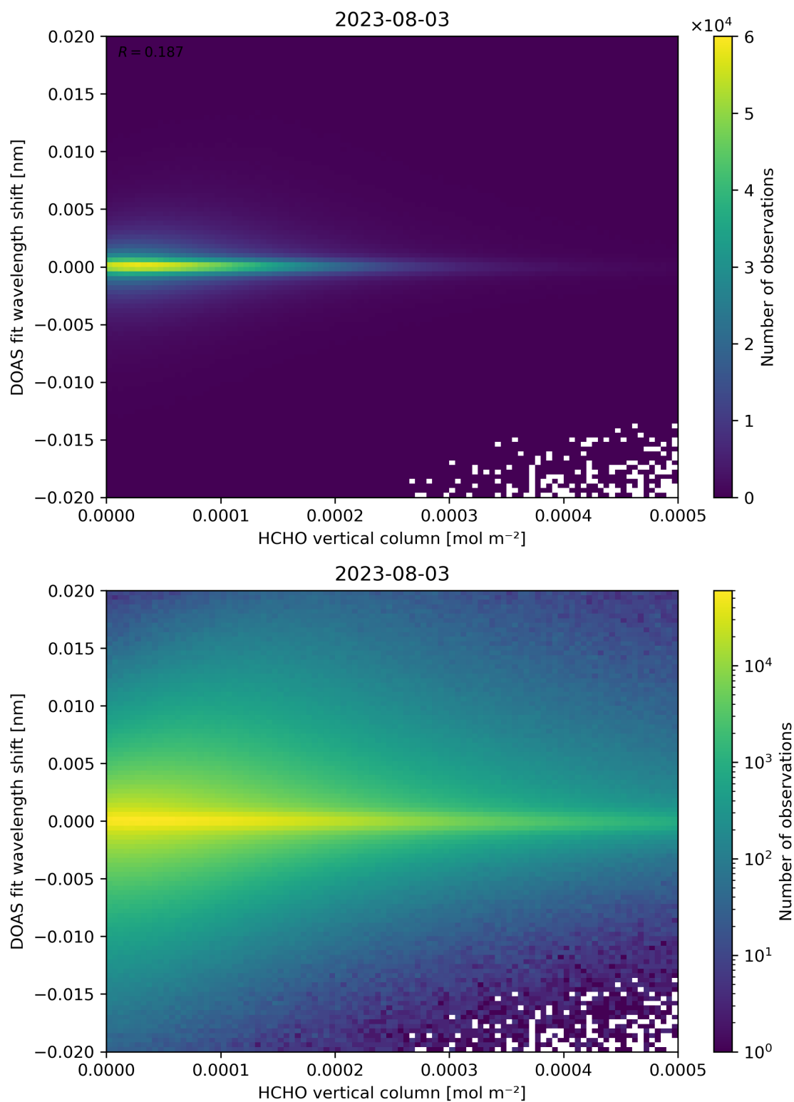
Figure 124: Scatter density plot of “HCHO vertical column” against “DOAS fit wavelength shift” for 2023-08-02 to 2023-08-04.
