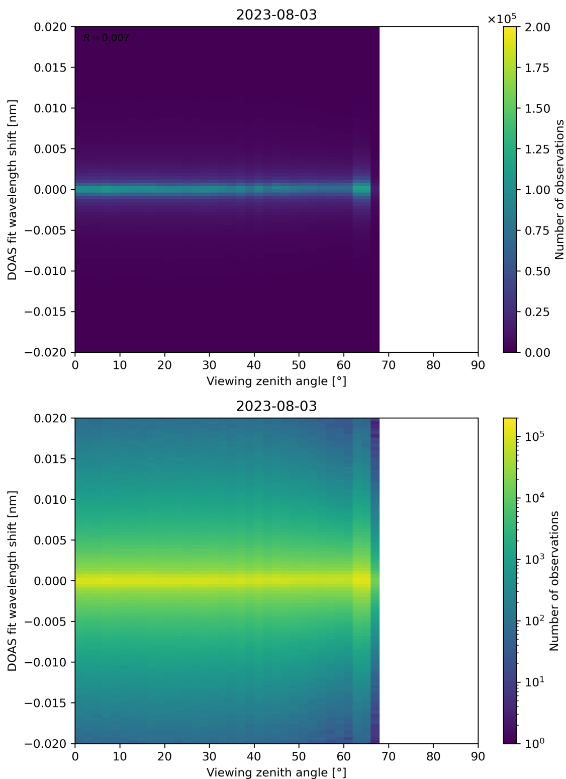
Figure 183: Scatter density plot of “Viewing zenith angle” against “DOAS fit wavelength shift” for 2023-08-02 to 2023-08-04.
