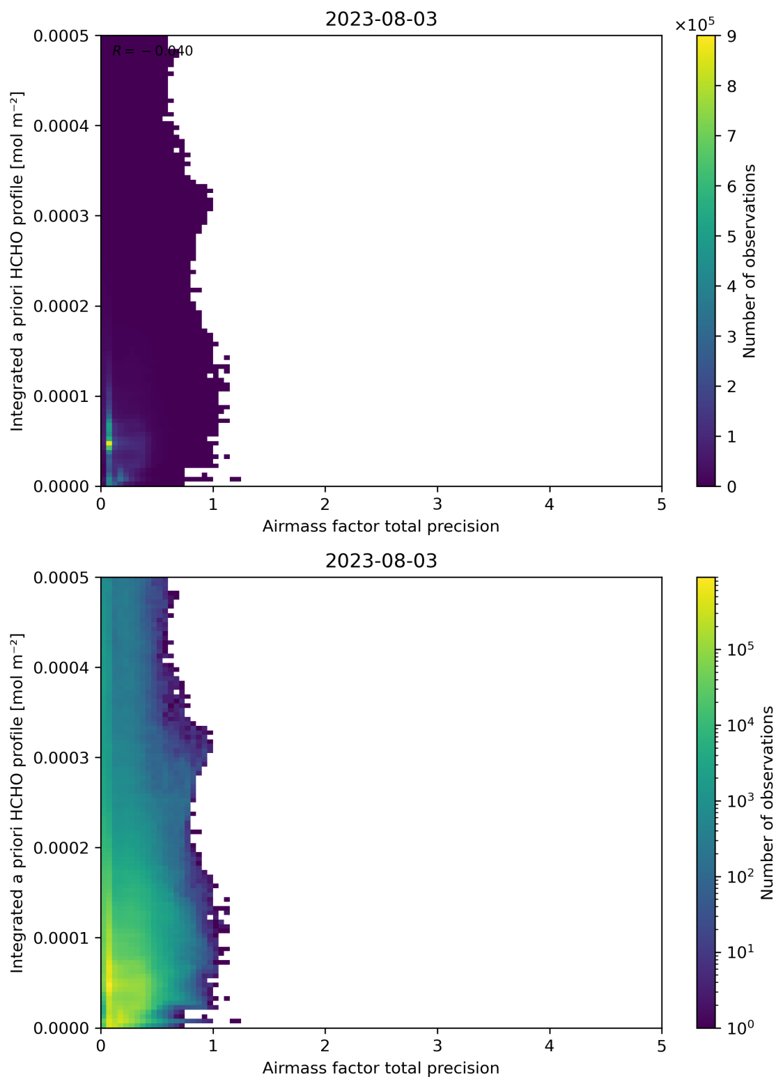
Figure 111: Scatter density plot of “Airmass factor total precision” against “Integrated a priori HCHO profile” for 2023-08-02 to 2023-08-04.
