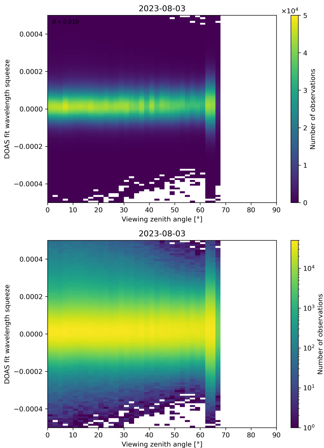
Figure 184: Scatter density plot of “Viewing zenith angle” against “DOAS fit wavelength squeeze” for 2023-08-02 to 2023-08-04.
