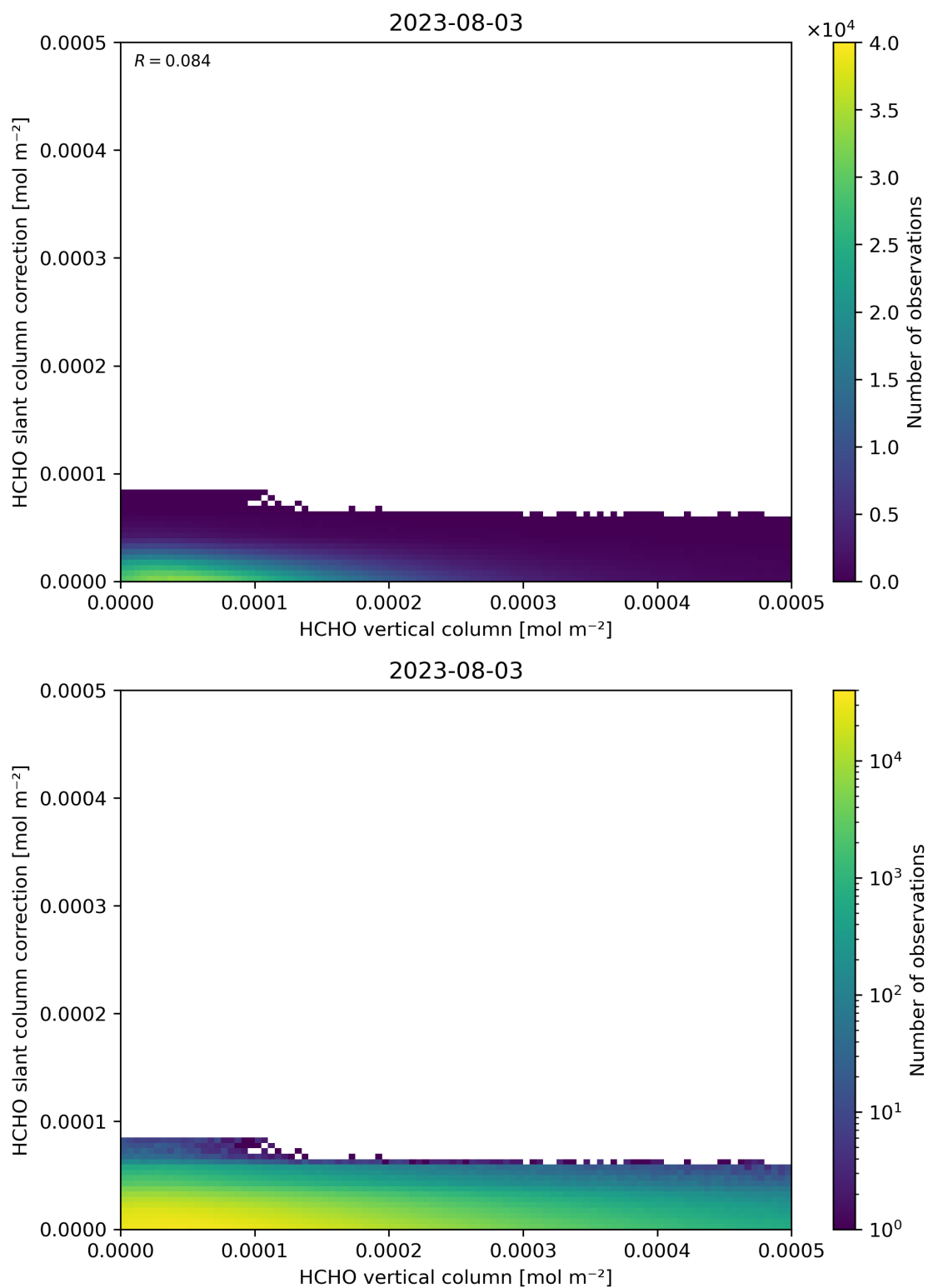
Figure 128: Scatter density plot of “HCHO vertical column” against “HCHO slant column correction” for 2023-08-02 to 2023-08-04.
