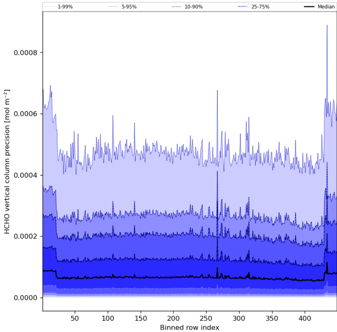
Figure 50: Along track statistics of “HCHO vertical column precision” for 2023-08-02 to 2023-08-04
