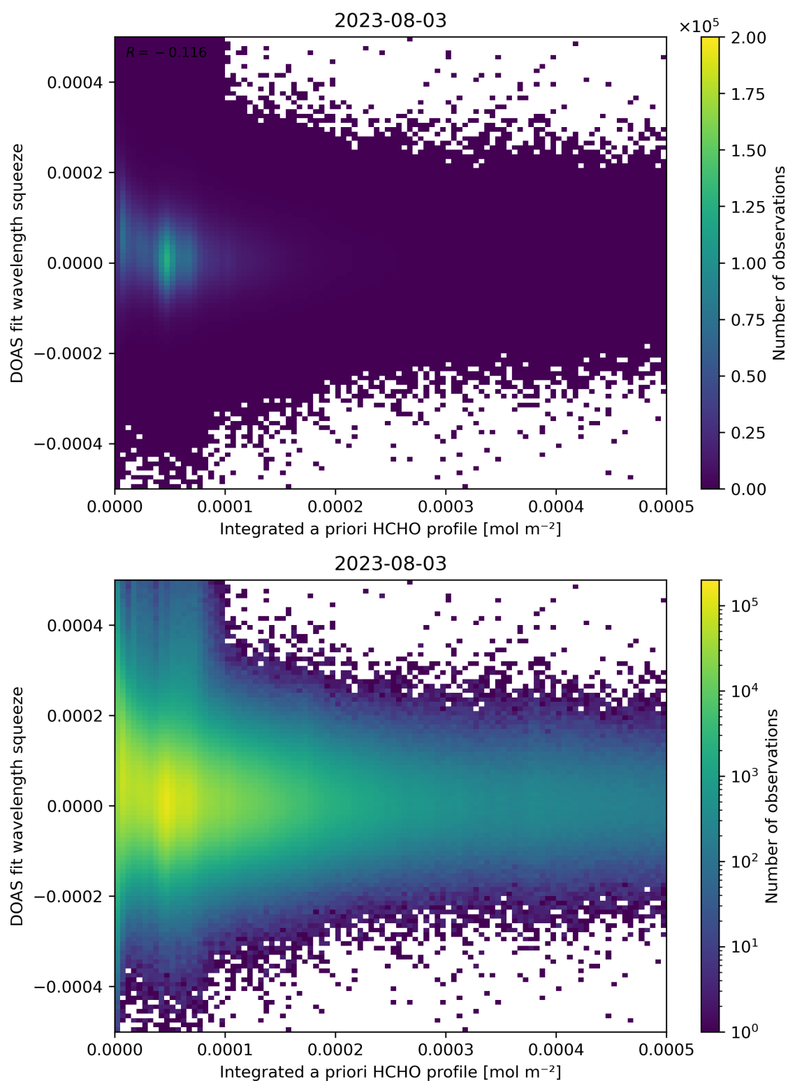
Figure 150: Scatter density plot of “Integrated a priori HCHO profile” against “DOAS fit wavelength squeeze” for 2023-08-02 to 2023-08-04.
