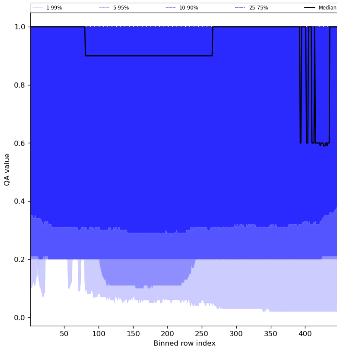
Figure 48: Along track statistics of “QA value” for 2023-08-02 to 2023-08-04
