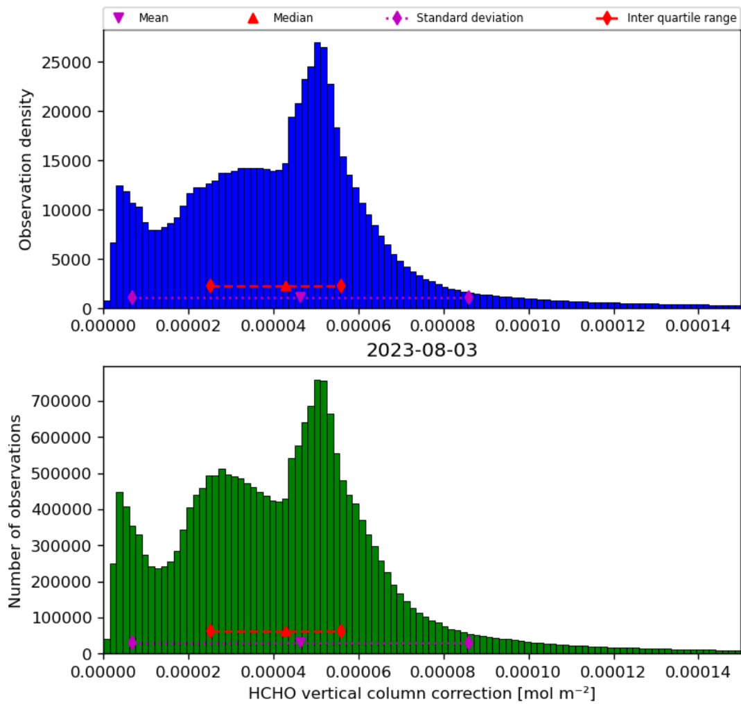
Figure 37: Histogram of “HCHO vertical column correction” for 2023-08-02 to 2023-08-04
