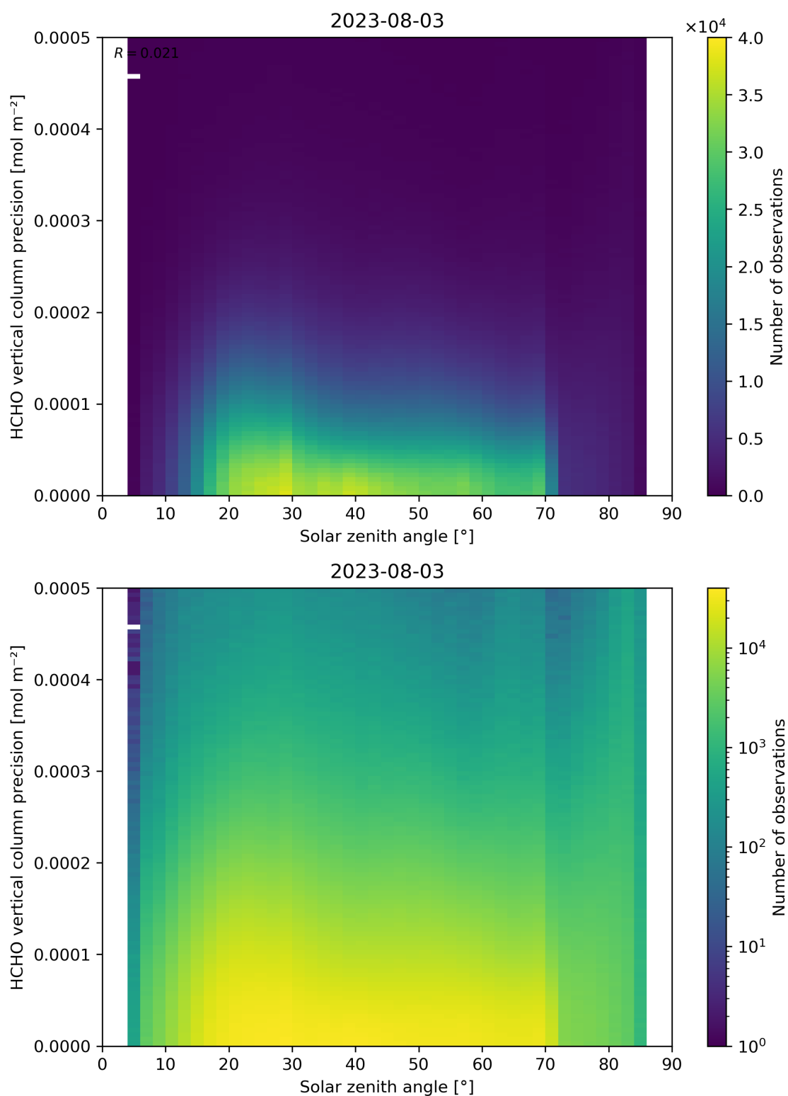
Figure 179: Scatter density plot of “Solar zenith angle” against “HCHO vertical column precision” for 2023-08-02 to 2023-08-04.
