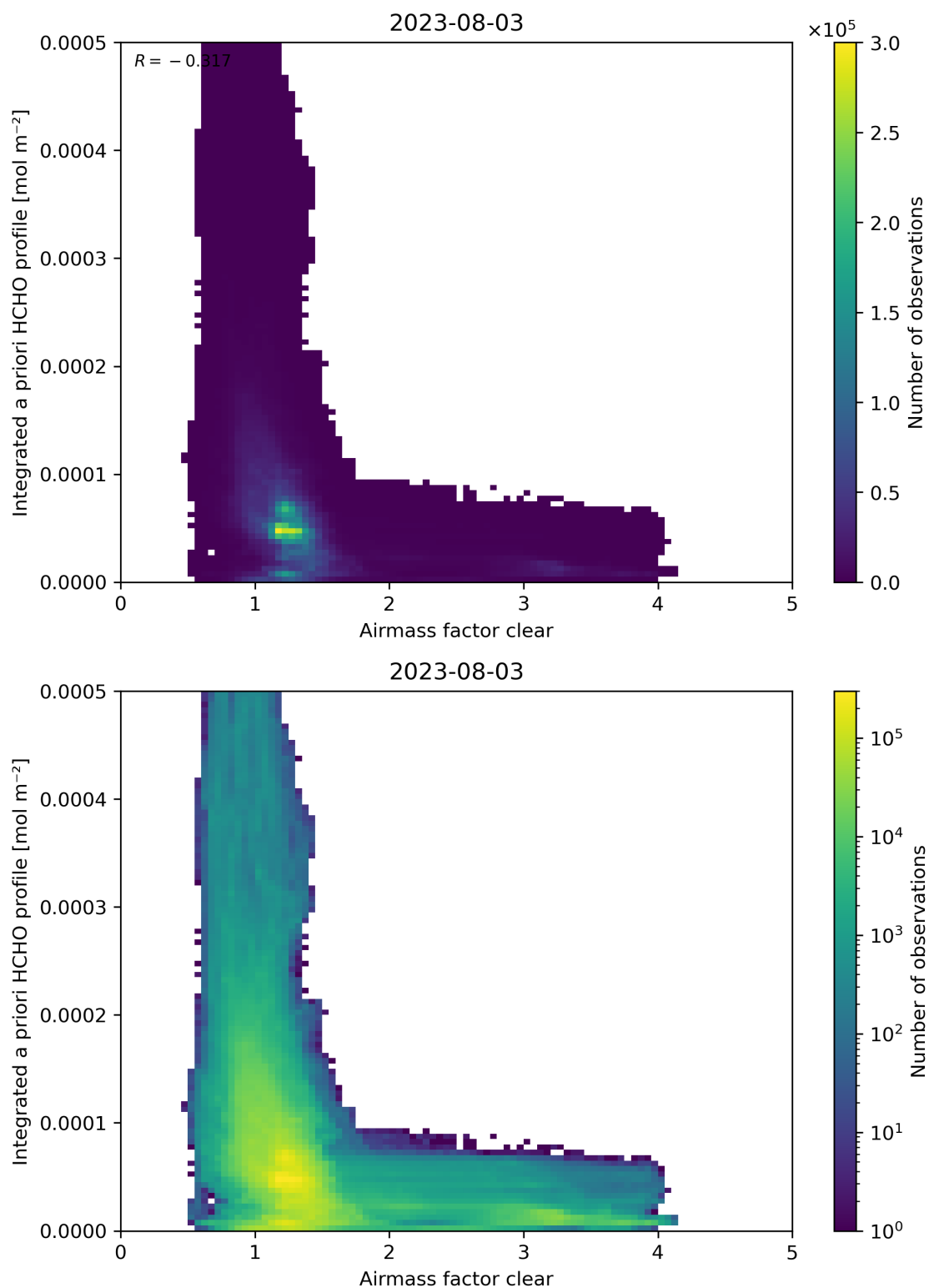
Figure 76: Scatter density plot of “Airmass factor clear” against “Integrated a priori HCHO profile” for 2023-08-02 to 2023-08-04.
