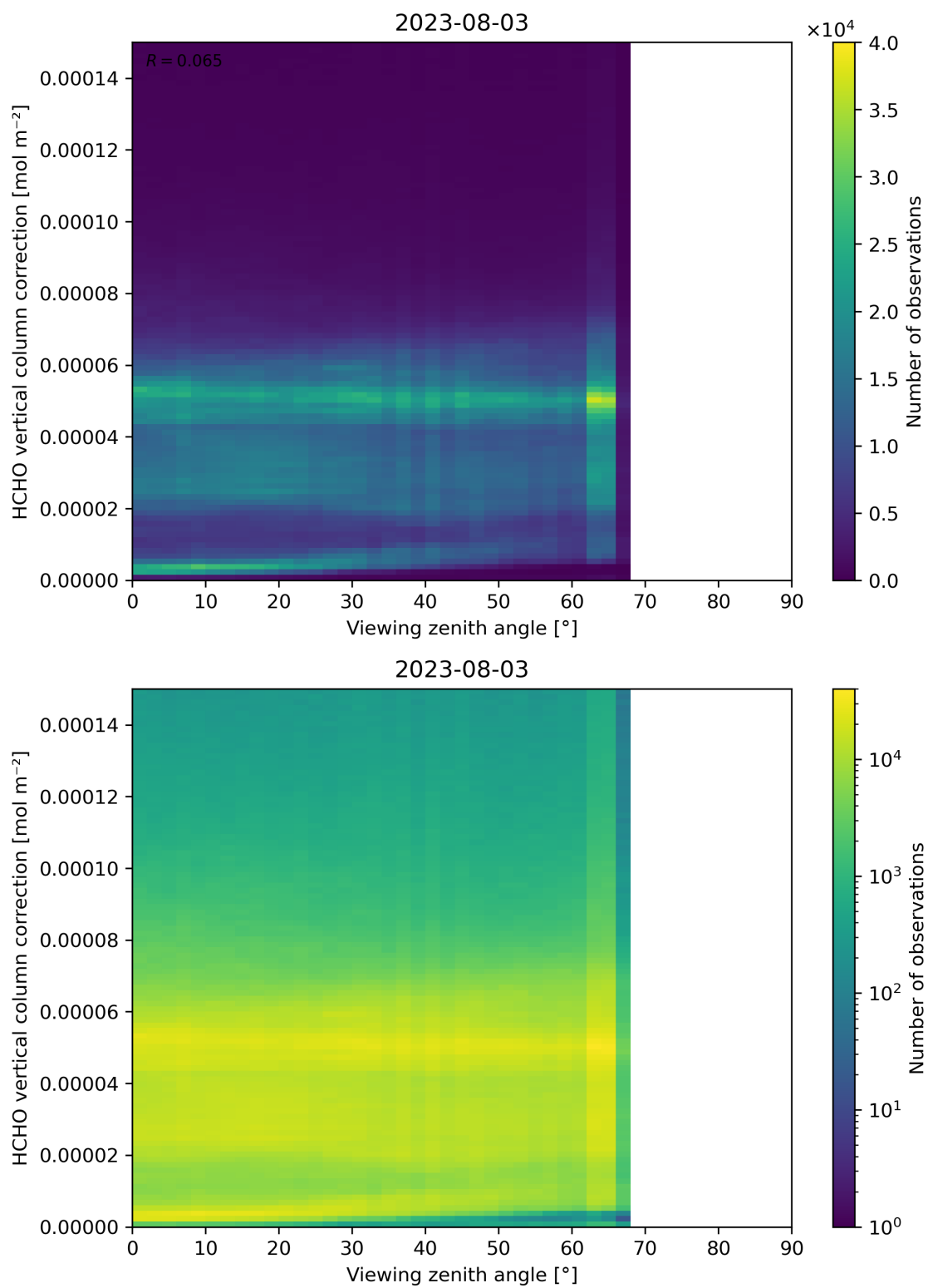
Figure 193: Scatter density plot of “Viewing zenith angle” against “HCHO vertical column correction” for 2023-08-02 to 2023-08-04.
