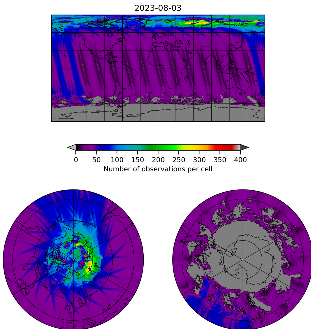
Figure 19: Map of the number of observations for 2023-08-02 to 2023-08-04
