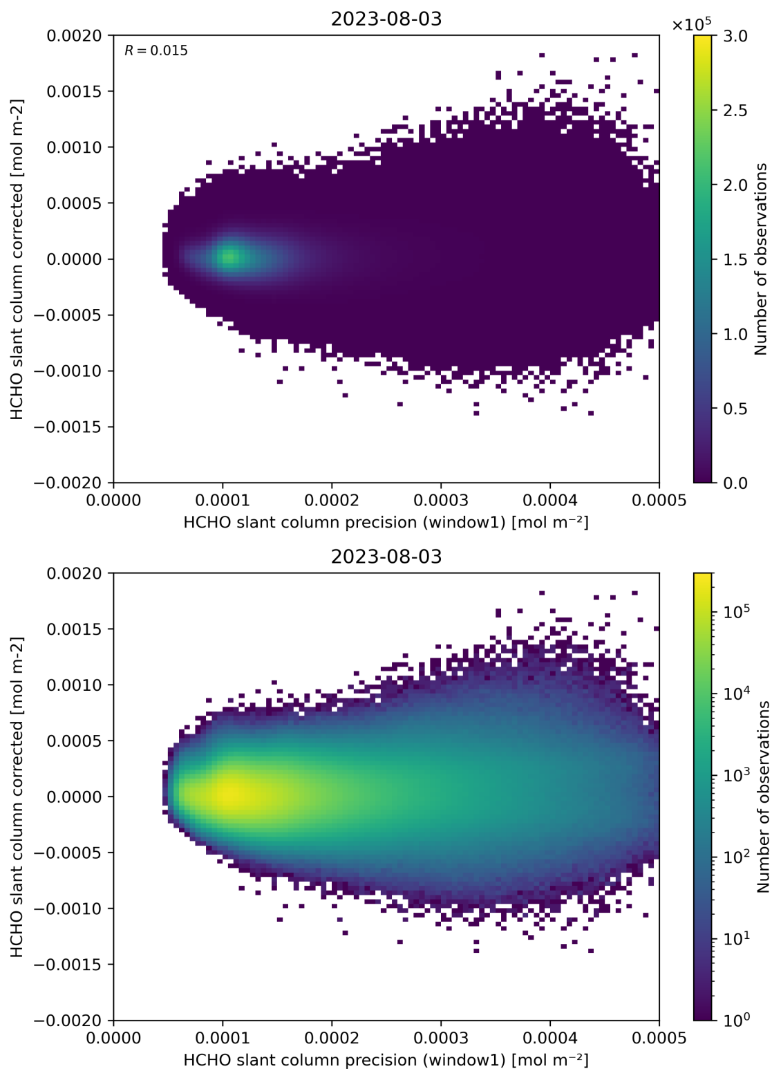
Figure 92: Scatter density plot of “HCHO slant column precision (window1)” against “HCHO slant column corrected” for 2023-08-02 to 2023-08-04.
