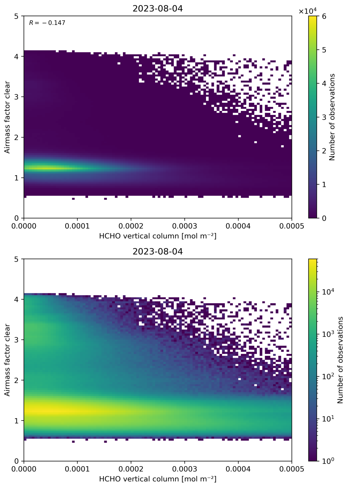
Figure 126: Scatter density plot of “HCHO vertical column” against “Airmass factor clear” for 2023-08-04 to 2023-08-05.
