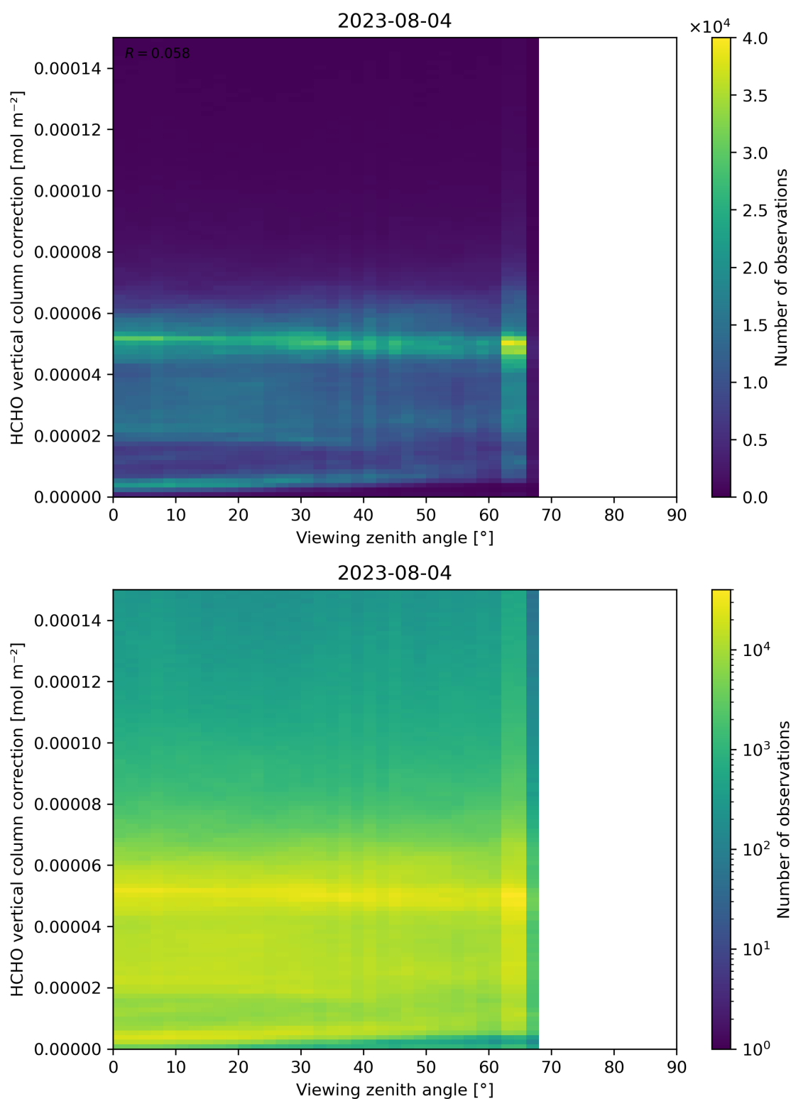
Figure 193: Scatter density plot of “Viewing zenith angle” against “HCHO vertical column correction” for 2023-08-04 to 2023-08-05.
