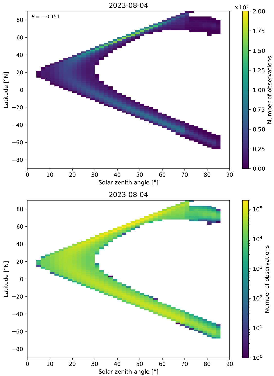
Figure 181: Scatter density plot of “Solar zenith angle” against “Latitude” for 2023-08-04 to 2023-08-05.
