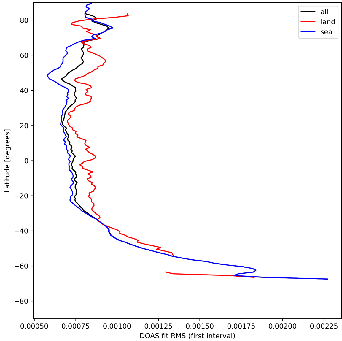
Figure 32: Zonal average of "DOAS fit RMS (first interval)" for 2023-08-04 to 2023-08-05.
