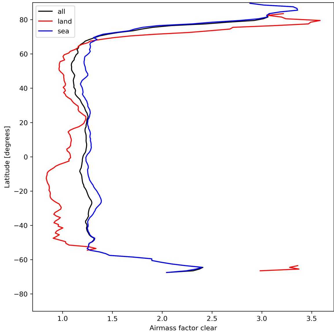
Figure 28: Zonal average of “Airmass factor clear” for 2023-08-04 to 2023-08-05.
