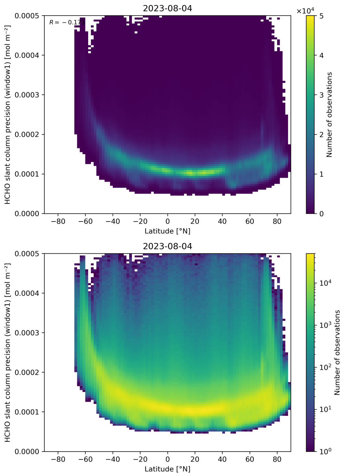
Figure 160: Scatter density plot of “Latitude” against “HCHO slant column precision (window1)” for 2023-08-04 to 2023-08-05.
