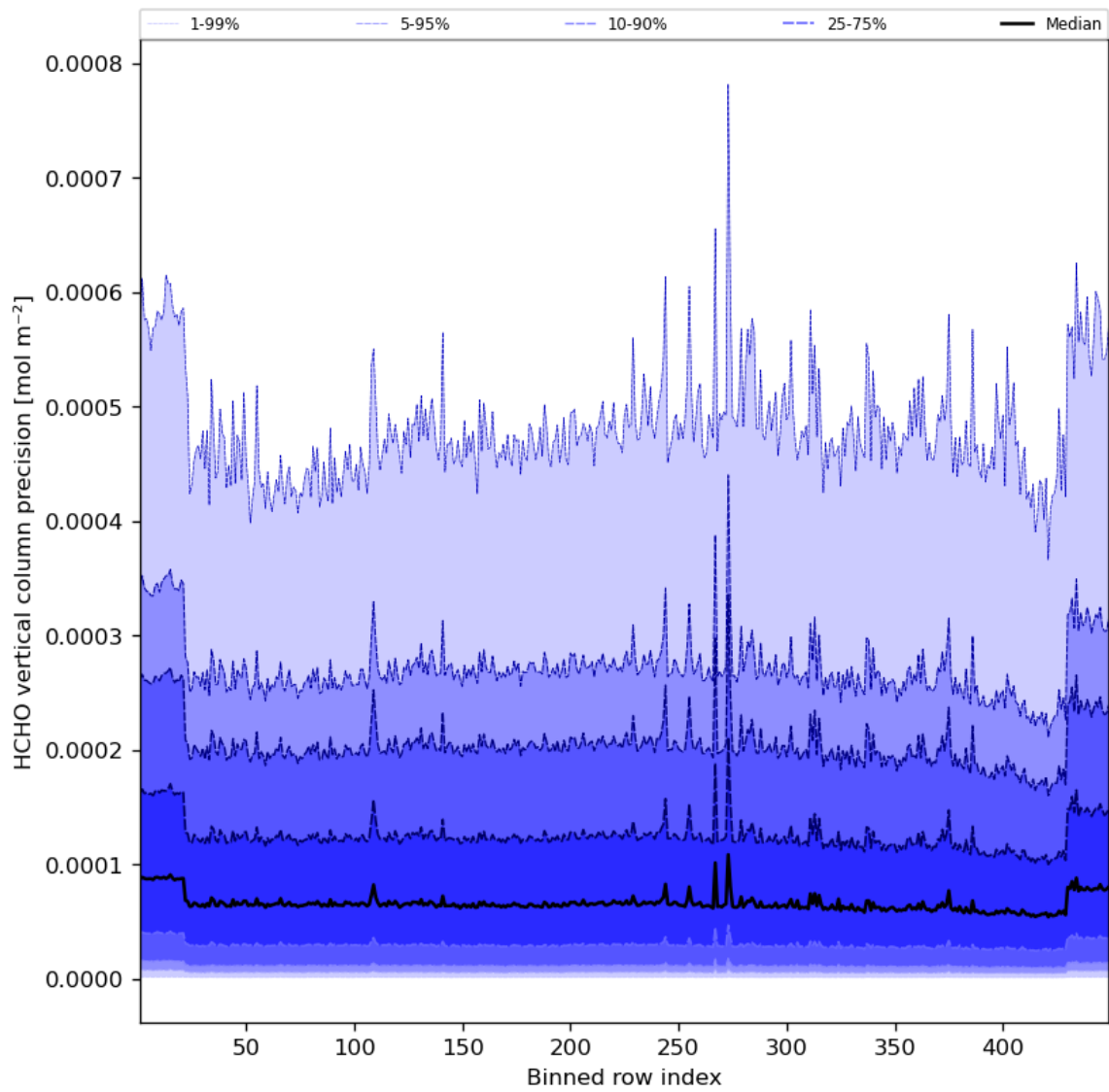
Figure 50: Along track statistics of “HCHO vertical column precision” for 2023-08-04 to 2023-08-05
