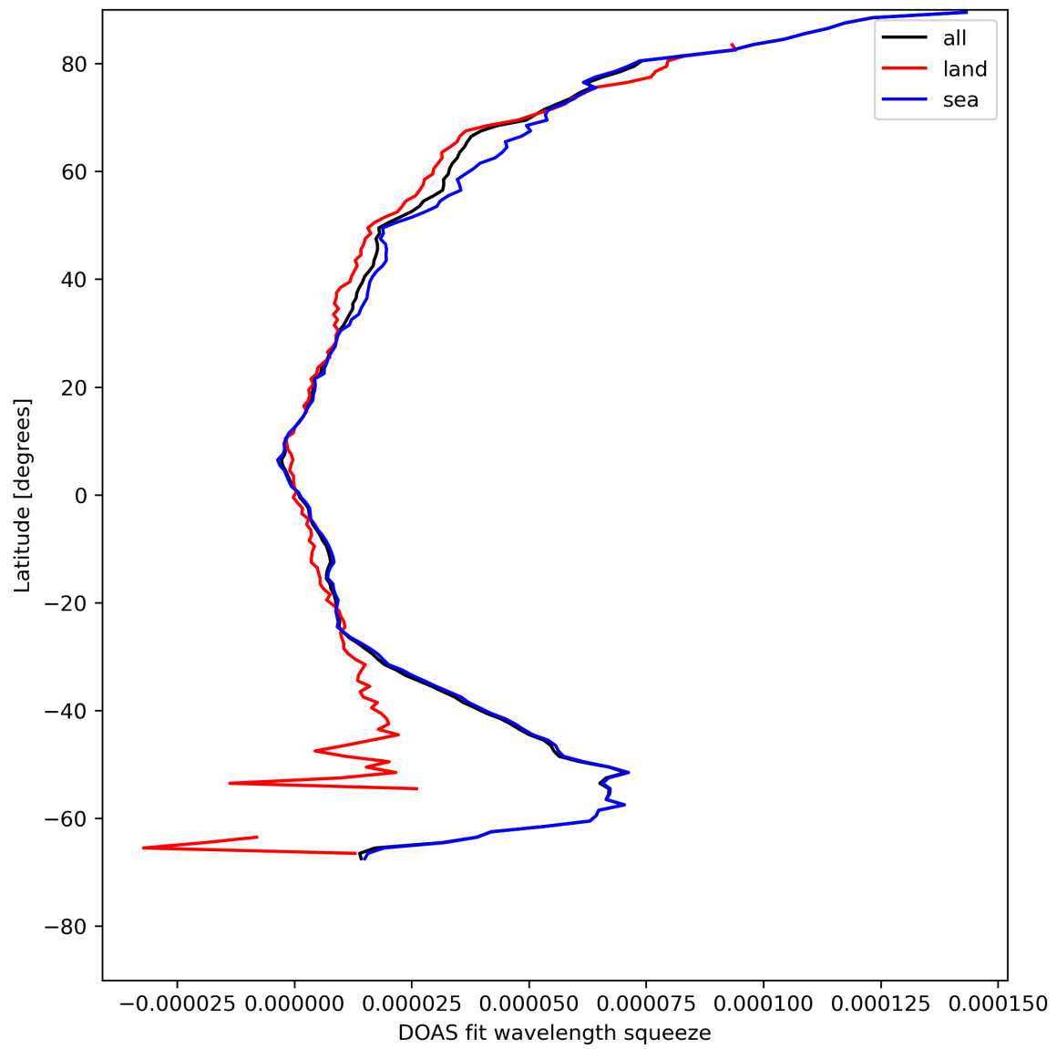
Figure 31: Zonal average of “DOAS fit wavelength squeeze” for 2023-08-04 to 2023-08-05.
