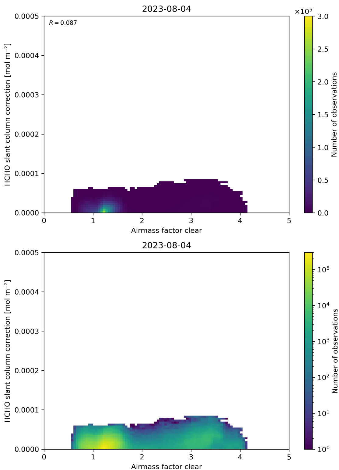
Figure 75: Scatter density plot of “Airmass factor clear” against “HCHO slant column correction” for 2023-08-04 to 2023-08-05.
