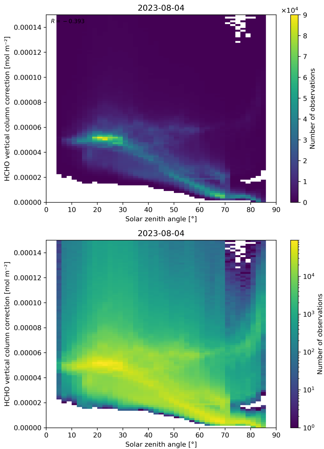
Figure 178: Scatter density plot of “Solar zenith angle” against “HCHO vertical column correction” for 2023-08-04 to 2023-08-05.
