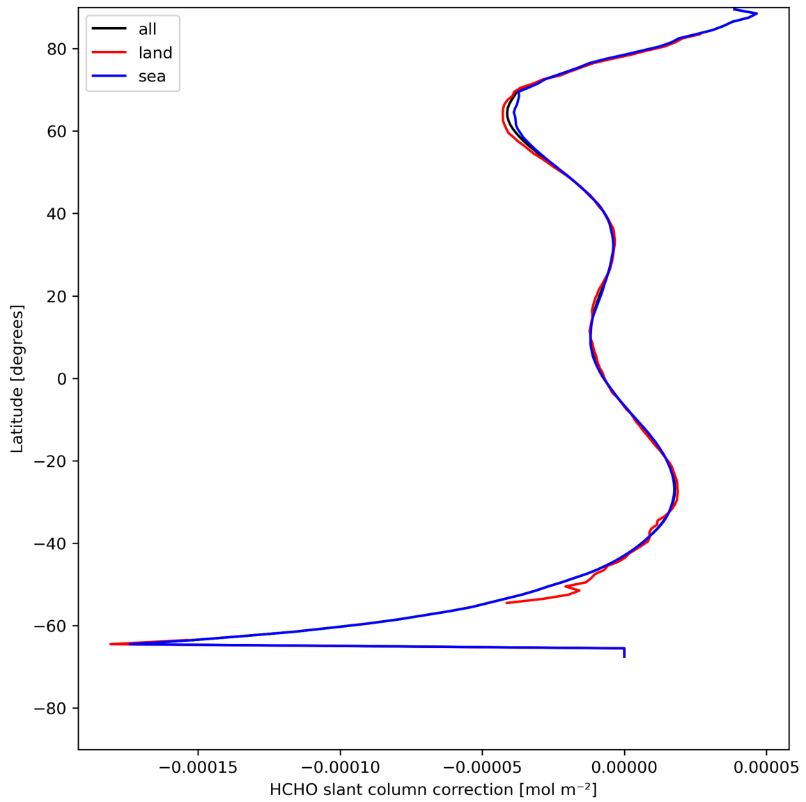
Figure 33: Zonal average of “HCHO slant column correction” for 2023-08-04 to 2023-08-05.
