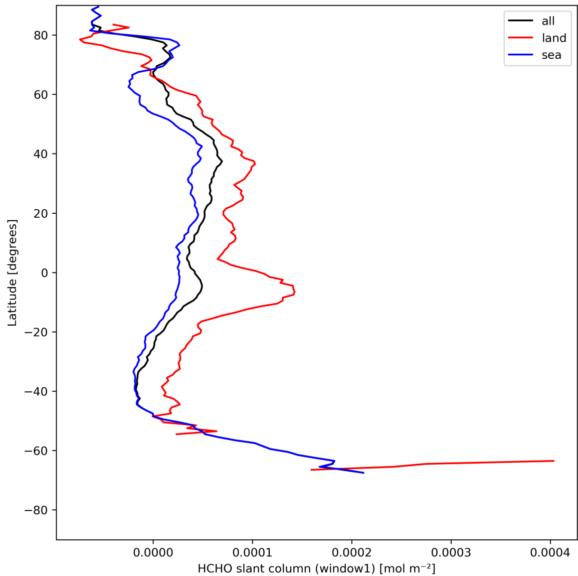
Figure 24: Zonal average of “HCHO slant column (window1)” for 2023-08-04 to 2023-08-05.
