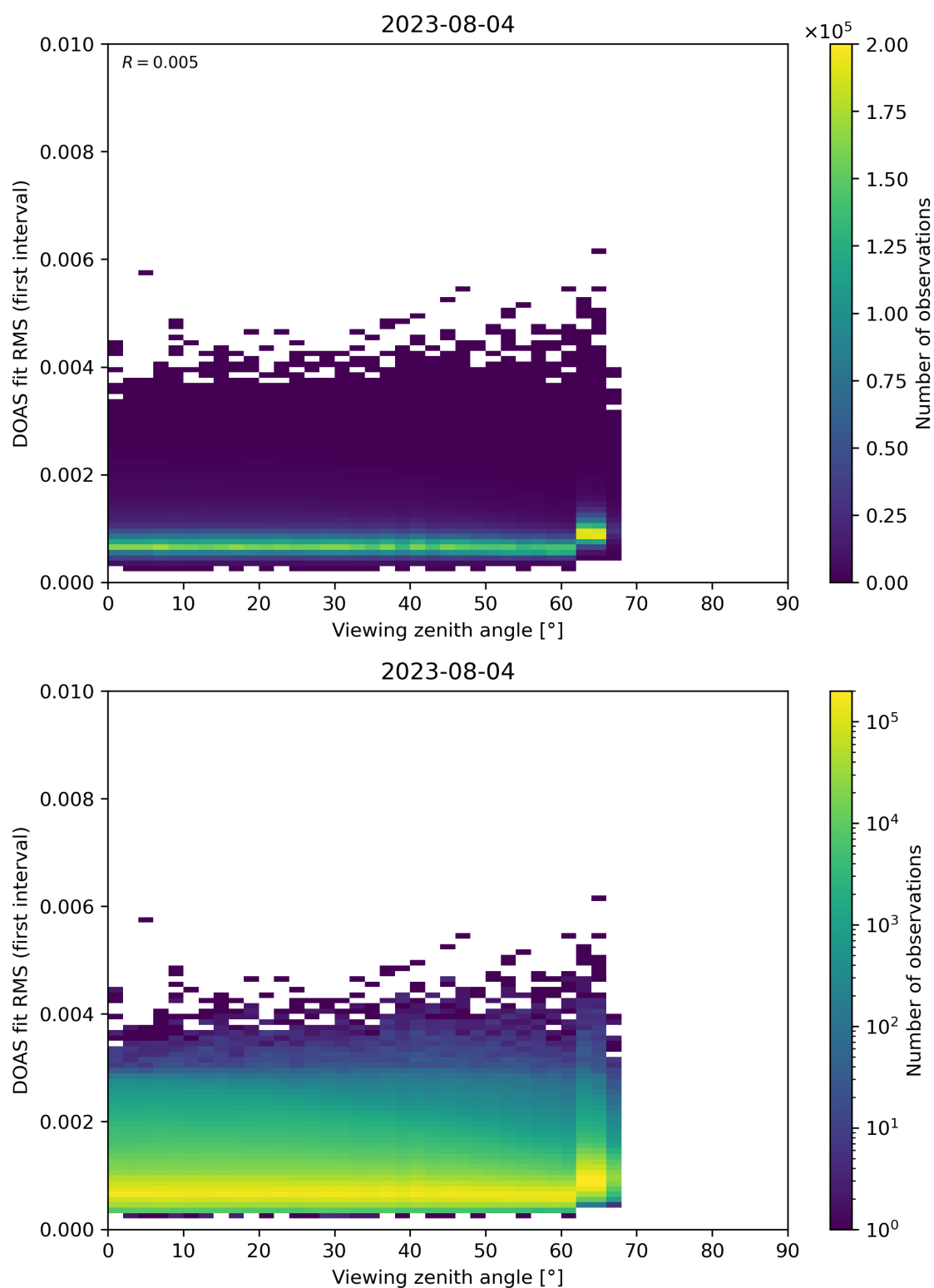
Figure 182: Scatter density plot of “Viewing zenith angle” against “DOAS fit RMS (first interval)” for 2023-08-04 to 2023-08-05.
