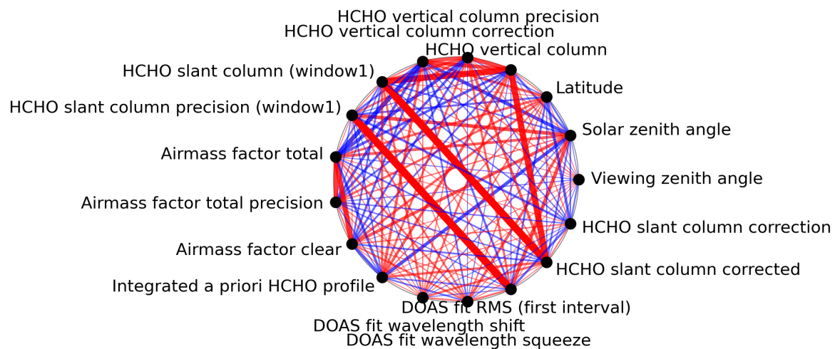
Figure 1: Map of correlation graph for 2023-08-04 to 2023-08-05.
