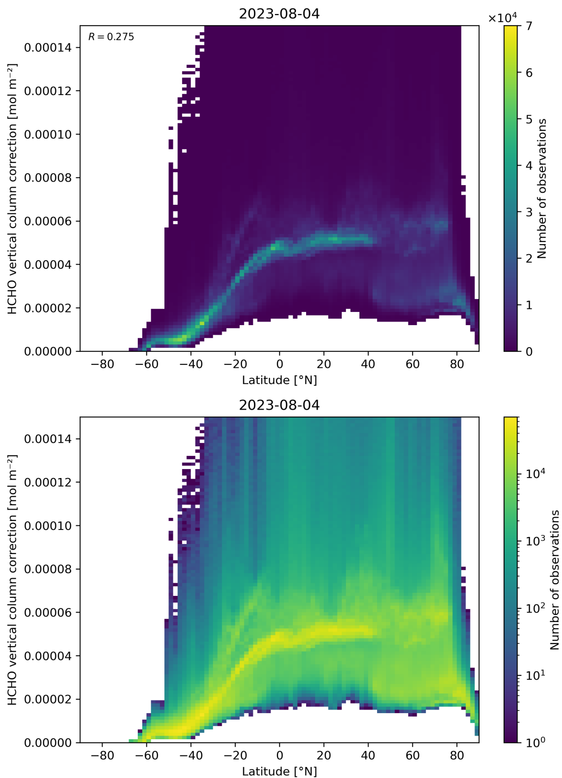
Figure 164: Scatter density plot of “Latitude” against “HCHO vertical column correction” for 2023-08-04 to 2023-08-05.
