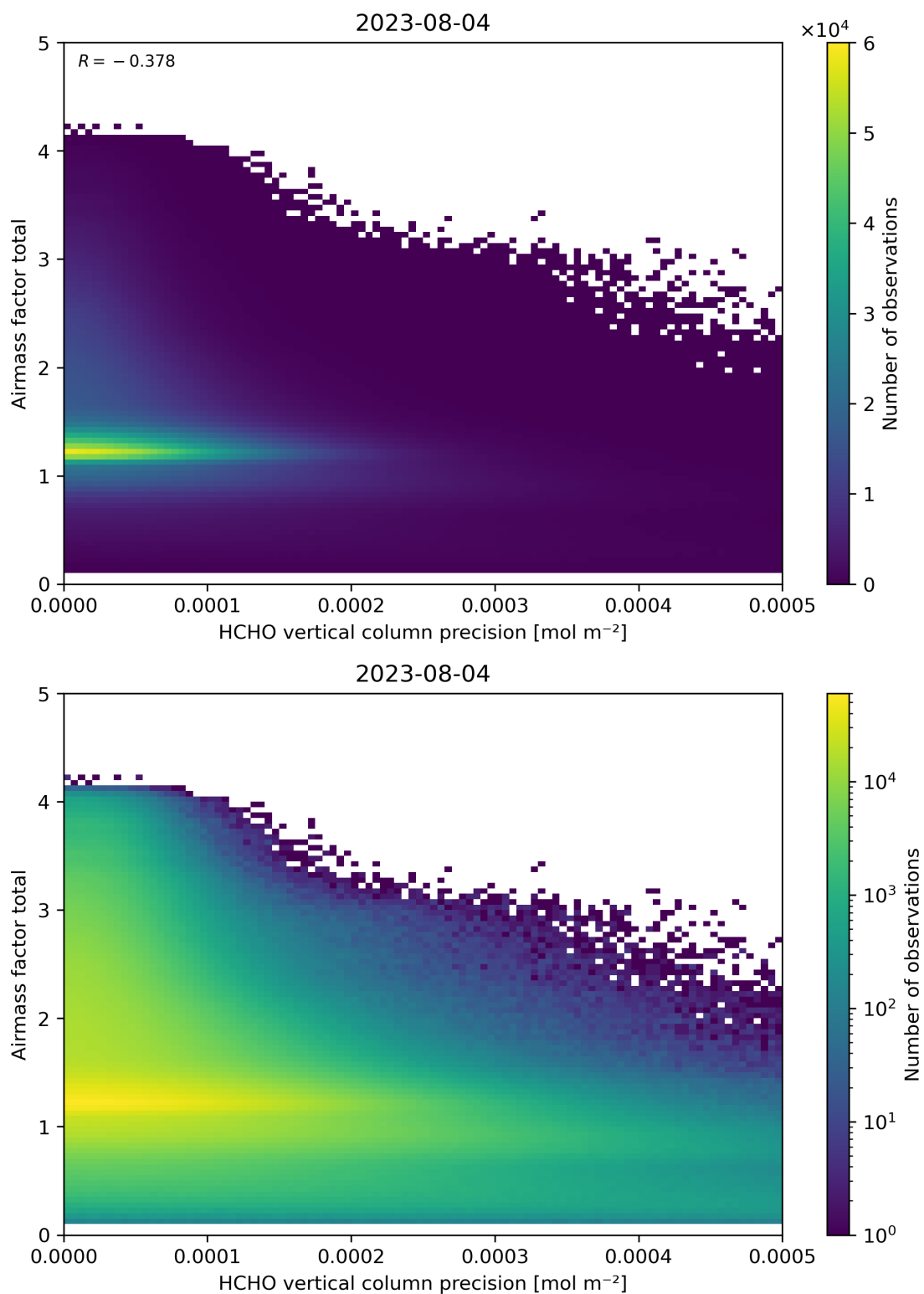
Figure 144: Scatter density plot of “HCHO vertical column precision” against “Airmass factor total” for 2023-08-04 to 2023-08-05.
