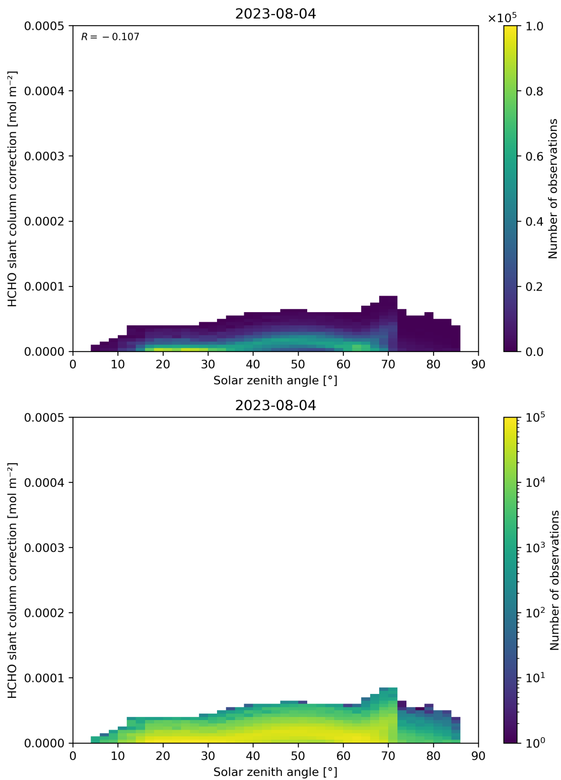
Figure 172: Scatter density plot of “Solar zenith angle” against “HCHO slant column correction” for 2023-08-04 to 2023-08-05.
