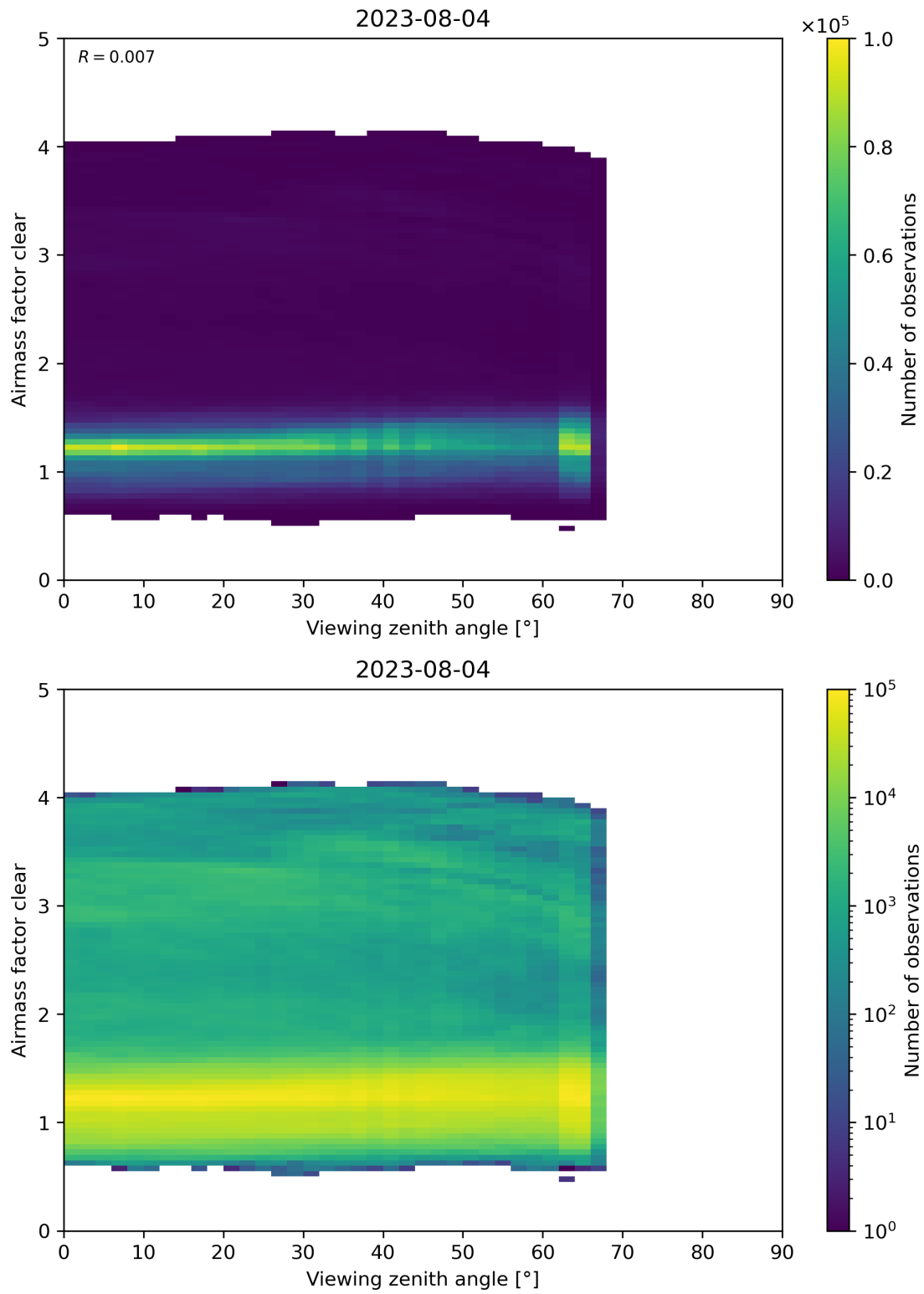
Figure 185: Scatter density plot of “Viewing zenith angle” against “Airmass factor clear” for 2023-08-04 to 2023-08-05.
