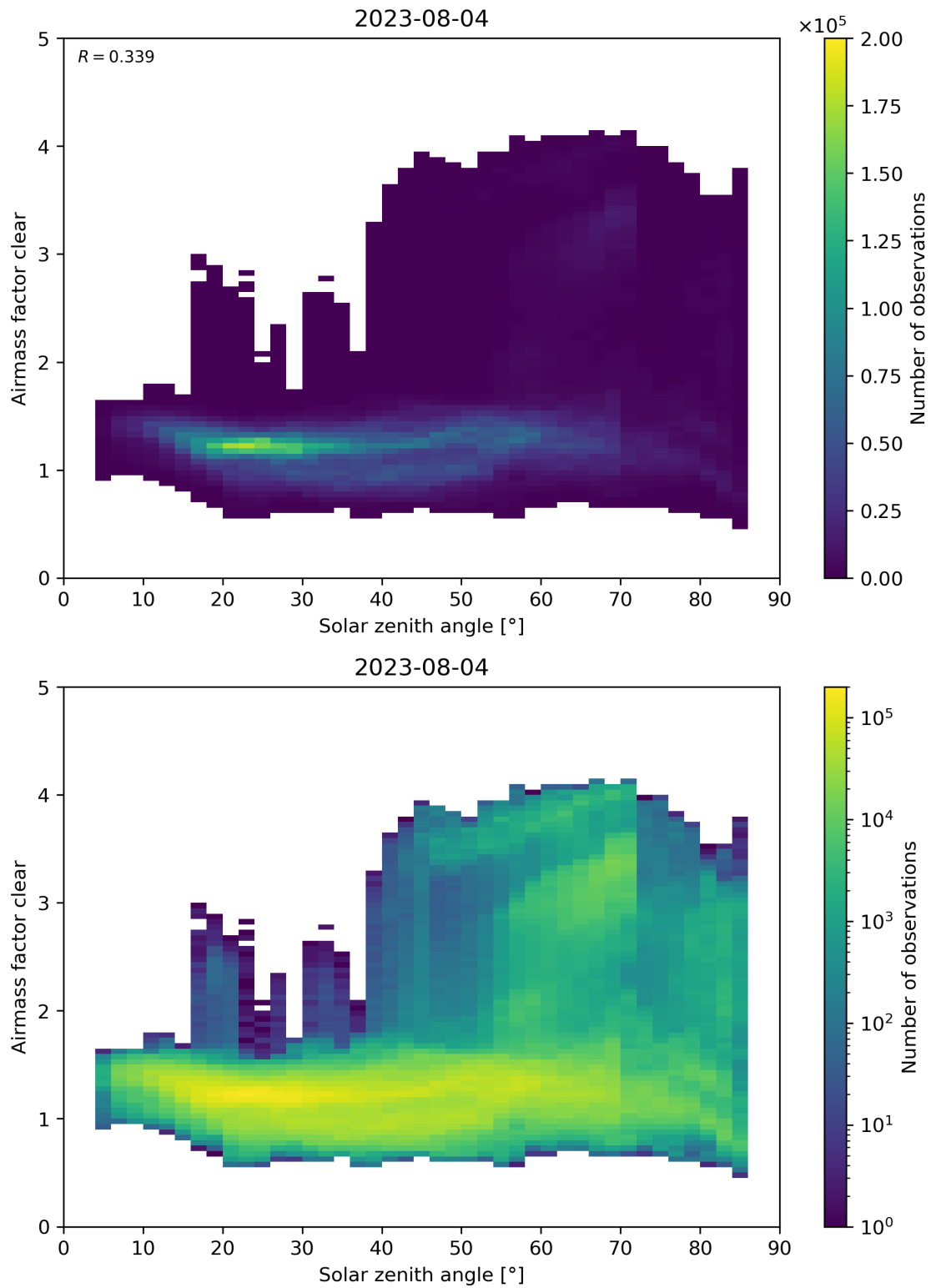
Figure 170: Scatter density plot of “Solar zenith angle” against “Airmass factor clear” for 2023-08-04 to 2023-08-05.
