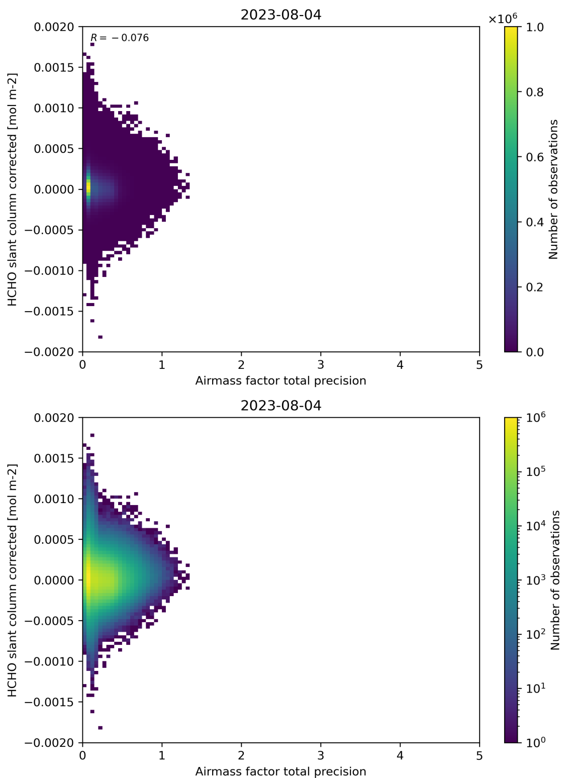
Figure 109: Scatter density plot of “Airmass factor total precision” against “HCHO slant column corrected” for 2023-08-04 to 2023-08-05.
