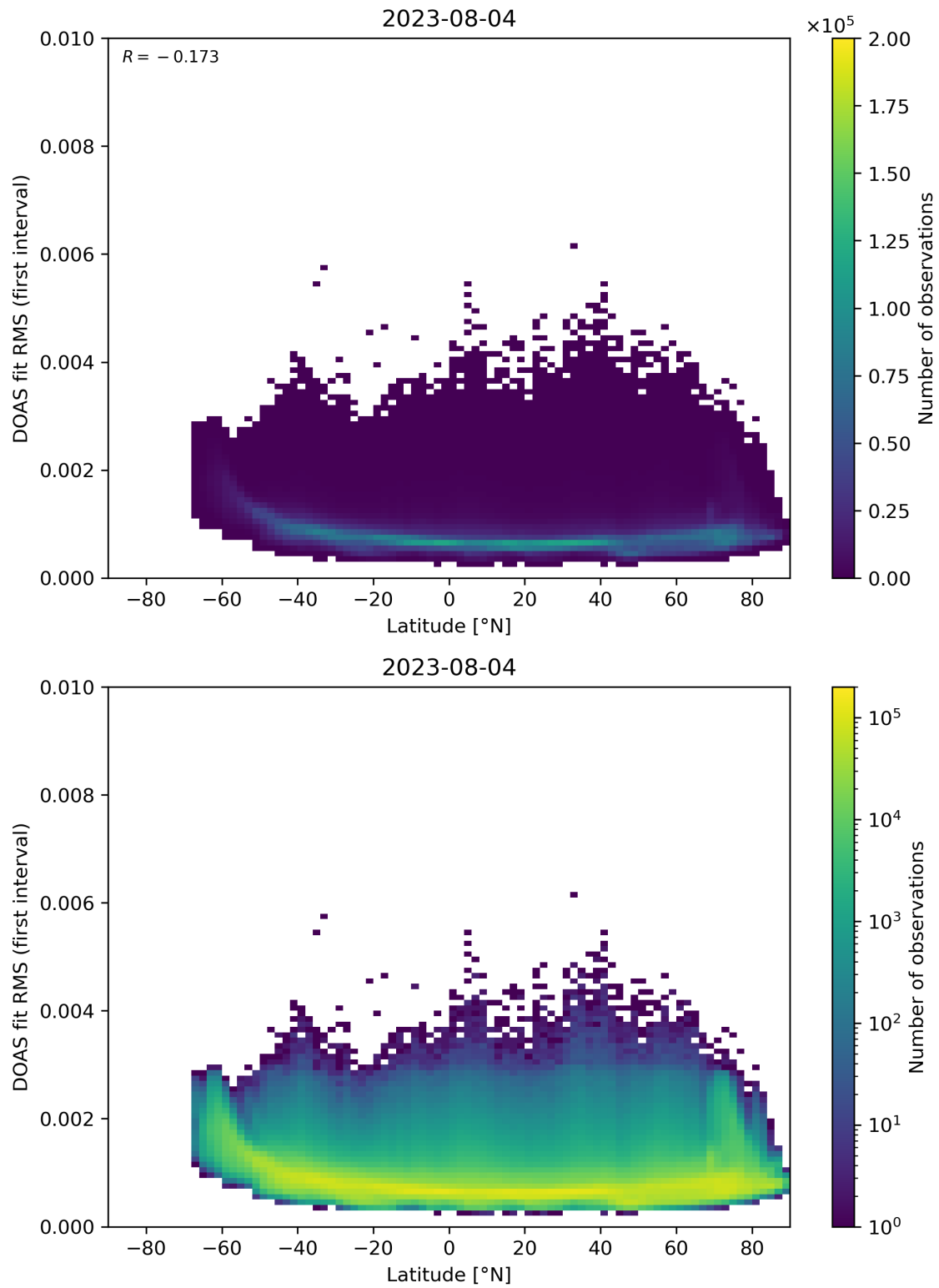
Figure 153: Scatter density plot of “Latitude” against “DOAS fit RMS (first interval)” for 2023-08-04 to 2023-08-05.
