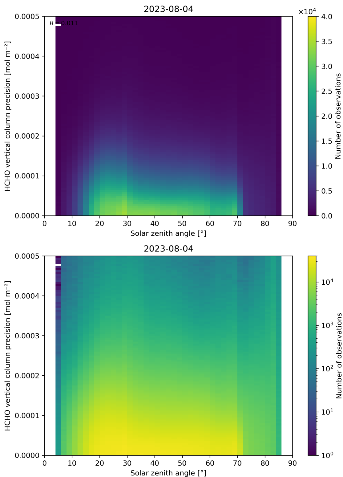
Figure 179: Scatter density plot of “Solar zenith angle” against “HCHO vertical column precision” for 2023-08-04 to 2023-08-05.
