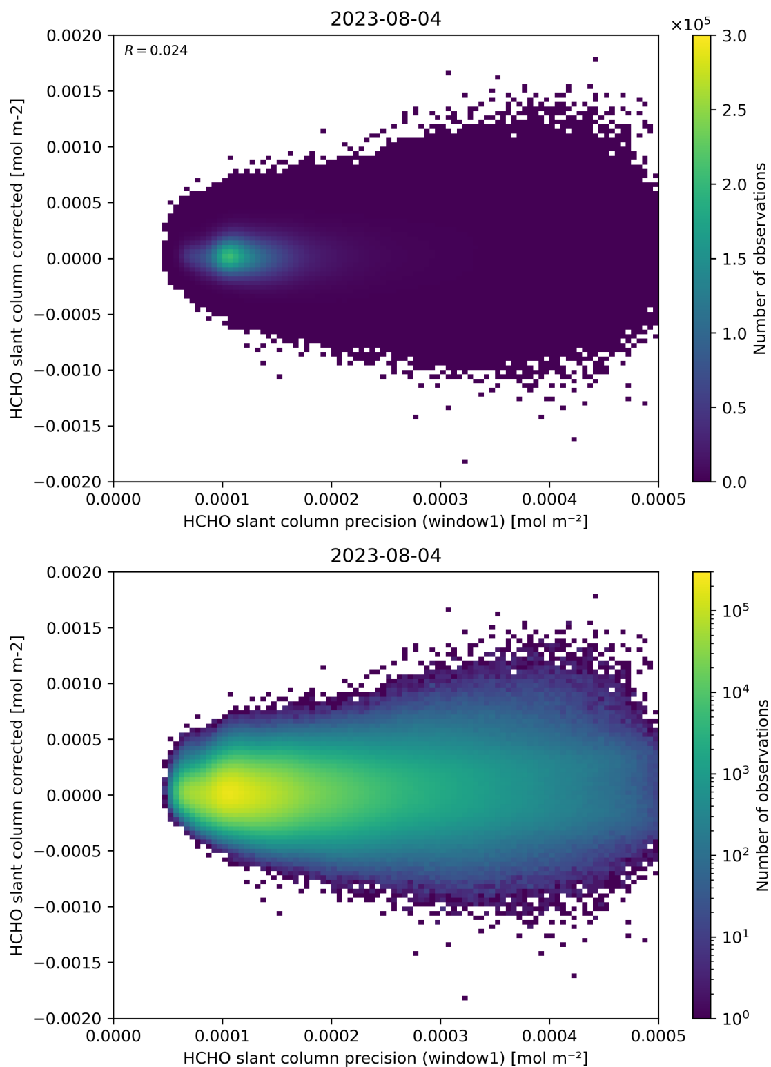
Figure 92: Scatter density plot of “HCHO slant column precision (window1)” against “HCHO slant column corrected” for 2023-08-04 to 2023-08-05.
