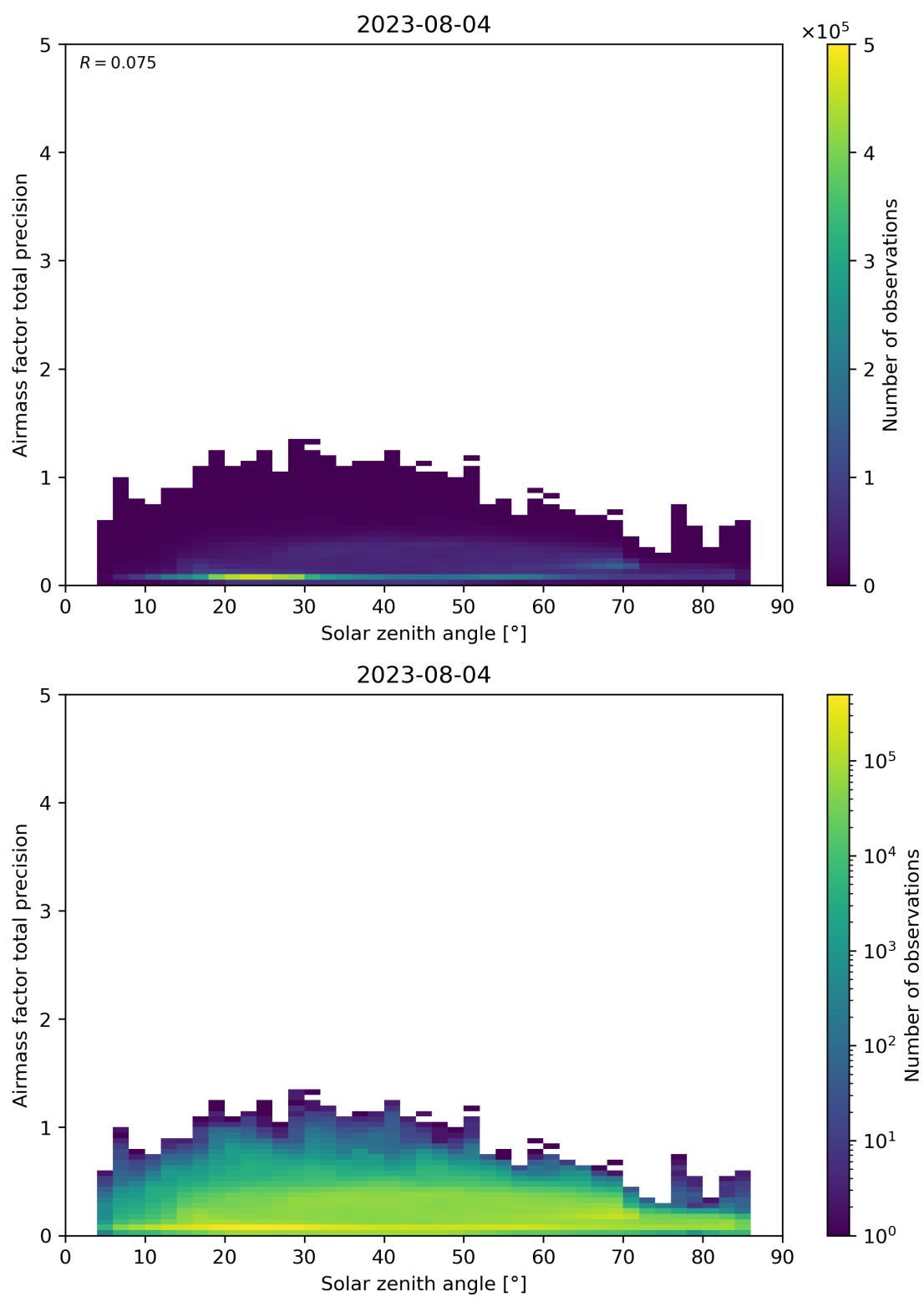
Figure 176: Scatter density plot of “Solar zenith angle” against “Airmass factor total precision” for 2023-08-04 to 2023-08-05.
