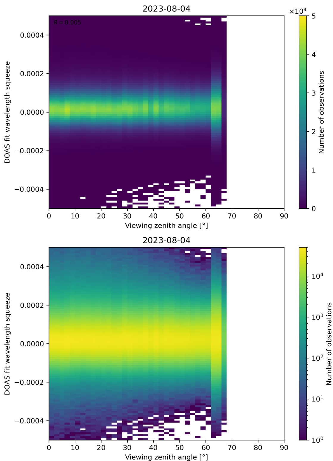
Figure 184: Scatter density plot of “Viewing zenith angle” against “DOAS fit wavelength squeeze” for 2023-08-04 to 2023-08-05.
