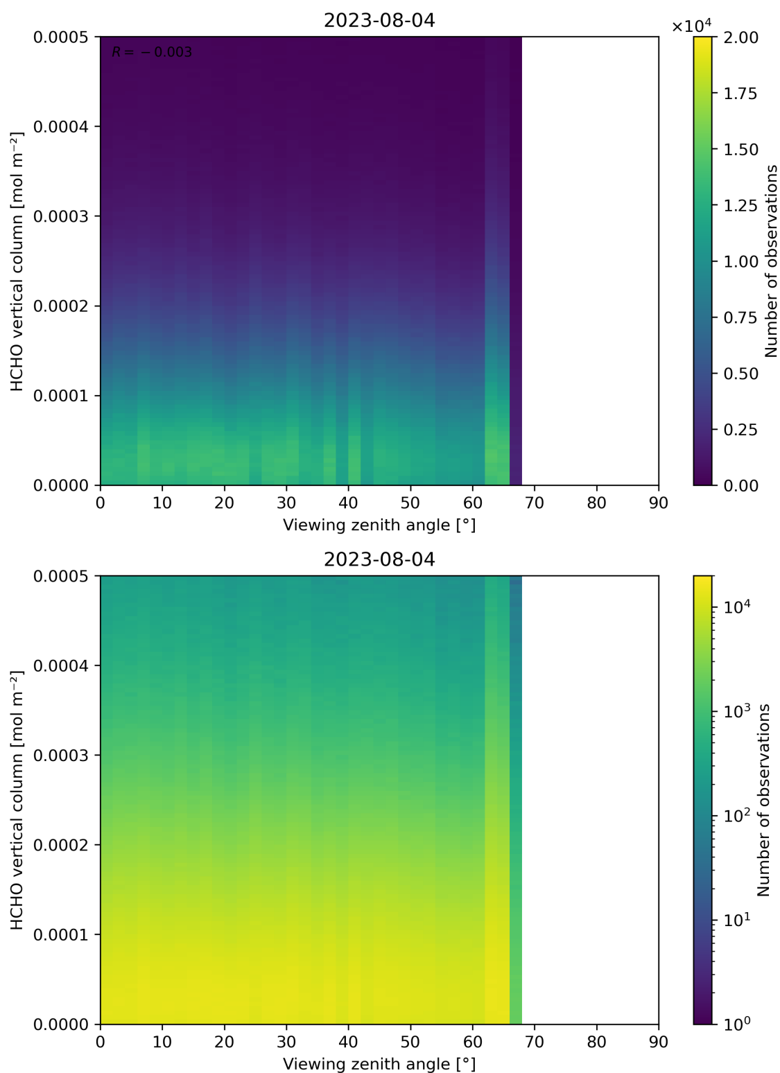
Figure 192: Scatter density plot of “Viewing zenith angle” against “HCHO vertical column” for 2023-08-04 to 2023-08-05.
