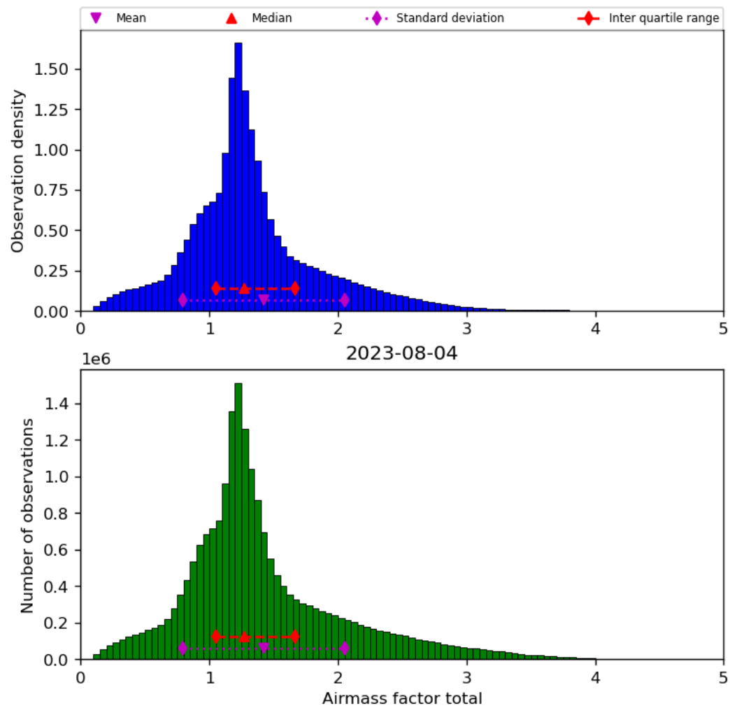
Figure 40: Histogram of “Airmass factor total” for 2023-08-04 to 2023-08-05
