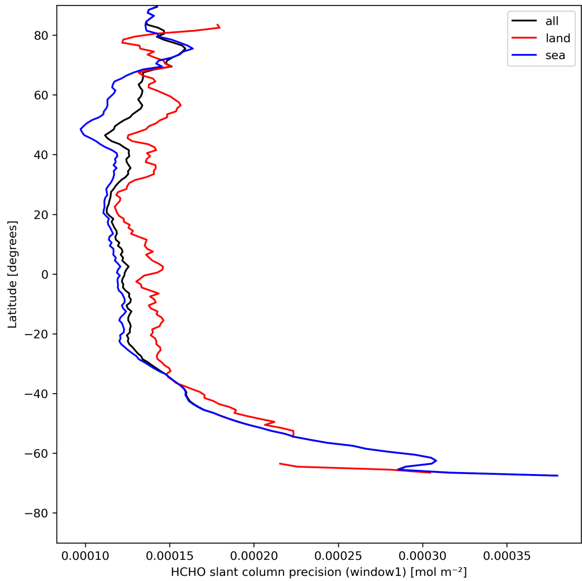
Figure 25: Zonal average of “HCHO slant column precision (window1)” for 2023-08-04 to 2023-08-05.
