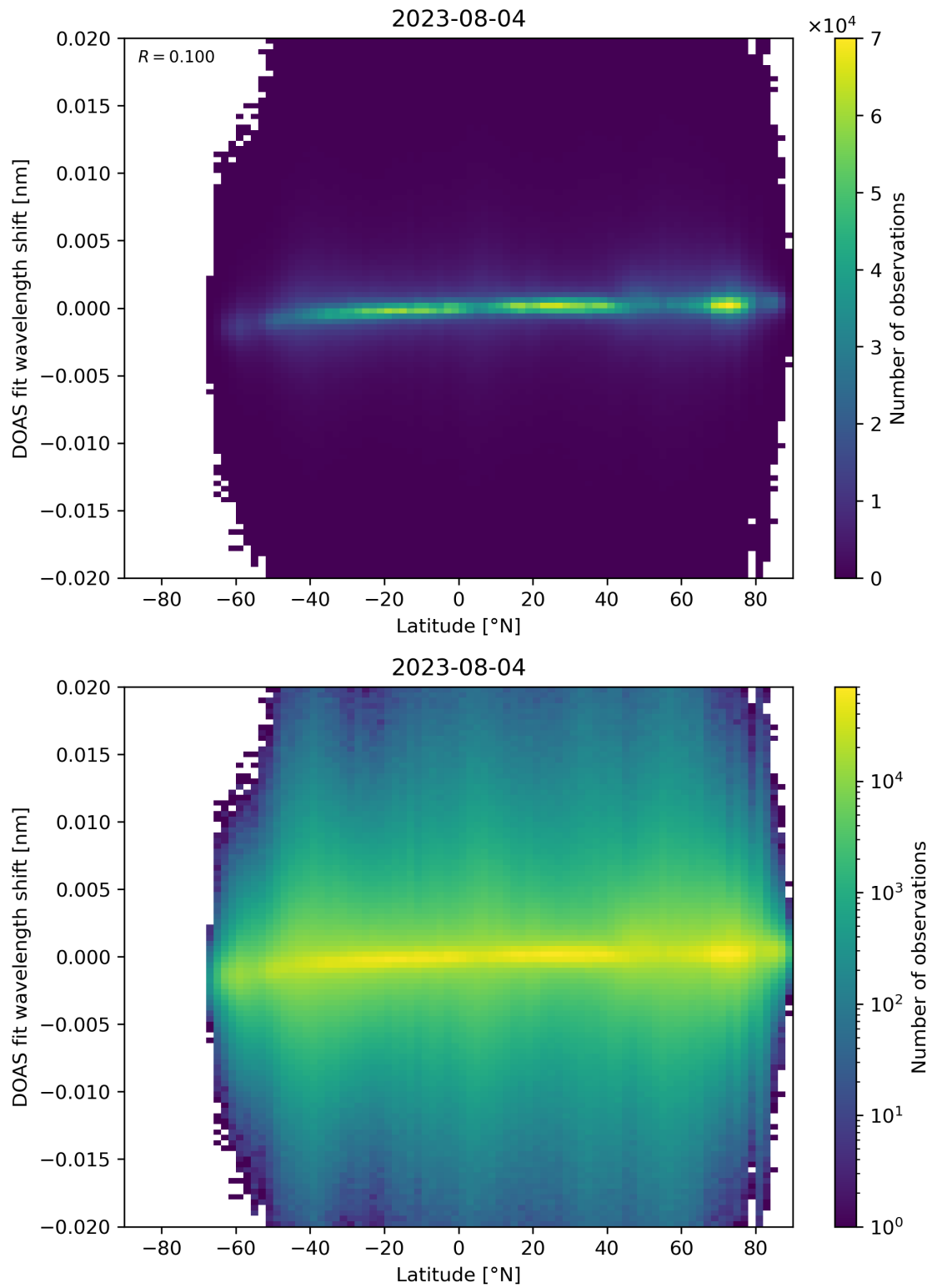
Figure 154: Scatter density plot of “Latitude” against “DOAS fit wavelength shift” for 2023-08-04 to 2023-08-05.
