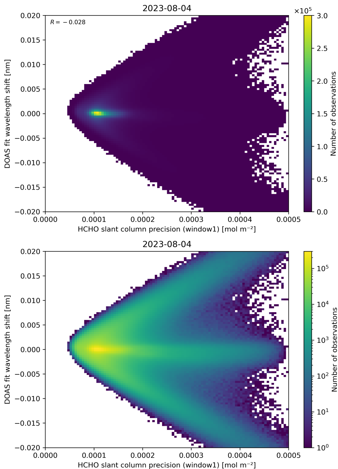
Figure 89: Scatter density plot of “HCHO slant column precision (window1)” against “DOAS fit wavelength shift” for 2023-08-04 to 2023-08-05.
