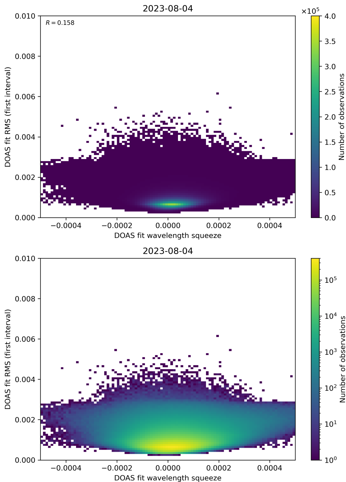
Figure 68: Scatter density plot of “DOAS fit wavelength squeeze” against “DOAS fit RMS (first interval)” for 2023-08-04 to 2023-08-05.
