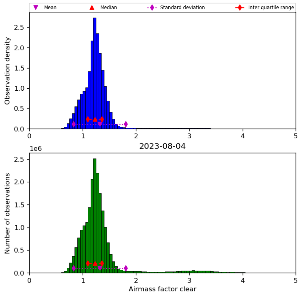
Figure 42: Histogram of “Airmass factor clear” for 2023-08-04 to 2023-08-05
