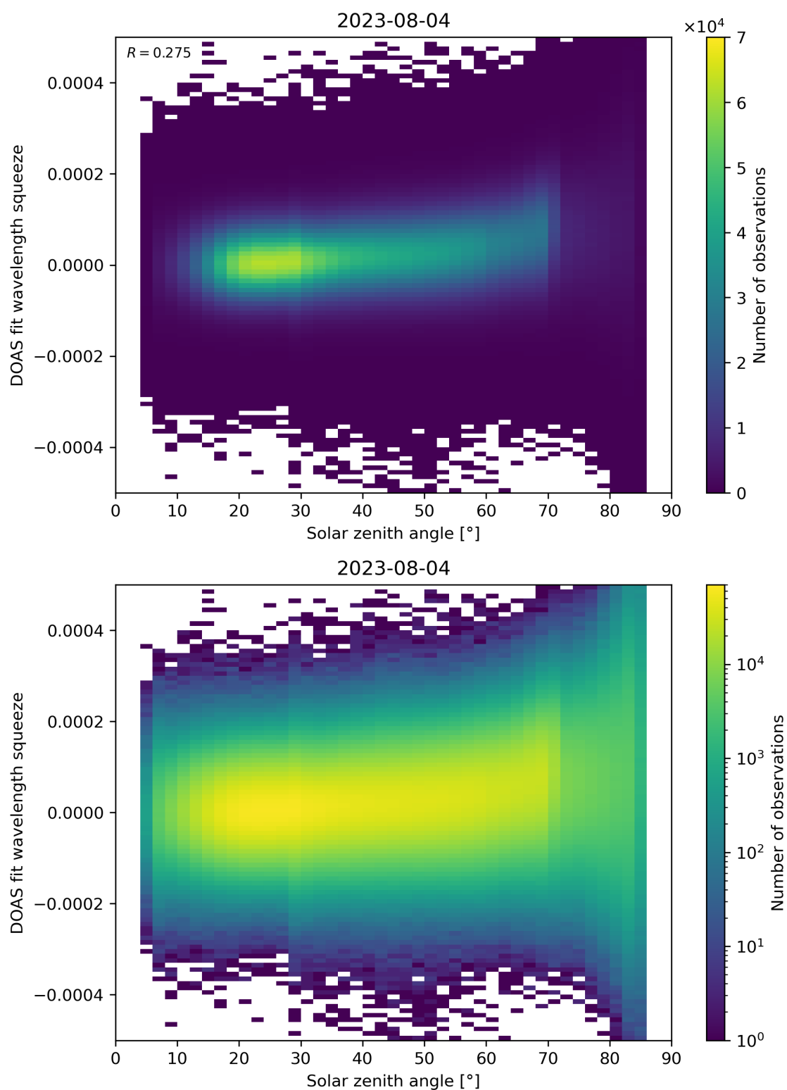
Figure 169: Scatter density plot of “Solar zenith angle” against “DOAS fit wavelength squeeze” for 2023-08-04 to 2023-08-05.
