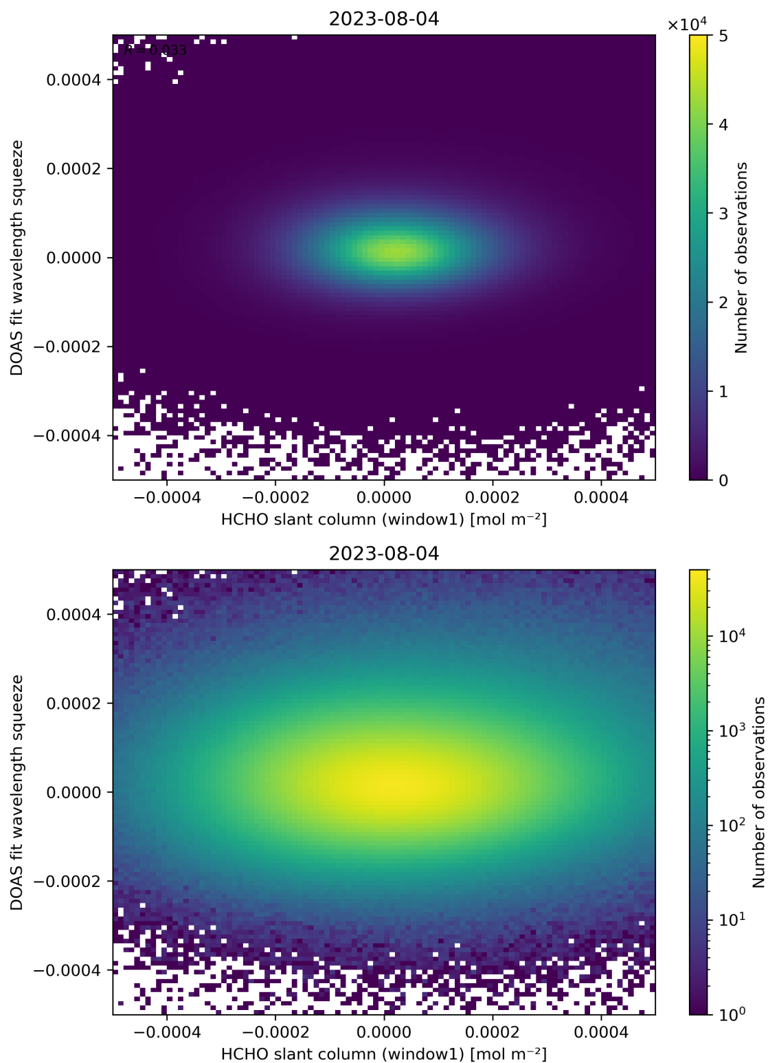
Figure 80: Scatter density plot of “HCHO slant column (window1)” against “DOAS fit wavelength squeeze” for 2023-08-04 to 2023-08-05.
