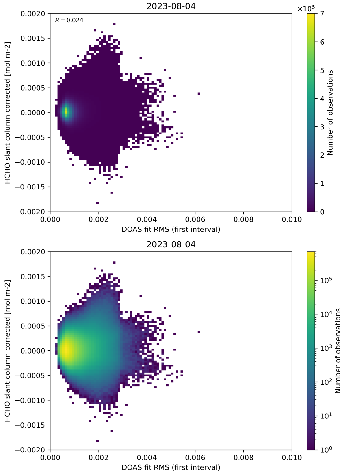
Figure 62: Scatter density plot of “DOAS fit RMS (first interval)” against “HCHO slant column corrected” for 2023-08-04 to 2023-08-05.
