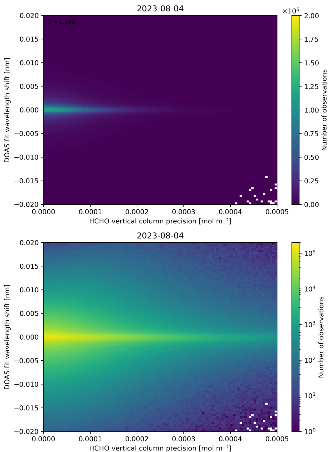
Figure 137: Scatter density plot of “HCHO vertical column precision” against “DOAS fit wavelength shift” for 2023-08-04 to 2023-08-05.
