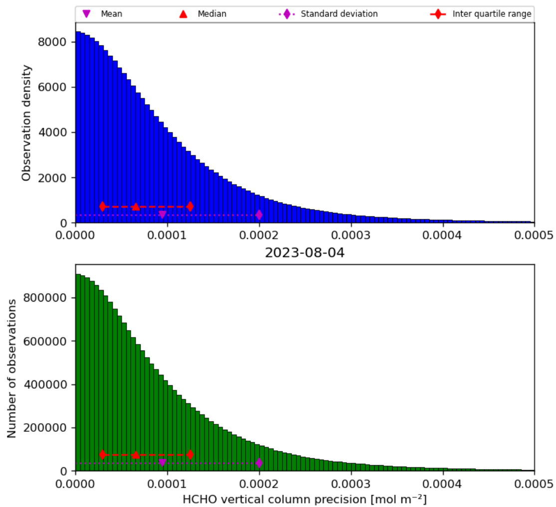
Figure 36: Histogram of “HCHO vertical column precision” for 2023-08-04 to 2023-08-05
