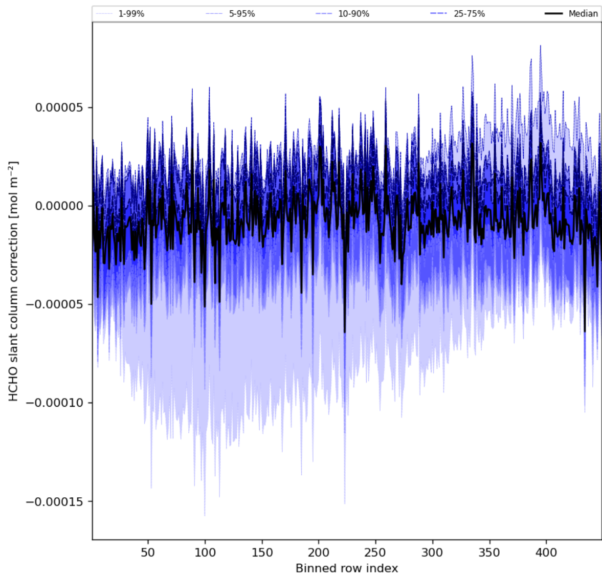
Figure 61: Along track statistics of “HCHO slant column correction” for 2023-08-04 to 2023-08-05
