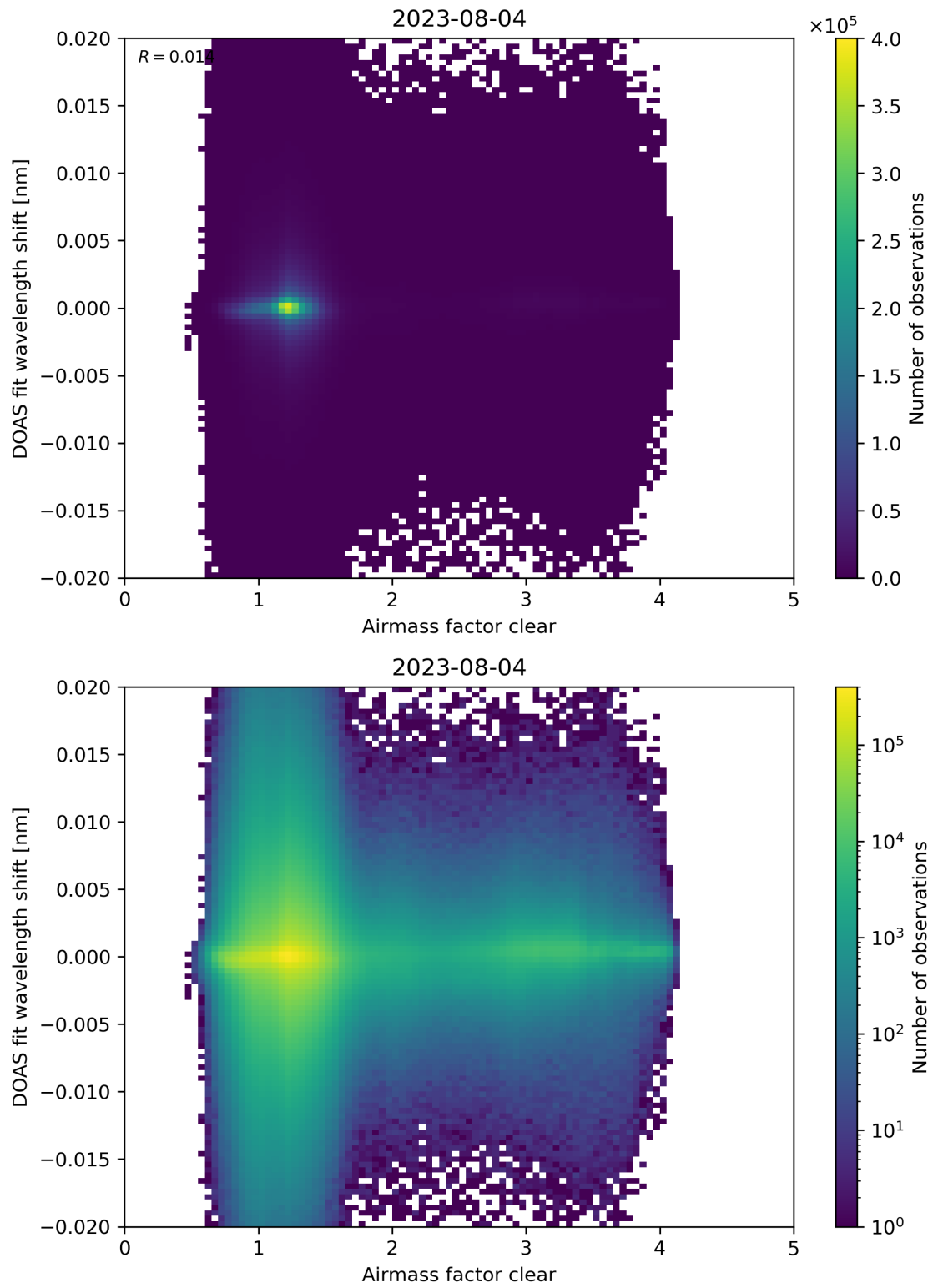
Figure 72: Scatter density plot of “Airmass factor clear” against “DOAS fit wavelength shift” for 2023-08-04 to 2023-08-05.
