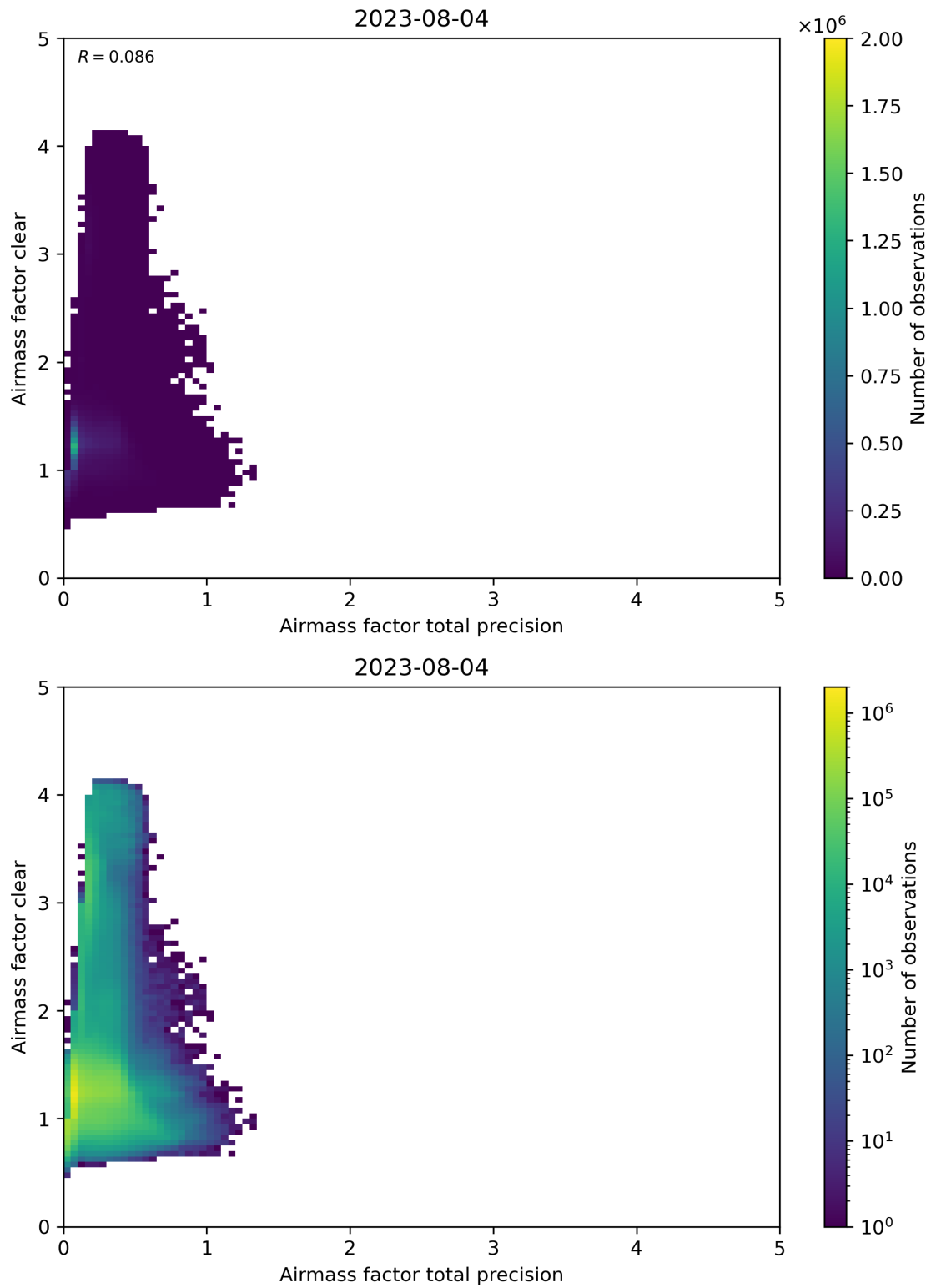
Figure 108: Scatter density plot of “Airmass factor total precision” against “Airmass factor clear” for 2023-08-04 to 2023-08-05.
