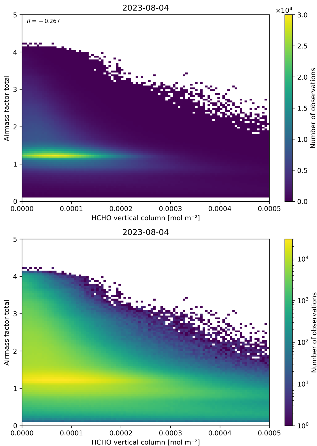
Figure 131: Scatter density plot of “HCHO vertical column” against “Airmass factor total” for 2023-08-04 to 2023-08-05.
