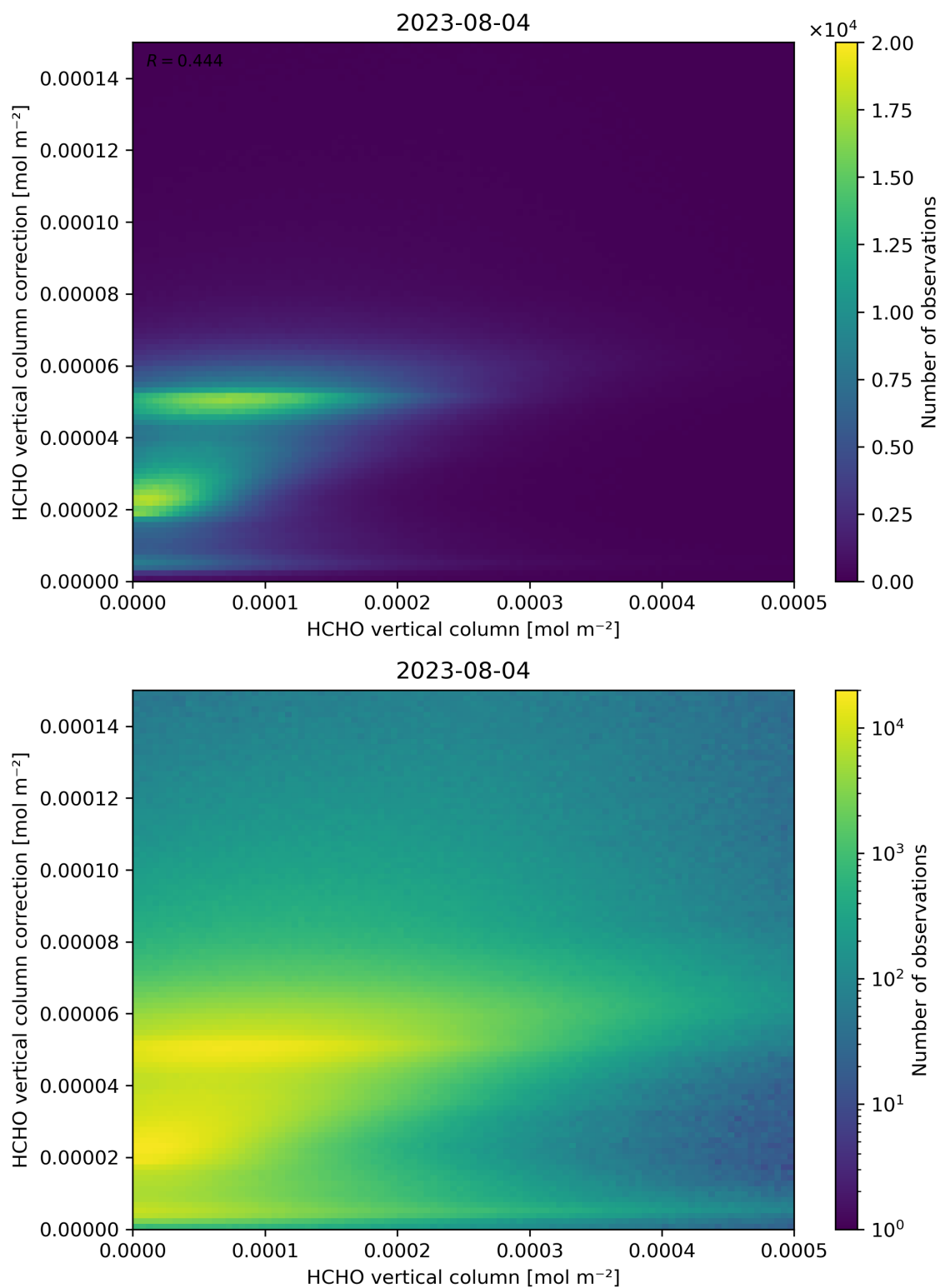
Figure 133: Scatter density plot of “HCHO vertical column” against “HCHO vertical column correction” for 2023-08-04 to 2023-08-05.
