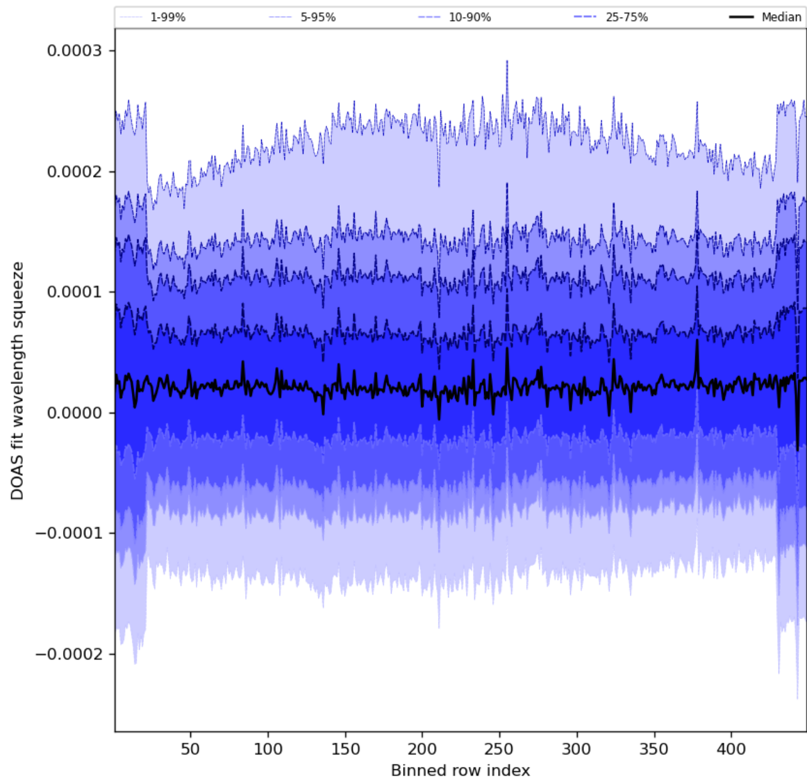
Figure 59: Along track statistics of “DOAS fit wavelength squeeze” for 2023-08-04 to 2023-08-05
