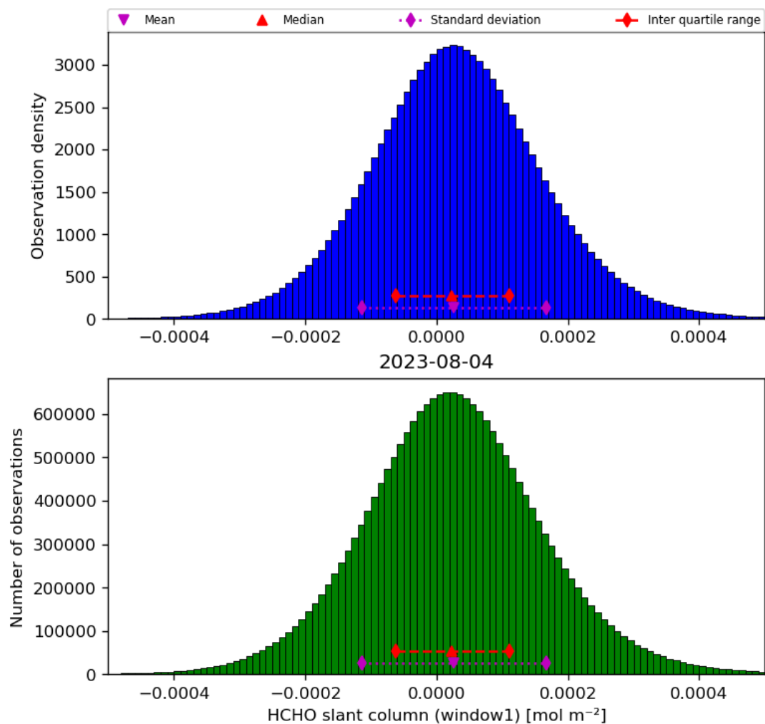
Figure 38: Histogram of “HCHO slant column (window1)” for 2023-08-04 to 2023-08-05
