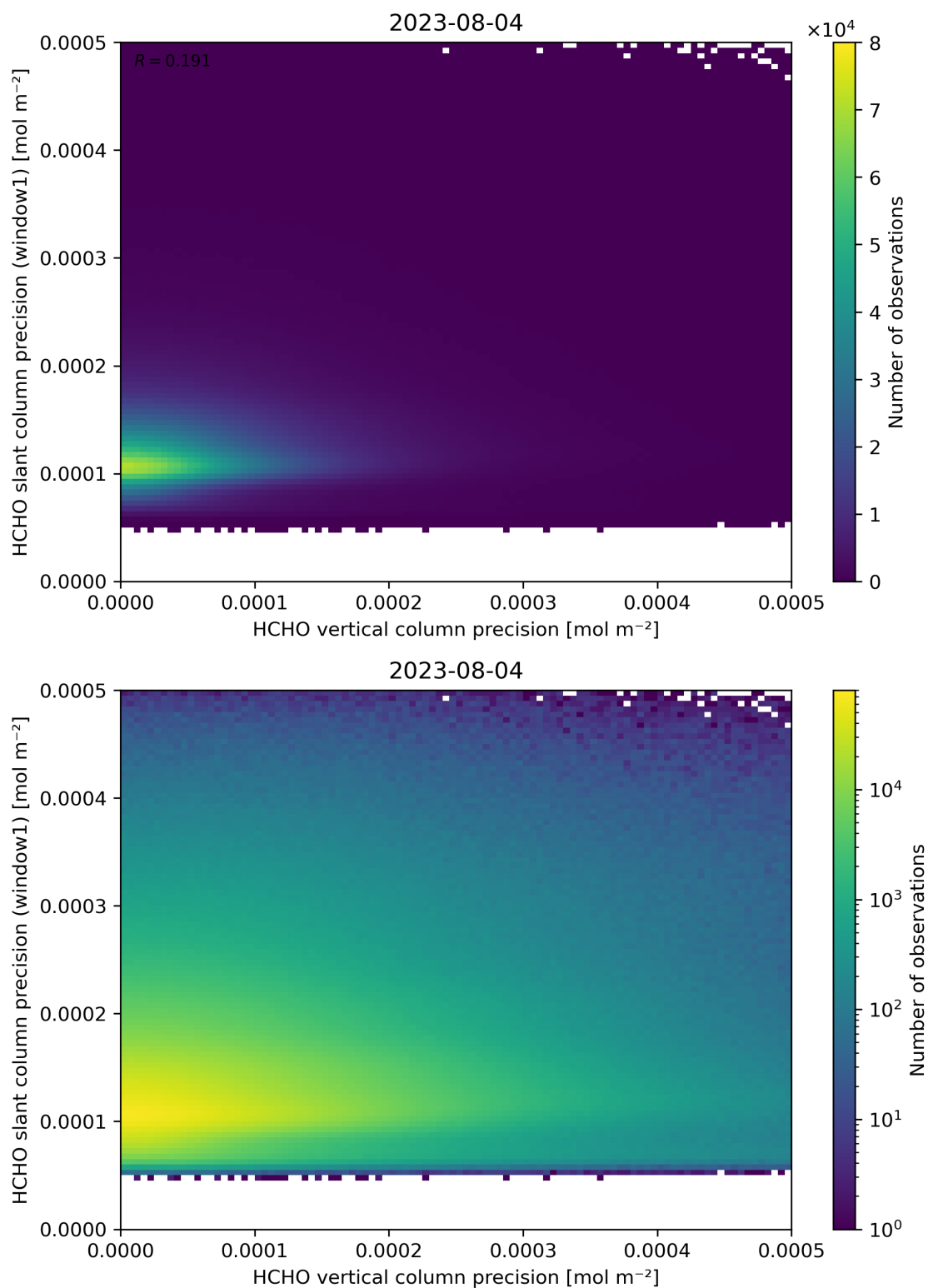
Figure 143: Scatter density plot of “HCHO vertical column precision” against “HCHO slant column precision (window1)” for 2023-08-04 to 2023-08-05.
