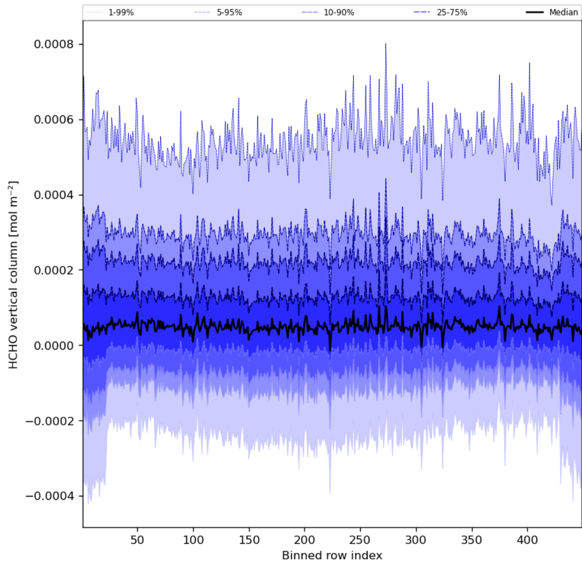
Figure 49: Along track statistics of “HCHO vertical column” for 2023-08-04 to 2023-08-05
