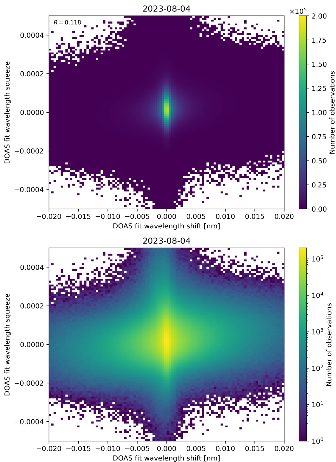
Figure 65: Scatter density plot of “DOAS fit wavelength shift” against “DOAS fit wavelength squeeze” for 2023-08-04 to 2023-08-05.
