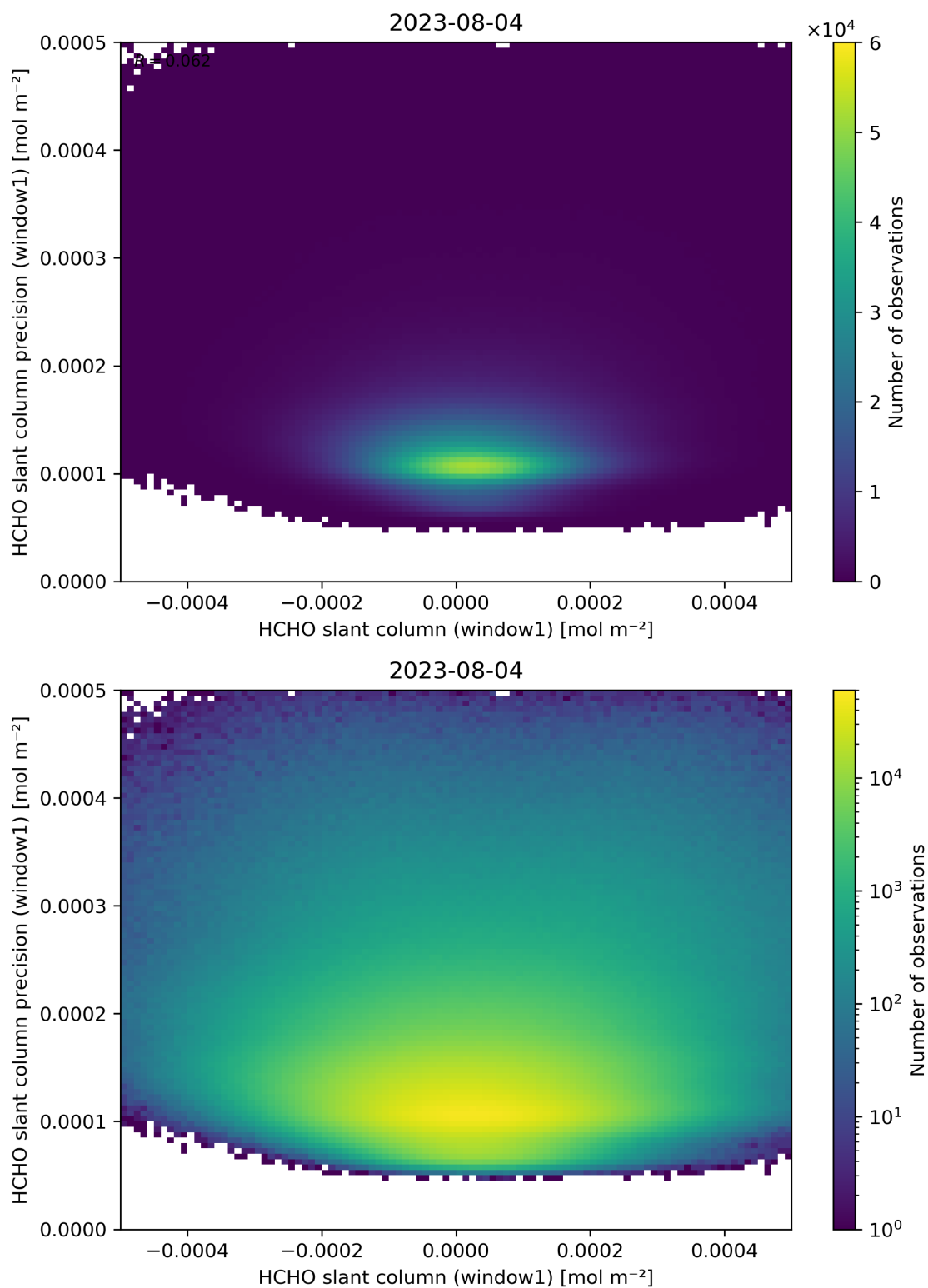
Figure 84: Scatter density plot of “HCHO slant column (window1)” against “HCHO slant column precision (window1)” for 2023-08-04 to 2023-08-05.
