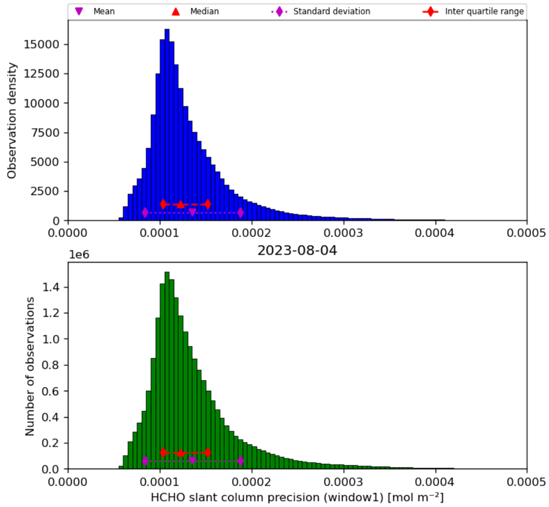
Figure 39: Histogram of “HCHO slant column precision (window1)” for 2023-08-04 to 2023-08-05
