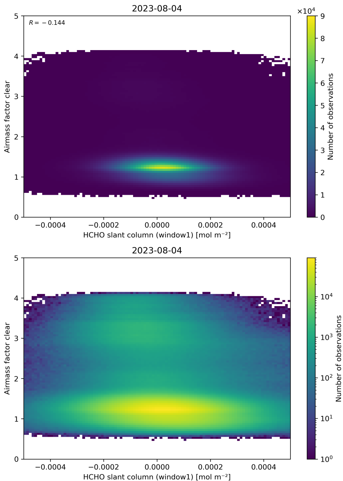
Figure 81: Scatter density plot of “HCHO slant column (window1)” against “Airmass factor clear” for 2023-08-04 to 2023-08-05.
