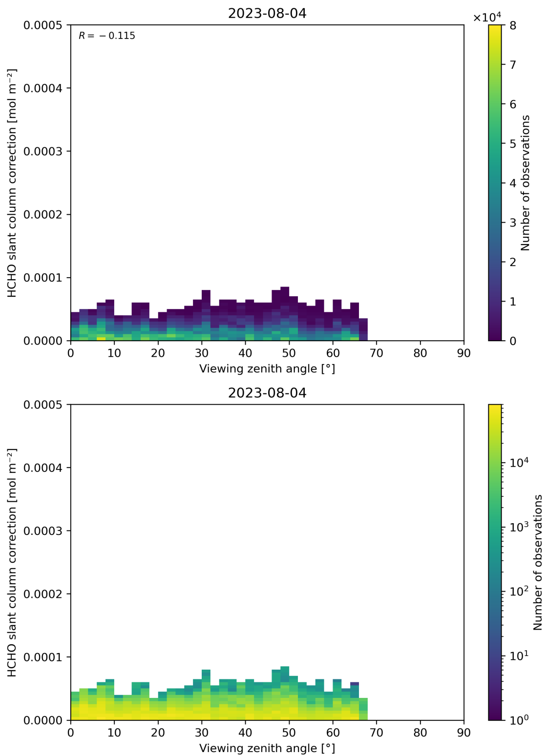
Figure 187: Scatter density plot of “Viewing zenith angle” against “HCHO slant column correction” for 2023-08-04 to 2023-08-05.
