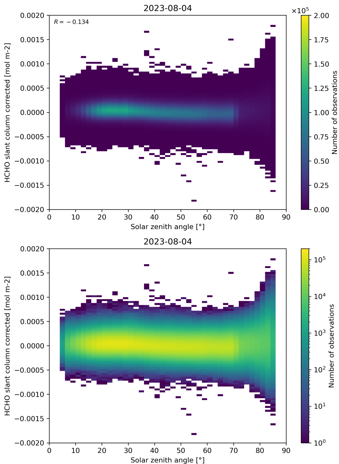
Figure 171: Scatter density plot of “Solar zenith angle” against “HCHO slant column corrected” for 2023-08-04 to 2023-08-05.
