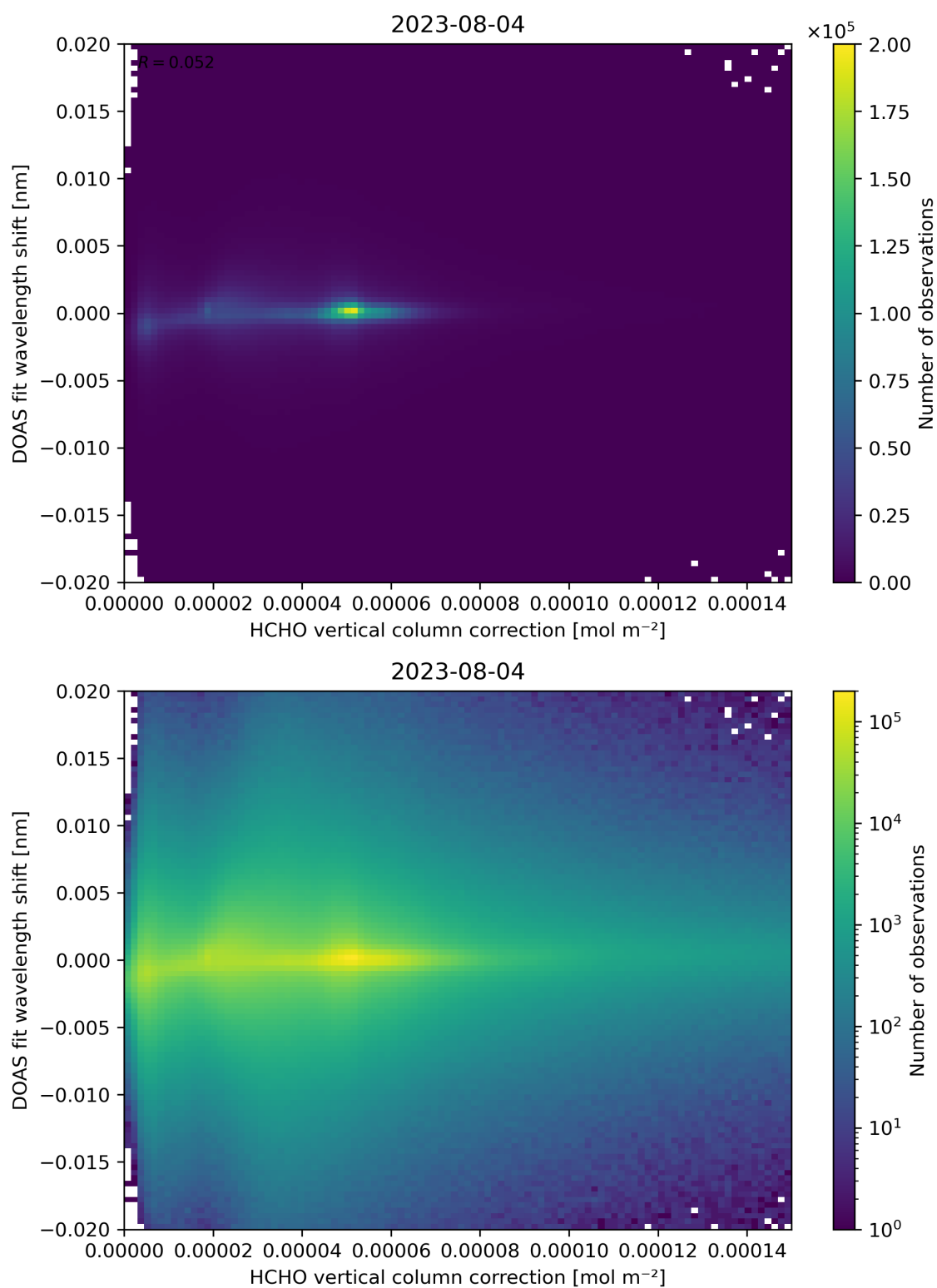
Figure 113: Scatter density plot of “HCHO vertical column correction” against “DOAS fit wavelength shift” for 2023-08-04 to 2023-08-05.
