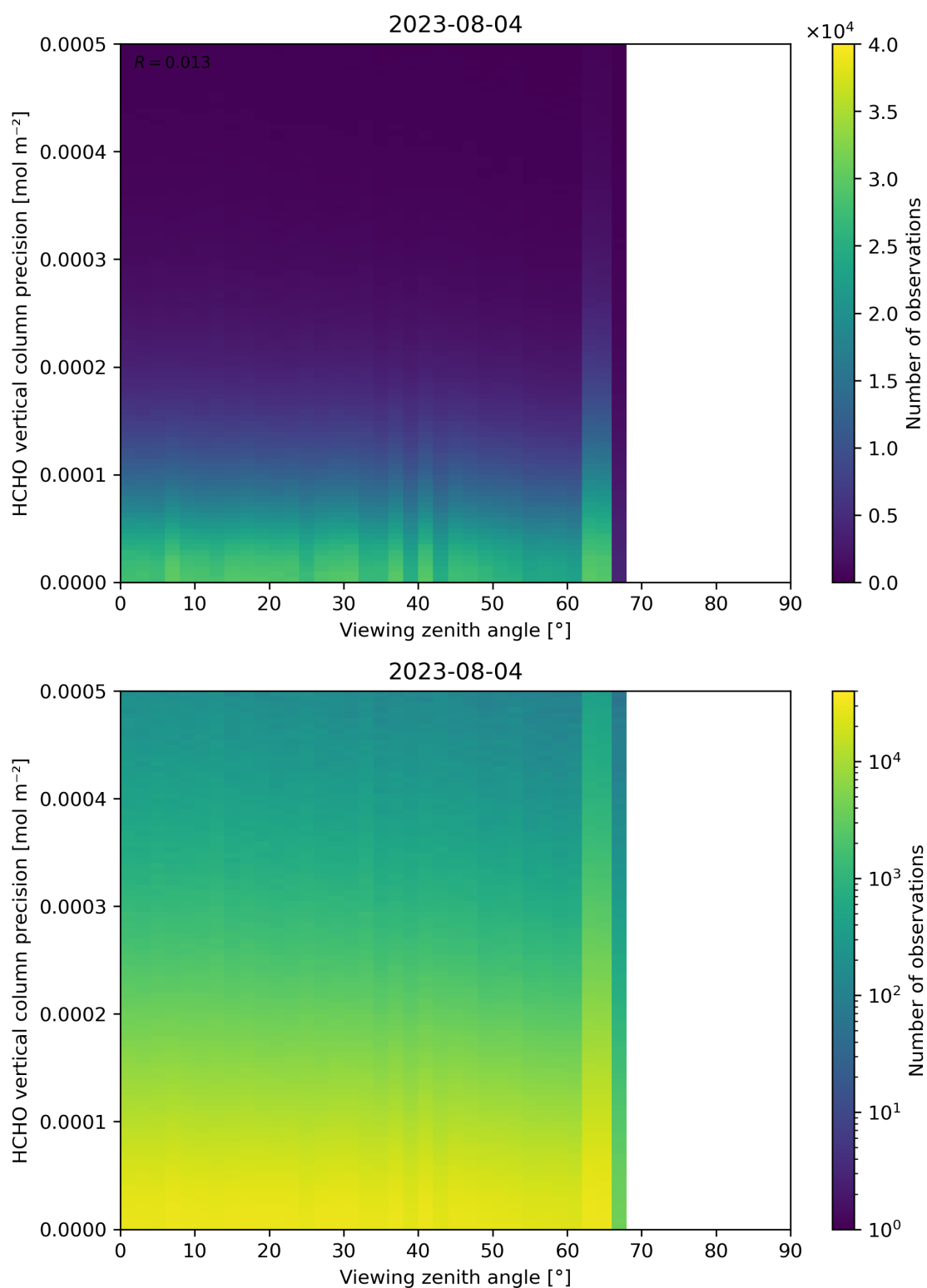
Figure 194: Scatter density plot of “Viewing zenith angle” against “HCHO vertical column precision” for 2023-08-04 to 2023-08-05.
