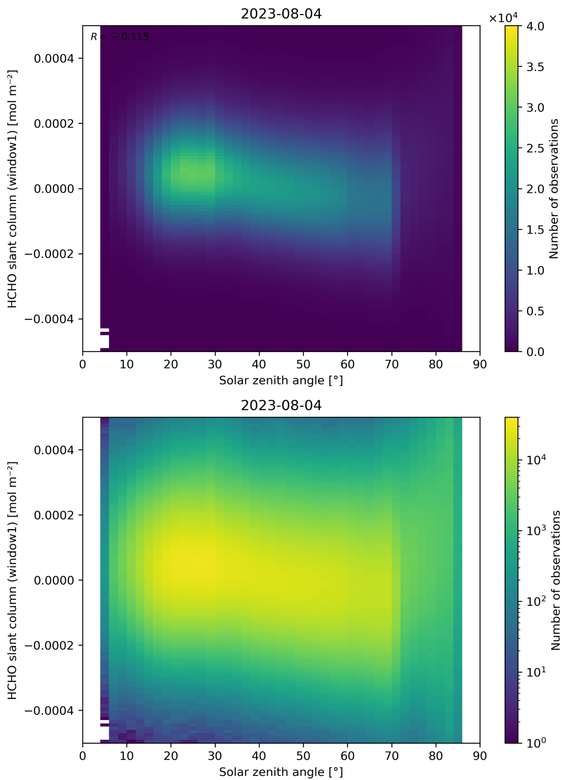
Figure 173: Scatter density plot of “Solar zenith angle” against “HCHO slant column (window1)” for 2023-08-04 to 2023-08-05.
