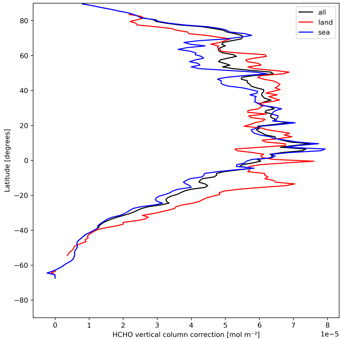
Figure 23: Zonal average of “HCHO vertical column correction” for 2023-08-04 to 2023-08-05.
