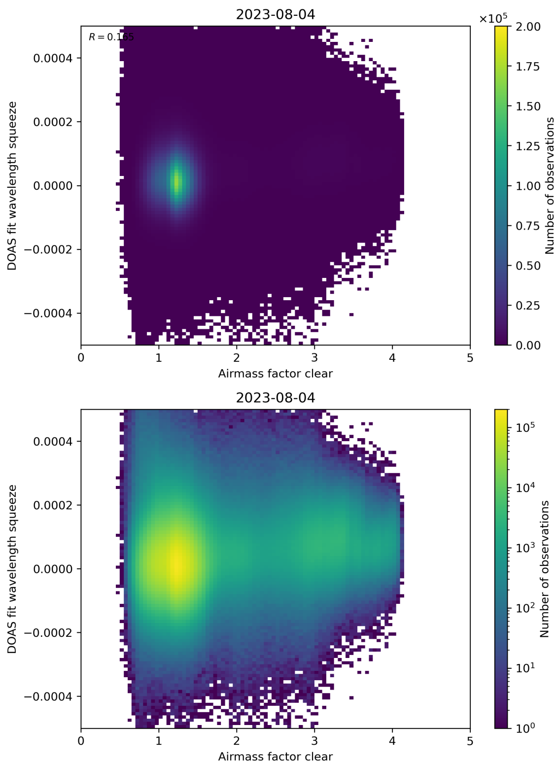
Figure 73: Scatter density plot of “Airmass factor clear” against “DOAS fit wavelength squeeze” for 2023-08-04 to 2023-08-05.
