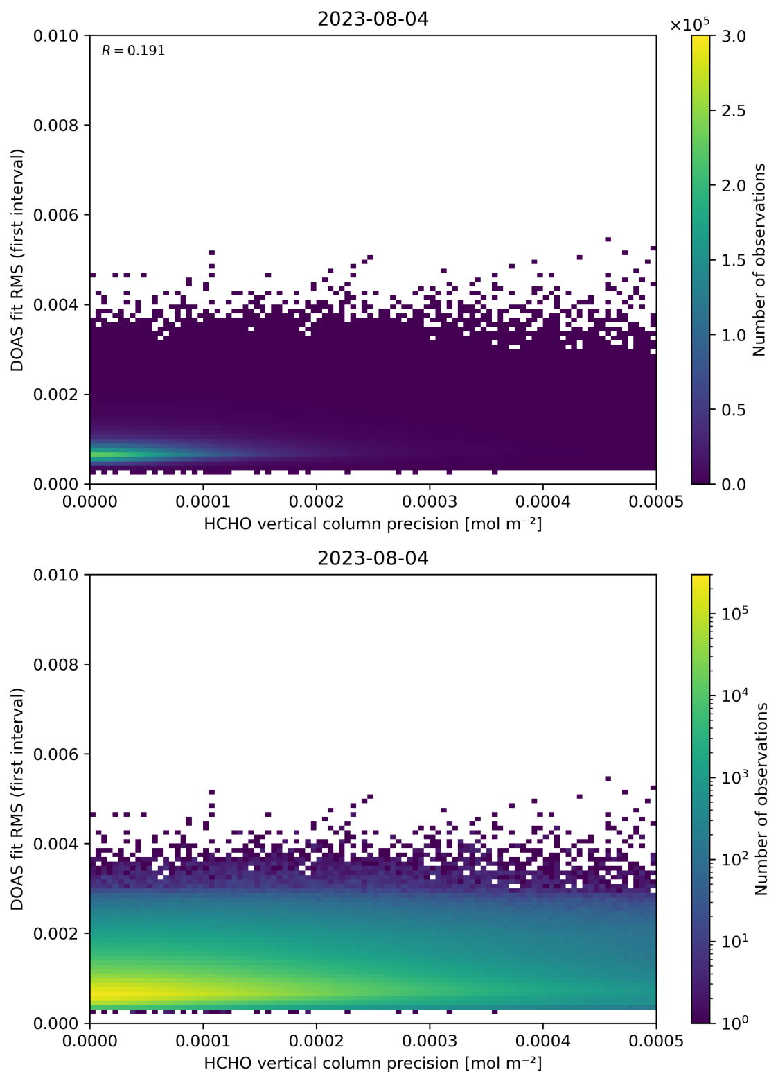
Figure 136: Scatter density plot of “HCHO vertical column precision” against “DOAS fit RMS (first interval)” for 2023-08-04 to 2023-08-05.
