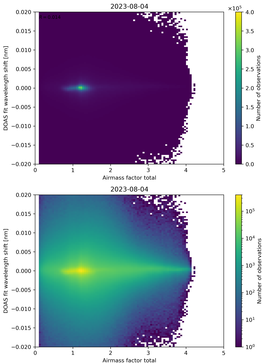
Figure 98: Scatter density plot of “Airmass factor total” against “DOAS fit wavelength shift” for 2023-08-04 to 2023-08-05.
