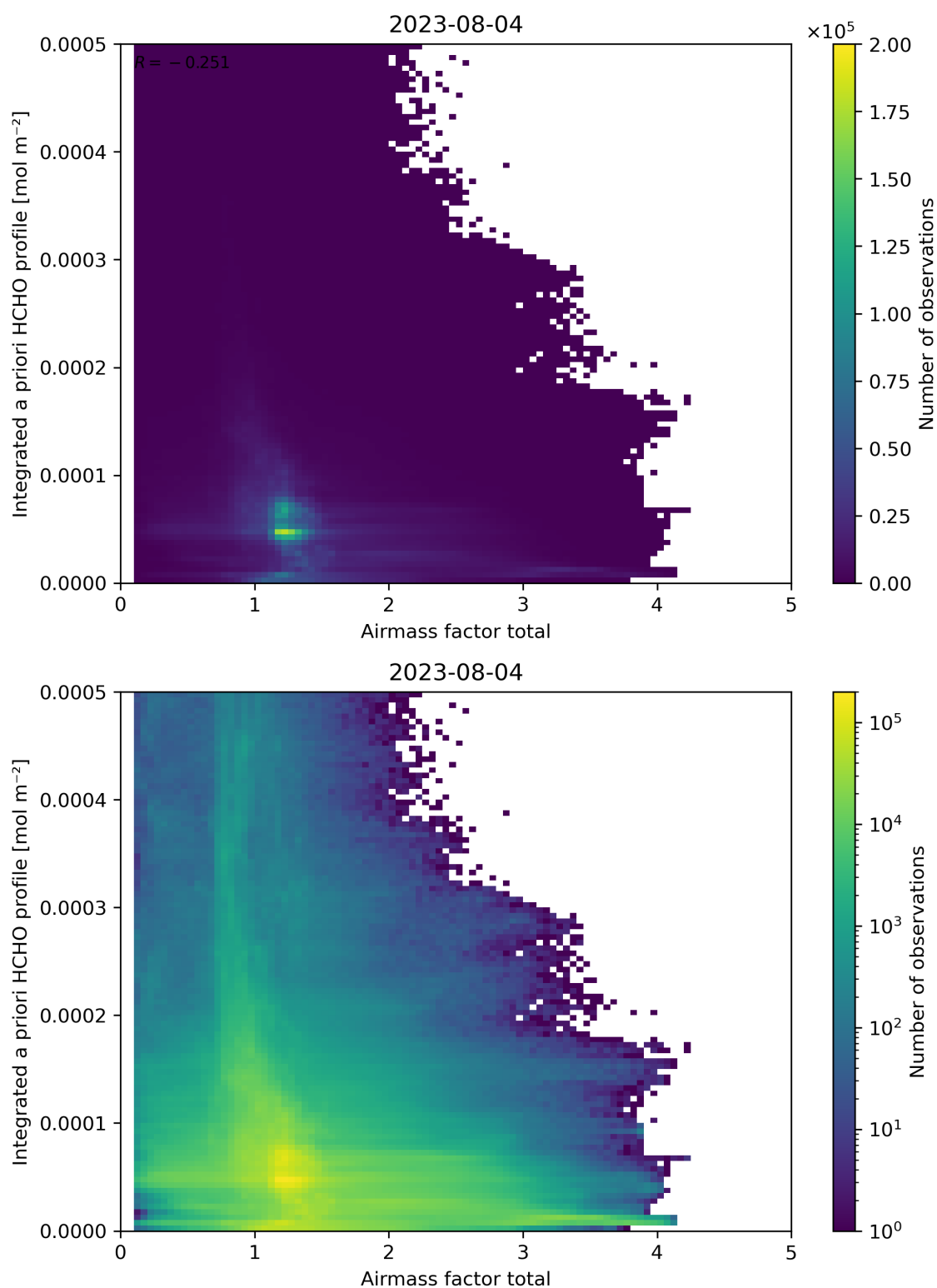
Figure 104: Scatter density plot of “Airmass factor total” against “Integrated a priori HCHO profile” for 2023-08-04 to 2023-08-05.
