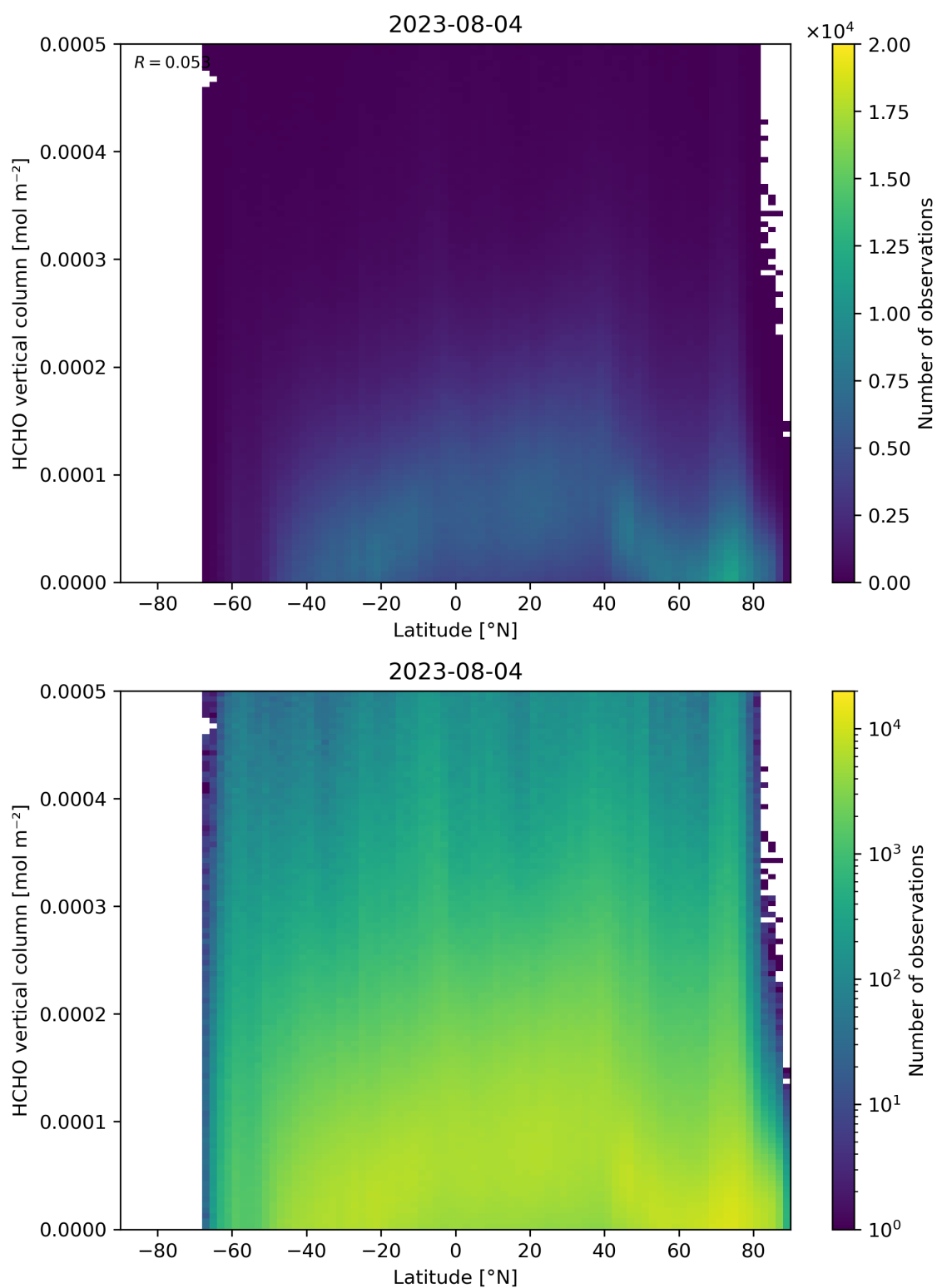
Figure 163: Scatter density plot of “Latitude” against “HCHO vertical column” for 2023-08-04 to 2023-08-05.
