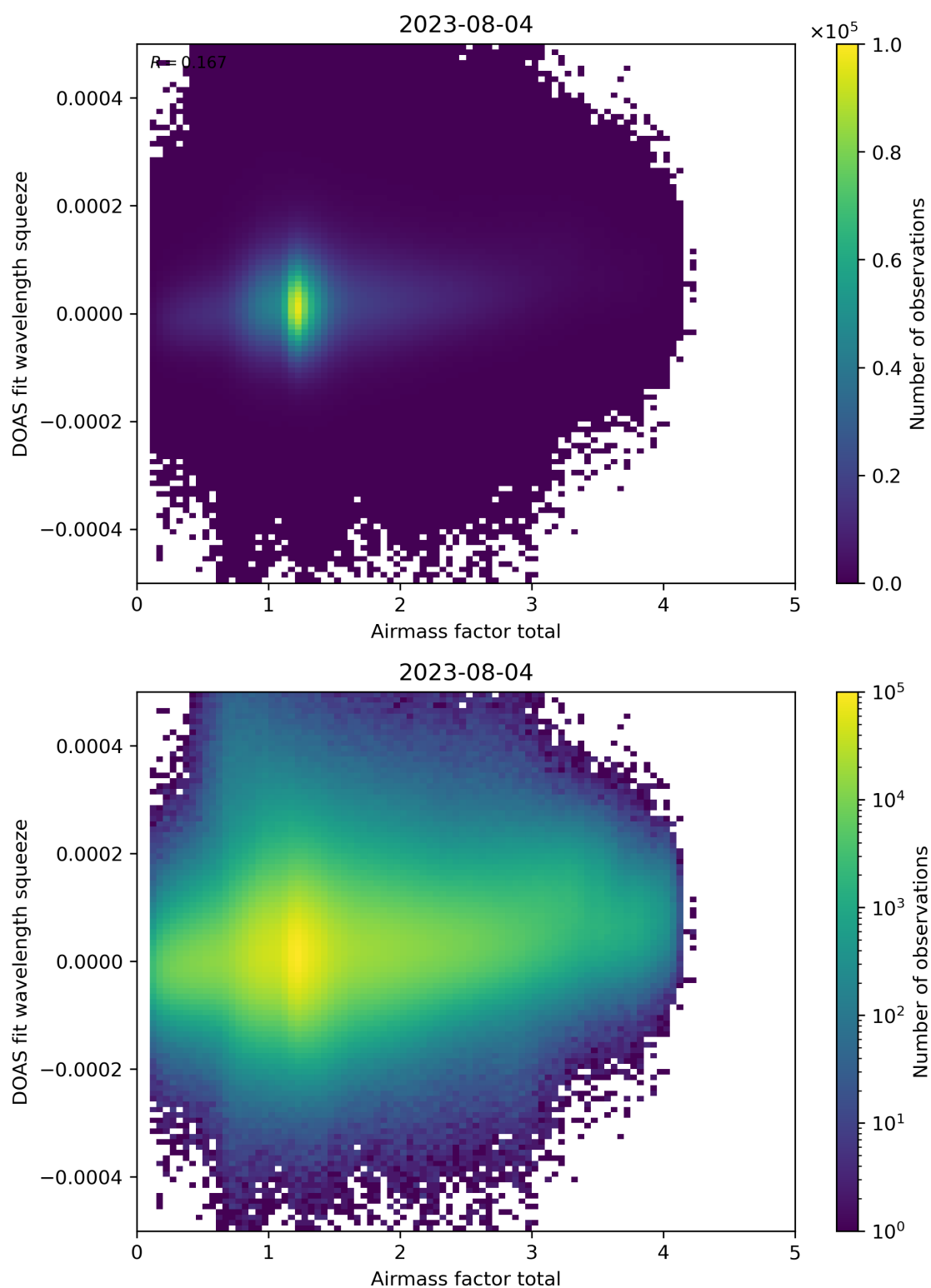
Figure 99: Scatter density plot of “Airmass factor total” against “DOAS fit wavelength squeeze” for 2023-08-04 to 2023-08-05.
