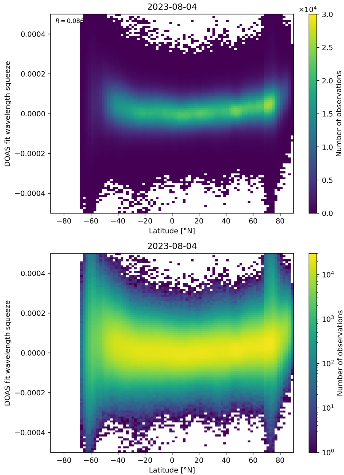
Figure 155: Scatter density plot of “Latitude” against “DOAS fit wavelength squeeze” for 2023-08-04 to 2023-08-05.
