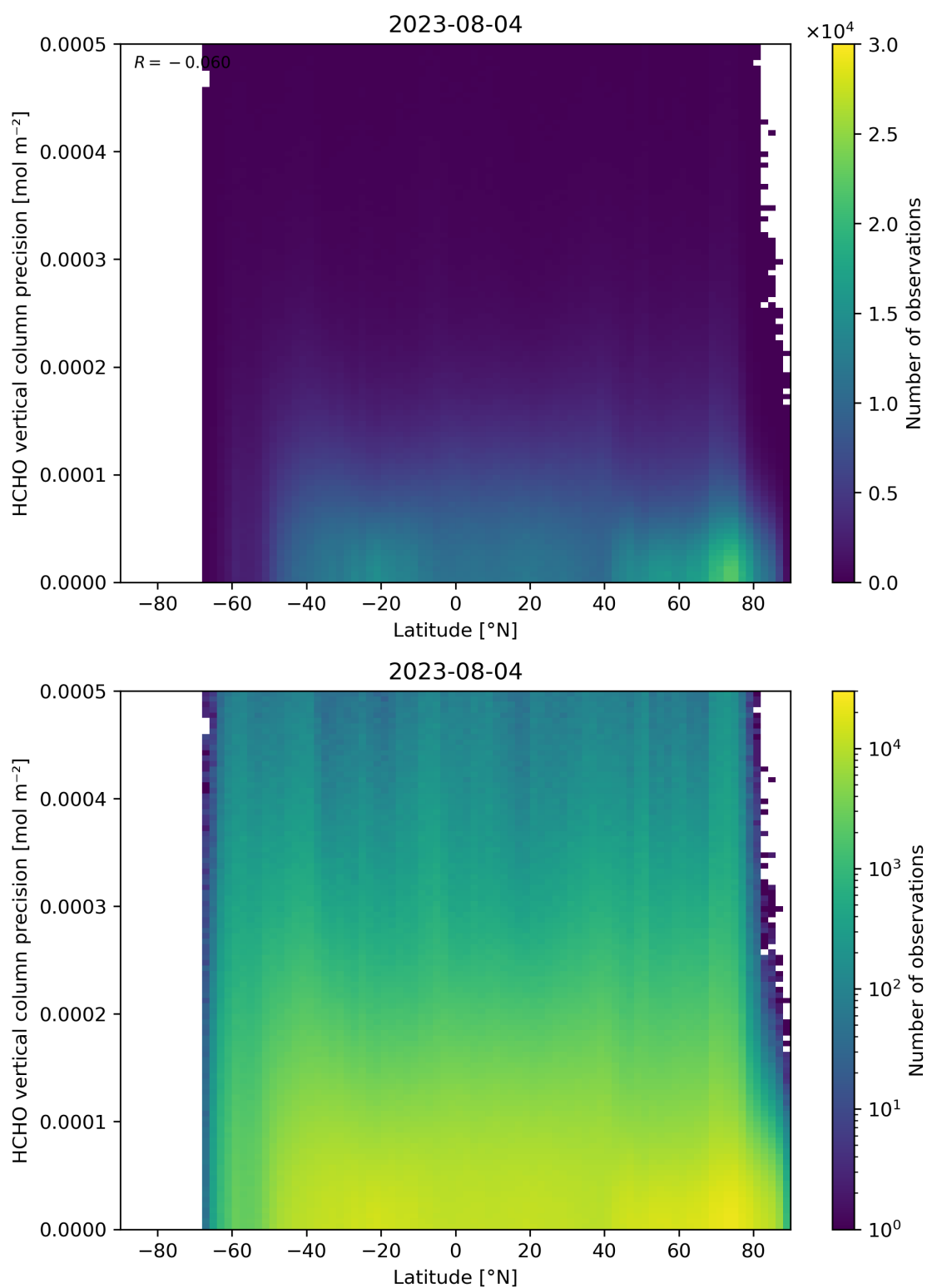
Figure 165: Scatter density plot of “Latitude” against “HCHO vertical column precision” for 2023-08-04 to 2023-08-05.
