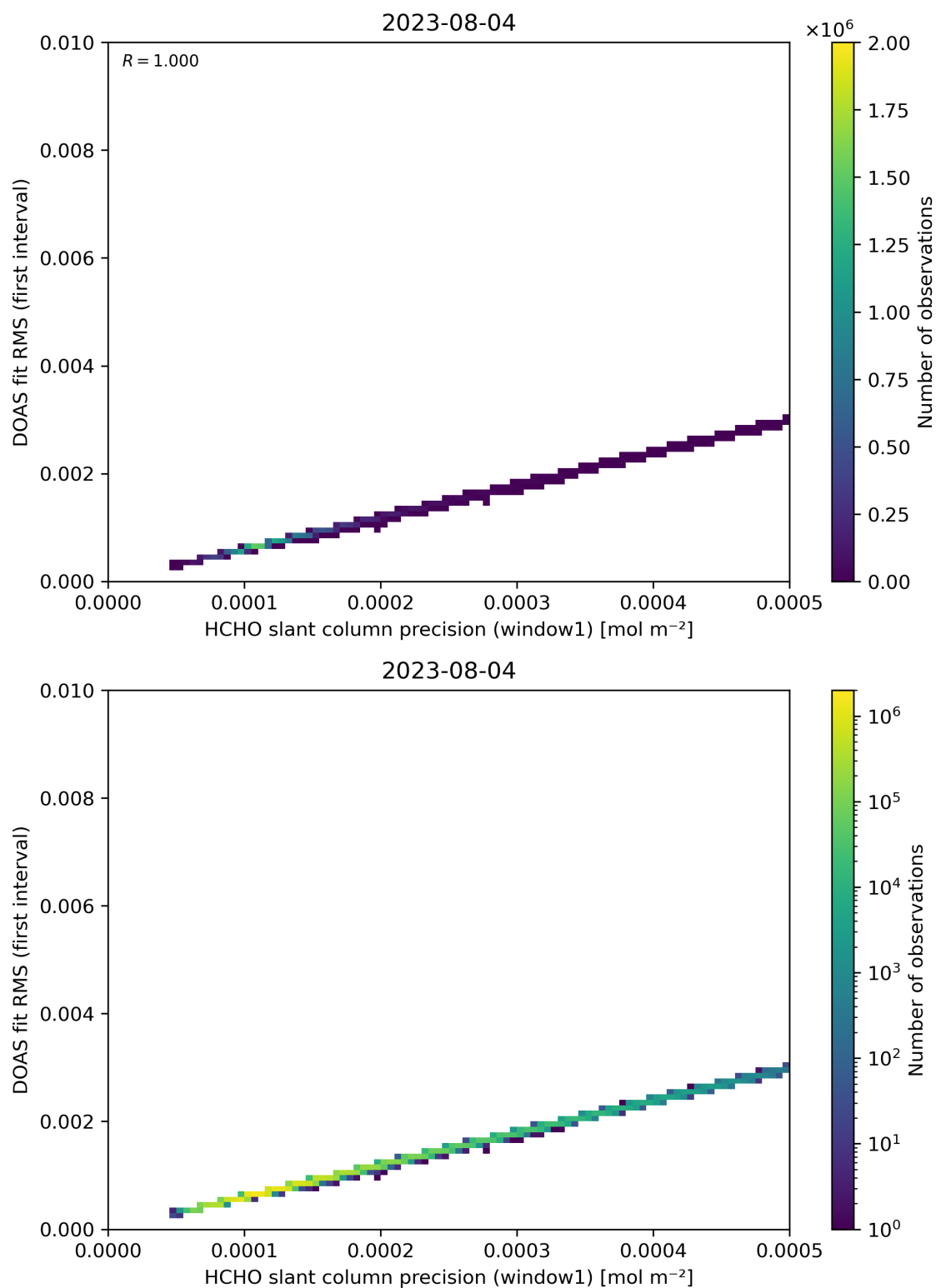
Figure 88: Scatter density plot of “HCHO slant column precision (window1)” against “DOAS fit RMS (first interval)” for 2023-08-04 to 2023-08-05.
