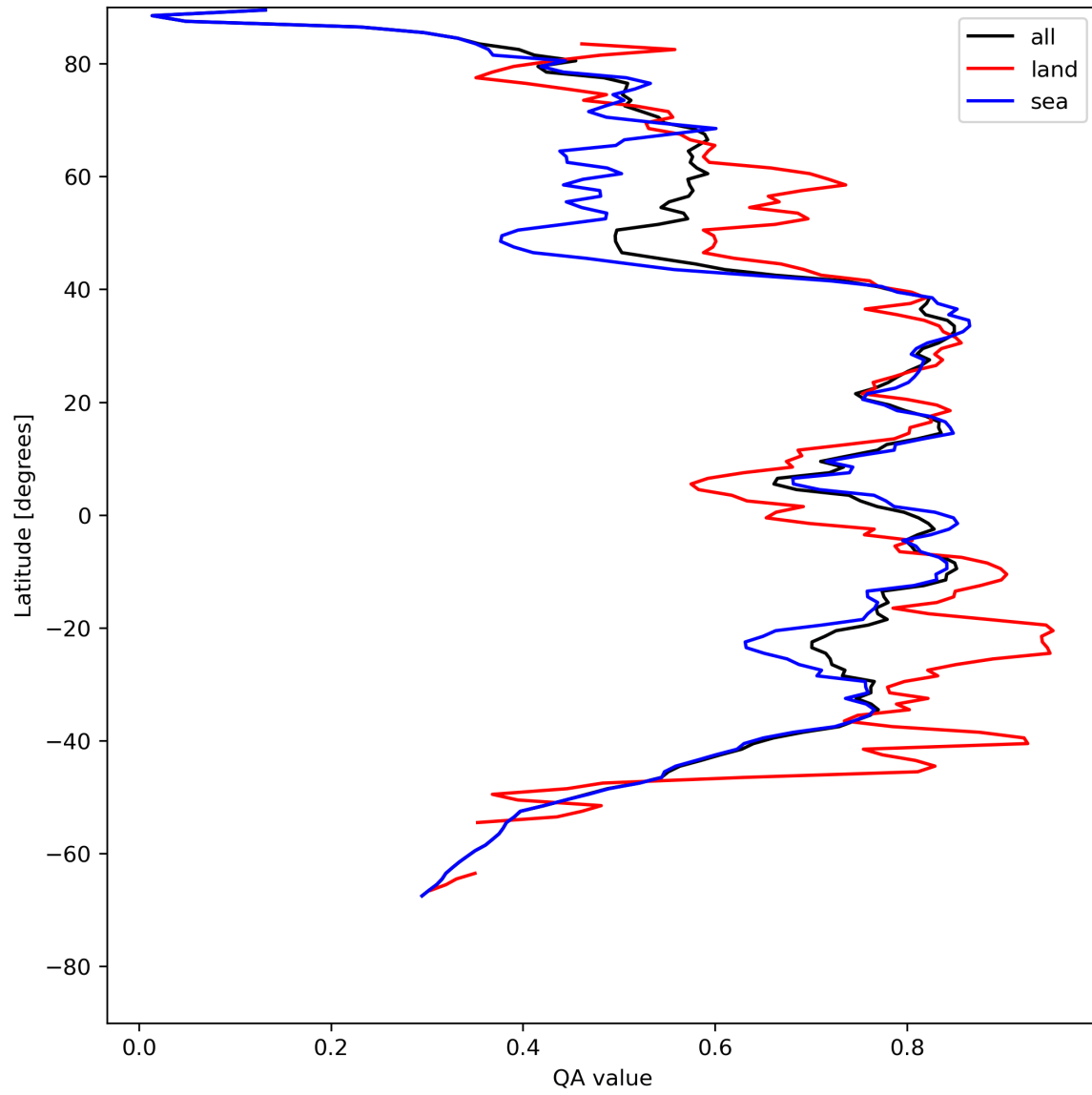
Figure 20: Zonal average of “QA value” for 2023-08-04 to 2023-08-05.
