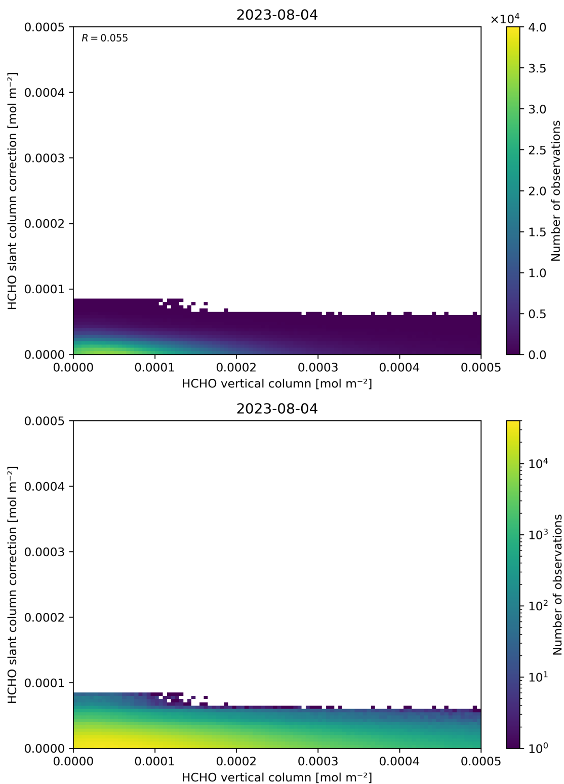
Figure 128: Scatter density plot of “HCHO vertical column” against “HCHO slant column correction” for 2023-08-04 to 2023-08-05.
