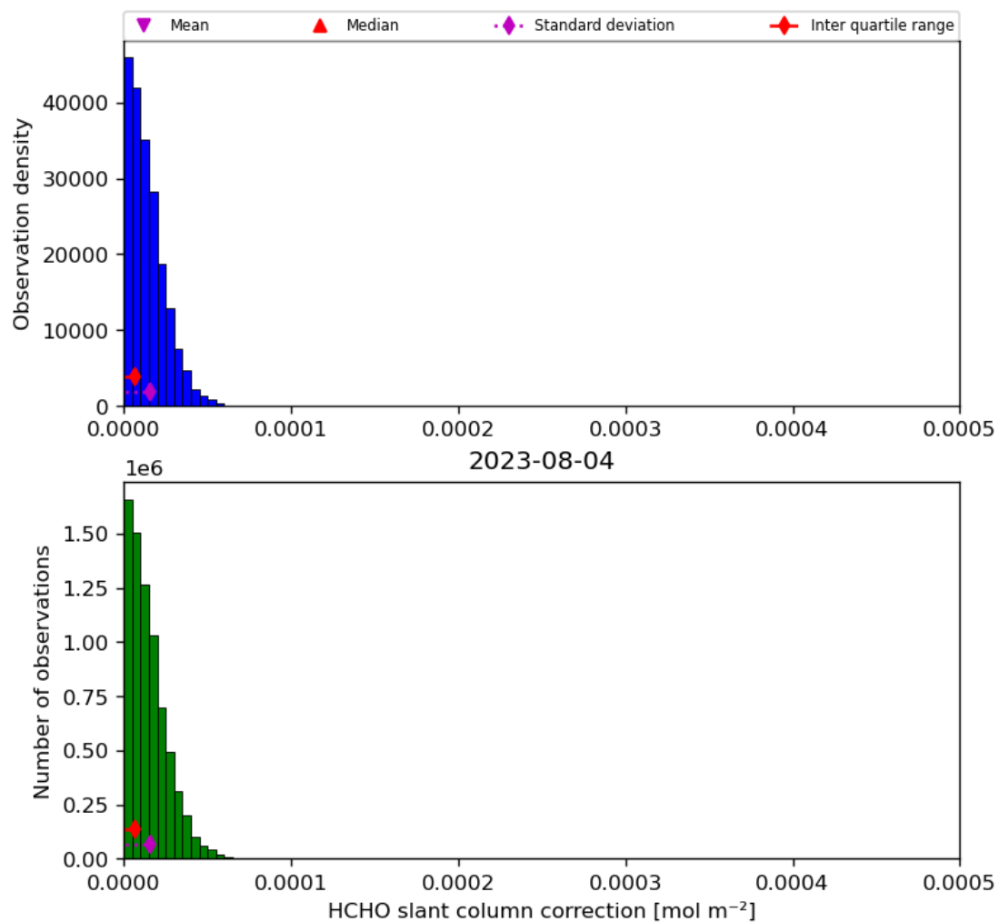
Figure 47: Histogram of “HCHO slant column correction” for 2023-08-04 to 2023-08-05
