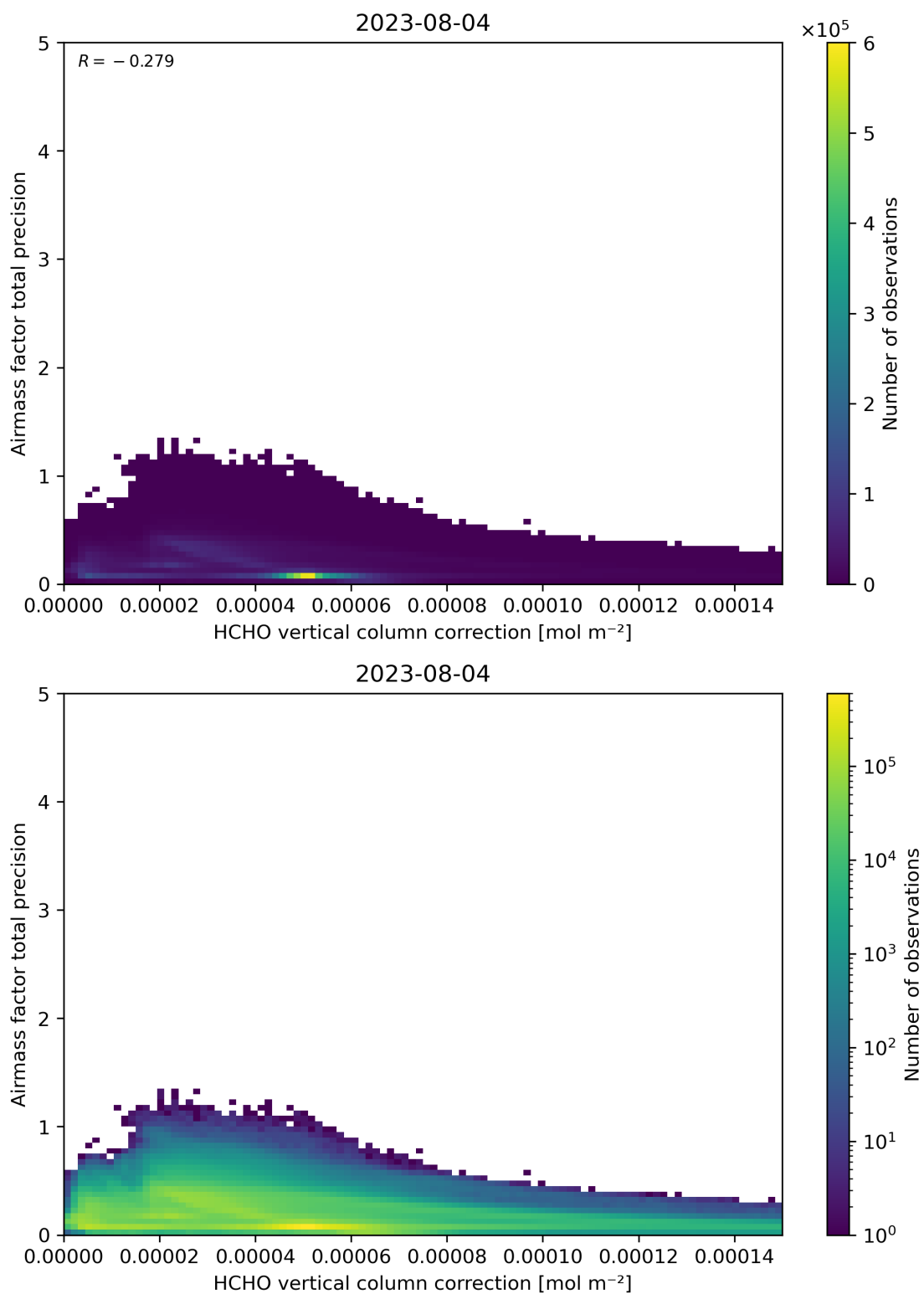
Figure 121: Scatter density plot of “HCHO vertical column correction” against “Airmass factor total precision” for 2023-08-04 to 2023-08-05.
