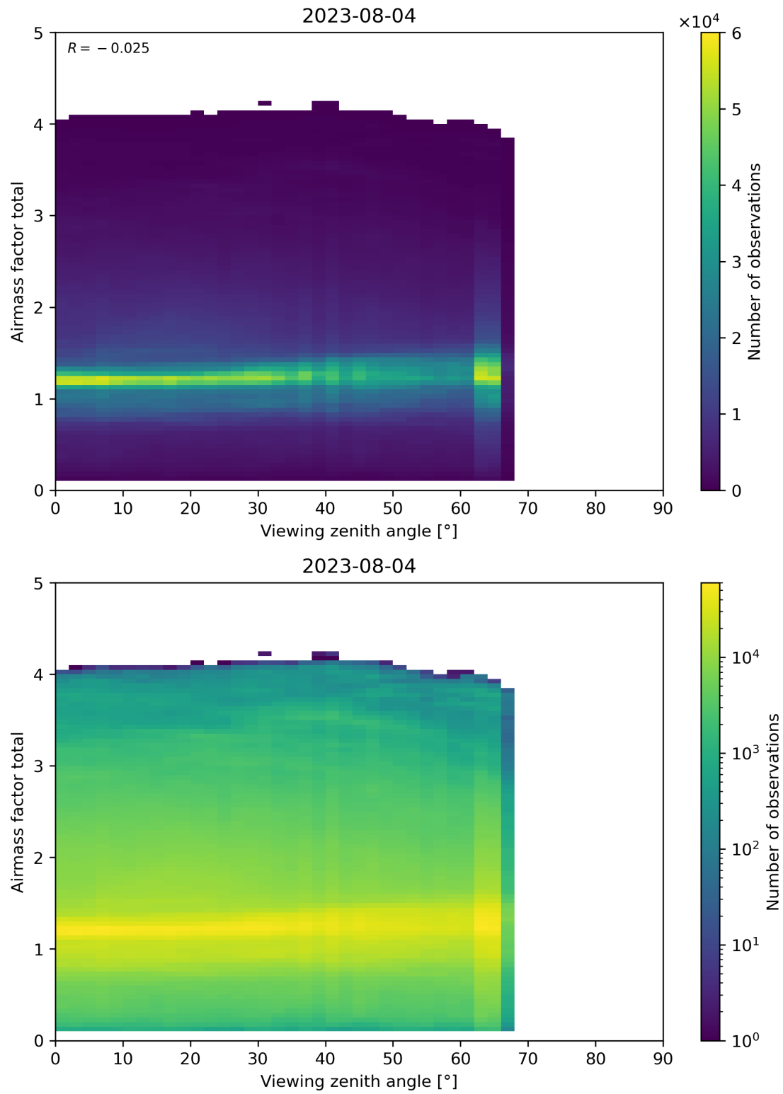
Figure 190: Scatter density plot of “Viewing zenith angle” against “Airmass factor total” for 2023-08-04 to 2023-08-05.
