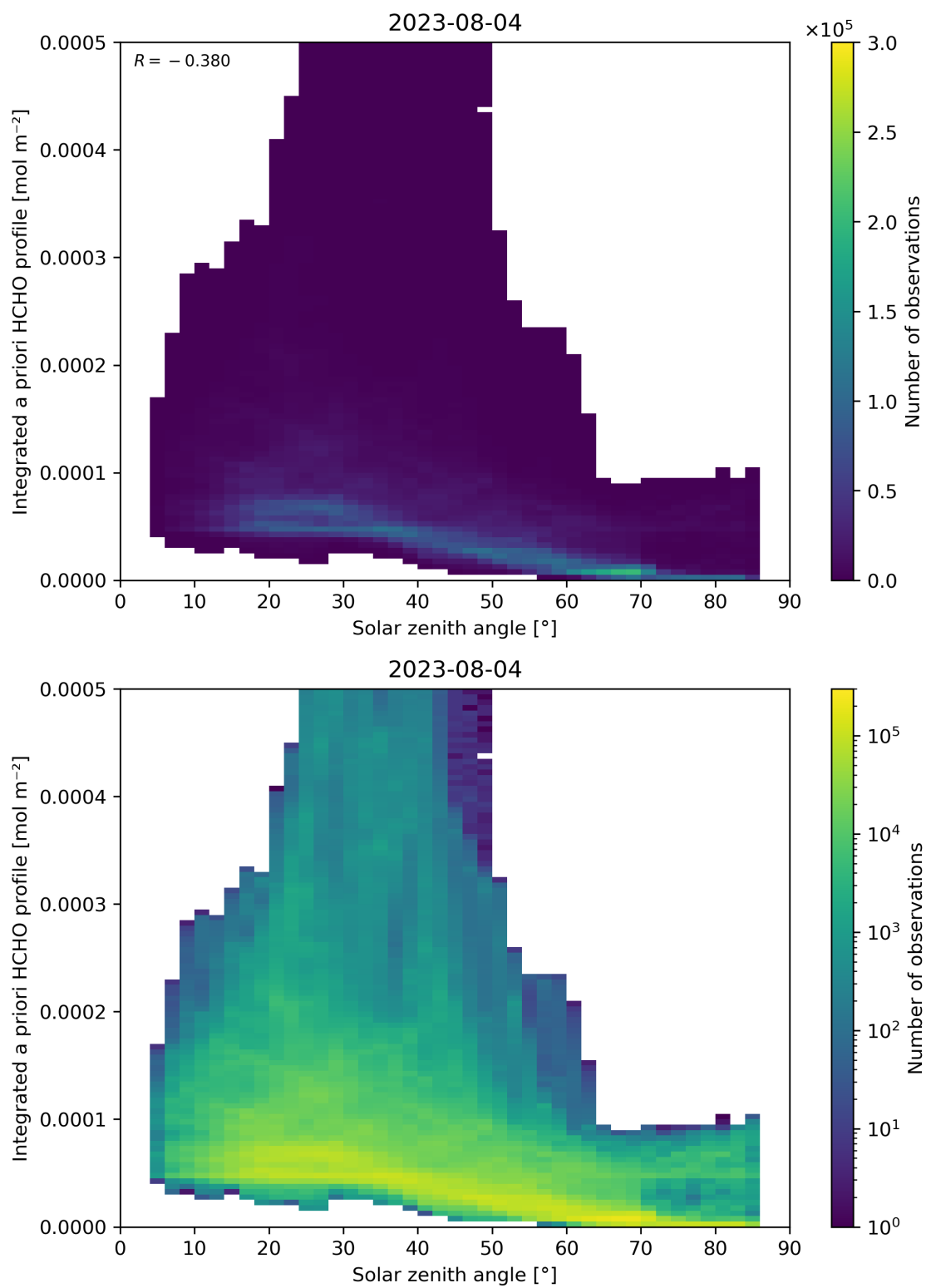
Figure 180: Scatter density plot of “Solar zenith angle” against “Integrated a priori HCHO profile” for 2023-08-04 to 2023-08-05.
