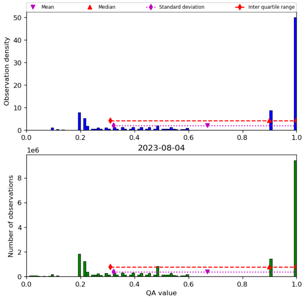
Figure 34: Histogram of “QA value” for 2023-08-04 to 2023-08-05
