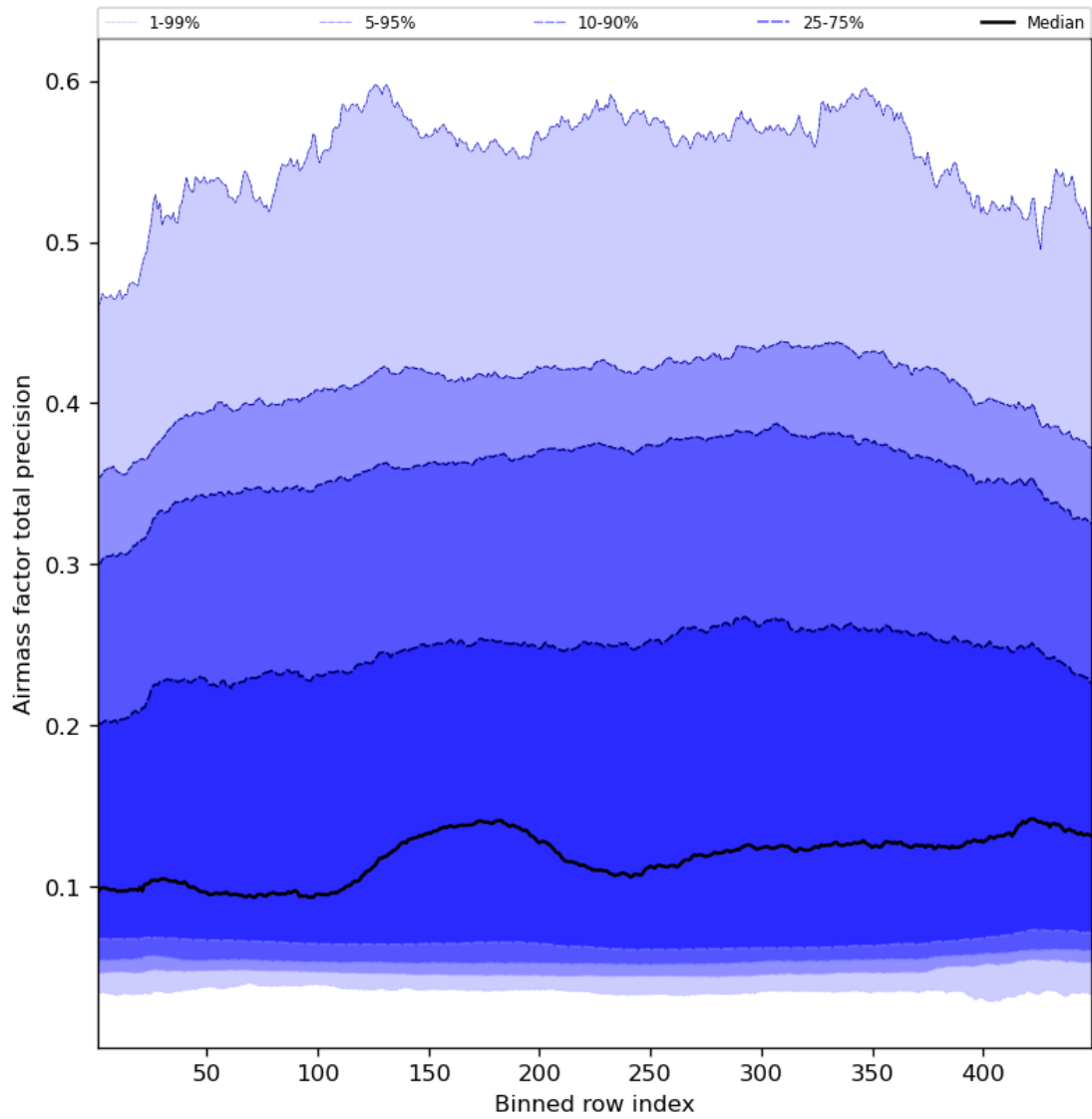
Figure 55: Along track statistics of “Airmass factor total precision” for 2023-08-04 to 2023-08-05
