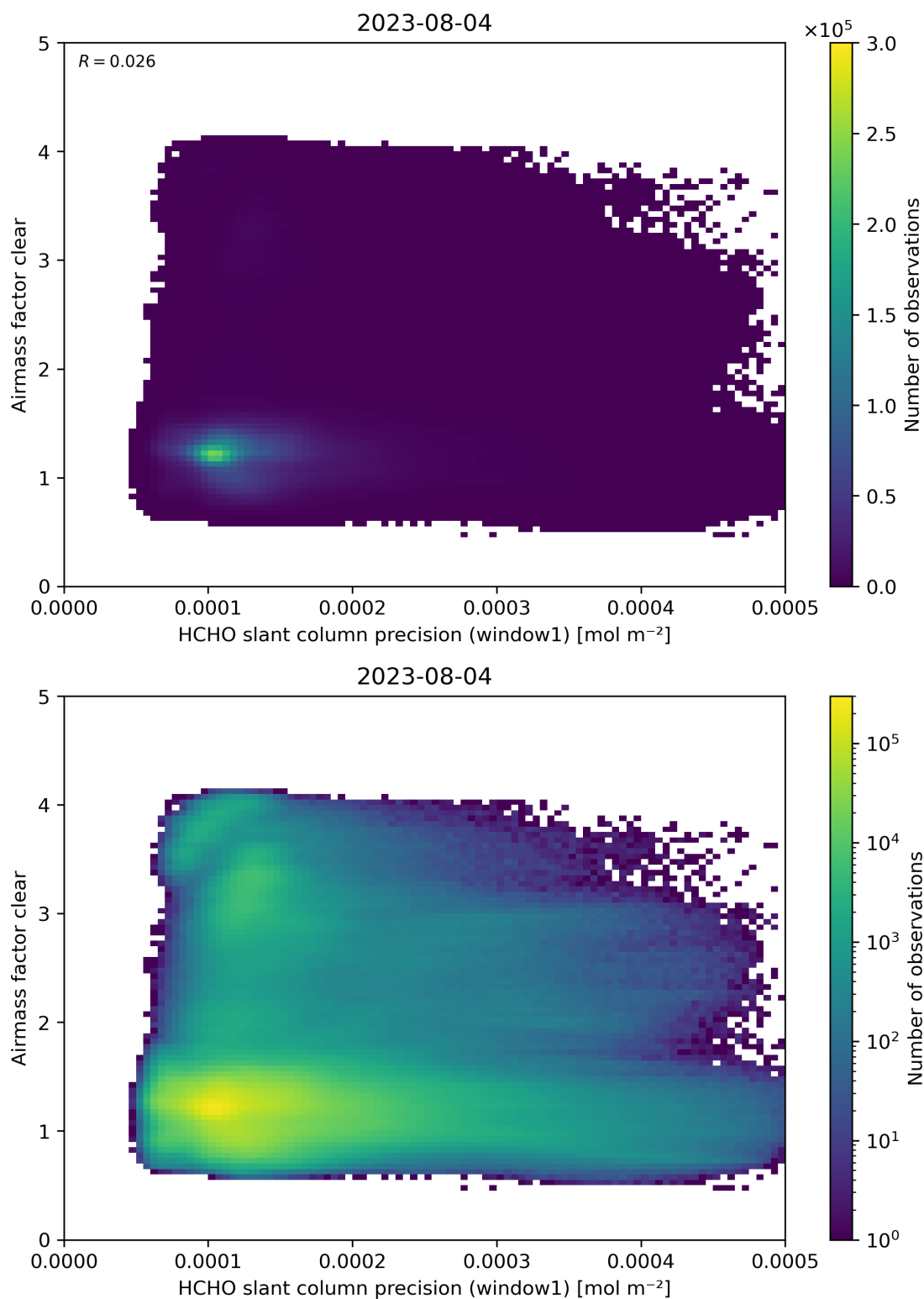
Figure 91: Scatter density plot of “HCHO slant column precision (window1)” against “Airmass factor clear” for 2023-08-04 to 2023-08-05.
