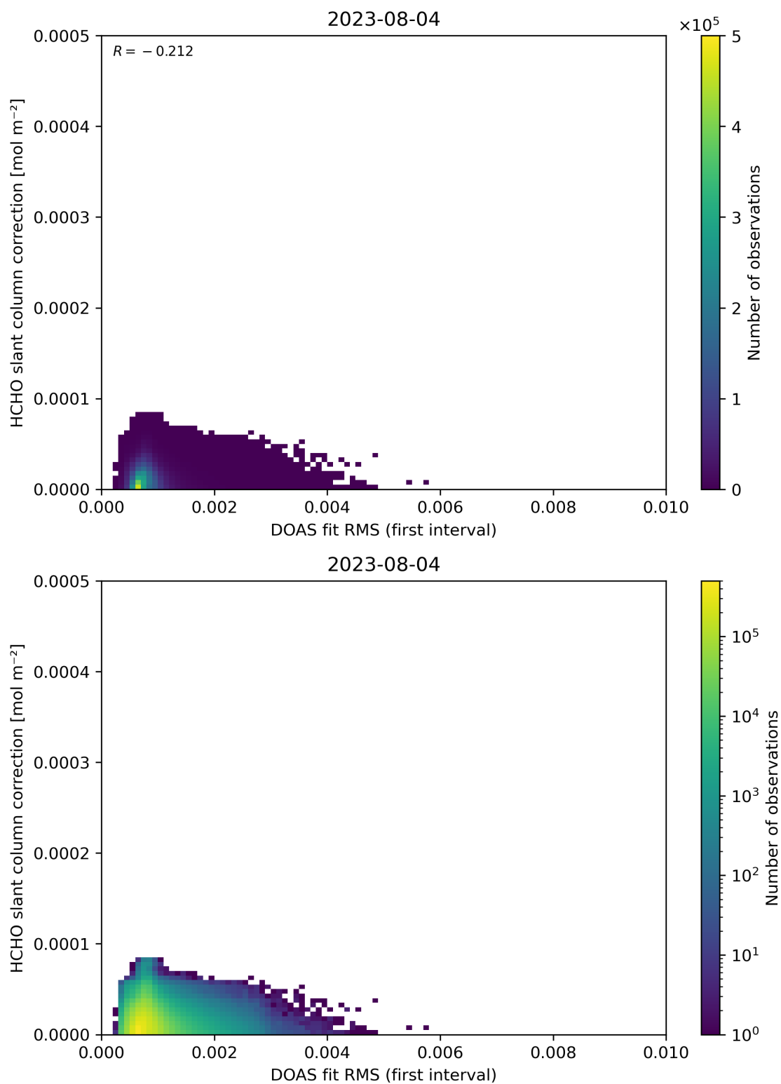
Figure 63: Scatter density plot of “DOAS fit RMS (first interval)” against “HCHO slant column correction” for 2023-08-04 to 2023-08-05.
