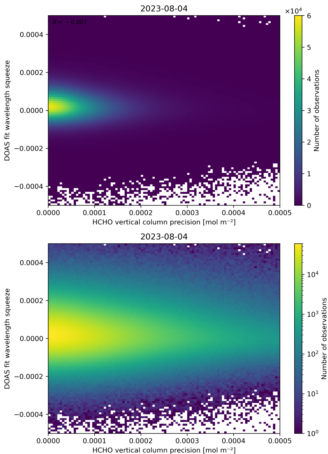
Figure 138: Scatter density plot of “HCHO vertical column precision” against “DOAS fit wavelength squeeze” for 2023-08-04 to 2023-08-05.
