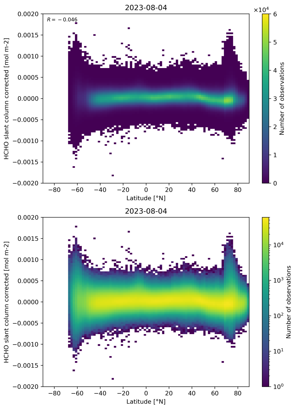
Figure 157: Scatter density plot of “Latitude” against “HCHO slant column corrected” for 2023-08-04 to 2023-08-05.
