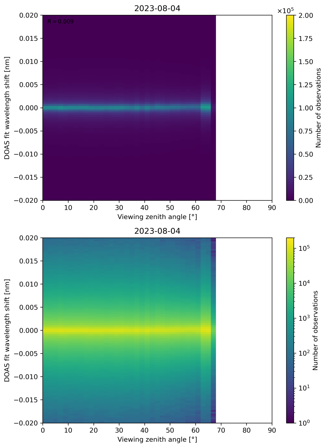
Figure 183: Scatter density plot of “Viewing zenith angle” against “DOAS fit wavelength shift” for 2023-08-04 to 2023-08-05.
