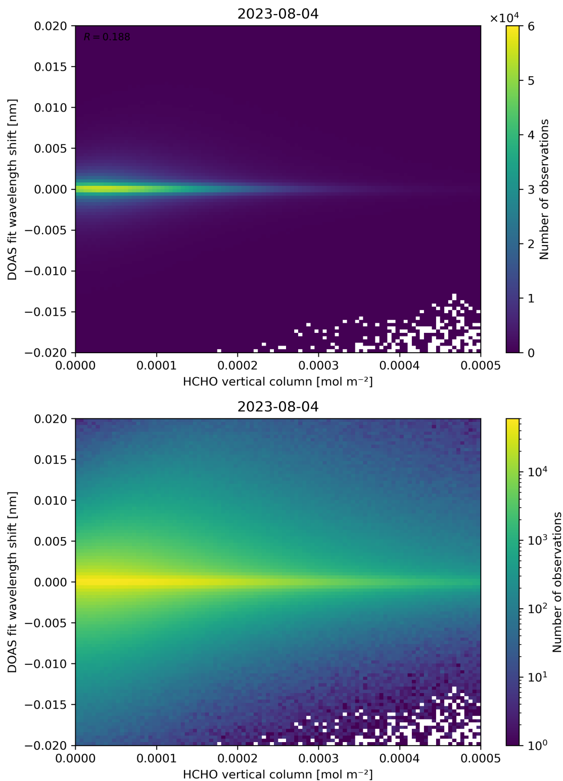
Figure 124: Scatter density plot of “HCHO vertical column” against “DOAS fit wavelength shift” for 2023-08-04 to 2023-08-05.
