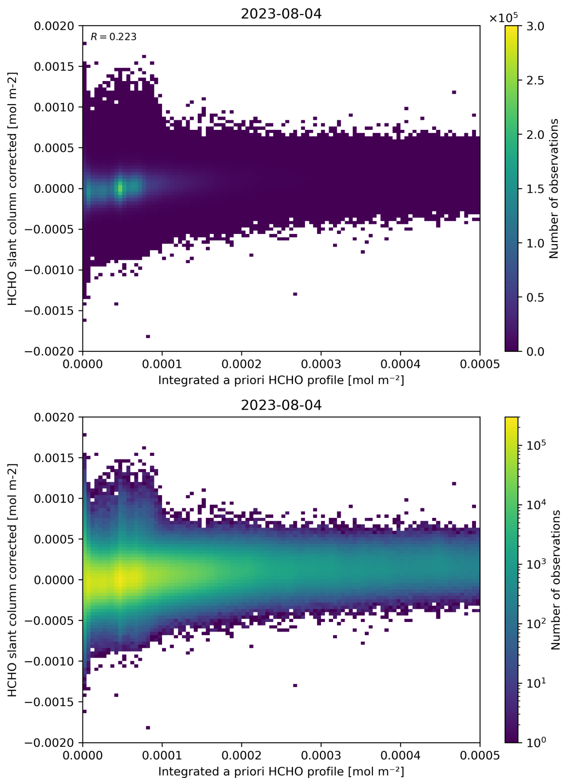
Figure 151: Scatter density plot of “Integrated a priori HCHO profile” against “HCHO slant column corrected” for 2023-08-04 to 2023-08-05.
