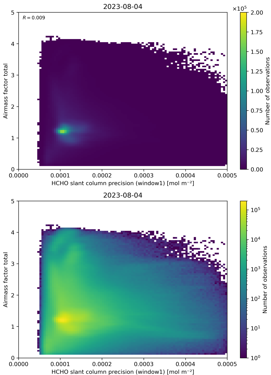
Figure 94: Scatter density plot of “HCHO slant column precision (window1)” against “Airmass factor total” for 2023-08-04 to 2023-08-05.
