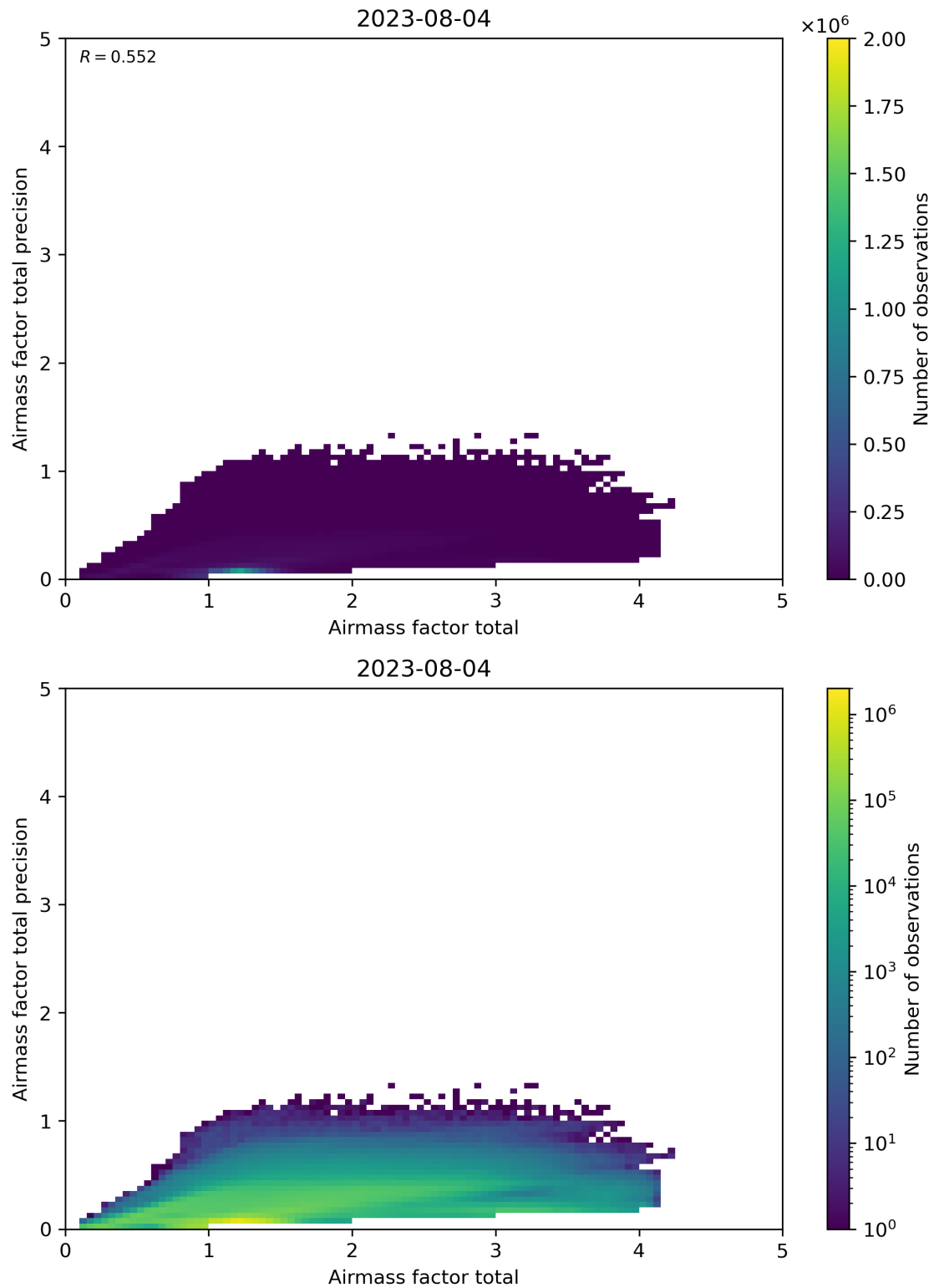
Figure 103: Scatter density plot of “Airmass factor total” against “Airmass factor total precision” for 2023-08-04 to 2023-08-05.
