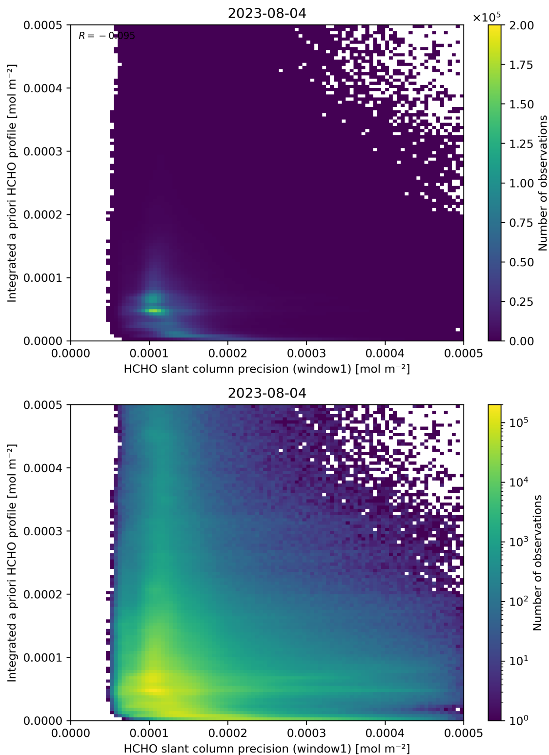
Figure 96: Scatter density plot of “HCHO slant column precision (window1)” against “Integrated a priori HCHO profile” for 2023-08-04 to 2023-08-05.
