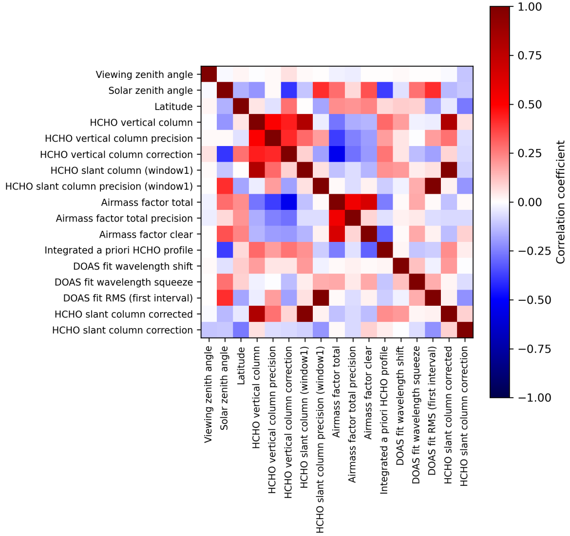
Figure 2: Map of correlation matrix for 2023-08-04 to 2023-08-05.
