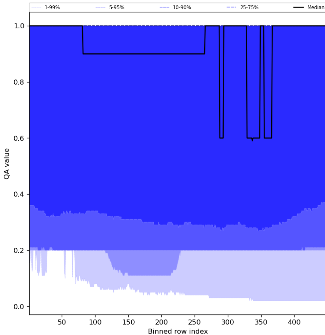
Figure 48: Along track statistics of “QA value” for 2023-08-04 to 2023-08-05
