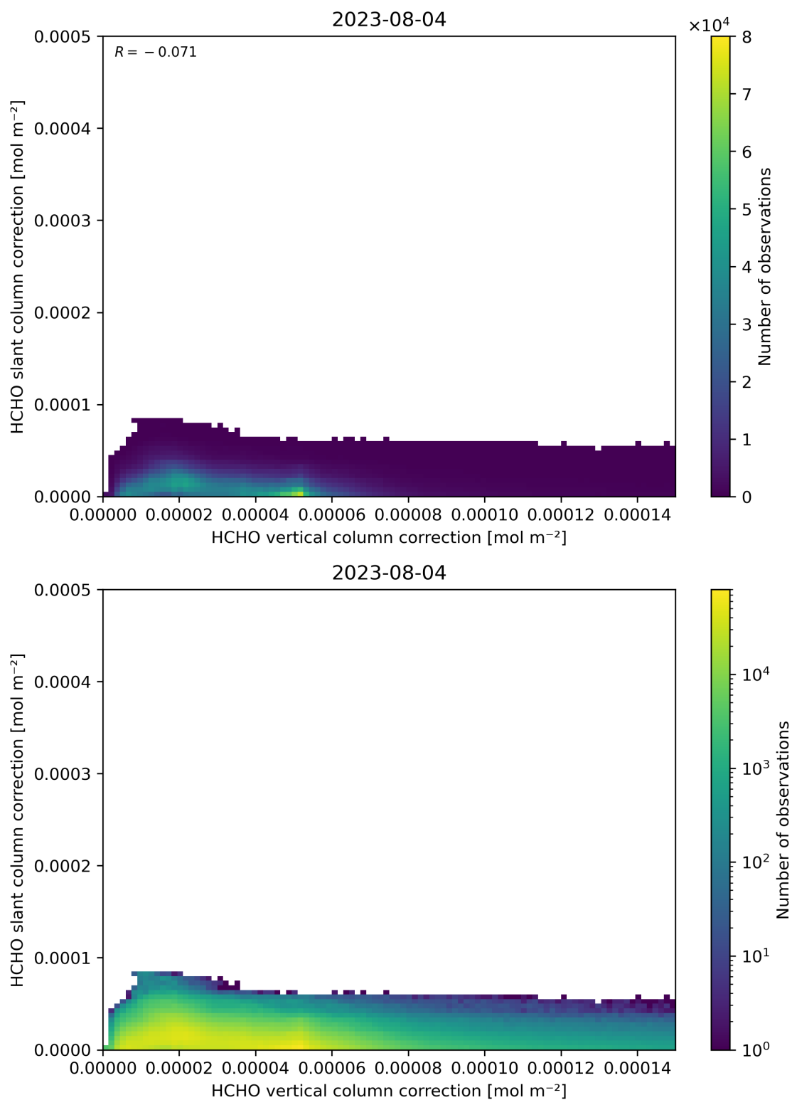
Figure 117: Scatter density plot of “HCHO vertical column correction” against “HCHO slant column correction” for 2023-08-04 to 2023-08-05.
