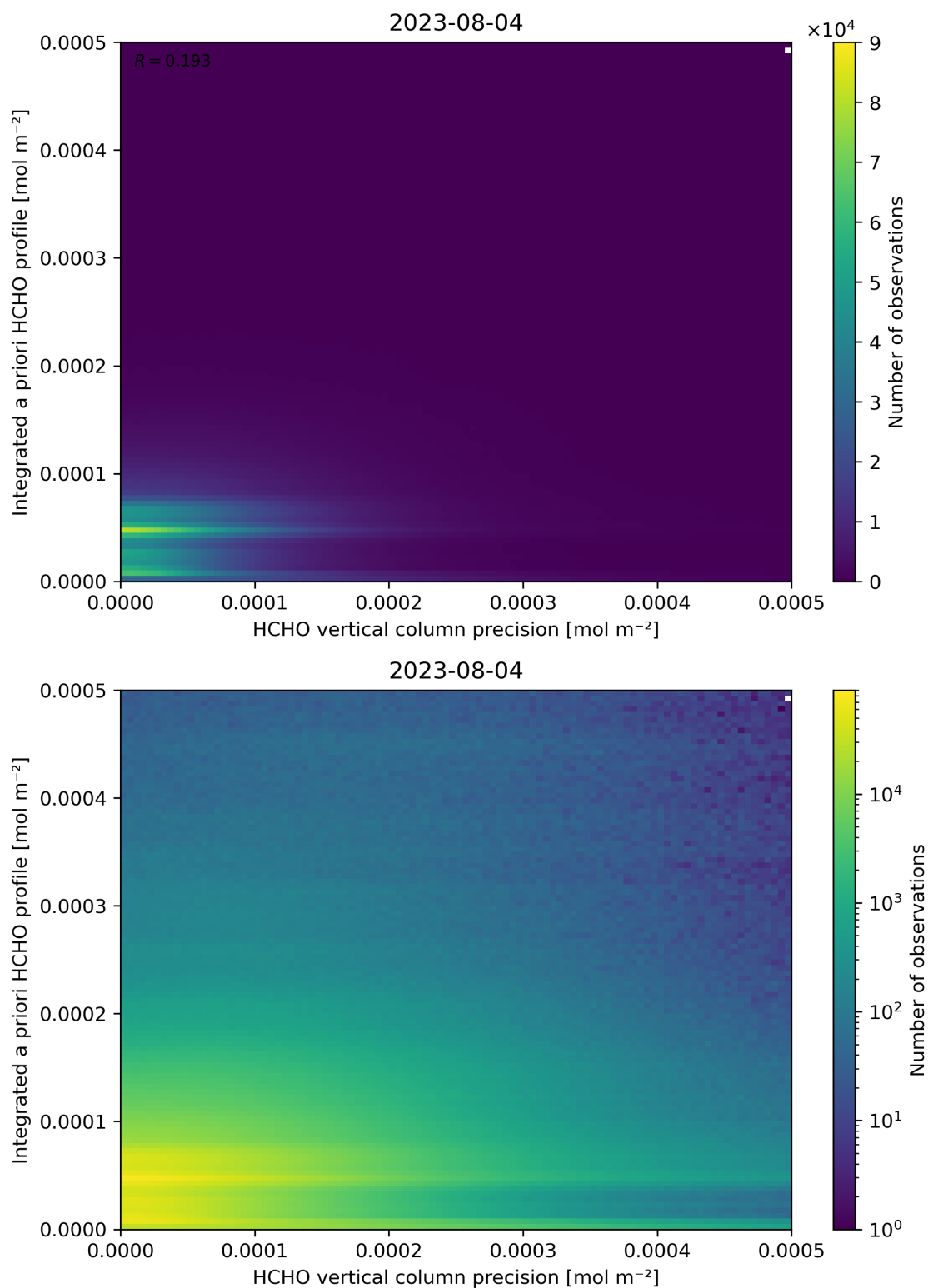
Figure 147: Scatter density plot of “HCHO vertical column precision” against “Integrated a priori HCHO profile” for 2023-08-04 to 2023-08-05.
