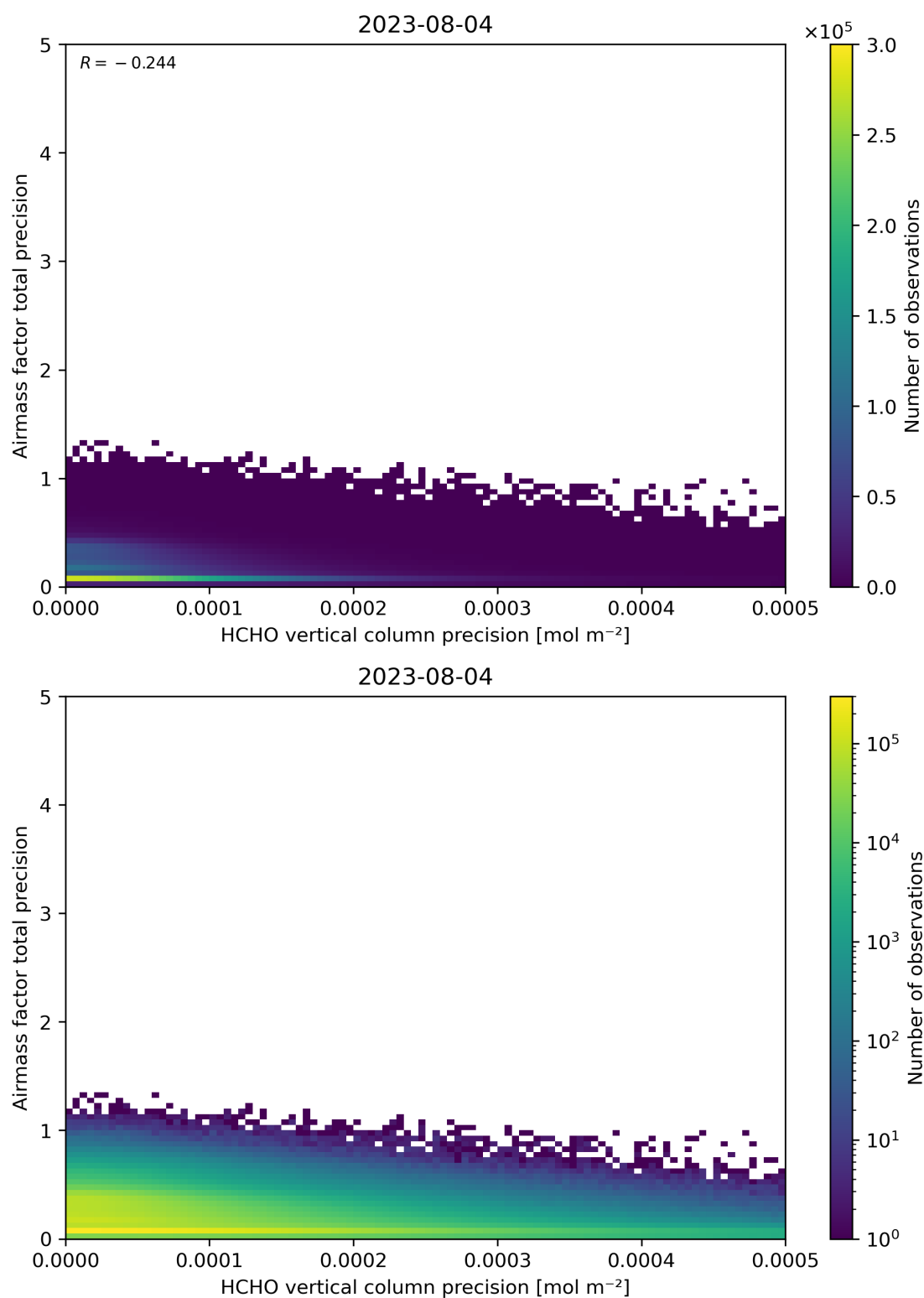
Figure 145: Scatter density plot of “HCHO vertical column precision” against “Airmass factor total precision” for 2023-08-04 to 2023-08-05.
