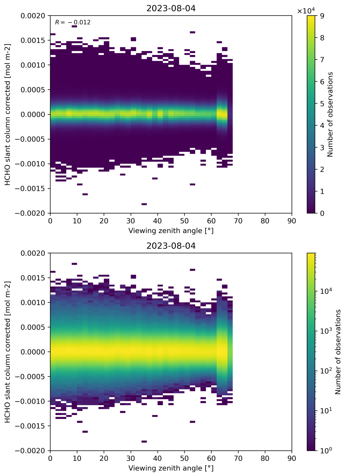
Figure 186: Scatter density plot of “Viewing zenith angle” against “HCHO slant column corrected” for 2023-08-04 to 2023-08-05.
