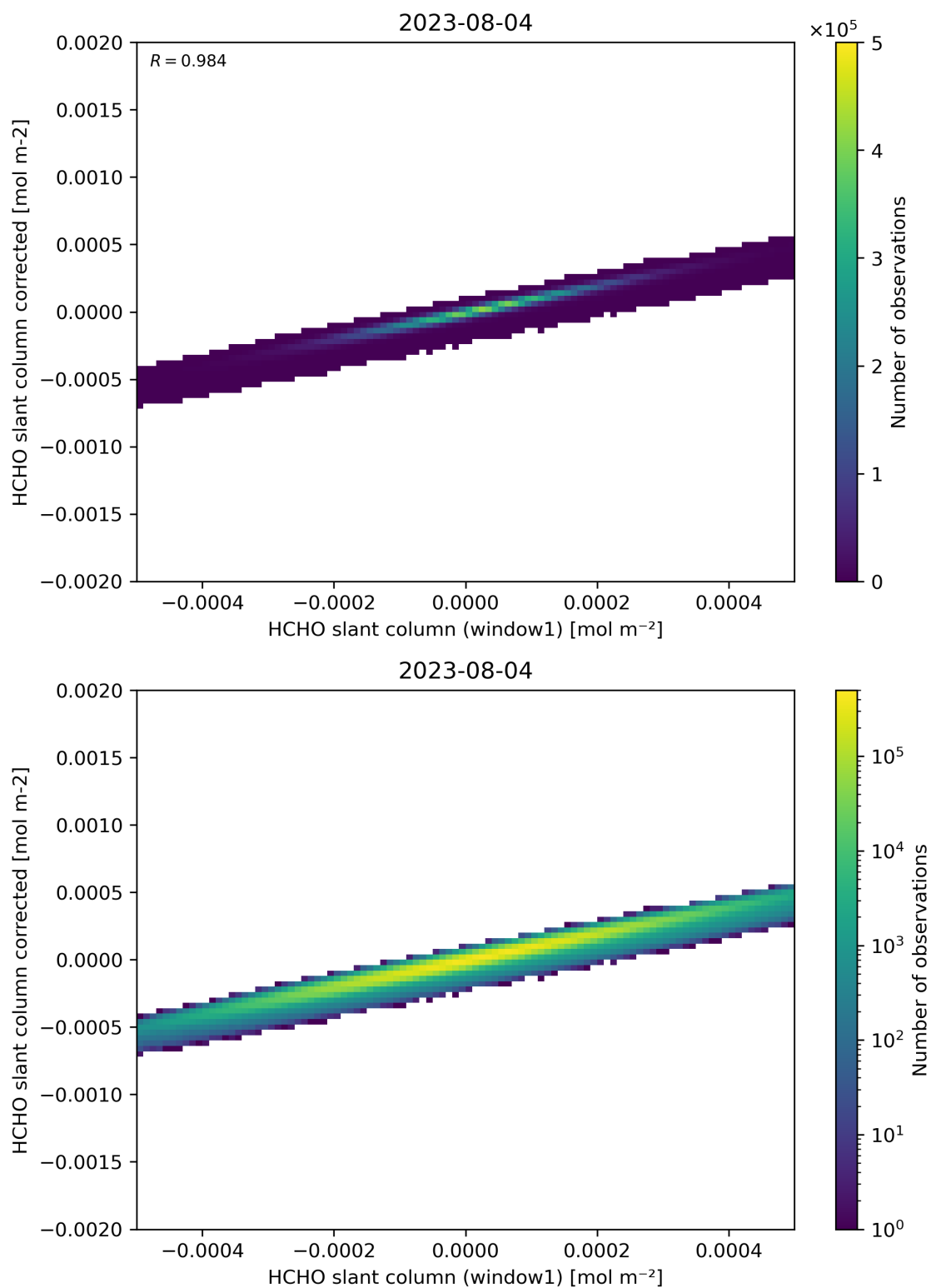
Figure 82: Scatter density plot of “HCHO slant column (window1)” against “HCHO slant column corrected” for 2023-08-04 to 2023-08-05.
