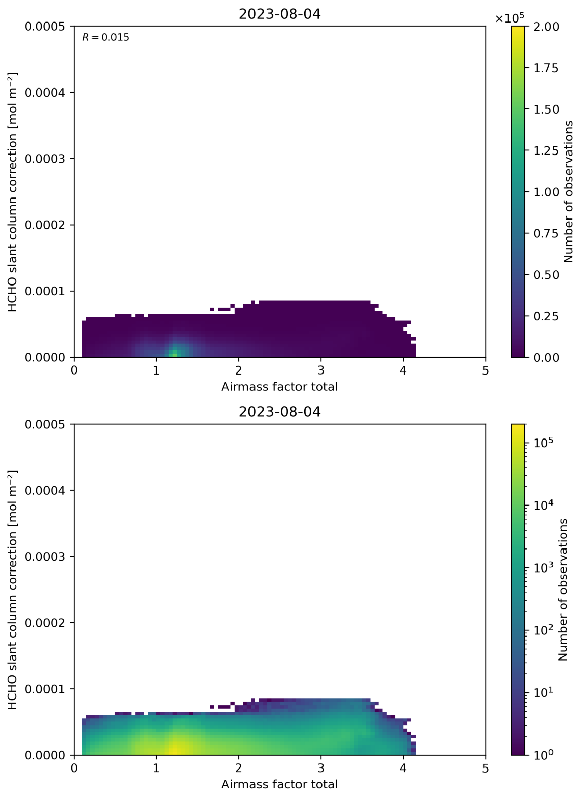
Figure 102: Scatter density plot of “Airmass factor total” against “HCHO slant column correction” for 2023-08-04 to 2023-08-05.
