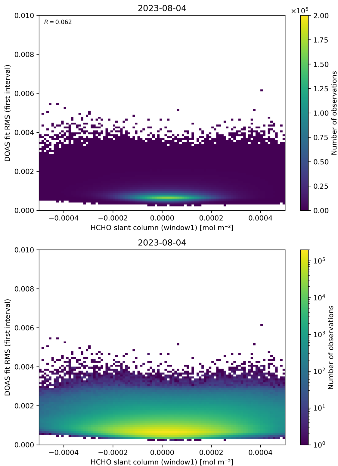
Figure 78: Scatter density plot of “HCHO slant column (window1)” against “DOAS fit RMS (first interval)” for 2023-08-04 to 2023-08-05.
