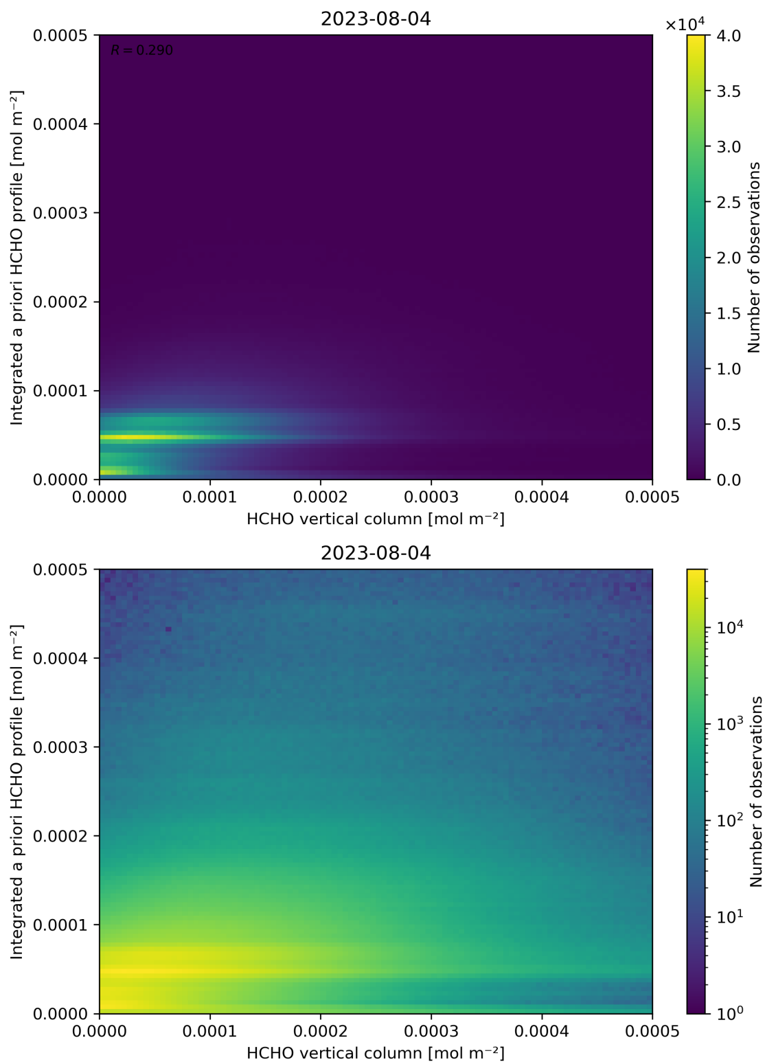
Figure 135: Scatter density plot of “HCHO vertical column” against “Integrated a priori HCHO profile” for 2023-08-04 to 2023-08-05.
