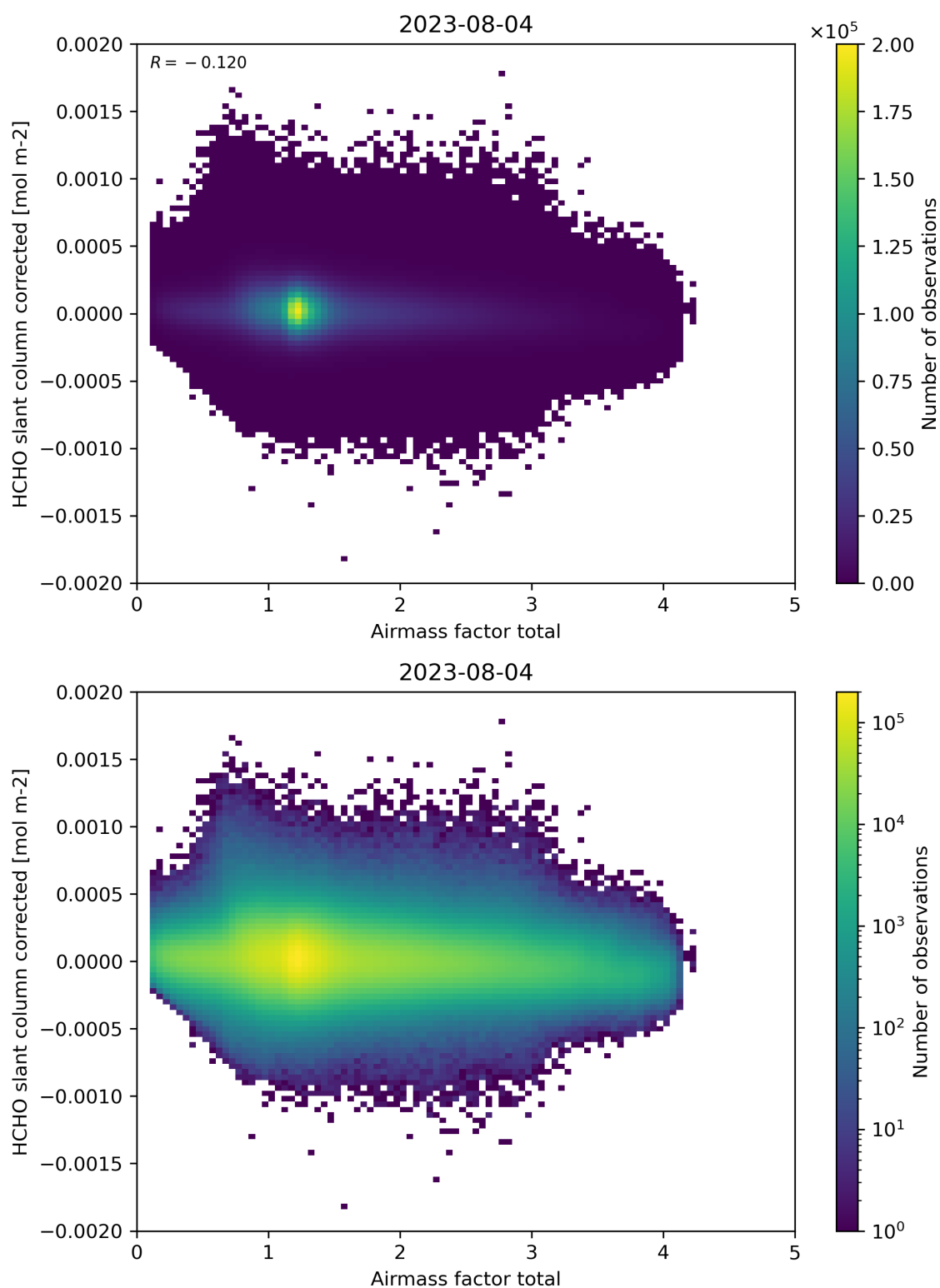
Figure 101: Scatter density plot of “Airmass factor total” against “HCHO slant column corrected” for 2023-08-04 to 2023-08-05.
