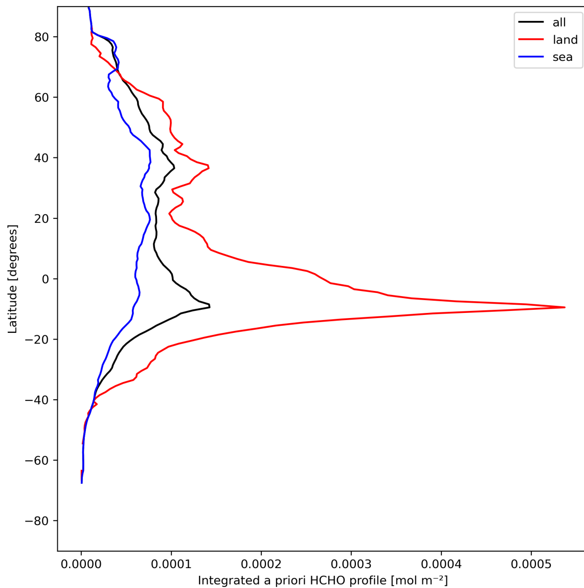
Figure 29: Zonal average of “Integrated a priori HCHO profile” for 2023-08-04 to 2023-08-05.
