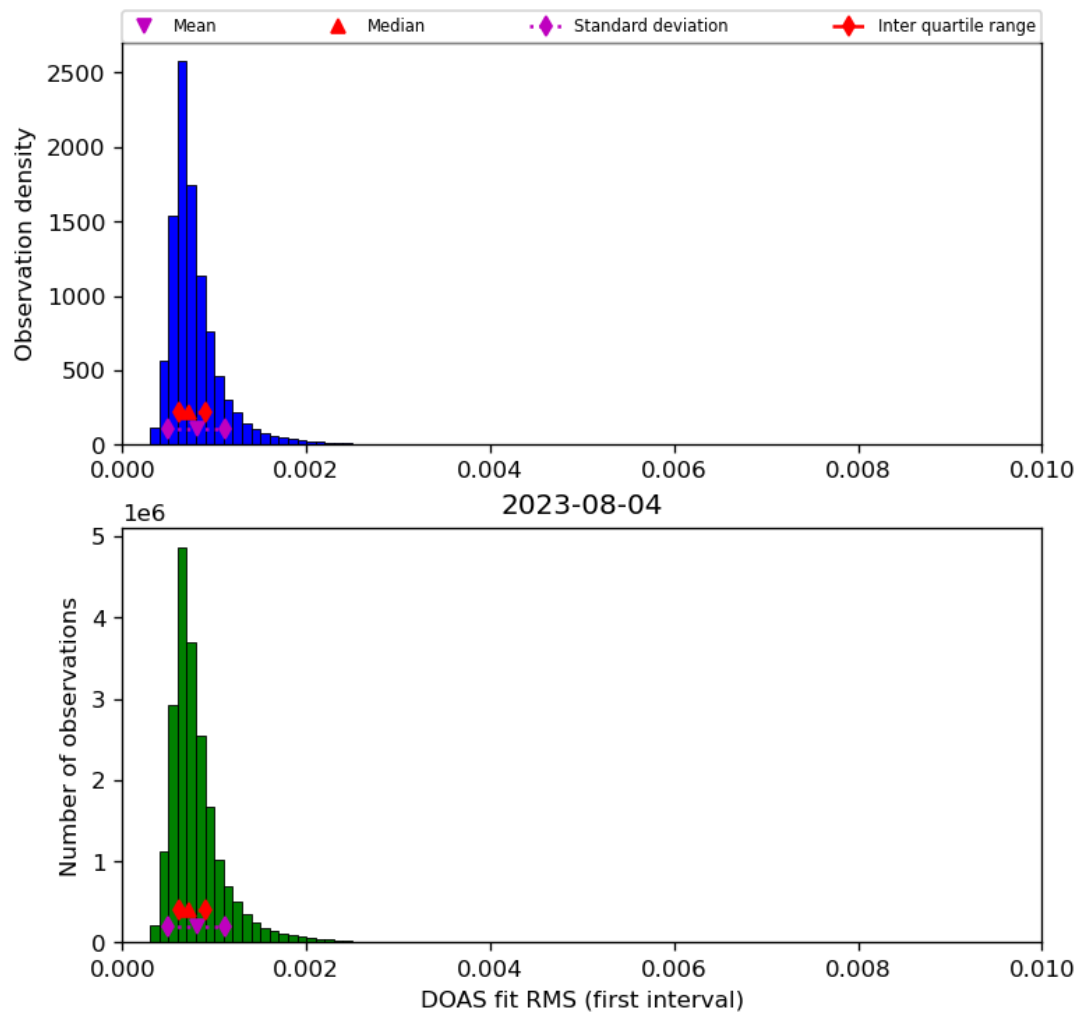
Figure 46: Histogram of “DOAS fit RMS (first interval)” for 2023-08-04 to 2023-08-05
