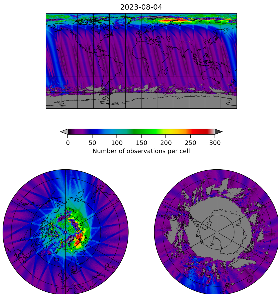
Figure 19: Map of the number of observations for 2023-08-04 to 2023-08-05
