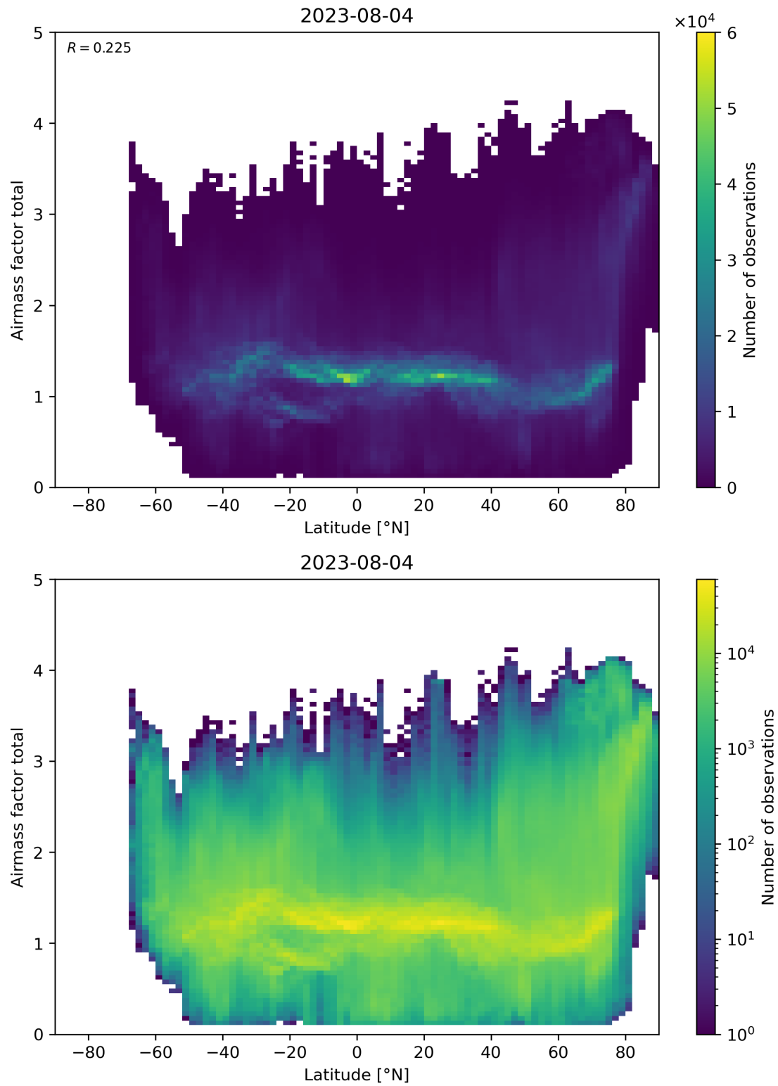
Figure 161: Scatter density plot of “Latitude” against “Airmass factor total” for 2023-08-04 to 2023-08-05.
