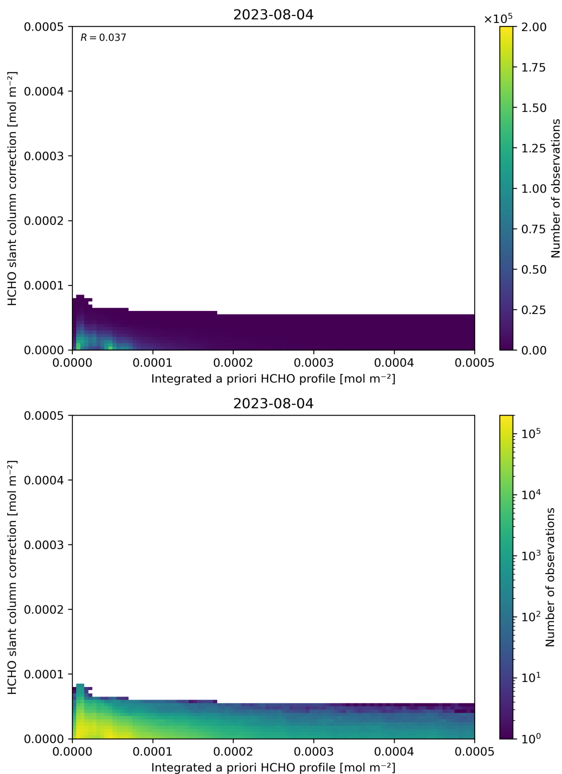
Figure 152: Scatter density plot of “Integrated a priori HCHO profile” against “HCHO slant column correction” for 2023-08-04 to 2023-08-05.
