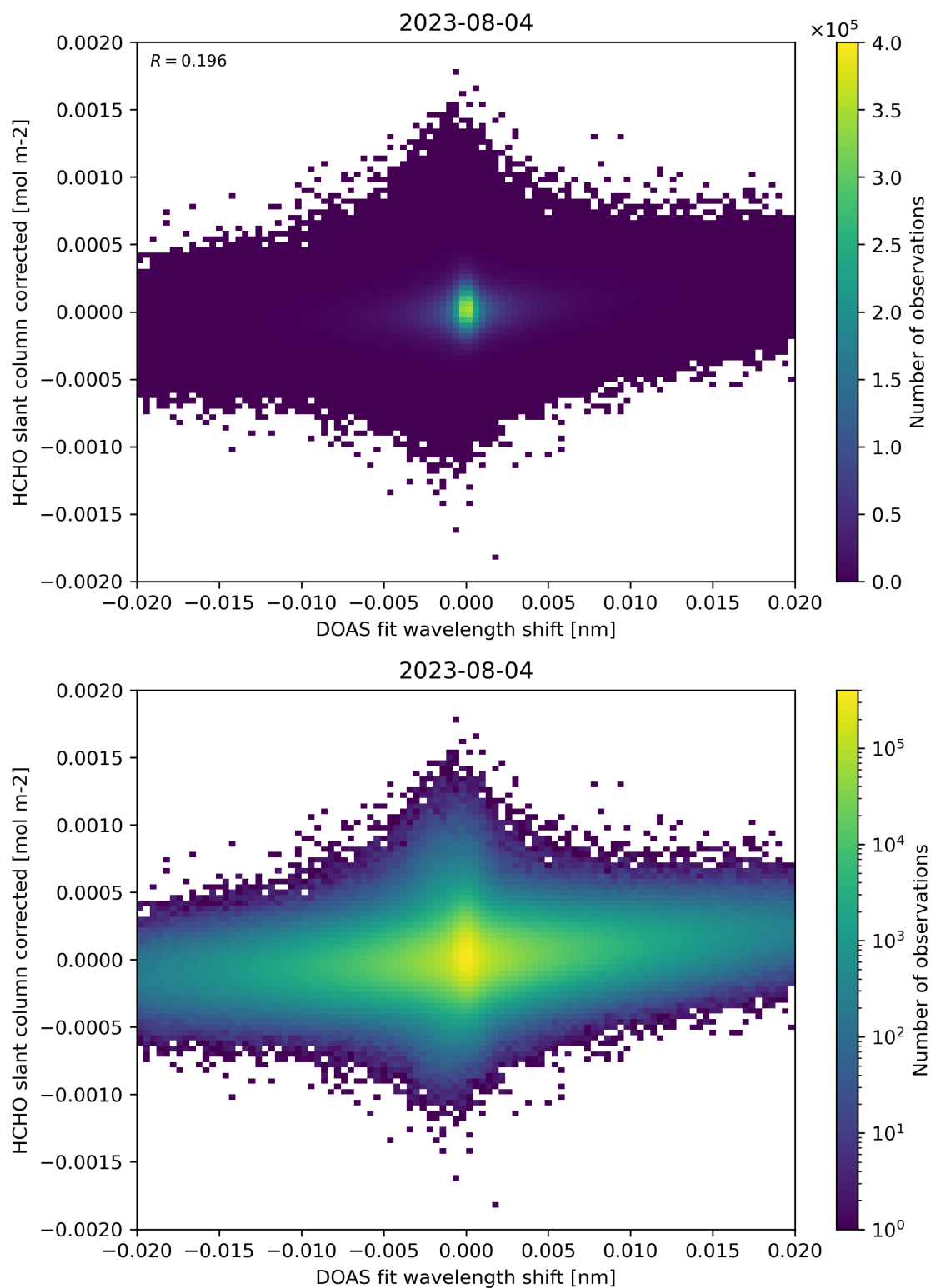
Figure 66: Scatter density plot of “DOAS fit wavelength shift” against “HCHO slant column corrected” for 2023-08-04 to 2023-08-05.
