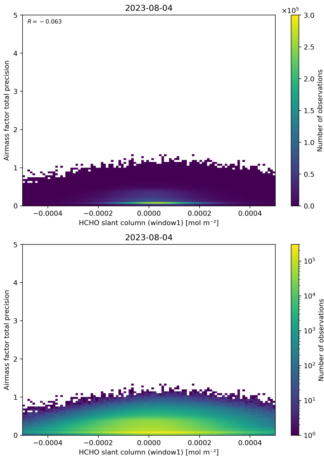
Figure 86: Scatter density plot of “HCHO slant column (window1)” against “Airmass factor total precision” for 2023-08-04 to 2023-08-05.
