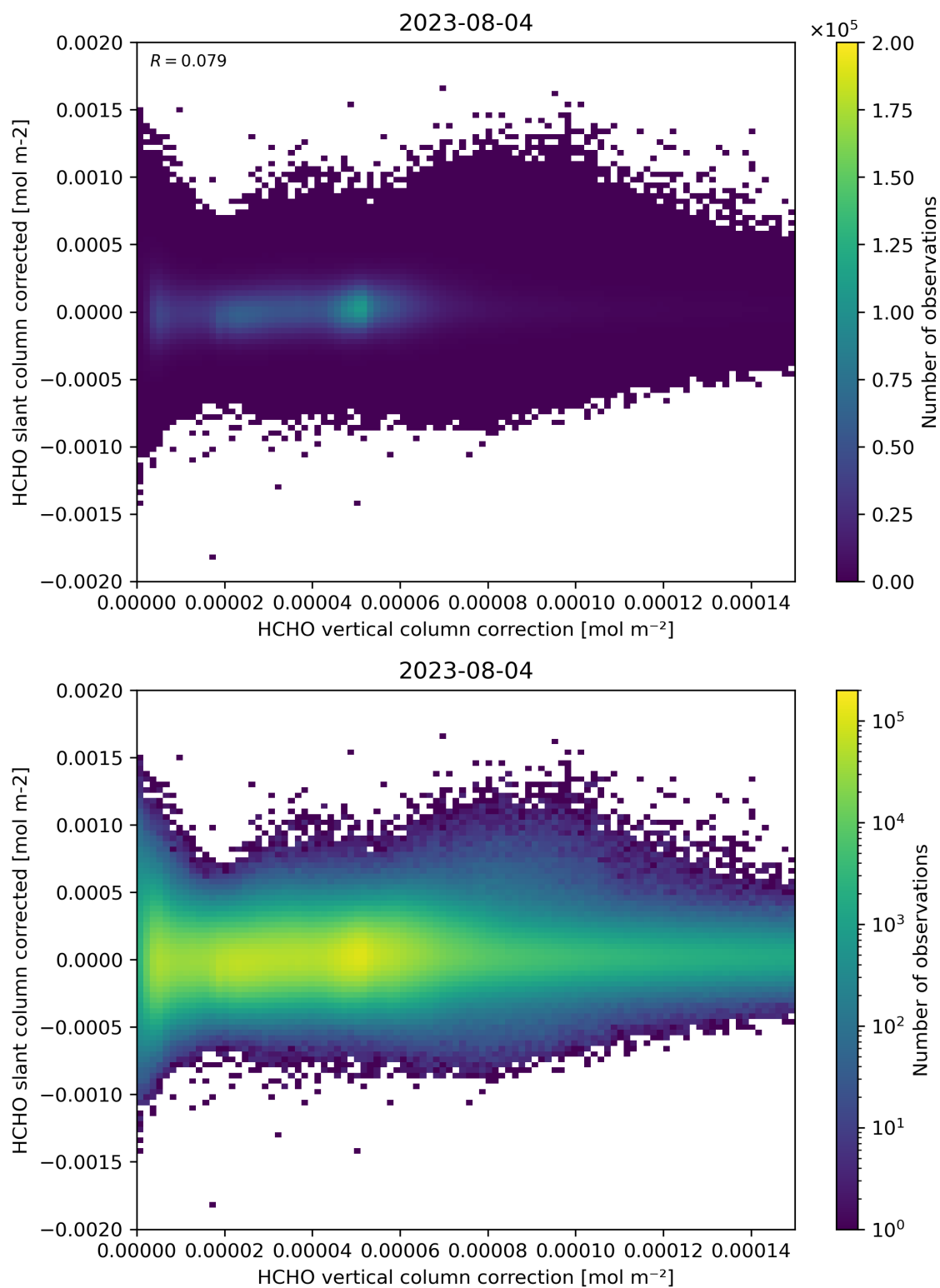
Figure 116: Scatter density plot of “HCHO vertical column correction” against “HCHO slant column corrected” for 2023-08-04 to 2023-08-05.
