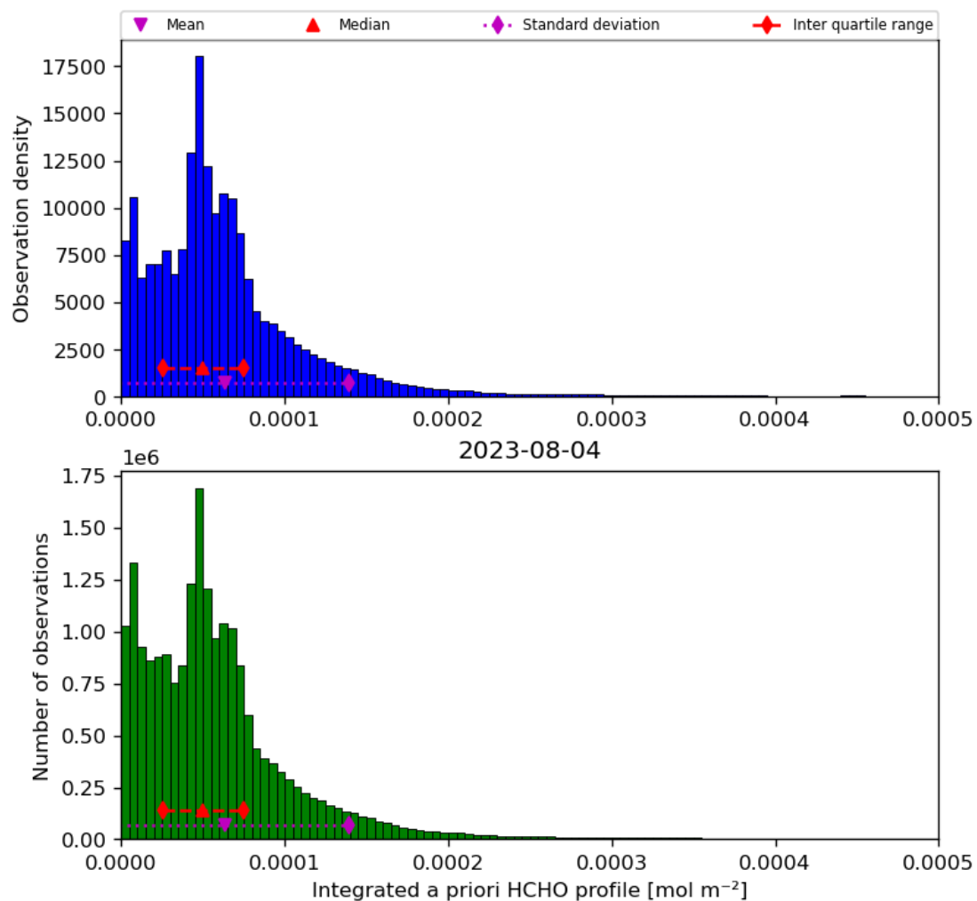
Figure 43: Histogram of “Integrated a priori HCHO profile” for 2023-08-04 to 2023-08-05
