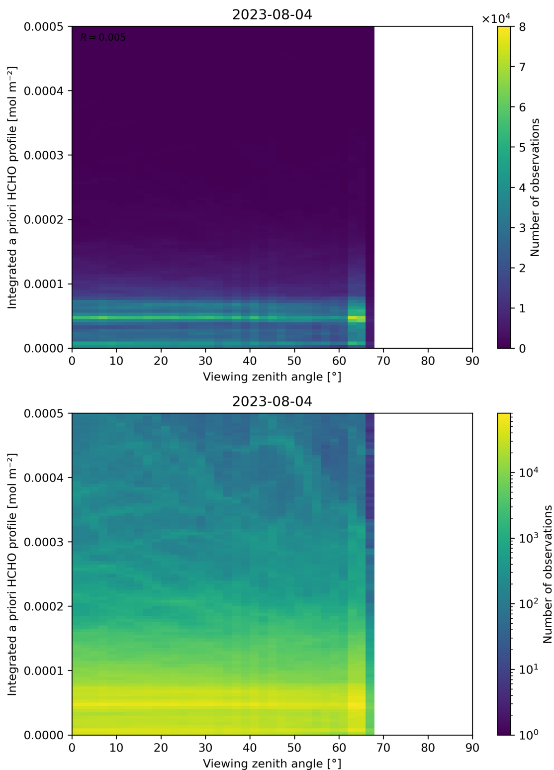
Figure 195: Scatter density plot of “Viewing zenith angle” against “Integrated a priori HCHO profile” for 2023-08-04 to 2023-08-05.
