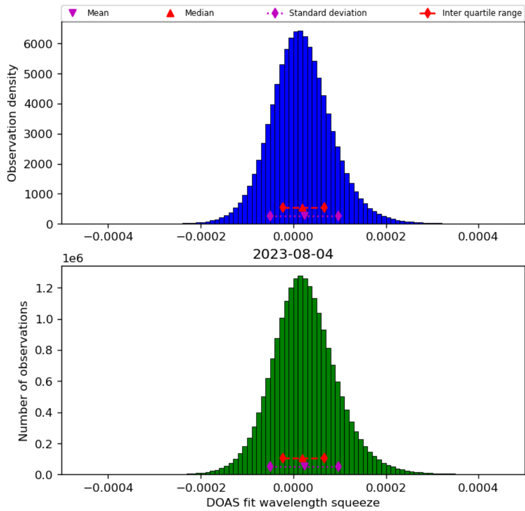
Figure 45: Histogram of “DOAS fit wavelength squeeze” for 2023-08-04 to 2023-08-05
