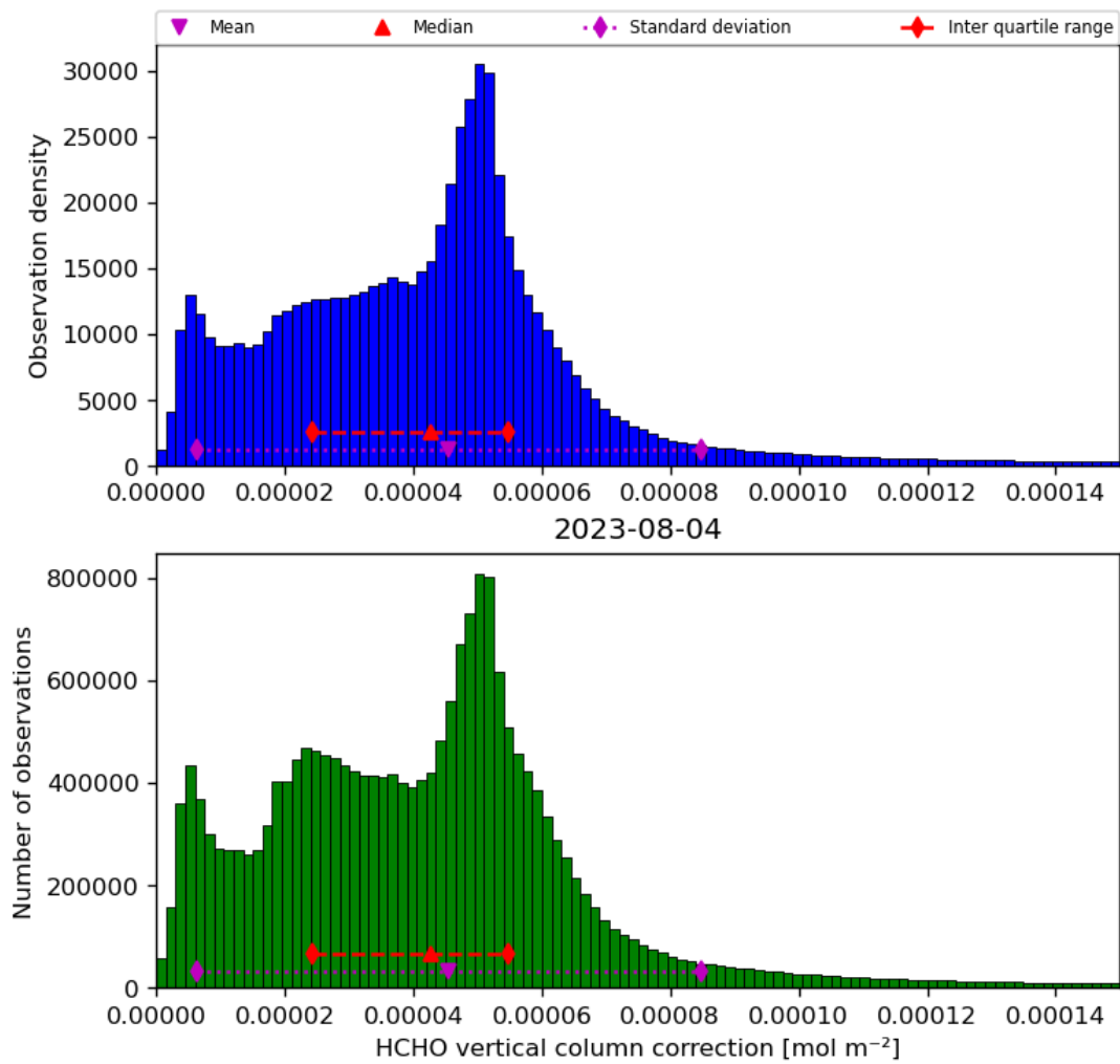
Figure 37: Histogram of “HCHO vertical column correction” for 2023-08-04 to 2023-08-05
