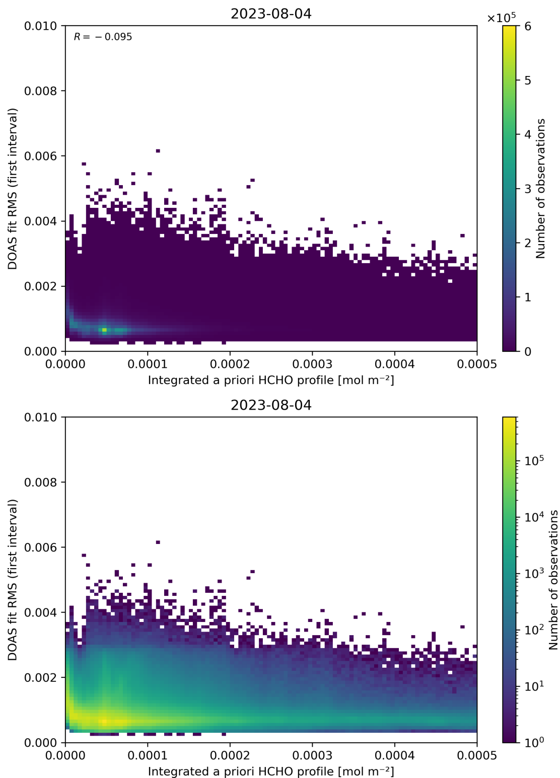
Figure 148: Scatter density plot of “Integrated a priori HCHO profile” against “DOAS fit RMS (first interval)” for 2023-08-04 to 2023-08-05.
