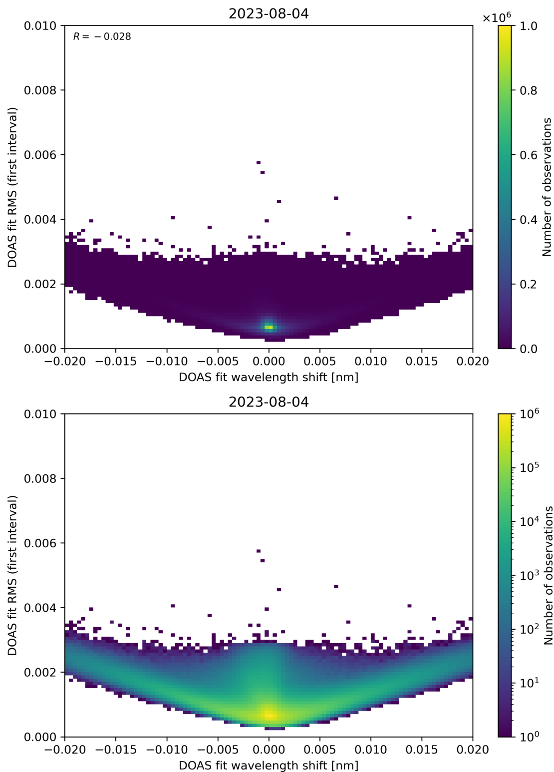
Figure 64: Scatter density plot of “DOAS fit wavelength shift” against “DOAS fit RMS (first interval)” for 2023-08-04 to 2023-08-05.
