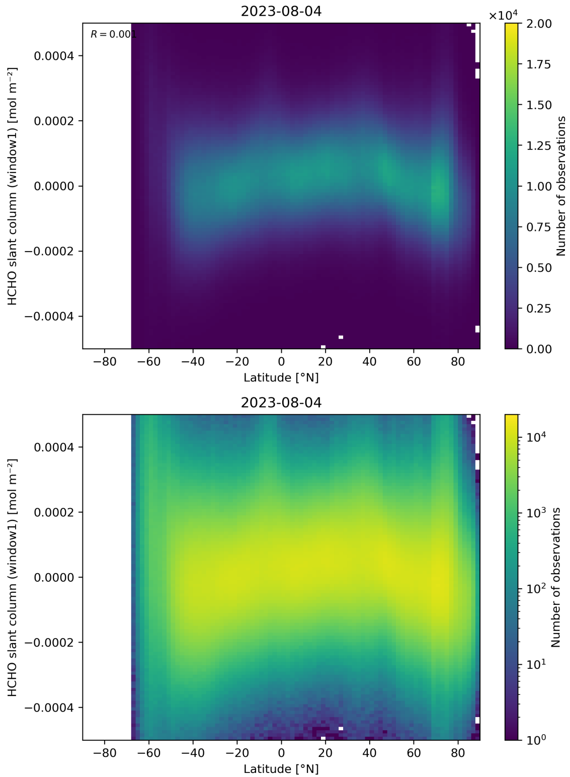
Figure 159: Scatter density plot of “Latitude” against “HCHO slant column (window1)” for 2023-08-04 to 2023-08-05.
