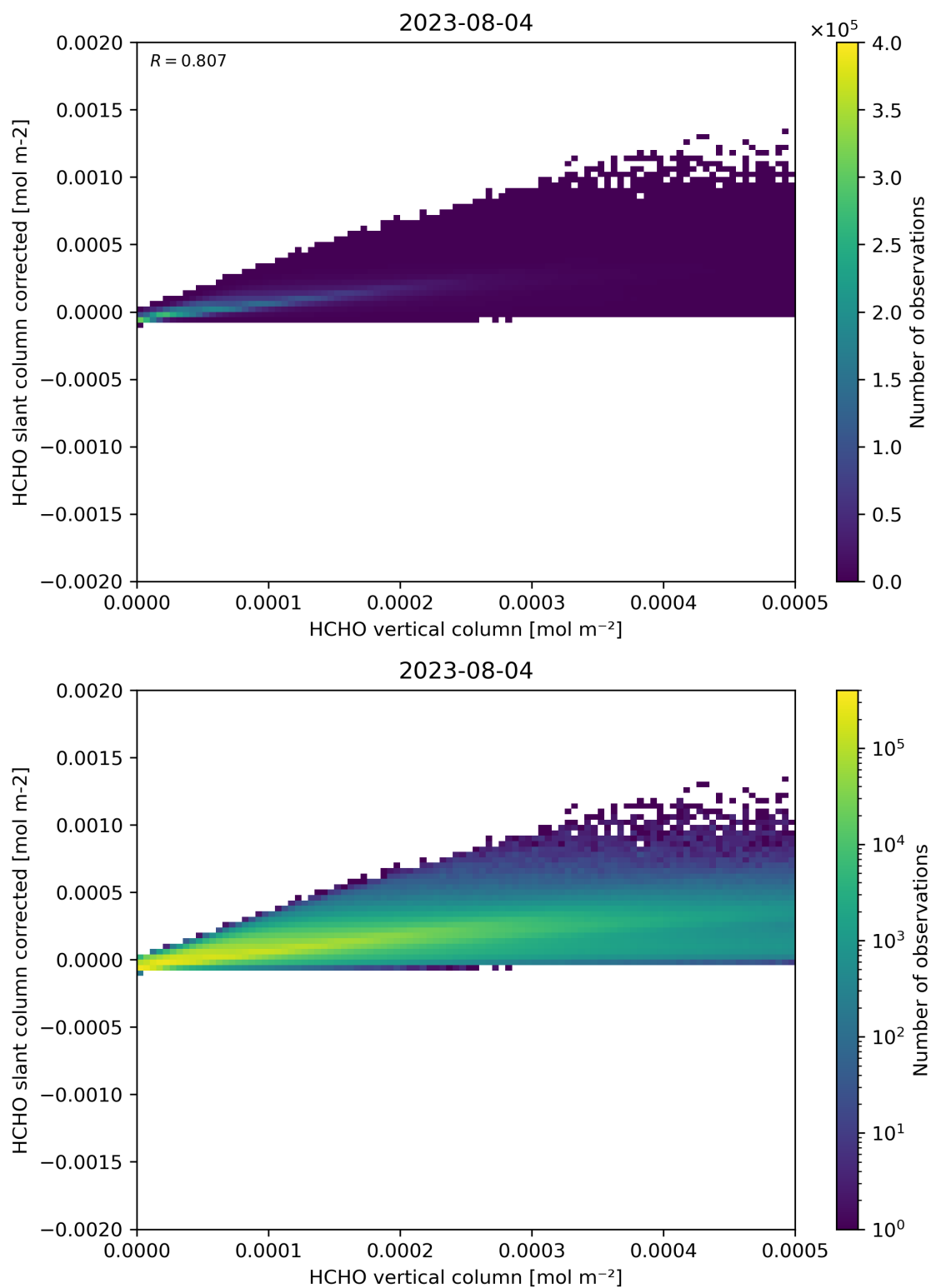
Figure 127: Scatter density plot of “HCHO vertical column” against “HCHO slant column corrected” for 2023-08-04 to 2023-08-05.
