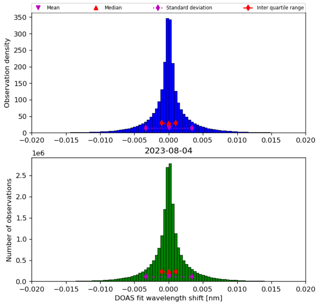
Figure 44: Histogram of “DOAS fit wavelength shift” for 2023-08-04 to 2023-08-05
