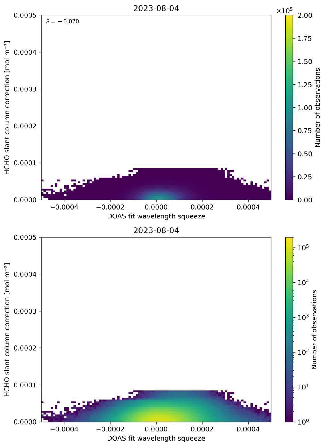
Figure 70: Scatter density plot of “DOAS fit wavelength squeeze” against “HCHO slant column correction” for 2023-08-04 to 2023-08-05.
