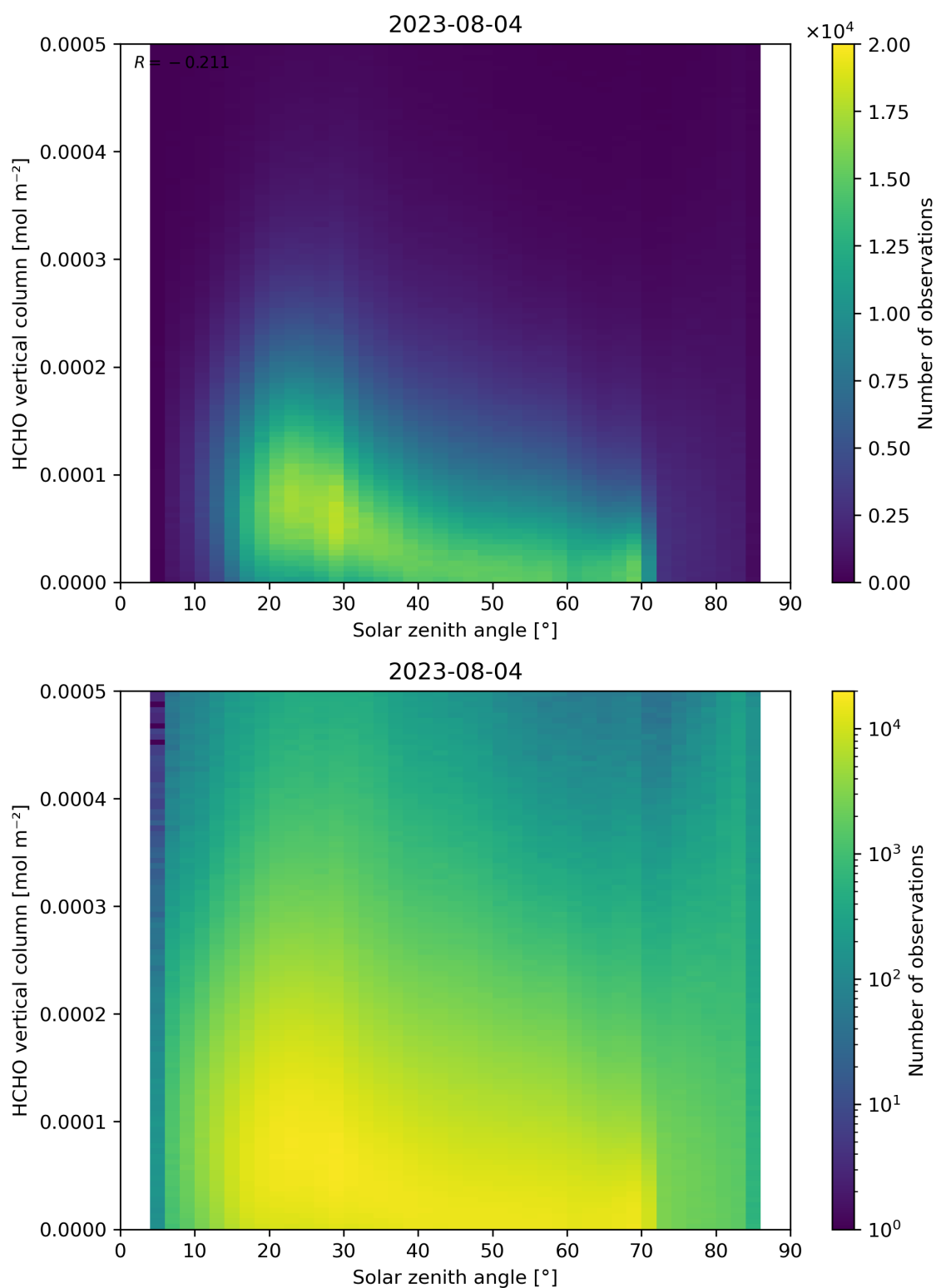
Figure 177: Scatter density plot of “Solar zenith angle” against “HCHO vertical column” for 2023-08-04 to 2023-08-05.
