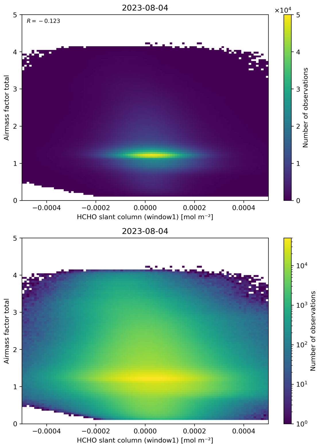
Figure 85: Scatter density plot of “HCHO slant column (window1)” against “Airmass factor total” for 2023-08-04 to 2023-08-05.
