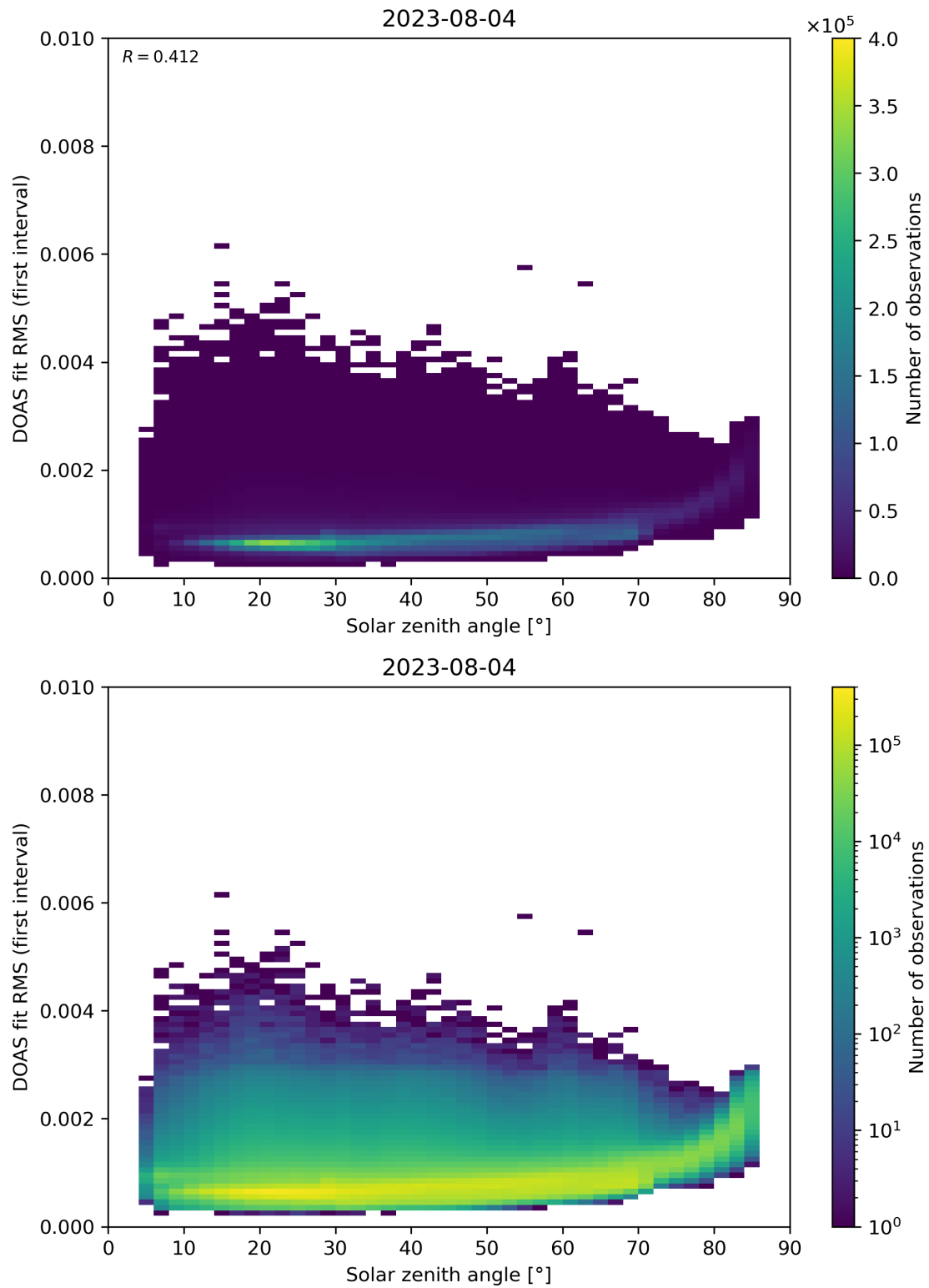
Figure 167: Scatter density plot of “Solar zenith angle” against “DOAS fit RMS (first interval)” for 2023-08-04 to 2023-08-05.
