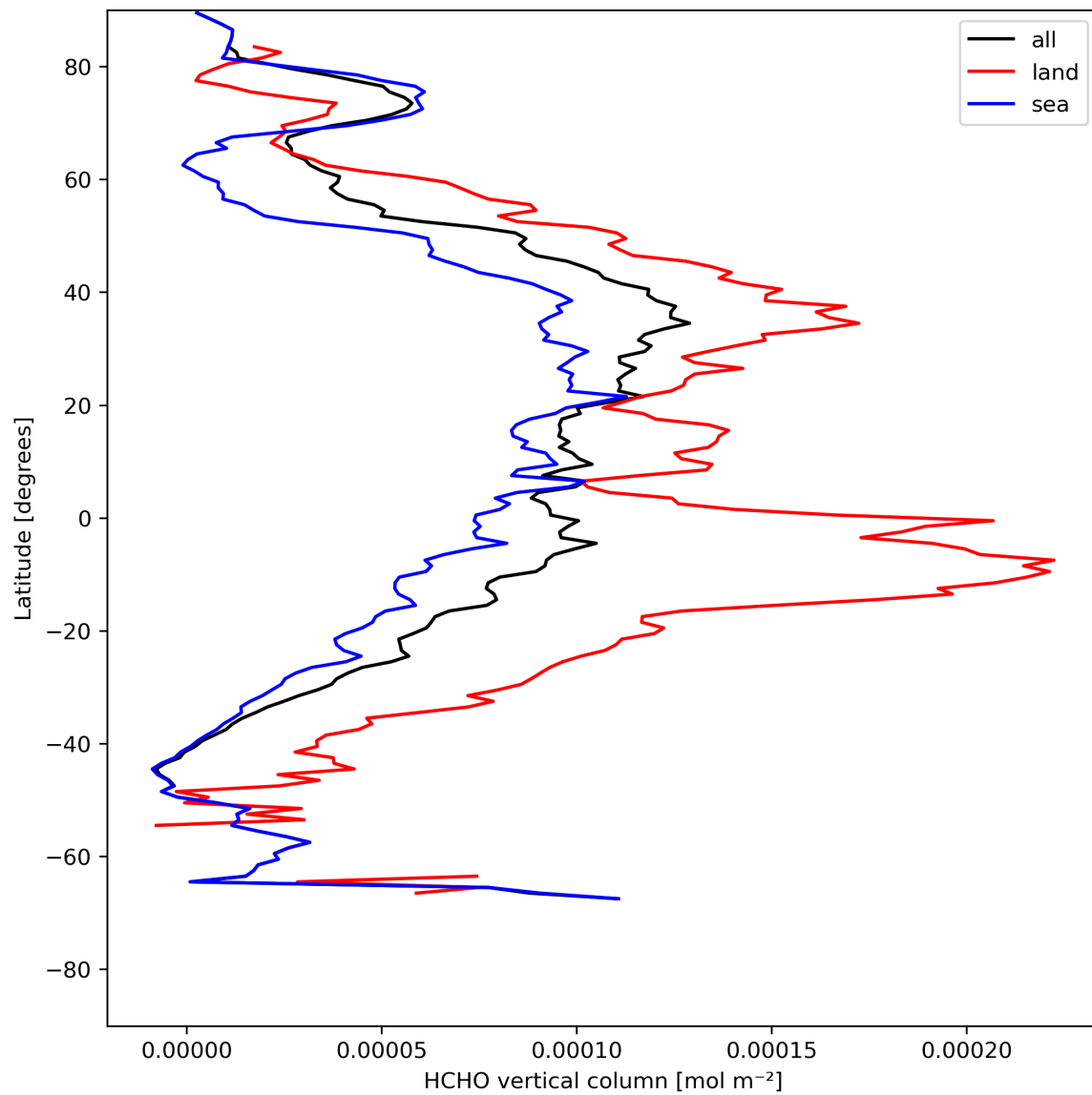
Figure 21: Zonal average of “HCHO vertical column” for 2023-08-04 to 2023-08-05.
