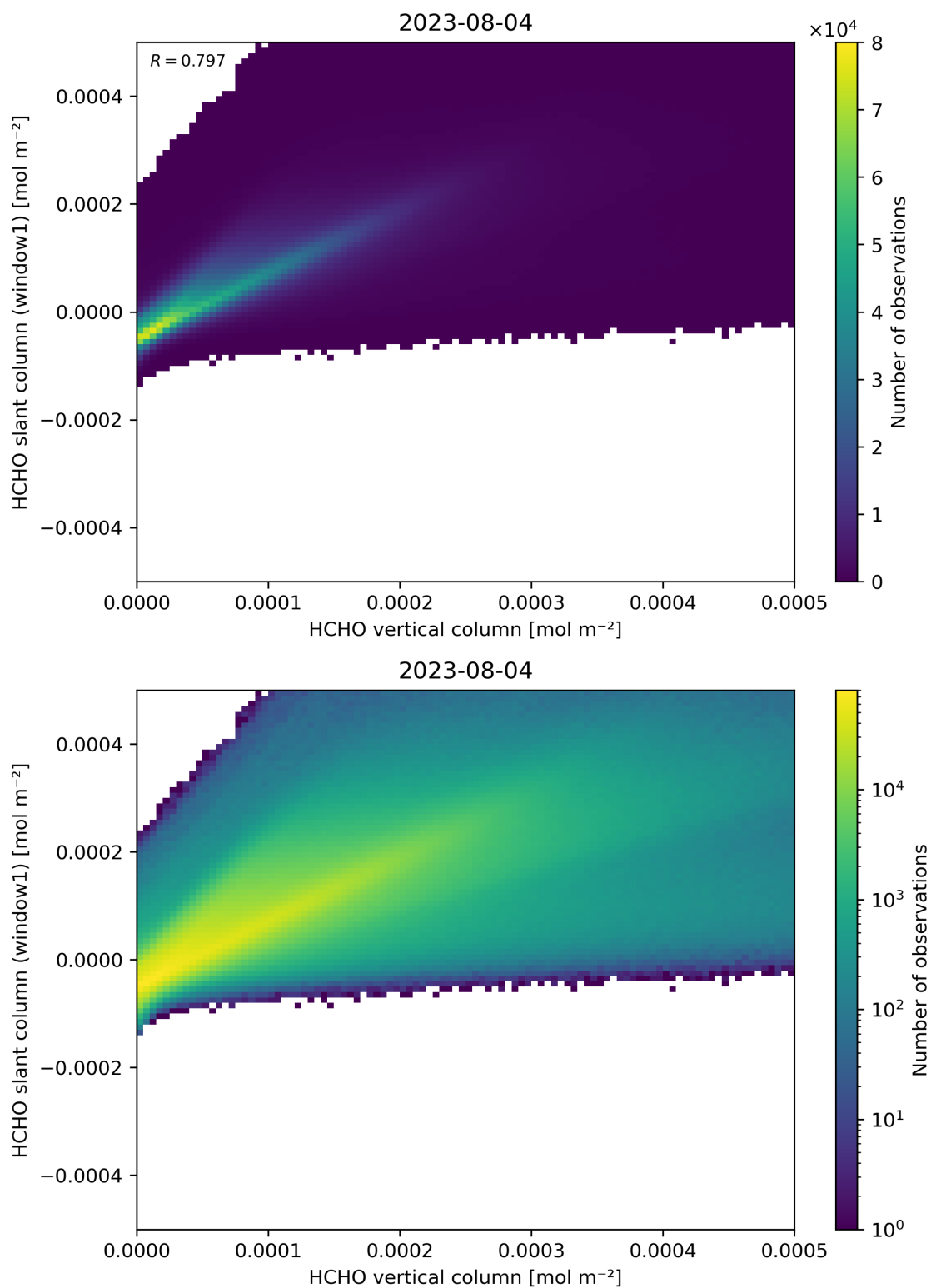
Figure 129: Scatter density plot of “HCHO vertical column” against “HCHO slant column (window1)” for 2023-08-04 to 2023-08-05.
