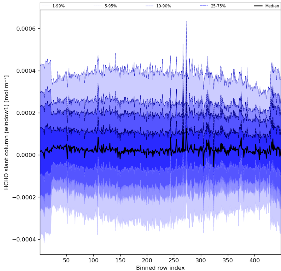
Figure 52: Along track statistics of “HCHO slant column (window1)” for 2023-08-04 to 2023-08-05
