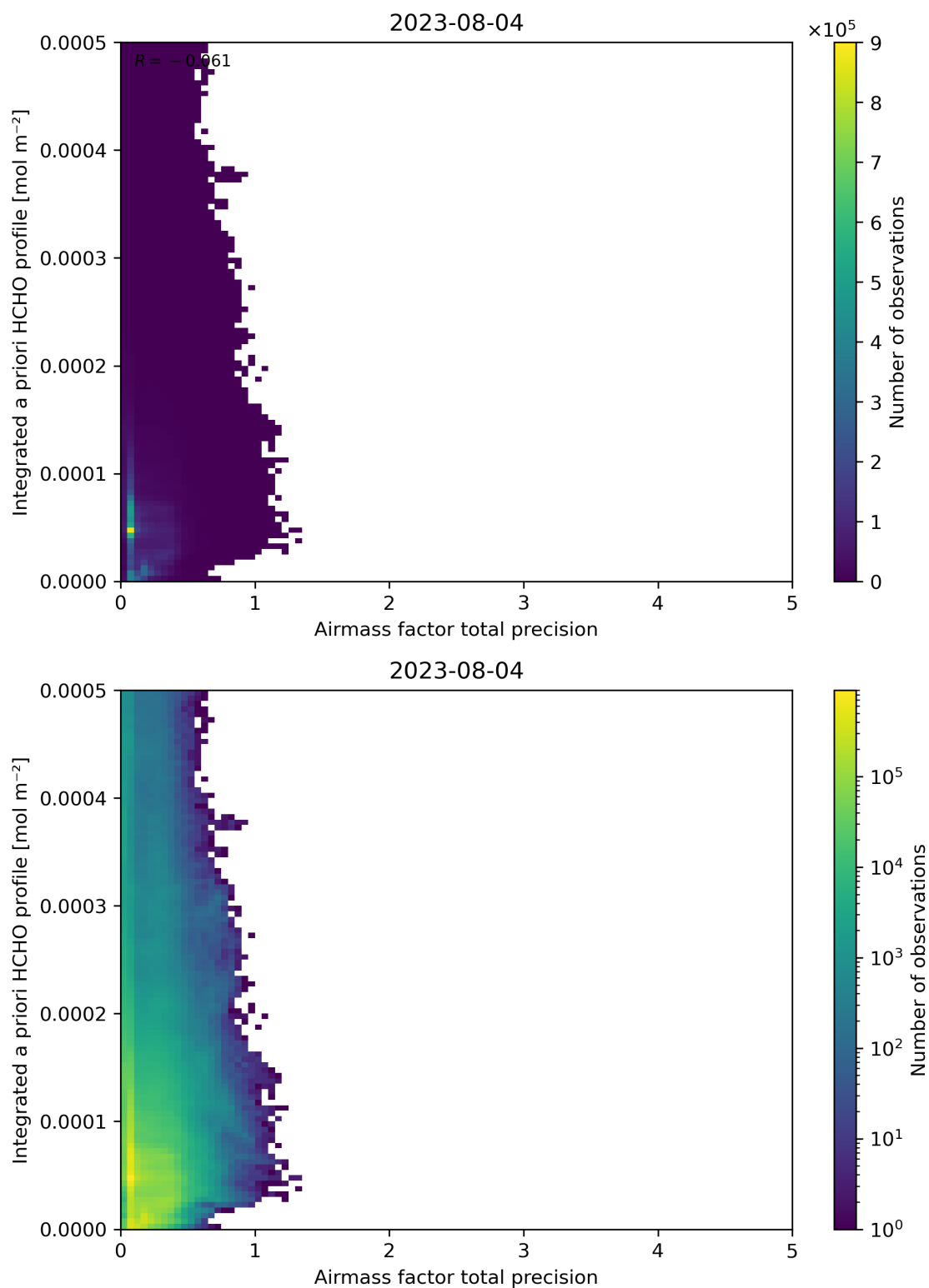
Figure 111: Scatter density plot of “Airmass factor total precision” against “Integrated a priori HCHO profile” for 2023-08-04 to 2023-08-05.
