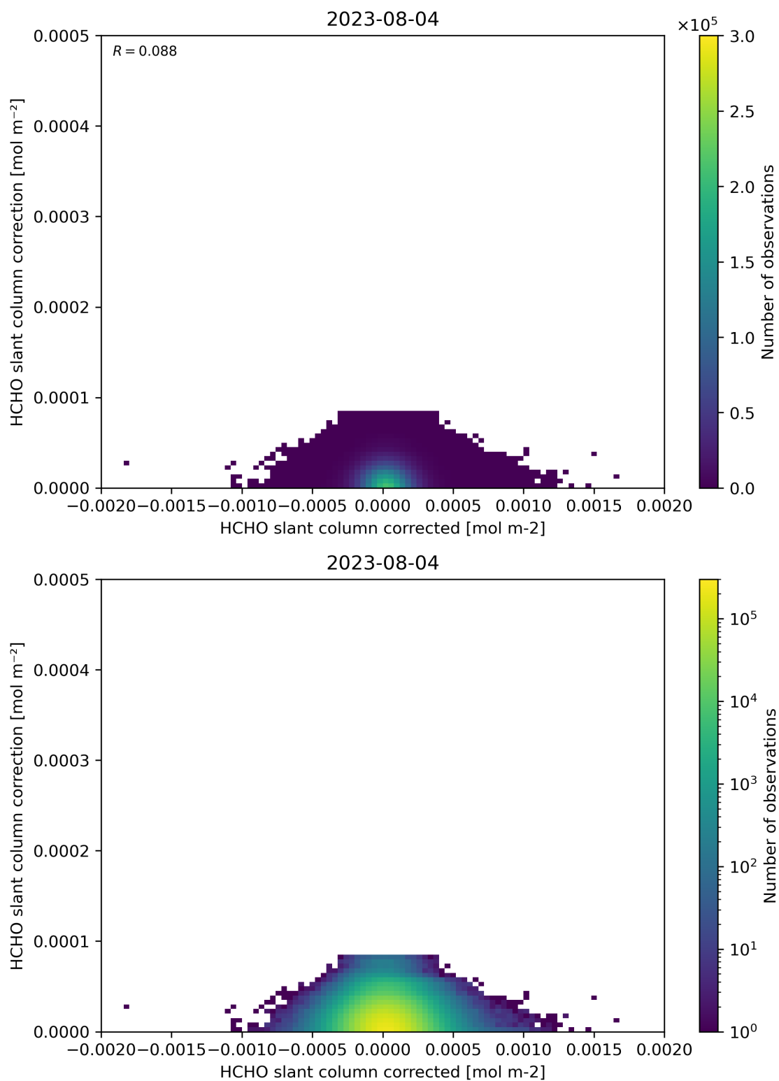
Figure 77: Scatter density plot of “HCHO slant column corrected” against “HCHO slant column correction” for 2023-08-04 to 2023-08-05.
