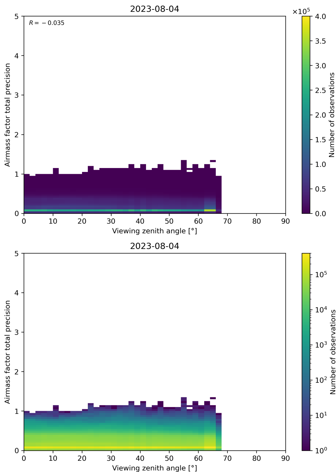
Figure 191: Scatter density plot of “Viewing zenith angle” against “Airmass factor total precision” for 2023-08-04 to 2023-08-05.
