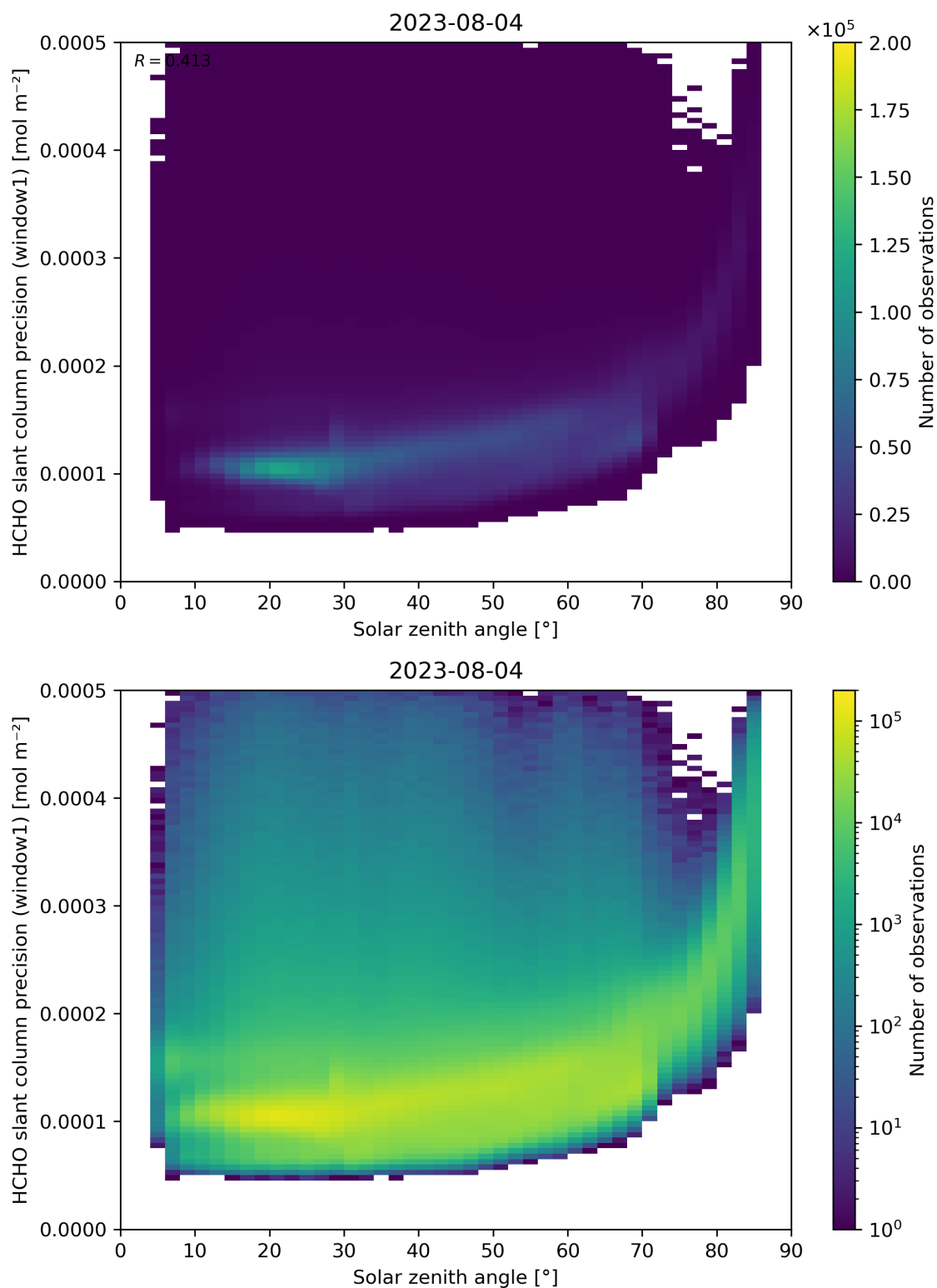
Figure 174: Scatter density plot of “Solar zenith angle” against “HCHO slant column precision (window1)” for 2023-08-04 to 2023-08-05.
