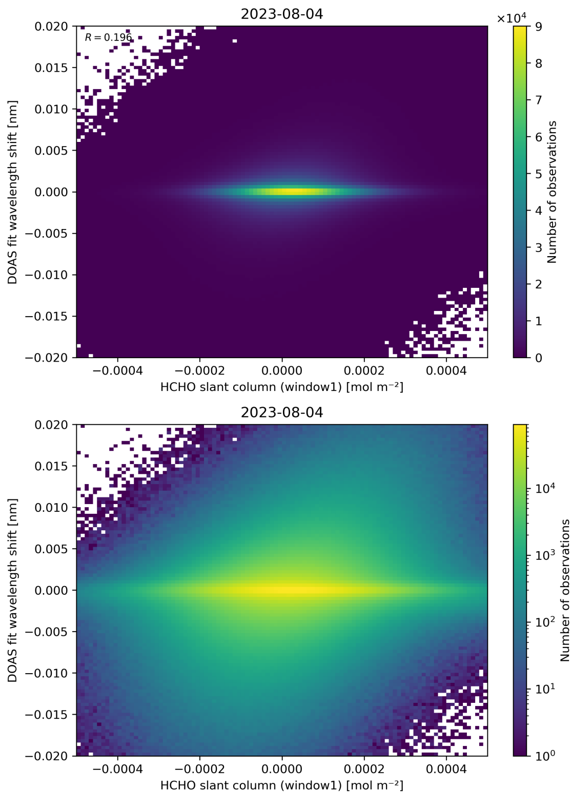
Figure 79: Scatter density plot of “HCHO slant column (window1)” against “DOAS fit wavelength shift” for 2023-08-04 to 2023-08-05.
