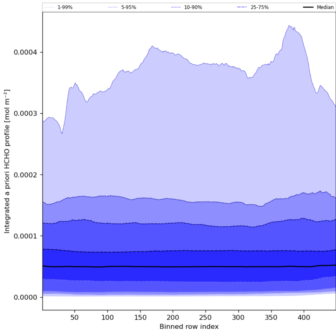
Figure 57: Along track statistics of "Integrated a priori HCHO profile" for 2023-08-04 to 2023-08-05
