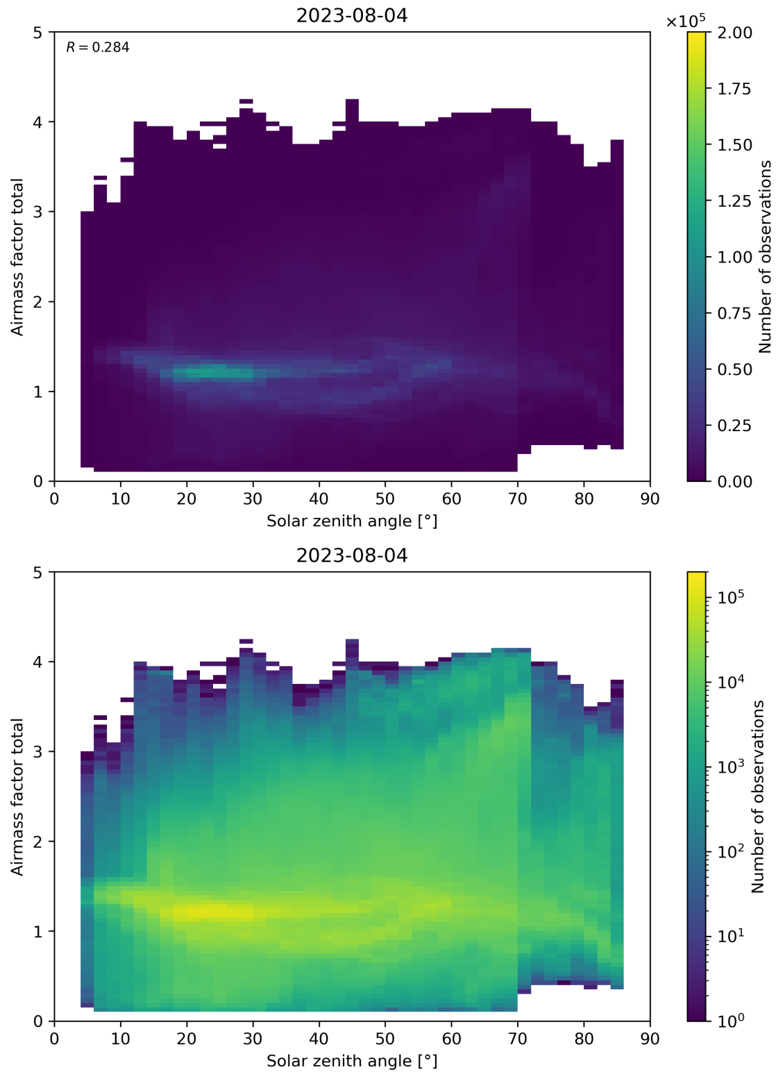
Figure 175: Scatter density plot of “Solar zenith angle” against “Airmass factor total” for 2023-08-04 to 2023-08-05.
