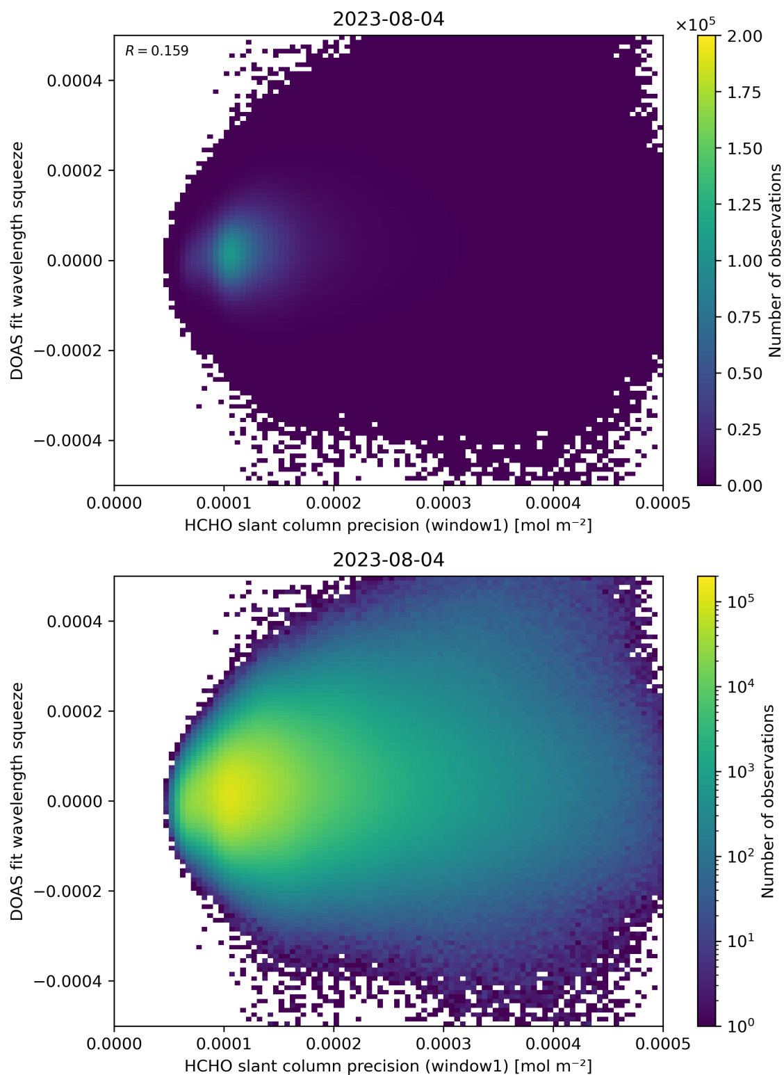
Figure 90: Scatter density plot of “HCHO slant column precision (window1)” against “DOAS fit wavelength squeeze” for 2023-08-04 to 2023-08-05.
