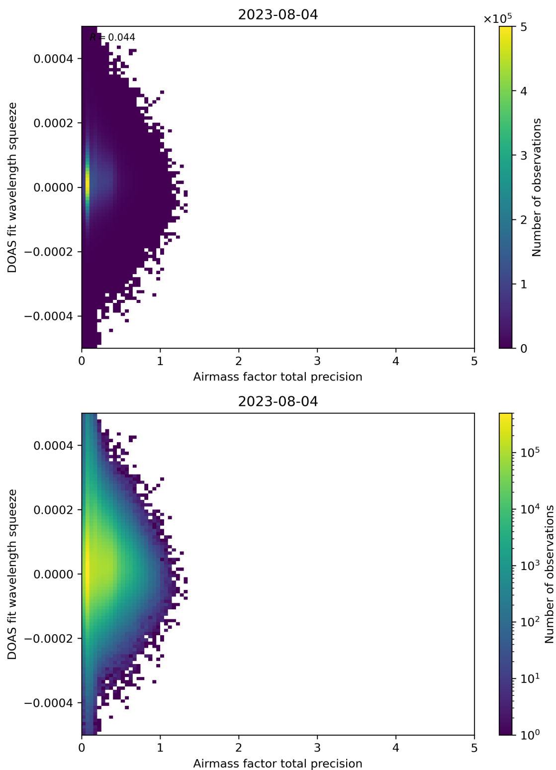
Figure 107: Scatter density plot of “Airmass factor total precision” against “DOAS fit wavelength squeeze” for 2023-08-04 to 2023-08-05.
