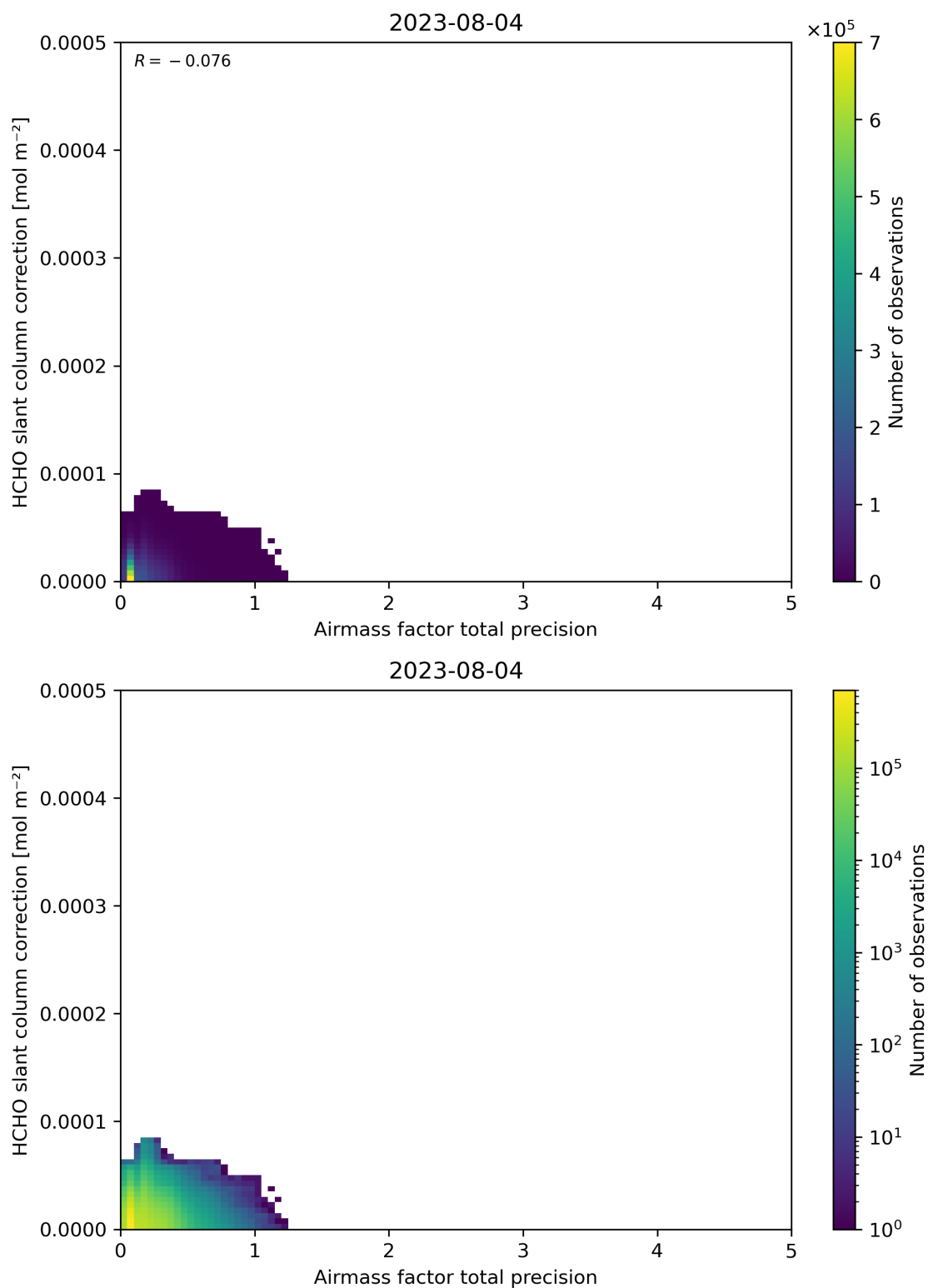
Figure 110: Scatter density plot of “Airmass factor total precision” against “HCHO slant column correction” for 2023-08-04 to 2023-08-05.
