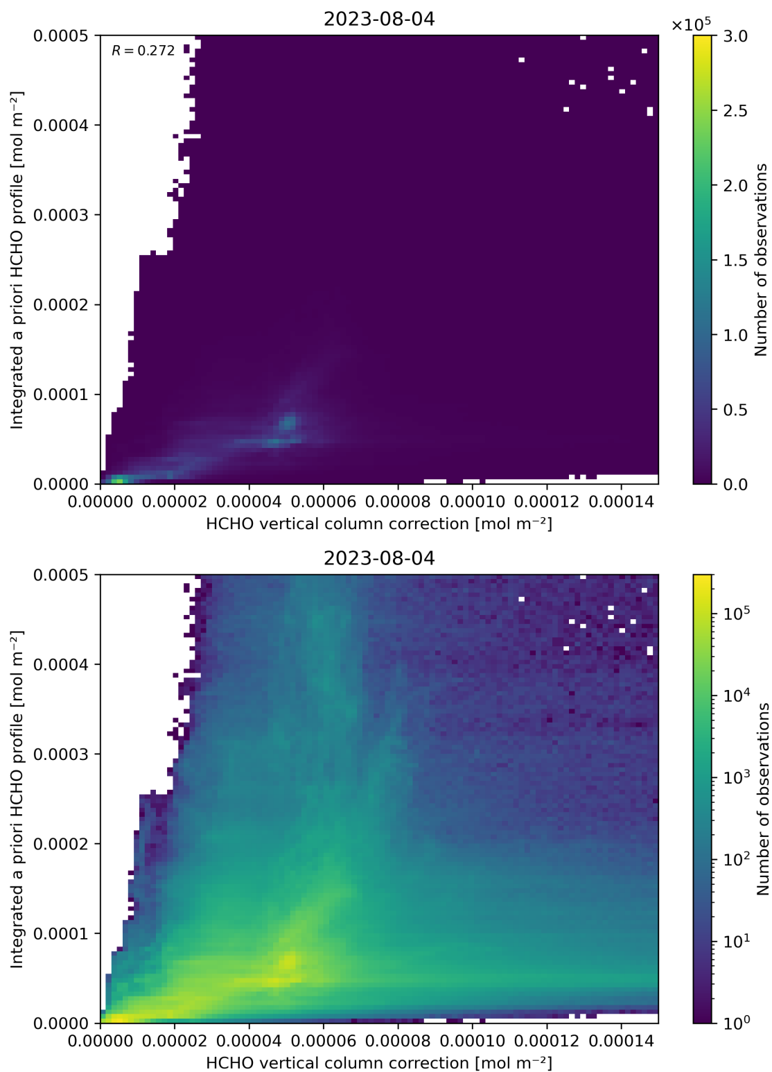
Figure 122: Scatter density plot of “HCHO vertical column correction” against “Integrated a priori HCHO profile” for 2023-08-04 to 2023-08-05.
