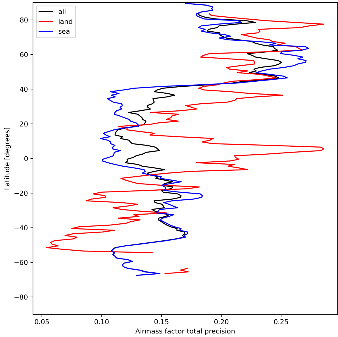
Figure 27: Zonal average of “Airmass factor total precision” for 2023-08-04 to 2023-08-05.
