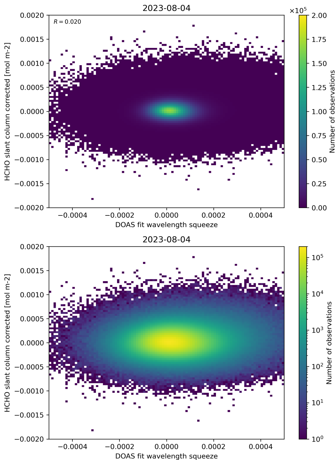
Figure 69: Scatter density plot of “DOAS fit wavelength squeeze” against “HCHO slant column corrected” for 2023-08-04 to 2023-08-05.
