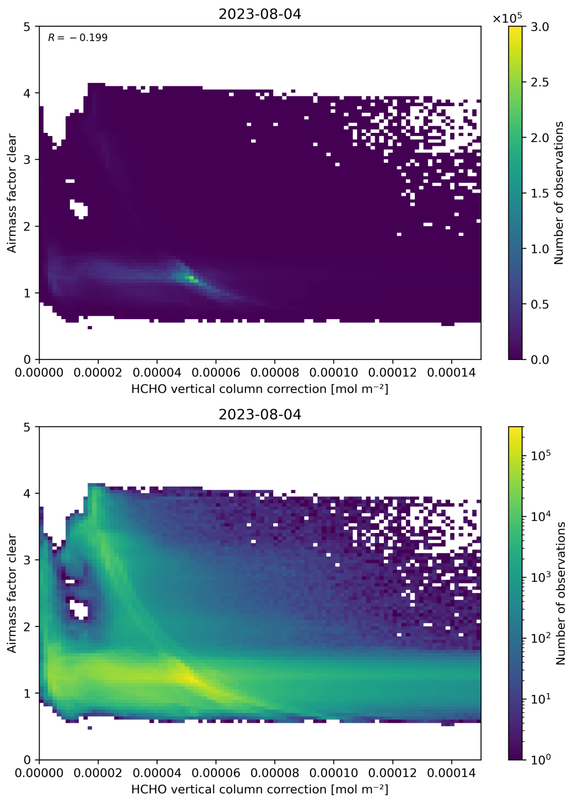
Figure 115: Scatter density plot of “HCHO vertical column correction” against “Airmass factor clear” for 2023-08-04 to 2023-08-05.
