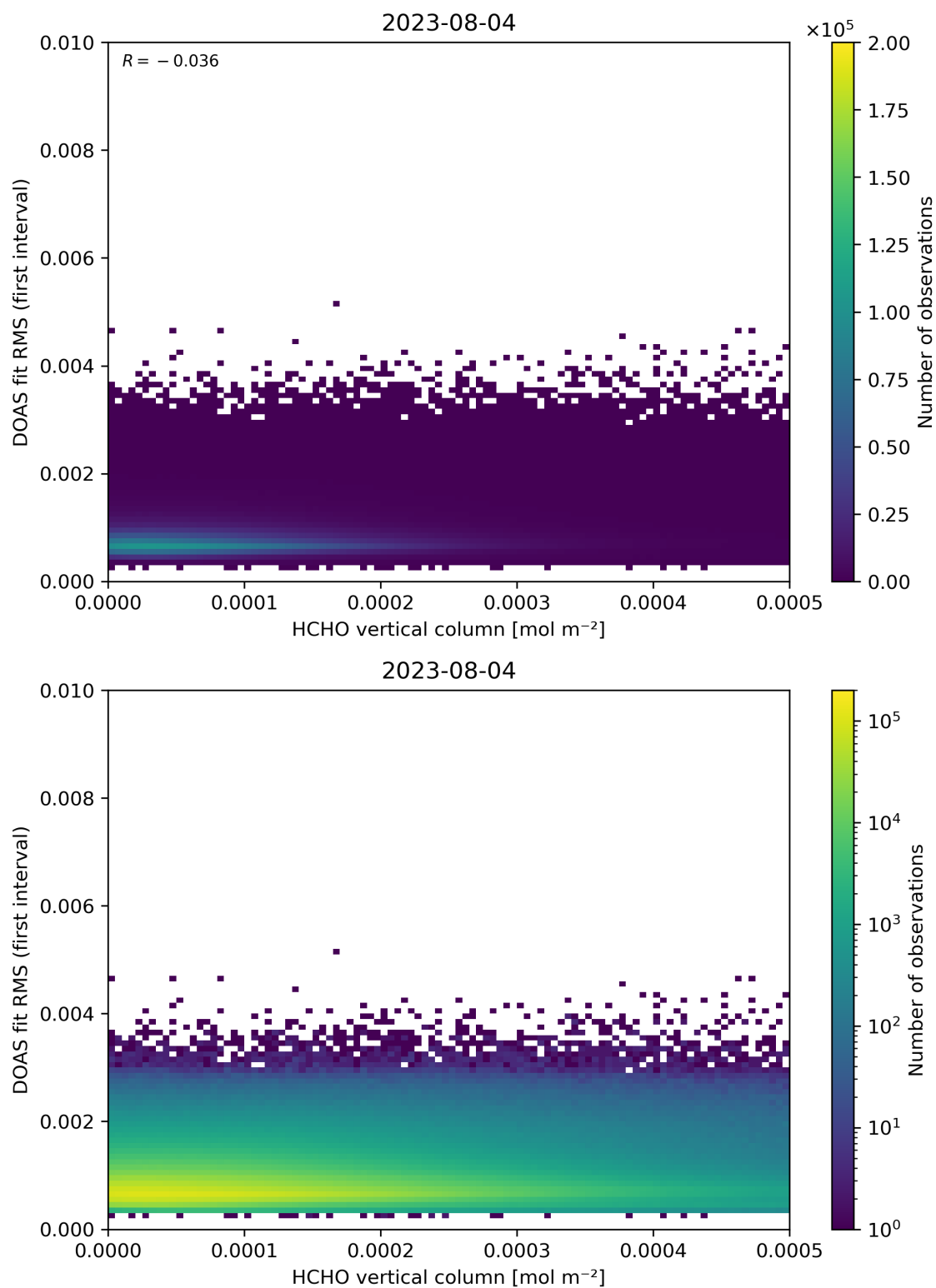
Figure 123: Scatter density plot of “HCHO vertical column” against “DOAS fit RMS (first interval)” for 2023-08-04 to 2023-08-05.
