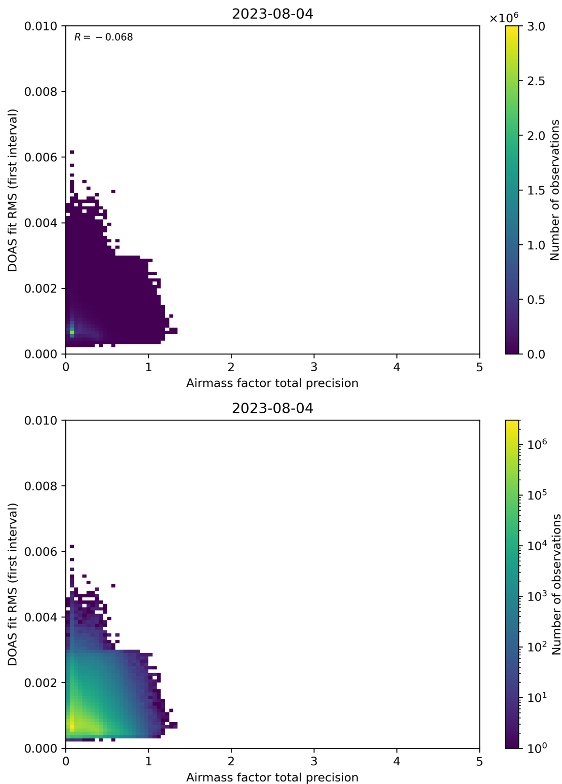
Figure 105: Scatter density plot of “Airmass factor total precision” against “DOAS fit RMS (first interval)” for 2023-08-04 to 2023-08-05.
