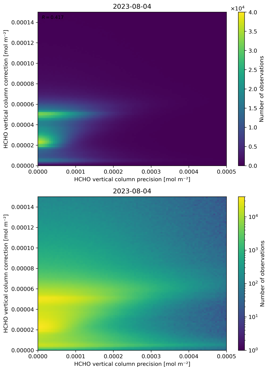
Figure 146: Scatter density plot of “HCHO vertical column precision” against “HCHO vertical column correction” for 2023-08-04 to 2023-08-05.
