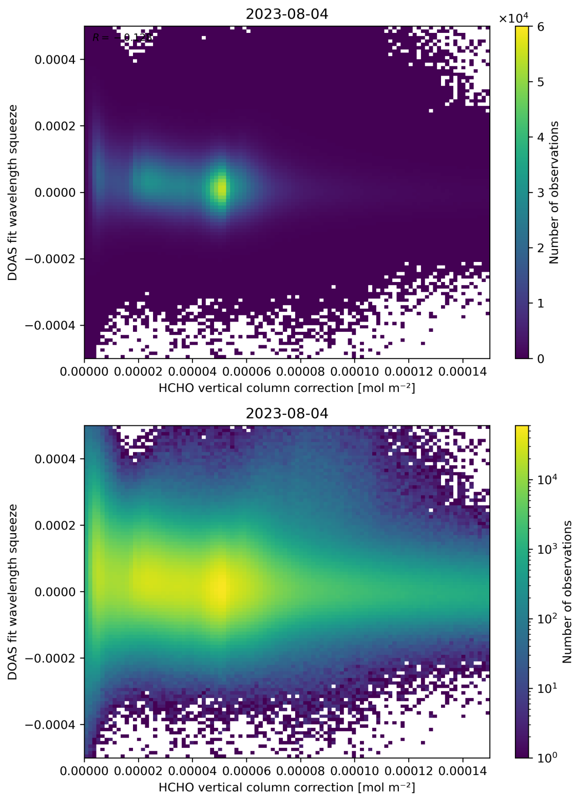
Figure 114: Scatter density plot of “HCHO vertical column correction” against “DOAS fit wavelength squeeze” for 2023-08-04 to 2023-08-05.
