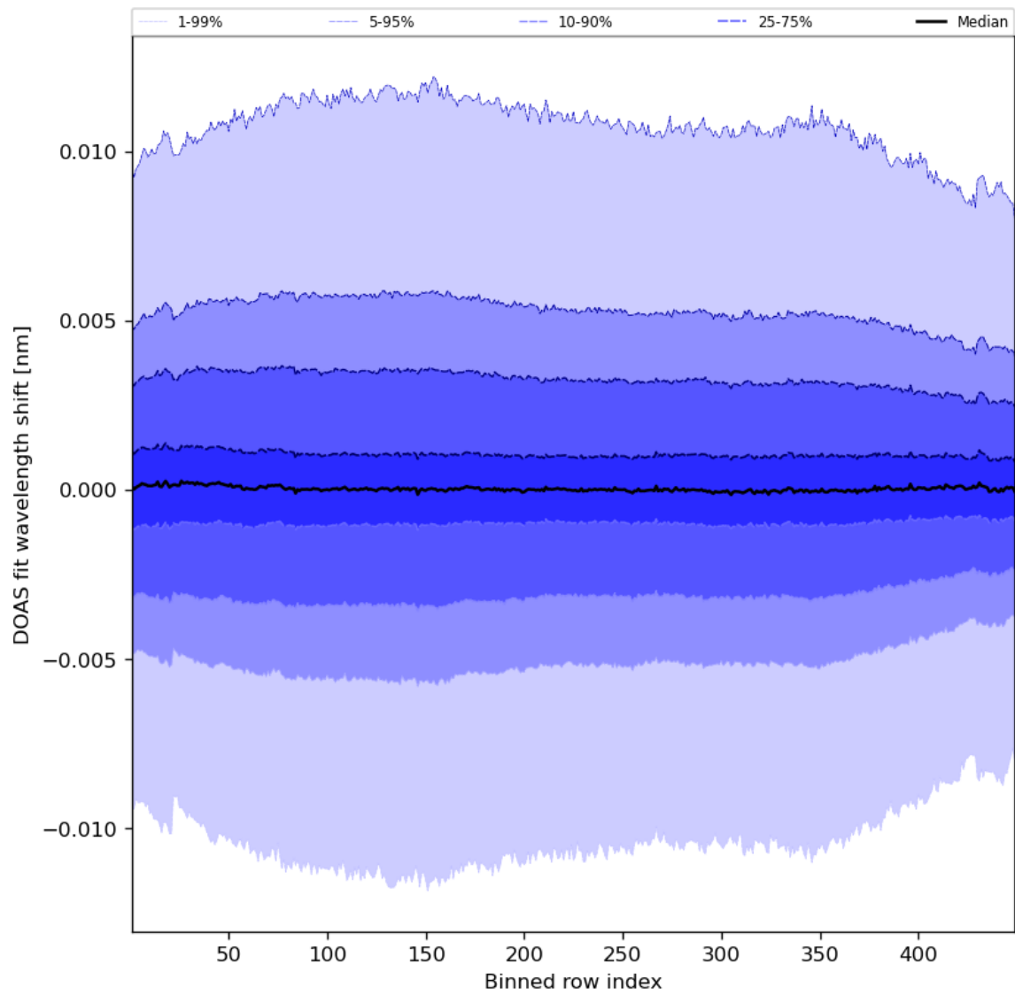
Figure 58: Along track statistics of “DOAS fit wavelength shift” for 2023-08-04 to 2023-08-05
