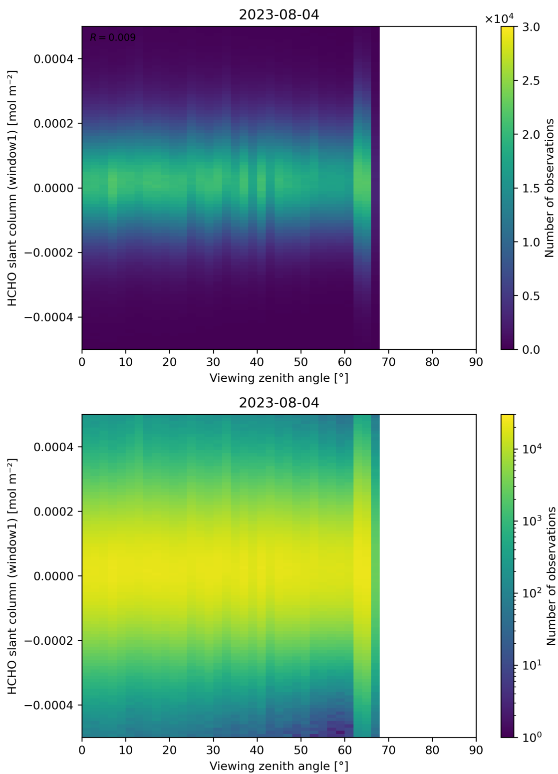
Figure 188: Scatter density plot of “Viewing zenith angle” against “HCHO slant column (window1)” for 2023-08-04 to 2023-08-05.
