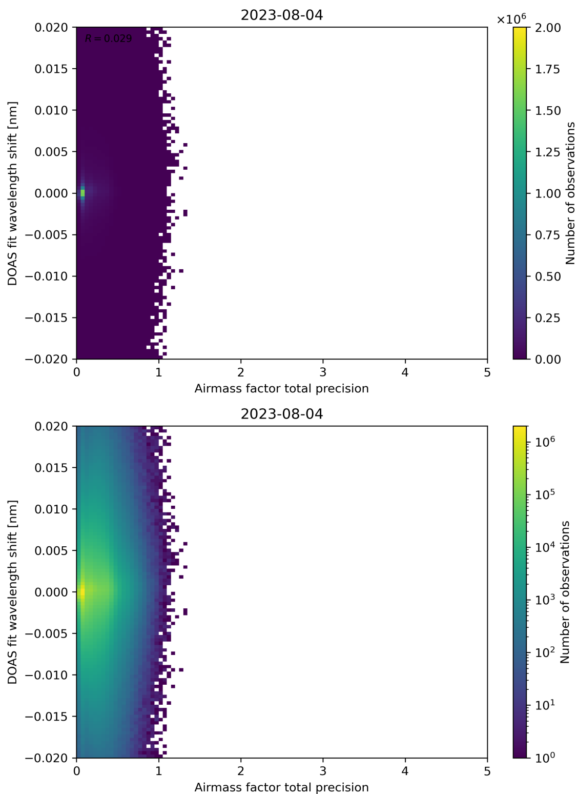
Figure 106: Scatter density plot of “Airmass factor total precision” against “DOAS fit wavelength shift” for 2023-08-04 to 2023-08-05.
