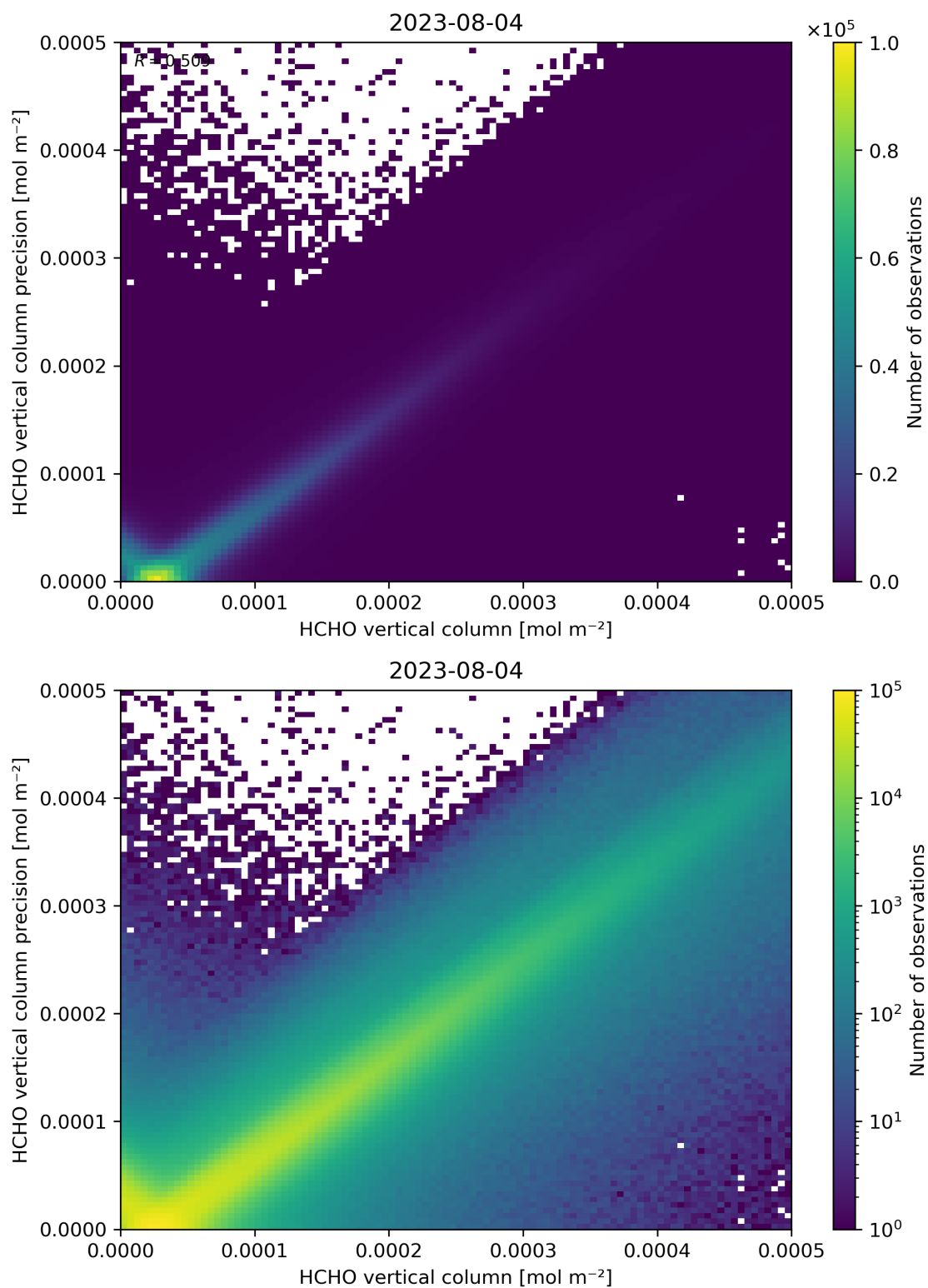
Figure 134: Scatter density plot of “HCHO vertical column” against “HCHO vertical column precision” for 2023-08-04 to 2023-08-05.
