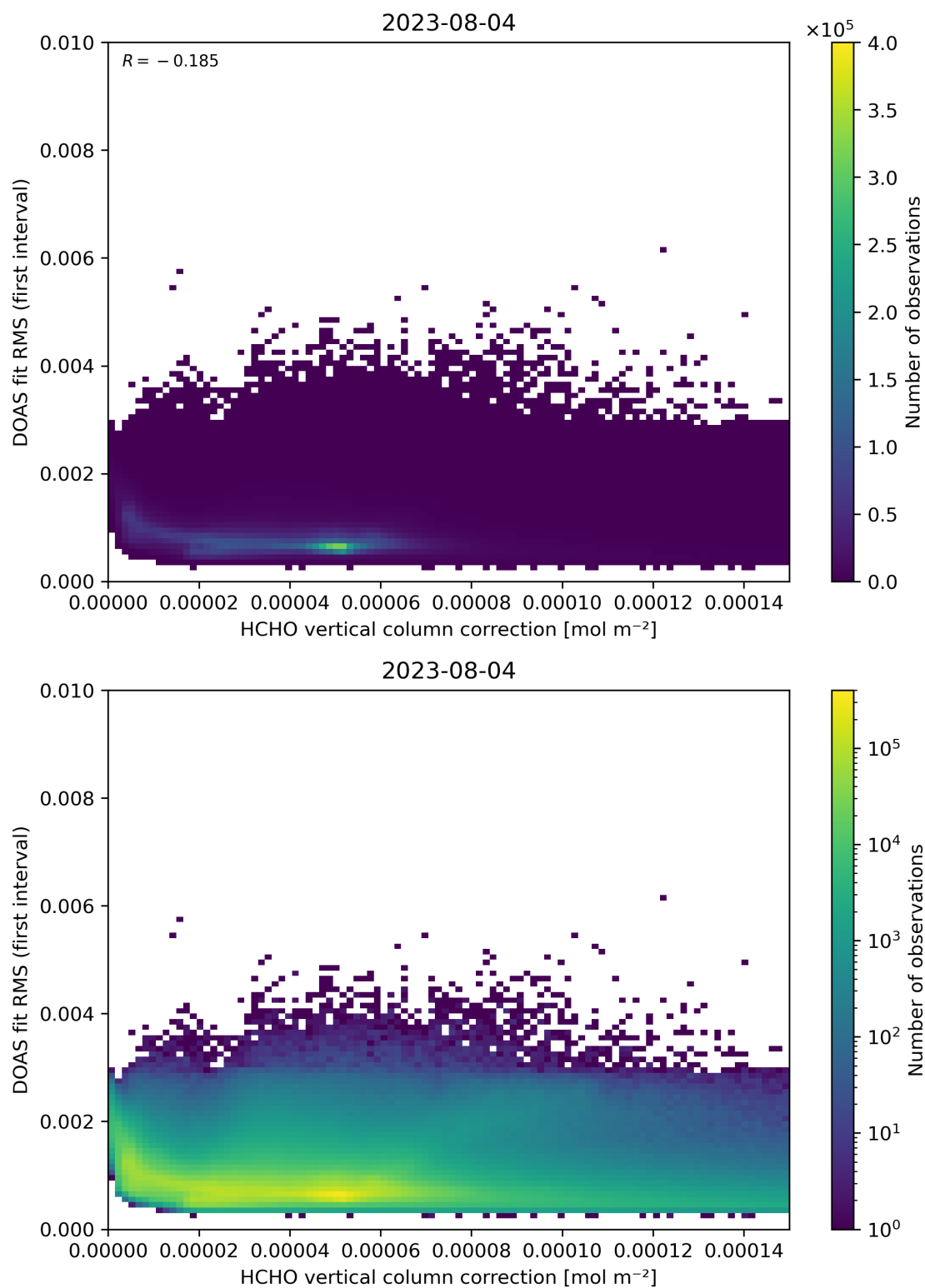
Figure 112: Scatter density plot of “HCHO vertical column correction” against “DOAS fit RMS (first interval)” for 2023-08-04 to 2023-08-05.
