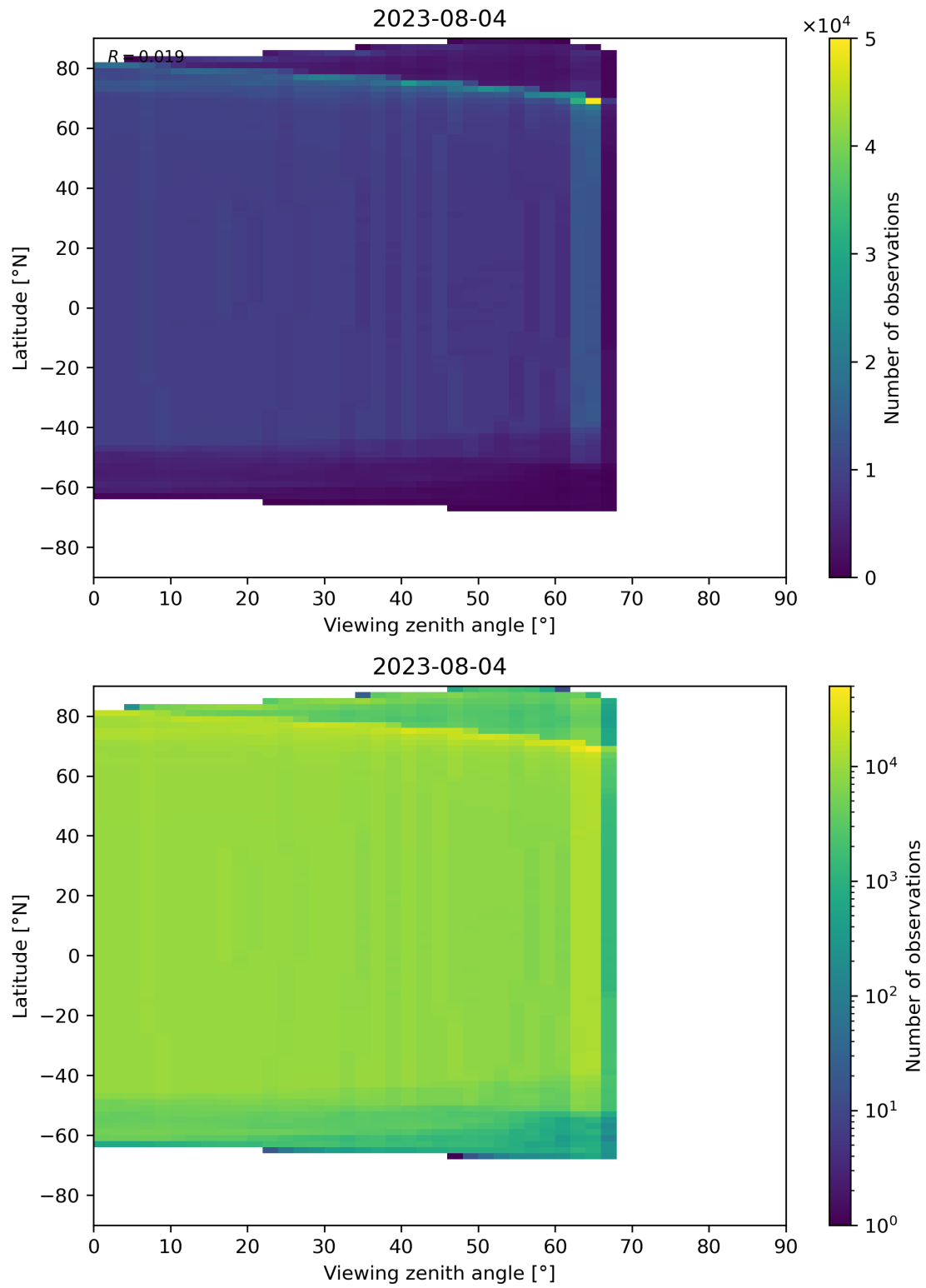
Figure 196: Scatter density plot of “Viewing zenith angle” against “Latitude” for 2023-08-04 to 2023-08-05.
