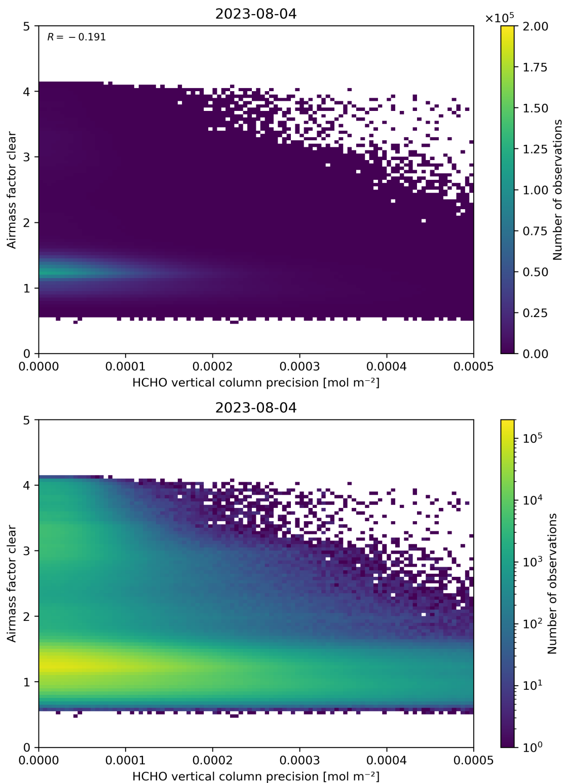
Figure 139: Scatter density plot of “HCHO vertical column precision” against “Airmass factor clear” for 2023-08-04 to 2023-08-05.
