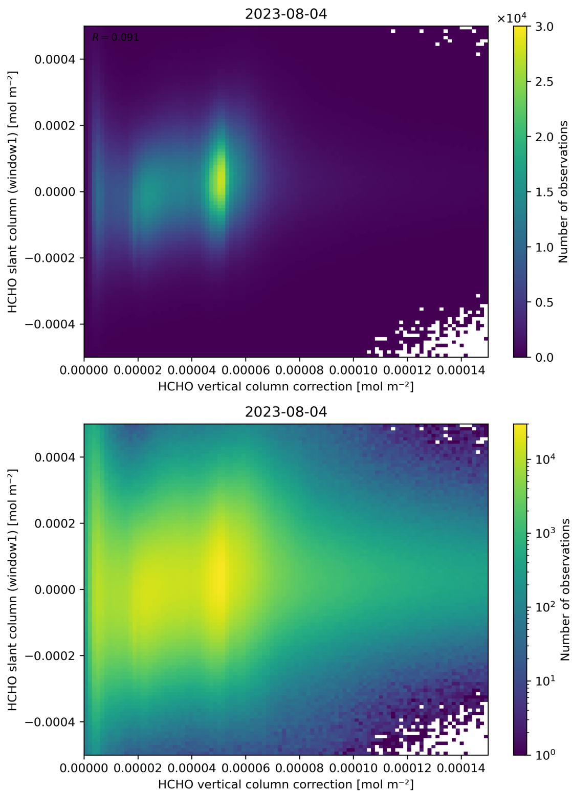
Figure 118: Scatter density plot of “HCHO vertical column correction” against “HCHO slant column (window1)” for 2023-08-04 to 2023-08-05.
