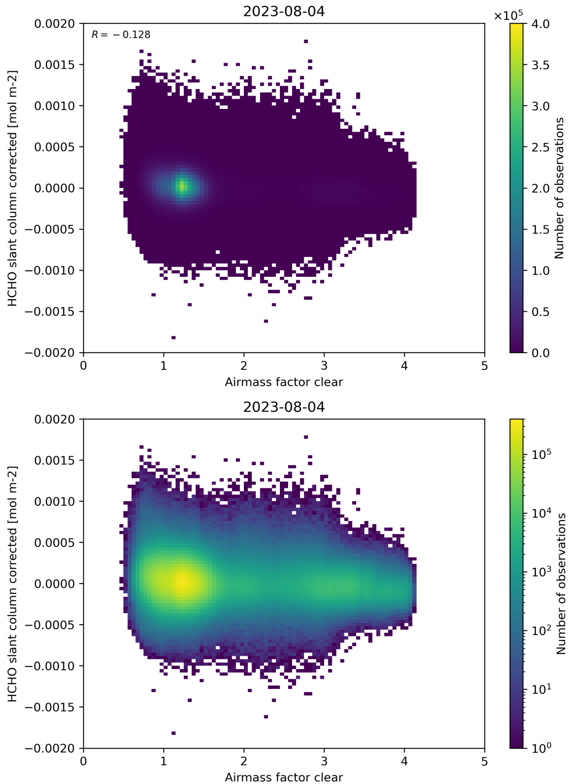
Figure 74: Scatter density plot of “Airmass factor clear” against “HCHO slant column corrected” for 2023-08-04 to 2023-08-05.
