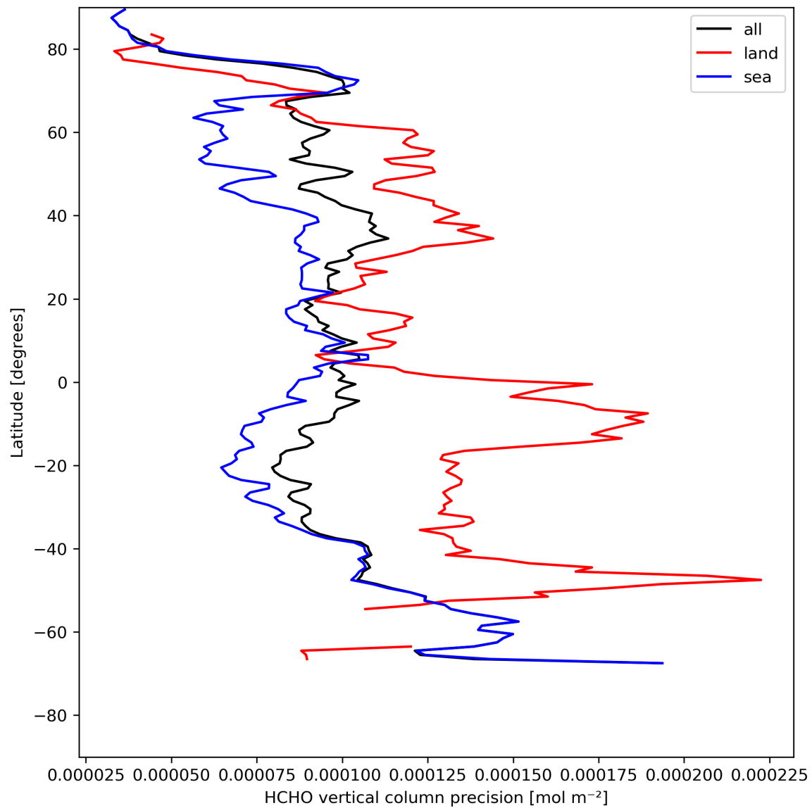
Figure 22: Zonal average of “HCHO vertical column precision” for 2023-08-04 to 2023-08-05.
