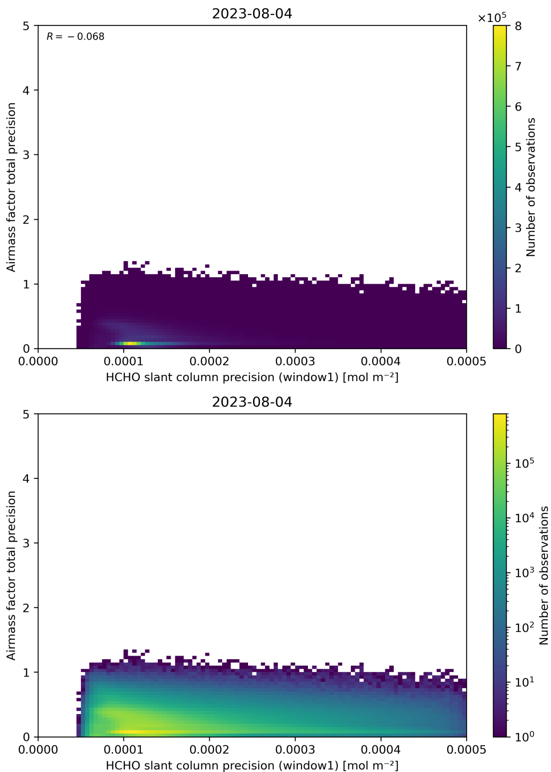
Figure 95: Scatter density plot of “HCHO slant column precision (window1)” against “Airmass factor total precision” for 2023-08-04 to 2023-08-05.
