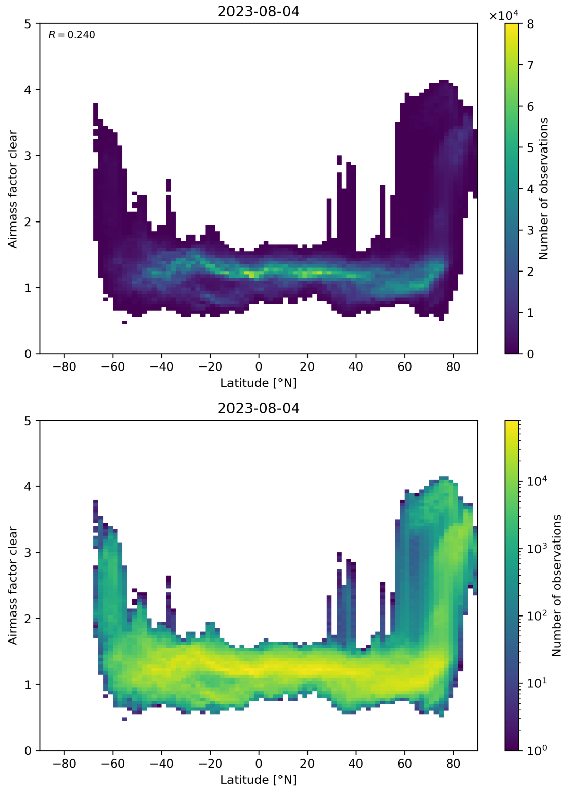
Figure 156: Scatter density plot of “Latitude” against “Airmass factor clear” for 2023-08-04 to 2023-08-05.
