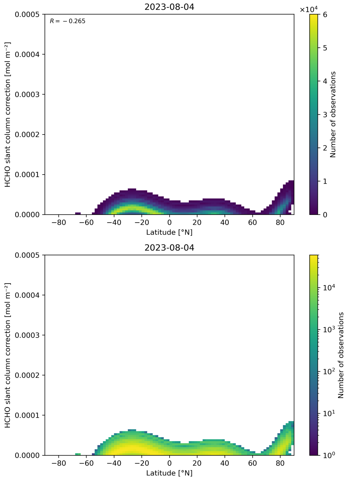
Figure 158: Scatter density plot of “Latitude” against “HCHO slant column correction” for 2023-08-04 to 2023-08-05.
