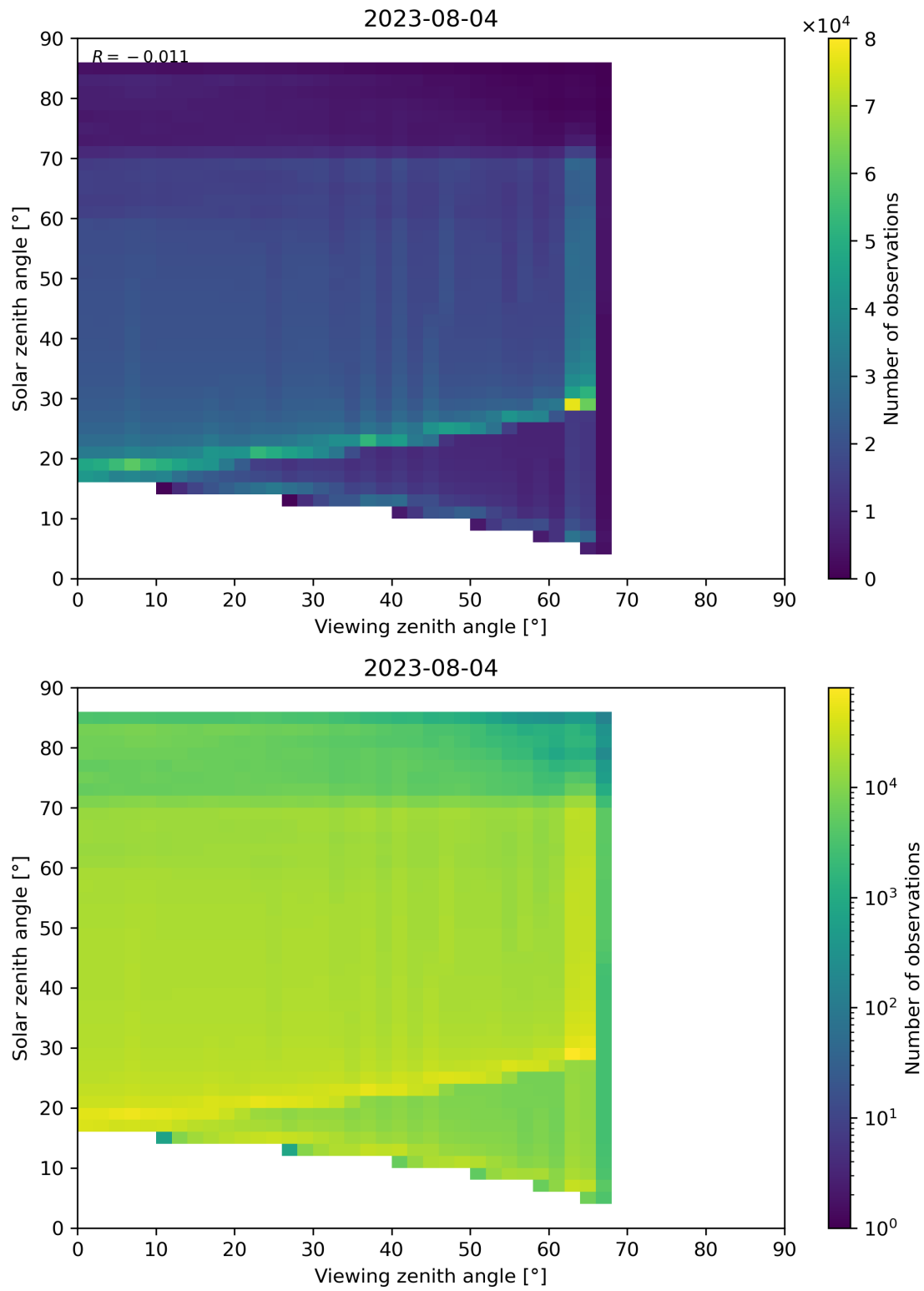
Figure 197: Scatter density plot of “Viewing zenith angle” against “Solar zenith angle” for 2023-08-04 to 2023-08-05.
