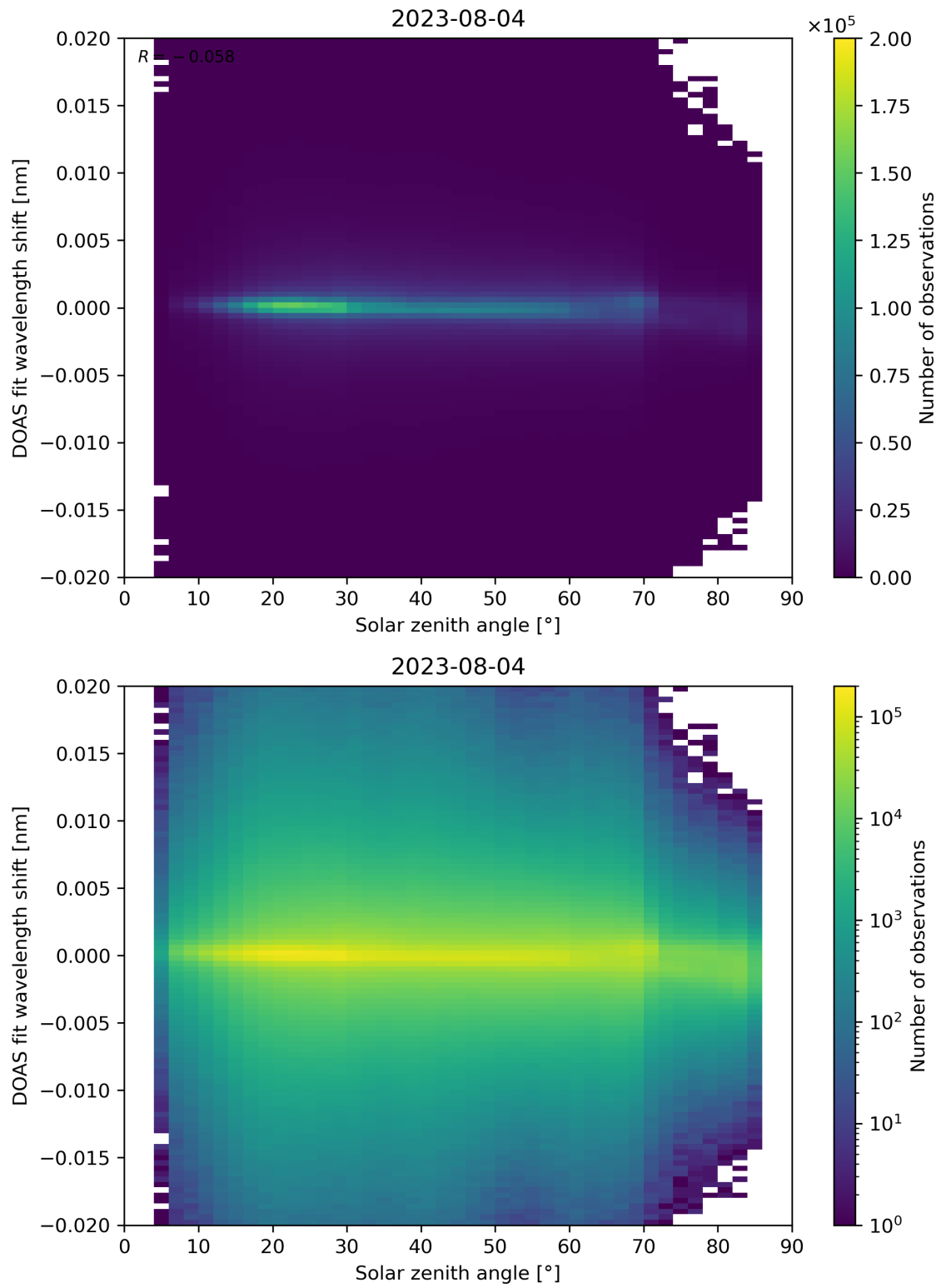
Figure 168: Scatter density plot of “Solar zenith angle” against “DOAS fit wavelength shift” for 2023-08-04 to 2023-08-05.
