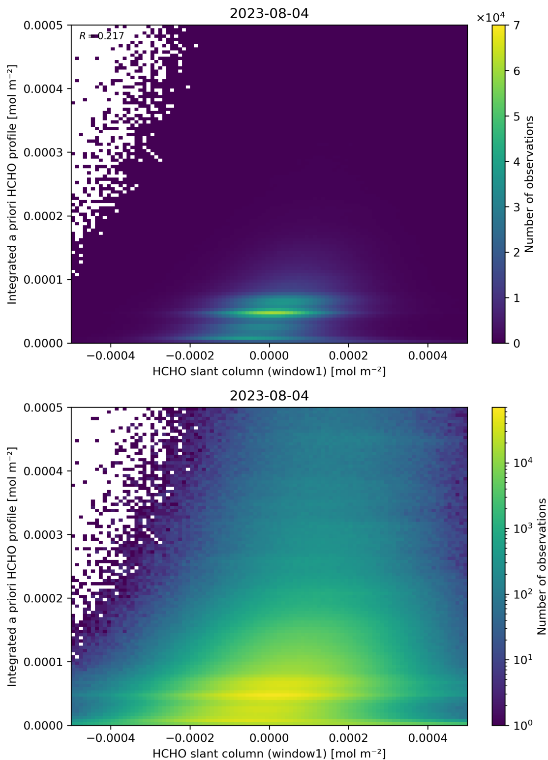
Figure 87: Scatter density plot of “HCHO slant column (window1)” against “Integrated a priori HCHO profile” for 2023-08-04 to 2023-08-05.
