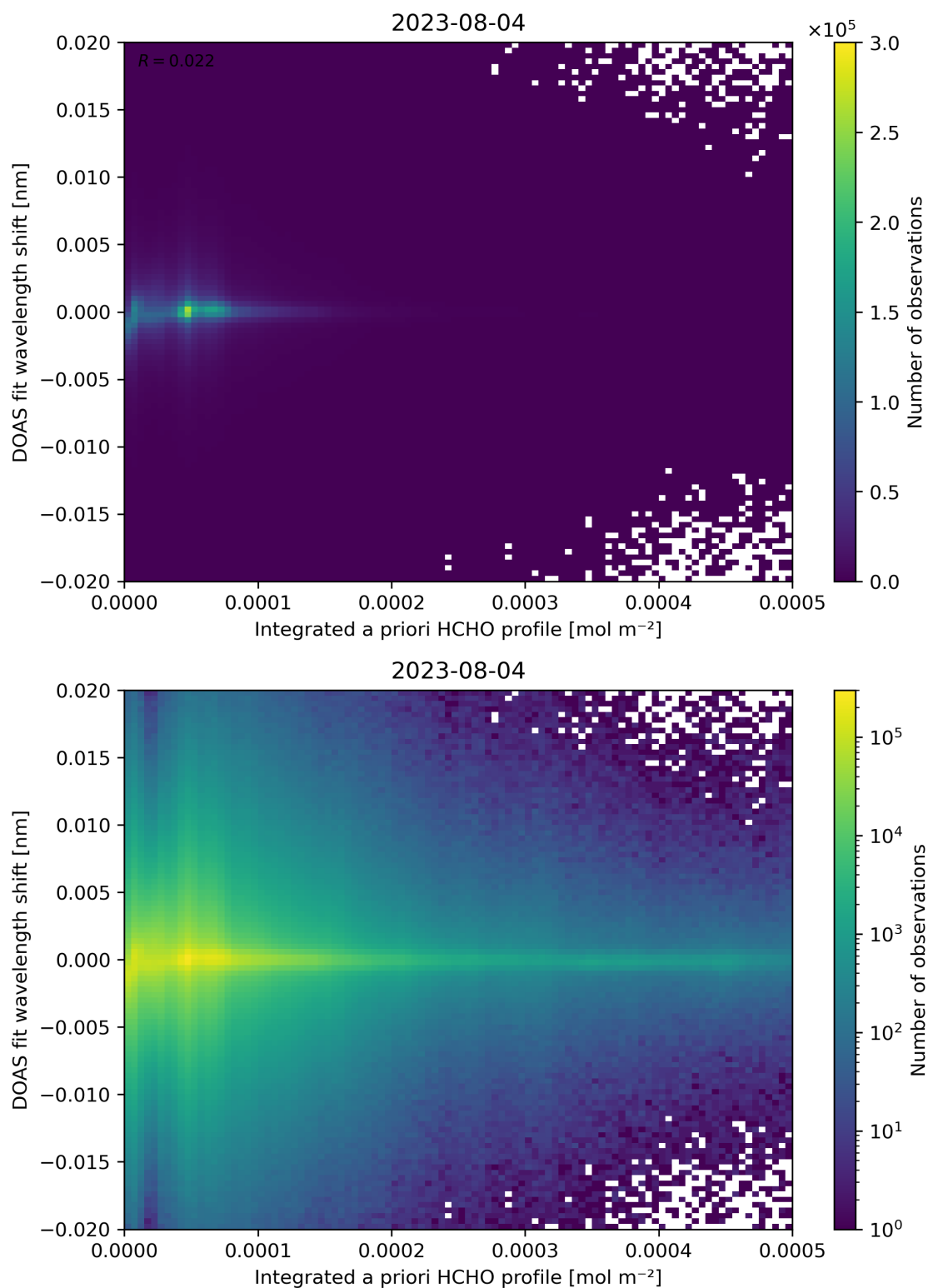
Figure 149: Scatter density plot of “Integrated a priori HCHO profile” against “DOAS fit wavelength shift” for 2023-08-04 to 2023-08-05.
