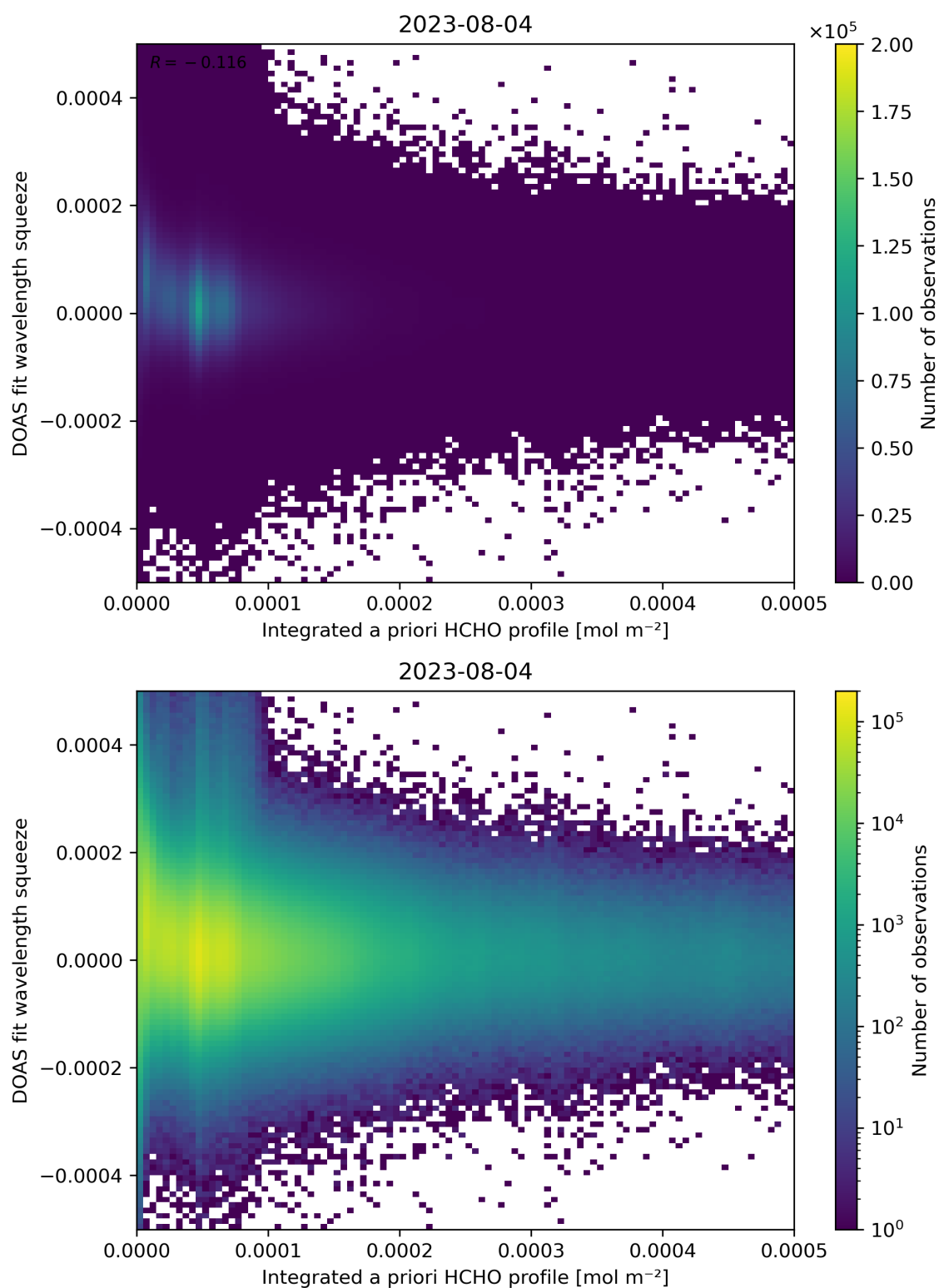
Figure 150: Scatter density plot of “Integrated a priori HCHO profile” against “DOAS fit wavelength squeeze” for 2023-08-04 to 2023-08-05.
