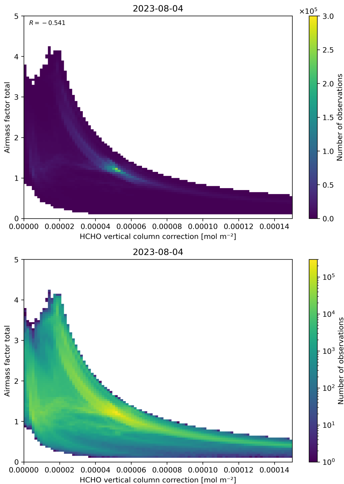
Figure 120: Scatter density plot of “HCHO vertical column correction” against “Airmass factor total” for 2023-08-04 to 2023-08-05.
