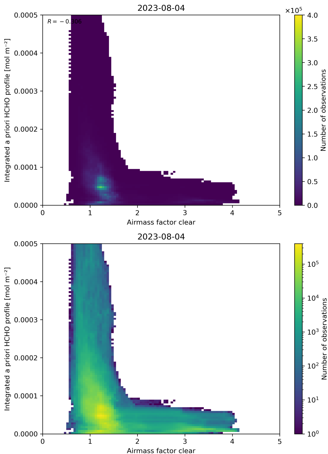
Figure 76: Scatter density plot of “Airmass factor clear” against “Integrated a priori HCHO profile” for 2023-08-04 to 2023-08-05.
