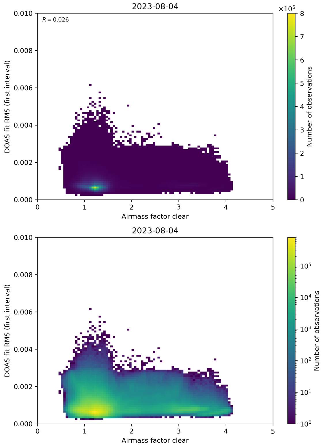
Figure 71: Scatter density plot of “Airmass factor clear” against “DOAS fit RMS (first interval)” for 2023-08-04 to 2023-08-05.
