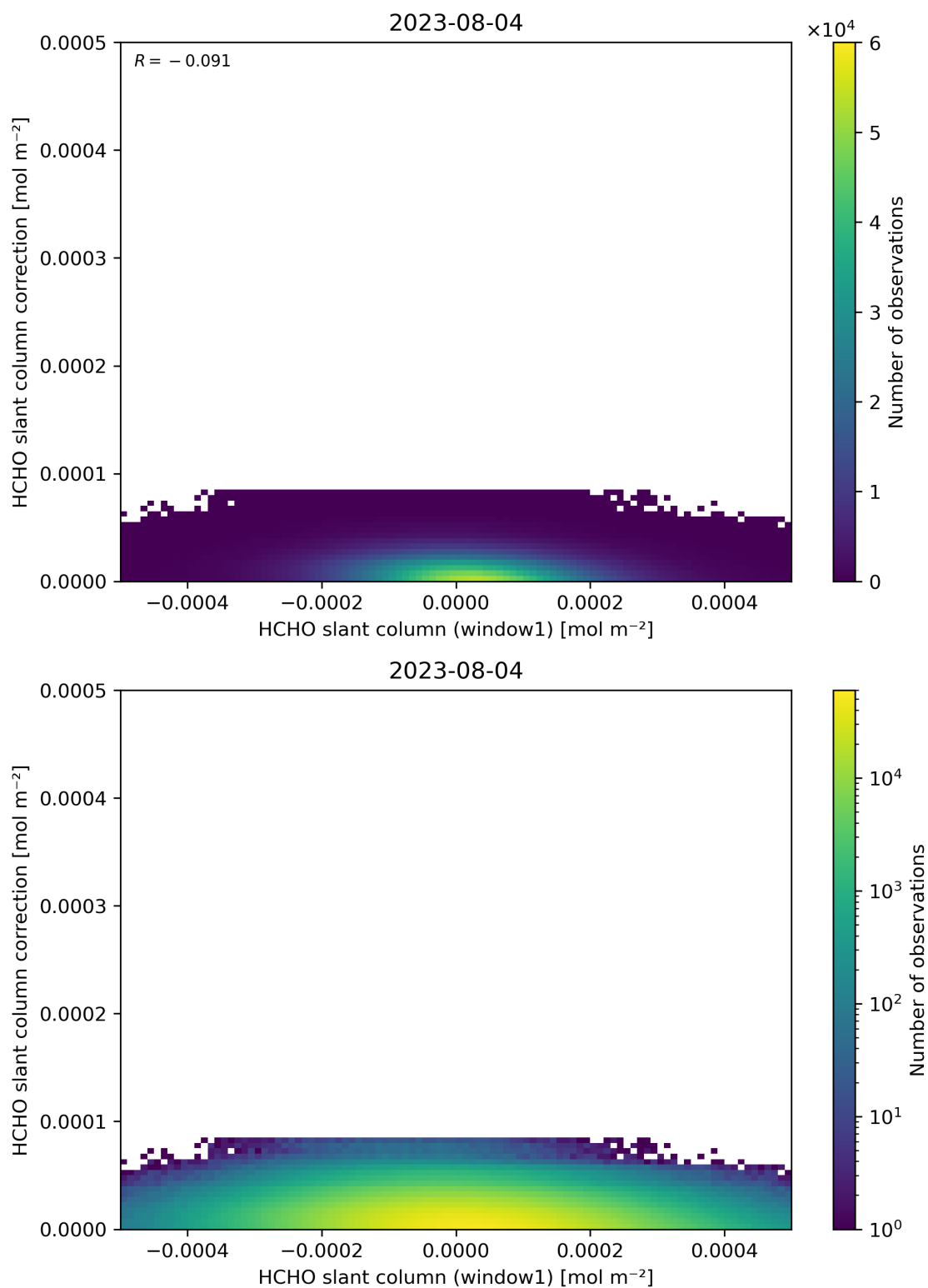
Figure 83: Scatter density plot of “HCHO slant column (window1)” against “HCHO slant column correction” for 2023-08-04 to 2023-08-05.
