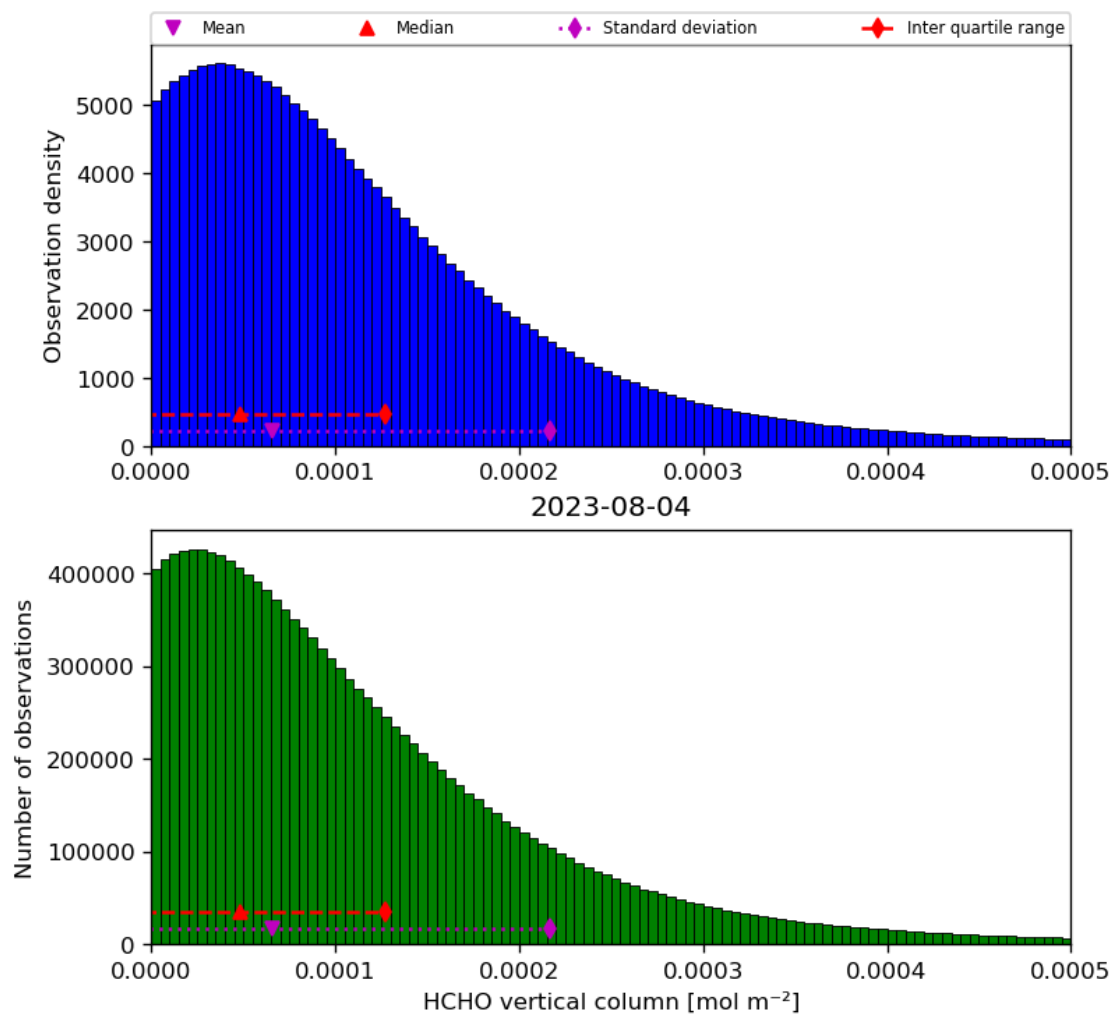
Figure 35: Histogram of “HCHO vertical column” for 2023-08-04 to 2023-08-05
