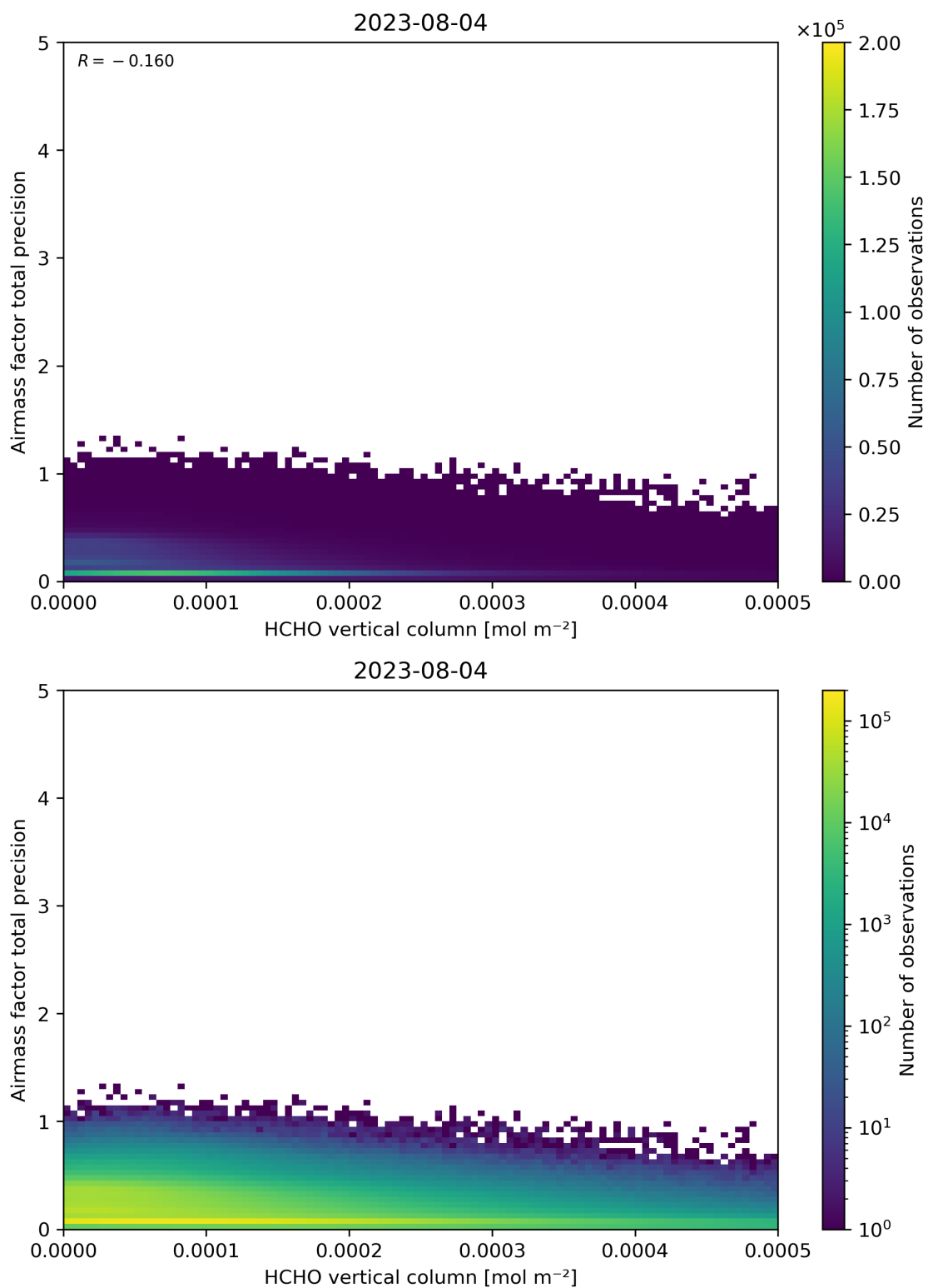
Figure 132: Scatter density plot of “HCHO vertical column” against “Airmass factor total precision” for 2023-08-04 to 2023-08-05.
