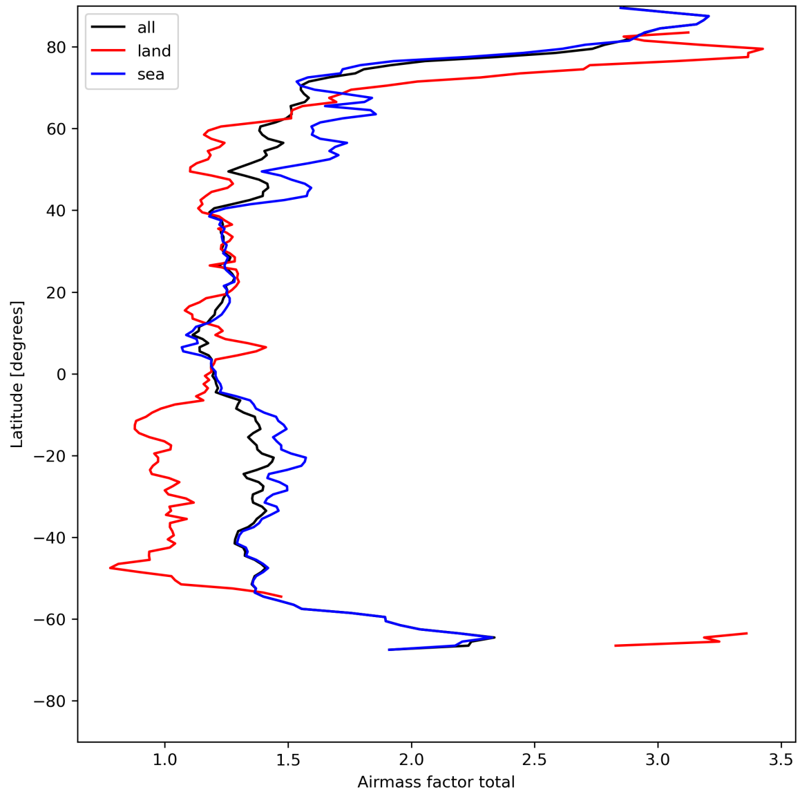
Figure 26: Zonal average of “Airmass factor total” for 2023-08-04 to 2023-08-05.
