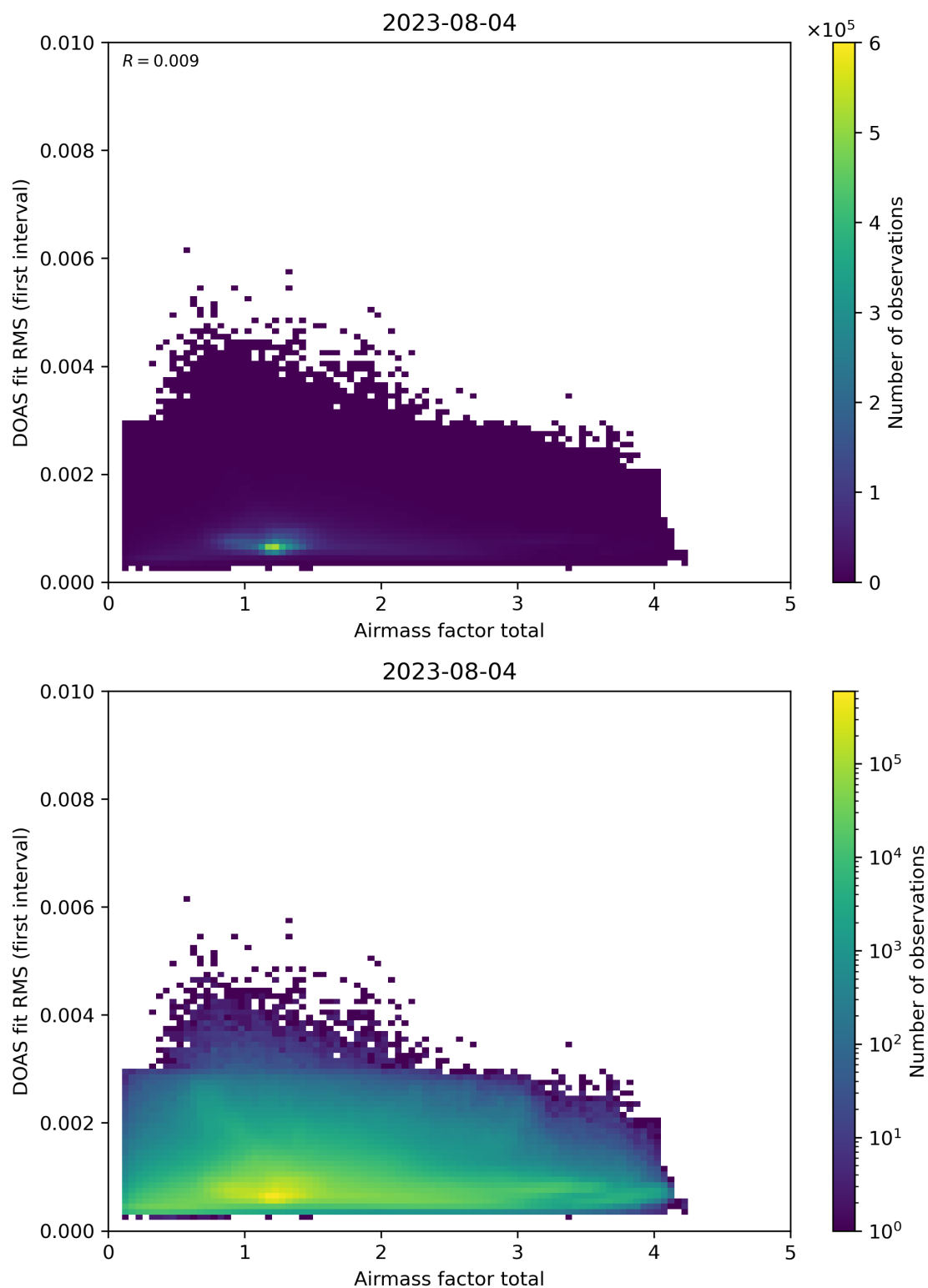
Figure 97: Scatter density plot of “Airmass factor total” against “DOAS fit RMS (first interval)” for 2023-08-04 to 2023-08-05.
