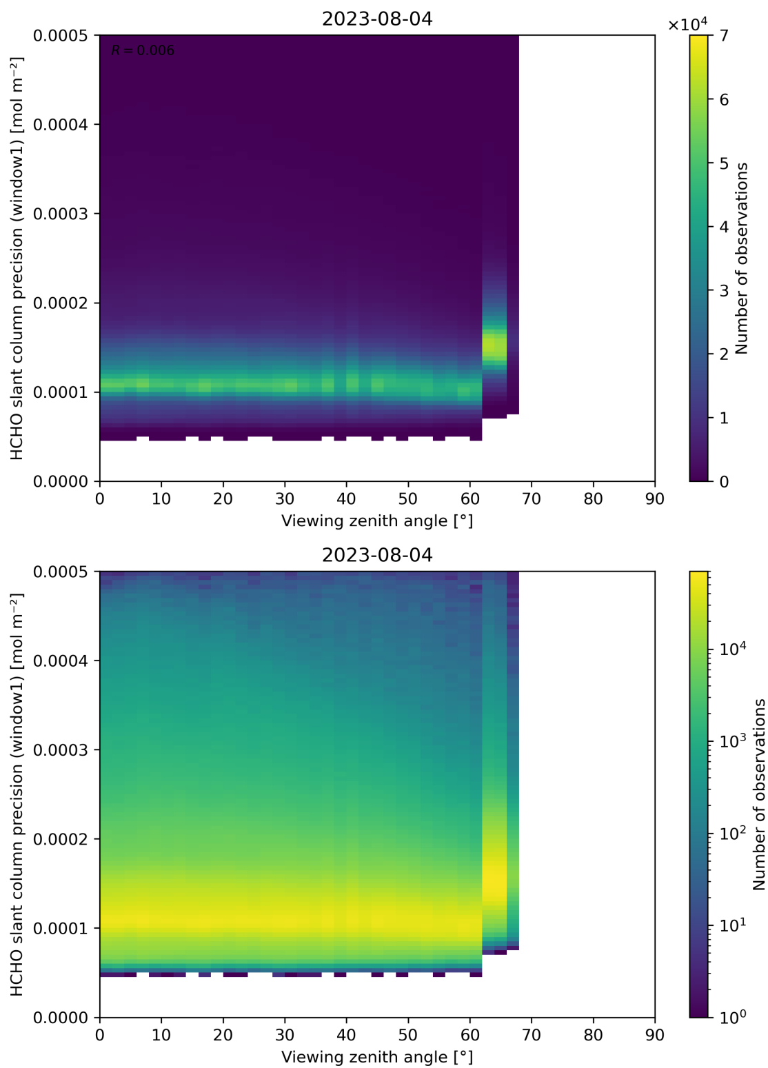
Figure 189: Scatter density plot of “Viewing zenith angle” against “HCHO slant column precision (window1)” for 2023-08-04 to 2023-08-05.
