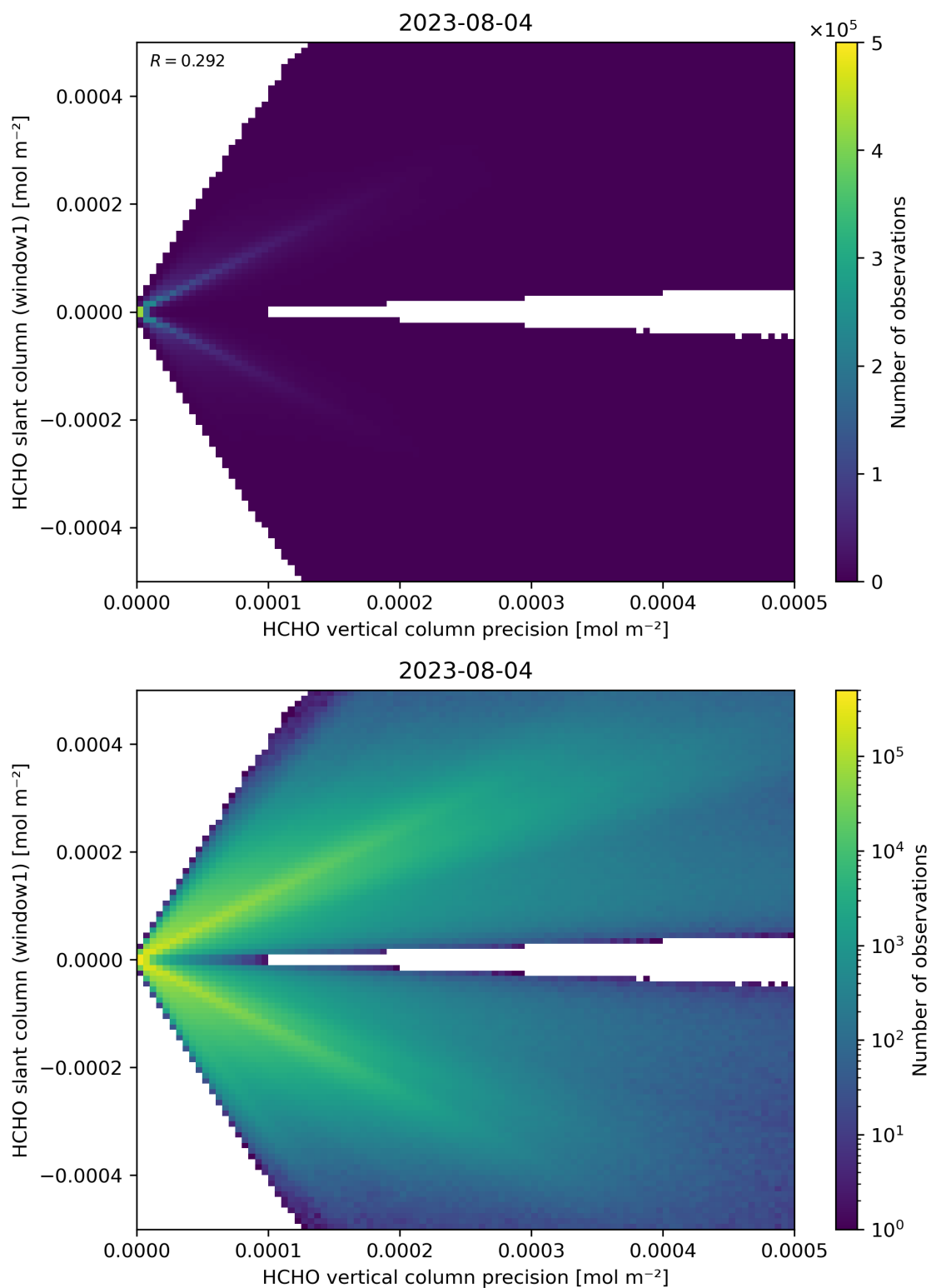
Figure 142: Scatter density plot of “HCHO vertical column precision” against “HCHO slant column (window1)” for 2023-08-04 to 2023-08-05.
