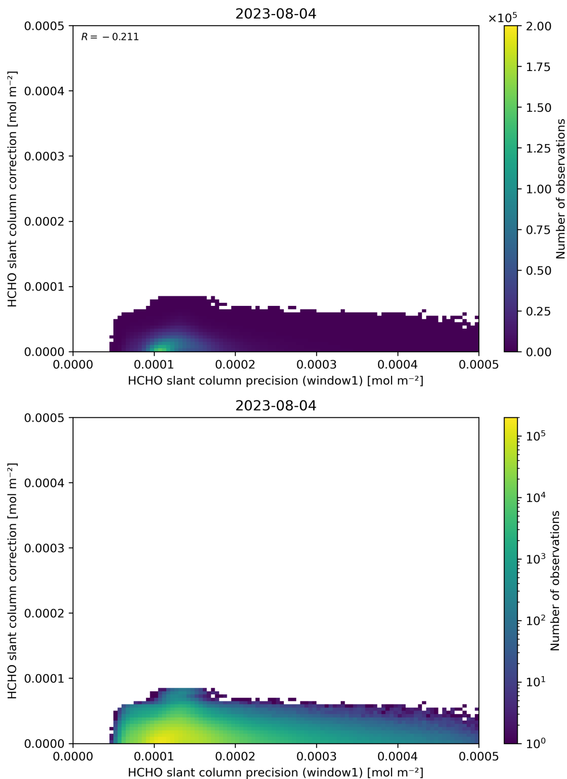
Figure 93: Scatter density plot of “HCHO slant column precision (window1)” against “HCHO slant column correction” for 2023-08-04 to 2023-08-05.
