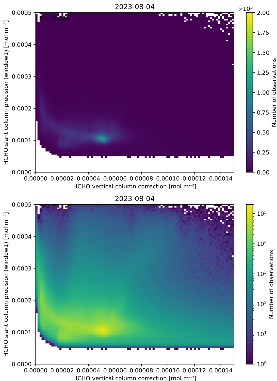
Figure 119: Scatter density plot of “HCHO vertical column correction” against “HCHO slant column precision (window1)” for 2023-08-04 to 2023-08-05.
