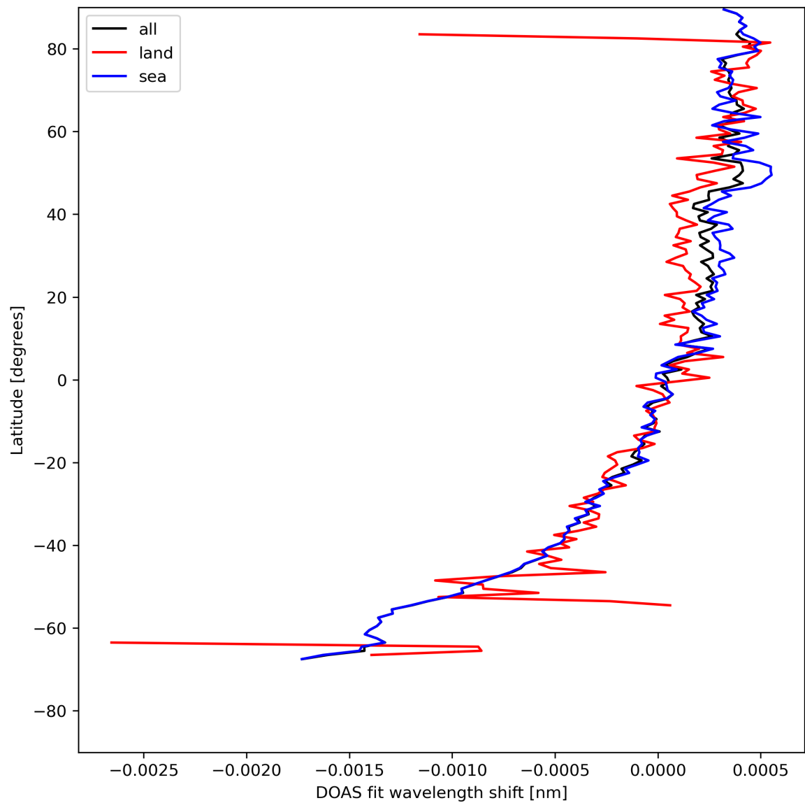
Figure 30: Zonal average of “DOAS fit wavelength shift” for 2023-08-04 to 2023-08-05.
