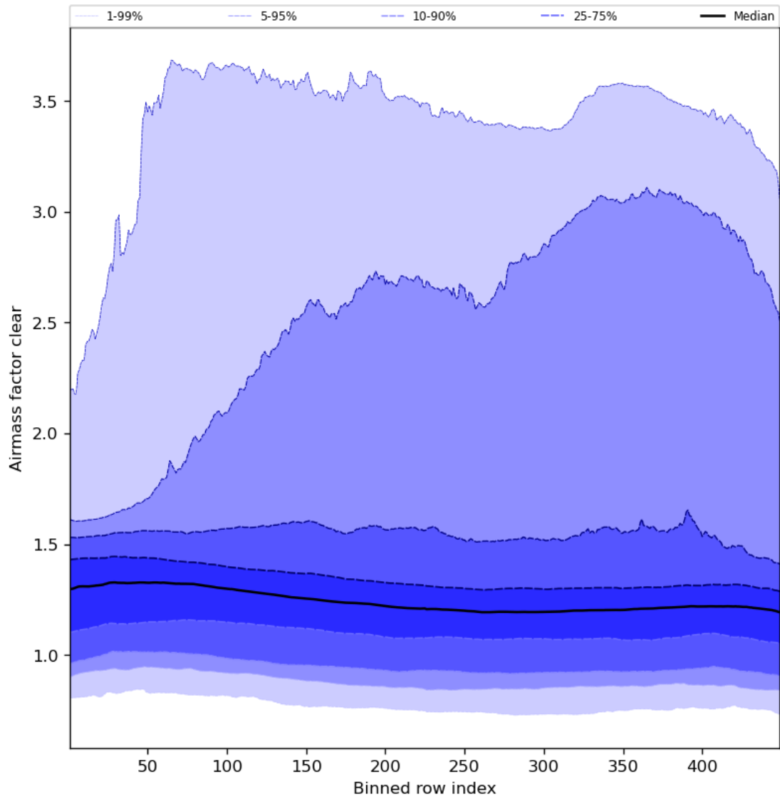
Figure 56: Along track statistics of “Airmass factor clear” for 2023-08-04 to 2023-08-05
