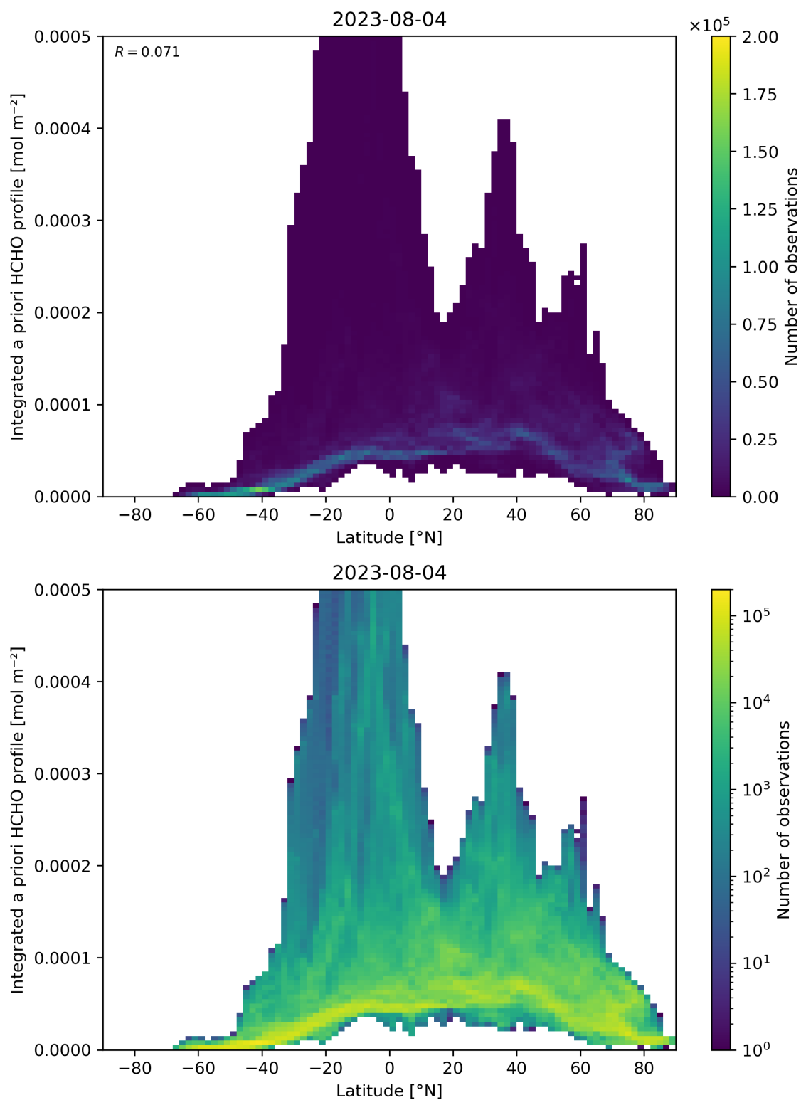
Figure 166: Scatter density plot of “Latitude” against “Integrated a priori HCHO profile” for 2023-08-04 to 2023-08-05.
