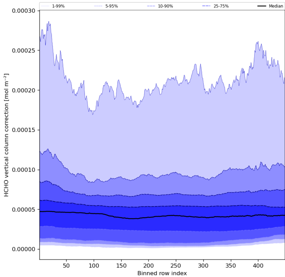
Figure 51: Along track statistics of “HCHO vertical column correction” for 2023-08-04 to 2023-08-05
