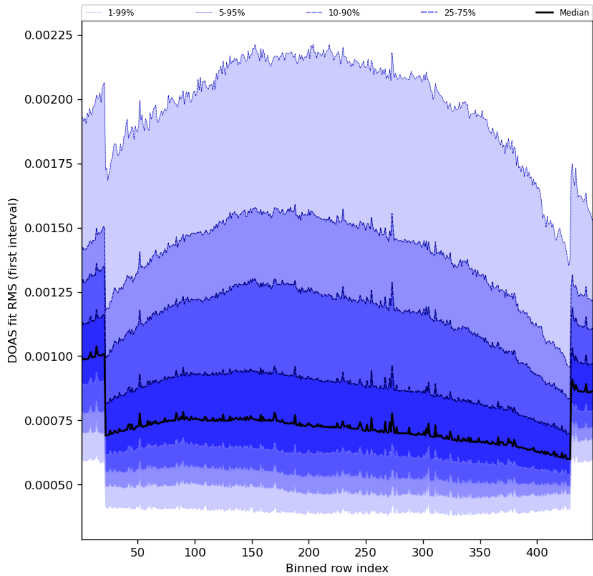
Figure 60: Along track statistics of “DOAS fit RMS (first interval)” for 2023-08-04 to 2023-08-05
