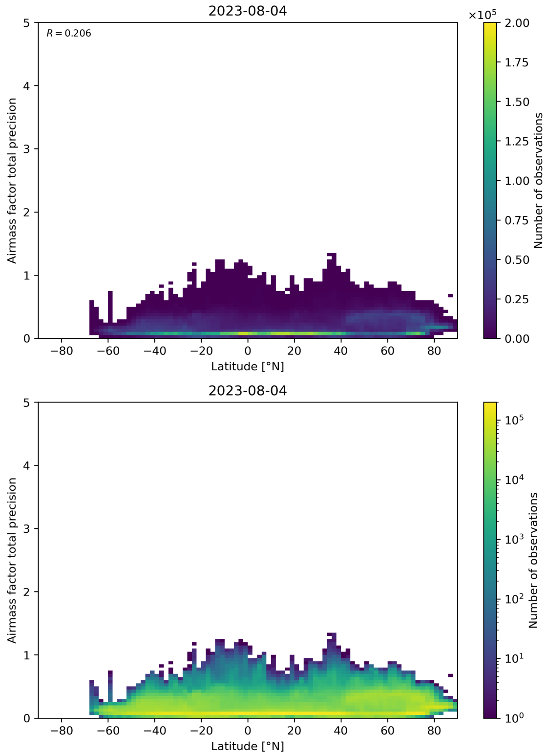
Figure 162: Scatter density plot of “Latitude” against “Airmass factor total precision” for 2023-08-04 to 2023-08-05.
