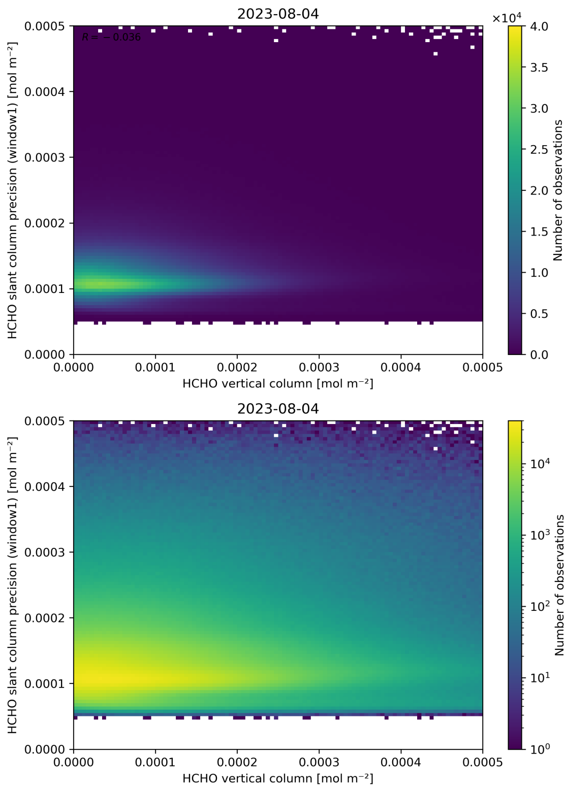
Figure 130: Scatter density plot of “HCHO vertical column” against “HCHO slant column precision (window1)” for 2023-08-04 to 2023-08-05.
