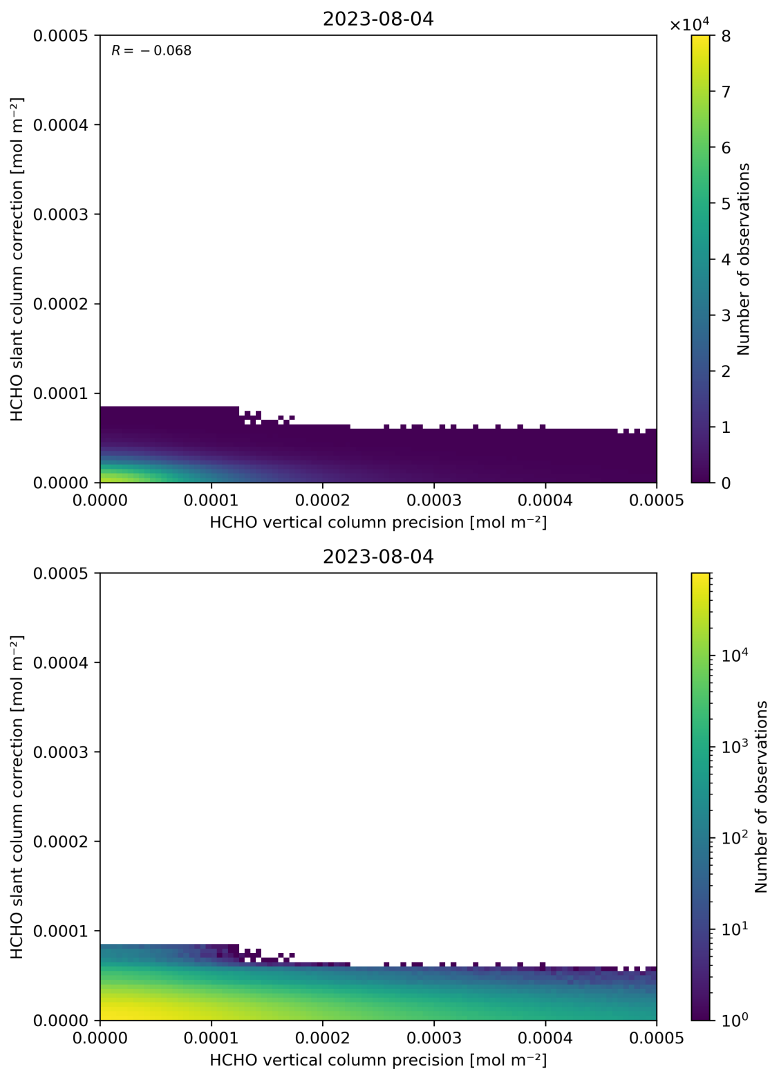
Figure 141: Scatter density plot of “HCHO vertical column precision” against “HCHO slant column correction” for 2023-08-04 to 2023-08-05.
