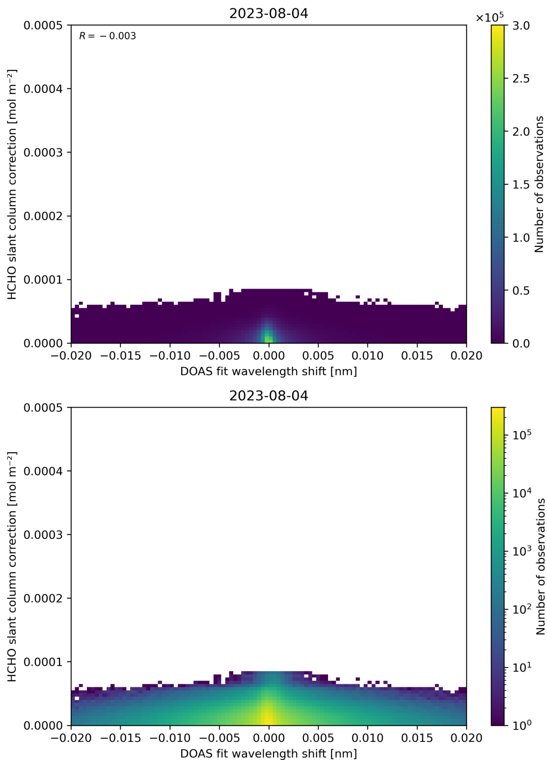
Figure 67: Scatter density plot of “DOAS fit wavelength shift” against “HCHO slant column correction” for 2023-08-04 to 2023-08-05.
