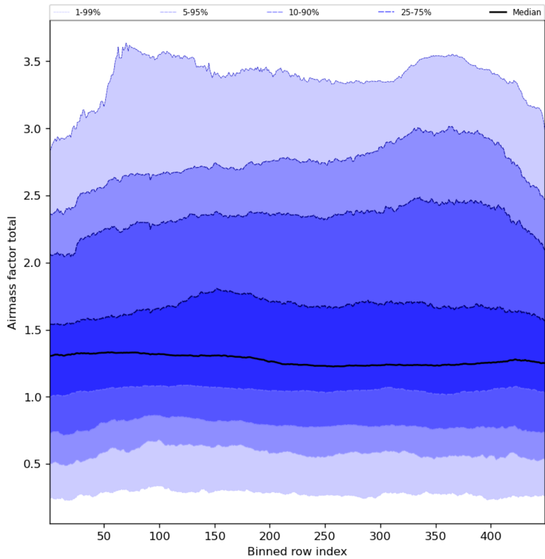
Figure 54: Along track statistics of “Airmass factor total” for 2023-08-04 to 2023-08-05
