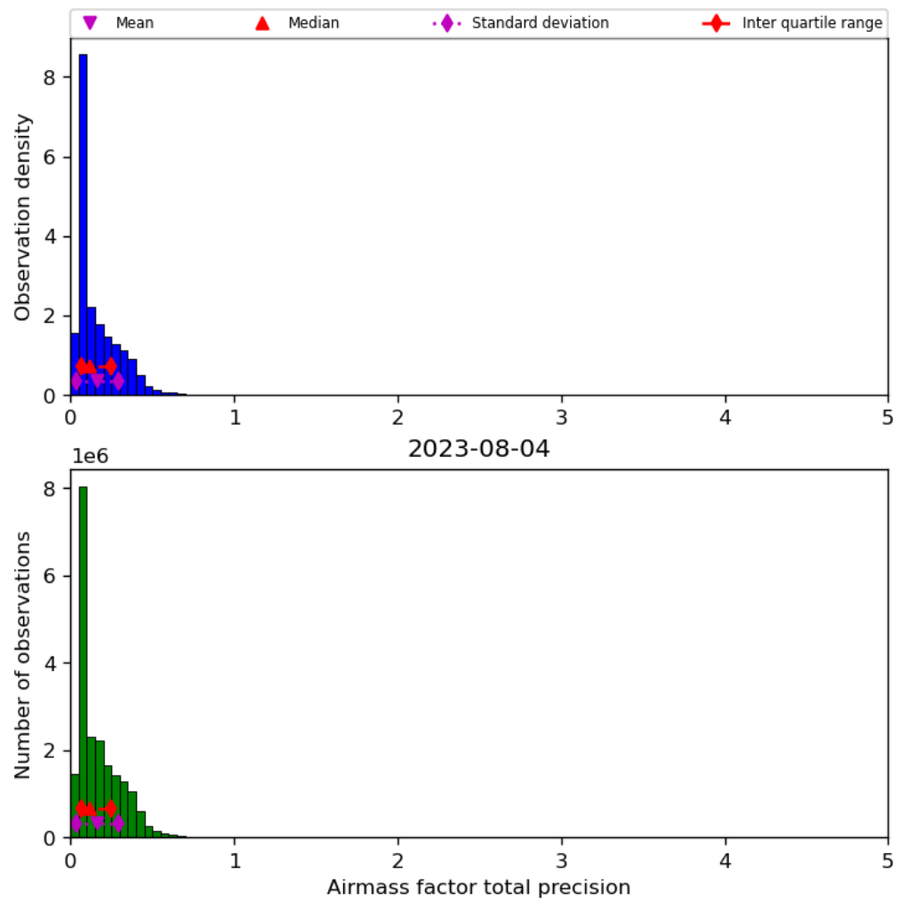
Figure 41: Histogram of “Airmass factor total precision” for 2023-08-04 to 2023-08-05
