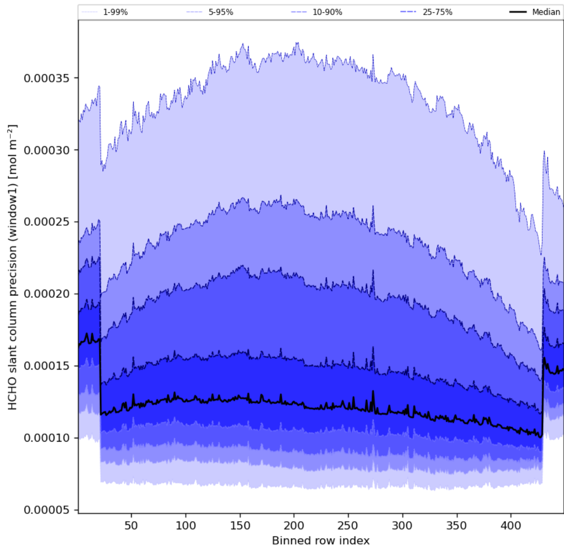
Figure 53: Along track statistics of “HCHO slant column precision (window1)” for 2023-08-04 to 2023-08-05
