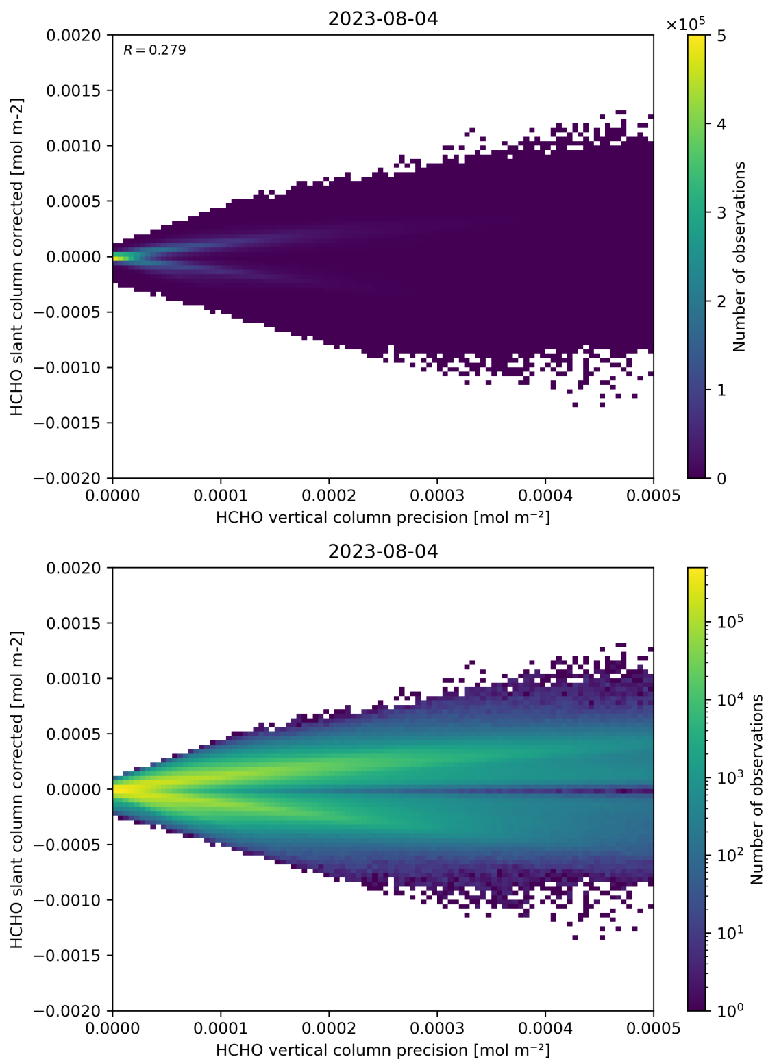
Figure 140: Scatter density plot of “HCHO vertical column precision” against “HCHO slant column corrected” for 2023-08-04 to 2023-08-05.
