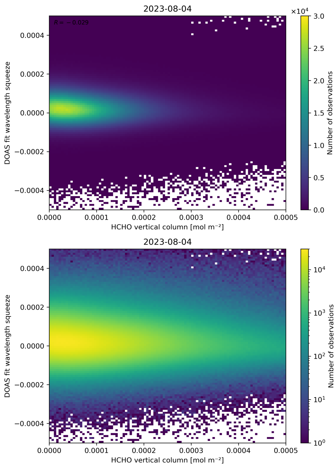
Figure 125: Scatter density plot of “HCHO vertical column” against “DOAS fit wavelength squeeze” for 2023-08-04 to 2023-08-05.
