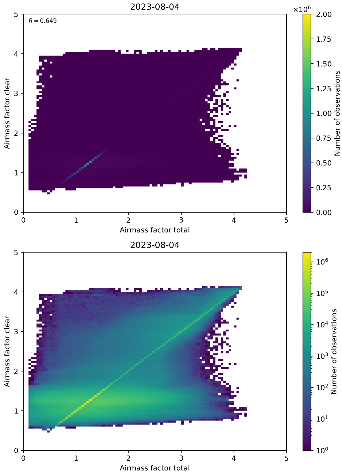
Figure 100: Scatter density plot of “Airmass factor total” against “Airmass factor clear” for 2023-08-04 to 2023-08-05.
