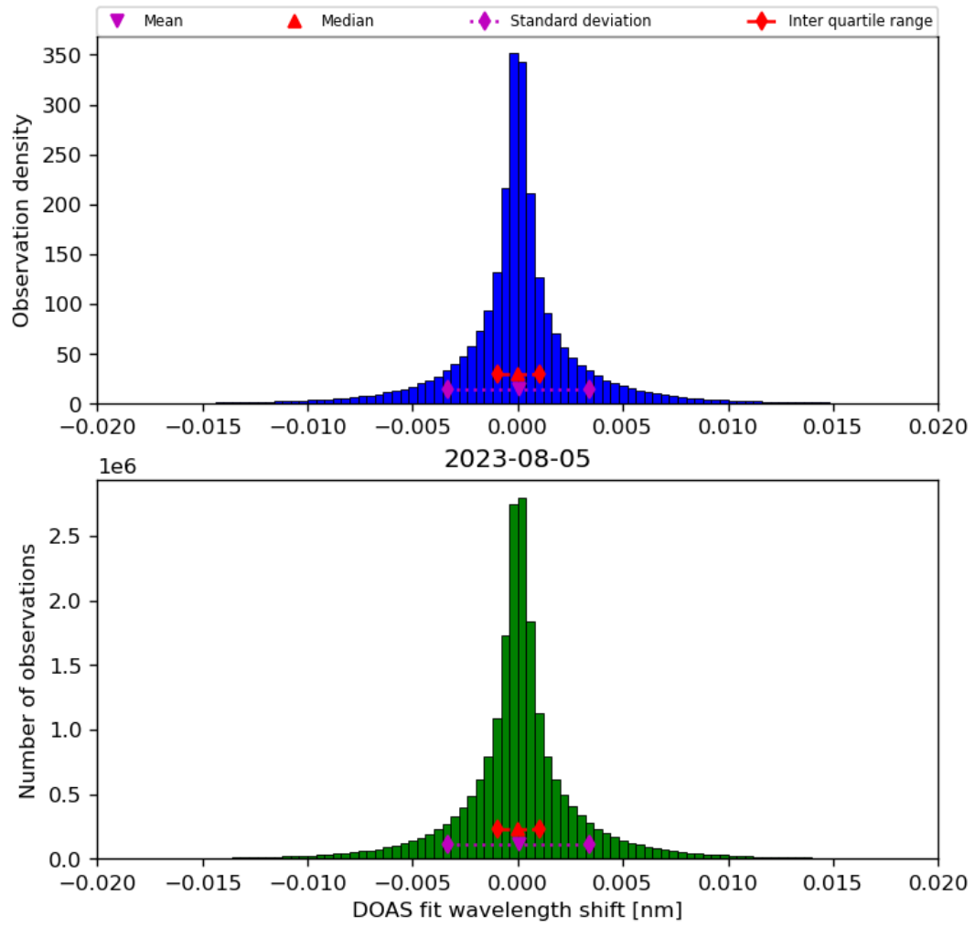
Figure 44: Histogram of “DOAS fit wavelength shift” for 2023-08-04 to 2023-08-06
