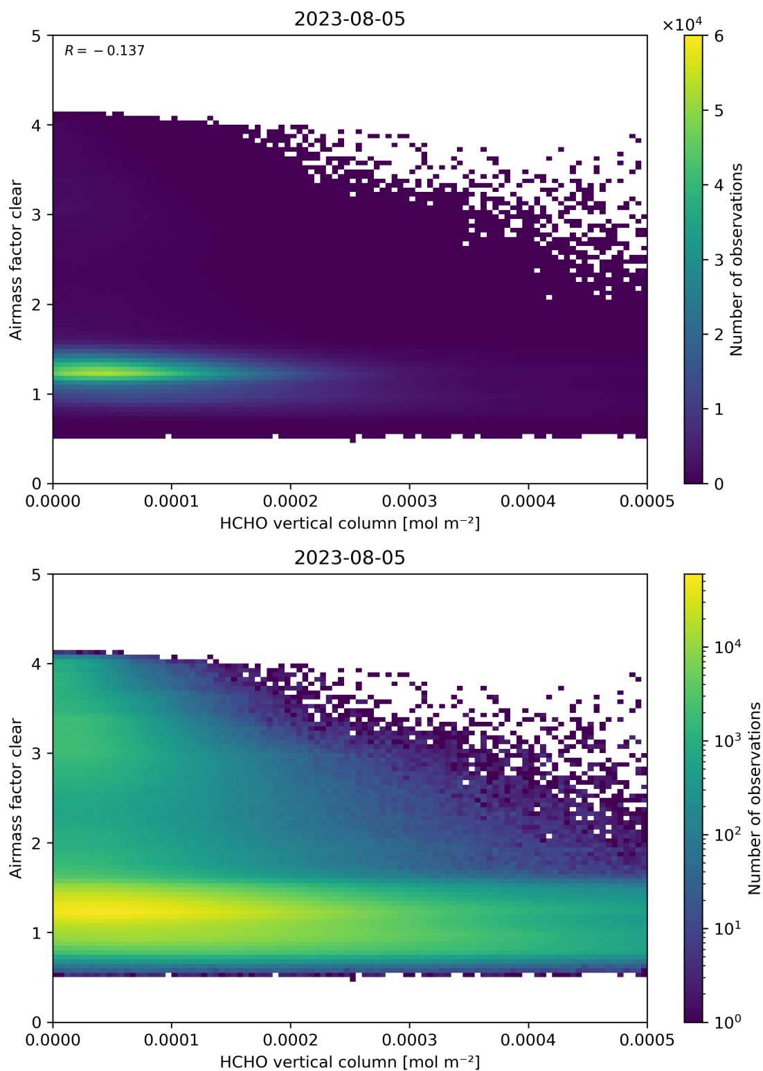
Figure 126: Scatter density plot of “HCHO vertical column” against “Airmass factor clear” for 2023-08-04 to 2023-08-06.
