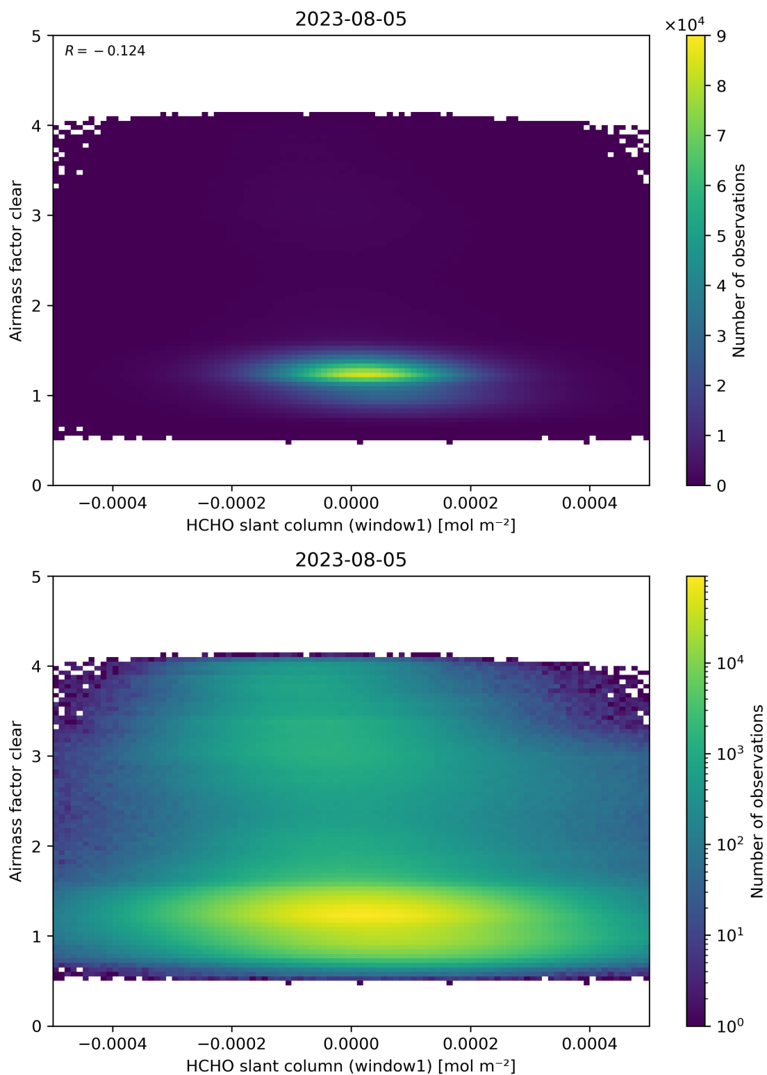
Figure 81: Scatter density plot of “HCHO slant column (window1)” against “Airmass factor clear” for 2023-08-04 to 2023-08-06.
