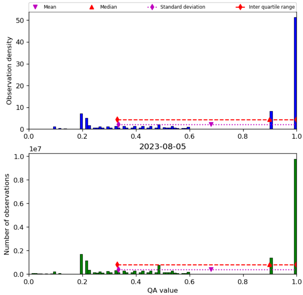
Figure 34: Histogram of “QA value” for 2023-08-04 to 2023-08-06
