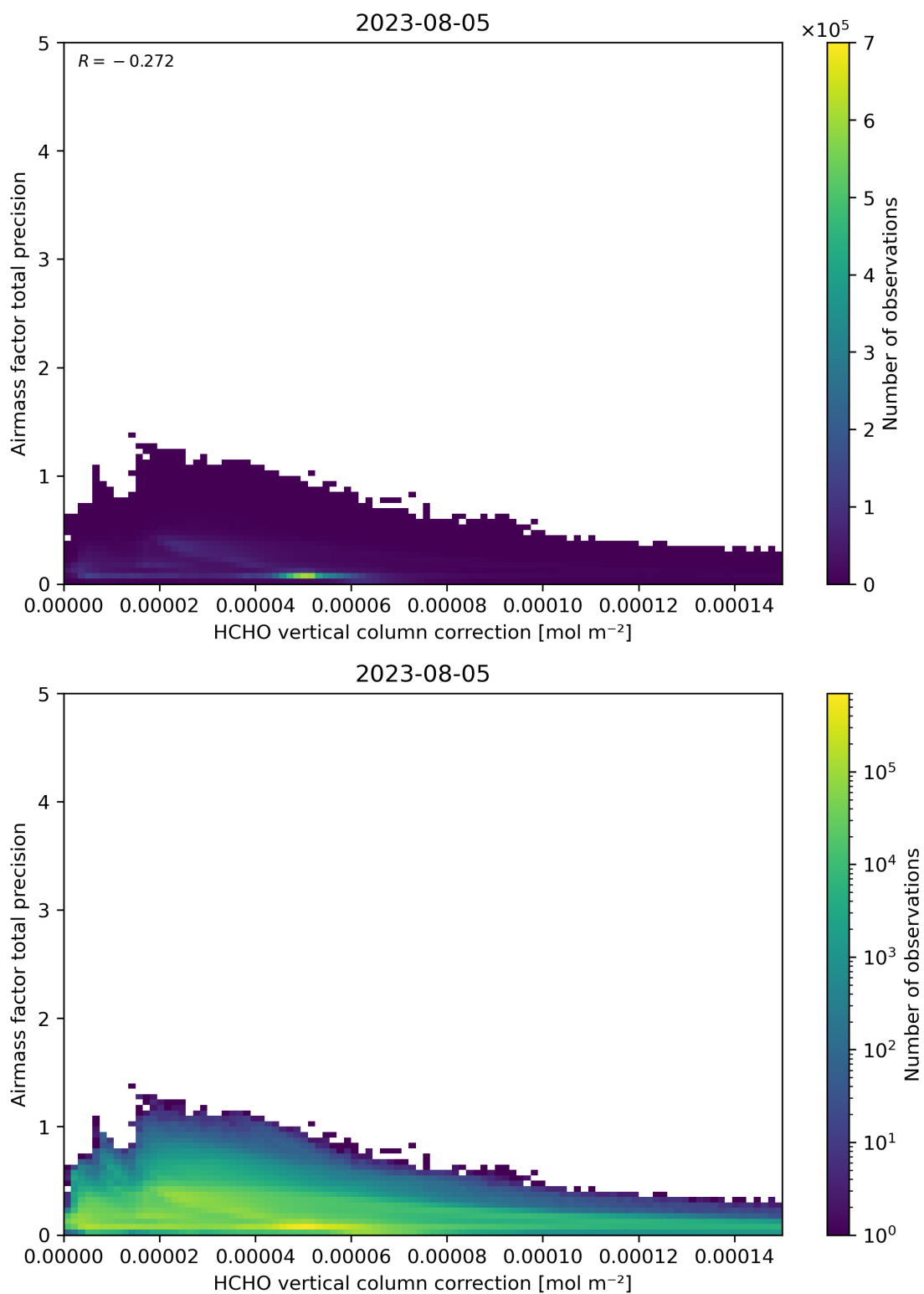
Figure 121: Scatter density plot of “HCHO vertical column correction” against “Airmass factor total precision” for 2023-08-04 to 2023-08-06.
