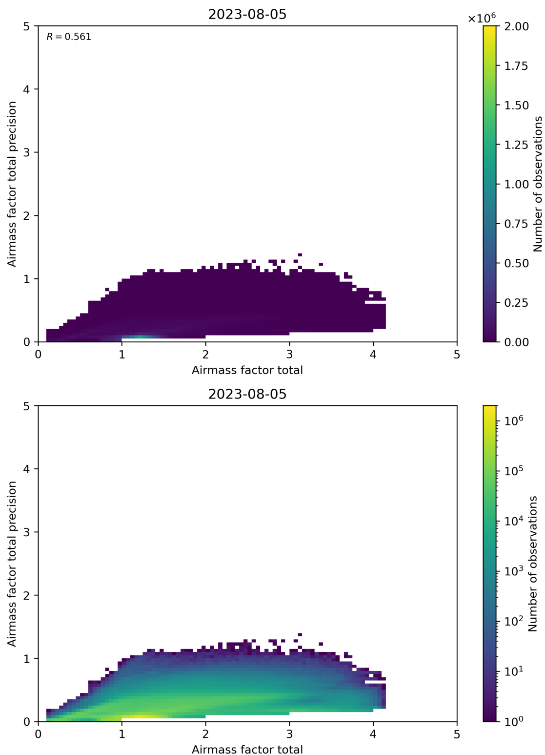
Figure 103: Scatter density plot of “Airmass factor total” against “Airmass factor total precision” for 2023-08-04 to 2023-08-06.
