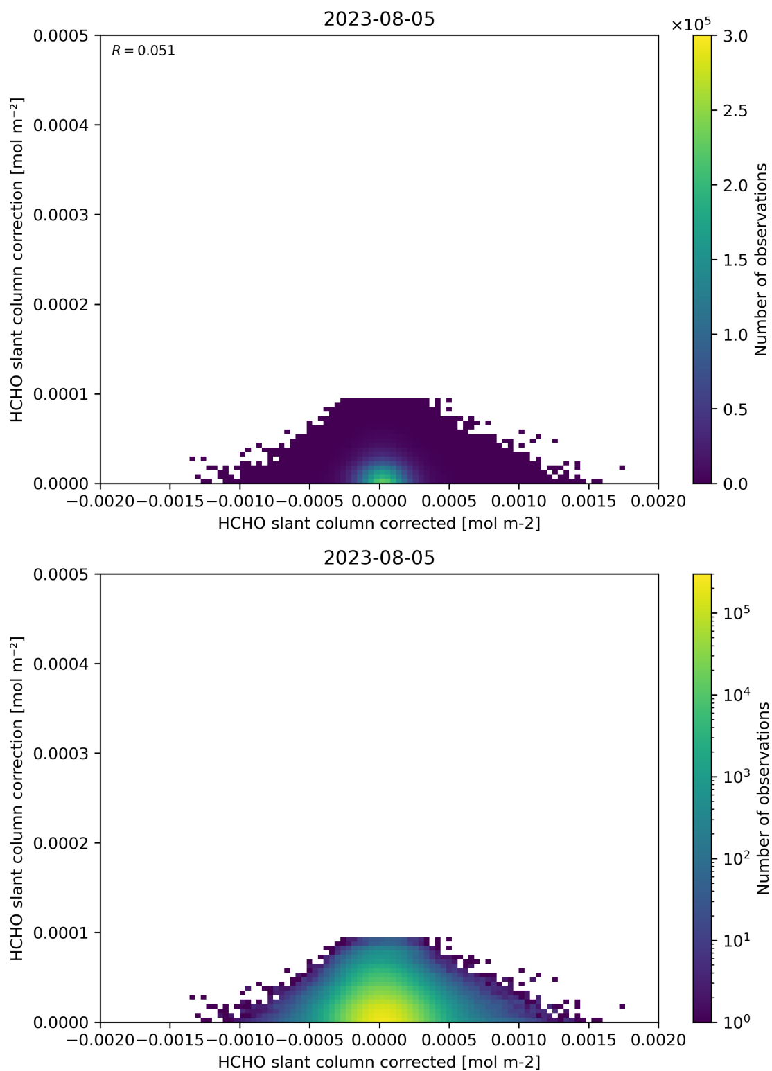
Figure 77: Scatter density plot of “HCHO slant column corrected” against “HCHO slant column correction” for 2023-08-04 to 2023-08-06.
