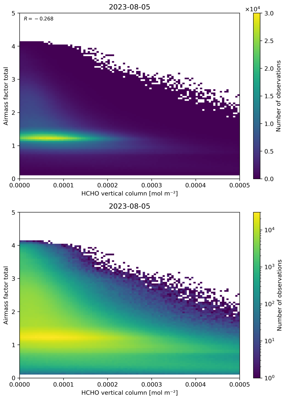
Figure 131: Scatter density plot of “HCHO vertical column” against “Airmass factor total” for 2023-08-04 to 2023-08-06.
