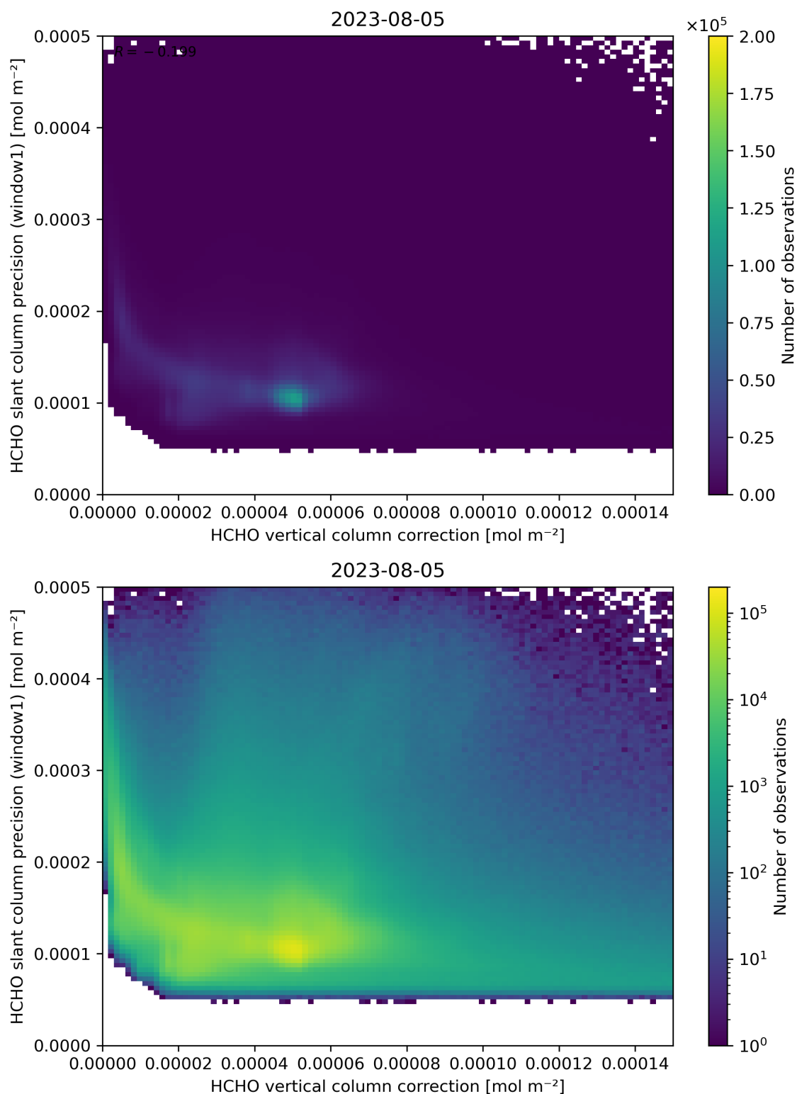
Figure 119: Scatter density plot of “HCHO vertical column correction” against “HCHO slant column precision (window1)” for 2023-08-04 to 2023-08-06.
