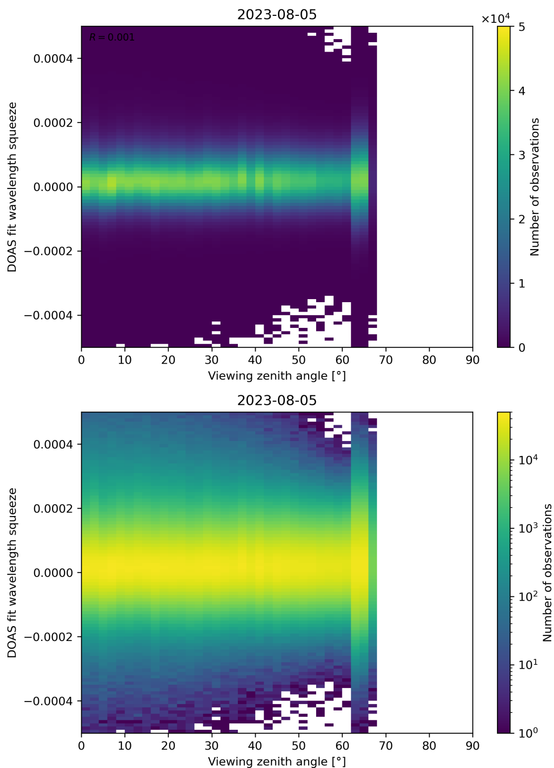
Figure 184: Scatter density plot of “Viewing zenith angle” against “DOAS fit wavelength squeeze” for 2023-08-04 to 2023-08-06.
