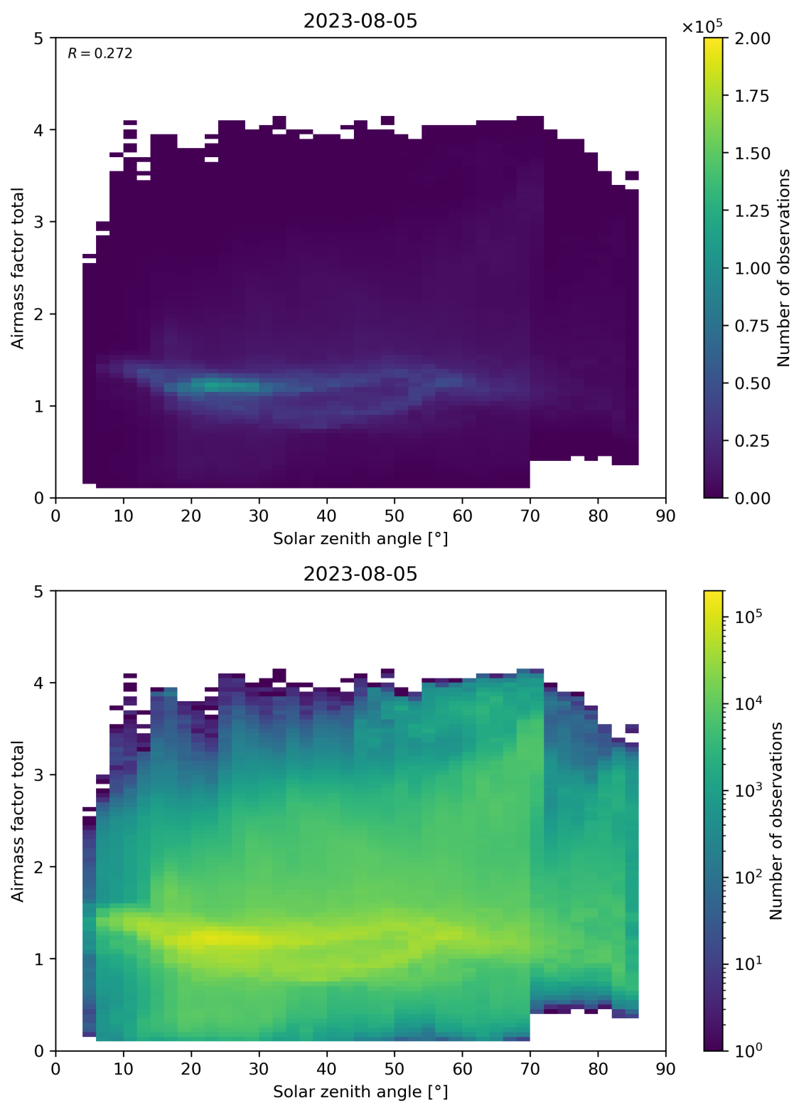
Figure 175: Scatter density plot of “Solar zenith angle” against “Airmass factor total” for 2023-08-04 to 2023-08-06.
