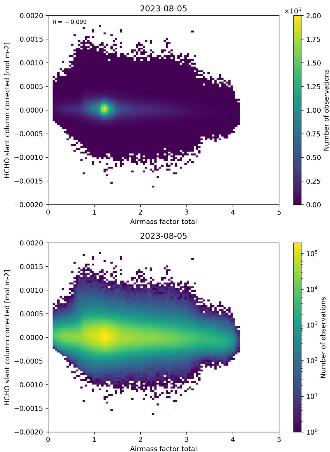
Figure 101: Scatter density plot of “Airmass factor total” against “HCHO slant column corrected” for 2023-08-04 to 2023-08-06.
