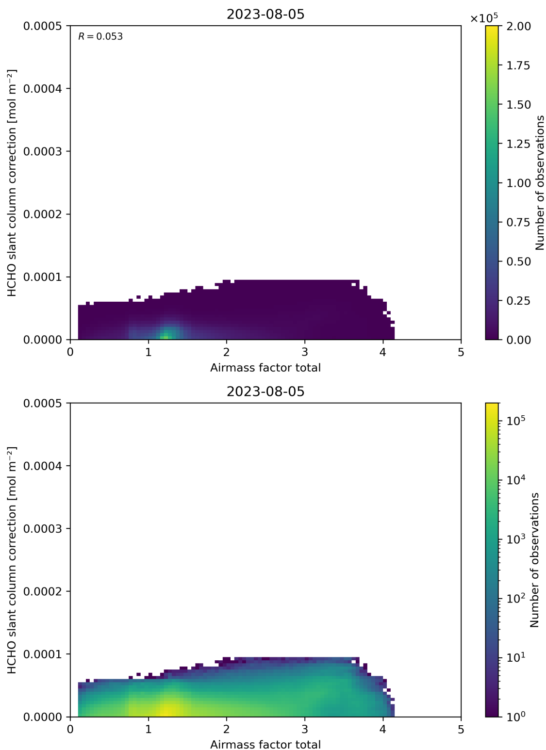
Figure 102: Scatter density plot of “Airmass factor total” against “HCHO slant column correction” for 2023-08-04 to 2023-08-06.
