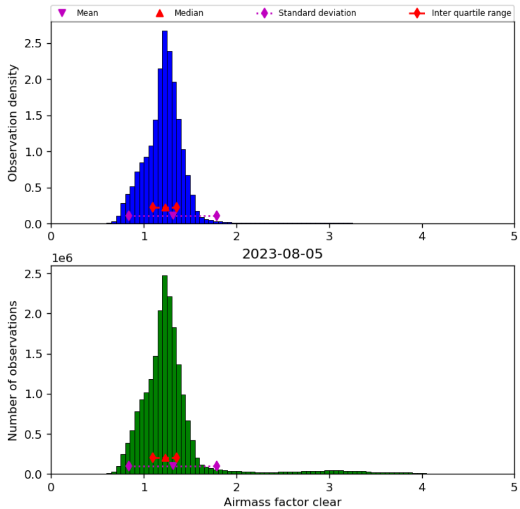
Figure 42: Histogram of “Airmass factor clear” for 2023-08-04 to 2023-08-06
