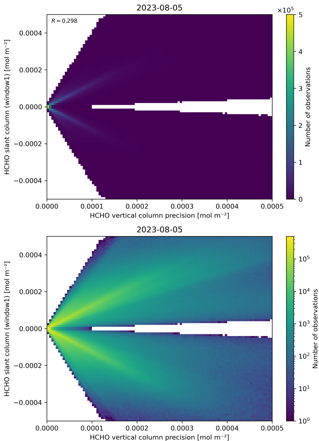
Figure 142: Scatter density plot of “HCHO vertical column precision” against “HCHO slant column (window1)” for 2023-08-04 to 2023-08-06.
