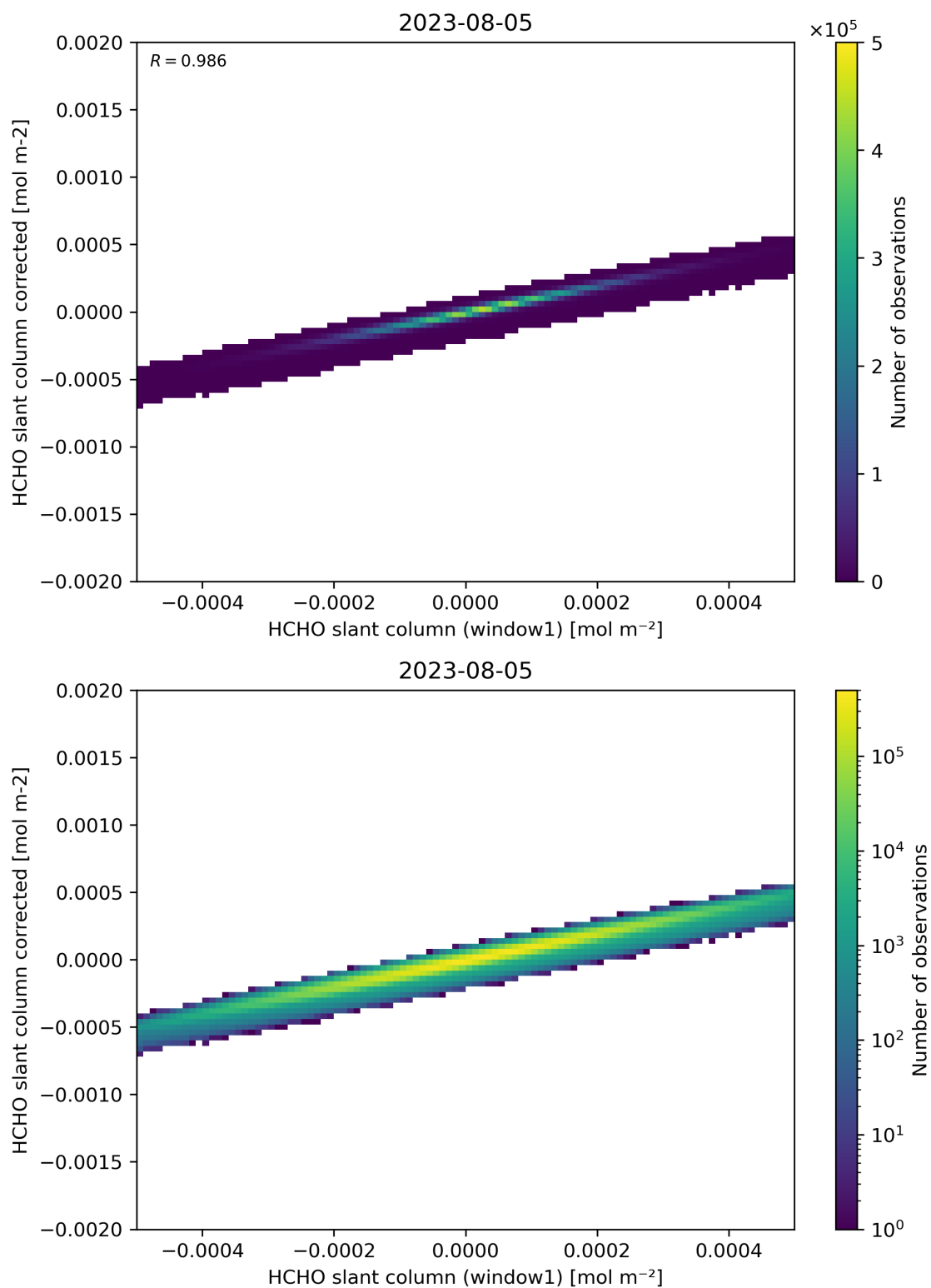
Figure 82: Scatter density plot of “HCHO slant column (window1)” against “HCHO slant column corrected” for 2023-08-04 to 2023-08-06.
