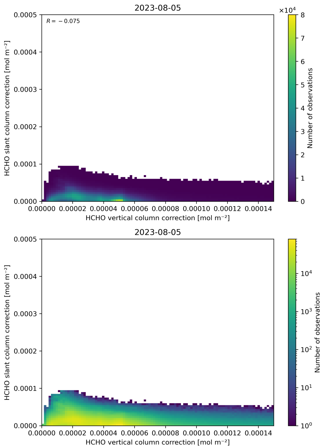
Figure 117: Scatter density plot of “HCHO vertical column correction” against “HCHO slant column correction” for 2023-08-04 to 2023-08-06.
