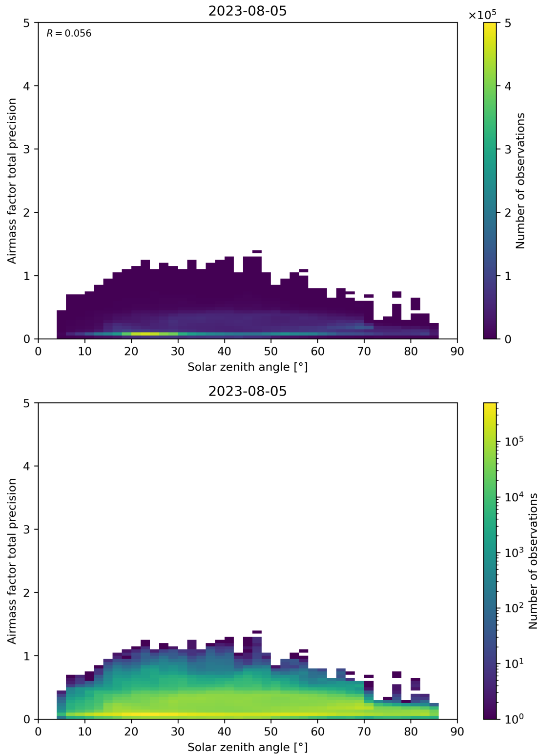
Figure 176: Scatter density plot of “Solar zenith angle” against “Airmass factor total precision” for 2023-08-04 to 2023-08-06.
