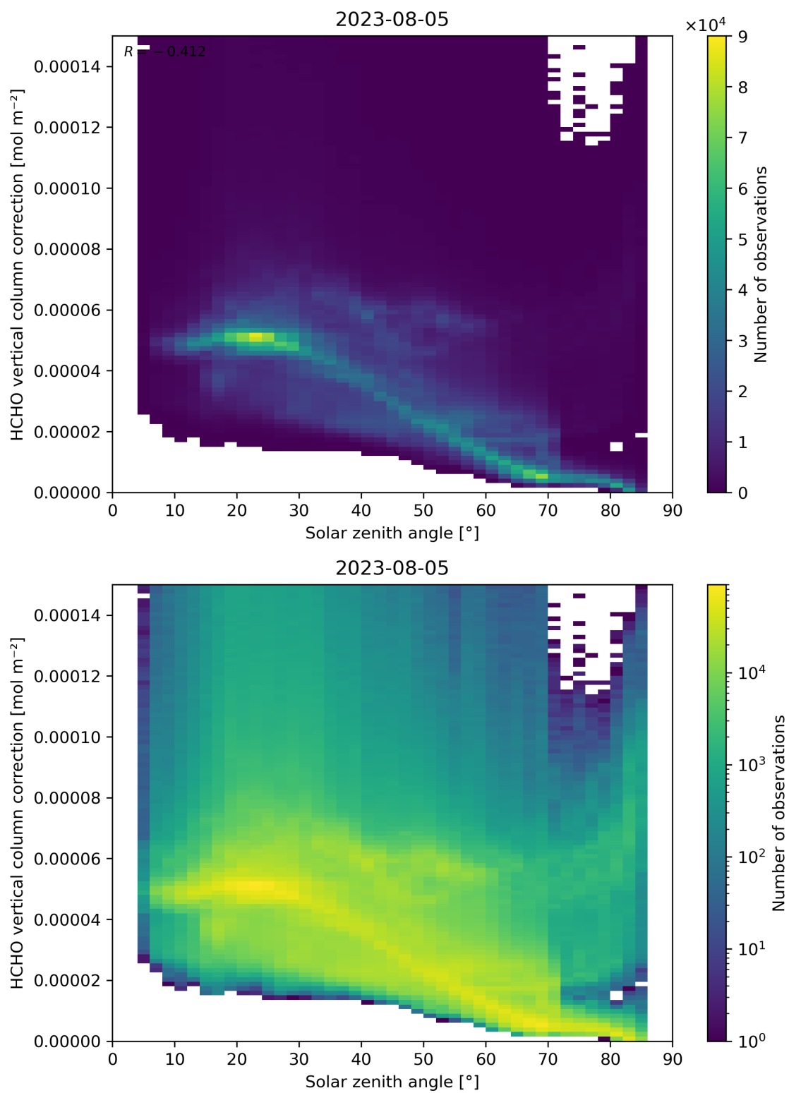
Figure 178: Scatter density plot of “Solar zenith angle” against “HCHO vertical column correction” for 2023-08-04 to 2023-08-06.
