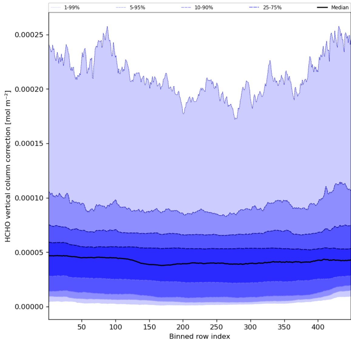
Figure 51: Along track statistics of “HCHO vertical column correction” for 2023-08-04 to 2023-08-06
