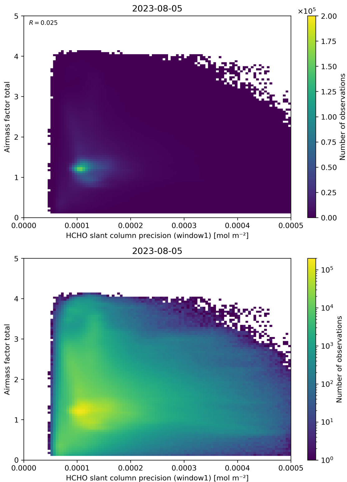
Figure 94: Scatter density plot of “HCHO slant column precision (window1)” against “Airmass factor total” for 2023-08-04 to 2023-08-06.
