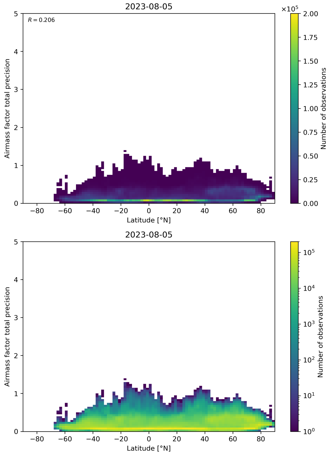
Figure 162: Scatter density plot of “Latitude” against “Airmass factor total precision” for 2023-08-04 to 2023-08-06.
