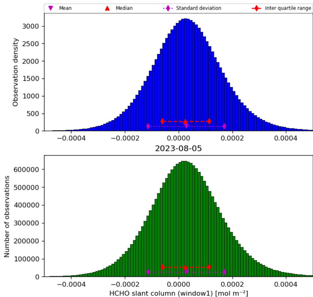
Figure 38: Histogram of “HCHO slant column (window1)” for 2023-08-04 to 2023-08-06
