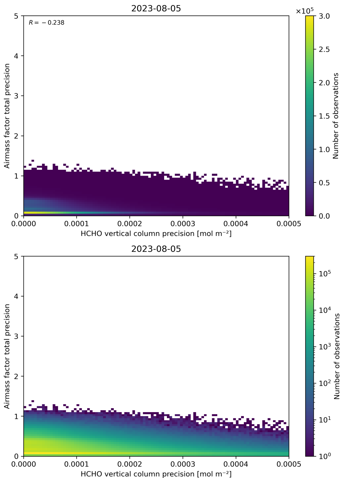
Figure 145: Scatter density plot of “HCHO vertical column precision” against “Airmass factor total precision” for 2023-08-04 to 2023-08-06.
