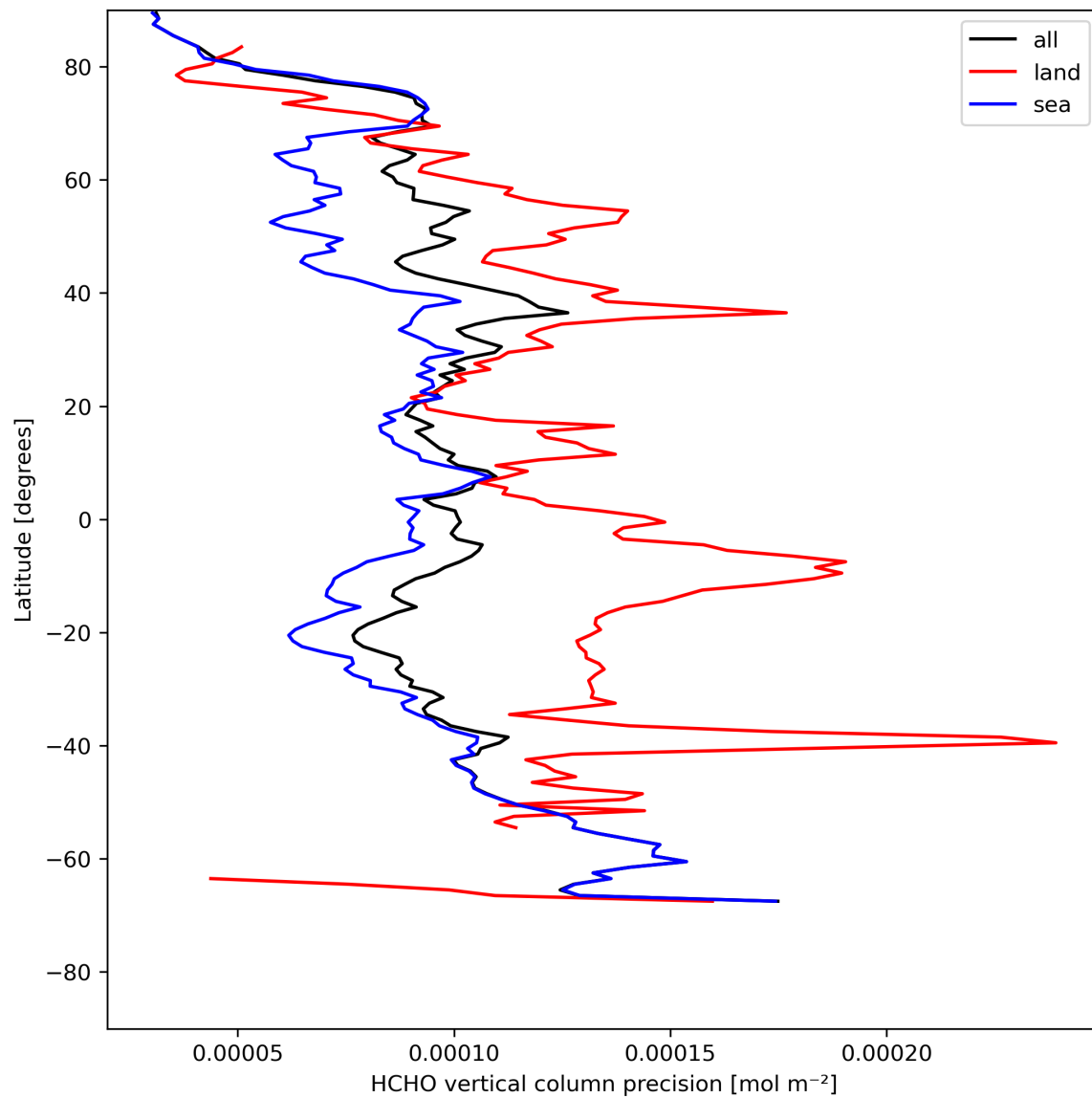
Figure 22: Zonal average of “HCHO vertical column precision” for 2023-08-04 to 2023-08-06.
