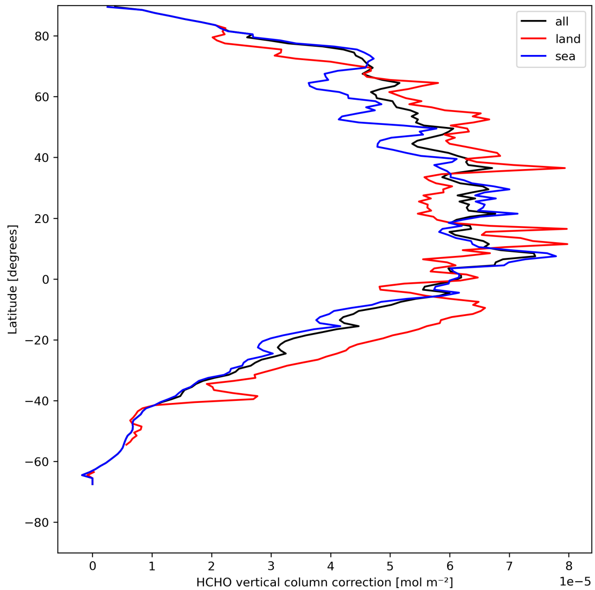
Figure 23: Zonal average of “HCHO vertical column correction” for 2023-08-04 to 2023-08-06.
