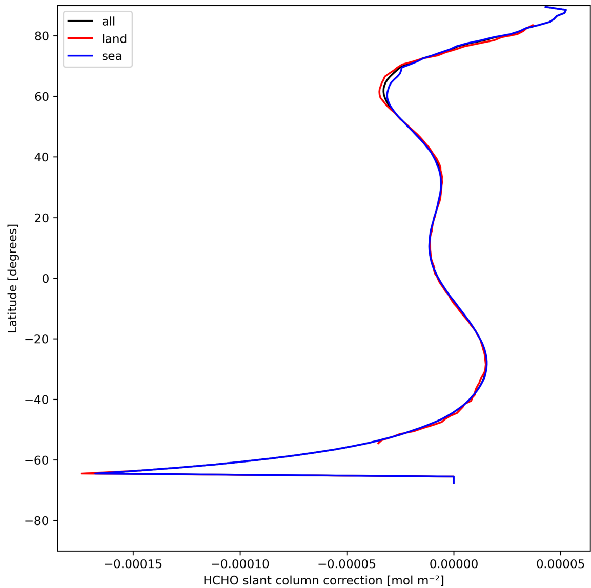
Figure 33: Zonal average of “HCHO slant column correction” for 2023-08-04 to 2023-08-06.
