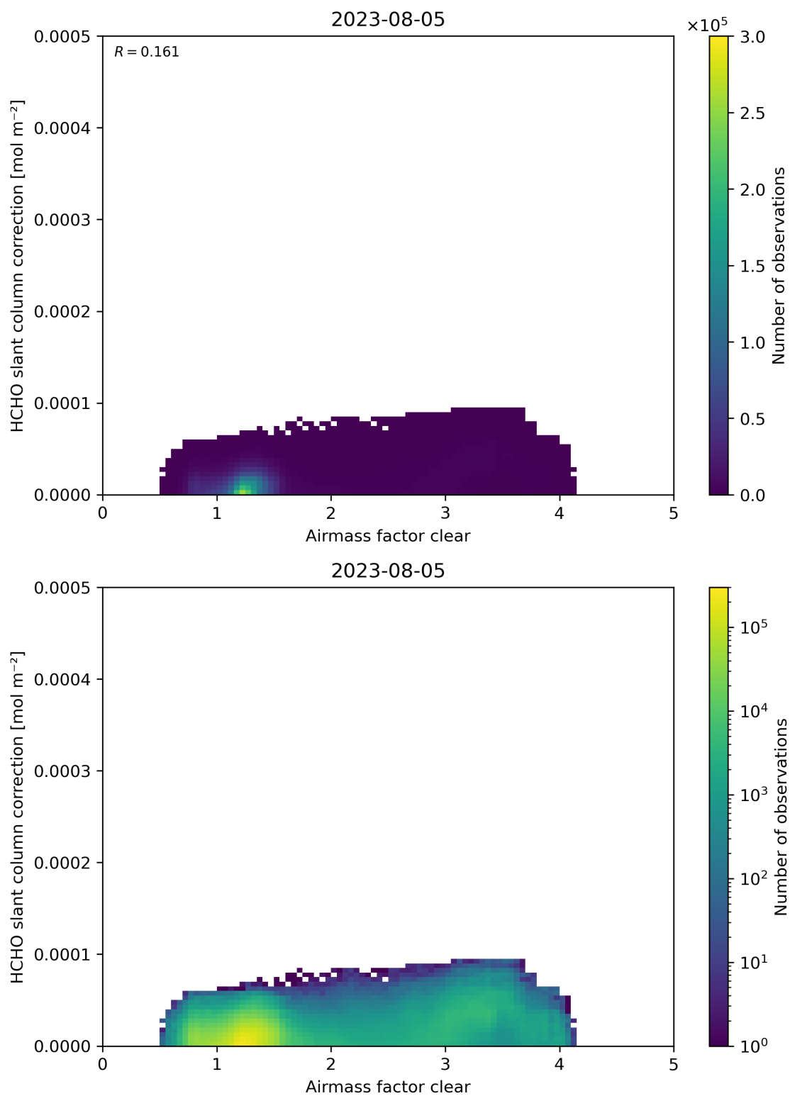
Figure 75: Scatter density plot of “Airmass factor clear” against “HCHO slant column correction” for 2023-08-04 to 2023-08-06.
