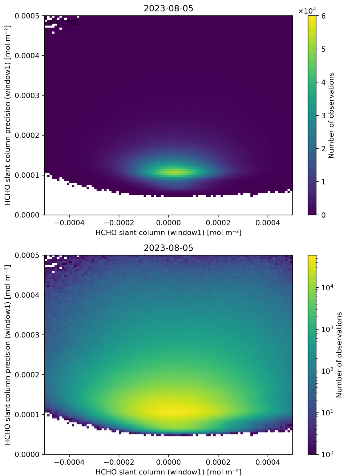
Figure 84: Scatter density plot of “HCHO slant column (window1)” against “HCHO slant column precision (window1)” for 2023-08-04 to 2023-08-06.
