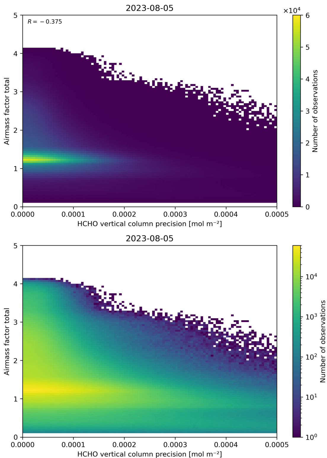
Figure 144: Scatter density plot of “HCHO vertical column precision” against “Airmass factor total” for 2023-08-04 to 2023-08-06.
