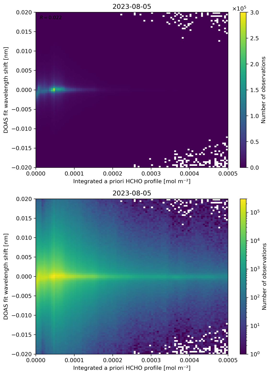
Figure 149: Scatter density plot of “Integrated a priori HCHO profile” against “DOAS fit wavelength shift” for 2023-08-04 to 2023-08-06.
