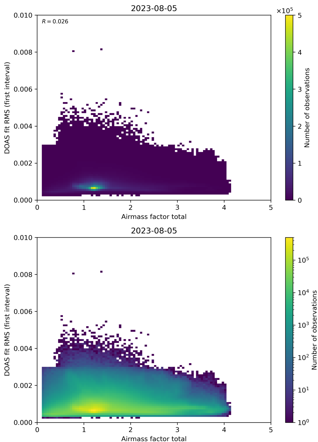
Figure 97: Scatter density plot of “Airmass factor total” against “DOAS fit RMS (first interval)” for 2023-08-04 to 2023-08-06.
