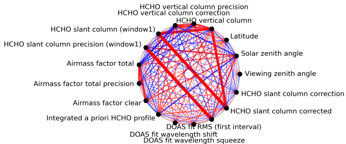
Figure 1: Map of correlation graph for 2023-08-04 to 2023-08-06.
