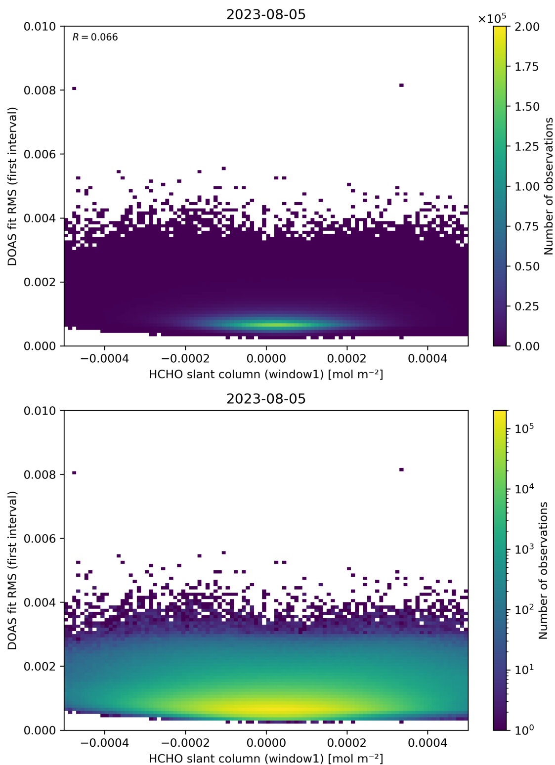
Figure 78: Scatter density plot of “HCHO slant column (window1)” against “DOAS fit RMS (first interval)” for 2023-08-04 to 2023-08-06.
