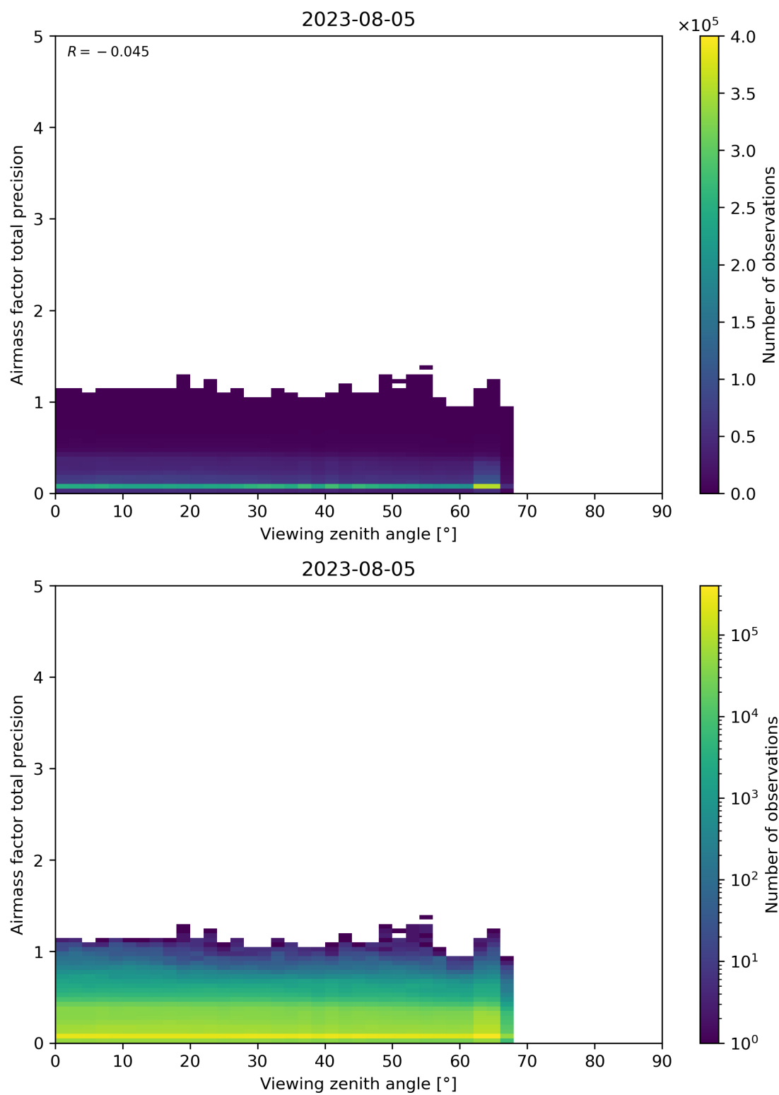
Figure 191: Scatter density plot of “Viewing zenith angle” against “Airmass factor total precision” for 2023-08-04 to 2023-08-06.
