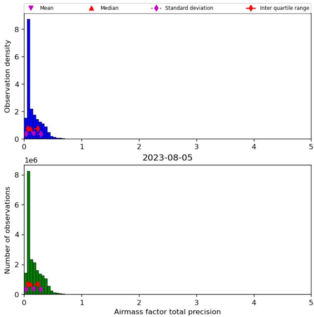
Figure 41: Histogram of “Airmass factor total precision” for 2023-08-04 to 2023-08-06
