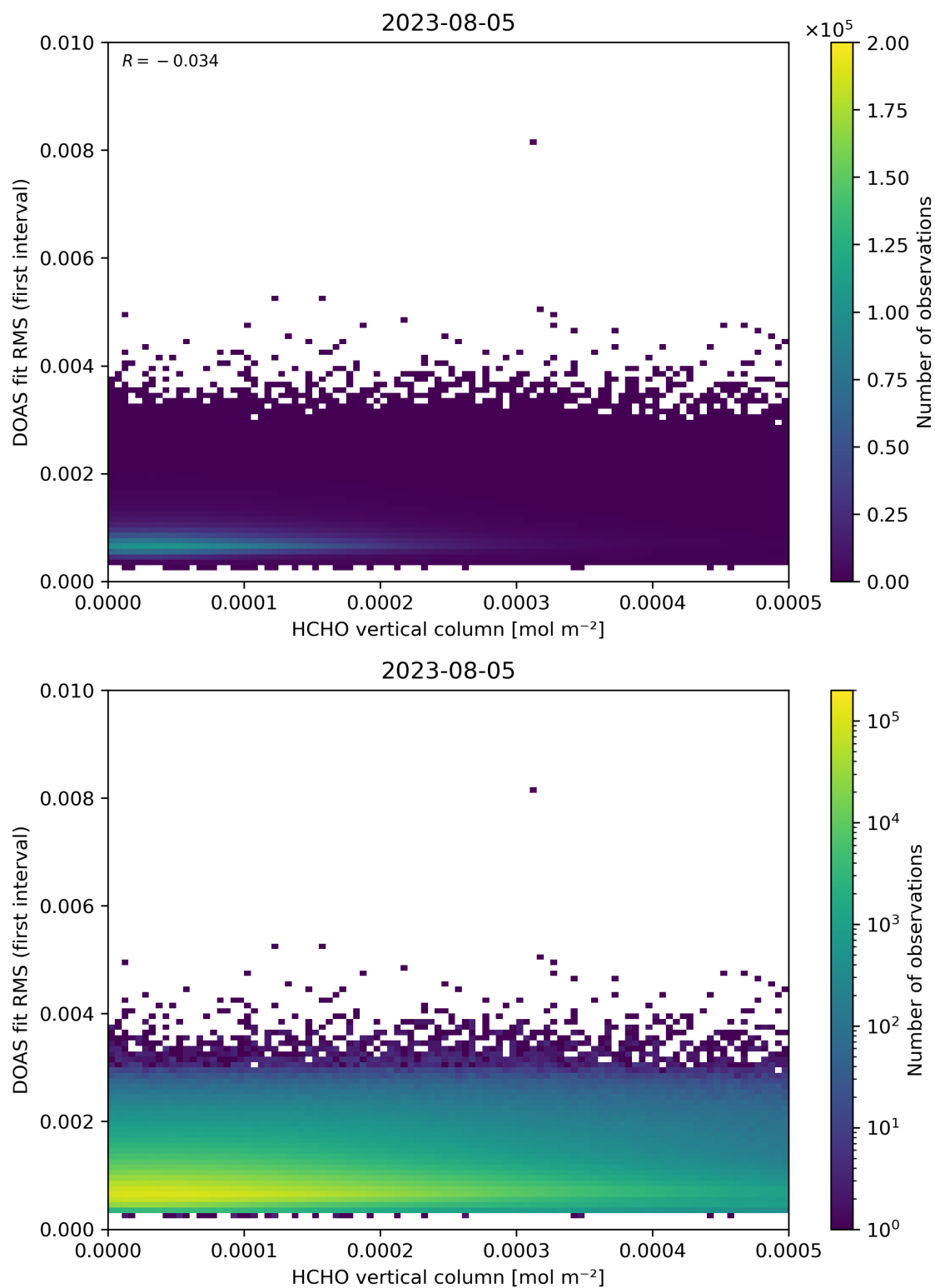
Figure 123: Scatter density plot of “HCHO vertical column” against “DOAS fit RMS (first interval)” for 2023-08-04 to 2023-08-06.
