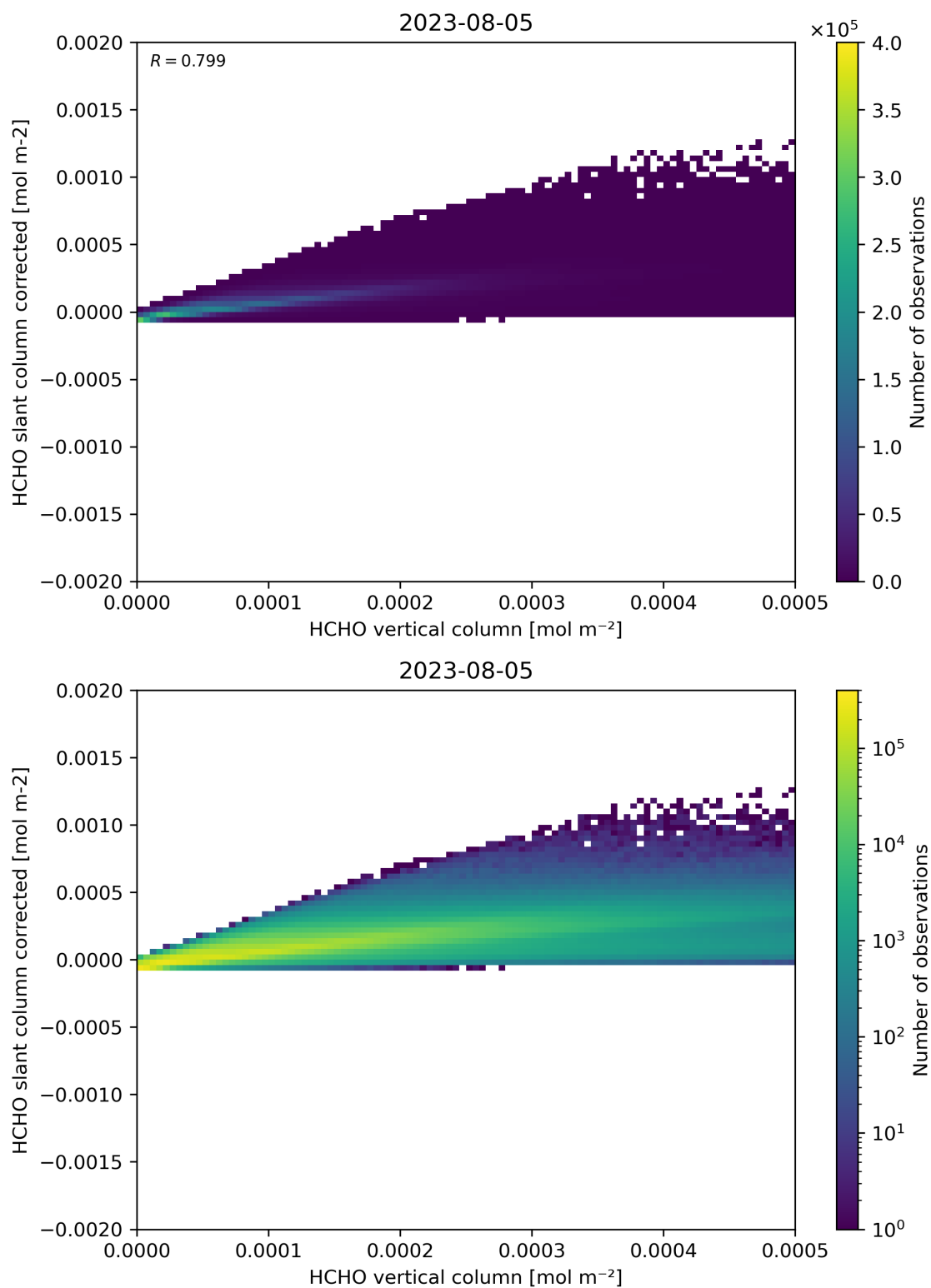
Figure 127: Scatter density plot of “HCHO vertical column” against “HCHO slant column corrected” for 2023-08-04 to 2023-08-06.
