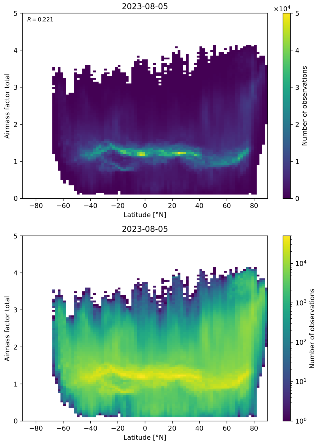
Figure 161: Scatter density plot of “Latitude” against “Airmass factor total” for 2023-08-04 to 2023-08-06.
