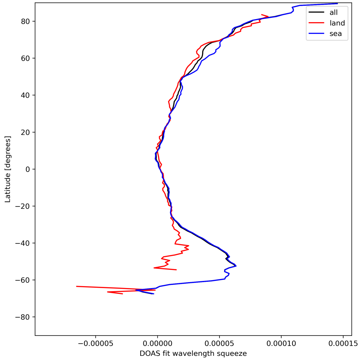
Figure 31: Zonal average of “DOAS fit wavelength squeeze” for 2023-08-04 to 2023-08-06.
