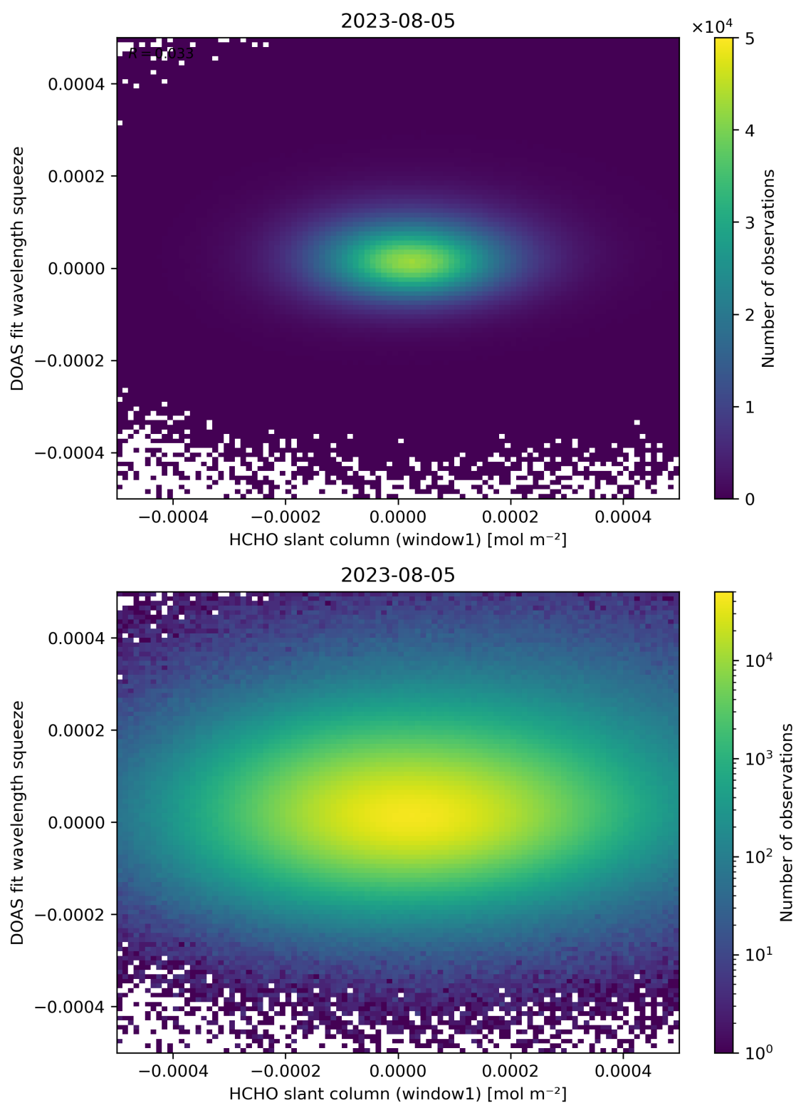
Figure 80: Scatter density plot of “HCHO slant column (window1)” against “DOAS fit wavelength squeeze” for 2023-08-04 to 2023-08-06.
