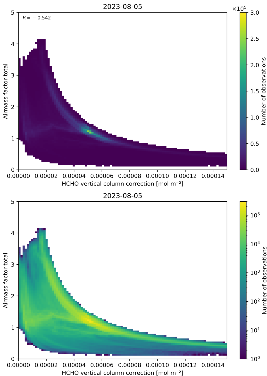
Figure 120: Scatter density plot of “HCHO vertical column correction” against “Airmass factor total” for 2023-08-04 to 2023-08-06.
