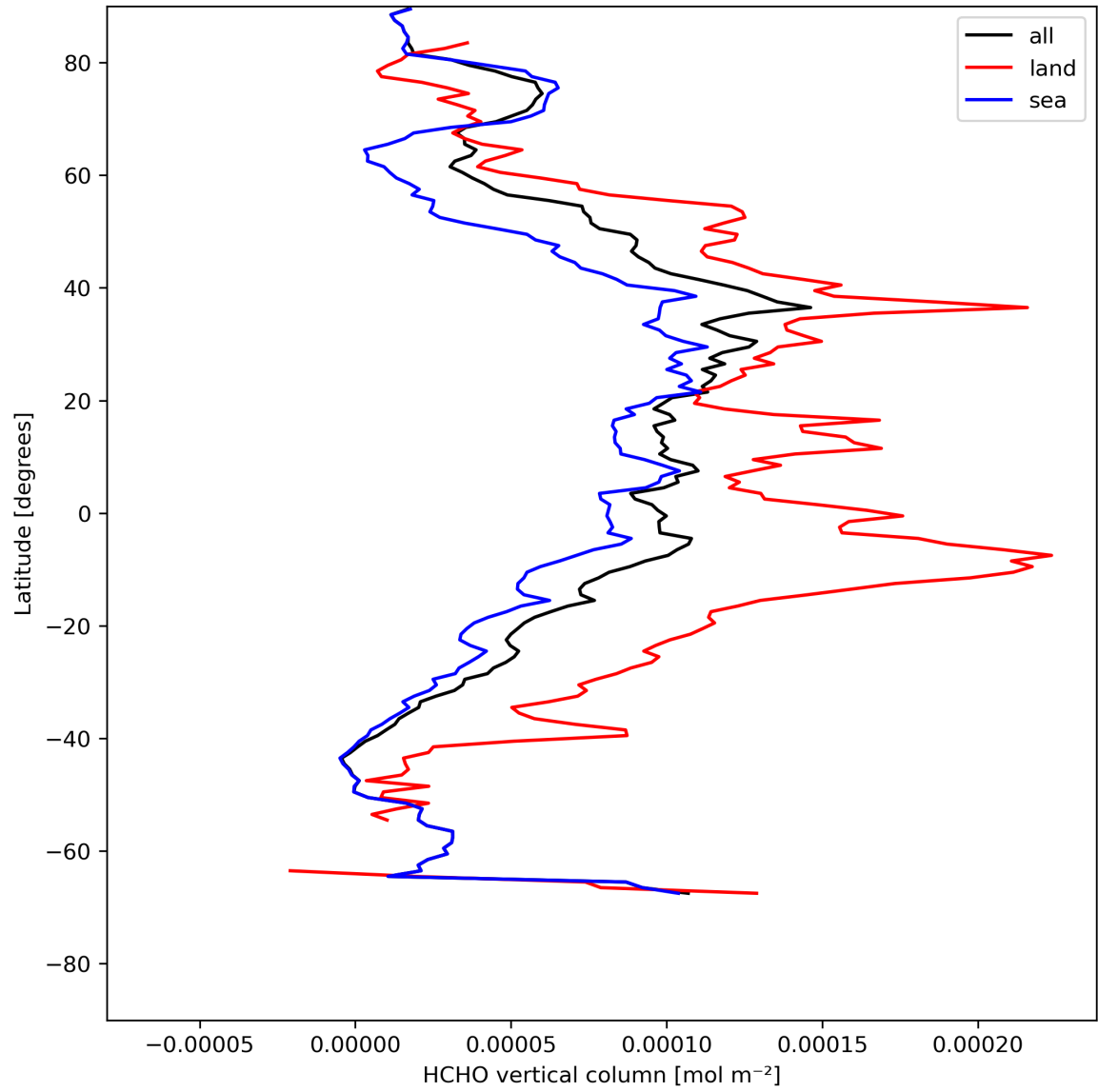
Figure 21: Zonal average of “HCHO vertical column” for 2023-08-04 to 2023-08-06.
