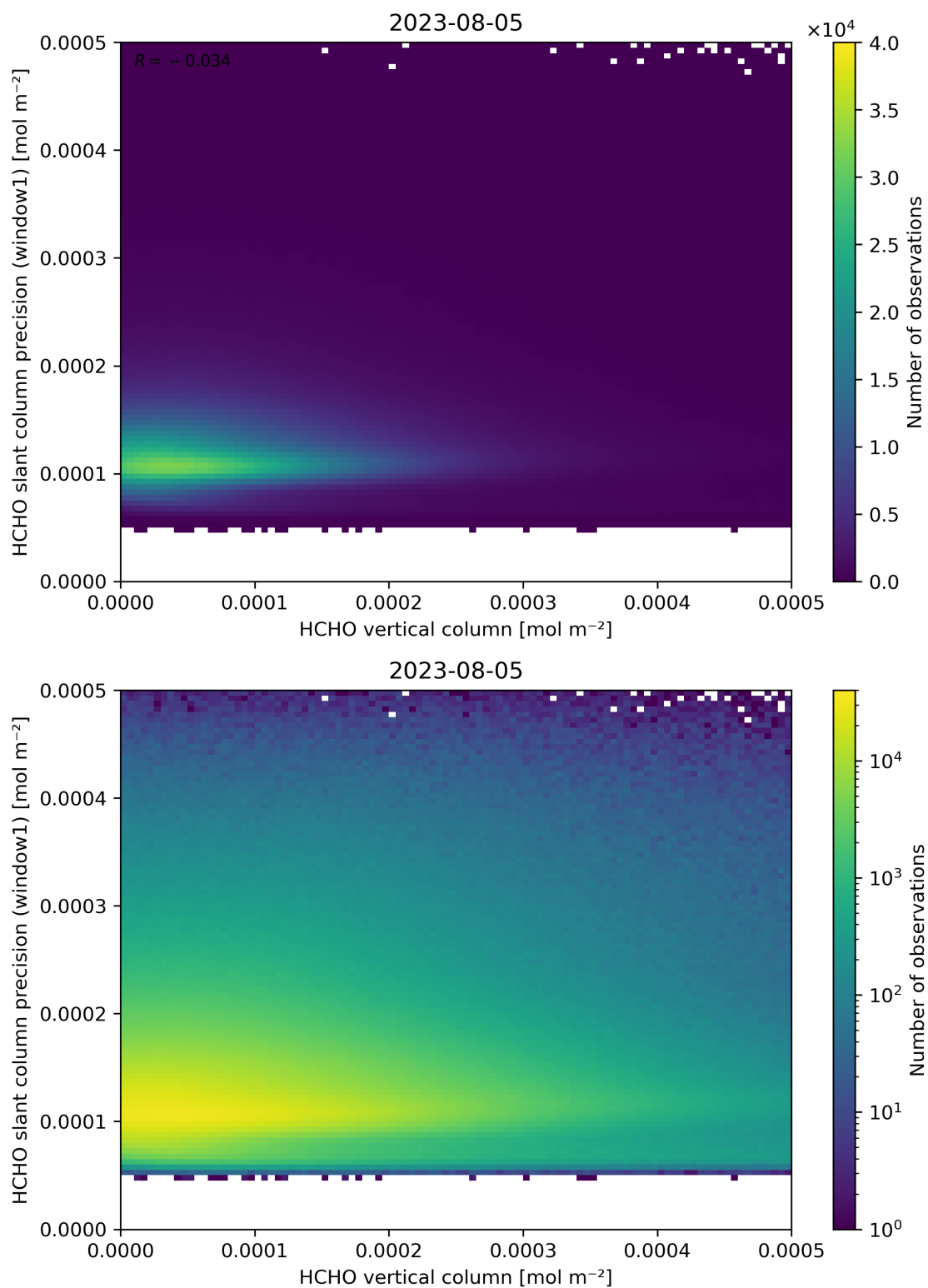
Figure 130: Scatter density plot of “HCHO vertical column” against “HCHO slant column precision (window1)” for 2023-08-04 to 2023-08-06.
