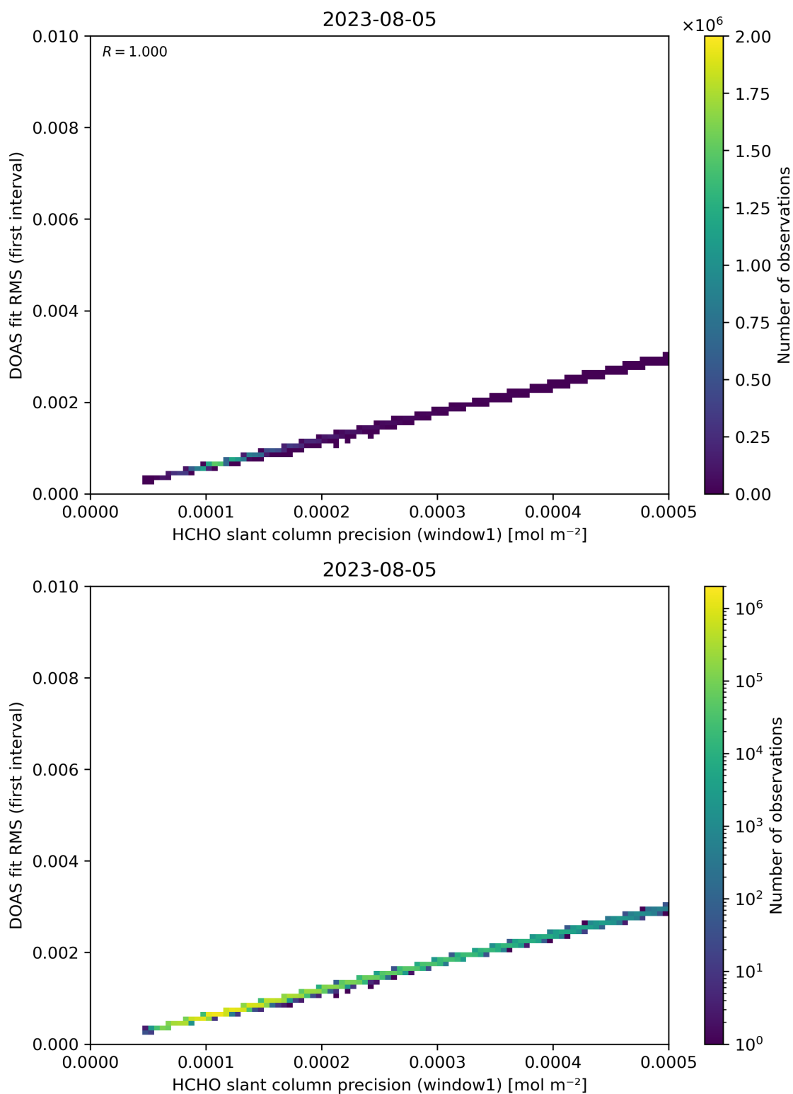
Figure 88: Scatter density plot of “HCHO slant column precision (window1)” against “DOAS fit RMS (first interval)” for 2023-08-04 to 2023-08-06.
