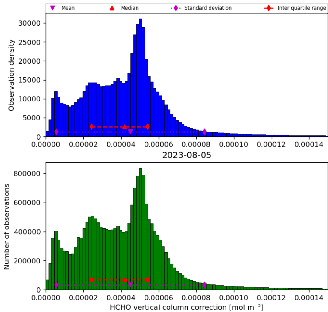
Figure 37: Histogram of “HCHO vertical column correction” for 2023-08-04 to 2023-08-06
