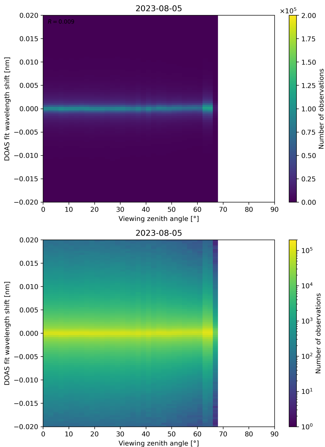
Figure 183: Scatter density plot of “Viewing zenith angle” against “DOAS fit wavelength shift” for 2023-08-04 to 2023-08-06.
