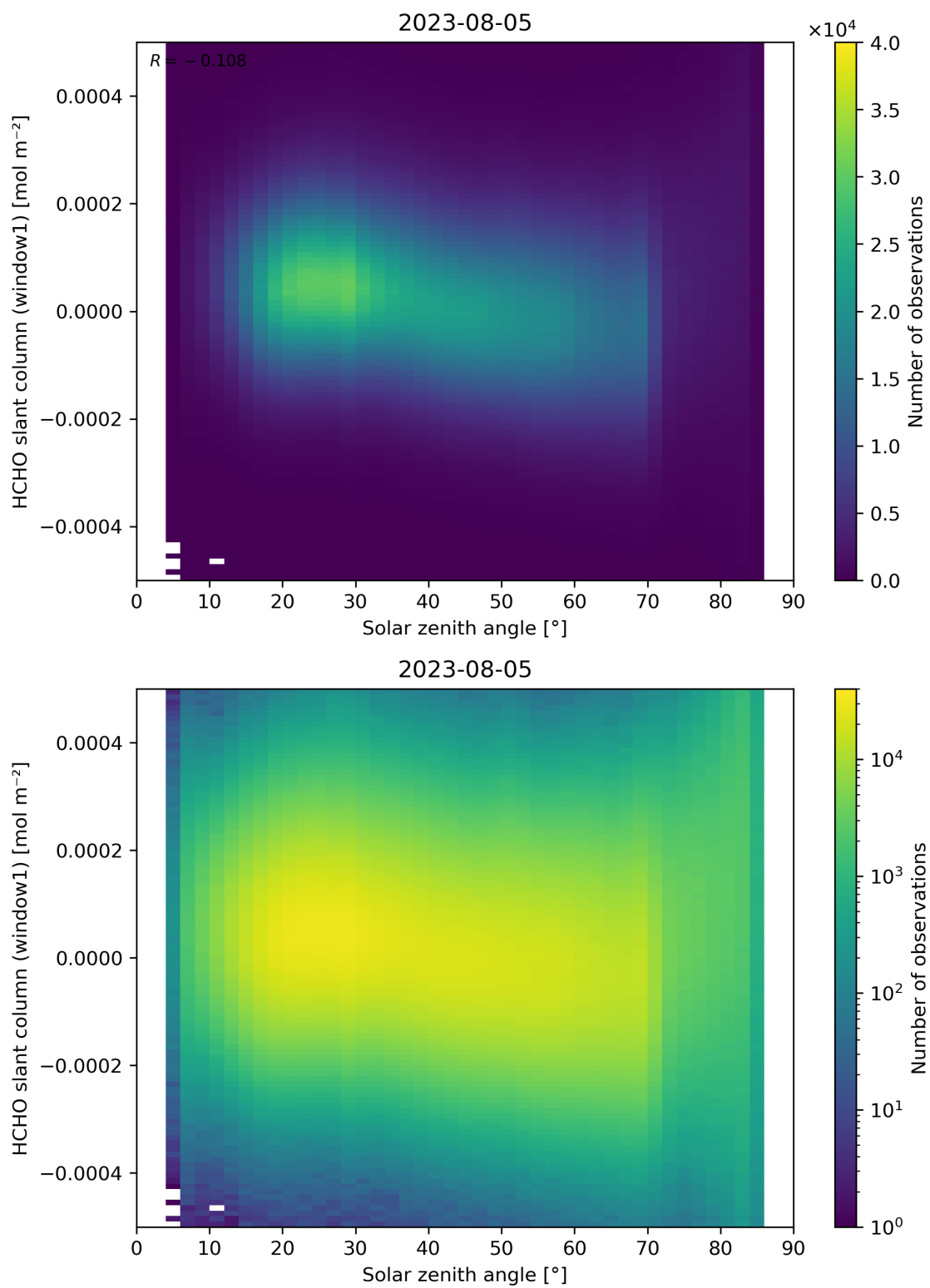
Figure 173: Scatter density plot of “Solar zenith angle” against “HCHO slant column (window1)” for 2023-08-04 to 2023-08-06.
