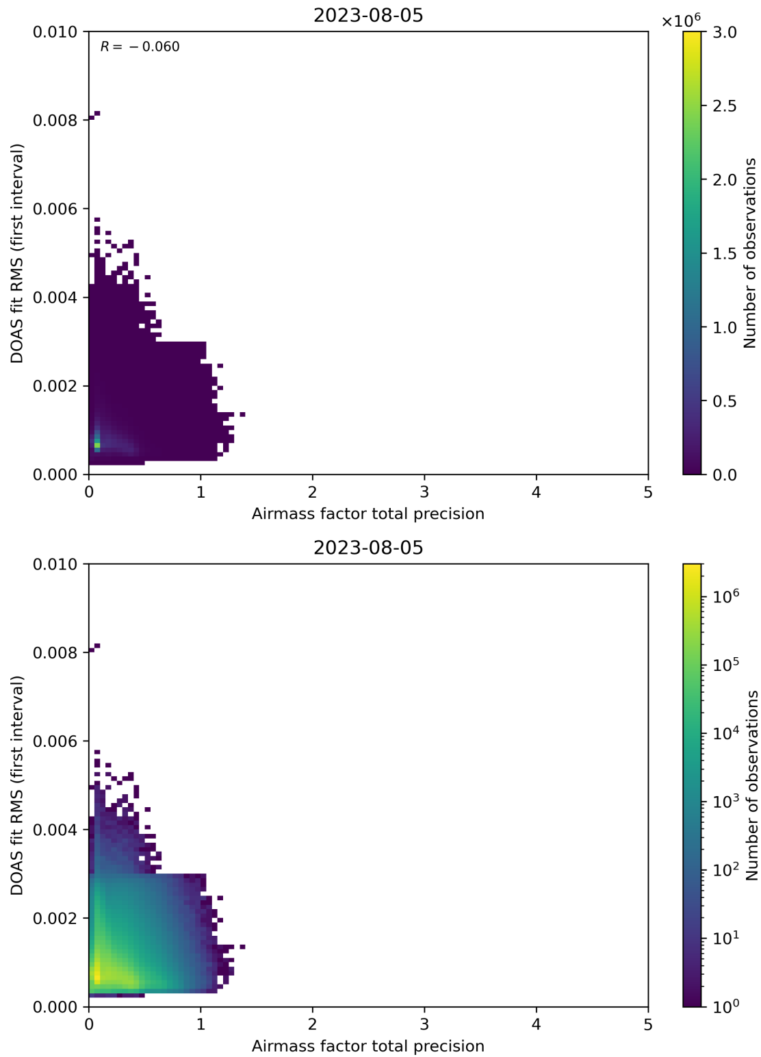
Figure 105: Scatter density plot of “Airmass factor total precision” against “DOAS fit RMS (first interval)” for 2023-08-04 to 2023-08-06.
