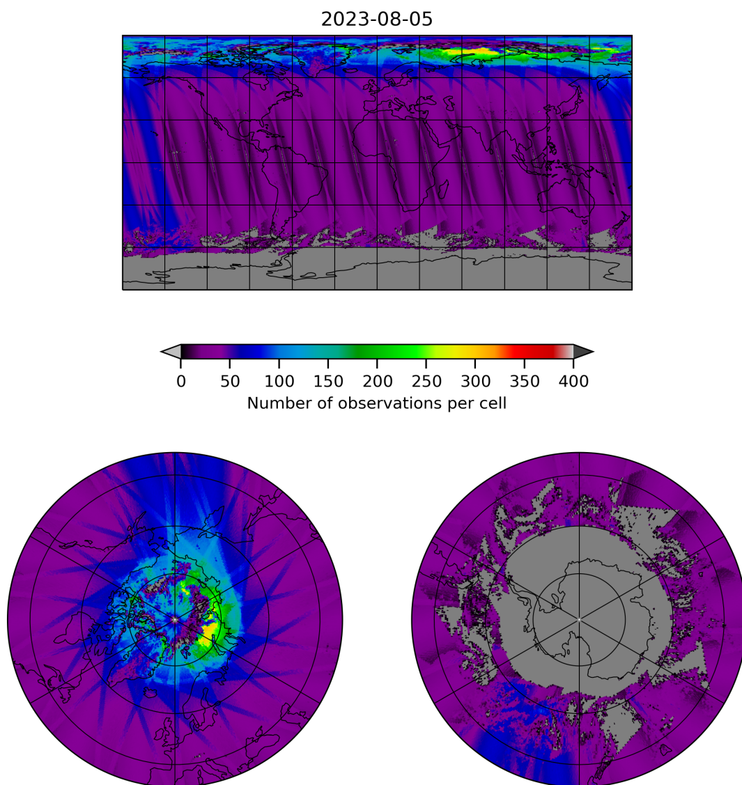
Figure 19: Map of the number of observations for 2023-08-04 to 2023-08-06
