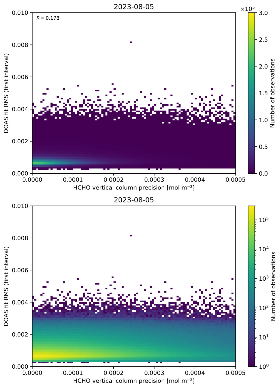
Figure 136: Scatter density plot of “HCHO vertical column precision” against “DOAS fit RMS (first interval)” for 2023-08-04 to 2023-08-06.
