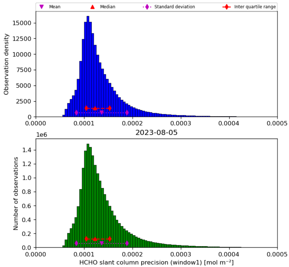
Figure 39: Histogram of “HCHO slant column precision (window1)” for 2023-08-04 to 2023-08-06
