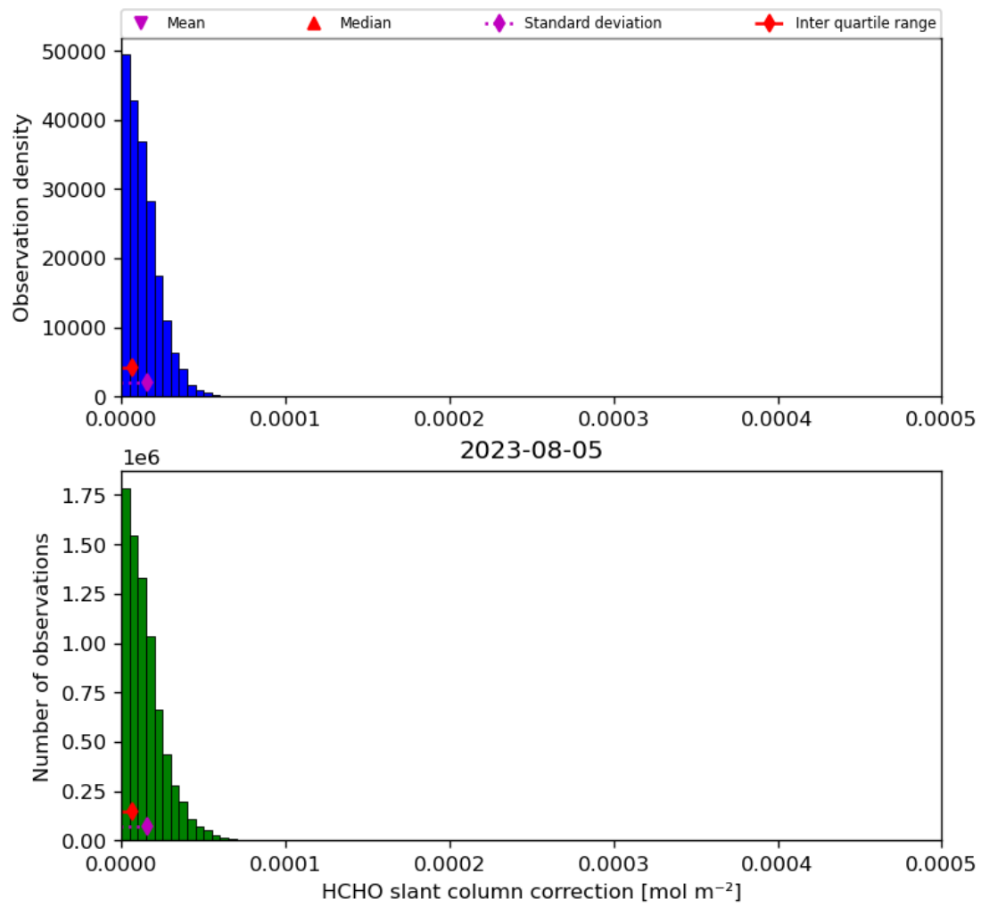
Figure 47: Histogram of “HCHO slant column correction” for 2023-08-04 to 2023-08-06
