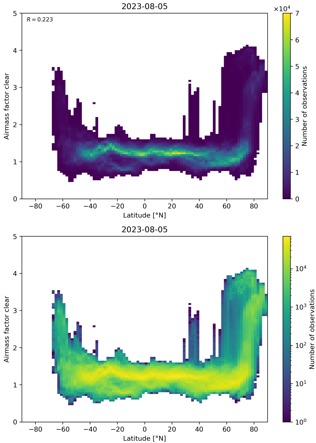
Figure 156: Scatter density plot of “Latitude” against “Airmass factor clear” for 2023-08-04 to 2023-08-06.
