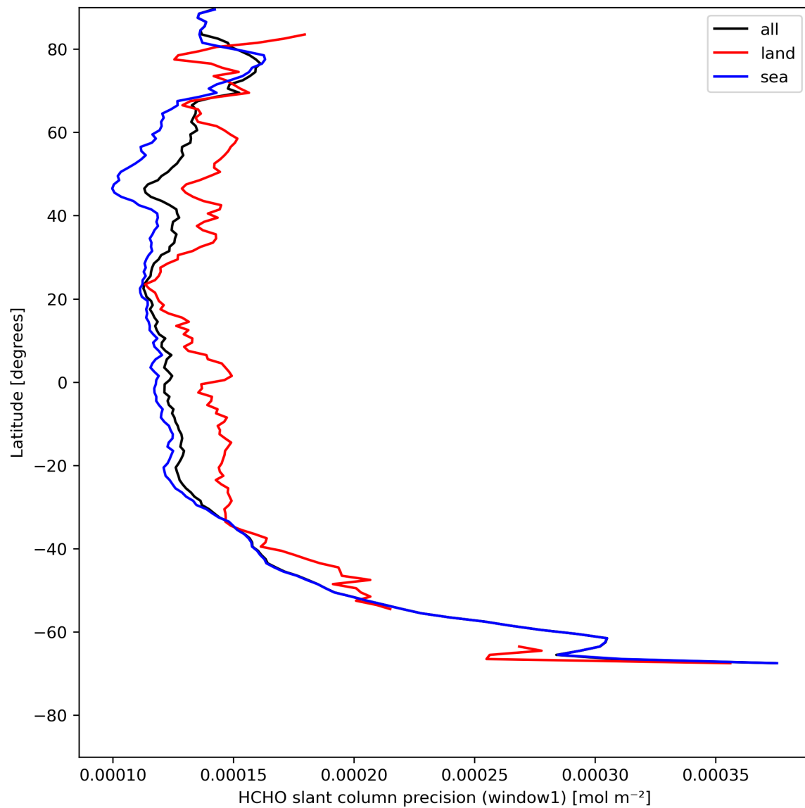
Figure 25: Zonal average of “HCHO slant column precision (window1)” for 2023-08-04 to 2023-08-06.
