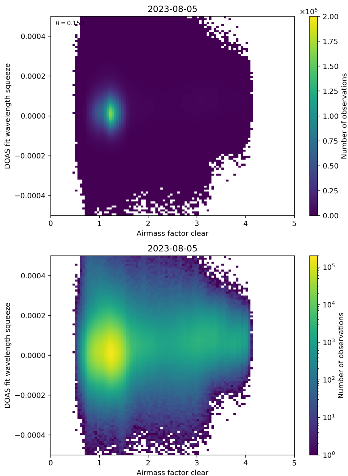
Figure 73: Scatter density plot of “Airmass factor clear” against “DOAS fit wavelength squeeze” for 2023-08-04 to 2023-08-06.
