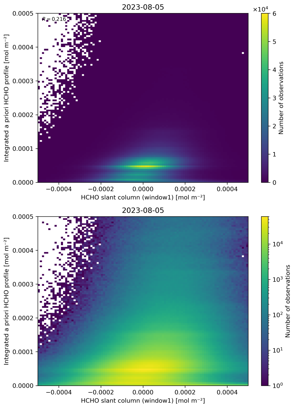
Figure 87: Scatter density plot of “HCHO slant column (window1)” against “Integrated a priori HCHO profile” for 2023-08-04 to 2023-08-06.
