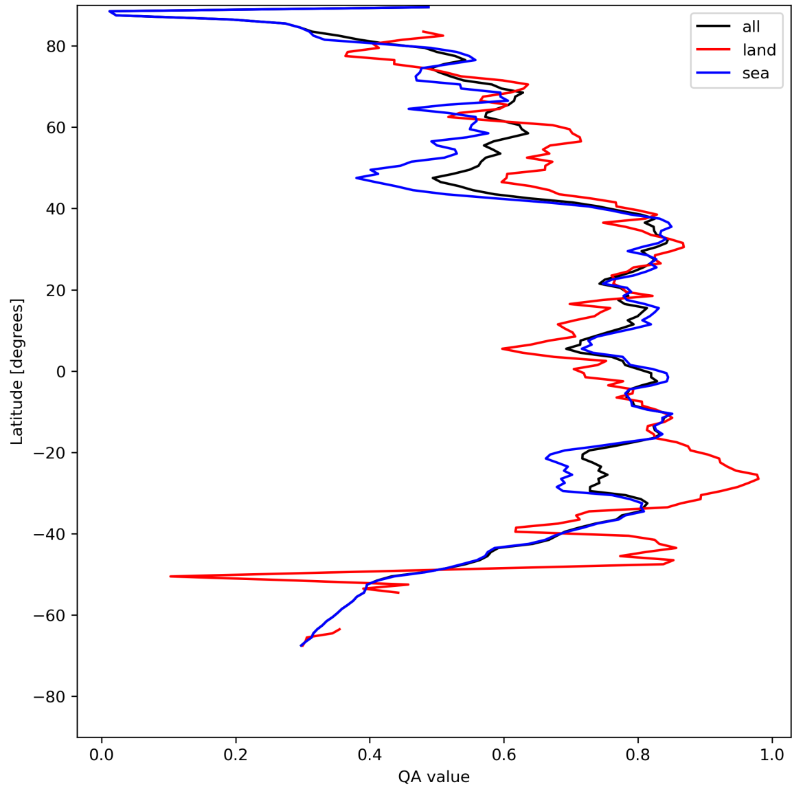
Figure 20: Zonal average of “QA value” for 2023-08-04 to 2023-08-06.
