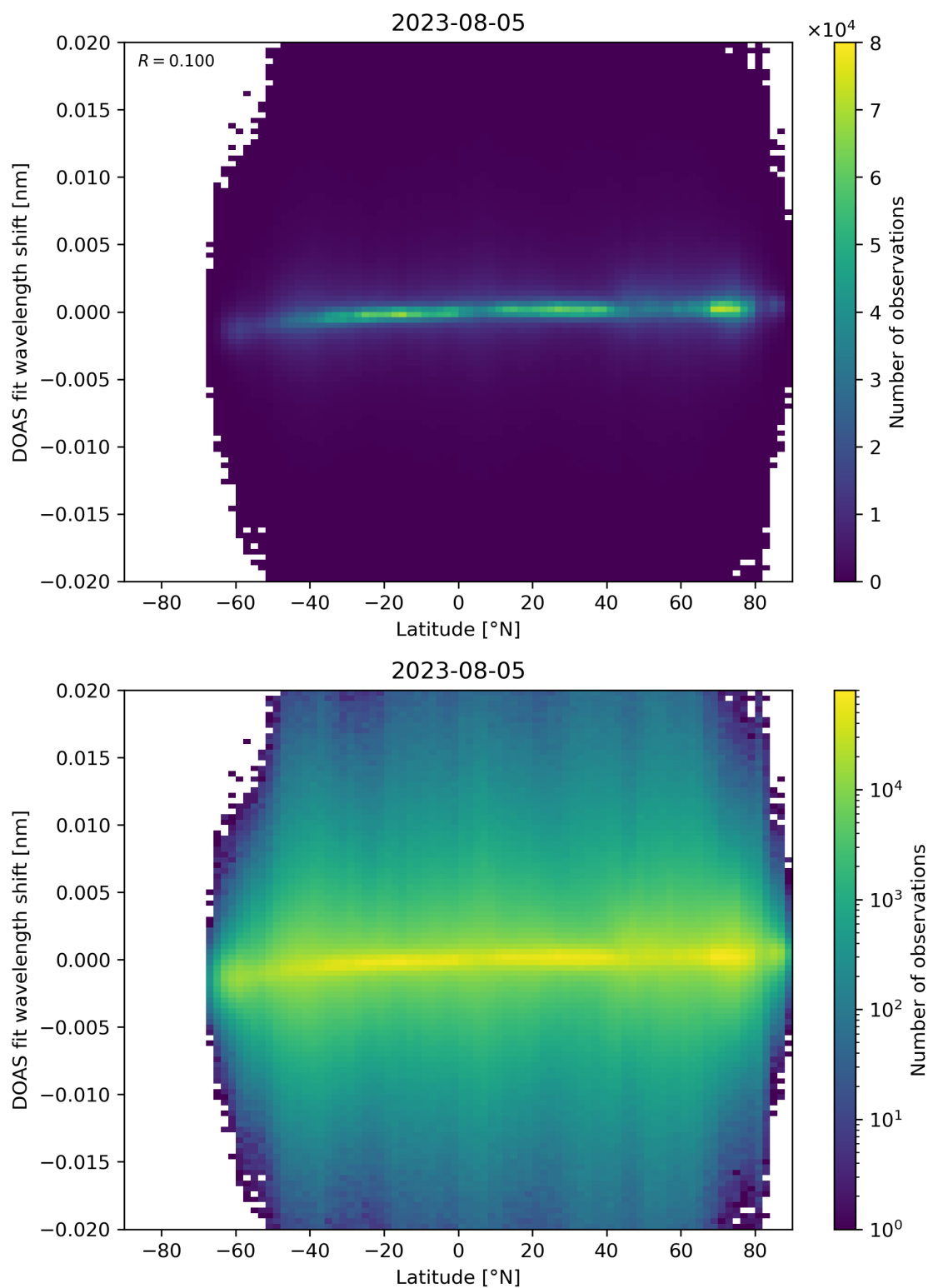
Figure 154: Scatter density plot of “Latitude” against “DOAS fit wavelength shift” for 2023-08-04 to 2023-08-06.
