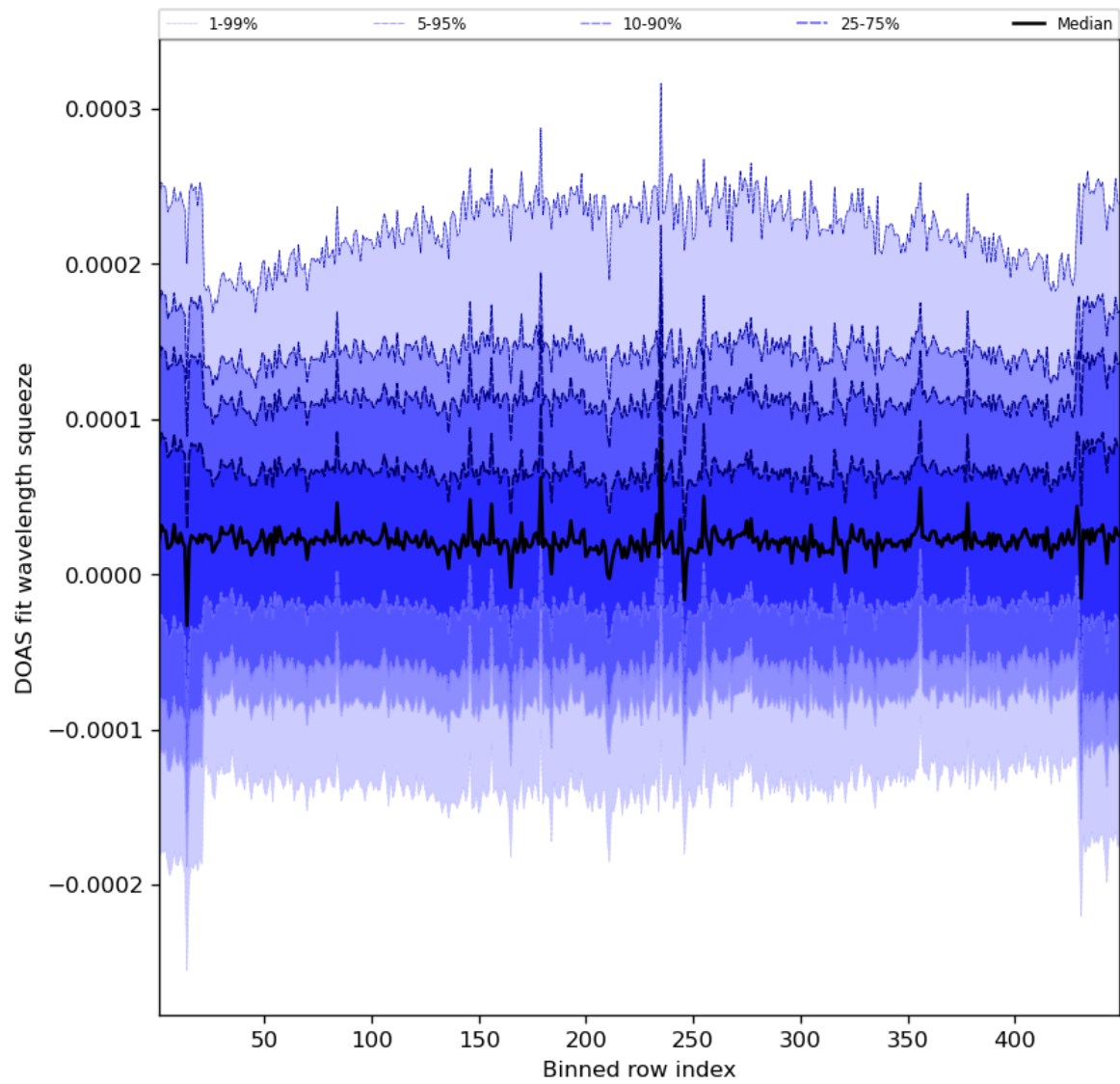
Figure 59: Along track statistics of “DOAS fit wavelength squeeze” for 2023-08-04 to 2023-08-06
