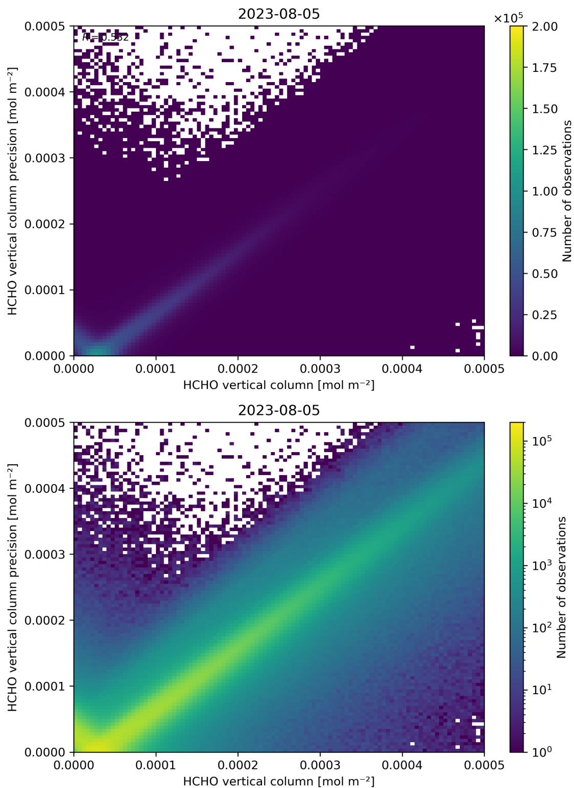
Figure 134: Scatter density plot of “HCHO vertical column” against “HCHO vertical column precision” for 2023-08-04 to 2023-08-06.
