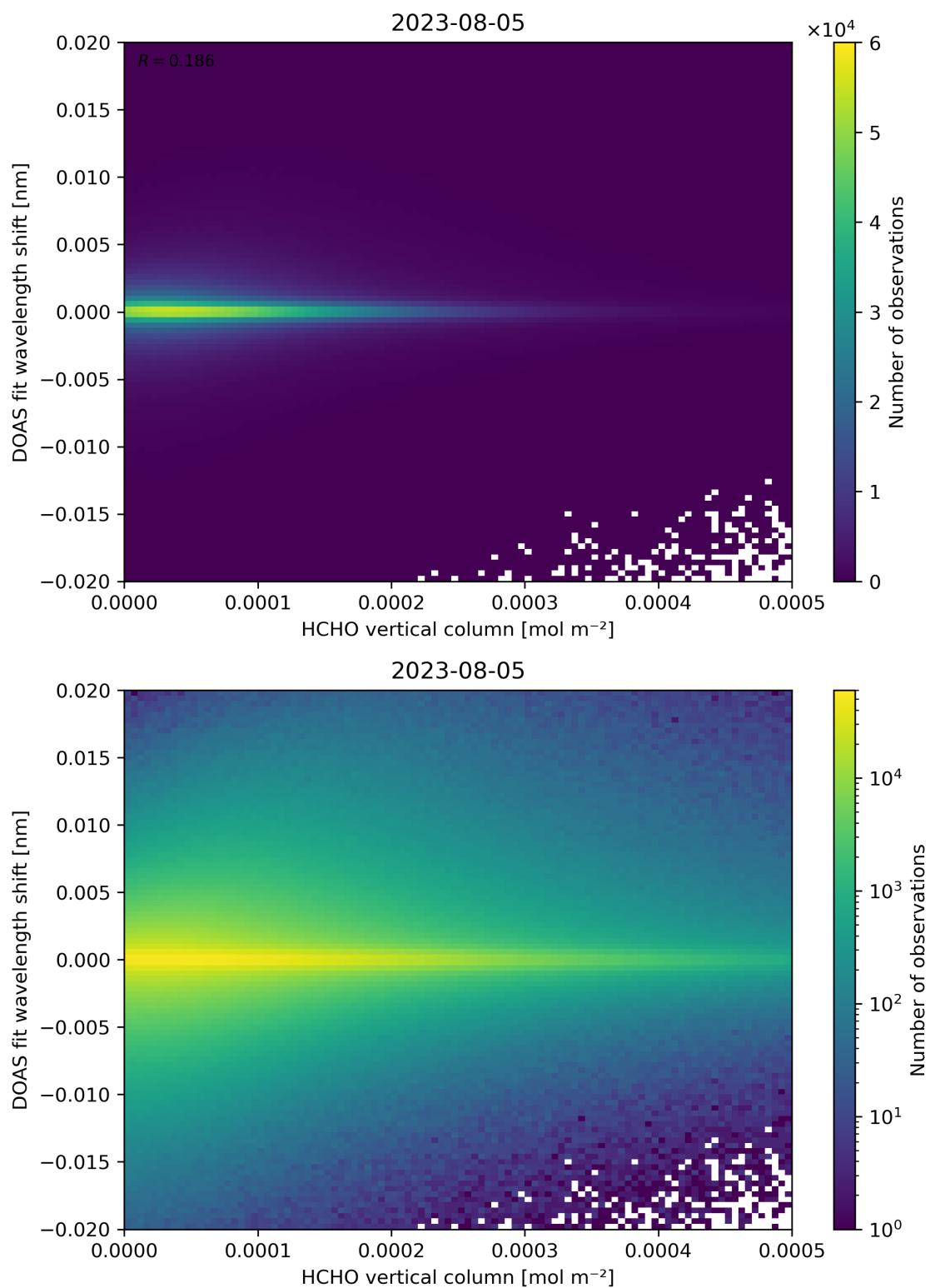
Figure 124: Scatter density plot of “HCHO vertical column” against “DOAS fit wavelength shift” for 2023-08-04 to 2023-08-06.
