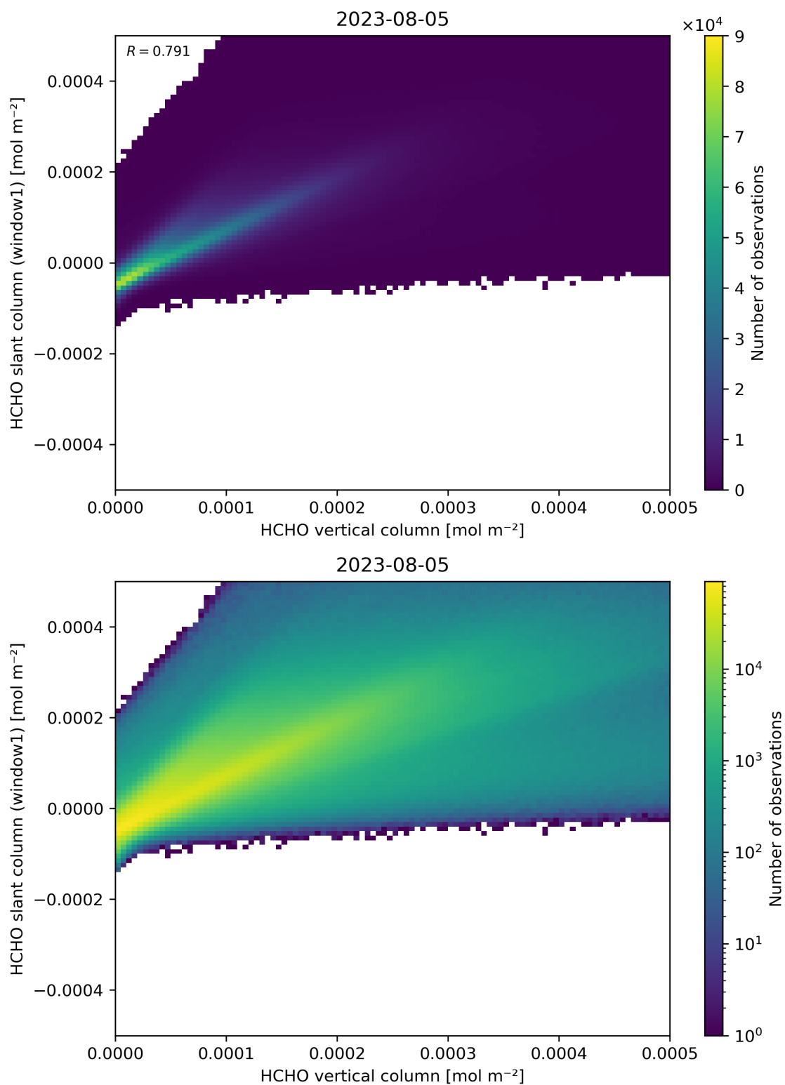
Figure 129: Scatter density plot of “HCHO vertical column” against “HCHO slant column (window1)” for 2023-08-04 to 2023-08-06.
