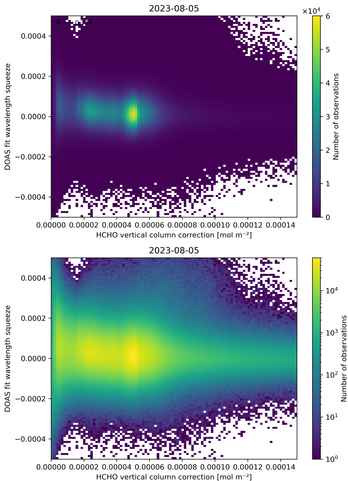
Figure 114: Scatter density plot of “HCHO vertical column correction” against “DOAS fit wavelength squeeze” for 2023-08-04 to 2023-08-06.
