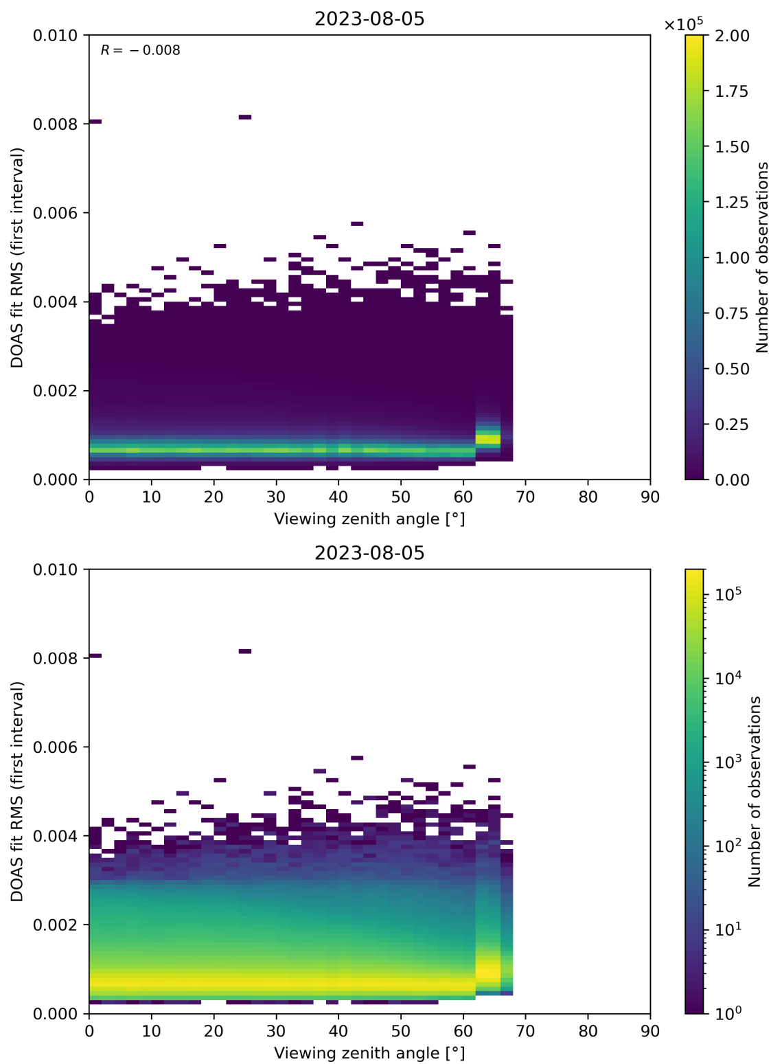
Figure 182: Scatter density plot of “Viewing zenith angle” against “DOAS fit RMS (first interval)” for 2023-08-04 to 2023-08-06.
