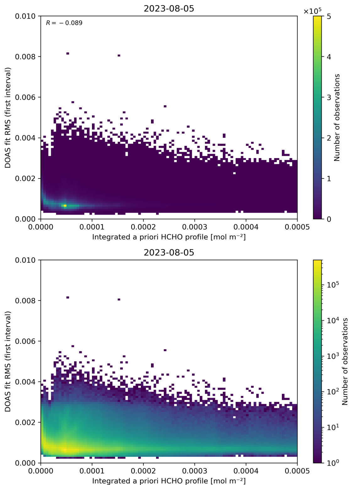
Figure 148: Scatter density plot of “Integrated a priori HCHO profile” against “DOAS fit RMS (first interval)” for 2023-08-04 to 2023-08-06.
