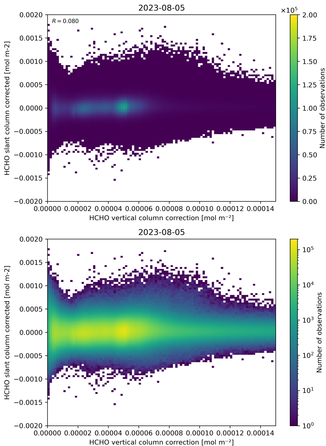
Figure 116: Scatter density plot of “HCHO vertical column correction” against “HCHO slant column corrected” for 2023-08-04 to 2023-08-06.
