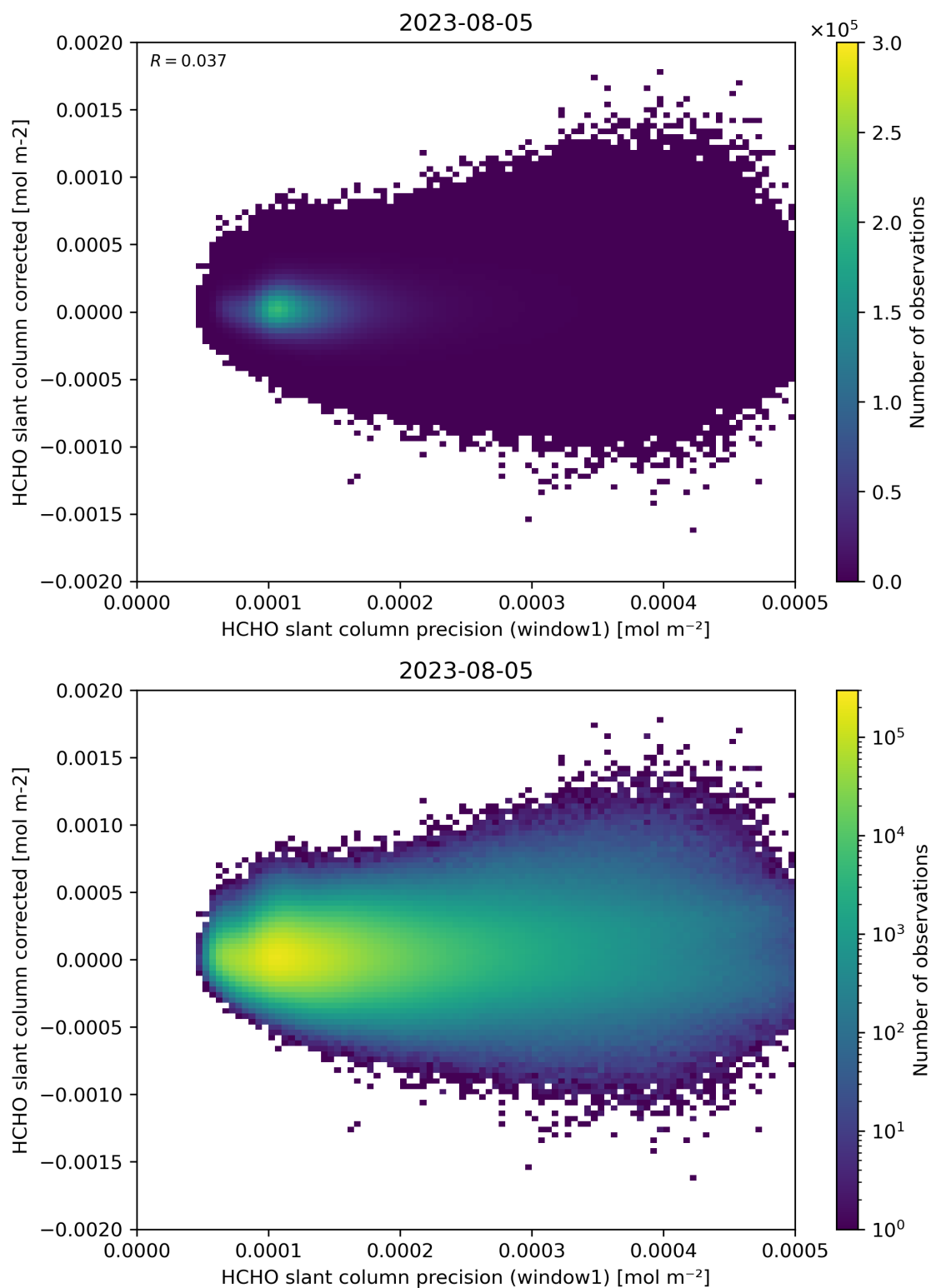
Figure 92: Scatter density plot of “HCHO slant column precision (window1)” against “HCHO slant column corrected” for 2023-08-04 to 2023-08-06.
