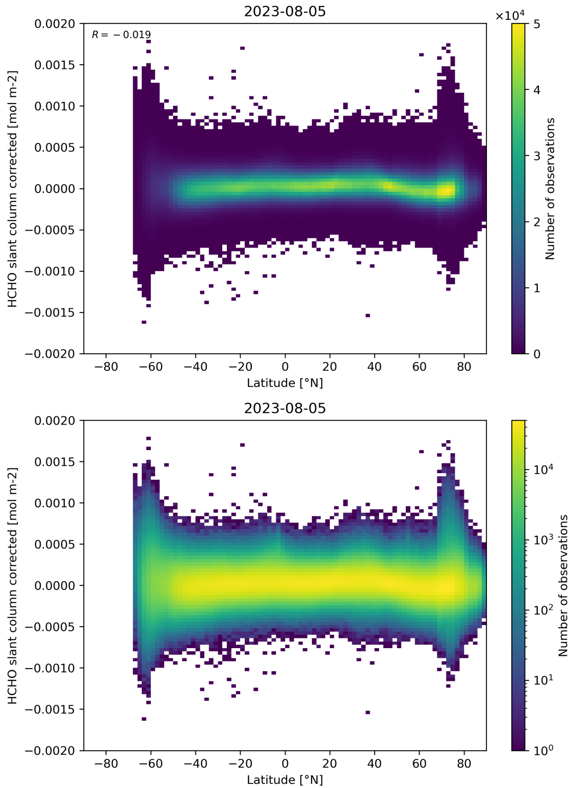
Figure 157: Scatter density plot of “Latitude” against “HCHO slant column corrected” for 2023-08-04 to 2023-08-06.
