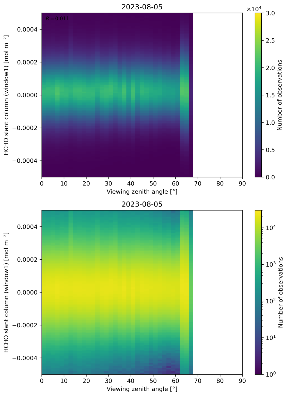
Figure 188: Scatter density plot of “Viewing zenith angle” against “HCHO slant column (window1)” for 2023-08-04 to 2023-08-06.
