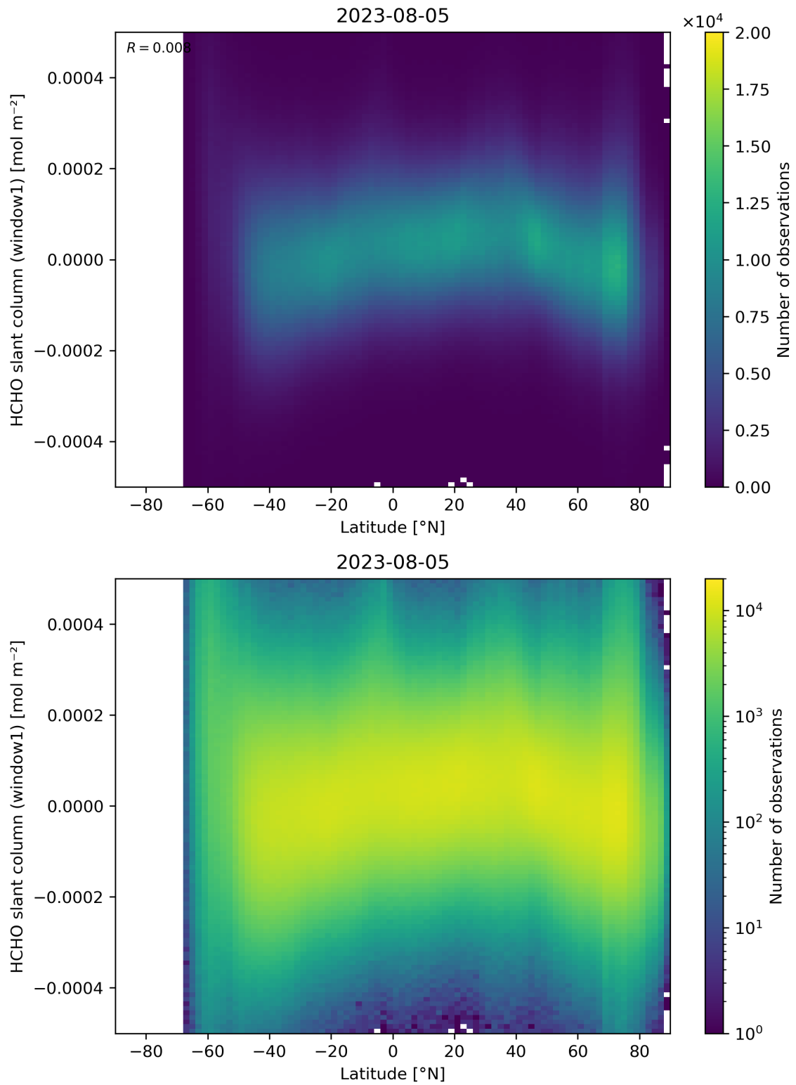
Figure 159: Scatter density plot of “Latitude” against “HCHO slant column (window1)” for 2023-08-04 to 2023-08-06.
