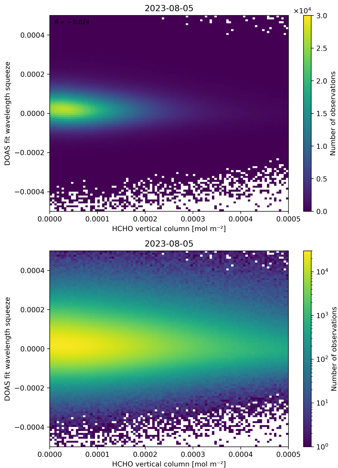
Figure 125: Scatter density plot of “HCHO vertical column” against “DOAS fit wavelength squeeze” for 2023-08-04 to 2023-08-06.
