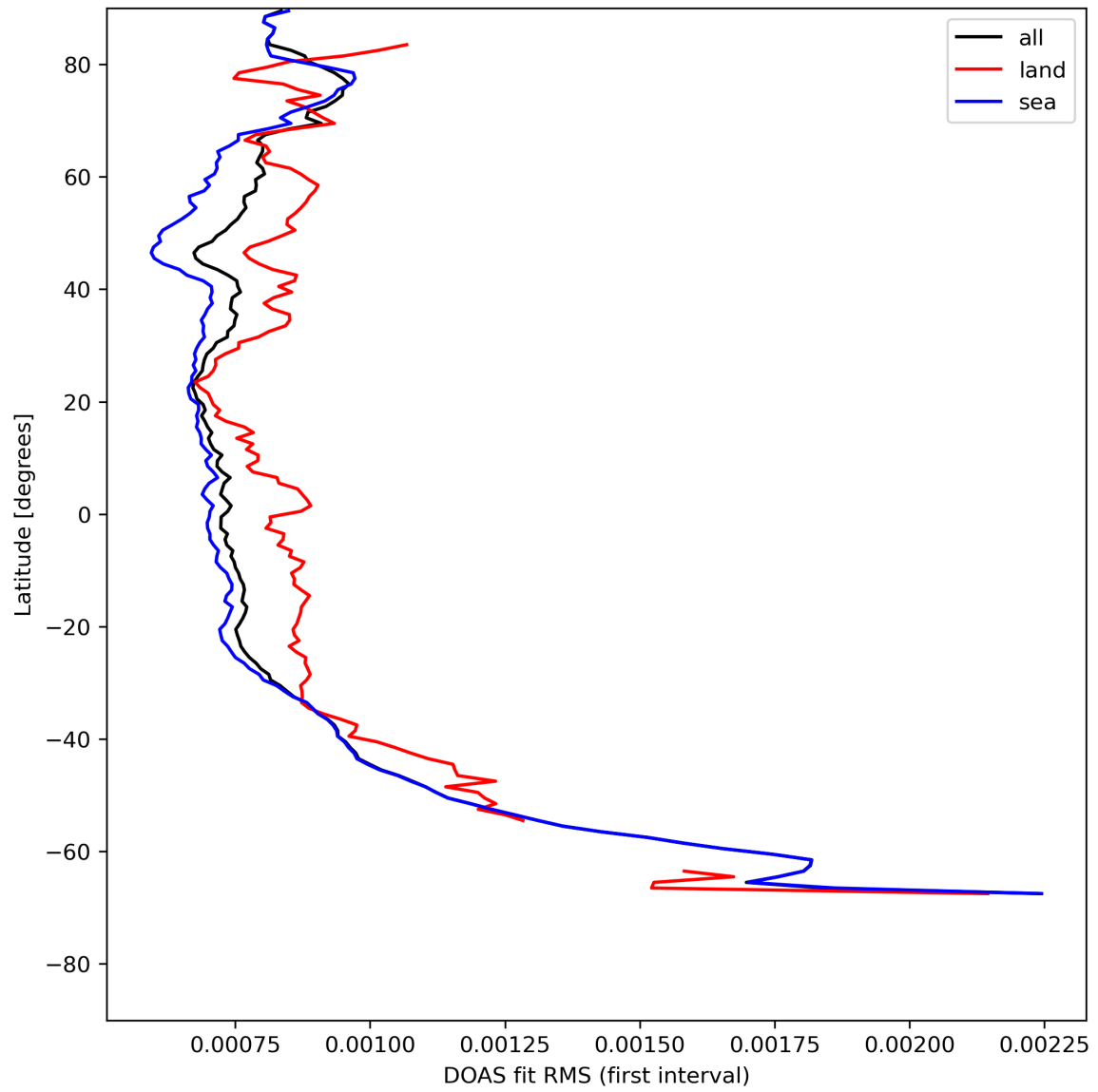
Figure 32: Zonal average of "DOAS fit RMS (first interval)" for 2023-08-04 to 2023-08-06.
