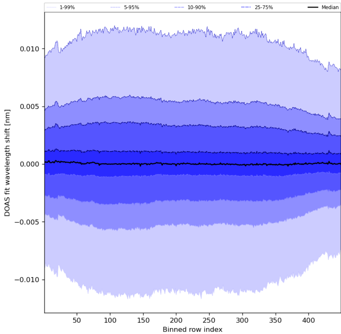
Figure 58: Along track statistics of “DOAS fit wavelength shift” for 2023-08-04 to 2023-08-06
