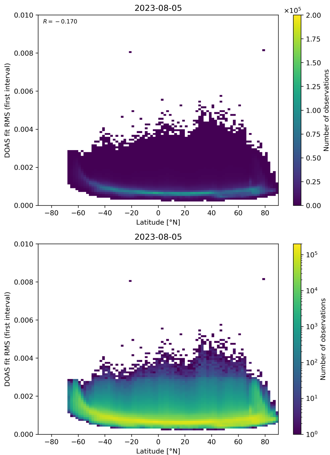
Figure 153: Scatter density plot of “Latitude” against “DOAS fit RMS (first interval)” for 2023-08-04 to 2023-08-06.
