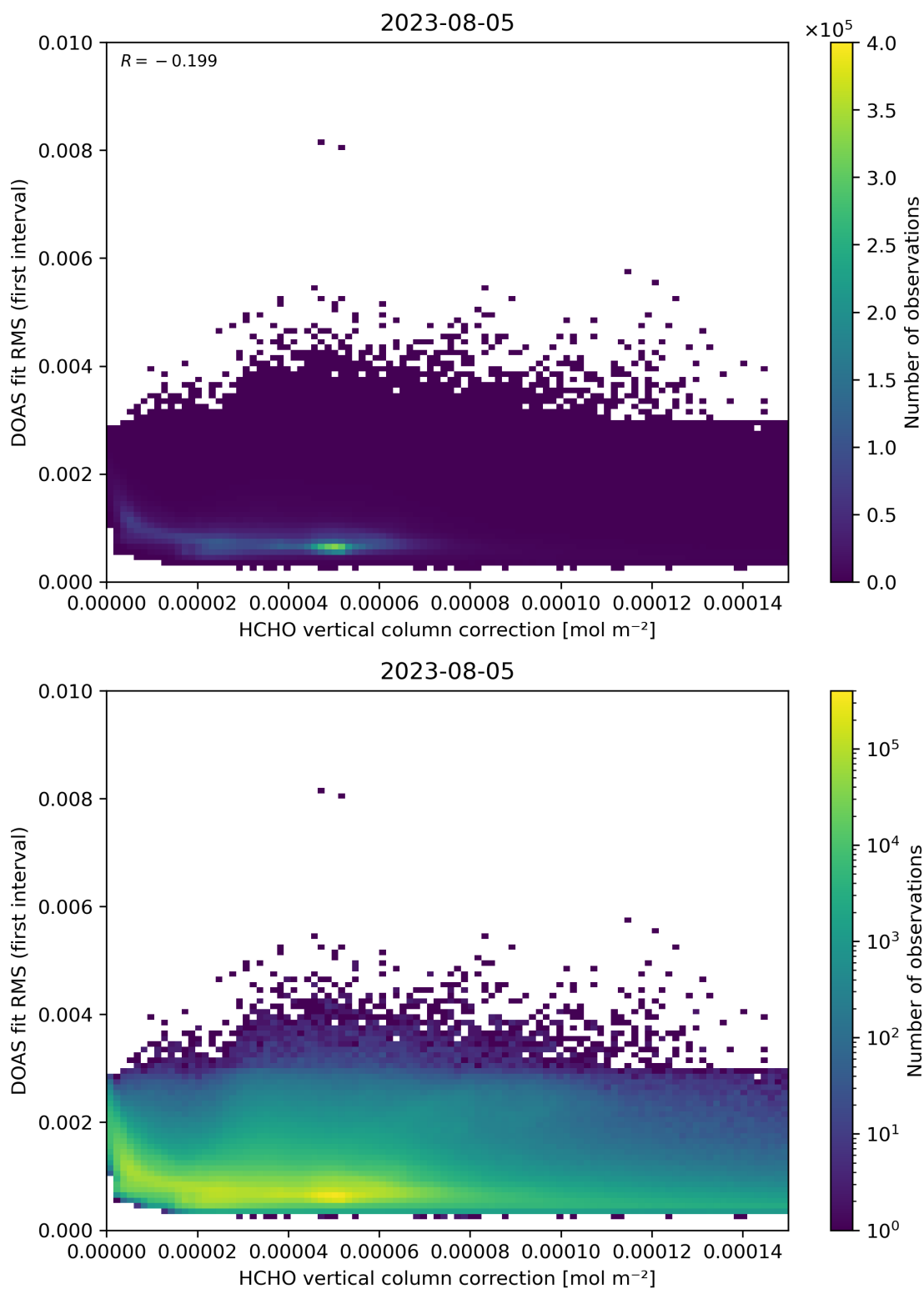
Figure 112: Scatter density plot of “HCHO vertical column correction” against “DOAS fit RMS (first interval)” for 2023-08-04 to 2023-08-06.
