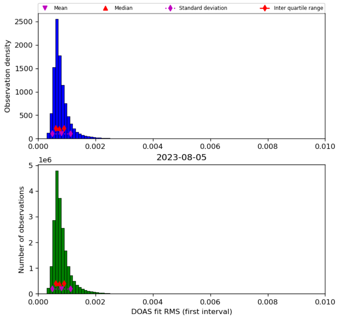
Figure 46: Histogram of “DOAS fit RMS (first interval)” for 2023-08-04 to 2023-08-06
