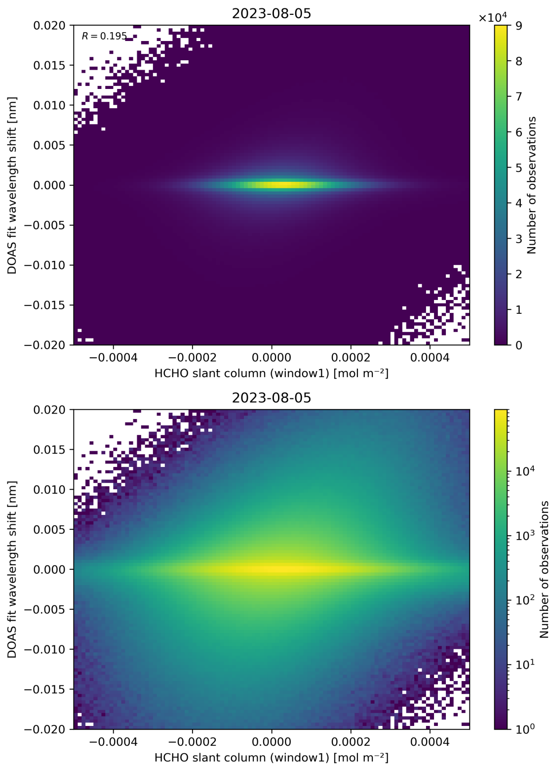
Figure 79: Scatter density plot of “HCHO slant column (window1)” against “DOAS fit wavelength shift” for 2023-08-04 to 2023-08-06.
