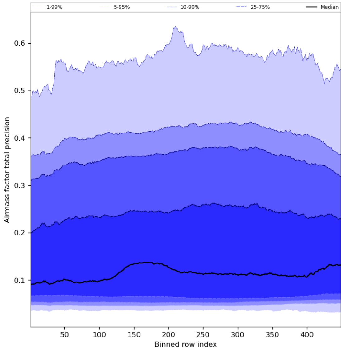
Figure 55: Along track statistics of “Airmass factor total precision” for 2023-08-04 to 2023-08-06
