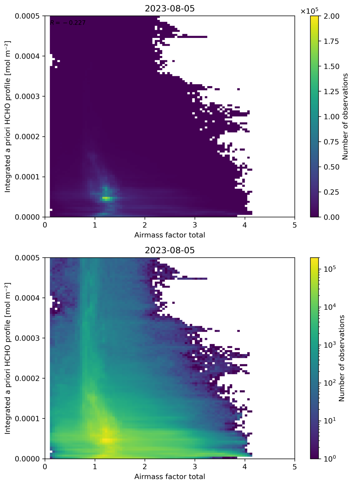
Figure 104: Scatter density plot of “Air mass factor total” against “Integrated a priori HCHO profile” for 2023-08-04 to 2023-08-06.
