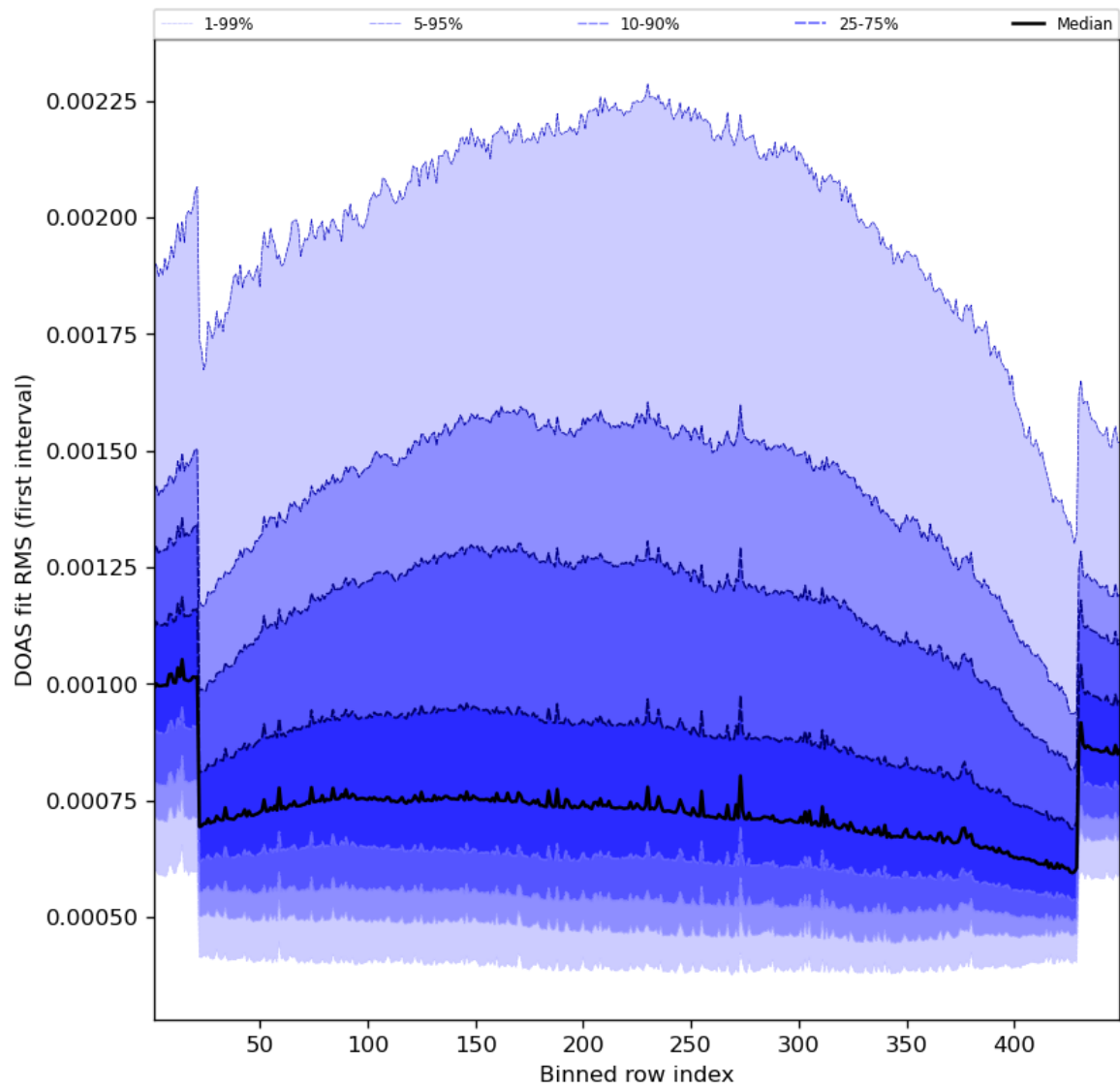
Figure 60: Along track statistics of “DOAS fit RMS (first interval)” for 2023-08-04 to 2023-08-06
