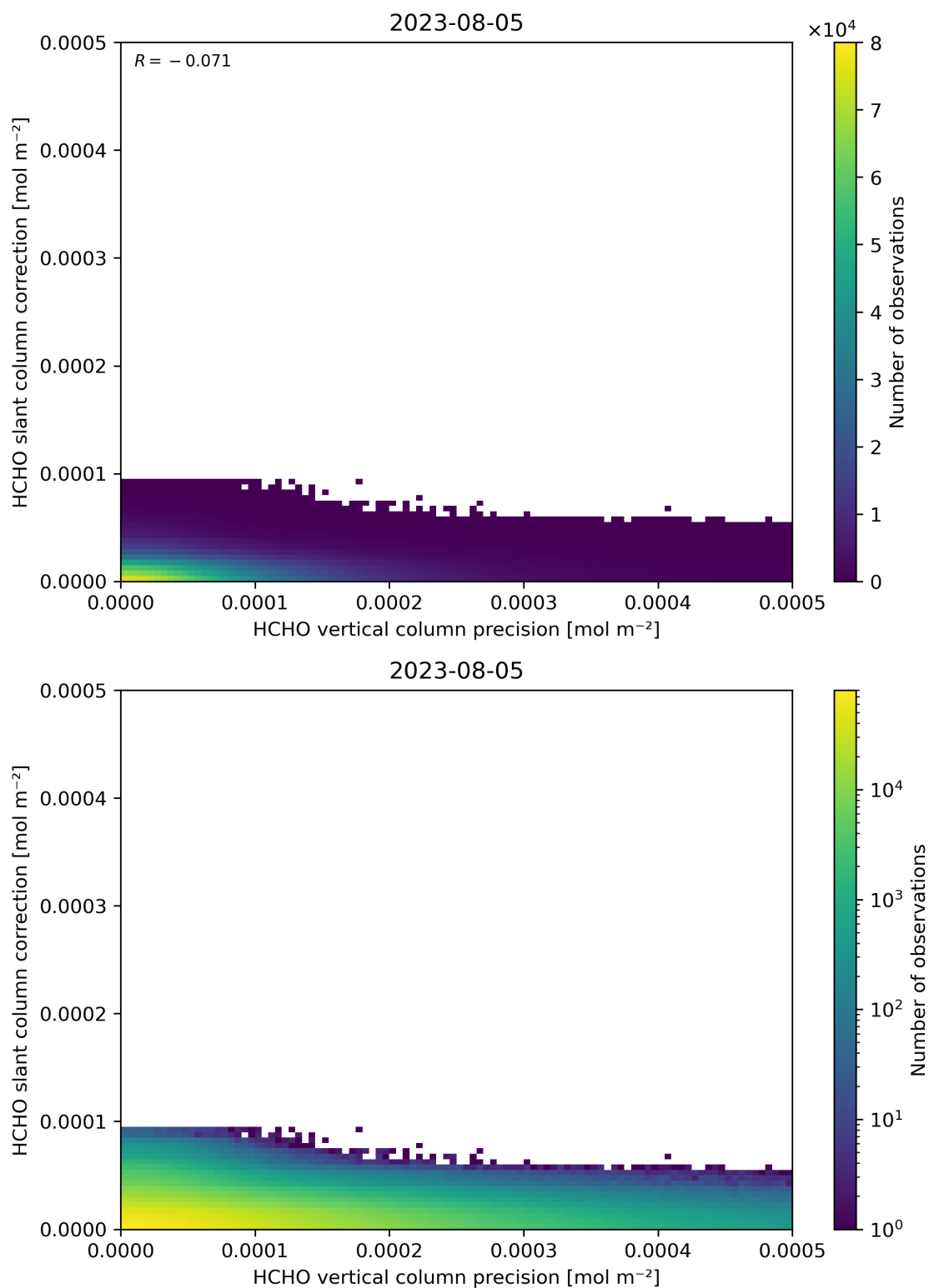
Figure 141: Scatter density plot of “HCHO vertical column precision” against “HCHO slant column correction” for 2023-08-04 to 2023-08-06.
