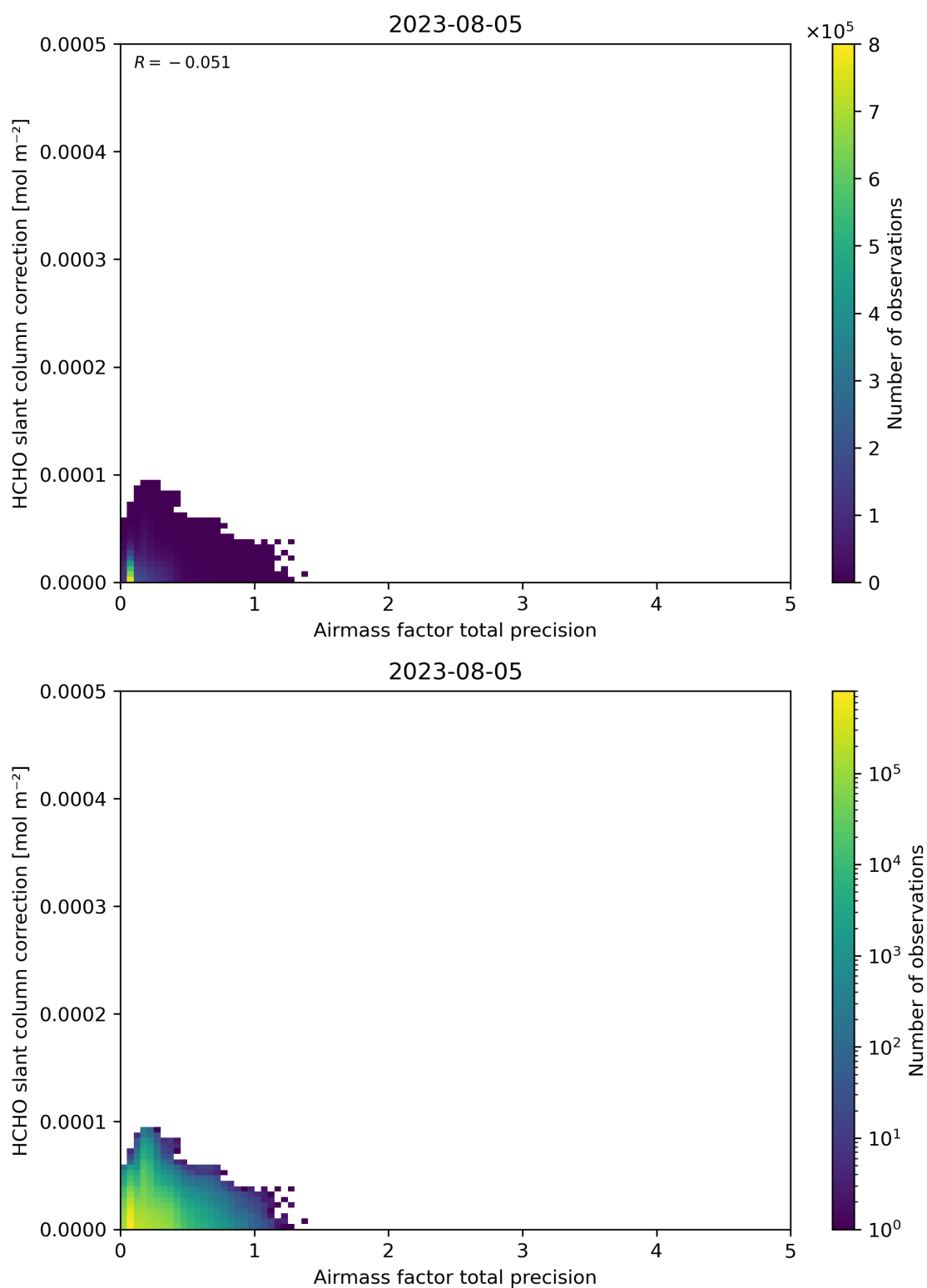
Figure 110: Scatter density plot of “Airmass factor total precision” against “HCHO slant column correction” for 2023-08-04 to 2023-08-06.
