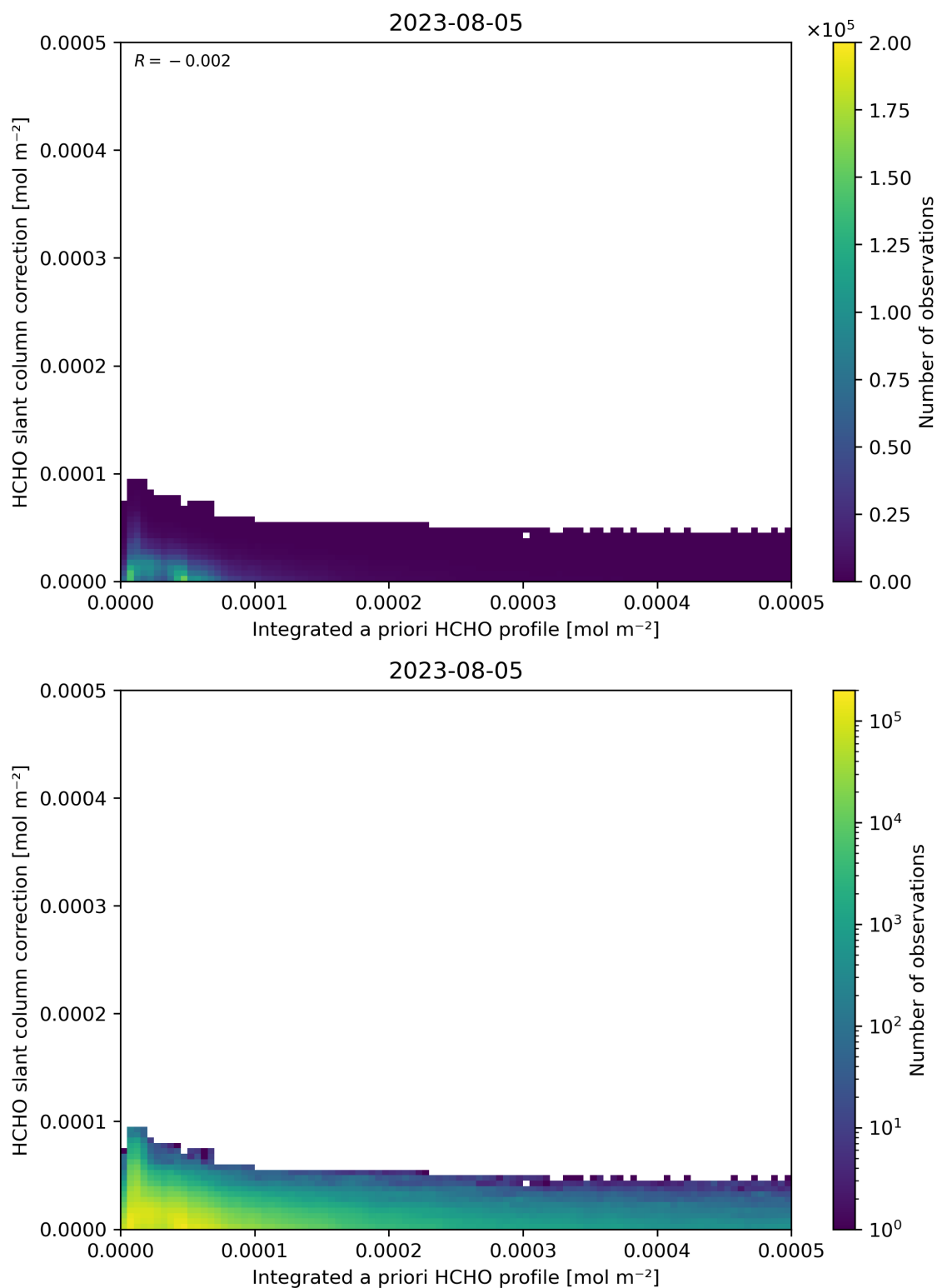
Figure 152: Scatter density plot of “Integrated a priori HCHO profile” against “HCHO slant column correction” for 2023-08-04 to 2023-08-06.
