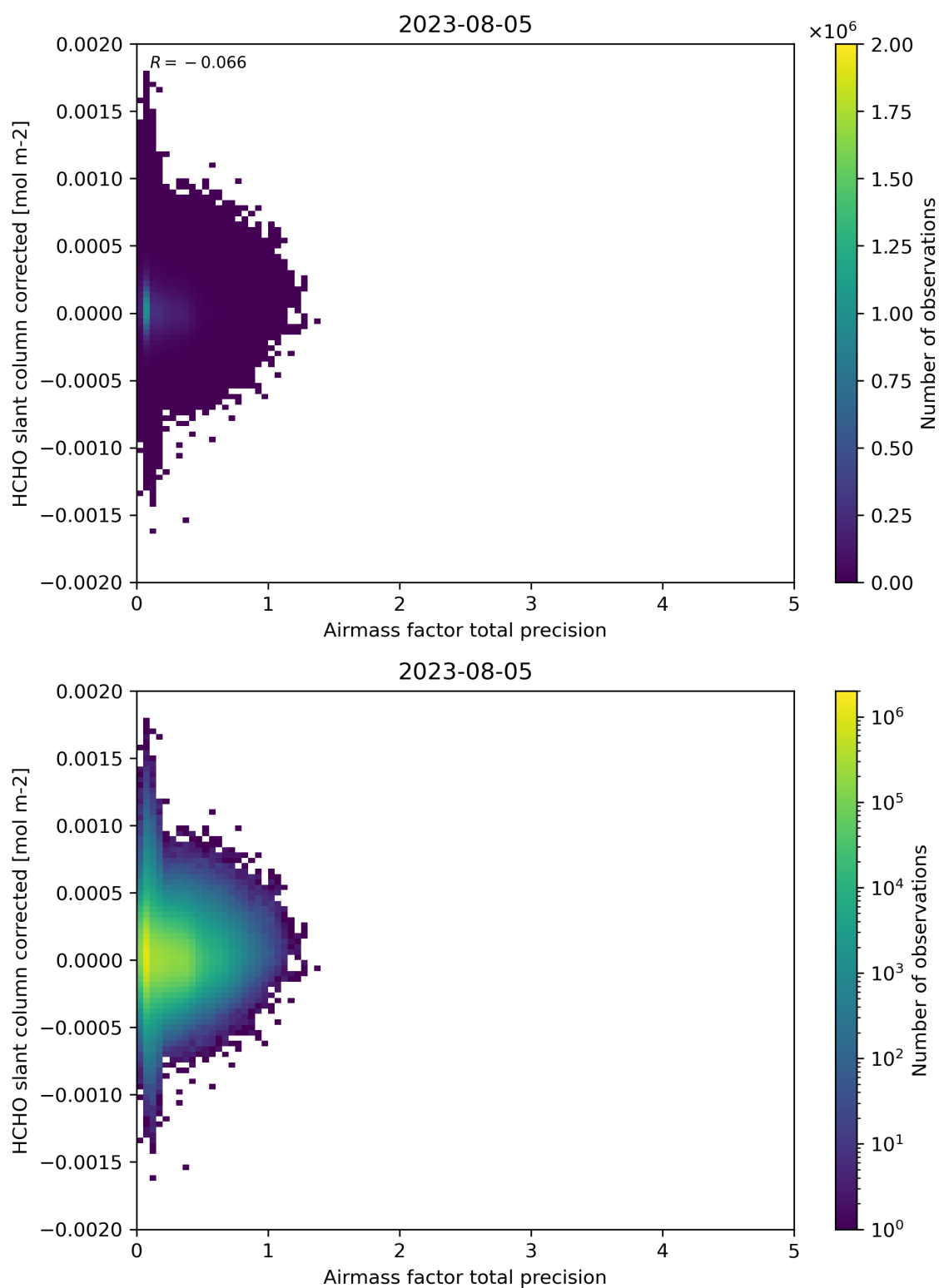
Figure 109: Scatter density plot of “Airmass factor total precision” against “HCHO slant column corrected” for 2023-08-04 to 2023-08-06.
