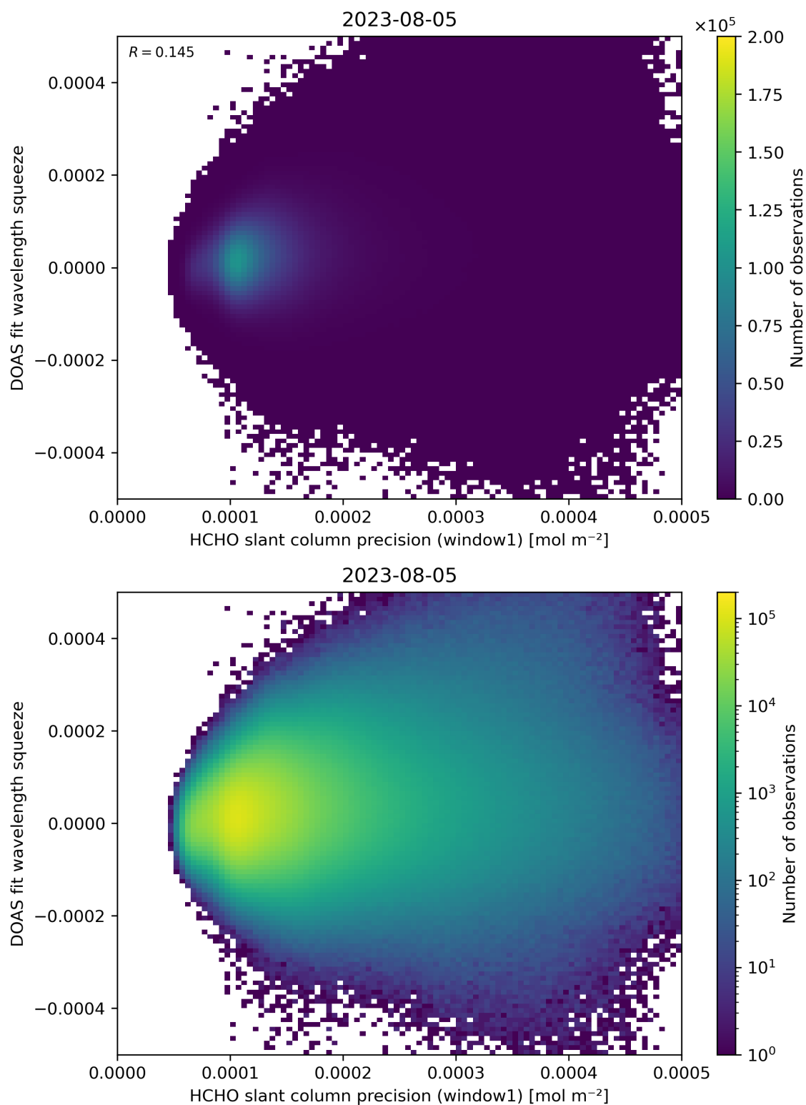
Figure 90: Scatter density plot of “HCHO slant column precision (window1)” against “DOAS fit wavelength squeeze” for 2023-08-04 to 2023-08-06.
