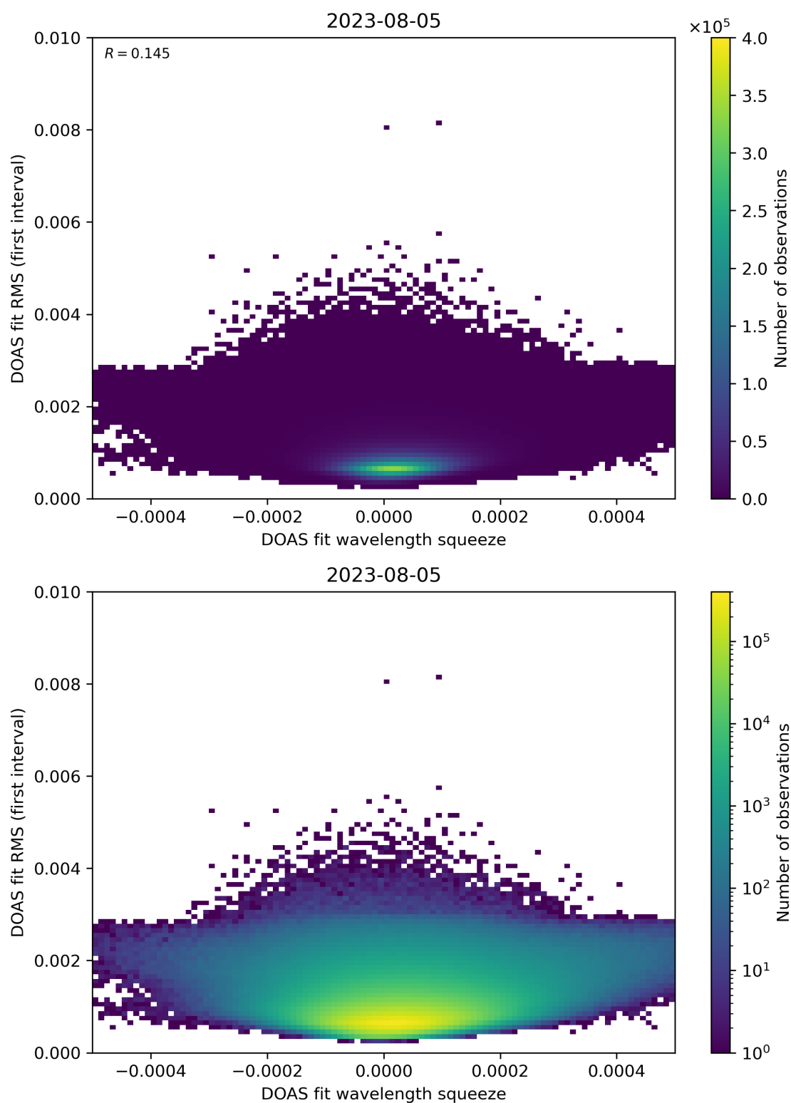
Figure 68: Scatter density plot of “DOAS fit wavelength squeeze” against “DOAS fit RMS (first interval)” for 2023-08-04 to 2023-08-06.
