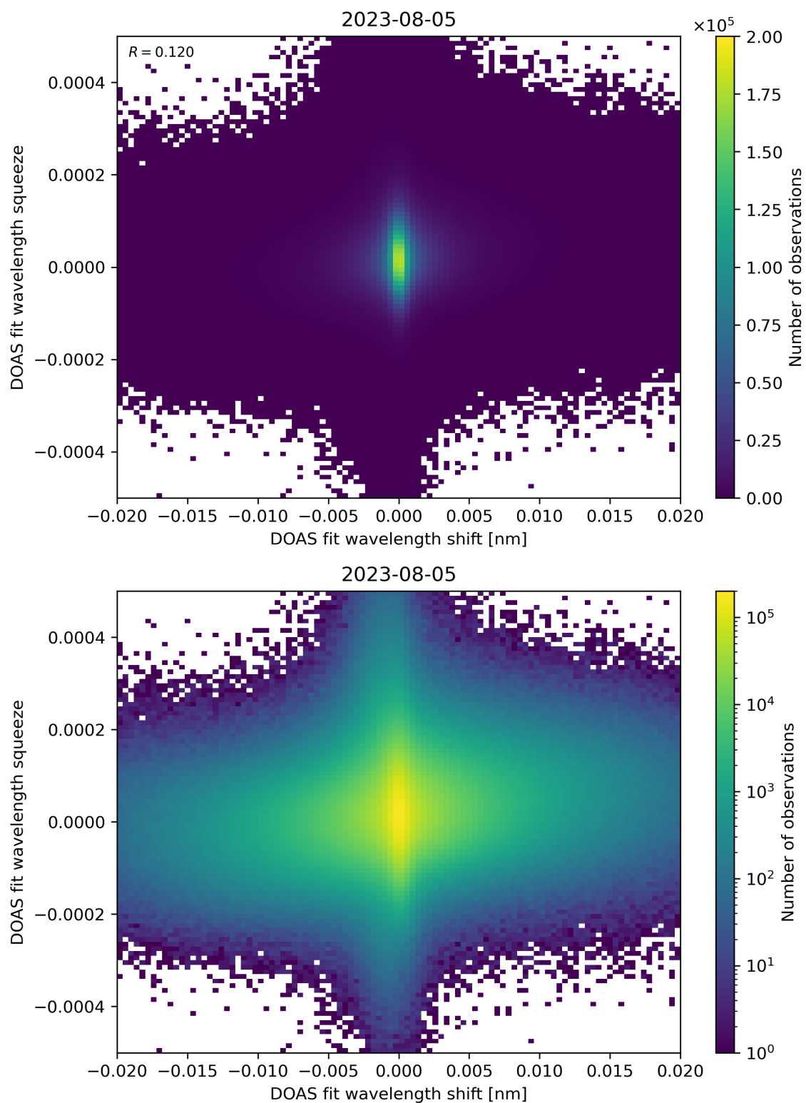
Figure 65: Scatter density plot of “DOAS fit wavelength shift” against “DOAS fit wavelength squeeze” for 2023-08-04 to 2023-08-06.
