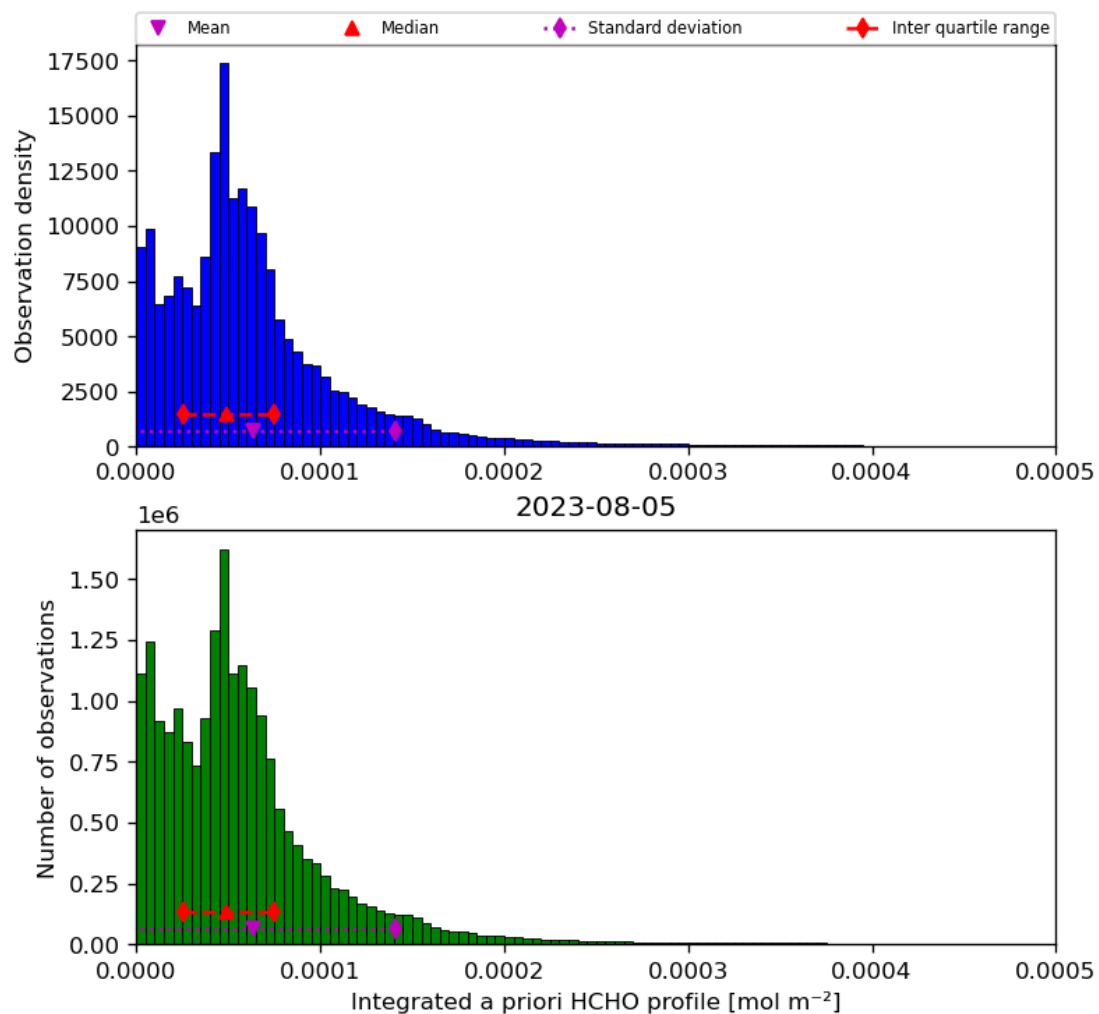
Figure 43: Histogram of “Integrated a priori HCHO profile” for 2023-08-04 to 2023-08-06
