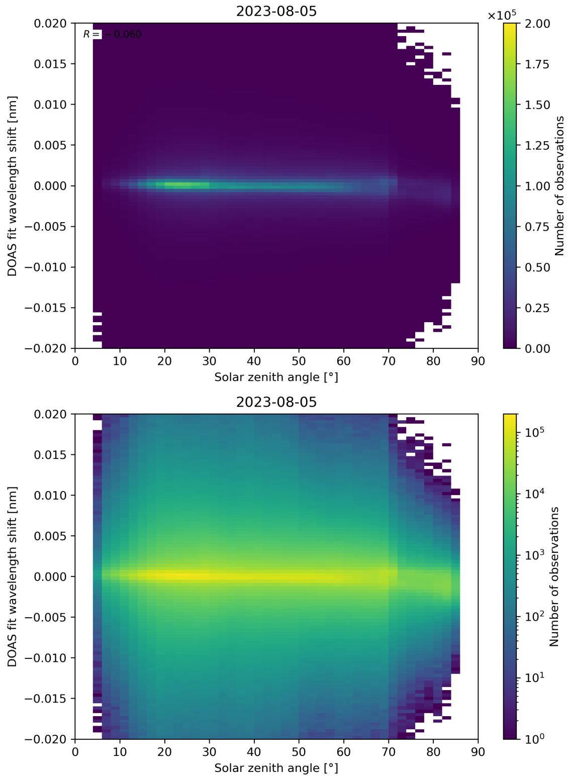
Figure 168: Scatter density plot of “Solar zenith angle” against “DOAS fit wavelength shift” for 2023-08-04 to 2023-08-06.
