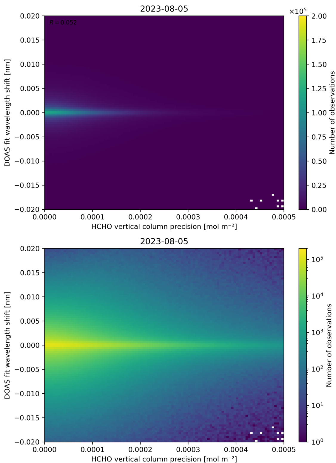
Figure 137: Scatter density plot of “HCHO vertical column precision” against “DOAS fit wavelength shift” for 2023-08-04 to 2023-08-06.
