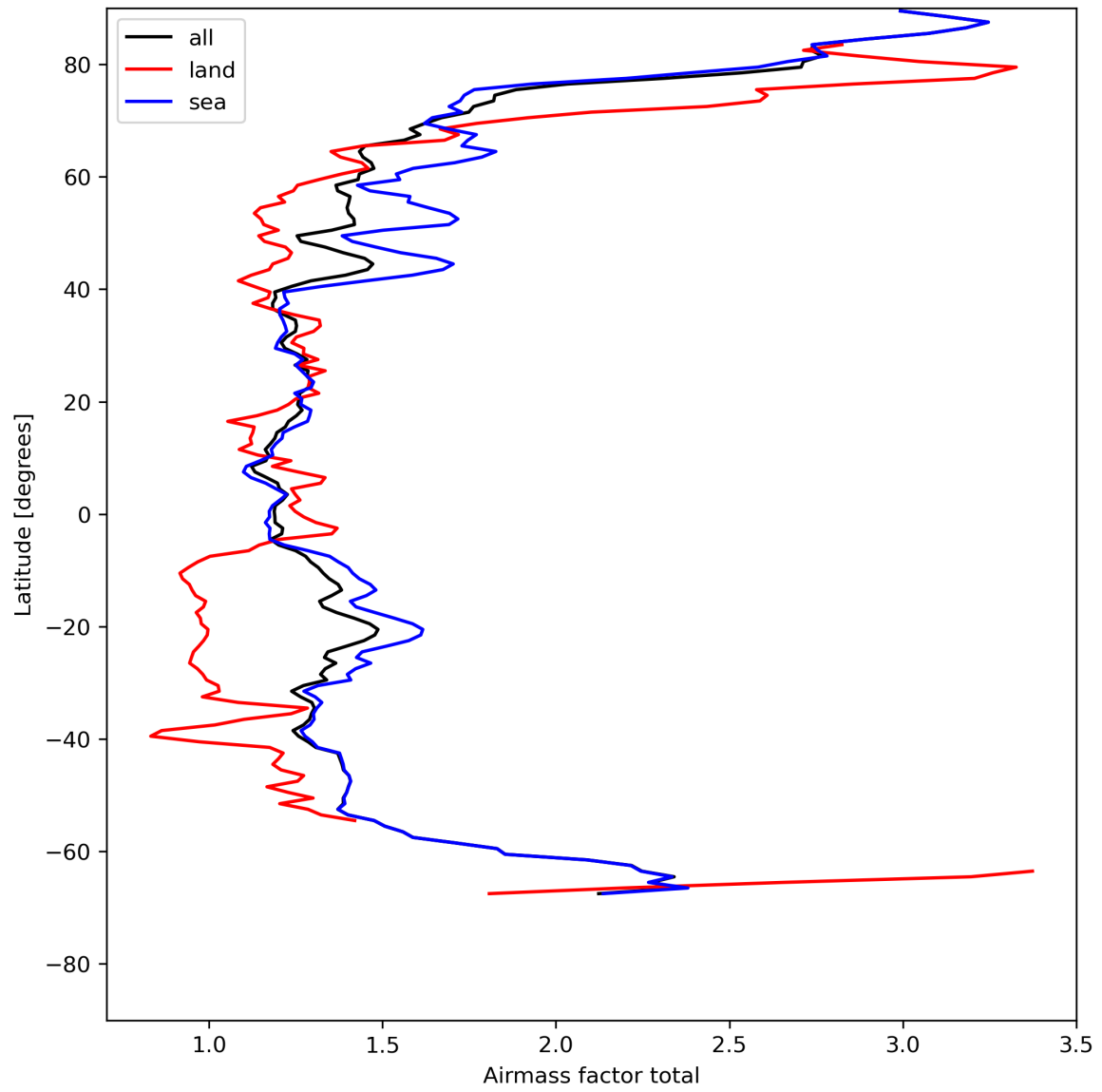
Figure 26: Zonal average of “Airmass factor total” for 2023-08-04 to 2023-08-06.
