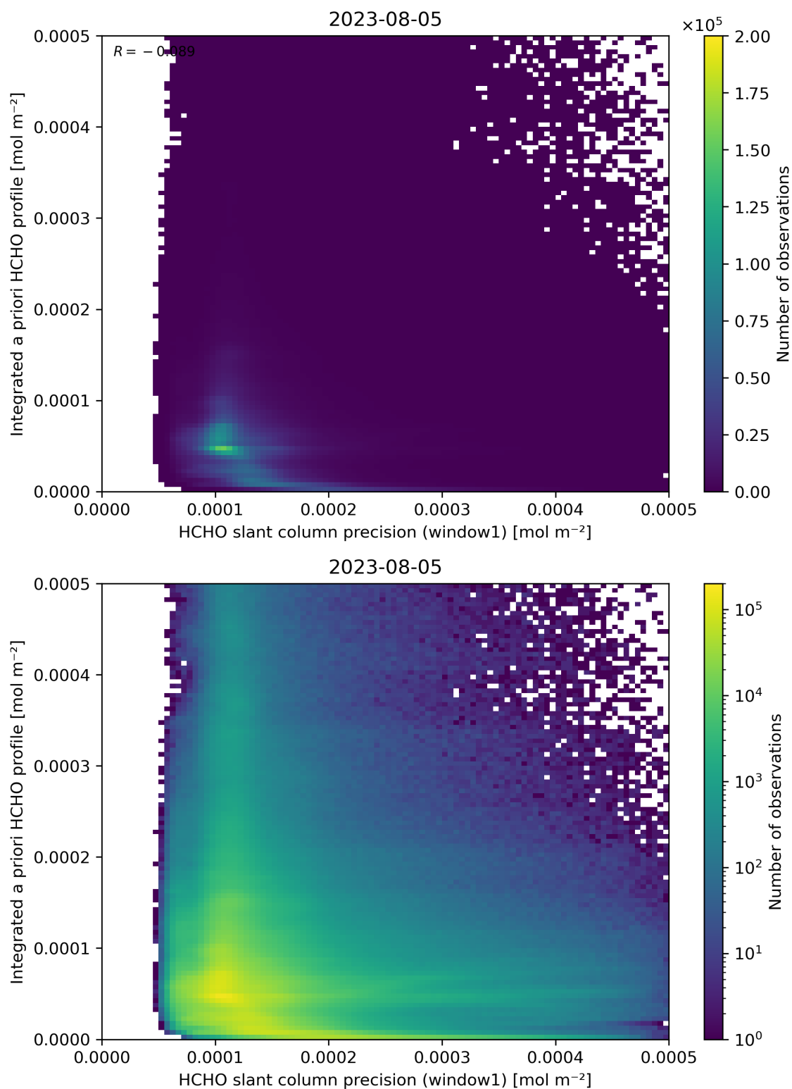
Figure 96: Scatter density plot of “HCHO slant column precision (window1)” against “Integrated a priori HCHO profile” for 2023-08-04 to 2023-08-06.
