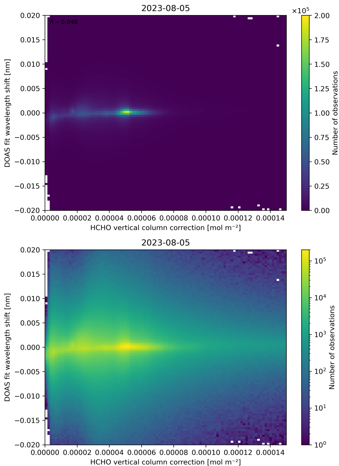
Figure 113: Scatter density plot of “HCHO vertical column correction” against “DOAS fit wavelength shift” for 2023-08-04 to 2023-08-06.
