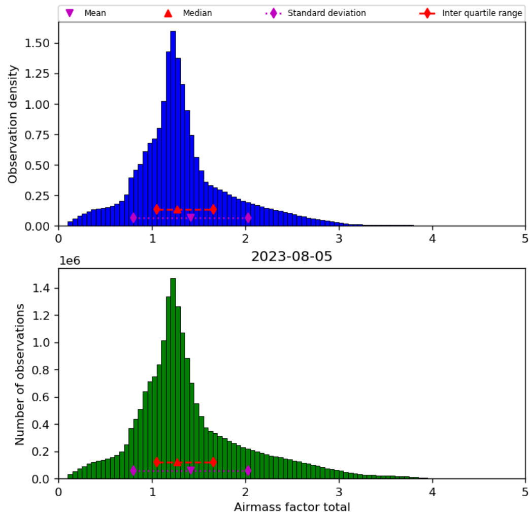
Figure 40: Histogram of “Airmass factor total” for 2023-08-04 to 2023-08-06
