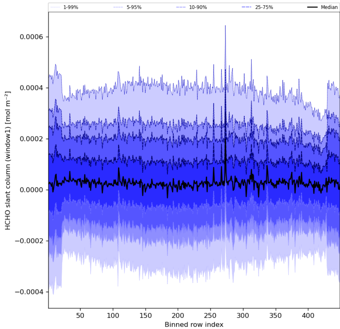
Figure 52: Along track statistics of “HCHO slant column (window1)” for 2023-08-04 to 2023-08-06
