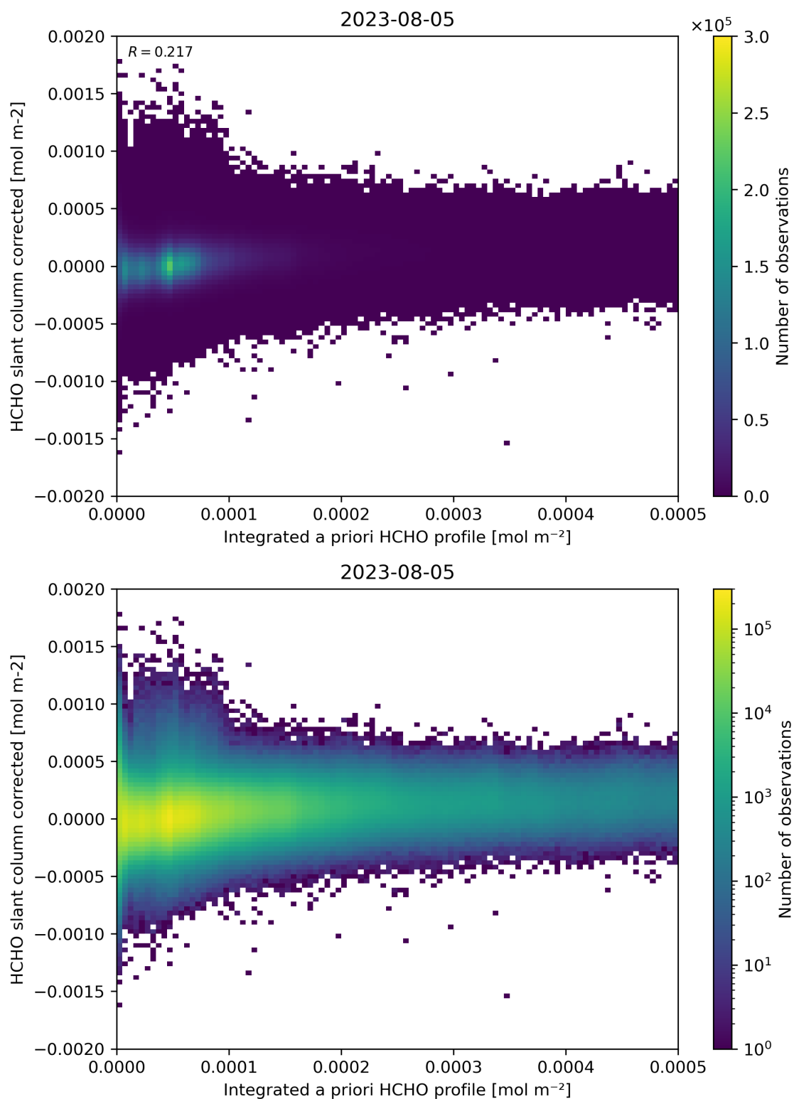
Figure 151: Scatter density plot of “Integrated a priori HCHO profile” against “HCHO slant column corrected” for 2023-08-04 to 2023-08-06.
