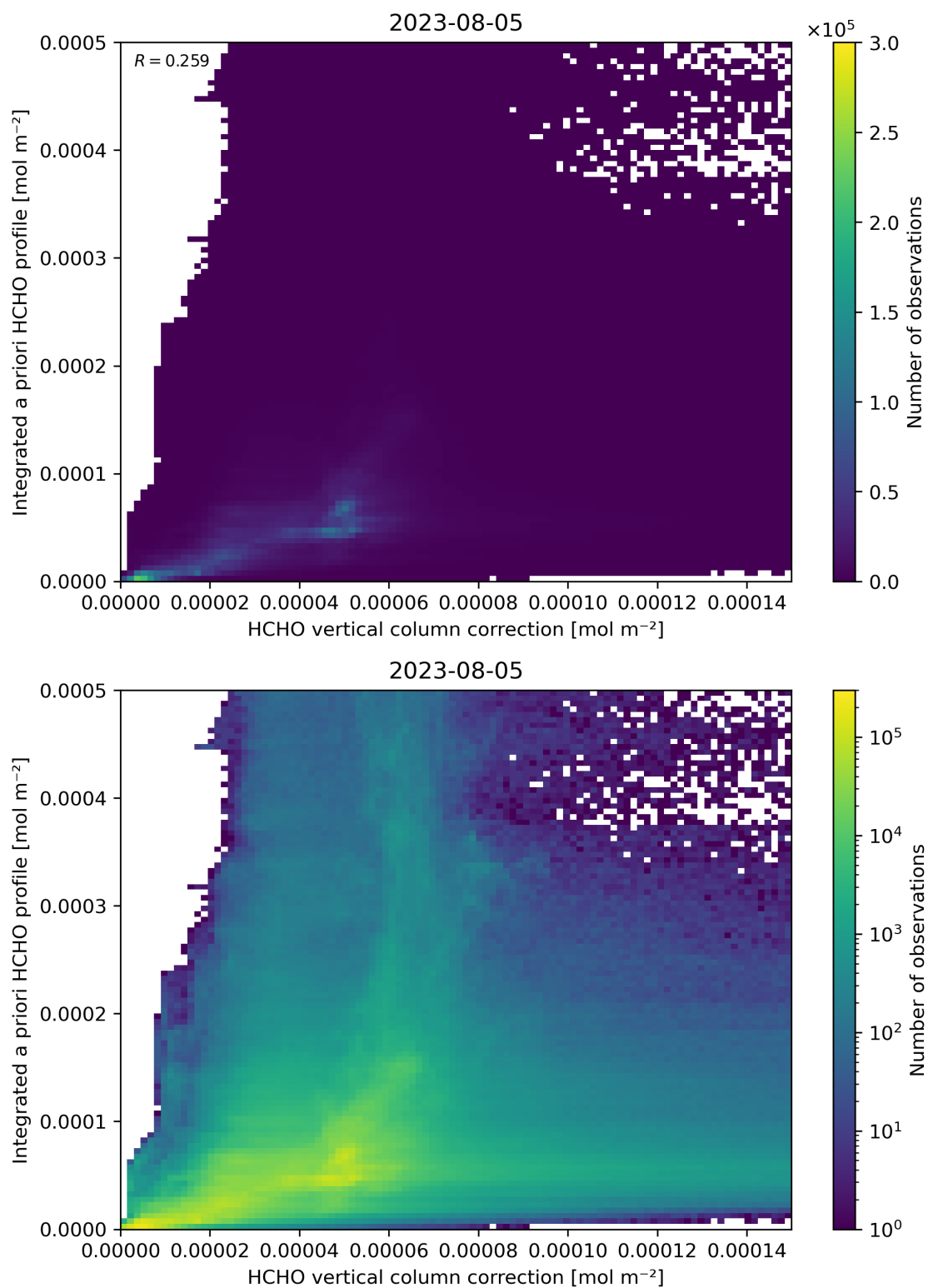
Figure 122: Scatter density plot of “HCHO vertical column correction” against “Integrated a priori HCHO profile” for 2023-08-04 to 2023-08-06.
