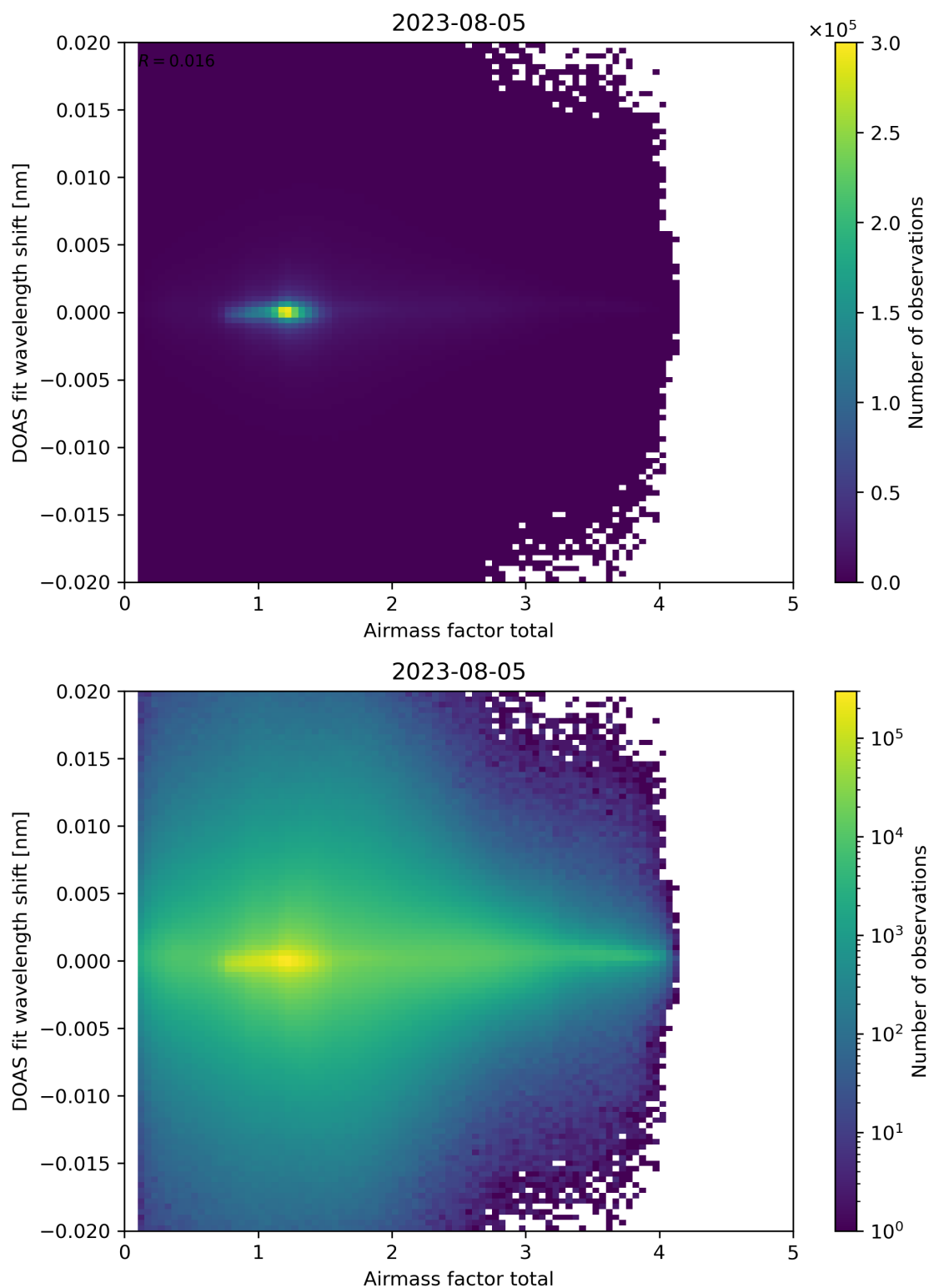
Figure 98: Scatter density plot of “Airmass factor total” against “DOAS fit wavelength shift” for 2023-08-04 to 2023-08-06.
