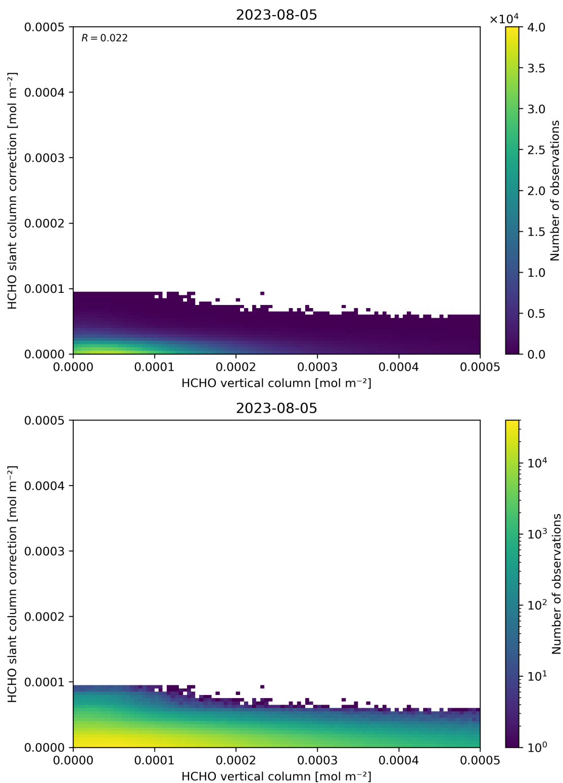
Figure 128: Scatter density plot of “HCHO vertical column” against “HCHO slant column correction” for 2023-08-04 to 2023-08-06.
