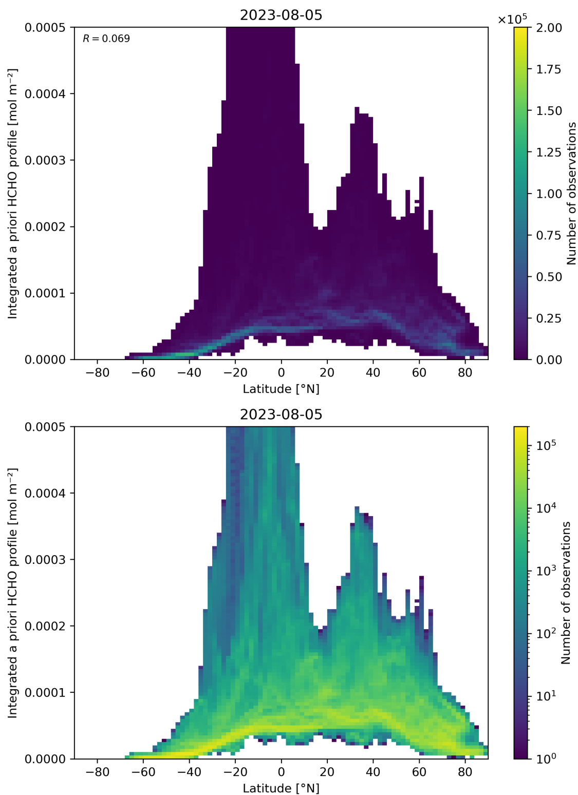
Figure 166: Scatter density plot of “Latitude” against “Integrated a priori HCHO profile” for 2023-08-04 to 2023-08-06.
