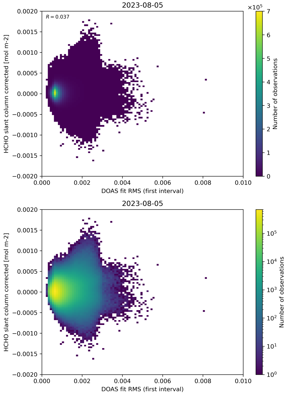
Figure 62: Scatter density plot of “DOAS fit RMS (first interval)” against “HCHO slant column corrected” for 2023-08-04 to 2023-08-06.
