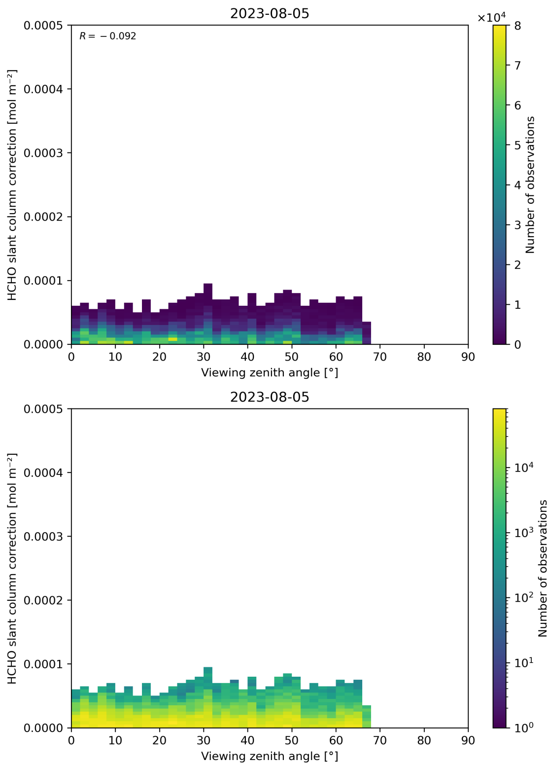
Figure 187: Scatter density plot of “Viewing zenith angle” against “HCHO slant column correction” for 2023-08-04 to 2023-08-06.
