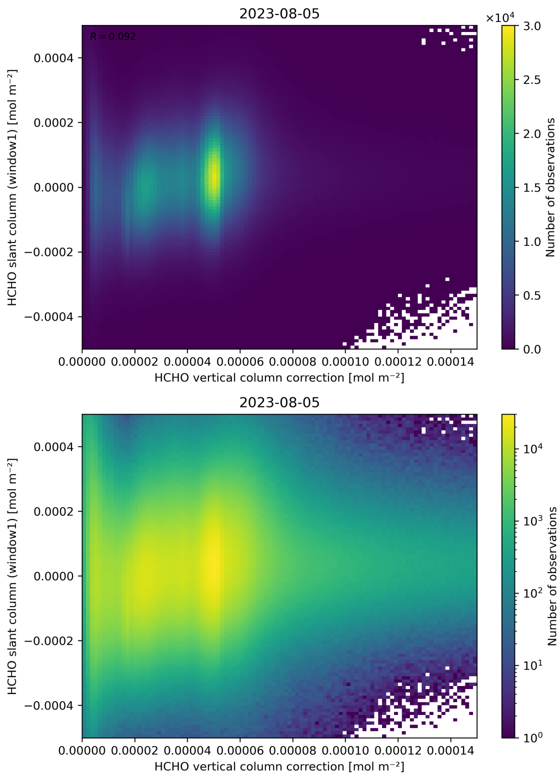
Figure 118: Scatter density plot of “HCHO vertical column correction” against “HCHO slant column (window1)” for 2023-08-04 to 2023-08-06.
