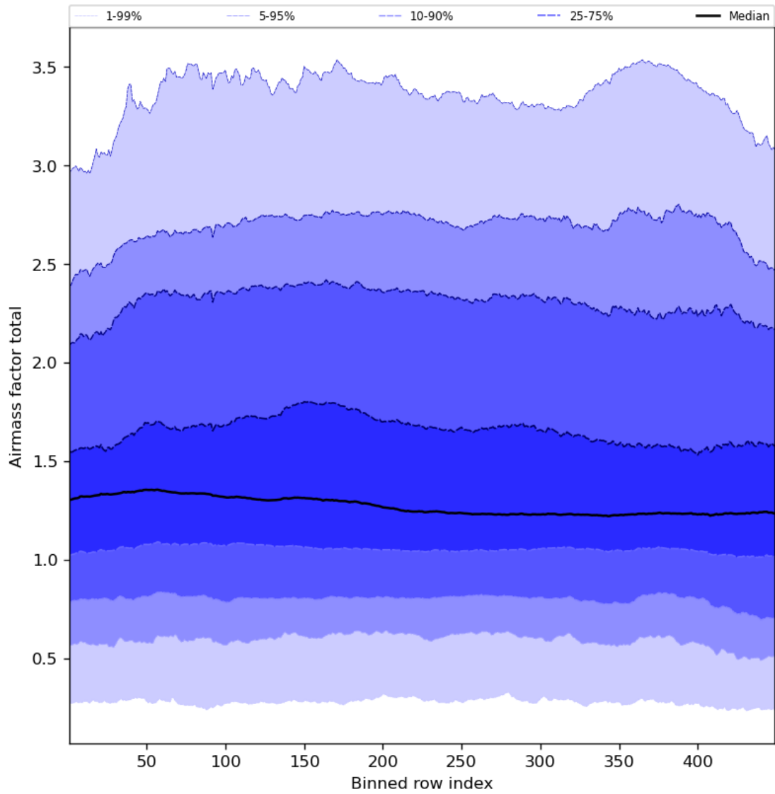
Figure 54: Along track statistics of “Airmass factor total” for 2023-08-04 to 2023-08-06
