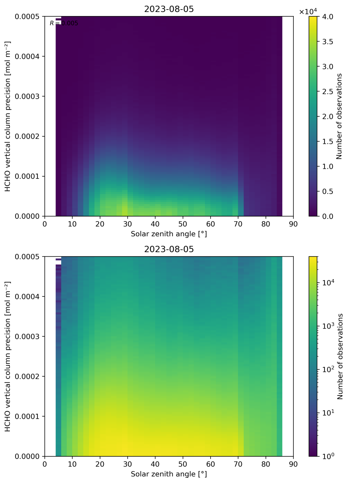
Figure 179: Scatter density plot of “Solar zenith angle” against “HCHO vertical column precision” for 2023-08-04 to 2023-08-06.
