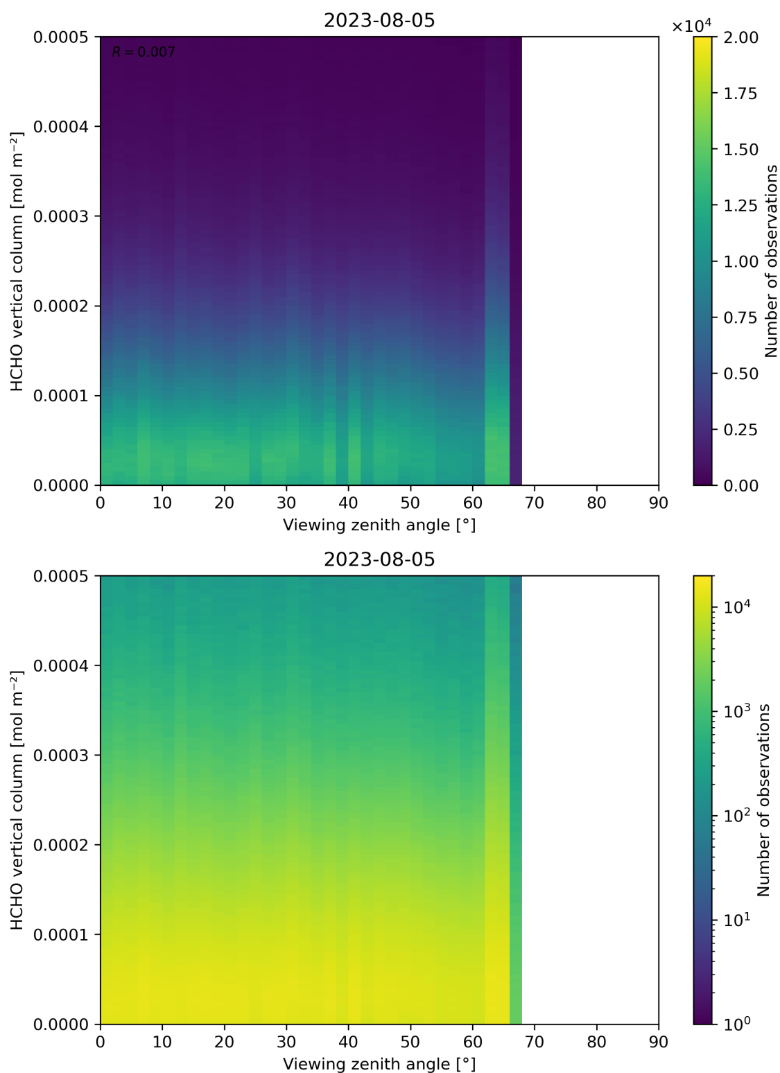
Figure 192: Scatter density plot of “Viewing zenith angle” against “HCHO vertical column” for 2023-08-04 to 2023-08-06.
