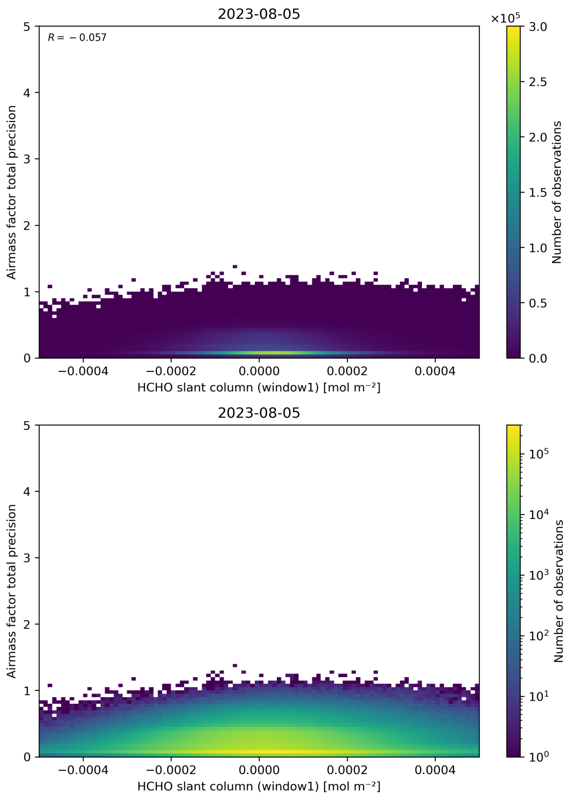
Figure 86: Scatter density plot of “HCHO slant column (window1)” against “Airmass factor total precision” for 2023-08-04 to 2023-08-06.
