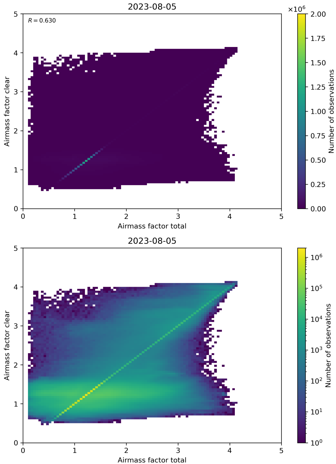
Figure 100: Scatter density plot of “Airmass factor total” against “Airmass factor clear” for 2023-08-04 to 2023-08-06.
