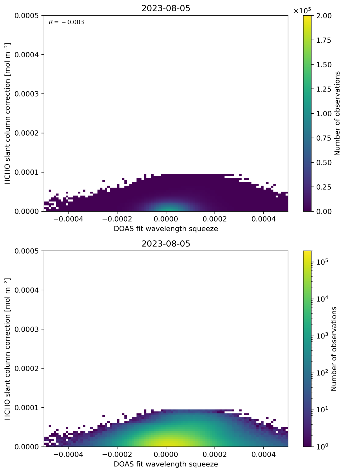
Figure 70: Scatter density plot of “DOAS fit wavelength squeeze” against “HCHO slant column correction” for 2023-08-04 to 2023-08-06.
