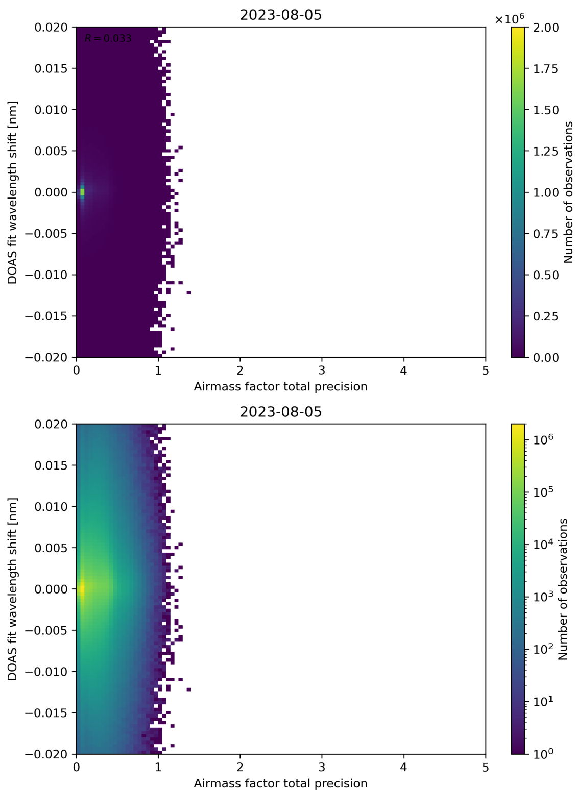
Figure 106: Scatter density plot of “Airmass factor total precision” against “DOAS fit wavelength shift” for 2023-08-04 to 2023-08-06.
