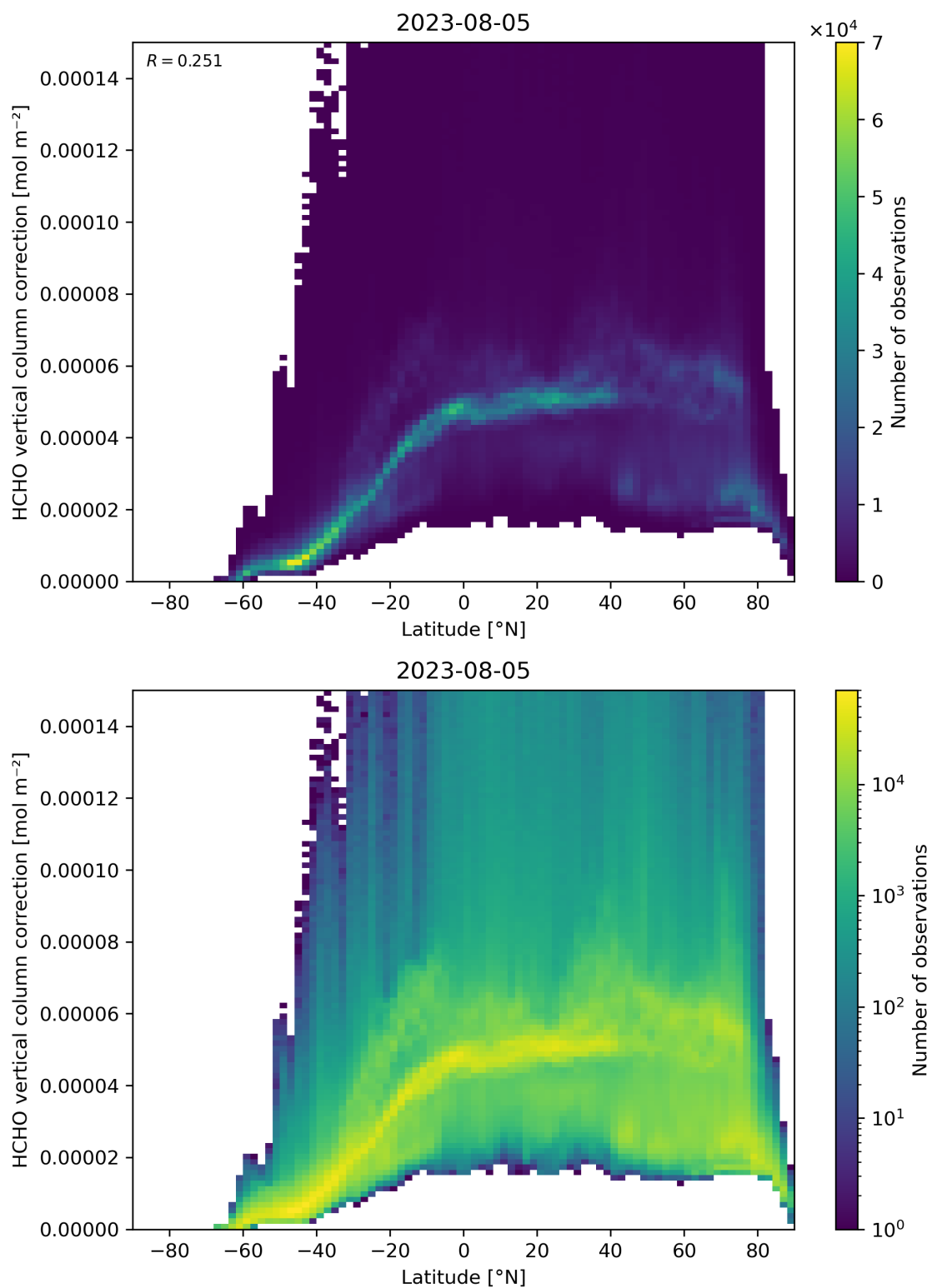
Figure 164: Scatter density plot of “Latitude” against “HCHO vertical column correction” for 2023-08-04 to 2023-08-06.
