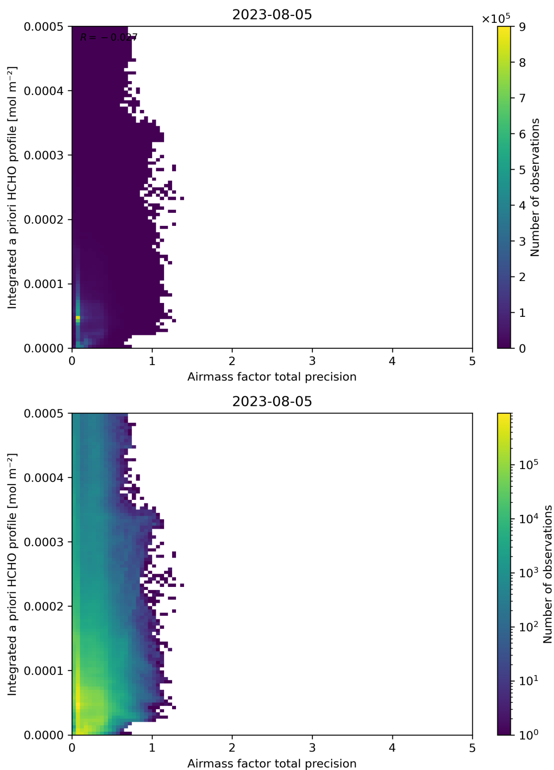
Figure 111: Scatter density plot of “Airmass factor total precision” against “Integrated a priori HCHO profile” for 2023-08-04 to 2023-08-06.
