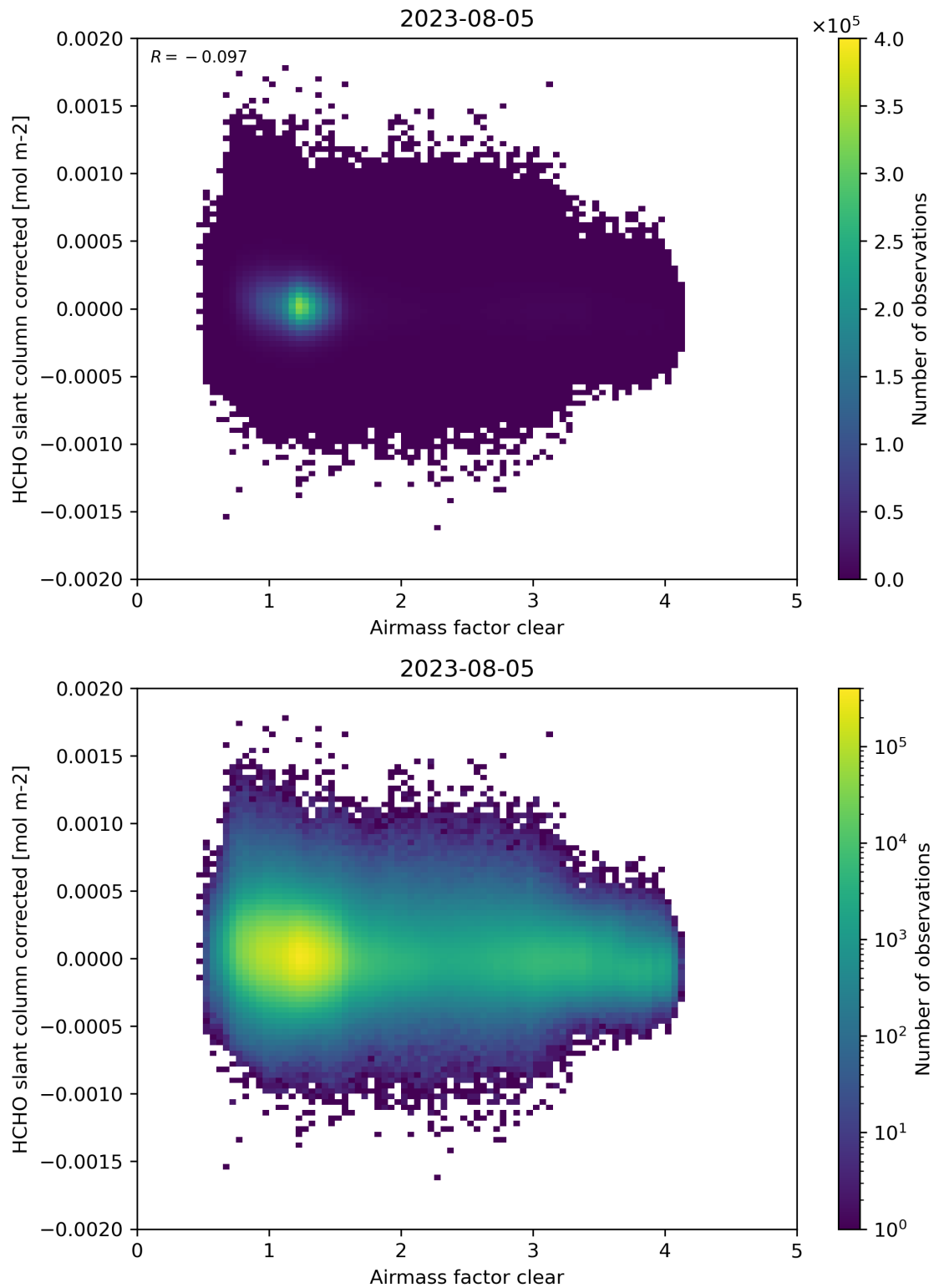
Figure 74: Scatter density plot of “Airmass factor clear” against “HCHO slant column corrected” for 2023-08-04 to 2023-08-06.
