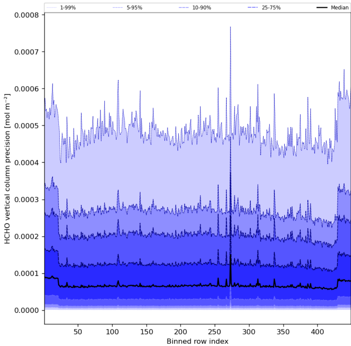
Figure 50: Along track statistics of "HCHO vertical column precision" for 2023-08-04 to 2023-08-06
