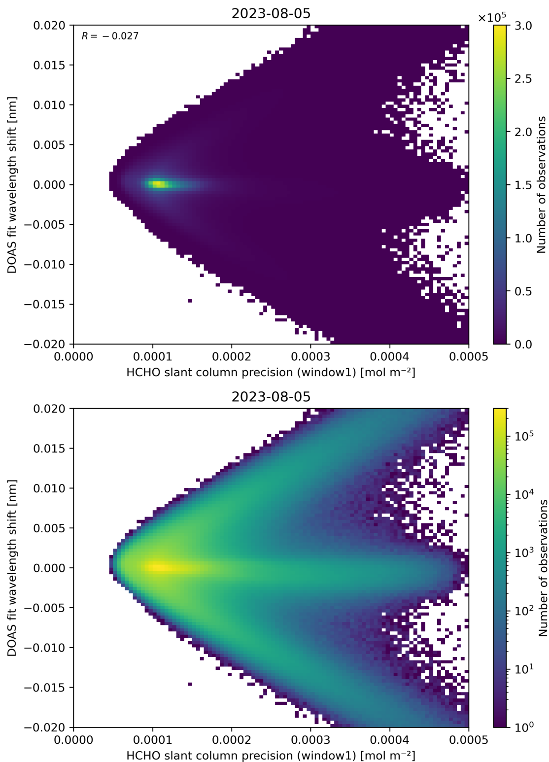
Figure 89: Scatter density plot of “HCHO slant column precision (window1)” against “DOAS fit wavelength shift” for 2023-08-04 to 2023-08-06.
