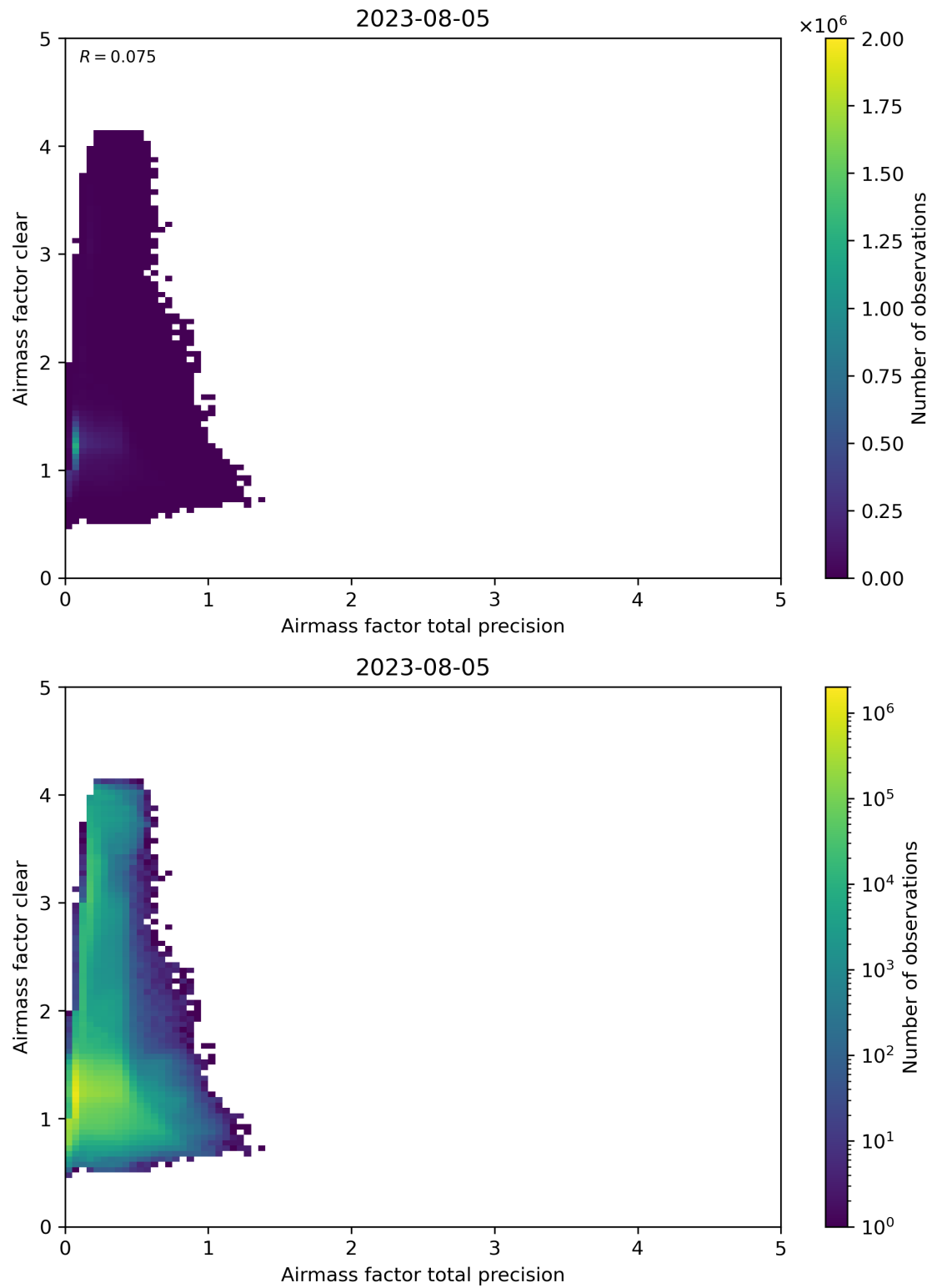
Figure 108: Scatter density plot of “Airmass factor total precision” against “Airmass factor clear” for 2023-08-04 to 2023-08-06.
