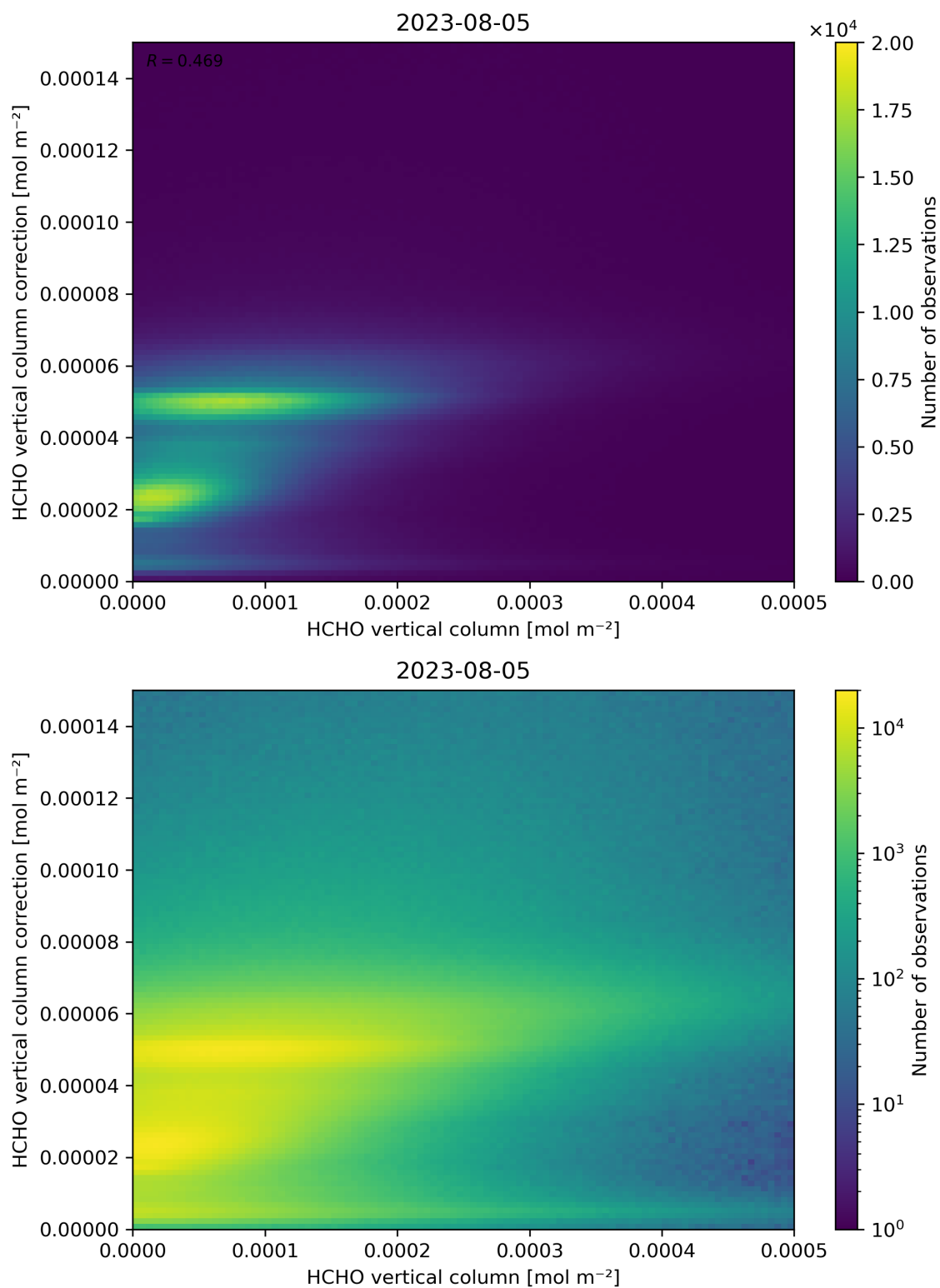
Figure 133: Scatter density plot of “HCHO vertical column” against “HCHO vertical column correction” for 2023-08-04 to 2023-08-06.
