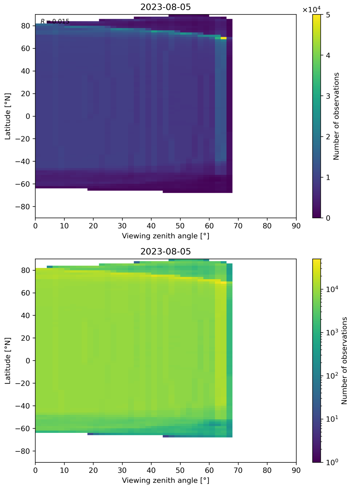
Figure 196: Scatter density plot of “Viewing zenith angle” against “Latitude” for 2023-08-04 to 2023-08-06.
