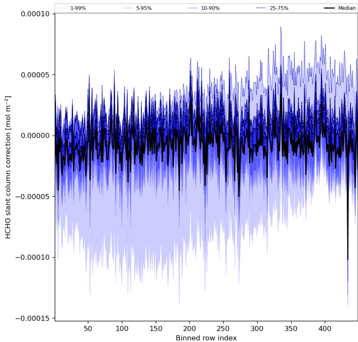
Figure 61: Along track statistics of “HCHO slant column correction” for 2023-08-04 to 2023-08-06
