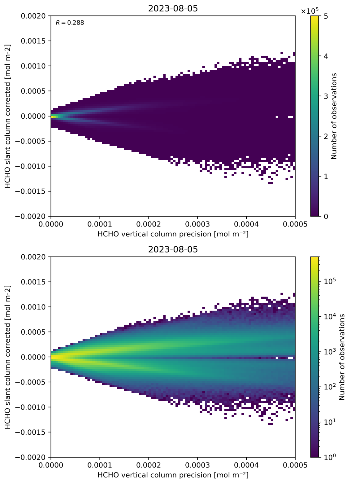
Figure 140: Scatter density plot of “HCHO vertical column precision” against “HCHO slant column corrected” for 2023-08-04 to 2023-08-06.
