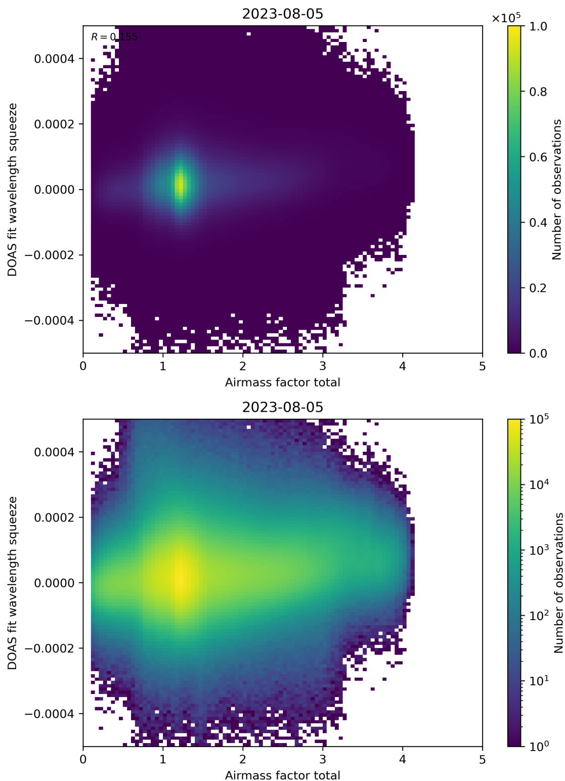
Figure 99: Scatter density plot of “Airmass factor total” against “DOAS fit wavelength squeeze” for 2023-08-04 to 2023-08-06.
