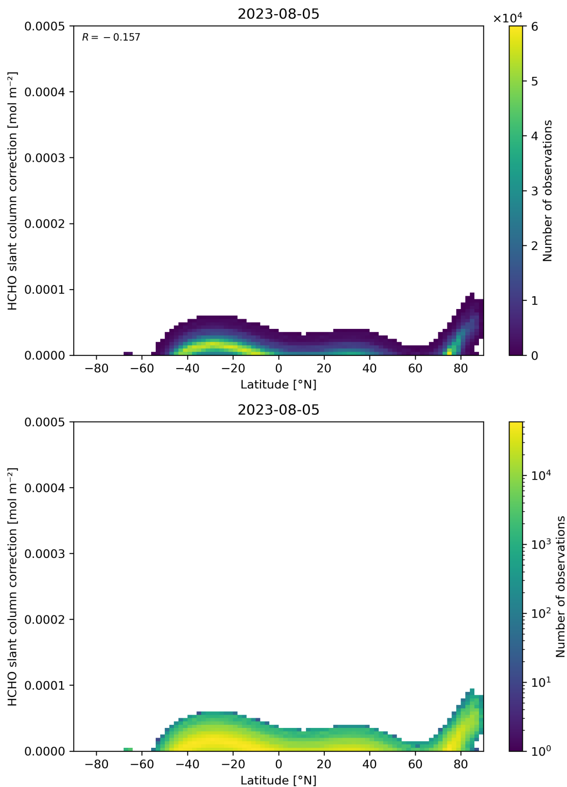
Figure 158: Scatter density plot of “Latitude” against “HCHO slant column correction” for 2023-08-04 to 2023-08-06.
