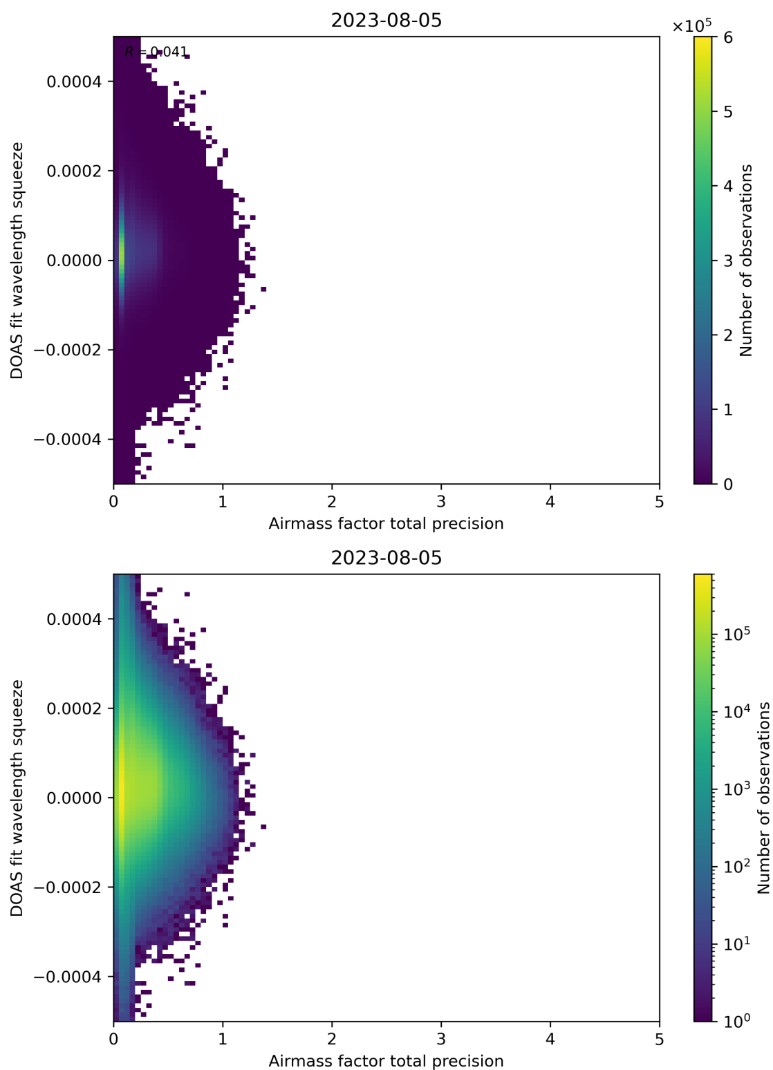
Figure 107: Scatter density plot of “Airmass factor total precision” against “DOAS fit wavelength squeeze” for 2023-08-04 to 2023-08-06.
