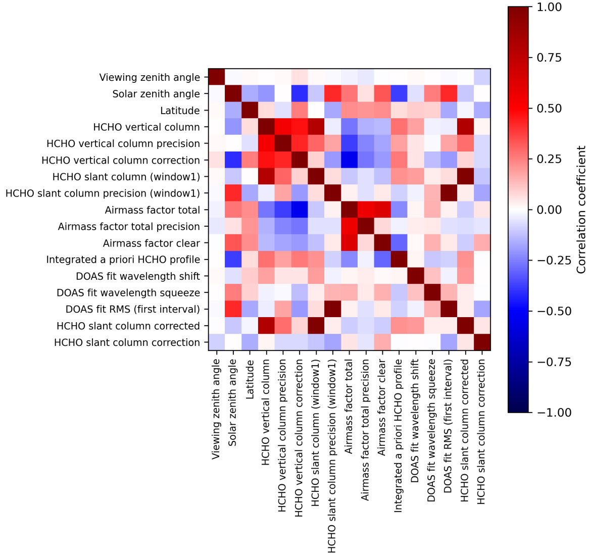
Figure 2: Map of correlation matrix for 2023-08-04 to 2023-08-06.
