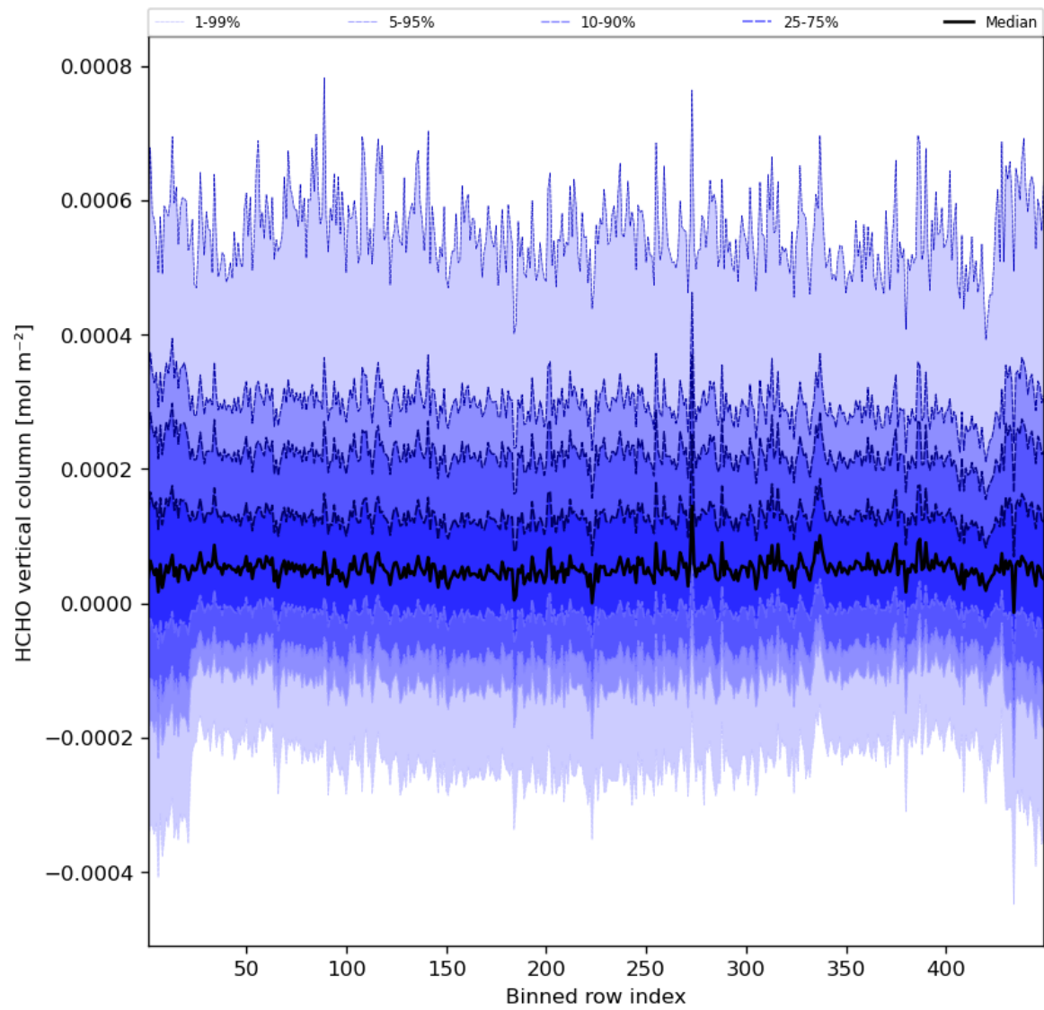
Figure 49: Along track statistics of “HCHO vertical column” for 2023-08-04 to 2023-08-06
