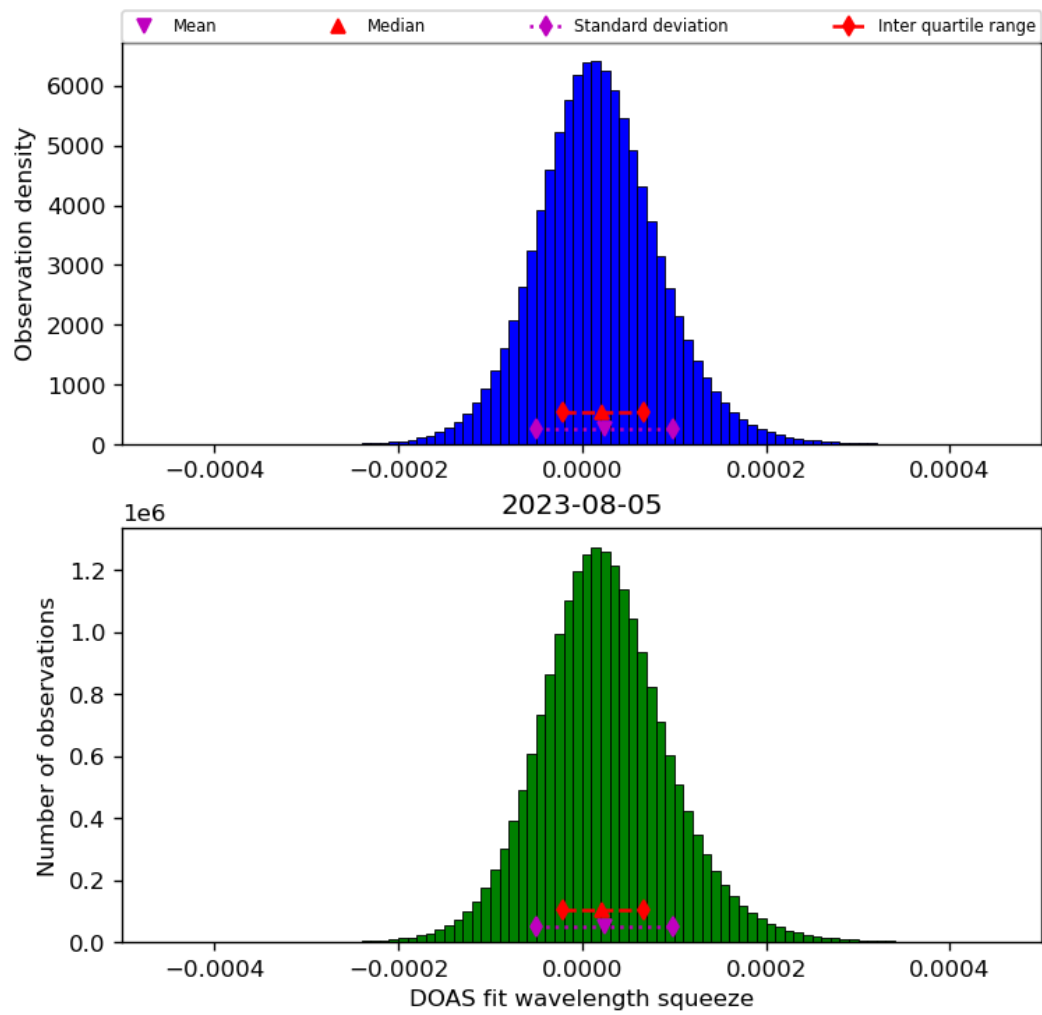
Figure 45: Histogram of “DOAS fit wavelength squeeze” for 2023-08-04 to 2023-08-06
