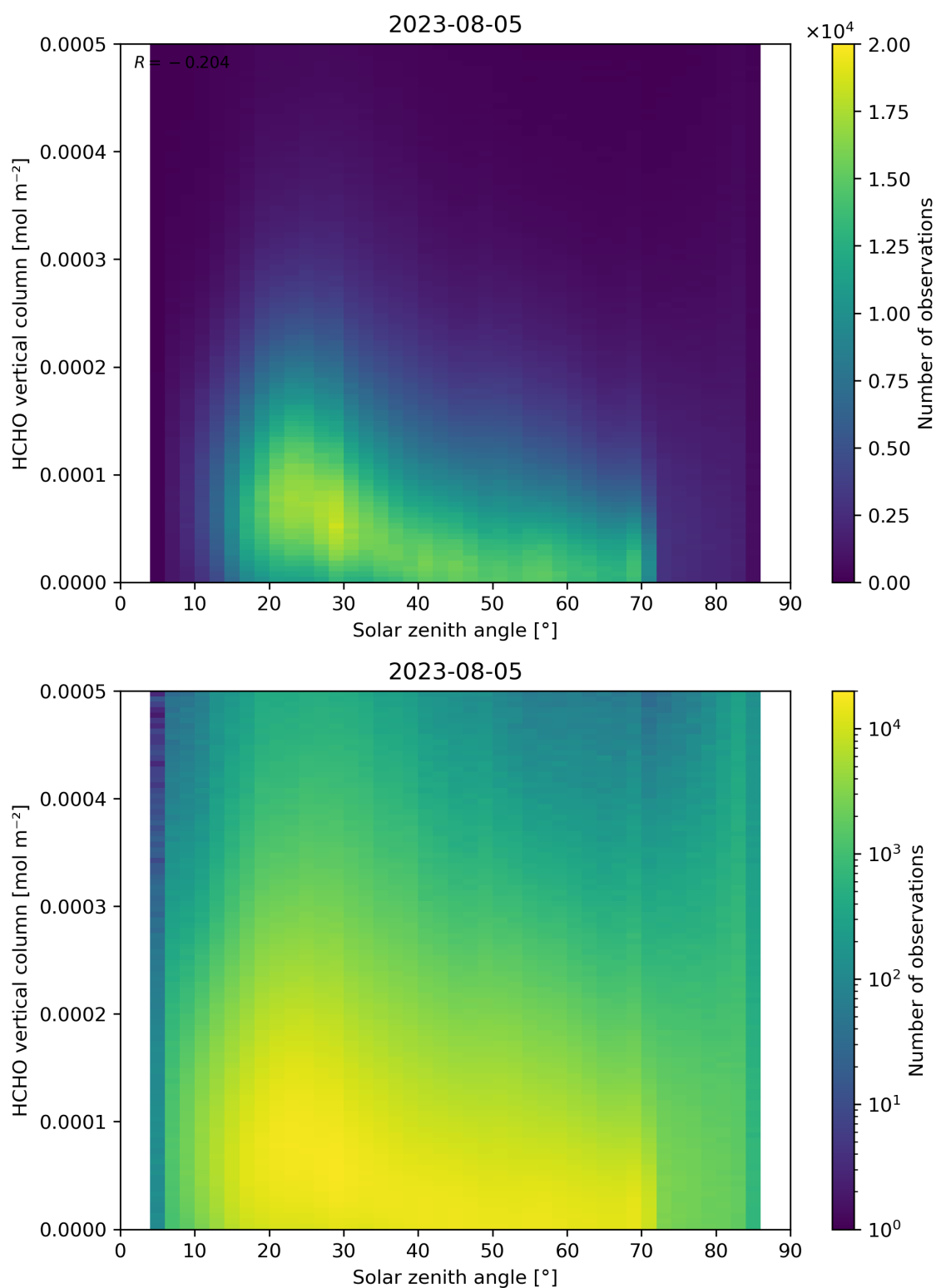
Figure 177: Scatter density plot of “Solar zenith angle” against “HCHO vertical column” for 2023-08-04 to 2023-08-06.
