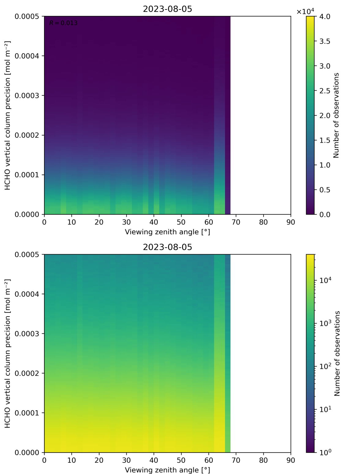
Figure 194: Scatter density plot of “Viewing zenith angle” against “HCHO vertical column precision” for 2023-08-04 to 2023-08-06.
