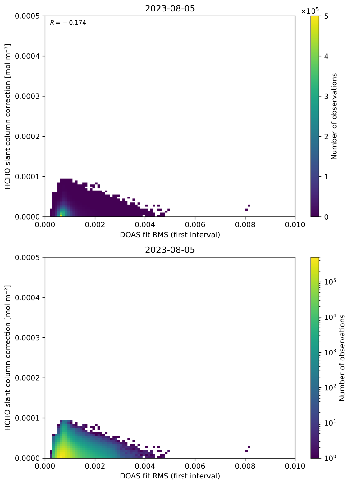
Figure 63: Scatter density plot of “DOAS fit RMS (first interval)” against “HCHO slant column correction” for 2023-08-04 to 2023-08-06.
