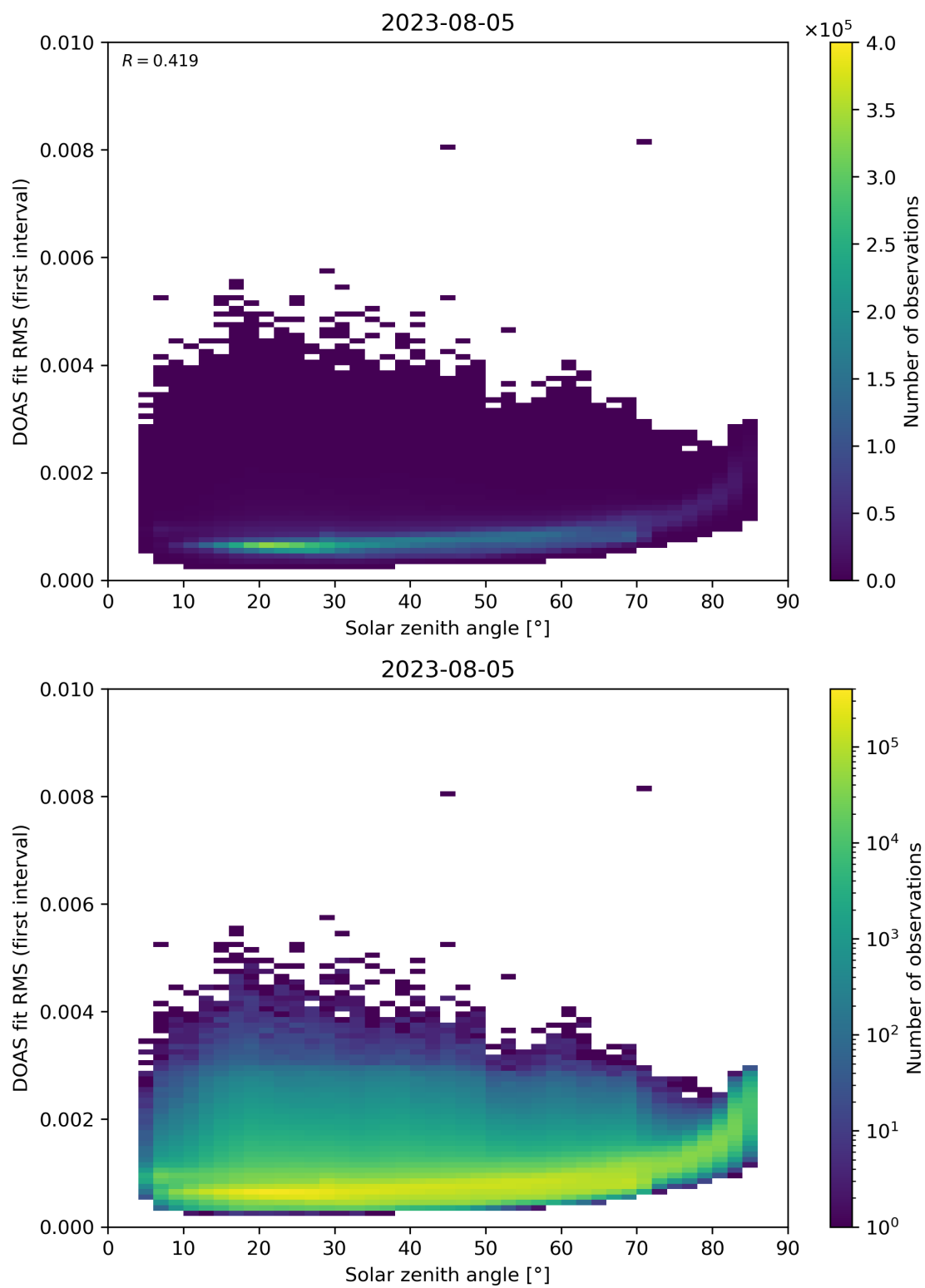
Figure 167: Scatter density plot of “Solar zenith angle” against “DOAS fit RMS (first interval)” for 2023-08-04 to 2023-08-06.
