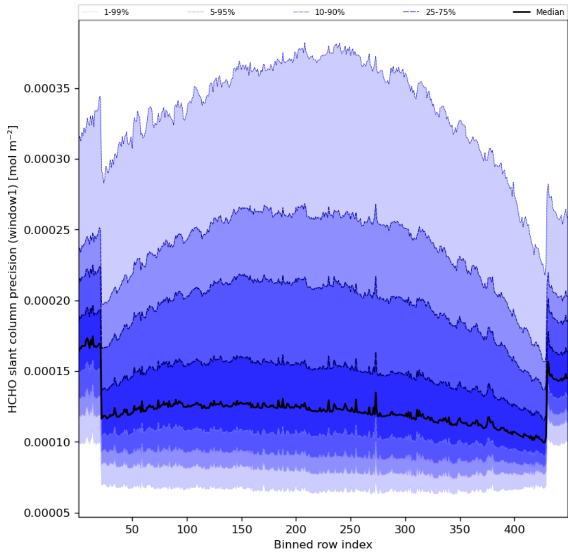
Figure 53: Along track statistics of “HCHO slant column precision (window1)” for 2023-08-04 to 2023-08-06
