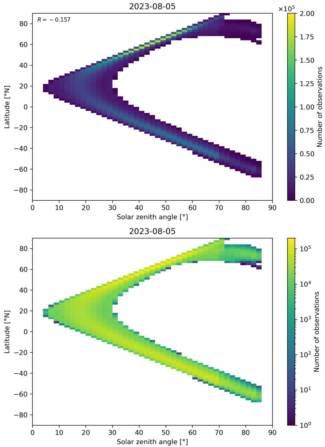
Figure 181: Scatter density plot of “Solar zenith angle” against “Latitude” for 2023-08-04 to 2023-08-06.
