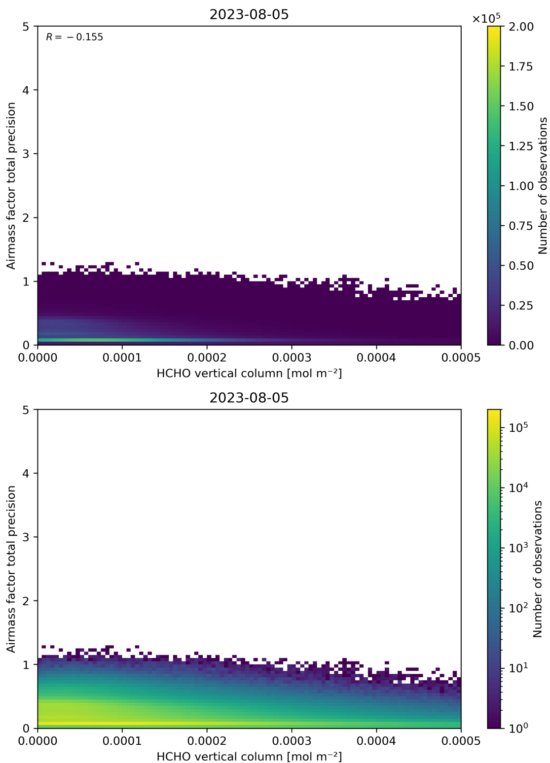
Figure 132: Scatter density plot of “HCHO vertical column” against “Airmass factor total precision” for 2023-08-04 to 2023-08-06.
