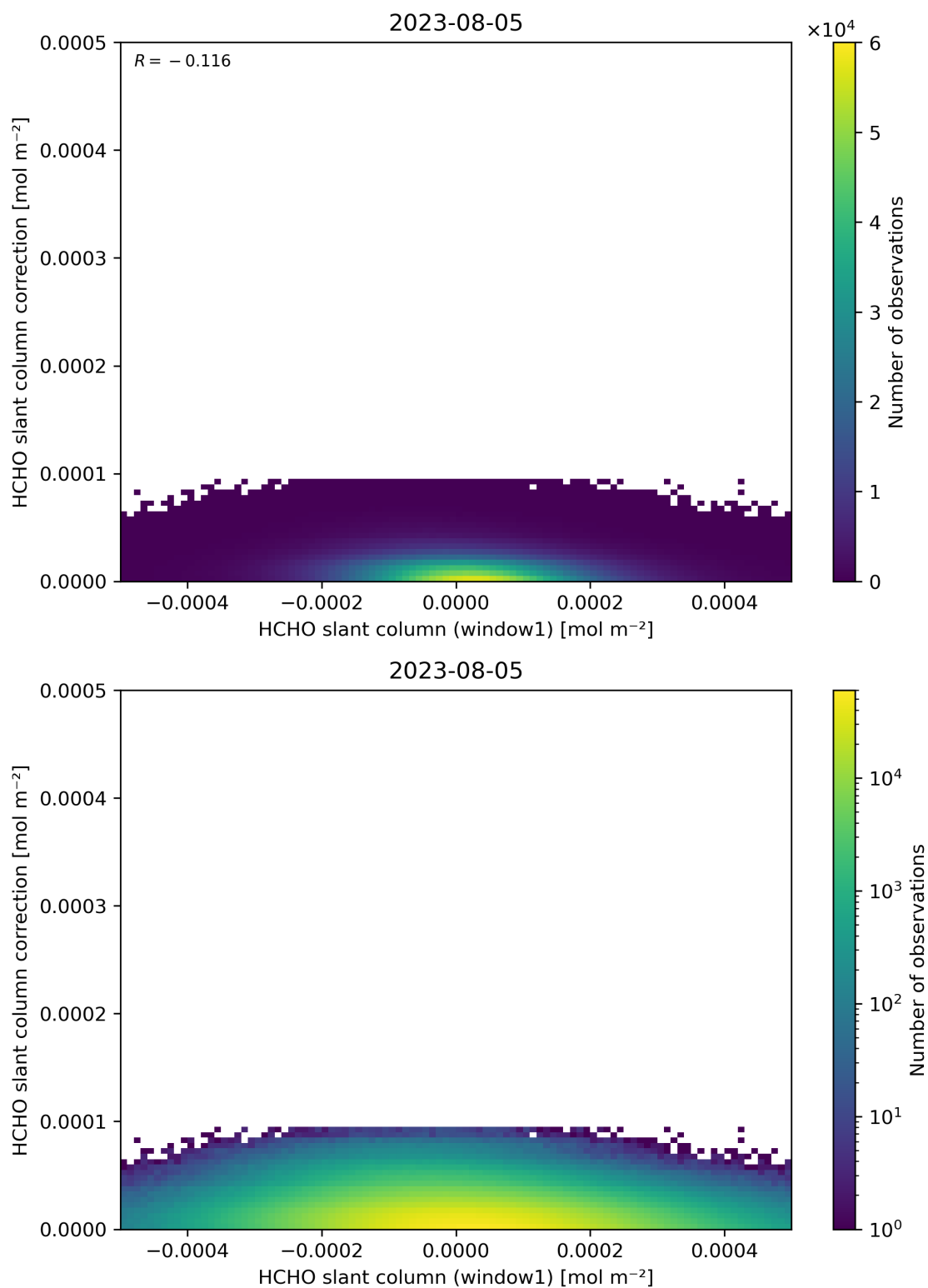
Figure 83: Scatter density plot of “HCHO slant column (window1)” against “HCHO slant column correction” for 2023-08-04 to 2023-08-06.
