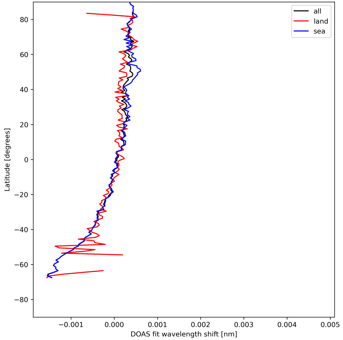
Figure 30: Zonal average of “DOAS fit wavelength shift” for 2023-08-04 to 2023-08-06.
