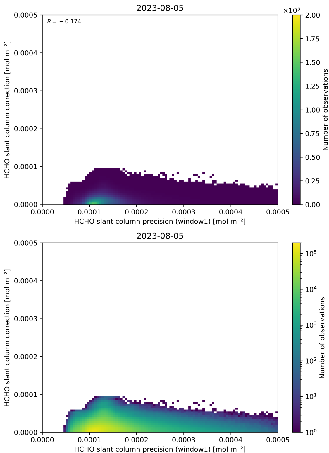
Figure 93: Scatter density plot of “HCHO slant column precision (window1)” against “HCHO slant column correction” for 2023-08-04 to 2023-08-06.
