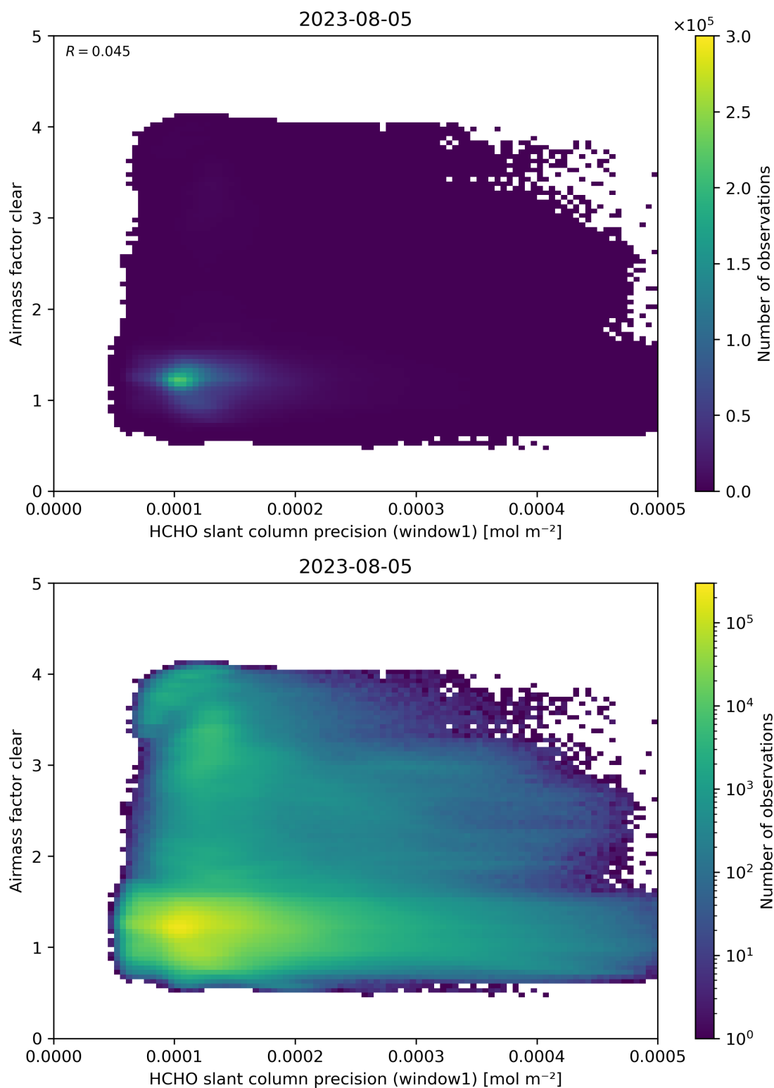
Figure 91: Scatter density plot of “HCHO slant column precision (window1)” against “Airmass factor clear” for 2023-08-04 to 2023-08-06.
