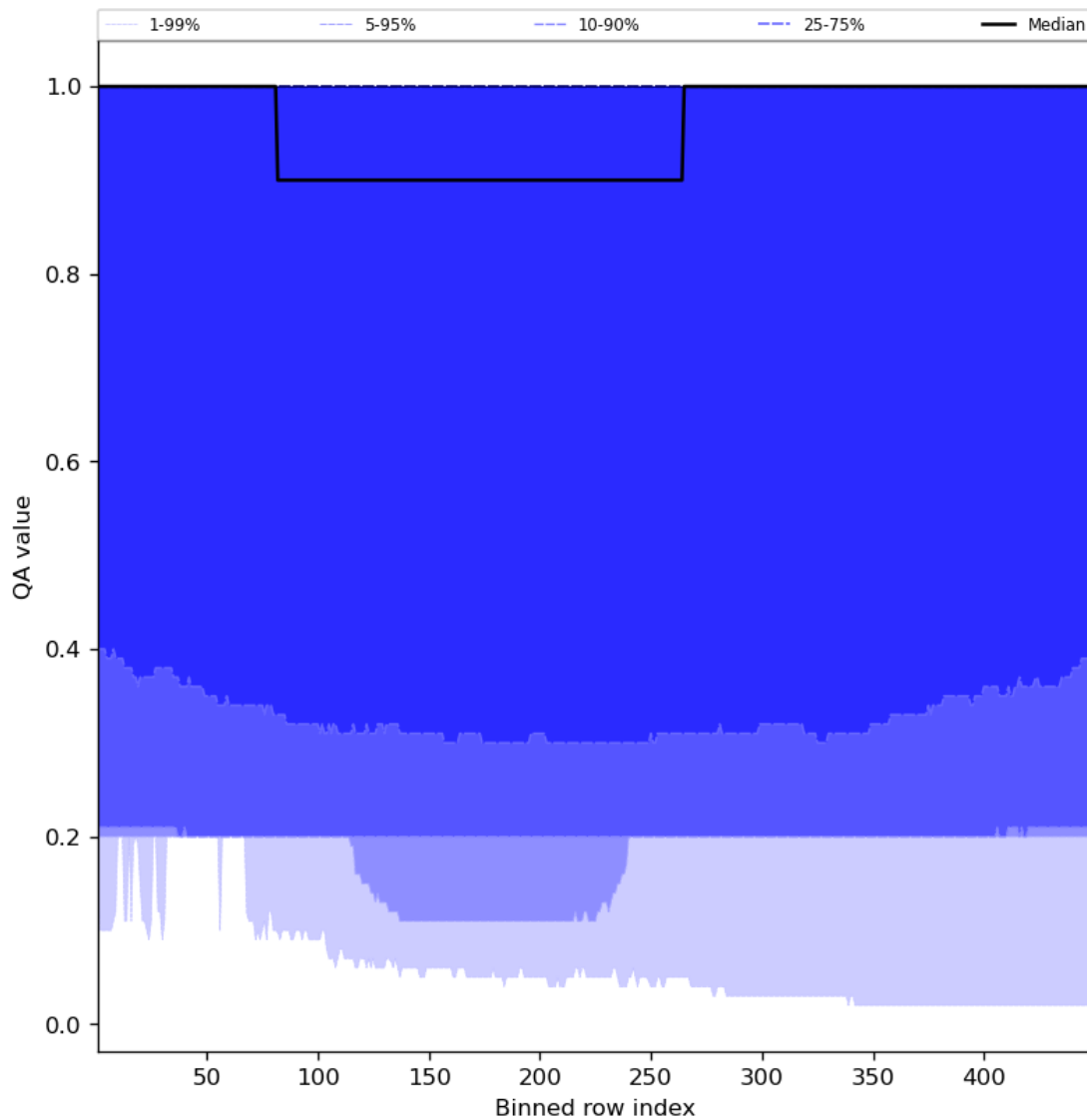
Figure 48: Along track statistics of “QA value” for 2023-08-04 to 2023-08-06
