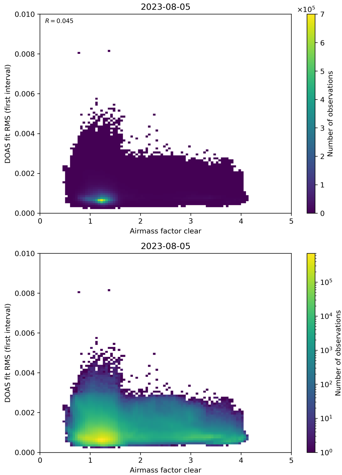
Figure 71: Scatter density plot of “Airmass factor clear” against “DOAS fit RMS (first interval)” for 2023-08-04 to 2023-08-06.
