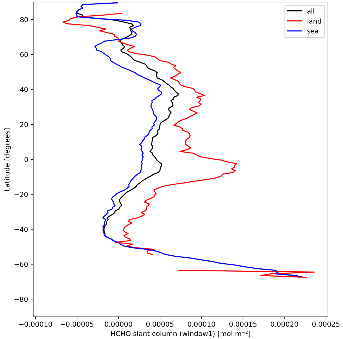
Figure 24: Zonal average of “HCHO slant column (window1)” for 2023-08-04 to 2023-08-06.
