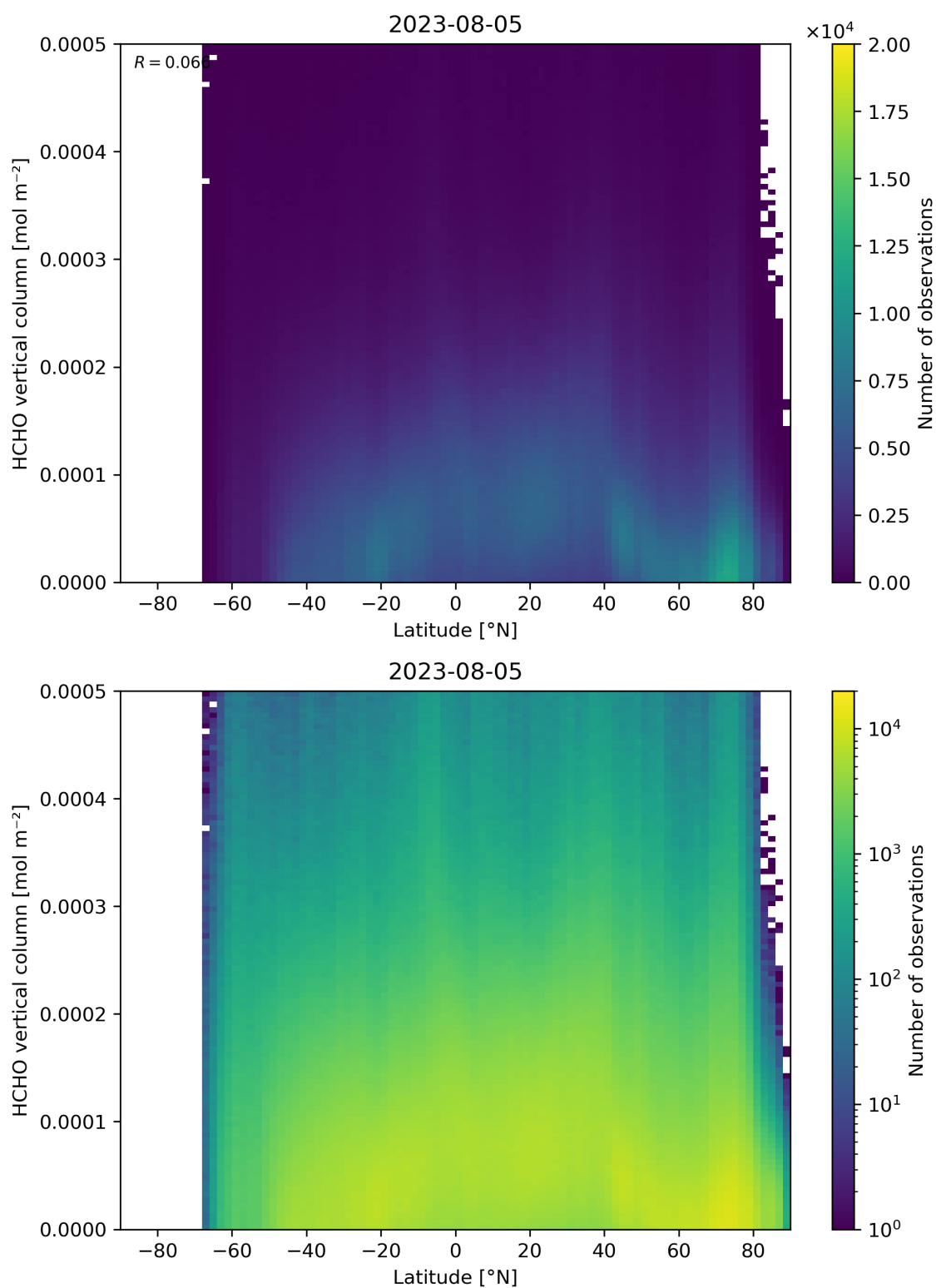
Figure 163: Scatter density plot of “Latitude” against “HCHO vertical column” for 2023-08-04 to 2023-08-06.
