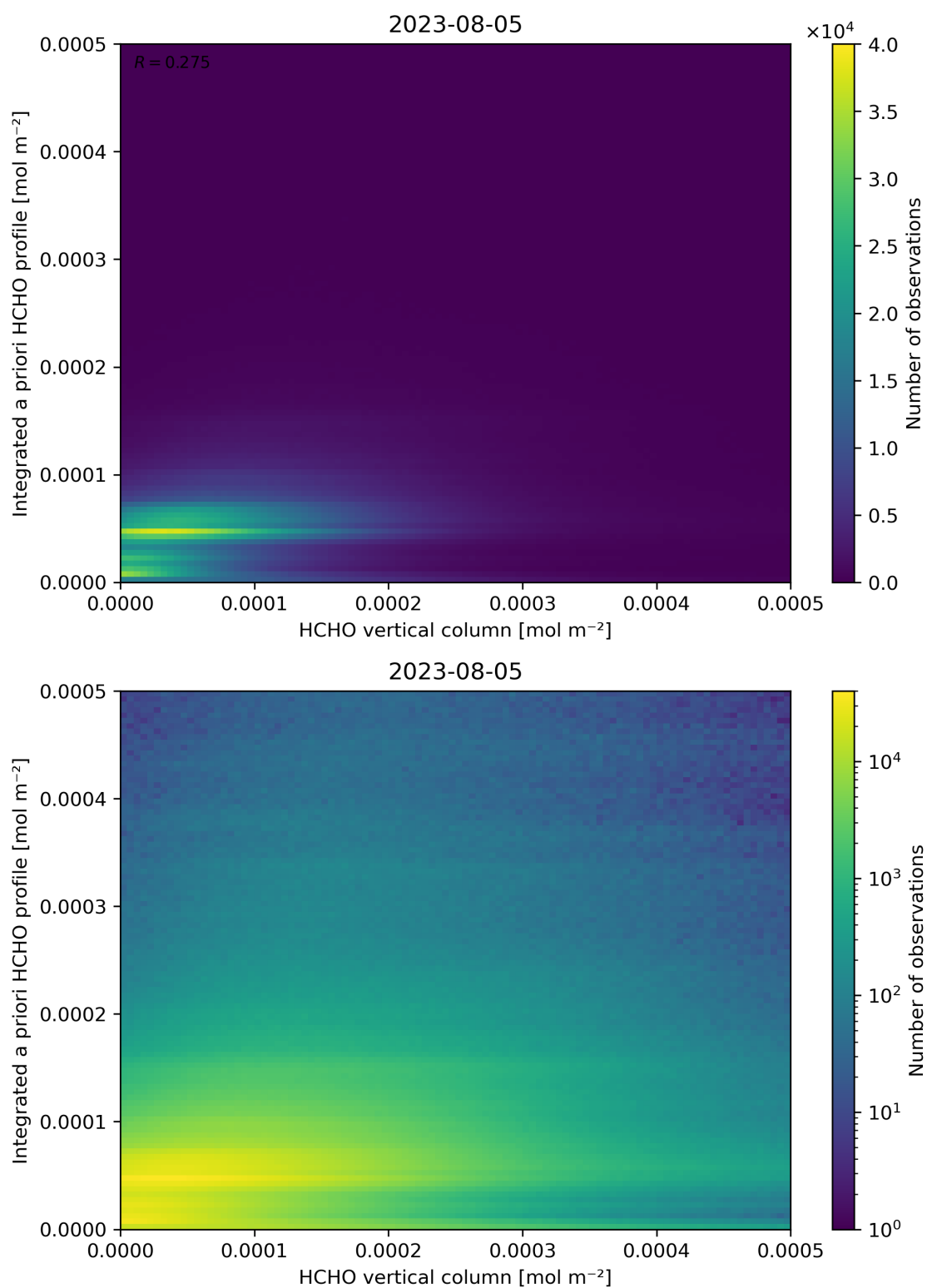
Figure 135: Scatter density plot of “HCHO vertical column” against “Integrated a priori HCHO profile” for 2023-08-04 to 2023-08-06.
