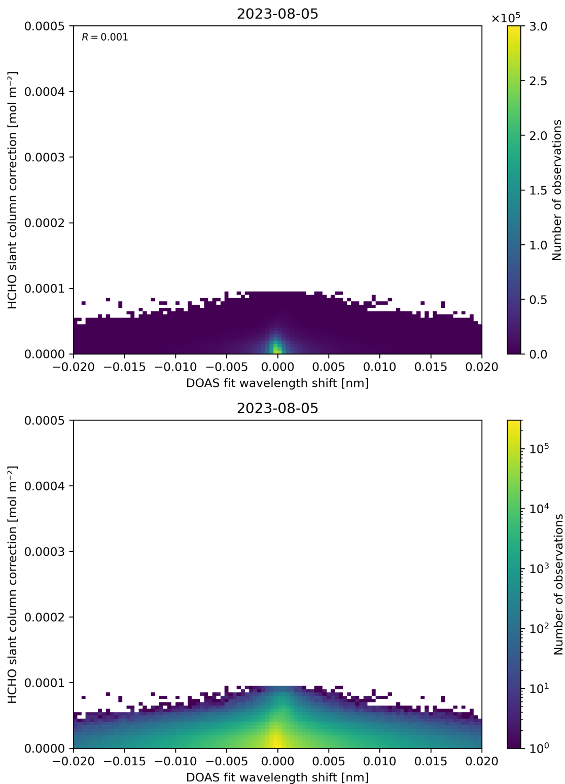
Figure 67: Scatter density plot of “DOAS fit wavelength shift” against “HCHO slant column correction” for 2023-08-04 to 2023-08-06.
