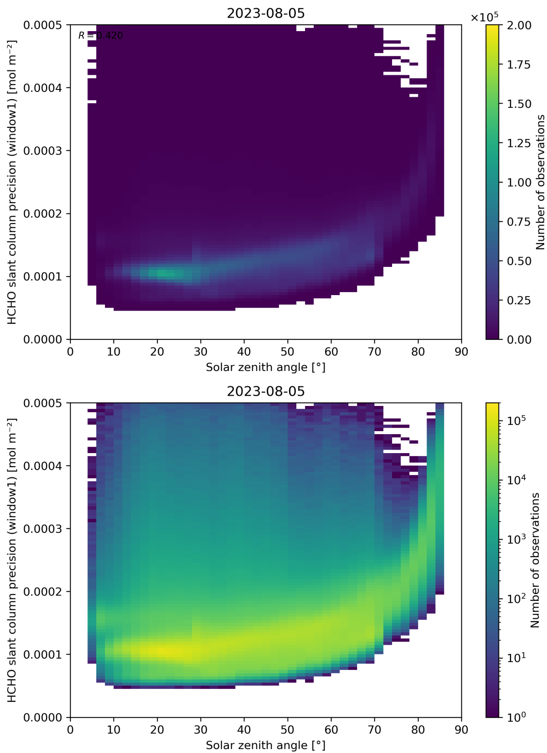
Figure 174: Scatter density plot of “Solar zenith angle” against “HCHO slant column precision (window1)” for 2023-08-04 to 2023-08-06.
