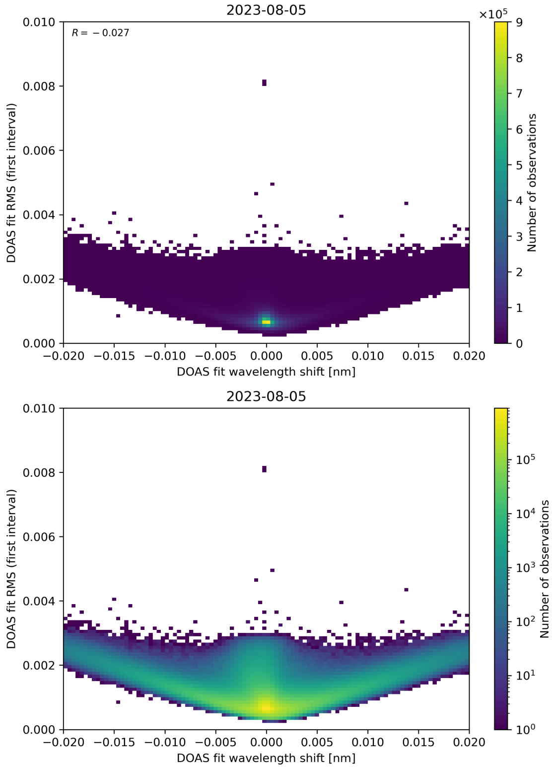
Figure 64: Scatter density plot of “DOAS fit wavelength shift” against “DOAS fit RMS (first interval)” for 2023-08-04 to 2023-08-06.
