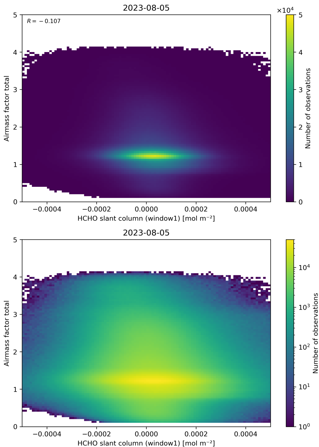
Figure 85: Scatter density plot of “HCHO slant column (window1)” against “Airmass factor total” for 2023-08-04 to 2023-08-06.
