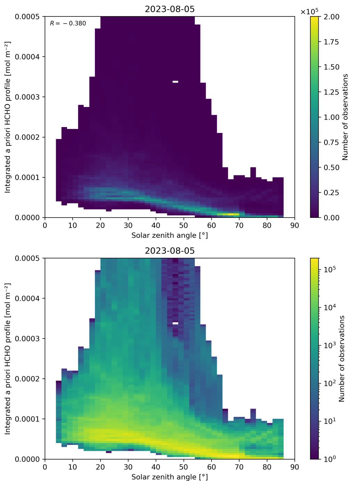
Figure 180: Scatter density plot of “Solar zenith angle” against “Integrated a priori HCHO profile” for 2023-08-04 to 2023-08-06.
