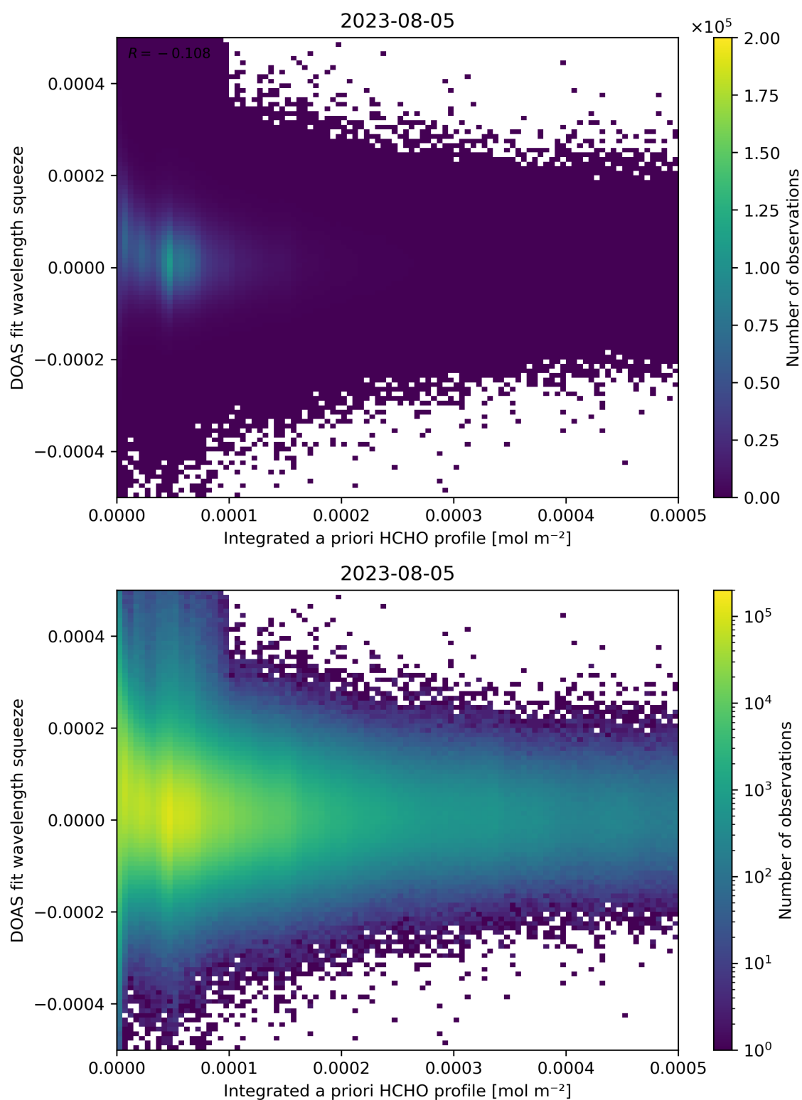
Figure 150: Scatter density plot of “Integrated a priori HCHO profile” against “DOAS fit wavelength squeeze” for 2023-08-04 to 2023-08-06.
