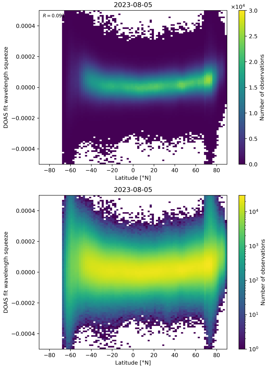
Figure 155: Scatter density plot of “Latitude” against “DOAS fit wavelength squeeze” for 2023-08-04 to 2023-08-06.
