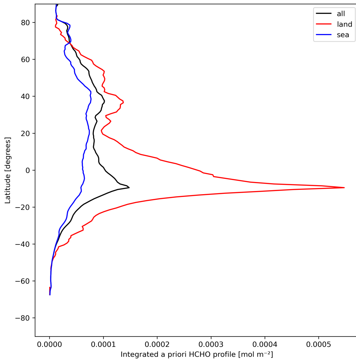
Figure 29: Zonal average of “Integrated a priori HCHO profile” for 2023-08-04 to 2023-08-06.
