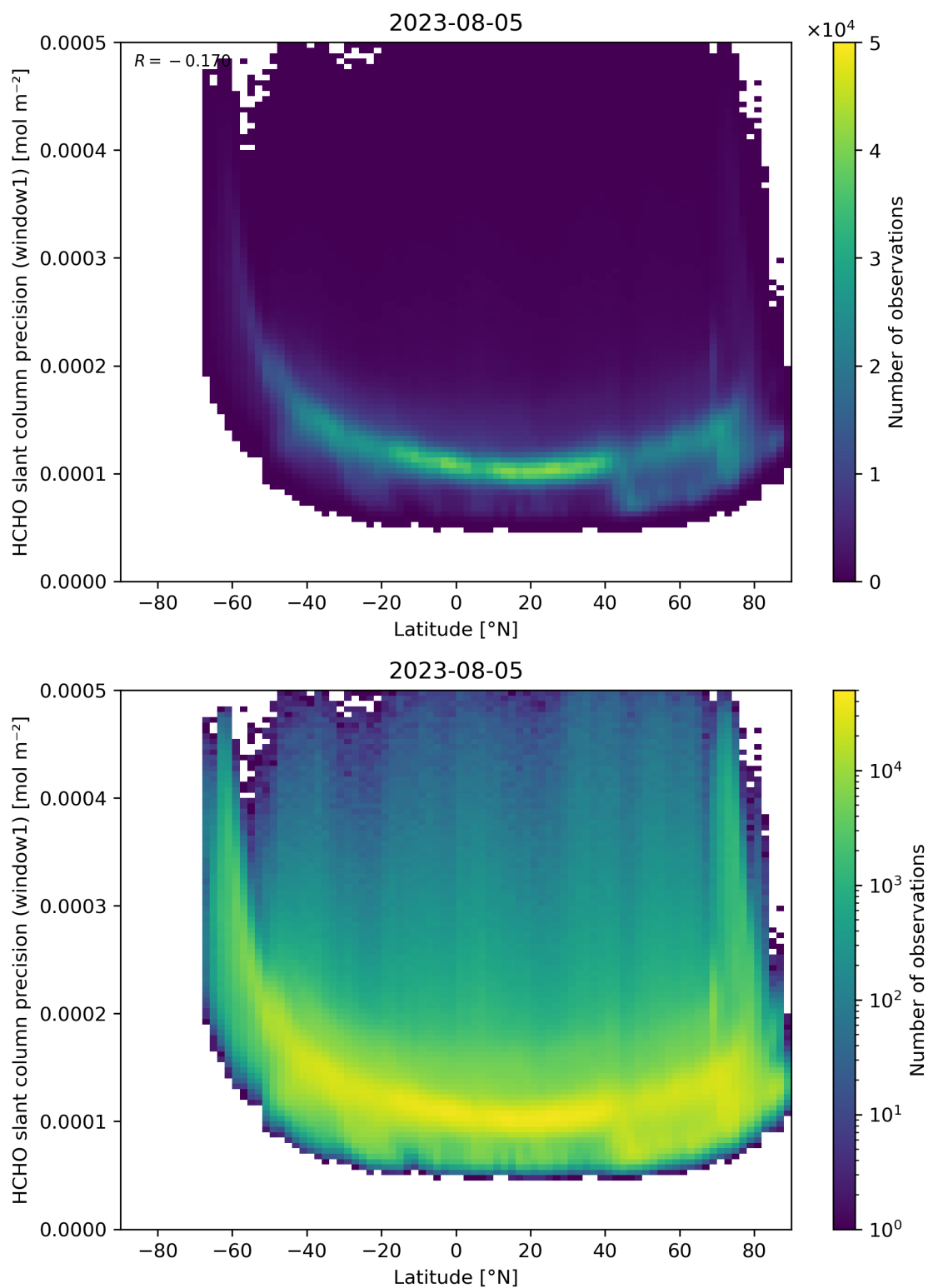
Figure 160: Scatter density plot of “Latitude” against “HCHO slant column precision (window1)” for 2023-08-04 to 2023-08-06.
