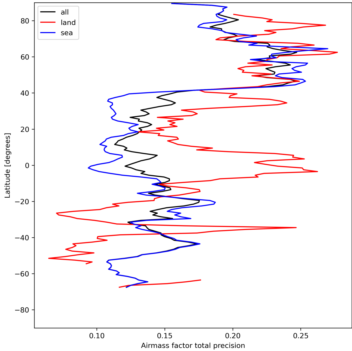
Figure 27: Zonal average of “Airmass factor total precision” for 2023-08-04 to 2023-08-06.
