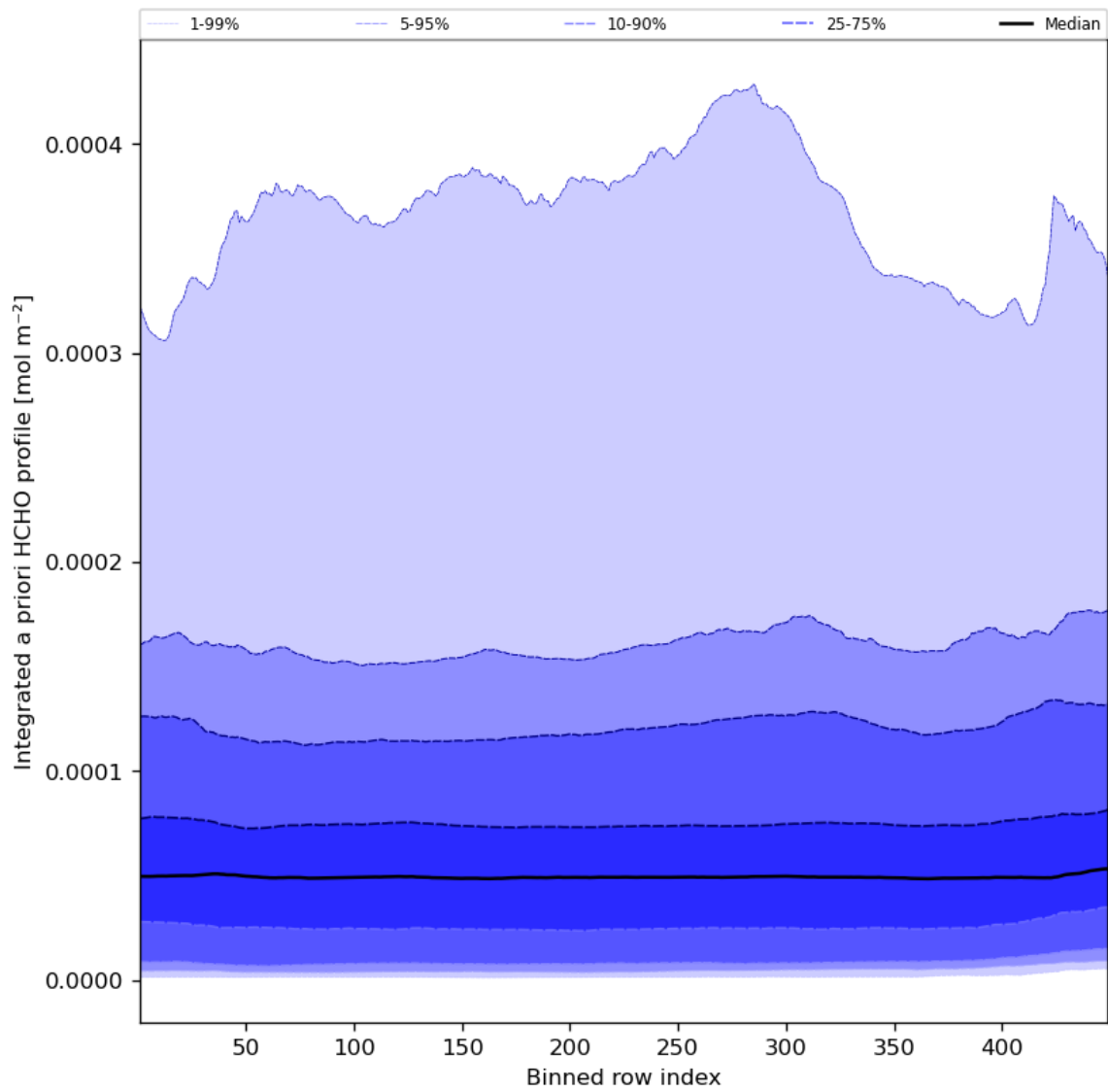
Figure 57: Along track statistics of “Integrated a priori HCHO profile” for 2023-08-04 to 2023-08-06
