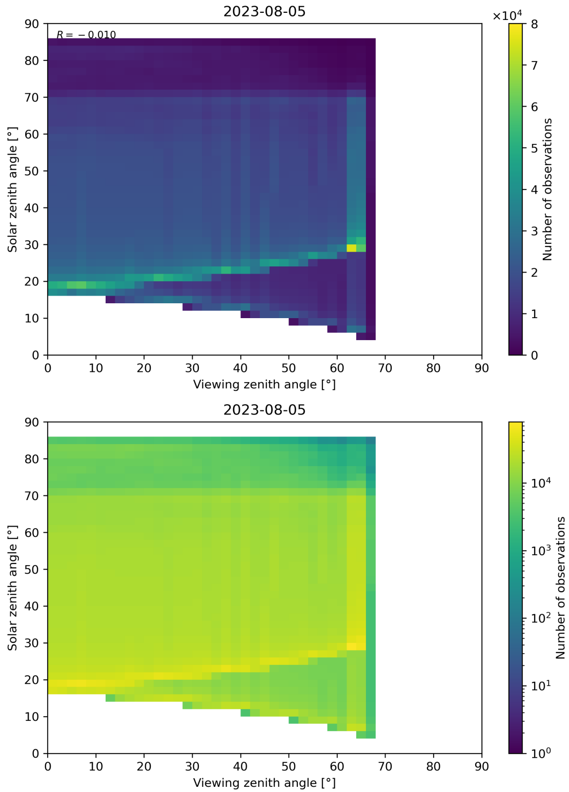
Figure 197: Scatter density plot of “Viewing zenith angle” against “Solar zenith angle” for 2023-08-04 to 2023-08-06.
