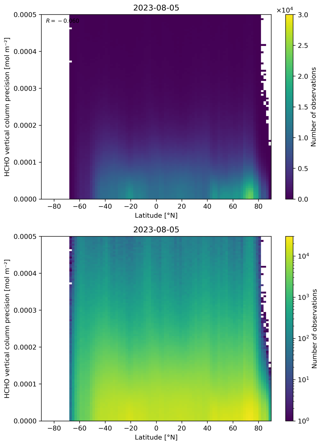
Figure 165: Scatter density plot of “Latitude” against “HCHO vertical column precision” for 2023-08-04 to 2023-08-06.
