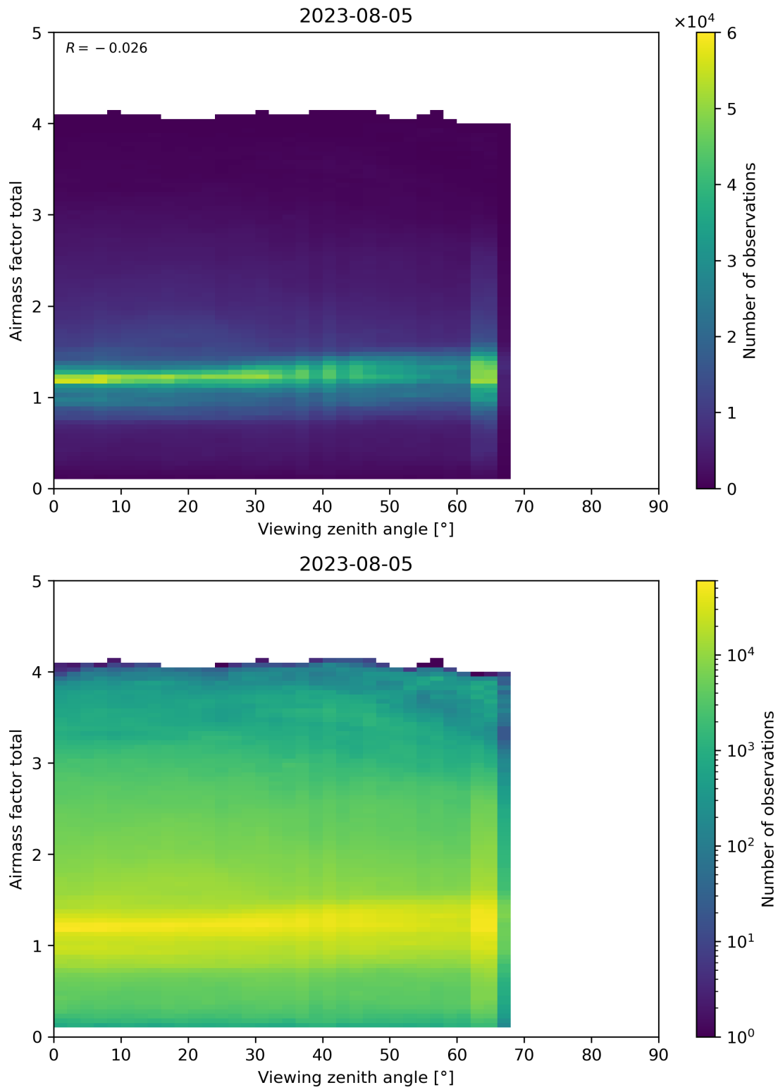
Figure 190: Scatter density plot of “Viewing zenith angle” against “Airmass factor total” for 2023-08-04 to 2023-08-06.
