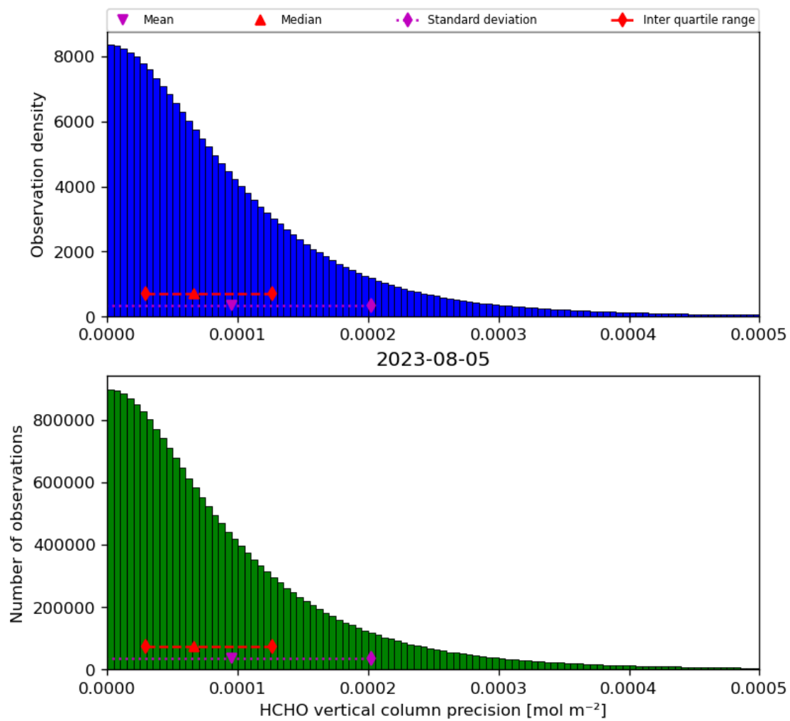
Figure 36: Histogram of “HCHO vertical column precision” for 2023-08-04 to 2023-08-06
