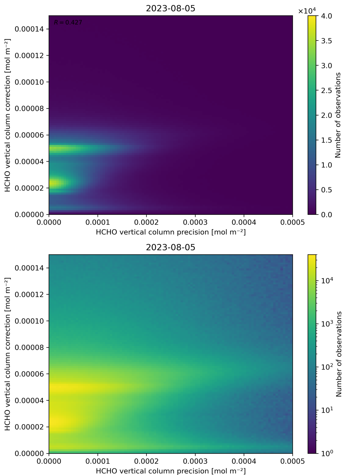
Figure 146: Scatter density plot of “HCHO vertical column precision” against “HCHO vertical column correction” for 2023-08-04 to 2023-08-06.
