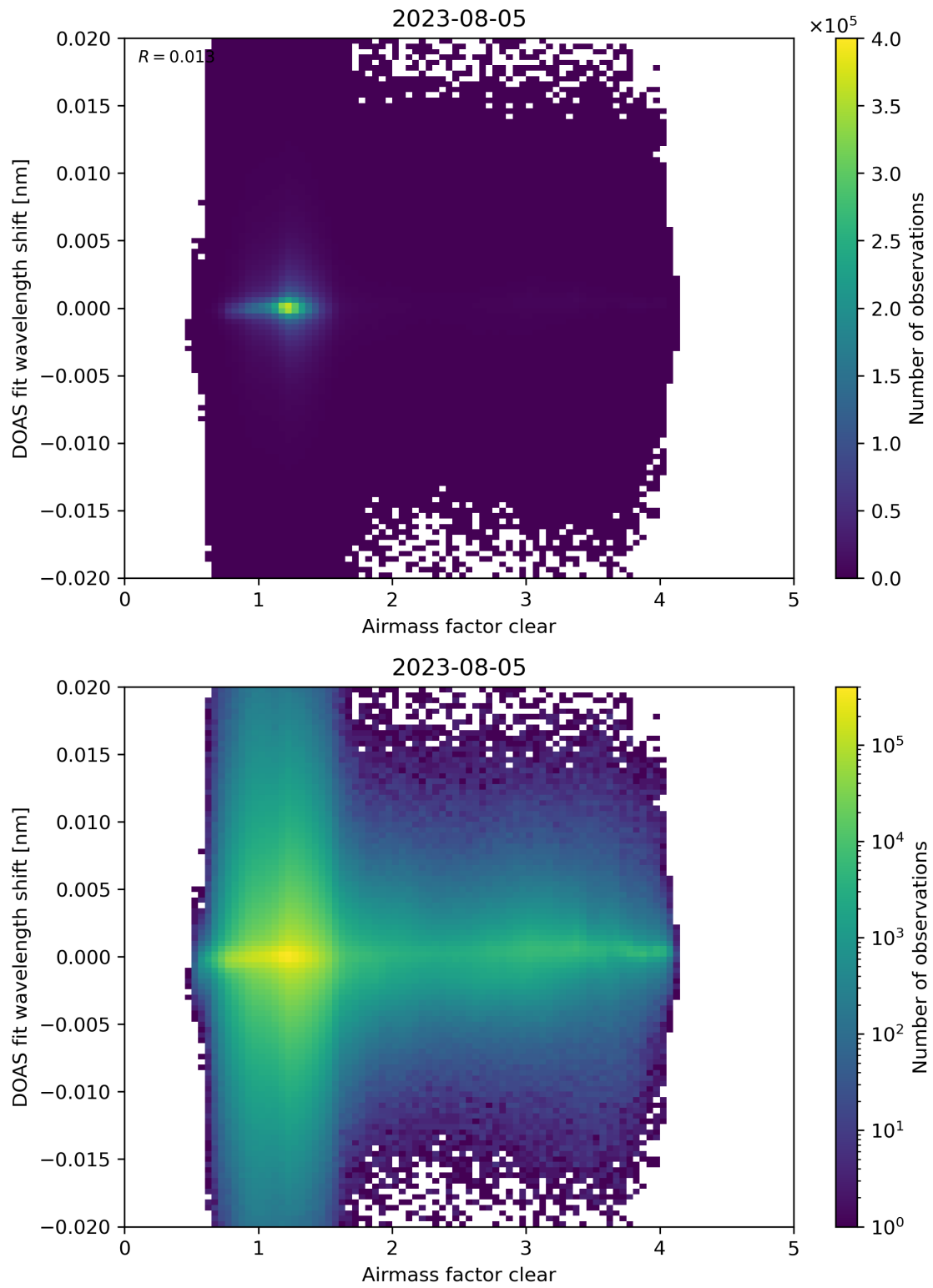
Figure 72: Scatter density plot of “Airmass factor clear” against “DOAS fit wavelength shift” for 2023-08-04 to 2023-08-06.
