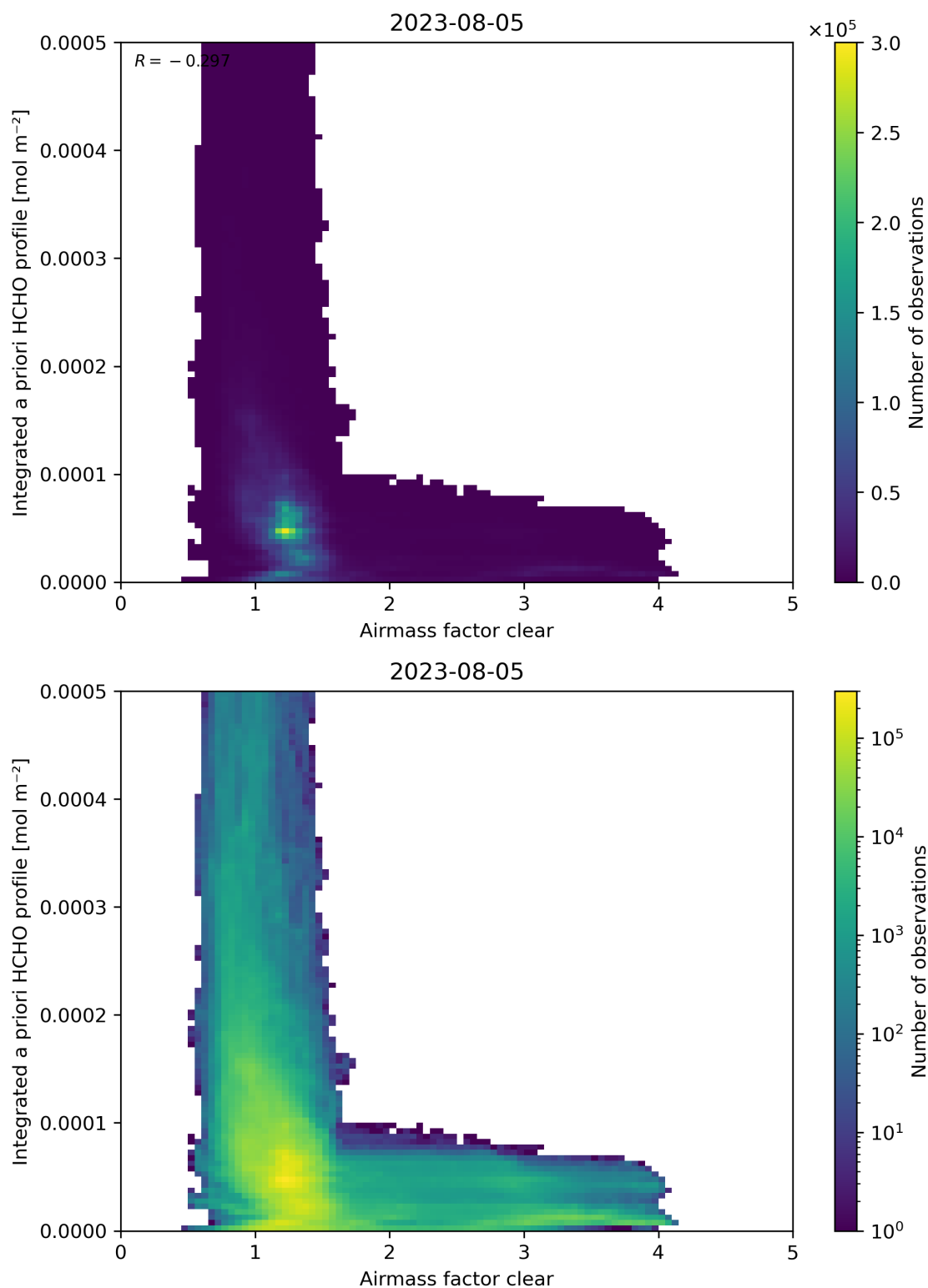
Figure 76: Scatter density plot of “Airmass factor clear” against “Integrated a priori HCHO profile” for 2023-08-04 to 2023-08-06.
