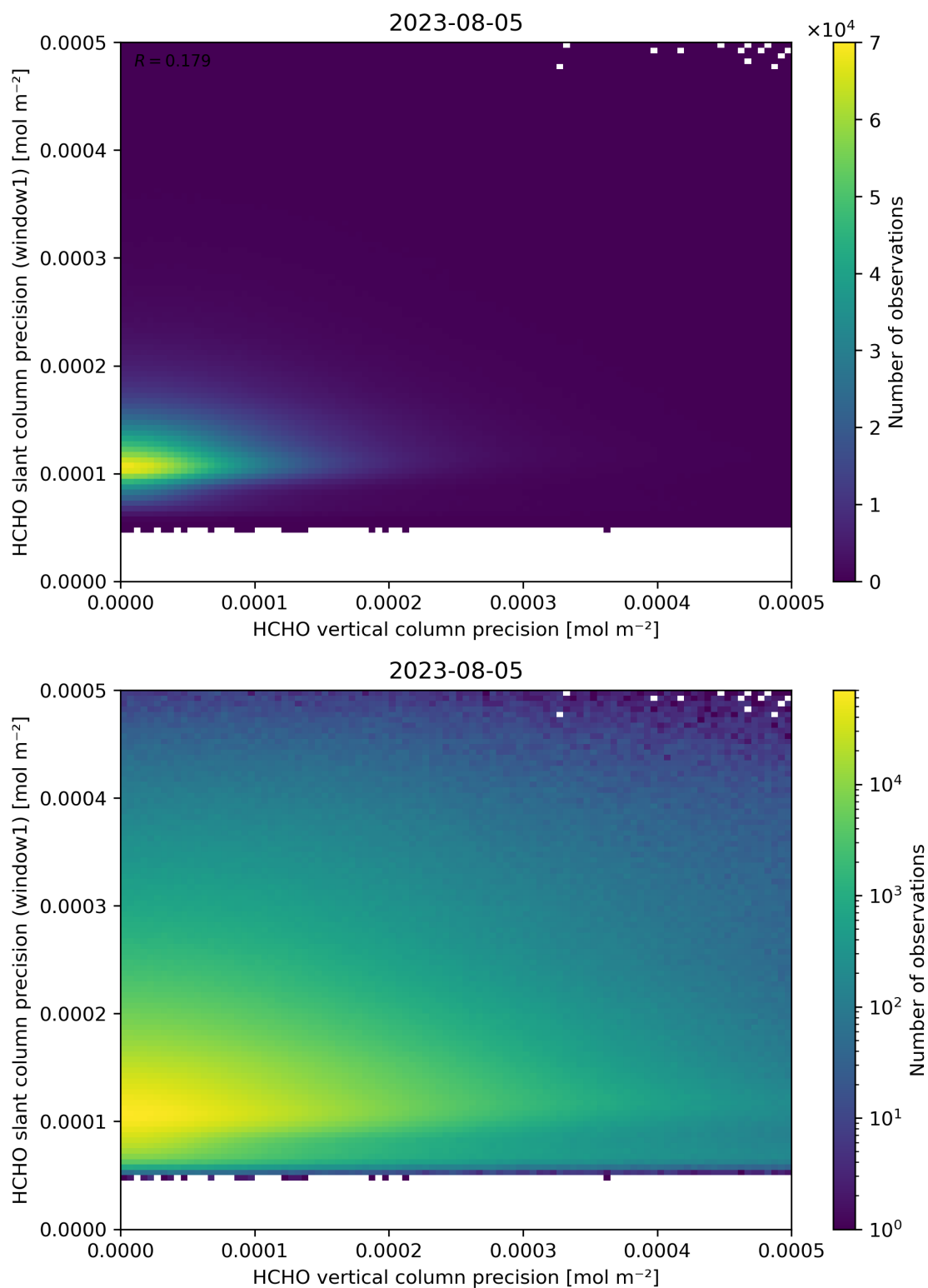
Figure 143: Scatter density plot of “HCHO vertical column precision” against “HCHO slant column precision (window1)” for 2023-08-04 to 2023-08-06.
