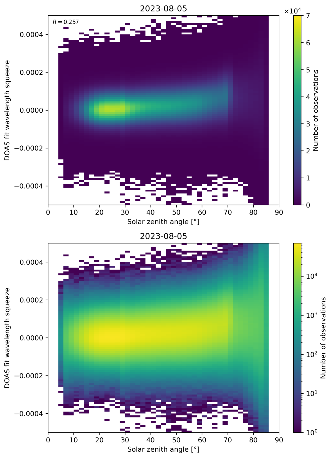
Figure 169: Scatter density plot of “Solar zenith angle” against “DOAS fit wavelength squeeze” for 2023-08-04 to 2023-08-06.
