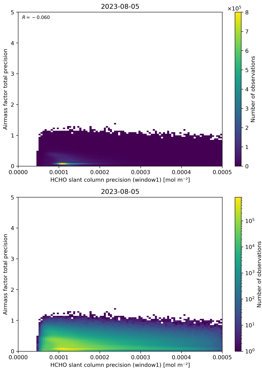
Figure 95: Scatter density plot of “HCHO slant column precision (window1)” against “Airmass factor total precision” for 2023-08-04 to 2023-08-06.
