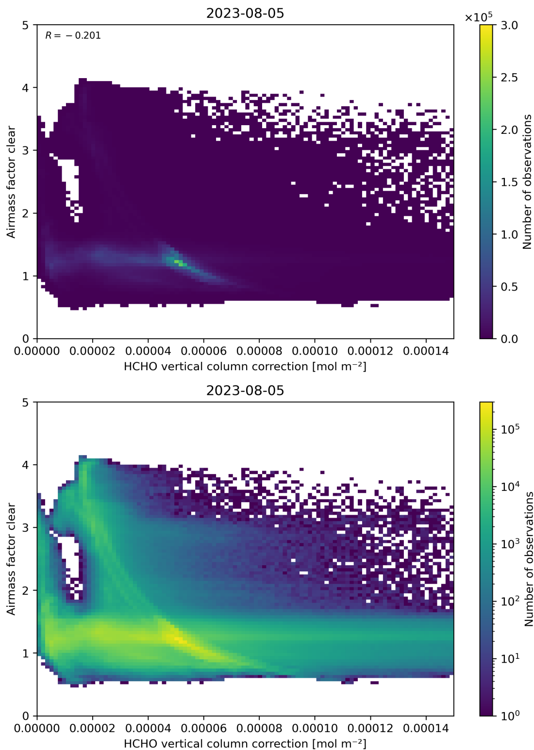
Figure 115: Scatter density plot of “HCHO vertical column correction” against “Airmass factor clear” for 2023-08-04 to 2023-08-06.
