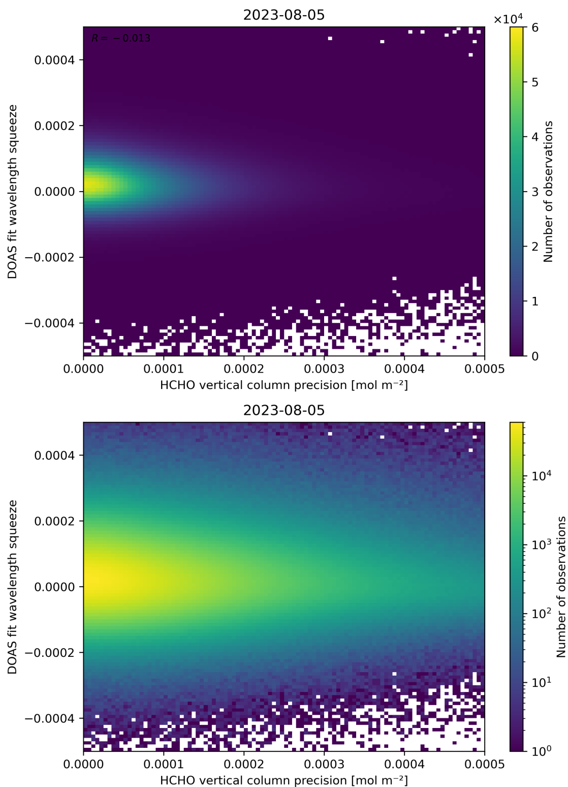
Figure 138: Scatter density plot of “HCHO vertical column precision” against “DOAS fit wavelength squeeze” for 2023-08-04 to 2023-08-06.
