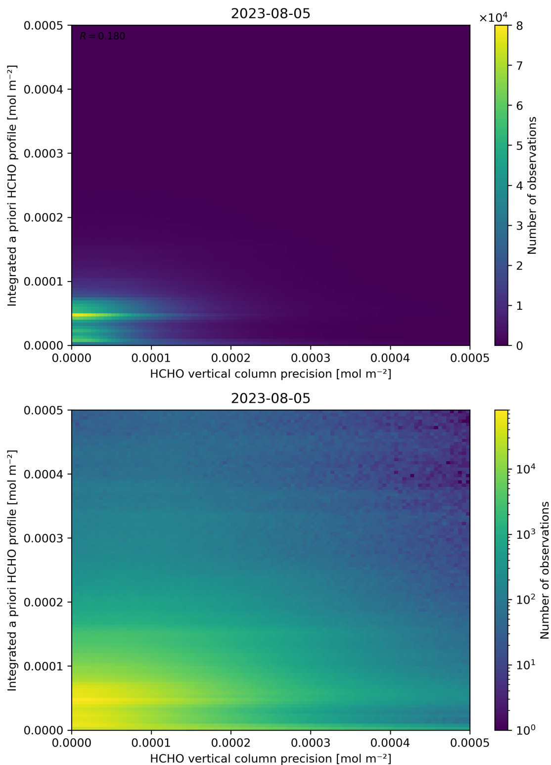
Figure 147: Scatter density plot of “HCHO vertical column precision” against “Integrated a priori HCHO profile” for 2023-08-04 to 2023-08-06.
