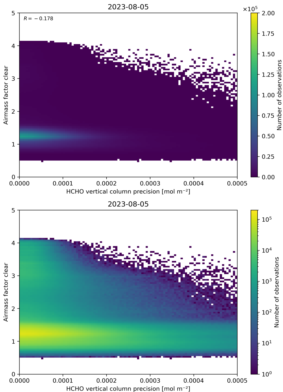
Figure 139: Scatter density plot of “HCHO vertical column precision” against “Airmass factor clear” for 2023-08-04 to 2023-08-06.
