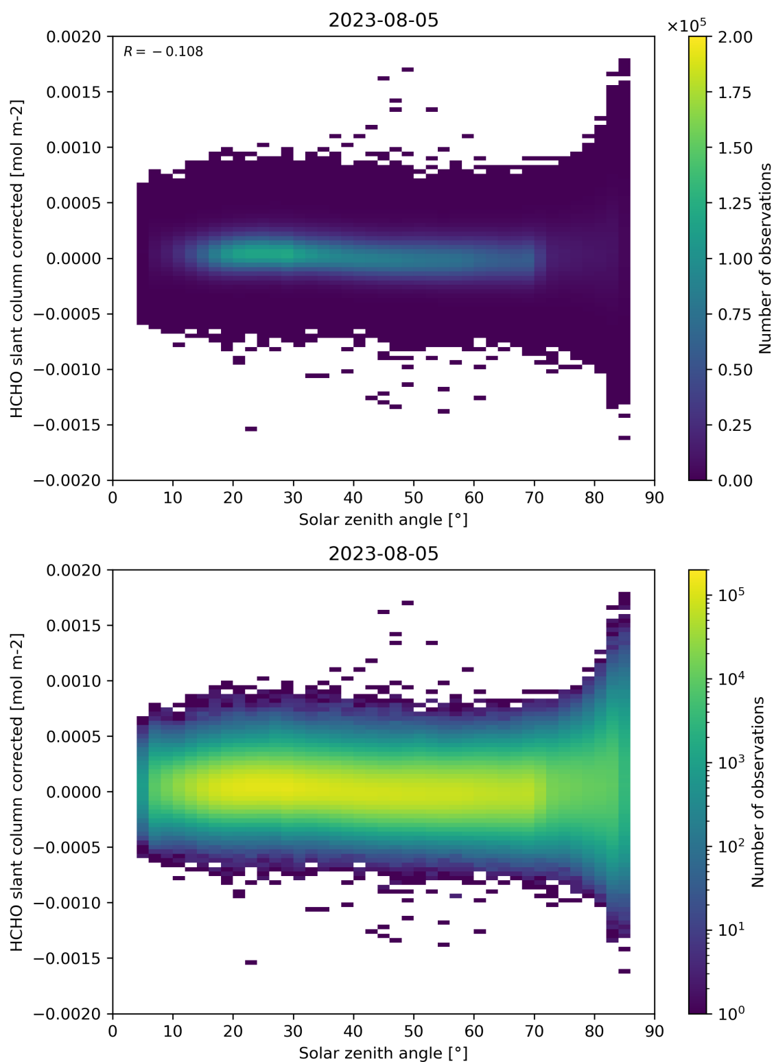
Figure 171: Scatter density plot of “Solar zenith angle” against “HCHO slant column corrected” for 2023-08-04 to 2023-08-06.
