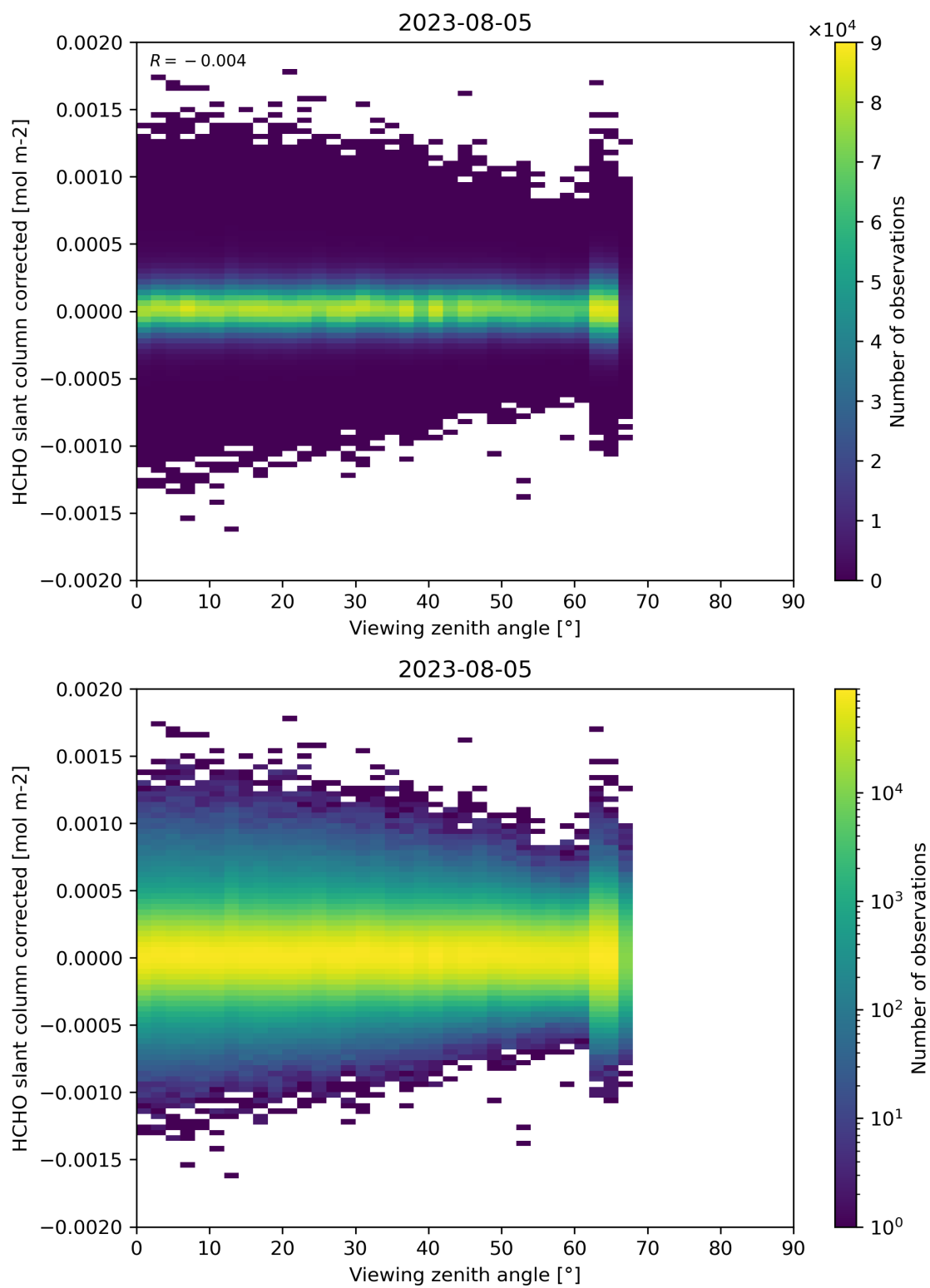
Figure 186: Scatter density plot of “Viewing zenith angle” against “HCHO slant column corrected” for 2023-08-04 to 2023-08-06.
