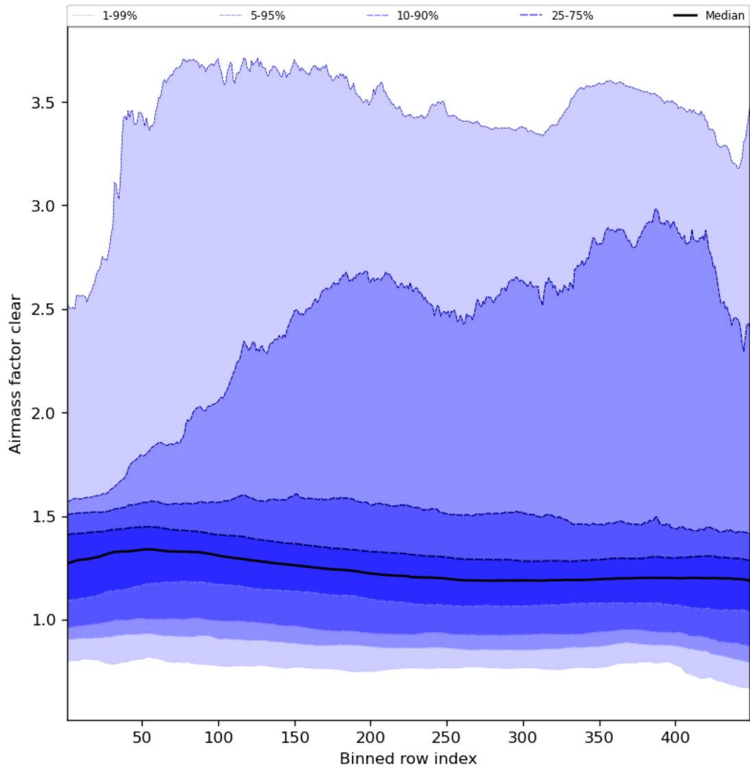
Figure 56: Along track statistics of “Airmass factor clear” for 2023-08-04 to 2023-08-06
