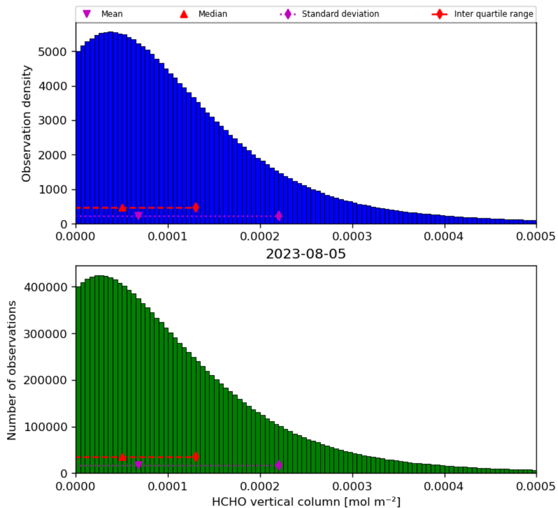
Figure 35: Histogram of “HCHO vertical column” for 2023-08-04 to 2023-08-06
