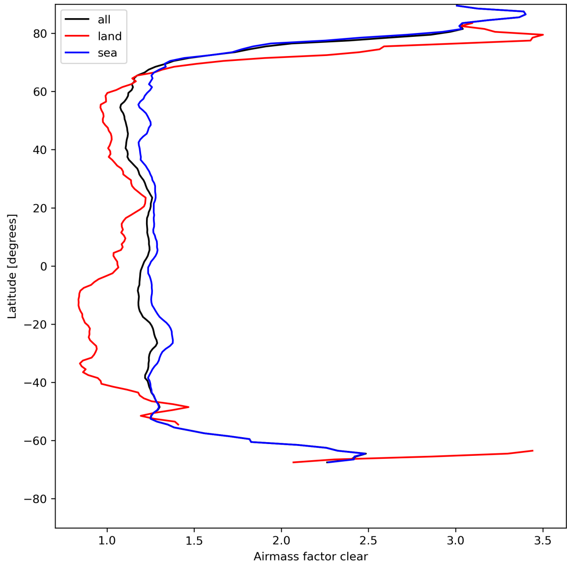
Figure 28: Zonal average of “Airmass factor clear” for 2023-08-04 to 2023-08-06.
