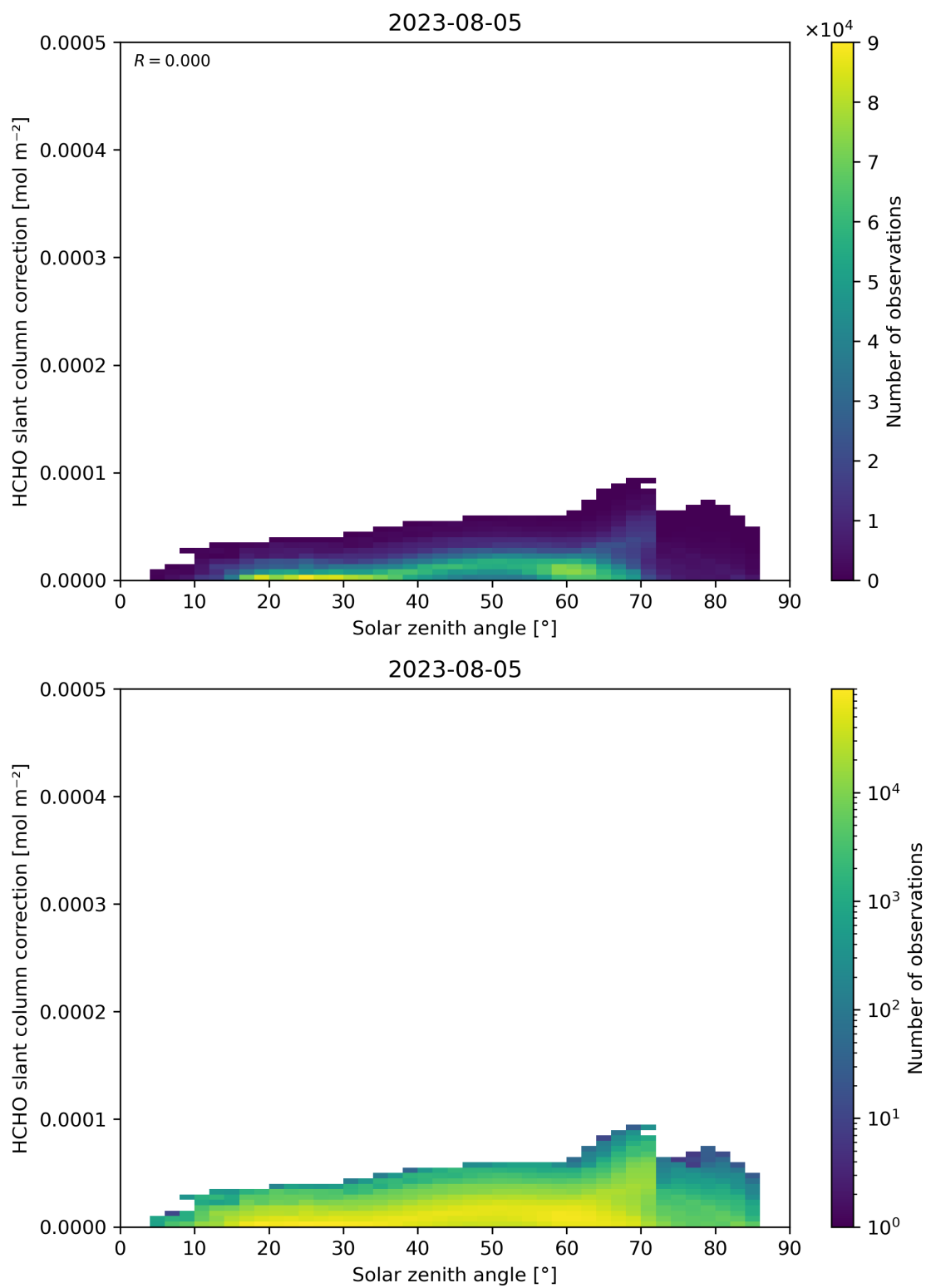
Figure 172: Scatter density plot of “Solar zenith angle” against “HCHO slant column correction” for 2023-08-04 to 2023-08-06.
