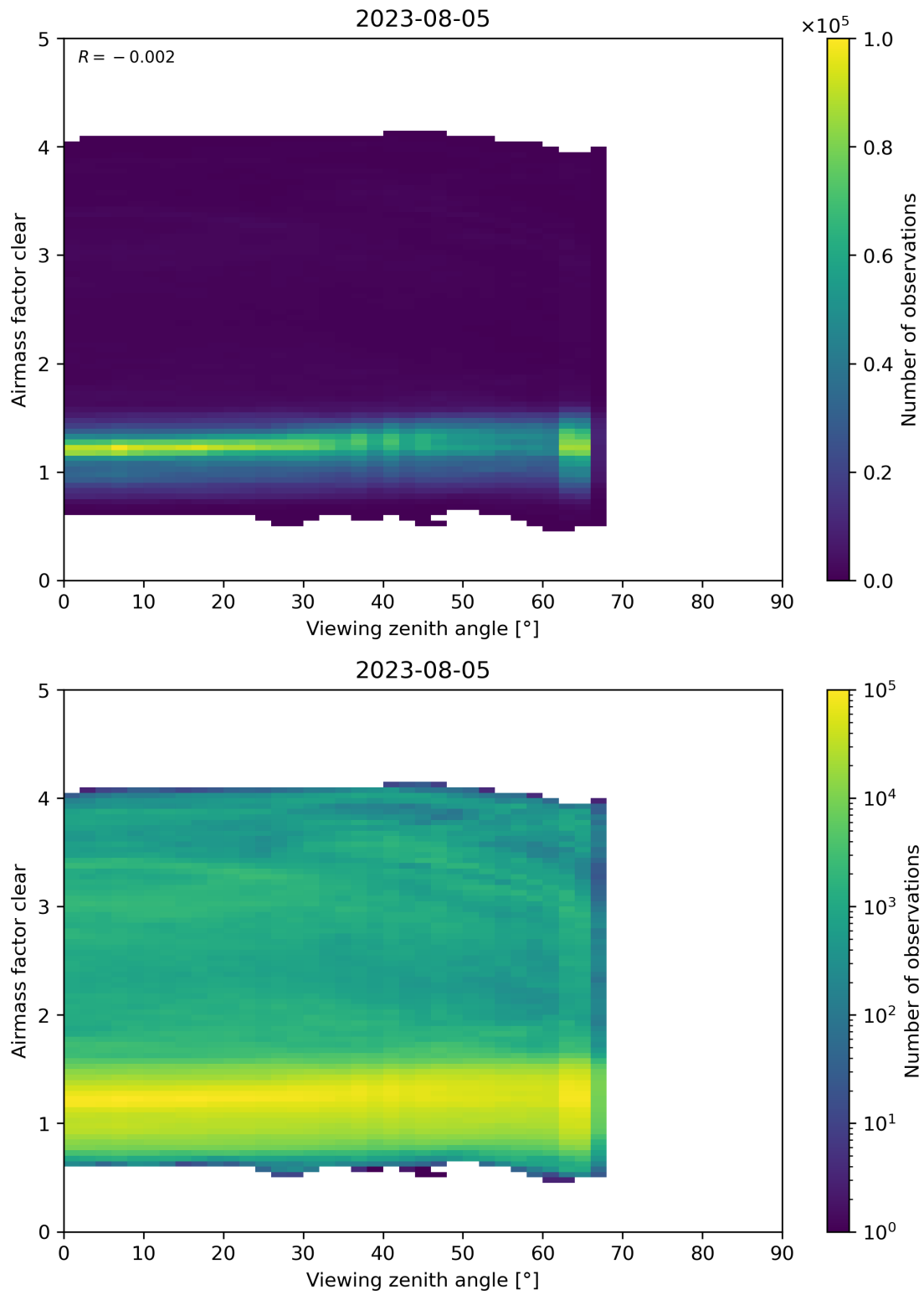
Figure 185: Scatter density plot of “Viewing zenith angle” against “Airmass factor clear” for 2023-08-04 to 2023-08-06.
