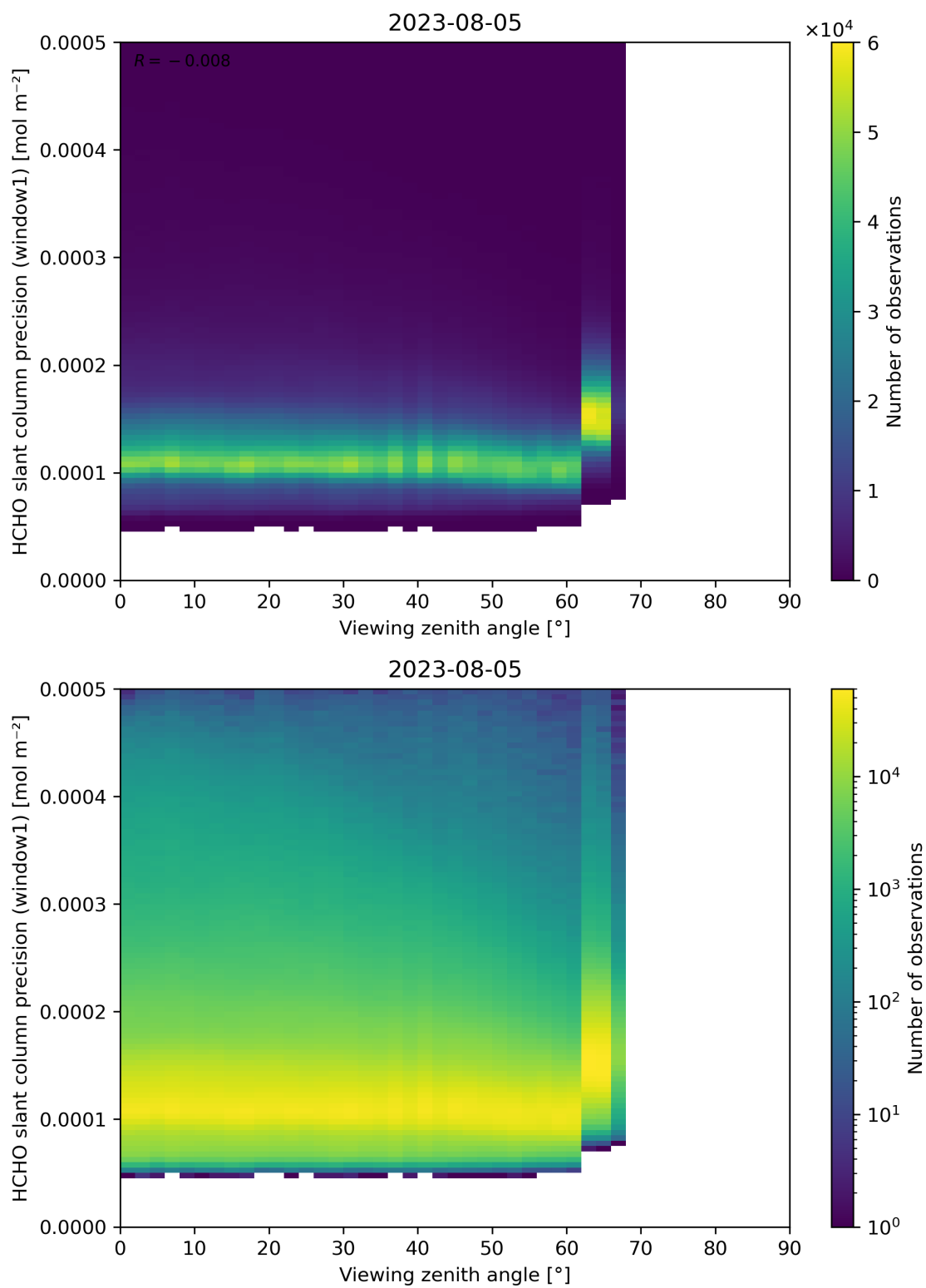
Figure 189: Scatter density plot of “Viewing zenith angle” against “HCHO slant column precision (window1)” for 2023-08-04 to 2023-08-06.
