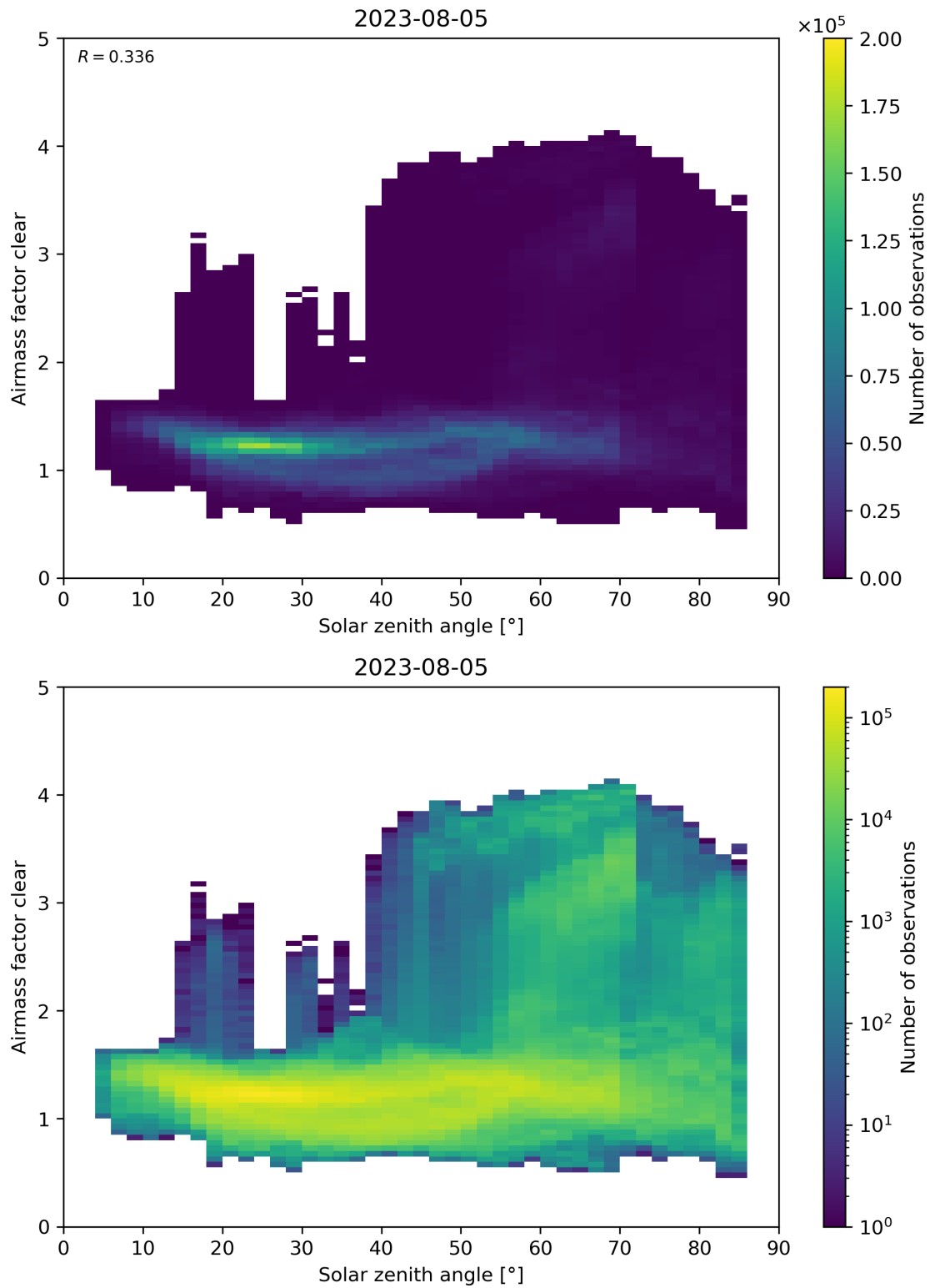
Figure 170: Scatter density plot of “Solar zenith angle” against “Airmass factor clear” for 2023-08-04 to 2023-08-06.
