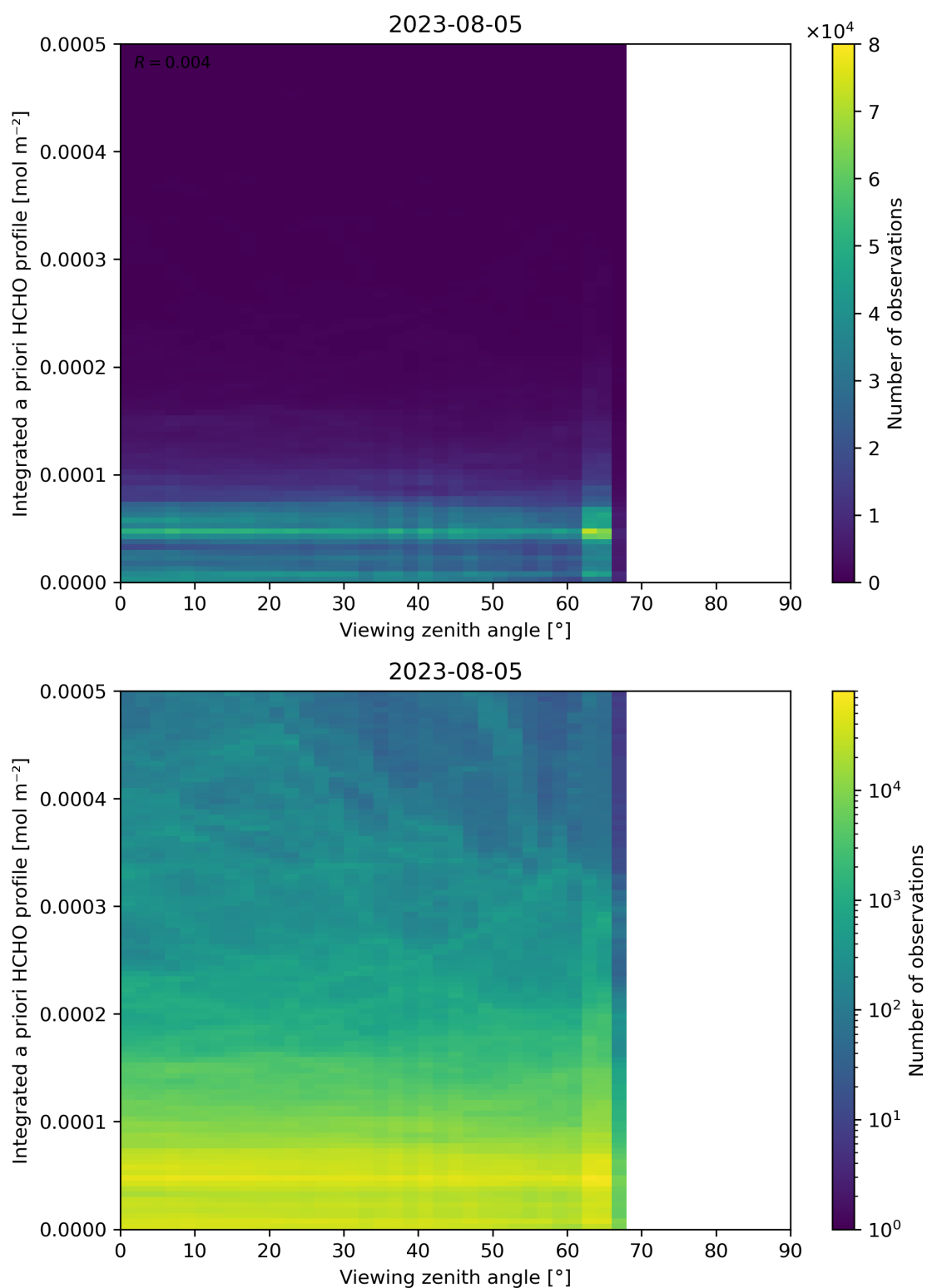
Figure 195: Scatter density plot of “Viewing zenith angle” against “Integrated a priori HCHO profile” for 2023-08-04 to 2023-08-06.
