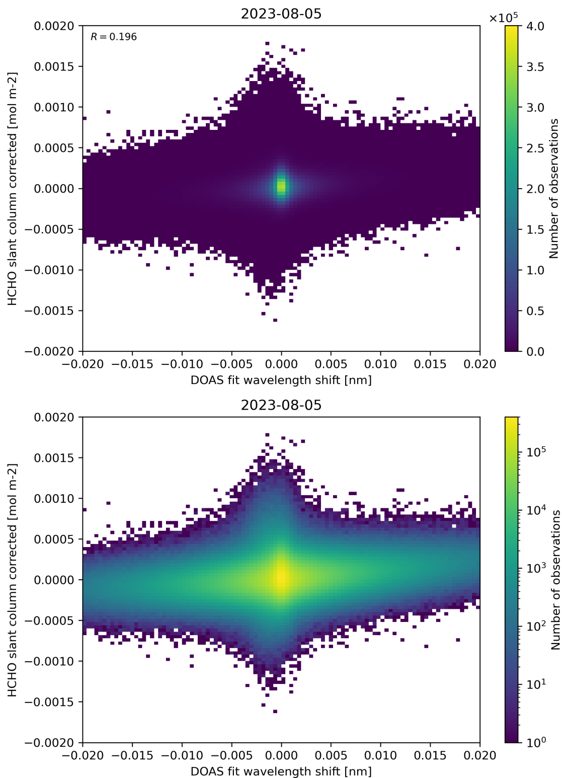
Figure 66: Scatter density plot of “DOAS fit wavelength shift” against “HCHO slant column corrected” for 2023-08-04 to 2023-08-06.
