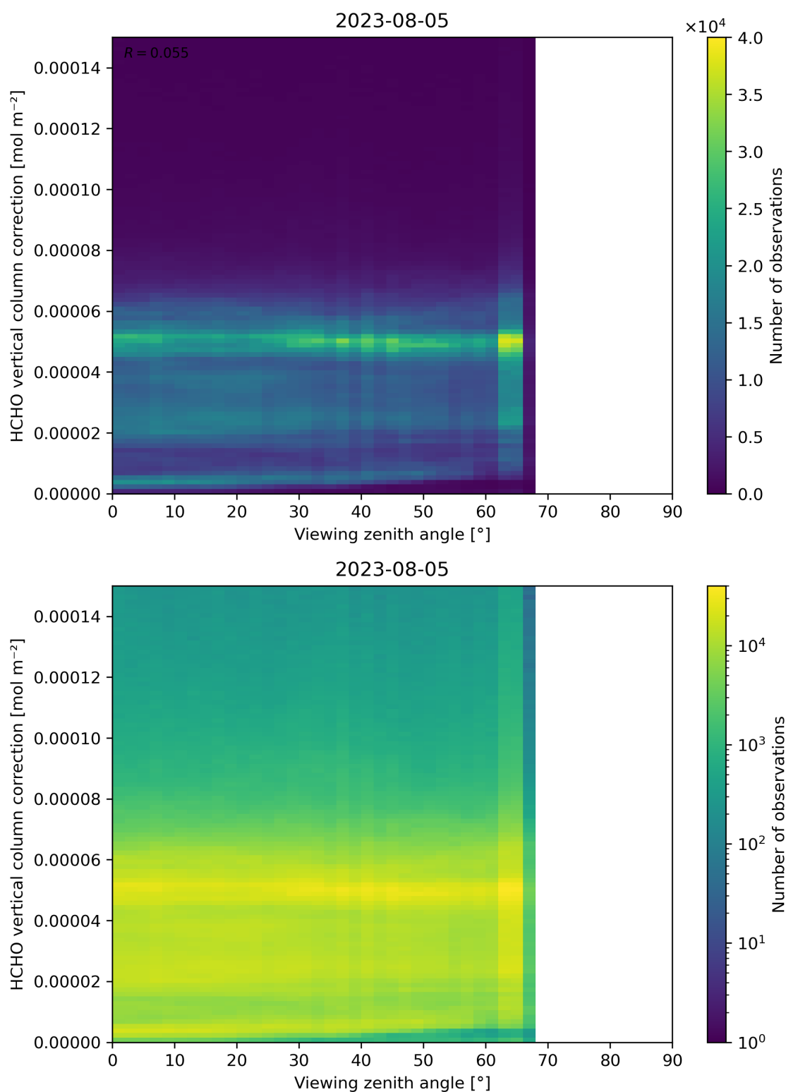
Figure 193: Scatter density plot of “Viewing zenith angle” against “HCHO vertical column correction” for 2023-08-04 to 2023-08-06.
