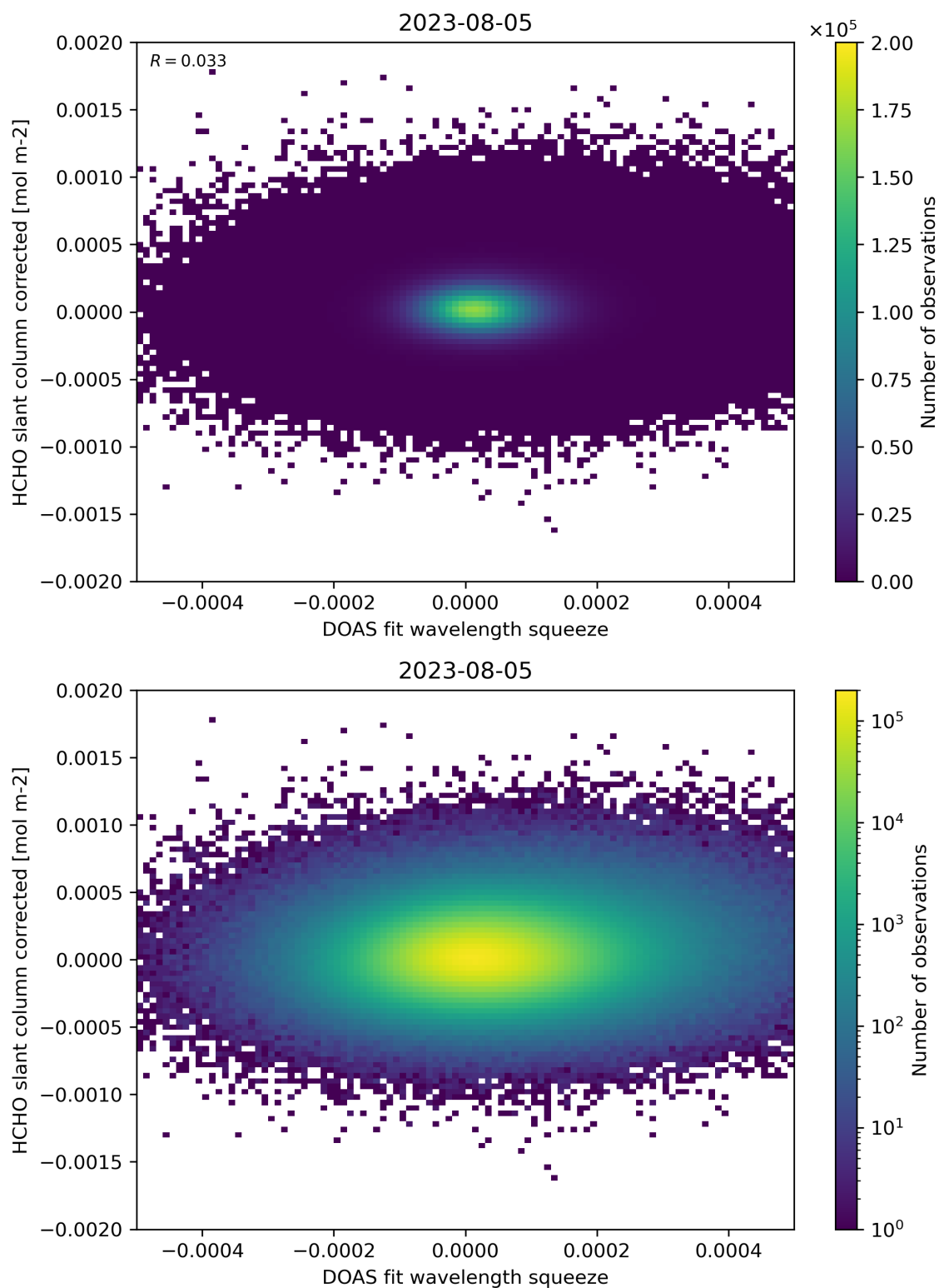
Figure 69: Scatter density plot of “DOAS fit wavelength squeeze” against “HCHO slant column corrected” for 2023-08-04 to 2023-08-06.
