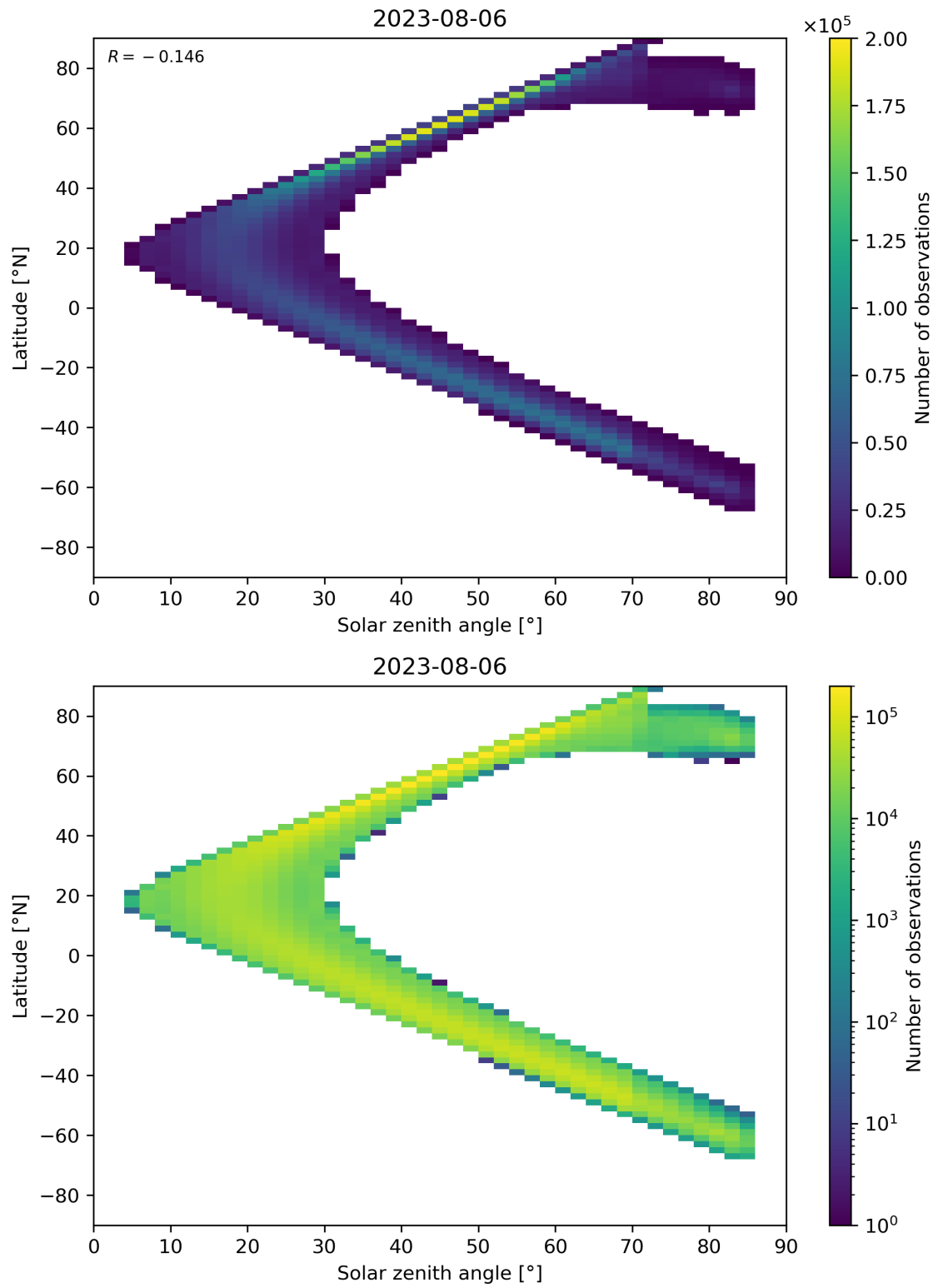
Figure 181: Scatter density plot of “Solar zenith angle” against “Latitude” for 2023-08-05 to 2023-08-07.
