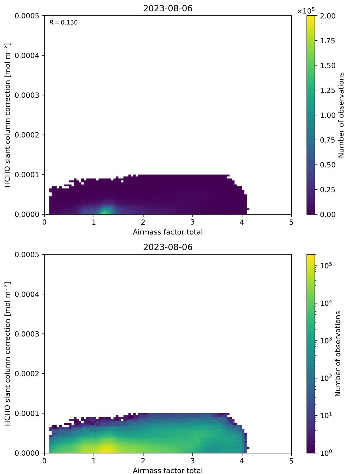
Figure 102: Scatter density plot of “Airmass factor total” against “HCHO slant column correction” for 2023-08-05 to 2023-08-07.
