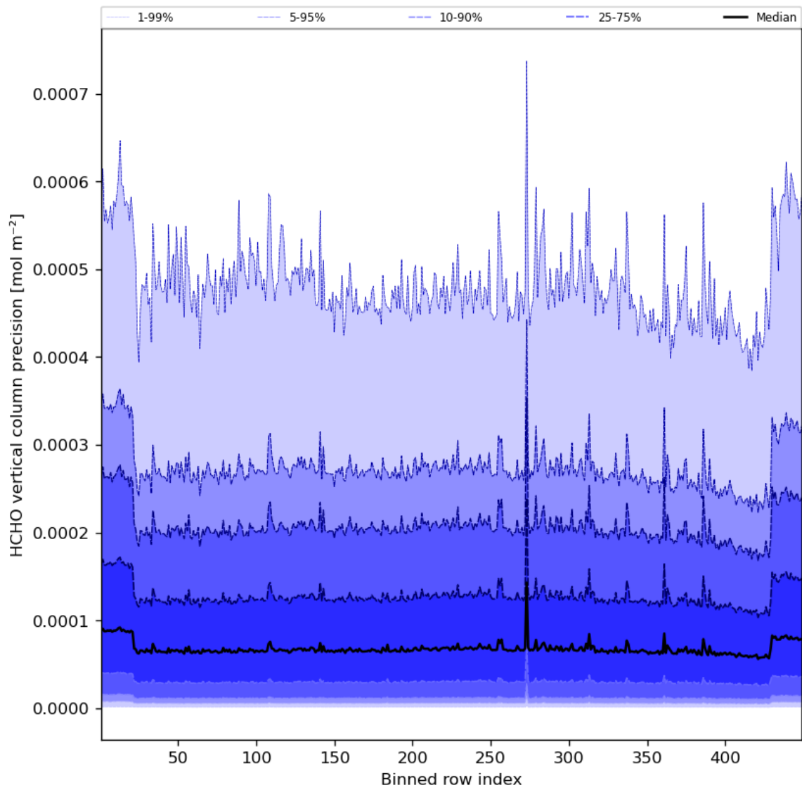
Figure 50: Along track statistics of “HCHO vertical column precision” for 2023-08-05 to 2023-08-07
