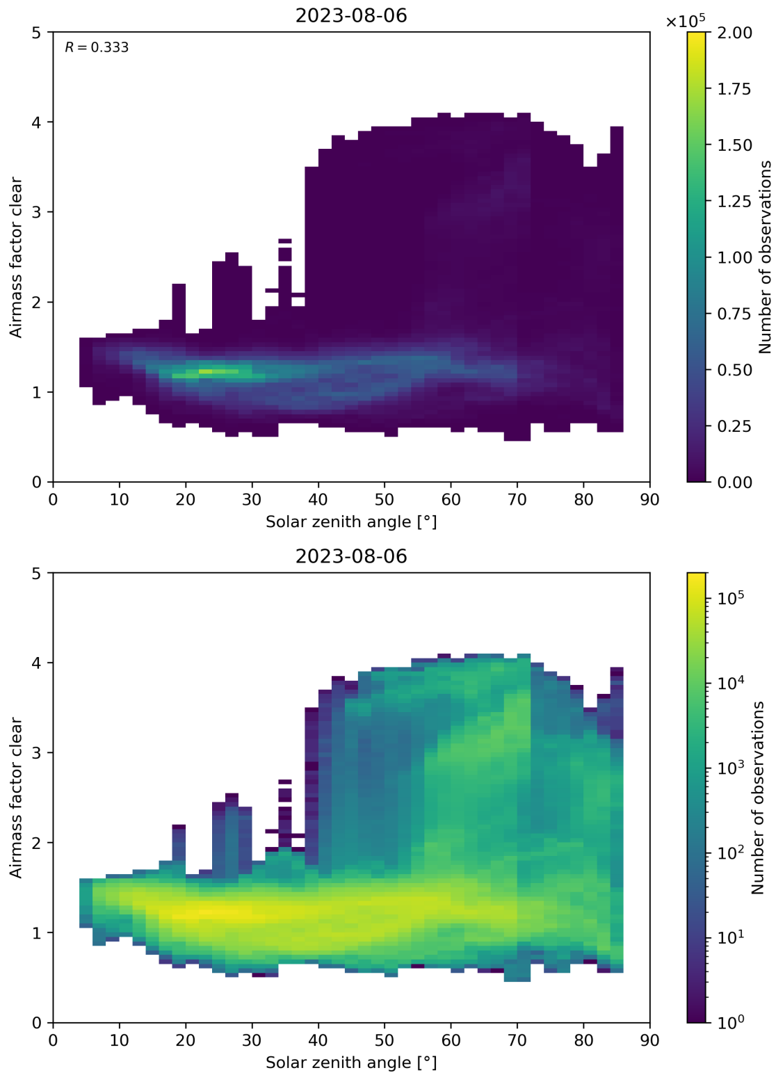
Figure 170: Scatter density plot of “Solar zenith angle” against “Airmass factor clear” for 2023-08-05 to 2023-08-07.
