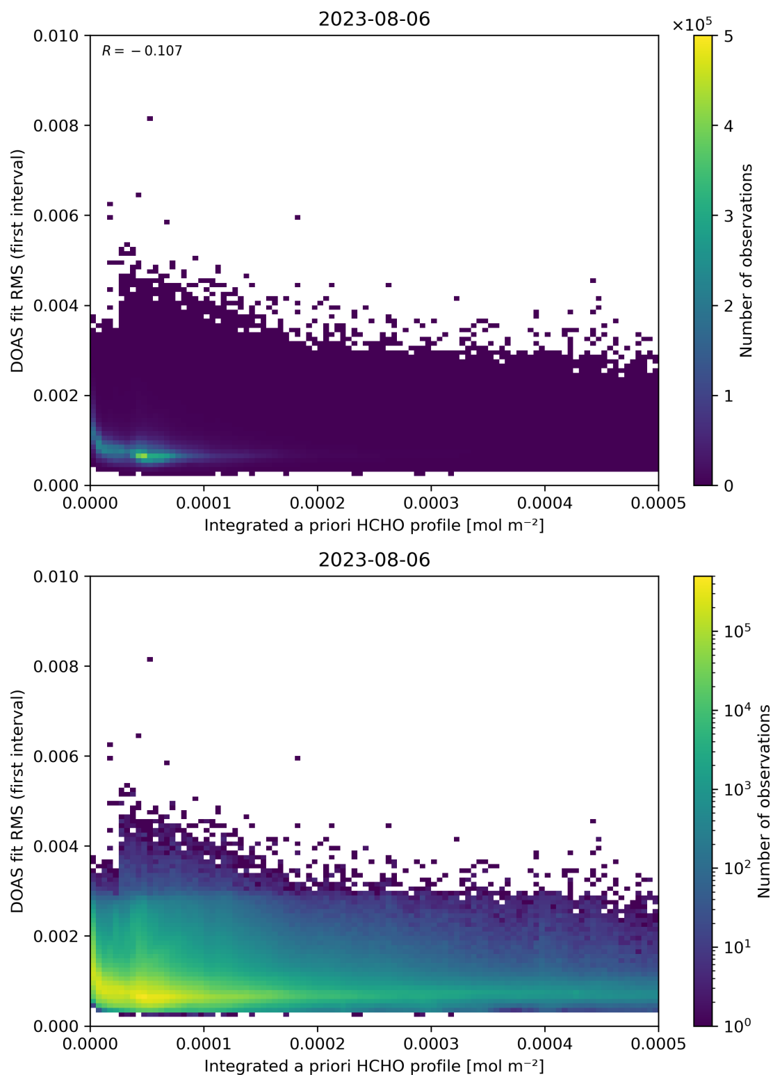
Figure 148: Scatter density plot of “Integrated a priori HCHO profile” against “DOAS fit RMS (first interval)” for 2023-08-05 to 2023-08-07.
