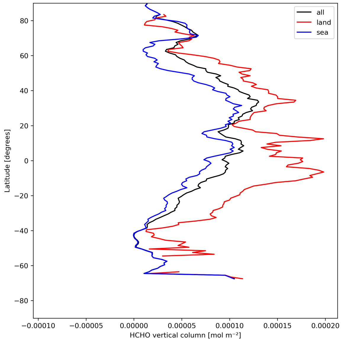
Figure 21: Zonal average of “HCHO vertical column” for 2023-08-05 to 2023-08-07.
