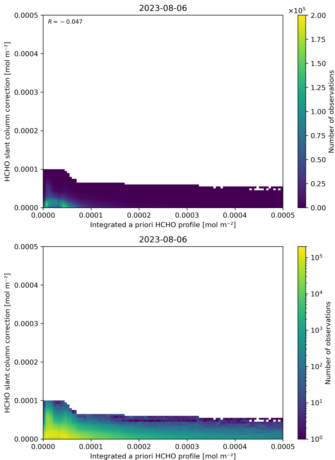
Figure 152: Scatter density plot of “Integrated a priori HCHO profile” against “HCHO slant column correction” for 2023-08-05 to 2023-08-07.
