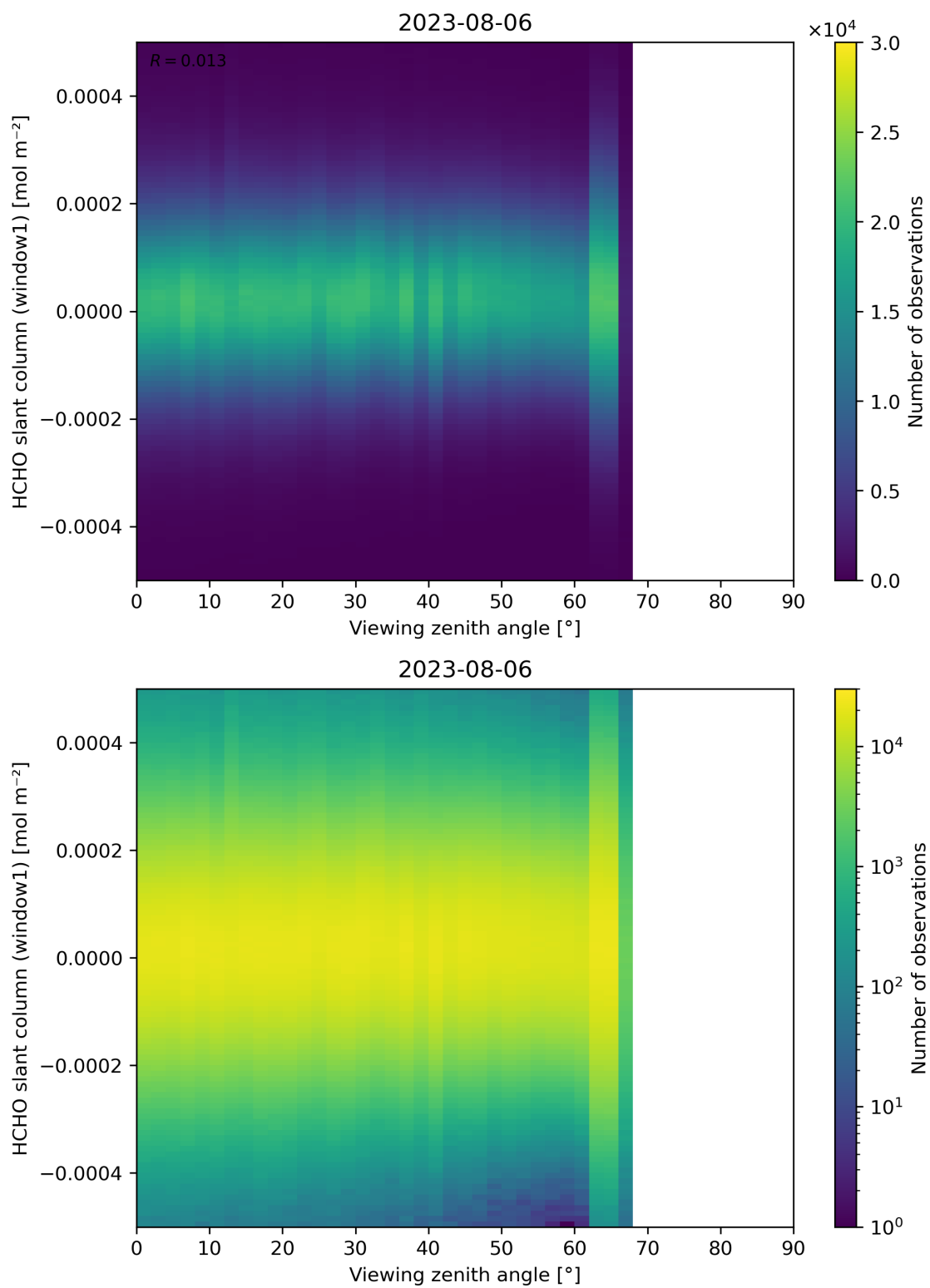
Figure 188: Scatter density plot of “Viewing zenith angle” against “HCHO slant column (window1)” for 2023-08-05 to 2023-08-07.
