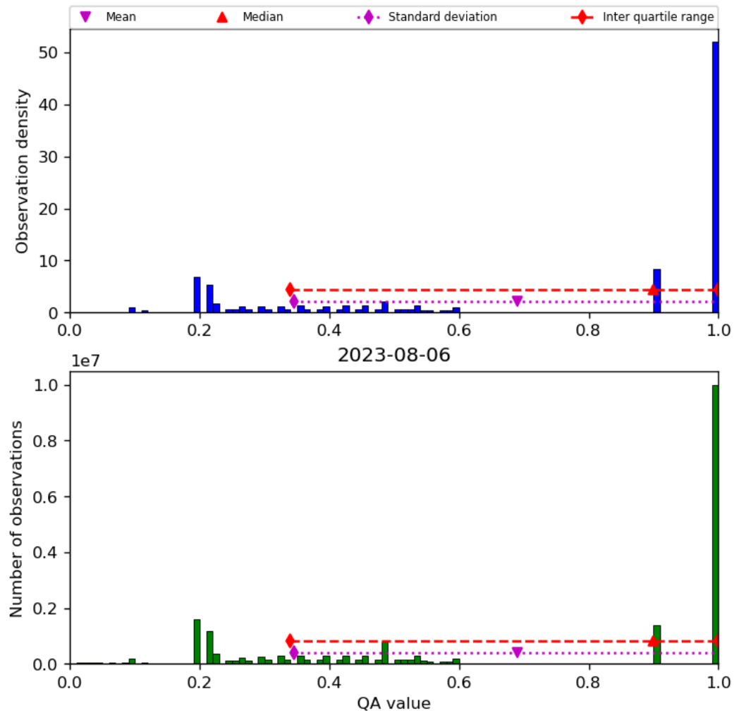
Figure 34: Histogram of “QA value” for 2023-08-05 to 2023-08-07
