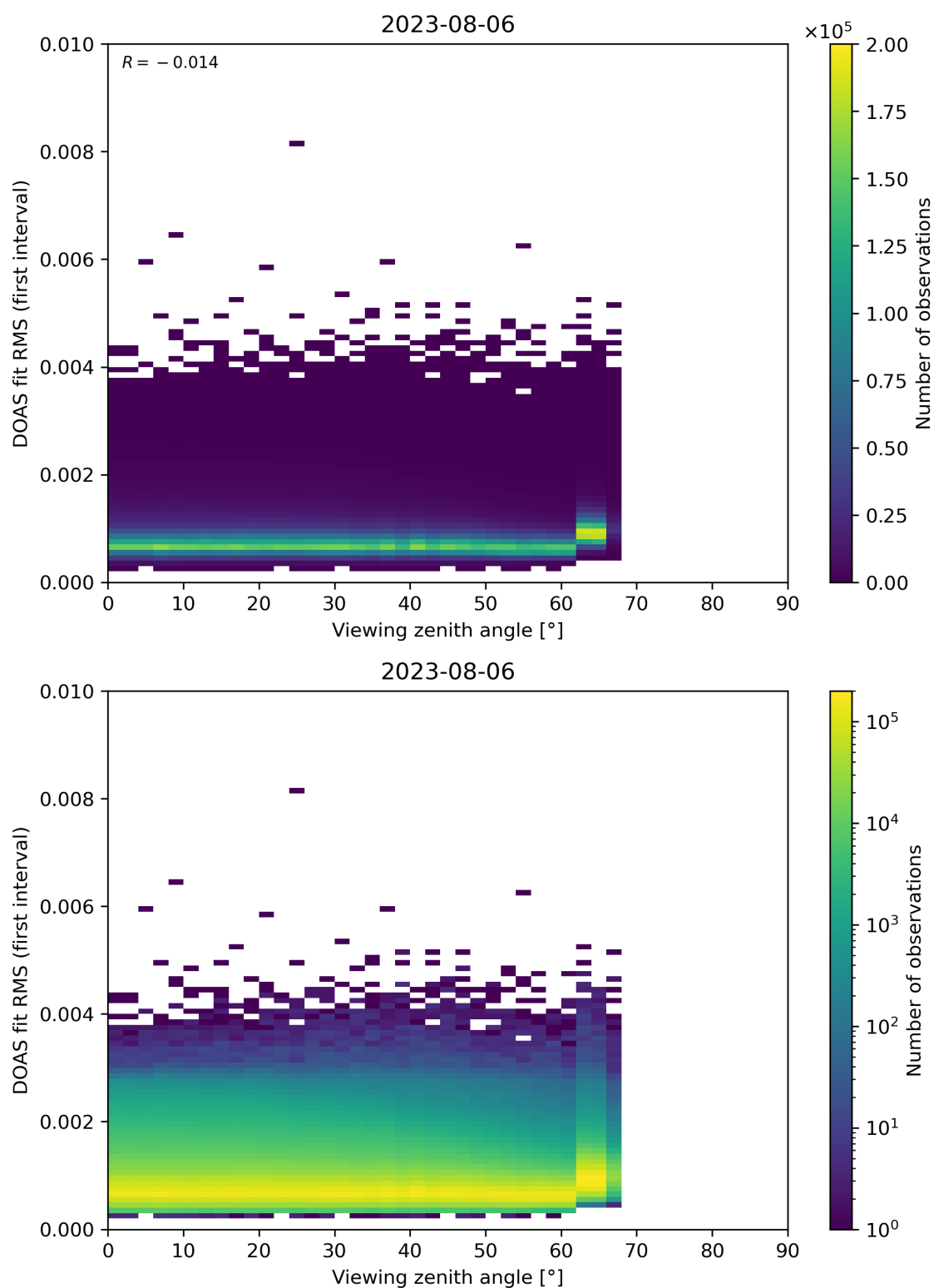
Figure 182: Scatter density plot of “Viewing zenith angle” against “DOAS fit RMS (first interval)” for 2023-08-05 to 2023-08-07.
