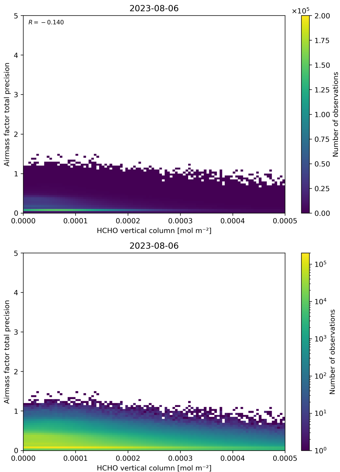
Figure 132: Scatter density plot of “HCHO vertical column” against “Airmass factor total precision” for 2023-08-05 to 2023-08-07.
