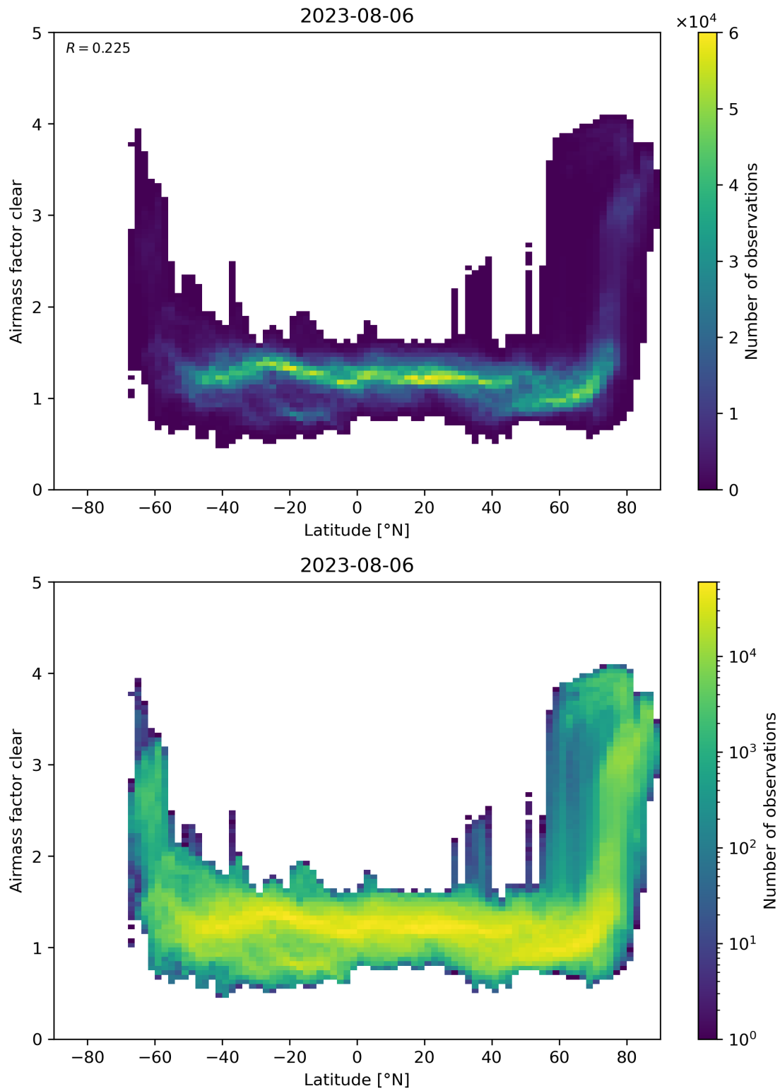
Figure 156: Scatter density plot of “Latitude” against “Airmass factor clear” for 2023-08-05 to 2023-08-07.
