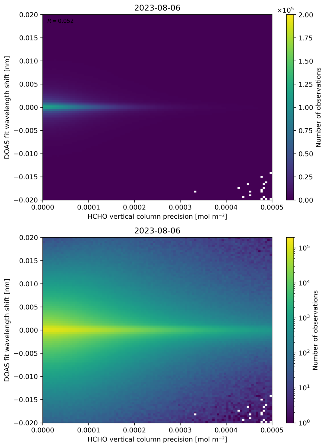
Figure 137: Scatter density plot of “HCHO vertical column precision” against “DOAS fit wavelength shift” for 2023-08-05 to 2023-08-07.
