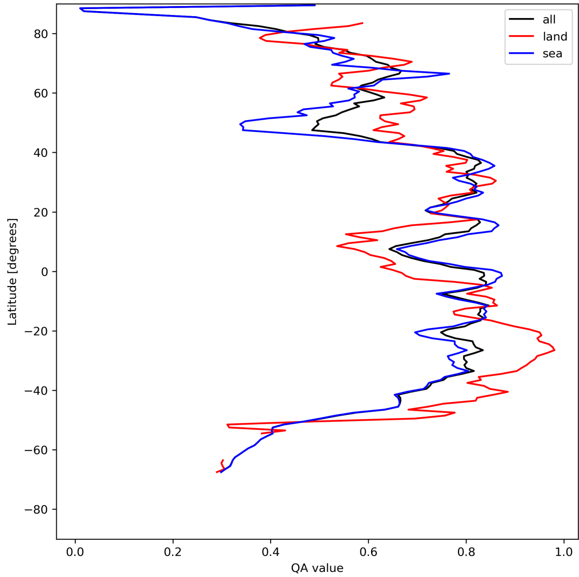
Figure 20: Zonal average of “QA value” for 2023-08-05 to 2023-08-07.
