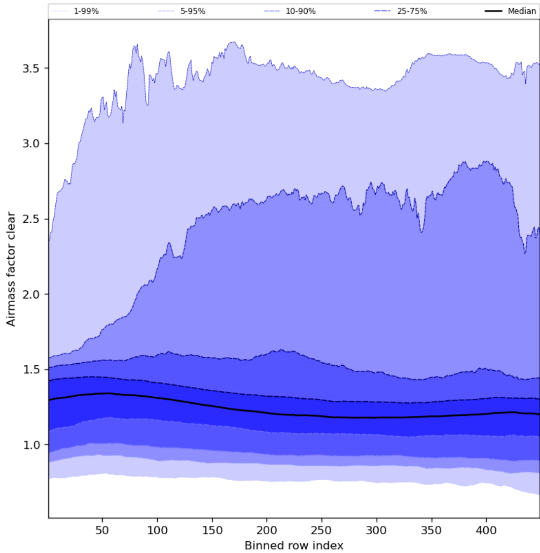
Figure 56: Along track statistics of “Airmass factor clear” for 2023-08-05 to 2023-08-07
