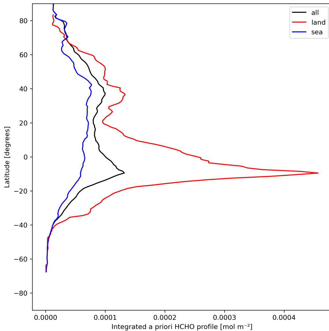
Figure 29: Zonal average of “Integrated a priori HCHO profile” for 2023-08-05 to 2023-08-07.
