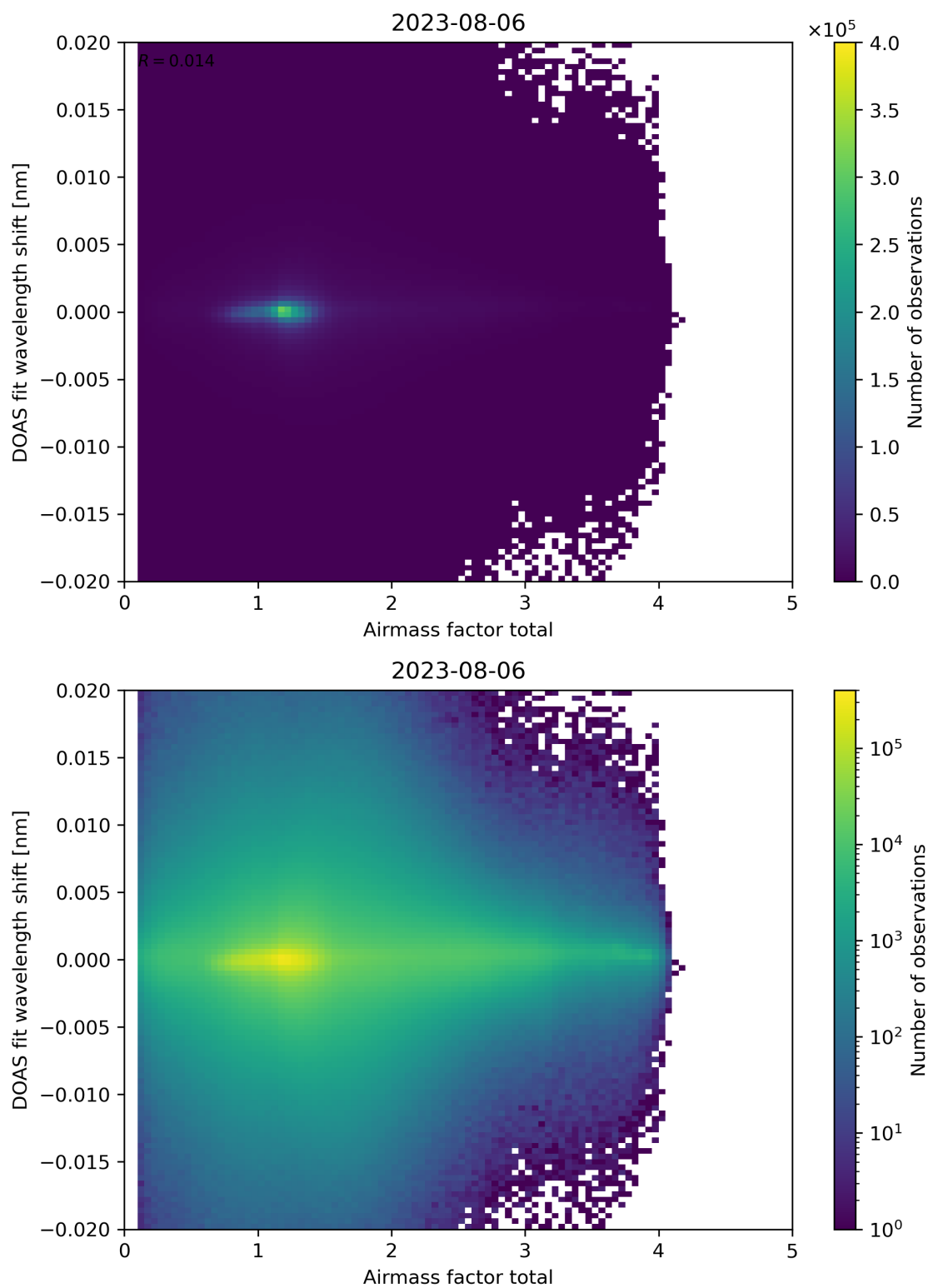
Figure 98: Scatter density plot of “Airmass factor total” against “DOAS fit wavelength shift” for 2023-08-05 to 2023-08-07.
