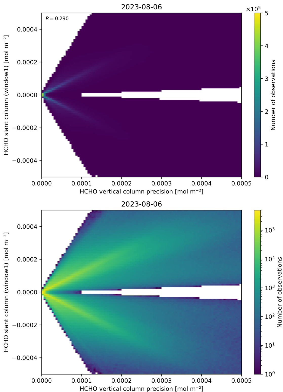
Figure 142: Scatter density plot of “HCHO vertical column precision” against “HCHO slant column (window1)” for 2023-08-05 to 2023-08-07.
