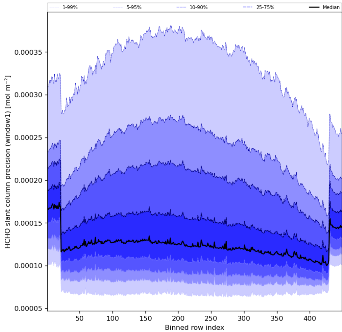
Figure 53: Along track statistics of “HCHO slant column precision (window1)” for 2023-08-05 to 2023-08-07
