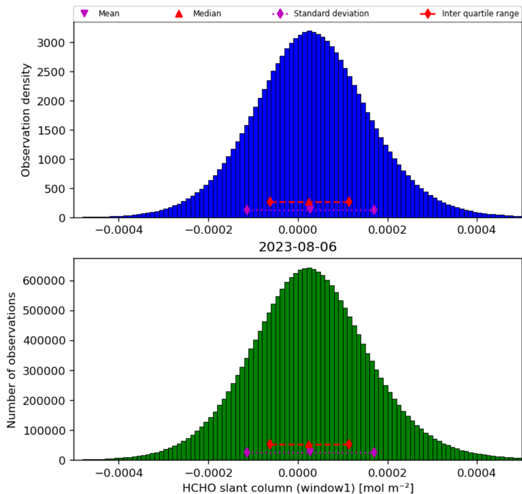
Figure 38: Histogram of “HCHO slant column (window1)” for 2023-08-05 to 2023-08-07
