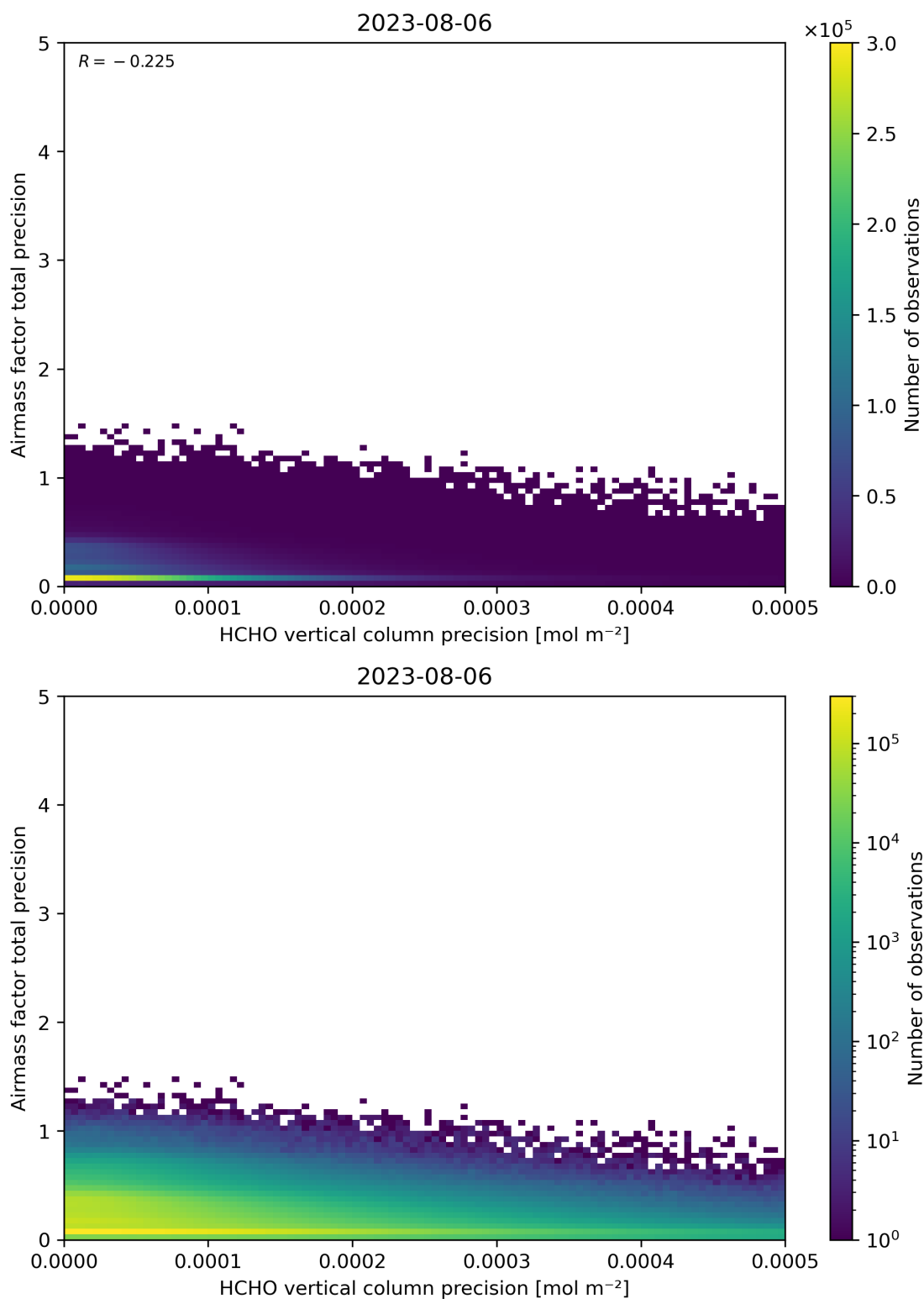
Figure 145: Scatter density plot of “HCHO vertical column precision” against “Airmass factor total precision” for 2023-08-05 to 2023-08-07.
