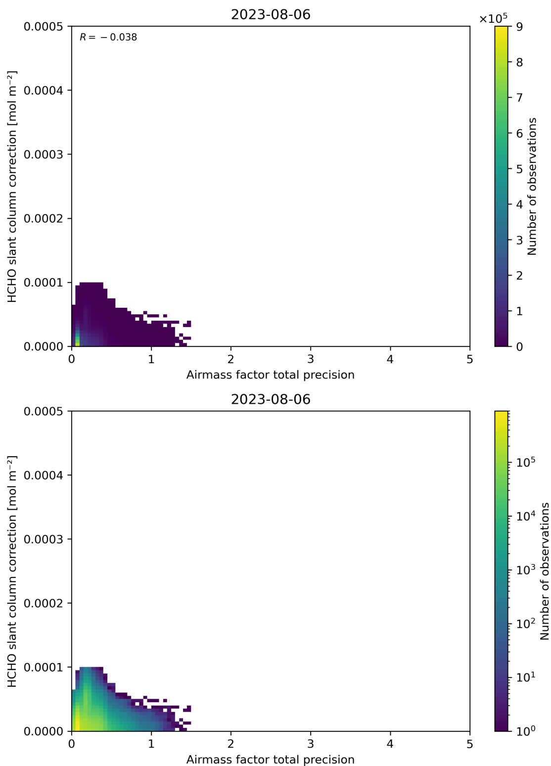
Figure 110: Scatter density plot of “Airmass factor total precision” against “HCHO slant column correction” for 2023-08-05 to 2023-08-07.
