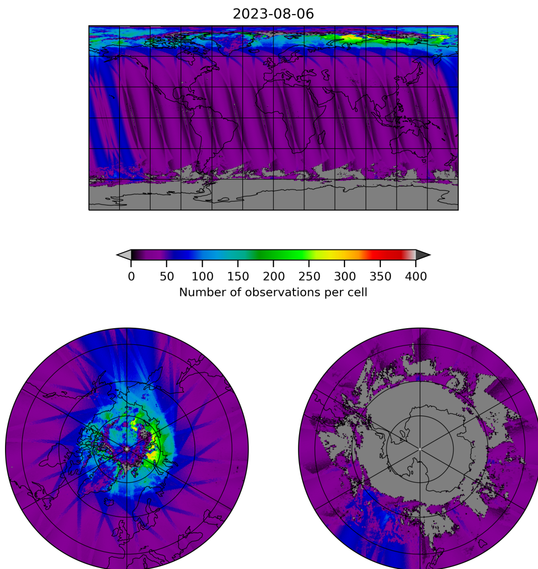
Figure 19: Map of the number of observations for 2023-08-05 to 2023-08-07
