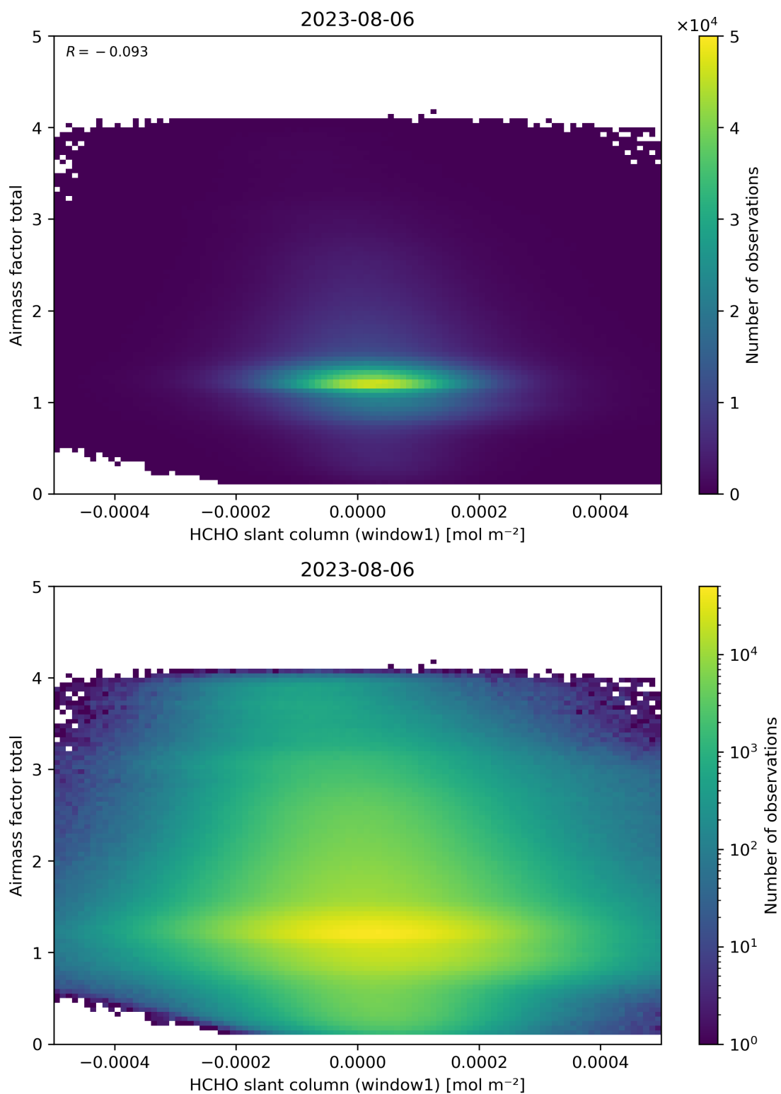
Figure 85: Scatter density plot of “HCHO slant column (window1)” against “Airmass factor total” for 2023-08-05 to 2023-08-07.
