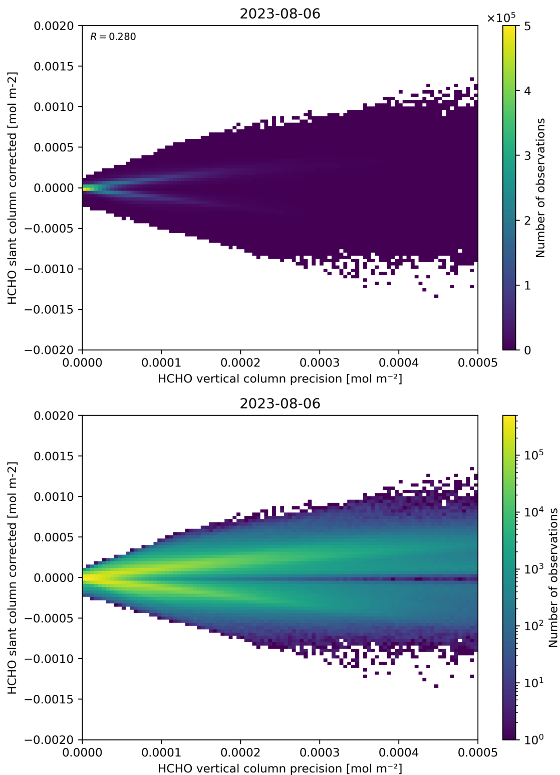
Figure 140: Scatter density plot of “HCHO vertical column precision” against “HCHO slant column corrected” for 2023-08-05 to 2023-08-07.
