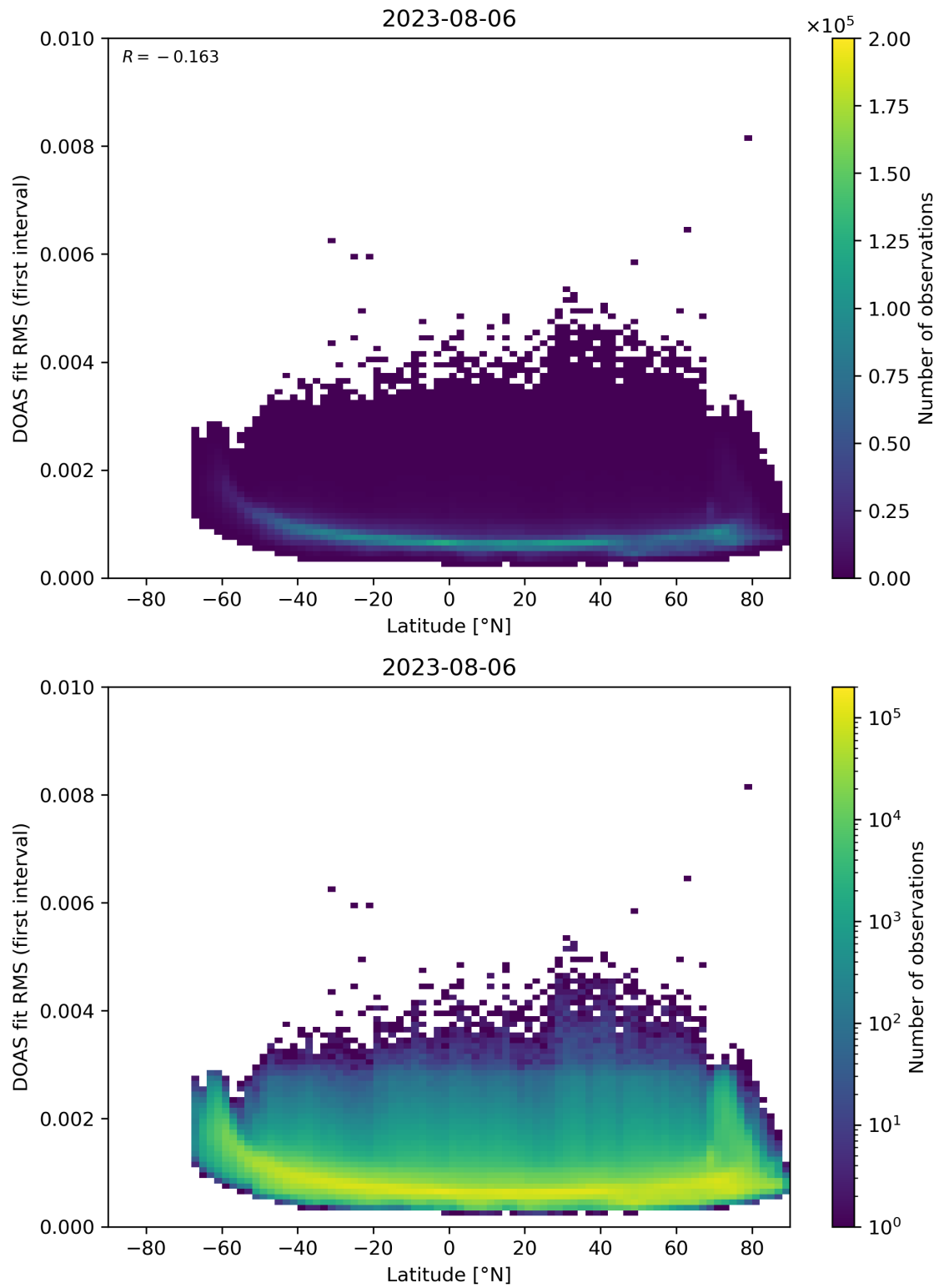
Figure 153: Scatter density plot of “Latitude” against “DOAS fit RMS (first interval)” for 2023-08-05 to 2023-08-07.
