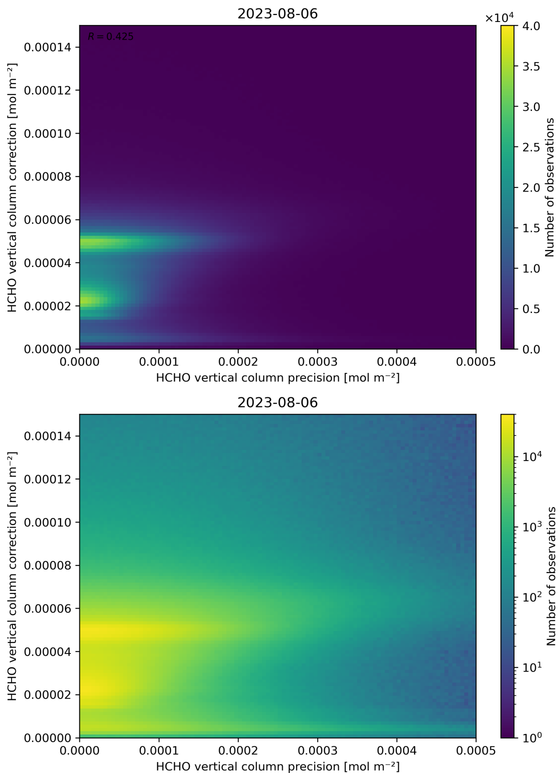
Figure 146: Scatter density plot of “HCHO vertical column precision” against “HCHO vertical column correction” for 2023-08-05 to 2023-08-07.
