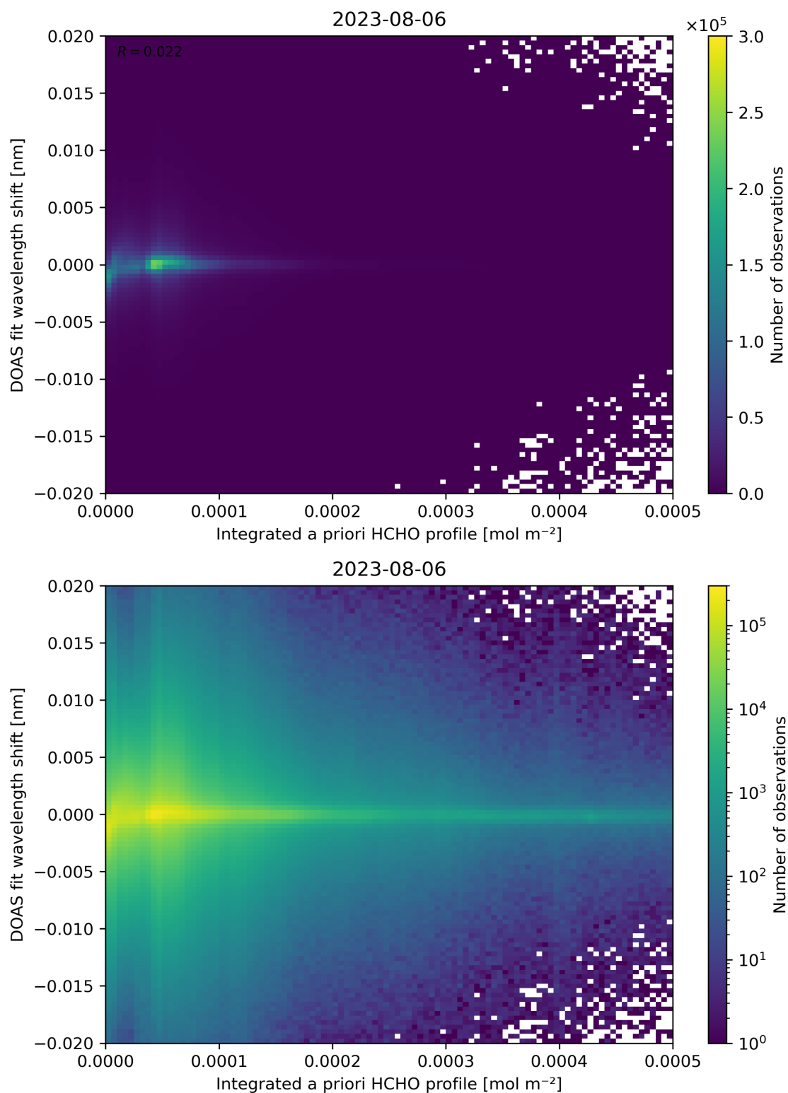
Figure 149: Scatter density plot of “Integrated a priori HCHO profile” against “DOAS fit wavelength shift” for 2023-08-05 to 2023-08-07.
