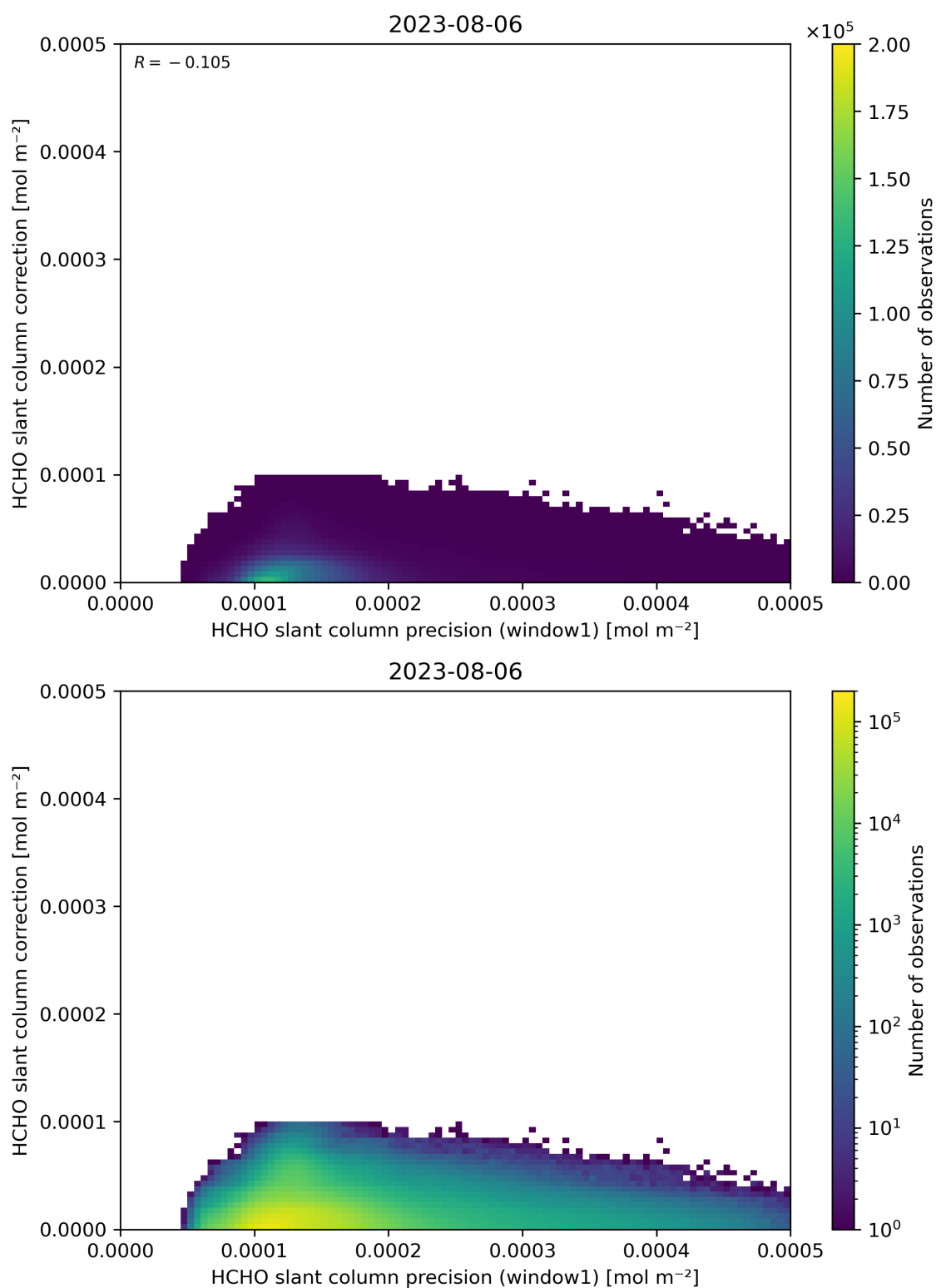
Figure 93: Scatter density plot of “HCHO slant column precision (window1)” against “HCHO slant column correction” for 2023-08-05 to 2023-08-07.
