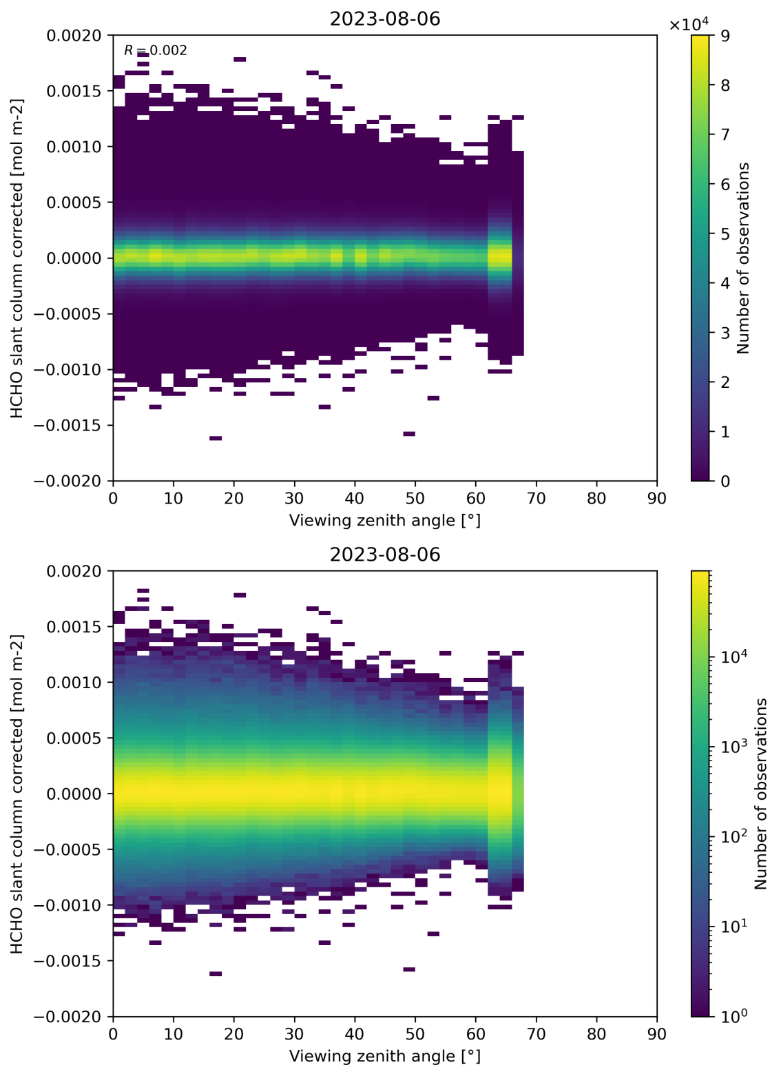
Figure 186: Scatter density plot of “Viewing zenith angle” against “HCHO slant column corrected” for 2023-08-05 to 2023-08-07.
