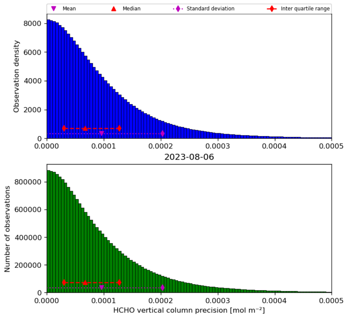
Figure 36: Histogram of “HCHO vertical column precision” for 2023-08-05 to 2023-08-07
