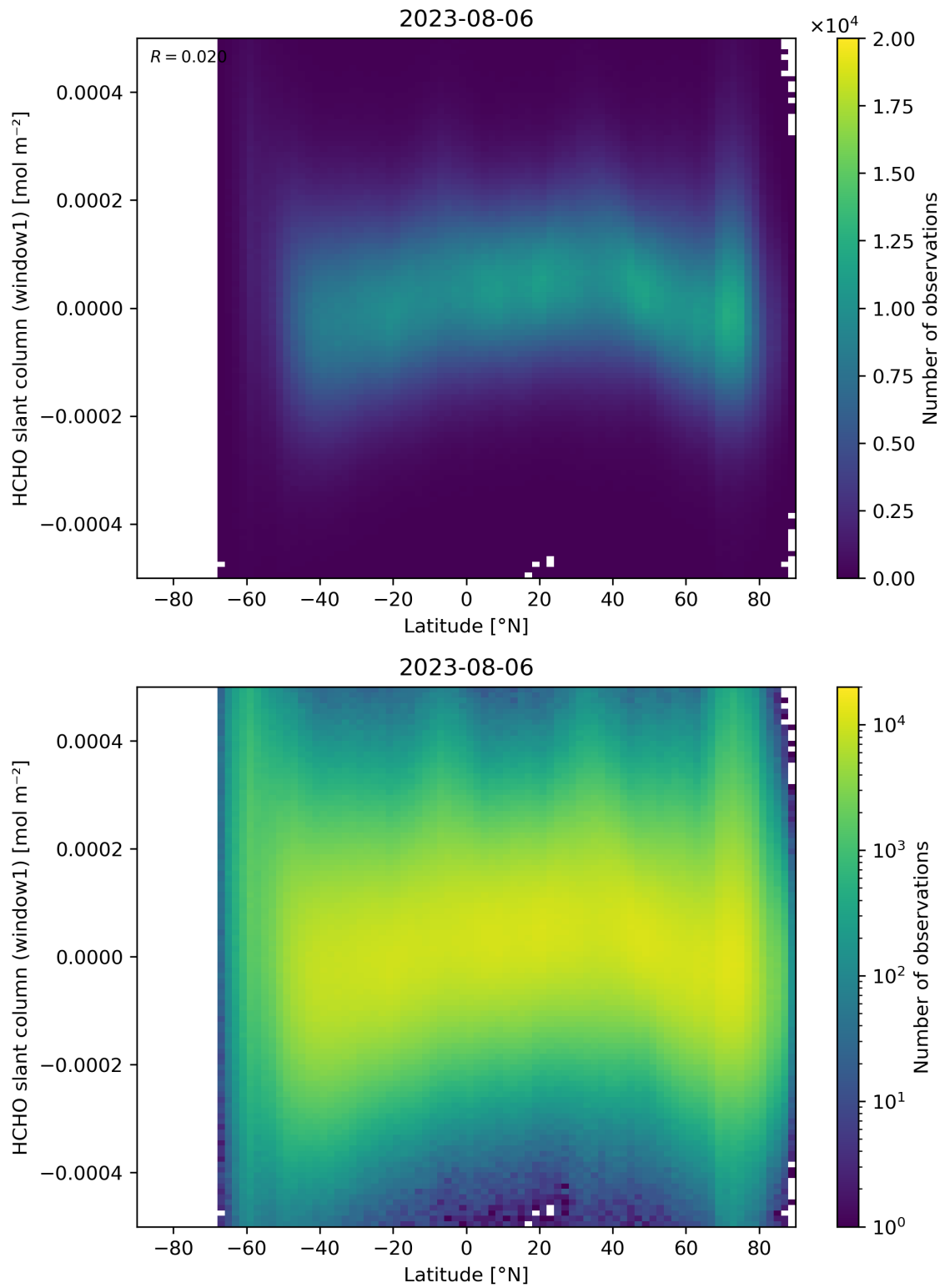
Figure 159: Scatter density plot of “Latitude” against “HCHO slant column (window1)” for 2023-08-05 to 2023-08-07.
