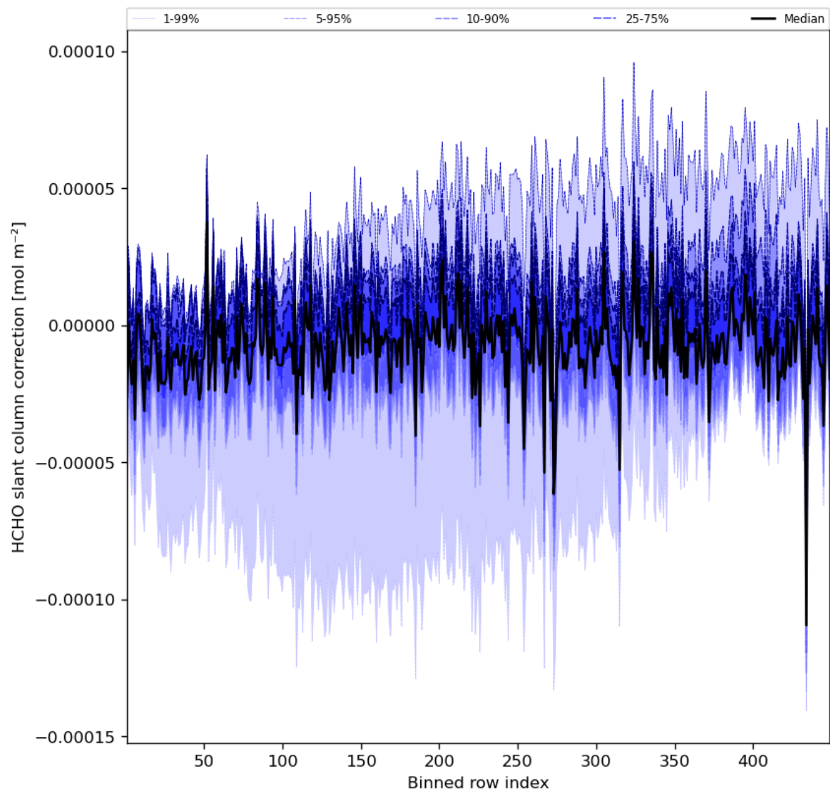
Figure 61: Along track statistics of “HCHO slant column correction” for 2023-08-05 to 2023-08-07
