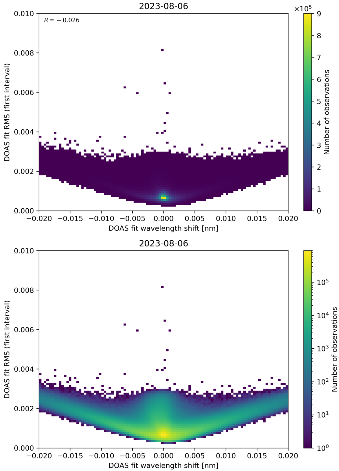
Figure 64: Scatter density plot of “DOAS fit wavelength shift” against “DOAS fit RMS (first interval)” for 2023-08-05 to 2023-08-07.
