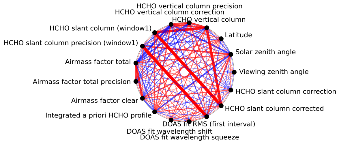
Figure 1: Map of correlation graph for 2023-08-05 to 2023-08-07.
