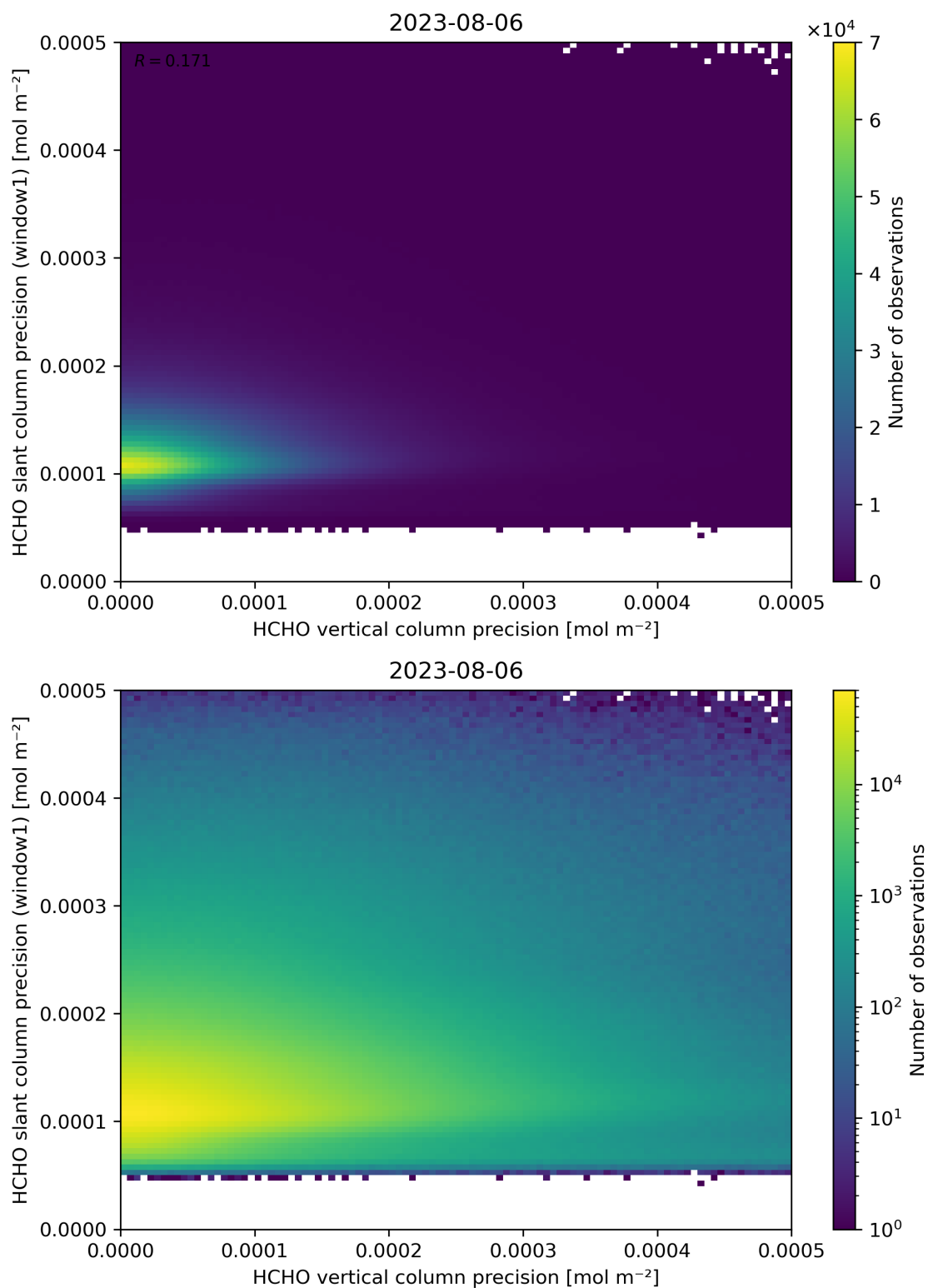
Figure 143: Scatter density plot of “HCHO vertical column precision” against “HCHO slant column precision (window1)” for 2023-08-05 to 2023-08-07.
