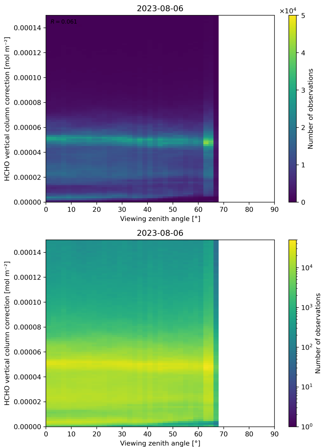
Figure 193: Scatter density plot of “Viewing zenith angle” against “HCHO vertical column correction” for 2023-08-05 to 2023-08-07.
