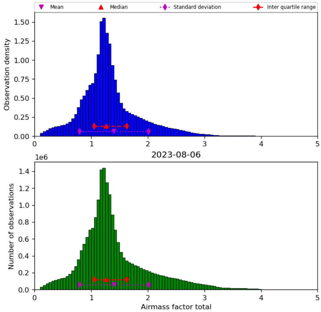
Figure 40: Histogram of “Airmass factor total” for 2023-08-05 to 2023-08-07
