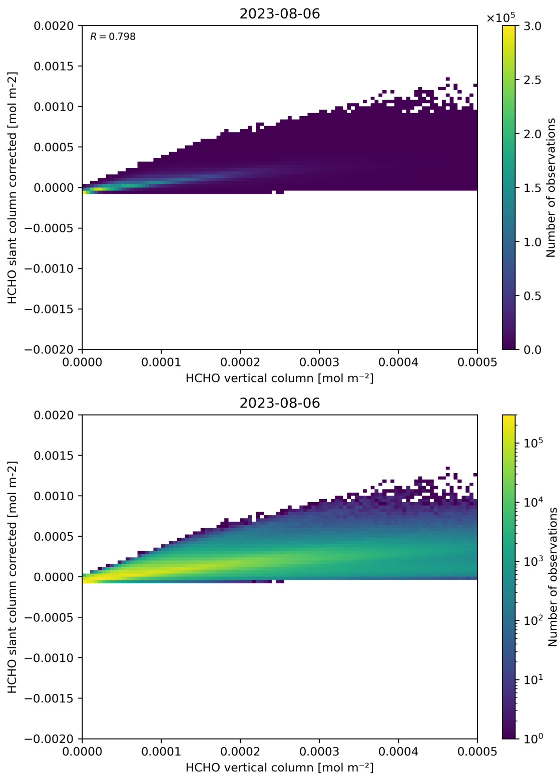
Figure 127: Scatter density plot of “HCHO vertical column” against “HCHO slant column corrected” for 2023-08-05 to 2023-08-07.
