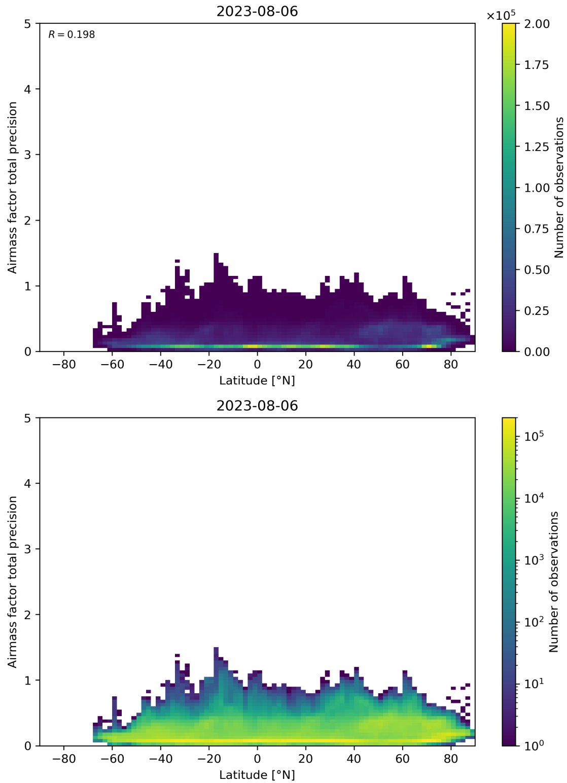
Figure 162: Scatter density plot of “Latitude” against “Airmass factor total precision” for 2023-08-05 to 2023-08-07.
