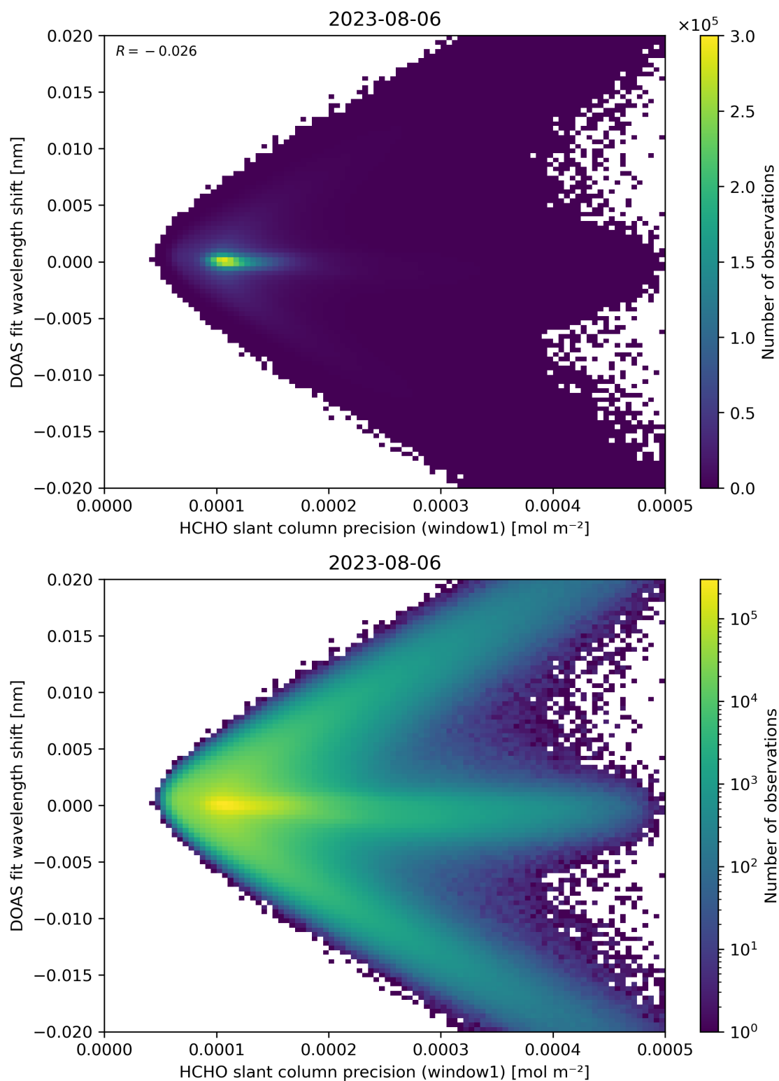
Figure 89: Scatter density plot of “HCHO slant column precision (window1)” against “DOAS fit wavelength shift” for 2023-08-05 to 2023-08-07.
