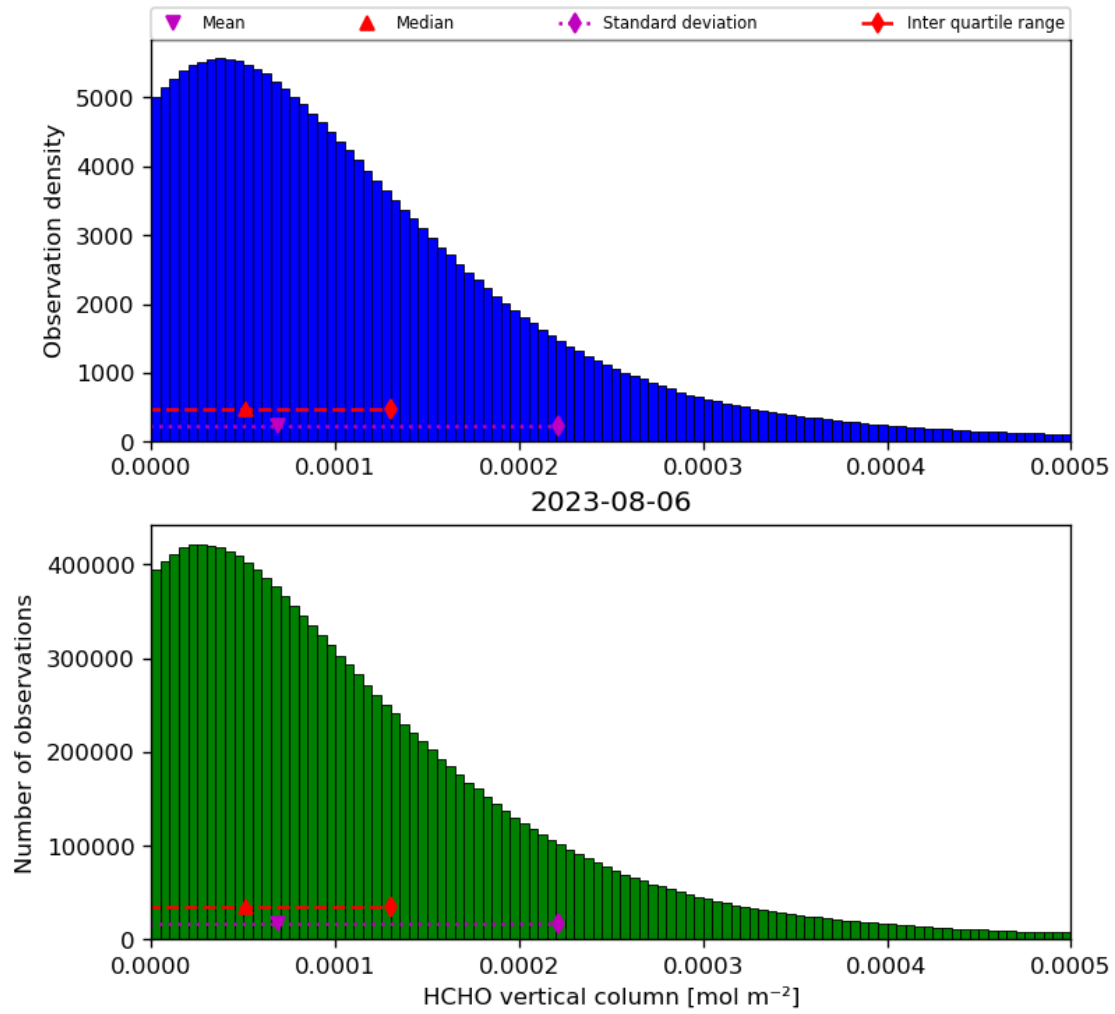
Figure 35: Histogram of “HCHO vertical column” for 2023-08-05 to 2023-08-07
