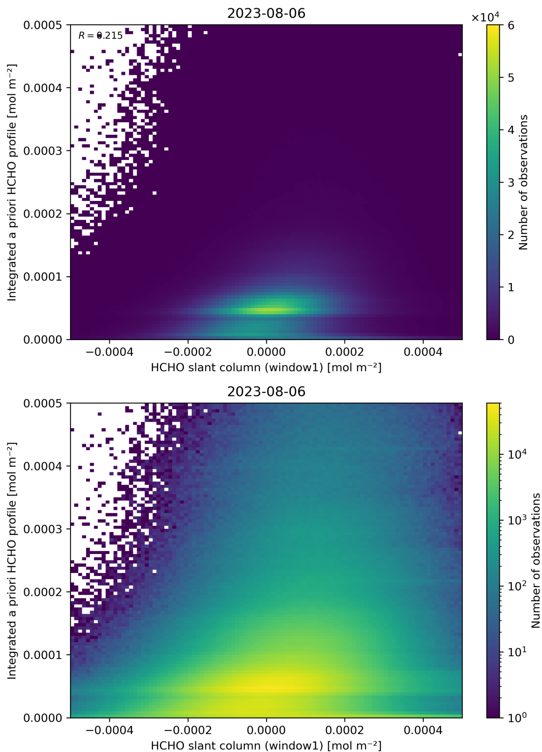
Figure 87: Scatter density plot of “HCHO slant column (window1)” against “Integrated a priori HCHO profile” for 2023-08-05 to 2023-08-07.
