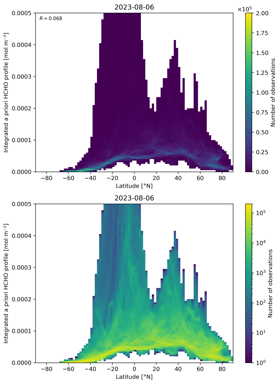
Figure 166: Scatter density plot of “Latitude” against “Integrated a priori HCHO profile” for 2023-08-05 to 2023-08-07.
