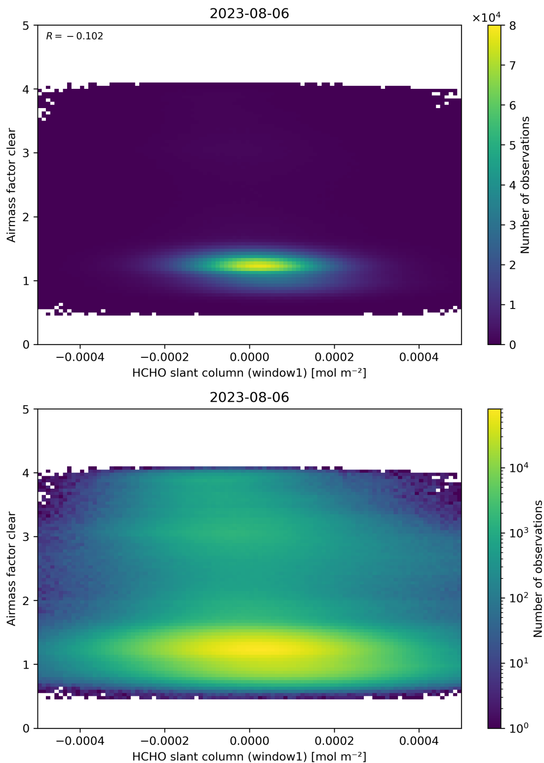
Figure 81: Scatter density plot of “HCHO slant column (window1)” against “Airmass factor clear” for 2023-08-05 to 2023-08-07.
