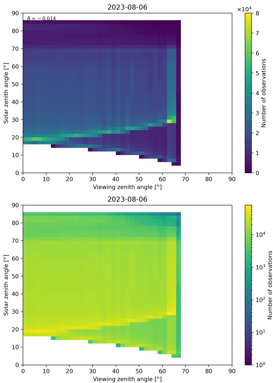
Figure 197: Scatter density plot of “Viewing zenith angle” against “Solar zenith angle” for 2023-08-05 to 2023-08-07.
