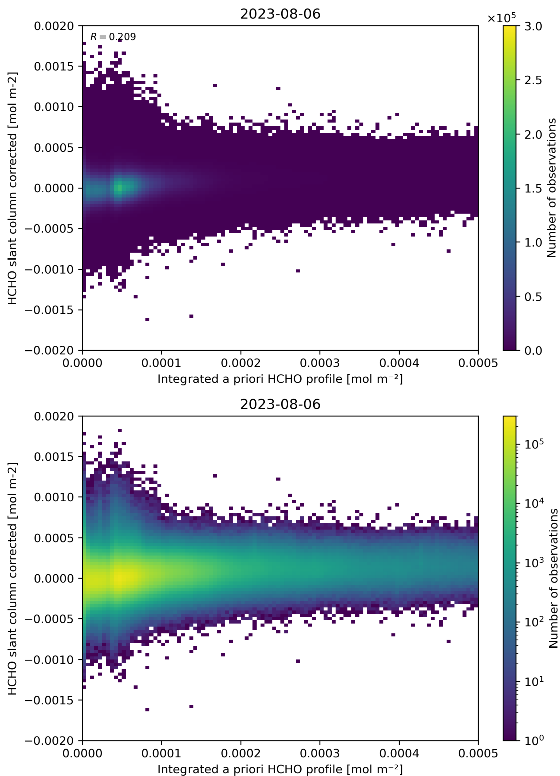
Figure 151: Scatter density plot of “Integrated a priori HCHO profile” against “HCHO slant column corrected” for 2023-08-05 to 2023-08-07.
