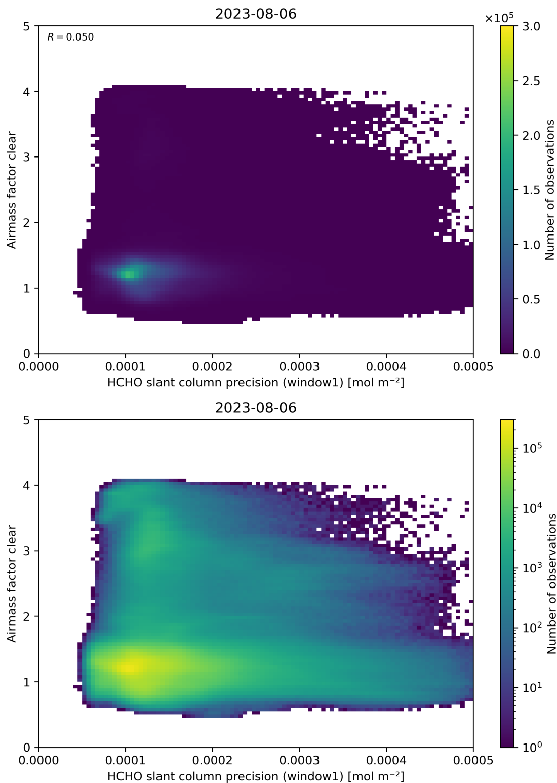
Figure 91: Scatter density plot of “HCHO slant column precision (window1)” against “Airmass factor clear” for 2023-08-05 to 2023-08-07.
