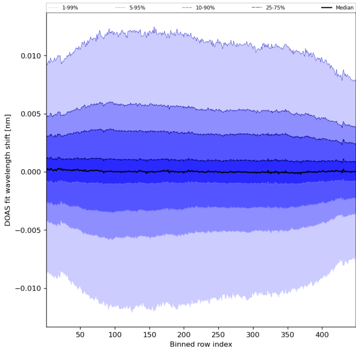
Figure 58: Along track statistics of “DOAS fit wavelength shift” for 2023-08-05 to 2023-08-07
