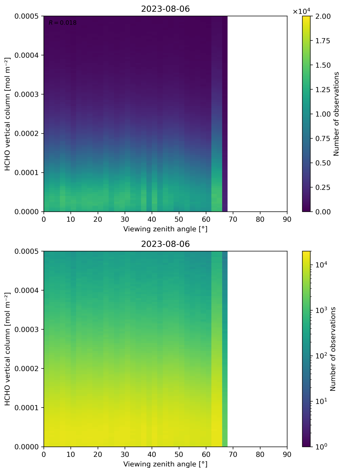
Figure 192: Scatter density plot of “Viewing zenith angle” against “HCHO vertical column” for 2023-08-05 to 2023-08-07.
