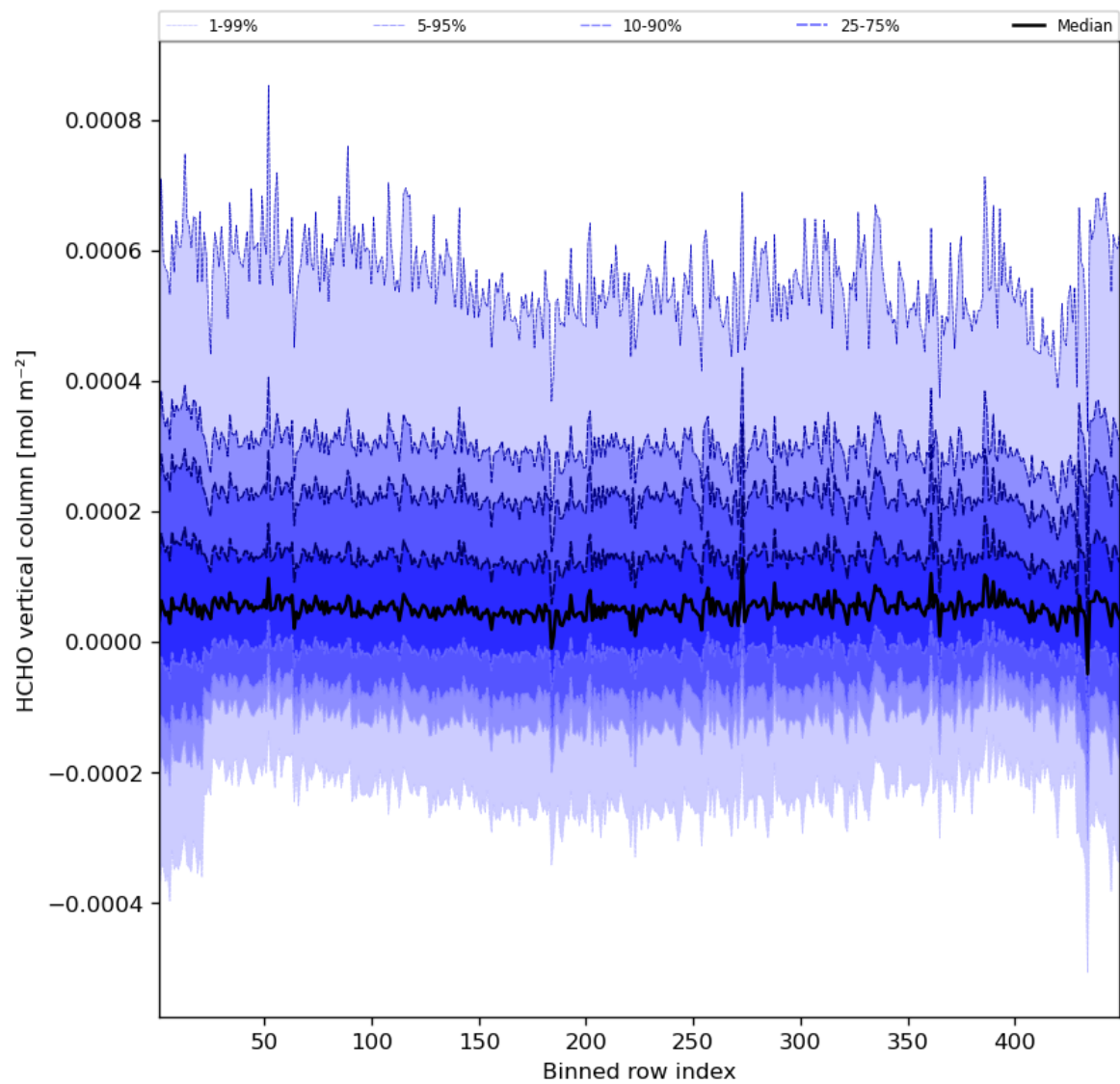
Figure 49: Along track statistics of "HCHO vertical column" for 2023-08-05 to 2023-08-07
