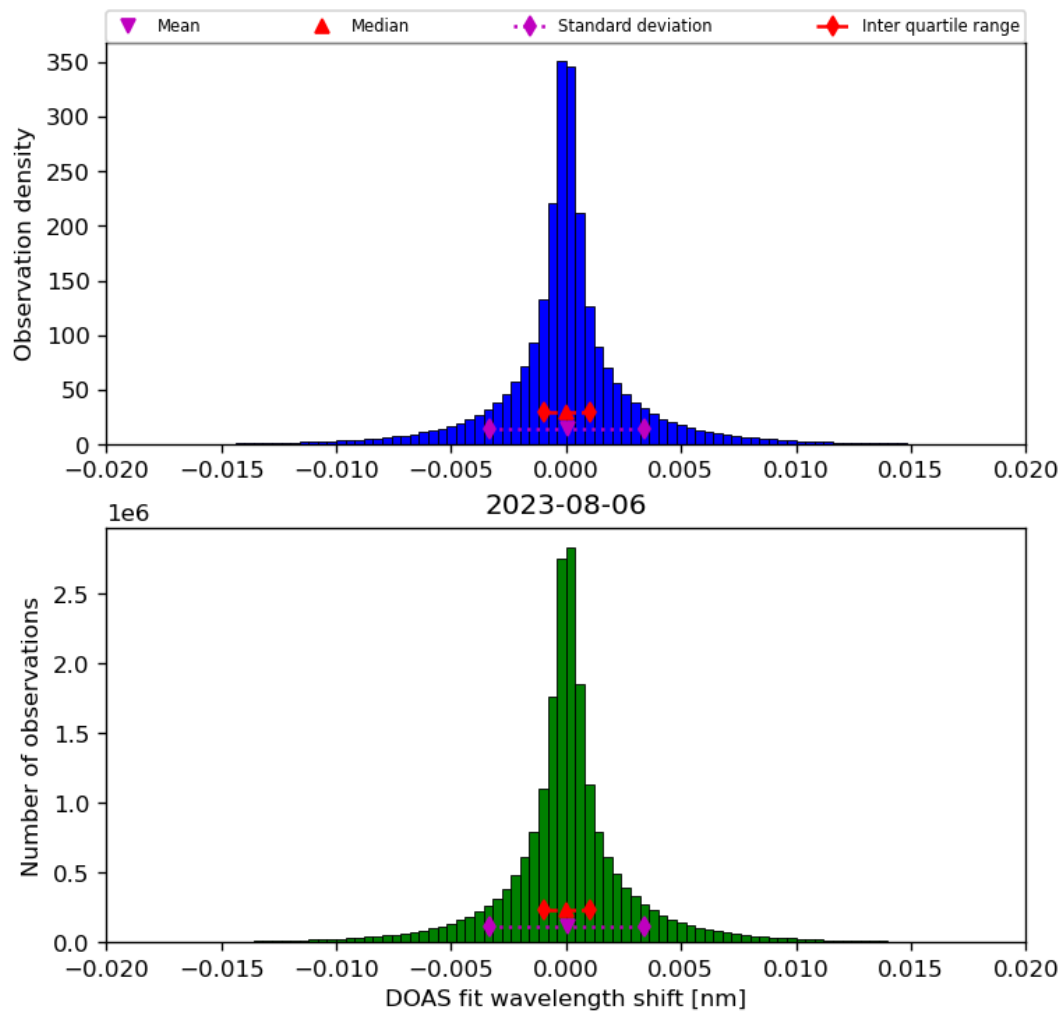
Figure 44: Histogram of “DOAS fit wavelength shift” for 2023-08-05 to 2023-08-07
