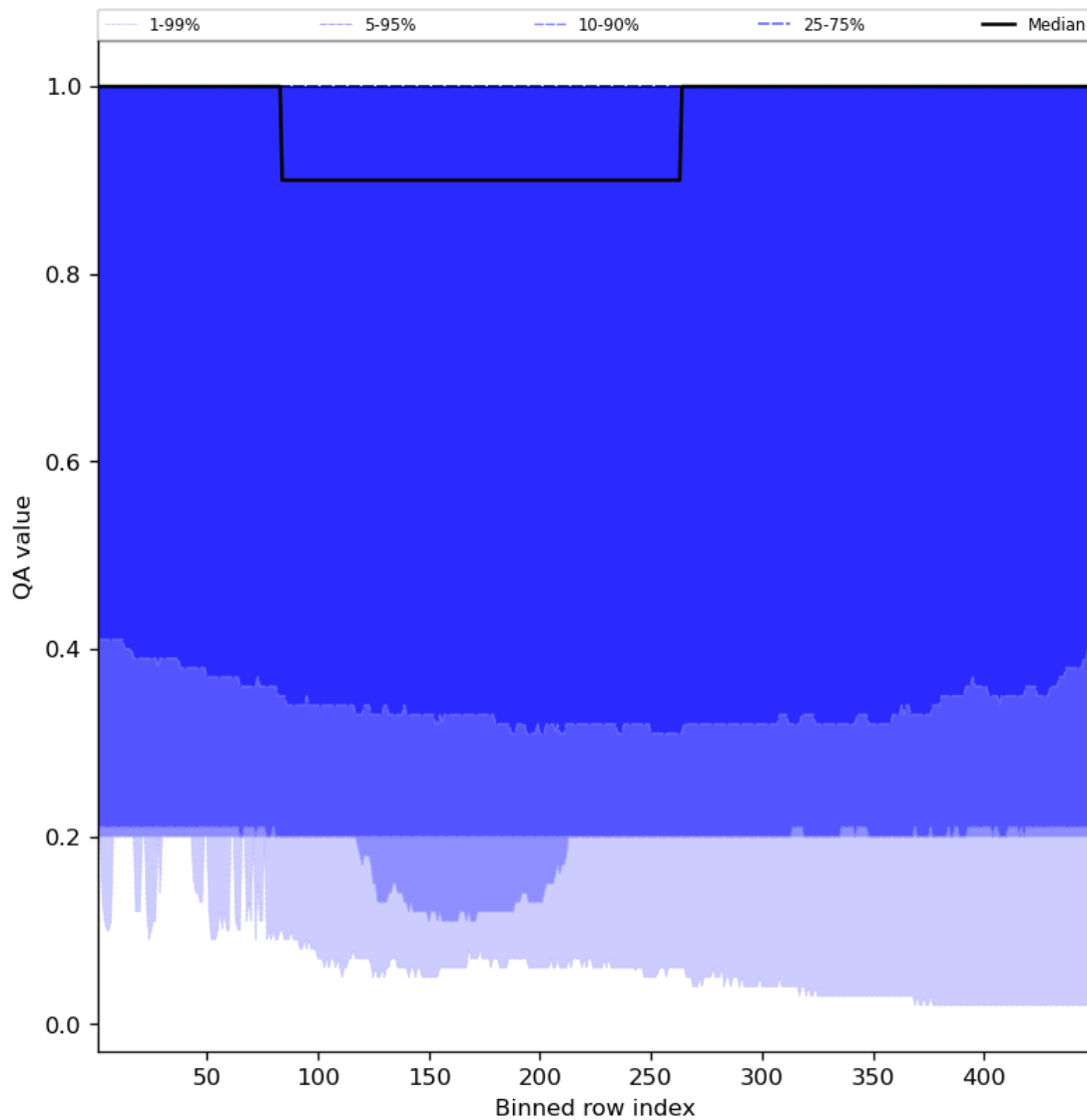
Figure 48: Along track statistics of “QA value” for 2023-08-05 to 2023-08-07
