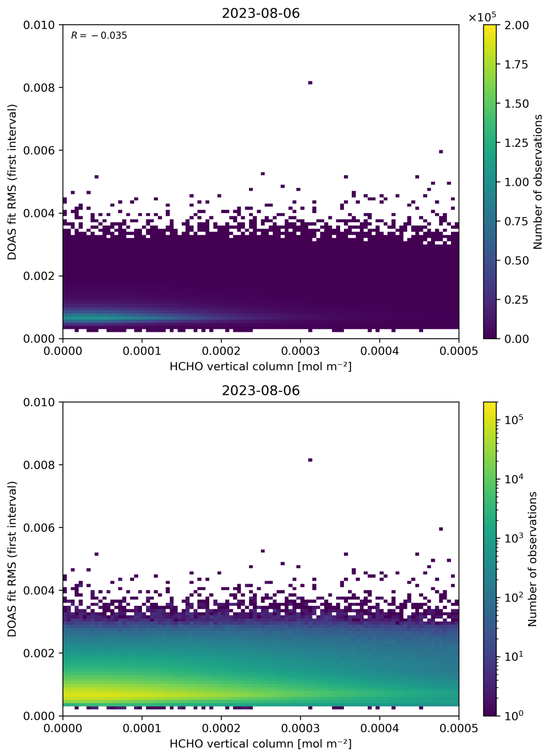
Figure 123: Scatter density plot of “HCHO vertical column” against “DOAS fit RMS (first interval)” for 2023-08-05 to 2023-08-07.
