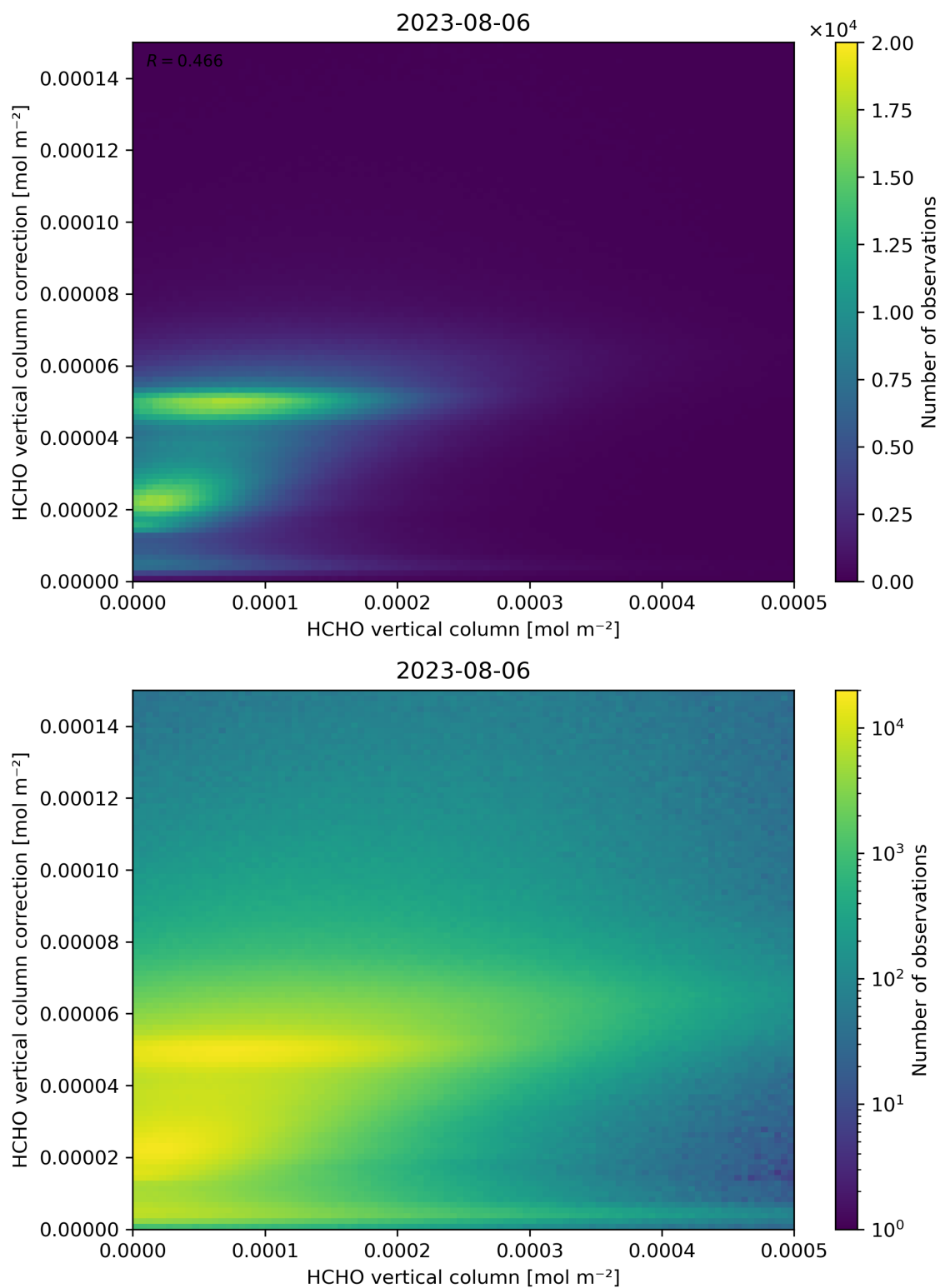
Figure 133: Scatter density plot of “HCHO vertical column” against “HCHO vertical column correction” for 2023-08-05 to 2023-08-07.
