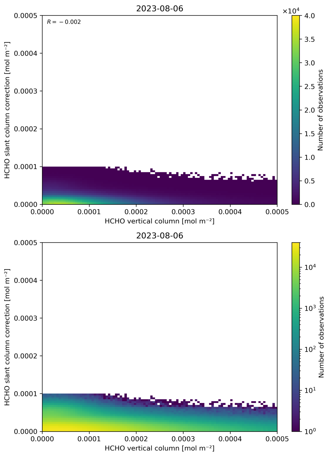
Figure 128: Scatter density plot of “HCHO vertical column” against “HCHO slant column correction” for 2023-08-05 to 2023-08-07.
