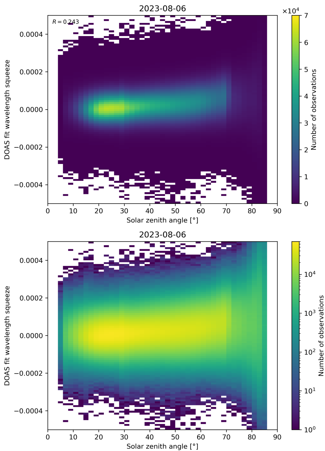
Figure 169: Scatter density plot of “Solar zenith angle” against “DOAS fit wavelength squeeze” for 2023-08-05 to 2023-08-07.
