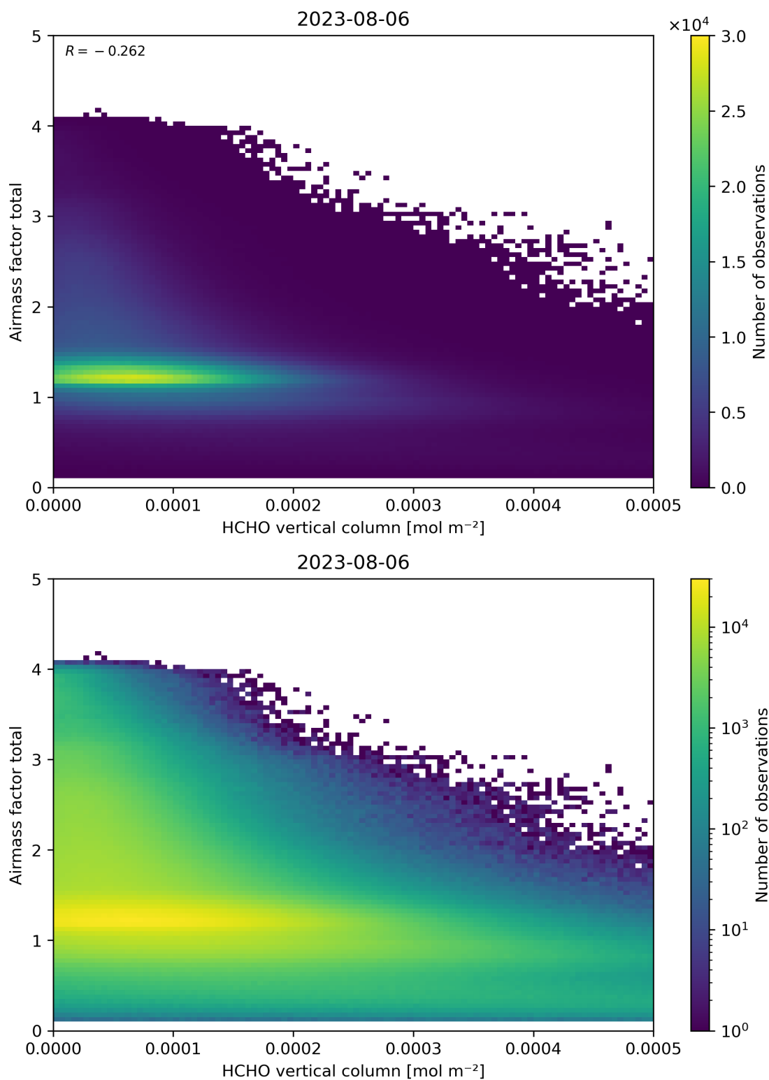
Figure 131: Scatter density plot of “HCHO vertical column” against “Airmass factor total” for 2023-08-05 to 2023-08-07.
