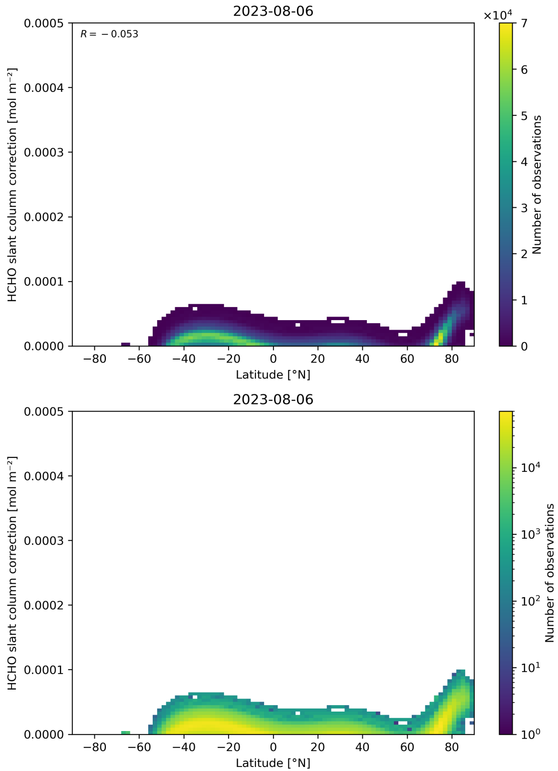
Figure 158: Scatter density plot of “Latitude” against “HCHO slant column correction” for 2023-08-05 to 2023-08-07.
