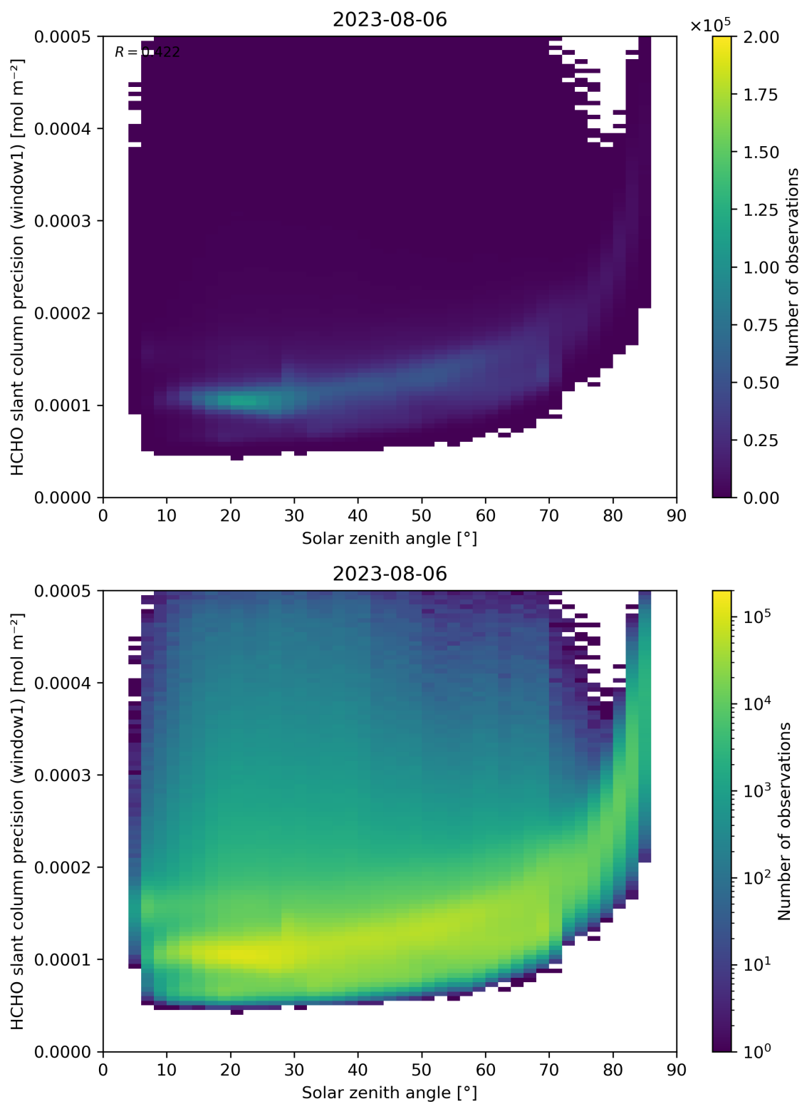
Figure 174: Scatter density plot of “Solar zenith angle” against “HCHO slant column precision (window1)” for 2023-08-05 to 2023-08-07.
