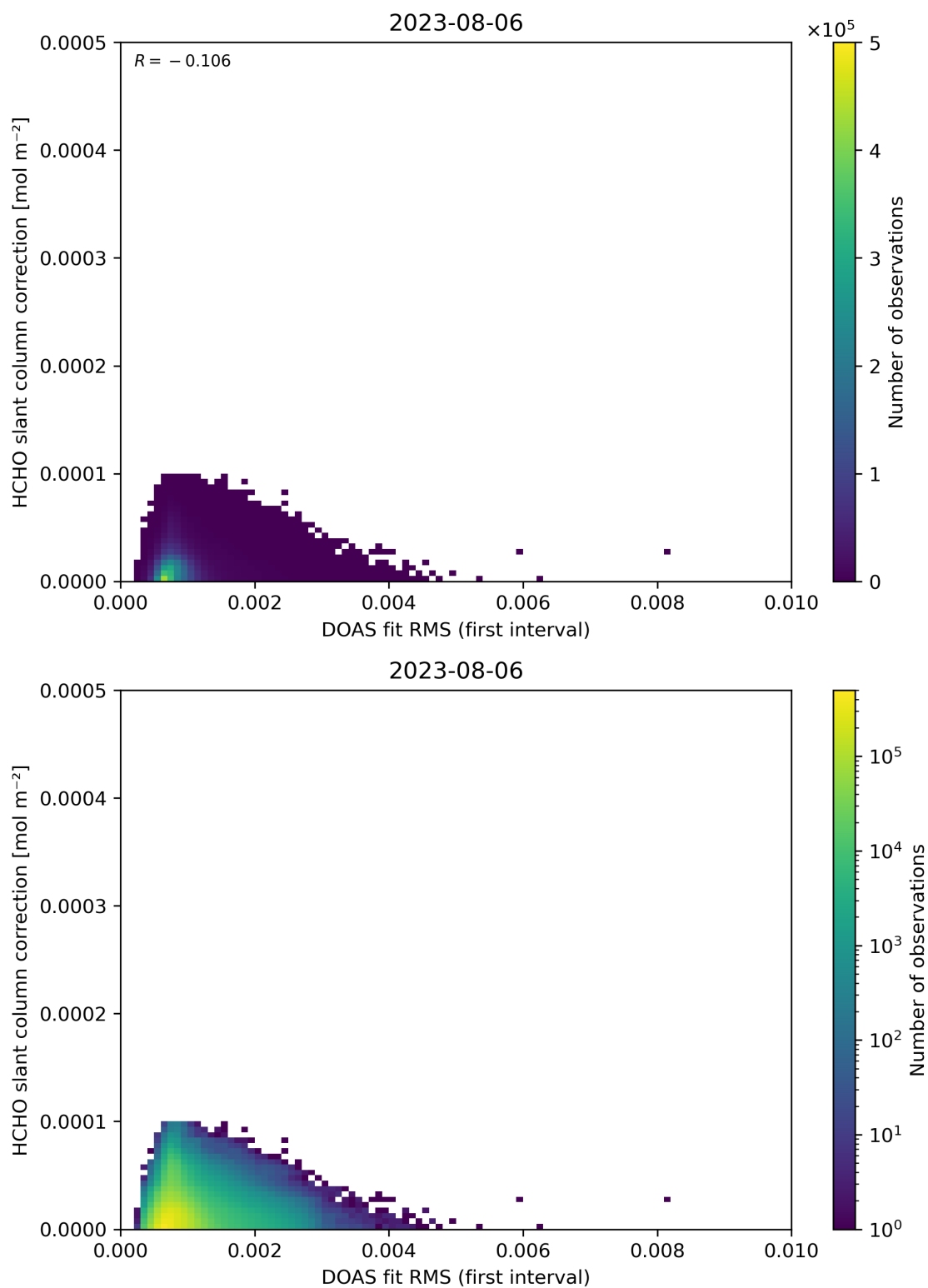
Figure 63: Scatter density plot of “DOAS fit RMS (first interval)” against “HCHO slant column correction” for 2023-08-05 to 2023-08-07.
