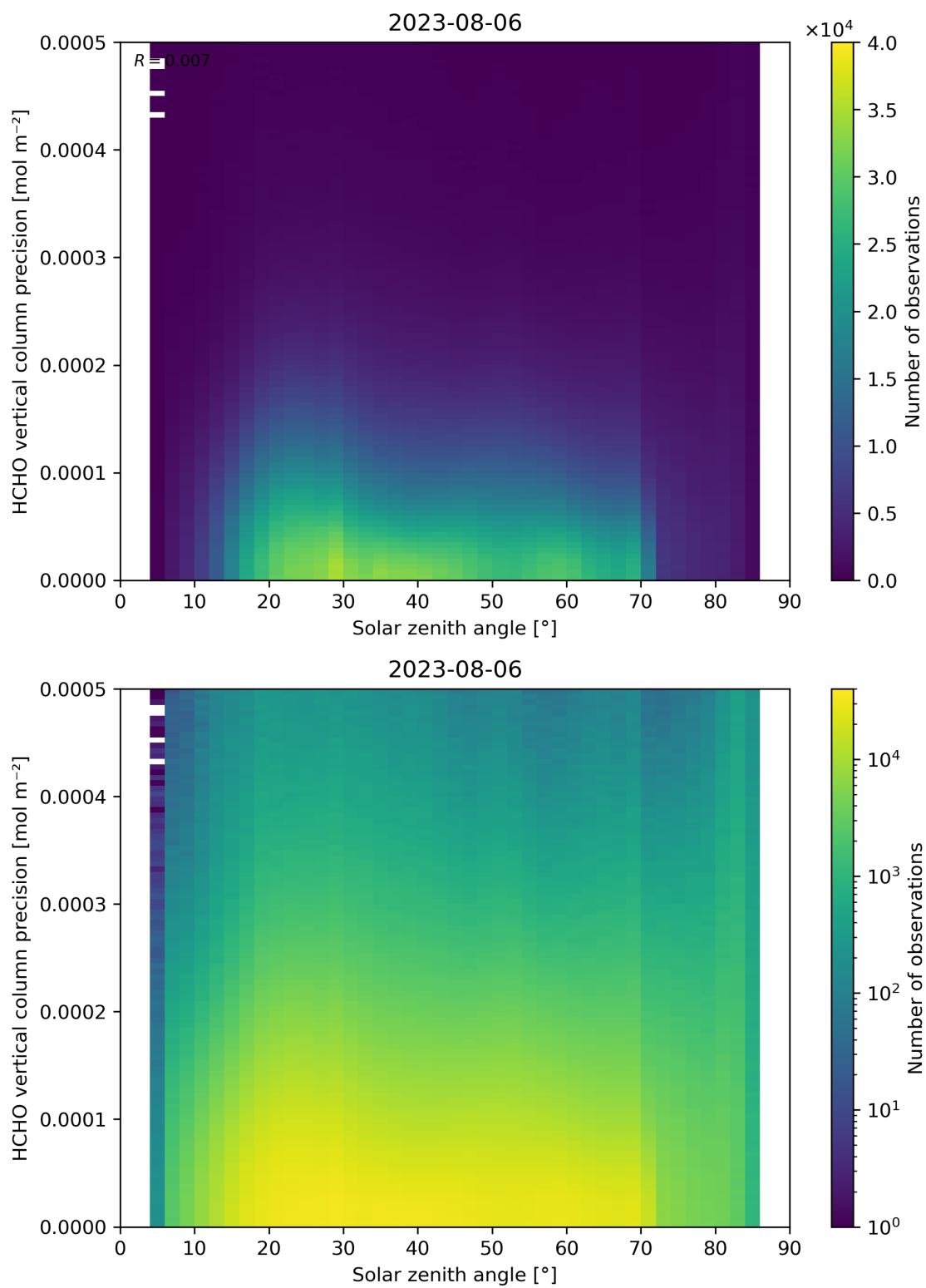
Figure 179: Scatter density plot of “Solar zenith angle” against “HCHO vertical column precision” for 2023-08-05 to 2023-08-07.
