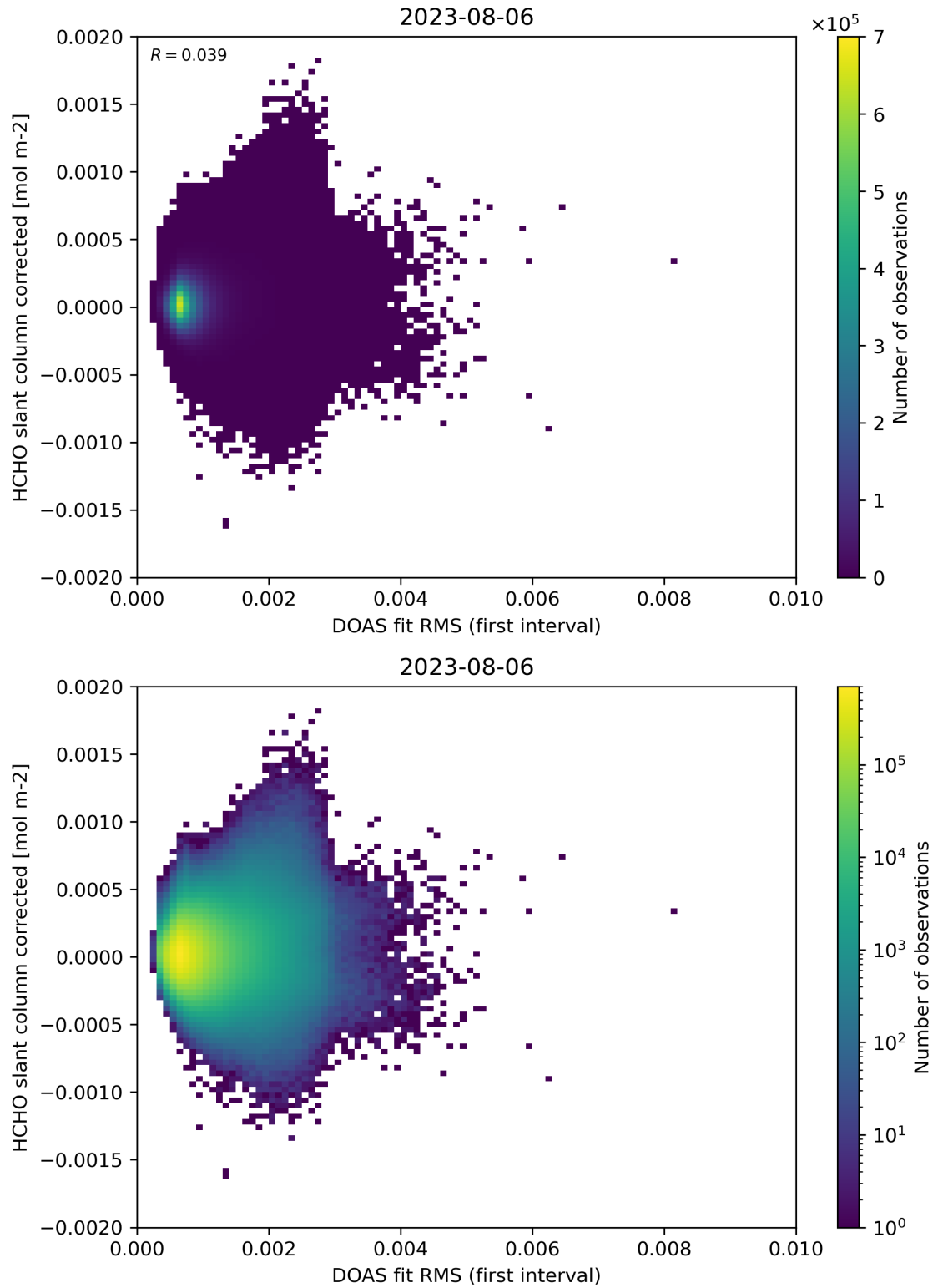
Figure 62: Scatter density plot of “DOAS fit RMS (first interval)” against “HCHO slant column corrected” for 2023-08-05 to 2023-08-07.
