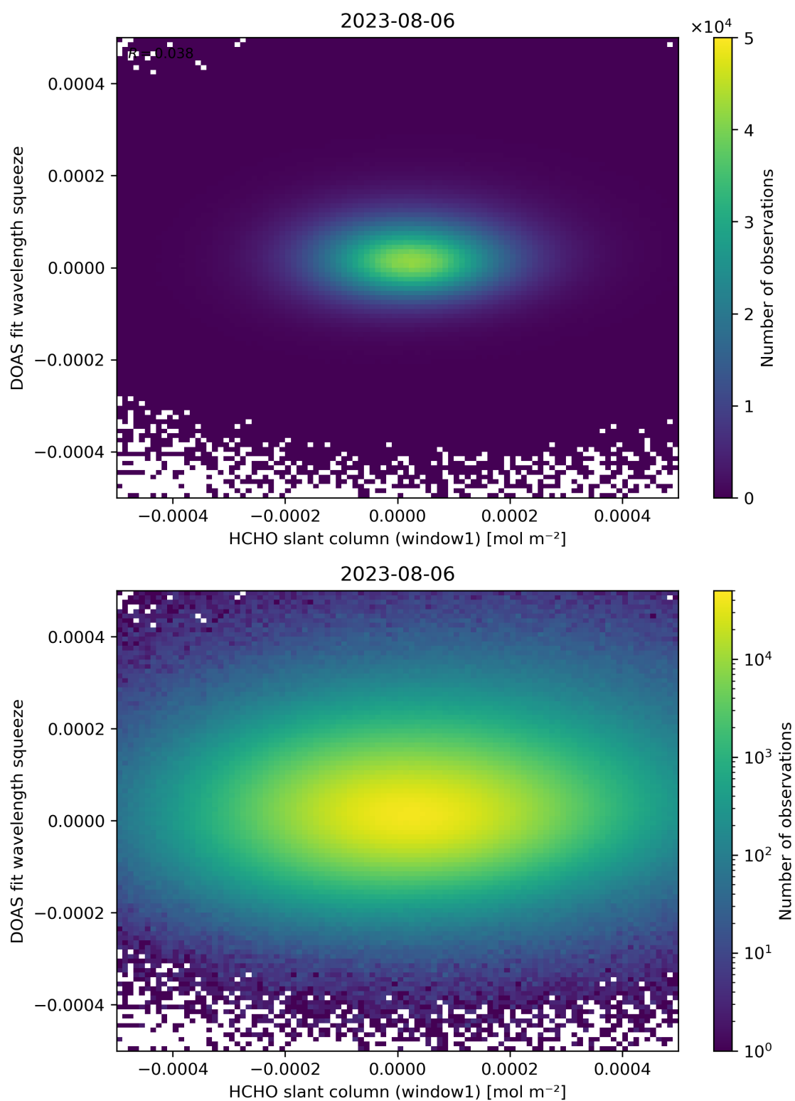
Figure 80: Scatter density plot of “HCHO slant column (window1)” against “DOAS fit wavelength squeeze” for 2023-08-05 to 2023-08-07.
