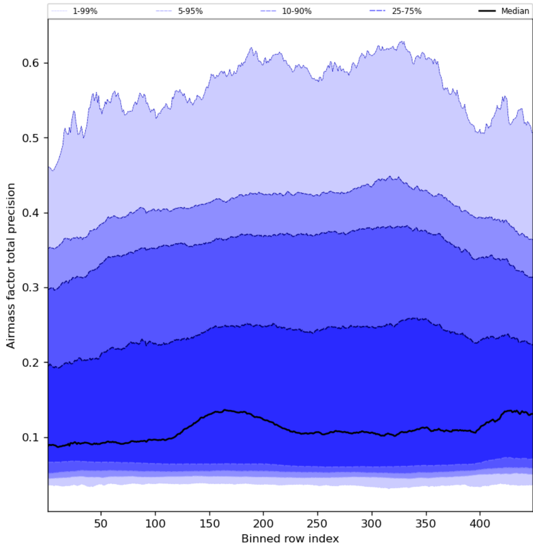
Figure 55: Along track statistics of “Airmass factor total precision” for 2023-08-05 to 2023-08-07
