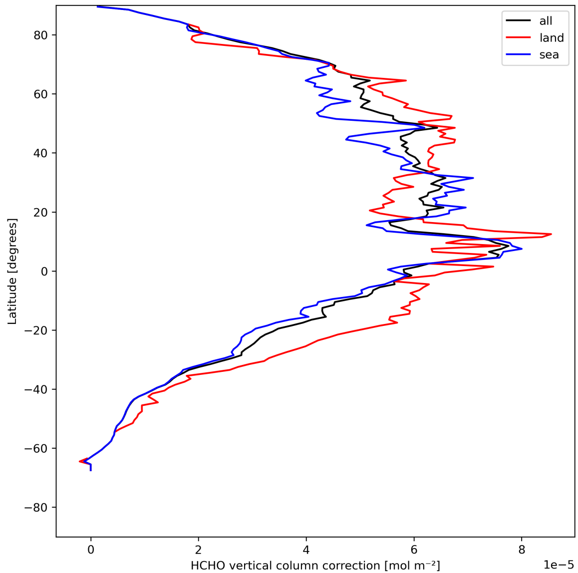
Figure 23: Zonal average of “HCHO vertical column correction” for 2023-08-05 to 2023-08-07.
