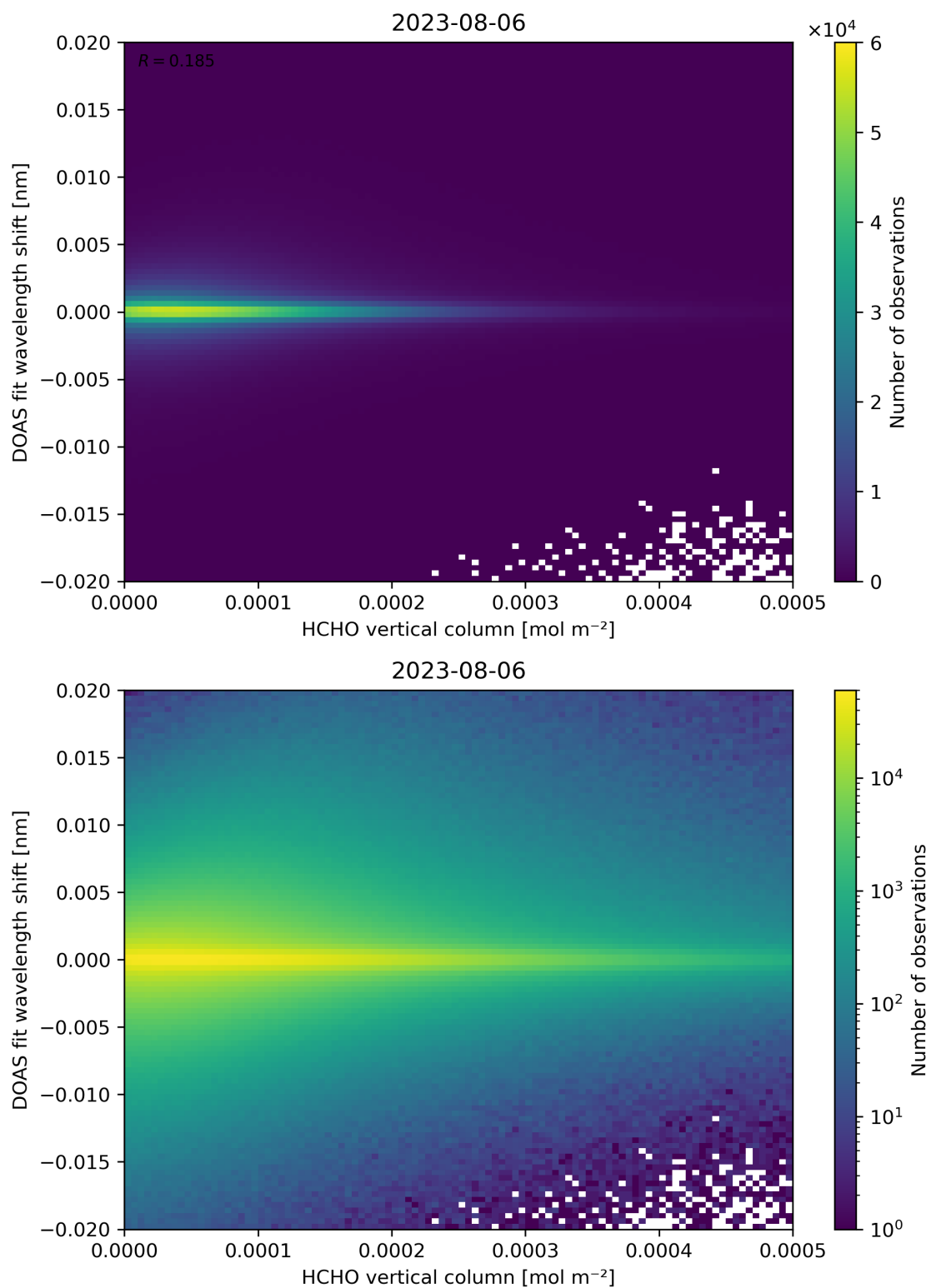
Figure 124: Scatter density plot of “HCHO vertical column” against “DOAS fit wavelength shift” for 2023-08-05 to 2023-08-07.
