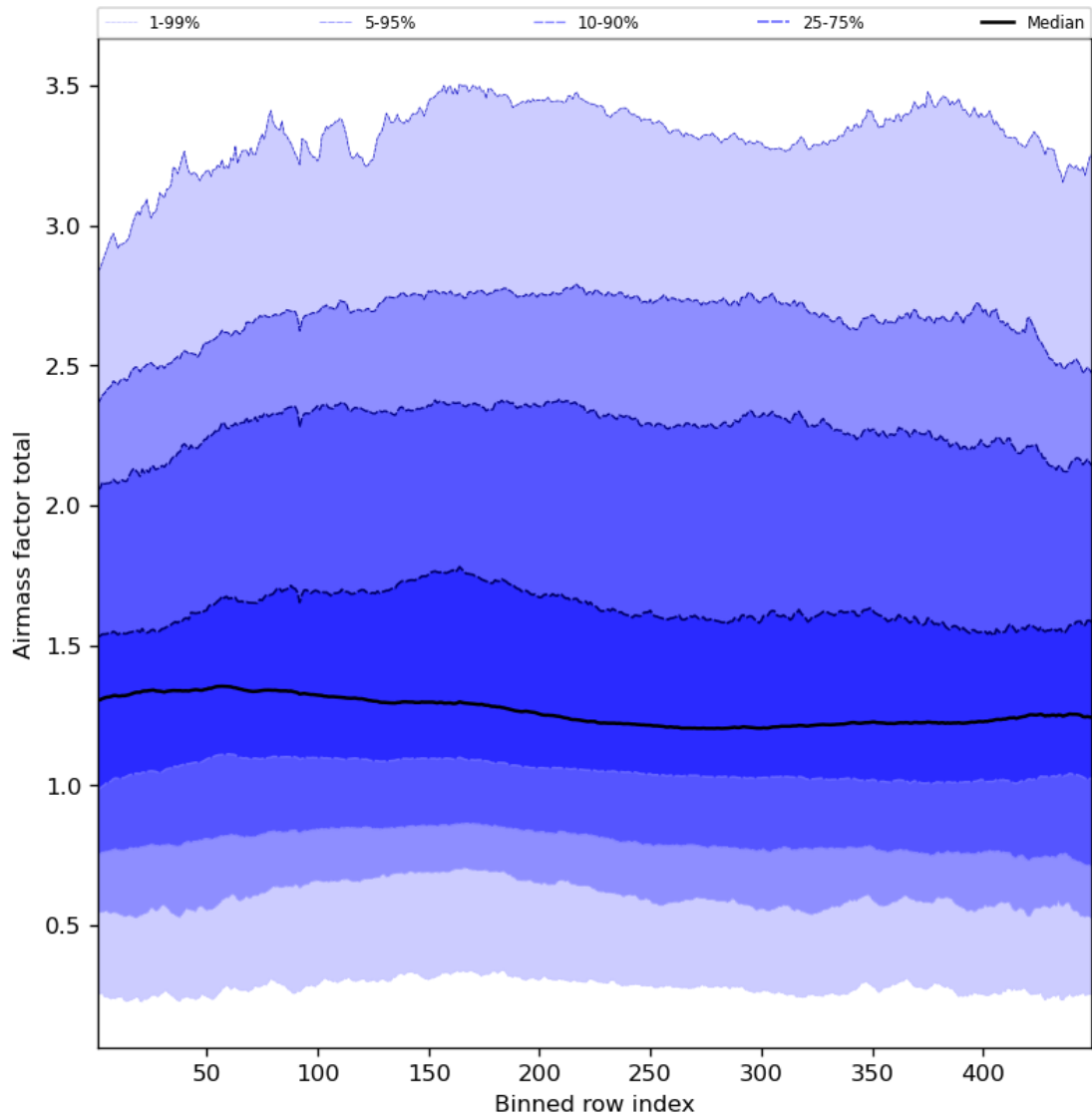
Figure 54: Along track statistics of “Airmass factor total” for 2023-08-05 to 2023-08-07
