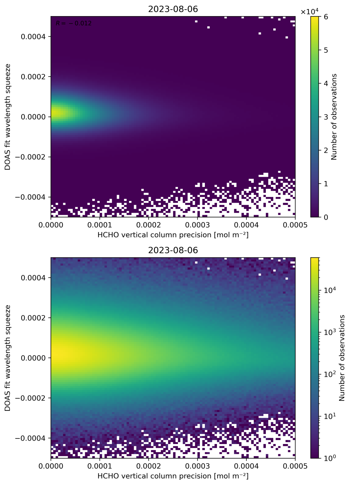
Figure 138: Scatter density plot of “HCHO vertical column precision” against “DOAS fit wavelength squeeze” for 2023-08-05 to 2023-08-07.
