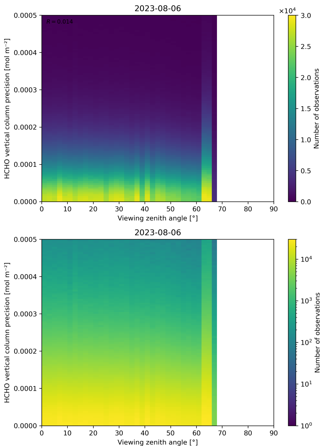
Figure 194: Scatter density plot of “Viewing zenith angle” against “HCHO vertical column precision” for 2023-08-05 to 2023-08-07.
