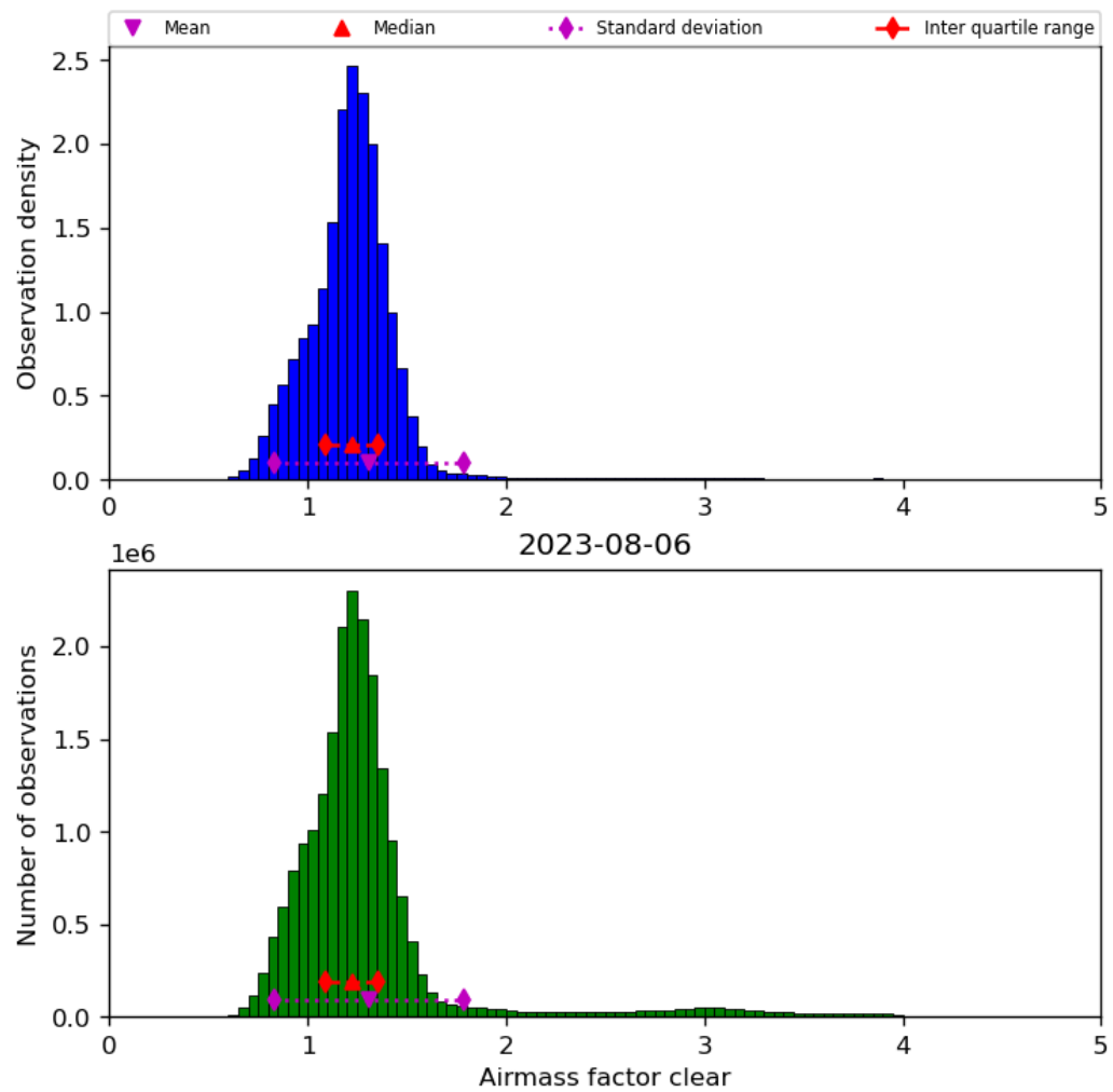
Figure 42: Histogram of “Airmass factor clear” for 2023-08-05 to 2023-08-07
