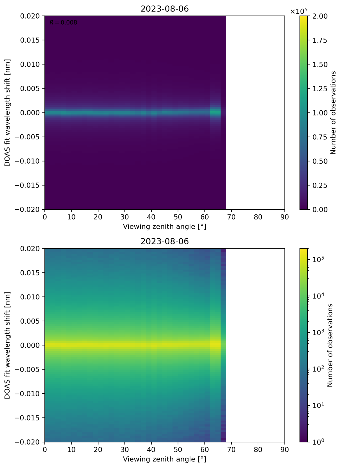
Figure 183: Scatter density plot of “Viewing zenith angle” against “DOAS fit wavelength shift” for 2023-08-05 to 2023-08-07.
