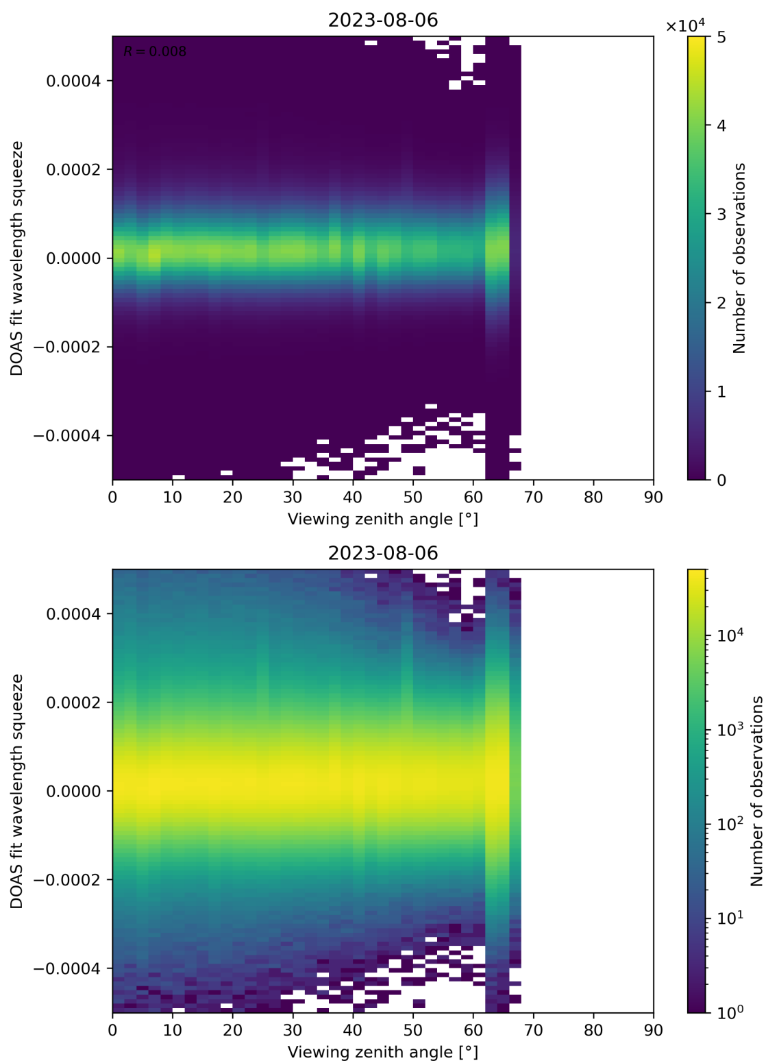
Figure 184: Scatter density plot of “Viewing zenith angle” against “DOAS fit wavelength squeeze” for 2023-08-05 to 2023-08-07.
