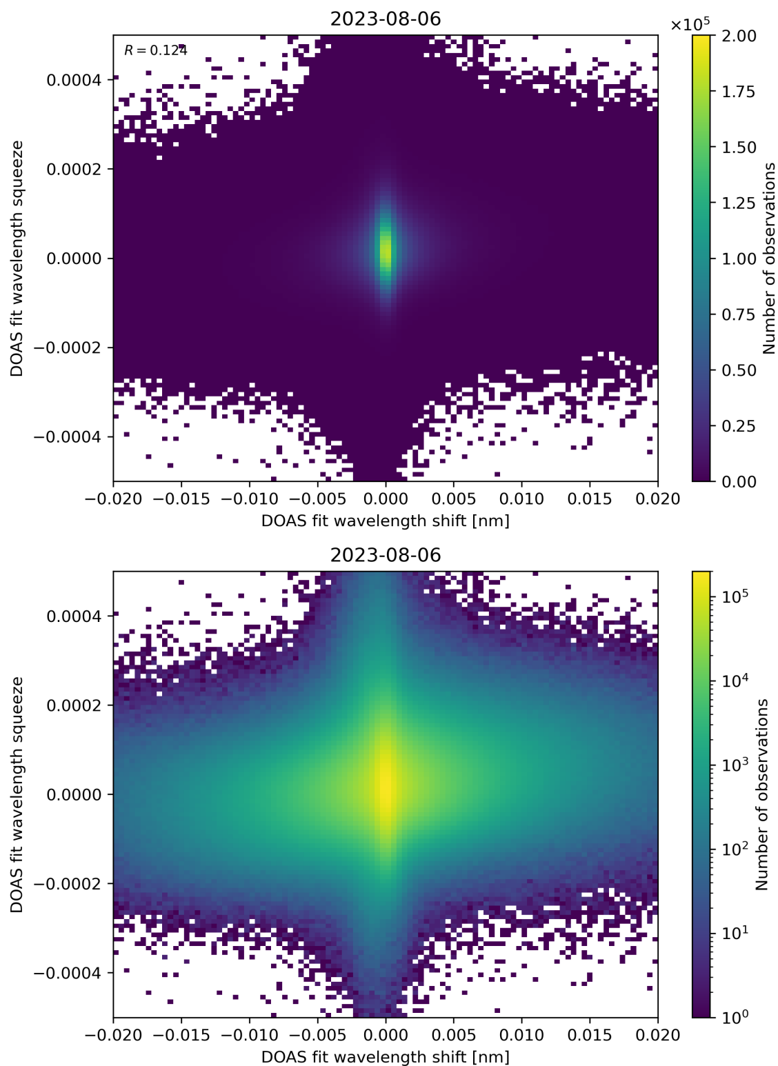
Figure 65: Scatter density plot of “DOAS fit wavelength shift” against “DOAS fit wavelength squeeze” for 2023-08-05 to 2023-08-07.
