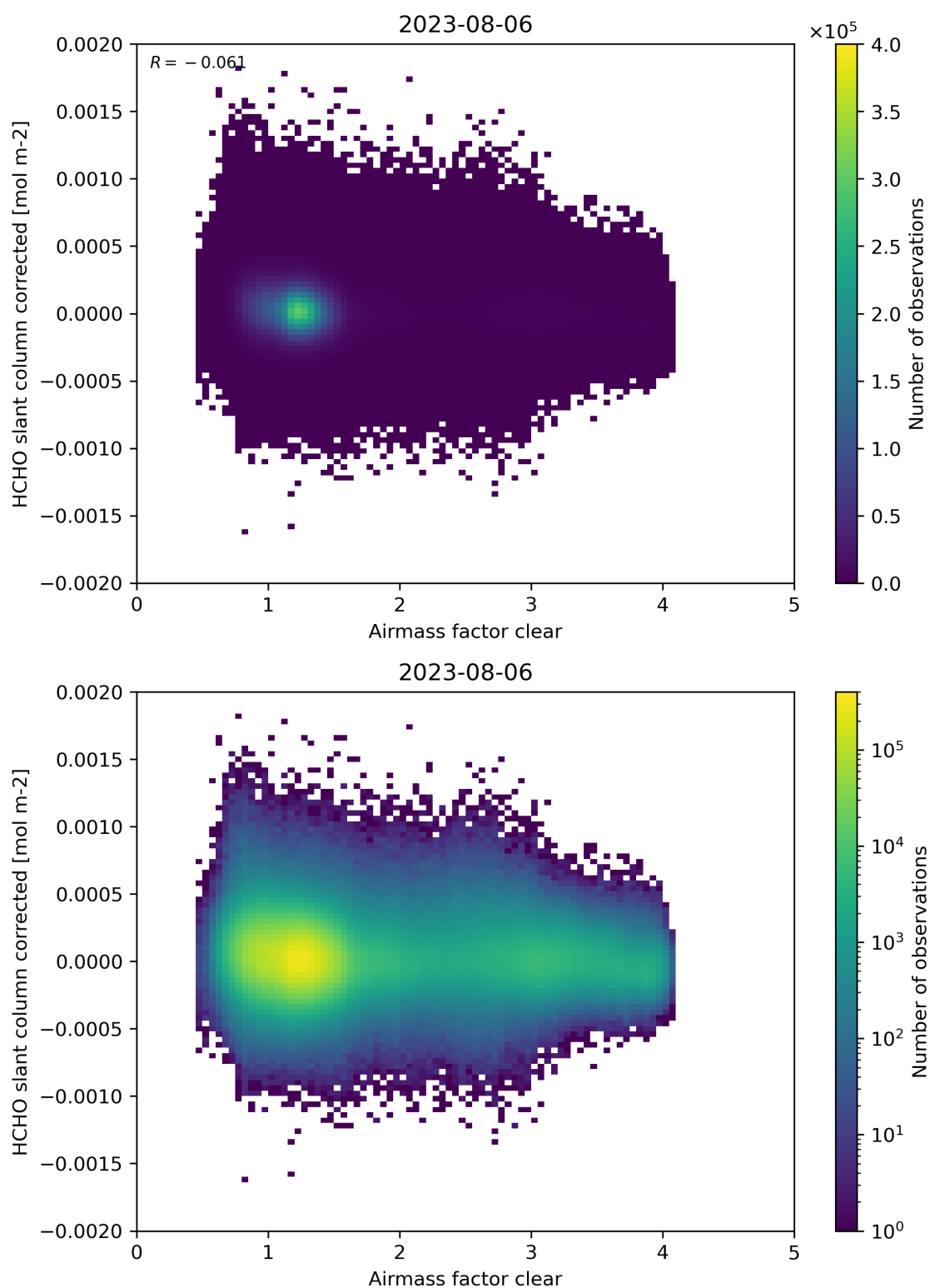
Figure 74: Scatter density plot of “Airmass factor clear” against “HCHO slant column corrected” for 2023-08-05 to 2023-08-07.
