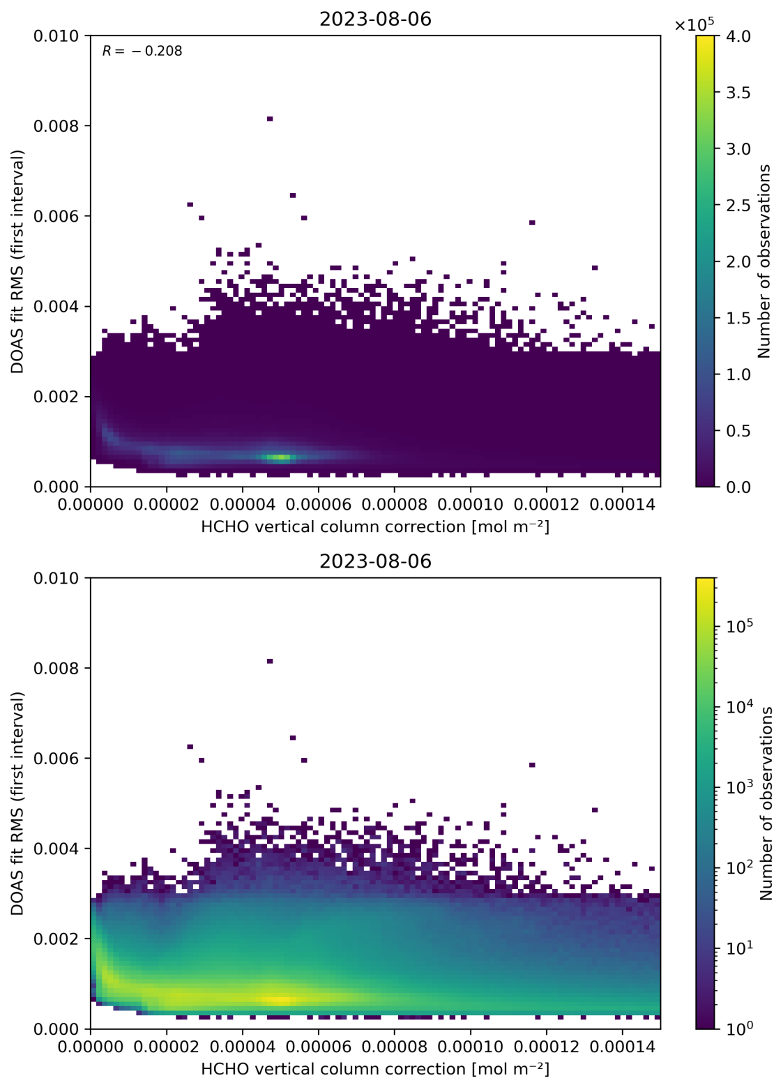
Figure 112: Scatter density plot of “HCHO vertical column correction” against “DOAS fit RMS (first interval)” for 2023-08-05 to 2023-08-07.
