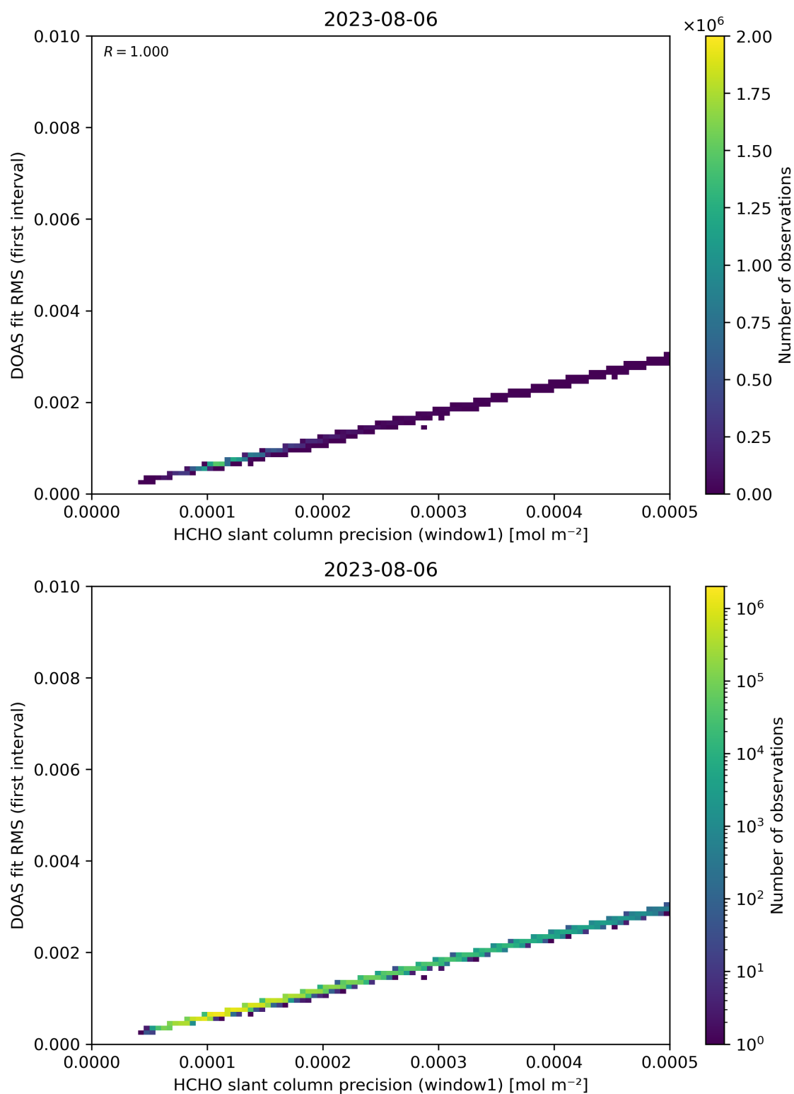
Figure 88: Scatter density plot of “HCHO slant column precision (window1)” against “DOAS fit RMS (first interval)” for 2023-08-05 to 2023-08-07.
