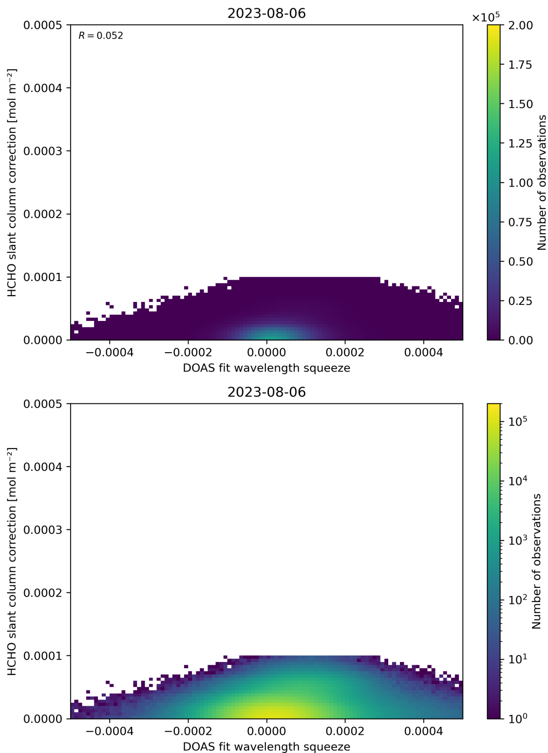
Figure 70: Scatter density plot of “DOAS fit wavelength squeeze” against “HCHO slant column correction” for 2023-08-05 to 2023-08-07.
