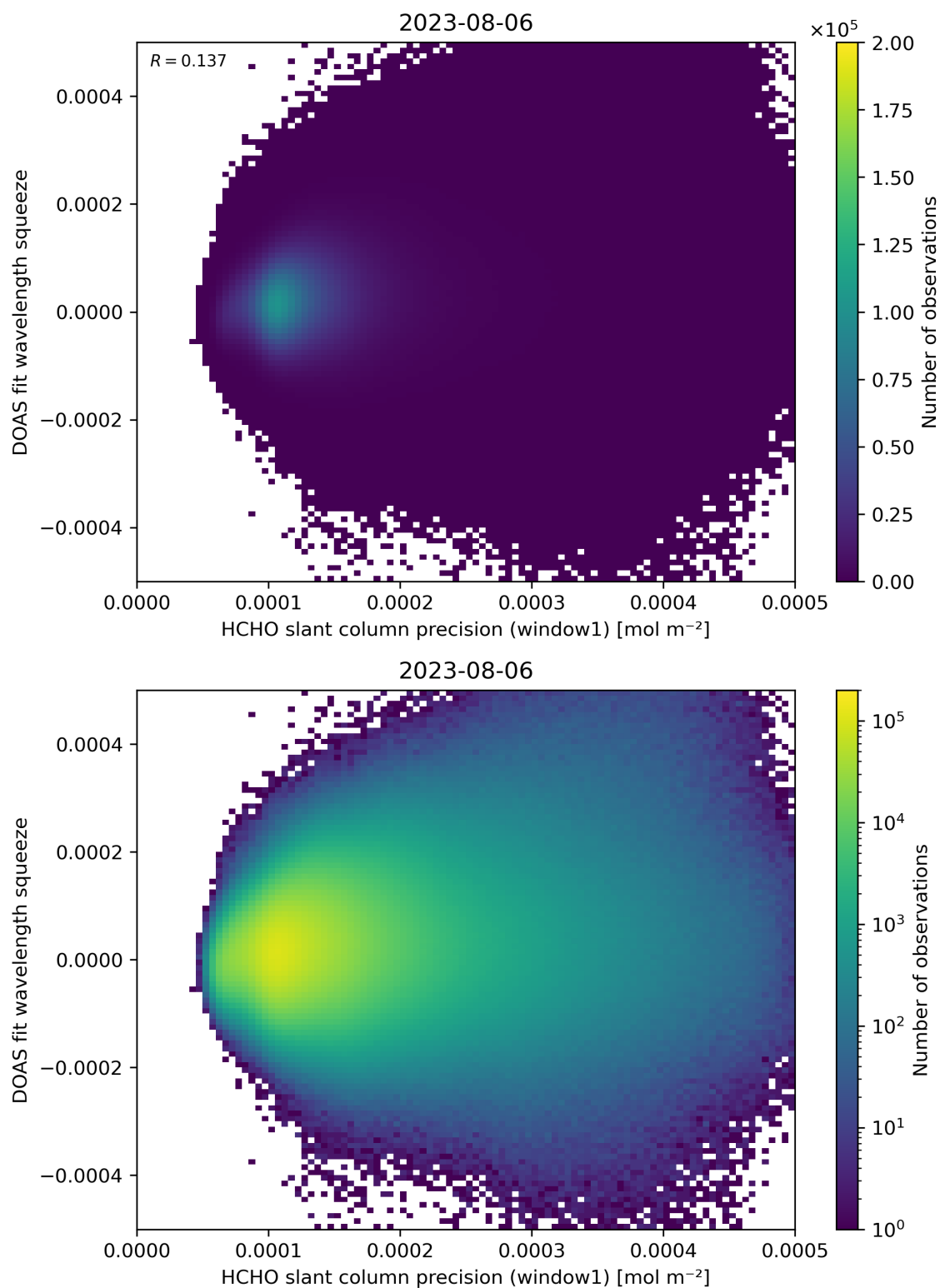
Figure 90: Scatter density plot of “HCHO slant column precision (window1)” against “DOAS fit wavelength squeeze” for 2023-08-05 to 2023-08-07.
