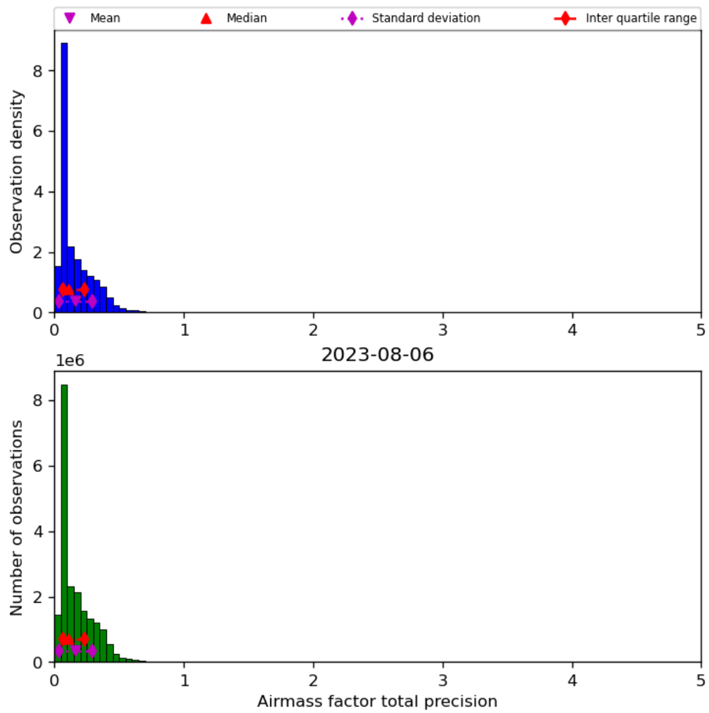
Figure 41: Histogram of "Airmass factor total precision" for 2023-08-05 to 2023-08-07
