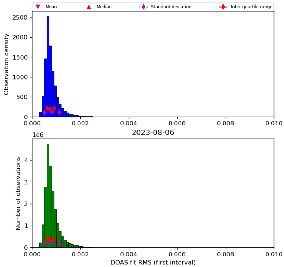
Figure 46: Histogram of “DOAS fit RMS (first interval)” for 2023-08-05 to 2023-08-07
