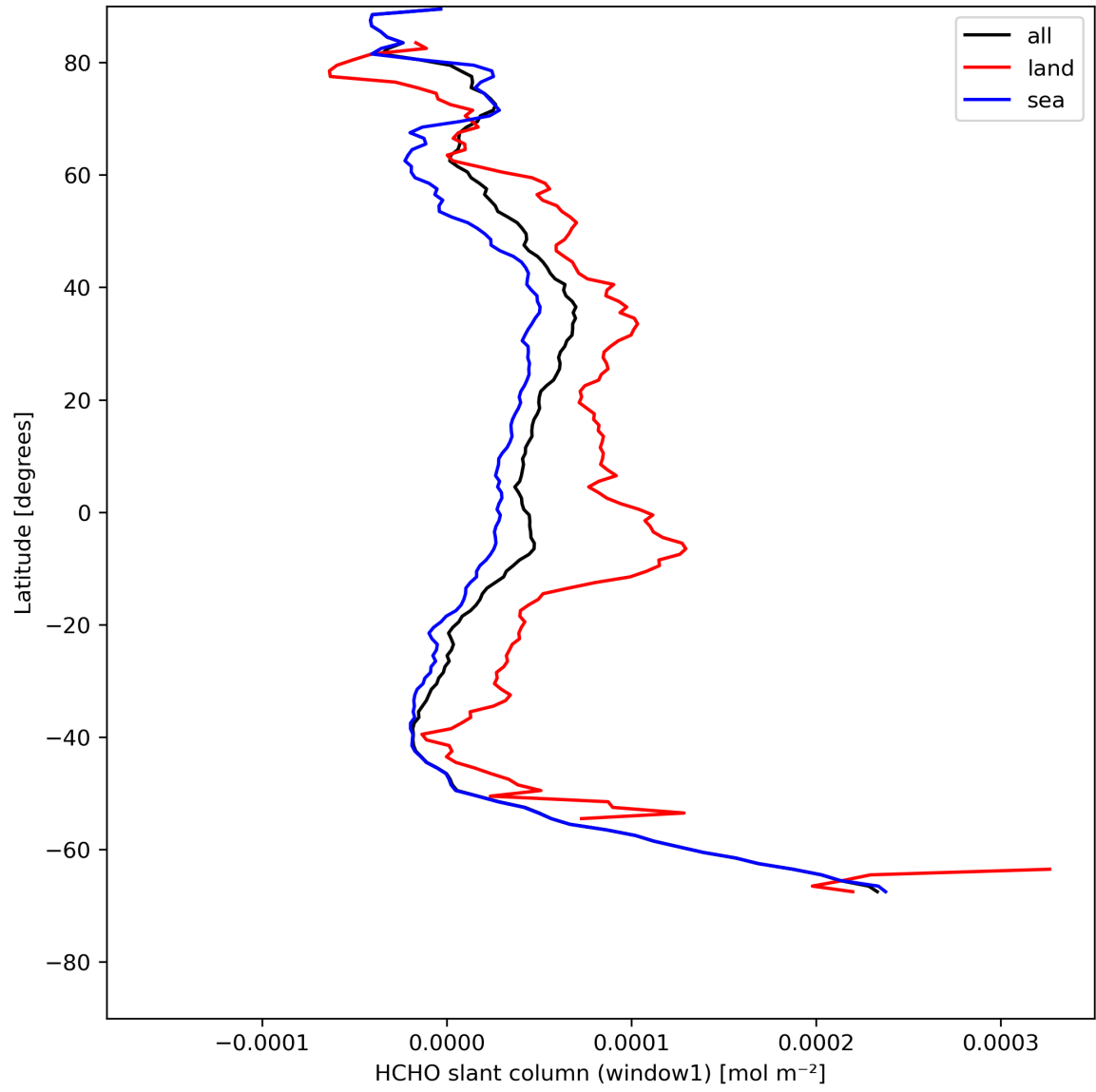
Figure 24: Zonal average of “HCHO slant column (window1)” for 2023-08-05 to 2023-08-07.
