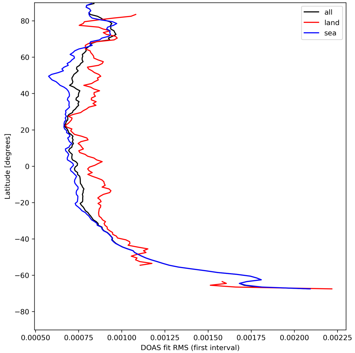
Figure 32: Zonal average of "DOAS fit RMS (first interval)" for 2023-08-05 to 2023-08-07.
