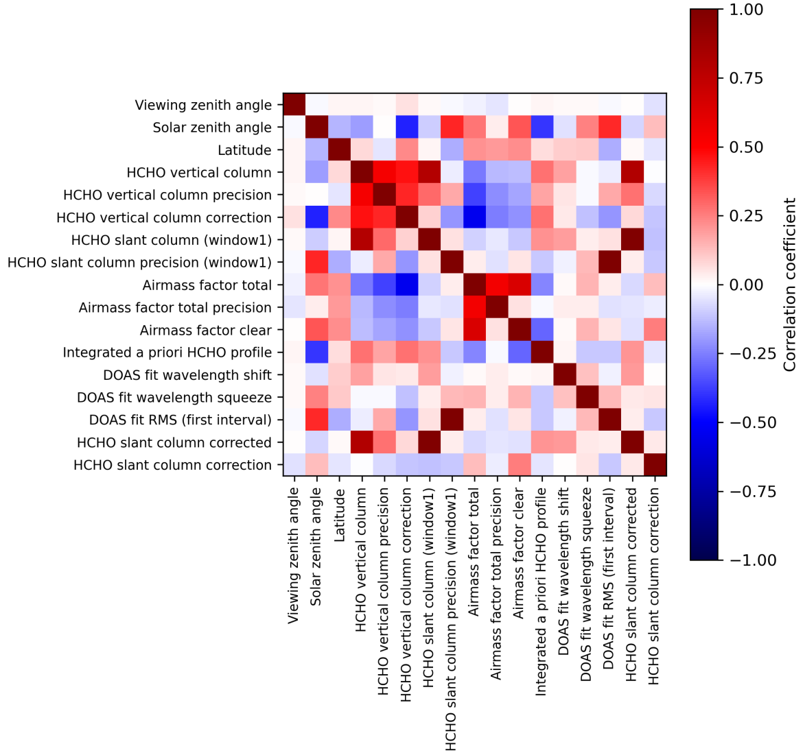
Figure 2: Map of correlation matrix for 2023-08-05 to 2023-08-07.
