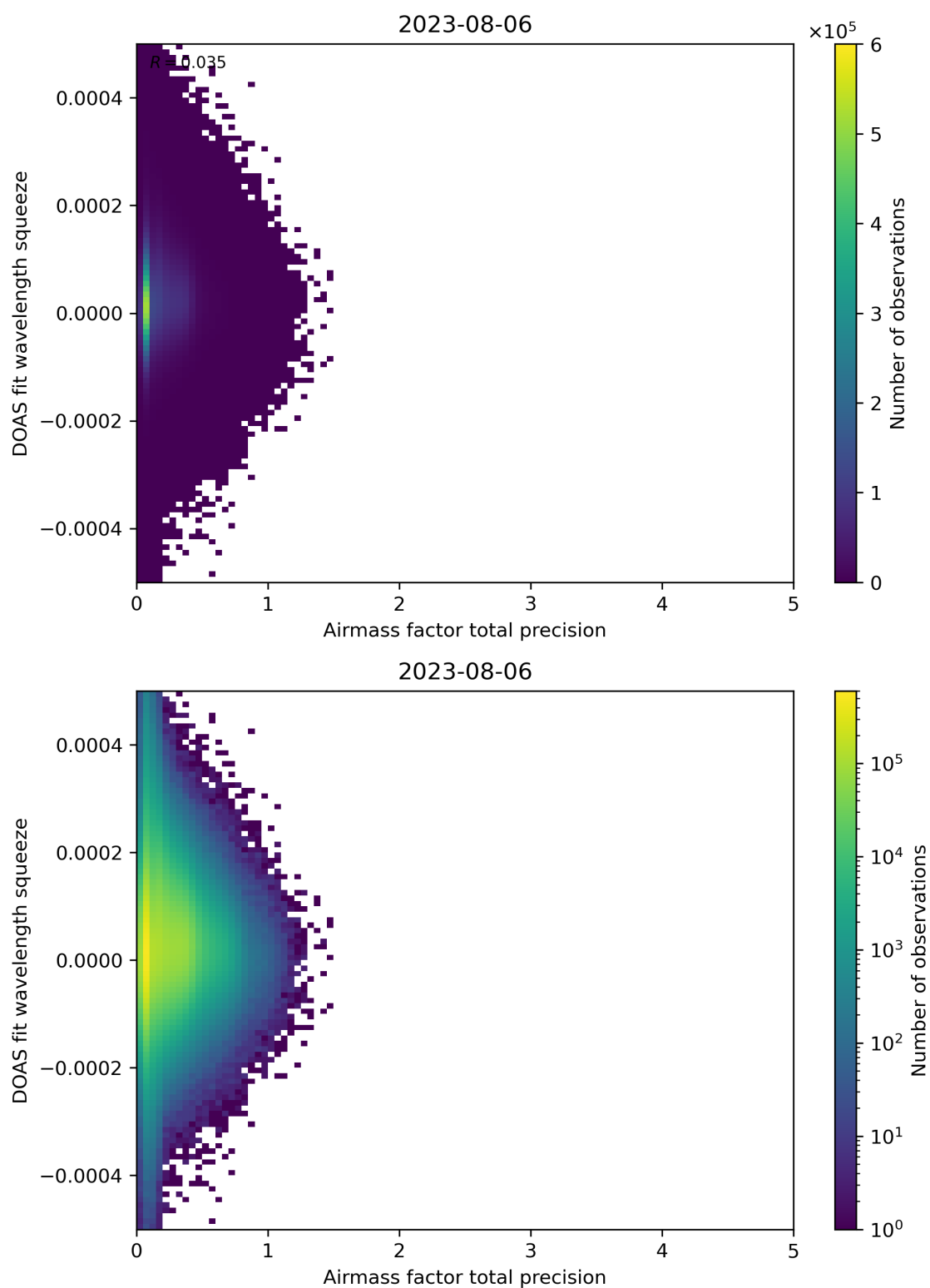
Figure 107: Scatter density plot of “Airmass factor total precision” against “DOAS fit wavelength squeeze” for 2023-08-05 to 2023-08-07.
