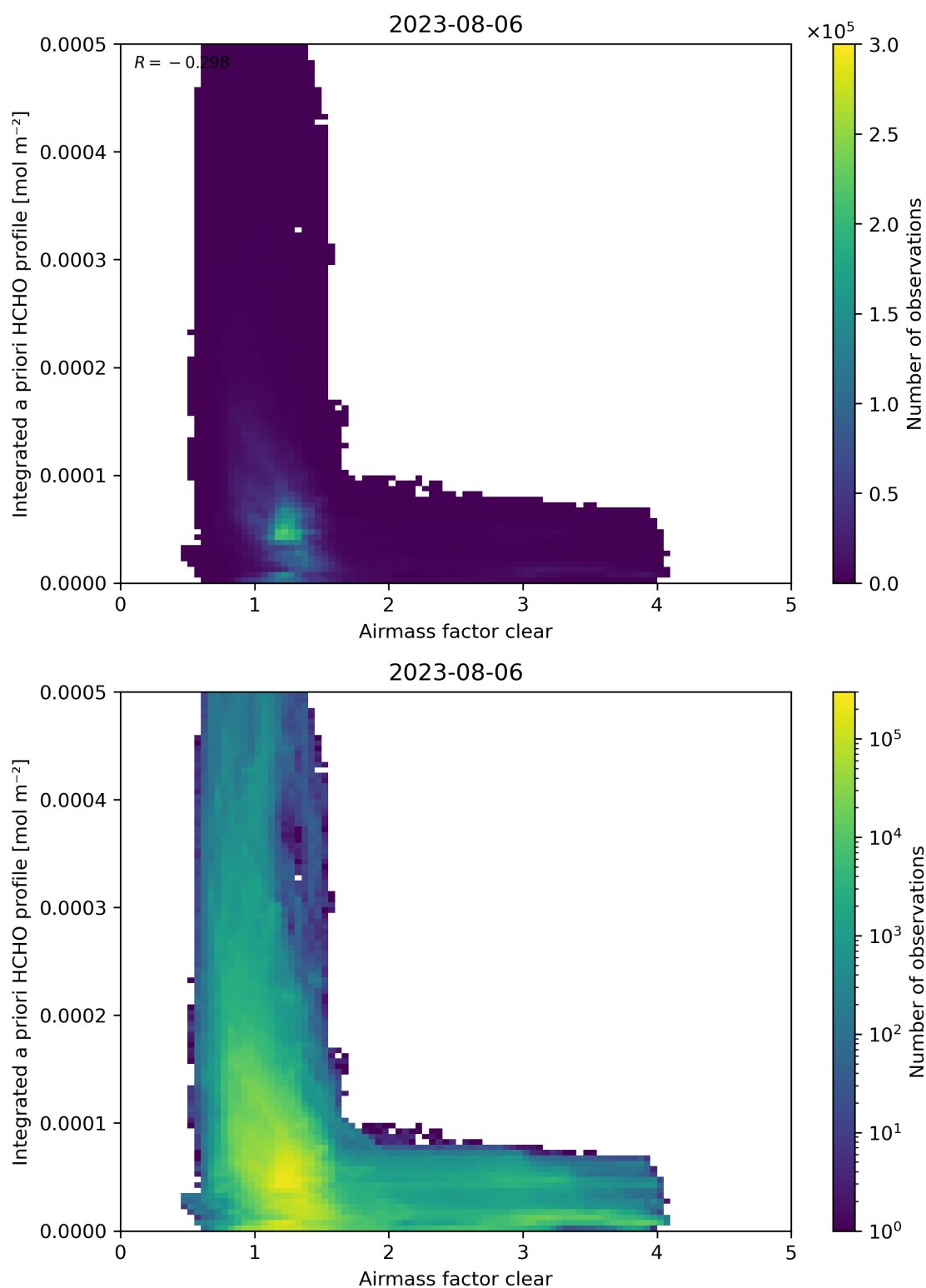
Figure 76: Scatter density plot of “Airmass factor clear” against “Integrated a priori HCHO profile” for 2023-08-05 to 2023-08-07.
