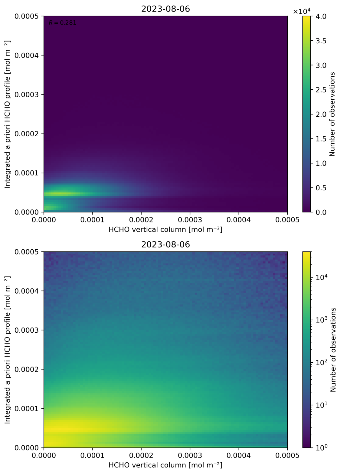
Figure 135: Scatter density plot of “HCHO vertical column” against “Integrated a priori HCHO profile” for 2023-08-05 to 2023-08-07.
