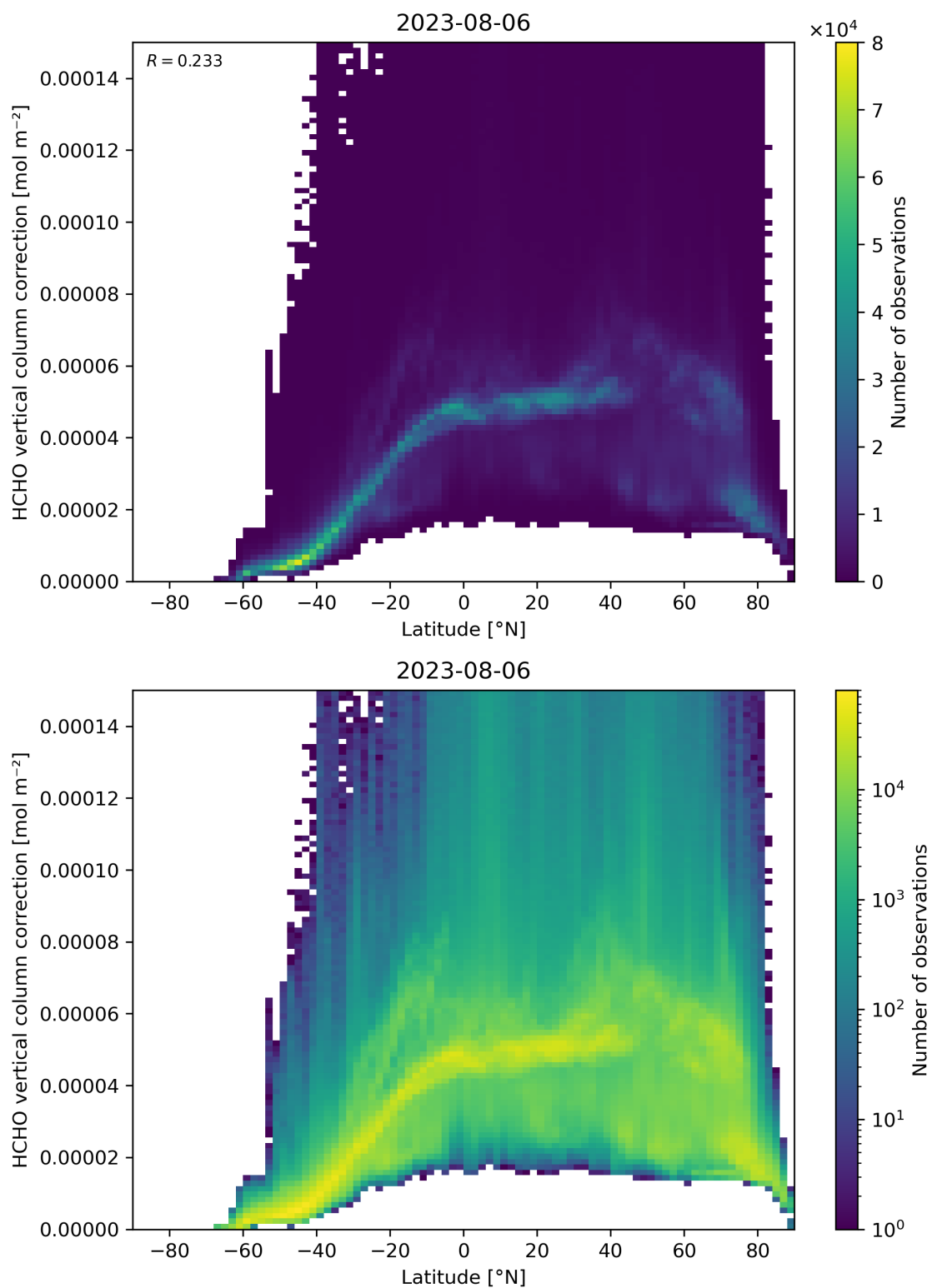
Figure 164: Scatter density plot of “Latitude” against “HCHO vertical column correction” for 2023-08-05 to 2023-08-07.
