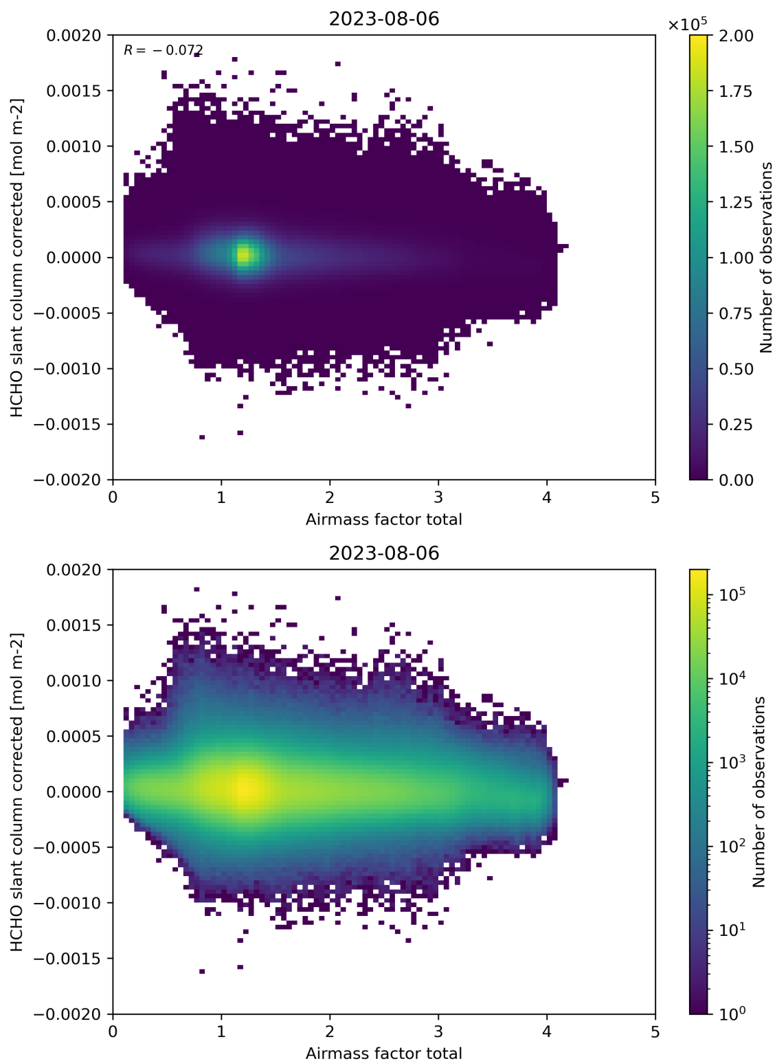
Figure 101: Scatter density plot of “Airmass factor total” against “HCHO slant column corrected” for 2023-08-05 to 2023-08-07.
