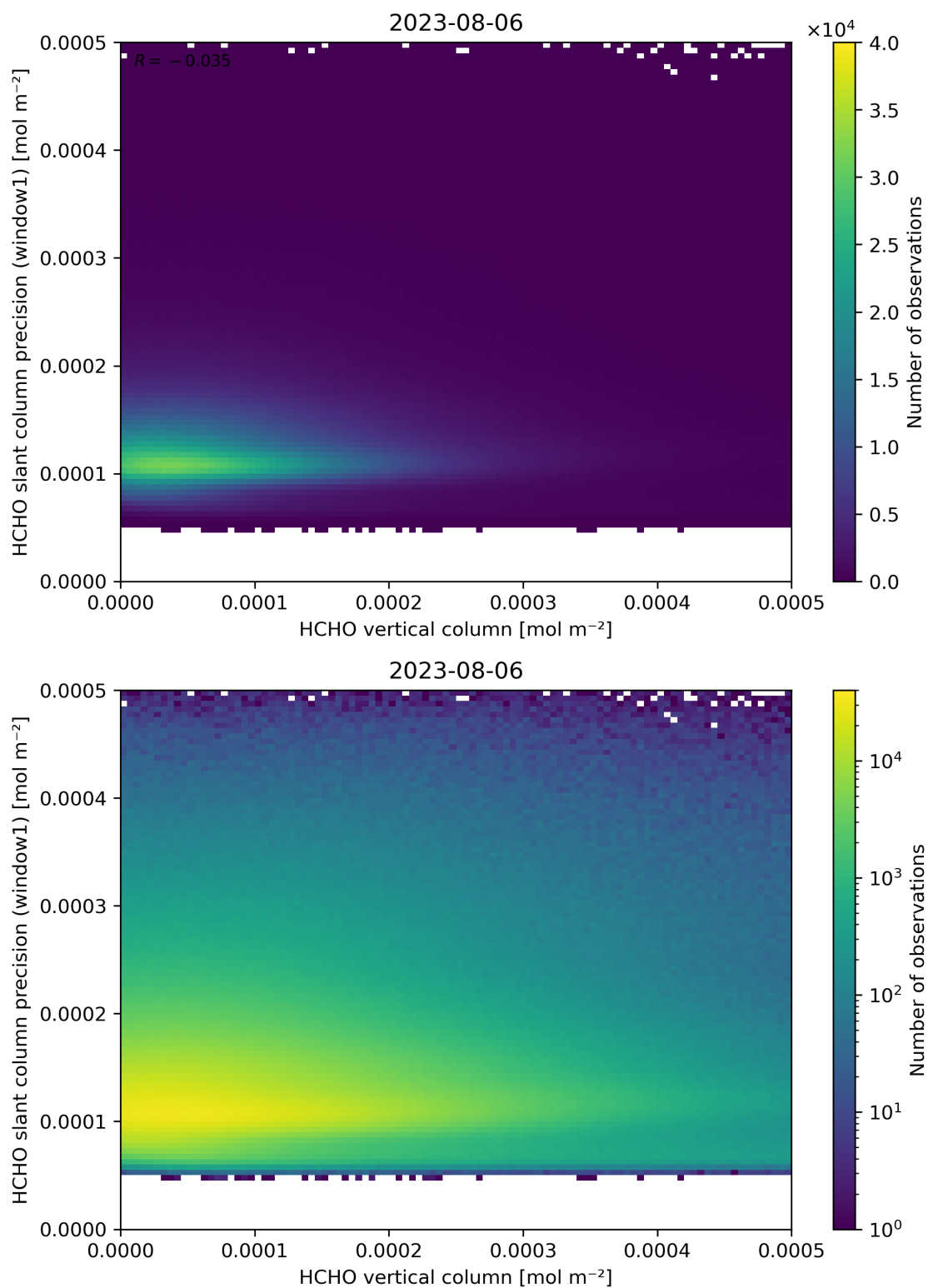
Figure 130: Scatter density plot of “HCHO vertical column” against “HCHO slant column precision (window1)” for 2023-08-05 to 2023-08-07.
