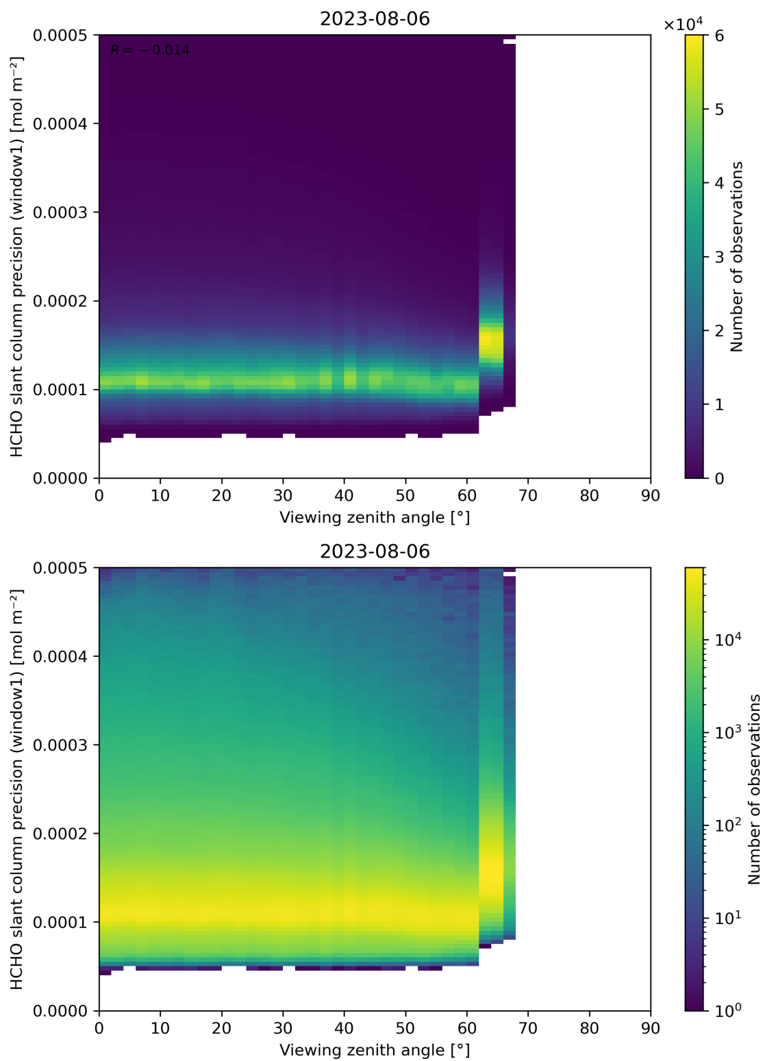
Figure 189: Scatter density plot of “Viewing zenith angle” against “HCHO slant column precision (window1)” for 2023-08-05 to 2023-08-07.
