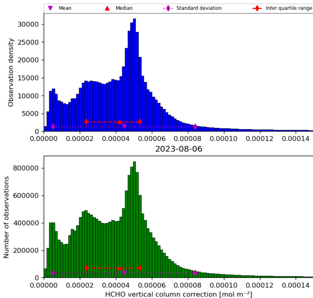
Figure 37: Histogram of “HCHO vertical column correction” for 2023-08-05 to 2023-08-07
