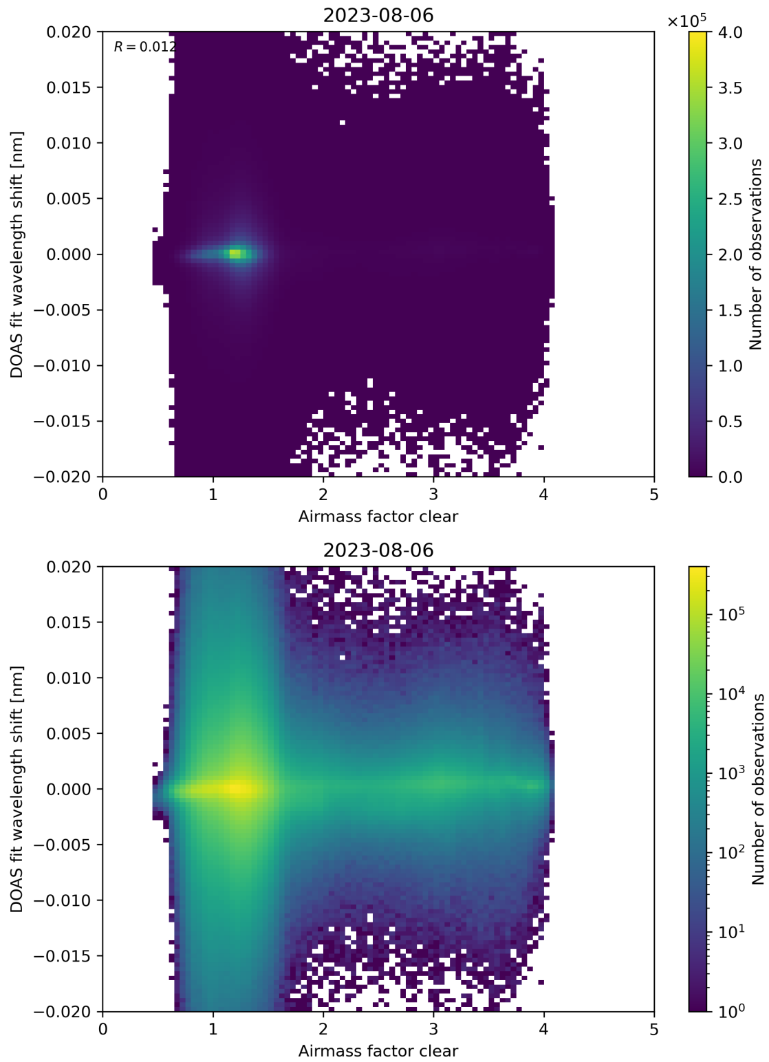
Figure 72: Scatter density plot of “Airmass factor clear” against “DOAS fit wavelength shift” for 2023-08-05 to 2023-08-07.
