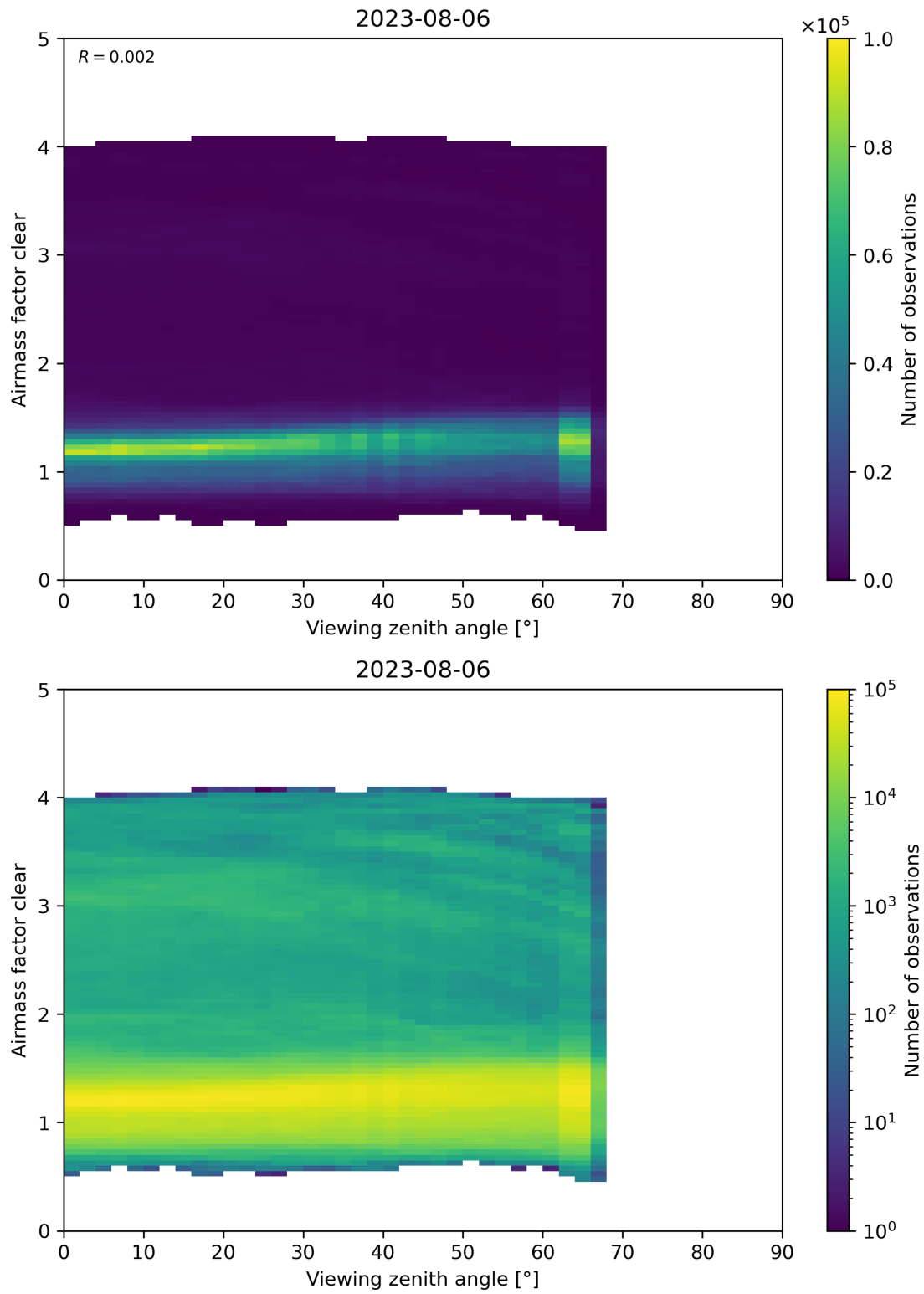
Figure 185: Scatter density plot of “Viewing zenith angle” against “Airmass factor clear” for 2023-08-05 to 2023-08-07.
