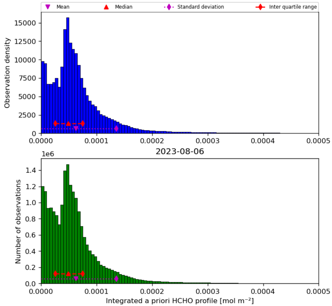
Figure 43: Histogram of “Integrated a priori HCHO profile” for 2023-08-05 to 2023-08-07
