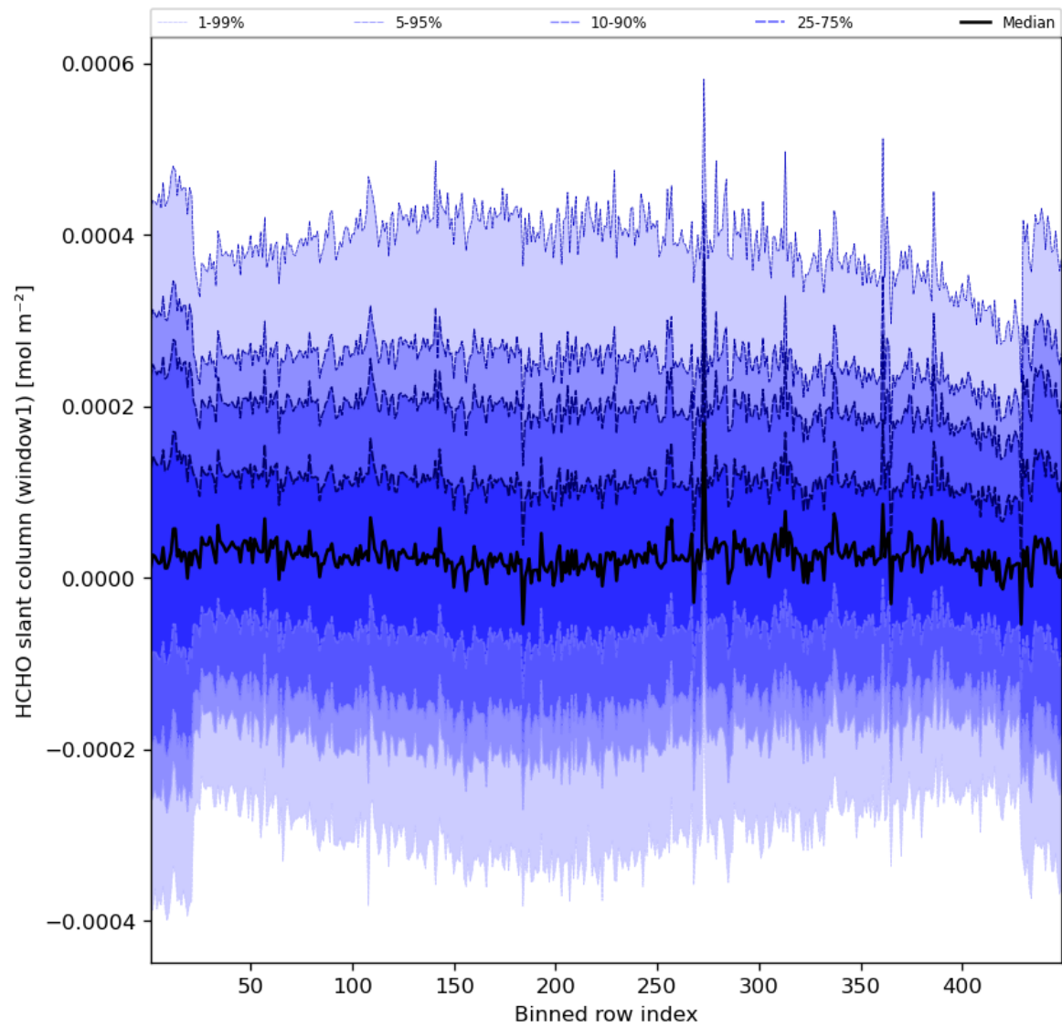
Figure 52: Along track statistics of “HCHO slant column (window1)” for 2023-08-05 to 2023-08-07
