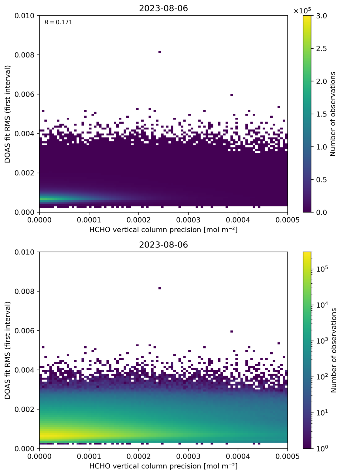
Figure 136: Scatter density plot of “HCHO vertical column precision” against “DOAS fit RMS (first interval)” for 2023-08-05 to 2023-08-07.
