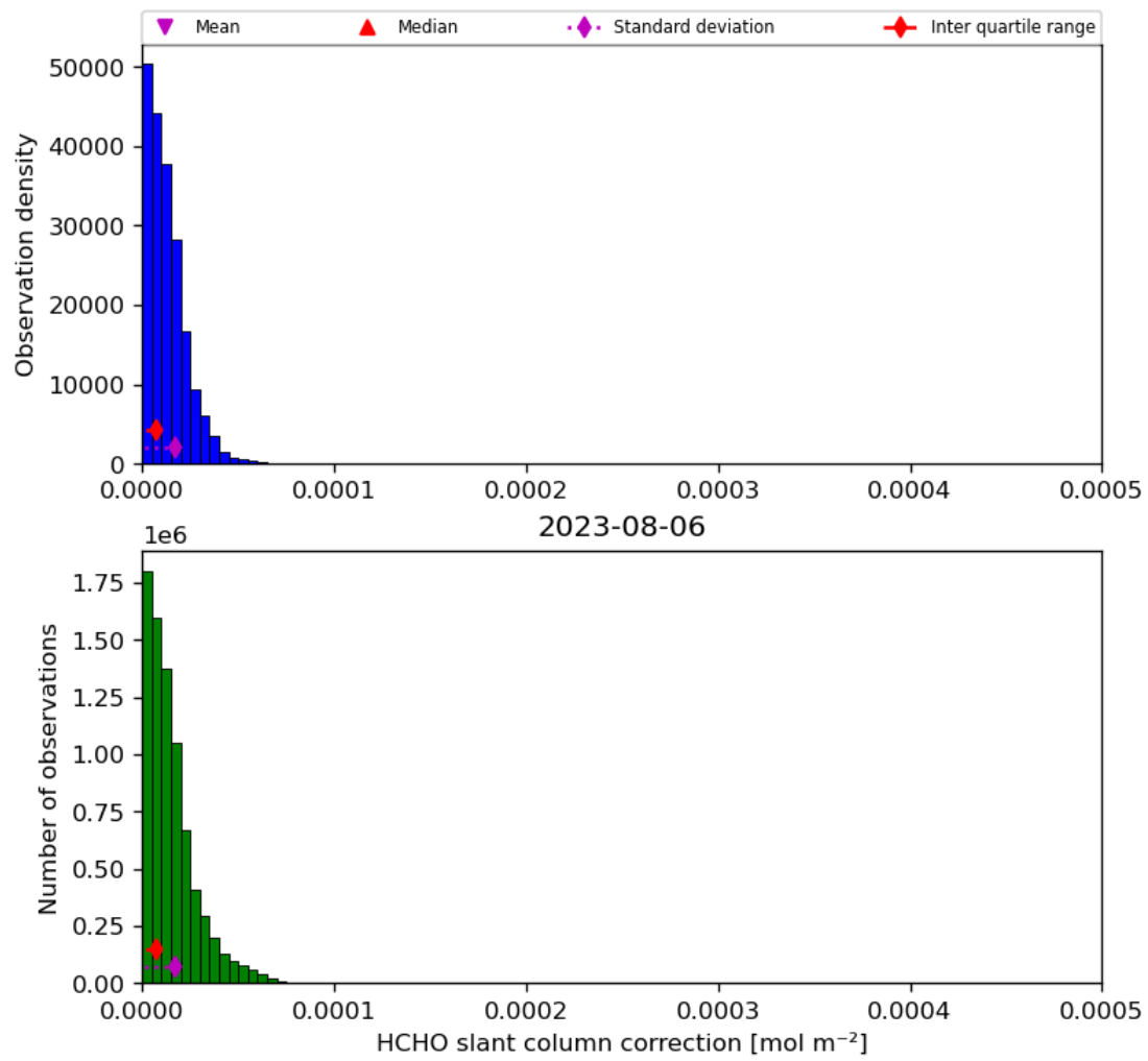
Figure 47: Histogram of “HCHO slant column correction” for 2023-08-05 to 2023-08-07
