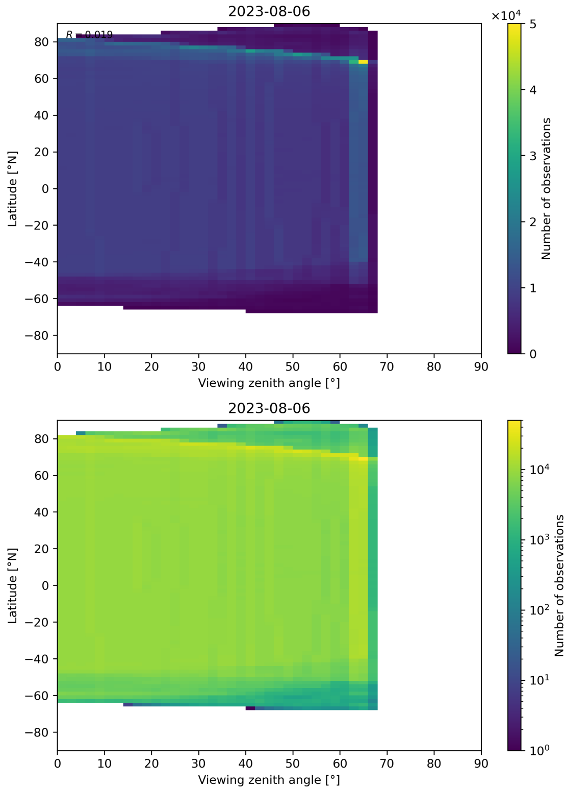
Figure 196: Scatter density plot of “Viewing zenith angle” against “Latitude” for 2023-08-05 to 2023-08-07.
