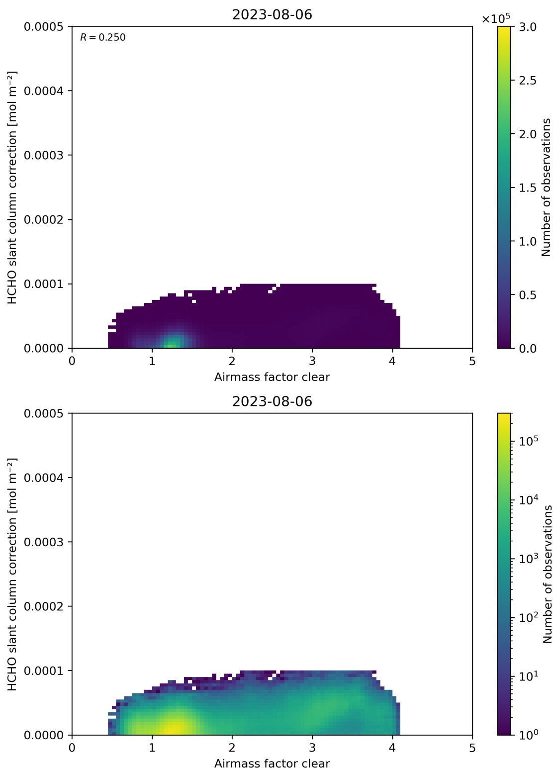
Figure 75: Scatter density plot of “Airmass factor clear” against “HCHO slant column correction” for 2023-08-05 to 2023-08-07.
