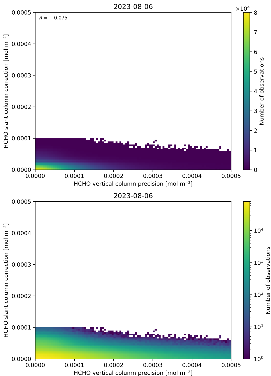
Figure 141: Scatter density plot of “HCHO vertical column precision” against “HCHO slant column correction” for 2023-08-05 to 2023-08-07.
