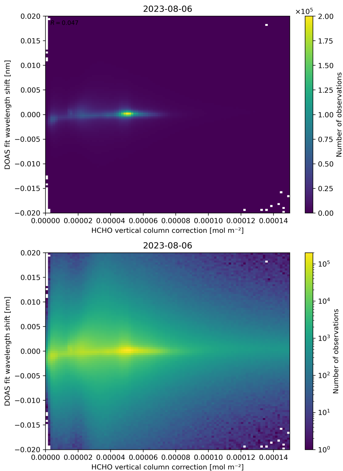
Figure 113: Scatter density plot of “HCHO vertical column correction” against “DOAS fit wavelength shift” for 2023-08-05 to 2023-08-07.
