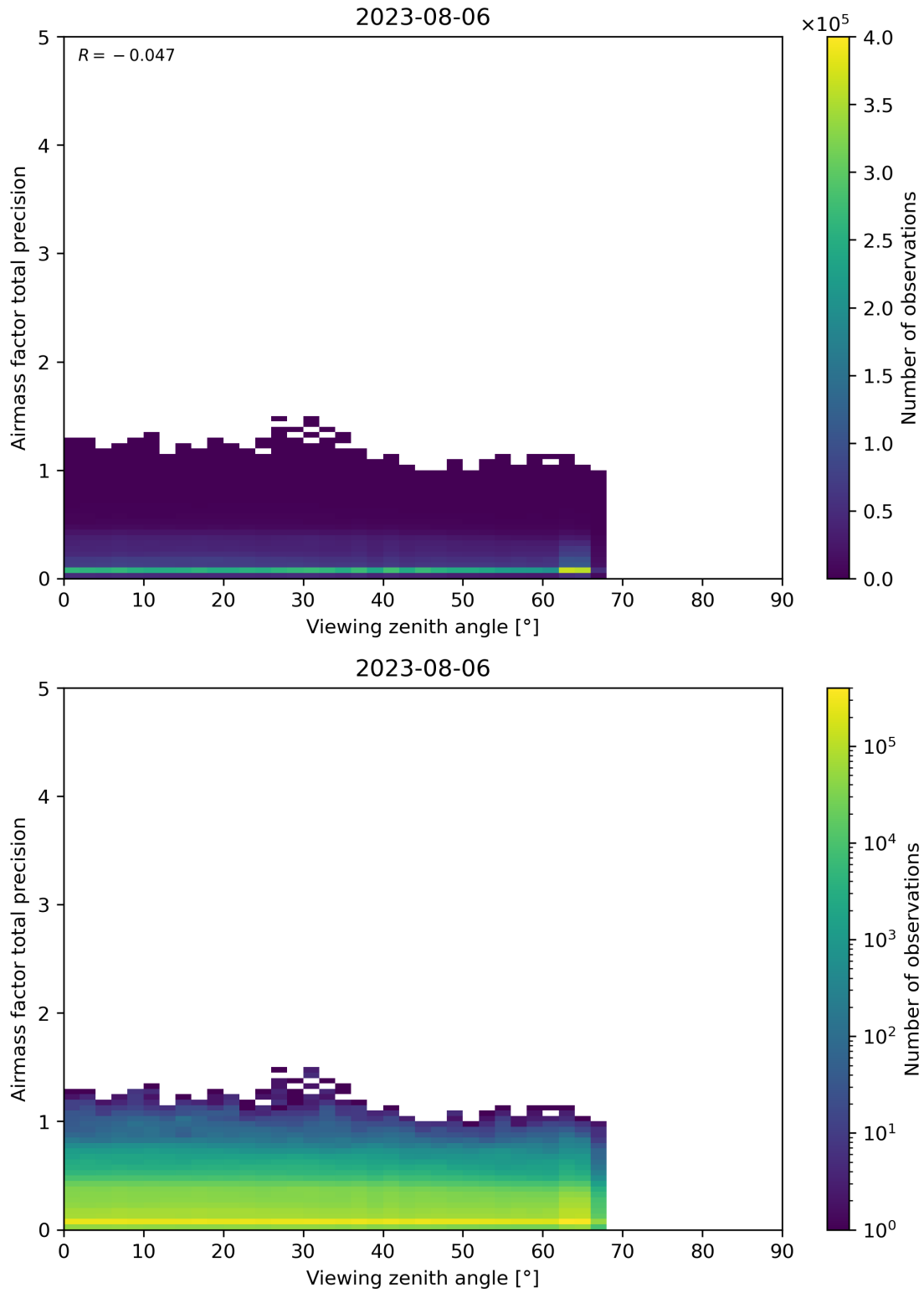
Figure 191: Scatter density plot of “Viewing zenith angle” against “Airmass factor total precision” for 2023-08-05 to 2023-08-07.
