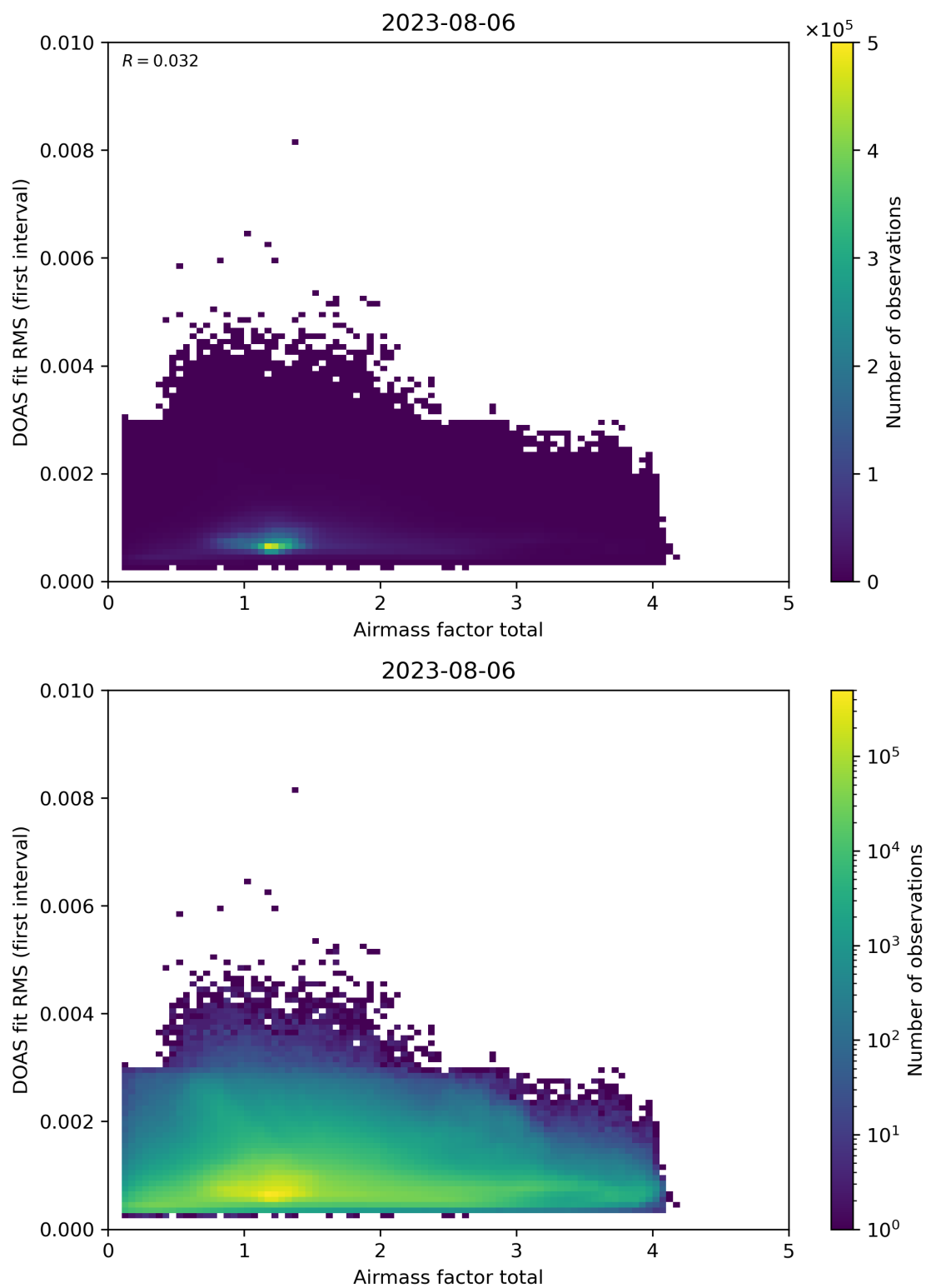
Figure 97: Scatter density plot of “Airmass factor total” against “DOAS fit RMS (first interval)” for 2023-08-05 to 2023-08-07.
