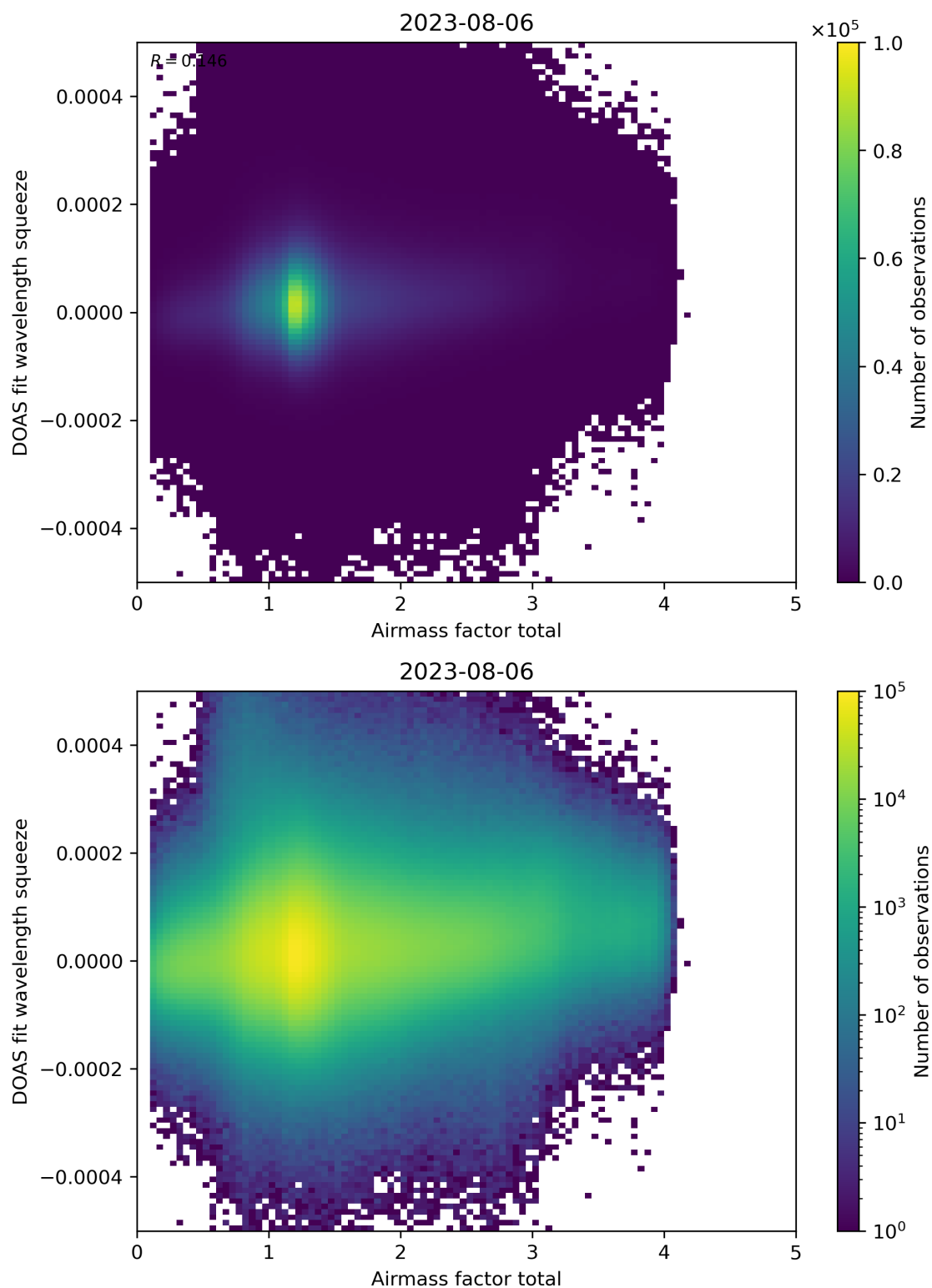
Figure 99: Scatter density plot of “Airmass factor total” against “DOAS fit wavelength squeeze” for 2023-08-05 to 2023-08-07.
