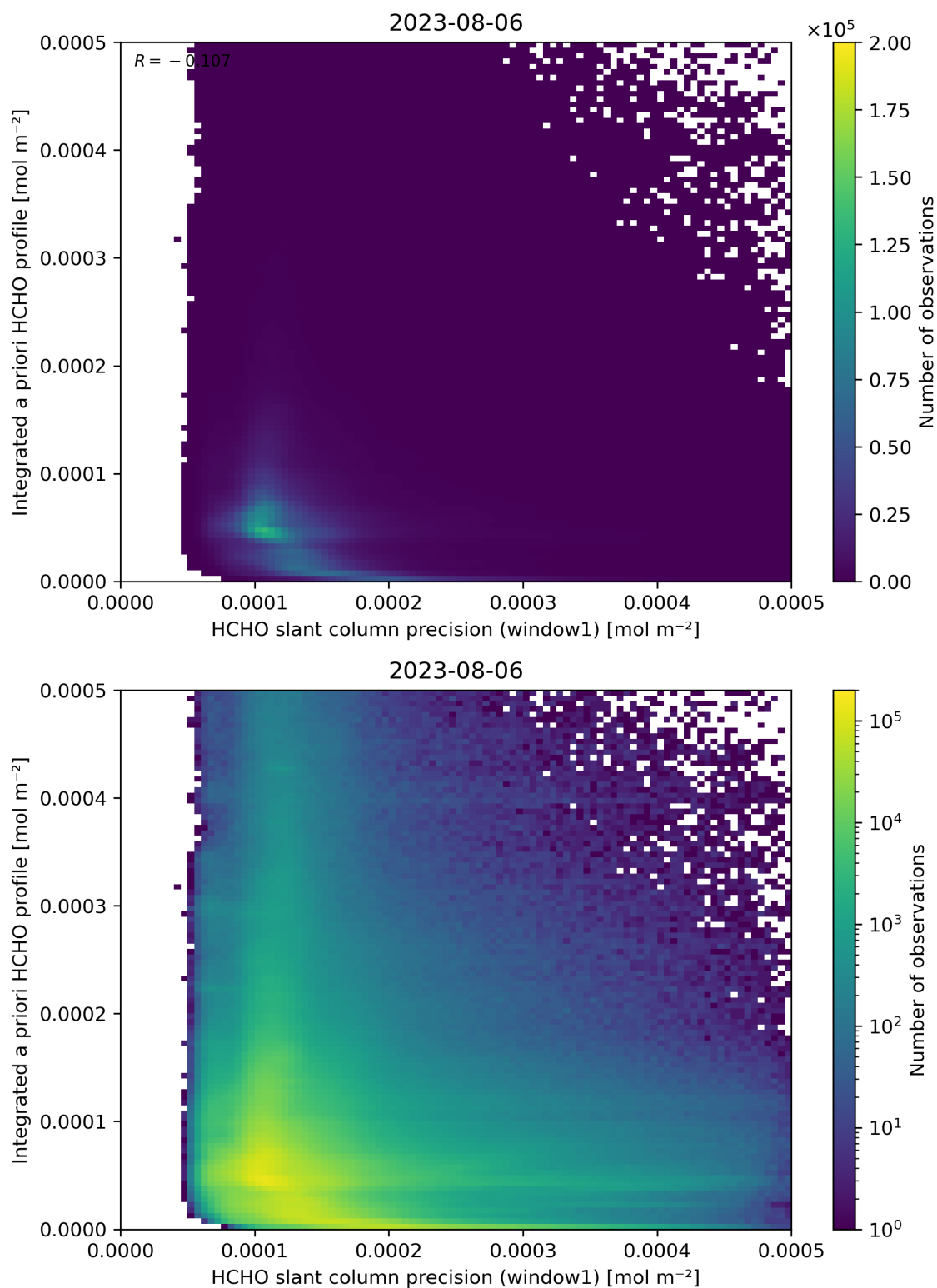
Figure 96: Scatter density plot of “HCHO slant column precision (window1)” against “Integrated a priori HCHO profile” for 2023-08-05 to 2023-08-07.
