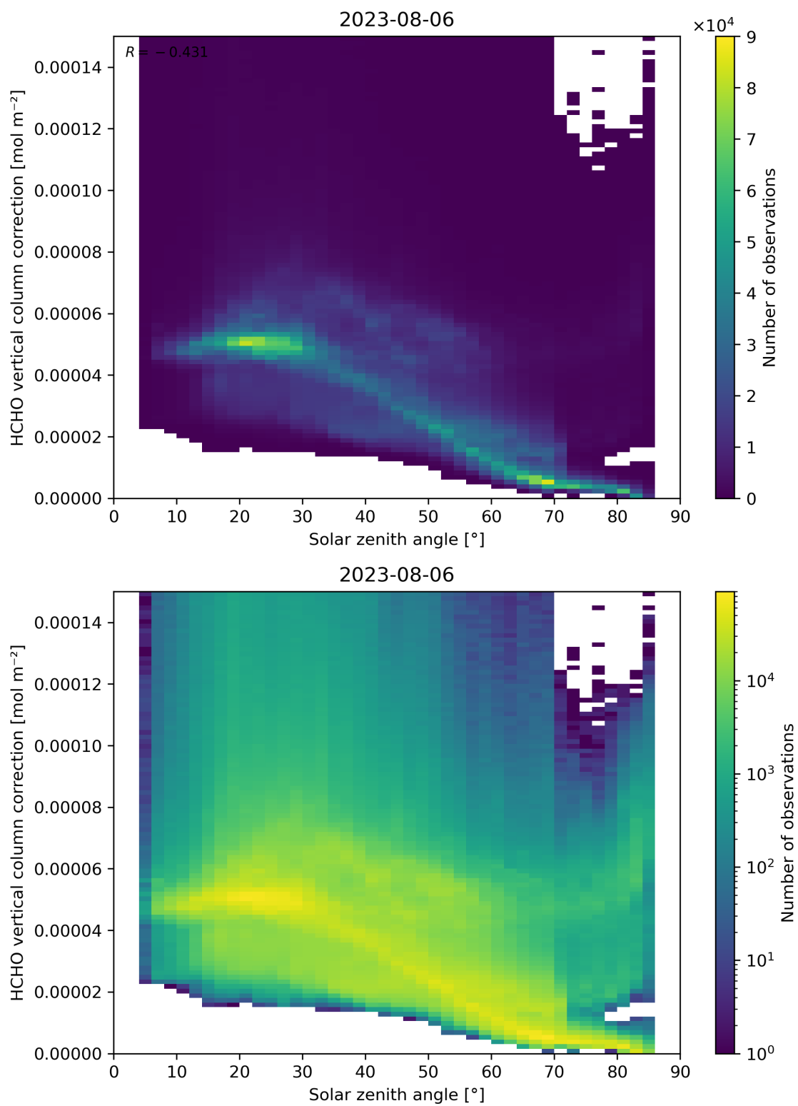
Figure 178: Scatter density plot of “Solar zenith angle” against “HCHO vertical column correction” for 2023-08-05 to 2023-08-07.
