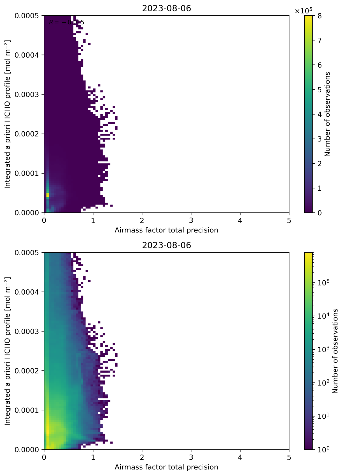
Figure 111: Scatter density plot of “Airmass factor total precision” against “Integrated a priori HCHO profile” for 2023-08-05 to 2023-08-07.
