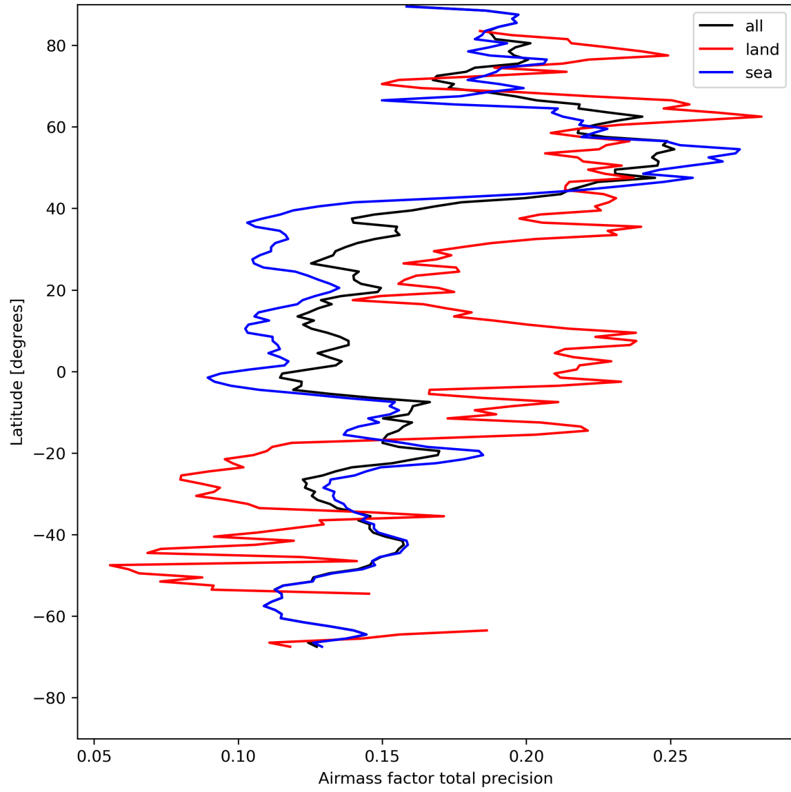
Figure 27: Zonal average of “Airmass factor total precision” for 2023-08-05 to 2023-08-07.
