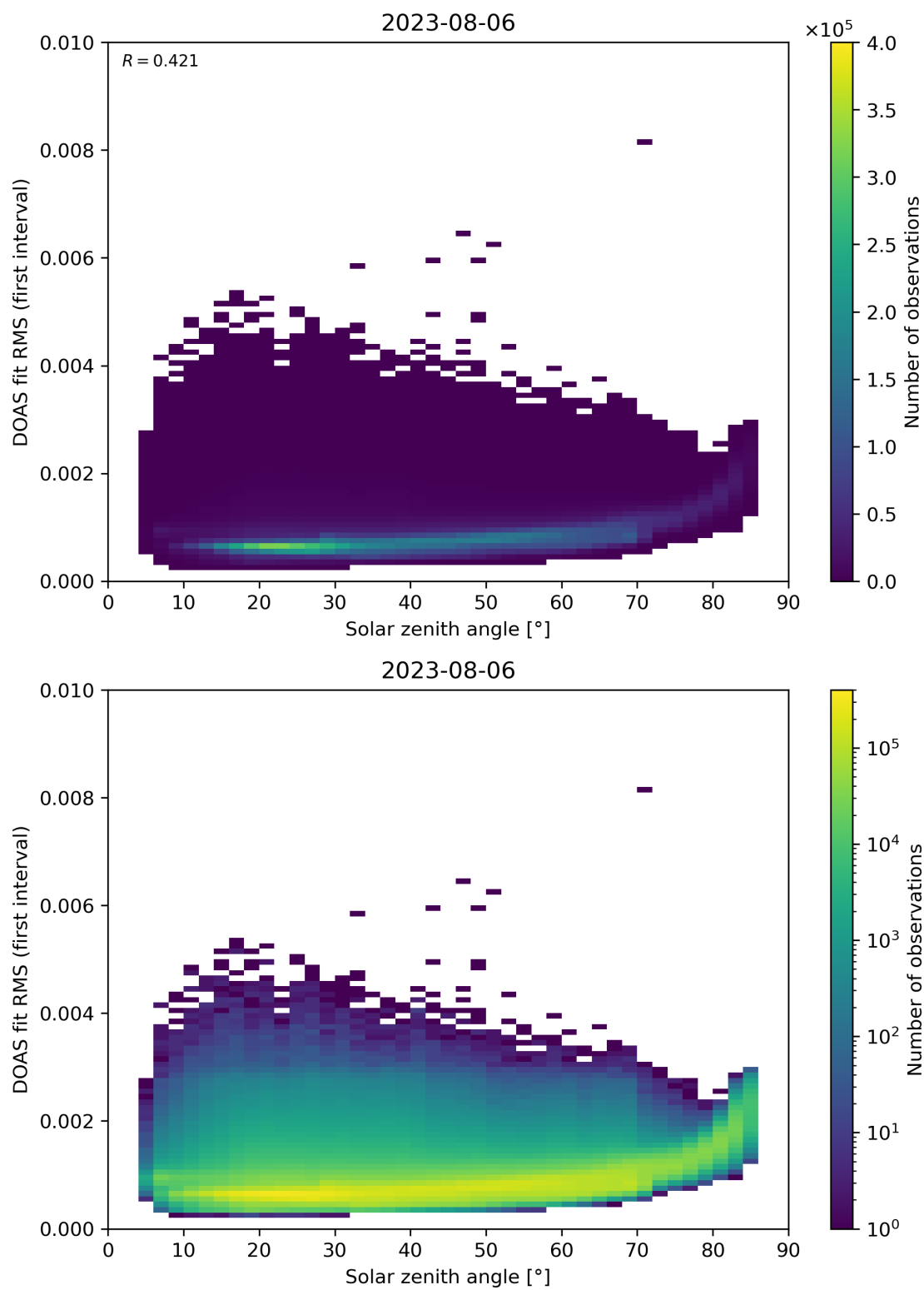
Figure 167: Scatter density plot of “Solar zenith angle” against “DOAS fit RMS (first interval)” for 2023-08-05 to 2023-08-07.
