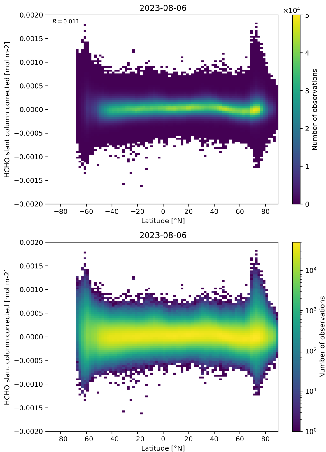
Figure 157: Scatter density plot of “Latitude” against “HCHO slant column corrected” for 2023-08-05 to 2023-08-07.
