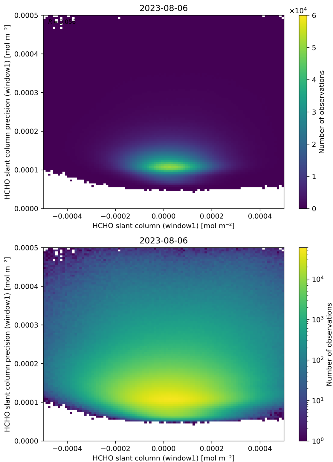
Figure 84: Scatter density plot of “HCHO slant column (window1)” against “HCHO slant column precision (window1)” for 2023-08-05 to 2023-08-07.
