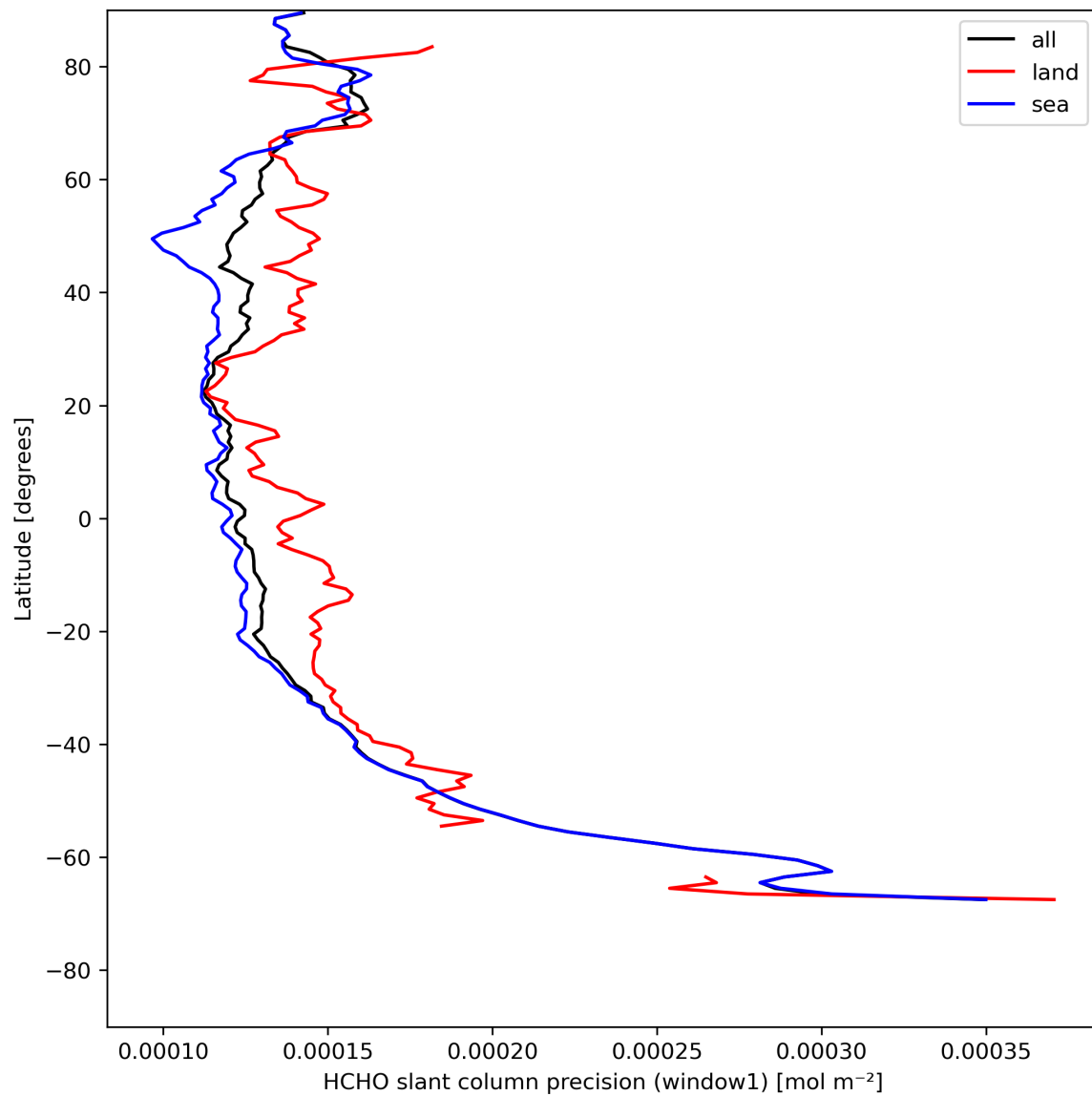
Figure 25: Zonal average of “HCHO slant column precision (window1)” for 2023-08-05 to 2023-08-07.
