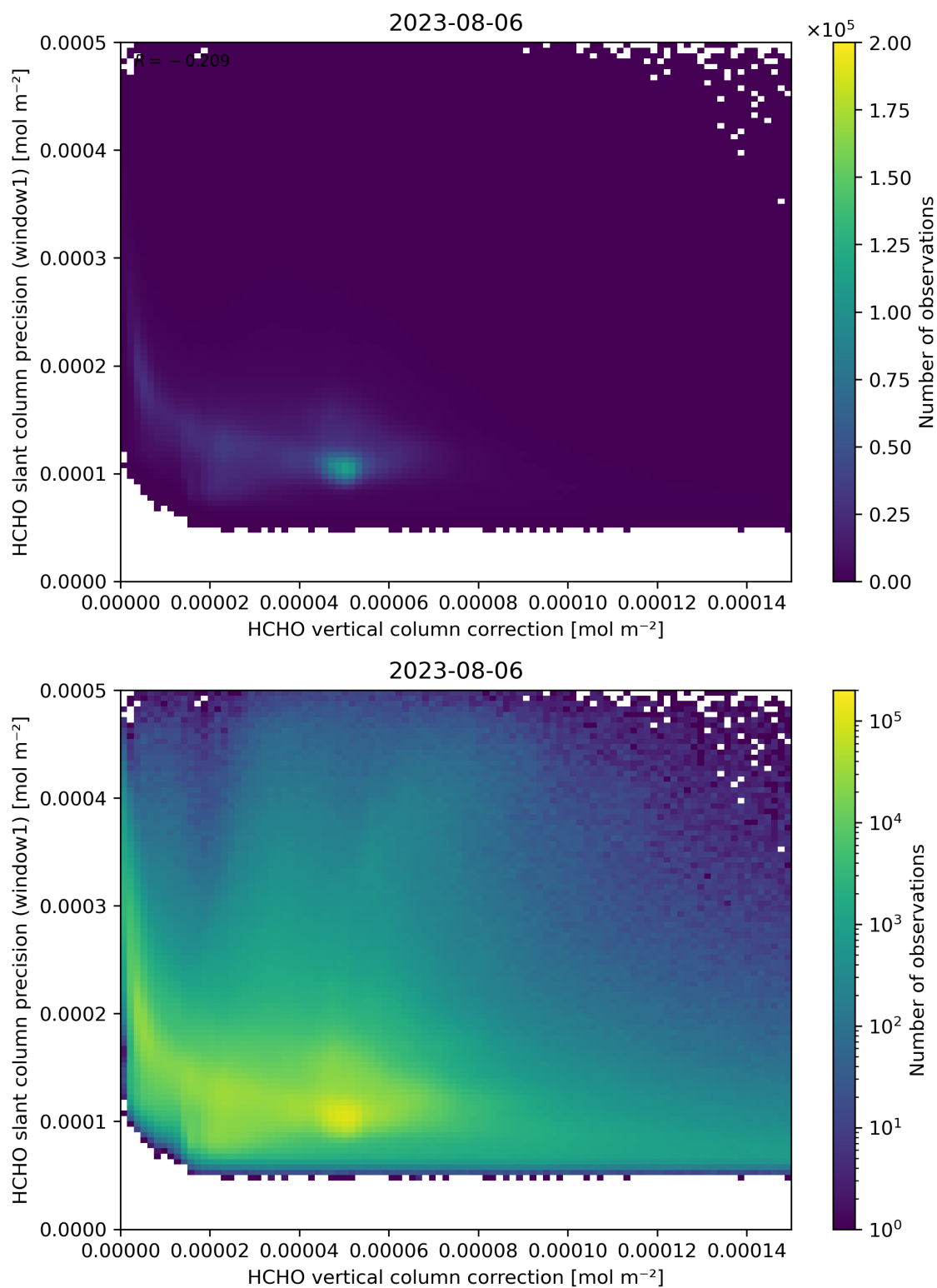
Figure 119: Scatter density plot of “HCHO vertical column correction” against “HCHO slant column precision (window1)” for 2023-08-05 to 2023-08-07.
