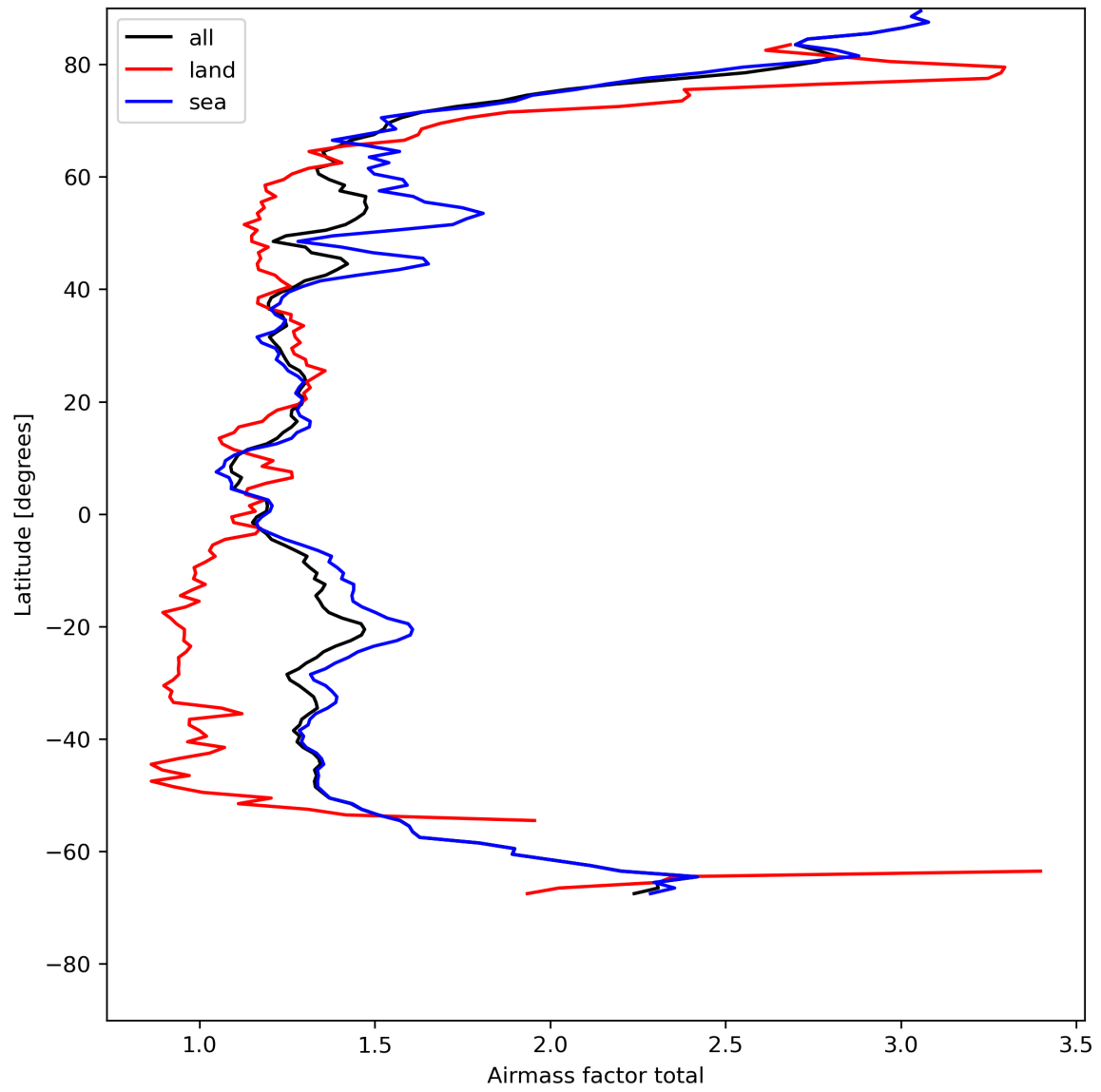
Figure 26: Zonal average of “Airmass factor total” for 2023-08-05 to 2023-08-07.
