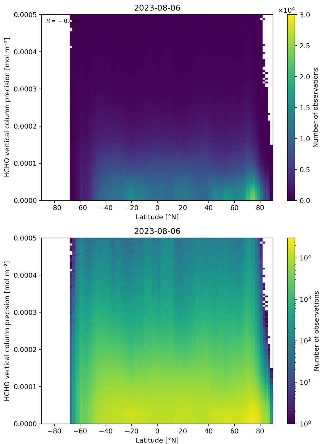
Figure 165: Scatter density plot of “Latitude” against “HCHO vertical column precision” for 2023-08-05 to 2023-08-07.
