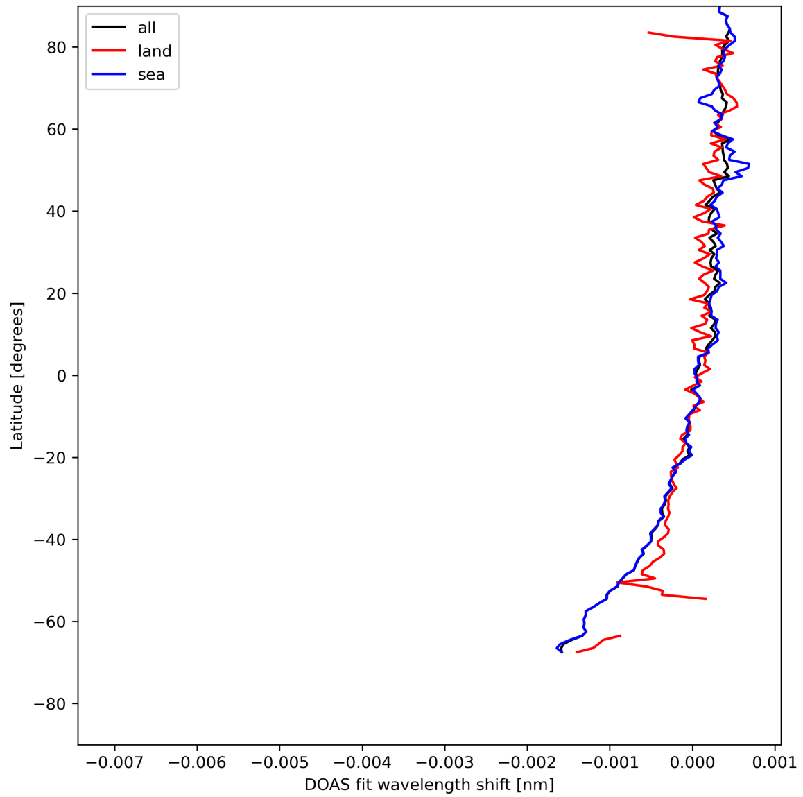
Figure 30: Zonal average of “DOAS fit wavelength shift” for 2023-08-05 to 2023-08-07.
