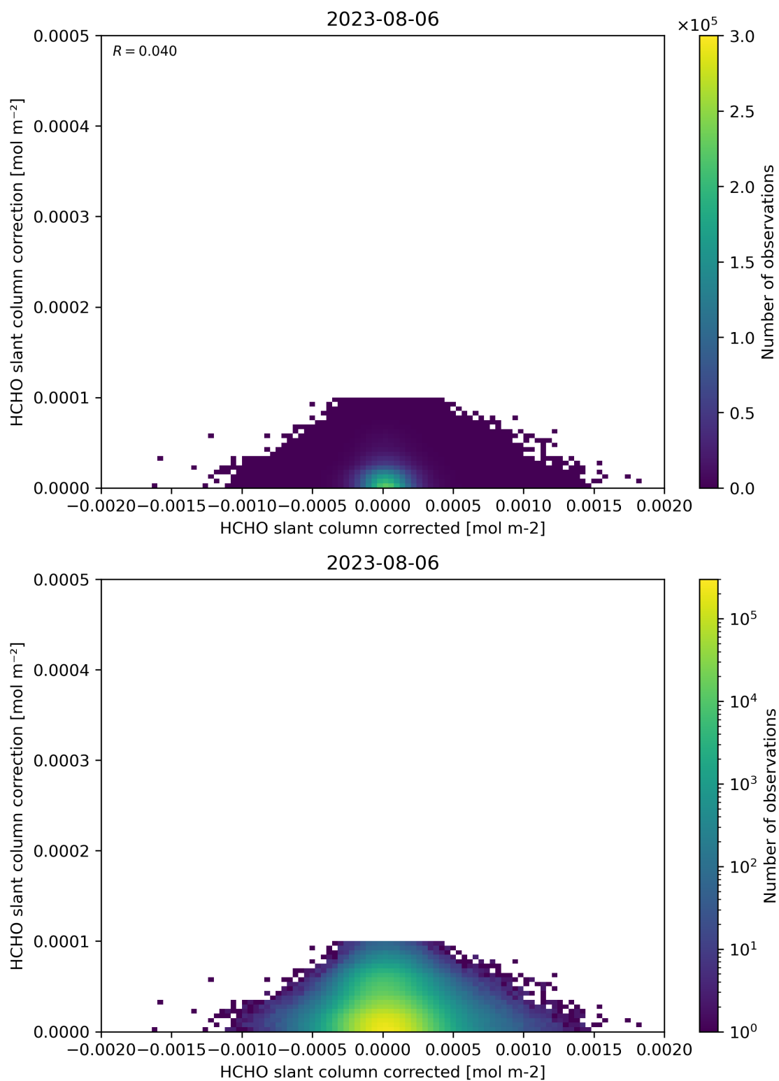
Figure 77: Scatter density plot of “HCHO slant column corrected” against “HCHO slant column correction” for 2023-08-05 to 2023-08-07.
