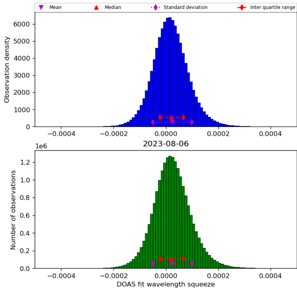
Figure 45: Histogram of “DOAS fit wavelength squeeze” for 2023-08-05 to 2023-08-07
