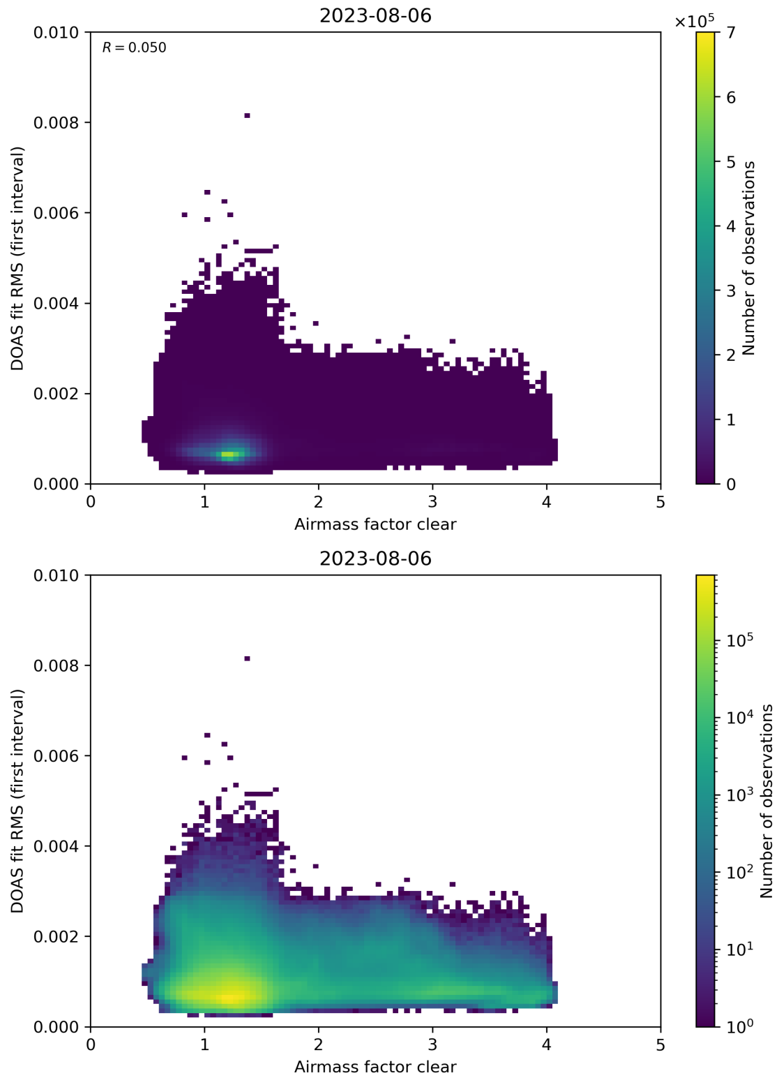
Figure 71: Scatter density plot of “Airmass factor clear” against “DOAS fit RMS (first interval)” for 2023-08-05 to 2023-08-07.
