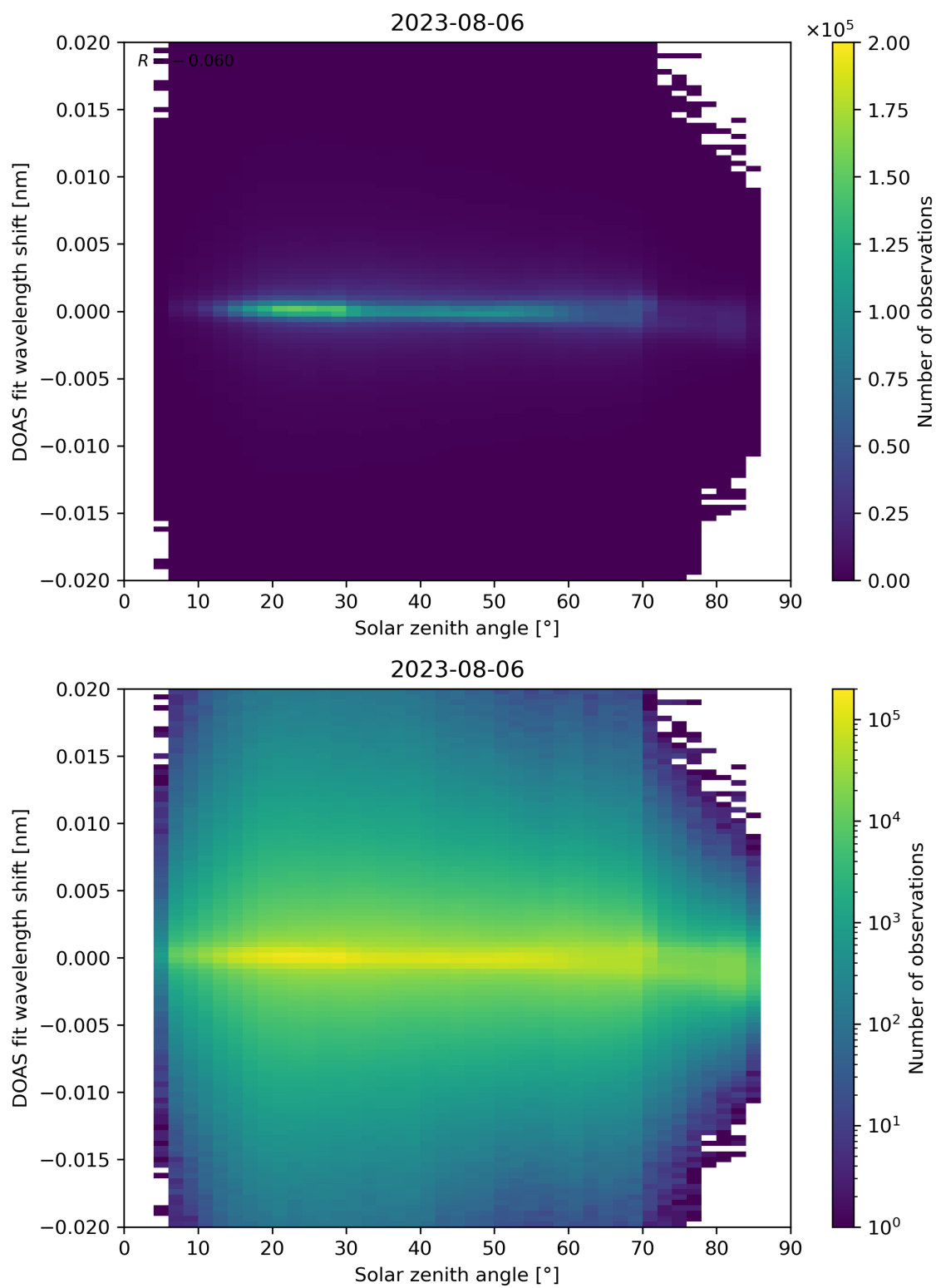
Figure 168: Scatter density plot of “Solar zenith angle” against “DOAS fit wavelength shift” for 2023-08-05 to 2023-08-07.
