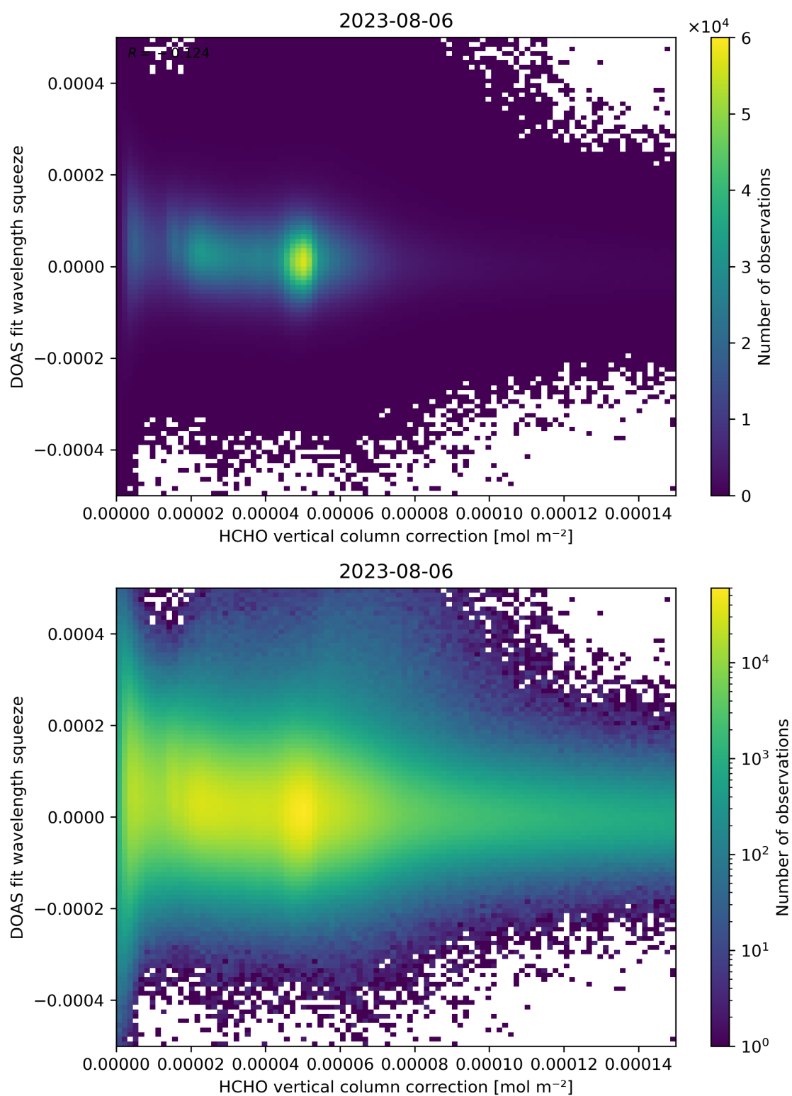
Figure 114: Scatter density plot of “HCHO vertical column correction” against “DOAS fit wavelength squeeze” for 2023-08-05 to 2023-08-07.
