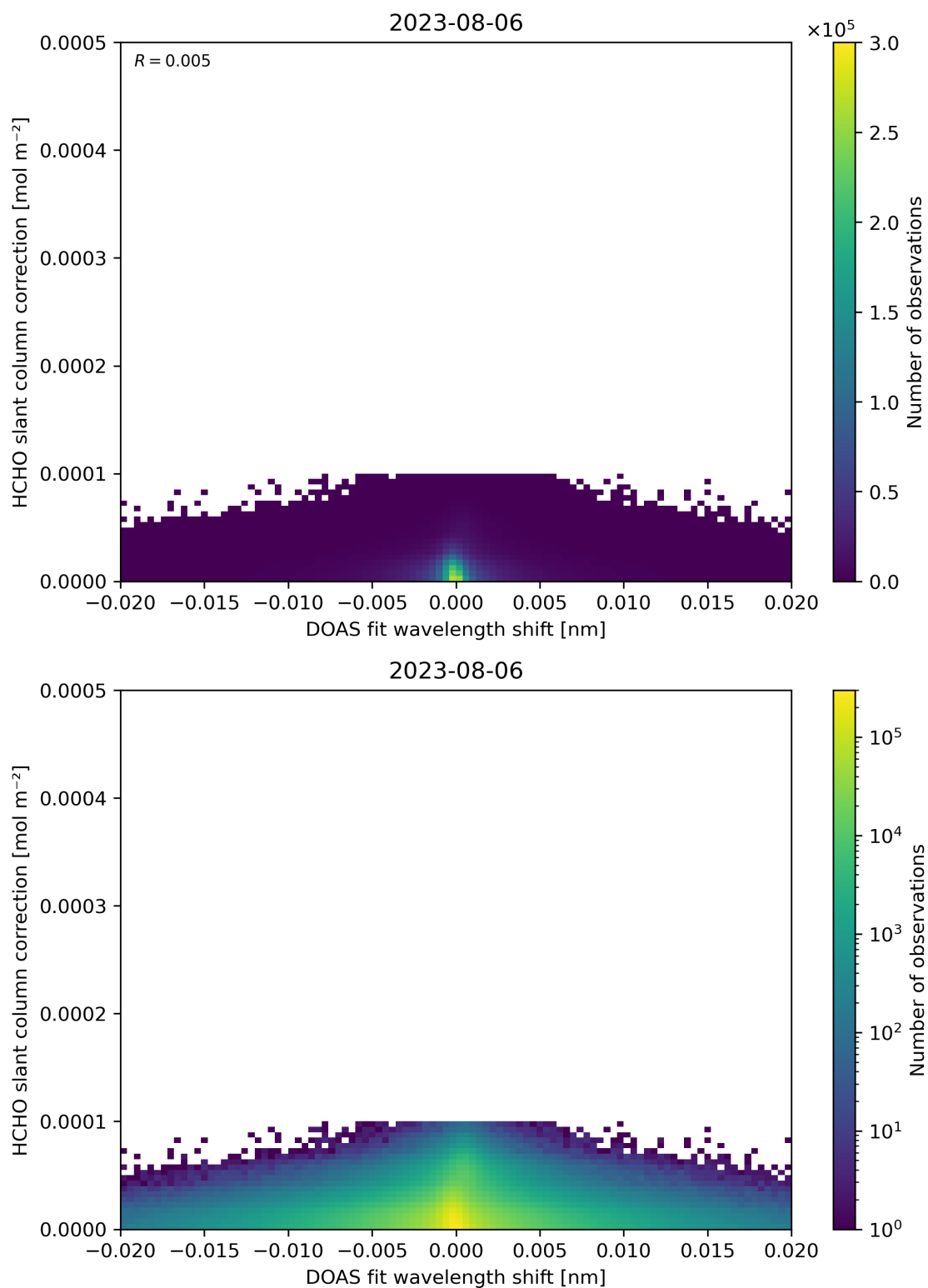
Figure 67: Scatter density plot of “DOAS fit wavelength shift” against “HCHO slant column correction” for 2023-08-05 to 2023-08-07.
