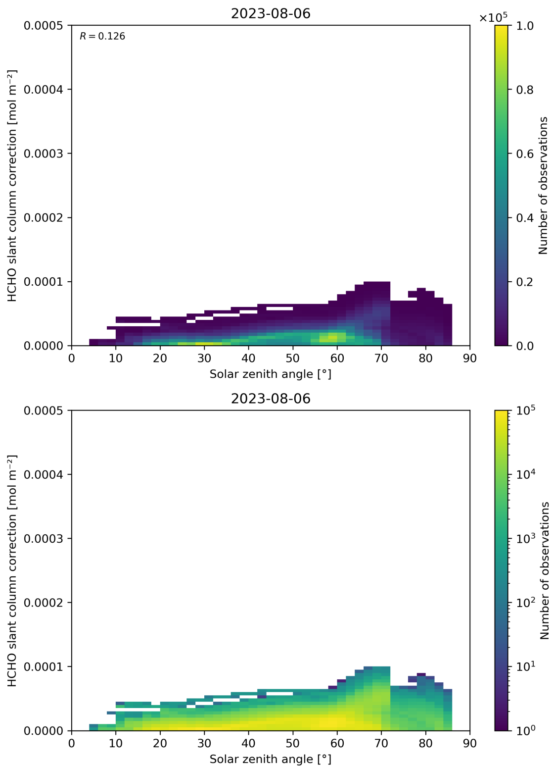
Figure 172: Scatter density plot of “Solar zenith angle” against “HCHO slant column correction” for 2023-08-05 to 2023-08-07.
