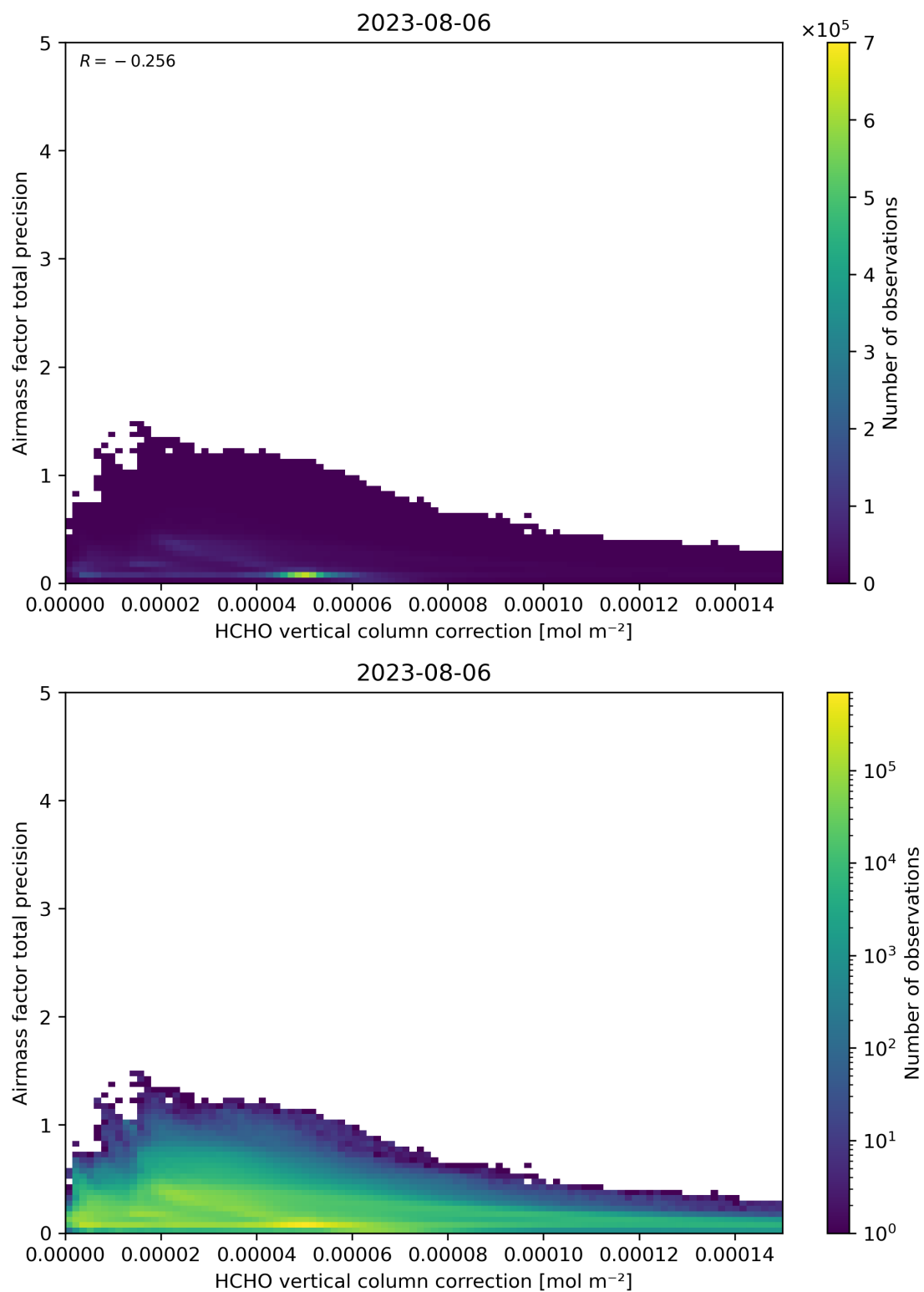
Figure 121: Scatter density plot of “HCHO vertical column correction” against “Airmass factor total precision” for 2023-08-05 to 2023-08-07.
