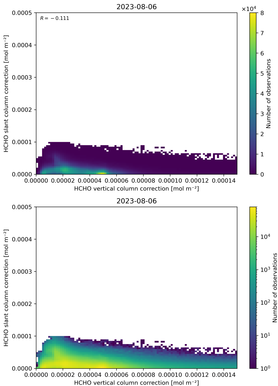
Figure 117: Scatter density plot of “HCHO vertical column correction” against “HCHO slant column correction” for 2023-08-05 to 2023-08-07.
