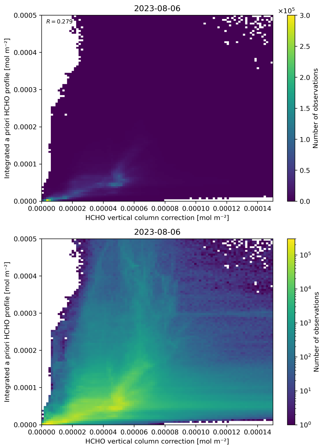
Figure 122: Scatter density plot of “HCHO vertical column correction” against “Integrated a priori HCHO profile” for 2023-08-05 to 2023-08-07.
