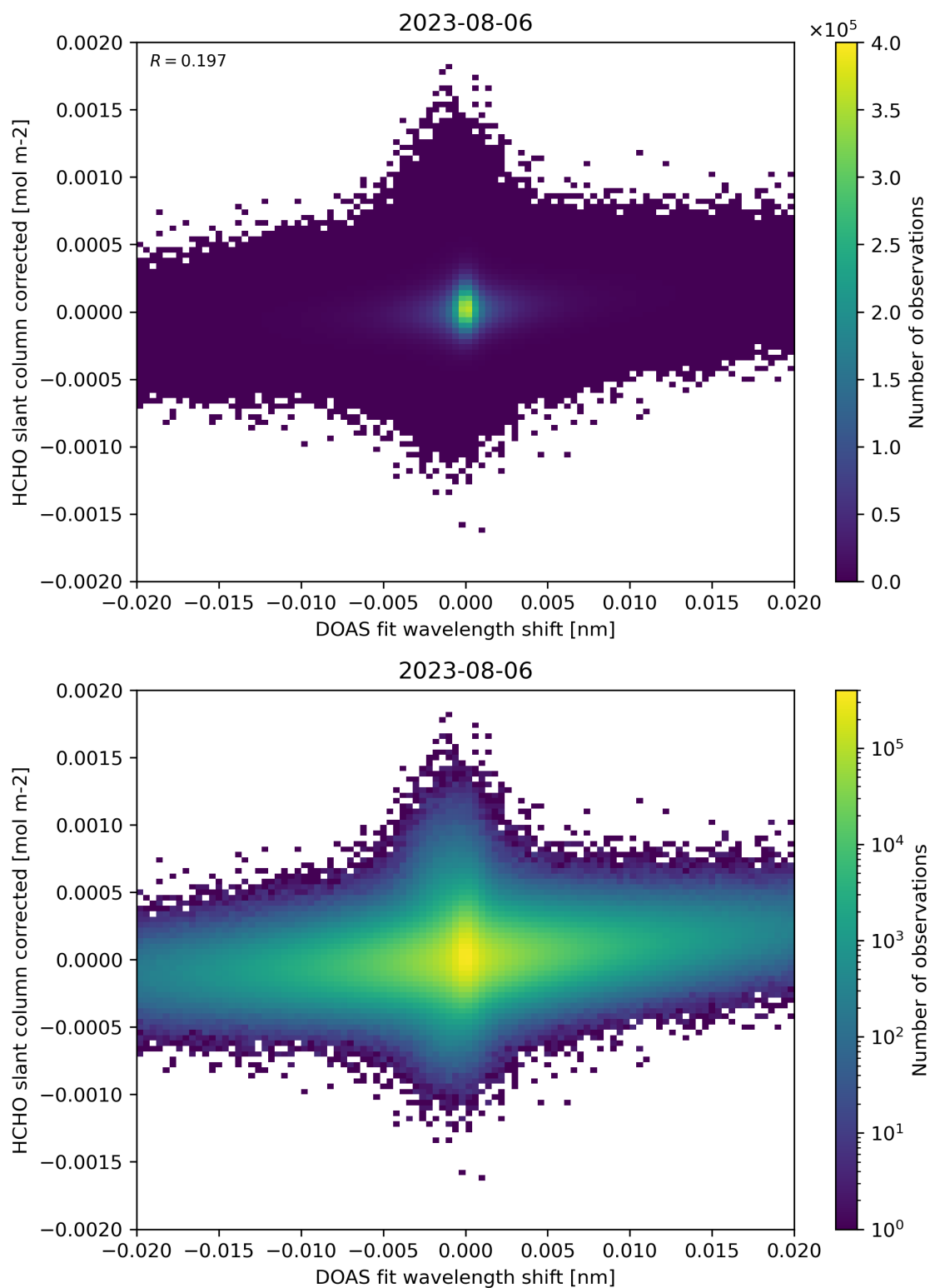
Figure 66: Scatter density plot of “DOAS fit wavelength shift” against “HCHO slant column corrected” for 2023-08-05 to 2023-08-07.
