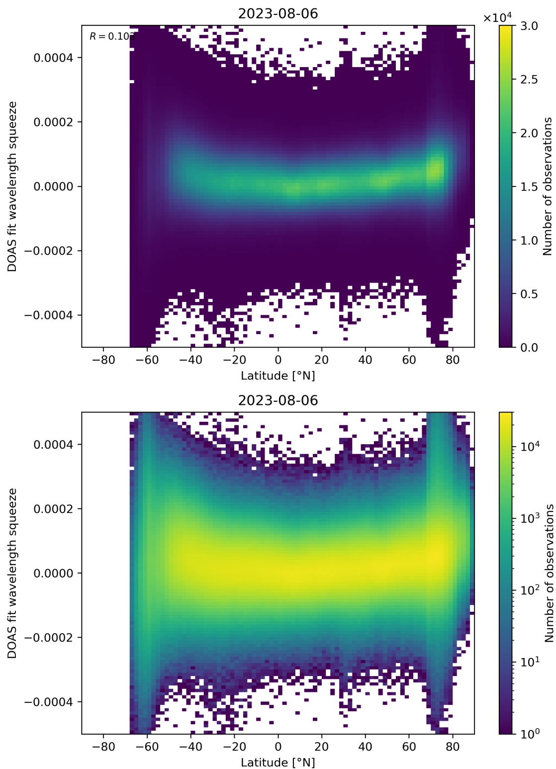
Figure 155: Scatter density plot of “Latitude” against “DOAS fit wavelength squeeze” for 2023-08-05 to 2023-08-07.
