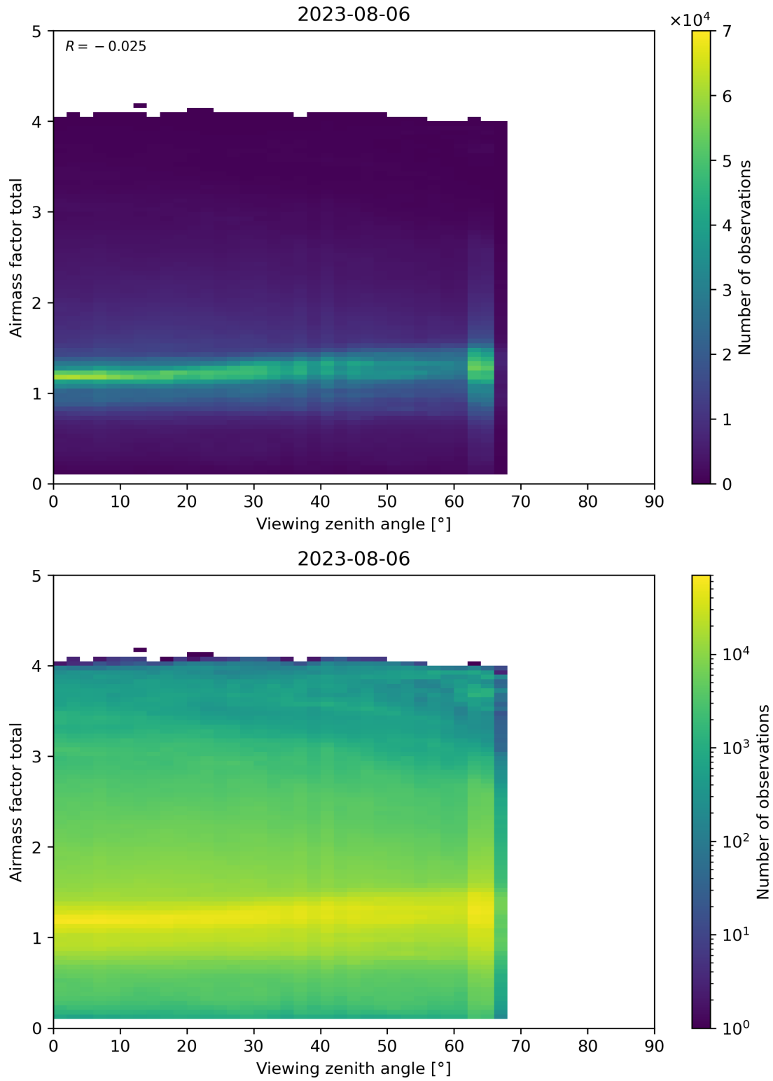
Figure 190: Scatter density plot of “Viewing zenith angle” against “Airmass factor total” for 2023-08-05 to 2023-08-07.
