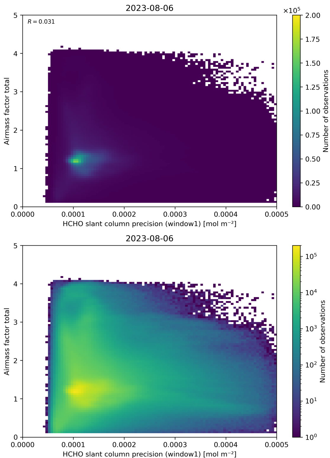
Figure 94: Scatter density plot of “HCHO slant column precision (window1)” against “Airmass factor total” for 2023-08-05 to 2023-08-07.
