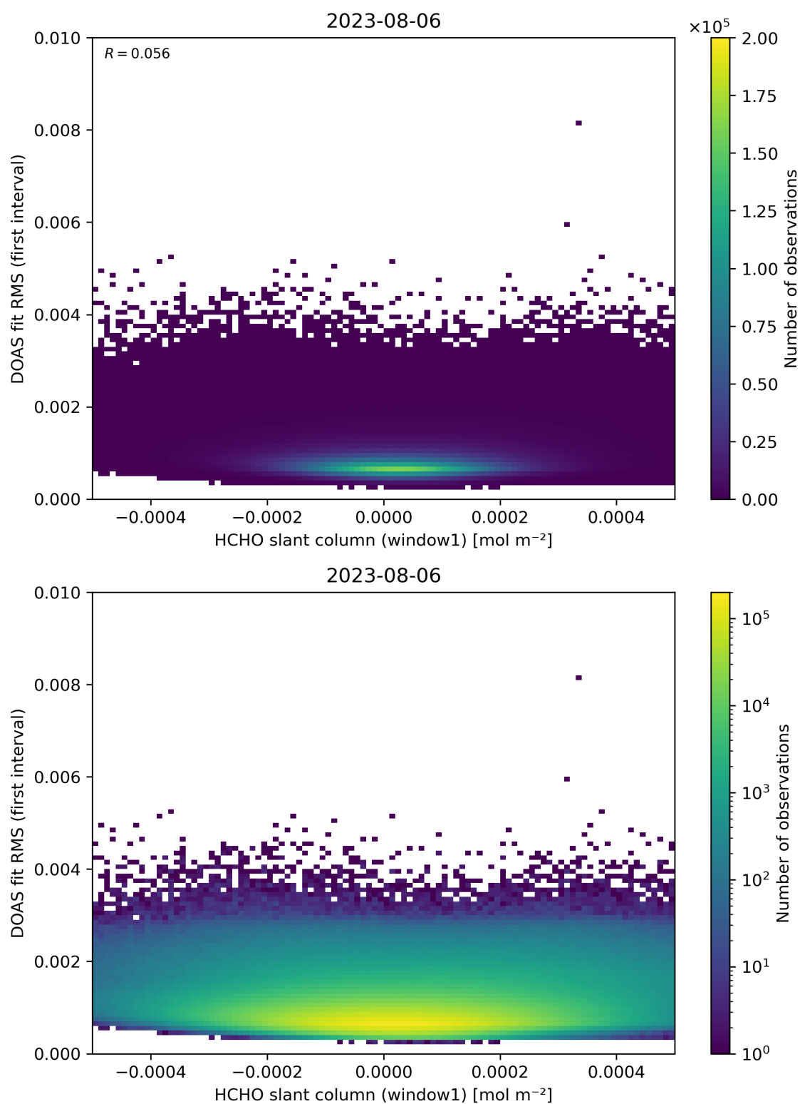
Figure 78: Scatter density plot of “HCHO slant column (window1)” against “DOAS fit RMS (first interval)” for 2023-08-05 to 2023-08-07.
