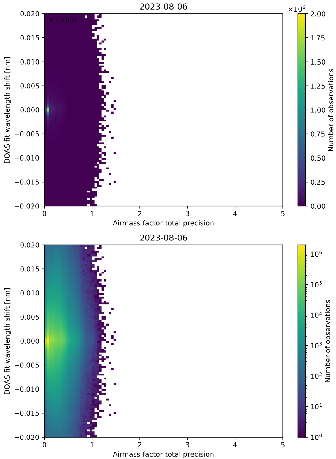
Figure 106: Scatter density plot of “Airmass factor total precision” against “DOAS fit wavelength shift” for 2023-08-05 to 2023-08-07.
