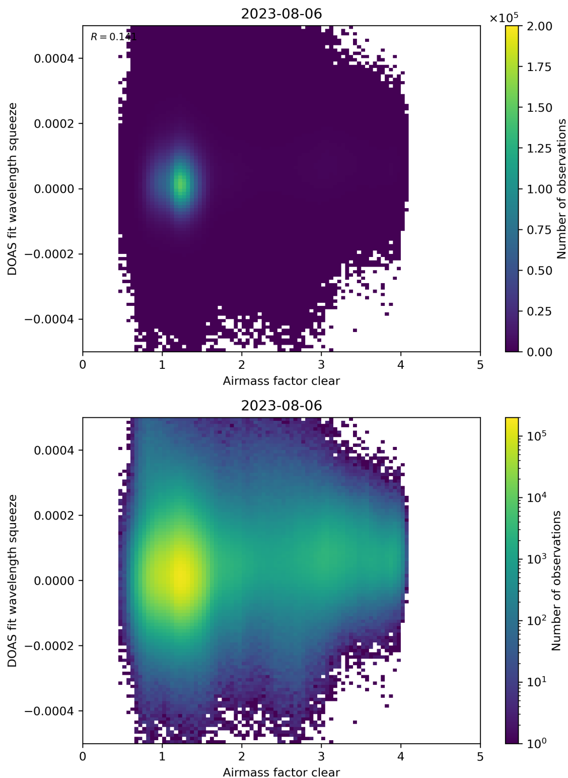
Figure 73: Scatter density plot of “Airmass factor clear” against “DOAS fit wavelength squeeze” for 2023-08-05 to 2023-08-07.
