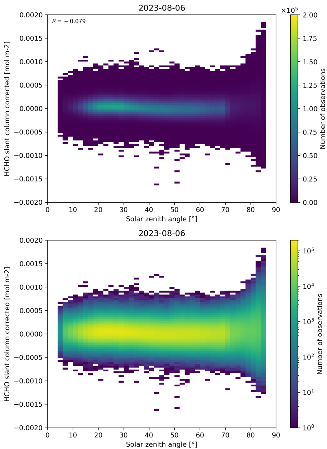
Figure 171: Scatter density plot of “Solar zenith angle” against “HCHO slant column corrected” for 2023-08-05 to 2023-08-07.
