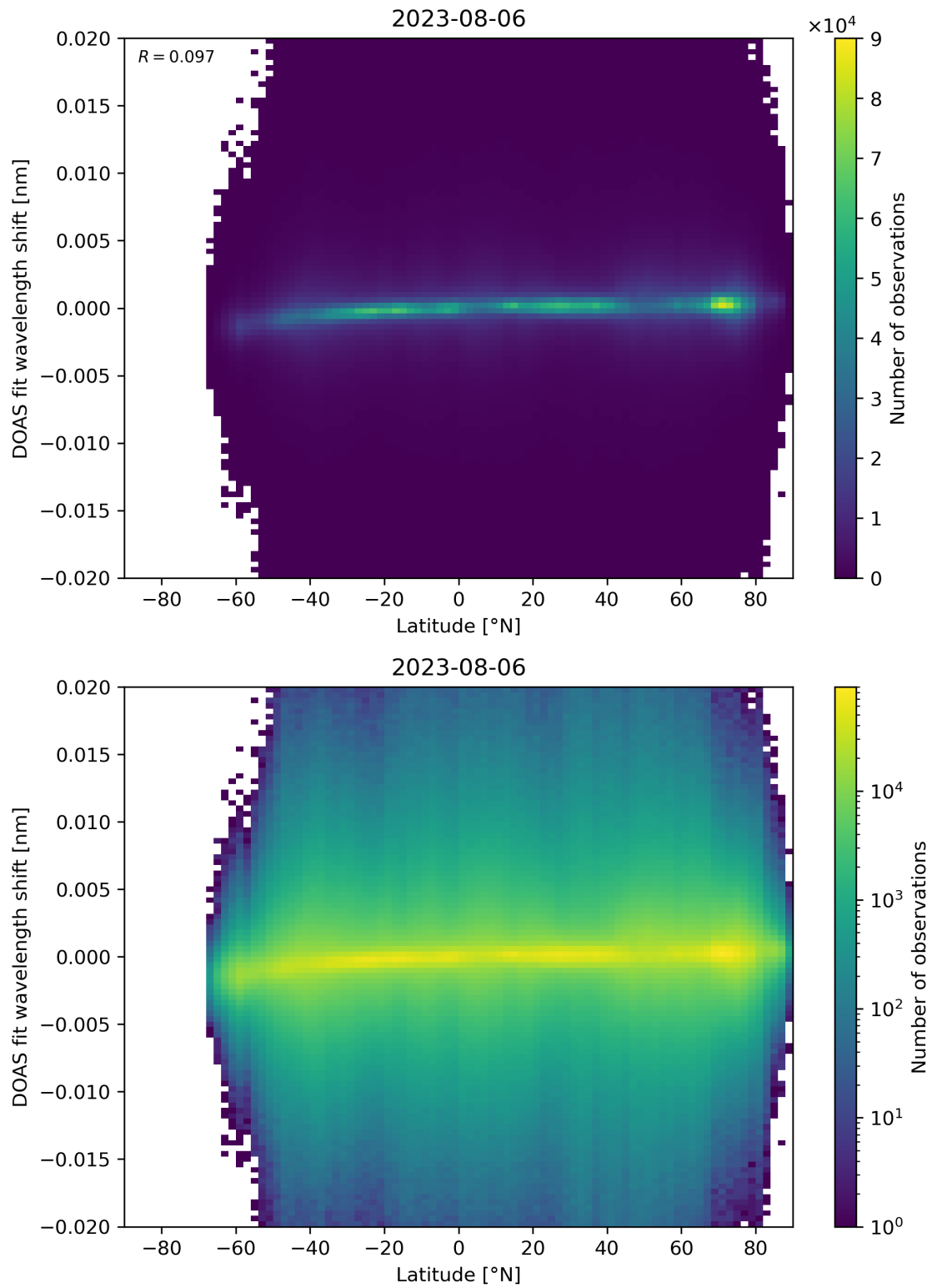
Figure 154: Scatter density plot of “Latitude” against “DOAS fit wavelength shift” for 2023-08-05 to 2023-08-07.
