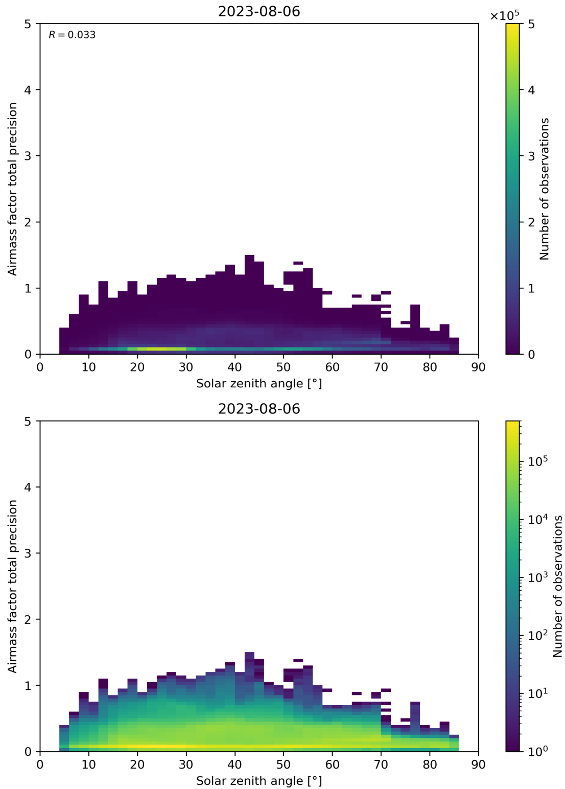
Figure 176: Scatter density plot of “Solar zenith angle” against “Airmass factor total precision” for 2023-08-05 to 2023-08-07.
