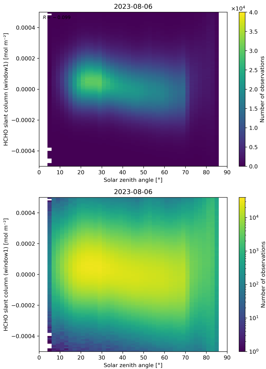
Figure 173: Scatter density plot of “Solar zenith angle” against “HCHO slant column (window1)” for 2023-08-05 to 2023-08-07.
