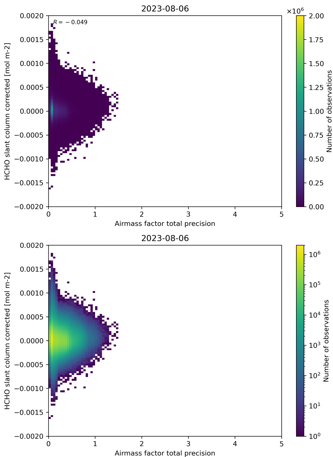
Figure 109: Scatter density plot of “Airmass factor total precision” against “HCHO slant column corrected” for 2023-08-05 to 2023-08-07.
