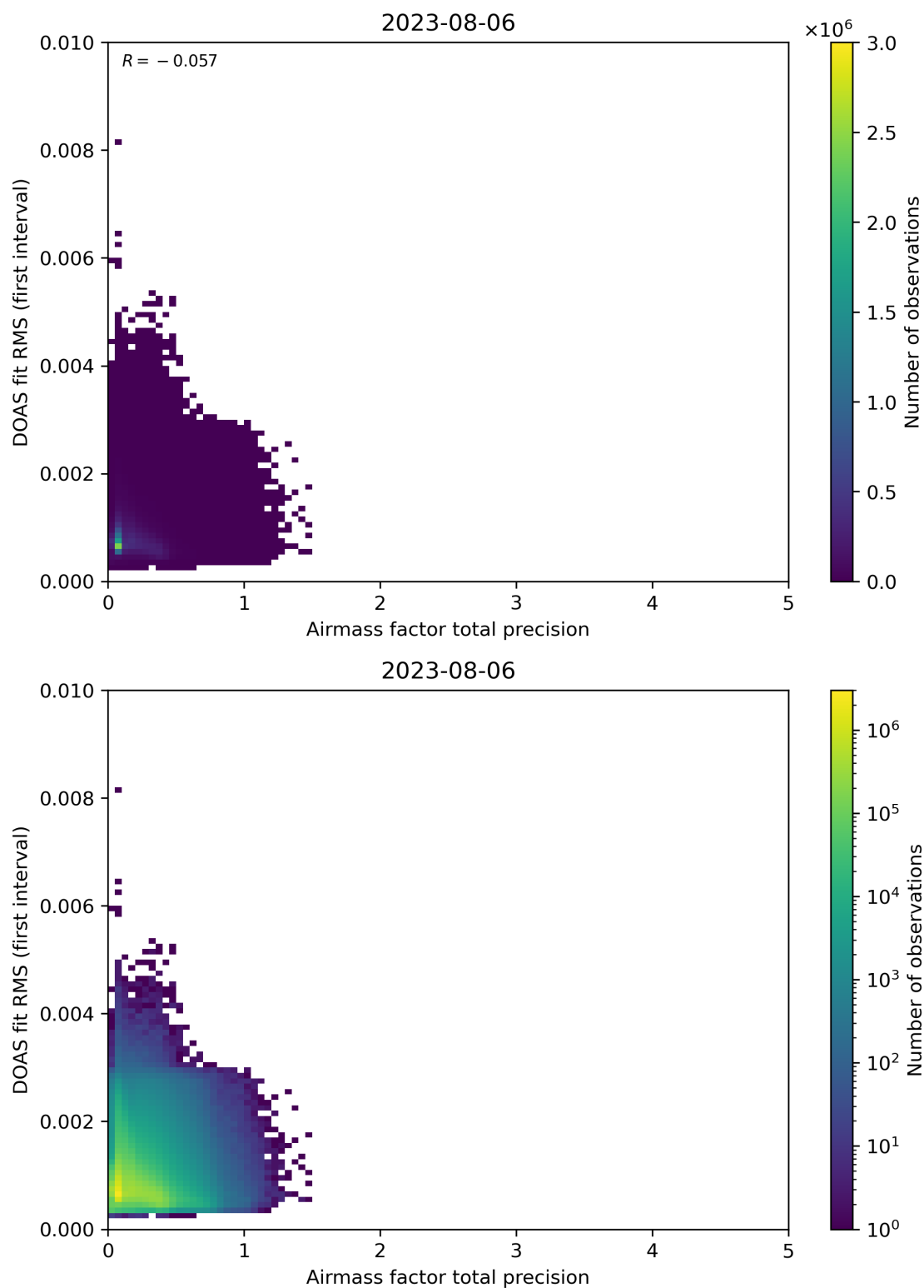
Figure 105: Scatter density plot of “Airmass factor total precision” against “DOAS fit RMS (first interval)” for 2023-08-05 to 2023-08-07.
