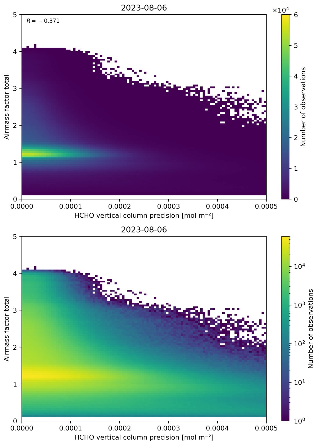
Figure 144: Scatter density plot of “HCHO vertical column precision” against “Airmass factor total” for 2023-08-05 to 2023-08-07.
