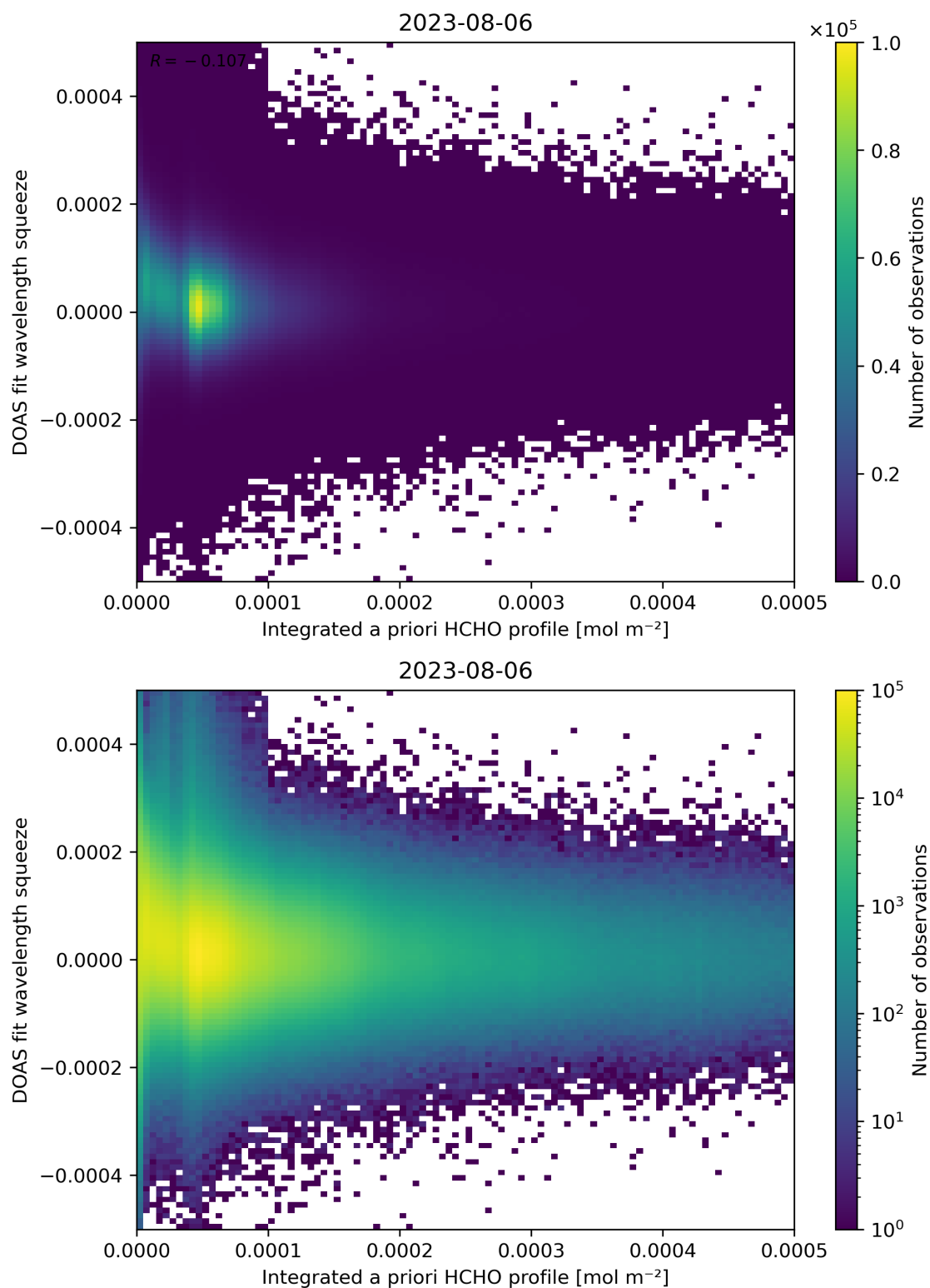
Figure 150: Scatter density plot of “Integrated a priori HCHO profile” against “DOAS fit wavelength squeeze” for 2023-08-05 to 2023-08-07.
