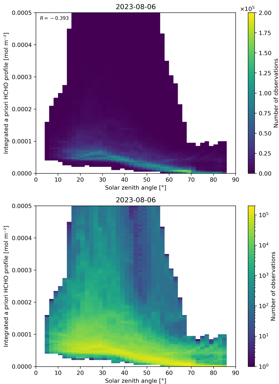
Figure 180: Scatter density plot of “Solar zenith angle” against “Integrated a priori HCHO profile” for 2023-08-05 to 2023-08-07.
