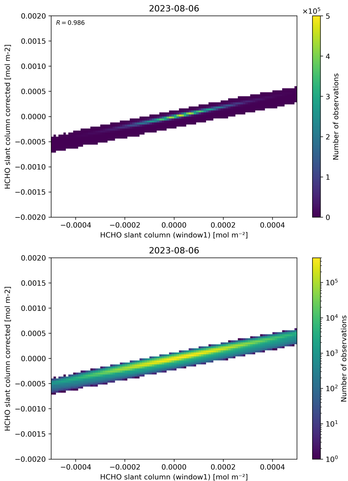
Figure 82: Scatter density plot of “HCHO slant column (window1)” against “HCHO slant column corrected” for 2023-08-05 to 2023-08-07.
