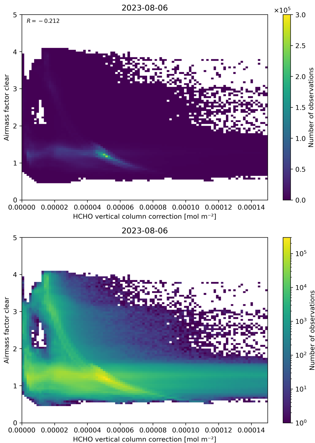
Figure 115: Scatter density plot of “HCHO vertical column correction” against “Airmass factor clear” for 2023-08-05 to 2023-08-07.
