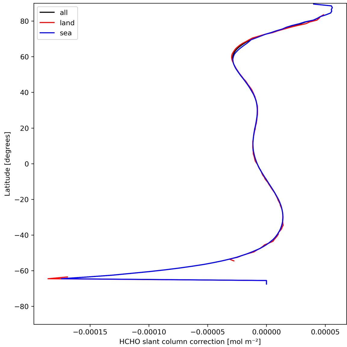
Figure 33: Zonal average of “HCHO slant column correction” for 2023-08-05 to 2023-08-07.
