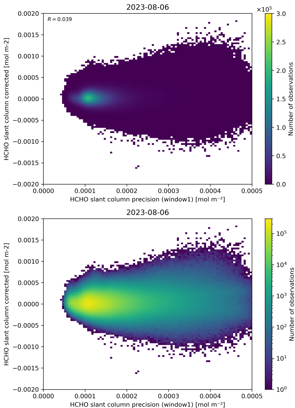
Figure 92: Scatter density plot of “HCHO slant column precision (window1)” against “HCHO slant column corrected” for 2023-08-05 to 2023-08-07.
