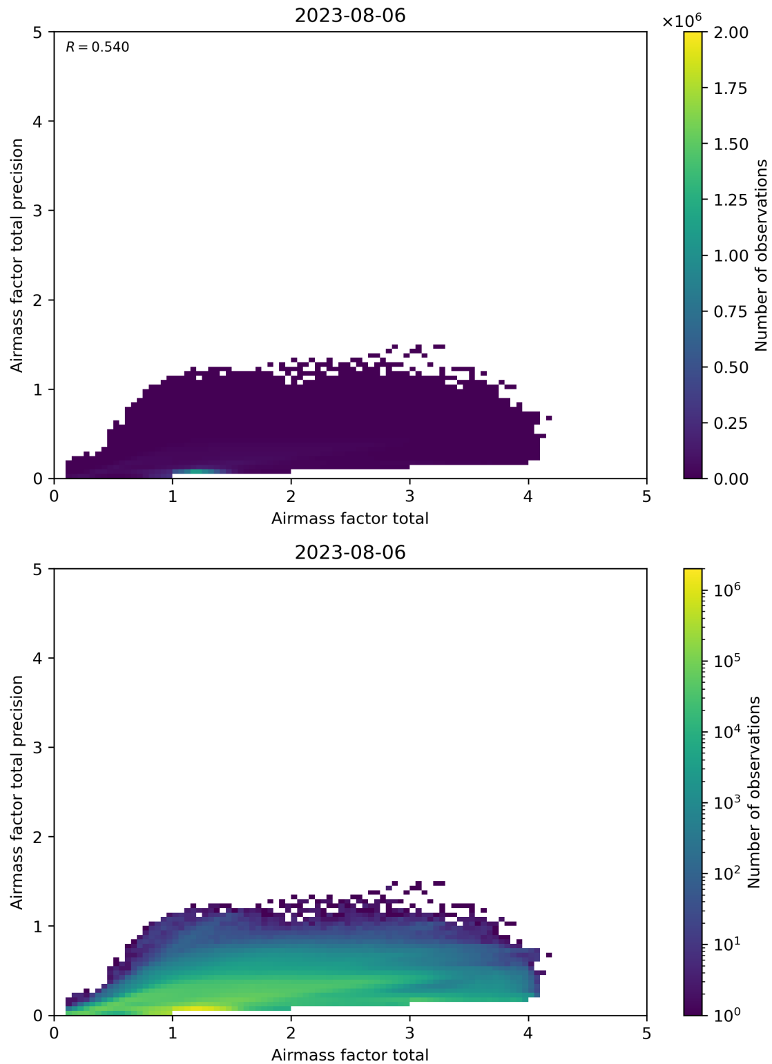
Figure 103: Scatter density plot of “Airmass factor total” against “Airmass factor total precision” for 2023-08-05 to 2023-08-07.
