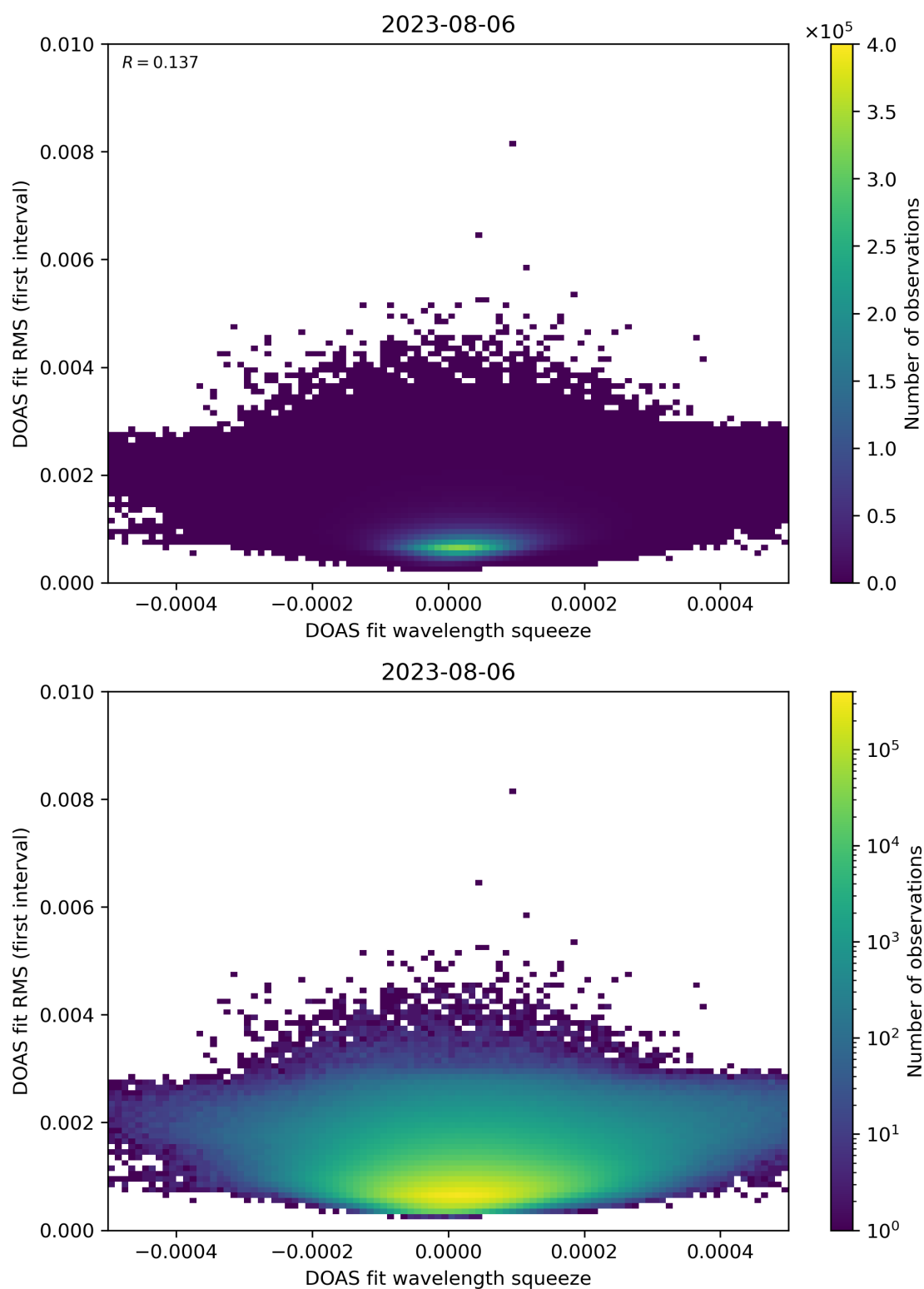
Figure 68: Scatter density plot of “DOAS fit wavelength squeeze” against “DOAS fit RMS (first interval)” for 2023-08-05 to 2023-08-07.
