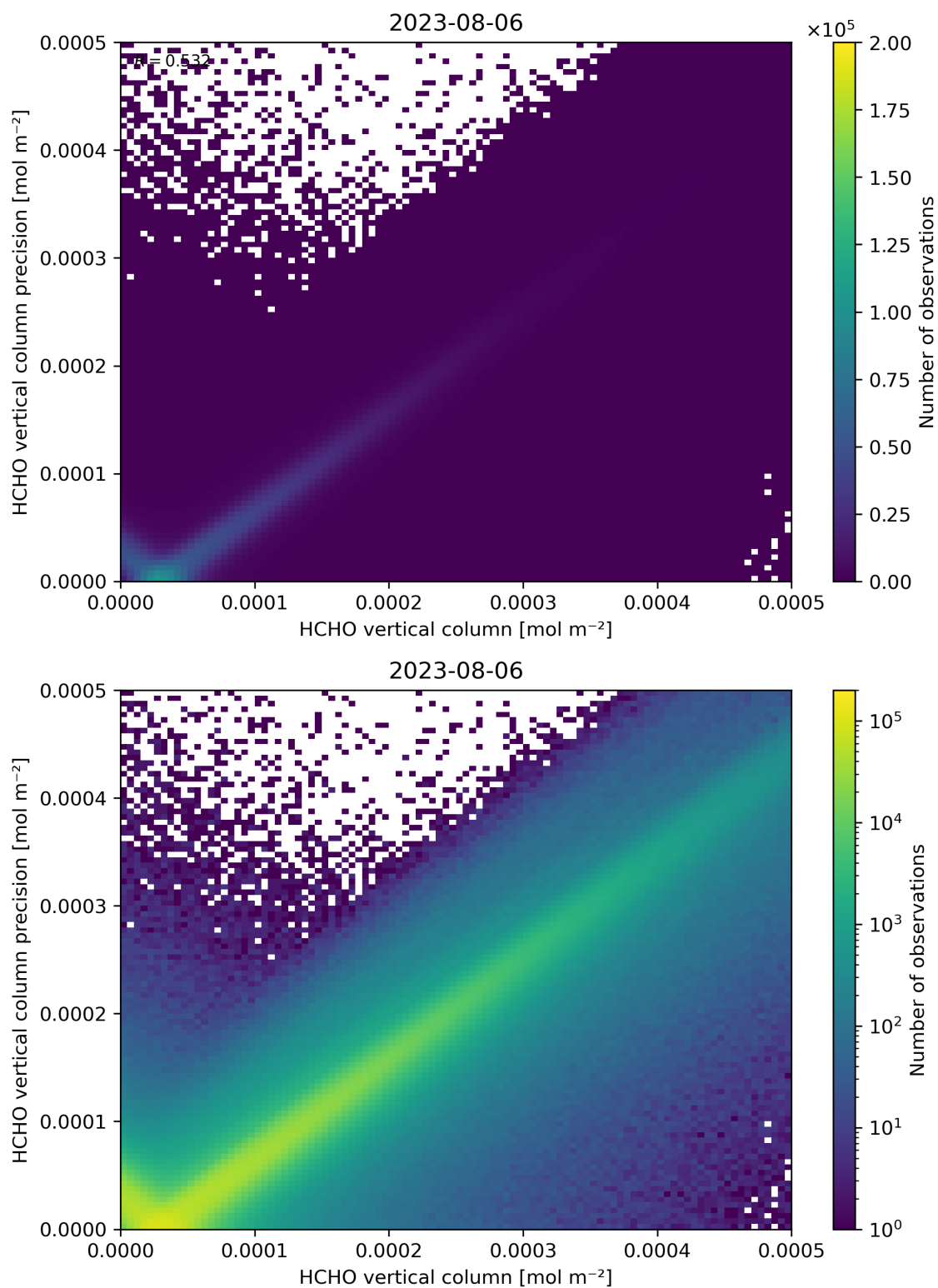
Figure 134: Scatter density plot of “HCHO vertical column” against “HCHO vertical column precision” for 2023-08-05 to 2023-08-07.
