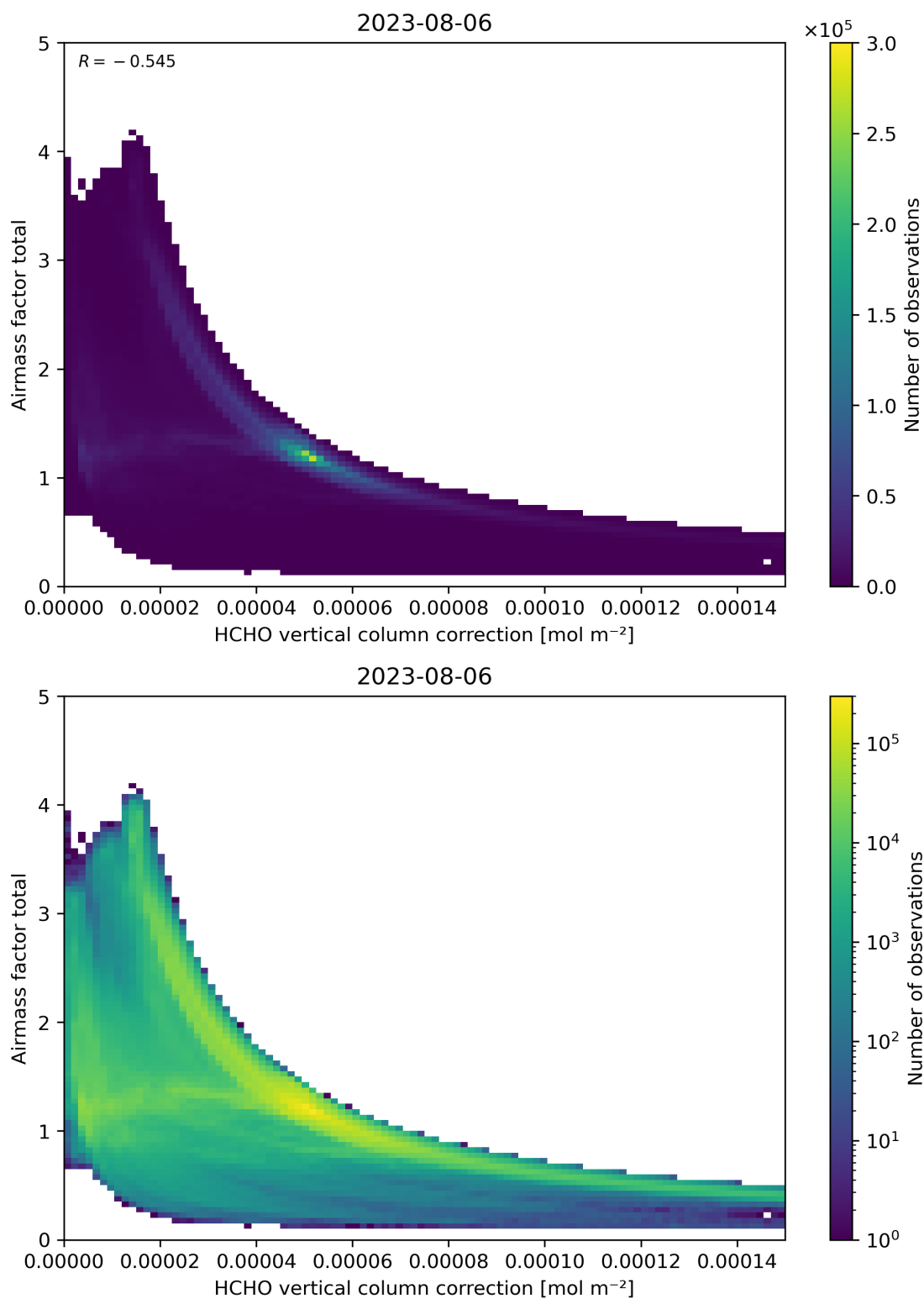
Figure 120: Scatter density plot of “HCHO vertical column correction” against “Airmass factor total” for 2023-08-05 to 2023-08-07.
