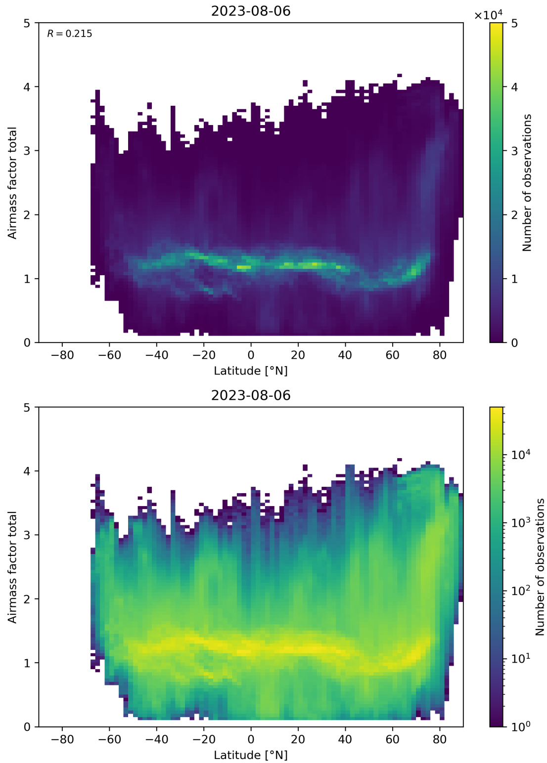
Figure 161: Scatter density plot of “Latitude” against “Airmass factor total” for 2023-08-05 to 2023-08-07.
