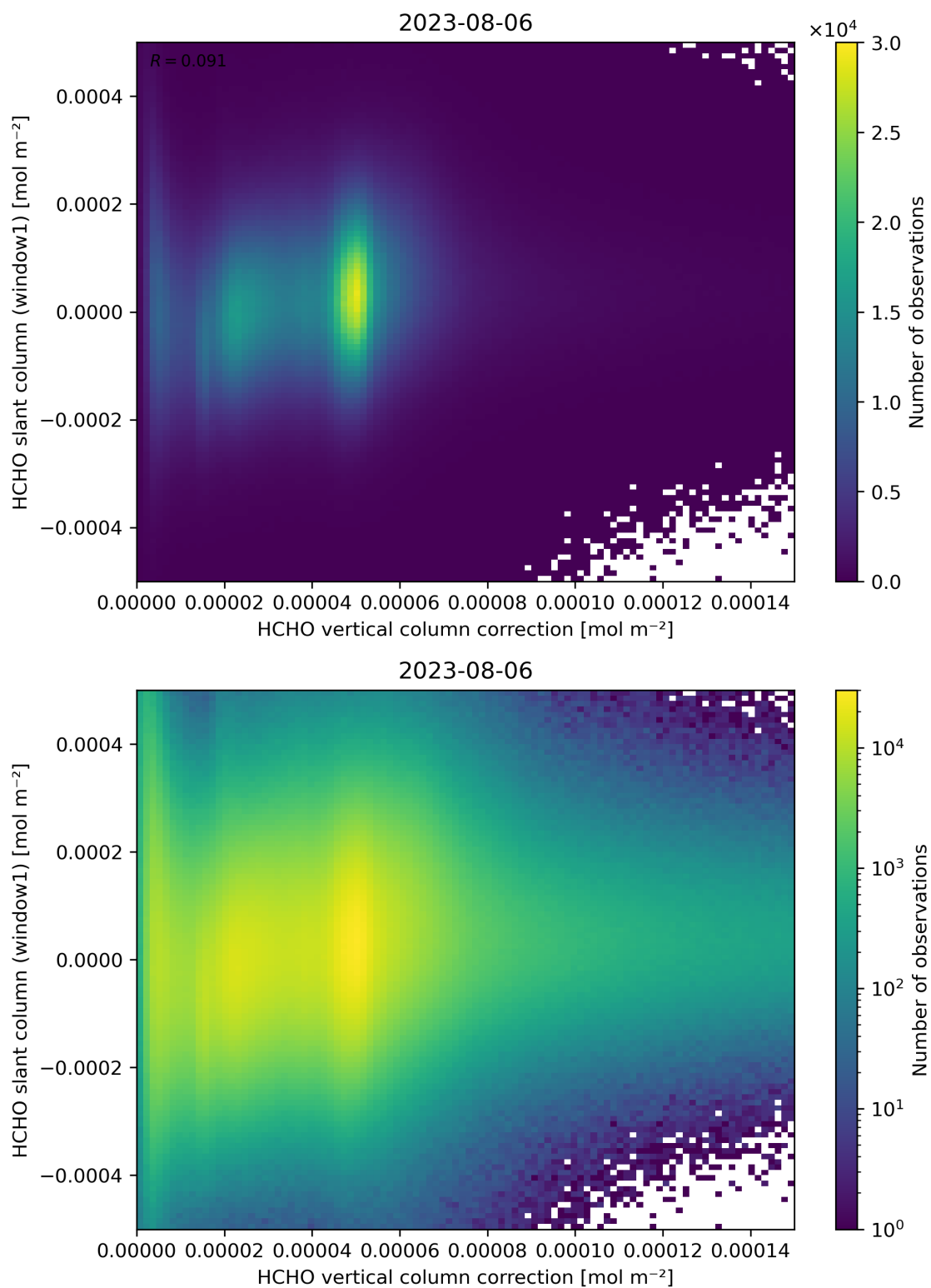
Figure 118: Scatter density plot of “HCHO vertical column correction” against “HCHO slant column (window1)” for 2023-08-05 to 2023-08-07.
