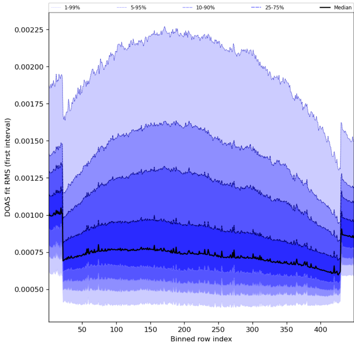
Figure 60: Along track statistics of “DOAS fit RMS (first interval)” for 2023-08-05 to 2023-08-07
