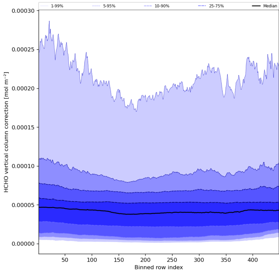
Figure 51: Along track statistics of "HCHO vertical column correction" for 2023-08-05 to 2023-08-07
