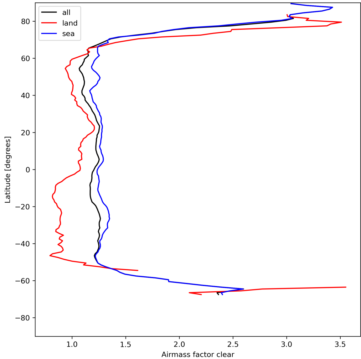
Figure 28: Zonal average of “Airmass factor clear” for 2023-08-05 to 2023-08-07.
