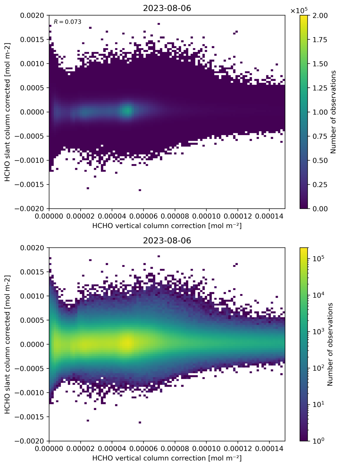
Figure 116: Scatter density plot of “HCHO vertical column correction” against “HCHO slant column corrected” for 2023-08-05 to 2023-08-07.
