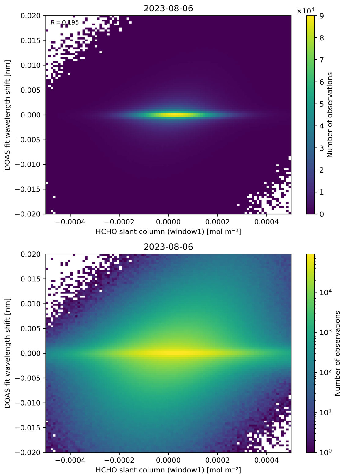
Figure 79: Scatter density plot of “HCHO slant column (window1)” against “DOAS fit wavelength shift” for 2023-08-05 to 2023-08-07.
