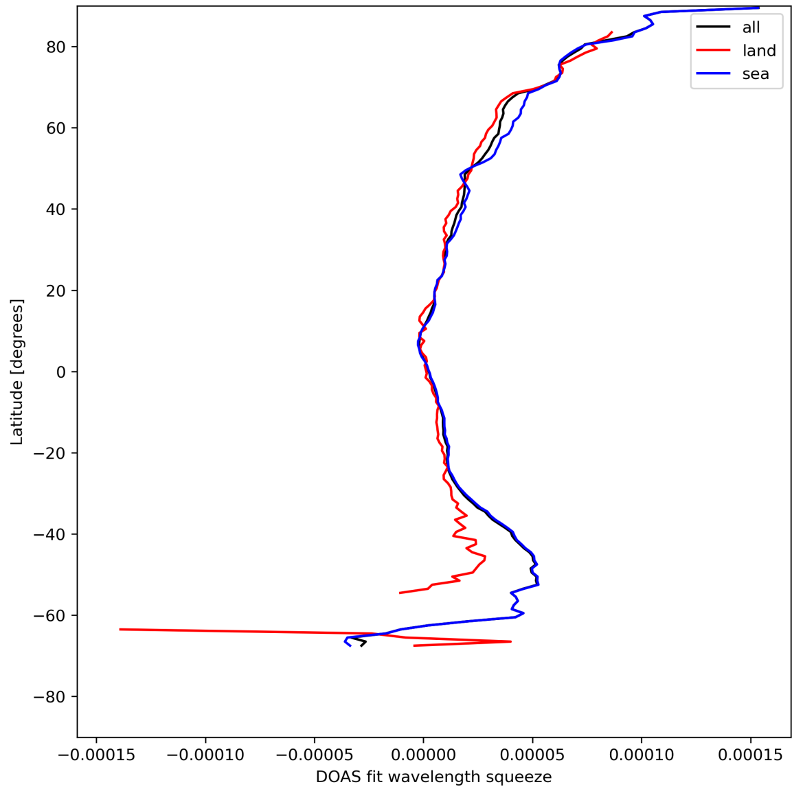
Figure 31: Zonal average of “DOAS fit wavelength squeeze” for 2023-08-05 to 2023-08-07.
