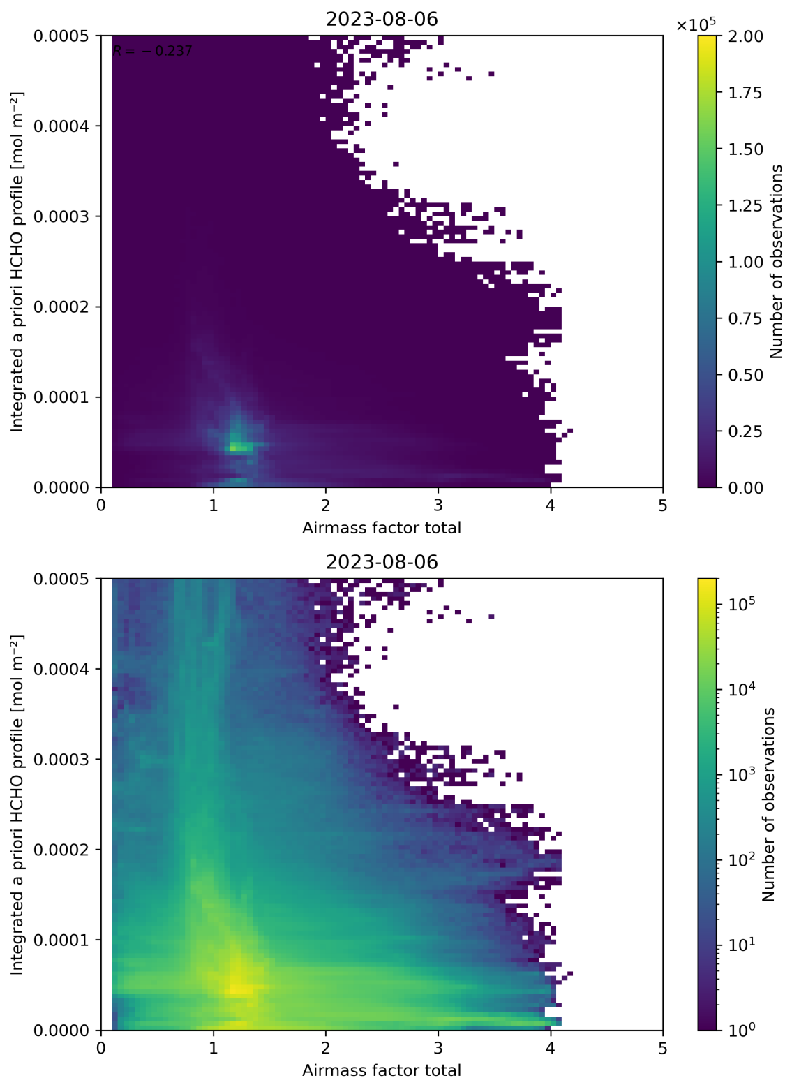
Figure 104: Scatter density plot of “Airmass factor total” against “Integrated a priori HCHO profile” for 2023-08-05 to 2023-08-07.
