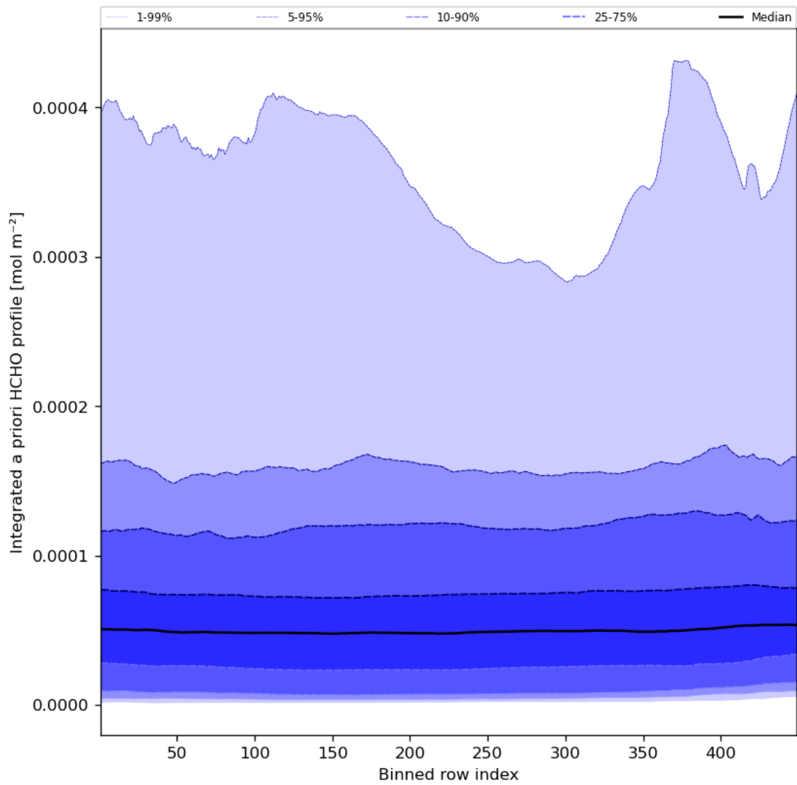
Figure 57: Along track statistics of “Integrated a priori HCHO profile” for 2023-08-05 to 2023-08-07
