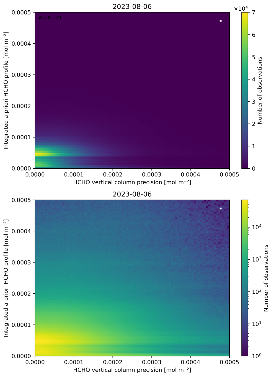
Figure 147: Scatter density plot of “HCHO vertical column precision” against “Integrated a priori HCHO profile” for 2023-08-05 to 2023-08-07.
