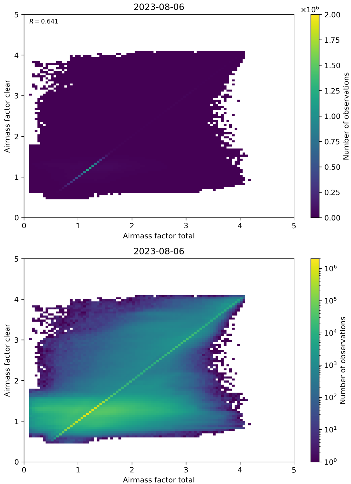
Figure 100: Scatter density plot of “Airmass factor total” against “Airmass factor clear” for 2023-08-05 to 2023-08-07.
