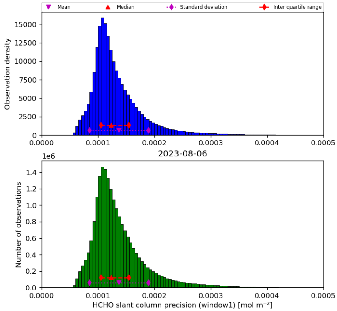
Figure 39: Histogram of “HCHO slant column precision (window1)” for 2023-08-05 to 2023-08-07
