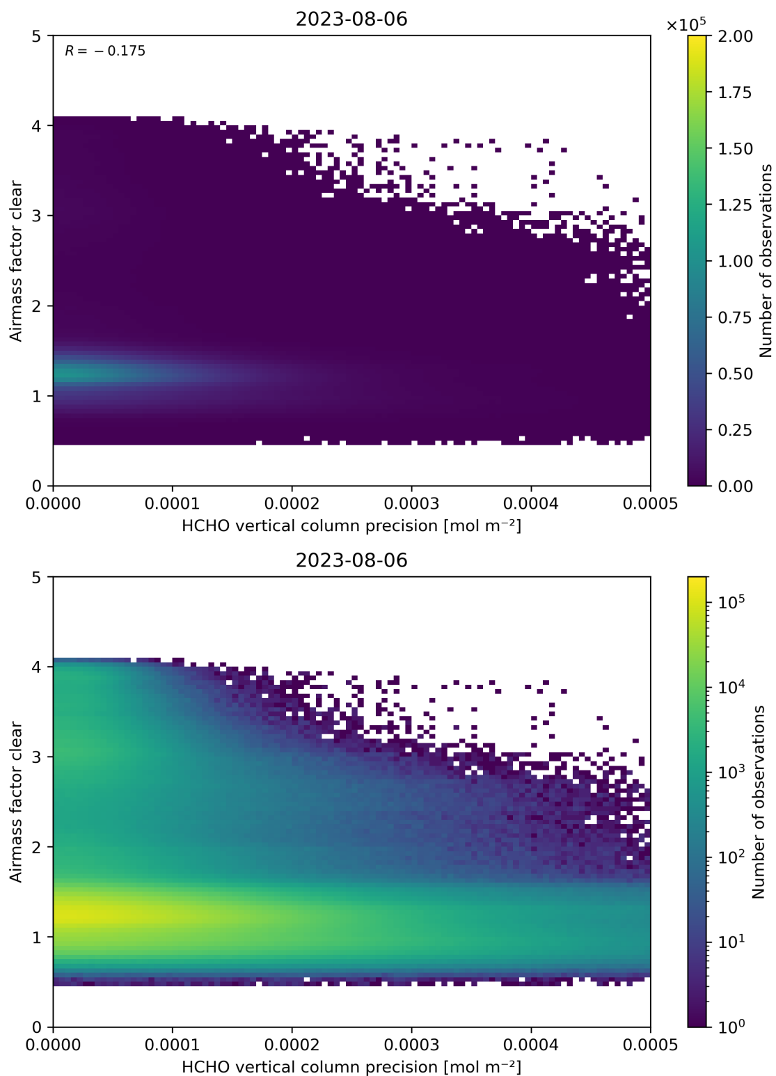
Figure 139: Scatter density plot of “HCHO vertical column precision” against “Airmass factor clear” for 2023-08-05 to 2023-08-07.
