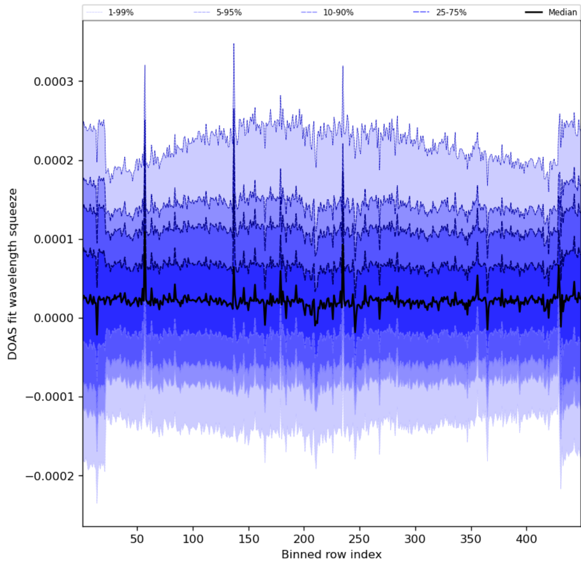
Figure 59: Along track statistics of “DOAS fit wavelength squeeze” for 2023-08-05 to 2023-08-07
