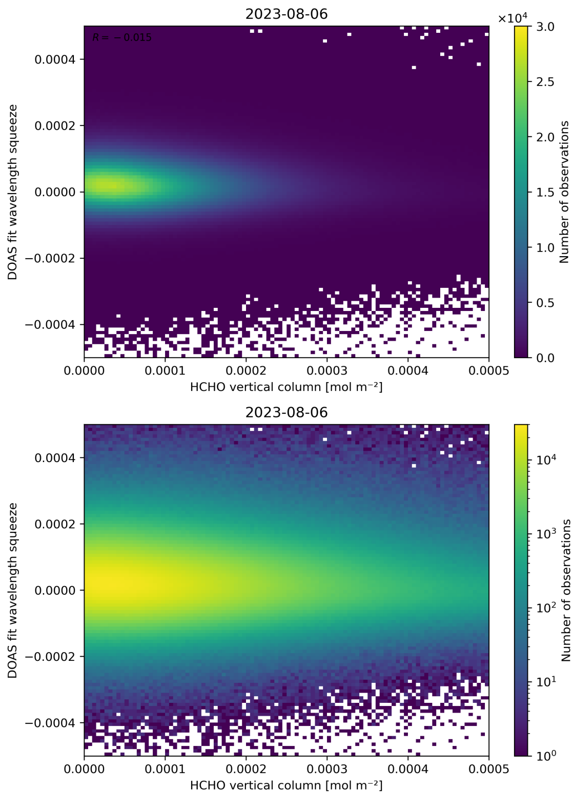
Figure 125: Scatter density plot of “HCHO vertical column” against “DOAS fit wavelength squeeze” for 2023-08-05 to 2023-08-07.
