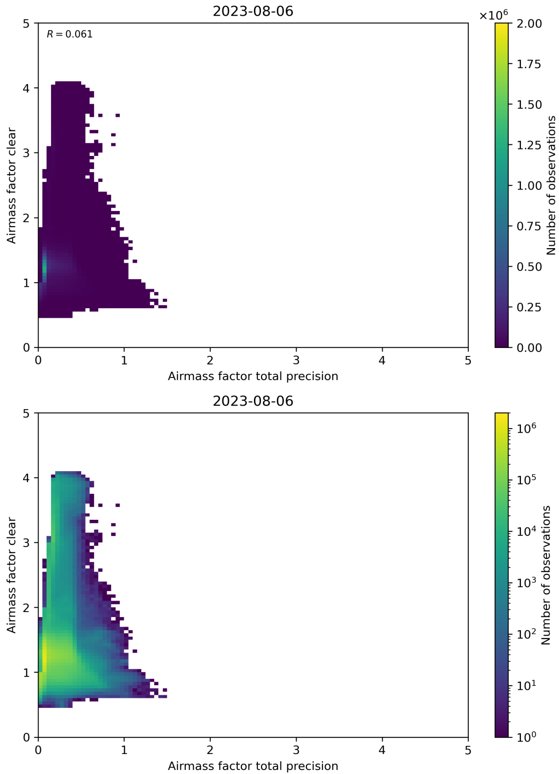
Figure 108: Scatter density plot of “Airmass factor total precision” against “Airmass factor clear” for 2023-08-05 to 2023-08-07.
