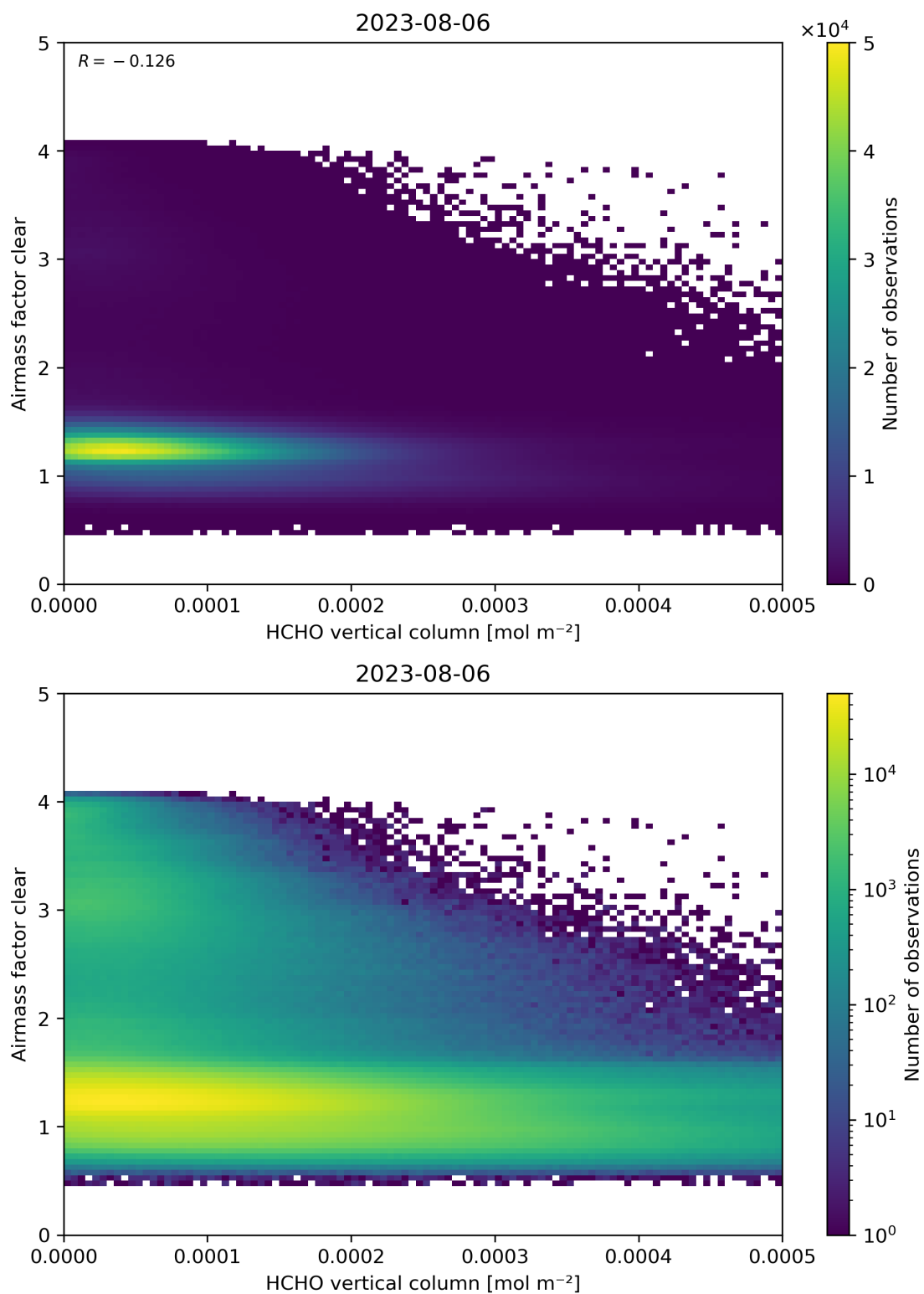
Figure 126: Scatter density plot of “HCHO vertical column” against “Airmass factor clear” for 2023-08-05 to 2023-08-07.
