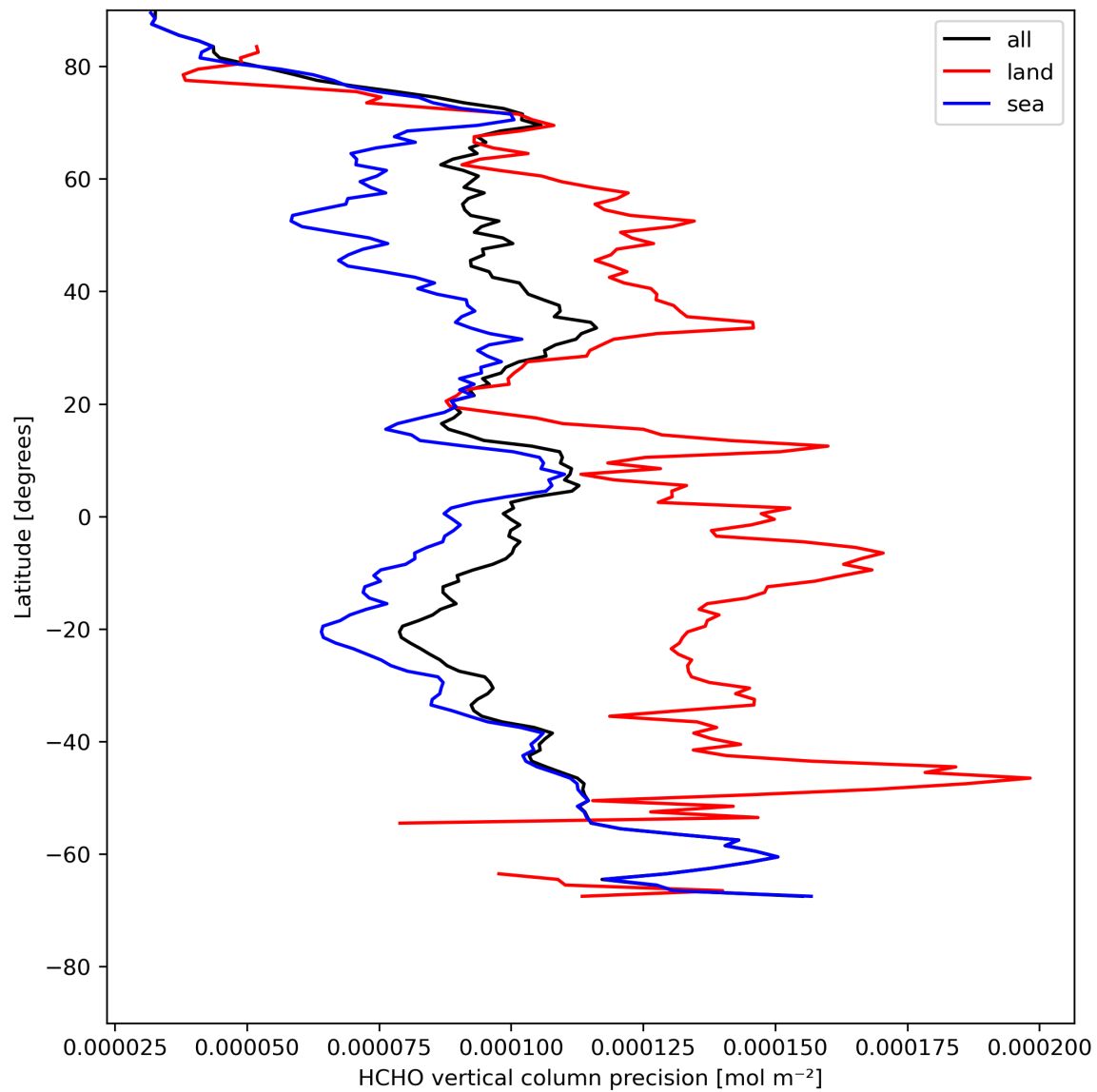
Figure 22: Zonal average of “HCHO vertical column precision” for 2023-08-05 to 2023-08-07.
