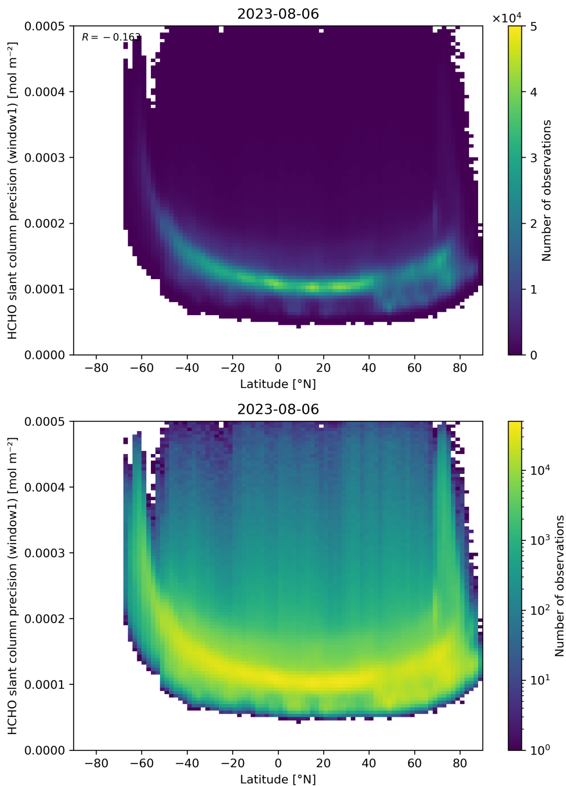
Figure 160: Scatter density plot of “Latitude” against “HCHO slant column precision (window1)” for 2023-08-05 to 2023-08-07.
