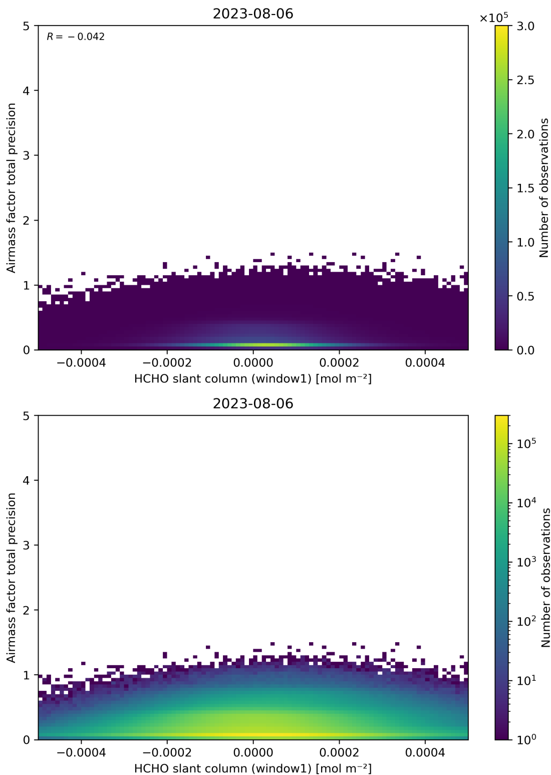
Figure 86: Scatter density plot of “HCHO slant column (window1)” against “Airmass factor total precision” for 2023-08-05 to 2023-08-07.
