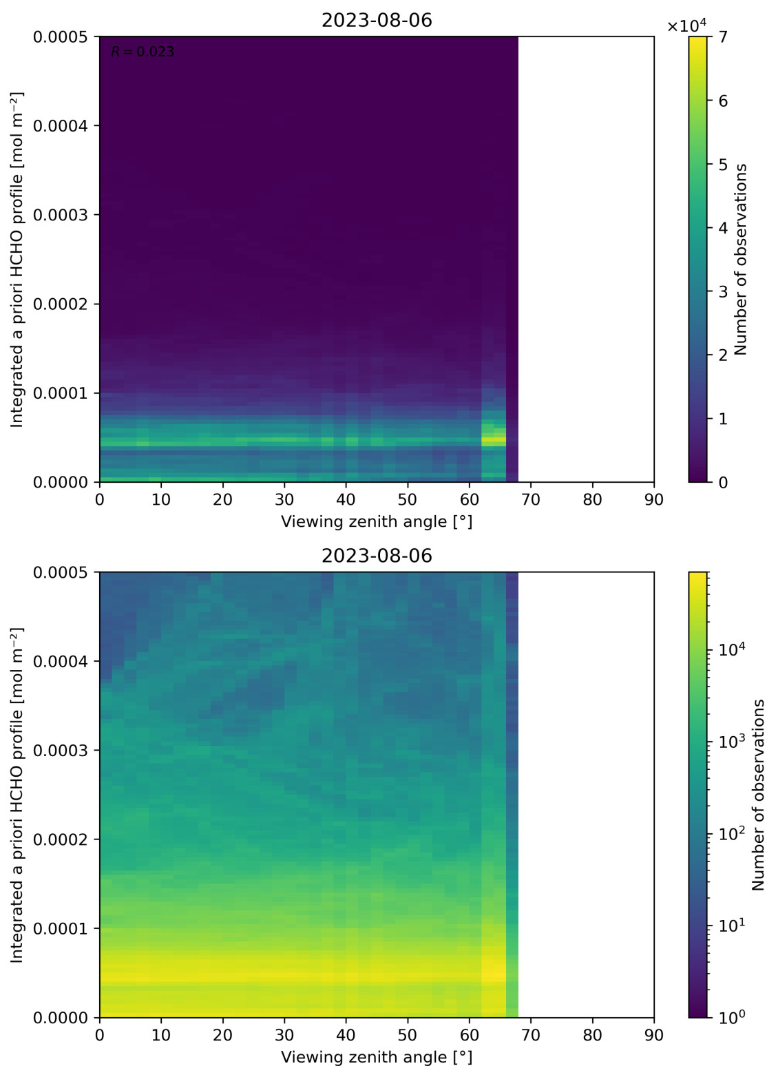
Figure 195: Scatter density plot of “Viewing zenith angle” against “Integrated a priori HCHO profile” for 2023-08-05 to 2023-08-07.
