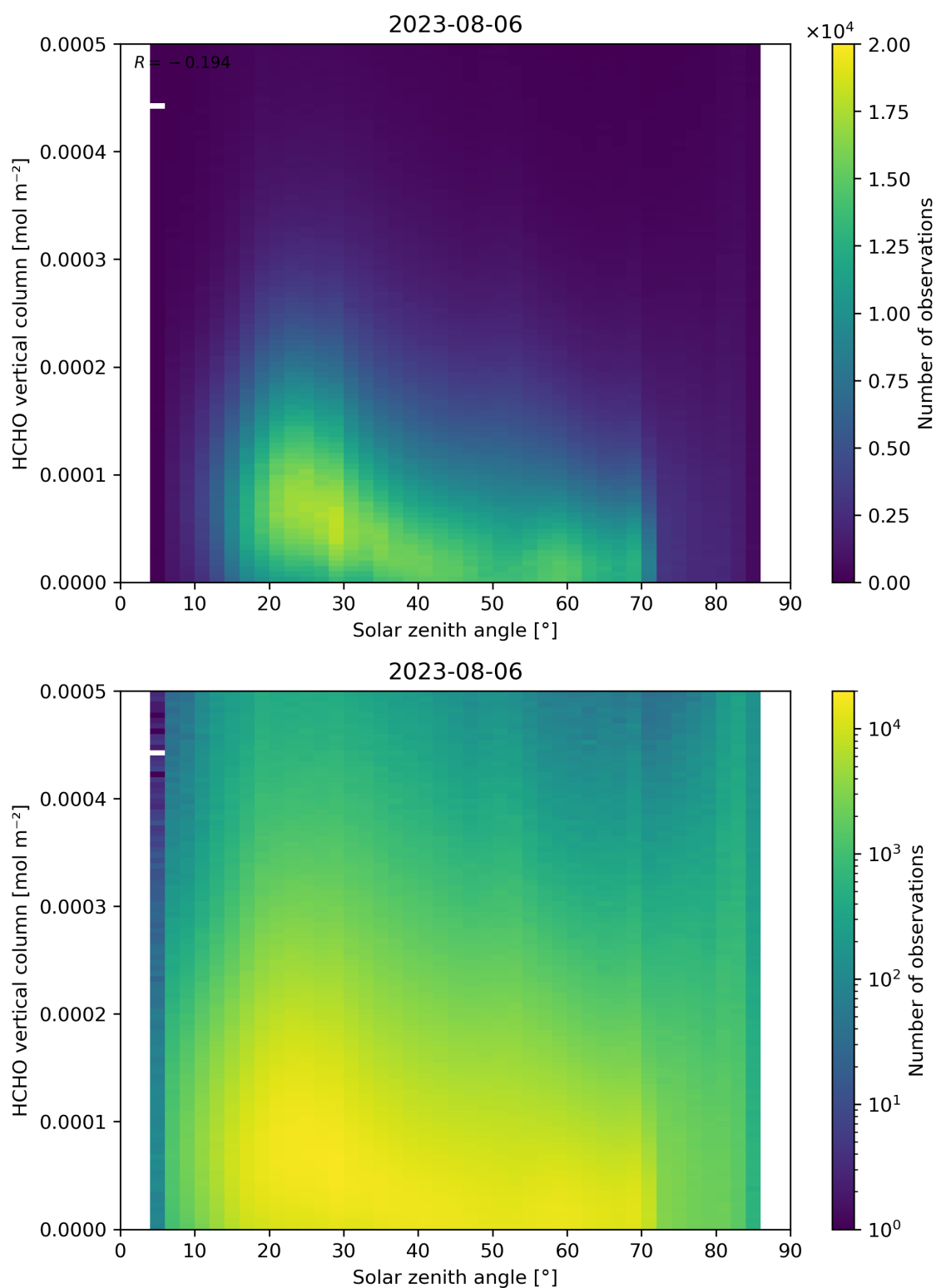
Figure 177: Scatter density plot of “Solar zenith angle” against “HCHO vertical column” for 2023-08-05 to 2023-08-07.
