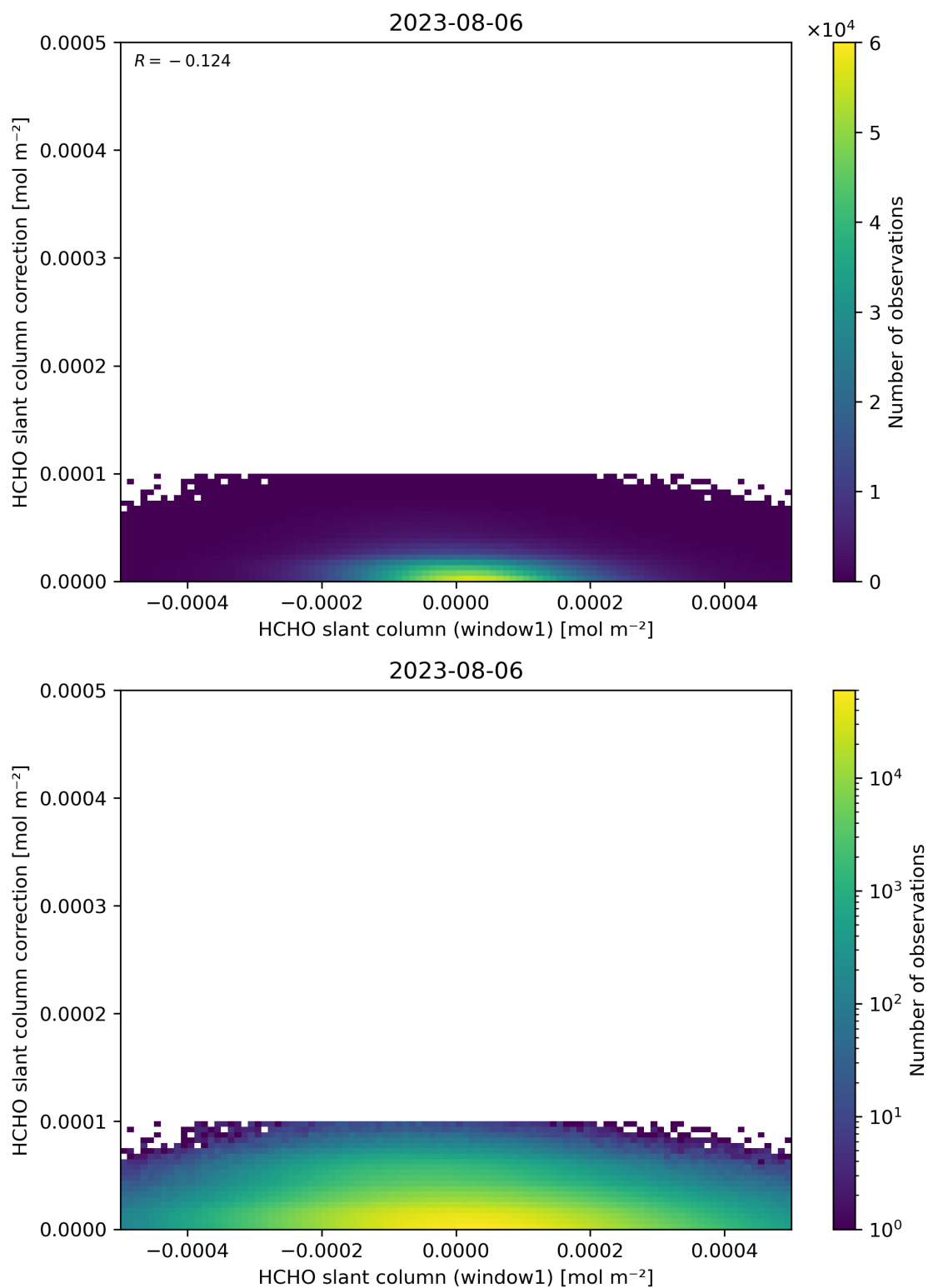
Figure 83: Scatter density plot of “HCHO slant column (window1)” against “HCHO slant column correction” for 2023-08-05 to 2023-08-07.
