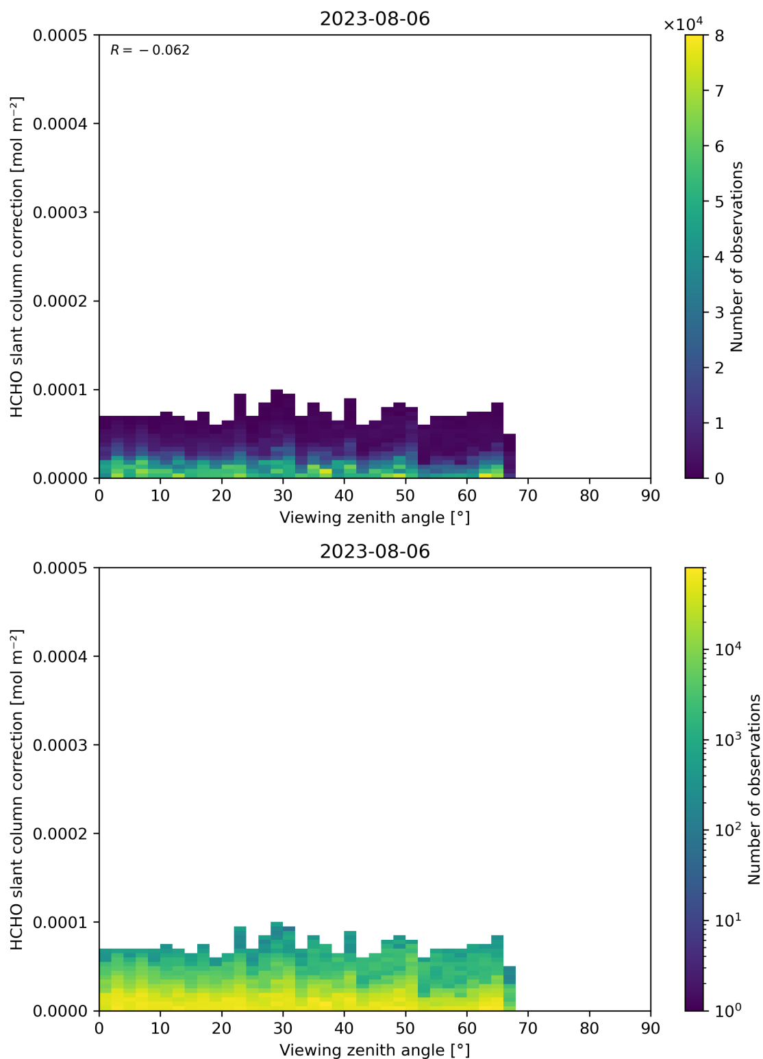
Figure 187: Scatter density plot of “Viewing zenith angle” against “HCHO slant column correction” for 2023-08-05 to 2023-08-07.
