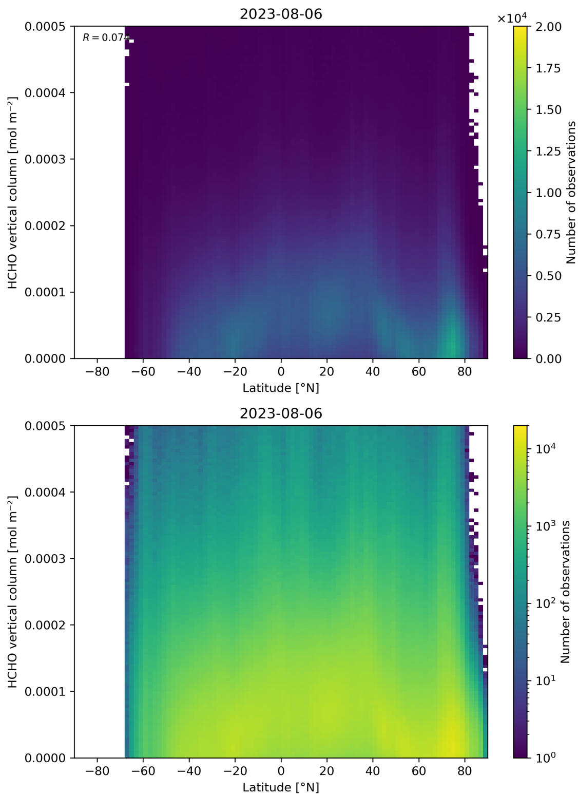
Figure 163: Scatter density plot of “Latitude” against “HCHO vertical column” for 2023-08-05 to 2023-08-07.
