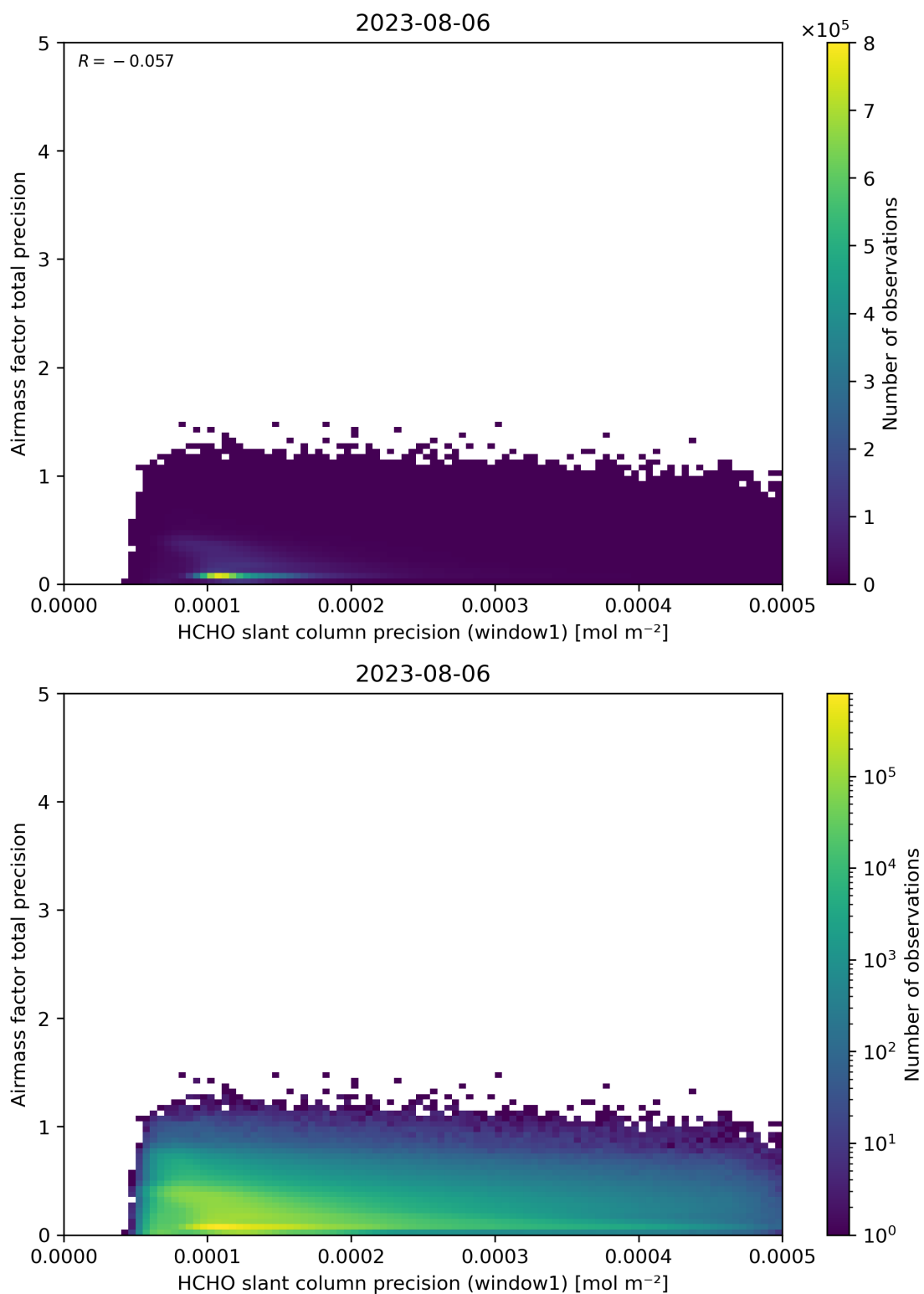
Figure 95: Scatter density plot of “HCHO slant column precision (window1)” against “Airmass factor total precision” for 2023-08-05 to 2023-08-07.
