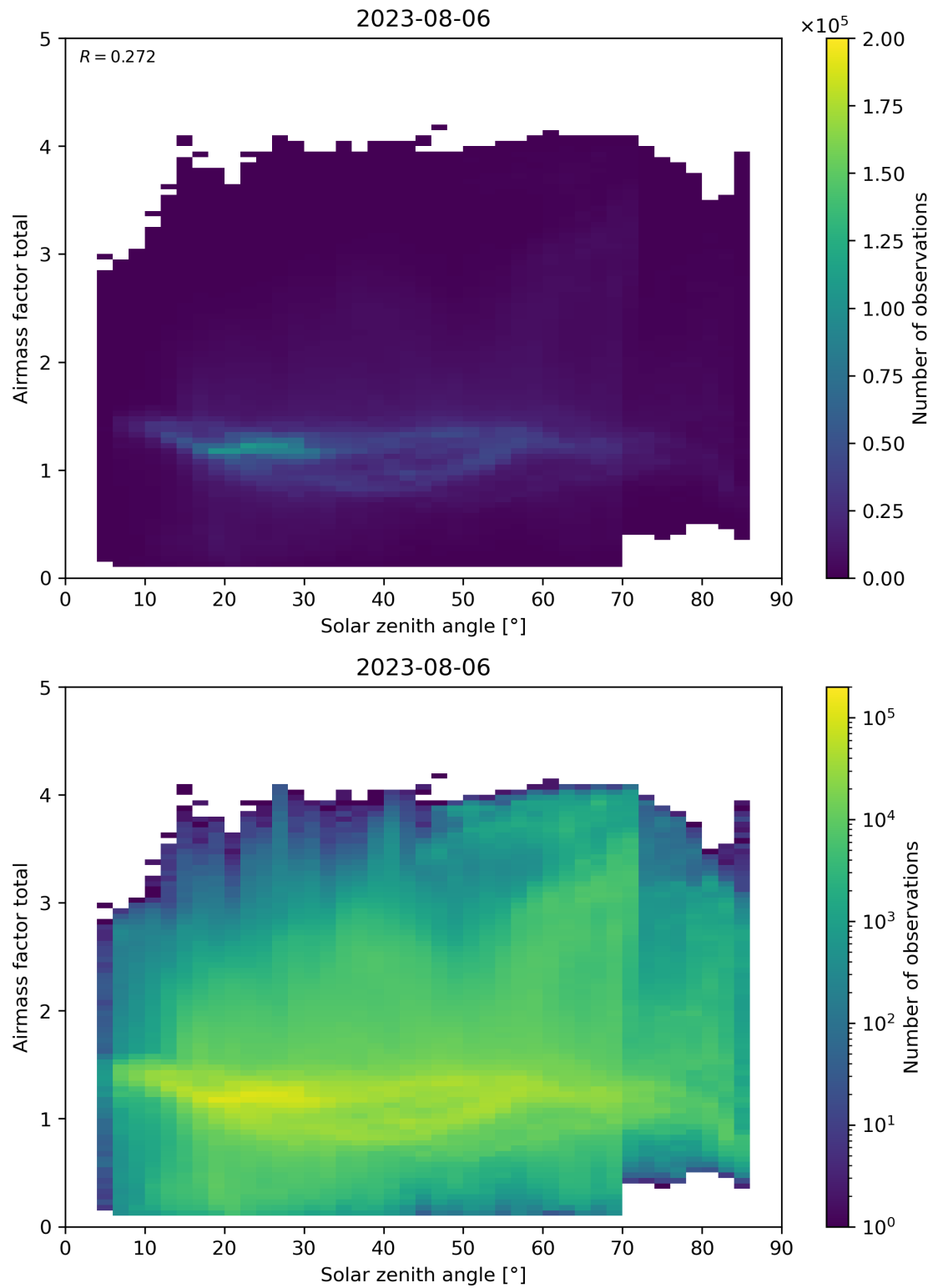
Figure 175: Scatter density plot of “Solar zenith angle” against “Airmass factor total” for 2023-08-05 to 2023-08-07.
