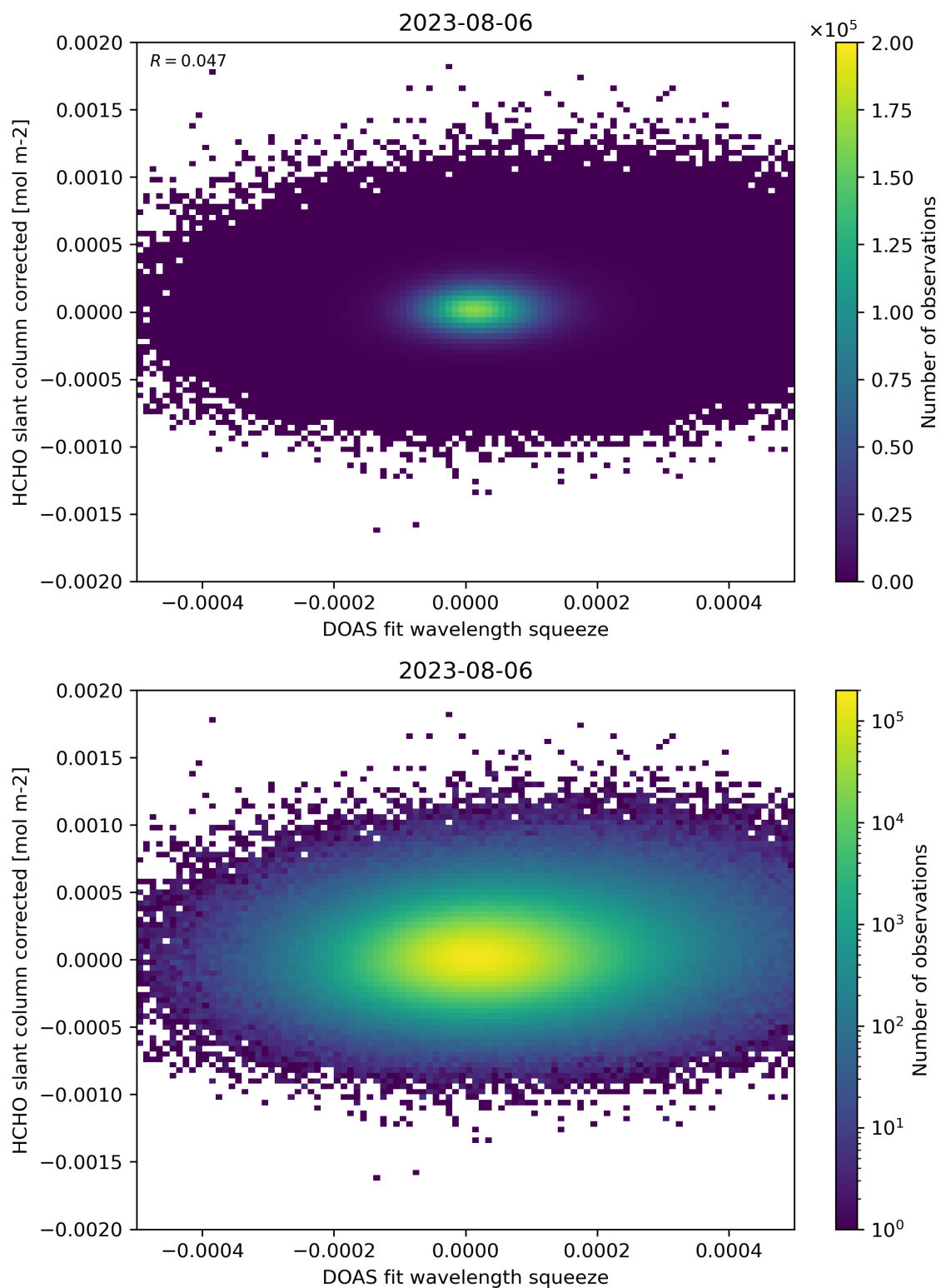
Figure 69: Scatter density plot of “DOAS fit wavelength squeeze” against “HCHO slant column corrected” for 2023-08-05 to 2023-08-07.
