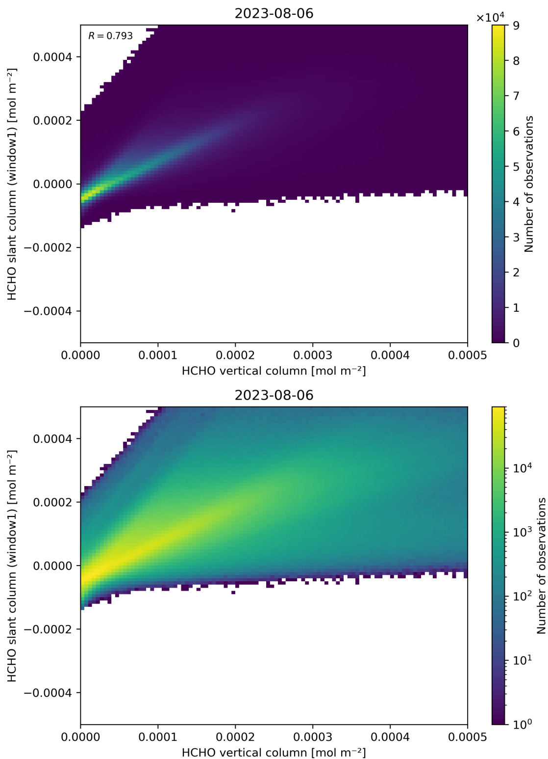
Figure 129: Scatter density plot of “HCHO vertical column” against “HCHO slant column (window1)” for 2023-08-05 to 2023-08-07.
