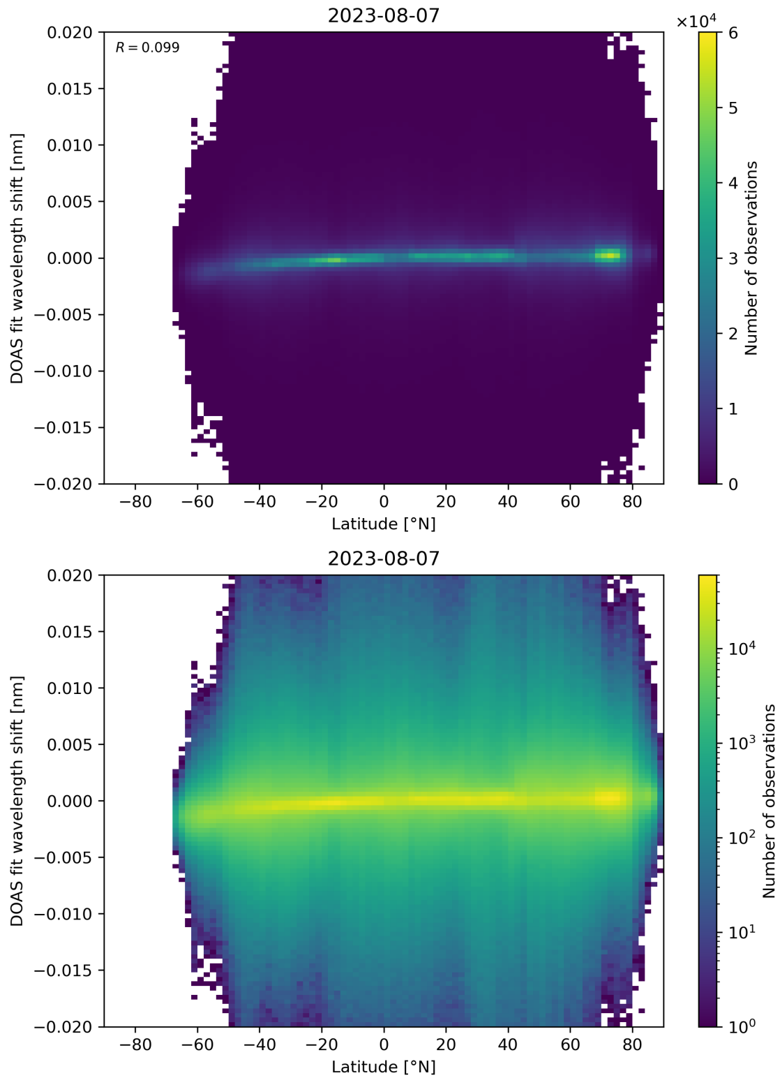
Figure 154: Scatter density plot of “Latitude” against “DOAS fit wavelength shift” for 2023-08-06 to 2023-08-08.
