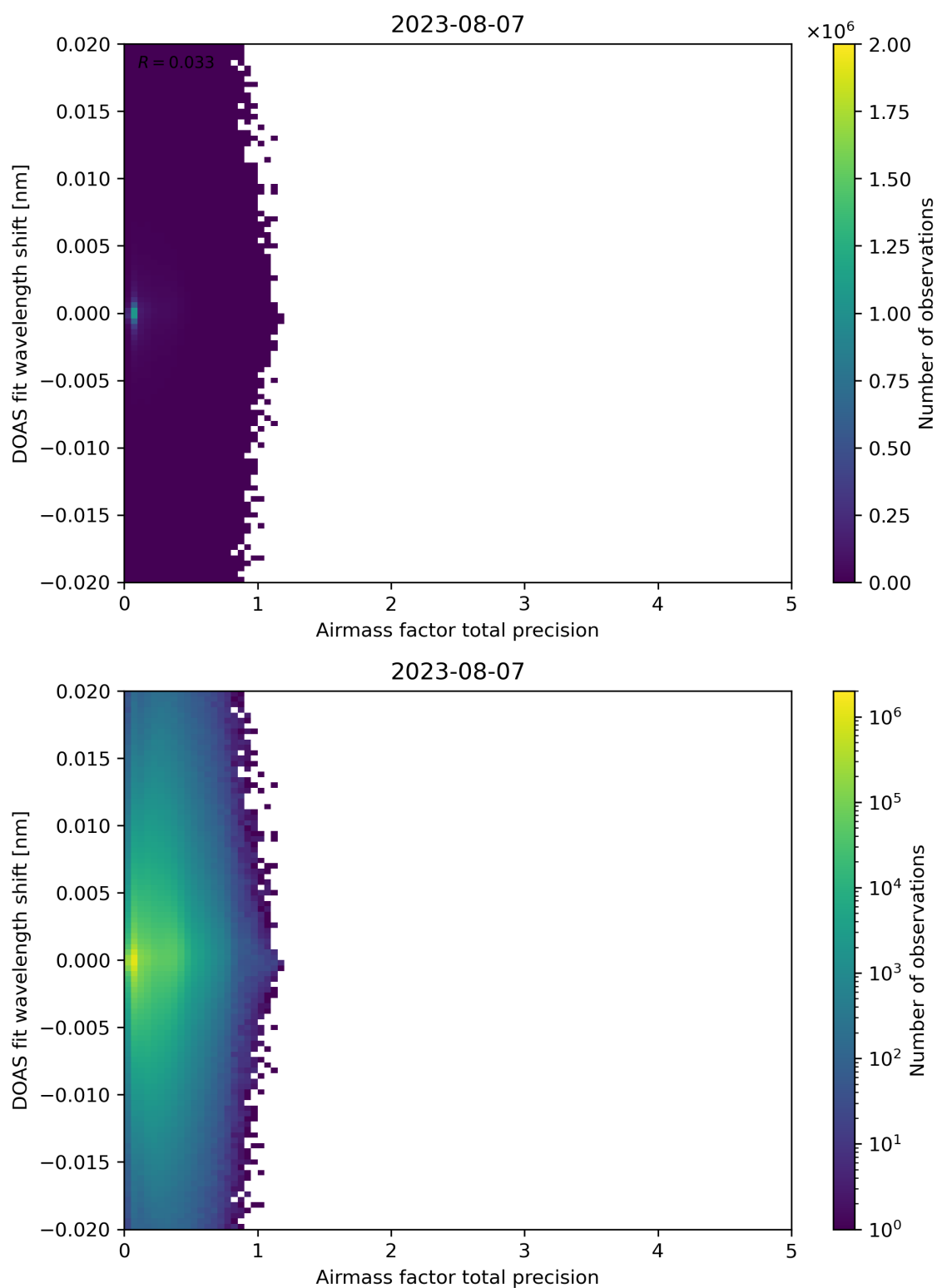
Figure 106: Scatter density plot of “Airmass factor total precision” against “DOAS fit wavelength shift” for 2023-08-06 to 2023-08-08.
