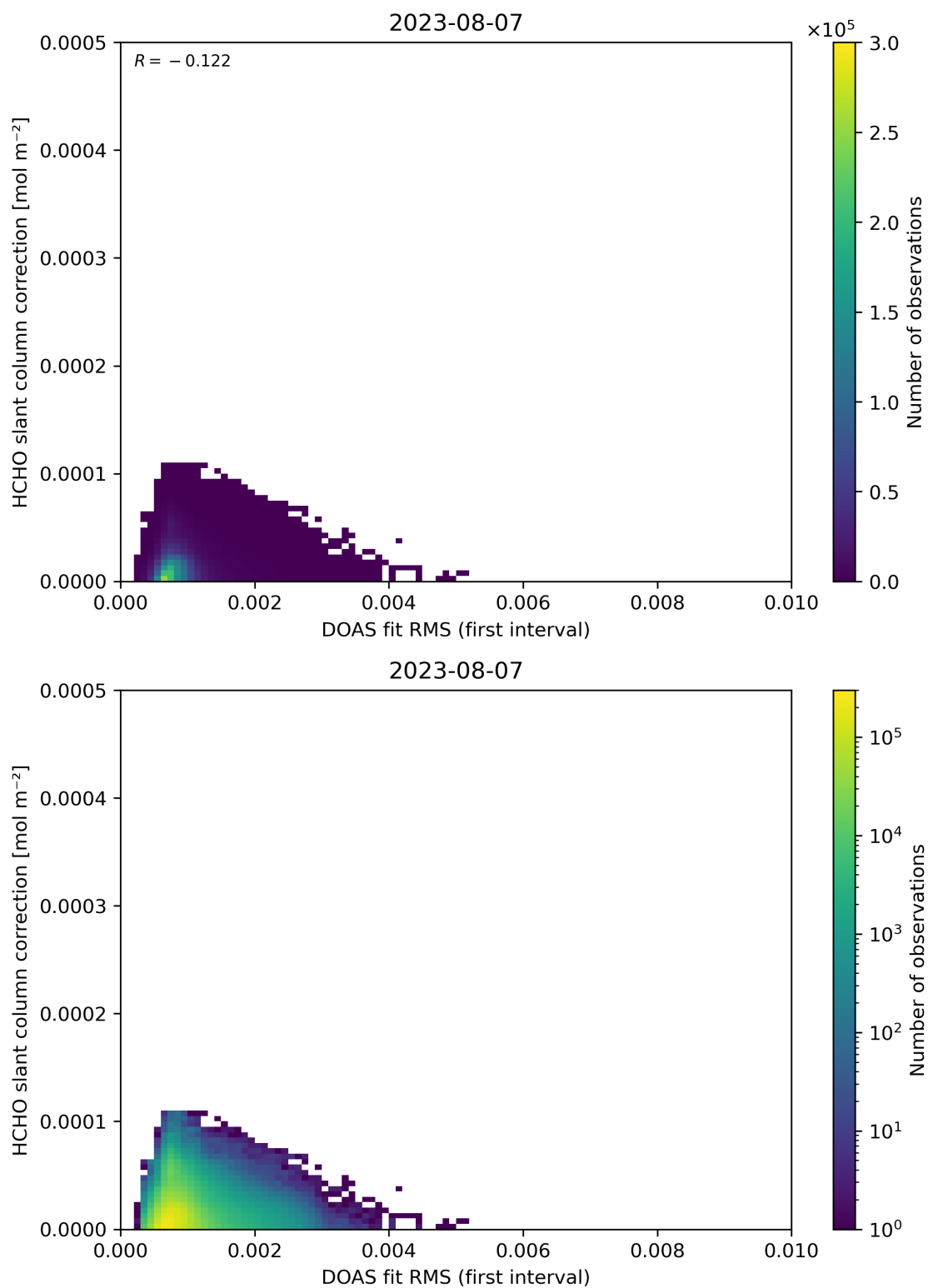
Figure 63: Scatter density plot of “DOAS fit RMS (first interval)” against “HCHO slant column correction” for 2023-08-06 to 2023-08-08.
