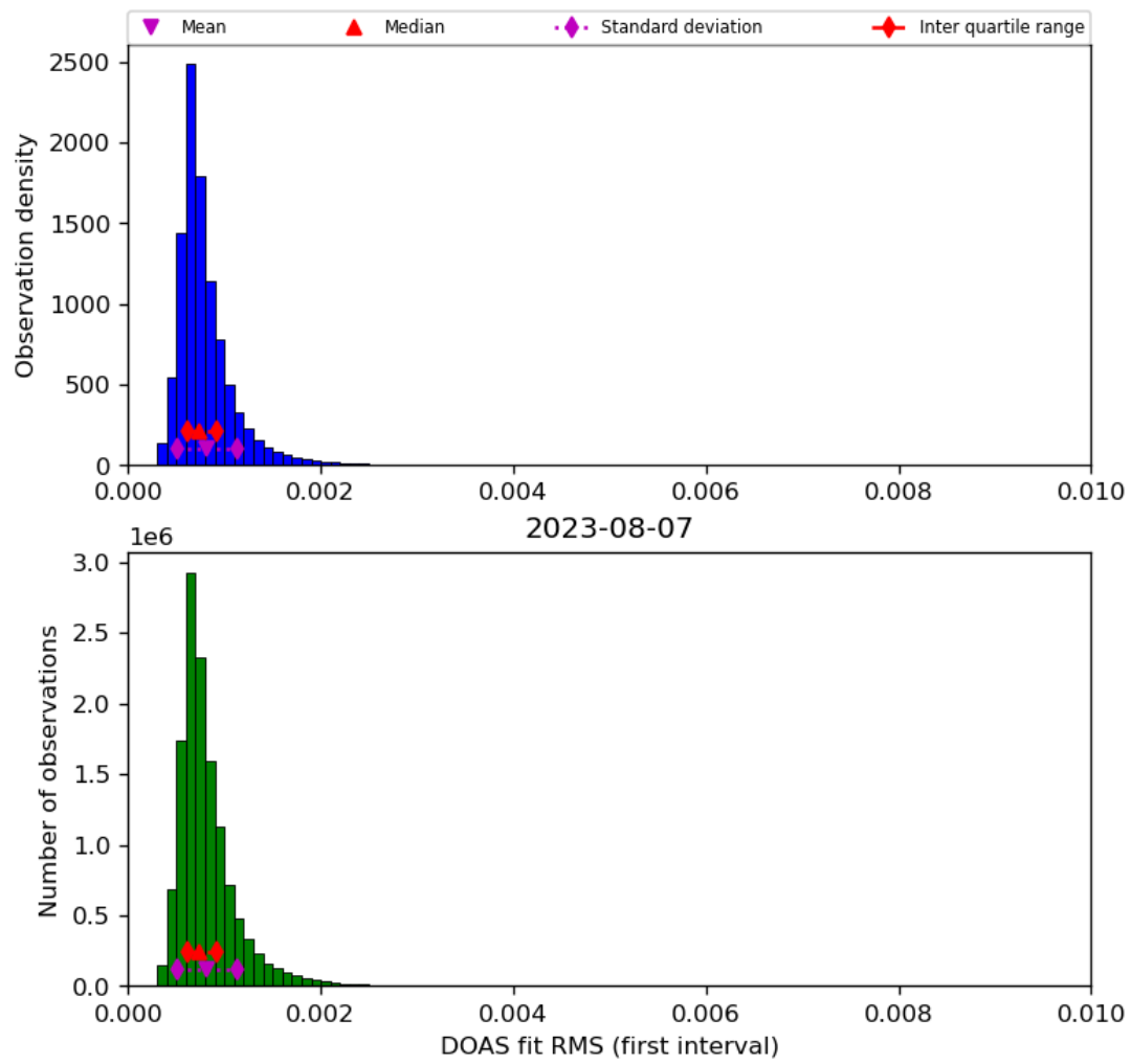
Figure 46: Histogram of “DOAS fit RMS (first interval)” for 2023-08-06 to 2023-08-08
