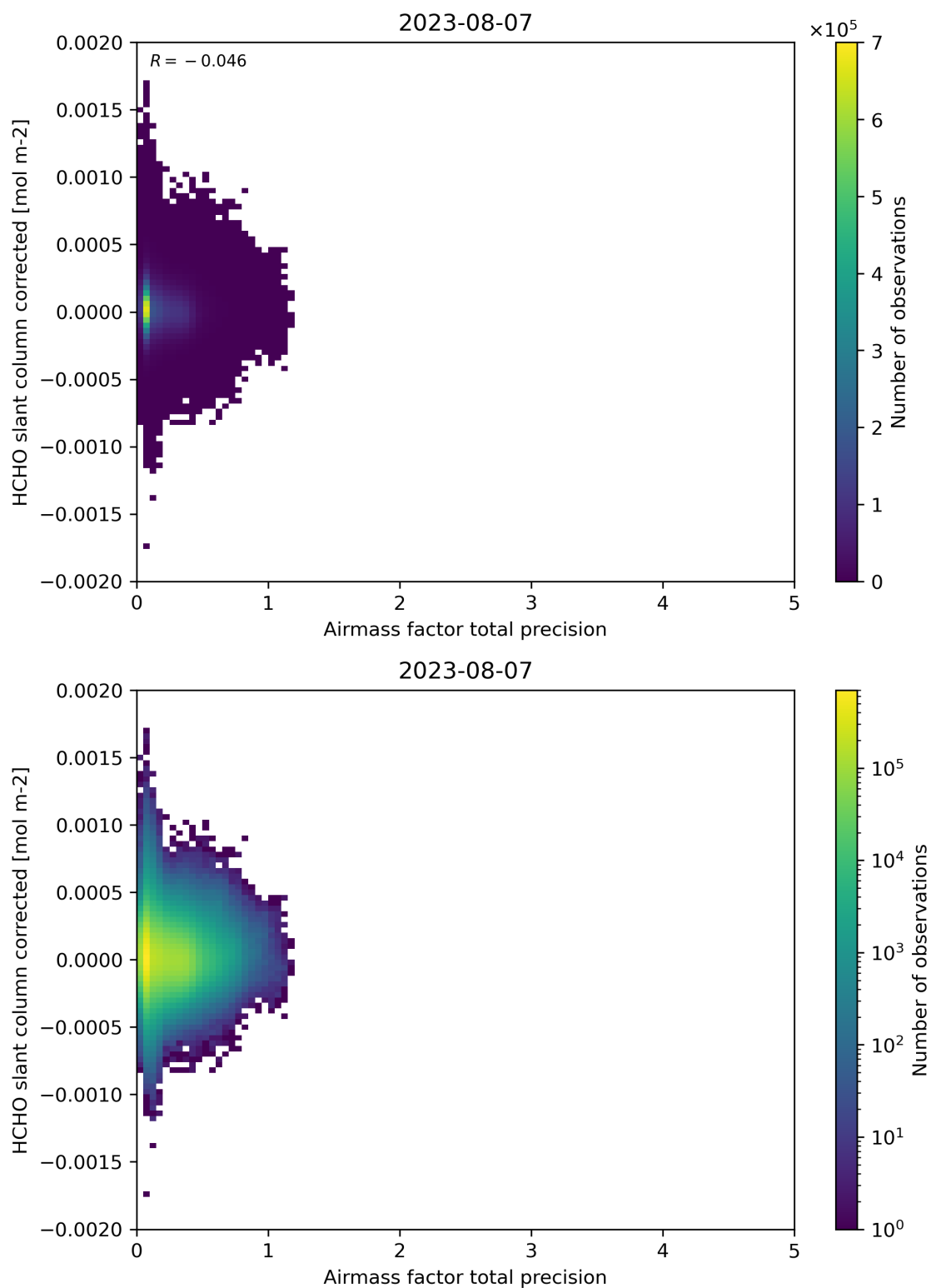
Figure 109: Scatter density plot of “Airmass factor total precision” against “HCHO slant column corrected” for 2023-08-06 to 2023-08-08.
