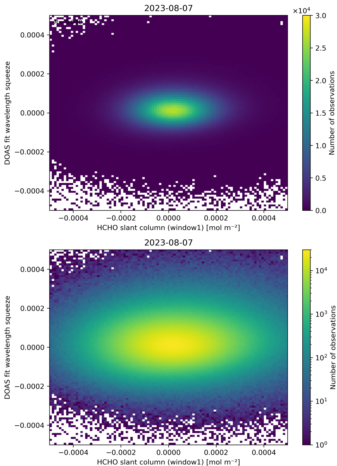
Figure 80: Scatter density plot of “HCHO slant column (window1)” against “DOAS fit wavelength squeeze” for 2023-08-06 to 2023-08-08.
