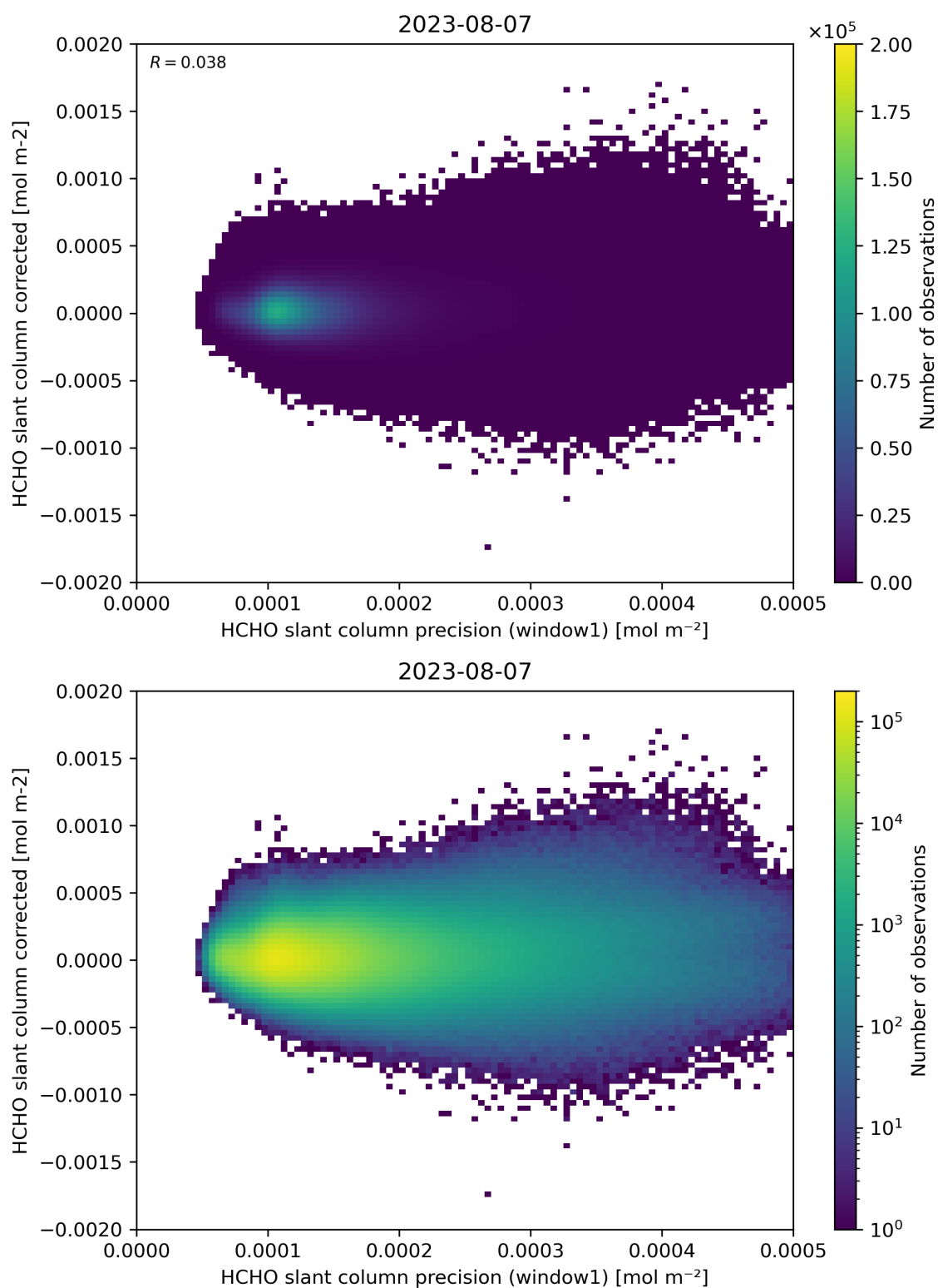
Figure 92: Scatter density plot of “HCHO slant column precision (window1)” against “HCHO slant column corrected” for 2023-08-06 to 2023-08-08.
