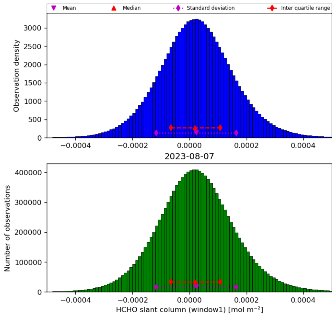
Figure 38: Histogram of “HCHO slant column (window1)” for 2023-08-06 to 2023-08-08
