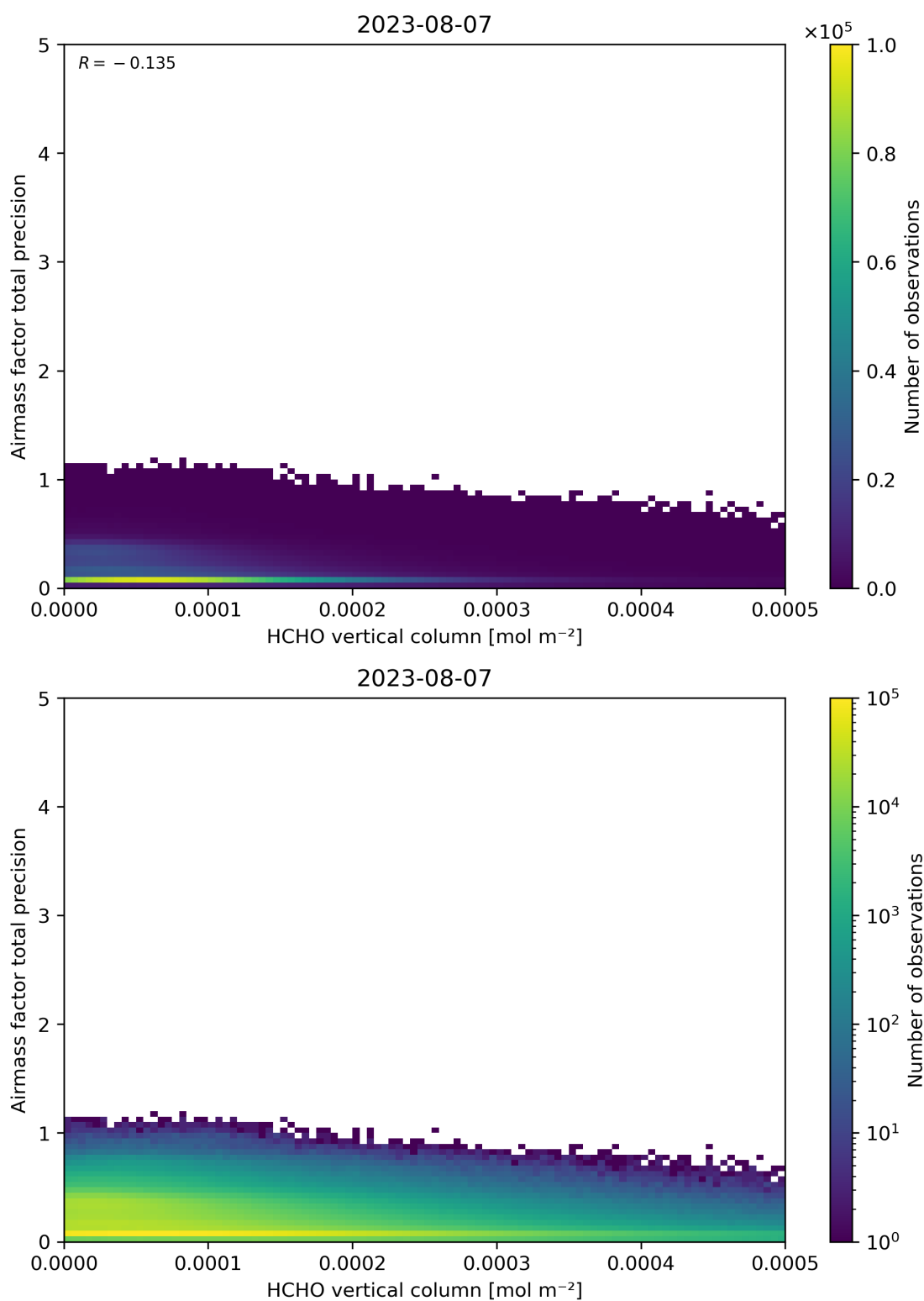
Figure 132: Scatter density plot of “HCHO vertical column” against “Airmass factor total precision” for 2023-08-06 to 2023-08-08.
