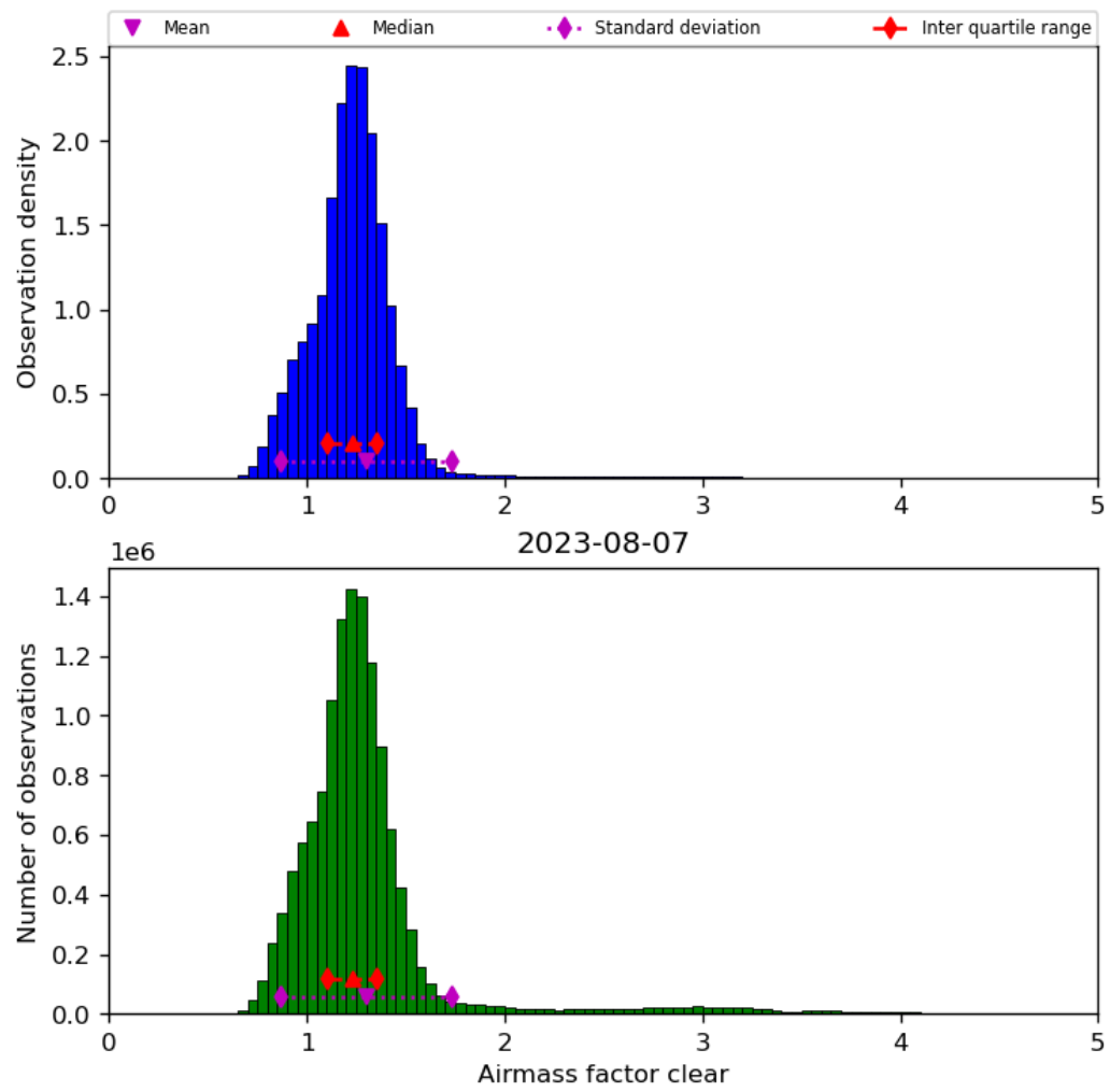
Figure 42: Histogram of “Airmass factor clear” for 2023-08-06 to 2023-08-08
