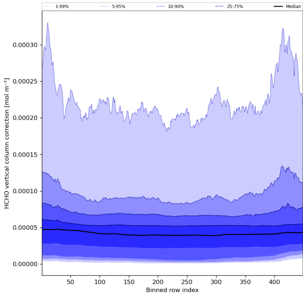
Figure 51: Along track statistics of “HCHO vertical column correction” for 2023-08-06 to 2023-08-08
