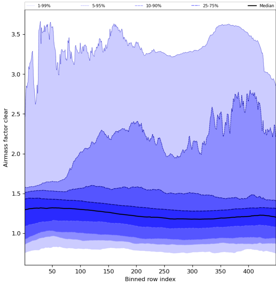
Figure 56: Along track statistics of “Airmass factor clear” for 2023-08-06 to 2023-08-08
