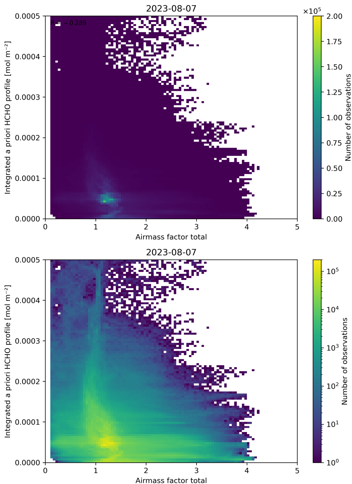
Figure 104: Scatter density plot of “Airmass factor total” against “Integrated a priori HCHO profile” for 2023-08-06 to 2023-08-08.
