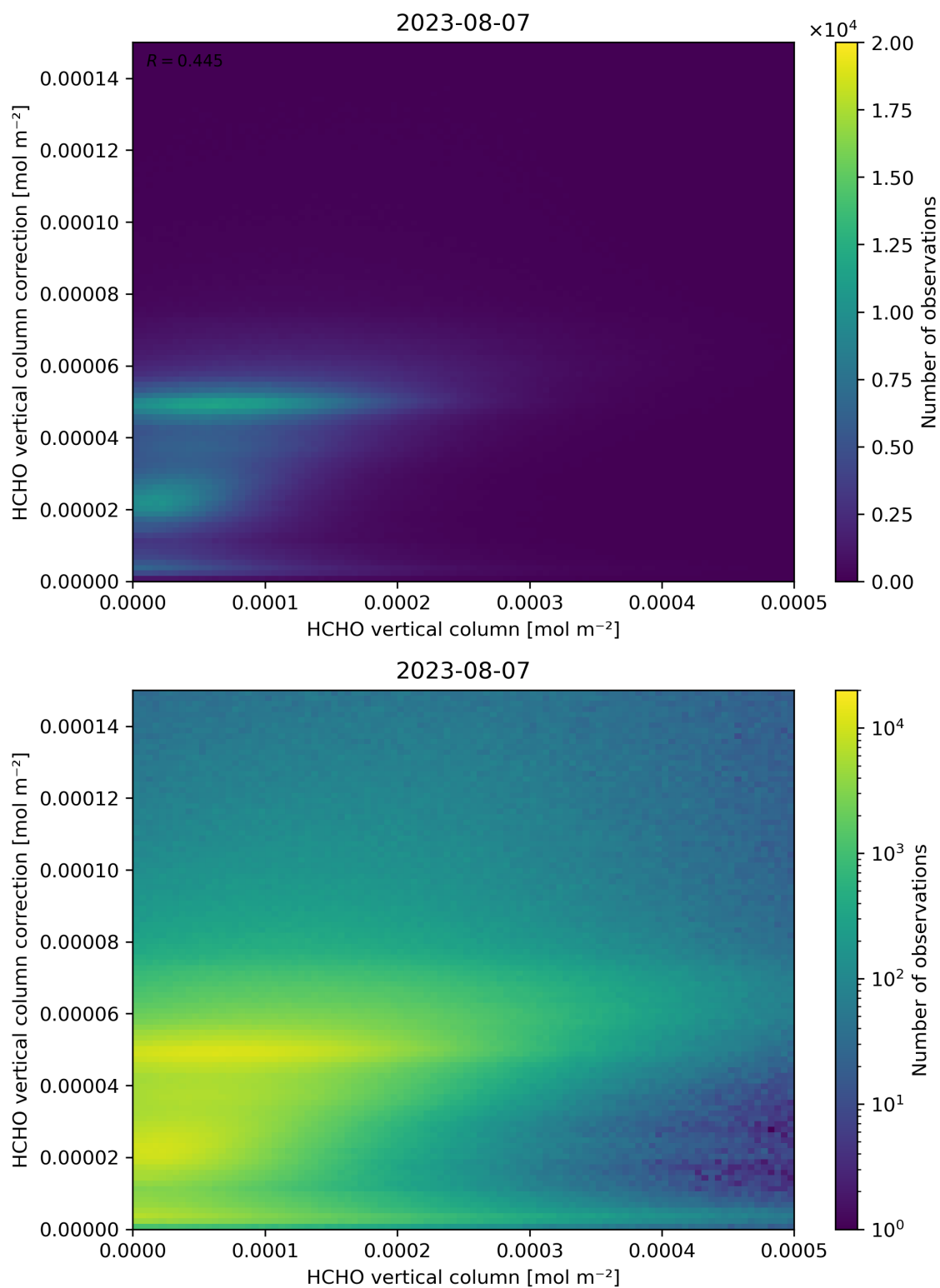
Figure 133: Scatter density plot of “HCHO vertical column” against “HCHO vertical column correction” for 2023-08-06 to 2023-08-08.
