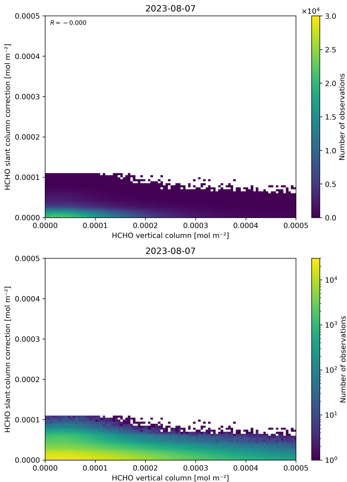
Figure 128: Scatter density plot of “HCHO vertical column” against “HCHO slant column correction” for 2023-08-06 to 2023-08-08.
