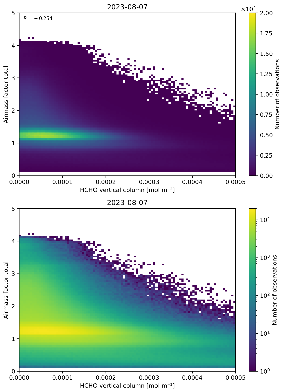
Figure 131: Scatter density plot of “HCHO vertical column” against “Airmass factor total” for 2023-08-06 to 2023-08-08.
