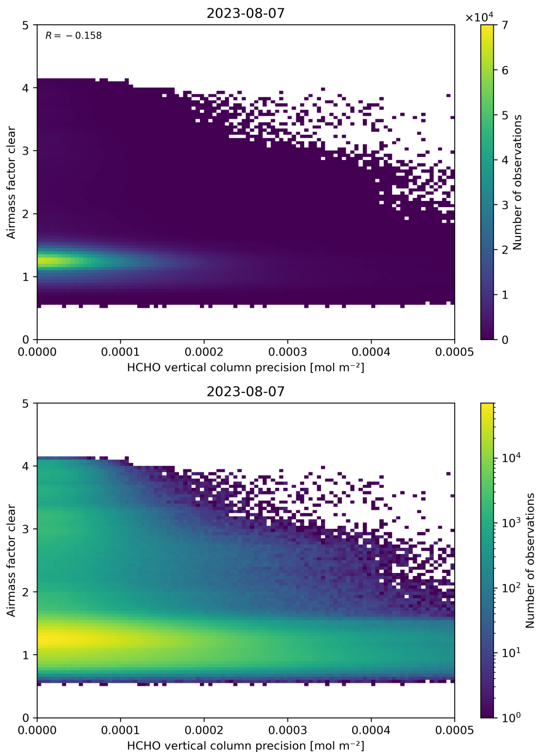
Figure 139: Scatter density plot of “HCHO vertical column precision” against “Airmass factor clear” for 2023-08-06 to 2023-08-08.
