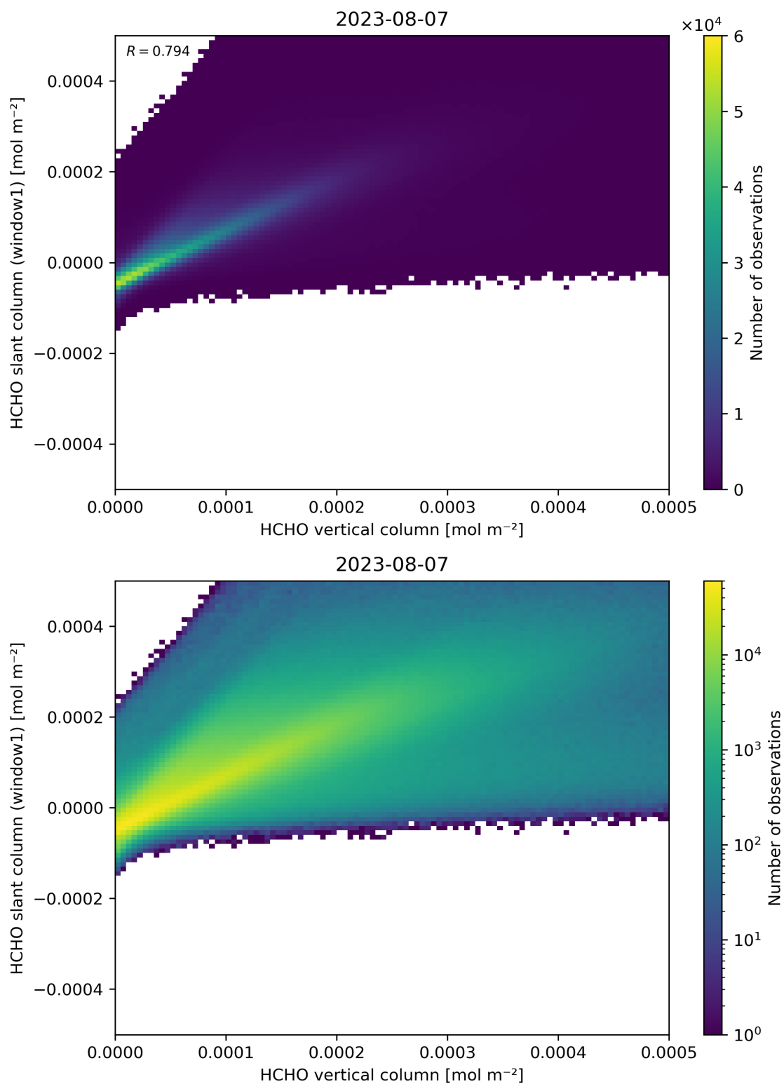
Figure 129: Scatter density plot of “HCHO vertical column” against “HCHO slant column (window1)” for 2023-08-06 to 2023-08-08.
