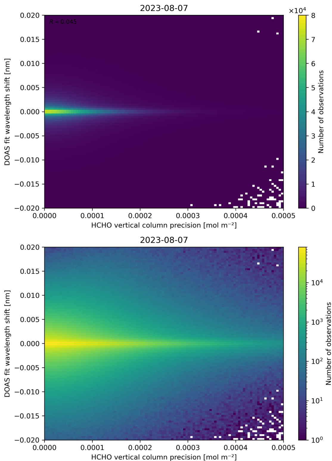
Figure 137: Scatter density plot of “HCHO vertical column precision” against “DOAS fit wavelength shift” for 2023-08-06 to 2023-08-08.
