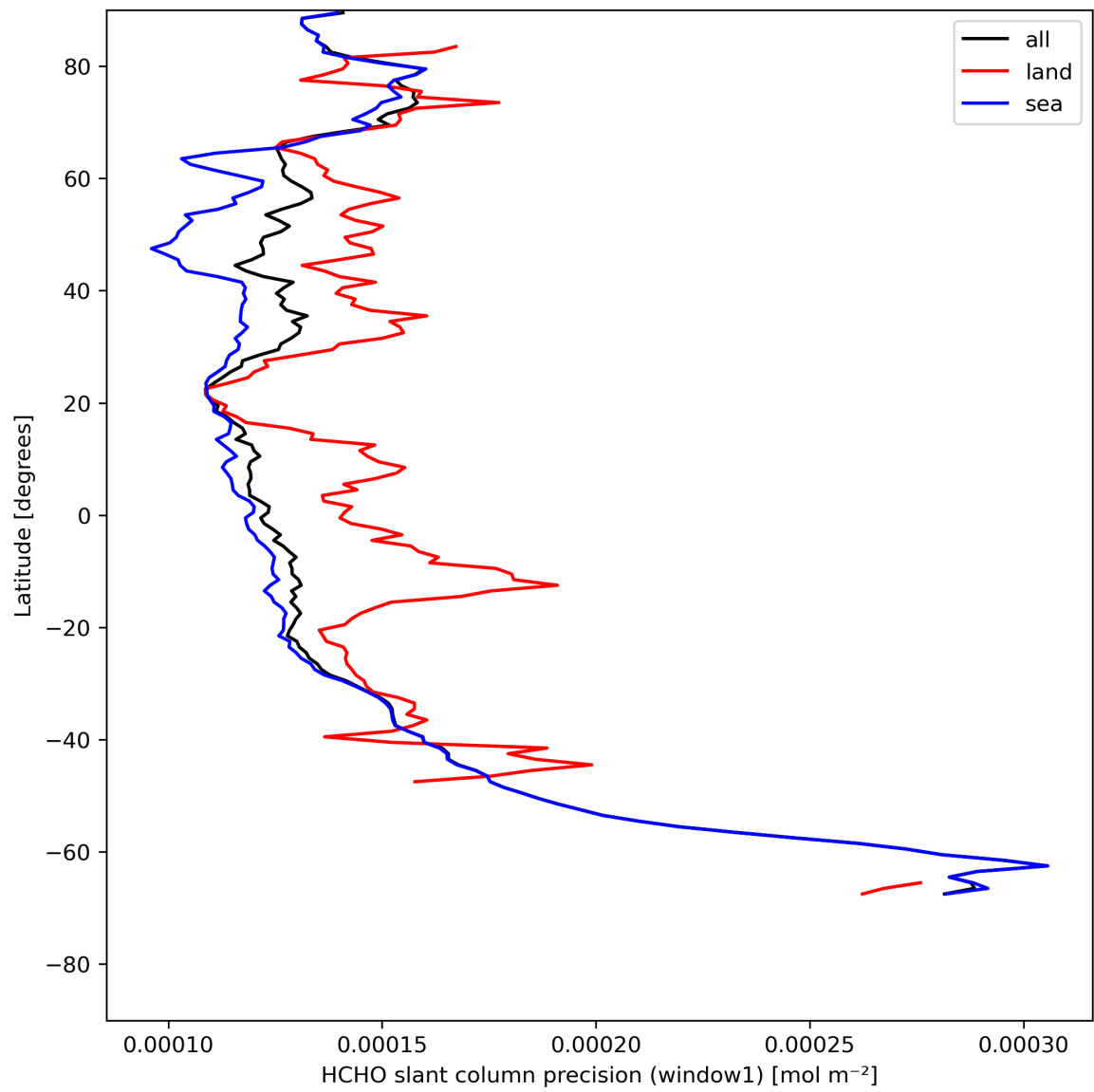
Figure 25: Zonal average of “HCHO slant column precision (window1)” for 2023-08-06 to 2023-08-08.
