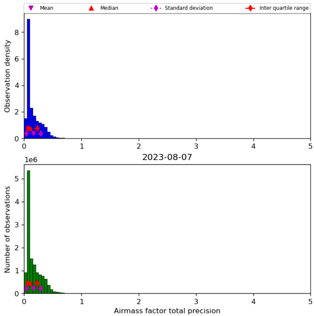
Figure 41: Histogram of “Airmass factor total precision” for 2023-08-06 to 2023-08-08
