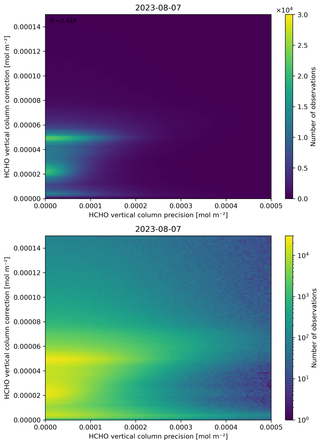
Figure 146: Scatter density plot of “HCHO vertical column precision” against “HCHO vertical column correction” for 2023-08-06 to 2023-08-08.
