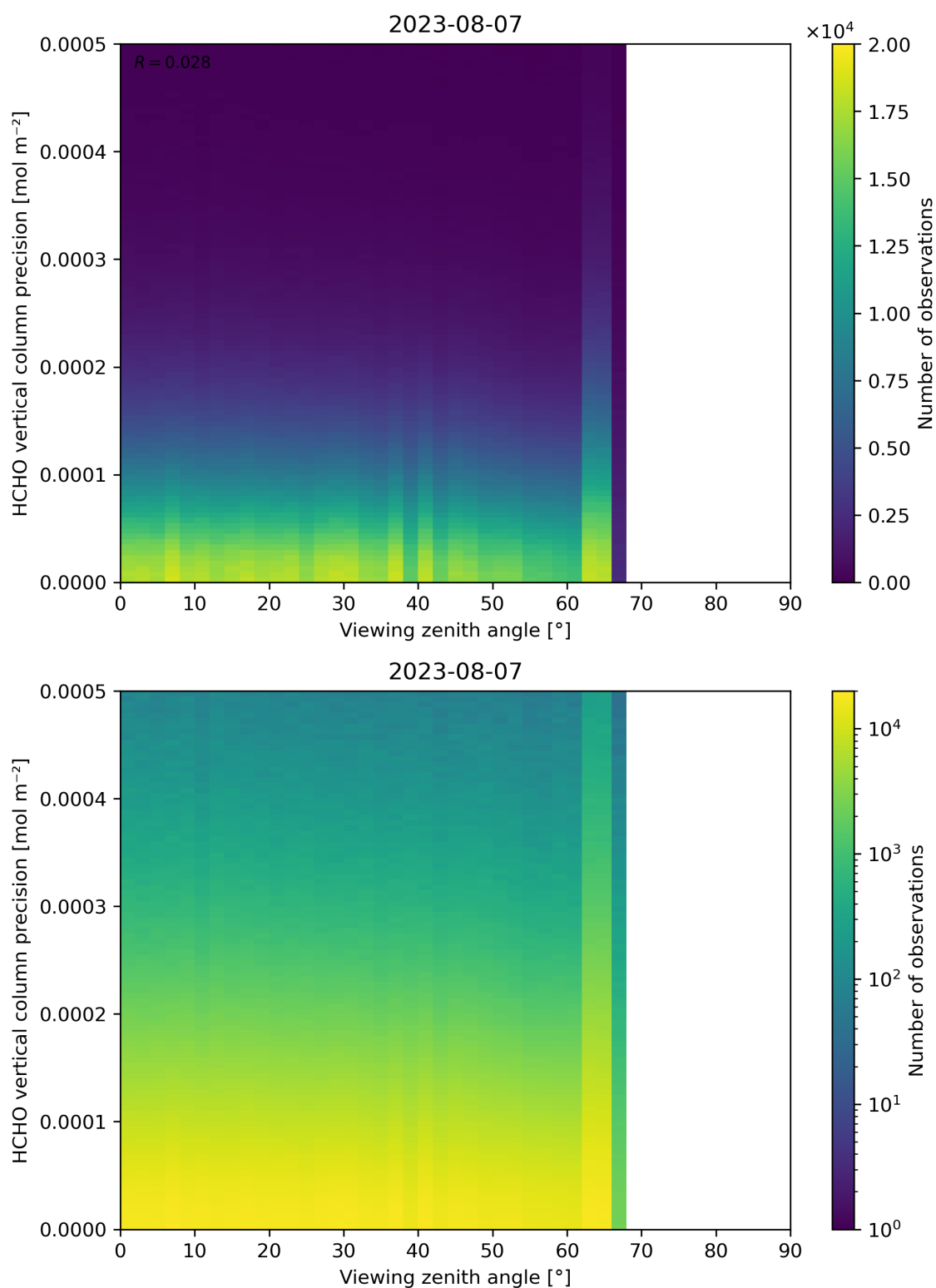
Figure 194: Scatter density plot of “Viewing zenith angle” against “HCHO vertical column precision” for 2023-08-06 to 2023-08-08.
