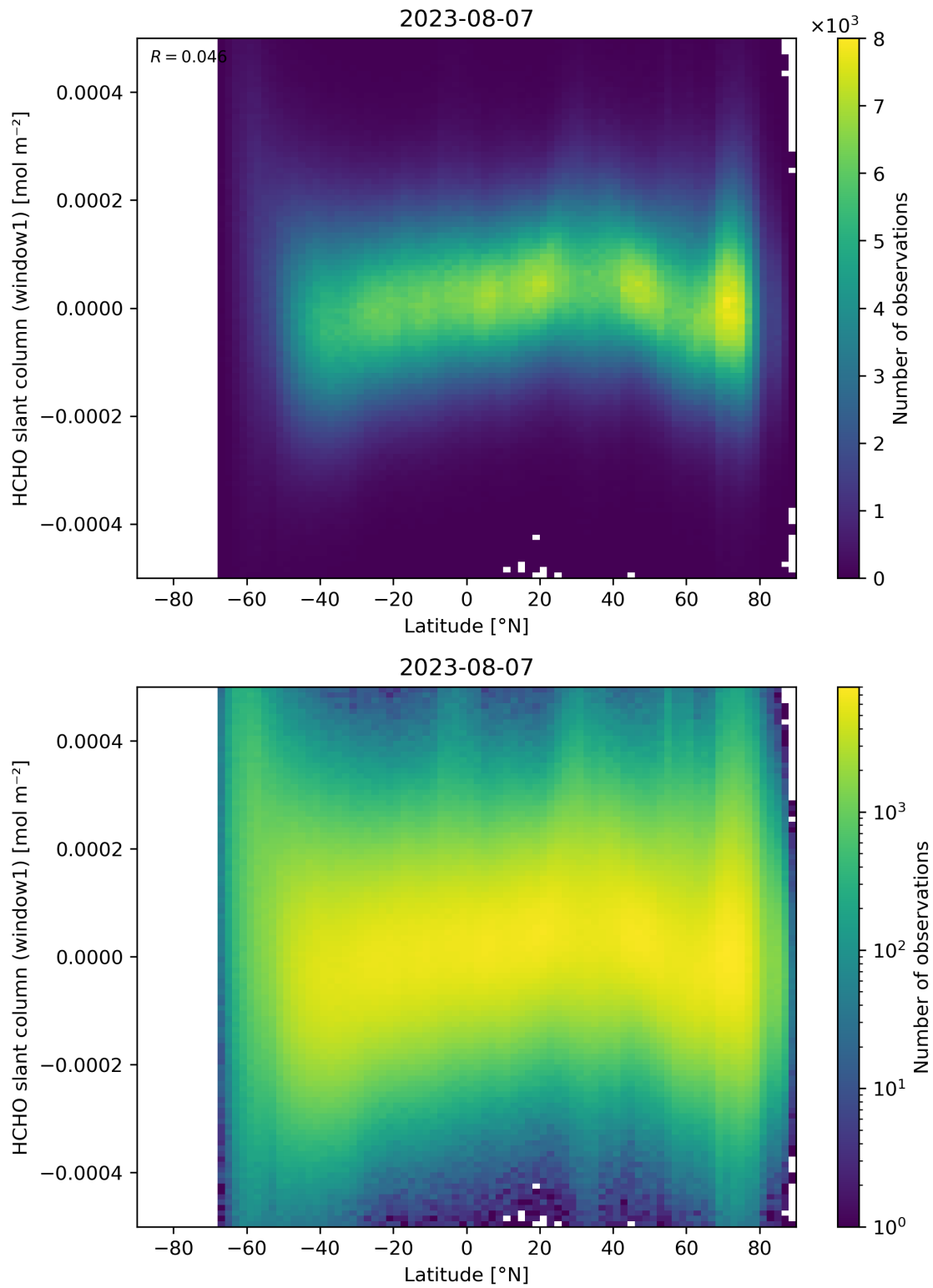
Figure 159: Scatter density plot of “Latitude” against “HCHO slant column (window1)” for 2023-08-06 to 2023-08-08.
