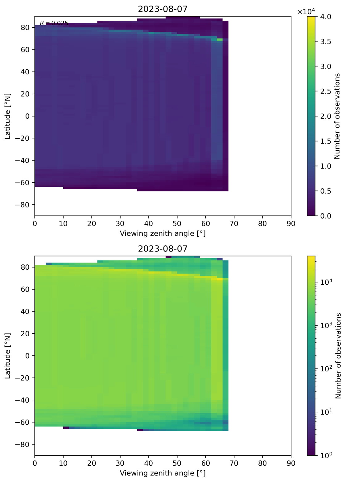
Figure 196: Scatter density plot of “Viewing zenith angle” against “Latitude” for 2023-08-06 to 2023-08-08.
