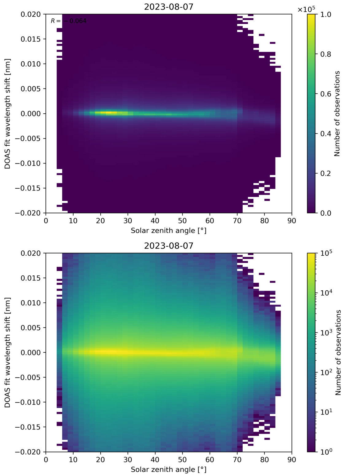
Figure 168: Scatter density plot of “Solar zenith angle” against “DOAS fit wavelength shift” for 2023-08-06 to 2023-08-08.
