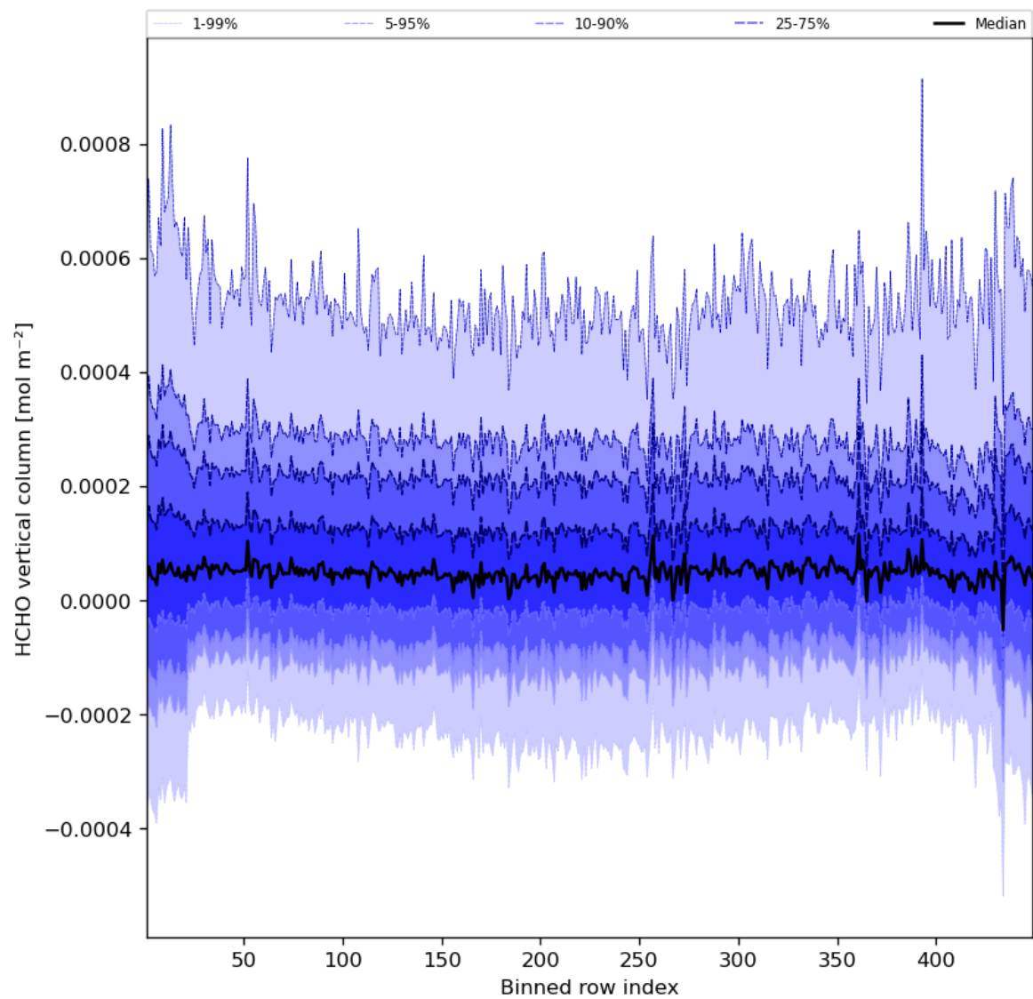
Figure 49: Along track statistics of “HCHO vertical column” for 2023-08-06 to 2023-08-08
