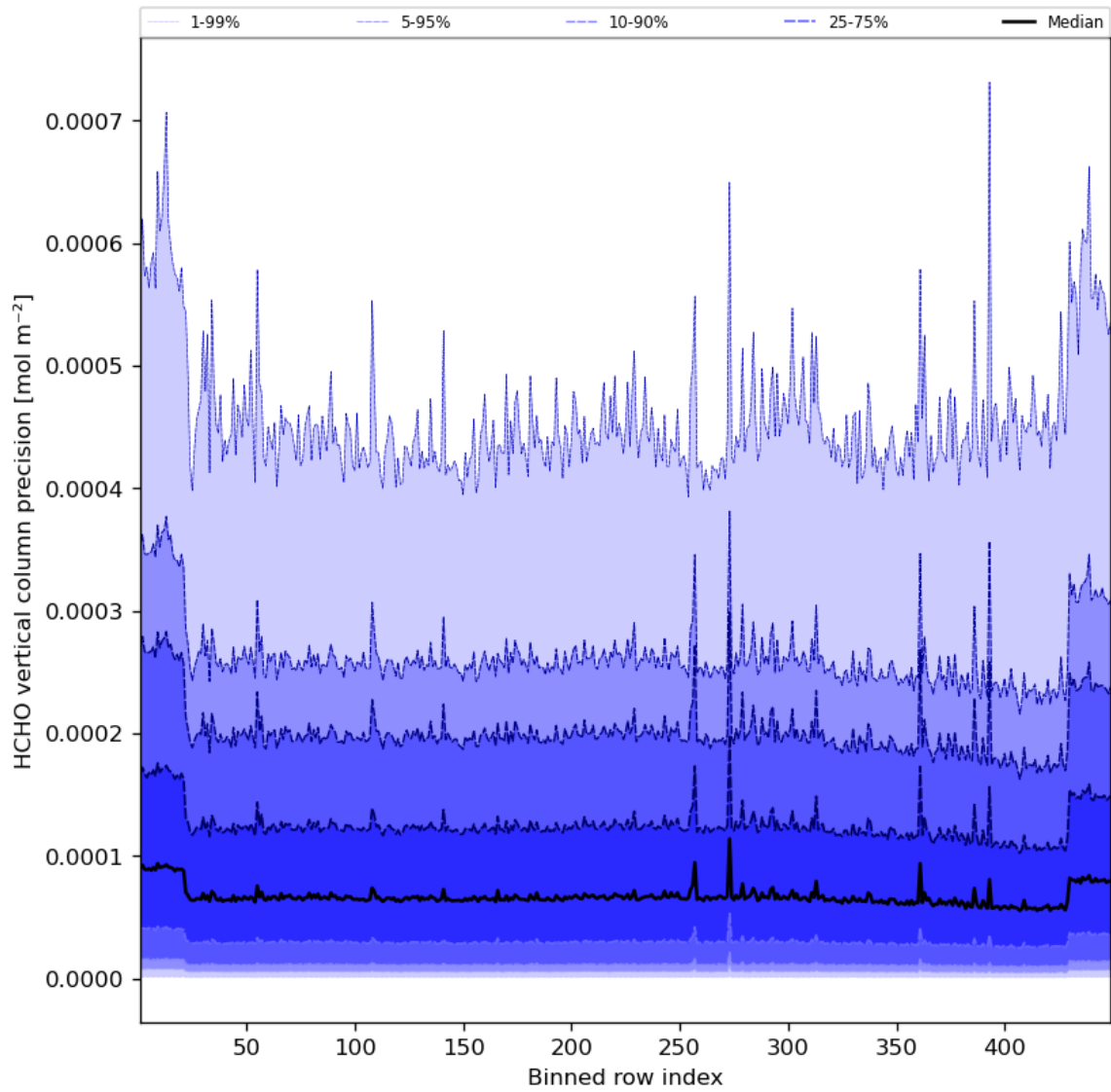
Figure 50: Along track statistics of “HCHO vertical column precision” for 2023-08-06 to 2023-08-08
