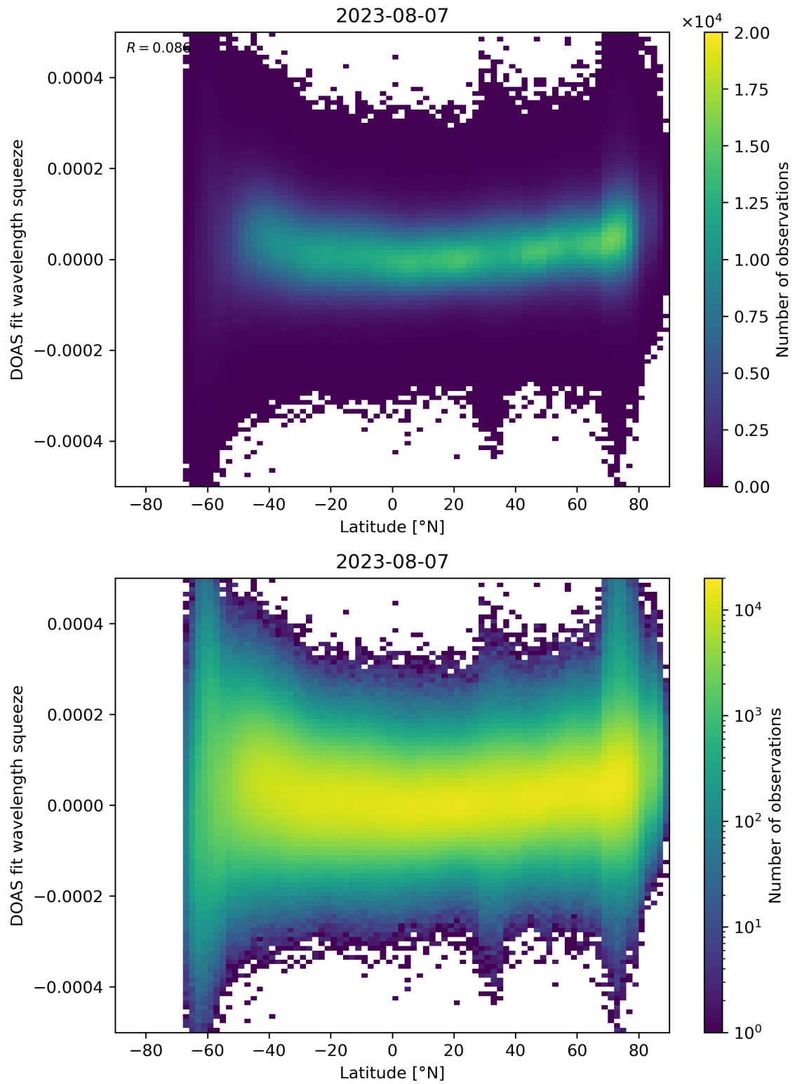
Figure 155: Scatter density plot of “Latitude” against “DOAS fit wavelength squeeze” for 2023-08-06 to 2023-08-08.
