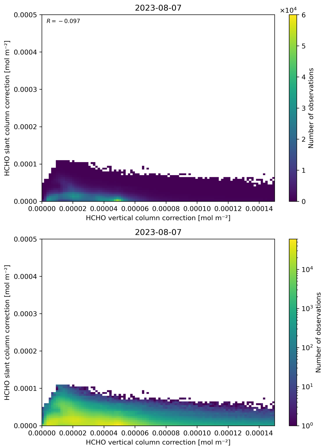
Figure 117: Scatter density plot of “HCHO vertical column correction” against “HCHO slant column correction” for 2023-08-06 to 2023-08-08.
