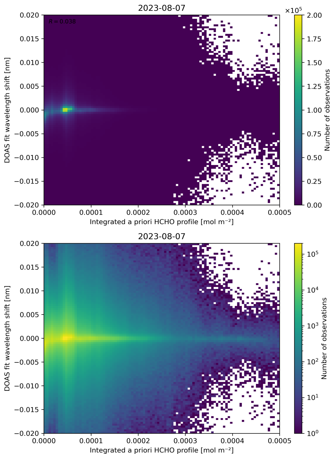
Figure 149: Scatter density plot of “Integrated a priori HCHO profile” against “DOAS fit wavelength shift” for 2023-08-06 to 2023-08-08.
