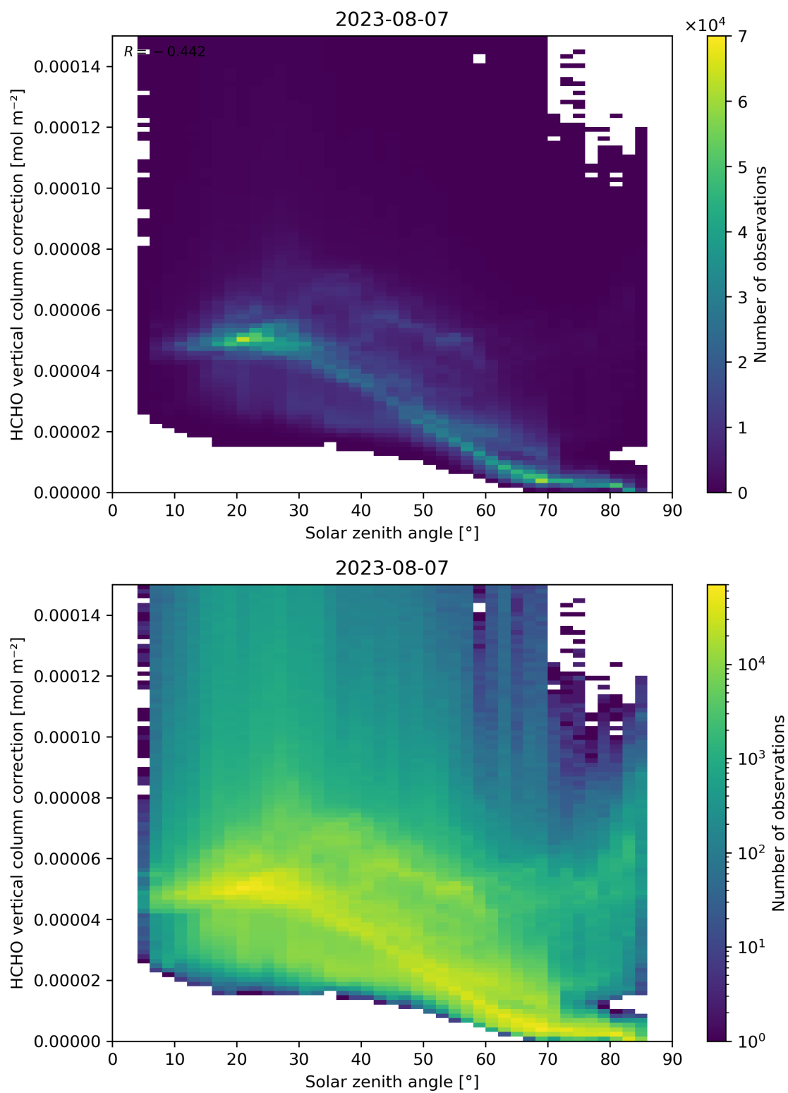
Figure 178: Scatter density plot of “Solar zenith angle” against “HCHO vertical column correction” for 2023-08-06 to 2023-08-08.
