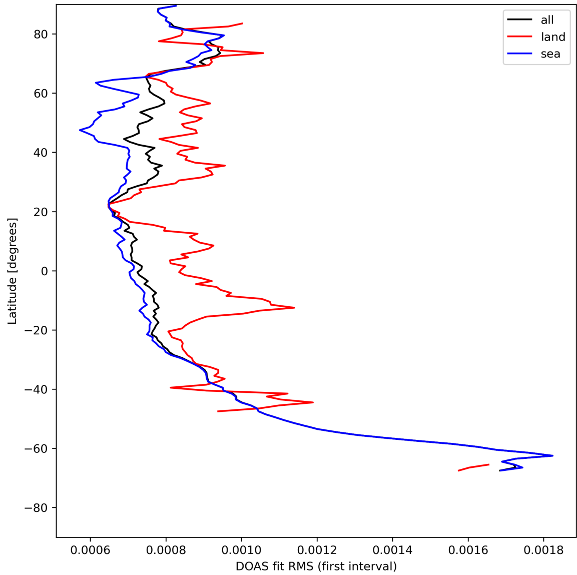
Figure 32: Zonal average of "DOAS fit RMS (first interval)" for 2023-08-06 to 2023-08-08.
