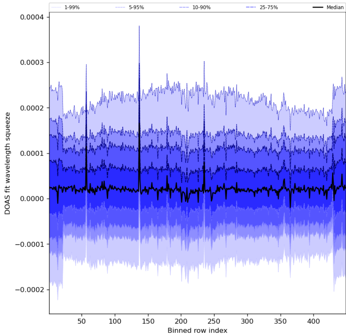
Figure 59: Along track statistics of “DOAS fit wavelength squeeze” for 2023-08-06 to 2023-08-08
