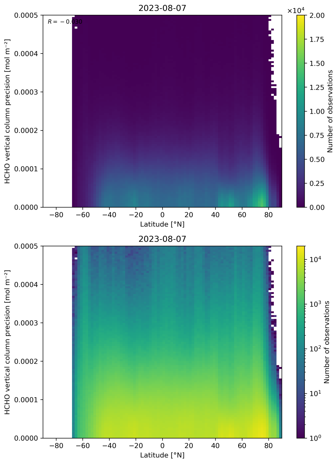
Figure 165: Scatter density plot of “Latitude” against “HCHO vertical column precision” for 2023-08-06 to 2023-08-08.
