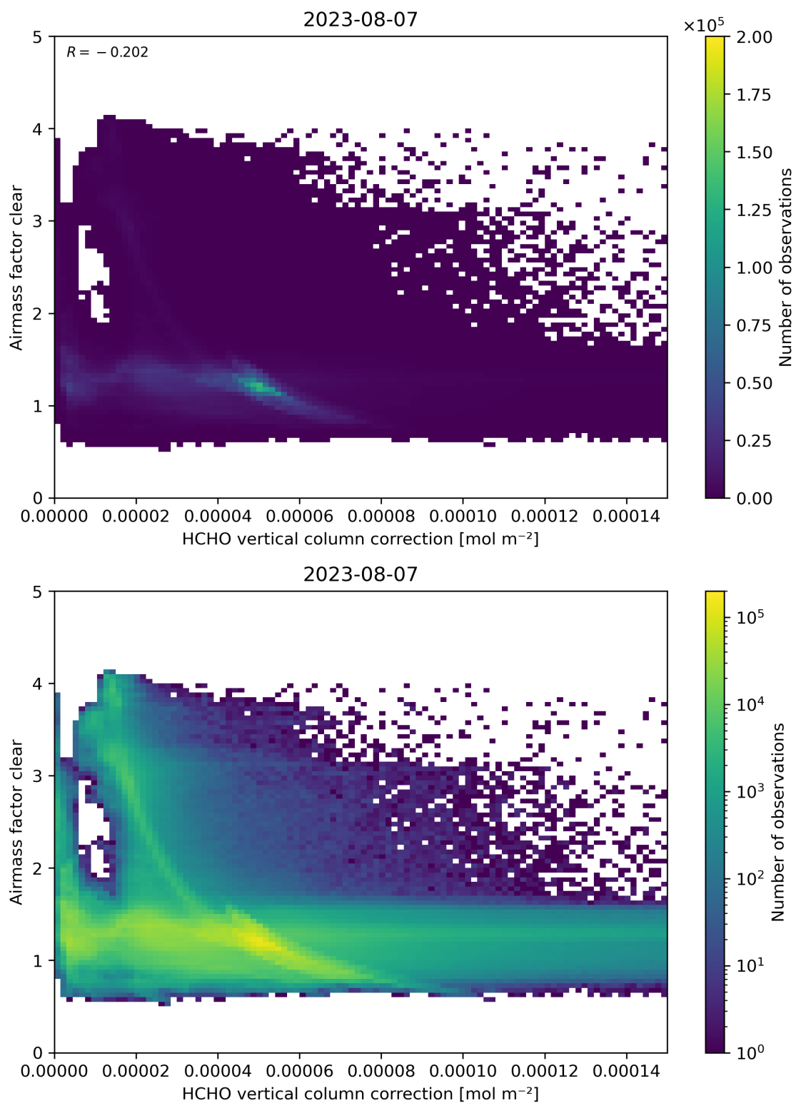
Figure 115: Scatter density plot of “HCHO vertical column correction” against “Airmass factor clear” for 2023-08-06 to 2023-08-08.
