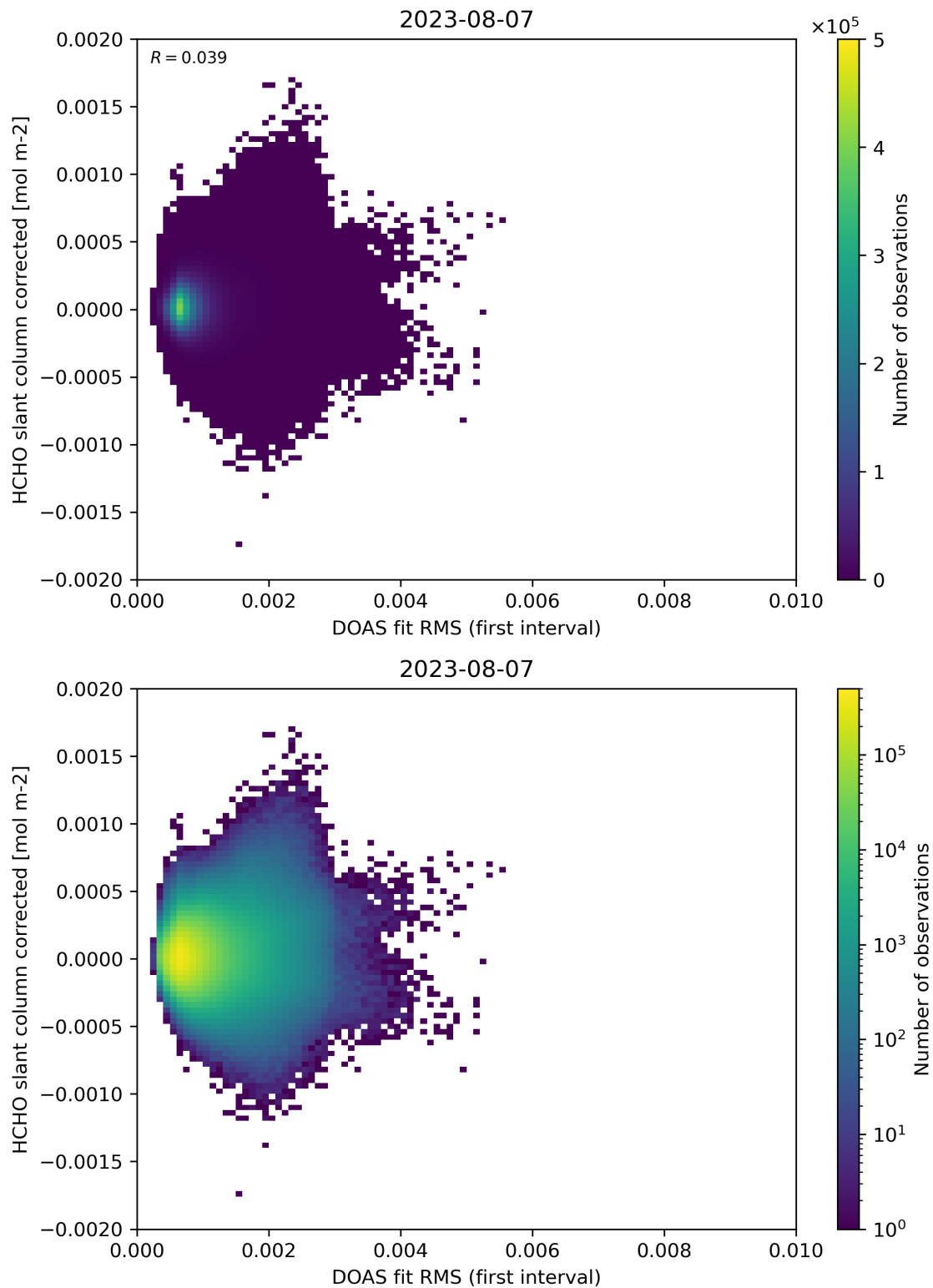
Figure 62: Scatter density plot of “DOAS fit RMS (first interval)” against “HCHO slant column corrected” for 2023-08-06 to 2023-08-08.
