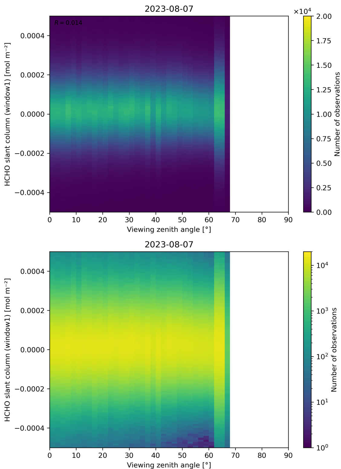
Figure 188: Scatter density plot of “Viewing zenith angle” against “HCHO slant column (window1)” for 2023-08-06 to 2023-08-08.
