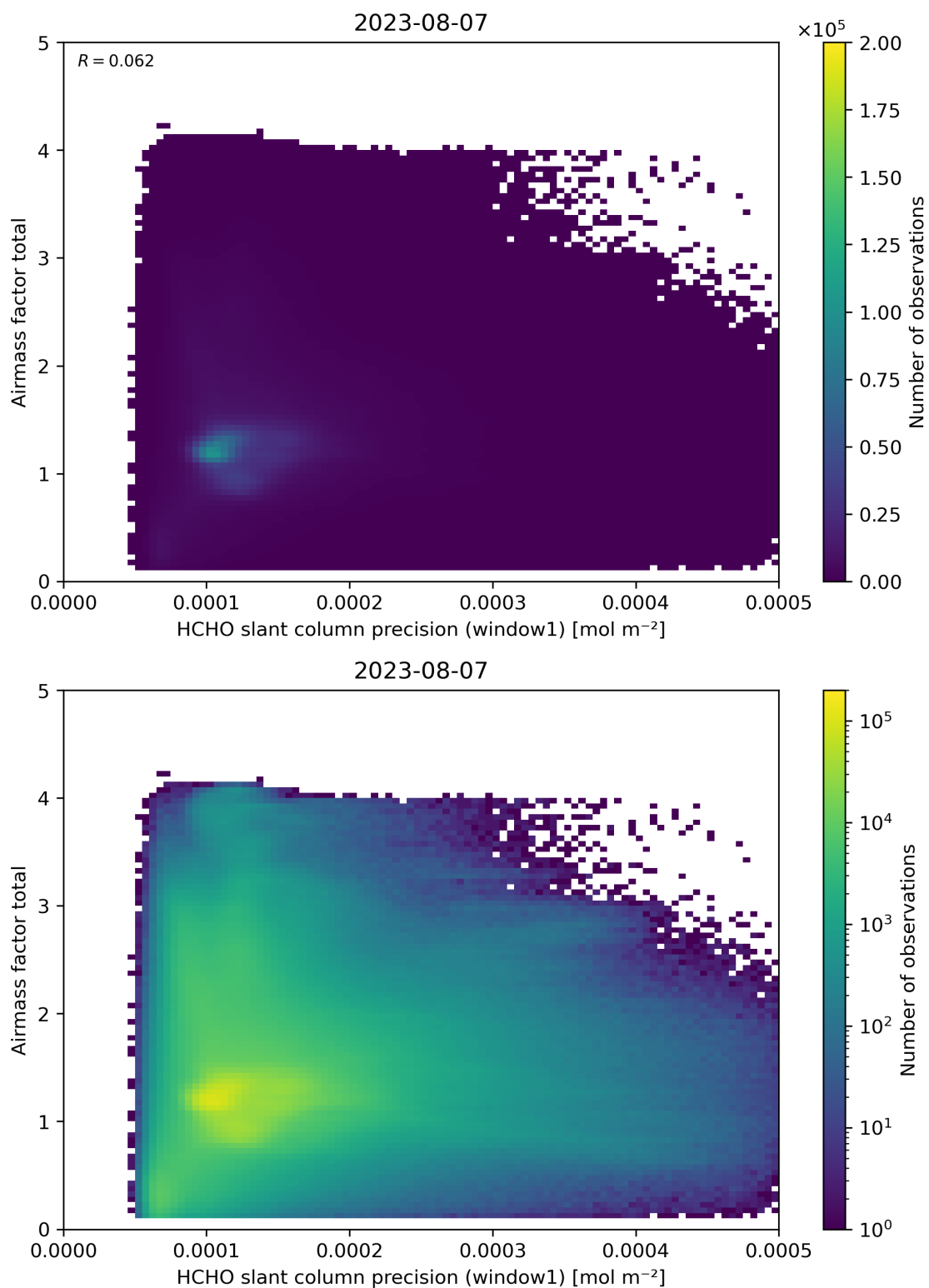
Figure 94: Scatter density plot of “HCHO slant column precision (window1)” against “Airmass factor total” for 2023-08-06 to 2023-08-08.
