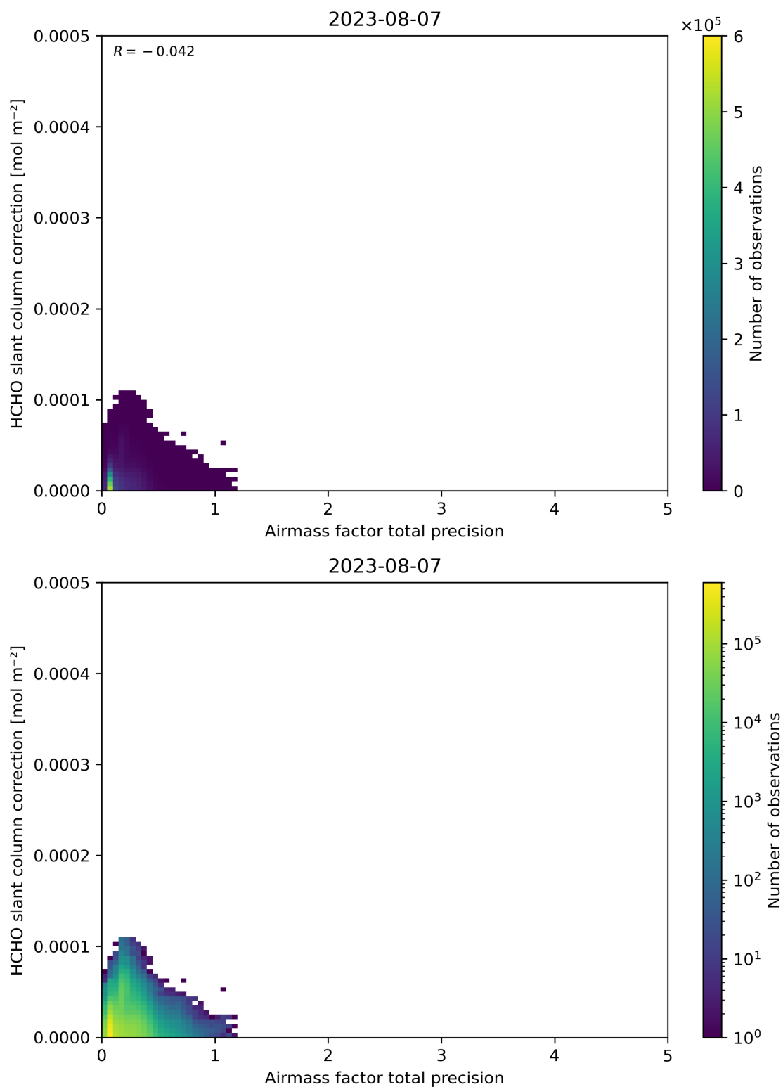
Figure 110: Scatter density plot of “Airmass factor total precision” against “HCHO slant column correction” for 2023-08-06 to 2023-08-08.
