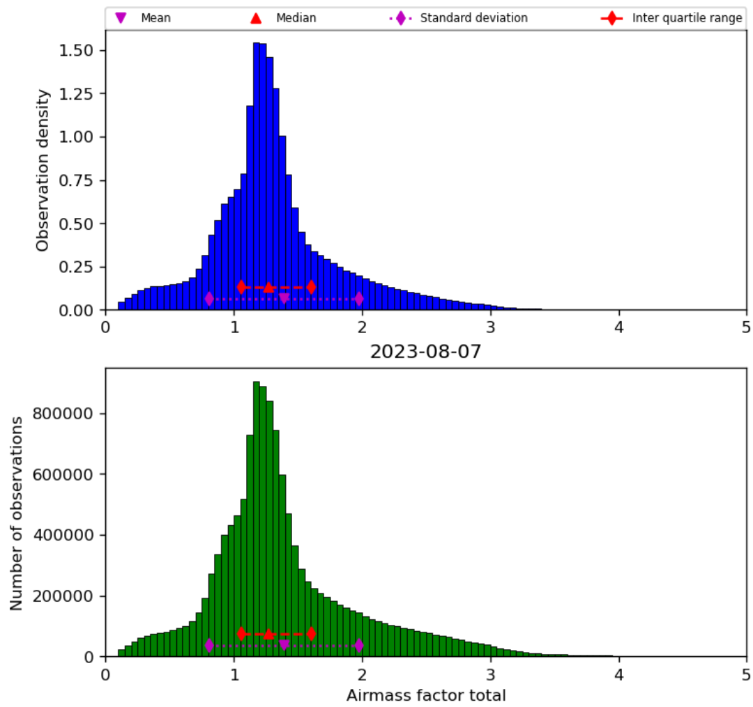
Figure 40: Histogram of “Airmass factor total” for 2023-08-06 to 2023-08-08
