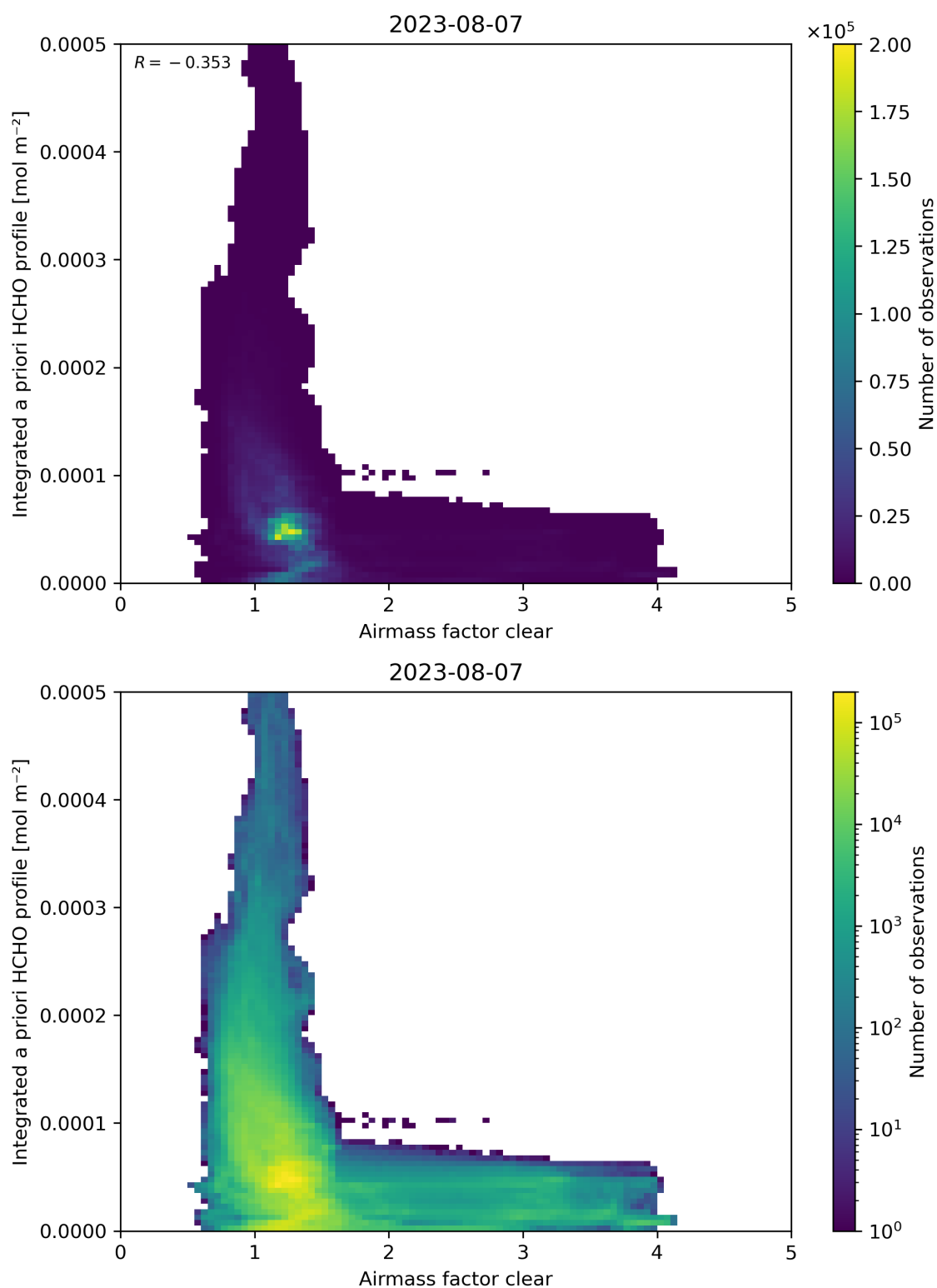
Figure 76: Scatter density plot of “Airmass factor clear” against “Integrated a priori HCHO profile” for 2023-08-06 to 2023-08-08.
