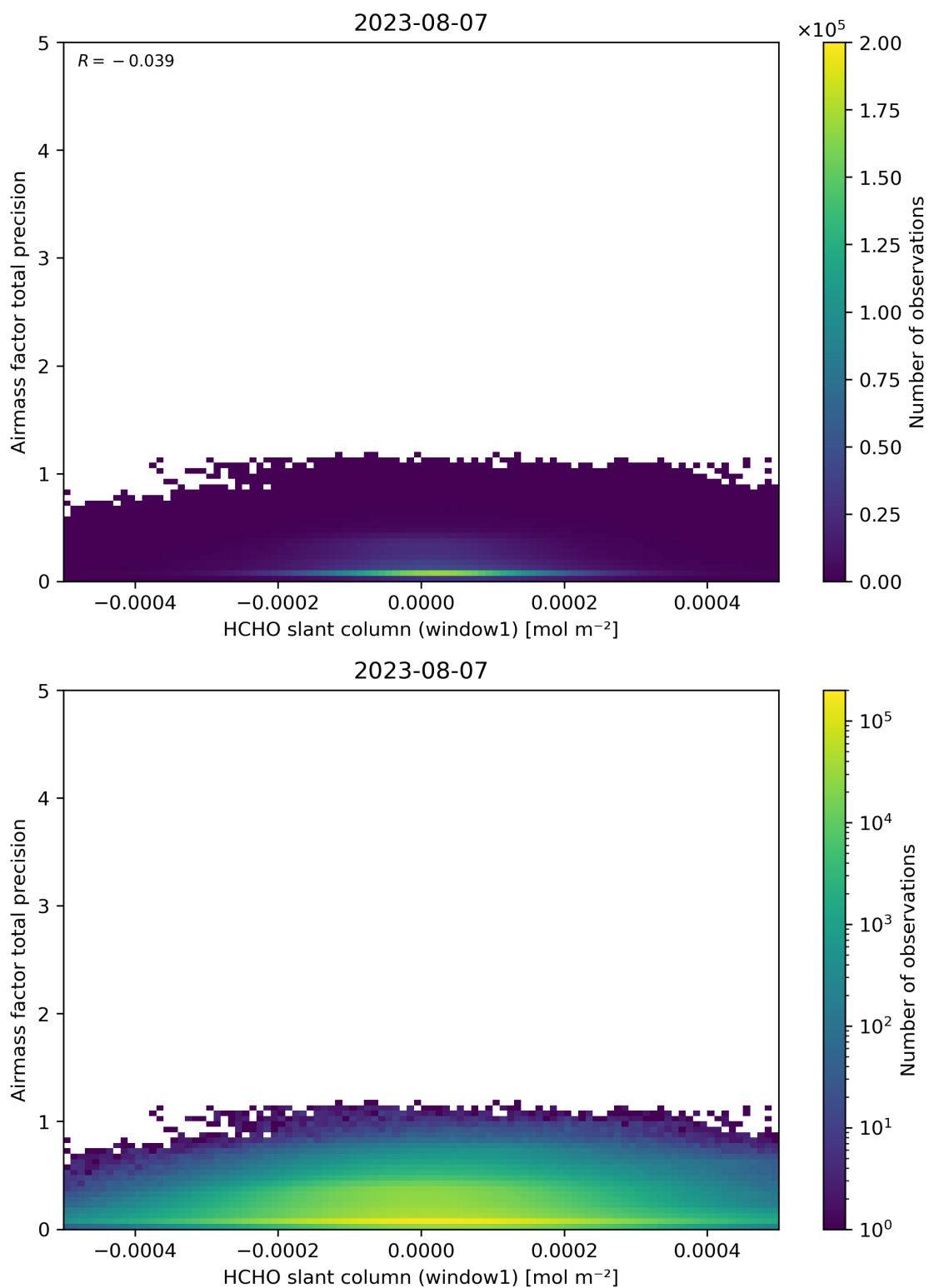
Figure 86: Scatter density plot of “HCHO slant column (window1)” against “Airmass factor total precision” for 2023-08-06 to 2023-08-08.
