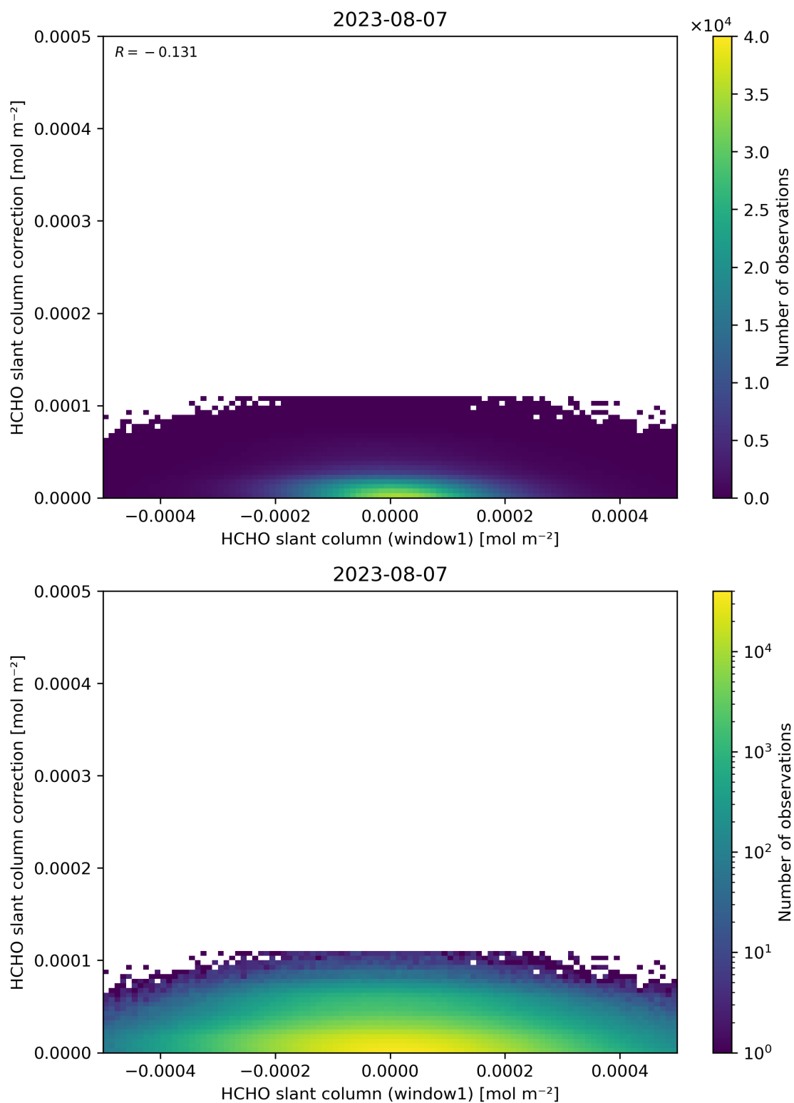
Figure 83: Scatter density plot of “HCHO slant column (window1)” against “HCHO slant column correction” for 2023-08-06 to 2023-08-08.
