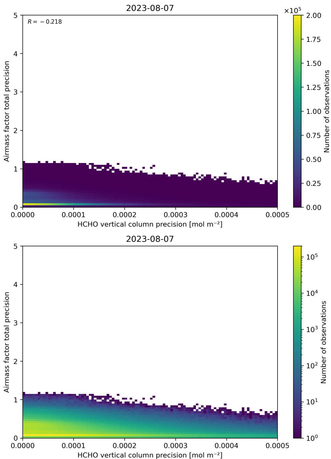
Figure 145: Scatter density plot of “HCHO vertical column precision” against “Airmass factor total precision” for 2023-08-06 to 2023-08-08.
