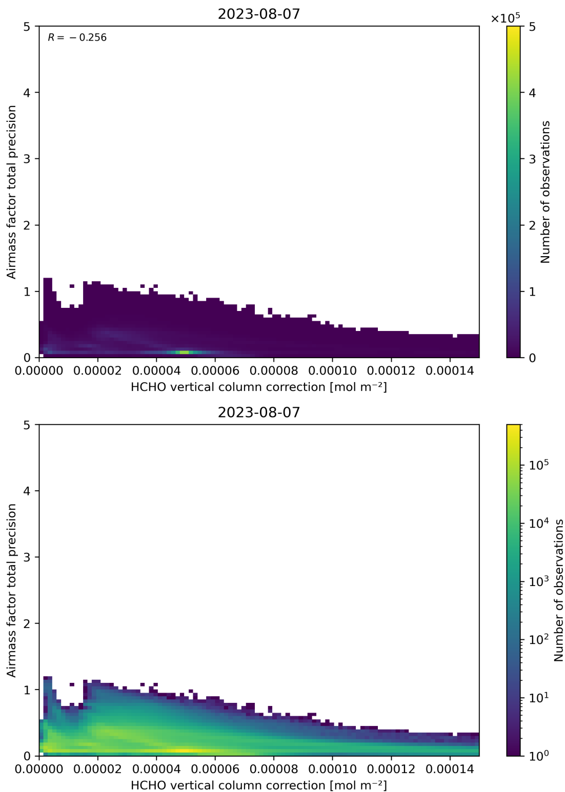
Figure 121: Scatter density plot of “HCHO vertical column correction” against “Airmass factor total precision” for 2023-08-06 to 2023-08-08.
