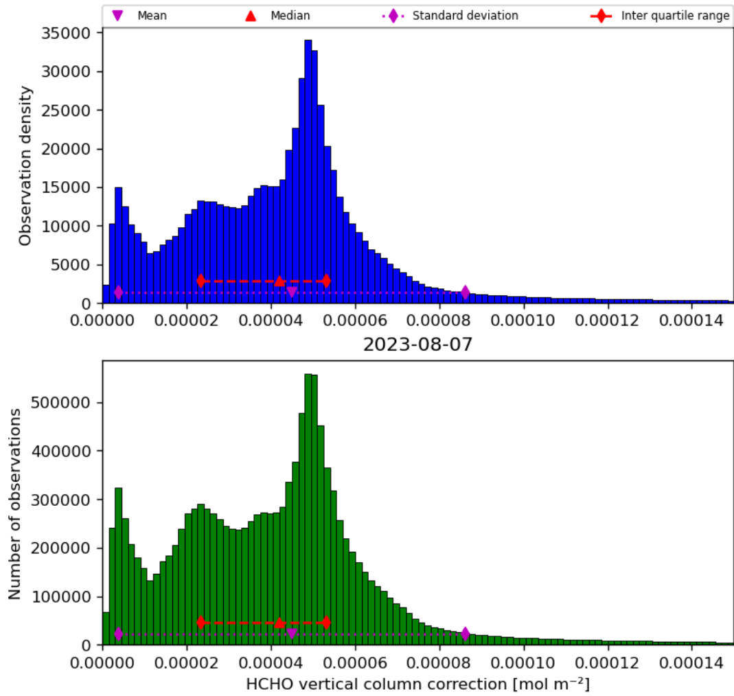
Figure 37: Histogram of “HCHO vertical column correction” for 2023-08-06 to 2023-08-08
