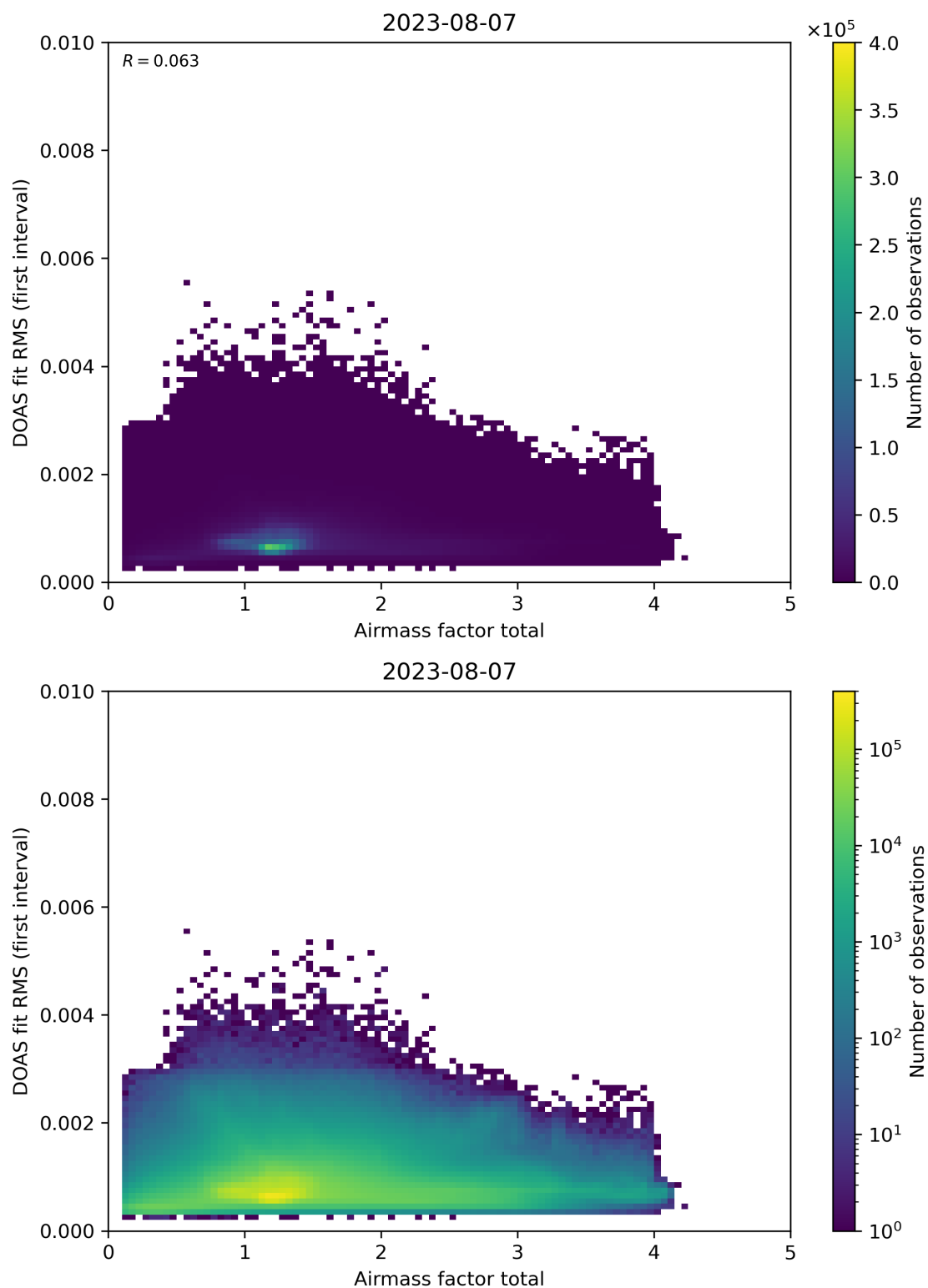
Figure 97: Scatter density plot of “Airmass factor total” against “DOAS fit RMS (first interval)” for 2023-08-06 to 2023-08-08.
