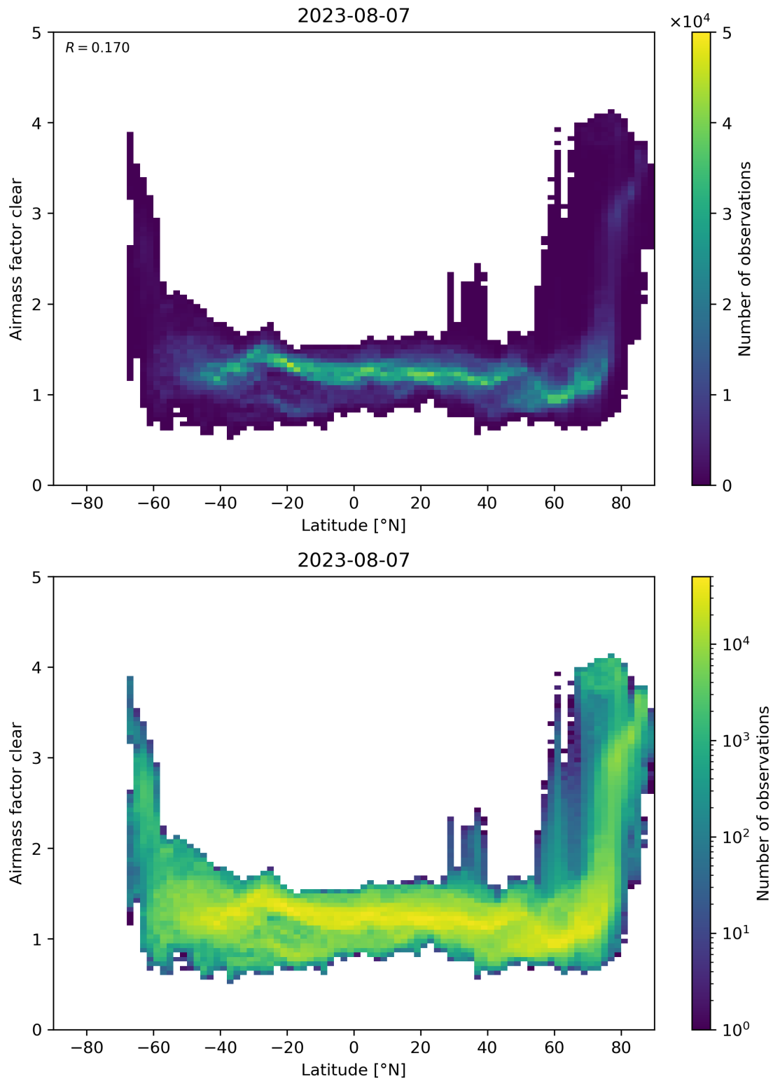
Figure 156: Scatter density plot of “Latitude” against “Airmass factor clear” for 2023-08-06 to 2023-08-08.
