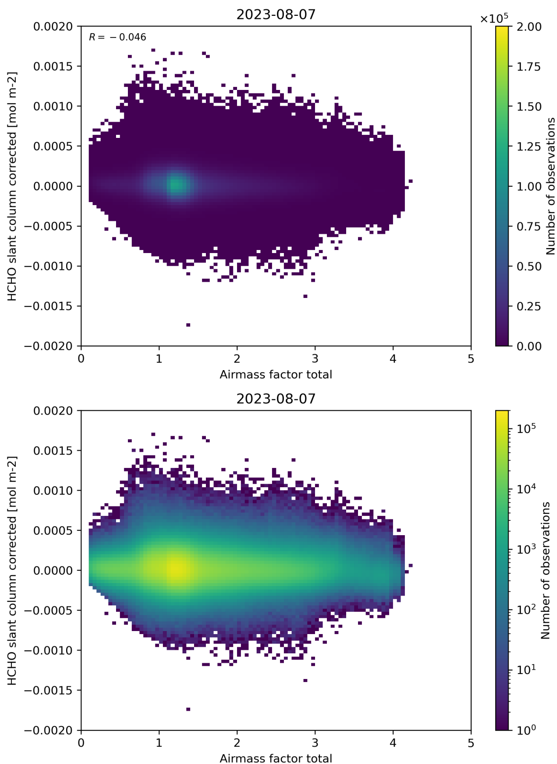
Figure 101: Scatter density plot of “Airmass factor total” against “HCHO slant column corrected” for 2023-08-06 to 2023-08-08.
