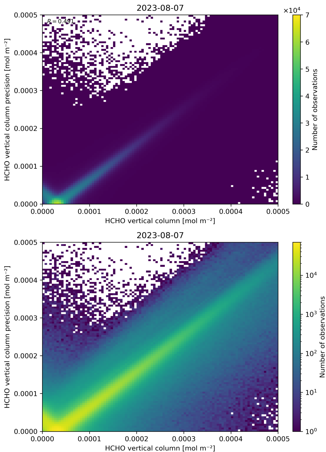
Figure 134: Scatter density plot of “HCHO vertical column” against “HCHO vertical column precision” for 2023-08-06 to 2023-08-08.
