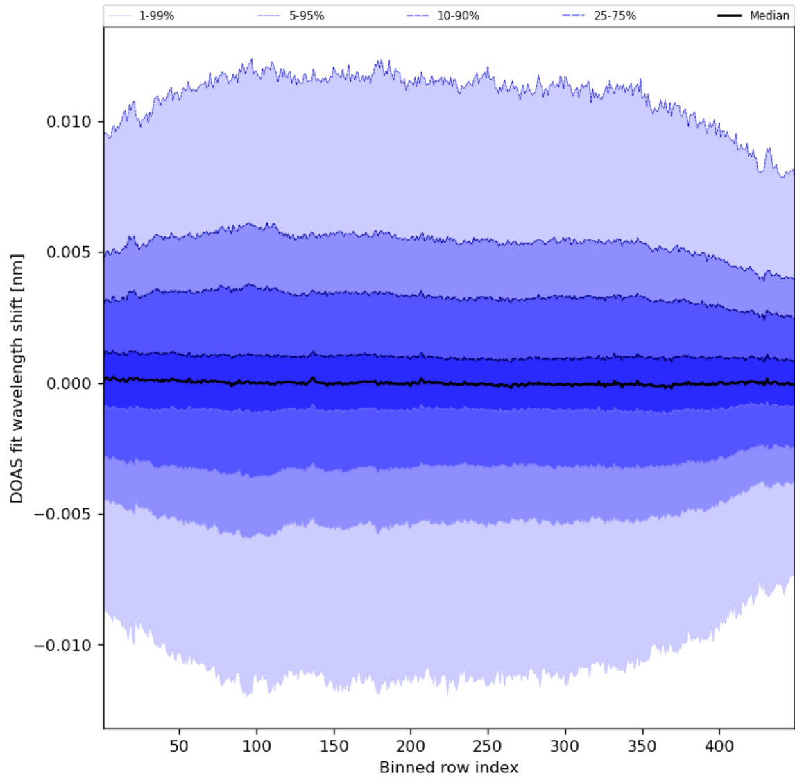
Figure 58: Along track statistics of “DOAS fit wavelength shift” for 2023-08-06 to 2023-08-08
