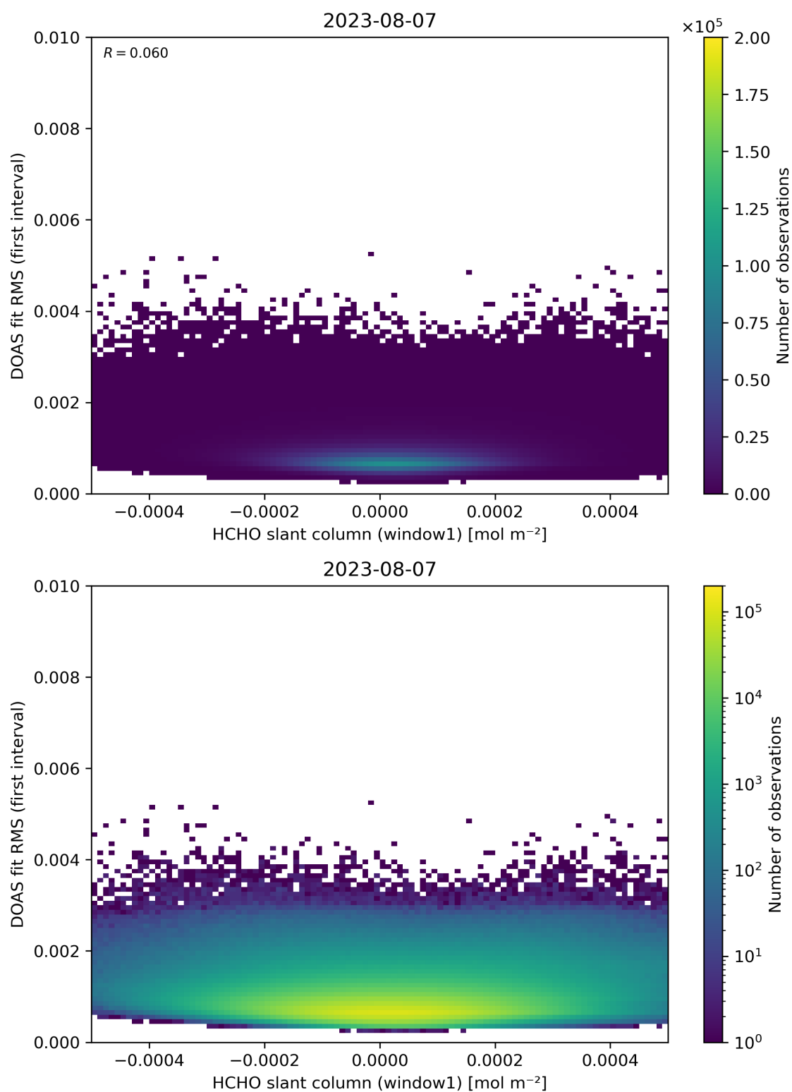
Figure 78: Scatter density plot of “HCHO slant column (window1)” against “DOAS fit RMS (first interval)” for 2023-08-06 to 2023-08-08.
