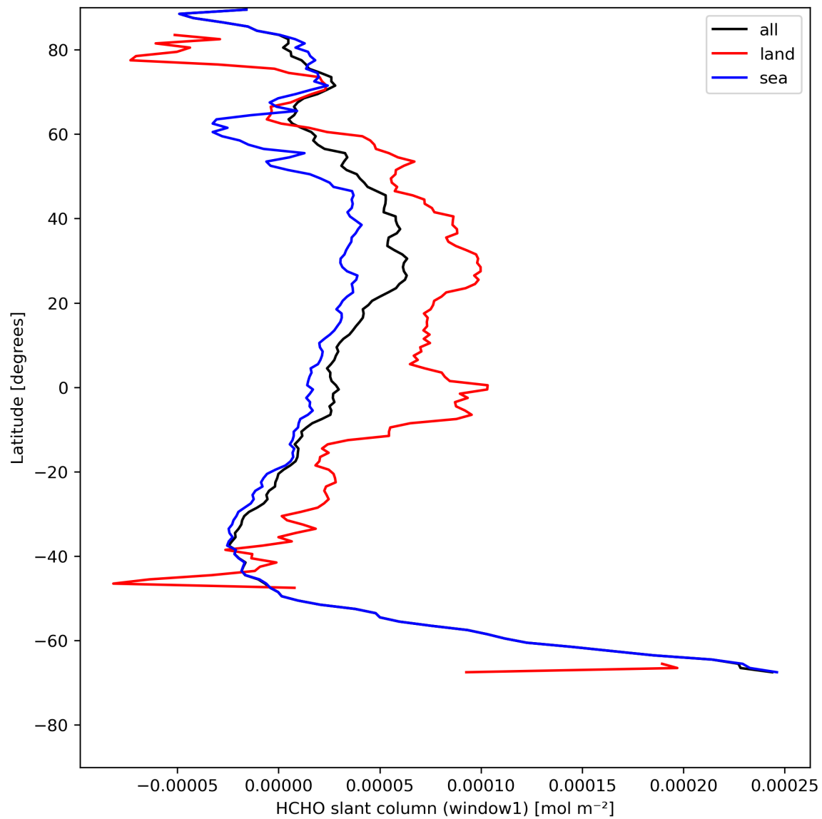
Figure 24: Zonal average of “HCHO slant column (window1)” for 2023-08-06 to 2023-08-08.
