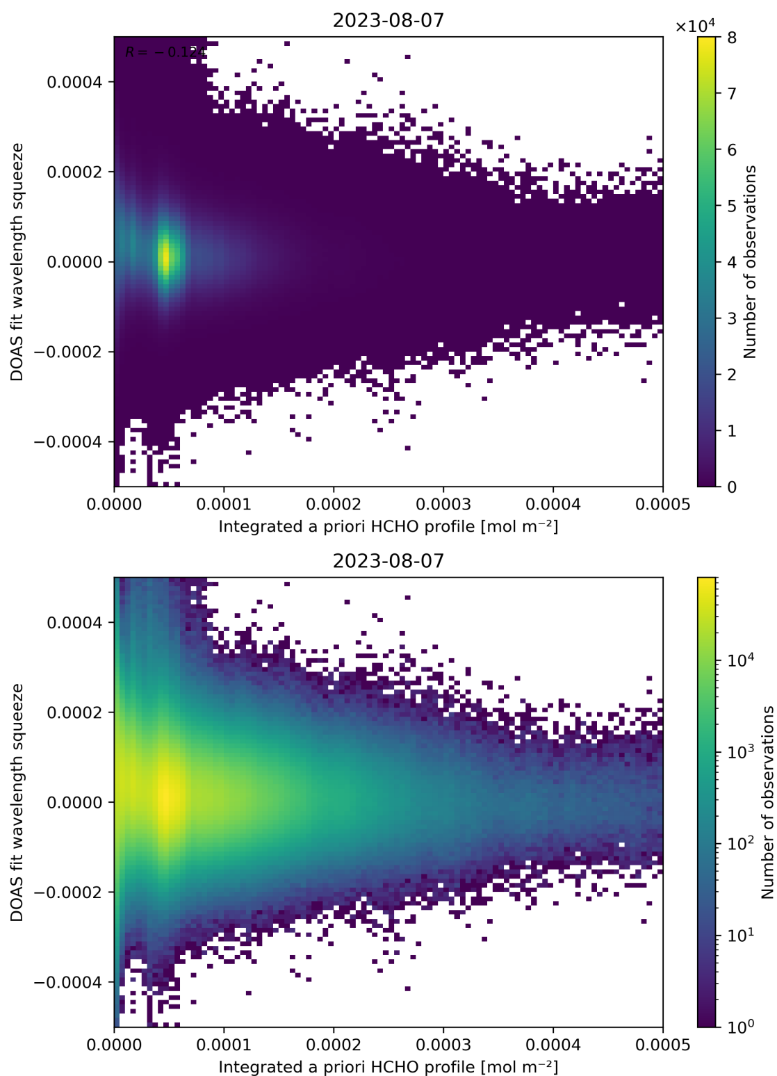
Figure 150: Scatter density plot of “Integrated a priori HCHO profile” against “DOAS fit wavelength squeeze” for 2023-08-06 to 2023-08-08.
