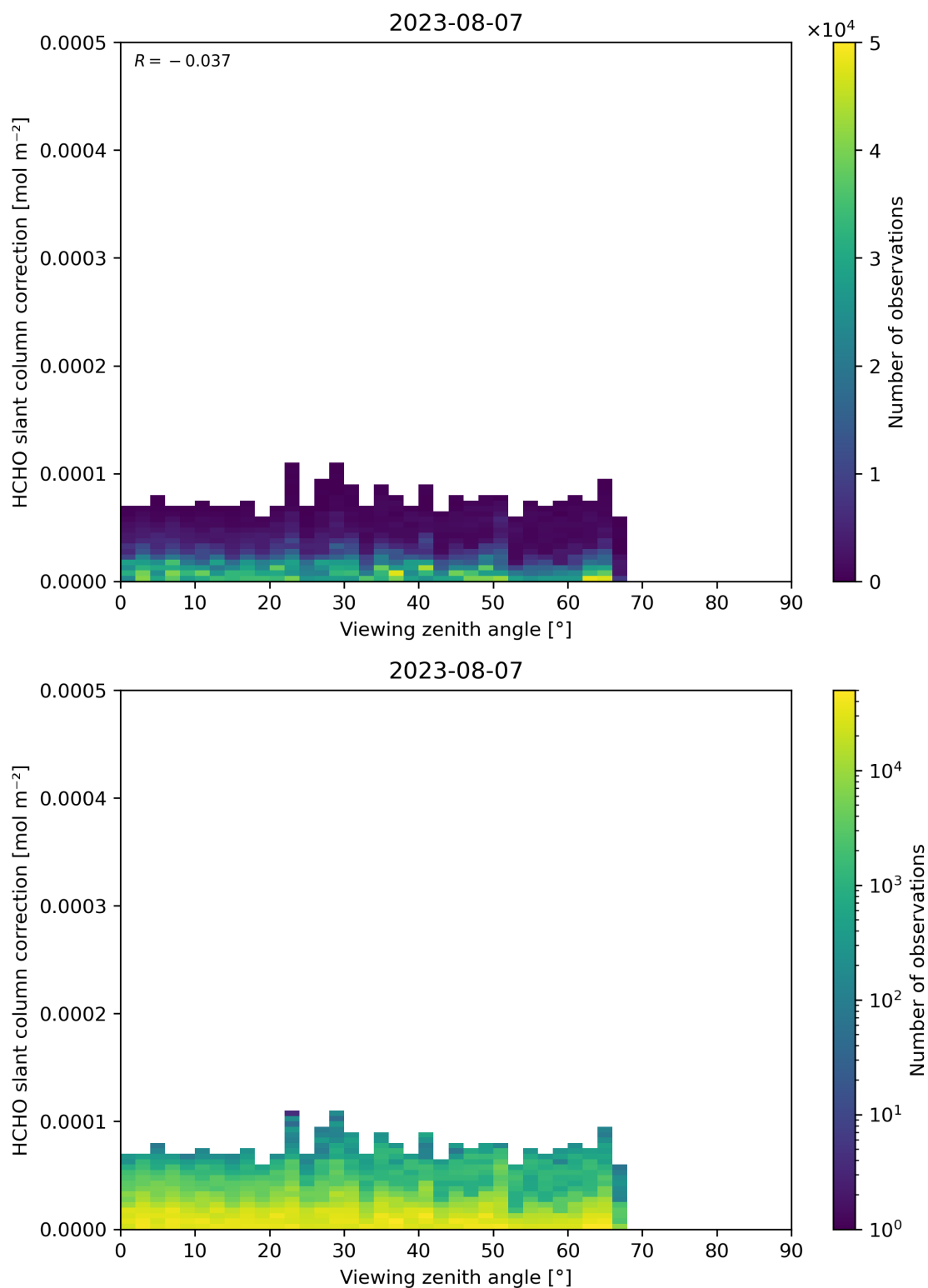
Figure 187: Scatter density plot of “Viewing zenith angle” against “HCHO slant column correction” for 2023-08-06 to 2023-08-08.
