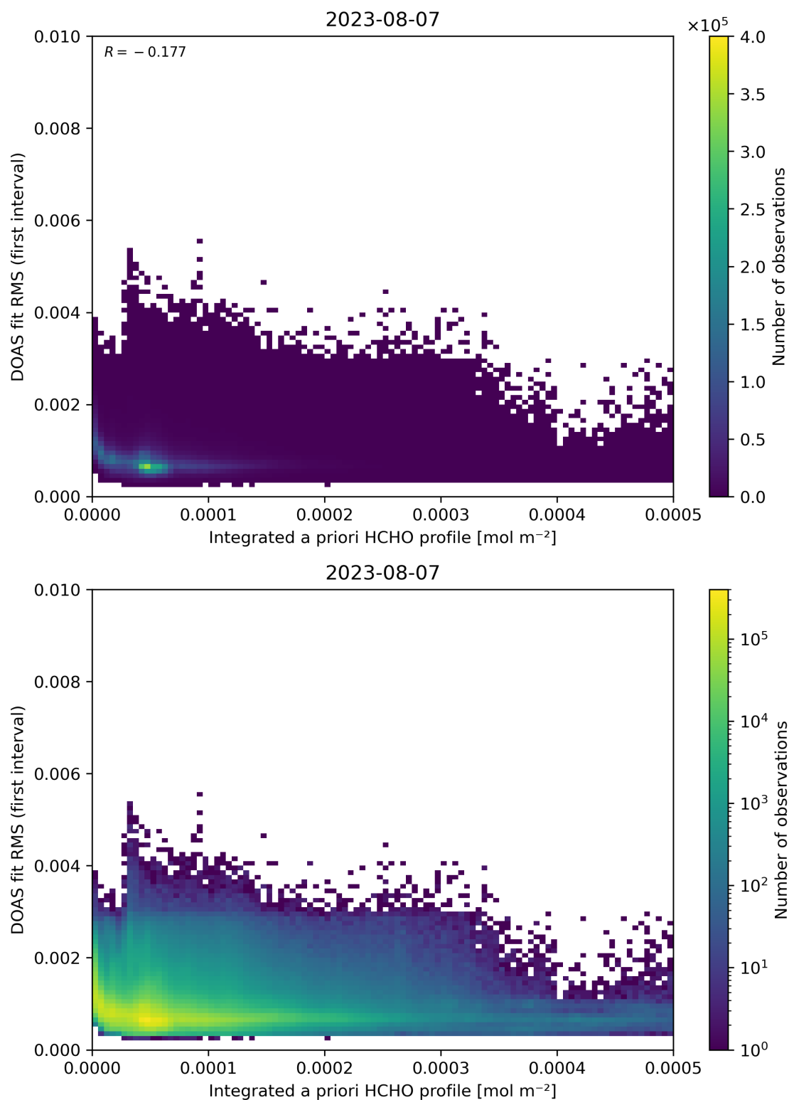
Figure 148: Scatter density plot of “Integrated a priori HCHO profile” against “DOAS fit RMS (first interval)” for 2023-08-06 to 2023-08-08.
