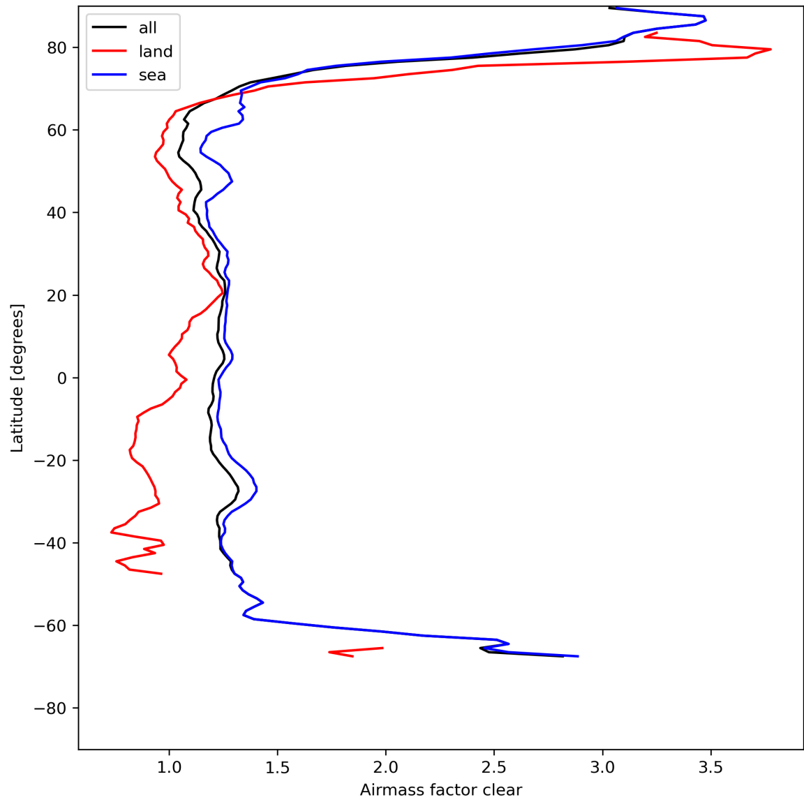
Figure 28: Zonal average of “Airmass factor clear” for 2023-08-06 to 2023-08-08.
