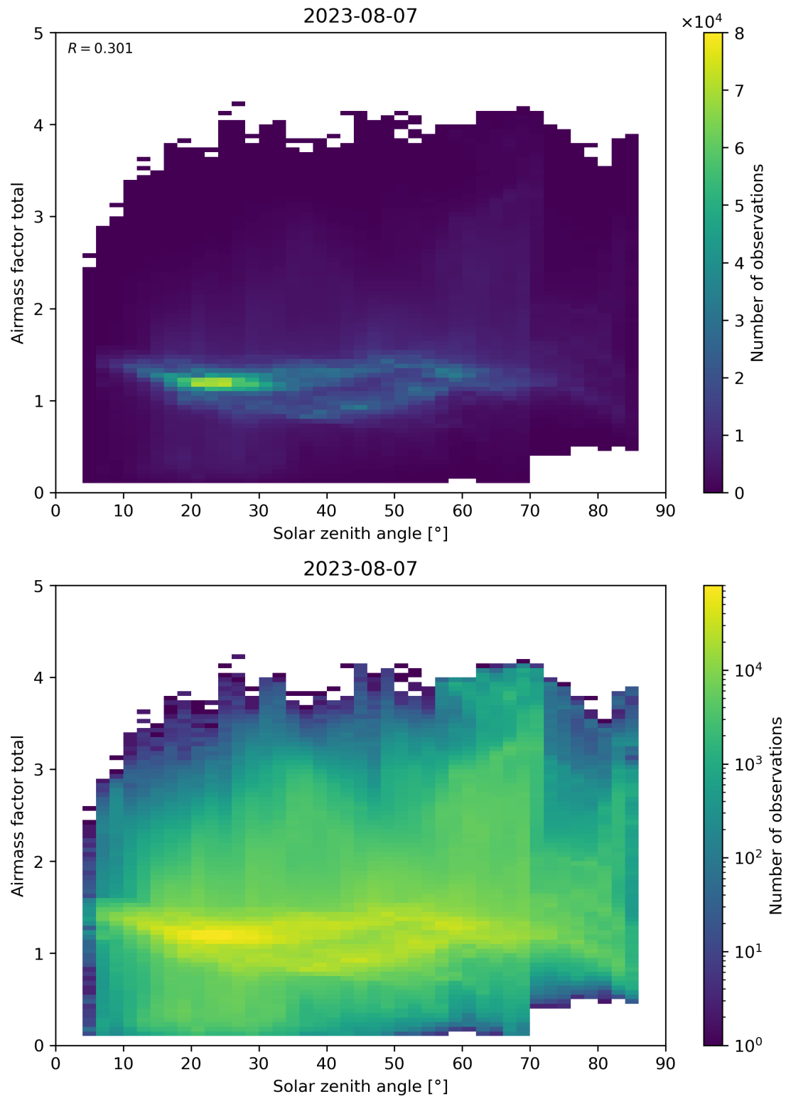
Figure 175: Scatter density plot of “Solar zenith angle” against “Airmass factor total” for 2023-08-06 to 2023-08-08.
