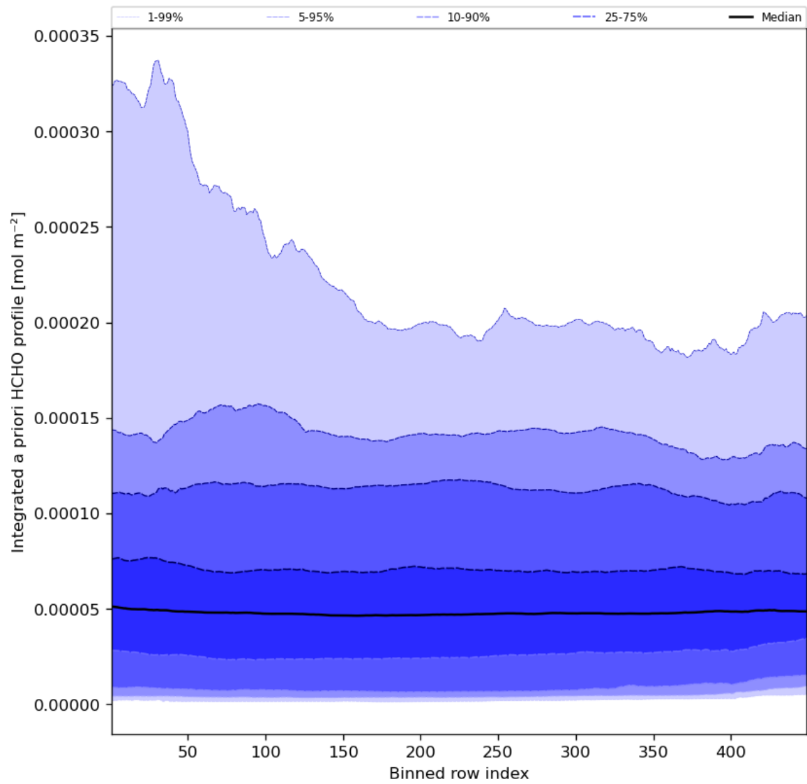
Figure 57: Along track statistics of “Integrated a priori HCHO profile” for 2023-08-06 to 2023-08-08
