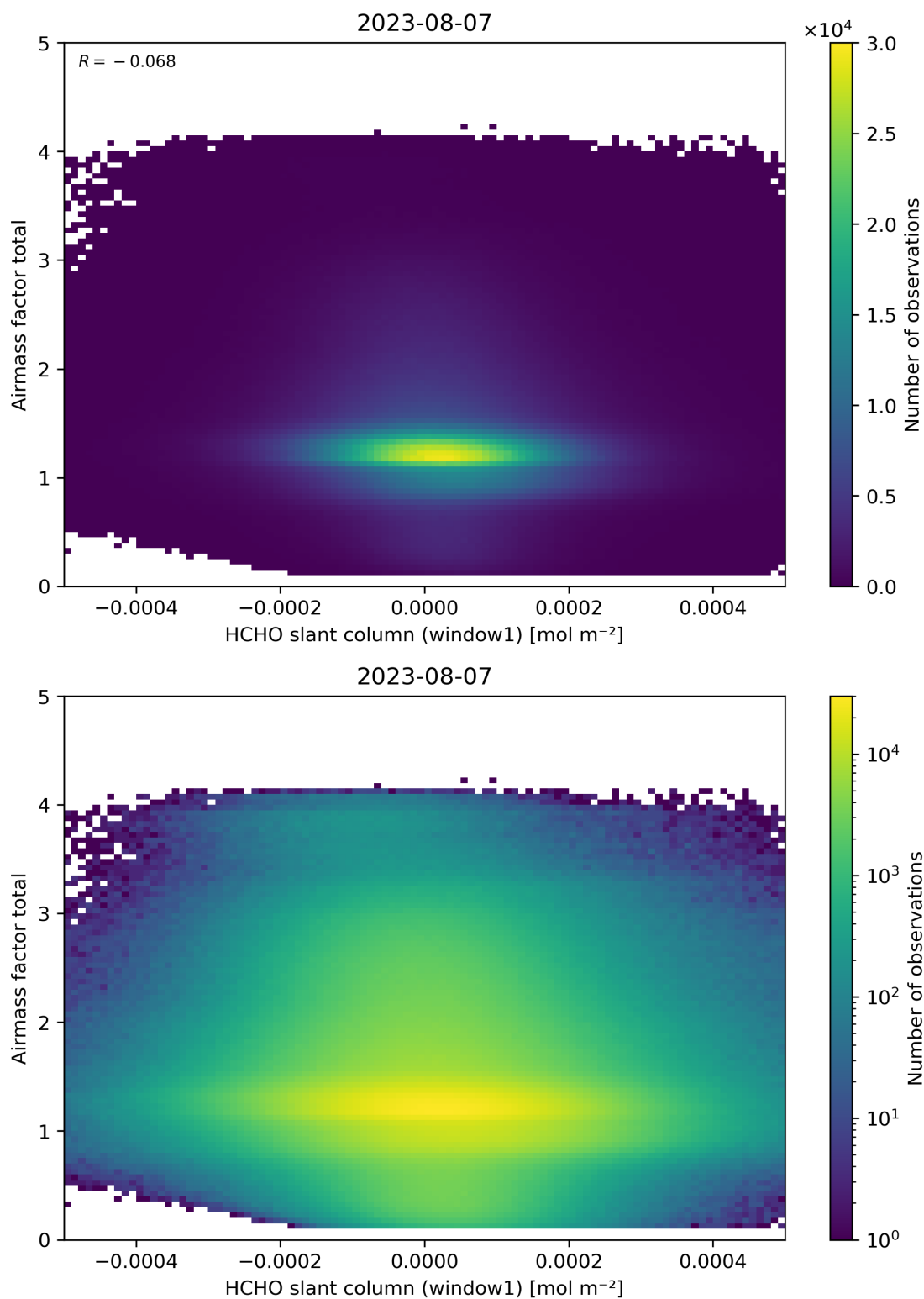
Figure 85: Scatter density plot of “HCHO slant column (window1)” against “Airmass factor total” for 2023-08-06 to 2023-08-08.
