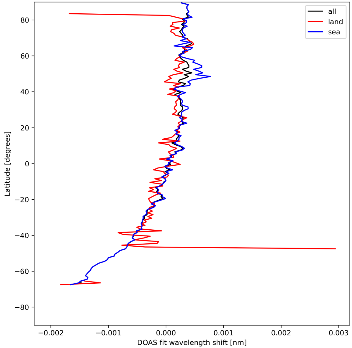
Figure 30: Zonal average of “DOAS fit wavelength shift” for 2023-08-06 to 2023-08-08.
