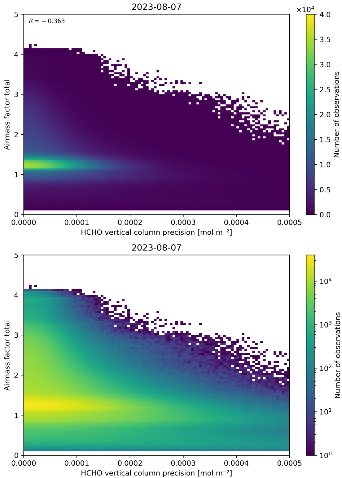
Figure 144: Scatter density plot of “HCHO vertical column precision” against “Airmass factor total” for 2023-08-06 to 2023-08-08.
