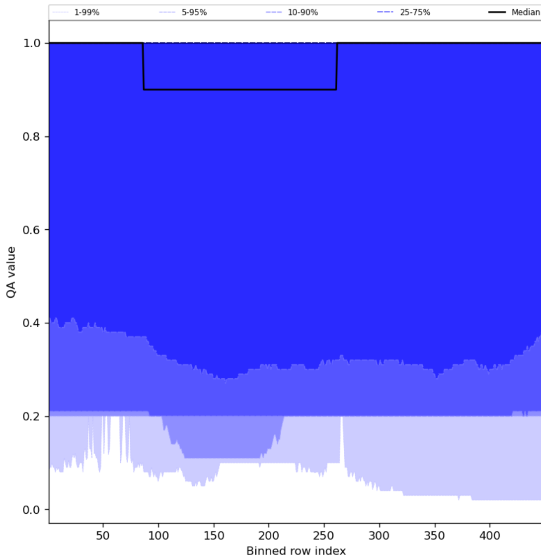
Figure 48: Along track statistics of “QA value” for 2023-08-06 to 2023-08-08
