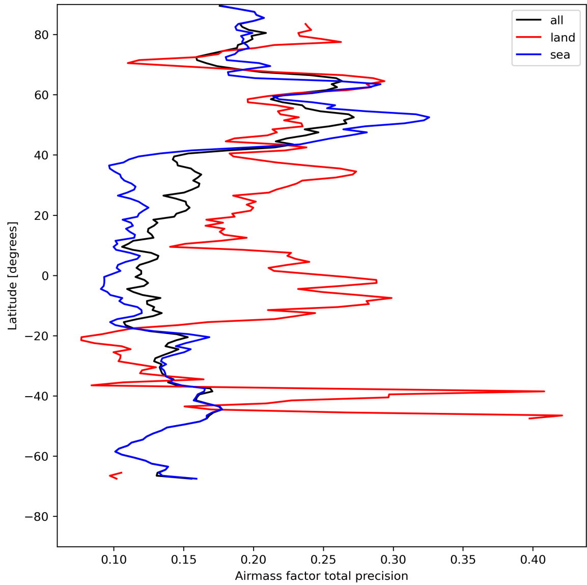
Figure 27: Zonal average of “Airmass factor total precision” for 2023-08-06 to 2023-08-08.
