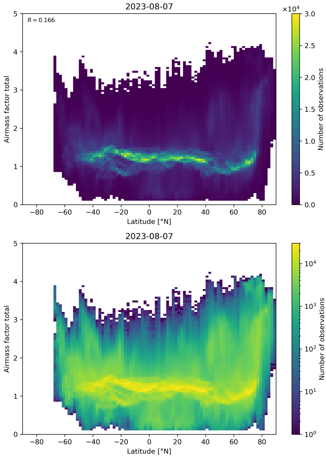
Figure 161: Scatter density plot of “Latitude” against “Airmass factor total” for 2023-08-06 to 2023-08-08.
