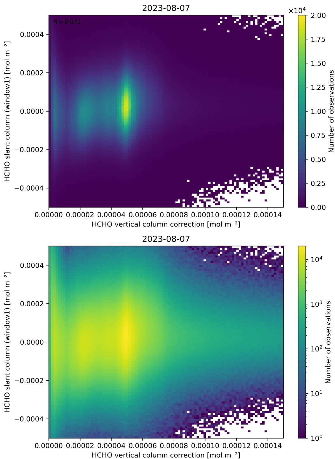
Figure 118: Scatter density plot of “HCHO vertical column correction” against “HCHO slant column (window1)” for 2023-08-06 to 2023-08-08.
