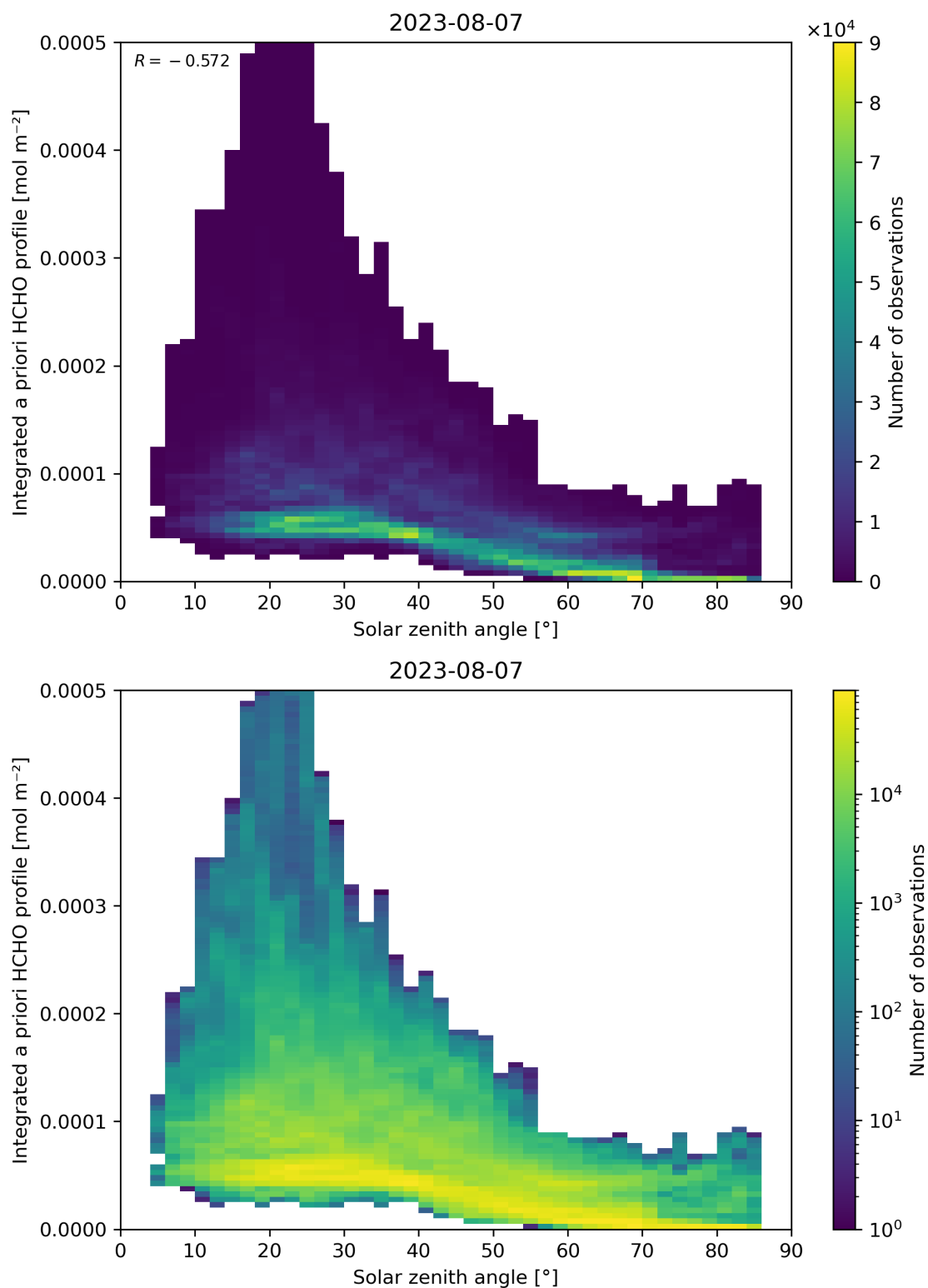
Figure 180: Scatter density plot of “Solar zenith angle” against “Integrated a priori HCHO profile” for 2023-08-06 to 2023-08-08.
