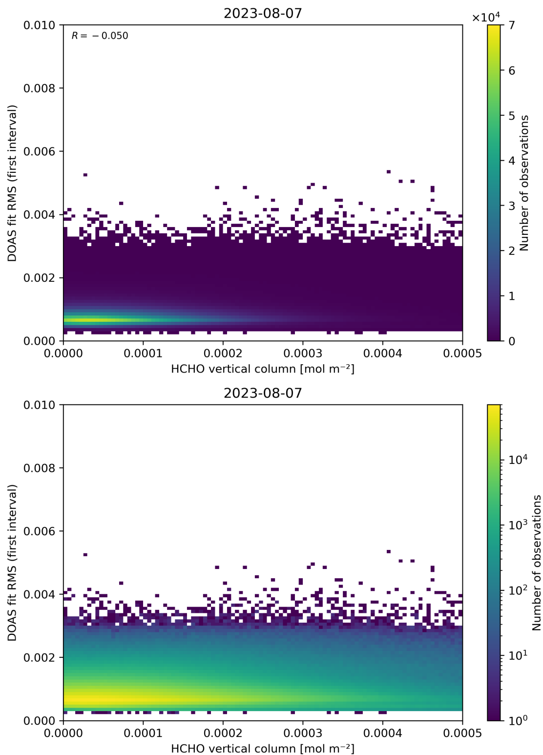
Figure 123: Scatter density plot of “HCHO vertical column” against “DOAS fit RMS (first interval)” for 2023-08-06 to 2023-08-08.
