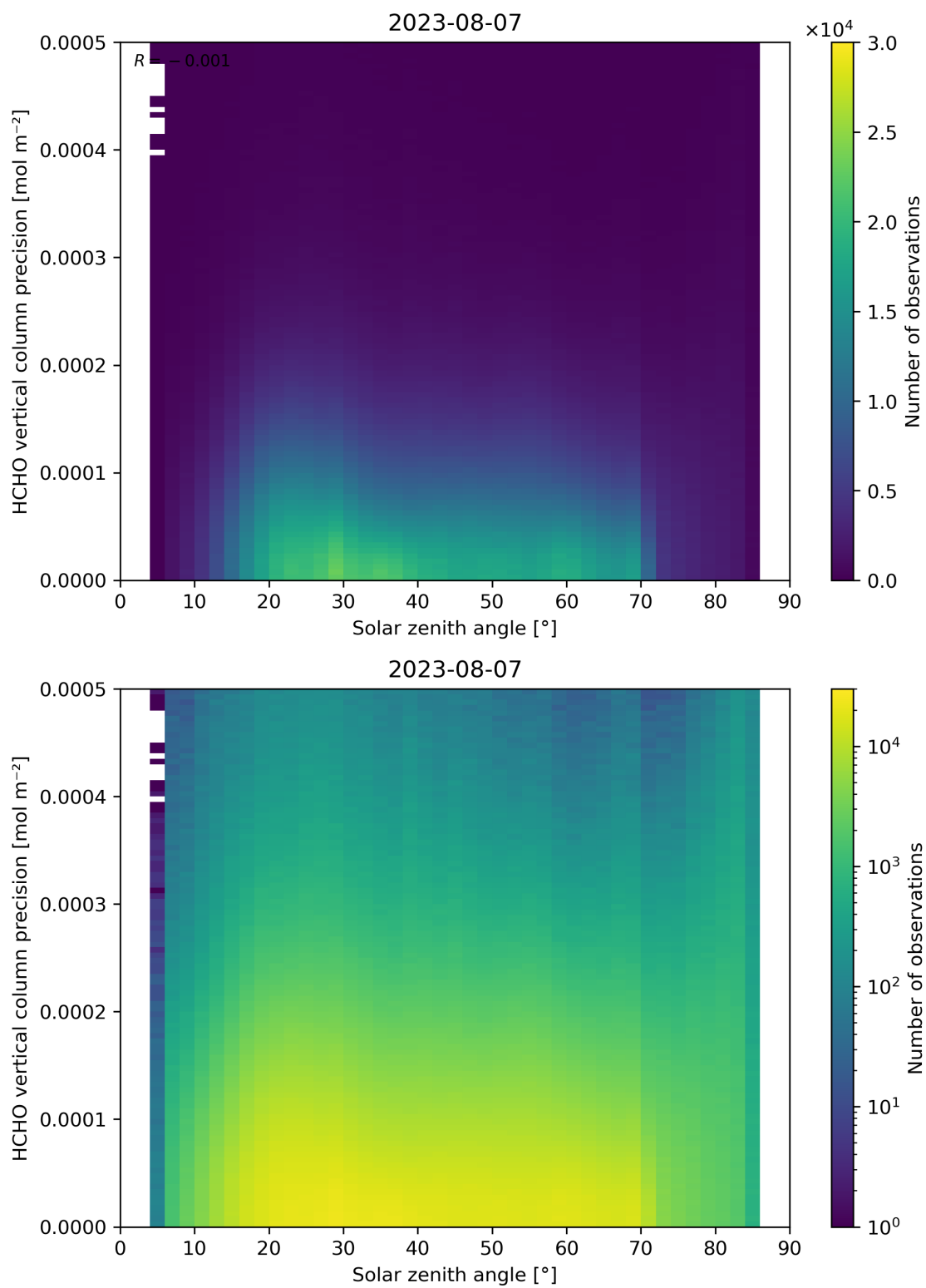
Figure 179: Scatter density plot of “Solar zenith angle” against “HCHO vertical column precision” for 2023-08-06 to 2023-08-08.
