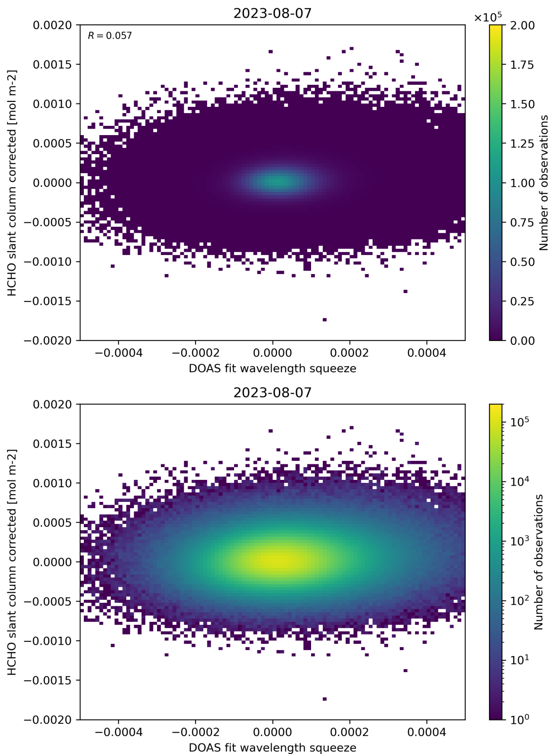
Figure 69: Scatter density plot of “DOAS fit wavelength squeeze” against “HCHO slant column corrected” for 2023-08-06 to 2023-08-08.
