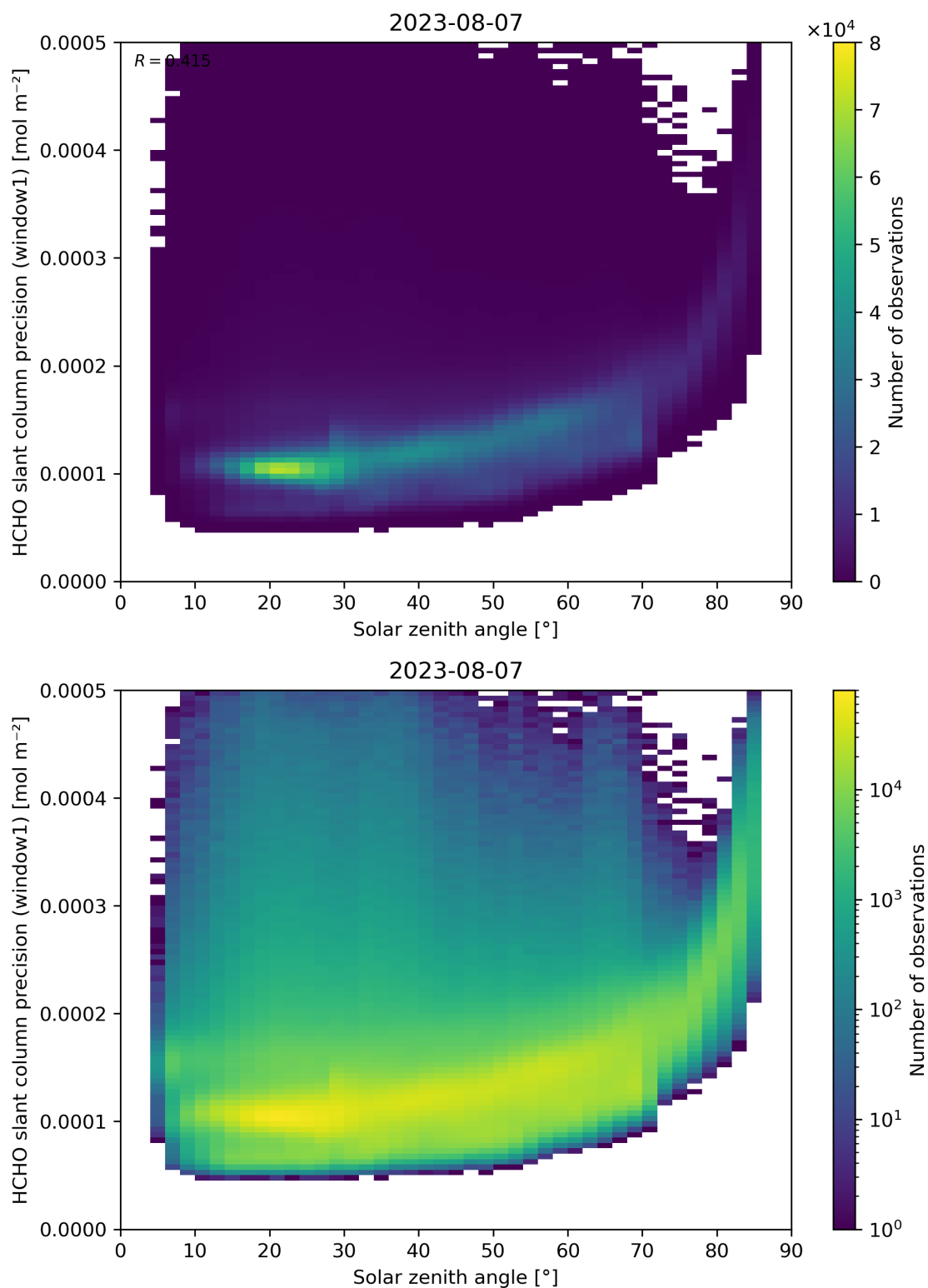
Figure 174: Scatter density plot of “Solar zenith angle” against “HCHO slant column precision (window1)” for 2023-08-06 to 2023-08-08.
