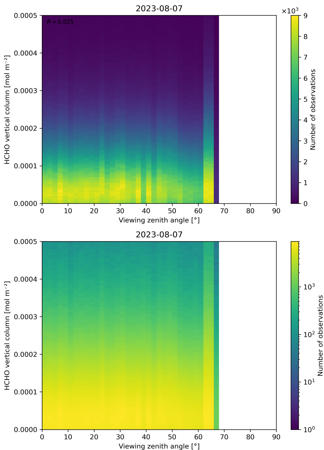
Figure 192: Scatter density plot of “Viewing zenith angle” against “HCHO vertical column” for 2023-08-06 to 2023-08-08.
