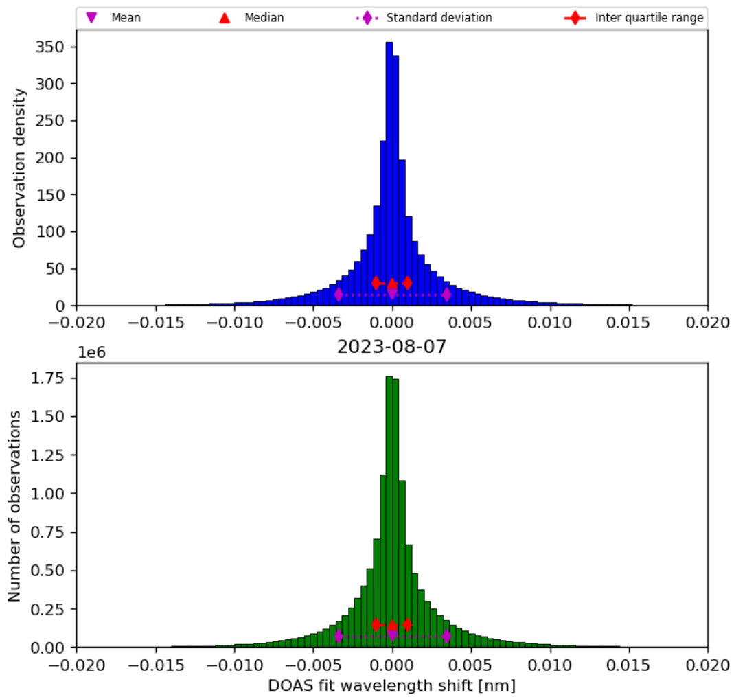
Figure 44: Histogram of “DOAS fit wavelength shift” for 2023-08-06 to 2023-08-08
