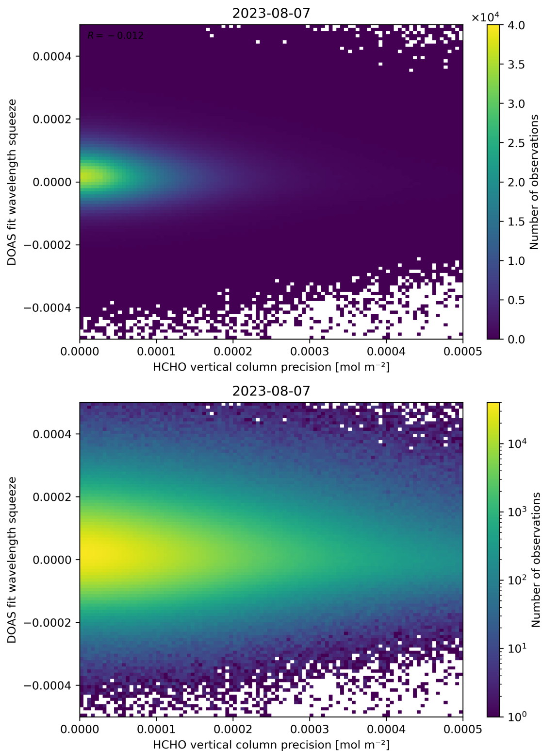
Figure 138: Scatter density plot of “HCHO vertical column precision” against “DOAS fit wavelength squeeze” for 2023-08-06 to 2023-08-08.
