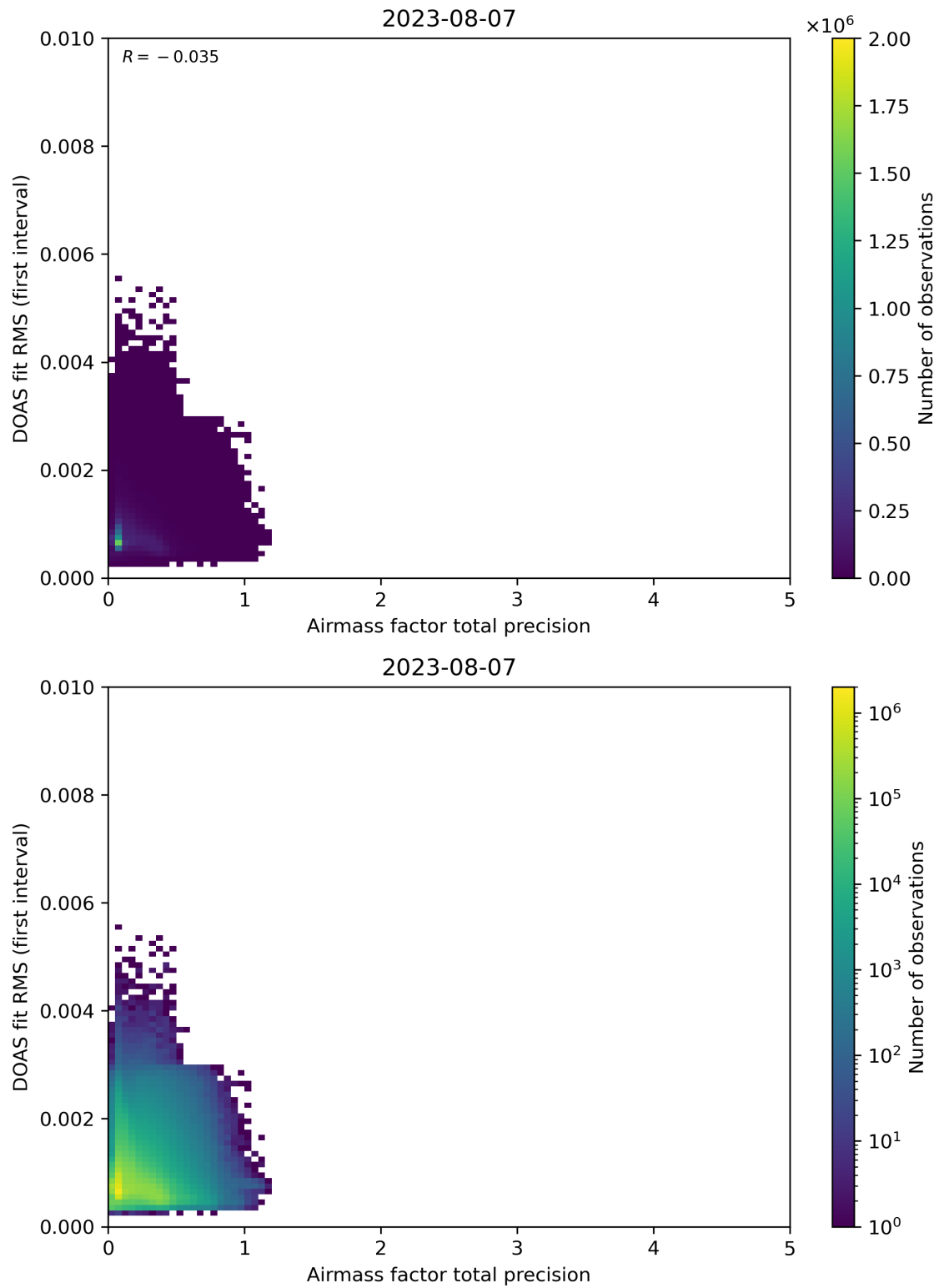
Figure 105: Scatter density plot of “Airmass factor total precision” against “DOAS fit RMS (first interval)” for 2023-08-06 to 2023-08-08.
