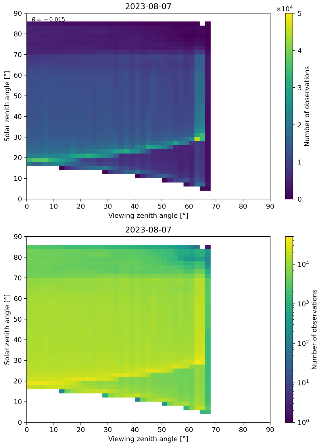
Figure 197: Scatter density plot of “Viewing zenith angle” against “Solar zenith angle” for 2023-08-06 to 2023-08-08.
