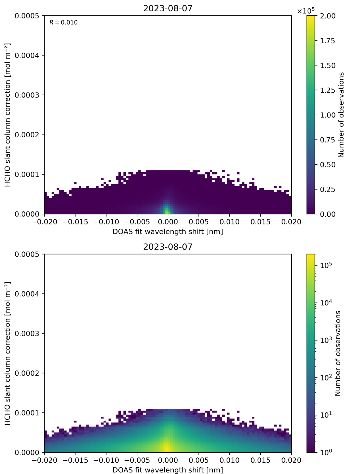
Figure 67: Scatter density plot of “DOAS fit wavelength shift” against “HCHO slant column correction” for 2023-08-06 to 2023-08-08.
