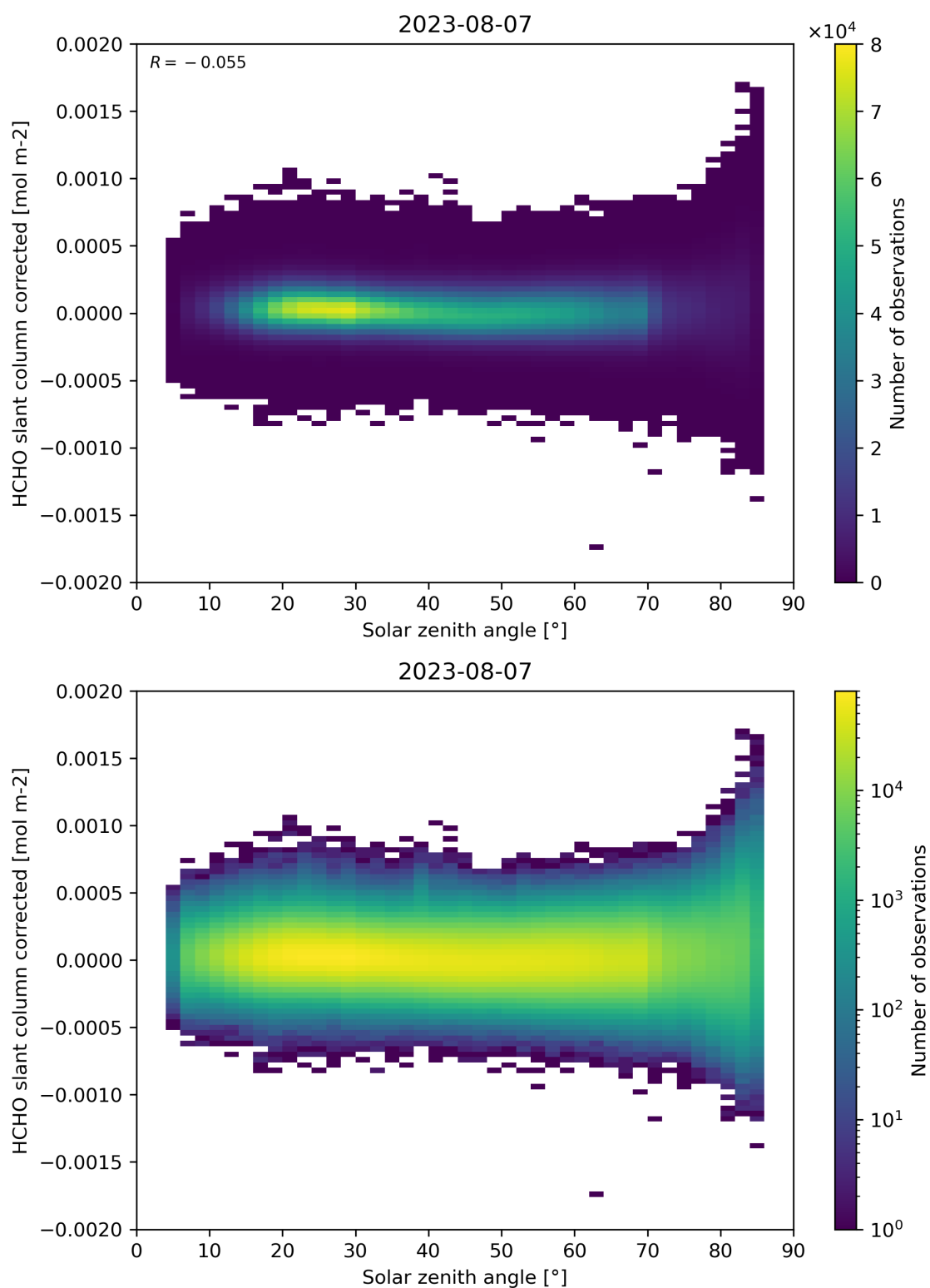
Figure 171: Scatter density plot of “Solar zenith angle” against “HCHO slant column corrected” for 2023-08-06 to 2023-08-08.
