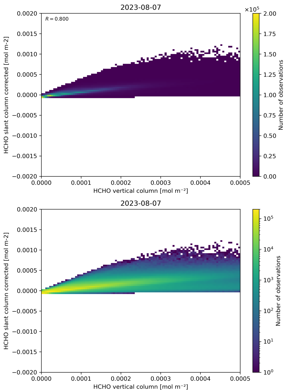
Figure 127: Scatter density plot of “HCHO vertical column” against “HCHO slant column corrected” for 2023-08-06 to 2023-08-08.
