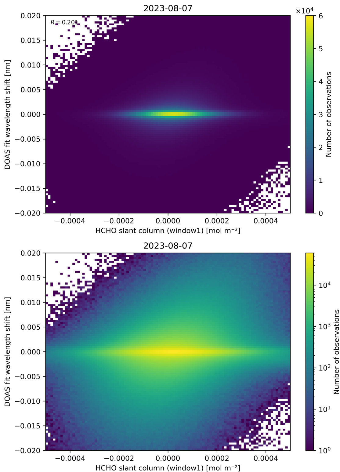
Figure 79: Scatter density plot of “HCHO slant column (window1)” against “DOAS fit wavelength shift” for 2023-08-06 to 2023-08-08.
