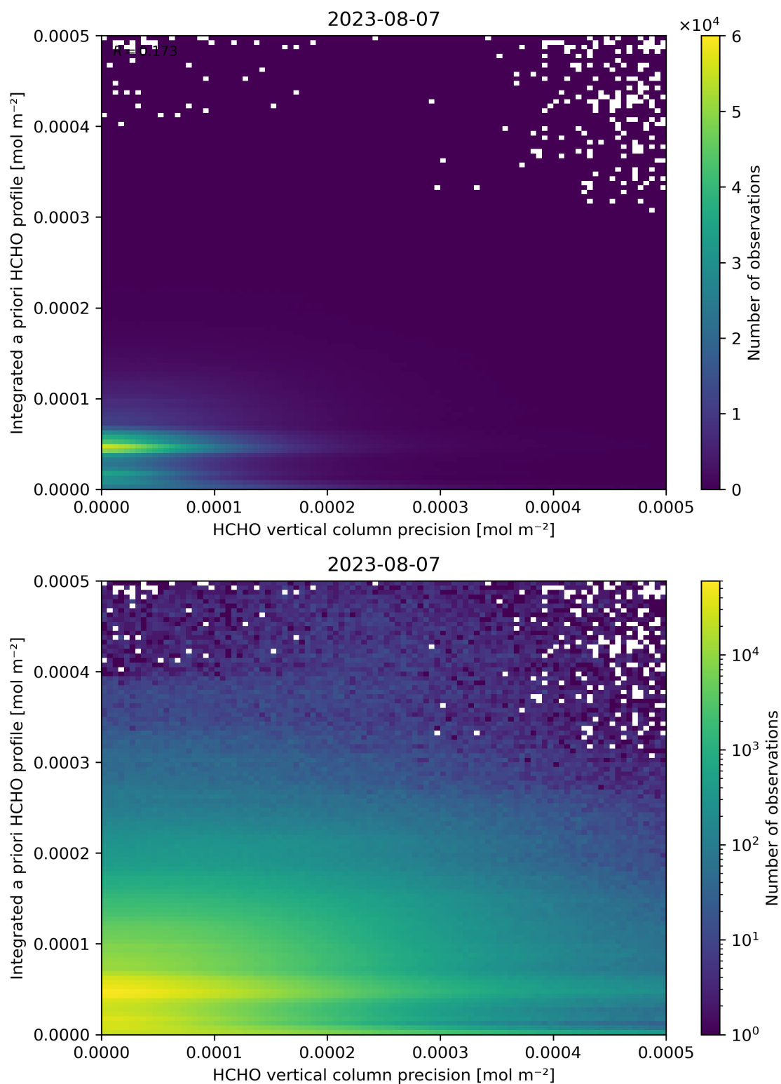
Figure 147: Scatter density plot of “HCHO vertical column precision” against “Integrated a priori HCHO profile” for 2023-08-06 to 2023-08-08.
