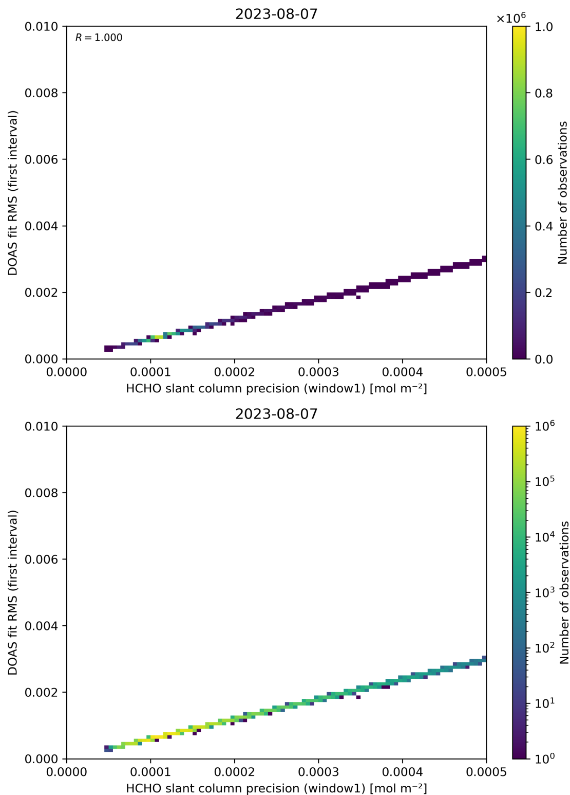
Figure 88: Scatter density plot of “HCHO slant column precision (window1)” against “DOAS fit RMS (first interval)” for 2023-08-06 to 2023-08-08.
