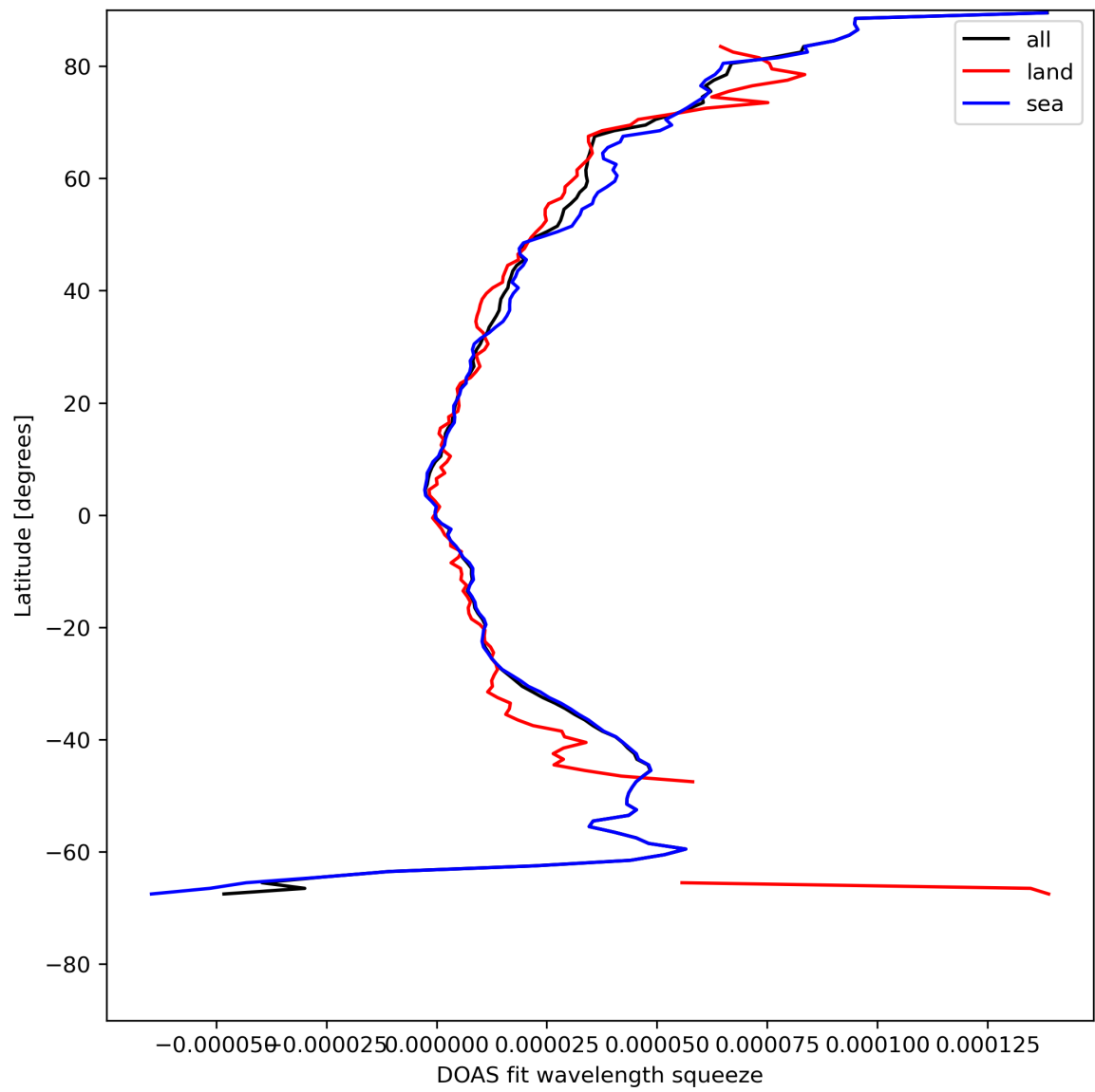
Figure 31: Zonal average of “DOAS fit wavelength squeeze” for 2023-08-06 to 2023-08-08.
