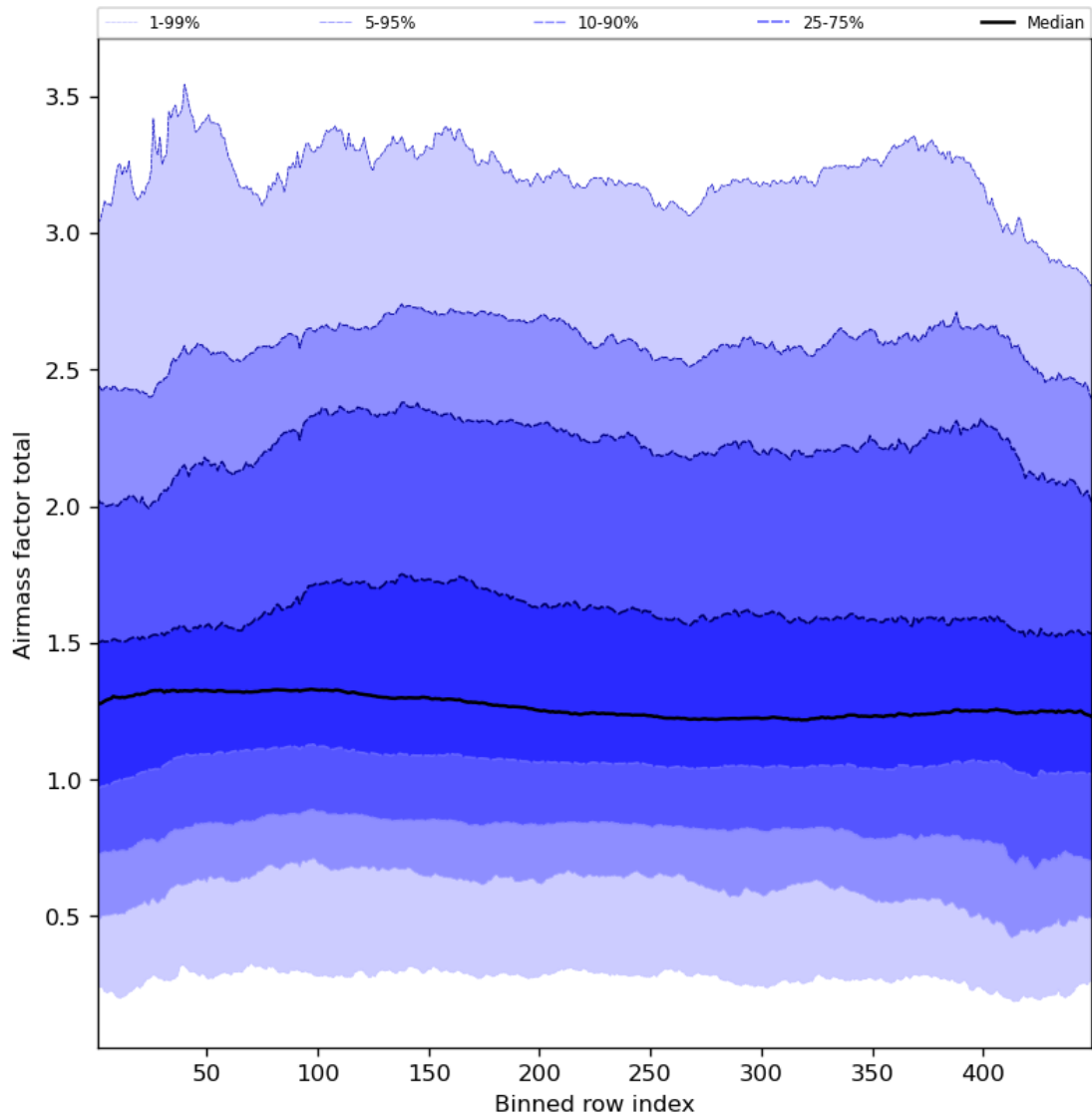
Figure 54: Along track statistics of “Airmass factor total” for 2023-08-06 to 2023-08-08
