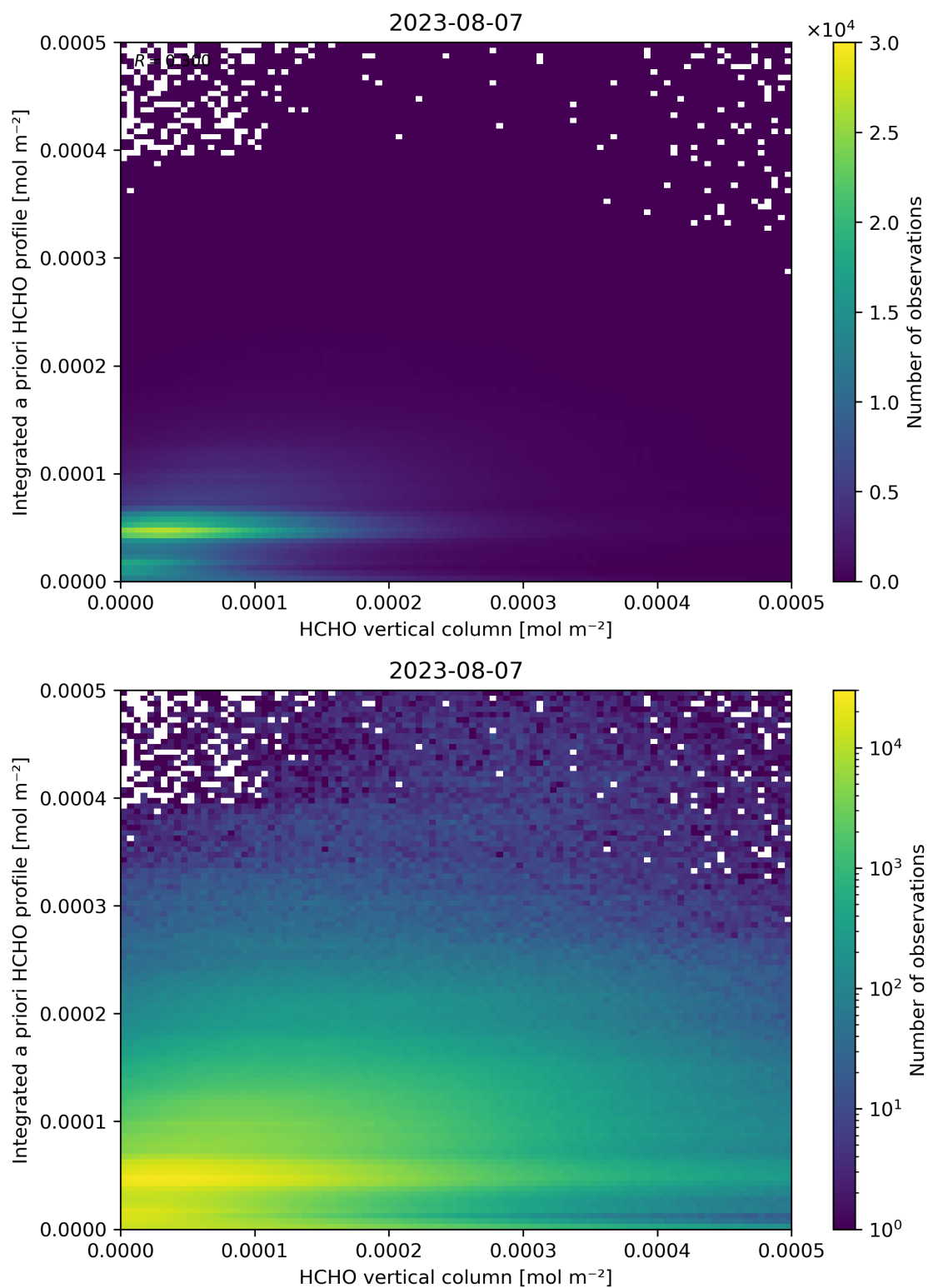
Figure 135: Scatter density plot of “HCHO vertical column” against “Integrated a priori HCHO profile” for 2023-08-06 to 2023-08-08.
