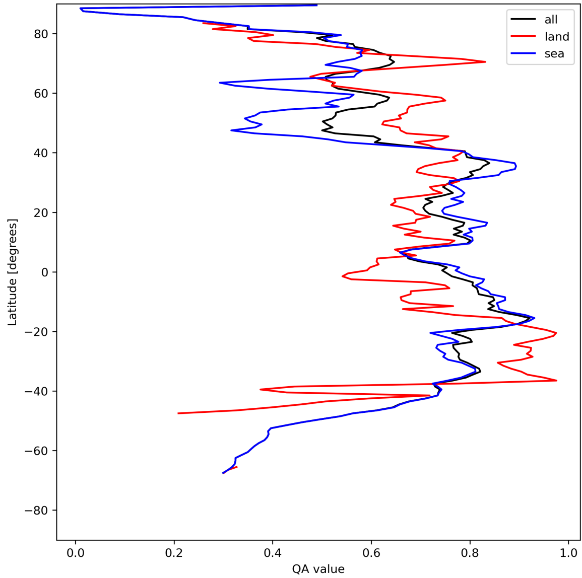
Figure 20: Zonal average of “QA value” for 2023-08-06 to 2023-08-08.
