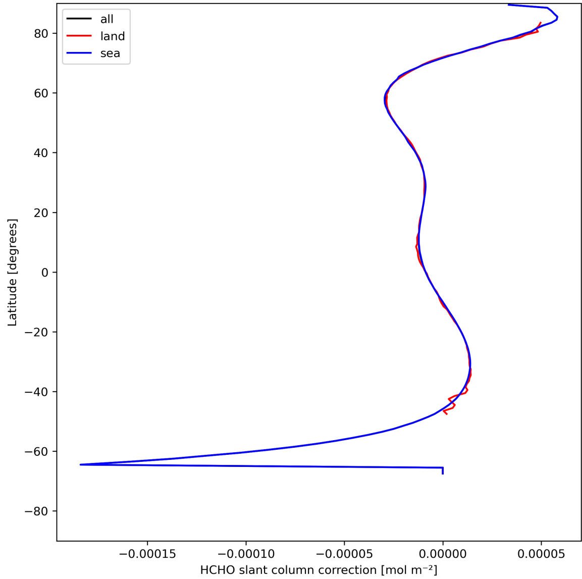
Figure 33: Zonal average of “HCHO slant column correction” for 2023-08-06 to 2023-08-08.
