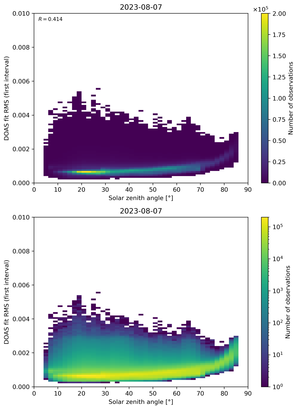
Figure 167: Scatter density plot of “Solar zenith angle” against “DOAS fit RMS (first interval)” for 2023-08-06 to 2023-08-08.
