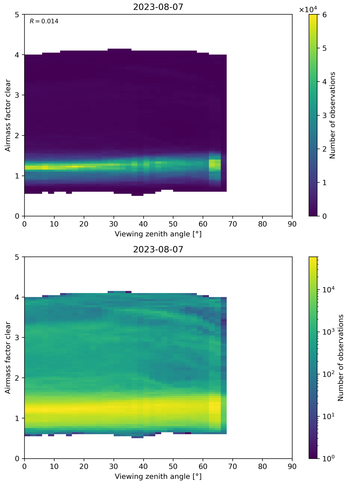
Figure 185: Scatter density plot of “Viewing zenith angle” against “Airmass factor clear” for 2023-08-06 to 2023-08-08.
