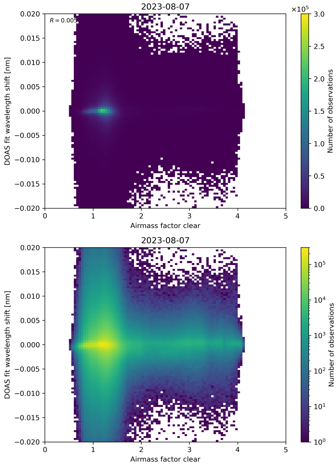
Figure 72: Scatter density plot of “Airmass factor clear” against “DOAS fit wavelength shift” for 2023-08-06 to 2023-08-08.
