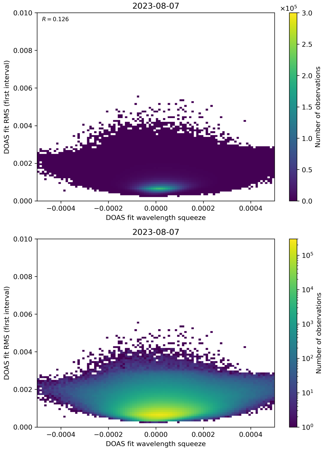
Figure 68: Scatter density plot of “DOAS fit wavelength squeeze” against “DOAS fit RMS (first interval)” for 2023-08-06 to 2023-08-08.
