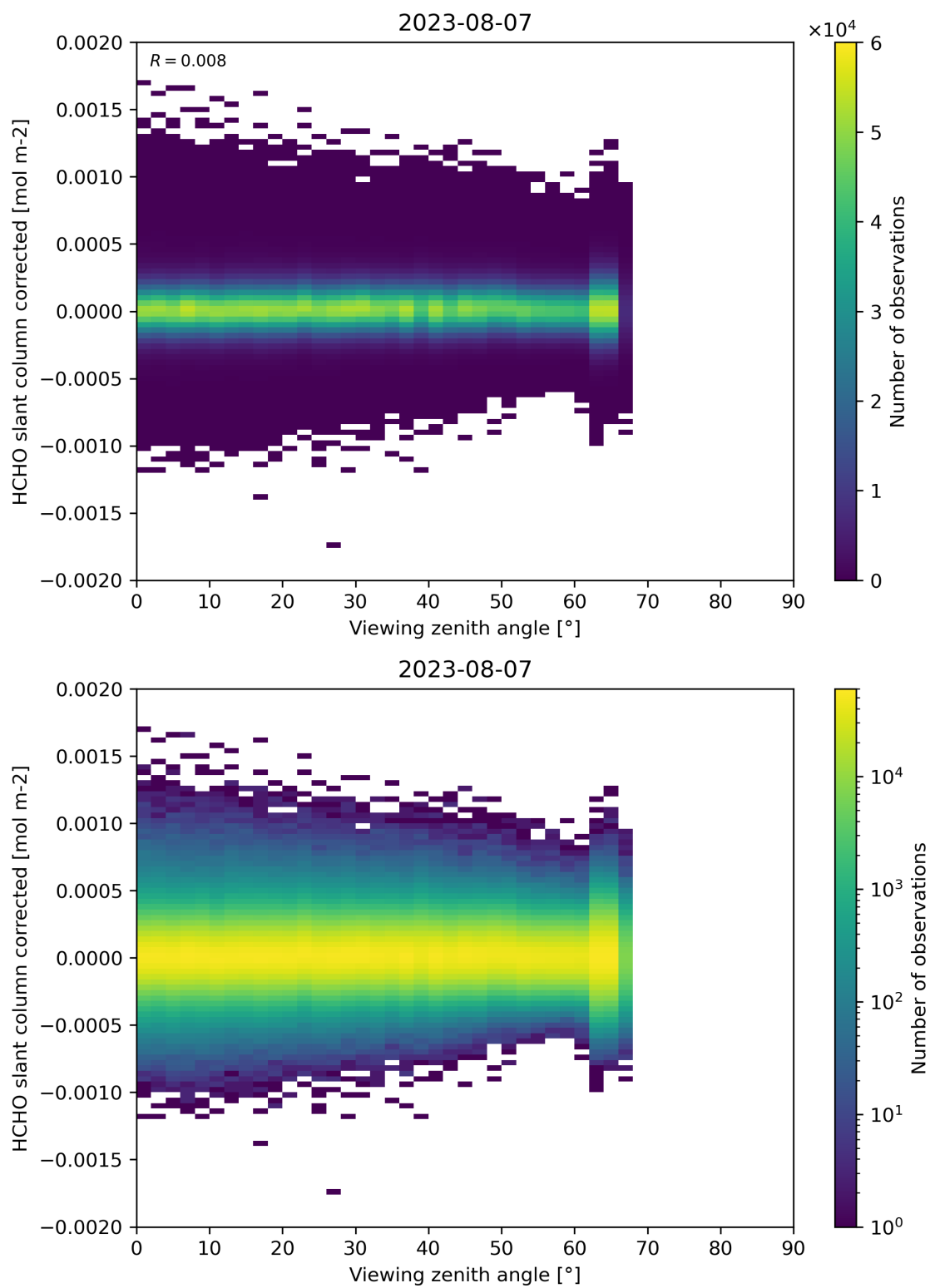
Figure 186: Scatter density plot of “Viewing zenith angle” against “HCHO slant column corrected” for 2023-08-06 to 2023-08-08.
