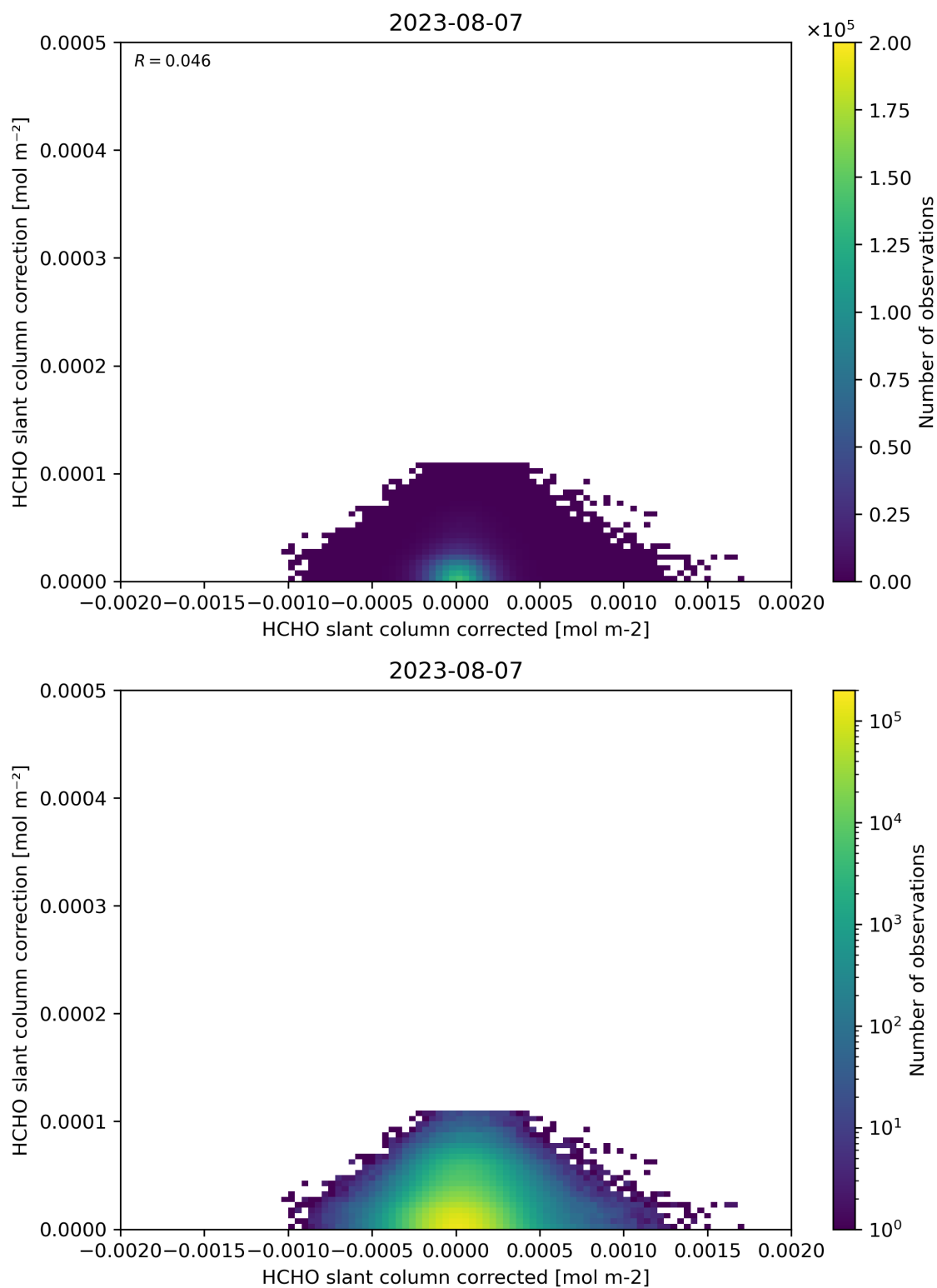
Figure 77: Scatter density plot of “HCHO slant column corrected” against “HCHO slant column correction” for 2023-08-06 to 2023-08-08.
