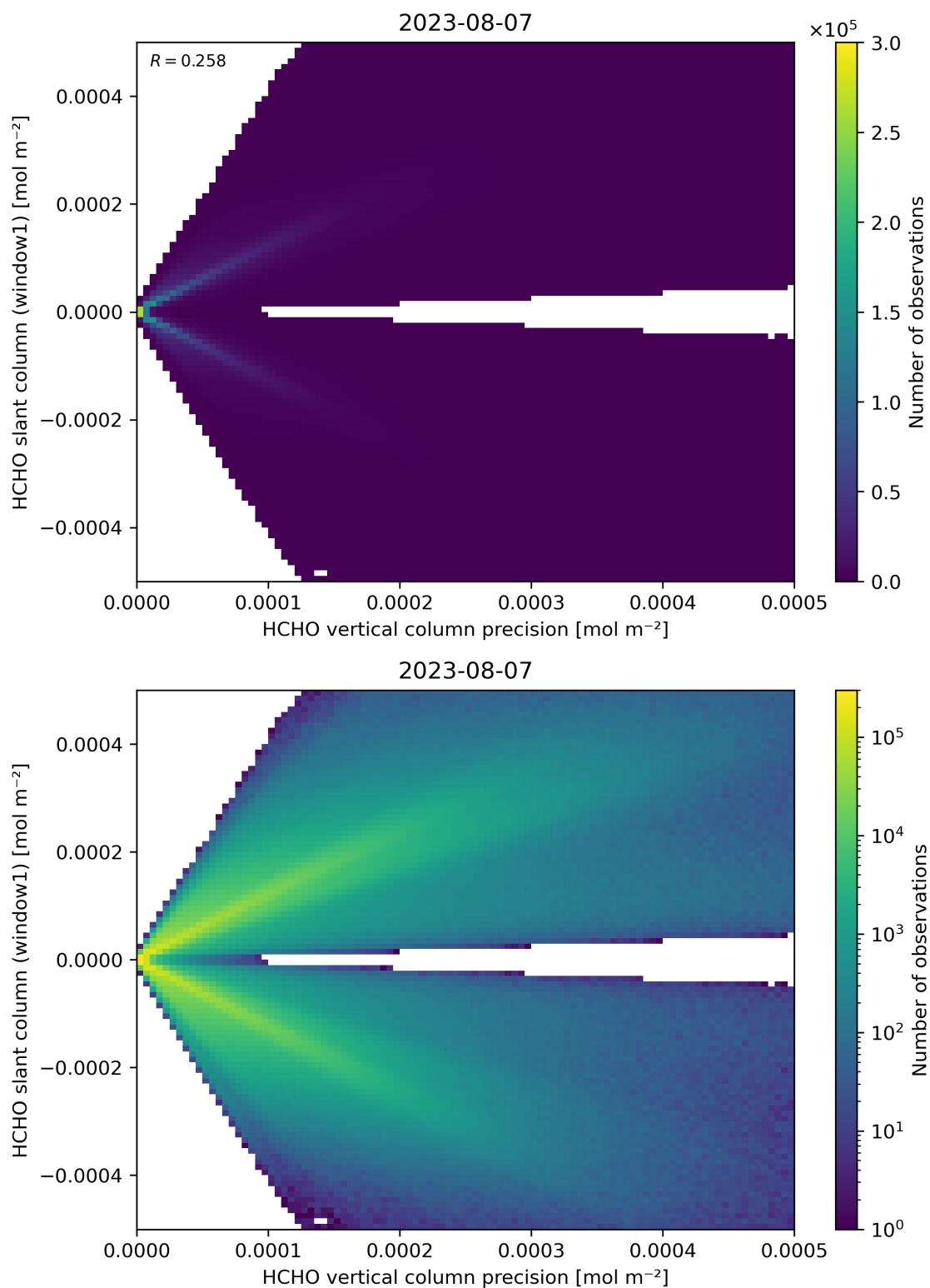
Figure 142: Scatter density plot of “HCHO vertical column precision” against “HCHO slant column (window1)” for 2023-08-06 to 2023-08-08.
