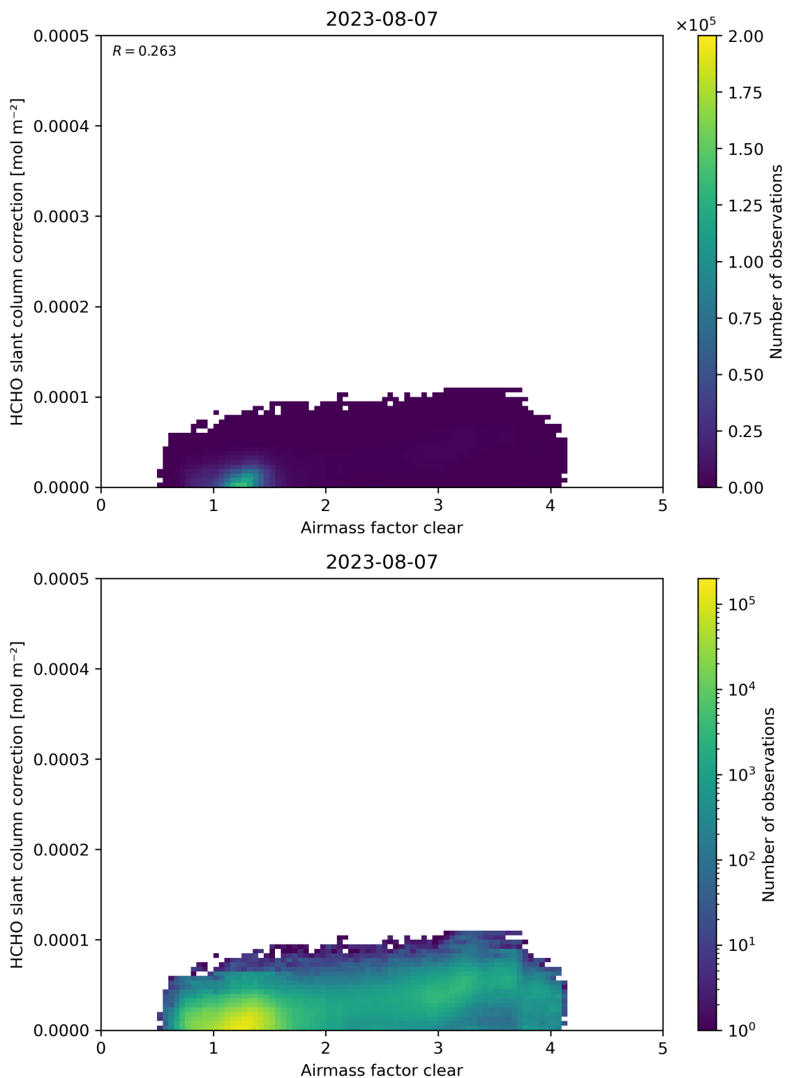
Figure 75: Scatter density plot of “Airmass factor clear” against “HCHO slant column correction” for 2023-08-06 to 2023-08-08.
