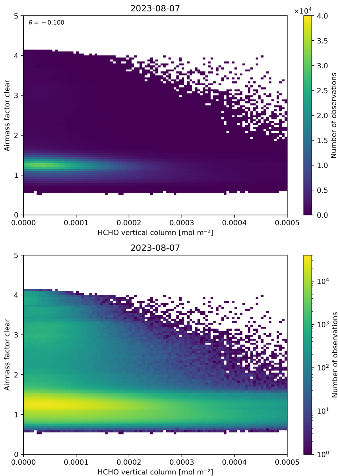
Figure 126: Scatter density plot of “HCHO vertical column” against “Airmass factor clear” for 2023-08-06 to 2023-08-08.
