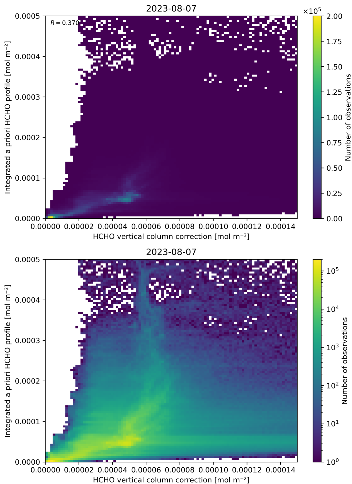
Figure 122: Scatter density plot of “HCHO vertical column correction” against “Integrated a priori HCHO profile” for 2023-08-06 to 2023-08-08.
