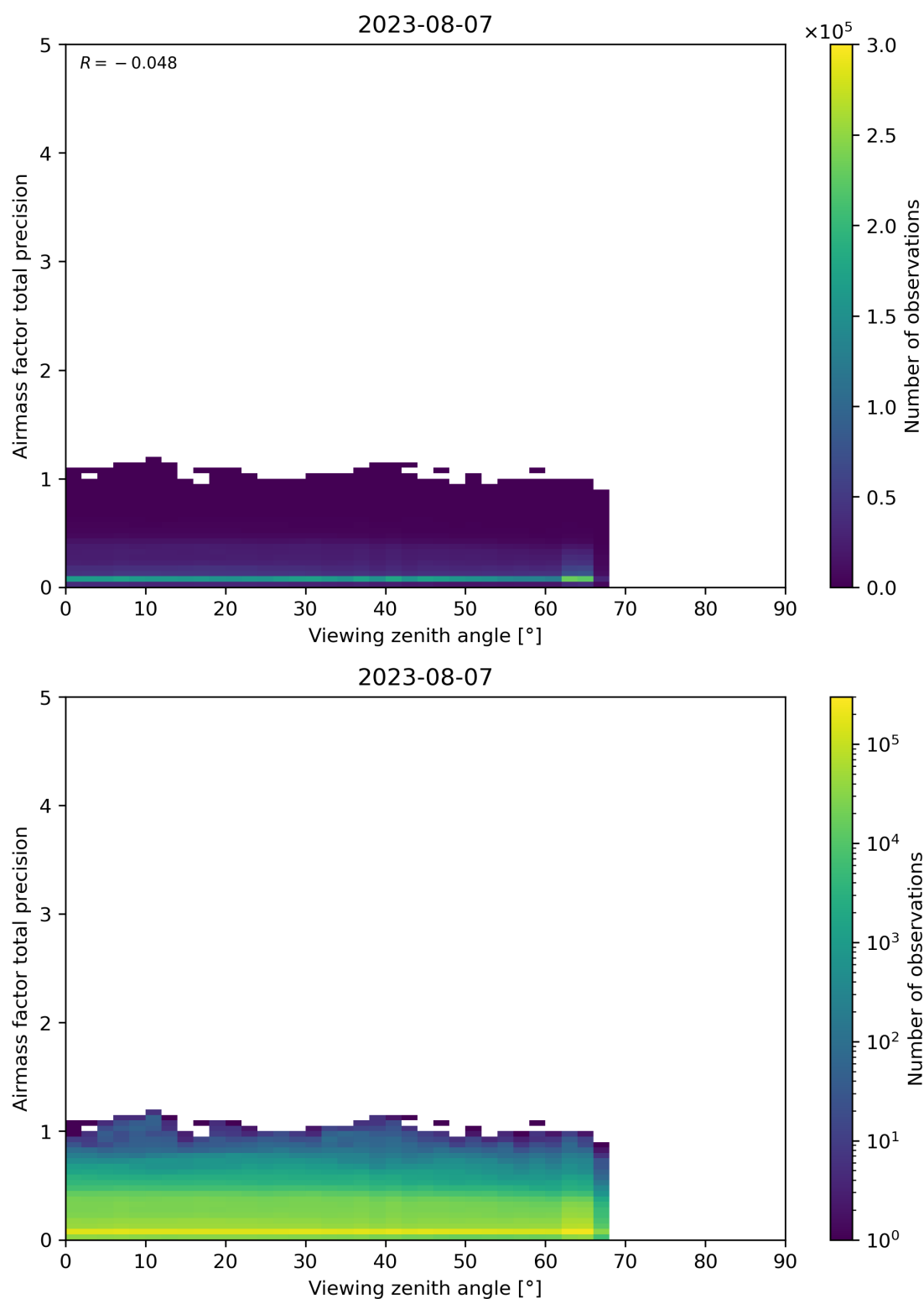
Figure 191: Scatter density plot of “Viewing zenith angle” against “Airmass factor total precision” for 2023-08-06 to 2023-08-08.
