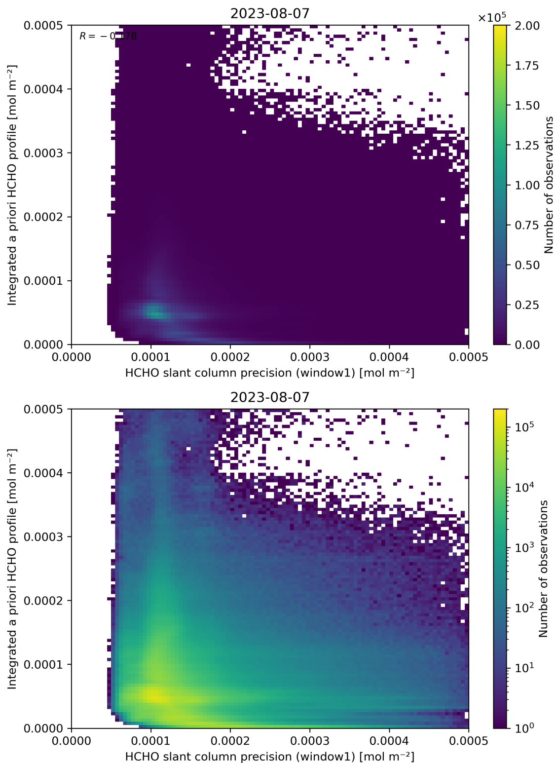
Figure 96: Scatter density plot of “HCHO slant column precision (window1)” against “Integrated a priori HCHO profile” for 2023-08-06 to 2023-08-08.
