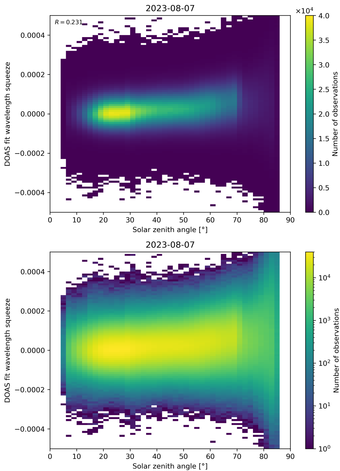
Figure 169: Scatter density plot of “Solar zenith angle” against “DOAS fit wavelength squeeze” for 2023-08-06 to 2023-08-08.
