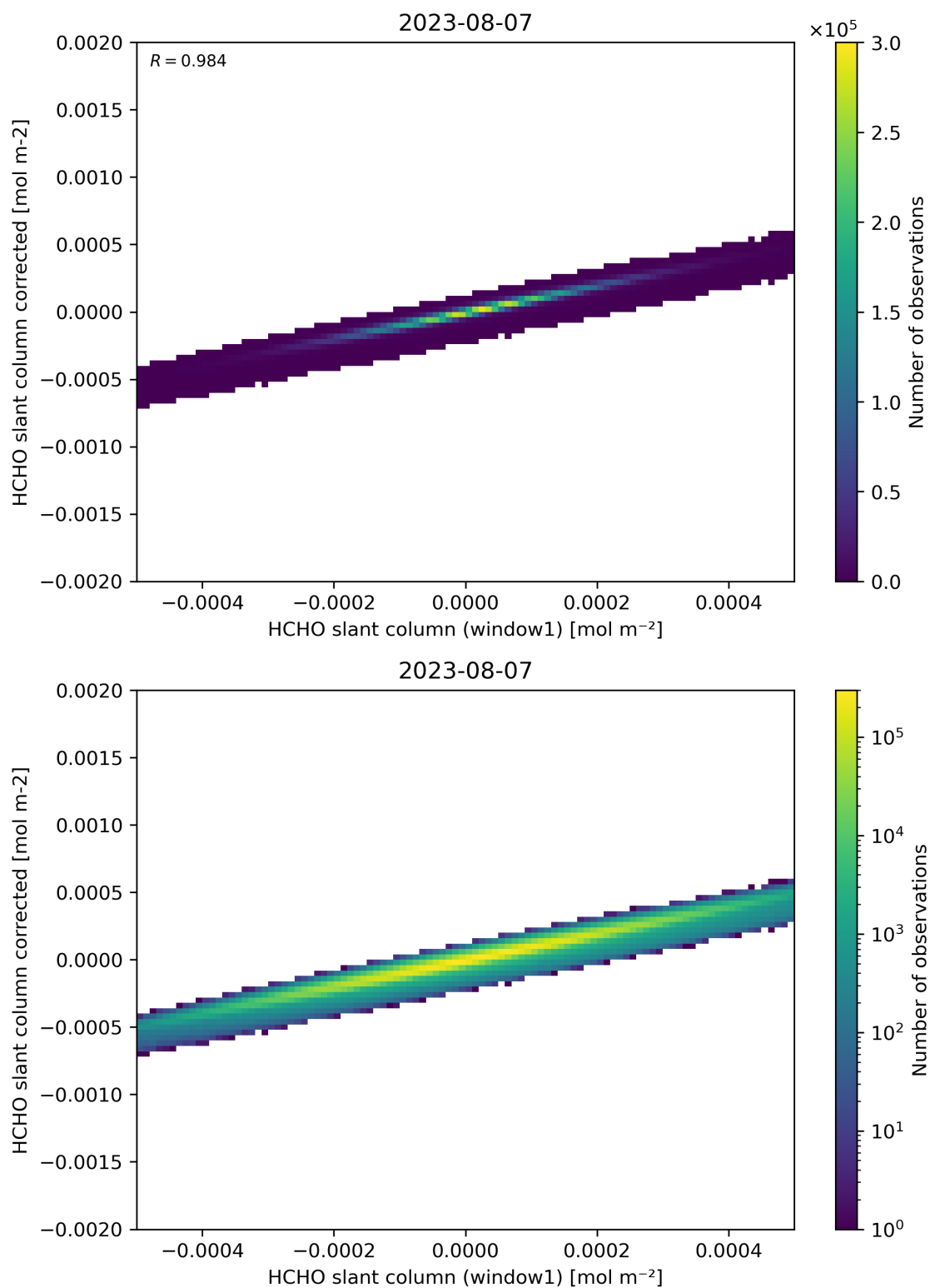
Figure 82: Scatter density plot of “HCHO slant column (window1)” against “HCHO slant column corrected” for 2023-08-06 to 2023-08-08.
