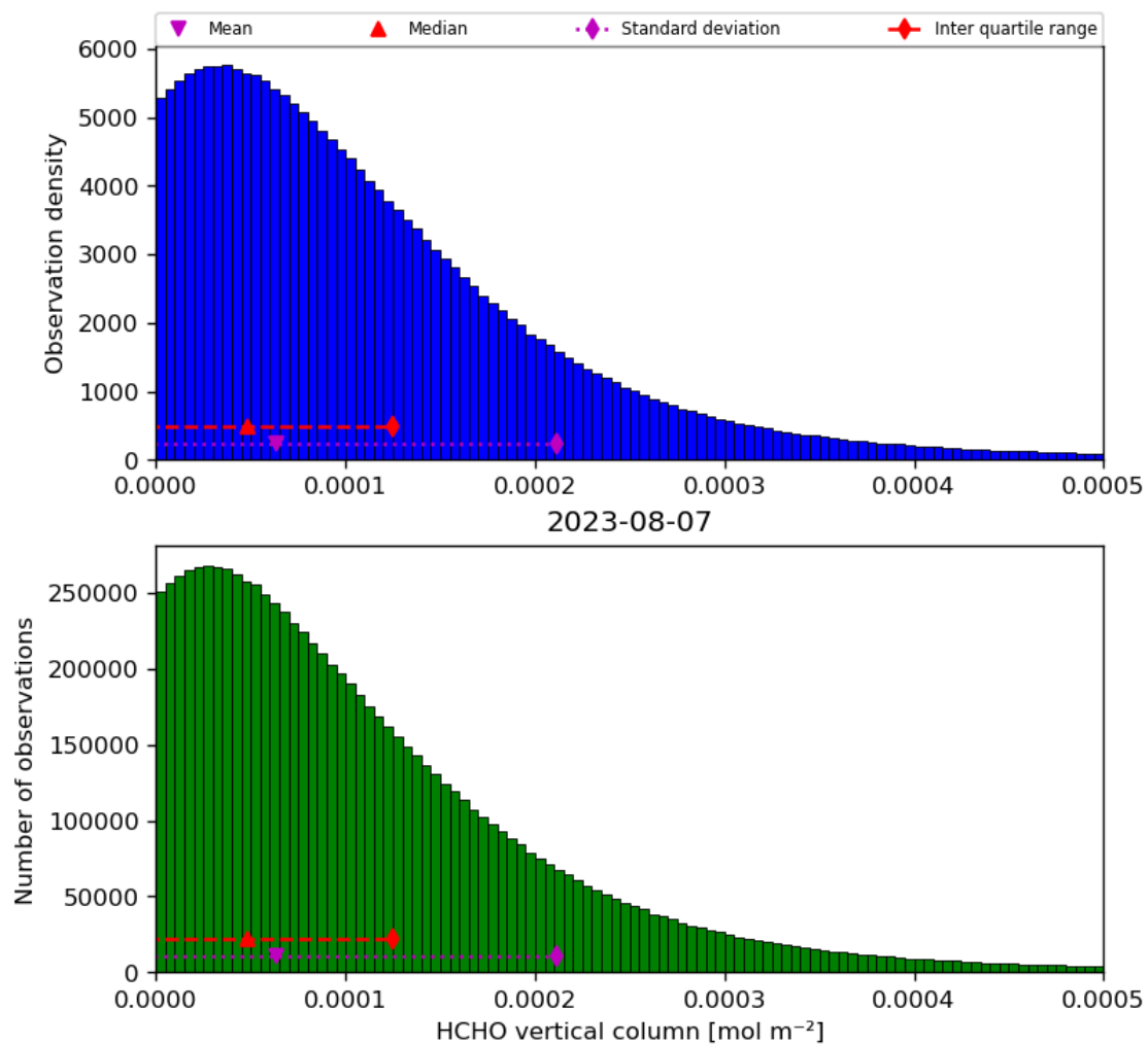
Figure 35: Histogram of “HCHO vertical column” for 2023-08-06 to 2023-08-08
