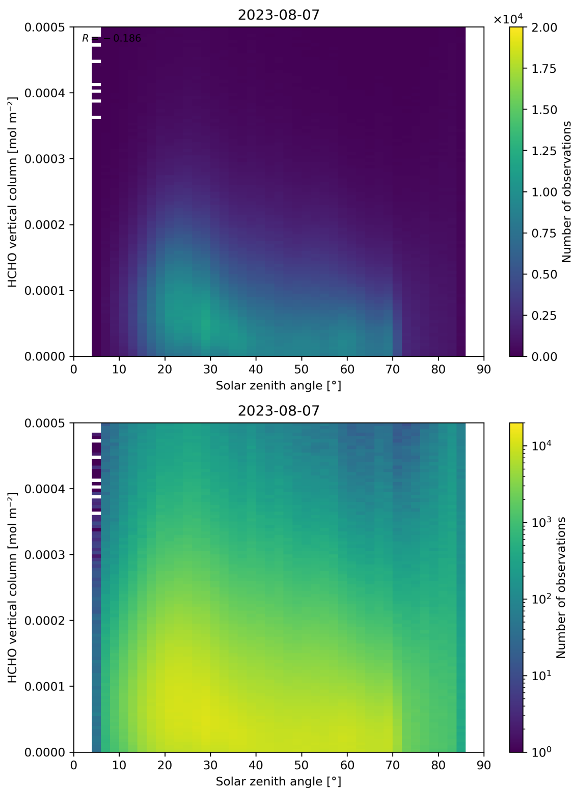
Figure 177: Scatter density plot of “Solar zenith angle” against “HCHO vertical column” for 2023-08-06 to 2023-08-08.
