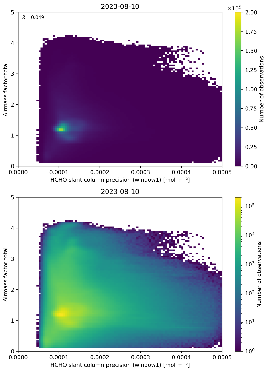
Figure 94: Scatter density plot of “HCHO slant column precision (window1)” against “Airmass factor total” for 2023-08-09 to 2023-08-11.
