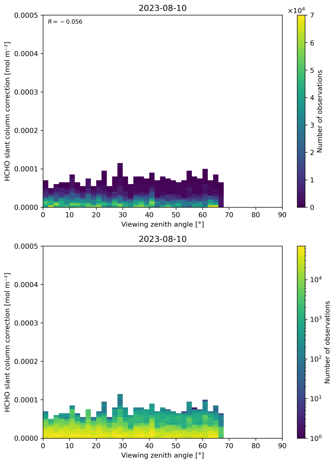
Figure 187: Scatter density plot of “Viewing zenith angle” against “HCHO slant column correction” for 2023-08-09 to 2023-08-11.
