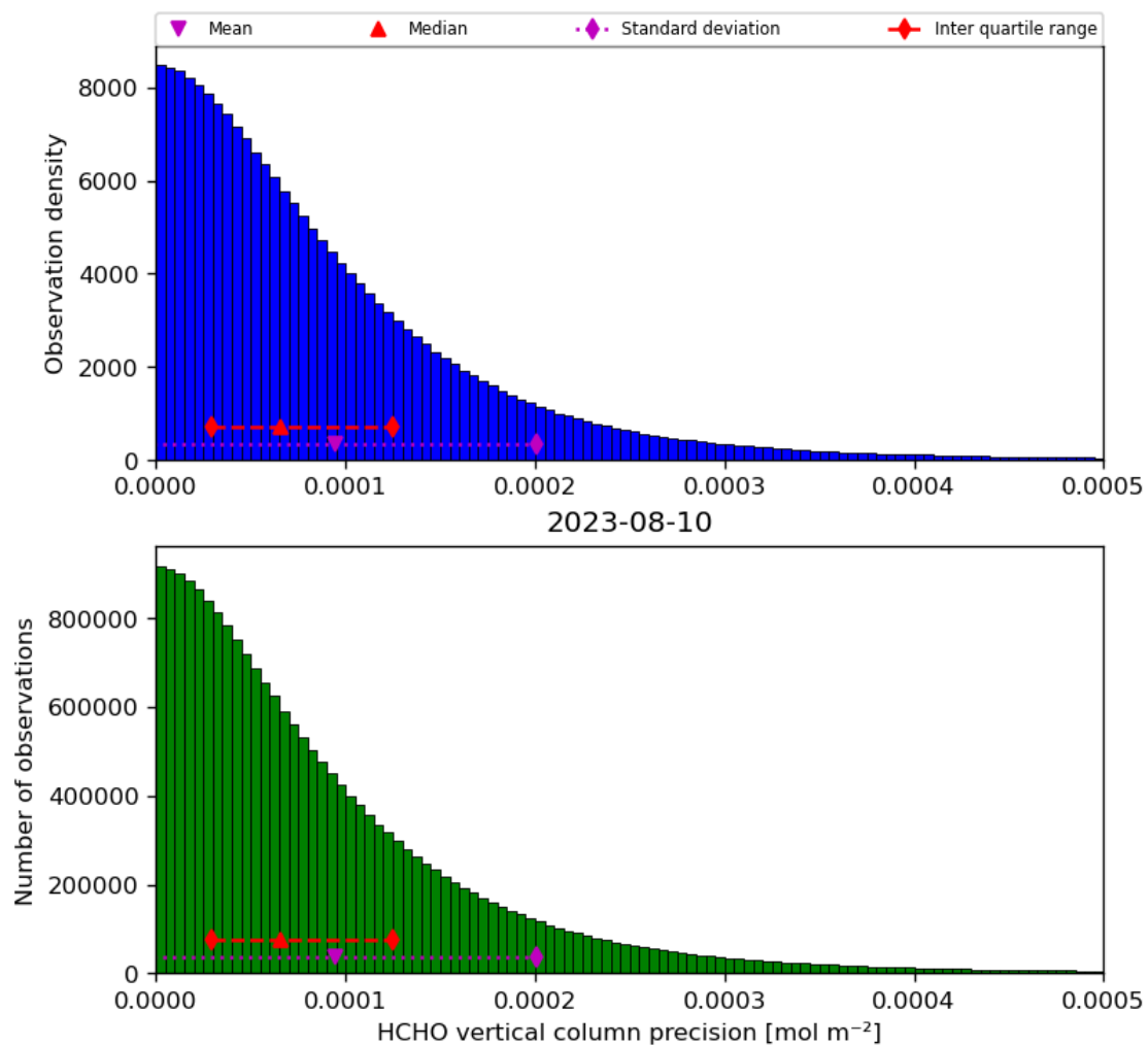
Figure 36: Histogram of “HCHO vertical column precision” for 2023-08-09 to 2023-08-11
