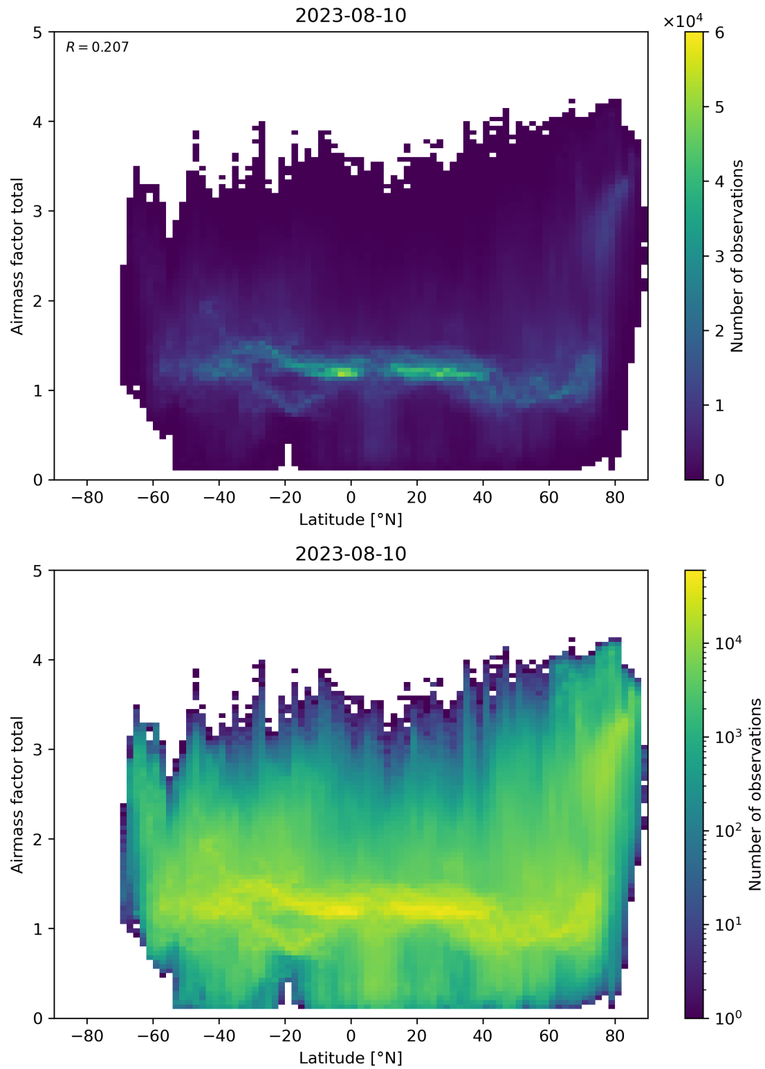
Figure 161: Scatter density plot of “Latitude” against “Airmass factor total” for 2023-08-09 to 2023-08-11.
