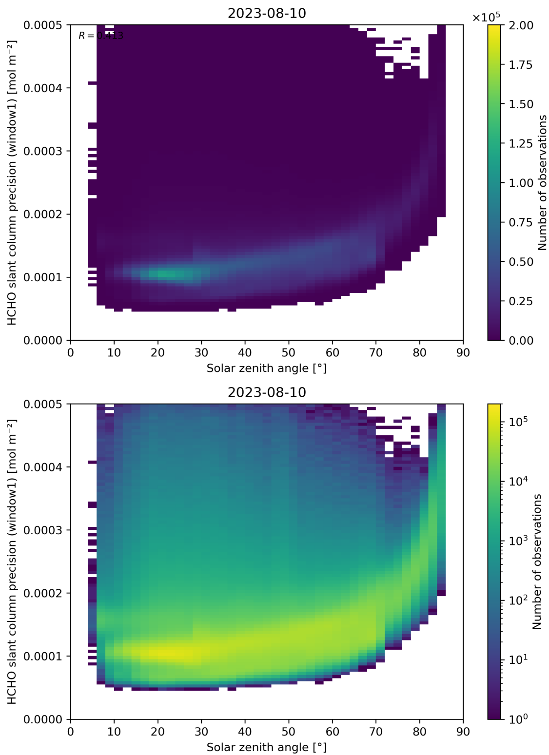
Figure 174: Scatter density plot of “Solar zenith angle” against “HCHO slant column precision (window1)” for 2023-08-09 to 2023-08-11.
