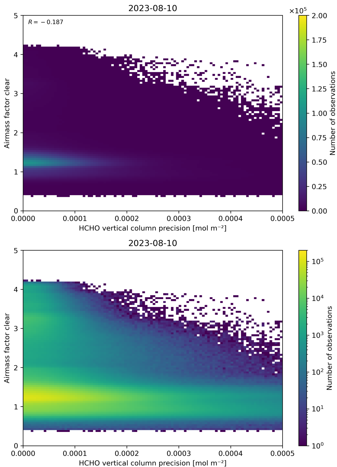
Figure 139: Scatter density plot of “HCHO vertical column precision” against “Airmass factor clear” for 2023-08-09 to 2023-08-11.
