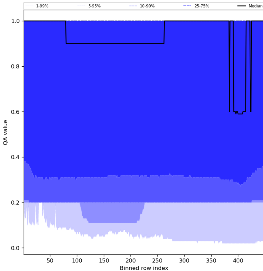
Figure 48: Along track statistics of “QA value” for 2023-08-09 to 2023-08-11
