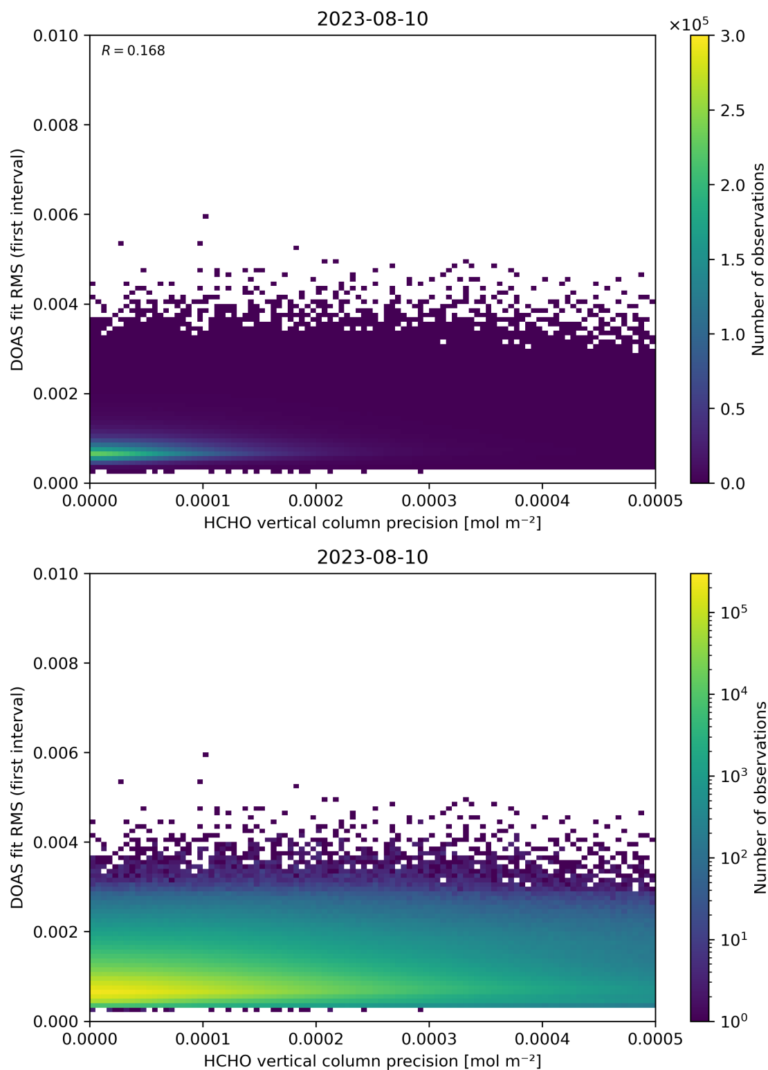
Figure 136: Scatter density plot of “HCHO vertical column precision” against “DOAS fit RMS (first interval)” for 2023-08-09 to 2023-08-11.
