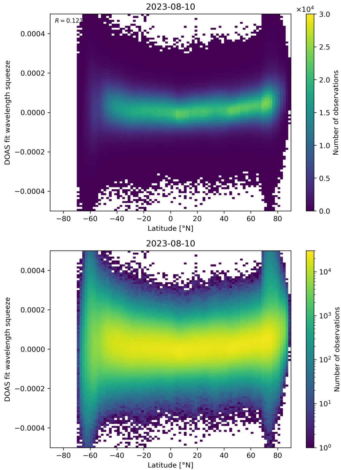
Figure 155: Scatter density plot of “Latitude” against “DOAS fit wavelength squeeze” for 2023-08-09 to 2023-08-11.
