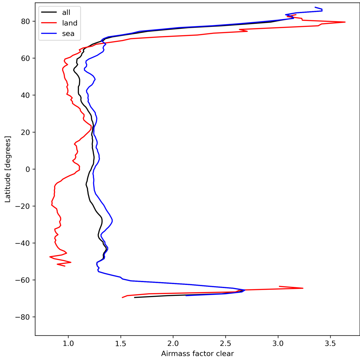
Figure 28: Zonal average of “Airmass factor clear” for 2023-08-09 to 2023-08-11.
