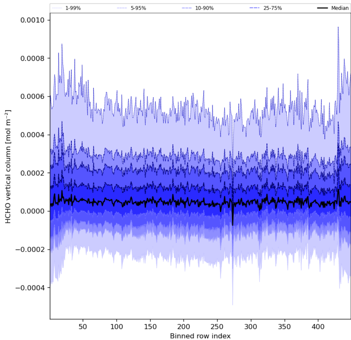
Figure 49: Along track statistics of “HCHO vertical column” for 2023-08-09 to 2023-08-11
