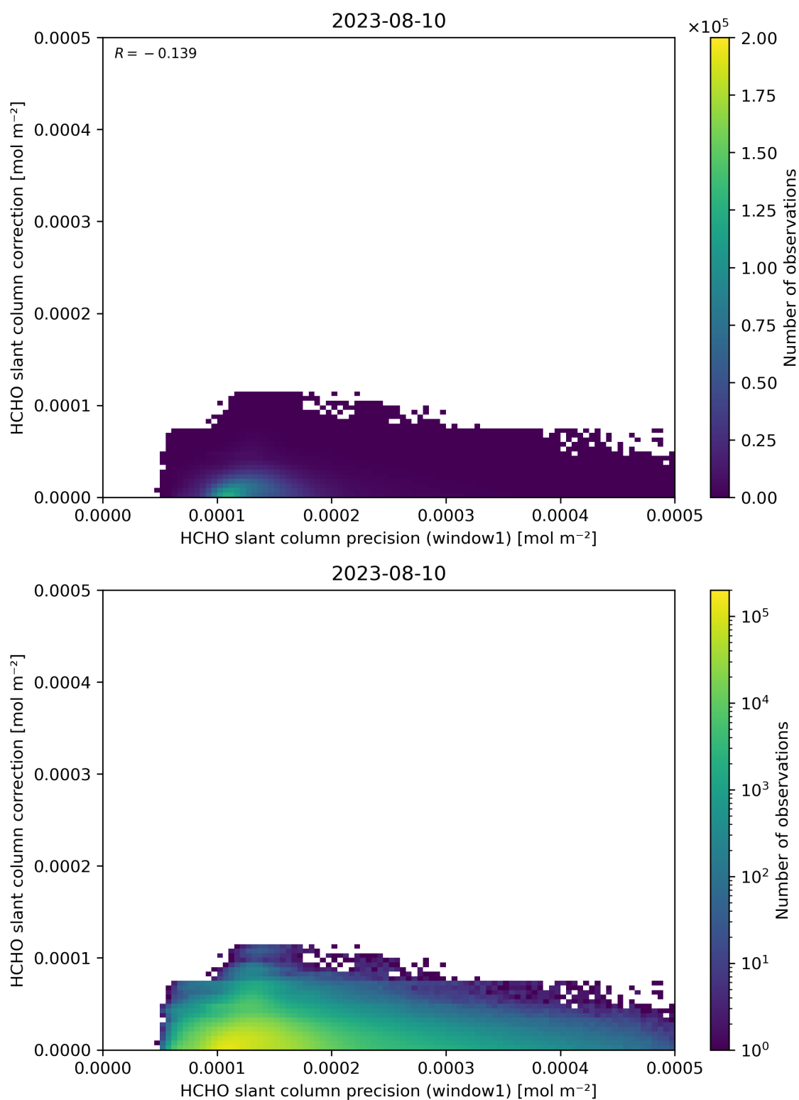
Figure 93: Scatter density plot of “HCHO slant column precision (window1)” against “HCHO slant column correction” for 2023-08-09 to 2023-08-11.
