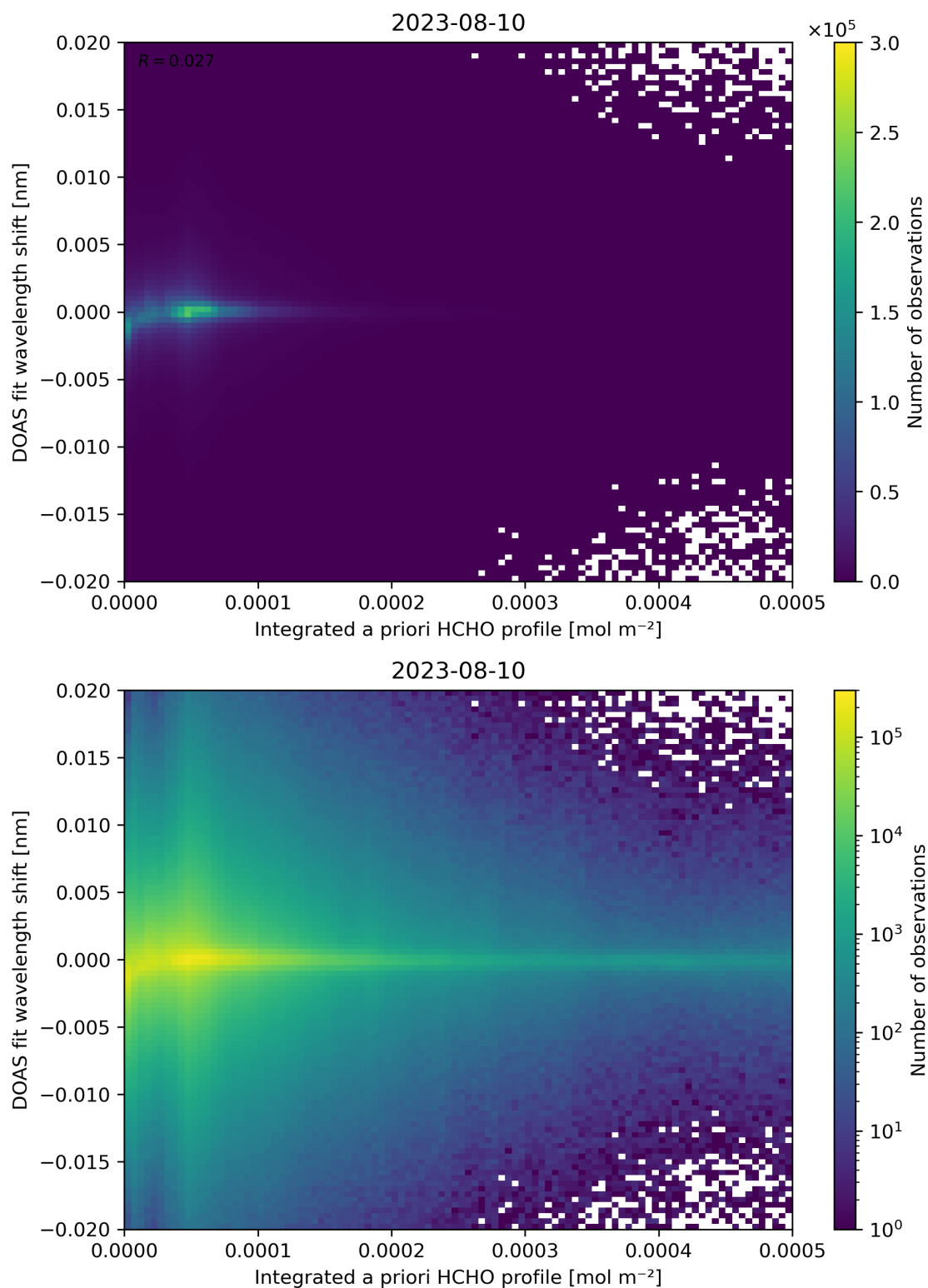
Figure 149: Scatter density plot of “Integrated a priori HCHO profile” against “DOAS fit wavelength shift” for 2023-08-09 to 2023-08-11.
