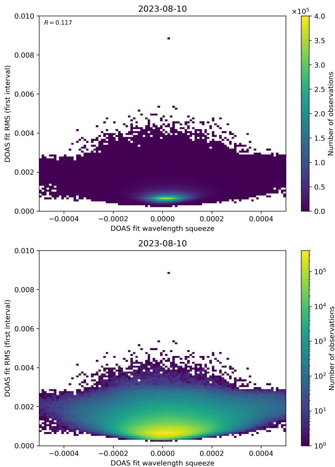
Figure 68: Scatter density plot of “DOAS fit wavelength squeeze” against “DOAS fit RMS (first interval)” for 2023-08-09 to 2023-08-11.
