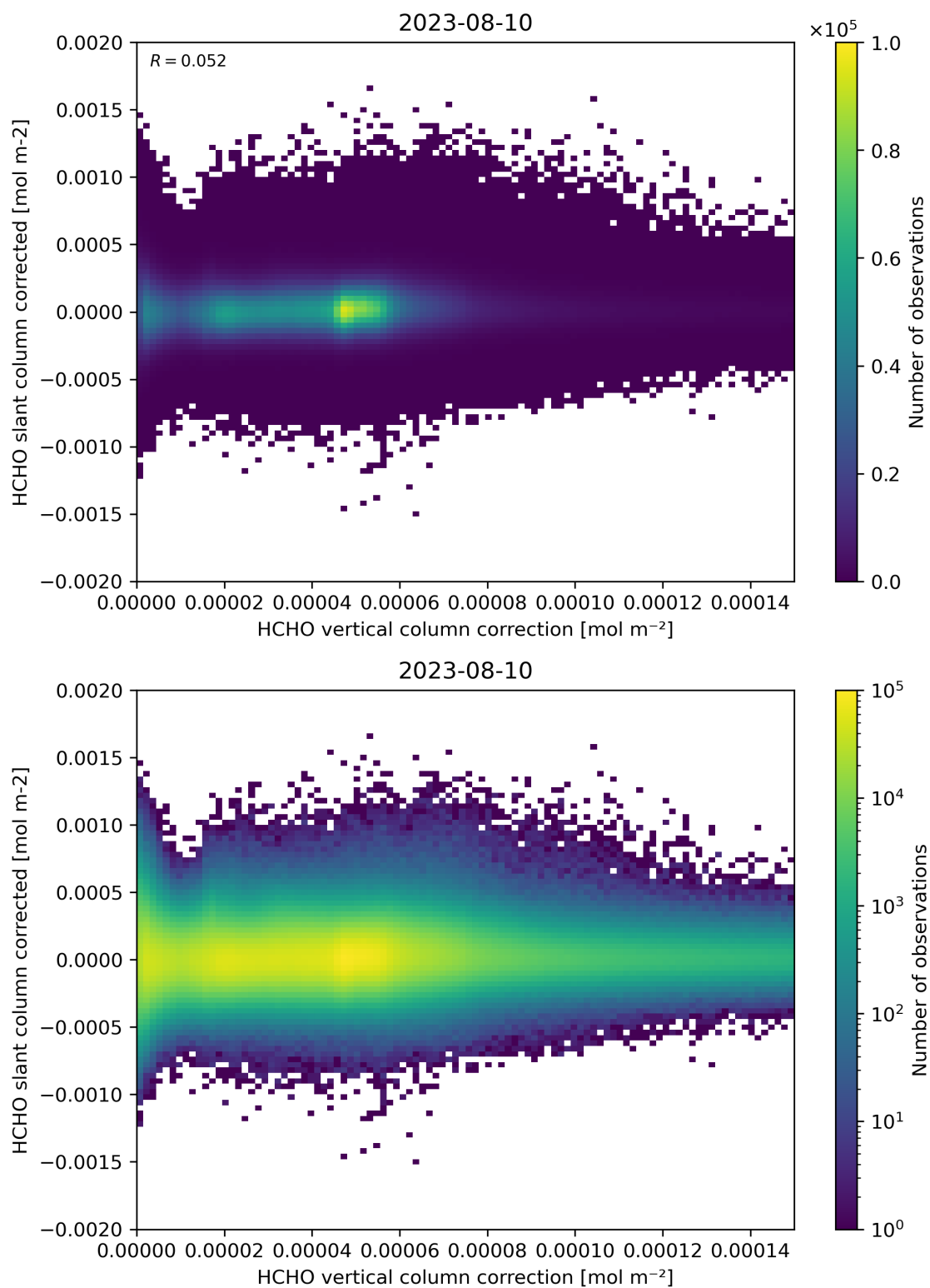
Figure 116: Scatter density plot of “HCHO vertical column correction” against “HCHO slant column corrected” for 2023-08-09 to 2023-08-11.
