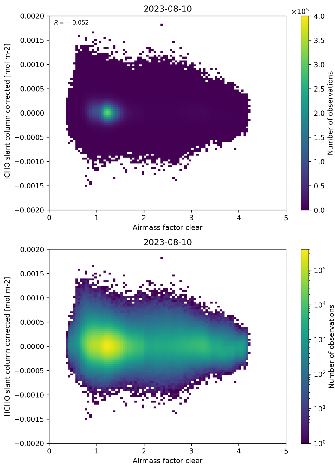
Figure 74: Scatter density plot of “Airmass factor clear” against “HCHO slant column corrected” for 2023-08-09 to 2023-08-11.
