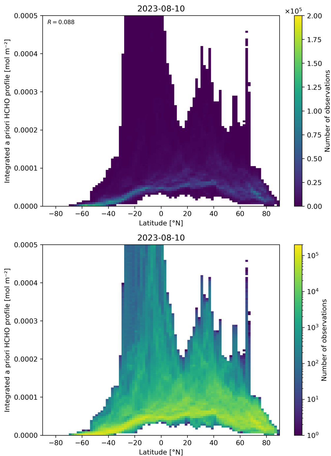
Figure 166: Scatter density plot of “Latitude” against “Integrated a priori HCHO profile” for 2023-08-09 to 2023-08-11.
