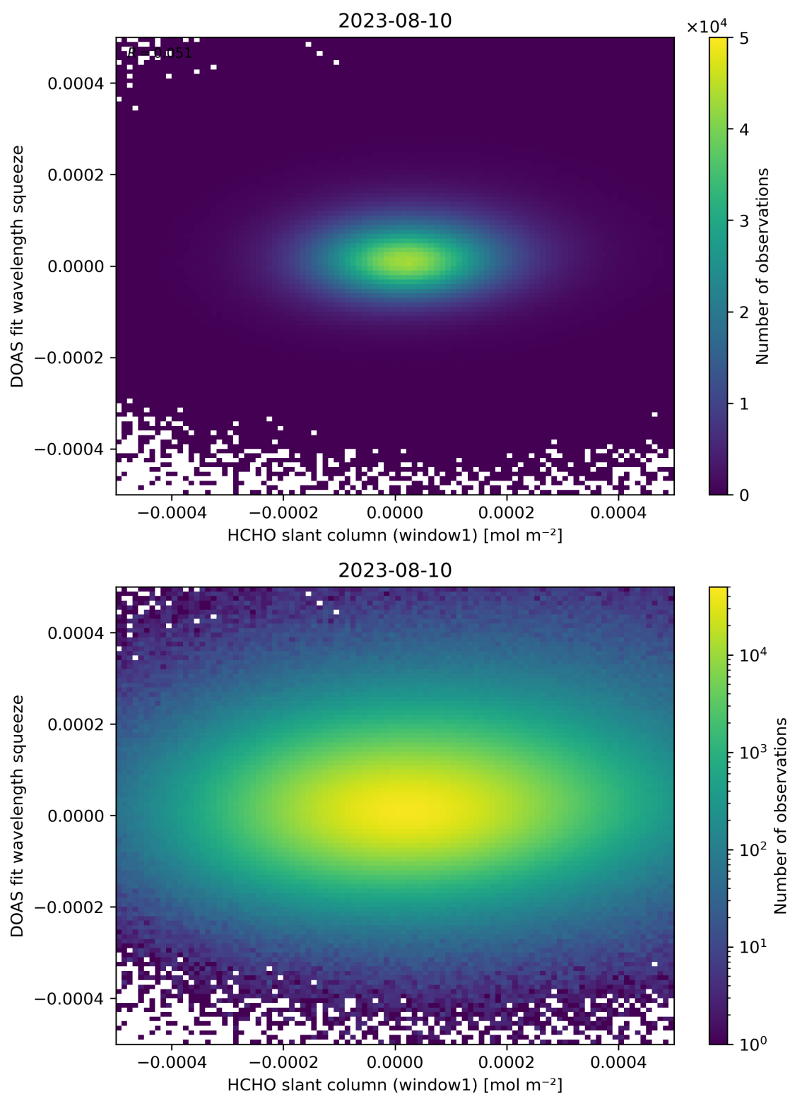
Figure 80: Scatter density plot of “HCHO slant column (window1)” against “DOAS fit wavelength squeeze” for 2023-08-09 to 2023-08-11.
