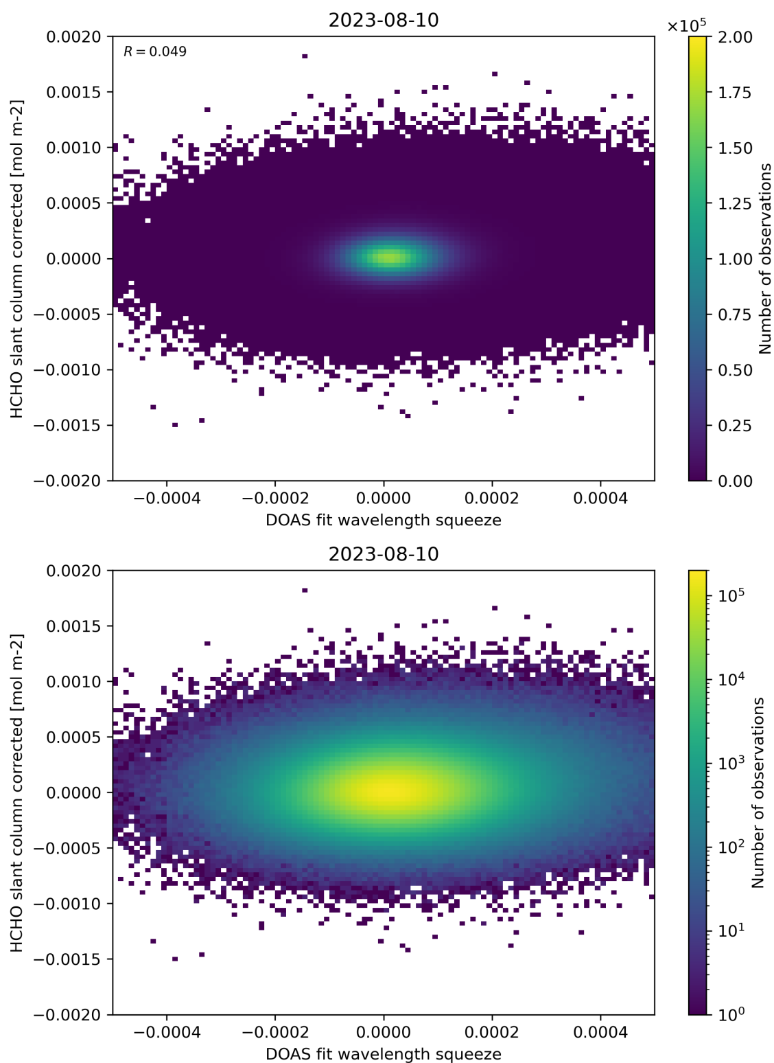
Figure 69: Scatter density plot of “DOAS fit wavelength squeeze” against “HCHO slant column corrected” for 2023-08-09 to 2023-08-11.
