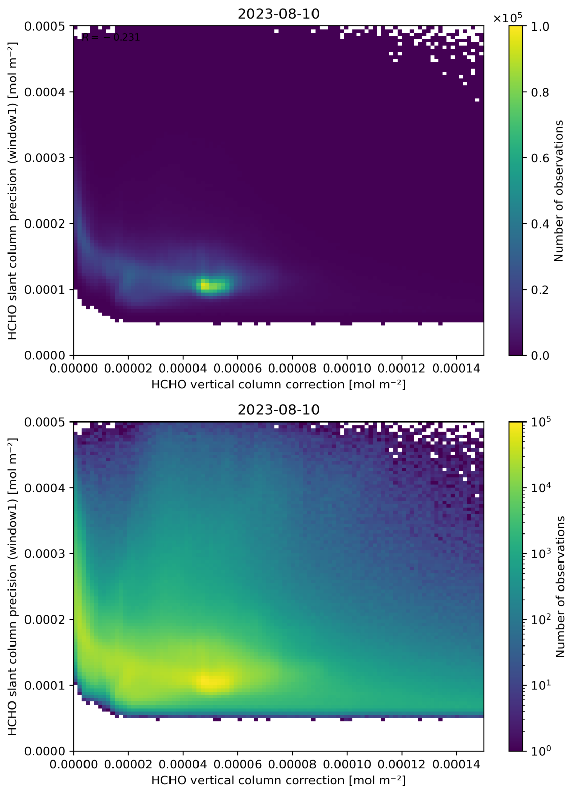
Figure 119: Scatter density plot of “HCHO vertical column correction” against “HCHO slant column precision (window1)” for 2023-08-09 to 2023-08-11.
