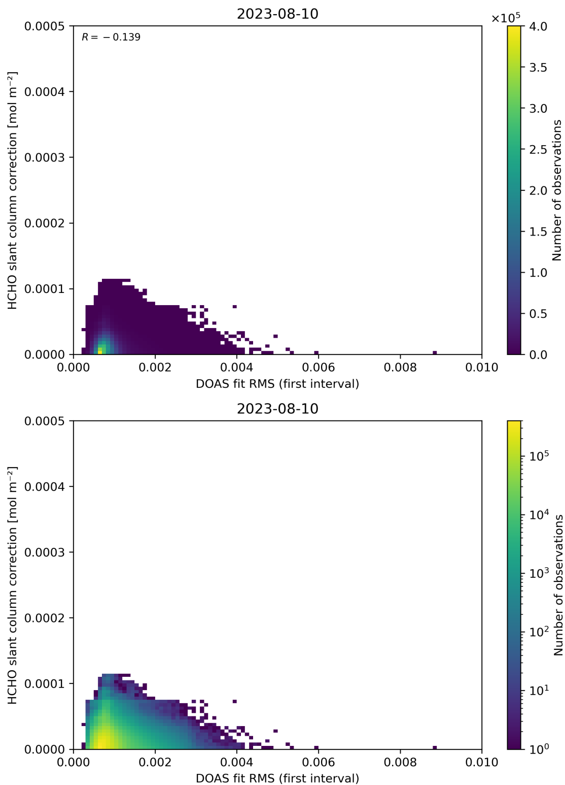
Figure 63: Scatter density plot of “DOAS fit RMS (first interval)” against “HCHO slant column correction” for 2023-08-09 to 2023-08-11.
