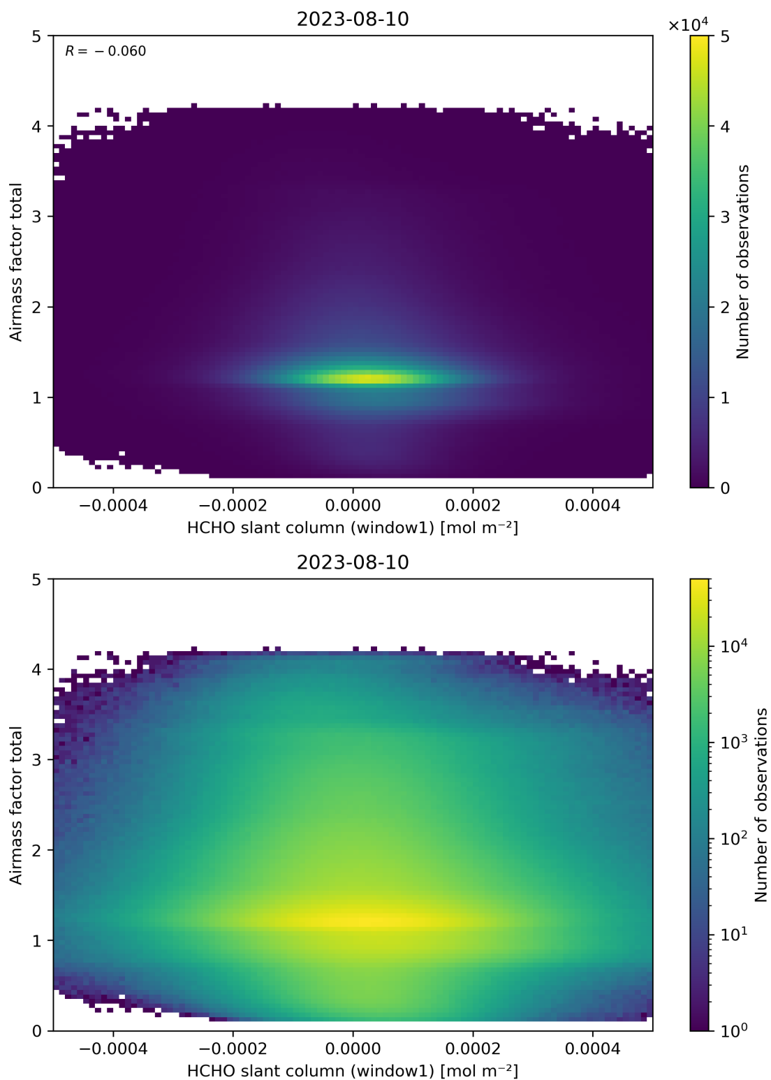
Figure 85: Scatter density plot of “HCHO slant column (window1)” against “Airmass factor total” for 2023-08-09 to 2023-08-11.
