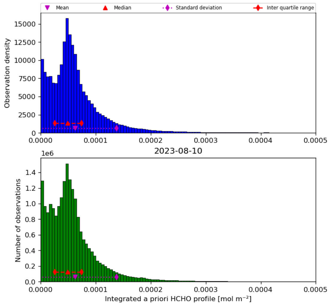
Figure 43: Histogram of “Integrated a priori HCHO profile” for 2023-08-09 to 2023-08-11
