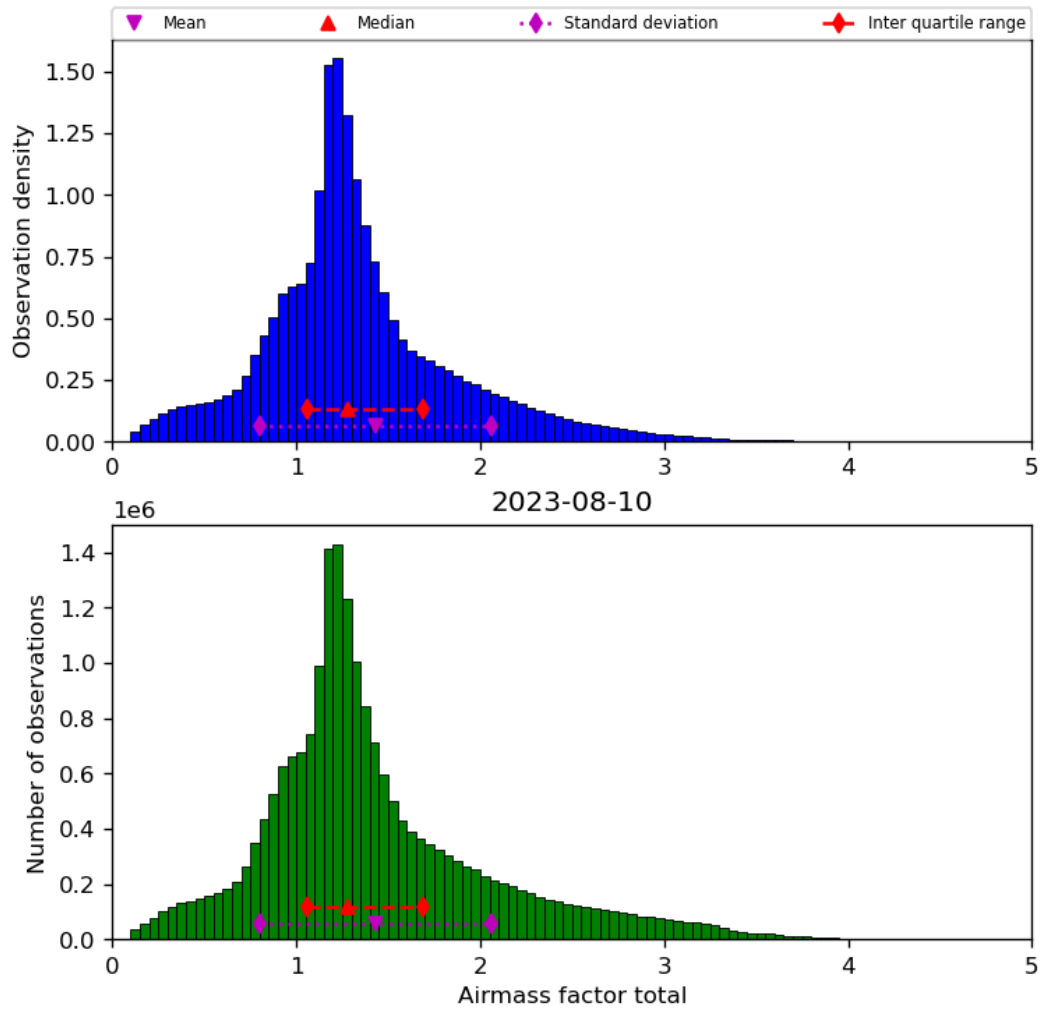
Figure 40: Histogram of “Airmass factor total” for 2023-08-09 to 2023-08-11
