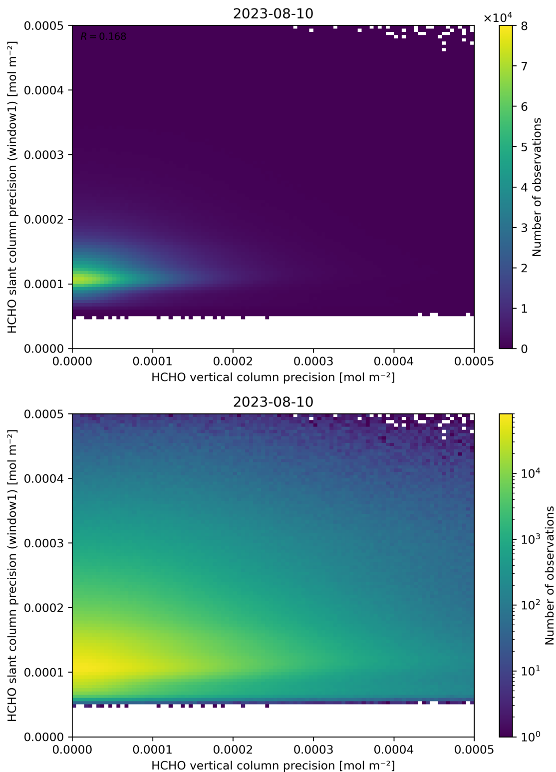
Figure 143: Scatter density plot of “HCHO vertical column precision” against “HCHO slant column precision (window1)” for 2023-08-09 to 2023-08-11.
