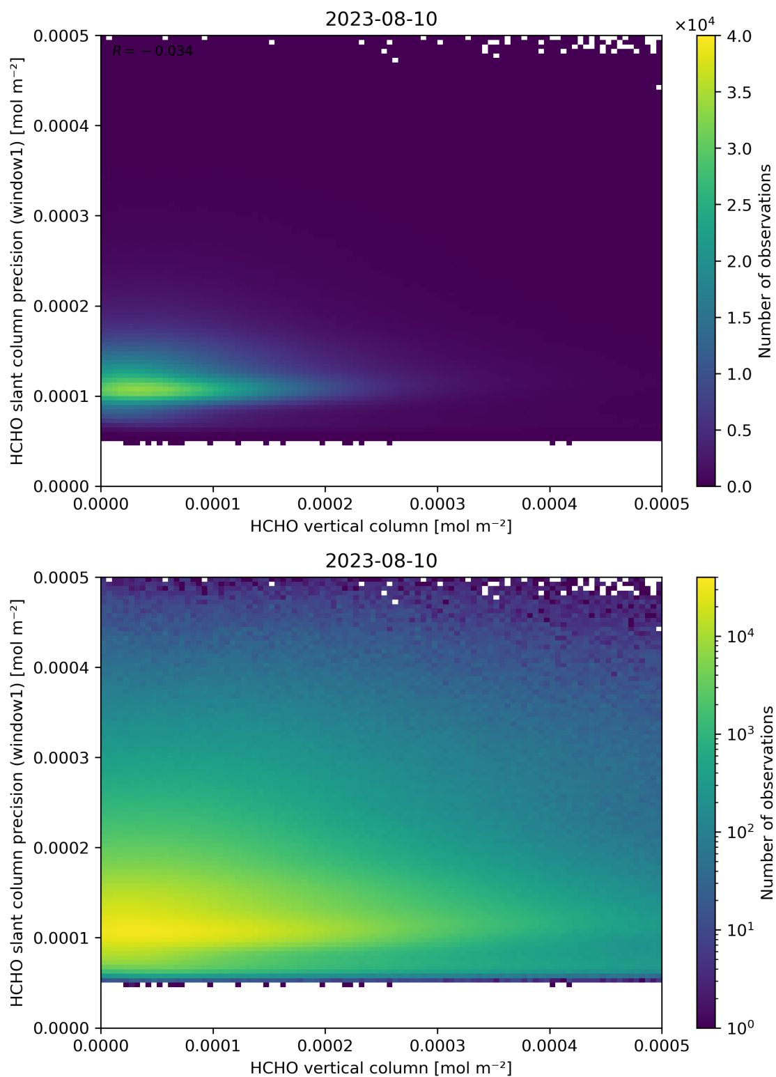
Figure 130: Scatter density plot of “HCHO vertical column” against “HCHO slant column precision (window1)” for 2023-08-09 to 2023-08-11.
