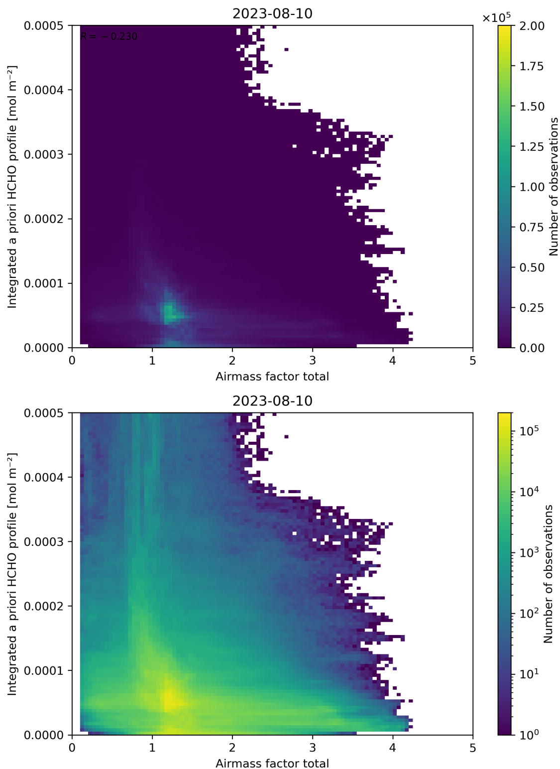
Figure 104: Scatter density plot of “Airmass factor total” against “Integrated a priori HCHO profile” for 2023-08-09 to 2023-08-11.
