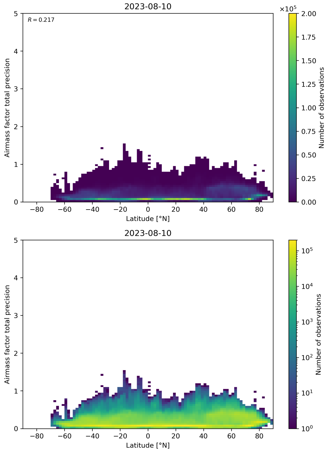
Figure 162: Scatter density plot of “Latitude” against “Airmass factor total precision” for 2023-08-09 to 2023-08-11.
