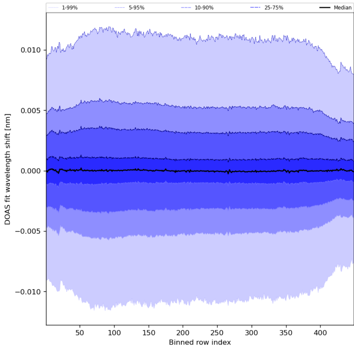
Figure 58: Along track statistics of “DOAS fit wavelength shift” for 2023-08-09 to 2023-08-11
