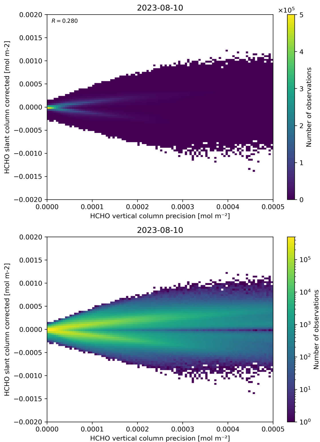
Figure 140: Scatter density plot of “HCHO vertical column precision” against “HCHO slant column corrected” for 2023-08-09 to 2023-08-11.
