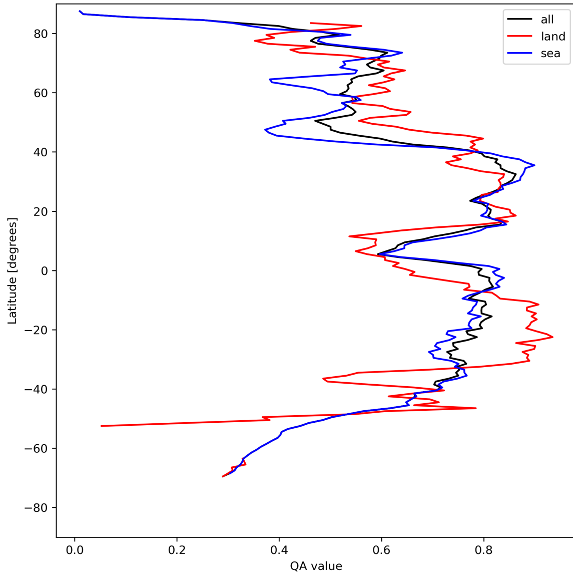
Figure 20: Zonal average of “QA value” for 2023-08-09 to 2023-08-11.
