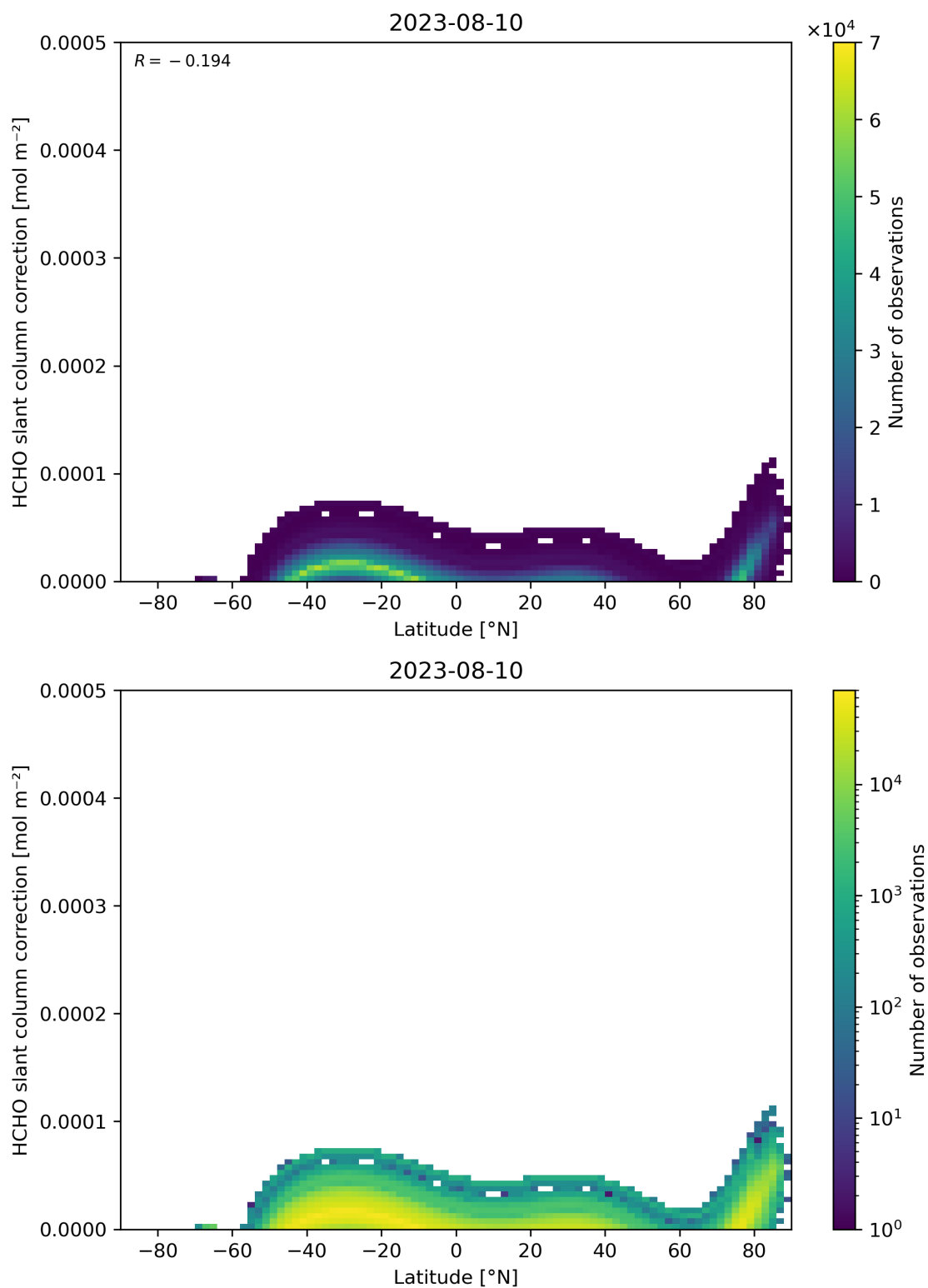
Figure 158: Scatter density plot of “Latitude” against “HCHO slant column correction” for 2023-08-09 to 2023-08-11.
