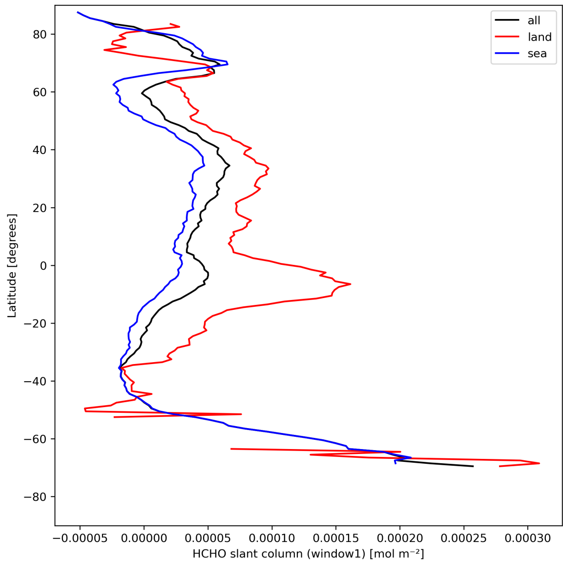
Figure 24: Zonal average of “HCHO slant column (window1)” for 2023-08-09 to 2023-08-11.
