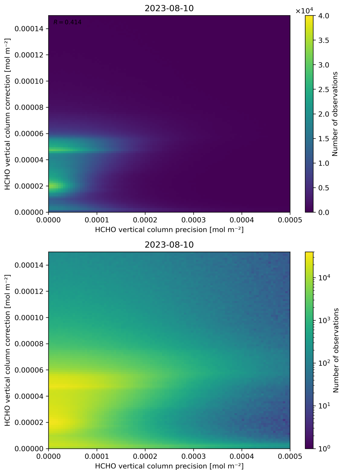
Figure 146: Scatter density plot of “HCHO vertical column precision” against “HCHO vertical column correction” for 2023-08-09 to 2023-08-11.
