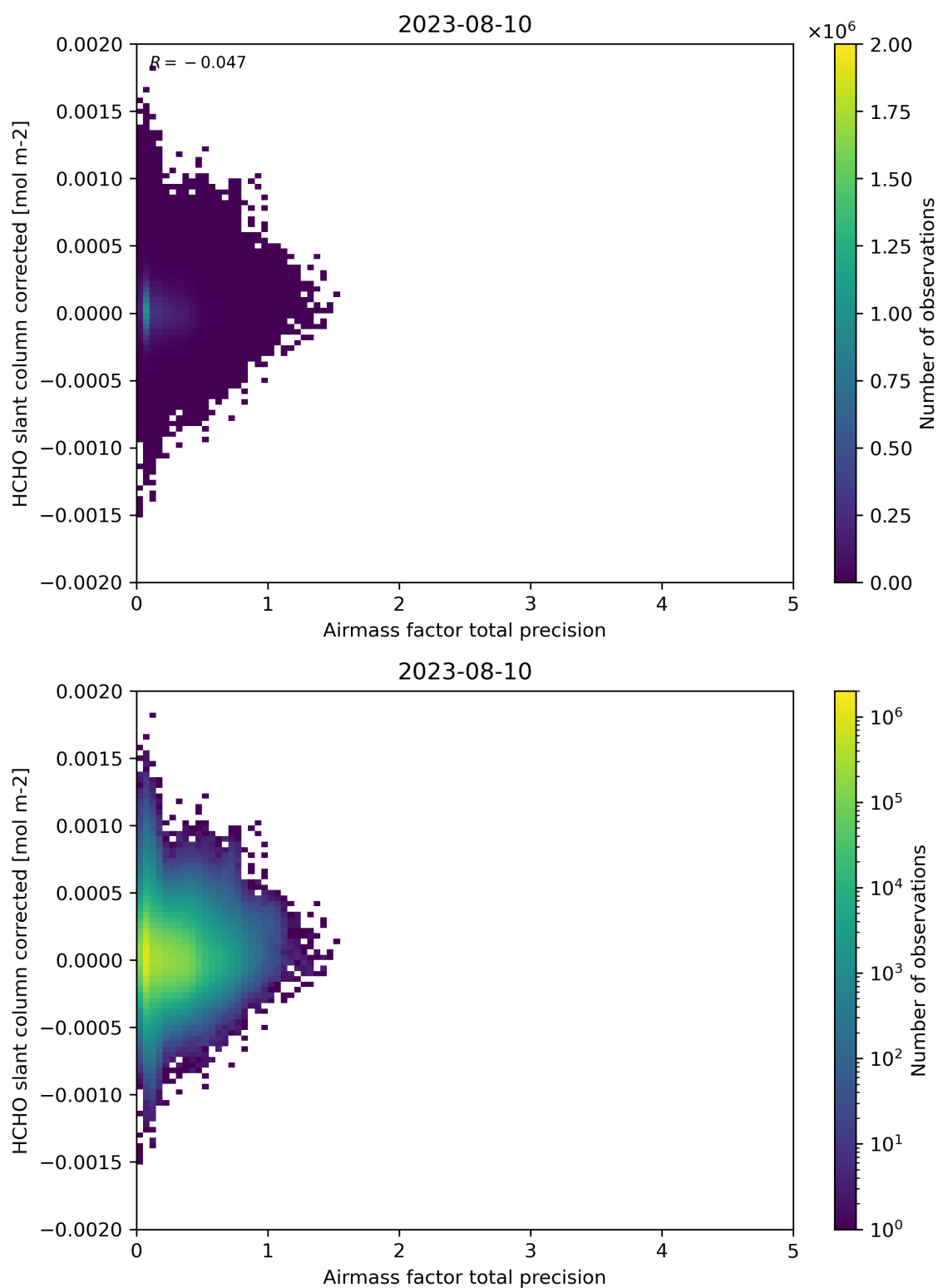
Figure 109: Scatter density plot of “Airmass factor total precision” against “HCHO slant column corrected” for 2023-08-09 to 2023-08-11.
