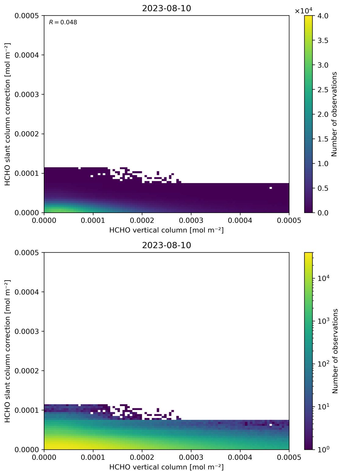
Figure 128: Scatter density plot of “HCHO vertical column” against “HCHO slant column correction” for 2023-08-09 to 2023-08-11.
