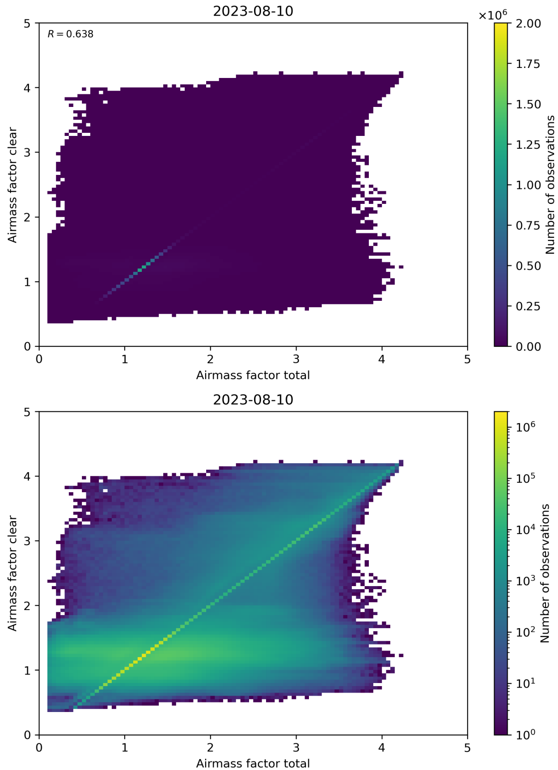
Figure 100: Scatter density plot of “Airmass factor total” against “Airmass factor clear” for 2023-08-09 to 2023-08-11.
