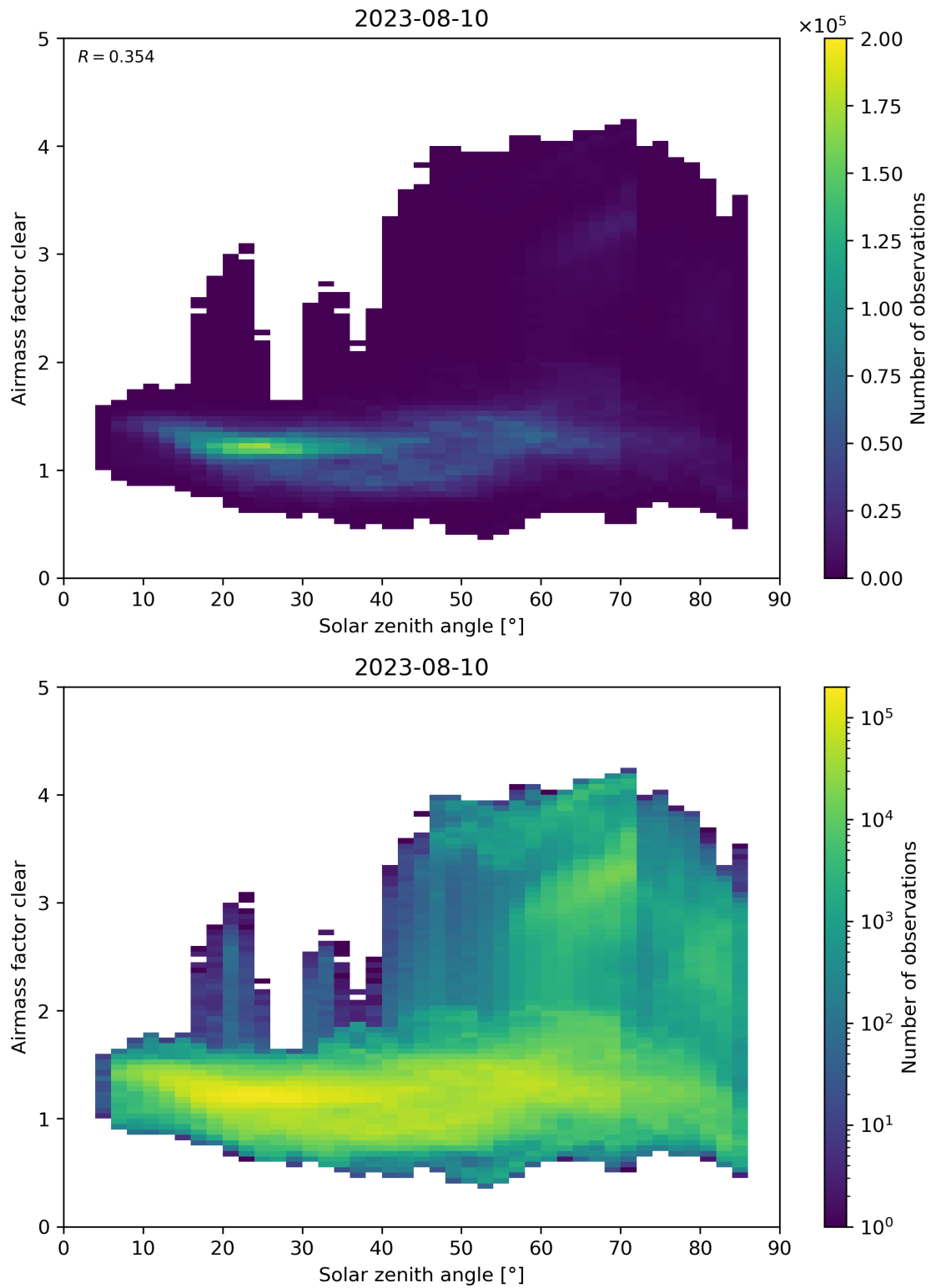
Figure 170: Scatter density plot of “Solar zenith angle” against “Airmass factor clear” for 2023-08-09 to 2023-08-11.
