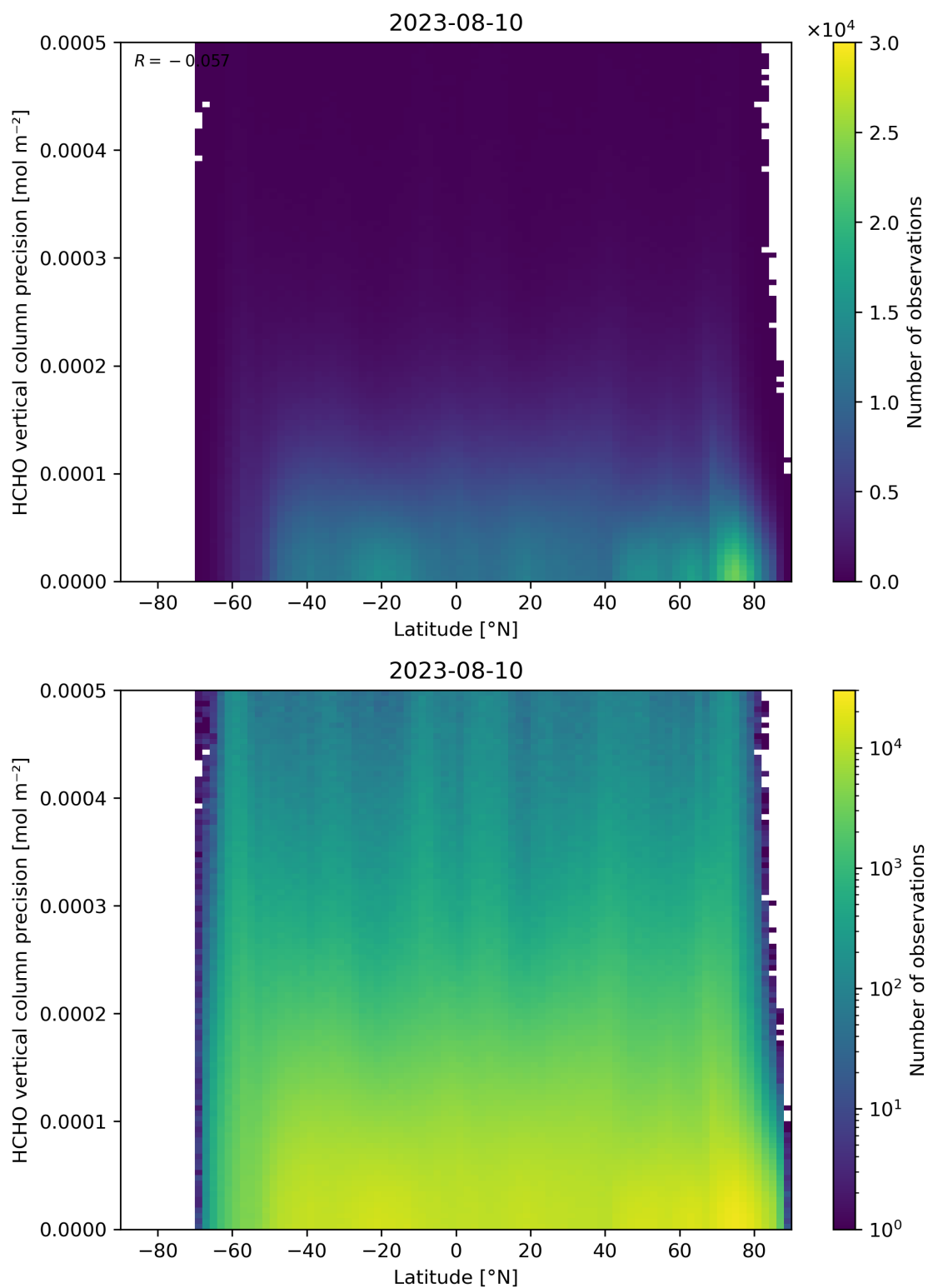
Figure 165: Scatter density plot of “Latitude” against “HCHO vertical column precision” for 2023-08-09 to 2023-08-11.
