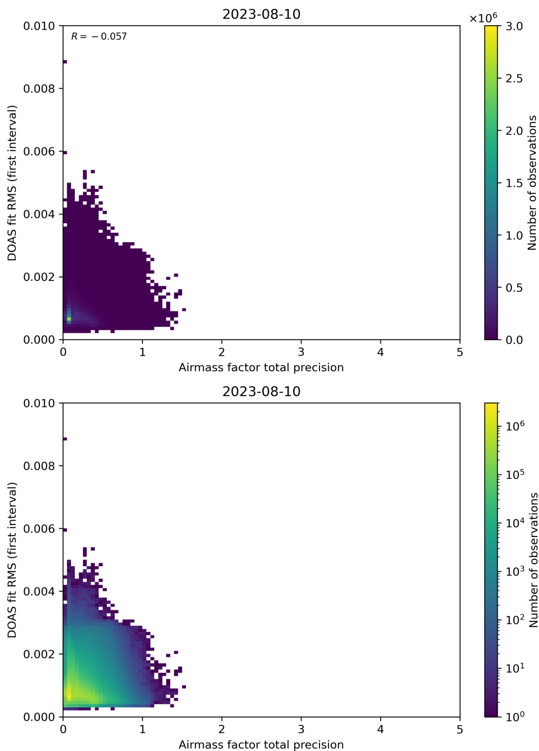
Figure 105: Scatter density plot of “Airmass factor total precision” against “DOAS fit RMS (first interval)” for 2023-08-09 to 2023-08-11.
