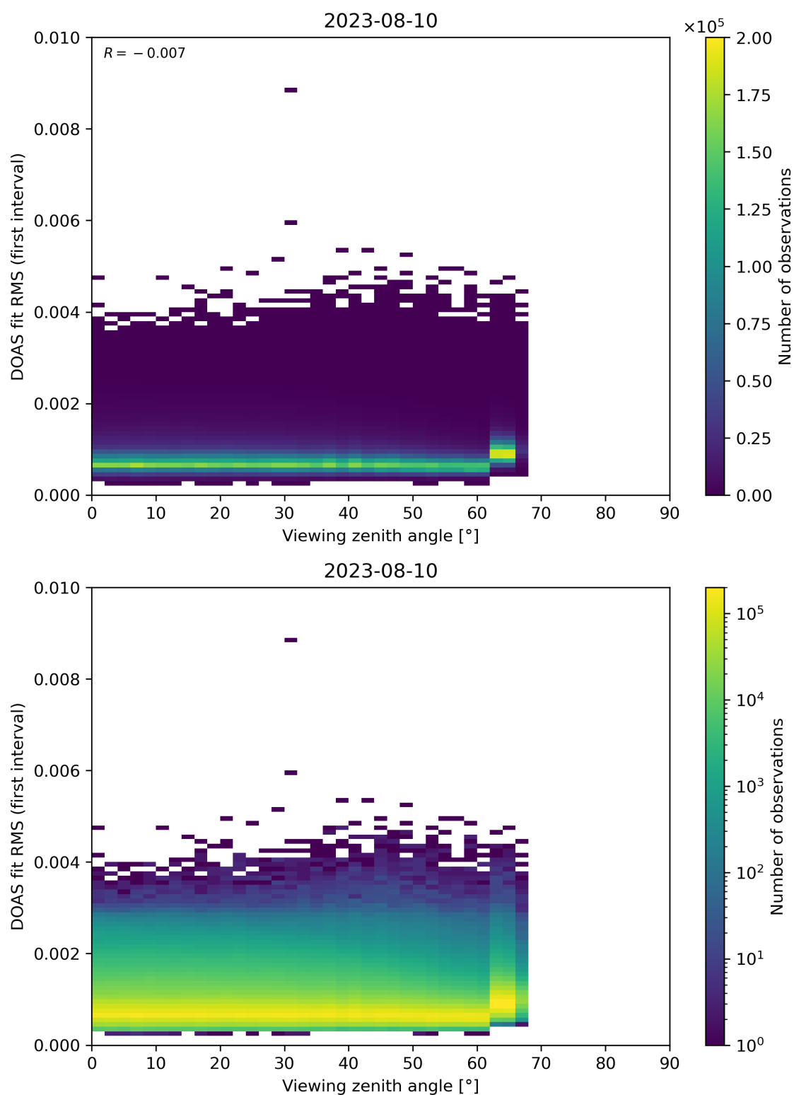
Figure 182: Scatter density plot of “Viewing zenith angle” against “DOAS fit RMS (first interval)” for 2023-08-09 to 2023-08-11.
