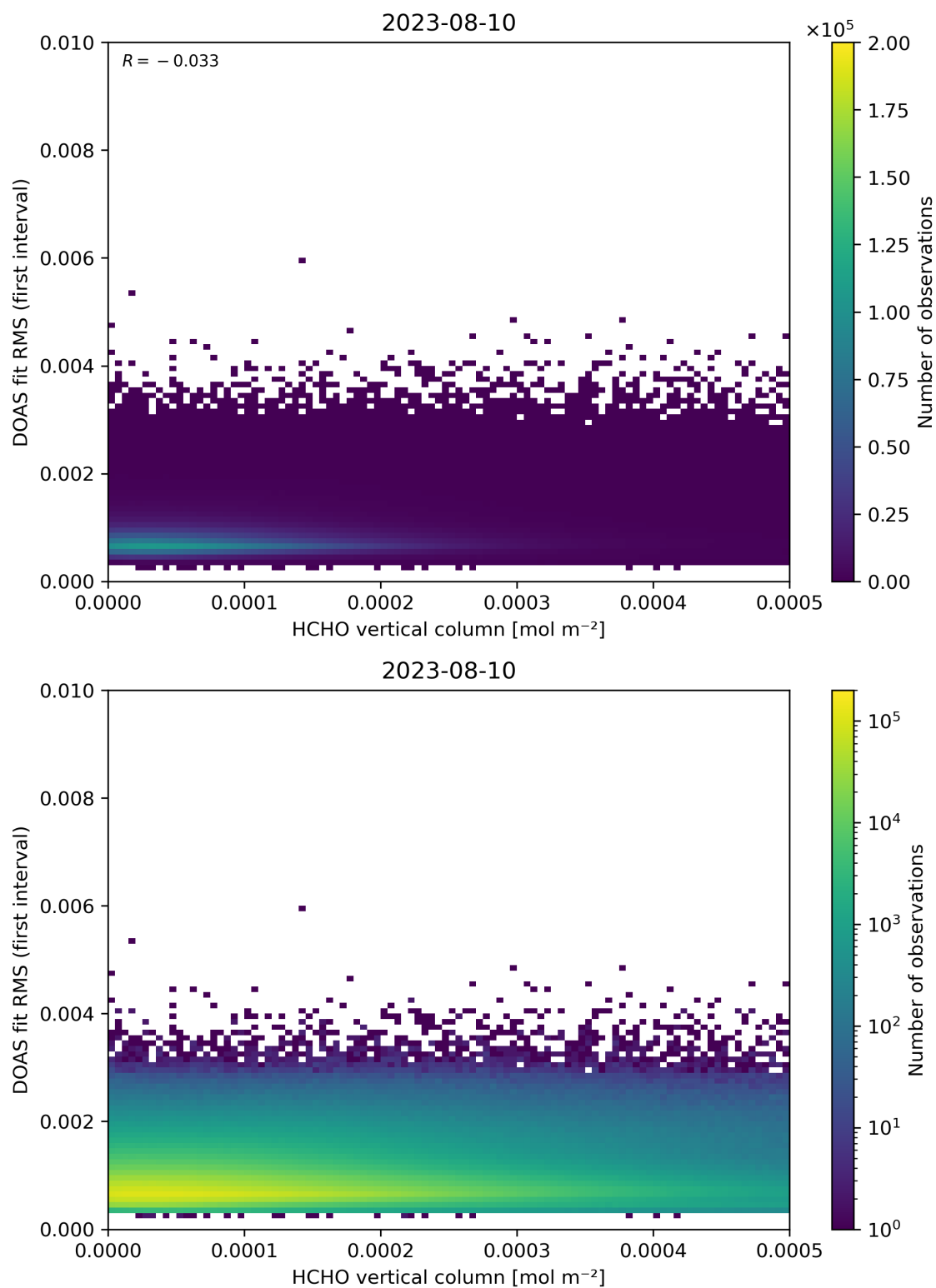
Figure 123: Scatter density plot of “HCHO vertical column” against “DOAS fit RMS (first interval)” for 2023-08-09 to 2023-08-11.
