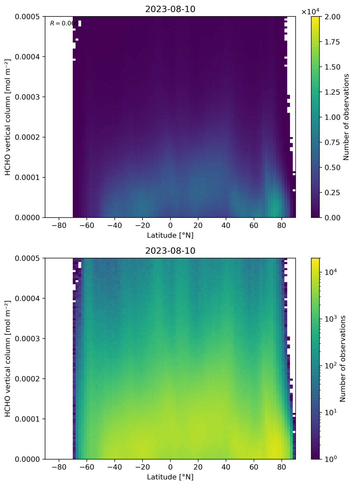
Figure 163: Scatter density plot of “Latitude” against “HCHO vertical column” for 2023-08-09 to 2023-08-11.
