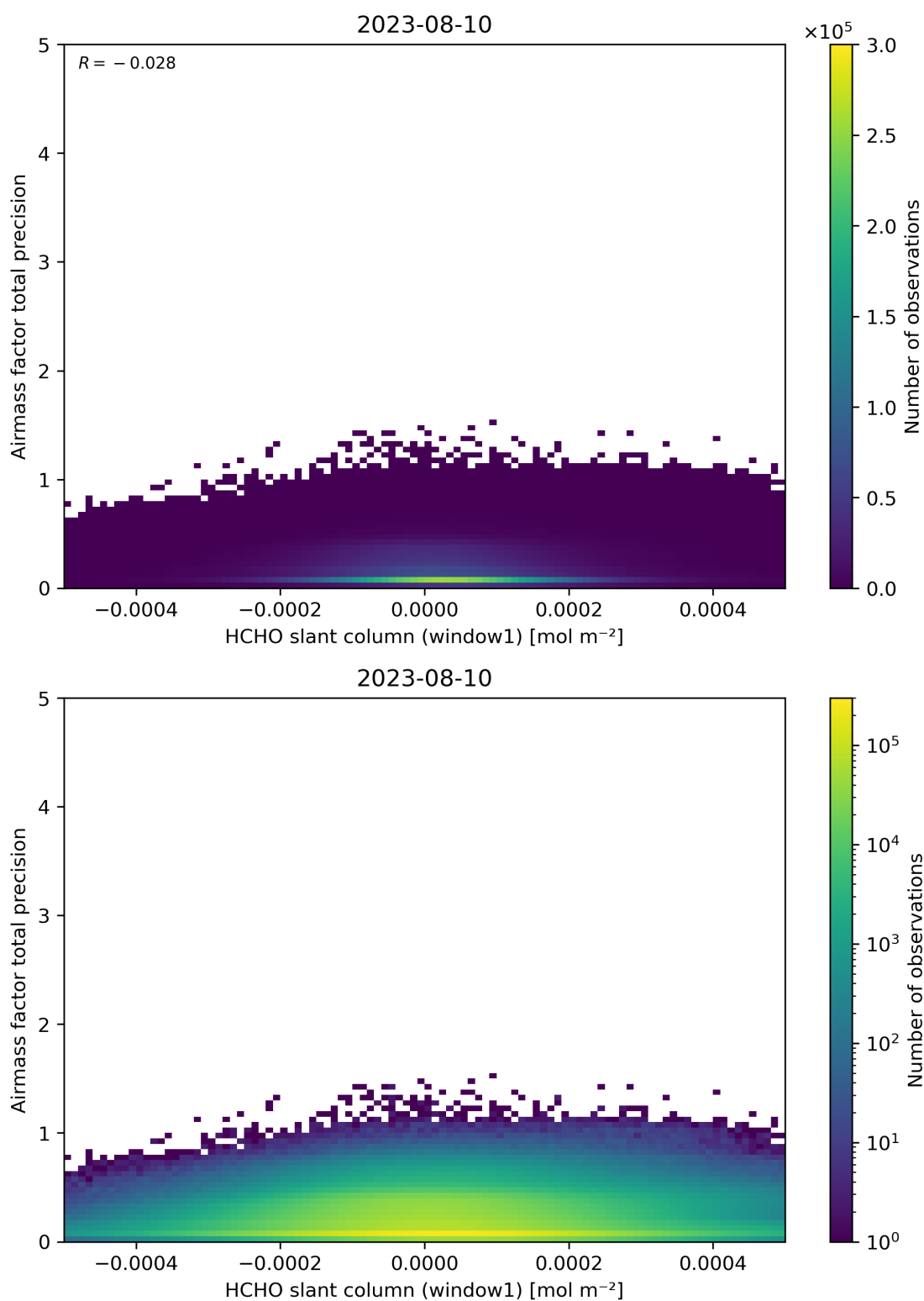
Figure 86: Scatter density plot of “HCHO slant column (window1)” against “Airmass factor total precision” for 2023-08-09 to 2023-08-11.
