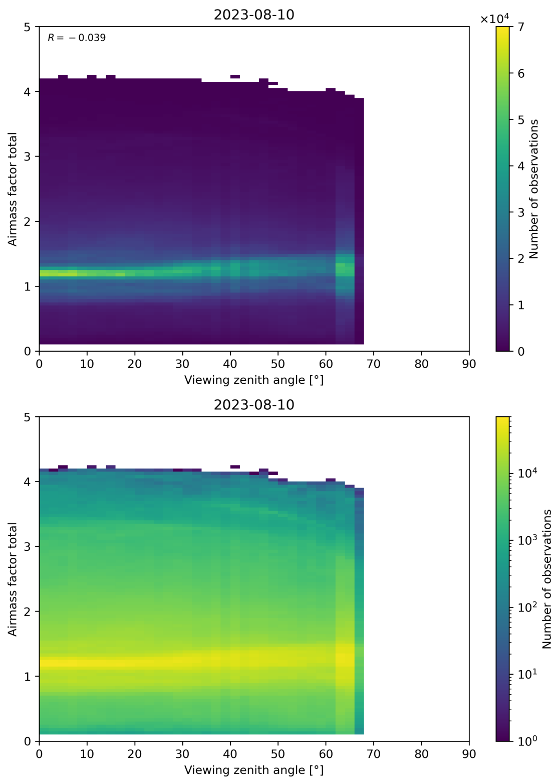
Figure 190: Scatter density plot of “Viewing zenith angle” against “Airmass factor total” for 2023-08-09 to 2023-08-11.
