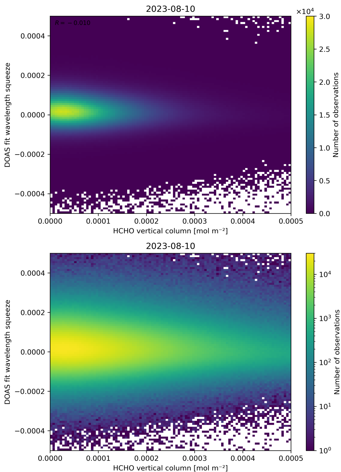
Figure 125: Scatter density plot of “HCHO vertical column” against “DOAS fit wavelength squeeze” for 2023-08-09 to 2023-08-11.
