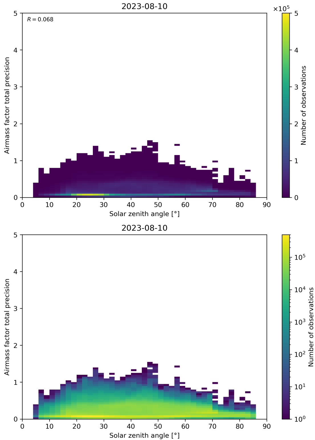
Figure 176: Scatter density plot of “Solar zenith angle” against “Airmass factor total precision” for 2023-08-09 to 2023-08-11.
