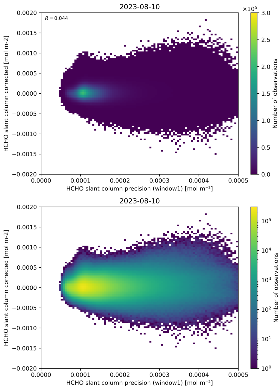
Figure 92: Scatter density plot of “HCHO slant column precision (window1)” against “HCHO slant column corrected” for 2023-08-09 to 2023-08-11.
