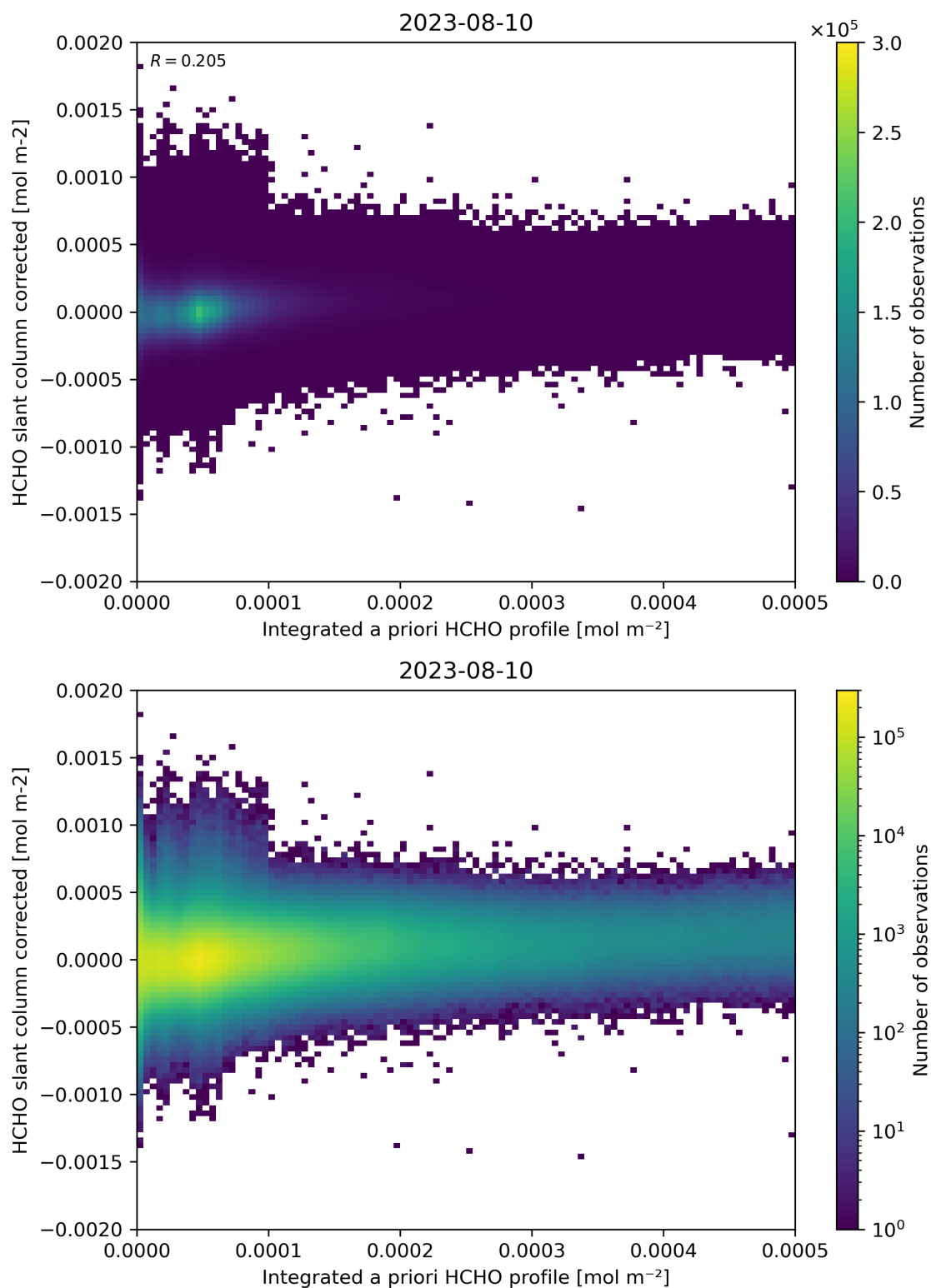
Figure 151: Scatter density plot of “Integrated a priori HCHO profile” against “HCHO slant column corrected” for 2023-08-09 to 2023-08-11.
