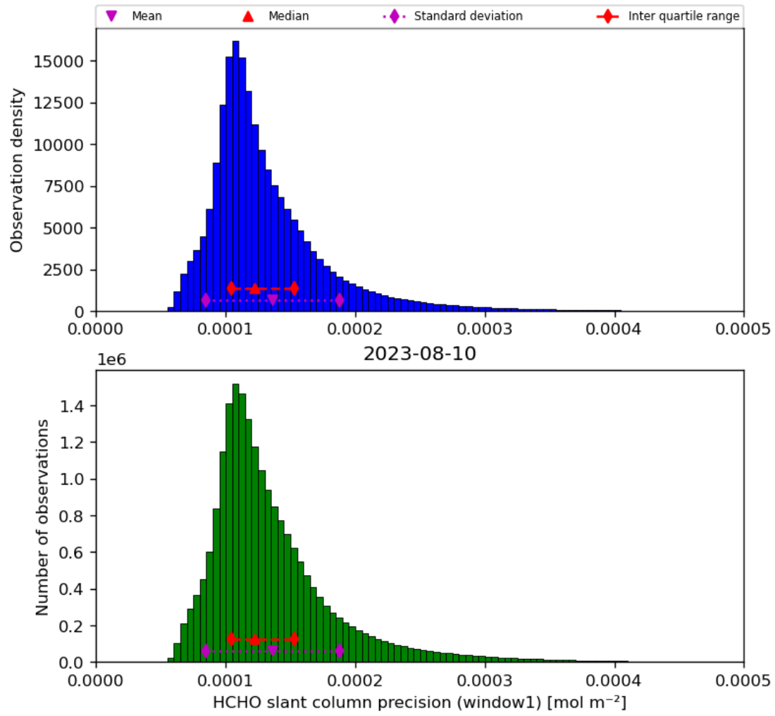
Figure 39: Histogram of “HCHO slant column precision (window1)” for 2023-08-09 to 2023-08-11
