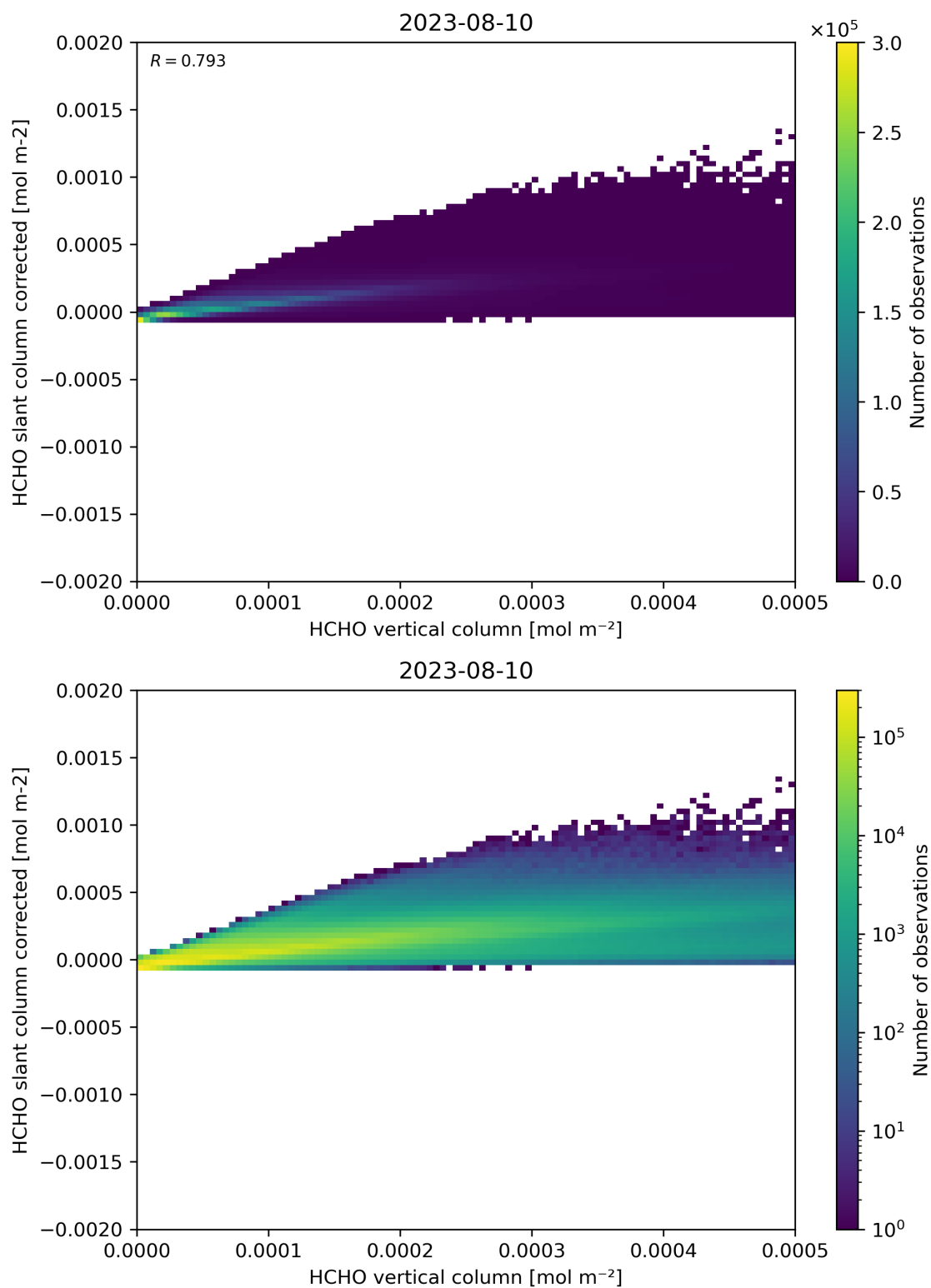
Figure 127: Scatter density plot of “HCHO vertical column” against “HCHO slant column corrected” for 2023-08-09 to 2023-08-11.
