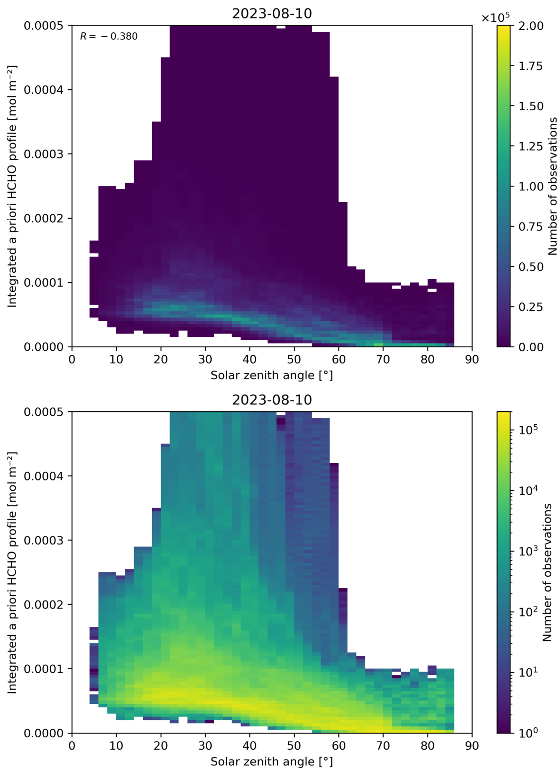
Figure 180: Scatter density plot of “Solar zenith angle” against “Integrated a priori HCHO profile” for 2023-08-09 to 2023-08-11.
