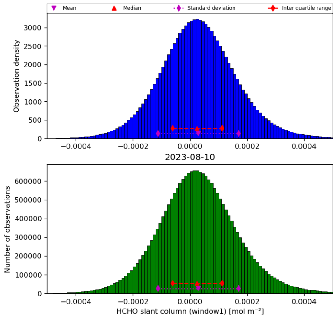
Figure 38: Histogram of “HCHO slant column (window1)” for 2023-08-09 to 2023-08-11
