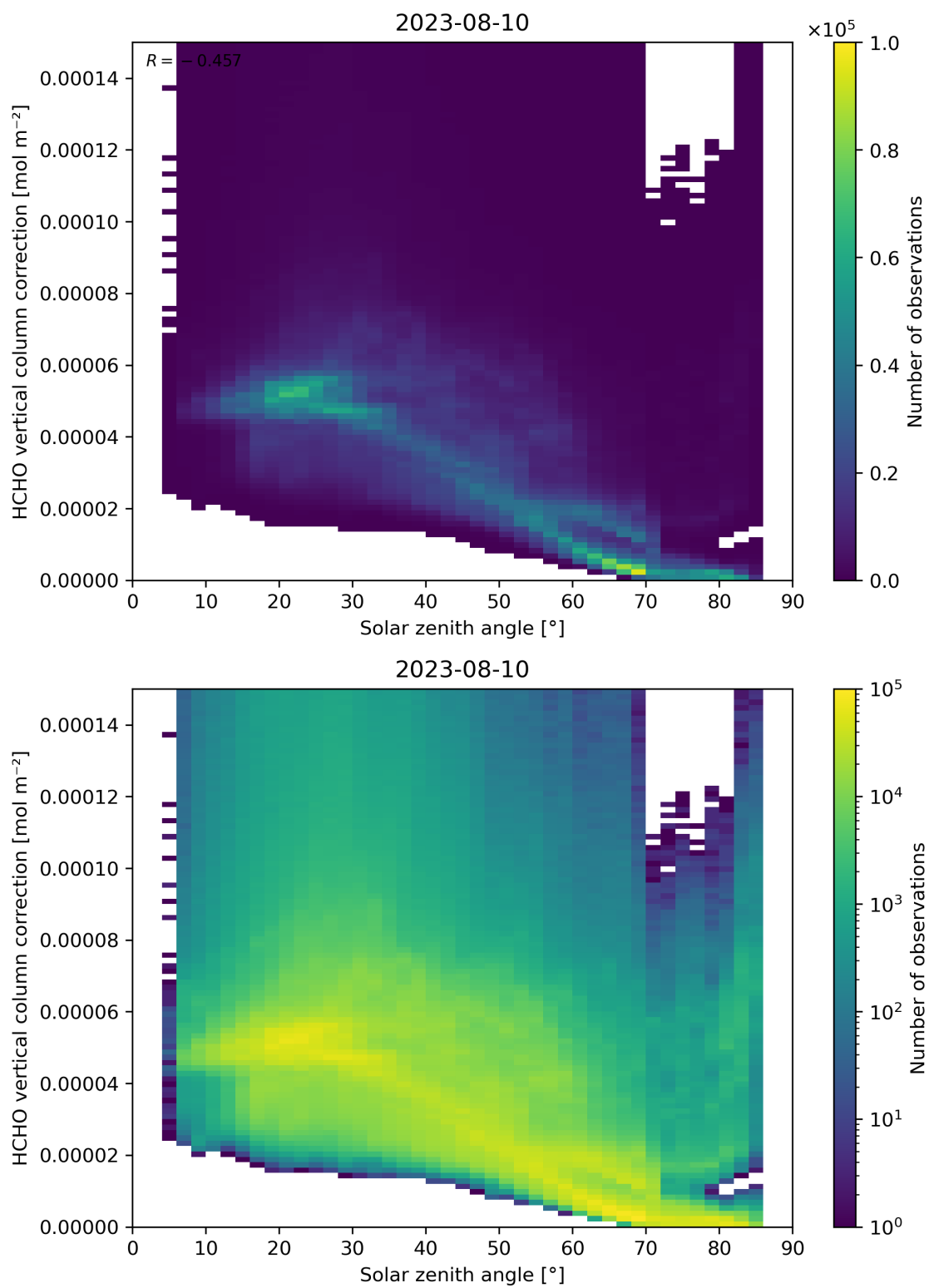
Figure 178: Scatter density plot of “Solar zenith angle” against “HCHO vertical column correction” for 2023-08-09 to 2023-08-11.
