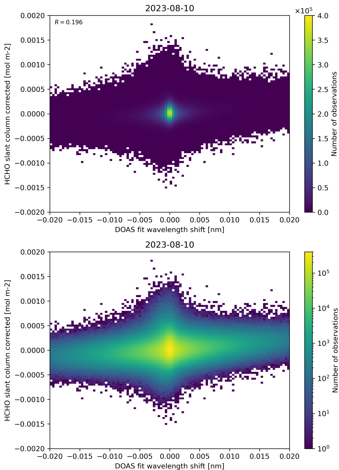
Figure 66: Scatter density plot of “DOAS fit wavelength shift” against “HCHO slant column corrected” for 2023-08-09 to 2023-08-11.
