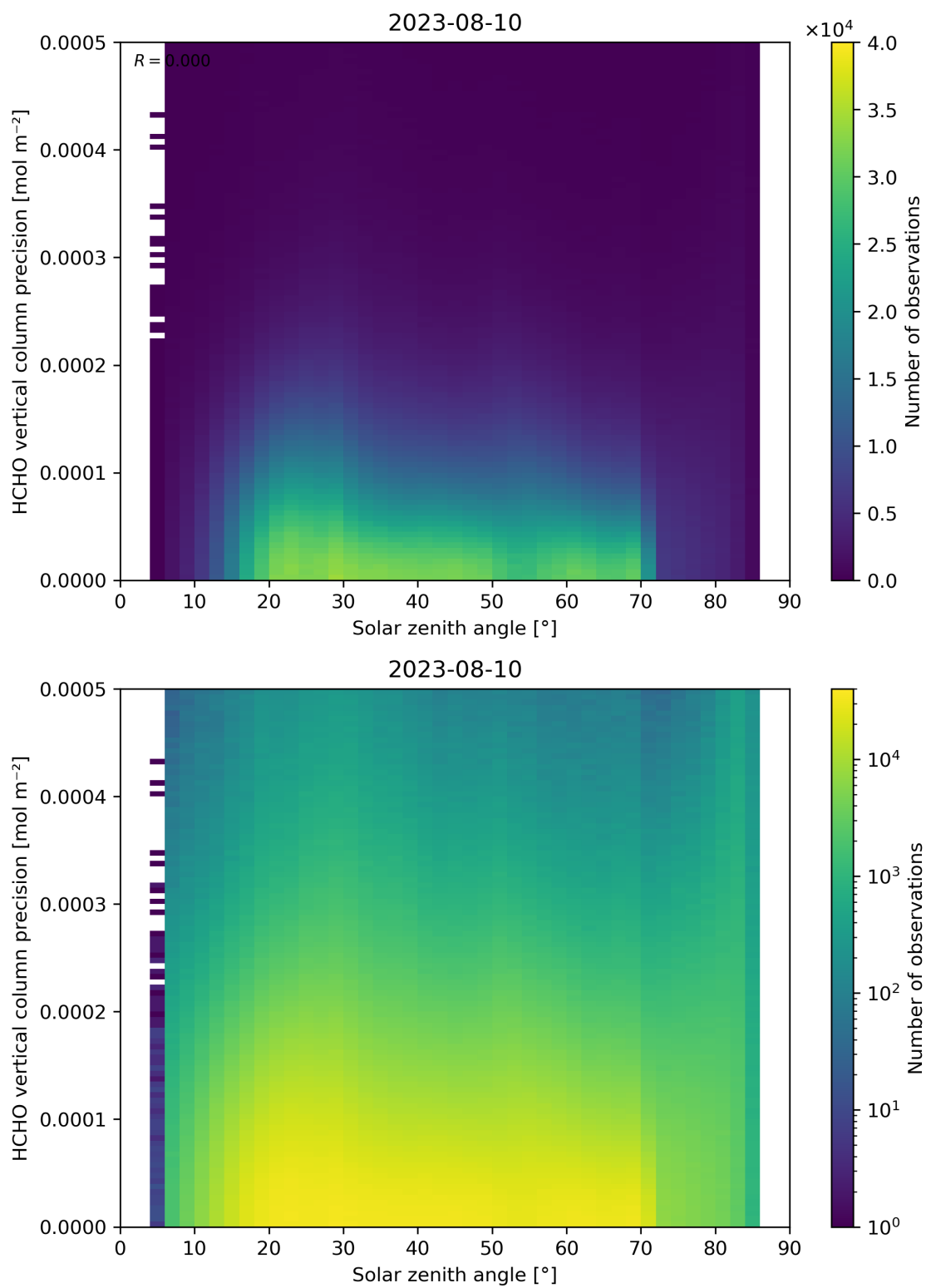
Figure 179: Scatter density plot of “Solar zenith angle” against “HCHO vertical column precision” for 2023-08-09 to 2023-08-11.
