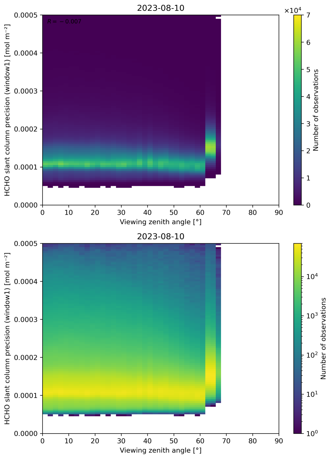
Figure 189: Scatter density plot of “Viewing zenith angle” against “HCHO slant column precision (window1)” for 2023-08-09 to 2023-08-11.
