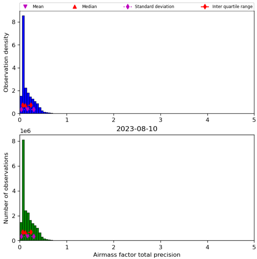
Figure 41: Histogram of “Airmass factor total precision” for 2023-08-09 to 2023-08-11
