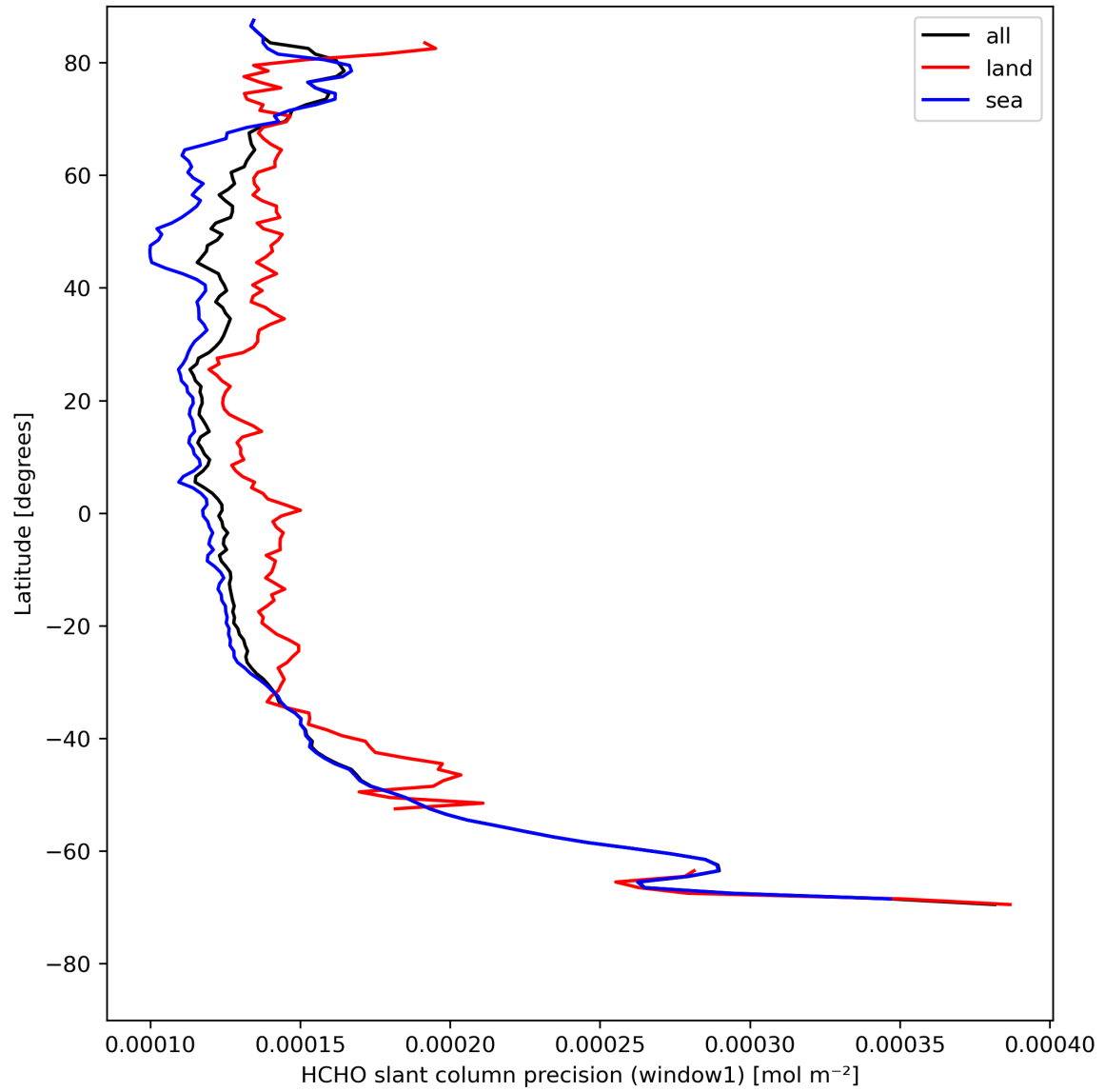
Figure 25: Zonal average of “HCHO slant column precision (window1)” for 2023-08-09 to 2023-08-11.
