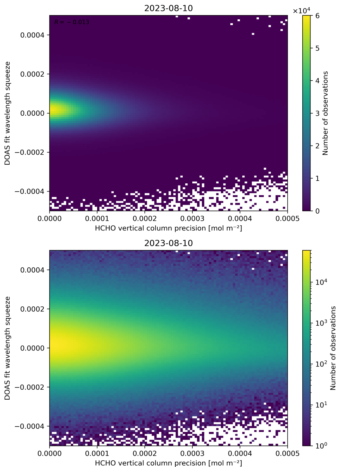
Figure 138: Scatter density plot of “HCHO vertical column precision” against “DOAS fit wavelength squeeze” for 2023-08-09 to 2023-08-11.
