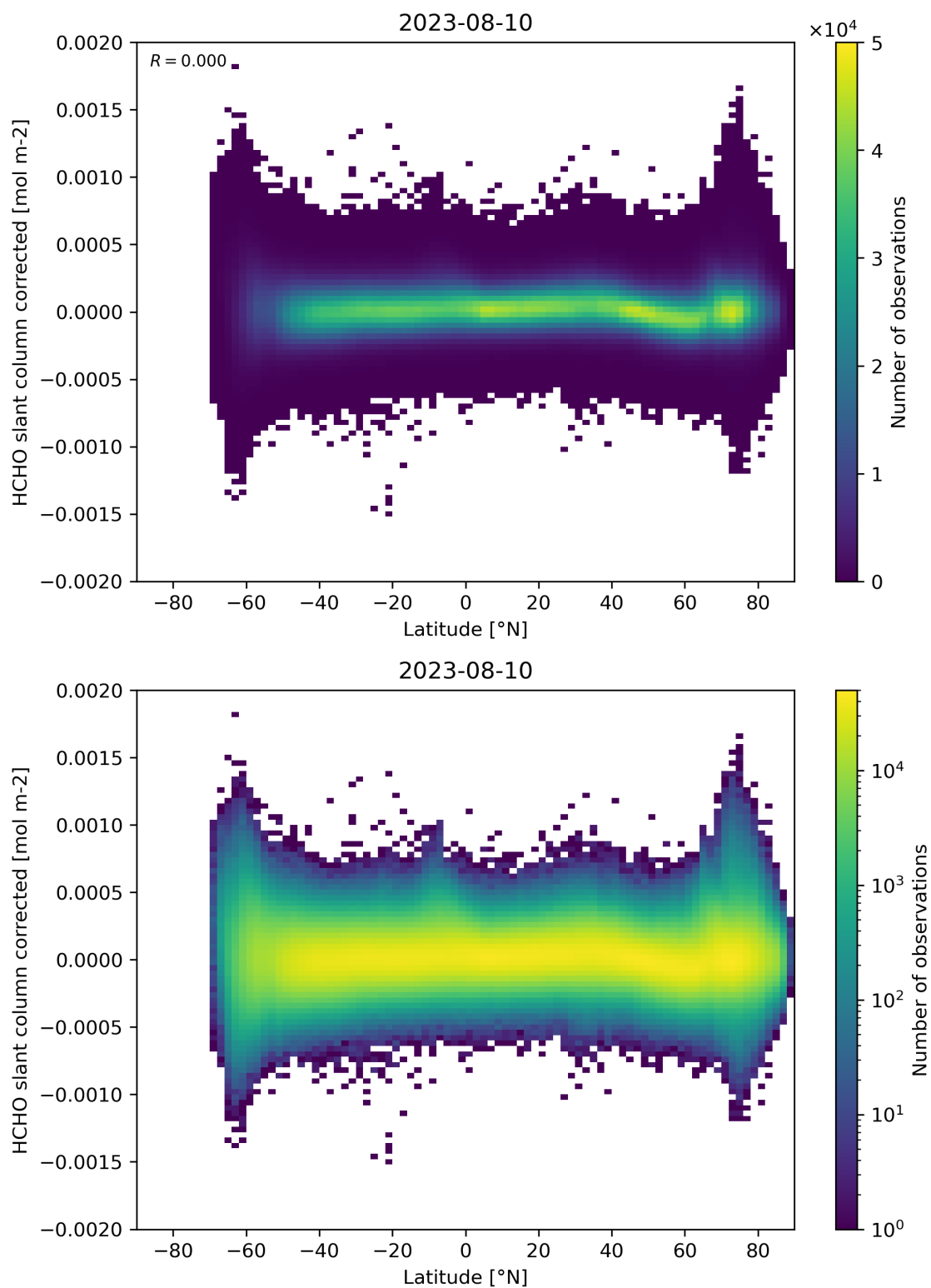
Figure 157: Scatter density plot of “Latitude” against “HCHO slant column corrected” for 2023-08-09 to 2023-08-11.
