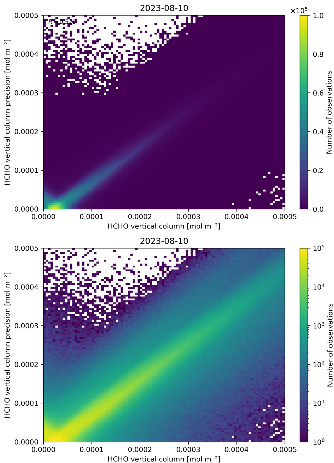
Figure 134: Scatter density plot of “HCHO vertical column” against “HCHO vertical column precision” for 2023-08-09 to 2023-08-11.
