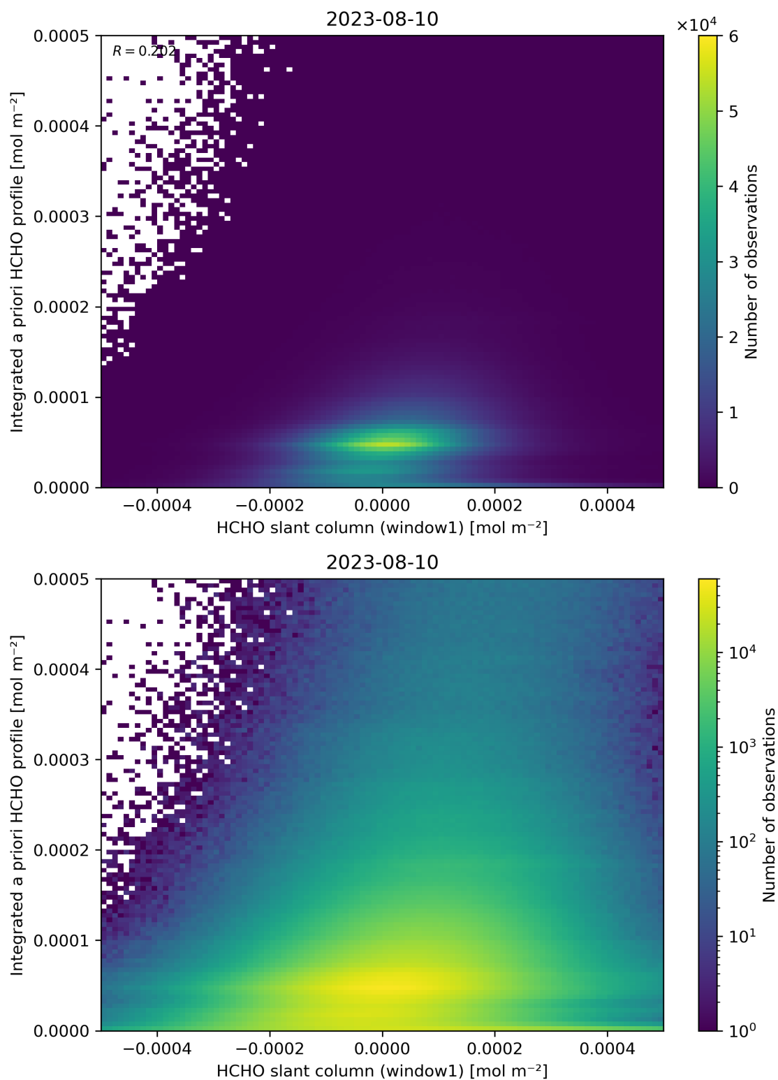
Figure 87: Scatter density plot of “HCHO slant column (window1)” against “Integrated a priori HCHO profile” for 2023-08-09 to 2023-08-11.
