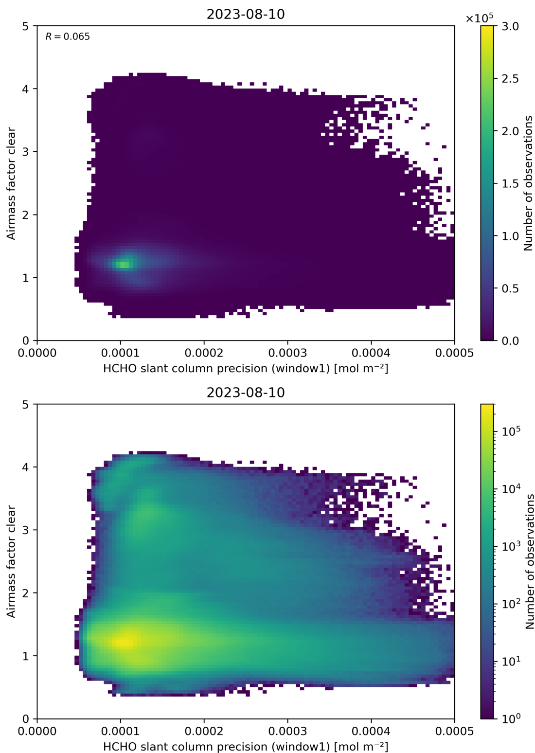
Figure 91: Scatter density plot of “HCHO slant column precision (window1)” against “Airmass factor clear” for 2023-08-09 to 2023-08-11.
