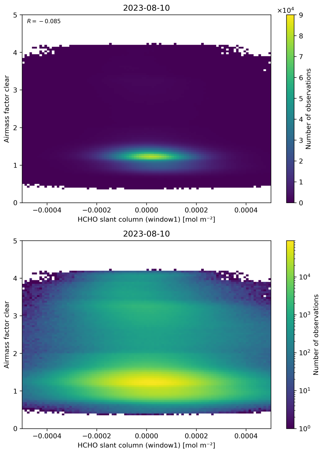
Figure 81: Scatter density plot of “HCHO slant column (window1)” against “Airmass factor clear” for 2023-08-09 to 2023-08-11.
