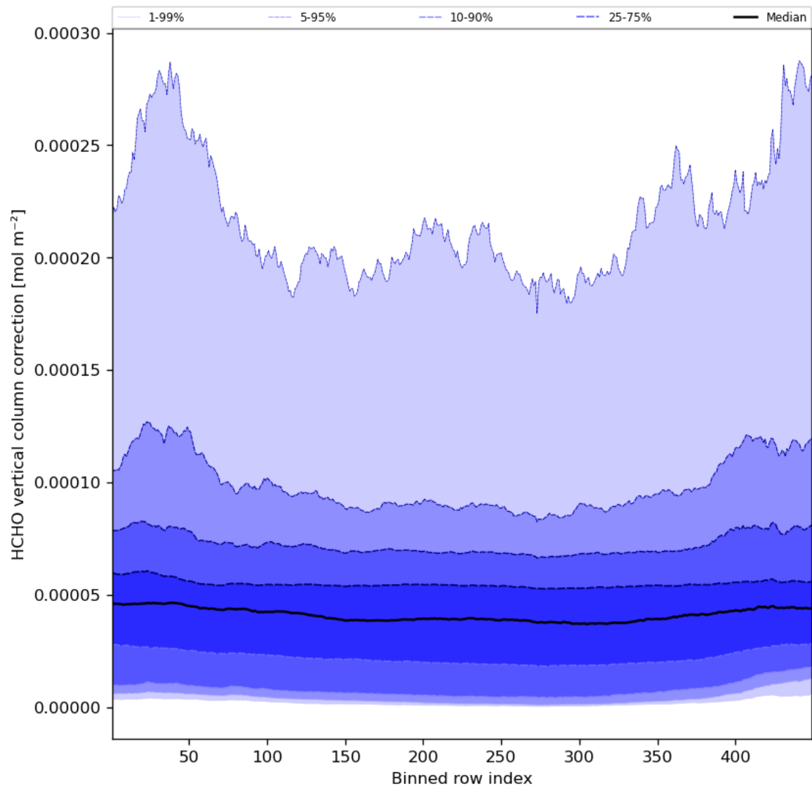
Figure 51: Along track statistics of “HCHO vertical column correction” for 2023-08-09 to 2023-08-11
