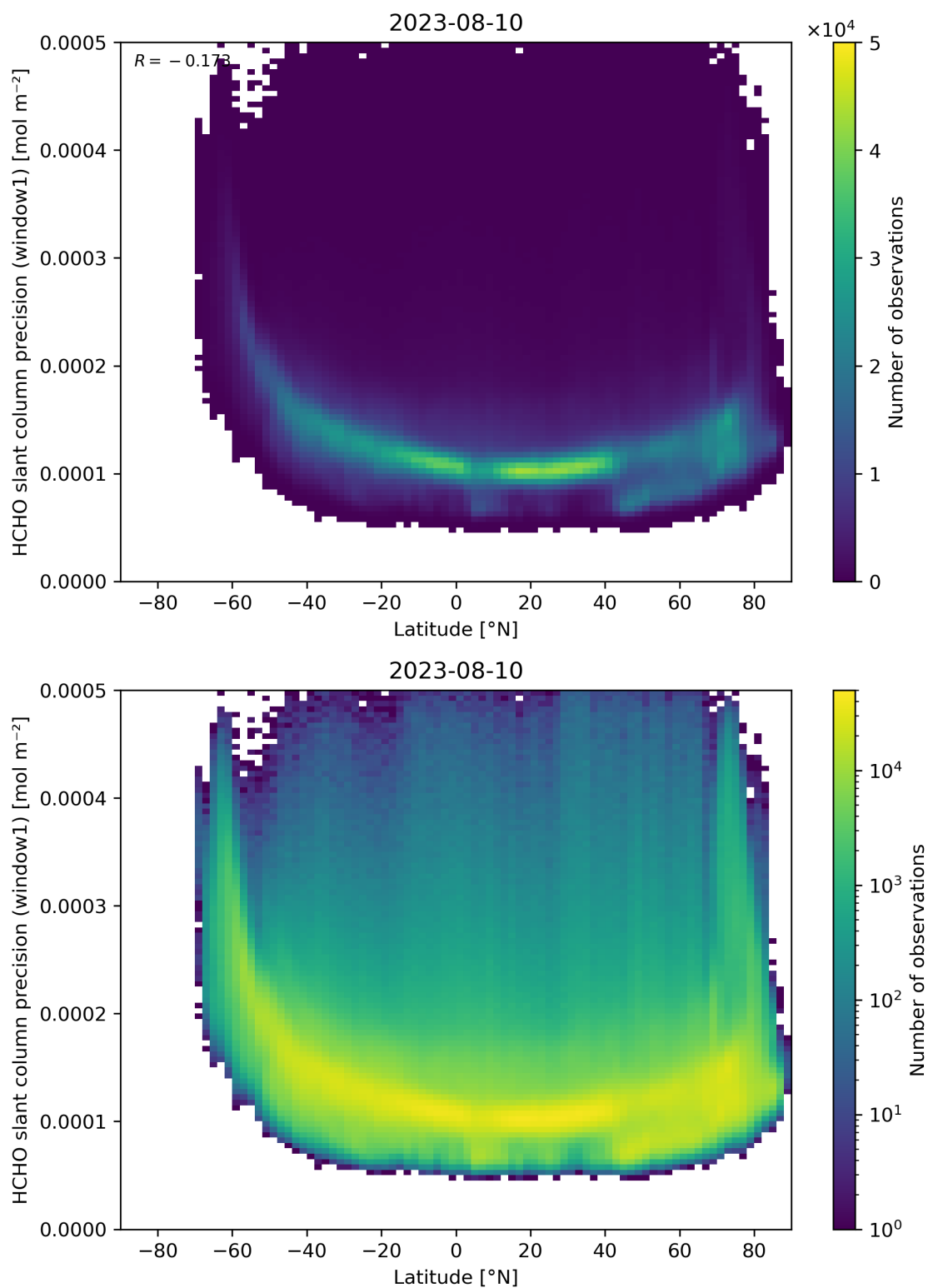
Figure 160: Scatter density plot of “Latitude” against “HCHO slant column precision (window1)” for 2023-08-09 to 2023-08-11.
