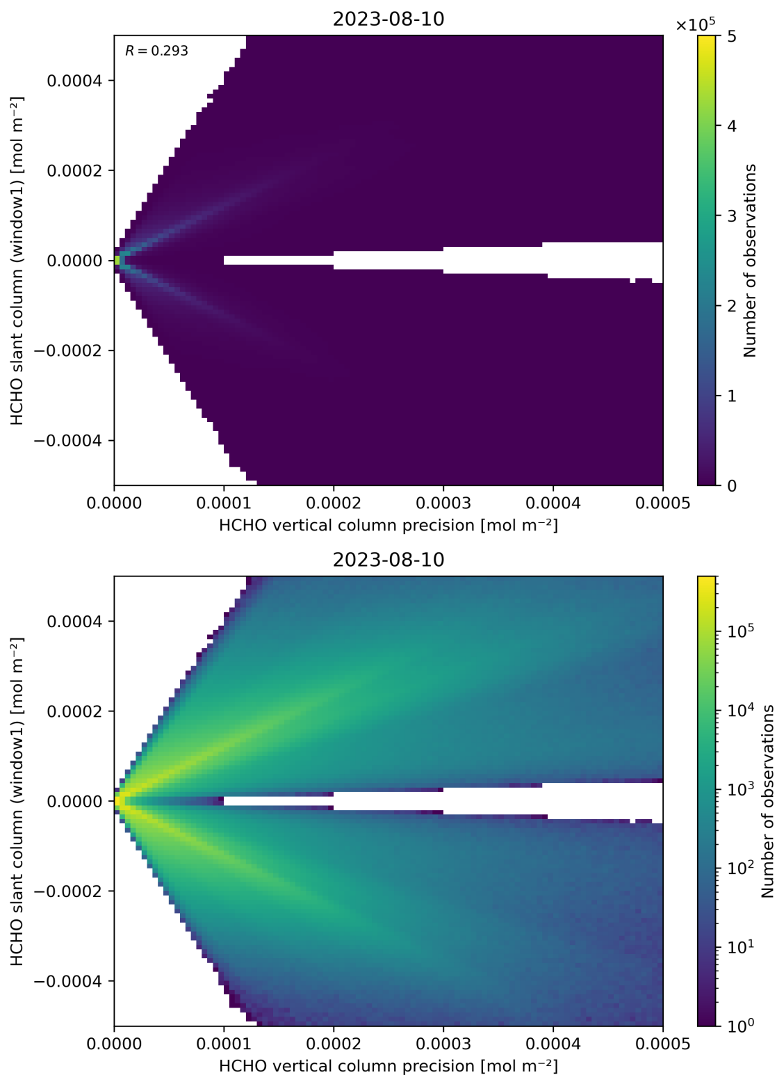
Figure 142: Scatter density plot of “HCHO vertical column precision” against “HCHO slant column (window1)” for 2023-08-09 to 2023-08-11.
