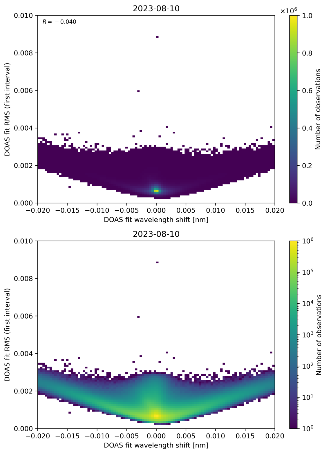
Figure 64: Scatter density plot of “DOAS fit wavelength shift” against “DOAS fit RMS (first interval)” for 2023-08-09 to 2023-08-11.
