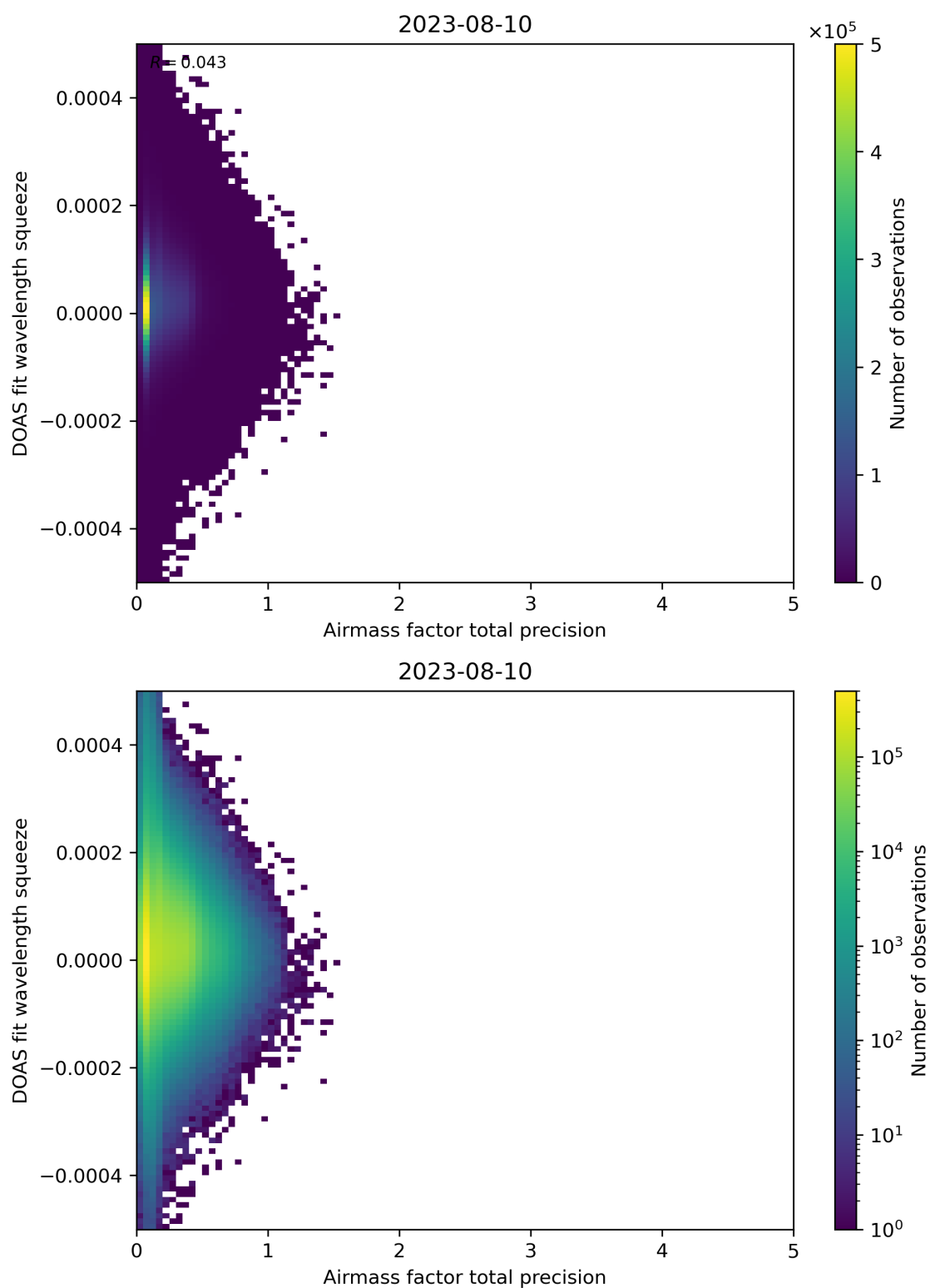
Figure 107: Scatter density plot of “Airmass factor total precision” against “DOAS fit wavelength squeeze” for 2023-08-09 to 2023-08-11.
