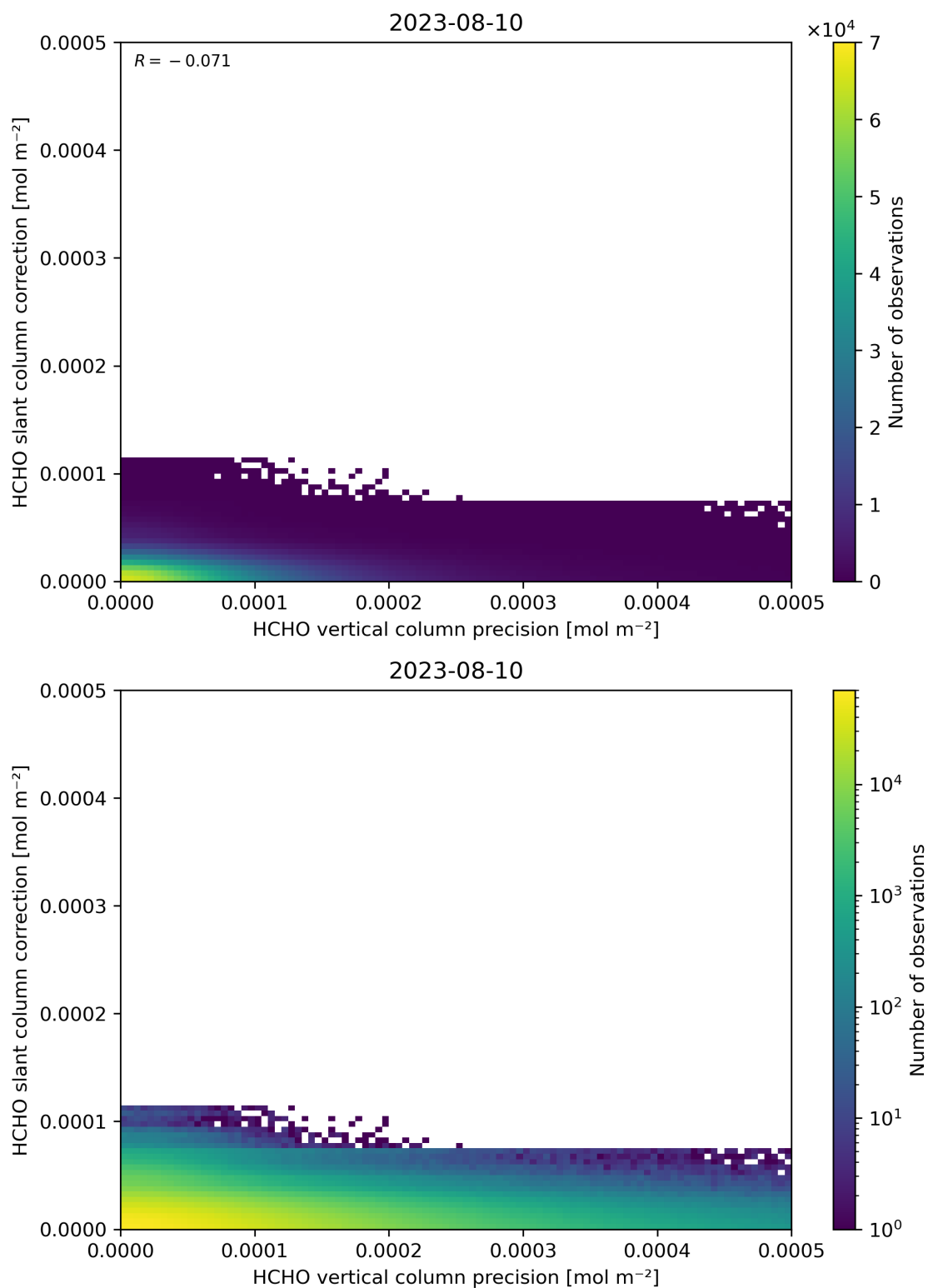
Figure 141: Scatter density plot of “HCHO vertical column precision” against “HCHO slant column correction” for 2023-08-09 to 2023-08-11.
