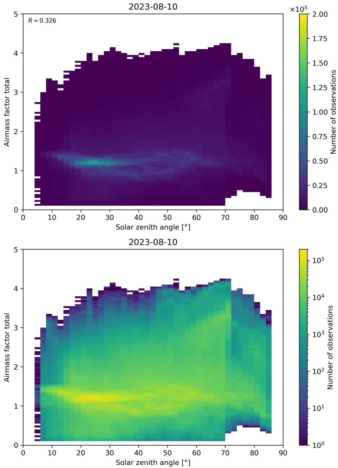
Figure 175: Scatter density plot of “Solar zenith angle” against “Airmass factor total” for 2023-08-09 to 2023-08-11.
