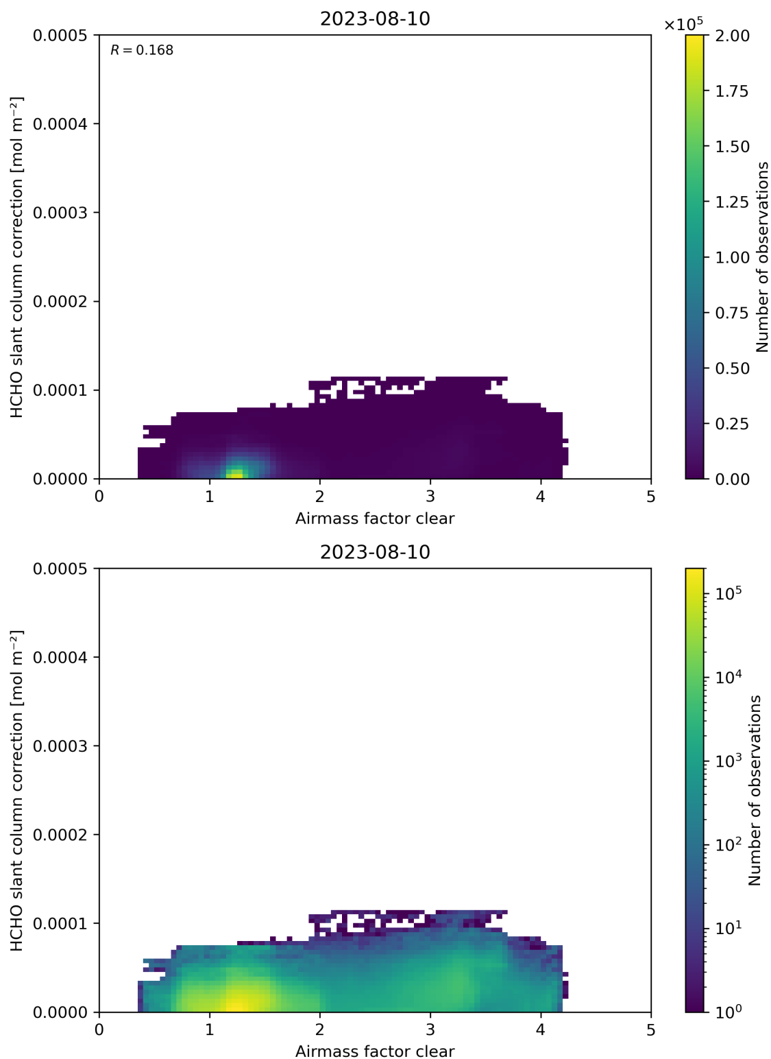
Figure 75: Scatter density plot of “Airmass factor clear” against “HCHO slant column correction” for 2023-08-09 to 2023-08-11.
