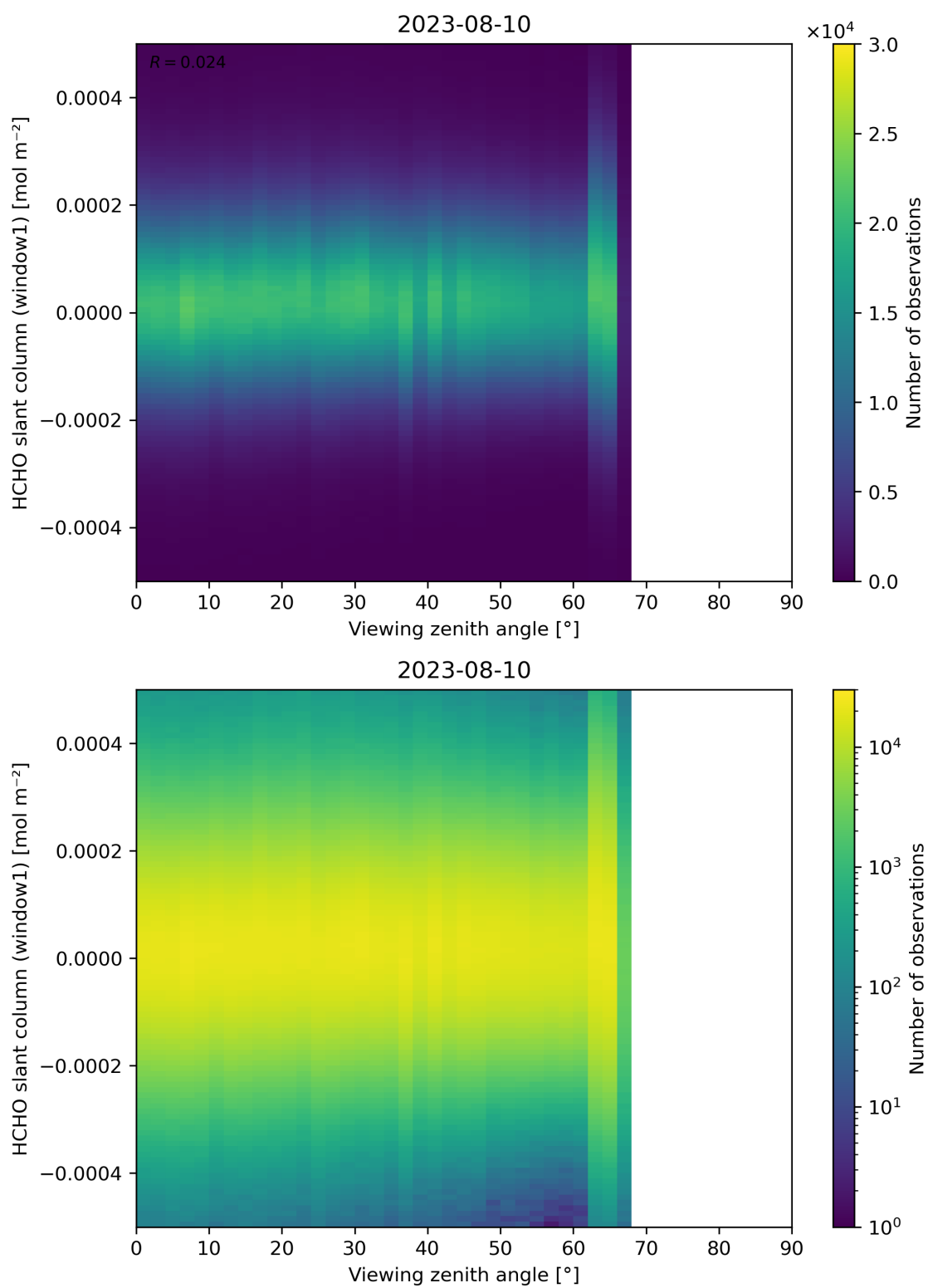
Figure 188: Scatter density plot of “Viewing zenith angle” against “HCHO slant column (window1)” for 2023-08-09 to 2023-08-11.
