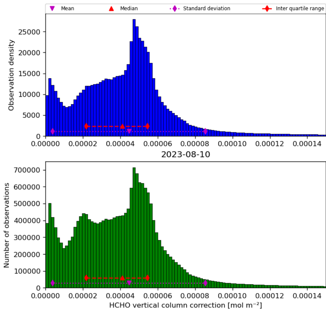
Figure 37: Histogram of “HCHO vertical column correction” for 2023-08-09 to 2023-08-11
