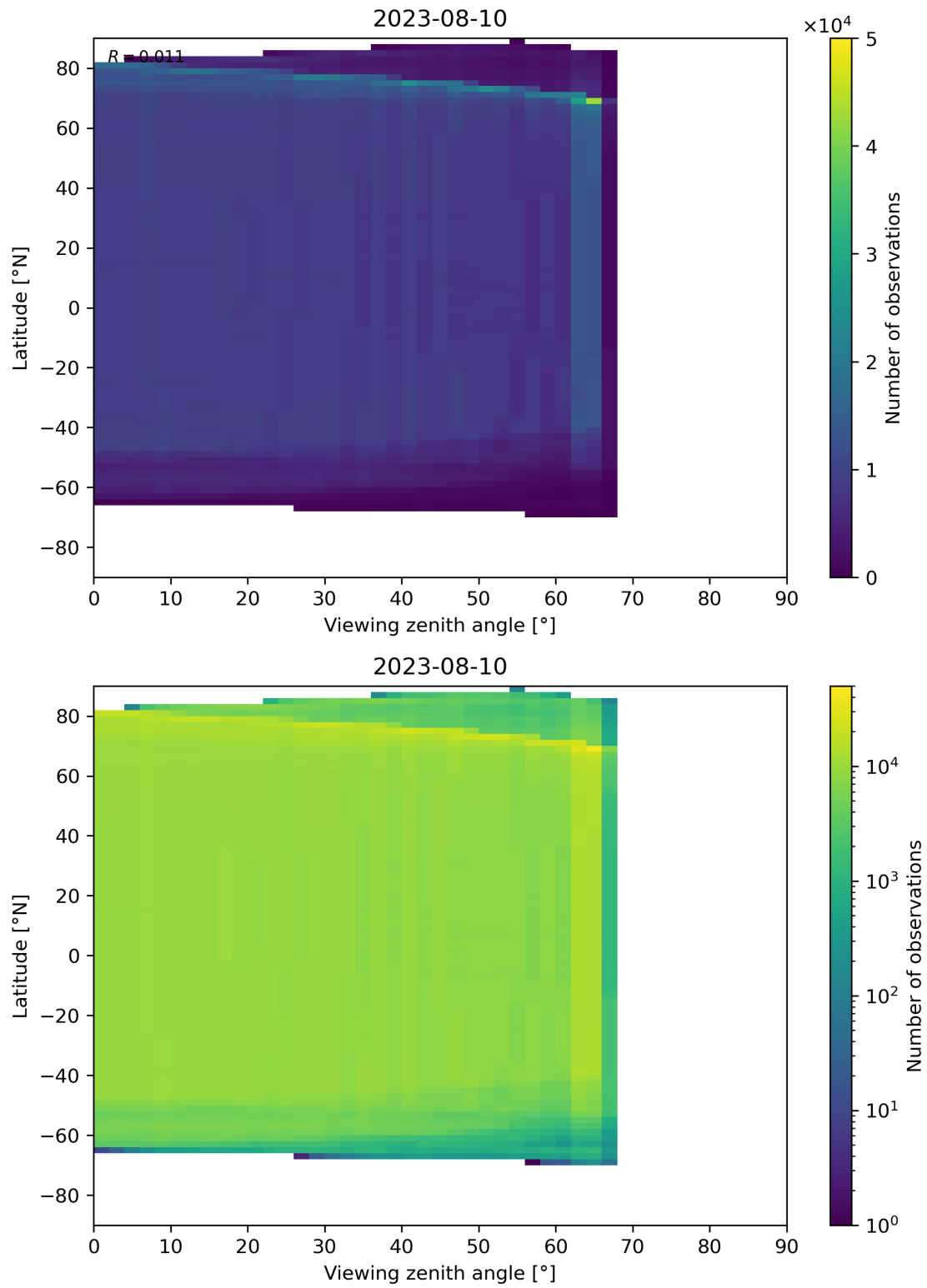
Figure 196: Scatter density plot of “Viewing zenith angle” against “Latitude” for 2023-08-09 to 2023-08-11.
