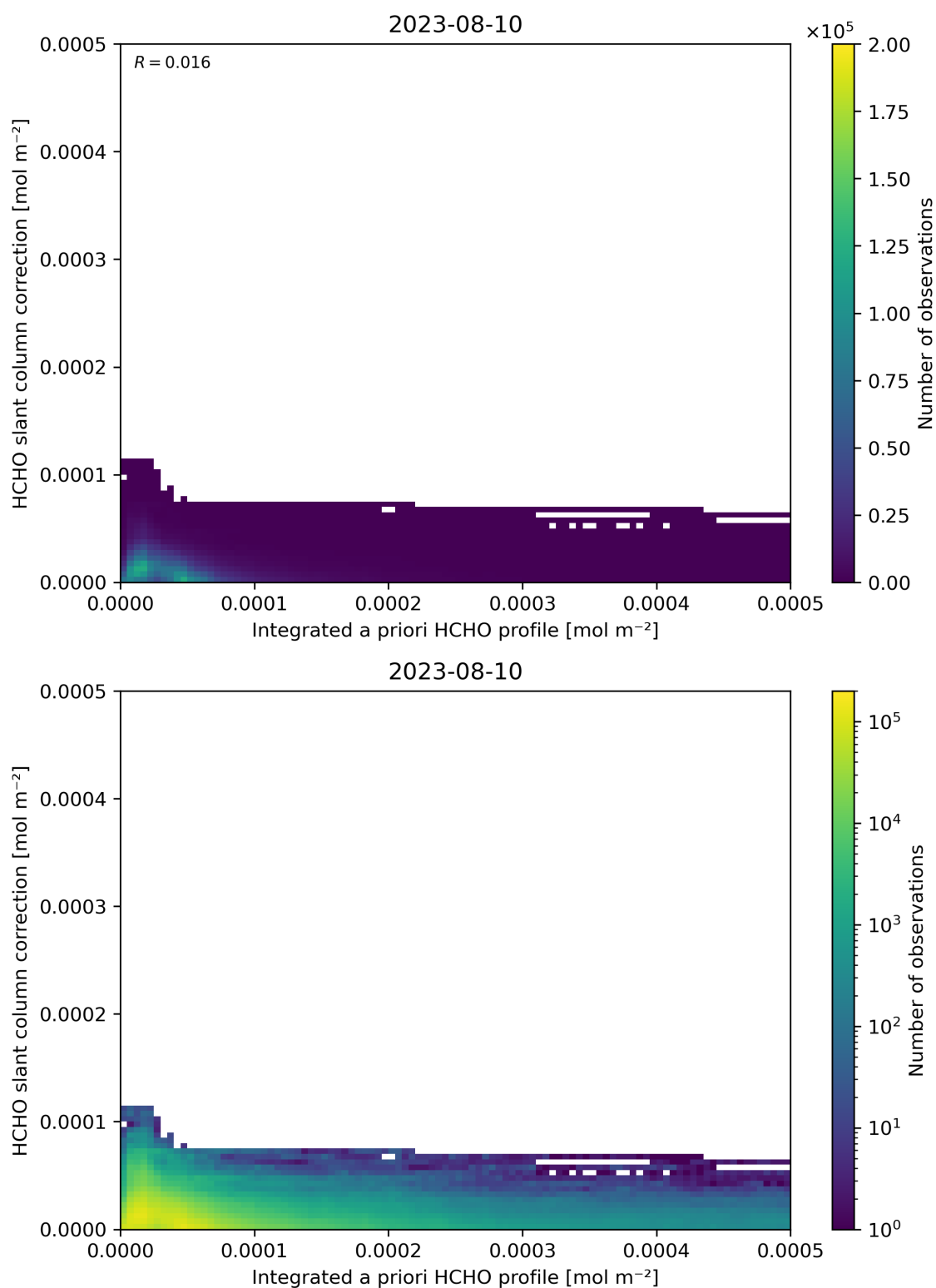
Figure 152: Scatter density plot of “Integrated a priori HCHO profile” against “HCHO slant column correction” for 2023-08-09 to 2023-08-11.
