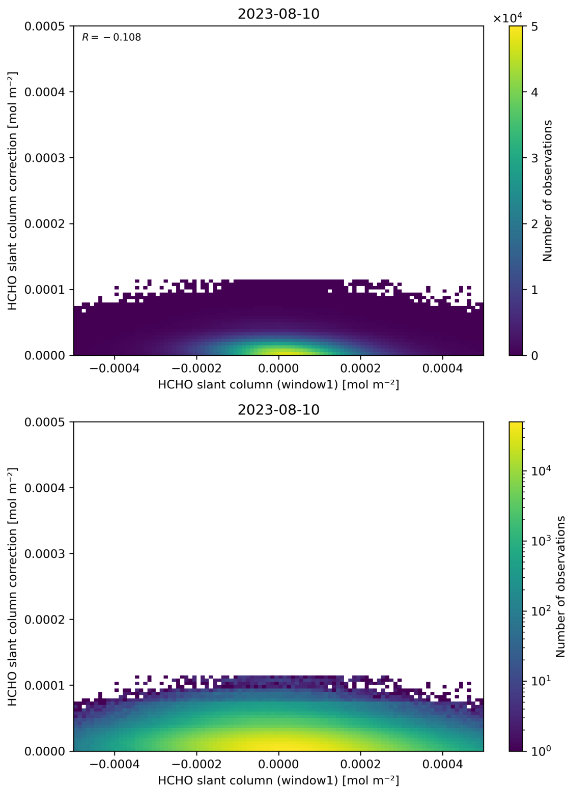
Figure 83: Scatter density plot of “HCHO slant column (window1)” against “HCHO slant column correction” for 2023-08-09 to 2023-08-11.
