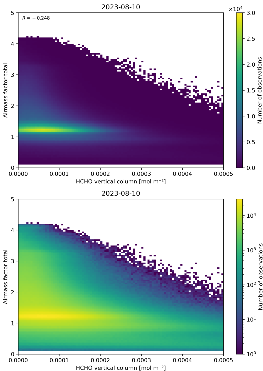
Figure 131: Scatter density plot of “HCHO vertical column” against “Airmass factor total” for 2023-08-09 to 2023-08-11.
