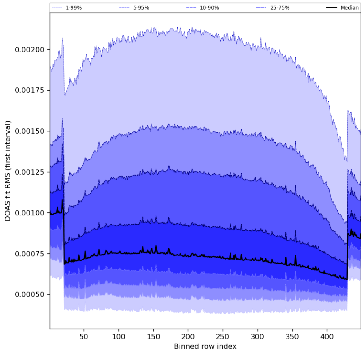
Figure 60: Along track statistics of “DOAS fit RMS (first interval)” for 2023-08-09 to 2023-08-11
