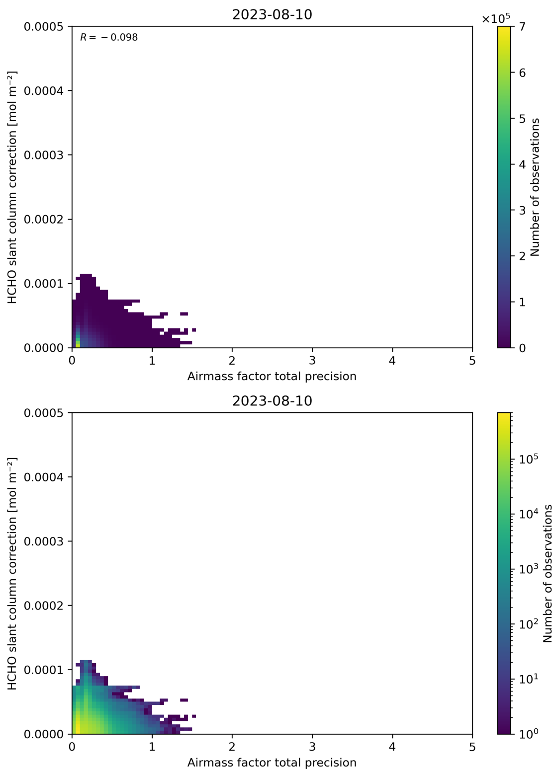
Figure 110: Scatter density plot of “Airmass factor total precision” against “HCHO slant column correction” for 2023-08-09 to 2023-08-11.
