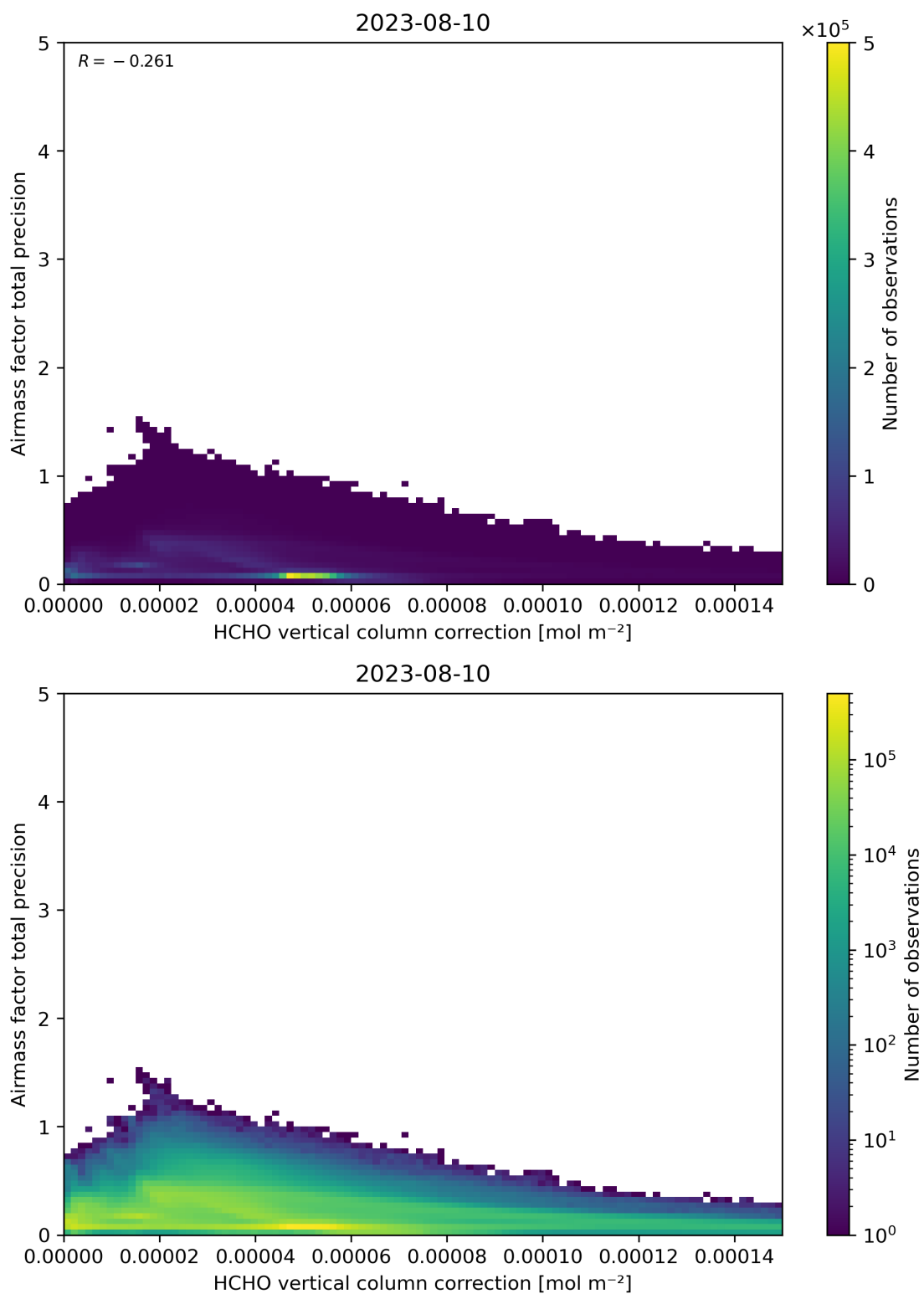
Figure 121: Scatter density plot of “HCHO vertical column correction” against “Airmass factor total precision” for 2023-08-09 to 2023-08-11.
