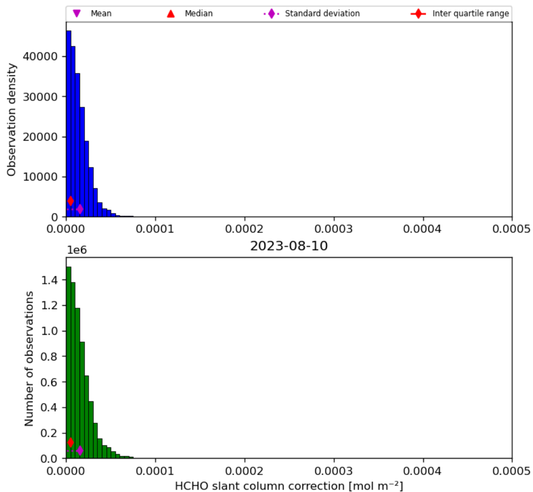
Figure 47: Histogram of “HCHO slant column correction” for 2023-08-09 to 2023-08-11
