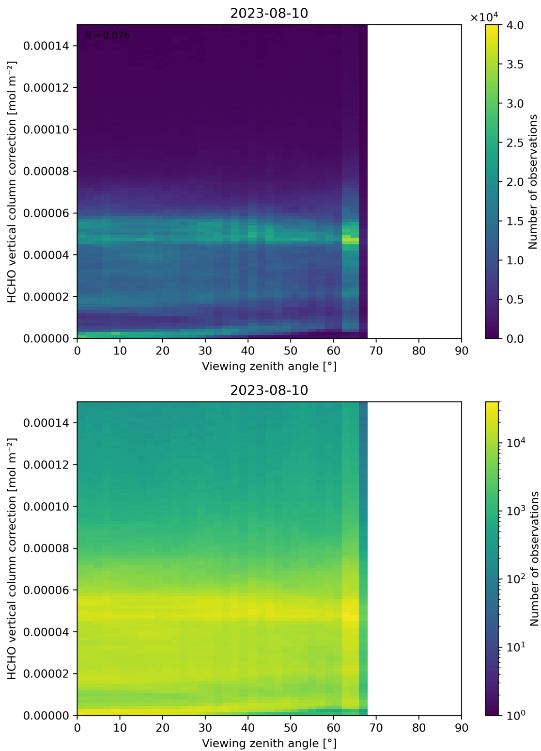
Figure 193: Scatter density plot of “Viewing zenith angle” against “HCHO vertical column correction” for 2023-08-09 to 2023-08-11.
