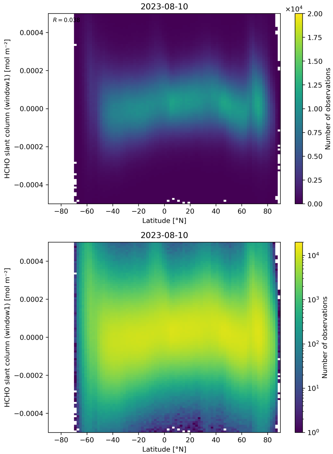
Figure 159: Scatter density plot of “Latitude” against “HCHO slant column (window1)” for 2023-08-09 to 2023-08-11.
