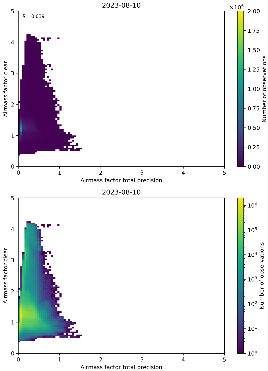
Figure 108: Scatter density plot of “Airmass factor total precision” against “Airmass factor clear” for 2023-08-09 to 2023-08-11.
