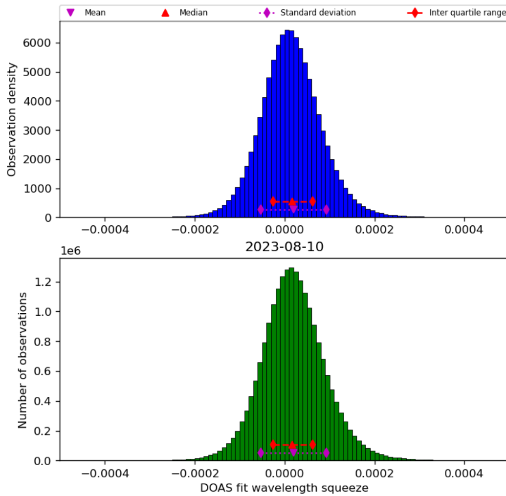
Figure 45: Histogram of “DOAS fit wavelength squeeze” for 2023-08-09 to 2023-08-11
