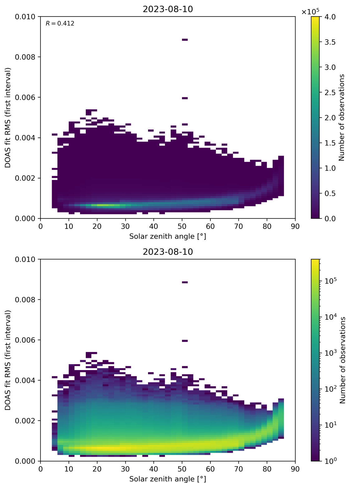
Figure 167: Scatter density plot of “Solar zenith angle” against “DOAS fit RMS (first interval)” for 2023-08-09 to 2023-08-11.
