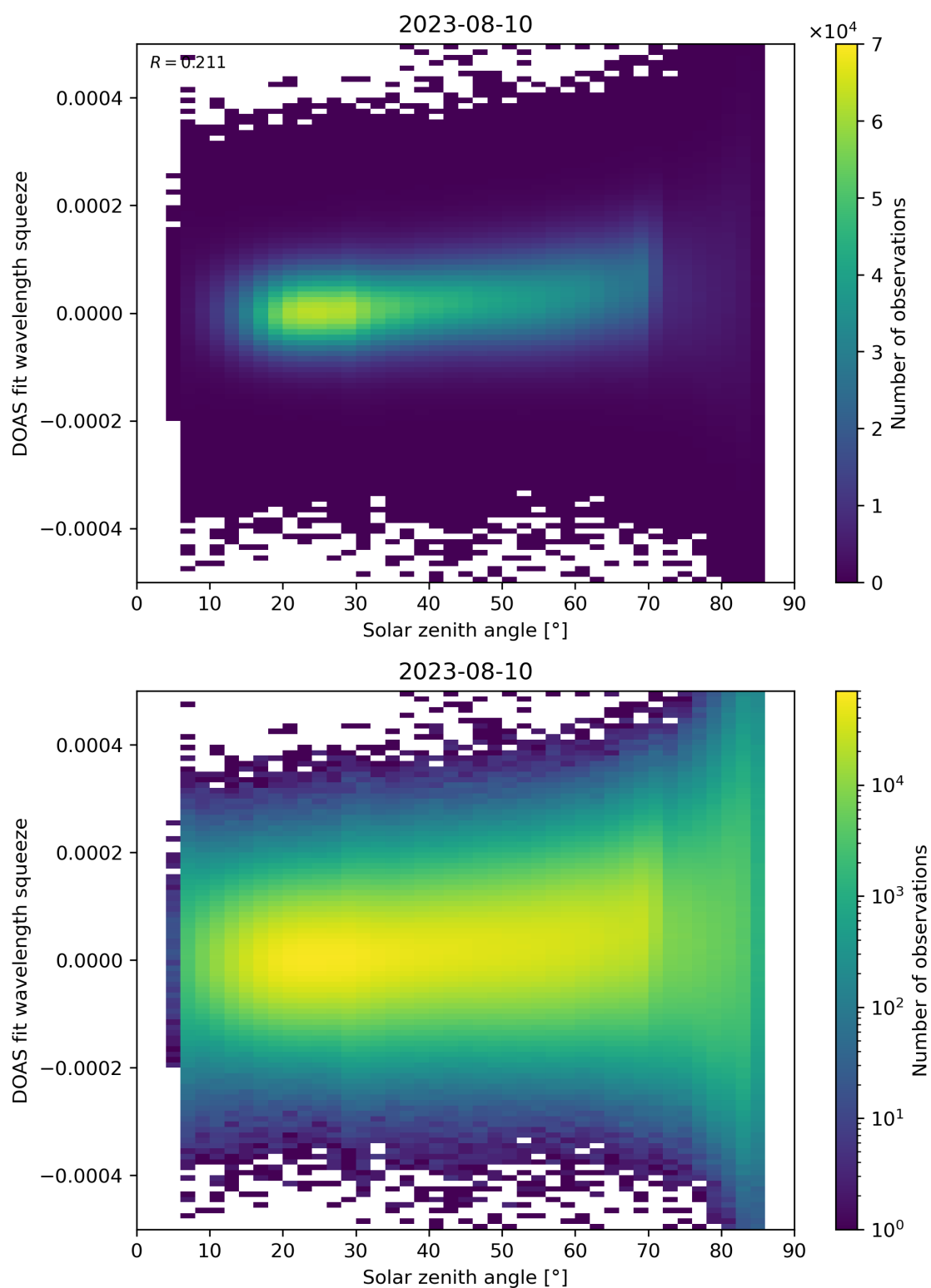
Figure 169: Scatter density plot of “Solar zenith angle” against “DOAS fit wavelength squeeze” for 2023-08-09 to 2023-08-11.
