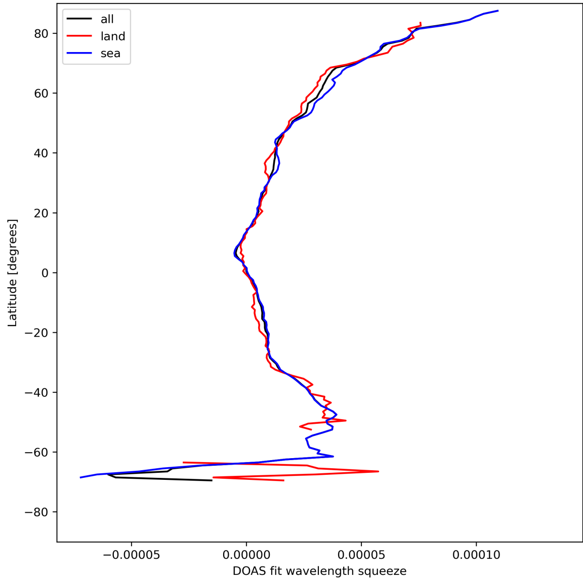
Figure 31: Zonal average of “DOAS fit wavelength squeeze” for 2023-08-09 to 2023-08-11.
