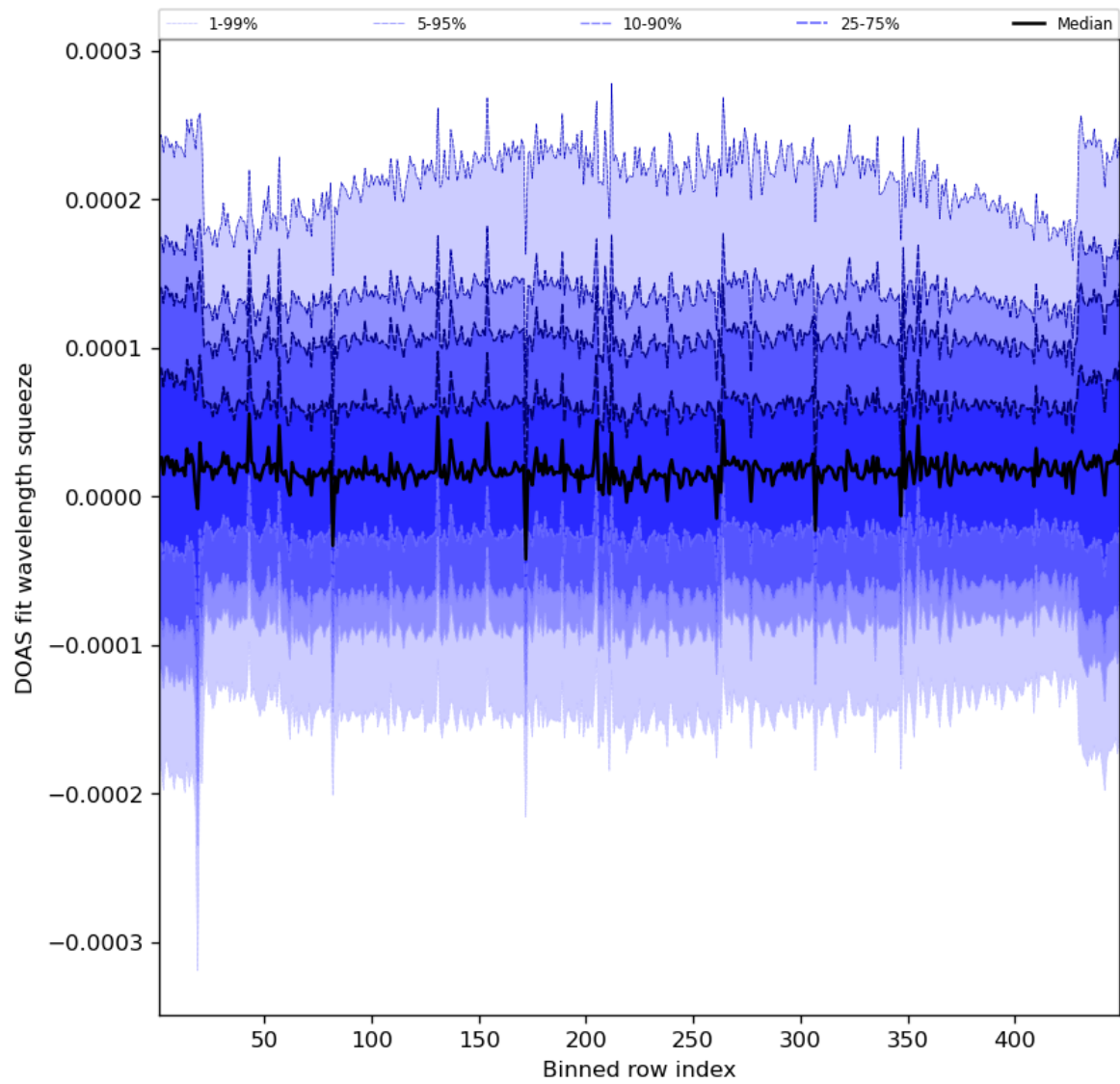
Figure 59: Along track statistics of “DOAS fit wavelength squeeze” for 2023-08-09 to 2023-08-11
