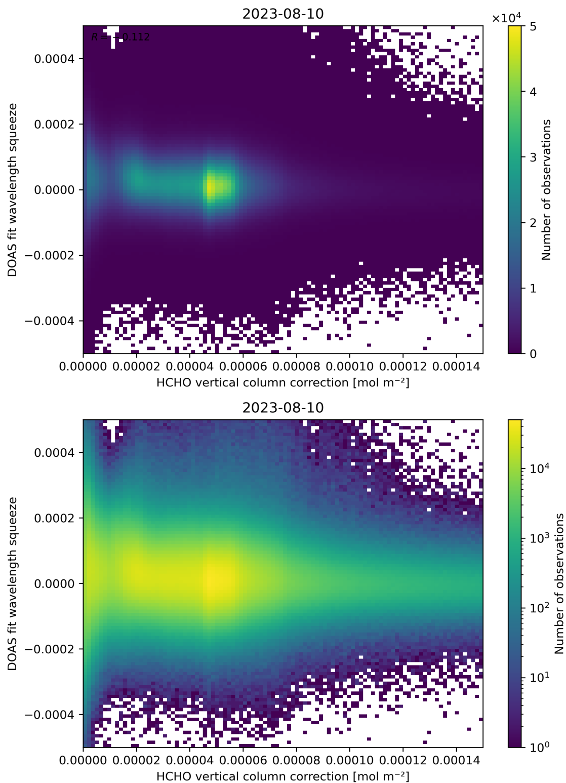
Figure 114: Scatter density plot of “HCHO vertical column correction” against “DOAS fit wavelength squeeze” for 2023-08-09 to 2023-08-11.
