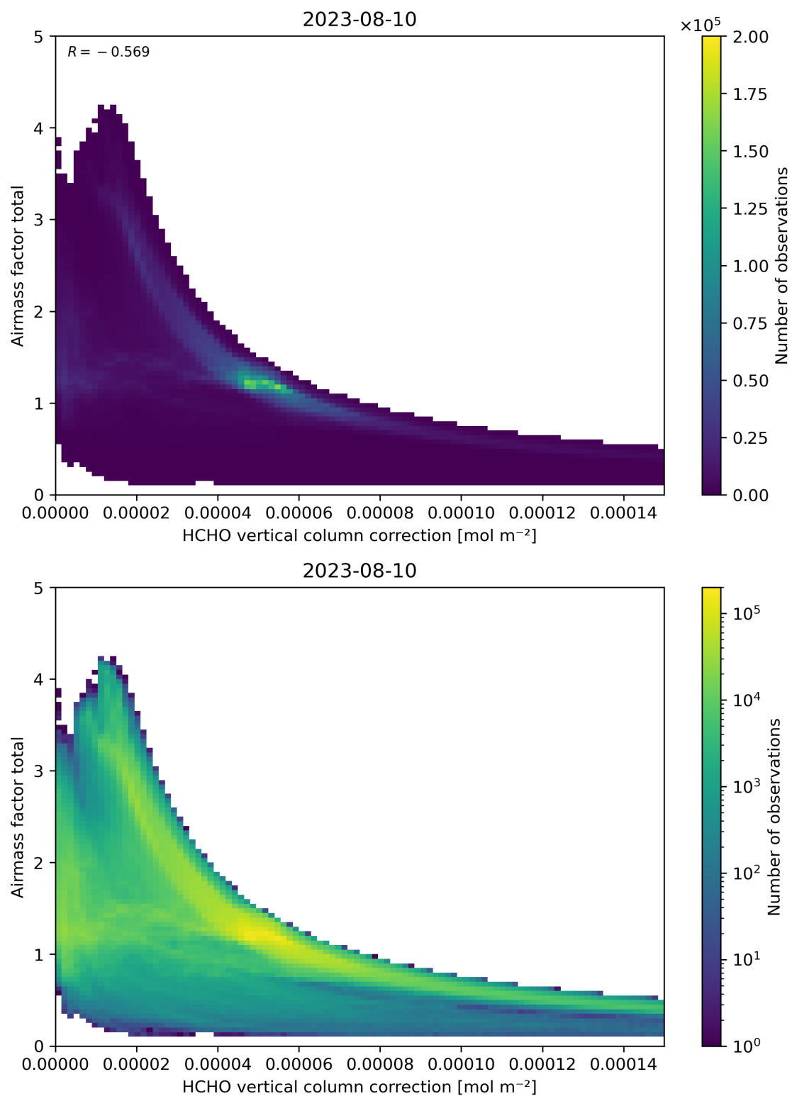
Figure 120: Scatter density plot of “HCHO vertical column correction” against “Airmass factor total” for 2023-08-09 to 2023-08-11.
