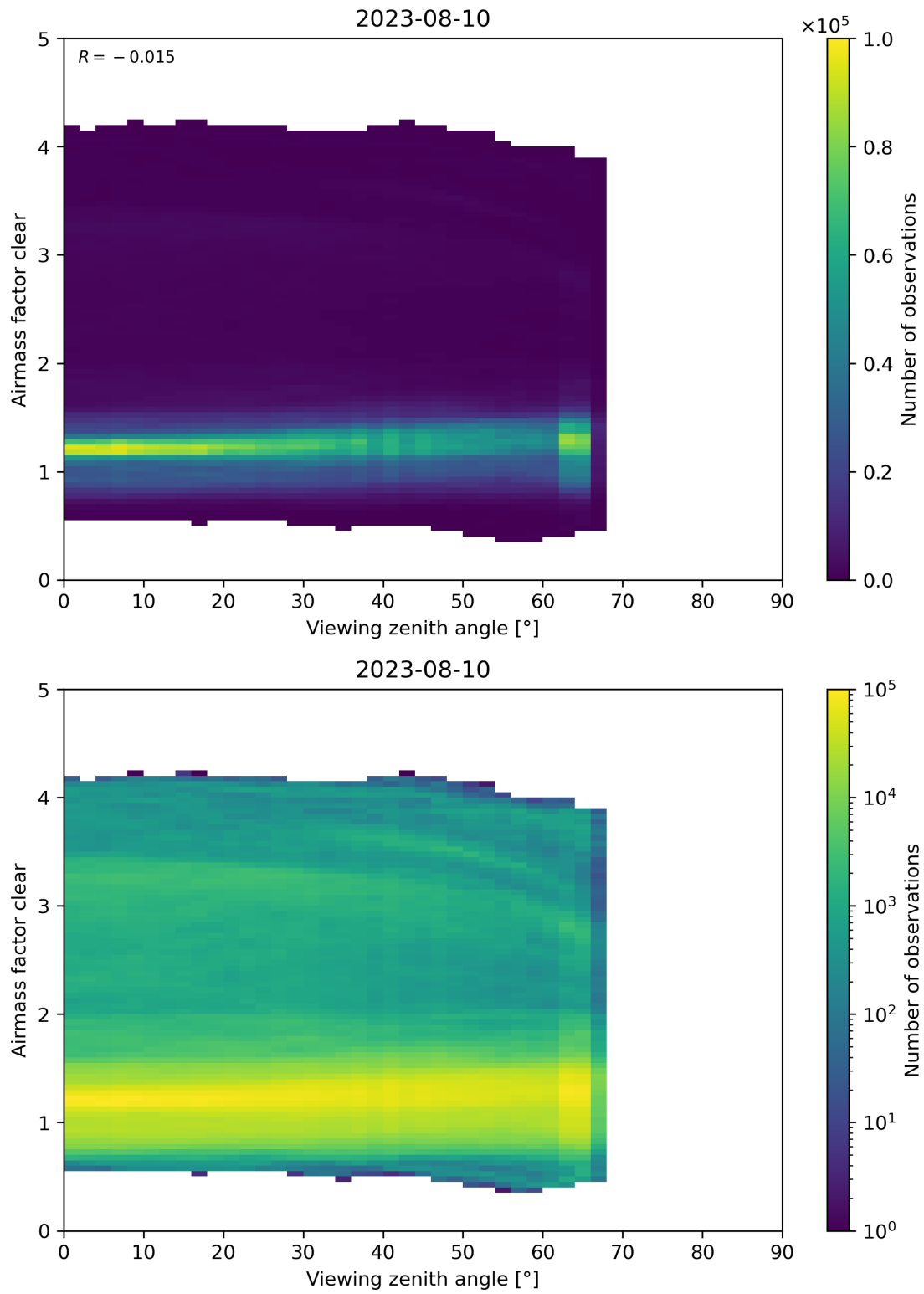
Figure 185: Scatter density plot of “Viewing zenith angle” against “Airmass factor clear” for 2023-08-09 to 2023-08-11.
