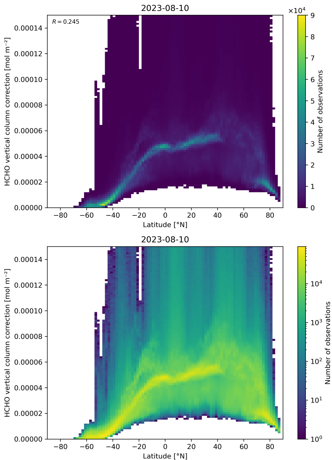
Figure 164: Scatter density plot of “Latitude” against “HCHO vertical column correction” for 2023-08-09 to 2023-08-11.
