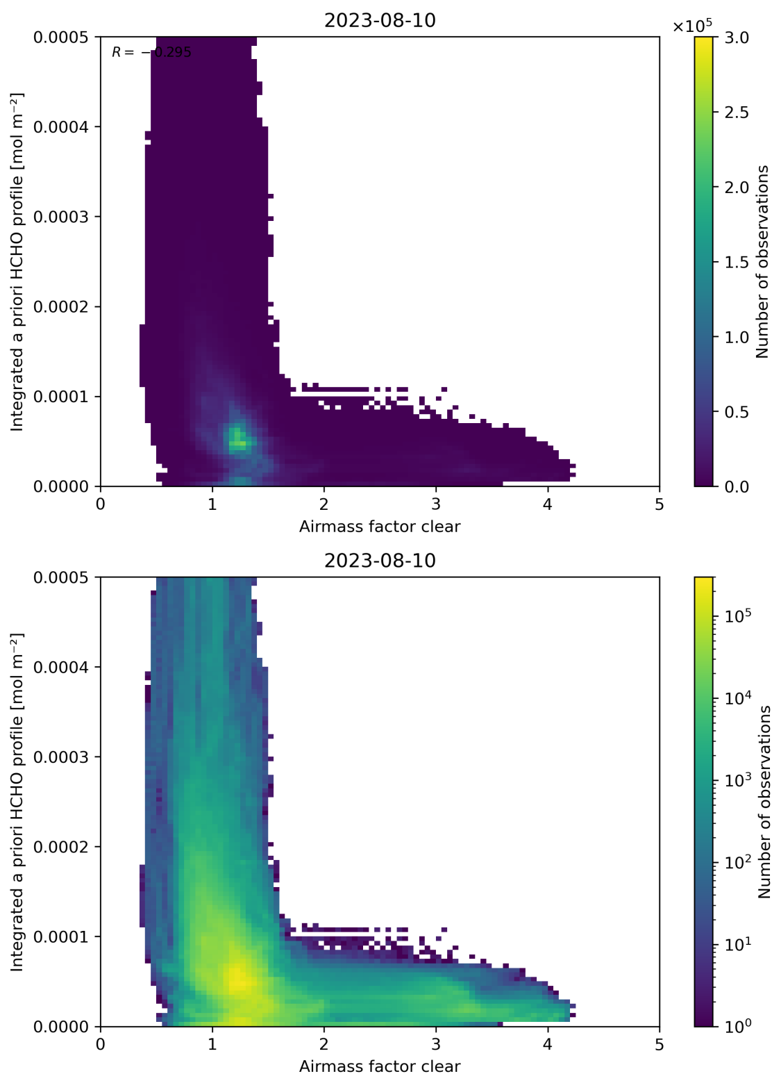
Figure 76: Scatter density plot of “Airmass factor clear” against “Integrated a priori HCHO profile” for 2023-08-09 to 2023-08-11.
