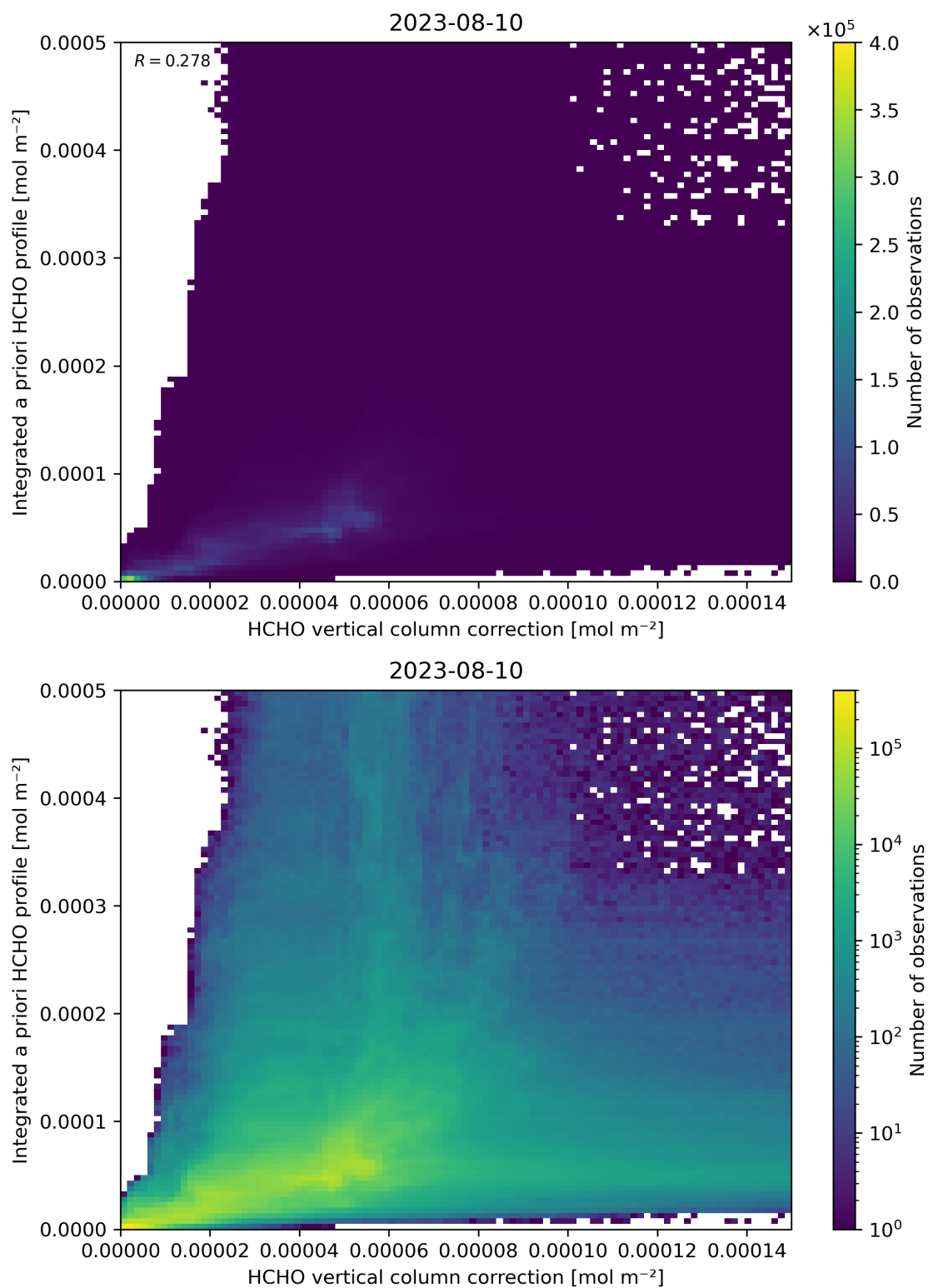
Figure 122: Scatter density plot of “HCHO vertical column correction” against “Integrated a priori HCHO profile” for 2023-08-09 to 2023-08-11.
