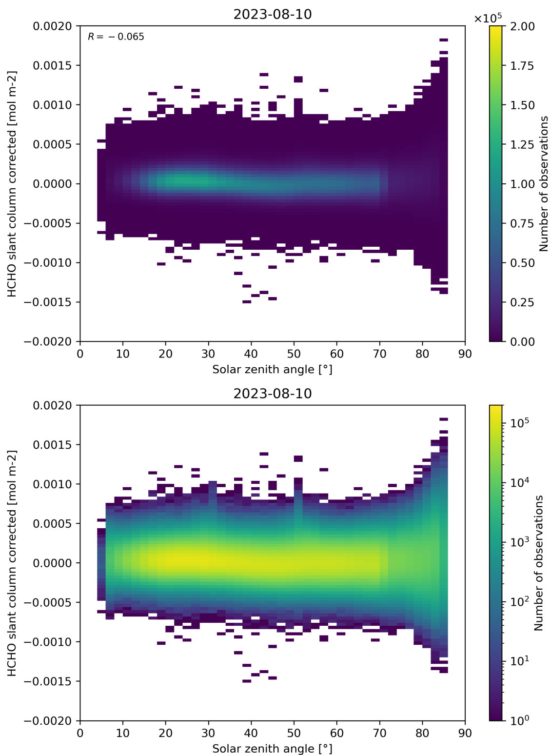
Figure 171: Scatter density plot of “Solar zenith angle” against “HCHO slant column corrected” for 2023-08-09 to 2023-08-11.
