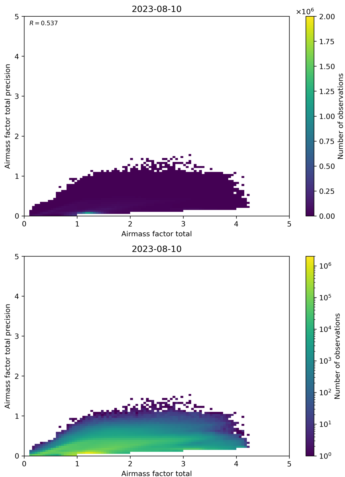
Figure 103: Scatter density plot of “Airmass factor total” against “Airmass factor total precision” for 2023-08-09 to 2023-08-11.
