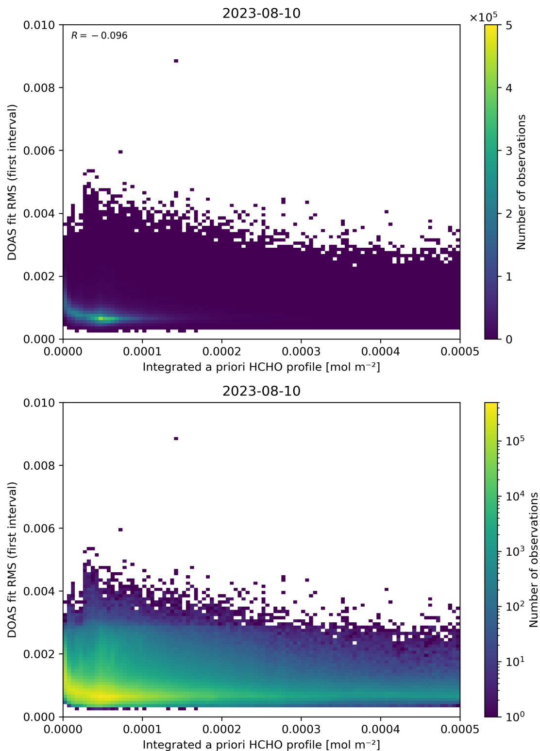
Figure 148: Scatter density plot of “Integrated a priori HCHO profile” against “DOAS fit RMS (first interval)” for 2023-08-09 to 2023-08-11.
