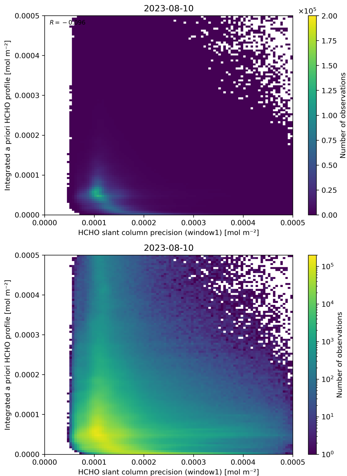
Figure 96: Scatter density plot of “HCHO slant column precision (window1)” against “Integrated a priori HCHO profile” for 2023-08-09 to 2023-08-11.
