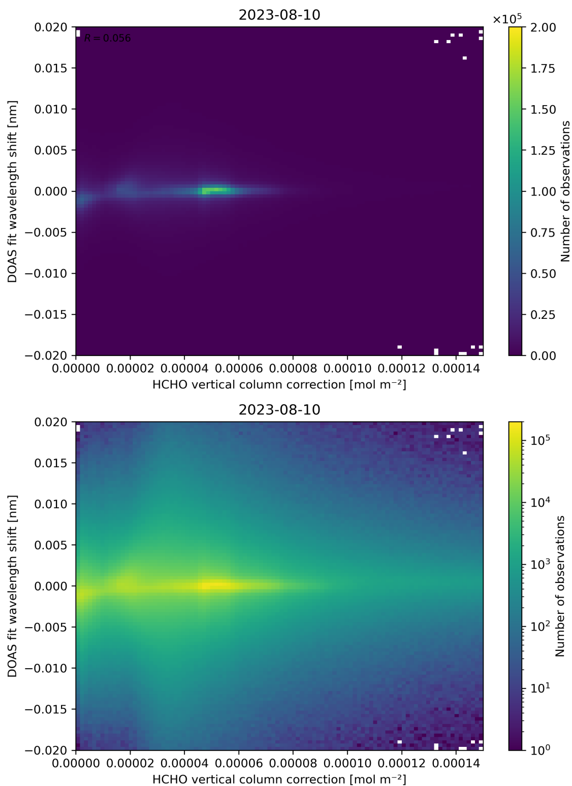
Figure 113: Scatter density plot of “HCHO vertical column correction” against “DOAS fit wavelength shift” for 2023-08-09 to 2023-08-11.
