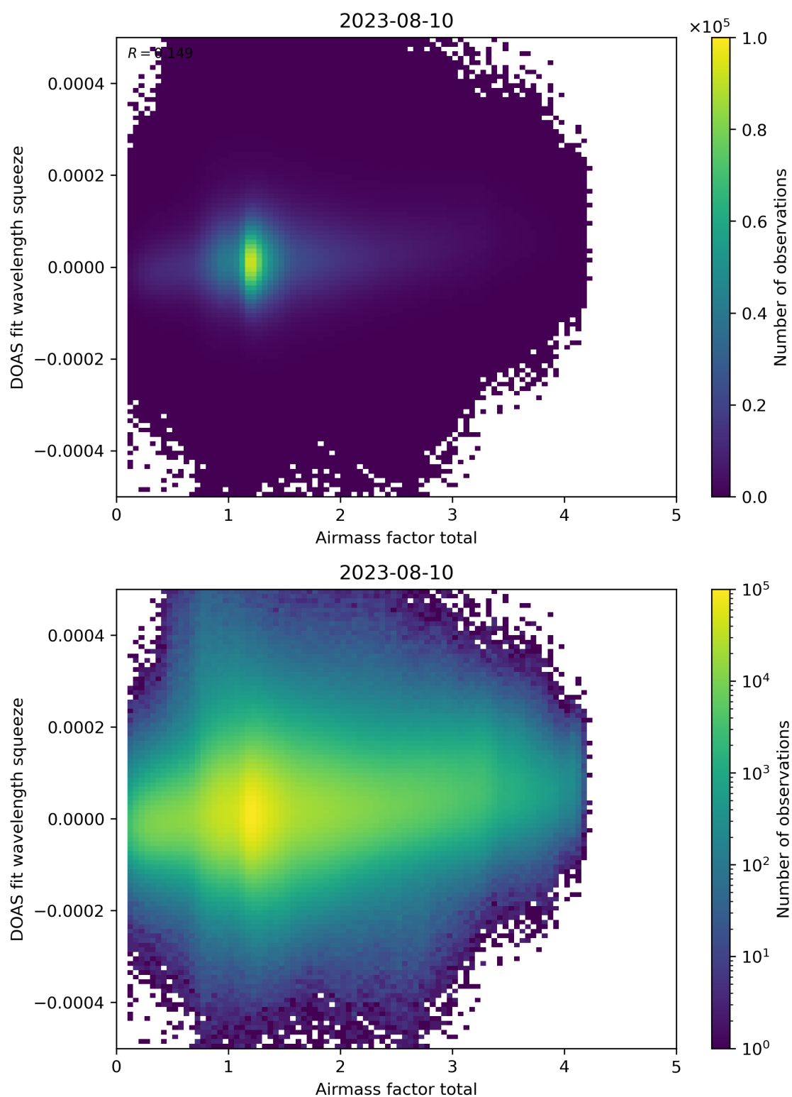
Figure 99: Scatter density plot of “Airmass factor total” against “DOAS fit wavelength squeeze” for 2023-08-09 to 2023-08-11.
