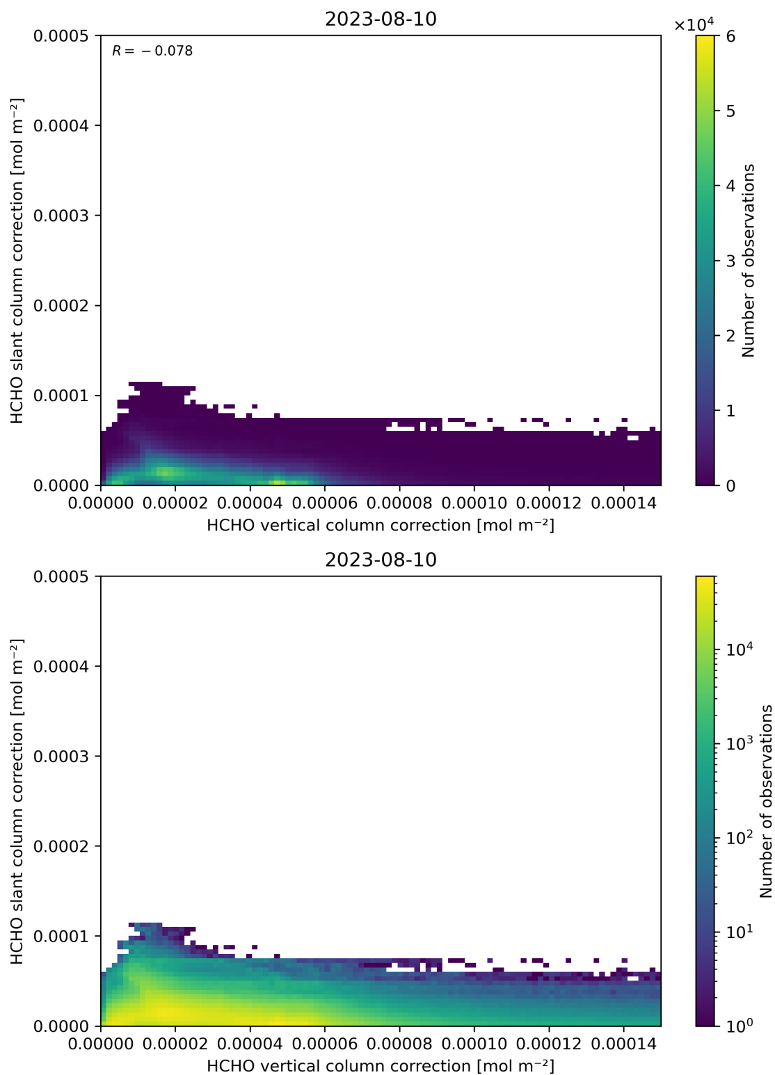
Figure 117: Scatter density plot of “HCHO vertical column correction” against “HCHO slant column correction” for 2023-08-09 to 2023-08-11.
