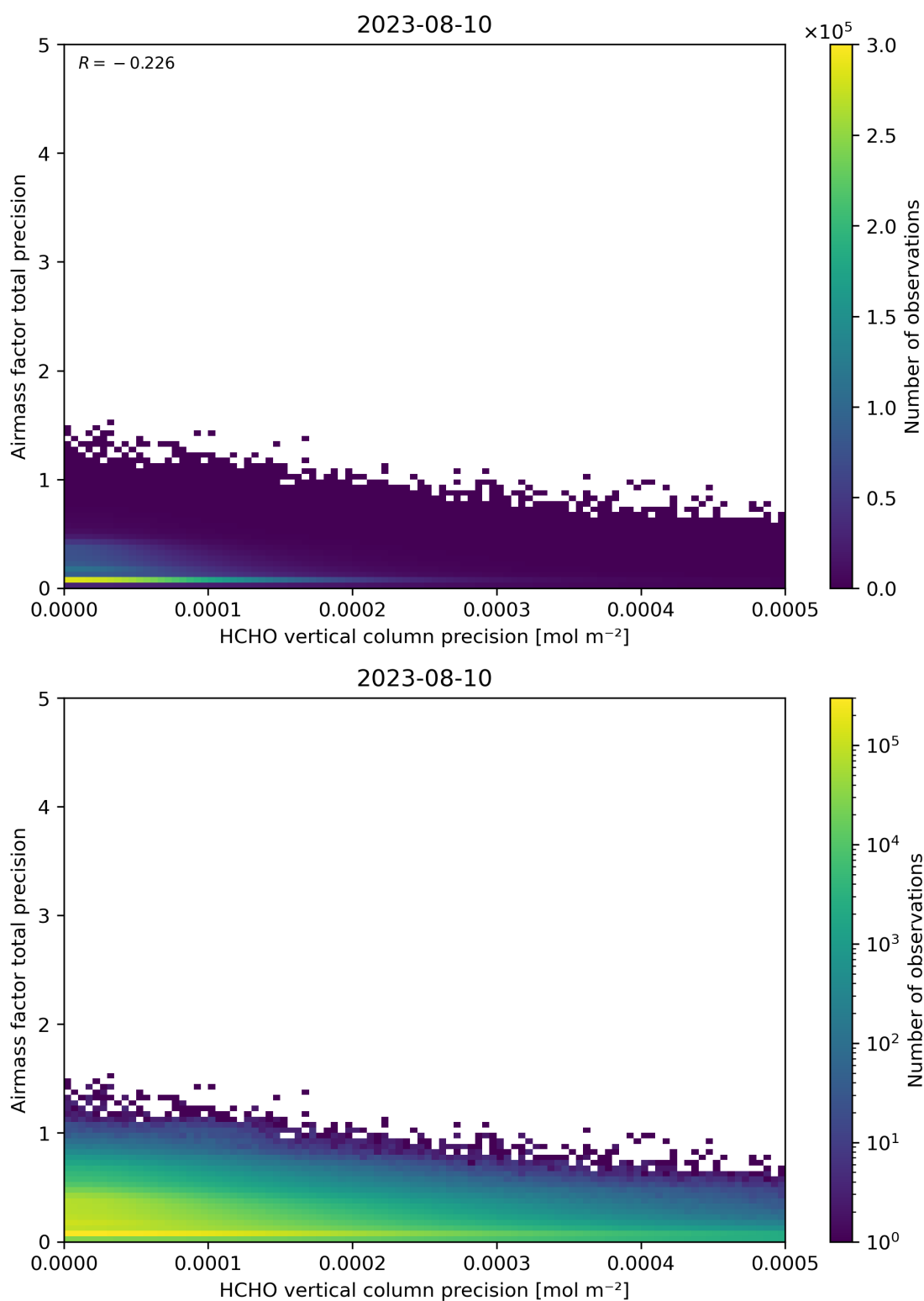
Figure 145: Scatter density plot of “HCHO vertical column precision” against “Airmass factor total precision” for 2023-08-09 to 2023-08-11.
