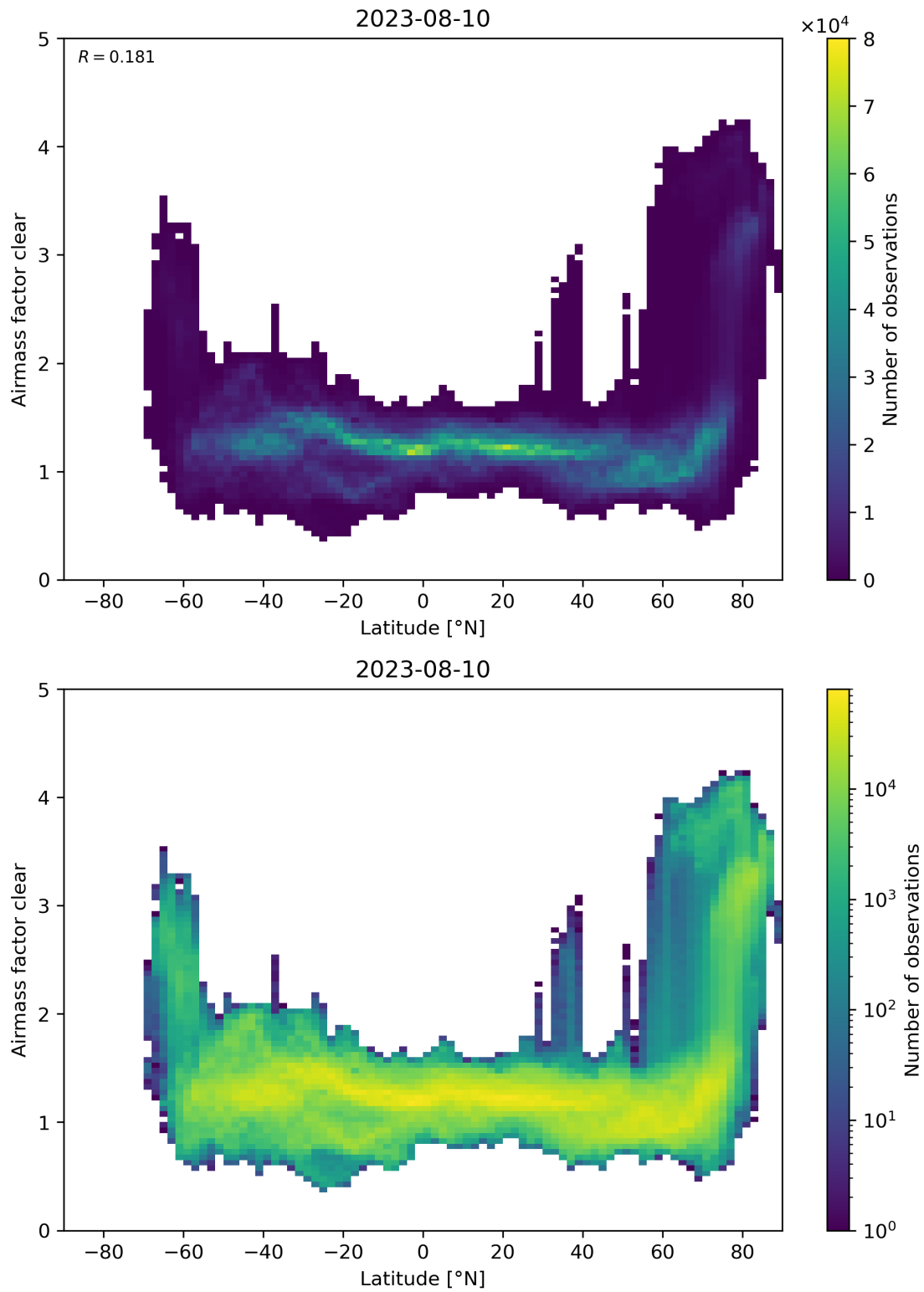
Figure 156: Scatter density plot of “Latitude” against “Airmass factor clear” for 2023-08-09 to 2023-08-11.
