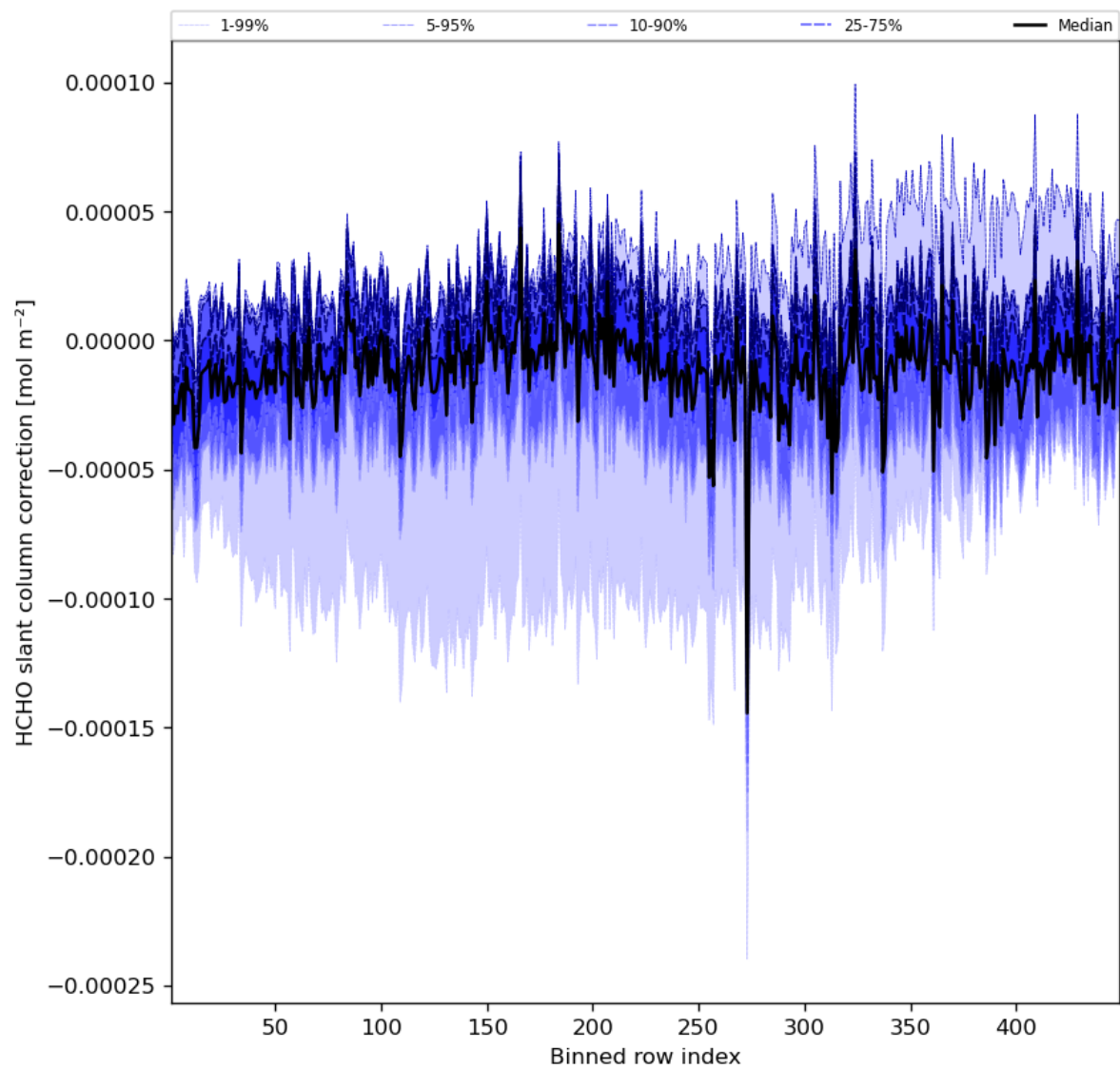
Figure 61: Along track statistics of “HCHO slant column correction” for 2023-08-09 to 2023-08-11
