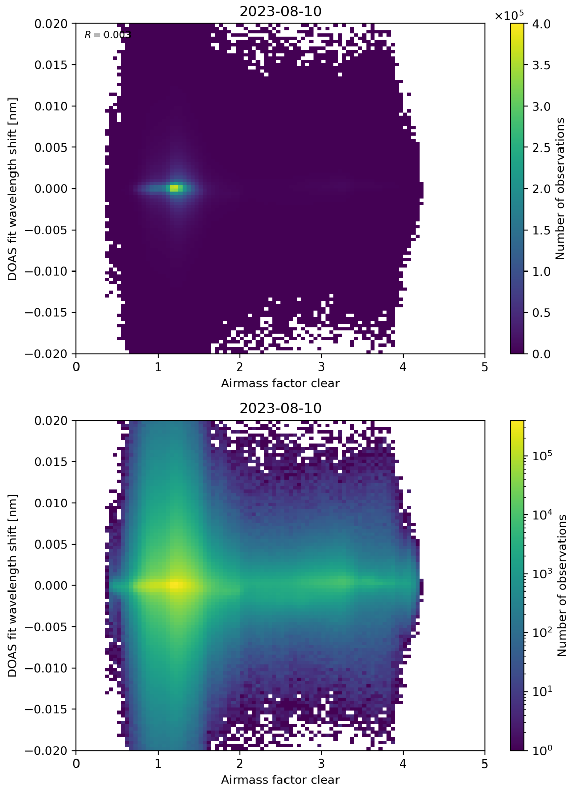
Figure 72: Scatter density plot of “Airmass factor clear” against “DOAS fit wavelength shift” for 2023-08-09 to 2023-08-11.
