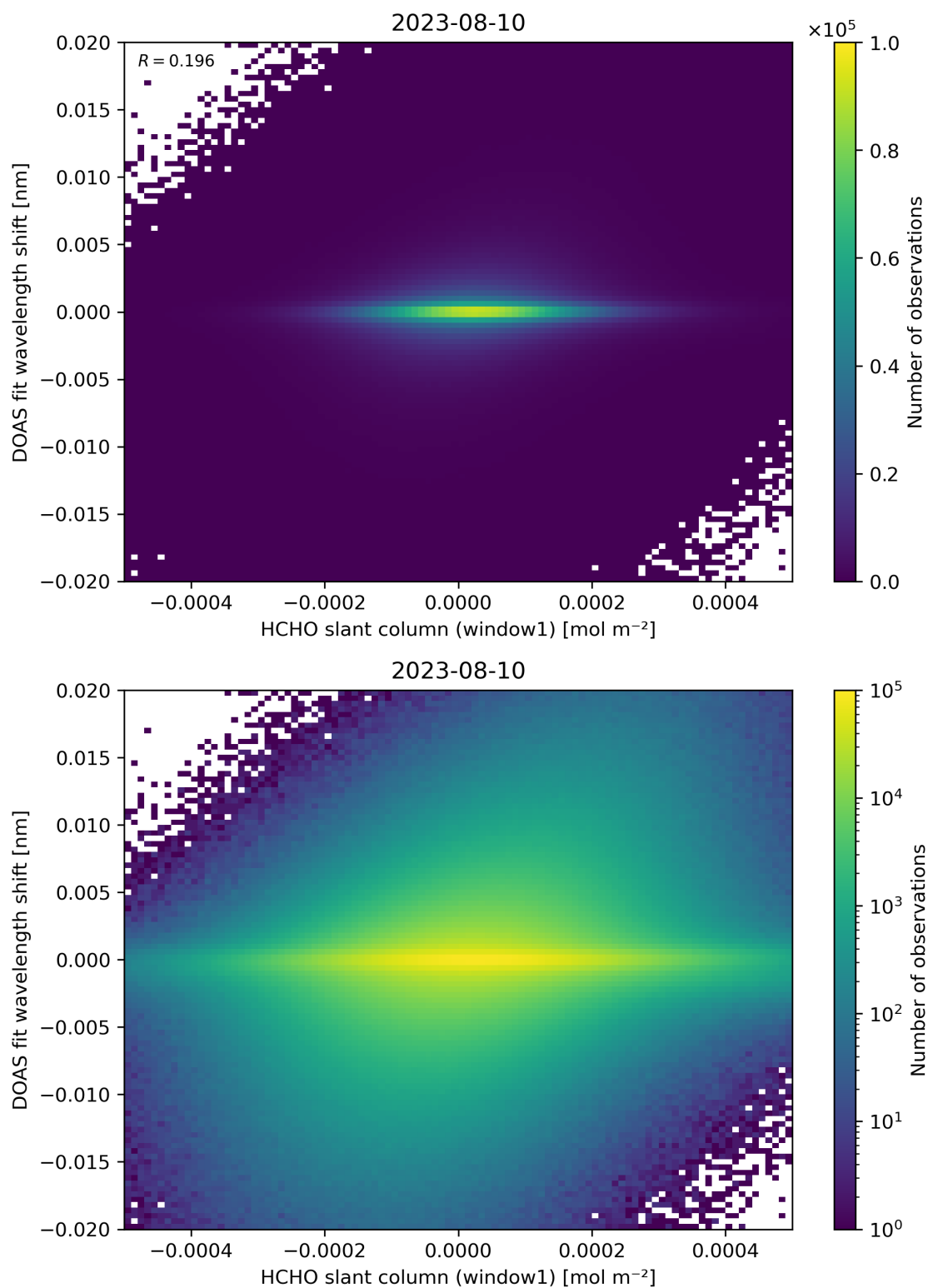
Figure 79: Scatter density plot of “HCHO slant column (window1)” against “DOAS fit wavelength shift” for 2023-08-09 to 2023-08-11.
