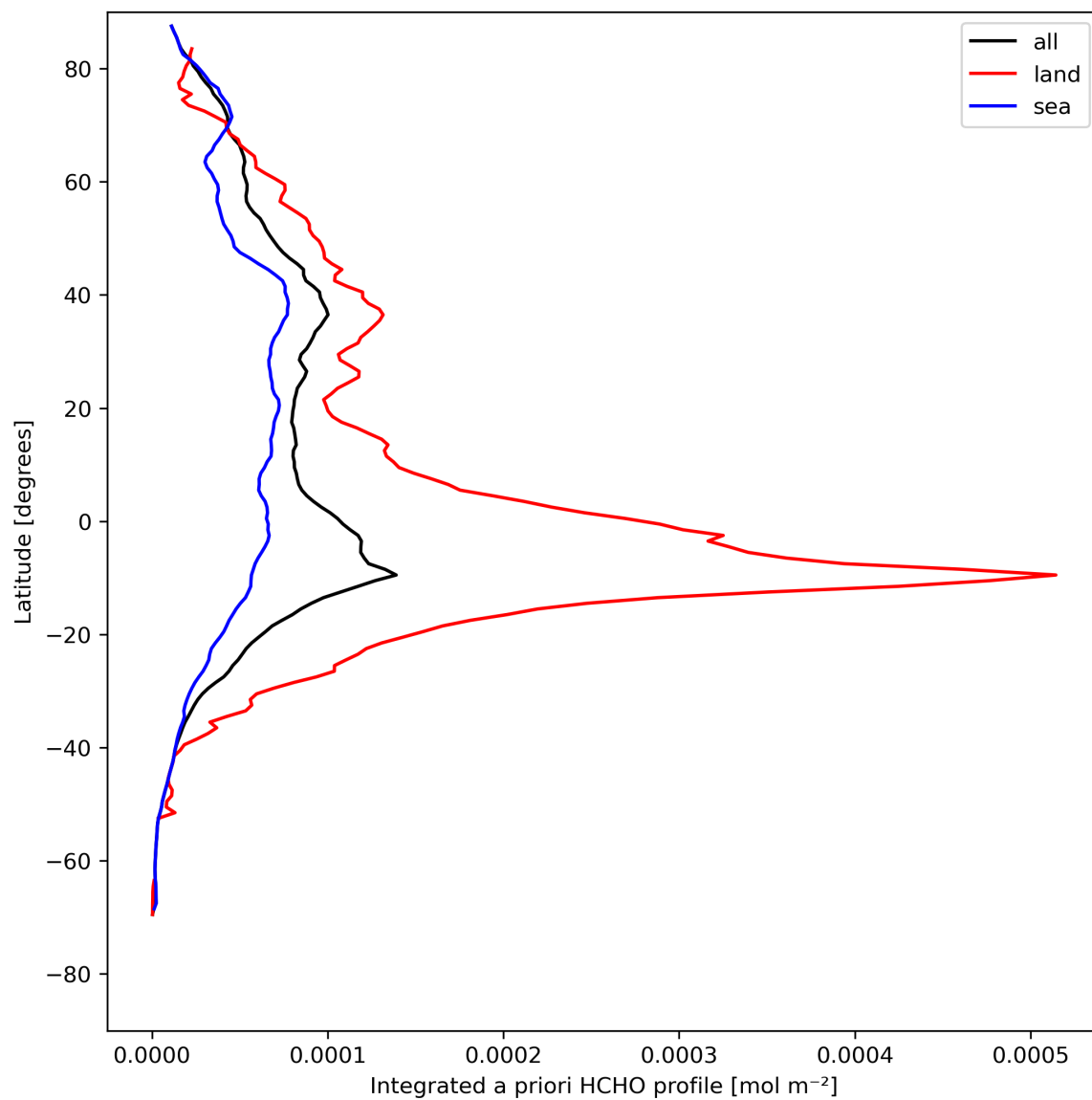
Figure 29: Zonal average of “Integrated a priori HCHO profile” for 2023-08-09 to 2023-08-11.
