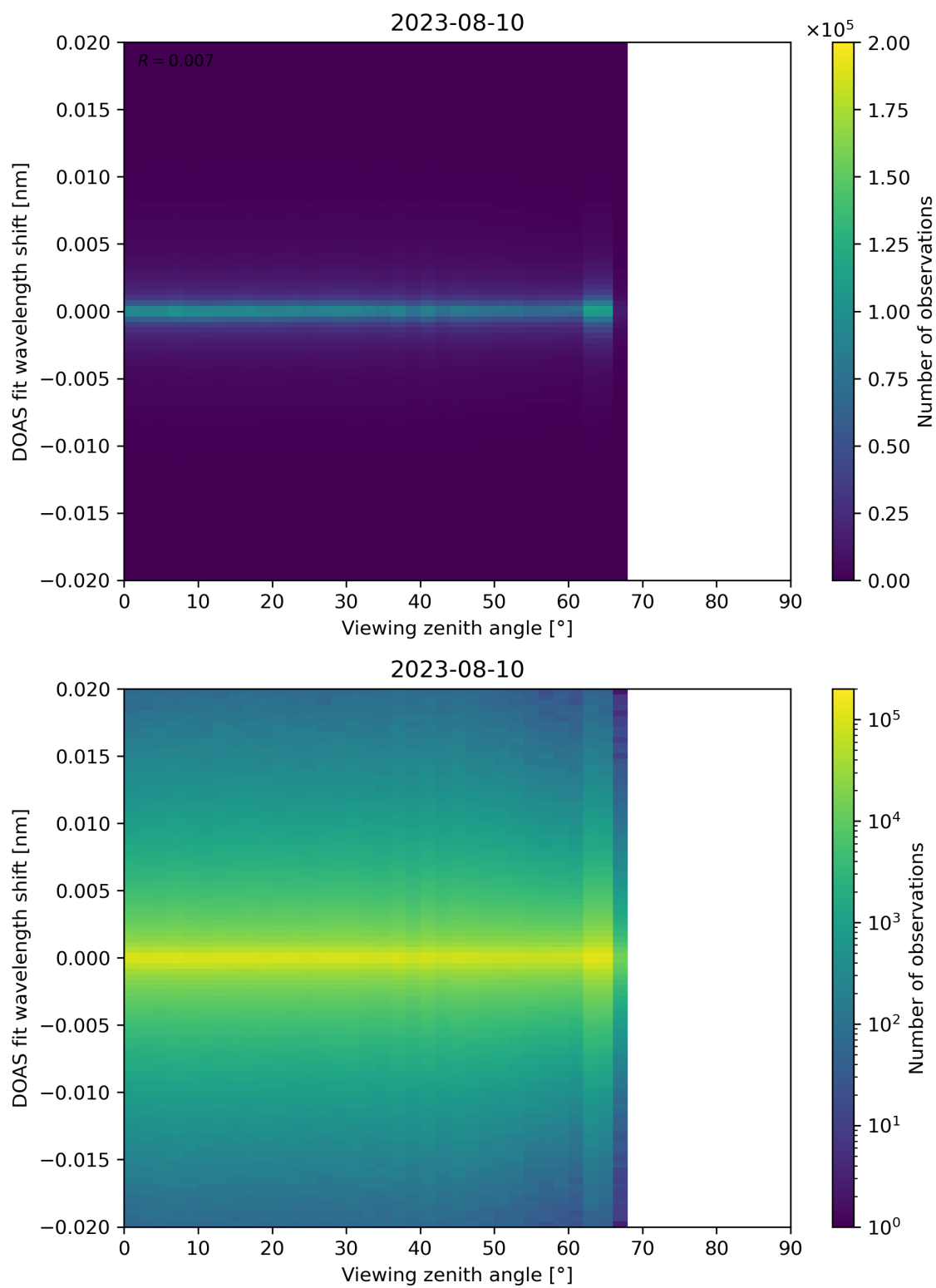
Figure 183: Scatter density plot of “Viewing zenith angle” against “DOAS fit wavelength shift” for 2023-08-09 to 2023-08-11.
