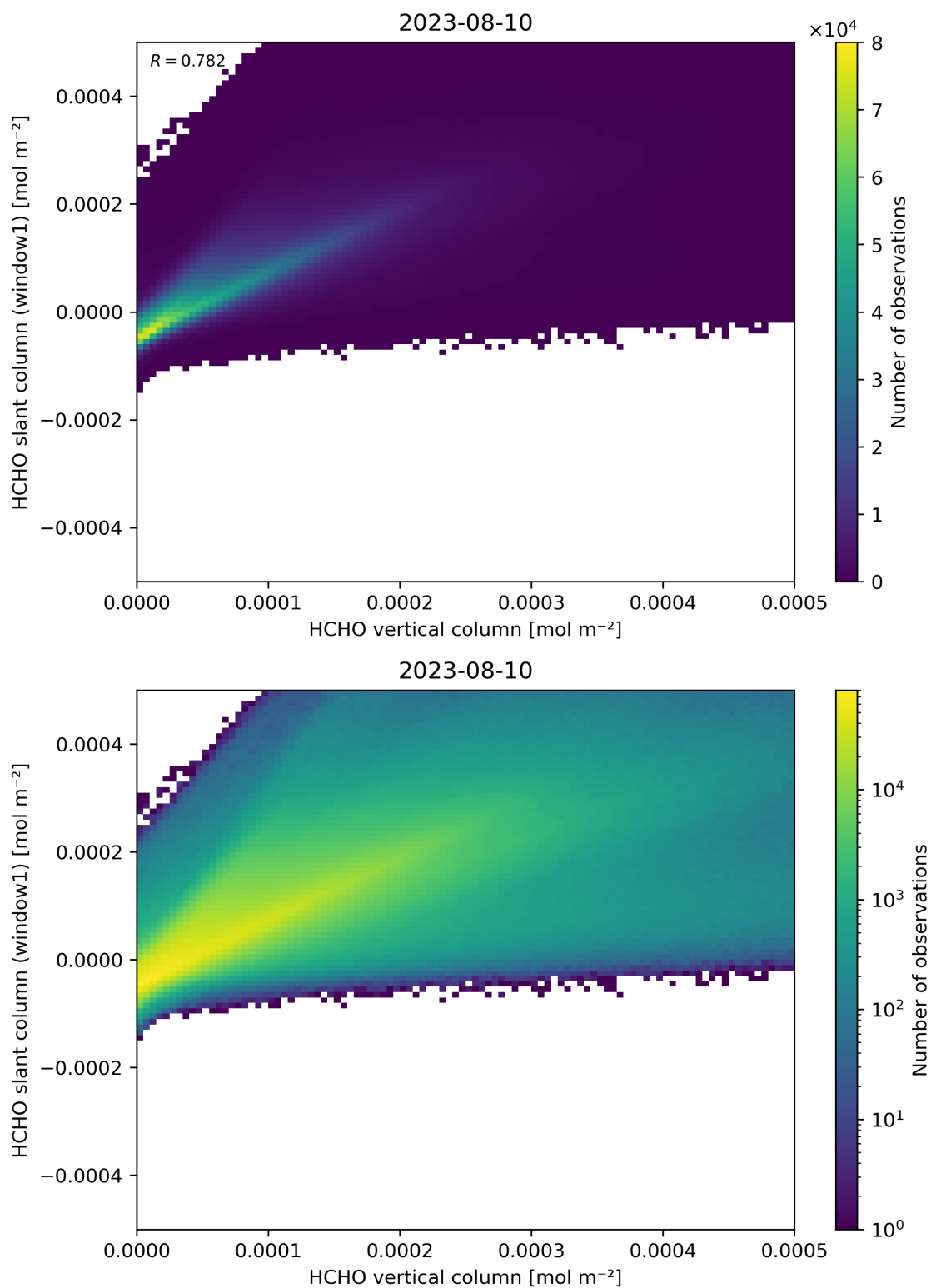
Figure 129: Scatter density plot of “HCHO vertical column” against “HCHO slant column (window1)” for 2023-08-09 to 2023-08-11.
