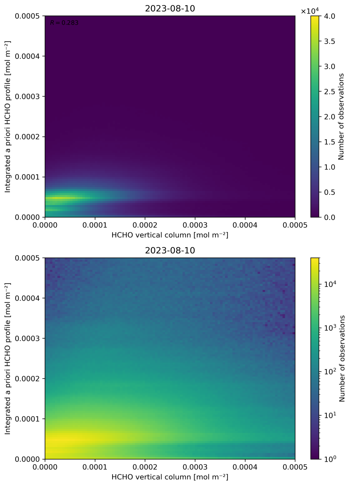
Figure 135: Scatter density plot of “HCHO vertical column” against “Integrated a priori HCHO profile” for 2023-08-09 to 2023-08-11.
