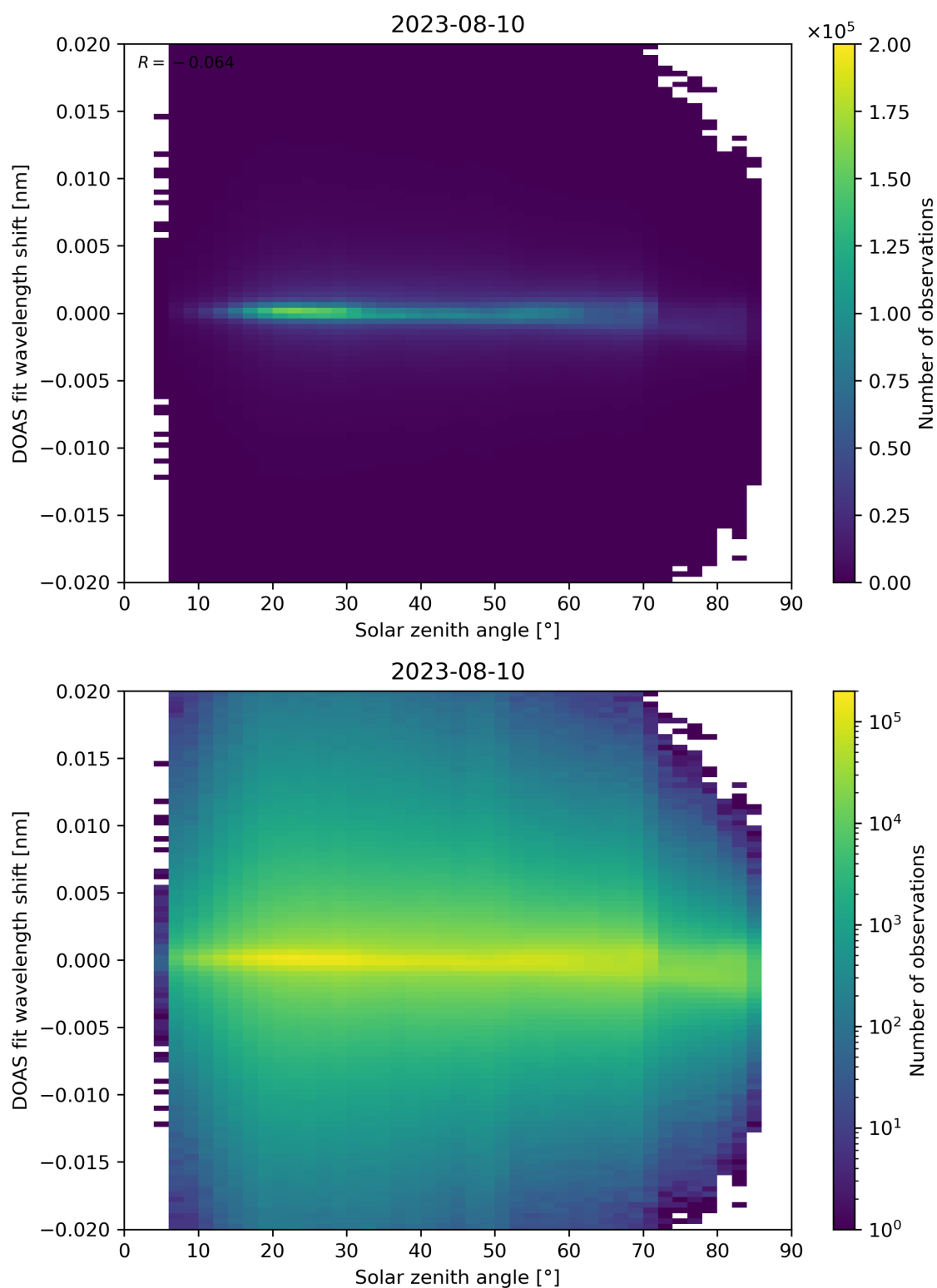
Figure 168: Scatter density plot of “Solar zenith angle” against “DOAS fit wavelength shift” for 2023-08-09 to 2023-08-11.
