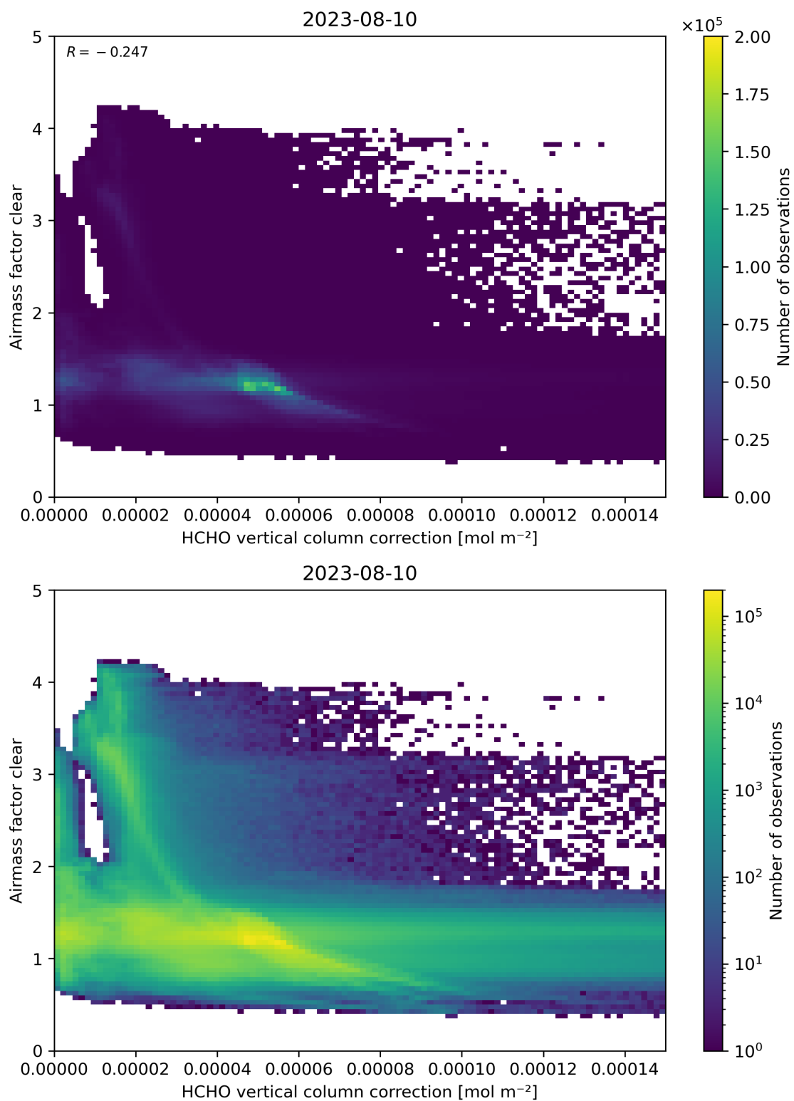
Figure 115: Scatter density plot of “HCHO vertical column correction” against “Airmass factor clear” for 2023-08-09 to 2023-08-11.
