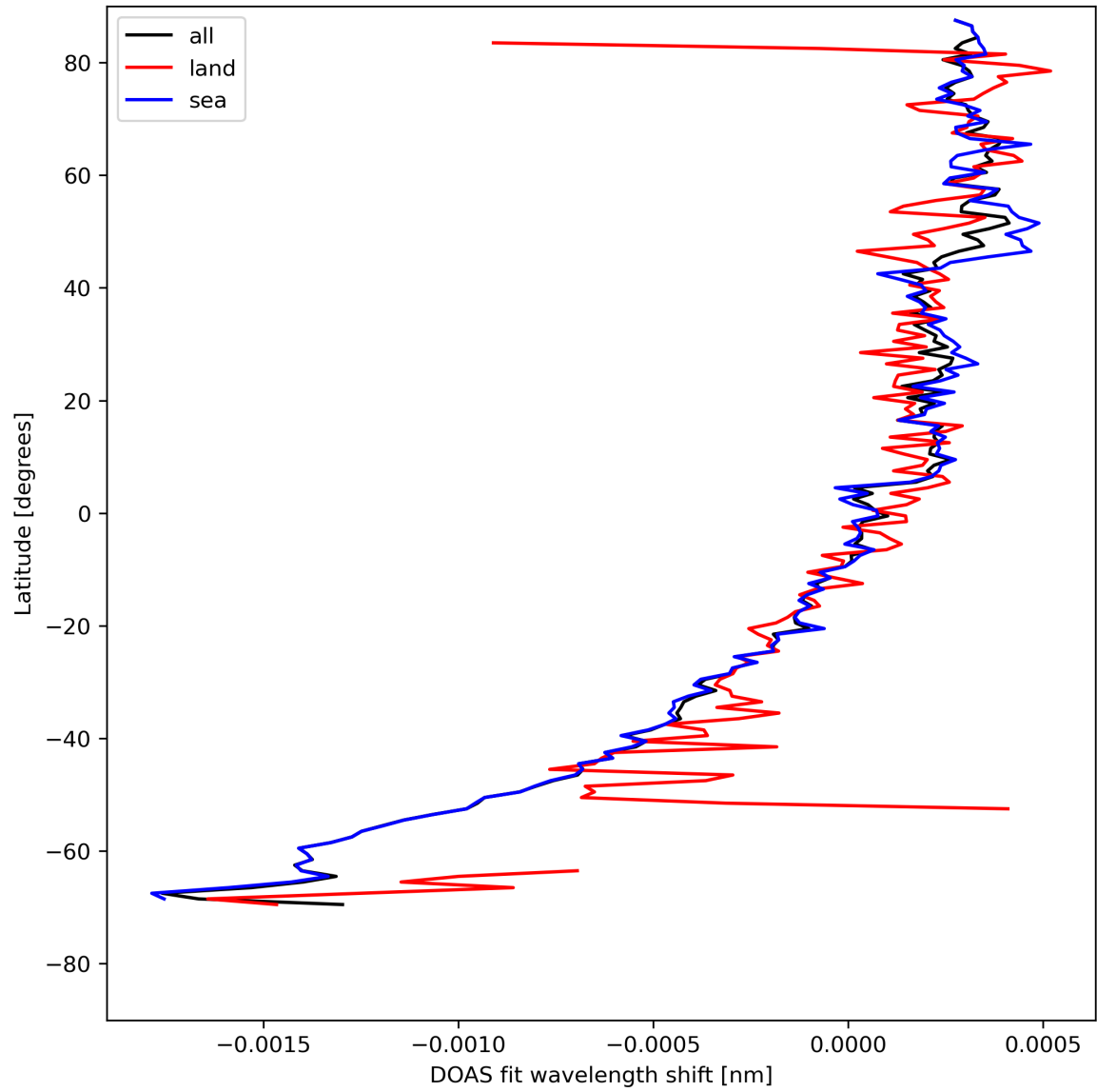
Figure 30: Zonal average of “DOAS fit wavelength shift” for 2023-08-09 to 2023-08-11.
