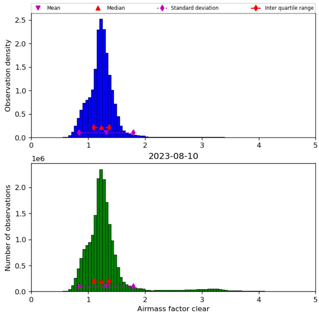
Figure 42: Histogram of “Airmass factor clear” for 2023-08-09 to 2023-08-11
