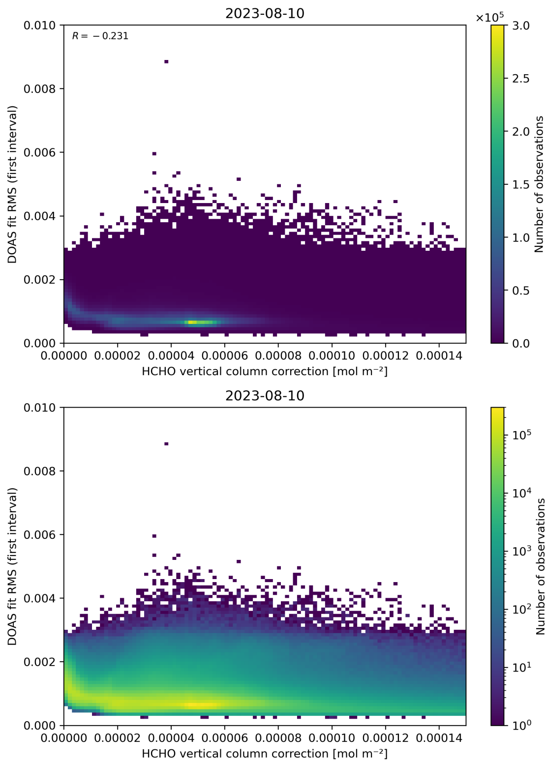
Figure 112: Scatter density plot of “HCHO vertical column correction” against “DOAS fit RMS (first interval)” for 2023-08-09 to 2023-08-11.
