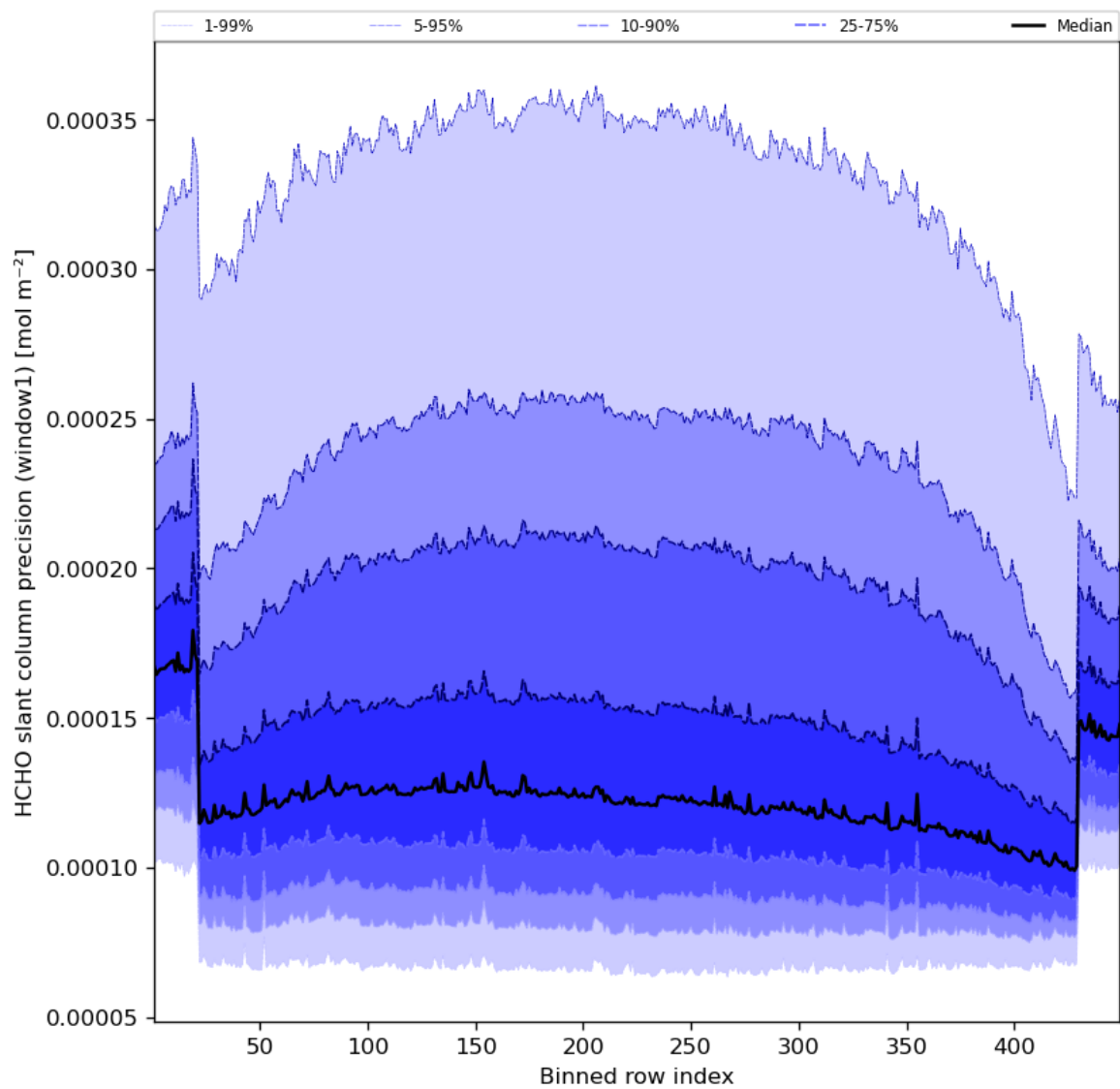
Figure 53: Along track statistics of “HCHO slant column precision (window1)” for 2023-08-09 to 2023-08-11
