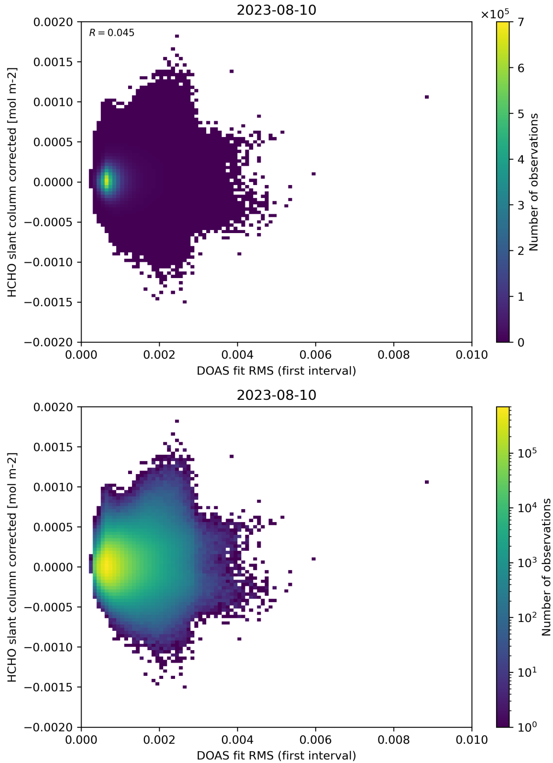
Figure 62: Scatter density plot of “DOAS fit RMS (first interval)” against “HCHO slant column corrected” for 2023-08-09 to 2023-08-11.
