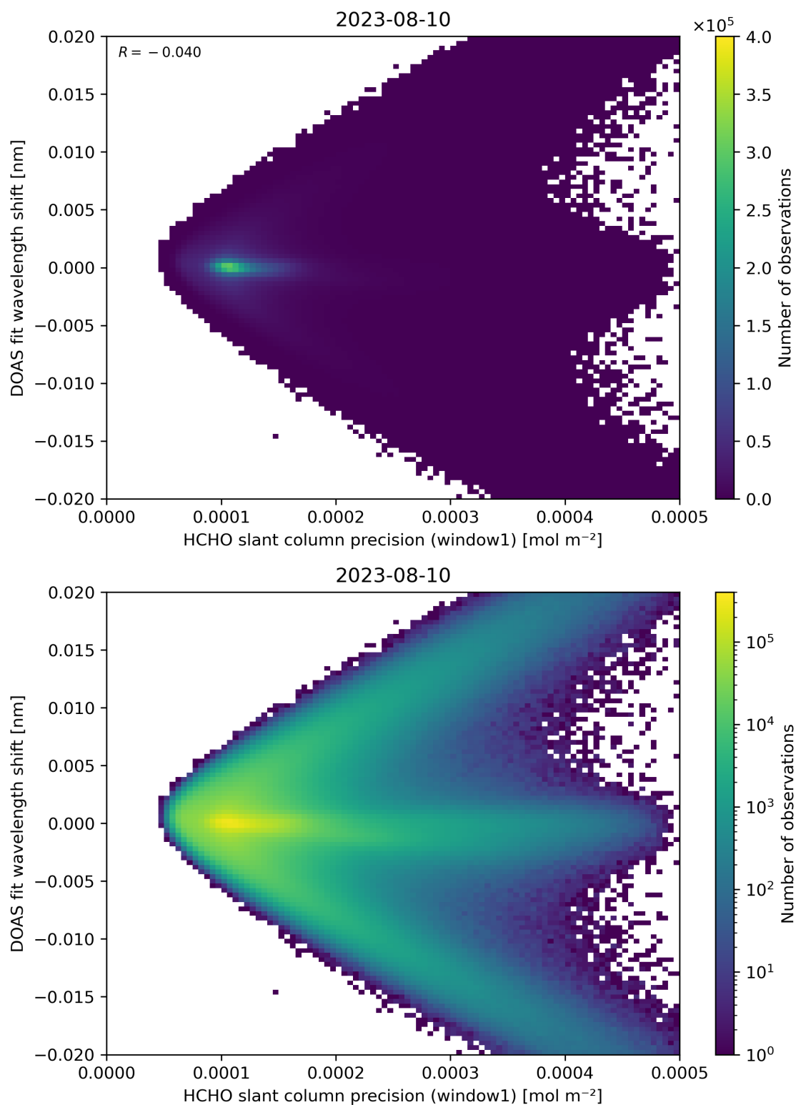
Figure 89: Scatter density plot of “HCHO slant column precision (window1)” against “DOAS fit wavelength shift” for 2023-08-09 to 2023-08-11.
