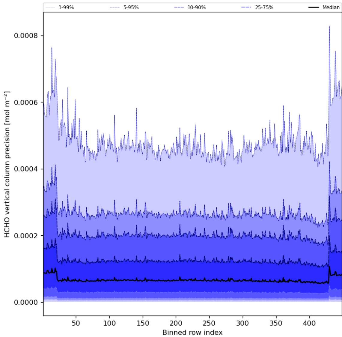
Figure 50: Along track statistics of “HCHO vertical column precision” for 2023-08-09 to 2023-08-11
