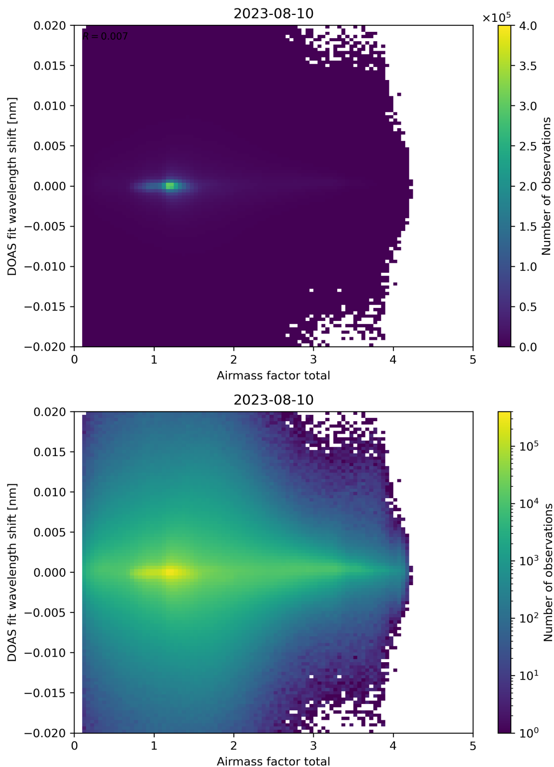
Figure 98: Scatter density plot of “Airmass factor total” against “DOAS fit wavelength shift” for 2023-08-09 to 2023-08-11.
