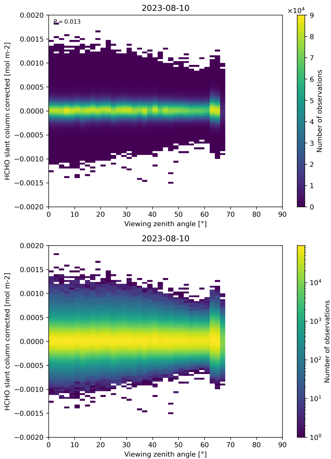
Figure 186: Scatter density plot of “Viewing zenith angle” against “HCHO slant column corrected” for 2023-08-09 to 2023-08-11.
