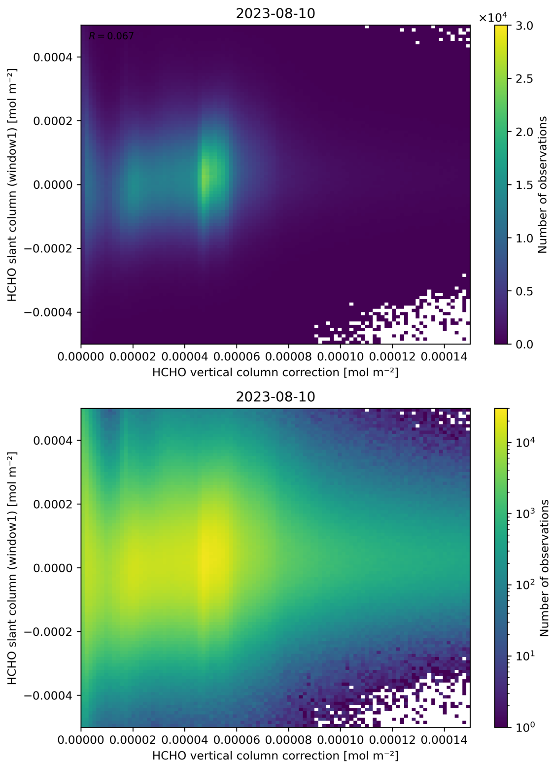
Figure 118: Scatter density plot of “HCHO vertical column correction” against “HCHO slant column (window1)” for 2023-08-09 to 2023-08-11.
