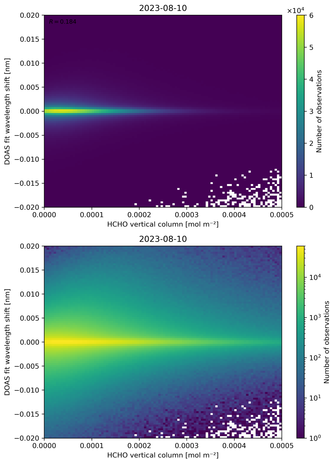
Figure 124: Scatter density plot of “HCHO vertical column” against “DOAS fit wavelength shift” for 2023-08-09 to 2023-08-11.
