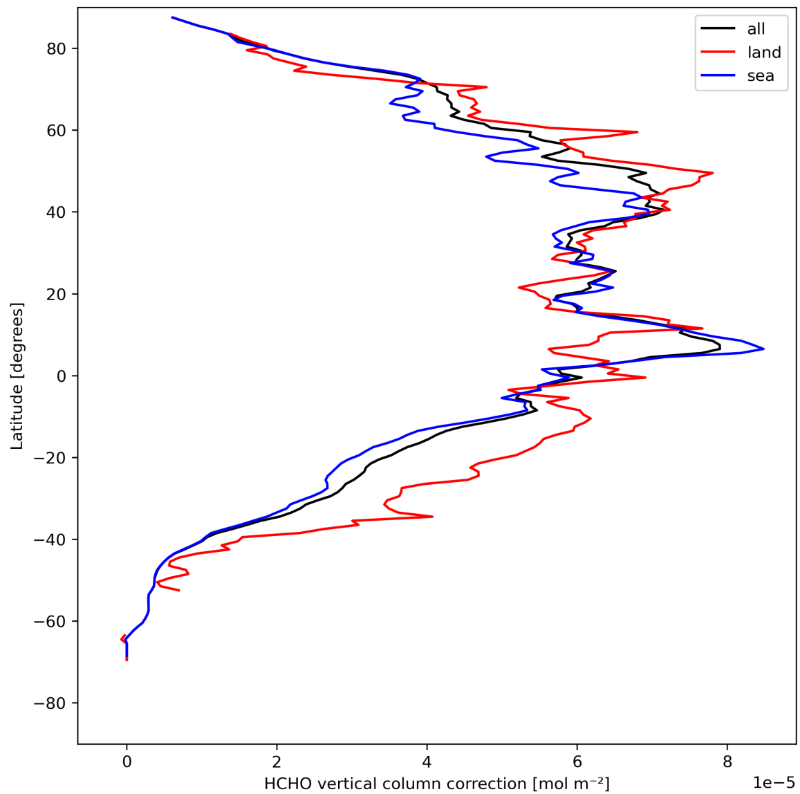
Figure 23: Zonal average of “HCHO vertical column correction” for 2023-08-09 to 2023-08-11.
