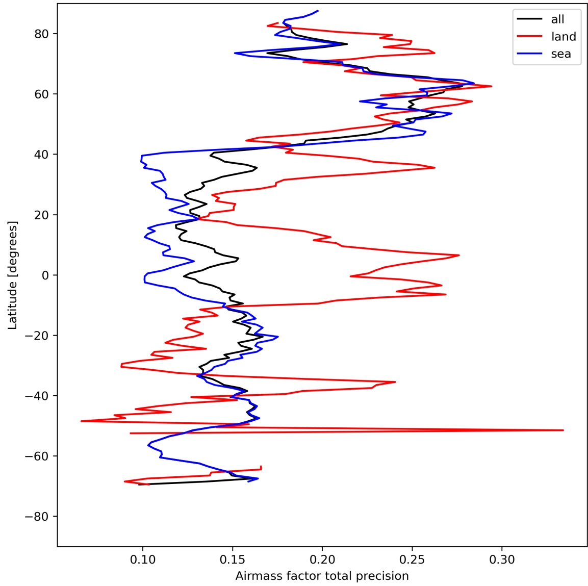
Figure 27: Zonal average of “Airmass factor total precision” for 2023-08-09 to 2023-08-11.
