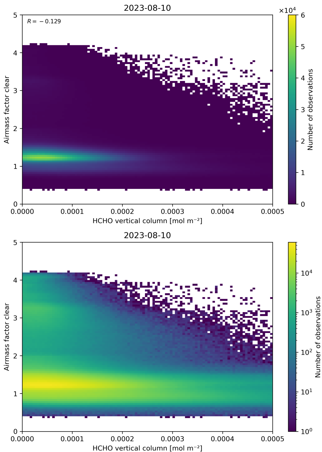
Figure 126: Scatter density plot of “HCHO vertical column” against “Airmass factor clear” for 2023-08-09 to 2023-08-11.
