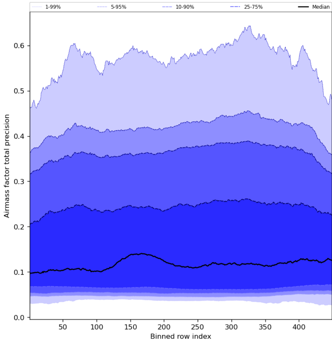
Figure 55: Along track statistics of “Airmass factor total precision” for 2023-08-09 to 2023-08-11
