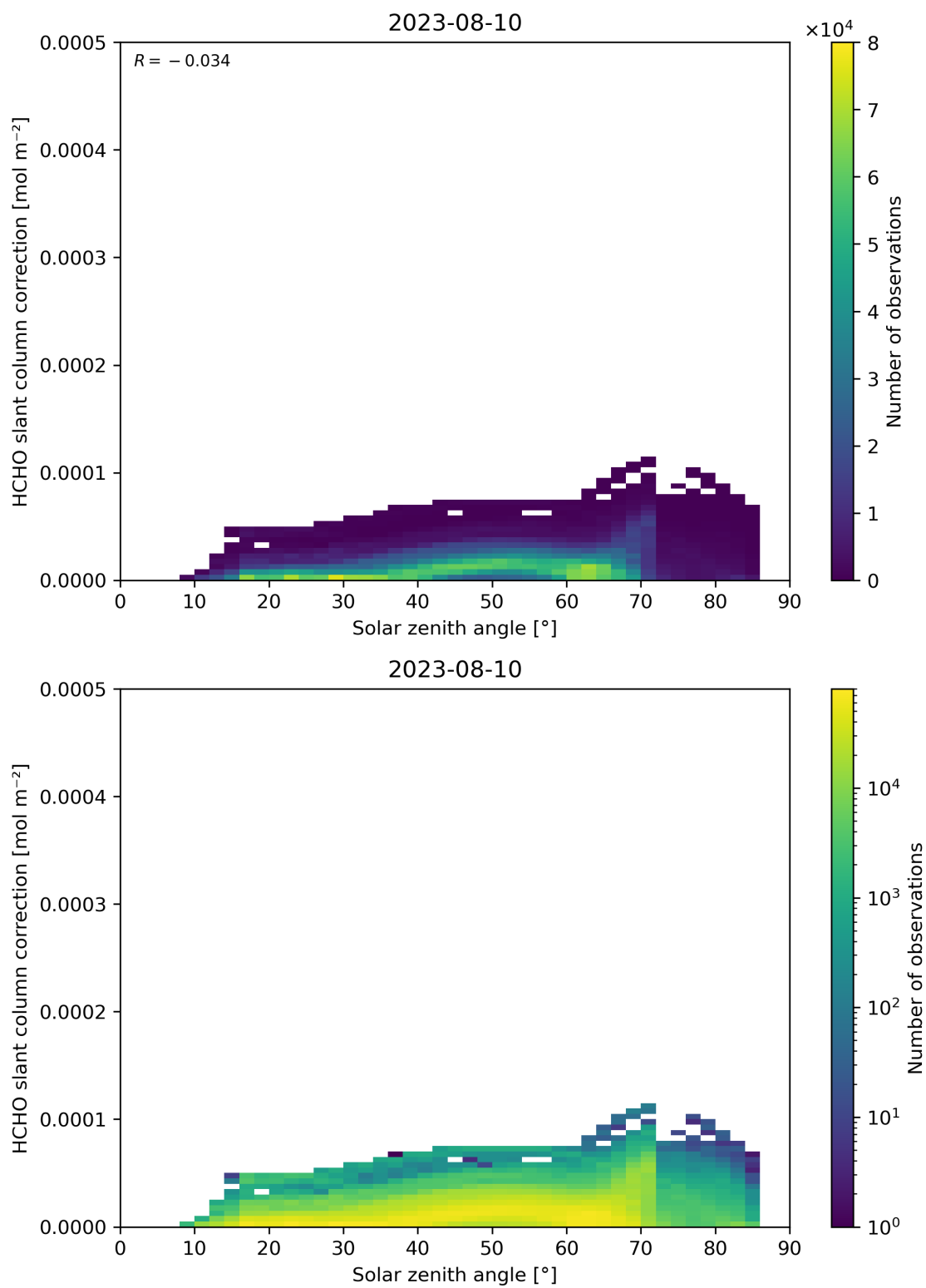
Figure 172: Scatter density plot of “Solar zenith angle” against “HCHO slant column correction” for 2023-08-09 to 2023-08-11.
