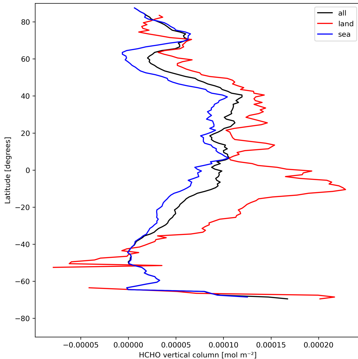
Figure 21: Zonal average of “HCHO vertical column” for 2023-08-09 to 2023-08-11.
