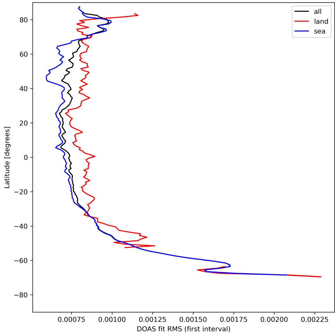
Figure 32: Zonal average of “DOAS fit RMS (first interval)” for 2023-08-09 to 2023-08-11.
