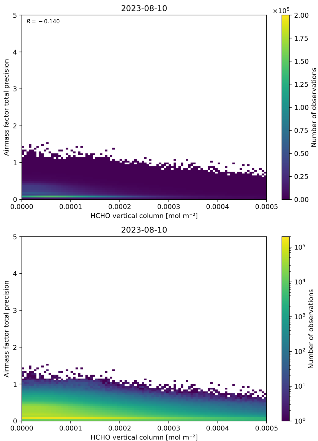
Figure 132: Scatter density plot of “HCHO vertical column” against “Airmass factor total precision” for 2023-08-09 to 2023-08-11.
