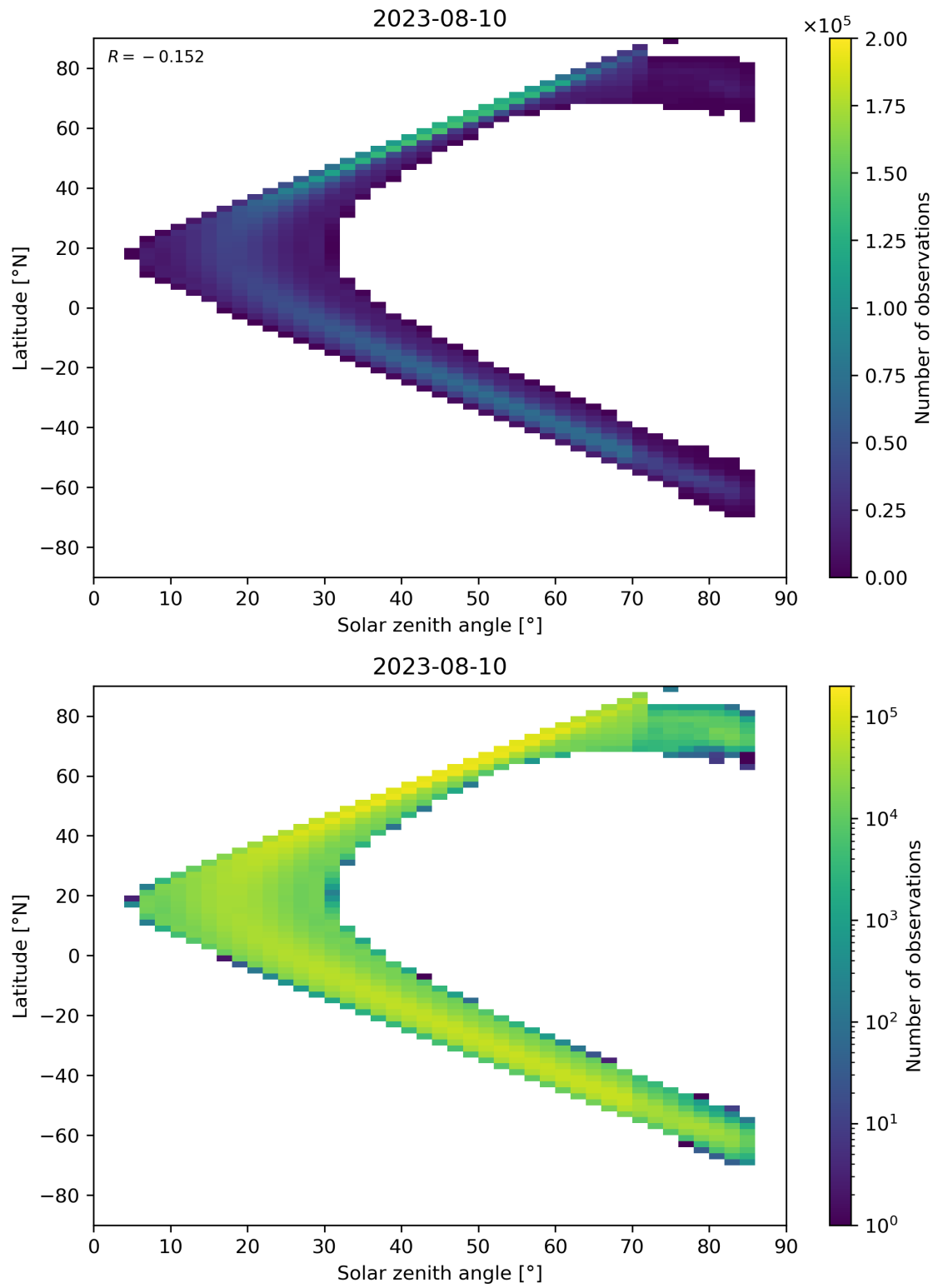
Figure 181: Scatter density plot of “Solar zenith angle” against “Latitude” for 2023-08-09 to 2023-08-11.
