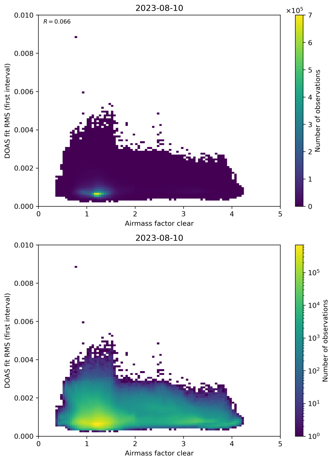
Figure 71: Scatter density plot of “Airmass factor clear” against “DOAS fit RMS (first interval)” for 2023-08-09 to 2023-08-11.
