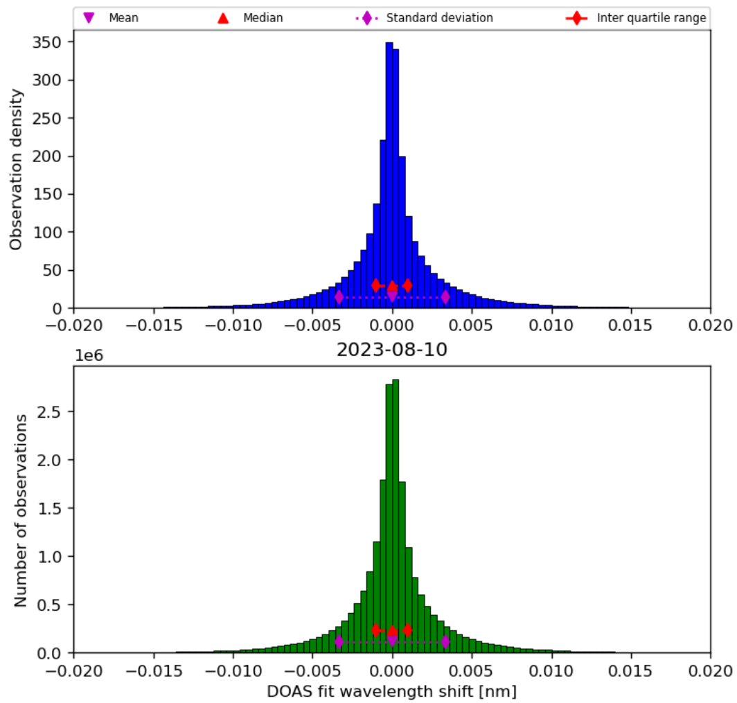
Figure 44: Histogram of “DOAS fit wavelength shift” for 2023-08-09 to 2023-08-11
