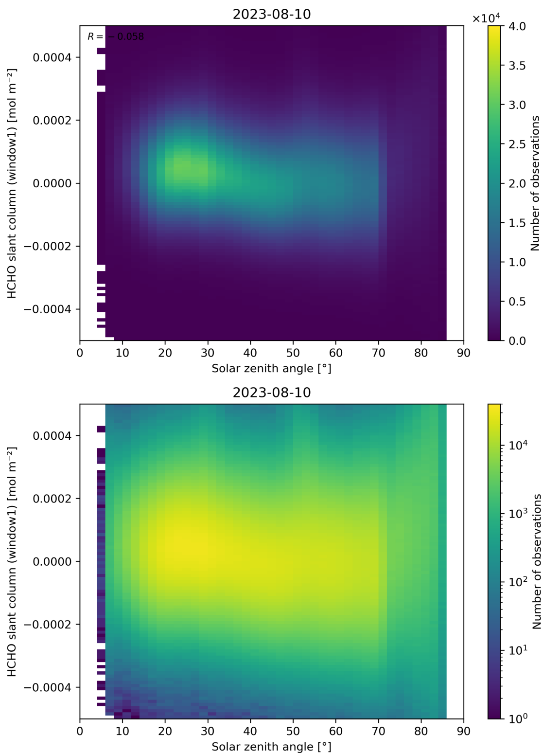
Figure 173: Scatter density plot of “Solar zenith angle” against “HCHO slant column (window1)” for 2023-08-09 to 2023-08-11.
