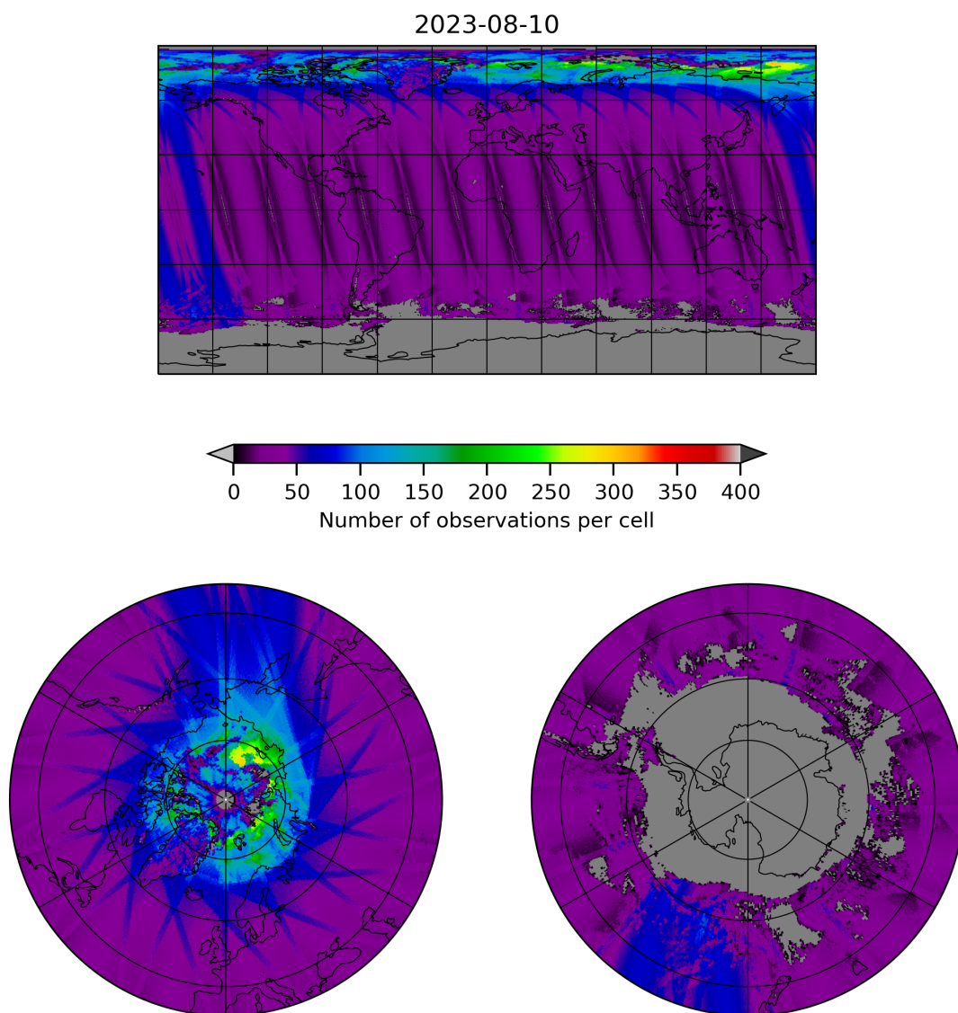
Figure 19: Map of the number of observations for 2023-08-09 to 2023-08-11
