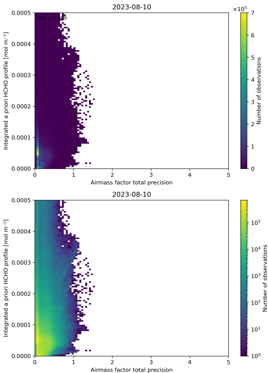
Figure 111: Scatter density plot of “Airmass factor total precision” against “Integrated a priori HCHO profile” for 2023-08-09 to 2023-08-11.
