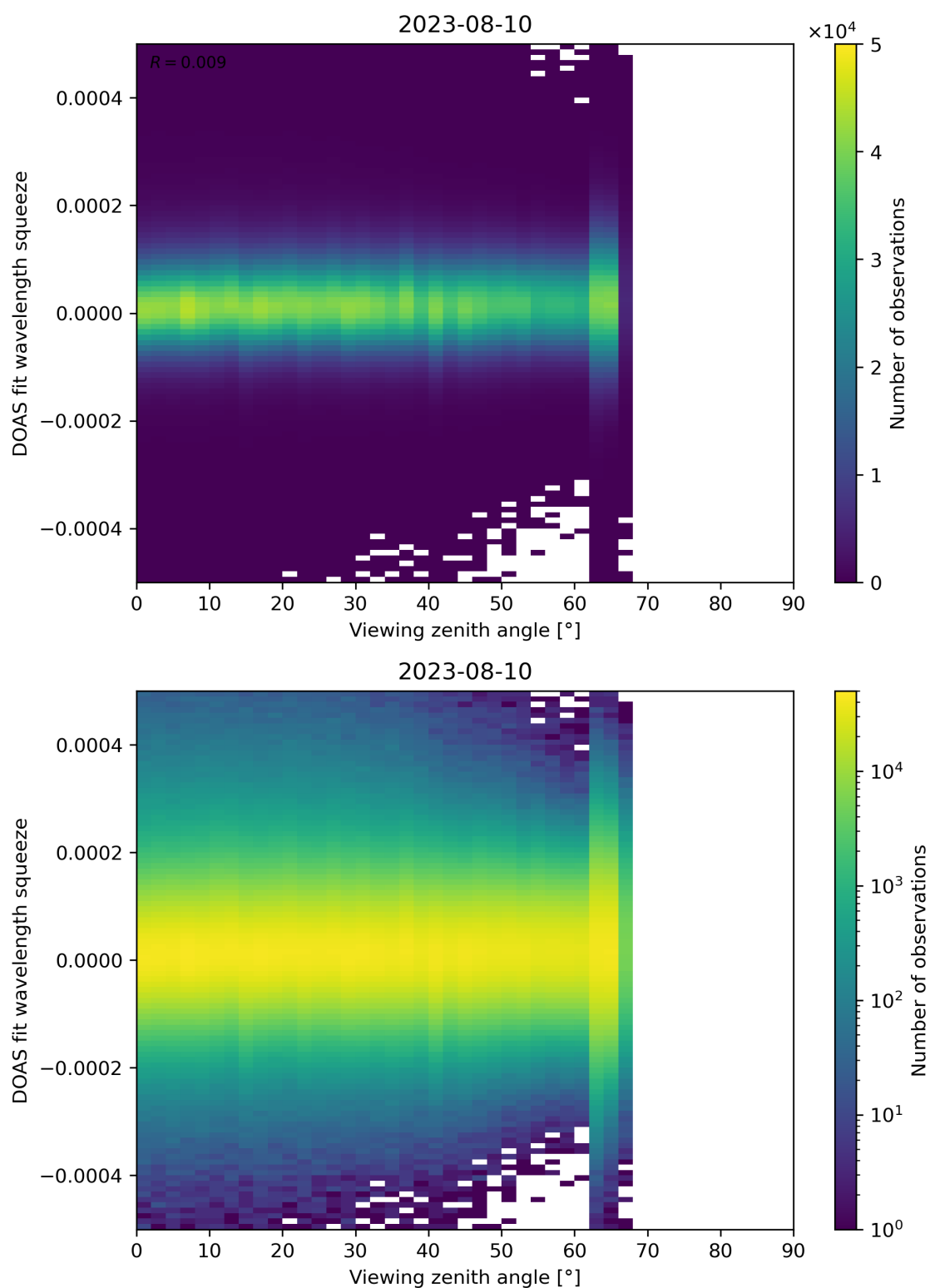
Figure 184: Scatter density plot of “Viewing zenith angle” against “DOAS fit wavelength squeeze” for 2023-08-09 to 2023-08-11.
