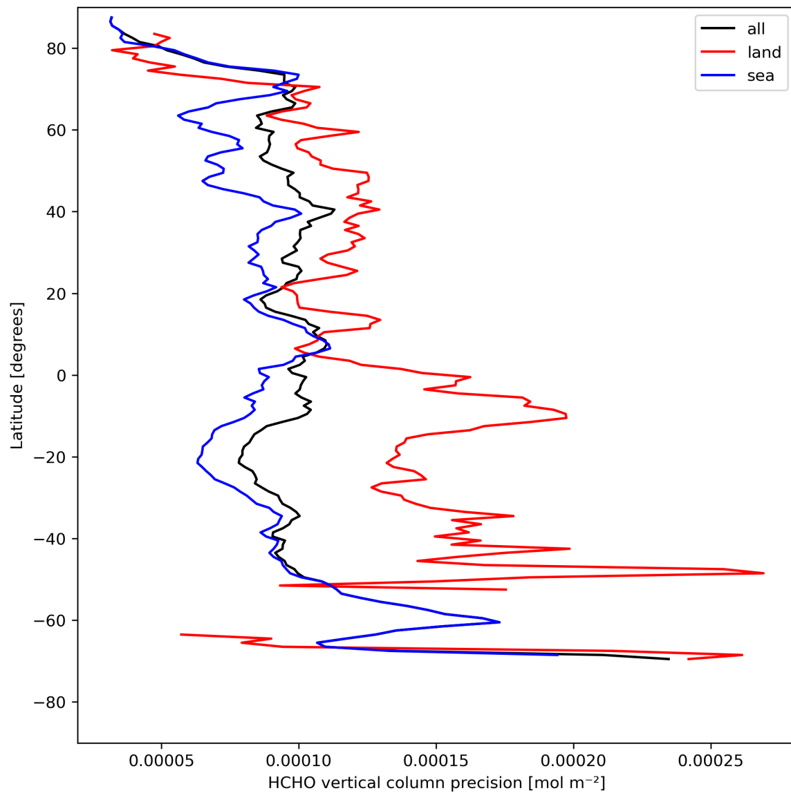
Figure 22: Zonal average of “HCHO vertical column precision” for 2023-08-09 to 2023-08-11.
