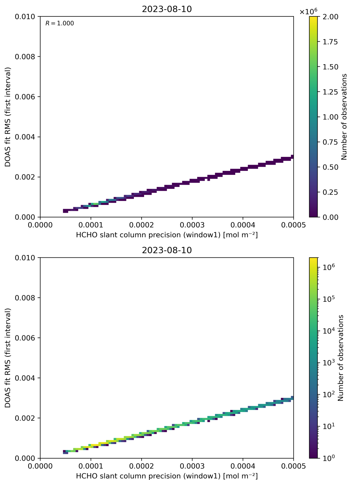
Figure 88: Scatter density plot of “HCHO slant column precision (window1)” against “DOAS fit RMS (first interval)” for 2023-08-09 to 2023-08-11.
