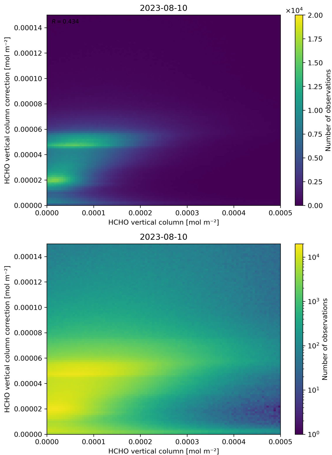
Figure 133: Scatter density plot of “HCHO vertical column” against “HCHO vertical column correction” for 2023-08-09 to 2023-08-11.
