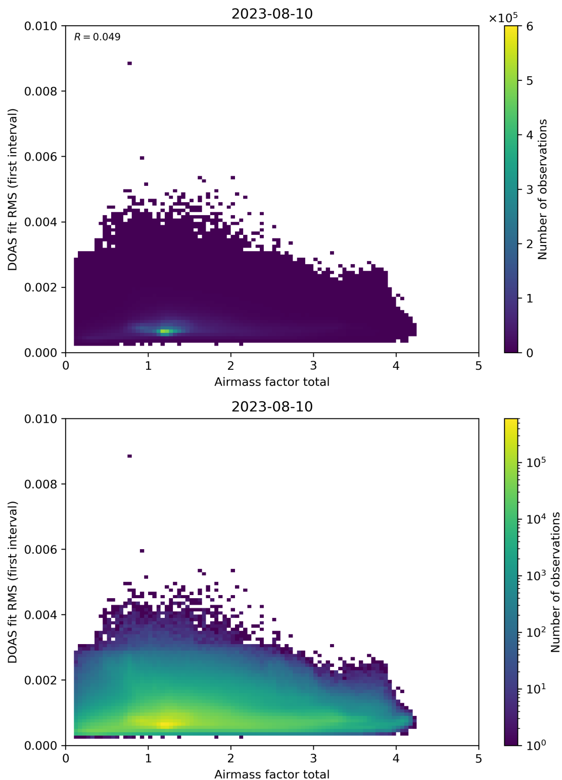
Figure 97: Scatter density plot of “Airmass factor total” against “DOAS fit RMS (first interval)” for 2023-08-09 to 2023-08-11.
