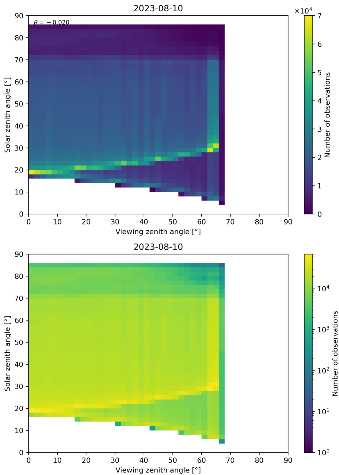
Figure 197: Scatter density plot of “Viewing zenith angle” against “Solar zenith angle” for 2023-08-09 to 2023-08-11.
