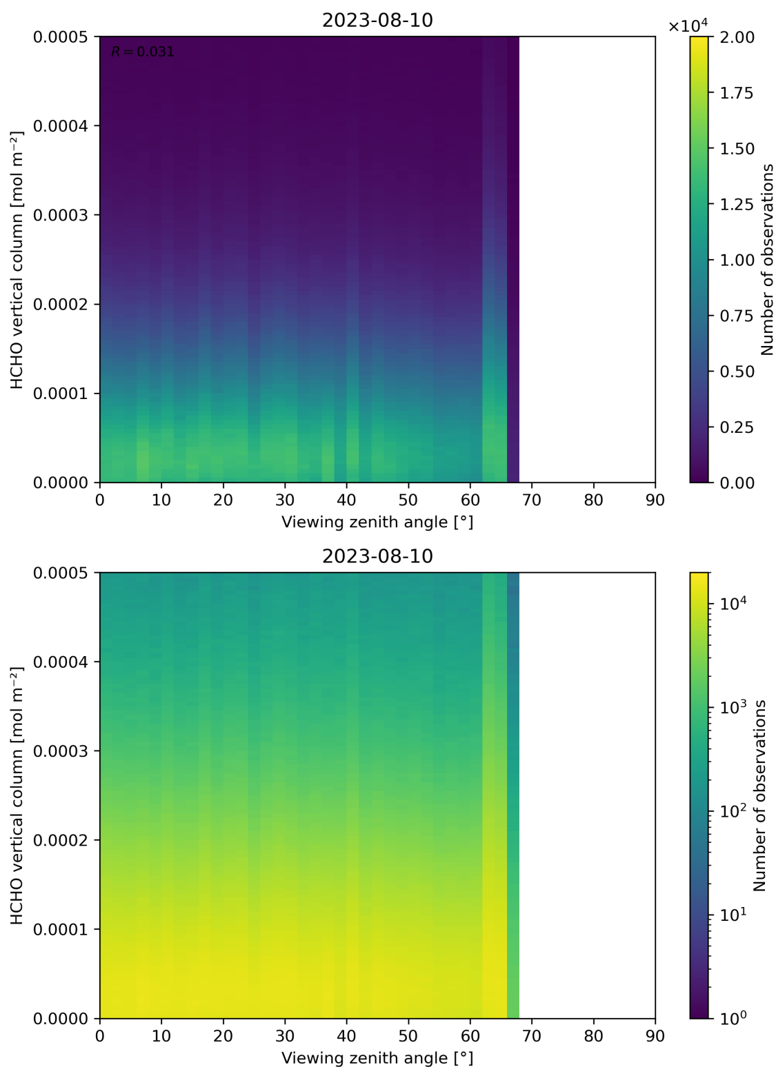
Figure 192: Scatter density plot of “Viewing zenith angle” against “HCHO vertical column” for 2023-08-09 to 2023-08-11.
