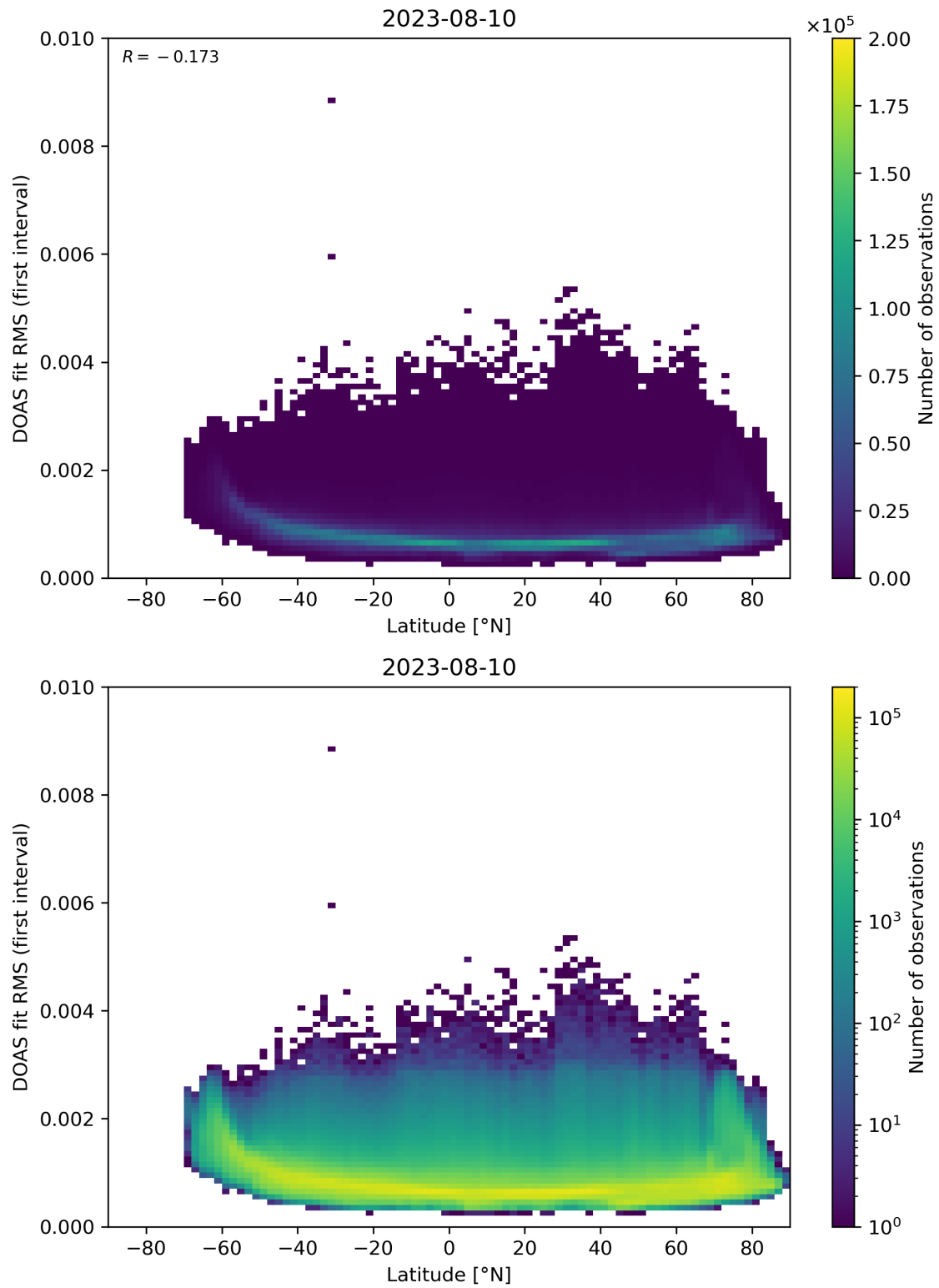
Figure 153: Scatter density plot of “Latitude” against “DOAS fit RMS (first interval)” for 2023-08-09 to 2023-08-11.
