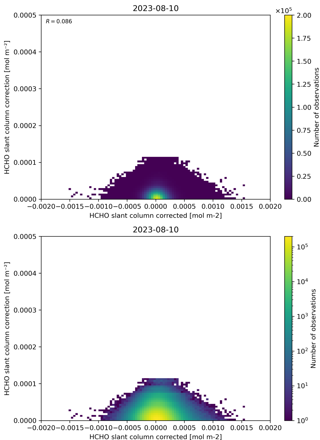
Figure 77: Scatter density plot of “HCHO slant column corrected” against “HCHO slant column correction” for 2023-08-09 to 2023-08-11.
