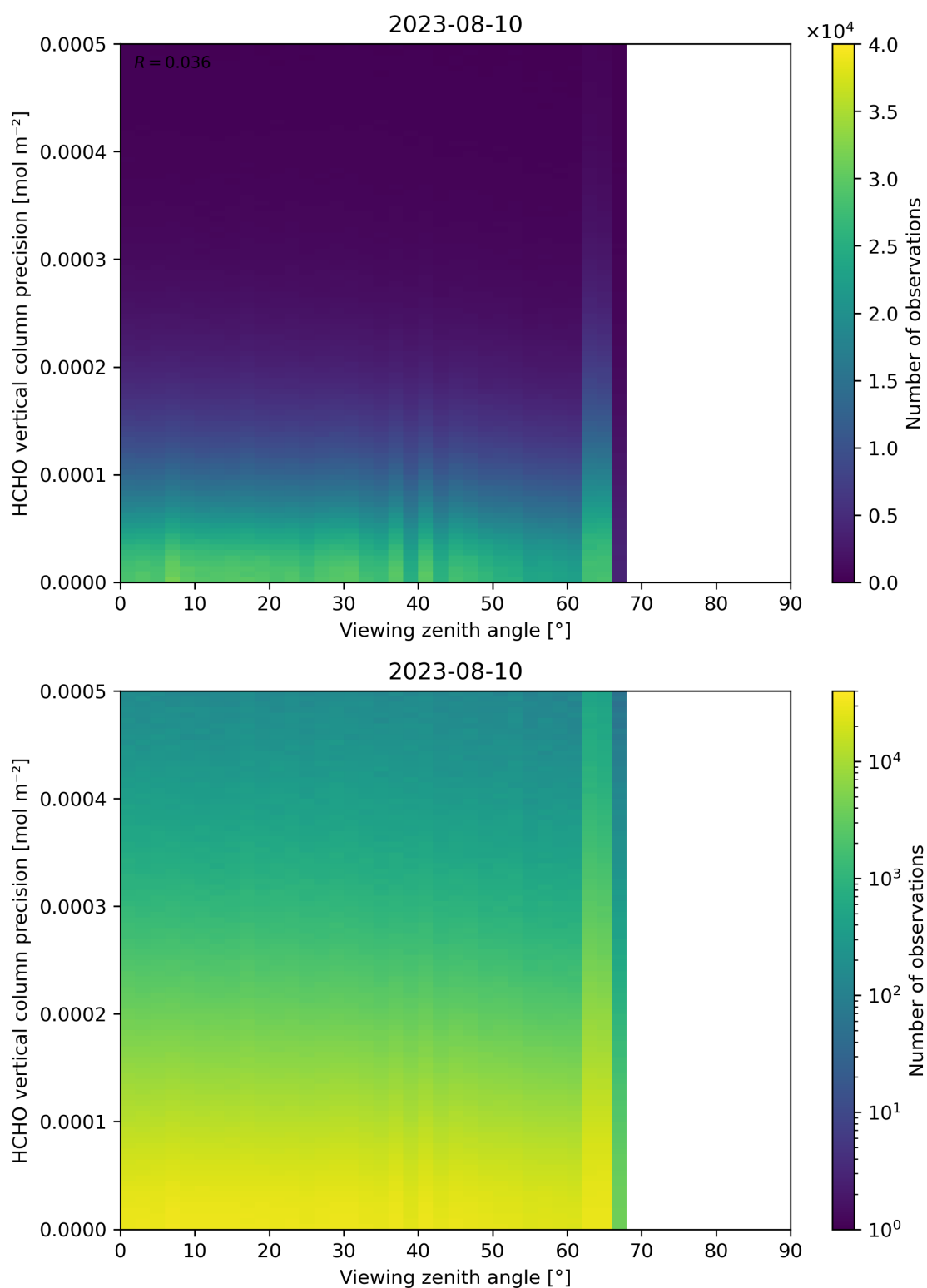
Figure 194: Scatter density plot of “Viewing zenith angle” against “HCHO vertical column precision” for 2023-08-09 to 2023-08-11.
