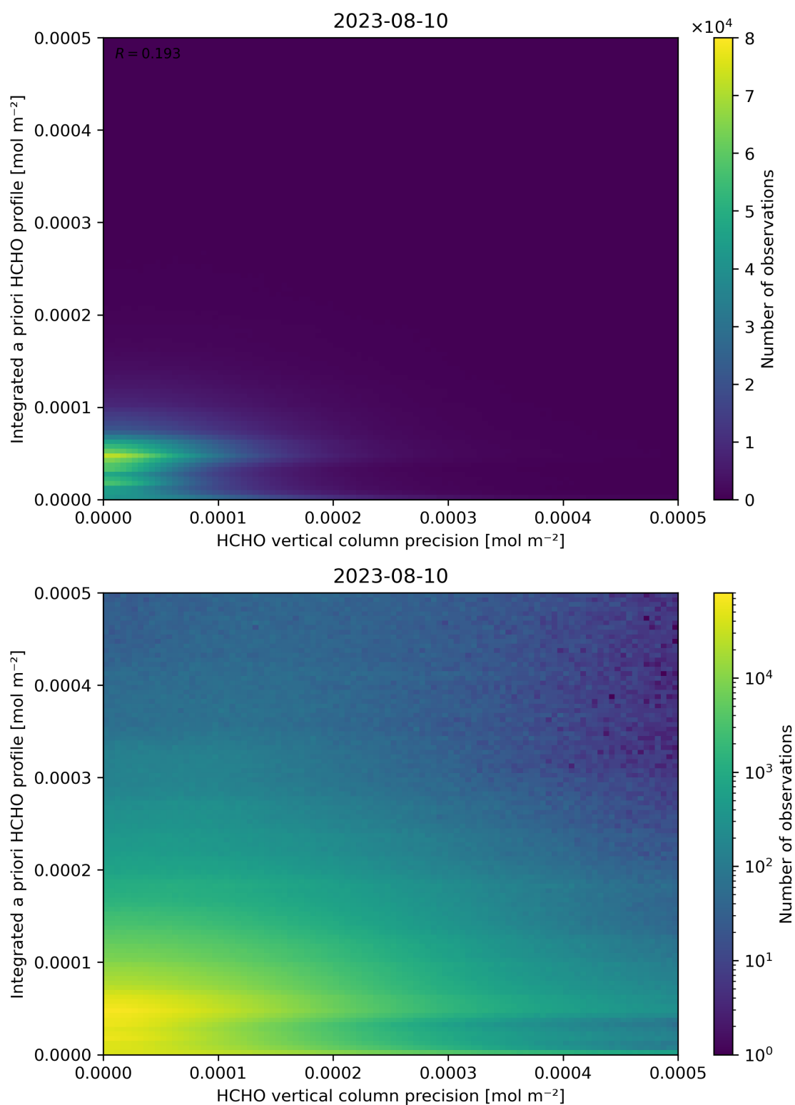
Figure 147: Scatter density plot of “HCHO vertical column precision” against “Integrated a priori HCHO profile” for 2023-08-09 to 2023-08-11.
