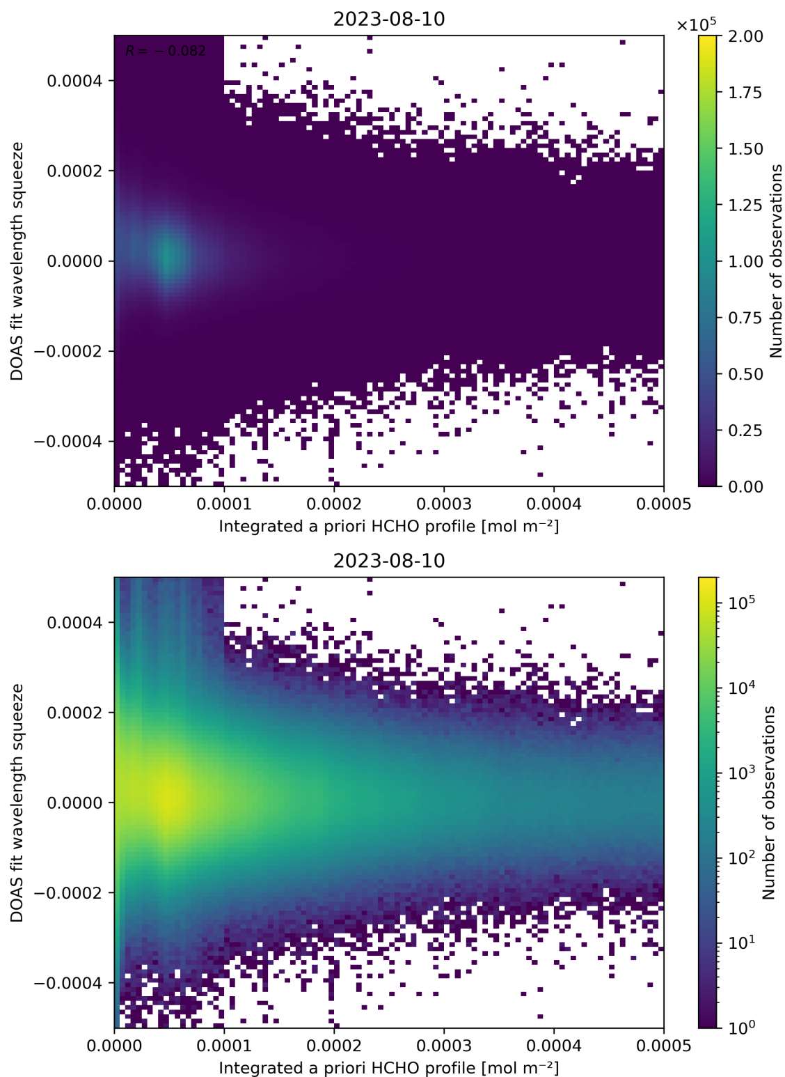
Figure 150: Scatter density plot of “Integrated a priori HCHO profile” against “DOAS fit wavelength squeeze” for 2023-08-09 to 2023-08-11.
