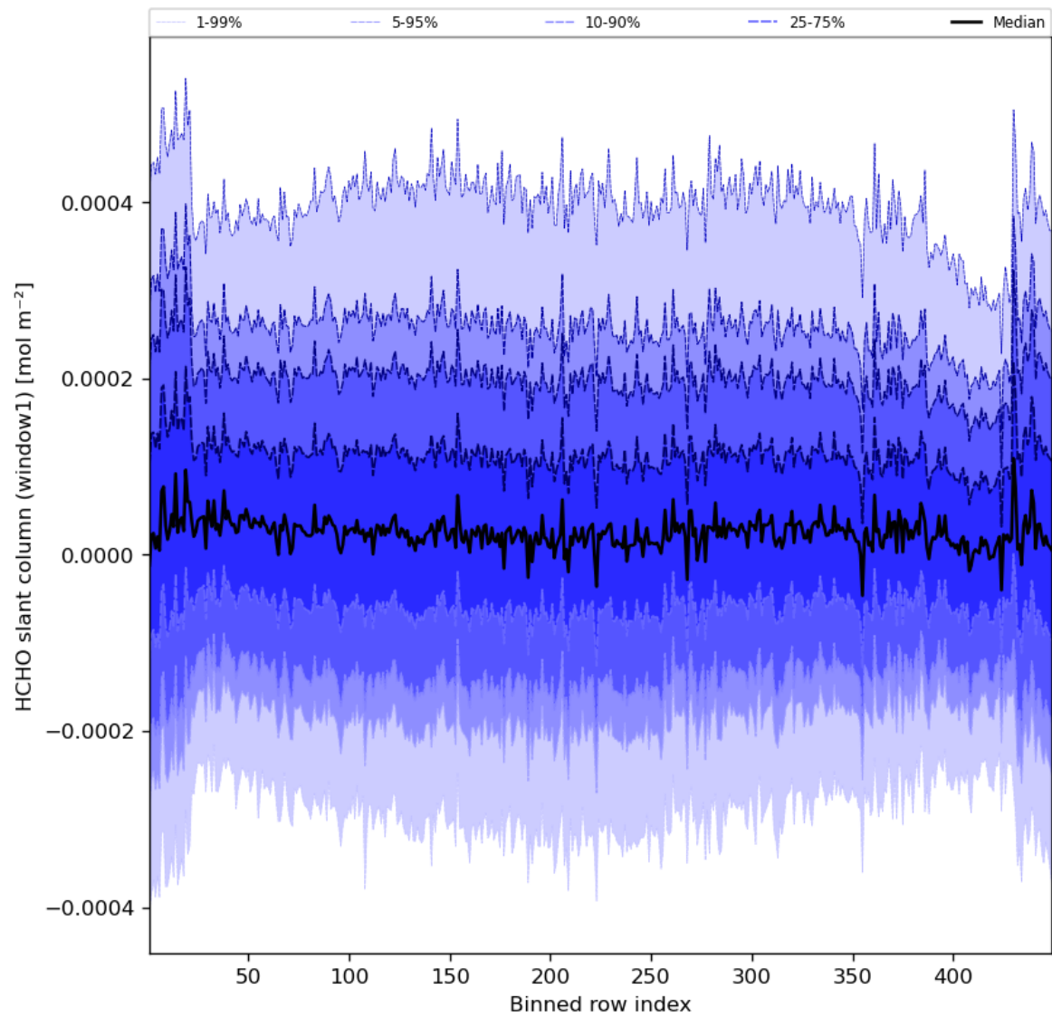
Figure 52: Along track statistics of “HCHO slant column (window1)” for 2023-08-09 to 2023-08-11
