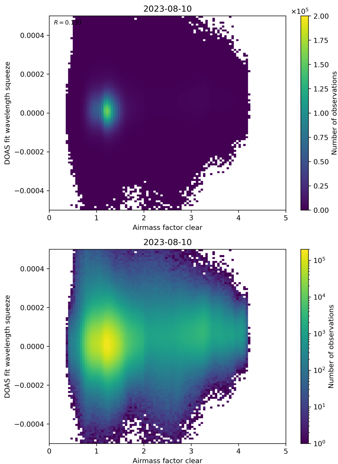
Figure 73: Scatter density plot of “Airmass factor clear” against “DOAS fit wavelength squeeze” for 2023-08-09 to 2023-08-11.
