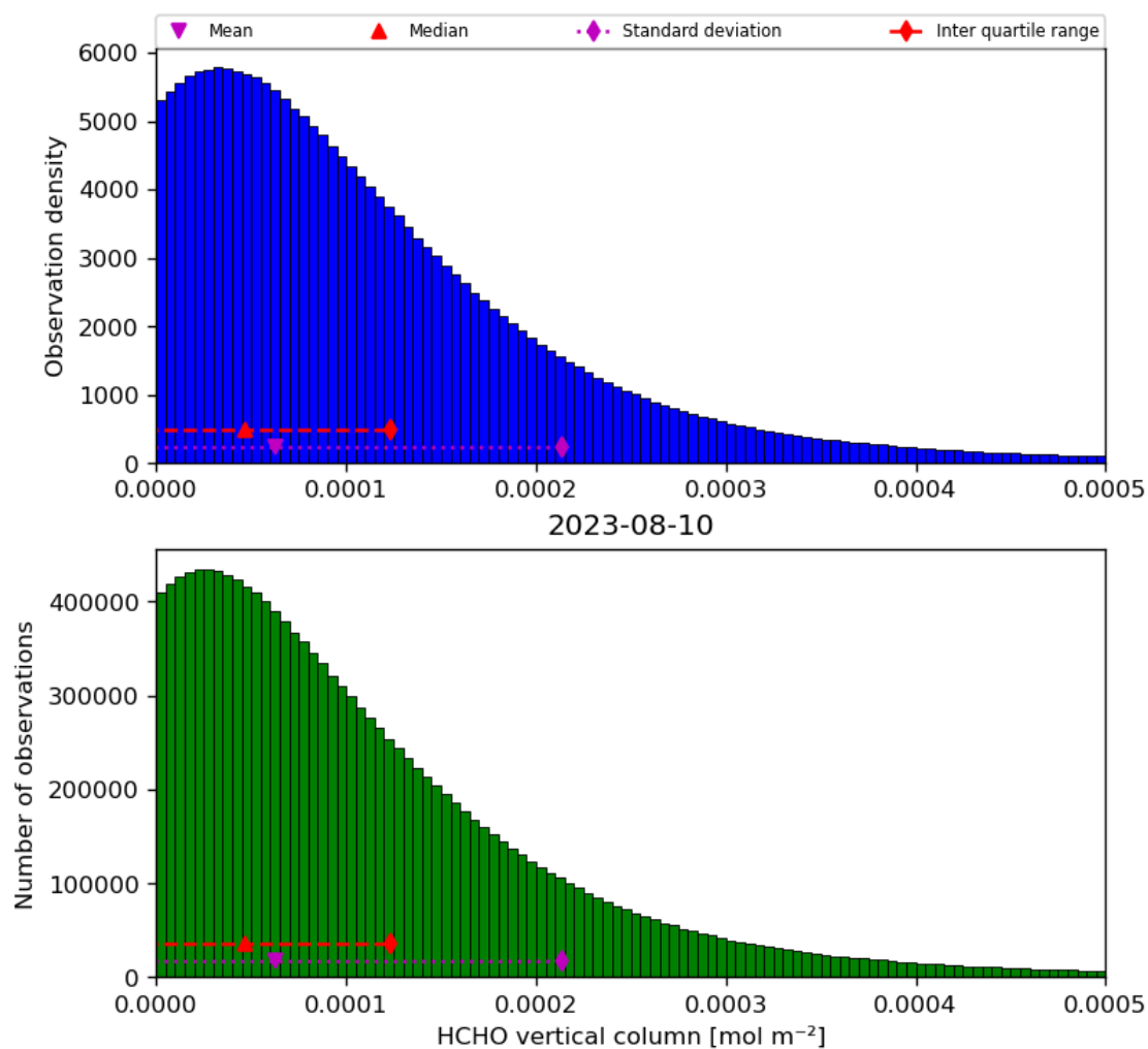
Figure 35: Histogram of “HCHO vertical column” for 2023-08-09 to 2023-08-11
