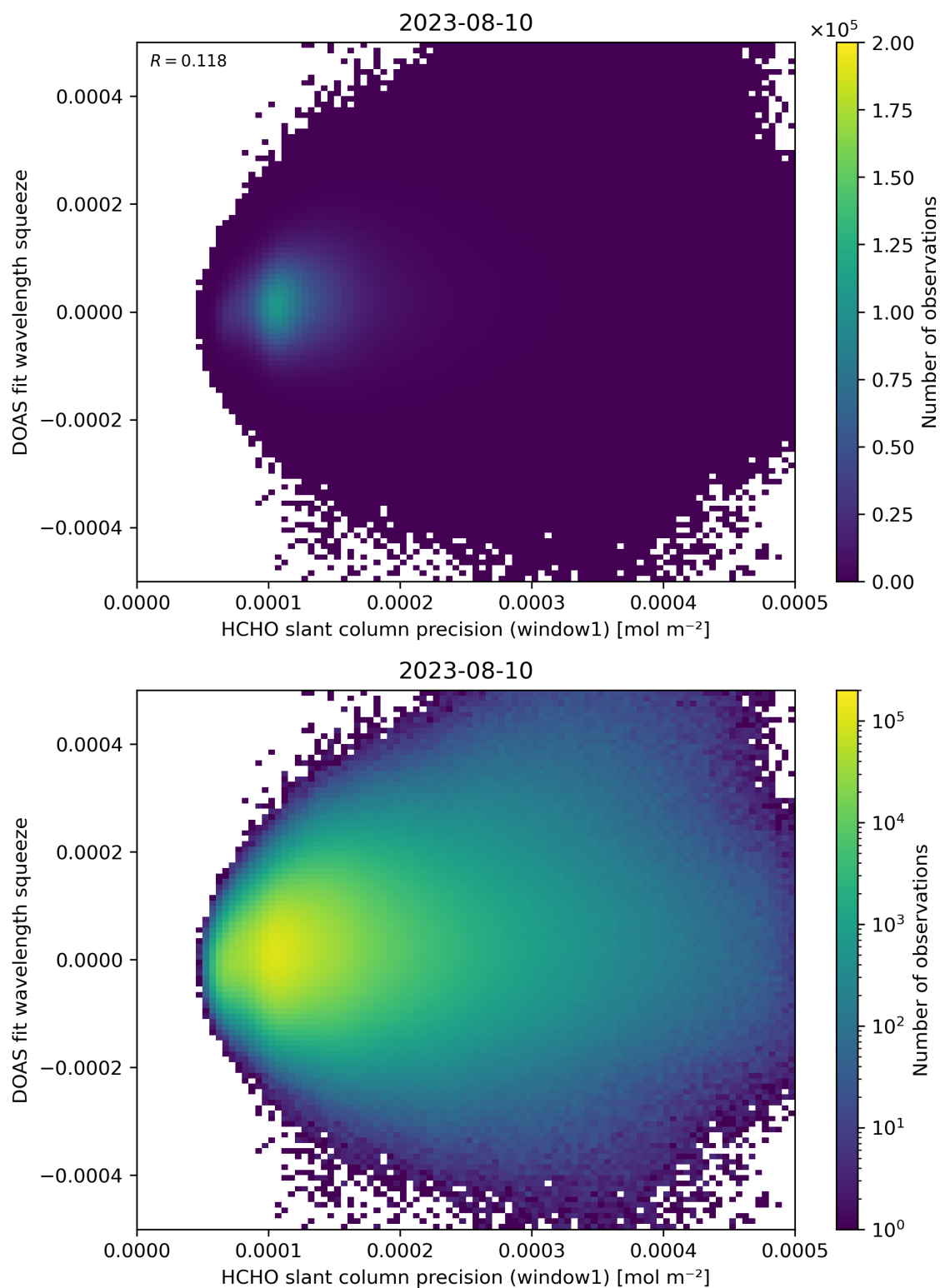
Figure 90: Scatter density plot of “HCHO slant column precision (window1)” against “DOAS fit wavelength squeeze” for 2023-08-09 to 2023-08-11.
