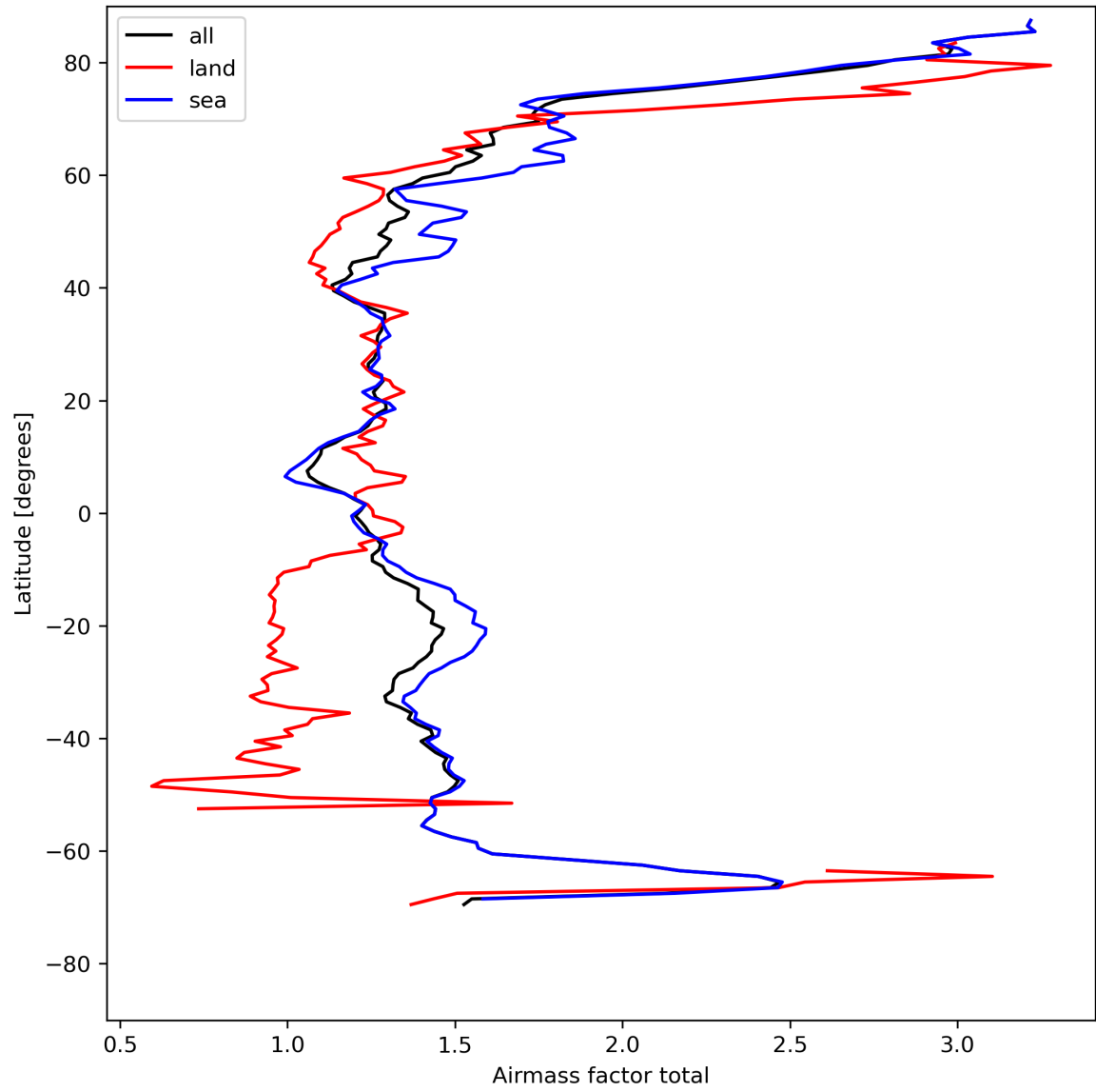
Figure 26: Zonal average of “Airmass factor total” for 2023-08-09 to 2023-08-11.
