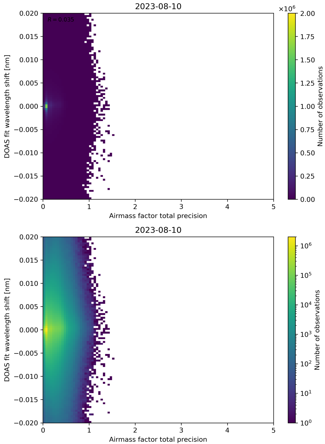
Figure 106: Scatter density plot of “Airmass factor total precision” against “DOAS fit wavelength shift” for 2023-08-09 to 2023-08-11.
