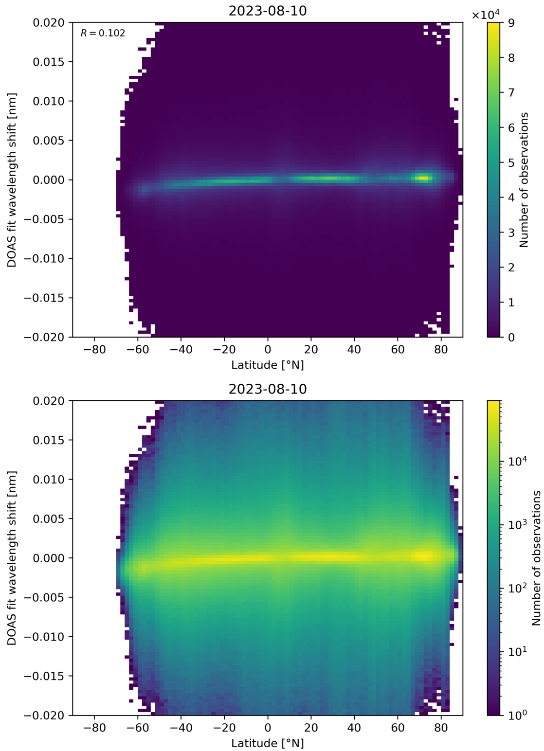
Figure 154: Scatter density plot of “Latitude” against “DOAS fit wavelength shift” for 2023-08-09 to 2023-08-11.
