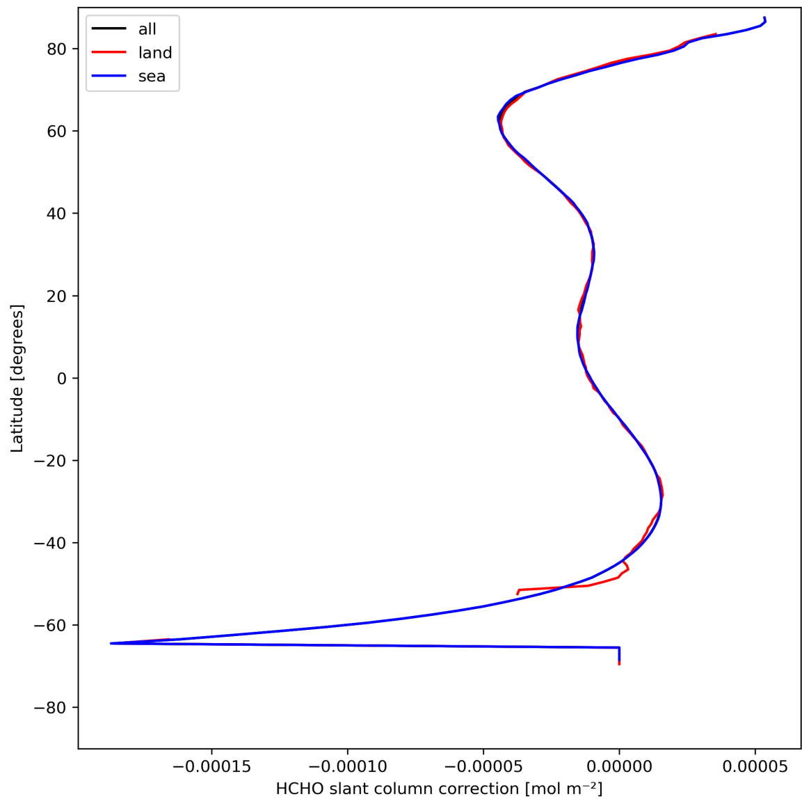
Figure 33: Zonal average of “HCHO slant column correction” for 2023-08-09 to 2023-08-11.
