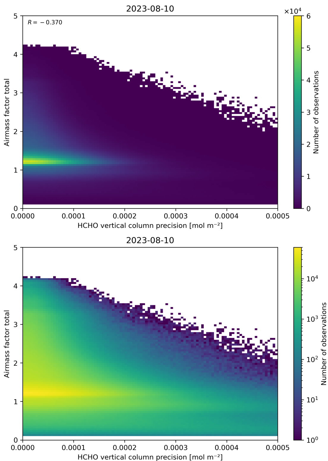
Figure 144: Scatter density plot of “HCHO vertical column precision” against “Airmass factor total” for 2023-08-09 to 2023-08-11.
