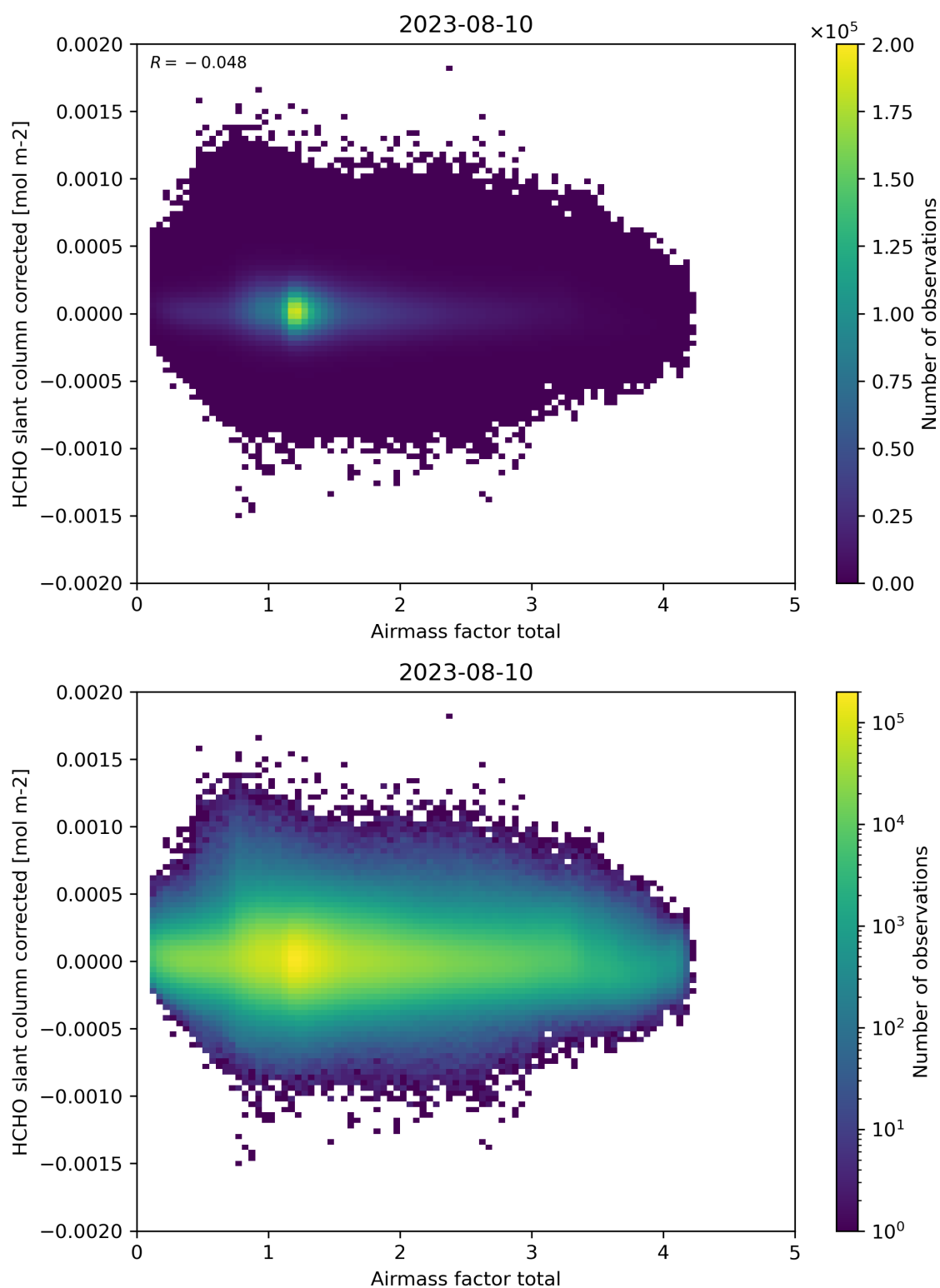
Figure 101: Scatter density plot of “Airmass factor total” against “HCHO slant column corrected” for 2023-08-09 to 2023-08-11.
