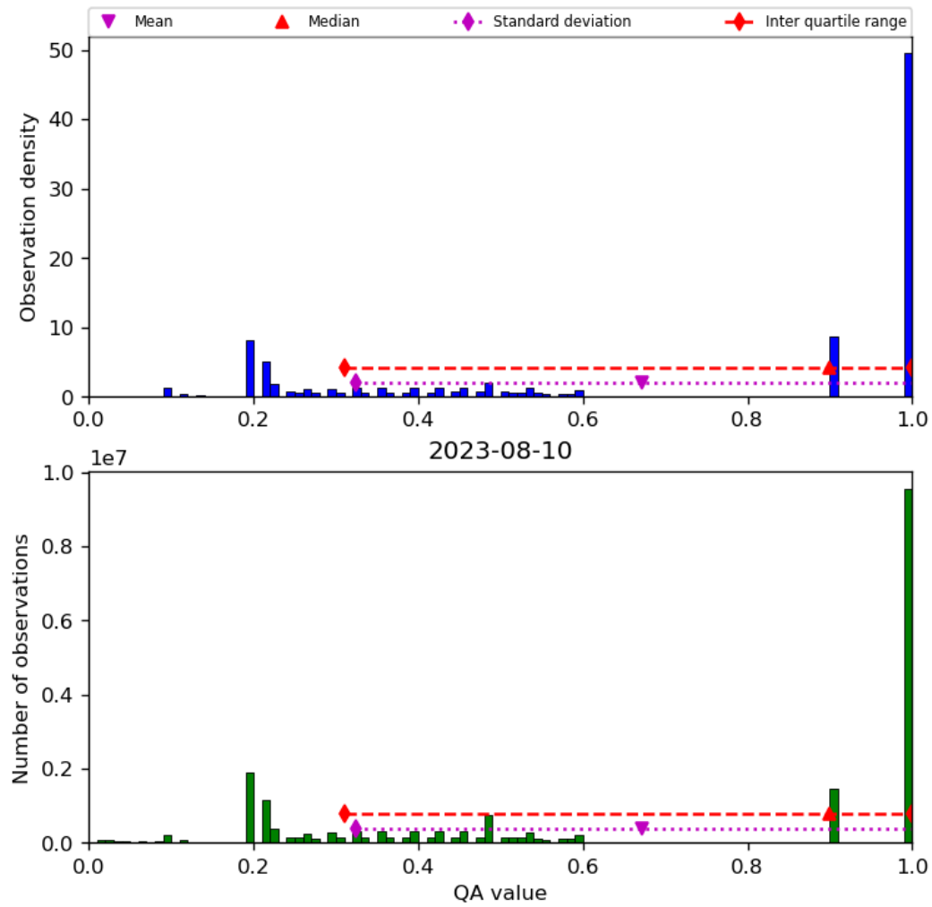
Figure 34: Histogram of “QA value” for 2023-08-09 to 2023-08-11
