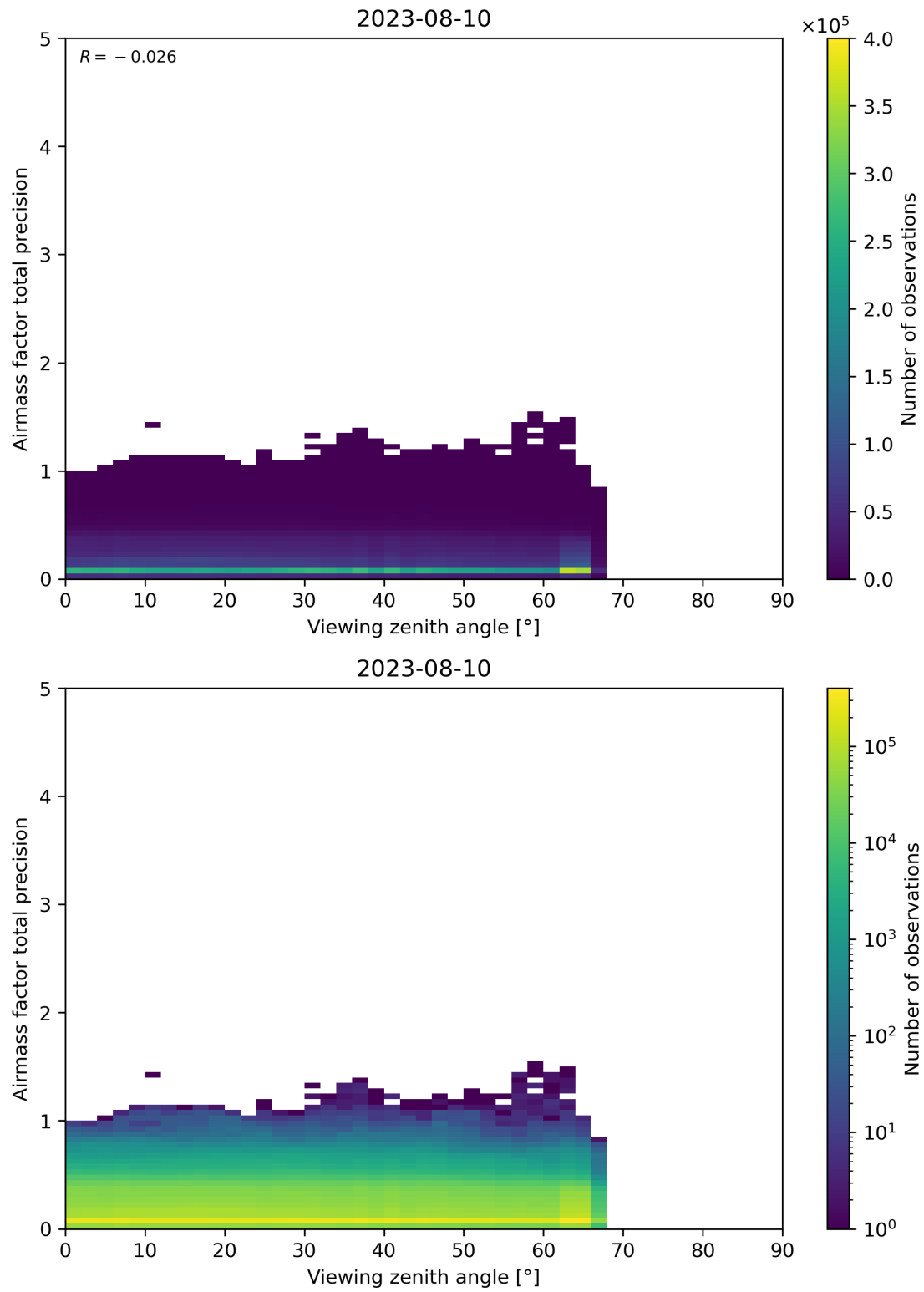
Figure 191: Scatter density plot of “Viewing zenith angle” against “Airmass factor total precision” for 2023-08-09 to 2023-08-11.
