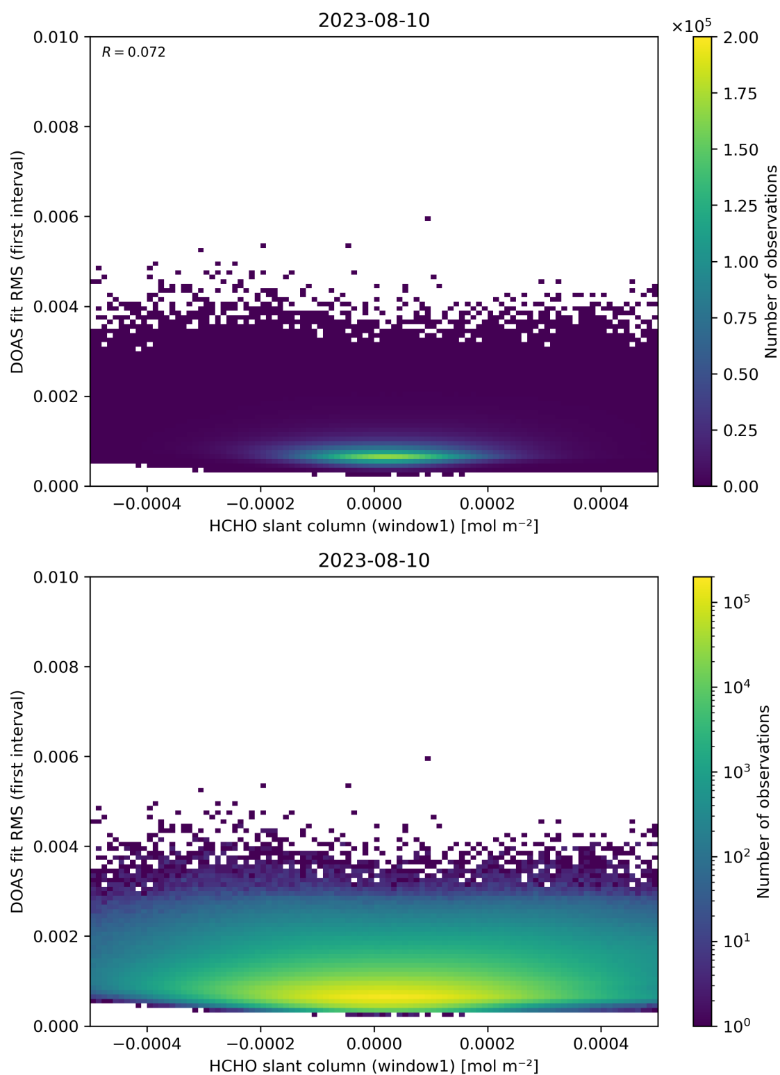
Figure 78: Scatter density plot of “HCHO slant column (window1)” against “DOAS fit RMS (first interval)” for 2023-08-09 to 2023-08-11.
