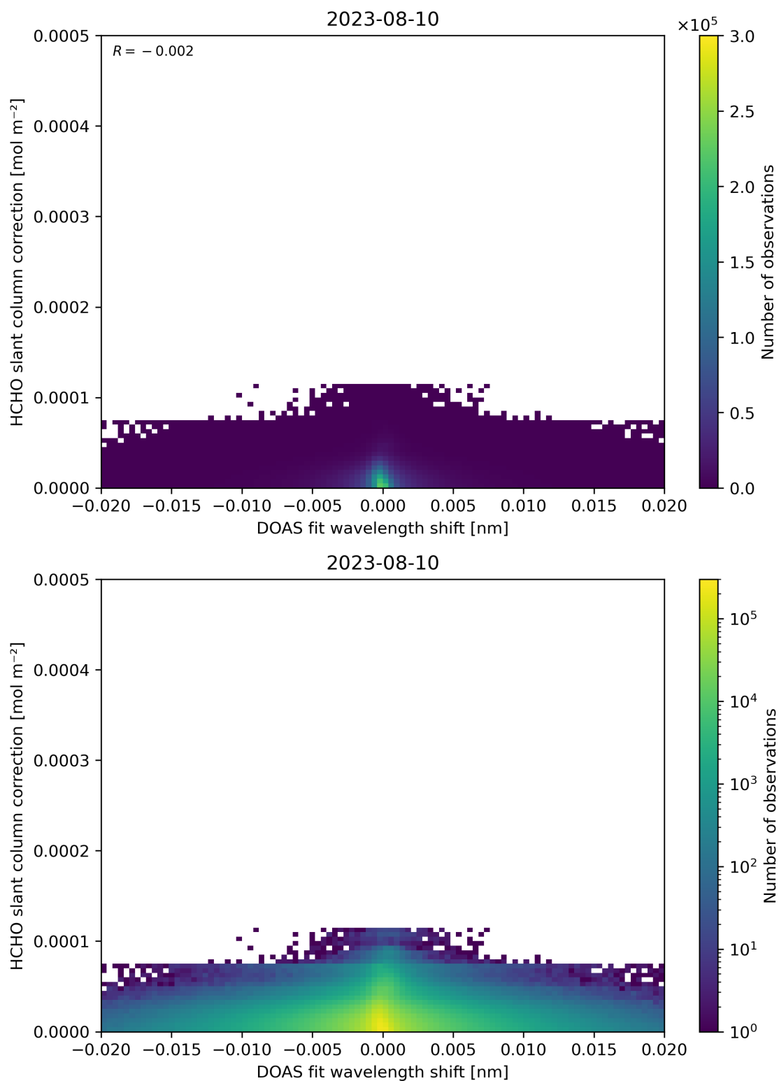
Figure 67: Scatter density plot of “DOAS fit wavelength shift” against “HCHO slant column correction” for 2023-08-09 to 2023-08-11.
