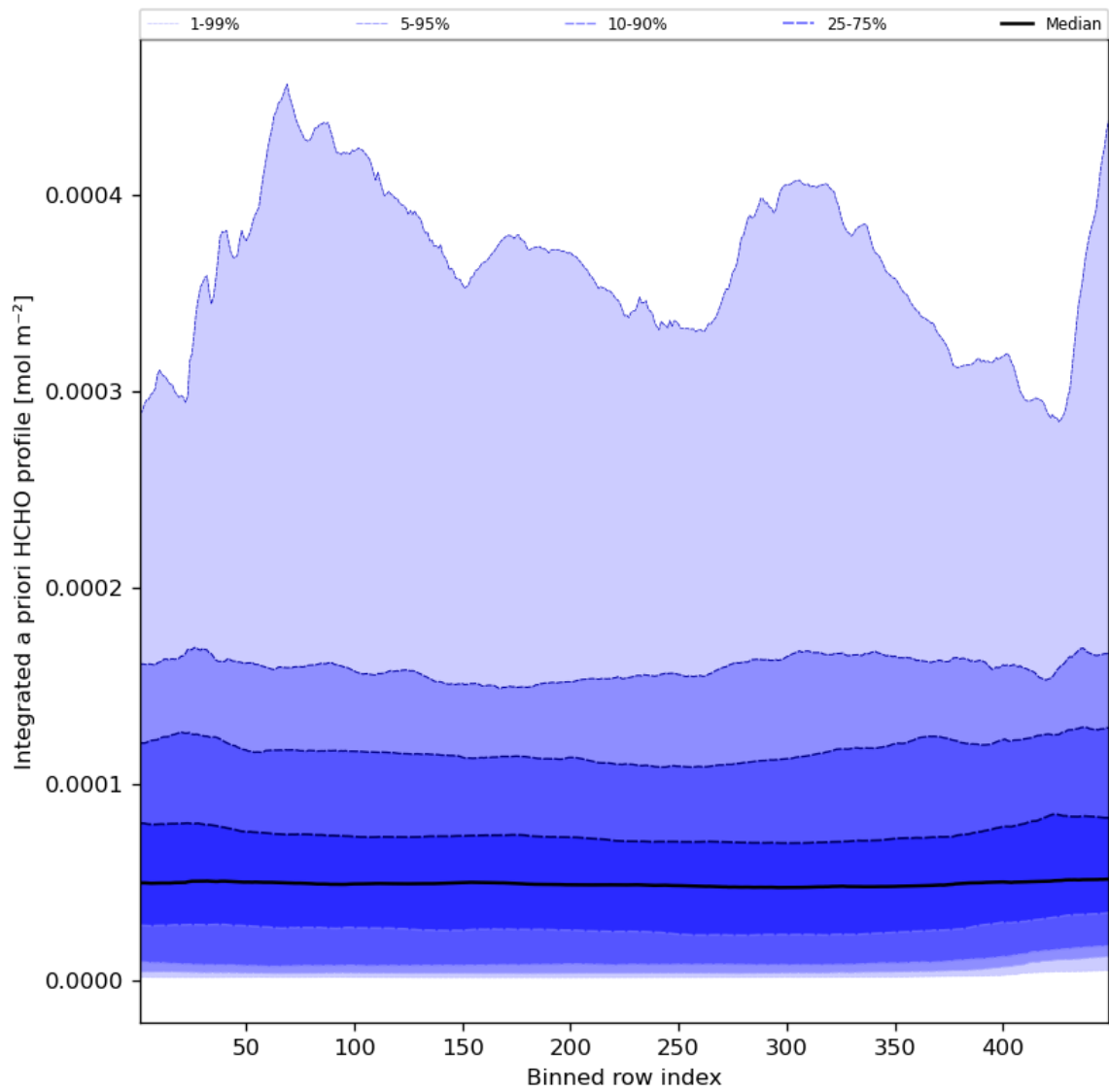
Figure 57: Along track statistics of “Integrated a priori HCHO profile” for 2023-08-09 to 2023-08-11
