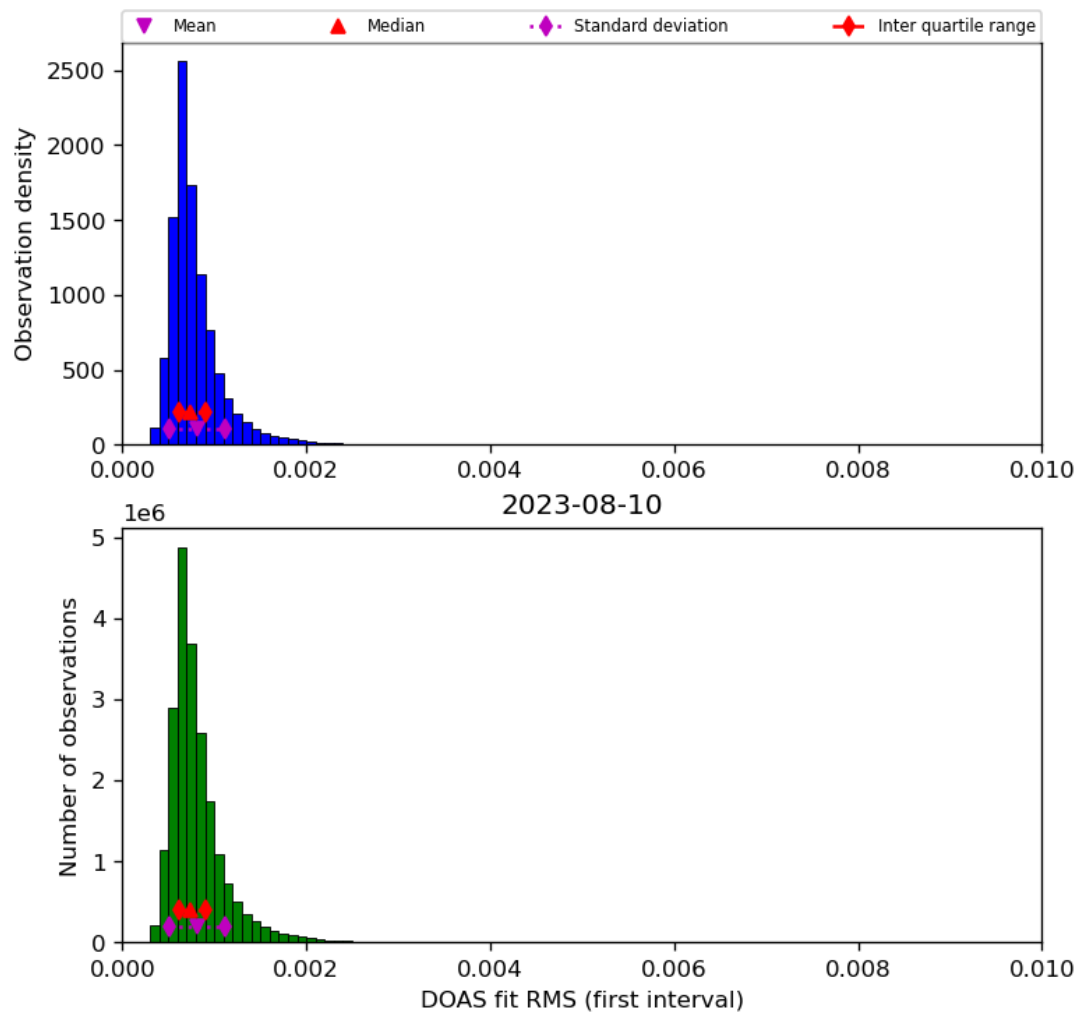
Figure 46: Histogram of “DOAS fit RMS (first interval)” for 2023-08-09 to 2023-08-11
