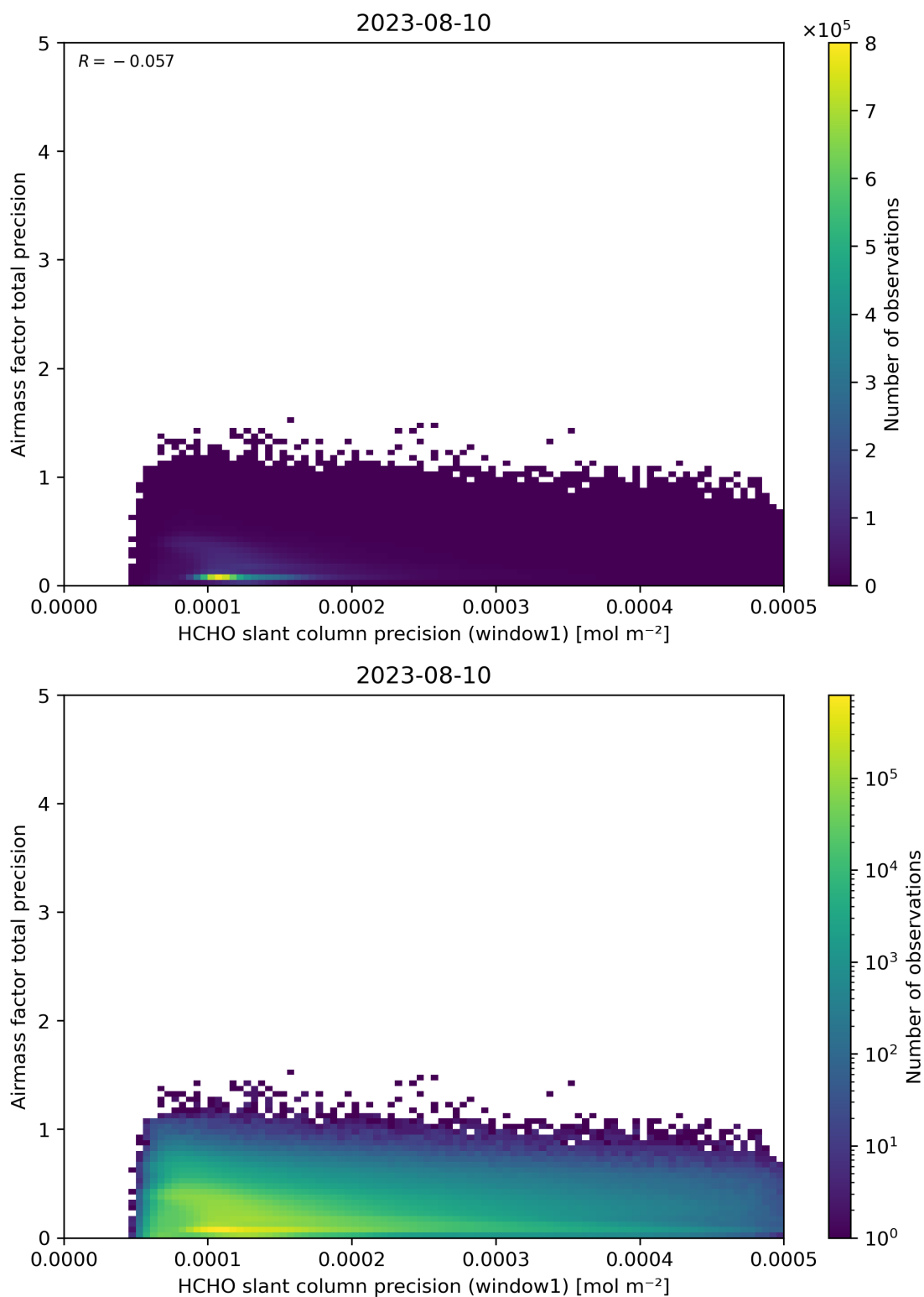
Figure 95: Scatter density plot of “HCHO slant column precision (window1)” against “Airmass factor total precision” for 2023-08-09 to 2023-08-11.
