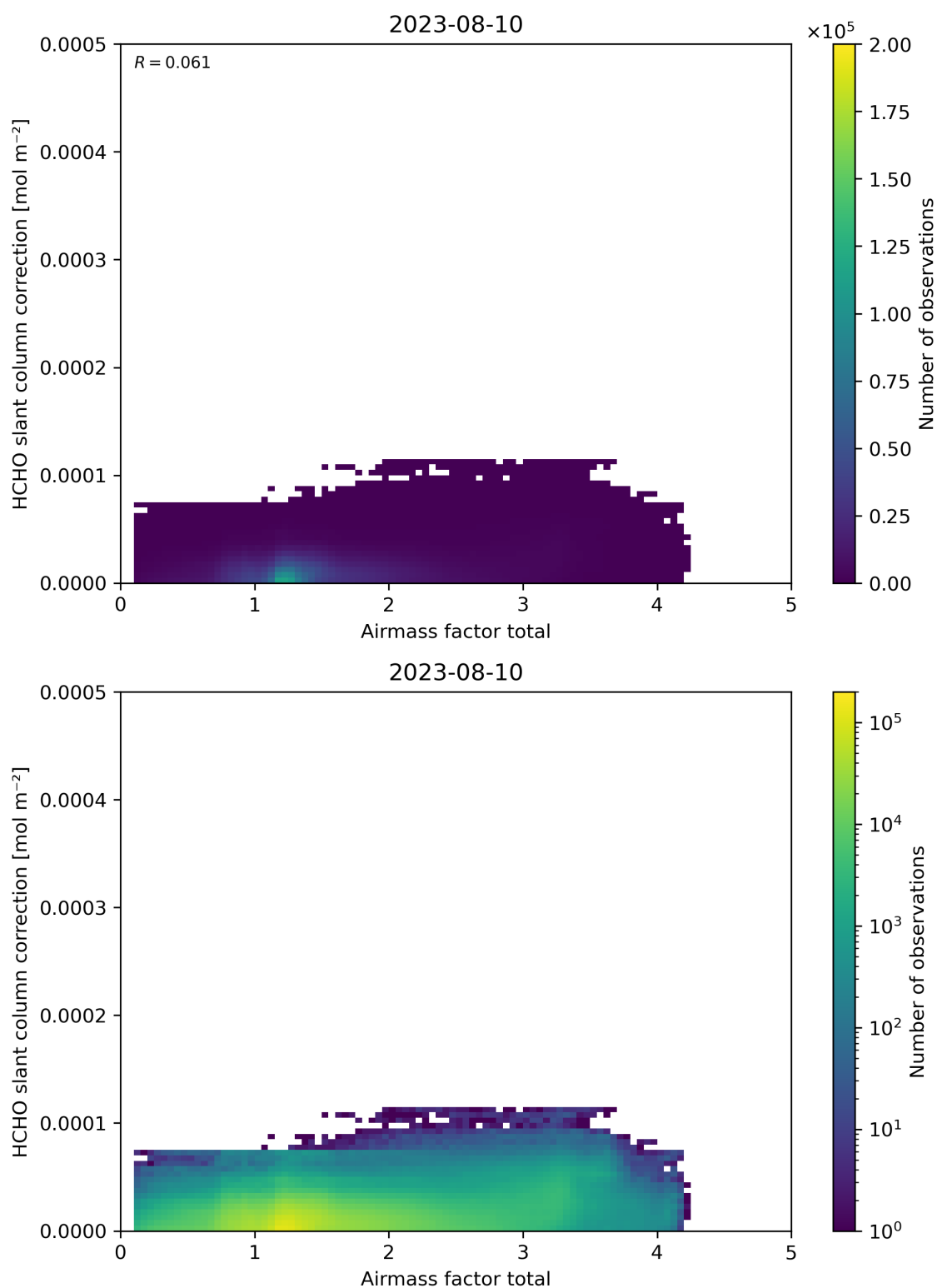
Figure 102: Scatter density plot of “Airmass factor total” against “HCHO slant column correction” for 2023-08-09 to 2023-08-11.
