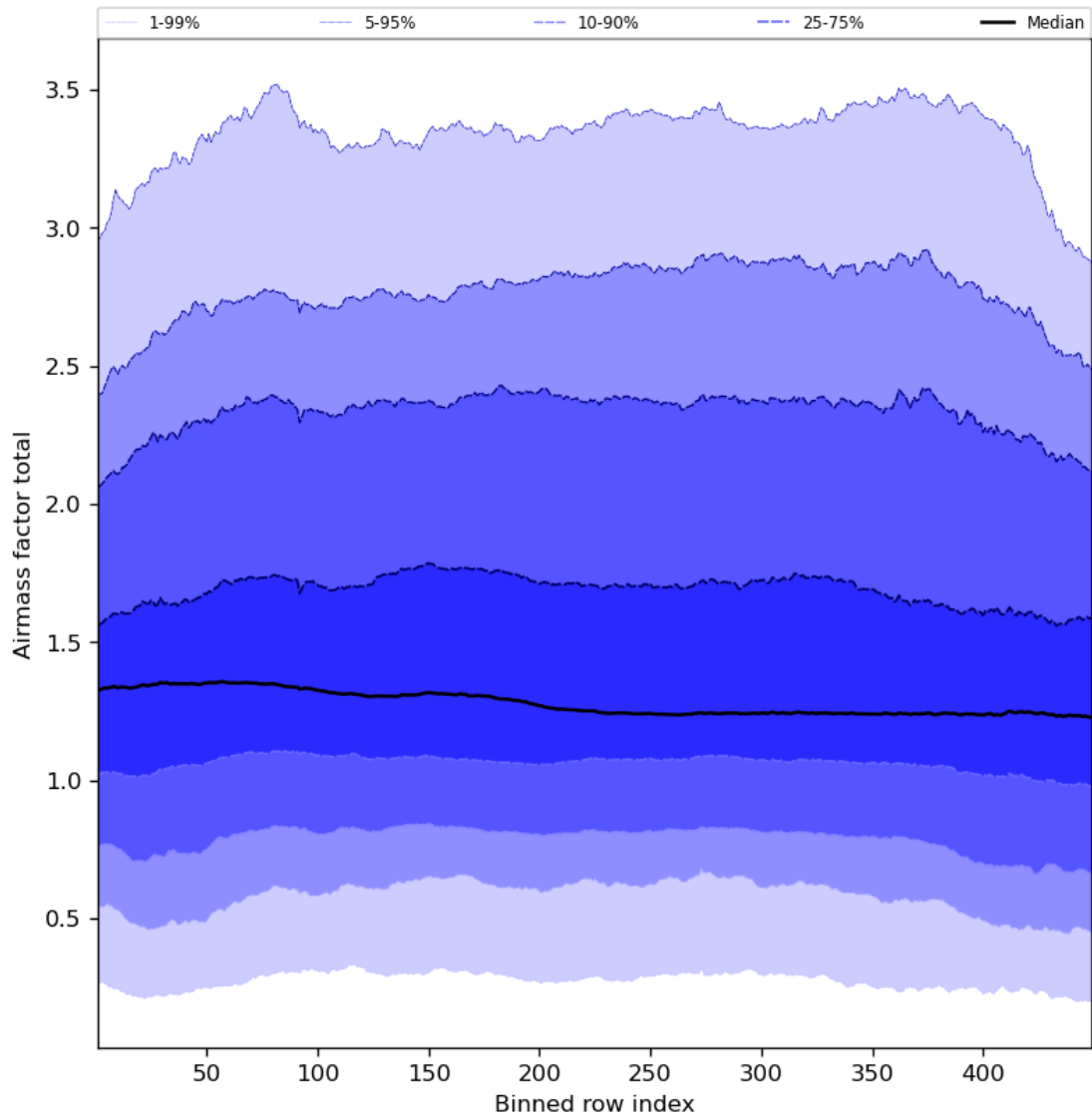
Figure 54: Along track statistics of “Airmass factor total” for 2023-08-09 to 2023-08-11
