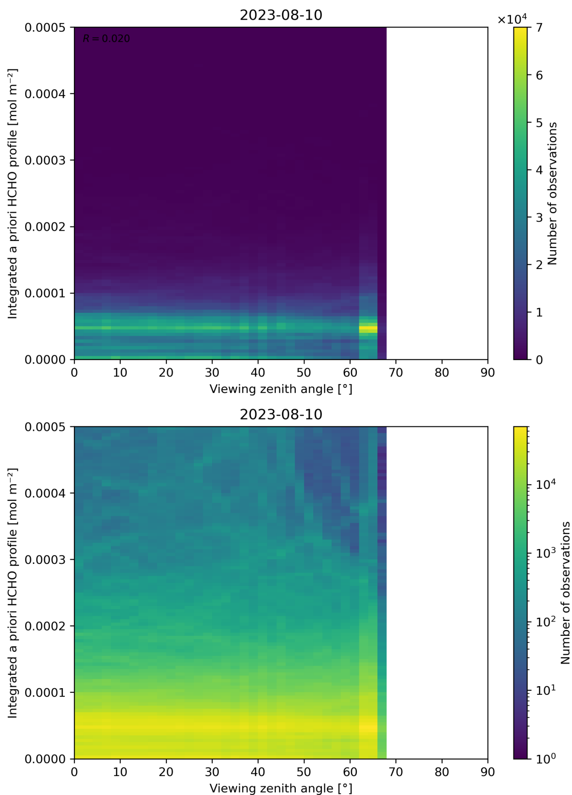
Figure 195: Scatter density plot of “Viewing zenith angle” against “Integrated a priori HCHO profile” for 2023-08-09 to 2023-08-11.
