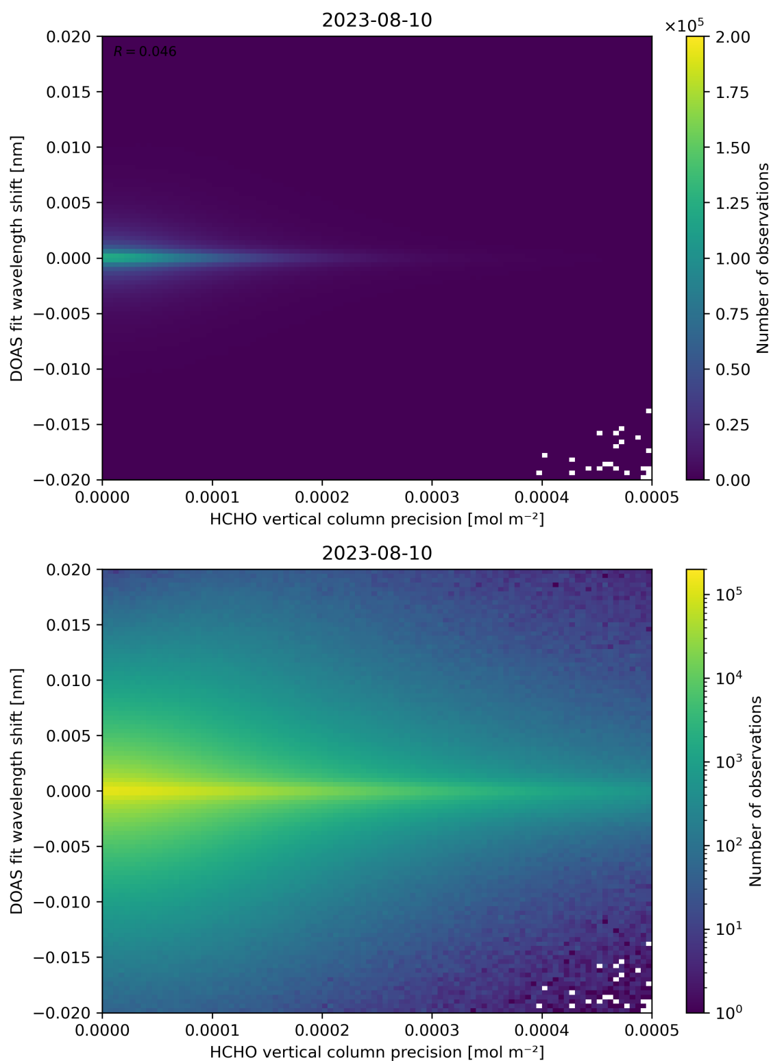
Figure 137: Scatter density plot of “HCHO vertical column precision” against “DOAS fit wavelength shift” for 2023-08-09 to 2023-08-11.
