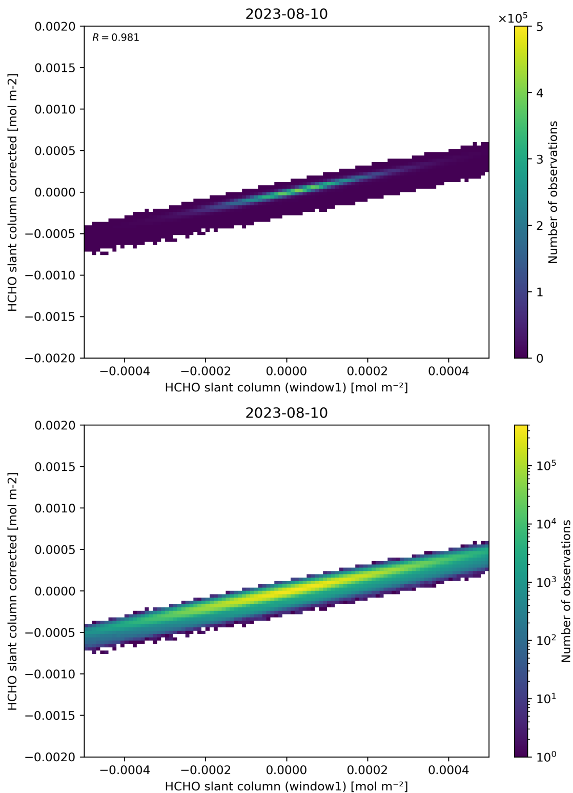
Figure 82: Scatter density plot of “HCHO slant column (window1)” against “HCHO slant column corrected” for 2023-08-09 to 2023-08-11.
