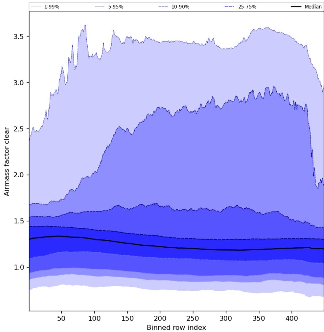
Figure 56: Along track statistics of “Airmass factor clear” for 2023-08-09 to 2023-08-11
