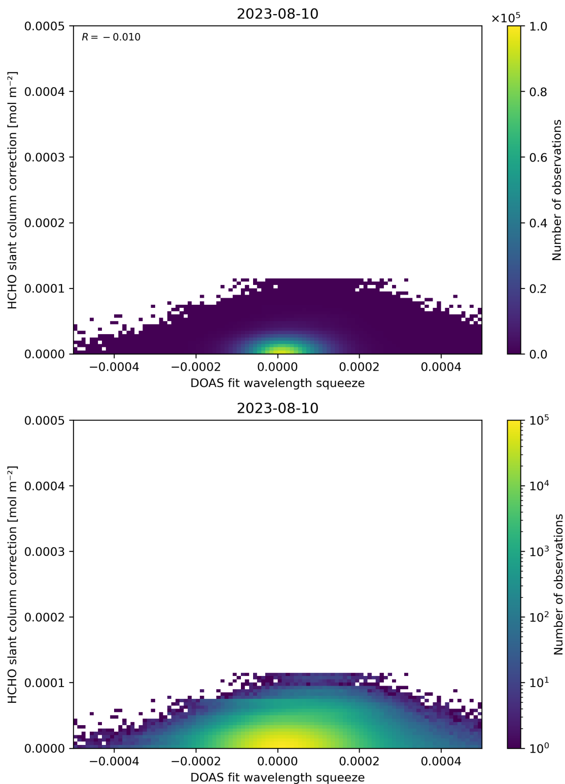
Figure 70: Scatter density plot of “DOAS fit wavelength squeeze” against “HCHO slant column correction” for 2023-08-09 to 2023-08-11.
