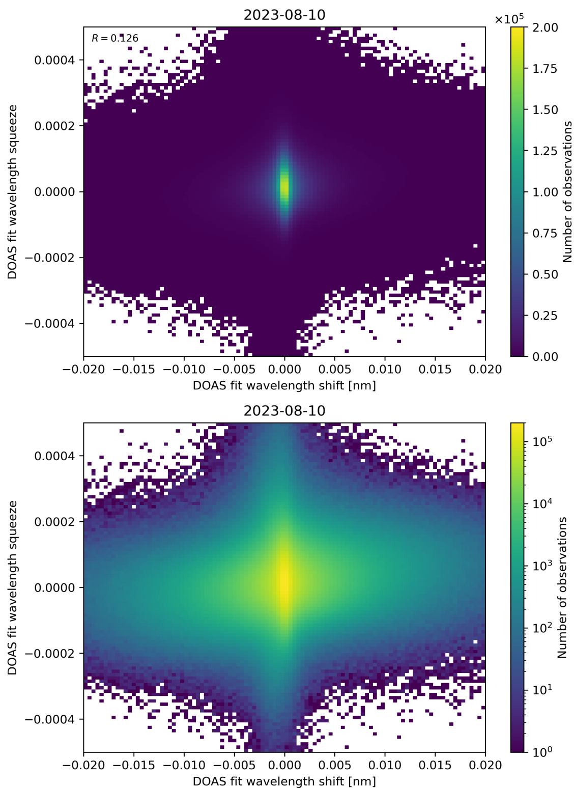
Figure 65: Scatter density plot of “DOAS fit wavelength shift” against “DOAS fit wavelength squeeze” for 2023-08-09 to 2023-08-11.
