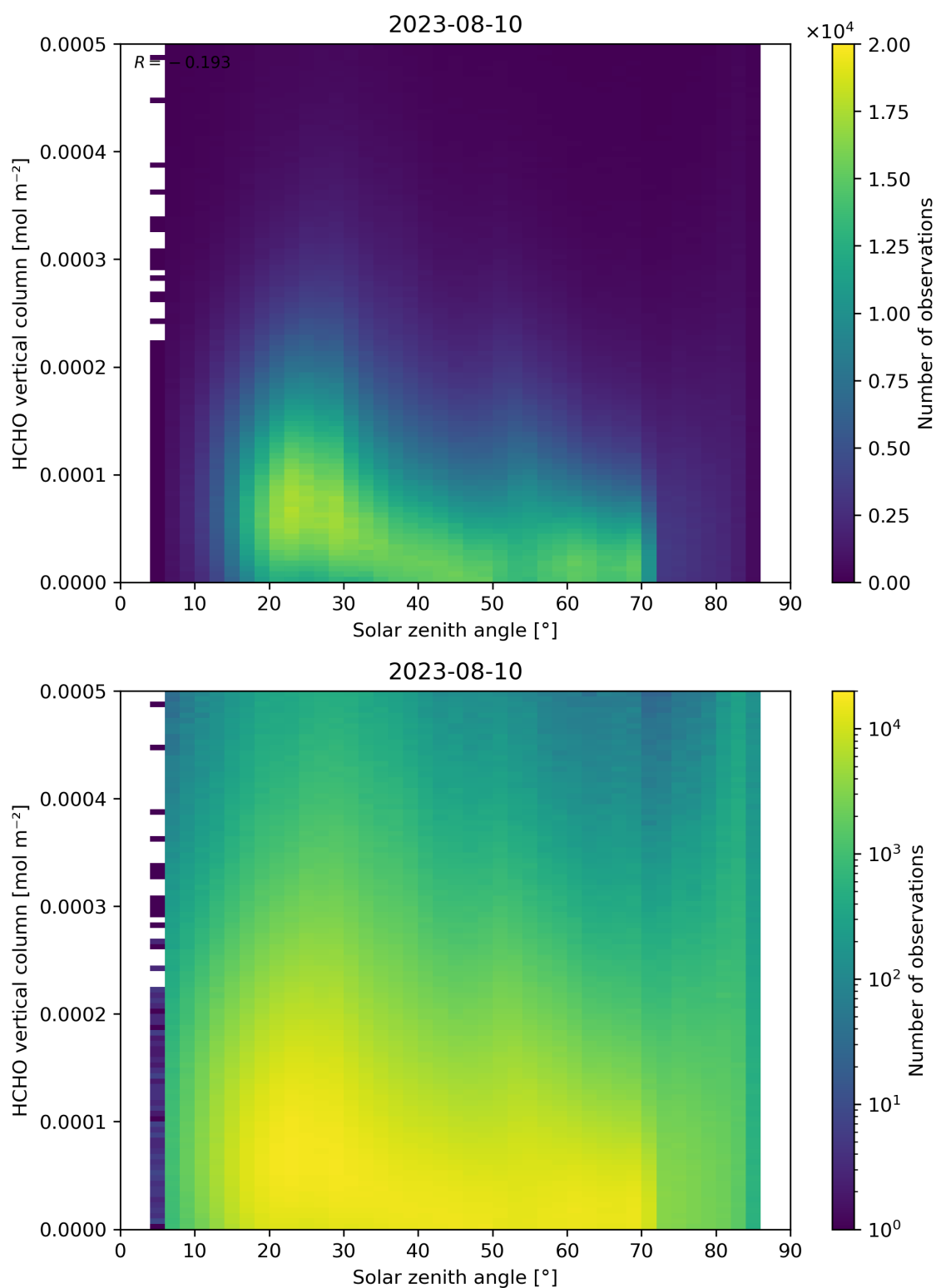
Figure 177: Scatter density plot of “Solar zenith angle” against “HCHO vertical column” for 2023-08-09 to 2023-08-11.
