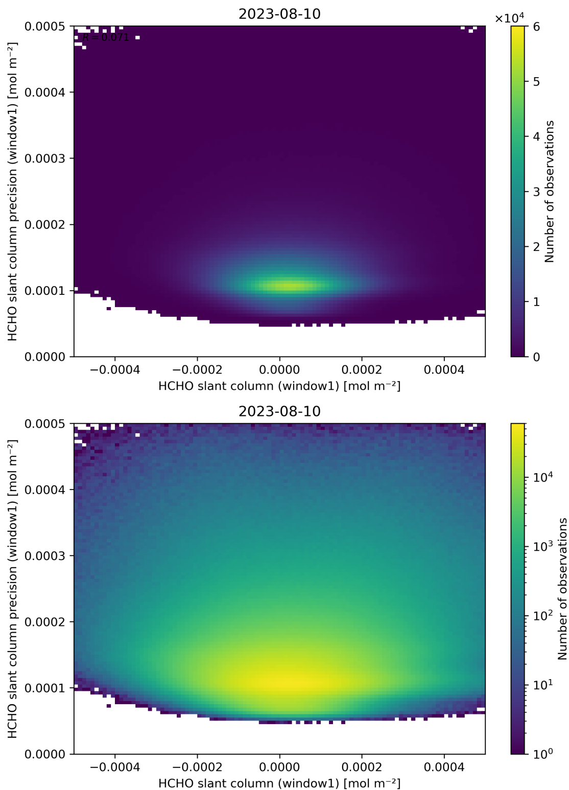
Figure 84: Scatter density plot of “HCHO slant column (window1)” against “HCHO slant column precision (window1)” for 2023-08-09 to 2023-08-11.
