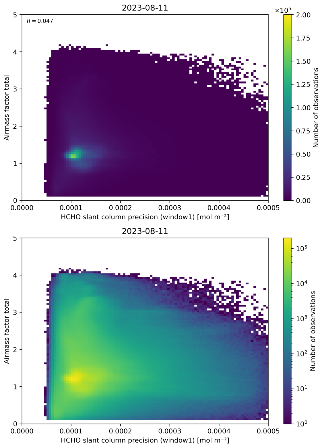
Figure 94: Scatter density plot of “HCHO slant column precision (window1)” against “Airmass factor total” for 2023-08-10 to 2023-08-12.
