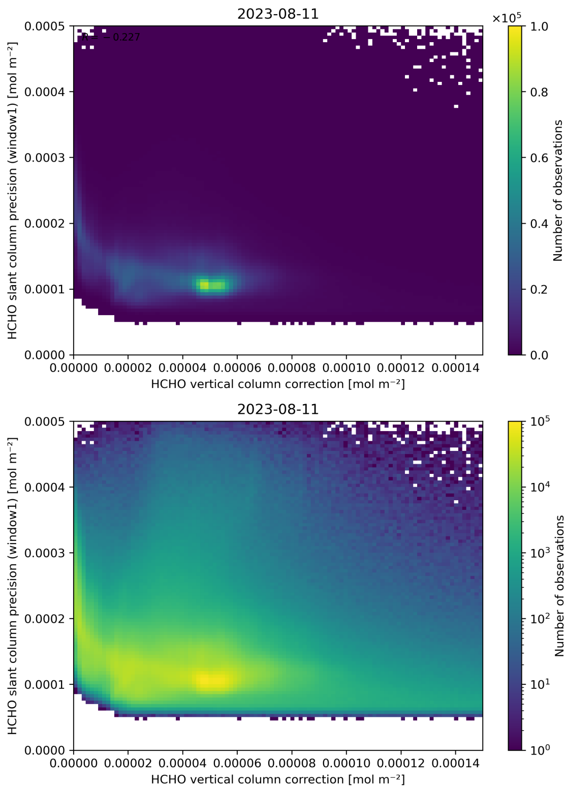
Figure 119: Scatter density plot of “HCHO vertical column correction” against “HCHO slant column precision (window1)” for 2023-08-10 to 2023-08-12.
