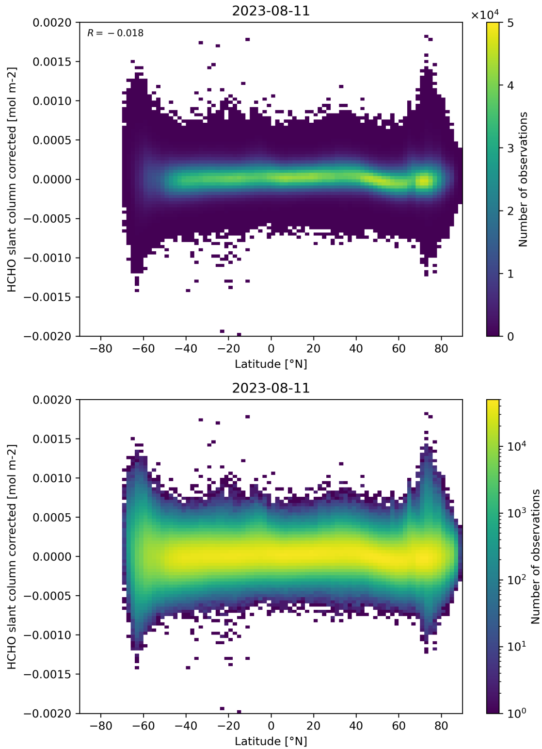
Figure 157: Scatter density plot of “Latitude” against “HCHO slant column corrected” for 2023-08-10 to 2023-08-12.
