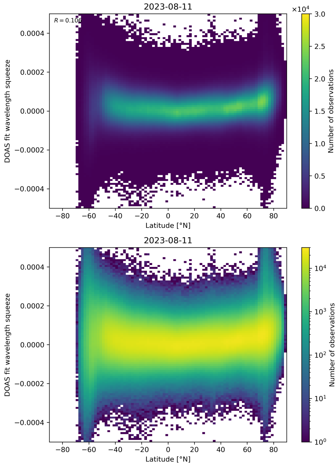
Figure 155: Scatter density plot of “Latitude” against “DOAS fit wavelength squeeze” for 2023-08-10 to 2023-08-12.
