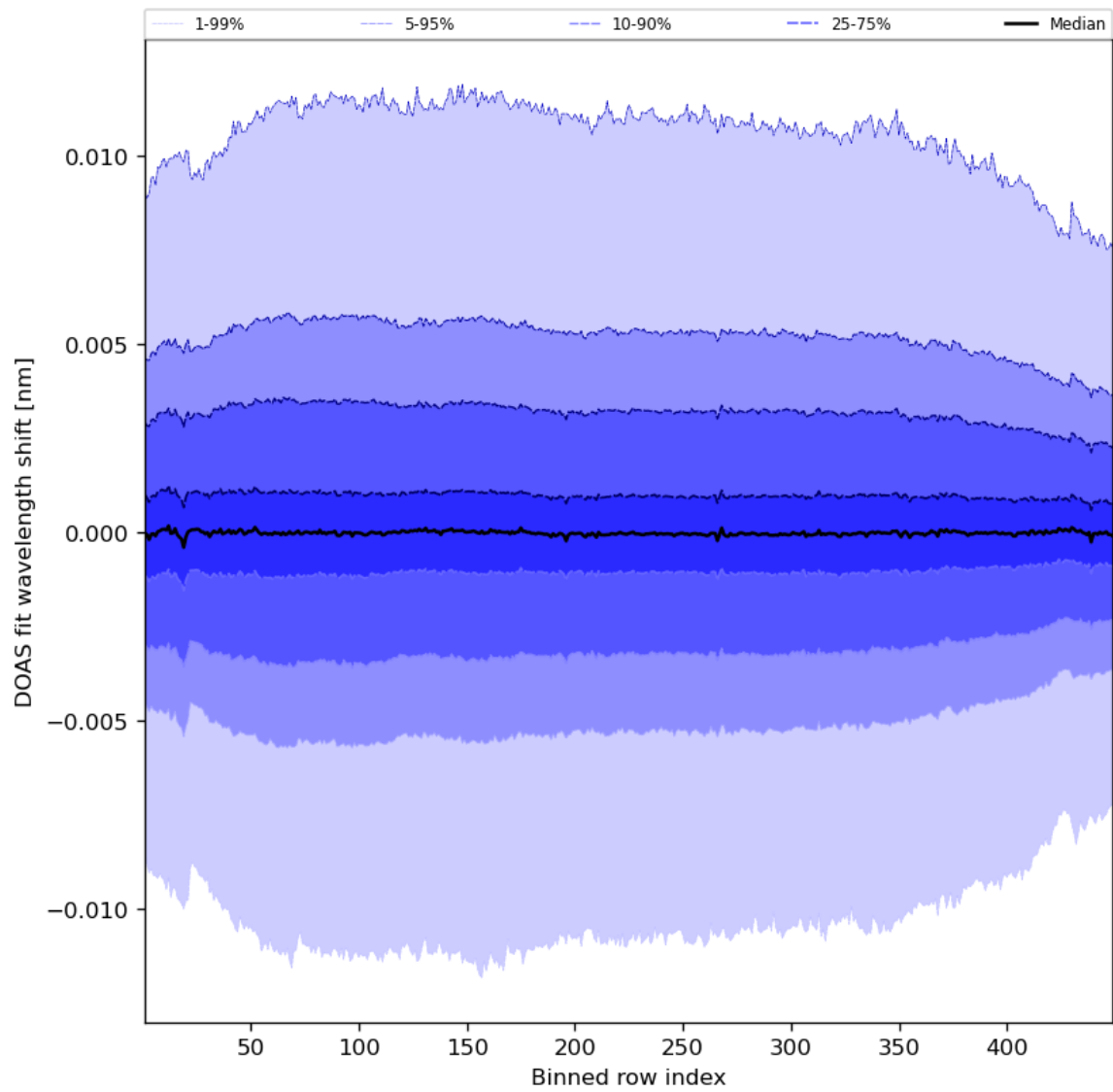
Figure 58: Along track statistics of “DOAS fit wavelength shift” for 2023-08-10 to 2023-08-12
