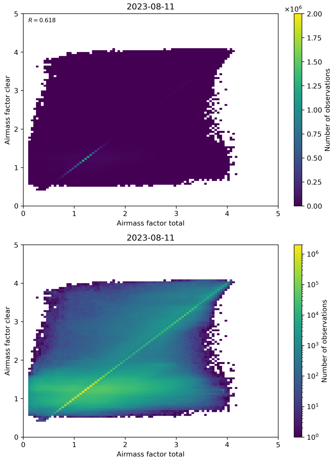
Figure 100: Scatter density plot of “Airmass factor total” against “Airmass factor clear” for 2023-08-10 to 2023-08-12.
