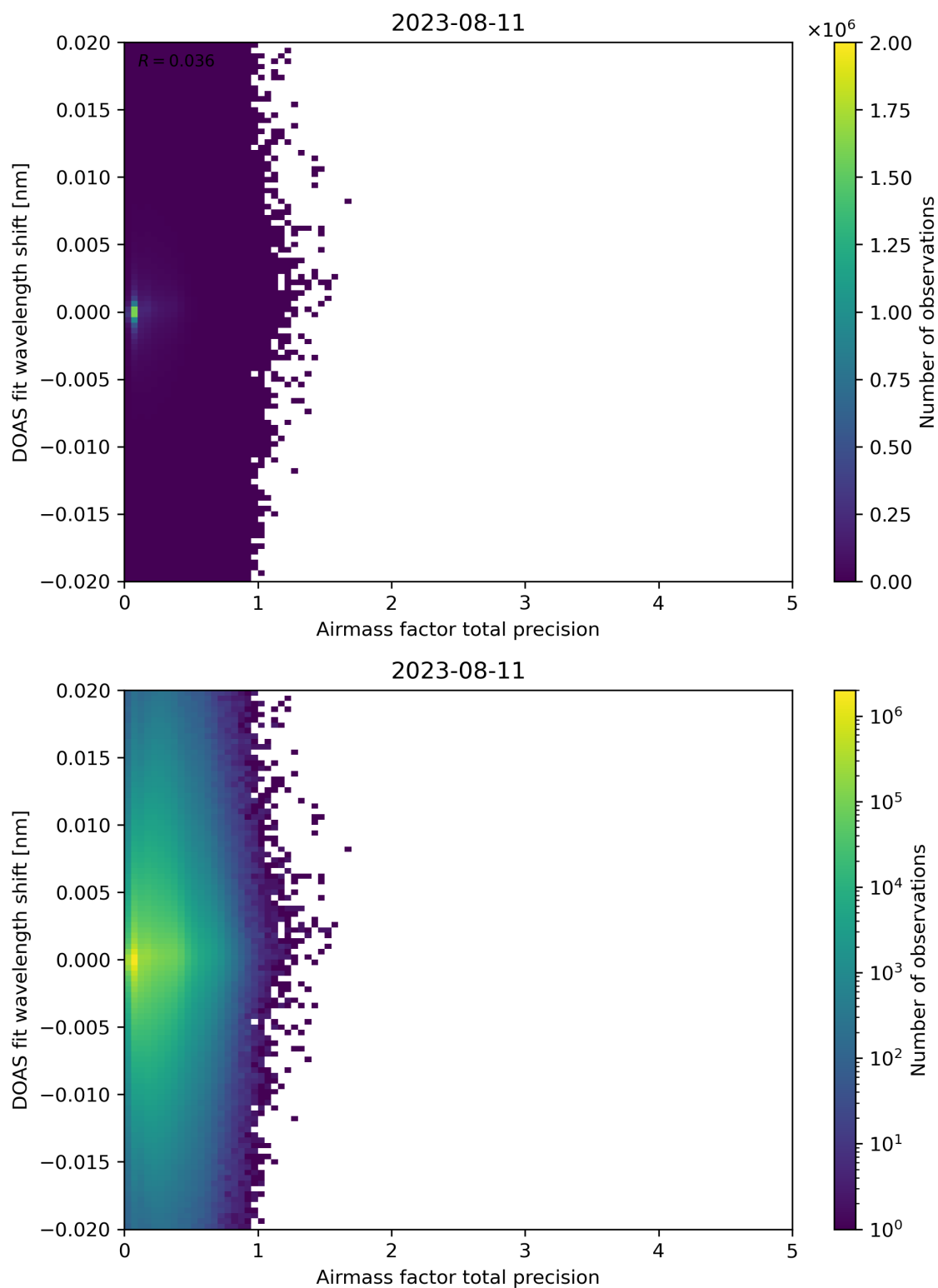
Figure 106: Scatter density plot of “Airmass factor total precision” against “DOAS fit wavelength shift” for 2023-08-10 to 2023-08-12.
