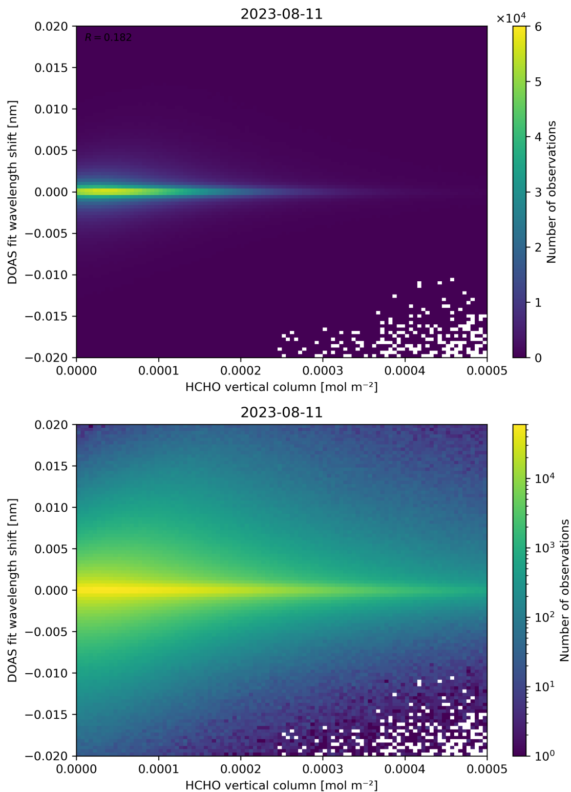
Figure 124: Scatter density plot of “HCHO vertical column” against “DOAS fit wavelength shift” for 2023-08-10 to 2023-08-12.
