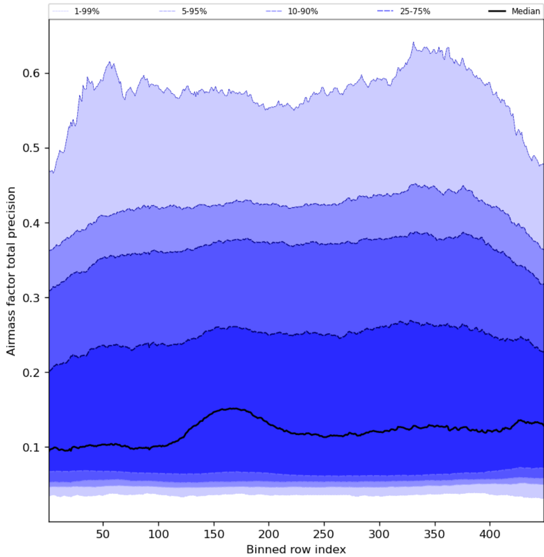
Figure 55: Along track statistics of “Airmass factor total precision” for 2023-08-10 to 2023-08-12
