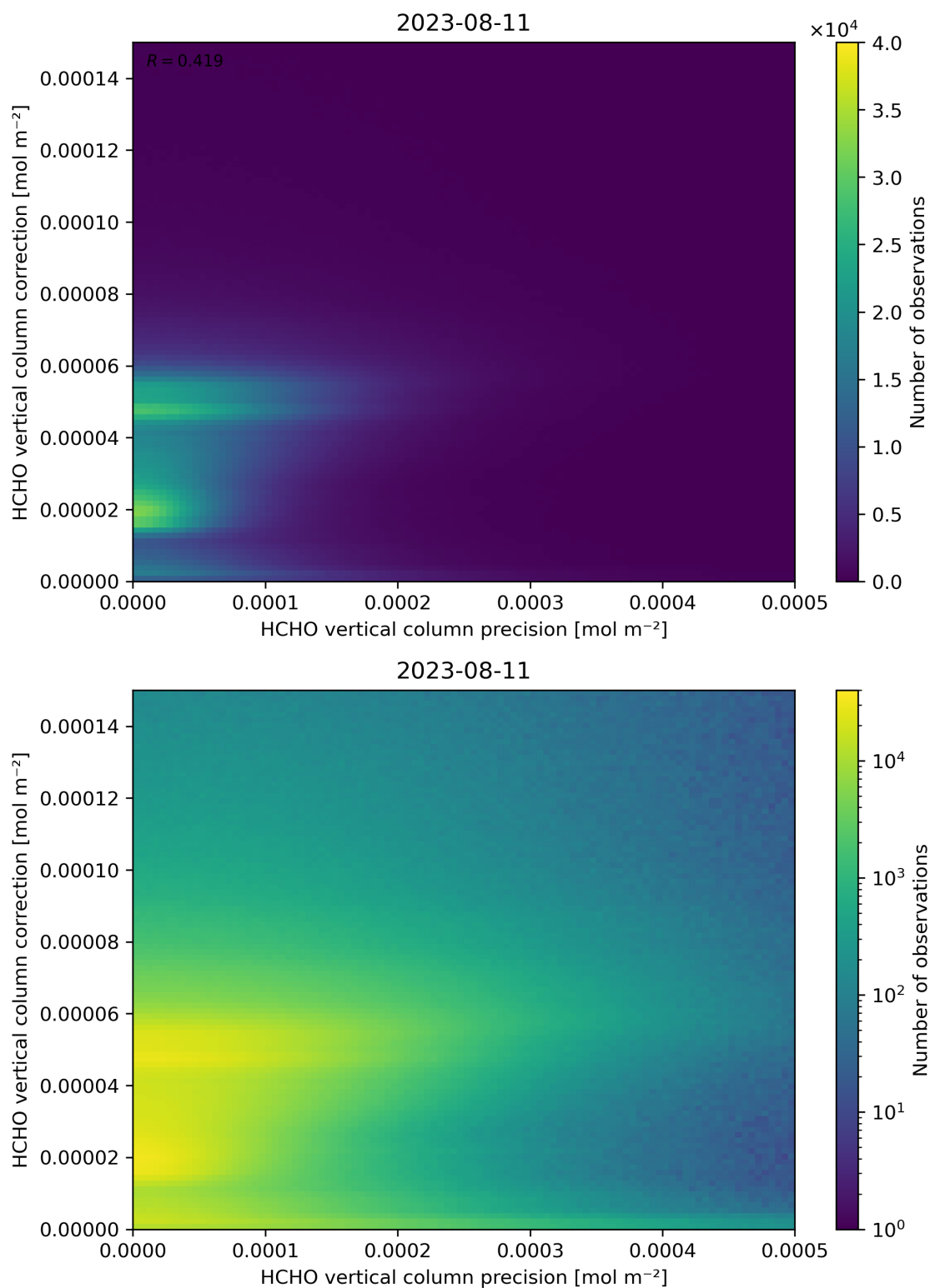
Figure 146: Scatter density plot of “HCHO vertical column precision” against “HCHO vertical column correction” for 2023-08-10 to 2023-08-12.
