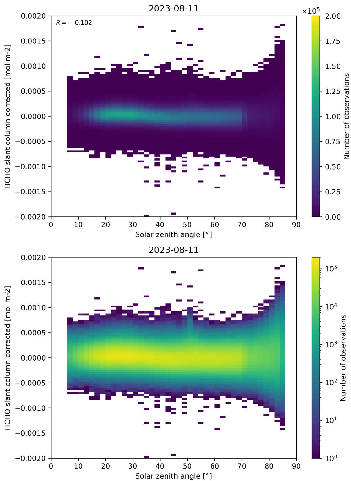
Figure 171: Scatter density plot of “Solar zenith angle” against “HCHO slant column corrected” for 2023-08-10 to 2023-08-12.
