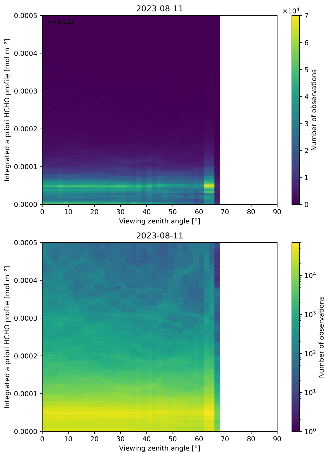
Figure 195: Scatter density plot of “Viewing zenith angle” against “Integrated a priori HCHO profile” for 2023-08-10 to 2023-08-12.
