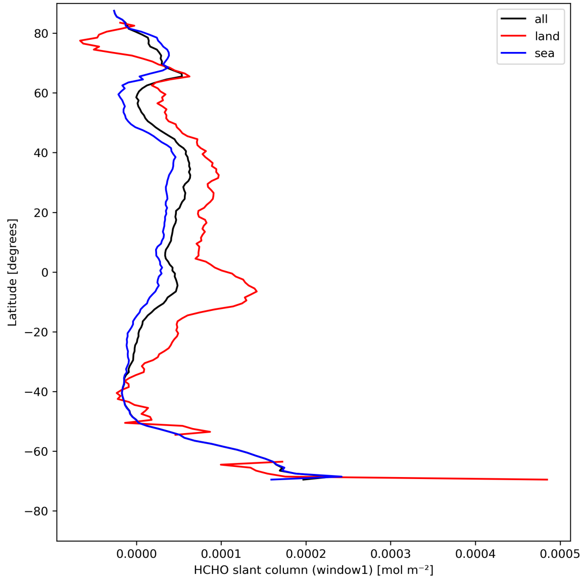
Figure 24: Zonal average of “HCHO slant column (window1)” for 2023-08-10 to 2023-08-12.
