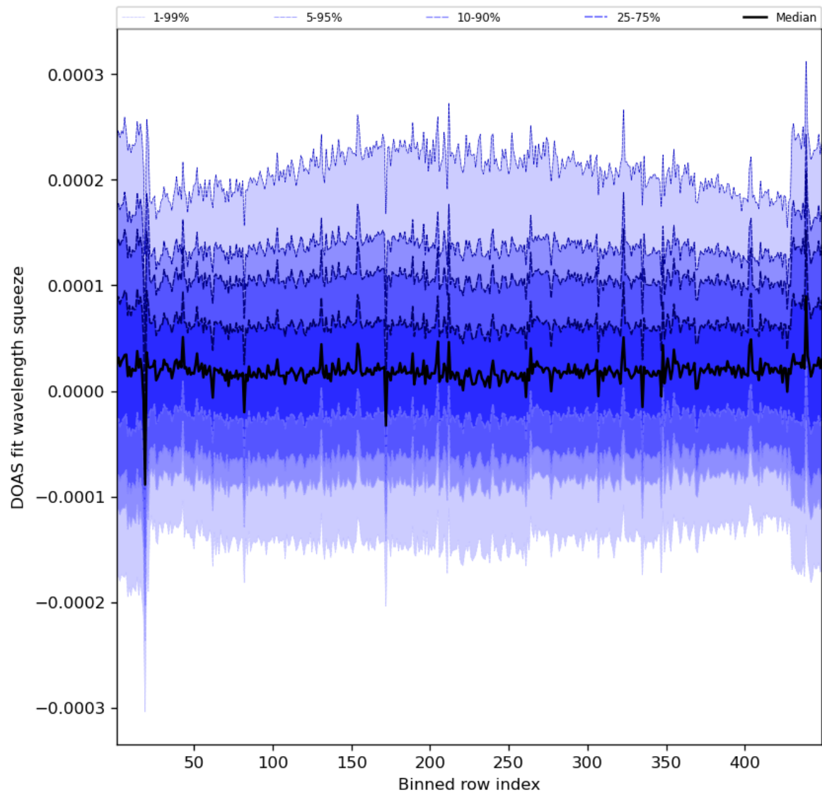
Figure 59: Along track statistics of “DOAS fit wavelength squeeze” for 2023-08-10 to 2023-08-12
