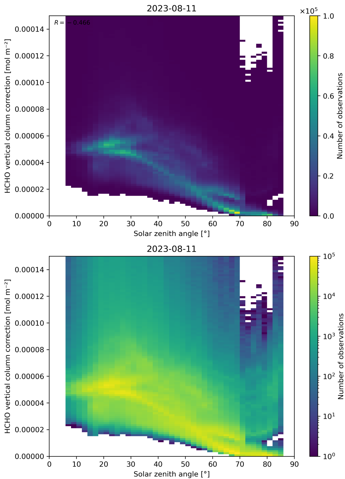
Figure 178: Scatter density plot of “Solar zenith angle” against “HCHO vertical column correction” for 2023-08-10 to 2023-08-12.
