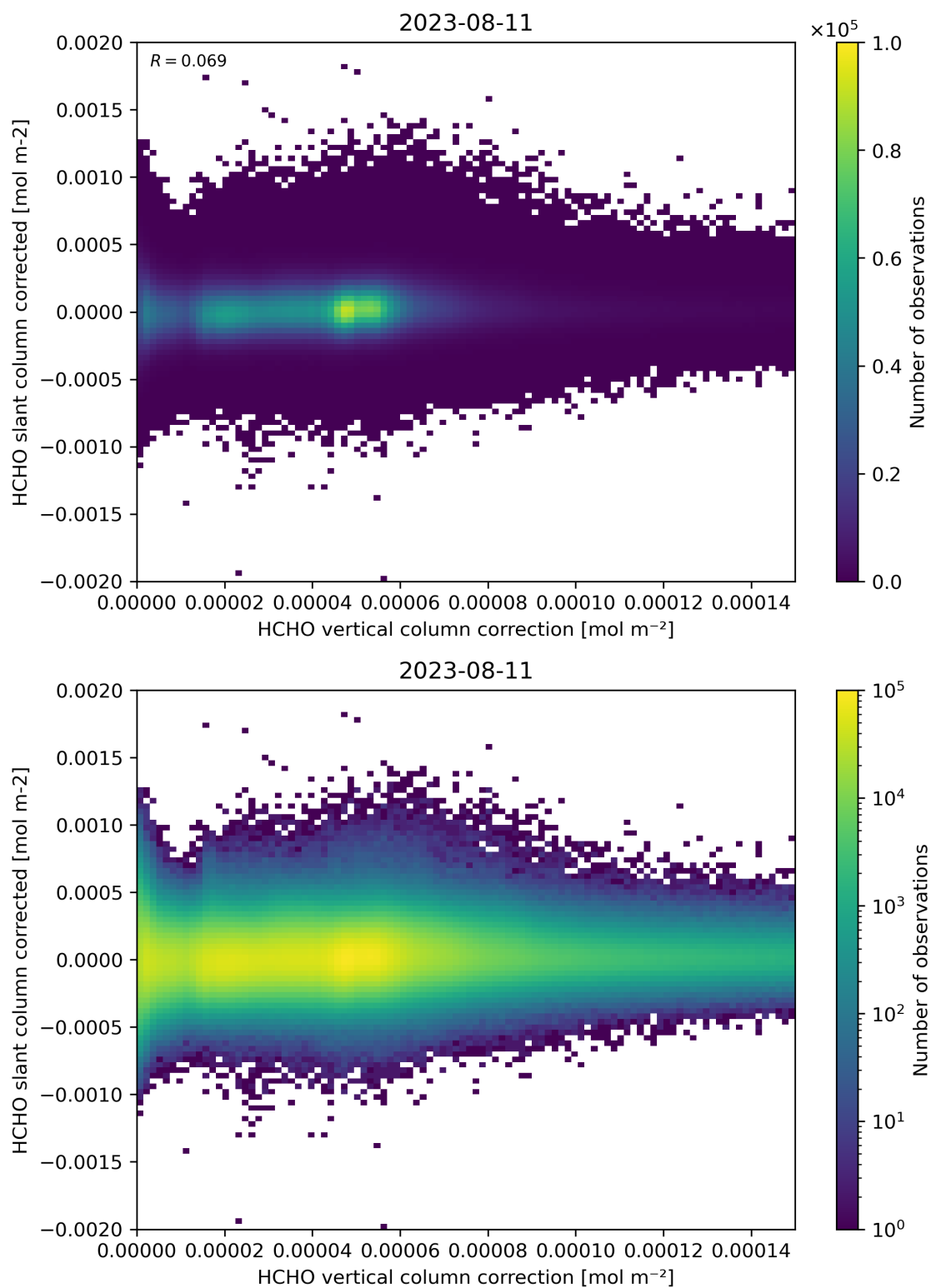
Figure 116: Scatter density plot of “HCHO vertical column correction” against “HCHO slant column corrected” for 2023-08-10 to 2023-08-12.
