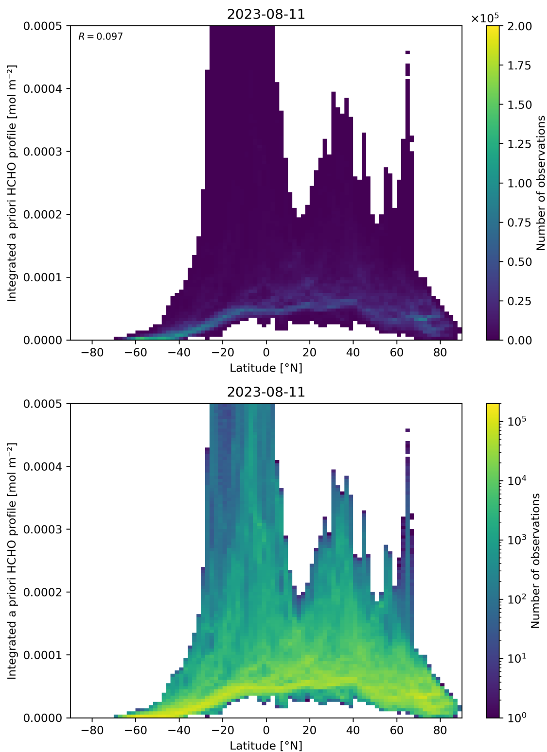
Figure 166: Scatter density plot of “Latitude” against “Integrated a priori HCHO profile” for 2023-08-10 to 2023-08-12.
