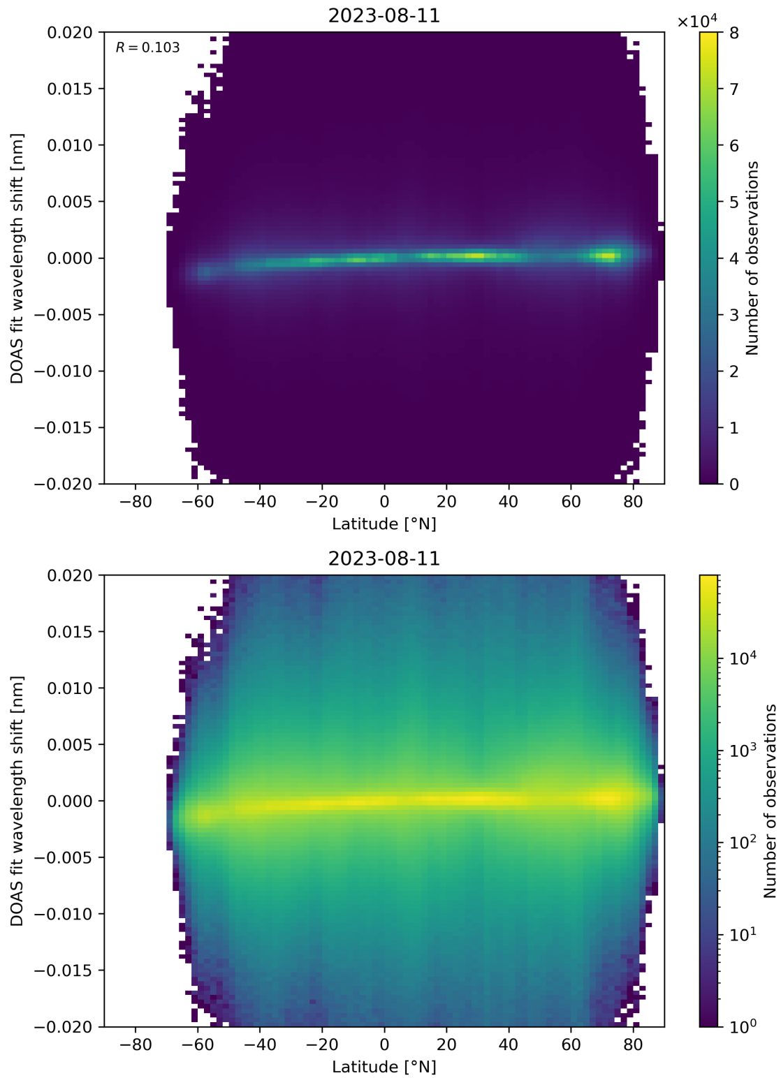
Figure 154: Scatter density plot of “Latitude” against “DOAS fit wavelength shift” for 2023-08-10 to 2023-08-12.
