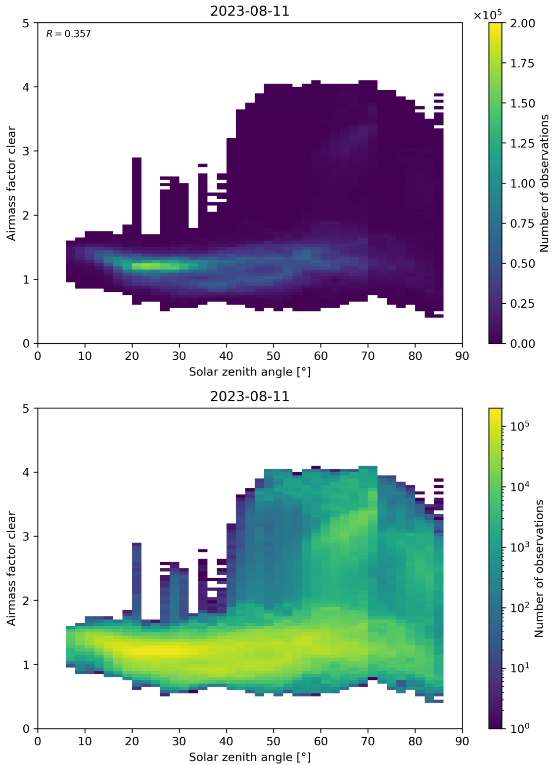
Figure 170: Scatter density plot of “Solar zenith angle” against “Airmass factor clear” for 2023-08-10 to 2023-08-12.
