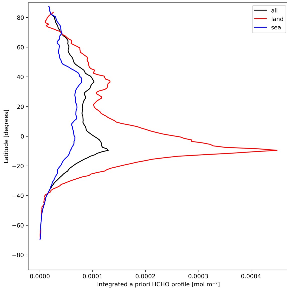
Figure 29: Zonal average of “Integrated a priori HCHO profile” for 2023-08-10 to 2023-08-12.
