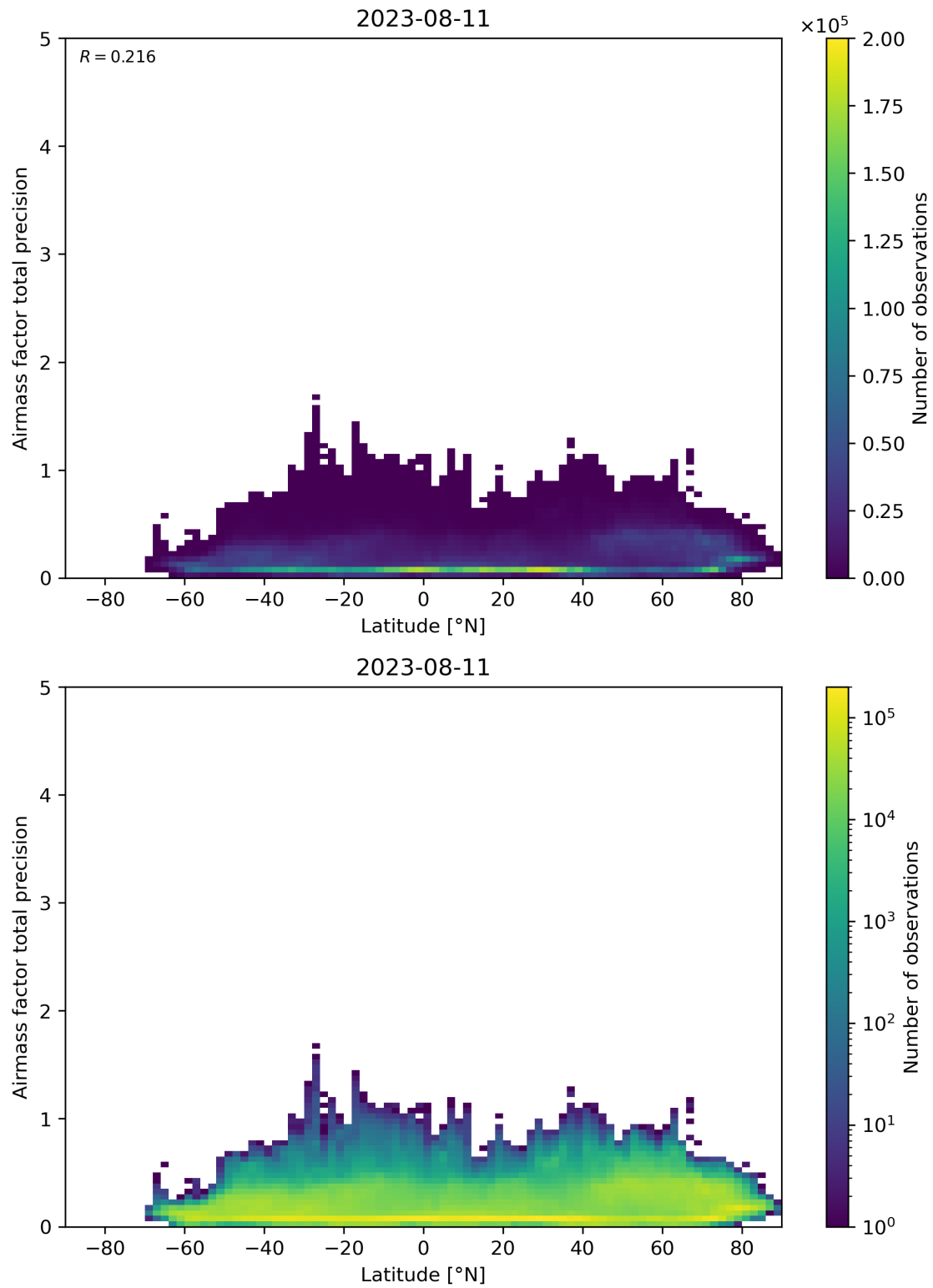
Figure 162: Scatter density plot of “Latitude” against “Airmass factor total precision” for 2023-08-10 to 2023-08-12.
