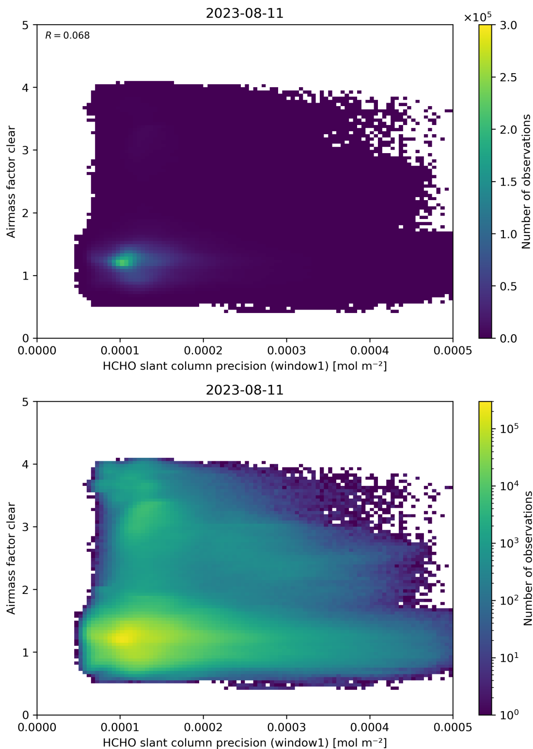
Figure 91: Scatter density plot of “HCHO slant column precision (window1)” against “Airmass factor clear” for 2023-08-10 to 2023-08-12.
