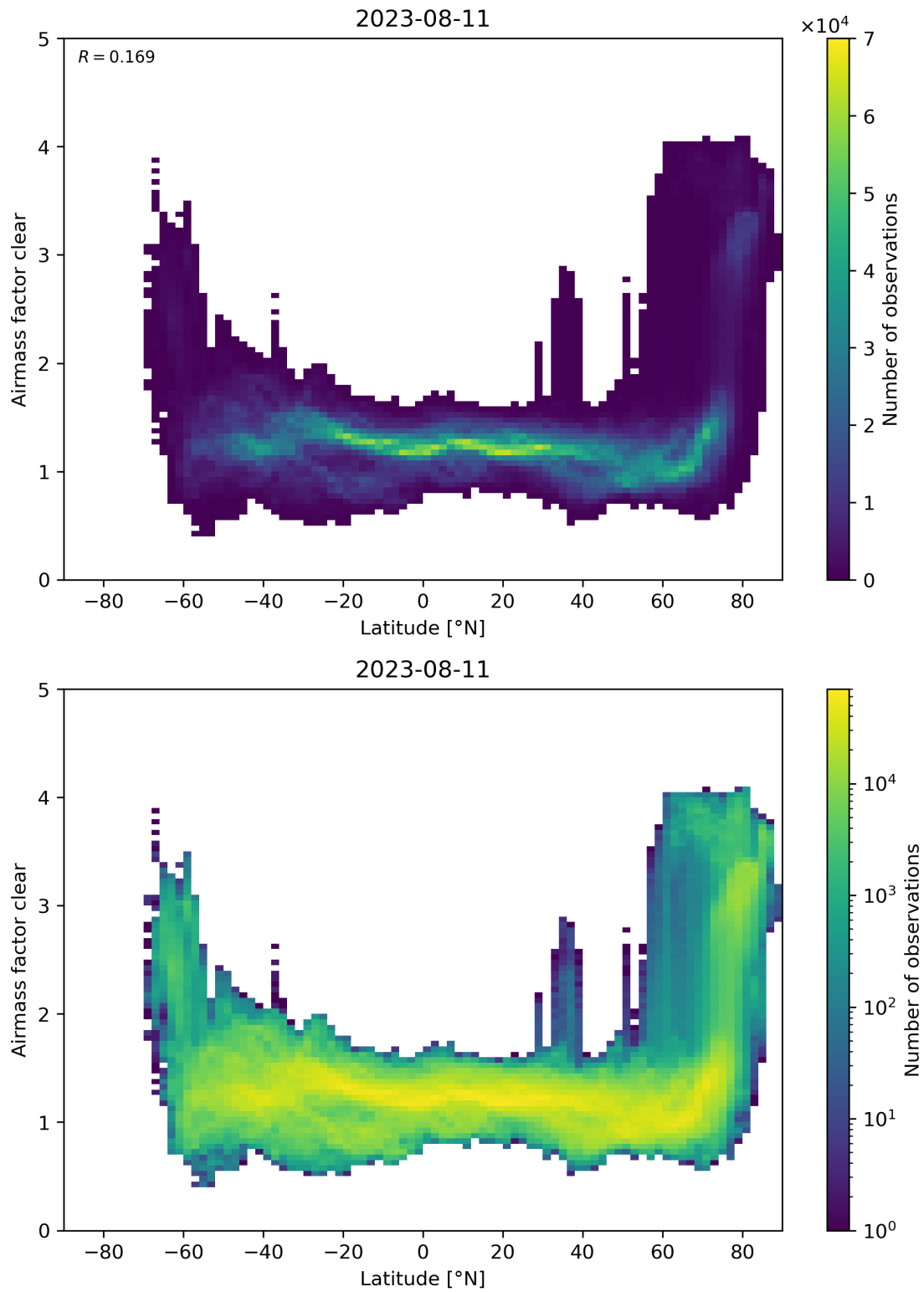
Figure 156: Scatter density plot of “Latitude” against “Airmass factor clear” for 2023-08-10 to 2023-08-12.
