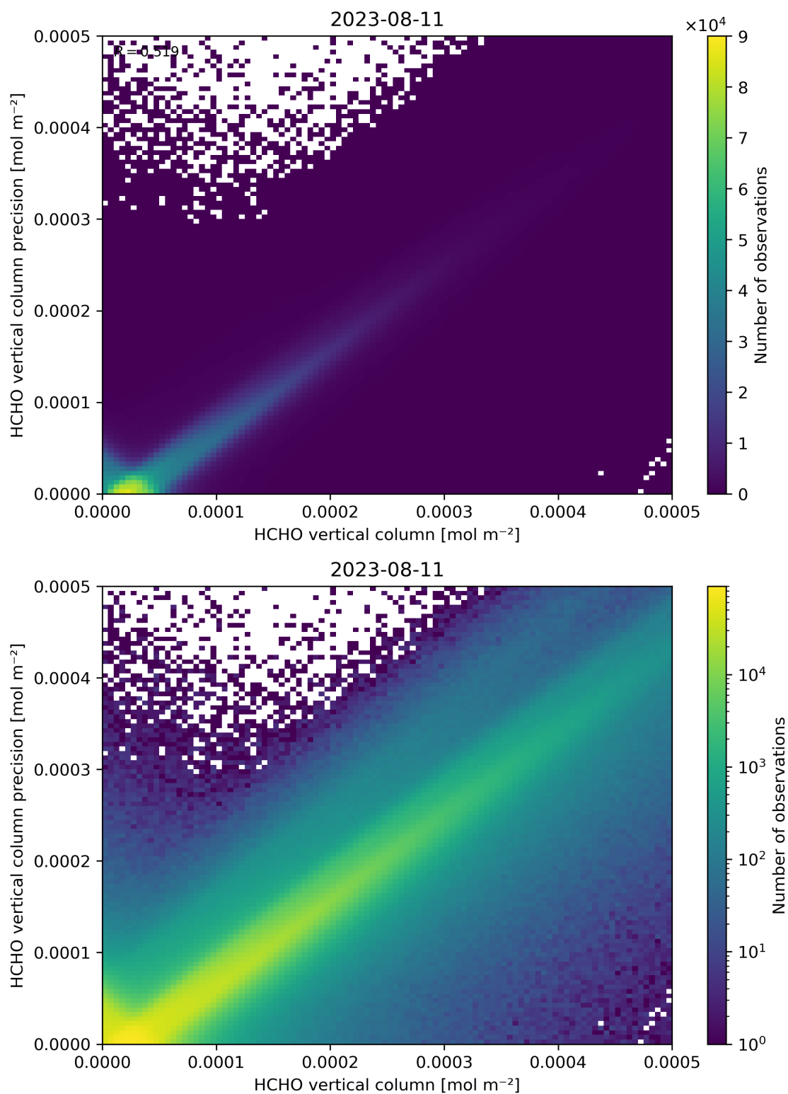
Figure 134: Scatter density plot of “HCHO vertical column” against “HCHO vertical column precision” for 2023-08-10 to 2023-08-12.
