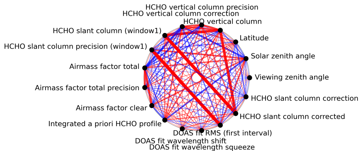
Figure 1: Map of correlation graph for 2023-08-10 to 2023-08-12.
