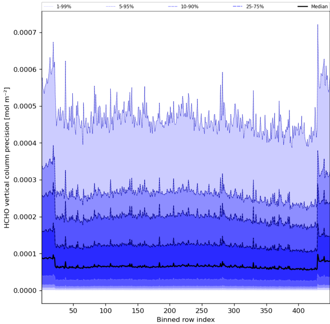
Figure 50: Along track statistics of “HCHO vertical column precision” for 2023-08-10 to 2023-08-12
