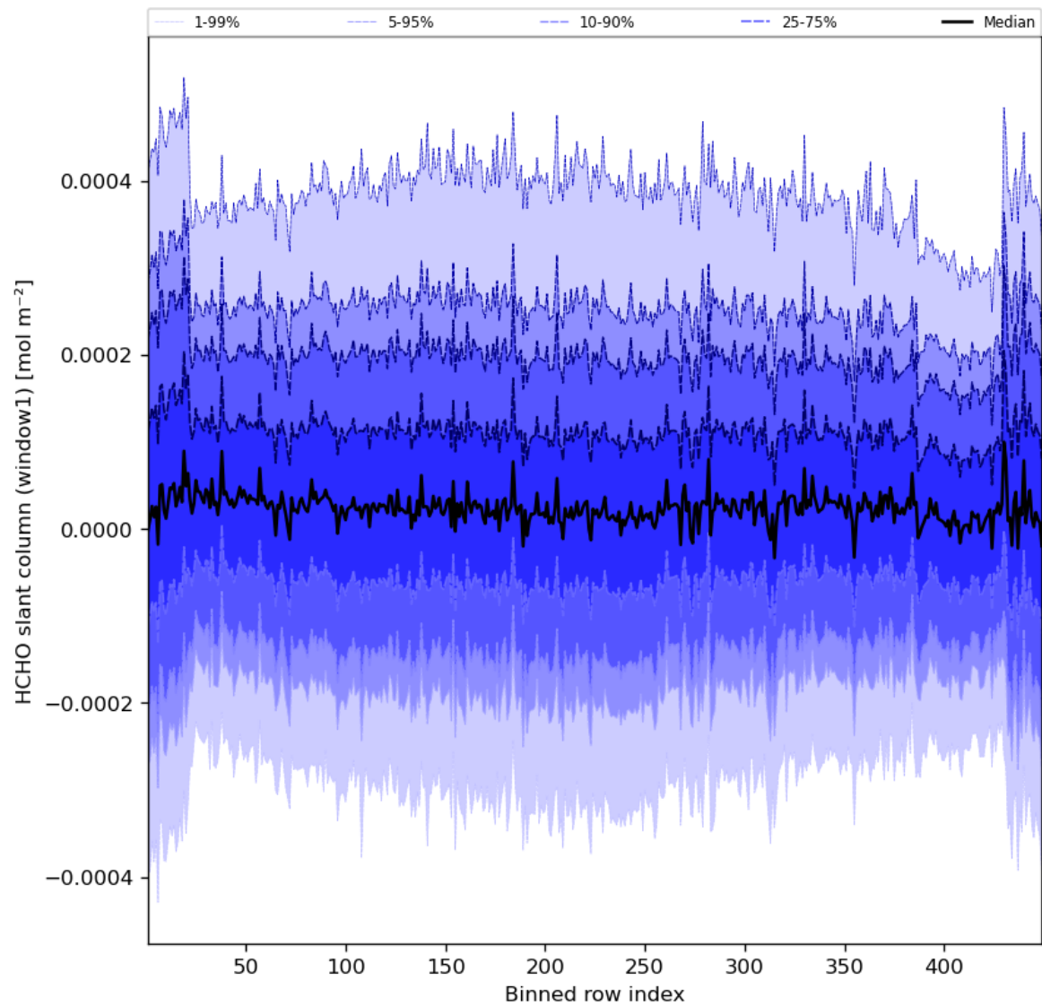
Figure 52: Along track statistics of “HCHO slant column (window1)” for 2023-08-10 to 2023-08-12
