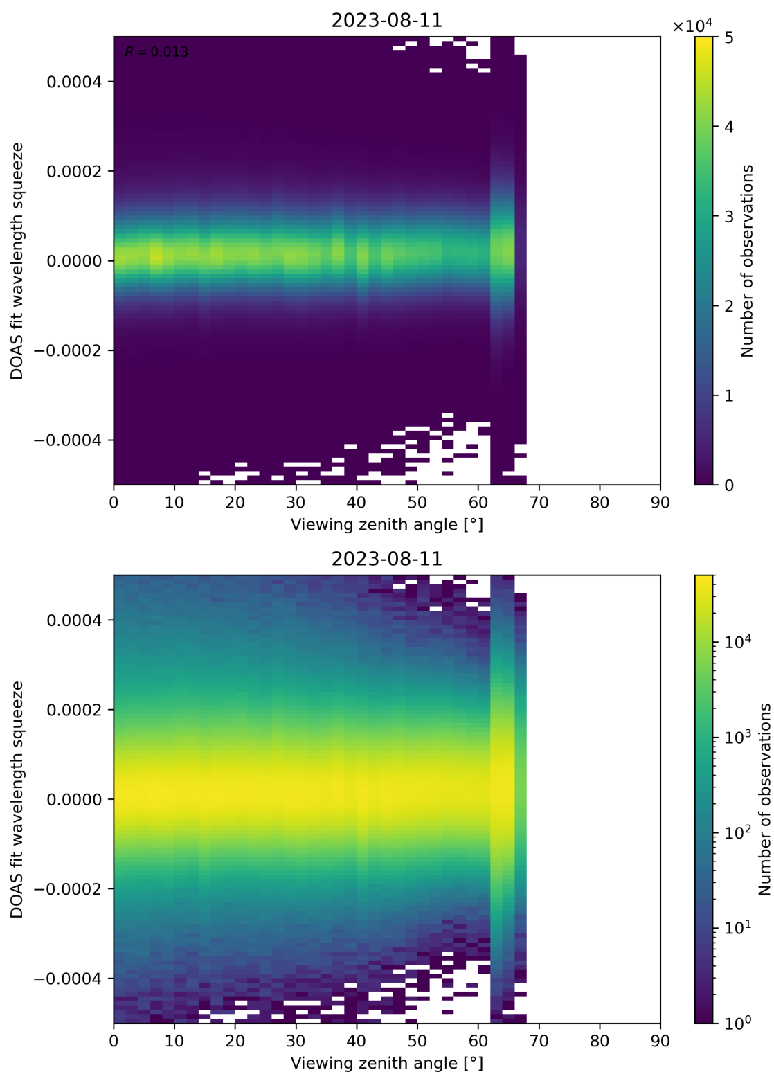
Figure 184: Scatter density plot of “Viewing zenith angle” against “DOAS fit wavelength squeeze” for 2023-08-10 to 2023-08-12.
