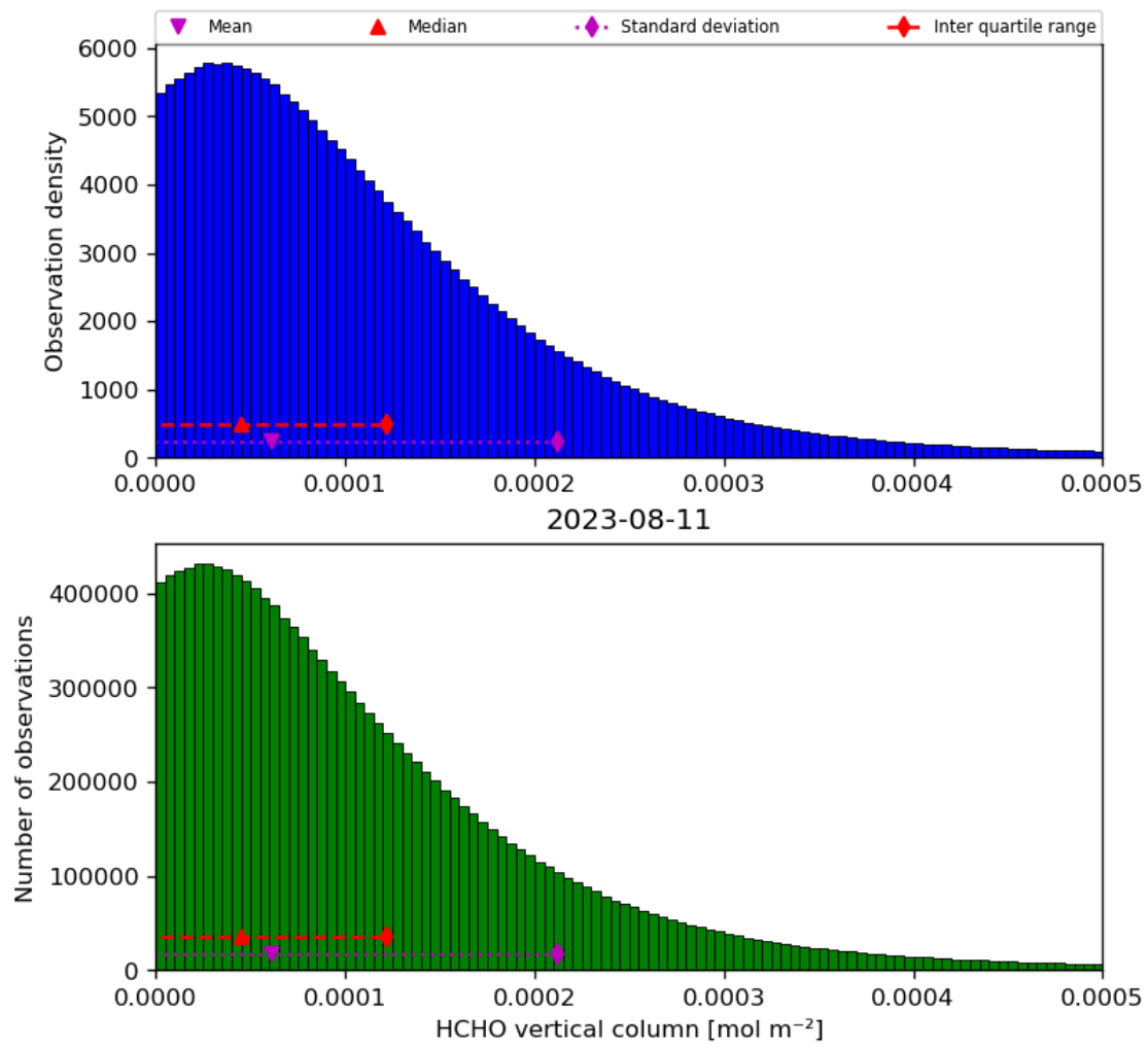
Figure 35: Histogram of “HCHO vertical column” for 2023-08-10 to 2023-08-12
