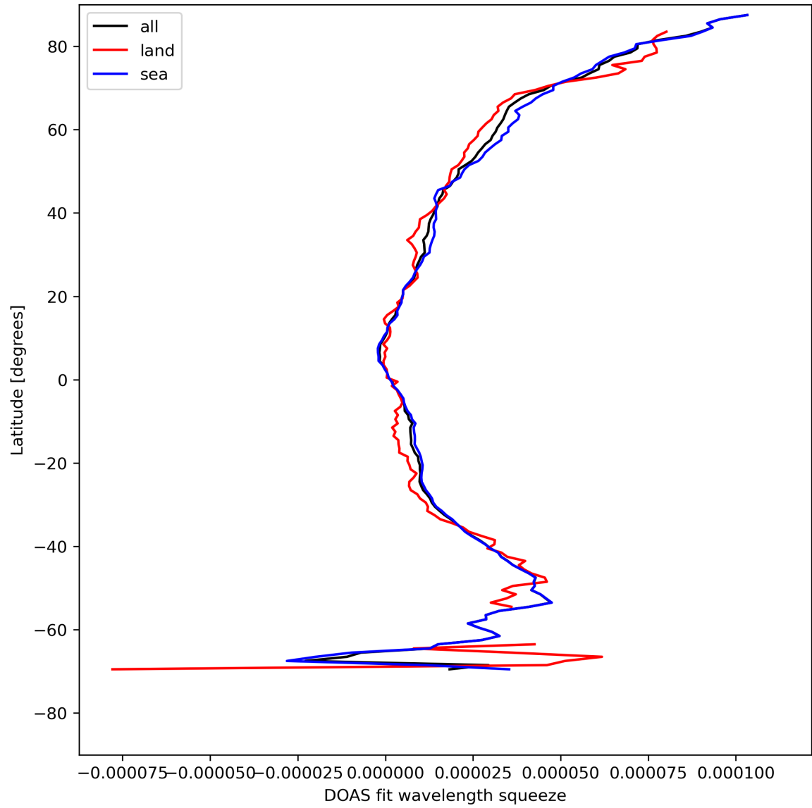
Figure 31: Zonal average of “DOAS fit wavelength squeeze” for 2023-08-10 to 2023-08-12.
