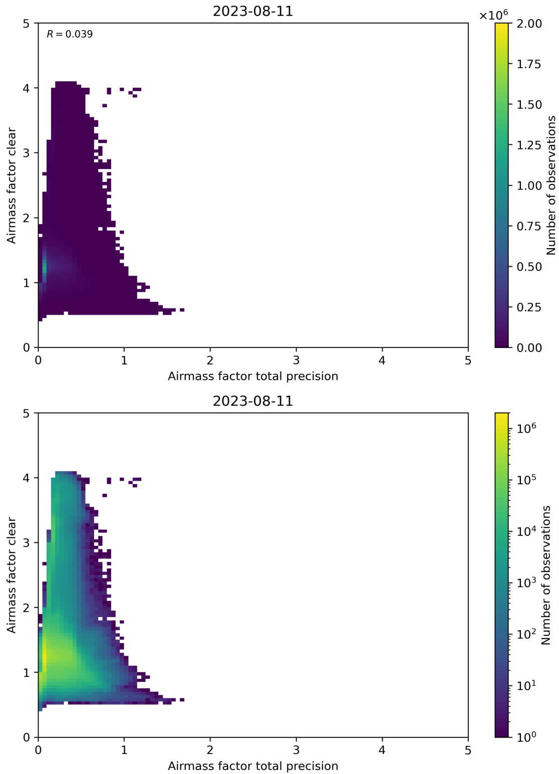
Figure 108: Scatter density plot of “Airmass factor total precision” against “Airmass factor clear” for 2023-08-10 to 2023-08-12.
