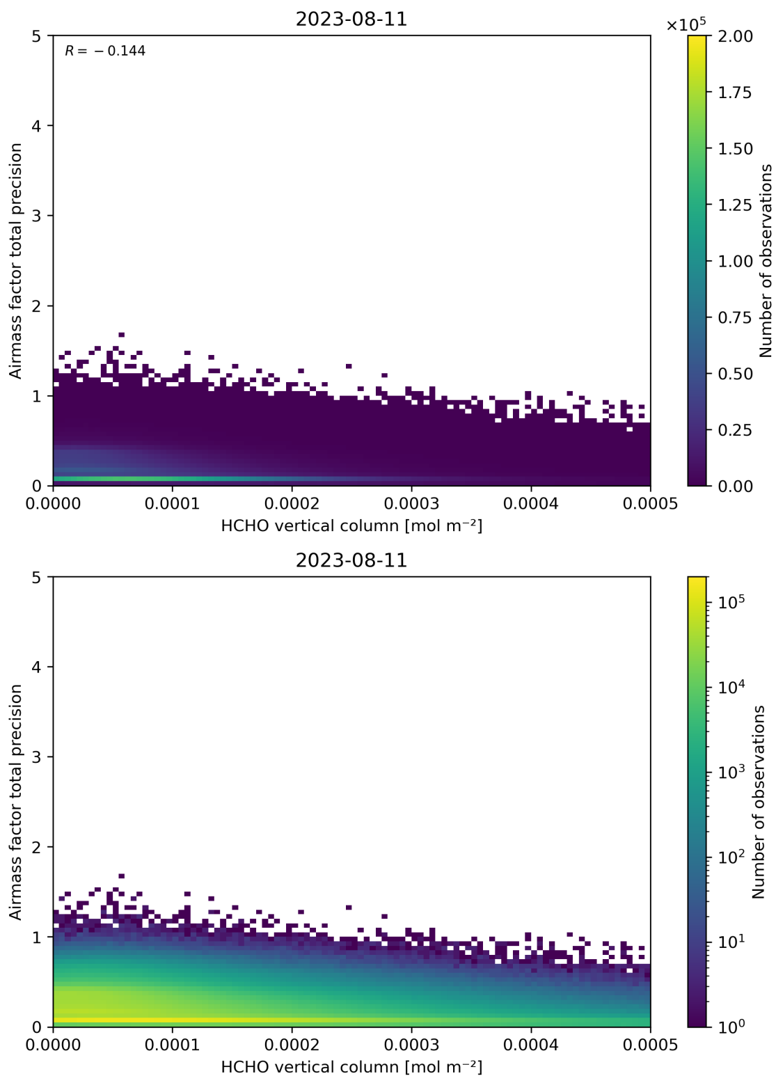
Figure 132: Scatter density plot of “HCHO vertical column” against “Airmass factor total precision” for 2023-08-10 to 2023-08-12.
