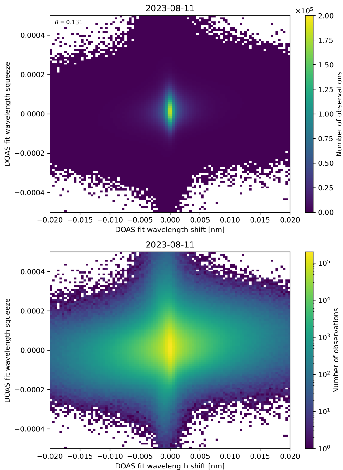
Figure 65: Scatter density plot of “DOAS fit wavelength shift” against “DOAS fit wavelength squeeze” for 2023-08-10 to 2023-08-12.
