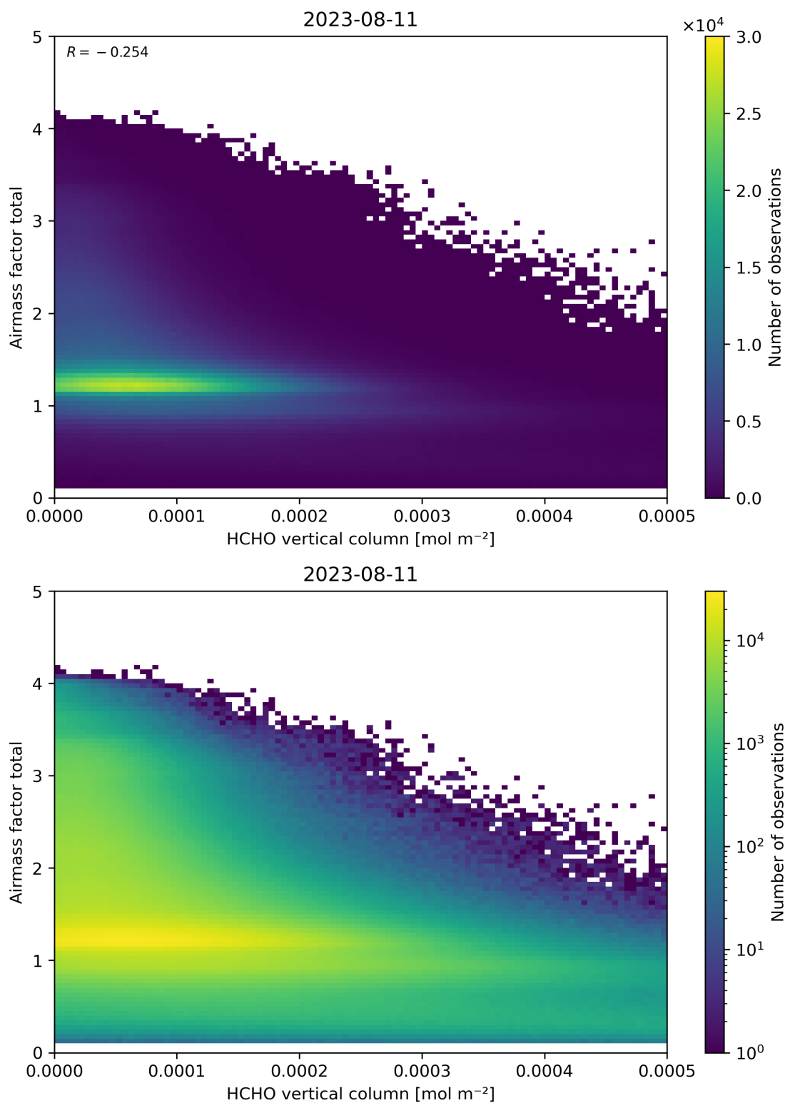
Figure 131: Scatter density plot of “HCHO vertical column” against “Airmass factor total” for 2023-08-10 to 2023-08-12.
