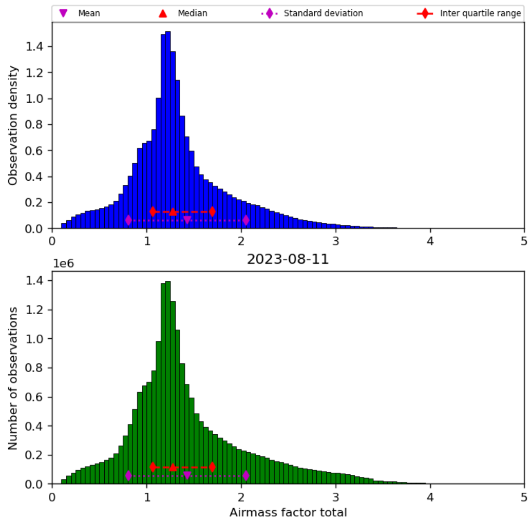
Figure 40: Histogram of “Airmass factor total” for 2023-08-10 to 2023-08-12
