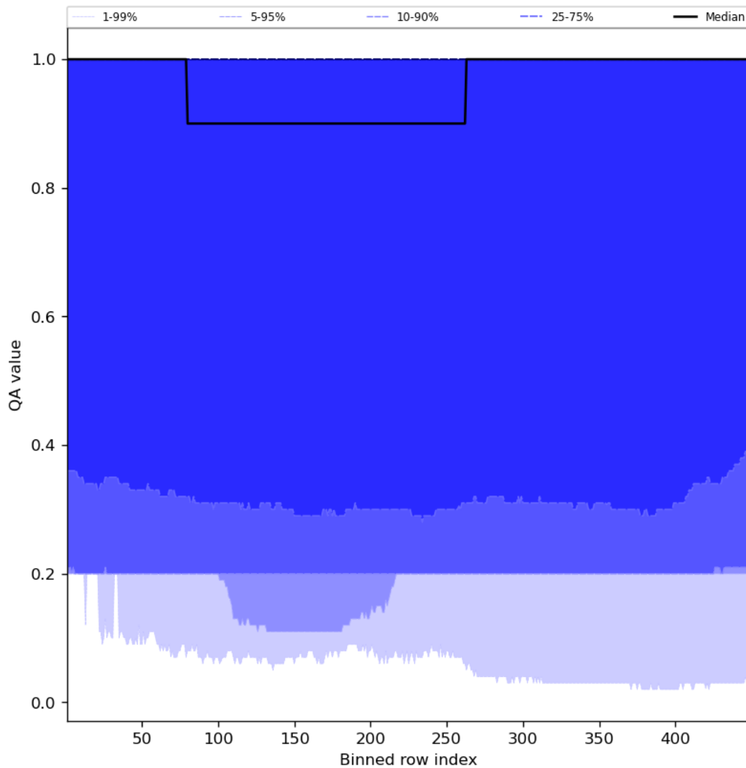
Figure 48: Along track statistics of “QA value” for 2023-08-10 to 2023-08-12
