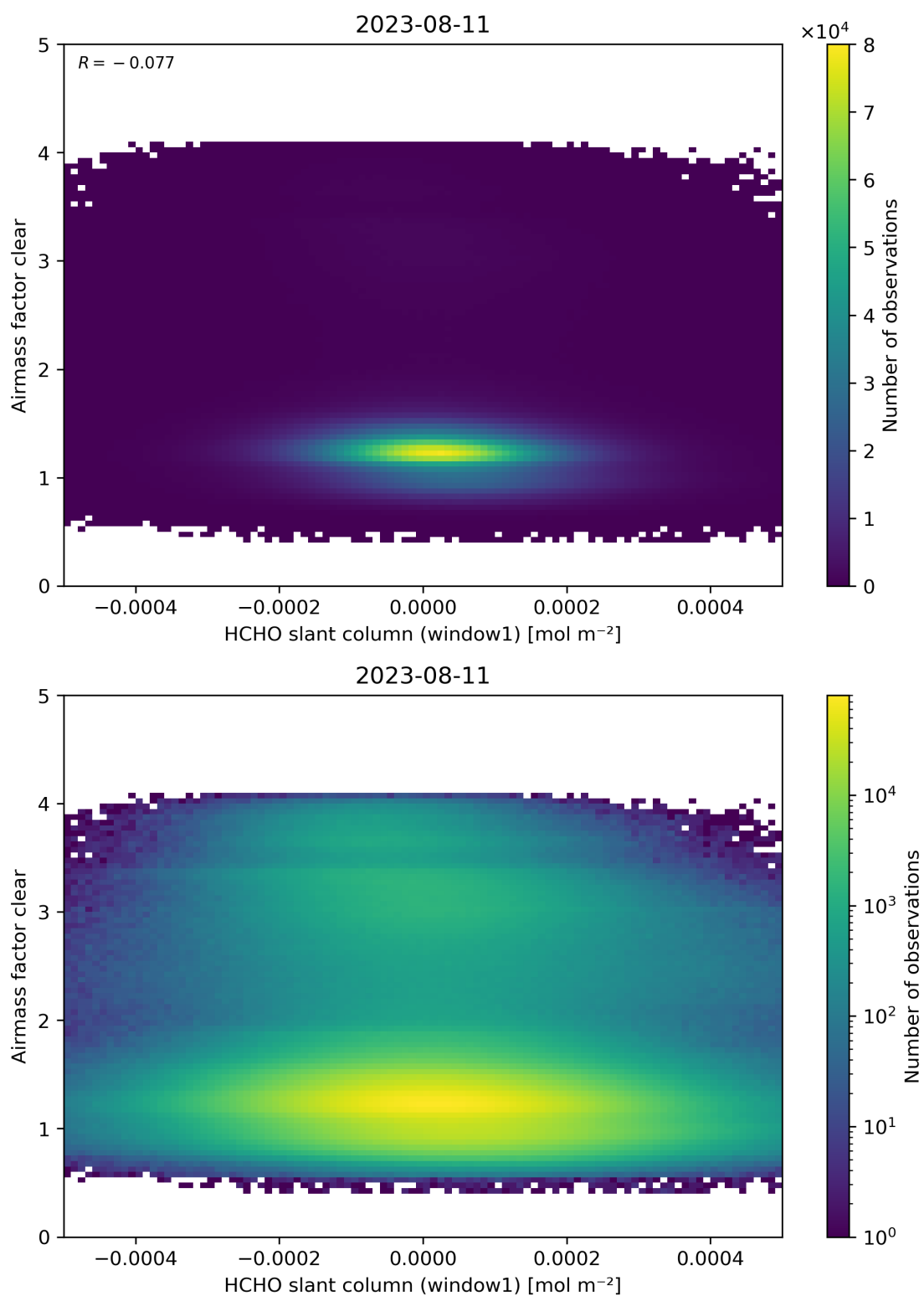
Figure 81: Scatter density plot of “HCHO slant column (window1)” against “Airmass factor clear” for 2023-08-10 to 2023-08-12.
