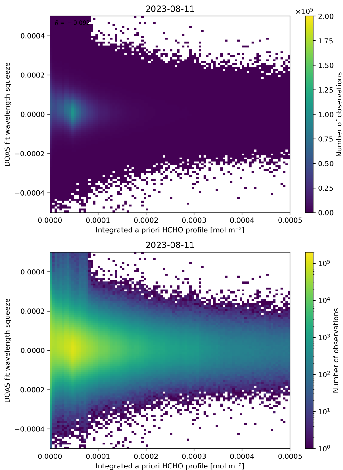
Figure 150: Scatter density plot of “Integrated a priori HCHO profile” against “DOAS fit wavelength squeeze” for 2023-08-10 to 2023-08-12.
