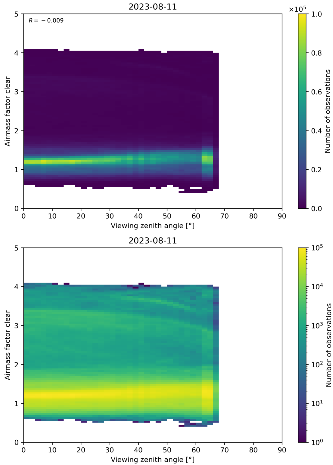
Figure 185: Scatter density plot of “Viewing zenith angle” against “Airmass factor clear” for 2023-08-10 to 2023-08-12.
