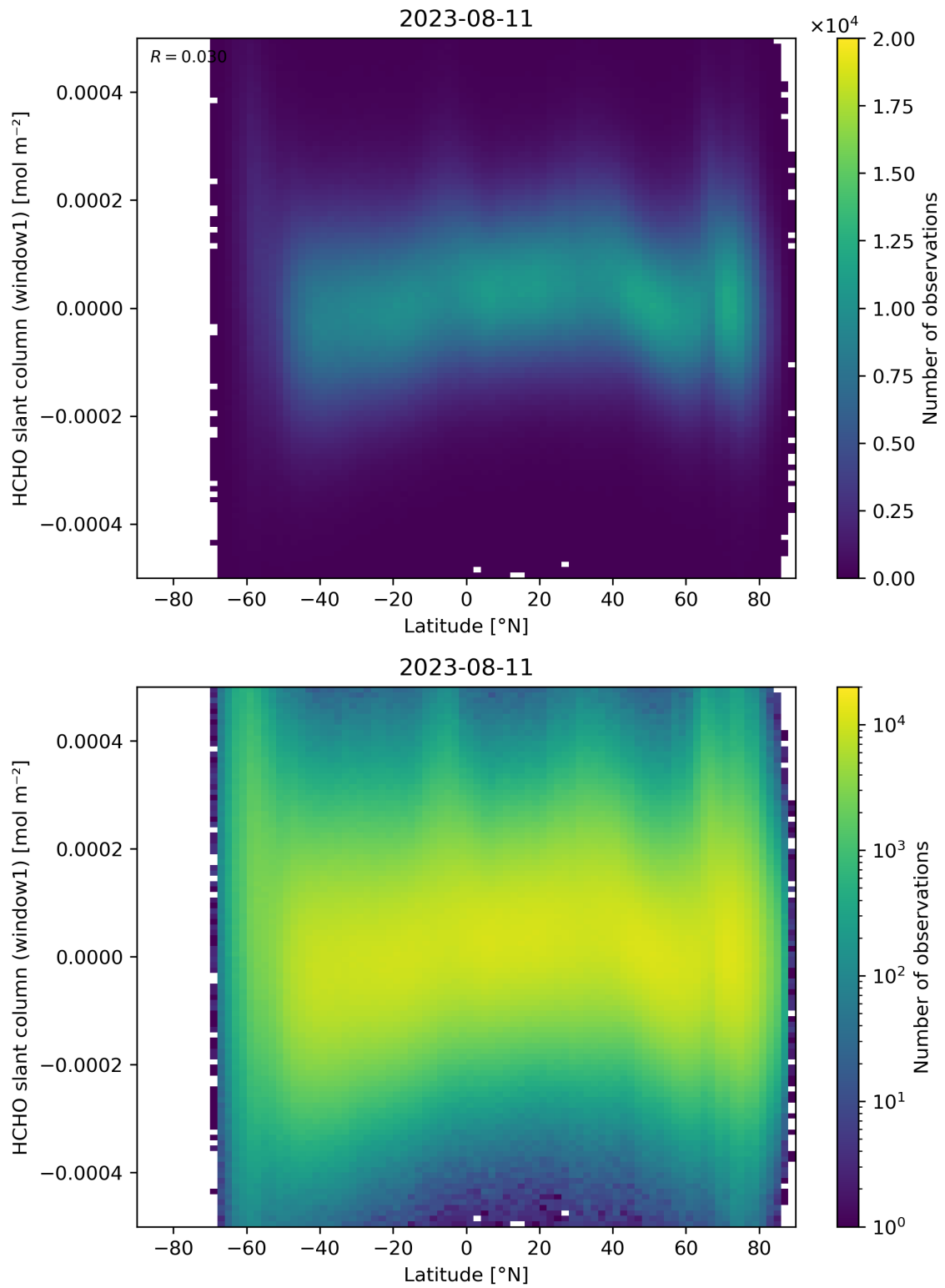
Figure 159: Scatter density plot of “Latitude” against “HCHO slant column (window1)” for 2023-08-10 to 2023-08-12.
