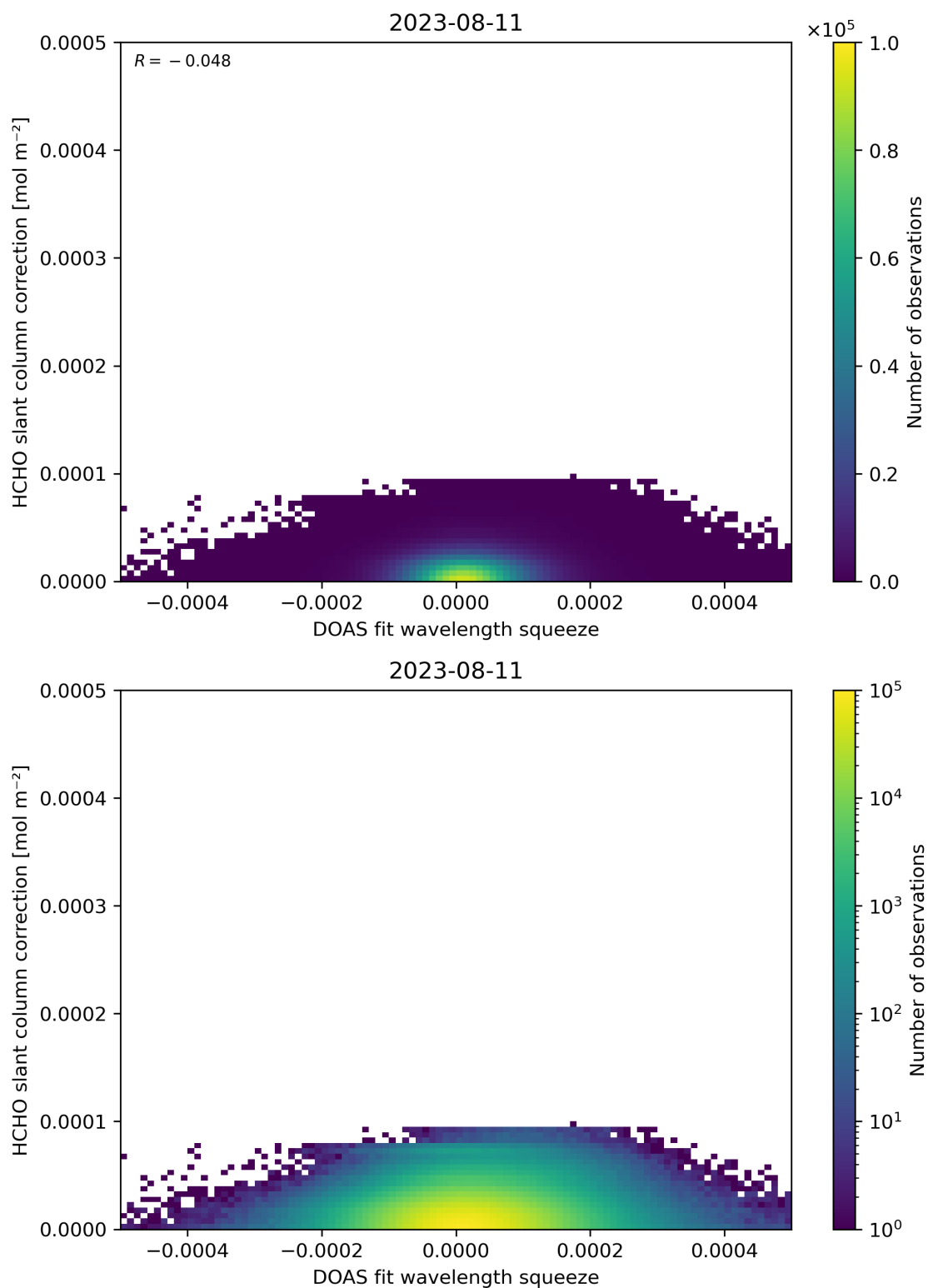
Figure 70: Scatter density plot of “DOAS fit wavelength squeeze” against “HCHO slant column correction” for 2023-08-10 to 2023-08-12.
