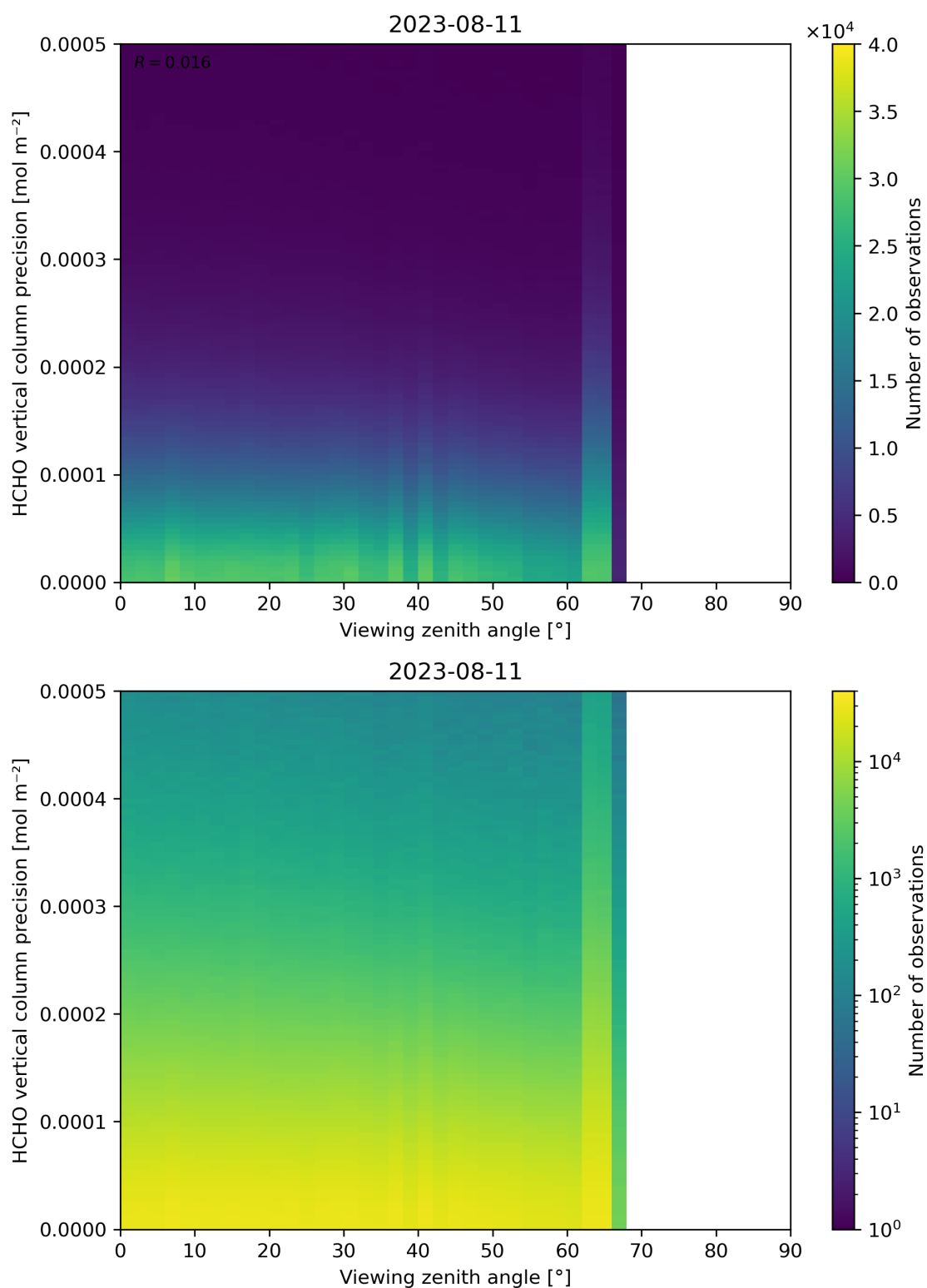
Figure 194: Scatter density plot of “Viewing zenith angle” against “HCHO vertical column precision” for 2023-08-10 to 2023-08-12.
