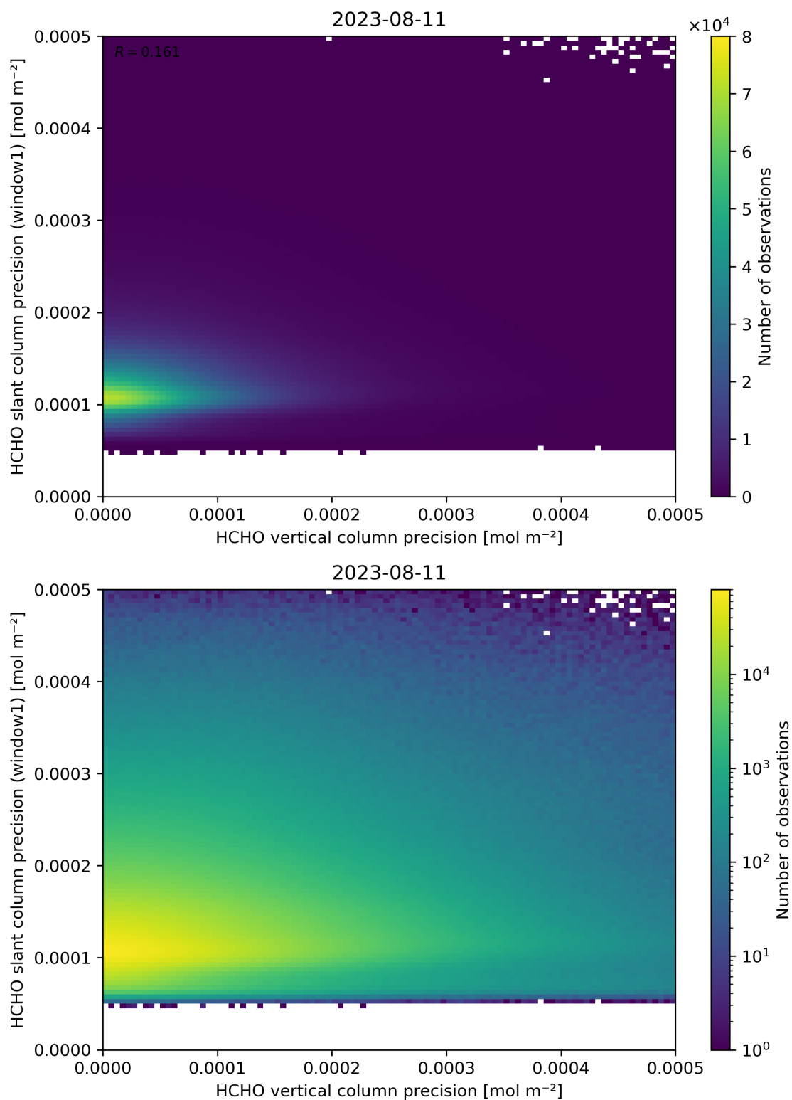
Figure 143: Scatter density plot of “HCHO vertical column precision” against “HCHO slant column precision (window1)” for 2023-08-10 to 2023-08-12.
