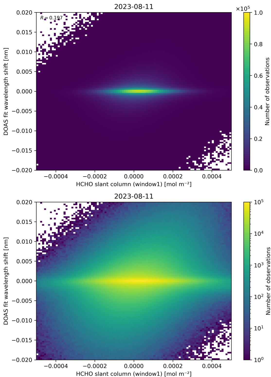
Figure 79: Scatter density plot of “HCHO slant column (window1)” against “DOAS fit wavelength shift” for 2023-08-10 to 2023-08-12.
