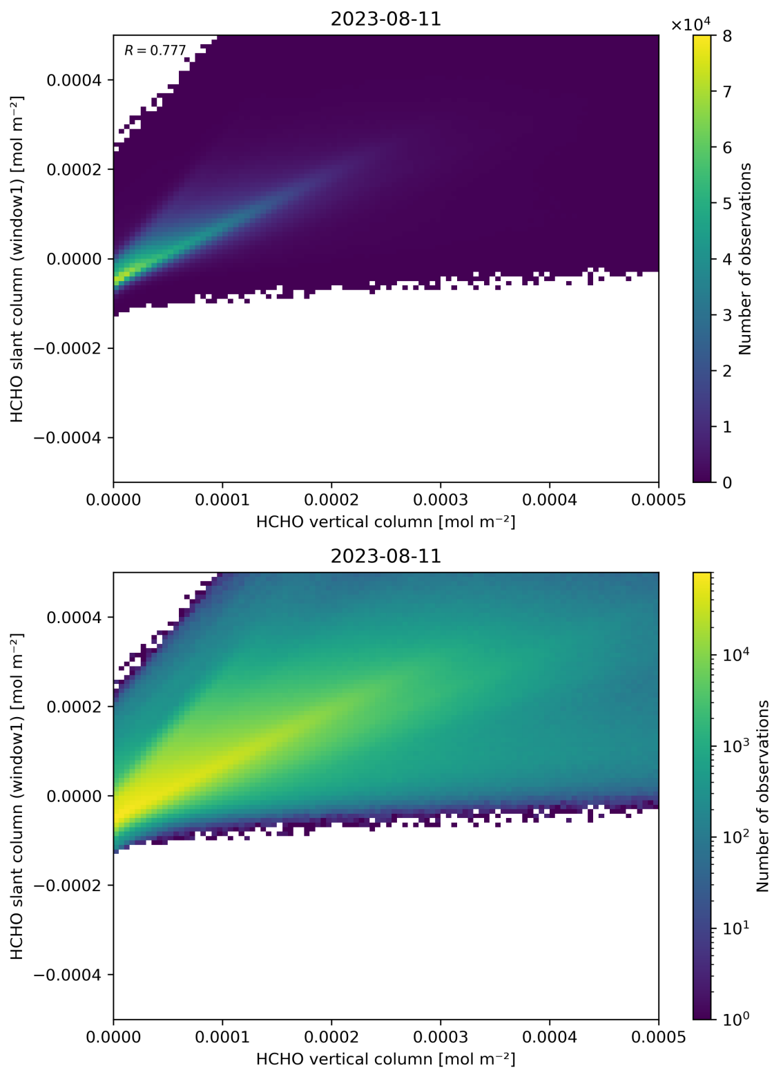
Figure 129: Scatter density plot of “HCHO vertical column” against “HCHO slant column (window1)” for 2023-08-10 to 2023-08-12.
