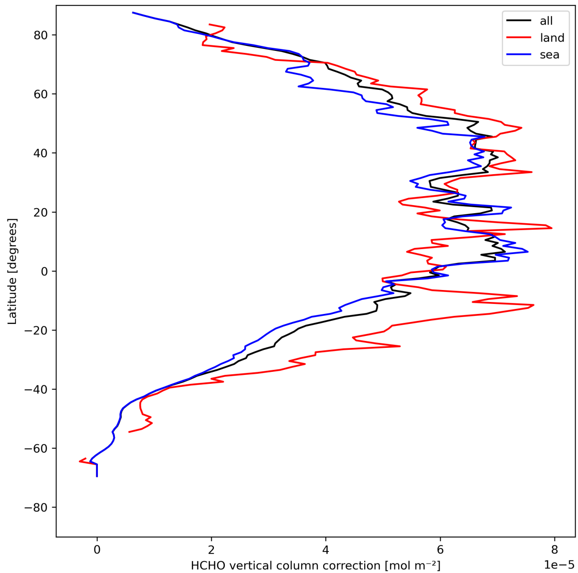
Figure 23: Zonal average of “HCHO vertical column correction” for 2023-08-10 to 2023-08-12.
