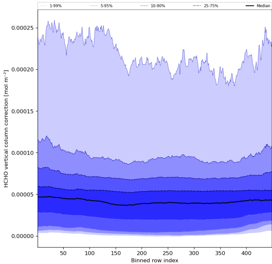
Figure 51: Along track statistics of “HCHO vertical column correction” for 2023-08-10 to 2023-08-12
