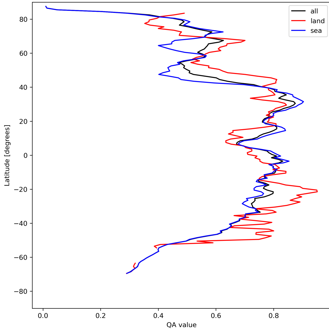
Figure 20: Zonal average of “QA value” for 2023-08-10 to 2023-08-12.
