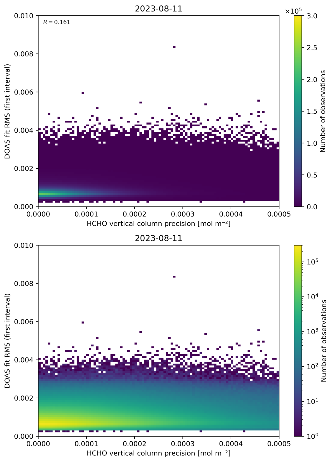
Figure 136: Scatter density plot of “HCHO vertical column precision” against “DOAS fit RMS (first interval)” for 2023-08-10 to 2023-08-12.
