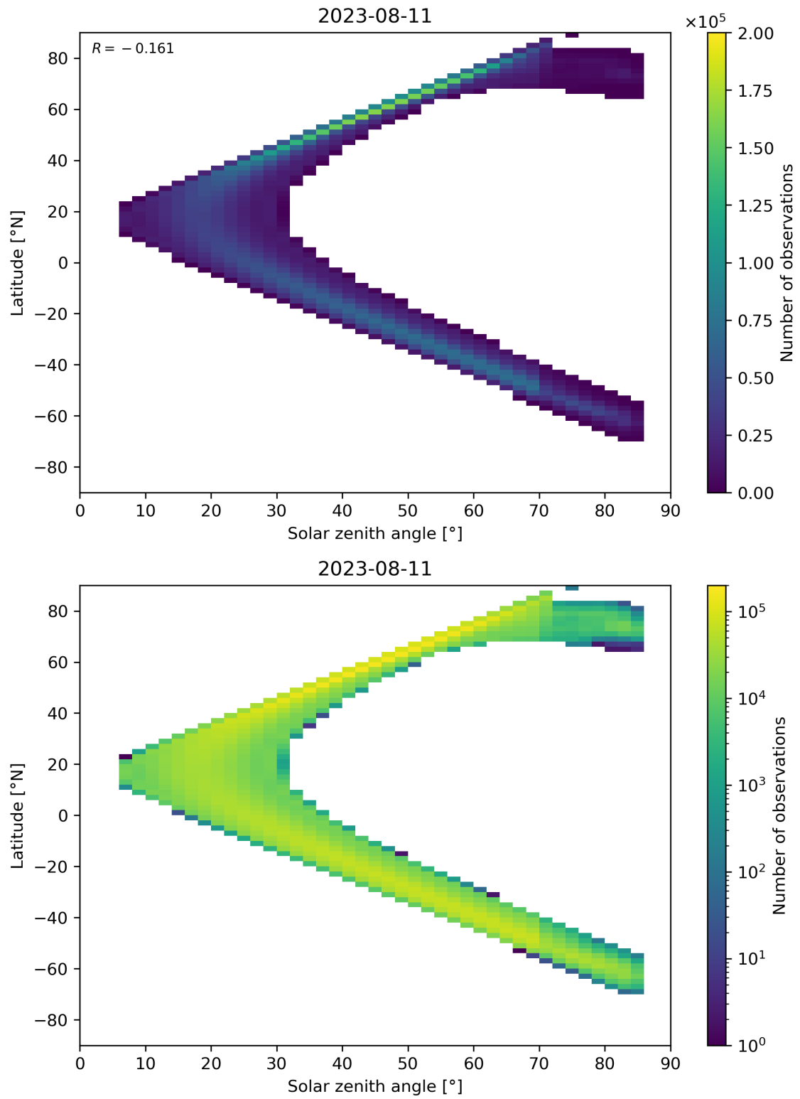
Figure 181: Scatter density plot of “Solar zenith angle” against “Latitude” for 2023-08-10 to 2023-08-12.
