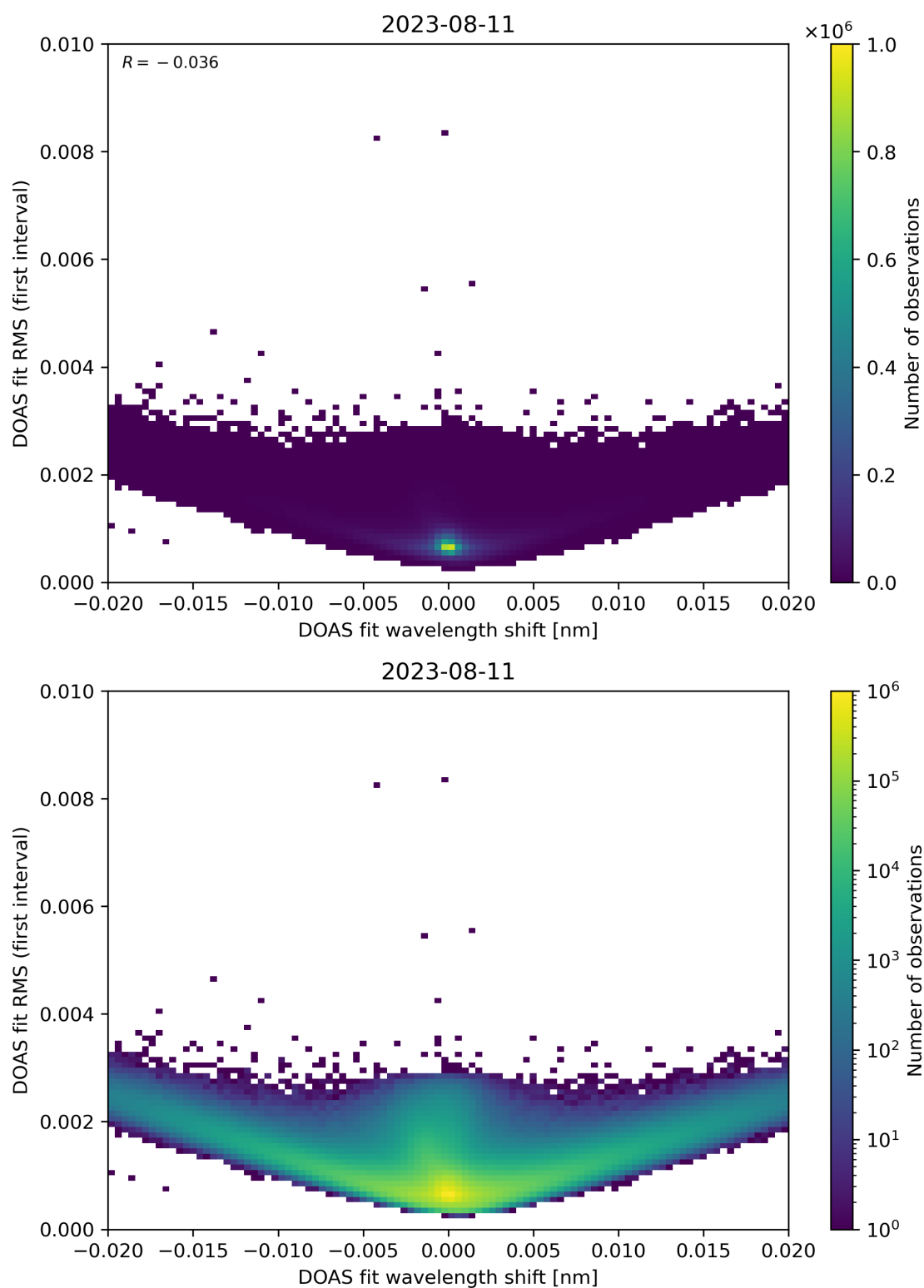
Figure 64: Scatter density plot of “DOAS fit wavelength shift” against “DOAS fit RMS (first interval)” for 2023-08-10 to 2023-08-12.
