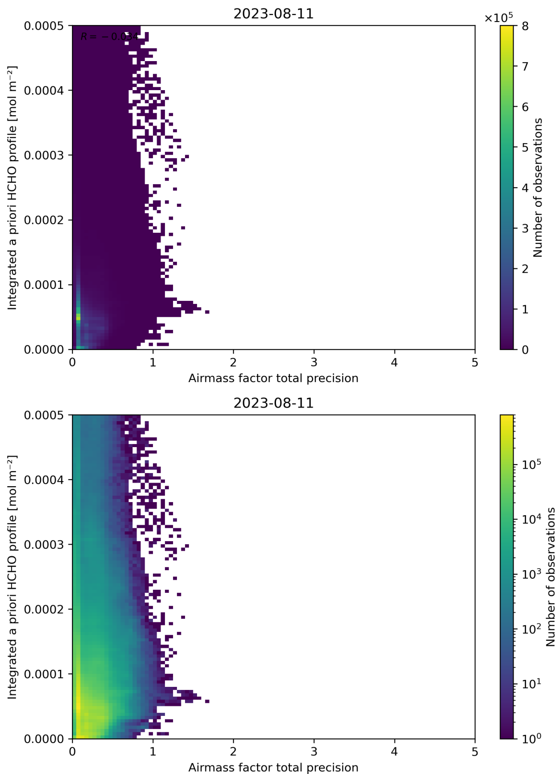
Figure 111: Scatter density plot of “Airmass factor total precision” against “Integrated a priori HCHO profile” for 2023-08-10 to 2023-08-12.
