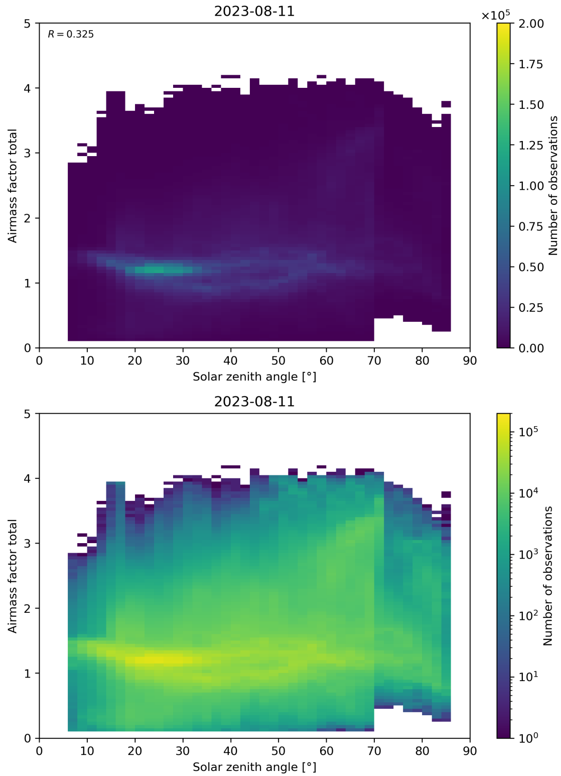
Figure 175: Scatter density plot of “Solar zenith angle” against “Airmass factor total” for 2023-08-10 to 2023-08-12.
