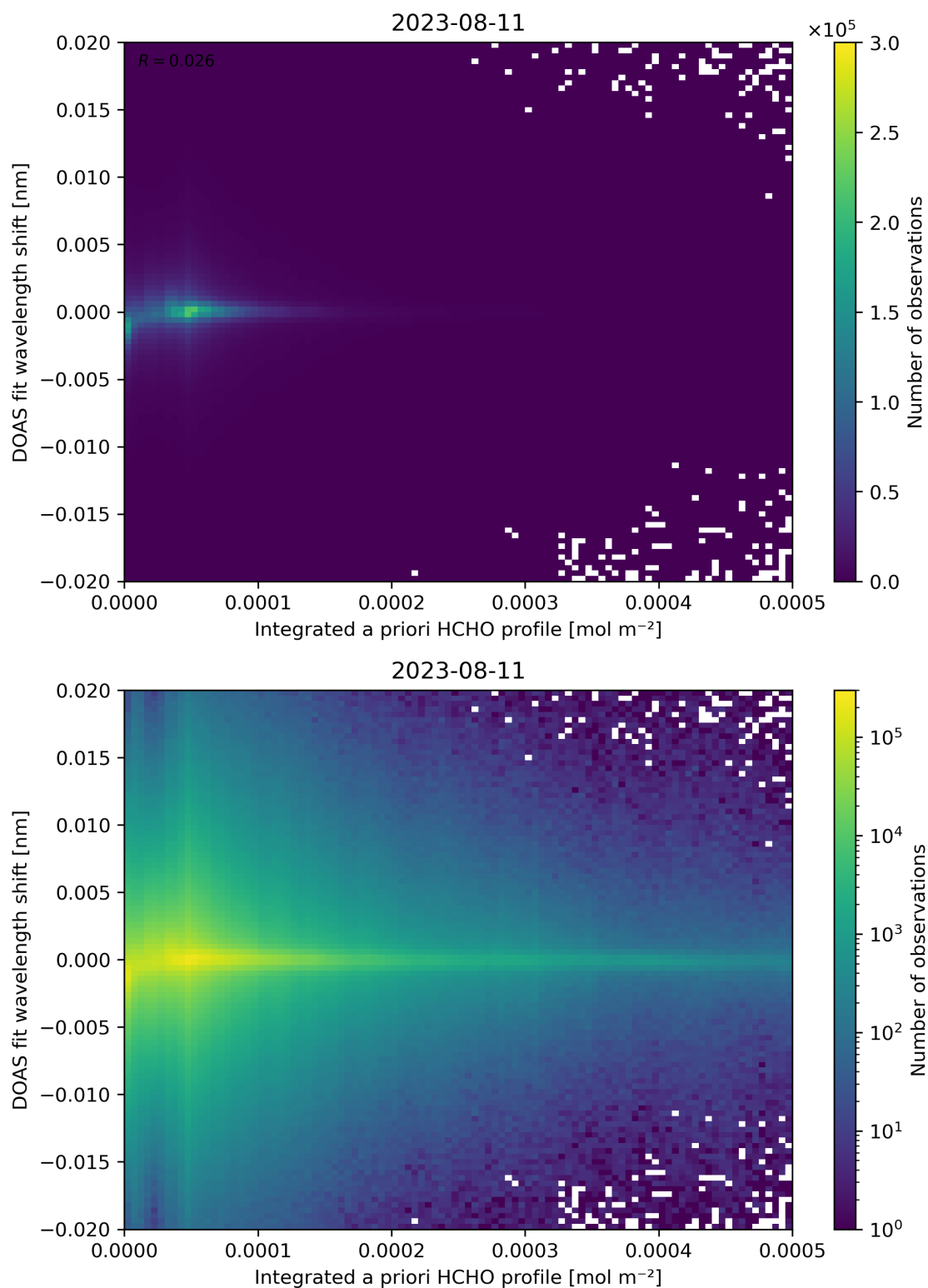
Figure 149: Scatter density plot of “Integrated a priori HCHO profile” against “DOAS fit wavelength shift” for 2023-08-10 to 2023-08-12.
