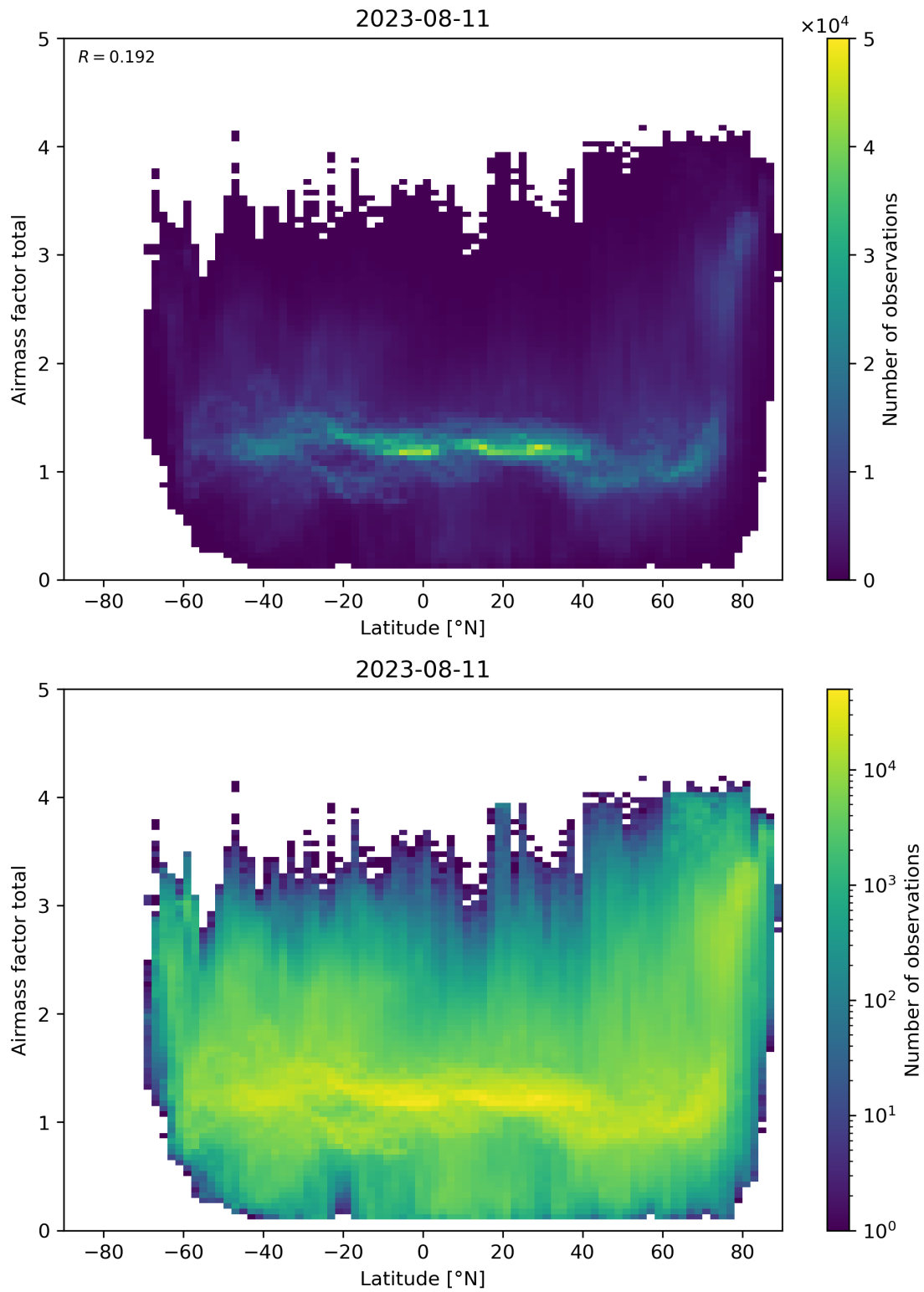
Figure 161: Scatter density plot of “Latitude” against “Airmass factor total” for 2023-08-10 to 2023-08-12.
