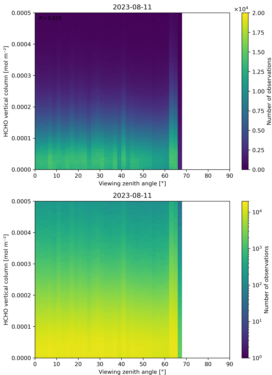
Figure 192: Scatter density plot of “Viewing zenith angle” against “HCHO vertical column” for 2023-08-10 to 2023-08-12.
