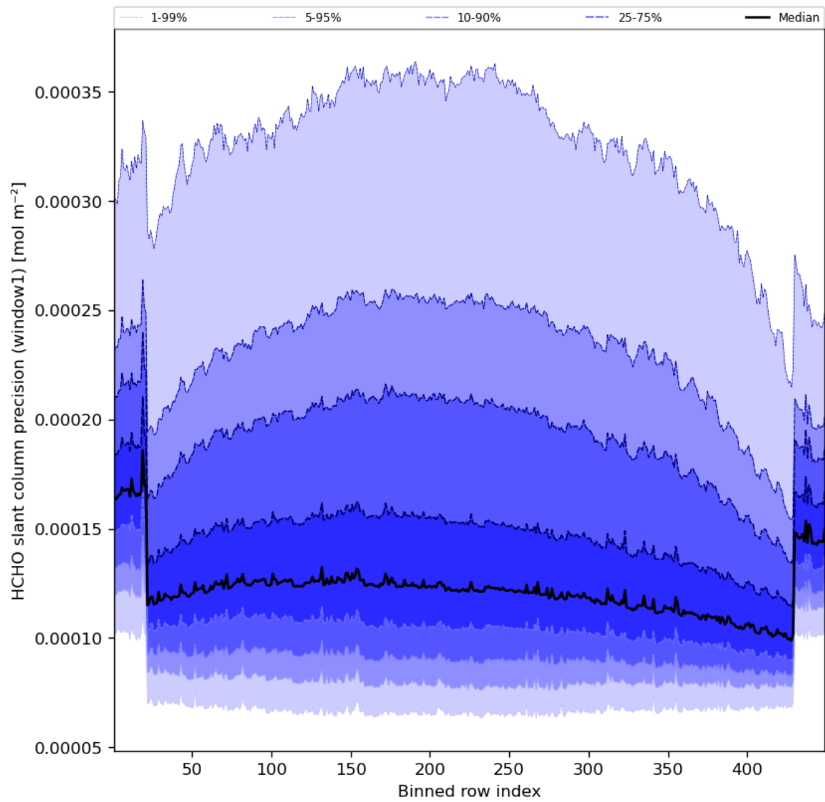
Figure 53: Along track statistics of “HCHO slant column precision (window1)” for 2023-08-10 to 2023-08-12
