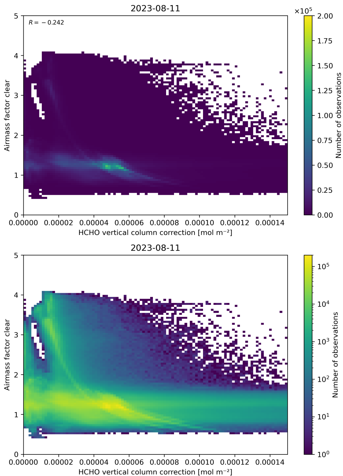
Figure 115: Scatter density plot of “HCHO vertical column correction” against “Airmass factor clear” for 2023-08-10 to 2023-08-12.
