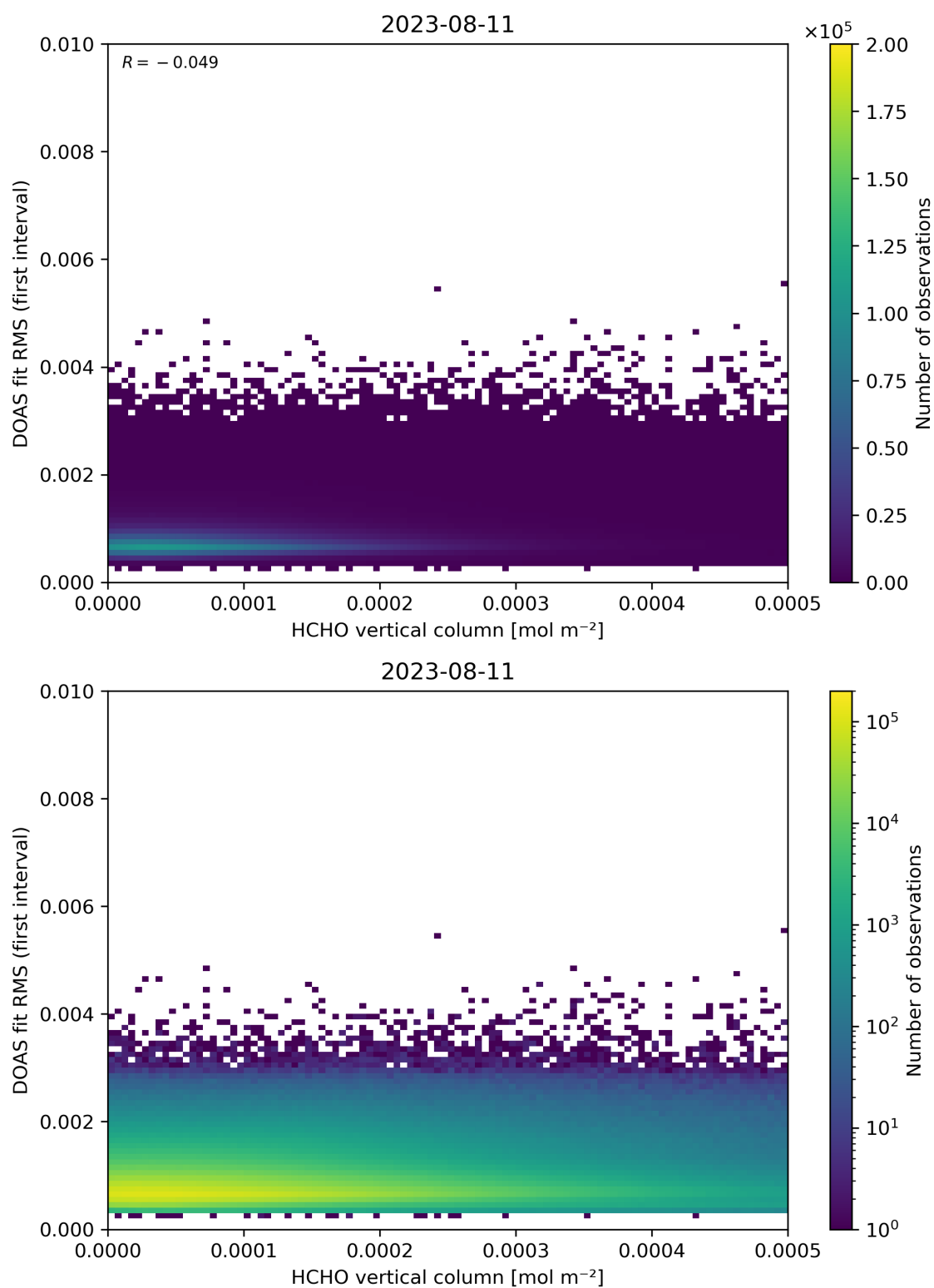
Figure 123: Scatter density plot of “HCHO vertical column” against “DOAS fit RMS (first interval)” for 2023-08-10 to 2023-08-12.
