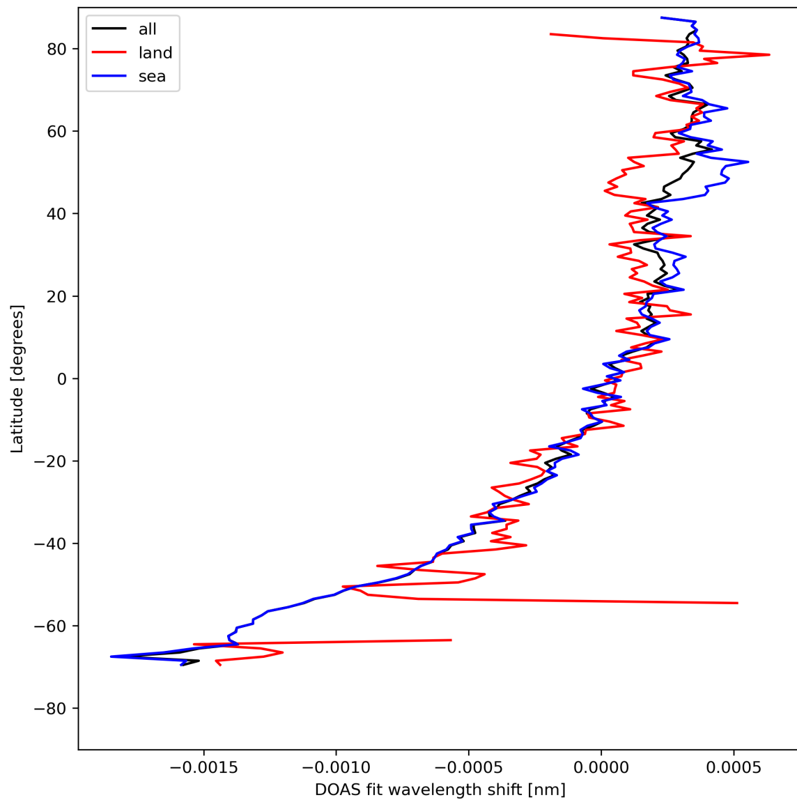
Figure 30: Zonal average of “DOAS fit wavelength shift” for 2023-08-10 to 2023-08-12.
