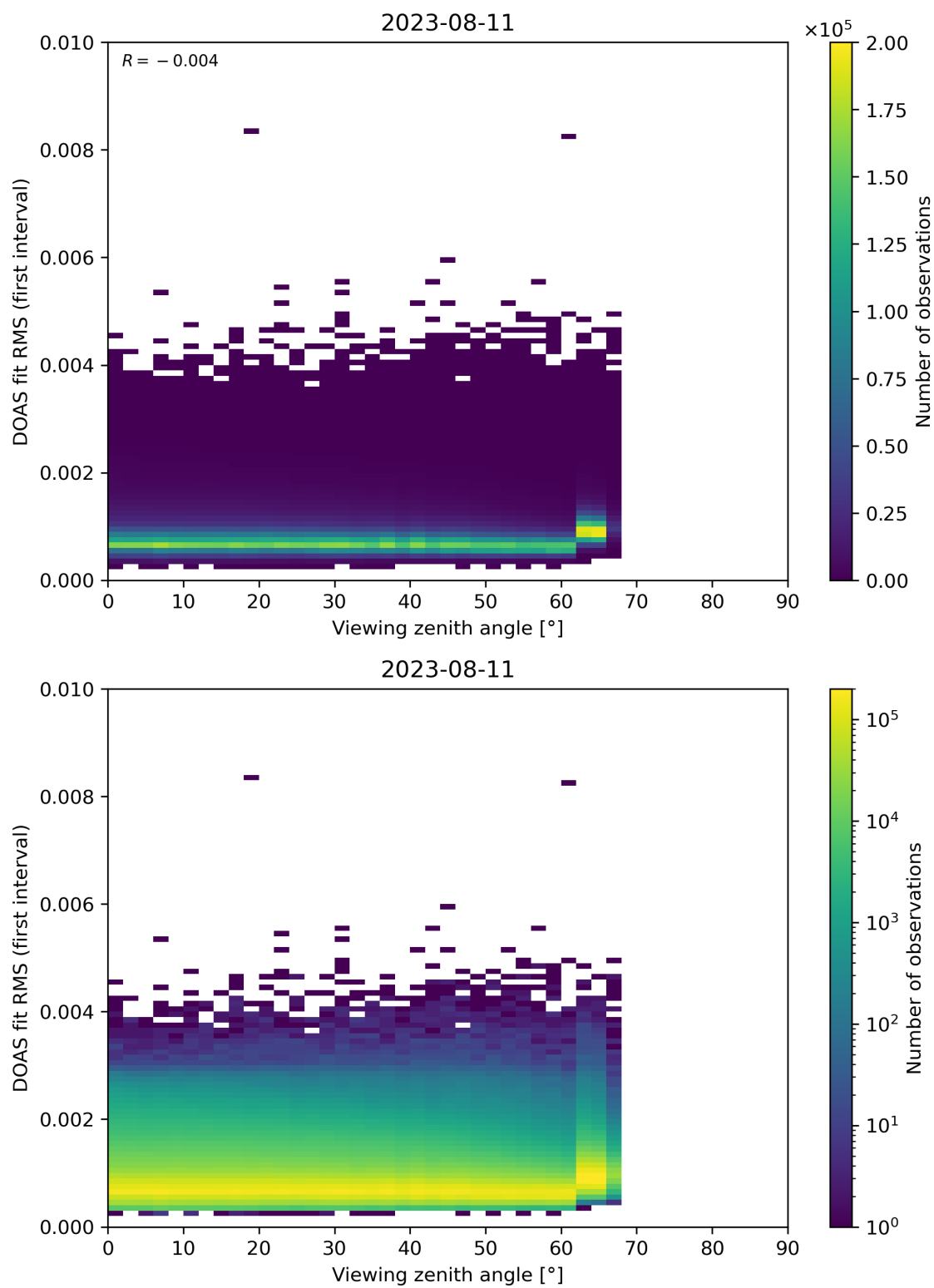
Figure 182: Scatter density plot of “Viewing zenith angle” against “DOAS fit RMS (first interval)” for 2023-08-10 to 2023-08-12.
