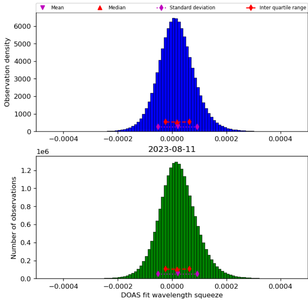
Figure 45: Histogram of “DOAS fit wavelength squeeze” for 2023-08-10 to 2023-08-12
