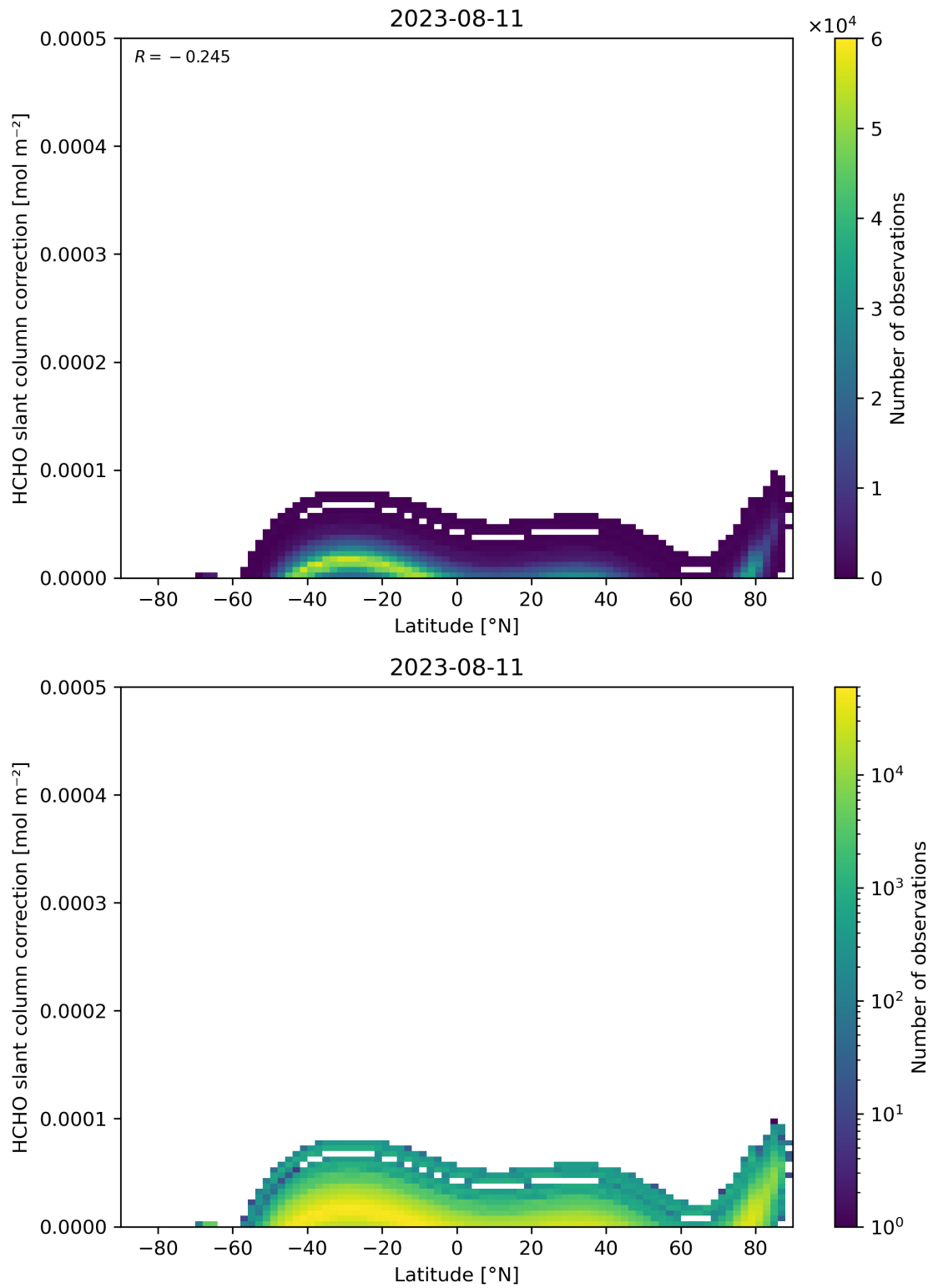
Figure 158: Scatter density plot of “Latitude” against “HCHO slant column correction” for 2023-08-10 to 2023-08-12.
