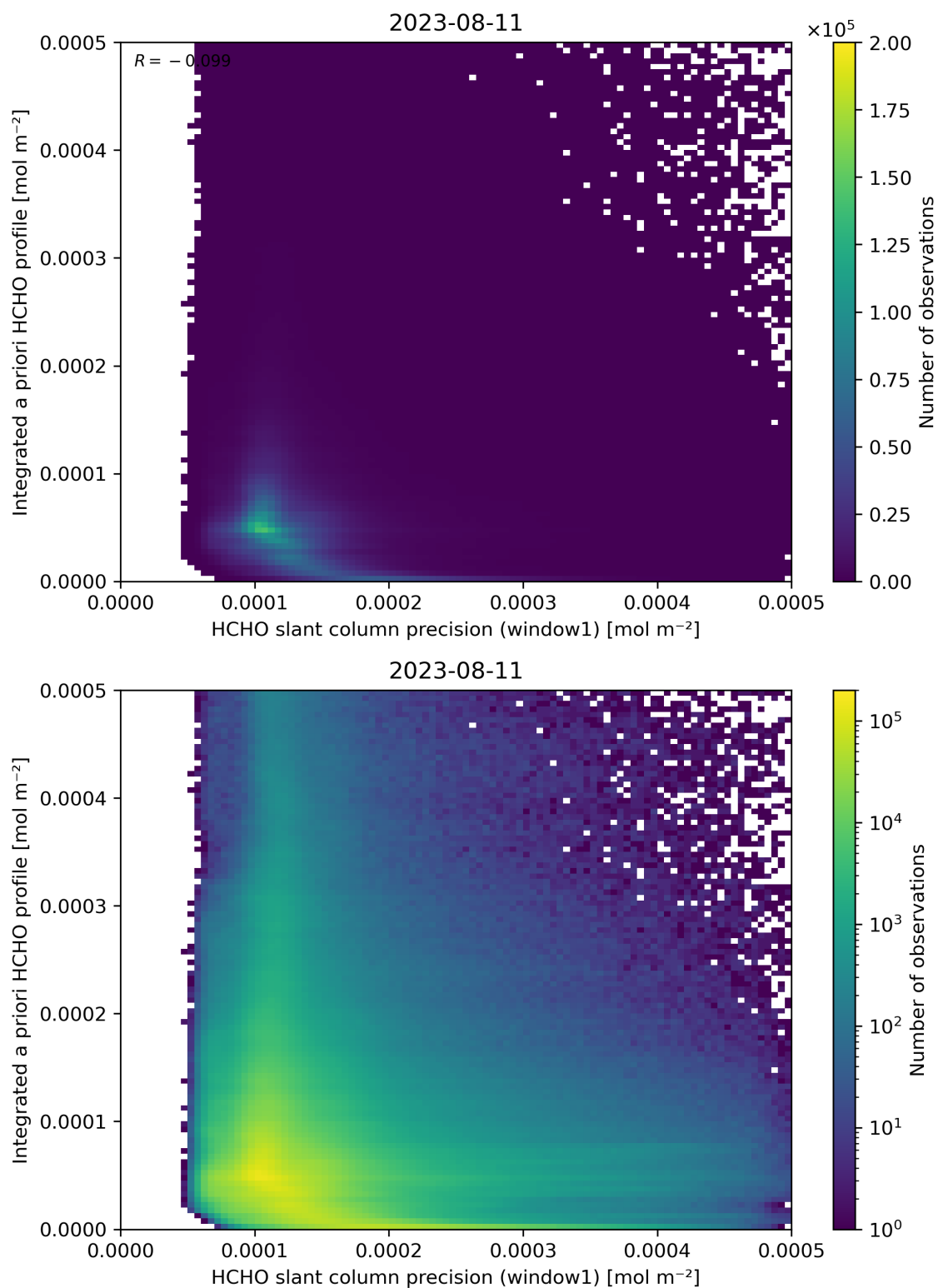
Figure 96: Scatter density plot of “HCHO slant column precision (window1)” against “Integrated a priori HCHO profile” for 2023-08-10 to 2023-08-12.
