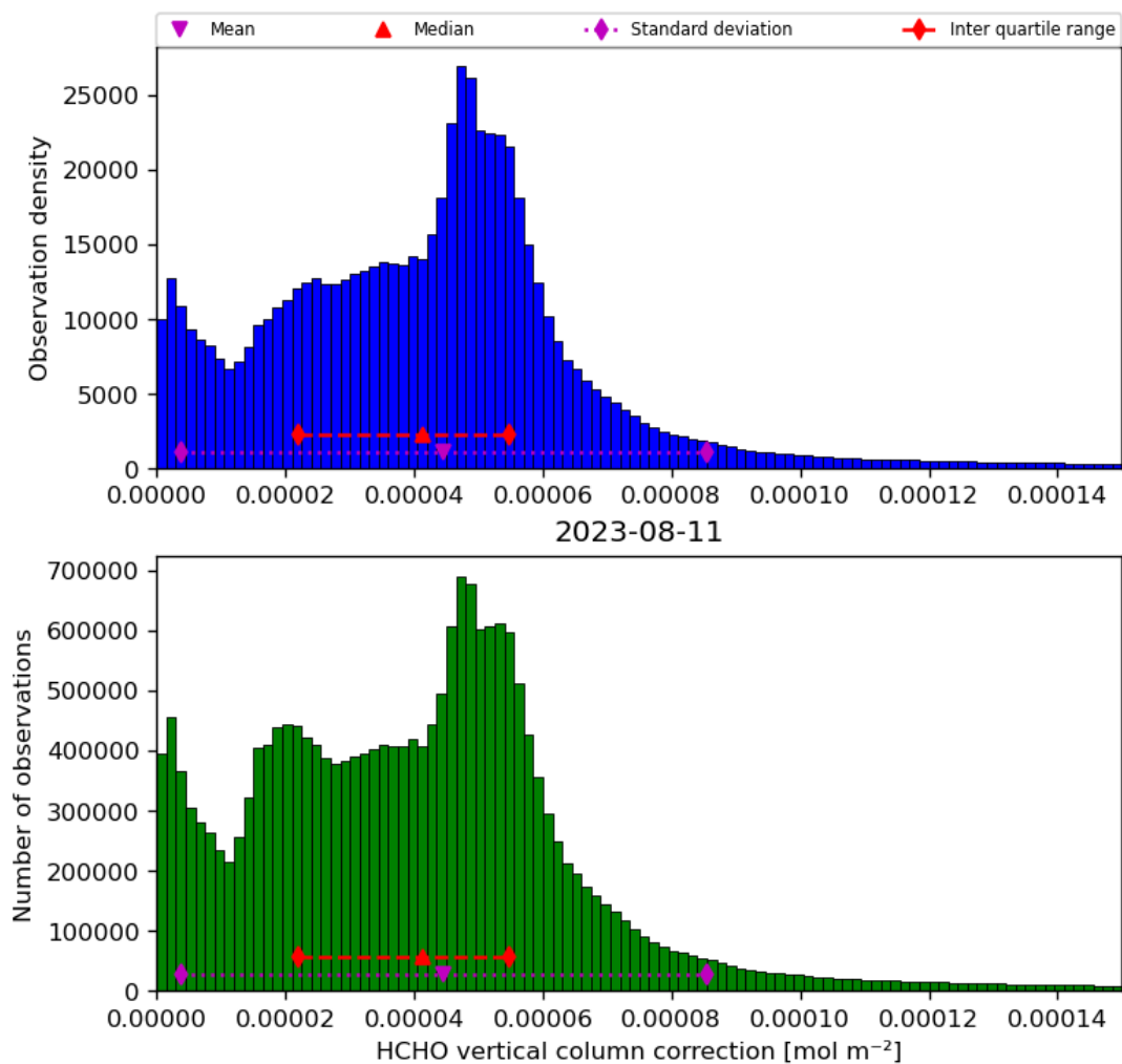
Figure 37: Histogram of “HCHO vertical column correction” for 2023-08-10 to 2023-08-12
