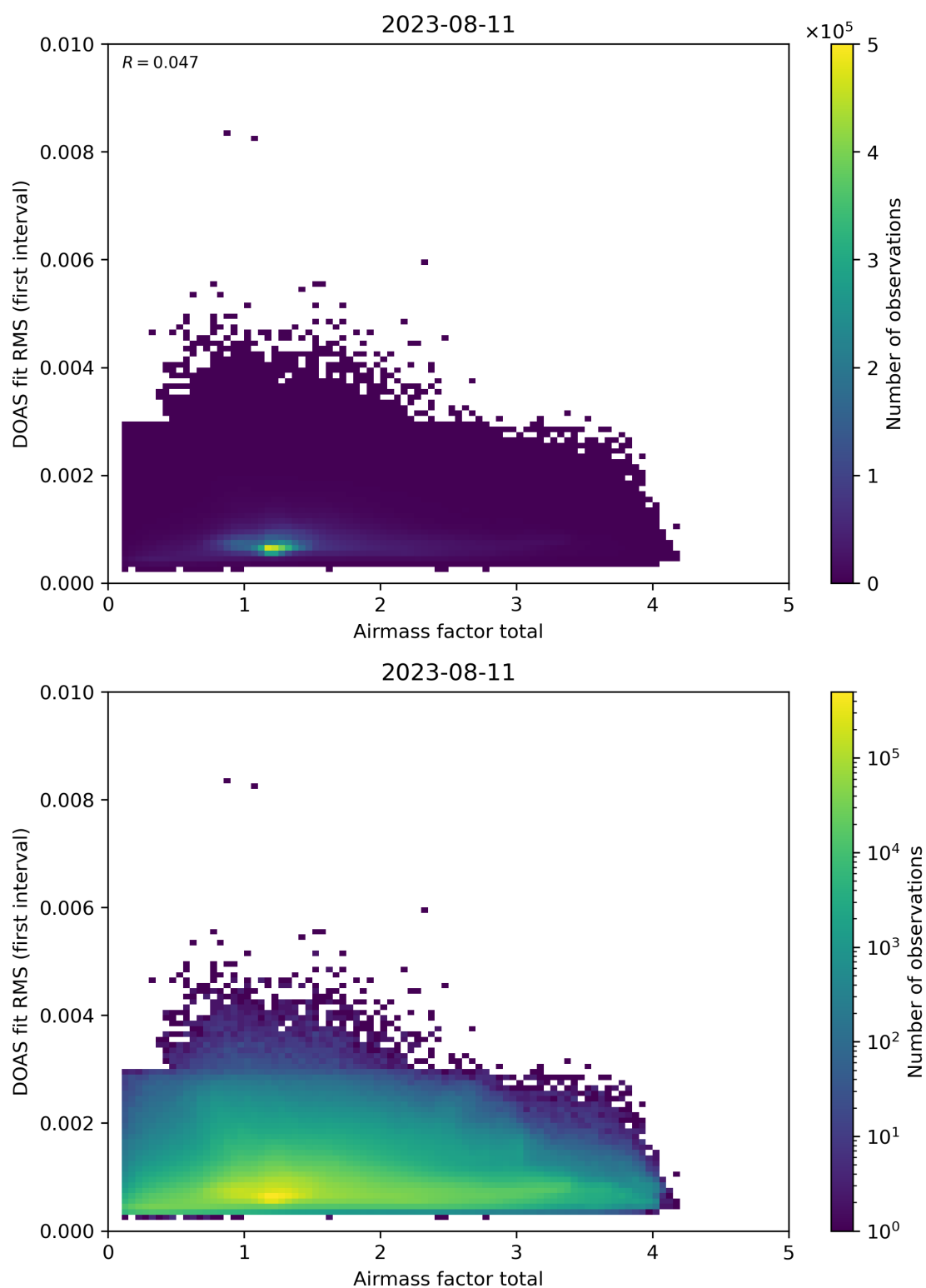
Figure 97: Scatter density plot of “Airmass factor total” against “DOAS fit RMS (first interval)” for 2023-08-10 to 2023-08-12.
