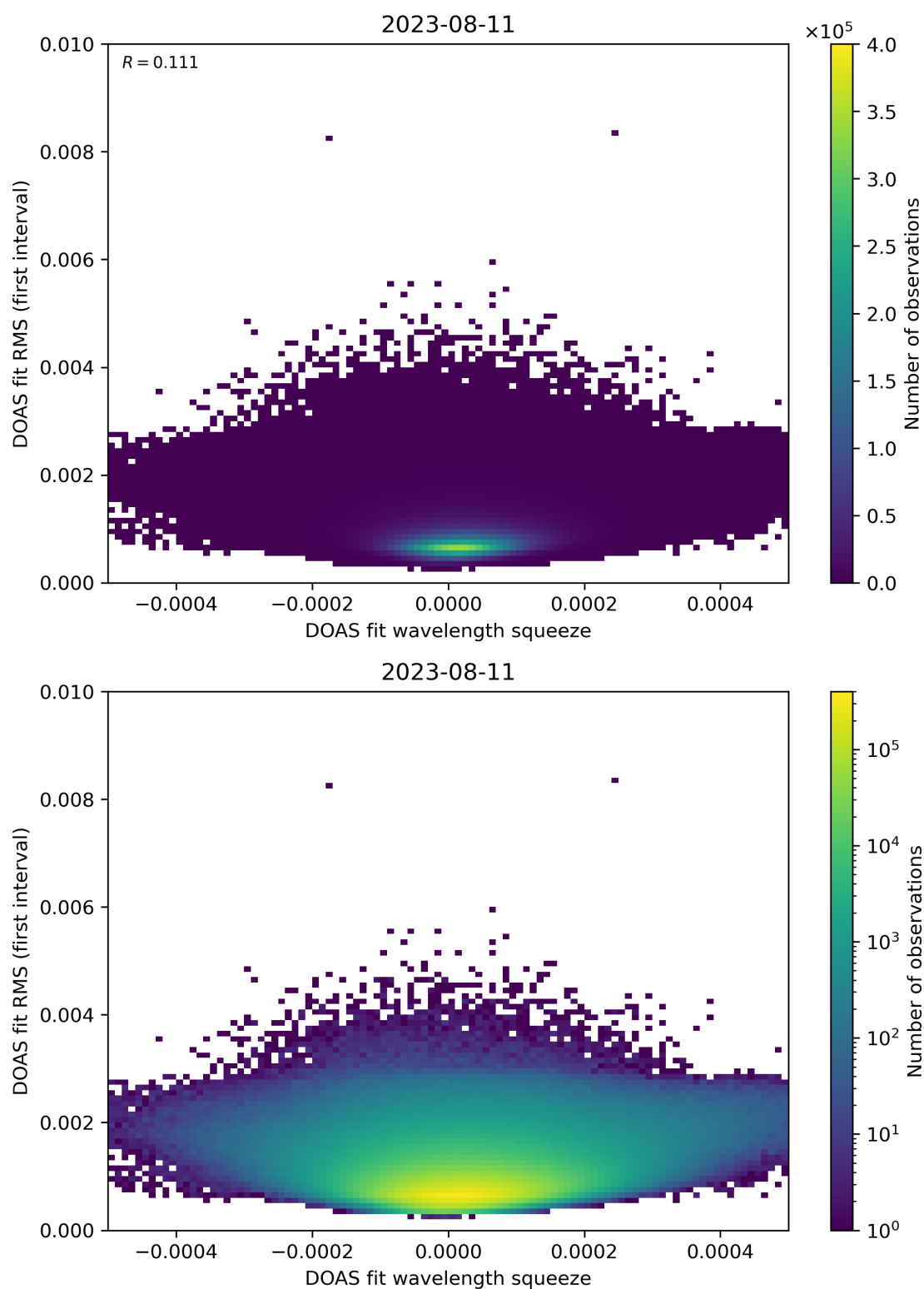
Figure 68: Scatter density plot of “DOAS fit wavelength squeeze” against “DOAS fit RMS (first interval)” for 2023-08-10 to 2023-08-12.
