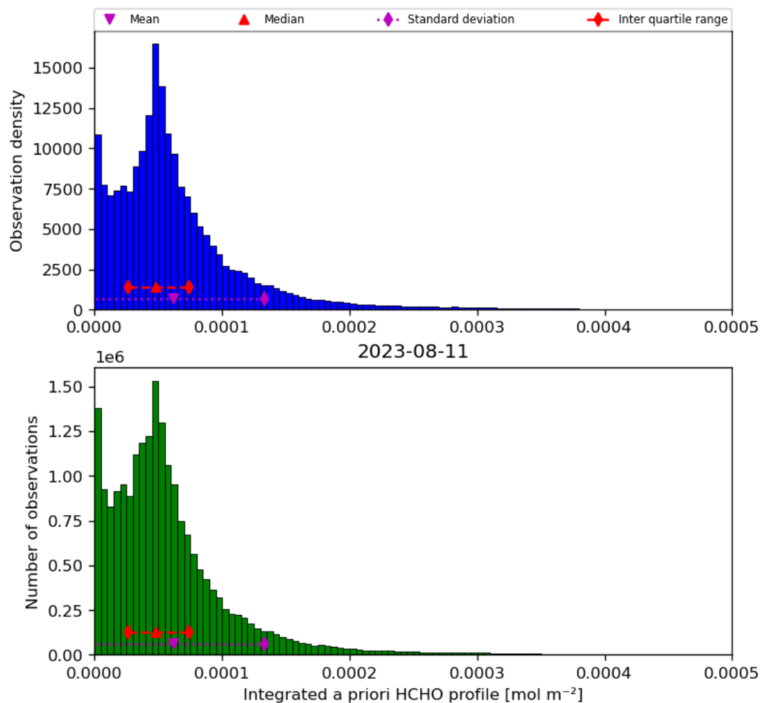
Figure 43: Histogram of “Integrated a priori HCHO profile” for 2023-08-10 to 2023-08-12
