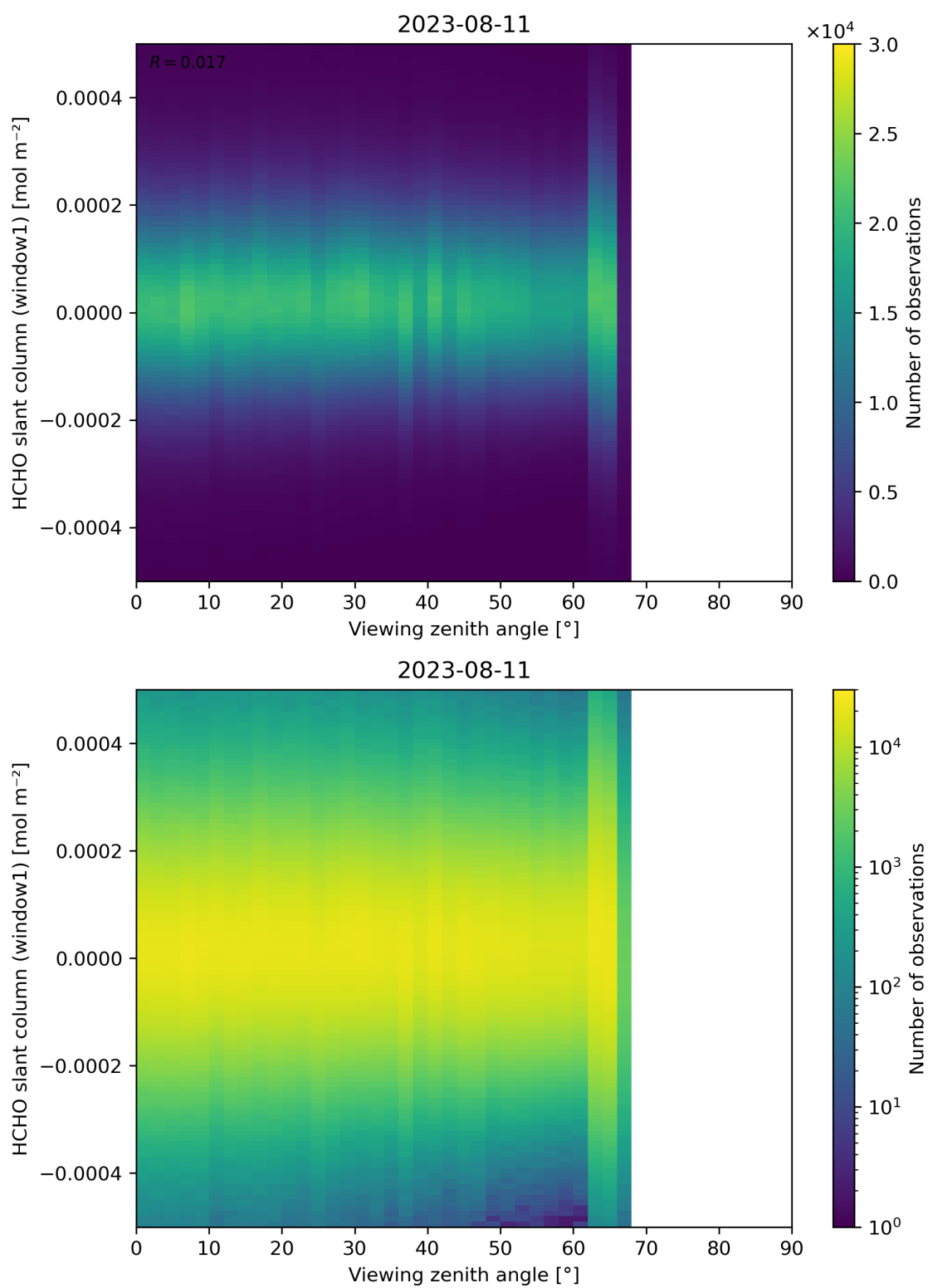
Figure 188: Scatter density plot of “Viewing zenith angle” against “HCHO slant column (window1)” for 2023-08-10 to 2023-08-12.
