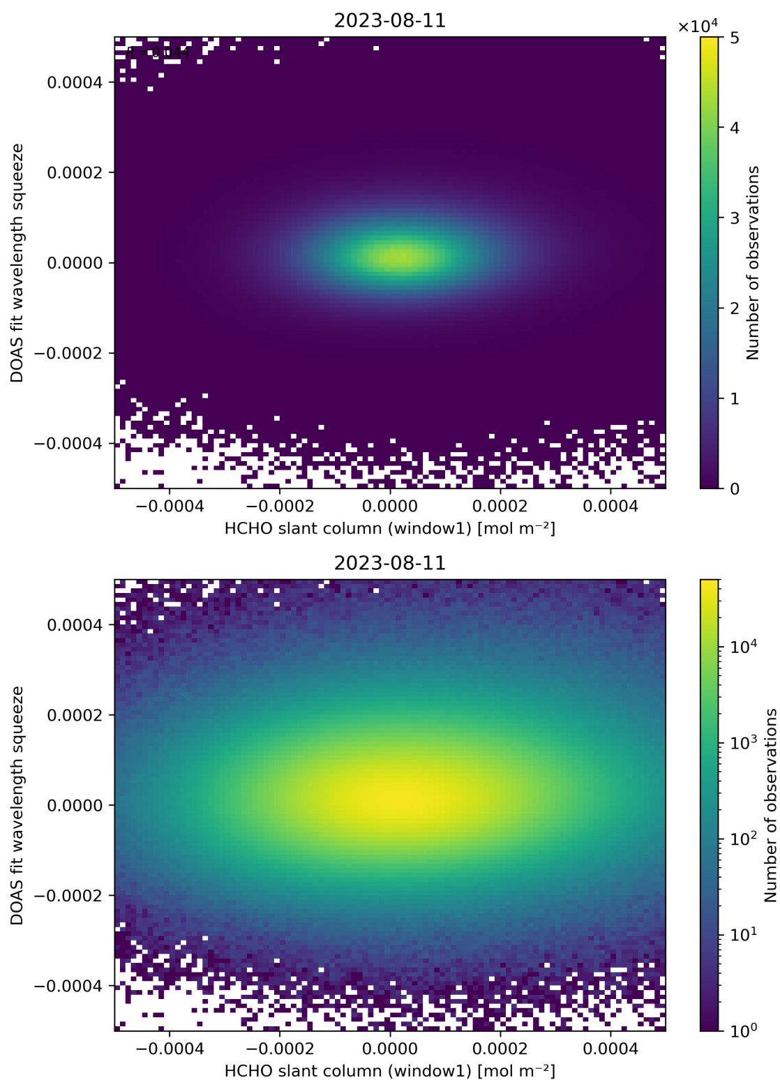
Figure 80: Scatter density plot of “HCHO slant column (window1)” against “DOAS fit wavelength squeeze” for 2023-08-10 to 2023-08-12.
