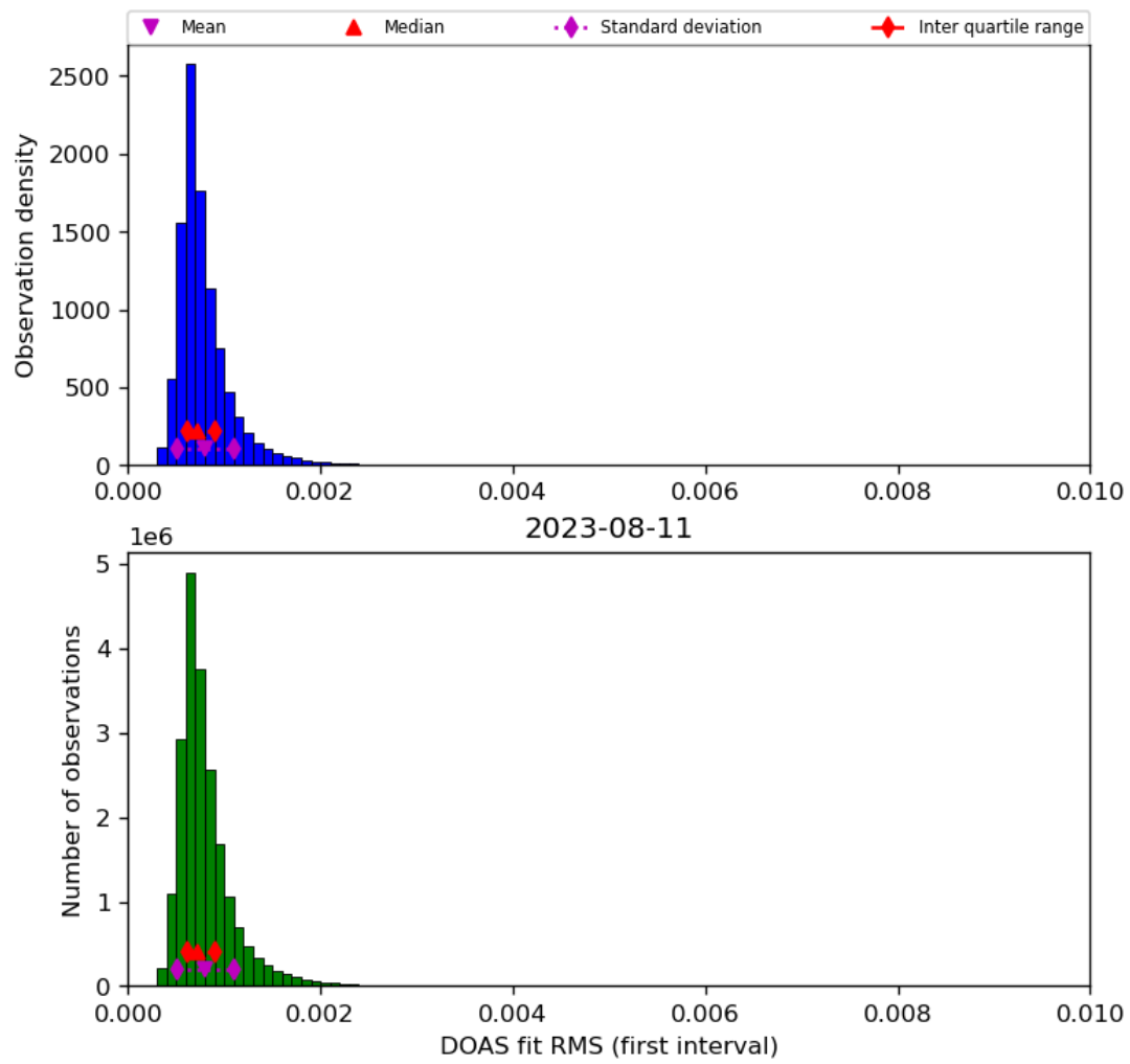
Figure 46: Histogram of “DOAS fit RMS (first interval)” for 2023-08-10 to 2023-08-12
