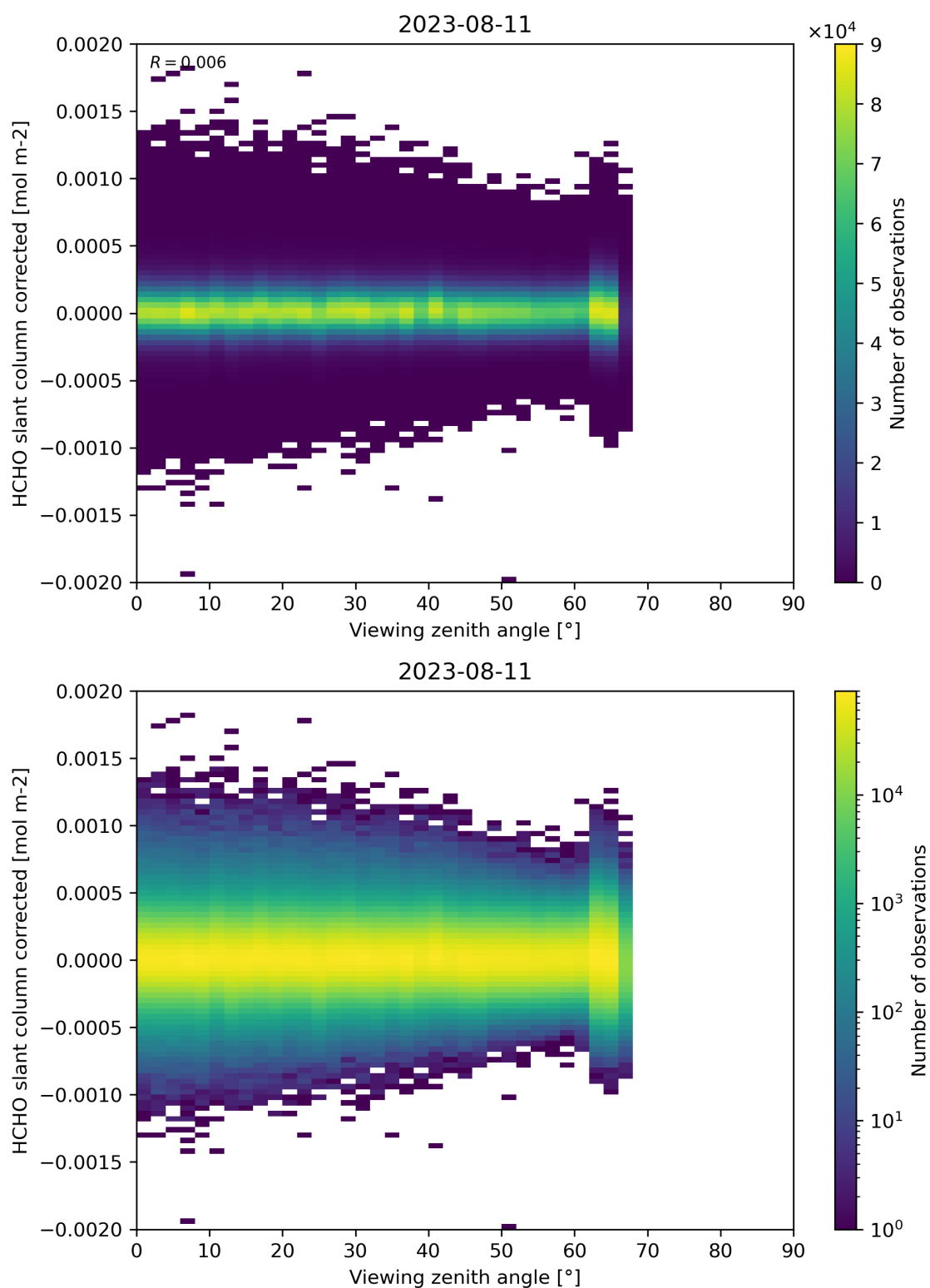
Figure 186: Scatter density plot of “Viewing zenith angle” against “HCHO slant column corrected” for 2023-08-10 to 2023-08-12.
