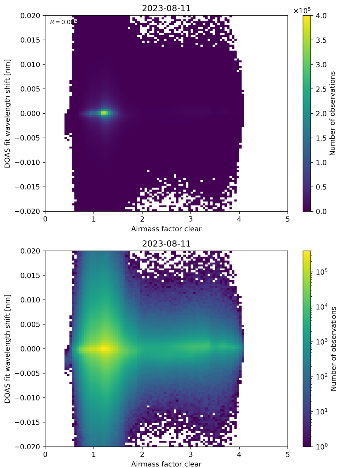
Figure 72: Scatter density plot of “Airmass factor clear” against “DOAS fit wavelength shift” for 2023-08-10 to 2023-08-12.
