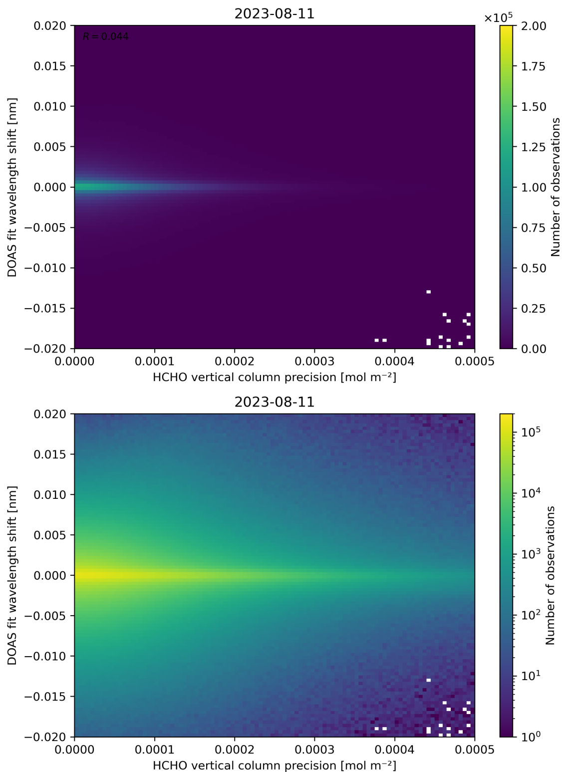
Figure 137: Scatter density plot of “HCHO vertical column precision” against “DOAS fit wavelength shift” for 2023-08-10 to 2023-08-12.
