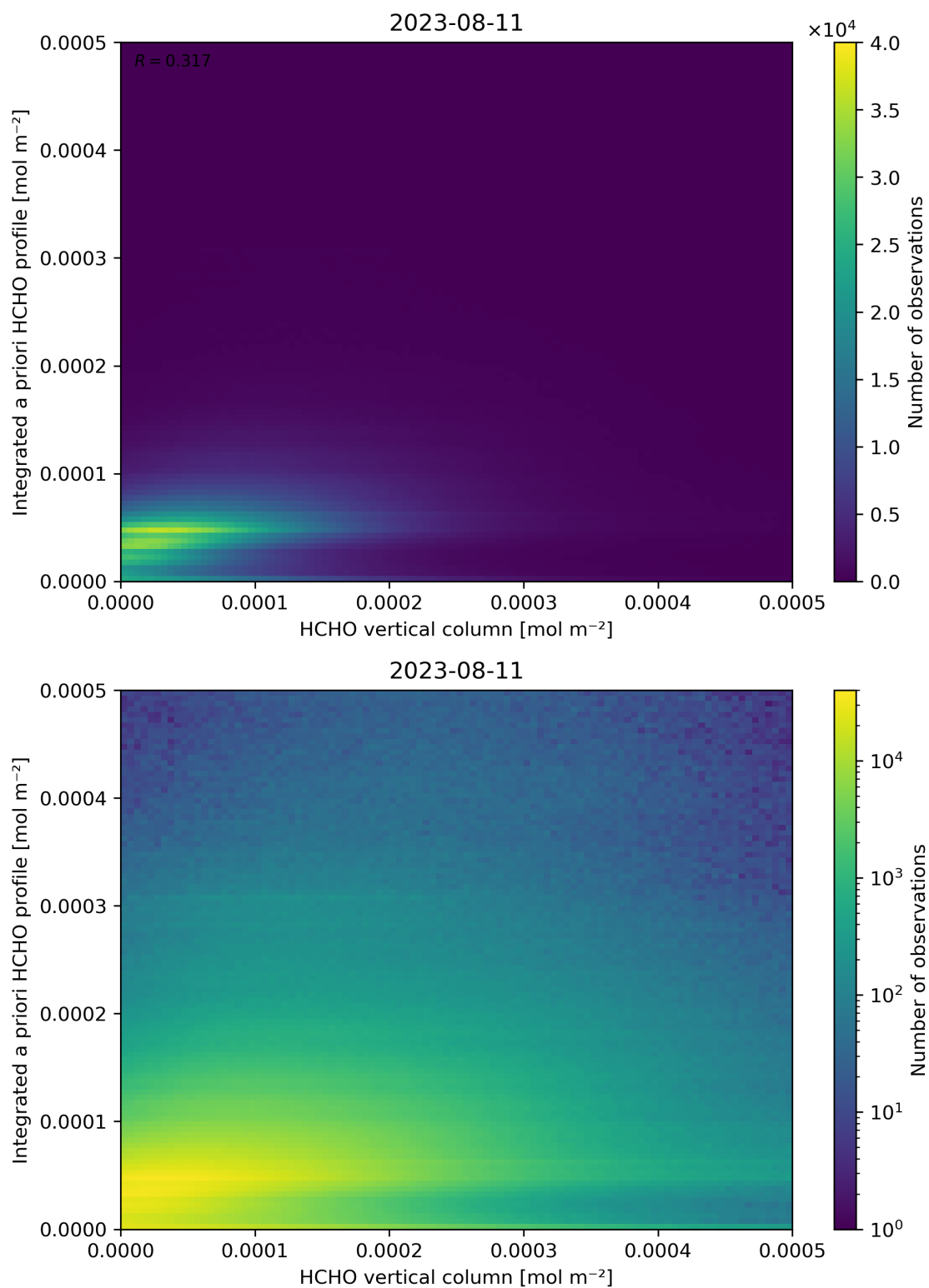
Figure 135: Scatter density plot of “HCHO vertical column” against “Integrated a priori HCHO profile” for 2023-08-10 to 2023-08-12.
