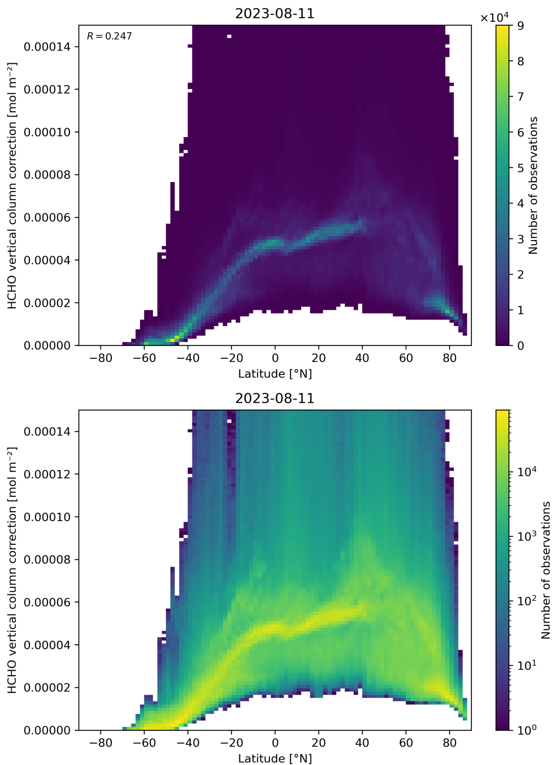
Figure 164: Scatter density plot of “Latitude” against “HCHO vertical column correction” for 2023-08-10 to 2023-08-12.
