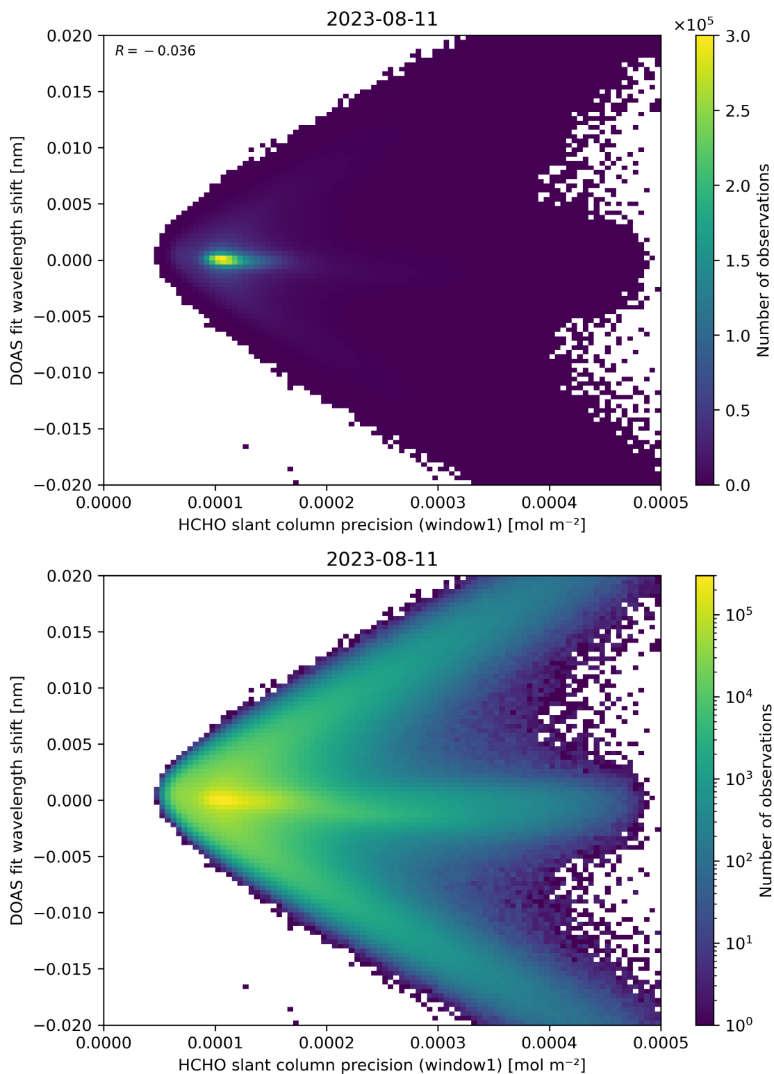
Figure 89: Scatter density plot of “HCHO slant column precision (window1)” against “DOAS fit wavelength shift” for 2023-08-10 to 2023-08-12.
