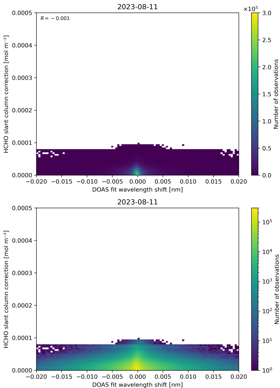
Figure 67: Scatter density plot of “DOAS fit wavelength shift” against “HCHO slant column correction” for 2023-08-10 to 2023-08-12.
