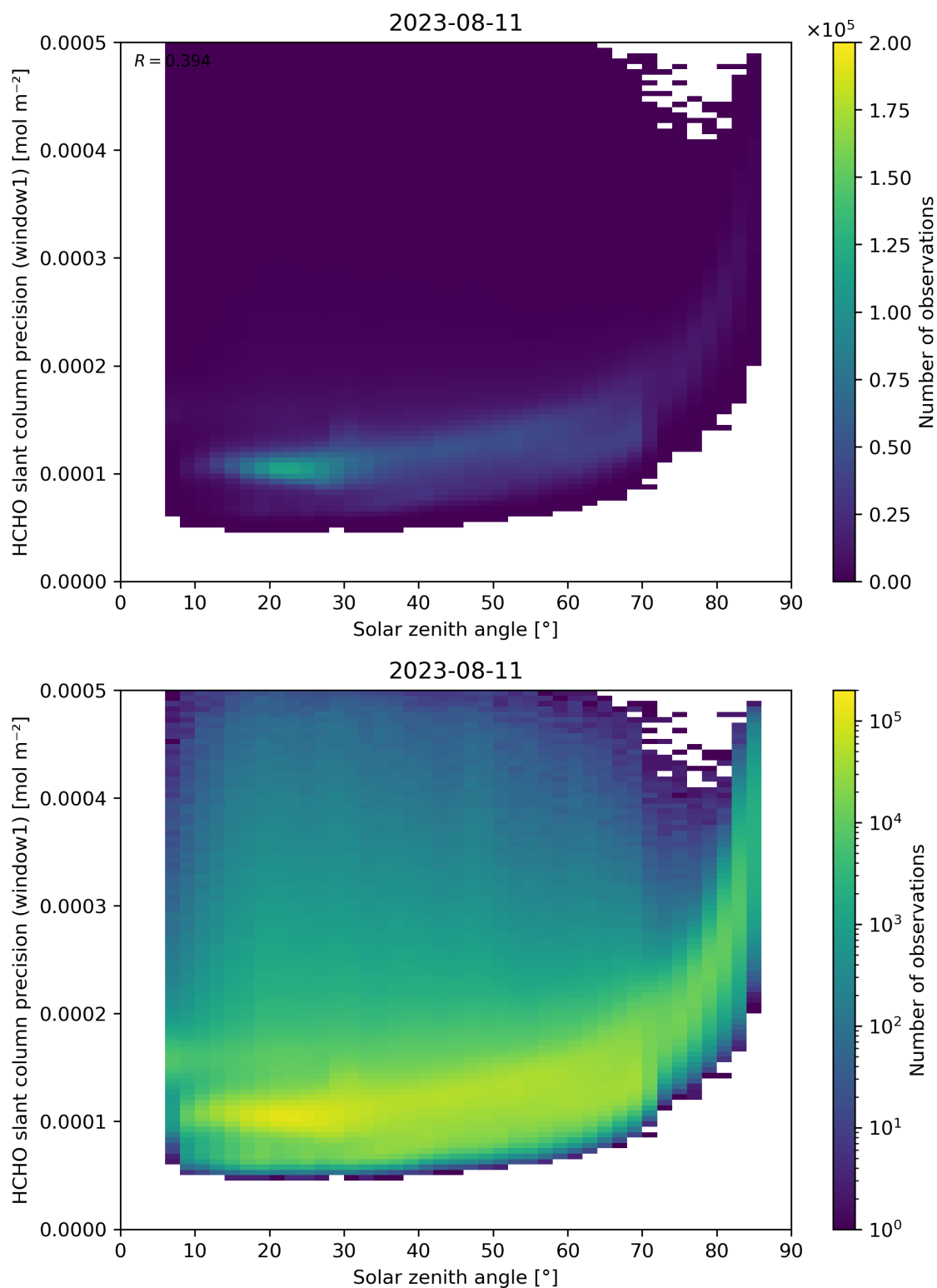
Figure 174: Scatter density plot of “Solar zenith angle” against “HCHO slant column precision (window1)” for 2023-08-10 to 2023-08-12.
