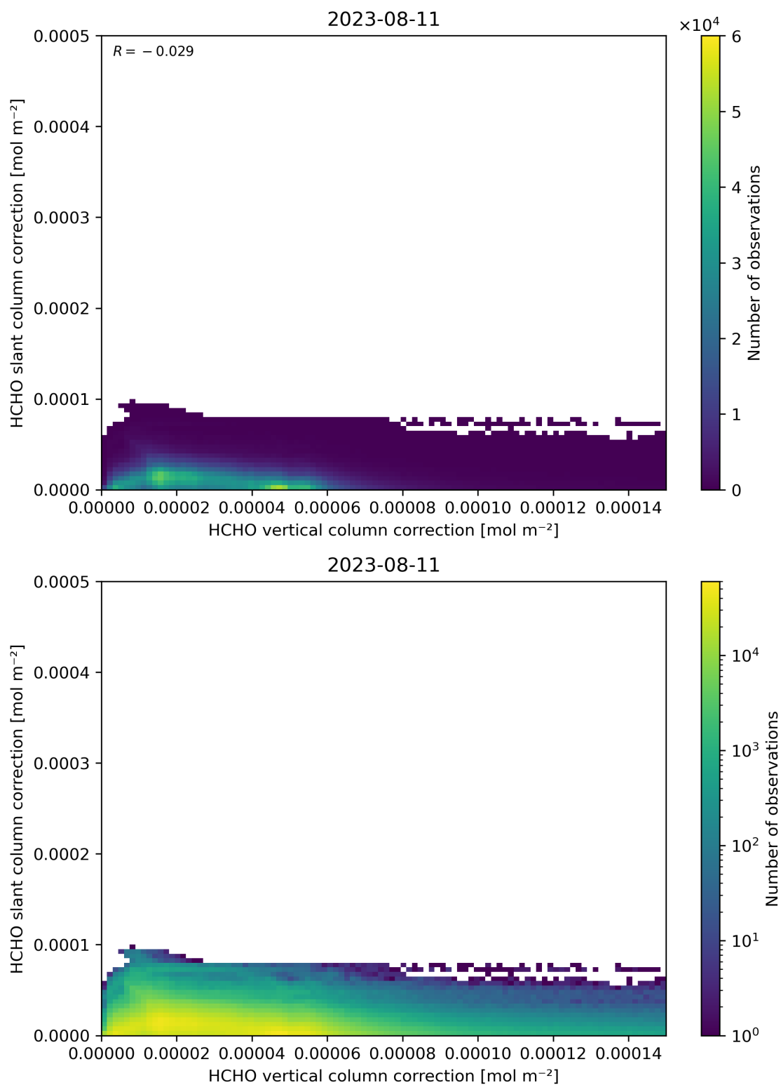
Figure 117: Scatter density plot of “HCHO vertical column correction” against “HCHO slant column correction” for 2023-08-10 to 2023-08-12.
