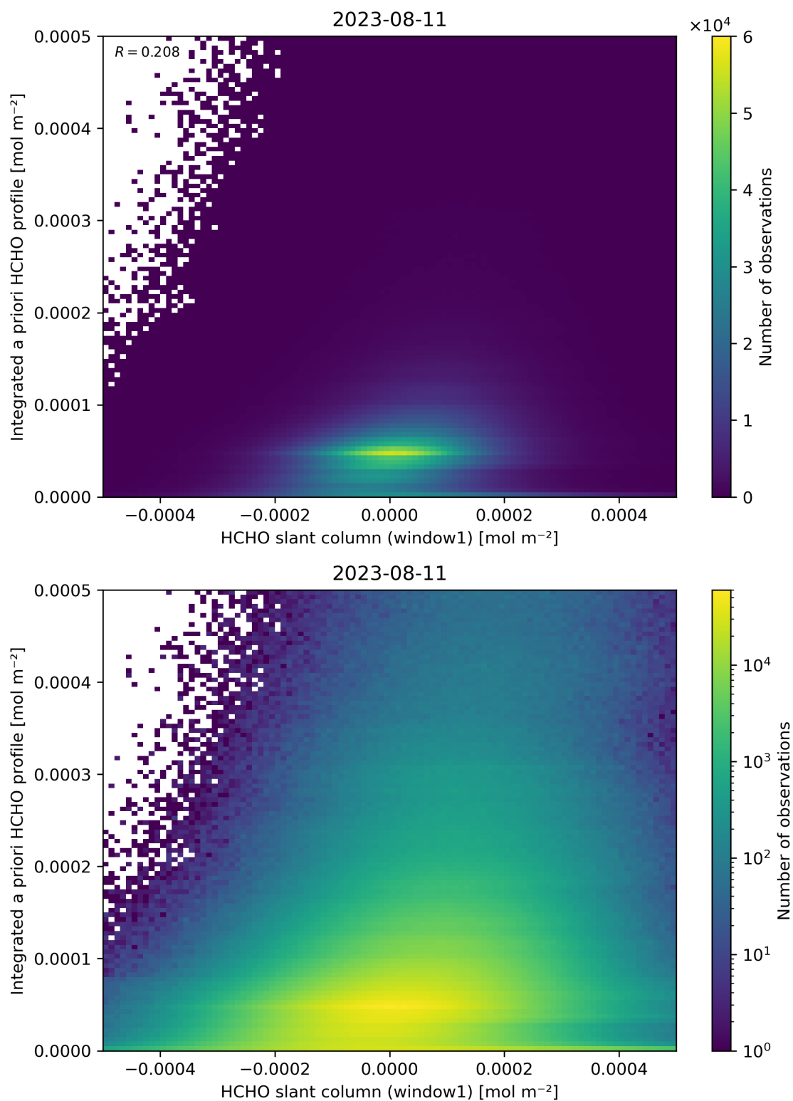
Figure 87: Scatter density plot of “HCHO slant column (window1)” against “Integrated a priori HCHO profile” for 2023-08-10 to 2023-08-12.
