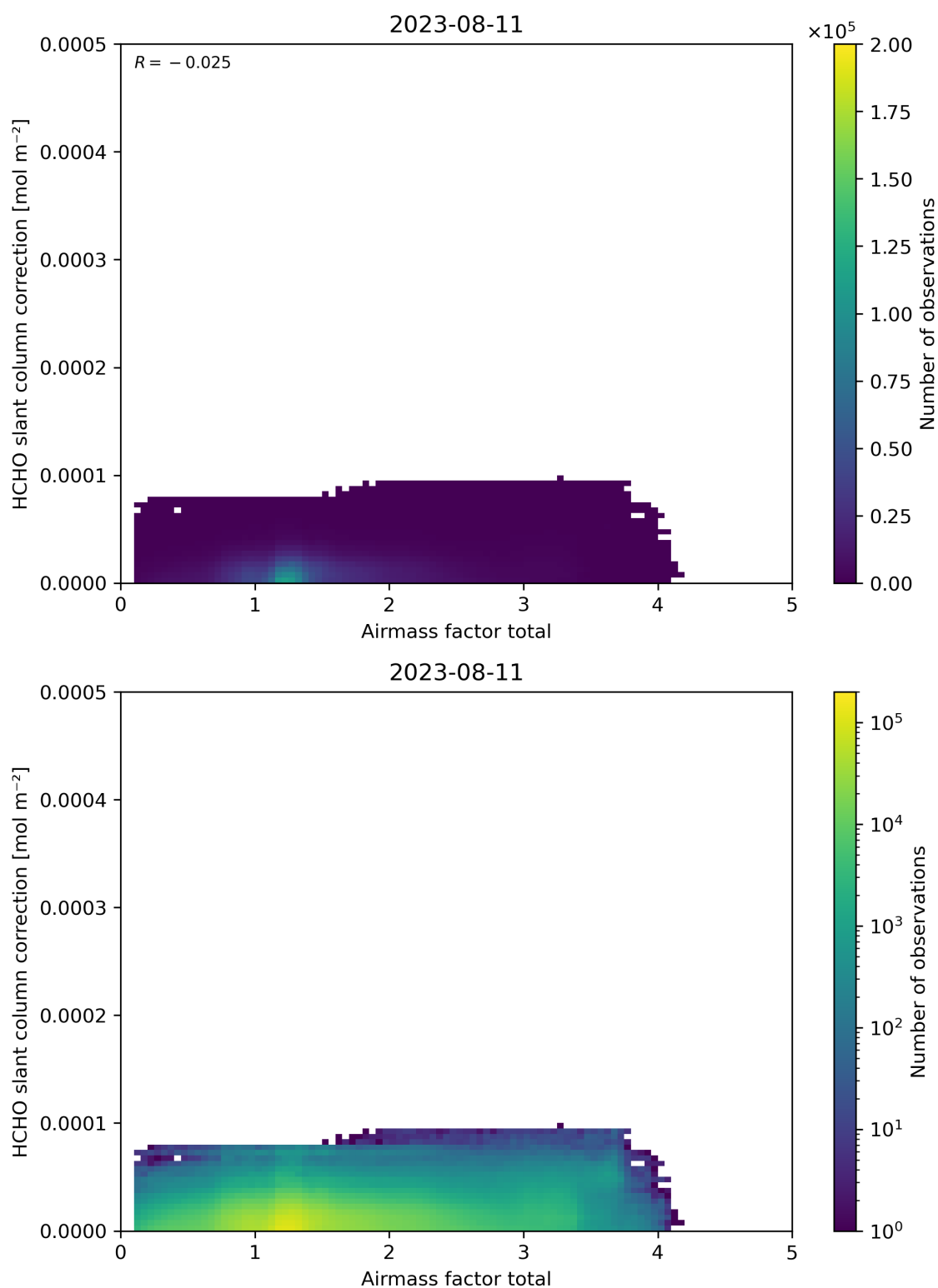
Figure 102: Scatter density plot of “Airmass factor total” against “HCHO slant column correction” for 2023-08-10 to 2023-08-12.
