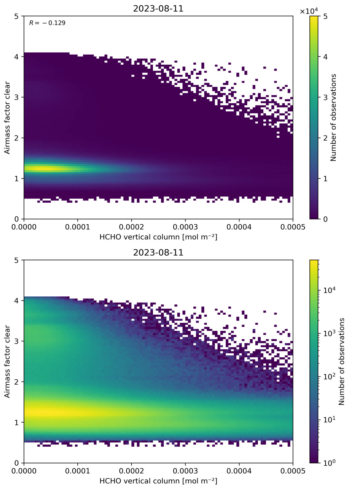
Figure 126: Scatter density plot of “HCHO vertical column” against “Airmass factor clear” for 2023-08-10 to 2023-08-12.
