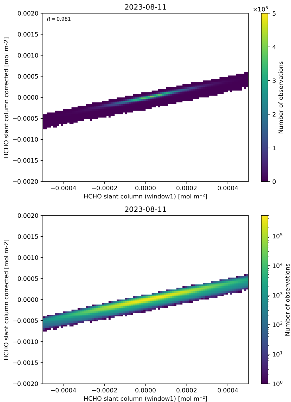
Figure 82: Scatter density plot of “HCHO slant column (window1)” against “HCHO slant column corrected” for 2023-08-10 to 2023-08-12.
