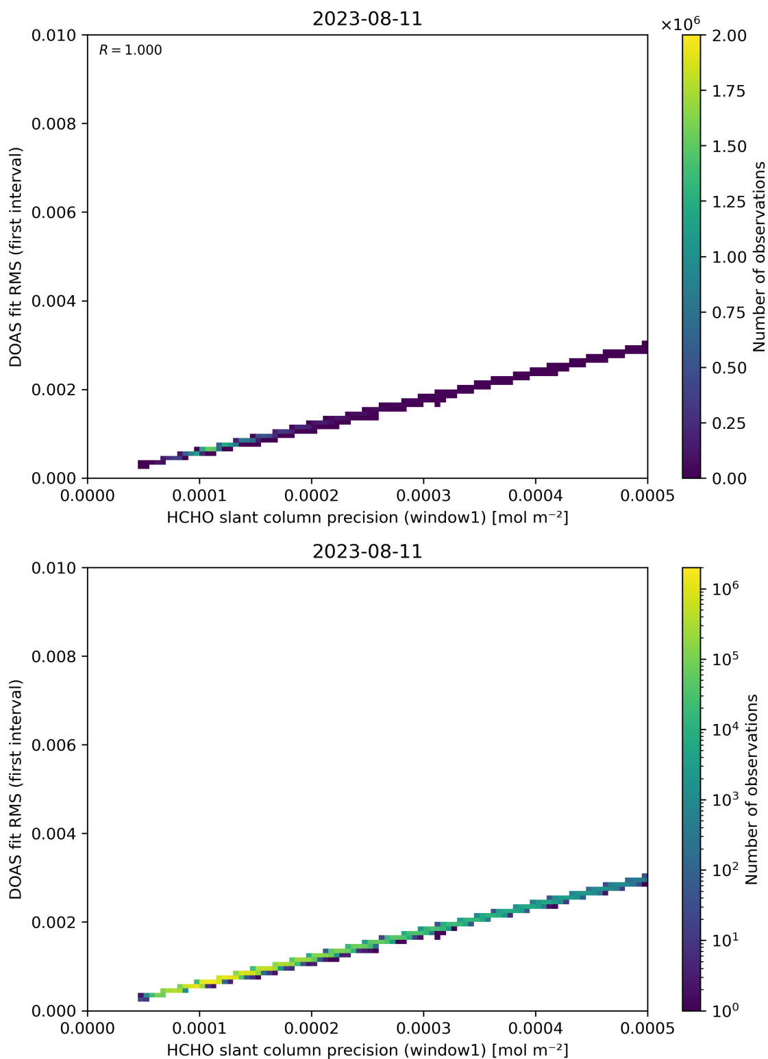
Figure 88: Scatter density plot of “HCHO slant column precision (window1)” against “DOAS fit RMS (first interval)” for 2023-08-10 to 2023-08-12.
