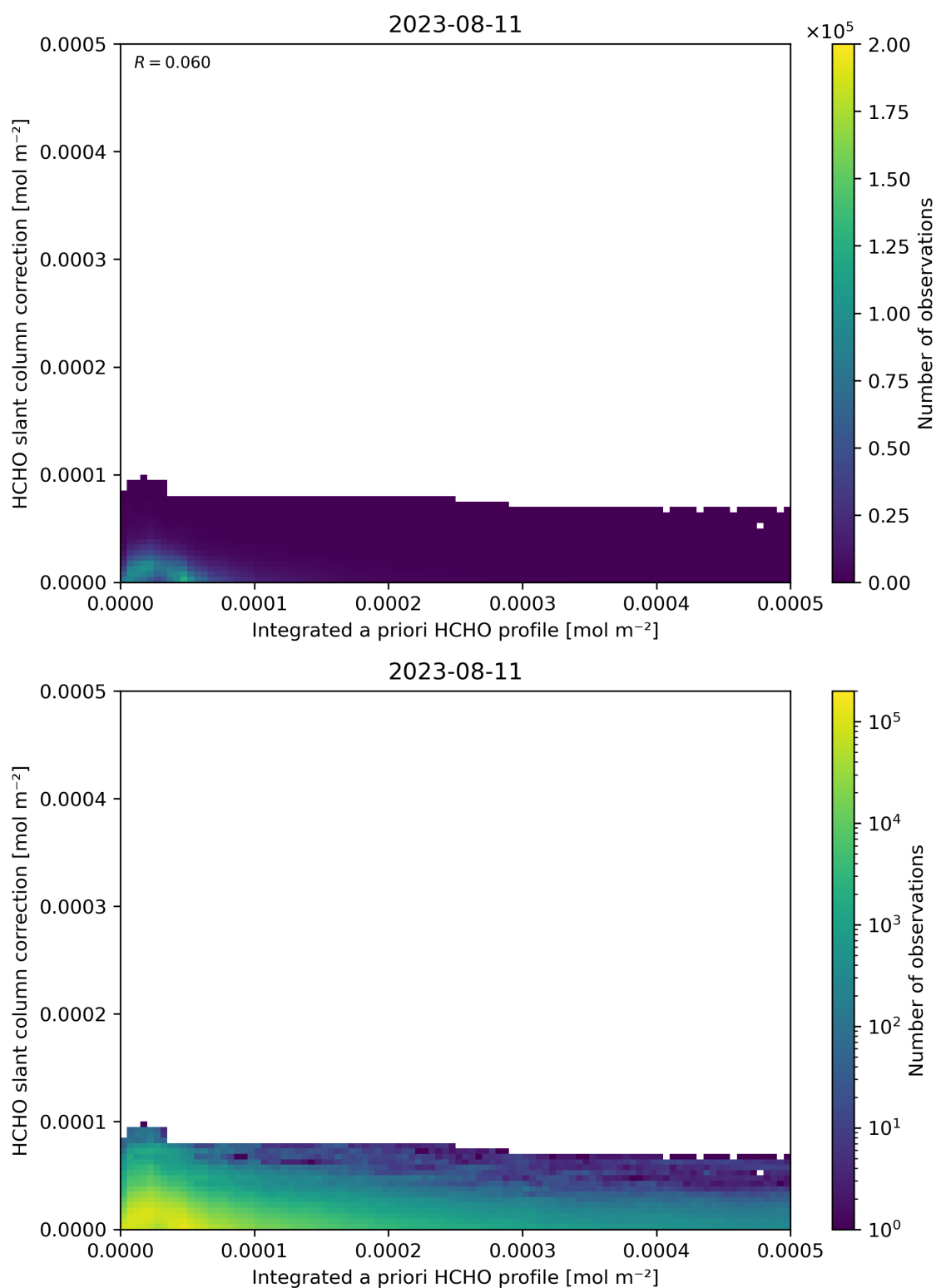
Figure 152: Scatter density plot of “Integrated a priori HCHO profile” against “HCHO slant column correction” for 2023-08-10 to 2023-08-12.
