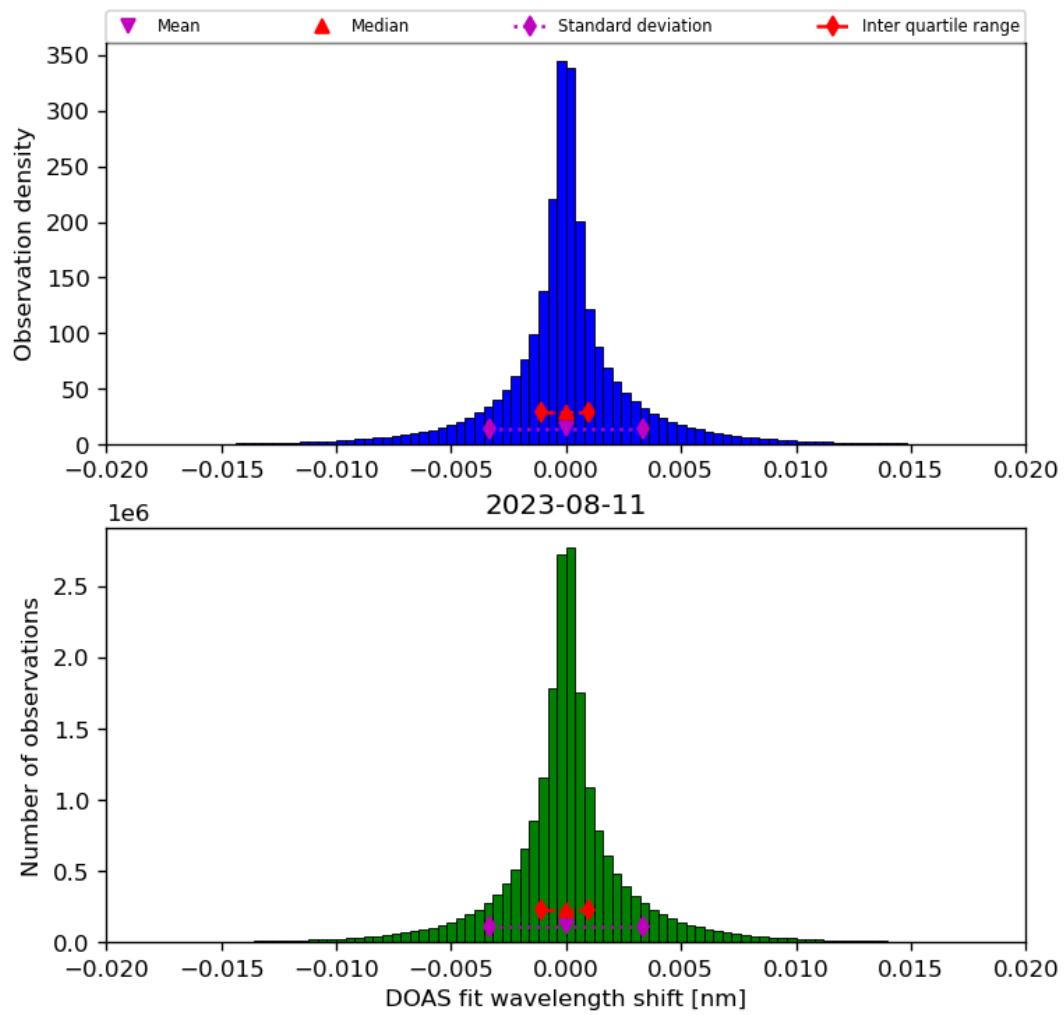
Figure 44: Histogram of “DOAS fit wavelength shift” for 2023-08-10 to 2023-08-12
