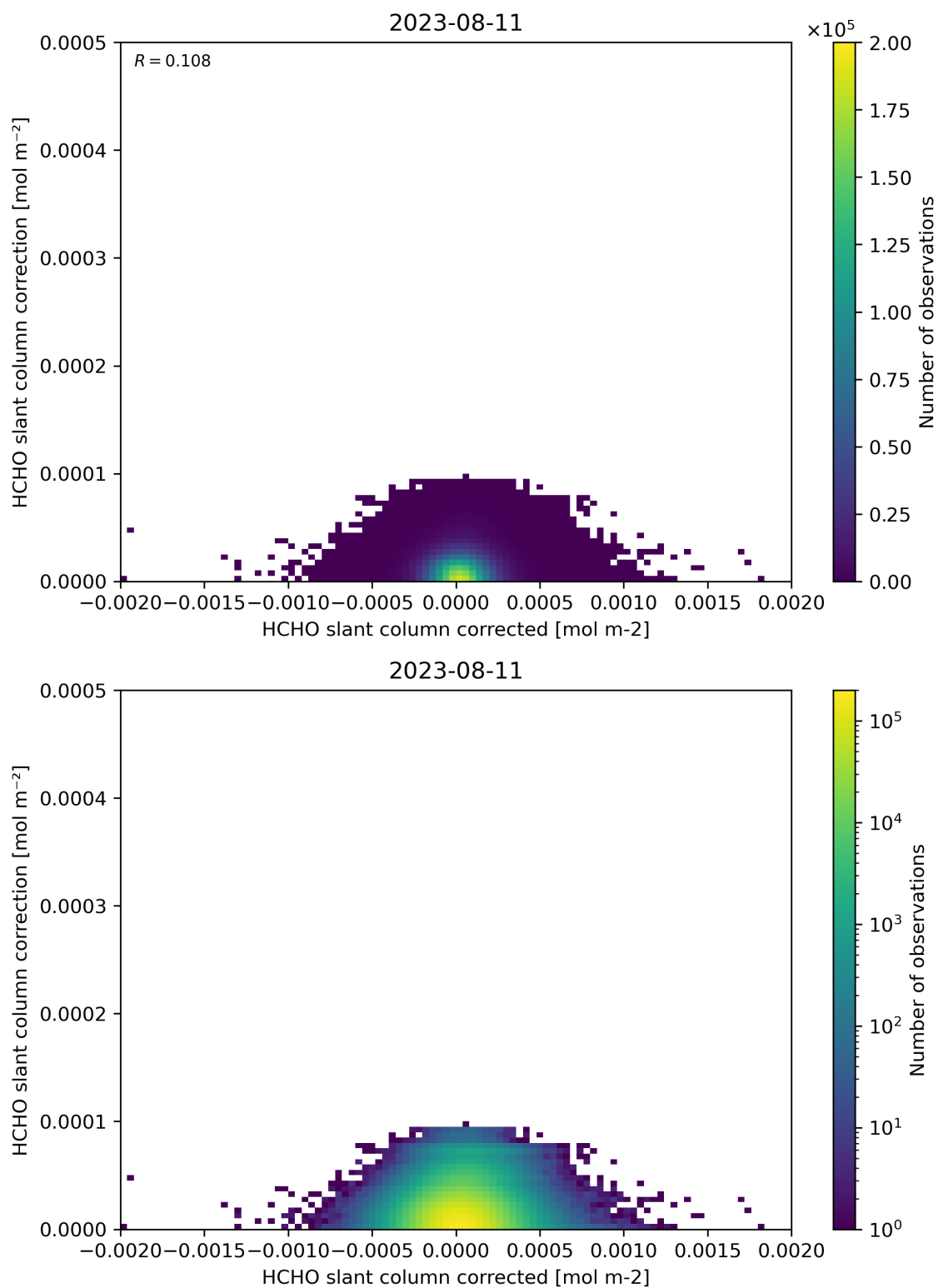
Figure 77: Scatter density plot of “HCHO slant column corrected” against “HCHO slant column correction” for 2023-08-10 to 2023-08-12.
