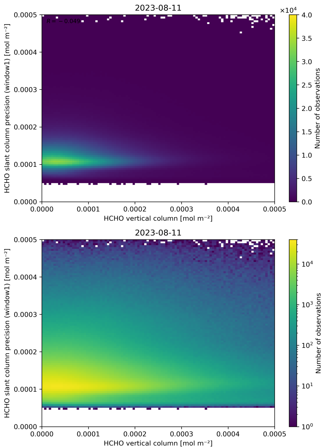
Figure 130: Scatter density plot of “HCHO vertical column” against “HCHO slant column precision (window1)” for 2023-08-10 to 2023-08-12.
