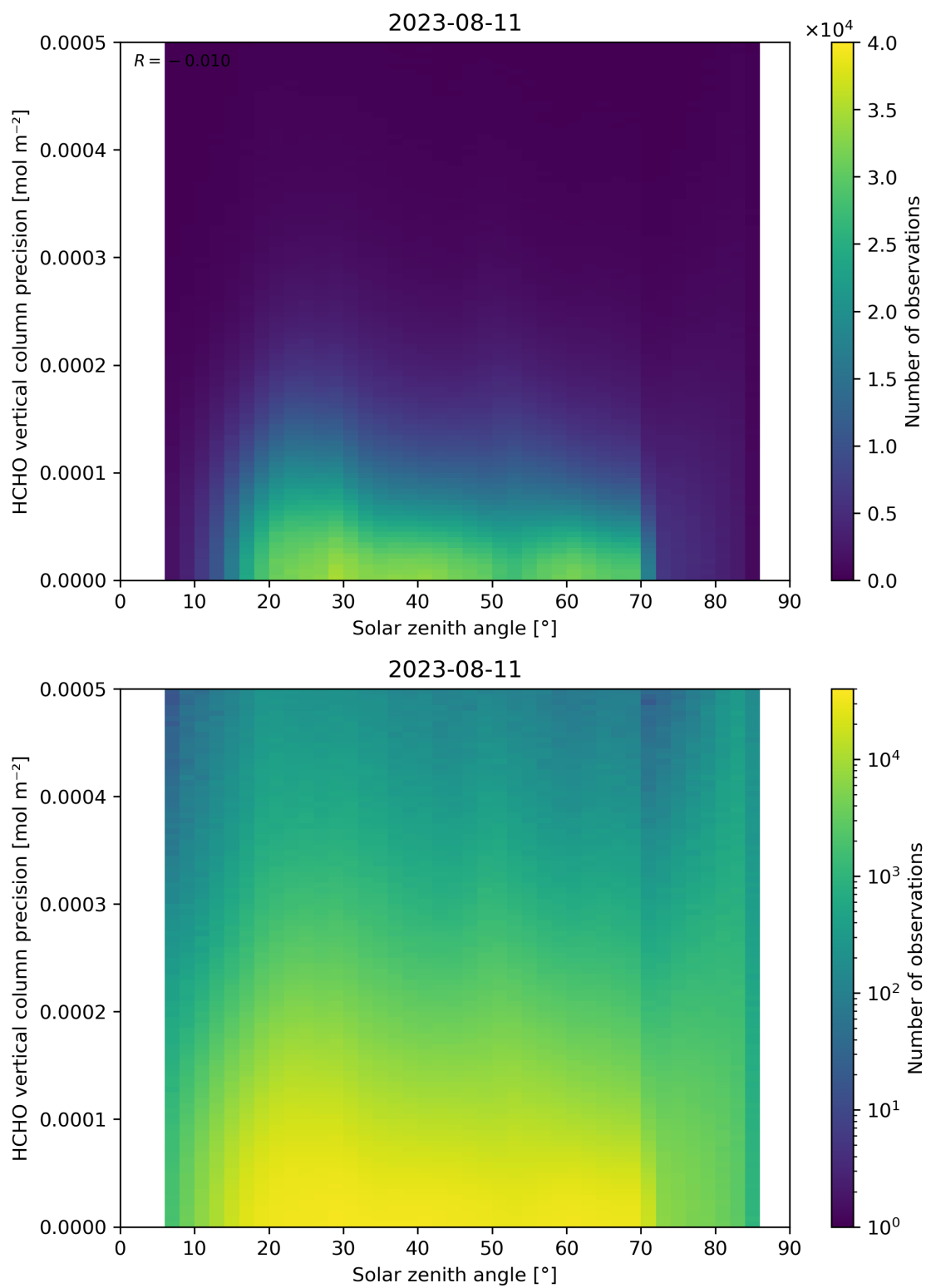
Figure 179: Scatter density plot of “Solar zenith angle” against “HCHO vertical column precision” for 2023-08-10 to 2023-08-12.
