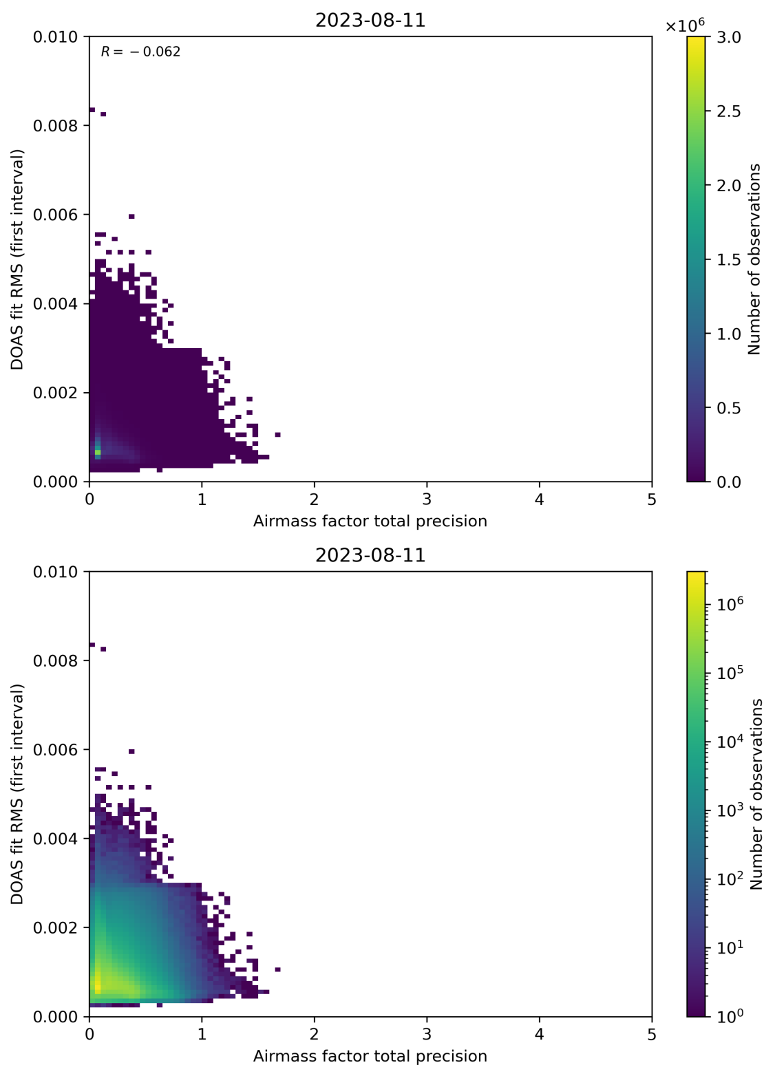
Figure 105: Scatter density plot of “Airmass factor total precision” against “DOAS fit RMS (first interval)” for 2023-08-10 to 2023-08-12.
