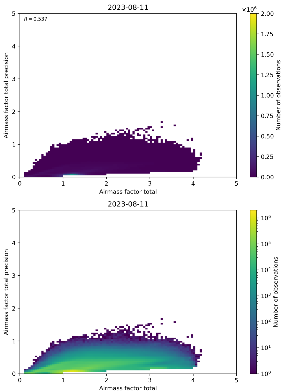
Figure 103: Scatter density plot of “Airmass factor total” against “Airmass factor total precision” for 2023-08-10 to 2023-08-12.
