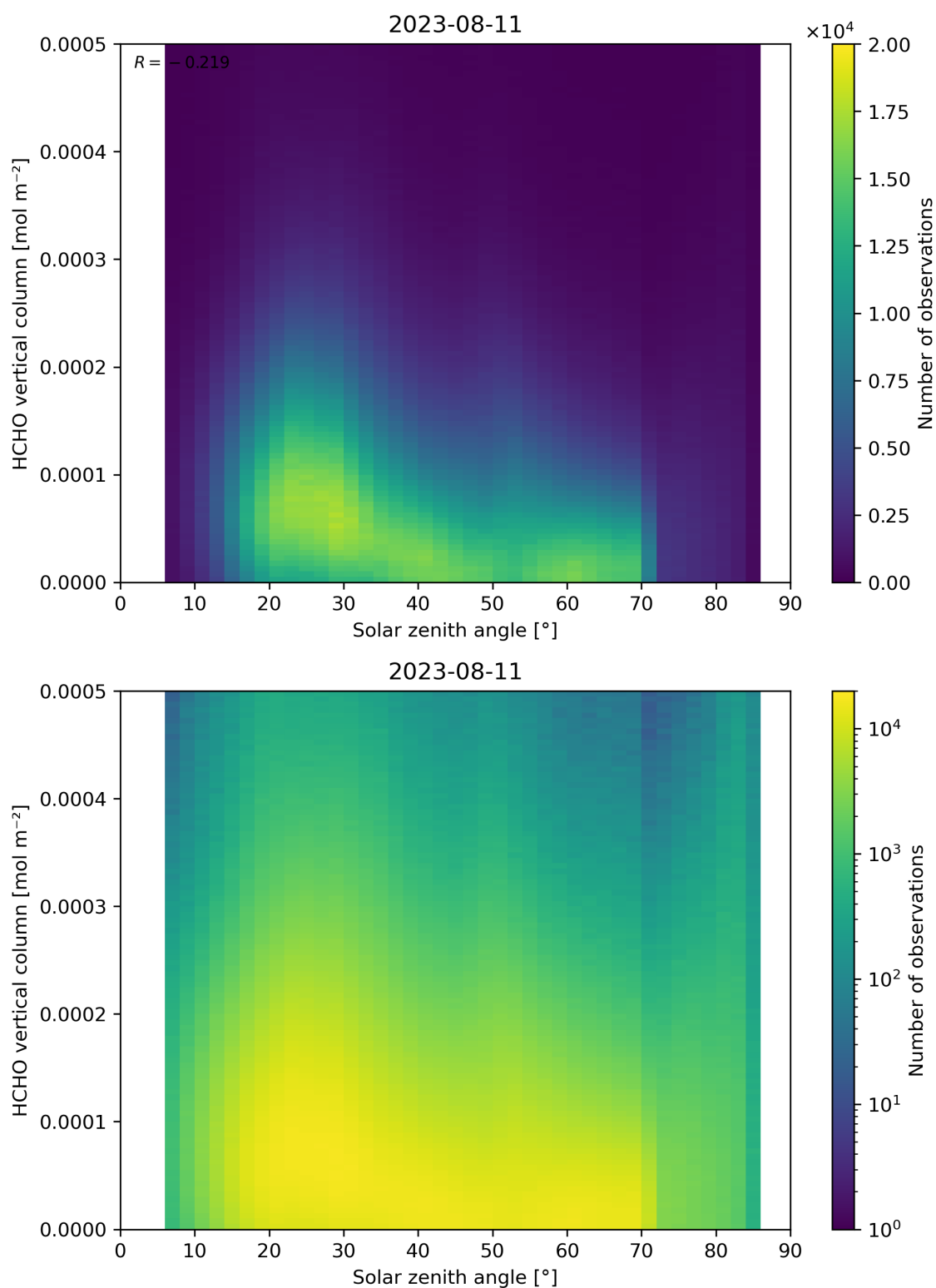
Figure 177: Scatter density plot of “Solar zenith angle” against “HCHO vertical column” for 2023-08-10 to 2023-08-12.
