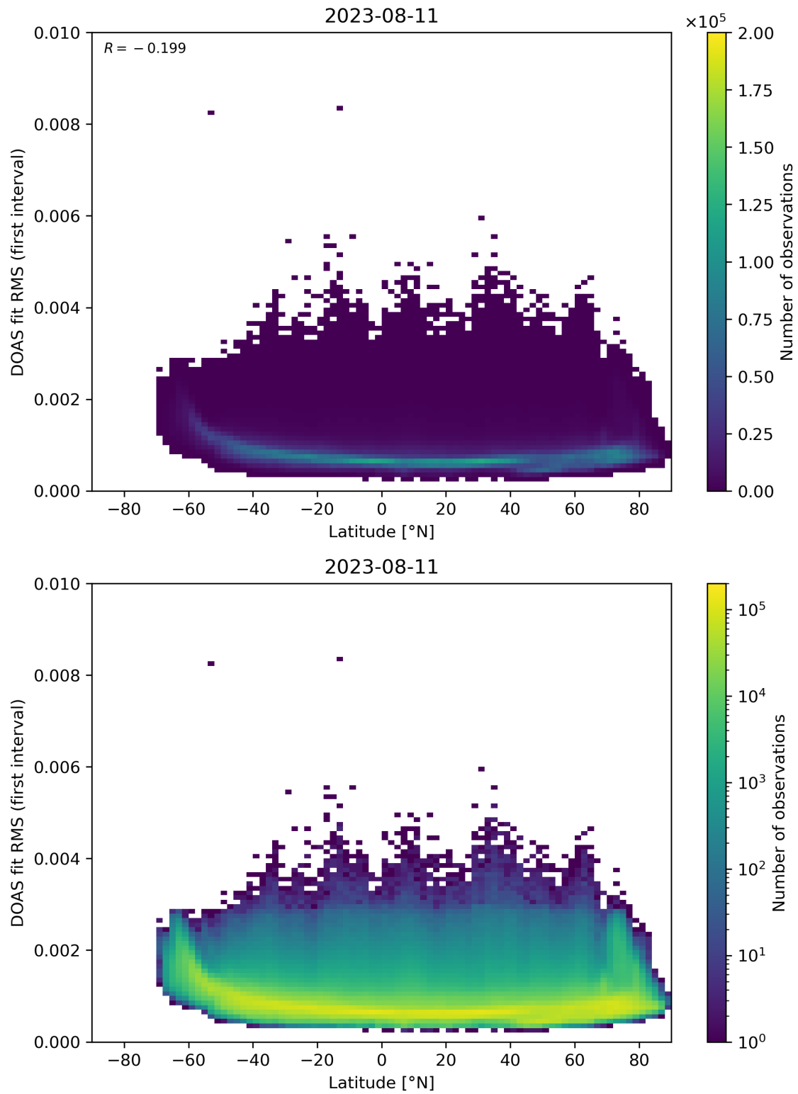
Figure 153: Scatter density plot of “Latitude” against “DOAS fit RMS (first interval)” for 2023-08-10 to 2023-08-12.
