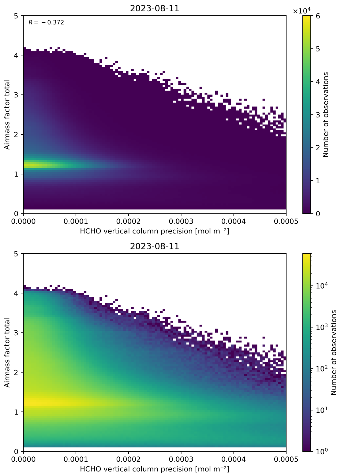
Figure 144: Scatter density plot of “HCHO vertical column precision” against “Airmass factor total” for 2023-08-10 to 2023-08-12.
