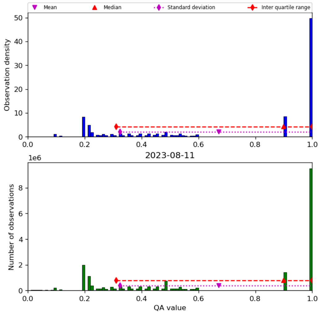
Figure 34: Histogram of “QA value” for 2023-08-10 to 2023-08-12
