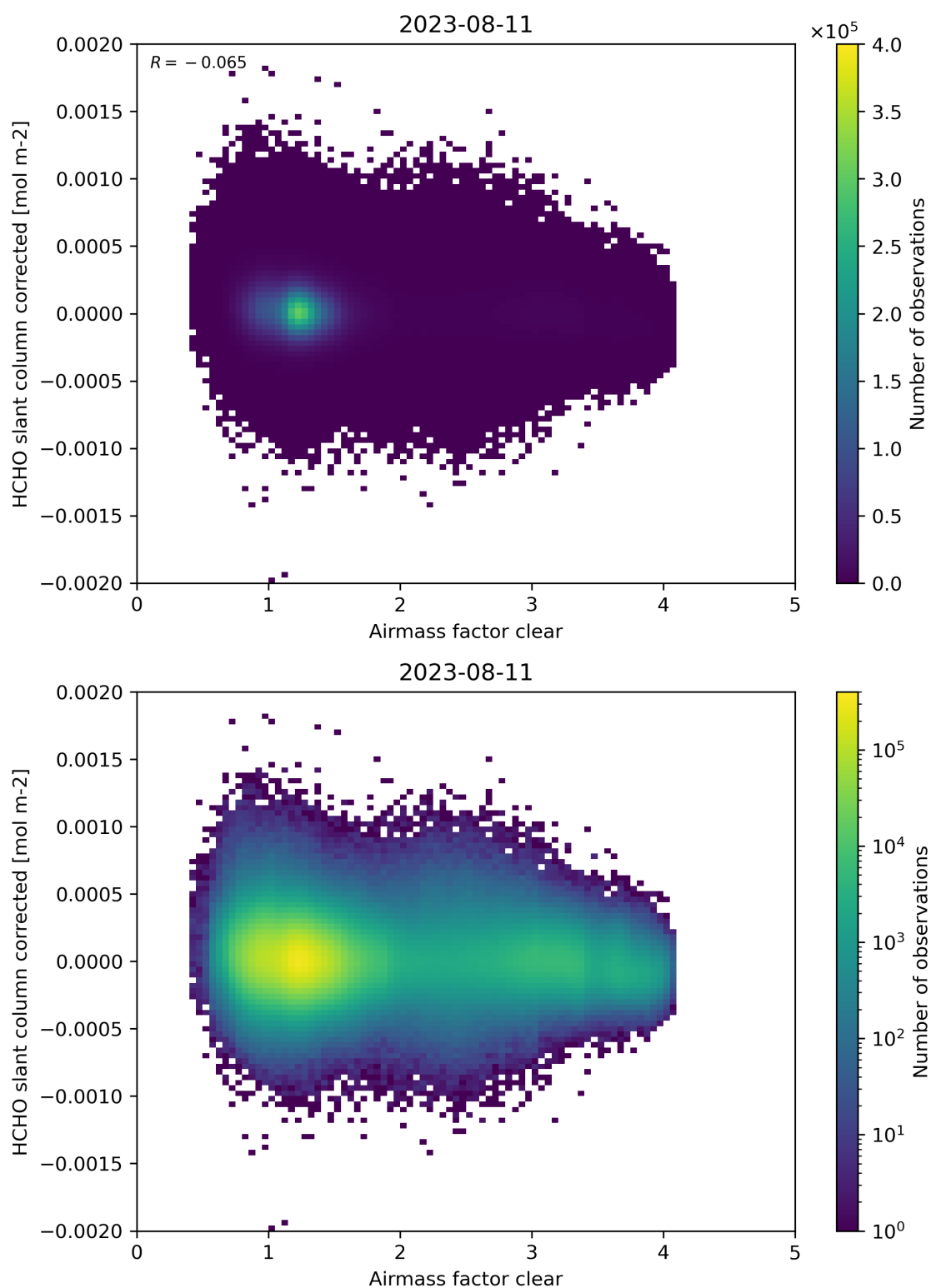
Figure 74: Scatter density plot of “Airmass factor clear” against “HCHO slant column corrected” for 2023-08-10 to 2023-08-12.
