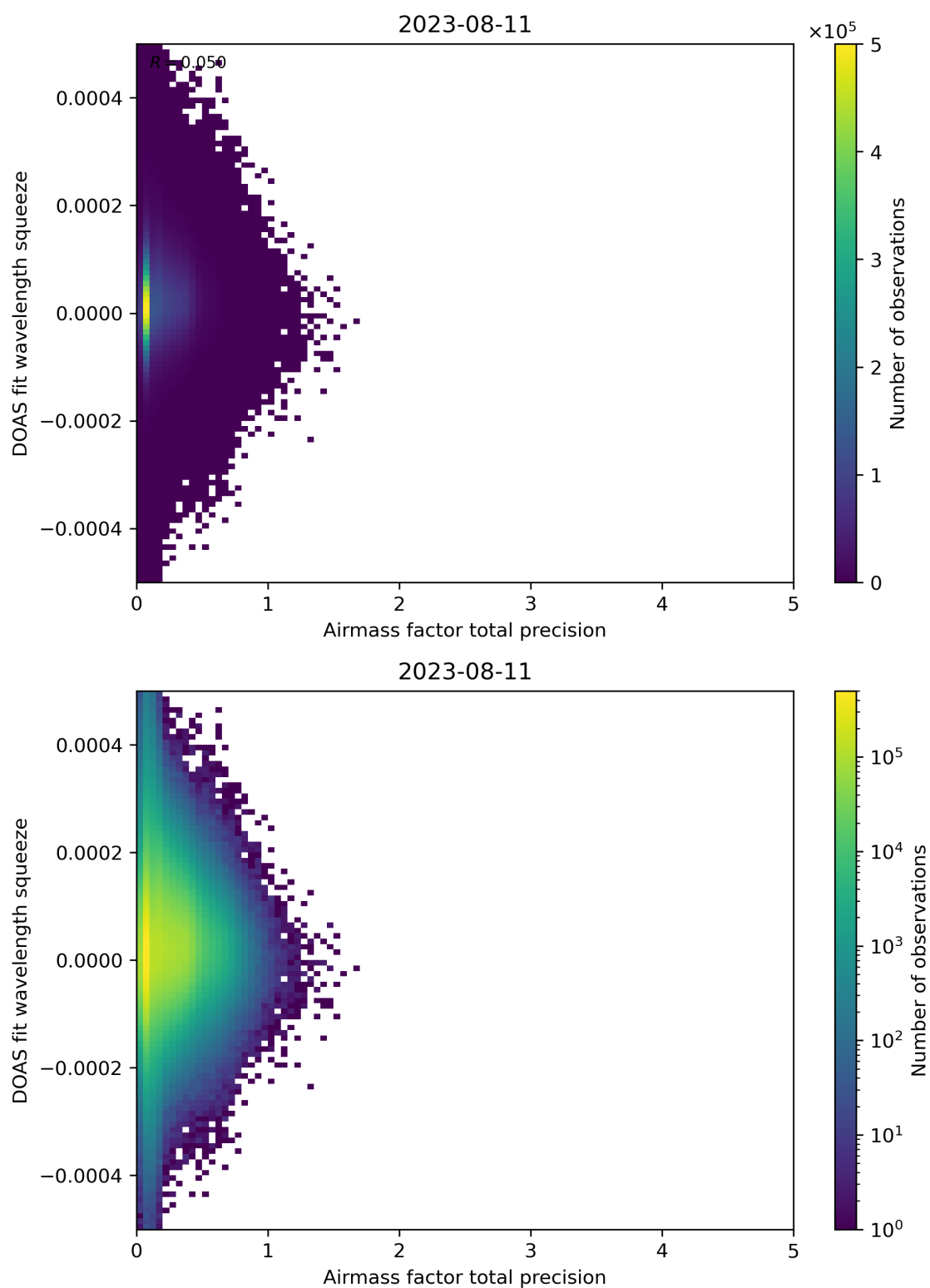
Figure 107: Scatter density plot of “Airmass factor total precision” against “DOAS fit wavelength squeeze” for 2023-08-10 to 2023-08-12.
