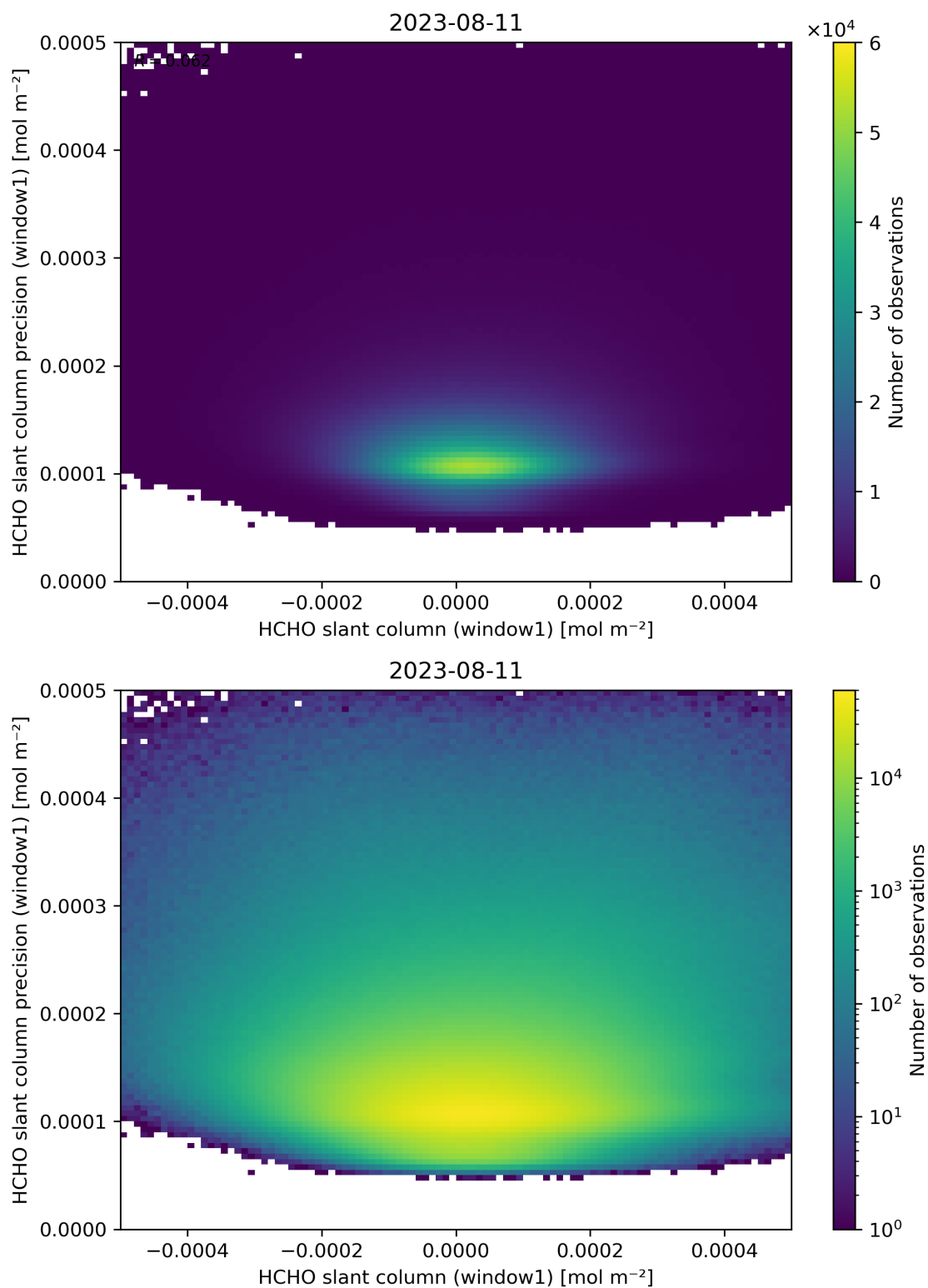
Figure 84: Scatter density plot of “HCHO slant column (window1)” against “HCHO slant column precision (window1)” for 2023-08-10 to 2023-08-12.
