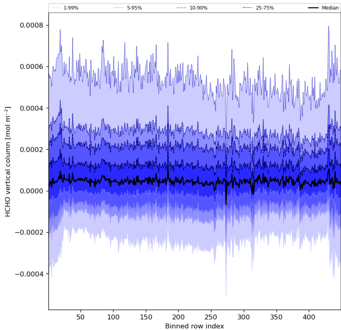
Figure 49: Along track statistics of “HCHO vertical column” for 2023-08-10 to 2023-08-12
