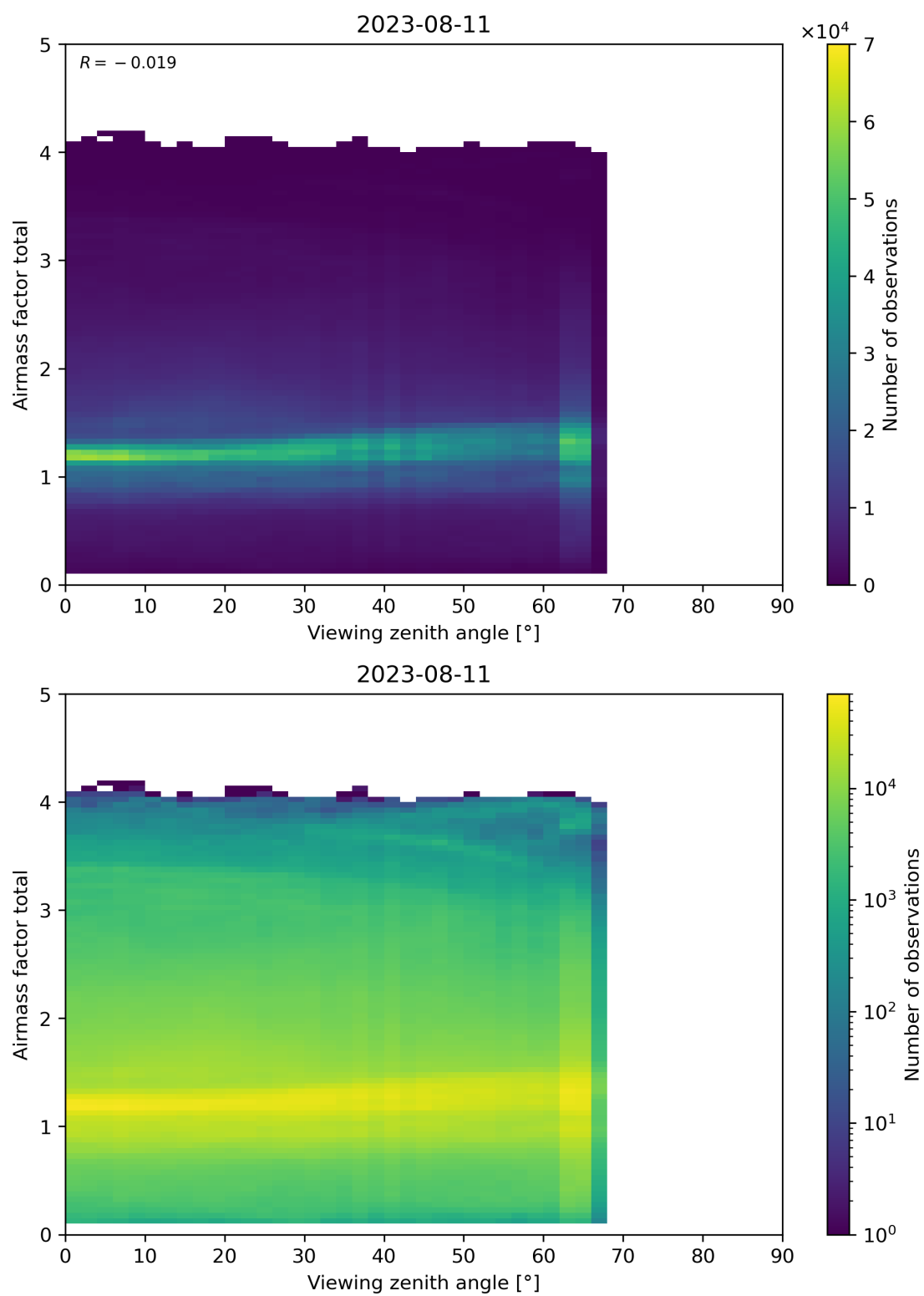
Figure 190: Scatter density plot of “Viewing zenith angle” against “Airmass factor total” for 2023-08-10 to 2023-08-12.
