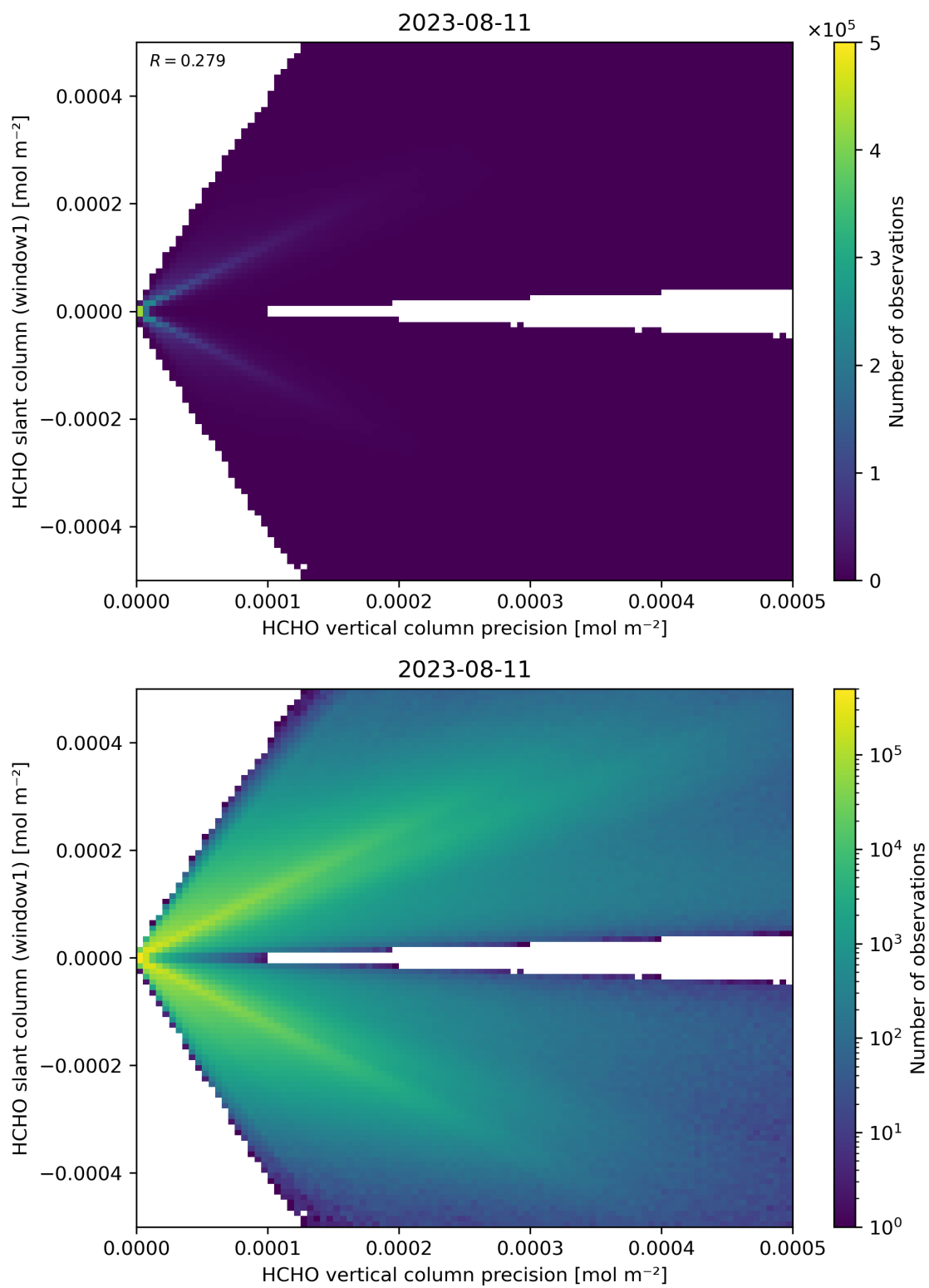
Figure 142: Scatter density plot of “HCHO vertical column precision” against “HCHO slant column (window1)” for 2023-08-10 to 2023-08-12.
