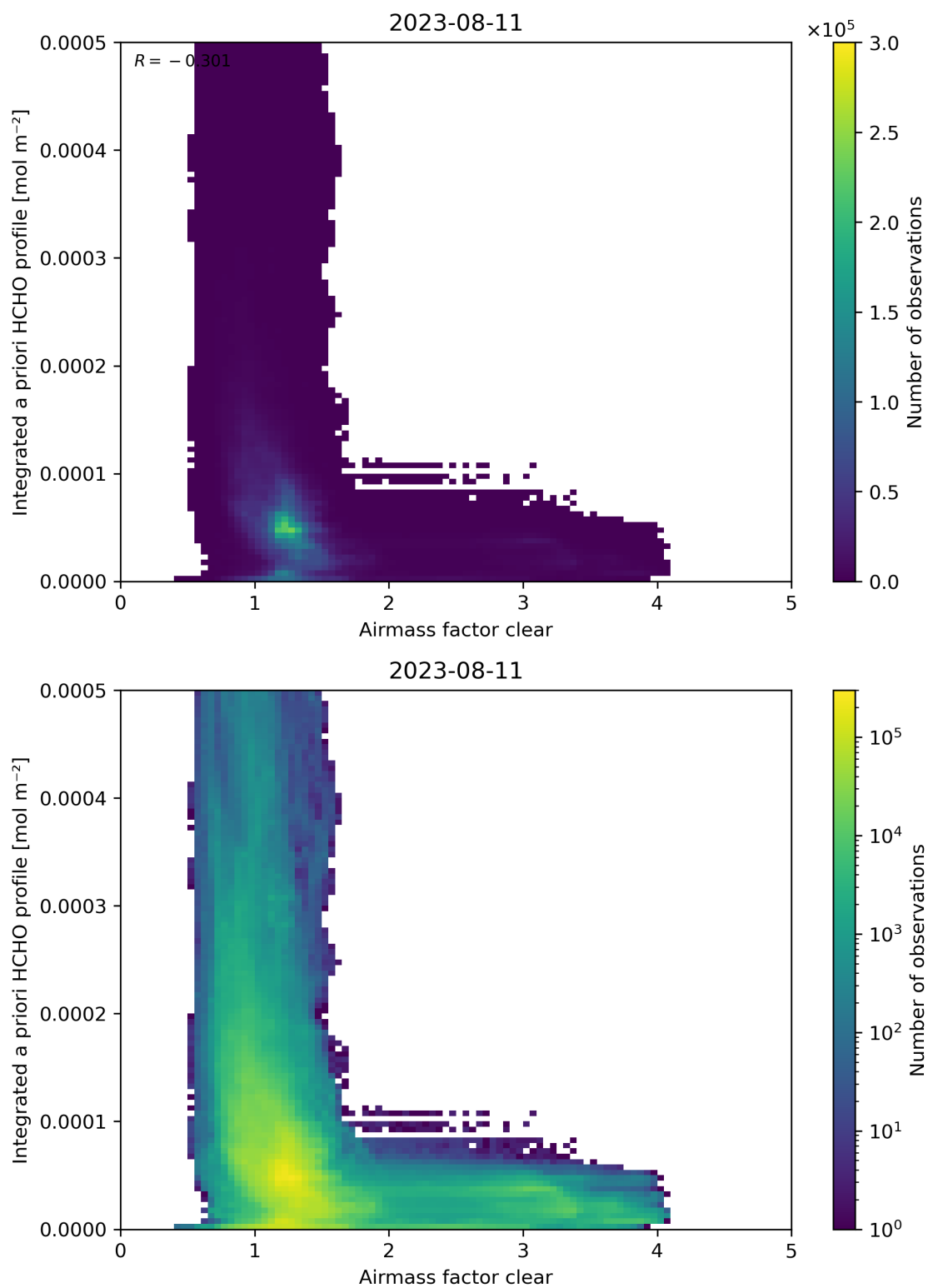
Figure 76: Scatter density plot of “Airmass factor clear” against “Integrated a priori HCHO profile” for 2023-08-10 to 2023-08-12.
