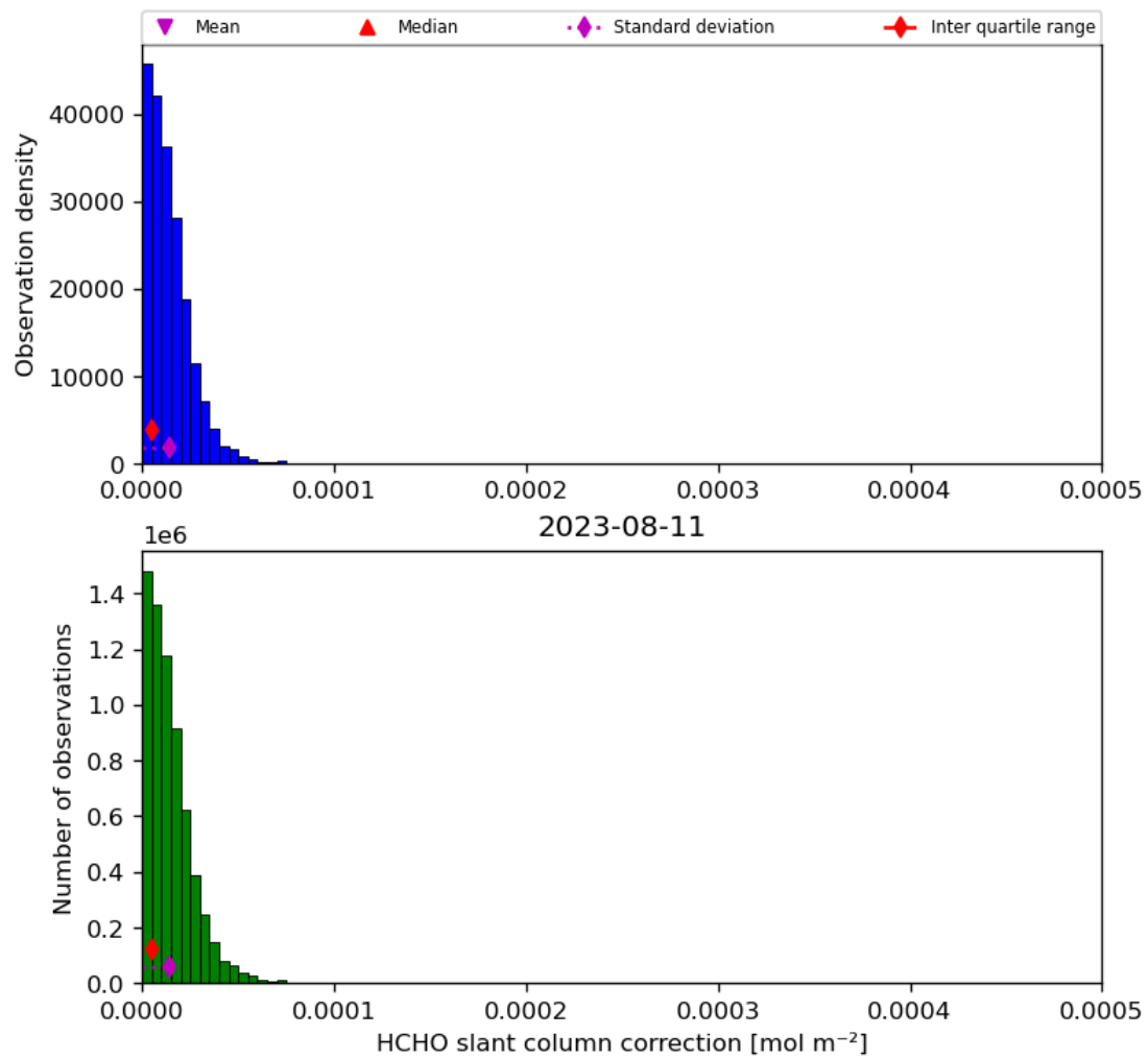
Figure 47: Histogram of “HCHO slant column correction” for 2023-08-10 to 2023-08-12
