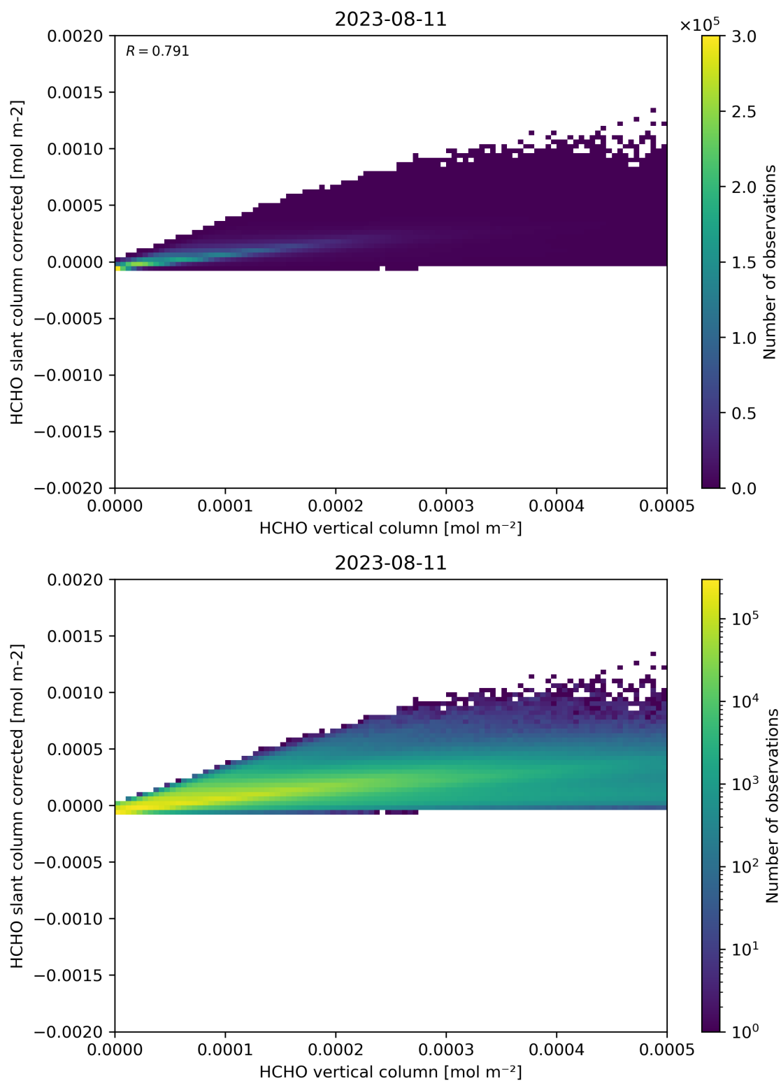
Figure 127: Scatter density plot of “HCHO vertical column” against “HCHO slant column corrected” for 2023-08-10 to 2023-08-12.
