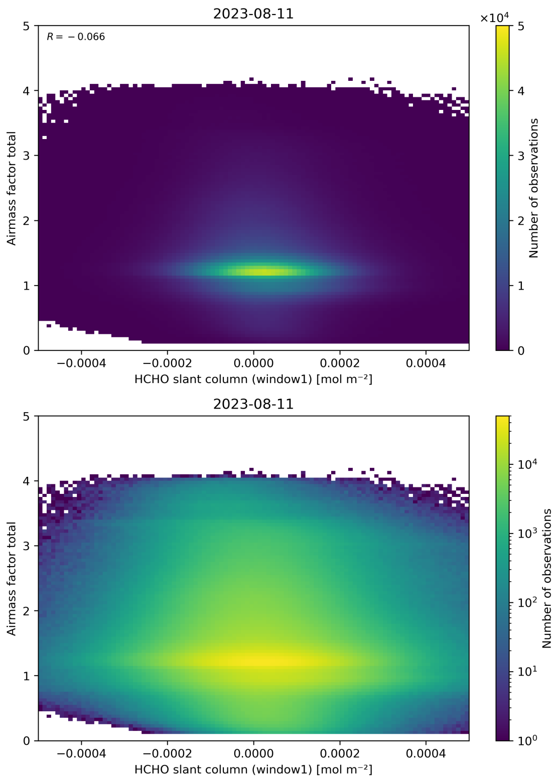
Figure 85: Scatter density plot of “HCHO slant column (window1)” against “Airmass factor total” for 2023-08-10 to 2023-08-12.
