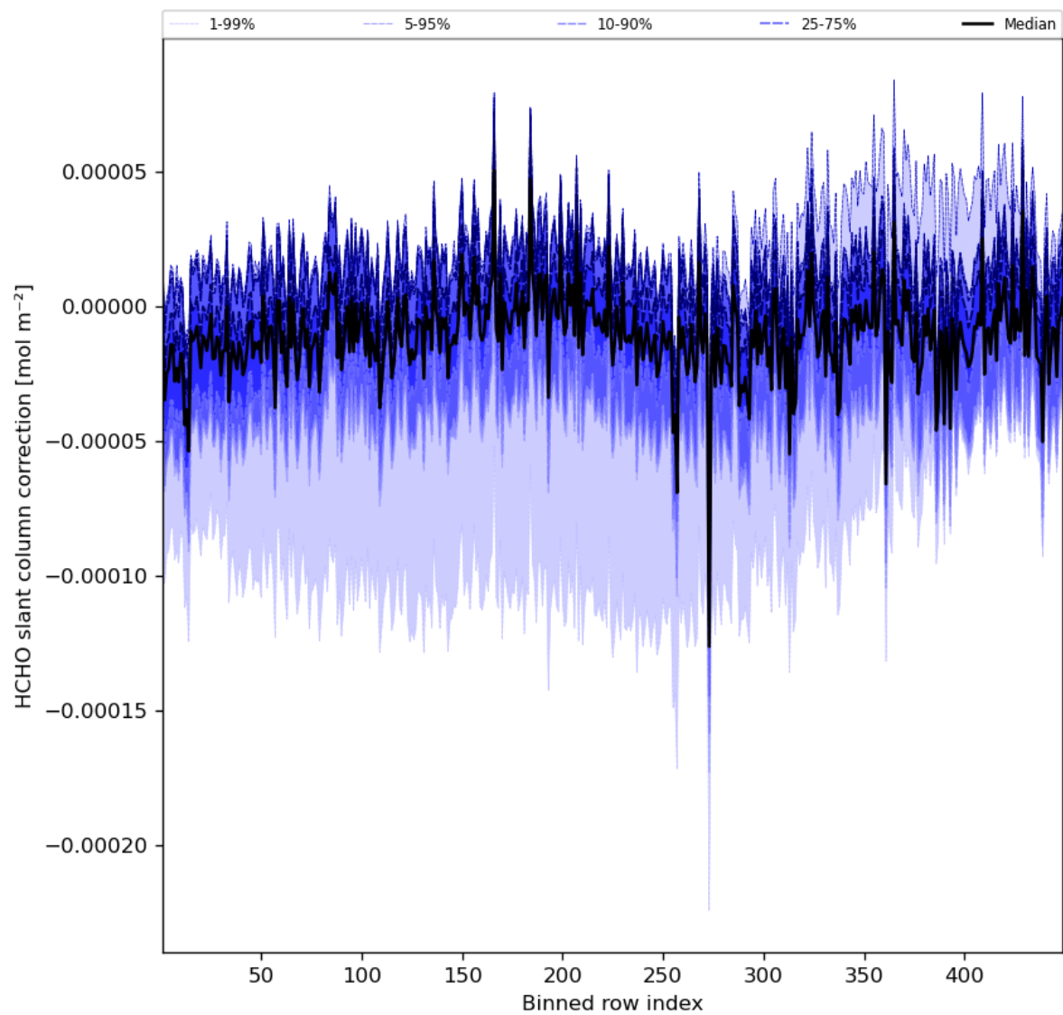
Figure 61: Along track statistics of “HCHO slant column correction” for 2023-08-10 to 2023-08-12
