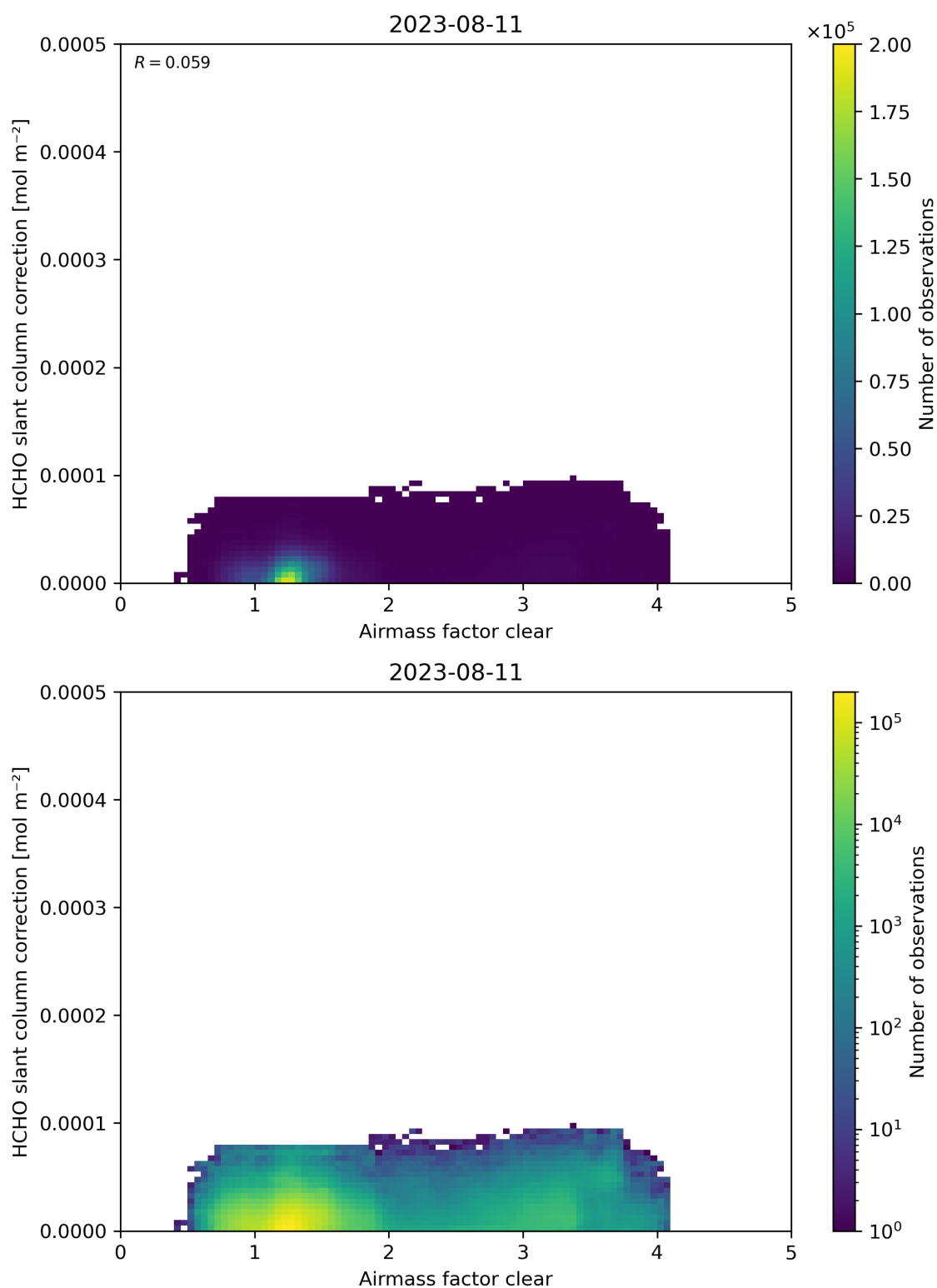
Figure 75: Scatter density plot of “Airmass factor clear” against “HCHO slant column correction” for 2023-08-10 to 2023-08-12.
