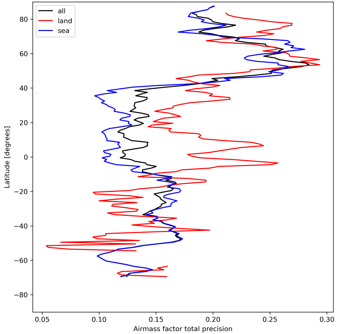
Figure 27: Zonal average of “Airmass factor total precision” for 2023-08-10 to 2023-08-12.
