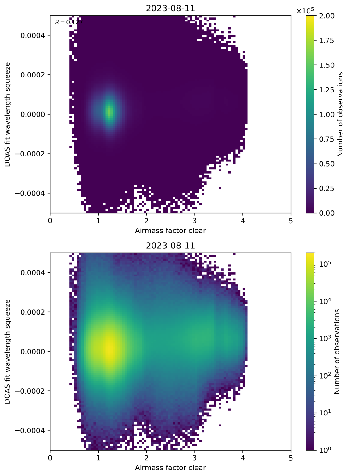
Figure 73: Scatter density plot of “Airmass factor clear” against “DOAS fit wavelength squeeze” for 2023-08-10 to 2023-08-12.
