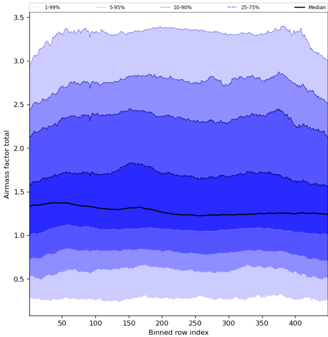
Figure 54: Along track statistics of “Airmass factor total” for 2023-08-10 to 2023-08-12
