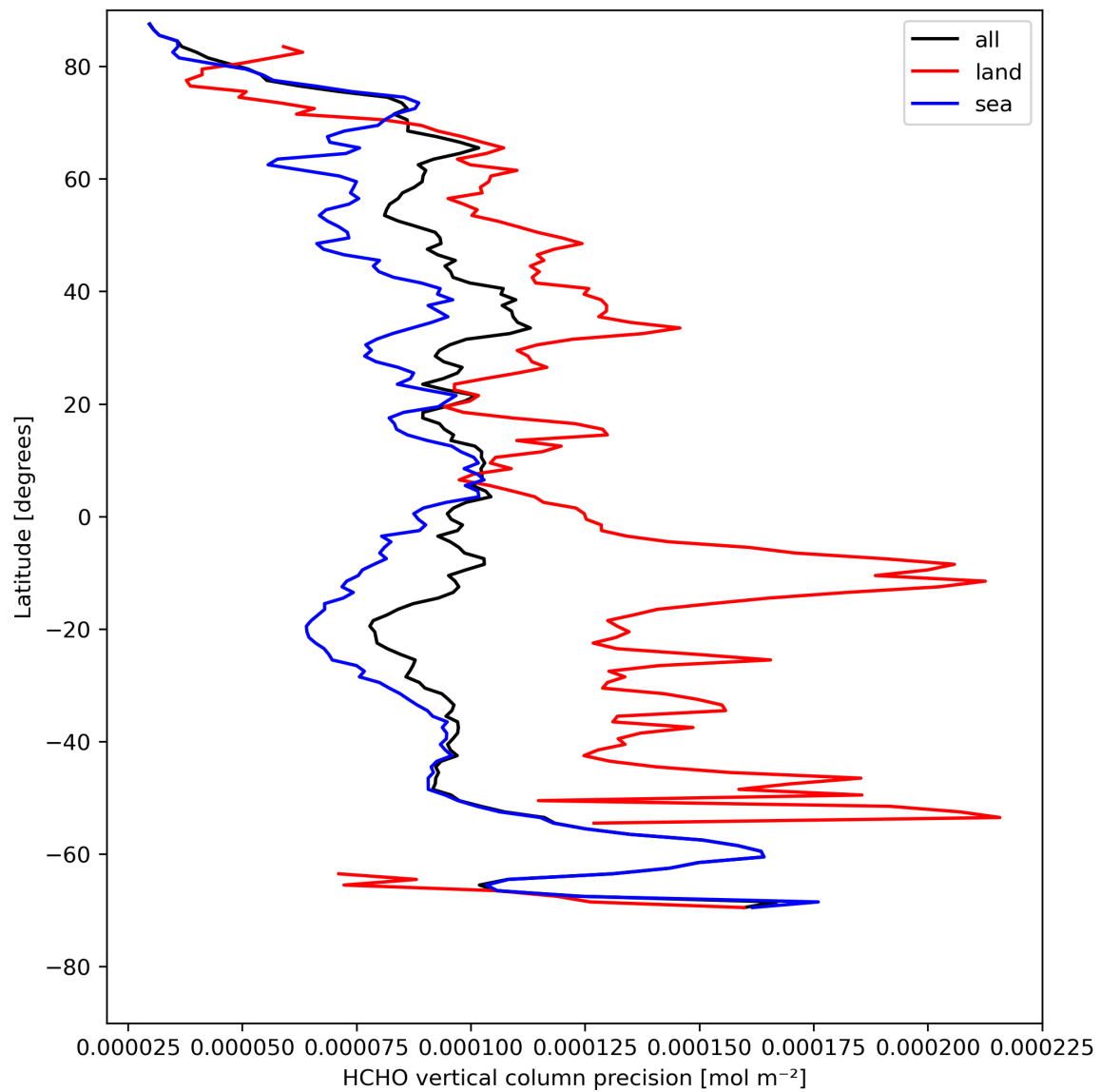
Figure 22: Zonal average of “HCHO vertical column precision” for 2023-08-10 to 2023-08-12.
