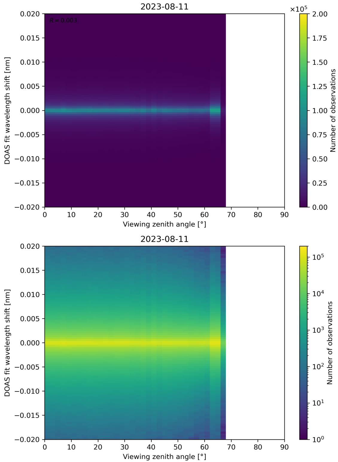
Figure 183: Scatter density plot of “Viewing zenith angle” against “DOAS fit wavelength shift” for 2023-08-10 to 2023-08-12.
