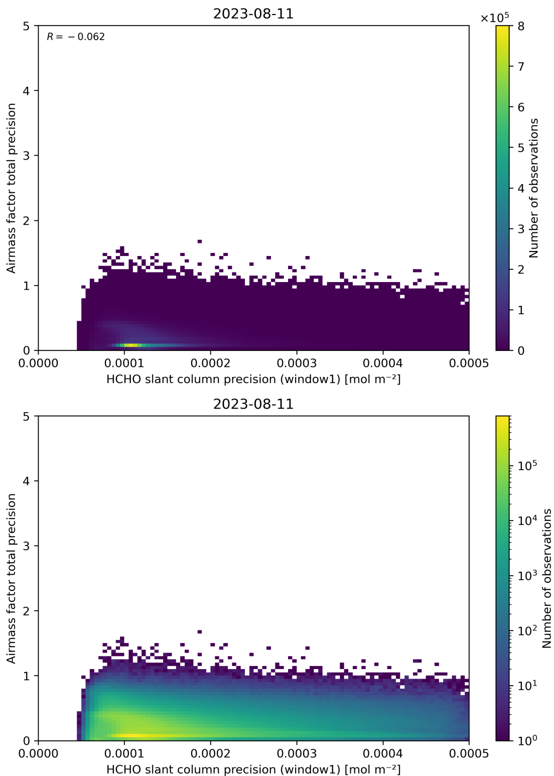
Figure 95: Scatter density plot of “HCHO slant column precision (window1)” against “Airmass factor total precision” for 2023-08-10 to 2023-08-12.
