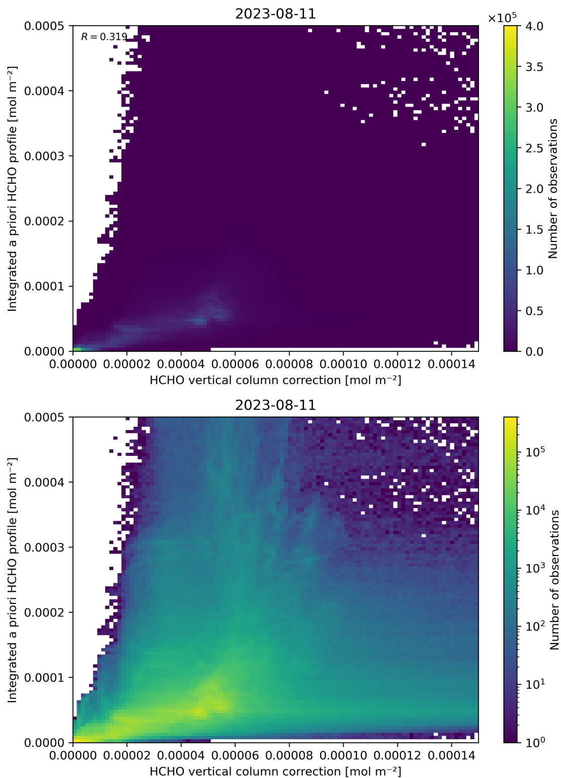
Figure 122: Scatter density plot of “HCHO vertical column correction” against “Integrated a priori HCHO profile” for 2023-08-10 to 2023-08-12.
