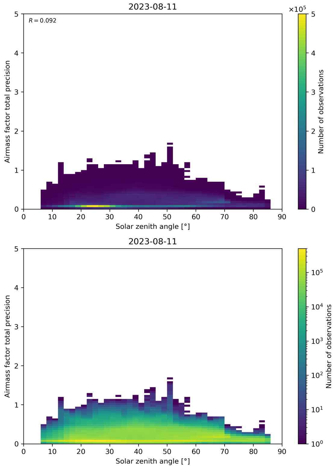
Figure 176: Scatter density plot of “Solar zenith angle” against “Airmass factor total precision” for 2023-08-10 to 2023-08-12.
