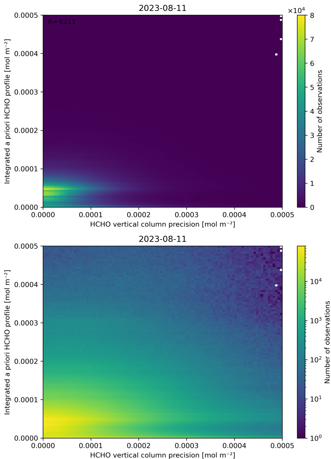
Figure 147: Scatter density plot of “HCHO vertical column precision” against “Integrated a priori HCHO profile” for 2023-08-10 to 2023-08-12.
