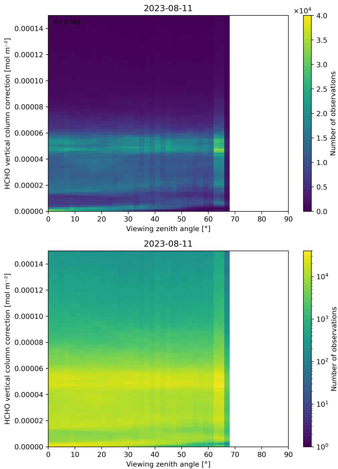
Figure 193: Scatter density plot of “Viewing zenith angle” against “HCHO vertical column correction” for 2023-08-10 to 2023-08-12.
