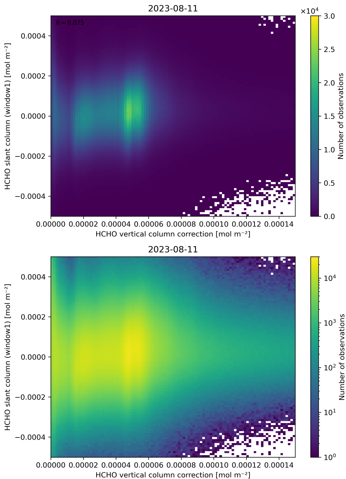
Figure 118: Scatter density plot of “HCHO vertical column correction” against “HCHO slant column (window1)” for 2023-08-10 to 2023-08-12.
