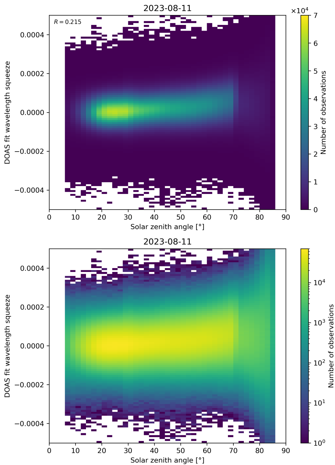
Figure 169: Scatter density plot of “Solar zenith angle” against “DOAS fit wavelength squeeze” for 2023-08-10 to 2023-08-12.
