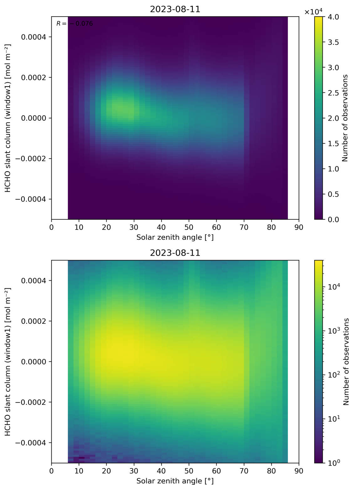
Figure 173: Scatter density plot of “Solar zenith angle” against “HCHO slant column (window1)” for 2023-08-10 to 2023-08-12.
