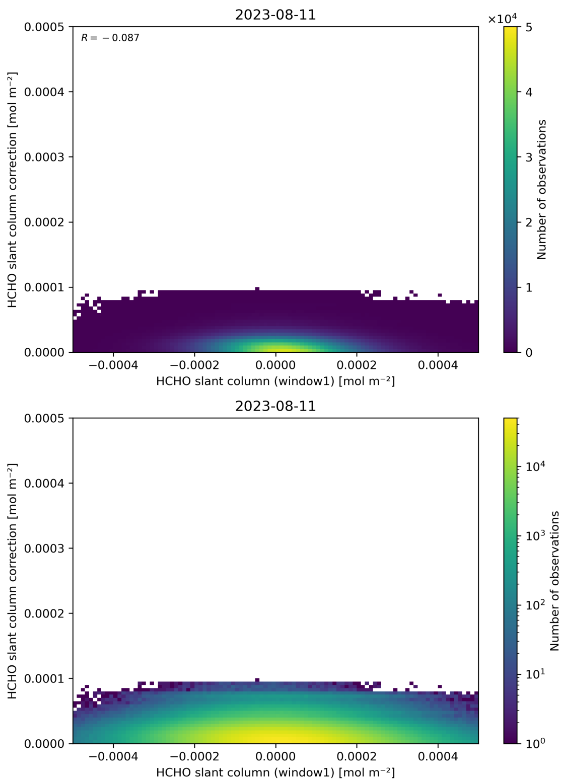
Figure 83: Scatter density plot of “HCHO slant column (window1)” against “HCHO slant column correction” for 2023-08-10 to 2023-08-12.
