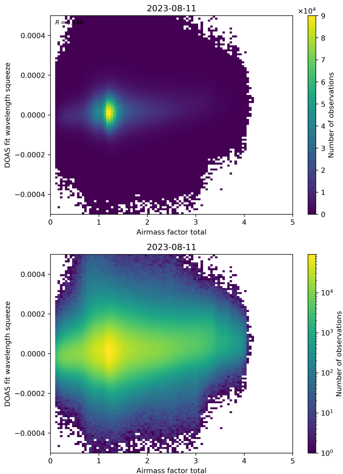
Figure 99: Scatter density plot of “Airmass factor total” against “DOAS fit wavelength squeeze” for 2023-08-10 to 2023-08-12.
