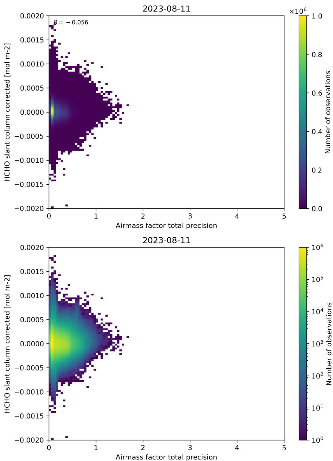
Figure 109: Scatter density plot of “Airmass factor total precision” against “HCHO slant column corrected” for 2023-08-10 to 2023-08-12.
