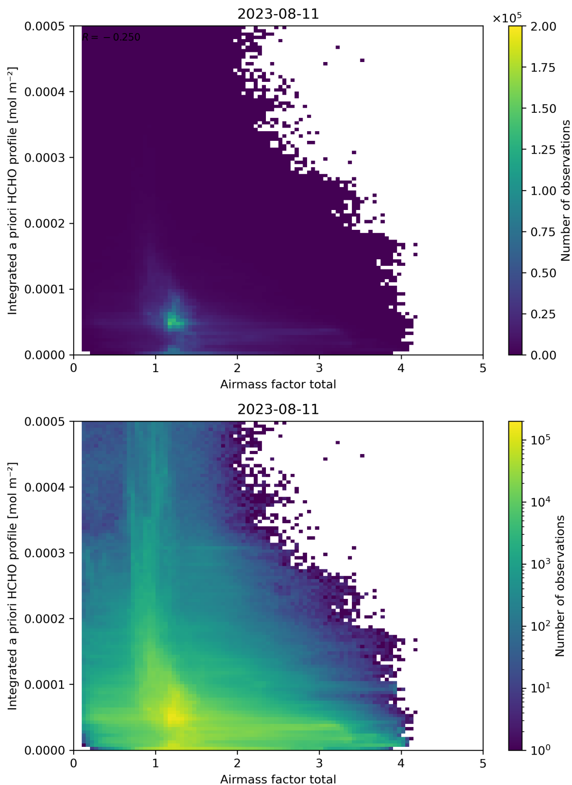
Figure 104: Scatter density plot of “Airmass factor total” against “Integrated a priori HCHO profile” for 2023-08-10 to 2023-08-12.
