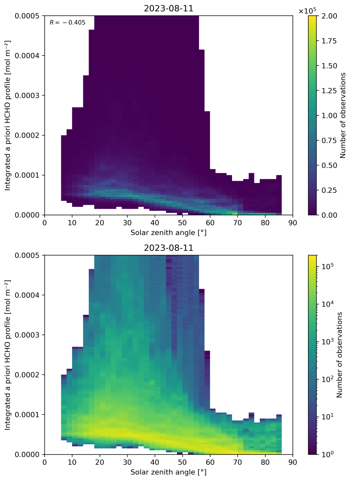
Figure 180: Scatter density plot of “Solar zenith angle” against “Integrated a priori HCHO profile” for 2023-08-10 to 2023-08-12.
