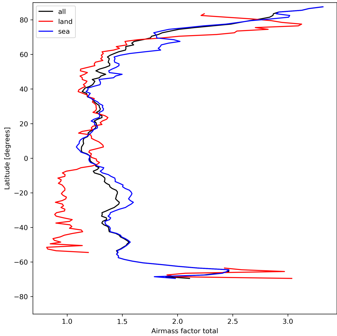
Figure 26: Zonal average of “Airmass factor total” for 2023-08-10 to 2023-08-12.
