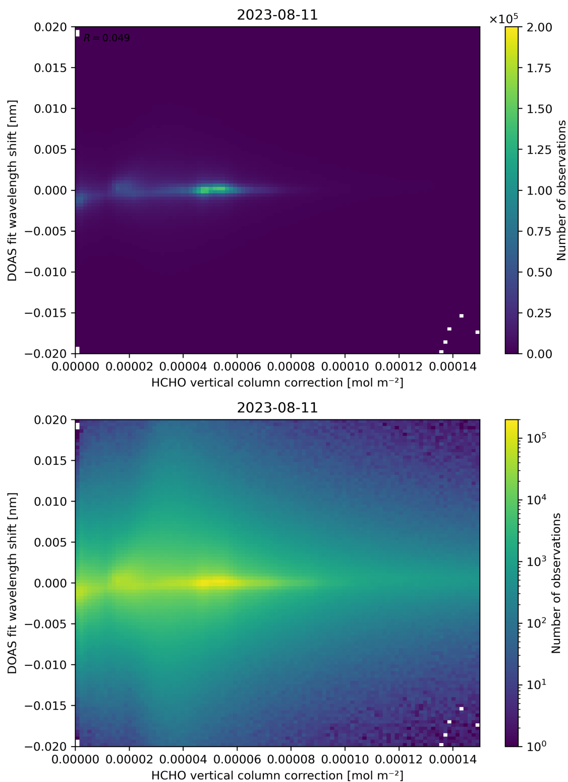
Figure 113: Scatter density plot of “HCHO vertical column correction” against “DOAS fit wavelength shift” for 2023-08-10 to 2023-08-12.
