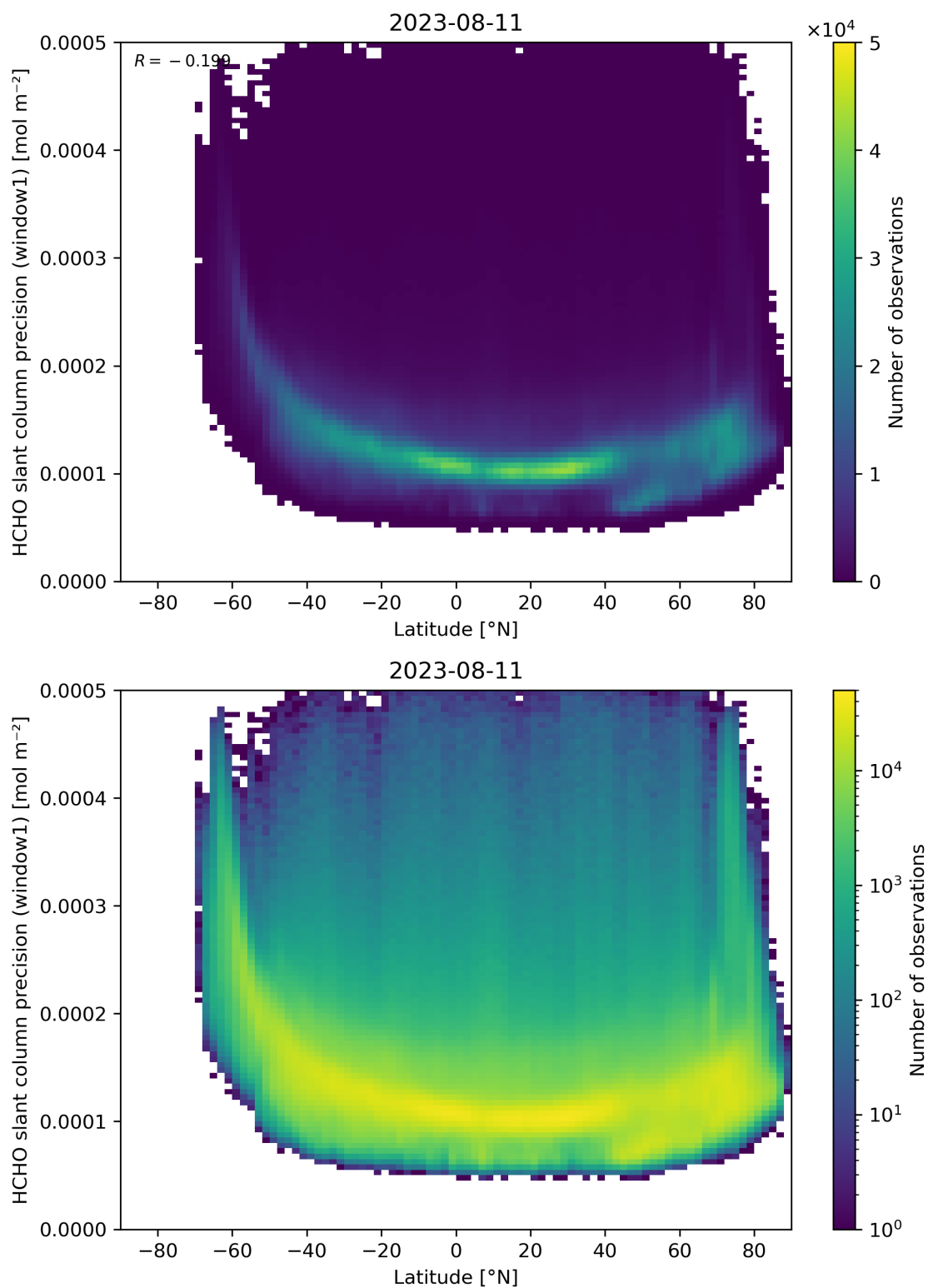
Figure 160: Scatter density plot of “Latitude” against “HCHO slant column precision (window1)” for 2023-08-10 to 2023-08-12.
