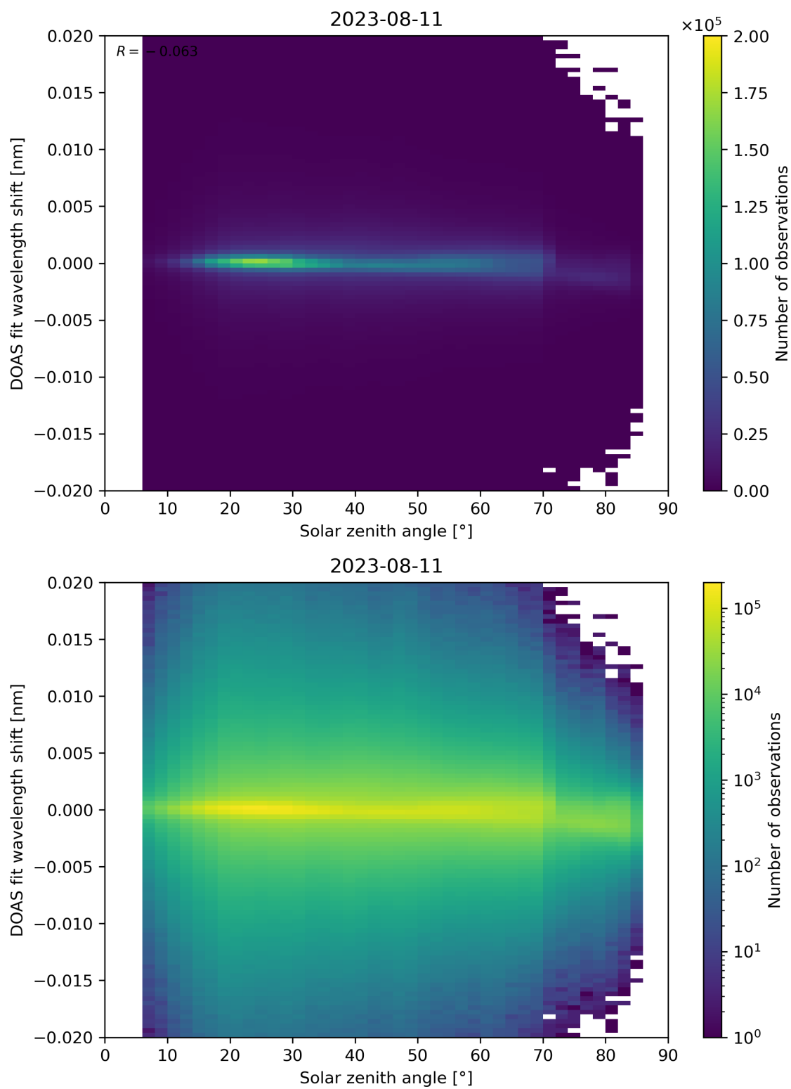
Figure 168: Scatter density plot of “Solar zenith angle” against “DOAS fit wavelength shift” for 2023-08-10 to 2023-08-12.
