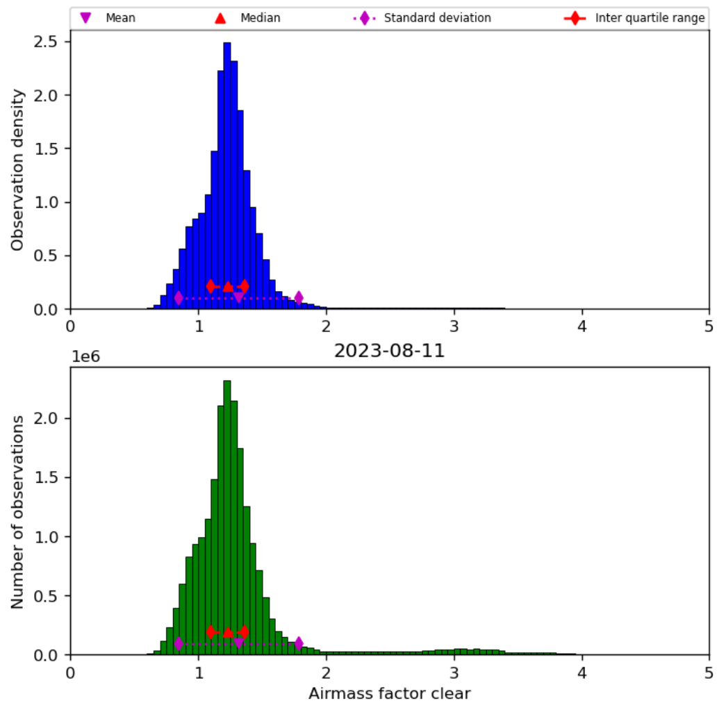
Figure 42: Histogram of “Airmass factor clear” for 2023-08-10 to 2023-08-12
