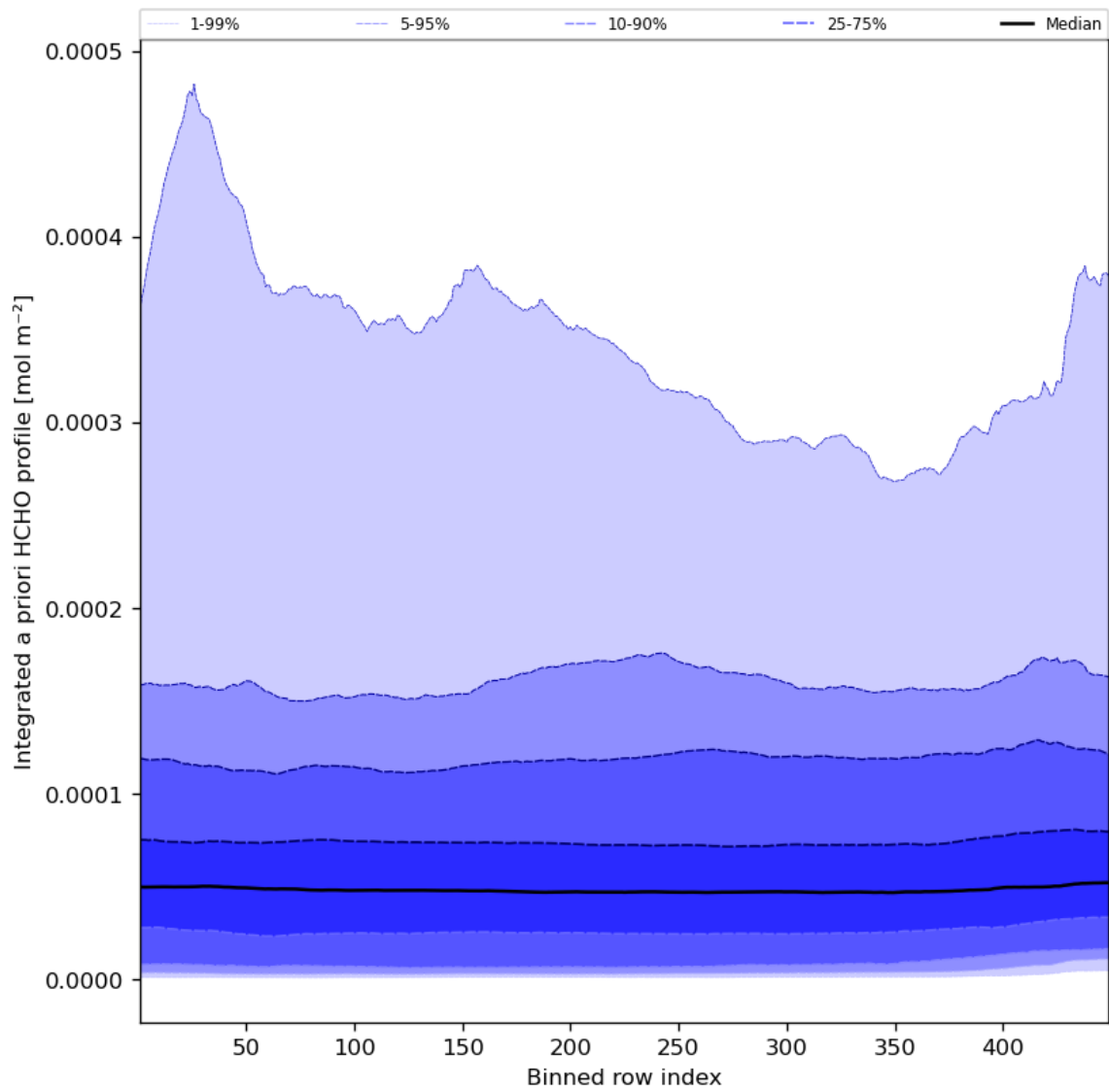
Figure 57: Along track statistics of "Integrated a priori HCHO profile" for 2023-08-10 to 2023-08-12
