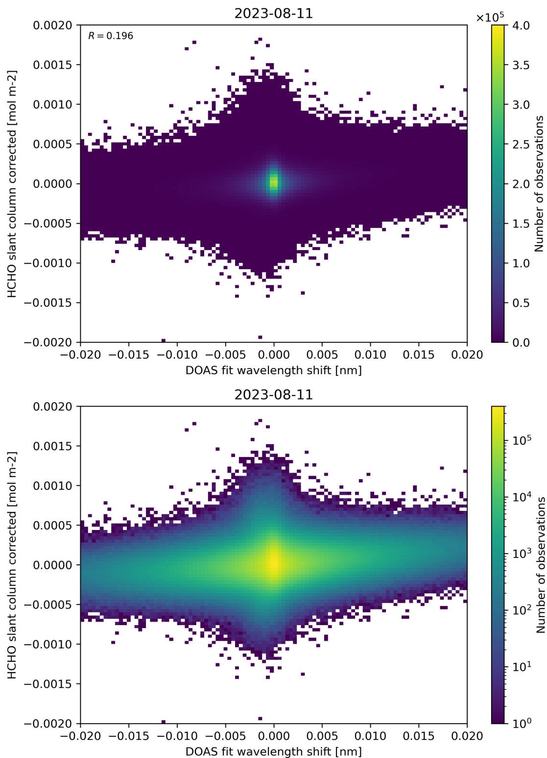
Figure 66: Scatter density plot of “DOAS fit wavelength shift” against “HCHO slant column corrected” for 2023-08-10 to 2023-08-12.
