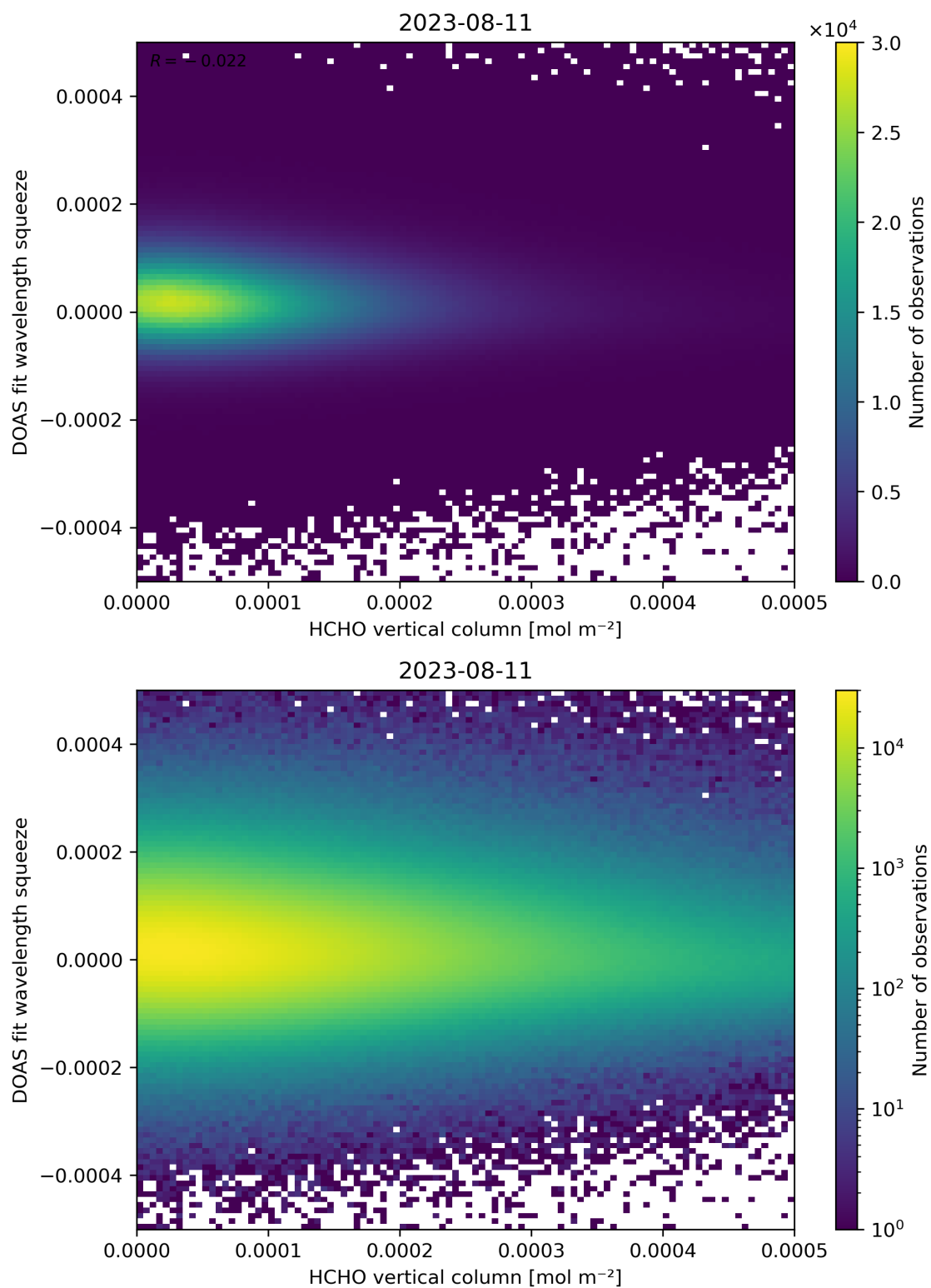
Figure 125: Scatter density plot of “HCHO vertical column” against “DOAS fit wavelength squeeze” for 2023-08-10 to 2023-08-12.
