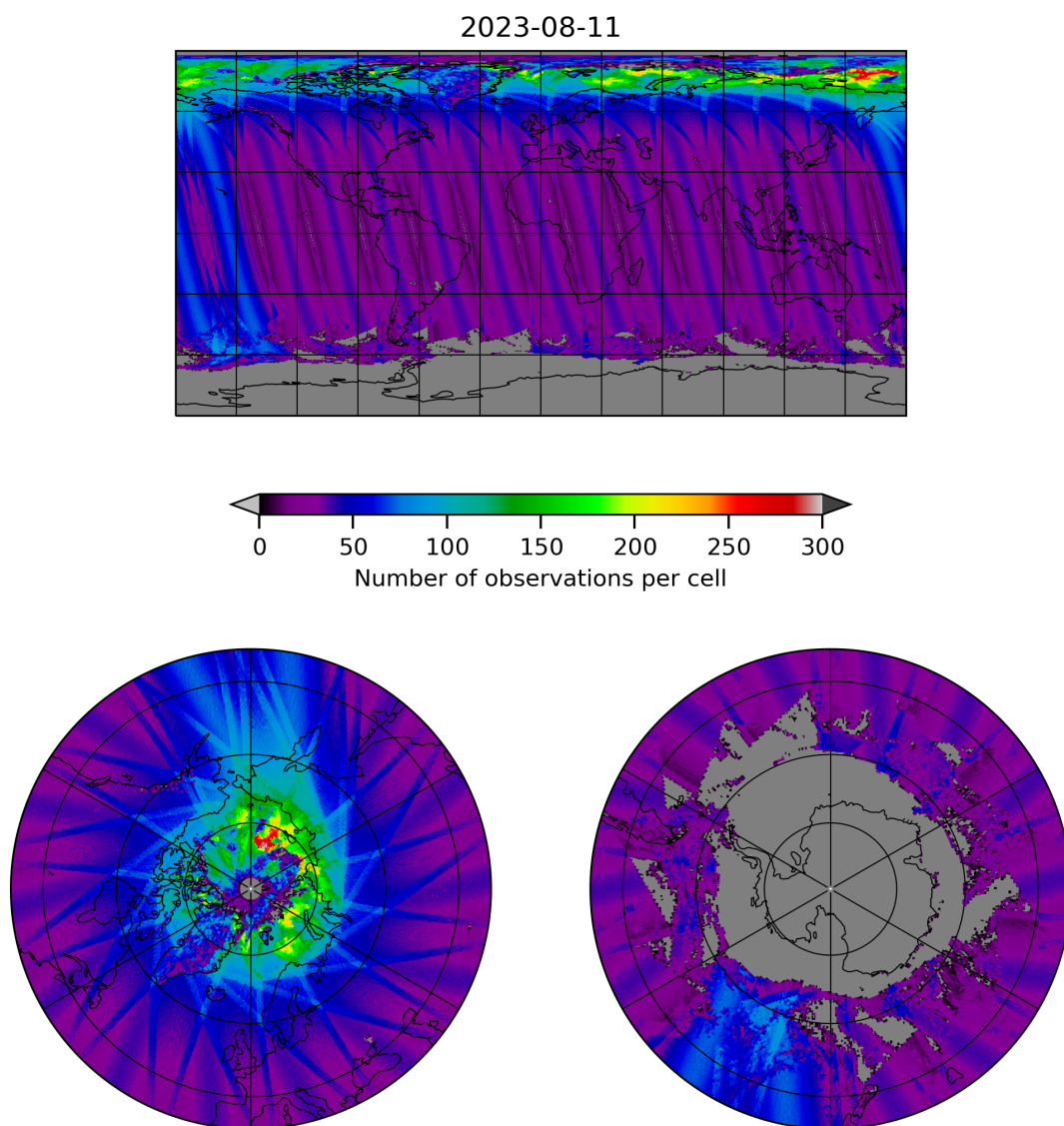
Figure 19: Map of the number of observations for 2023-08-10 to 2023-08-12
