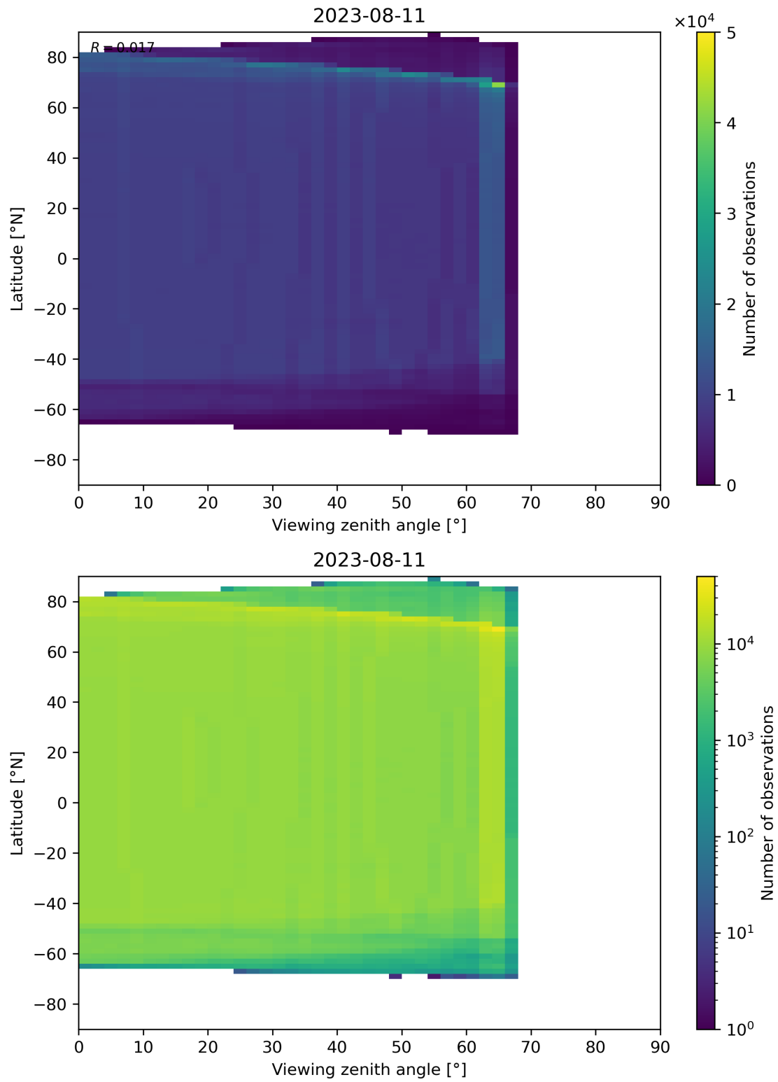
Figure 196: Scatter density plot of “Viewing zenith angle” against “Latitude” for 2023-08-10 to 2023-08-12.
