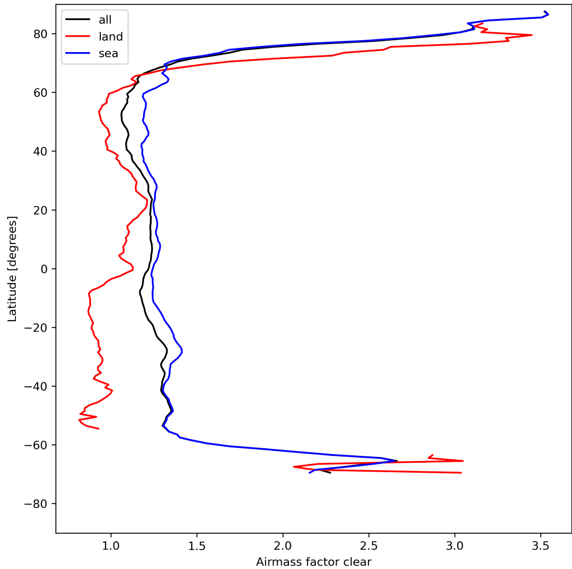
Figure 28: Zonal average of “Airmass factor clear” for 2023-08-10 to 2023-08-12.
