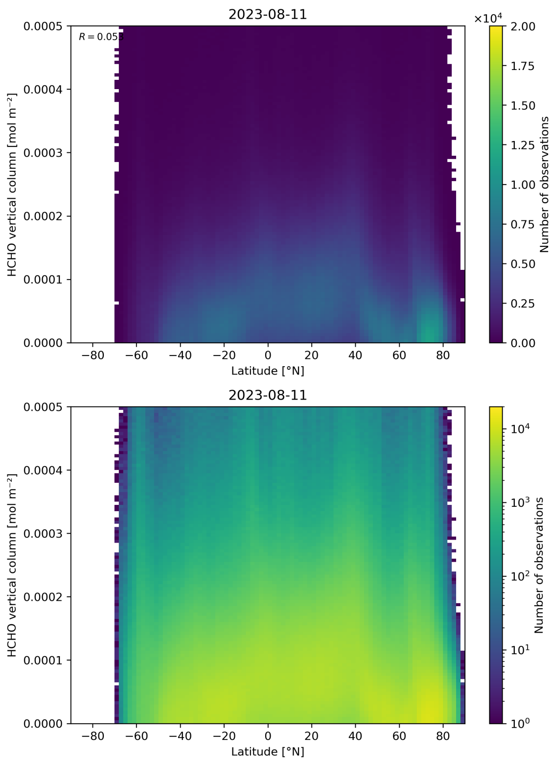
Figure 163: Scatter density plot of “Latitude” against “HCHO vertical column” for 2023-08-10 to 2023-08-12.
