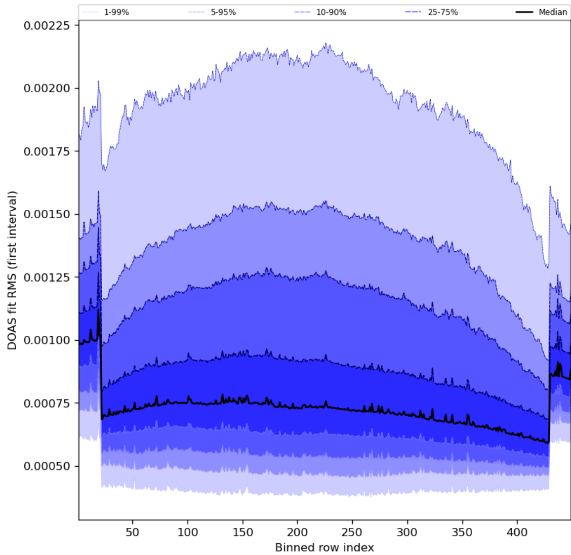
Figure 60: Along track statistics of “DOAS fit RMS (first interval)” for 2023-08-10 to 2023-08-12
