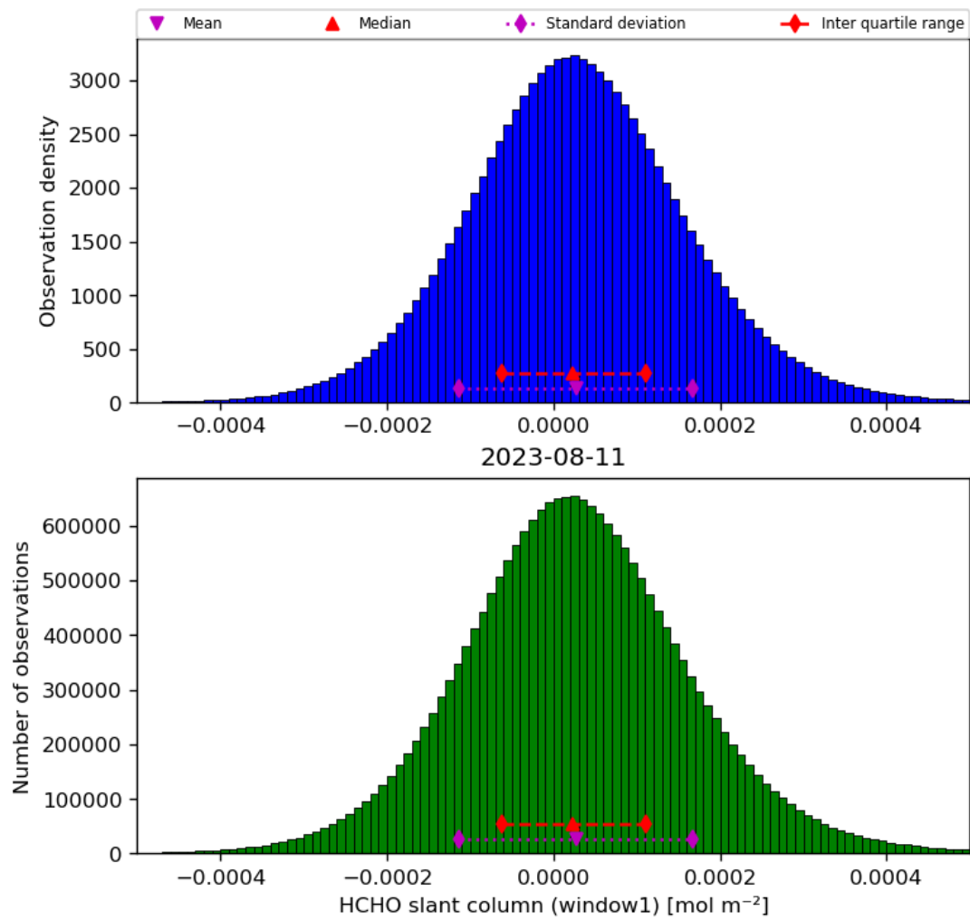
Figure 38: Histogram of “HCHO slant column (window1)” for 2023-08-10 to 2023-08-12
