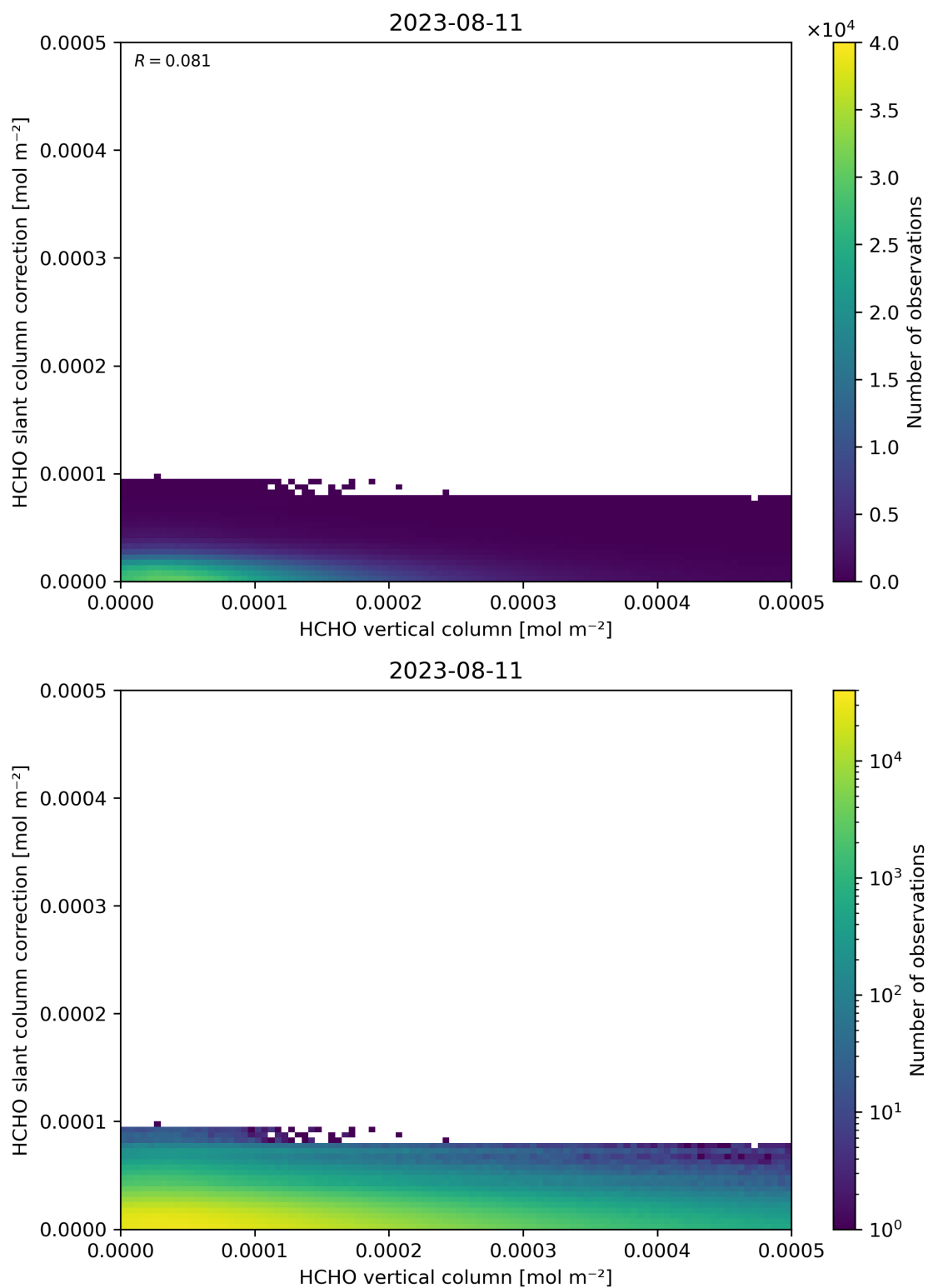
Figure 128: Scatter density plot of “HCHO vertical column” against “HCHO slant column correction” for 2023-08-10 to 2023-08-12.
