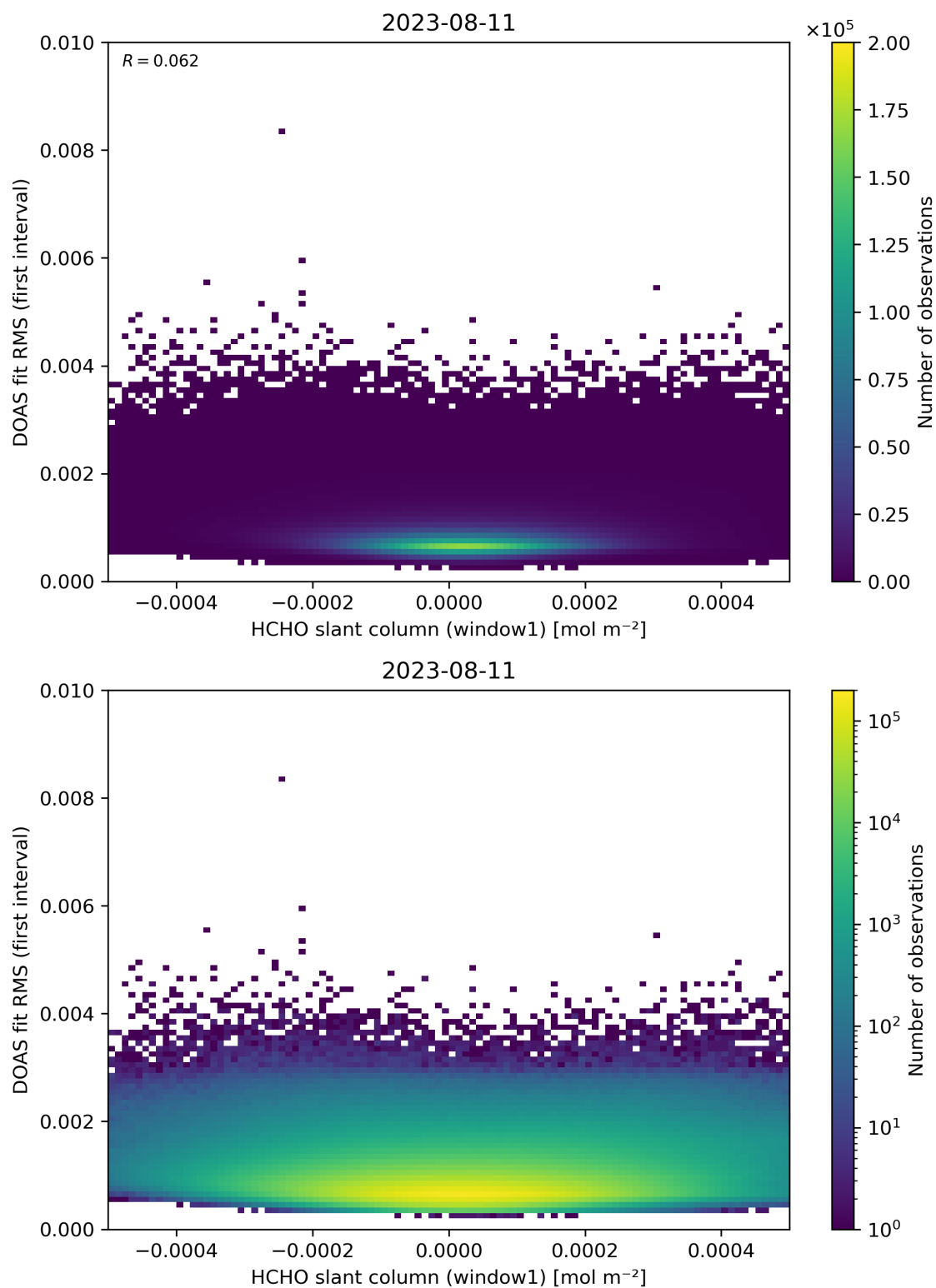
Figure 78: Scatter density plot of “HCHO slant column (window1)” against “DOAS fit RMS (first interval)” for 2023-08-10 to 2023-08-12.
