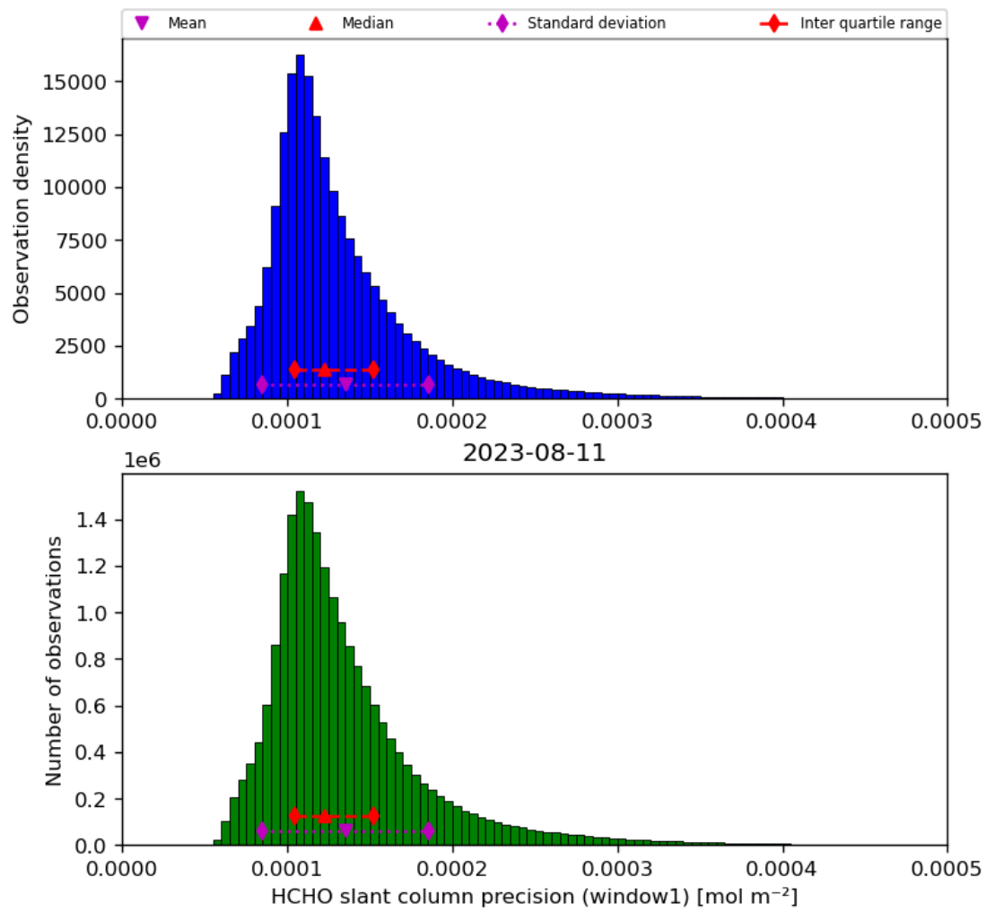
Figure 39: Histogram of “HCHO slant column precision (window1)” for 2023-08-10 to 2023-08-12
