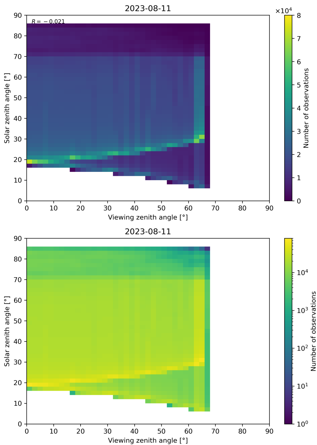
Figure 197: Scatter density plot of “Viewing zenith angle” against “Solar zenith angle” for 2023-08-10 to 2023-08-12.
