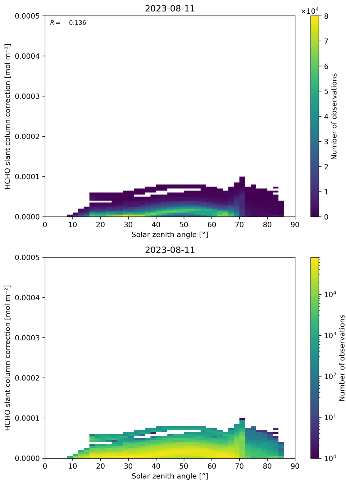
Figure 172: Scatter density plot of “Solar zenith angle” against “HCHO slant column correction” for 2023-08-10 to 2023-08-12.
