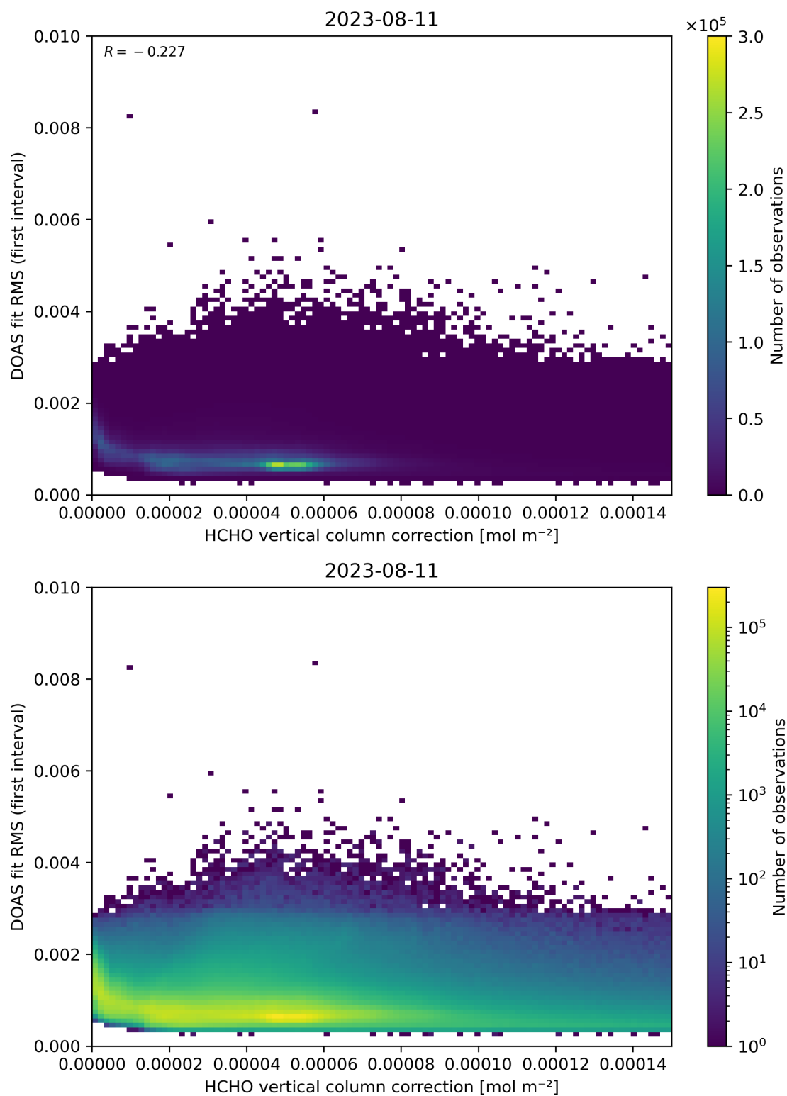
Figure 112: Scatter density plot of “HCHO vertical column correction” against “DOAS fit RMS (first interval)” for 2023-08-10 to 2023-08-12.
