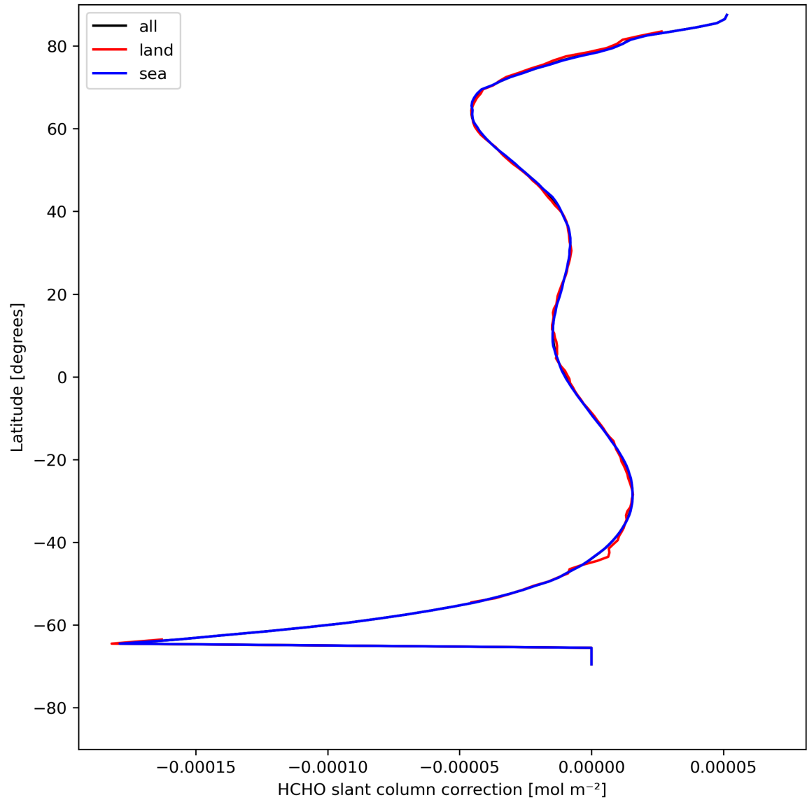
Figure 33: Zonal average of “HCHO slant column correction” for 2023-08-10 to 2023-08-12.
