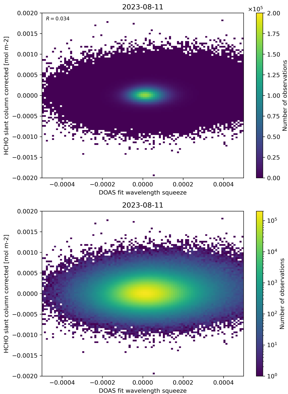
Figure 69: Scatter density plot of “DOAS fit wavelength squeeze” against “HCHO slant column corrected” for 2023-08-10 to 2023-08-12.
