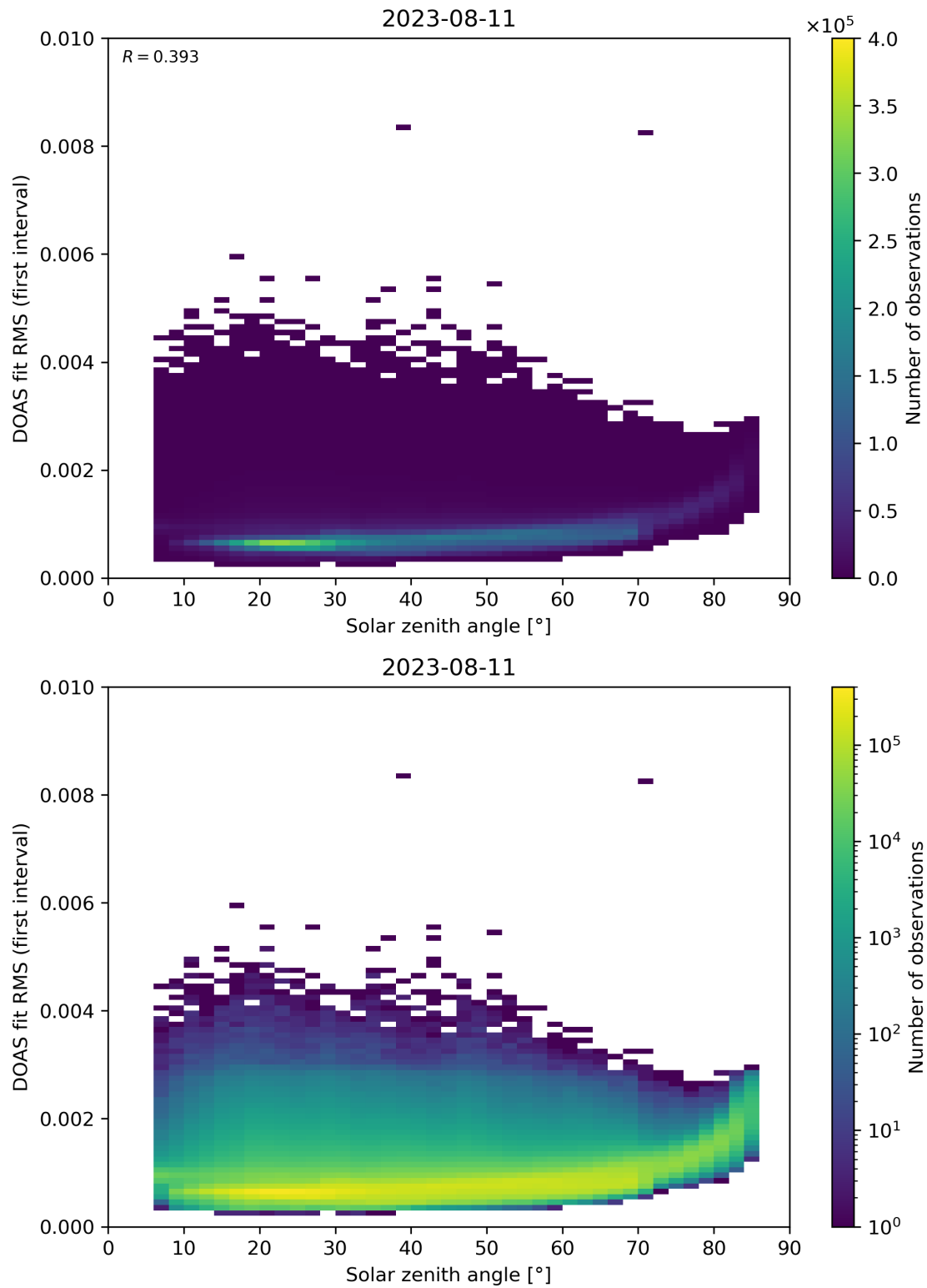
Figure 167: Scatter density plot of “Solar zenith angle” against “DOAS fit RMS (first interval)” for 2023-08-10 to 2023-08-12.
