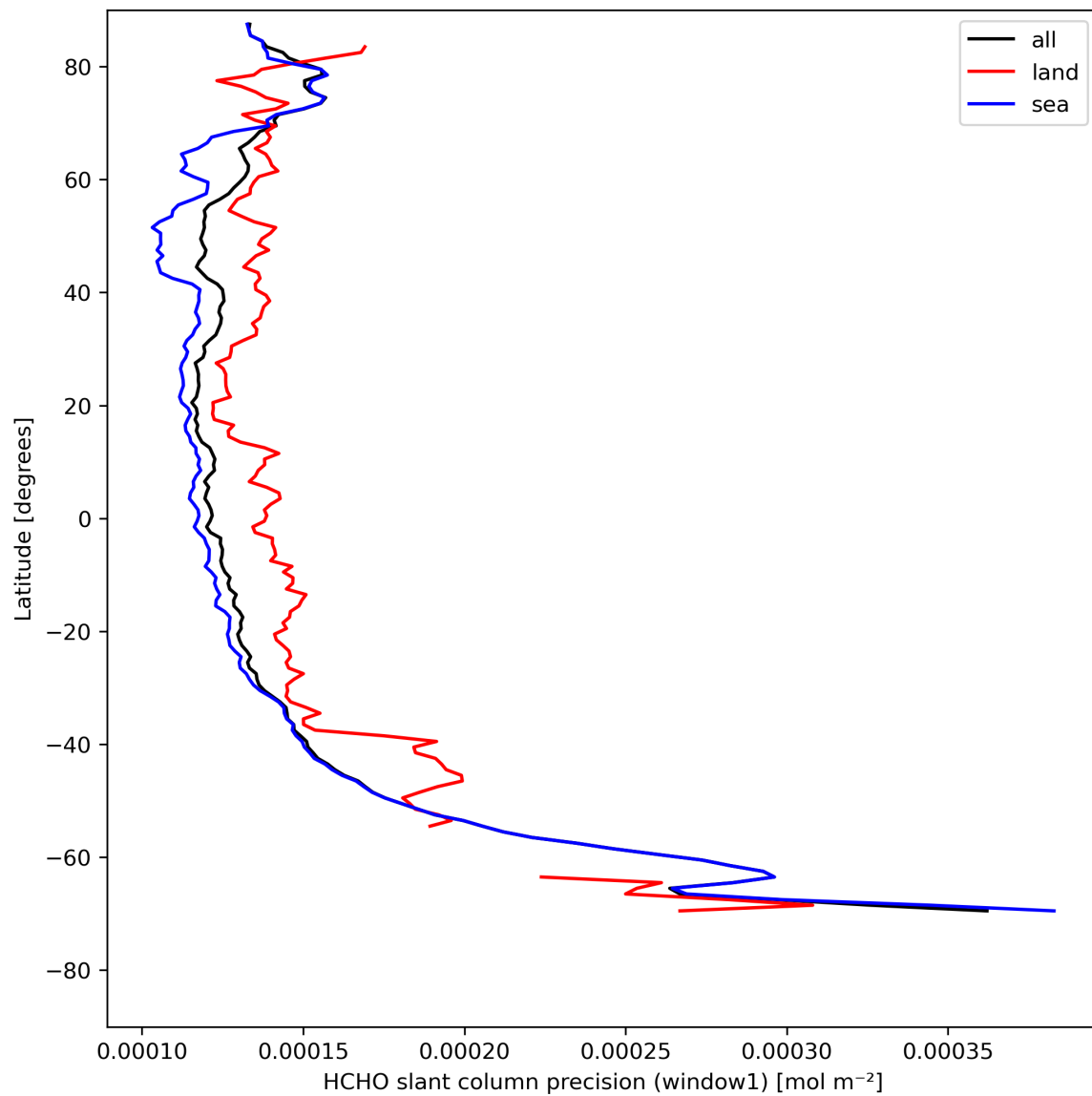
Figure 25: Zonal average of “HCHO slant column precision (window1)” for 2023-08-10 to 2023-08-12.
