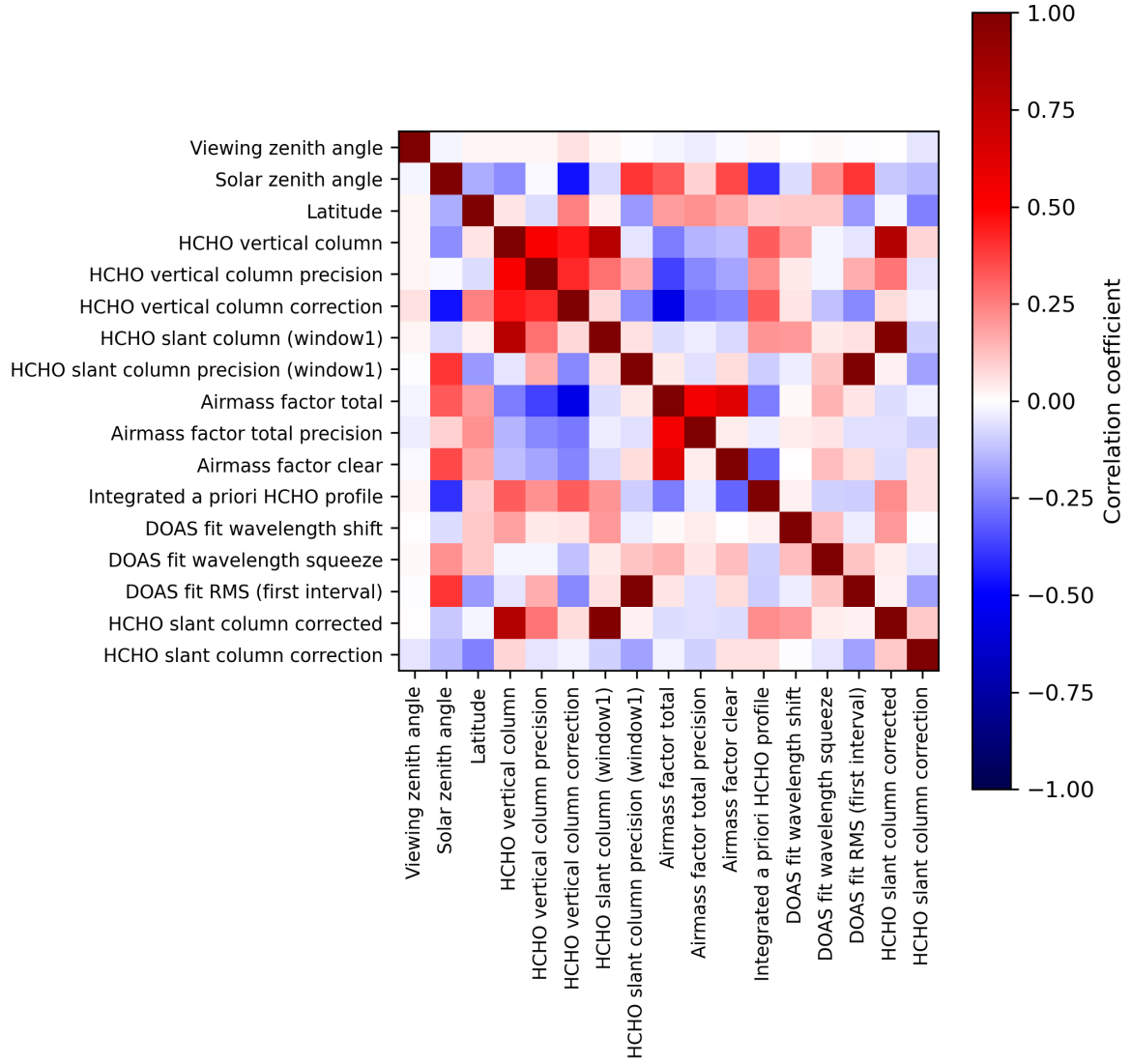
Figure 2: Map of correlation matrix for 2023-08-10 to 2023-08-12.
