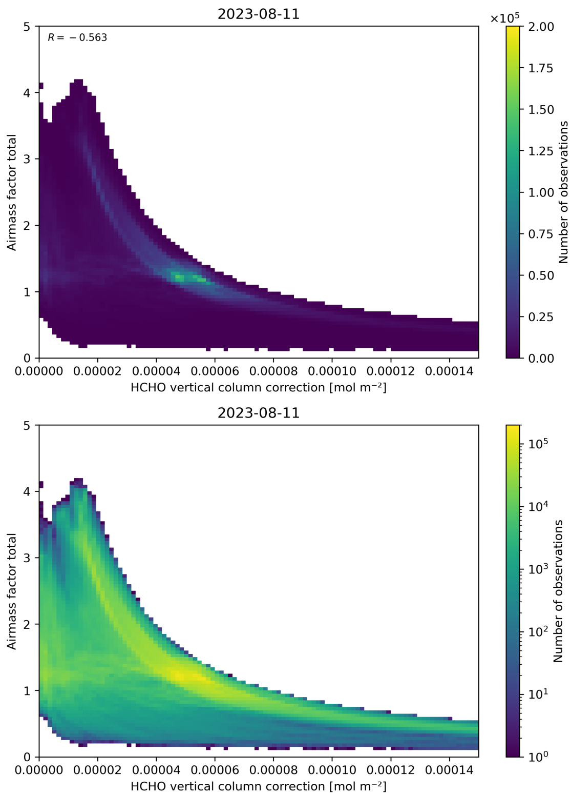
Figure 120: Scatter density plot of “HCHO vertical column correction” against “Airmass factor total” for 2023-08-10 to 2023-08-12.
