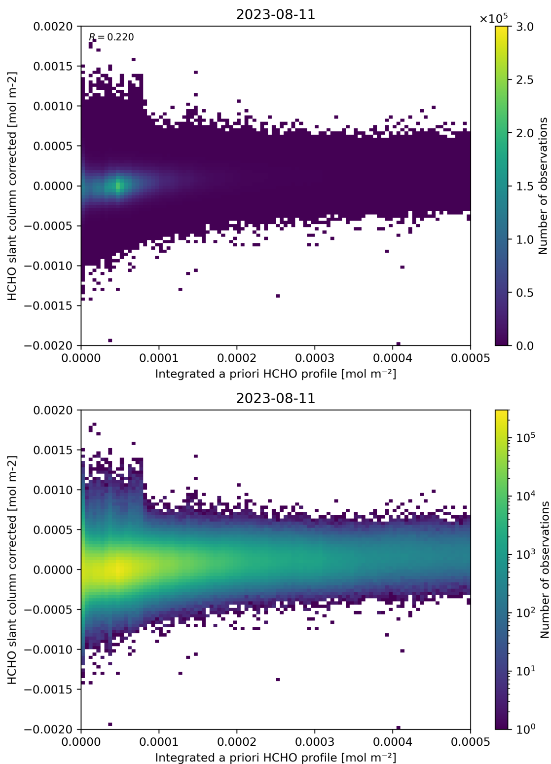
Figure 151: Scatter density plot of “Integrated a priori HCHO profile” against “HCHO slant column corrected” for 2023-08-10 to 2023-08-12.
