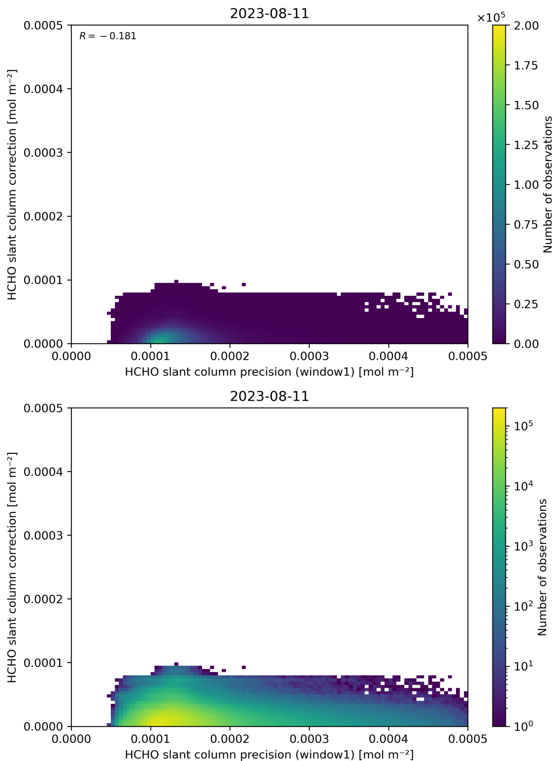
Figure 93: Scatter density plot of “HCHO slant column precision (window1)” against “HCHO slant column correction” for 2023-08-10 to 2023-08-12.
