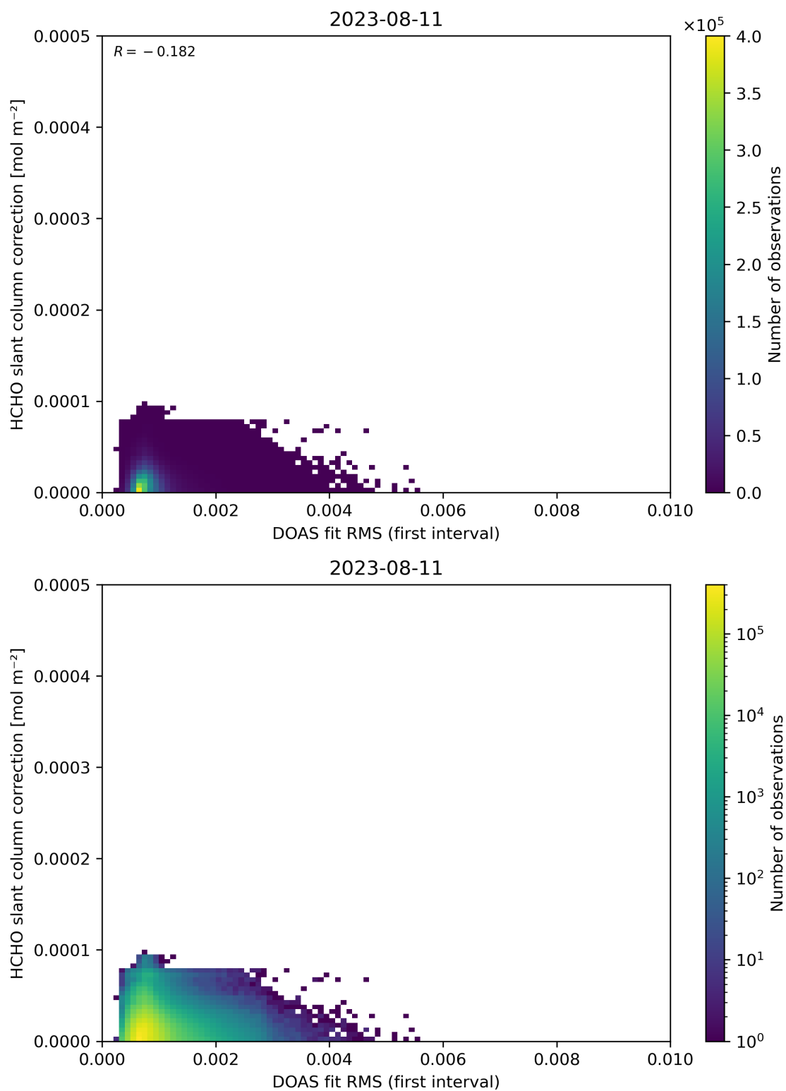
Figure 63: Scatter density plot of “DOAS fit RMS (first interval)” against “HCHO slant column correction” for 2023-08-10 to 2023-08-12.
