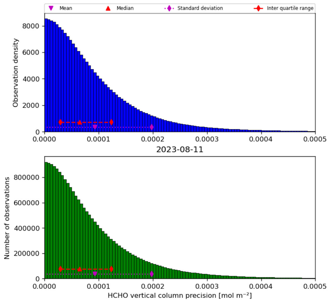
Figure 36: Histogram of “HCHO vertical column precision” for 2023-08-10 to 2023-08-12
