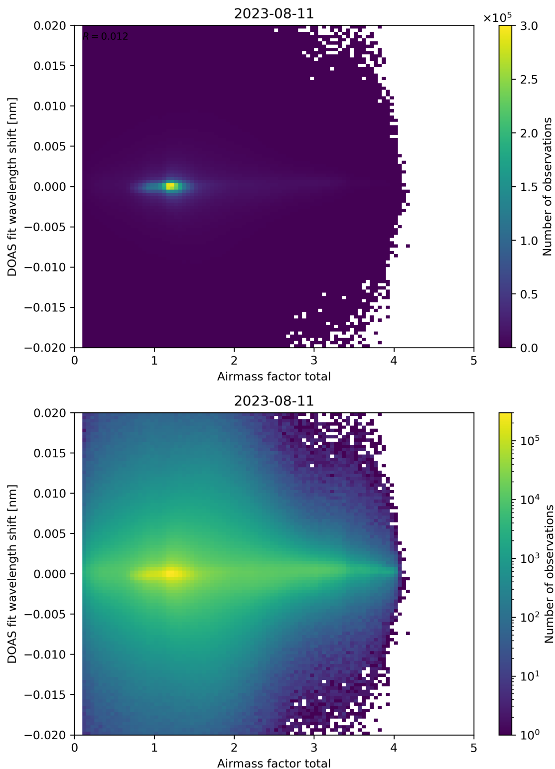
Figure 98: Scatter density plot of “Airmass factor total” against “DOAS fit wavelength shift” for 2023-08-10 to 2023-08-12.
