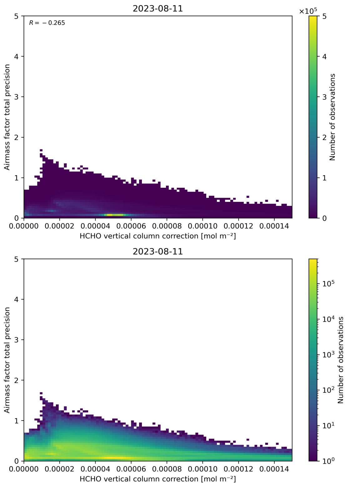
Figure 121: Scatter density plot of “HCHO vertical column correction” against “Airmass factor total precision” for 2023-08-10 to 2023-08-12.
