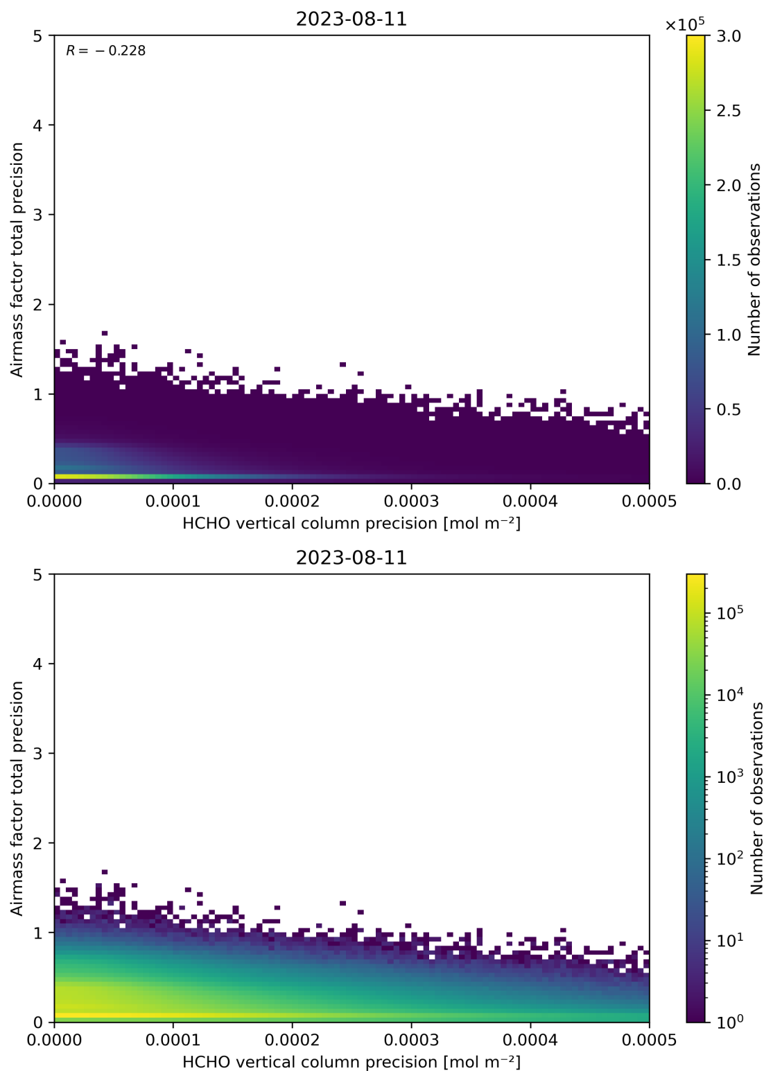
Figure 145: Scatter density plot of “HCHO vertical column precision” against “Airmass factor total precision” for 2023-08-10 to 2023-08-12.
