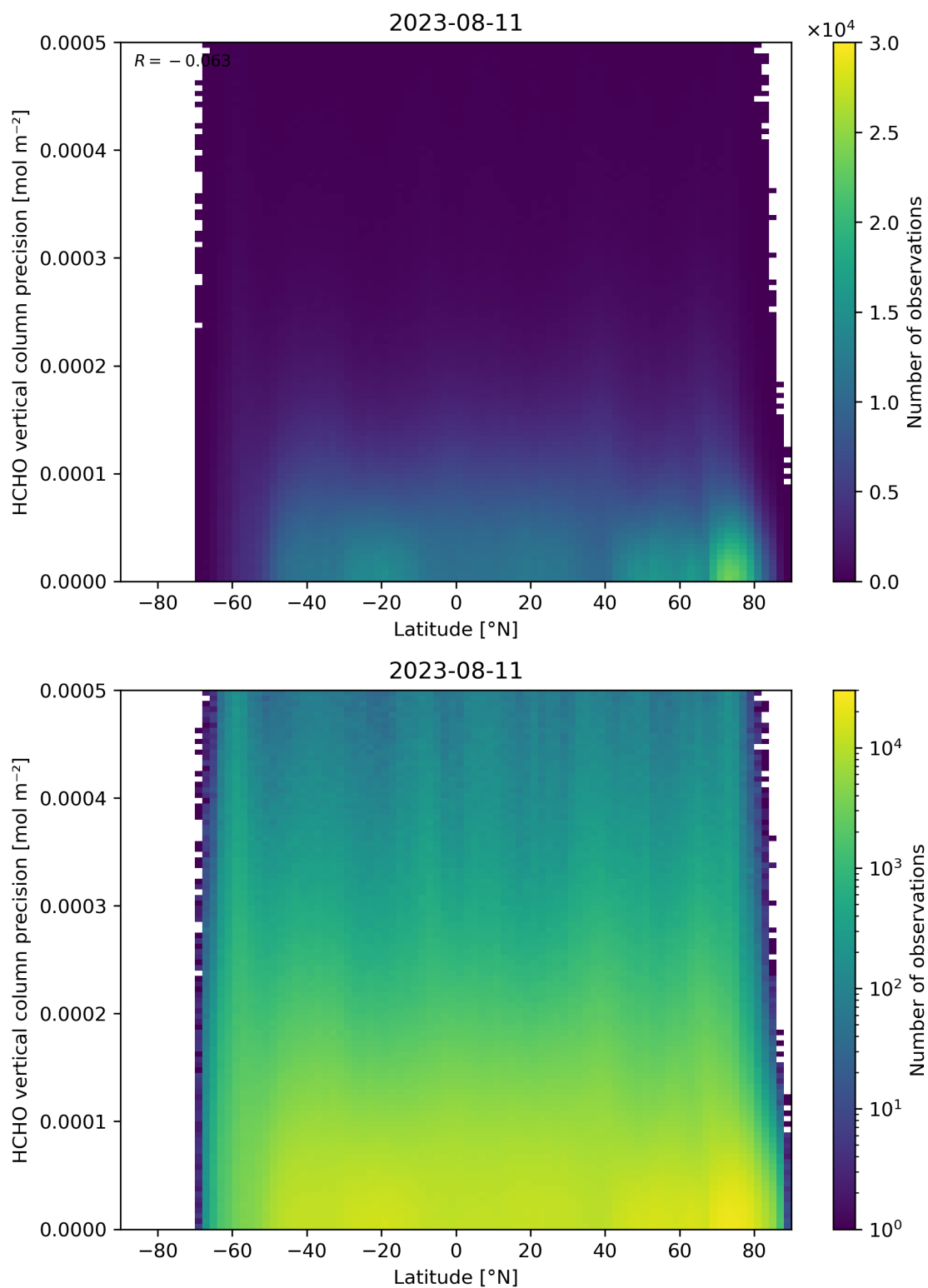
Figure 165: Scatter density plot of “Latitude” against “HCHO vertical column precision” for 2023-08-10 to 2023-08-12.
