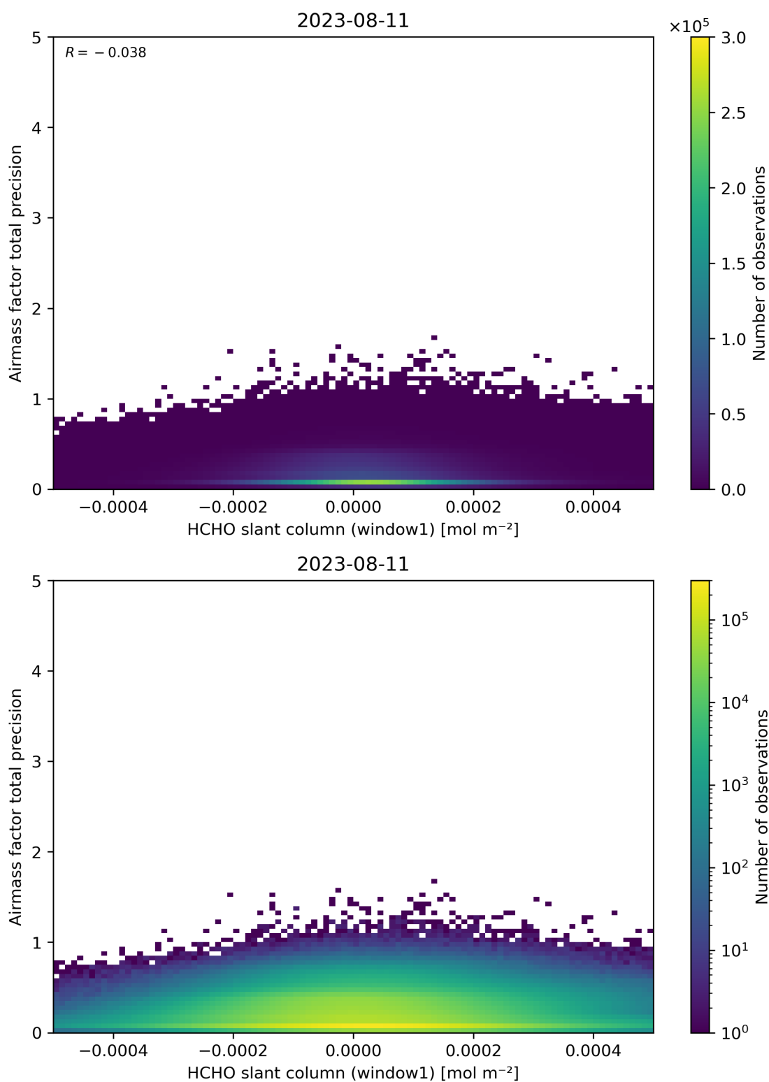
Figure 86: Scatter density plot of “HCHO slant column (window1)” against “Airmass factor total precision” for 2023-08-10 to 2023-08-12.
