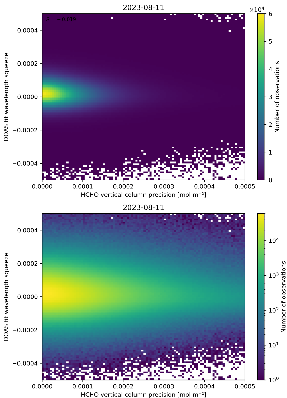
Figure 138: Scatter density plot of “HCHO vertical column precision” against “DOAS fit wavelength squeeze” for 2023-08-10 to 2023-08-12.
