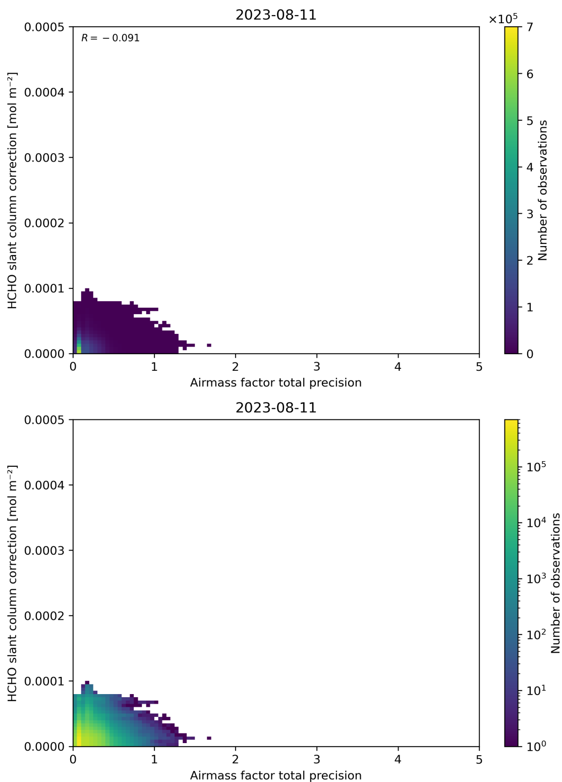
Figure 110: Scatter density plot of “Airmass factor total precision” against “HCHO slant column correction” for 2023-08-10 to 2023-08-12.
