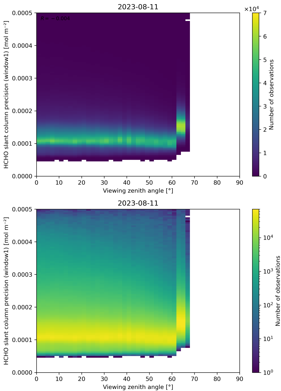
Figure 189: Scatter density plot of “Viewing zenith angle” against “HCHO slant column precision (window1)” for 2023-08-10 to 2023-08-12.
