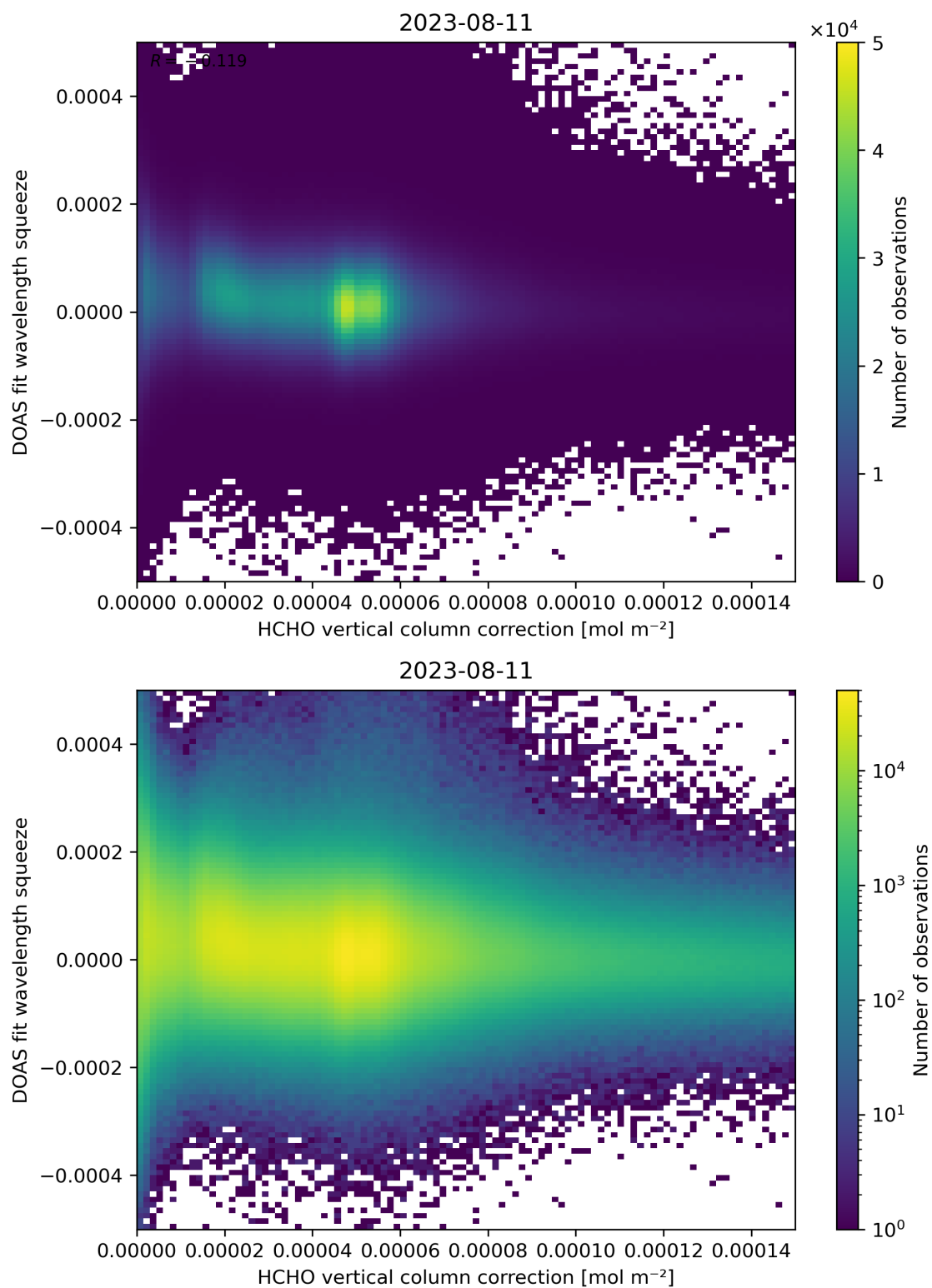
Figure 114: Scatter density plot of “HCHO vertical column correction” against “DOAS fit wavelength squeeze” for 2023-08-10 to 2023-08-12.
