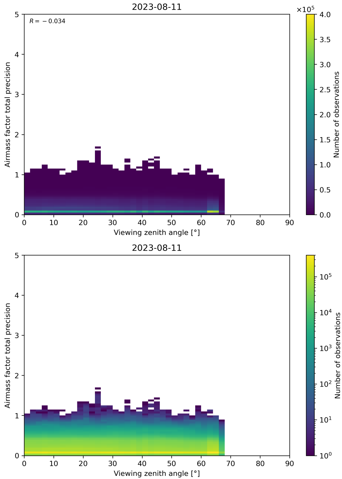
Figure 191: Scatter density plot of “Viewing zenith angle” against “Airmass factor total precision” for 2023-08-10 to 2023-08-12.
