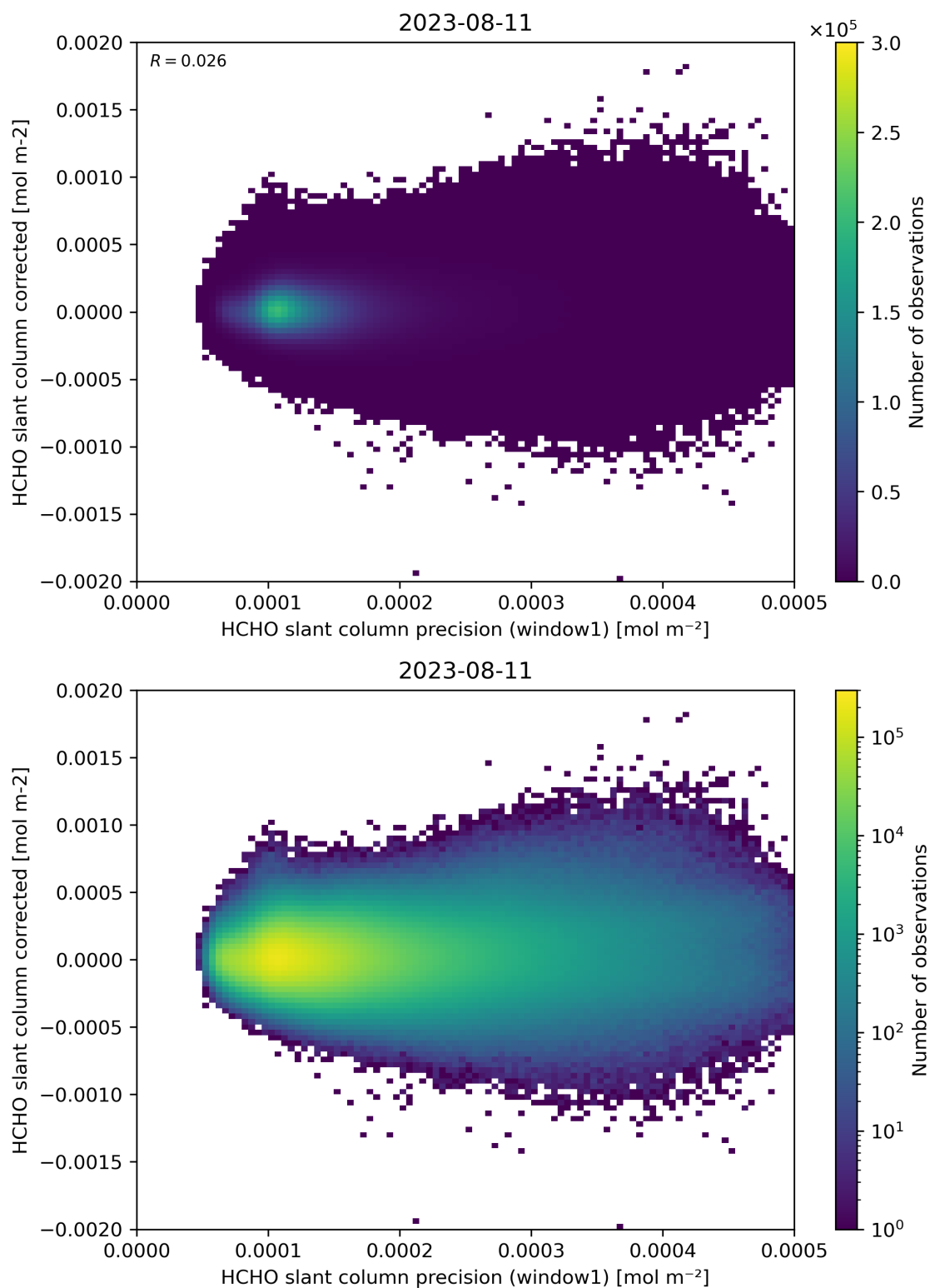
Figure 92: Scatter density plot of “HCHO slant column precision (window1)” against “HCHO slant column corrected” for 2023-08-10 to 2023-08-12.
