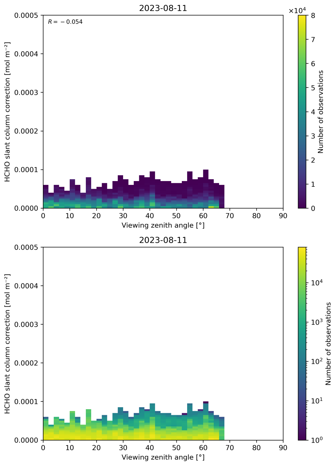
Figure 187: Scatter density plot of “Viewing zenith angle” against “HCHO slant column correction” for 2023-08-10 to 2023-08-12.
