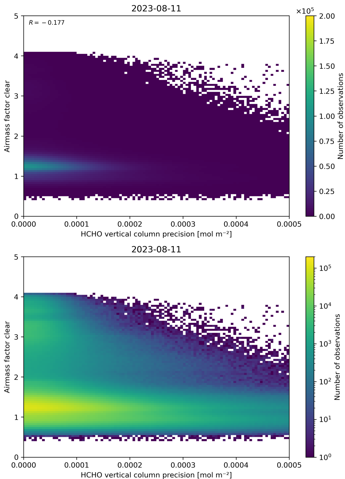
Figure 139: Scatter density plot of “HCHO vertical column precision” against “Airmass factor clear” for 2023-08-10 to 2023-08-12.
