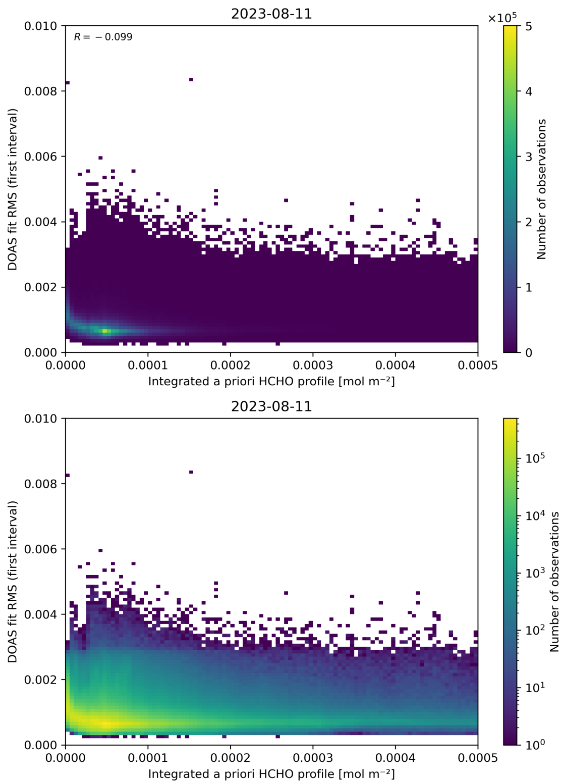
Figure 148: Scatter density plot of “Integrated a priori HCHO profile” against “DOAS fit RMS (first interval)” for 2023-08-10 to 2023-08-12.
