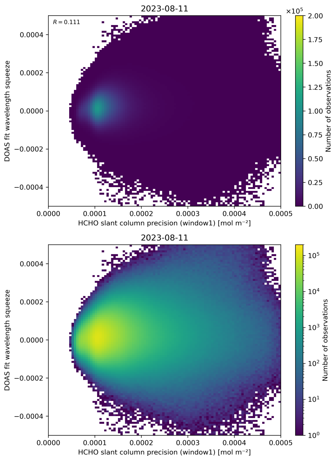
Figure 90: Scatter density plot of “HCHO slant column precision (window1)” against “DOAS fit wavelength squeeze” for 2023-08-10 to 2023-08-12.
