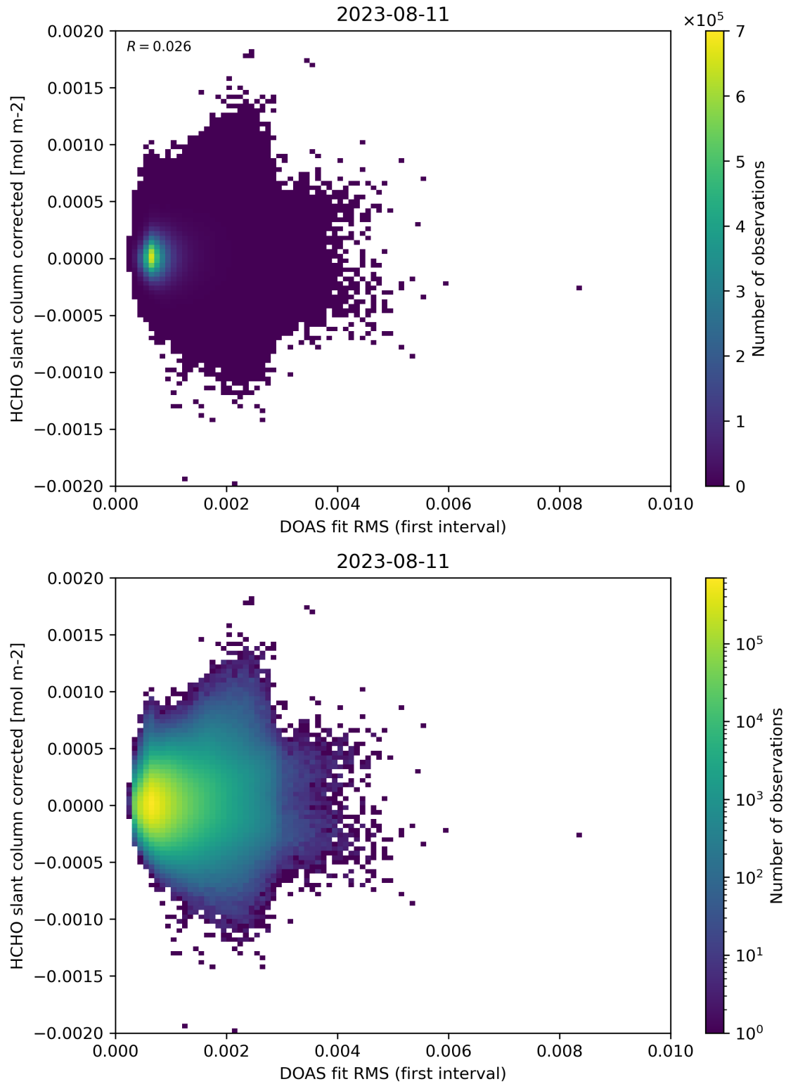
Figure 62: Scatter density plot of “DOAS fit RMS (first interval)” against “HCHO slant column corrected” for 2023-08-10 to 2023-08-12.
