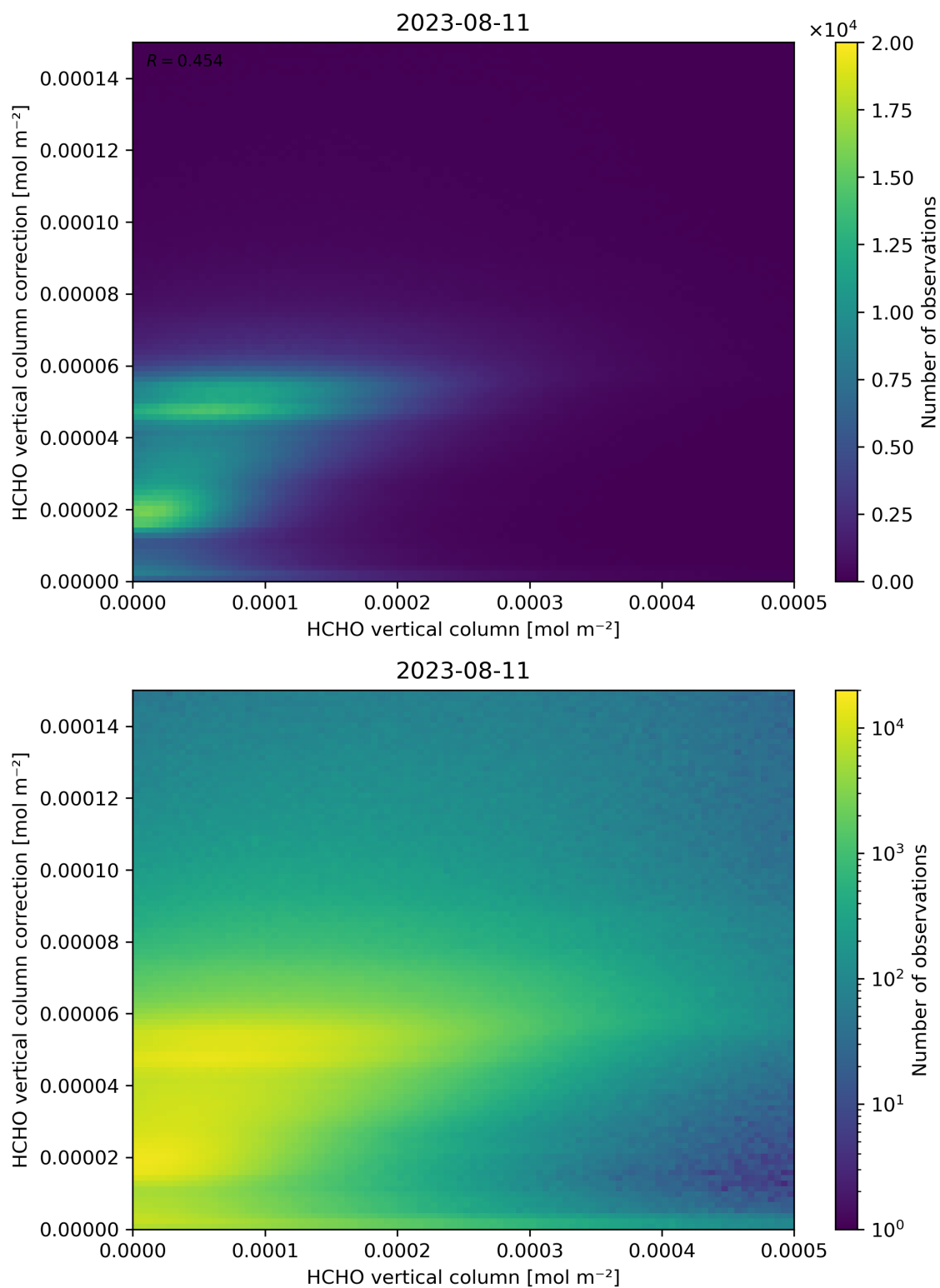
Figure 133: Scatter density plot of “HCHO vertical column” against “HCHO vertical column correction” for 2023-08-10 to 2023-08-12.
