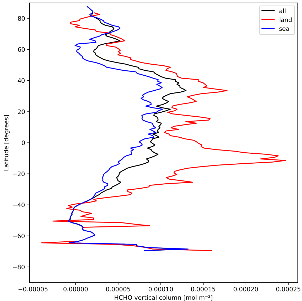
Figure 21: Zonal average of “HCHO vertical column” for 2023-08-10 to 2023-08-12.
