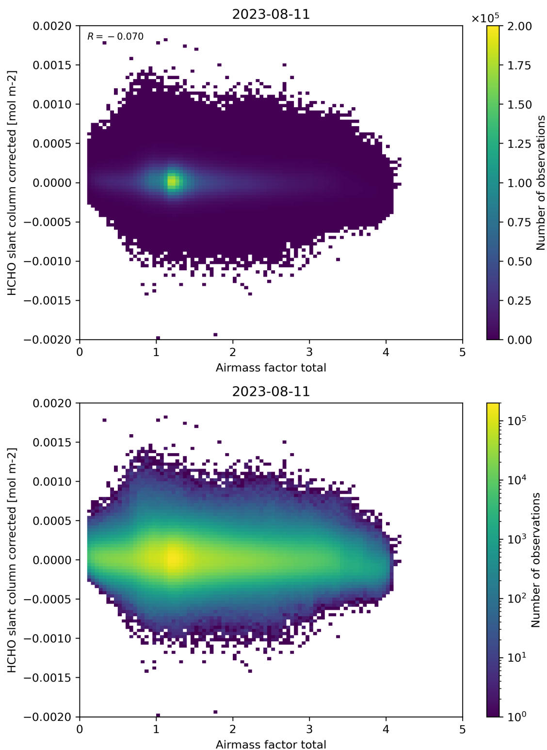
Figure 101: Scatter density plot of “Airmass factor total” against “HCHO slant column corrected” for 2023-08-10 to 2023-08-12.
