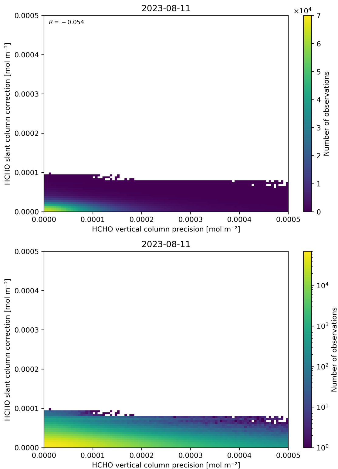
Figure 141: Scatter density plot of “HCHO vertical column precision” against “HCHO slant column correction” for 2023-08-10 to 2023-08-12.
