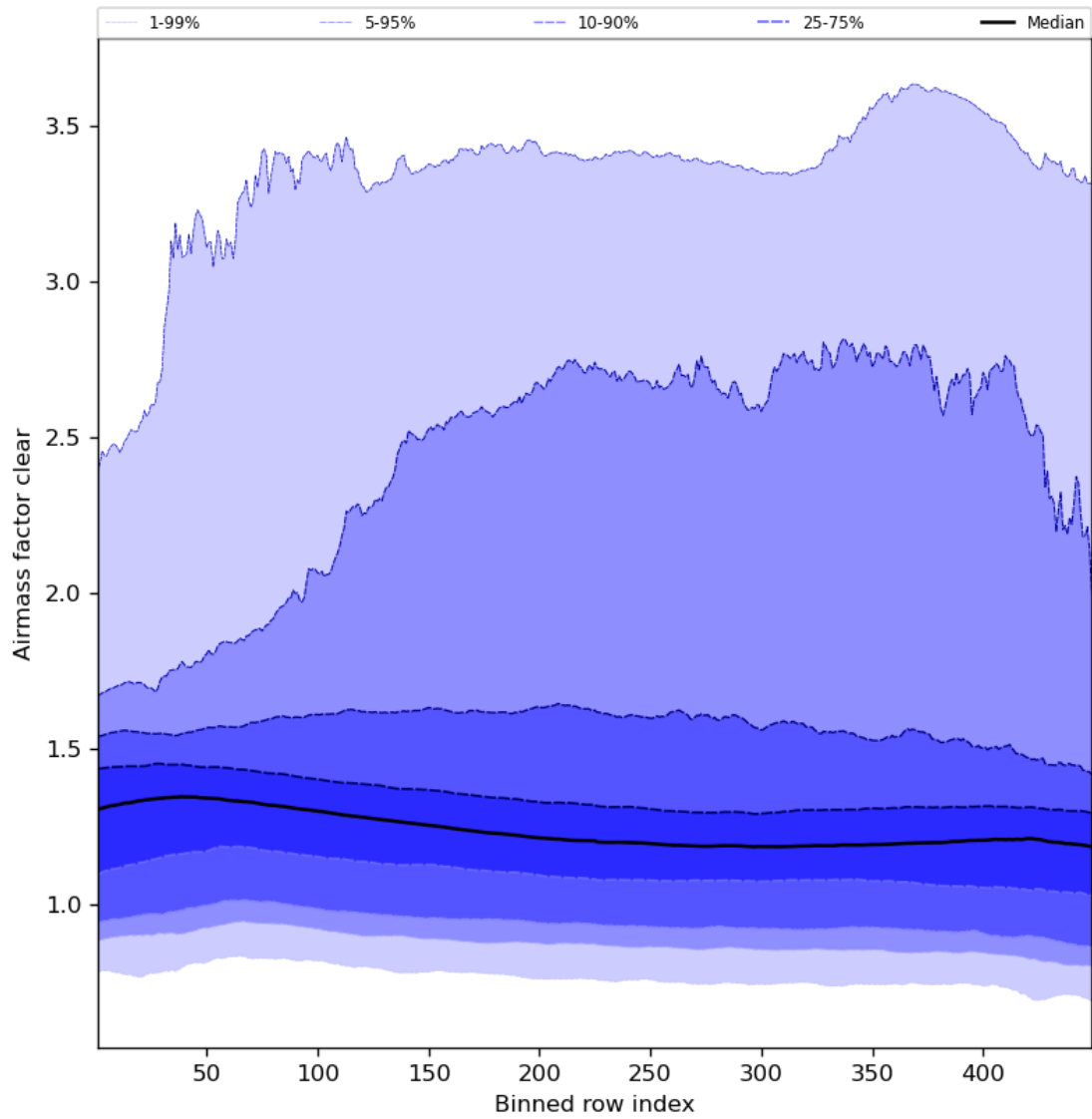
Figure 56: Along track statistics of “Airmass factor clear” for 2023-08-10 to 2023-08-12
