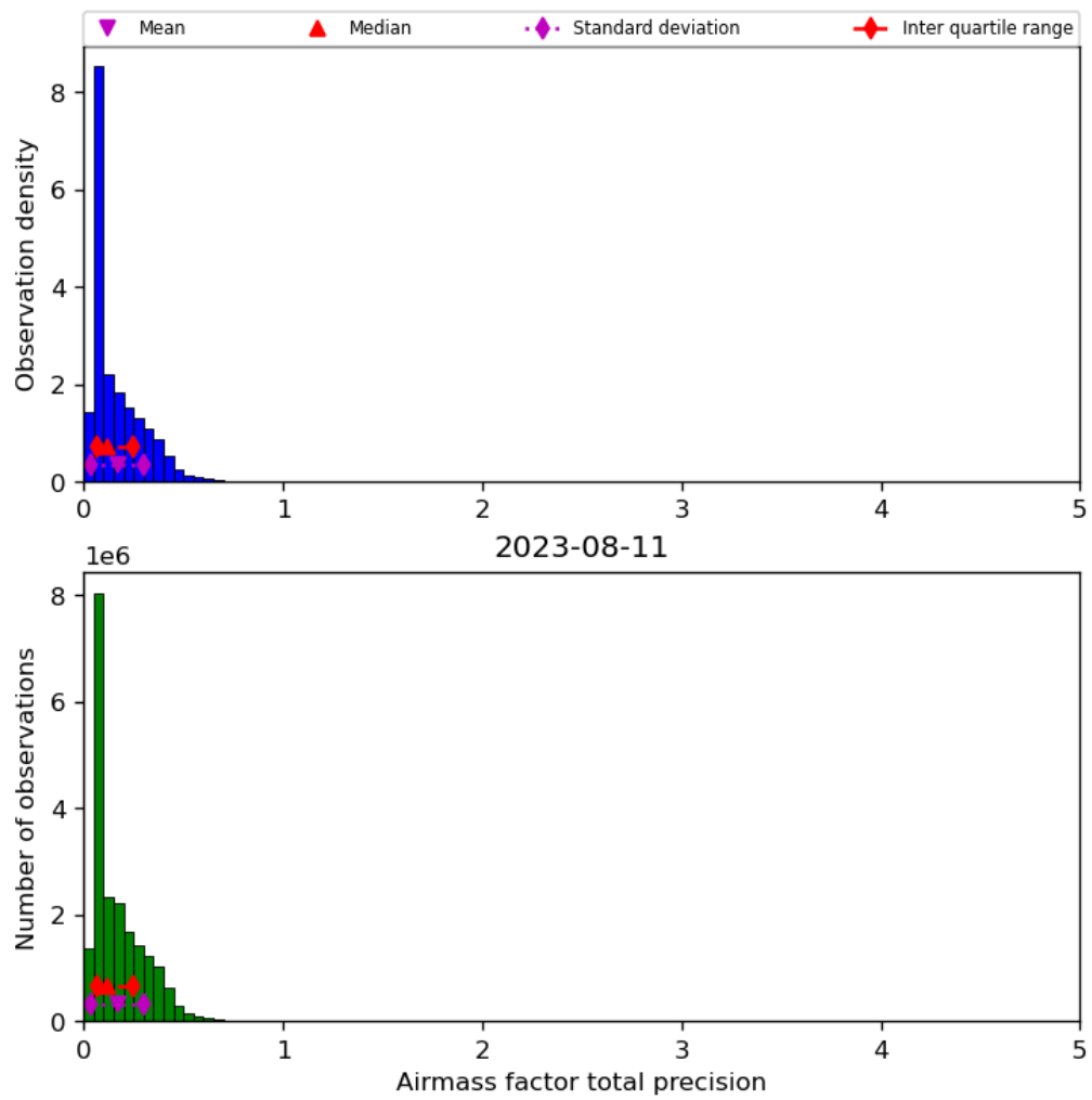
Figure 41: Histogram of “Airmass factor total precision” for 2023-08-10 to 2023-08-12
