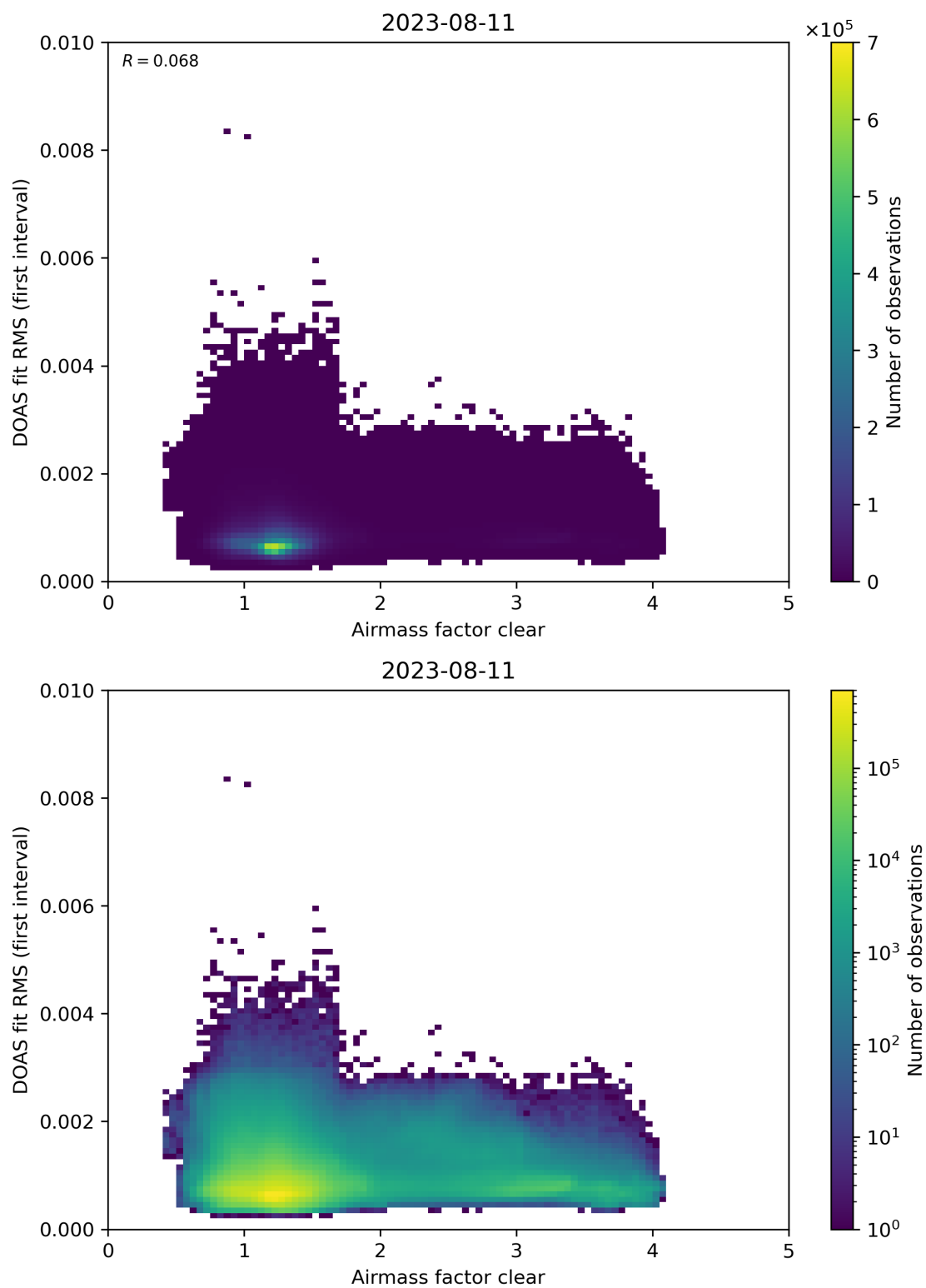
Figure 71: Scatter density plot of “Airmass factor clear” against “DOAS fit RMS (first interval)” for 2023-08-10 to 2023-08-12.
