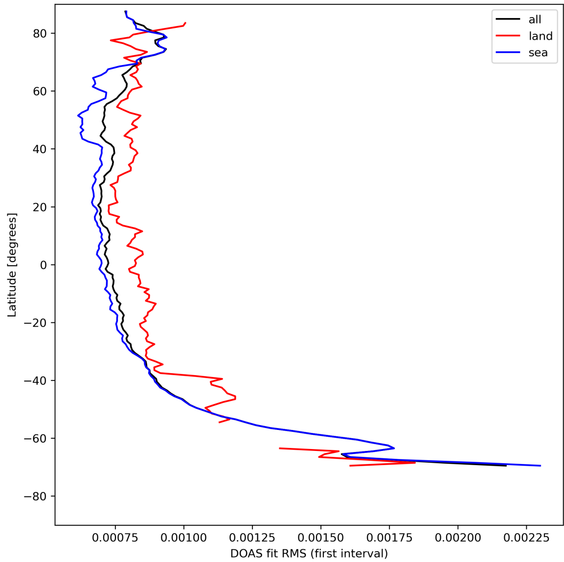
Figure 32: Zonal average of “DOAS fit RMS (first interval)” for 2023-08-10 to 2023-08-12.
