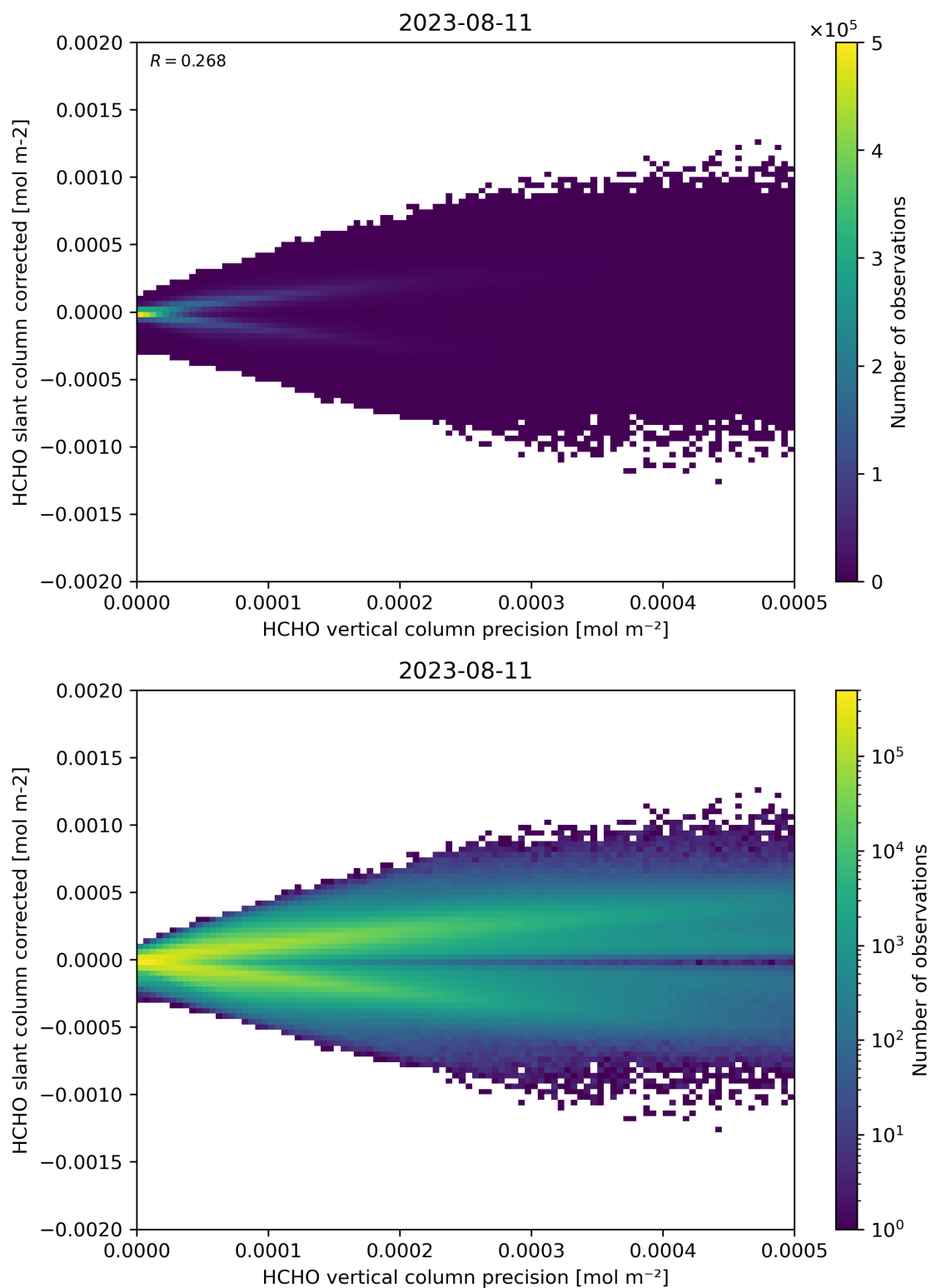
Figure 140: Scatter density plot of “HCHO vertical column precision” against “HCHO slant column corrected” for 2023-08-10 to 2023-08-12.
