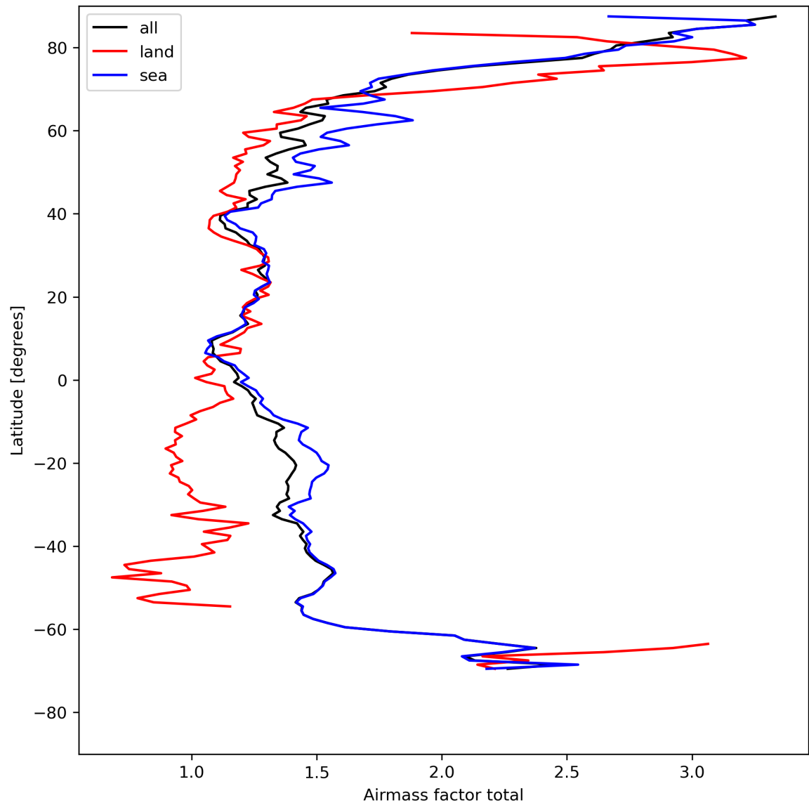
Figure 26: Zonal average of “Airmass factor total” for 2023-08-11 to 2023-08-13.
