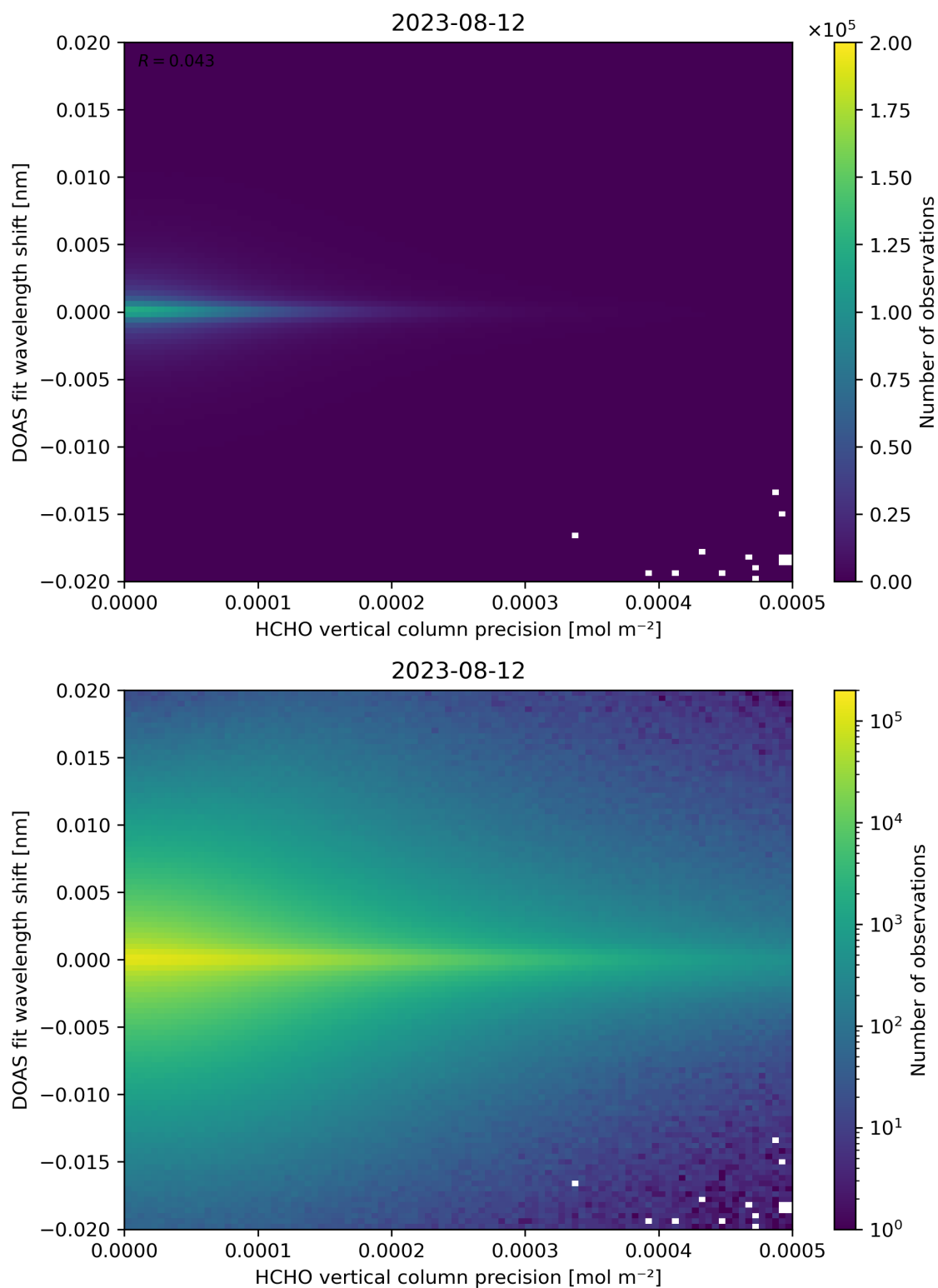
Figure 137: Scatter density plot of “HCHO vertical column precision” against “DOAS fit wavelength shift” for 2023-08-11 to 2023-08-13.
