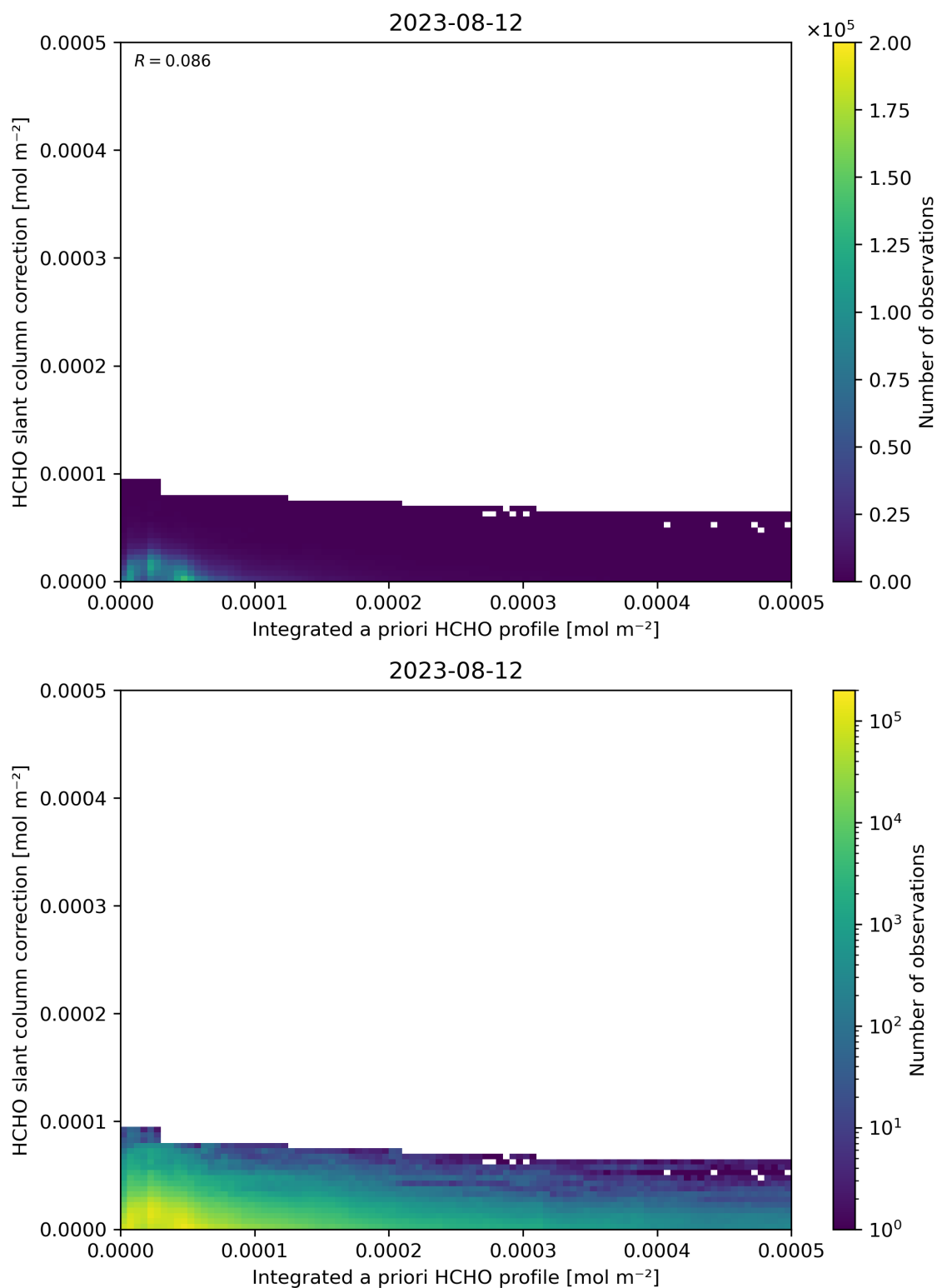
Figure 152: Scatter density plot of “Integrated a priori HCHO profile” against “HCHO slant column correction” for 2023-08-11 to 2023-08-13.
