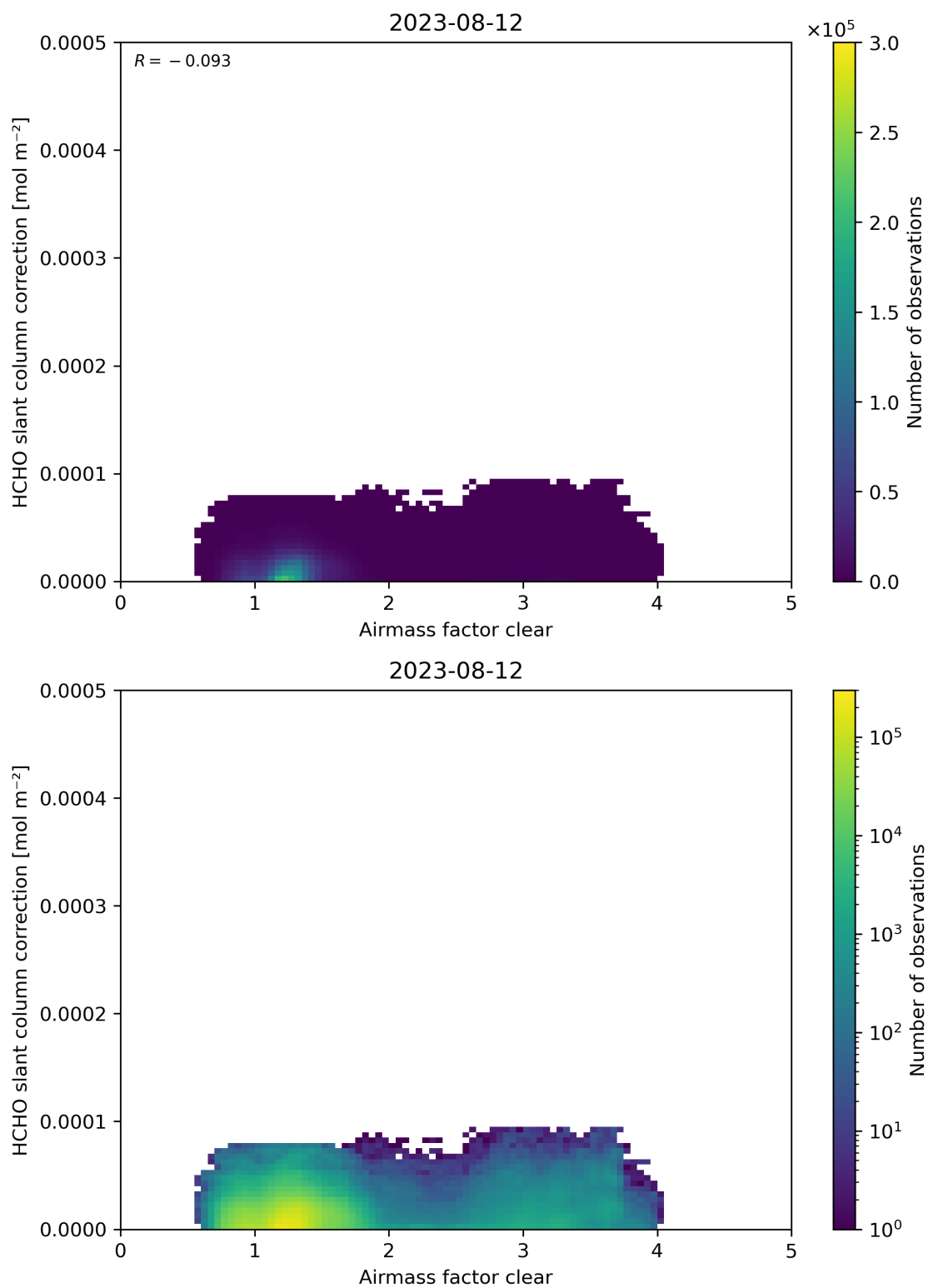
Figure 75: Scatter density plot of “Airmass factor clear” against “HCHO slant column correction” for 2023-08-11 to 2023-08-13.
