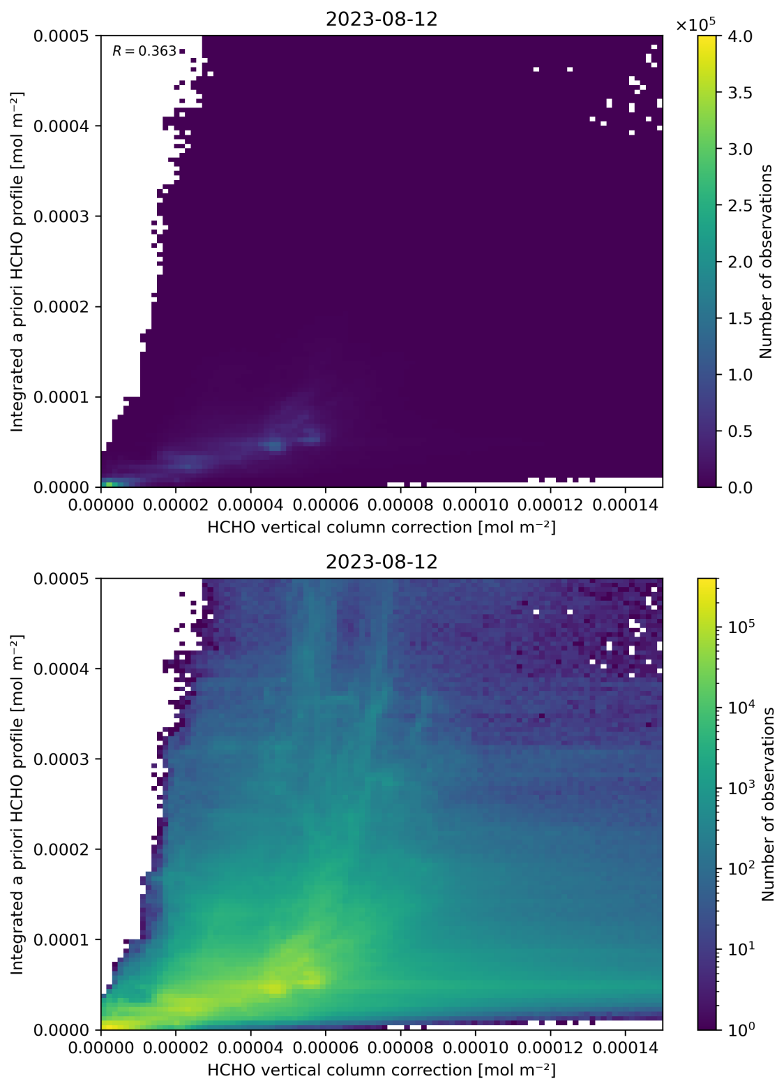
Figure 122: Scatter density plot of “HCHO vertical column correction” against “Integrated a priori HCHO profile” for 2023-08-11 to 2023-08-13.
