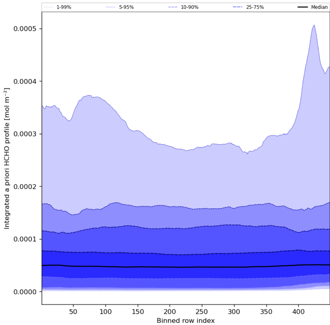
Figure 57: Along track statistics of "Integrated a priori HCHO profile" for 2023-08-11 to 2023-08-13
