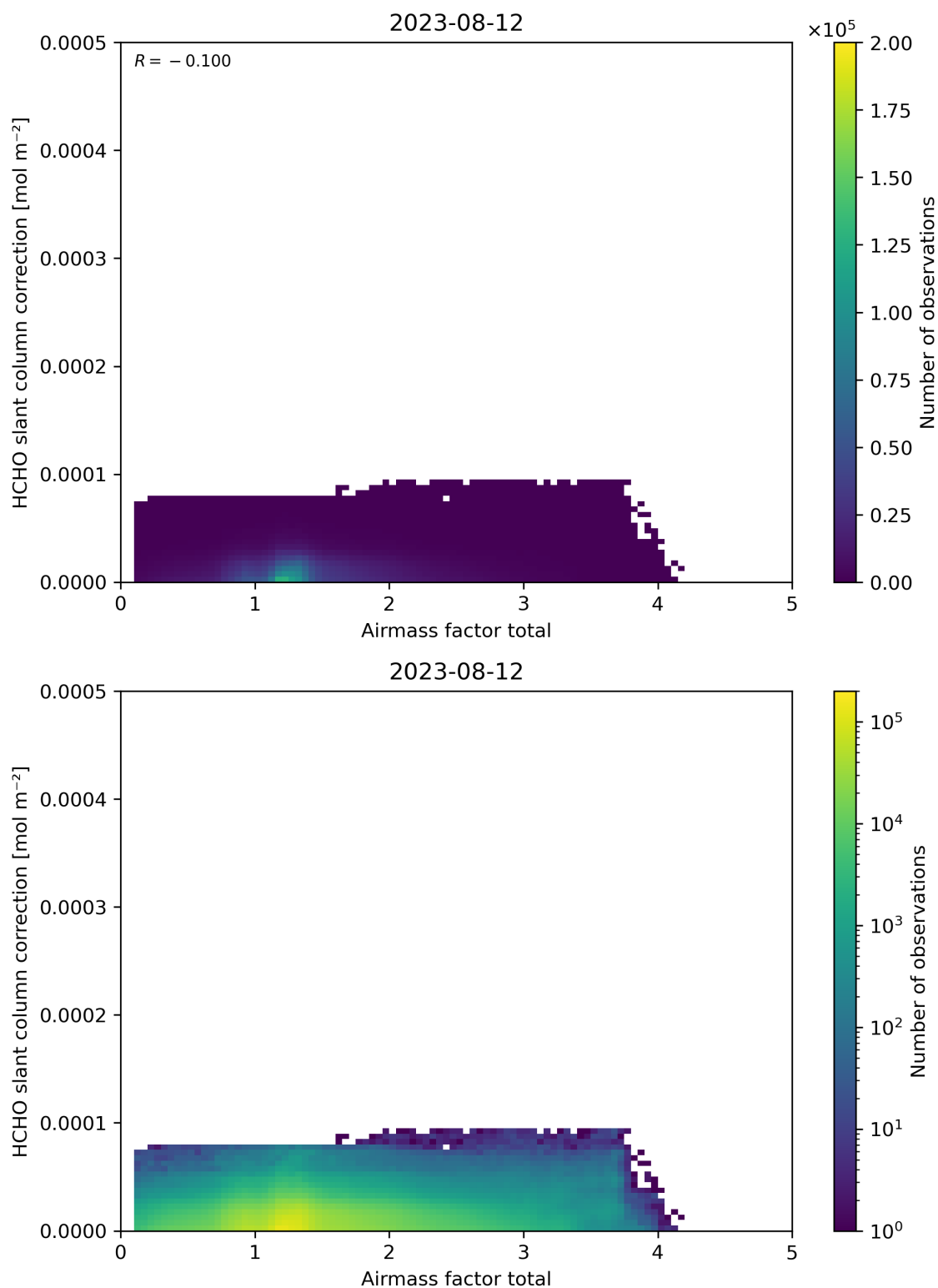
Figure 102: Scatter density plot of “Airmass factor total” against “HCHO slant column correction” for 2023-08-11 to 2023-08-13.
