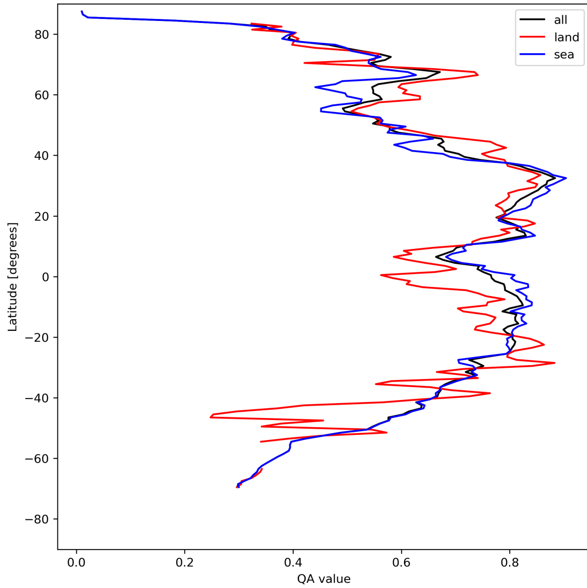
Figure 20: Zonal average of “QA value” for 2023-08-11 to 2023-08-13.
