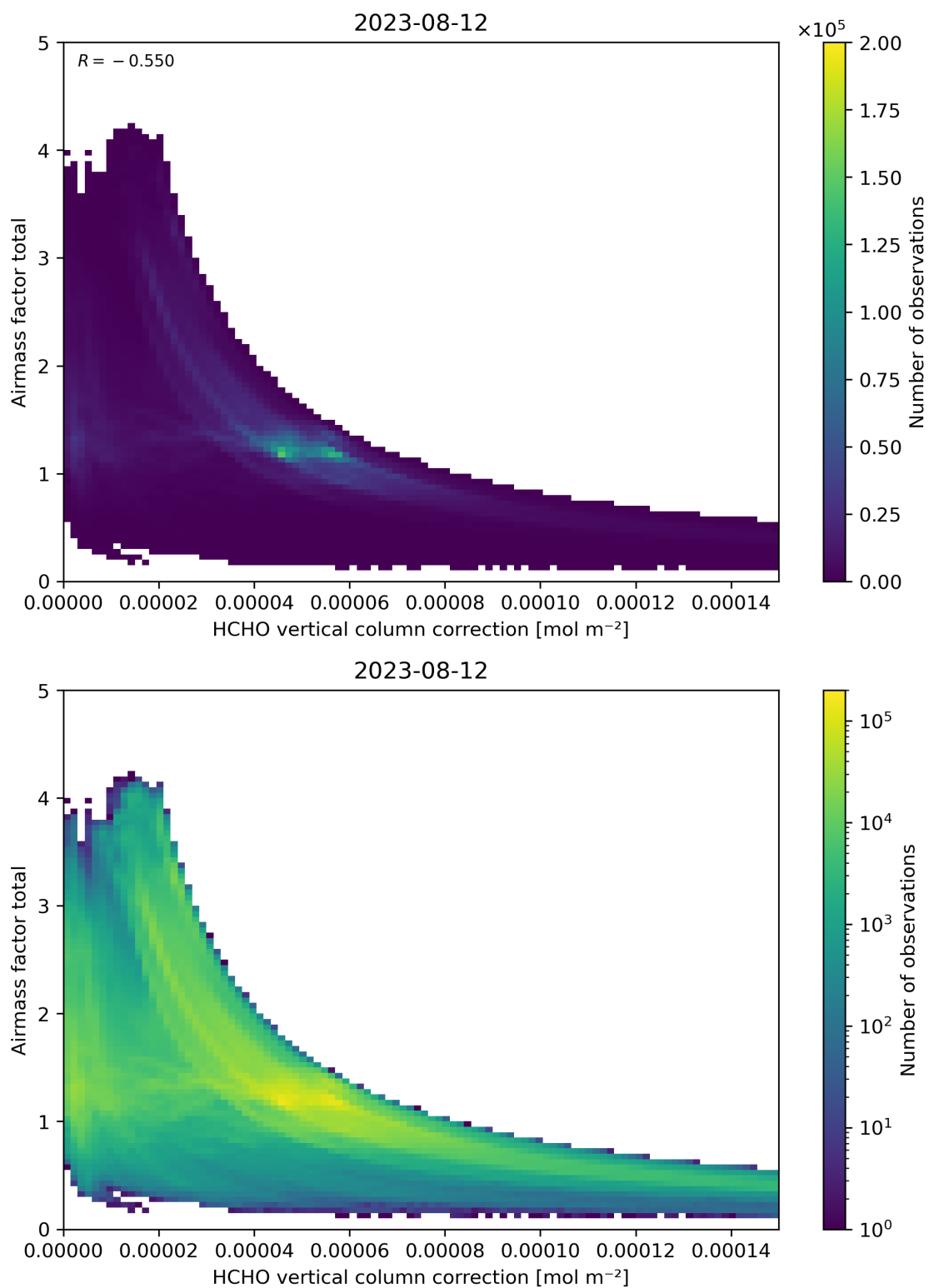
Figure 120: Scatter density plot of “HCHO vertical column correction” against “Airmass factor total” for 2023-08-11 to 2023-08-13.
