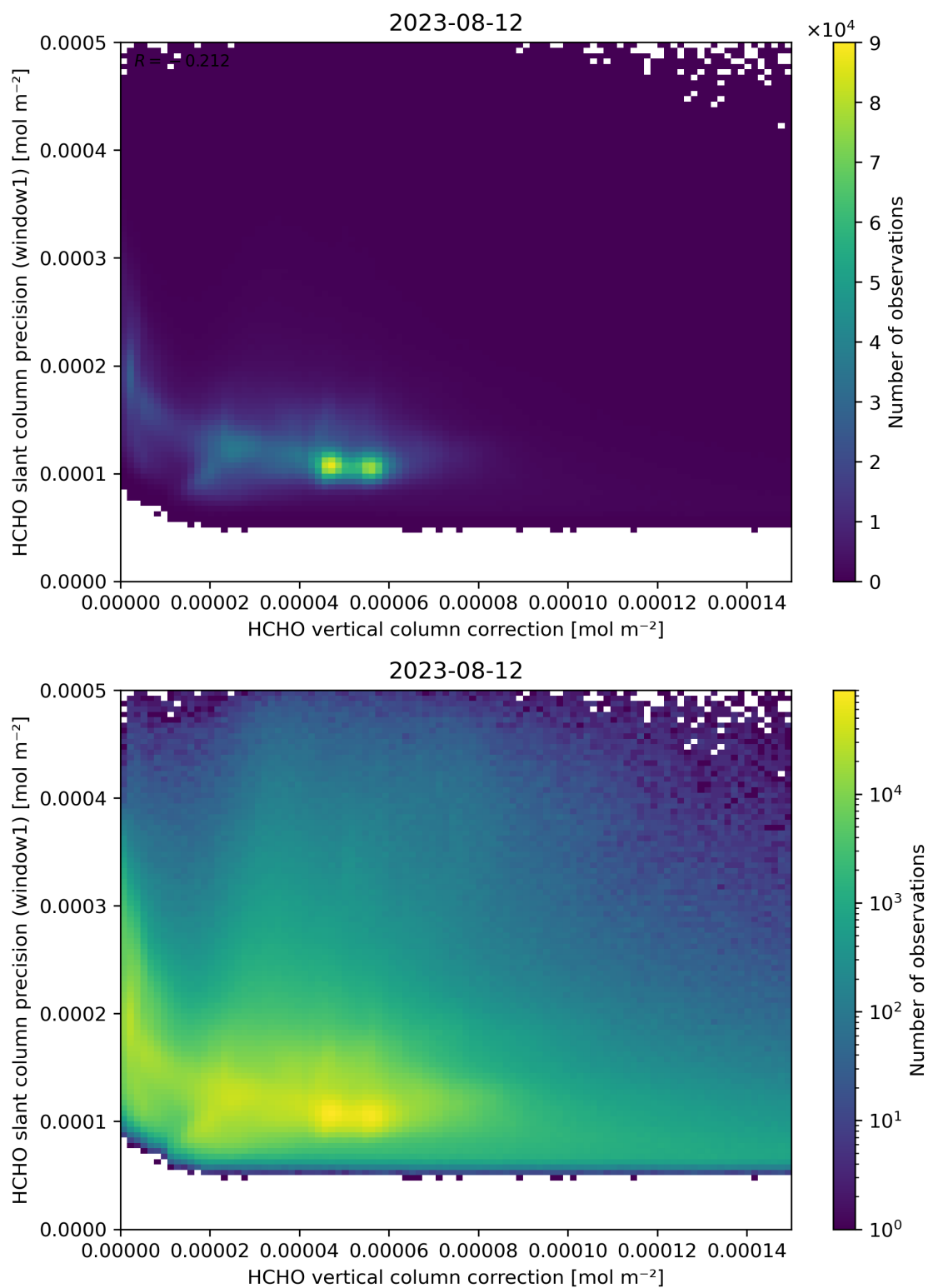
Figure 119: Scatter density plot of “HCHO vertical column correction” against “HCHO slant column precision (window1)” for 2023-08-11 to 2023-08-13.
