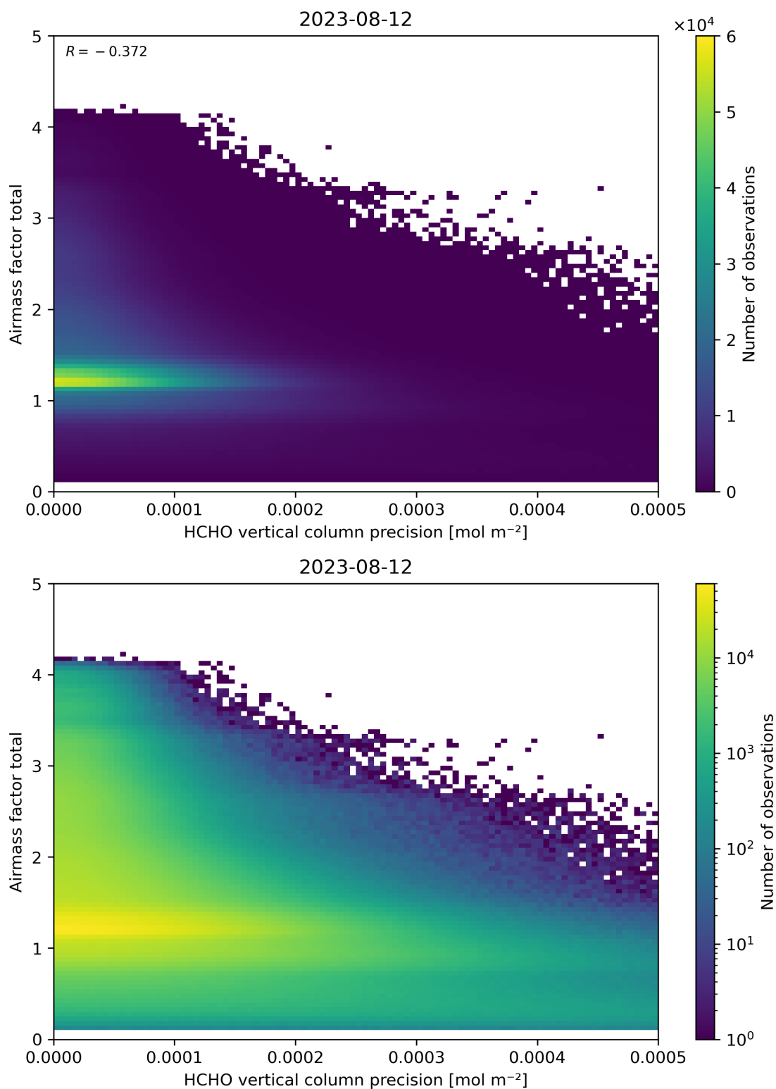
Figure 144: Scatter density plot of “HCHO vertical column precision” against “Airmass factor total” for 2023-08-11 to 2023-08-13.
