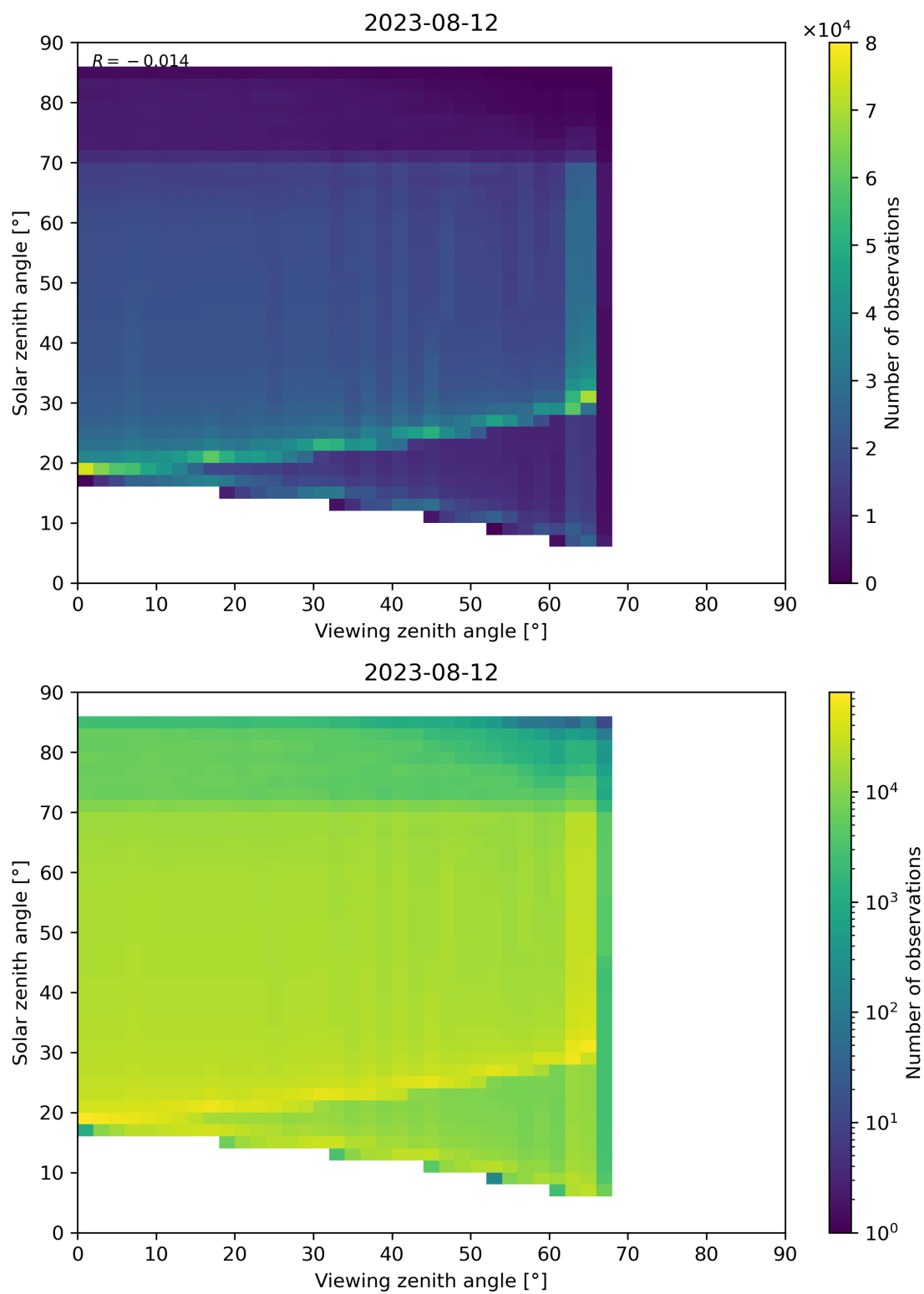
Figure 197: Scatter density plot of “Viewing zenith angle” against “Solar zenith angle” for 2023-08-11 to 2023-08-13.
