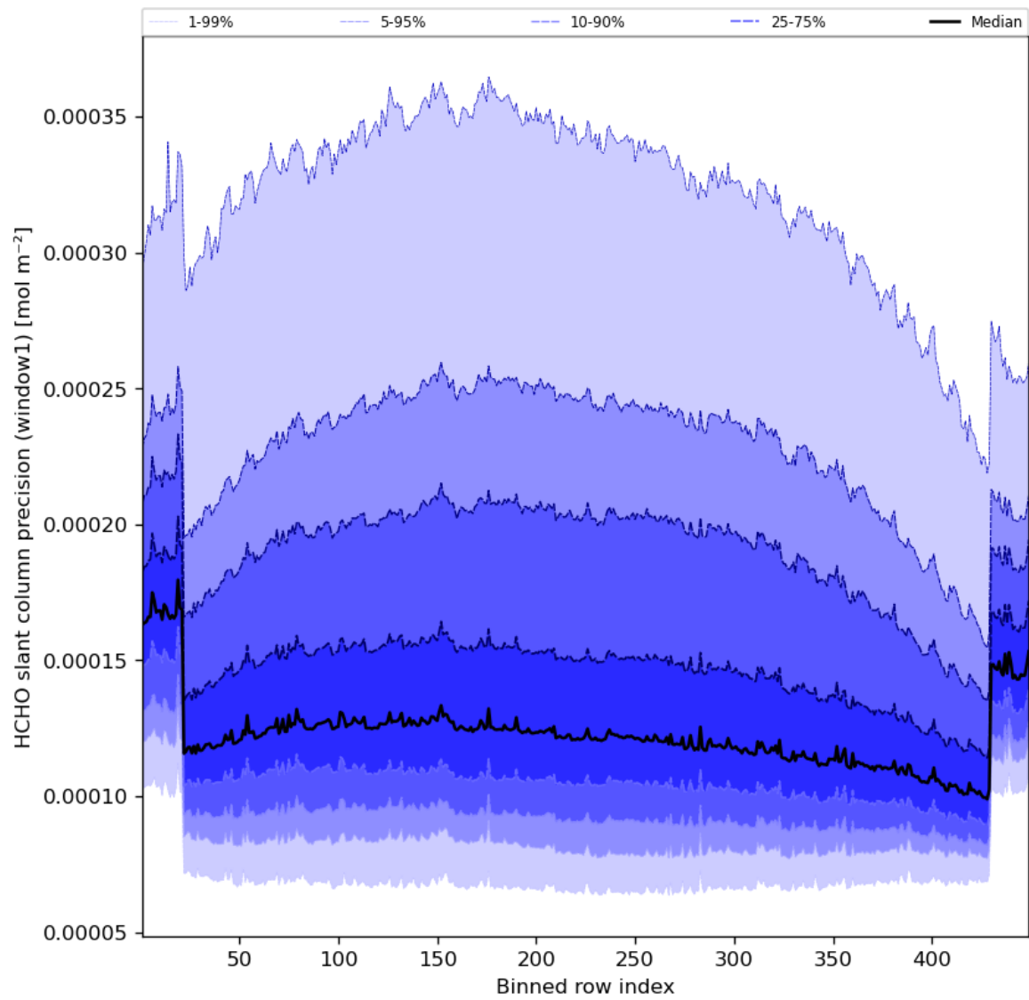
Figure 53: Along track statistics of “HCHO slant column precision (window1)” for 2023-08-11 to 2023-08-13
