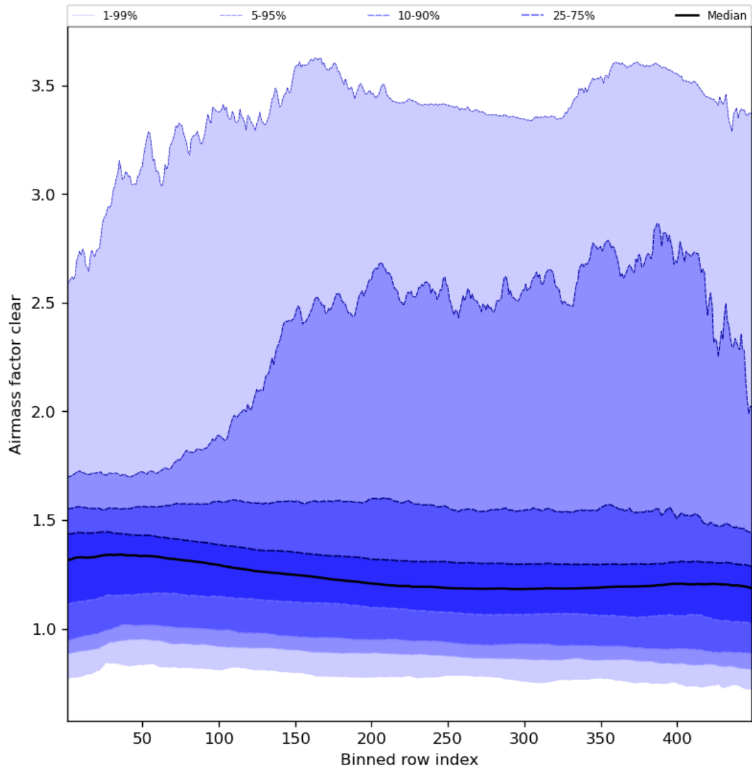
Figure 56: Along track statistics of “Airmass factor clear” for 2023-08-11 to 2023-08-13
