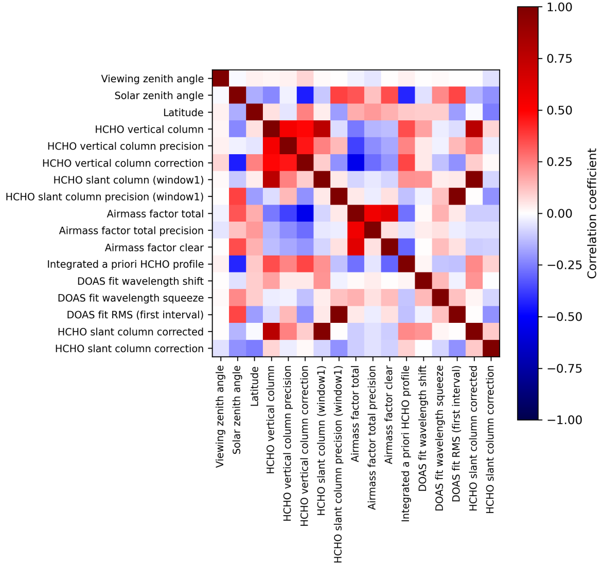
Figure 2: Map of correlation matrix for 2023-08-11 to 2023-08-13.
