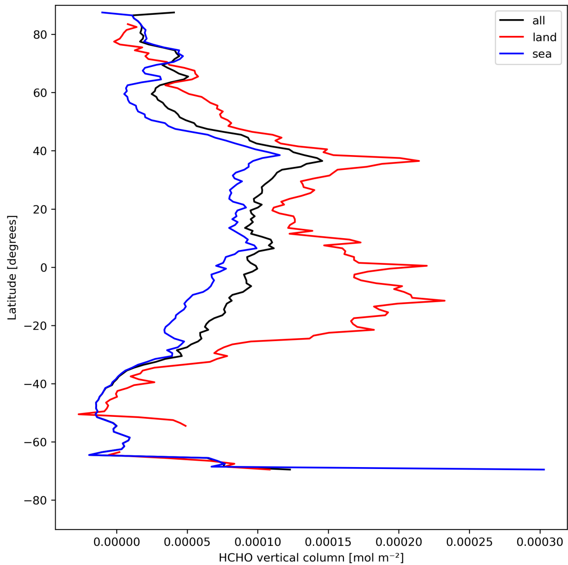
Figure 21: Zonal average of “HCHO vertical column” for 2023-08-11 to 2023-08-13.
