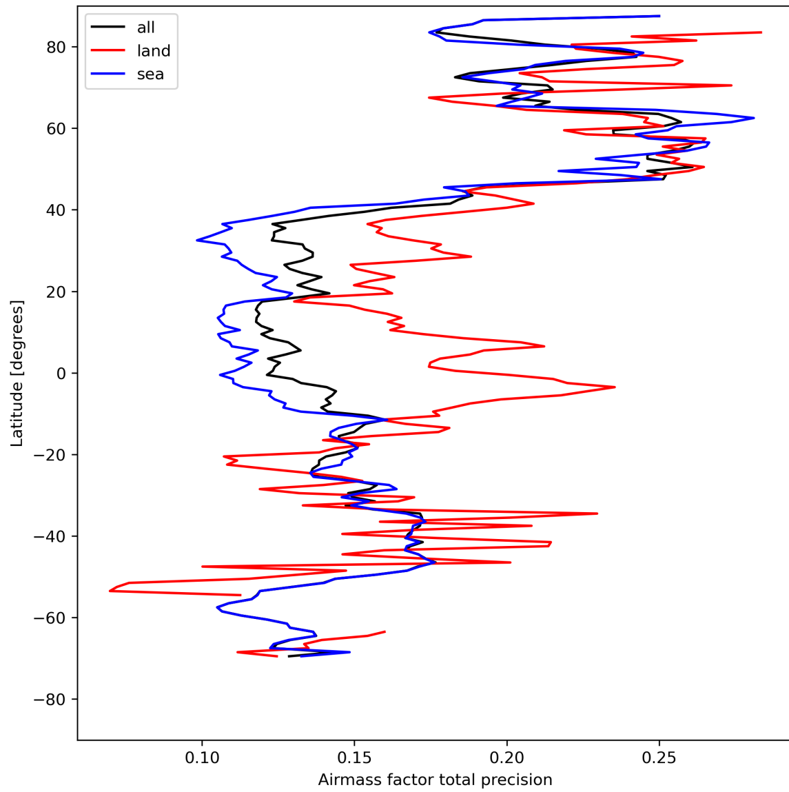
Figure 27: Zonal average of “Airmass factor total precision” for 2023-08-11 to 2023-08-13.
