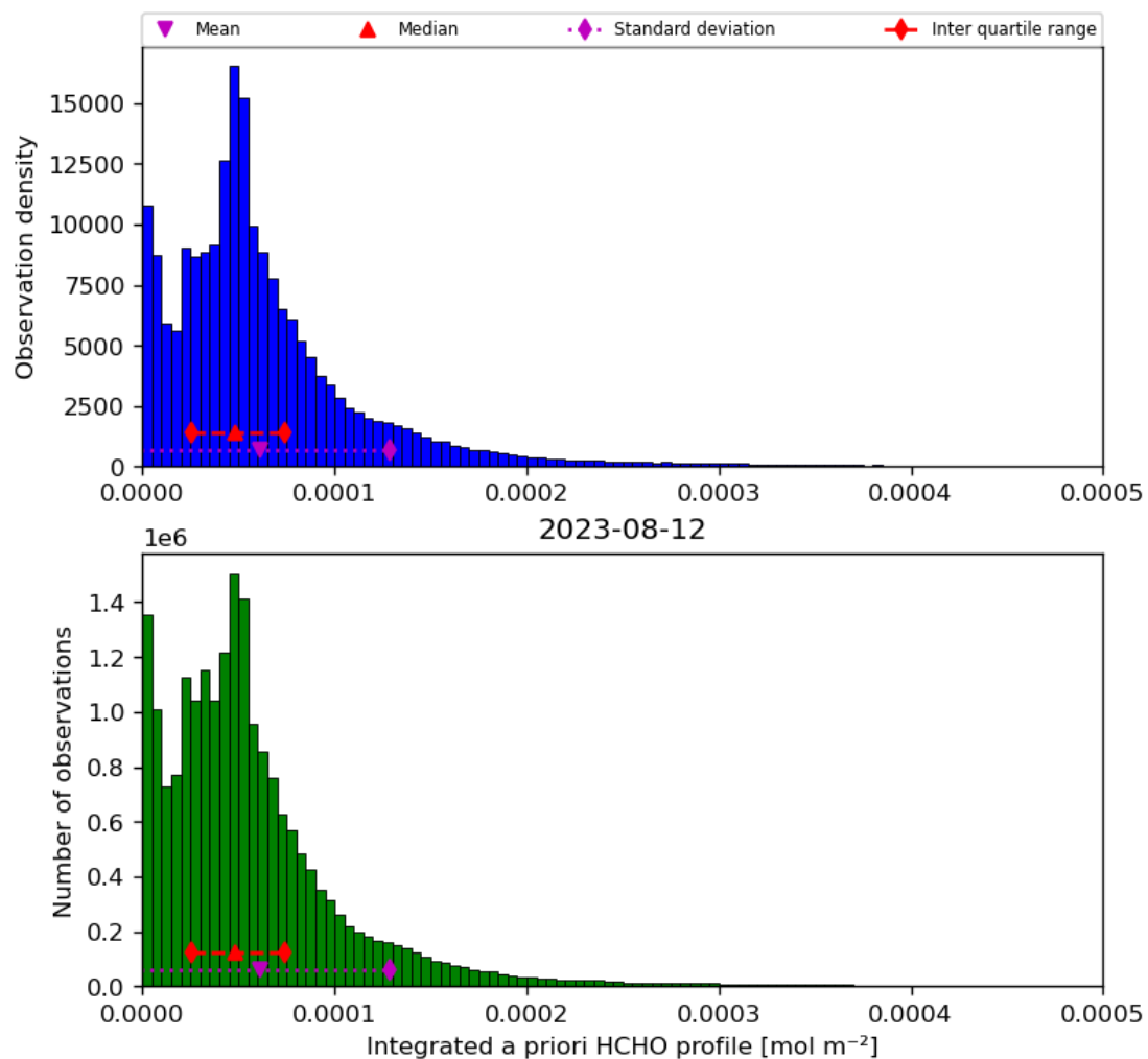
Figure 43: Histogram of “Integrated a priori HCHO profile” for 2023-08-11 to 2023-08-13
