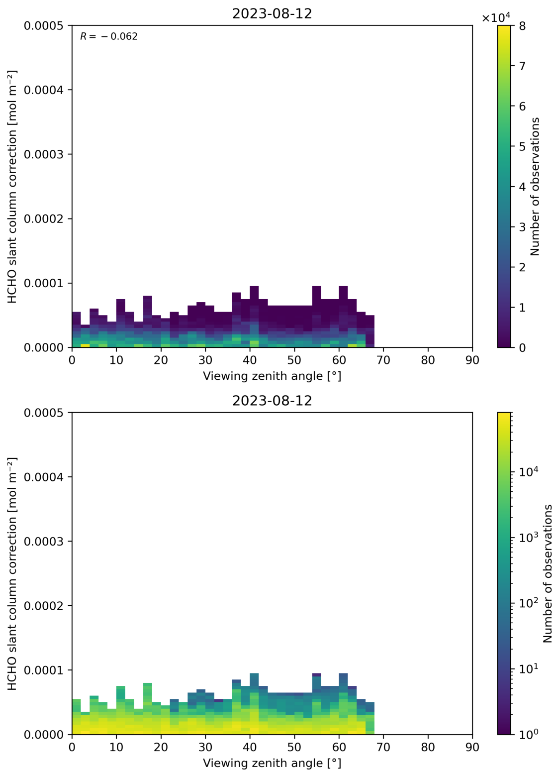
Figure 187: Scatter density plot of “Viewing zenith angle” against “HCHO slant column correction” for 2023-08-11 to 2023-08-13.
