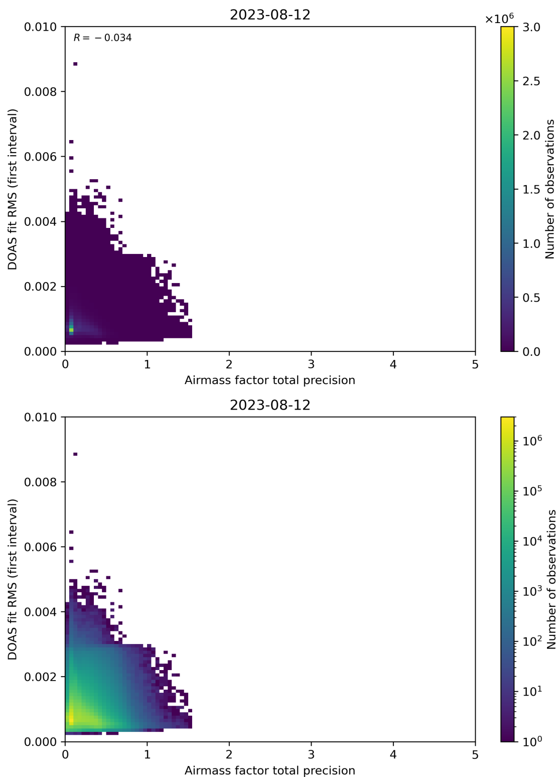
Figure 105: Scatter density plot of “Airmass factor total precision” against “DOAS fit RMS (first interval)” for 2023-08-11 to 2023-08-13.
