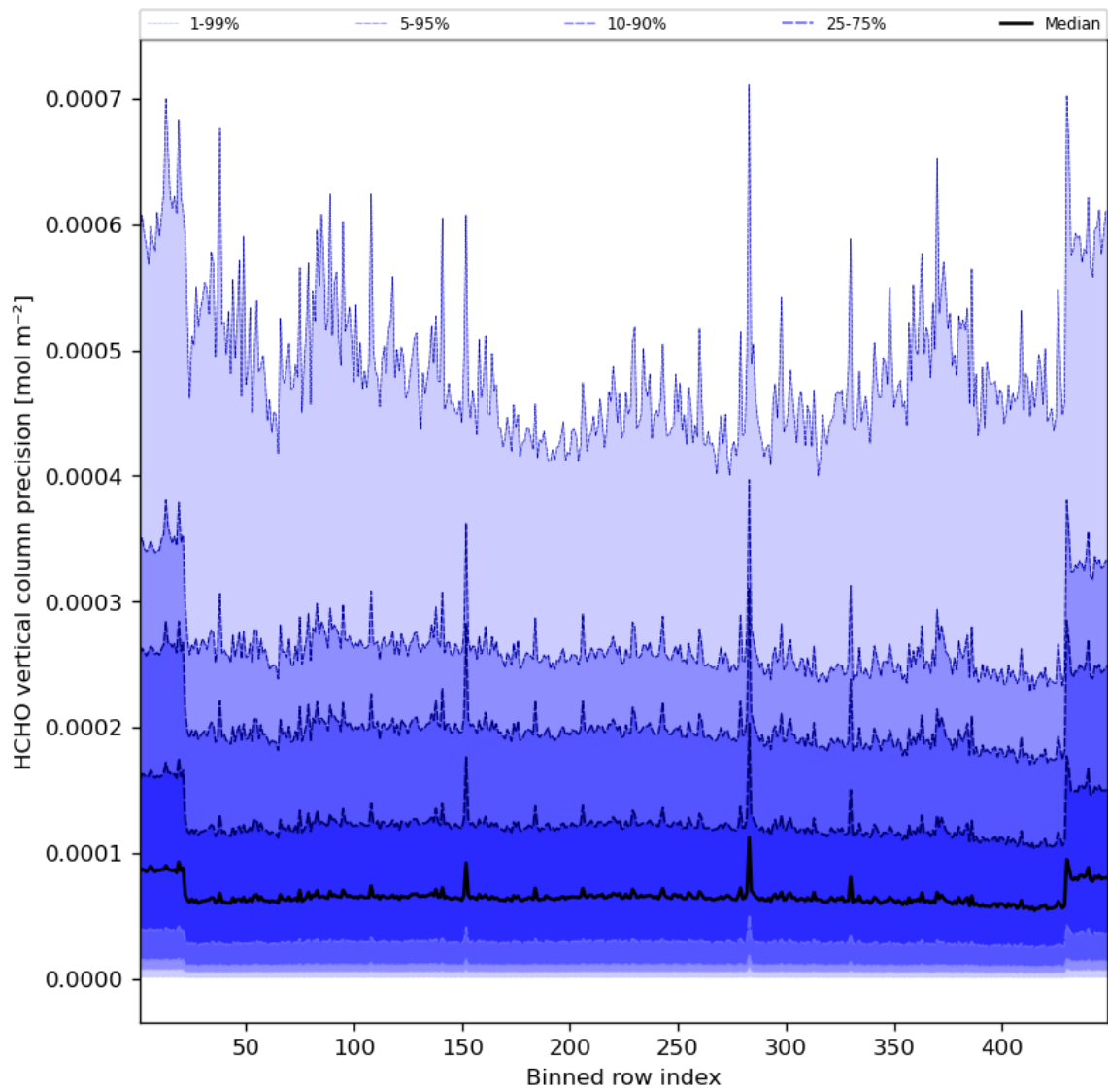
Figure 50: Along track statistics of “HCHO vertical column precision” for 2023-08-11 to 2023-08-13
