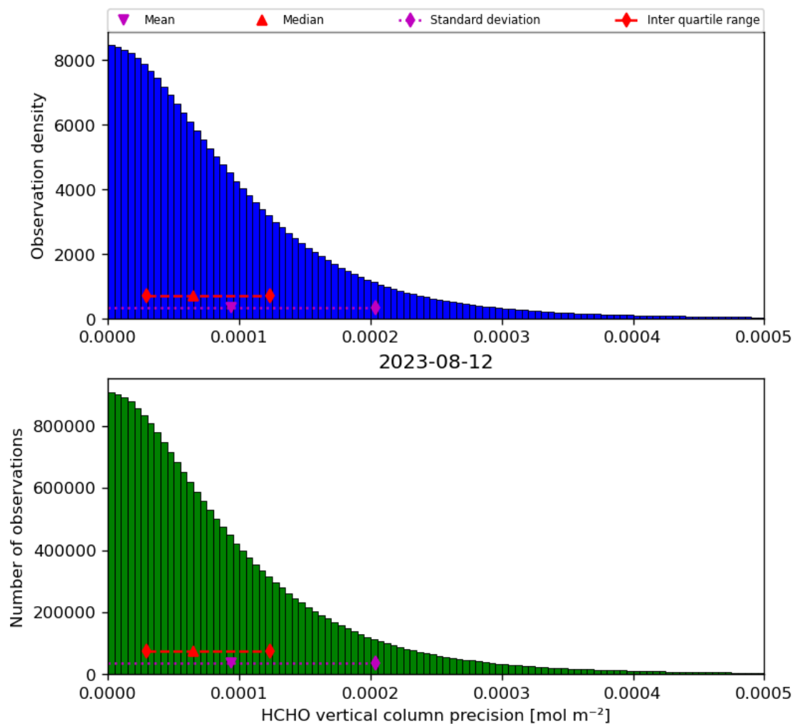
Figure 36: Histogram of “HCHO vertical column precision” for 2023-08-11 to 2023-08-13
