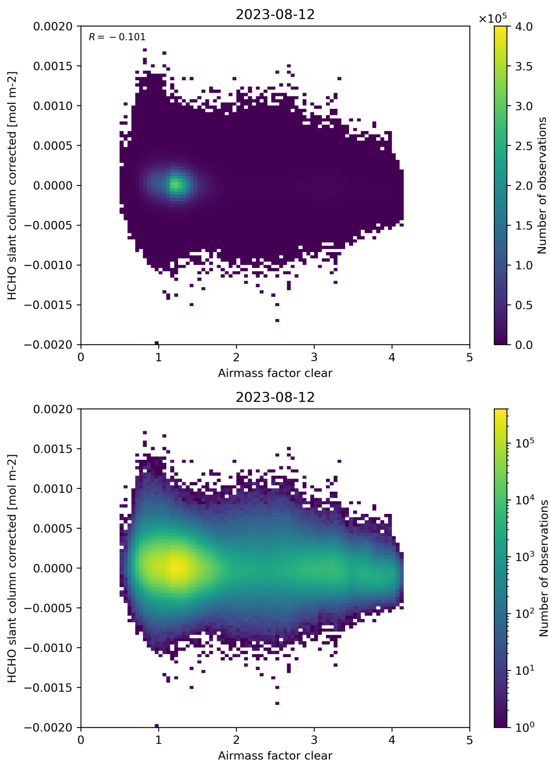
Figure 74: Scatter density plot of “Airmass factor clear” against “HCHO slant column corrected” for 2023-08-11 to 2023-08-13.
