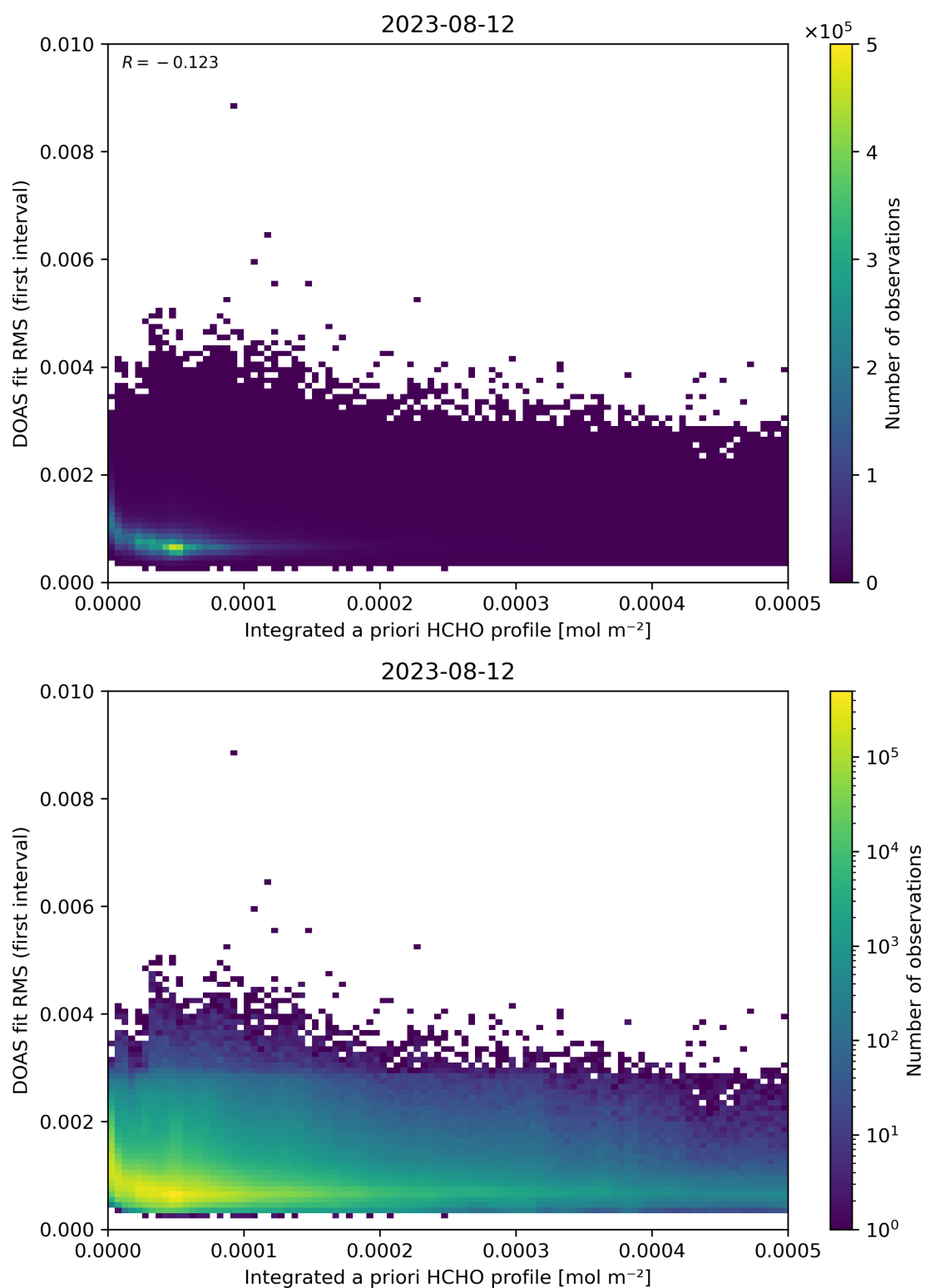
Figure 148: Scatter density plot of “Integrated a priori HCHO profile” against “DOAS fit RMS (first interval)” for 2023-08-11 to 2023-08-13.
