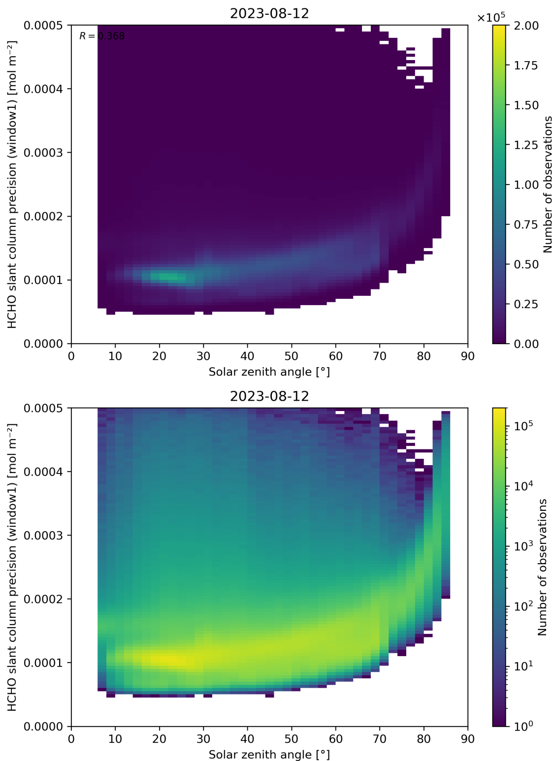
Figure 174: Scatter density plot of “Solar zenith angle” against “HCHO slant column precision (window1)” for 2023-08-11 to 2023-08-13.
