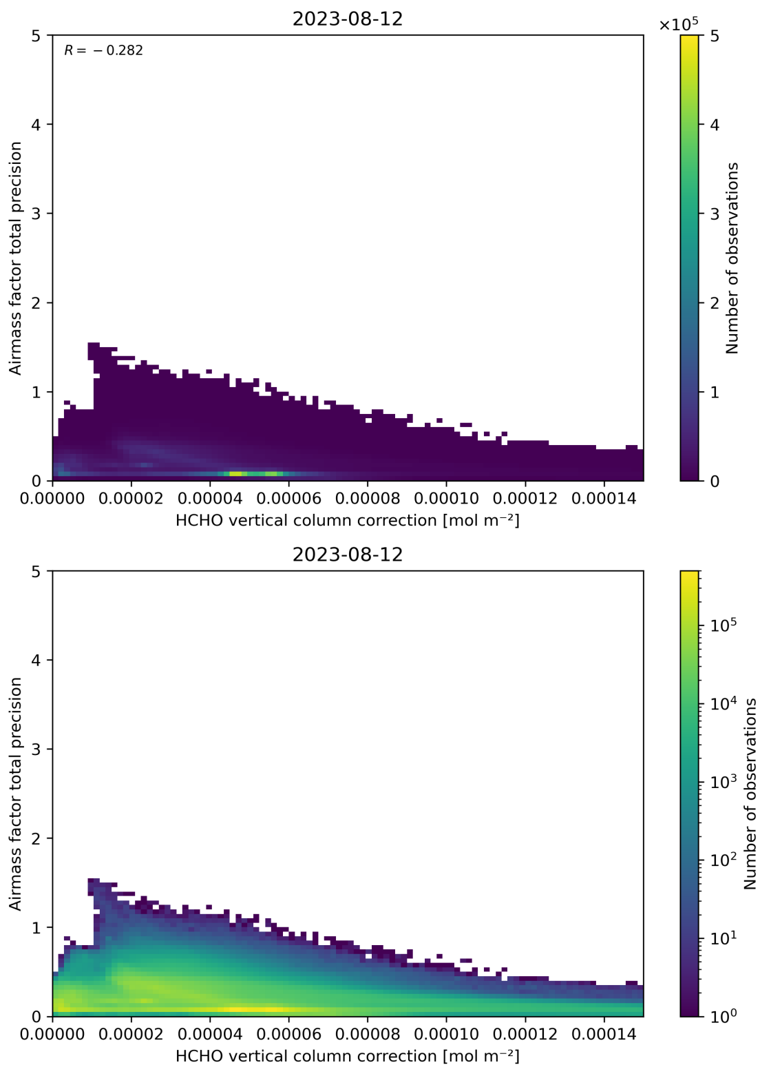
Figure 121: Scatter density plot of “HCHO vertical column correction” against “Airmass factor total precision” for 2023-08-11 to 2023-08-13.
