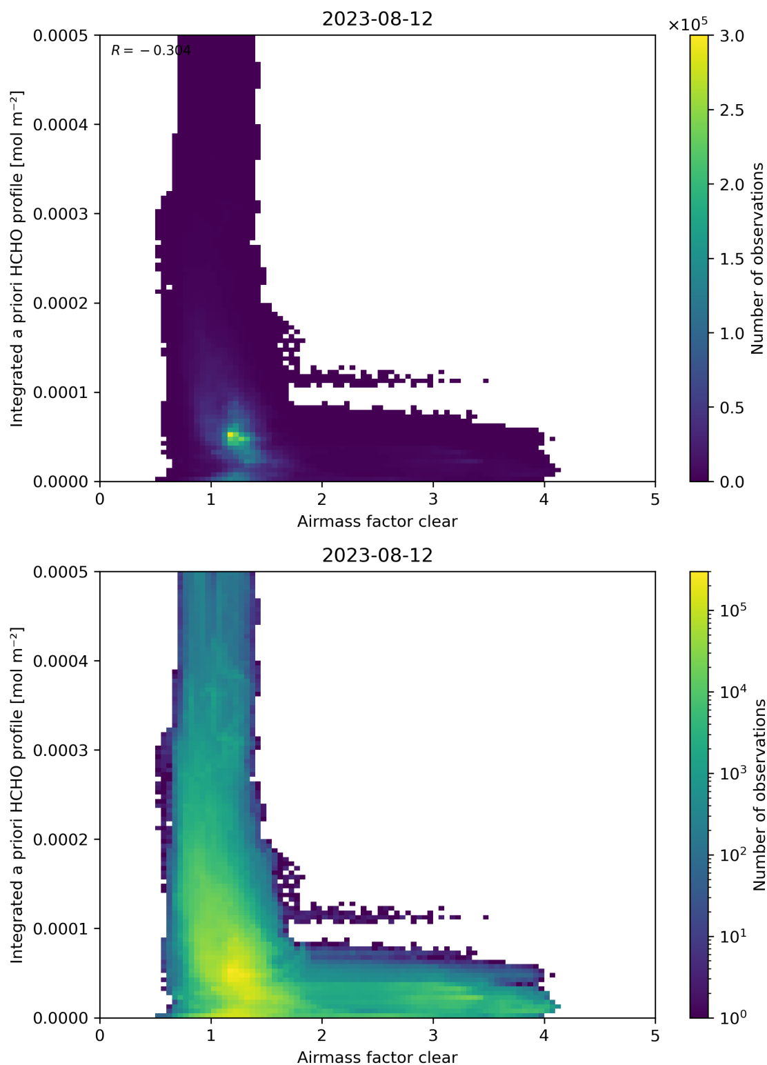
Figure 76: Scatter density plot of “Airmass factor clear” against “Integrated a priori HCHO profile” for 2023-08-11 to 2023-08-13.
