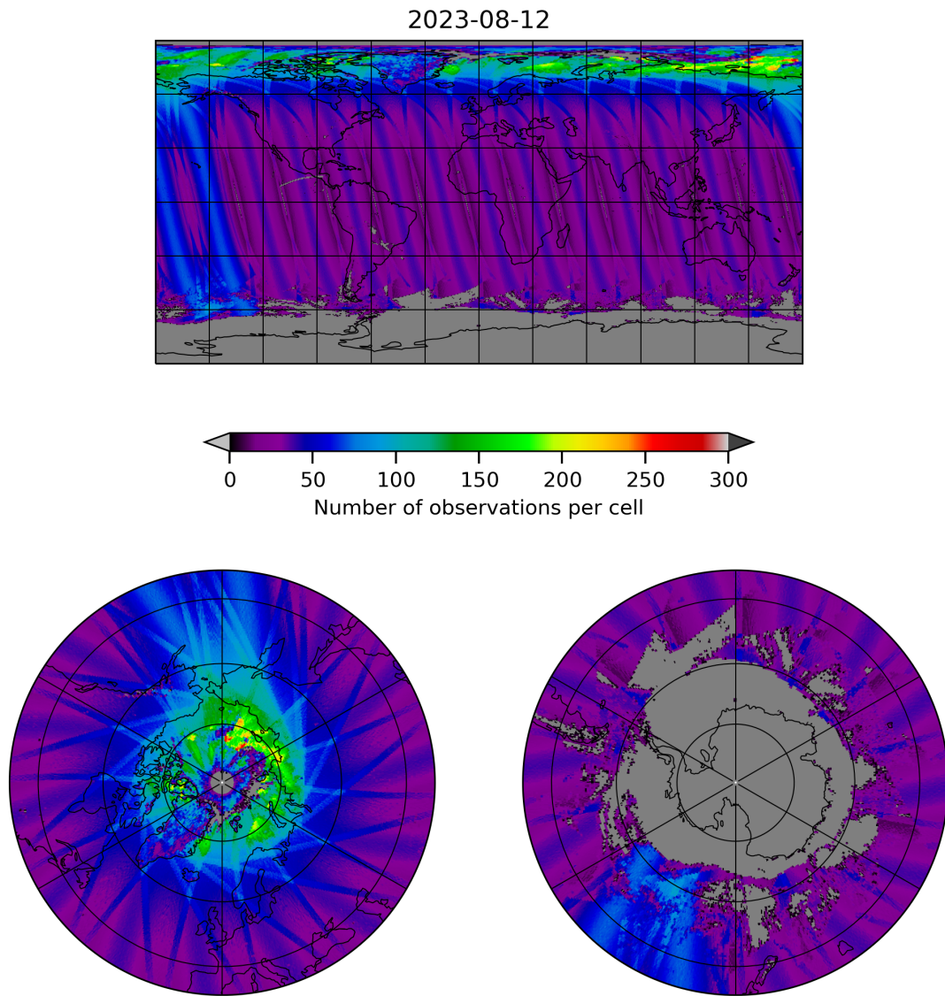
Figure 19: Map of the number of observations for 2023-08-11 to 2023-08-13
