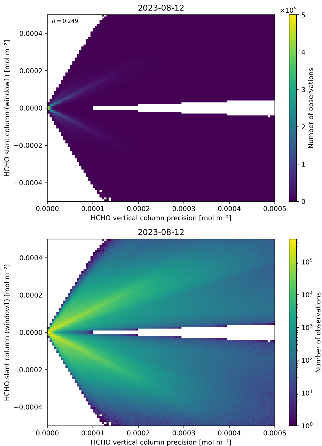
Figure 142: Scatter density plot of “HCHO vertical column precision” against “HCHO slant column (window1)” for 2023-08-11 to 2023-08-13.
