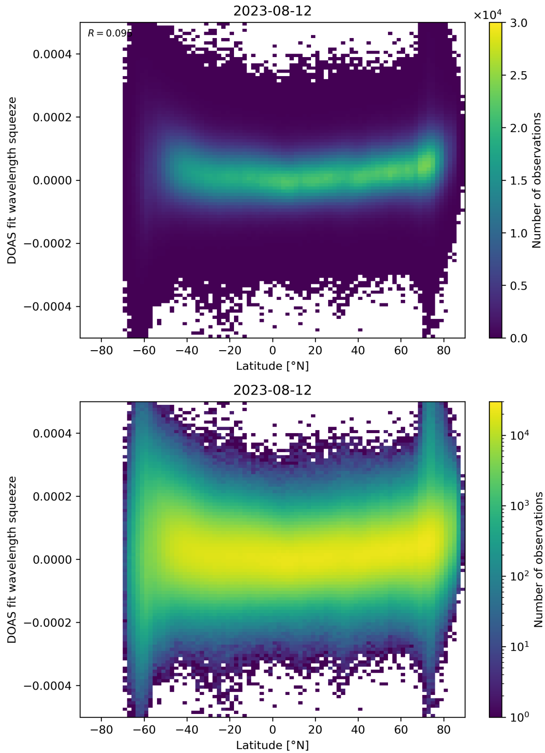
Figure 155: Scatter density plot of “Latitude” against “DOAS fit wavelength squeeze” for 2023-08-11 to 2023-08-13.
