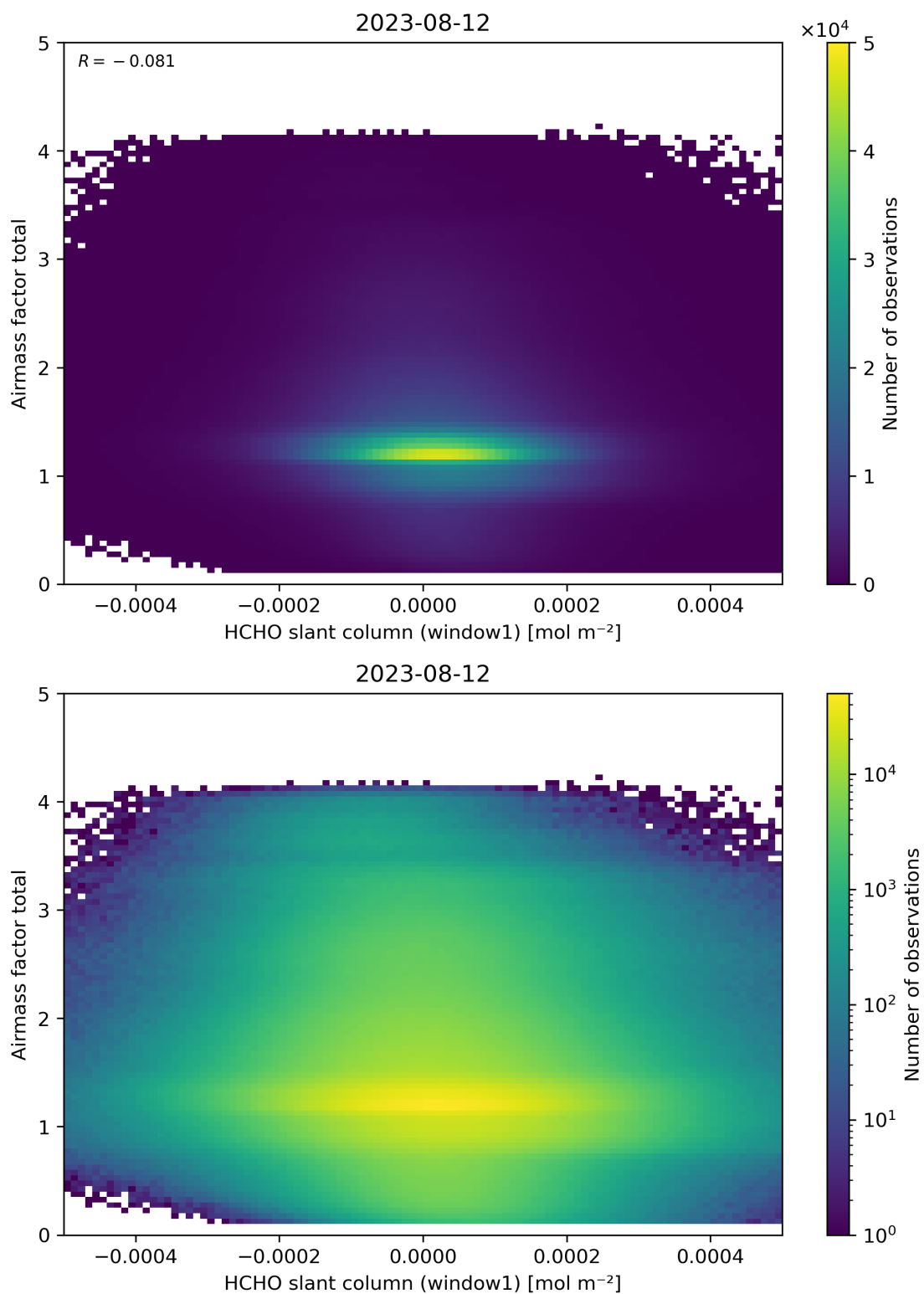
Figure 85: Scatter density plot of “HCHO slant column (window1)” against “Airmass factor total” for 2023-08-11 to 2023-08-13.
