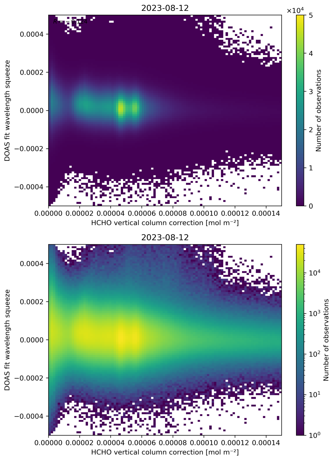
Figure 114: Scatter density plot of “HCHO vertical column correction” against “DOAS fit wavelength squeeze” for 2023-08-11 to 2023-08-13.
