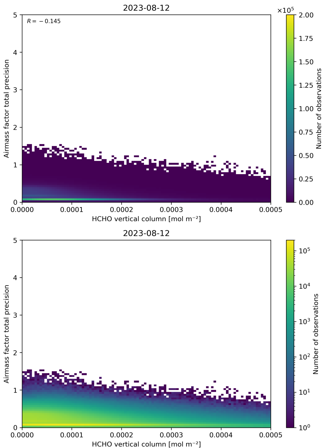
Figure 132: Scatter density plot of “HCHO vertical column” against “Airmass factor total precision” for 2023-08-11 to 2023-08-13.
