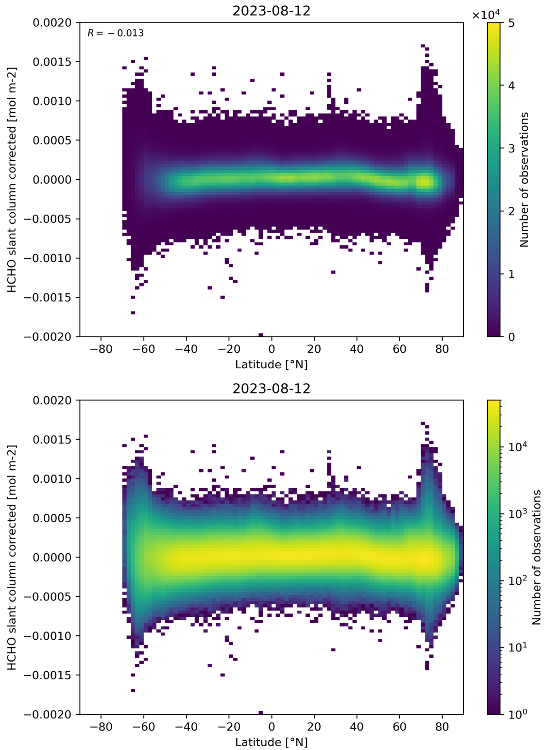
Figure 157: Scatter density plot of “Latitude” against “HCHO slant column corrected” for 2023-08-11 to 2023-08-13.
