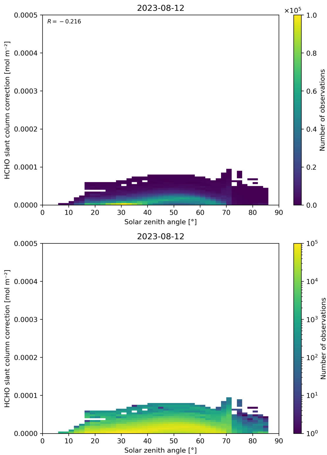
Figure 172: Scatter density plot of “Solar zenith angle” against “HCHO slant column correction” for 2023-08-11 to 2023-08-13.
