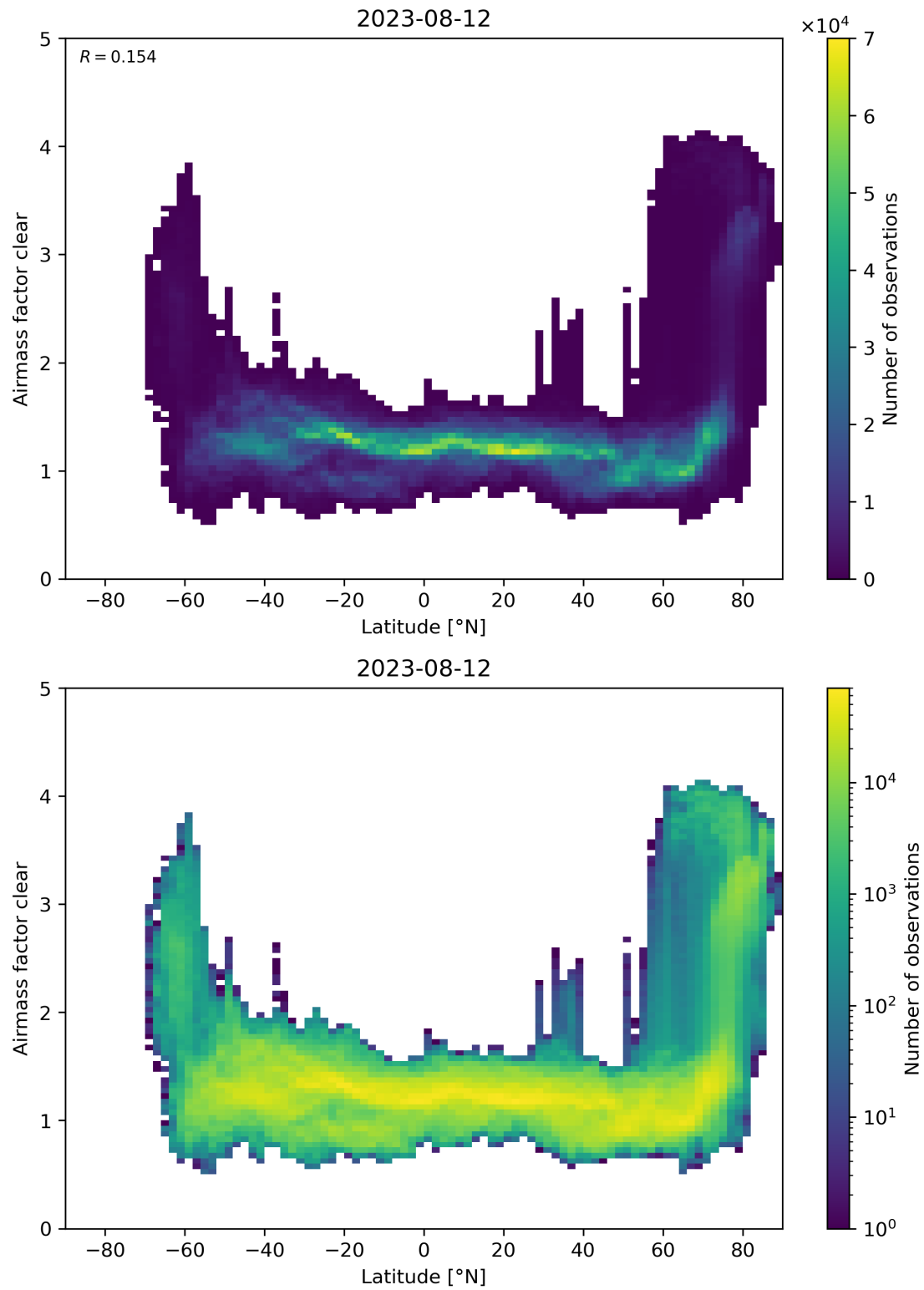
Figure 156: Scatter density plot of “Latitude” against “Airmass factor clear” for 2023-08-11 to 2023-08-13.
