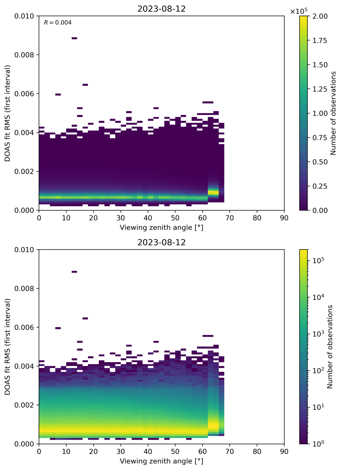
Figure 182: Scatter density plot of “Viewing zenith angle” against “DOAS fit RMS (first interval)” for 2023-08-11 to 2023-08-13.
