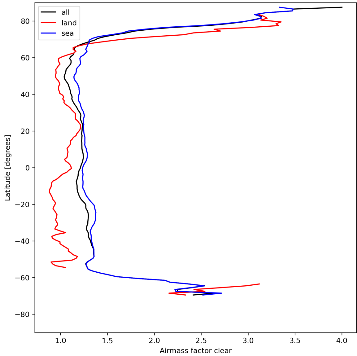
Figure 28: Zonal average of “Airmass factor clear” for 2023-08-11 to 2023-08-13.
