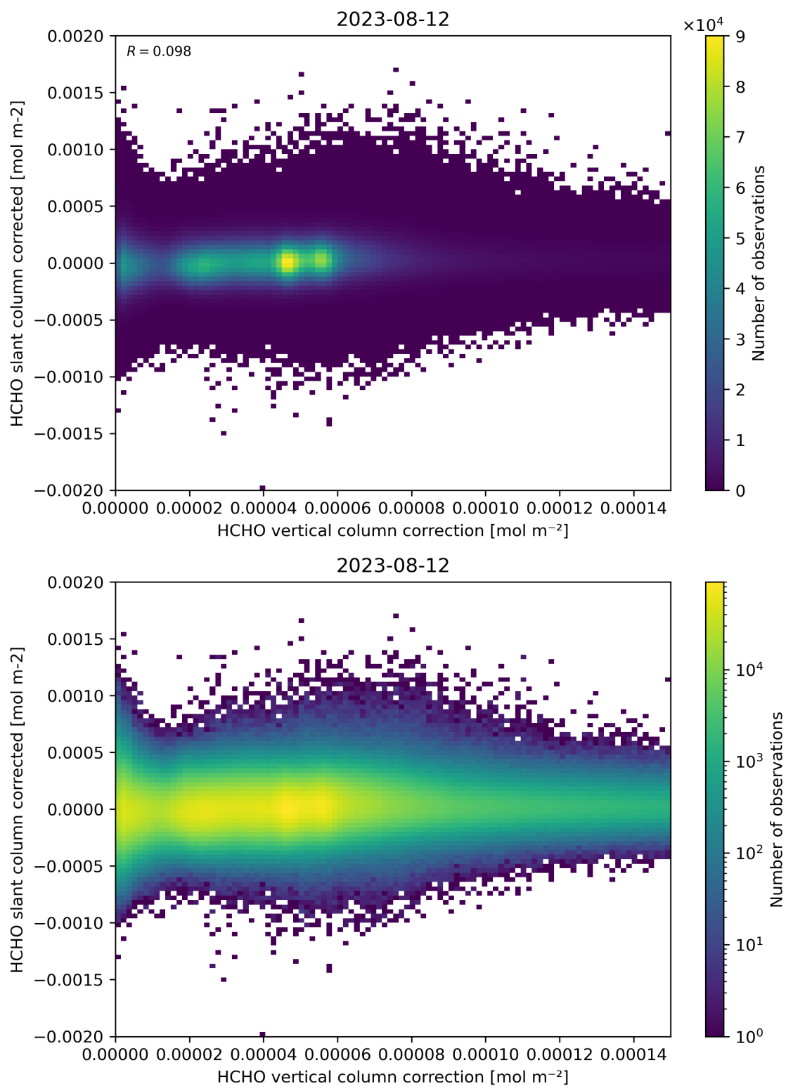
Figure 116: Scatter density plot of “HCHO vertical column correction” against “HCHO slant column corrected” for 2023-08-11 to 2023-08-13.
