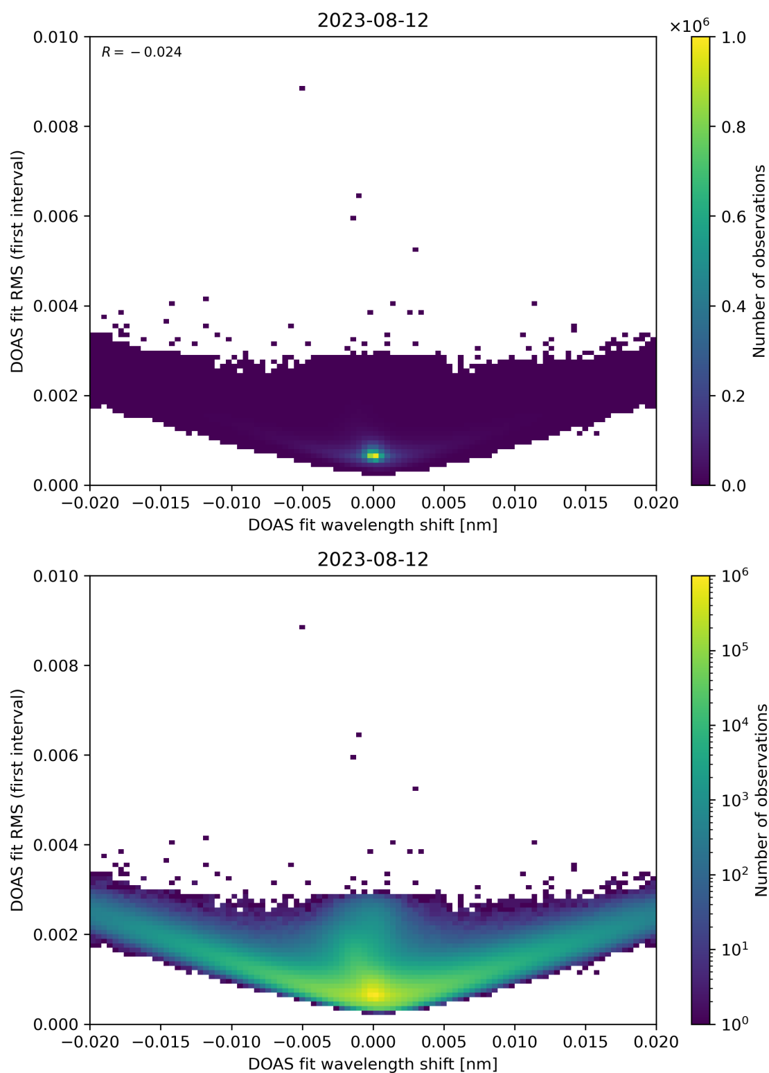
Figure 64: Scatter density plot of “DOAS fit wavelength shift” against “DOAS fit RMS (first interval)” for 2023-08-11 to 2023-08-13.
