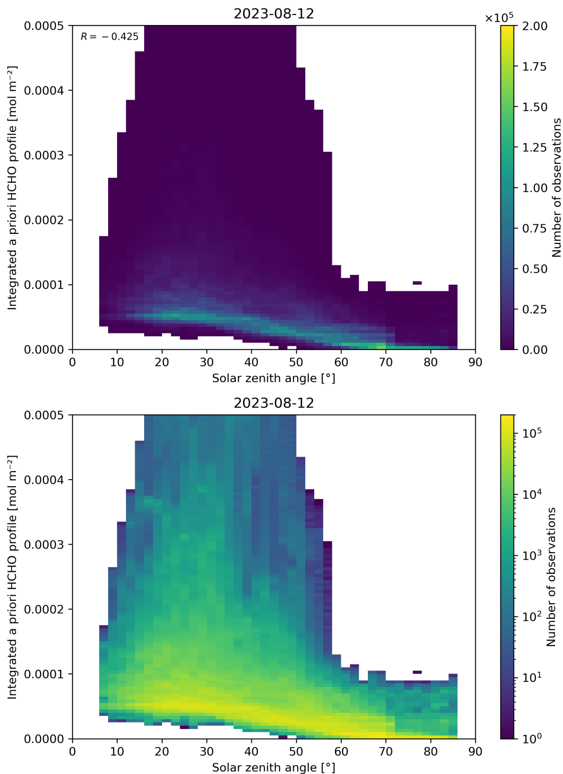
Figure 180: Scatter density plot of “Solar zenith angle” against “Integrated a priori HCHO profile” for 2023-08-11 to 2023-08-13.
