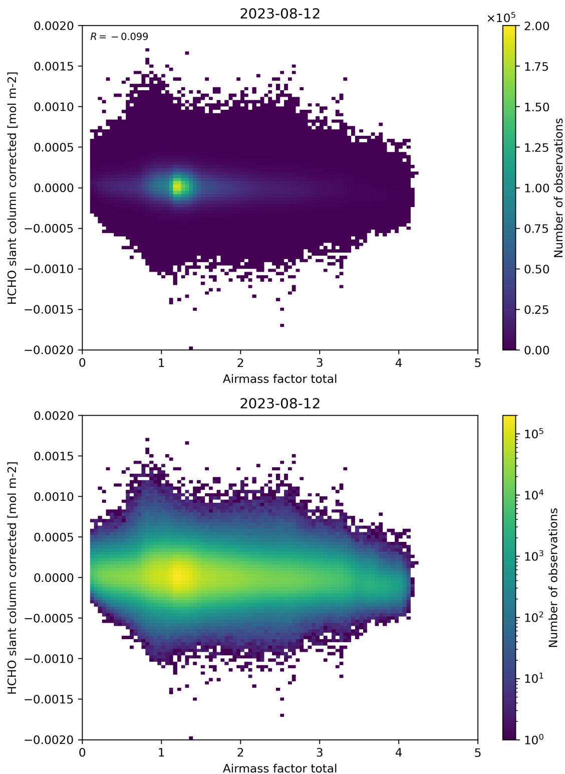
Figure 101: Scatter density plot of “Airmass factor total” against “HCHO slant column corrected” for 2023-08-11 to 2023-08-13.
