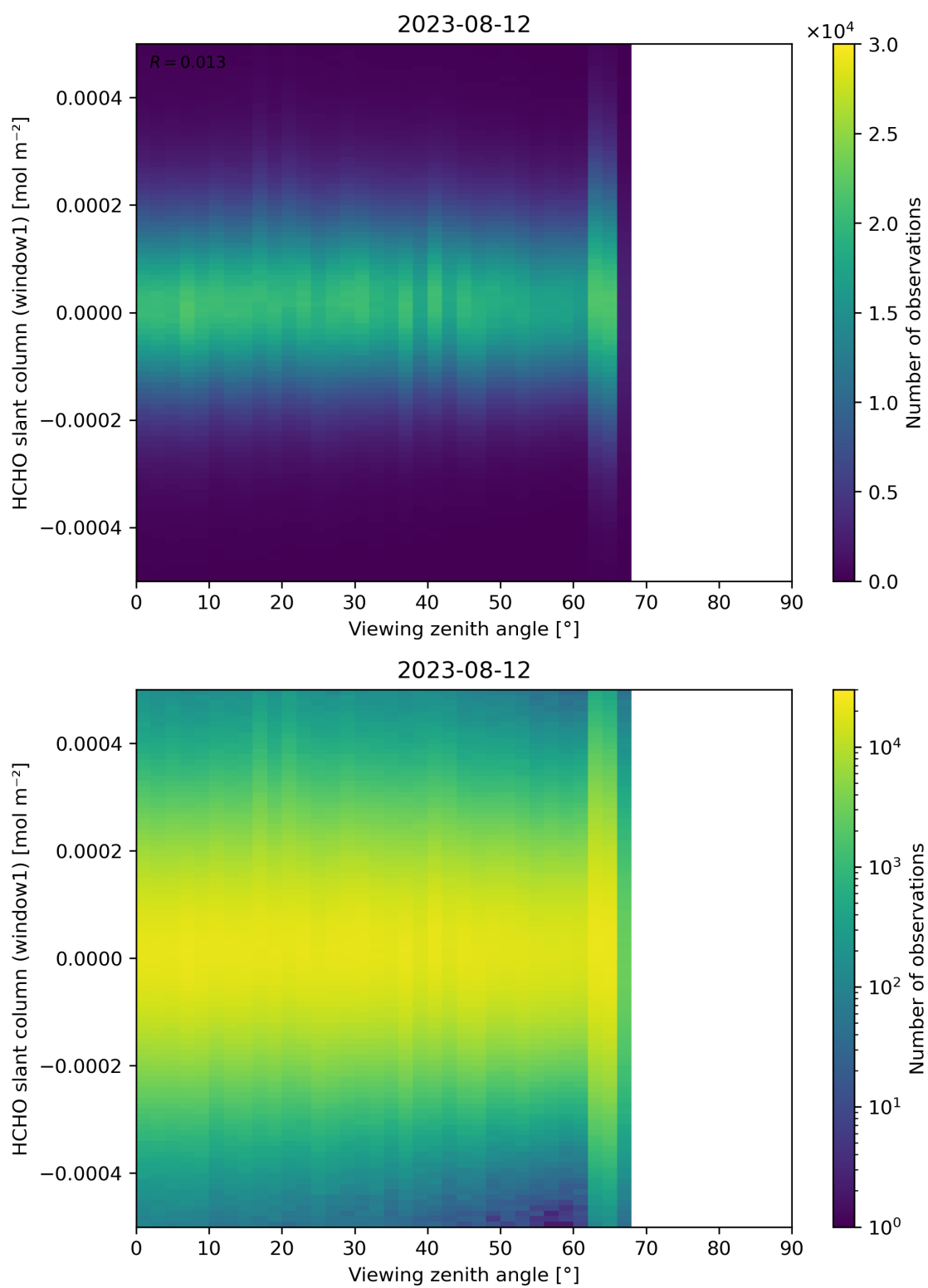
Figure 188: Scatter density plot of “Viewing zenith angle” against “HCHO slant column (window1)” for 2023-08-11 to 2023-08-13.
