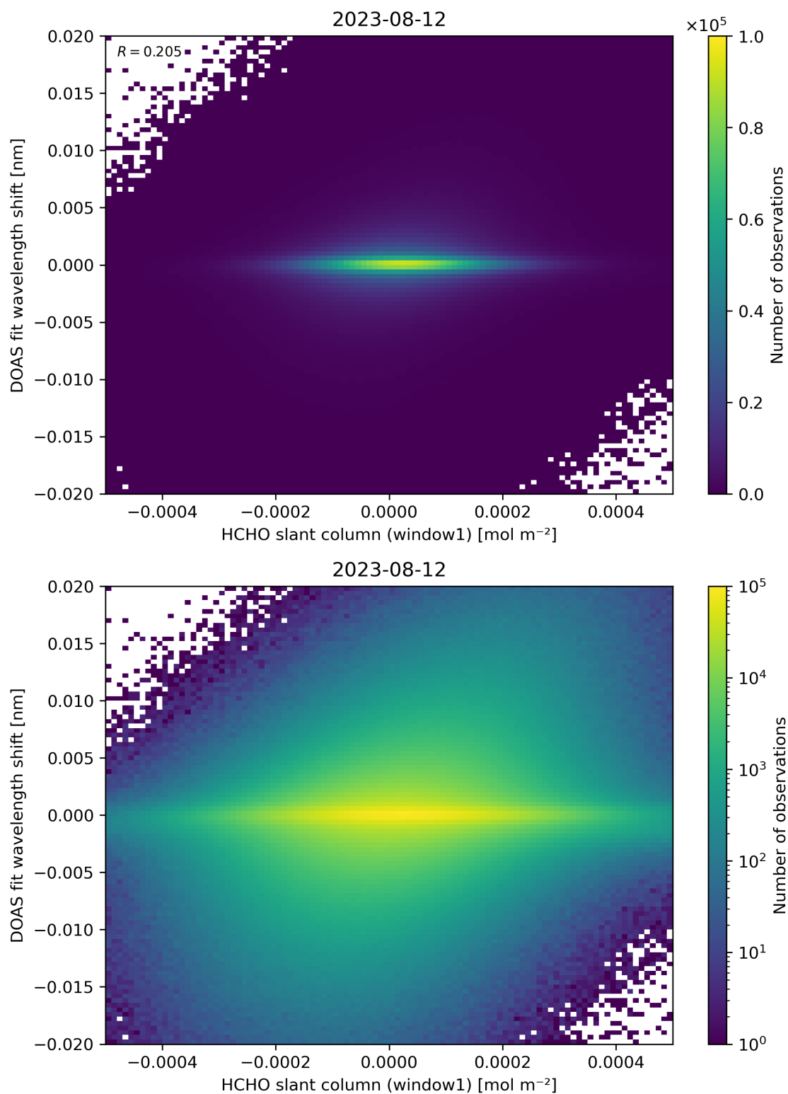
Figure 79: Scatter density plot of “HCHO slant column (window1)” against “DOAS fit wavelength shift” for 2023-08-11 to 2023-08-13.
