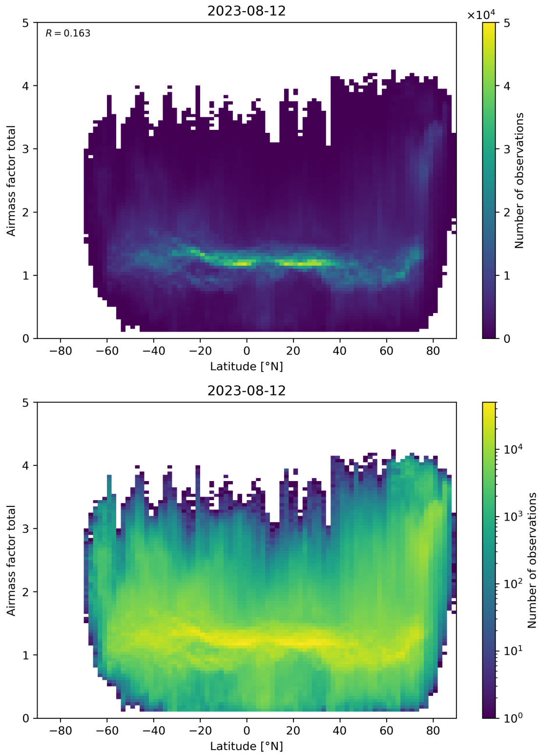
Figure 161: Scatter density plot of “Latitude” against “Airmass factor total” for 2023-08-11 to 2023-08-13.
