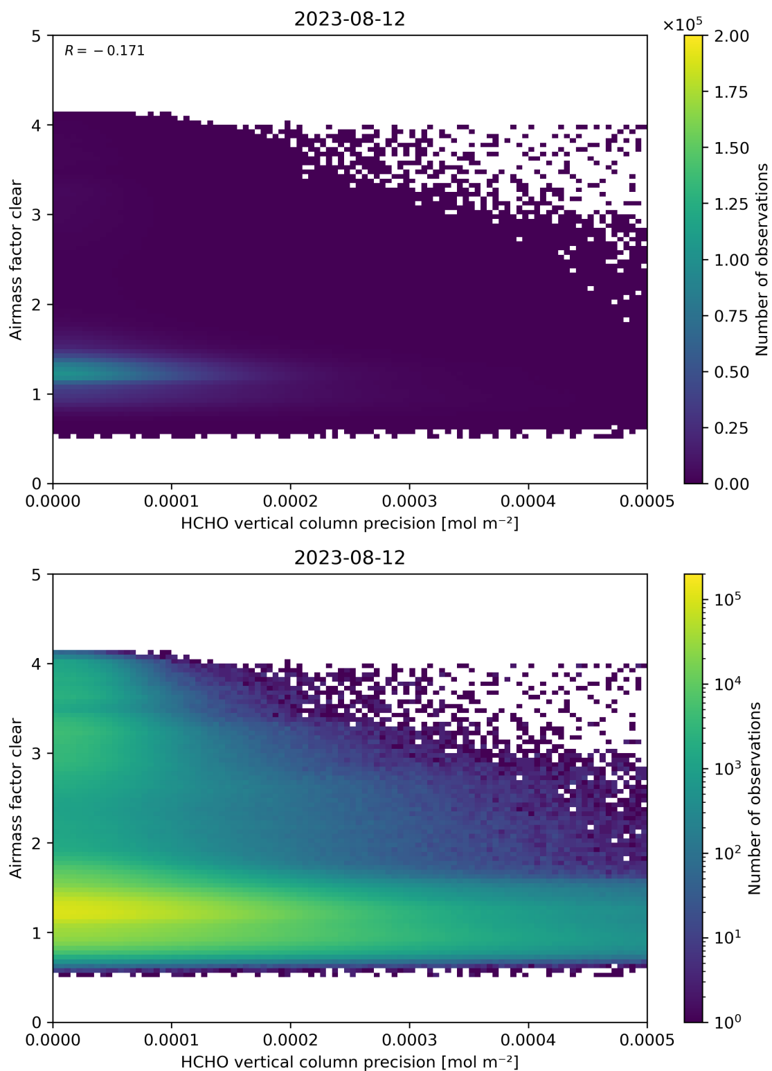
Figure 139: Scatter density plot of “HCHO vertical column precision” against “Airmass factor clear” for 2023-08-11 to 2023-08-13.
