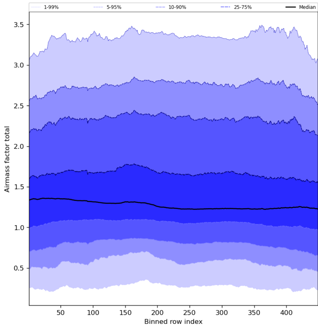
Figure 54: Along track statistics of “Airmass factor total” for 2023-08-11 to 2023-08-13
