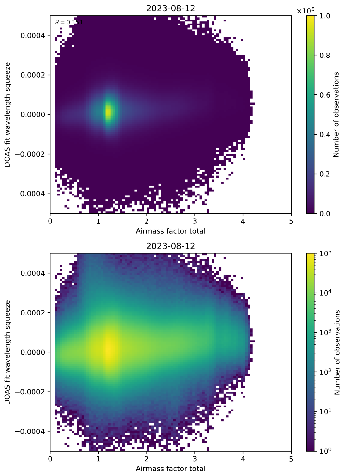
Figure 99: Scatter density plot of “Airmass factor total” against “DOAS fit wavelength squeeze” for 2023-08-11 to 2023-08-13.
