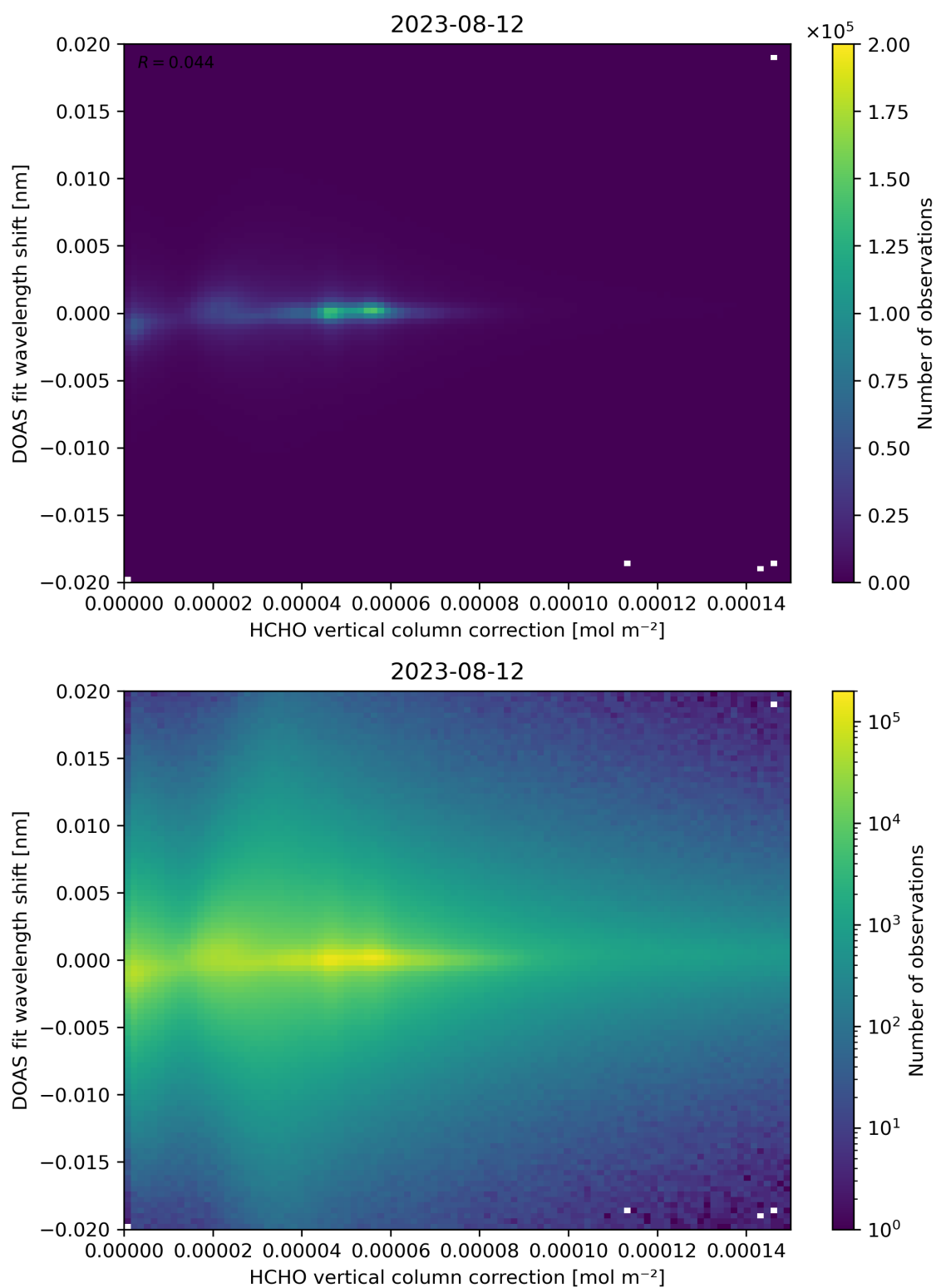
Figure 113: Scatter density plot of “HCHO vertical column correction” against “DOAS fit wavelength shift” for 2023-08-11 to 2023-08-13.
