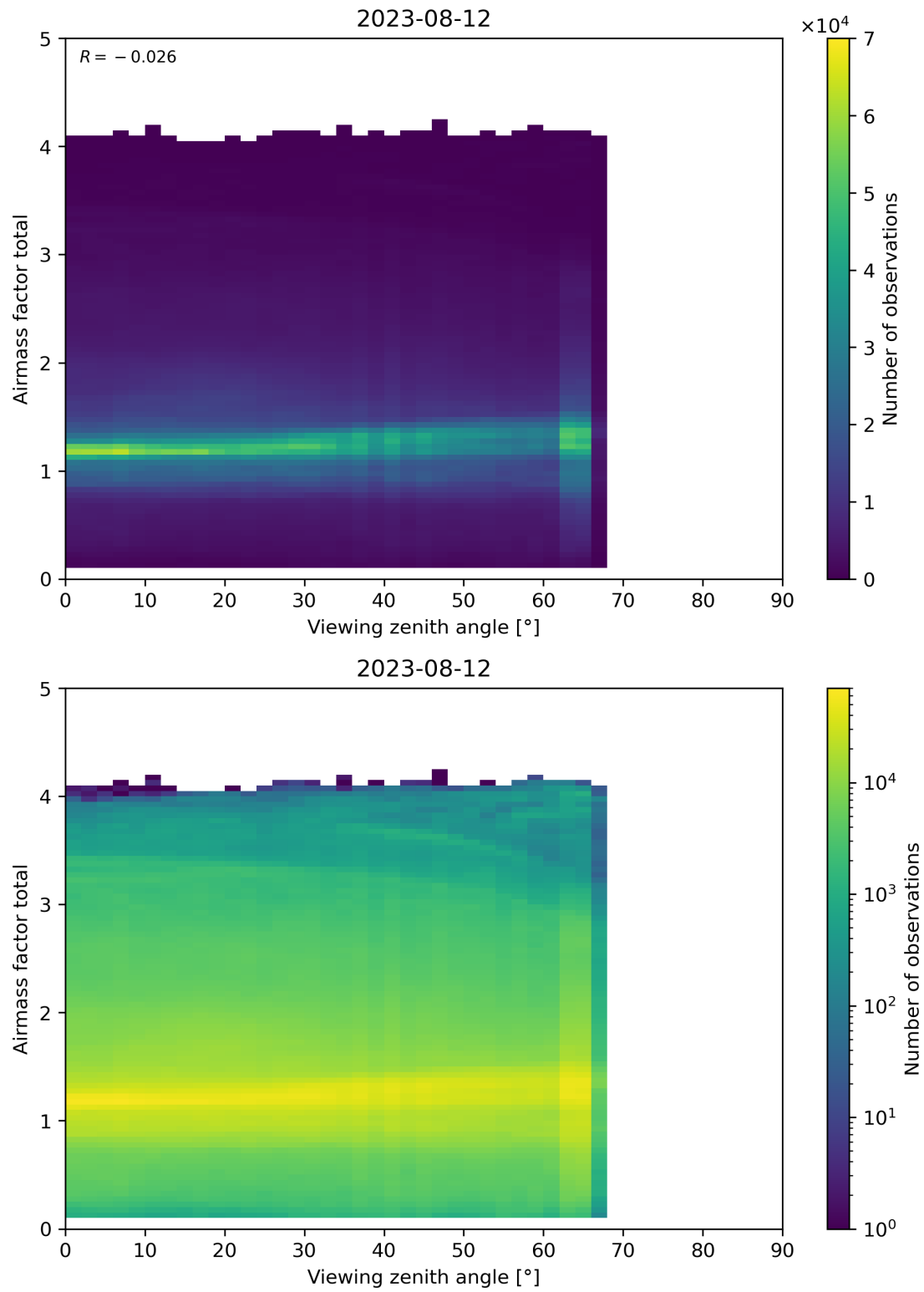
Figure 190: Scatter density plot of “Viewing zenith angle” against “Airmass factor total” for 2023-08-11 to 2023-08-13.
