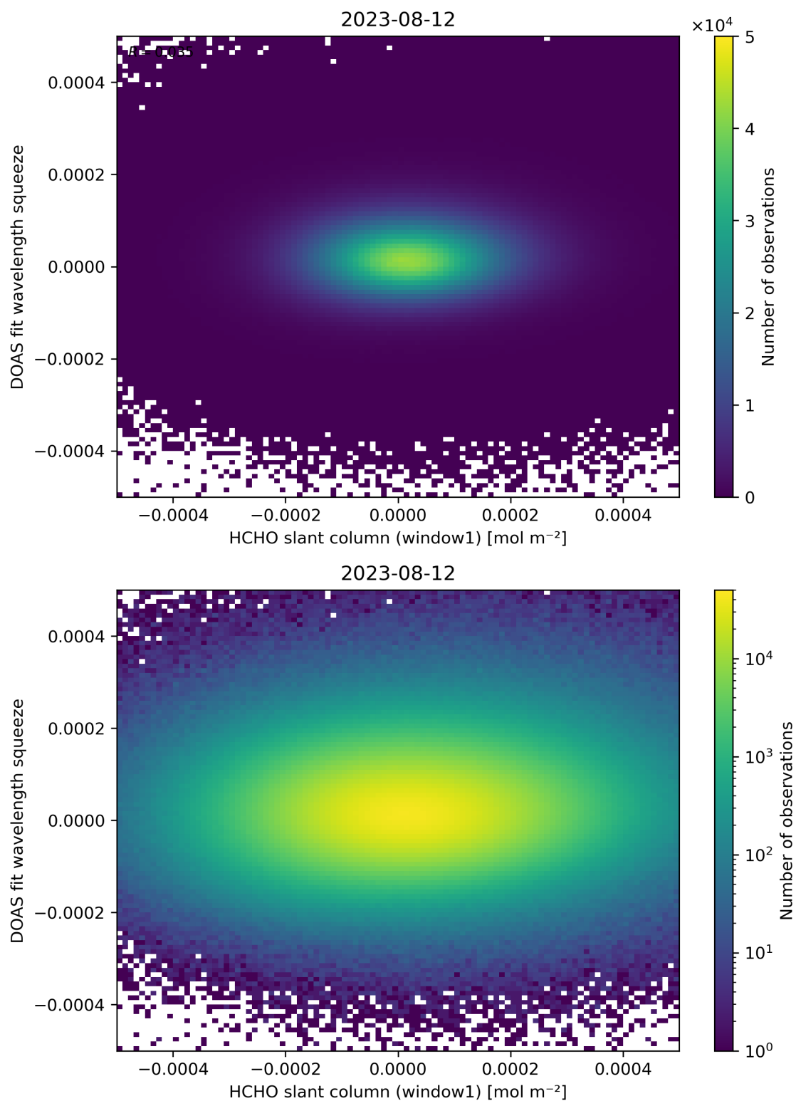
Figure 80: Scatter density plot of “HCHO slant column (window1)” against “DOAS fit wavelength squeeze” for 2023-08-11 to 2023-08-13.
