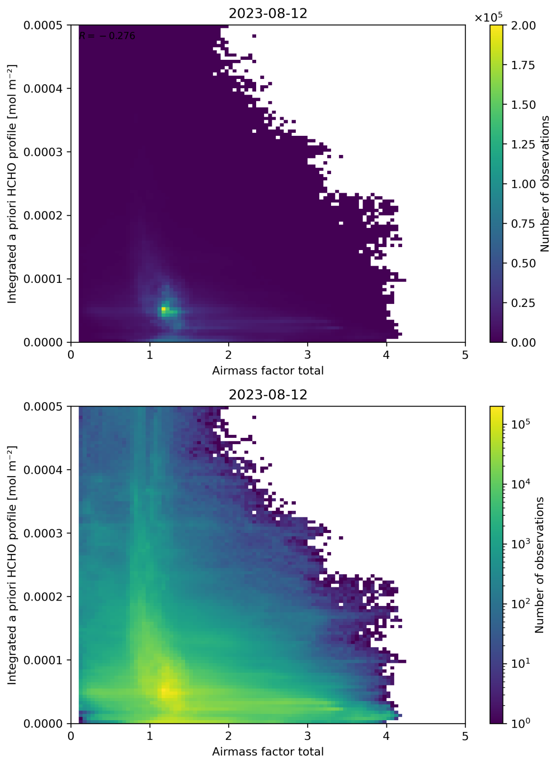
Figure 104: Scatter density plot of “Airmass factor total” against “Integrated a priori HCHO profile” for 2023-08-11 to 2023-08-13.
