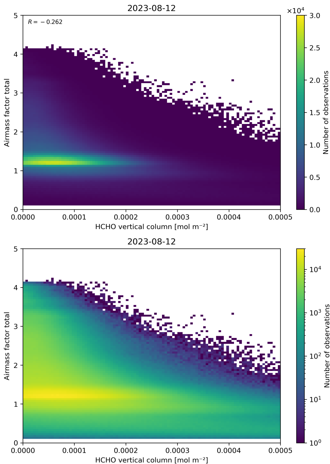
Figure 131: Scatter density plot of “HCHO vertical column” against “Airmass factor total” for 2023-08-11 to 2023-08-13.
