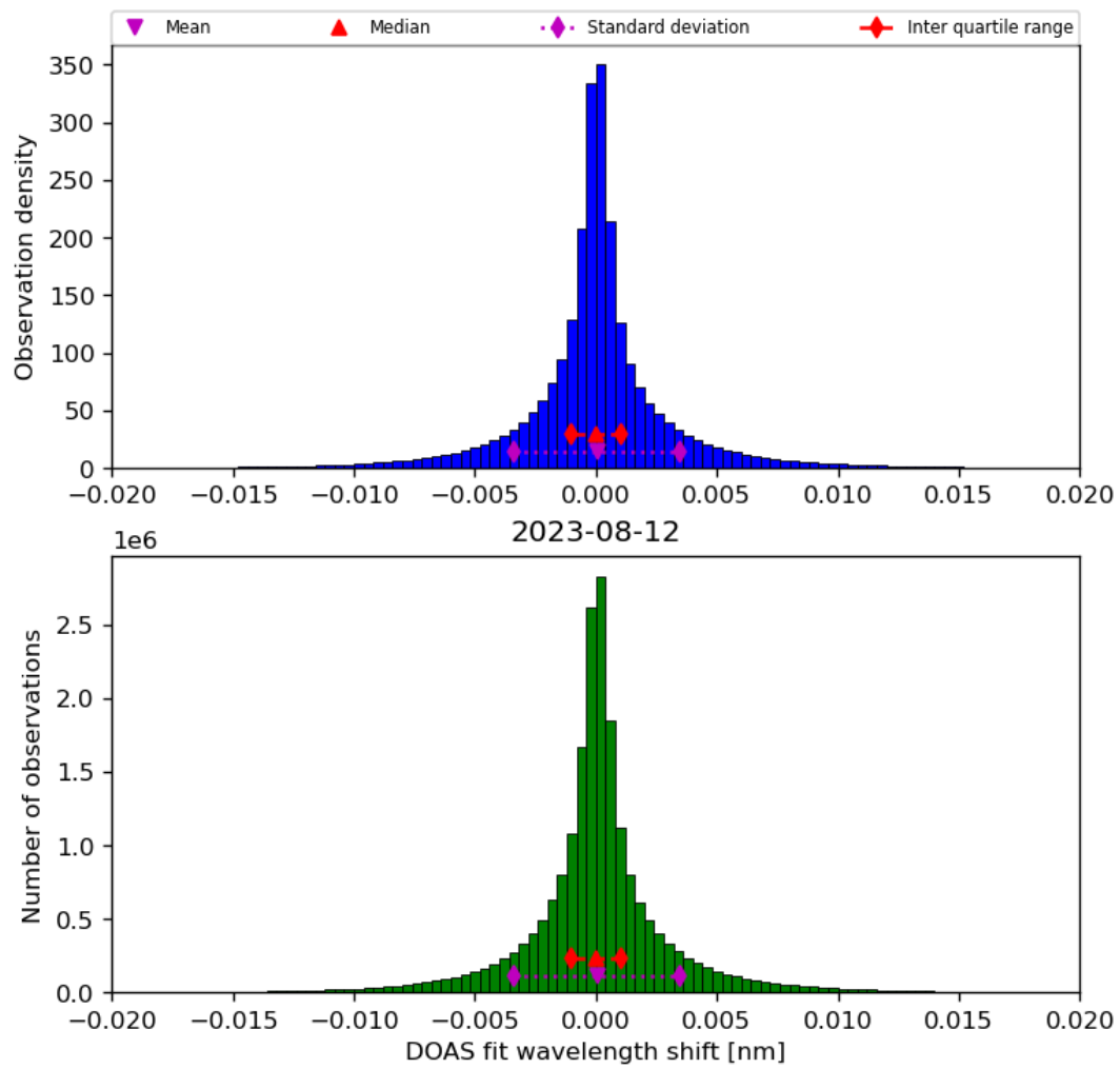
Figure 44: Histogram of “DOAS fit wavelength shift” for 2023-08-11 to 2023-08-13
