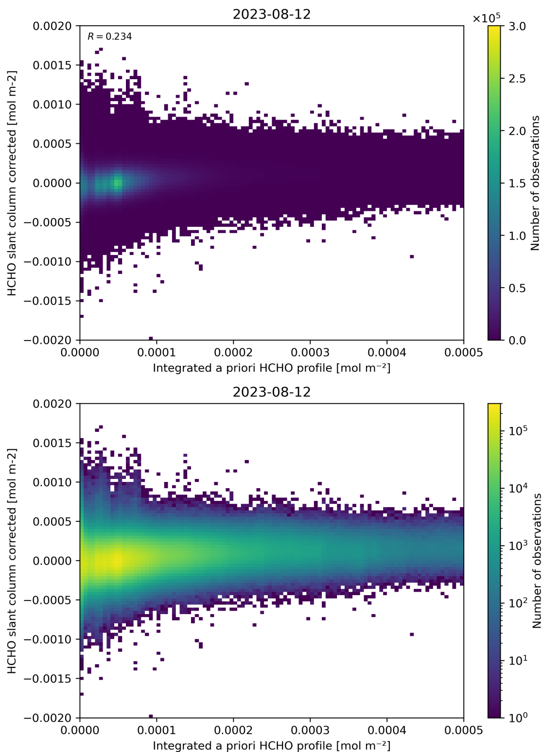
Figure 151: Scatter density plot of “Integrated a priori HCHO profile” against “HCHO slant column corrected” for 2023-08-11 to 2023-08-13.
