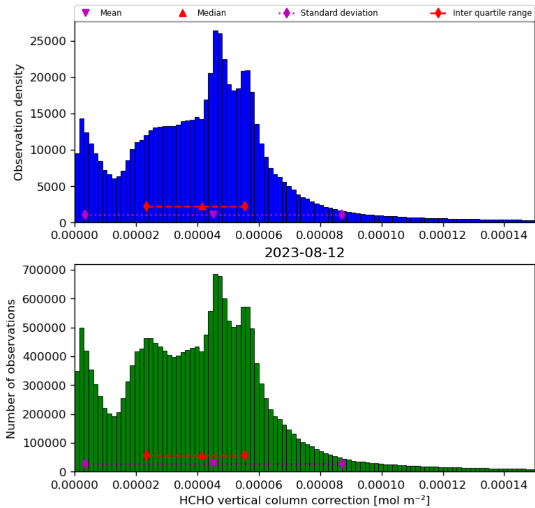
Figure 37: Histogram of “HCHO vertical column correction” for 2023-08-11 to 2023-08-13
