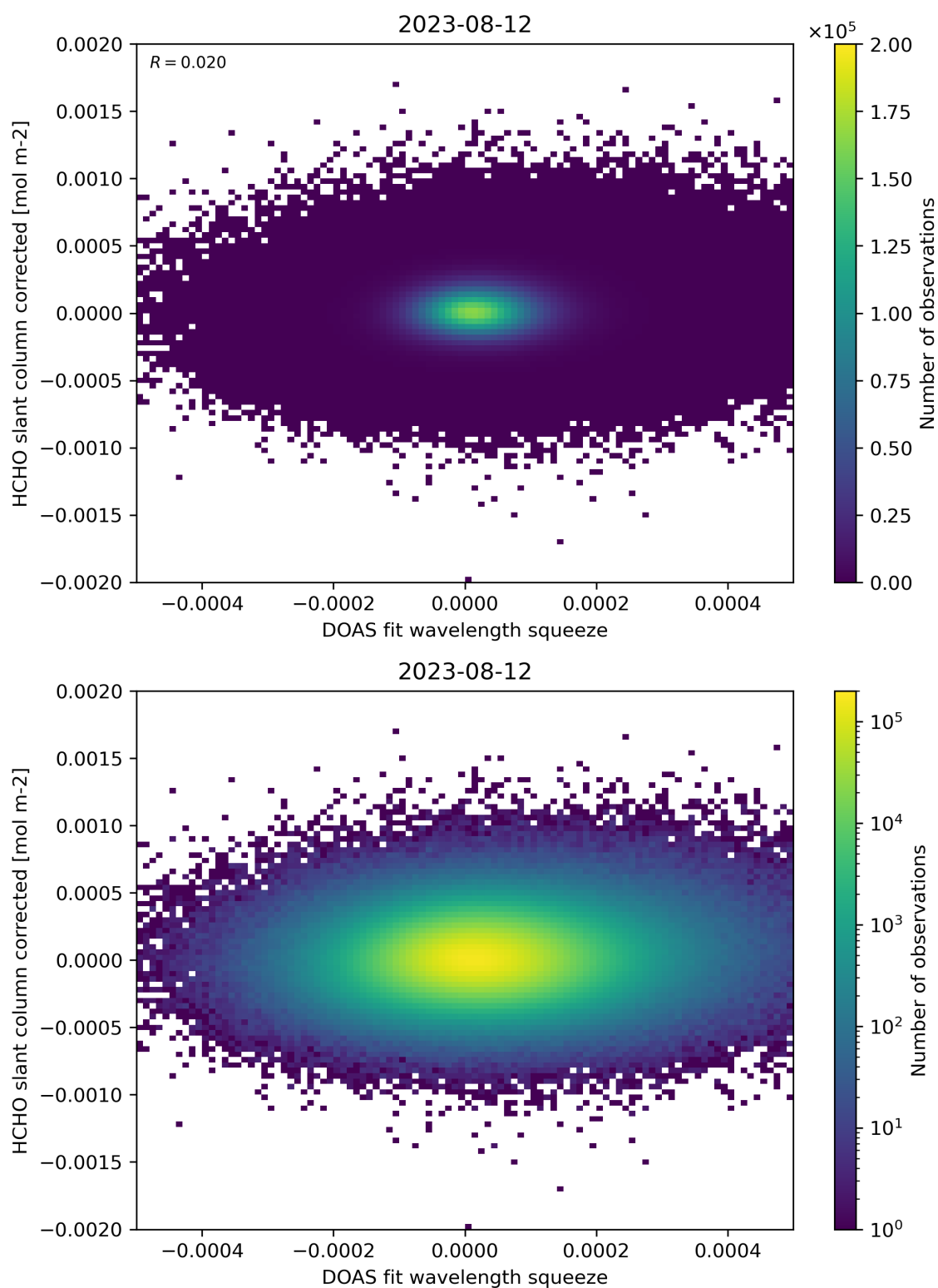
Figure 69: Scatter density plot of “DOAS fit wavelength squeeze” against “HCHO slant column corrected” for 2023-08-11 to 2023-08-13.
