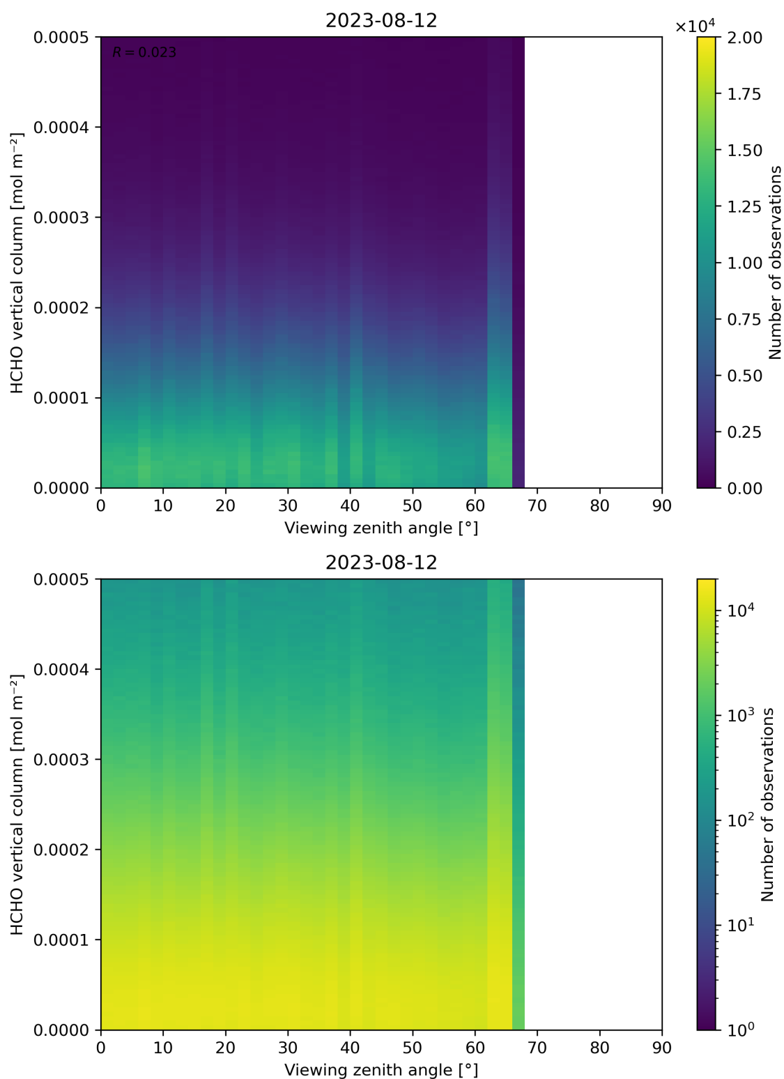
Figure 192: Scatter density plot of “Viewing zenith angle” against “HCHO vertical column” for 2023-08-11 to 2023-08-13.
