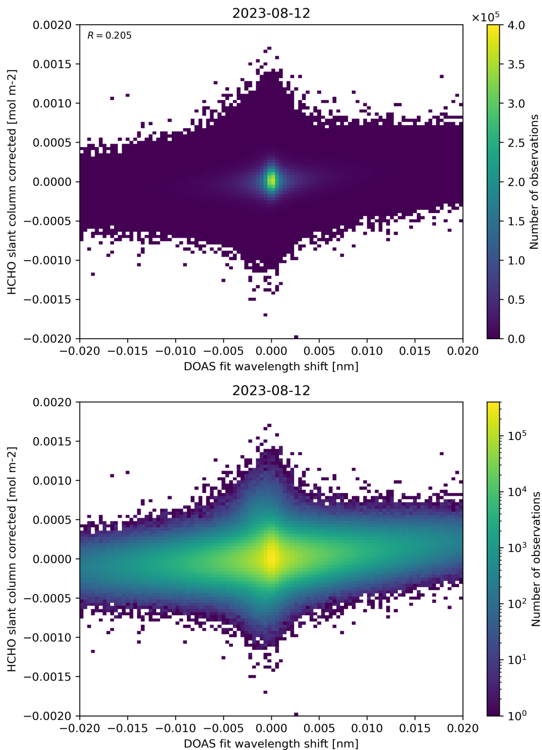
Figure 66: Scatter density plot of “DOAS fit wavelength shift” against “HCHO slant column corrected” for 2023-08-11 to 2023-08-13.
