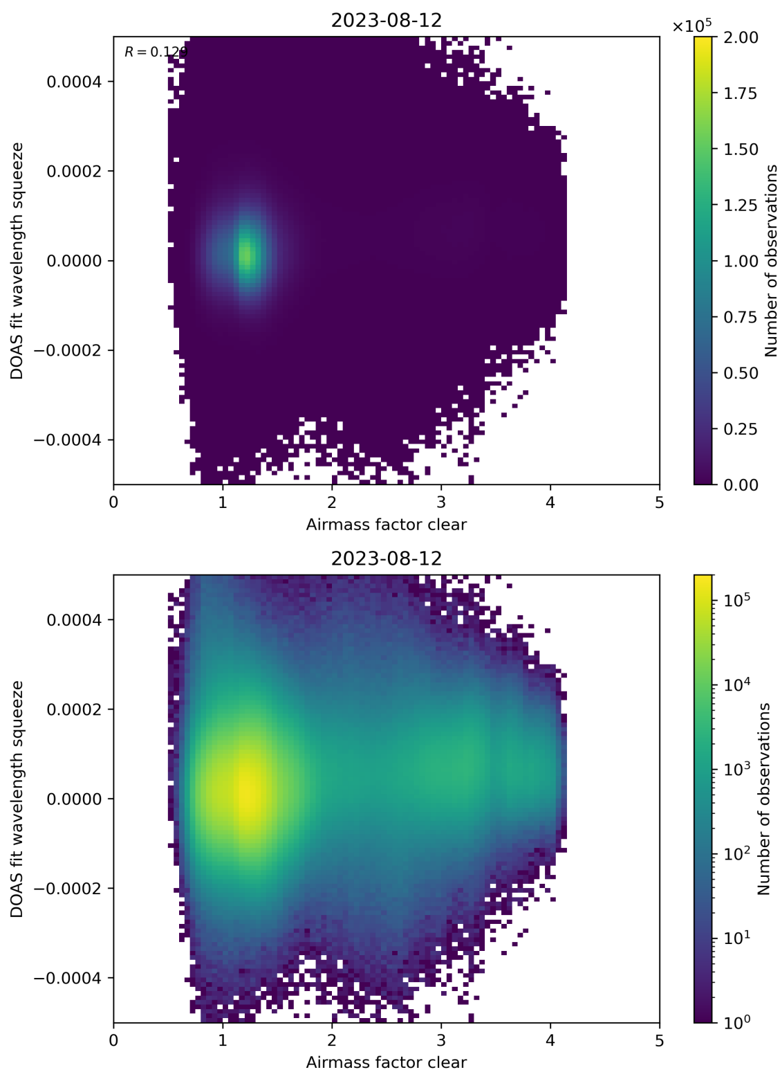
Figure 73: Scatter density plot of “Airmass factor clear” against “DOAS fit wavelength squeeze” for 2023-08-11 to 2023-08-13.
