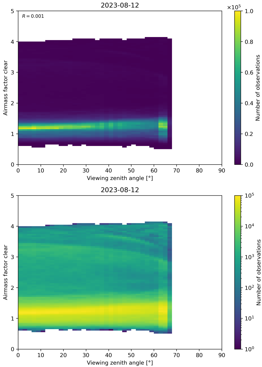
Figure 185: Scatter density plot of “Viewing zenith angle” against “Airmass factor clear” for 2023-08-11 to 2023-08-13.
