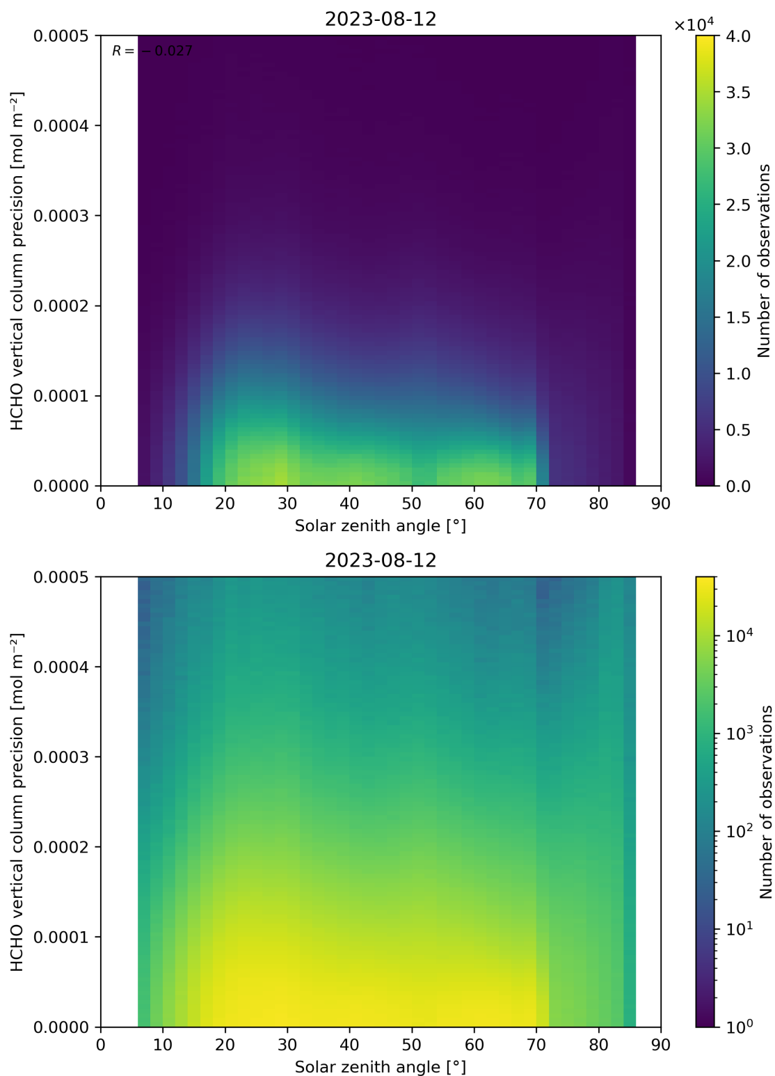
Figure 179: Scatter density plot of “Solar zenith angle” against “HCHO vertical column precision” for 2023-08-11 to 2023-08-13.
