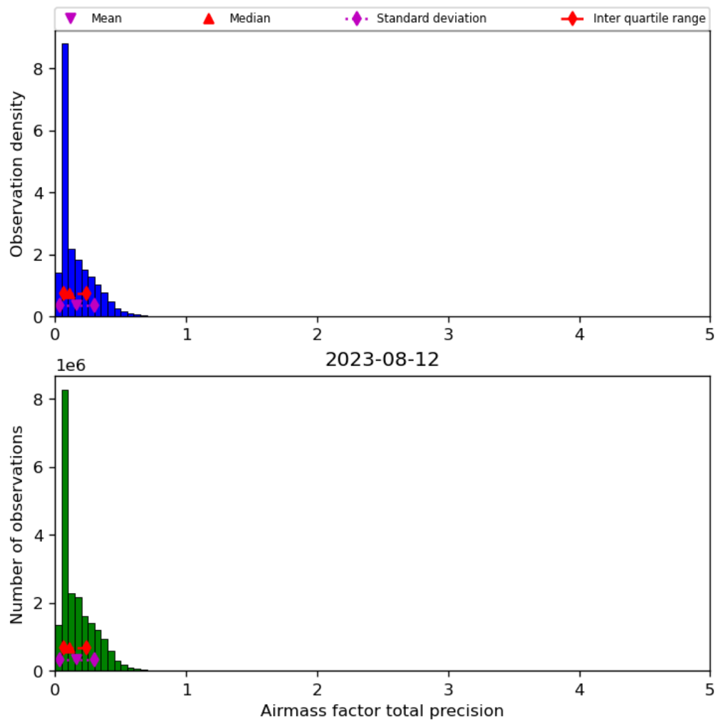
Figure 41: Histogram of “Airmass factor total precision” for 2023-08-11 to 2023-08-13
