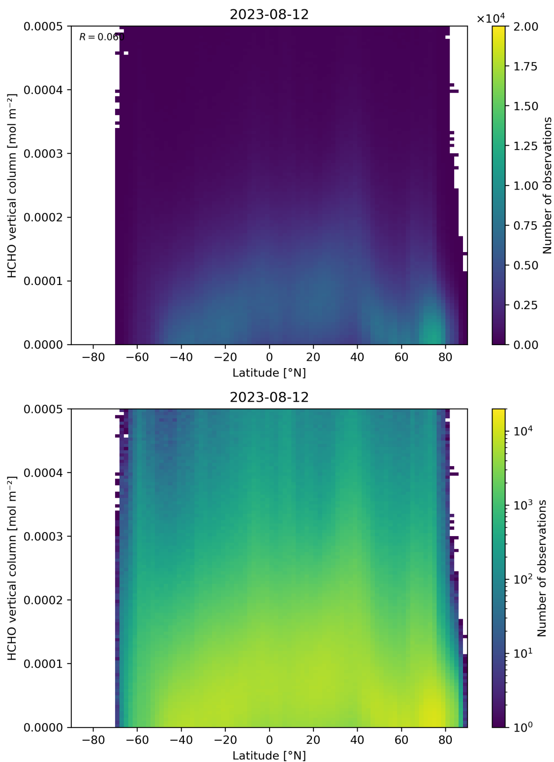
Figure 163: Scatter density plot of “Latitude” against “HCHO vertical column” for 2023-08-11 to 2023-08-13.
