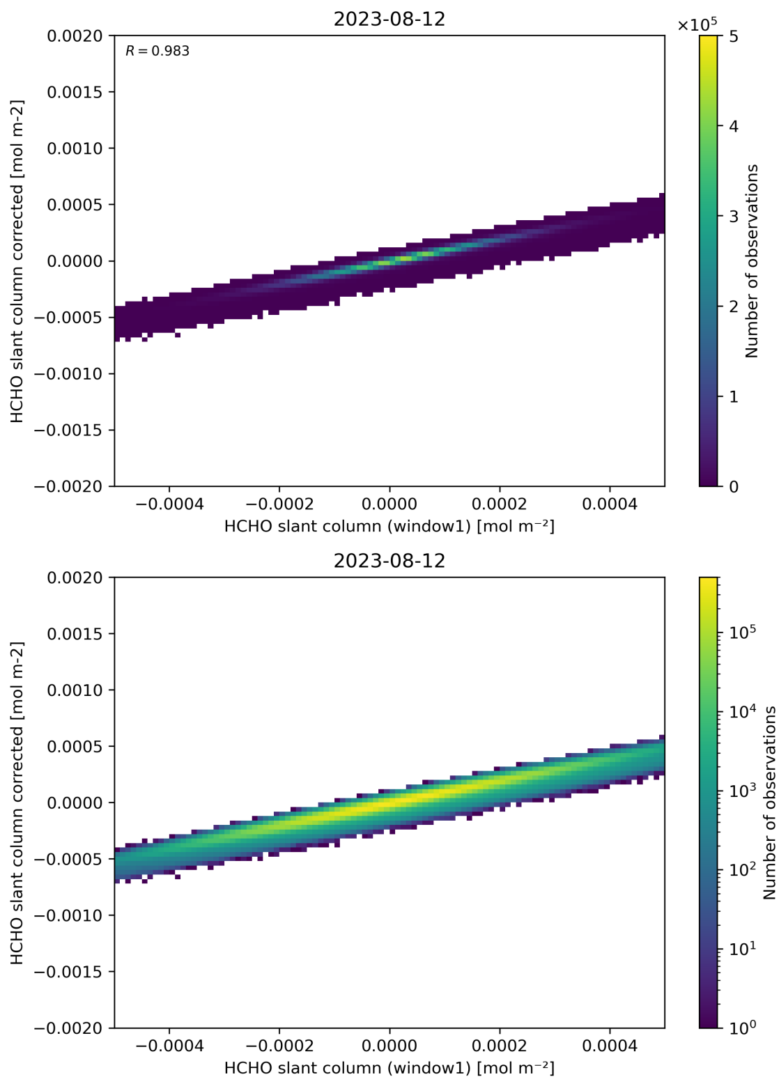
Figure 82: Scatter density plot of “HCHO slant column (window1)” against “HCHO slant column corrected” for 2023-08-11 to 2023-08-13.
