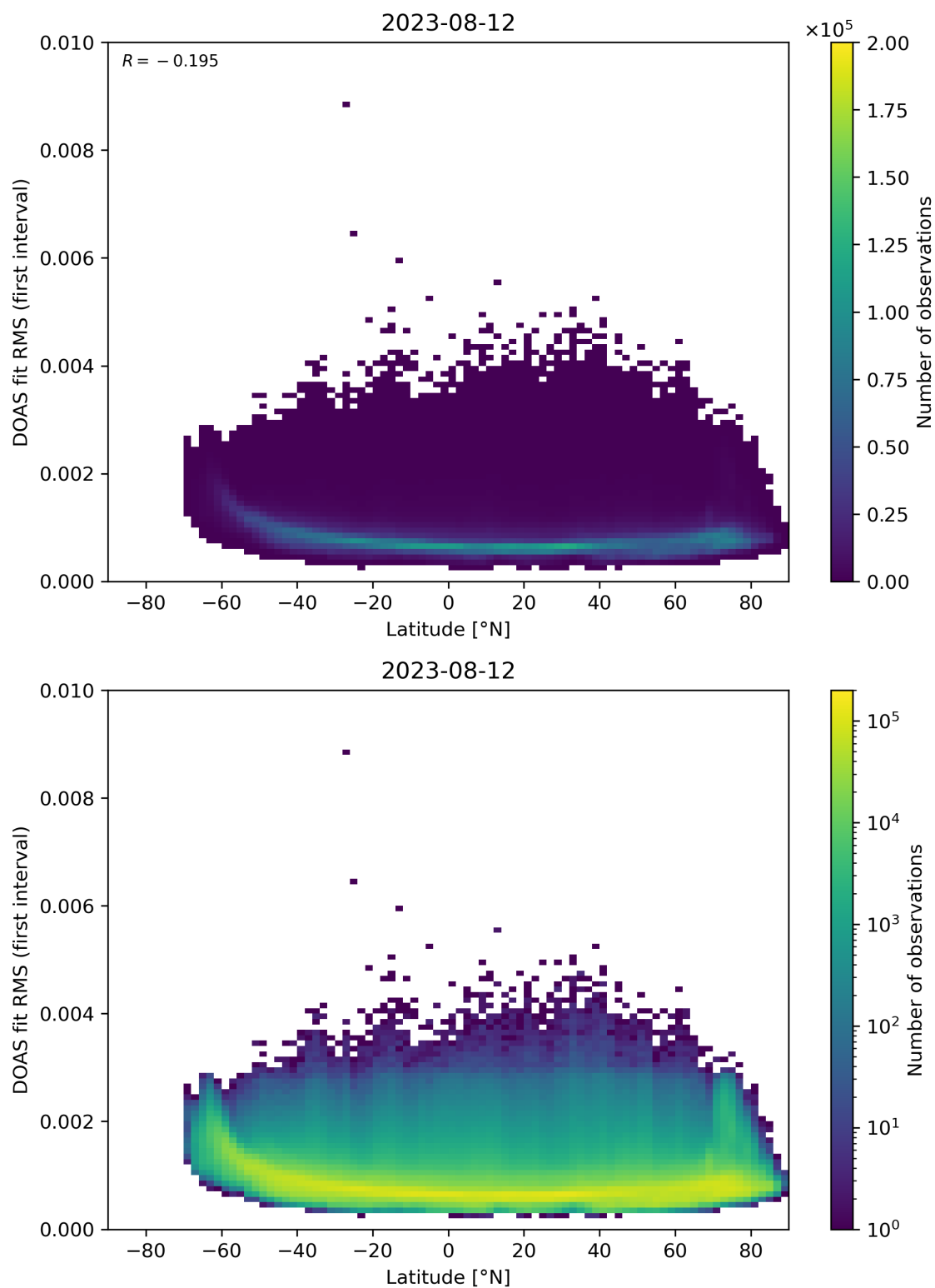
Figure 153: Scatter density plot of “Latitude” against “DOAS fit RMS (first interval)” for 2023-08-11 to 2023-08-13.
