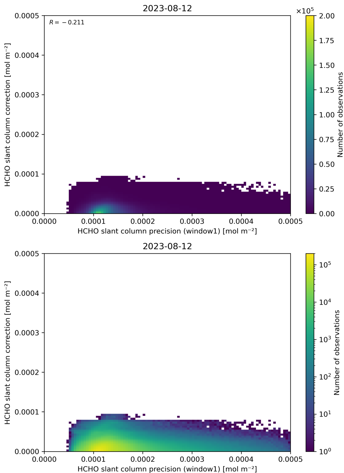
Figure 93: Scatter density plot of “HCHO slant column precision (window1)” against “HCHO slant column correction” for 2023-08-11 to 2023-08-13.
