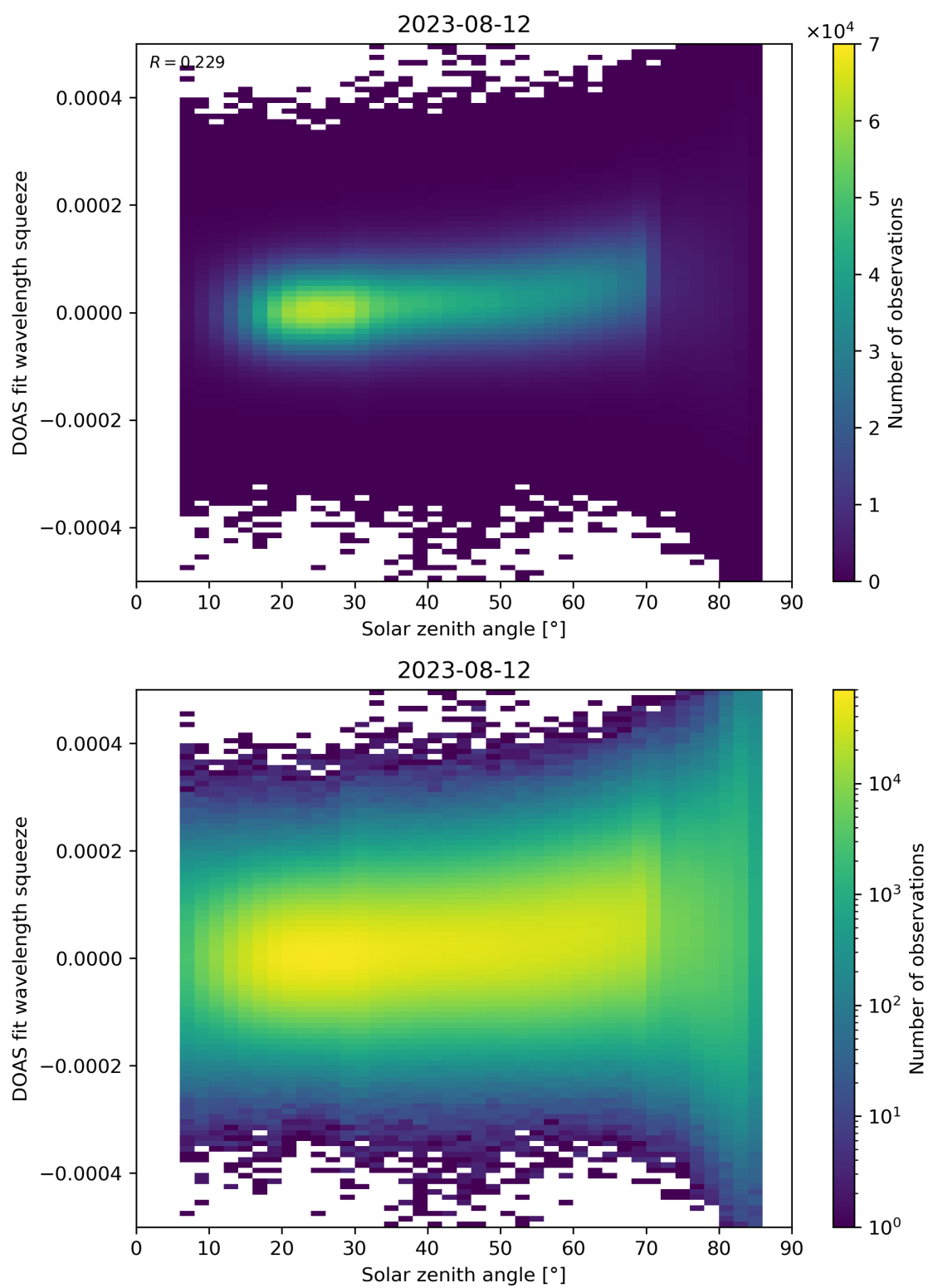
Figure 169: Scatter density plot of “Solar zenith angle” against “DOAS fit wavelength squeeze” for 2023-08-11 to 2023-08-13.
