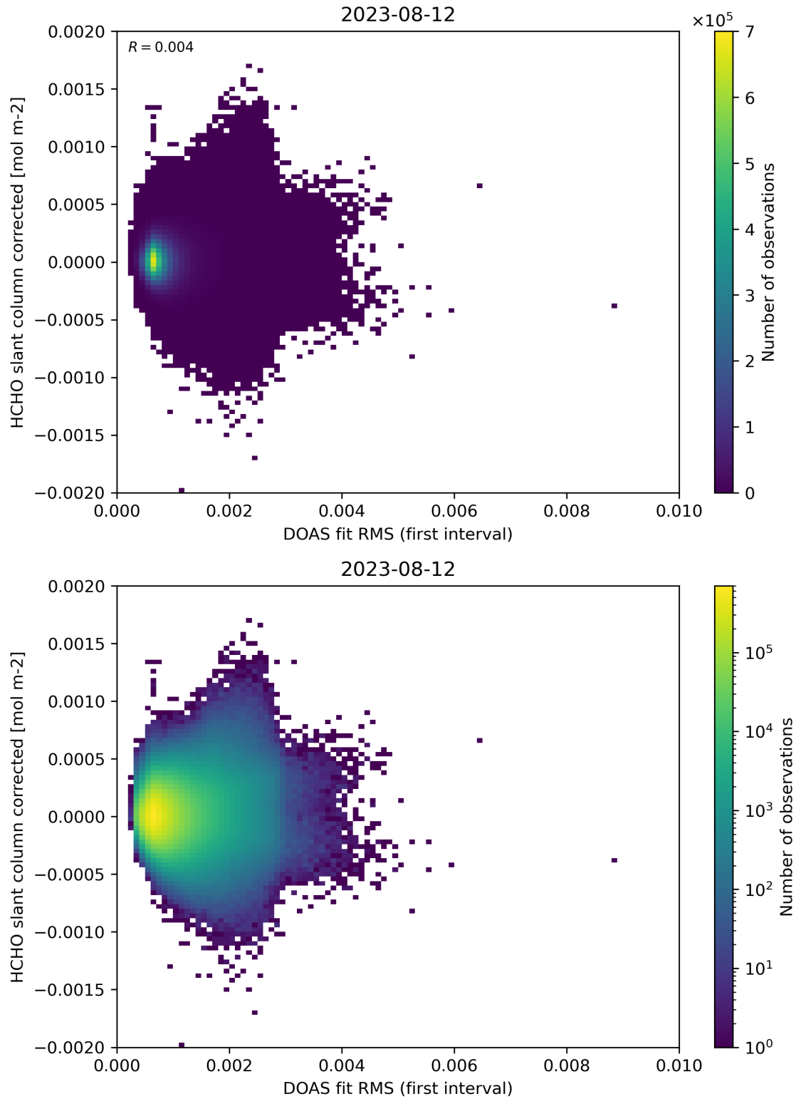
Figure 62: Scatter density plot of “DOAS fit RMS (first interval)” against “HCHO slant column corrected” for 2023-08-11 to 2023-08-13.
