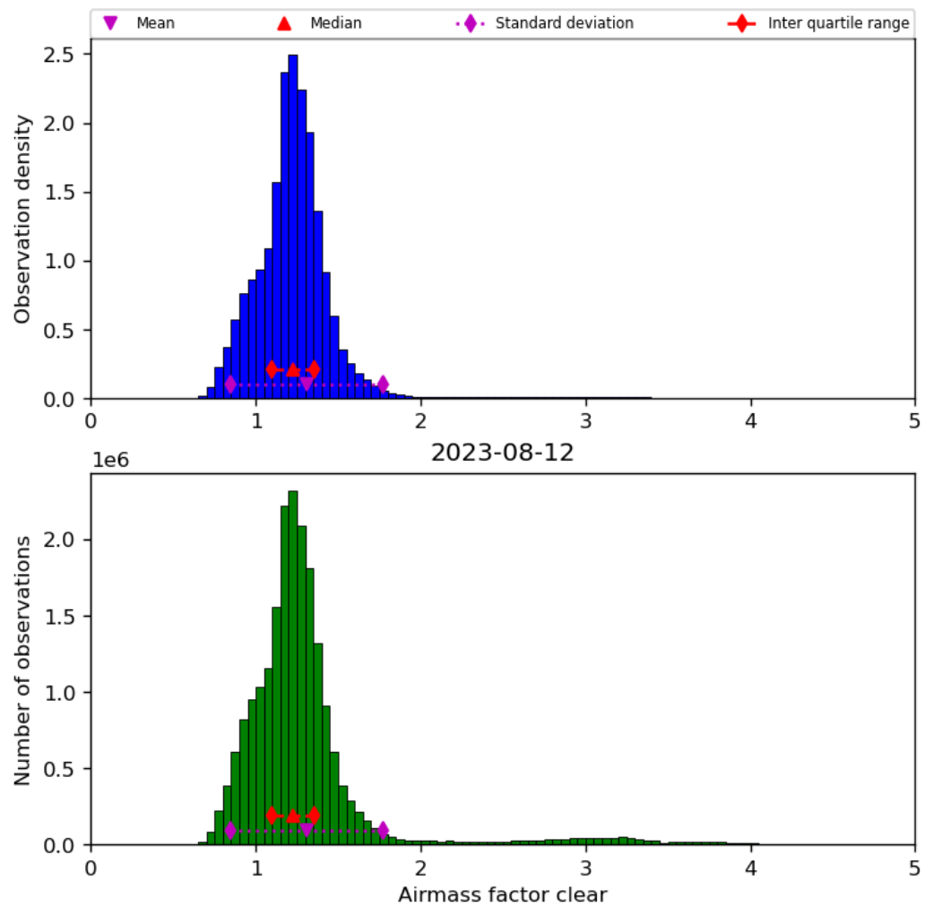
Figure 42: Histogram of “Airmass factor clear” for 2023-08-11 to 2023-08-13
