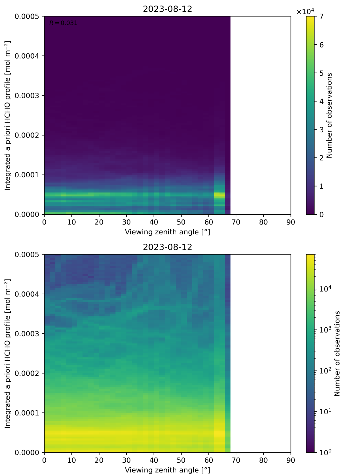
Figure 195: Scatter density plot of “Viewing zenith angle” against “Integrated a priori HCHO profile” for 2023-08-11 to 2023-08-13.
