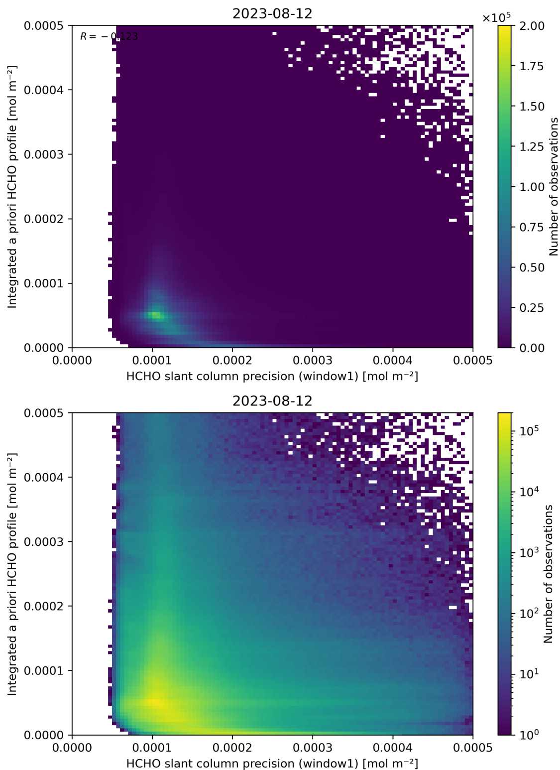
Figure 96: Scatter density plot of “HCHO slant column precision (window1)” against “Integrated a priori HCHO profile” for 2023-08-11 to 2023-08-13.
