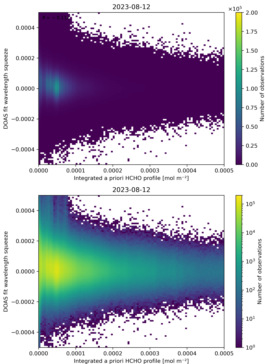
Figure 150: Scatter density plot of “Integrated a priori HCHO profile” against “DOAS fit wavelength squeeze” for 2023-08-11 to 2023-08-13.
