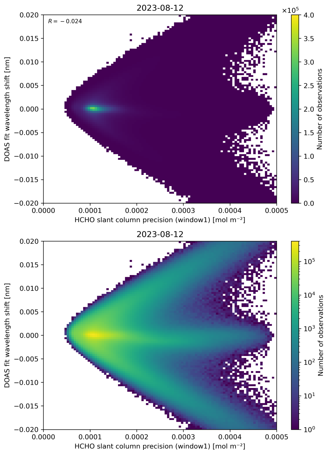
Figure 89: Scatter density plot of “HCHO slant column precision (window1)” against “DOAS fit wavelength shift” for 2023-08-11 to 2023-08-13.
