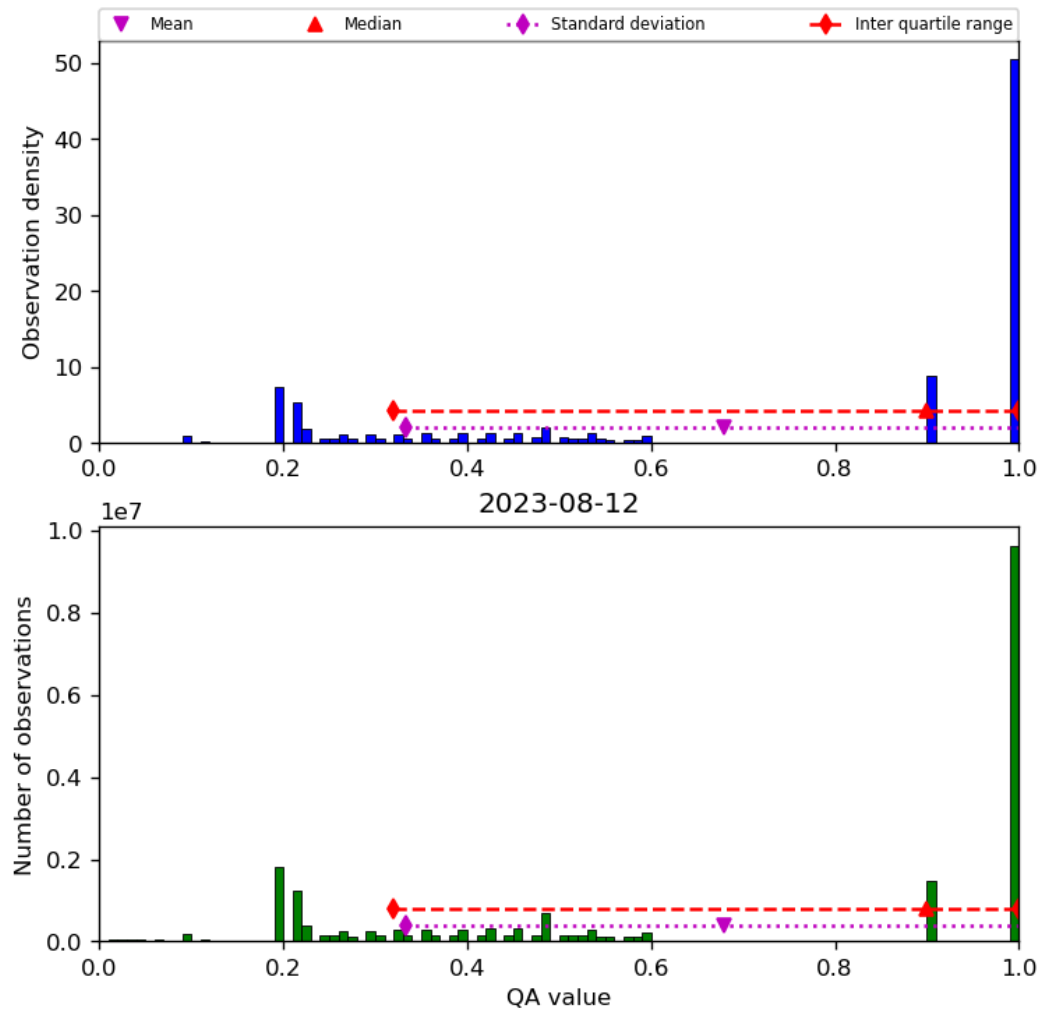
Figure 34: Histogram of “QA value” for 2023-08-11 to 2023-08-13
