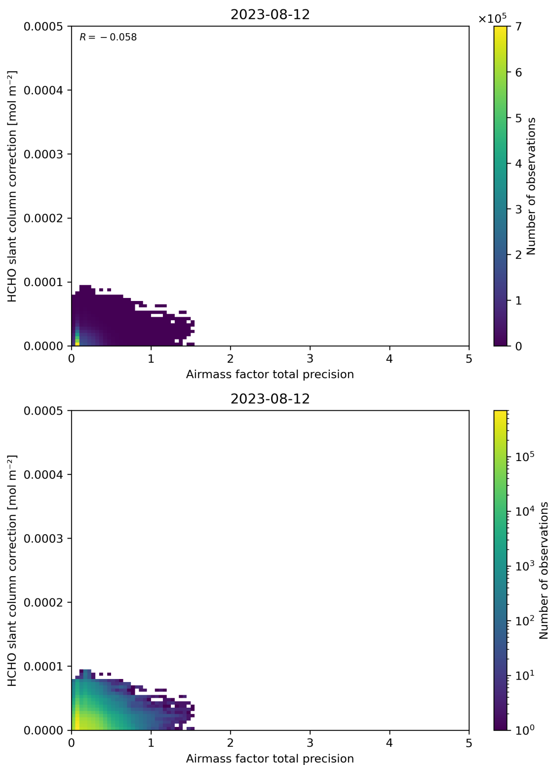
Figure 110: Scatter density plot of “Airmass factor total precision” against “HCHO slant column correction” for 2023-08-11 to 2023-08-13.
