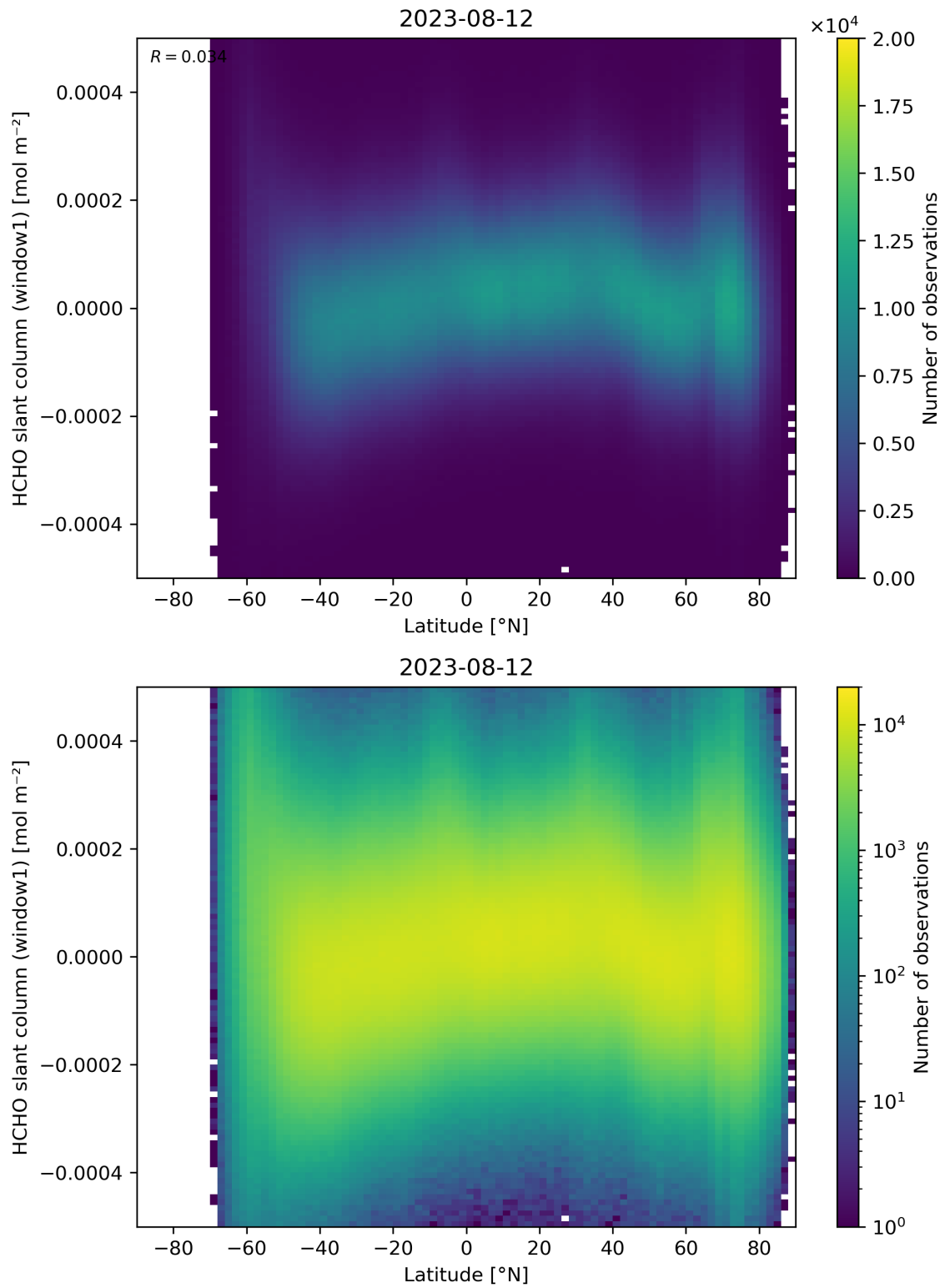
Figure 159: Scatter density plot of “Latitude” against “HCHO slant column (window1)” for 2023-08-11 to 2023-08-13.
