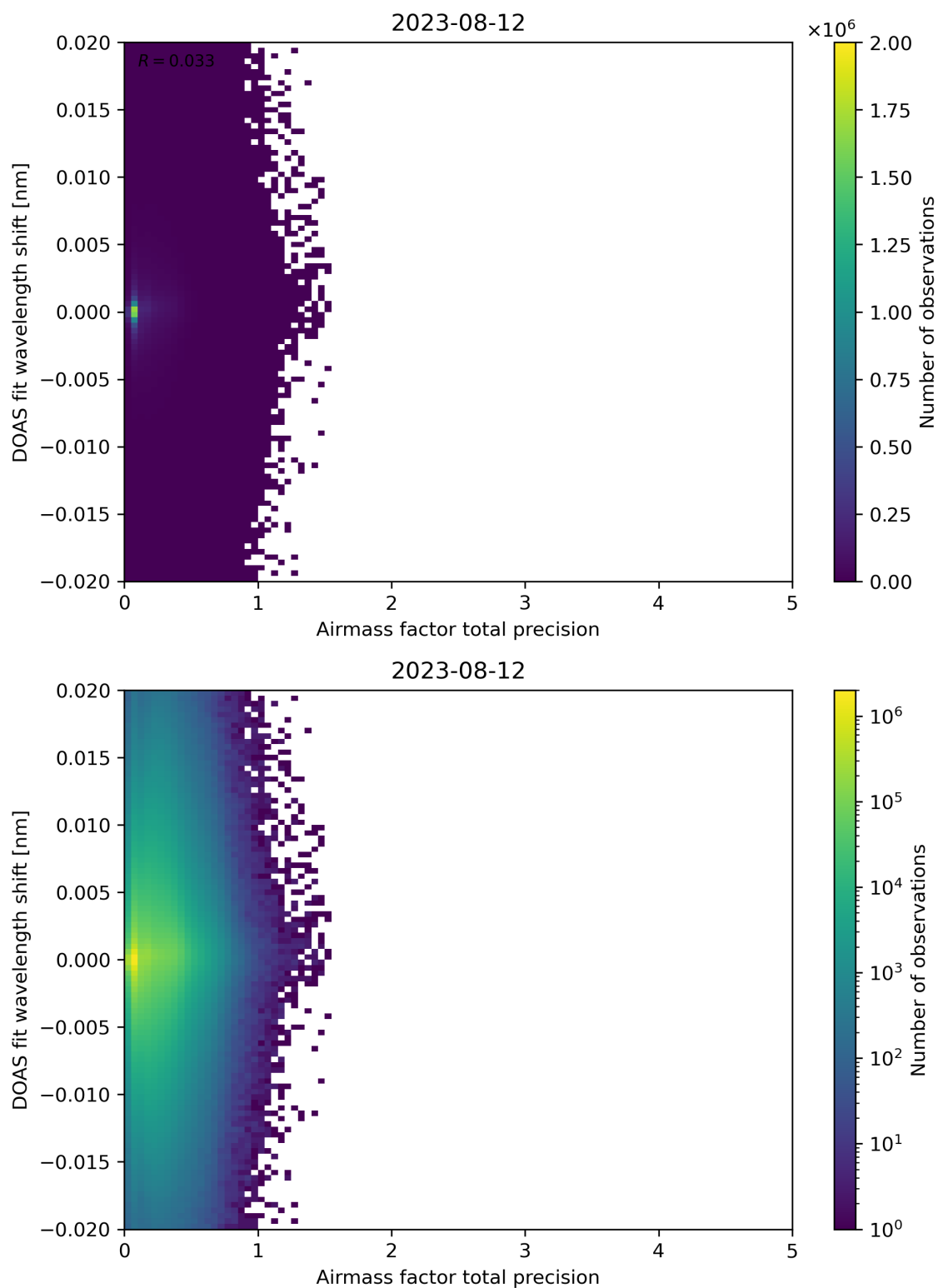
Figure 106: Scatter density plot of “Airmass factor total precision” against “DOAS fit wavelength shift” for 2023-08-11 to 2023-08-13.
