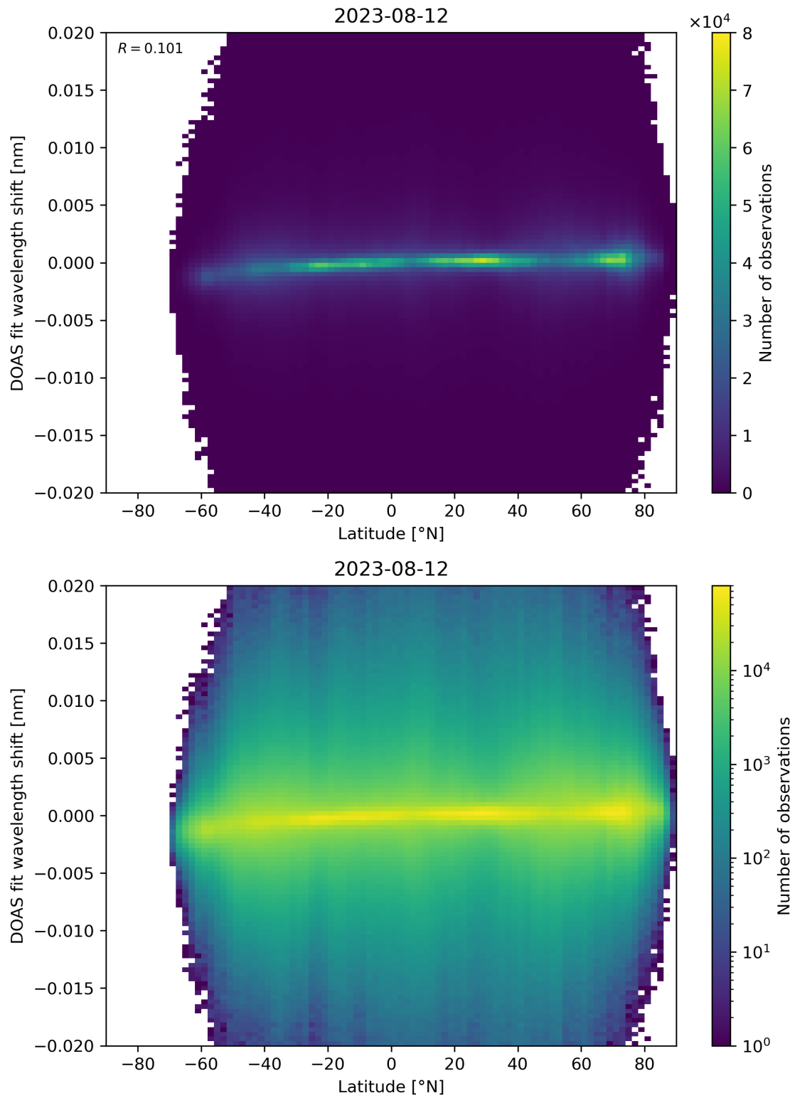
Figure 154: Scatter density plot of “Latitude” against “DOAS fit wavelength shift” for 2023-08-11 to 2023-08-13.
