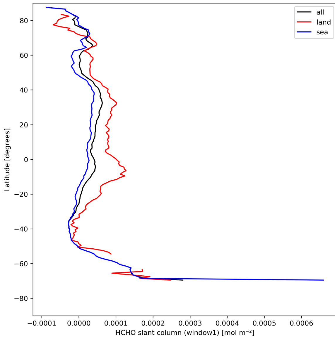
Figure 24: Zonal average of “HCHO slant column (window1)” for 2023-08-11 to 2023-08-13.
