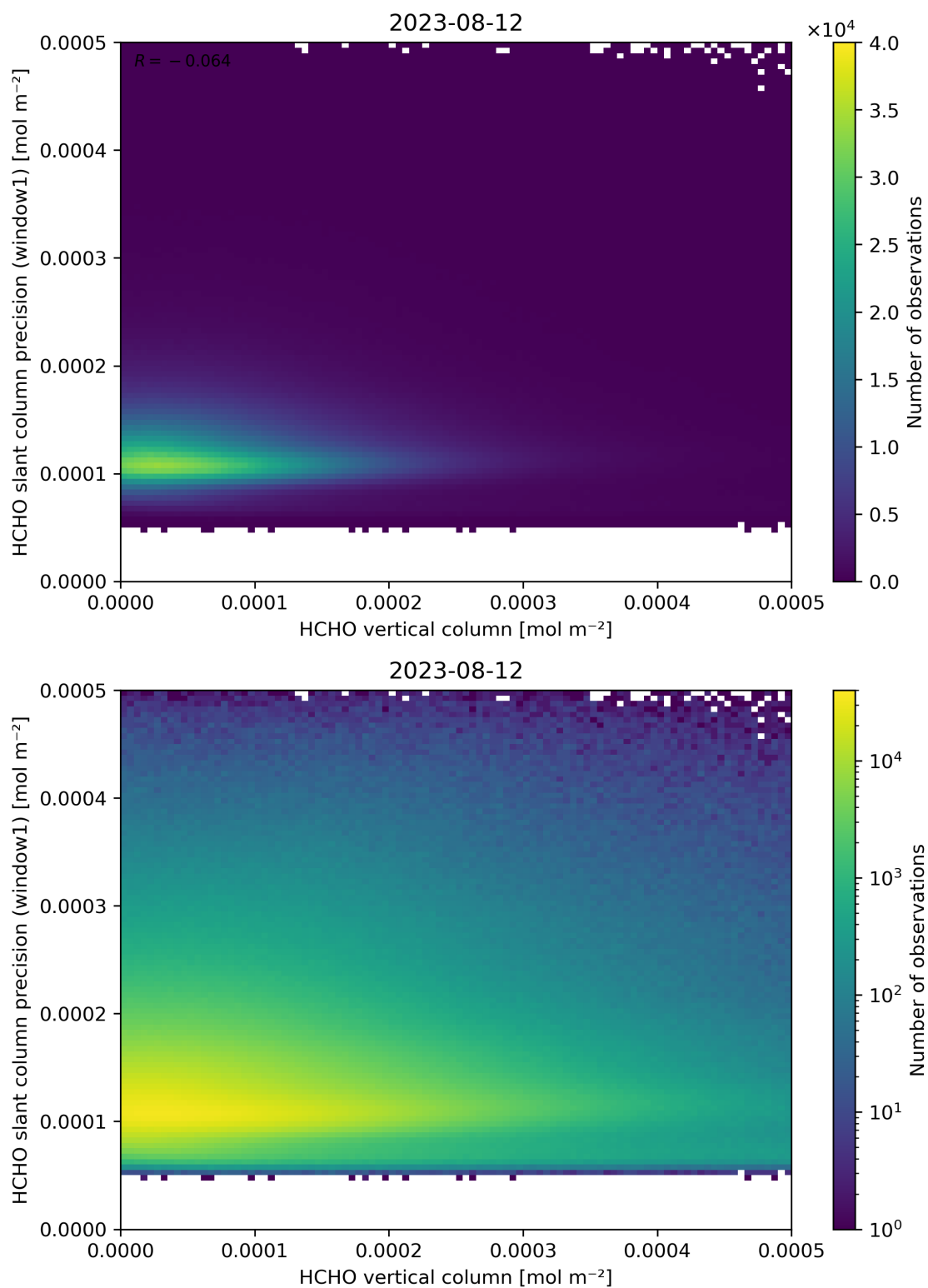
Figure 130: Scatter density plot of “HCHO vertical column” against “HCHO slant column precision (window1)” for 2023-08-11 to 2023-08-13.
