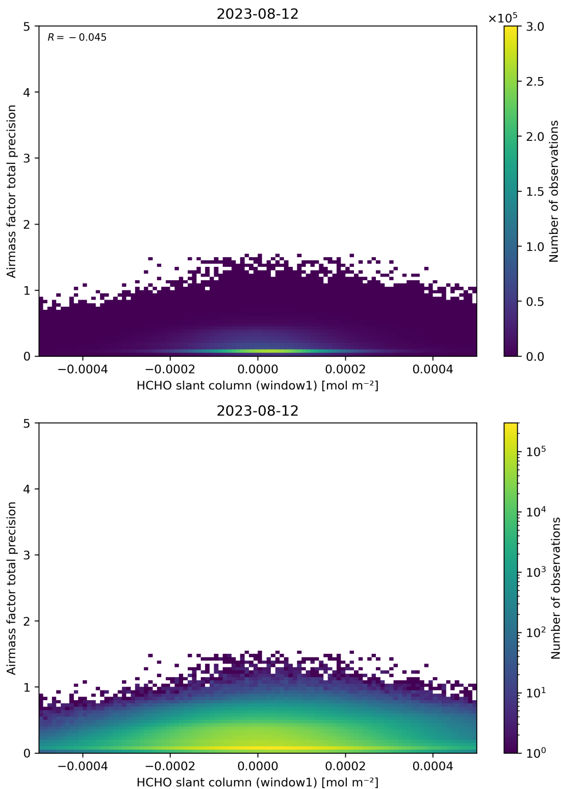
Figure 86: Scatter density plot of “HCHO slant column (window1)” against “Airmass factor total precision” for 2023-08-11 to 2023-08-13.
