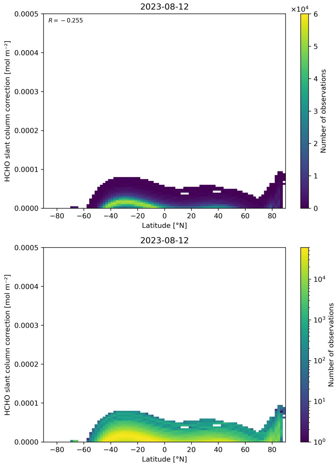
Figure 158: Scatter density plot of “Latitude” against “HCHO slant column correction” for 2023-08-11 to 2023-08-13.
