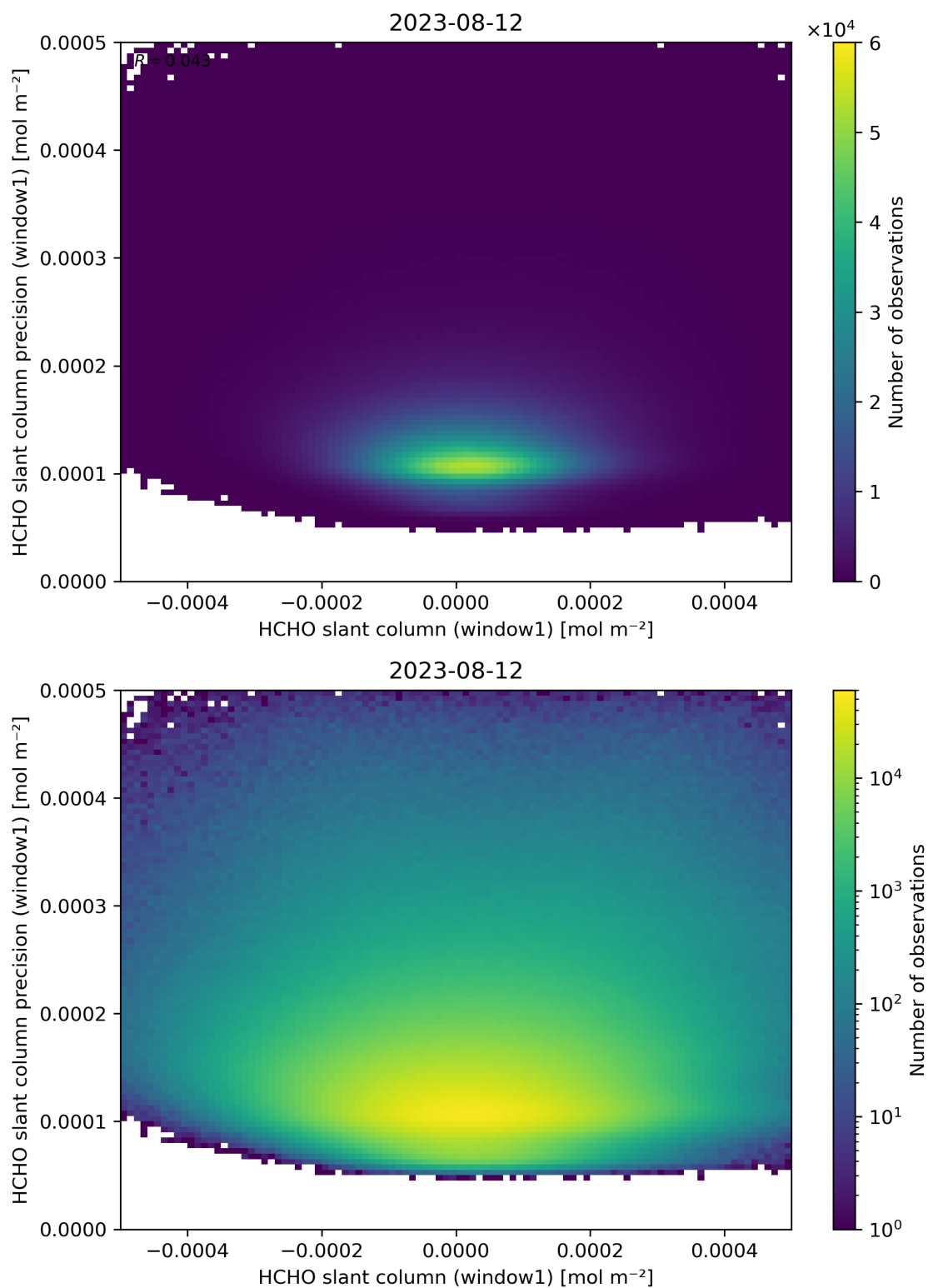
Figure 84: Scatter density plot of “HCHO slant column (window1)” against “HCHO slant column precision (window1)” for 2023-08-11 to 2023-08-13.
