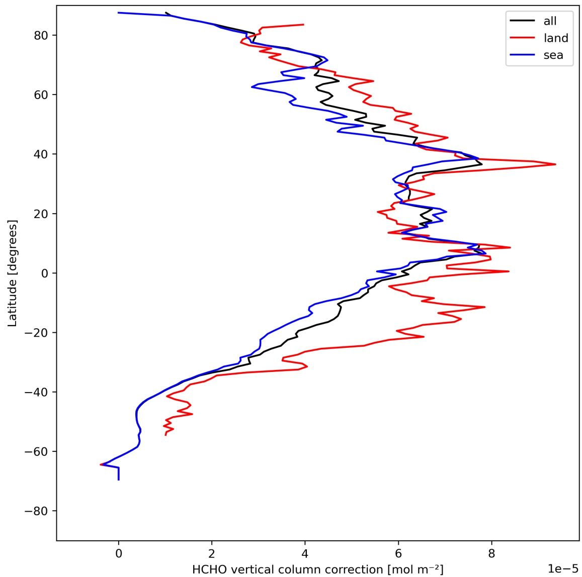
Figure 23: Zonal average of “HCHO vertical column correction” for 2023-08-11 to 2023-08-13.
