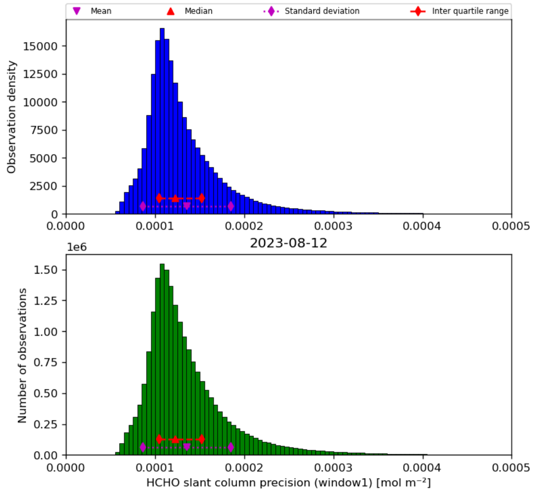
Figure 39: Histogram of “HCHO slant column precision (window1)” for 2023-08-11 to 2023-08-13
