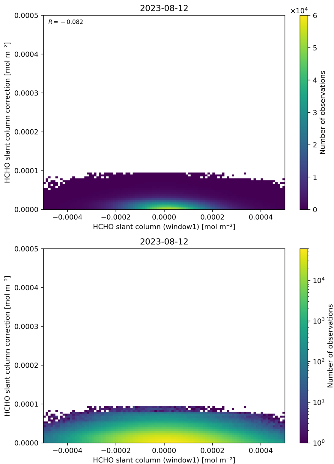
Figure 83: Scatter density plot of “HCHO slant column (window1)” against “HCHO slant column correction” for 2023-08-11 to 2023-08-13.
