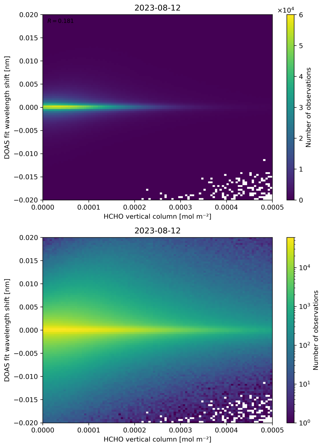
Figure 124: Scatter density plot of “HCHO vertical column” against “DOAS fit wavelength shift” for 2023-08-11 to 2023-08-13.
