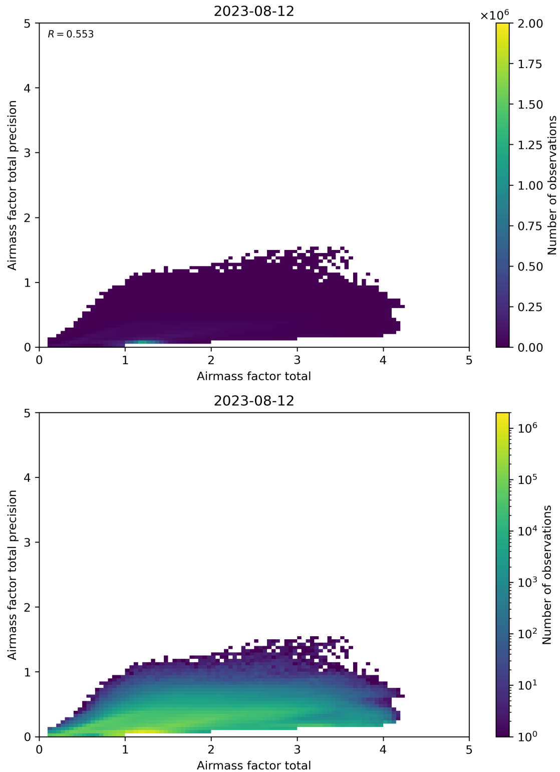
Figure 103: Scatter density plot of “Airmass factor total” against “Airmass factor total precision” for 2023-08-11 to 2023-08-13.
