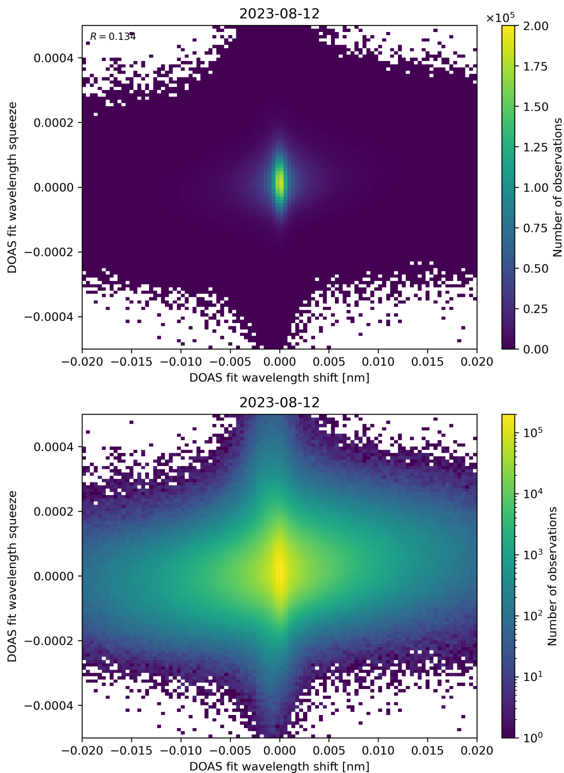
Figure 65: Scatter density plot of “DOAS fit wavelength shift” against “DOAS fit wavelength squeeze” for 2023-08-11 to 2023-08-13.
