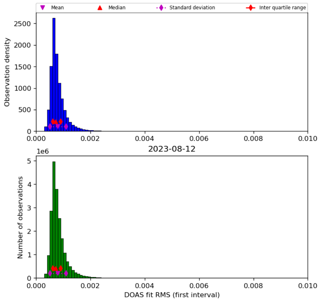
Figure 46: Histogram of “DOAS fit RMS (first interval)” for 2023-08-11 to 2023-08-13
