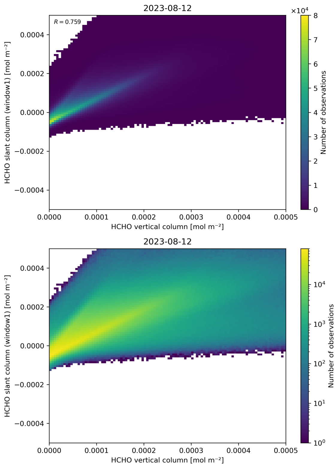
Figure 129: Scatter density plot of “HCHO vertical column” against “HCHO slant column (window1)” for 2023-08-11 to 2023-08-13.
