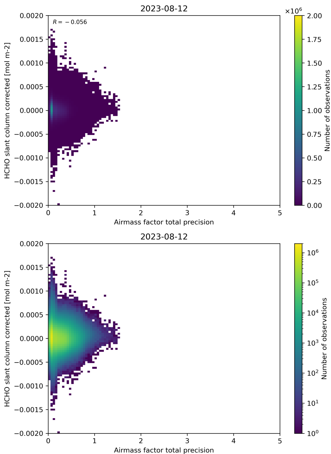
Figure 109: Scatter density plot of “Airmass factor total precision” against “HCHO slant column corrected” for 2023-08-11 to 2023-08-13.
