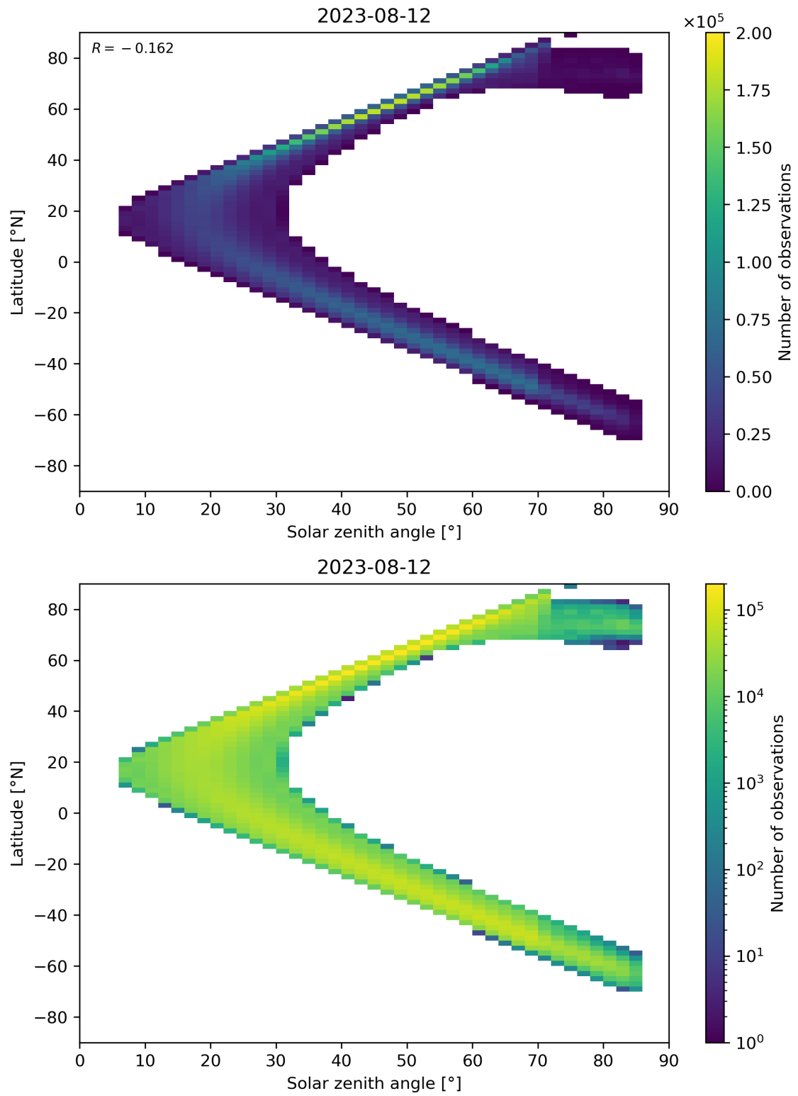
Figure 181: Scatter density plot of “Solar zenith angle” against “Latitude” for 2023-08-11 to 2023-08-13.
