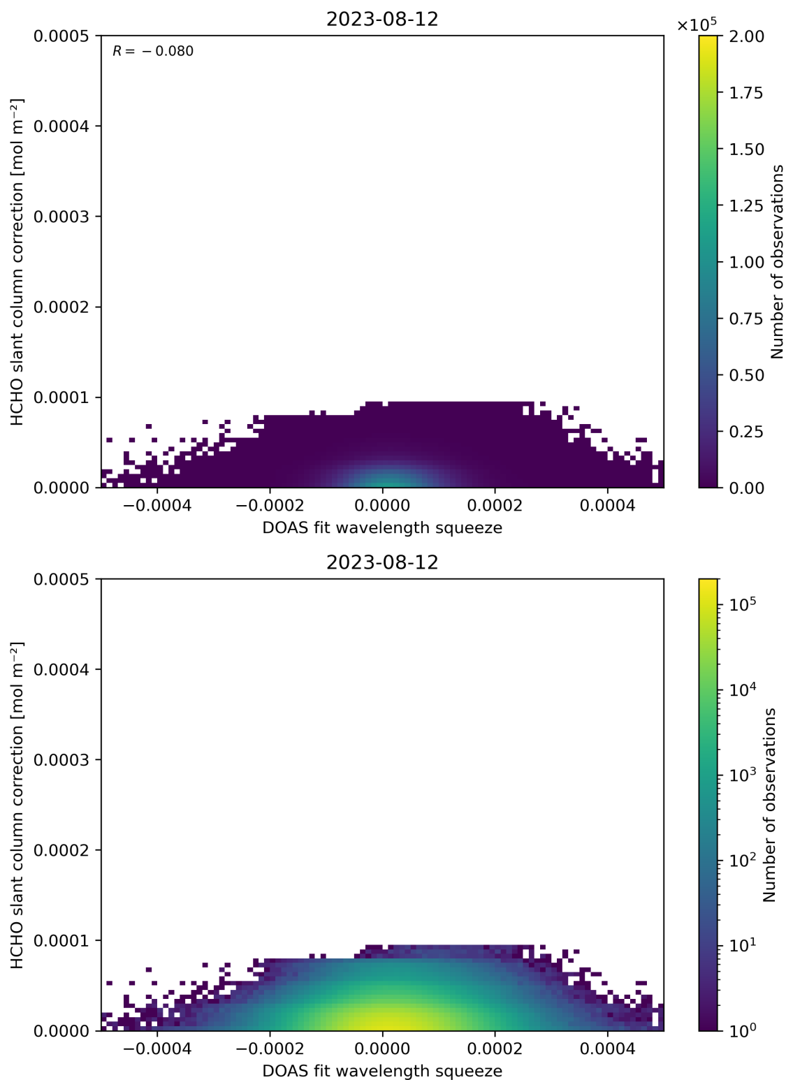
Figure 70: Scatter density plot of “DOAS fit wavelength squeeze” against “HCHO slant column correction” for 2023-08-11 to 2023-08-13.
