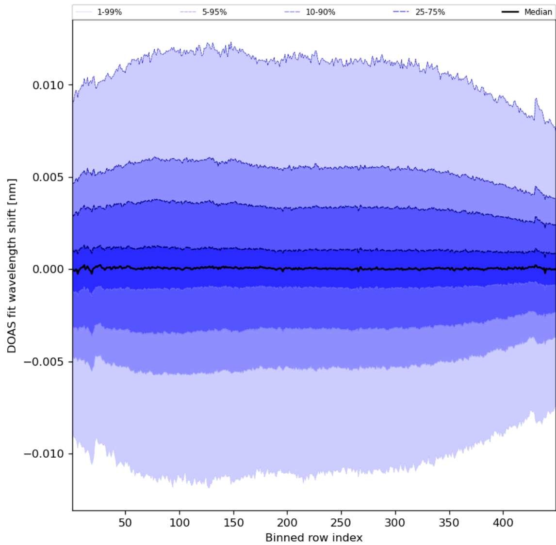
Figure 58: Along track statistics of “DOAS fit wavelength shift” for 2023-08-11 to 2023-08-13
