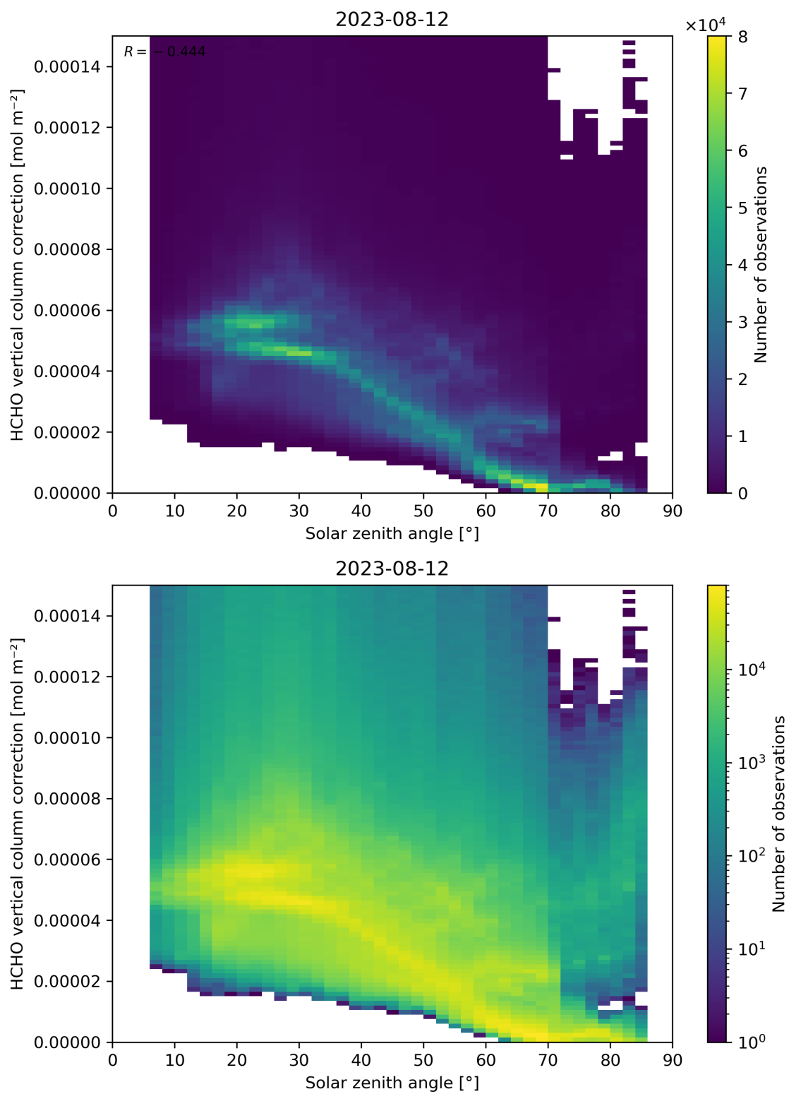
Figure 178: Scatter density plot of “Solar zenith angle” against “HCHO vertical column correction” for 2023-08-11 to 2023-08-13.
