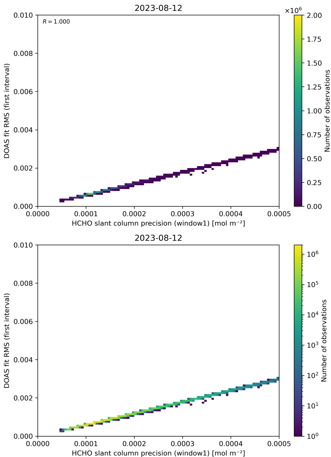
Figure 88: Scatter density plot of “HCHO slant column precision (window1)” against “DOAS fit RMS (first interval)” for 2023-08-11 to 2023-08-13.
