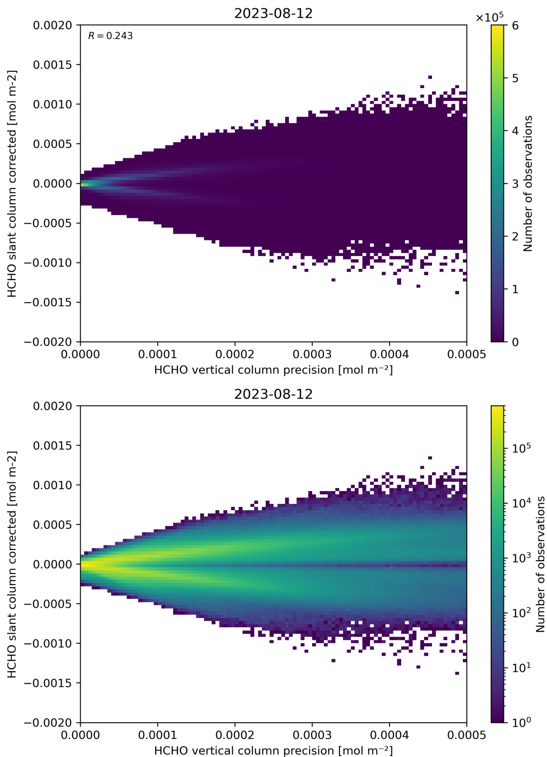
Figure 140: Scatter density plot of “HCHO vertical column precision” against “HCHO slant column corrected” for 2023-08-11 to 2023-08-13.
