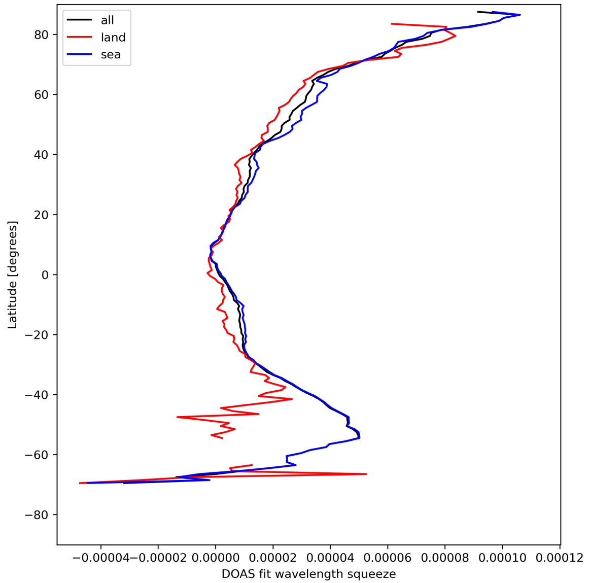
Figure 31: Zonal average of “DOAS fit wavelength squeeze” for 2023-08-11 to 2023-08-13.
