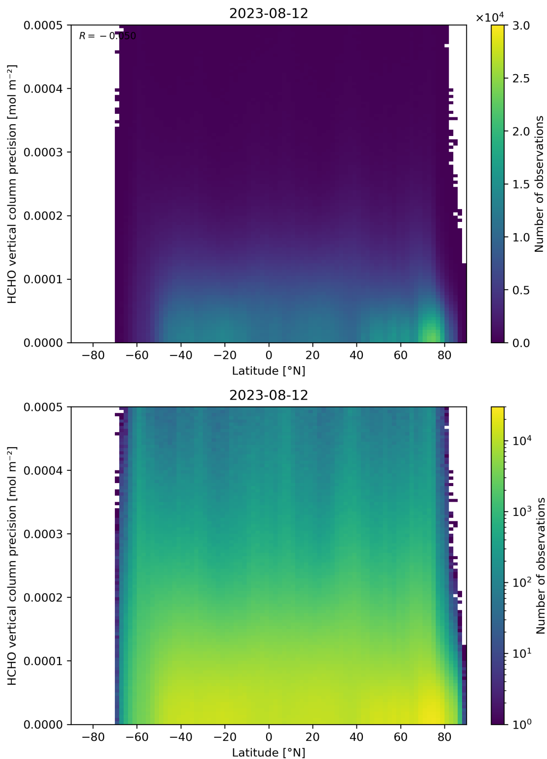
Figure 165: Scatter density plot of “Latitude” against “HCHO vertical column precision” for 2023-08-11 to 2023-08-13.
