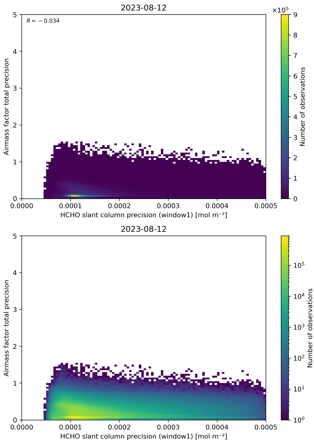
Figure 95: Scatter density plot of “HCHO slant column precision (window1)” against “Airmass factor total precision” for 2023-08-11 to 2023-08-13.
