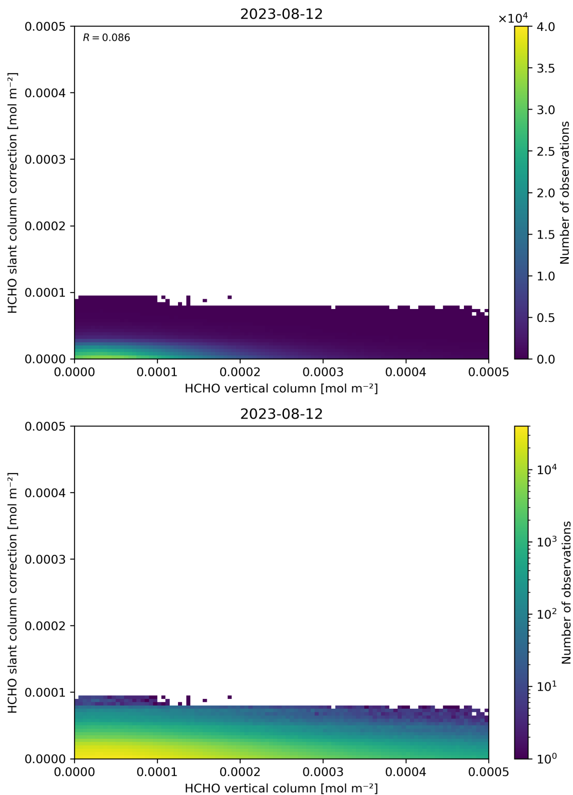
Figure 128: Scatter density plot of “HCHO vertical column” against “HCHO slant column correction” for 2023-08-11 to 2023-08-13.
