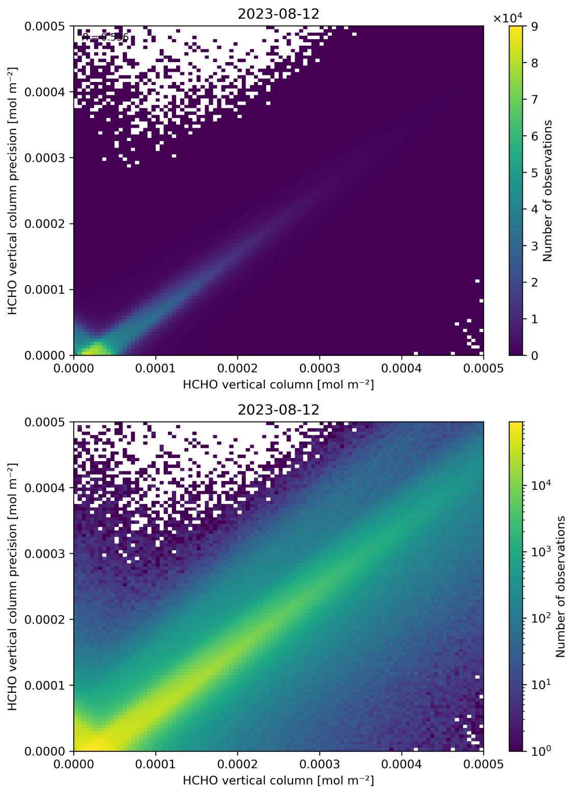
Figure 134: Scatter density plot of “HCHO vertical column” against “HCHO vertical column precision” for 2023-08-11 to 2023-08-13.
