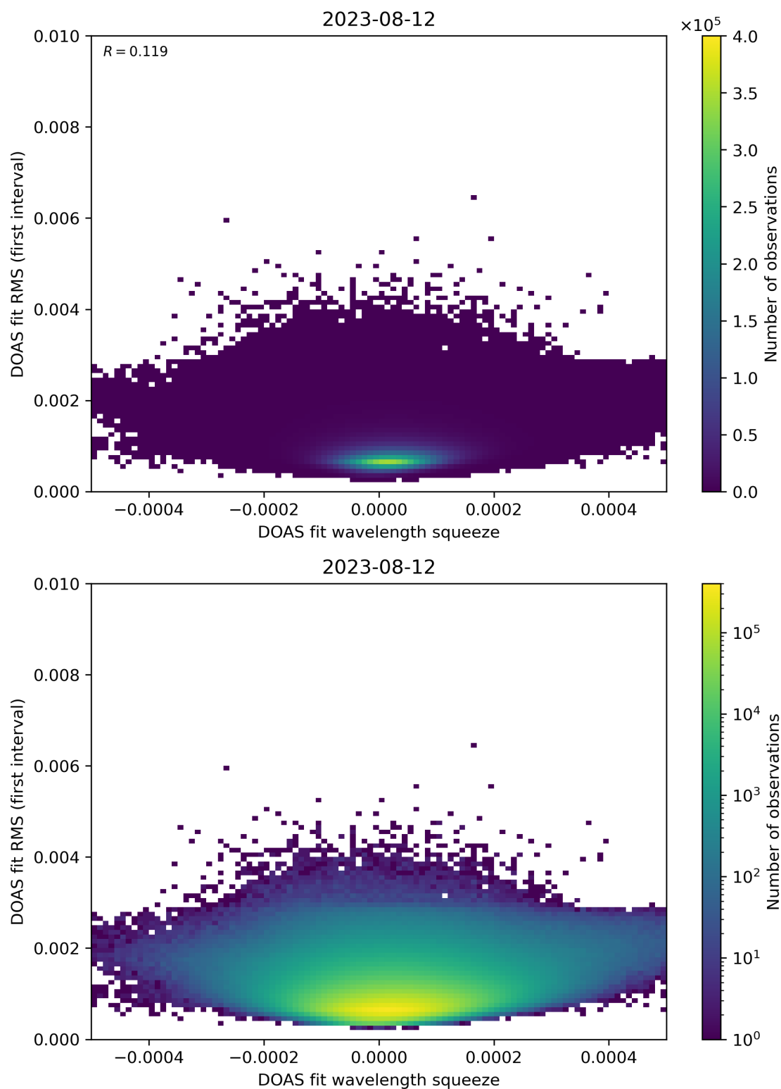
Figure 68: Scatter density plot of “DOAS fit wavelength squeeze” against “DOAS fit RMS (first interval)” for 2023-08-11 to 2023-08-13.
