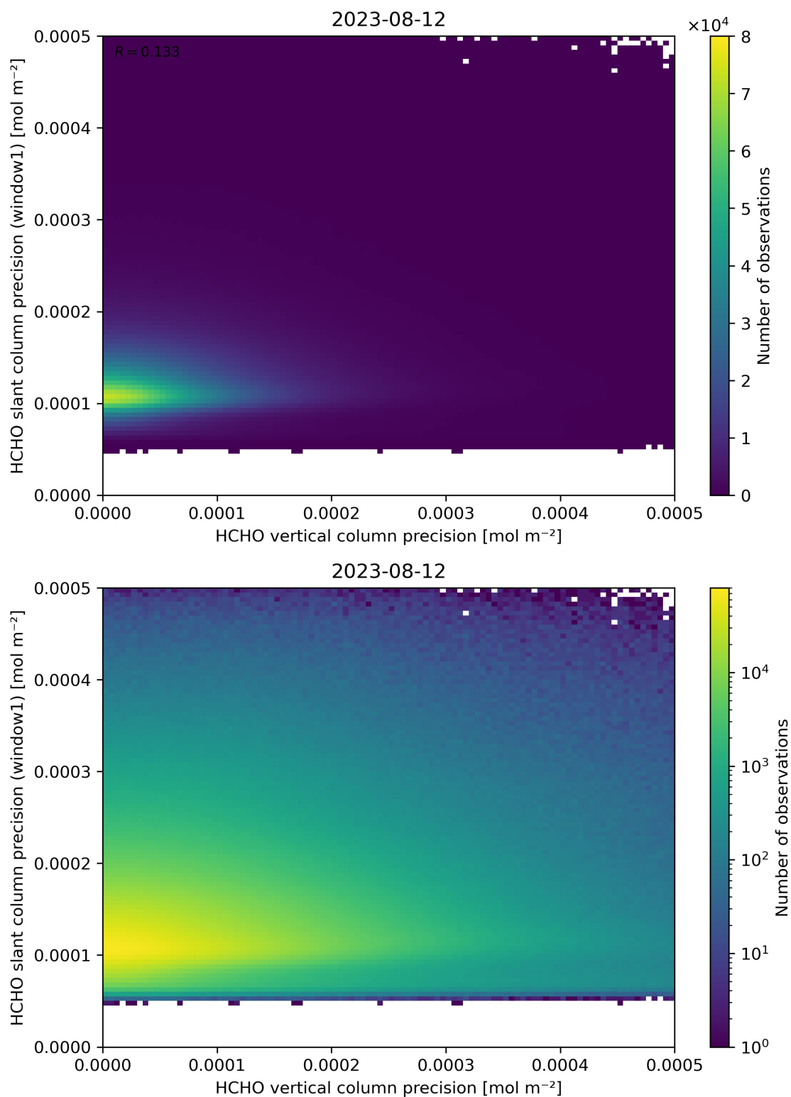
Figure 143: Scatter density plot of “HCHO vertical column precision” against “HCHO slant column precision (window1)” for 2023-08-11 to 2023-08-13.
