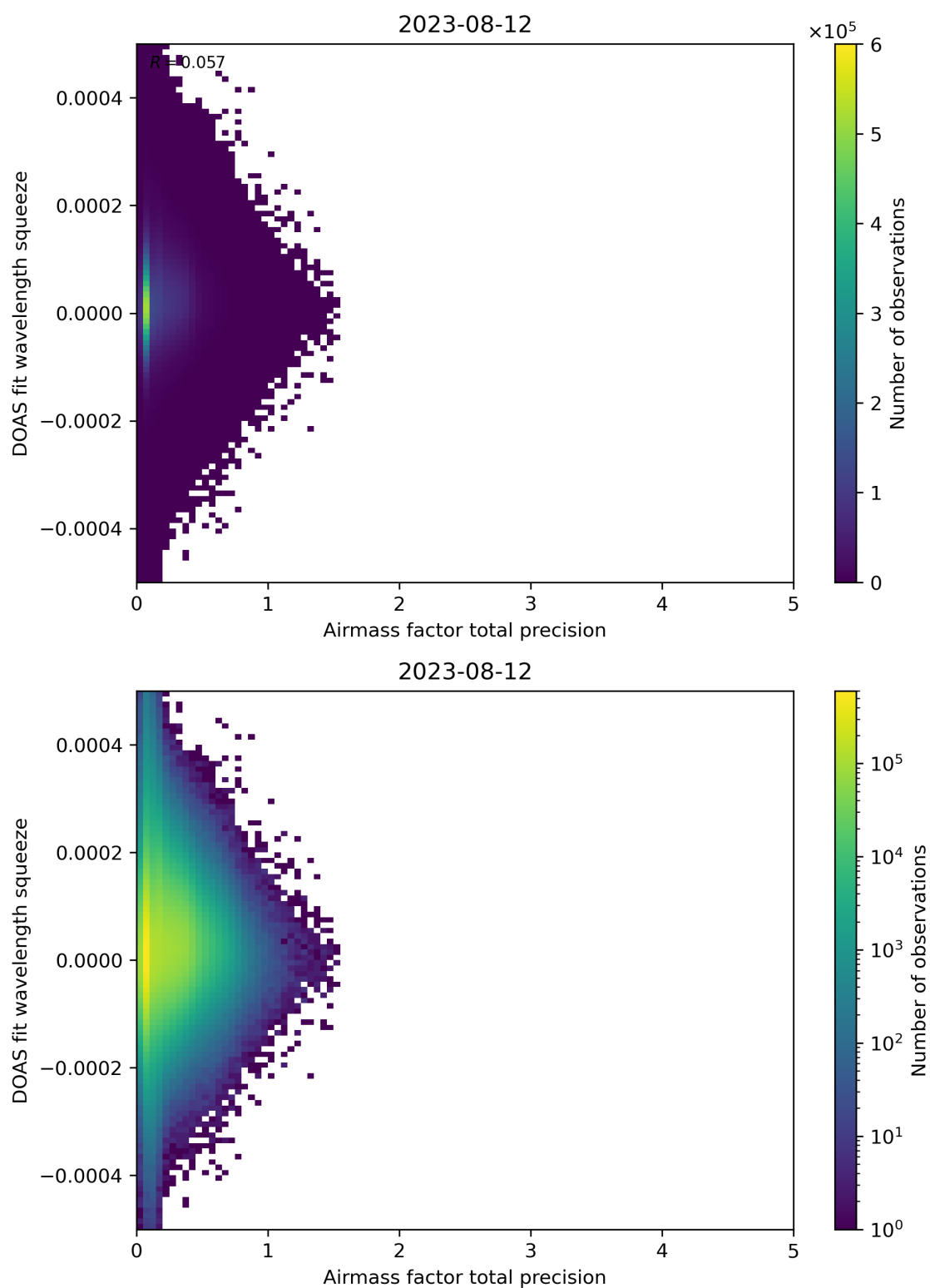
Figure 107: Scatter density plot of “Airmass factor total precision” against “DOAS fit wavelength squeeze” for 2023-08-11 to 2023-08-13.
