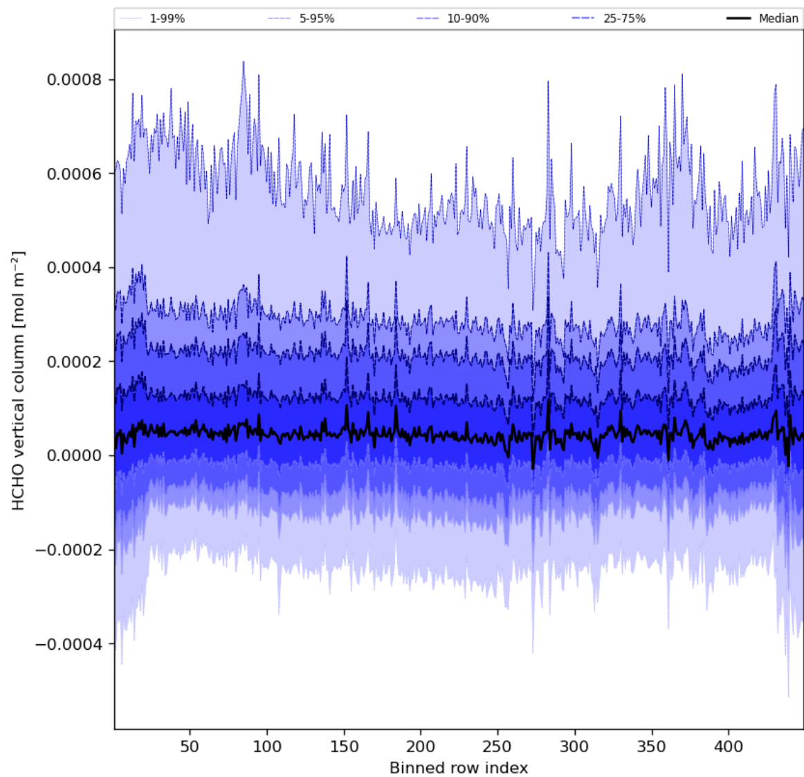
Figure 49: Along track statistics of “HCHO vertical column” for 2023-08-11 to 2023-08-13
