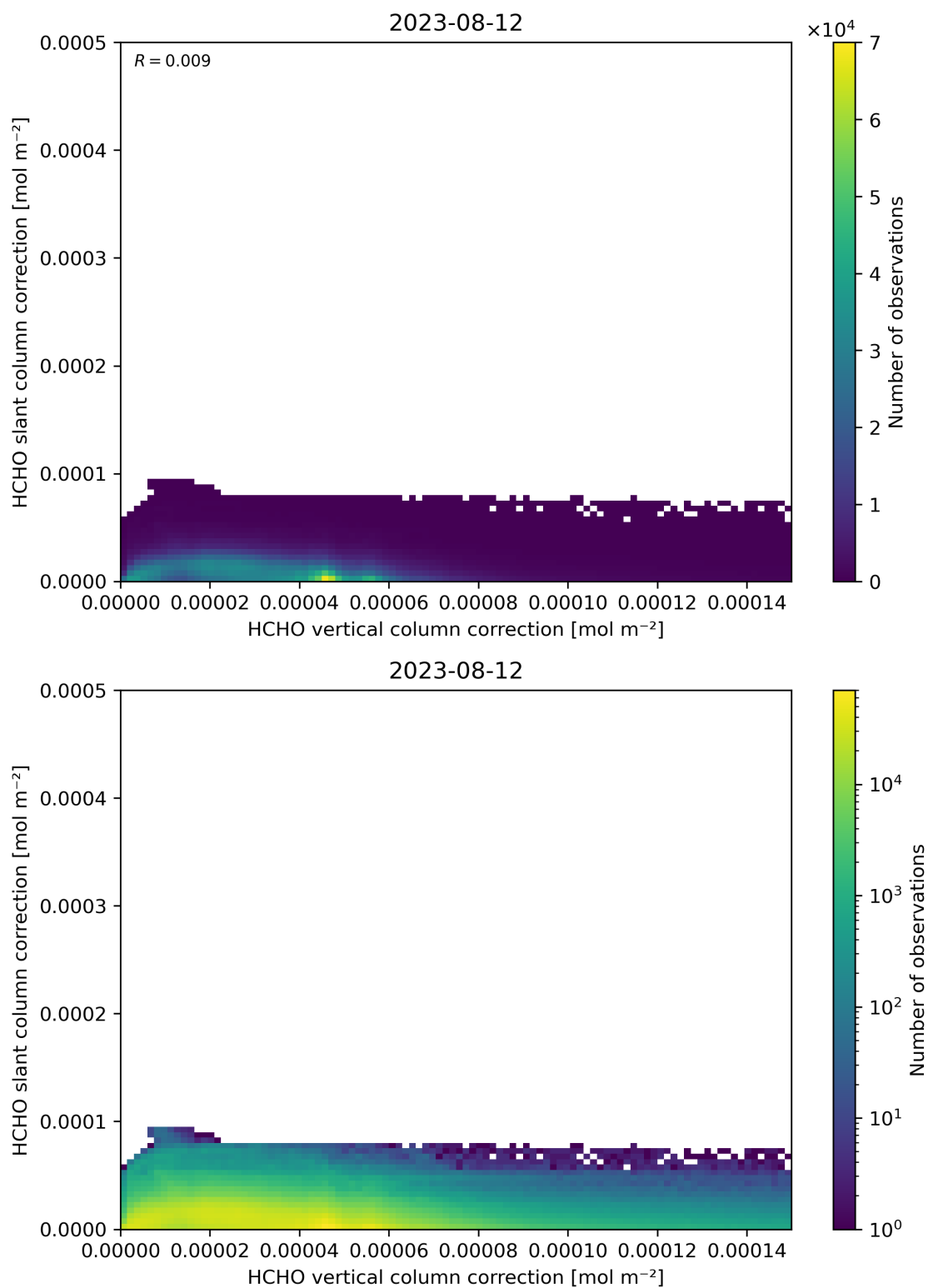
Figure 117: Scatter density plot of “HCHO vertical column correction” against “HCHO slant column correction” for 2023-08-11 to 2023-08-13.
