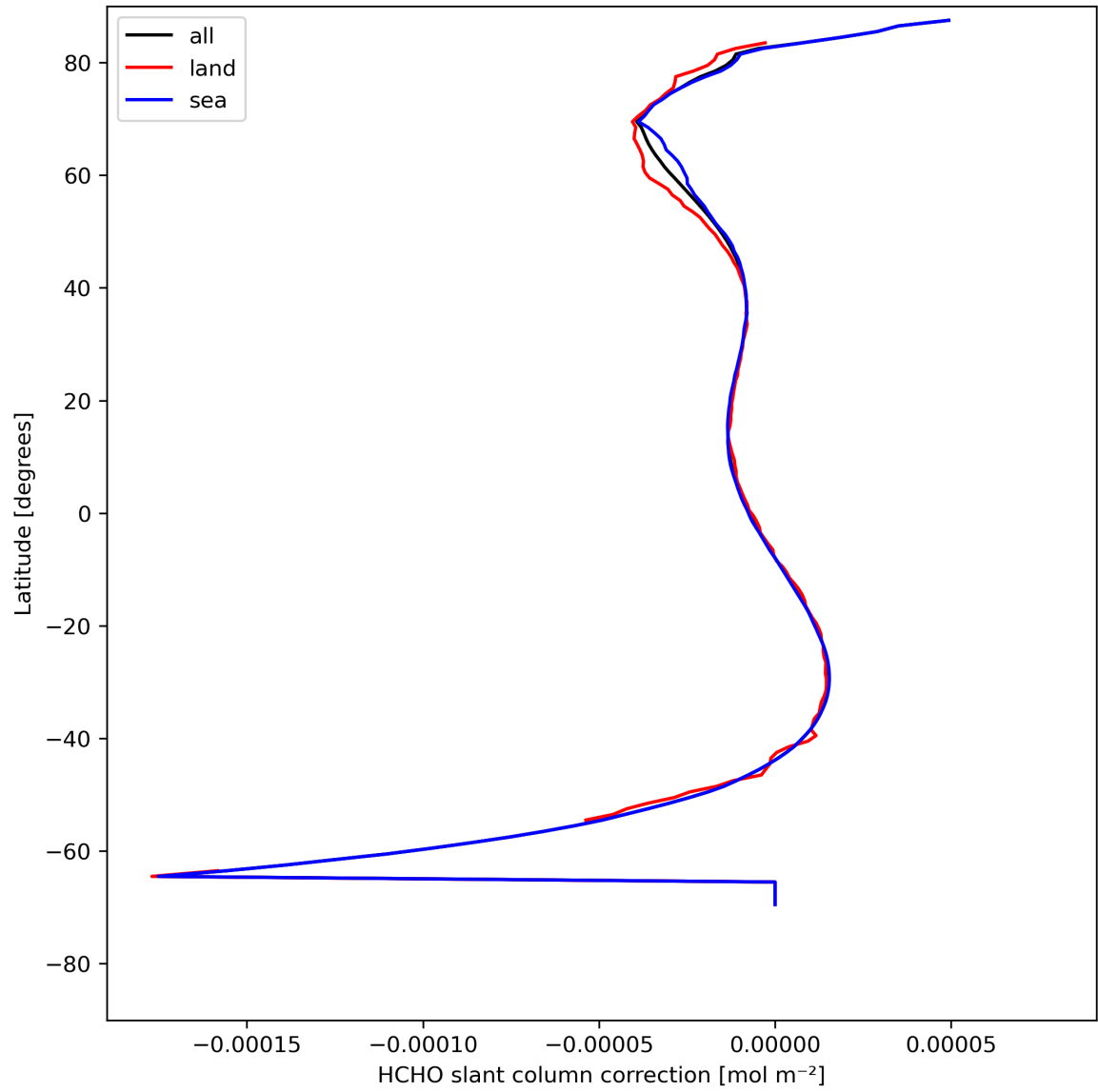
Figure 33: Zonal average of “HCHO slant column correction” for 2023-08-11 to 2023-08-13.
