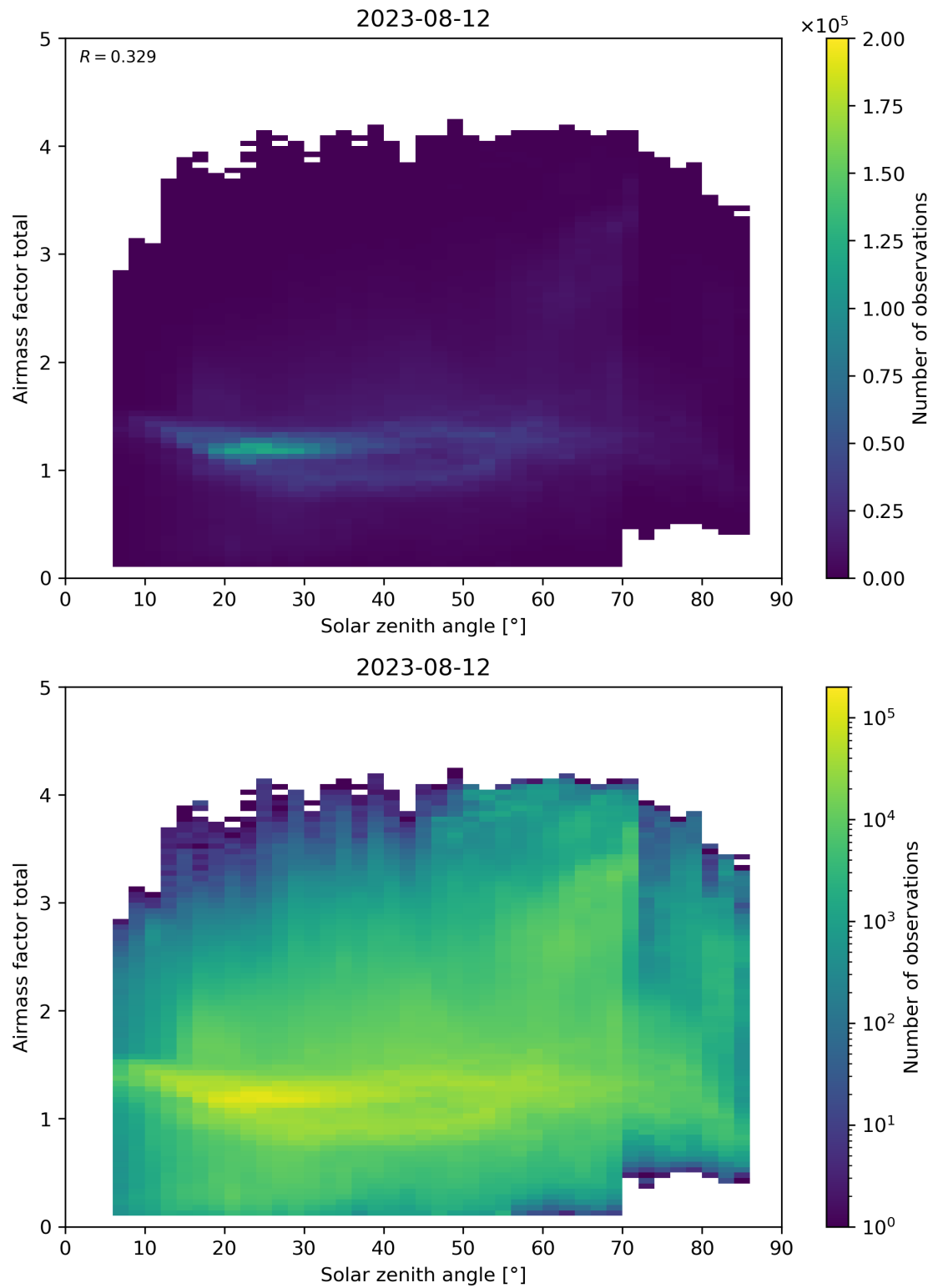
Figure 175: Scatter density plot of “Solar zenith angle” against “Airmass factor total” for 2023-08-11 to 2023-08-13.
