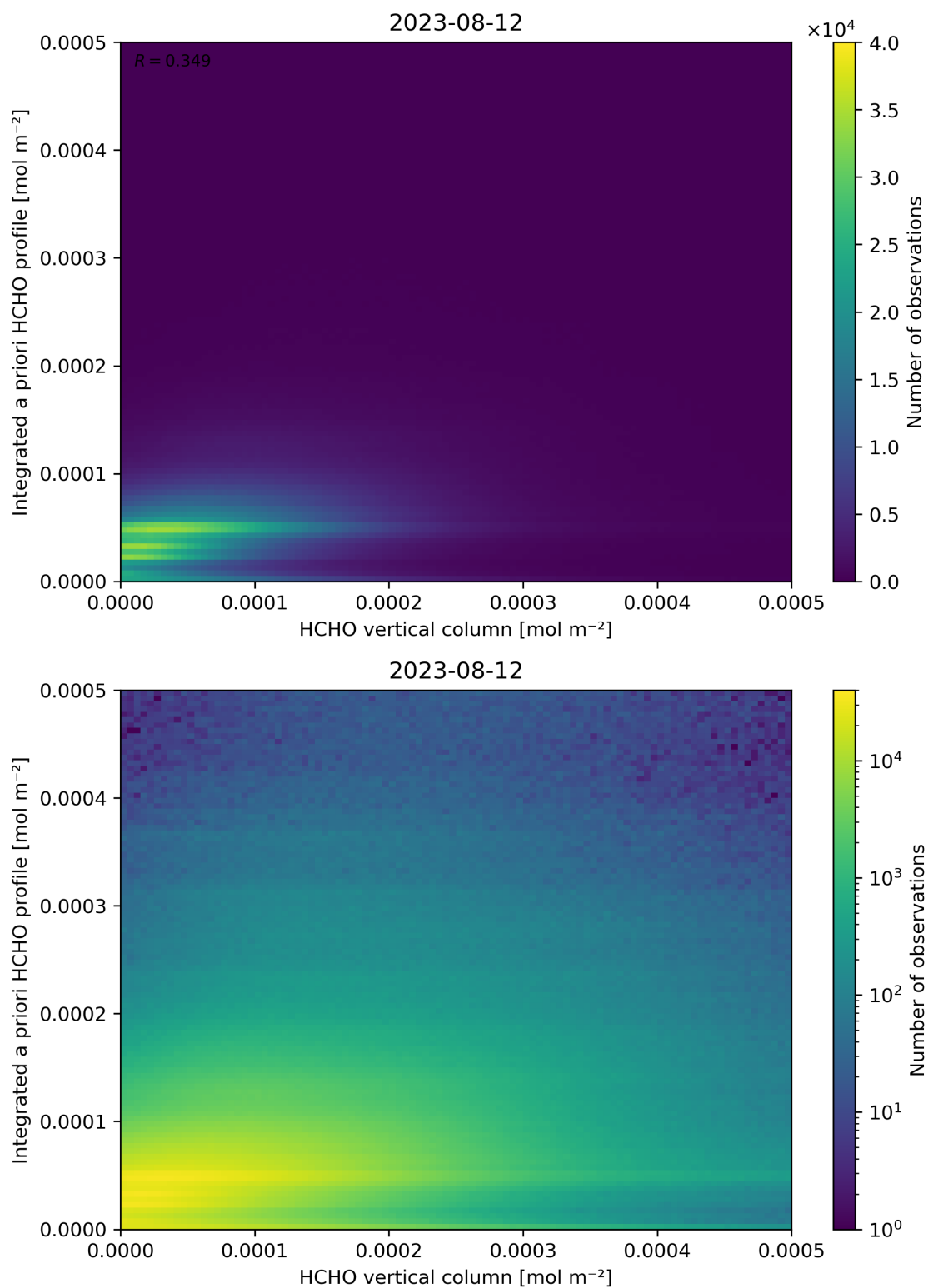
Figure 135: Scatter density plot of “HCHO vertical column” against “Integrated a priori HCHO profile” for 2023-08-11 to 2023-08-13.
