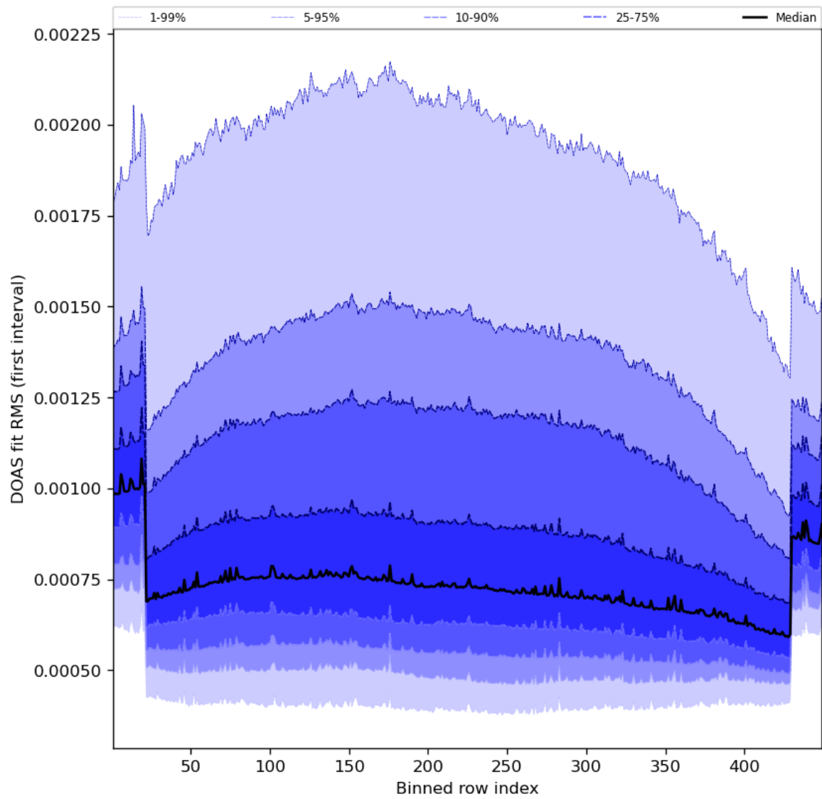
Figure 60: Along track statistics of “DOAS fit RMS (first interval)” for 2023-08-11 to 2023-08-13
