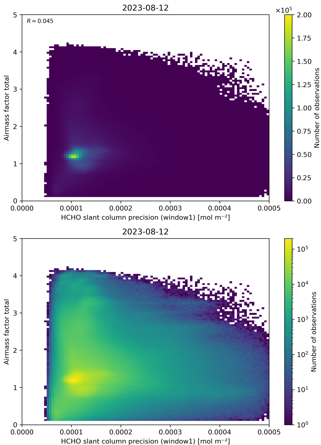
Figure 94: Scatter density plot of “HCHO slant column precision (window1)” against “Airmass factor total” for 2023-08-11 to 2023-08-13.
