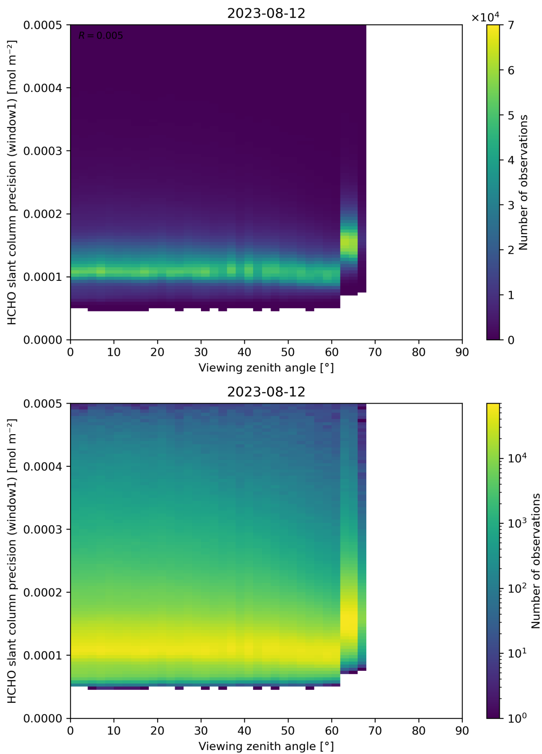
Figure 189: Scatter density plot of “Viewing zenith angle” against “HCHO slant column precision (window1)” for 2023-08-11 to 2023-08-13.
