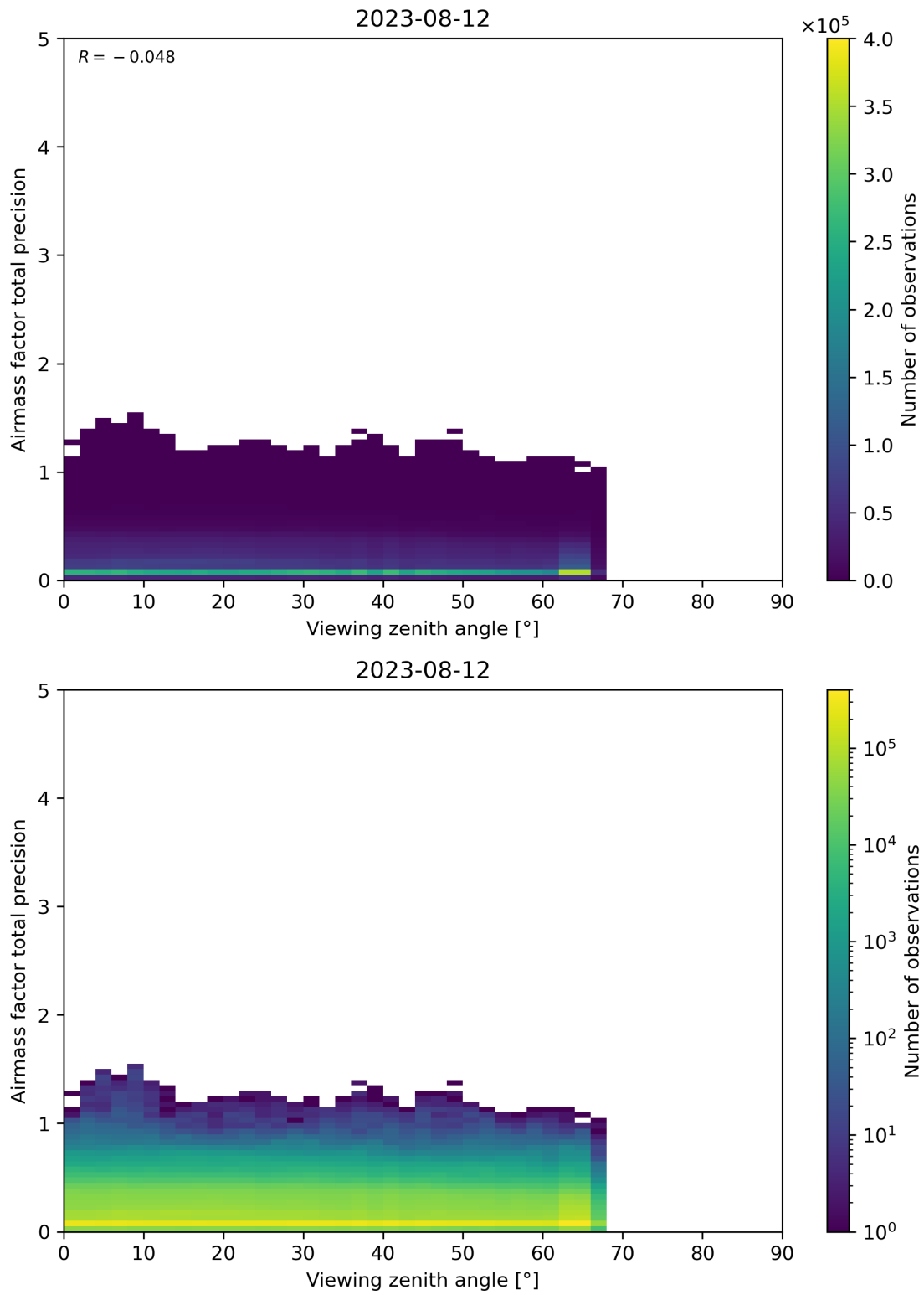
Figure 191: Scatter density plot of “Viewing zenith angle” against “Airmass factor total precision” for 2023-08-11 to 2023-08-13.
