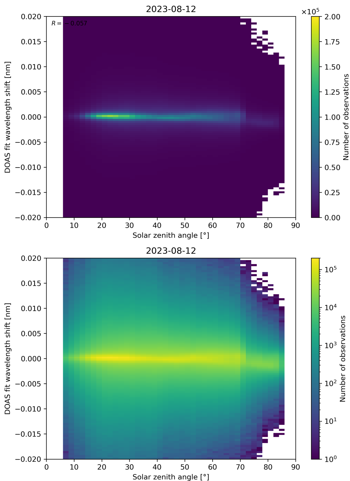
Figure 168: Scatter density plot of “Solar zenith angle” against “DOAS fit wavelength shift” for 2023-08-11 to 2023-08-13.
