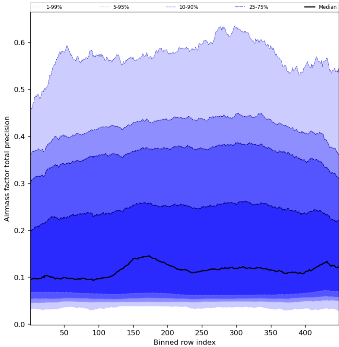
Figure 55: Along track statistics of “Airmass factor total precision” for 2023-08-11 to 2023-08-13
