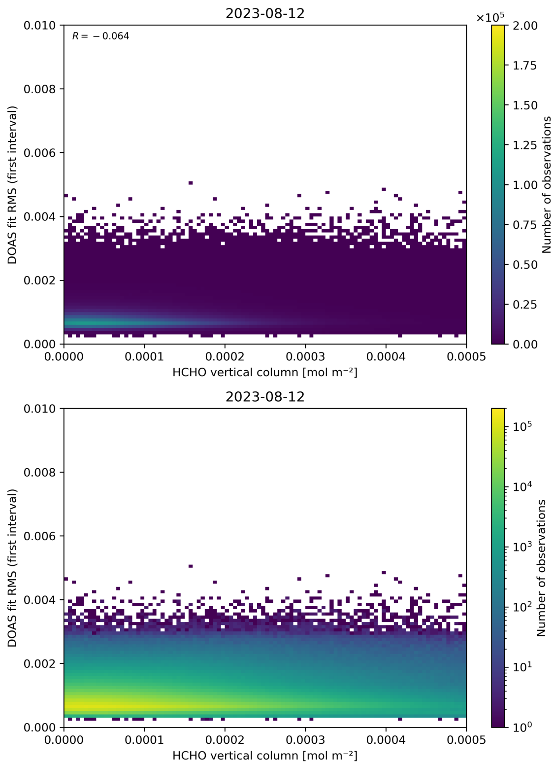
Figure 123: Scatter density plot of “HCHO vertical column” against “DOAS fit RMS (first interval)” for 2023-08-11 to 2023-08-13.
