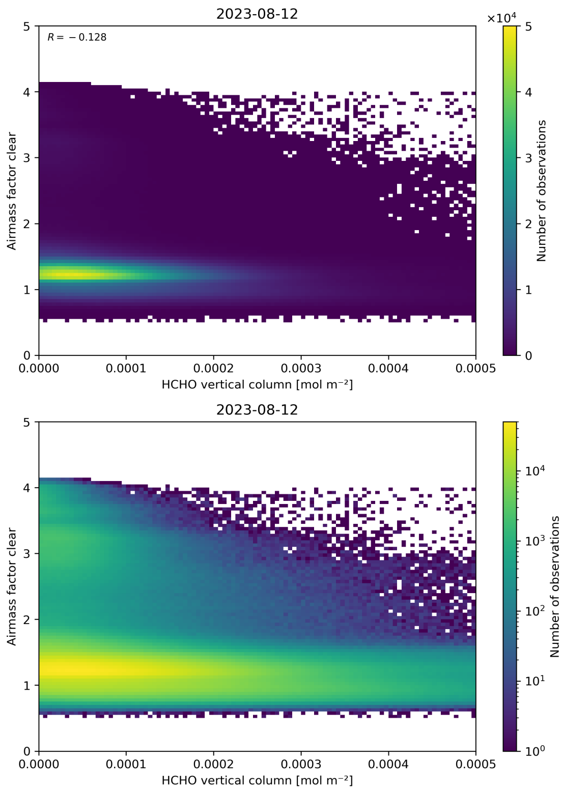
Figure 126: Scatter density plot of “HCHO vertical column” against “Airmass factor clear” for 2023-08-11 to 2023-08-13.
