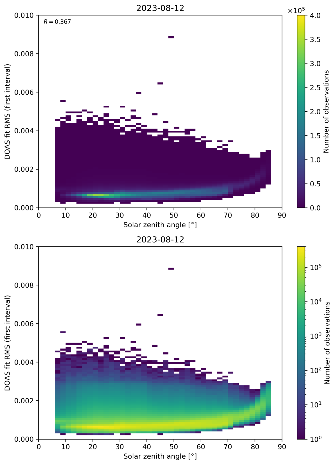
Figure 167: Scatter density plot of “Solar zenith angle” against “DOAS fit RMS (first interval)” for 2023-08-11 to 2023-08-13.
