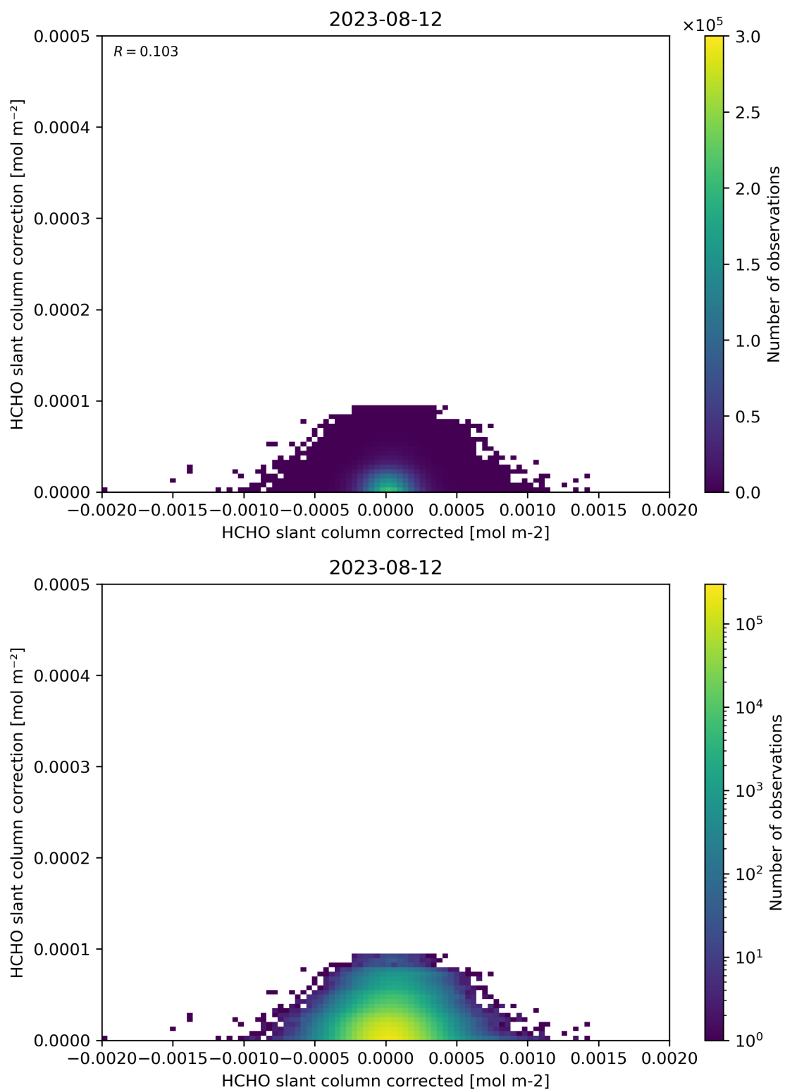
Figure 77: Scatter density plot of “HCHO slant column corrected” against “HCHO slant column correction” for 2023-08-11 to 2023-08-13.
