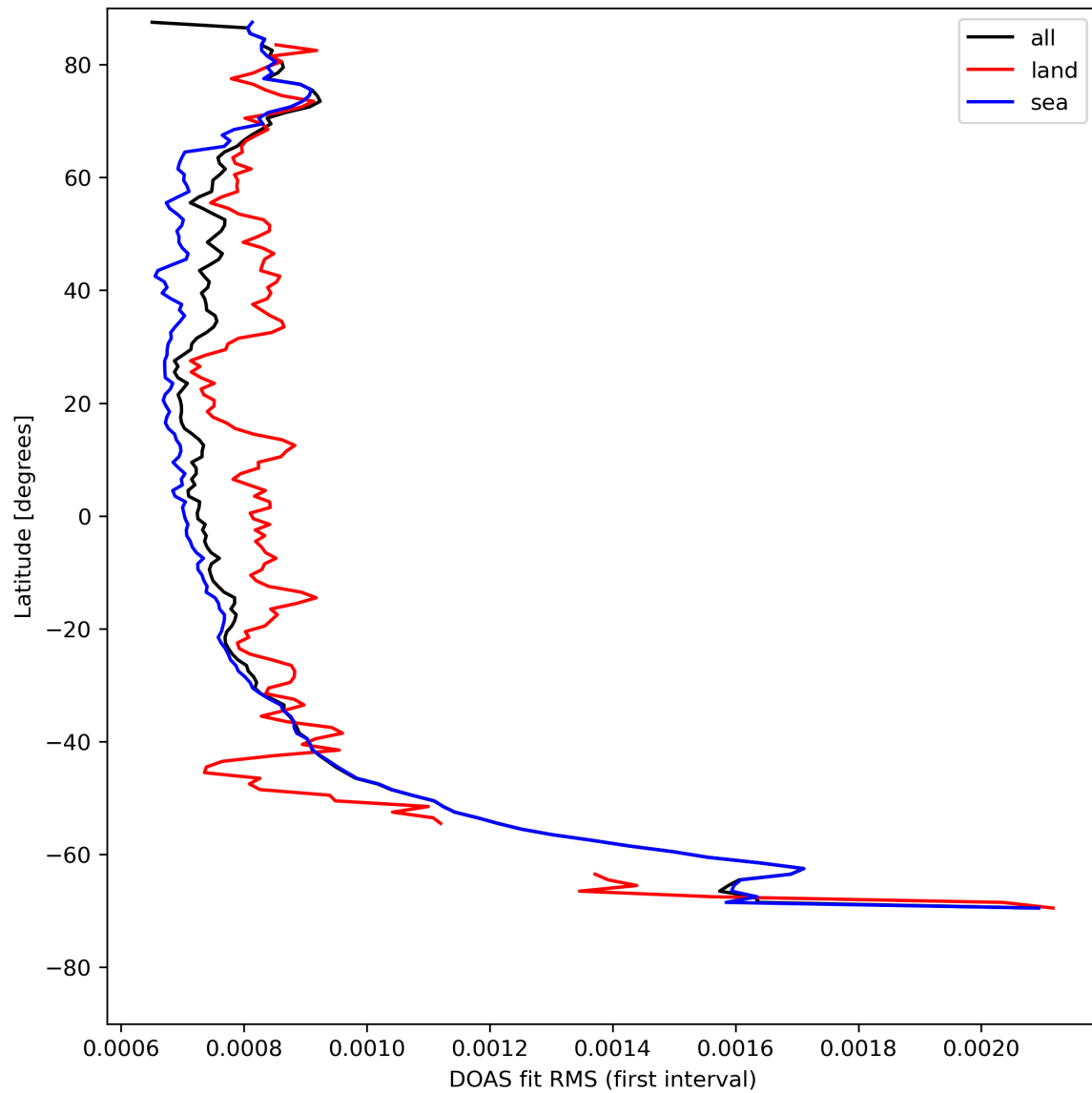
Figure 32: Zonal average of “DOAS fit RMS (first interval)” for 2023-08-11 to 2023-08-13.
