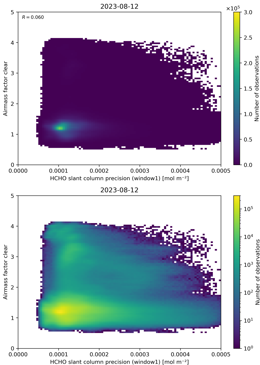
Figure 91: Scatter density plot of “HCHO slant column precision (window1)” against “Airmass factor clear” for 2023-08-11 to 2023-08-13.
