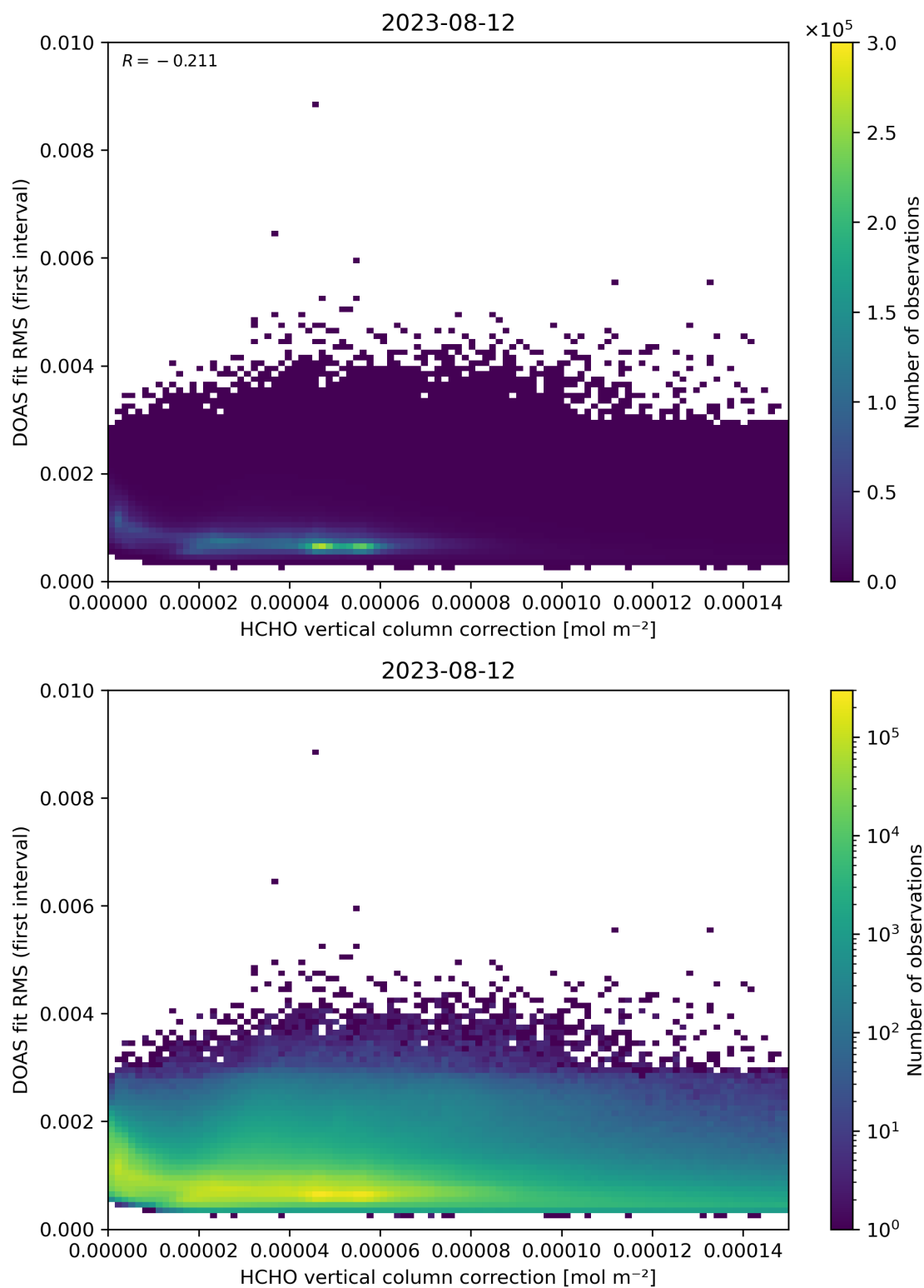
Figure 112: Scatter density plot of “HCHO vertical column correction” against “DOAS fit RMS (first interval)” for 2023-08-11 to 2023-08-13.
