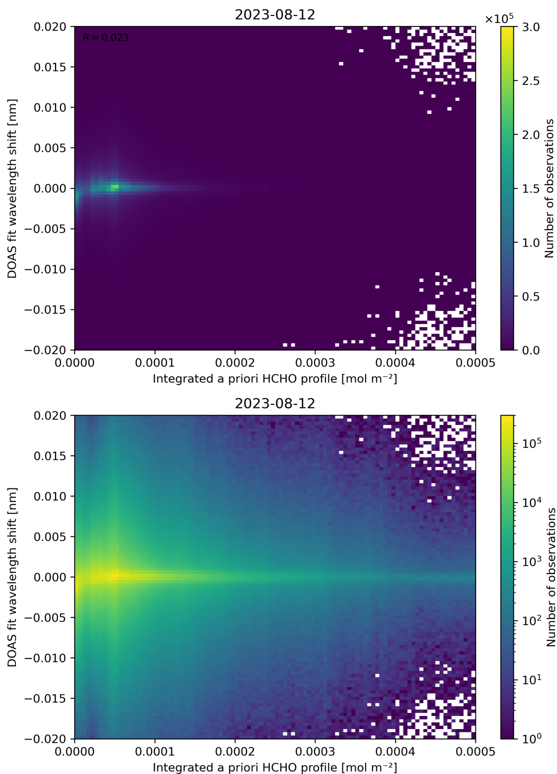
Figure 149: Scatter density plot of “Integrated a priori HCHO profile” against “DOAS fit wavelength shift” for 2023-08-11 to 2023-08-13.
