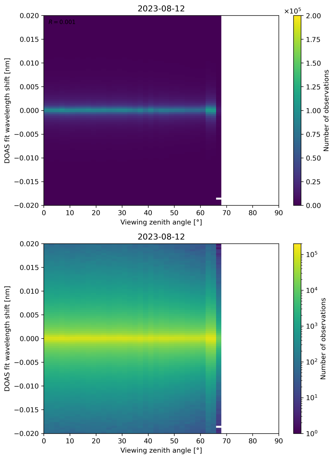
Figure 183: Scatter density plot of “Viewing zenith angle” against “DOAS fit wavelength shift” for 2023-08-11 to 2023-08-13.
