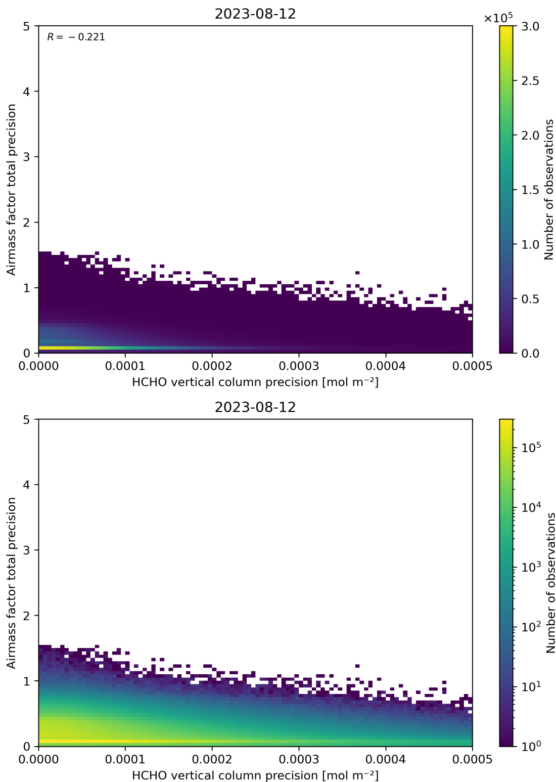
Figure 145: Scatter density plot of “HCHO vertical column precision” against “Airmass factor total precision” for 2023-08-11 to 2023-08-13.
