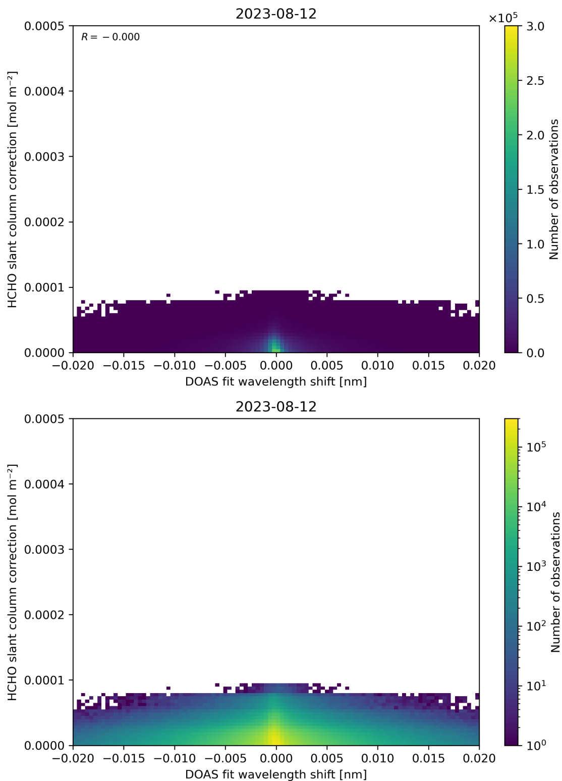
Figure 67: Scatter density plot of “DOAS fit wavelength shift” against “HCHO slant column correction” for 2023-08-11 to 2023-08-13.
