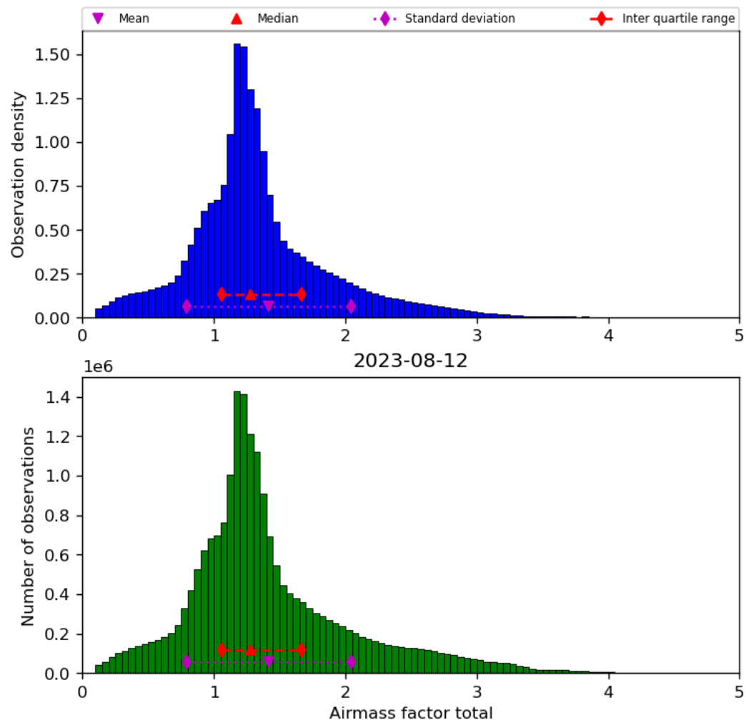
Figure 40: Histogram of “Airmass factor total” for 2023-08-11 to 2023-08-13
