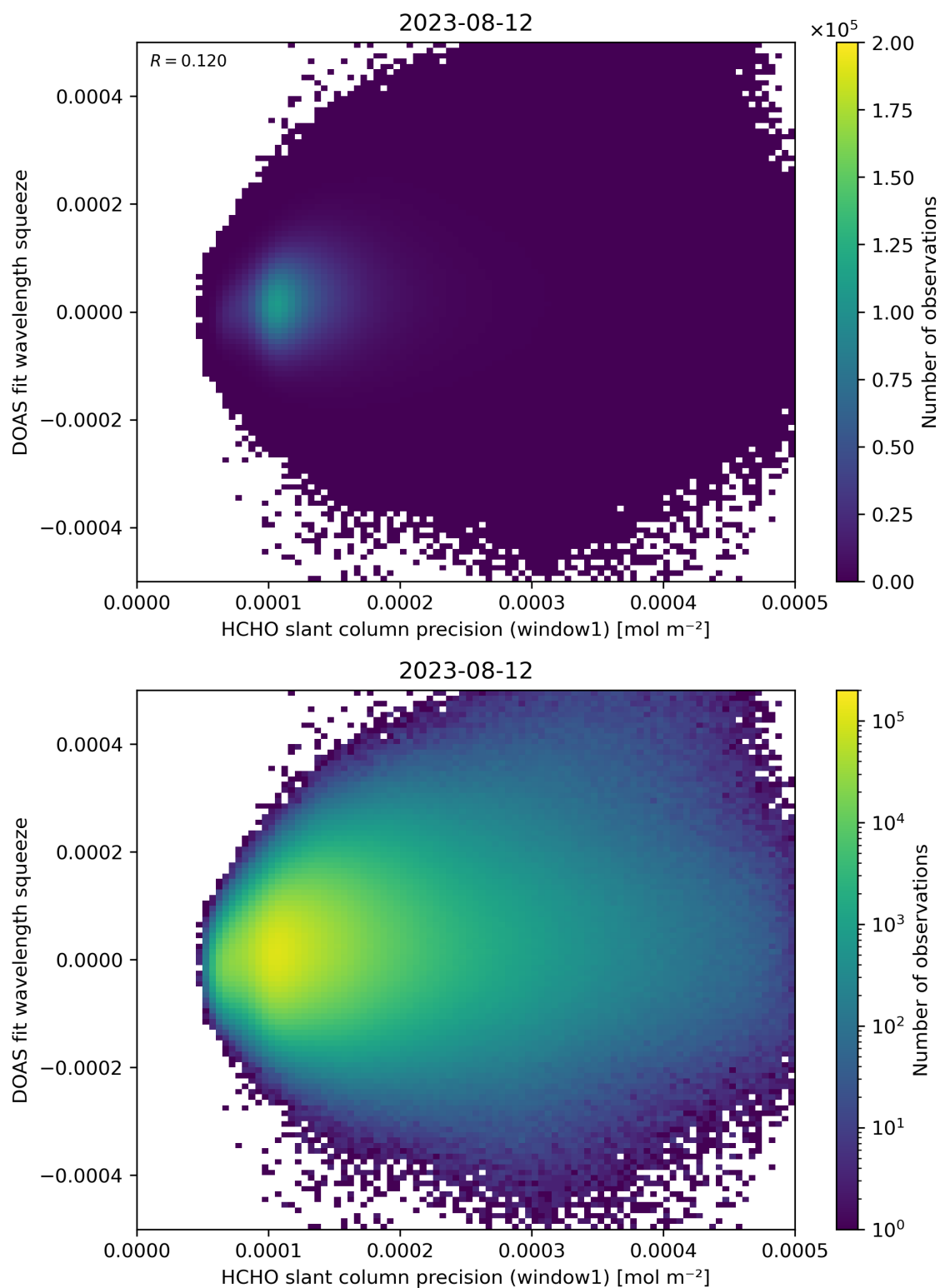
Figure 90: Scatter density plot of “HCHO slant column precision (window1)” against “DOAS fit wavelength squeeze” for 2023-08-11 to 2023-08-13.
