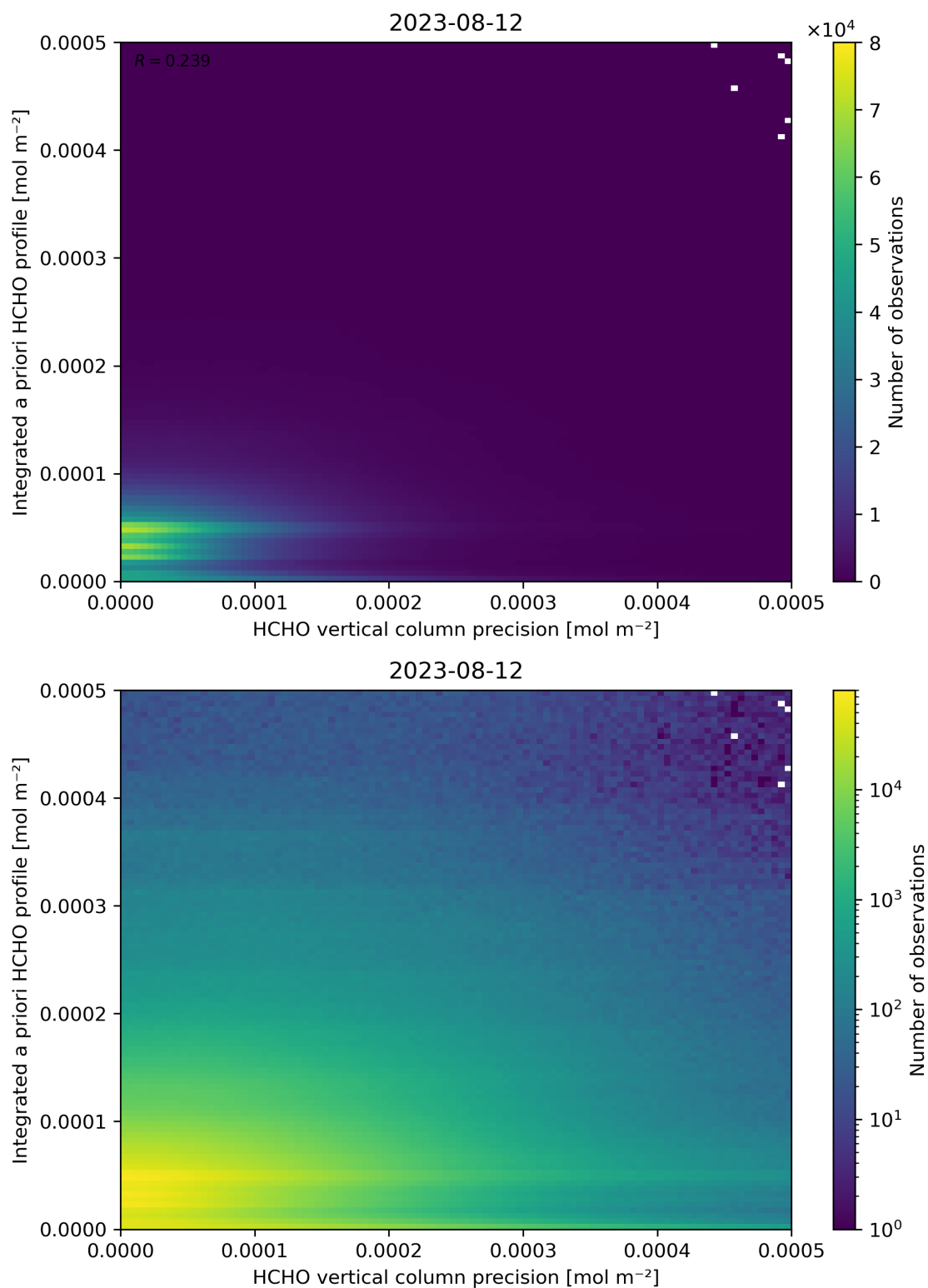
Figure 147: Scatter density plot of “HCHO vertical column precision” against “Integrated a priori HCHO profile” for 2023-08-11 to 2023-08-13.
