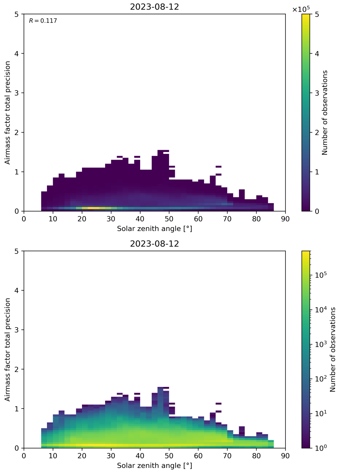
Figure 176: Scatter density plot of “Solar zenith angle” against “Airmass factor total precision” for 2023-08-11 to 2023-08-13.
