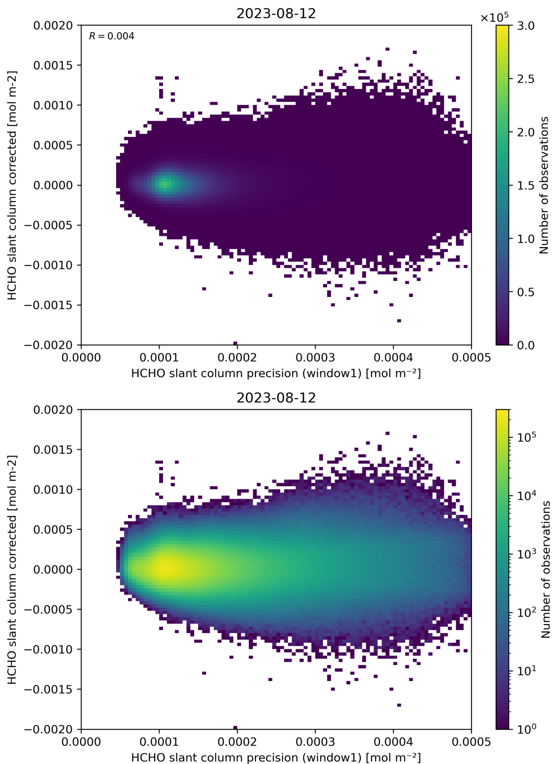
Figure 92: Scatter density plot of “HCHO slant column precision (window1)” against “HCHO slant column corrected” for 2023-08-11 to 2023-08-13.
