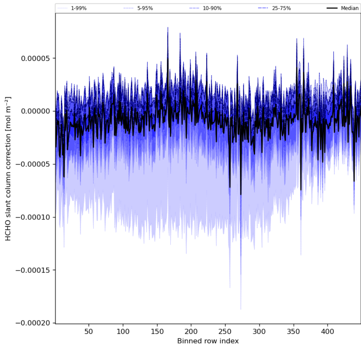
Figure 61: Along track statistics of “HCHO slant column correction” for 2023-08-11 to 2023-08-13
