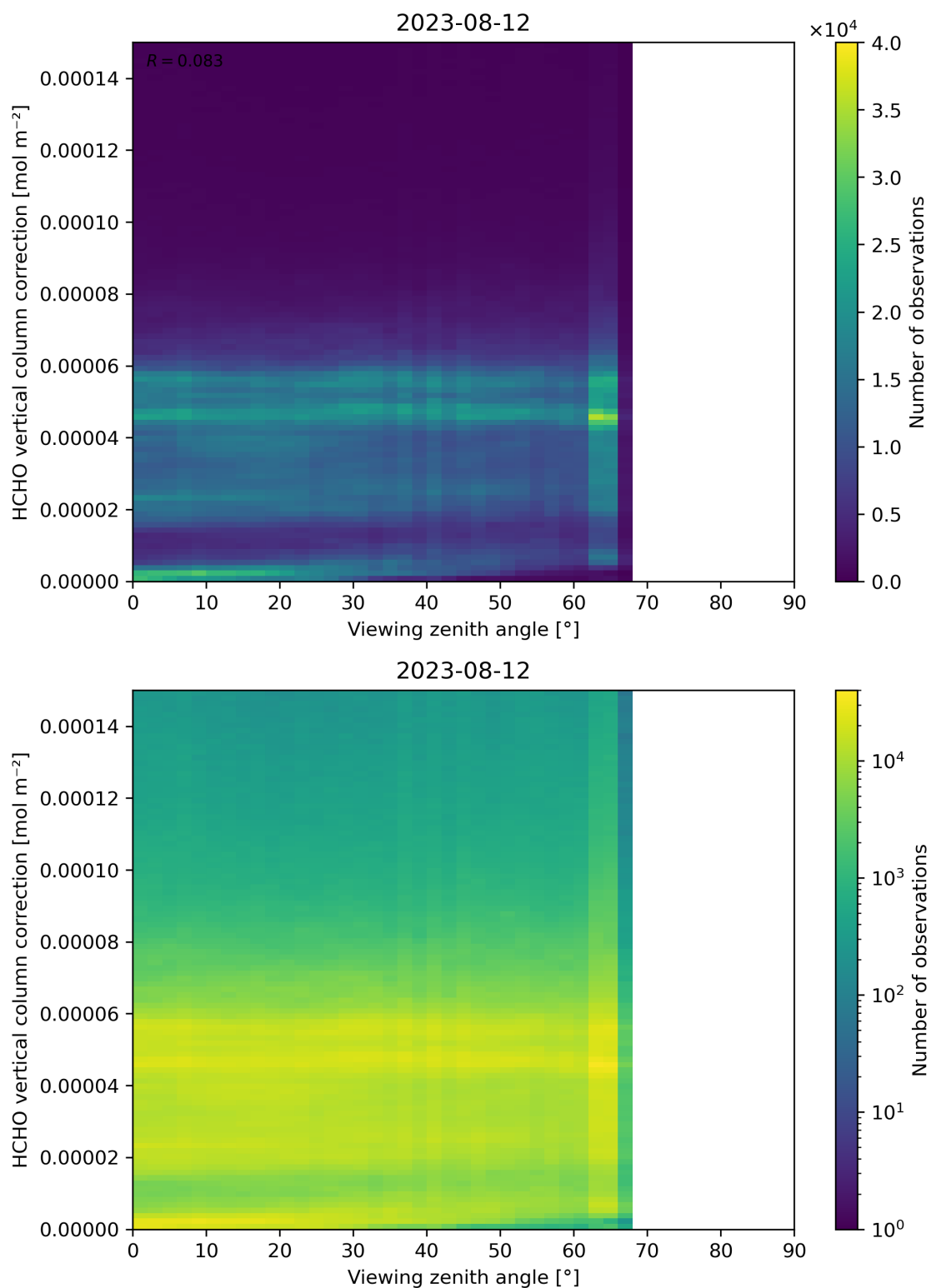
Figure 193: Scatter density plot of “Viewing zenith angle” against “HCHO vertical column correction” for 2023-08-11 to 2023-08-13.
