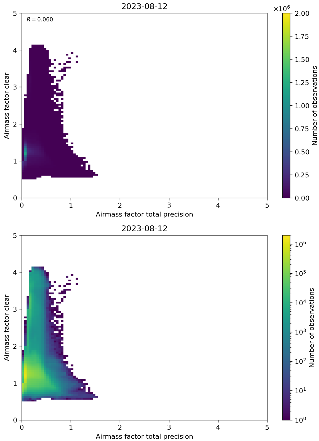
Figure 108: Scatter density plot of “Airmass factor total precision” against “Airmass factor clear” for 2023-08-11 to 2023-08-13.
