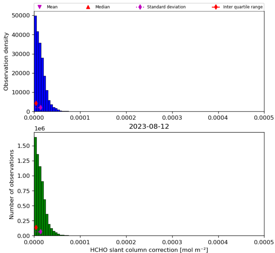
Figure 47: Histogram of “HCHO slant column correction” for 2023-08-11 to 2023-08-13
