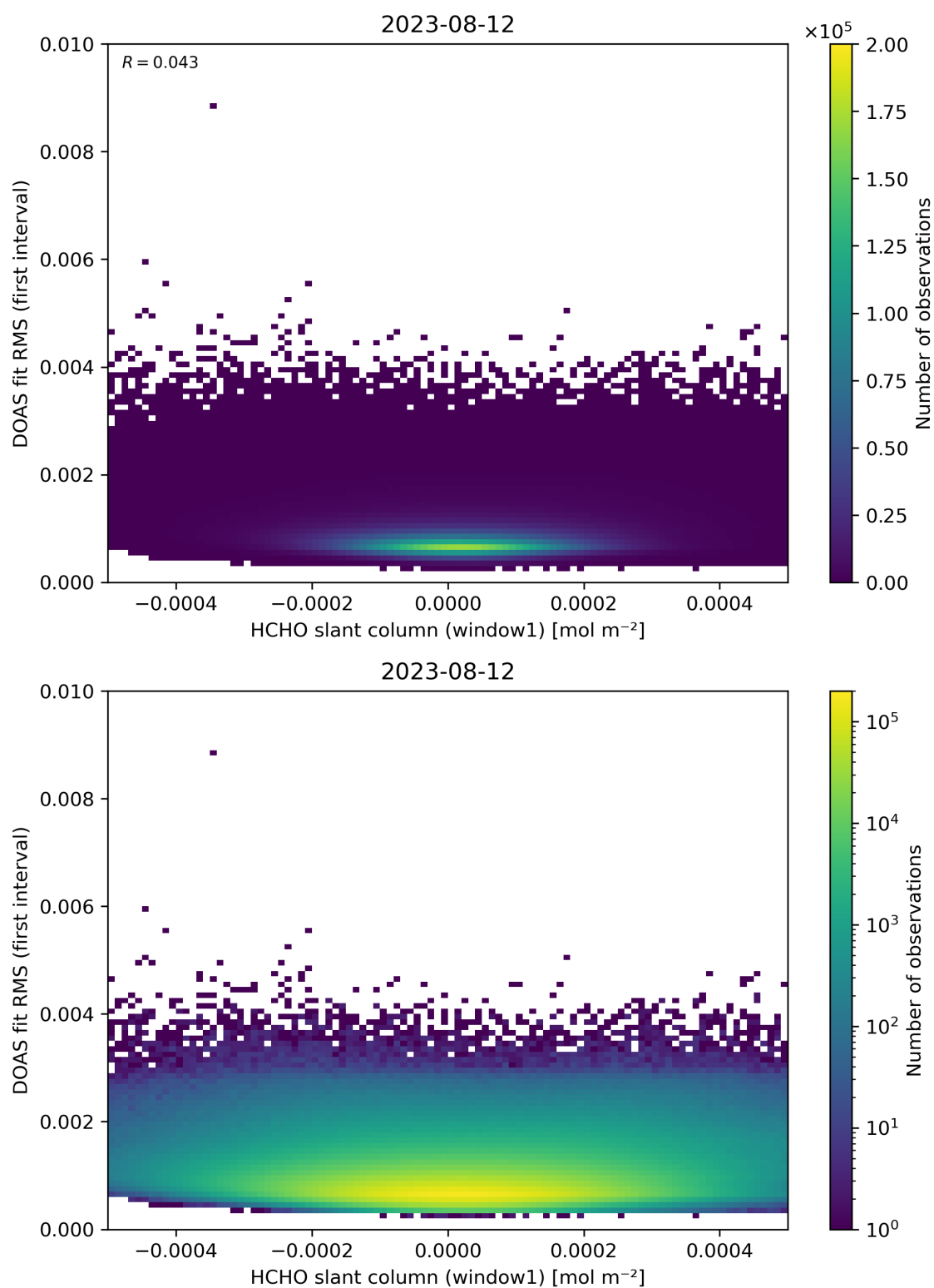
Figure 78: Scatter density plot of “HCHO slant column (window1)” against “DOAS fit RMS (first interval)” for 2023-08-11 to 2023-08-13.
