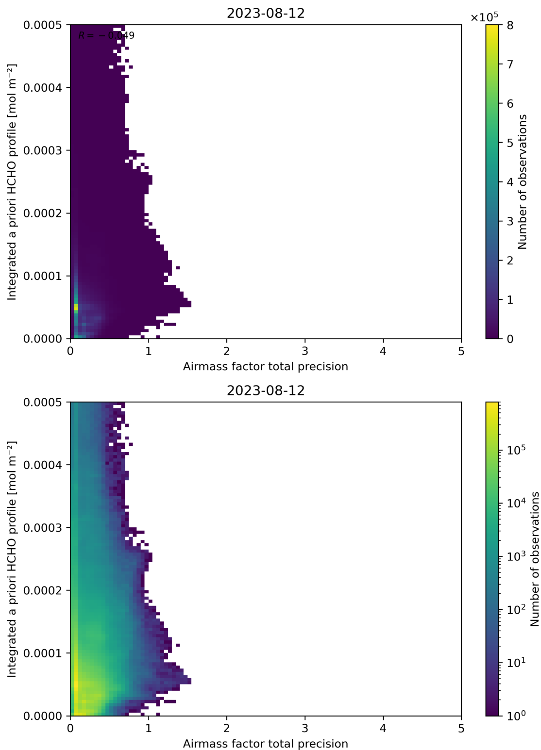
Figure 111: Scatter density plot of “Airmass factor total precision” against “Integrated a priori HCHO profile” for 2023-08-11 to 2023-08-13.
