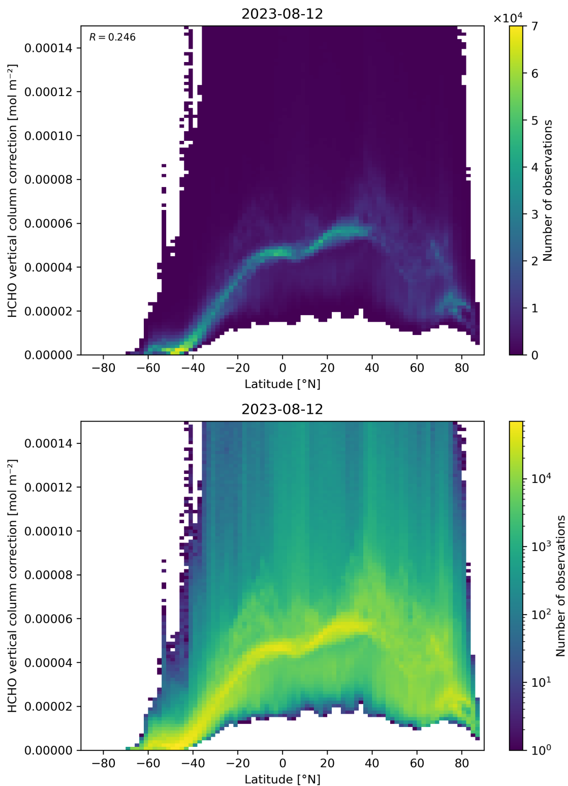
Figure 164: Scatter density plot of “Latitude” against “HCHO vertical column correction” for 2023-08-11 to 2023-08-13.
