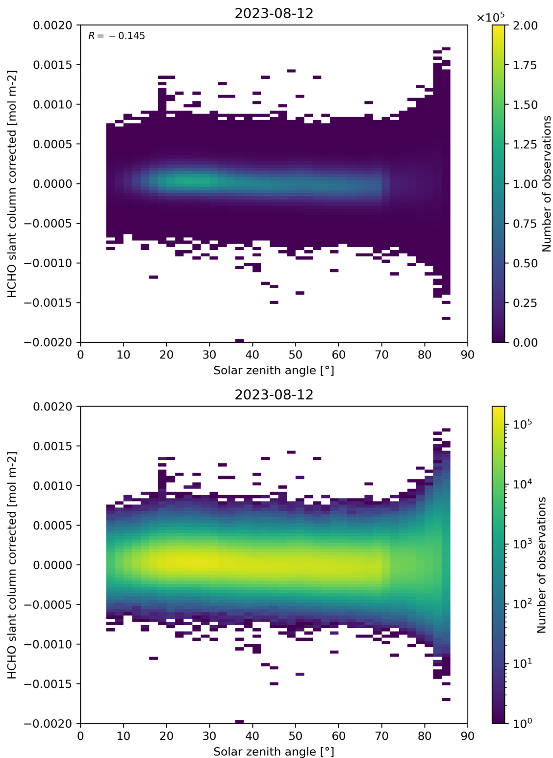
Figure 171: Scatter density plot of “Solar zenith angle” against “HCHO slant column corrected” for 2023-08-11 to 2023-08-13.
