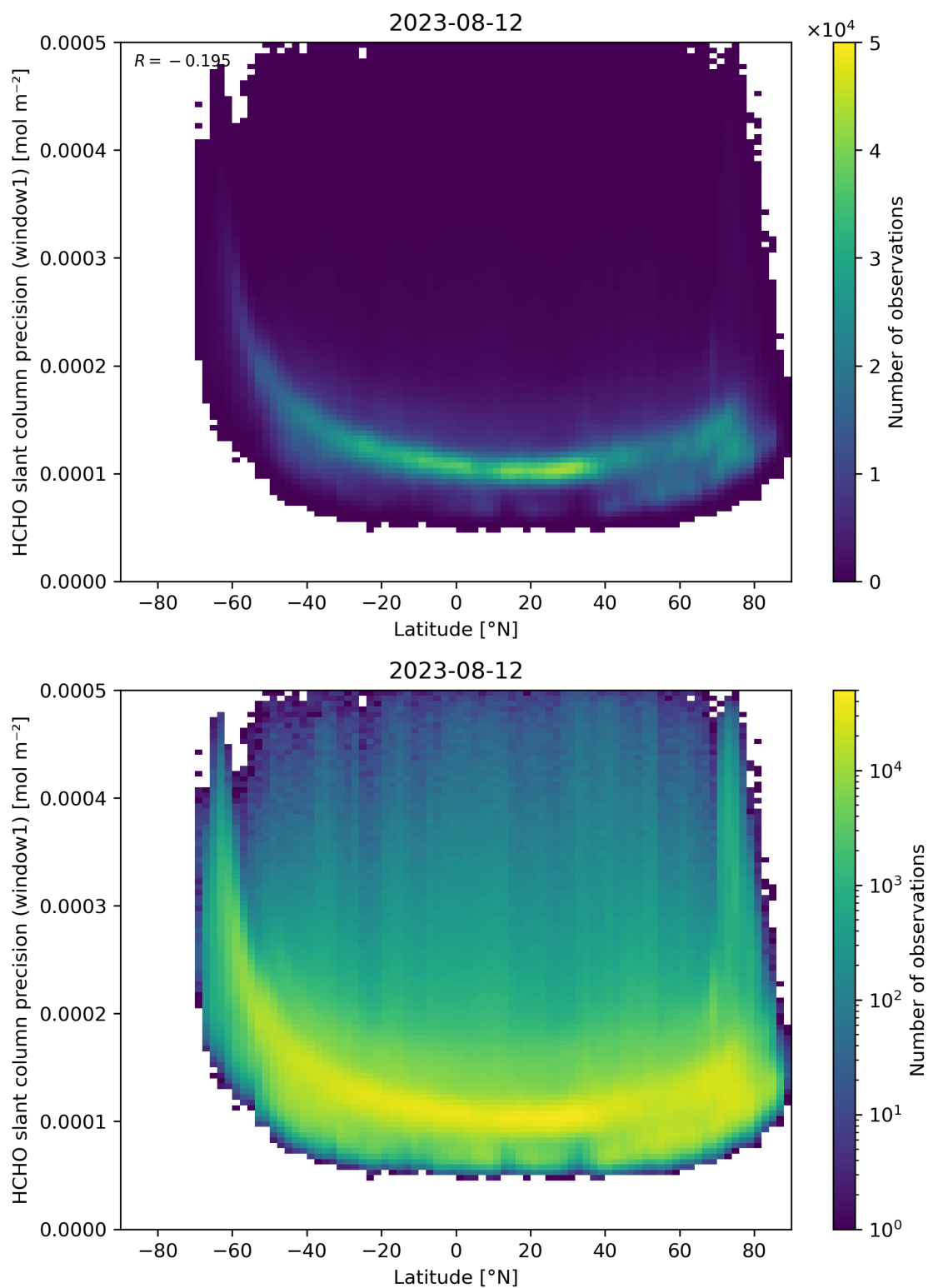
Figure 160: Scatter density plot of “Latitude” against “HCHO slant column precision (window1)” for 2023-08-11 to 2023-08-13.
