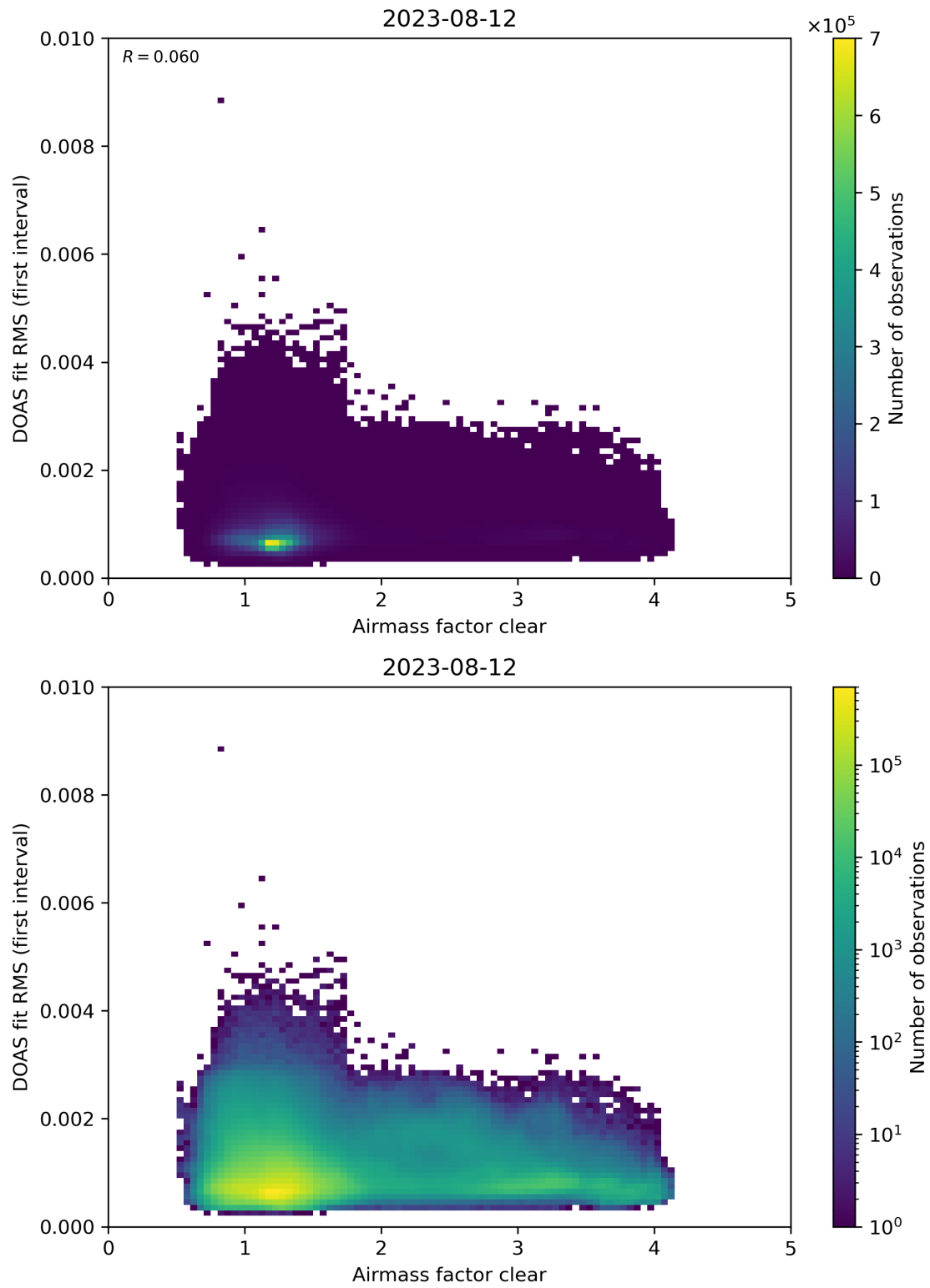
Figure 71: Scatter density plot of “Airmass factor clear” against “DOAS fit RMS (first interval)” for 2023-08-11 to 2023-08-13.
