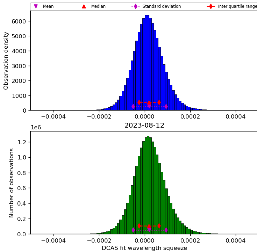
Figure 45: Histogram of “DOAS fit wavelength squeeze” for 2023-08-11 to 2023-08-13
