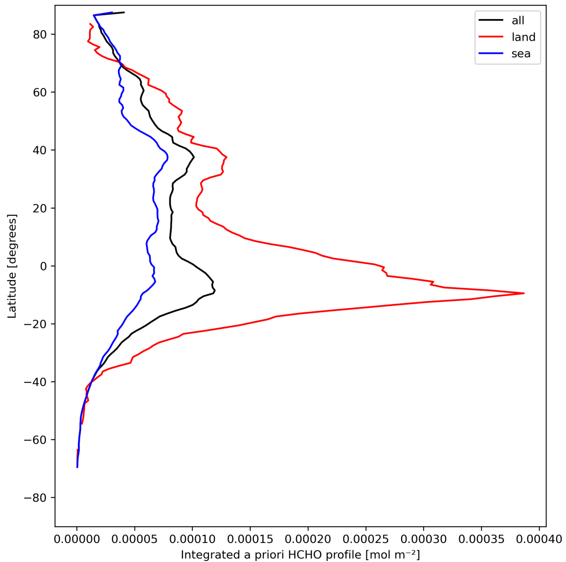
Figure 29: Zonal average of “Integrated a priori HCHO profile” for 2023-08-11 to 2023-08-13.
