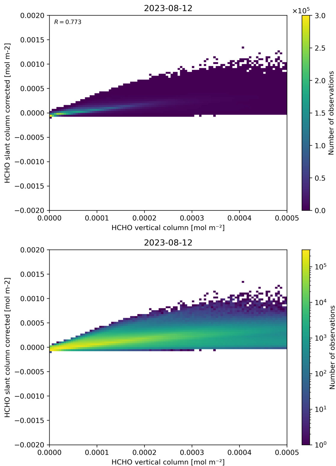
Figure 127: Scatter density plot of “HCHO vertical column” against “HCHO slant column corrected” for 2023-08-11 to 2023-08-13.
