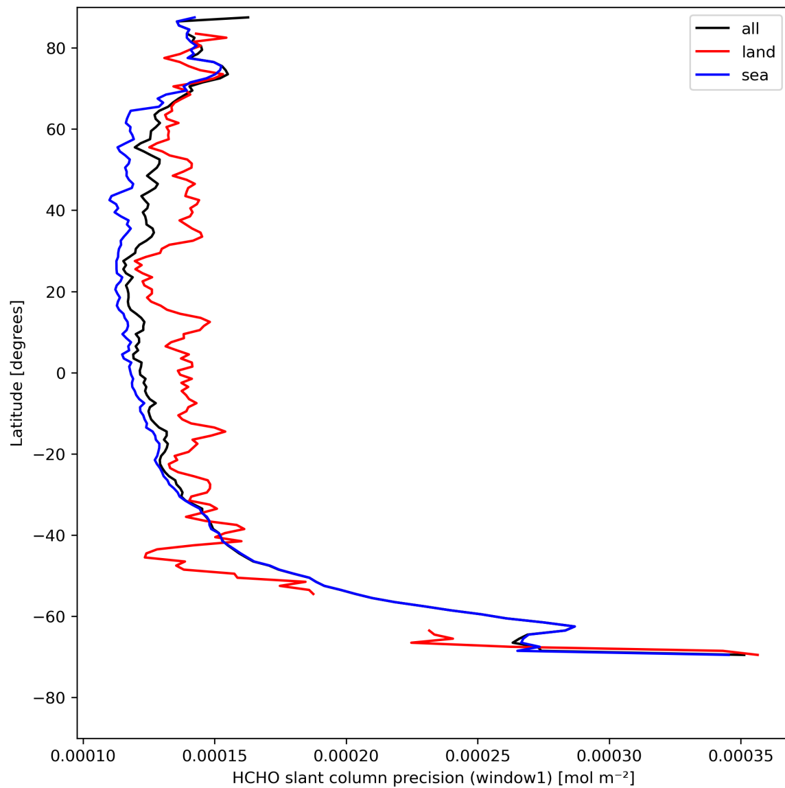
Figure 25: Zonal average of "HCHO slant column precision (window1)" for 2023-08-11 to 2023-08-13.
