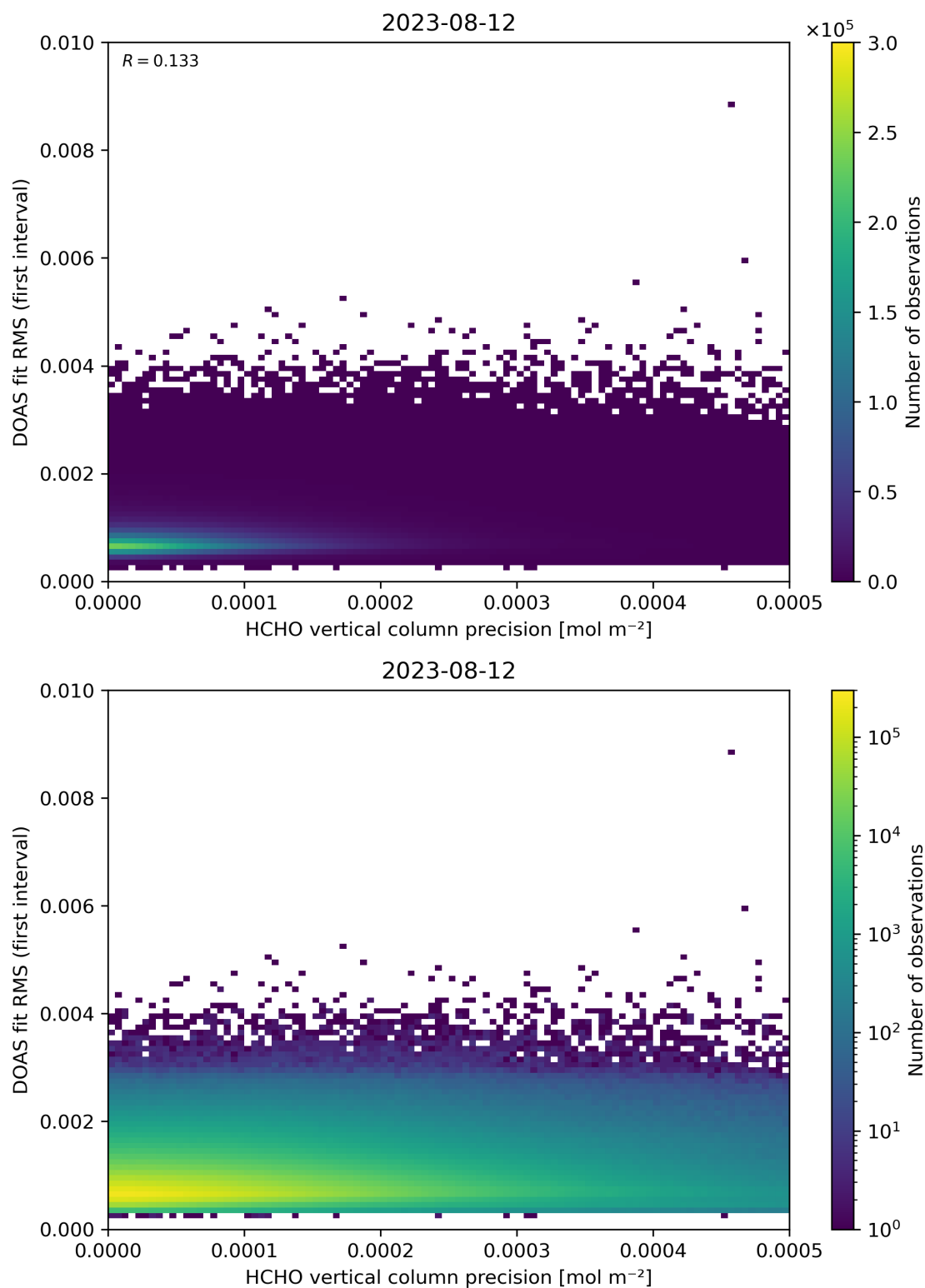
Figure 136: Scatter density plot of “HCHO vertical column precision” against “DOAS fit RMS (first interval)” for 2023-08-11 to 2023-08-13.
