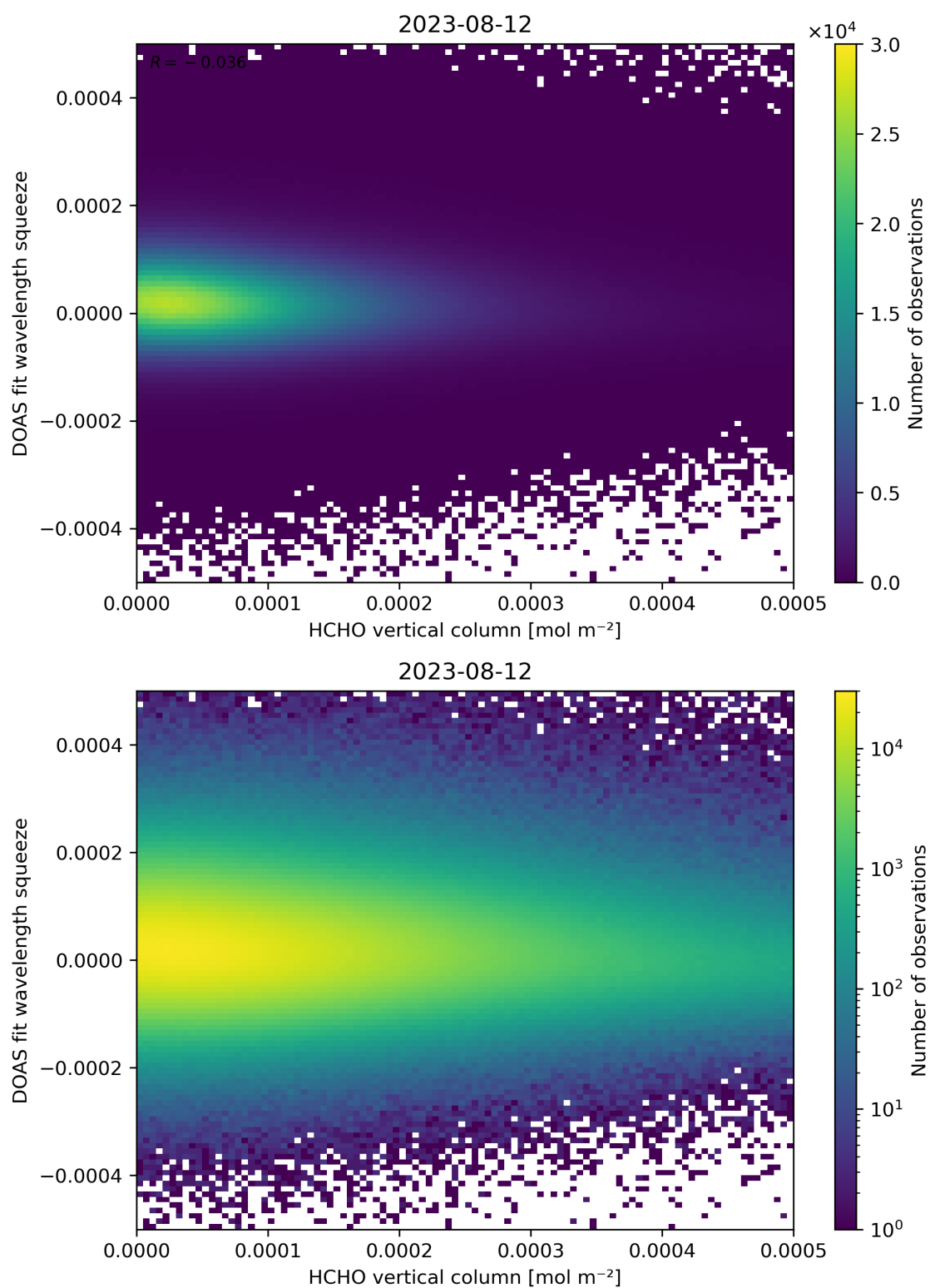
Figure 125: Scatter density plot of “HCHO vertical column” against “DOAS fit wavelength squeeze” for 2023-08-11 to 2023-08-13.
