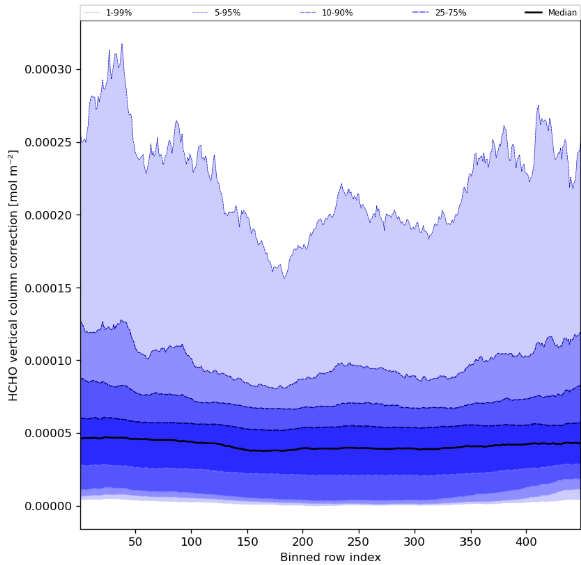
Figure 51: Along track statistics of “HCHO vertical column correction” for 2023-08-11 to 2023-08-13
