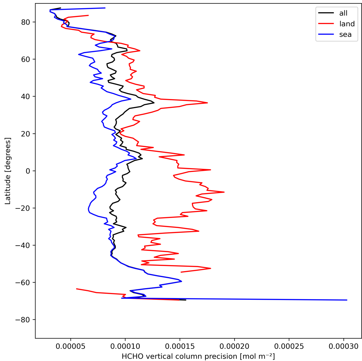
Figure 22: Zonal average of “HCHO vertical column precision” for 2023-08-11 to 2023-08-13.
