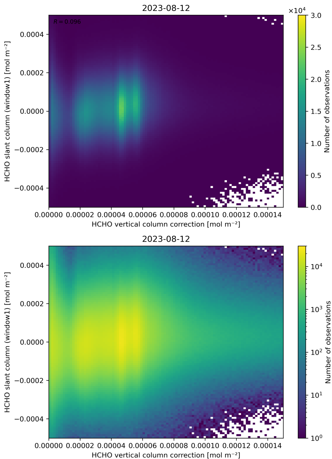
Figure 118: Scatter density plot of “HCHO vertical column correction” against “HCHO slant column (window1)” for 2023-08-11 to 2023-08-13.
