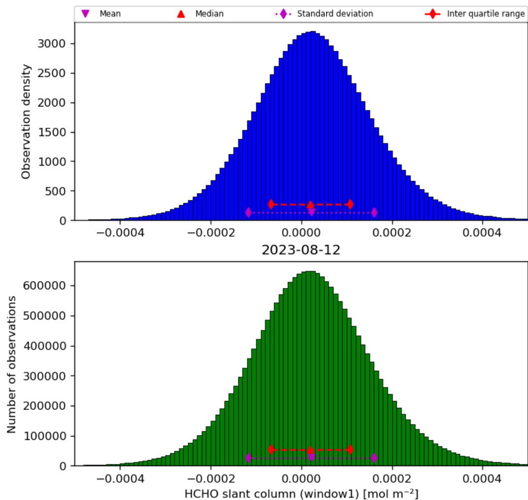
Figure 38: Histogram of “HCHO slant column (window1)” for 2023-08-11 to 2023-08-13
