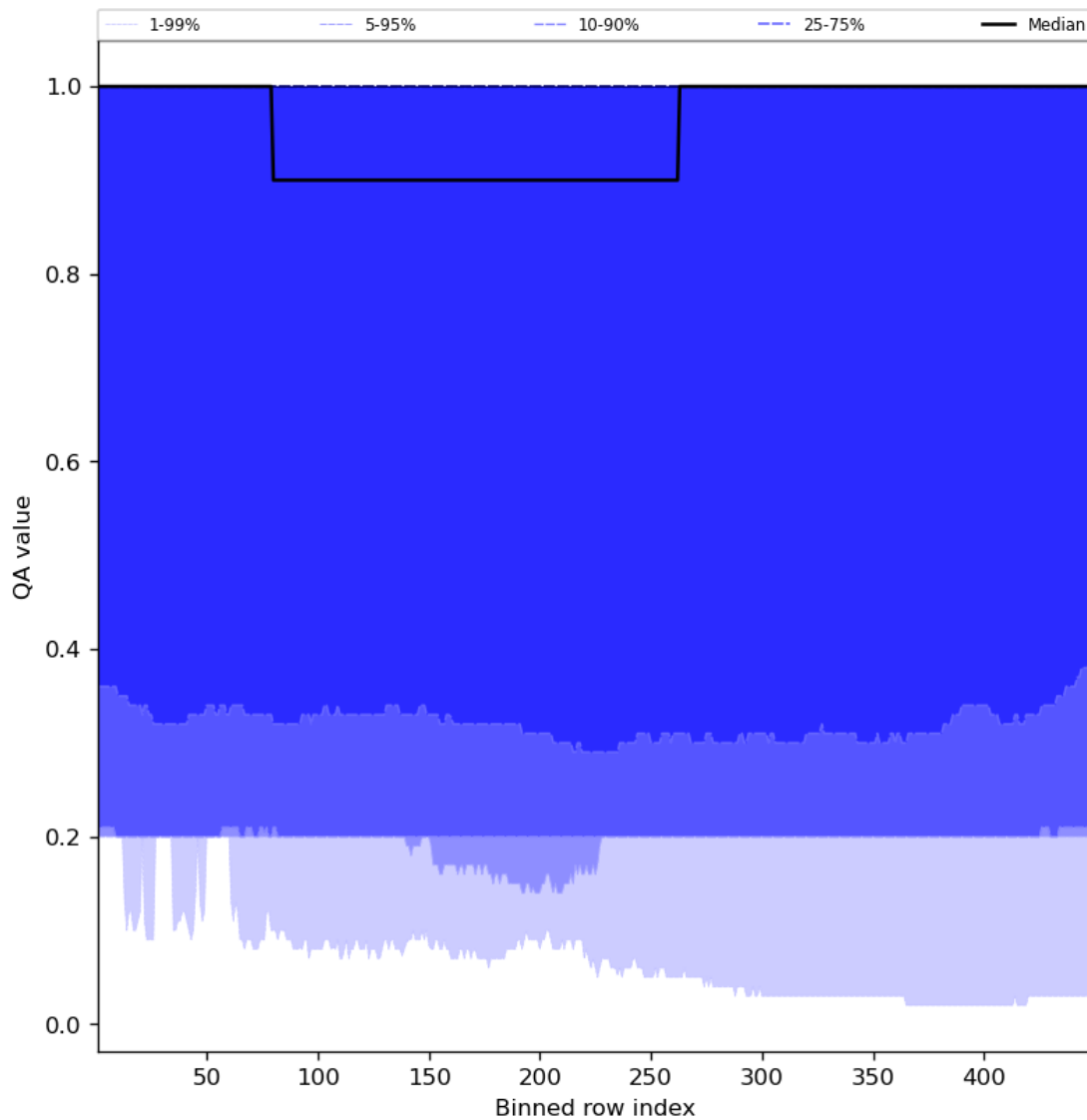
Figure 48: Along track statistics of “QA value” for 2023-08-11 to 2023-08-13
