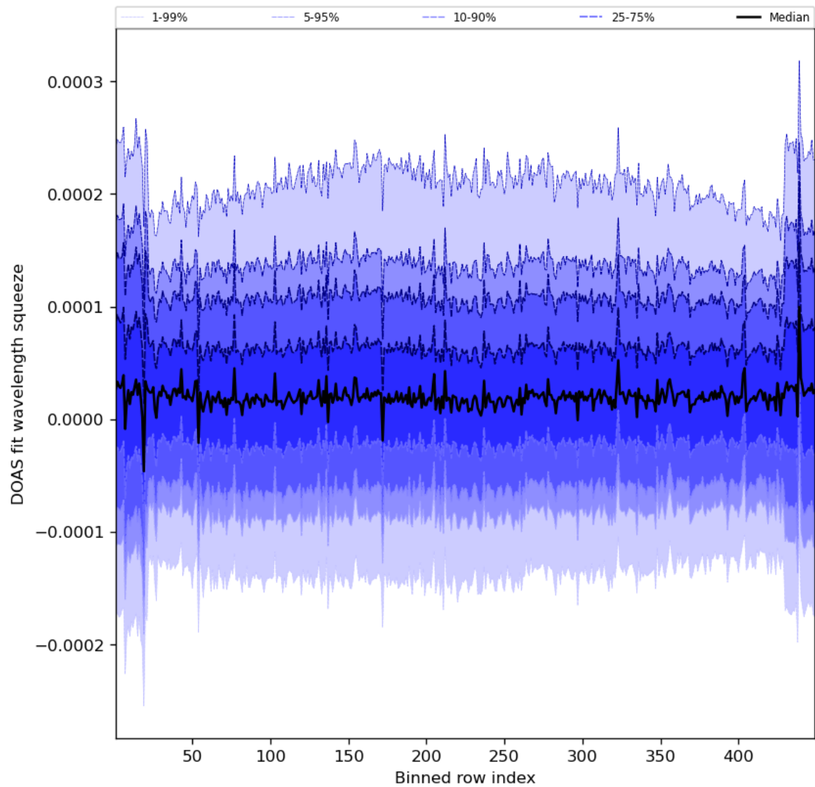
Figure 59: Along track statistics of “DOAS fit wavelength squeeze” for 2023-08-11 to 2023-08-13
