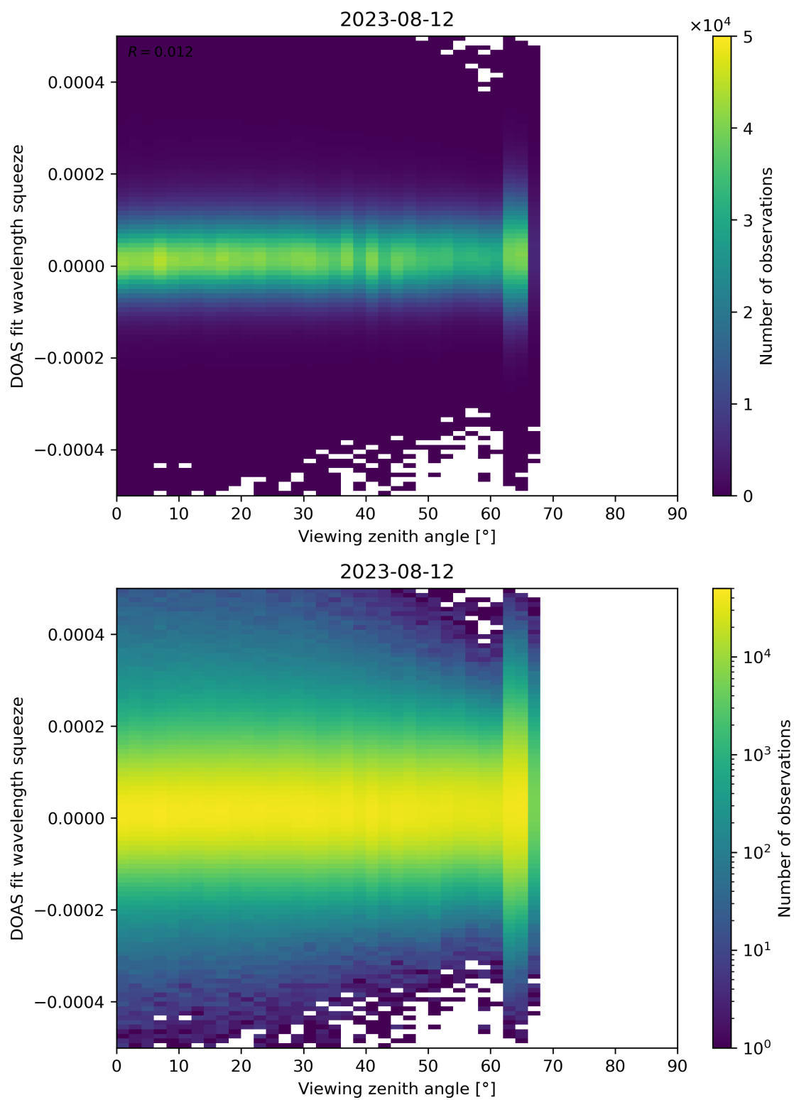
Figure 184: Scatter density plot of “Viewing zenith angle” against “DOAS fit wavelength squeeze” for 2023-08-11 to 2023-08-13.
