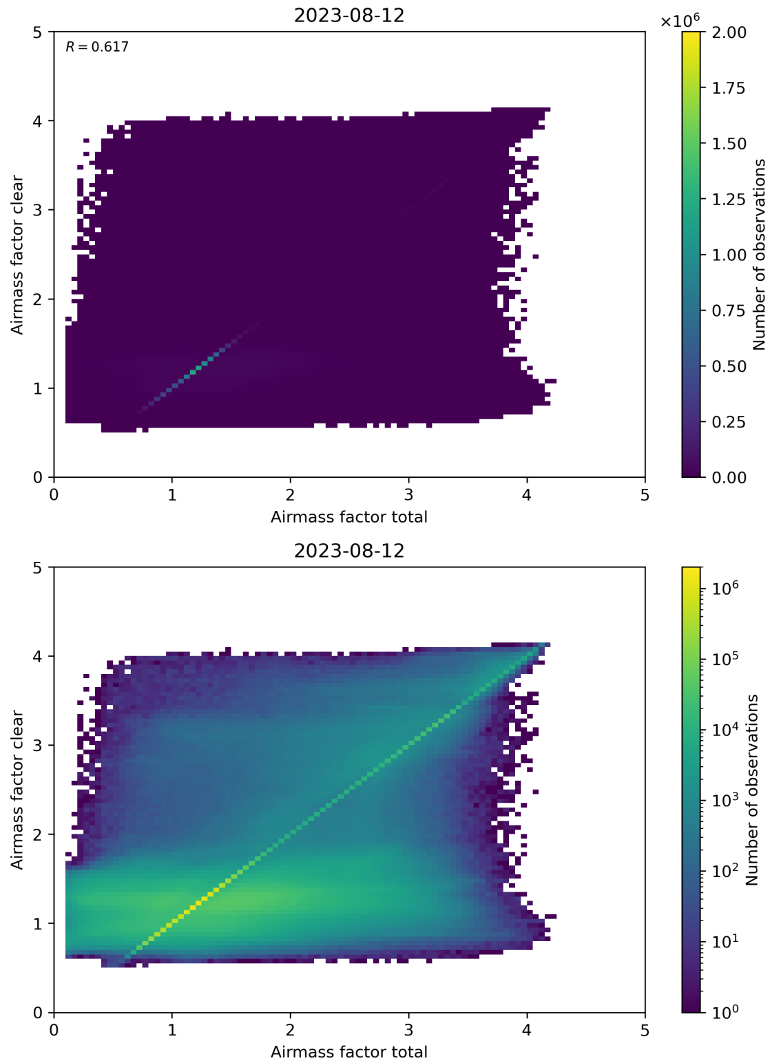
Figure 100: Scatter density plot of “Airmass factor total” against “Airmass factor clear” for 2023-08-11 to 2023-08-13.
