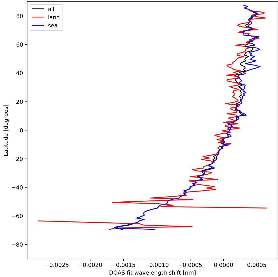
Figure 30: Zonal average of “DOAS fit wavelength shift” for 2023-08-11 to 2023-08-13.
