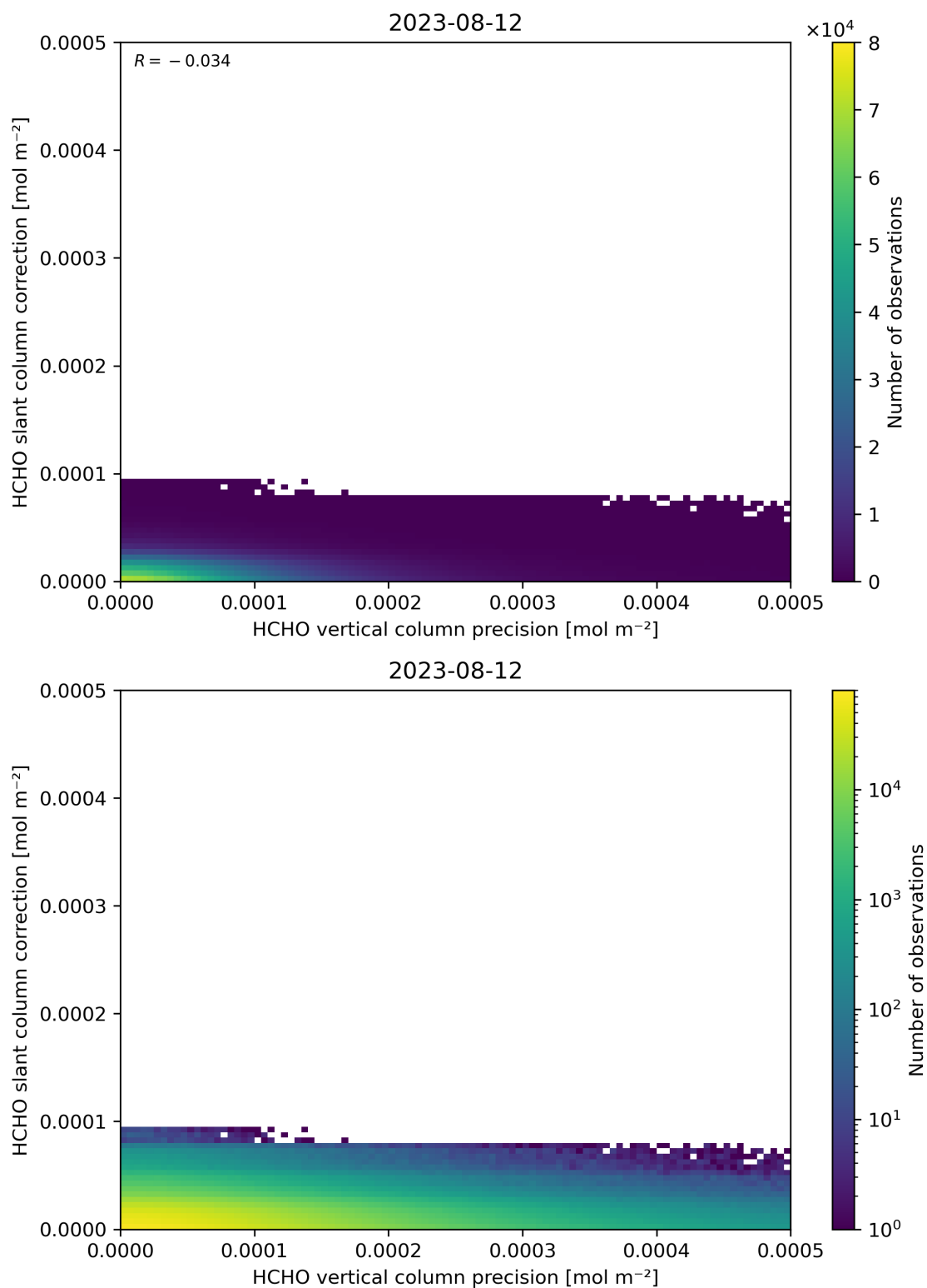
Figure 141: Scatter density plot of “HCHO vertical column precision” against “HCHO slant column correction” for 2023-08-11 to 2023-08-13.
