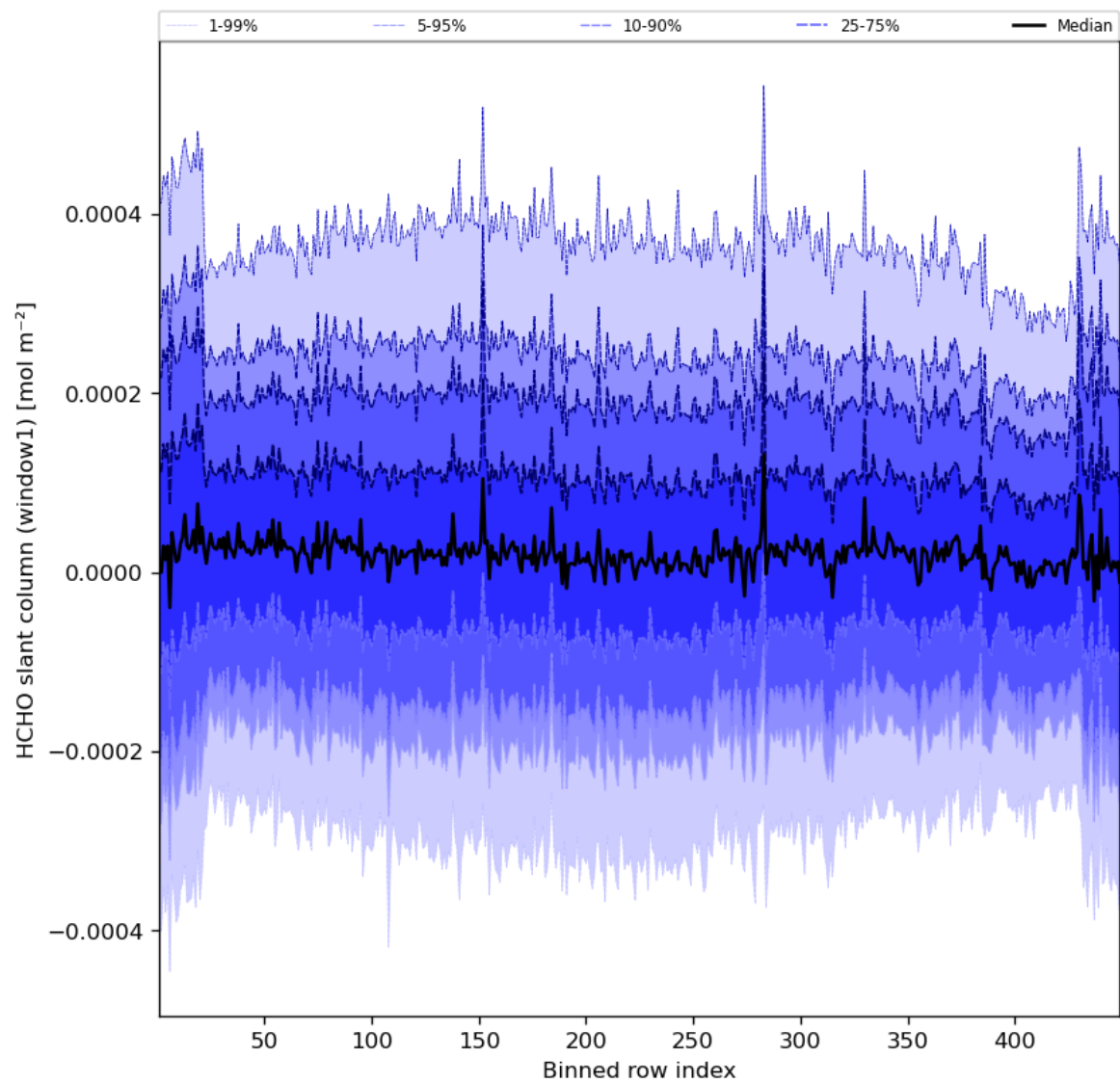
Figure 52: Along track statistics of “HCHO slant column (window1)” for 2023-08-11 to 2023-08-13
