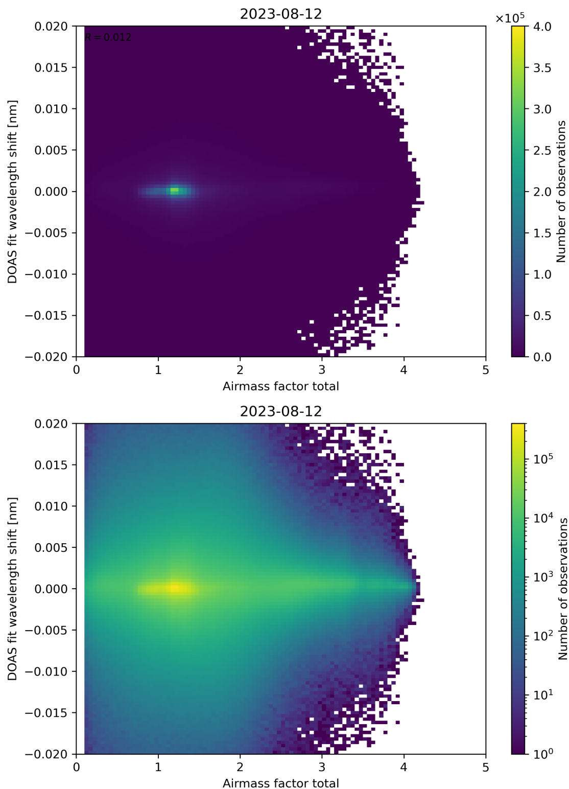
Figure 98: Scatter density plot of “Airmass factor total” against “DOAS fit wavelength shift” for 2023-08-11 to 2023-08-13.
