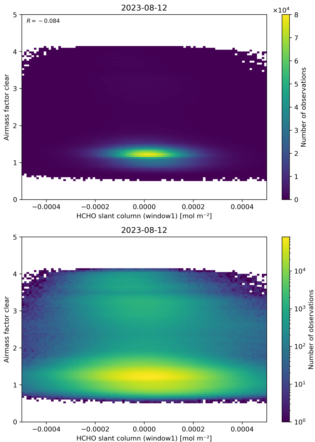
Figure 81: Scatter density plot of “HCHO slant column (window1)” against “Airmass factor clear” for 2023-08-11 to 2023-08-13.
