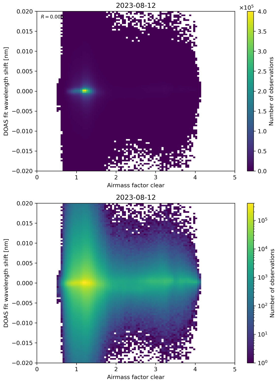
Figure 72: Scatter density plot of “Airmass factor clear” against “DOAS fit wavelength shift” for 2023-08-11 to 2023-08-13.
