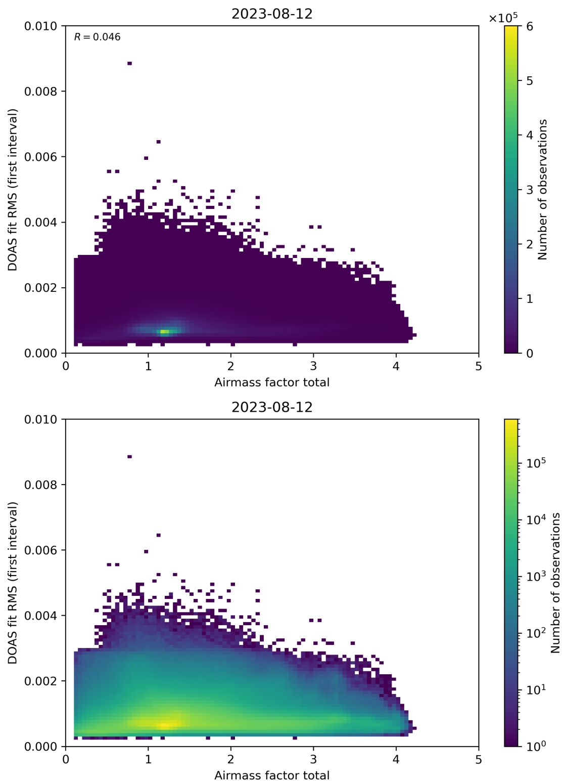
Figure 97: Scatter density plot of “Airmass factor total” against “DOAS fit RMS (first interval)” for 2023-08-11 to 2023-08-13.
