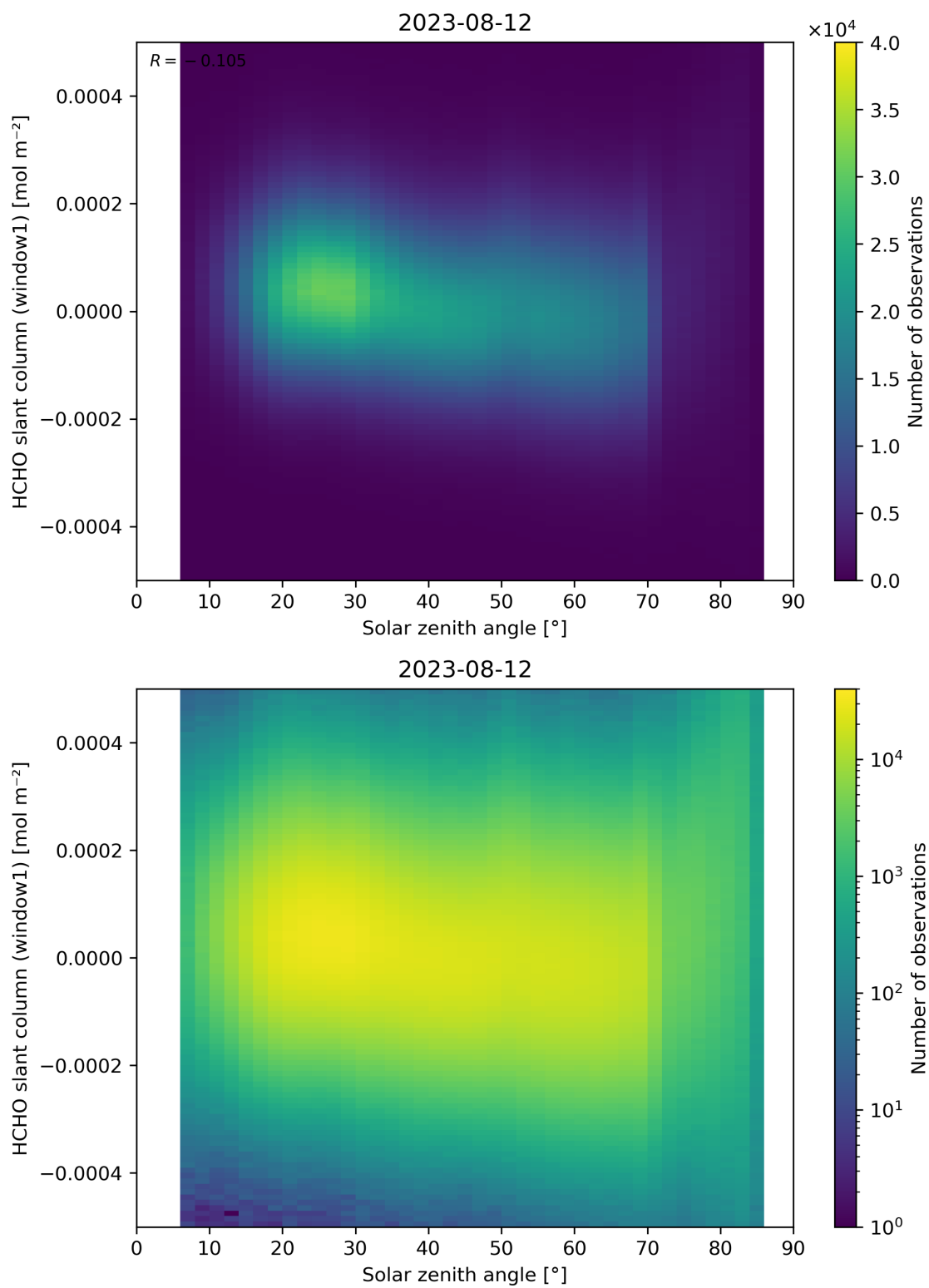
Figure 173: Scatter density plot of “Solar zenith angle” against “HCHO slant column (window1)” for 2023-08-11 to 2023-08-13.
