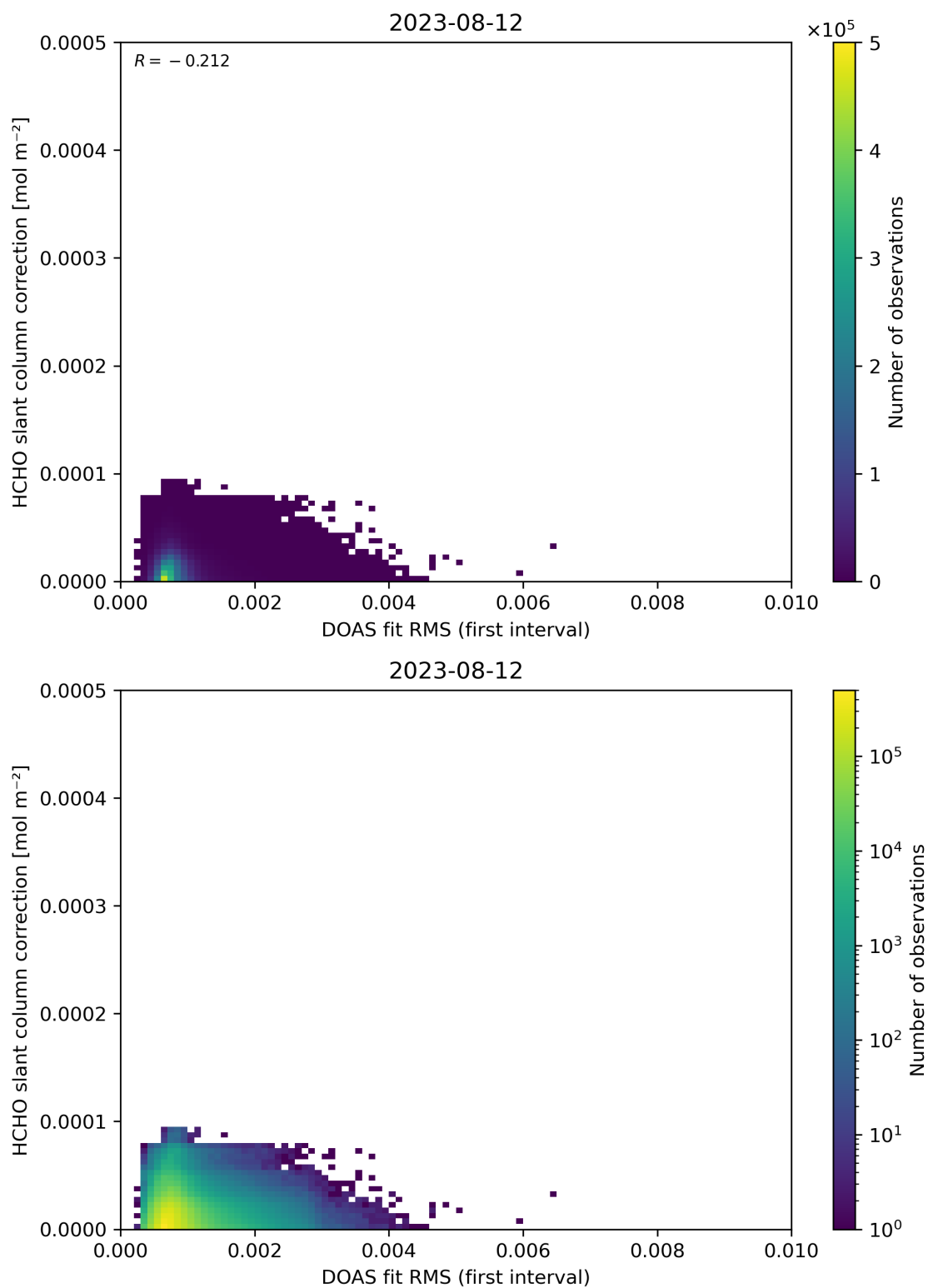
Figure 63: Scatter density plot of “DOAS fit RMS (first interval)” against “HCHO slant column correction” for 2023-08-11 to 2023-08-13.
