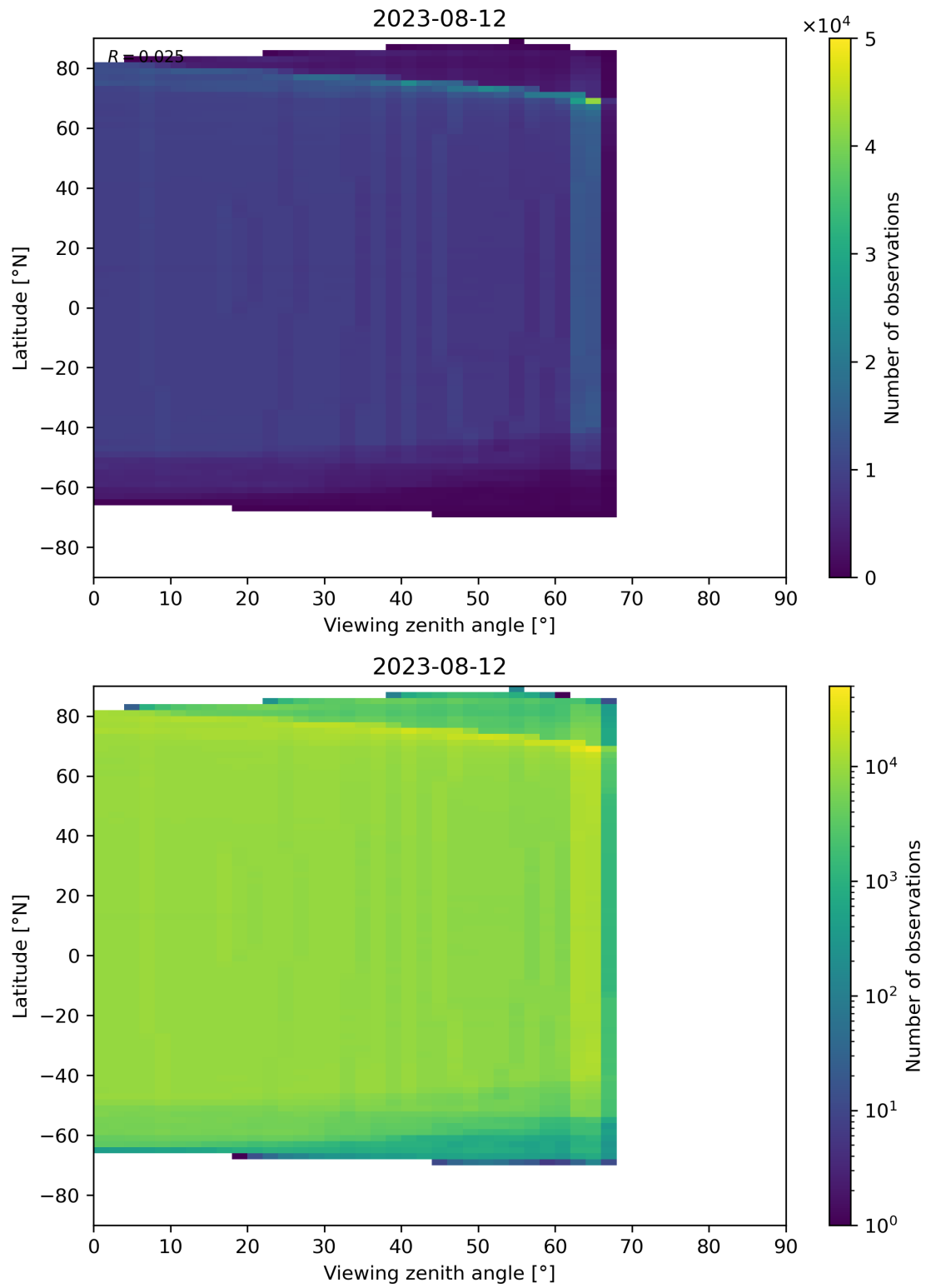
Figure 196: Scatter density plot of “Viewing zenith angle” against “Latitude” for 2023-08-11 to 2023-08-13.
