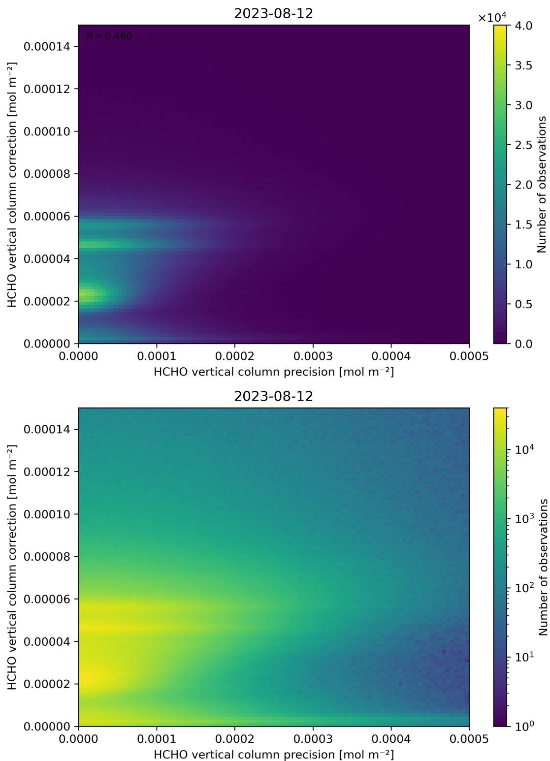
Figure 146: Scatter density plot of “HCHO vertical column precision” against “HCHO vertical column correction” for 2023-08-11 to 2023-08-13.
