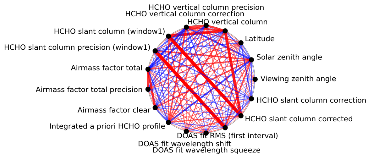
Figure 1: Map of correlation graph for 2023-08-11 to 2023-08-13.
