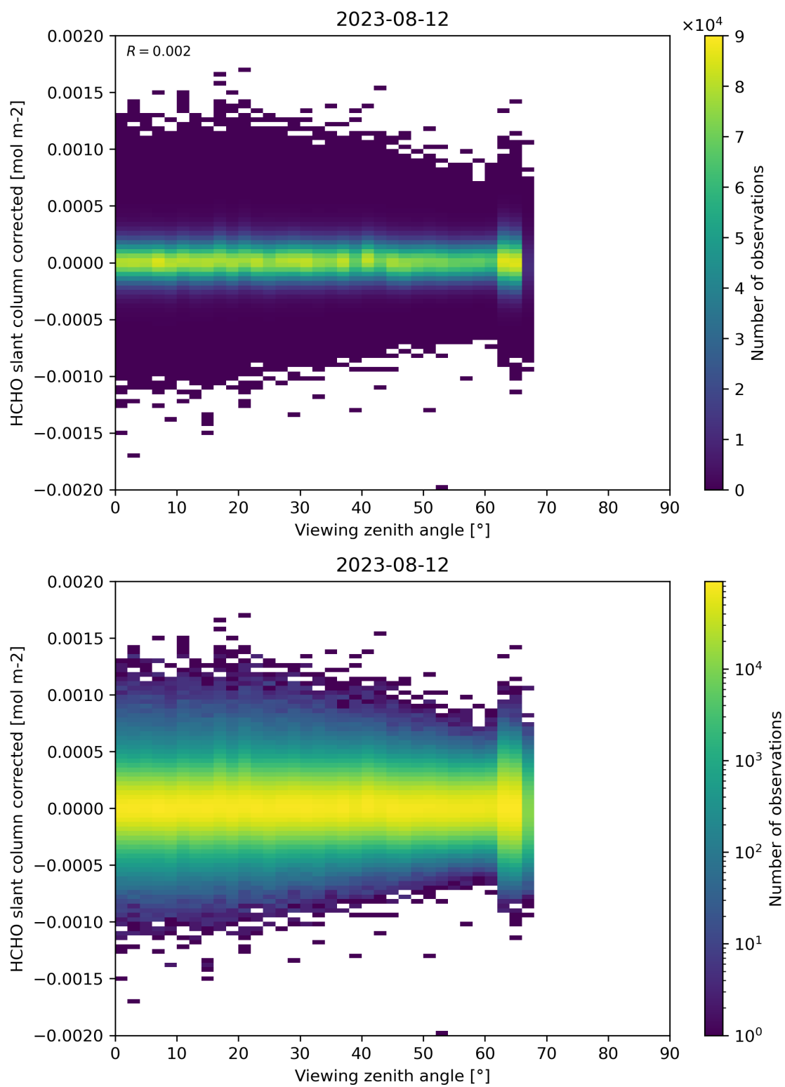
Figure 186: Scatter density plot of “Viewing zenith angle” against “HCHO slant column corrected” for 2023-08-11 to 2023-08-13.
