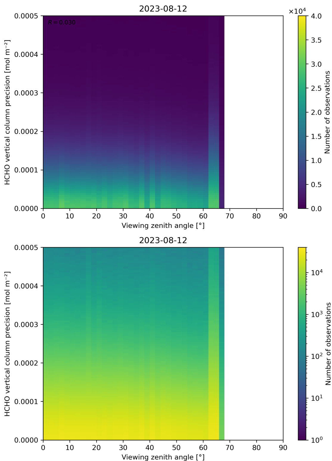
Figure 194: Scatter density plot of “Viewing zenith angle” against “HCHO vertical column precision” for 2023-08-11 to 2023-08-13.
