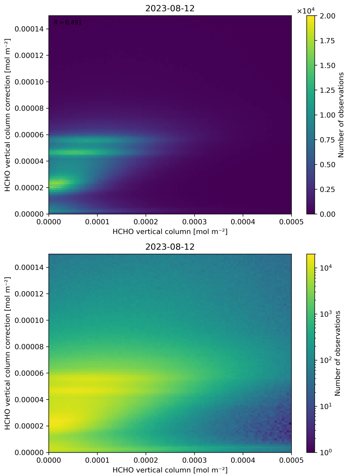
Figure 133: Scatter density plot of “HCHO vertical column” against “HCHO vertical column correction” for 2023-08-11 to 2023-08-13.
