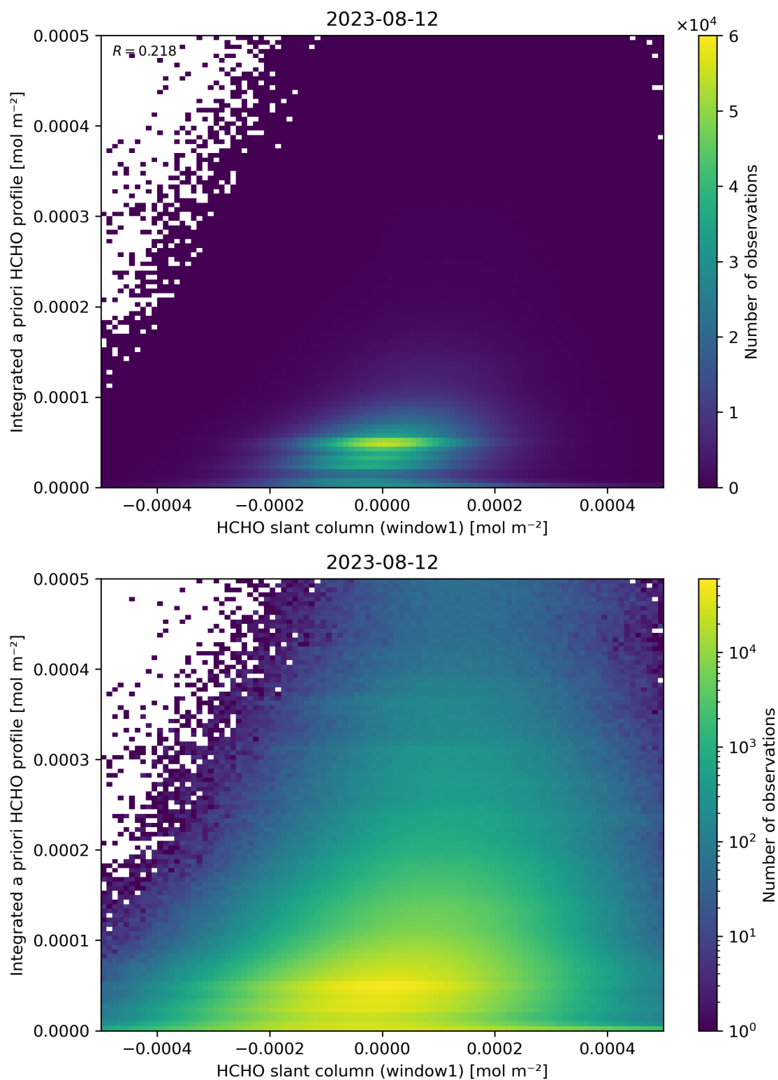
Figure 87: Scatter density plot of “HCHO slant column (window1)” against “Integrated a priori HCHO profile” for 2023-08-11 to 2023-08-13.
