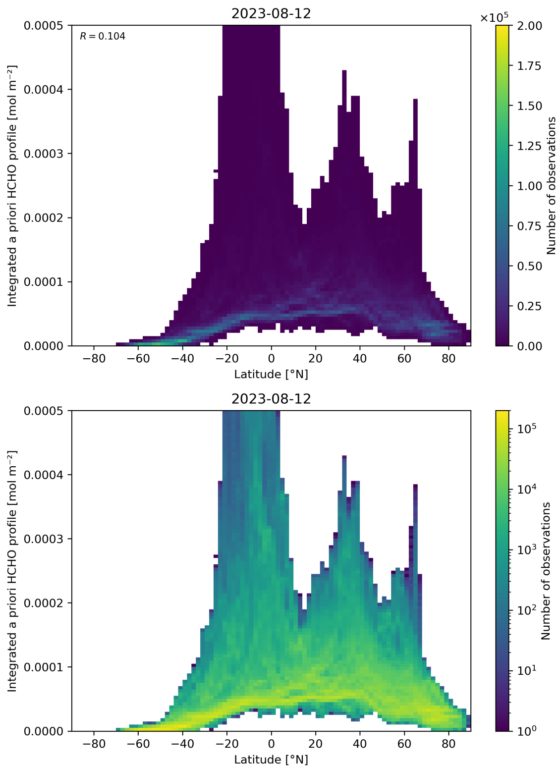
Figure 166: Scatter density plot of “Latitude” against “Integrated a priori HCHO profile” for 2023-08-11 to 2023-08-13.
