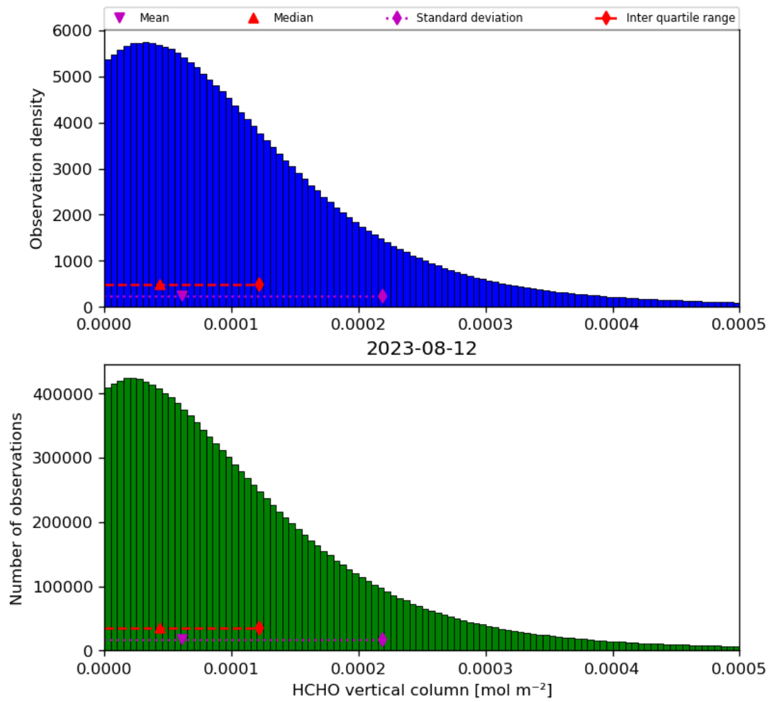
Figure 35: Histogram of “HCHO vertical column” for 2023-08-11 to 2023-08-13
