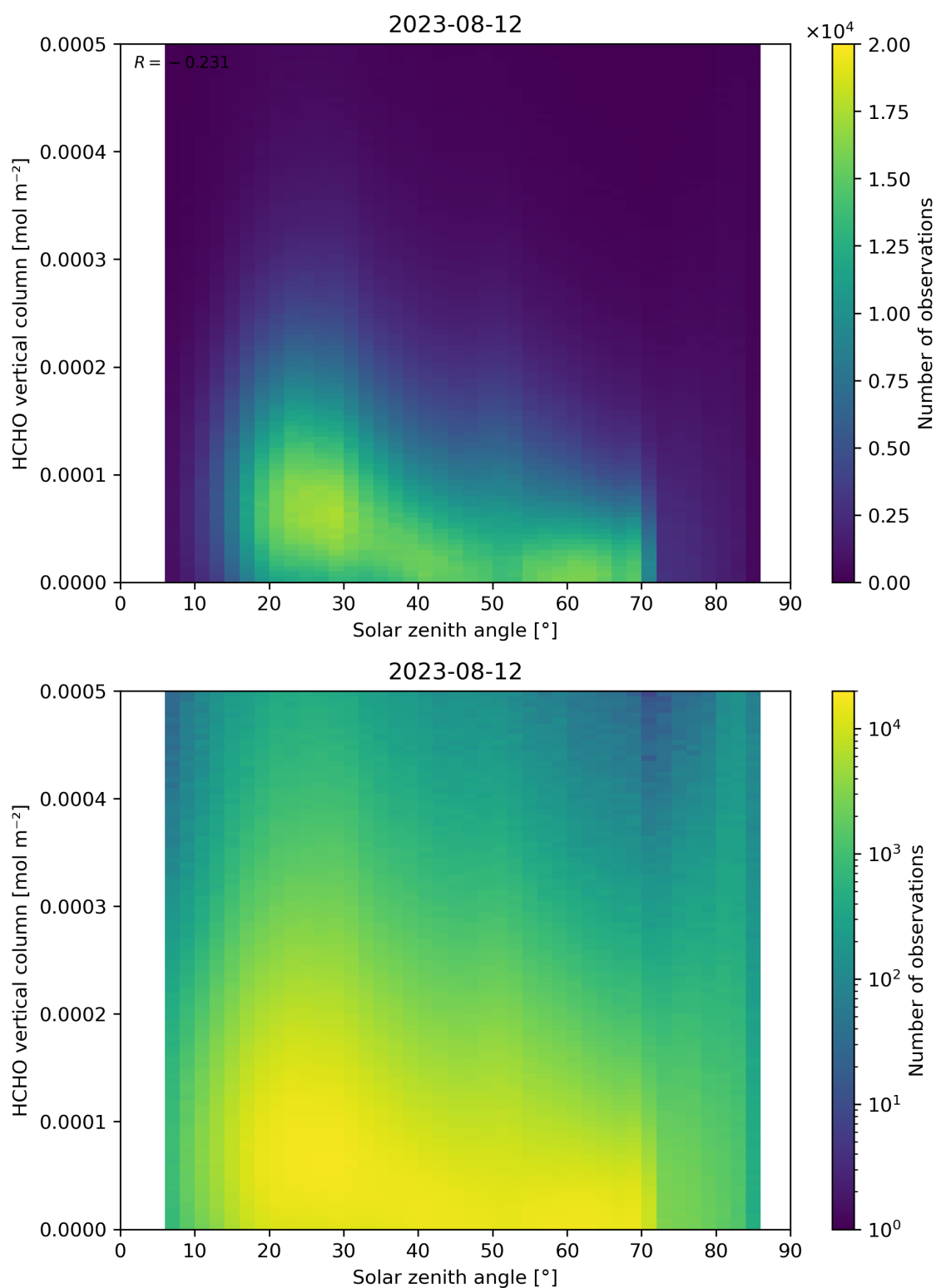
Figure 177: Scatter density plot of “Solar zenith angle” against “HCHO vertical column” for 2023-08-11 to 2023-08-13.
