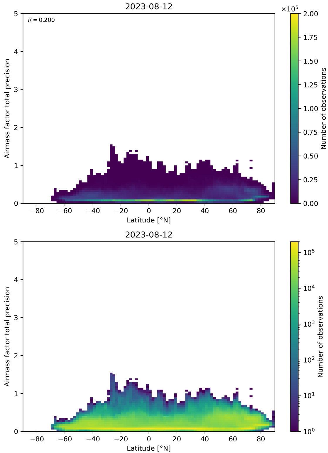
Figure 162: Scatter density plot of “Latitude” against “Airmass factor total precision” for 2023-08-11 to 2023-08-13.
