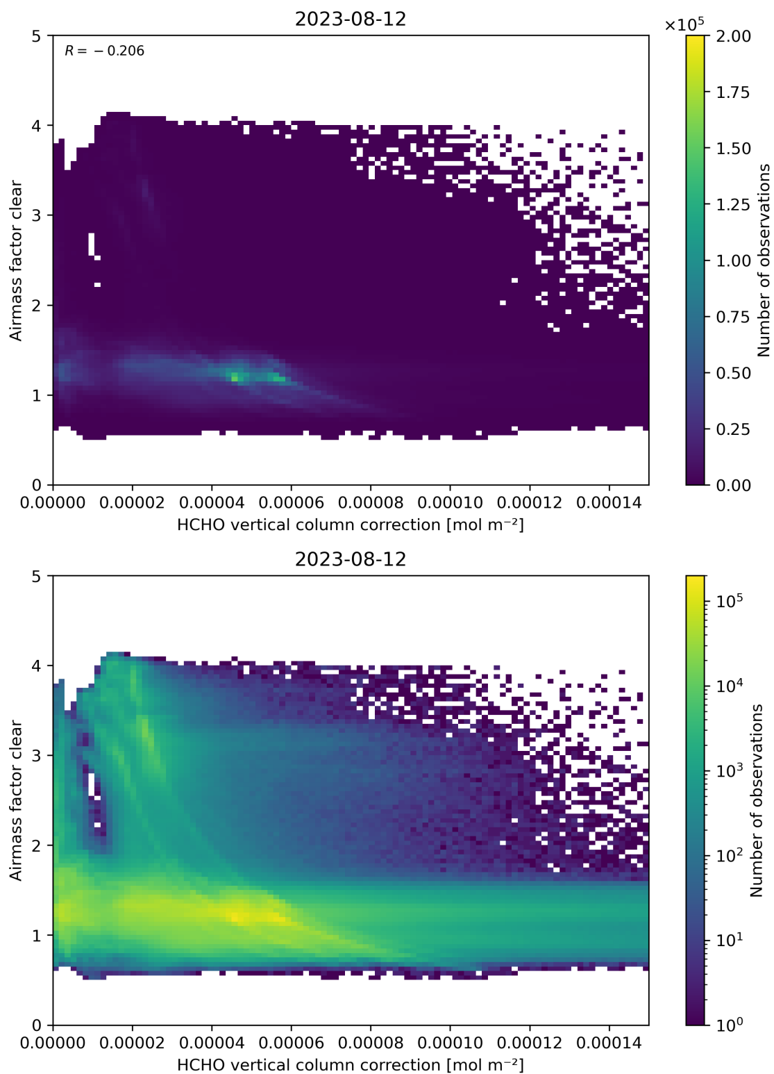
Figure 115: Scatter density plot of “HCHO vertical column correction” against “Airmass factor clear” for 2023-08-11 to 2023-08-13.
