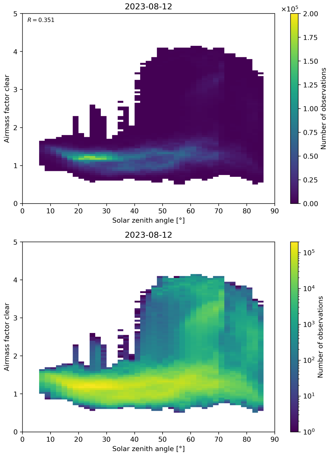
Figure 170: Scatter density plot of “Solar zenith angle” against “Airmass factor clear” for 2023-08-11 to 2023-08-13.
