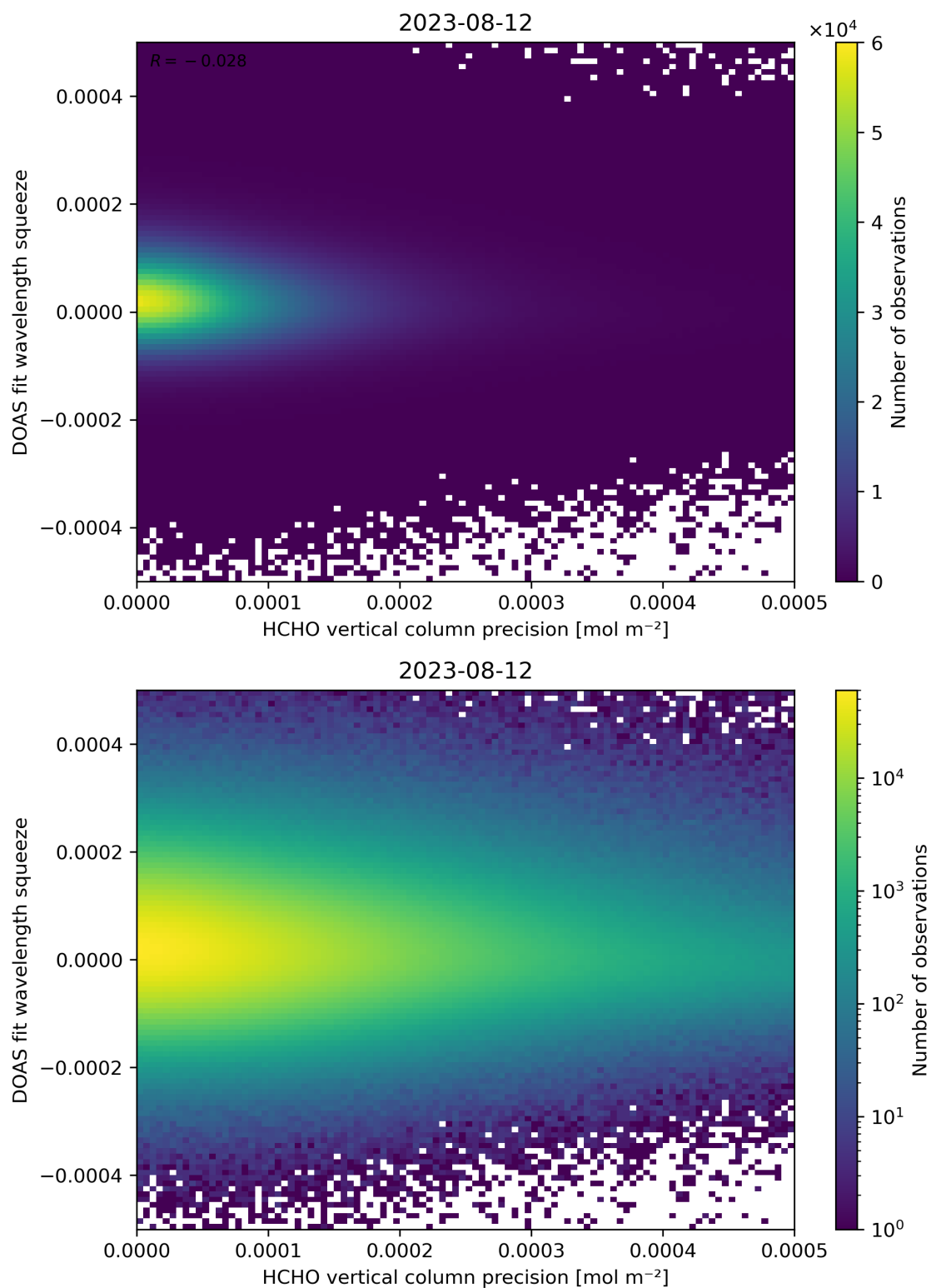
Figure 138: Scatter density plot of “HCHO vertical column precision” against “DOAS fit wavelength squeeze” for 2023-08-11 to 2023-08-13.
