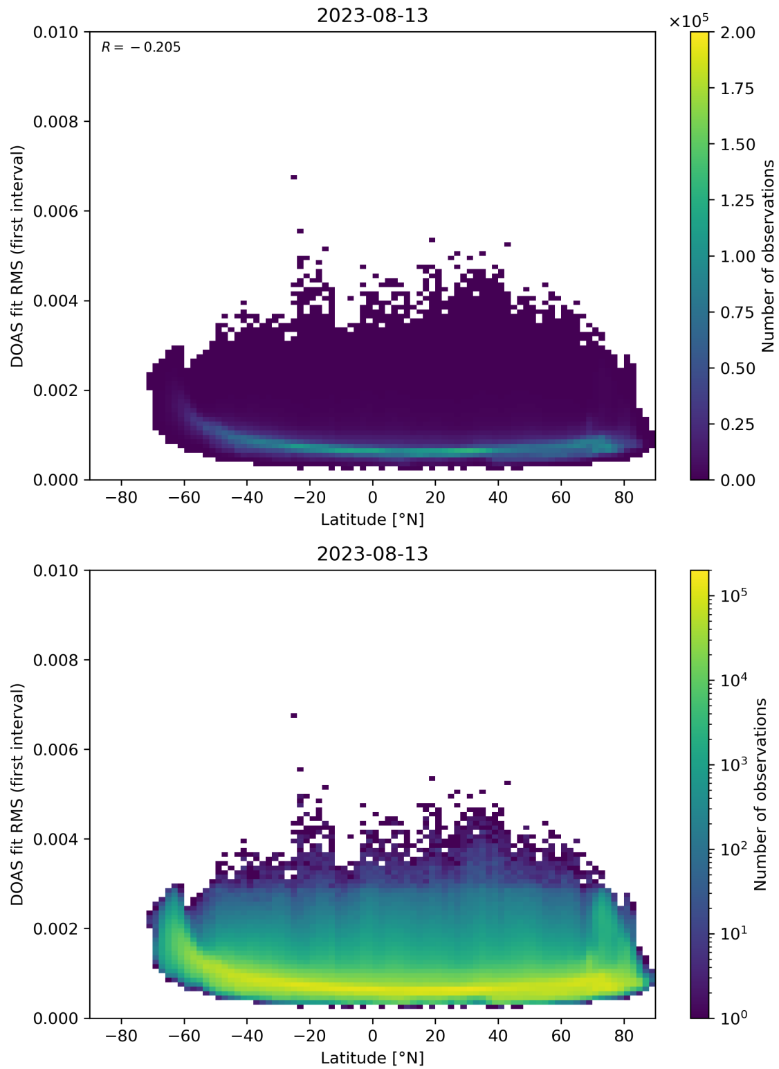
Figure 153: Scatter density plot of “Latitude” against “DOAS fit RMS (first interval)” for 2023-08-12 to 2023-08-14.
