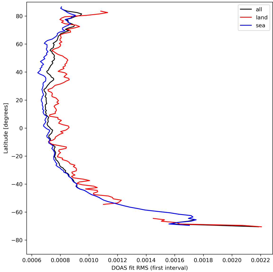
Figure 32: Zonal average of "DOAS fit RMS (first interval)" for 2023-08-12 to 2023-08-14.
