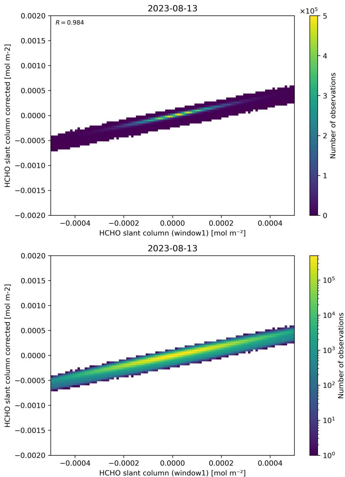
Figure 82: Scatter density plot of “HCHO slant column (window1)” against “HCHO slant column corrected” for 2023-08-12 to 2023-08-14.
