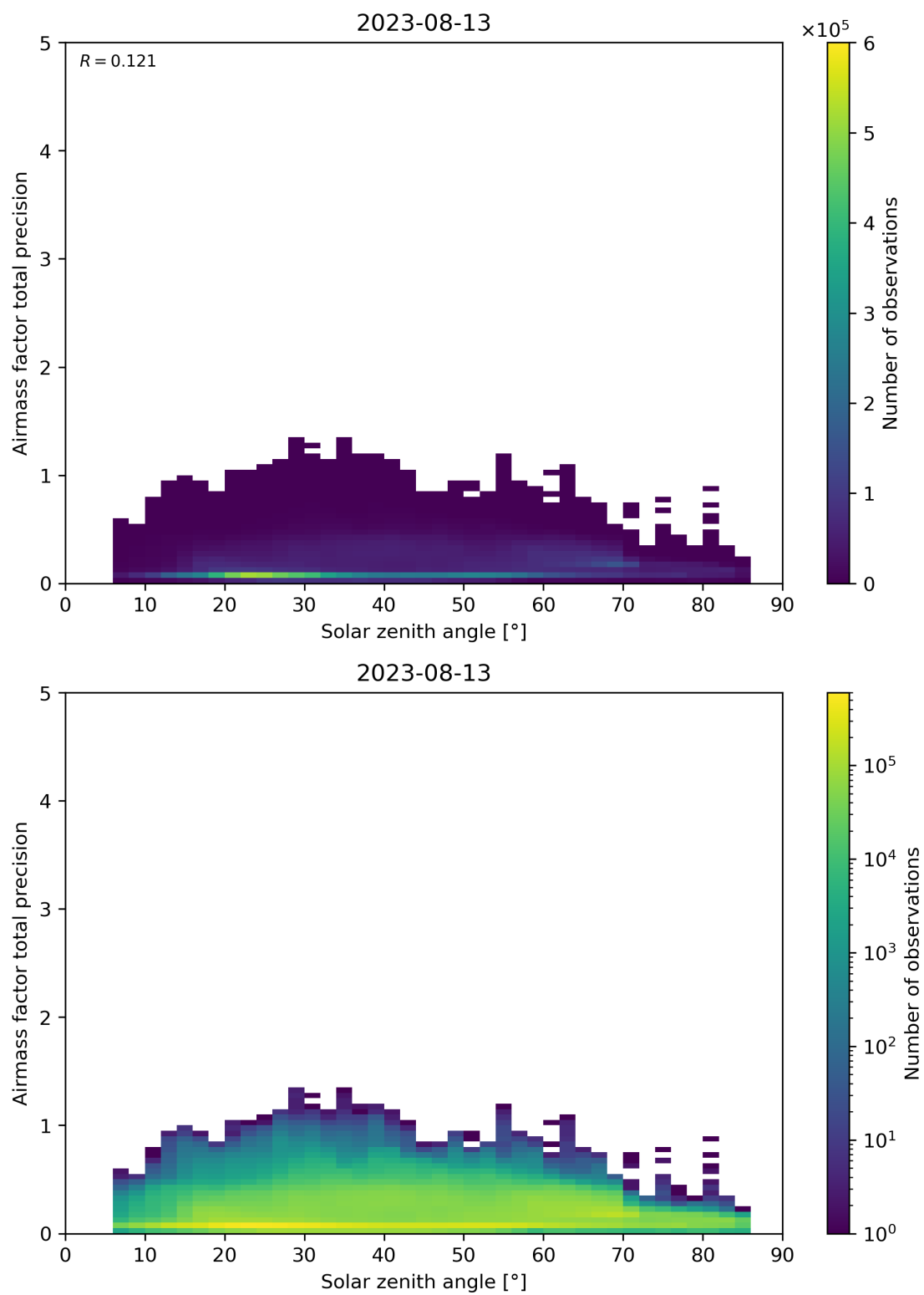
Figure 176: Scatter density plot of “Solar zenith angle” against “Airmass factor total precision” for 2023-08-12 to 2023-08-14.
