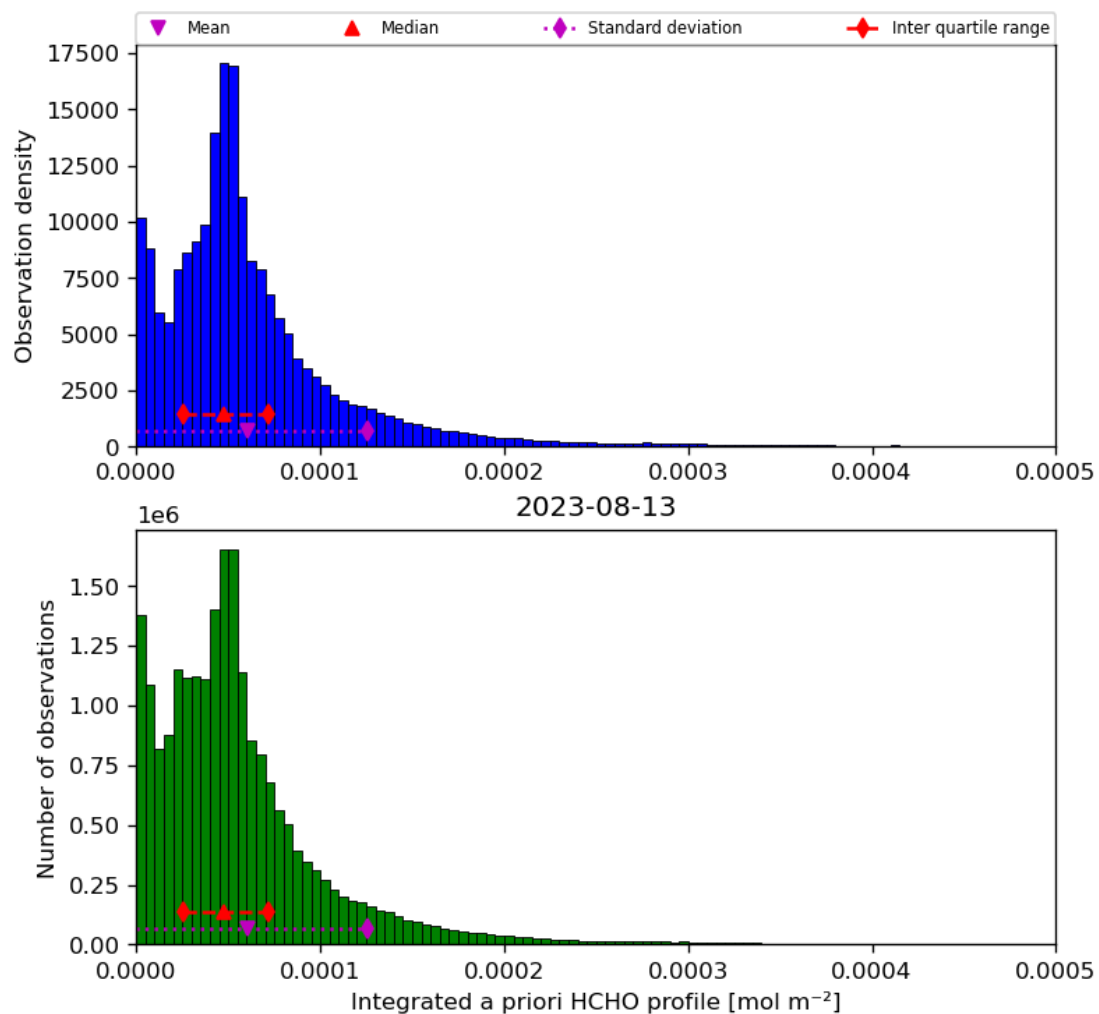
Figure 43: Histogram of “Integrated a priori HCHO profile” for 2023-08-12 to 2023-08-14
