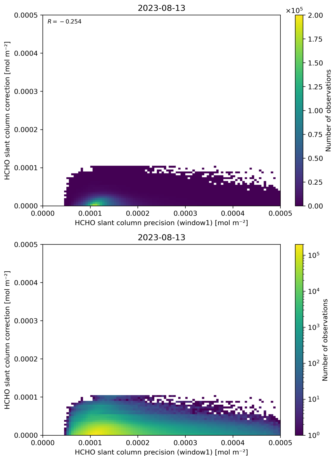
Figure 93: Scatter density plot of “HCHO slant column precision (window1)” against “HCHO slant column correction” for 2023-08-12 to 2023-08-14.
