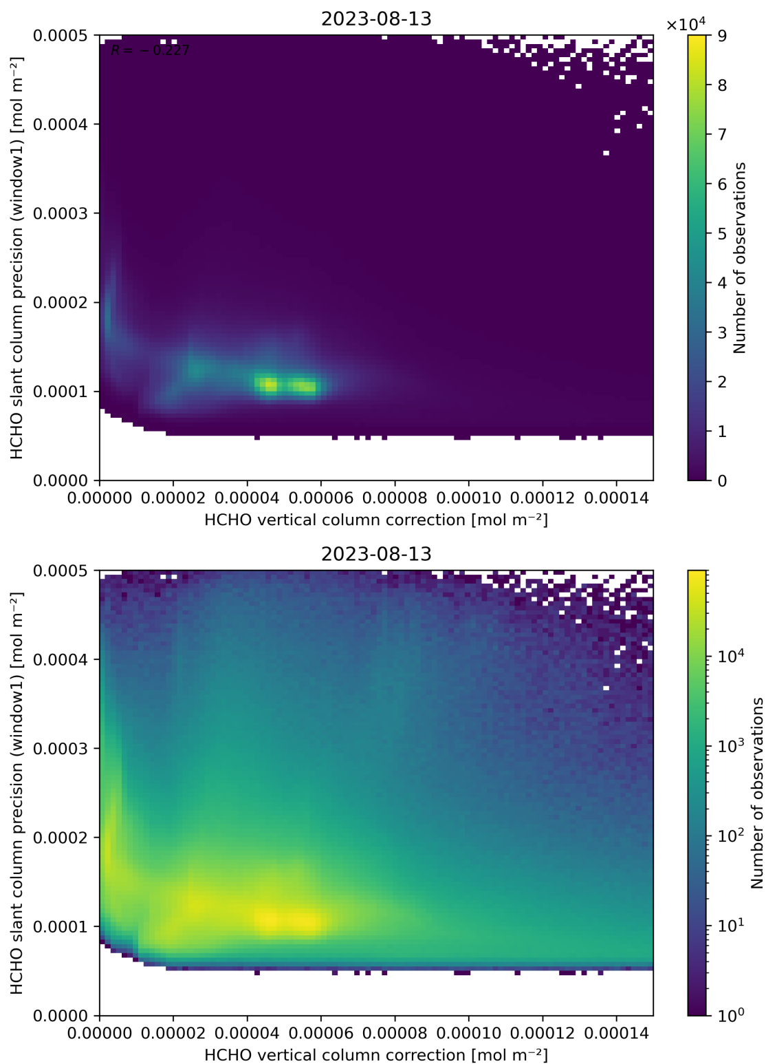
Figure 119: Scatter density plot of “HCHO vertical column correction” against “HCHO slant column precision (window1)” for 2023-08-12 to 2023-08-14.
