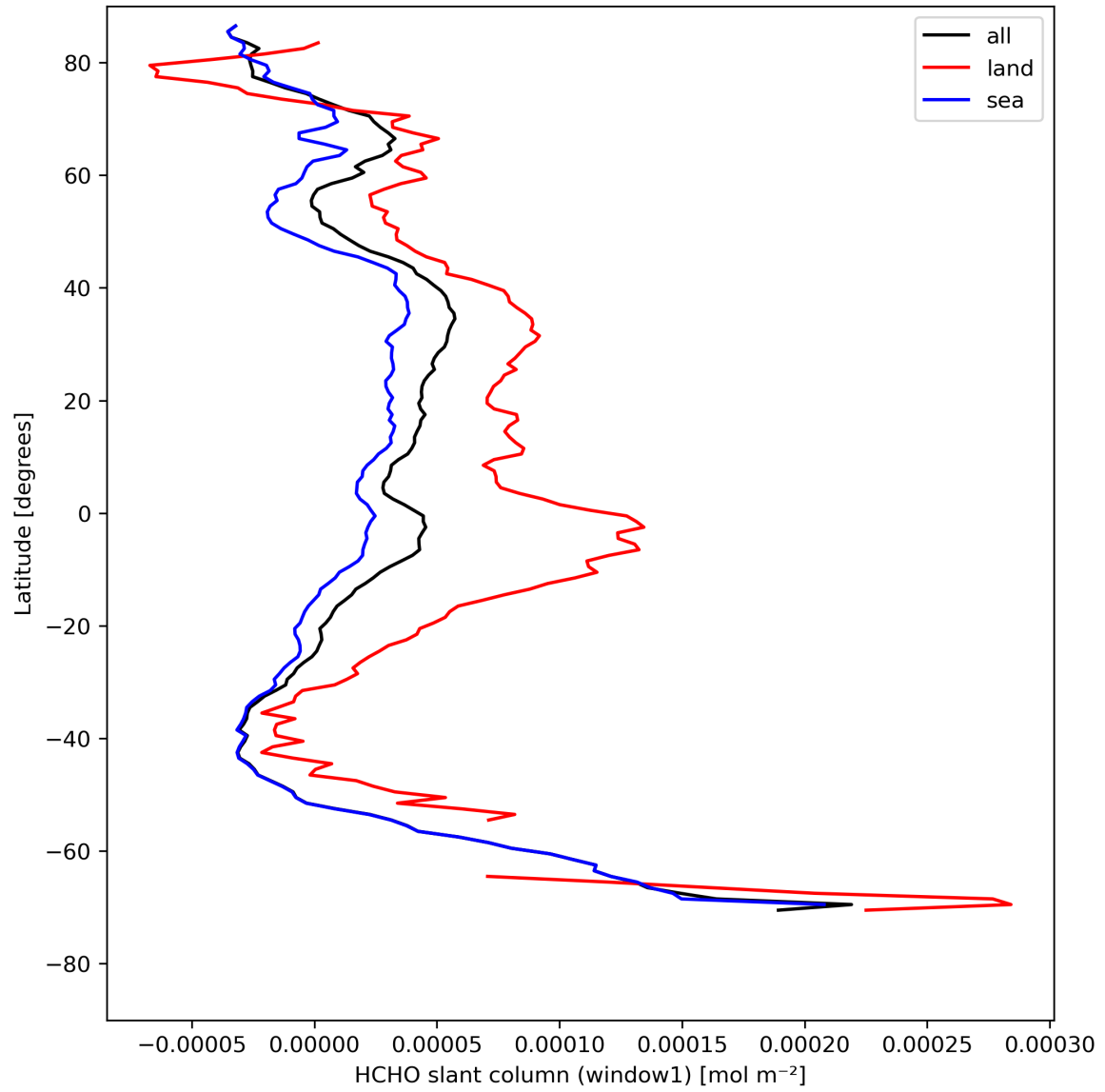
Figure 24: Zonal average of “HCHO slant column (window1)” for 2023-08-12 to 2023-08-14.
