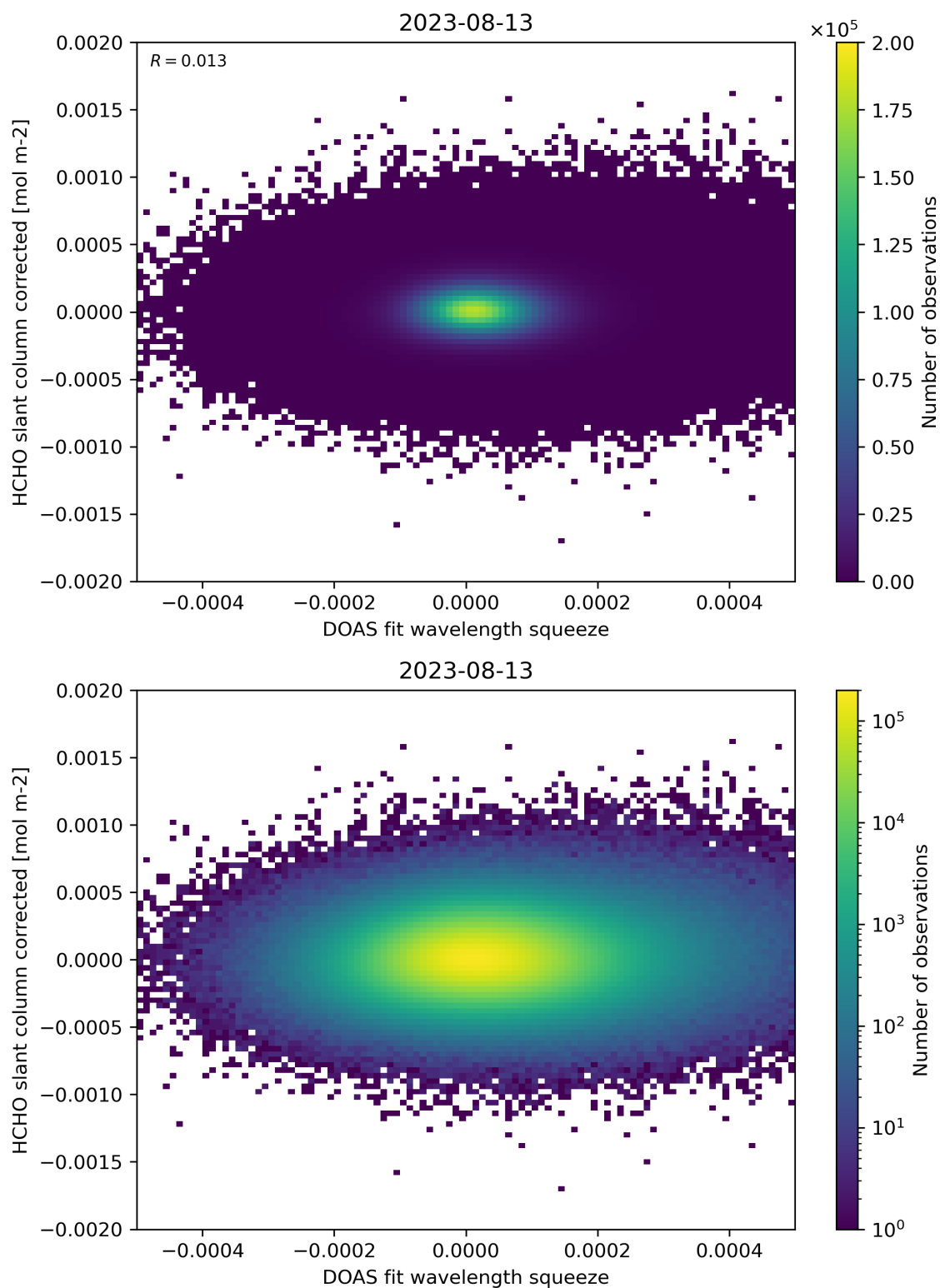
Figure 69: Scatter density plot of “DOAS fit wavelength squeeze” against “HCHO slant column corrected” for 2023-08-12 to 2023-08-14.
