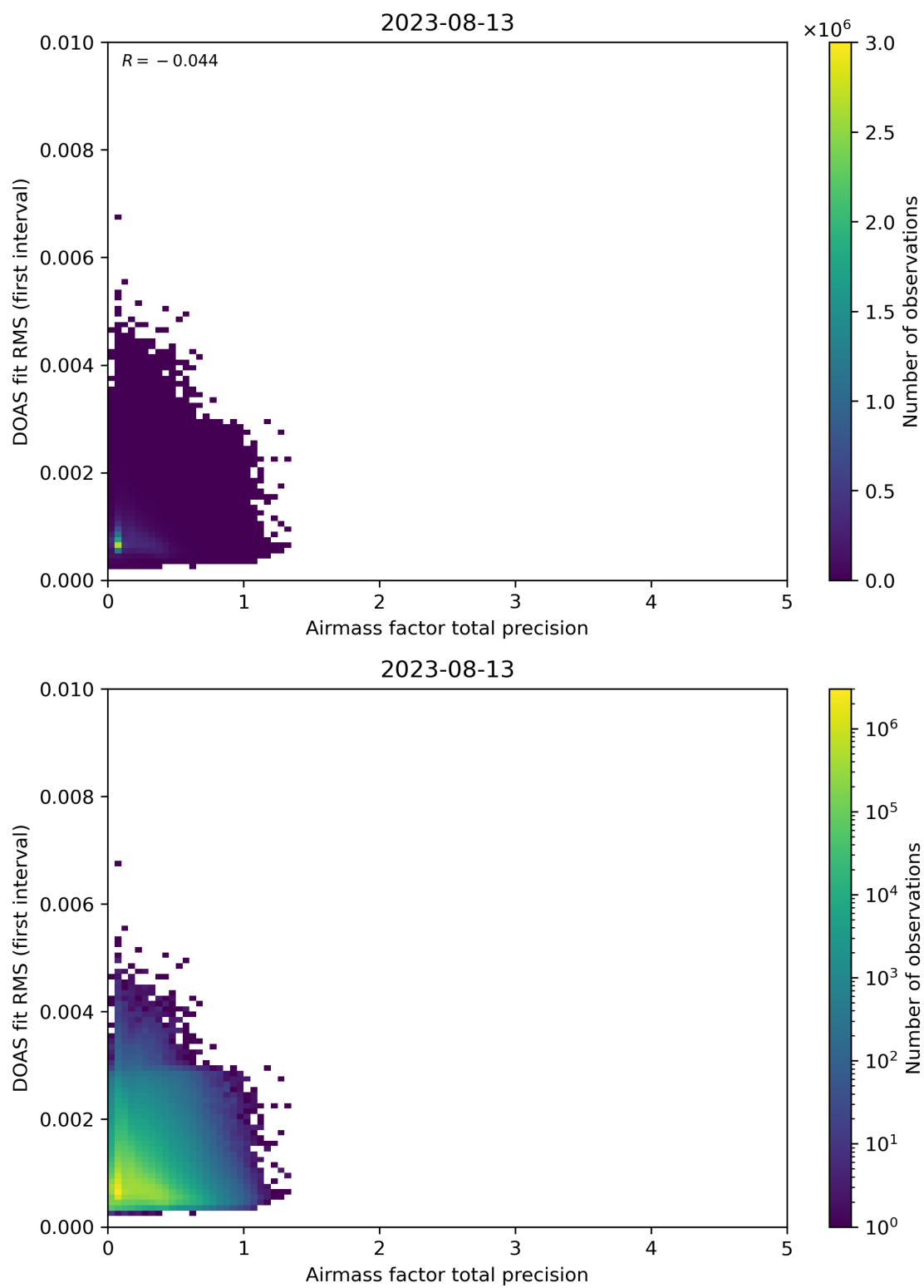
Figure 105: Scatter density plot of “Airmass factor total precision” against “DOAS fit RMS (first interval)” for 2023-08-12 to 2023-08-14.
