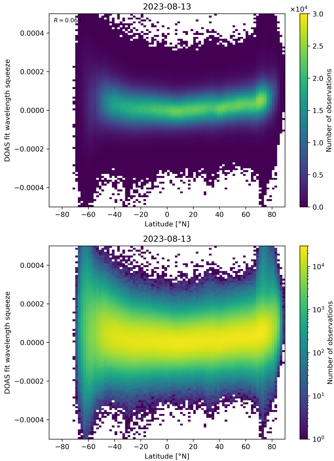
Figure 155: Scatter density plot of “Latitude” against “DOAS fit wavelength squeeze” for 2023-08-12 to 2023-08-14.
