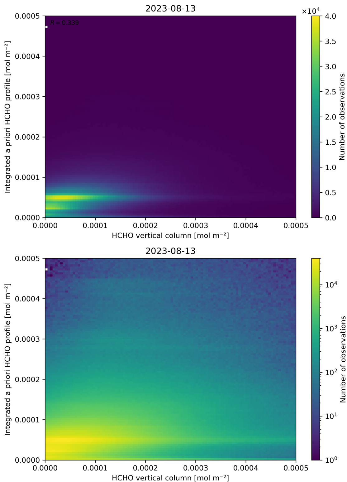
Figure 135: Scatter density plot of “HCHO vertical column” against “Integrated a priori HCHO profile” for 2023-08-12 to 2023-08-14.
