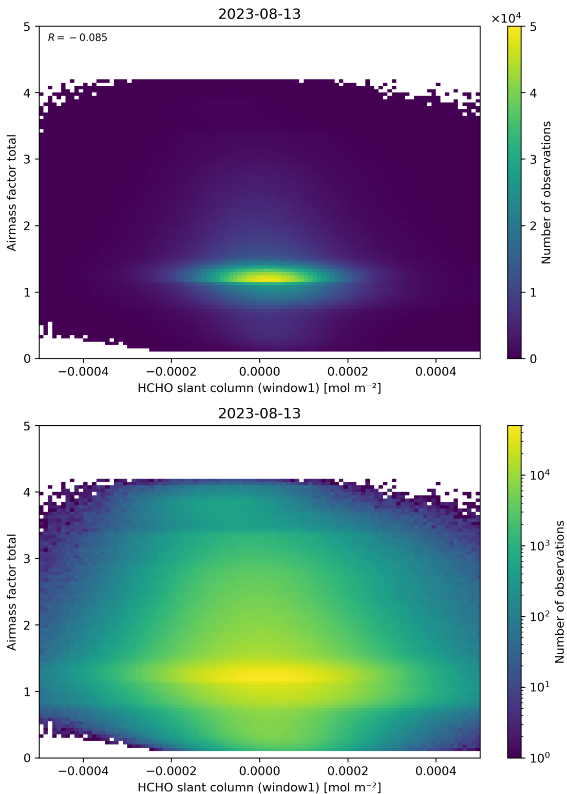
Figure 85: Scatter density plot of “HCHO slant column (window1)” against “Airmass factor total” for 2023-08-12 to 2023-08-14.
