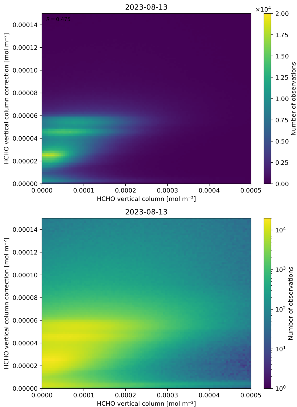
Figure 133: Scatter density plot of “HCHO vertical column” against “HCHO vertical column correction” for 2023-08-12 to 2023-08-14.
