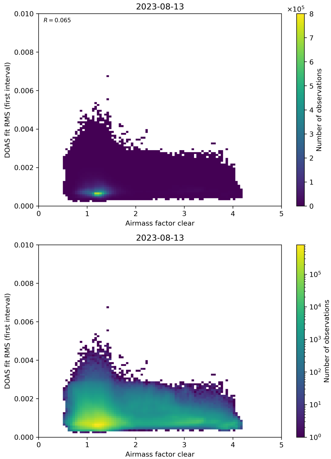
Figure 71: Scatter density plot of “Airmass factor clear” against “DOAS fit RMS (first interval)” for 2023-08-12 to 2023-08-14.
