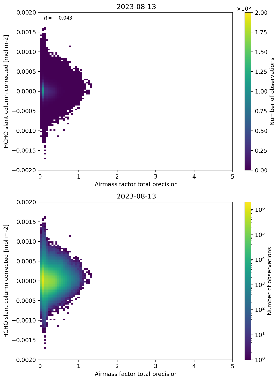
Figure 109: Scatter density plot of “Airmass factor total precision” against “HCHO slant column corrected” for 2023-08-12 to 2023-08-14.
