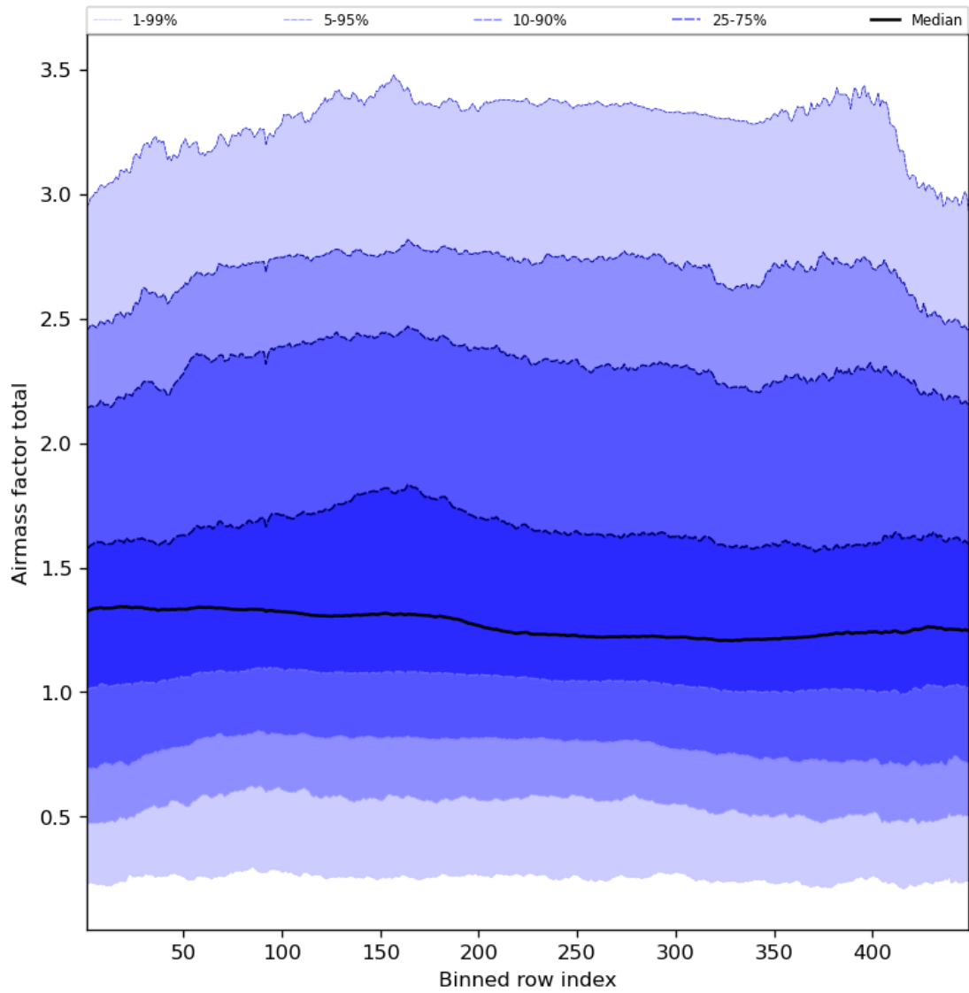
Figure 54: Along track statistics of “Airmass factor total” for 2023-08-12 to 2023-08-14
