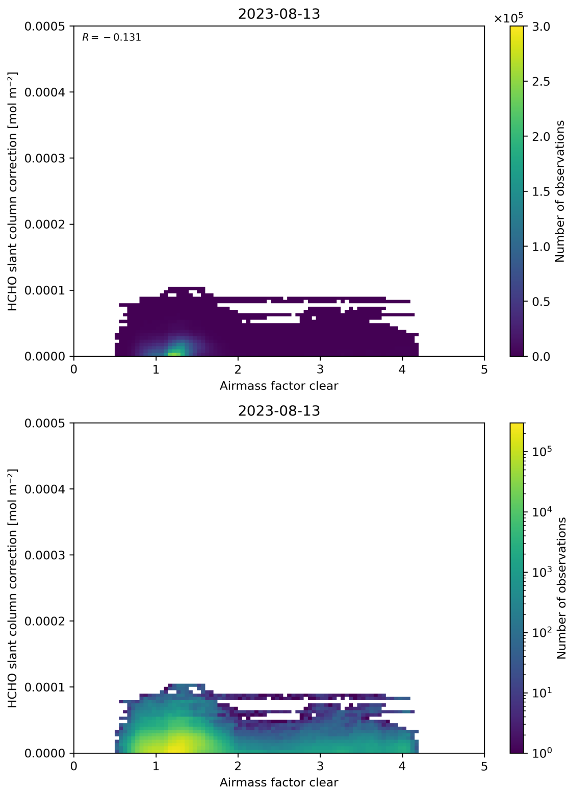
Figure 75: Scatter density plot of “Airmass factor clear” against “HCHO slant column correction” for 2023-08-12 to 2023-08-14.
