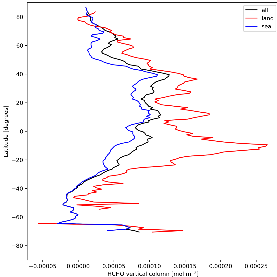
Figure 21: Zonal average of “HCHO vertical column” for 2023-08-12 to 2023-08-14.
