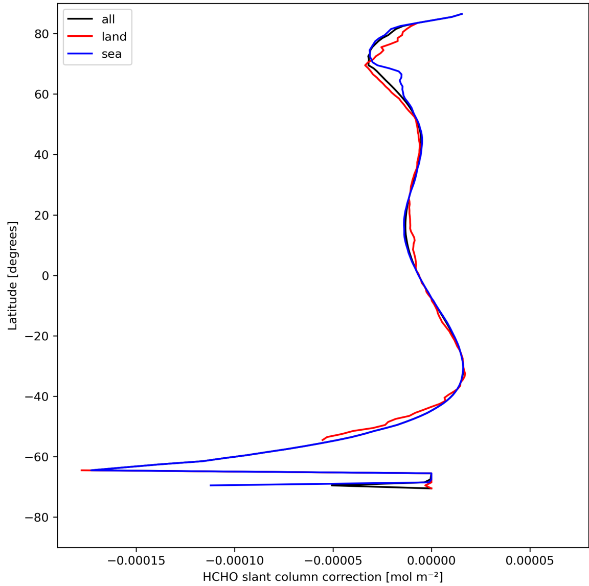
Figure 33: Zonal average of “HCHO slant column correction” for 2023-08-12 to 2023-08-14.
