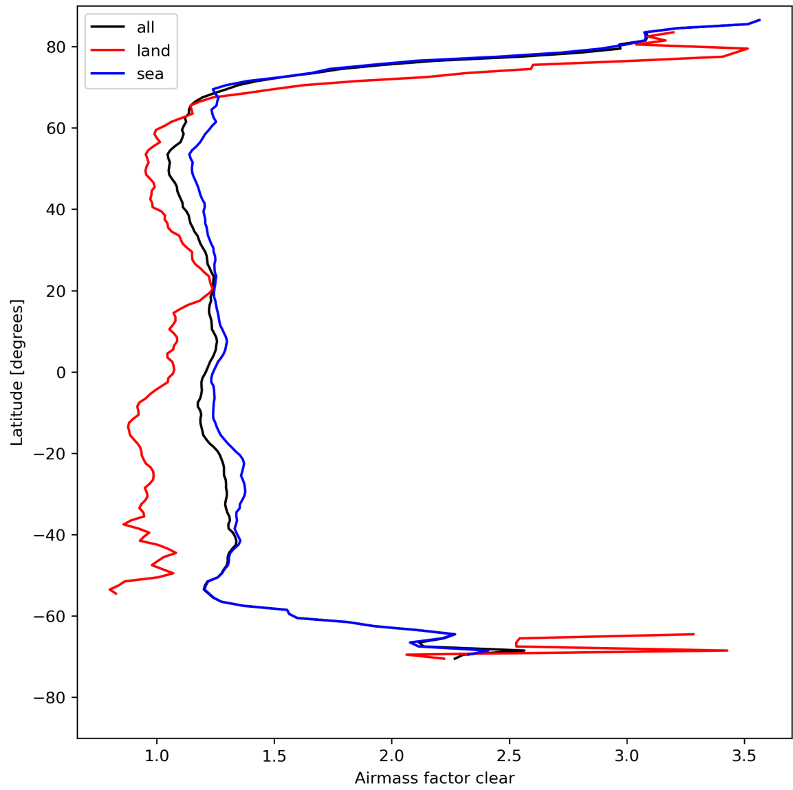
Figure 28: Zonal average of “Airmass factor clear” for 2023-08-12 to 2023-08-14.
