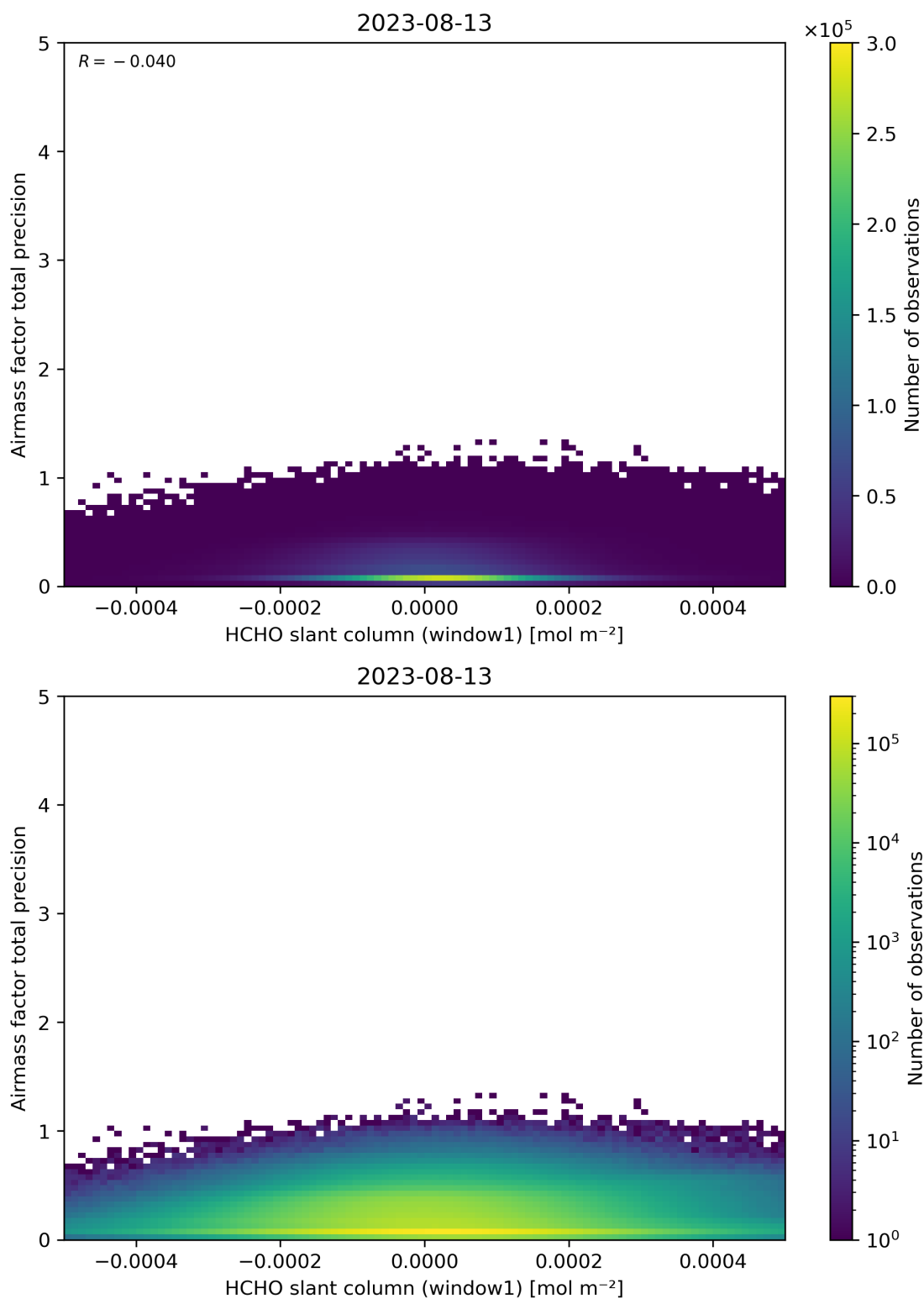
Figure 86: Scatter density plot of “HCHO slant column (window1)” against “Airmass factor total precision” for 2023-08-12 to 2023-08-14.
