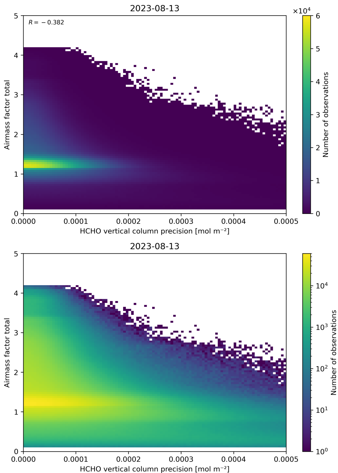
Figure 144: Scatter density plot of “HCHO vertical column precision” against “Airmass factor total” for 2023-08-12 to 2023-08-14.
