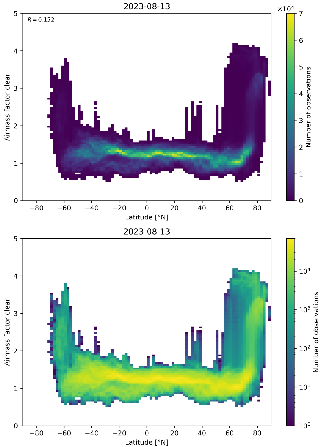
Figure 156: Scatter density plot of “Latitude” against “Airmass factor clear” for 2023-08-12 to 2023-08-14.
