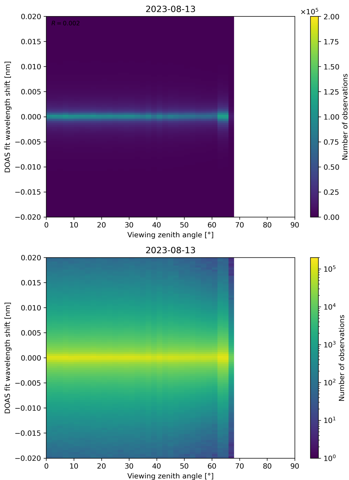
Figure 183: Scatter density plot of “Viewing zenith angle” against “DOAS fit wavelength shift” for 2023-08-12 to 2023-08-14.
