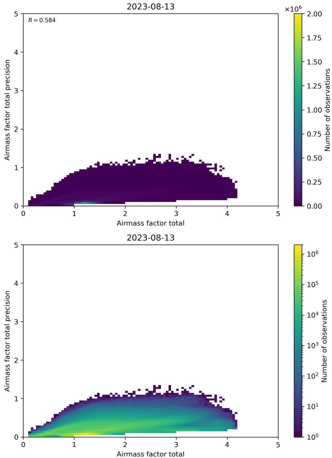
Figure 103: Scatter density plot of “Airmass factor total” against “Airmass factor total precision” for 2023-08-12 to 2023-08-14.
