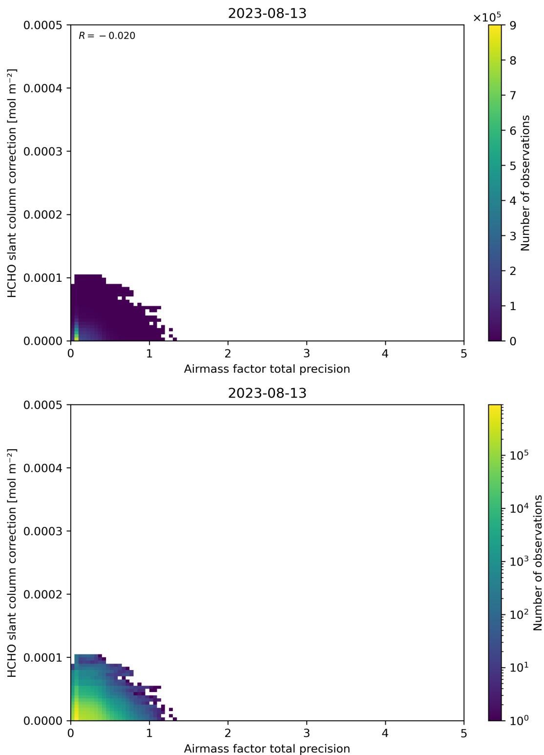
Figure 110: Scatter density plot of “Airmass factor total precision” against “HCHO slant column correction” for 2023-08-12 to 2023-08-14.
