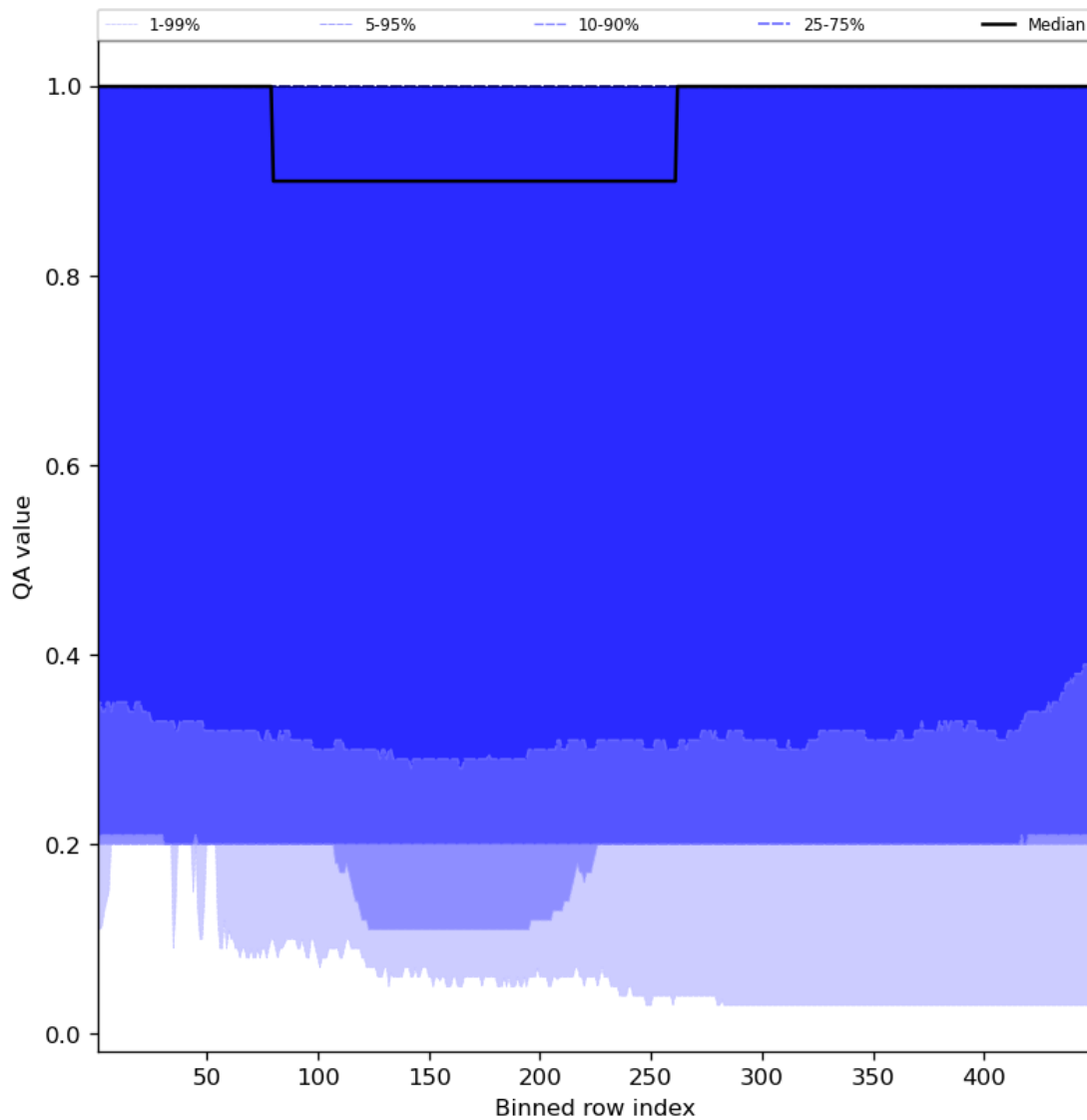
Figure 48: Along track statistics of “QA value” for 2023-08-12 to 2023-08-14
