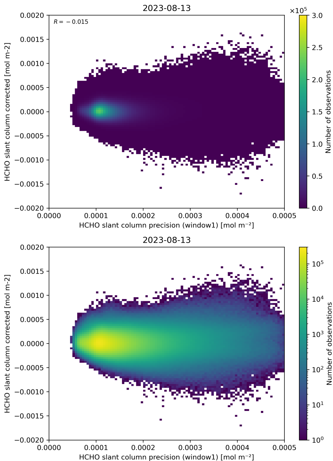
Figure 92: Scatter density plot of “HCHO slant column precision (window1)” against “HCHO slant column corrected” for 2023-08-12 to 2023-08-14.
