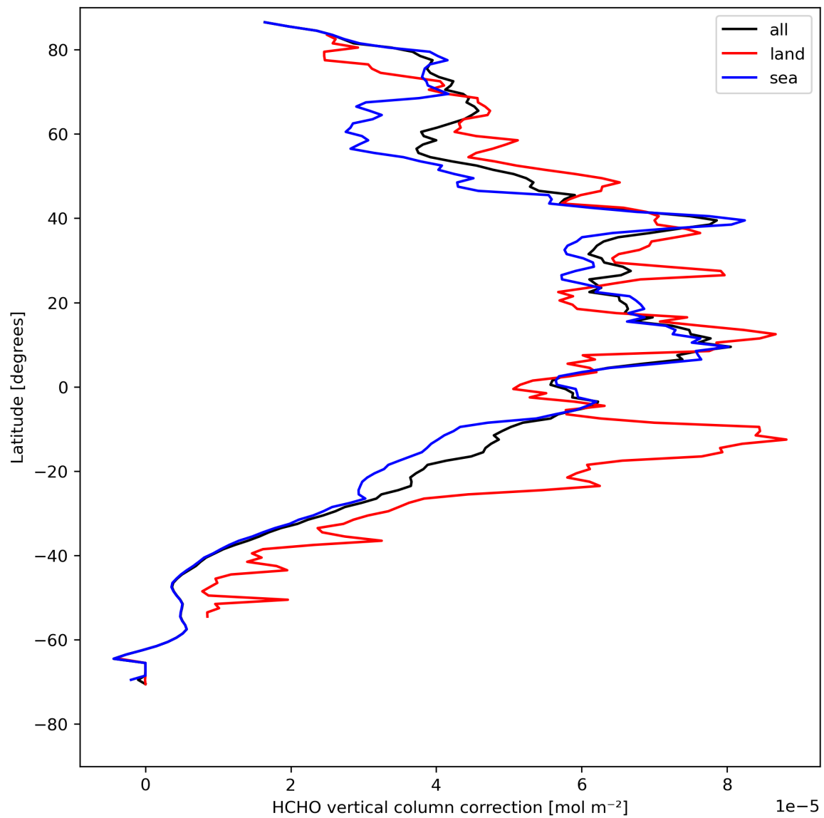
Figure 23: Zonal average of “HCHO vertical column correction” for 2023-08-12 to 2023-08-14.
