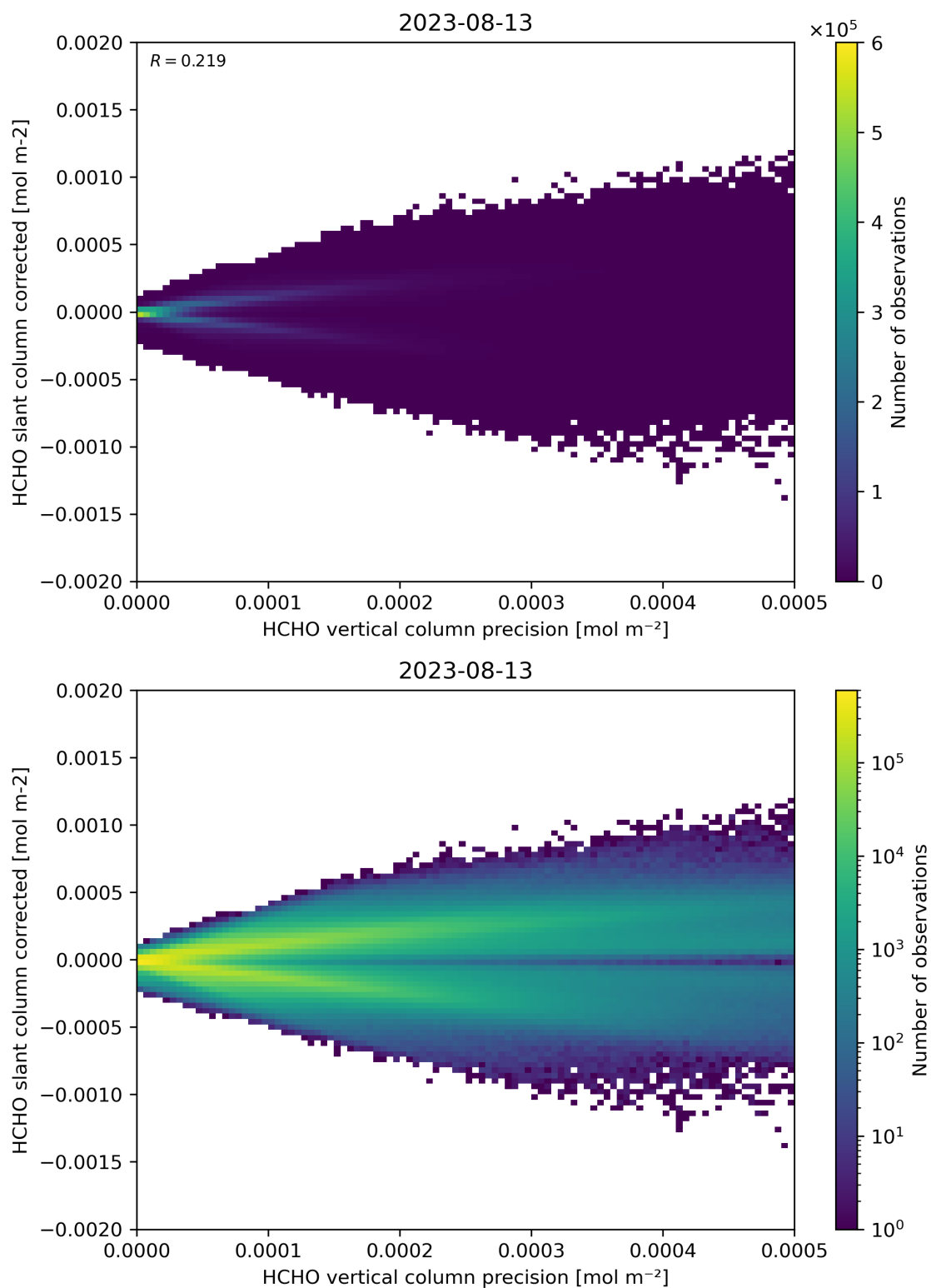
Figure 140: Scatter density plot of “HCHO vertical column precision” against “HCHO slant column corrected” for 2023-08-12 to 2023-08-14.
