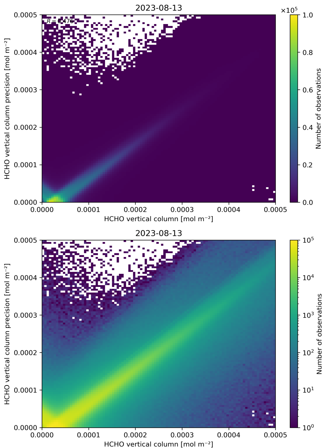
Figure 134: Scatter density plot of “HCHO vertical column” against “HCHO vertical column precision” for 2023-08-12 to 2023-08-14.
