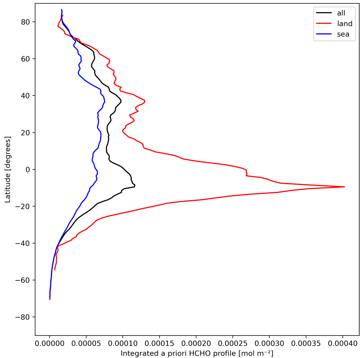
Figure 29: Zonal average of “Integrated a priori HCHO profile” for 2023-08-12 to 2023-08-14.
