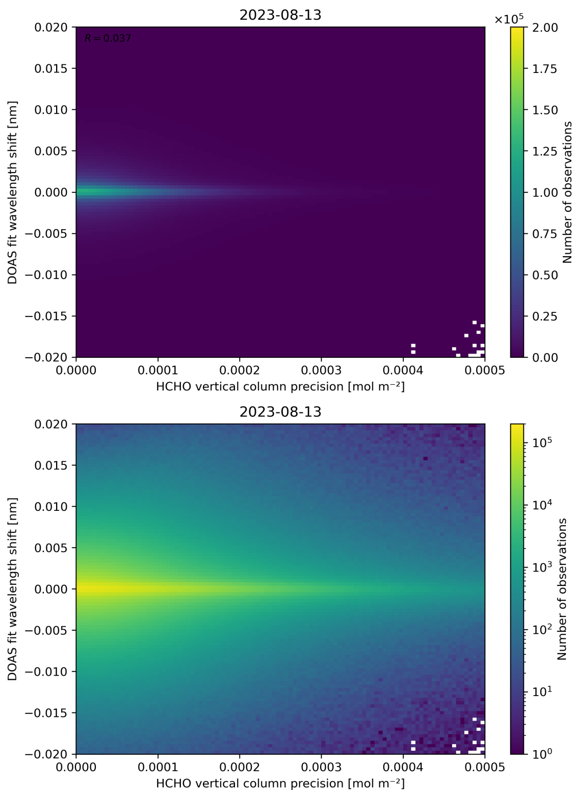
Figure 137: Scatter density plot of “HCHO vertical column precision” against “DOAS fit wavelength shift” for 2023-08-12 to 2023-08-14.
