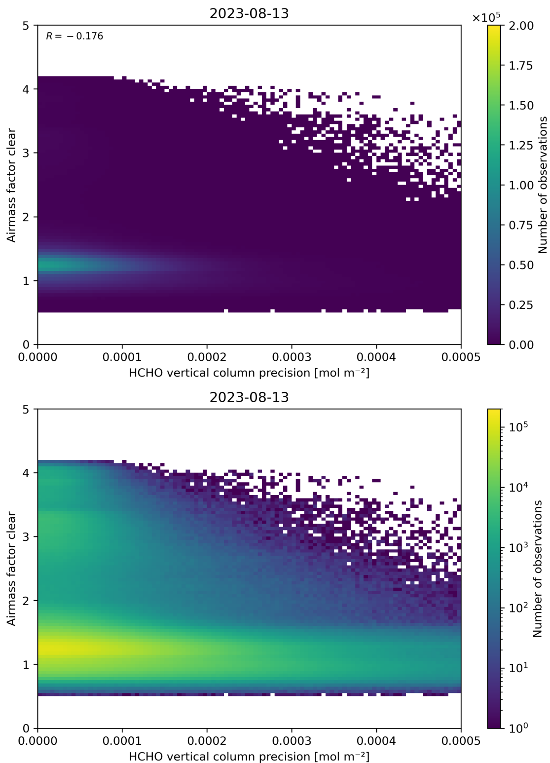
Figure 139: Scatter density plot of “HCHO vertical column precision” against “Airmass factor clear” for 2023-08-12 to 2023-08-14.
