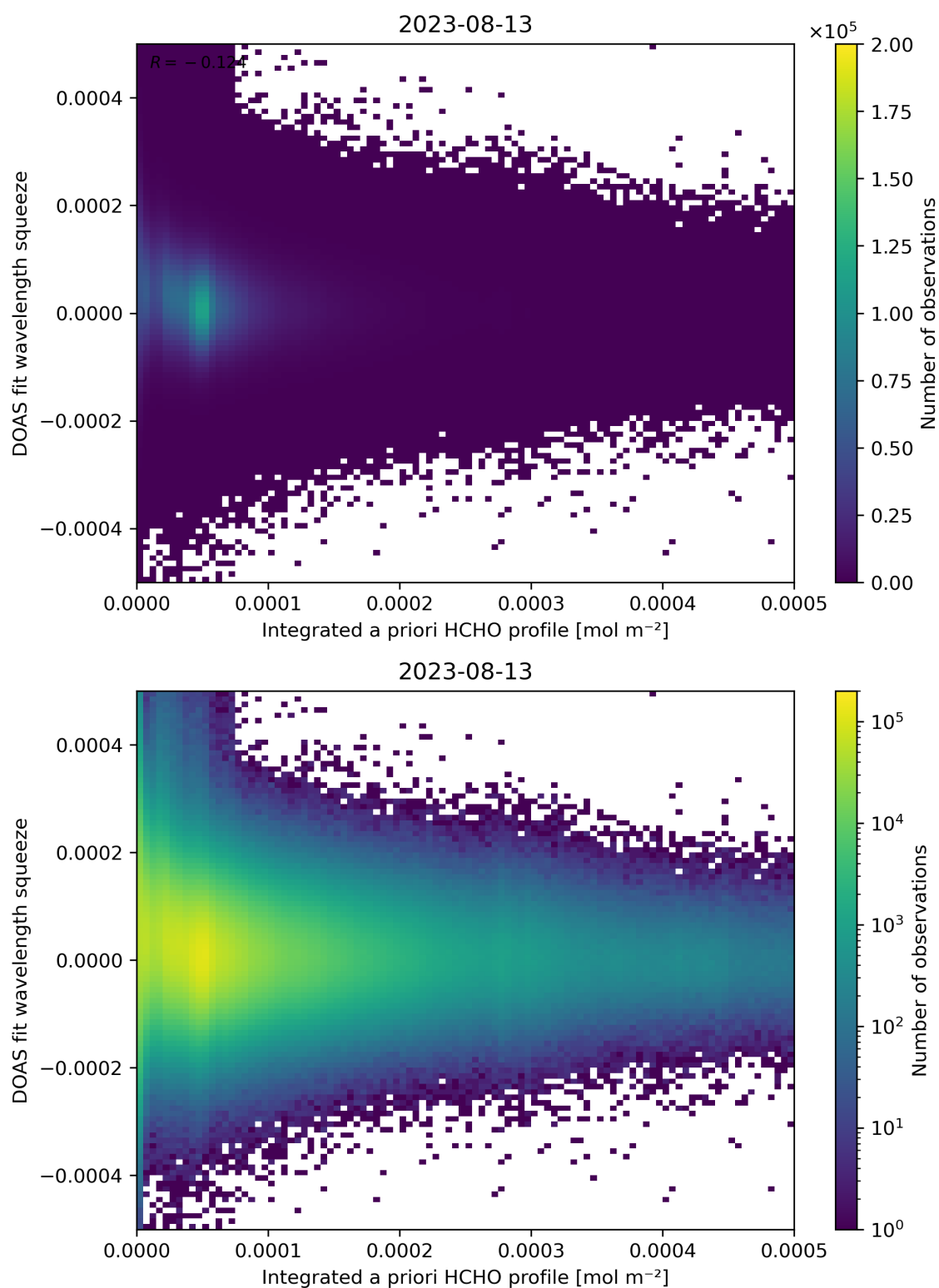
Figure 150: Scatter density plot of “Integrated a priori HCHO profile” against “DOAS fit wavelength squeeze” for 2023-08-12 to 2023-08-14.
