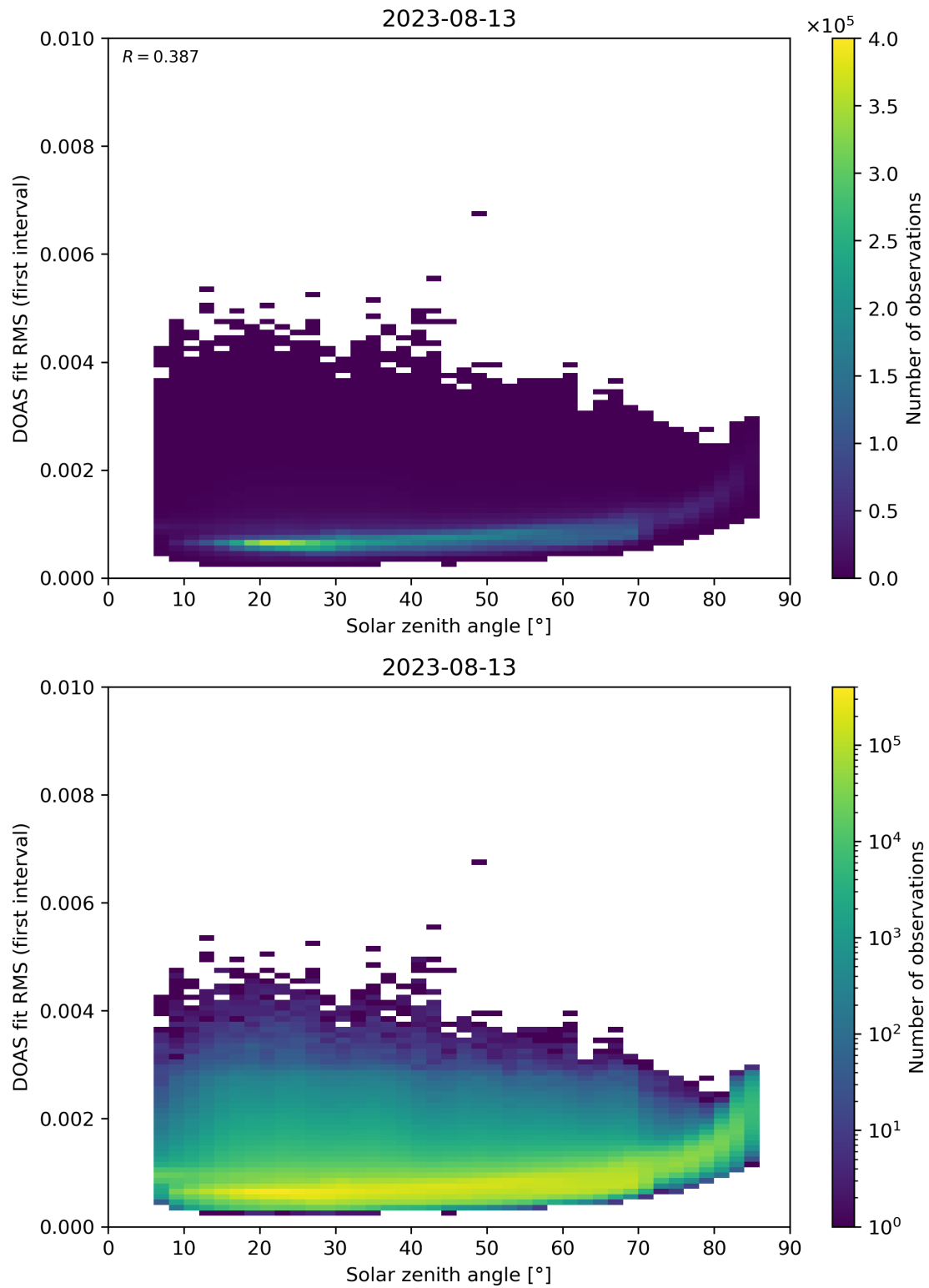
Figure 167: Scatter density plot of “Solar zenith angle” against “DOAS fit RMS (first interval)” for 2023-08-12 to 2023-08-14.
