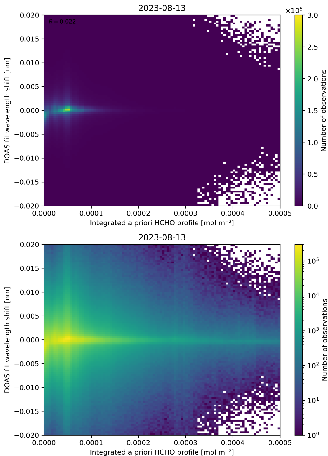
Figure 149: Scatter density plot of “Integrated a priori HCHO profile” against “DOAS fit wavelength shift” for 2023-08-12 to 2023-08-14.
