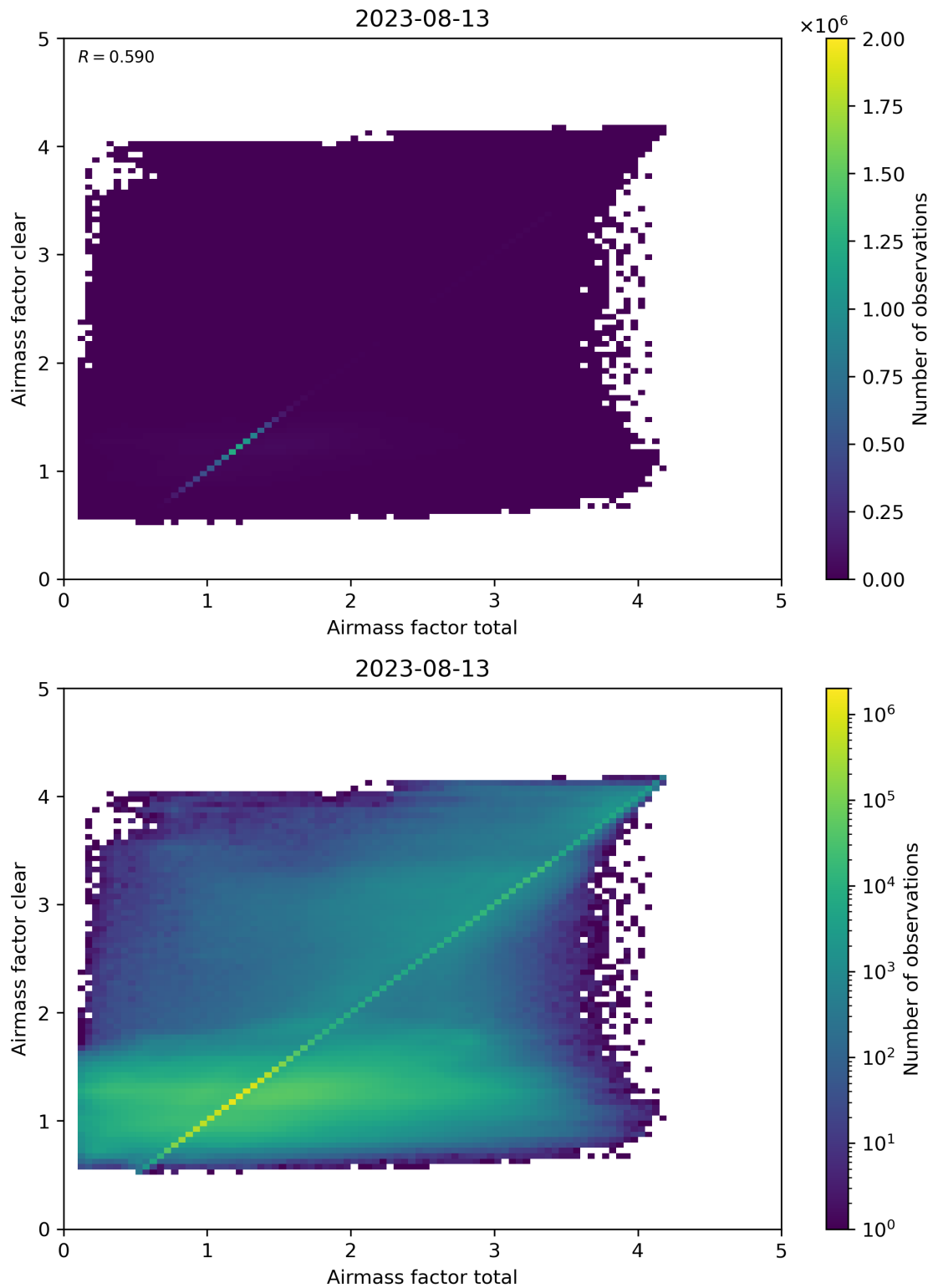
Figure 100: Scatter density plot of “Airmass factor total” against “Airmass factor clear” for 2023-08-12 to 2023-08-14.
