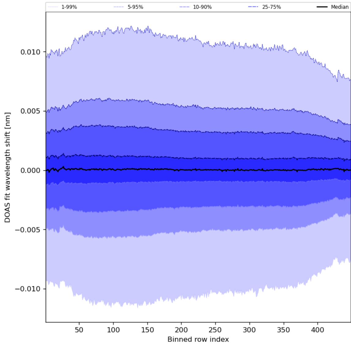
Figure 58: Along track statistics of “DOAS fit wavelength shift” for 2023-08-12 to 2023-08-14
