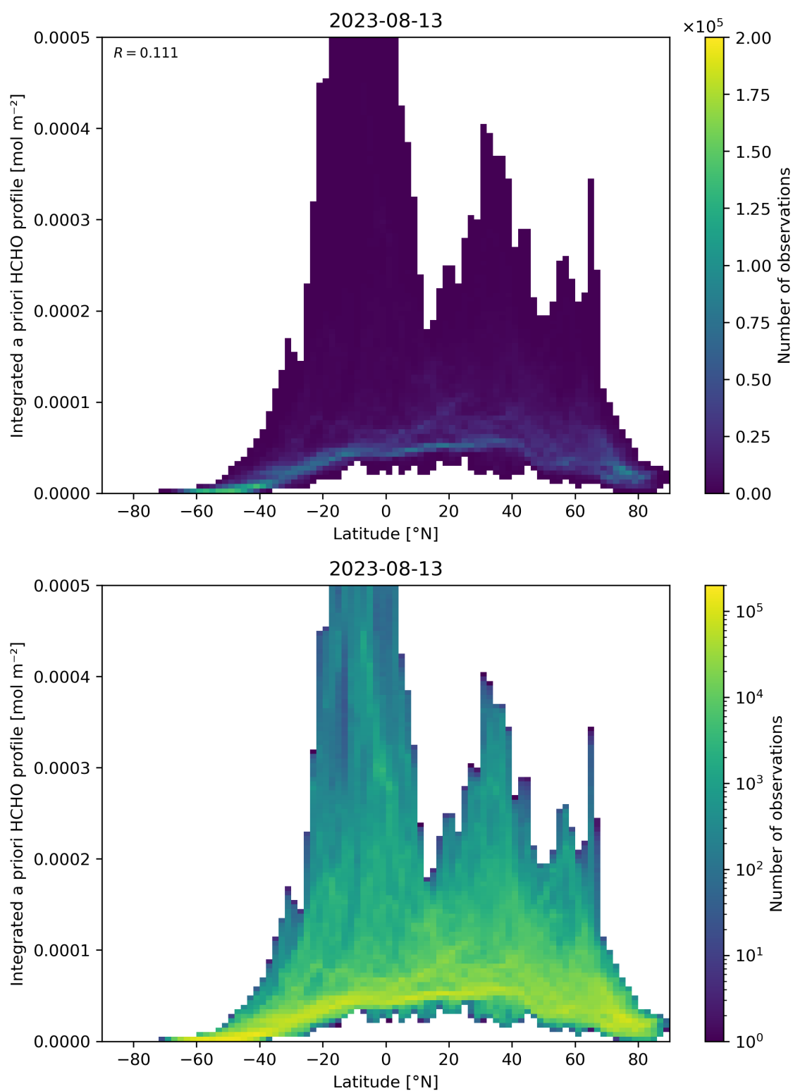
Figure 166: Scatter density plot of “Latitude” against “Integrated a priori HCHO profile” for 2023-08-12 to 2023-08-14.
