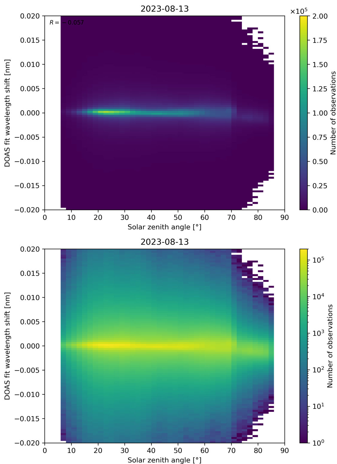
Figure 168: Scatter density plot of “Solar zenith angle” against “DOAS fit wavelength shift” for 2023-08-12 to 2023-08-14.
