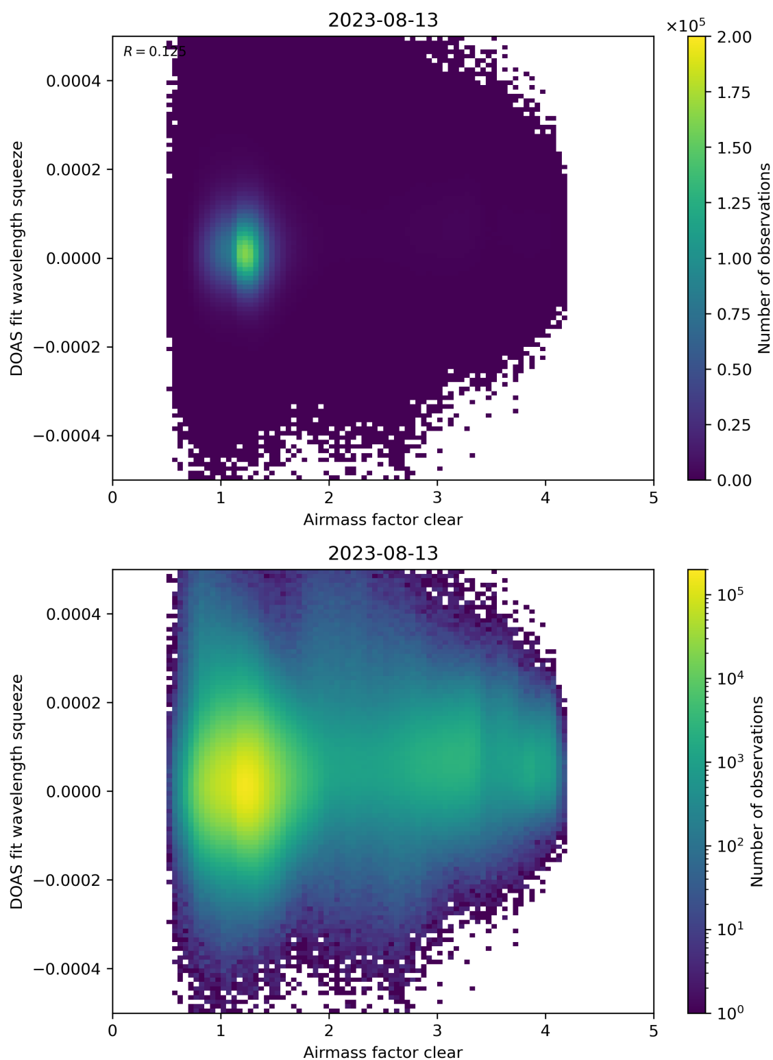
Figure 73: Scatter density plot of “Airmass factor clear” against “DOAS fit wavelength squeeze” for 2023-08-12 to 2023-08-14.
