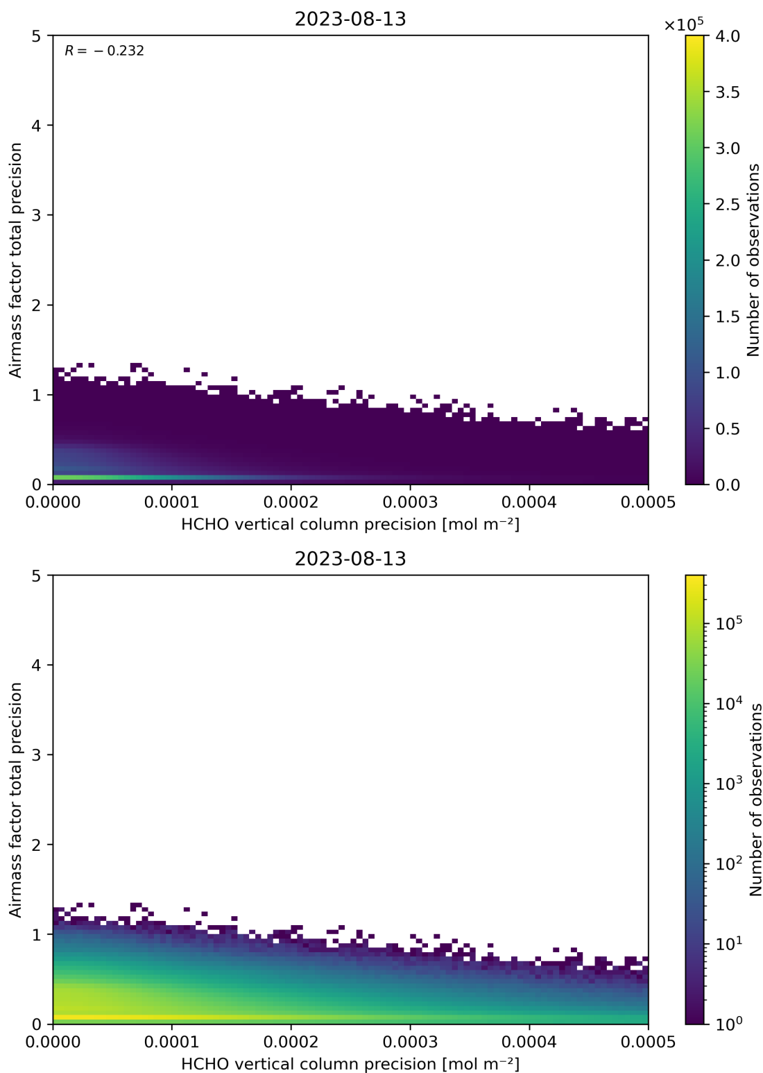
Figure 145: Scatter density plot of “HCHO vertical column precision” against “Airmass factor total precision” for 2023-08-12 to 2023-08-14.
