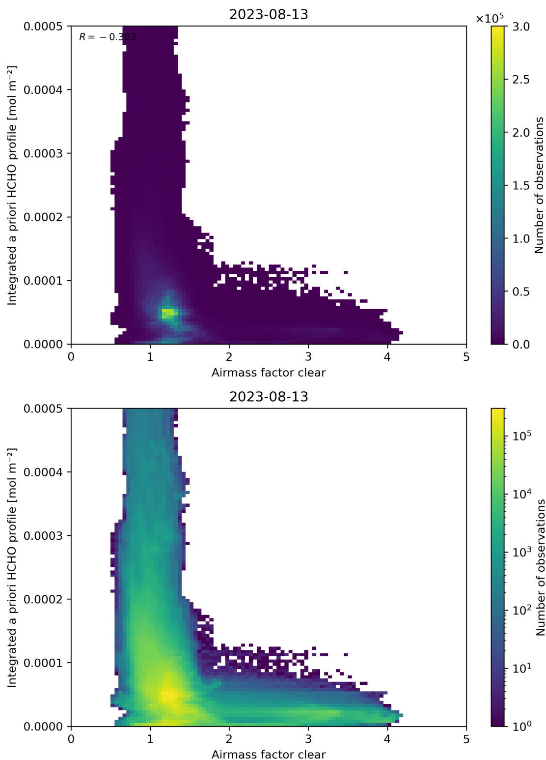
Figure 76: Scatter density plot of “Airmass factor clear” against “Integrated a priori HCHO profile” for 2023-08-12 to 2023-08-14.
