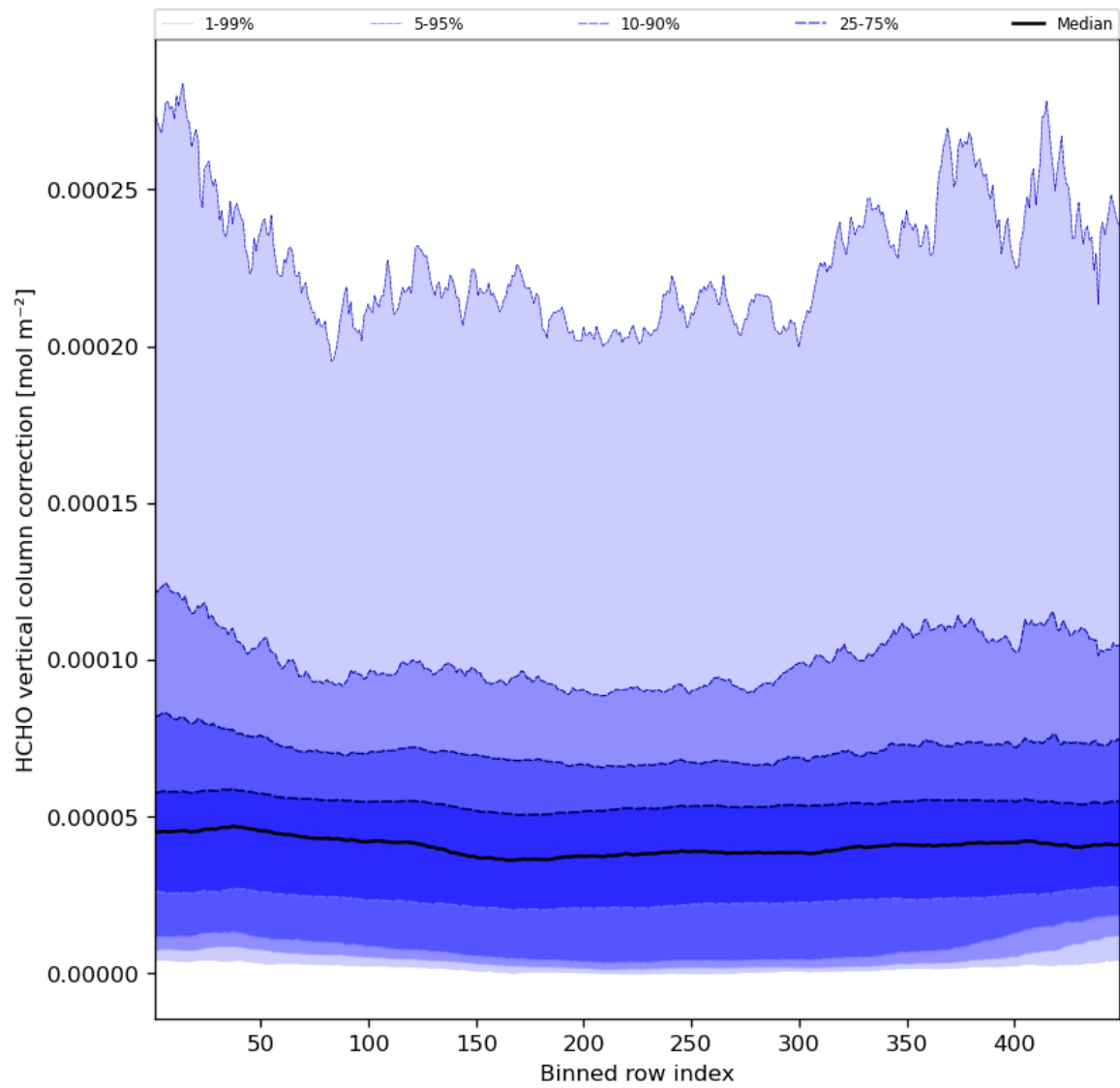
Figure 51: Along track statistics of “HCHO vertical column correction” for 2023-08-12 to 2023-08-14
