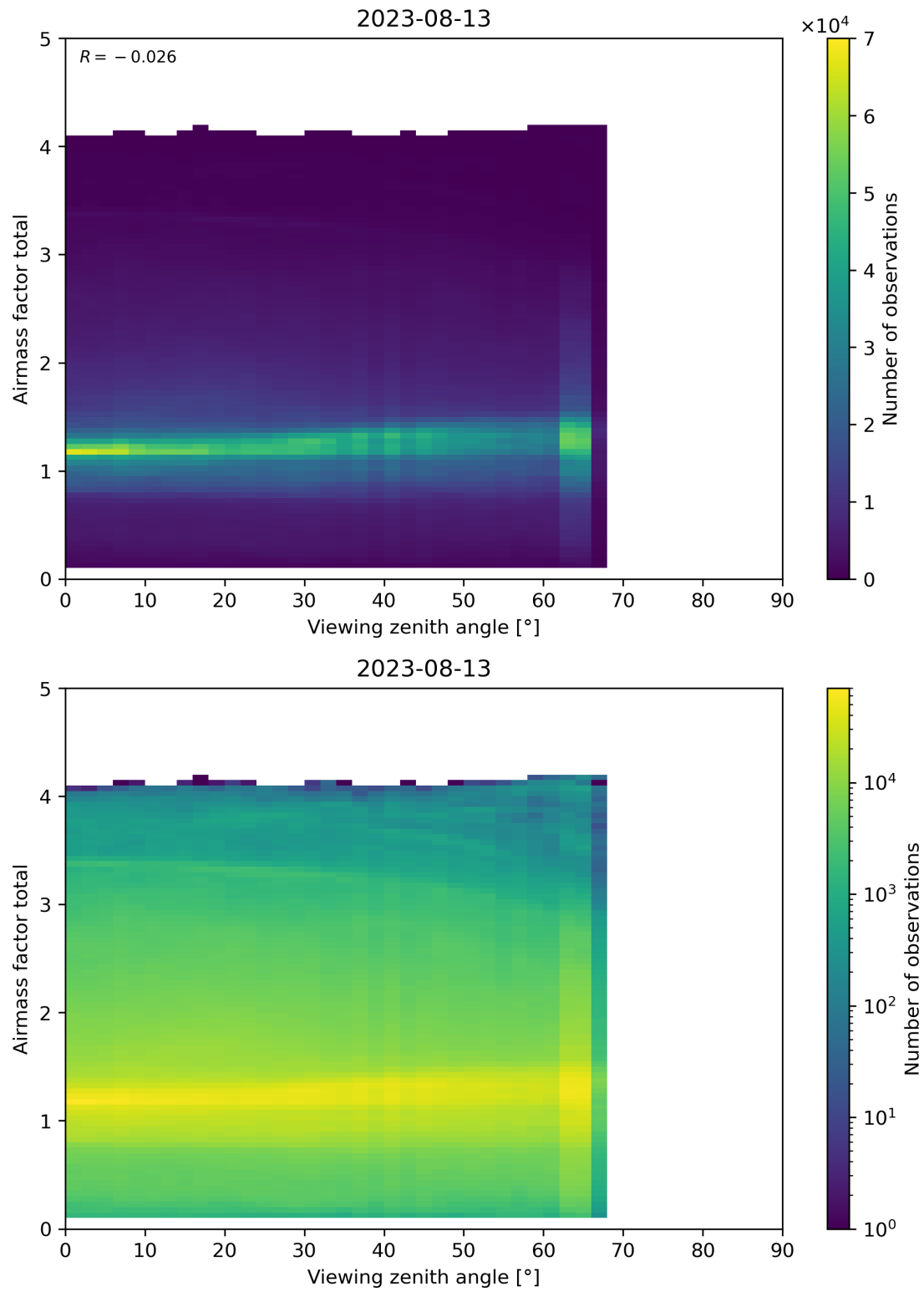
Figure 190: Scatter density plot of “Viewing zenith angle” against “Airmass factor total” for 2023-08-12 to 2023-08-14.
