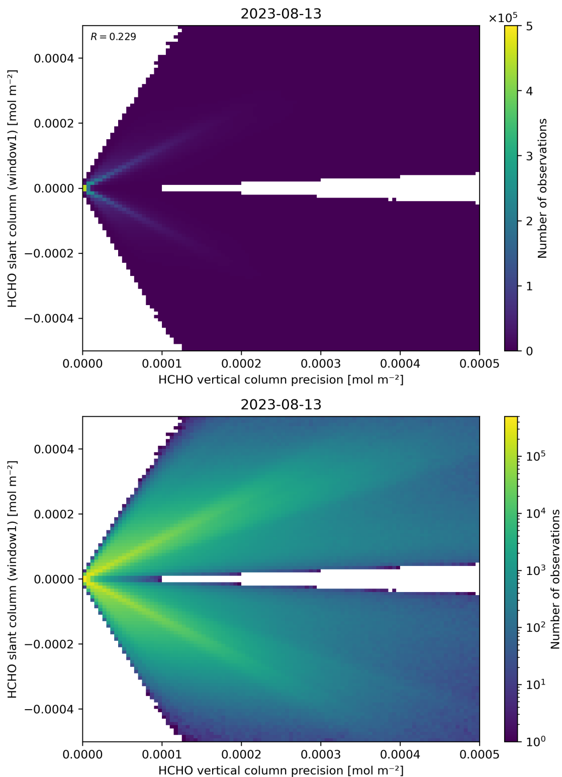
Figure 142: Scatter density plot of “HCHO vertical column precision” against “HCHO slant column (window1)” for 2023-08-12 to 2023-08-14.
