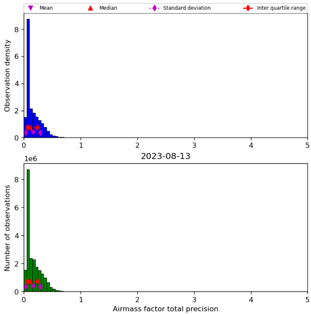
Figure 41: Histogram of “Airmass factor total precision” for 2023-08-12 to 2023-08-14
