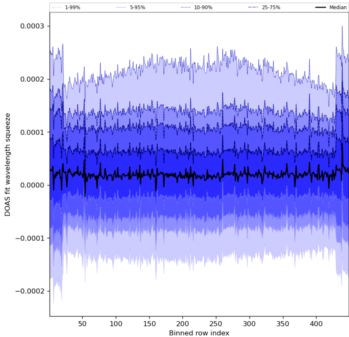
Figure 59: Along track statistics of “DOAS fit wavelength squeeze” for 2023-08-12 to 2023-08-14
