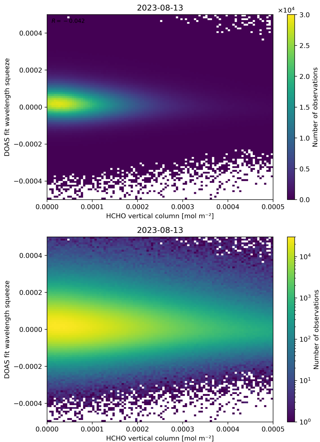
Figure 125: Scatter density plot of “HCHO vertical column” against “DOAS fit wavelength squeeze” for 2023-08-12 to 2023-08-14.
