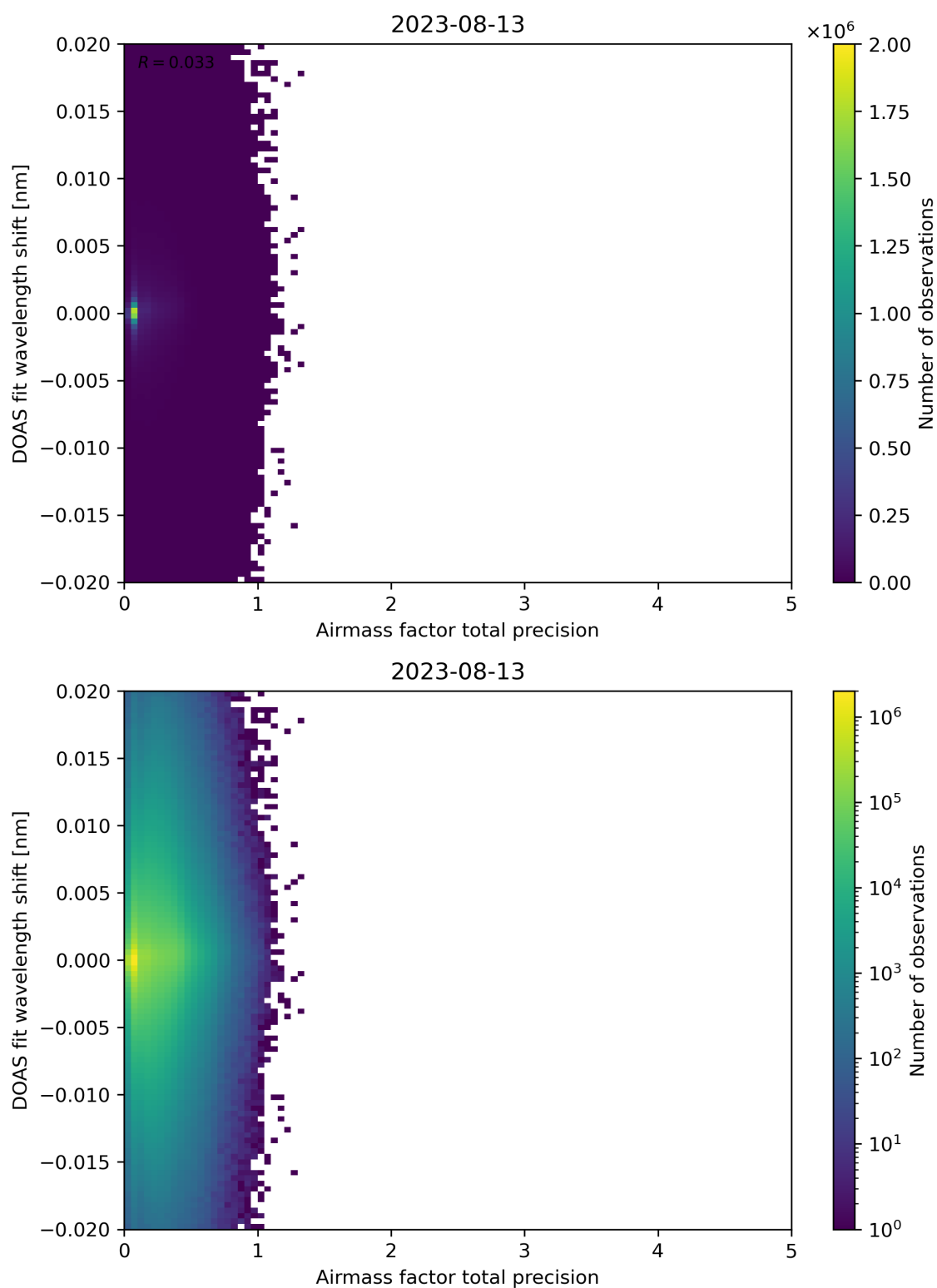
Figure 106: Scatter density plot of “Airmass factor total precision” against “DOAS fit wavelength shift” for 2023-08-12 to 2023-08-14.
