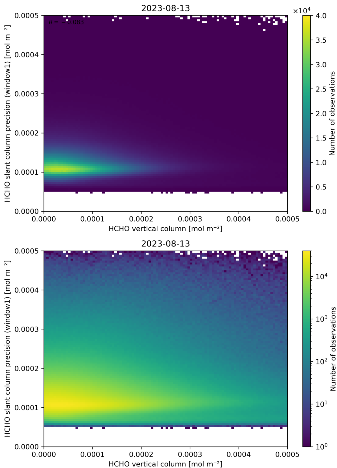
Figure 130: Scatter density plot of “HCHO vertical column” against “HCHO slant column precision (window1)” for 2023-08-12 to 2023-08-14.
