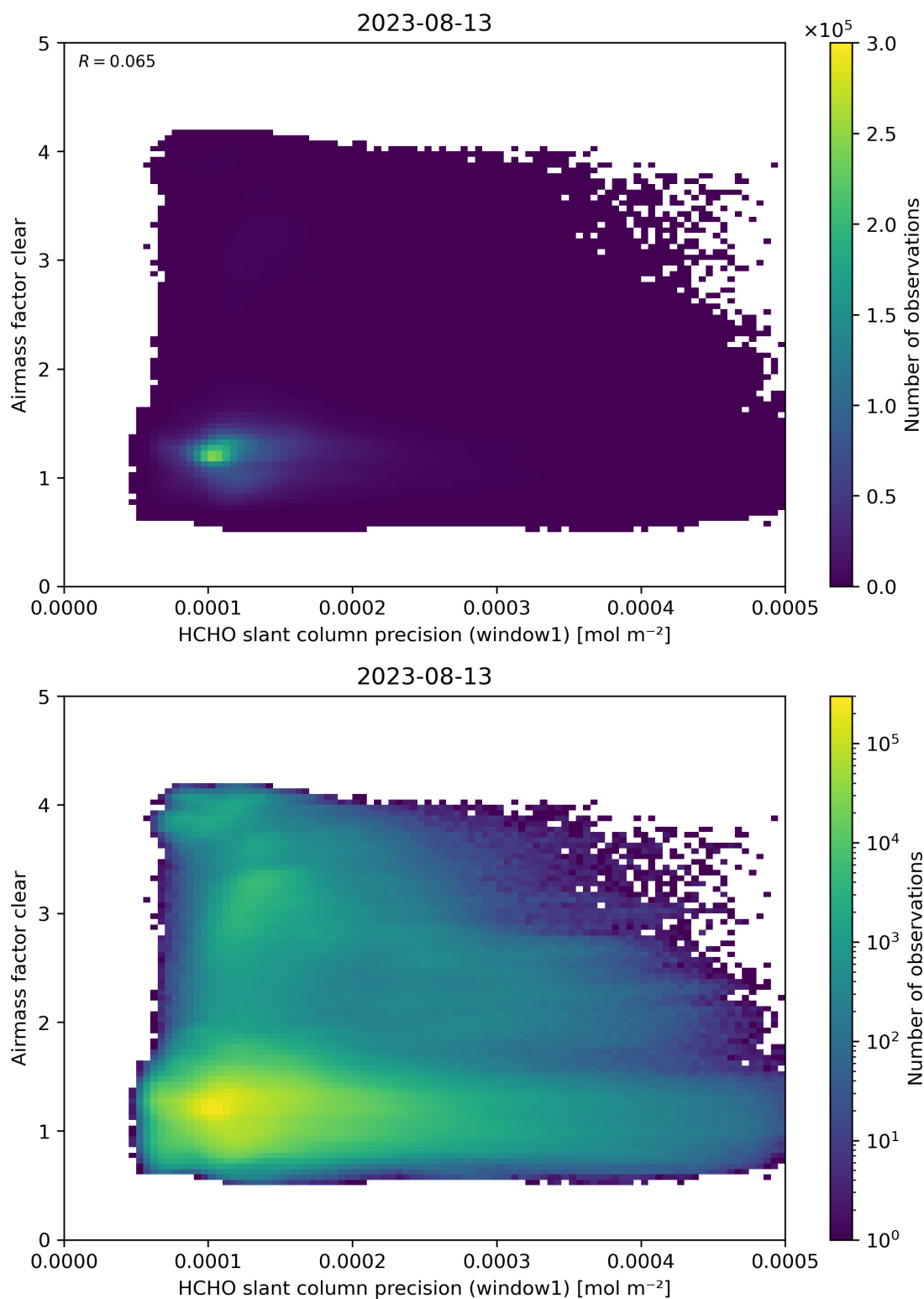
Figure 91: Scatter density plot of “HCHO slant column precision (window1)” against “Airmass factor clear” for 2023-08-12 to 2023-08-14.
