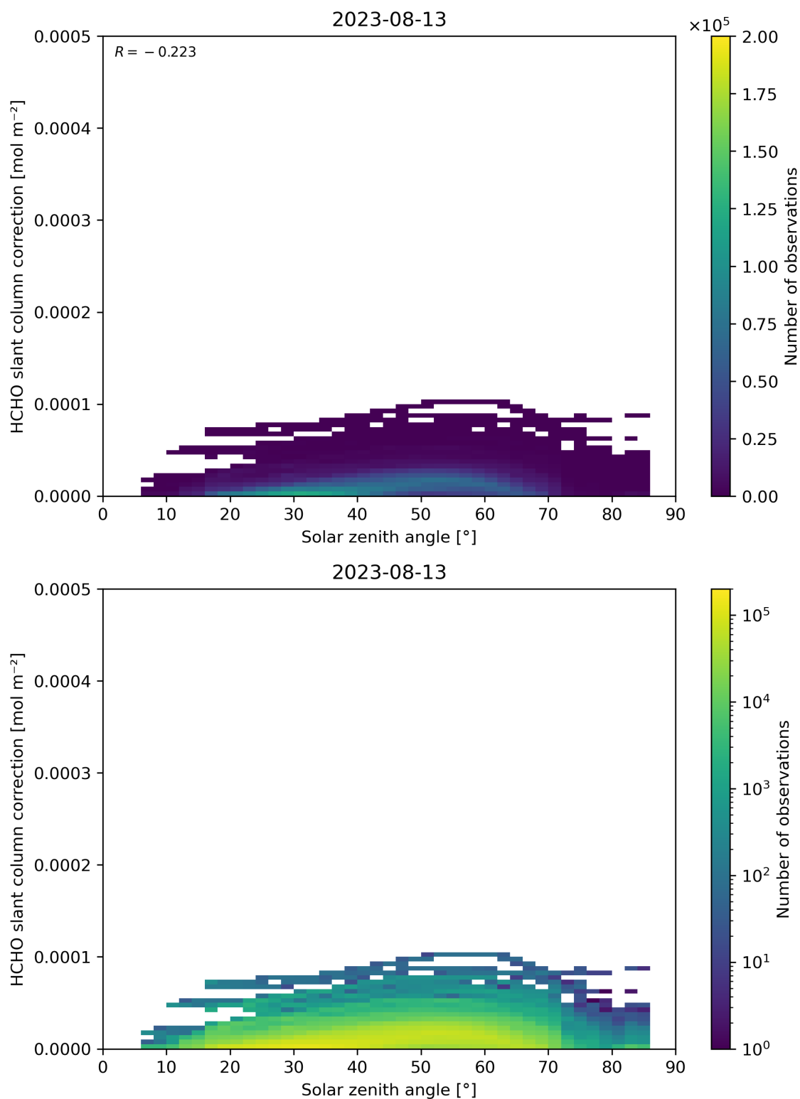
Figure 172: Scatter density plot of “Solar zenith angle” against “HCHO slant column correction” for 2023-08-12 to 2023-08-14.
