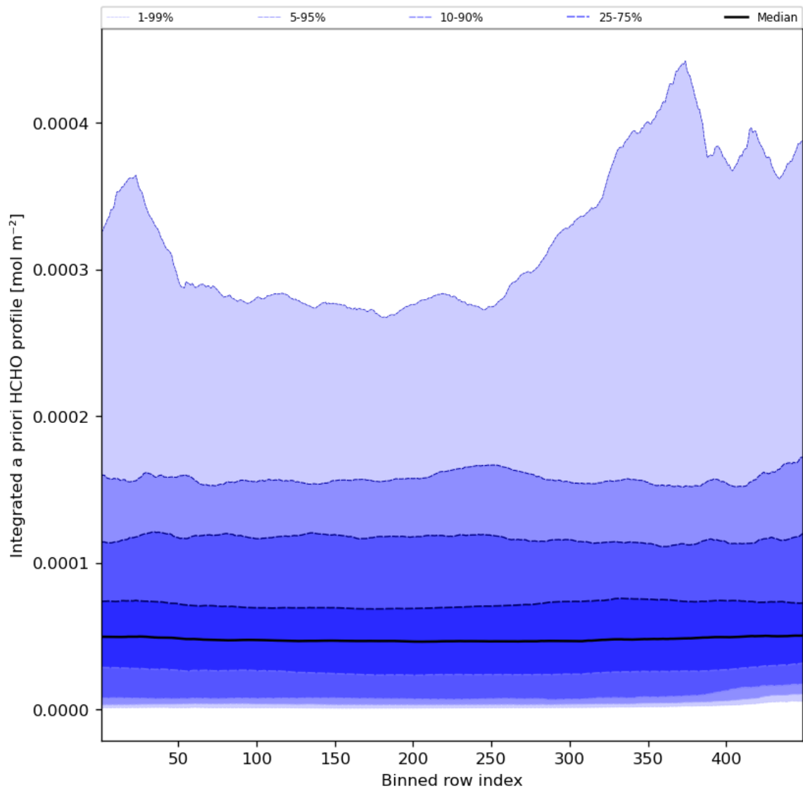
Figure 57: Along track statistics of “Integrated a priori HCHO profile” for 2023-08-12 to 2023-08-14
