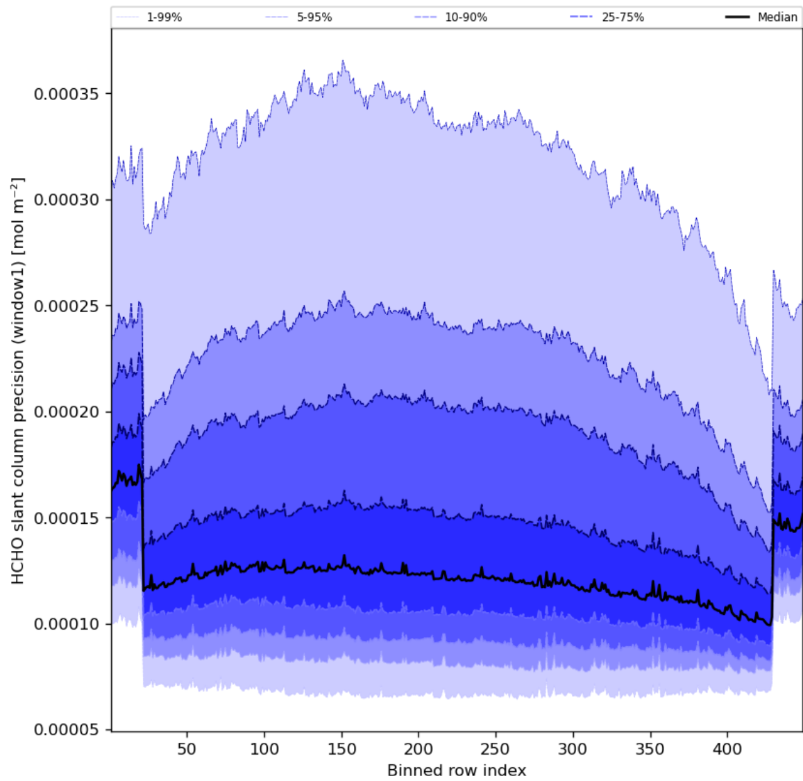
Figure 53: Along track statistics of “HCHO slant column precision (window1)” for 2023-08-12 to 2023-08-14
