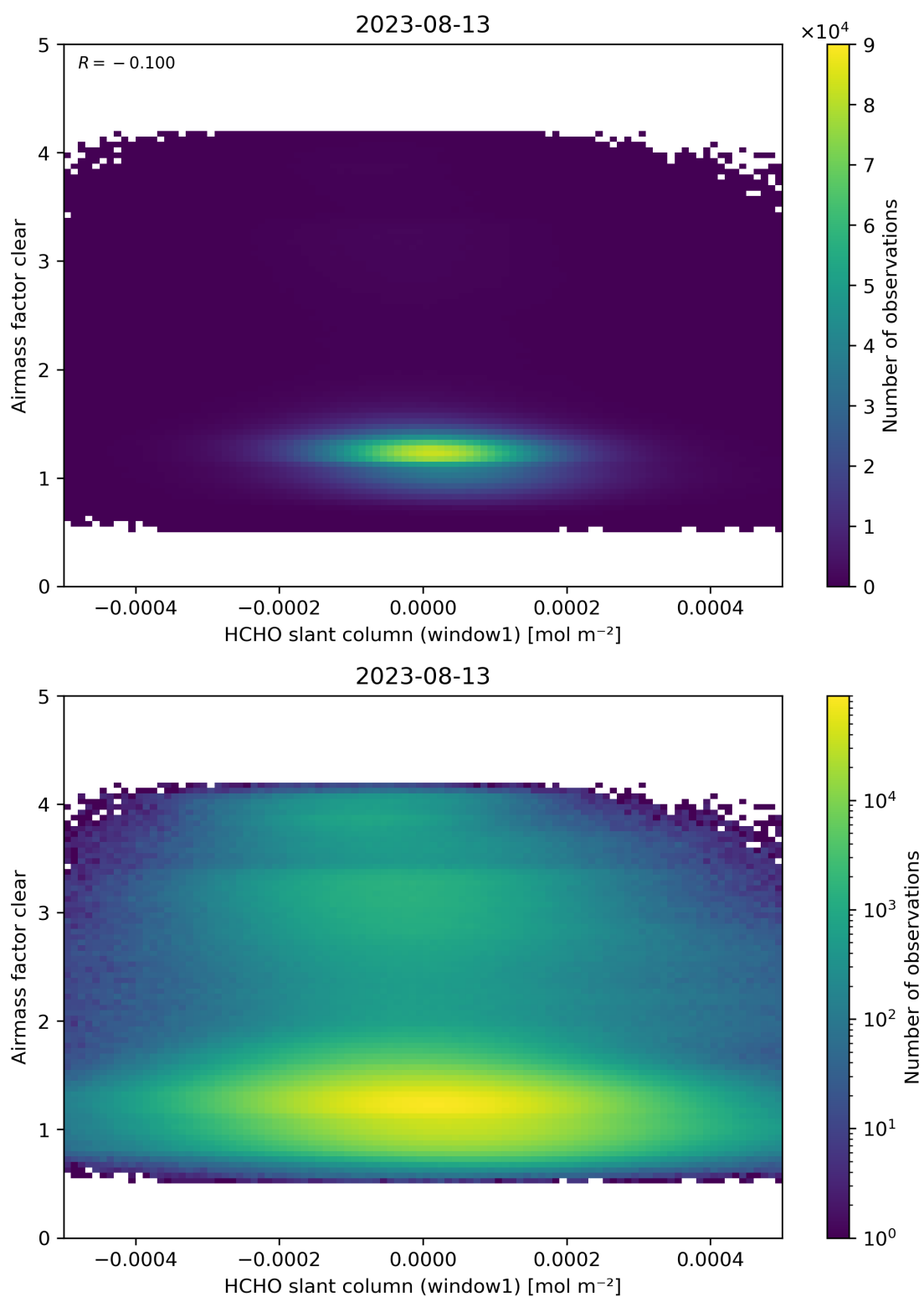
Figure 81: Scatter density plot of “HCHO slant column (window1)” against “Airmass factor clear” for 2023-08-12 to 2023-08-14.
