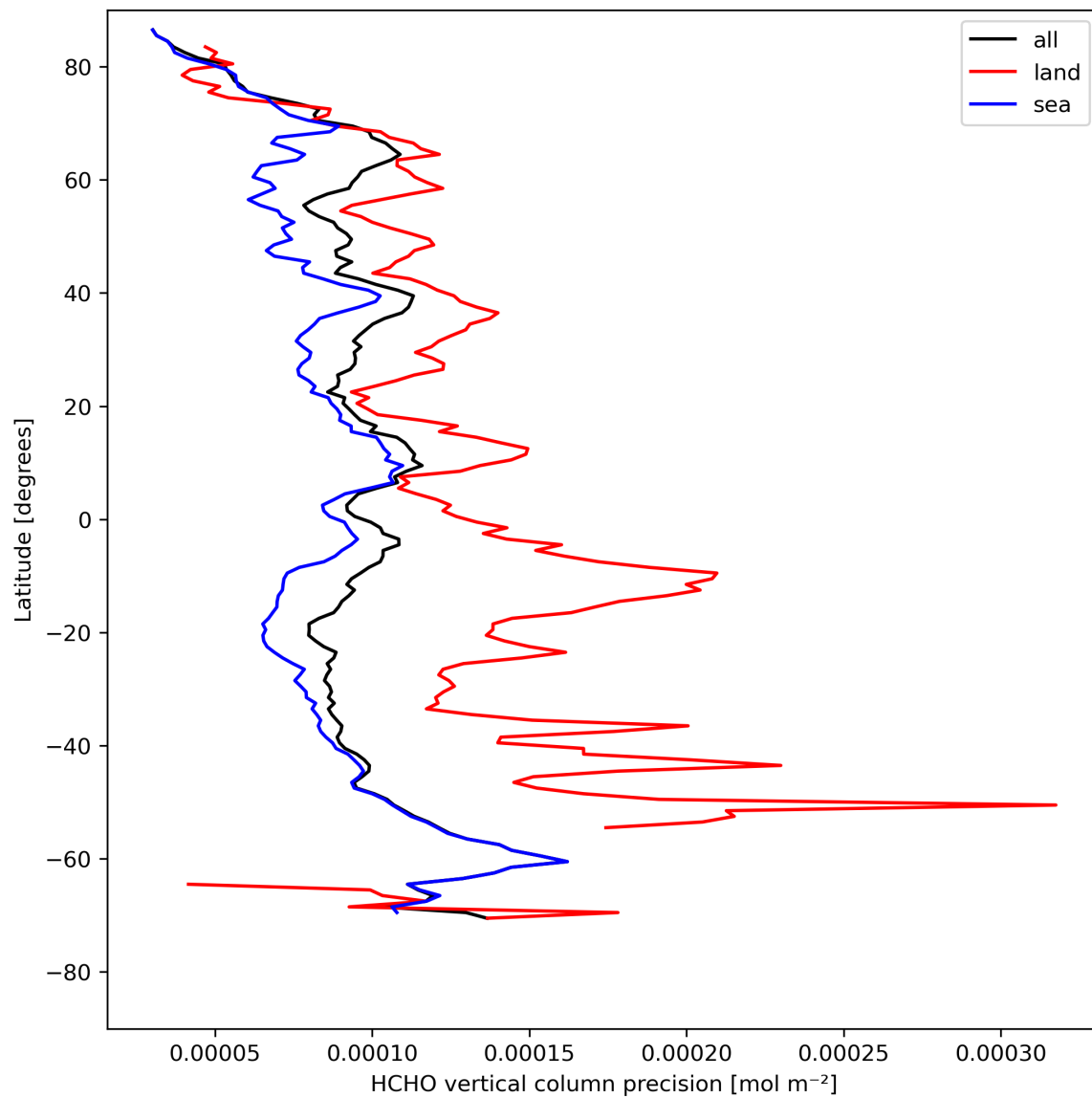
Figure 22: Zonal average of “HCHO vertical column precision” for 2023-08-12 to 2023-08-14.
