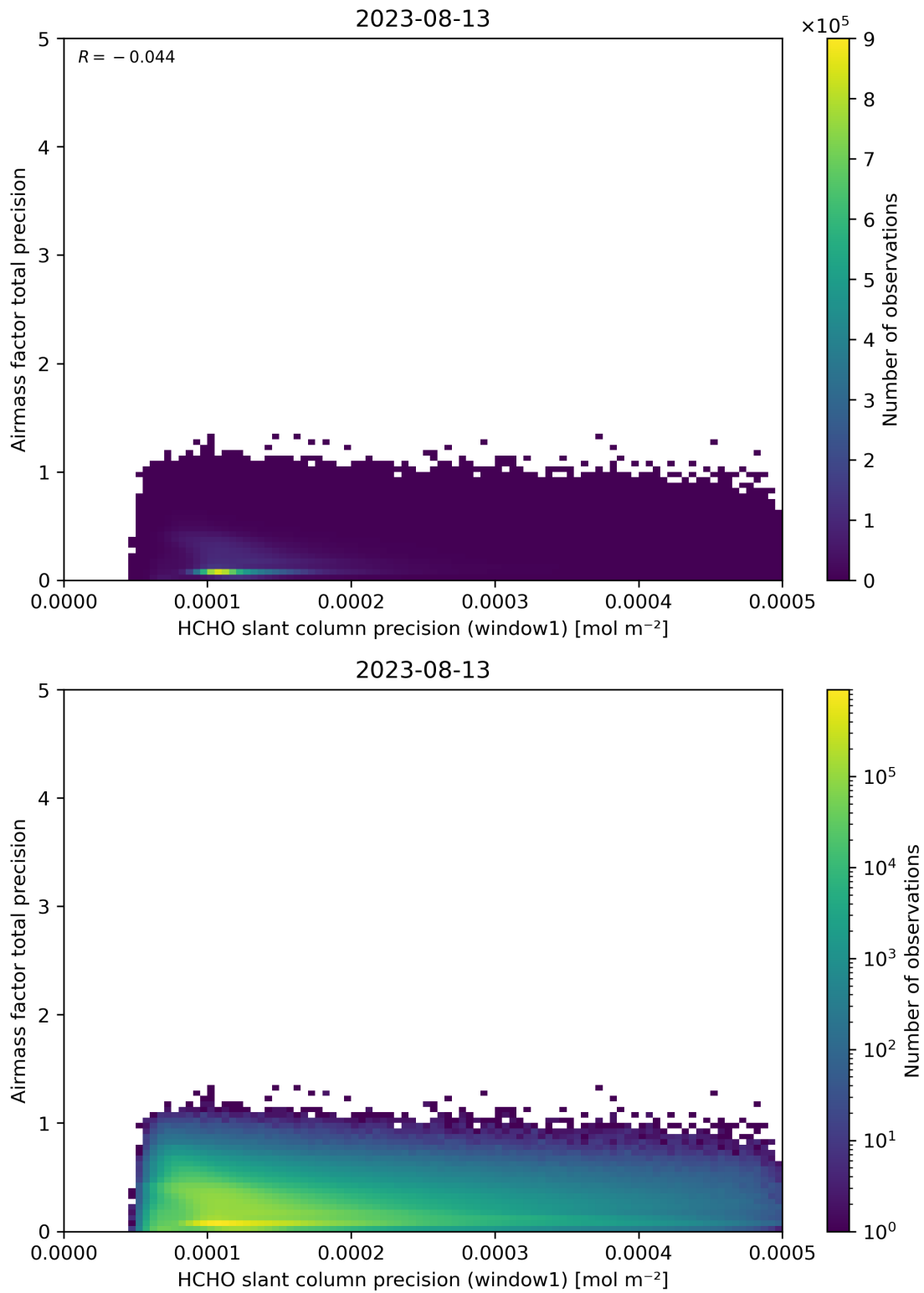
Figure 95: Scatter density plot of “HCHO slant column precision (window1)” against “Airmass factor total precision” for 2023-08-12 to 2023-08-14.
