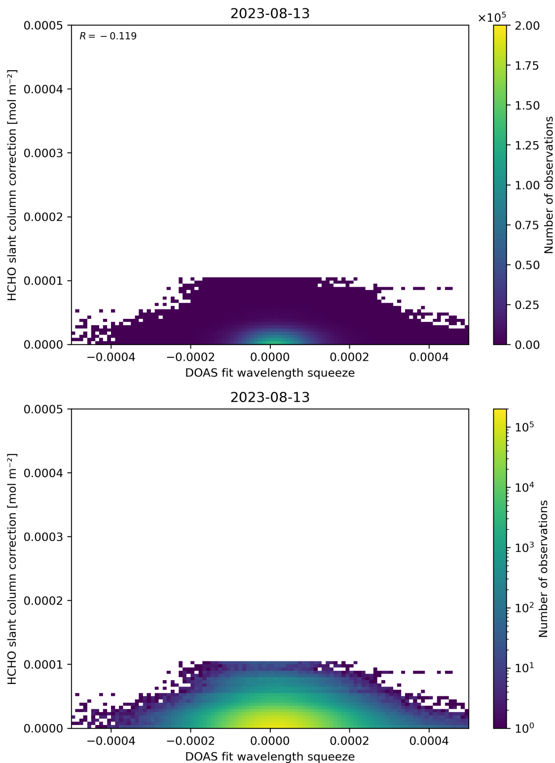
Figure 70: Scatter density plot of “DOAS fit wavelength squeeze” against “HCHO slant column correction” for 2023-08-12 to 2023-08-14.
