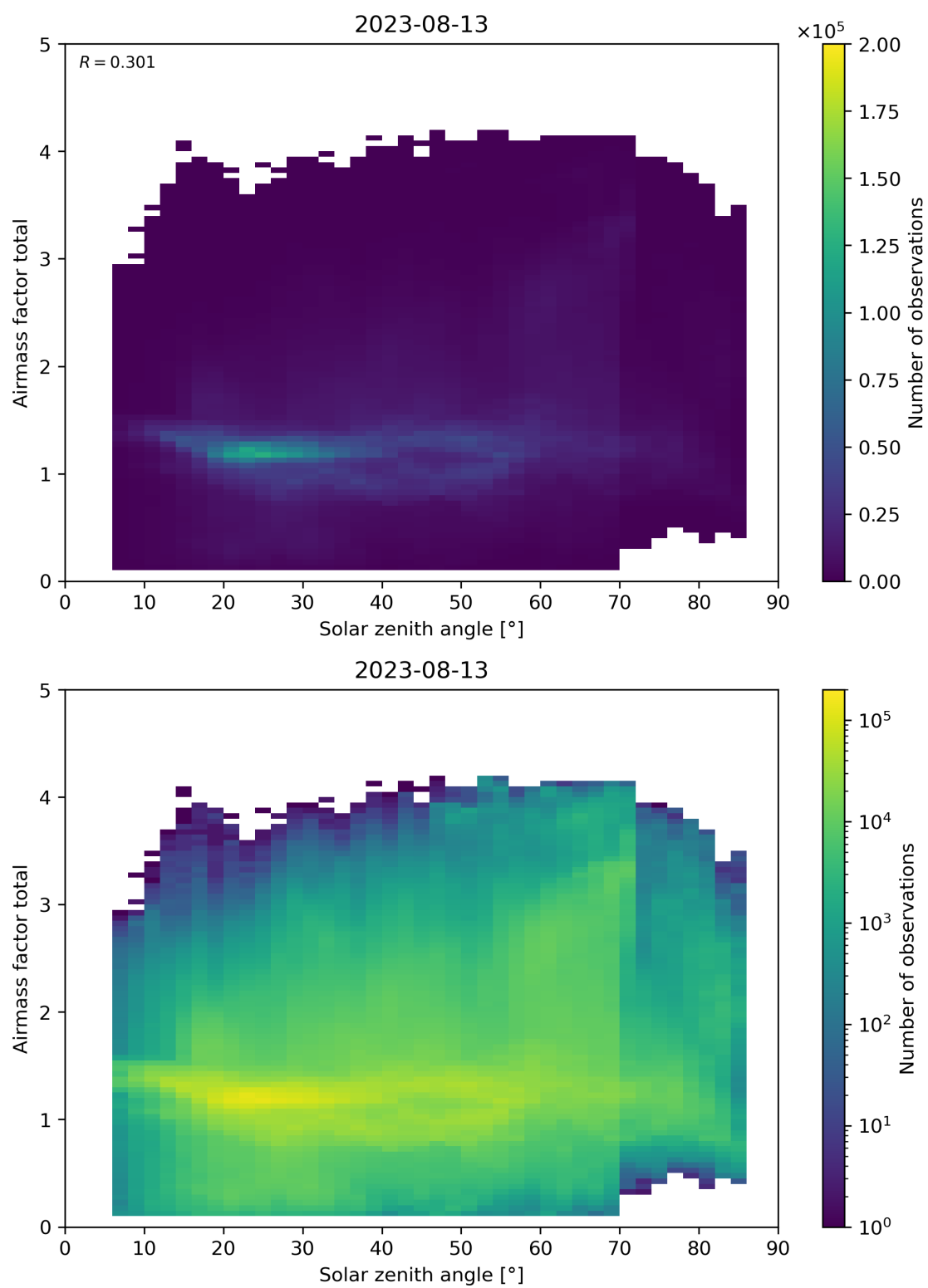
Figure 175: Scatter density plot of “Solar zenith angle” against “Airmass factor total” for 2023-08-12 to 2023-08-14.
