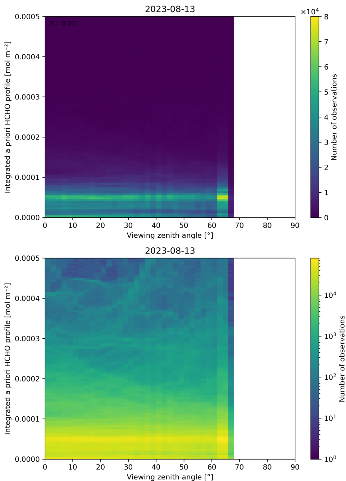
Figure 195: Scatter density plot of “Viewing zenith angle” against “Integrated a priori HCHO profile” for 2023-08-12 to 2023-08-14.
