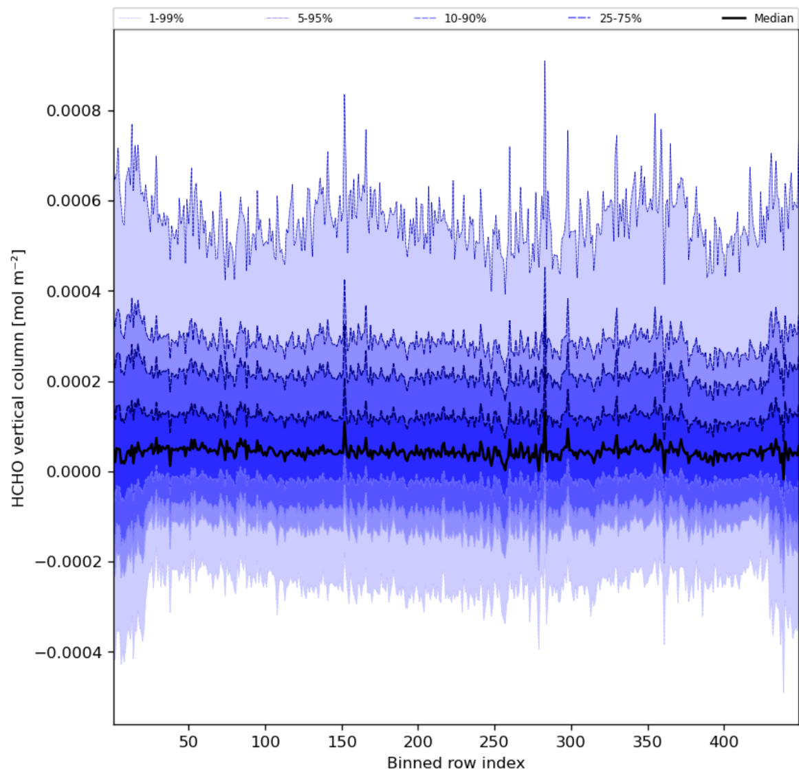
Figure 49: Along track statistics of “HCHO vertical column” for 2023-08-12 to 2023-08-14
