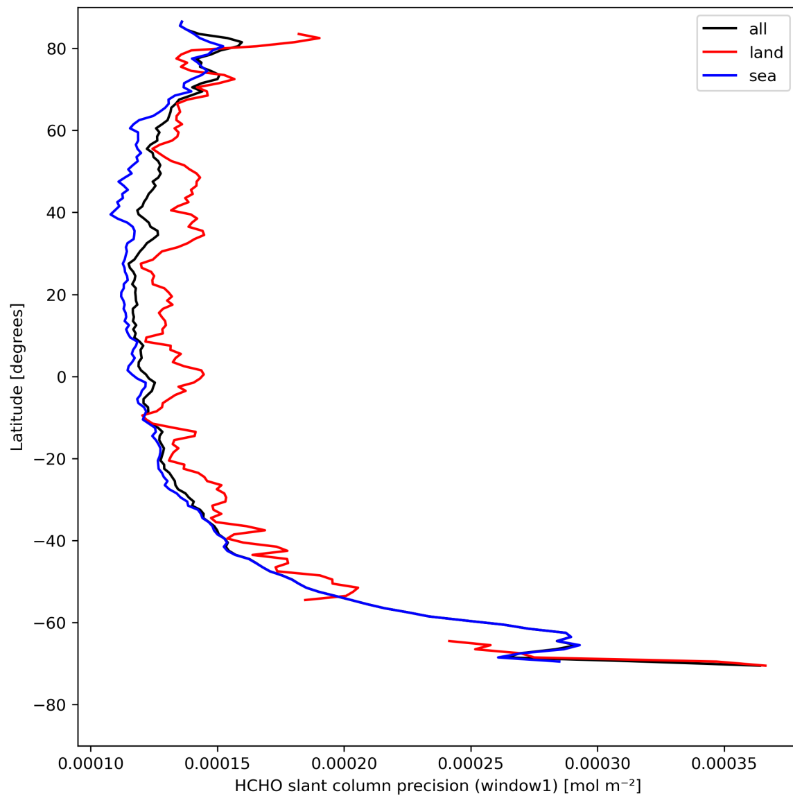
Figure 25: Zonal average of “HCHO slant column precision (window1)” for 2023-08-12 to 2023-08-14.
