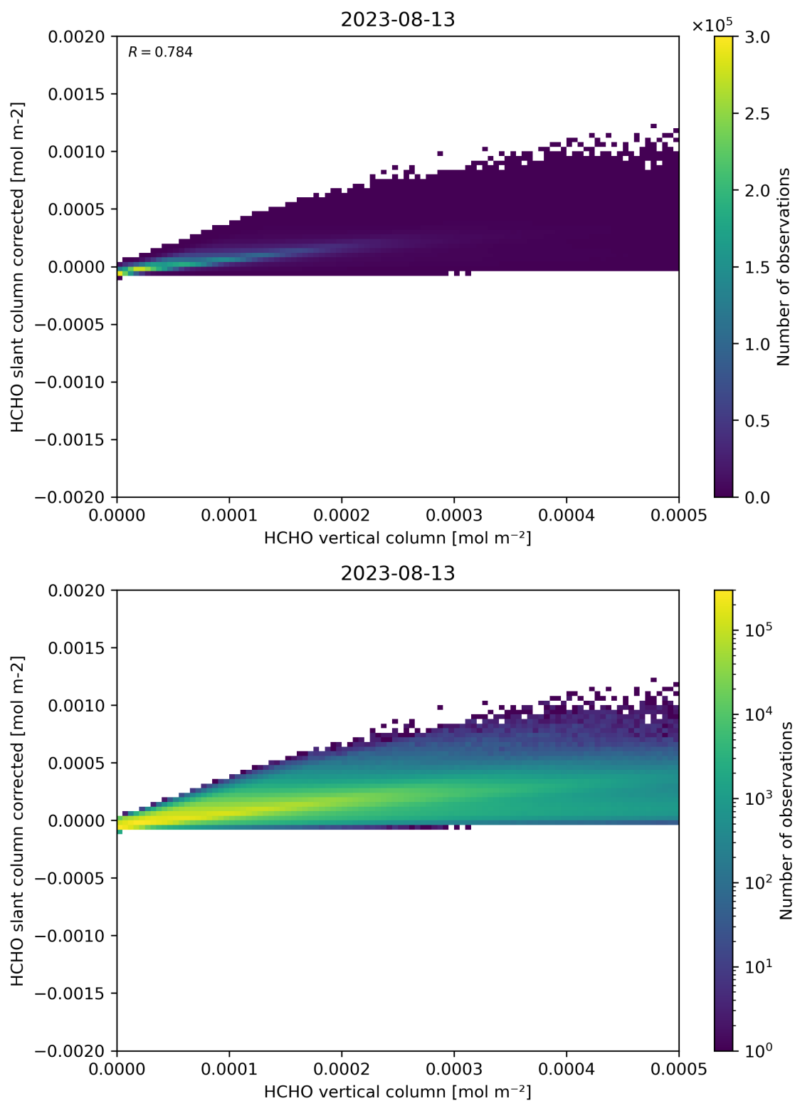
Figure 127: Scatter density plot of “HCHO vertical column” against “HCHO slant column corrected” for 2023-08-12 to 2023-08-14.
