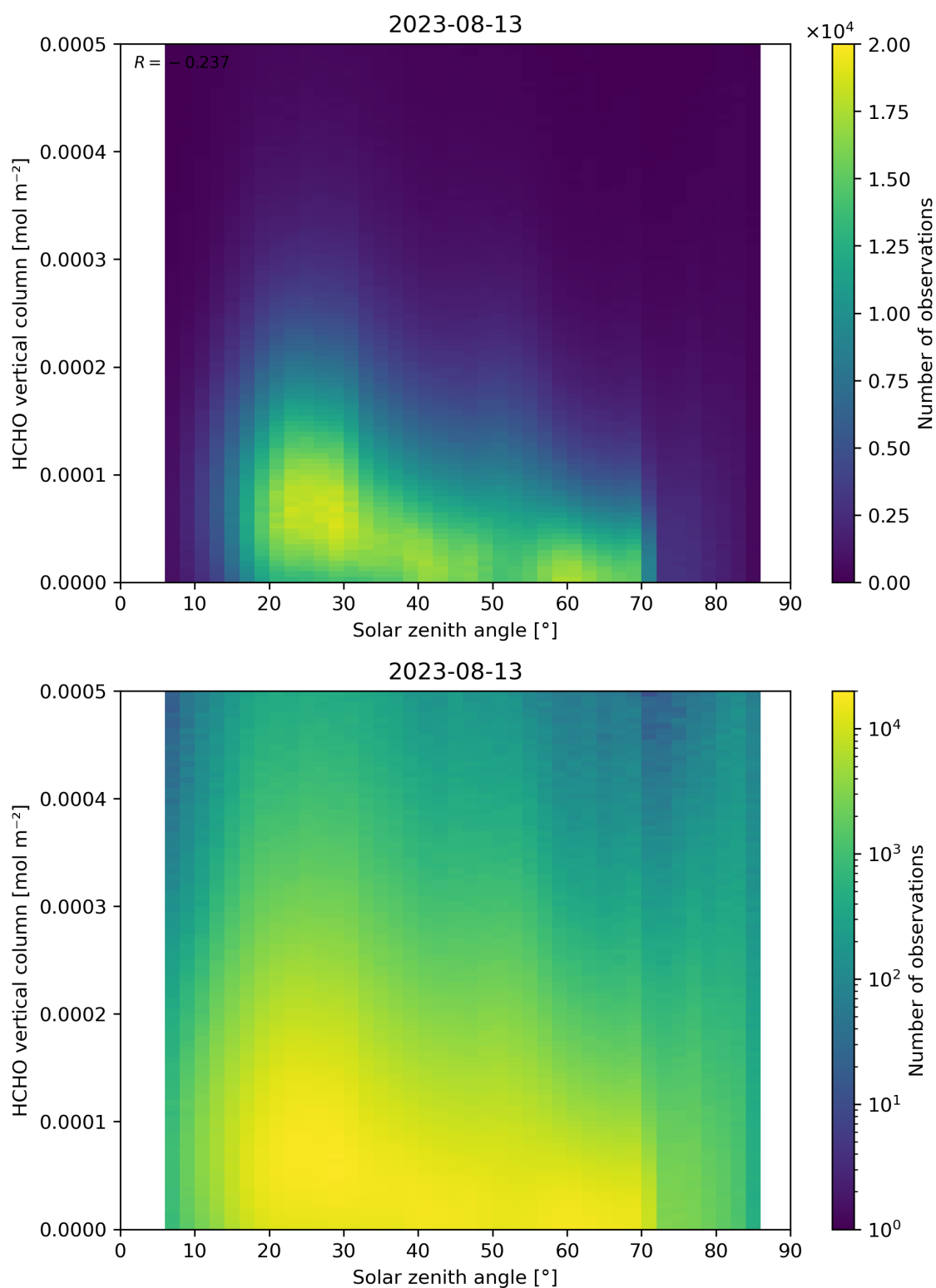
Figure 177: Scatter density plot of “Solar zenith angle” against “HCHO vertical column” for 2023-08-12 to 2023-08-14.
