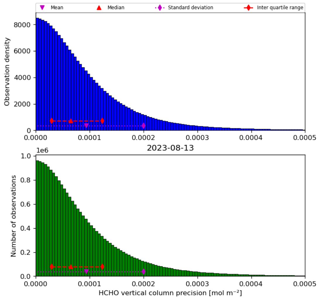
Figure 36: Histogram of “HCHO vertical column precision” for 2023-08-12 to 2023-08-14
