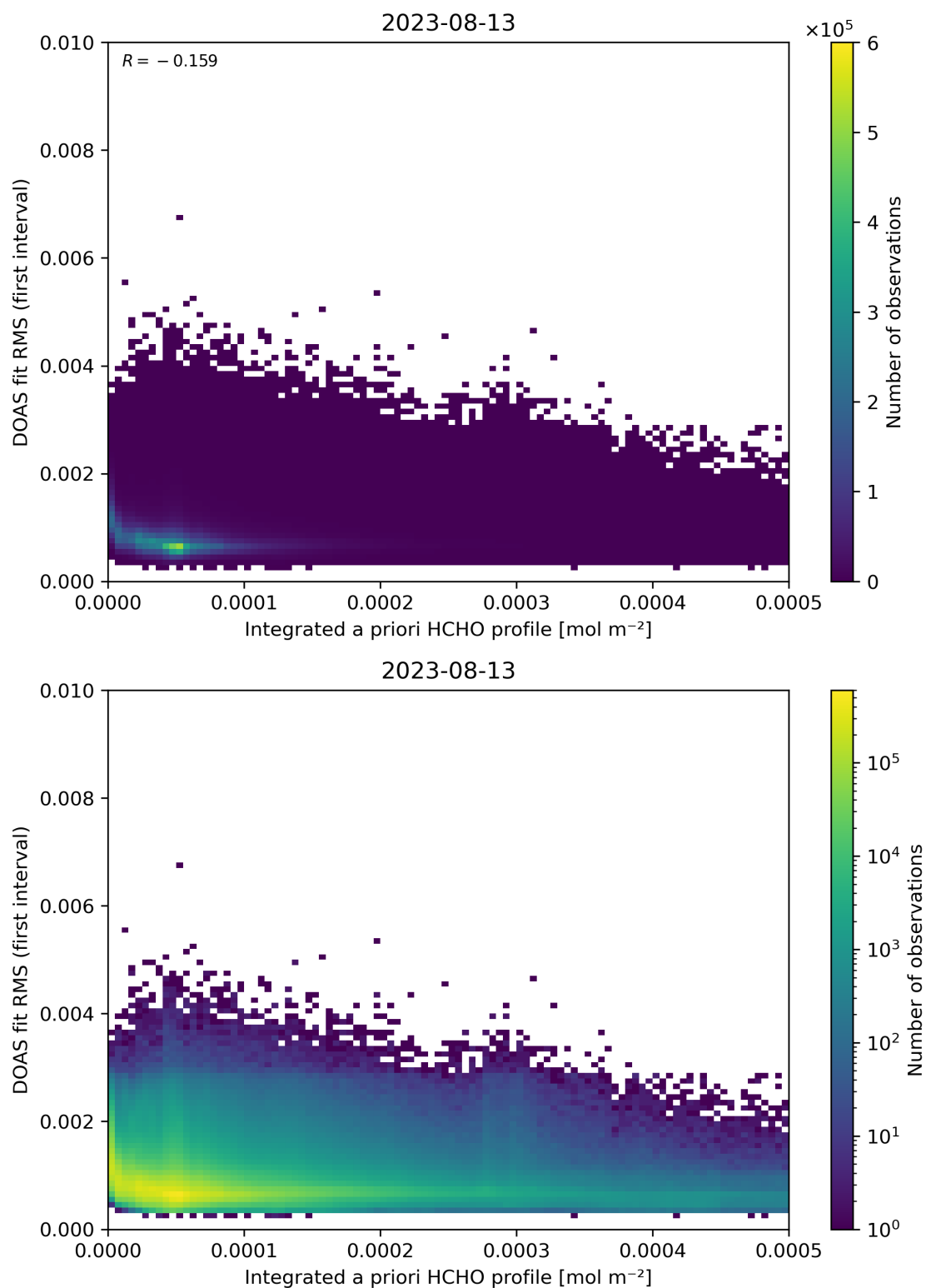
Figure 148: Scatter density plot of “Integrated a priori HCHO profile” against “DOAS fit RMS (first interval)” for 2023-08-12 to 2023-08-14.
