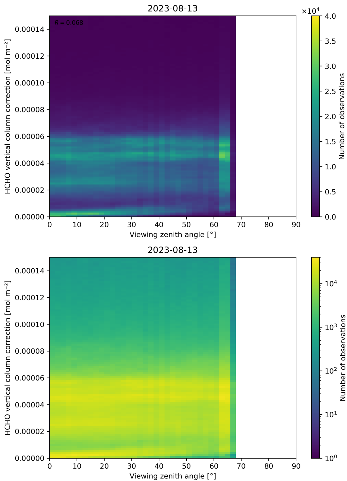
Figure 193: Scatter density plot of “Viewing zenith angle” against “HCHO vertical column correction” for 2023-08-12 to 2023-08-14.
