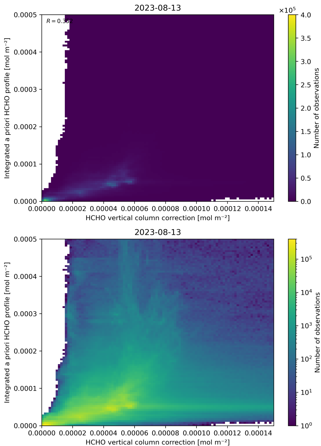
Figure 122: Scatter density plot of “HCHO vertical column correction” against “Integrated a priori HCHO profile” for 2023-08-12 to 2023-08-14.
