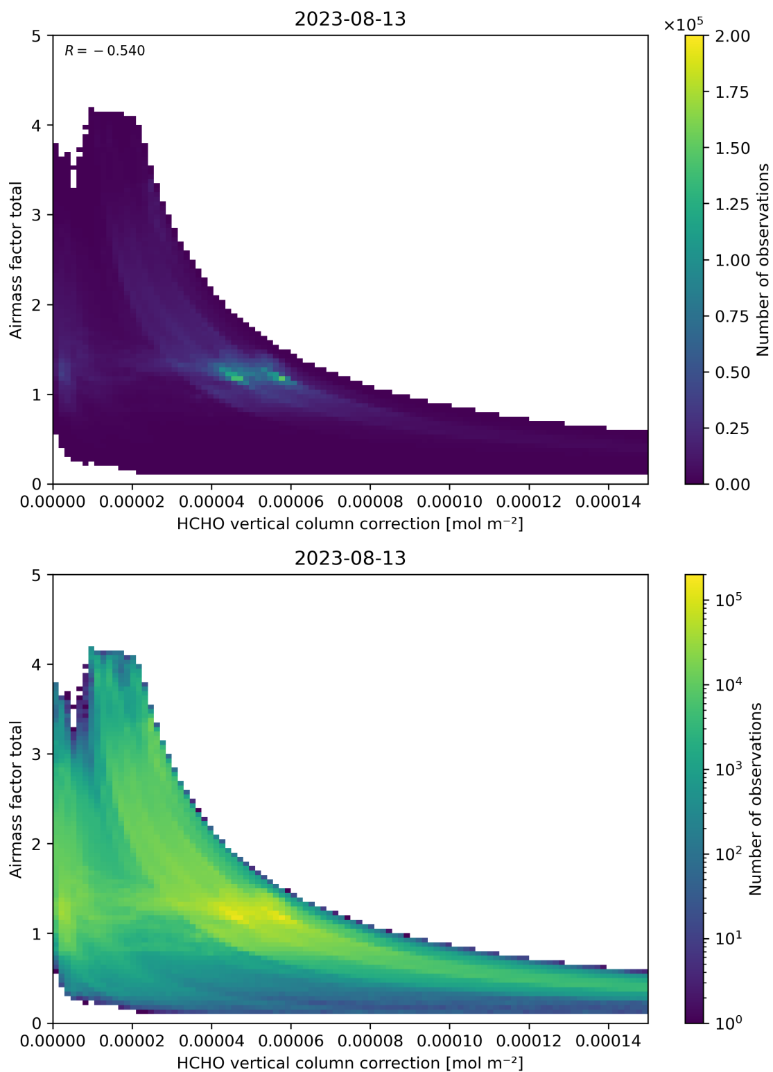
Figure 120: Scatter density plot of “HCHO vertical column correction” against “Airmass factor total” for 2023-08-12 to 2023-08-14.
