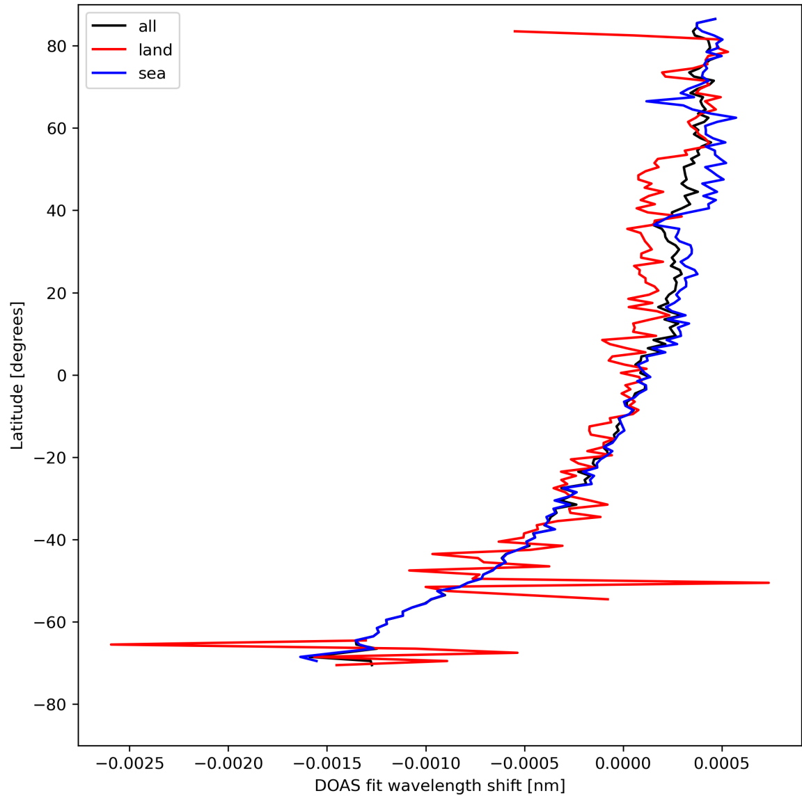
Figure 30: Zonal average of "DOAS fit wavelength shift" for 2023-08-12 to 2023-08-14.
