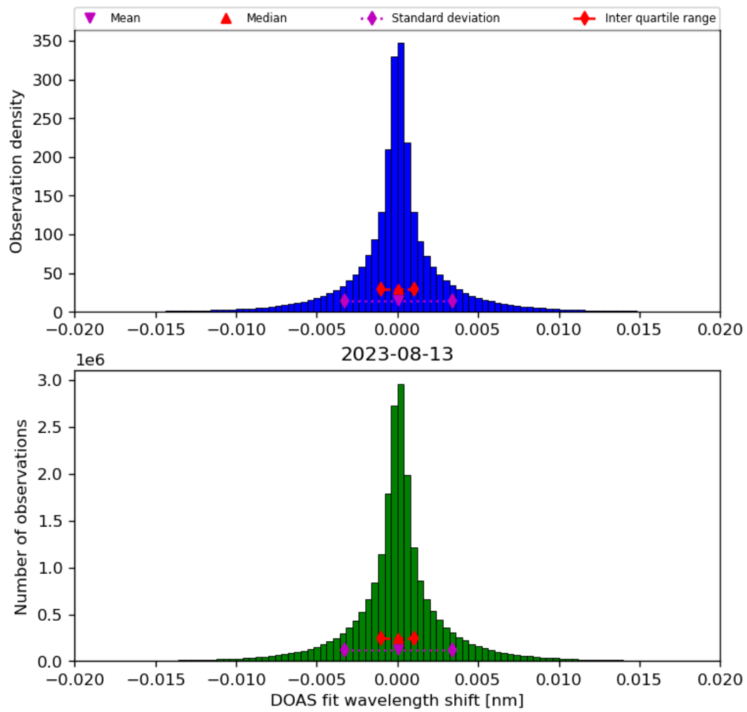
Figure 44: Histogram of “DOAS fit wavelength shift” for 2023-08-12 to 2023-08-14
