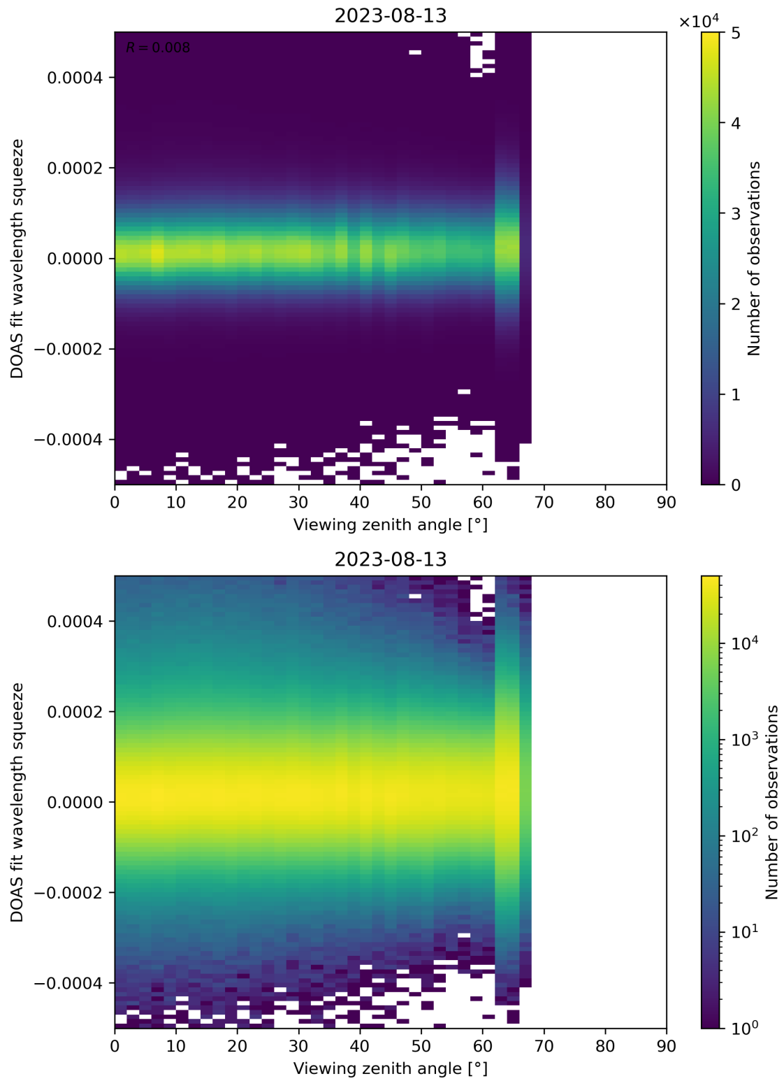
Figure 184: Scatter density plot of “Viewing zenith angle” against “DOAS fit wavelength squeeze” for 2023-08-12 to 2023-08-14.
