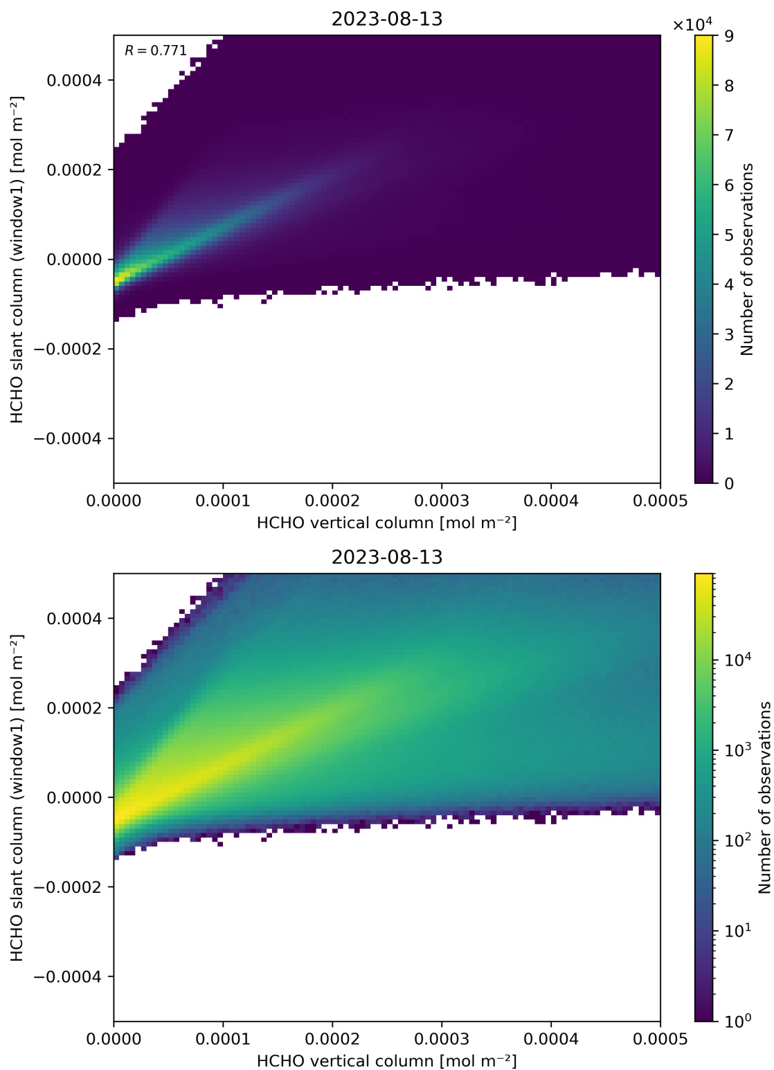
Figure 129: Scatter density plot of “HCHO vertical column” against “HCHO slant column (window1)” for 2023-08-12 to 2023-08-14.
