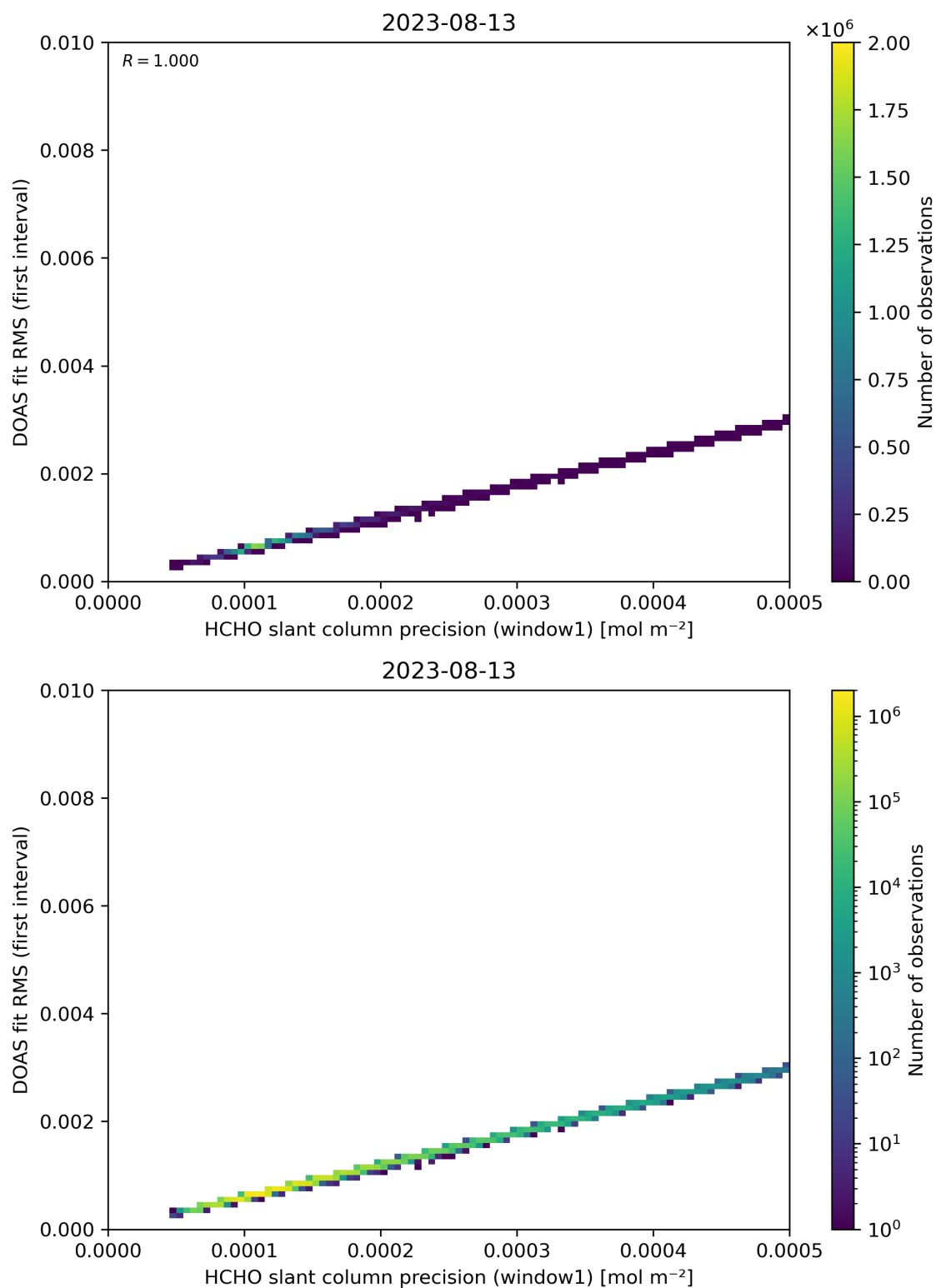
Figure 88: Scatter density plot of “HCHO slant column precision (window1)” against “DOAS fit RMS (first interval)” for 2023-08-12 to 2023-08-14.
