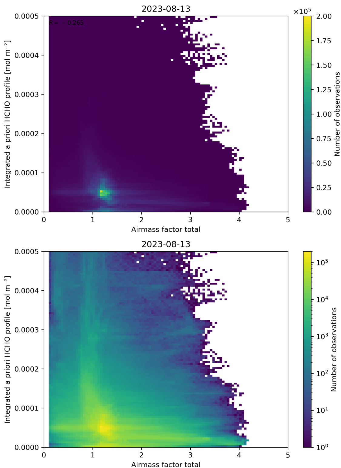
Figure 104: Scatter density plot of “Airmass factor total” against “Integrated a priori HCHO profile” for 2023-08-12 to 2023-08-14.
