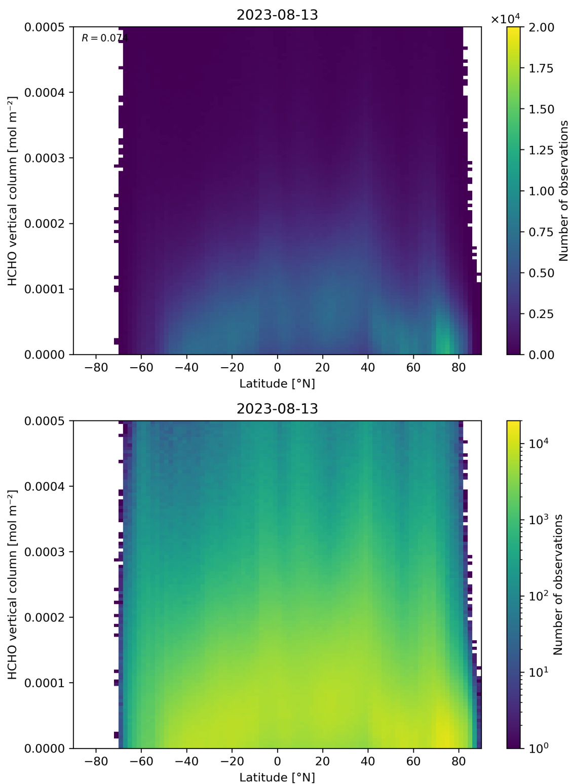
Figure 163: Scatter density plot of “Latitude” against “HCHO vertical column” for 2023-08-12 to 2023-08-14.
