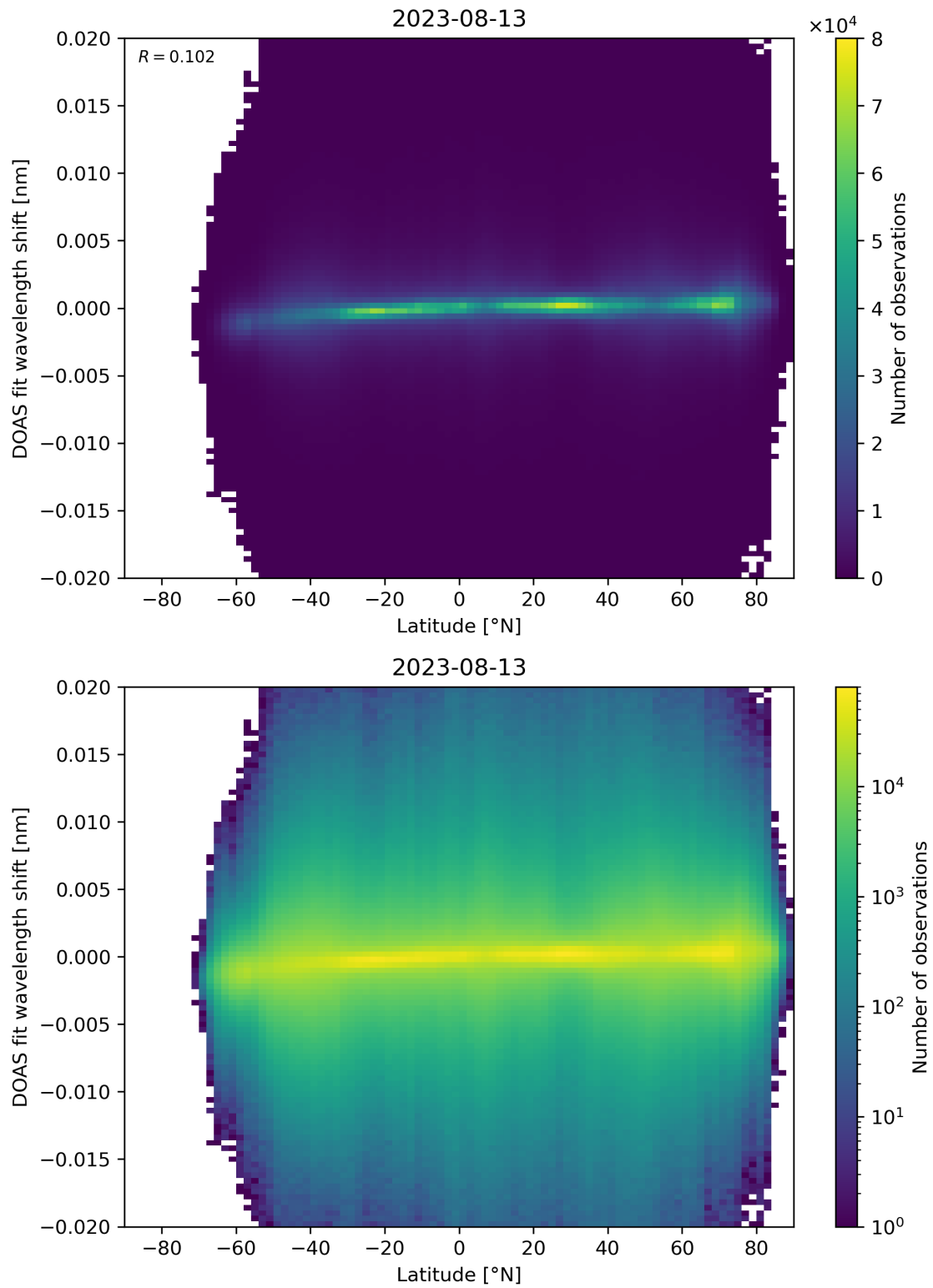
Figure 154: Scatter density plot of “Latitude” against “DOAS fit wavelength shift” for 2023-08-12 to 2023-08-14.
