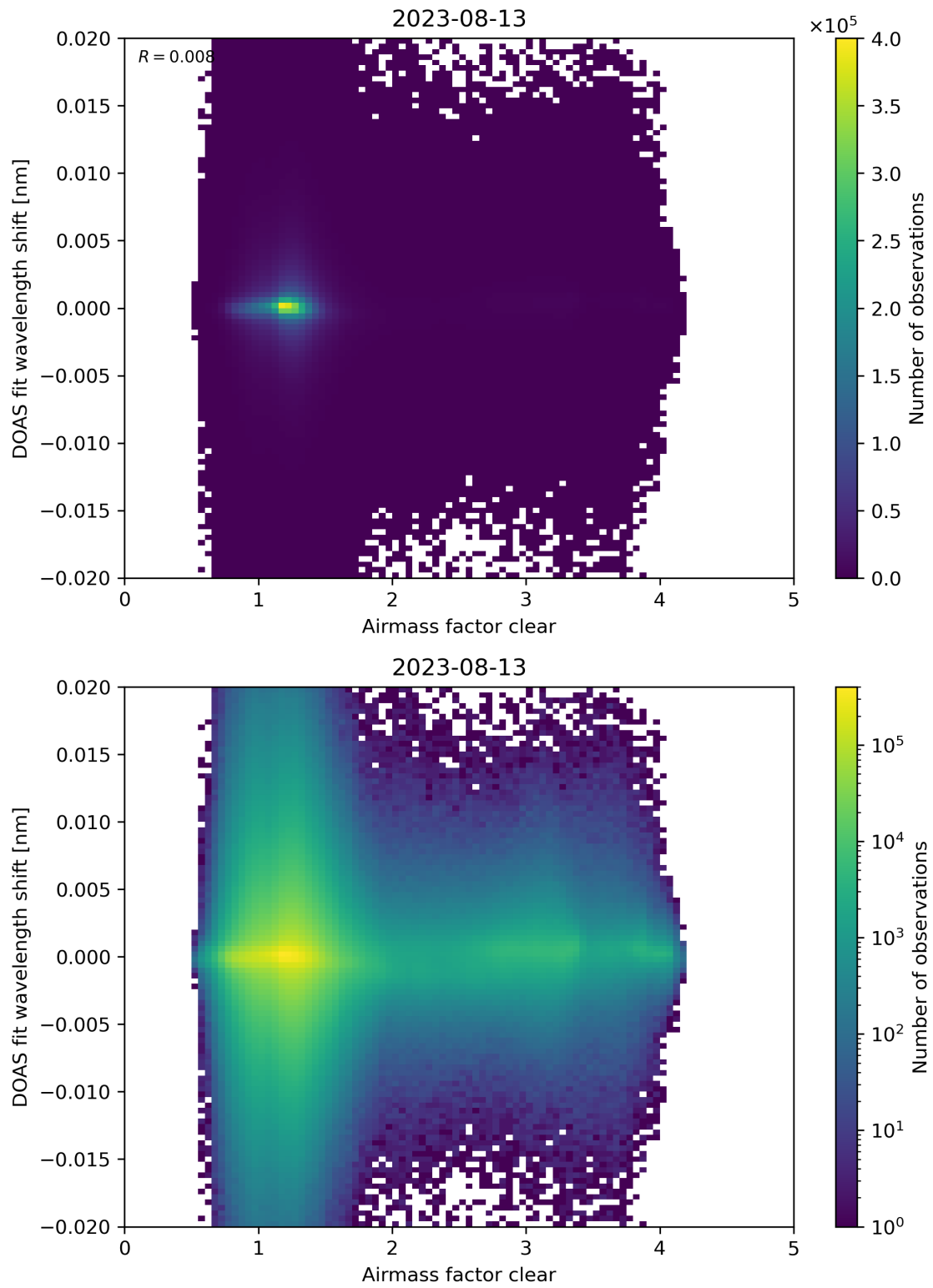
Figure 72: Scatter density plot of “Airmass factor clear” against “DOAS fit wavelength shift” for 2023-08-12 to 2023-08-14.
