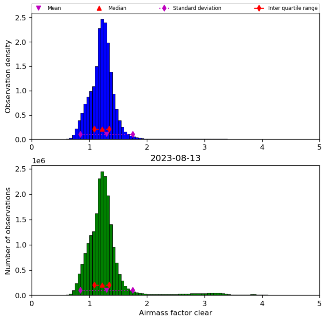
Figure 42: Histogram of “Airmass factor clear” for 2023-08-12 to 2023-08-14
