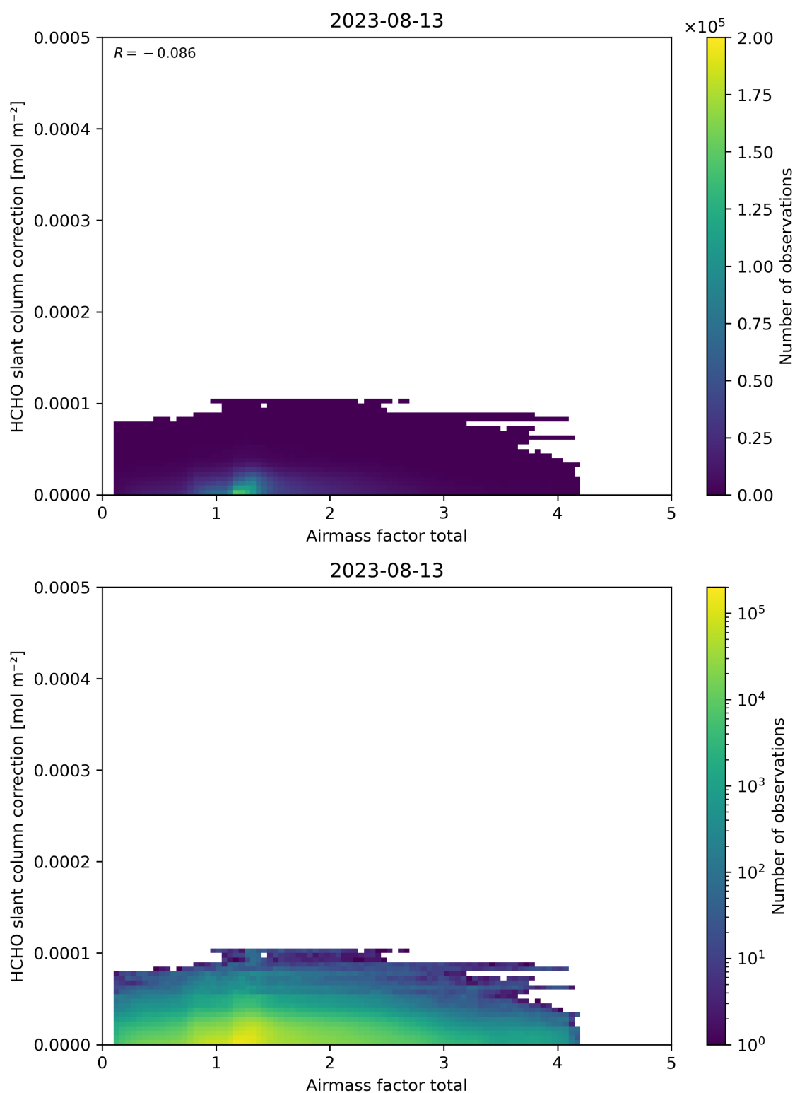
Figure 102: Scatter density plot of “Airmass factor total” against “HCHO slant column correction” for 2023-08-12 to 2023-08-14.
