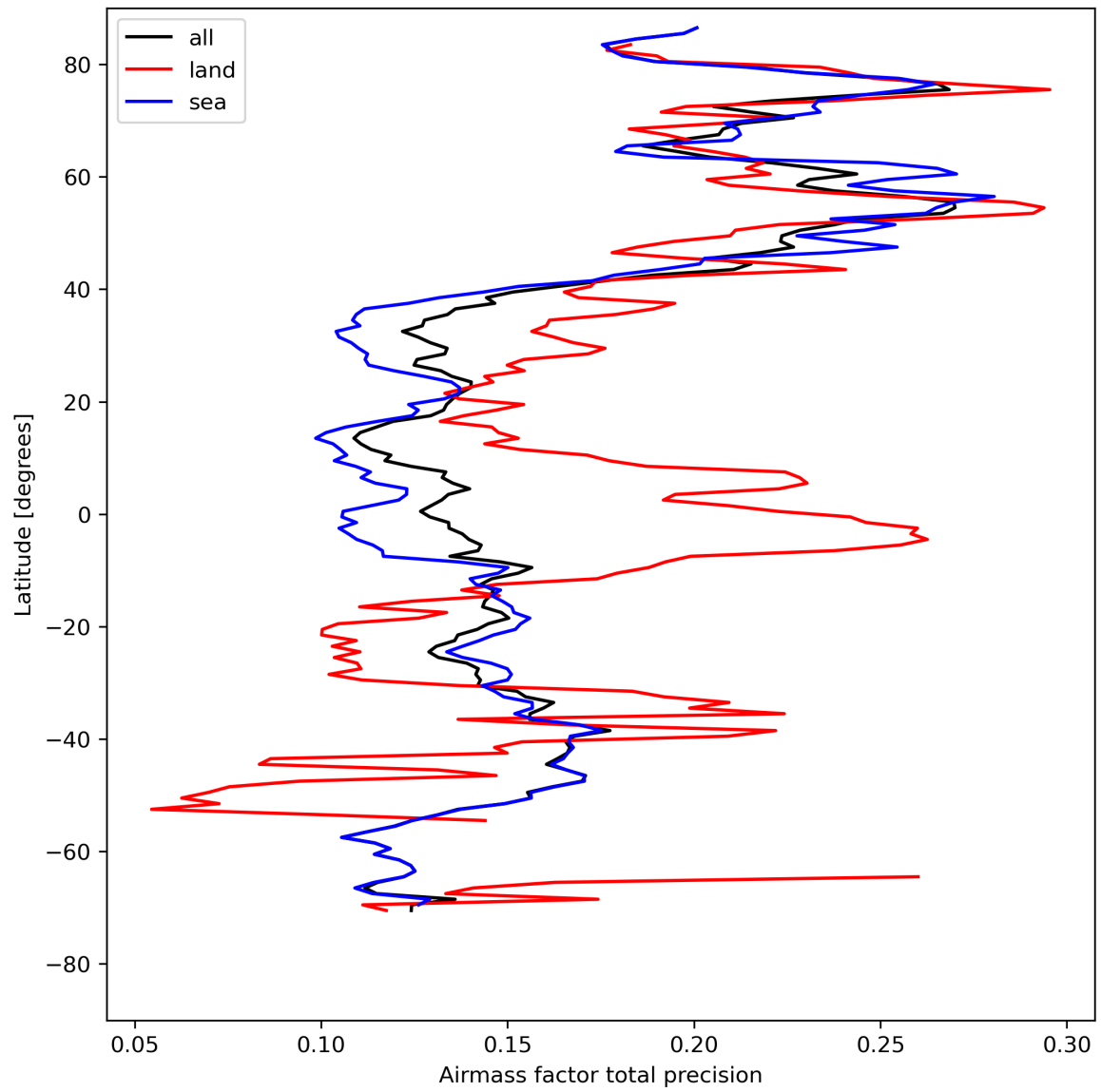
Figure 27: Zonal average of “Airmass factor total precision” for 2023-08-12 to 2023-08-14.
