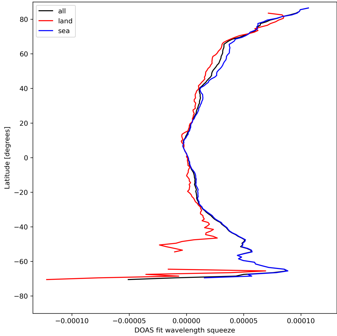
Figure 31: Zonal average of “DOAS fit wavelength squeeze” for 2023-08-12 to 2023-08-14.
