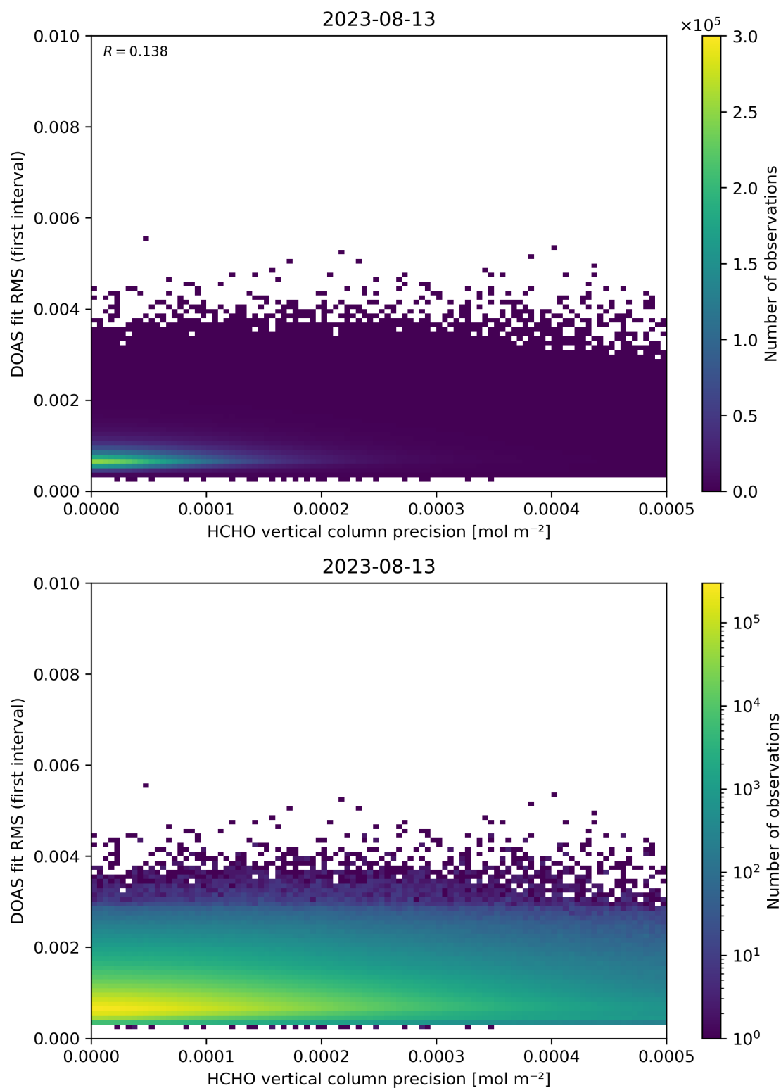
Figure 136: Scatter density plot of “HCHO vertical column precision” against “DOAS fit RMS (first interval)” for 2023-08-12 to 2023-08-14.
