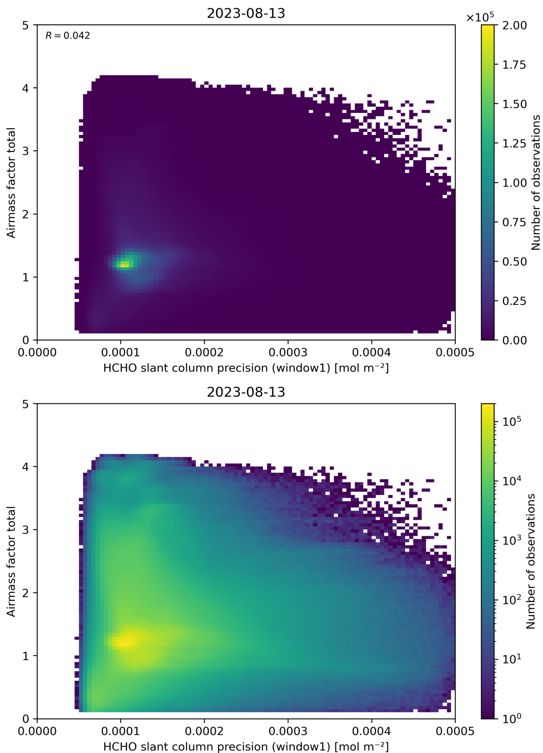
Figure 94: Scatter density plot of “HCHO slant column precision (window1)” against “Airmass factor total” for 2023-08-12 to 2023-08-14.
