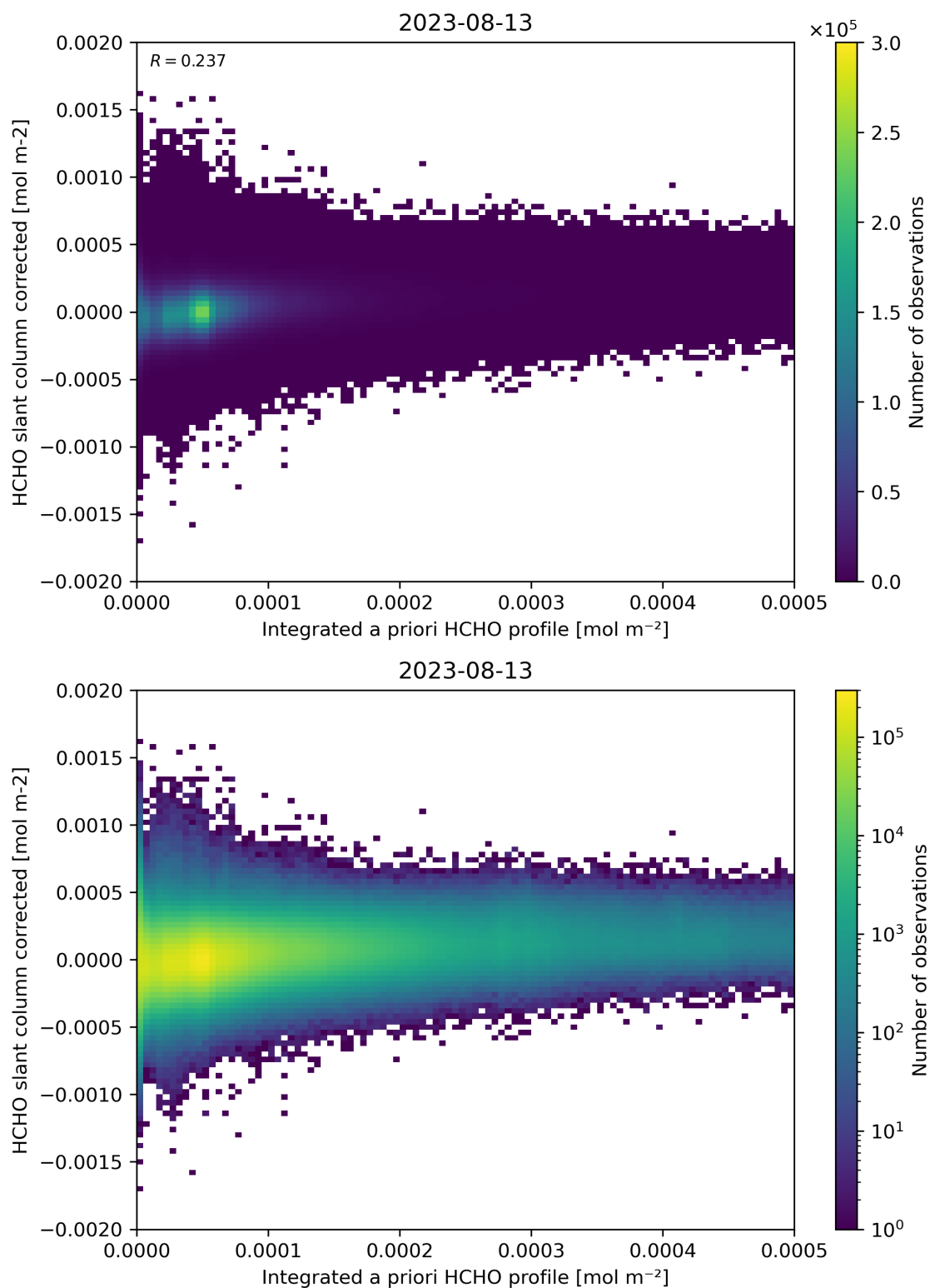
Figure 151: Scatter density plot of “Integrated a priori HCHO profile” against “HCHO slant column corrected” for 2023-08-12 to 2023-08-14.
