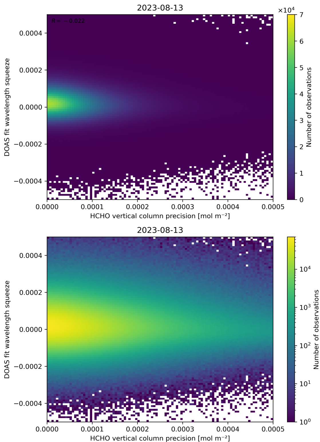
Figure 138: Scatter density plot of “HCHO vertical column precision” against “DOAS fit wavelength squeeze” for 2023-08-12 to 2023-08-14.
