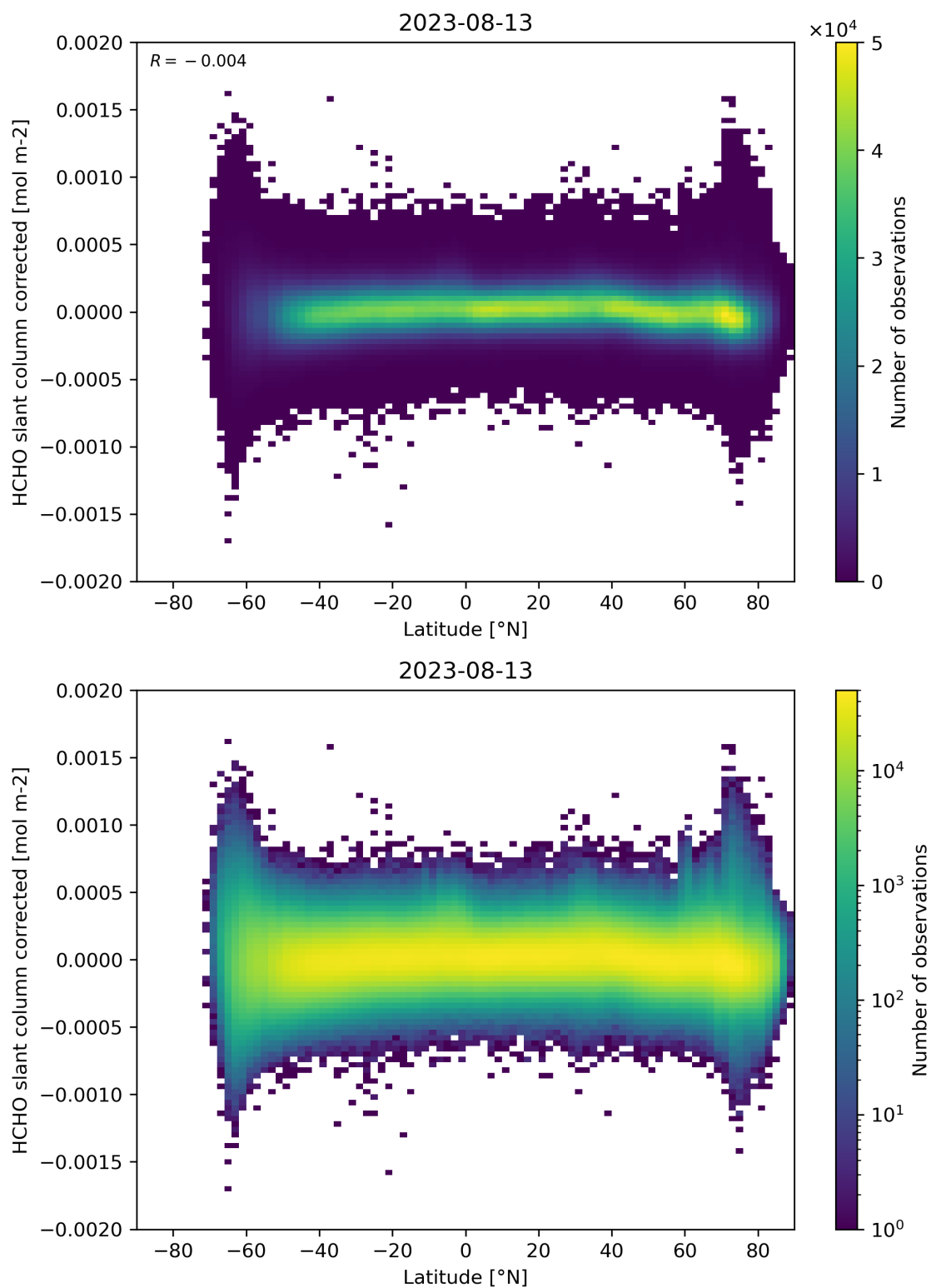
Figure 157: Scatter density plot of “Latitude” against “HCHO slant column corrected” for 2023-08-12 to 2023-08-14.
