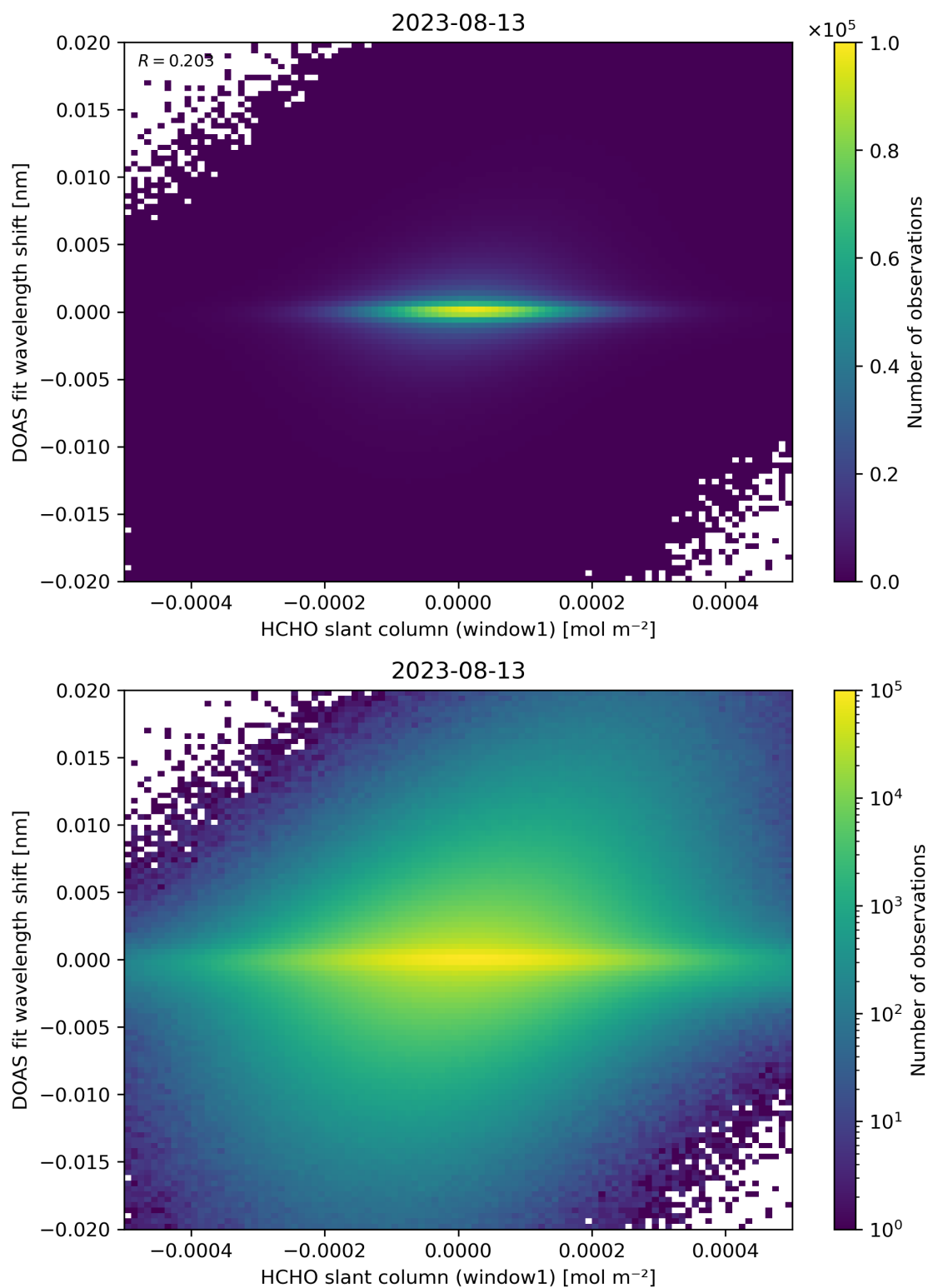
Figure 79: Scatter density plot of “HCHO slant column (window1)” against “DOAS fit wavelength shift” for 2023-08-12 to 2023-08-14.
