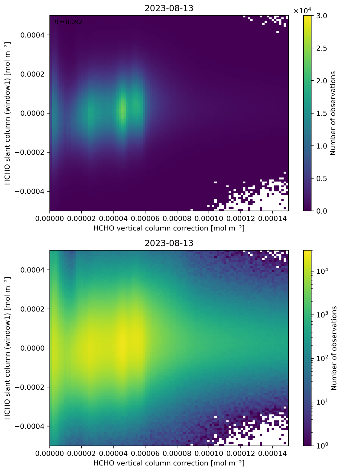
Figure 118: Scatter density plot of “HCHO vertical column correction” against “HCHO slant column (window1)” for 2023-08-12 to 2023-08-14.
