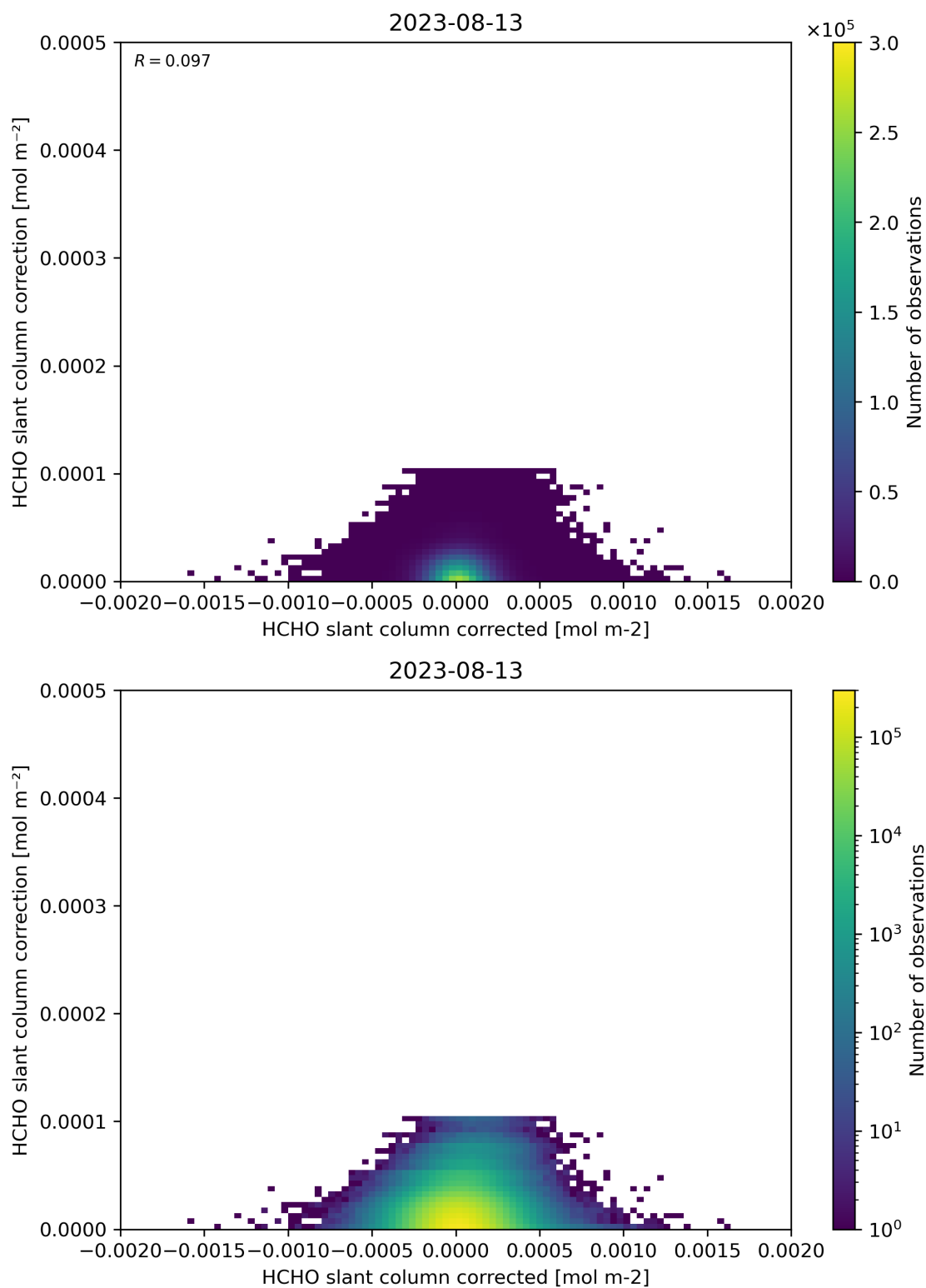
Figure 77: Scatter density plot of “HCHO slant column corrected” against “HCHO slant column correction” for 2023-08-12 to 2023-08-14.
