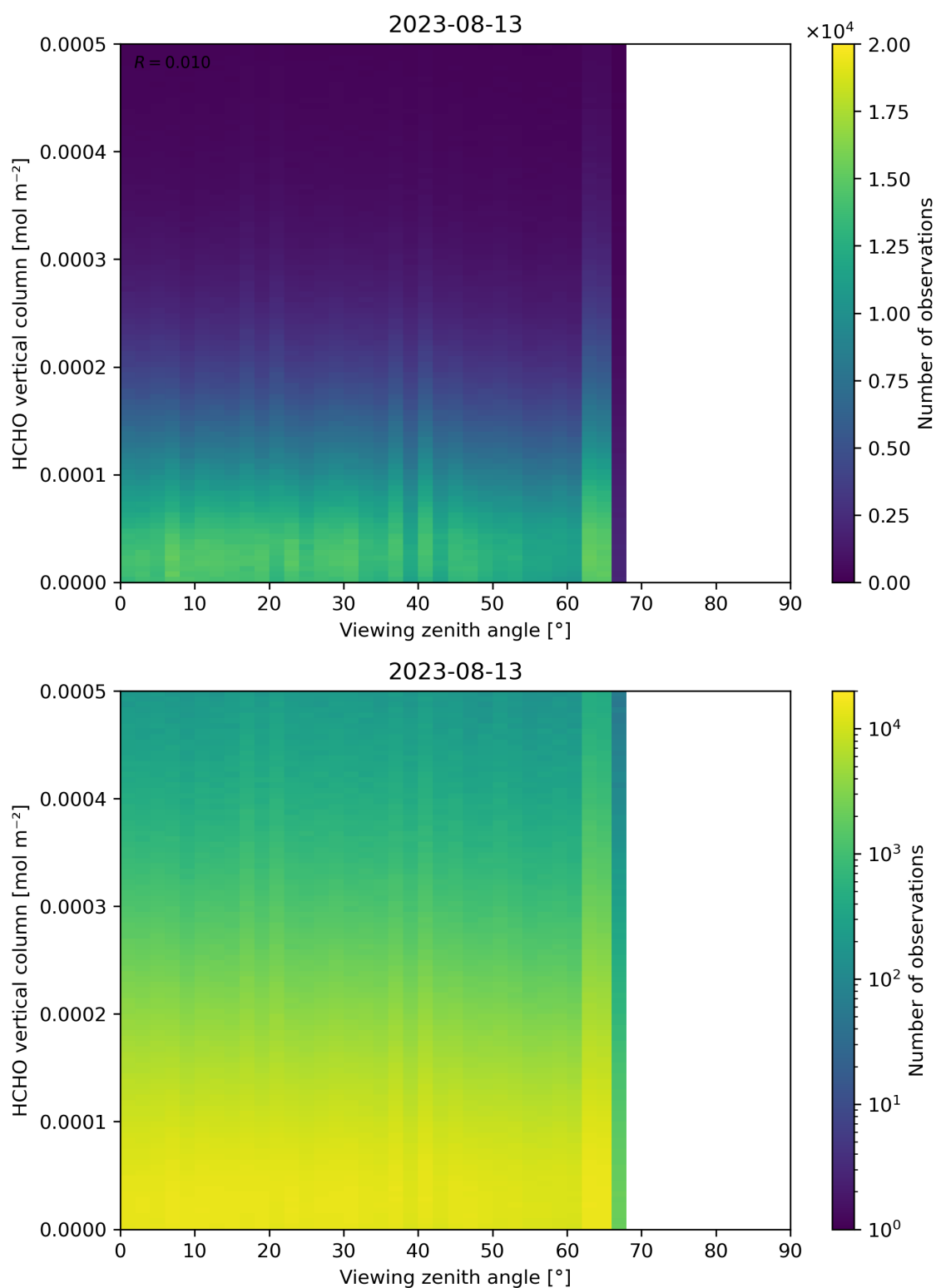
Figure 192: Scatter density plot of “Viewing zenith angle” against “HCHO vertical column” for 2023-08-12 to 2023-08-14.
