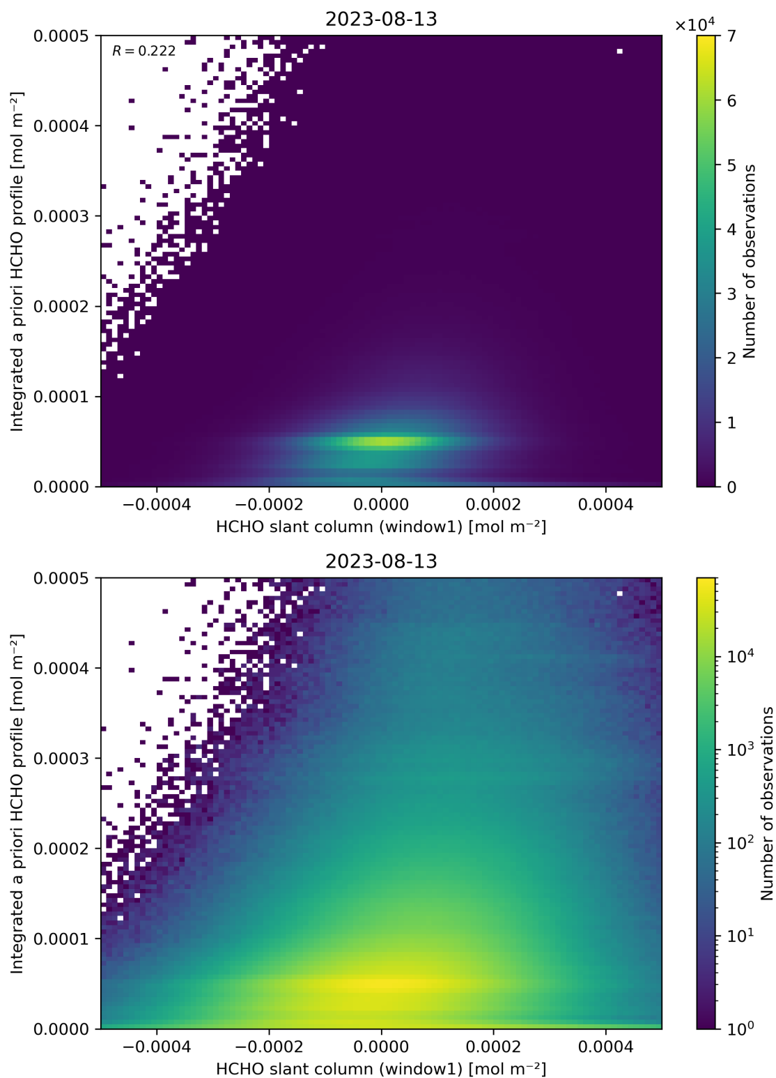
Figure 87: Scatter density plot of “HCHO slant column (window1)” against “Integrated a priori HCHO profile” for 2023-08-12 to 2023-08-14.
