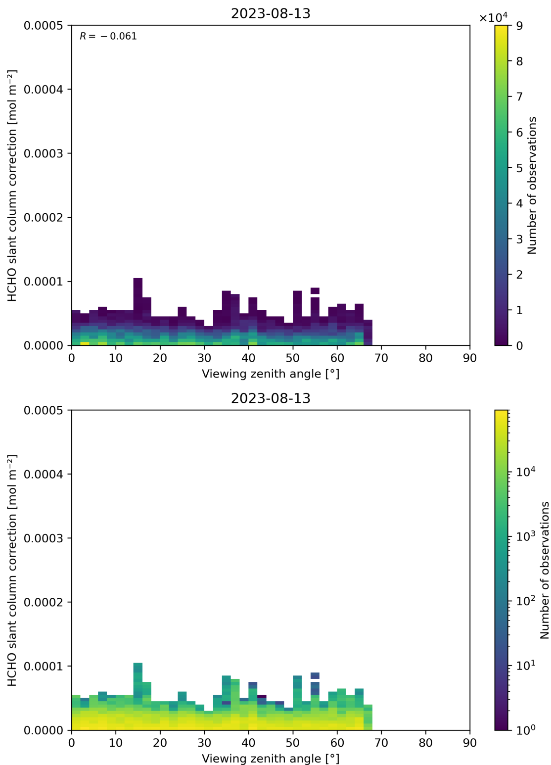
Figure 187: Scatter density plot of “Viewing zenith angle” against “HCHO slant column correction” for 2023-08-12 to 2023-08-14.
