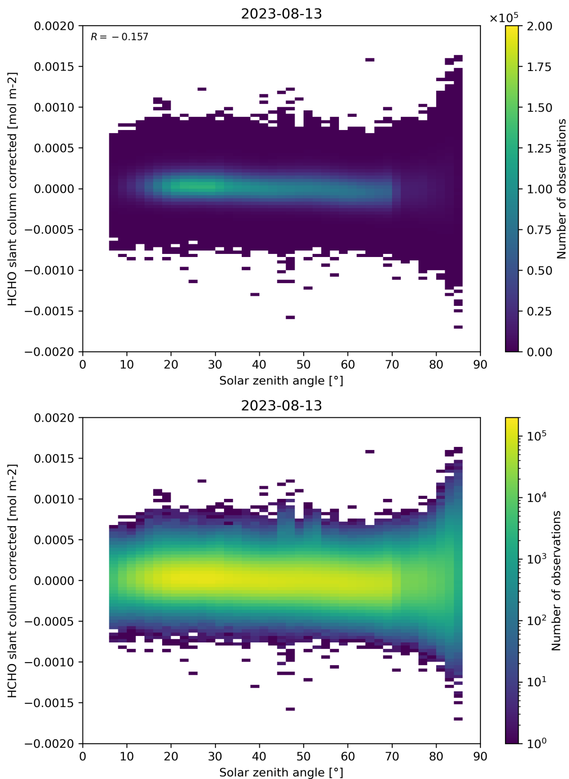
Figure 171: Scatter density plot of “Solar zenith angle” against “HCHO slant column corrected” for 2023-08-12 to 2023-08-14.
