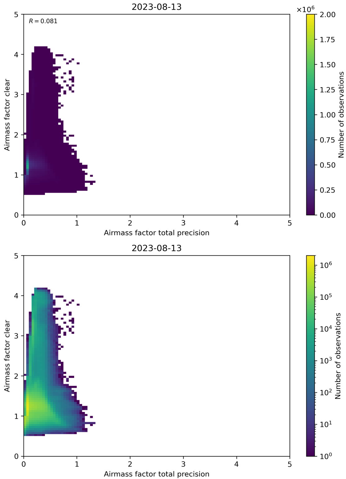
Figure 108: Scatter density plot of “Airmass factor total precision” against “Airmass factor clear” for 2023-08-12 to 2023-08-14.
