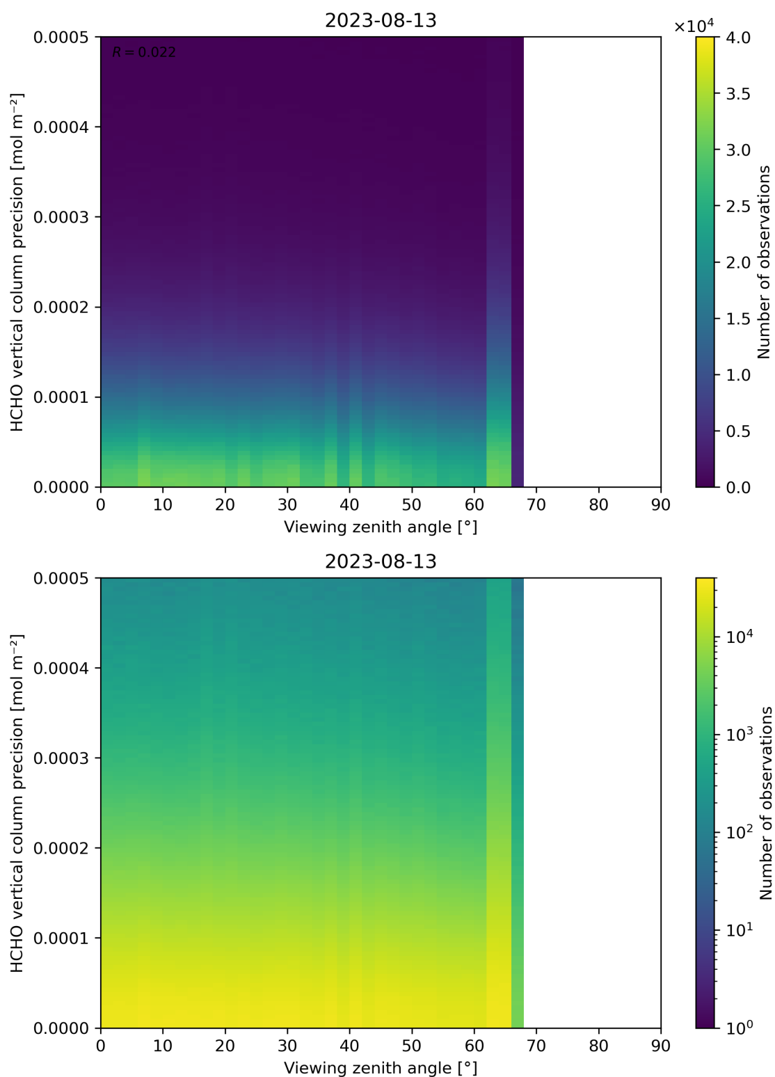
Figure 194: Scatter density plot of “Viewing zenith angle” against “HCHO vertical column precision” for 2023-08-12 to 2023-08-14.
