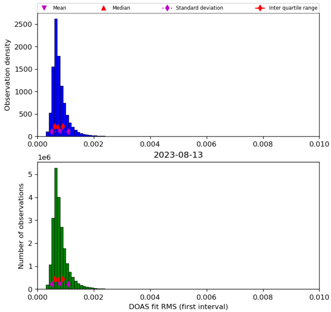
Figure 46: Histogram of “DOAS fit RMS (first interval)” for 2023-08-12 to 2023-08-14
