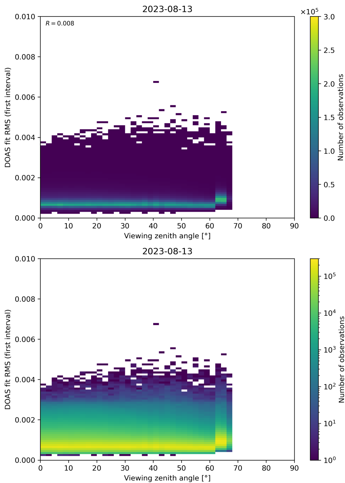
Figure 182: Scatter density plot of “Viewing zenith angle” against “DOAS fit RMS (first interval)” for 2023-08-12 to 2023-08-14.
