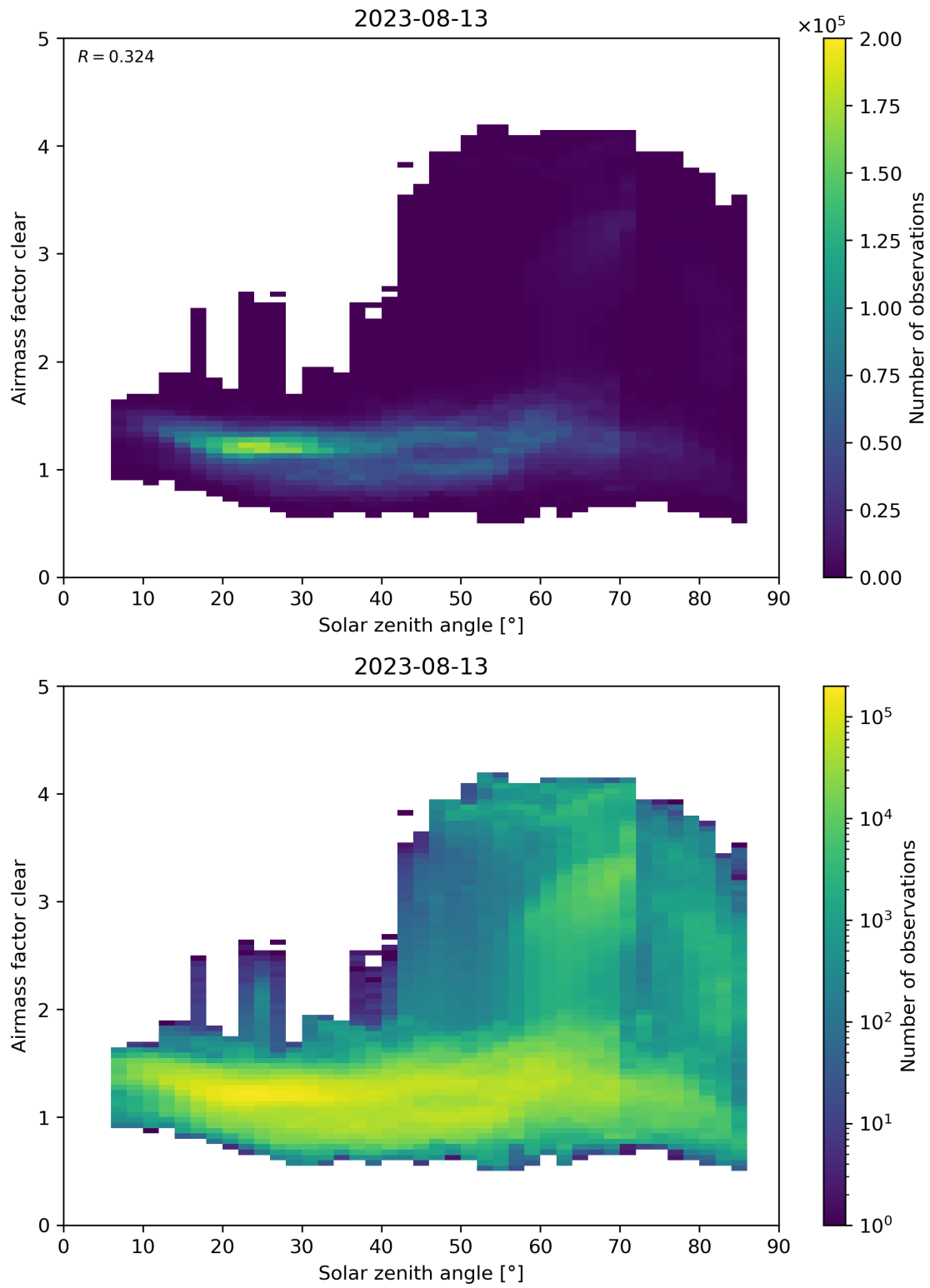
Figure 170: Scatter density plot of “Solar zenith angle” against “Airmass factor clear” for 2023-08-12 to 2023-08-14.
