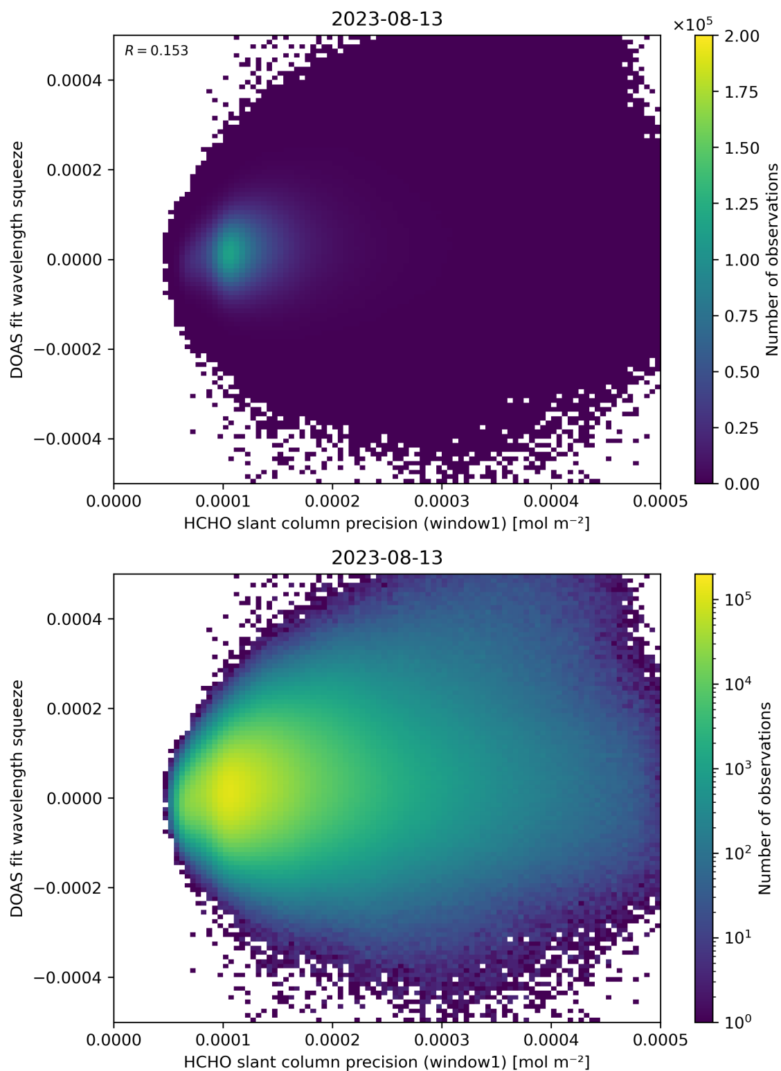
Figure 90: Scatter density plot of “HCHO slant column precision (window1)” against “DOAS fit wavelength squeeze” for 2023-08-12 to 2023-08-14.
