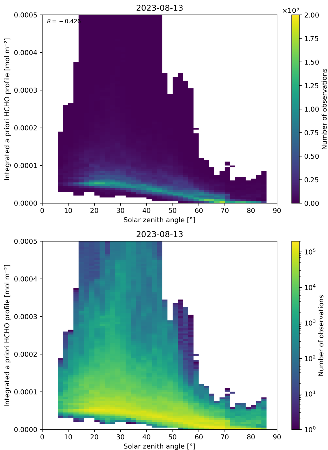
Figure 180: Scatter density plot of “Solar zenith angle” against “Integrated a priori HCHO profile” for 2023-08-12 to 2023-08-14.
