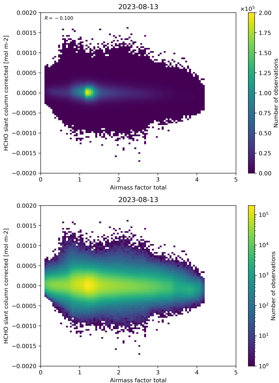
Figure 101: Scatter density plot of “Airmass factor total” against “HCHO slant column corrected” for 2023-08-12 to 2023-08-14.
