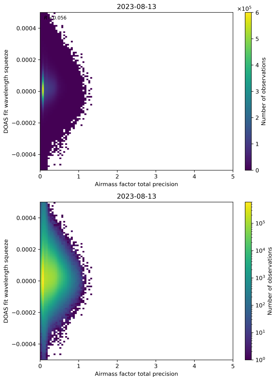
Figure 107: Scatter density plot of “Airmass factor total precision” against “DOAS fit wavelength squeeze” for 2023-08-12 to 2023-08-14.
