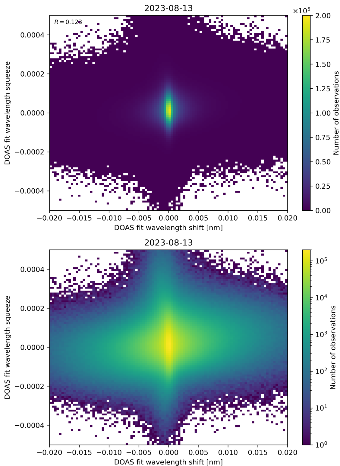
Figure 65: Scatter density plot of “DOAS fit wavelength shift” against “DOAS fit wavelength squeeze” for 2023-08-12 to 2023-08-14.
