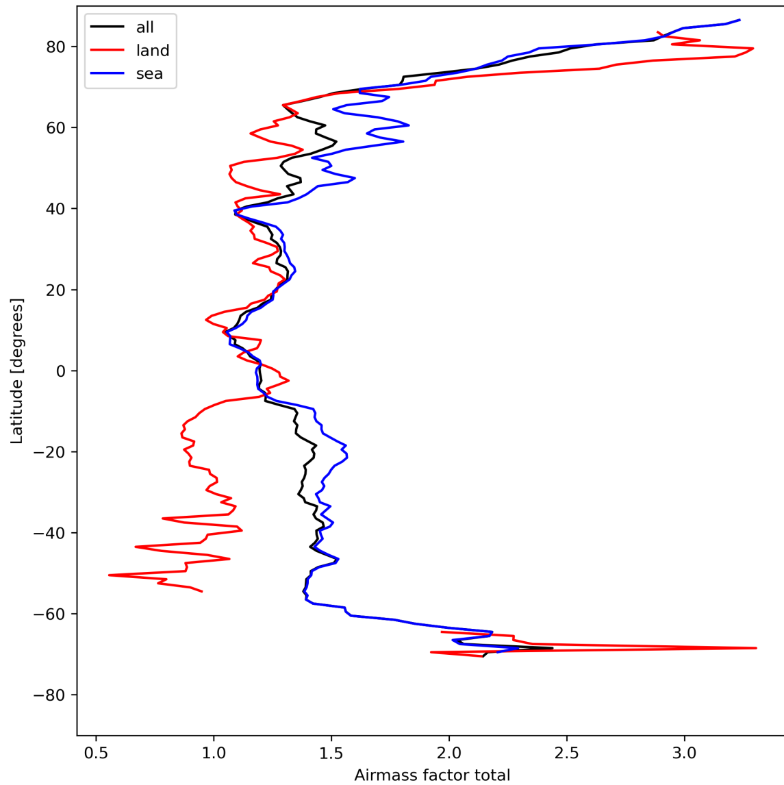
Figure 26: Zonal average of “Airmass factor total” for 2023-08-12 to 2023-08-14.
