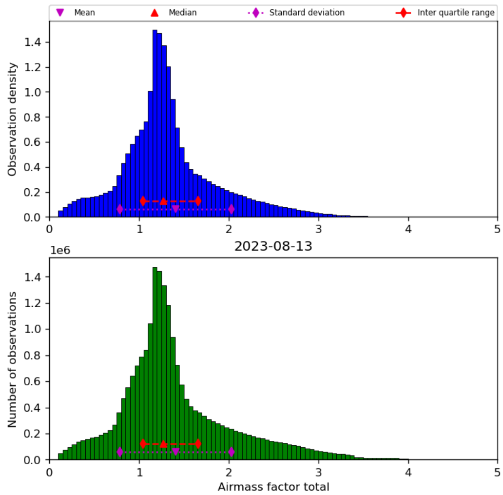
Figure 40: Histogram of “Airmass factor total” for 2023-08-12 to 2023-08-14
