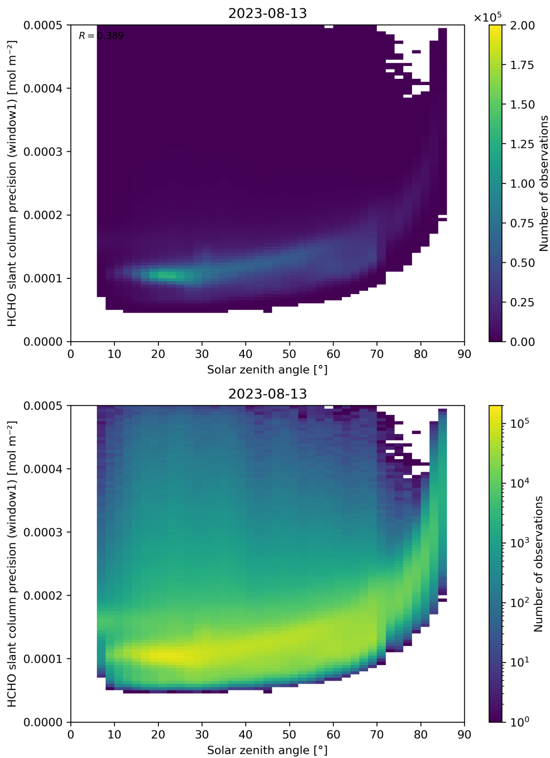
Figure 174: Scatter density plot of “Solar zenith angle” against “HCHO slant column precision (window1)” for 2023-08-12 to 2023-08-14.
