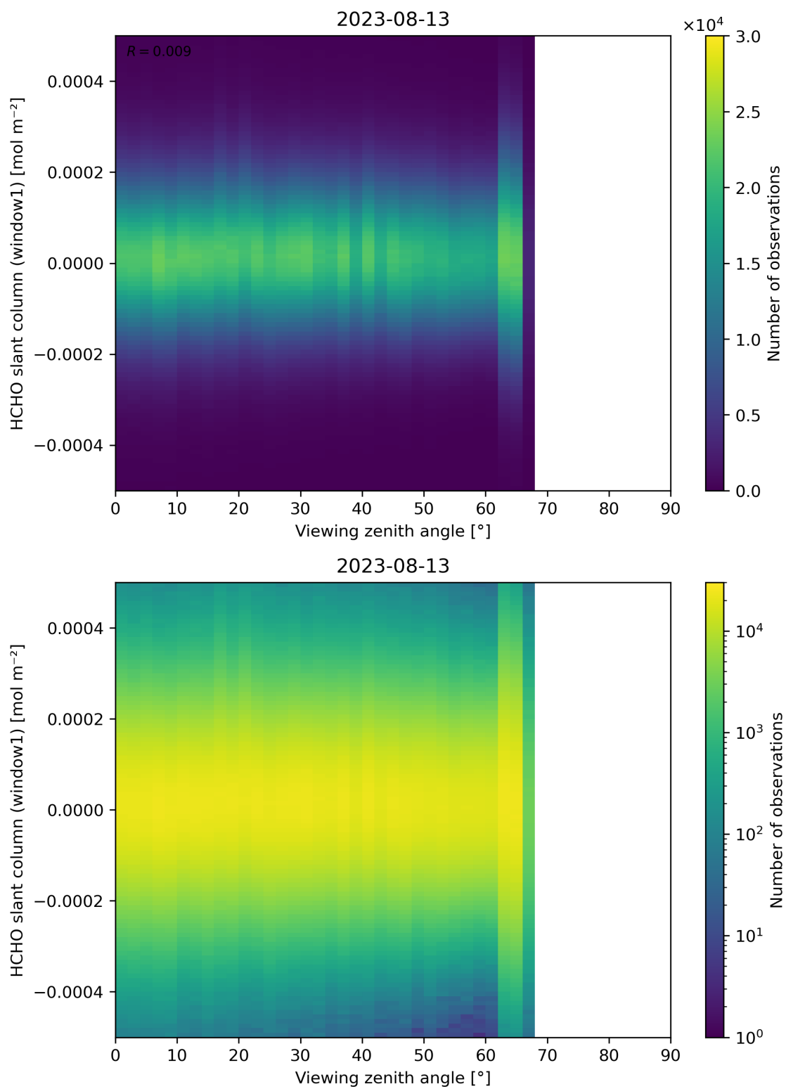
Figure 188: Scatter density plot of “Viewing zenith angle” against “HCHO slant column (window1)” for 2023-08-12 to 2023-08-14.
