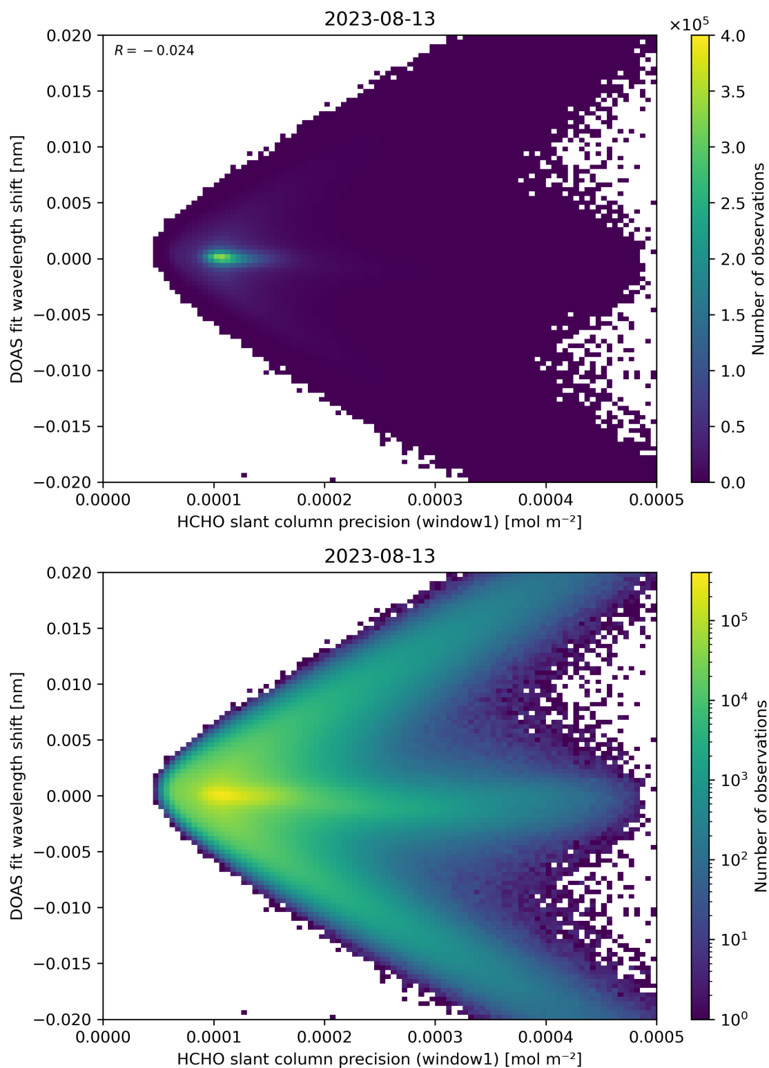
Figure 89: Scatter density plot of “HCHO slant column precision (window1)” against “DOAS fit wavelength shift” for 2023-08-12 to 2023-08-14.
