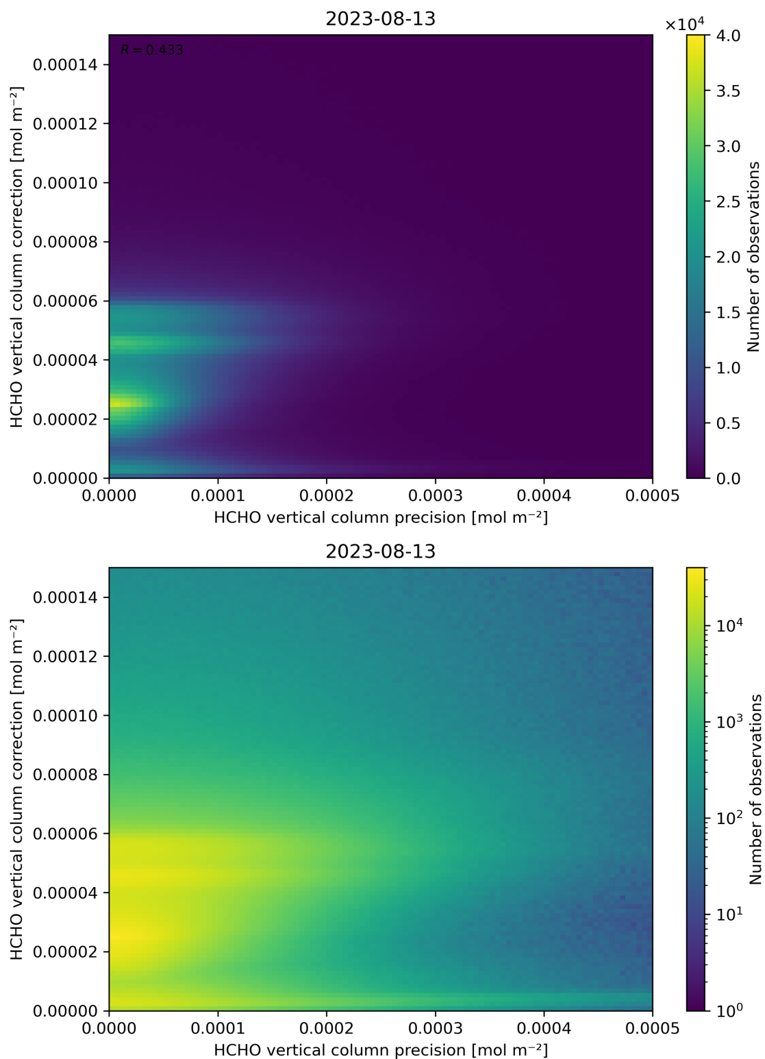
Figure 146: Scatter density plot of “HCHO vertical column precision” against “HCHO vertical column correction” for 2023-08-12 to 2023-08-14.
