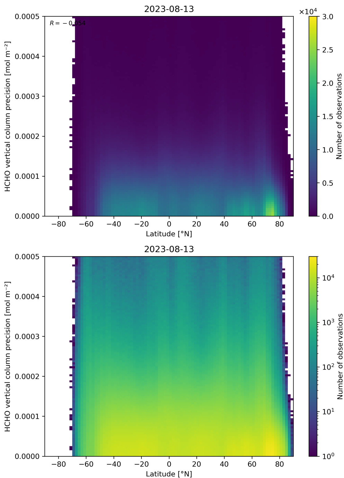
Figure 165: Scatter density plot of “Latitude” against “HCHO vertical column precision” for 2023-08-12 to 2023-08-14.
