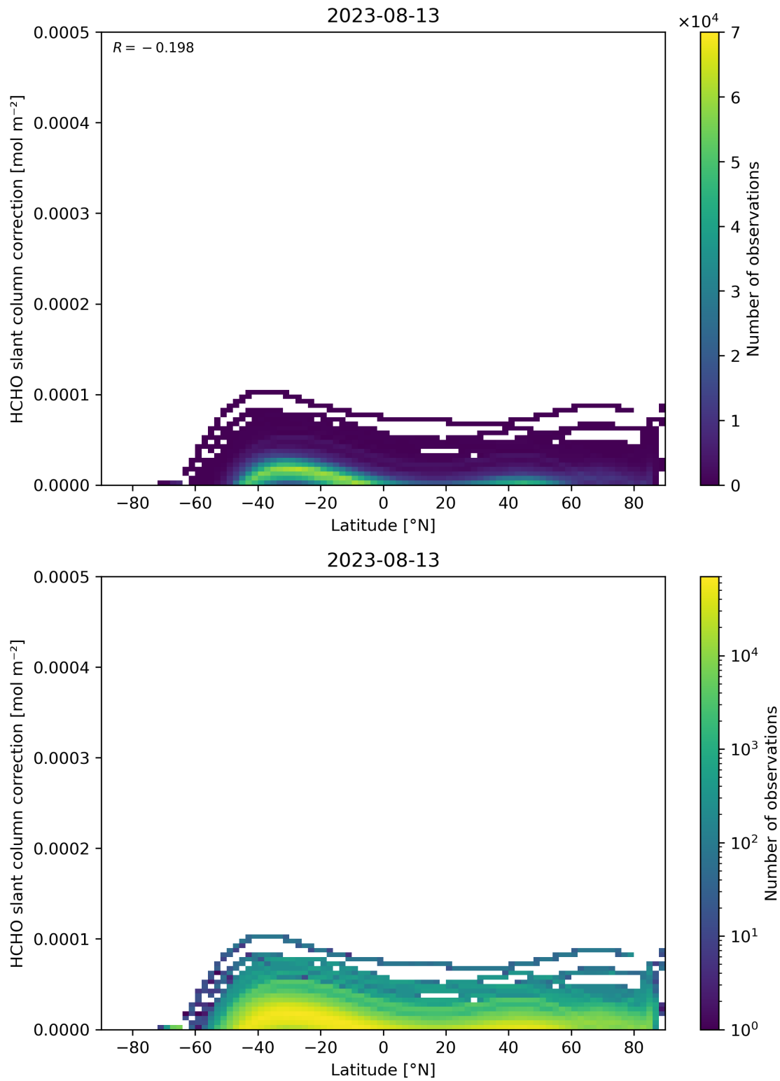
Figure 158: Scatter density plot of “Latitude” against “HCHO slant column correction” for 2023-08-12 to 2023-08-14.
