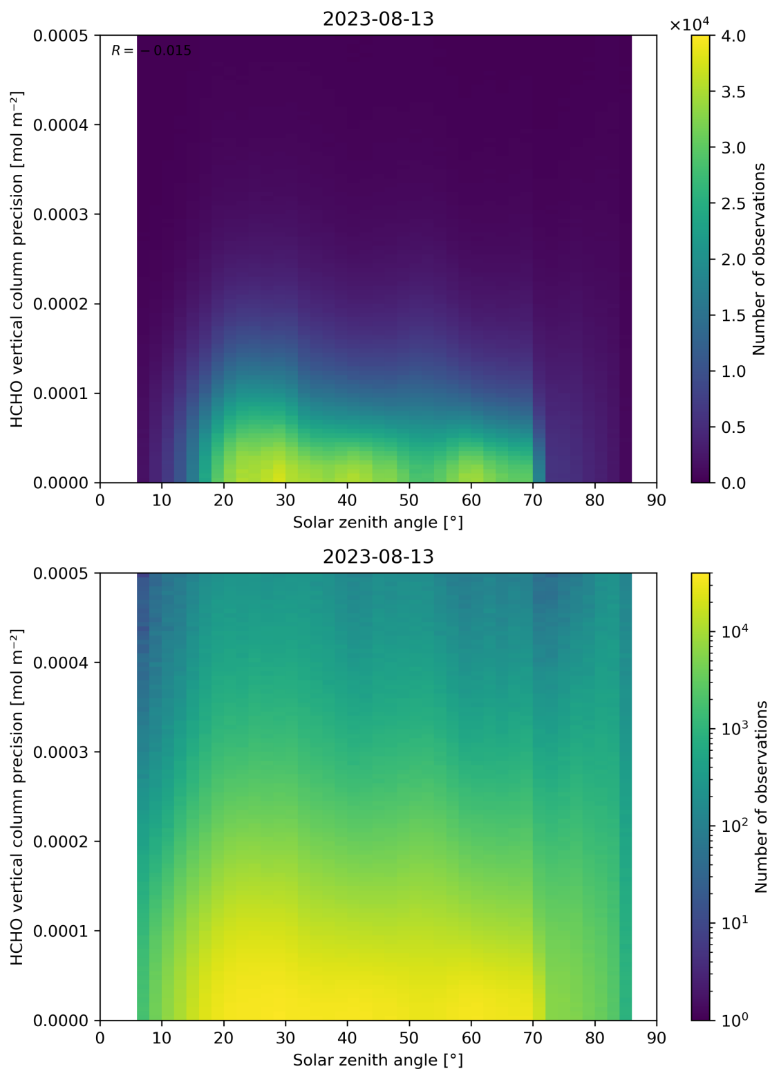
Figure 179: Scatter density plot of “Solar zenith angle” against “HCHO vertical column precision” for 2023-08-12 to 2023-08-14.
