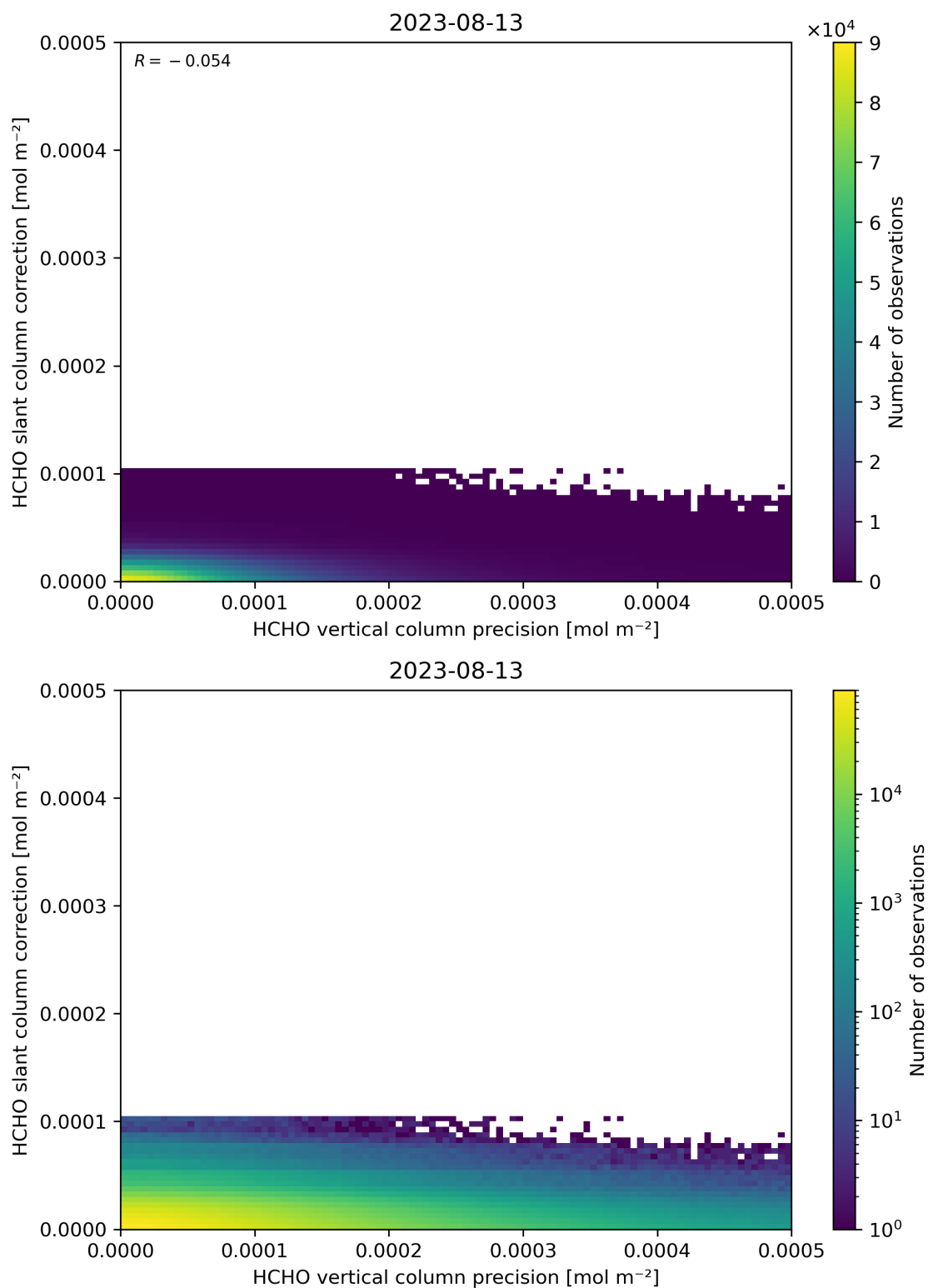
Figure 141: Scatter density plot of “HCHO vertical column precision” against “HCHO slant column correction” for 2023-08-12 to 2023-08-14.
