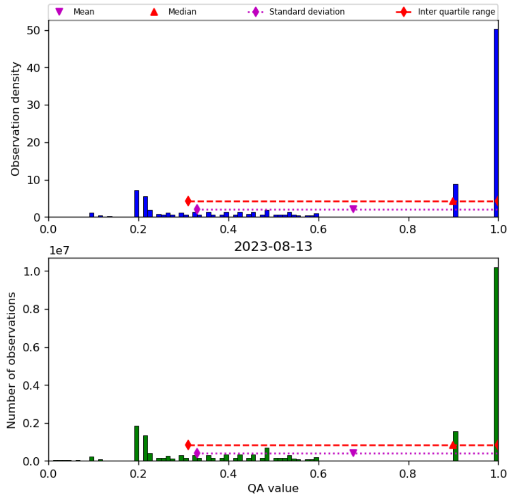
Figure 34: Histogram of “QA value” for 2023-08-12 to 2023-08-14
