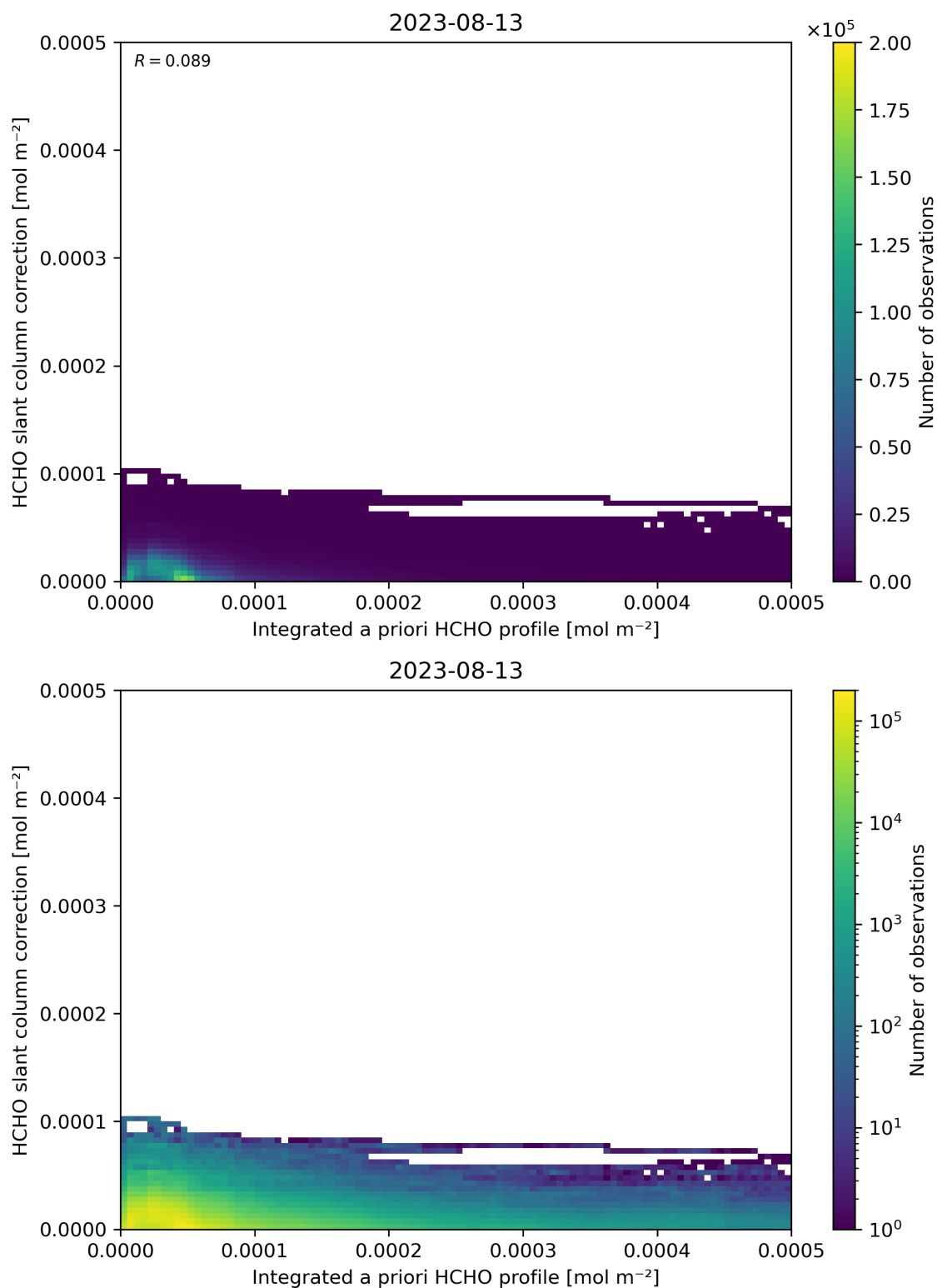
Figure 152: Scatter density plot of “Integrated a priori HCHO profile” against “HCHO slant column correction” for 2023-08-12 to 2023-08-14.
