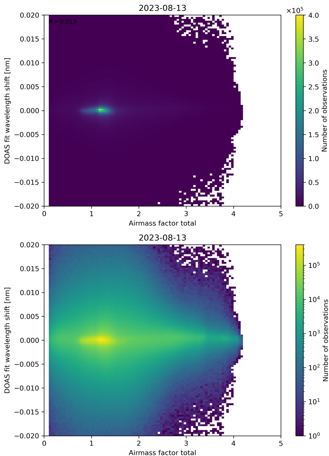
Figure 98: Scatter density plot of “Airmass factor total” against “DOAS fit wavelength shift” for 2023-08-12 to 2023-08-14.
