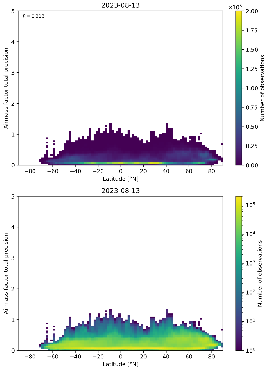
Figure 162: Scatter density plot of “Latitude” against “Airmass factor total precision” for 2023-08-12 to 2023-08-14.
