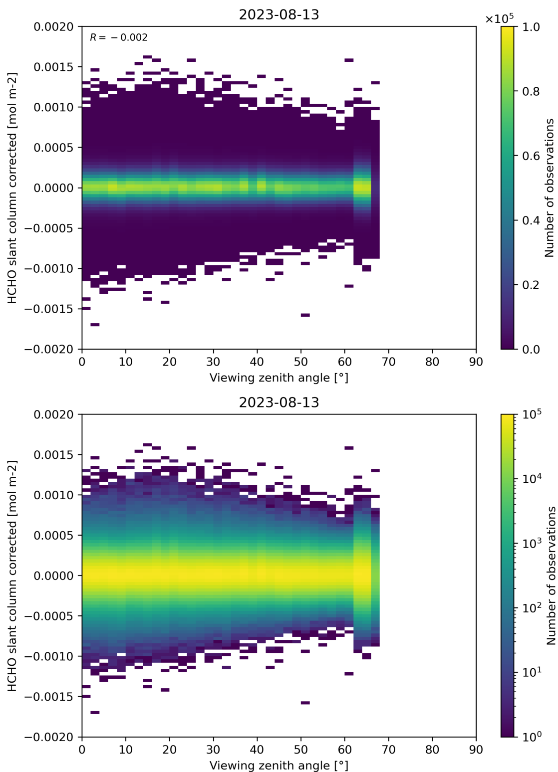
Figure 186: Scatter density plot of “Viewing zenith angle” against “HCHO slant column corrected” for 2023-08-12 to 2023-08-14.
