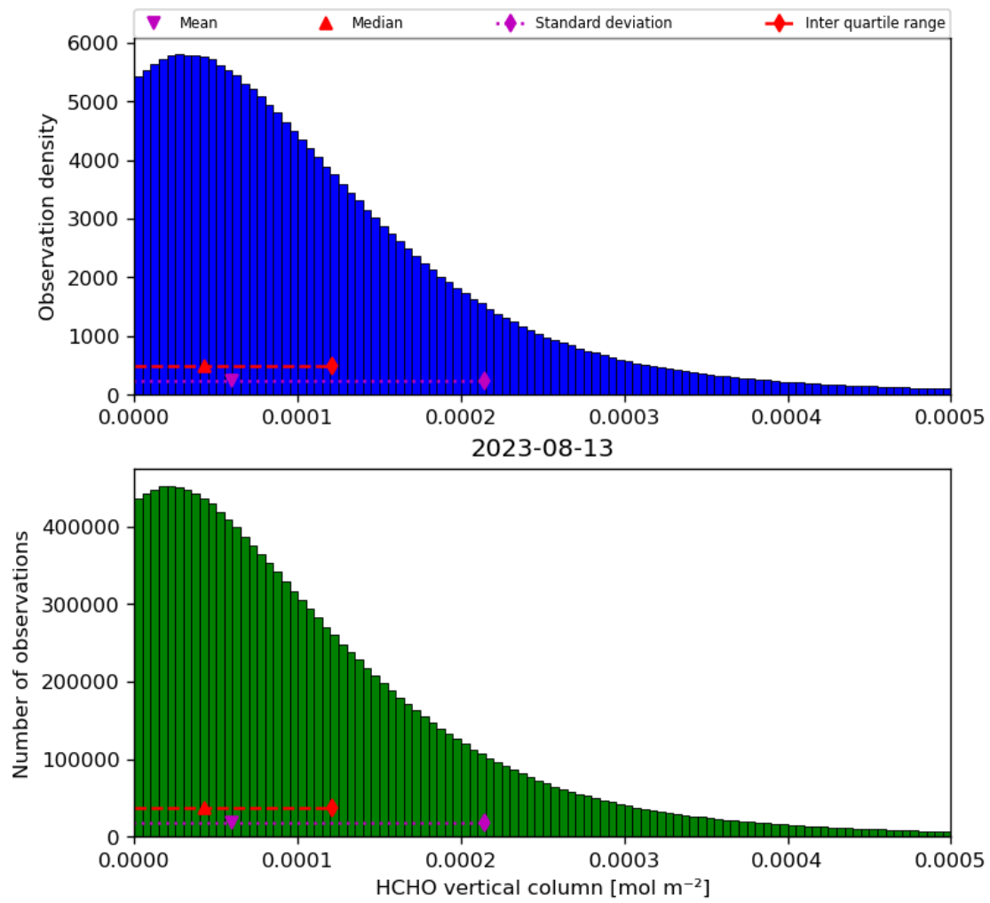
Figure 35: Histogram of “HCHO vertical column” for 2023-08-12 to 2023-08-14
