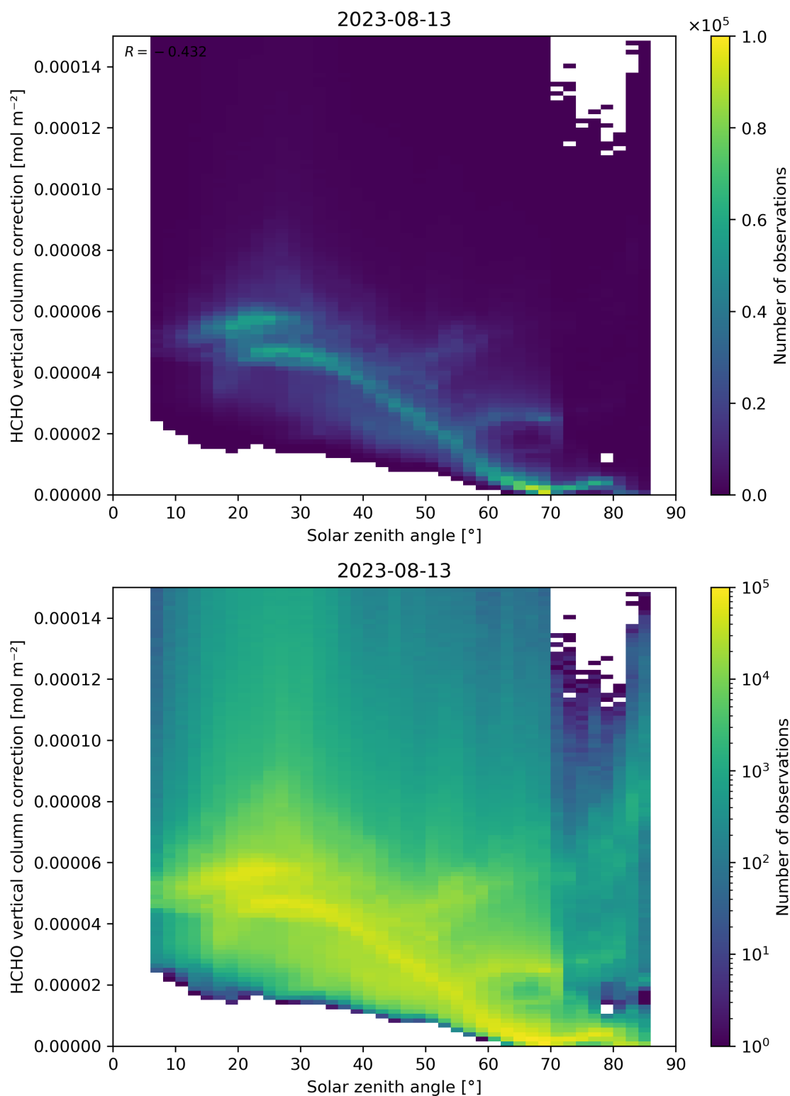
Figure 178: Scatter density plot of “Solar zenith angle” against “HCHO vertical column correction” for 2023-08-12 to 2023-08-14.
