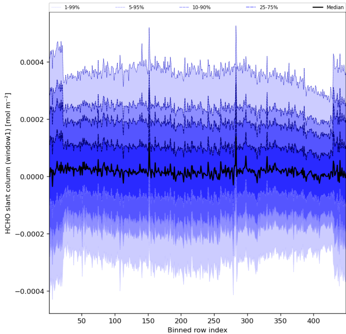
Figure 52: Along track statistics of “HCHO slant column (window1)” for 2023-08-12 to 2023-08-14
