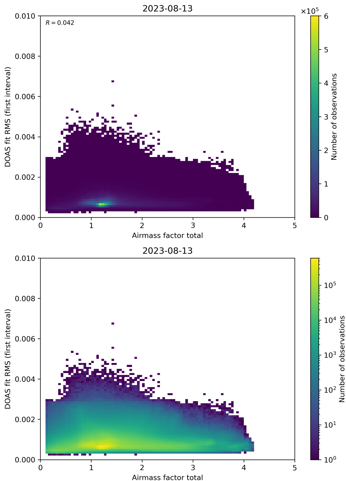
Figure 97: Scatter density plot of “Airmass factor total” against “DOAS fit RMS (first interval)” for 2023-08-12 to 2023-08-14.
