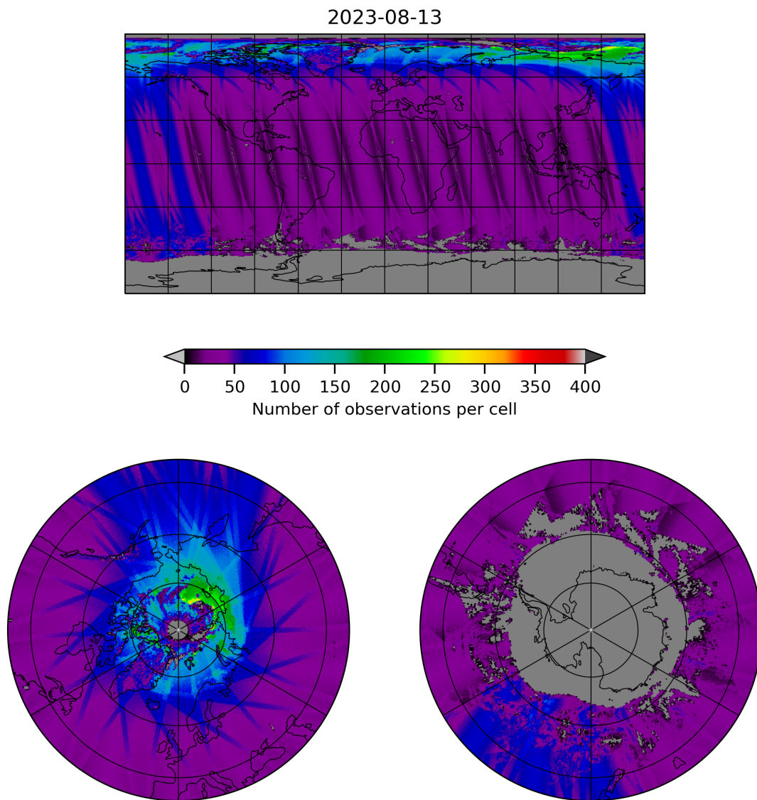
Figure 19: Map of the number of observations for 2023-08-12 to 2023-08-14
