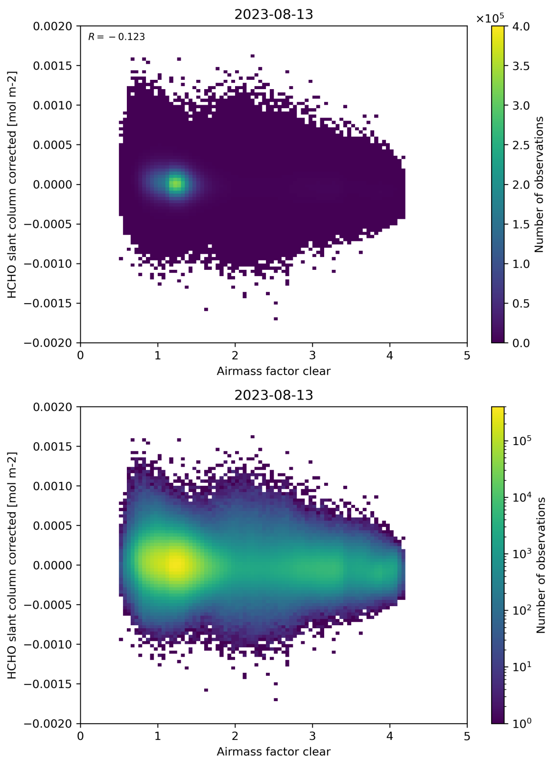
Figure 74: Scatter density plot of “Airmass factor clear” against “HCHO slant column corrected” for 2023-08-12 to 2023-08-14.
