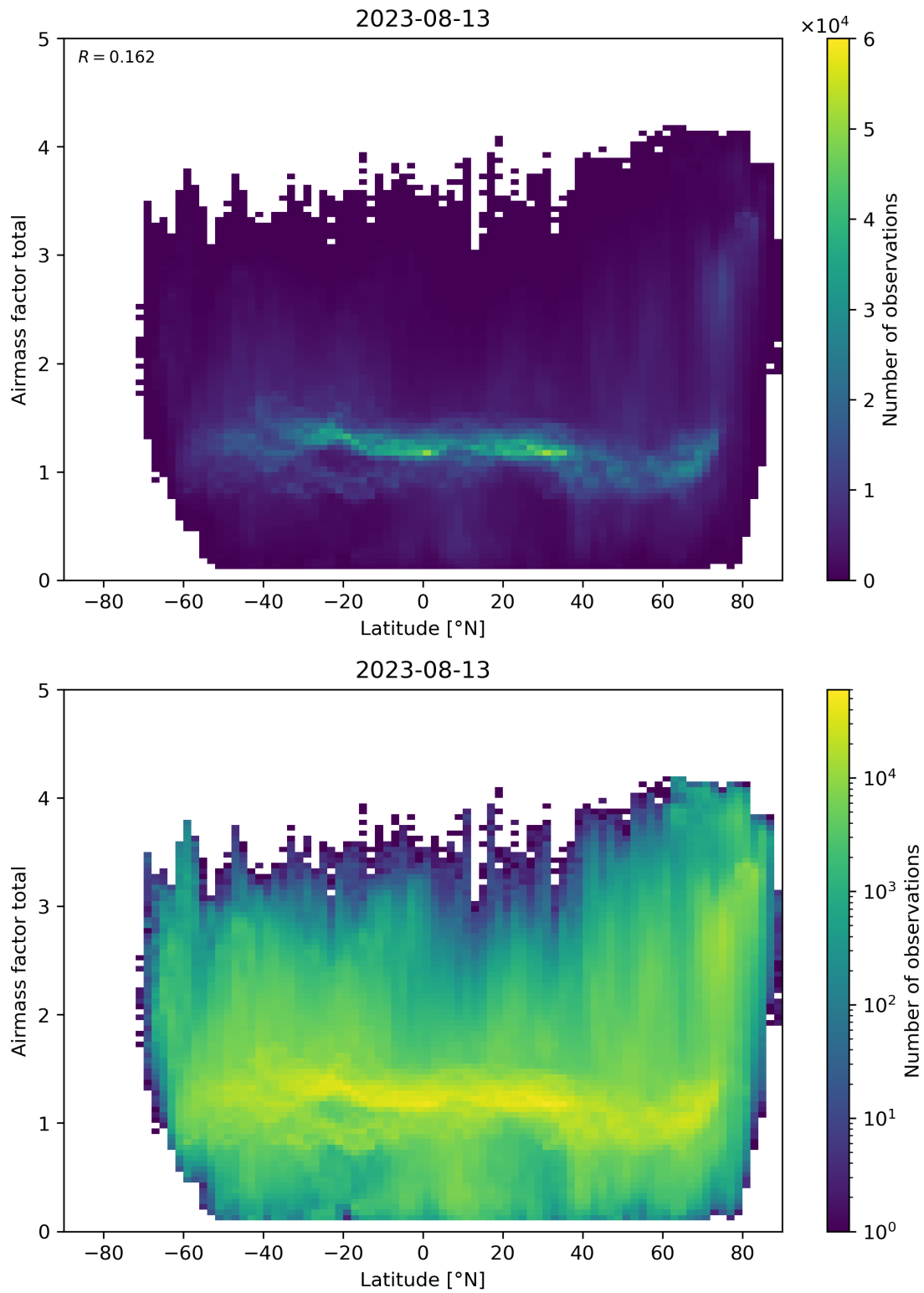
Figure 161: Scatter density plot of “Latitude” against “Airmass factor total” for 2023-08-12 to 2023-08-14.
