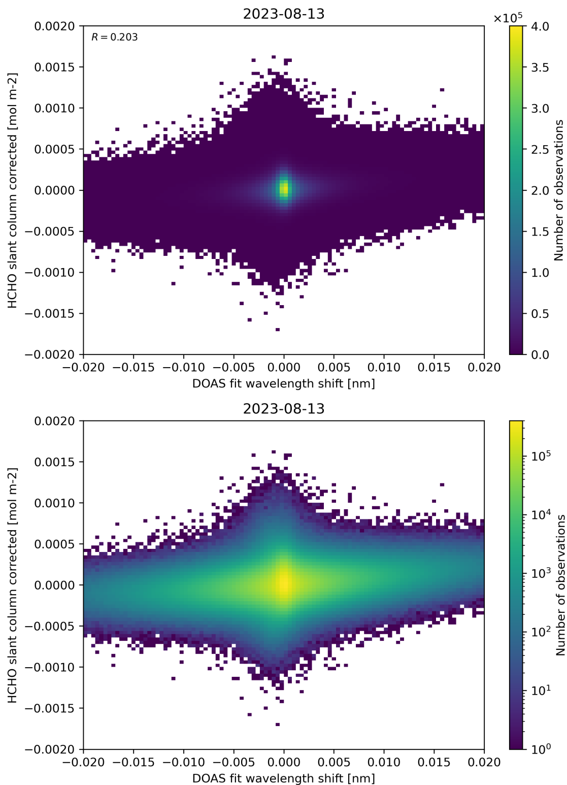
Figure 66: Scatter density plot of “DOAS fit wavelength shift” against “HCHO slant column corrected” for 2023-08-12 to 2023-08-14.
