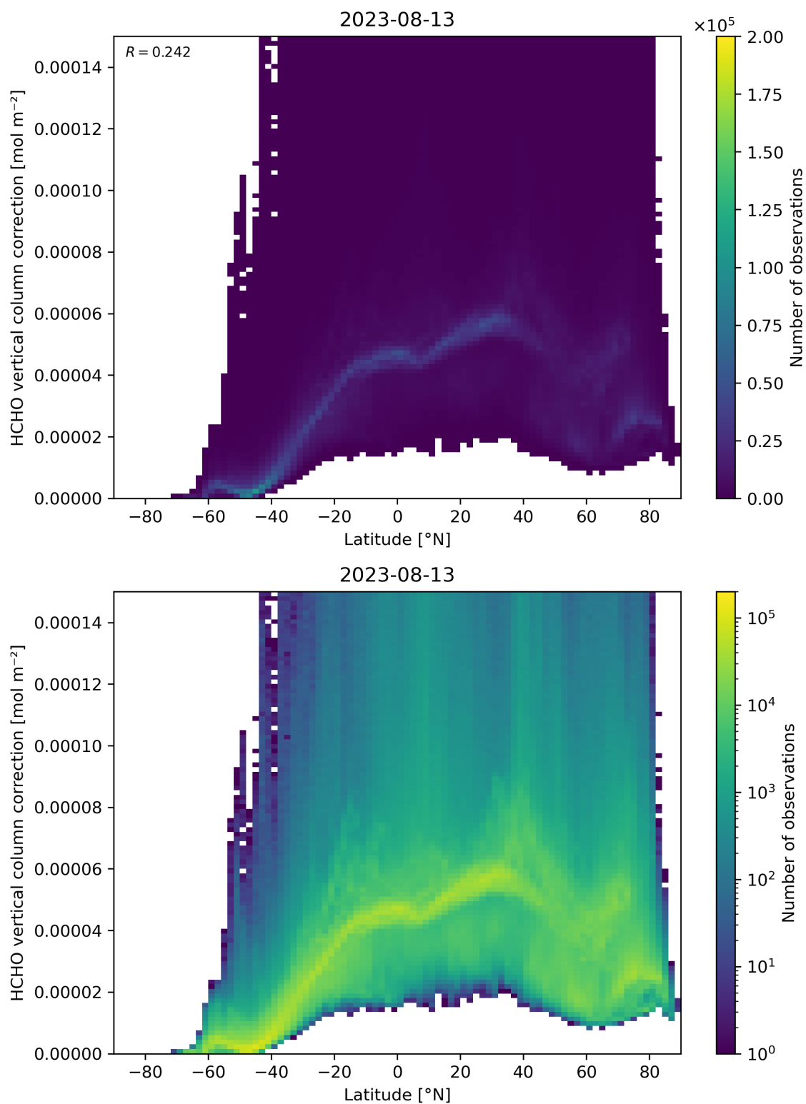
Figure 164: Scatter density plot of “Latitude” against “HCHO vertical column correction” for 2023-08-12 to 2023-08-14.
