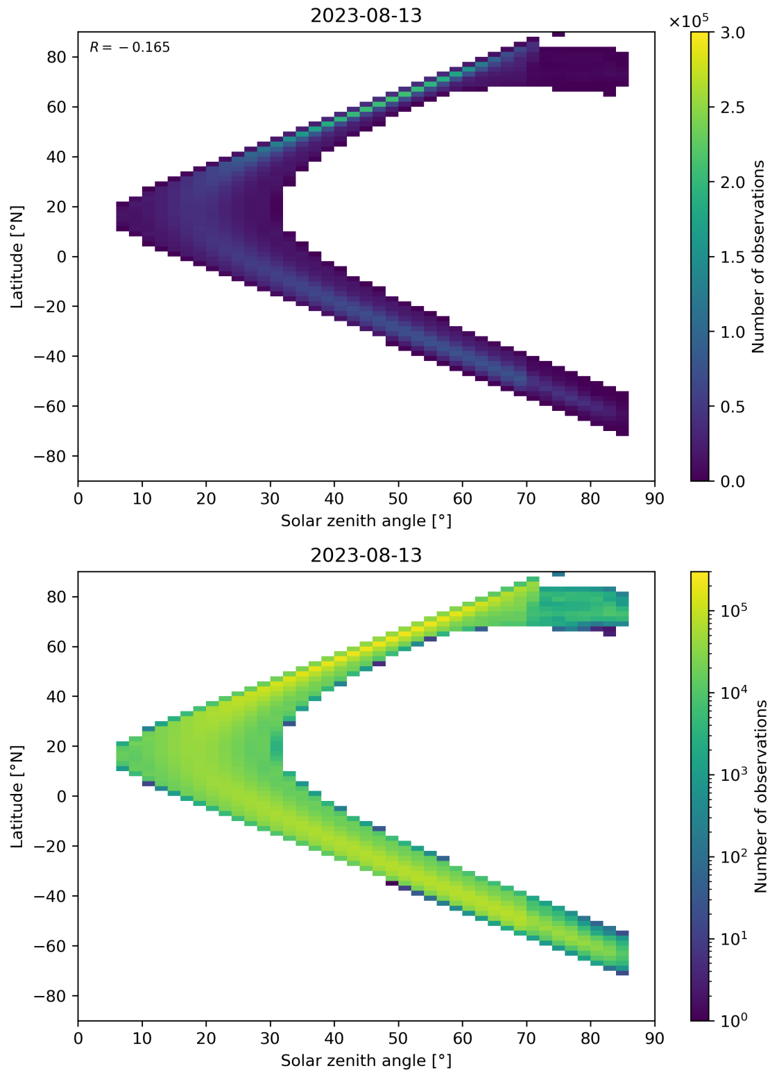
Figure 181: Scatter density plot of “Solar zenith angle” against “Latitude” for 2023-08-12 to 2023-08-14.
