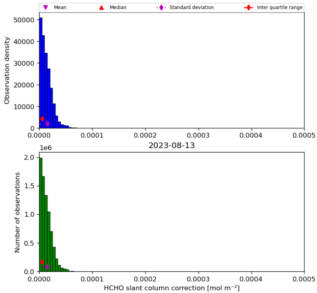
Figure 47: Histogram of “HCHO slant column correction” for 2023-08-12 to 2023-08-14
