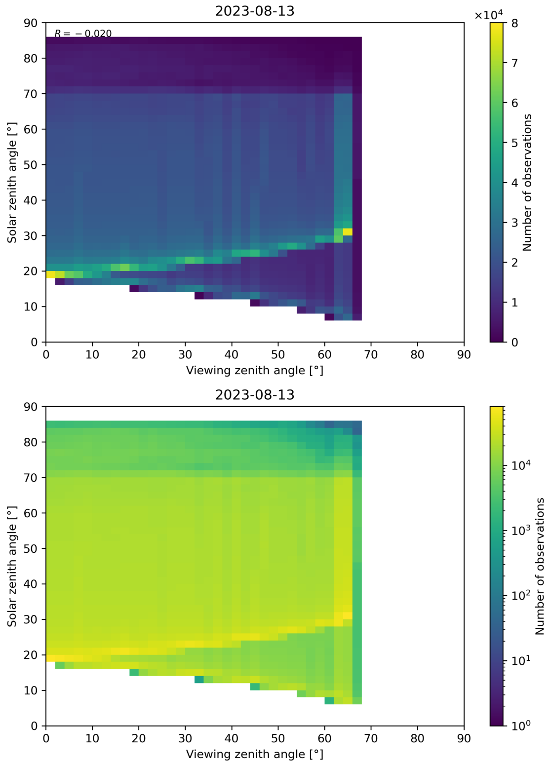
Figure 197: Scatter density plot of “Viewing zenith angle” against “Solar zenith angle” for 2023-08-12 to 2023-08-14.
