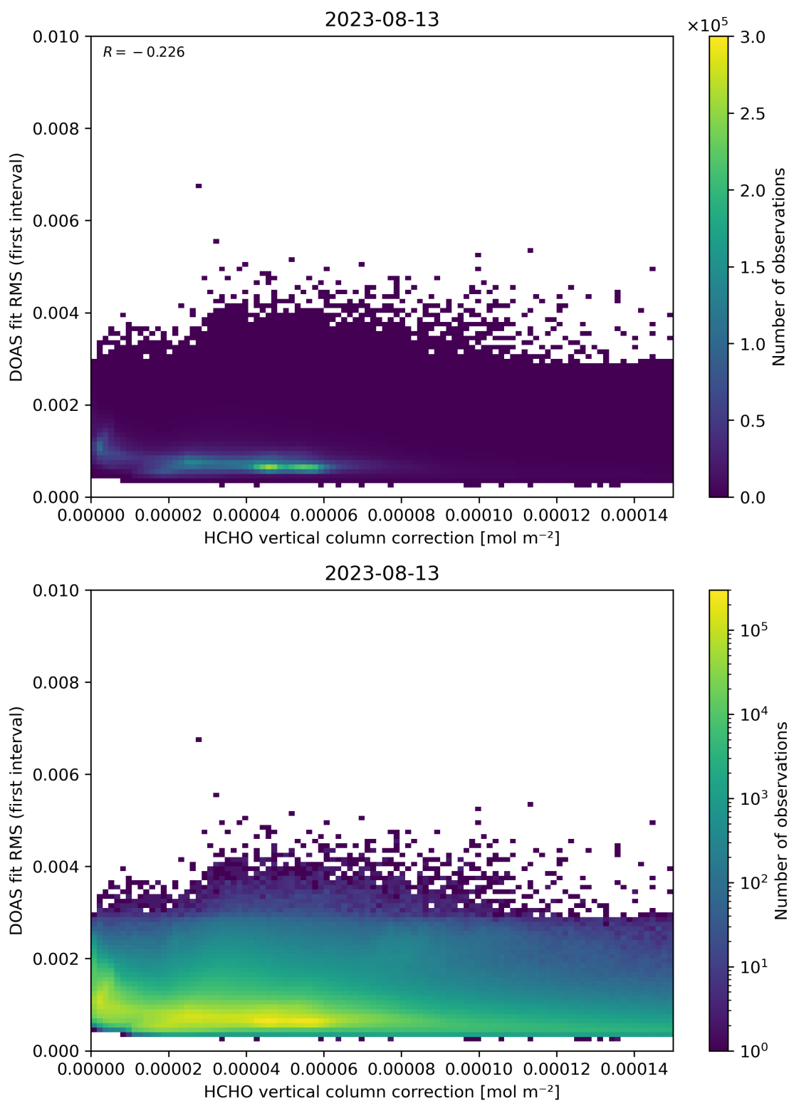
Figure 112: Scatter density plot of “HCHO vertical column correction” against “DOAS fit RMS (first interval)” for 2023-08-12 to 2023-08-14.
