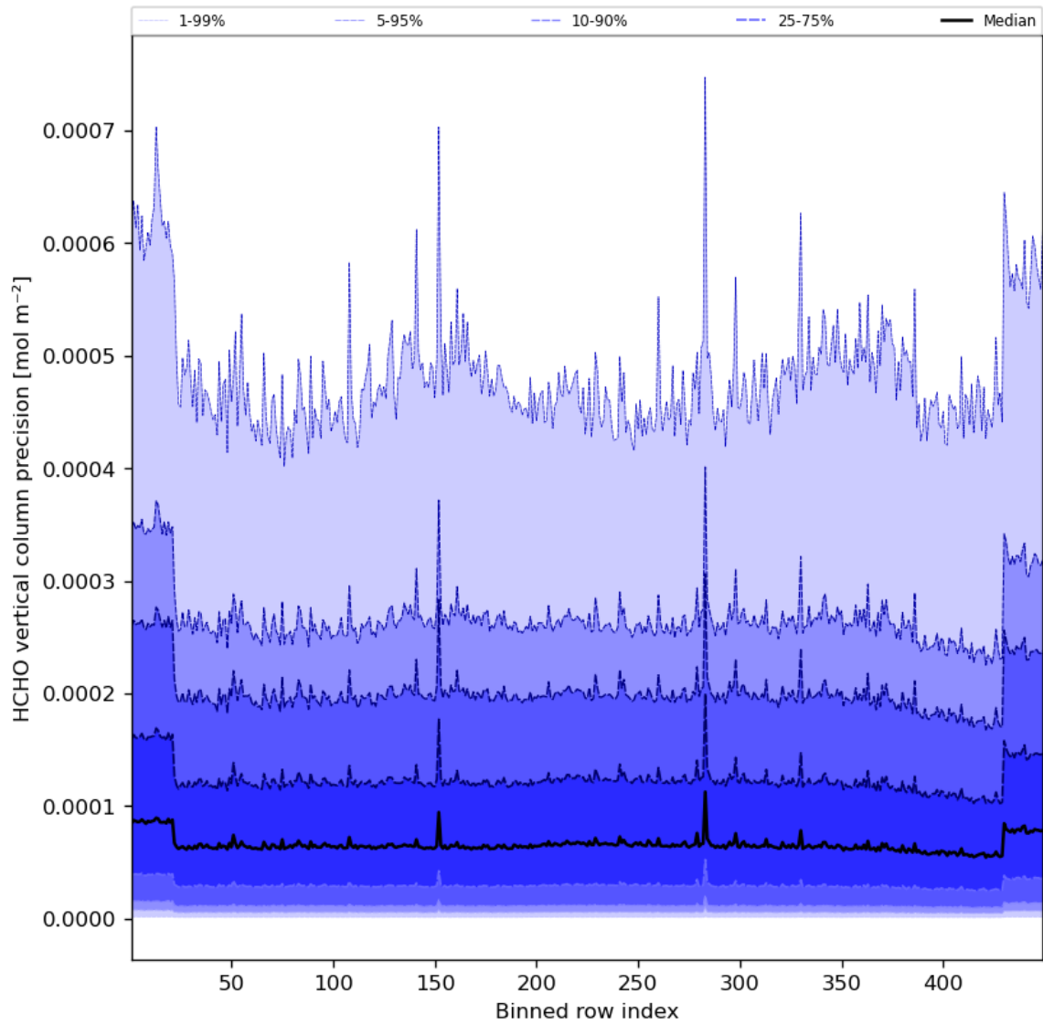
Figure 50: Along track statistics of “HCHO vertical column precision” for 2023-08-12 to 2023-08-14
