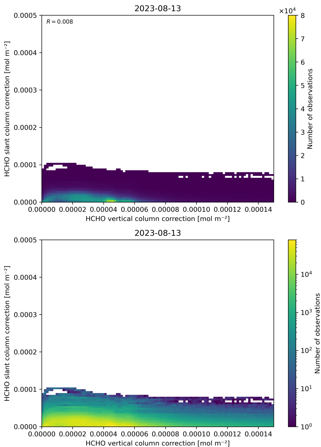
Figure 117: Scatter density plot of “HCHO vertical column correction” against “HCHO slant column correction” for 2023-08-12 to 2023-08-14.
