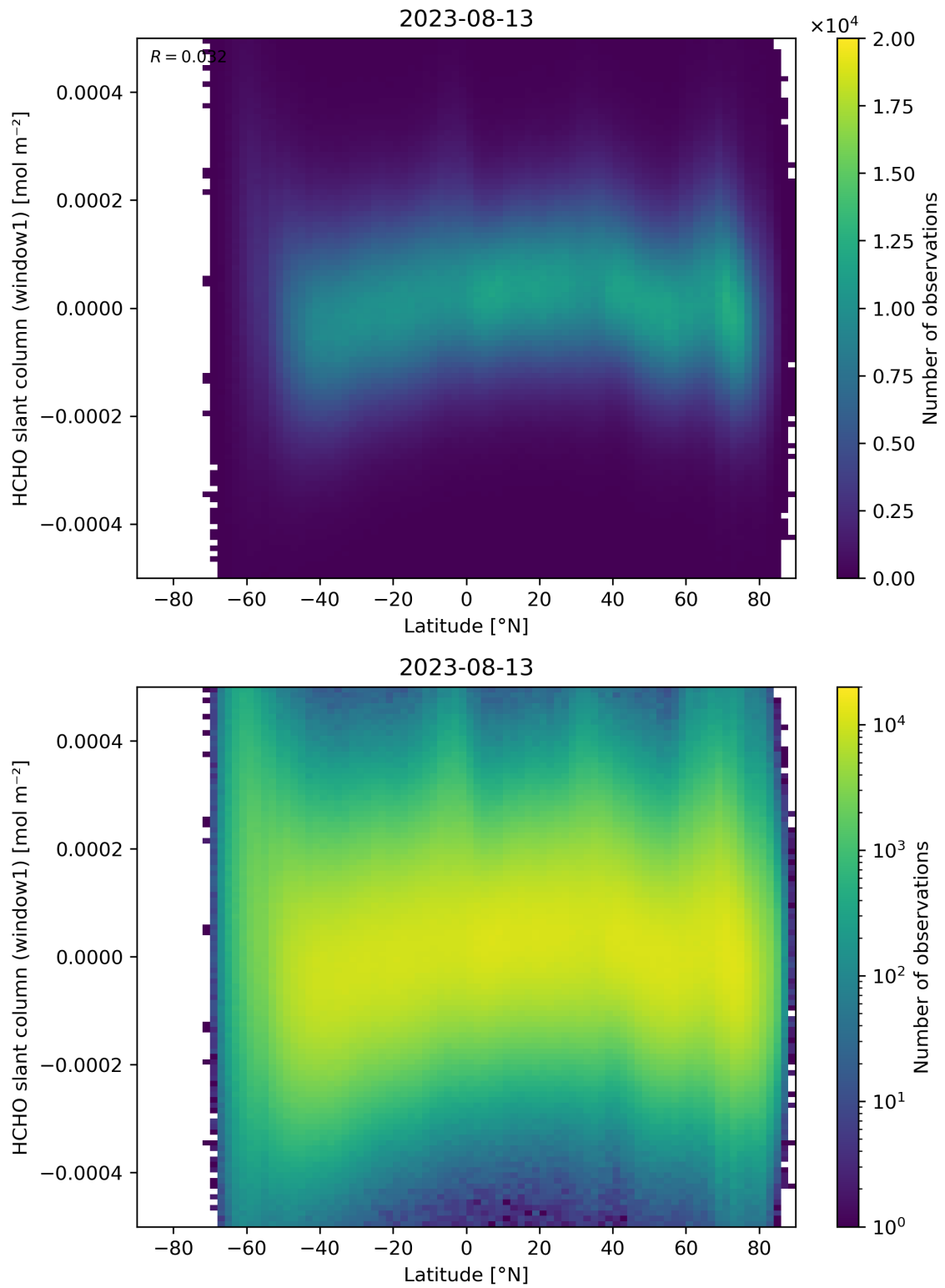
Figure 159: Scatter density plot of “Latitude” against “HCHO slant column (window1)” for 2023-08-12 to 2023-08-14.
