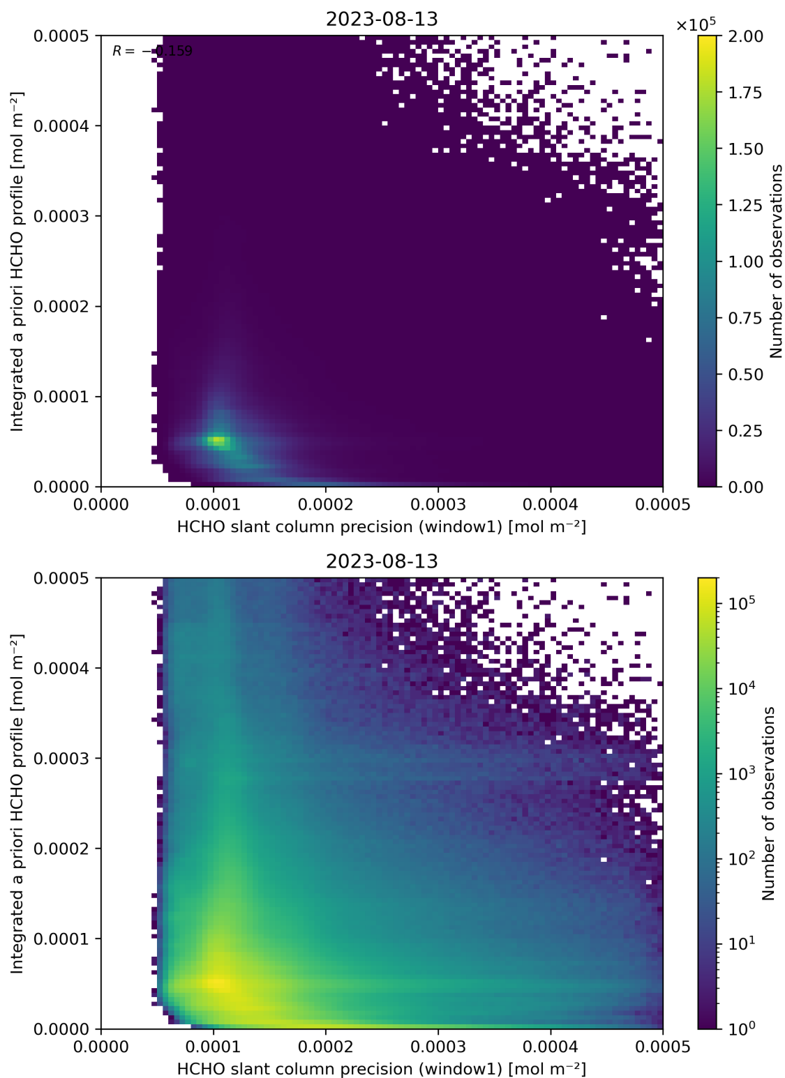
Figure 96: Scatter density plot of “HCHO slant column precision (window1)” against “Integrated a priori HCHO profile” for 2023-08-12 to 2023-08-14.
