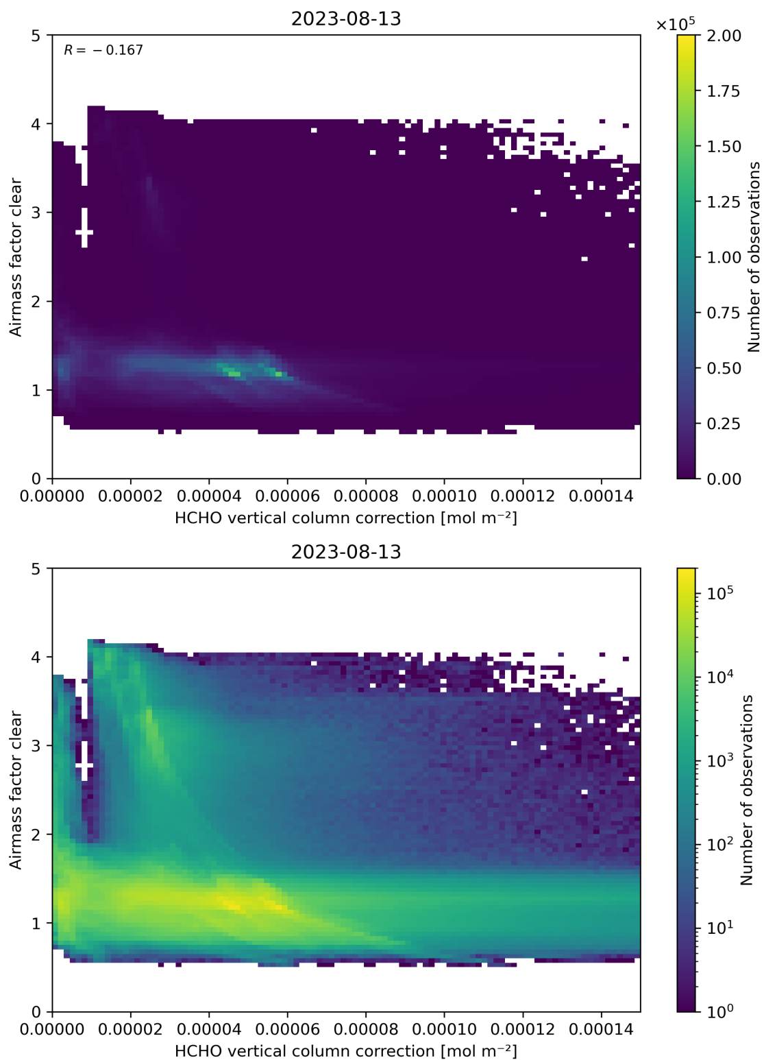
Figure 115: Scatter density plot of “HCHO vertical column correction” against “Airmass factor clear” for 2023-08-12 to 2023-08-14.
