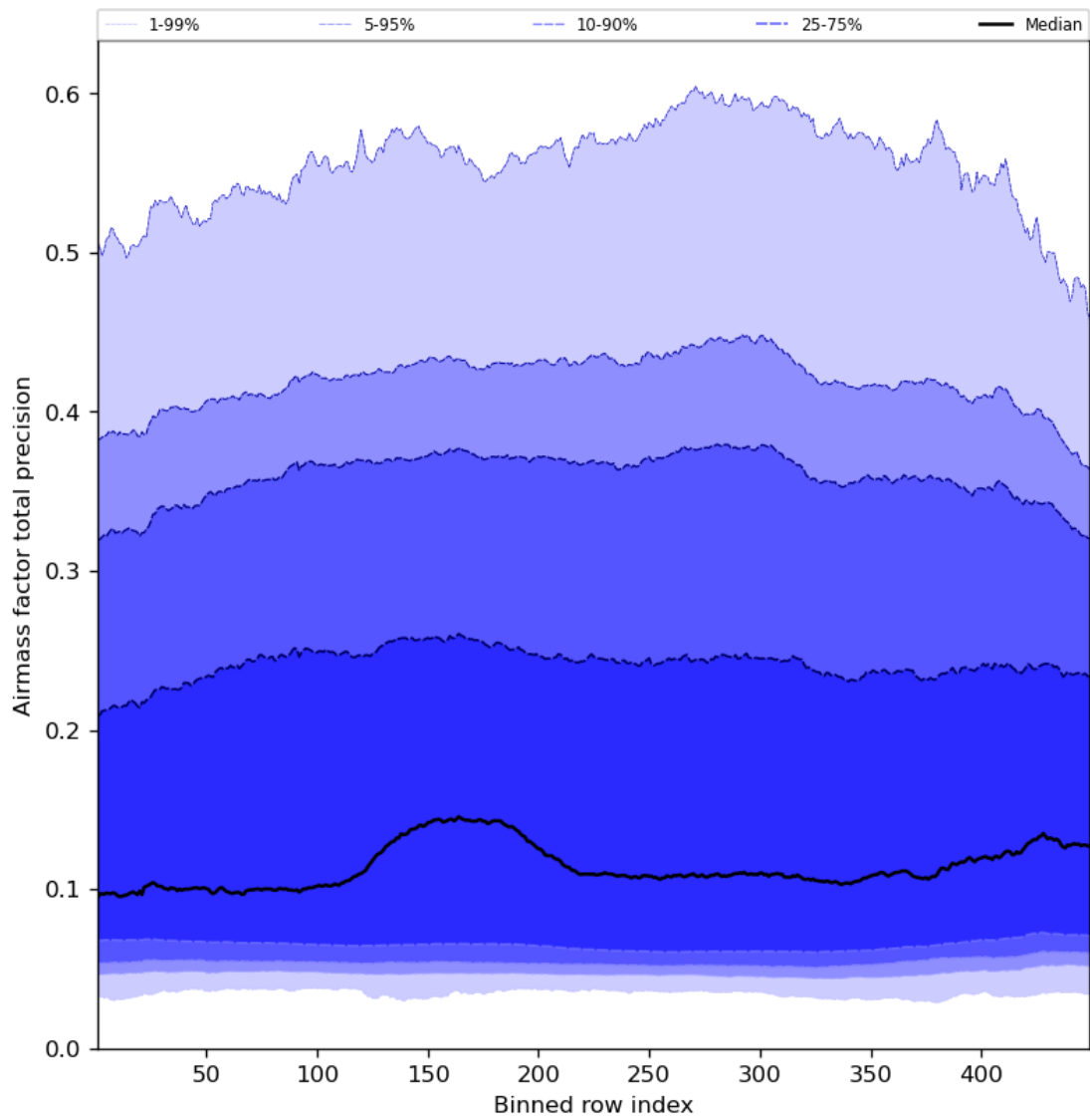
Figure 55: Along track statistics of “Airmass factor total precision” for 2023-08-12 to 2023-08-14
