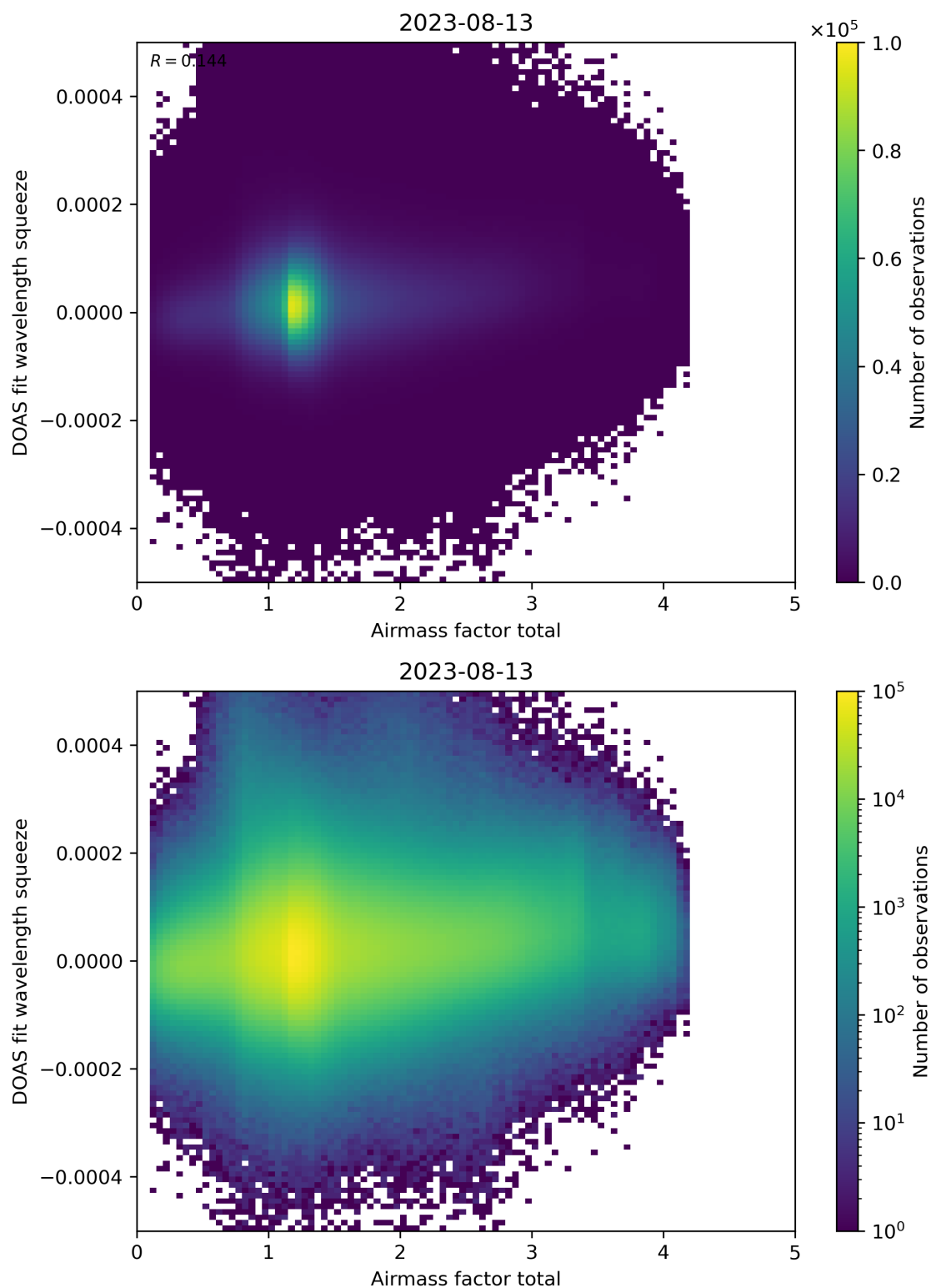
Figure 99: Scatter density plot of “Airmass factor total” against “DOAS fit wavelength squeeze” for 2023-08-12 to 2023-08-14.
