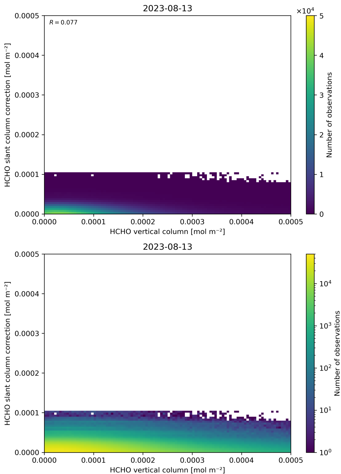
Figure 128: Scatter density plot of “HCHO vertical column” against “HCHO slant column correction” for 2023-08-12 to 2023-08-14.
