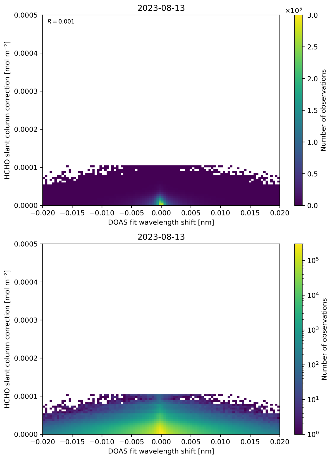
Figure 67: Scatter density plot of “DOAS fit wavelength shift” against “HCHO slant column correction” for 2023-08-12 to 2023-08-14.
