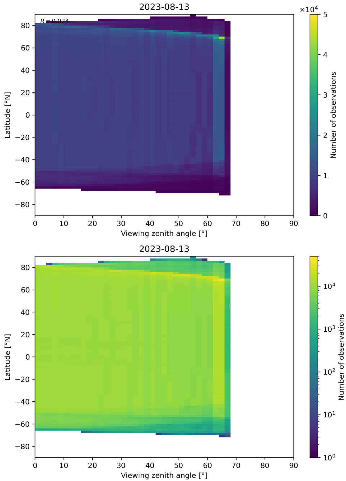
Figure 196: Scatter density plot of “Viewing zenith angle” against “Latitude” for 2023-08-12 to 2023-08-14.
