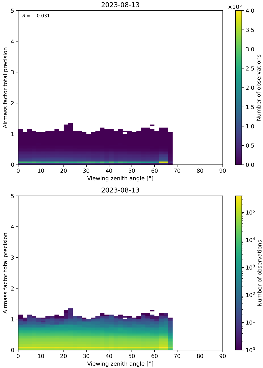
Figure 191: Scatter density plot of “Viewing zenith angle” against “Airmass factor total precision” for 2023-08-12 to 2023-08-14.
