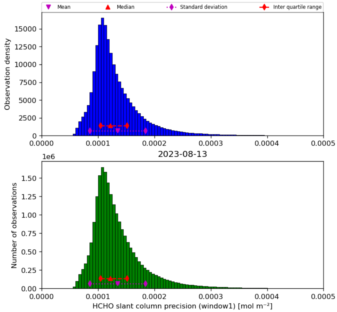
Figure 39: Histogram of “HCHO slant column precision (window1)” for 2023-08-12 to 2023-08-14
