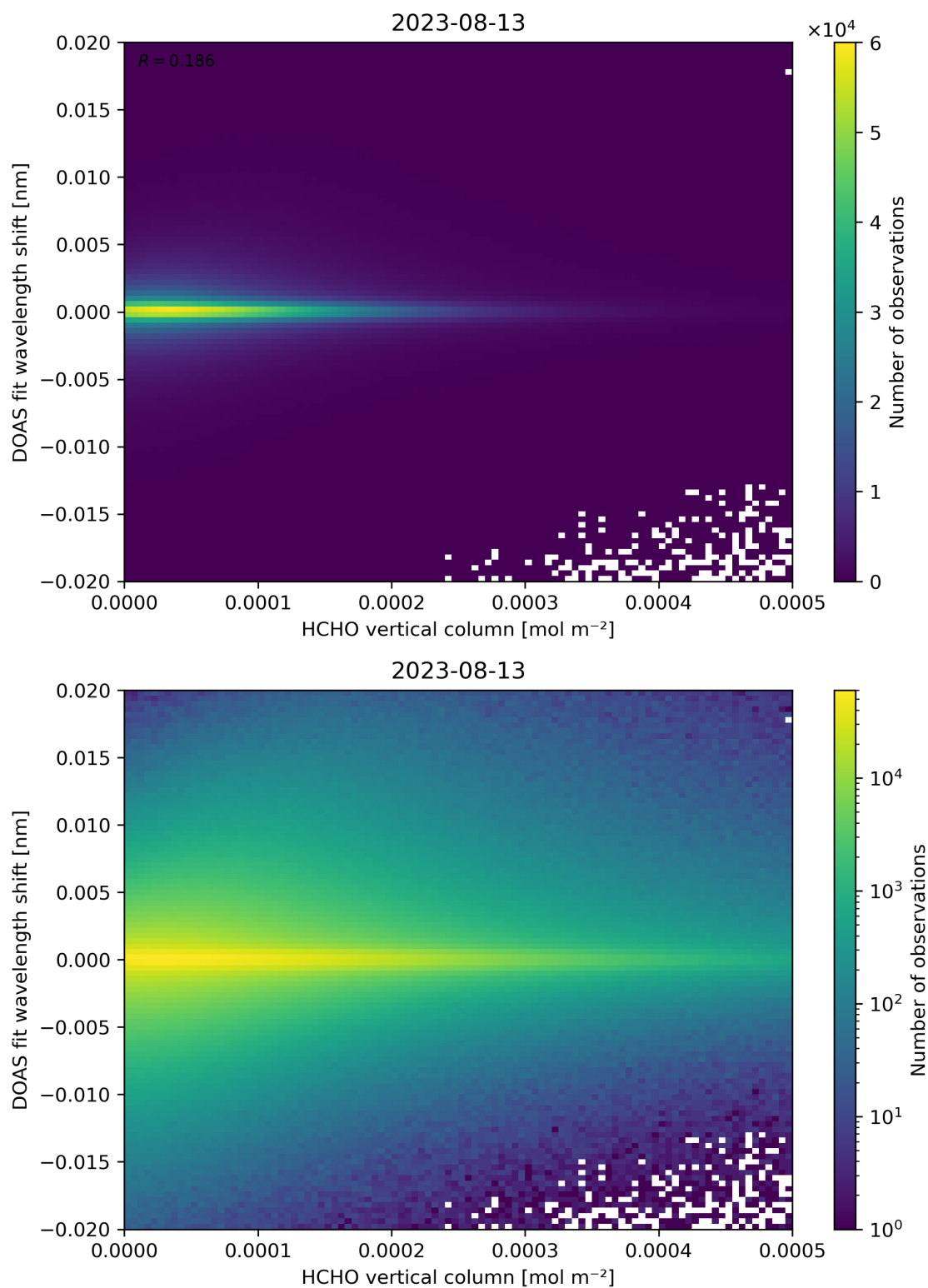
Figure 124: Scatter density plot of “HCHO vertical column” against “DOAS fit wavelength shift” for 2023-08-12 to 2023-08-14.
