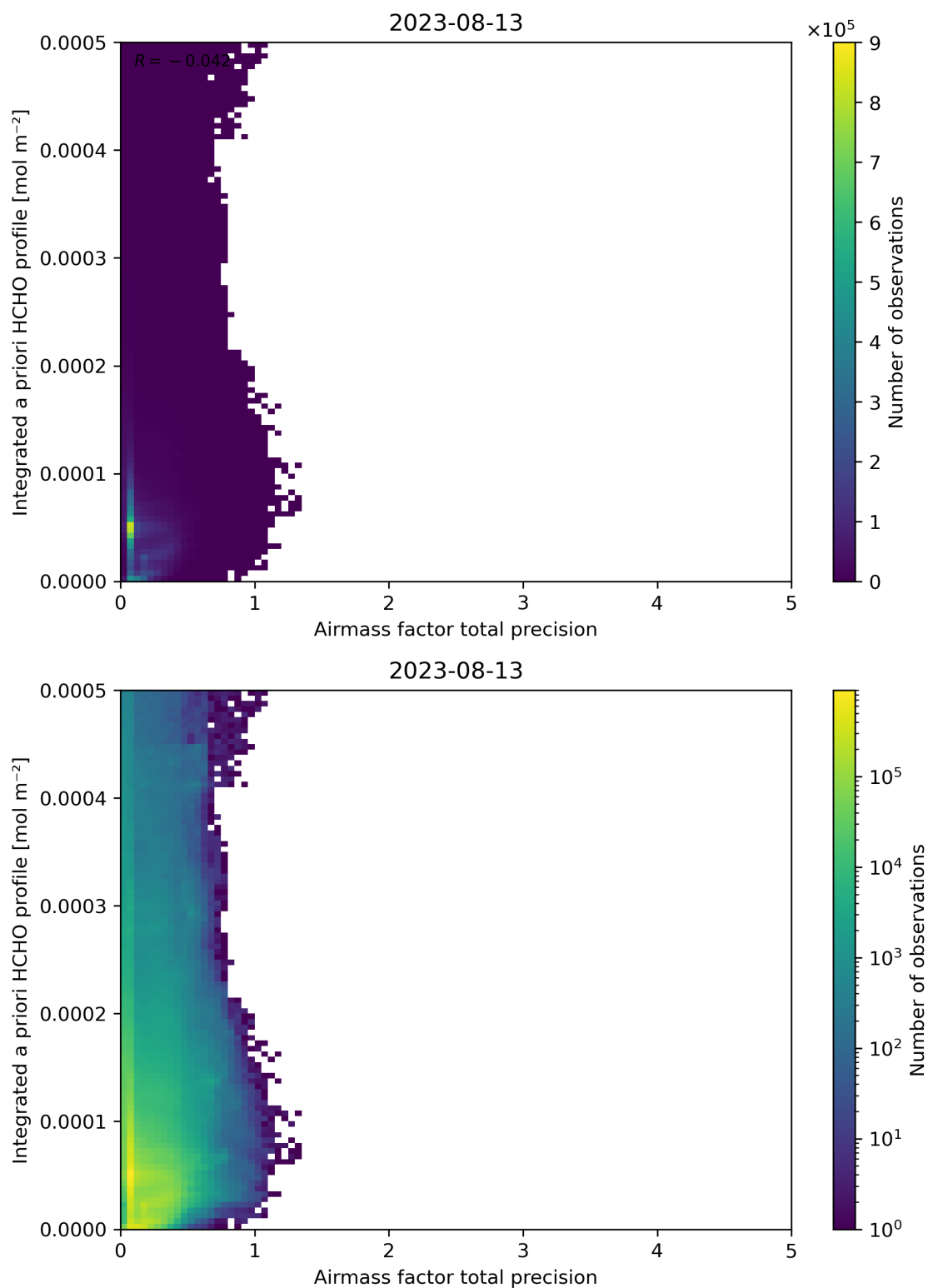
Figure 111: Scatter density plot of “Airmass factor total precision” against “Integrated a priori HCHO profile” for 2023-08-12 to 2023-08-14.
