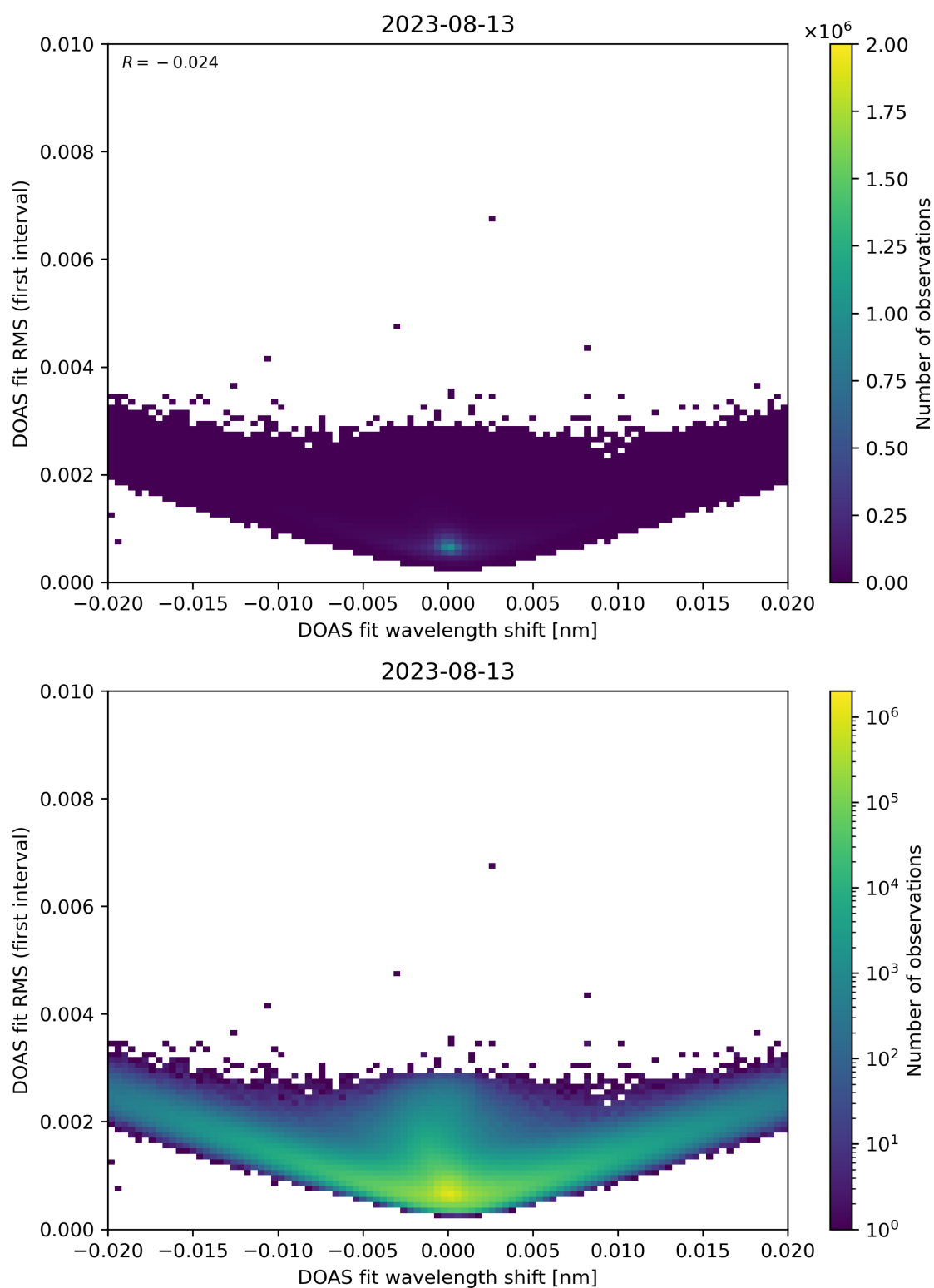
Figure 64: Scatter density plot of “DOAS fit wavelength shift” against “DOAS fit RMS (first interval)” for 2023-08-12 to 2023-08-14.
