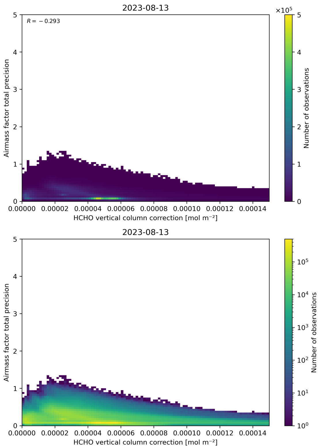
Figure 121: Scatter density plot of “HCHO vertical column correction” against “Airmass factor total precision” for 2023-08-12 to 2023-08-14.
