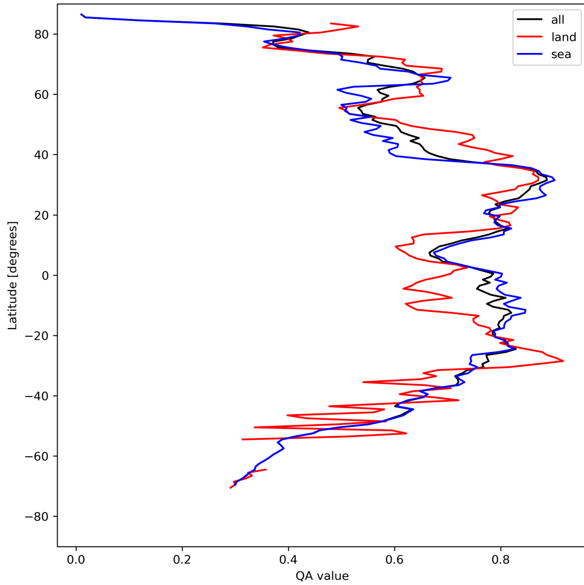
Figure 20: Zonal average of “QA value” for 2023-08-12 to 2023-08-14.
