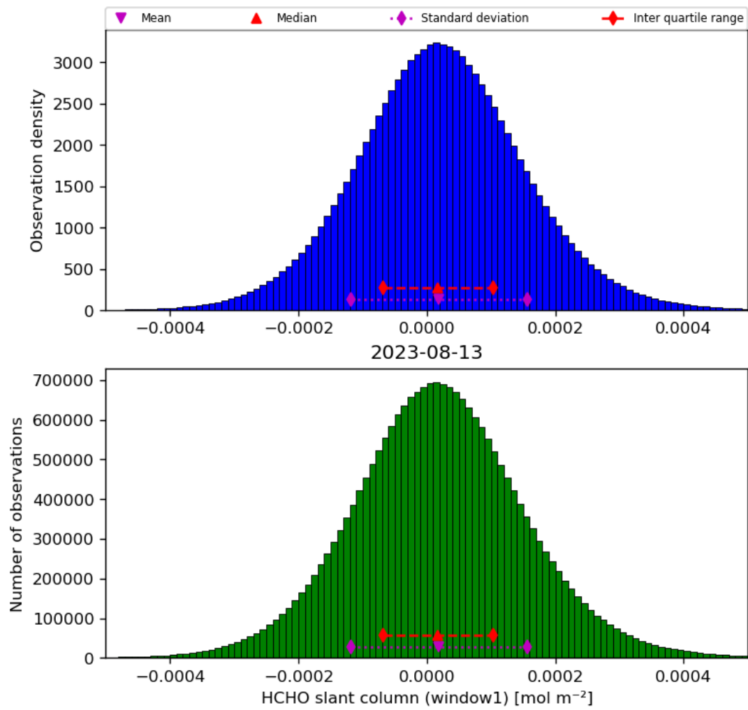
Figure 38: Histogram of “HCHO slant column (window1)” for 2023-08-12 to 2023-08-14
