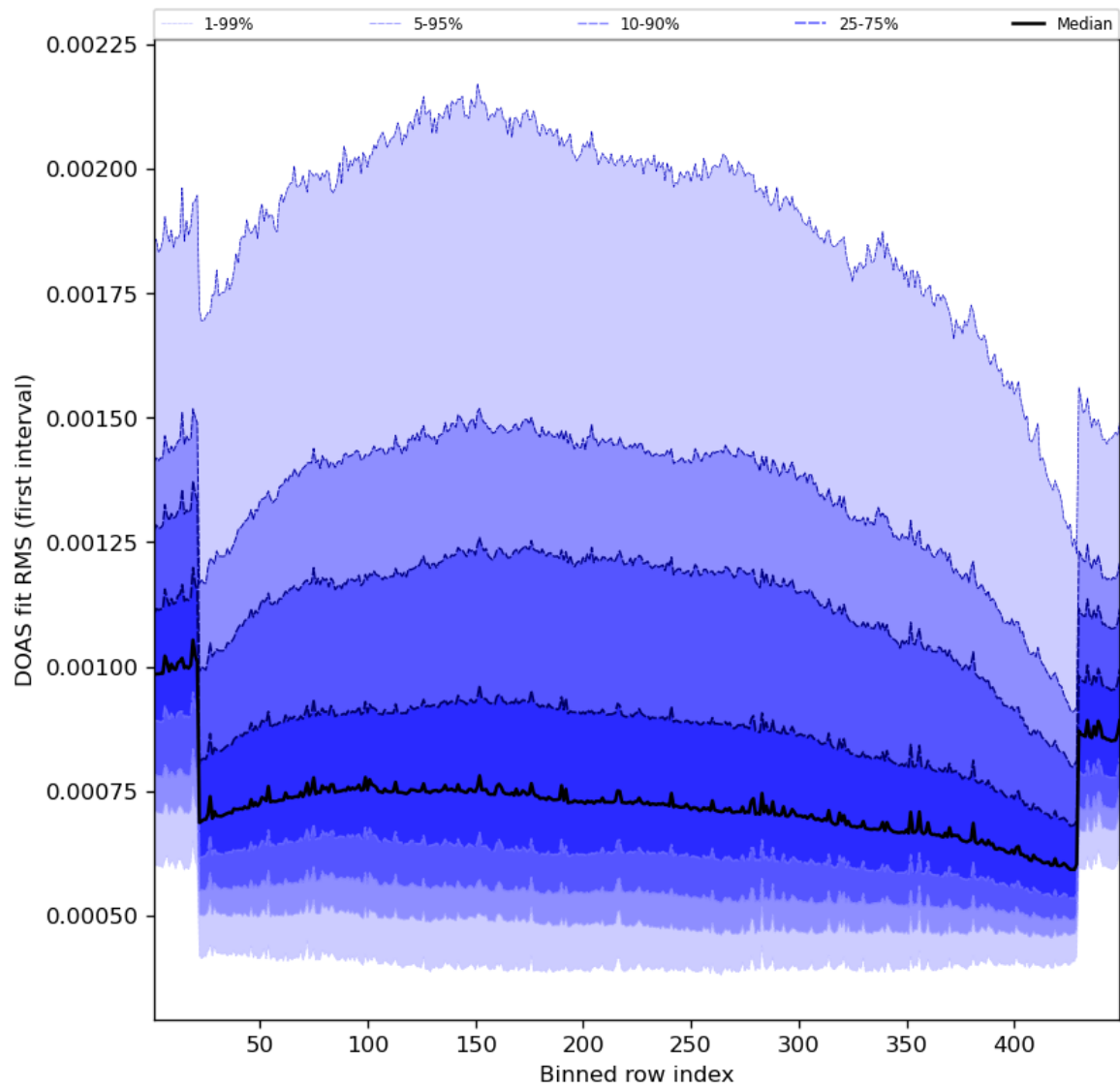
Figure 60: Along track statistics of “DOAS fit RMS (first interval)” for 2023-08-12 to 2023-08-14
