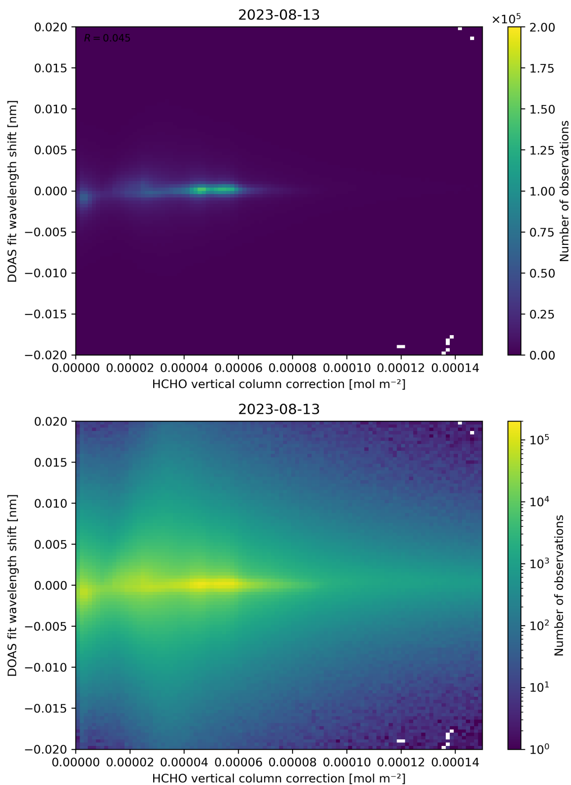
Figure 113: Scatter density plot of “HCHO vertical column correction” against “DOAS fit wavelength shift” for 2023-08-12 to 2023-08-14.
