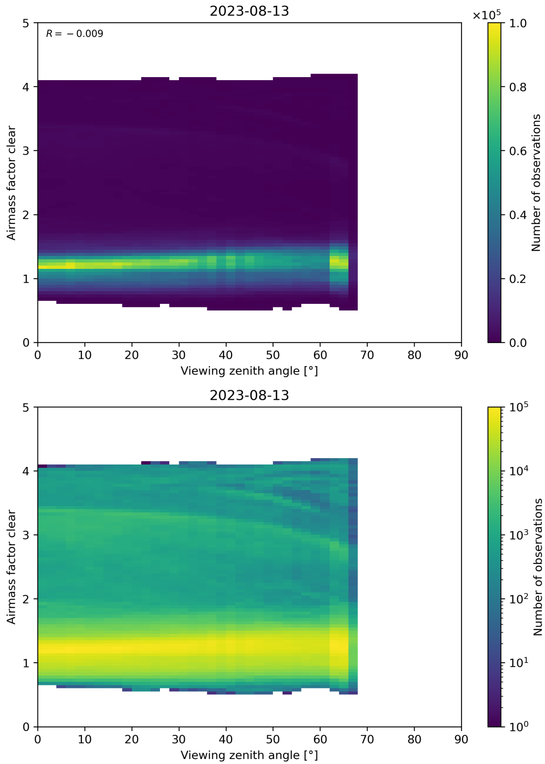
Figure 185: Scatter density plot of “Viewing zenith angle” against “Airmass factor clear” for 2023-08-12 to 2023-08-14.
