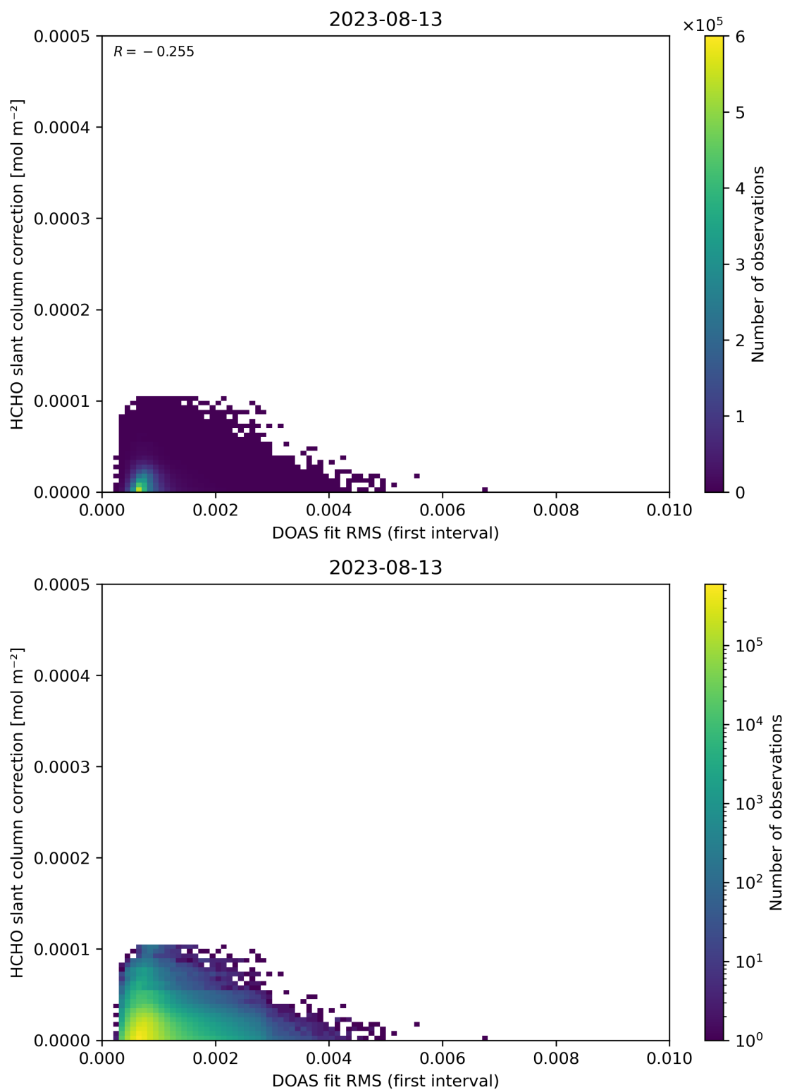
Figure 63: Scatter density plot of “DOAS fit RMS (first interval)” against “HCHO slant column correction” for 2023-08-12 to 2023-08-14.
