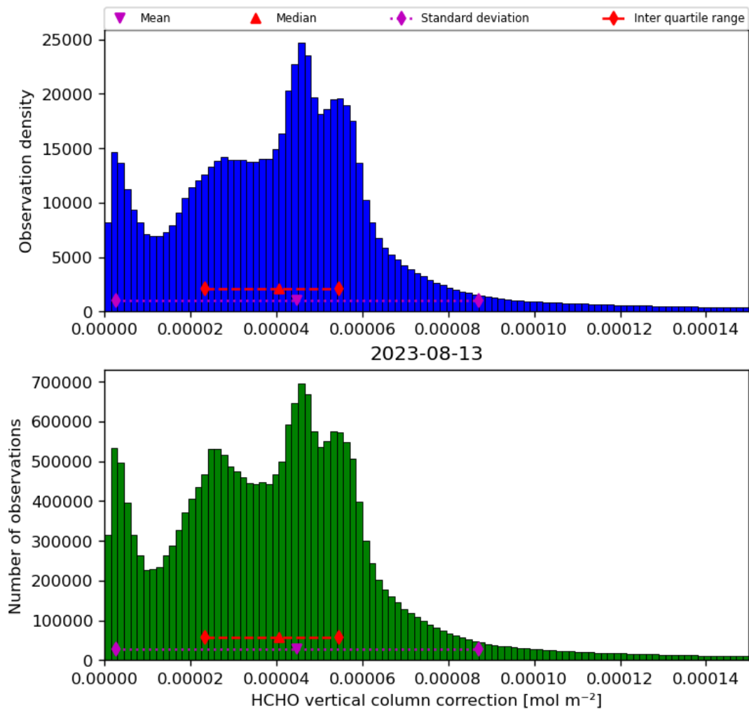
Figure 37: Histogram of “HCHO vertical column correction” for 2023-08-12 to 2023-08-14
