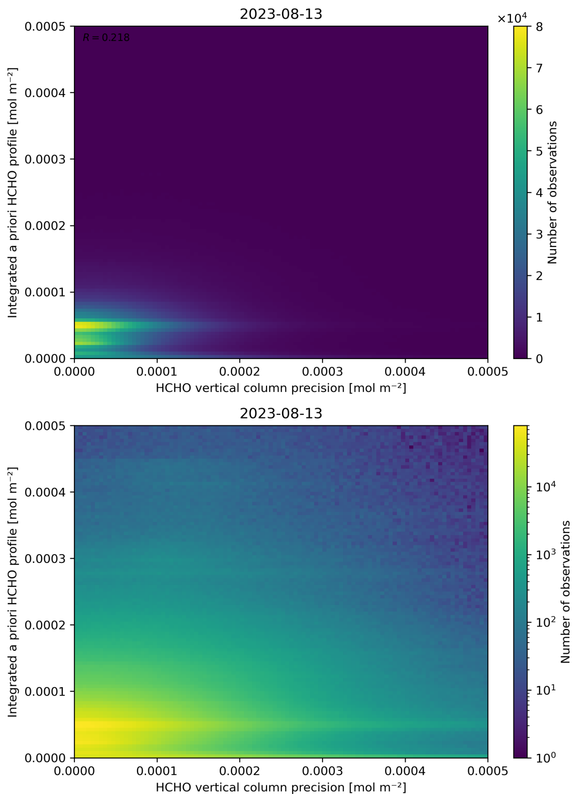
Figure 147: Scatter density plot of “HCHO vertical column precision” against “Integrated a priori HCHO profile” for 2023-08-12 to 2023-08-14.
