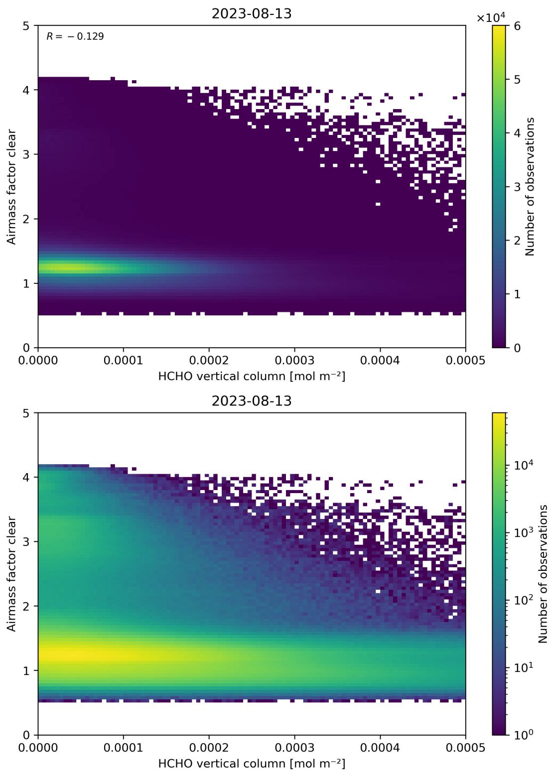
Figure 126: Scatter density plot of “HCHO vertical column” against “Airmass factor clear” for 2023-08-12 to 2023-08-14.
