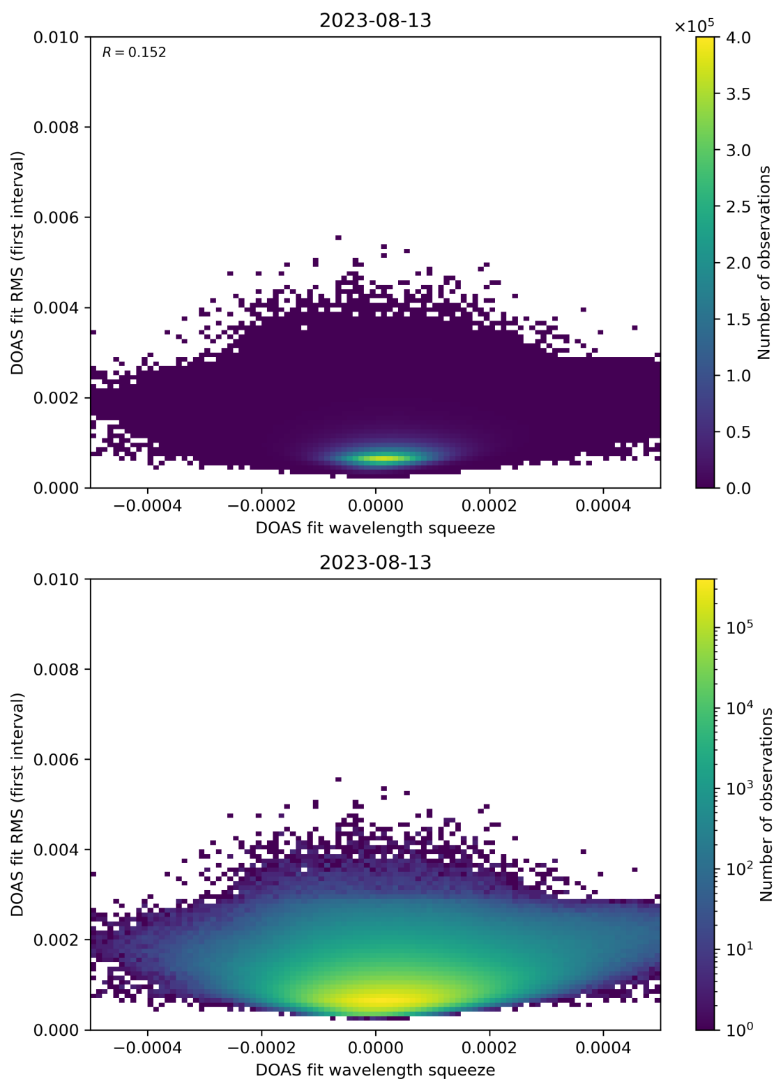
Figure 68: Scatter density plot of “DOAS fit wavelength squeeze” against “DOAS fit RMS (first interval)” for 2023-08-12 to 2023-08-14.
