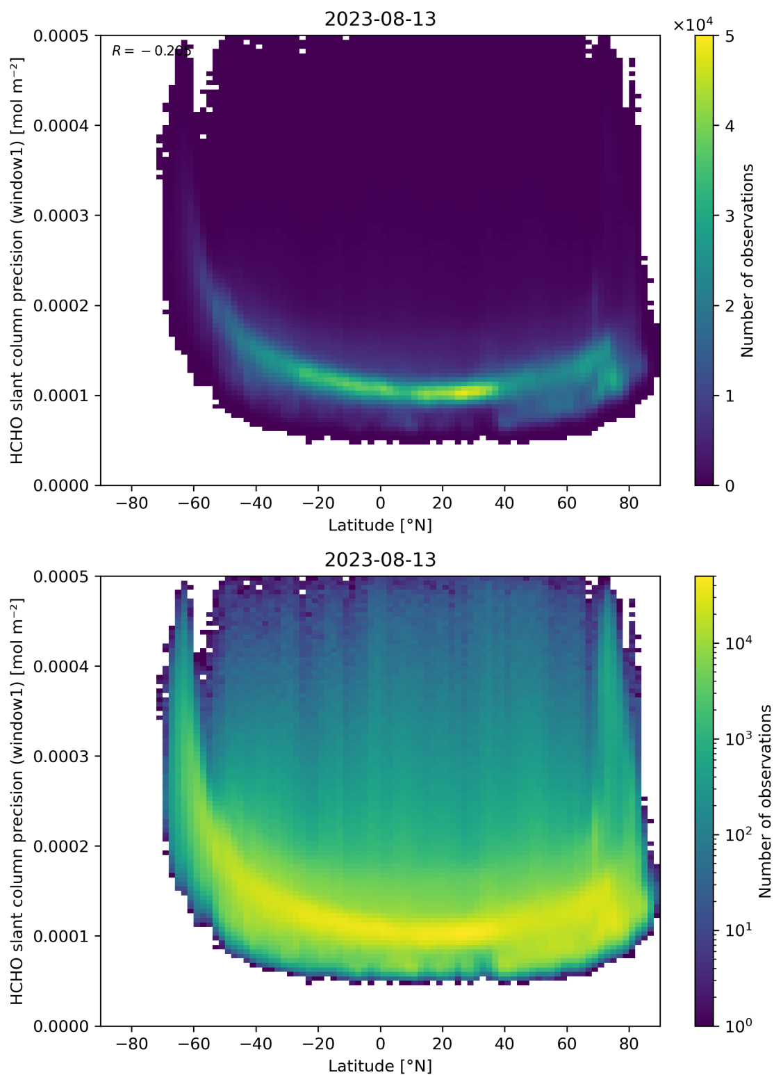
Figure 160: Scatter density plot of “Latitude” against “HCHO slant column precision (window1)” for 2023-08-12 to 2023-08-14.
