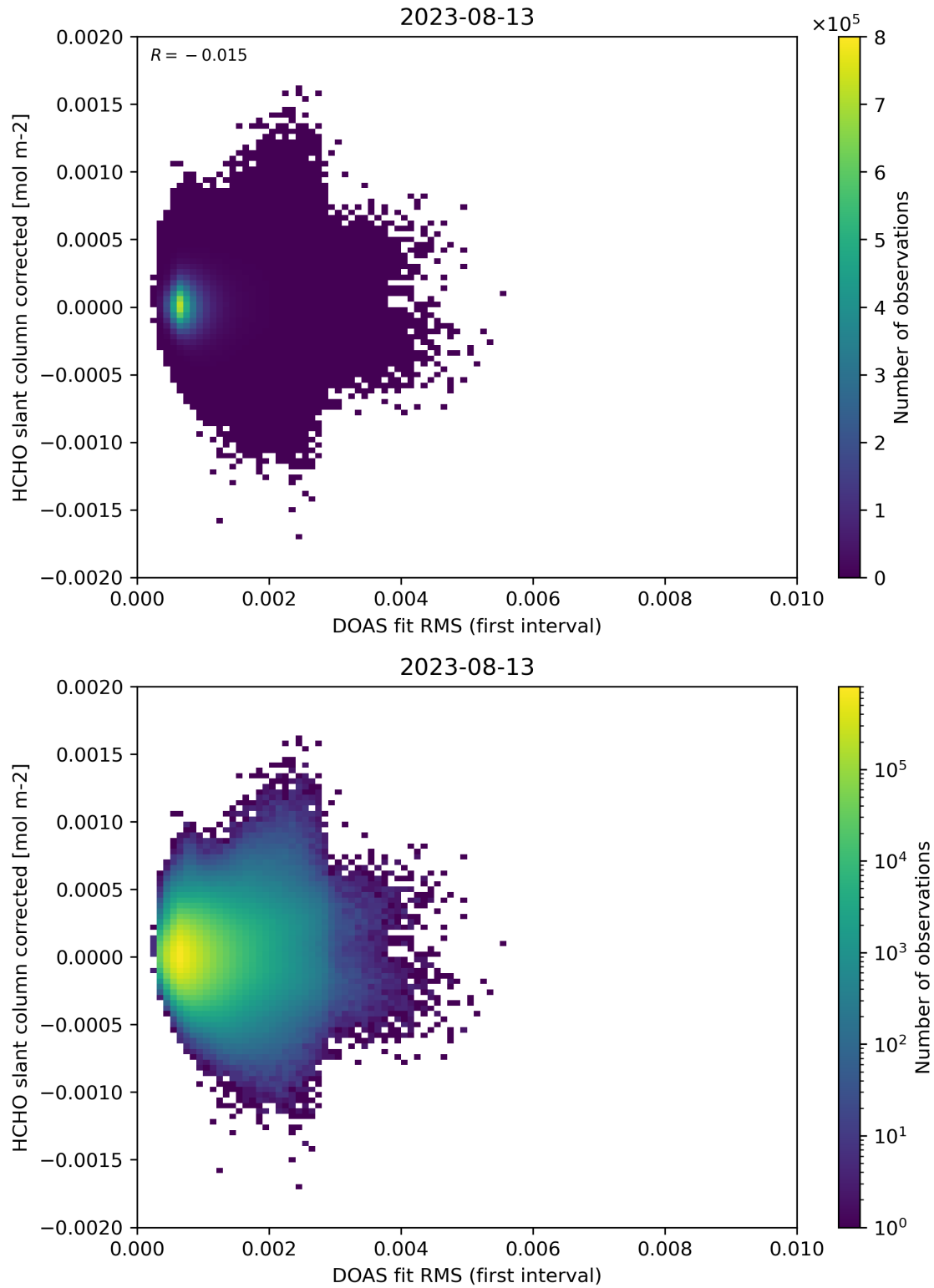
Figure 62: Scatter density plot of “DOAS fit RMS (first interval)” against “HCHO slant column corrected” for 2023-08-12 to 2023-08-14.
