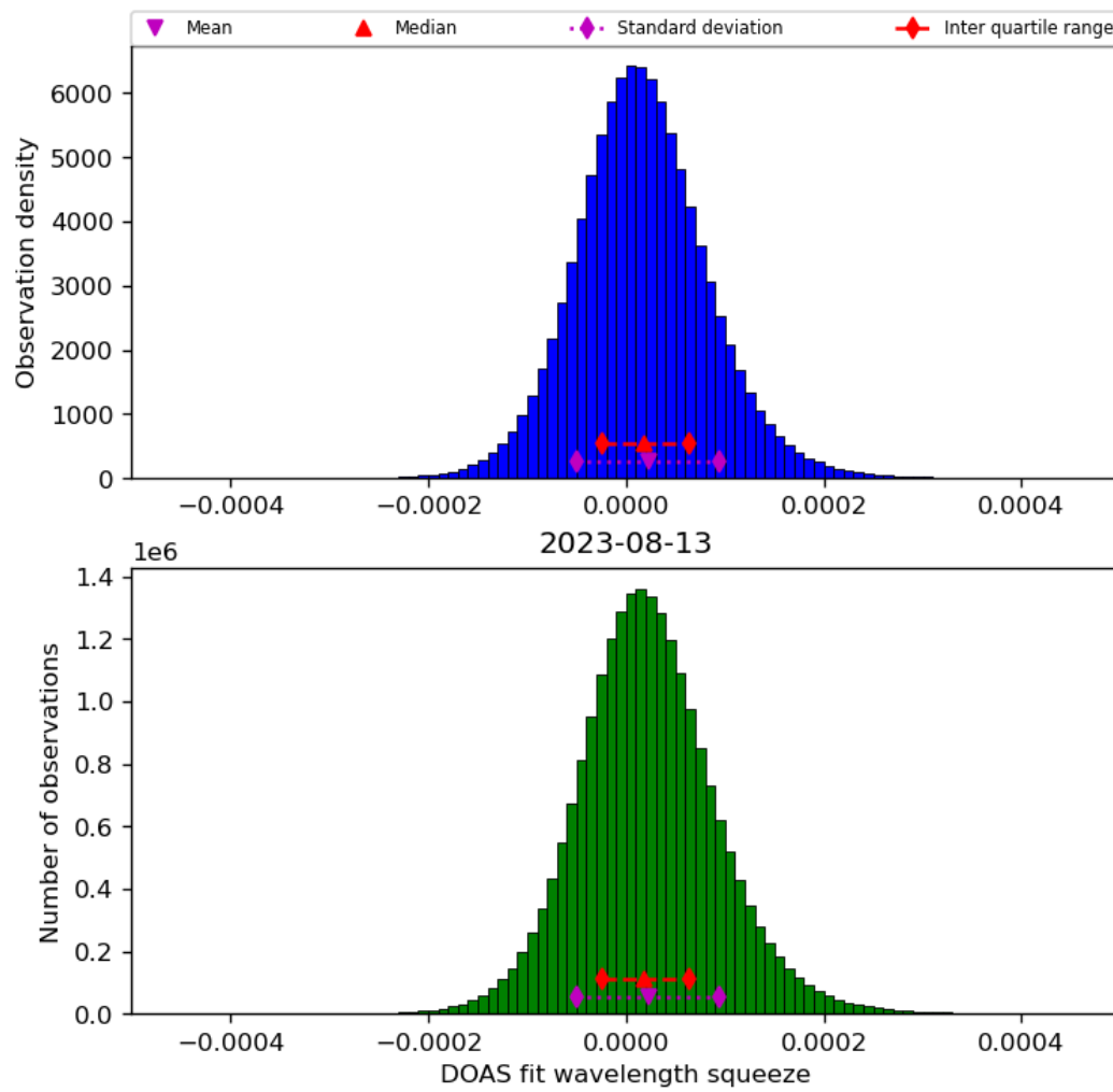
Figure 45: Histogram of “DOAS fit wavelength squeeze” for 2023-08-12 to 2023-08-14
