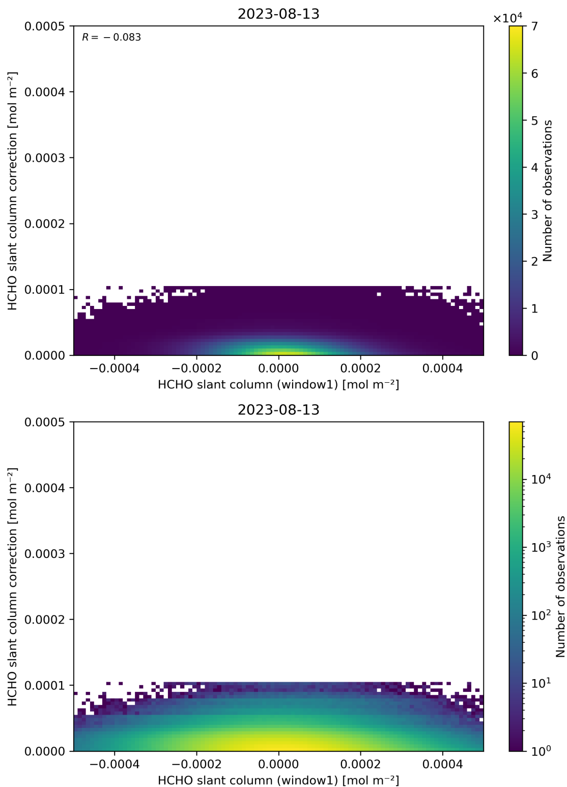
Figure 83: Scatter density plot of “HCHO slant column (window1)” against “HCHO slant column correction” for 2023-08-12 to 2023-08-14.
