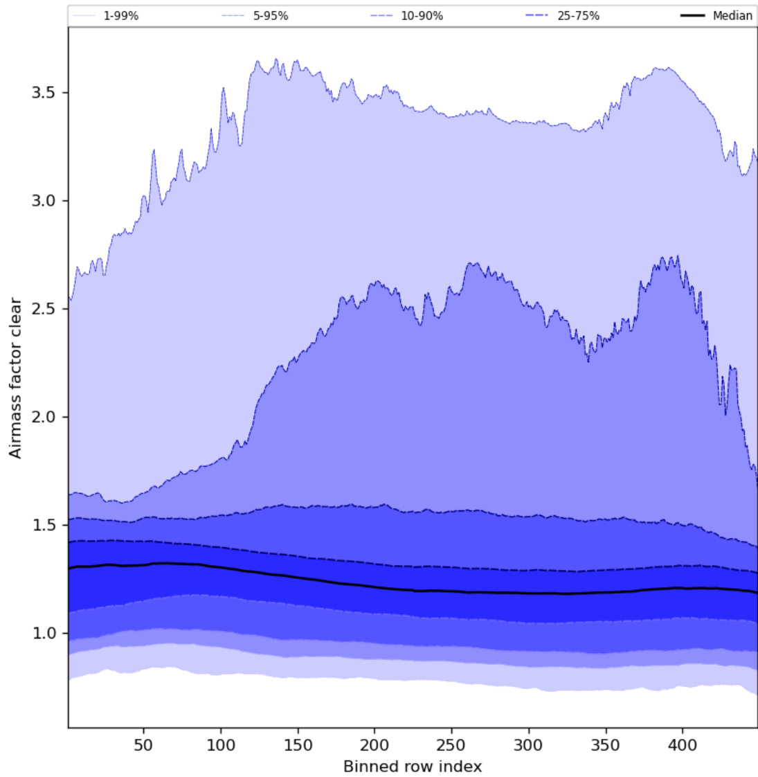
Figure 56: Along track statistics of “Airmass factor clear” for 2023-08-12 to 2023-08-14
