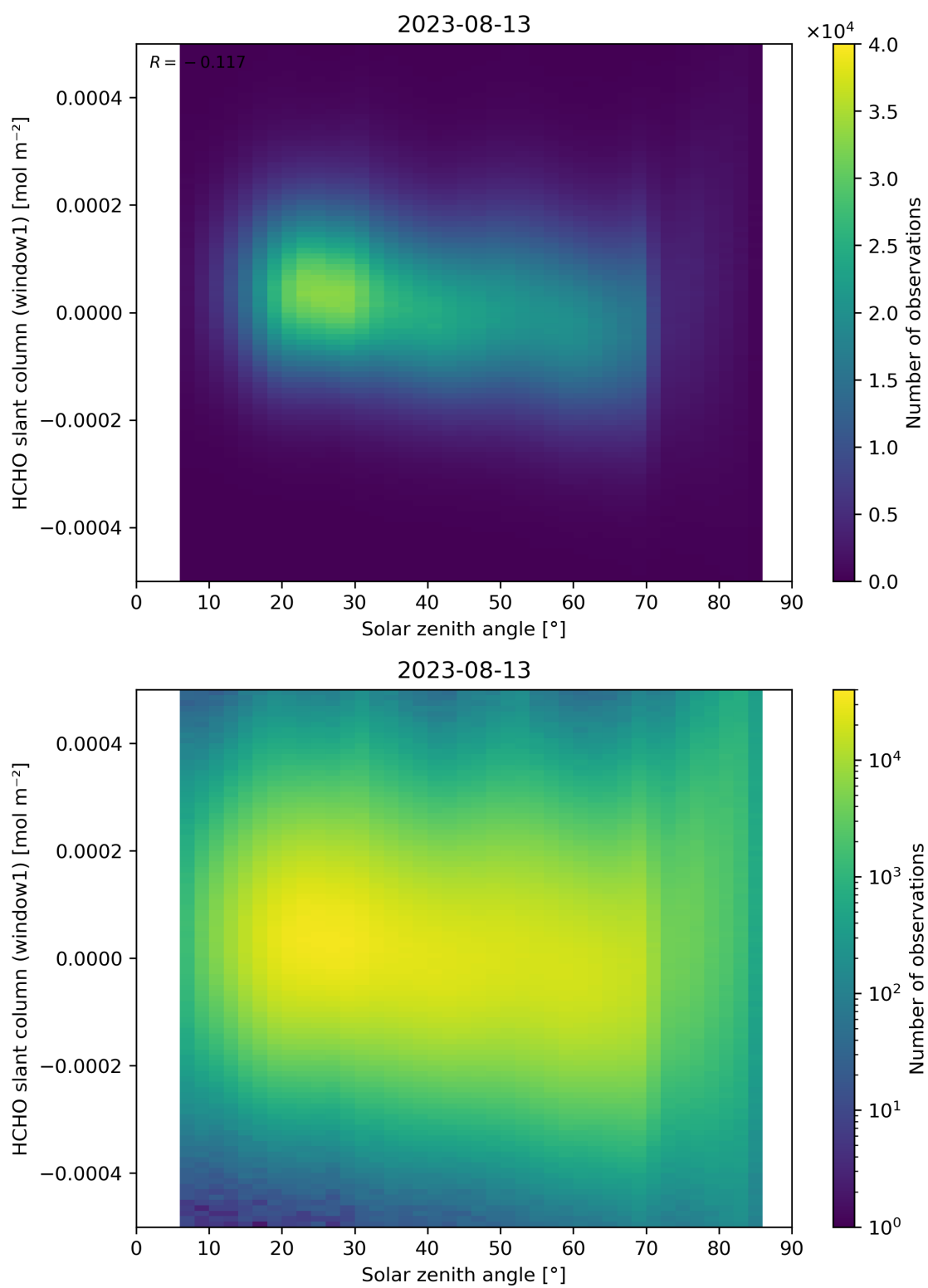
Figure 173: Scatter density plot of “Solar zenith angle” against “HCHO slant column (window1)” for 2023-08-12 to 2023-08-14.
