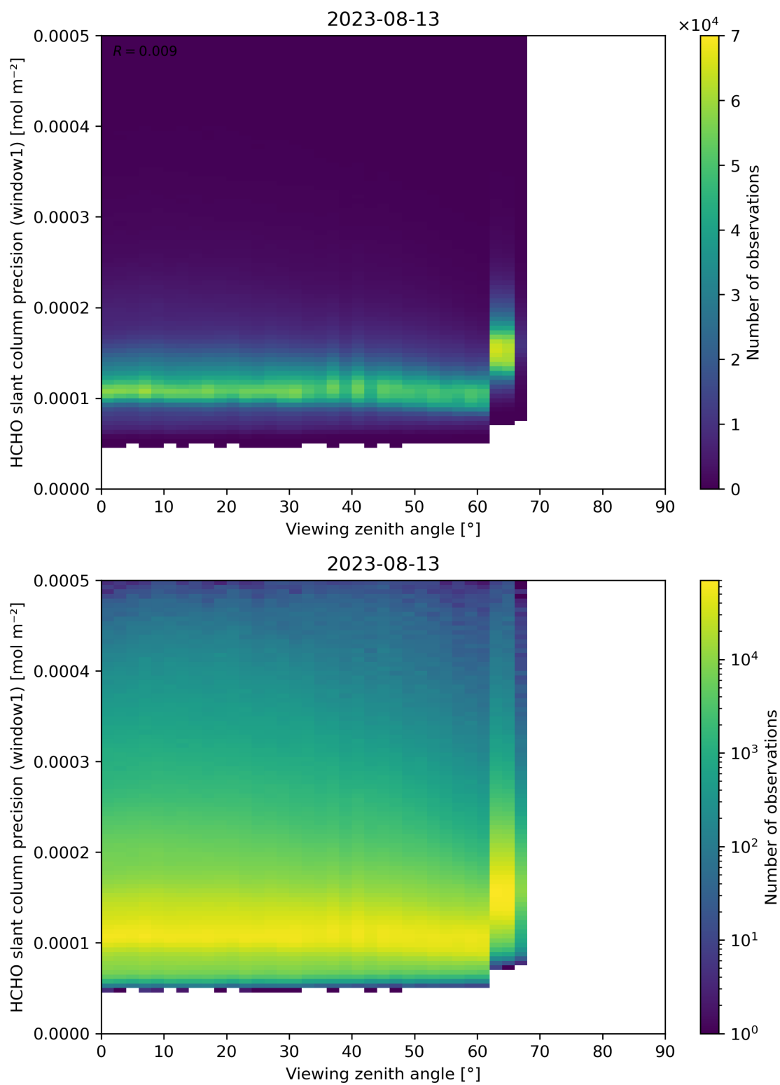
Figure 189: Scatter density plot of “Viewing zenith angle” against “HCHO slant column precision (window1)” for 2023-08-12 to 2023-08-14.
