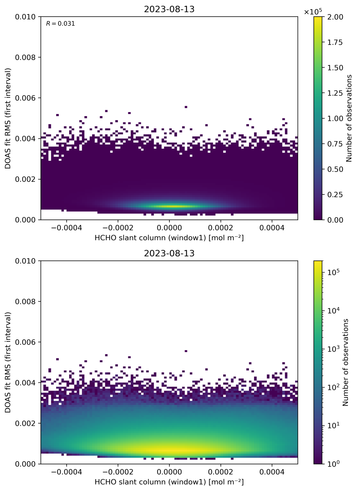
Figure 78: Scatter density plot of “HCHO slant column (window1)” against “DOAS fit RMS (first interval)” for 2023-08-12 to 2023-08-14.
