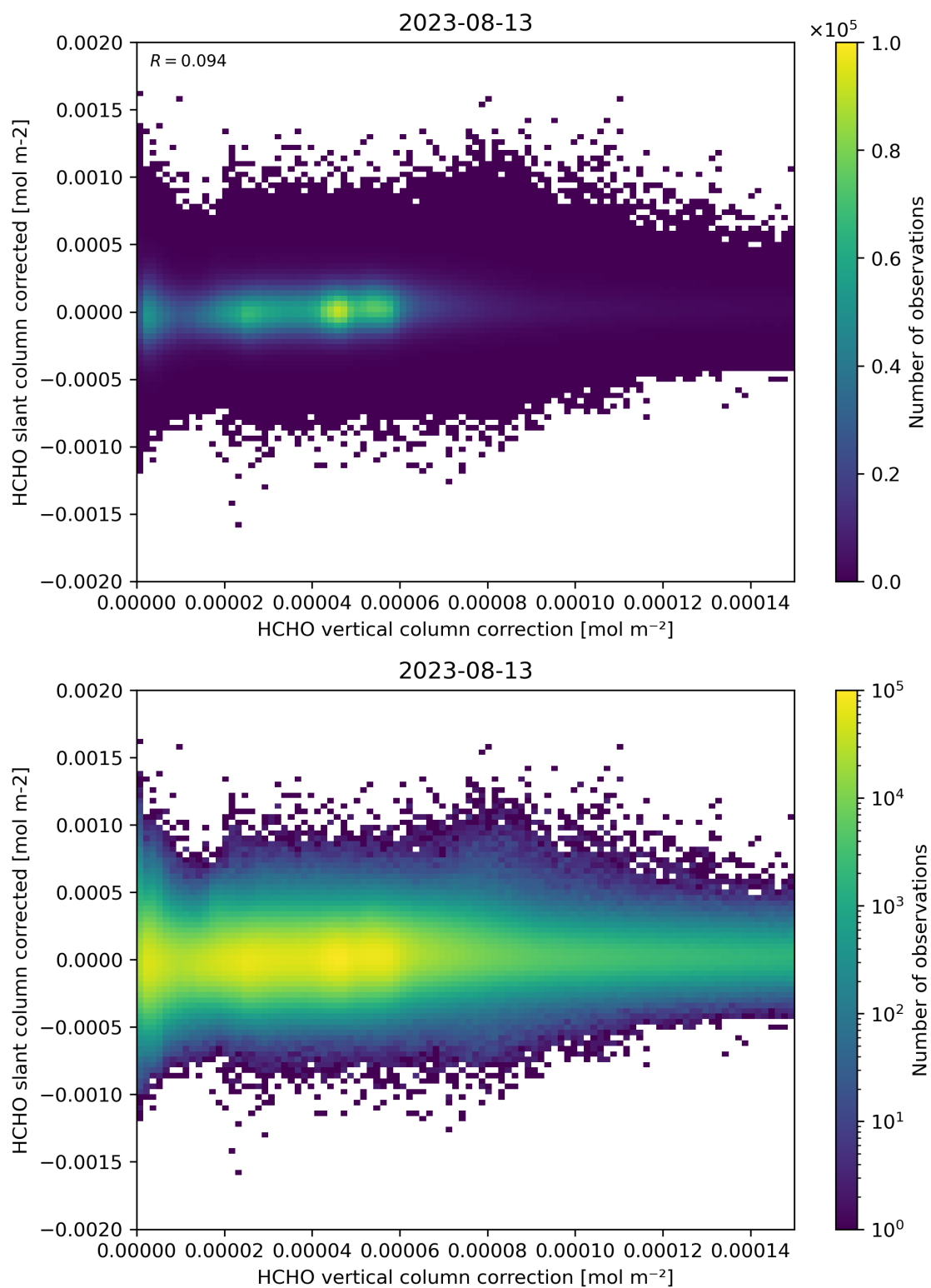
Figure 116: Scatter density plot of “HCHO vertical column correction” against “HCHO slant column corrected” for 2023-08-12 to 2023-08-14.
