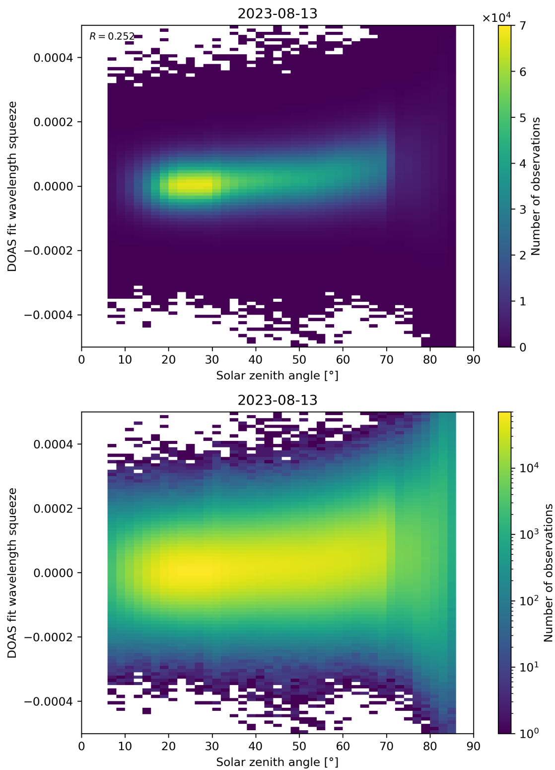
Figure 169: Scatter density plot of “Solar zenith angle” against “DOAS fit wavelength squeeze” for 2023-08-12 to 2023-08-14.
