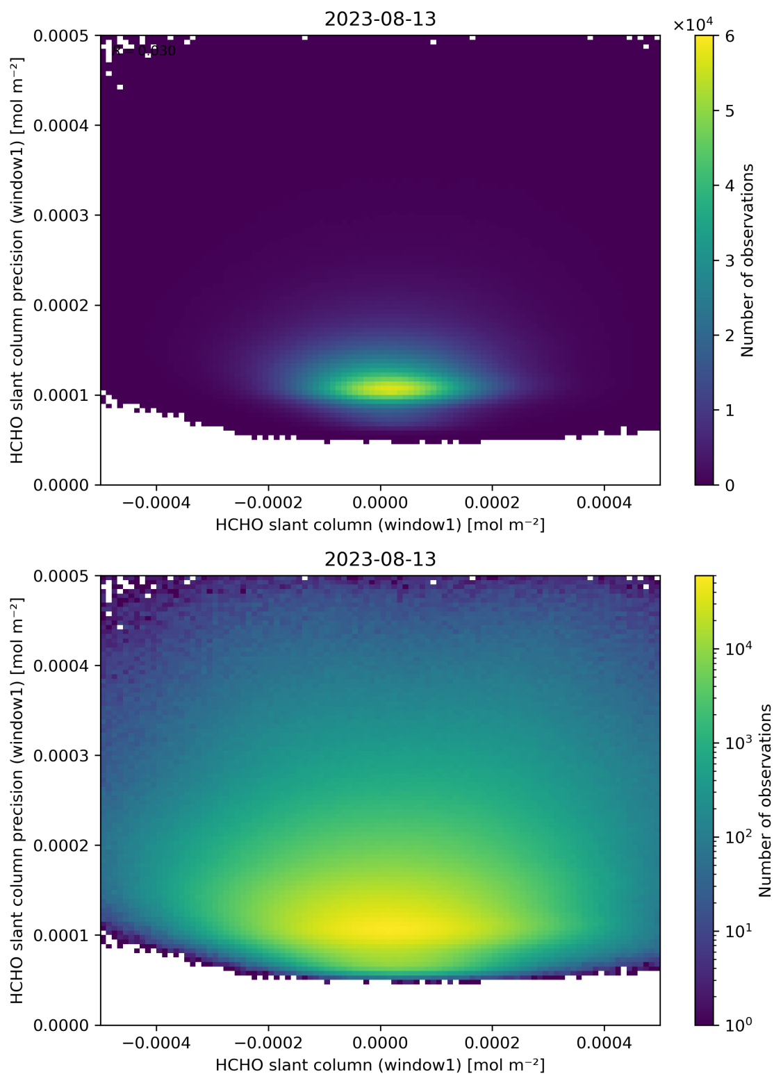
Figure 84: Scatter density plot of “HCHO slant column (window1)” against “HCHO slant column precision (window1)” for 2023-08-12 to 2023-08-14.
