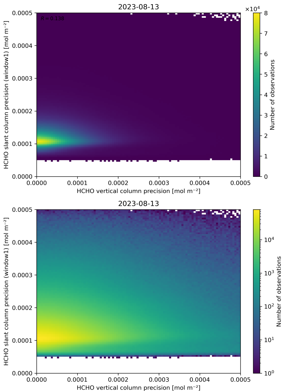
Figure 143: Scatter density plot of “HCHO vertical column precision” against “HCHO slant column precision (window1)” for 2023-08-12 to 2023-08-14.
