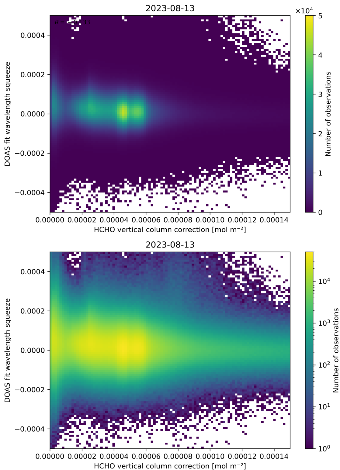
Figure 114: Scatter density plot of “HCHO vertical column correction” against “DOAS fit wavelength squeeze” for 2023-08-12 to 2023-08-14.
