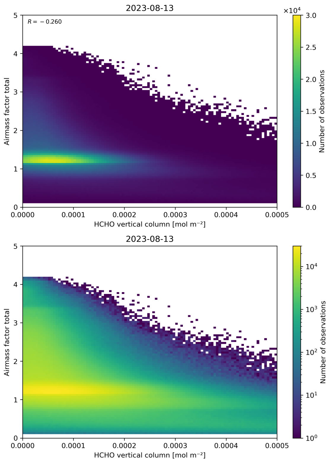
Figure 131: Scatter density plot of “HCHO vertical column” against “Airmass factor total” for 2023-08-12 to 2023-08-14.
