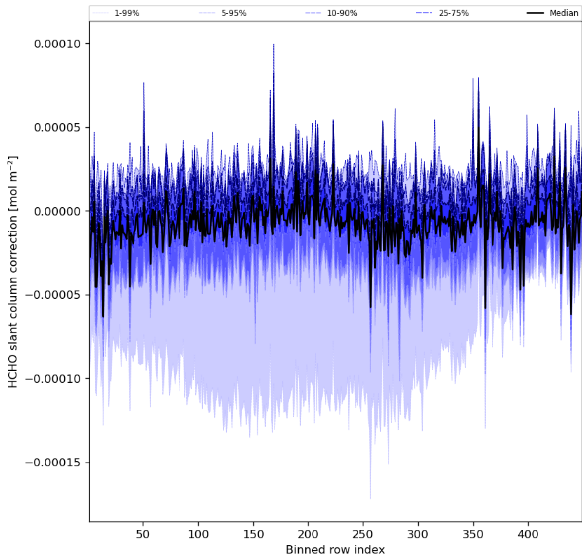
Figure 61: Along track statistics of “HCHO slant column correction” for 2023-08-12 to 2023-08-14
