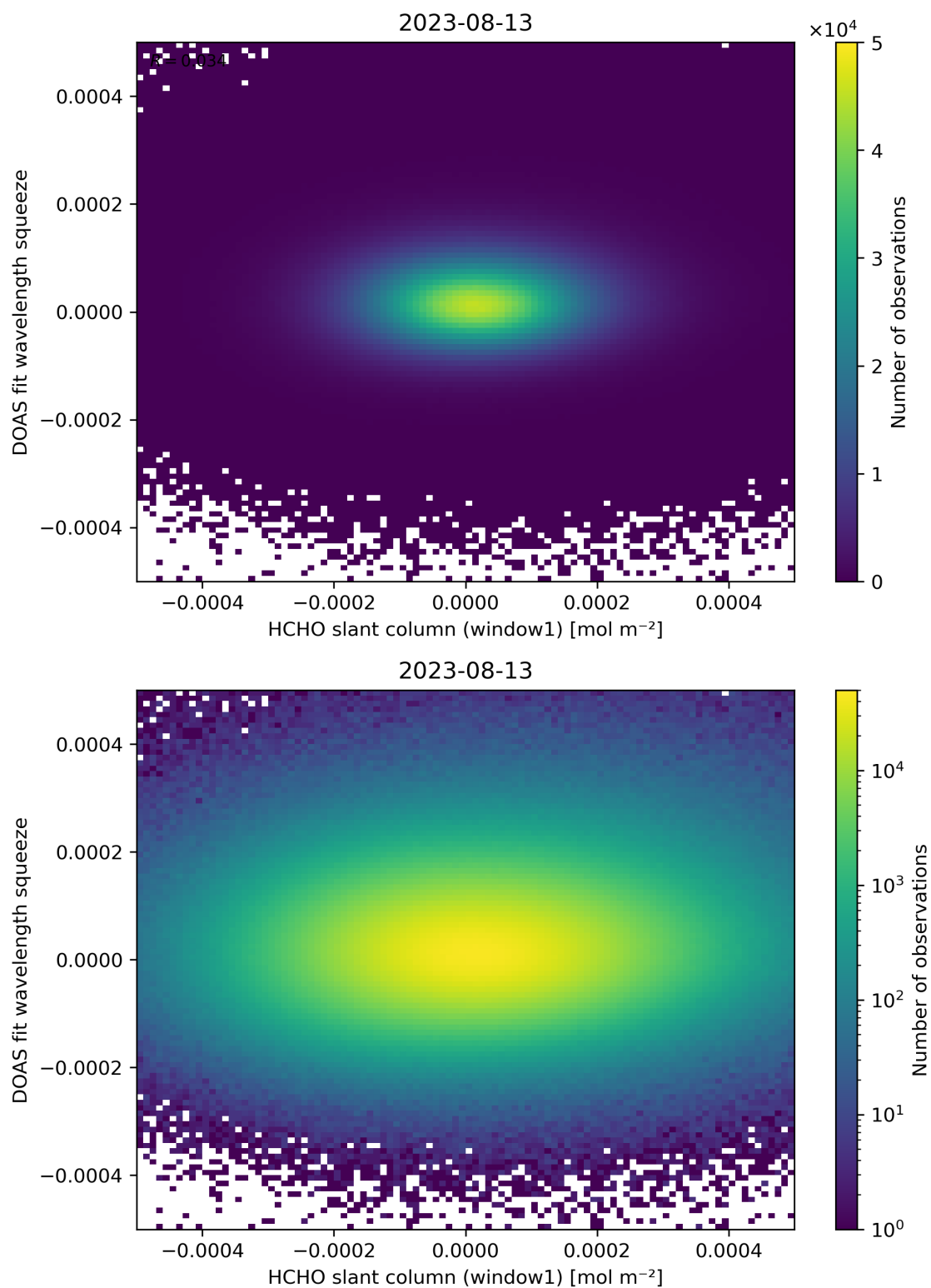
Figure 80: Scatter density plot of “HCHO slant column (window1)” against “DOAS fit wavelength squeeze” for 2023-08-12 to 2023-08-14.
