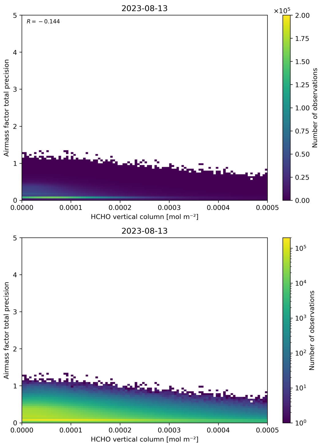
Figure 132: Scatter density plot of “HCHO vertical column” against “Airmass factor total precision” for 2023-08-12 to 2023-08-14.
