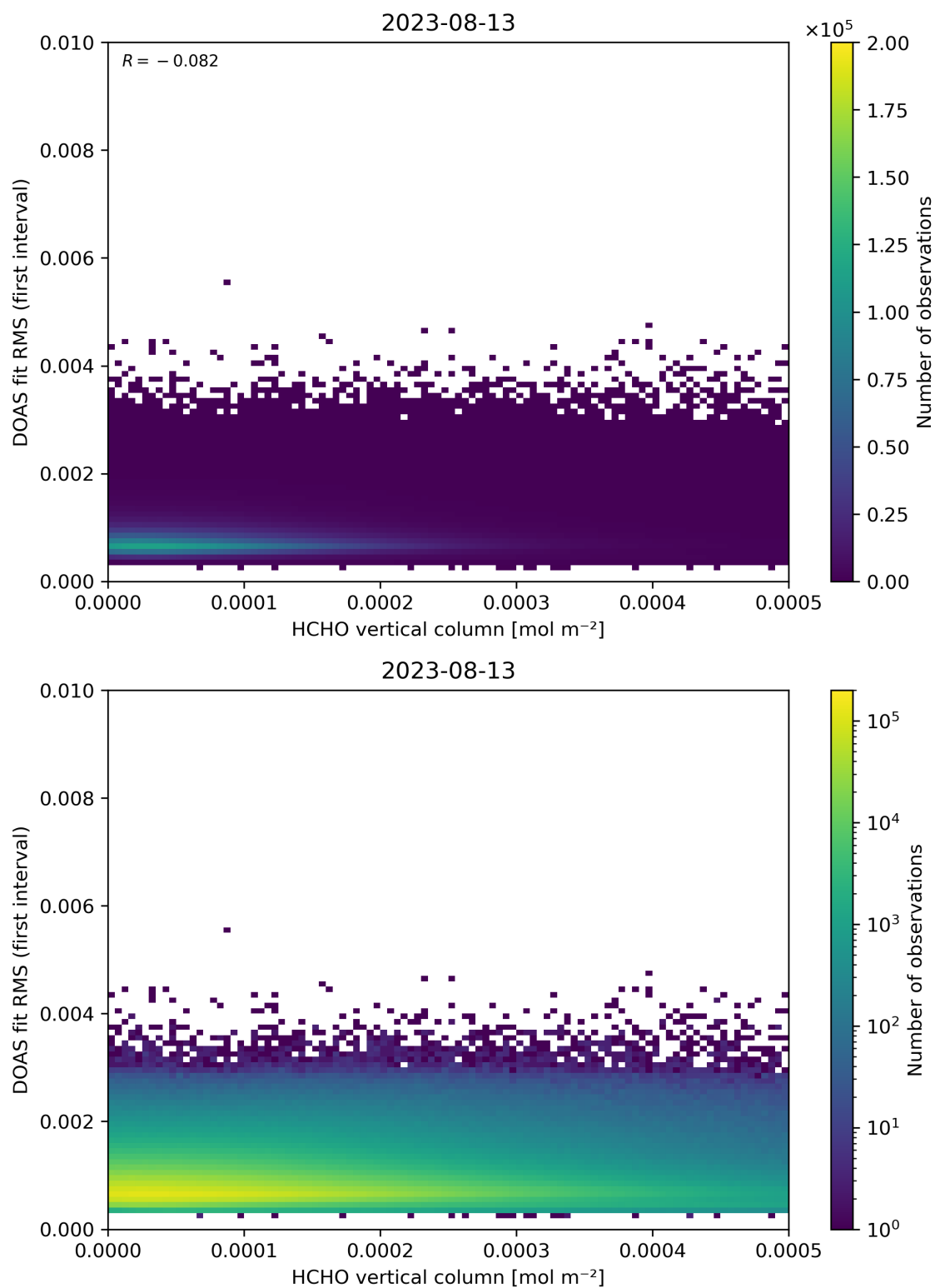
Figure 123: Scatter density plot of “HCHO vertical column” against “DOAS fit RMS (first interval)” for 2023-08-12 to 2023-08-14.
