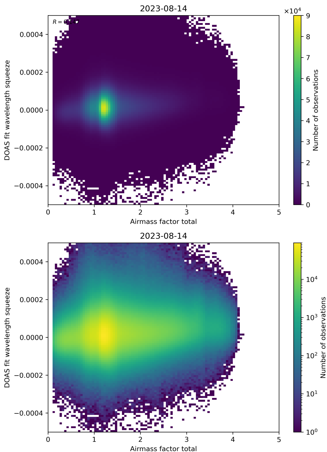
Figure 99: Scatter density plot of “Airmass factor total” against “DOAS fit wavelength squeeze” for 2023-08-14 to 2023-08-15.
