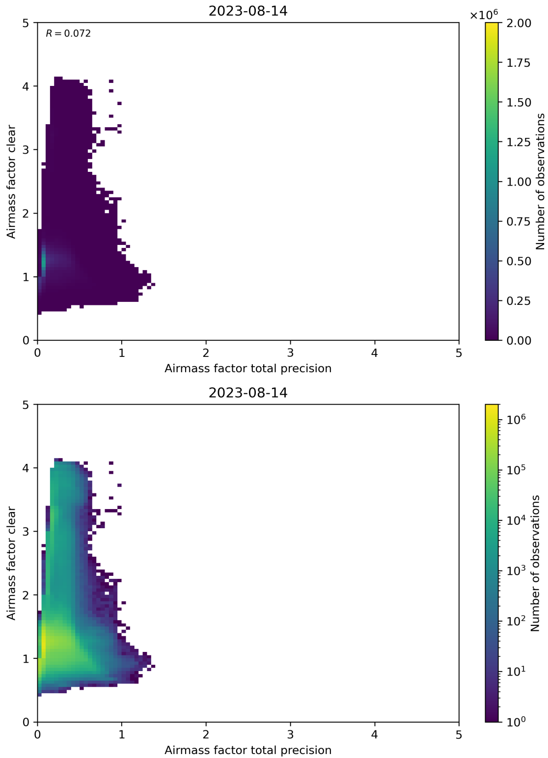
Figure 108: Scatter density plot of “Airmass factor total precision” against “Airmass factor clear” for 2023-08-14 to 2023-08-15.
