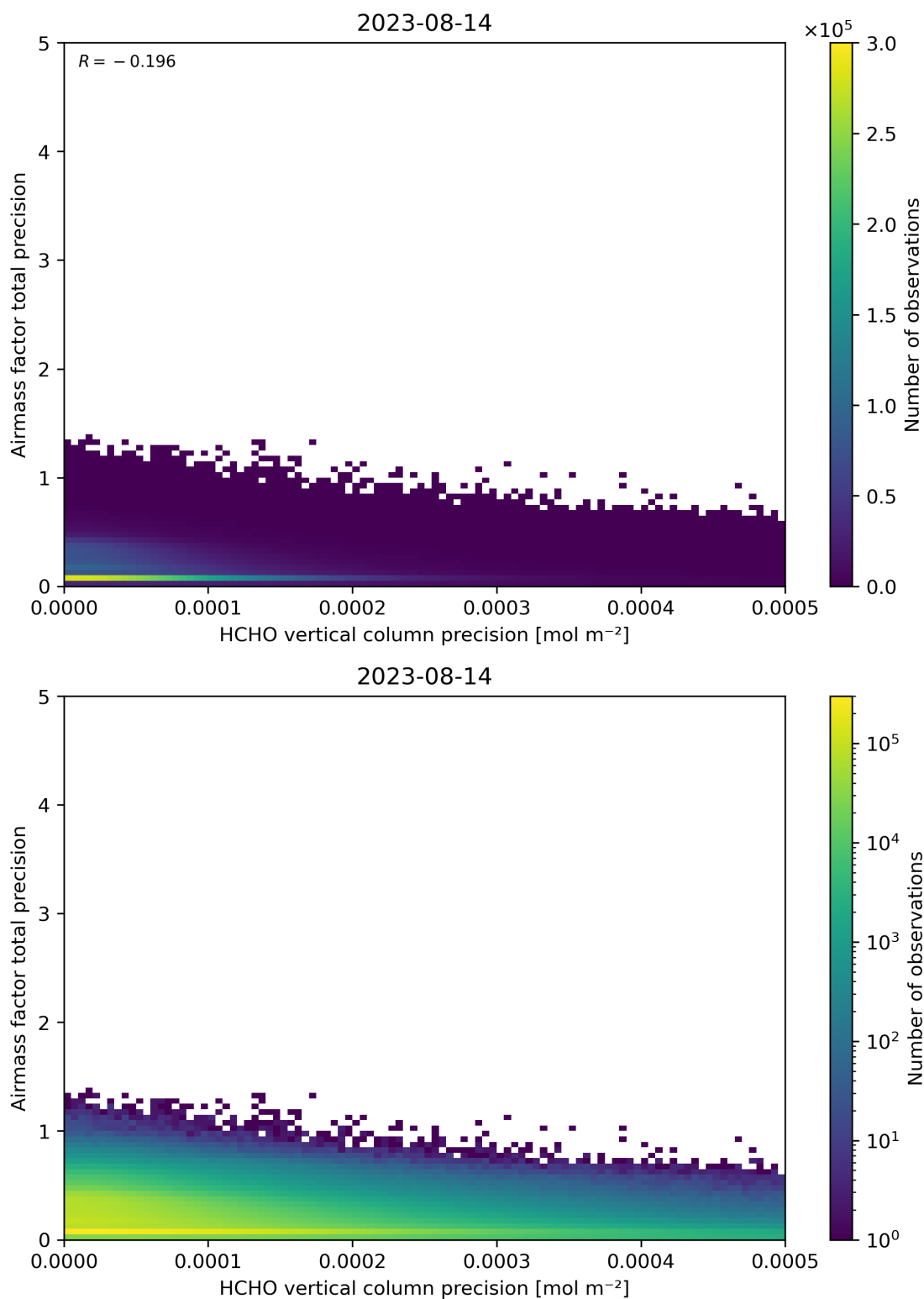
Figure 145: Scatter density plot of “HCHO vertical column precision” against “Airmass factor total precision” for 2023-08-14 to 2023-08-15.
