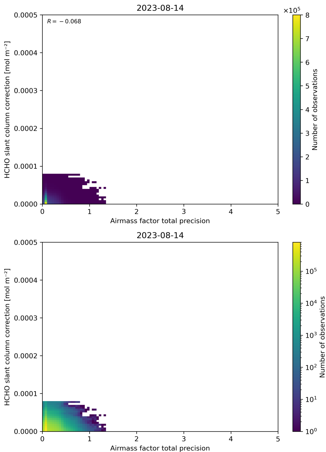
Figure 110: Scatter density plot of “Airmass factor total precision” against “HCHO slant column correction” for 2023-08-14 to 2023-08-15.
