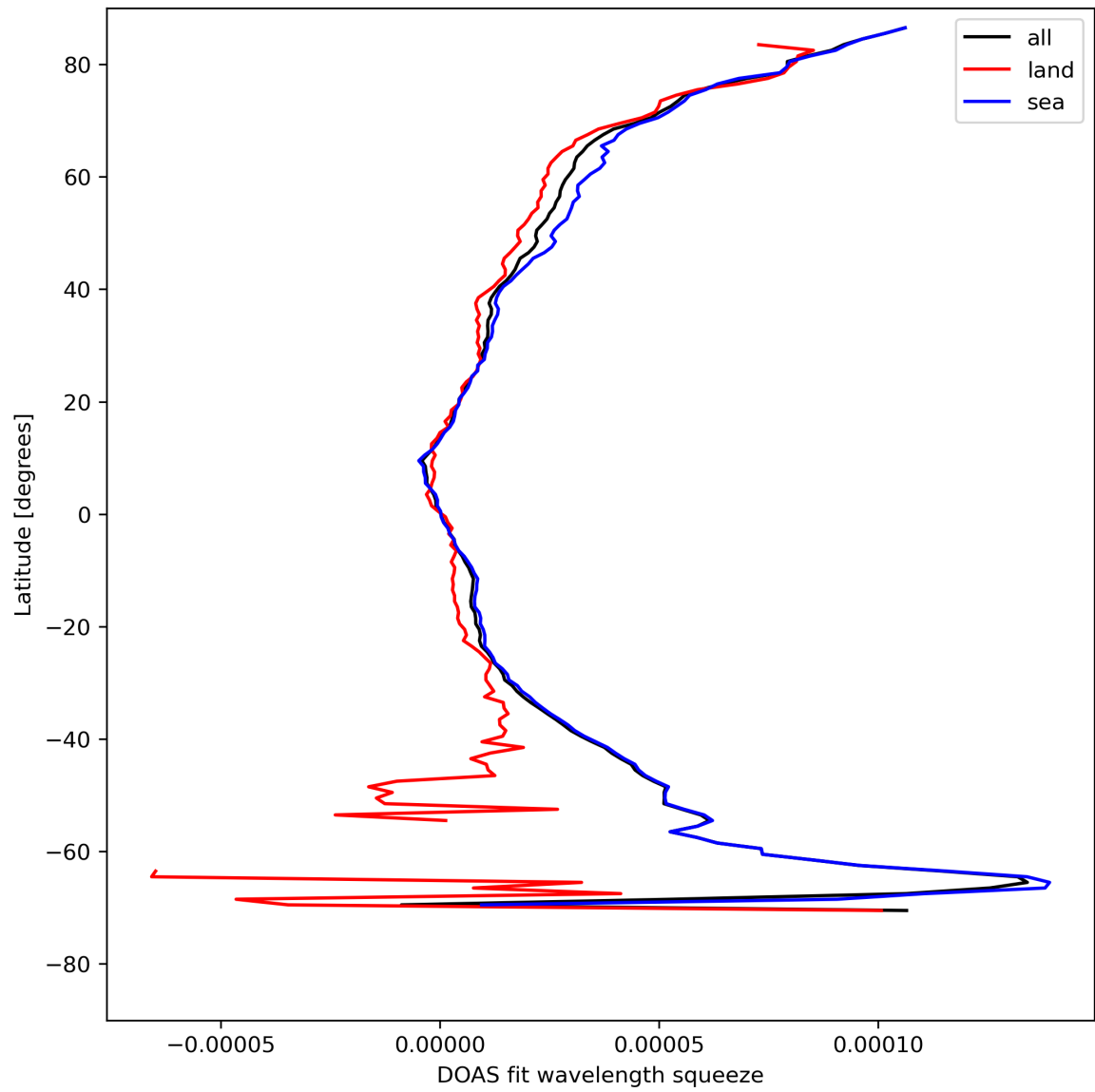
Figure 31: Zonal average of “DOAS fit wavelength squeeze” for 2023-08-14 to 2023-08-15.
