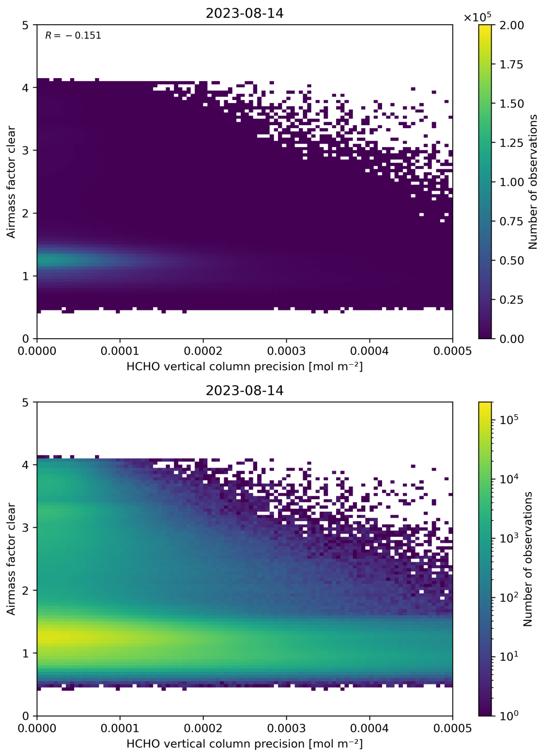
Figure 139: Scatter density plot of “HCHO vertical column precision” against “Airmass factor clear” for 2023-08-14 to 2023-08-15.
