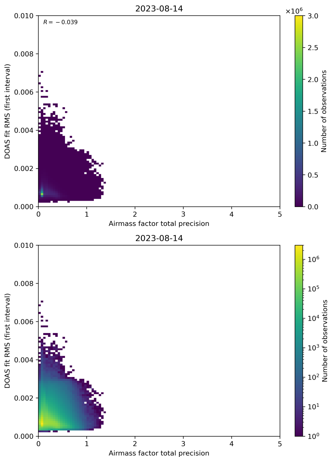
Figure 105: Scatter density plot of “Airmass factor total precision” against “DOAS fit RMS (first interval)” for 2023-08-14 to 2023-08-15.
