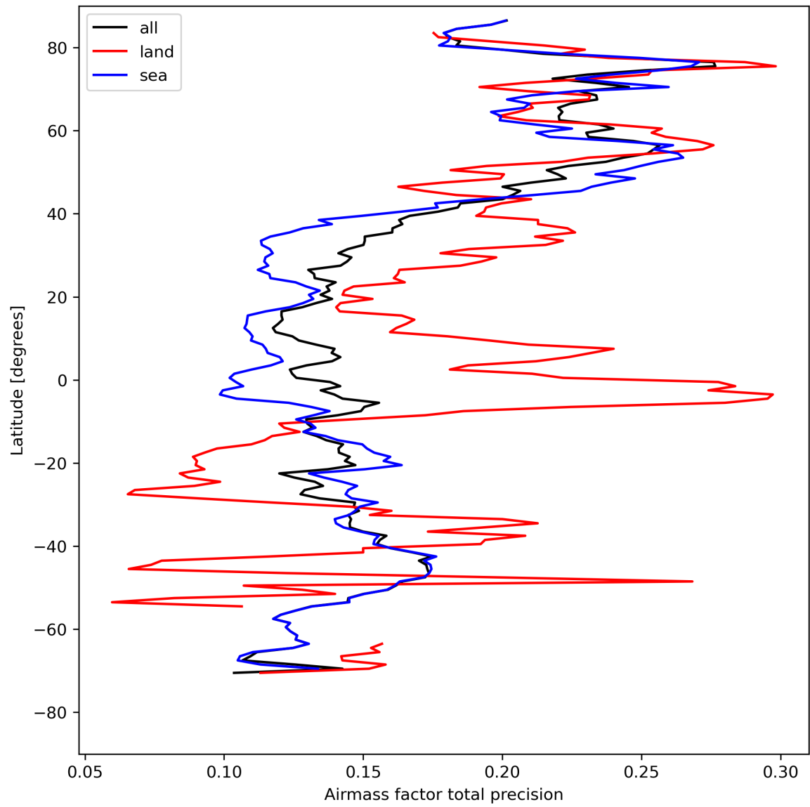
Figure 27: Zonal average of “Airmass factor total precision” for 2023-08-14 to 2023-08-15.
