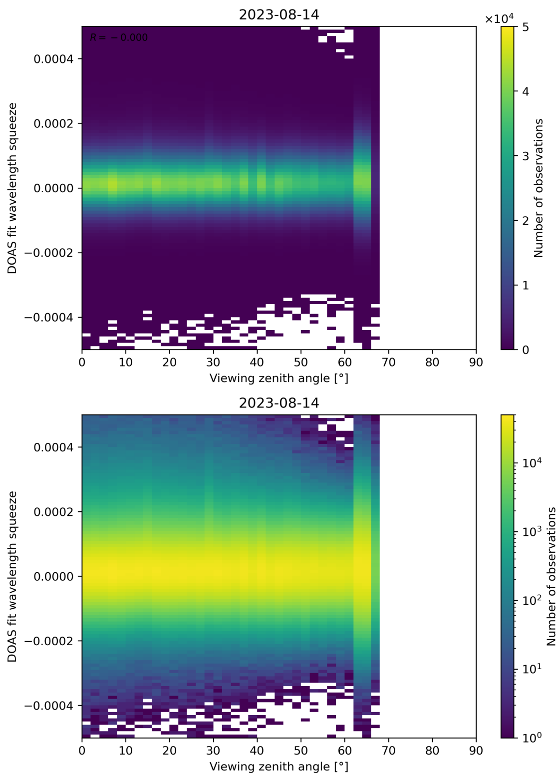
Figure 184: Scatter density plot of “Viewing zenith angle” against “DOAS fit wavelength squeeze” for 2023-08-14 to 2023-08-15.
