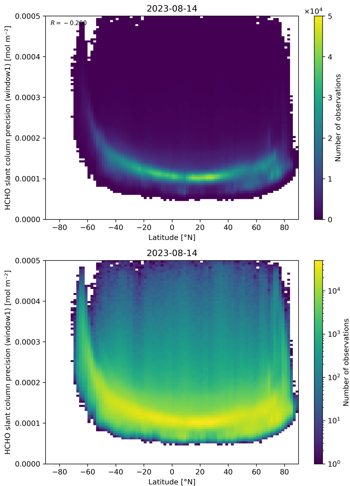
Figure 160: Scatter density plot of “Latitude” against “HCHO slant column precision (window1)” for 2023-08-14 to 2023-08-15.
