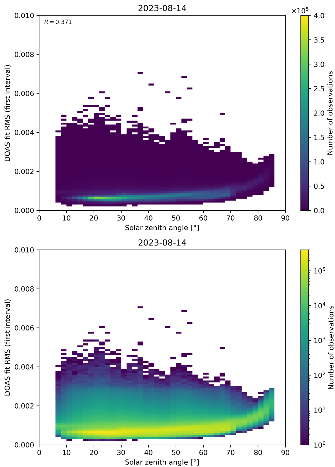
Figure 167: Scatter density plot of “Solar zenith angle” against “DOAS fit RMS (first interval)” for 2023-08-14 to 2023-08-15.
