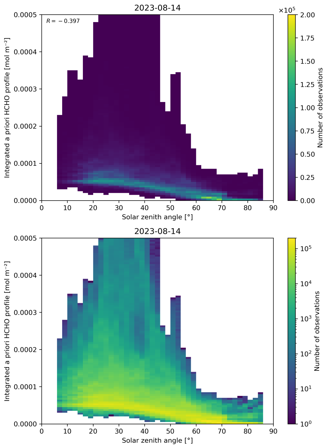
Figure 180: Scatter density plot of “Solar zenith angle” against “Integrated a priori HCHO profile” for 2023-08-14 to 2023-08-15.
