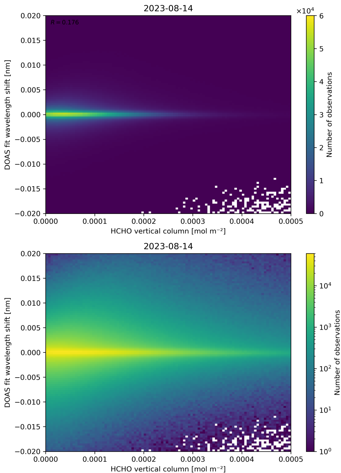
Figure 124: Scatter density plot of “HCHO vertical column” against “DOAS fit wavelength shift” for 2023-08-14 to 2023-08-15.
