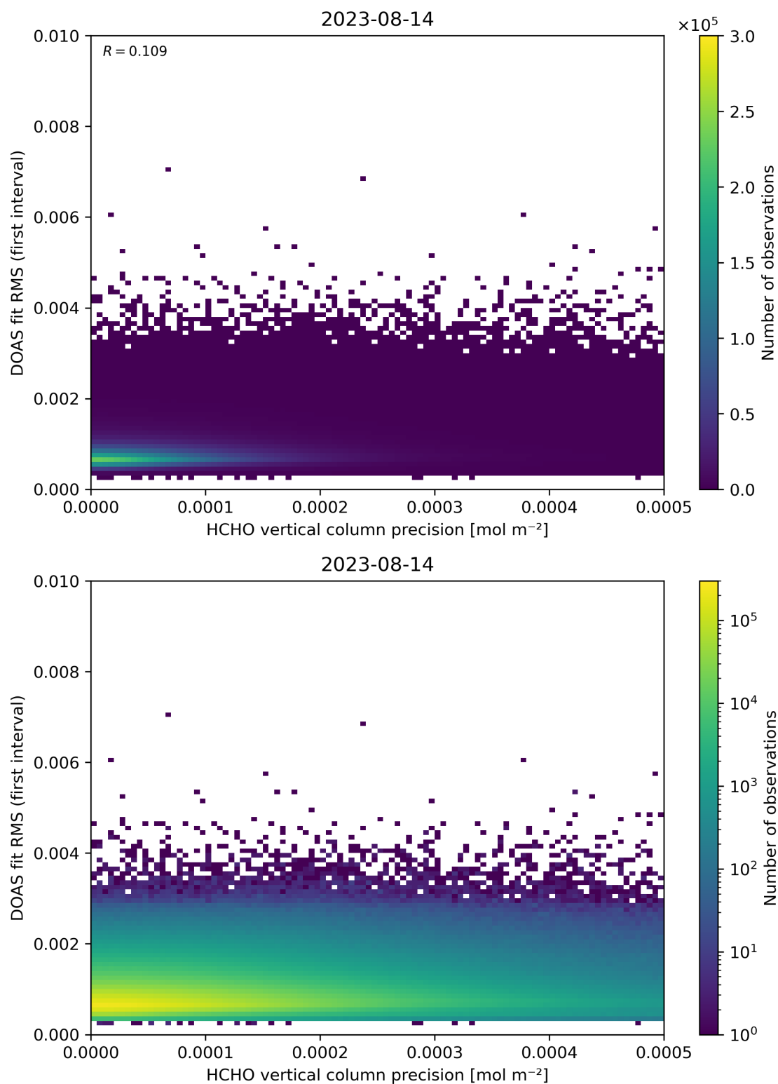
Figure 136: Scatter density plot of “HCHO vertical column precision” against “DOAS fit RMS (first interval)” for 2023-08-14 to 2023-08-15.
