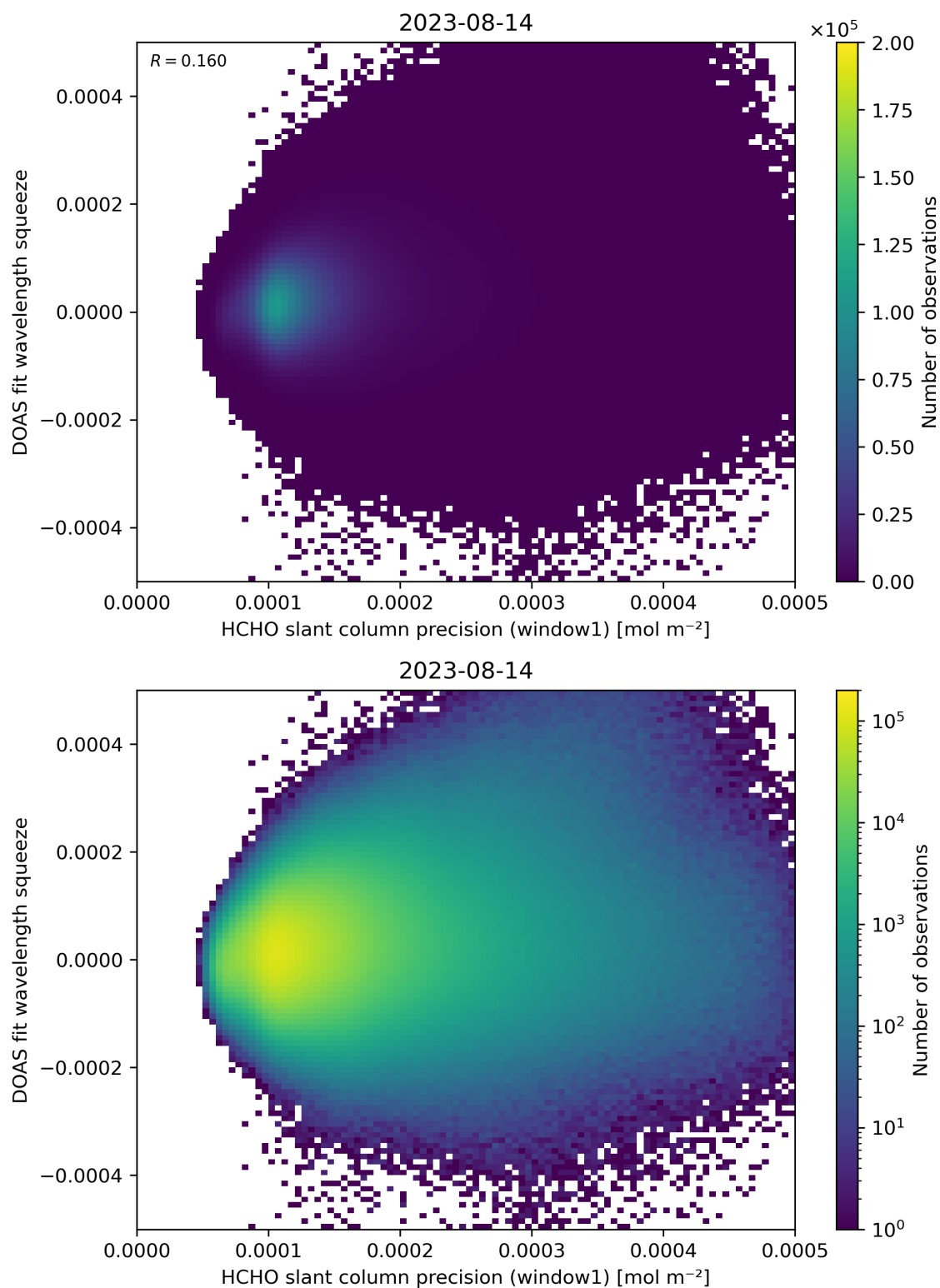
Figure 90: Scatter density plot of “HCHO slant column precision (window1)” against “DOAS fit wavelength squeeze” for 2023-08-14 to 2023-08-15.
