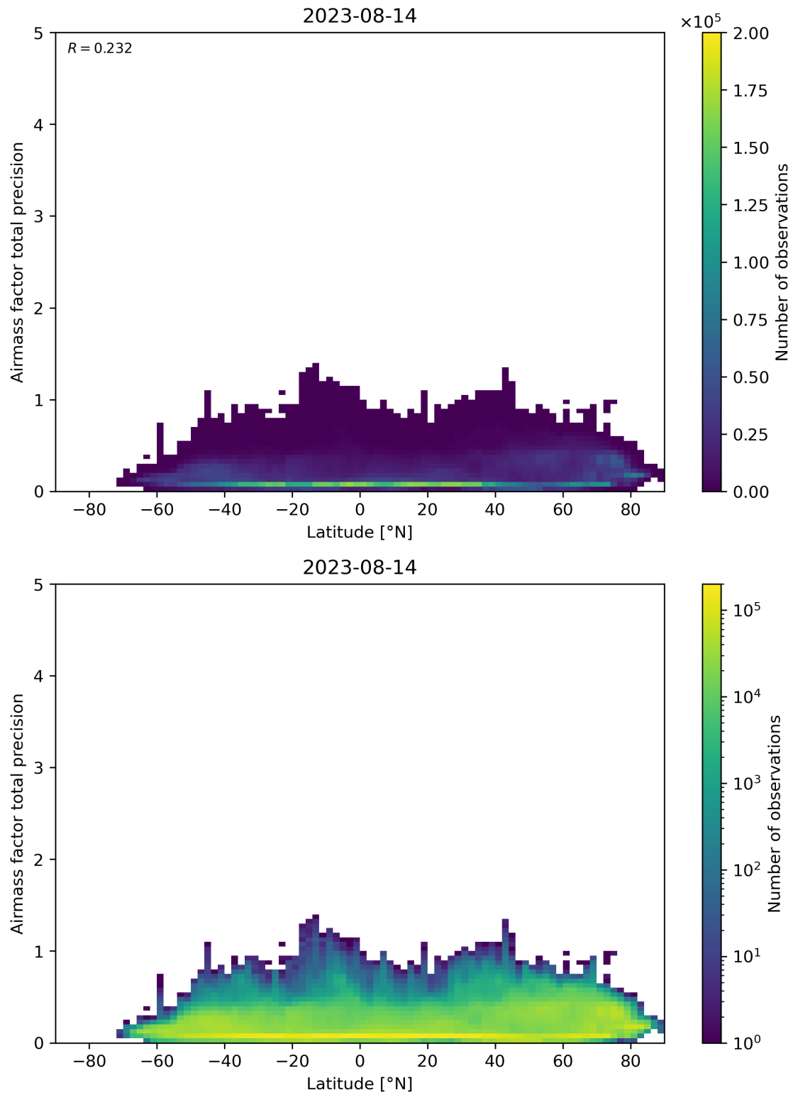
Figure 162: Scatter density plot of “Latitude” against “Airmass factor total precision” for 2023-08-14 to 2023-08-15.
