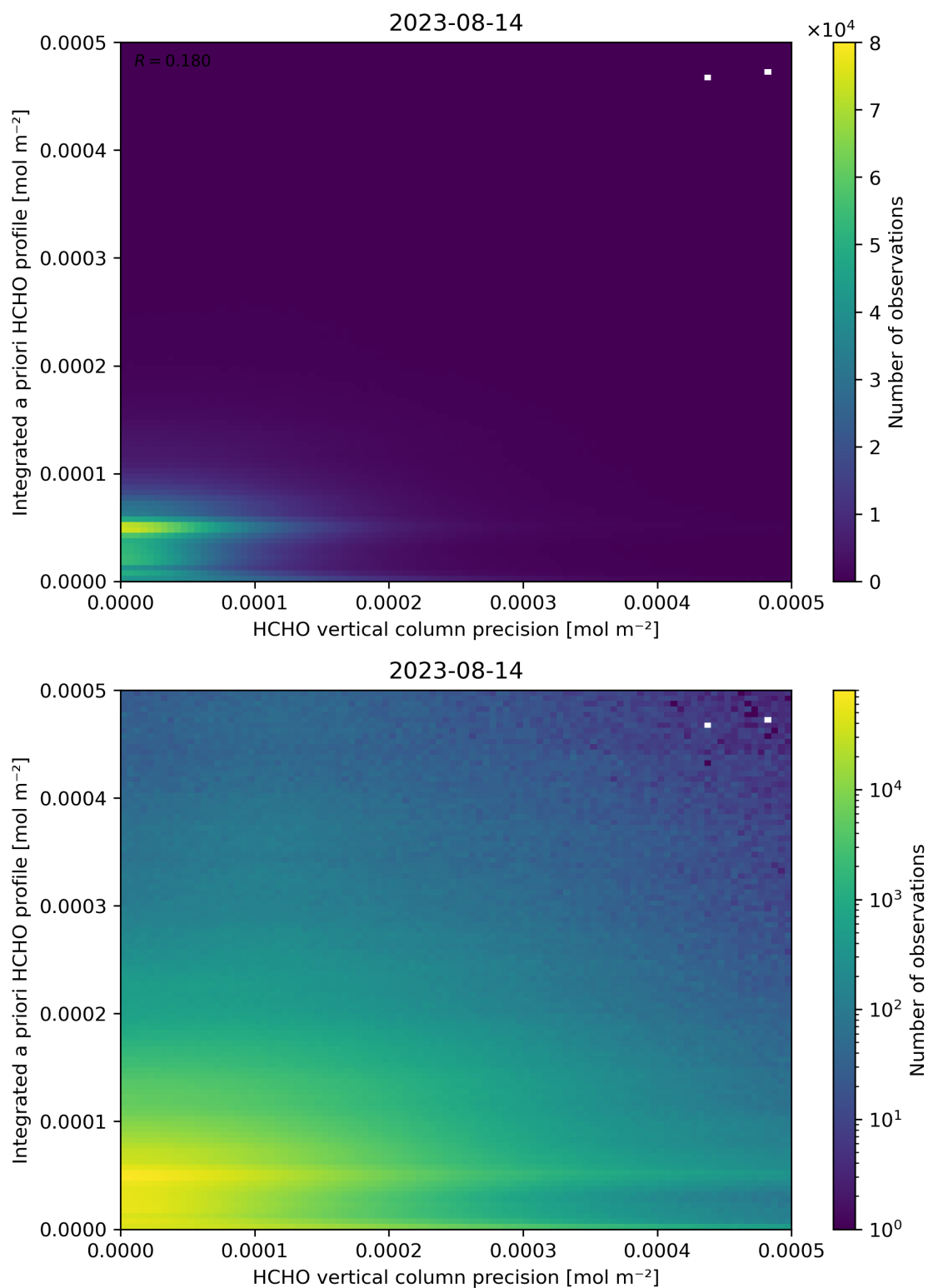
Figure 147: Scatter density plot of “HCHO vertical column precision” against “Integrated a priori HCHO profile” for 2023-08-14 to 2023-08-15.
