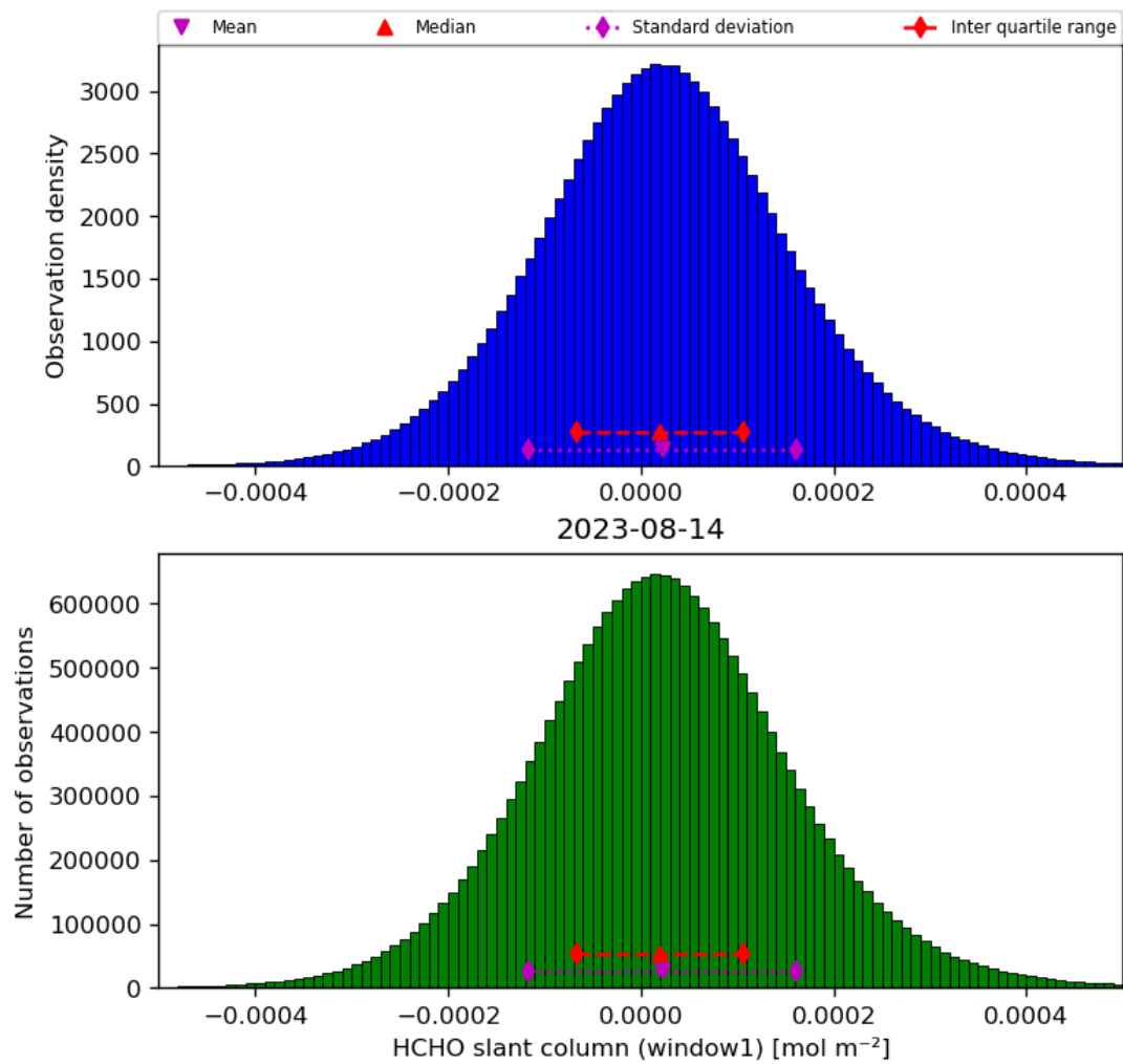
Figure 38: Histogram of “HCHO slant column (window1)” for 2023-08-14 to 2023-08-15
