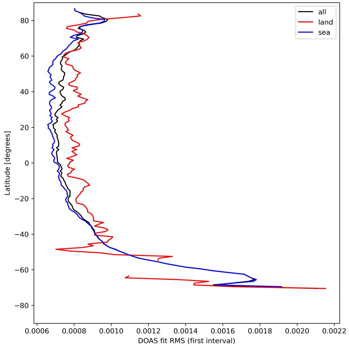
Figure 32: Zonal average of “DOAS fit RMS (first interval)” for 2023-08-14 to 2023-08-15.
