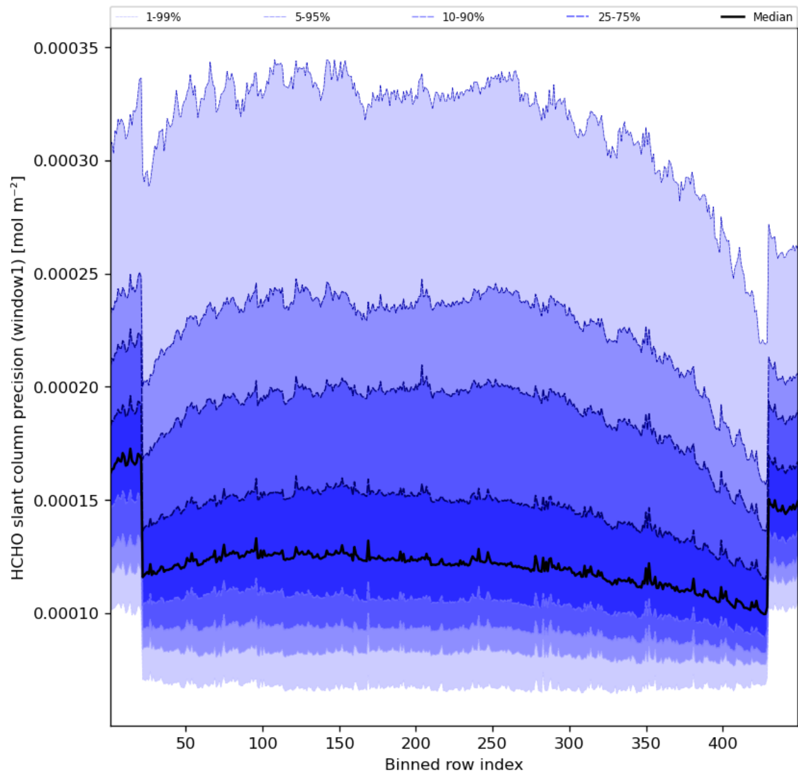
Figure 53: Along track statistics of “HCHO slant column precision (window1)” for 2023-08-14 to 2023-08-15
