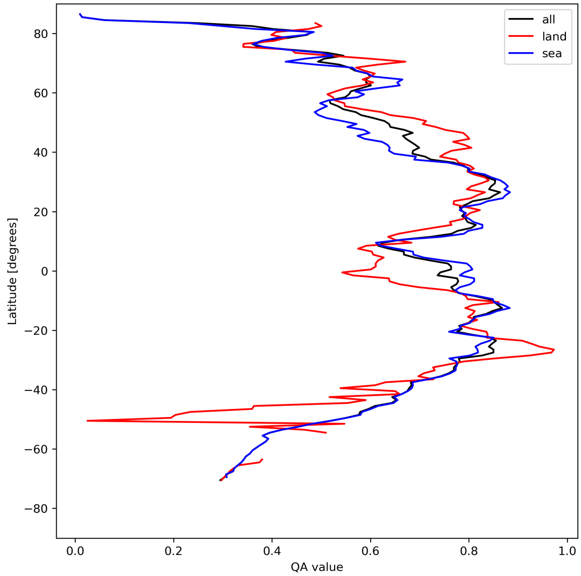
Figure 20: Zonal average of “QA value” for 2023-08-14 to 2023-08-15.
