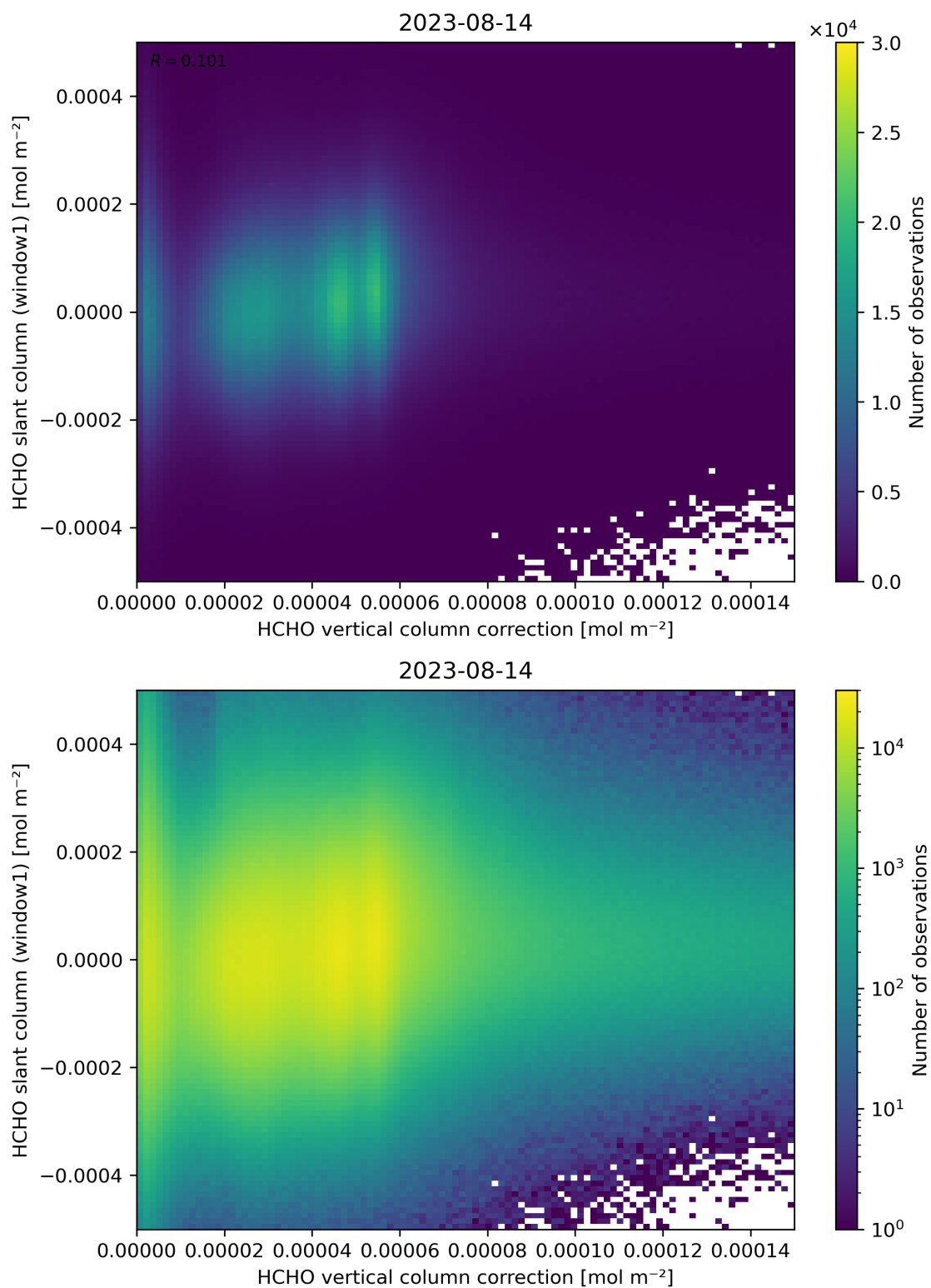
Figure 118: Scatter density plot of “HCHO vertical column correction” against “HCHO slant column (window1)” for 2023-08-14 to 2023-08-15.
