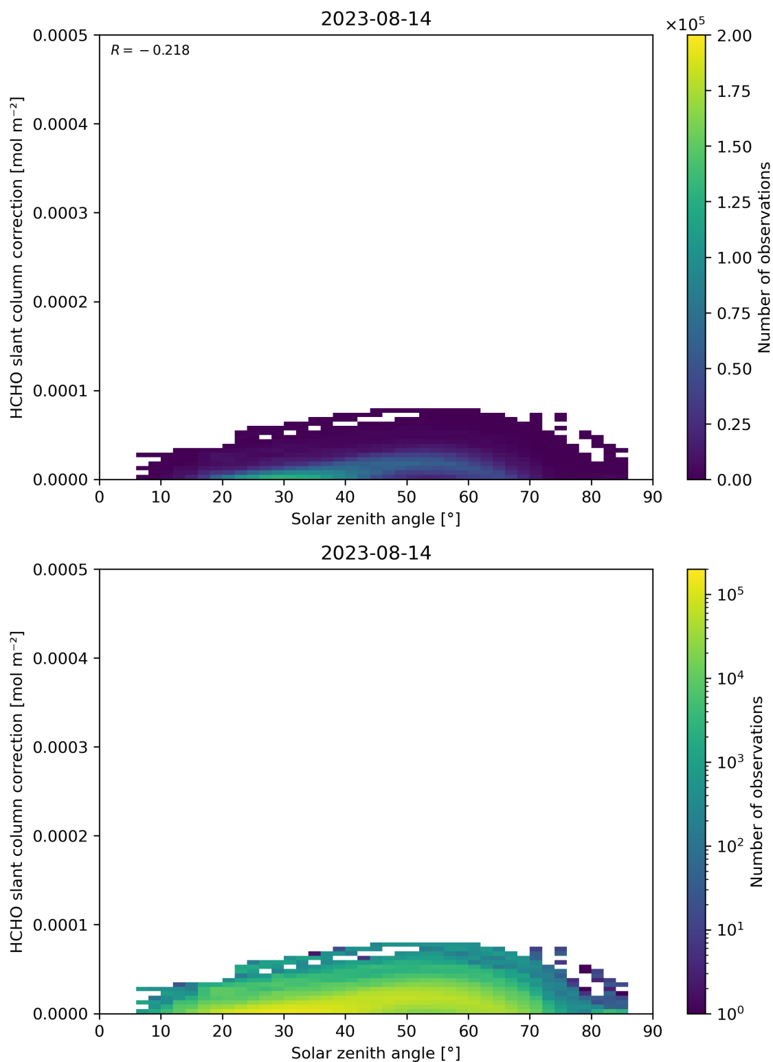
Figure 172: Scatter density plot of “Solar zenith angle” against “HCHO slant column correction” for 2023-08-14 to 2023-08-15.
