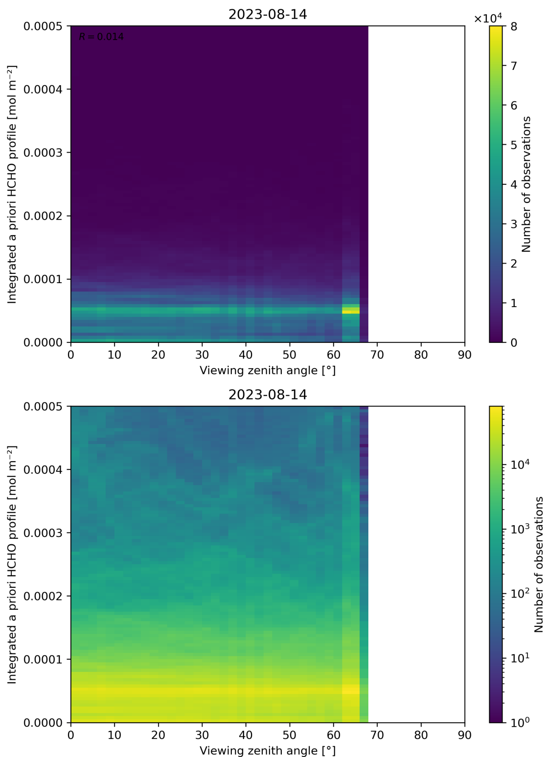
Figure 195: Scatter density plot of “Viewing zenith angle” against “Integrated a priori HCHO profile” for 2023-08-14 to 2023-08-15.
