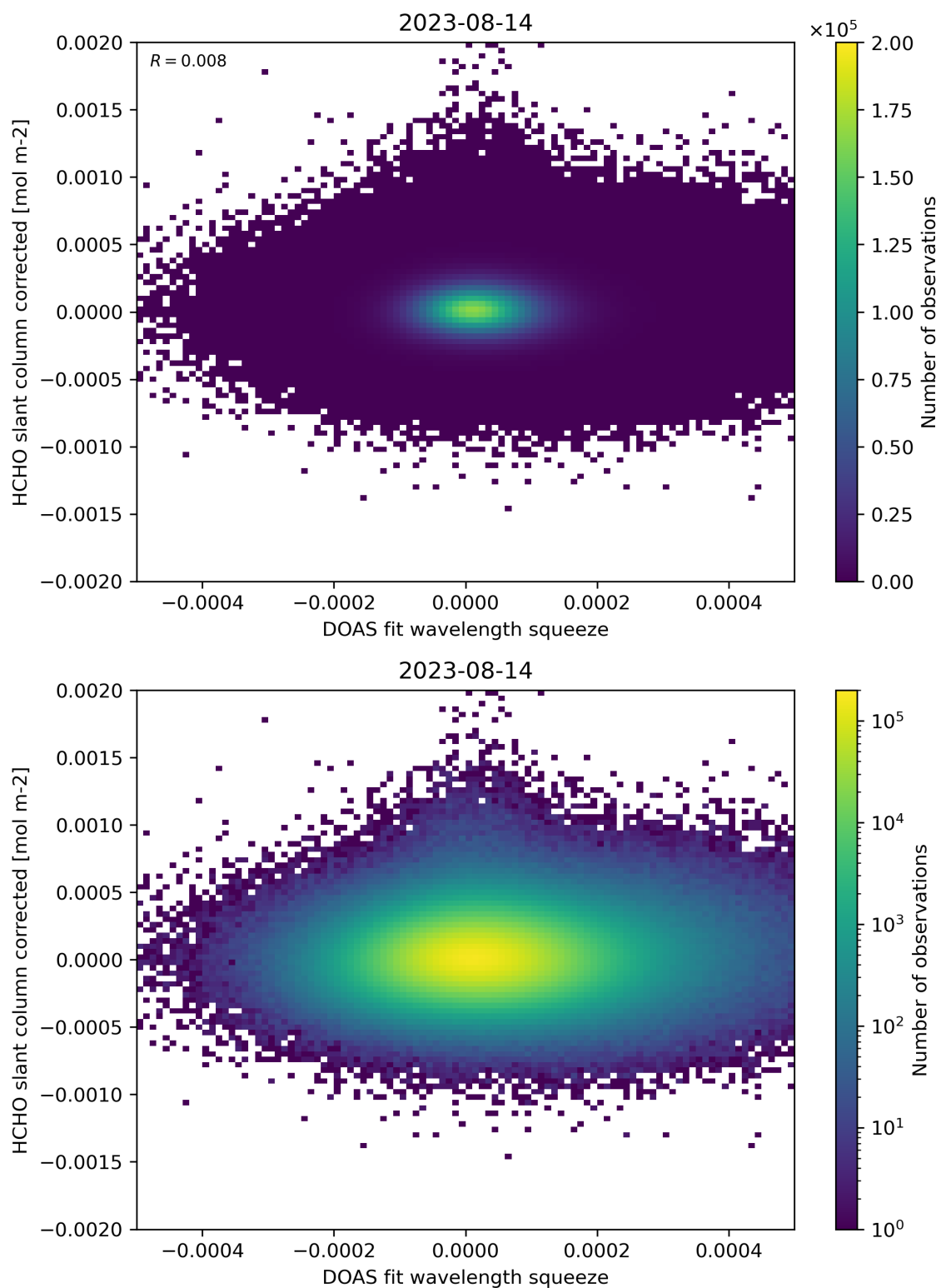
Figure 69: Scatter density plot of “DOAS fit wavelength squeeze” against “HCHO slant column corrected” for 2023-08-14 to 2023-08-15.
