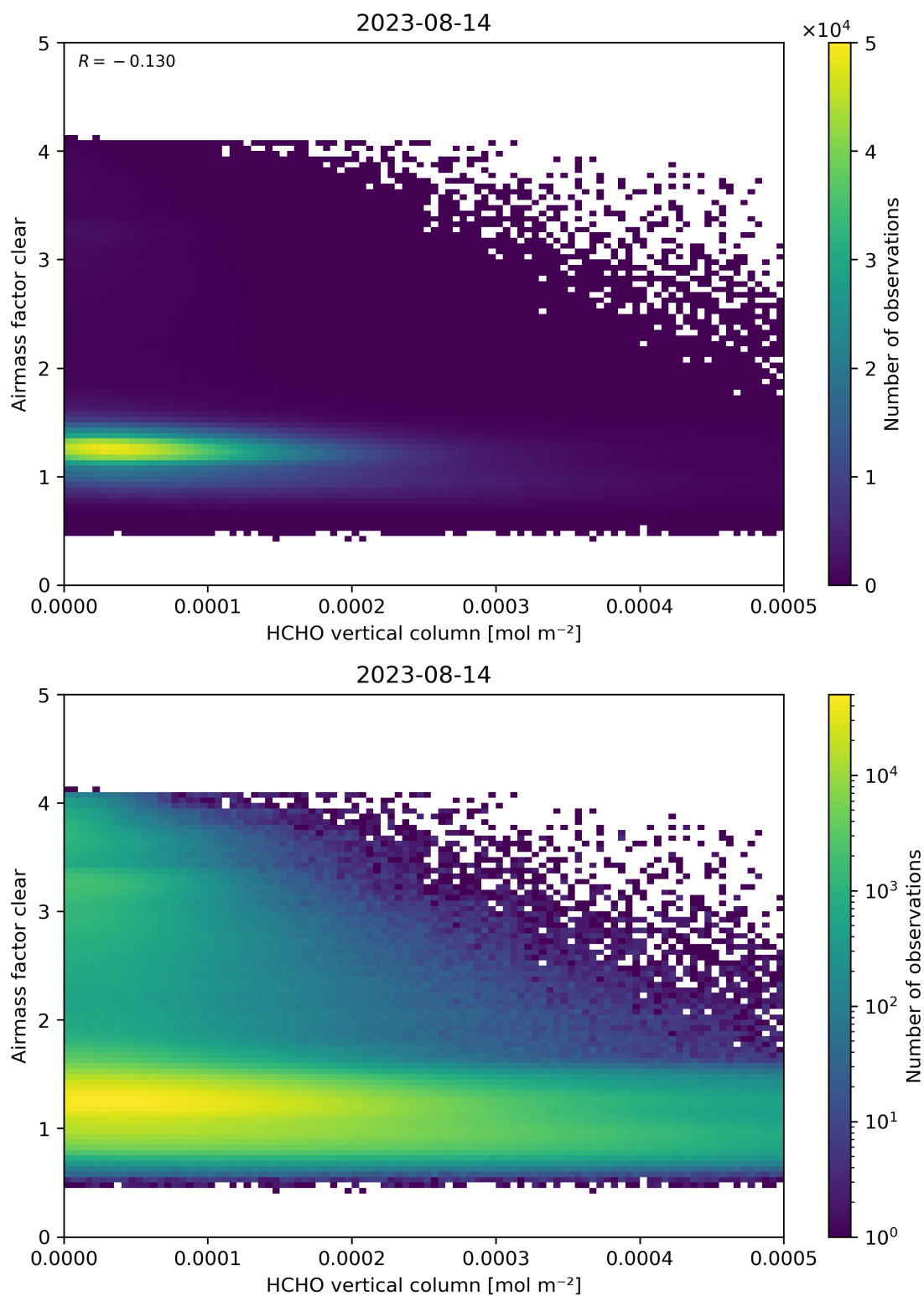
Figure 126: Scatter density plot of “HCHO vertical column” against “Airmass factor clear” for 2023-08-14 to 2023-08-15.
