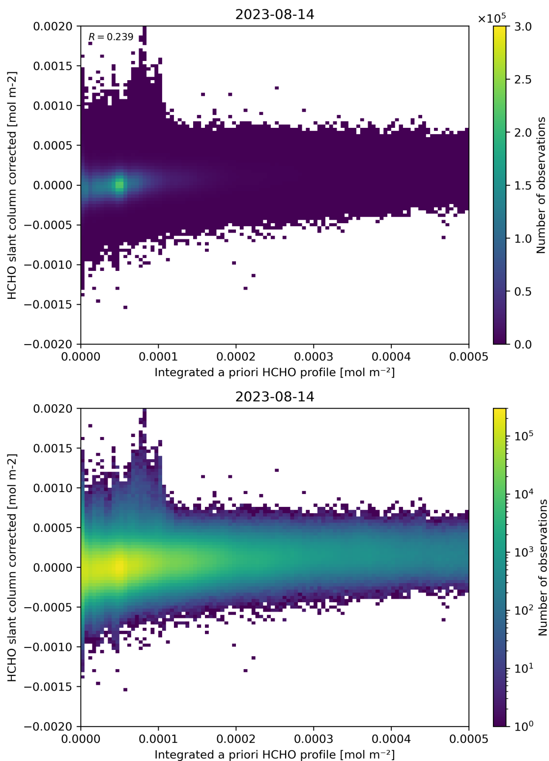
Figure 151: Scatter density plot of “Integrated a priori HCHO profile” against “HCHO slant column corrected” for 2023-08-14 to 2023-08-15.
