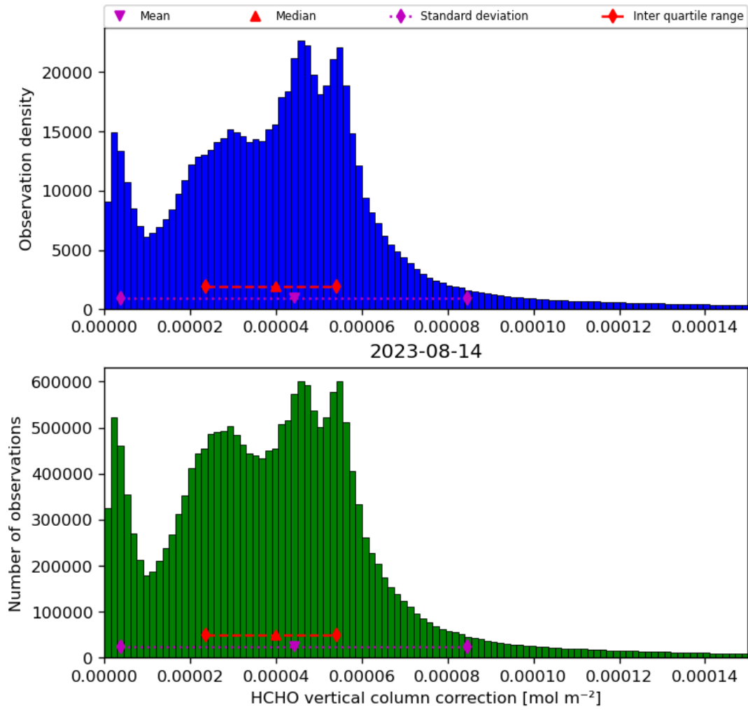
Figure 37: Histogram of “HCHO vertical column correction” for 2023-08-14 to 2023-08-15
