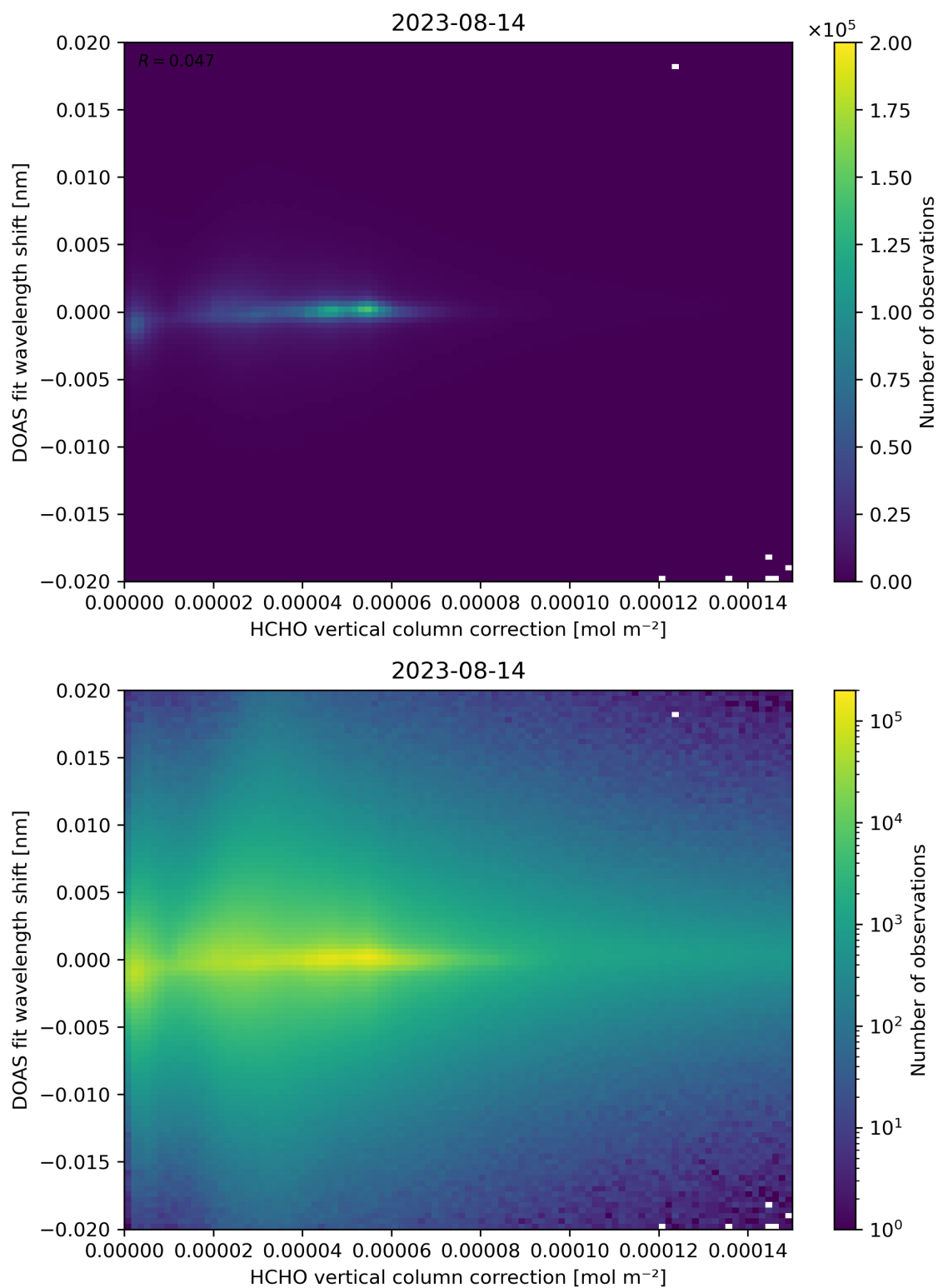
Figure 113: Scatter density plot of “HCHO vertical column correction” against “DOAS fit wavelength shift” for 2023-08-14 to 2023-08-15.
