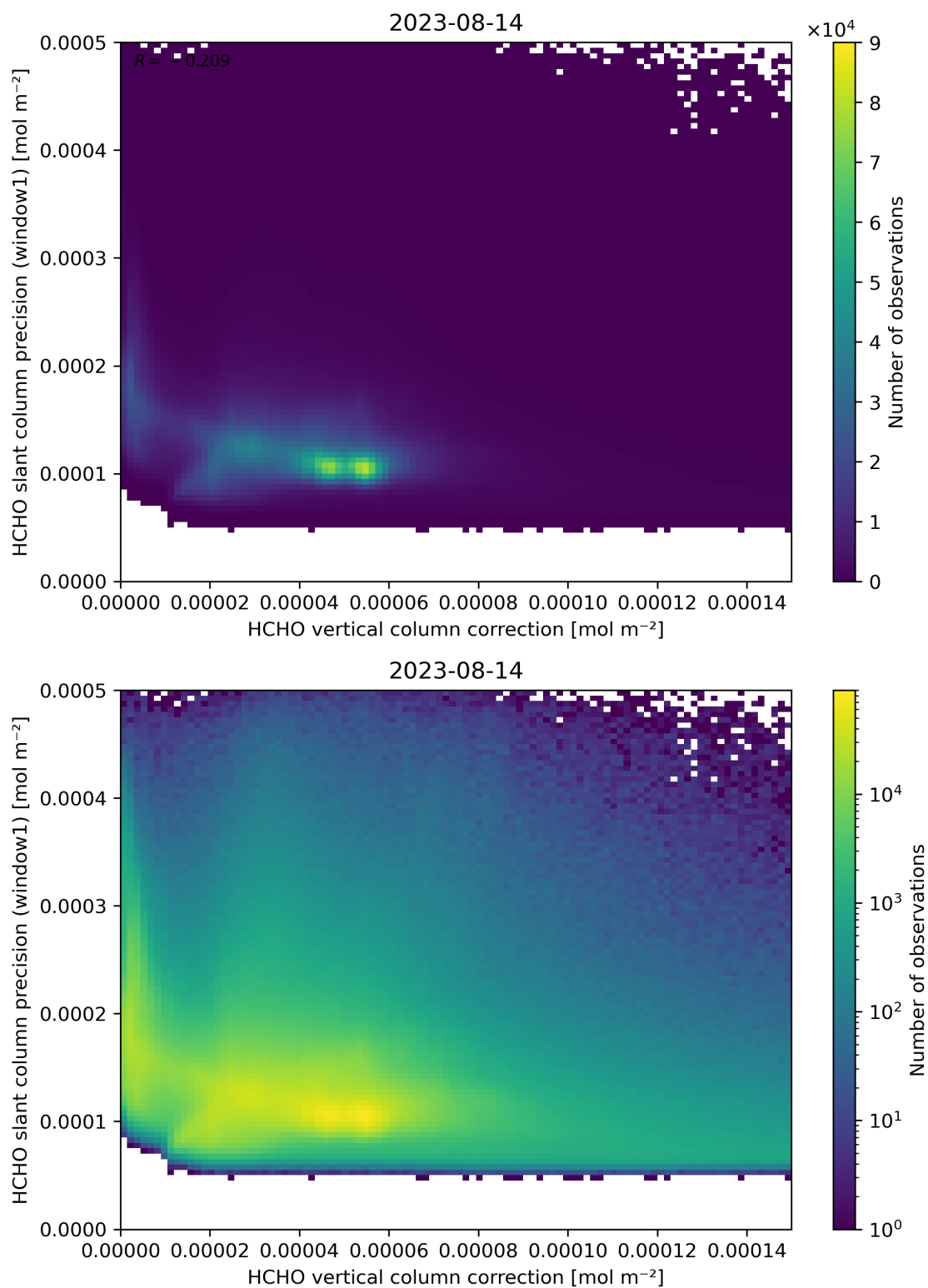
Figure 119: Scatter density plot of “HCHO vertical column correction” against “HCHO slant column precision (window1)” for 2023-08-14 to 2023-08-15.
