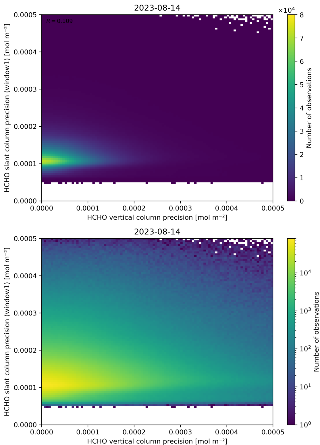
Figure 143: Scatter density plot of “HCHO vertical column precision” against “HCHO slant column precision (window1)” for 2023-08-14 to 2023-08-15.
