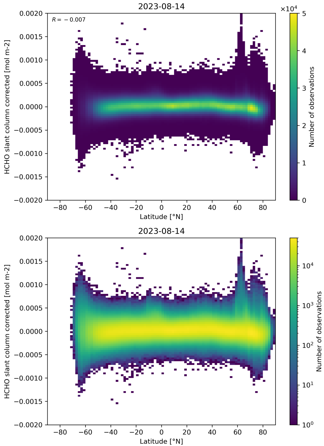
Figure 157: Scatter density plot of “Latitude” against “HCHO slant column corrected” for 2023-08-14 to 2023-08-15.
