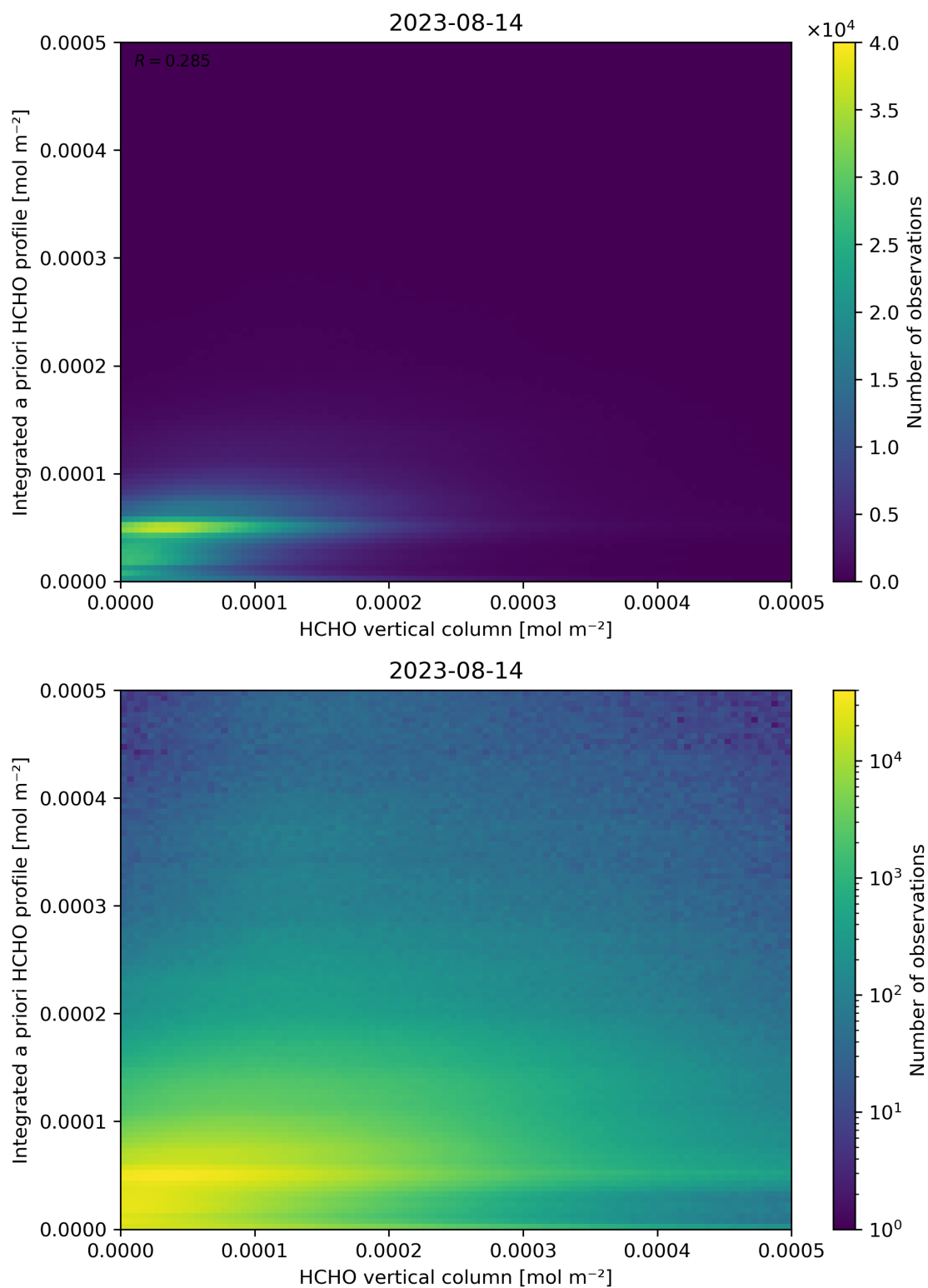
Figure 135: Scatter density plot of “HCHO vertical column” against “Integrated a priori HCHO profile” for 2023-08-14 to 2023-08-15.
