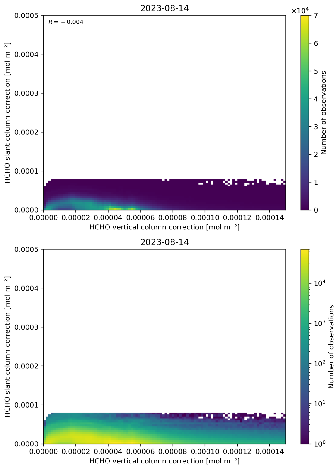
Figure 117: Scatter density plot of “HCHO vertical column correction” against “HCHO slant column correction” for 2023-08-14 to 2023-08-15.
