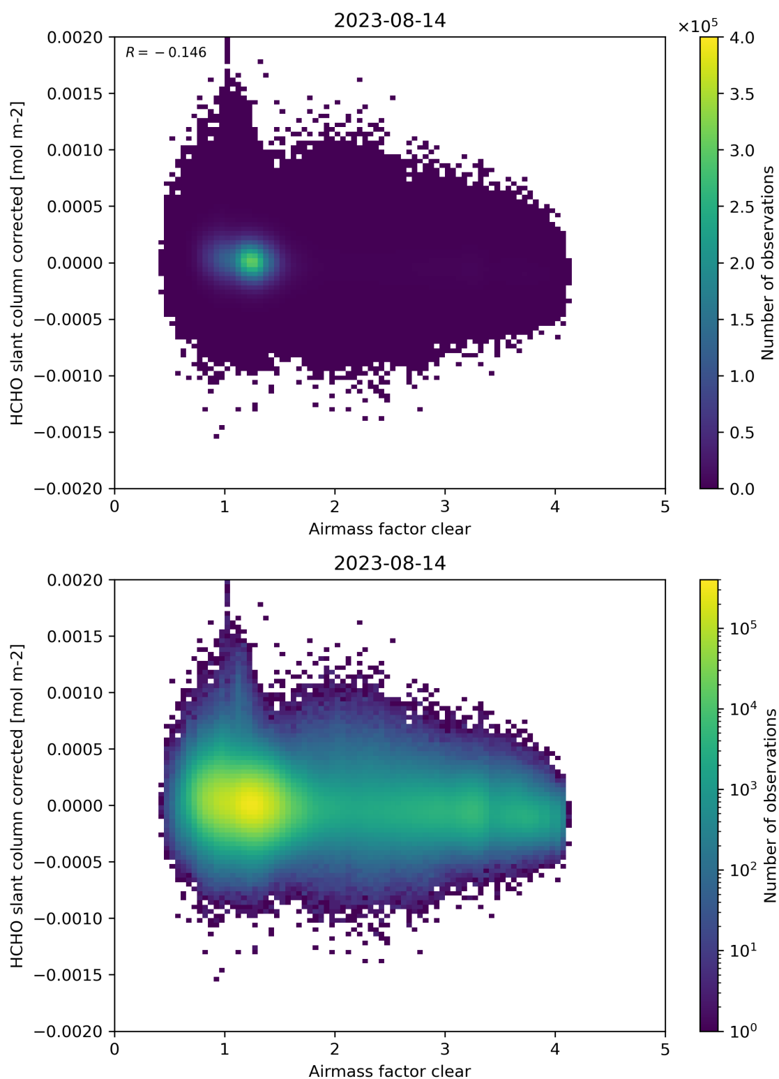
Figure 74: Scatter density plot of “Airmass factor clear” against “HCHO slant column corrected” for 2023-08-14 to 2023-08-15.
