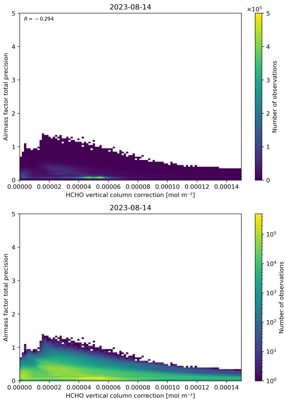
Figure 121: Scatter density plot of “HCHO vertical column correction” against “Airmass factor total precision” for 2023-08-14 to 2023-08-15.
