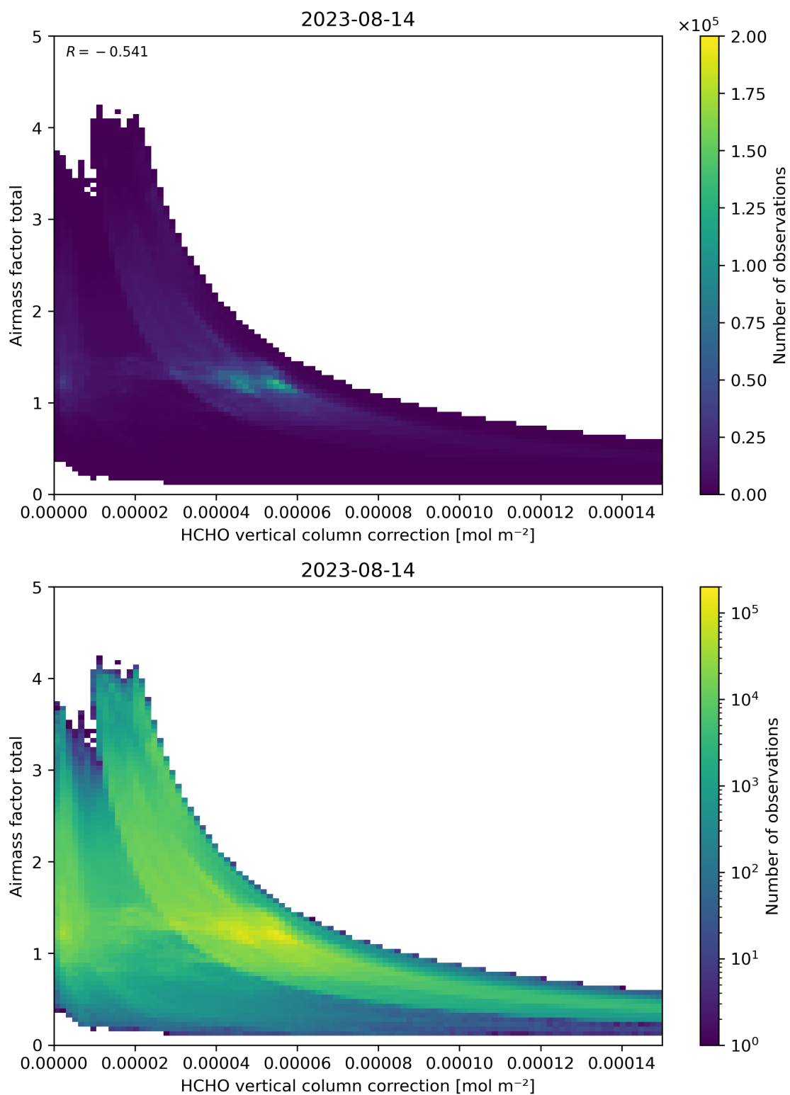
Figure 120: Scatter density plot of “HCHO vertical column correction” against “Airmass factor total” for 2023-08-14 to 2023-08-15.
