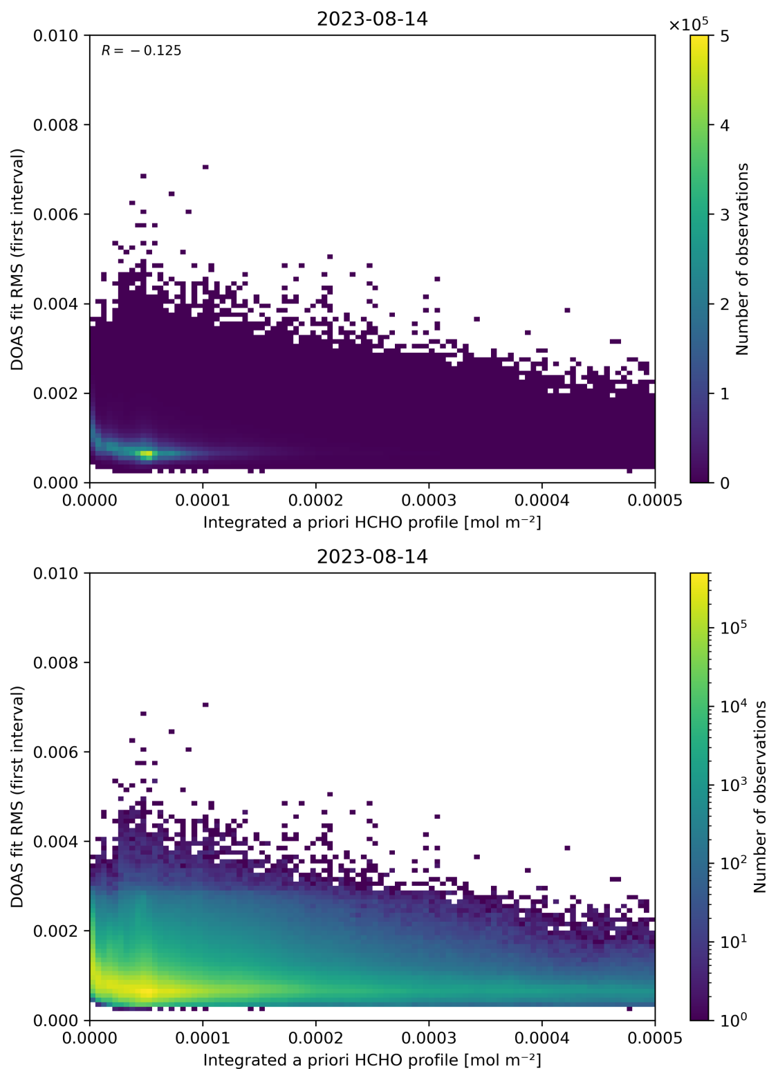
Figure 148: Scatter density plot of “Integrated a priori HCHO profile” against “DOAS fit RMS (first interval)” for 2023-08-14 to 2023-08-15.
