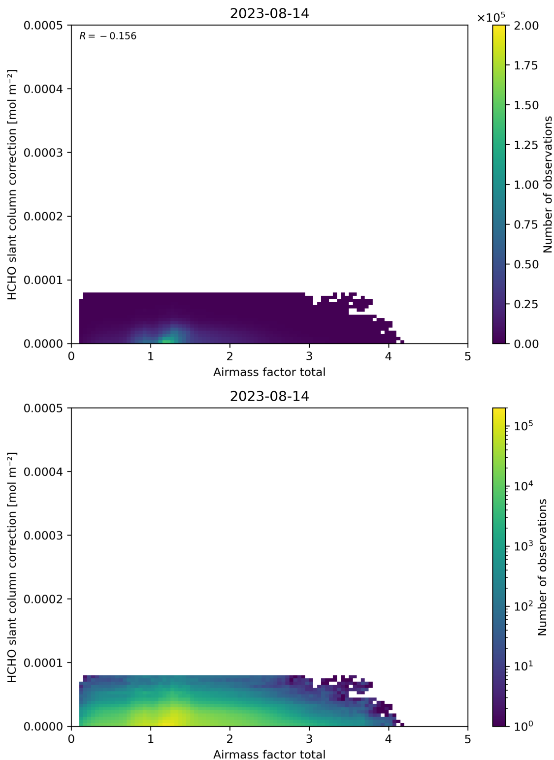
Figure 102: Scatter density plot of “Airmass factor total” against “HCHO slant column correction” for 2023-08-14 to 2023-08-15.
