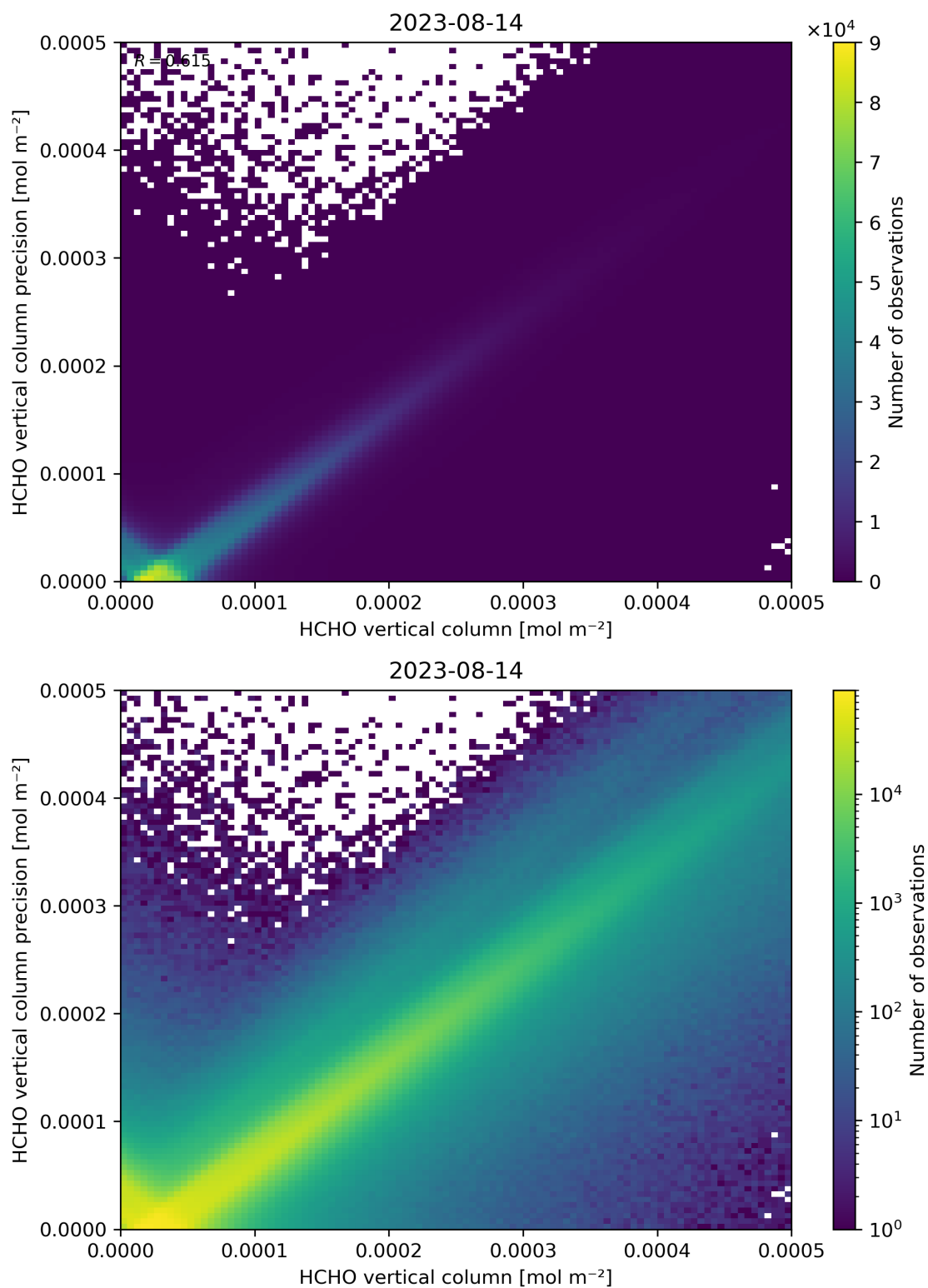
Figure 134: Scatter density plot of “HCHO vertical column” against “HCHO vertical column precision” for 2023-08-14 to 2023-08-15.
