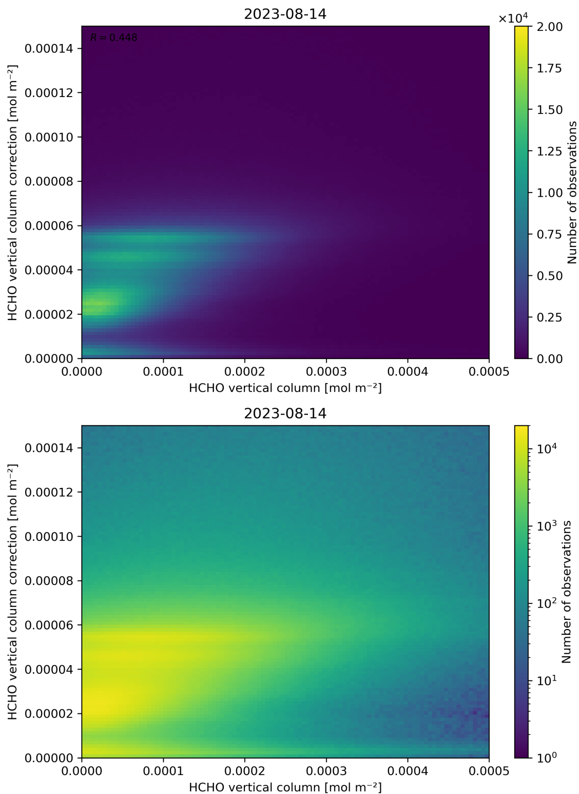
Figure 133: Scatter density plot of “HCHO vertical column” against “HCHO vertical column correction” for 2023-08-14 to 2023-08-15.
