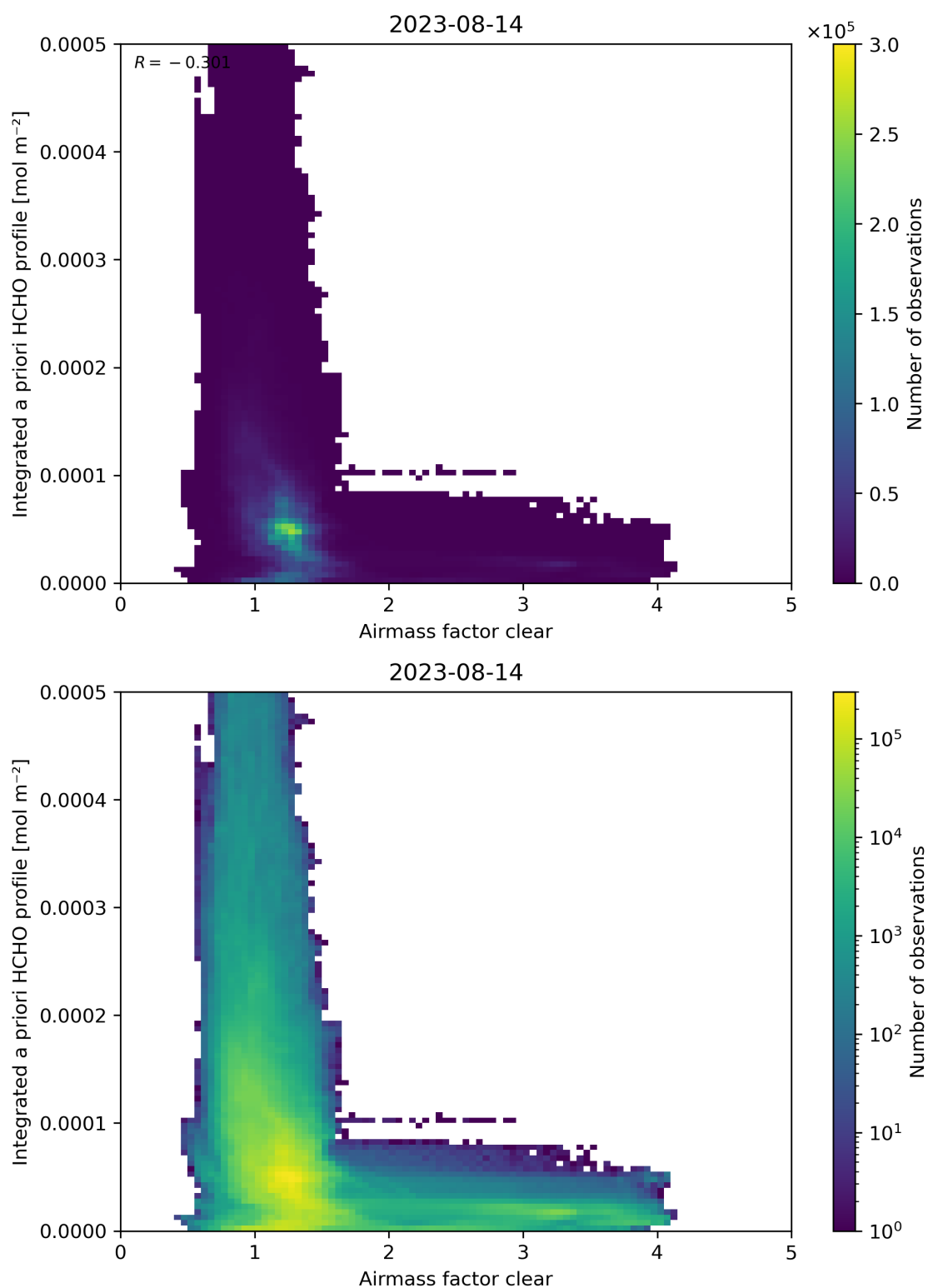
Figure 76: Scatter density plot of “Airmass factor clear” against “Integrated a priori HCHO profile” for 2023-08-14 to 2023-08-15.
