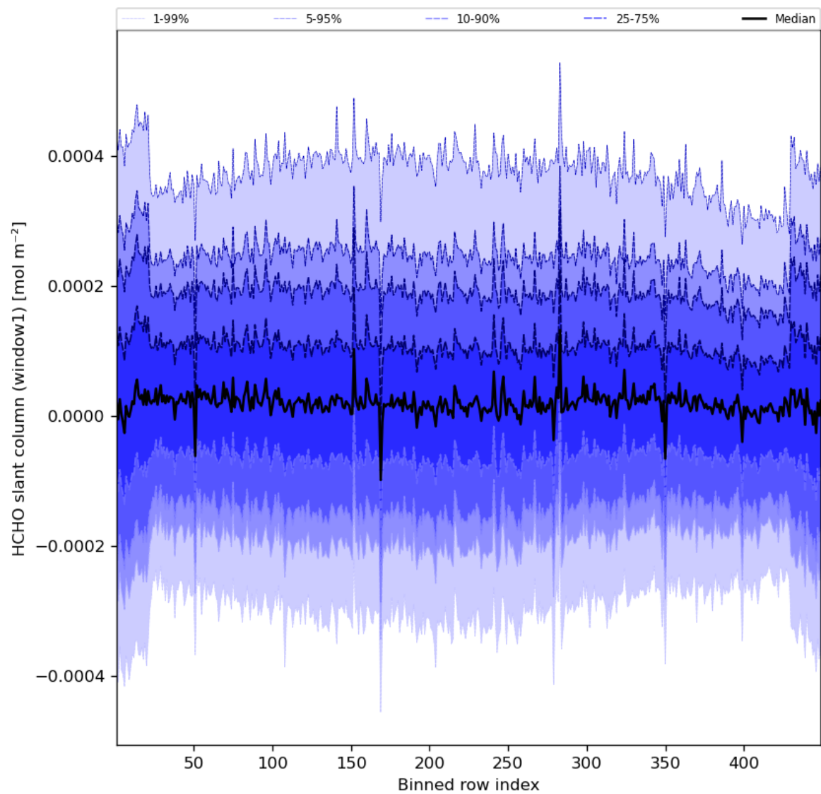
Figure 52: Along track statistics of “HCHO slant column (window1)” for 2023-08-14 to 2023-08-15
