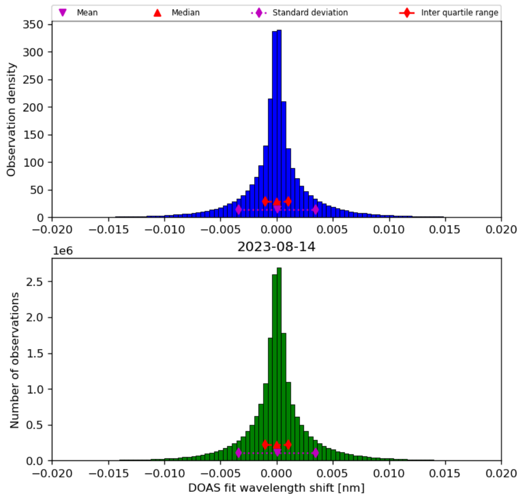
Figure 44: Histogram of “DOAS fit wavelength shift” for 2023-08-14 to 2023-08-15
