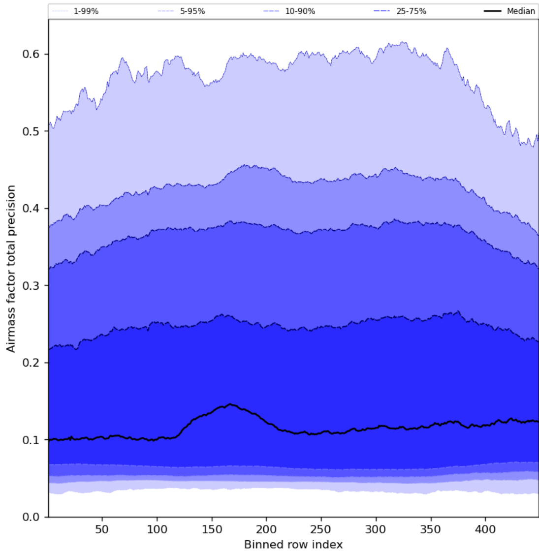
Figure 55: Along track statistics of “Airmass factor total precision” for 2023-08-14 to 2023-08-15
