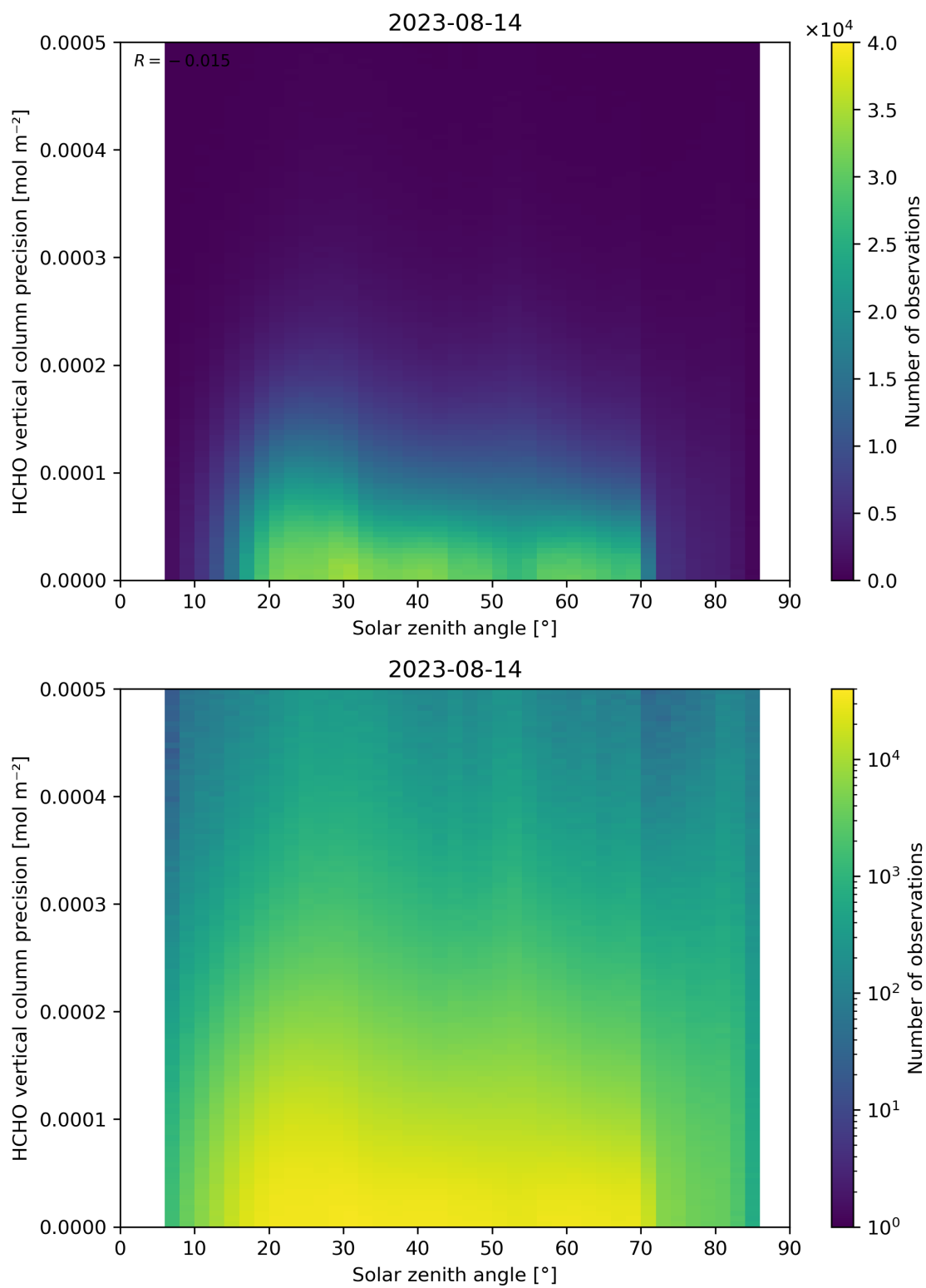
Figure 179: Scatter density plot of “Solar zenith angle” against “HCHO vertical column precision” for 2023-08-14 to 2023-08-15.
