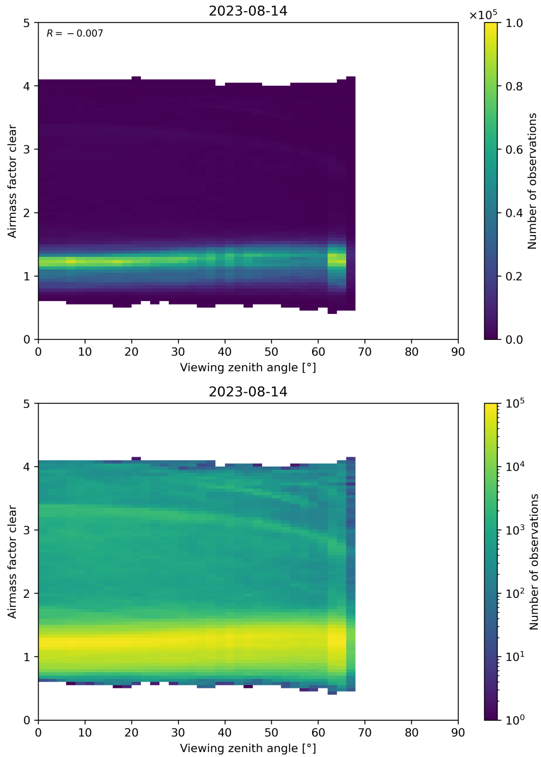
Figure 185: Scatter density plot of “Viewing zenith angle” against “Airmass factor clear” for 2023-08-14 to 2023-08-15.
