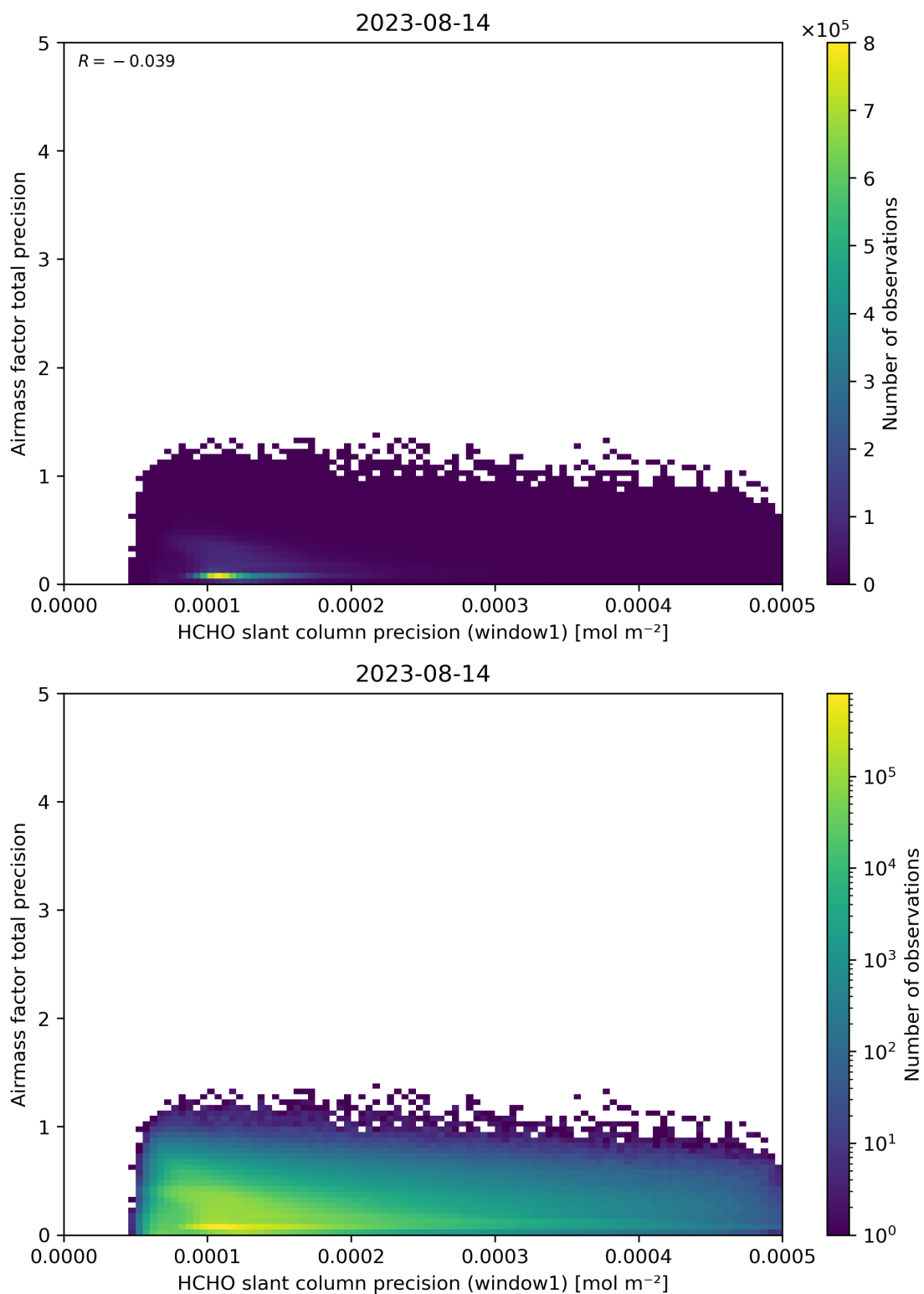
Figure 95: Scatter density plot of “HCHO slant column precision (window1)” against “Airmass factor total precision” for 2023-08-14 to 2023-08-15.
