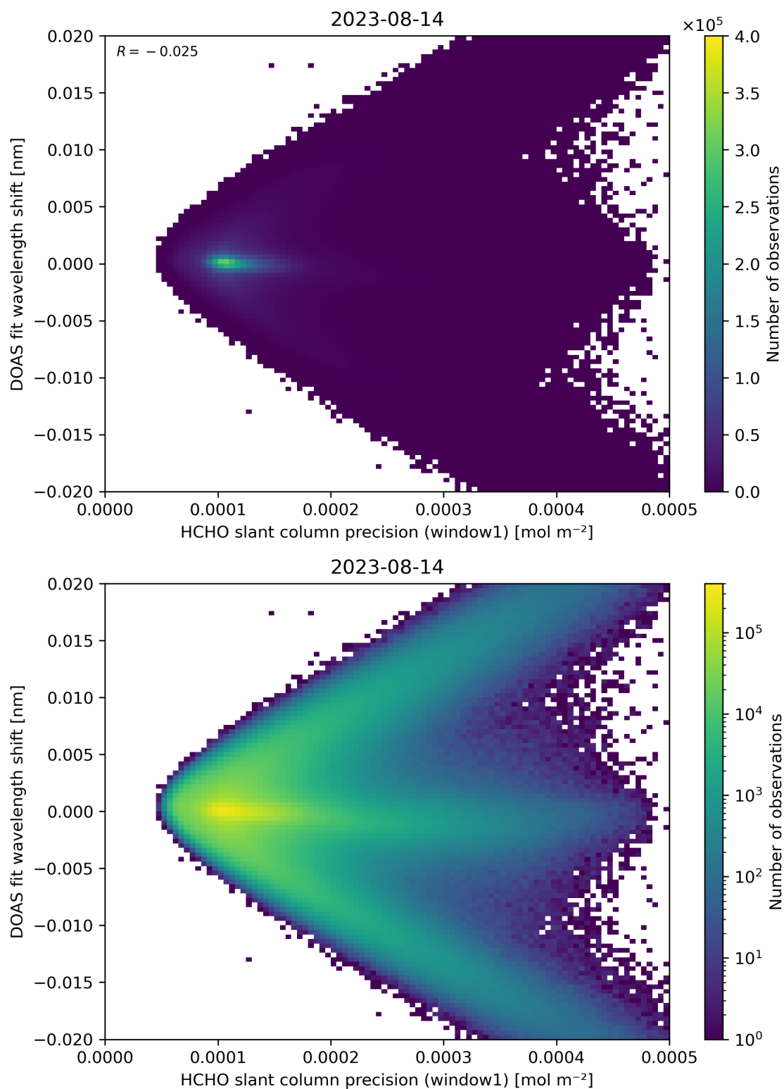
Figure 89: Scatter density plot of “HCHO slant column precision (window1)” against “DOAS fit wavelength shift” for 2023-08-14 to 2023-08-15.
