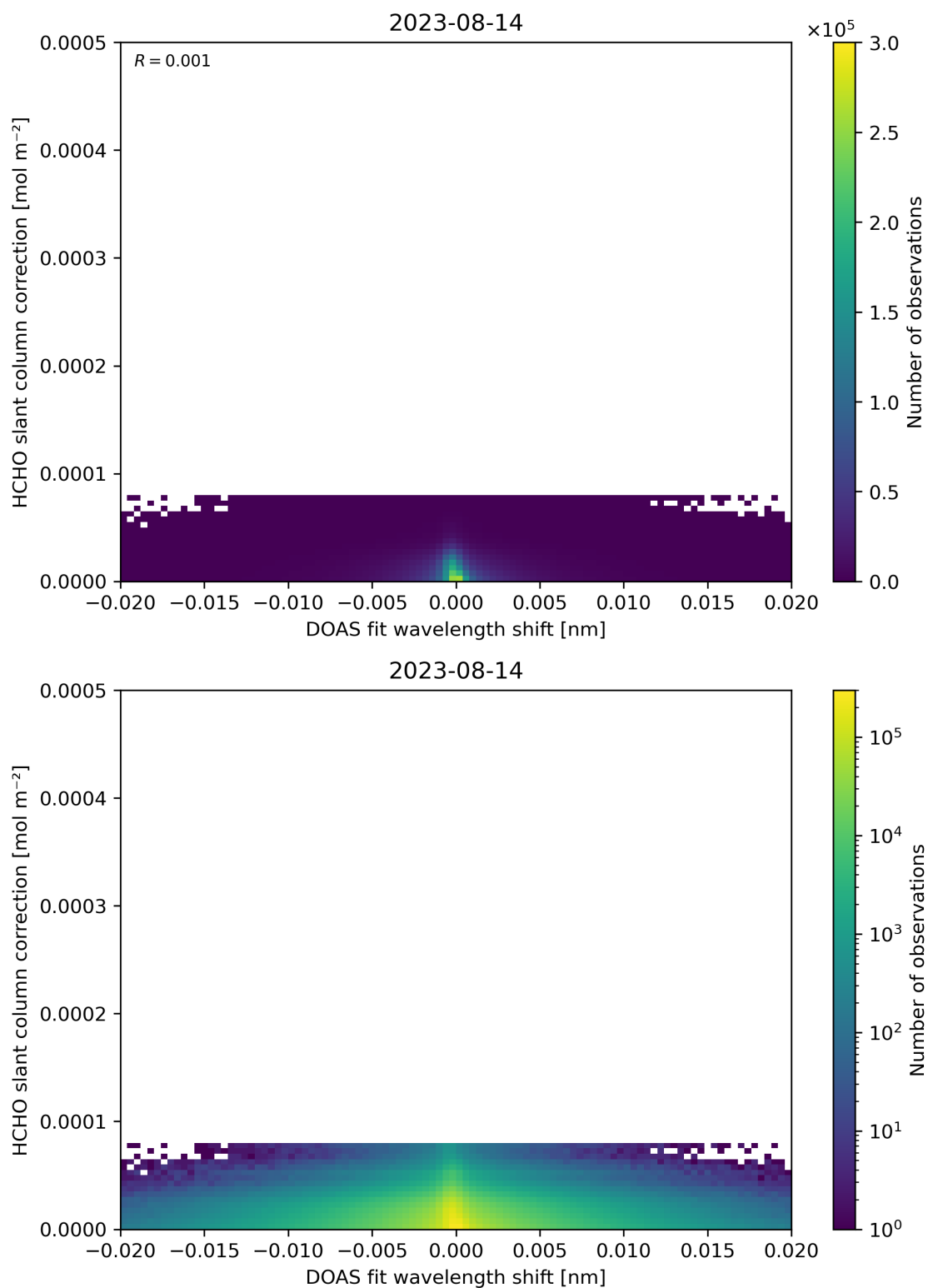
Figure 67: Scatter density plot of “DOAS fit wavelength shift” against “HCHO slant column correction” for 2023-08-14 to 2023-08-15.
