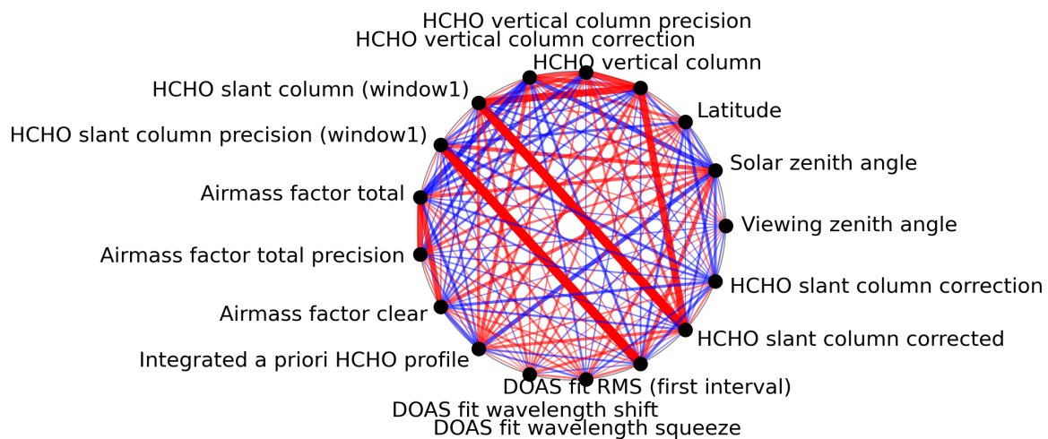
Figure 1: Map of correlation graph for 2023-08-14 to 2023-08-15.
