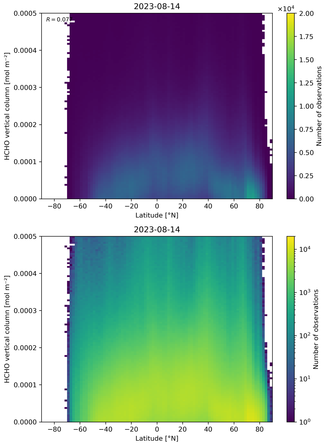
Figure 163: Scatter density plot of “Latitude” against “HCHO vertical column” for 2023-08-14 to 2023-08-15.
