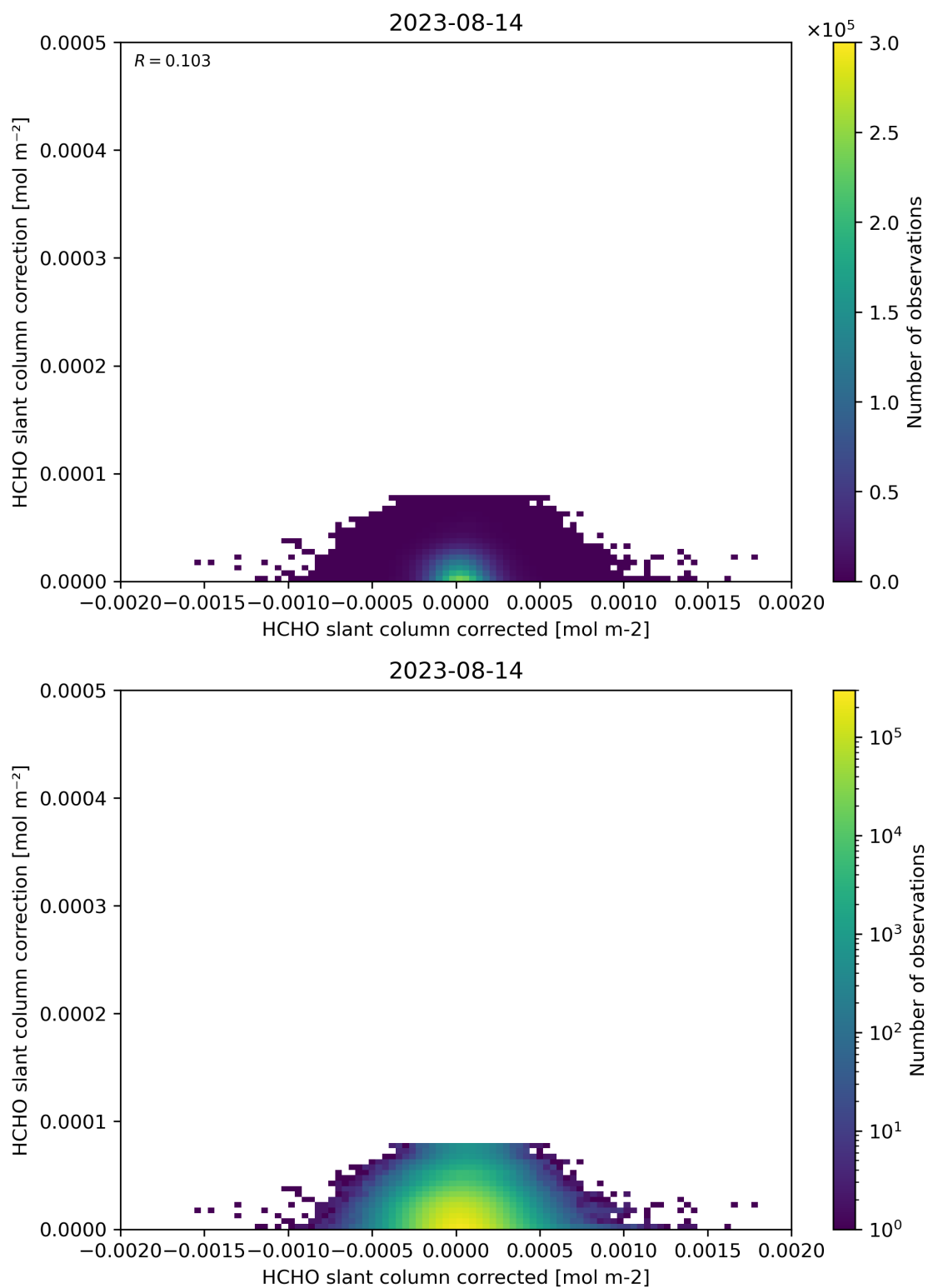
Figure 77: Scatter density plot of “HCHO slant column corrected” against “HCHO slant column correction” for 2023-08-14 to 2023-08-15.
