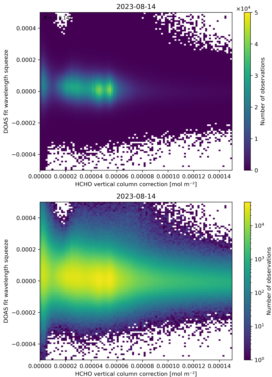
Figure 114: Scatter density plot of “HCHO vertical column correction” against “DOAS fit wavelength squeeze” for 2023-08-14 to 2023-08-15.
