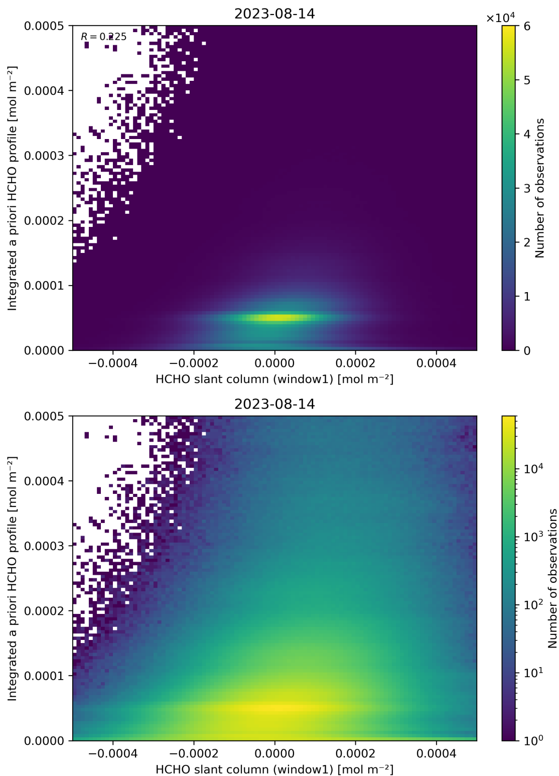
Figure 87: Scatter density plot of “HCHO slant column (window1)” against “Integrated a priori HCHO profile” for 2023-08-14 to 2023-08-15.
