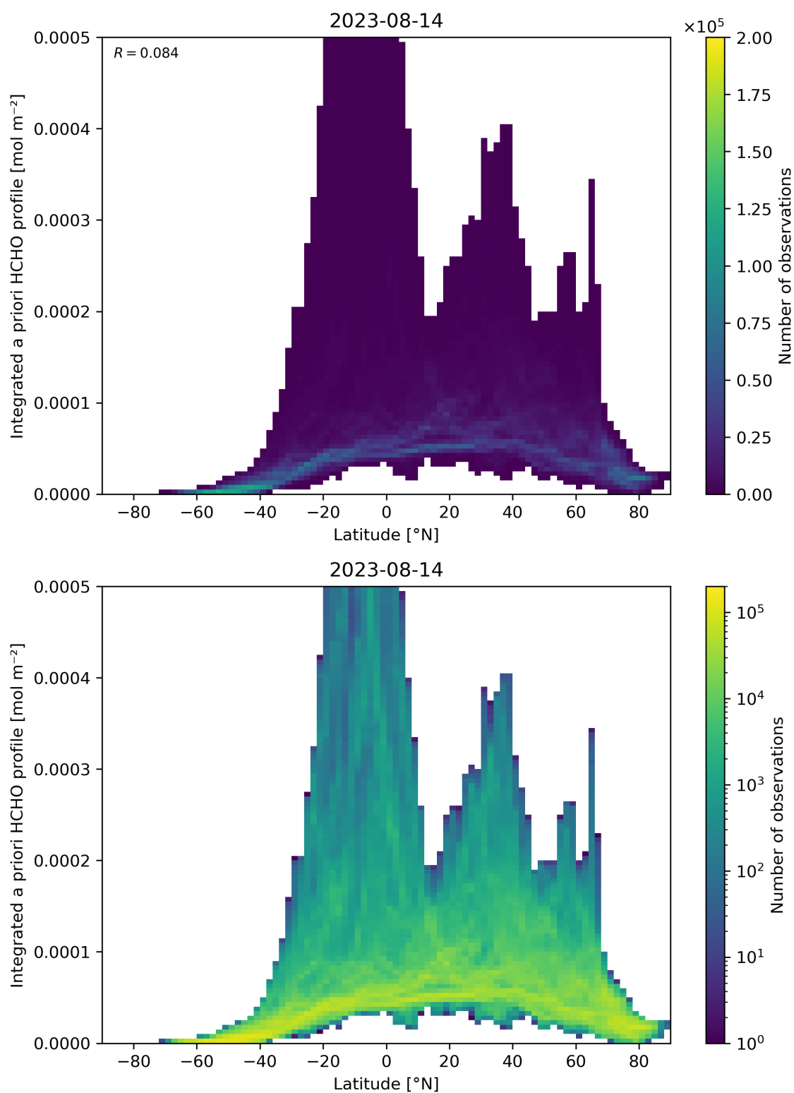
Figure 166: Scatter density plot of “Latitude” against “Integrated a priori HCHO profile” for 2023-08-14 to 2023-08-15.
