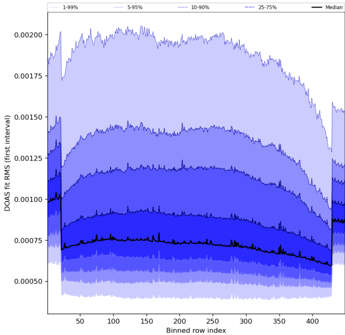
Figure 60: Along track statistics of “DOAS fit RMS (first interval)” for 2023-08-14 to 2023-08-15
