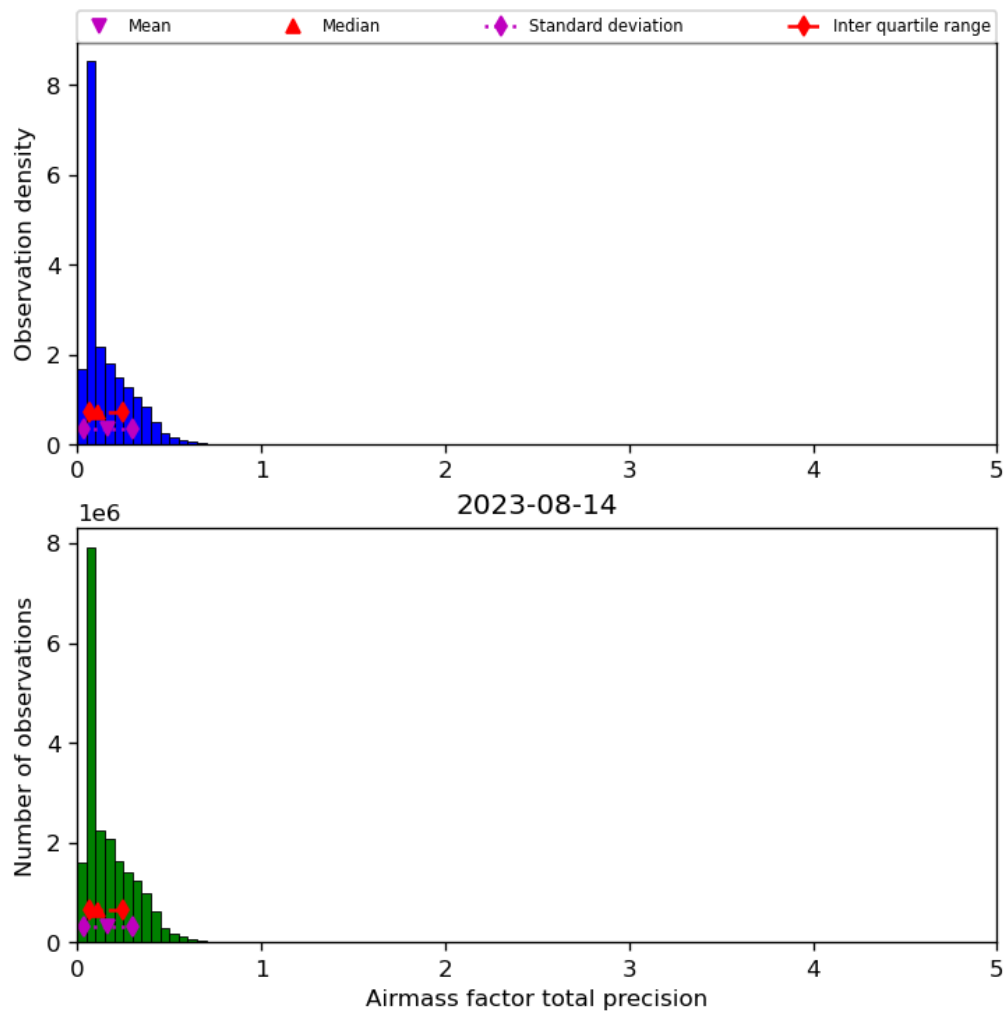
Figure 41: Histogram of “Airmass factor total precision” for 2023-08-14 to 2023-08-15
