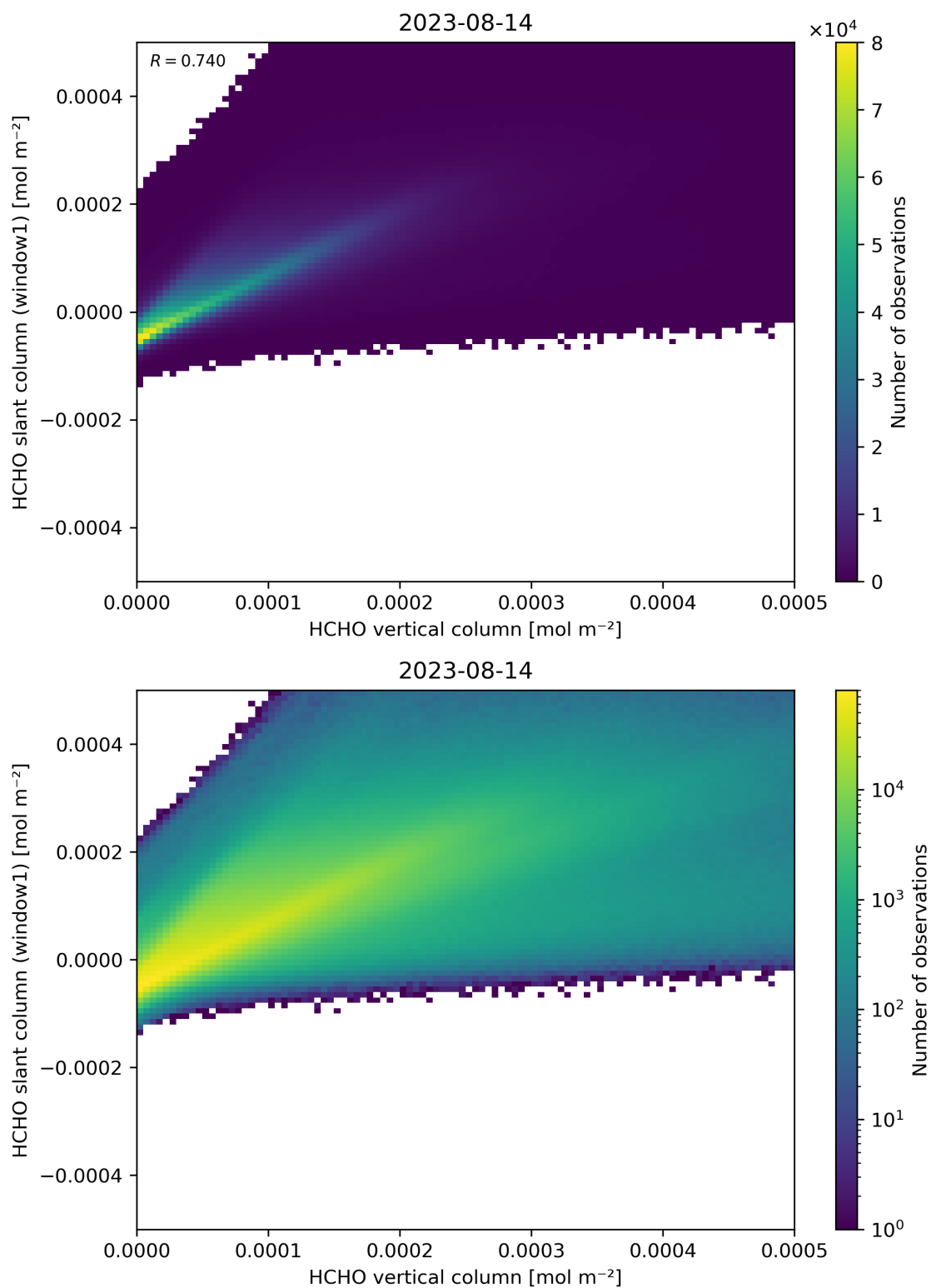
Figure 129: Scatter density plot of “HCHO vertical column” against “HCHO slant column (window1)” for 2023-08-14 to 2023-08-15.
