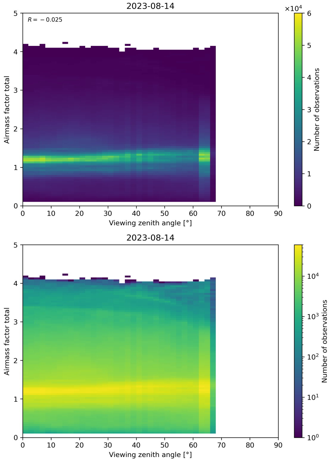
Figure 190: Scatter density plot of “Viewing zenith angle” against “Airmass factor total” for 2023-08-14 to 2023-08-15.
