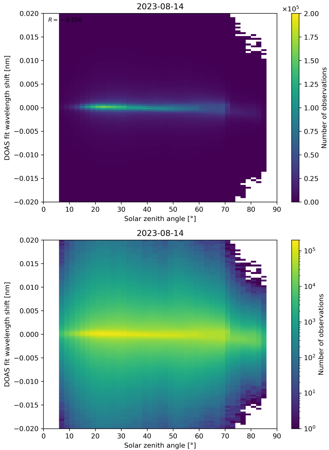
Figure 168: Scatter density plot of “Solar zenith angle” against “DOAS fit wavelength shift” for 2023-08-14 to 2023-08-15.
