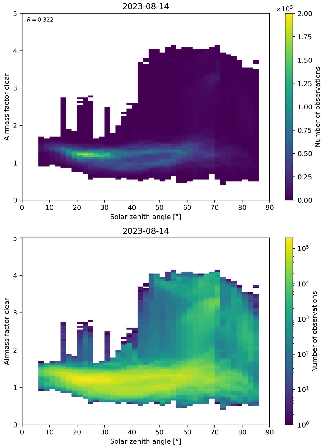
Figure 170: Scatter density plot of “Solar zenith angle” against “Airmass factor clear” for 2023-08-14 to 2023-08-15.
