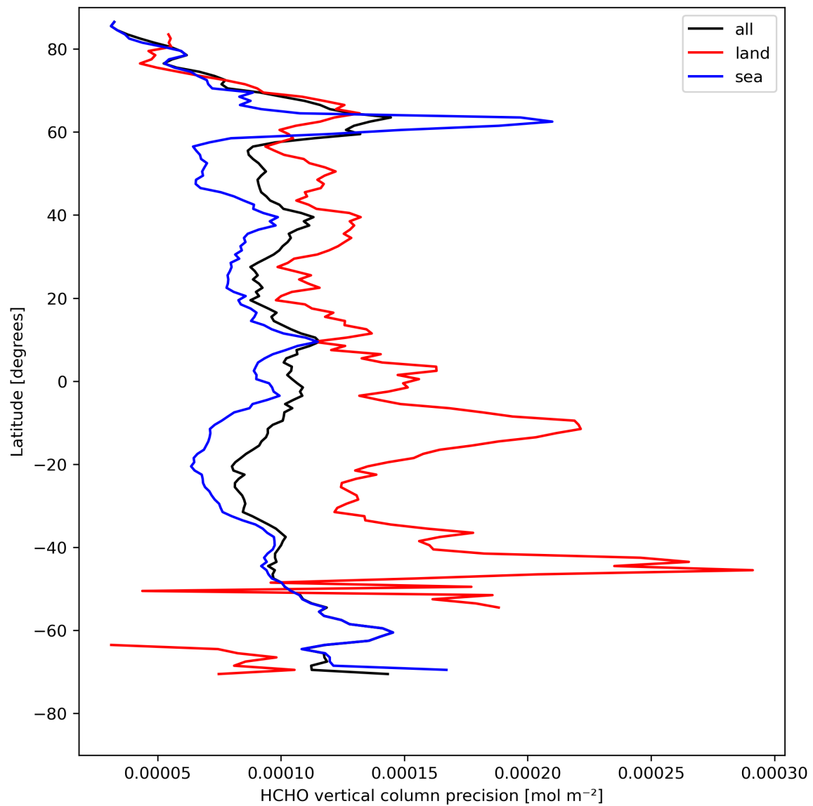
Figure 22: Zonal average of “HCHO vertical column precision” for 2023-08-14 to 2023-08-15.
