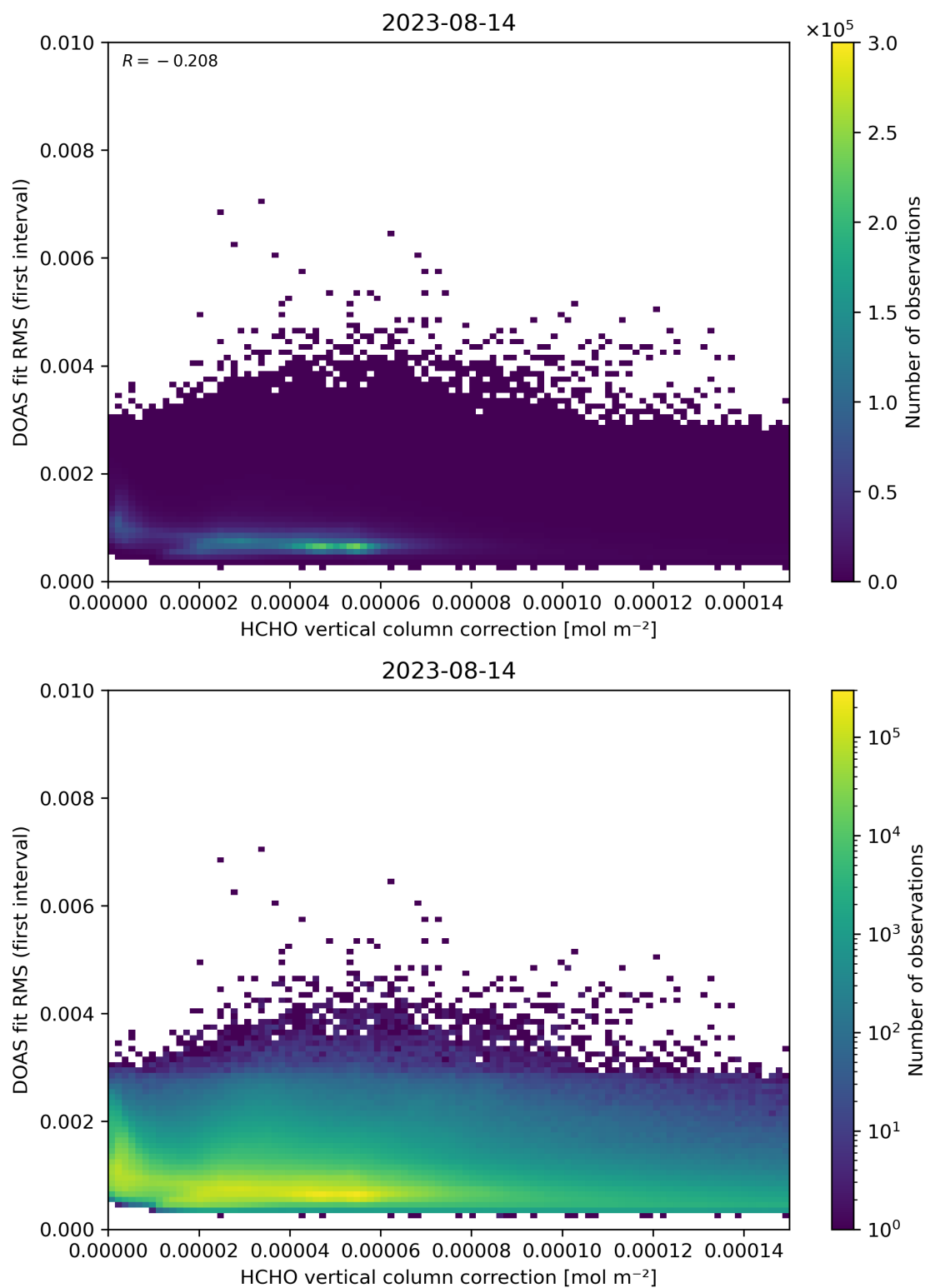
Figure 112: Scatter density plot of “HCHO vertical column correction” against “DOAS fit RMS (first interval)” for 2023-08-14 to 2023-08-15.
