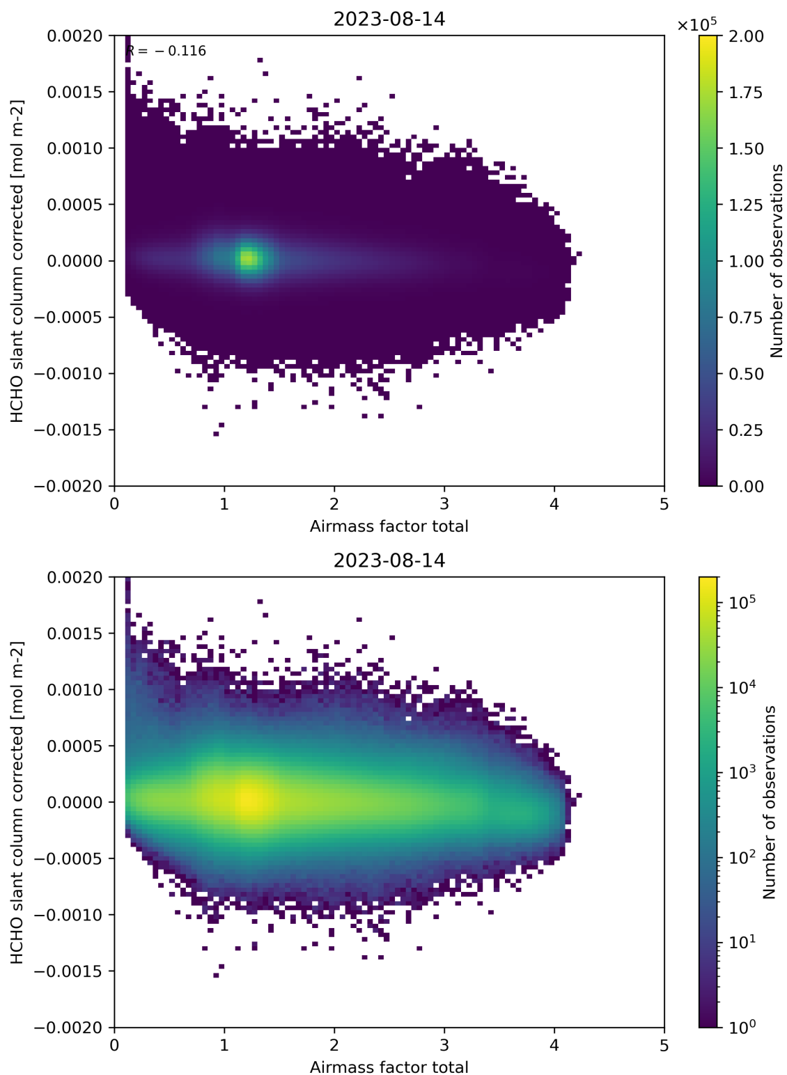
Figure 101: Scatter density plot of “Airmass factor total” against “HCHO slant column corrected” for 2023-08-14 to 2023-08-15.
