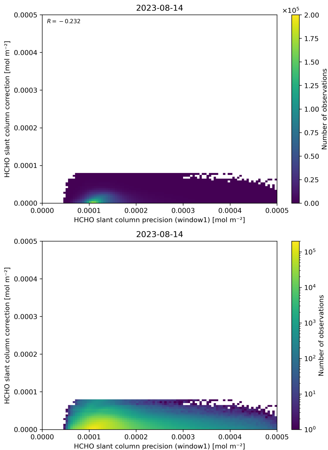
Figure 93: Scatter density plot of “HCHO slant column precision (window1)” against “HCHO slant column correction” for 2023-08-14 to 2023-08-15.
