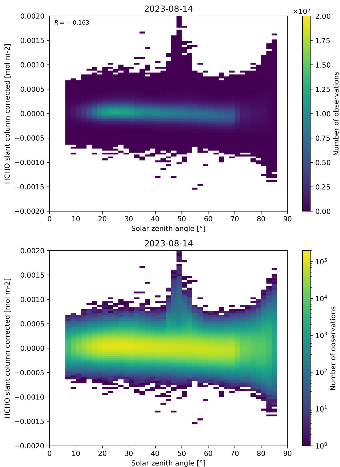
Figure 171: Scatter density plot of “Solar zenith angle” against “HCHO slant column corrected” for 2023-08-14 to 2023-08-15.
