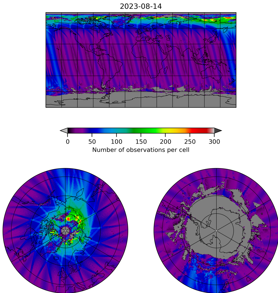
Figure 19: Map of the number of observations for 2023-08-14 to 2023-08-15
