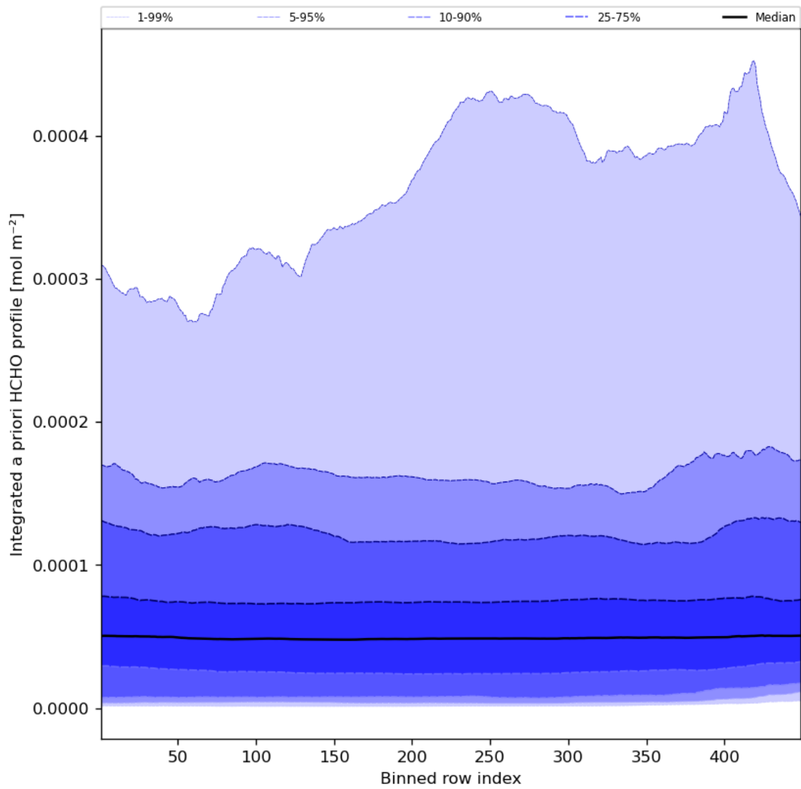
Figure 57: Along track statistics of “Integrated a priori HCHO profile” for 2023-08-14 to 2023-08-15
