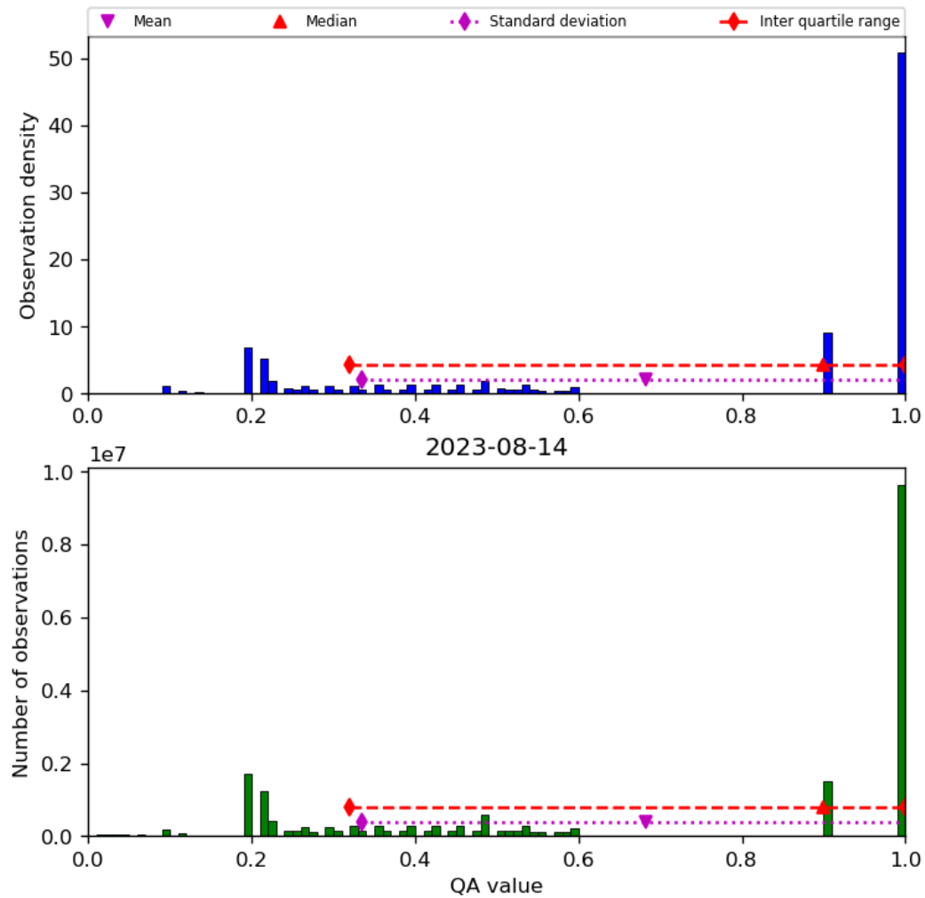
Figure 34: Histogram of “QA value” for 2023-08-14 to 2023-08-15
