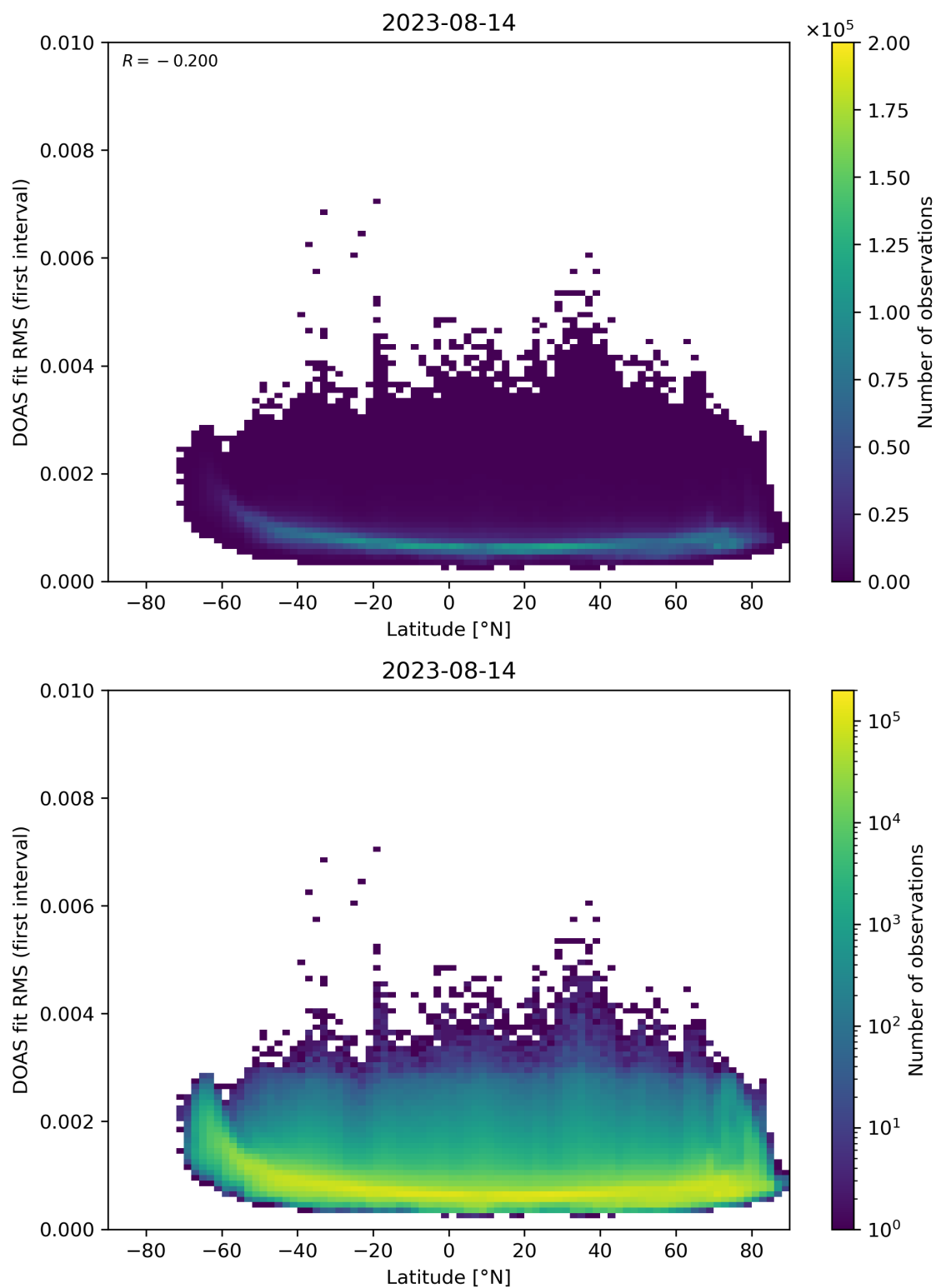
Figure 153: Scatter density plot of “Latitude” against “DOAS fit RMS (first interval)” for 2023-08-14 to 2023-08-15.
