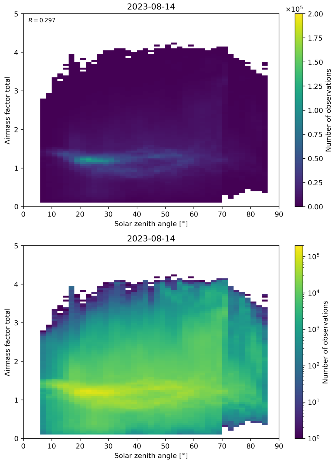
Figure 175: Scatter density plot of “Solar zenith angle” against “Airmass factor total” for 2023-08-14 to 2023-08-15.
