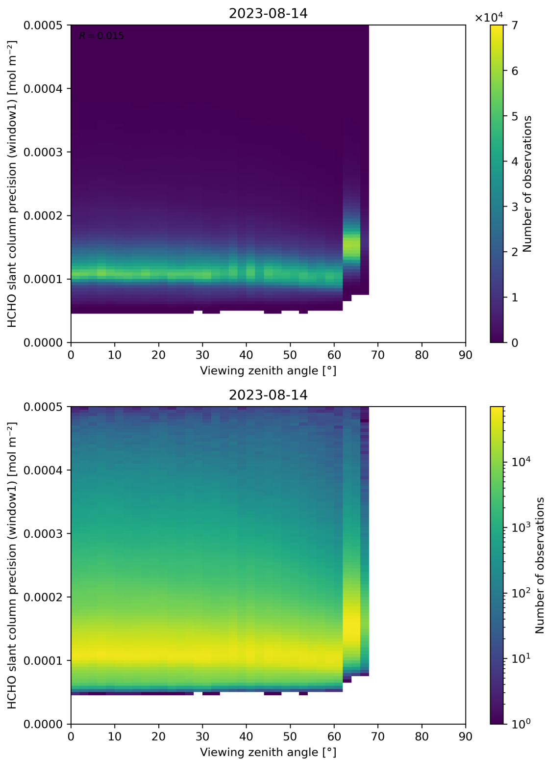
Figure 189: Scatter density plot of “Viewing zenith angle” against “HCHO slant column precision (window1)” for 2023-08-14 to 2023-08-15.
