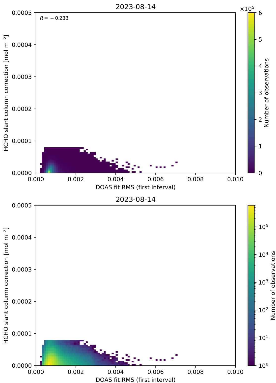
Figure 63: Scatter density plot of “DOAS fit RMS (first interval)” against “HCHO slant column correction” for 2023-08-14 to 2023-08-15.
