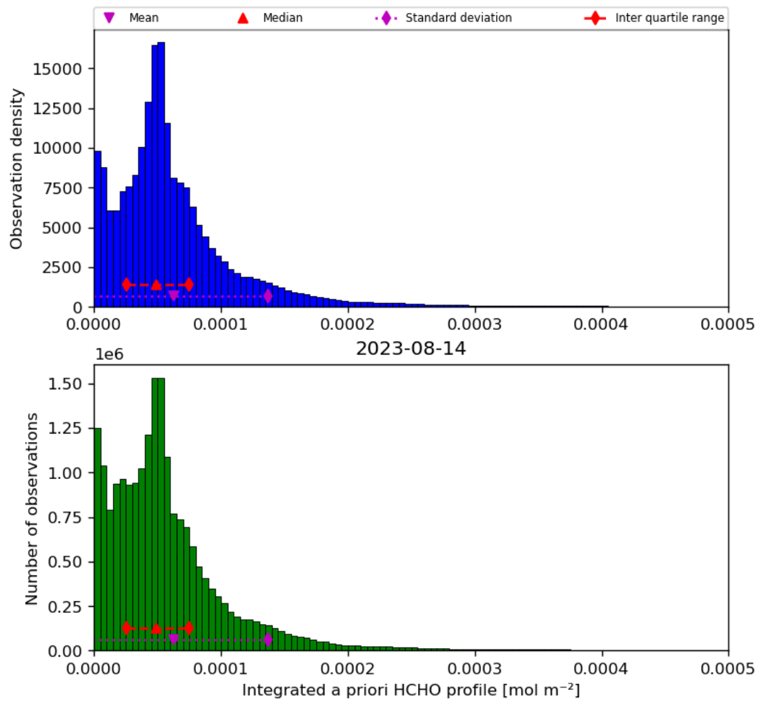
Figure 43: Histogram of “Integrated a priori HCHO profile” for 2023-08-14 to 2023-08-15
