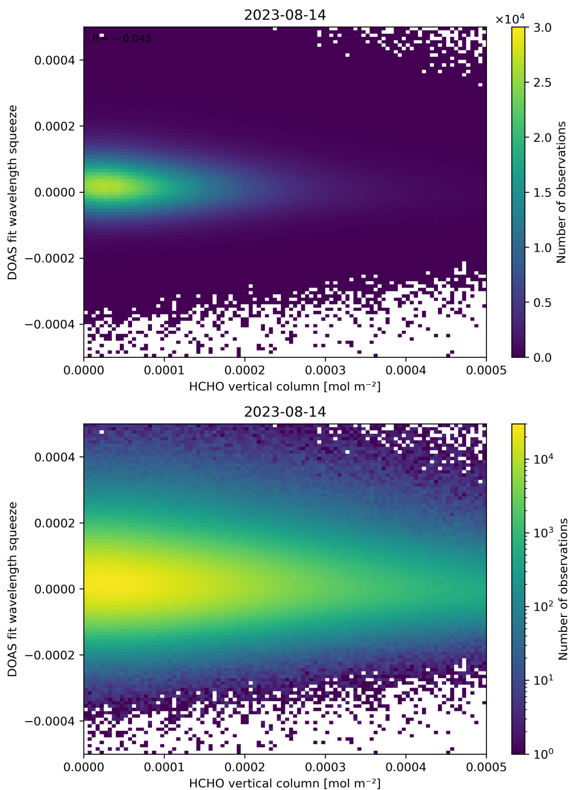
Figure 125: Scatter density plot of “HCHO vertical column” against “DOAS fit wavelength squeeze” for 2023-08-14 to 2023-08-15.
