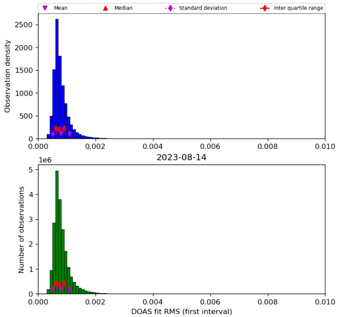
Figure 46: Histogram of “DOAS fit RMS (first interval)” for 2023-08-14 to 2023-08-15
