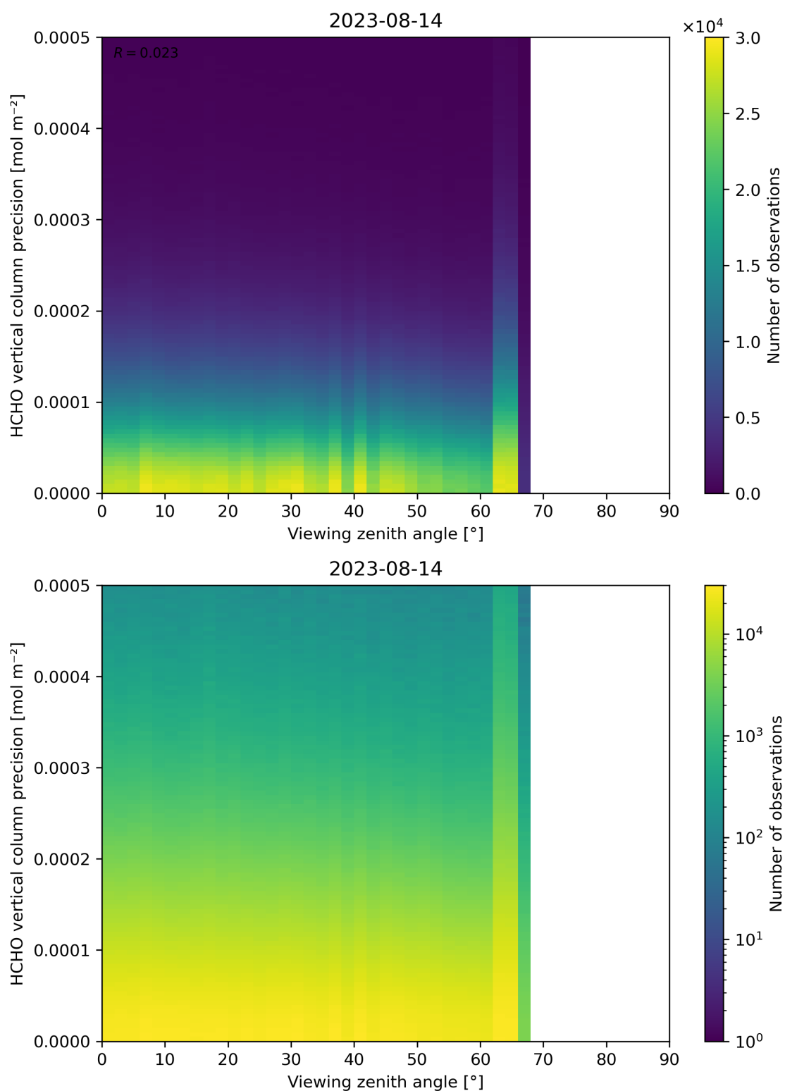
Figure 194: Scatter density plot of “Viewing zenith angle” against “HCHO vertical column precision” for 2023-08-14 to 2023-08-15.
