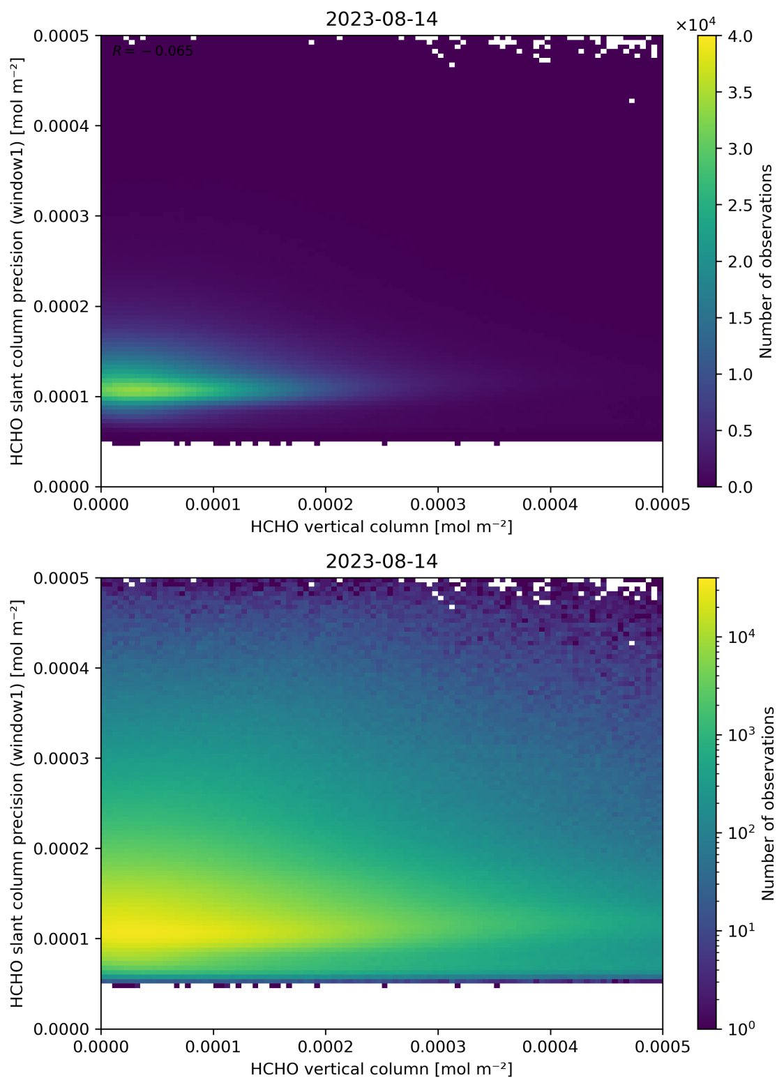
Figure 130: Scatter density plot of “HCHO vertical column” against “HCHO slant column precision (window1)” for 2023-08-14 to 2023-08-15.
