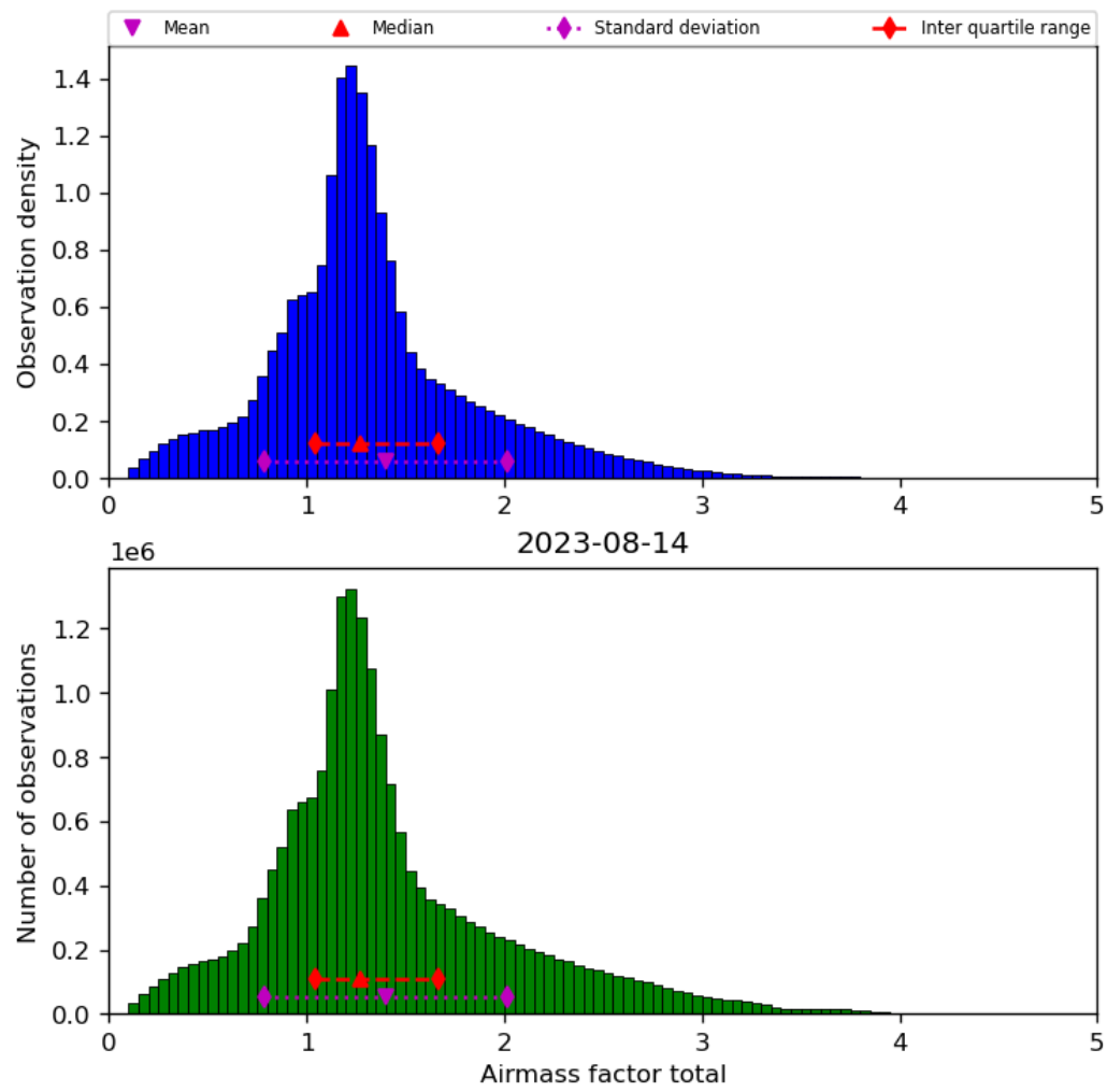
Figure 40: Histogram of “Airmass factor total” for 2023-08-14 to 2023-08-15
