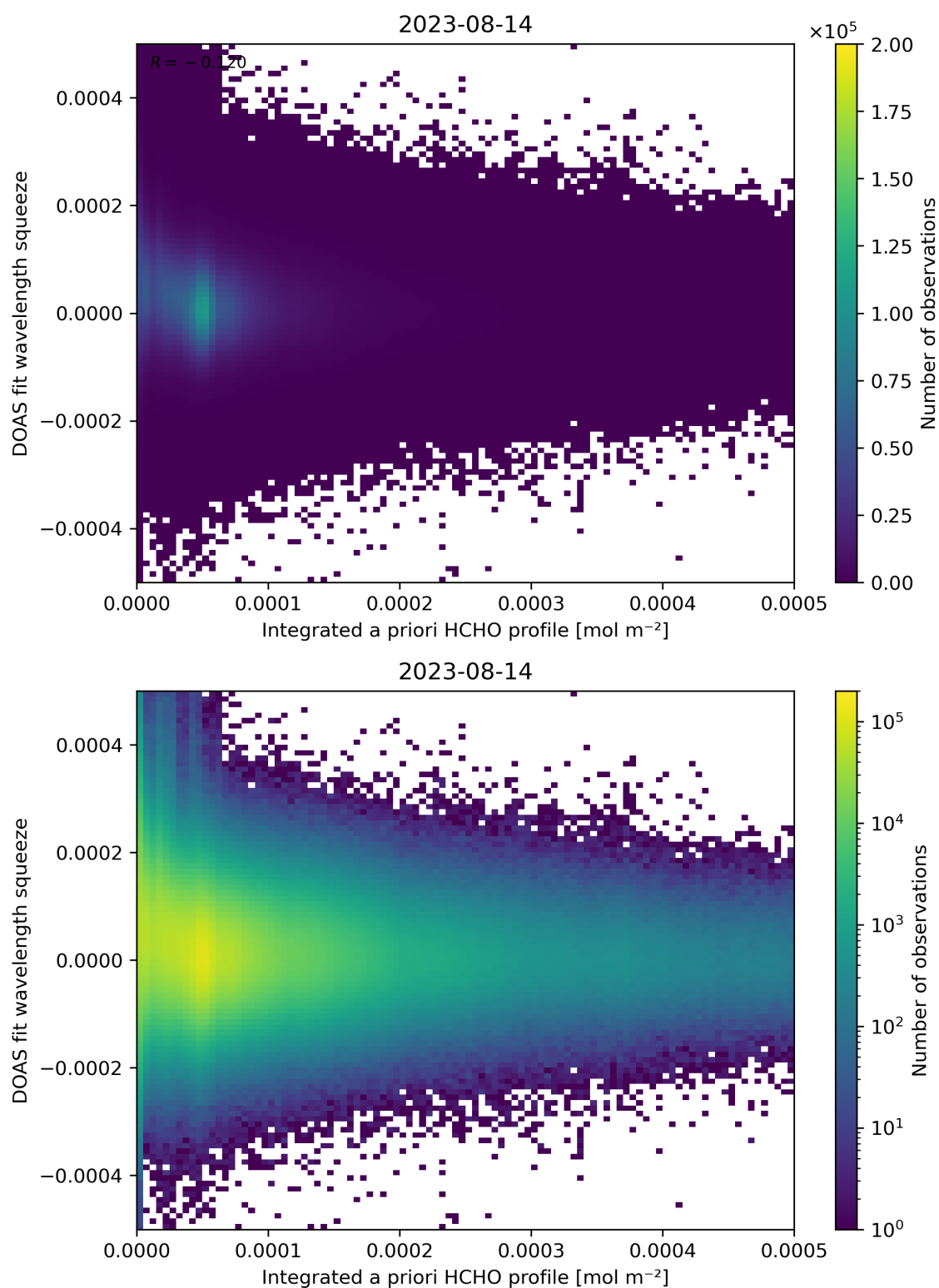
Figure 150: Scatter density plot of “Integrated a priori HCHO profile” against “DOAS fit wavelength squeeze” for 2023-08-14 to 2023-08-15.
