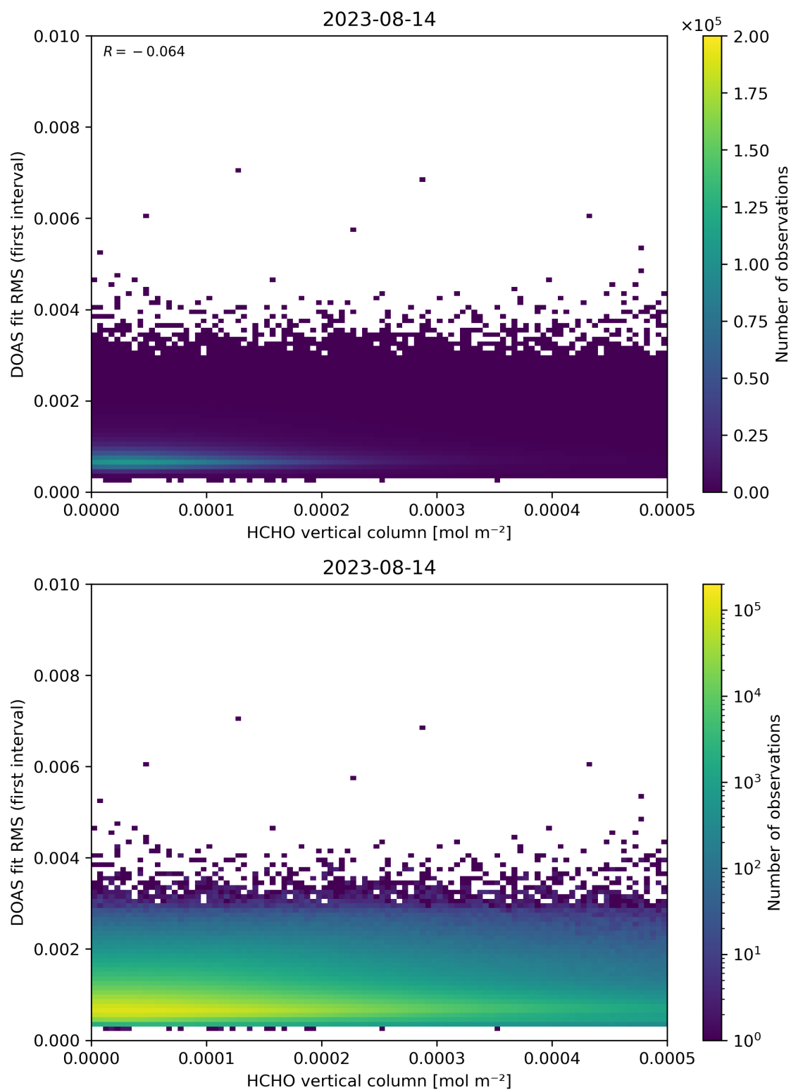
Figure 123: Scatter density plot of “HCHO vertical column” against “DOAS fit RMS (first interval)” for 2023-08-14 to 2023-08-15.
