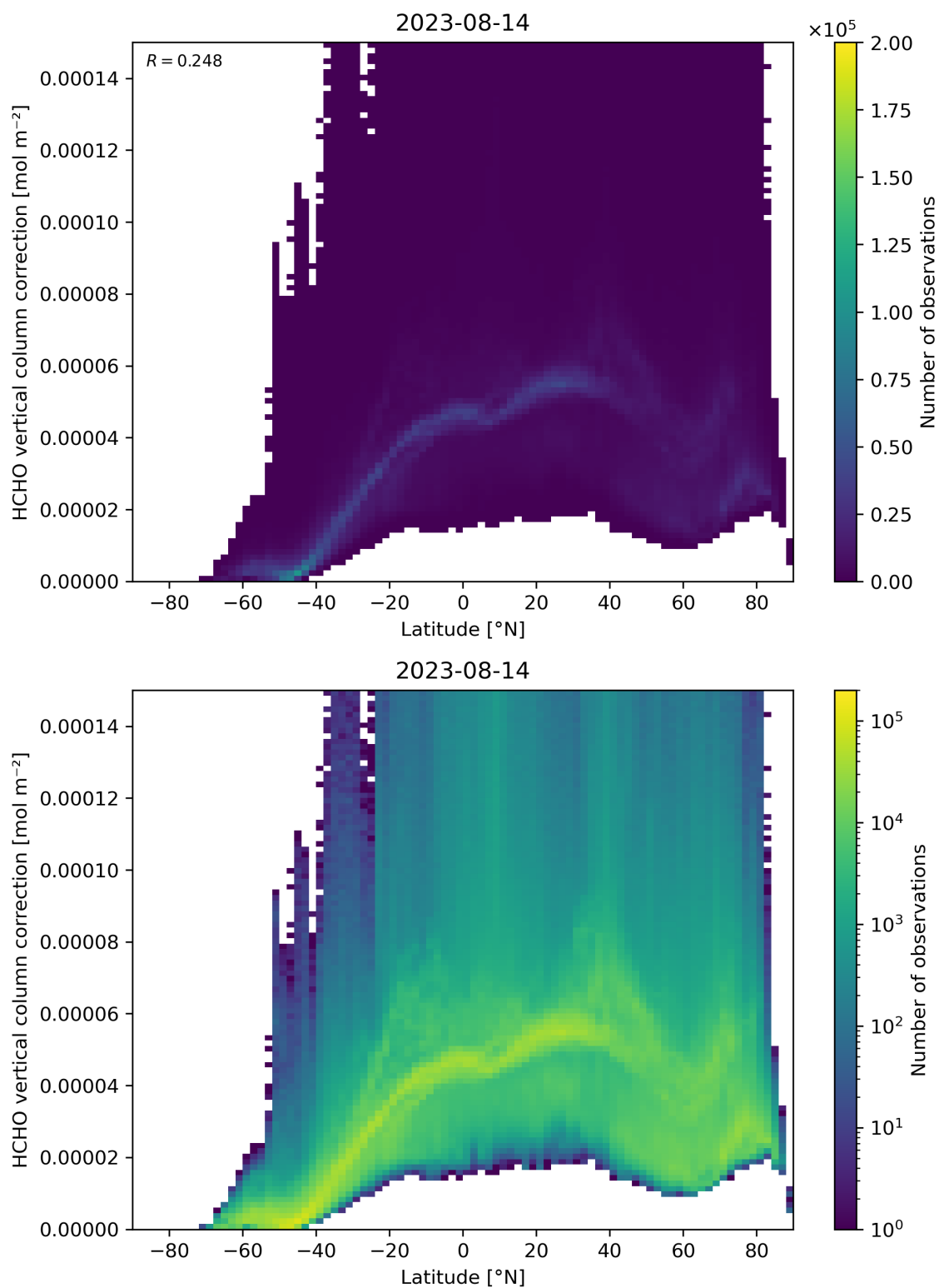
Figure 164: Scatter density plot of “Latitude” against “HCHO vertical column correction” for 2023-08-14 to 2023-08-15.
