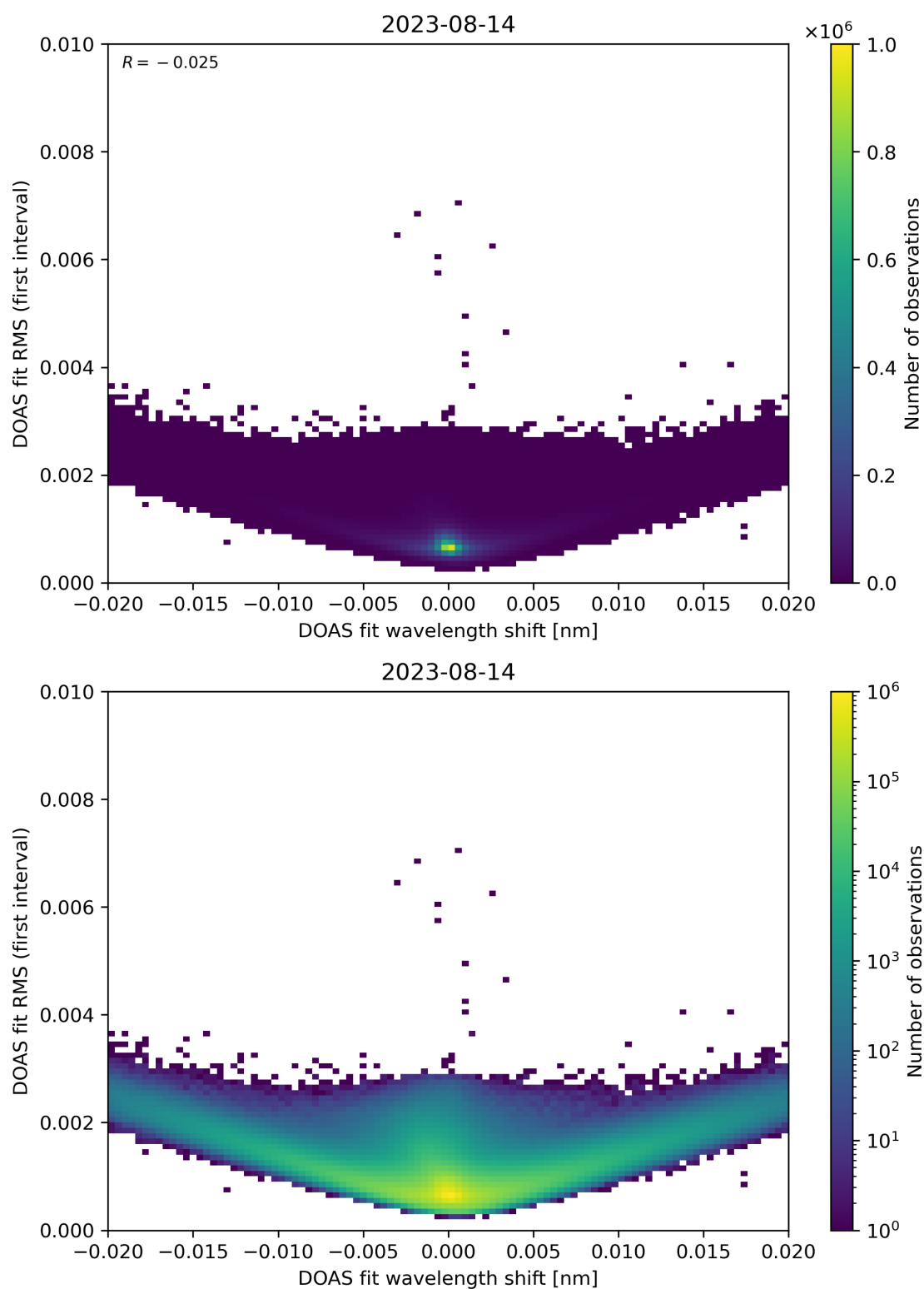
Figure 64: Scatter density plot of “DOAS fit wavelength shift” against “DOAS fit RMS (first interval)” for 2023-08-14 to 2023-08-15.
