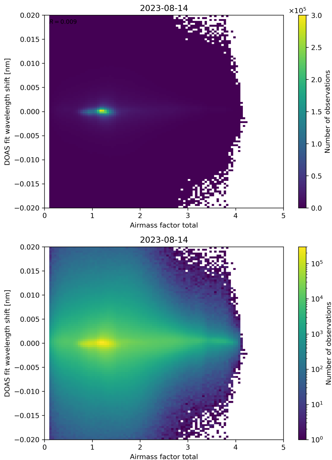
Figure 98: Scatter density plot of “Airmass factor total” against “DOAS fit wavelength shift” for 2023-08-14 to 2023-08-15.
