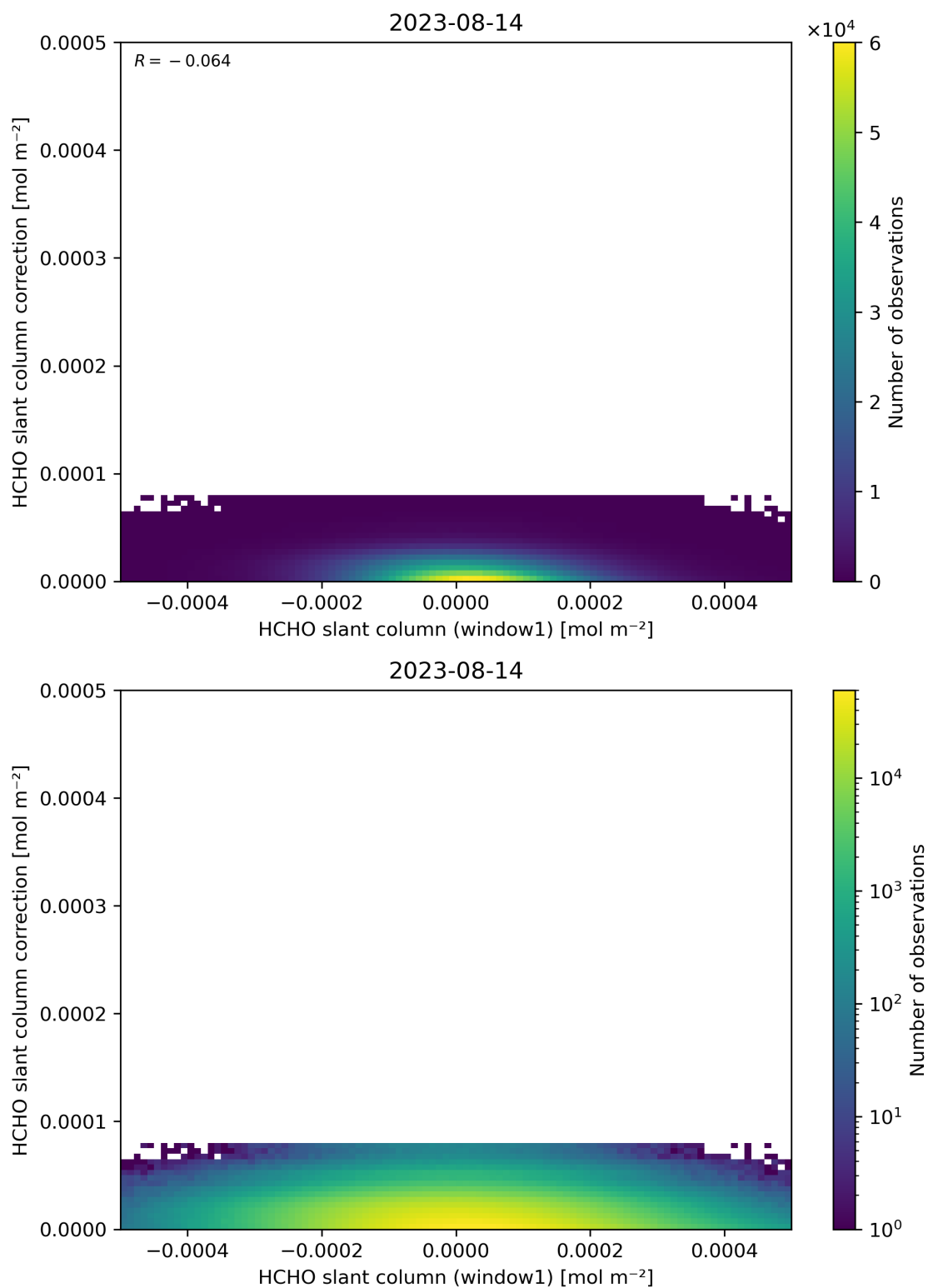
Figure 83: Scatter density plot of “HCHO slant column (window1)” against “HCHO slant column correction” for 2023-08-14 to 2023-08-15.
