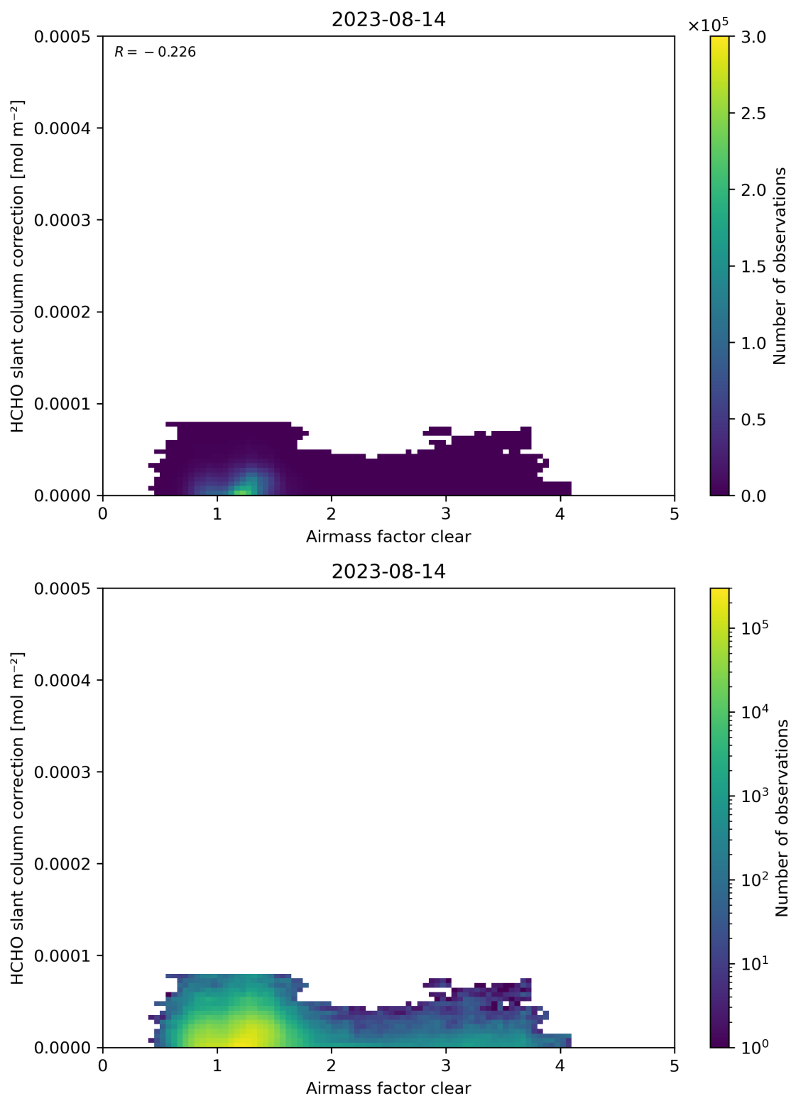
Figure 75: Scatter density plot of “Airmass factor clear” against “HCHO slant column correction” for 2023-08-14 to 2023-08-15.
