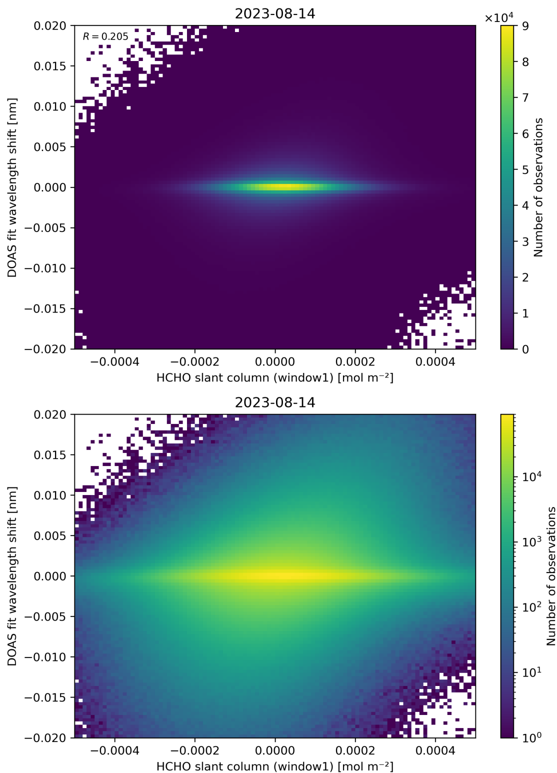
Figure 79: Scatter density plot of “HCHO slant column (window1)” against “DOAS fit wavelength shift” for 2023-08-14 to 2023-08-15.
