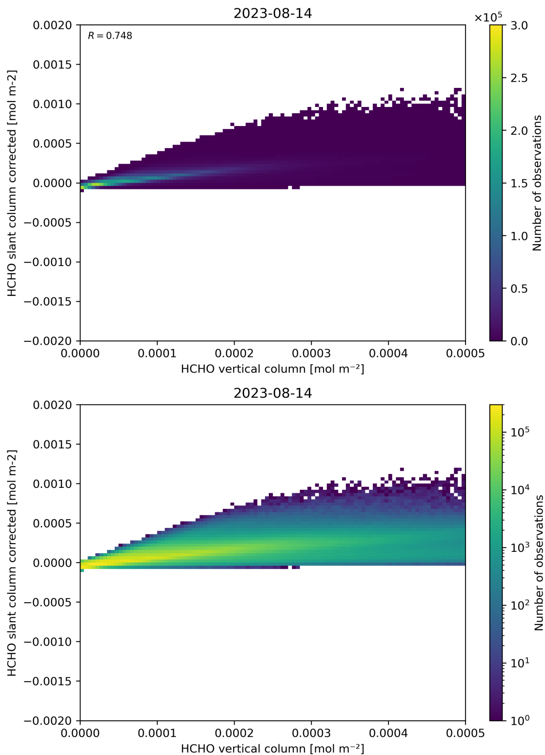
Figure 127: Scatter density plot of “HCHO vertical column” against “HCHO slant column corrected” for 2023-08-14 to 2023-08-15.
