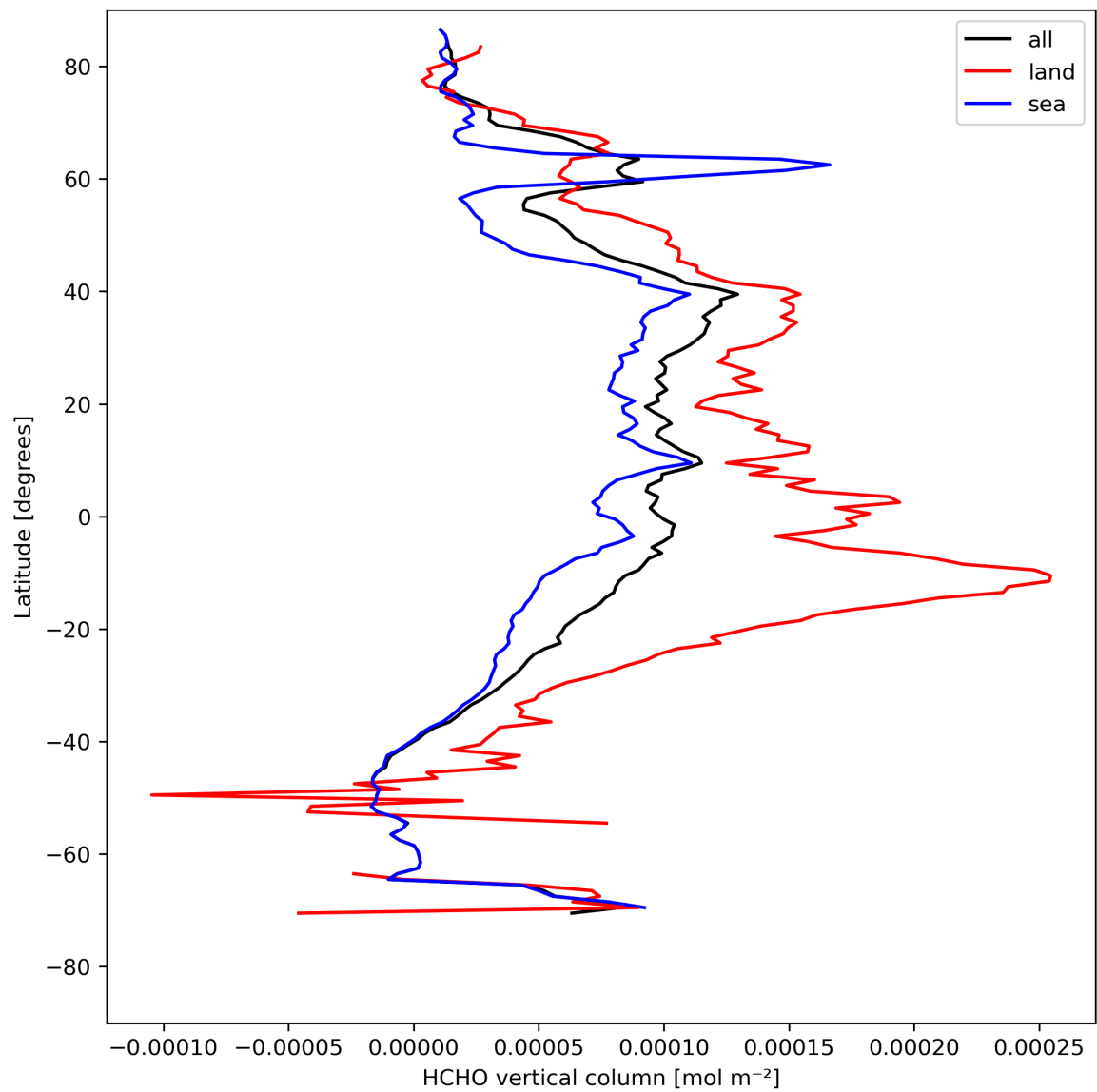
Figure 21: Zonal average of “HCHO vertical column” for 2023-08-14 to 2023-08-15.
