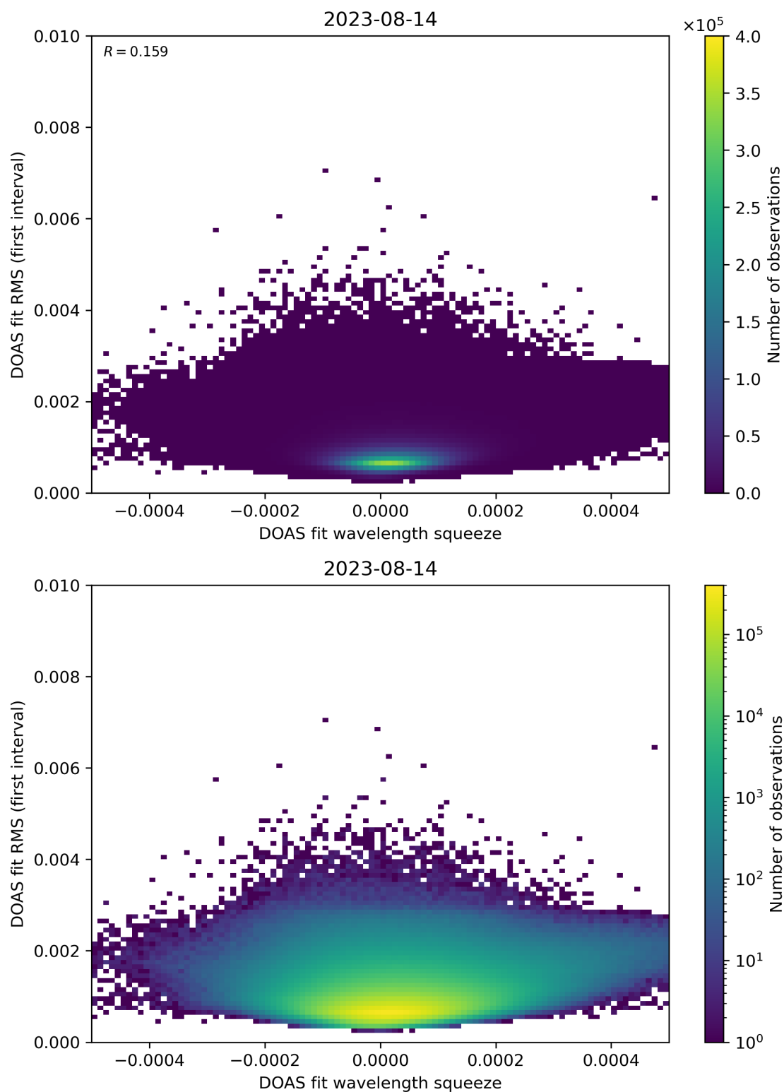
Figure 68: Scatter density plot of “DOAS fit wavelength squeeze” against “DOAS fit RMS (first interval)” for 2023-08-14 to 2023-08-15.
