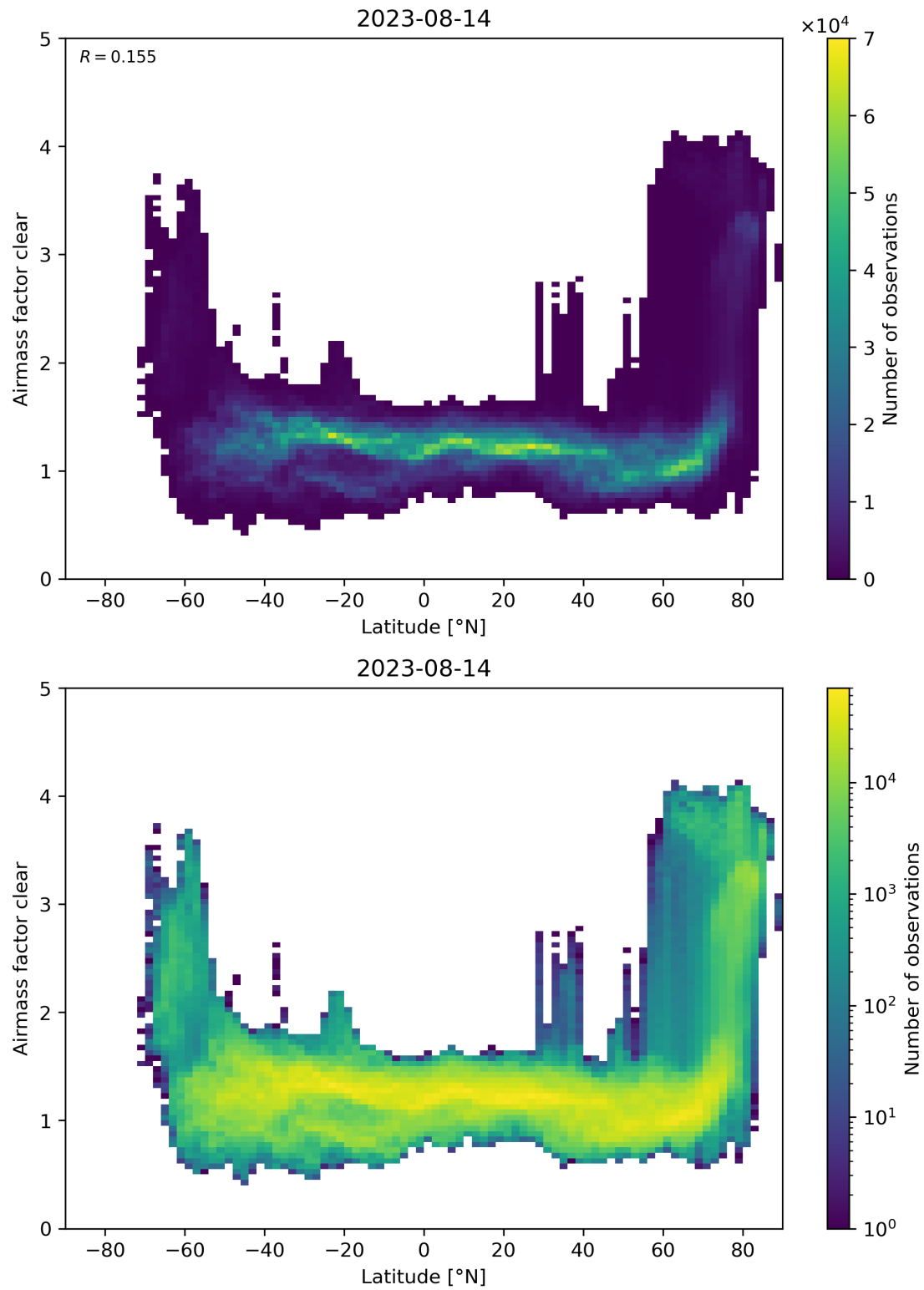
Figure 156: Scatter density plot of “Latitude” against “Airmass factor clear” for 2023-08-14 to 2023-08-15.
