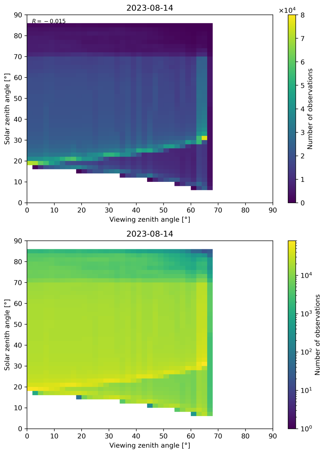
Figure 197: Scatter density plot of “Viewing zenith angle” against “Solar zenith angle” for 2023-08-14 to 2023-08-15.
