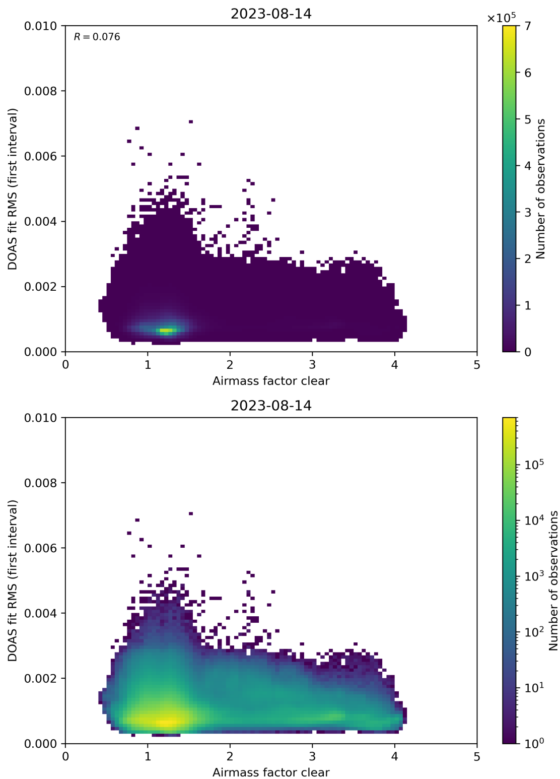
Figure 71: Scatter density plot of “Airmass factor clear” against “DOAS fit RMS (first interval)” for 2023-08-14 to 2023-08-15.
