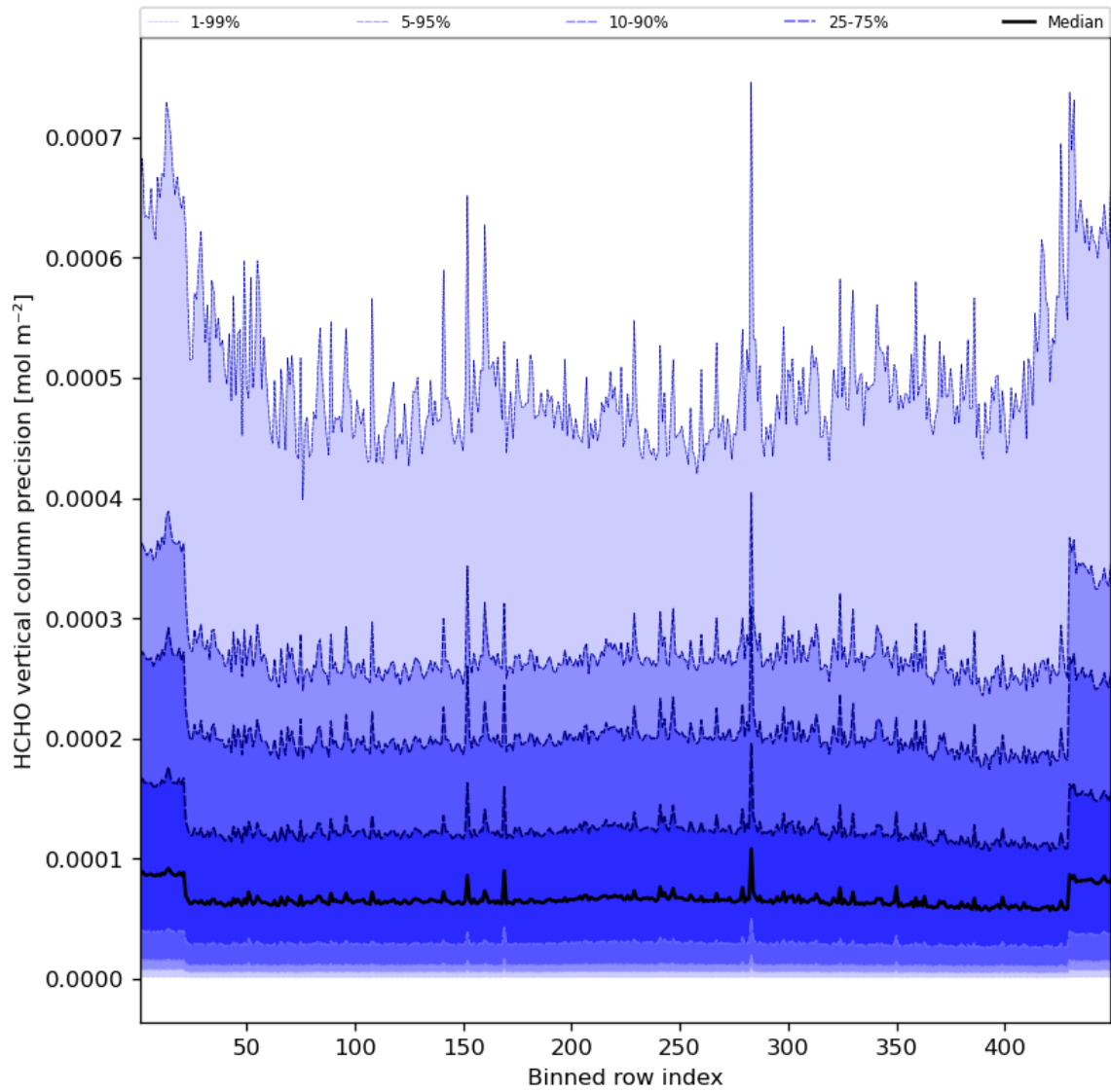
Figure 50: Along track statistics of “HCHO vertical column precision” for 2023-08-14 to 2023-08-15
