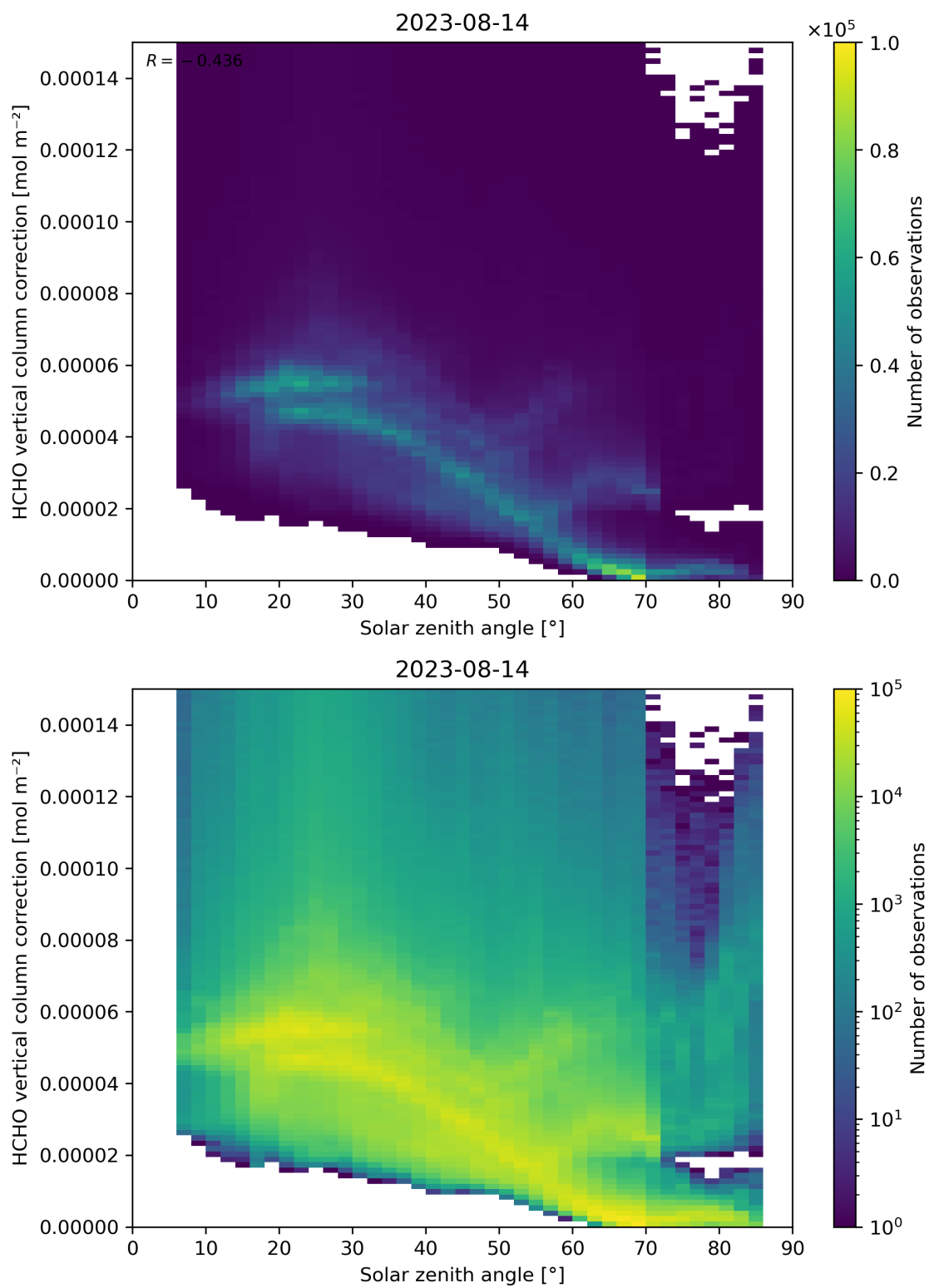
Figure 178: Scatter density plot of “Solar zenith angle” against “HCHO vertical column correction” for 2023-08-14 to 2023-08-15.
