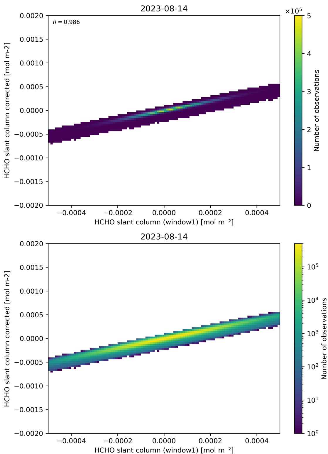
Figure 82: Scatter density plot of “HCHO slant column (window1)” against “HCHO slant column corrected” for 2023-08-14 to 2023-08-15.
