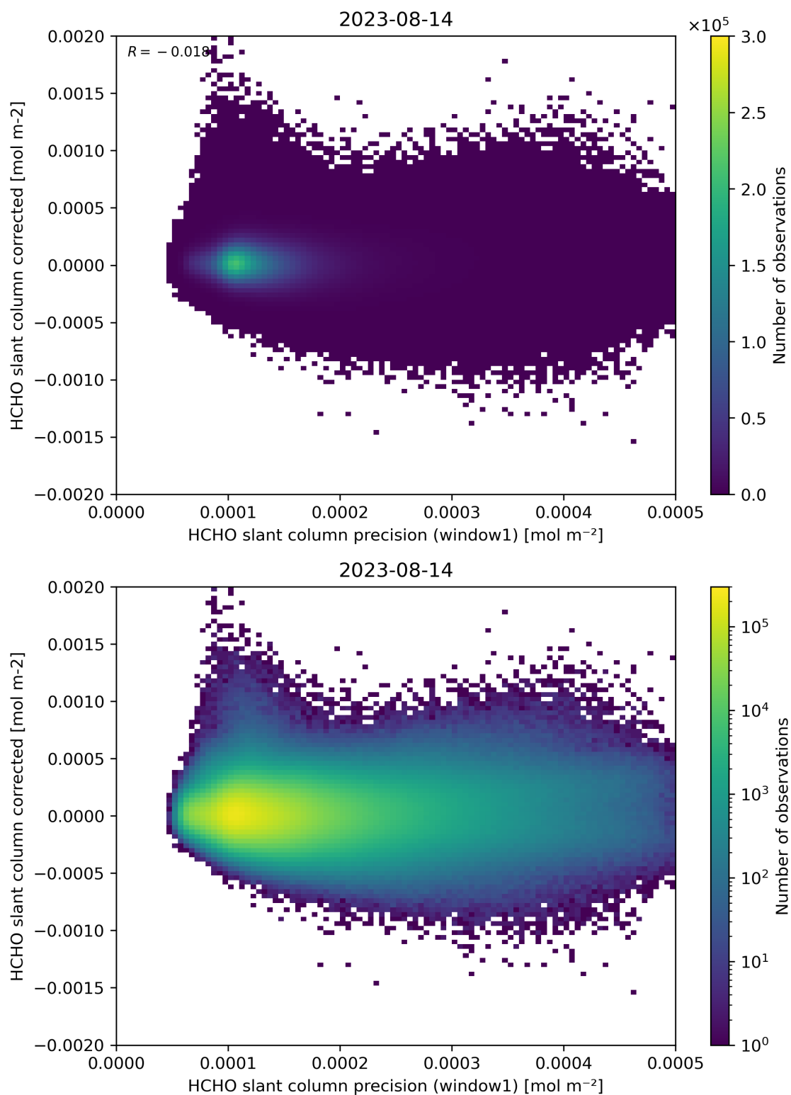
Figure 92: Scatter density plot of “HCHO slant column precision (window1)” against “HCHO slant column corrected” for 2023-08-14 to 2023-08-15.
