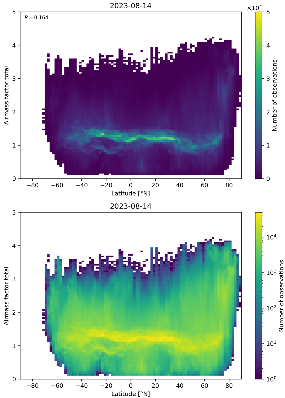
Figure 161: Scatter density plot of “Latitude” against “Airmass factor total” for 2023-08-14 to 2023-08-15.
