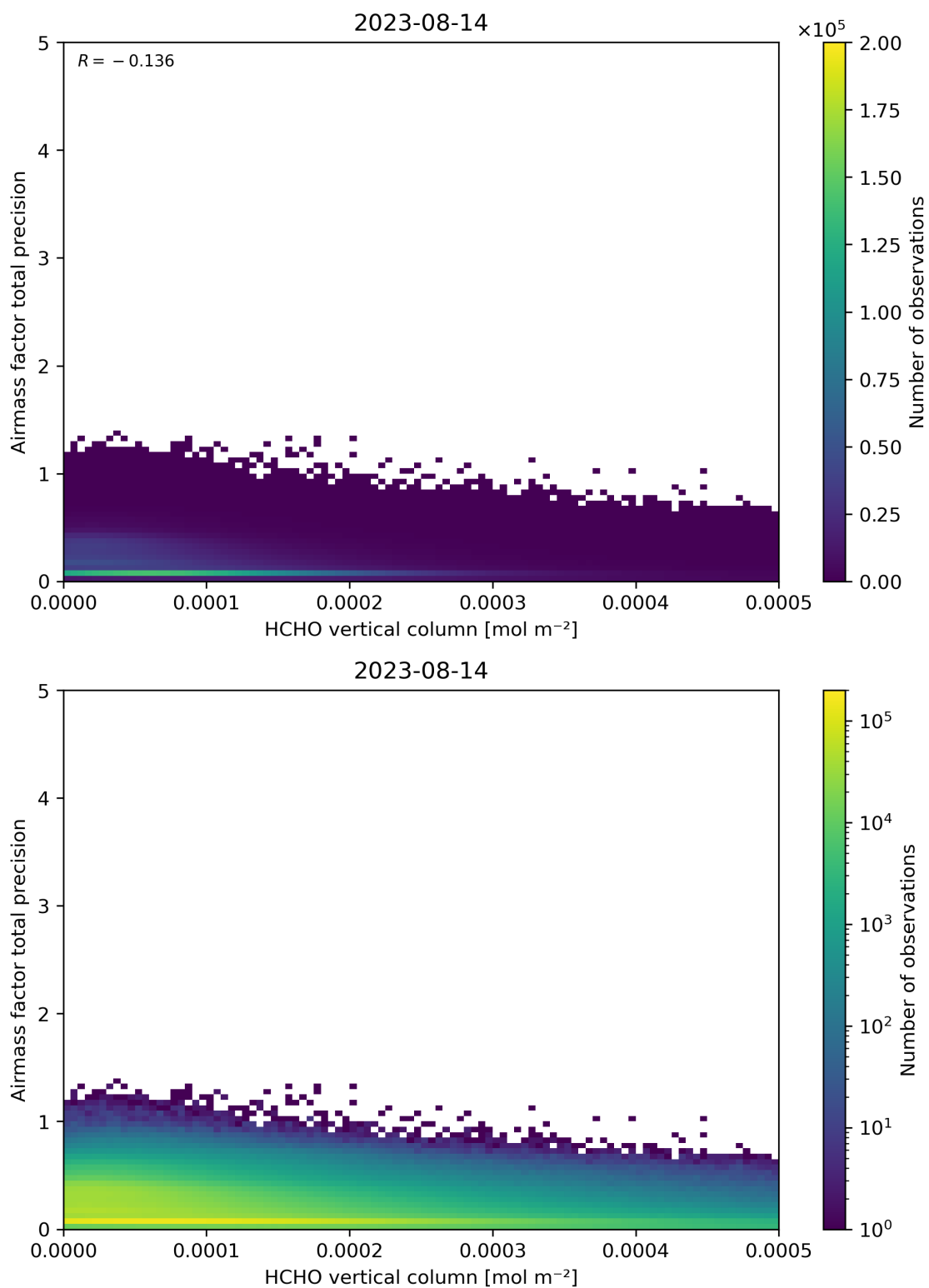
Figure 132: Scatter density plot of “HCHO vertical column” against “Airmass factor total precision” for 2023-08-14 to 2023-08-15.
