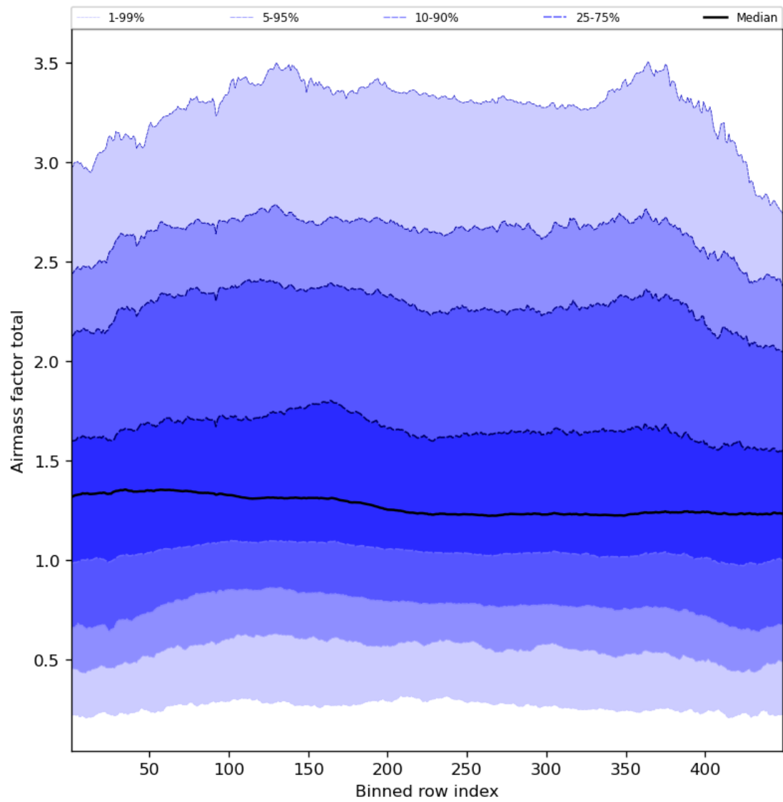
Figure 54: Along track statistics of “Airmass factor total” for 2023-08-14 to 2023-08-15
