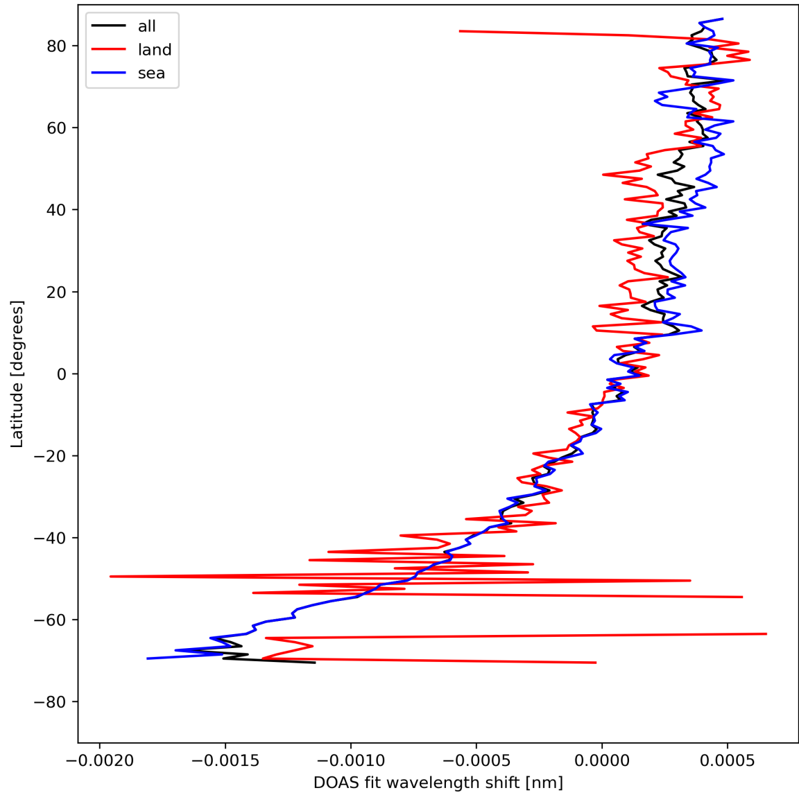
Figure 30: Zonal average of “DOAS fit wavelength shift” for 2023-08-14 to 2023-08-15.
