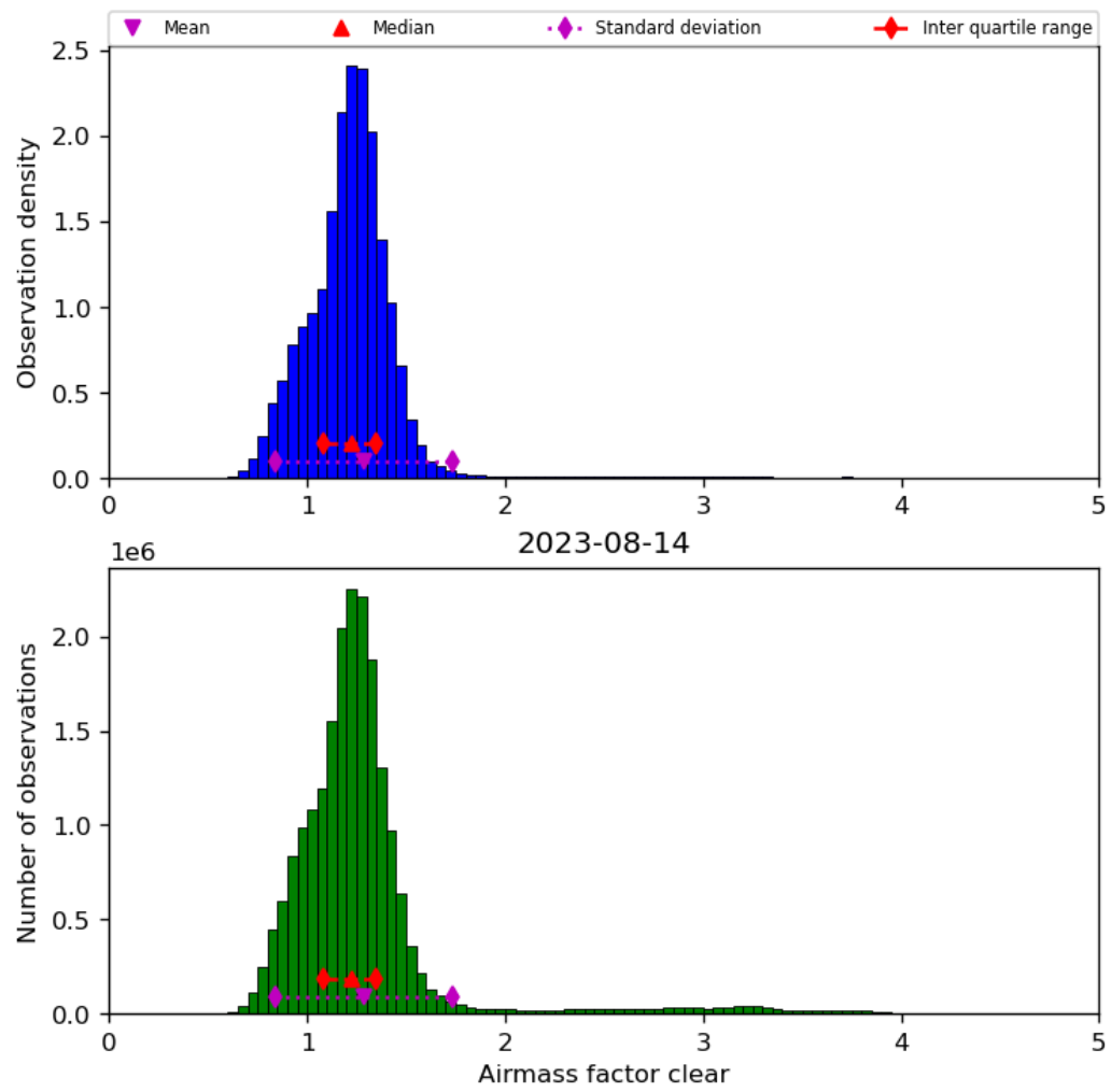
Figure 42: Histogram of “Airmass factor clear” for 2023-08-14 to 2023-08-15
