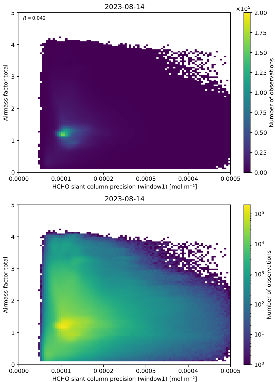
Figure 94: Scatter density plot of “HCHO slant column precision (window1)” against “Airmass factor total” for 2023-08-14 to 2023-08-15.
