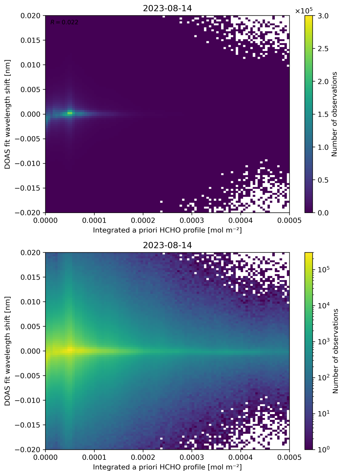
Figure 149: Scatter density plot of “Integrated a priori HCHO profile” against “DOAS fit wavelength shift” for 2023-08-14 to 2023-08-15.
