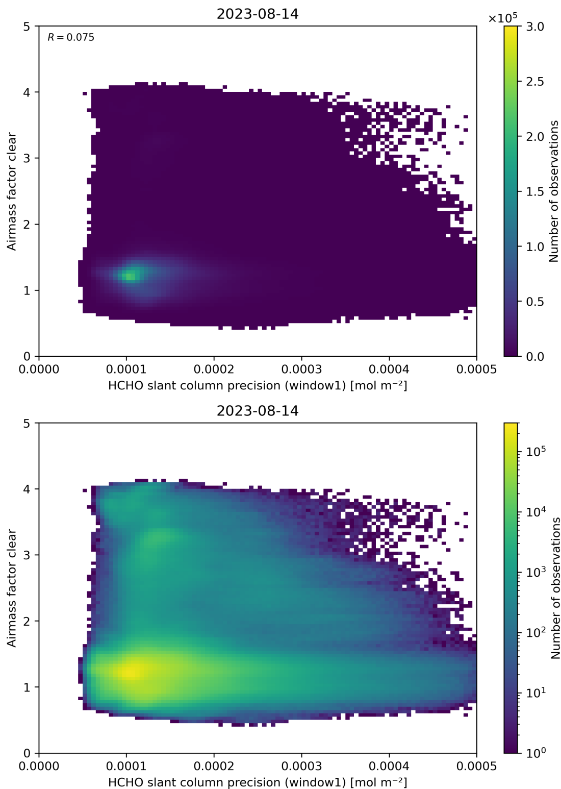
Figure 91: Scatter density plot of “HCHO slant column precision (window1)” against “Airmass factor clear” for 2023-08-14 to 2023-08-15.
