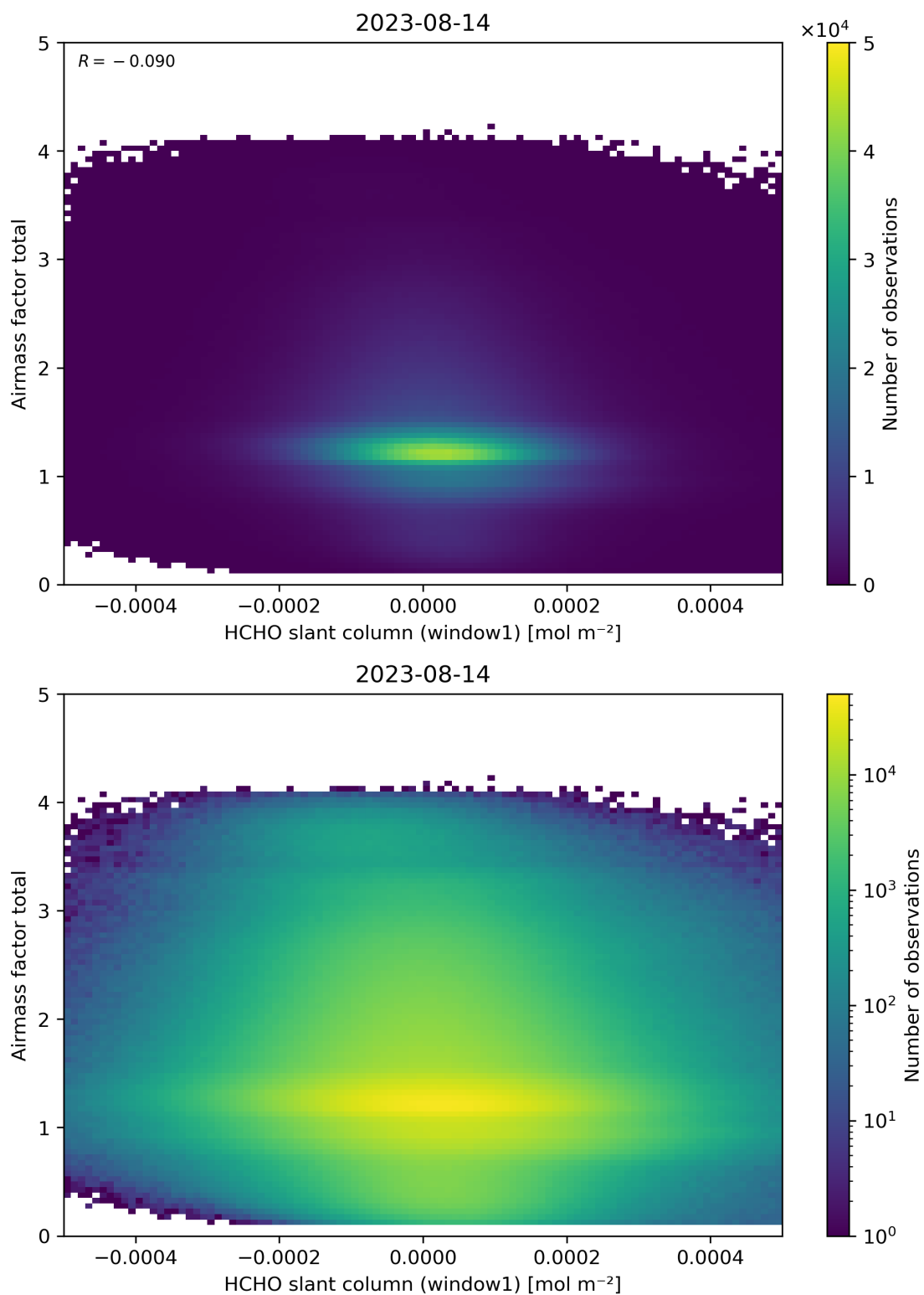
Figure 85: Scatter density plot of “HCHO slant column (window1)” against “Airmass factor total” for 2023-08-14 to 2023-08-15.
