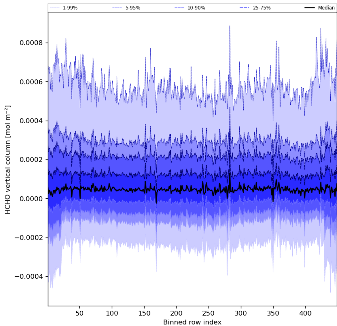
Figure 49: Along track statistics of “HCHO vertical column” for 2023-08-14 to 2023-08-15
