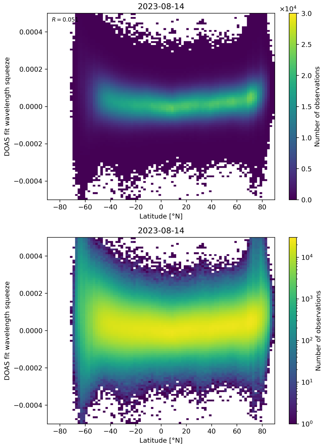
Figure 155: Scatter density plot of “Latitude” against “DOAS fit wavelength squeeze” for 2023-08-14 to 2023-08-15.
