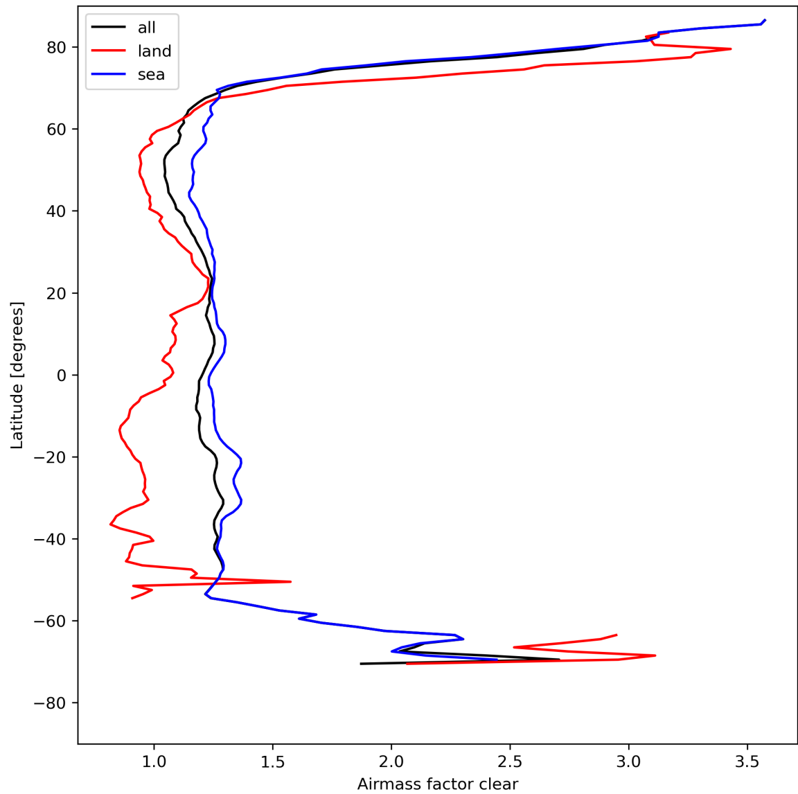
Figure 28: Zonal average of “Airmass factor clear” for 2023-08-14 to 2023-08-15.
