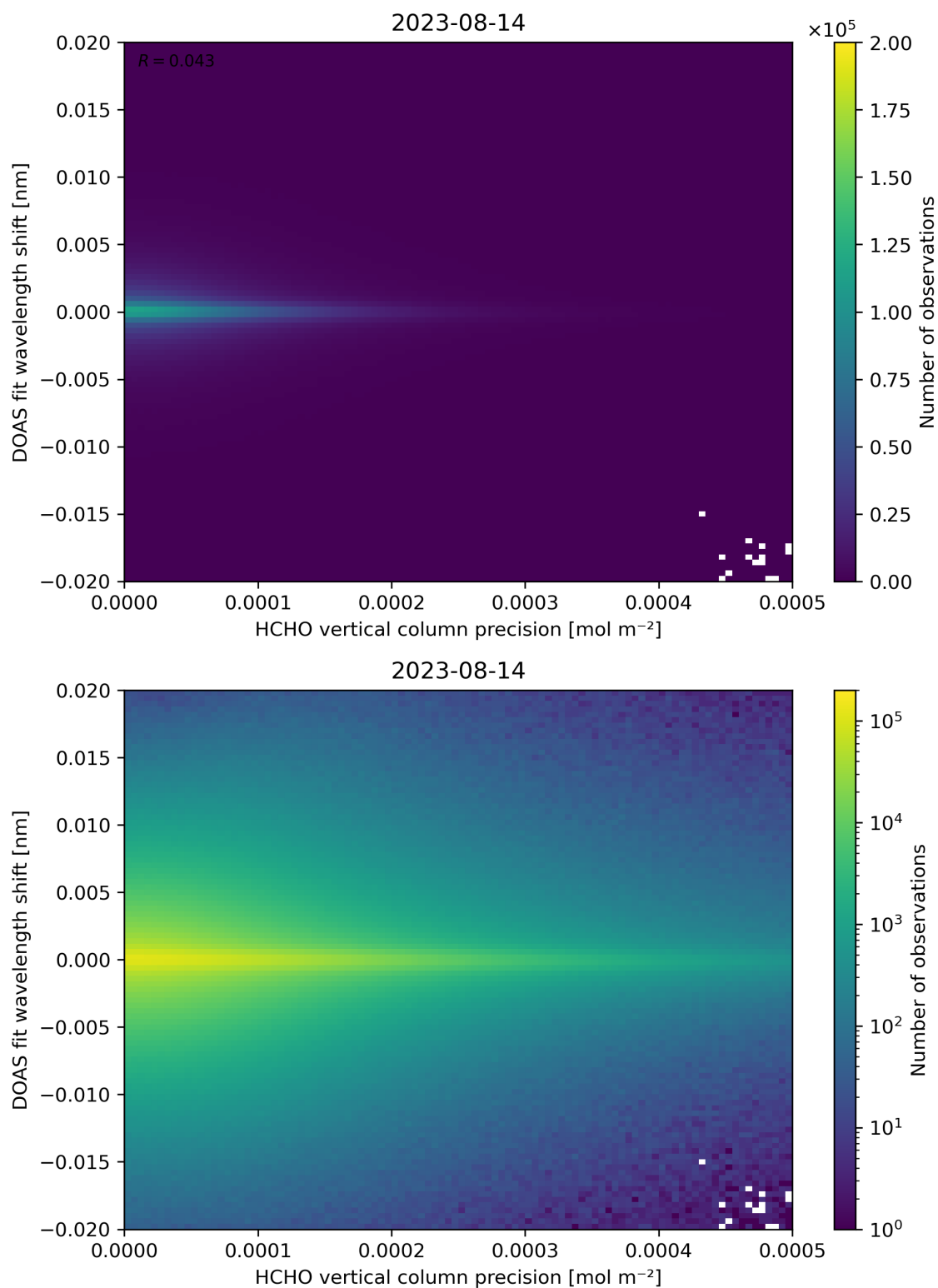
Figure 137: Scatter density plot of “HCHO vertical column precision” against “DOAS fit wavelength shift” for 2023-08-14 to 2023-08-15.
