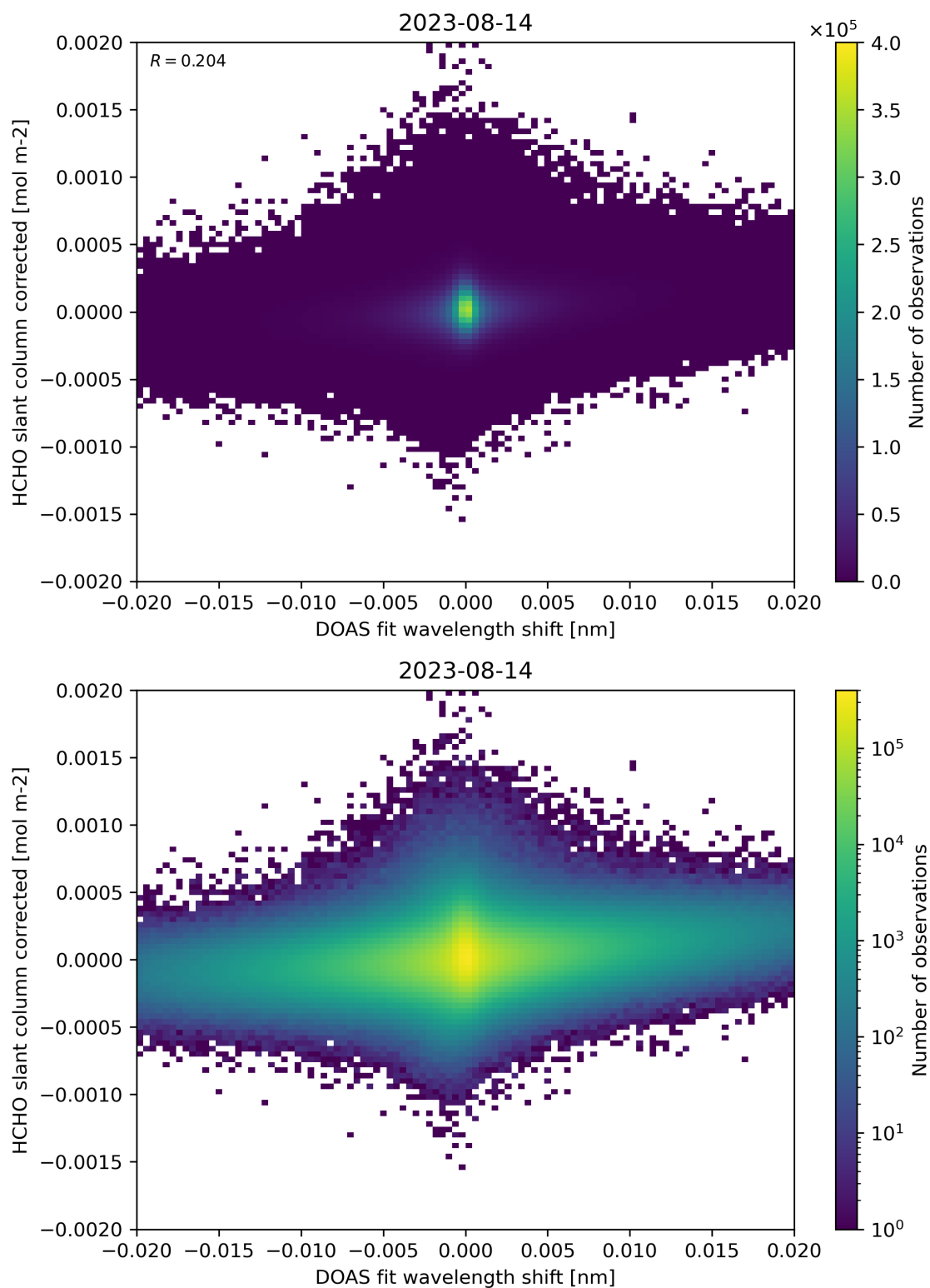
Figure 66: Scatter density plot of “DOAS fit wavelength shift” against “HCHO slant column corrected” for 2023-08-14 to 2023-08-15.
