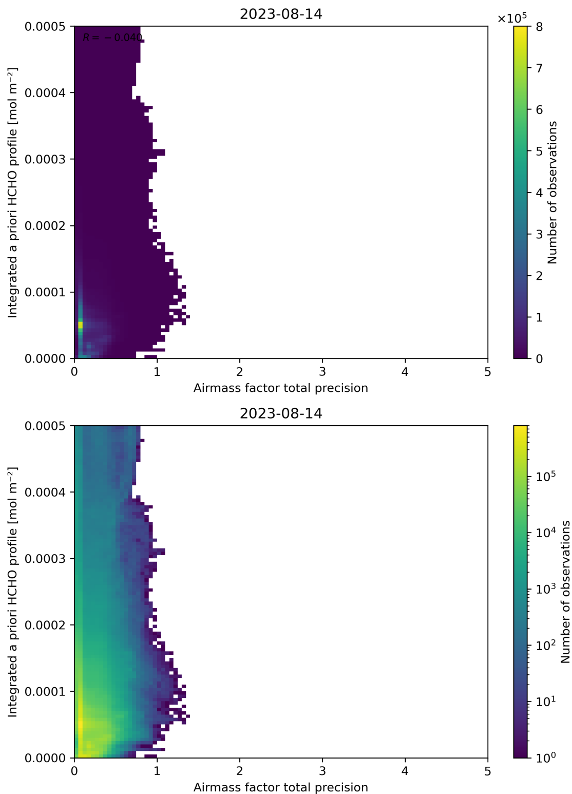
Figure 111: Scatter density plot of “Airmass factor total precision” against “Integrated a priori HCHO profile” for 2023-08-14 to 2023-08-15.
