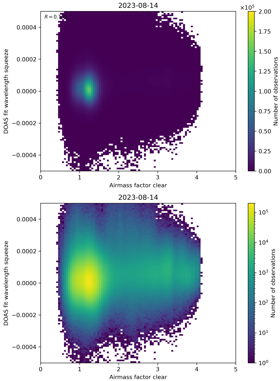
Figure 73: Scatter density plot of “Airmass factor clear” against “DOAS fit wavelength squeeze” for 2023-08-14 to 2023-08-15.
