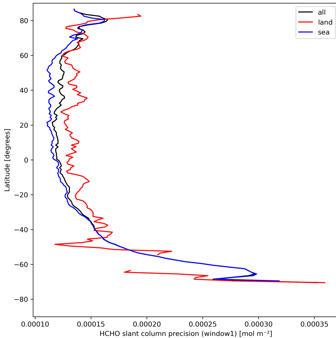
Figure 25: Zonal average of “HCHO slant column precision (window1)” for 2023-08-14 to 2023-08-15.
