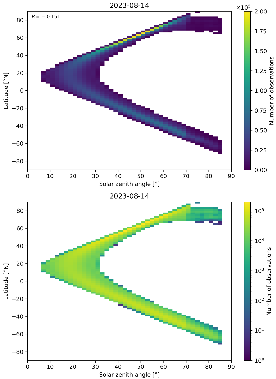
Figure 181: Scatter density plot of “Solar zenith angle” against “Latitude” for 2023-08-14 to 2023-08-15.
