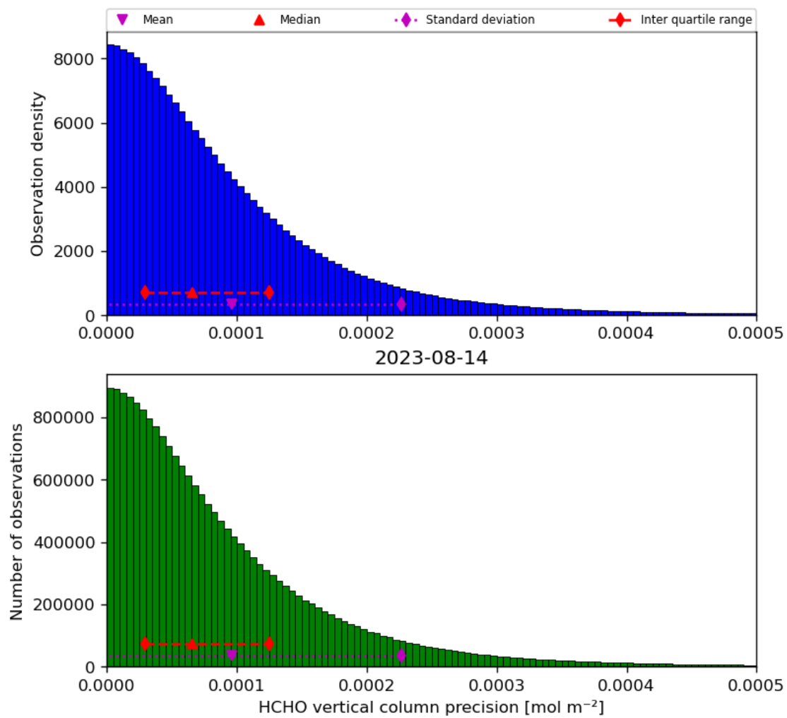
Figure 36: Histogram of “HCHO vertical column precision” for 2023-08-14 to 2023-08-15
