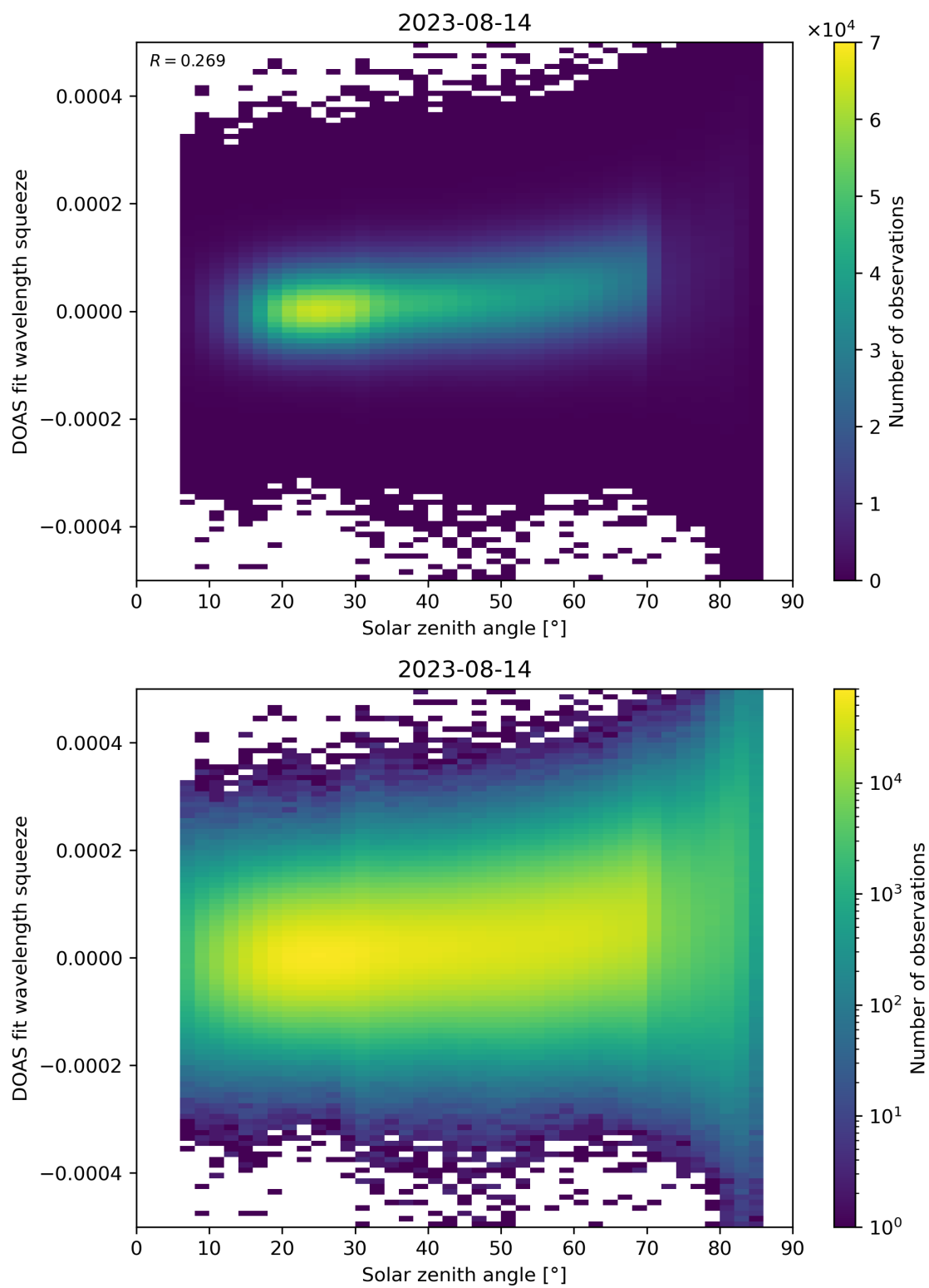
Figure 169: Scatter density plot of “Solar zenith angle” against “DOAS fit wavelength squeeze” for 2023-08-14 to 2023-08-15.
