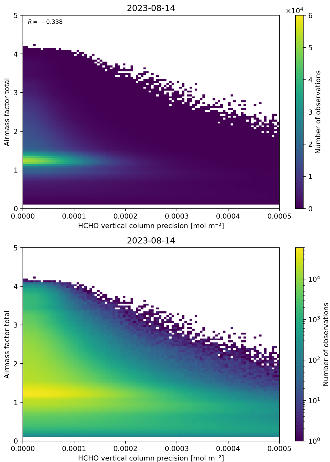
Figure 144: Scatter density plot of “HCHO vertical column precision” against “Airmass factor total” for 2023-08-14 to 2023-08-15.
