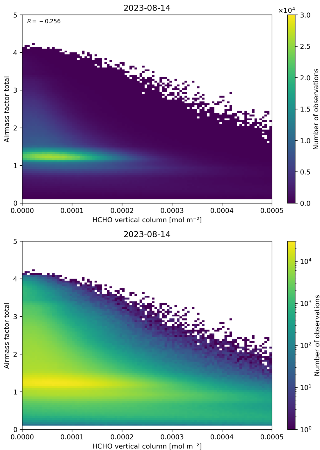
Figure 131: Scatter density plot of “HCHO vertical column” against “Airmass factor total” for 2023-08-14 to 2023-08-15.
