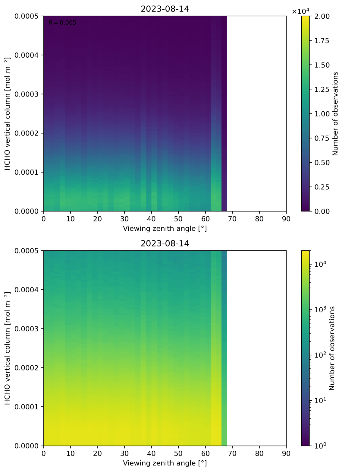
Figure 192: Scatter density plot of “Viewing zenith angle” against “HCHO vertical column” for 2023-08-14 to 2023-08-15.
