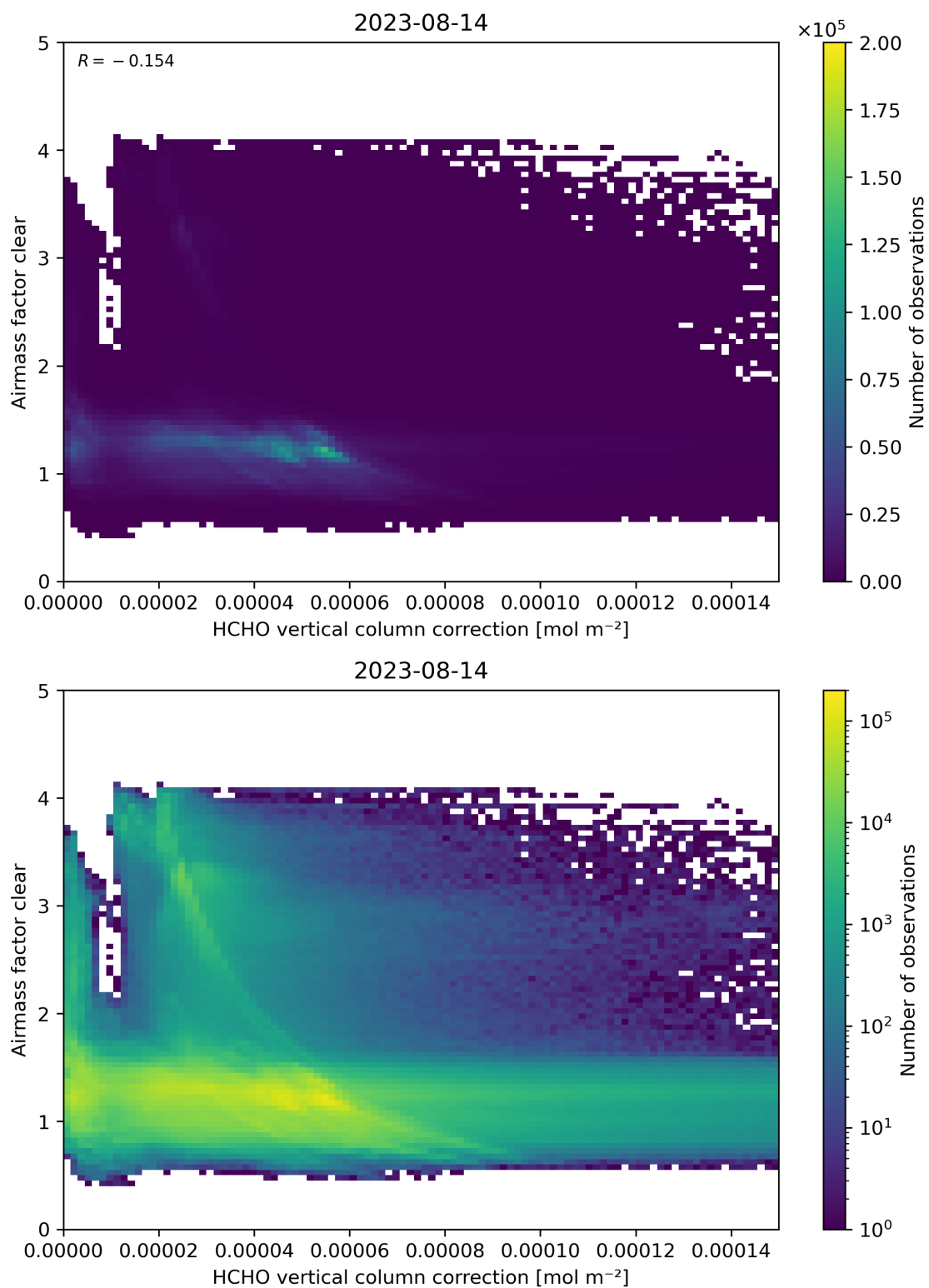
Figure 115: Scatter density plot of “HCHO vertical column correction” against “Airmass factor clear” for 2023-08-14 to 2023-08-15.
