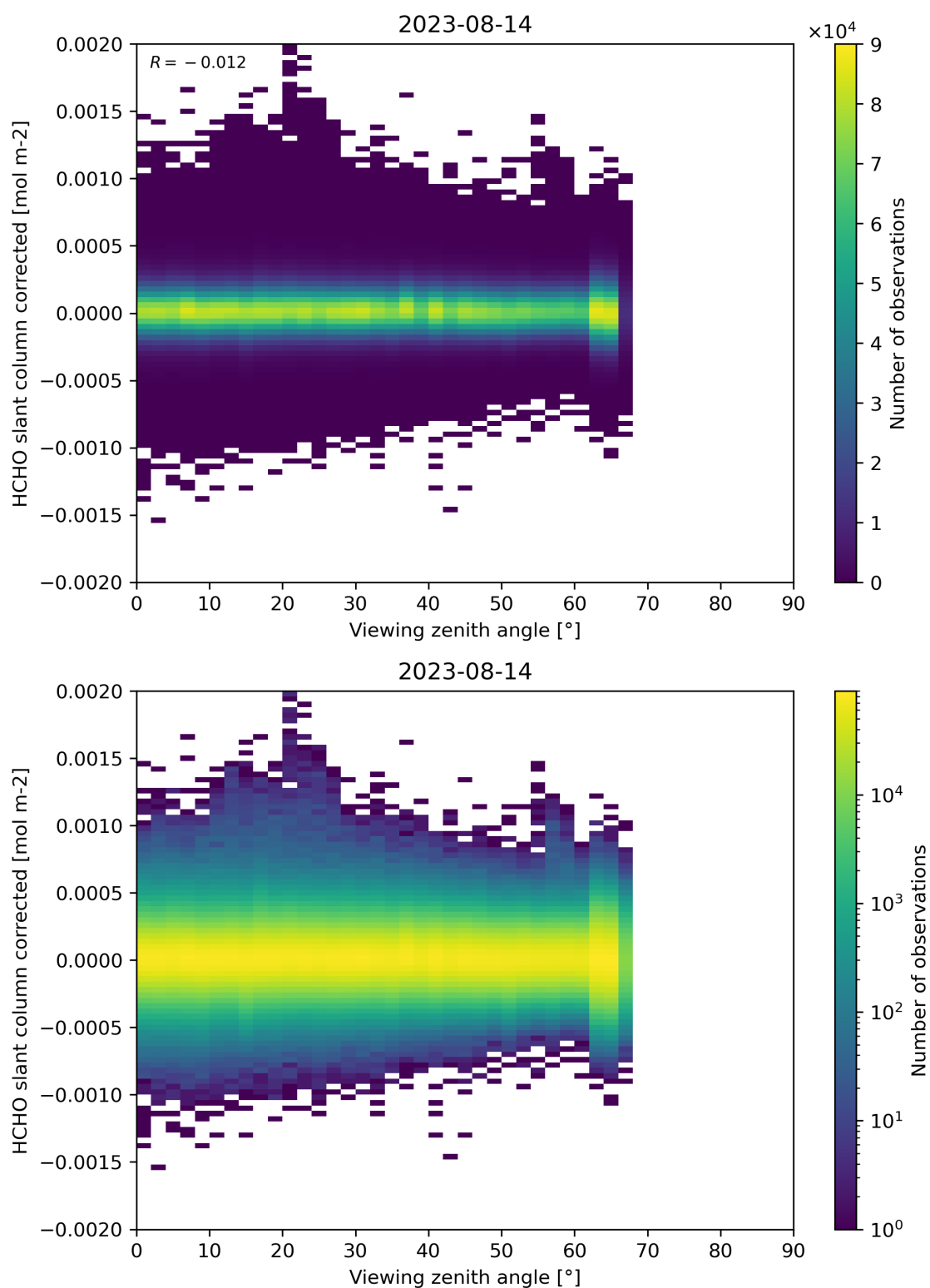
Figure 186: Scatter density plot of “Viewing zenith angle” against “HCHO slant column corrected” for 2023-08-14 to 2023-08-15.
