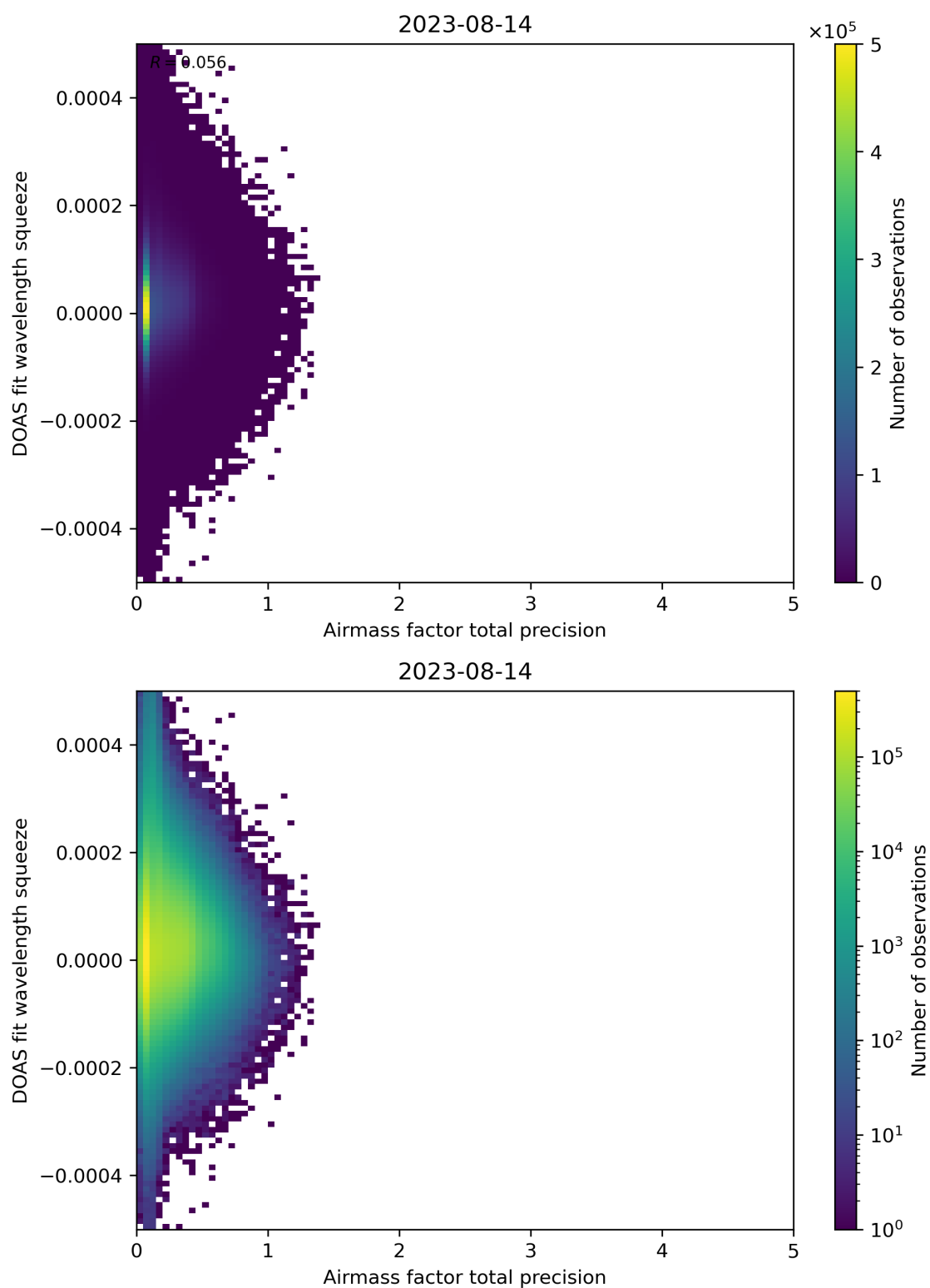
Figure 107: Scatter density plot of “Airmass factor total precision” against “DOAS fit wavelength squeeze” for 2023-08-14 to 2023-08-15.
