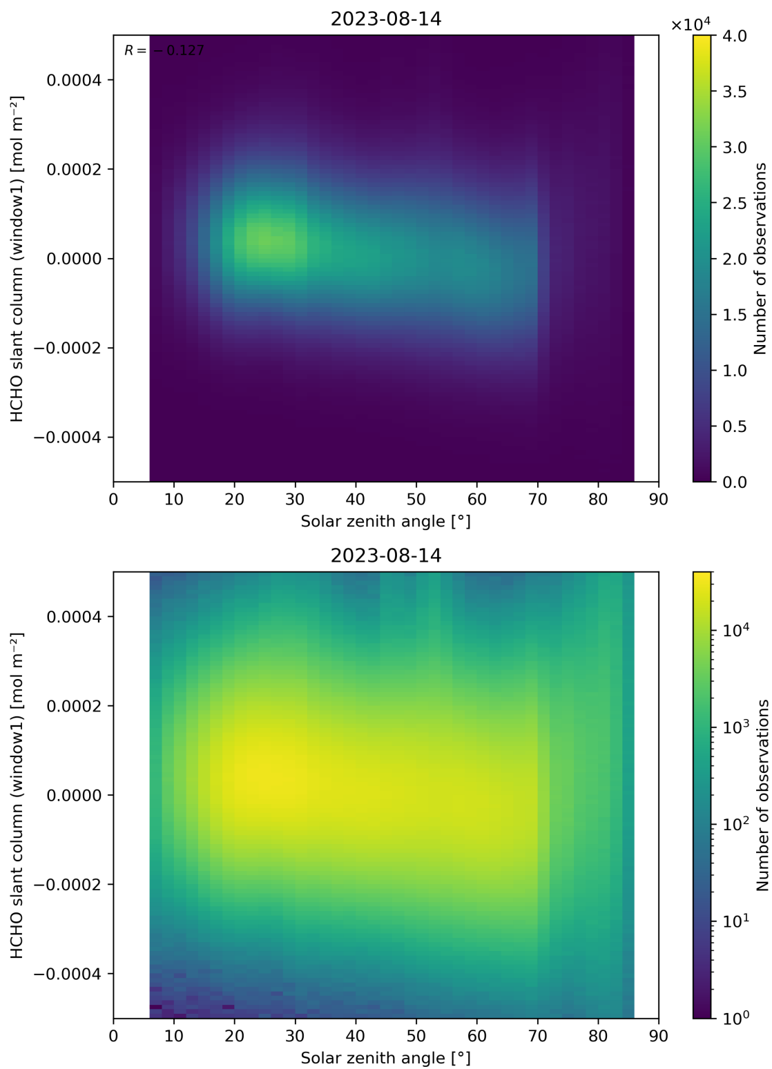
Figure 173: Scatter density plot of “Solar zenith angle” against “HCHO slant column (window1)” for 2023-08-14 to 2023-08-15.
