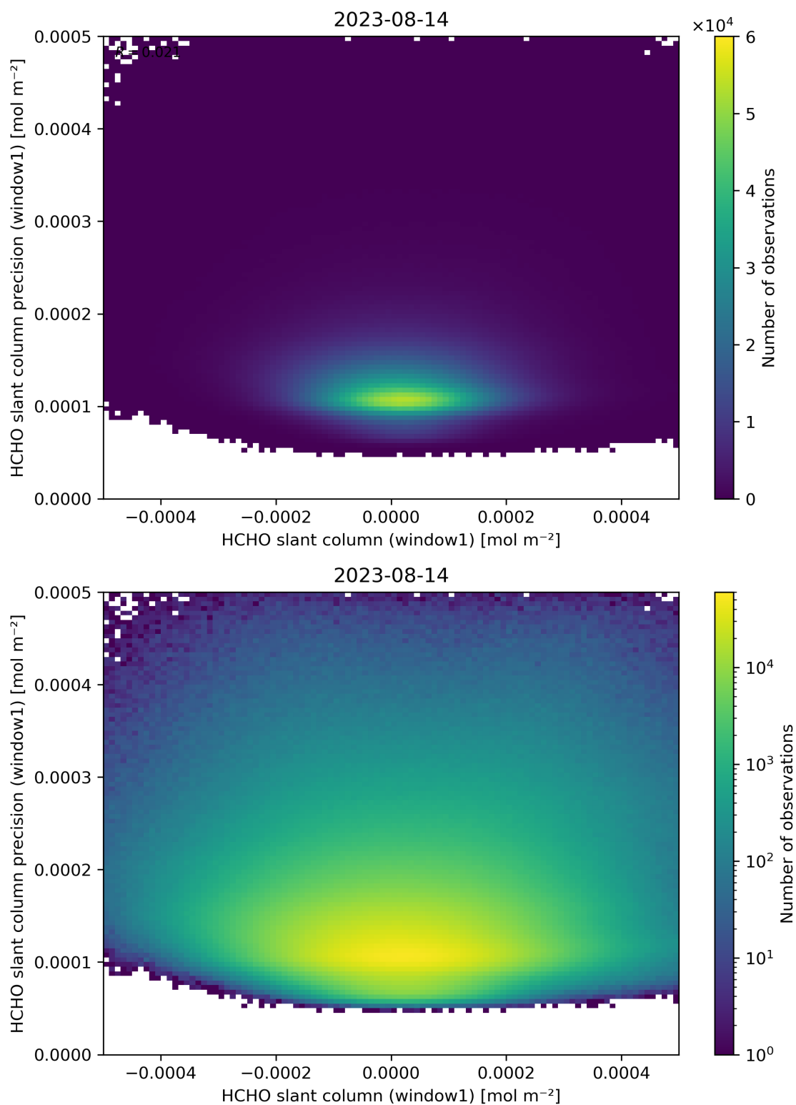
Figure 84: Scatter density plot of “HCHO slant column (window1)” against “HCHO slant column precision (window1)” for 2023-08-14 to 2023-08-15.
