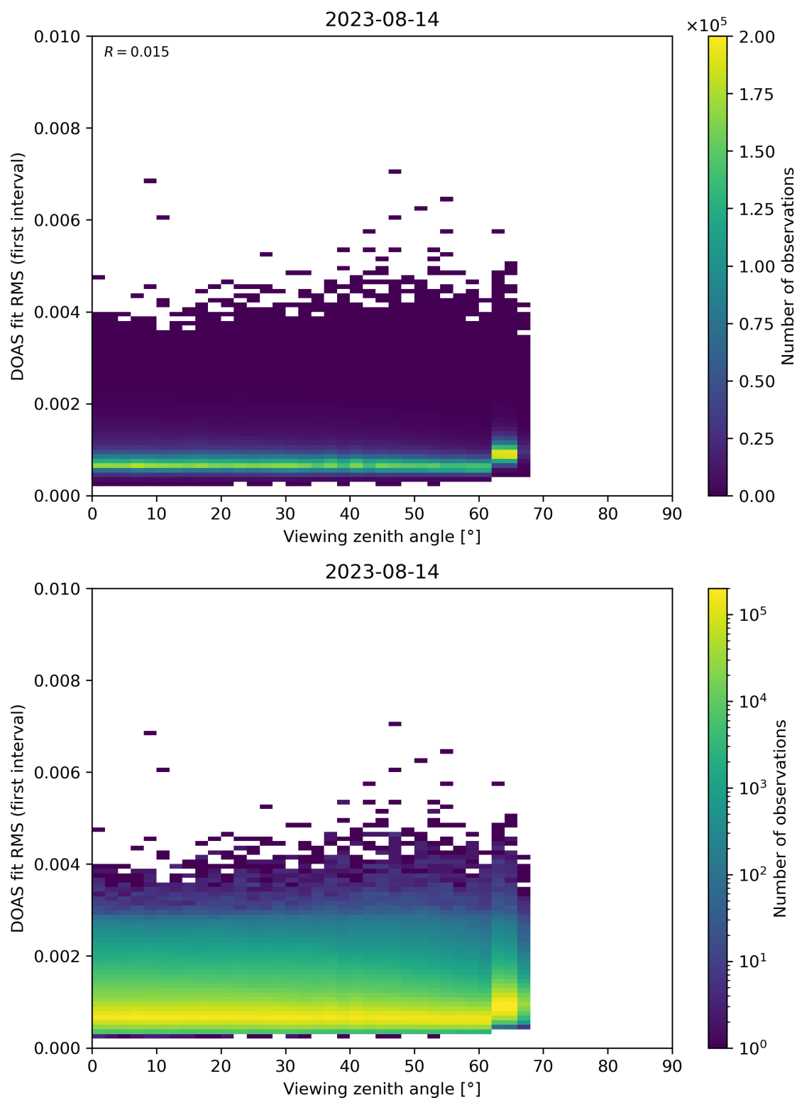
Figure 182: Scatter density plot of “Viewing zenith angle” against “DOAS fit RMS (first interval)” for 2023-08-14 to 2023-08-15.
