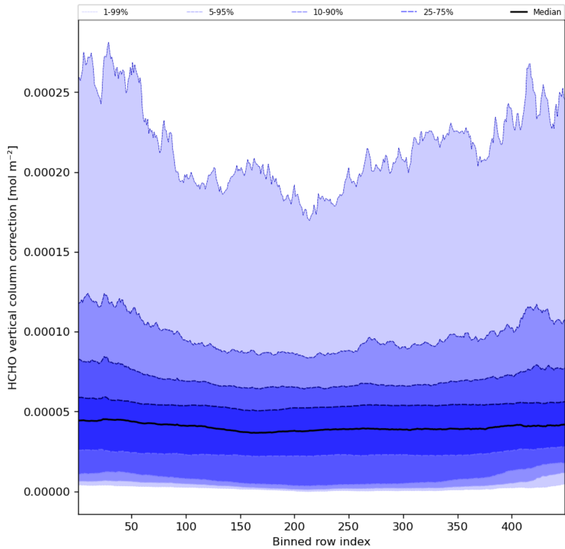
Figure 51: Along track statistics of “HCHO vertical column correction” for 2023-08-14 to 2023-08-15
