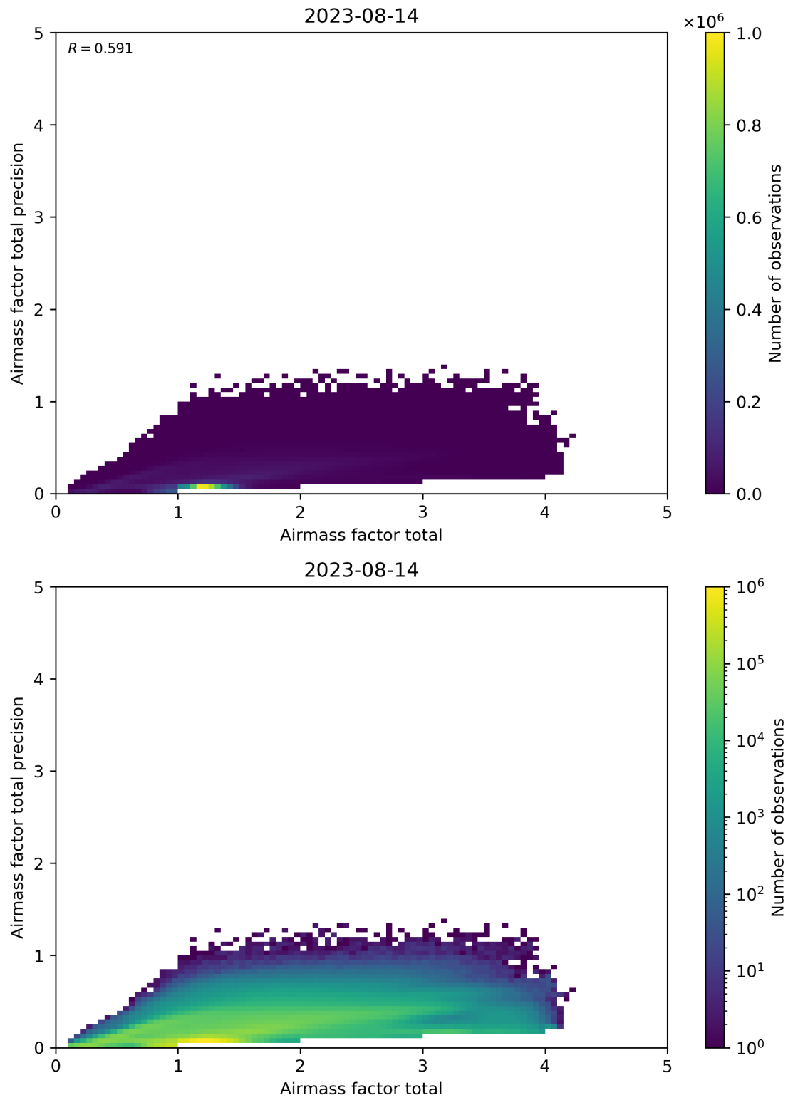
Figure 103: Scatter density plot of “Airmass factor total” against “Airmass factor total precision” for 2023-08-14 to 2023-08-15.
