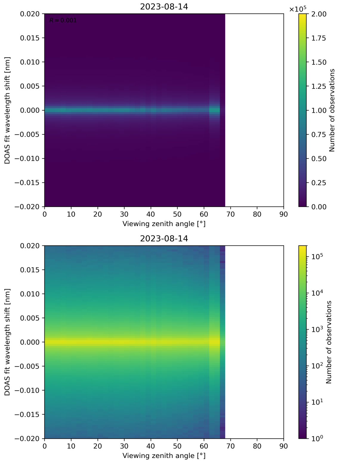
Figure 183: Scatter density plot of “Viewing zenith angle” against “DOAS fit wavelength shift” for 2023-08-14 to 2023-08-15.
