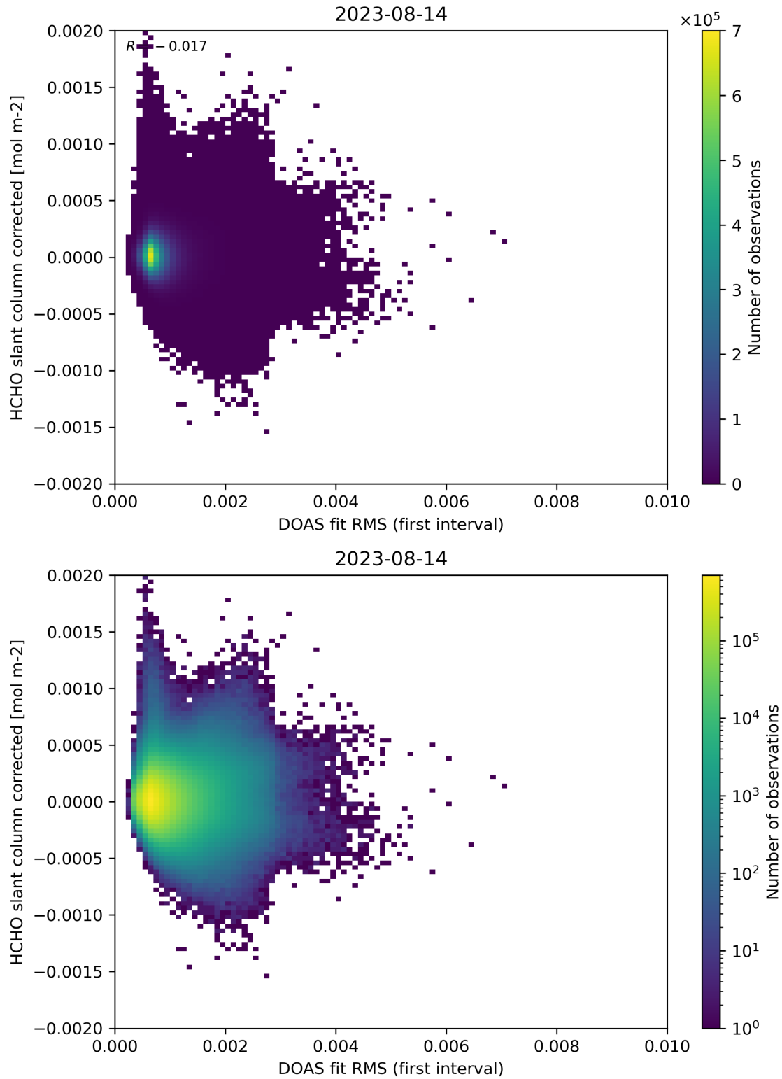
Figure 62: Scatter density plot of “DOAS fit RMS (first interval)” against “HCHO slant column corrected” for 2023-08-14 to 2023-08-15.
