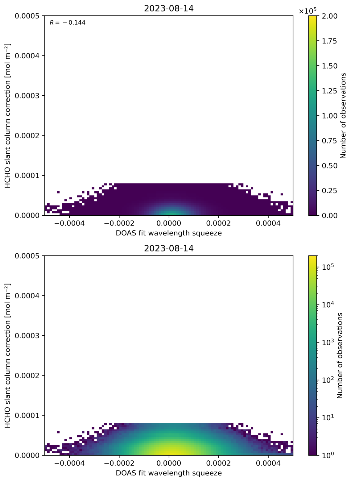
Figure 70: Scatter density plot of “DOAS fit wavelength squeeze” against “HCHO slant column correction” for 2023-08-14 to 2023-08-15.
