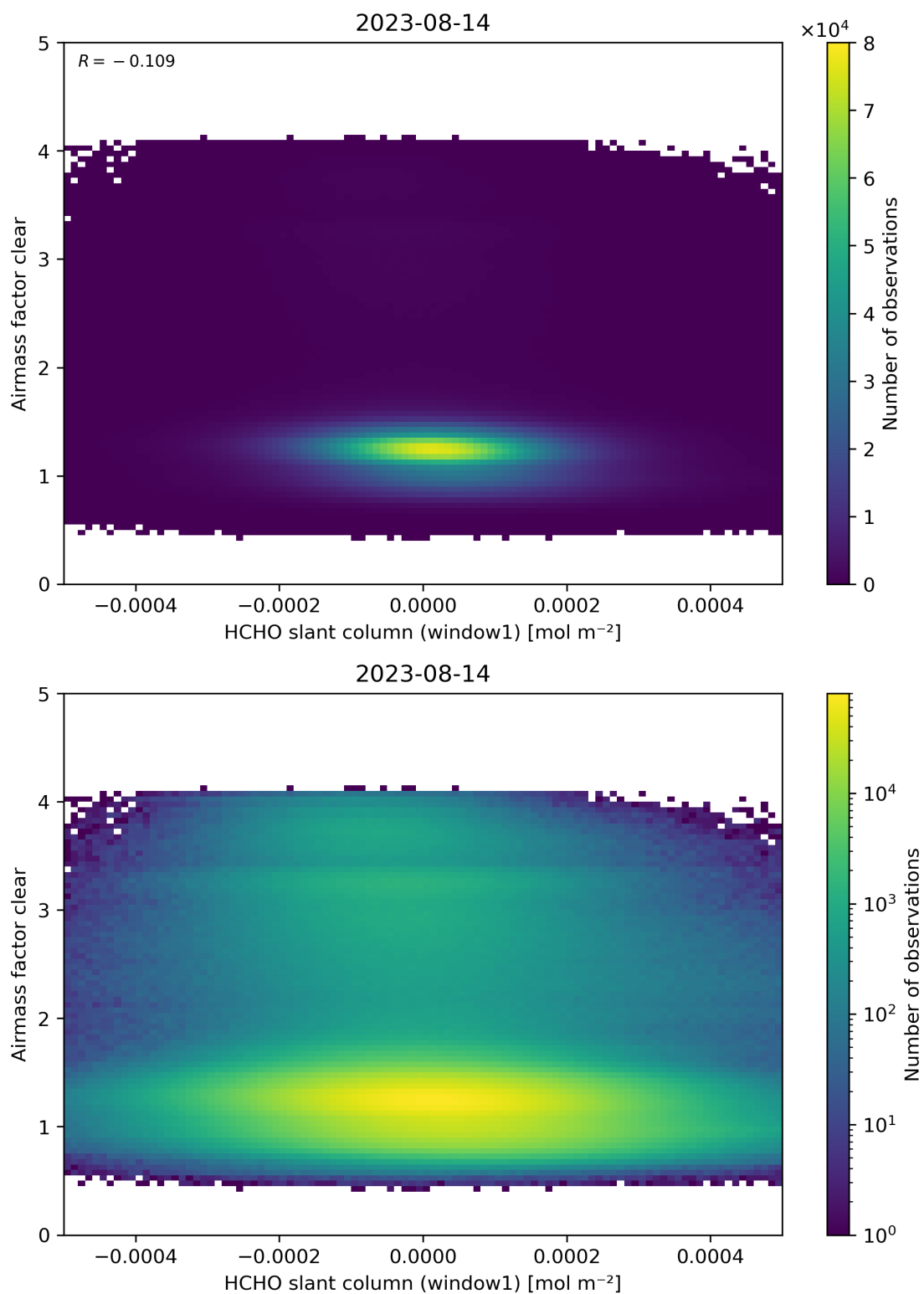
Figure 81: Scatter density plot of “HCHO slant column (window1)” against “Airmass factor clear” for 2023-08-14 to 2023-08-15.
