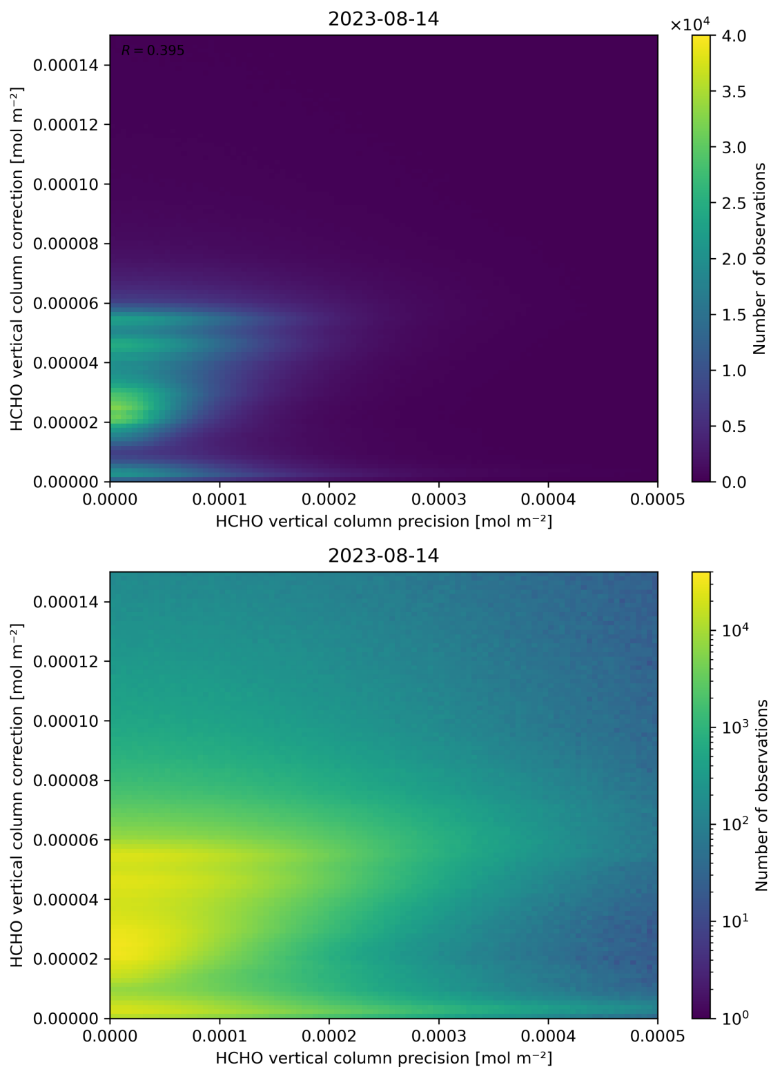
Figure 146: Scatter density plot of “HCHO vertical column precision” against “HCHO vertical column correction” for 2023-08-14 to 2023-08-15.
