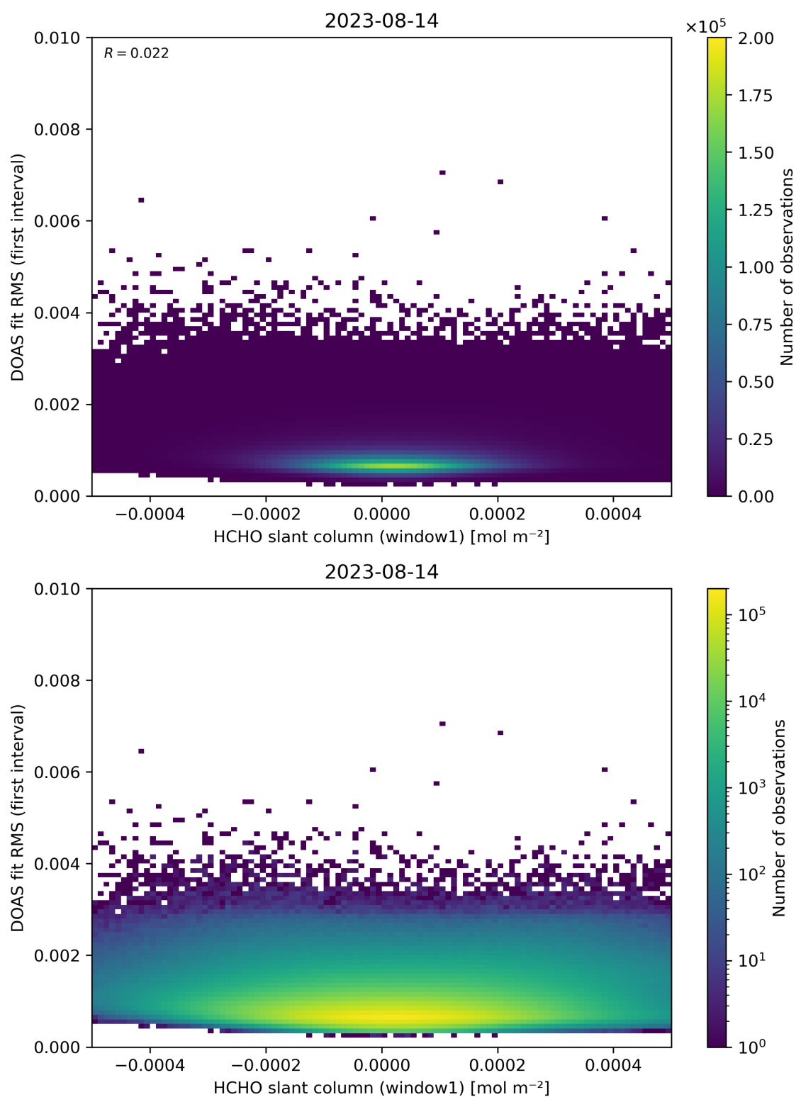
Figure 78: Scatter density plot of “HCHO slant column (window1)” against “DOAS fit RMS (first interval)” for 2023-08-14 to 2023-08-15.
