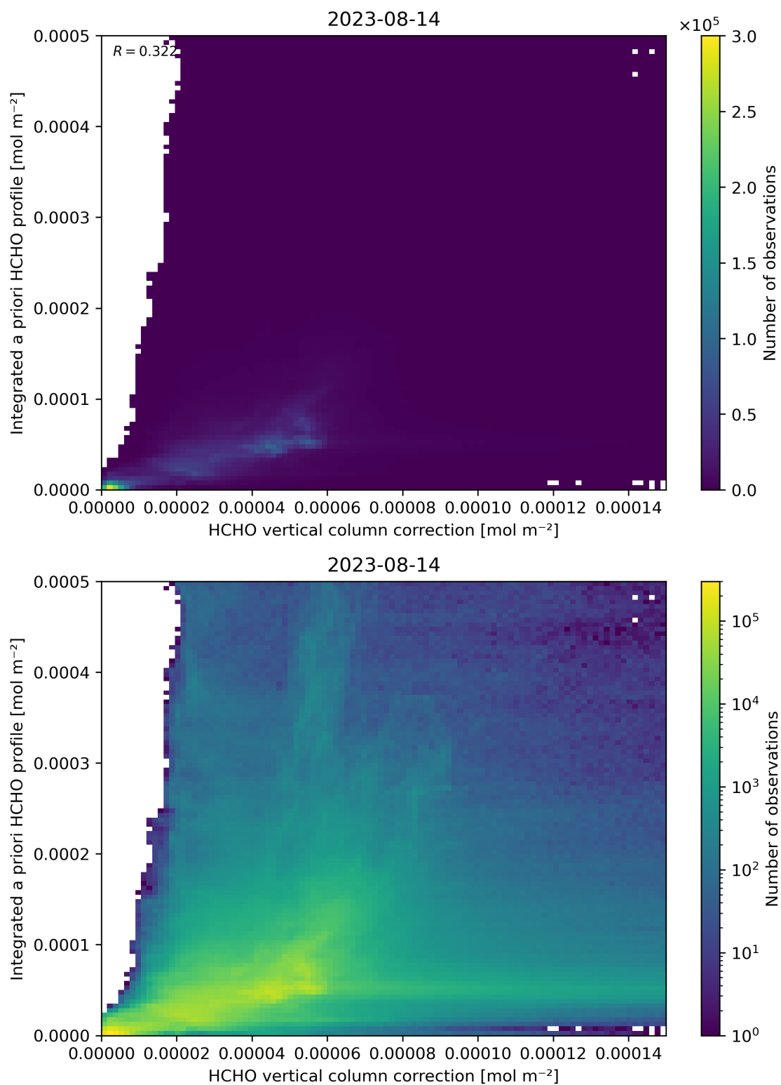
Figure 122: Scatter density plot of “HCHO vertical column correction” against “Integrated a priori HCHO profile” for 2023-08-14 to 2023-08-15.
