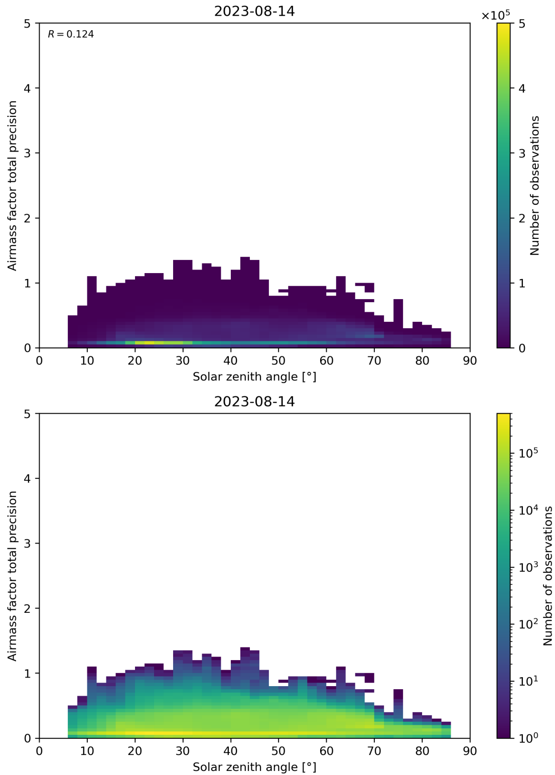
Figure 176: Scatter density plot of “Solar zenith angle” against “Airmass factor total precision” for 2023-08-14 to 2023-08-15.
