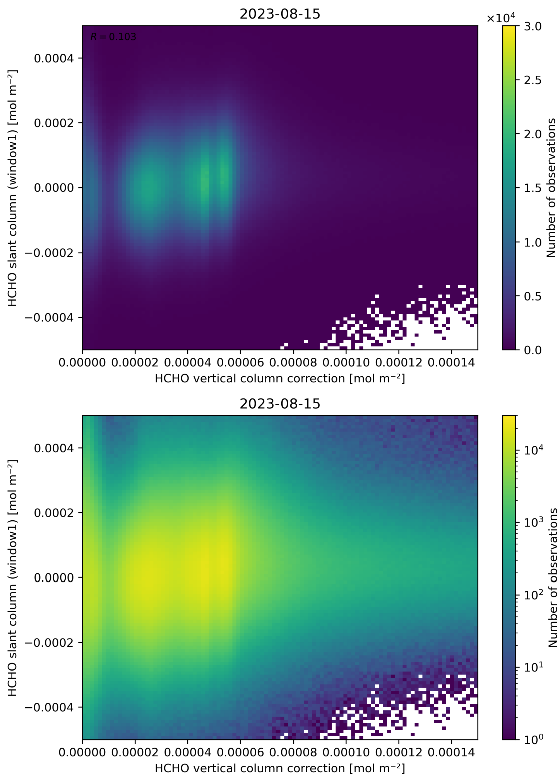
Figure 118: Scatter density plot of “HCHO vertical column correction” against “HCHO slant column (window1)” for 2023-08-14 to 2023-08-16.
