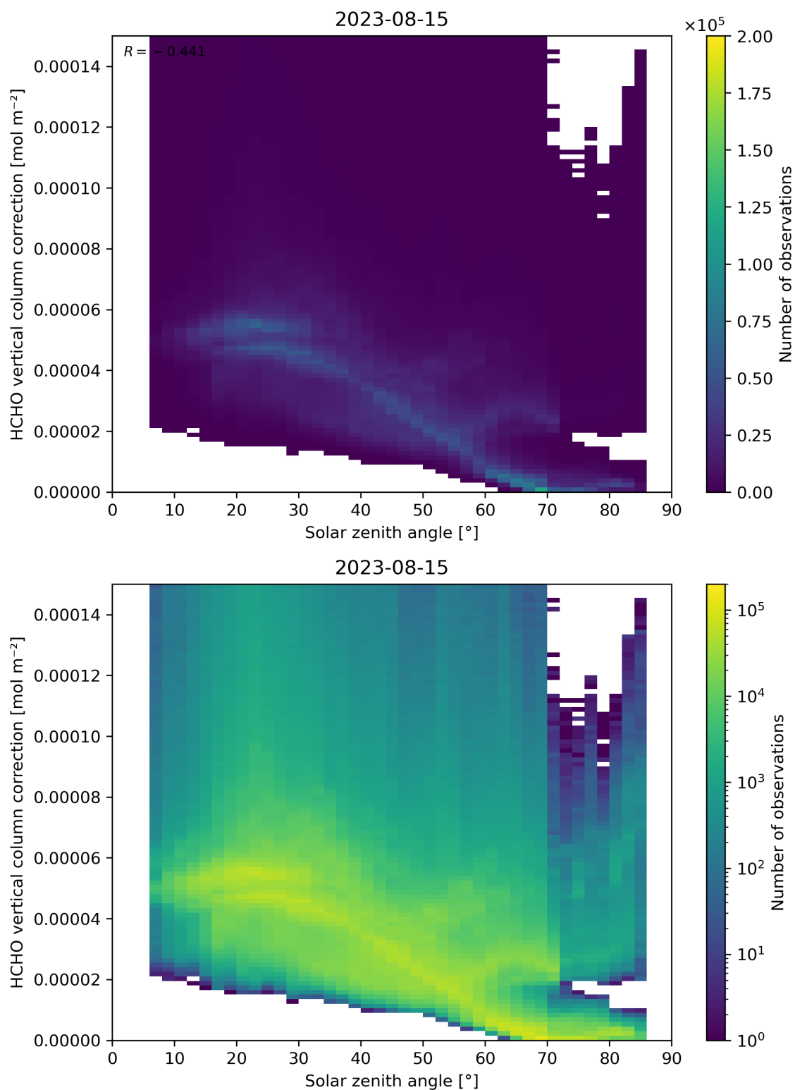
Figure 178: Scatter density plot of “Solar zenith angle” against “HCHO vertical column correction” for 2023-08-14 to 2023-08-16.
