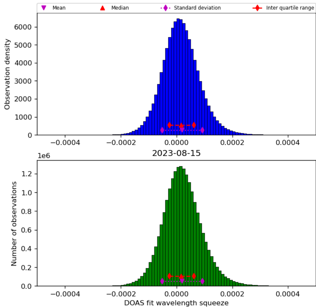
Figure 45: Histogram of “DOAS fit wavelength squeeze” for 2023-08-14 to 2023-08-16
