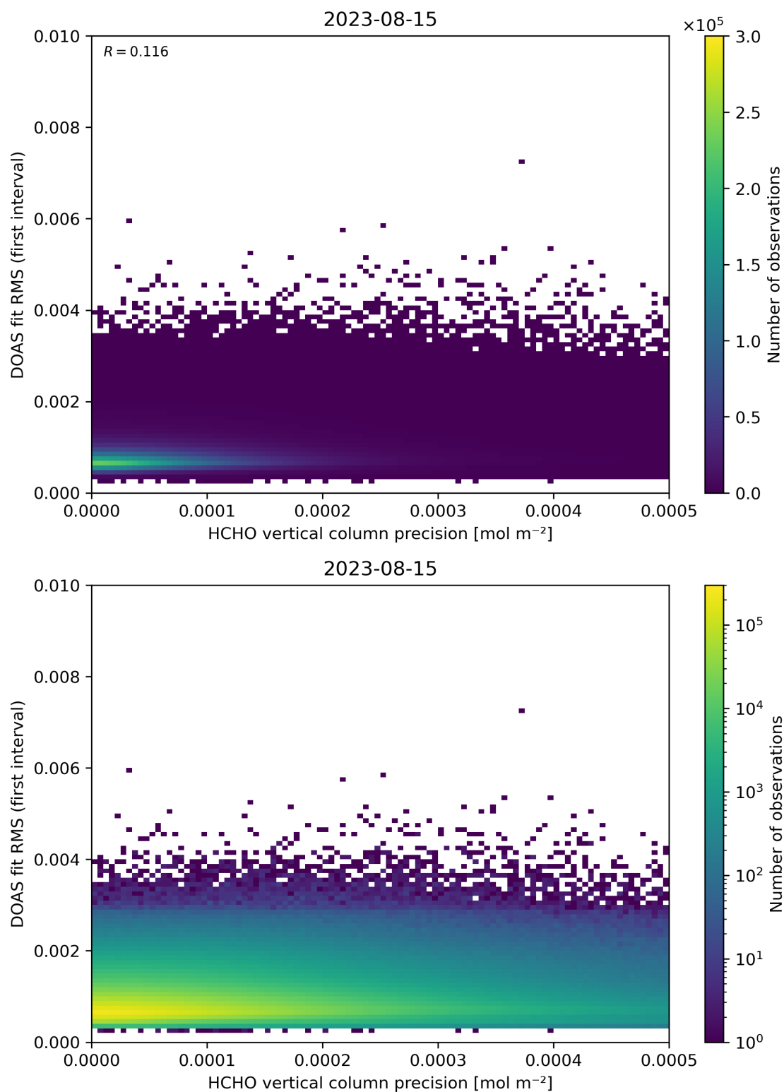
Figure 136: Scatter density plot of “HCHO vertical column precision” against “DOAS fit RMS (first interval)” for 2023-08-14 to 2023-08-16.
