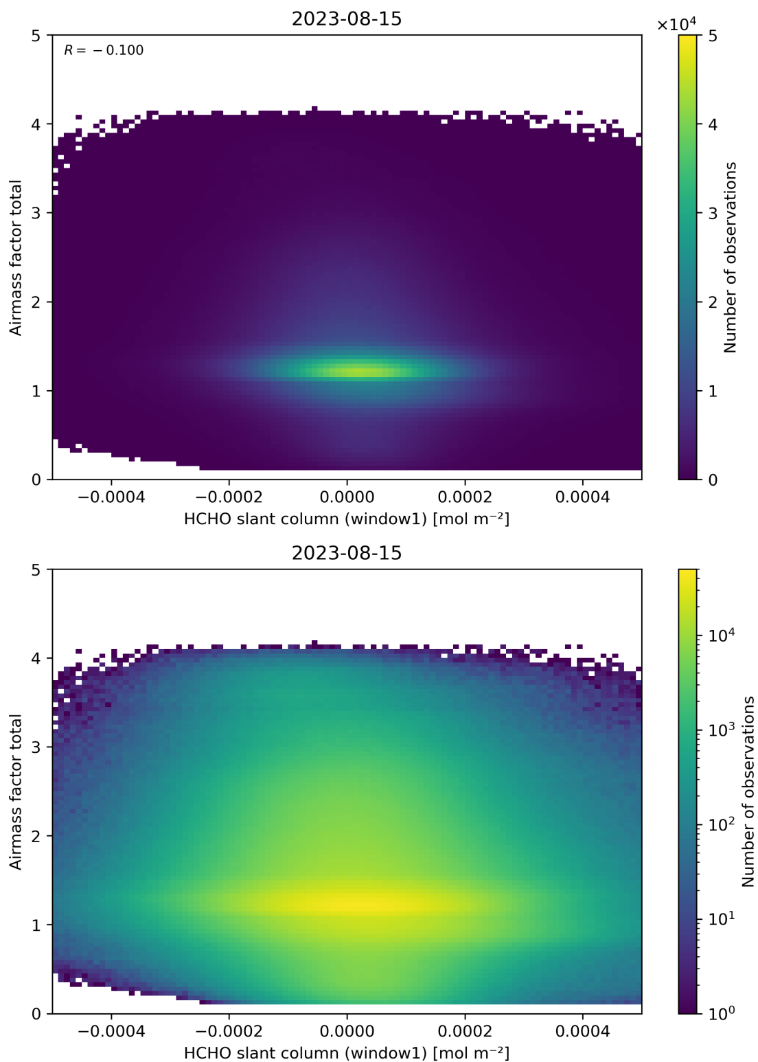
Figure 85: Scatter density plot of “HCHO slant column (window1)” against “Airmass factor total” for 2023-08-14 to 2023-08-16.
