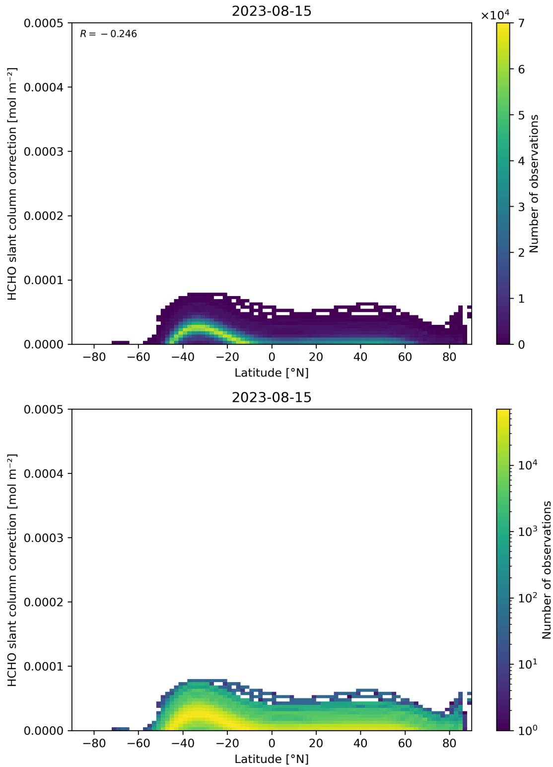
Figure 158: Scatter density plot of “Latitude” against “HCHO slant column correction” for 2023-08-14 to 2023-08-16.
