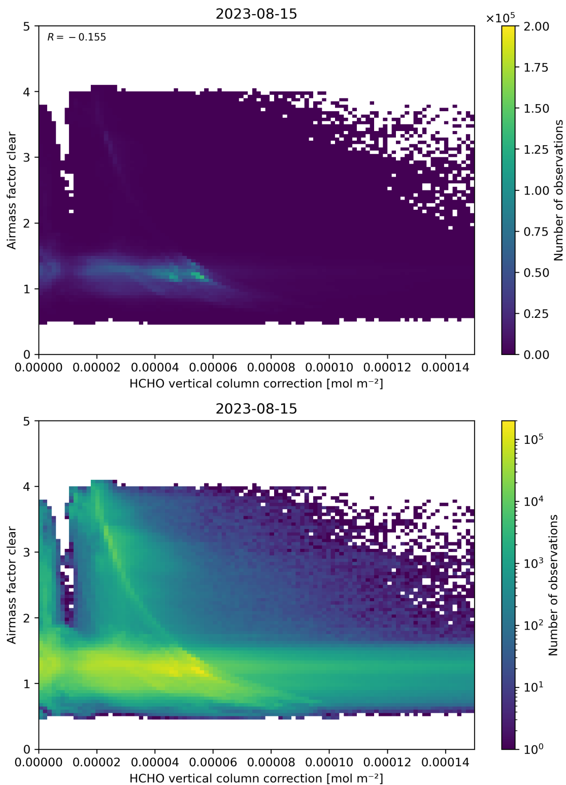
Figure 115: Scatter density plot of “HCHO vertical column correction” against “Airmass factor clear” for 2023-08-14 to 2023-08-16.
