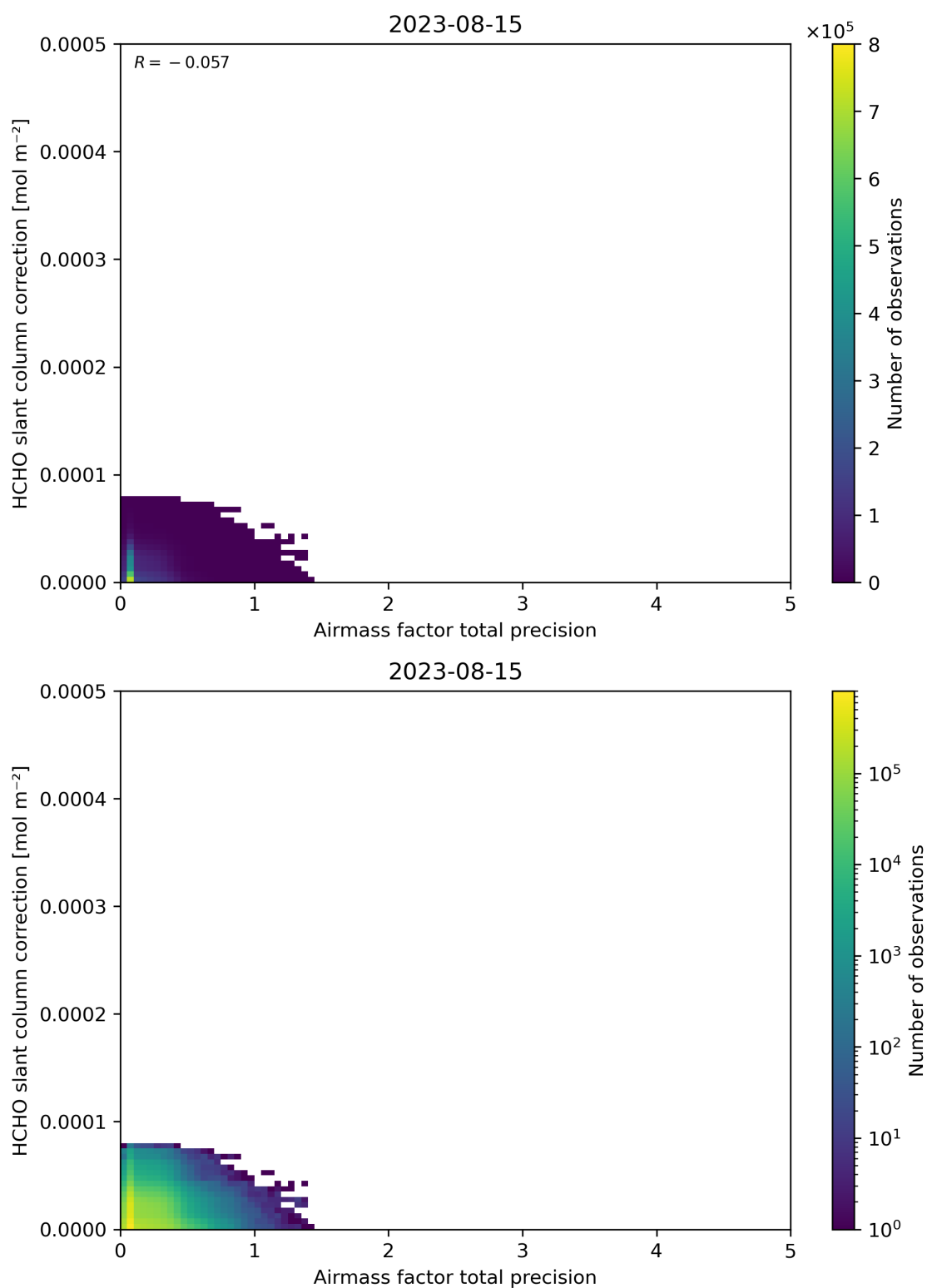
Figure 110: Scatter density plot of “Airmass factor total precision” against “HCHO slant column correction” for 2023-08-14 to 2023-08-16.
