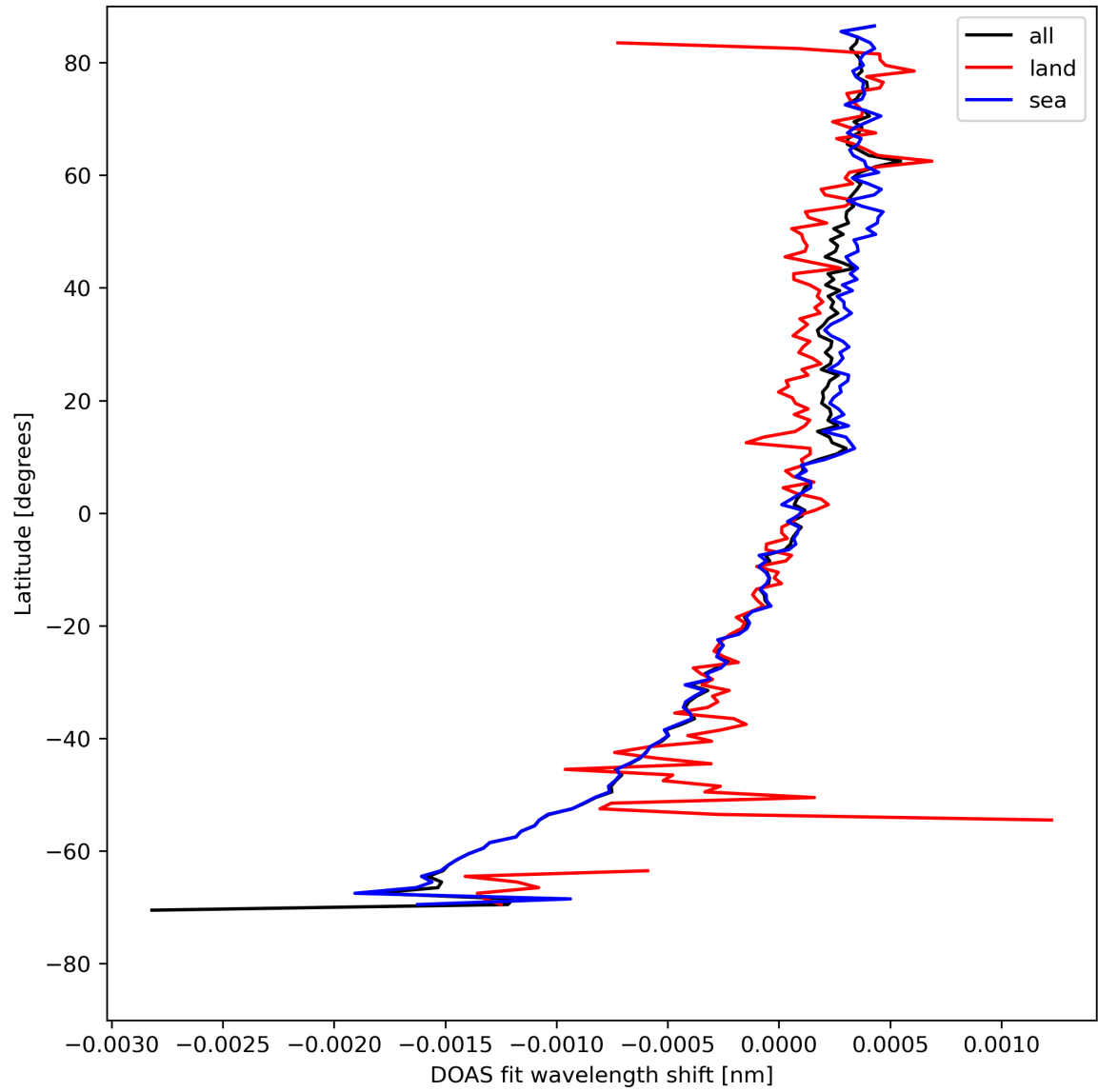
Figure 30: Zonal average of “DOAS fit wavelength shift” for 2023-08-14 to 2023-08-16.
