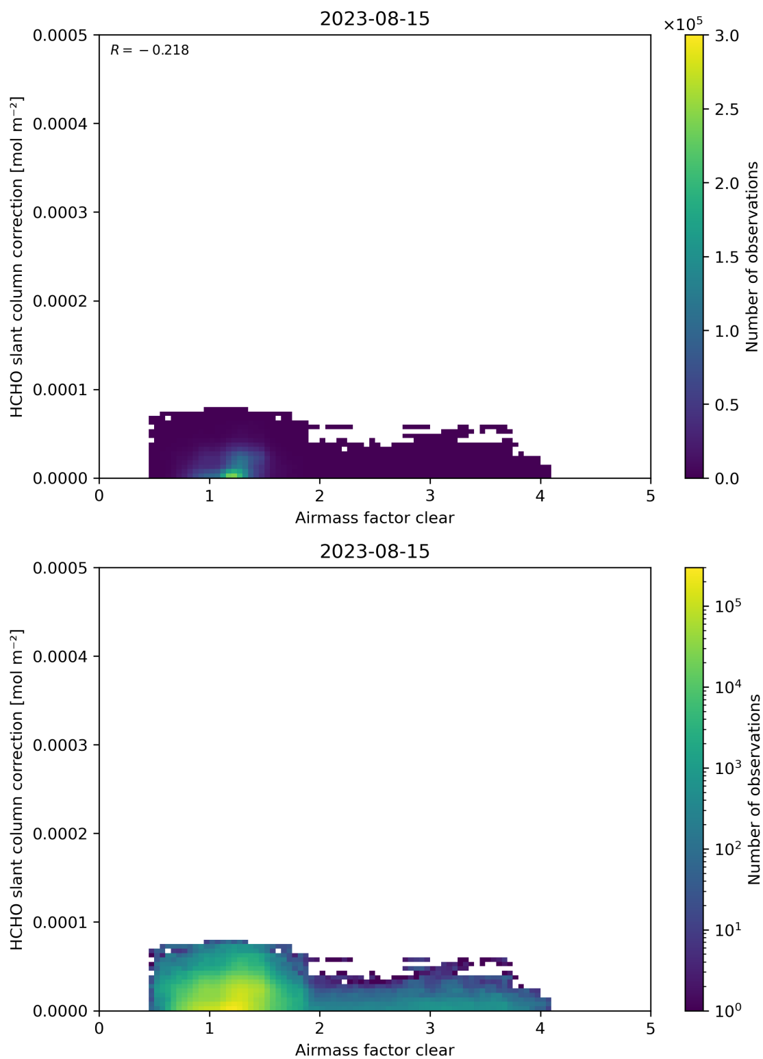
Figure 75: Scatter density plot of “Airmass factor clear” against “HCHO slant column correction” for 2023-08-14 to 2023-08-16.
