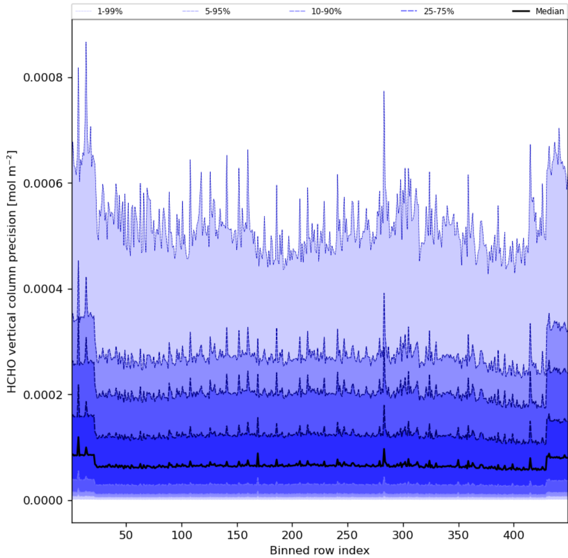
Figure 50: Along track statistics of “HCHO vertical column precision” for 2023-08-14 to 2023-08-16
