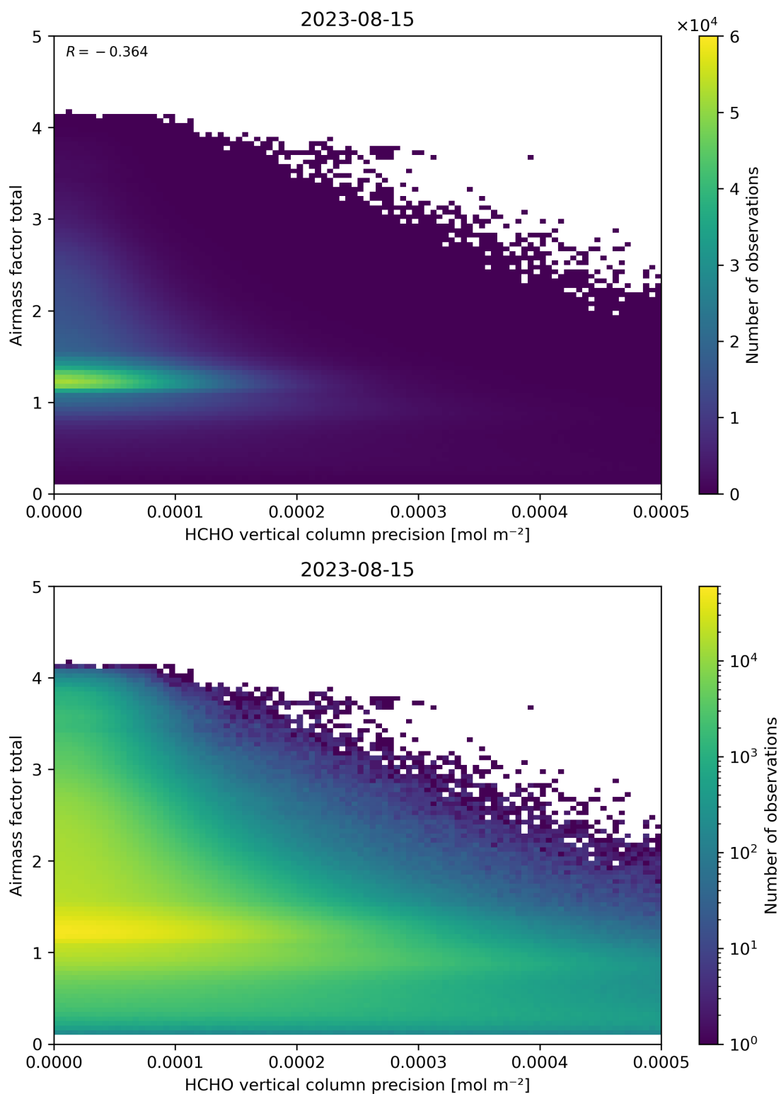
Figure 144: Scatter density plot of “HCHO vertical column precision” against “Airmass factor total” for 2023-08-14 to 2023-08-16.
