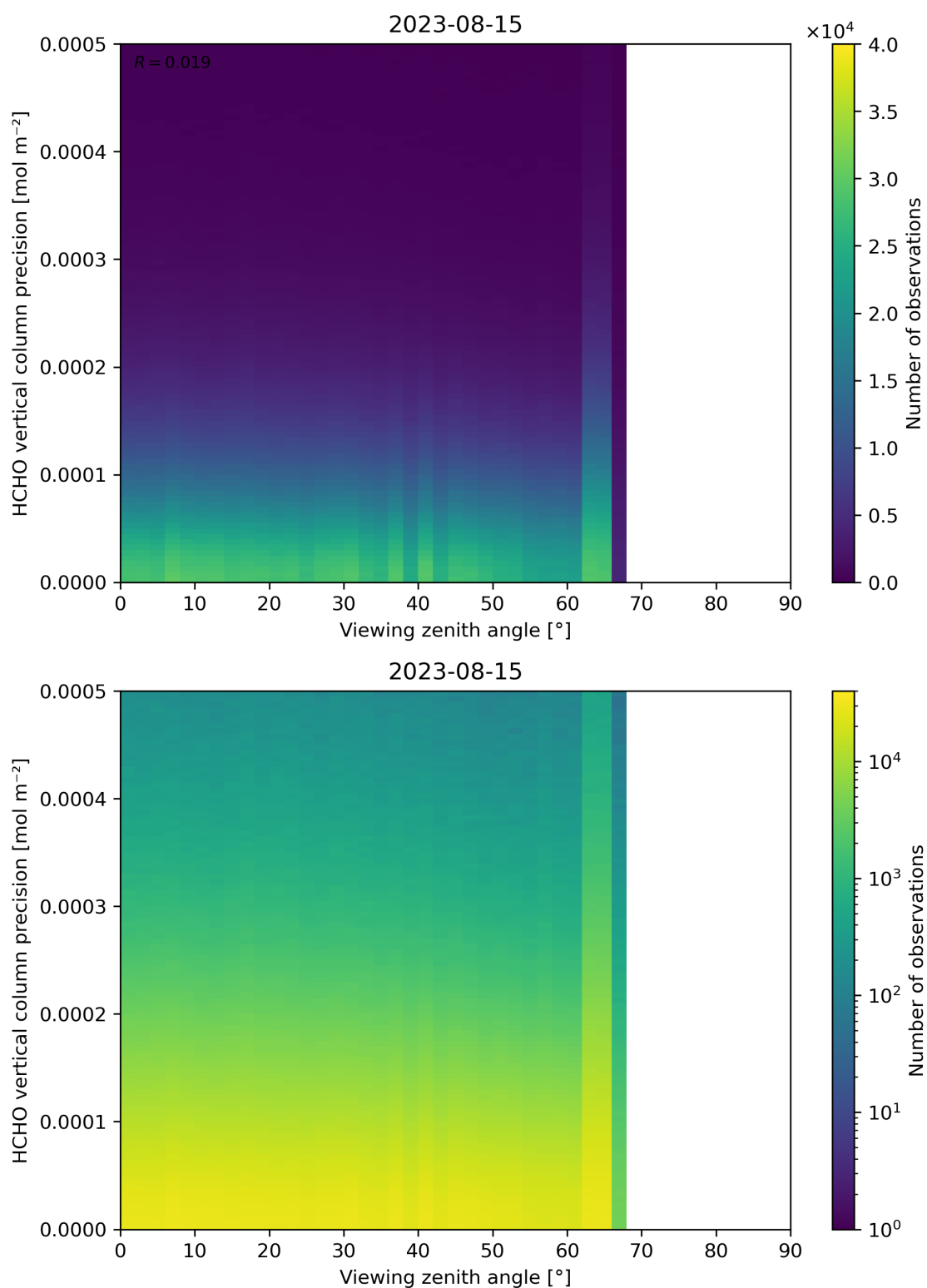
Figure 194: Scatter density plot of “Viewing zenith angle” against “HCHO vertical column precision” for 2023-08-14 to 2023-08-16.
