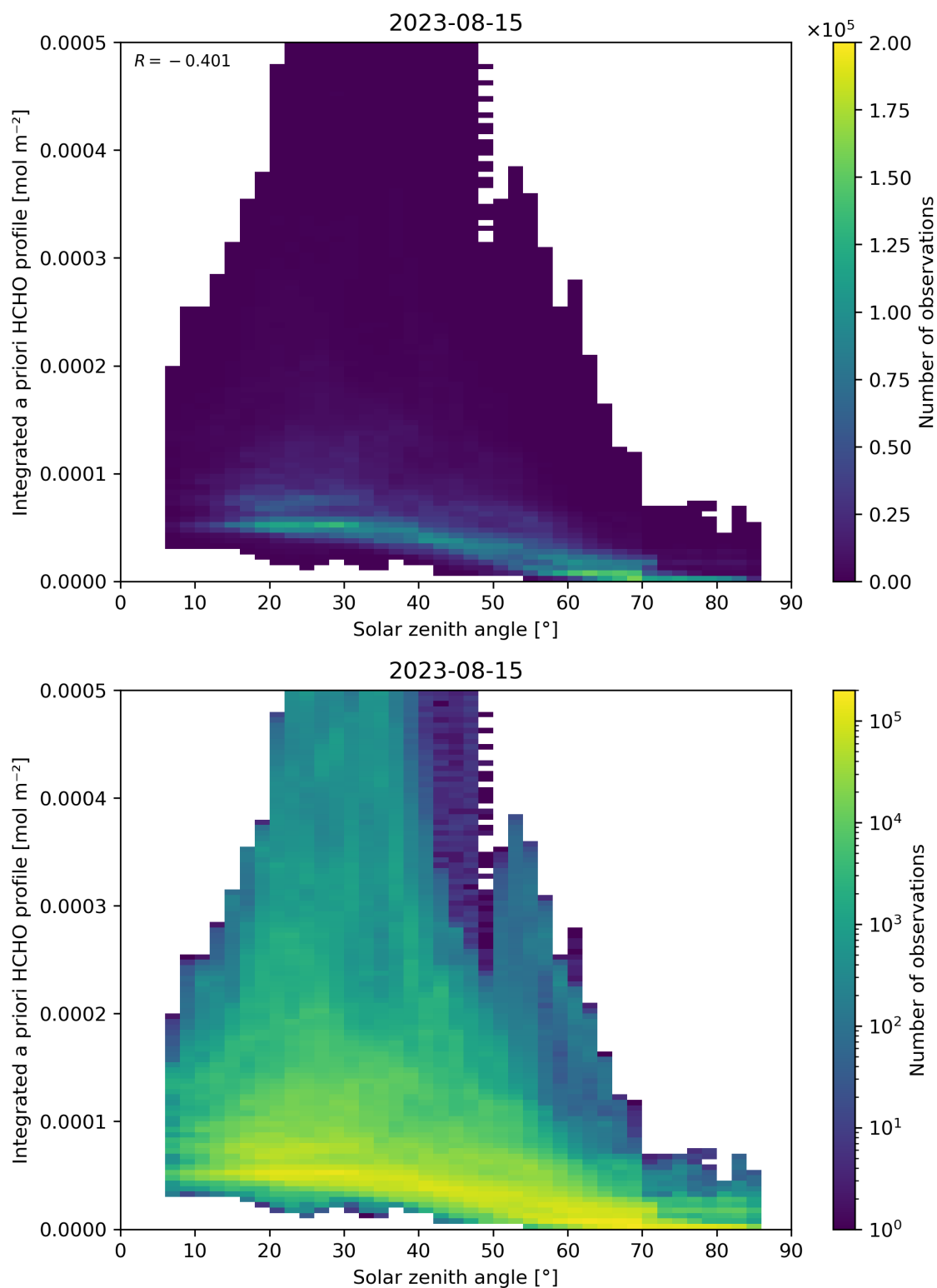
Figure 180: Scatter density plot of “Solar zenith angle” against “Integrated a priori HCHO profile” for 2023-08-14 to 2023-08-16.
