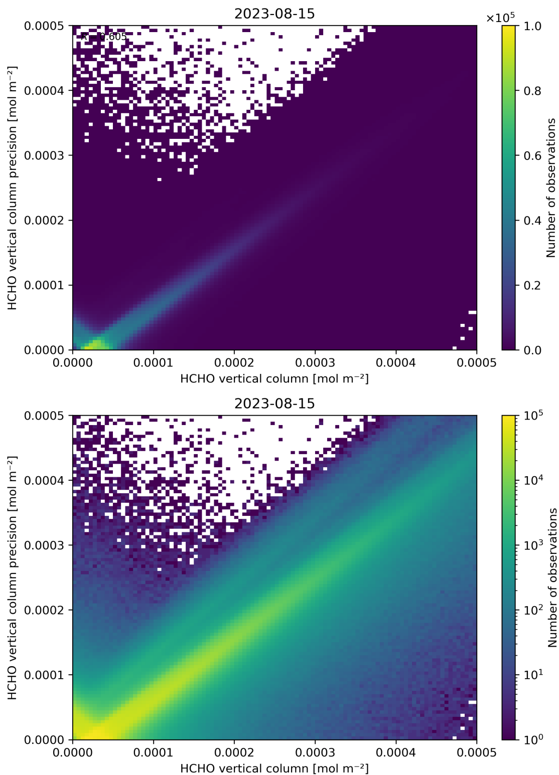
Figure 134: Scatter density plot of “HCHO vertical column” against “HCHO vertical column precision” for 2023-08-14 to 2023-08-16.
