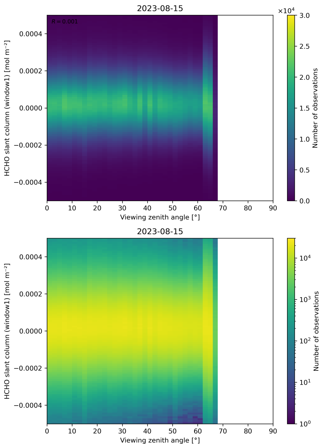
Figure 188: Scatter density plot of “Viewing zenith angle” against “HCHO slant column (window1)” for 2023-08-14 to 2023-08-16.
