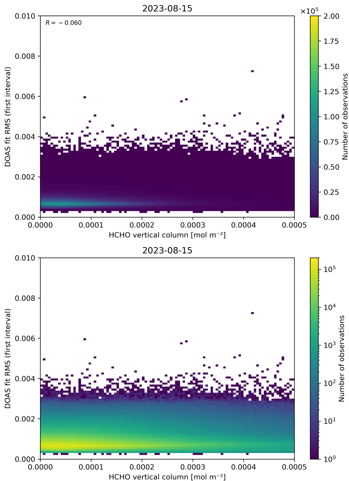
Figure 123: Scatter density plot of “HCHO vertical column” against “DOAS fit RMS (first interval)” for 2023-08-14 to 2023-08-16.
