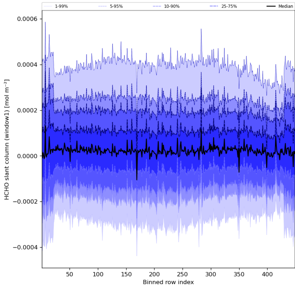
Figure 52: Along track statistics of “HCHO slant column (window1)” for 2023-08-14 to 2023-08-16
