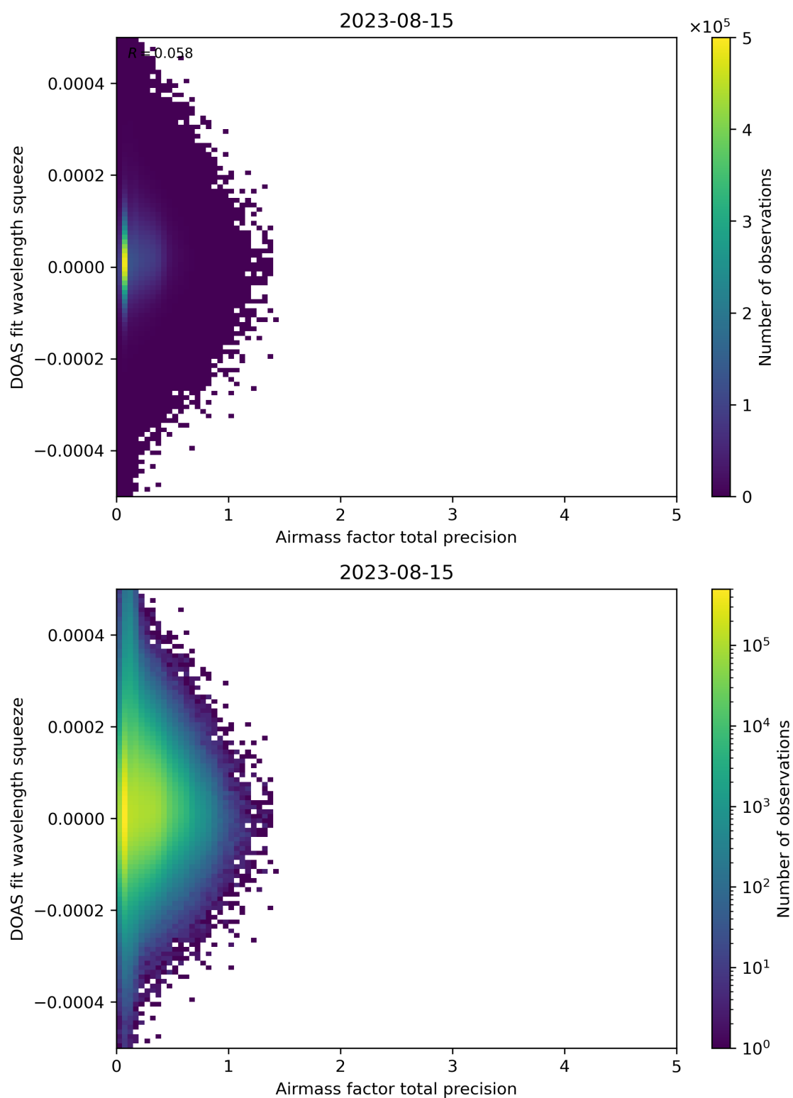
Figure 107: Scatter density plot of “Airmass factor total precision” against “DOAS fit wavelength squeeze” for 2023-08-14 to 2023-08-16.
