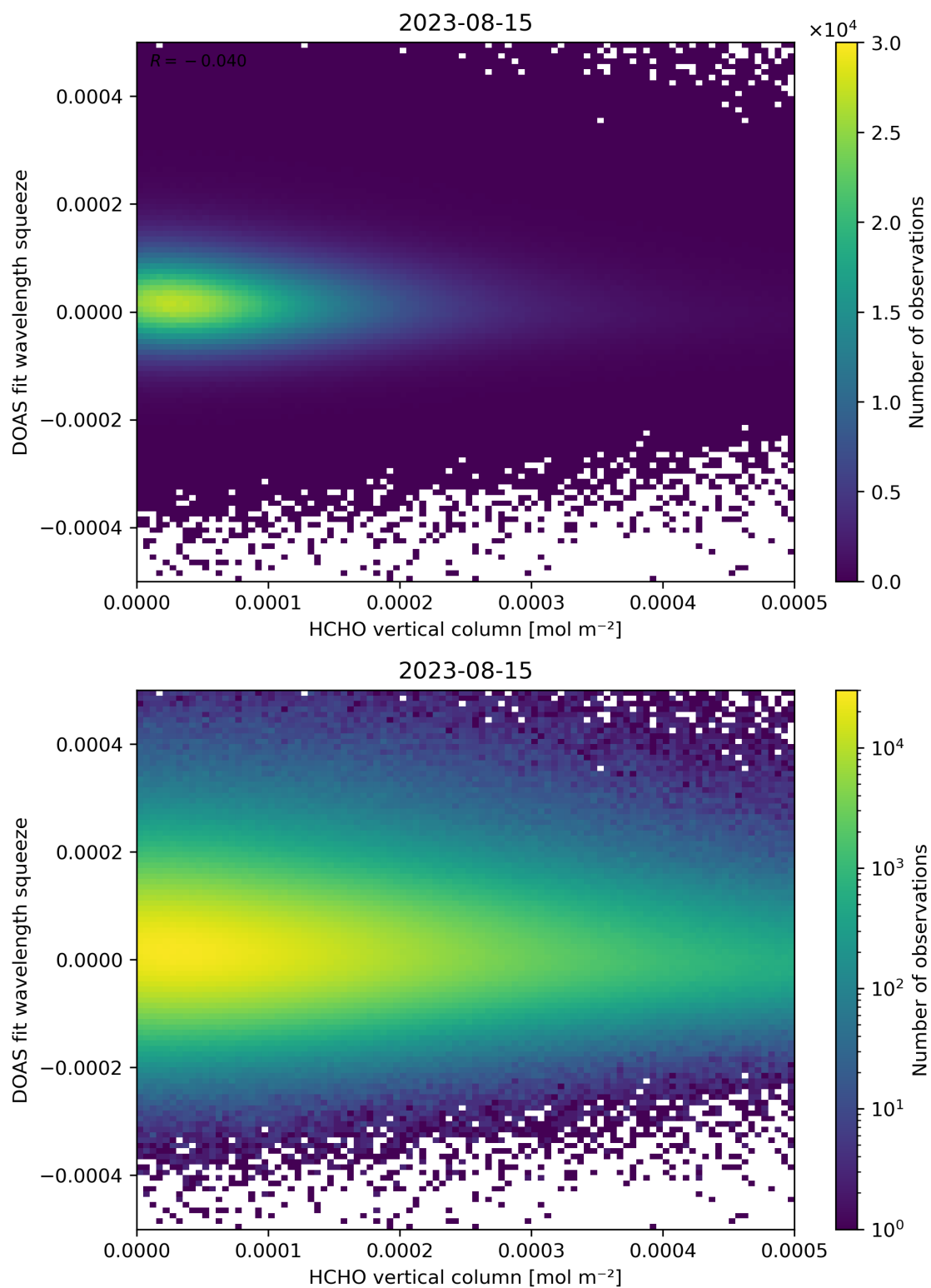
Figure 125: Scatter density plot of “HCHO vertical column” against “DOAS fit wavelength squeeze” for 2023-08-14 to 2023-08-16.
