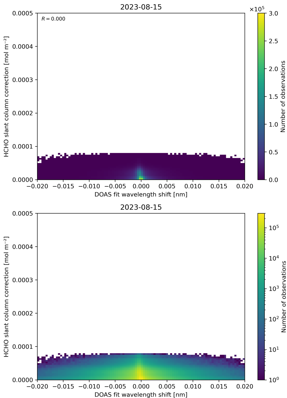
Figure 67: Scatter density plot of “DOAS fit wavelength shift” against “HCHO slant column correction” for 2023-08-14 to 2023-08-16.
