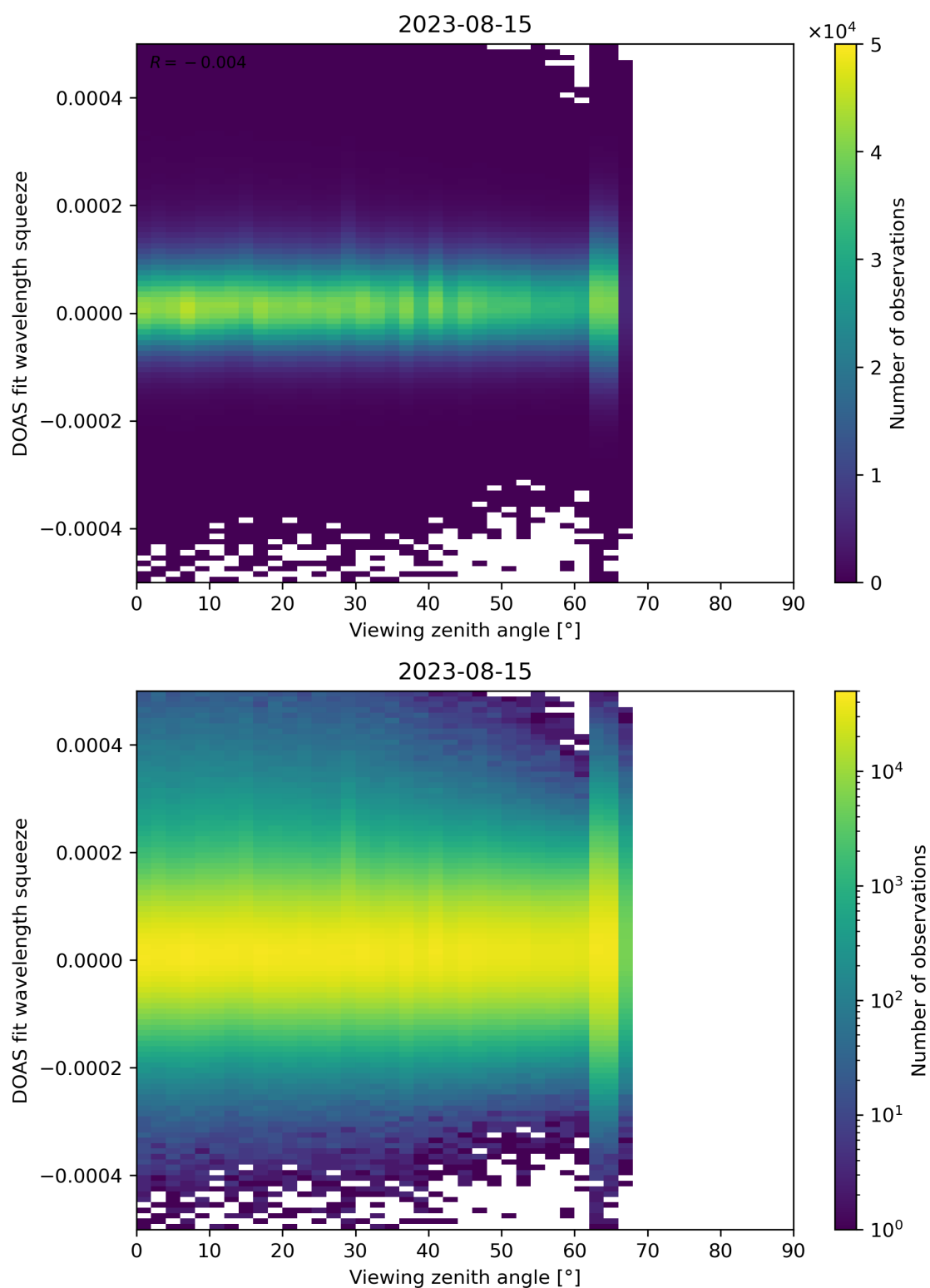
Figure 184: Scatter density plot of “Viewing zenith angle” against “DOAS fit wavelength squeeze” for 2023-08-14 to 2023-08-16.
