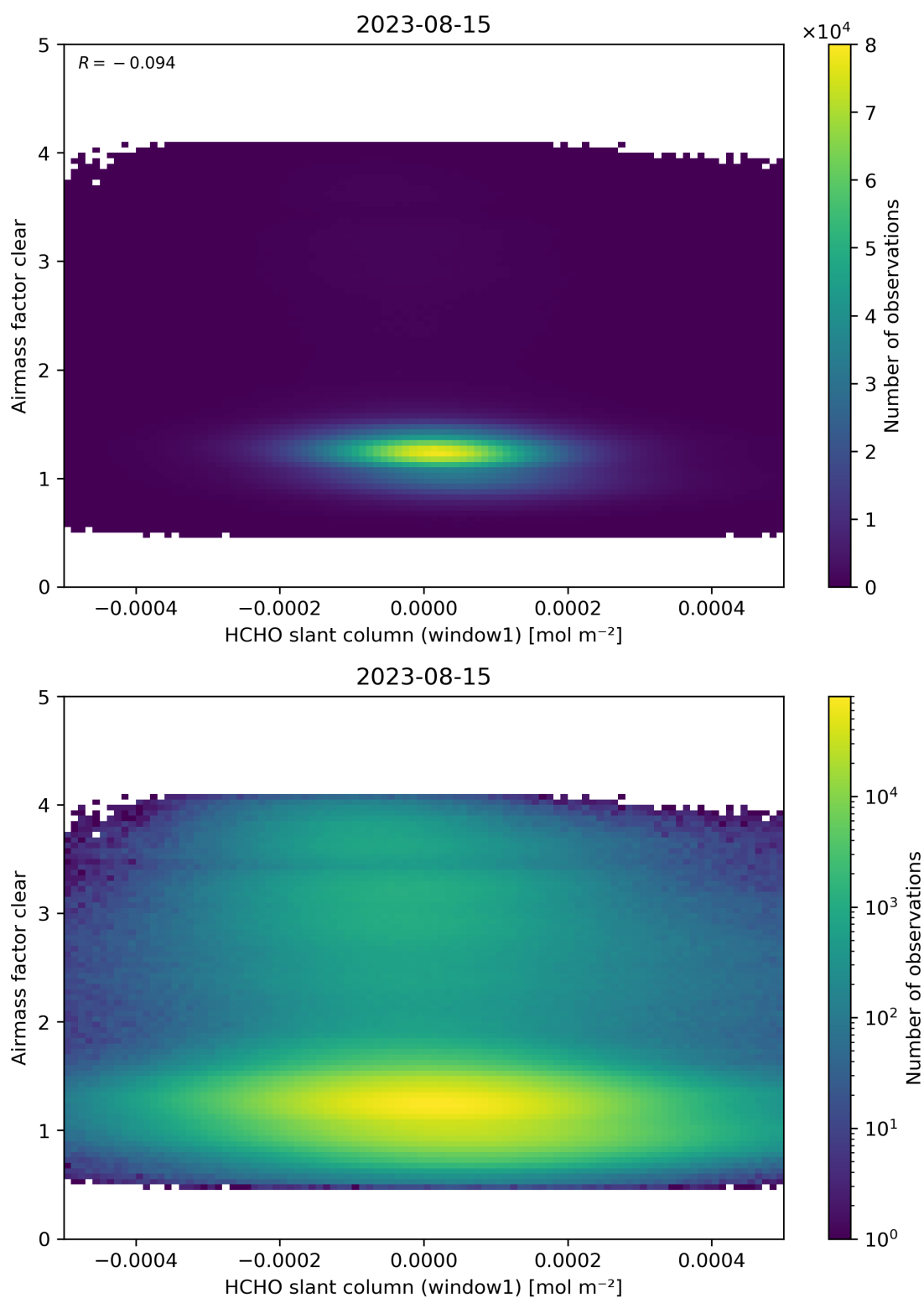
Figure 81: Scatter density plot of “HCHO slant column (window1)” against “Airmass factor clear” for 2023-08-14 to 2023-08-16.
