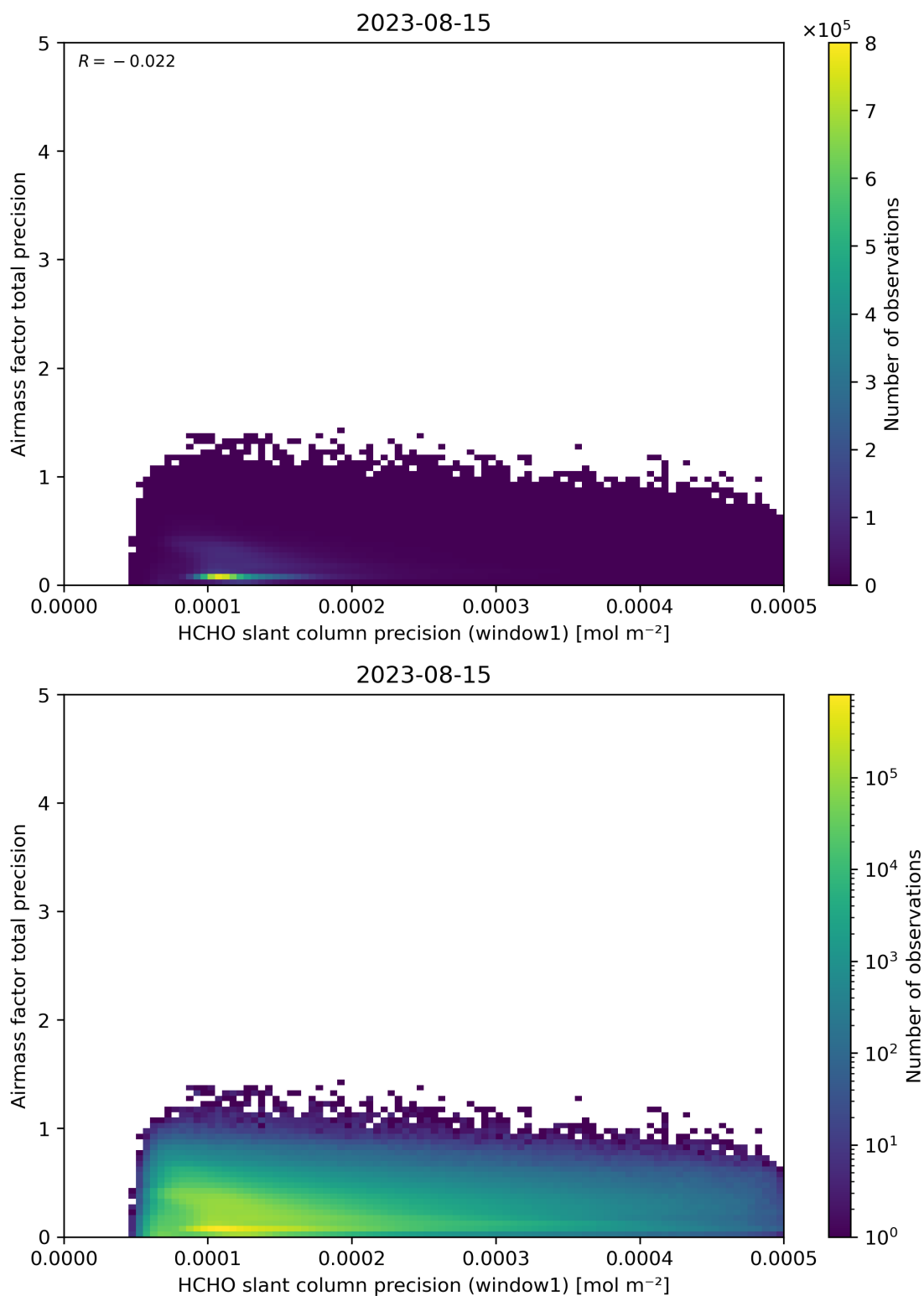
Figure 95: Scatter density plot of “HCHO slant column precision (window1)” against “Airmass factor total precision” for 2023-08-14 to 2023-08-16.
