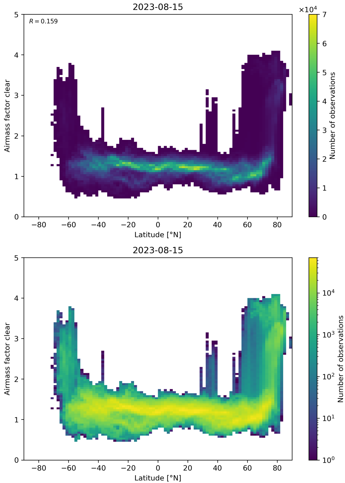
Figure 156: Scatter density plot of “Latitude” against “Airmass factor clear” for 2023-08-14 to 2023-08-16.
