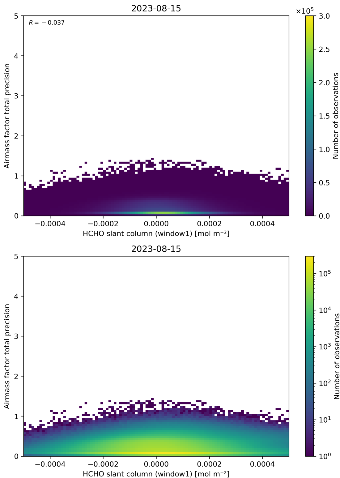
Figure 86: Scatter density plot of “HCHO slant column (window1)” against “Airmass factor total precision” for 2023-08-14 to 2023-08-16.
