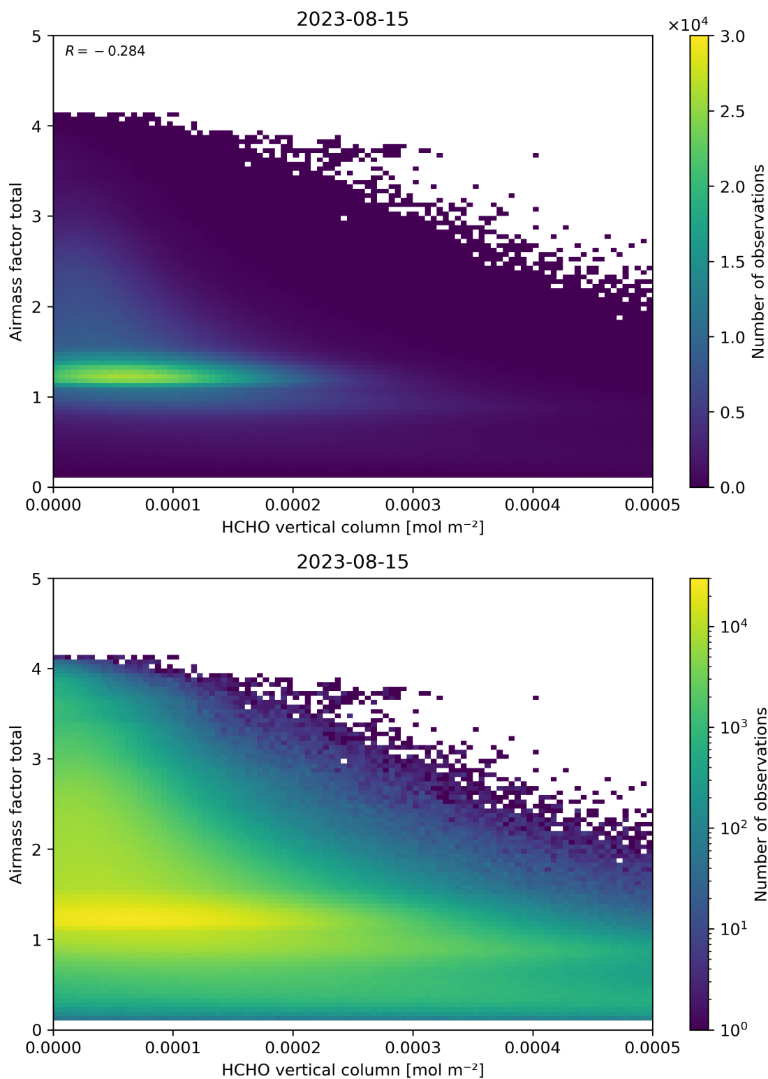
Figure 131: Scatter density plot of “HCHO vertical column” against “Airmass factor total” for 2023-08-14 to 2023-08-16.
