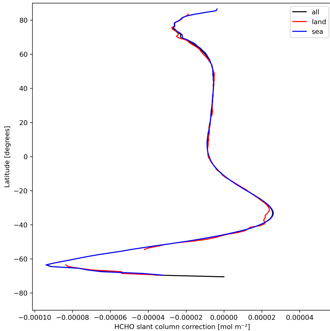
Figure 33: Zonal average of “HCHO slant column correction” for 2023-08-14 to 2023-08-16.
