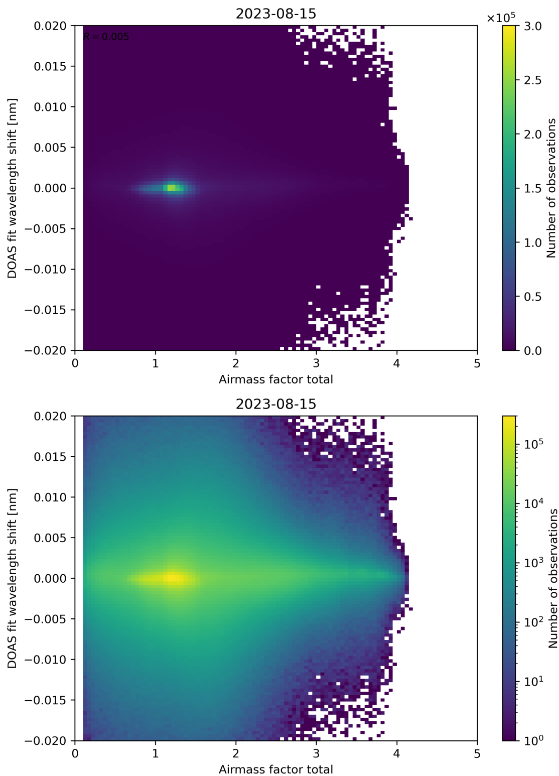
Figure 98: Scatter density plot of “Airmass factor total” against “DOAS fit wavelength shift” for 2023-08-14 to 2023-08-16.
