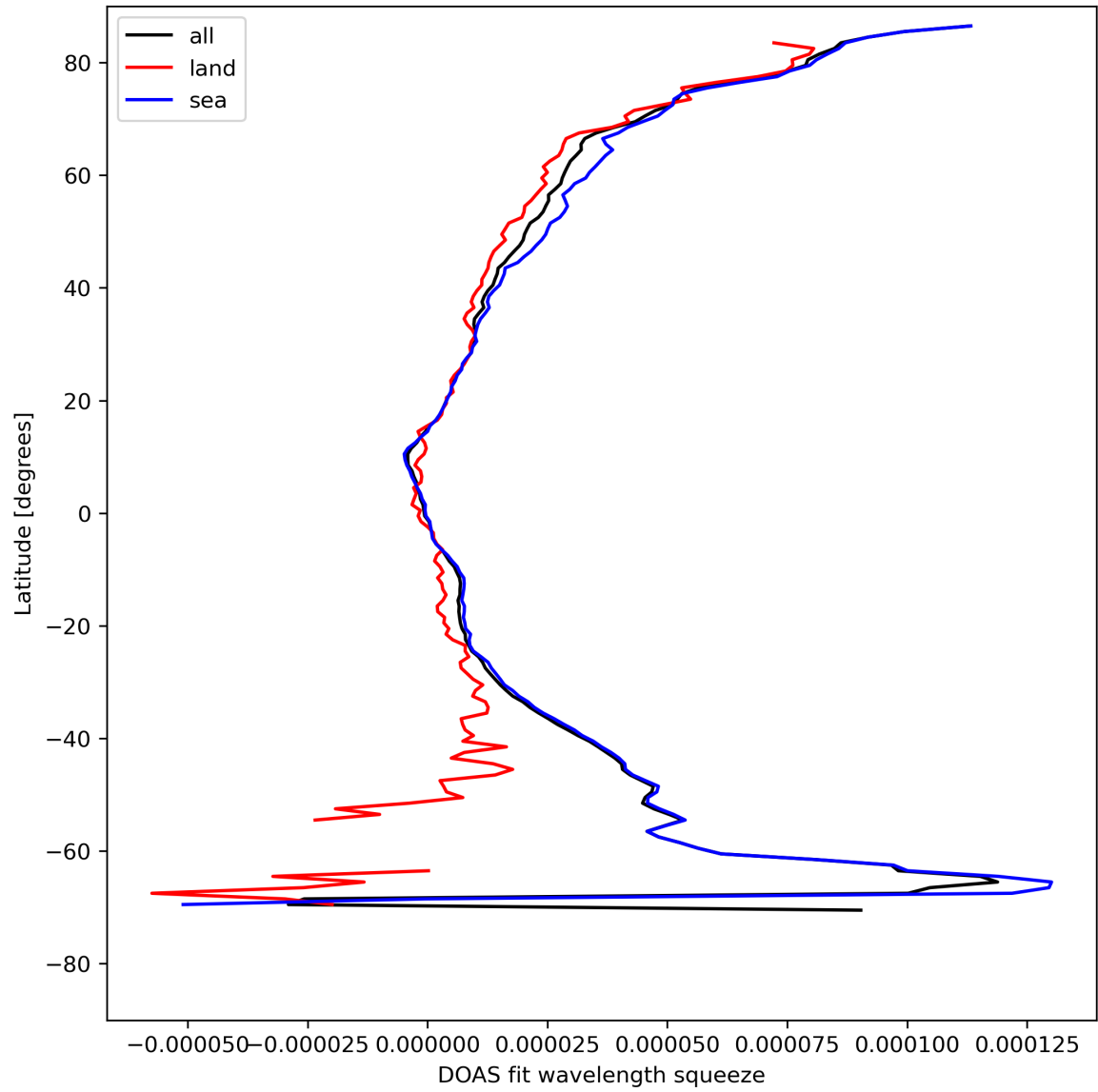
Figure 31: Zonal average of “DOAS fit wavelength squeeze” for 2023-08-14 to 2023-08-16.
