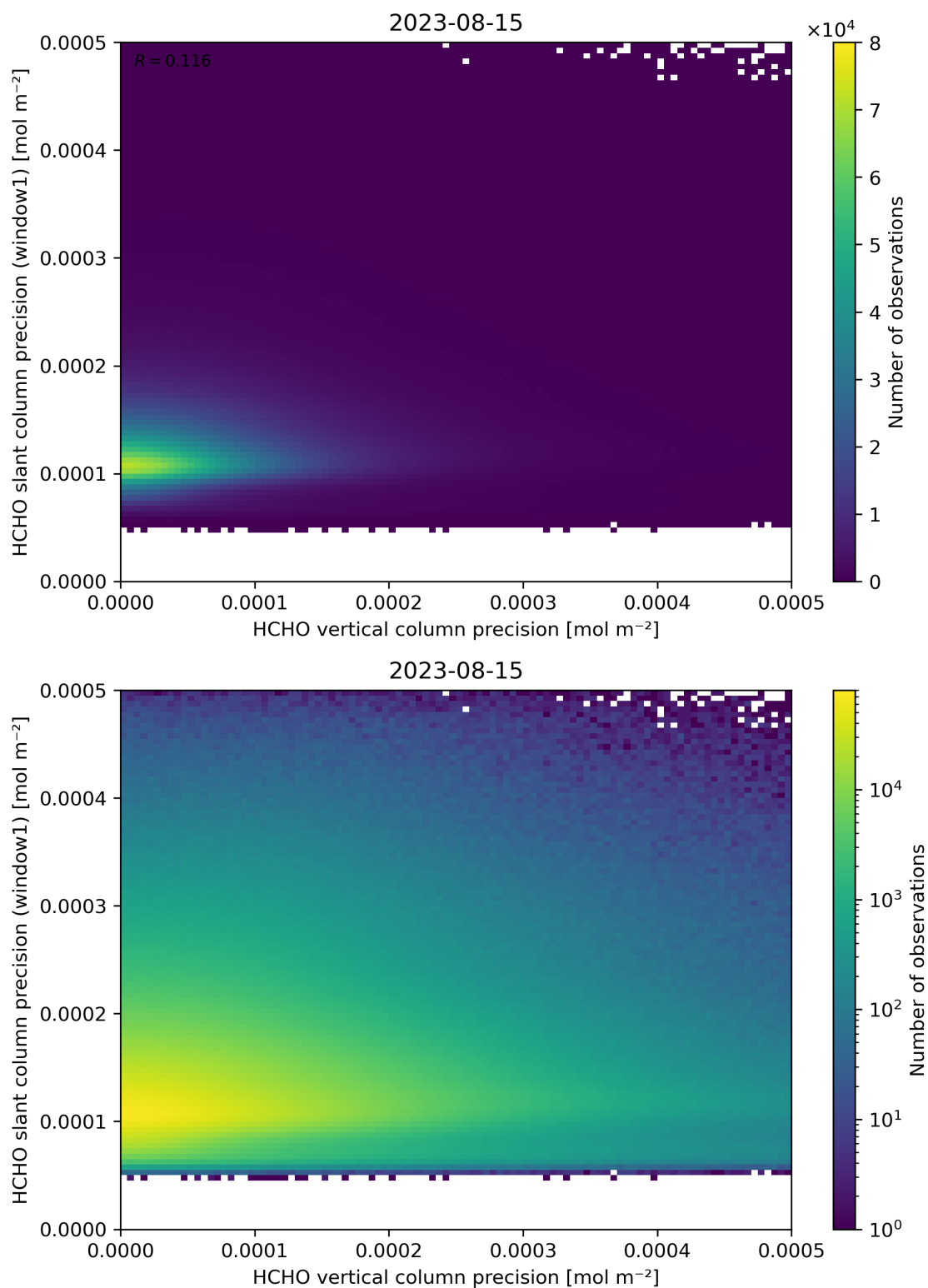
Figure 143: Scatter density plot of “HCHO vertical column precision” against “HCHO slant column precision (window1)” for 2023-08-14 to 2023-08-16.
