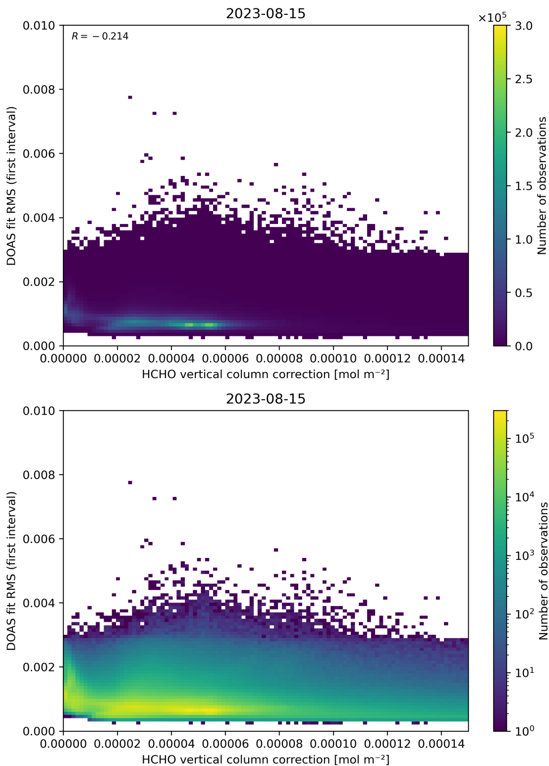
Figure 112: Scatter density plot of “HCHO vertical column correction” against “DOAS fit RMS (first interval)” for 2023-08-14 to 2023-08-16.
