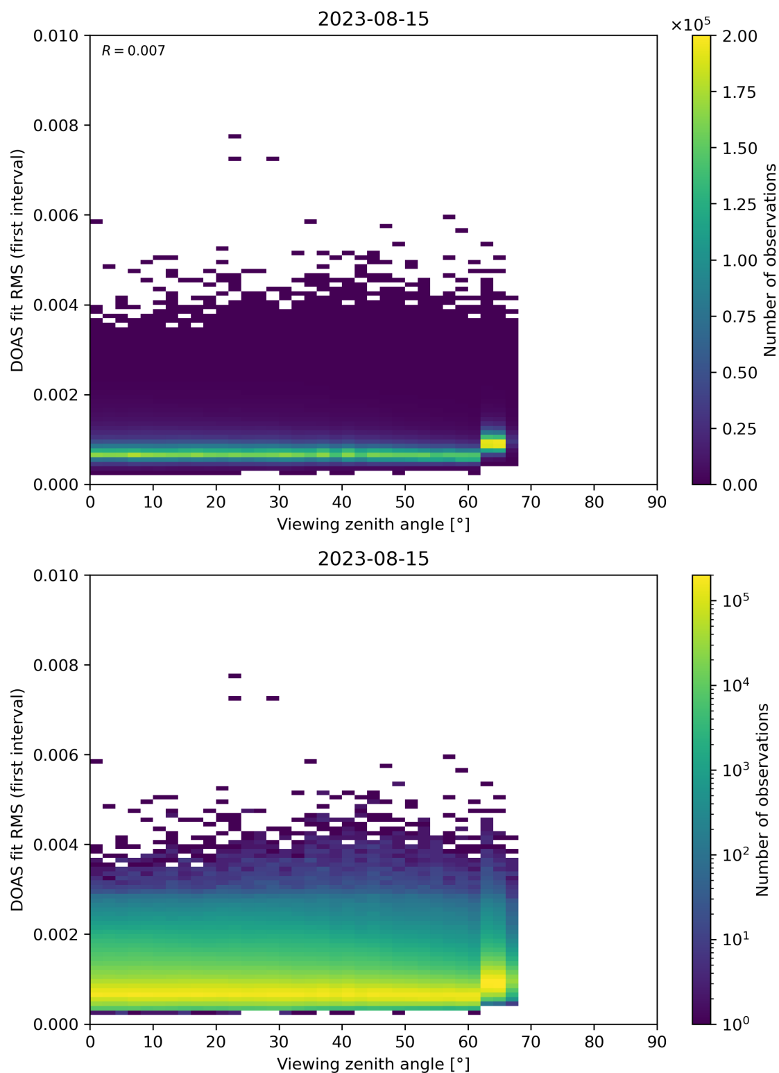
Figure 182: Scatter density plot of “Viewing zenith angle” against “DOAS fit RMS (first interval)” for 2023-08-14 to 2023-08-16.
