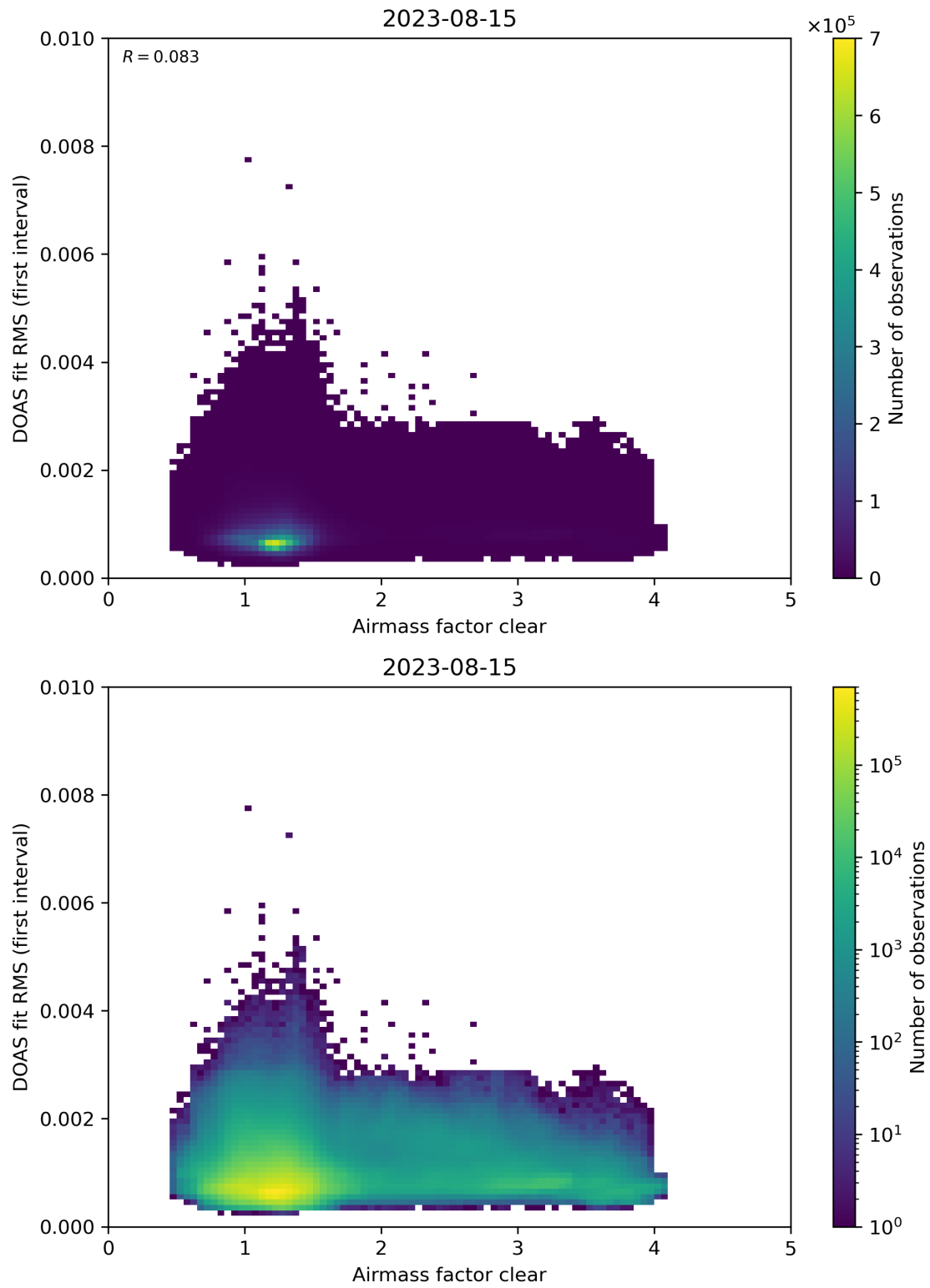
Figure 71: Scatter density plot of “Airmass factor clear” against “DOAS fit RMS (first interval)” for 2023-08-14 to 2023-08-16.
