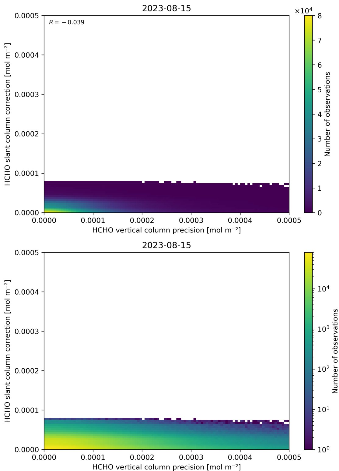
Figure 141: Scatter density plot of “HCHO vertical column precision” against “HCHO slant column correction” for 2023-08-14 to 2023-08-16.
