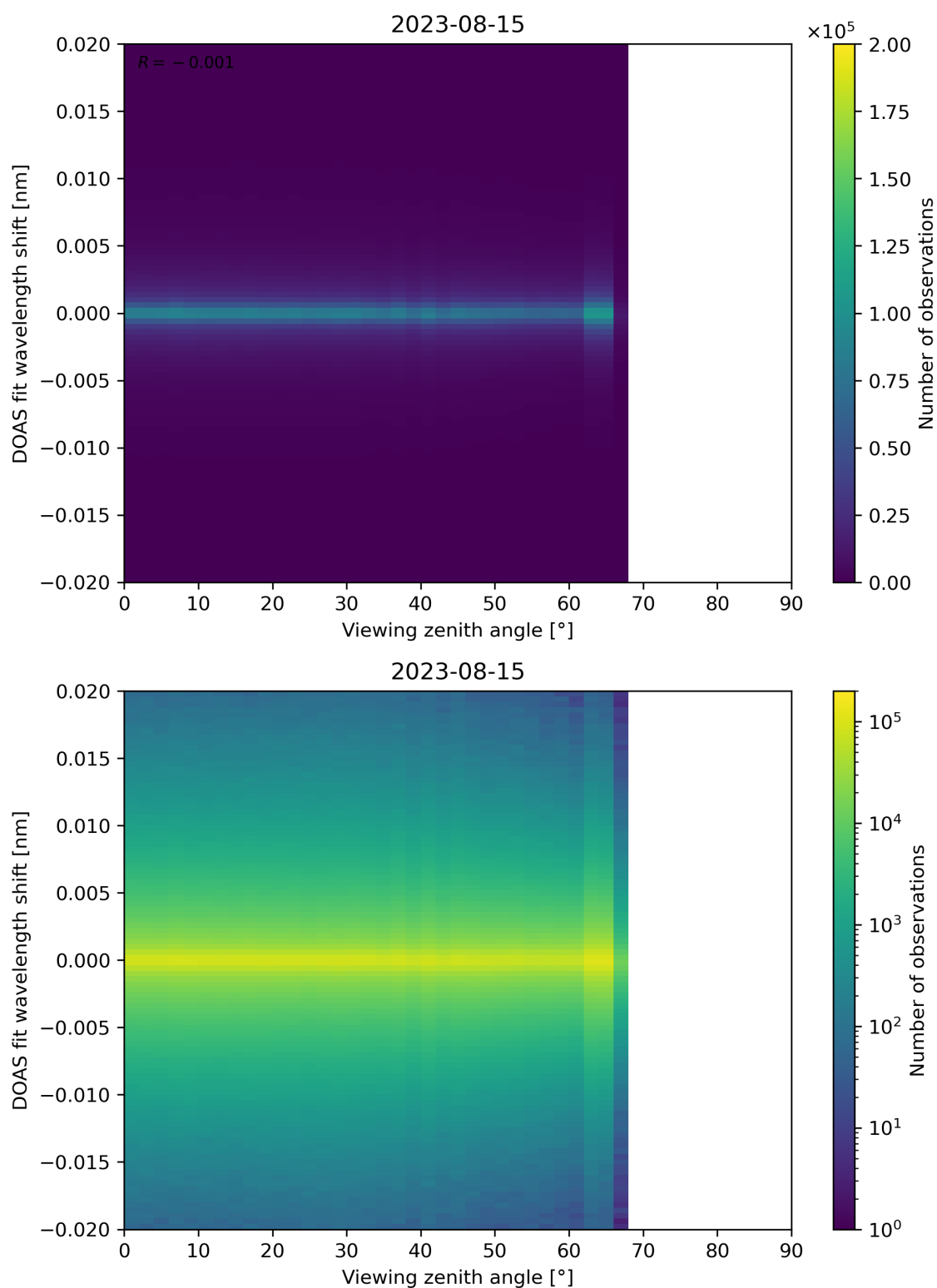
Figure 183: Scatter density plot of “Viewing zenith angle” against “DOAS fit wavelength shift” for 2023-08-14 to 2023-08-16.
