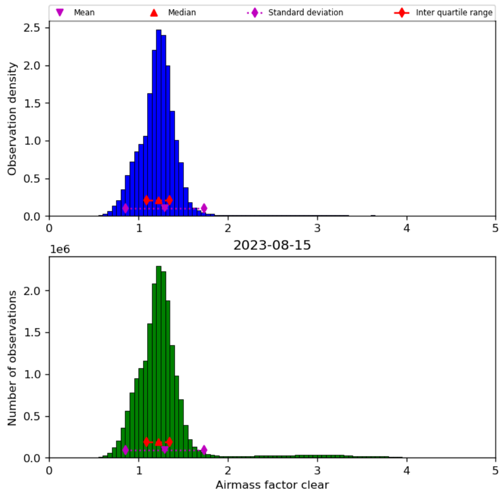
Figure 42: Histogram of “Airmass factor clear” for 2023-08-14 to 2023-08-16
