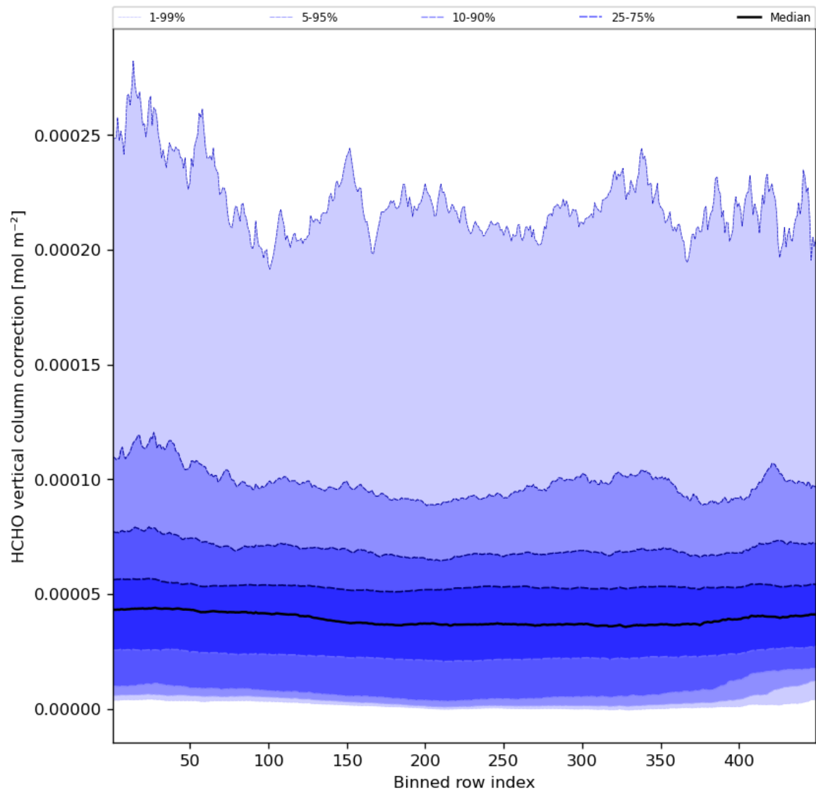
Figure 51: Along track statistics of “HCHO vertical column correction” for 2023-08-14 to 2023-08-16
