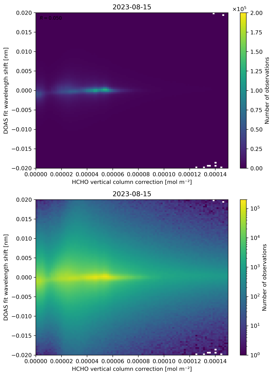
Figure 113: Scatter density plot of “HCHO vertical column correction” against “DOAS fit wavelength shift” for 2023-08-14 to 2023-08-16.
