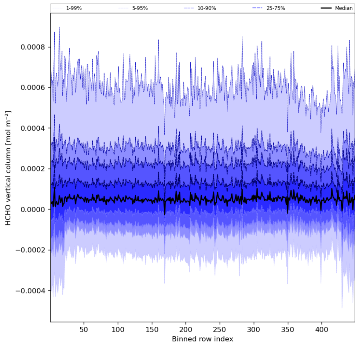
Figure 49: Along track statistics of “HCHO vertical column” for 2023-08-14 to 2023-08-16
