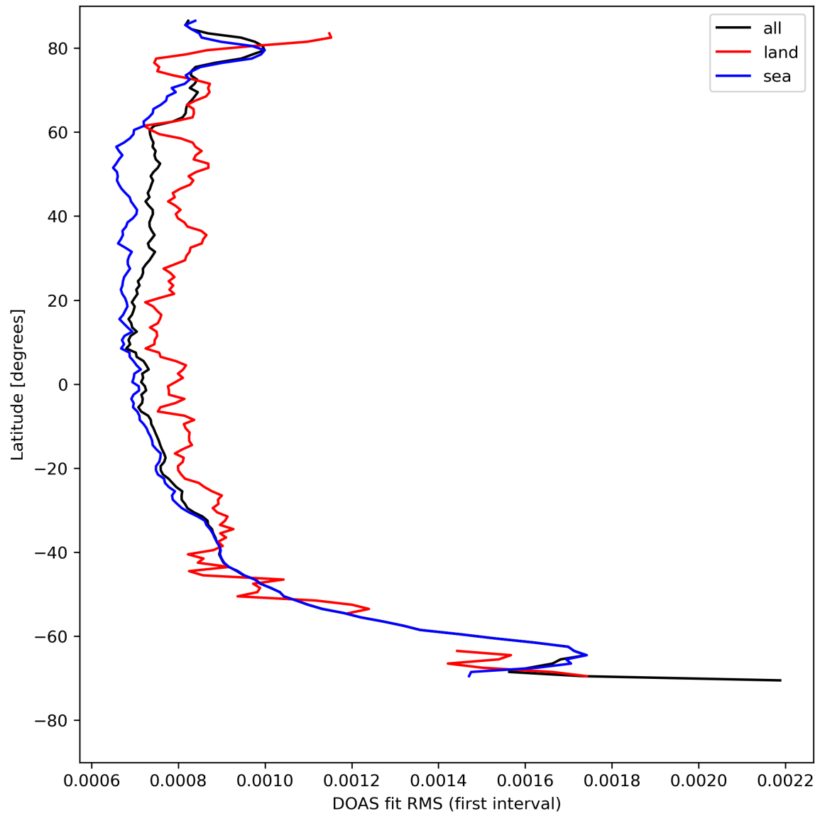
Figure 32: Zonal average of “DOAS fit RMS (first interval)” for 2023-08-14 to 2023-08-16.
