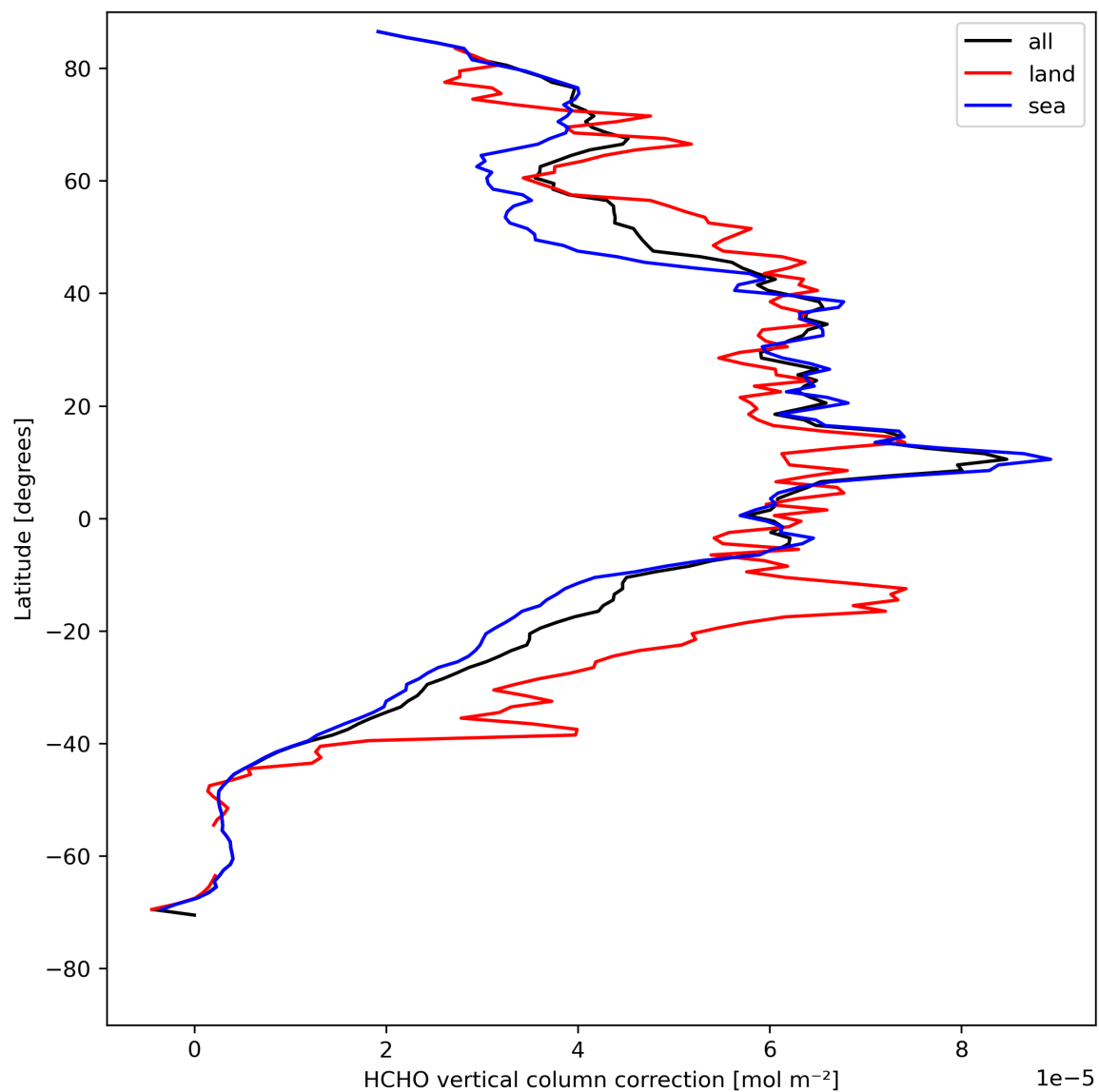
Figure 23: Zonal average of “HCHO vertical column correction” for 2023-08-14 to 2023-08-16.
