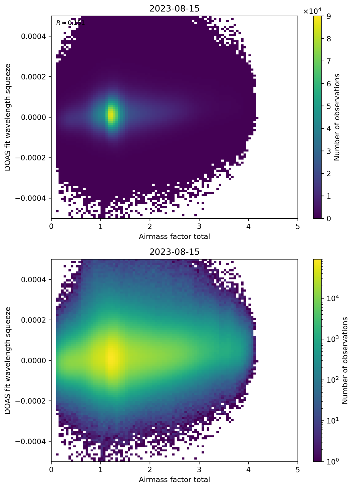
Figure 99: Scatter density plot of “Airmass factor total” against “DOAS fit wavelength squeeze” for 2023-08-14 to 2023-08-16.
