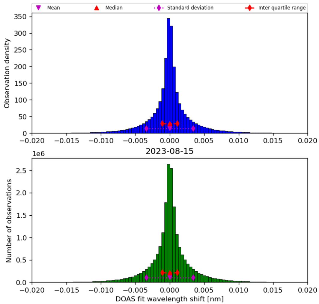
Figure 44: Histogram of “DOAS fit wavelength shift” for 2023-08-14 to 2023-08-16
