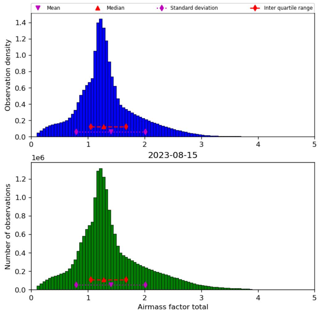
Figure 40: Histogram of “Airmass factor total” for 2023-08-14 to 2023-08-16
