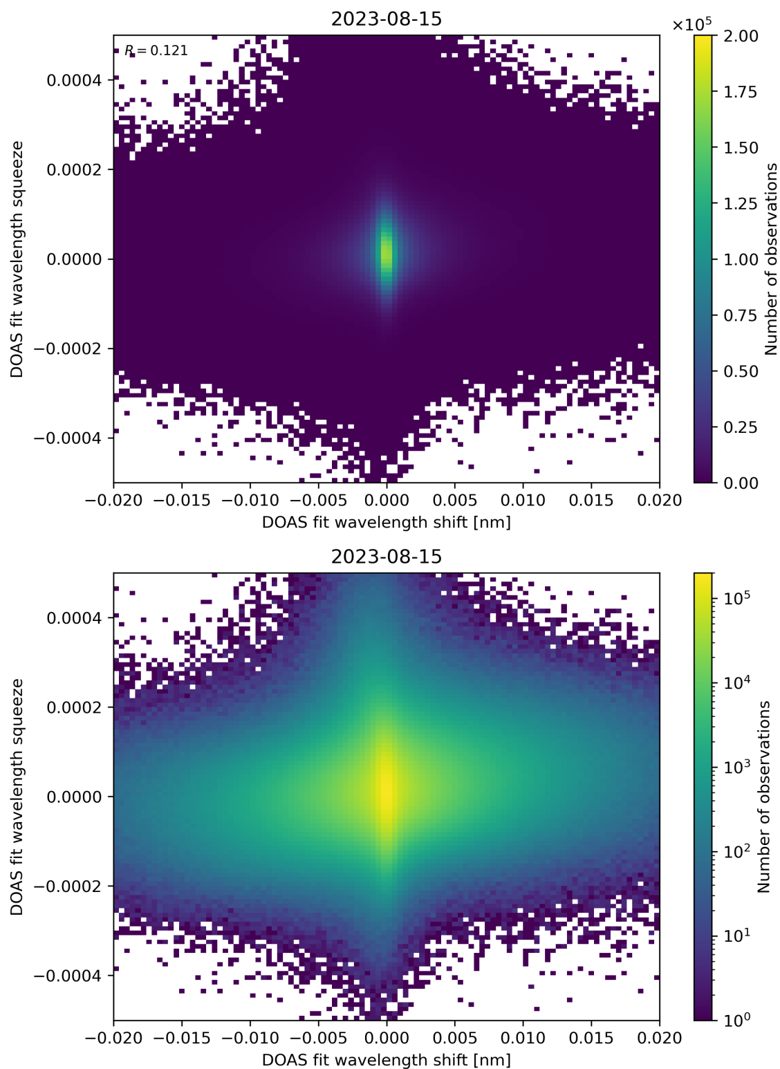
Figure 65: Scatter density plot of “DOAS fit wavelength shift” against “DOAS fit wavelength squeeze” for 2023-08-14 to 2023-08-16.
