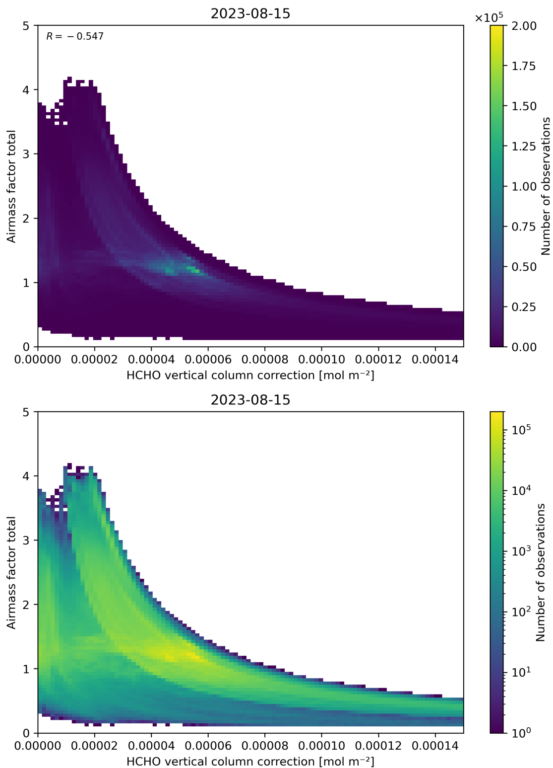
Figure 120: Scatter density plot of “HCHO vertical column correction” against “Airmass factor total” for 2023-08-14 to 2023-08-16.
