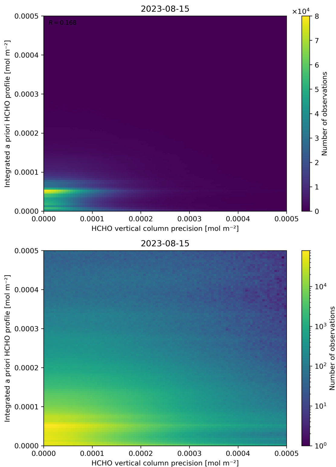
Figure 147: Scatter density plot of “HCHO vertical column precision” against “Integrated a priori HCHO profile” for 2023-08-14 to 2023-08-16.
