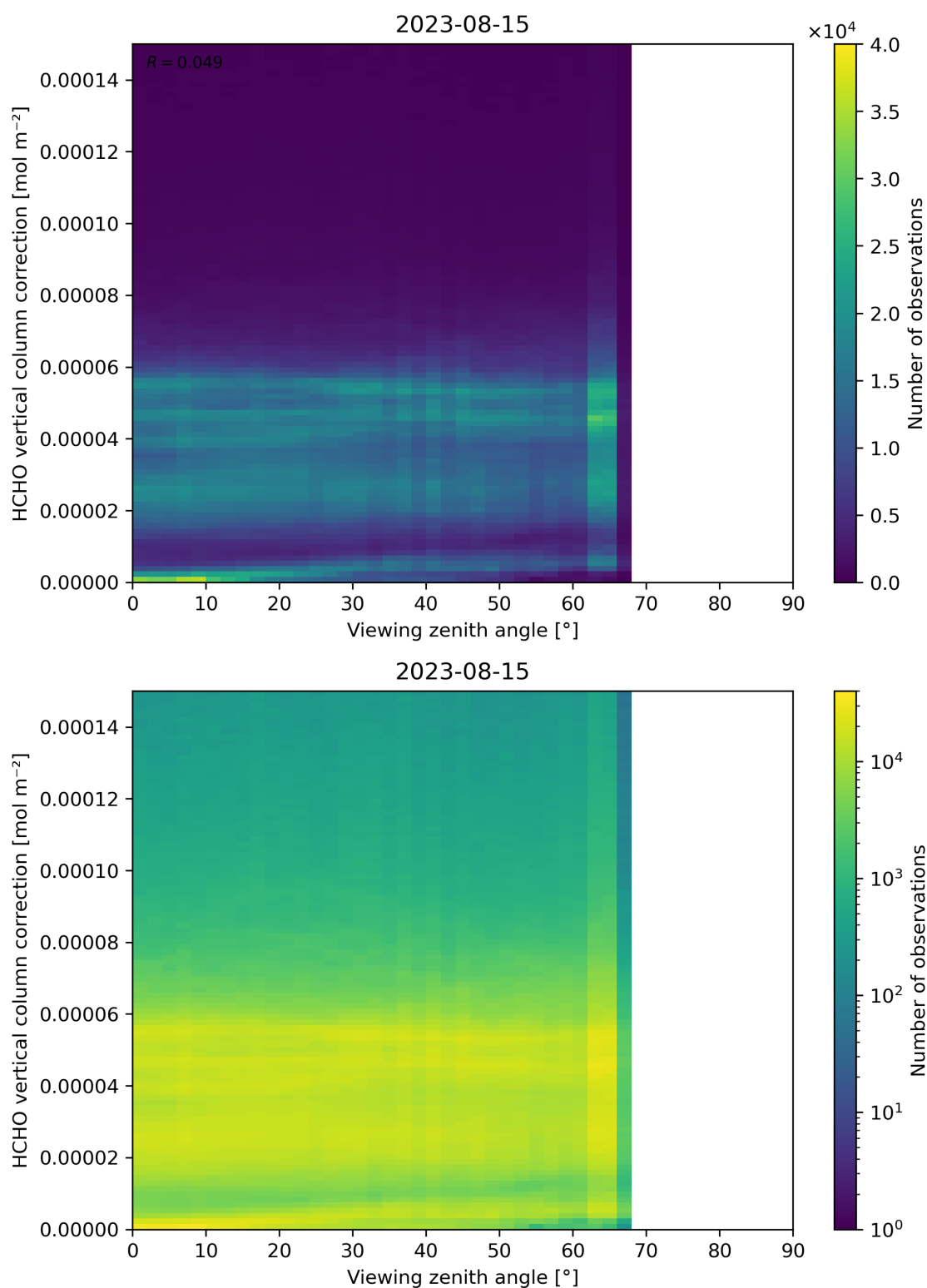
Figure 193: Scatter density plot of “Viewing zenith angle” against “HCHO vertical column correction” for 2023-08-14 to 2023-08-16.
