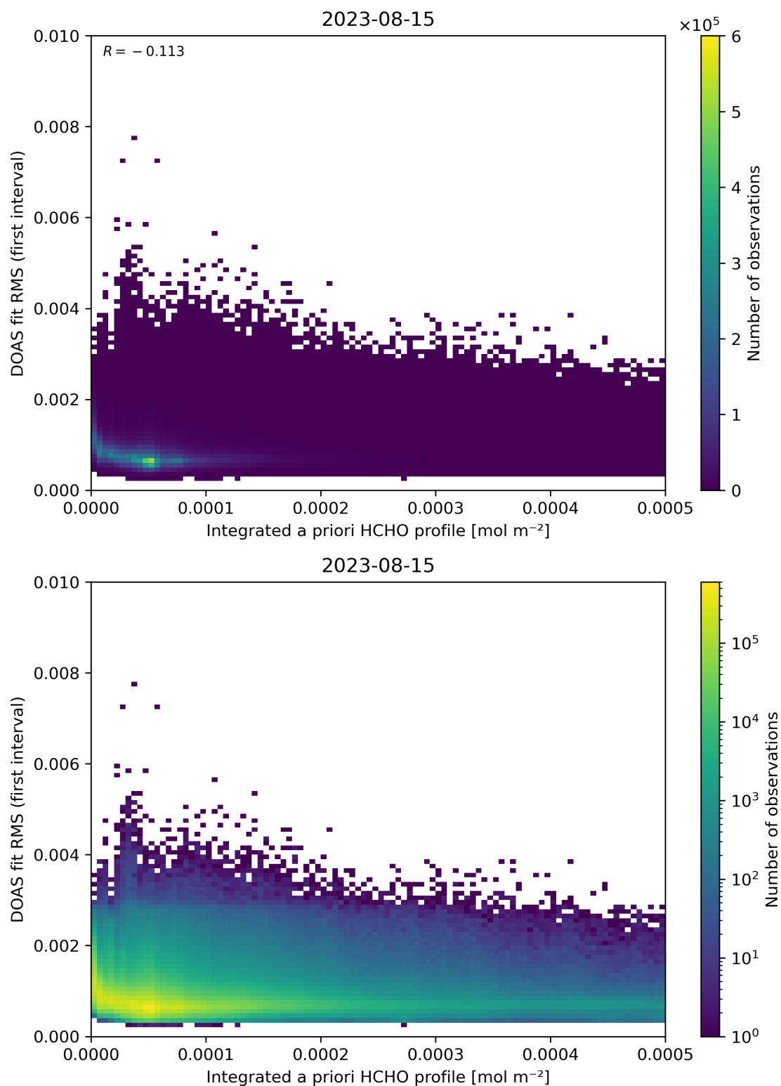
Figure 148: Scatter density plot of “Integrated a priori HCHO profile” against “DOAS fit RMS (first interval)” for 2023-08-14 to 2023-08-16.
