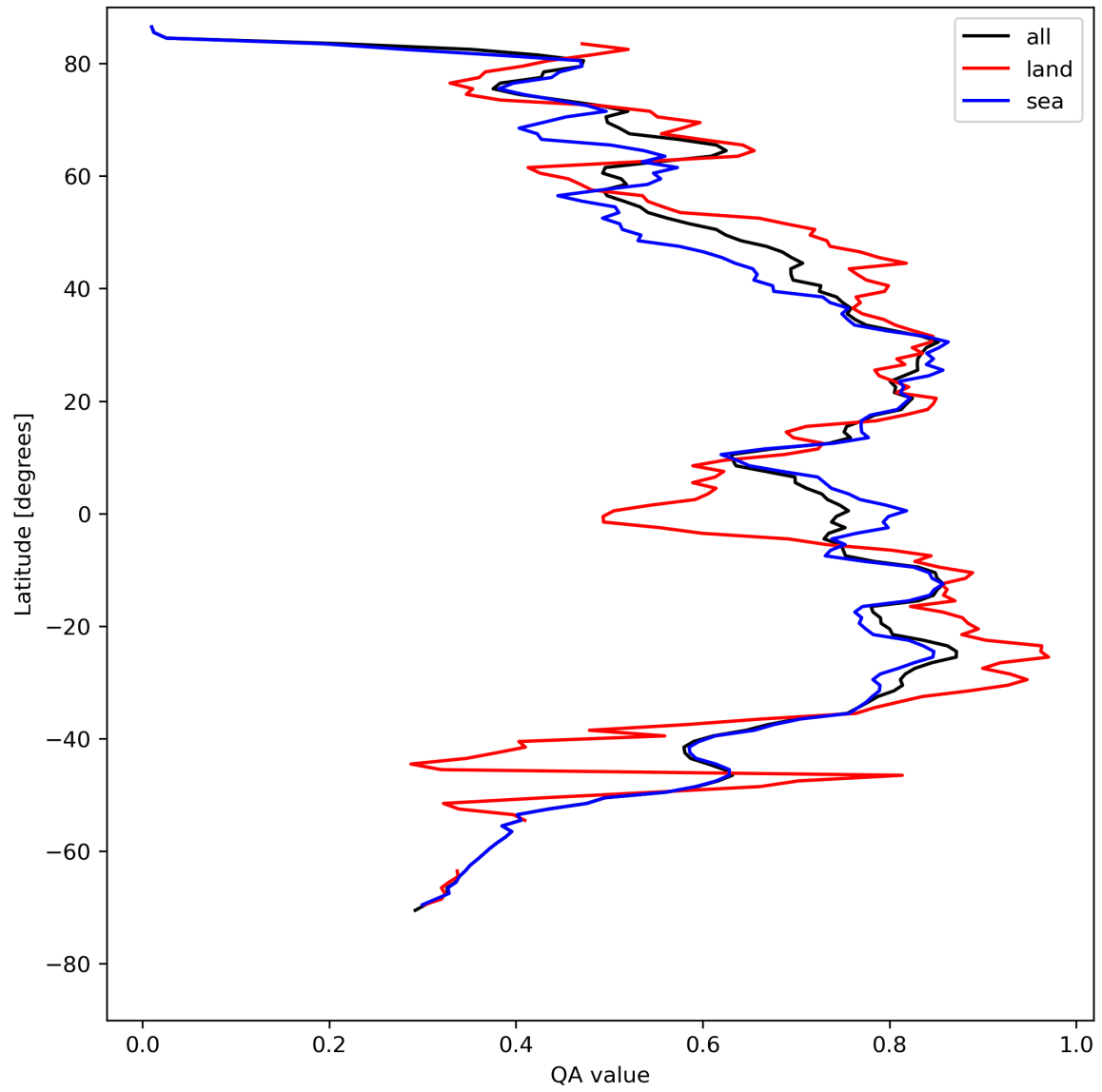
Figure 20: Zonal average of “QA value” for 2023-08-14 to 2023-08-16.
