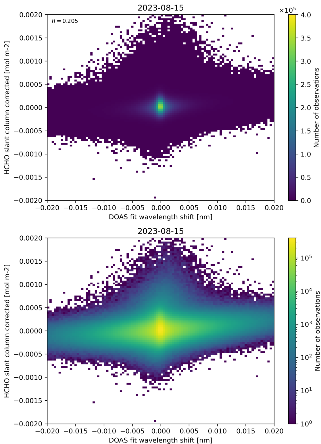
Figure 66: Scatter density plot of “DOAS fit wavelength shift” against “HCHO slant column corrected” for 2023-08-14 to 2023-08-16.
