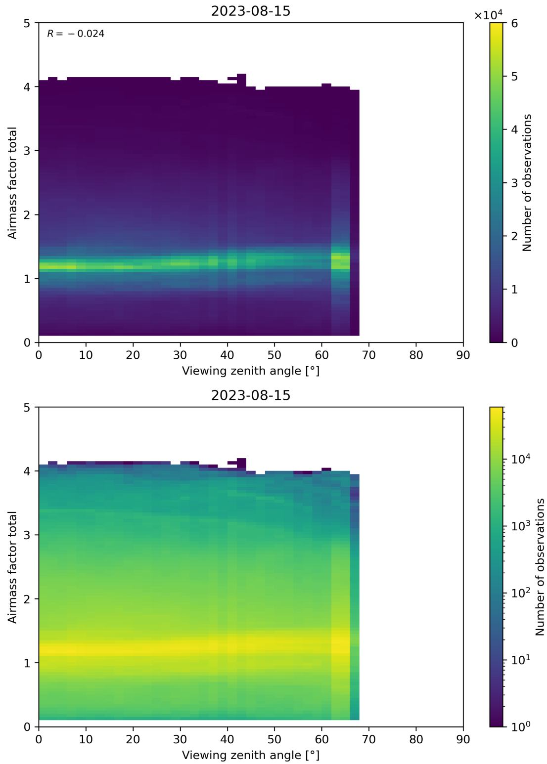
Figure 190: Scatter density plot of “Viewing zenith angle” against “Airmass factor total” for 2023-08-14 to 2023-08-16.
