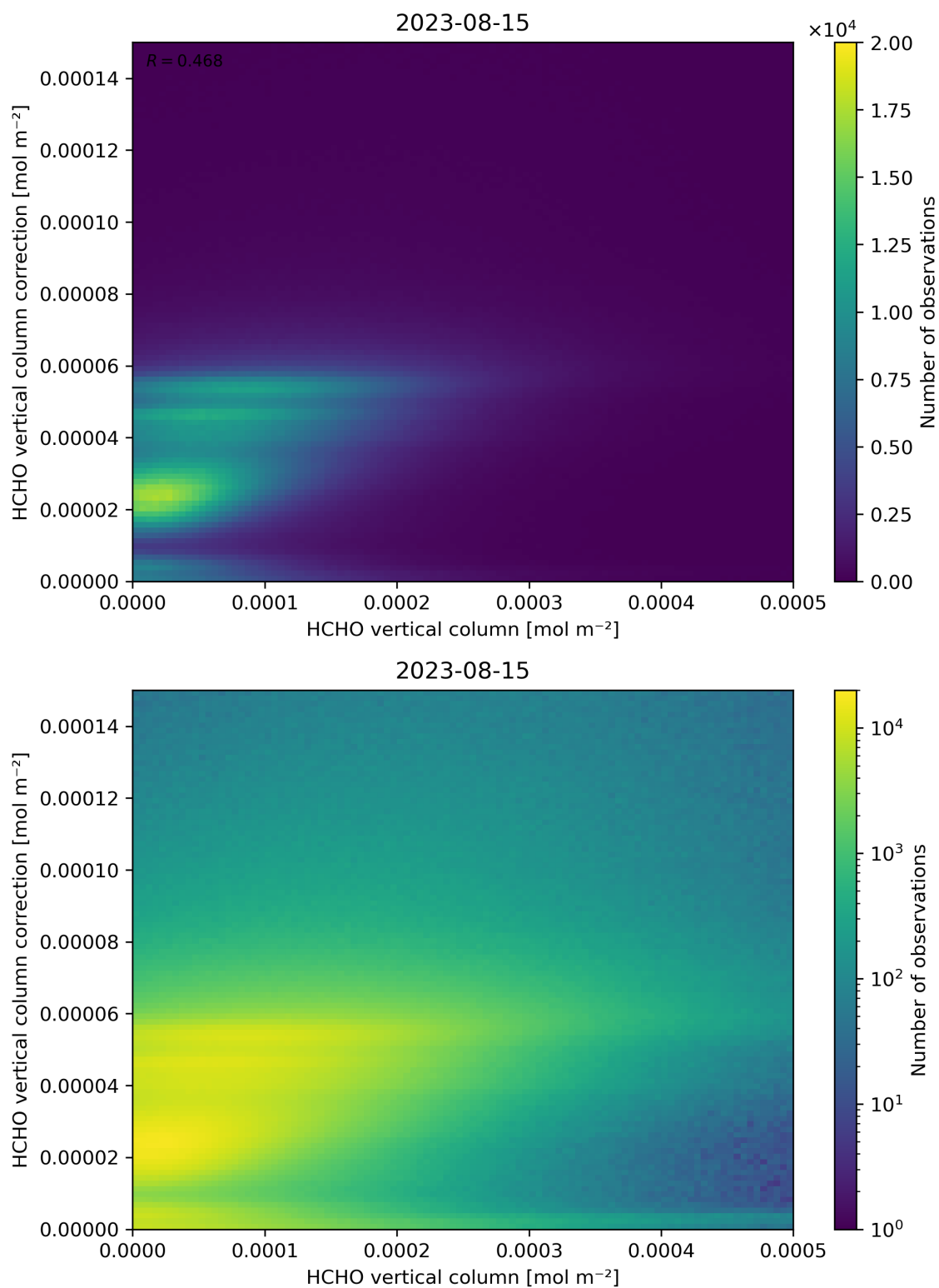
Figure 133: Scatter density plot of “HCHO vertical column” against “HCHO vertical column correction” for 2023-08-14 to 2023-08-16.
