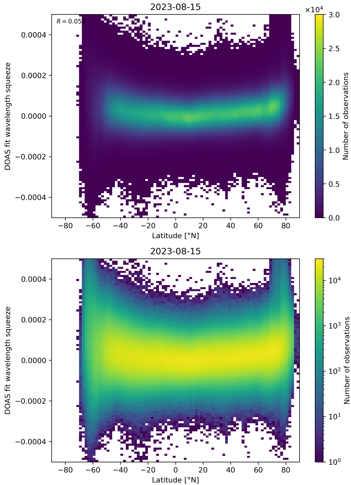
Figure 155: Scatter density plot of “Latitude” against “DOAS fit wavelength squeeze” for 2023-08-14 to 2023-08-16.
