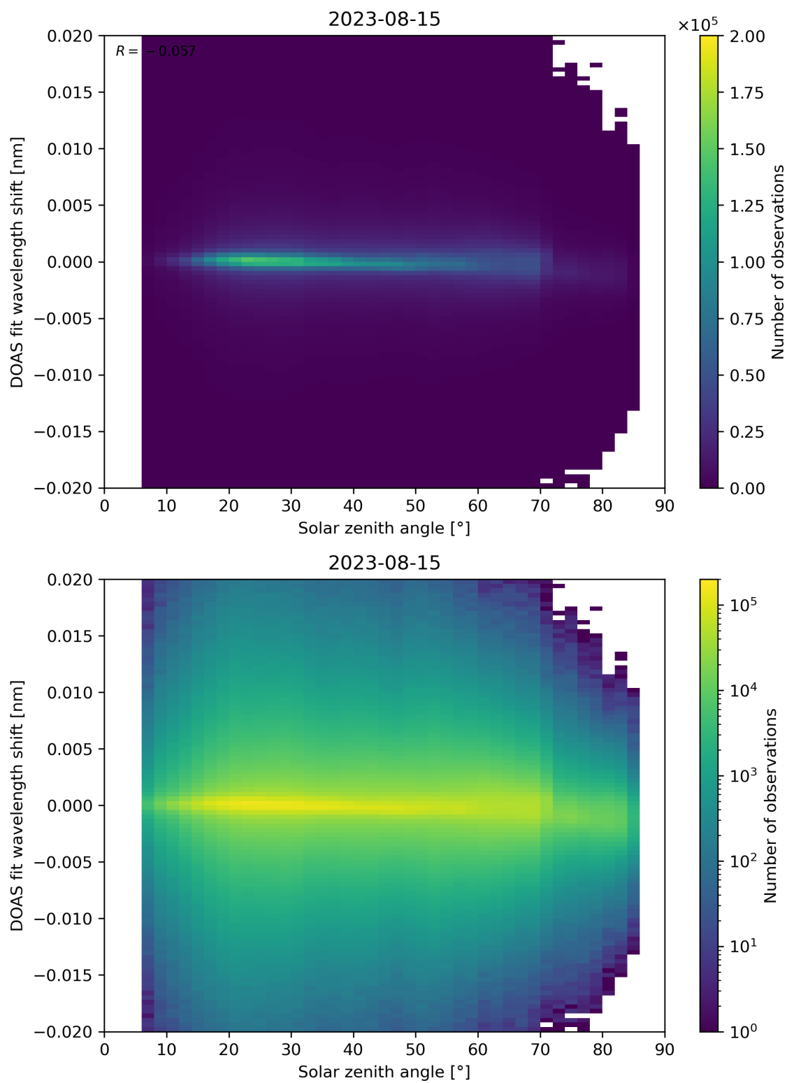
Figure 168: Scatter density plot of “Solar zenith angle” against “DOAS fit wavelength shift” for 2023-08-14 to 2023-08-16.
