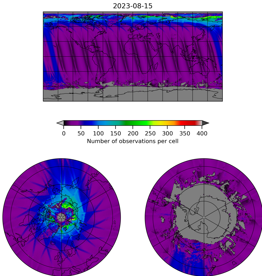
Figure 19: Map of the number of observations for 2023-08-14 to 2023-08-16
