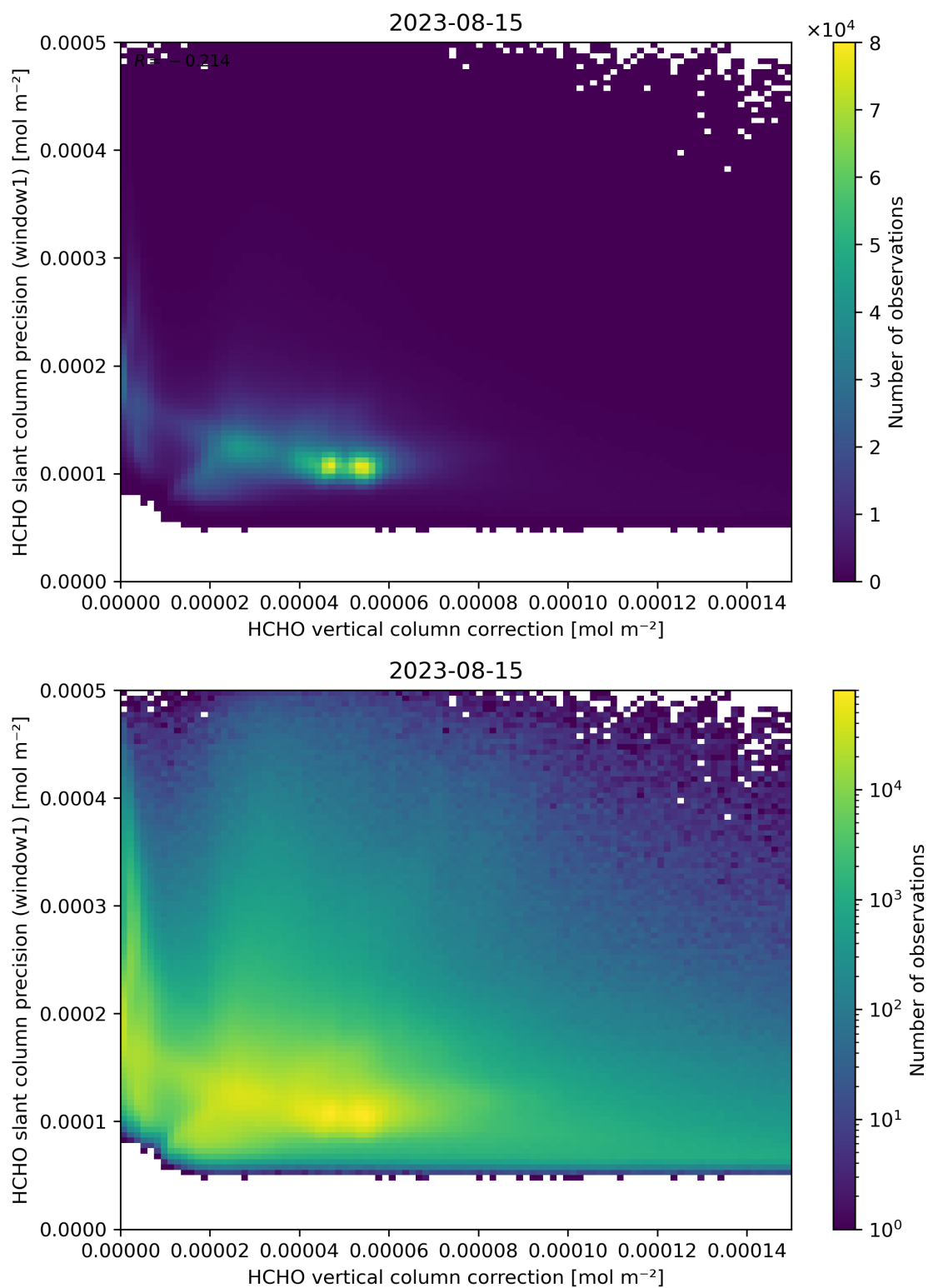
Figure 119: Scatter density plot of “HCHO vertical column correction” against “HCHO slant column precision (window1)” for 2023-08-14 to 2023-08-16.
