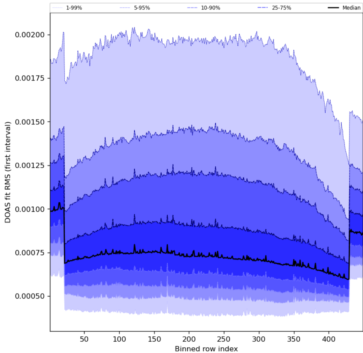
Figure 60: Along track statistics of “DOAS fit RMS (first interval)” for 2023-08-14 to 2023-08-16
