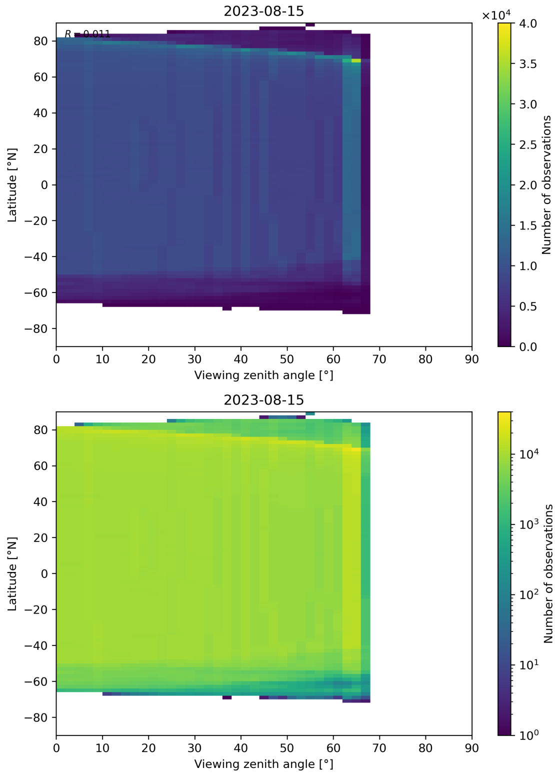
Figure 196: Scatter density plot of “Viewing zenith angle” against “Latitude” for 2023-08-14 to 2023-08-16.
