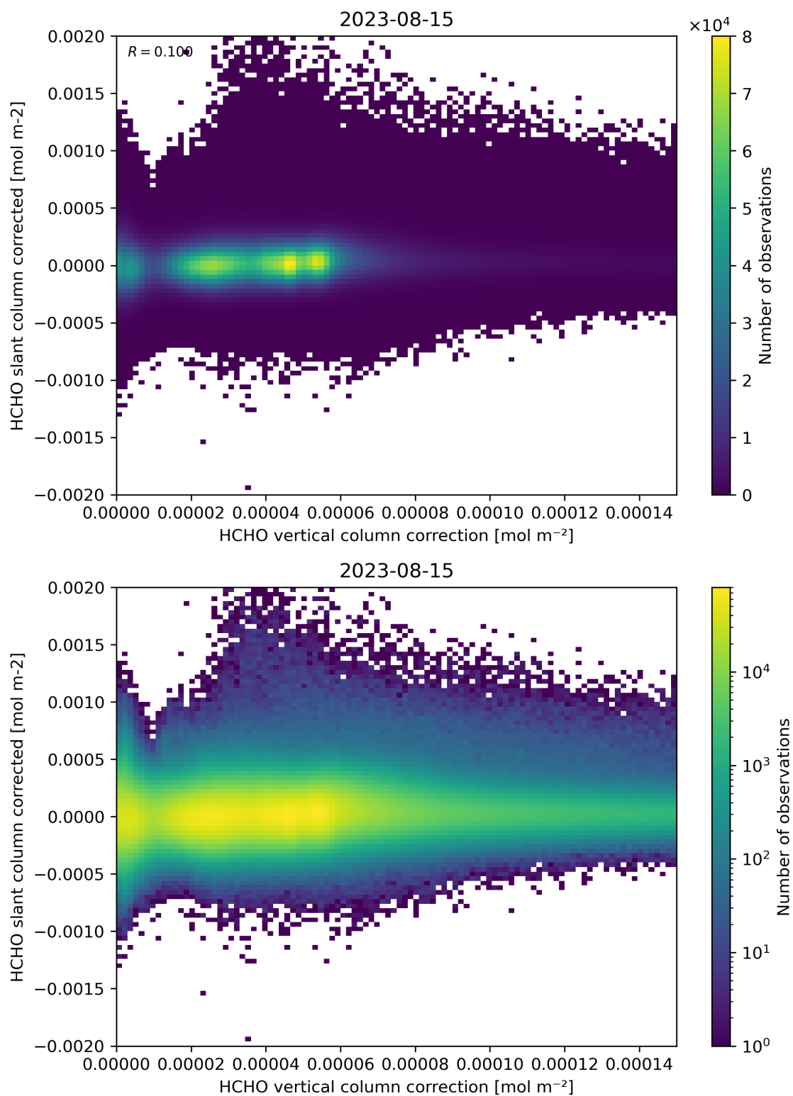
Figure 116: Scatter density plot of “HCHO vertical column correction” against “HCHO slant column corrected” for 2023-08-14 to 2023-08-16.
