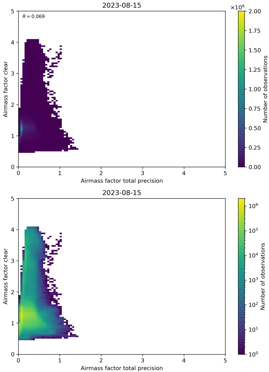
Figure 108: Scatter density plot of “Airmass factor total precision” against “Airmass factor clear” for 2023-08-14 to 2023-08-16.
