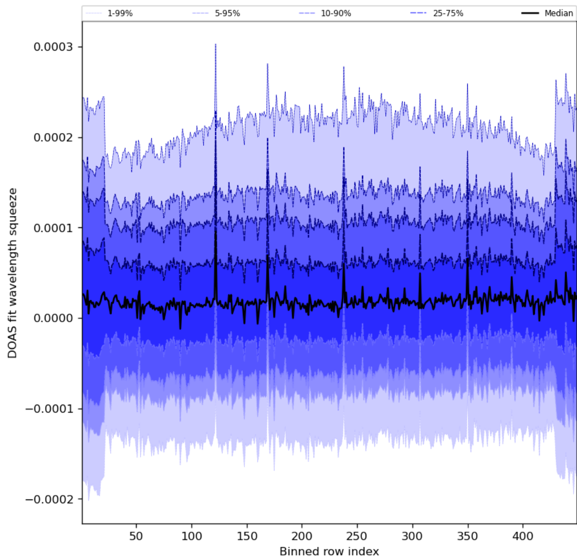
Figure 59: Along track statistics of “DOAS fit wavelength squeeze” for 2023-08-14 to 2023-08-16
