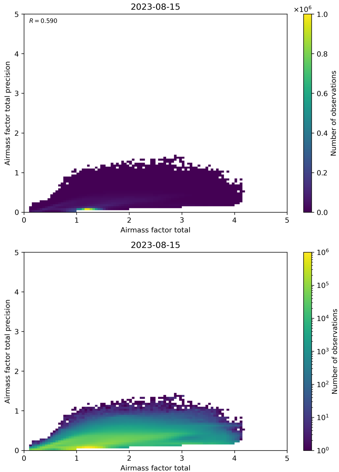
Figure 103: Scatter density plot of “Airmass factor total” against “Airmass factor total precision” for 2023-08-14 to 2023-08-16.
