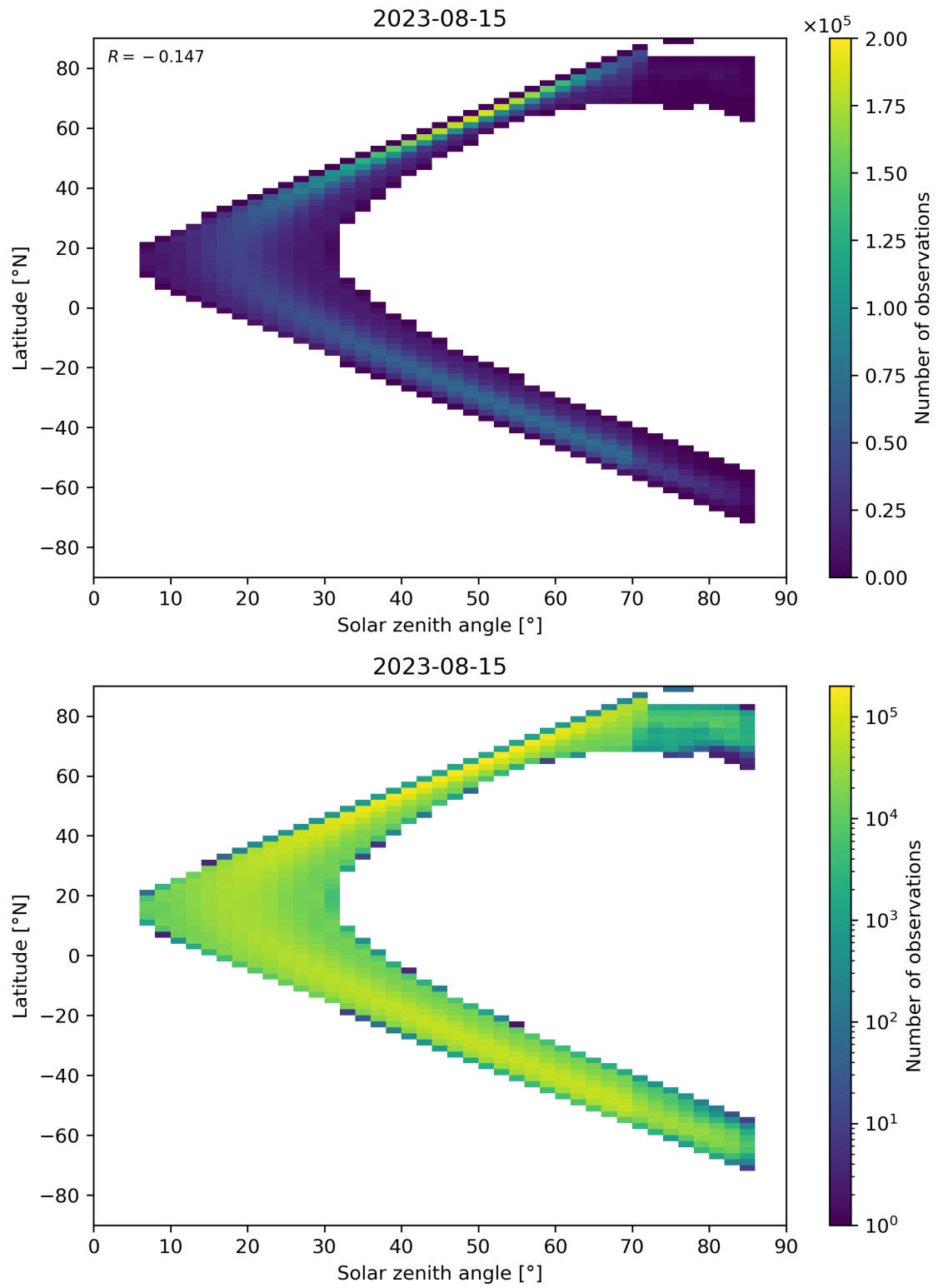
Figure 181: Scatter density plot of “Solar zenith angle” against “Latitude” for 2023-08-14 to 2023-08-16.
