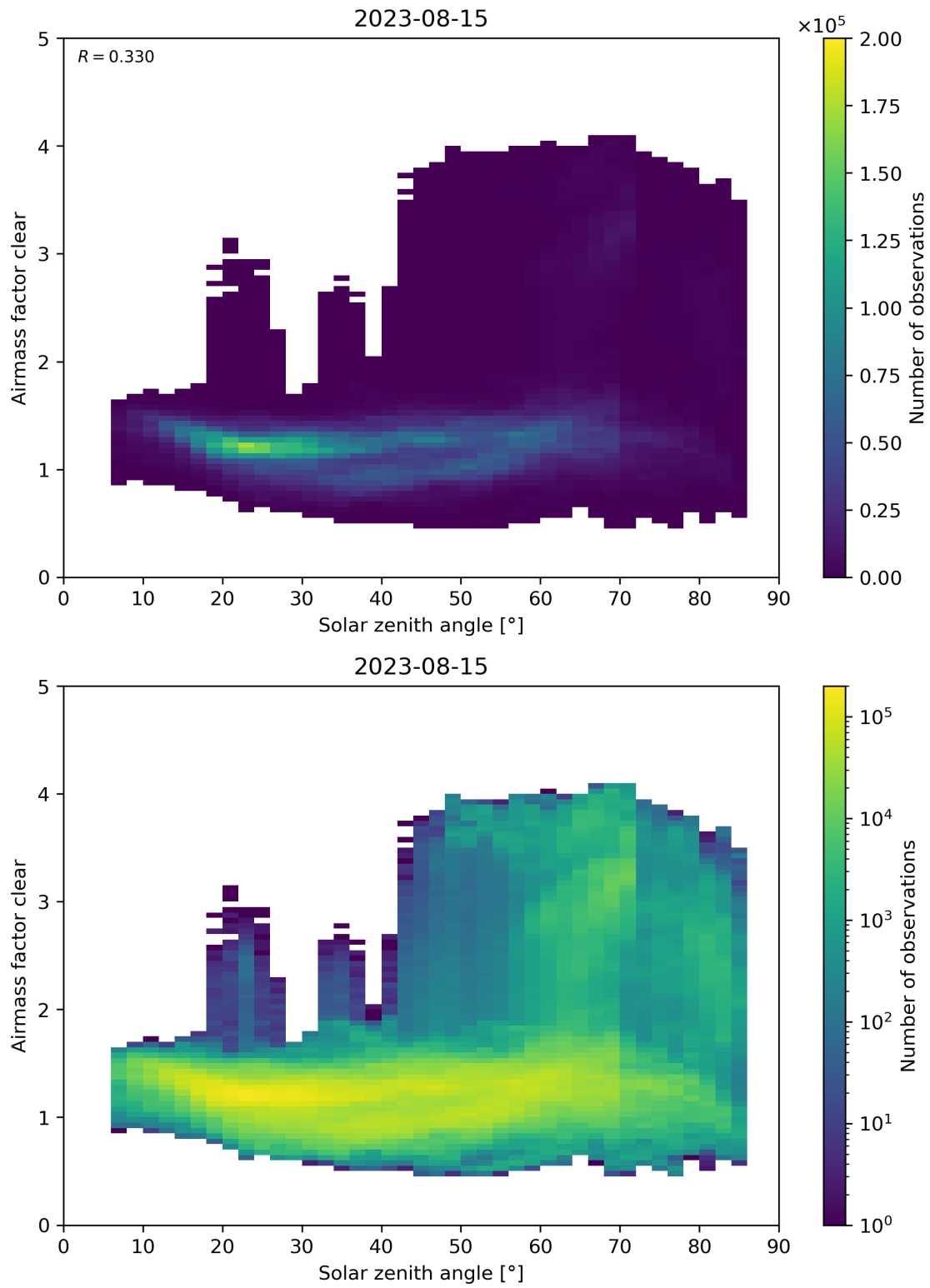
Figure 170: Scatter density plot of “Solar zenith angle” against “Airmass factor clear” for 2023-08-14 to 2023-08-16.
