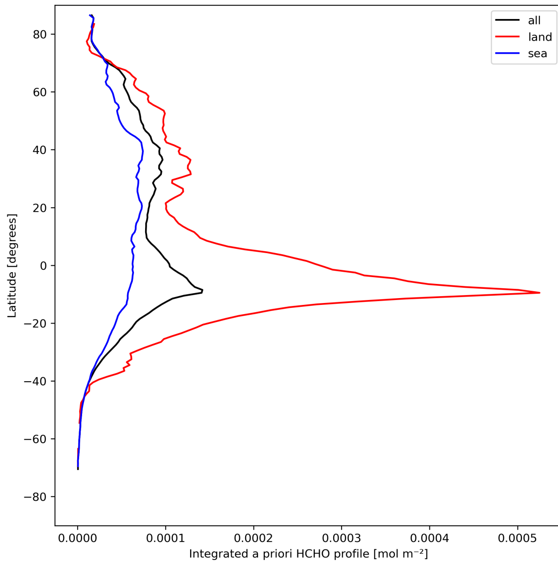
Figure 29: Zonal average of “Integrated a priori HCHO profile” for 2023-08-14 to 2023-08-16.
