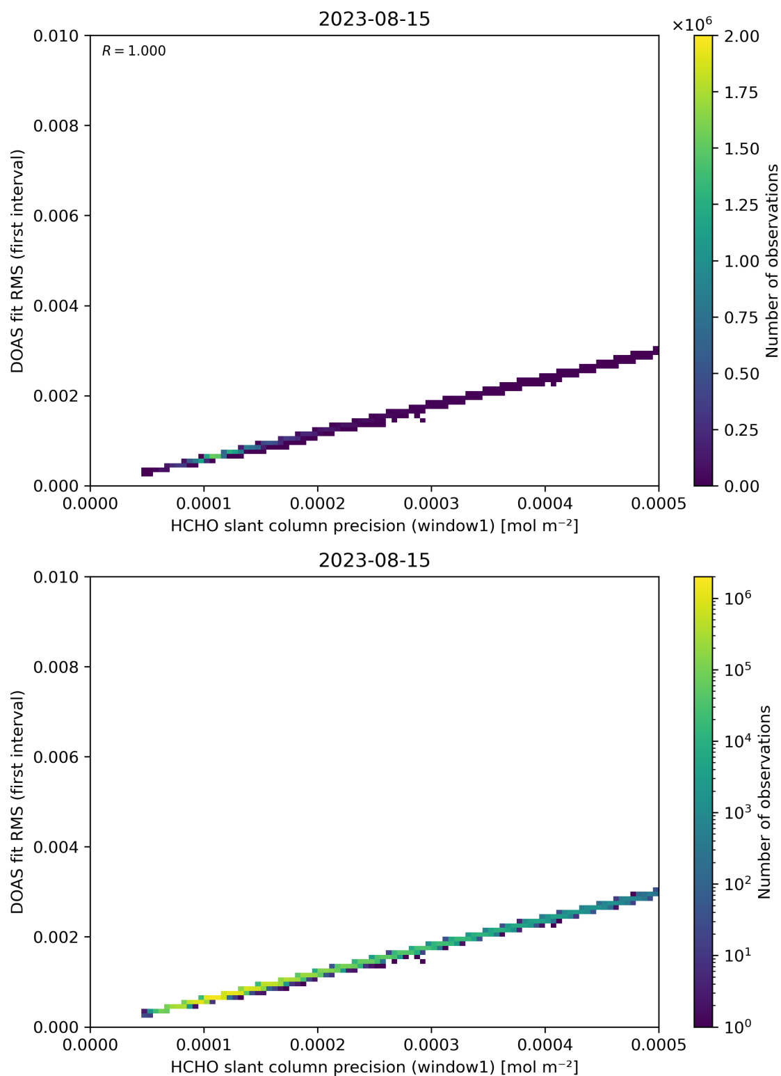
Figure 88: Scatter density plot of “HCHO slant column precision (window1)” against “DOAS fit RMS (first interval)” for 2023-08-14 to 2023-08-16.
