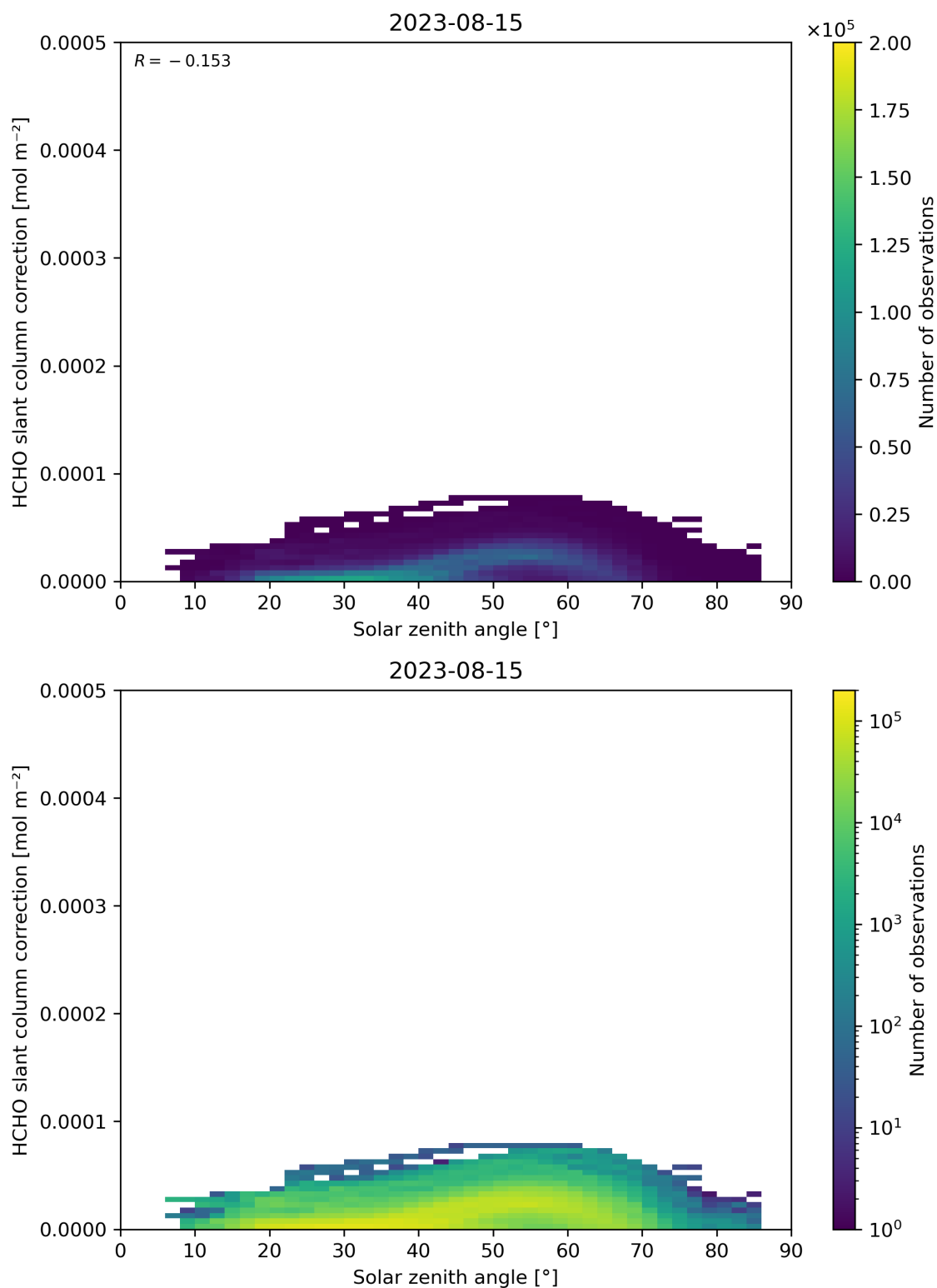
Figure 172: Scatter density plot of “Solar zenith angle” against “HCHO slant column correction” for 2023-08-14 to 2023-08-16.
