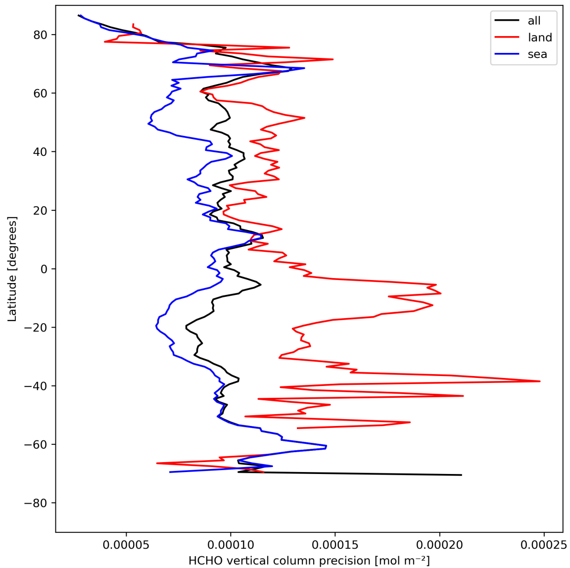
Figure 22: Zonal average of “HCHO vertical column precision” for 2023-08-14 to 2023-08-16.
