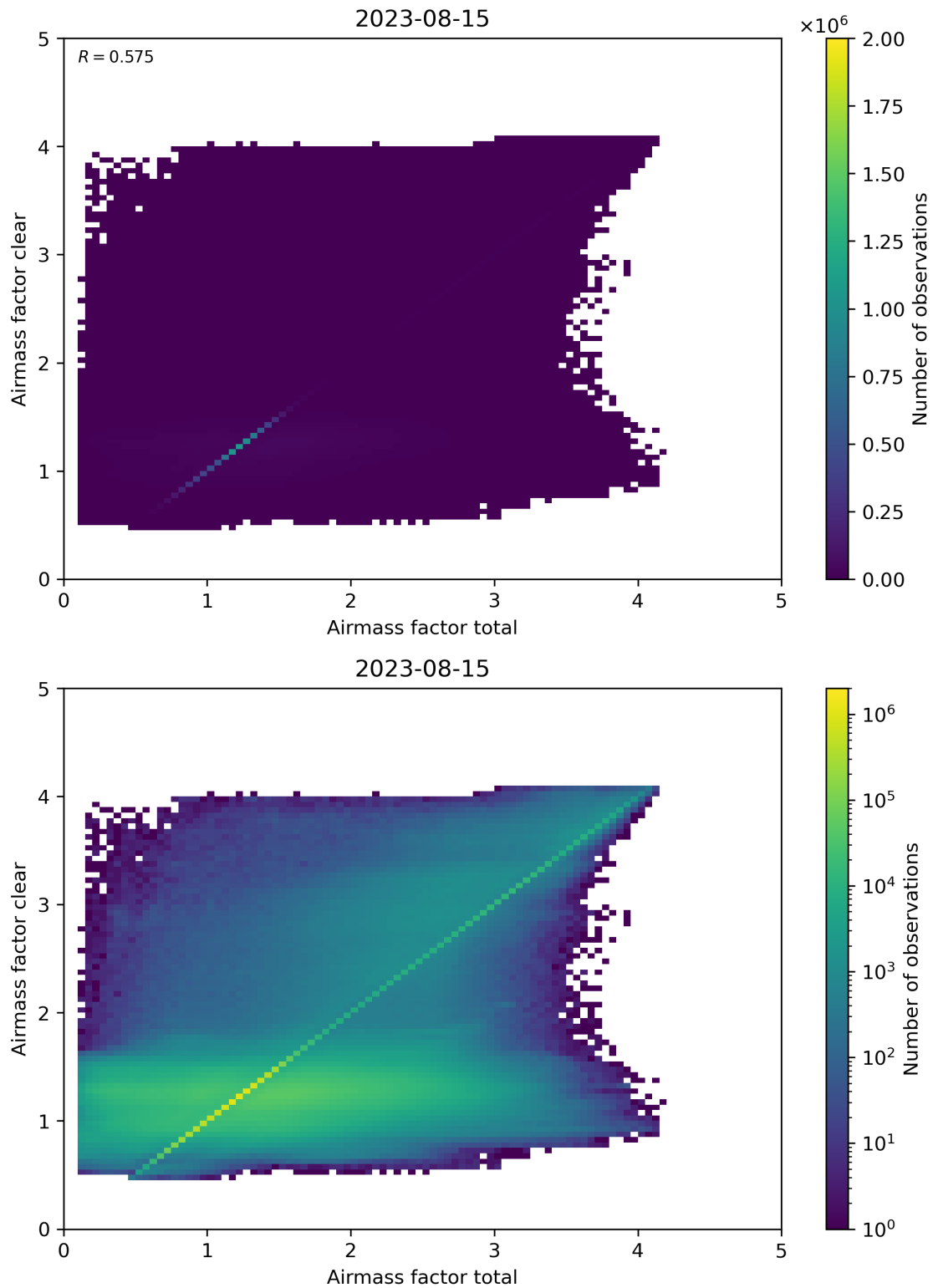
Figure 100: Scatter density plot of “Airmass factor total” against “Airmass factor clear” for 2023-08-14 to 2023-08-16.
