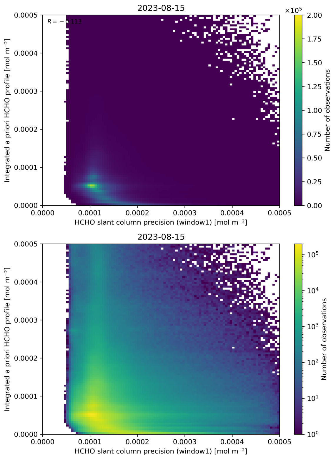
Figure 96: Scatter density plot of “HCHO slant column precision (window1)” against “Integrated a priori HCHO profile” for 2023-08-14 to 2023-08-16.
