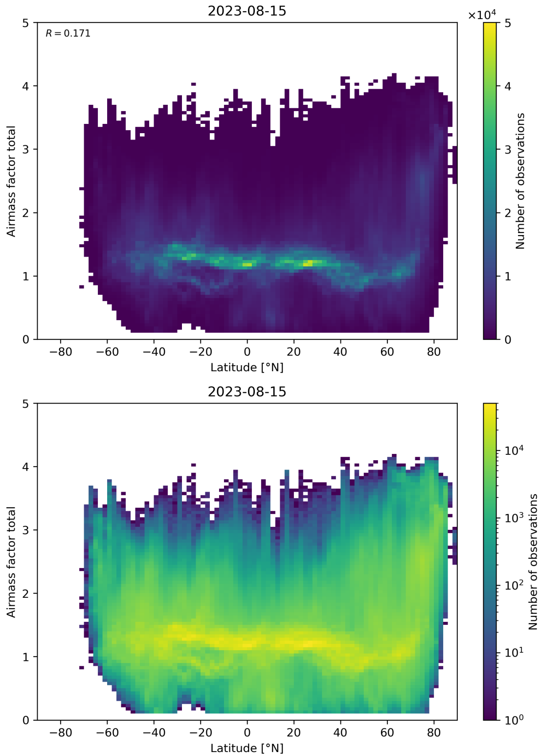
Figure 161: Scatter density plot of “Latitude” against “Airmass factor total” for 2023-08-14 to 2023-08-16.
