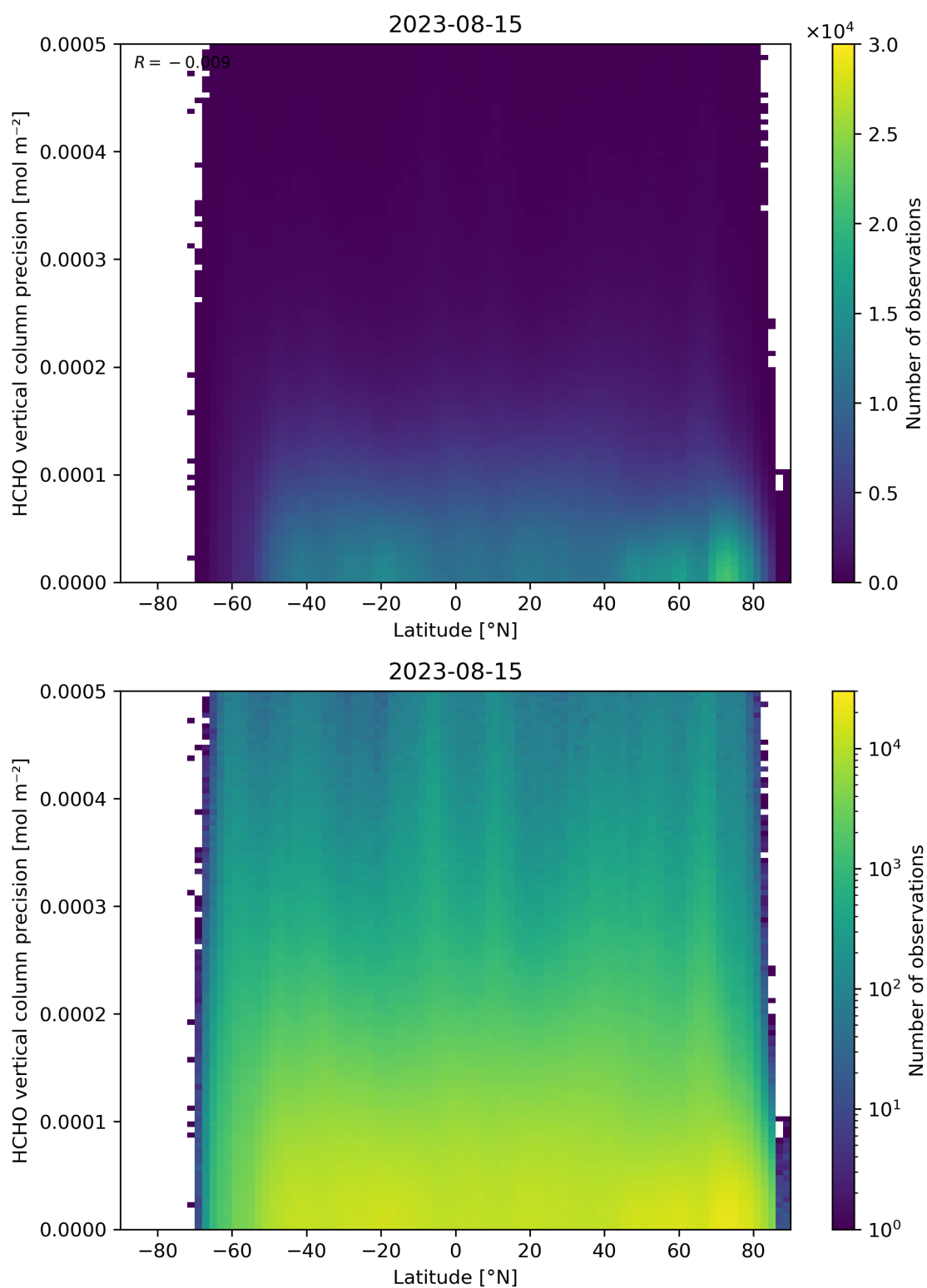
Figure 165: Scatter density plot of “Latitude” against “HCHO vertical column precision” for 2023-08-14 to 2023-08-16.
