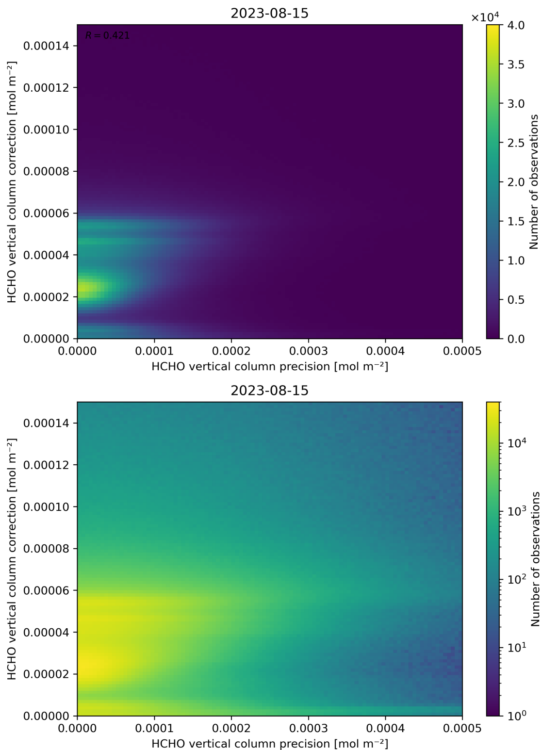
Figure 146: Scatter density plot of “HCHO vertical column precision” against “HCHO vertical column correction” for 2023-08-14 to 2023-08-16.
