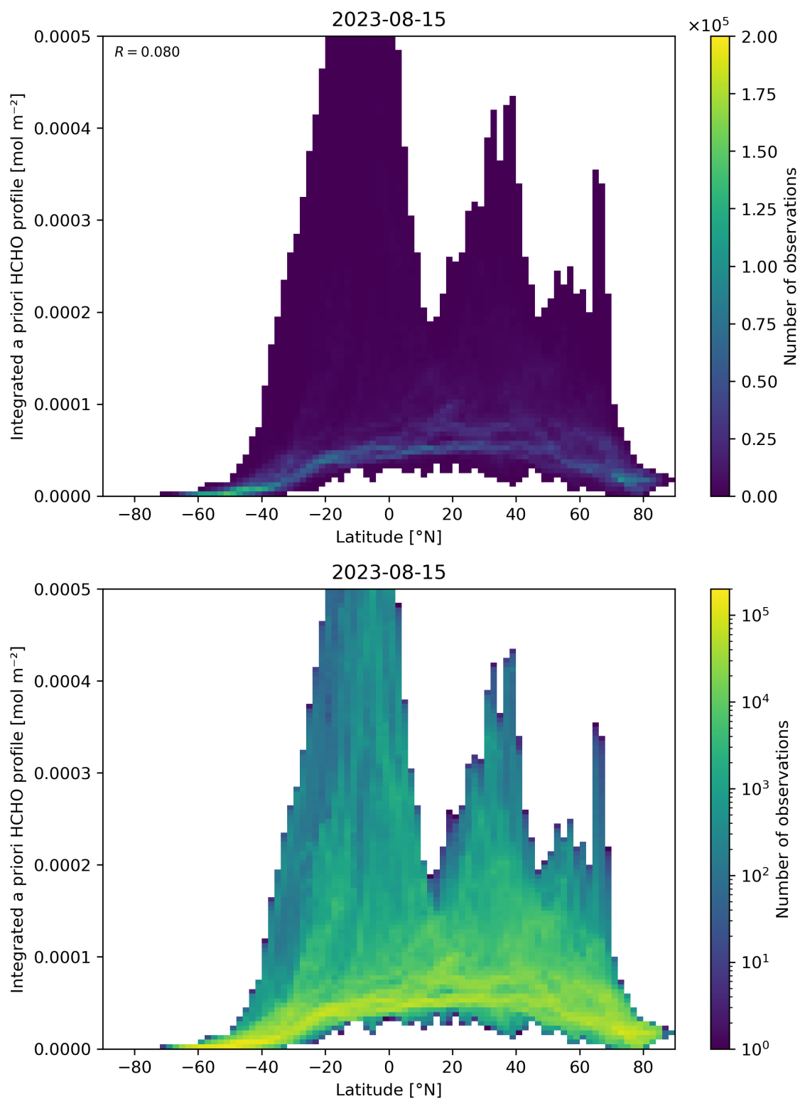
Figure 166: Scatter density plot of “Latitude” against “Integrated a priori HCHO profile” for 2023-08-14 to 2023-08-16.
