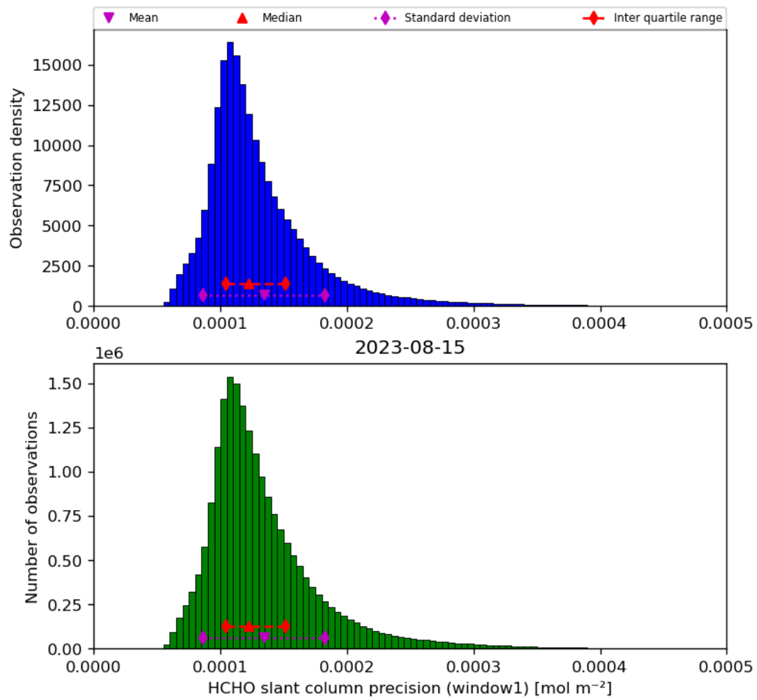
Figure 39: Histogram of “HCHO slant column precision (window1)” for 2023-08-14 to 2023-08-16
