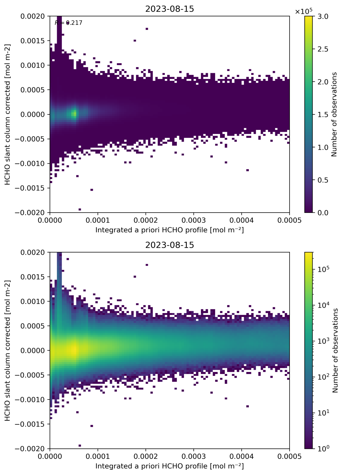
Figure 151: Scatter density plot of “Integrated a priori HCHO profile” against “HCHO slant column corrected” for 2023-08-14 to 2023-08-16.
