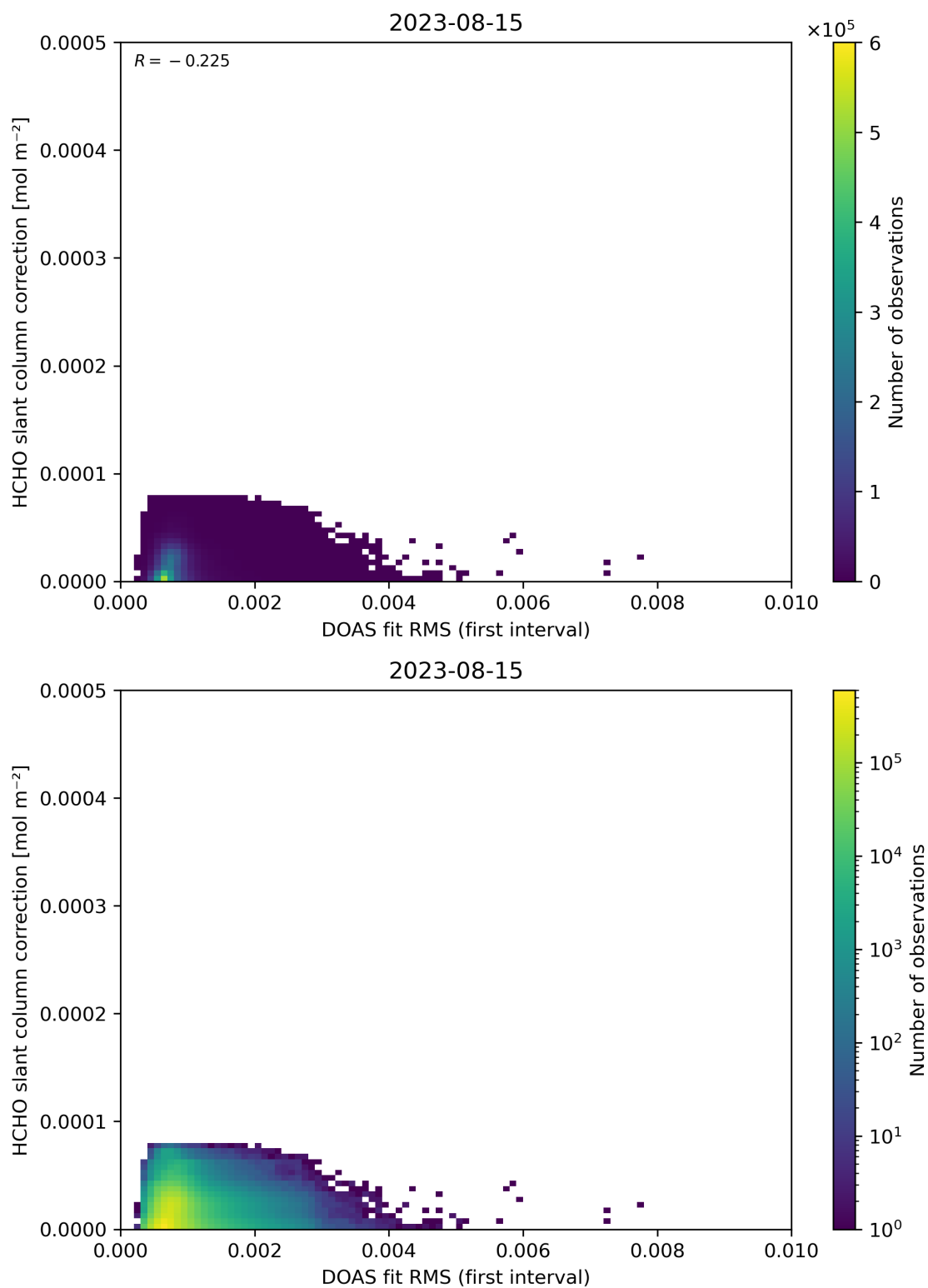
Figure 63: Scatter density plot of “DOAS fit RMS (first interval)” against “HCHO slant column correction” for 2023-08-14 to 2023-08-16.
