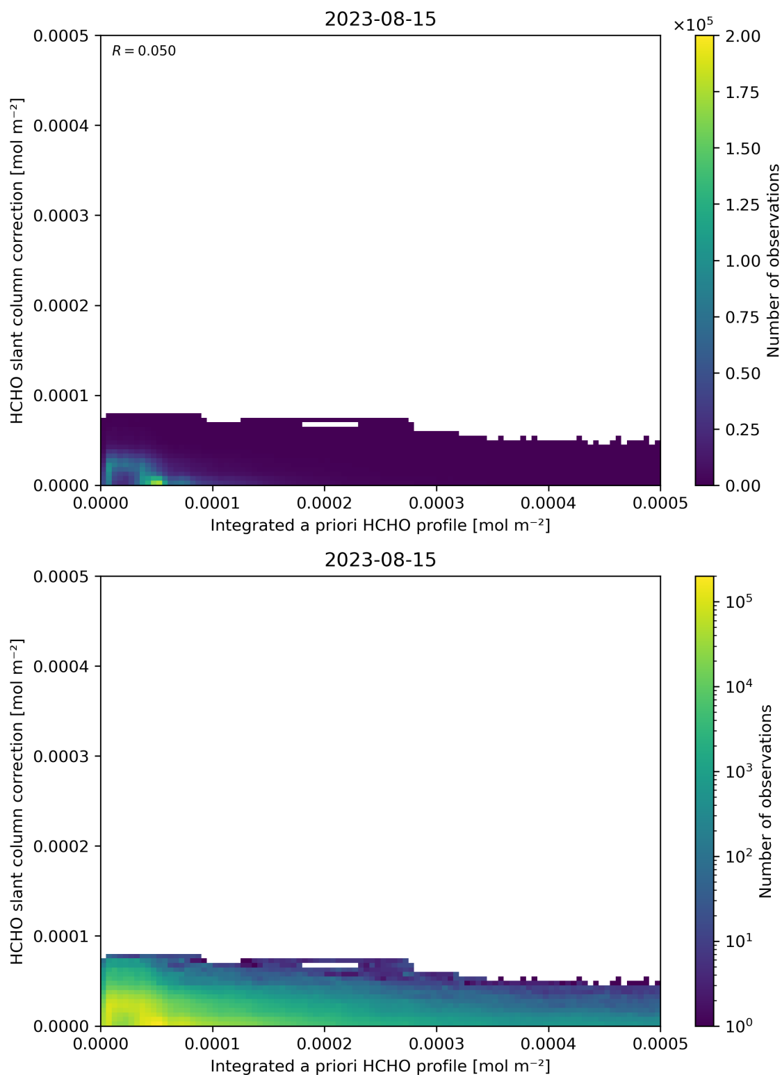
Figure 152: Scatter density plot of “Integrated a priori HCHO profile” against “HCHO slant column correction” for 2023-08-14 to 2023-08-16.
