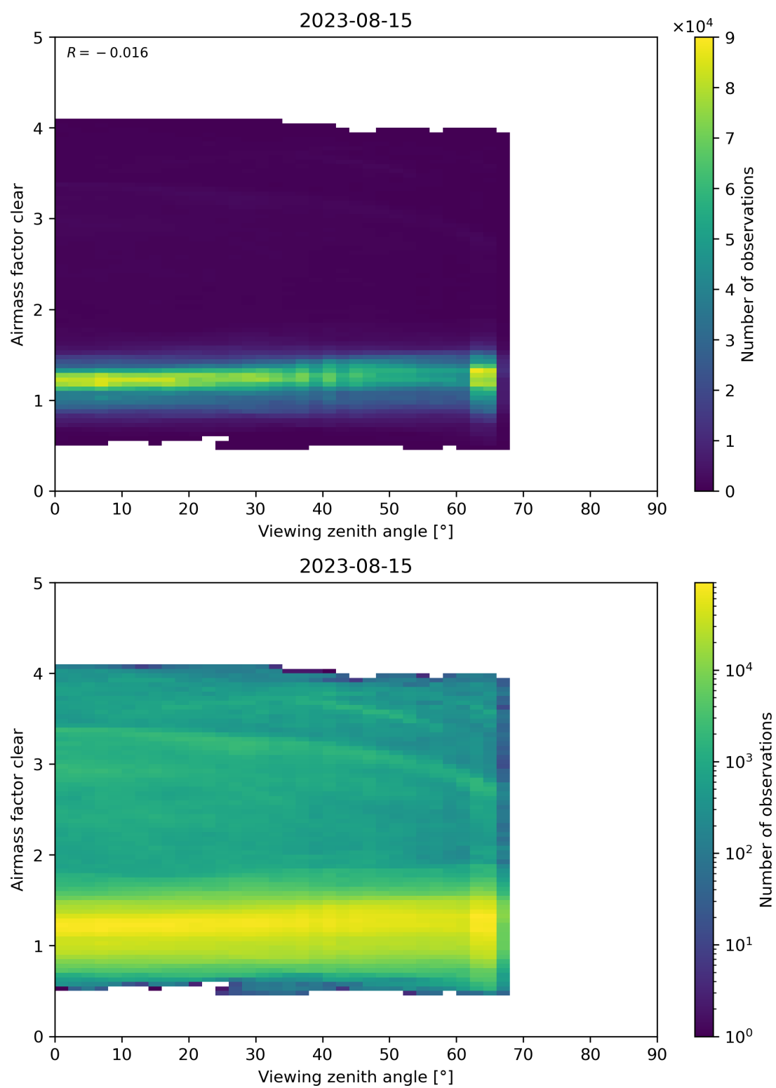
Figure 185: Scatter density plot of “Viewing zenith angle” against “Airmass factor clear” for 2023-08-14 to 2023-08-16.
