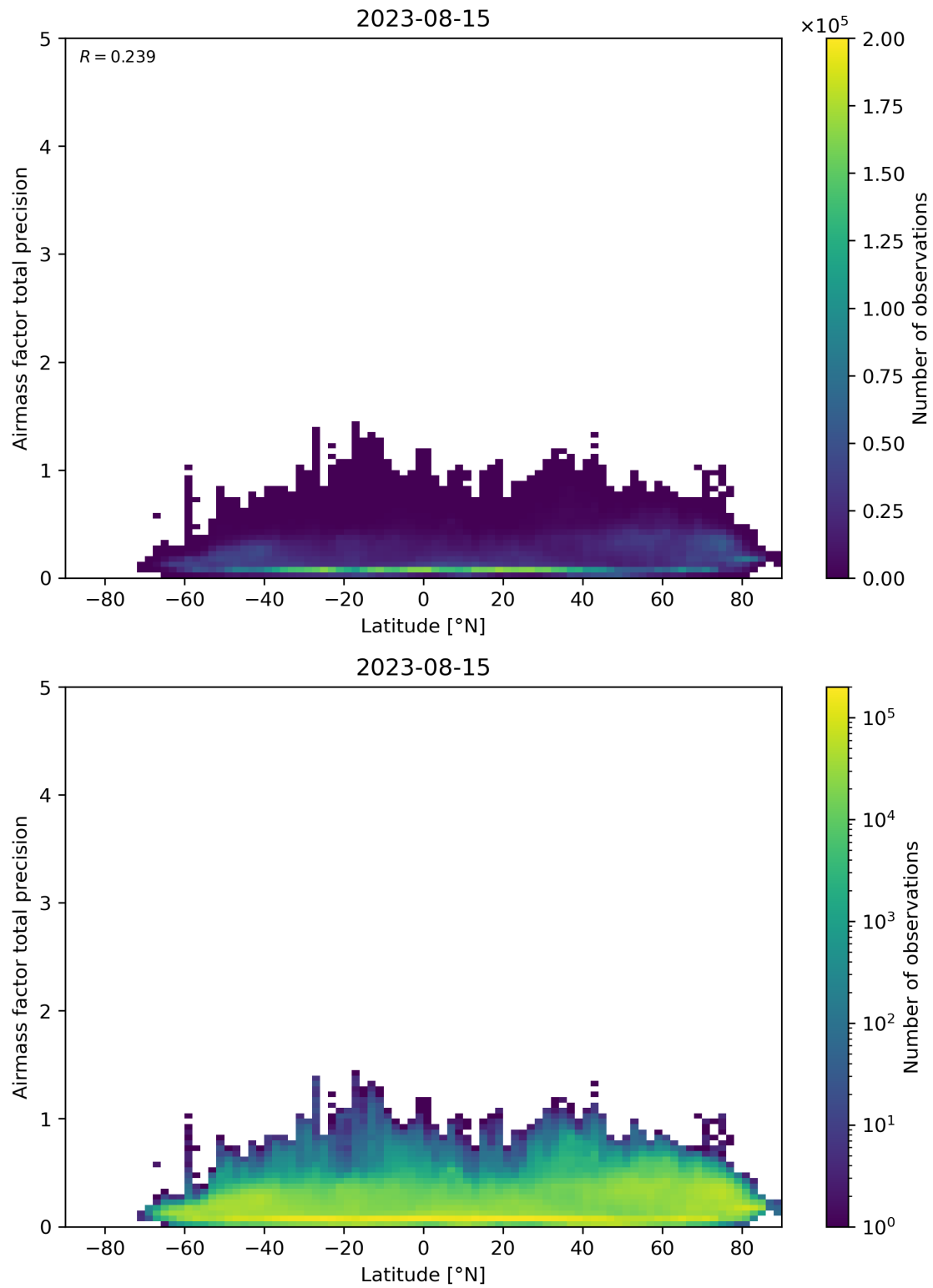
Figure 162: Scatter density plot of “Latitude” against “Airmass factor total precision” for 2023-08-14 to 2023-08-16.
