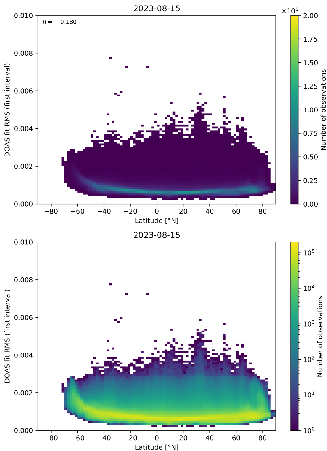
Figure 153: Scatter density plot of “Latitude” against “DOAS fit RMS (first interval)” for 2023-08-14 to 2023-08-16.
