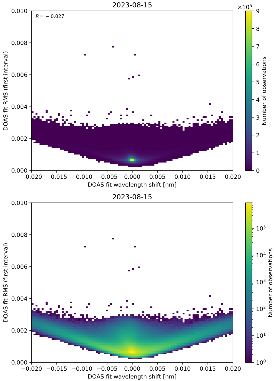
Figure 64: Scatter density plot of “DOAS fit wavelength shift” against “DOAS fit RMS (first interval)” for 2023-08-14 to 2023-08-16.
