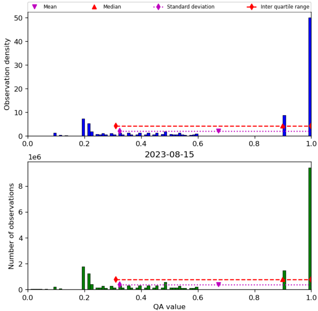
Figure 34: Histogram of “QA value” for 2023-08-14 to 2023-08-16
