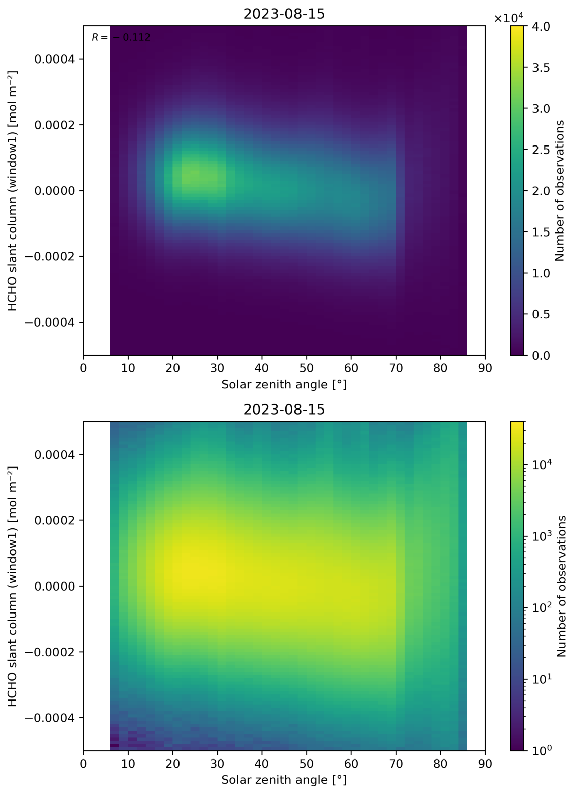
Figure 173: Scatter density plot of “Solar zenith angle” against “HCHO slant column (window1)” for 2023-08-14 to 2023-08-16.
