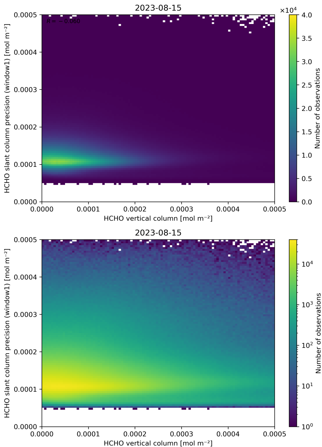
Figure 130: Scatter density plot of “HCHO vertical column” against “HCHO slant column precision (window1)” for 2023-08-14 to 2023-08-16.
