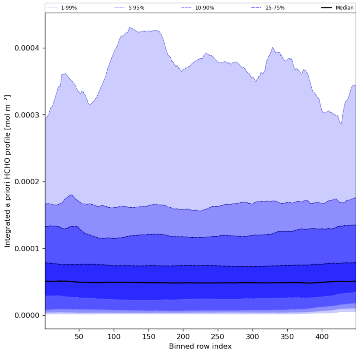
Figure 57: Along track statistics of “Integrated a priori HCHO profile” for 2023-08-14 to 2023-08-16
