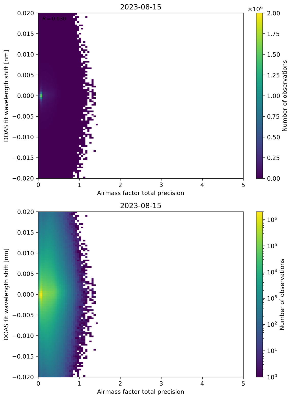
Figure 106: Scatter density plot of “Airmass factor total precision” against “DOAS fit wavelength shift” for 2023-08-14 to 2023-08-16.
