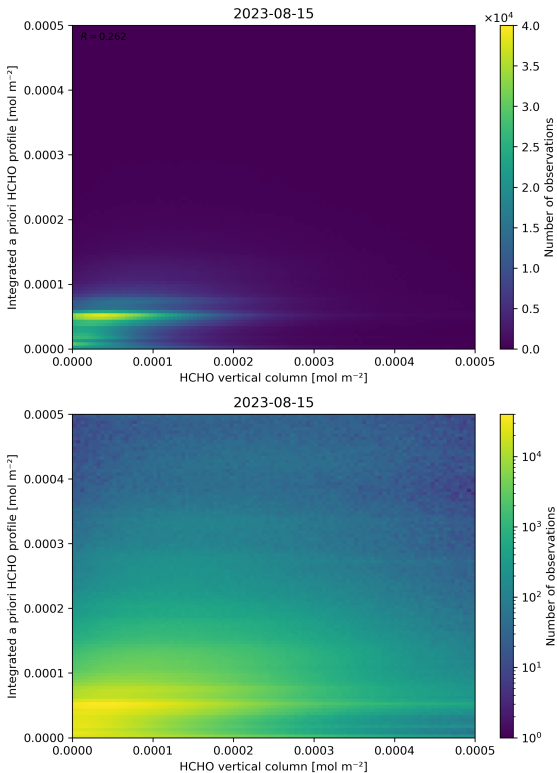
Figure 135: Scatter density plot of “HCHO vertical column” against “Integrated a priori HCHO profile” for 2023-08-14 to 2023-08-16.
