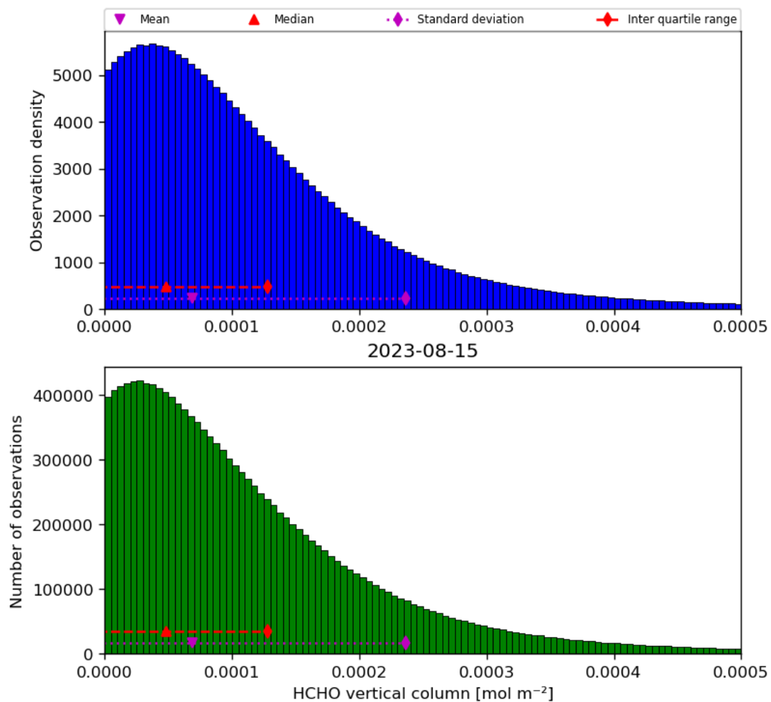
Figure 35: Histogram of “HCHO vertical column” for 2023-08-14 to 2023-08-16
