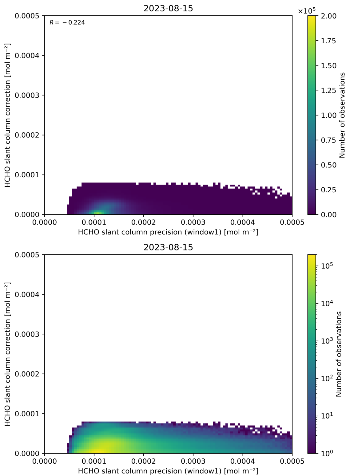
Figure 93: Scatter density plot of “HCHO slant column precision (window1)” against “HCHO slant column correction” for 2023-08-14 to 2023-08-16.
