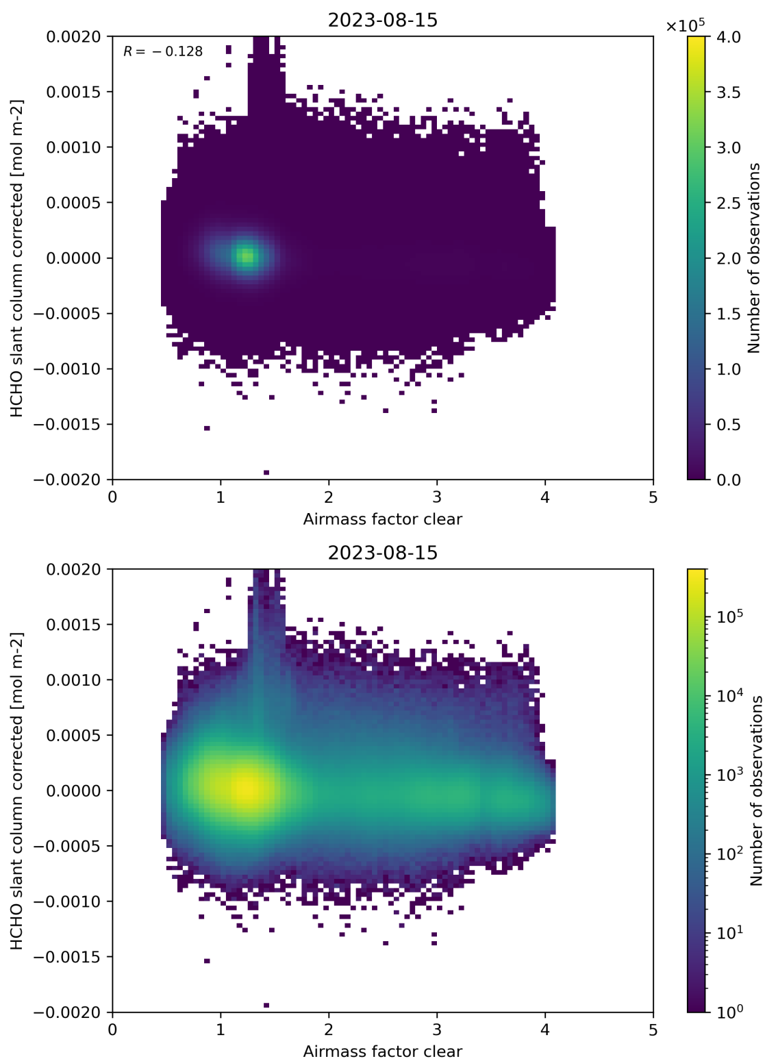
Figure 74: Scatter density plot of “Airmass factor clear” against “HCHO slant column corrected” for 2023-08-14 to 2023-08-16.
