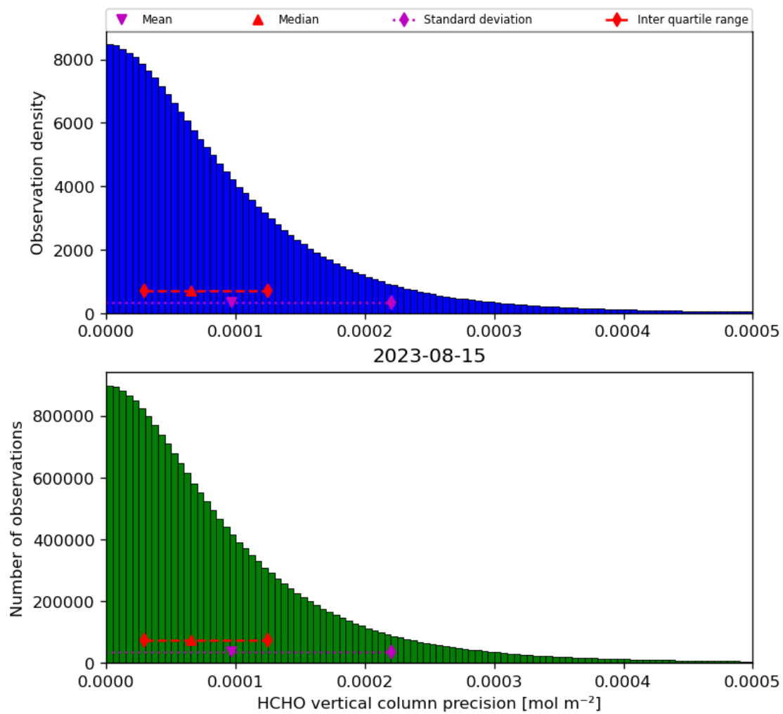
Figure 36: Histogram of “HCHO vertical column precision” for 2023-08-14 to 2023-08-16
