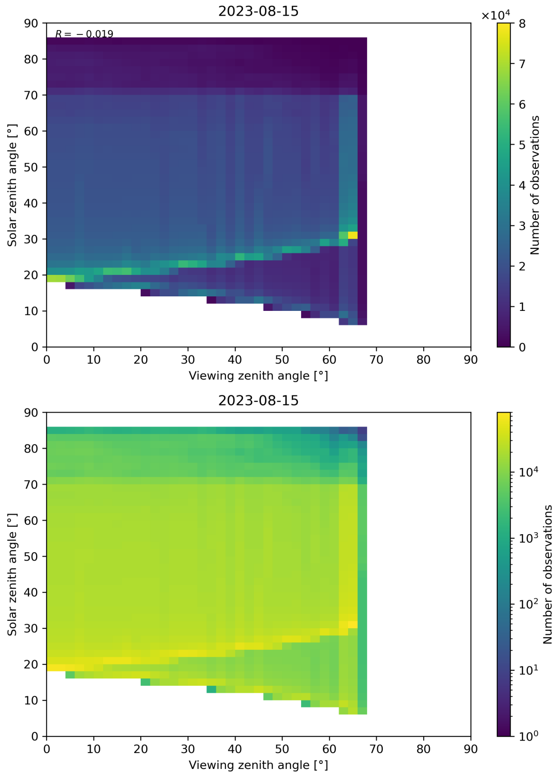
Figure 197: Scatter density plot of “Viewing zenith angle” against “Solar zenith angle” for 2023-08-14 to 2023-08-16.
