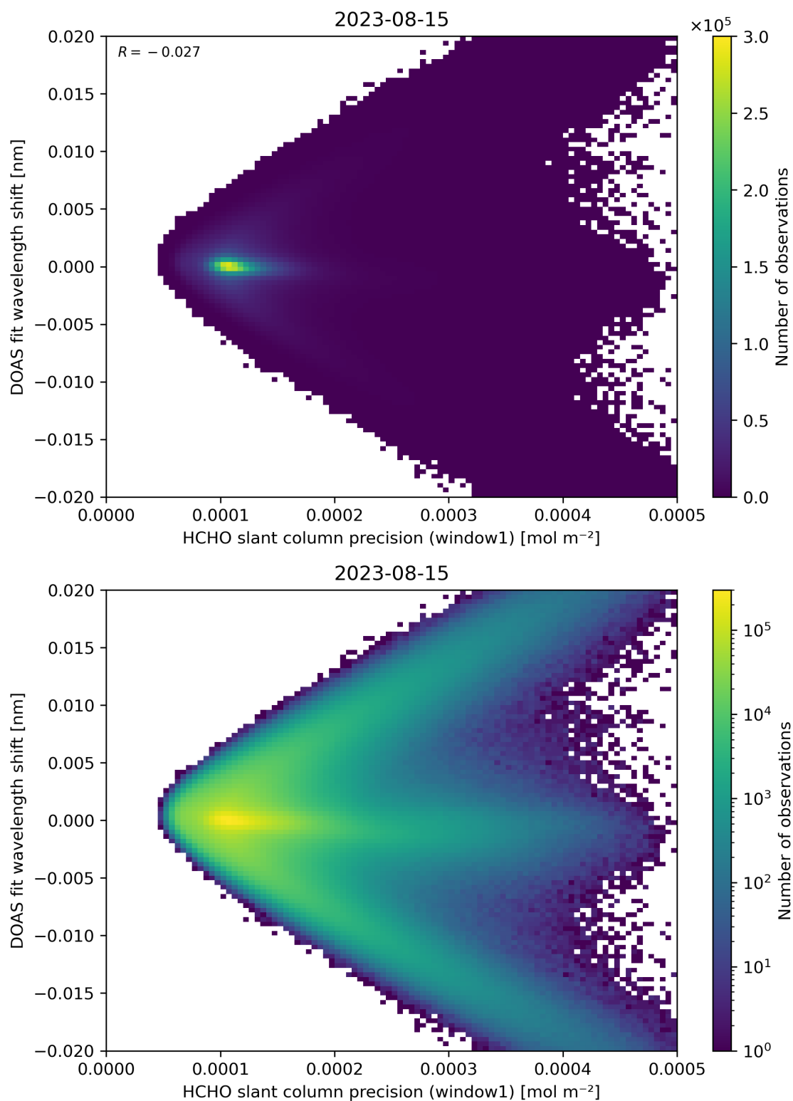
Figure 89: Scatter density plot of “HCHO slant column precision (window1)” against “DOAS fit wavelength shift” for 2023-08-14 to 2023-08-16.
