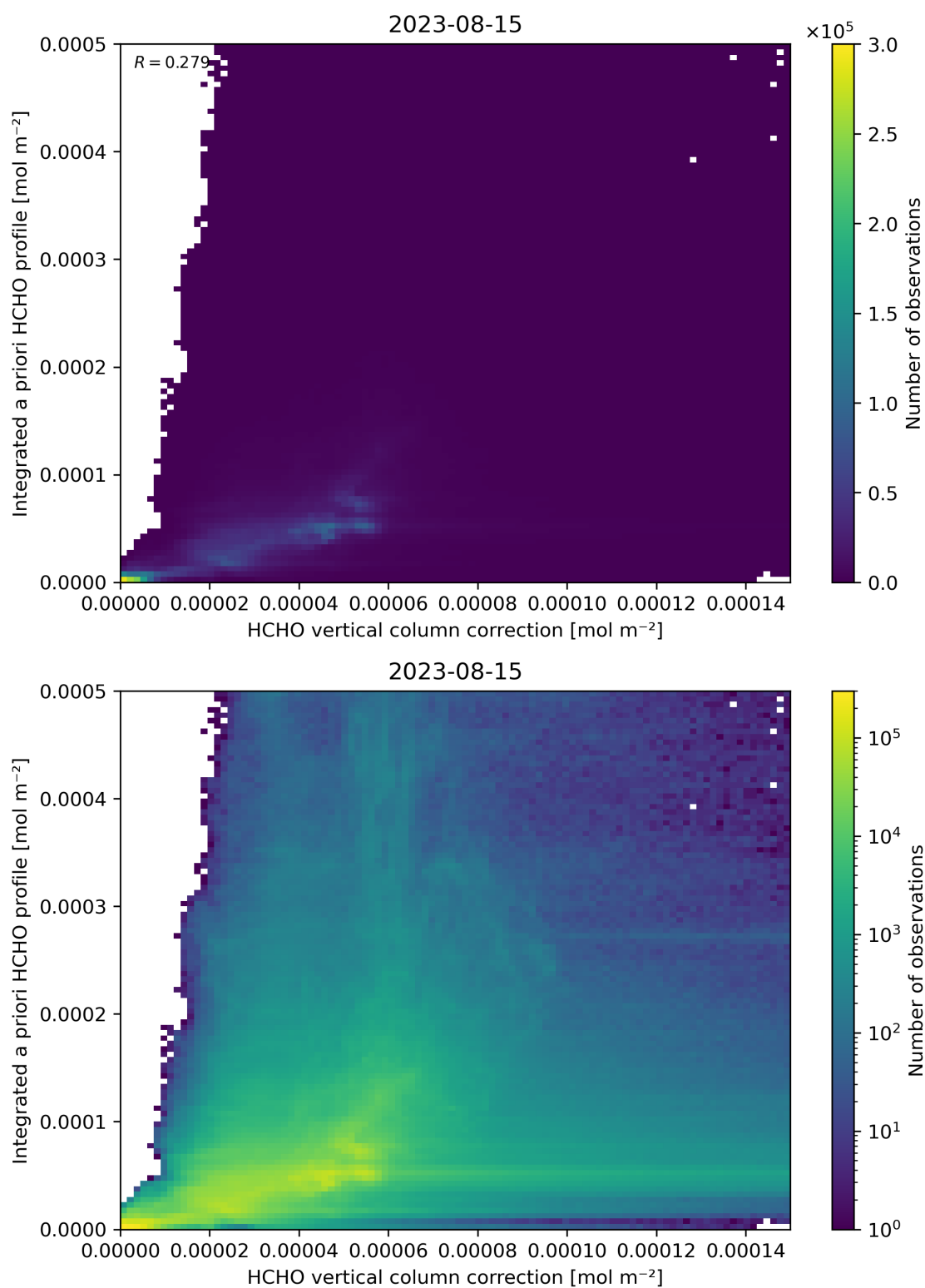
Figure 122: Scatter density plot of “HCHO vertical column correction” against “Integrated a priori HCHO profile” for 2023-08-14 to 2023-08-16.
