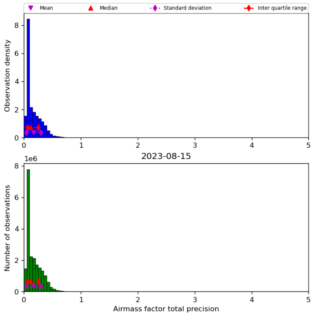
Figure 41: Histogram of “Airmass factor total precision” for 2023-08-14 to 2023-08-16
