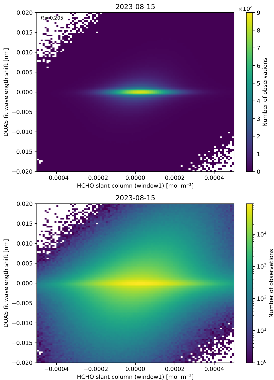
Figure 79: Scatter density plot of “HCHO slant column (window1)” against “DOAS fit wavelength shift” for 2023-08-14 to 2023-08-16.
