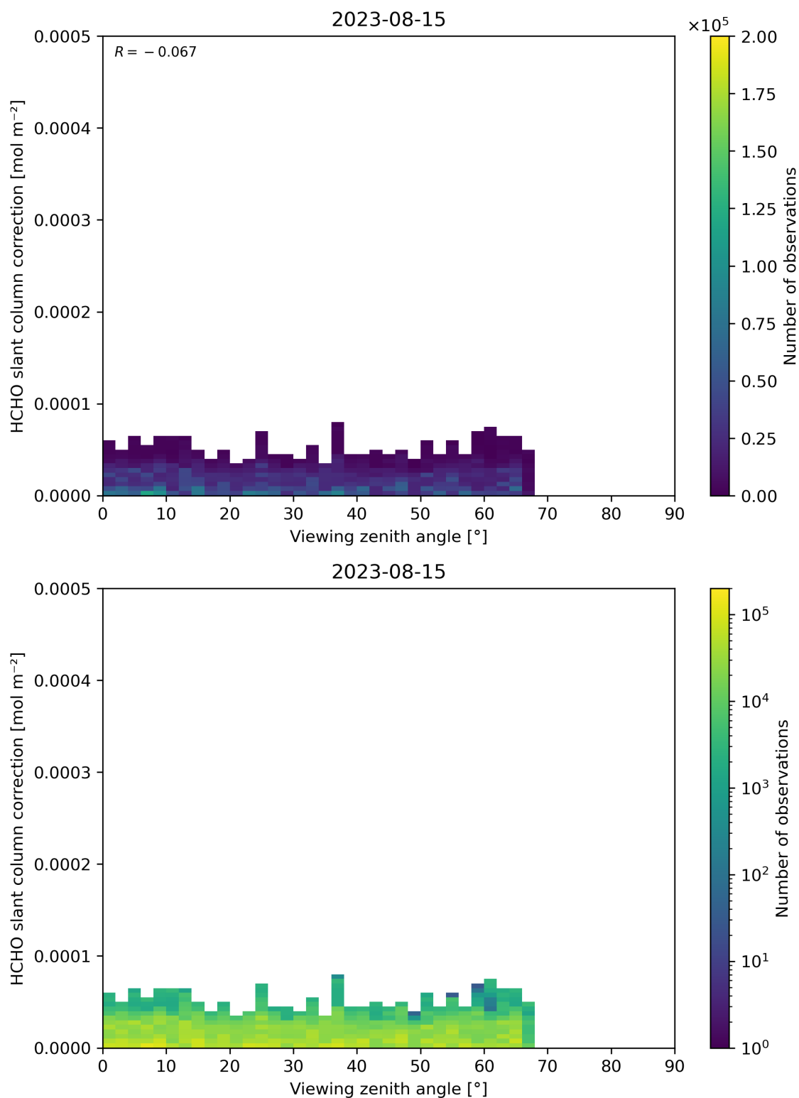
Figure 187: Scatter density plot of “Viewing zenith angle” against “HCHO slant column correction” for 2023-08-14 to 2023-08-16.
