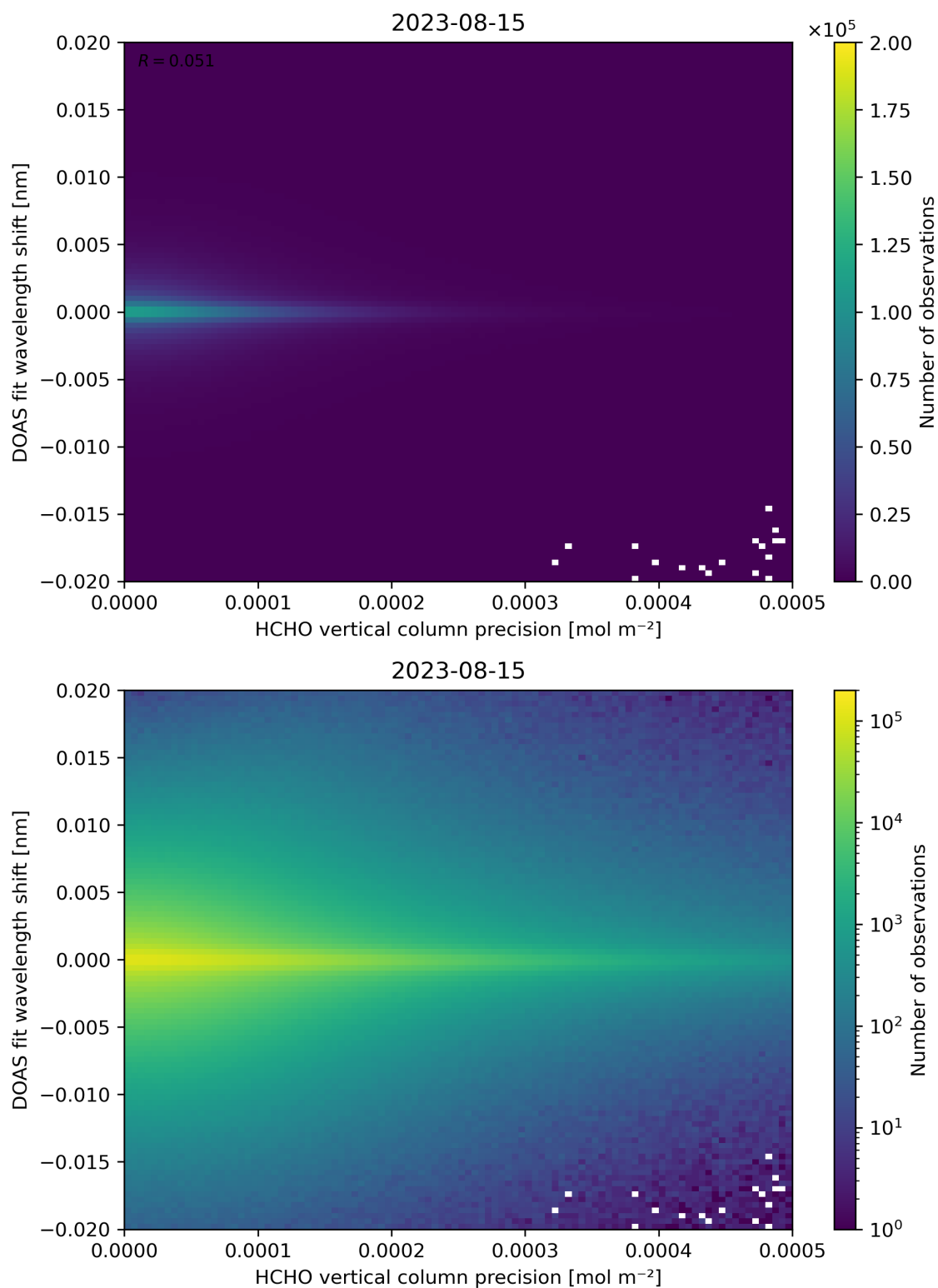
Figure 137: Scatter density plot of “HCHO vertical column precision” against “DOAS fit wavelength shift” for 2023-08-14 to 2023-08-16.
