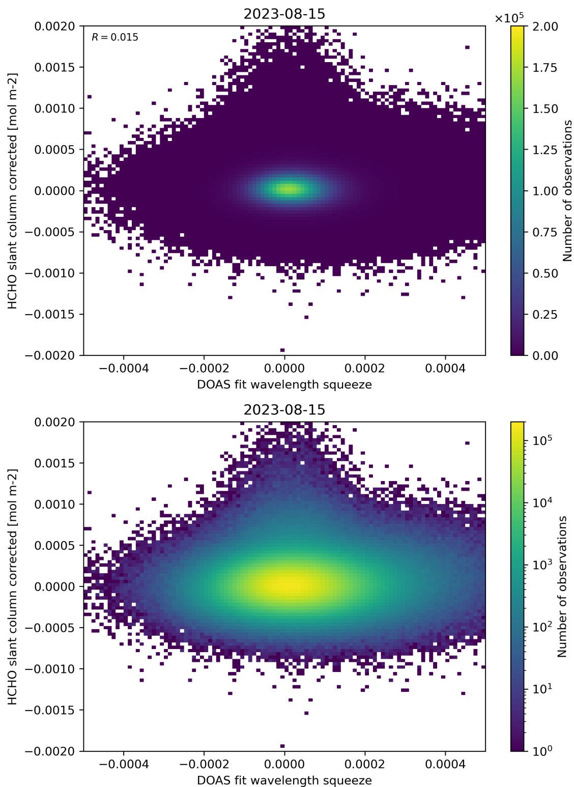
Figure 69: Scatter density plot of “DOAS fit wavelength squeeze” against “HCHO slant column corrected” for 2023-08-14 to 2023-08-16.
