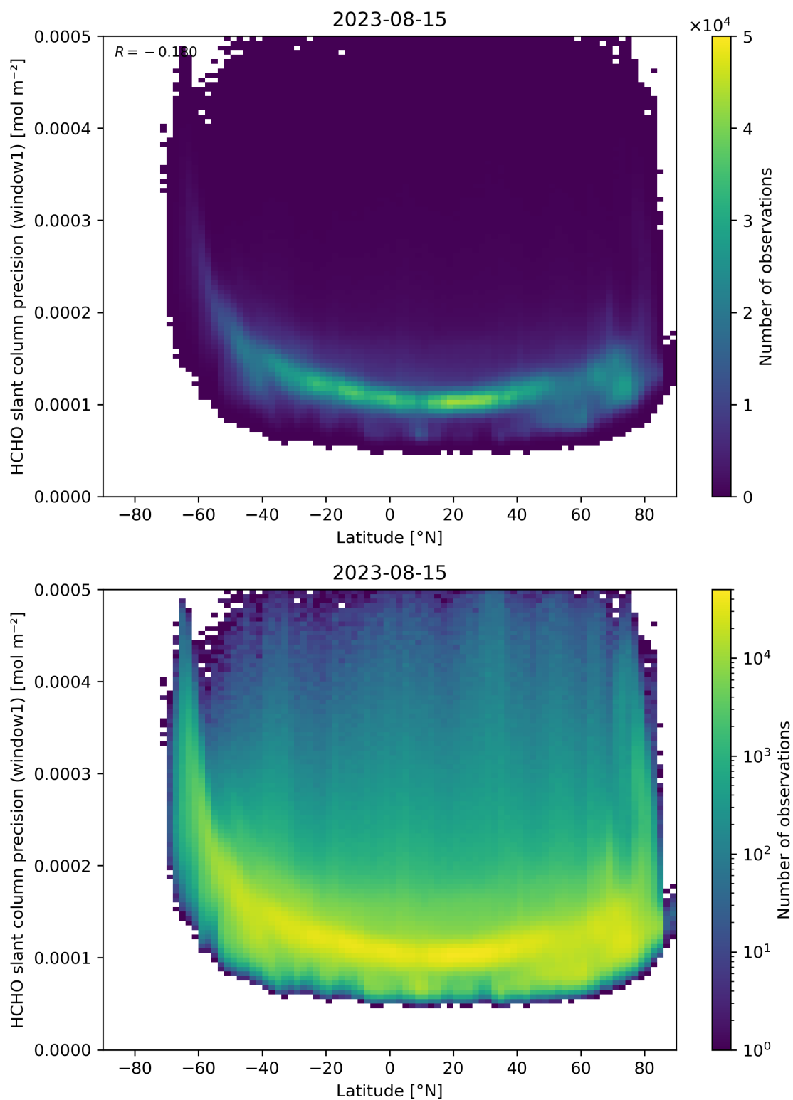
Figure 160: Scatter density plot of “Latitude” against “HCHO slant column precision (window1)” for 2023-08-14 to 2023-08-16.
