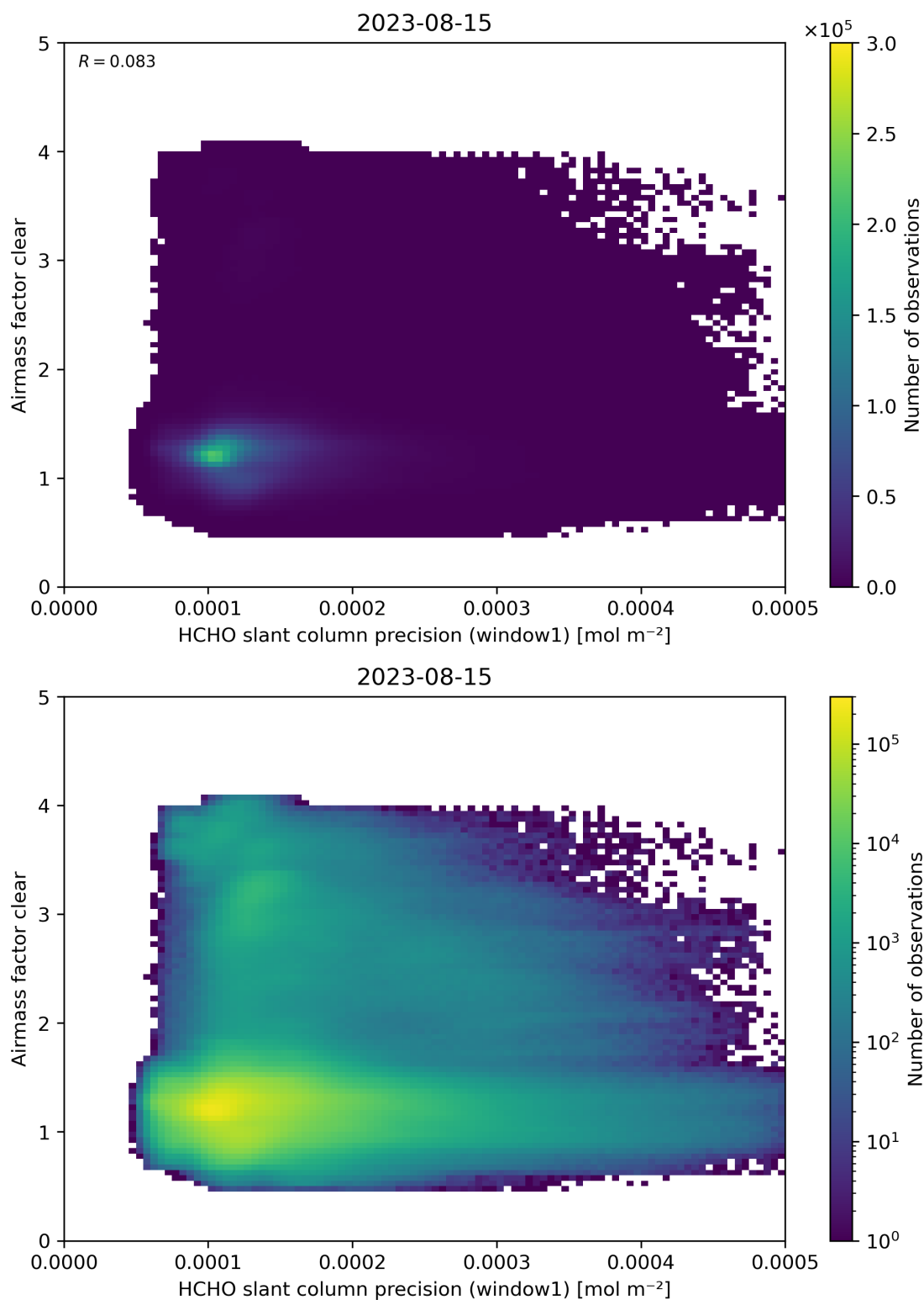
Figure 91: Scatter density plot of “HCHO slant column precision (window1)” against “Airmass factor clear” for 2023-08-14 to 2023-08-16.
