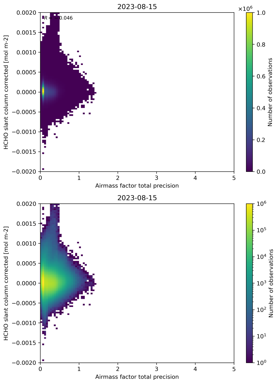
Figure 109: Scatter density plot of “Airmass factor total precision” against “HCHO slant column corrected” for 2023-08-14 to 2023-08-16.
