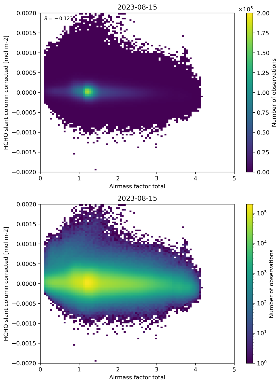
Figure 101: Scatter density plot of “Airmass factor total” against “HCHO slant column corrected” for 2023-08-14 to 2023-08-16.
