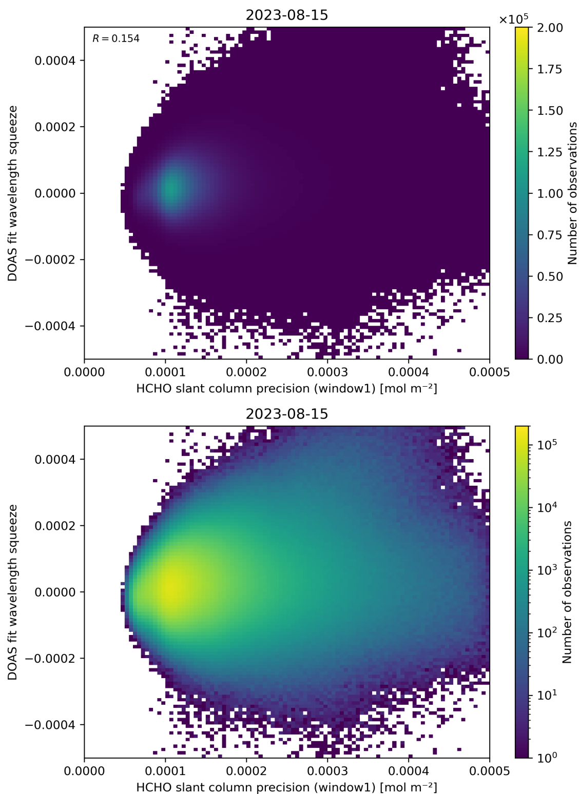
Figure 90: Scatter density plot of “HCHO slant column precision (window1)” against “DOAS fit wavelength squeeze” for 2023-08-14 to 2023-08-16.
