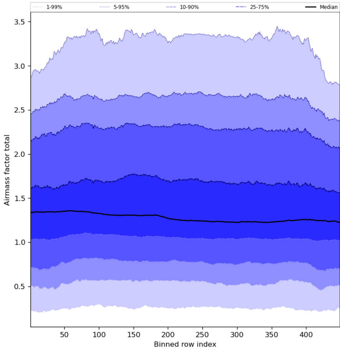
Figure 54: Along track statistics of “Airmass factor total” for 2023-08-14 to 2023-08-16
