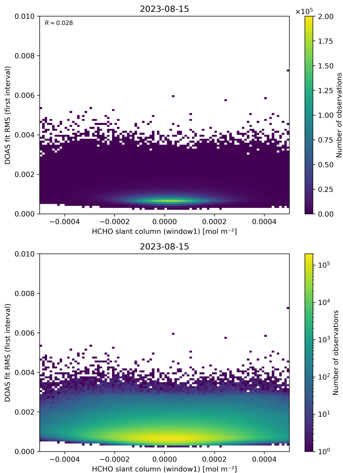
Figure 78: Scatter density plot of “HCHO slant column (window1)” against “DOAS fit RMS (first interval)” for 2023-08-14 to 2023-08-16.
