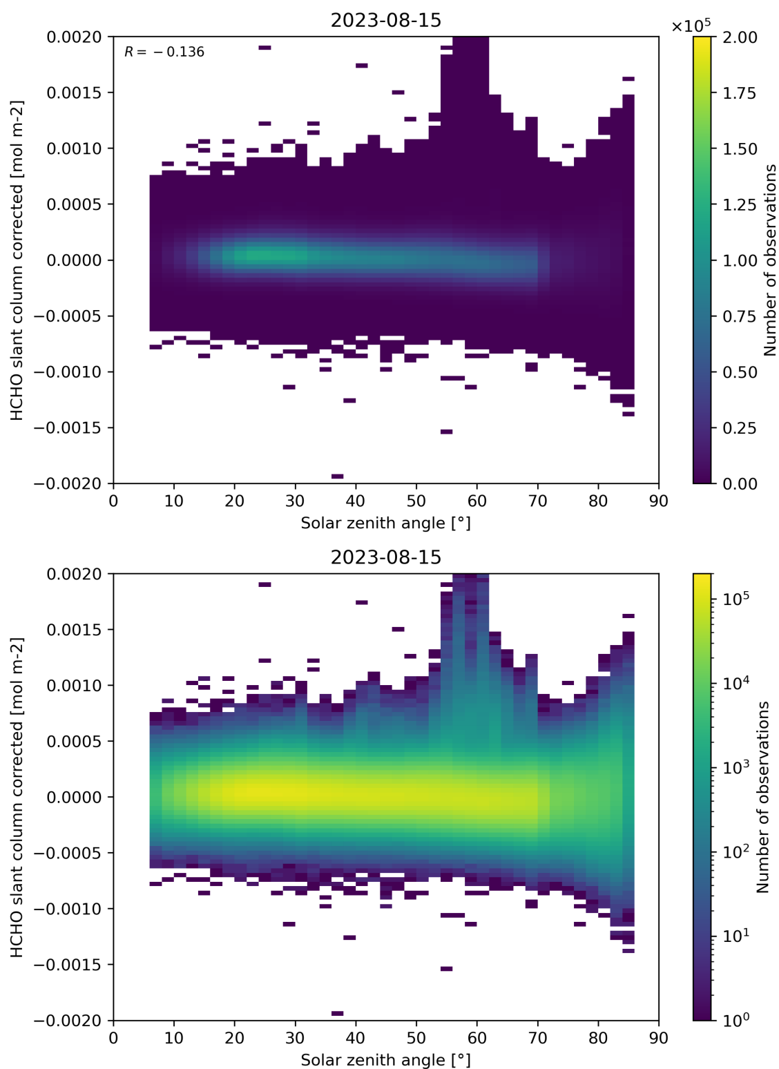
Figure 171: Scatter density plot of “Solar zenith angle” against “HCHO slant column corrected” for 2023-08-14 to 2023-08-16.
