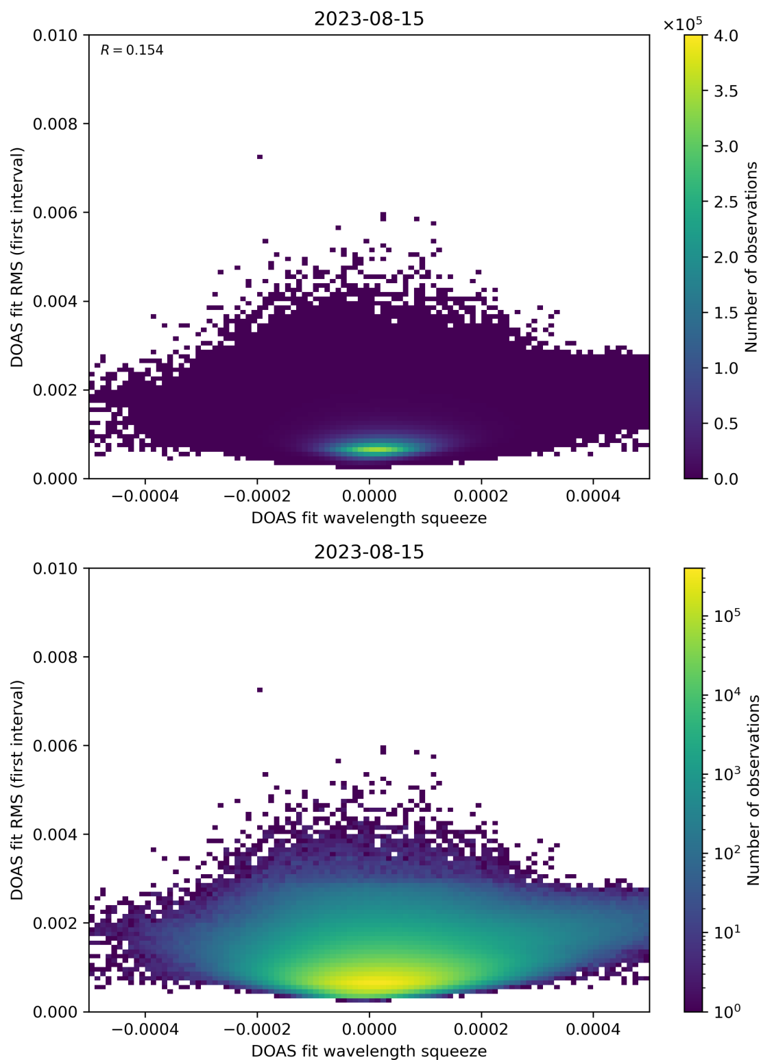
Figure 68: Scatter density plot of “DOAS fit wavelength squeeze” against “DOAS fit RMS (first interval)” for 2023-08-14 to 2023-08-16.
