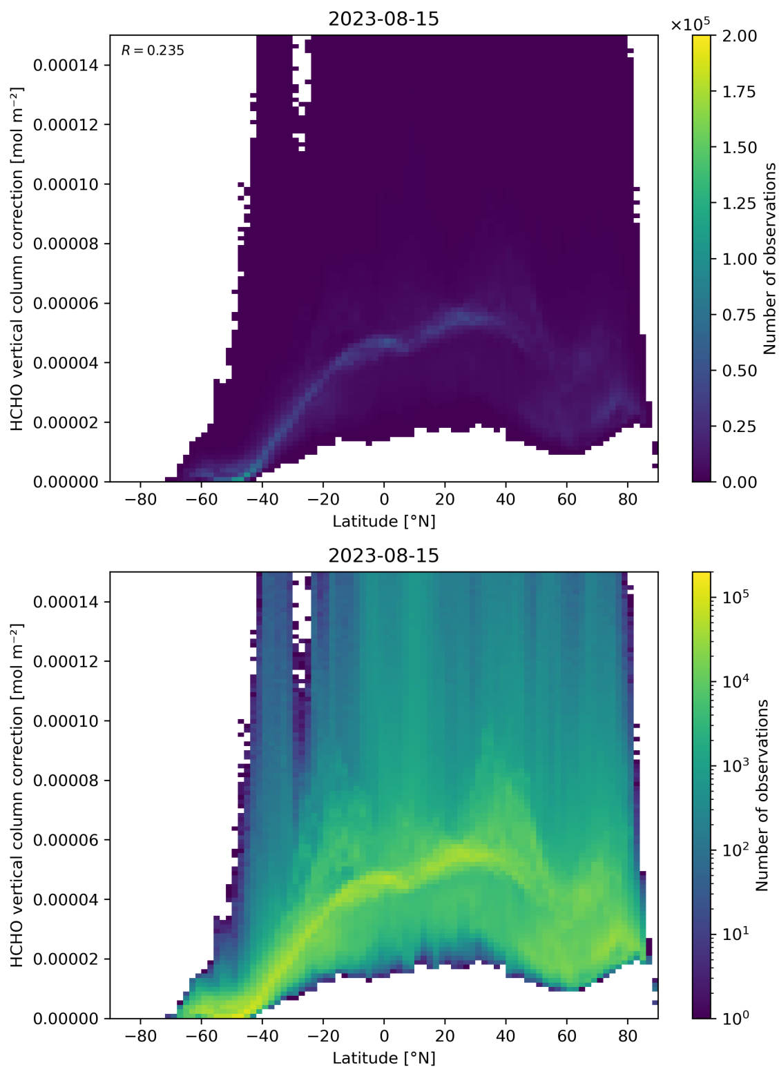
Figure 164: Scatter density plot of “Latitude” against “HCHO vertical column correction” for 2023-08-14 to 2023-08-16.
