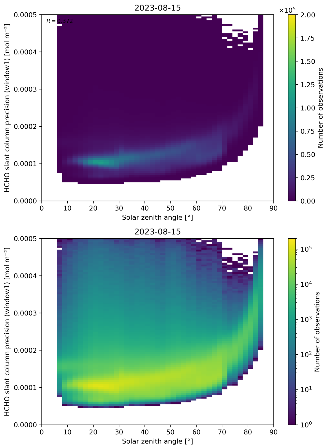
Figure 174: Scatter density plot of “Solar zenith angle” against “HCHO slant column precision (window1)” for 2023-08-14 to 2023-08-16.
