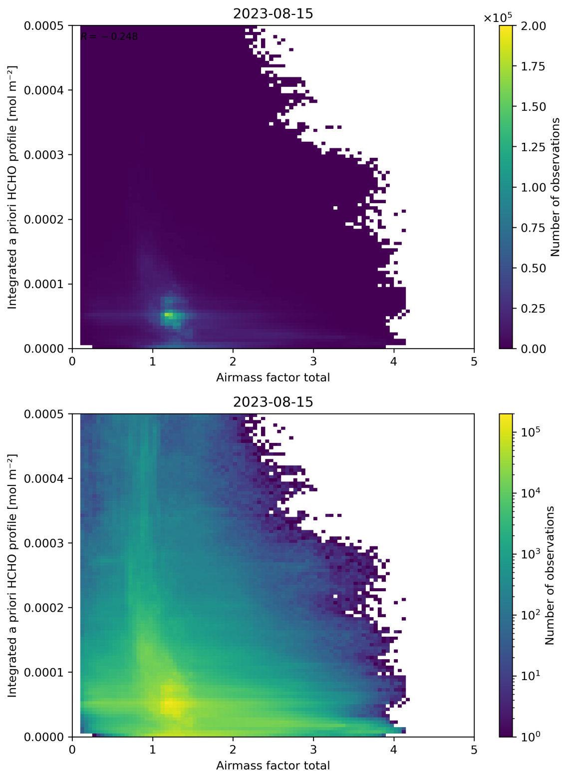
Figure 104: Scatter density plot of “Airmass factor total” against “Integrated a priori HCHO profile” for 2023-08-14 to 2023-08-16.
