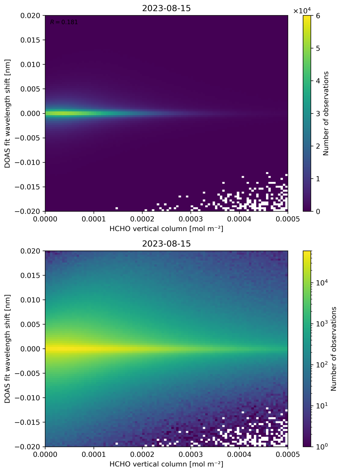
Figure 124: Scatter density plot of “HCHO vertical column” against “DOAS fit wavelength shift” for 2023-08-14 to 2023-08-16.
