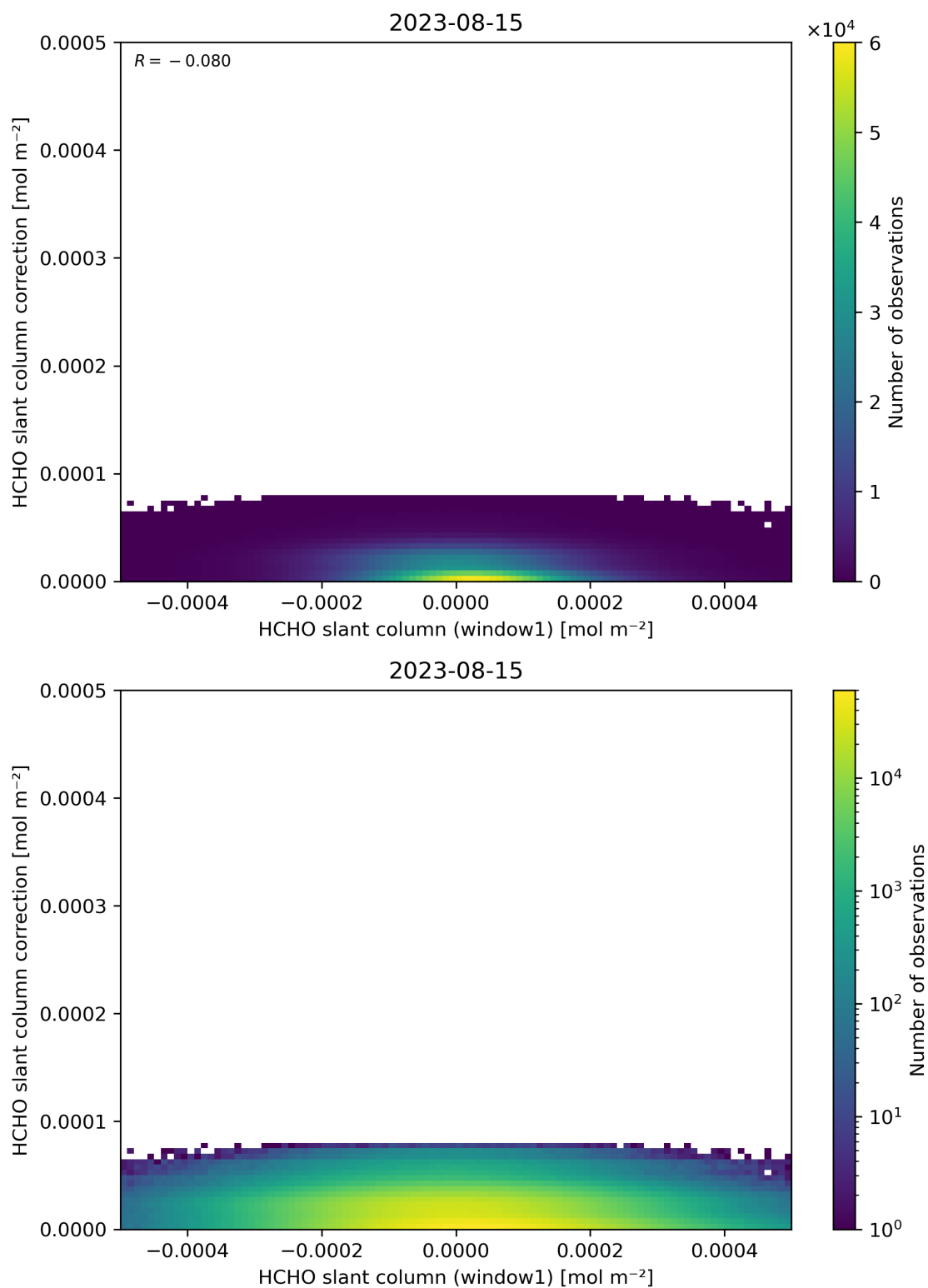
Figure 83: Scatter density plot of “HCHO slant column (window1)” against “HCHO slant column correction” for 2023-08-14 to 2023-08-16.
