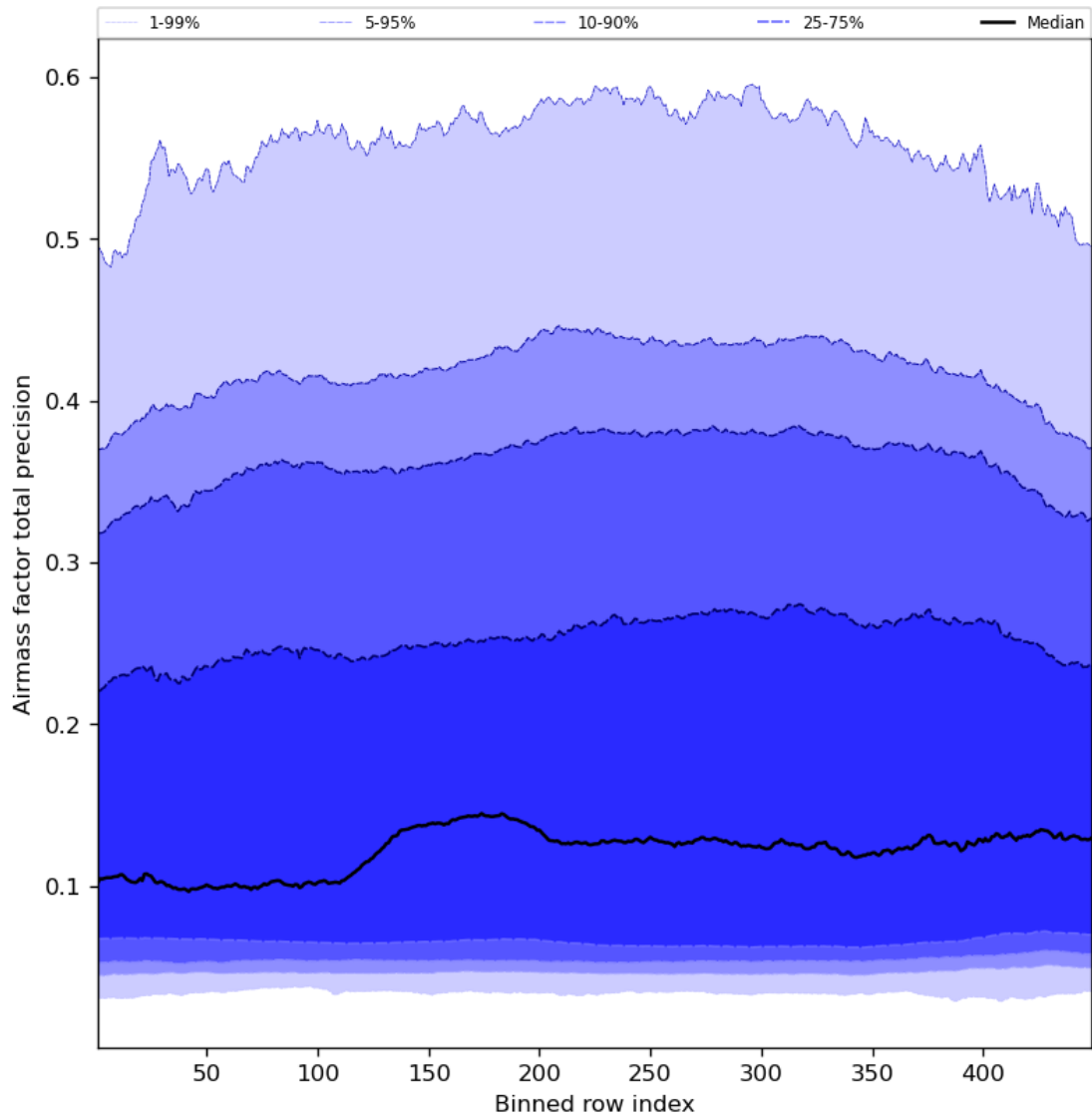
Figure 55: Along track statistics of “Airmass factor total precision” for 2023-08-14 to 2023-08-16
