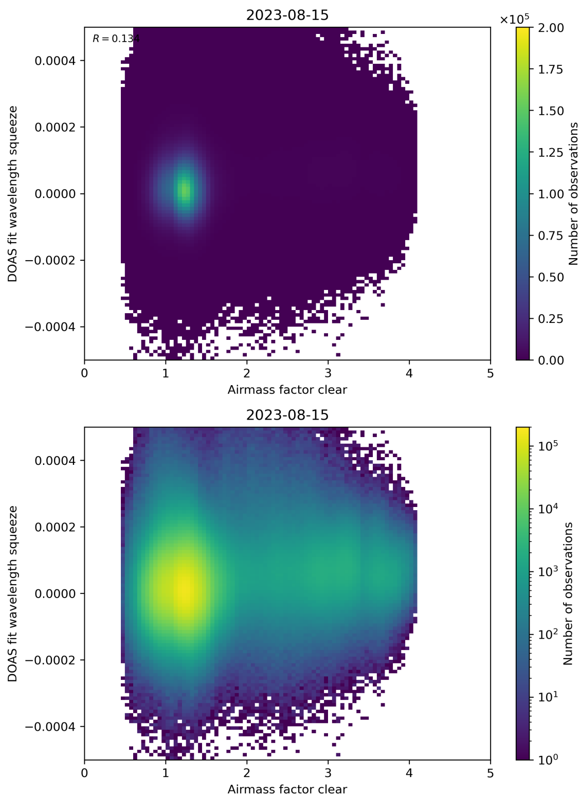
Figure 73: Scatter density plot of “Airmass factor clear” against “DOAS fit wavelength squeeze” for 2023-08-14 to 2023-08-16.
