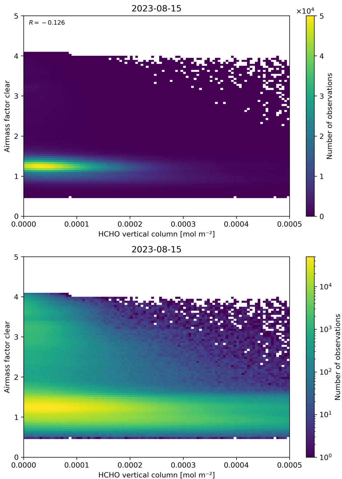
Figure 126: Scatter density plot of “HCHO vertical column” against “Airmass factor clear” for 2023-08-14 to 2023-08-16.
