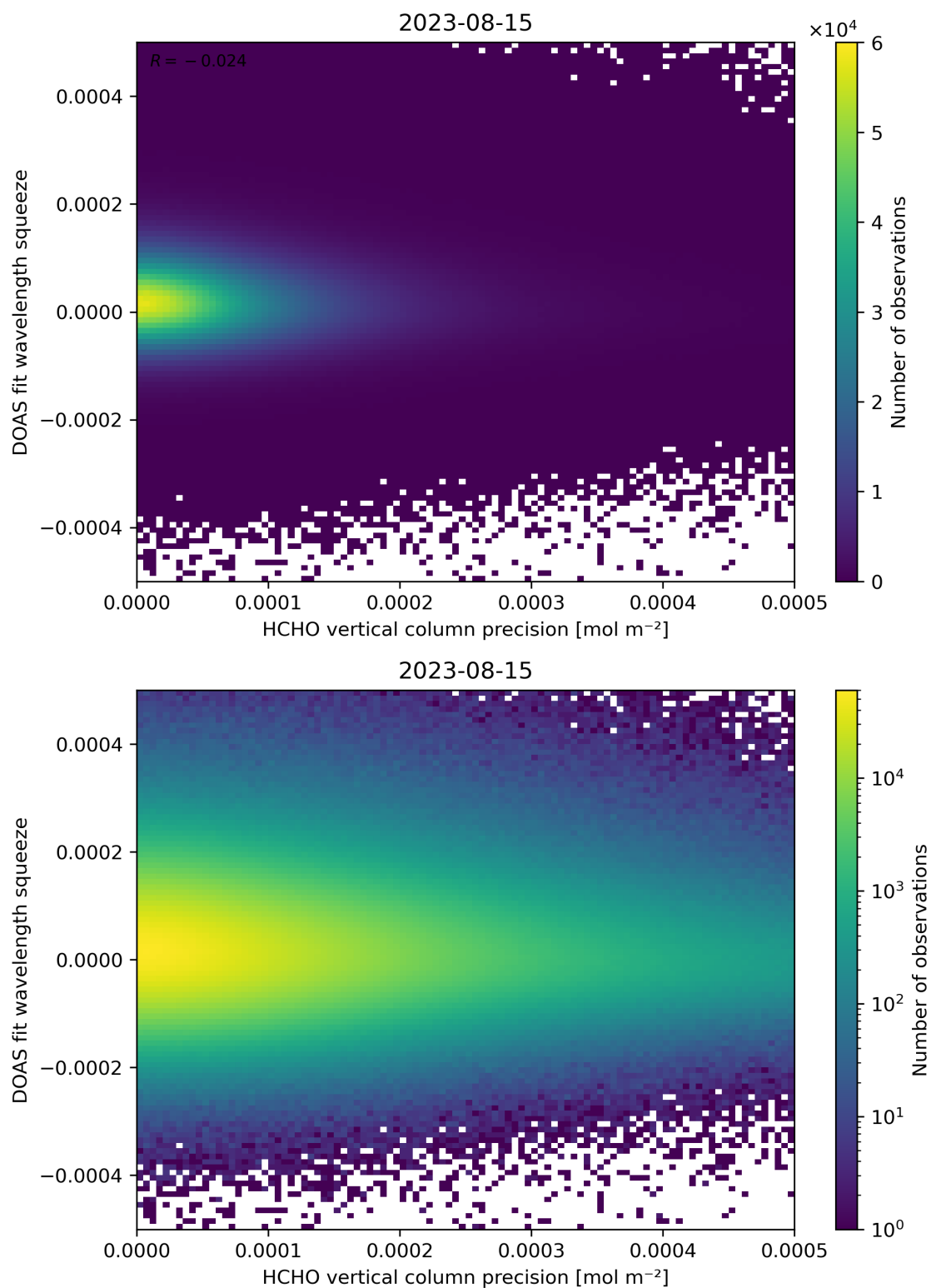
Figure 138: Scatter density plot of “HCHO vertical column precision” against “DOAS fit wavelength squeeze” for 2023-08-14 to 2023-08-16.
