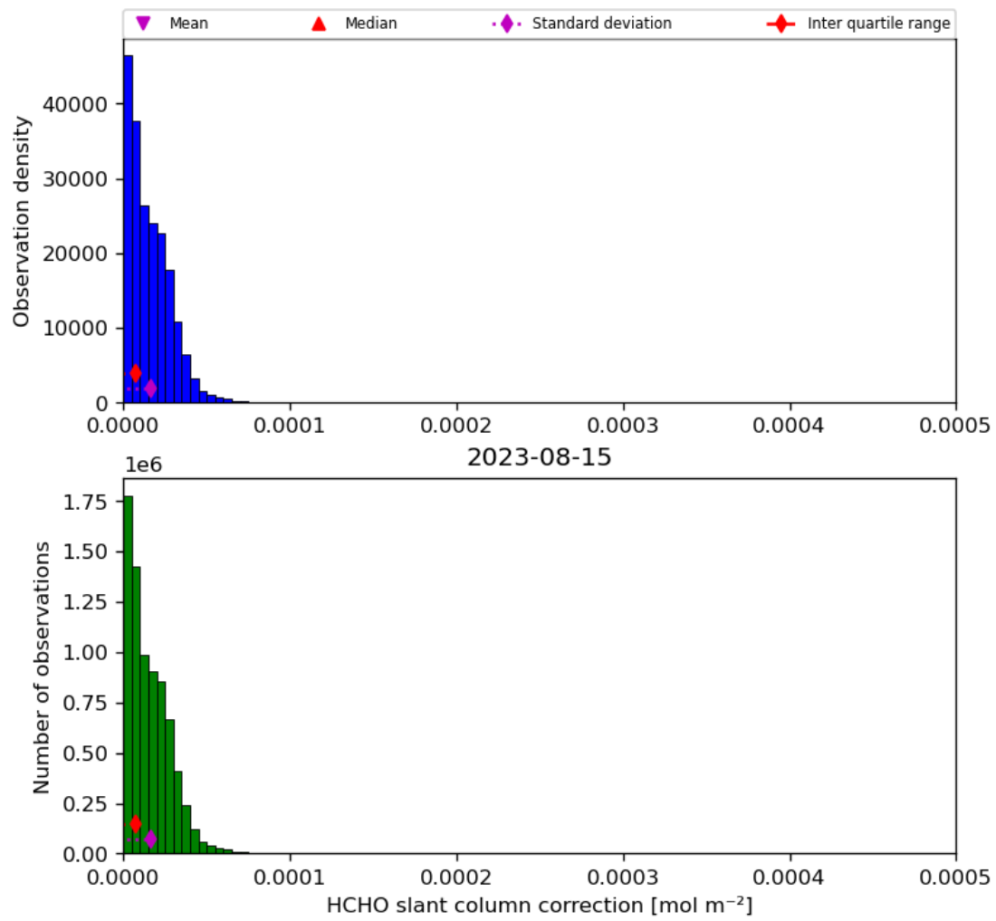
Figure 47: Histogram of “HCHO slant column correction” for 2023-08-14 to 2023-08-16
