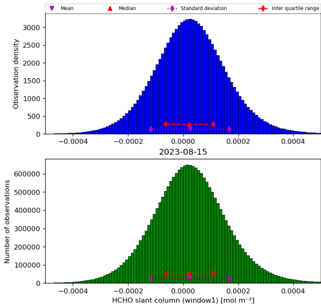
Figure 38: Histogram of “HCHO slant column (window1)” for 2023-08-14 to 2023-08-16
