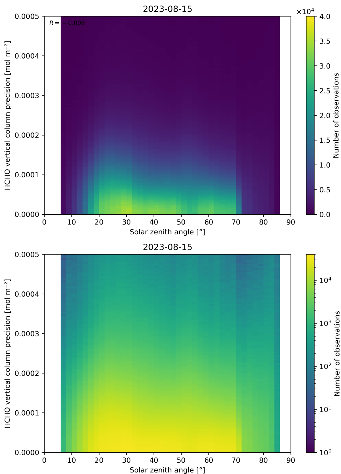
Figure 179: Scatter density plot of “Solar zenith angle” against “HCHO vertical column precision” for 2023-08-14 to 2023-08-16.
