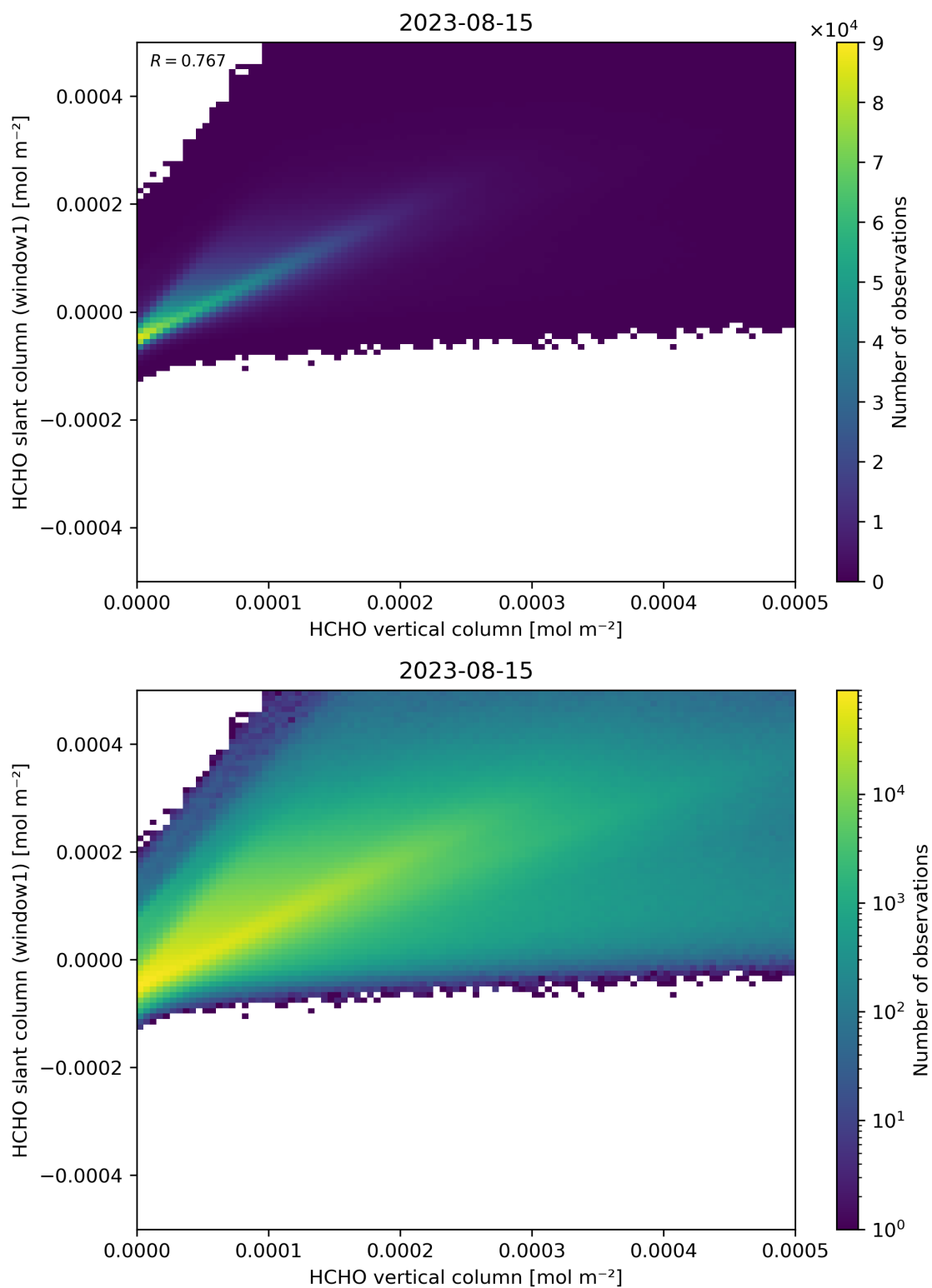
Figure 129: Scatter density plot of “HCHO vertical column” against “HCHO slant column (window1)” for 2023-08-14 to 2023-08-16.
