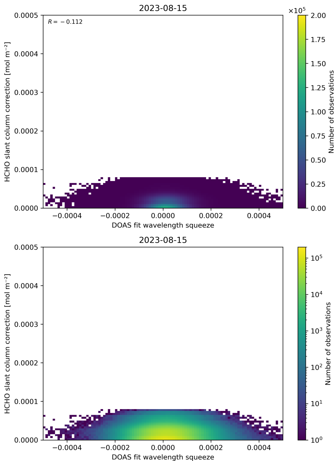
Figure 70: Scatter density plot of “DOAS fit wavelength squeeze” against “HCHO slant column correction” for 2023-08-14 to 2023-08-16.
