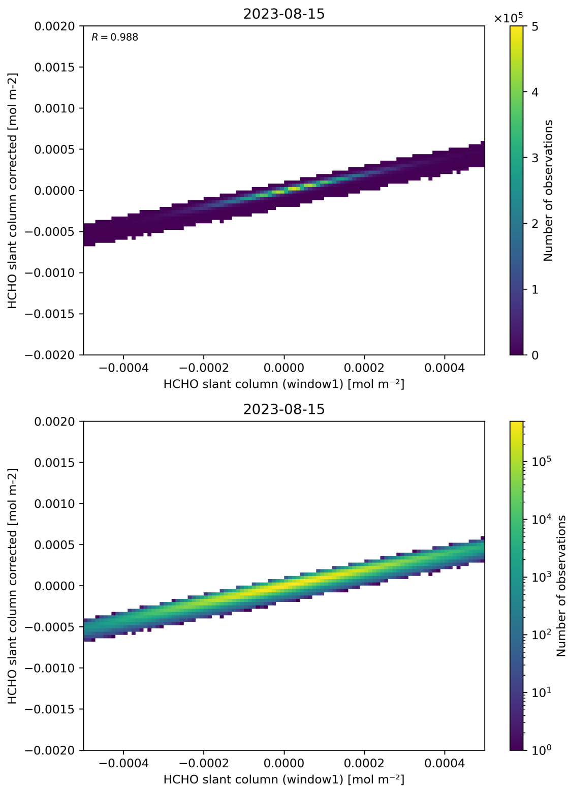
Figure 82: Scatter density plot of “HCHO slant column (window1)” against “HCHO slant column corrected” for 2023-08-14 to 2023-08-16.
