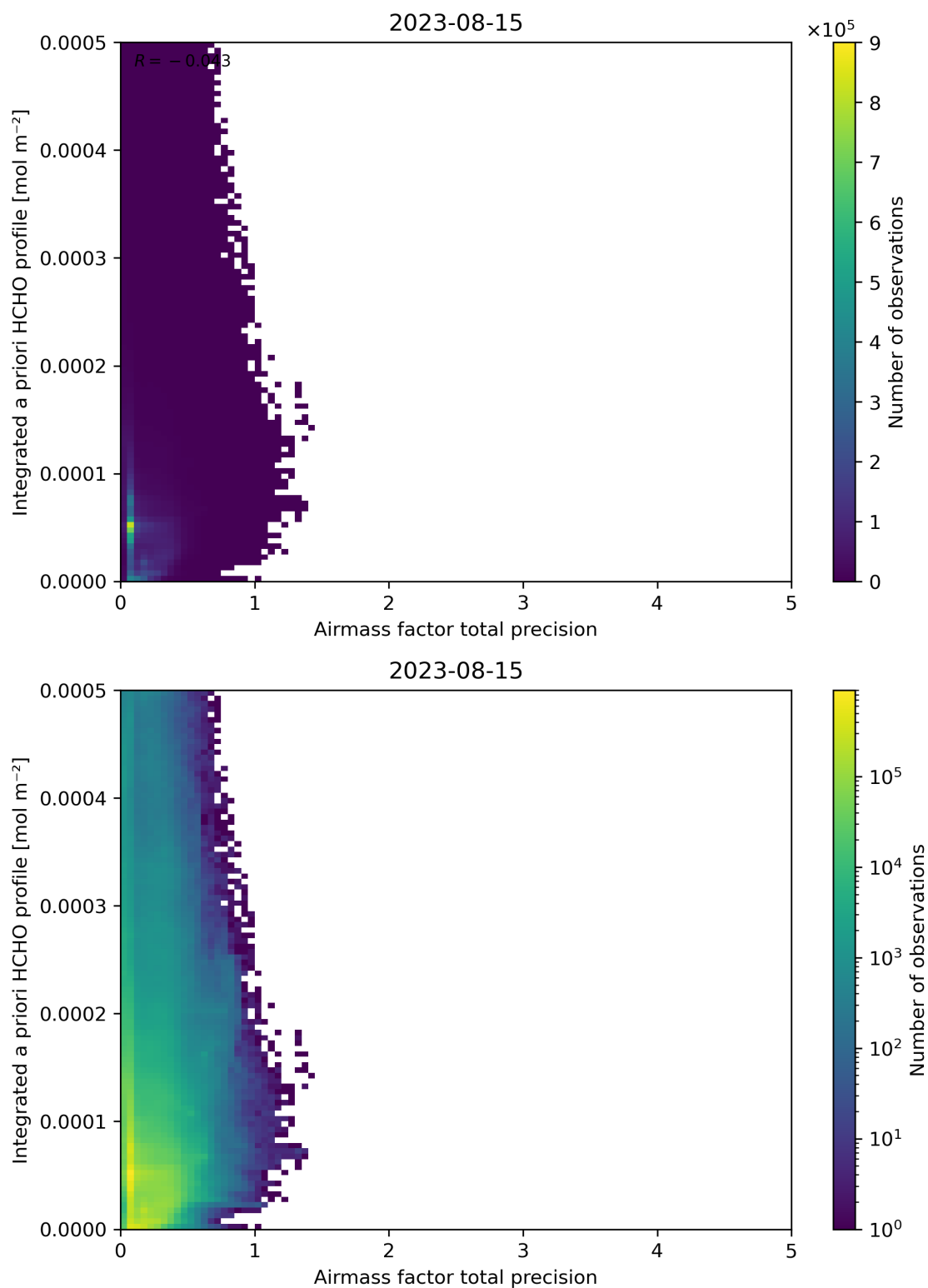
Figure 111: Scatter density plot of “Airmass factor total precision” against “Integrated a priori HCHO profile” for 2023-08-14 to 2023-08-16.
