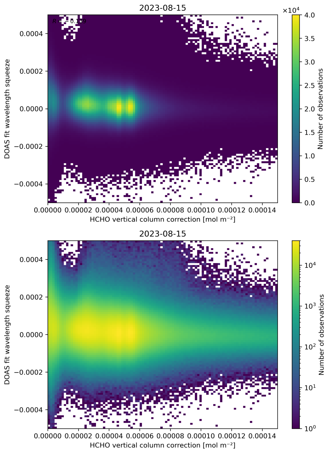
Figure 114: Scatter density plot of “HCHO vertical column correction” against “DOAS fit wavelength squeeze” for 2023-08-14 to 2023-08-16.
