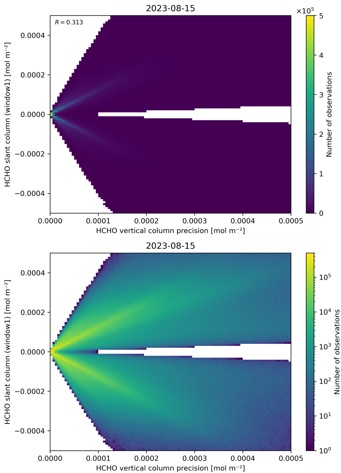
Figure 142: Scatter density plot of “HCHO vertical column precision” against “HCHO slant column (window1)” for 2023-08-14 to 2023-08-16.
