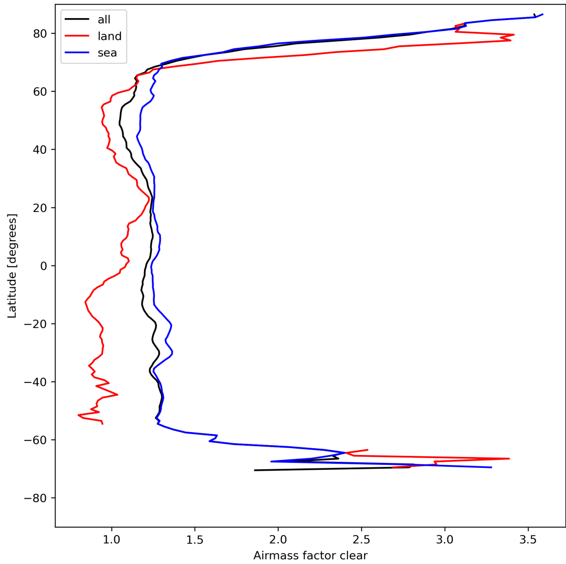
Figure 28: Zonal average of “Airmass factor clear” for 2023-08-14 to 2023-08-16.
