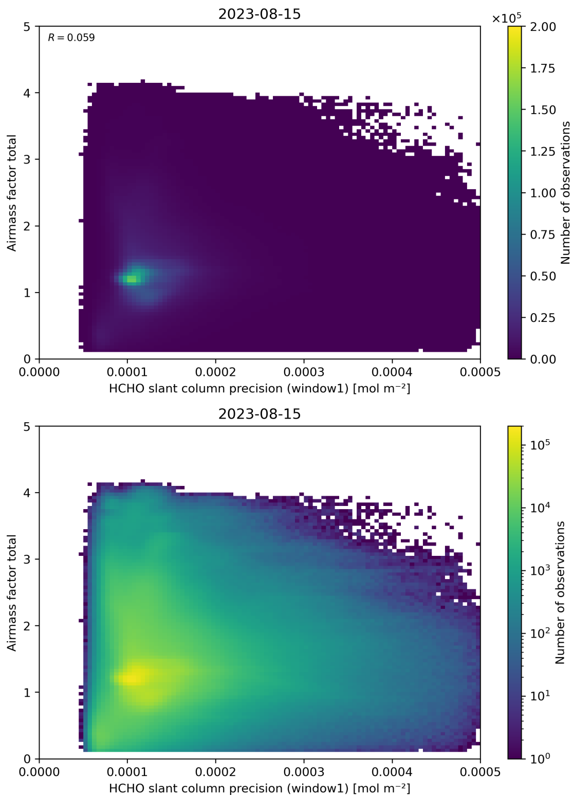
Figure 94: Scatter density plot of “HCHO slant column precision (window1)” against “Airmass factor total” for 2023-08-14 to 2023-08-16.
