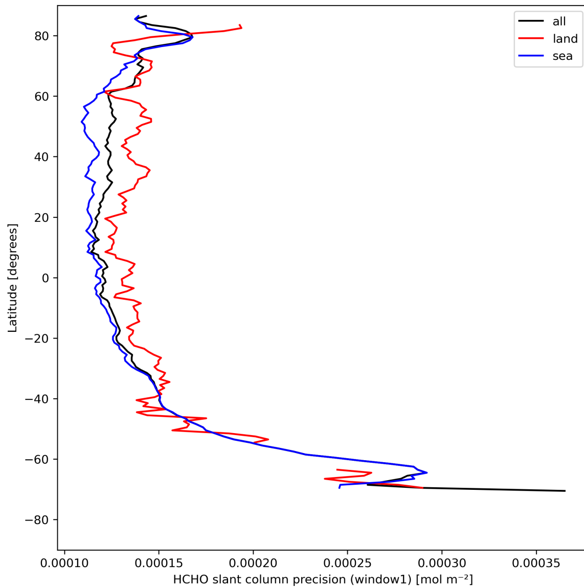
Figure 25: Zonal average of “HCHO slant column precision (window1)” for 2023-08-14 to 2023-08-16.
