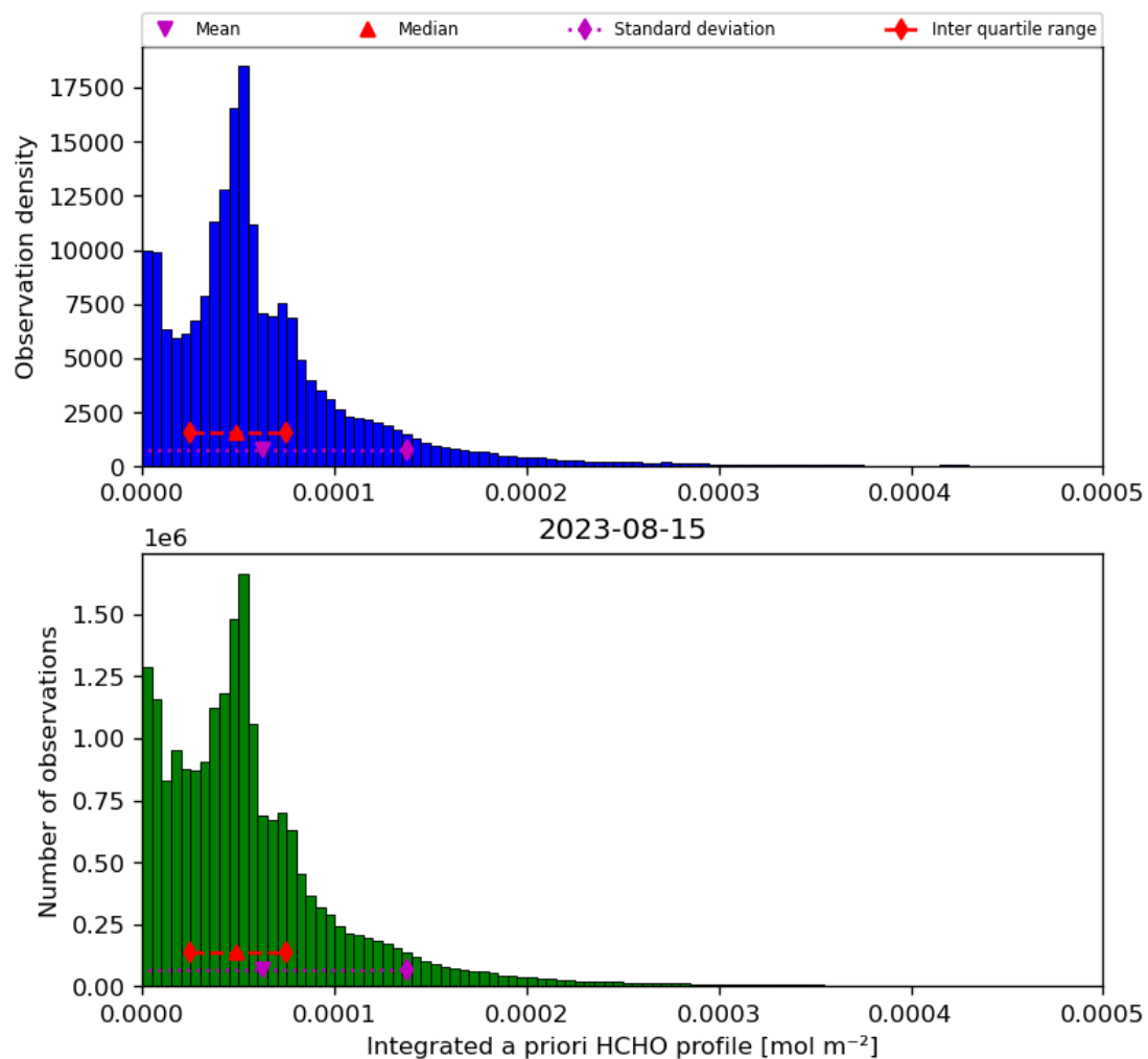
Figure 43: Histogram of “Integrated a priori HCHO profile” for 2023-08-14 to 2023-08-16
