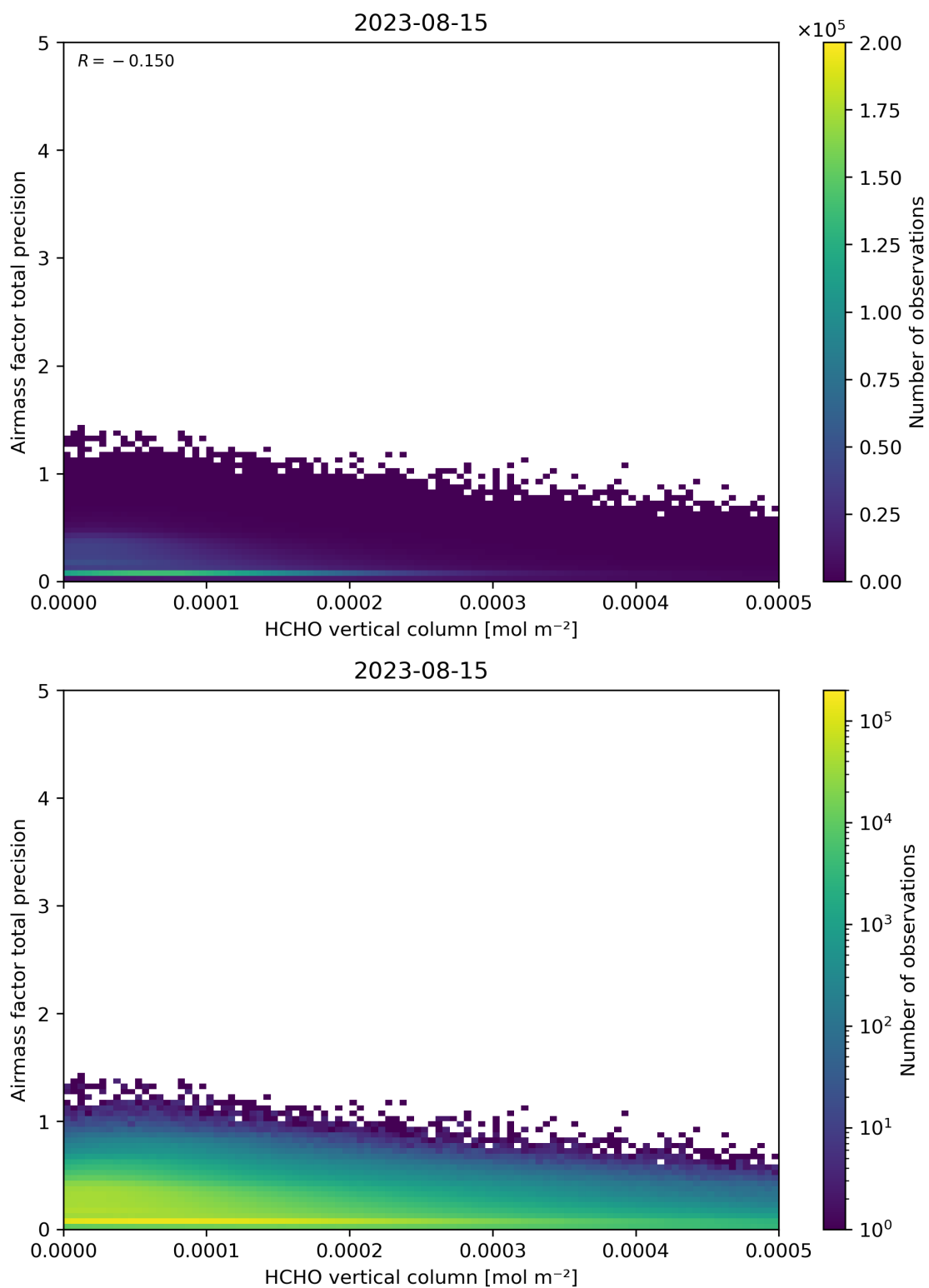
Figure 132: Scatter density plot of “HCHO vertical column” against “Airmass factor total precision” for 2023-08-14 to 2023-08-16.
