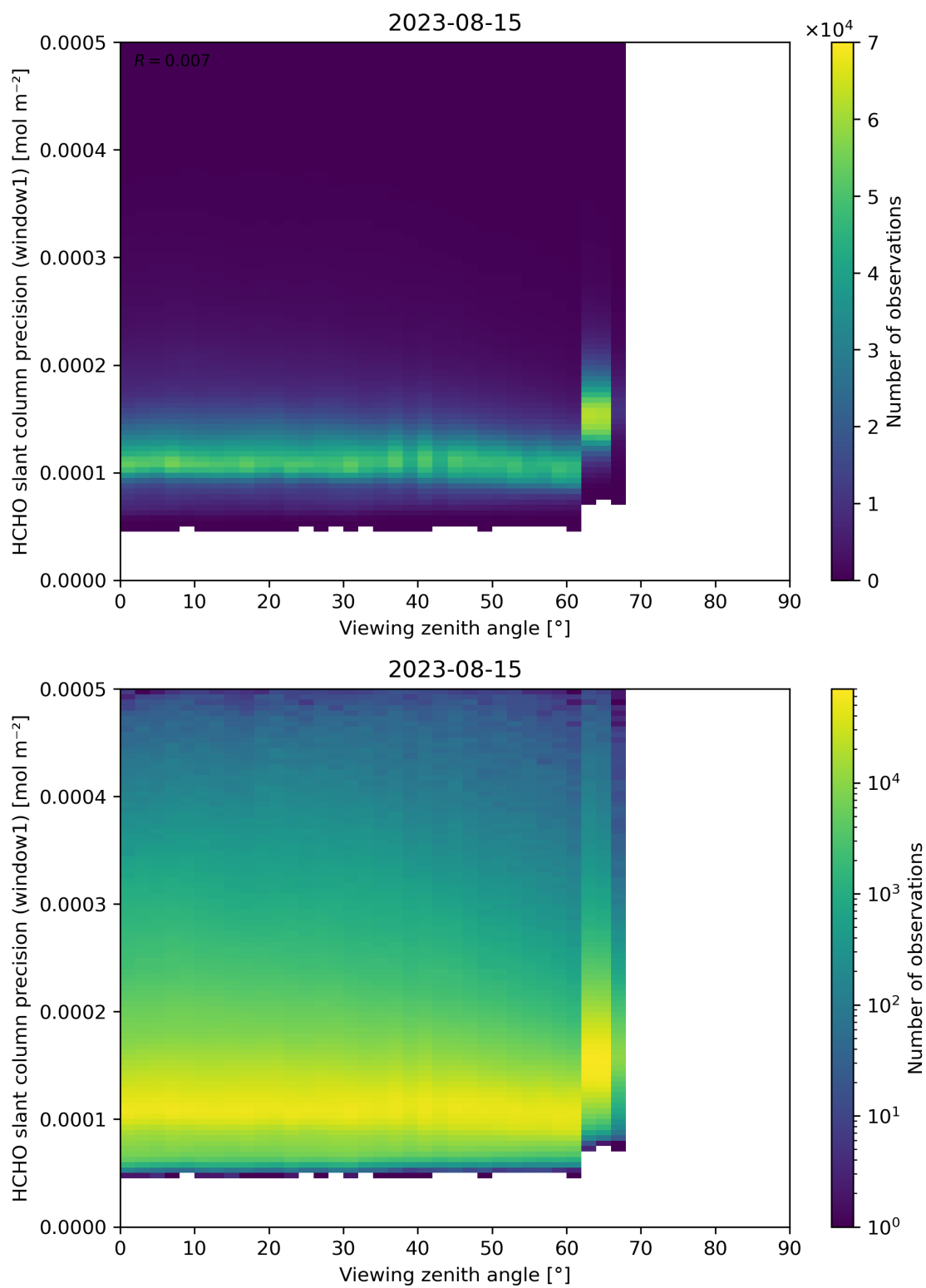
Figure 189: Scatter density plot of “Viewing zenith angle” against “HCHO slant column precision (window1)” for 2023-08-14 to 2023-08-16.
