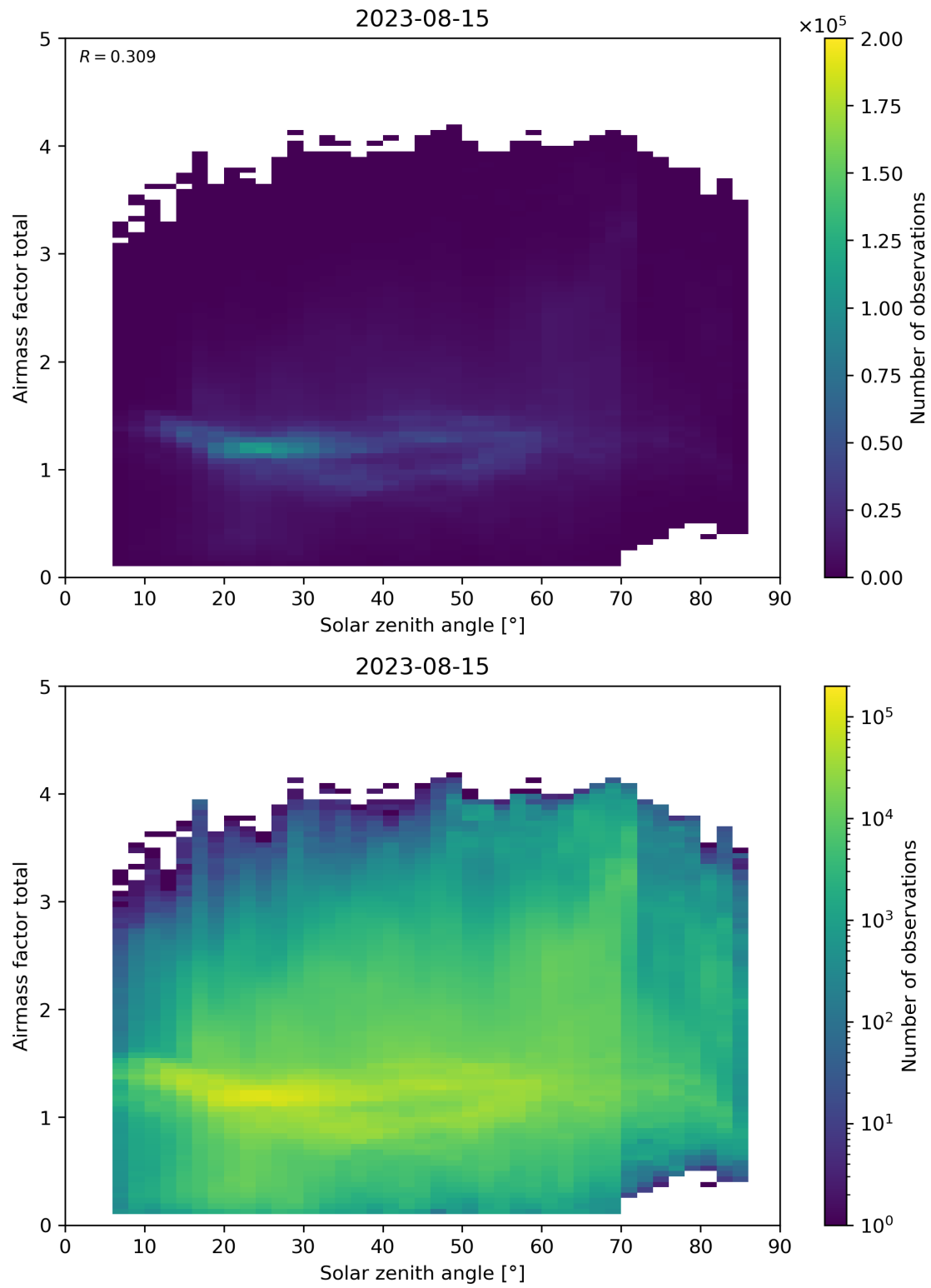
Figure 175: Scatter density plot of “Solar zenith angle” against “Airmass factor total” for 2023-08-14 to 2023-08-16.
