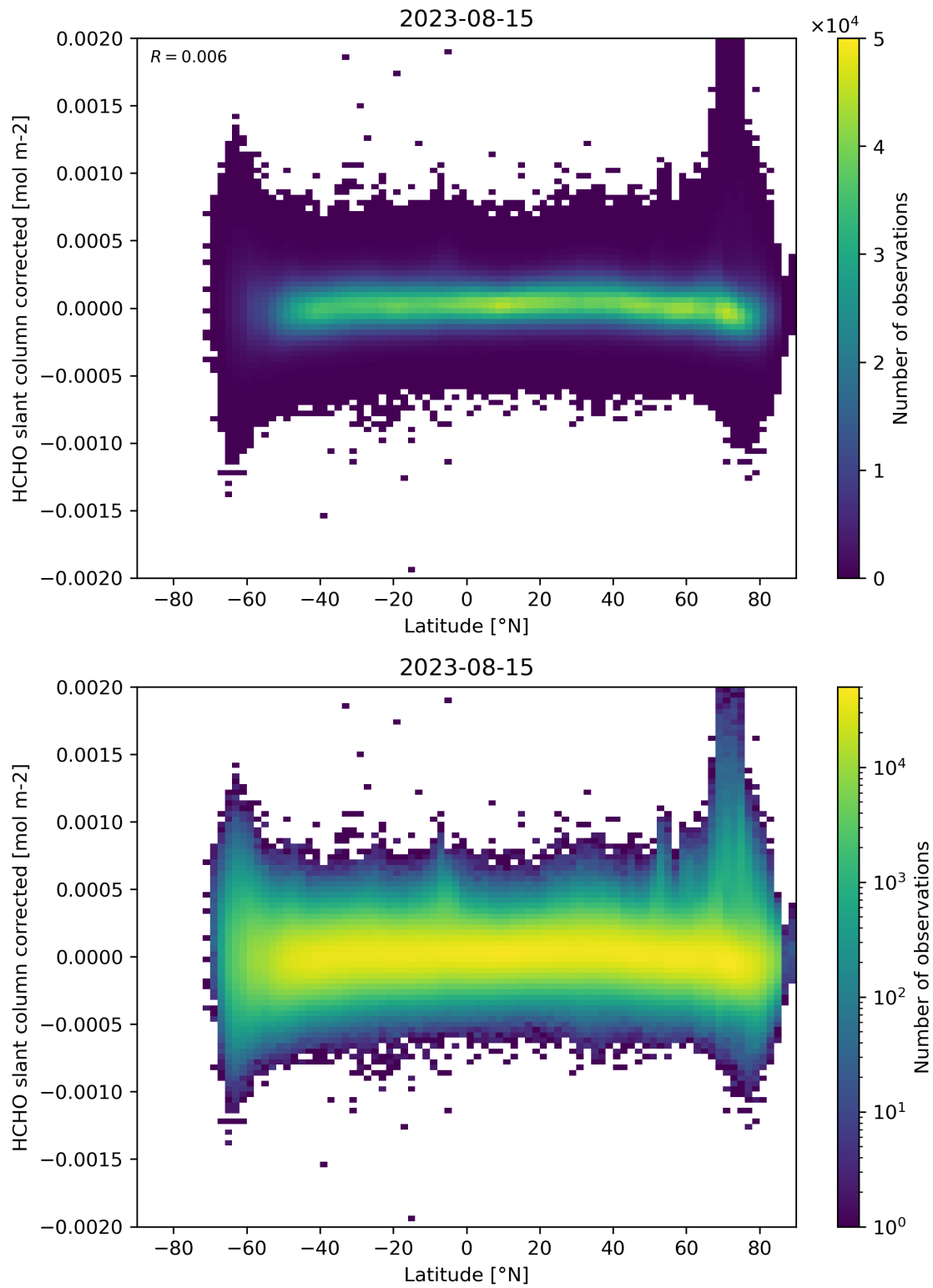
Figure 157: Scatter density plot of “Latitude” against “HCHO slant column corrected” for 2023-08-14 to 2023-08-16.
