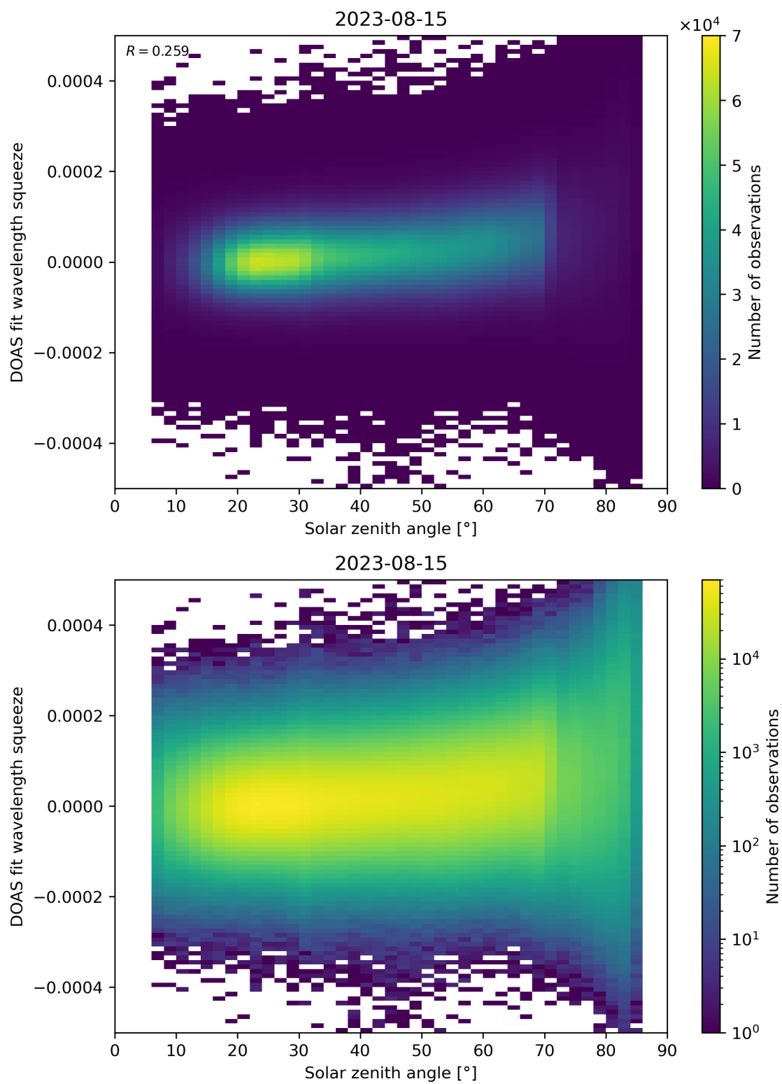
Figure 169: Scatter density plot of “Solar zenith angle” against “DOAS fit wavelength squeeze” for 2023-08-14 to 2023-08-16.
