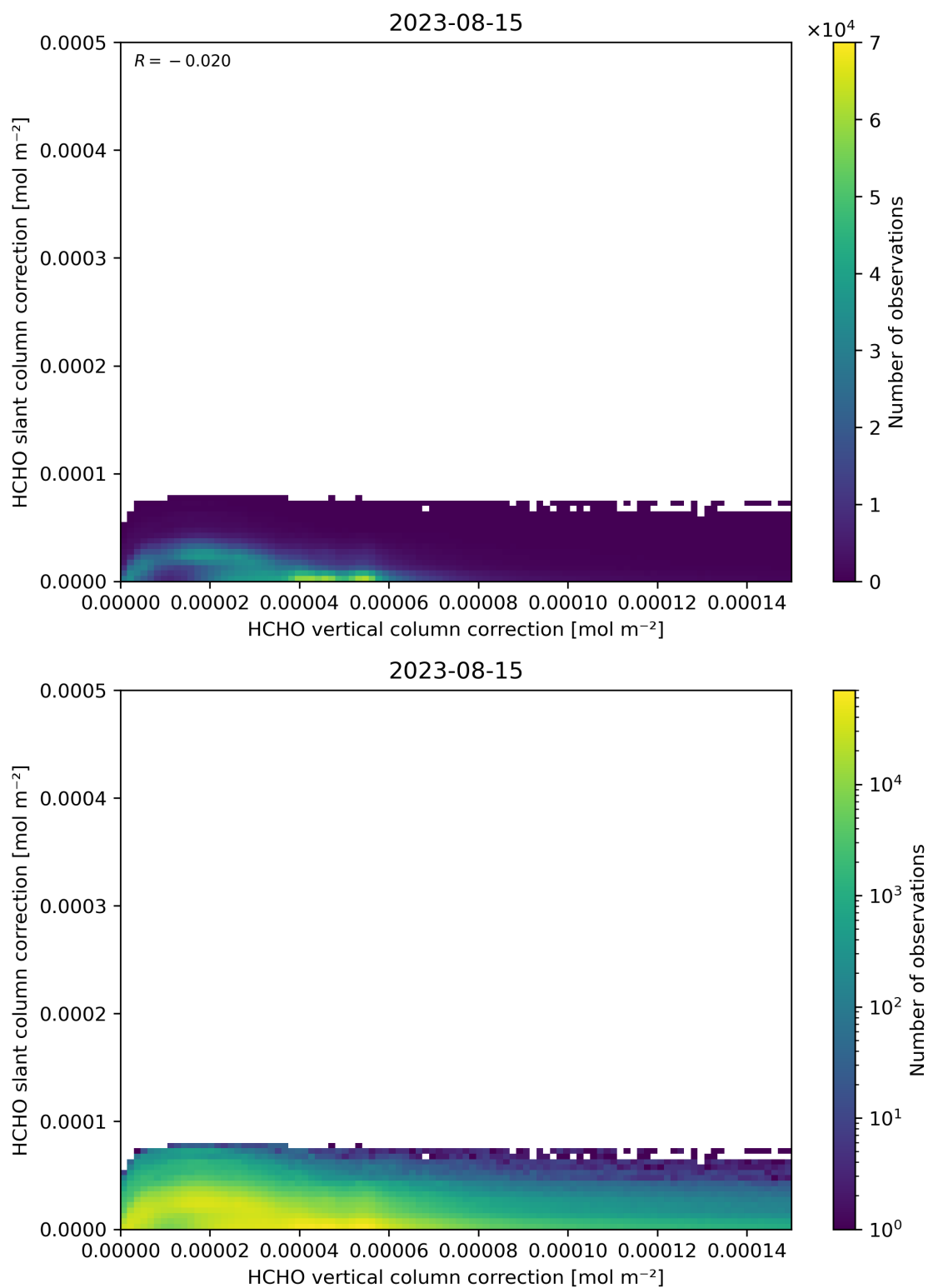
Figure 117: Scatter density plot of “HCHO vertical column correction” against “HCHO slant column correction” for 2023-08-14 to 2023-08-16.
