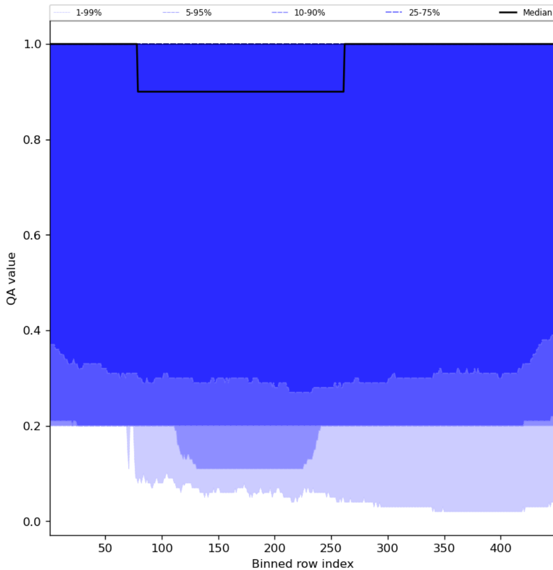
Figure 48: Along track statistics of “QA value” for 2023-08-14 to 2023-08-16
