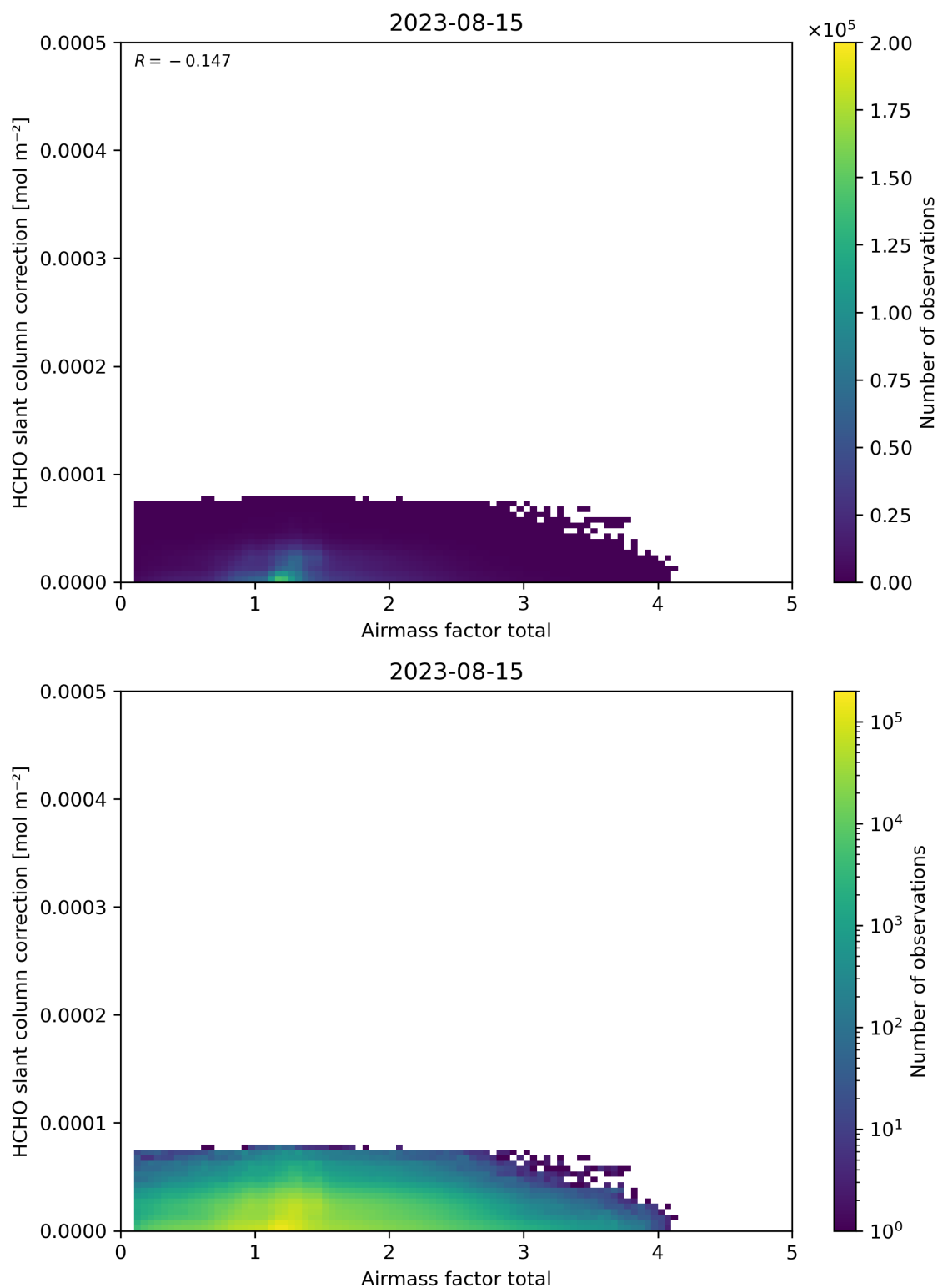
Figure 102: Scatter density plot of “Airmass factor total” against “HCHO slant column correction” for 2023-08-14 to 2023-08-16.
