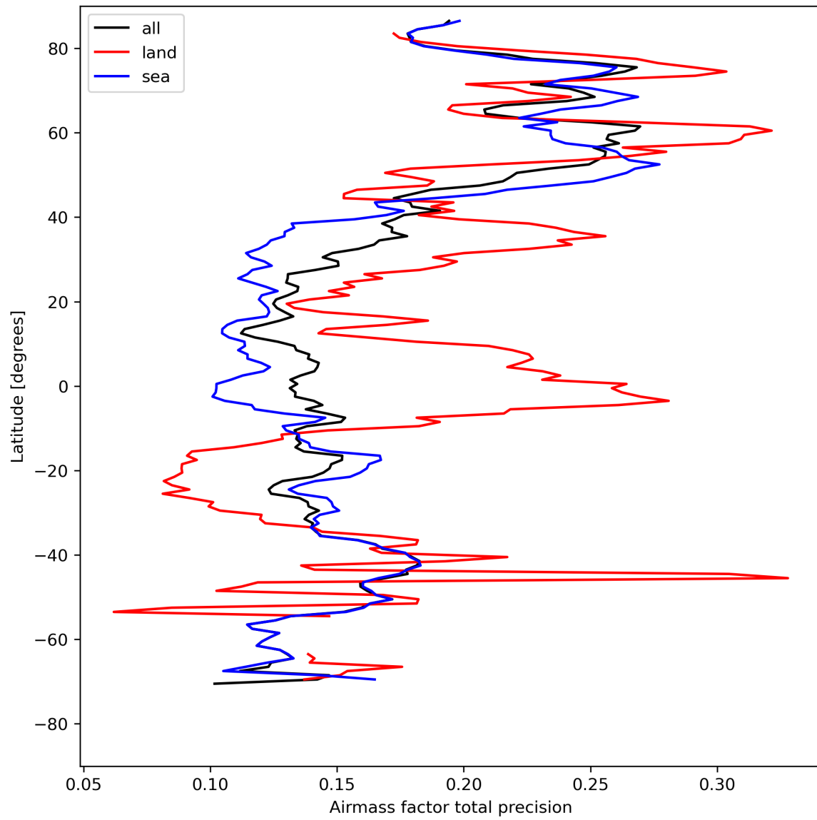
Figure 27: Zonal average of “Airmass factor total precision” for 2023-08-14 to 2023-08-16.
