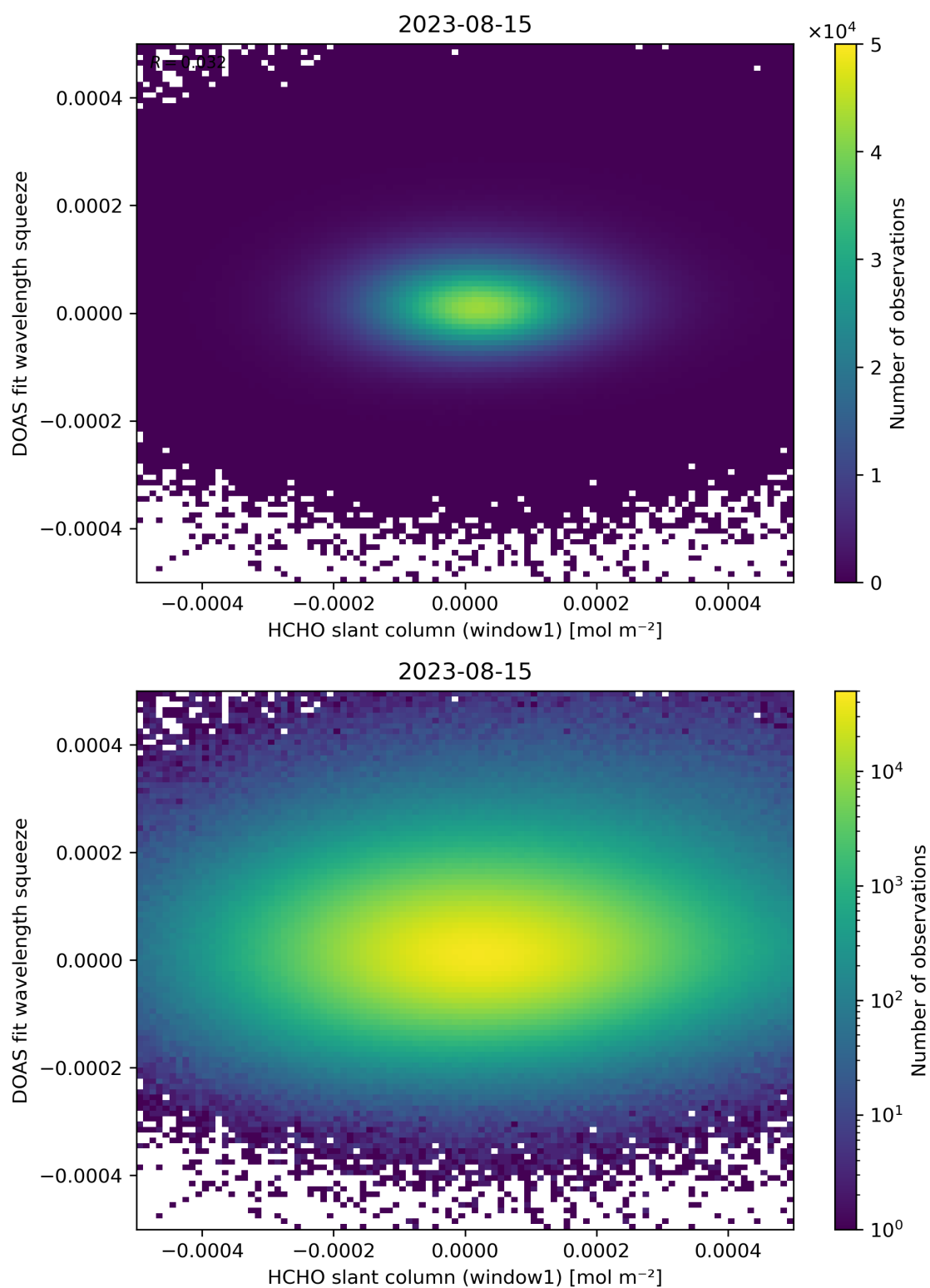
Figure 80: Scatter density plot of “HCHO slant column (window1)” against “DOAS fit wavelength squeeze” for 2023-08-14 to 2023-08-16.
