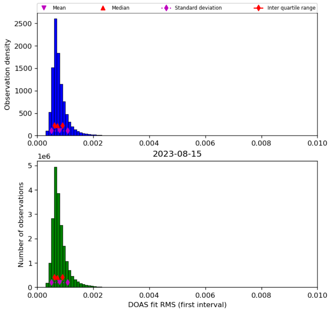
Figure 46: Histogram of “DOAS fit RMS (first interval)” for 2023-08-14 to 2023-08-16
