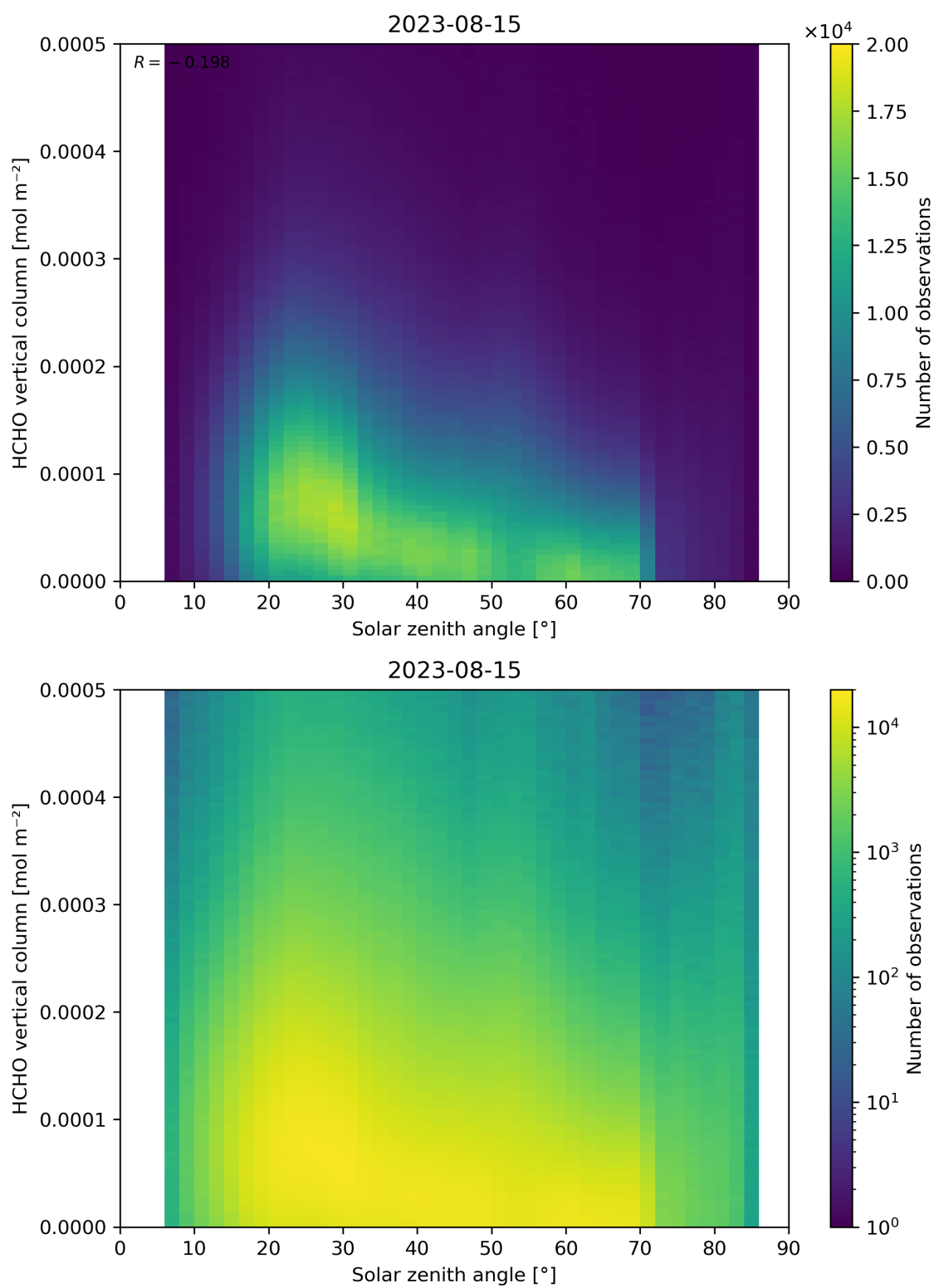
Figure 177: Scatter density plot of “Solar zenith angle” against “HCHO vertical column” for 2023-08-14 to 2023-08-16.
