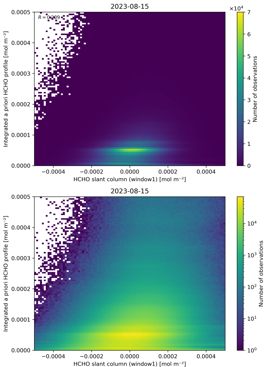
Figure 87: Scatter density plot of “HCHO slant column (window1)” against “Integrated a priori HCHO profile” for 2023-08-14 to 2023-08-16.
