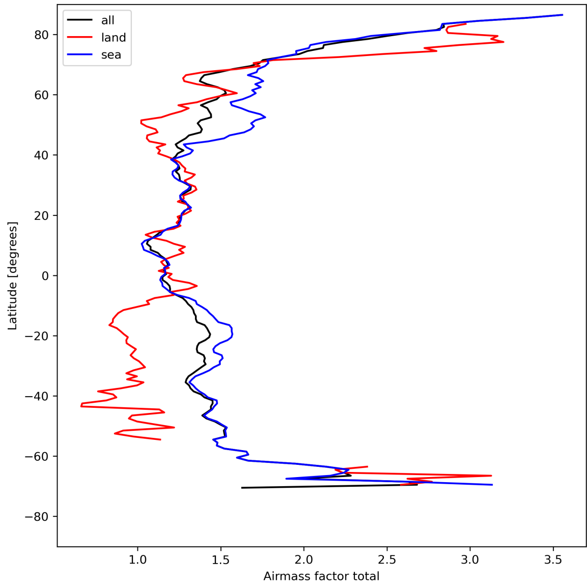
Figure 26: Zonal average of “Airmass factor total” for 2023-08-14 to 2023-08-16.
