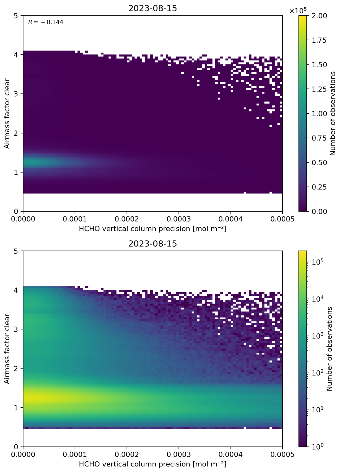
Figure 139: Scatter density plot of “HCHO vertical column precision” against “Airmass factor clear” for 2023-08-14 to 2023-08-16.
