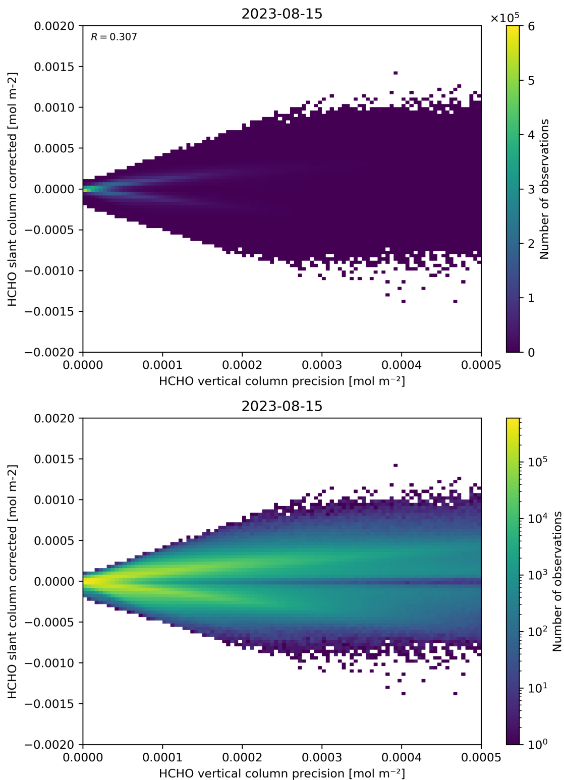
Figure 140: Scatter density plot of “HCHO vertical column precision” against “HCHO slant column corrected” for 2023-08-14 to 2023-08-16.
