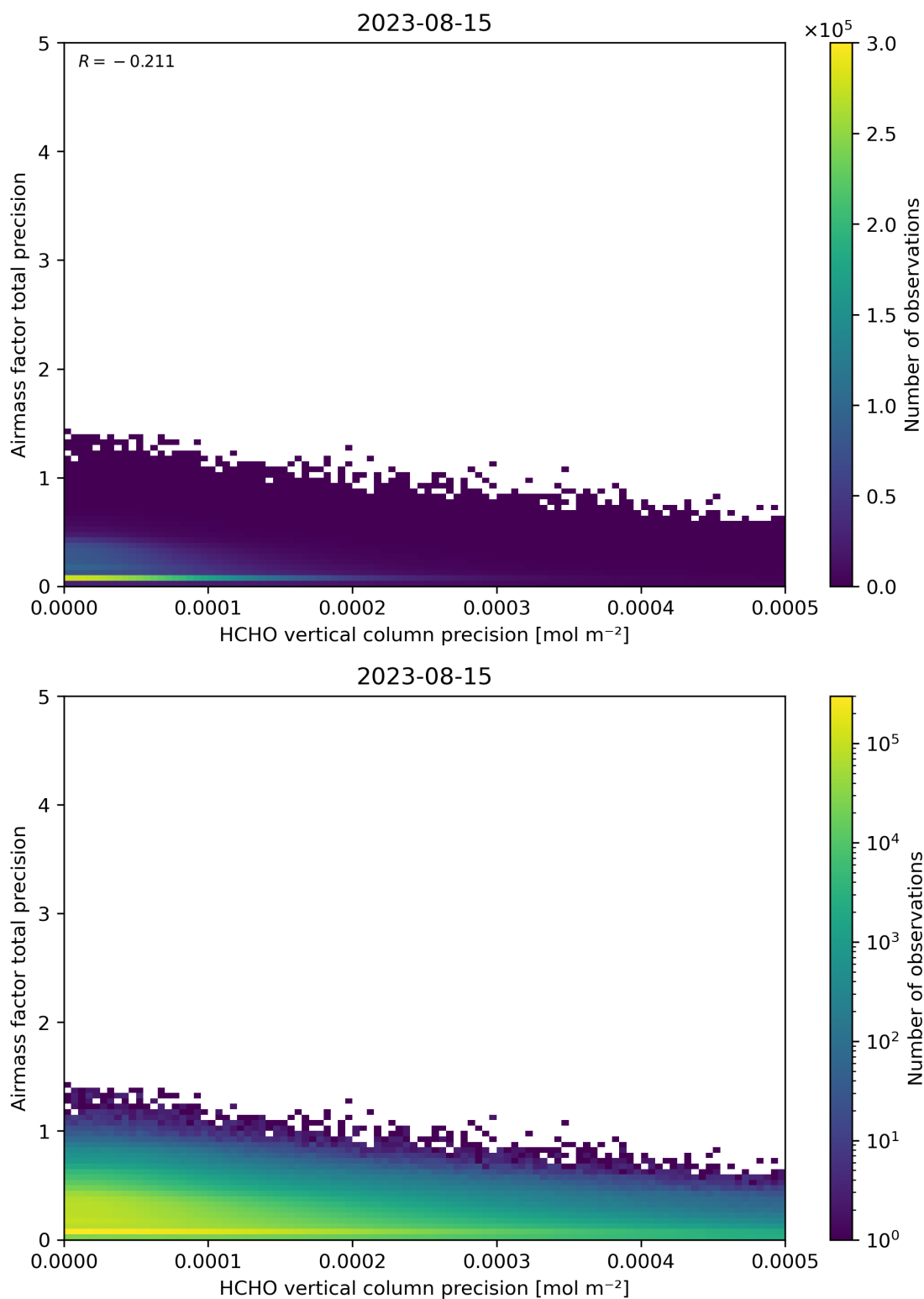
Figure 145: Scatter density plot of “HCHO vertical column precision” against “Airmass factor total precision” for 2023-08-14 to 2023-08-16.
