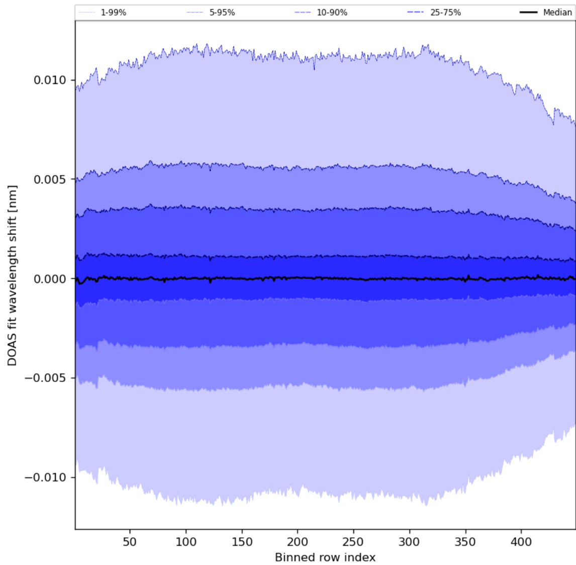
Figure 58: Along track statistics of “DOAS fit wavelength shift” for 2023-08-14 to 2023-08-16
