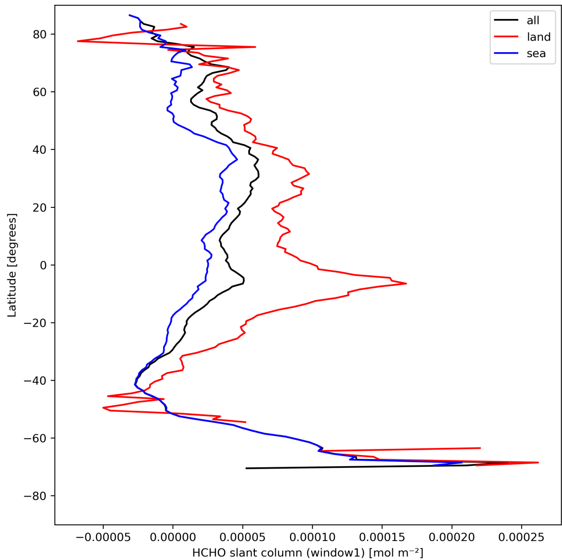
Figure 24: Zonal average of “HCHO slant column (window1)” for 2023-08-14 to 2023-08-16.
