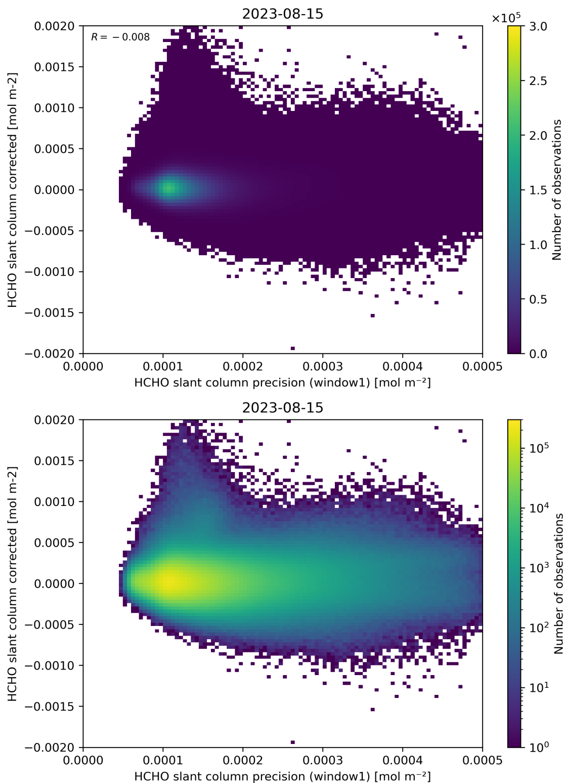
Figure 92: Scatter density plot of “HCHO slant column precision (window1)” against “HCHO slant column corrected” for 2023-08-14 to 2023-08-16.
