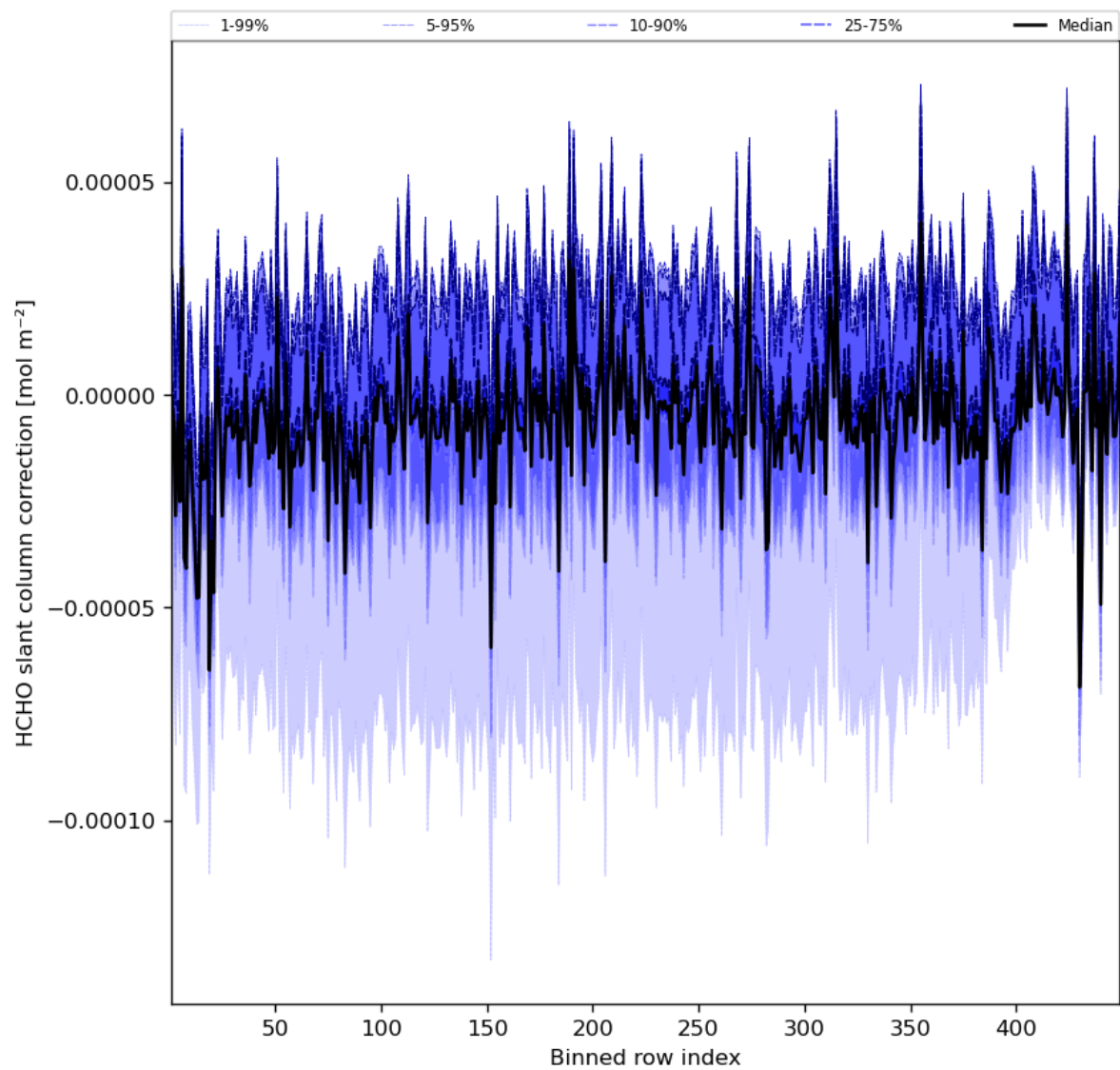
Figure 61: Along track statistics of “HCHO slant column correction” for 2023-08-14 to 2023-08-16
