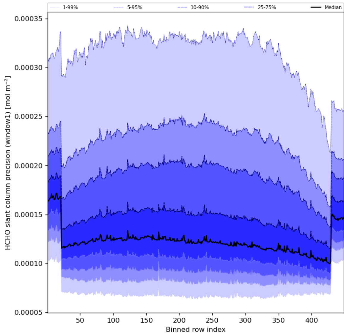
Figure 53: Along track statistics of “HCHO slant column precision (window1)” for 2023-08-14 to 2023-08-16
