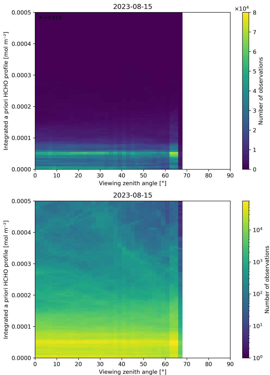
Figure 195: Scatter density plot of “Viewing zenith angle” against “Integrated a priori HCHO profile” for 2023-08-14 to 2023-08-16.
