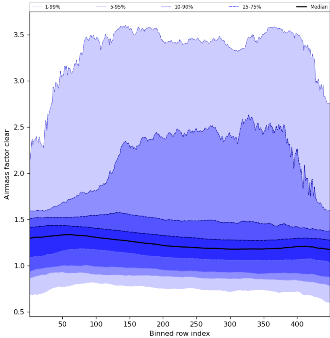
Figure 56: Along track statistics of “Airmass factor clear” for 2023-08-14 to 2023-08-16
