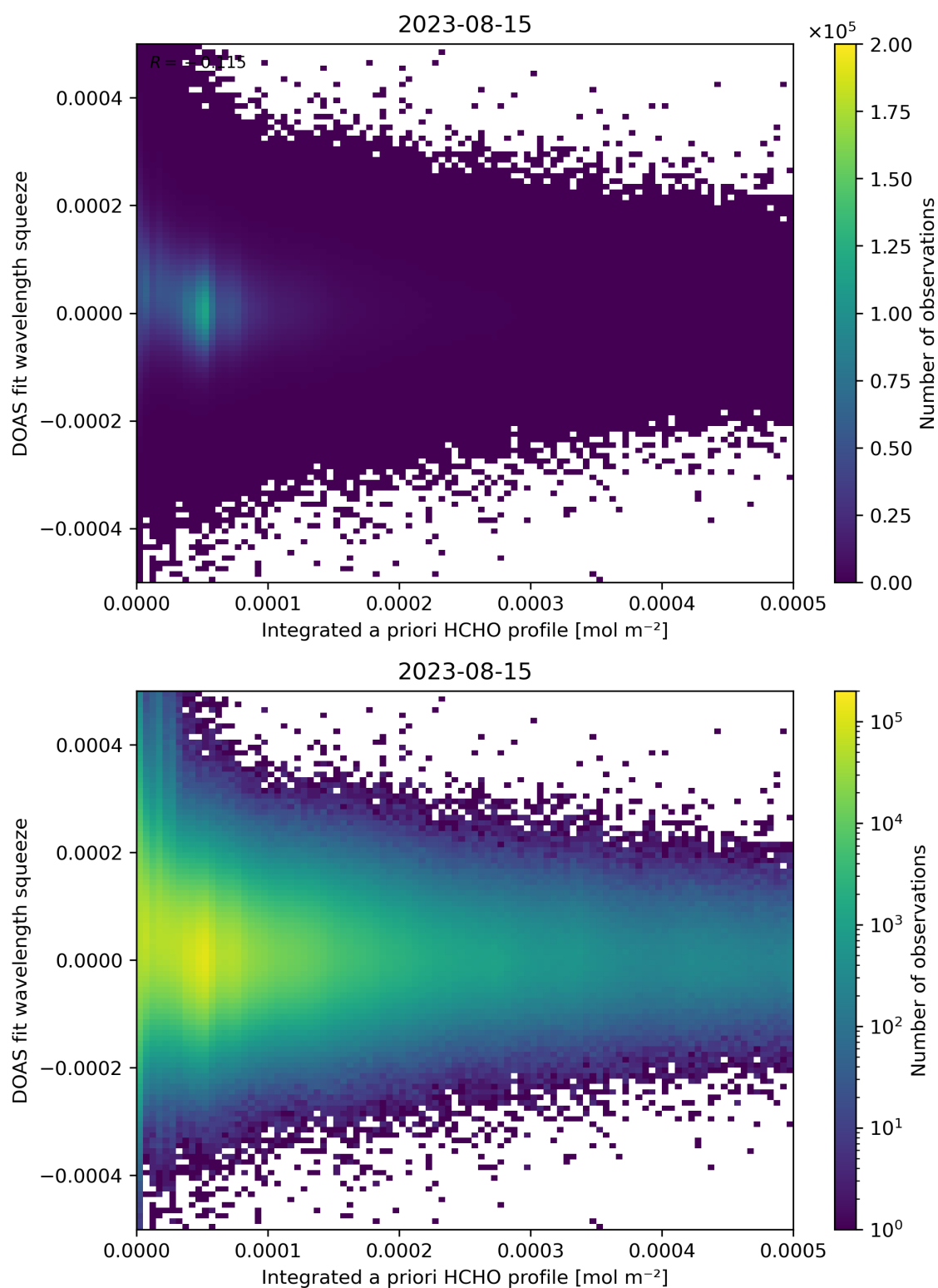
Figure 150: Scatter density plot of “Integrated a priori HCHO profile” against “DOAS fit wavelength squeeze” for 2023-08-14 to 2023-08-16.
