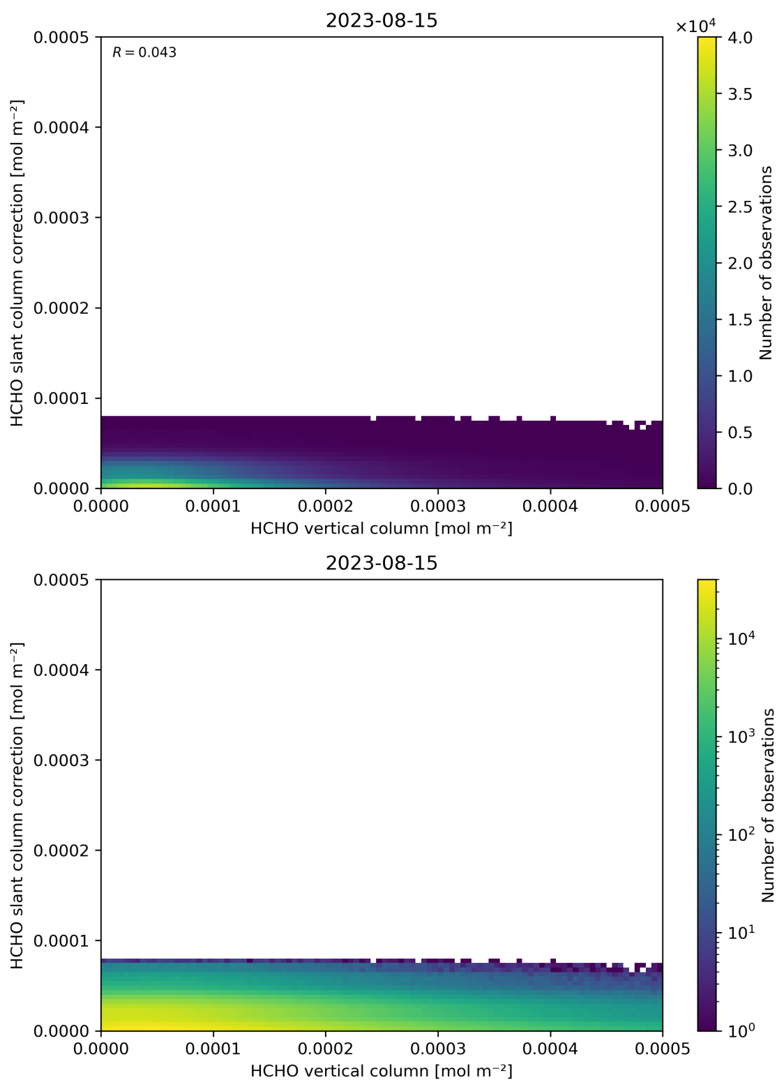
Figure 128: Scatter density plot of “HCHO vertical column” against “HCHO slant column correction” for 2023-08-14 to 2023-08-16.
