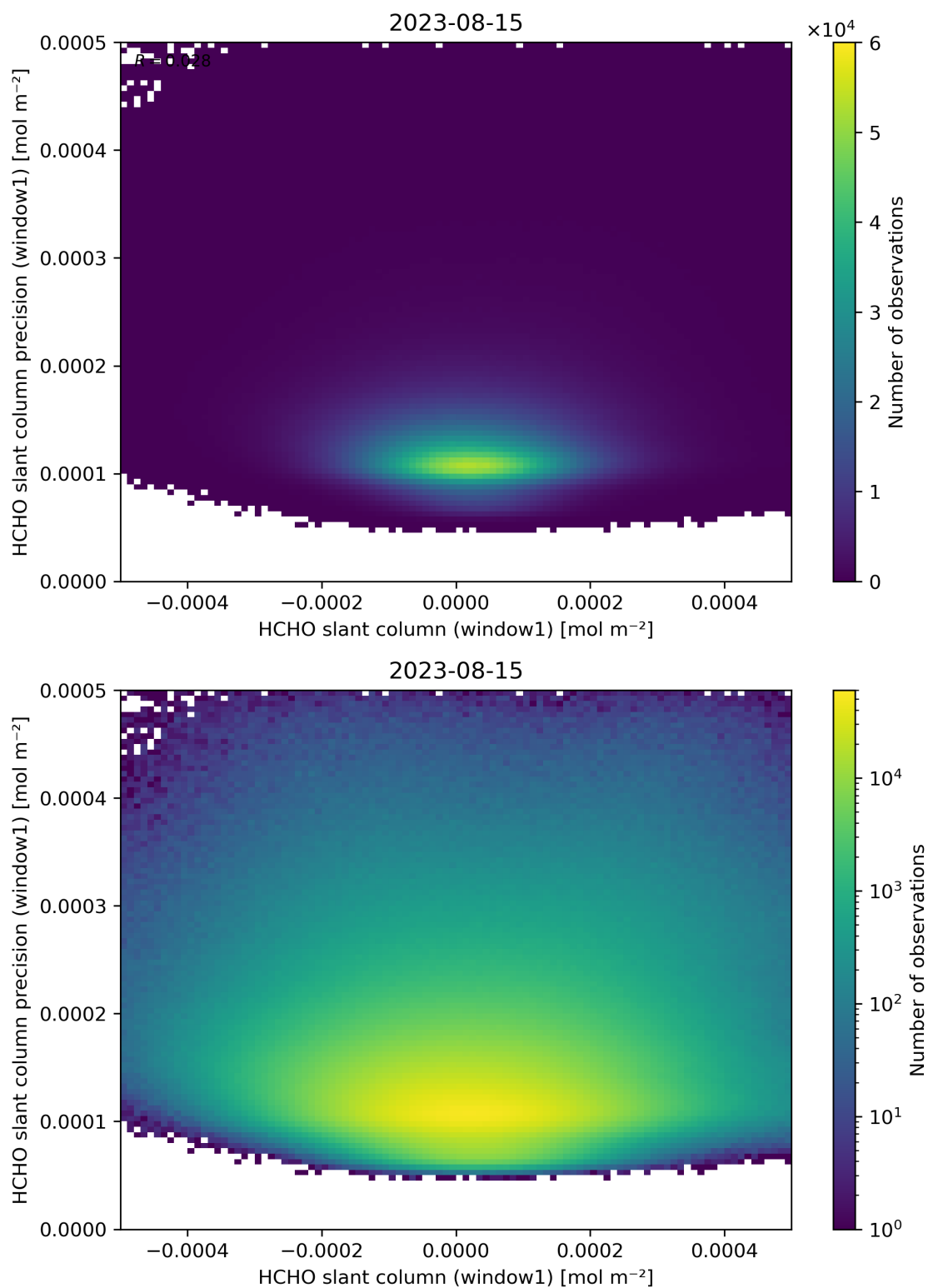
Figure 84: Scatter density plot of “HCHO slant column (window1)” against “HCHO slant column precision (window1)” for 2023-08-14 to 2023-08-16.
