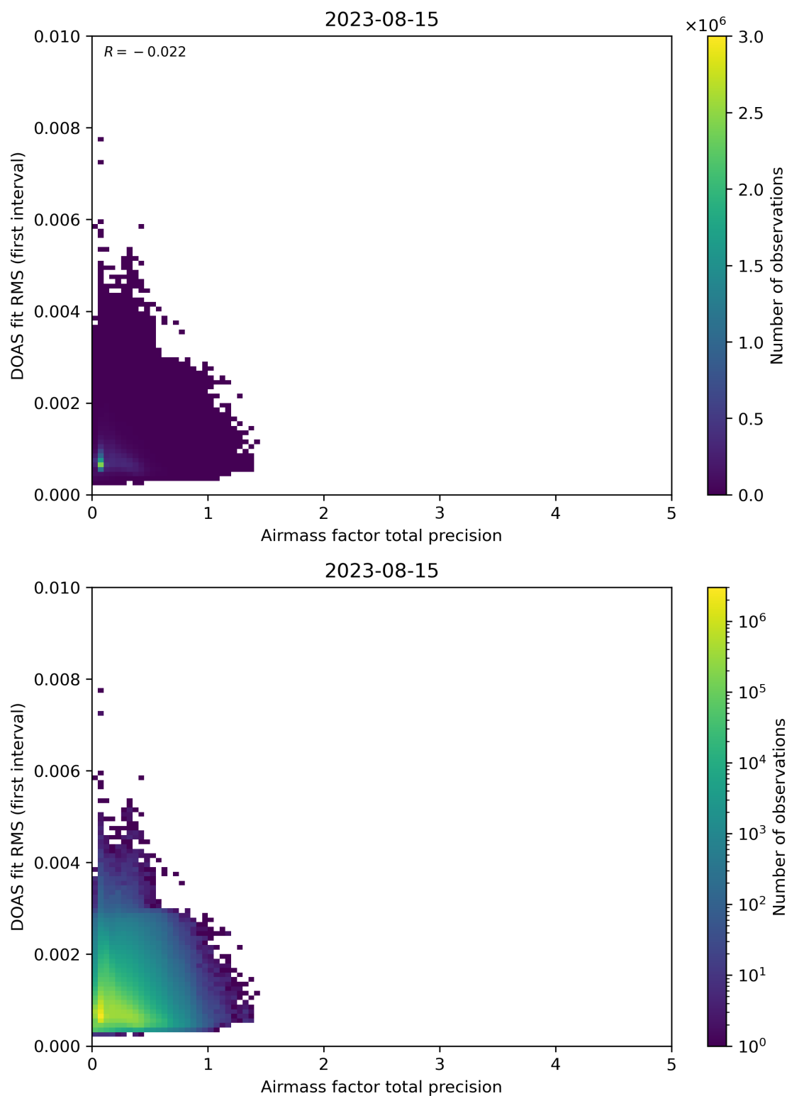
Figure 105: Scatter density plot of “Airmass factor total precision” against “DOAS fit RMS (first interval)” for 2023-08-14 to 2023-08-16.
