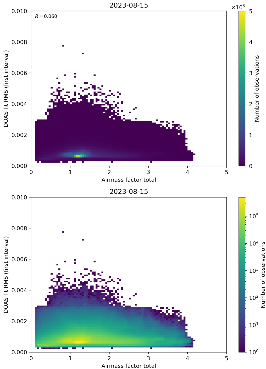
Figure 97: Scatter density plot of “Airmass factor total” against “DOAS fit RMS (first interval)” for 2023-08-14 to 2023-08-16.
