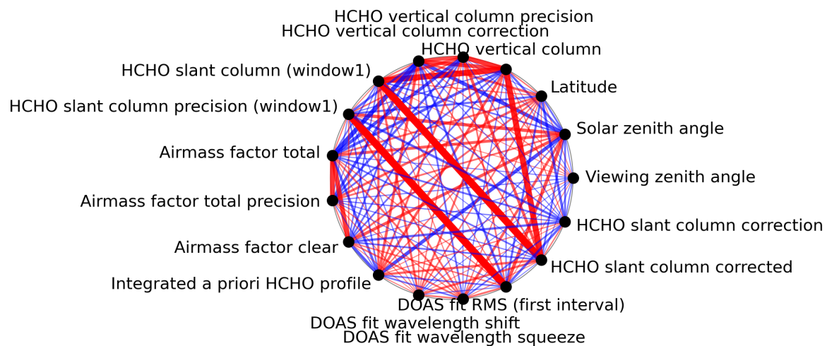
Figure 1: Map of correlation graph for 2023-08-14 to 2023-08-16.
