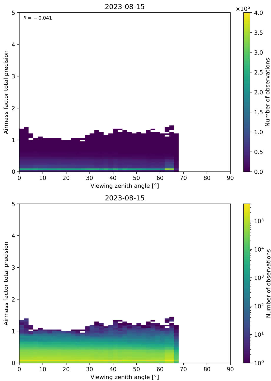
Figure 191: Scatter density plot of “Viewing zenith angle” against “Airmass factor total precision” for 2023-08-14 to 2023-08-16.
