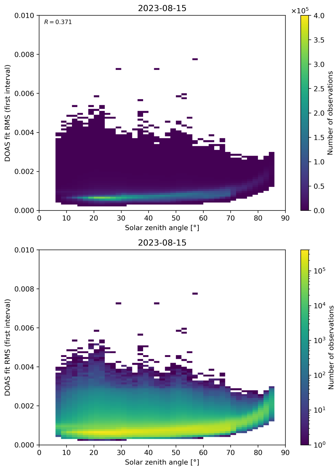
Figure 167: Scatter density plot of “Solar zenith angle” against “DOAS fit RMS (first interval)” for 2023-08-14 to 2023-08-16.
