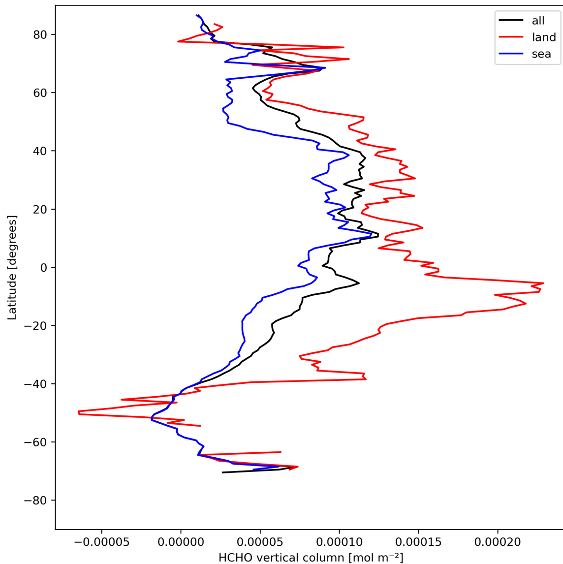
Figure 21: Zonal average of “HCHO vertical column” for 2023-08-14 to 2023-08-16.
