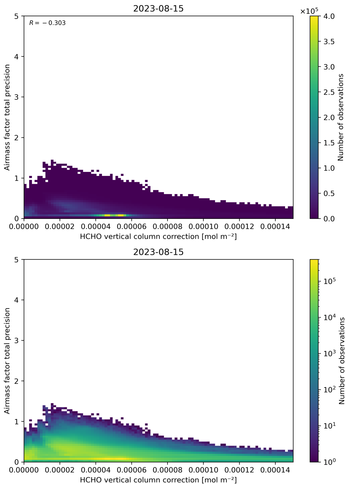
Figure 121: Scatter density plot of “HCHO vertical column correction” against “Airmass factor total precision” for 2023-08-14 to 2023-08-16.
