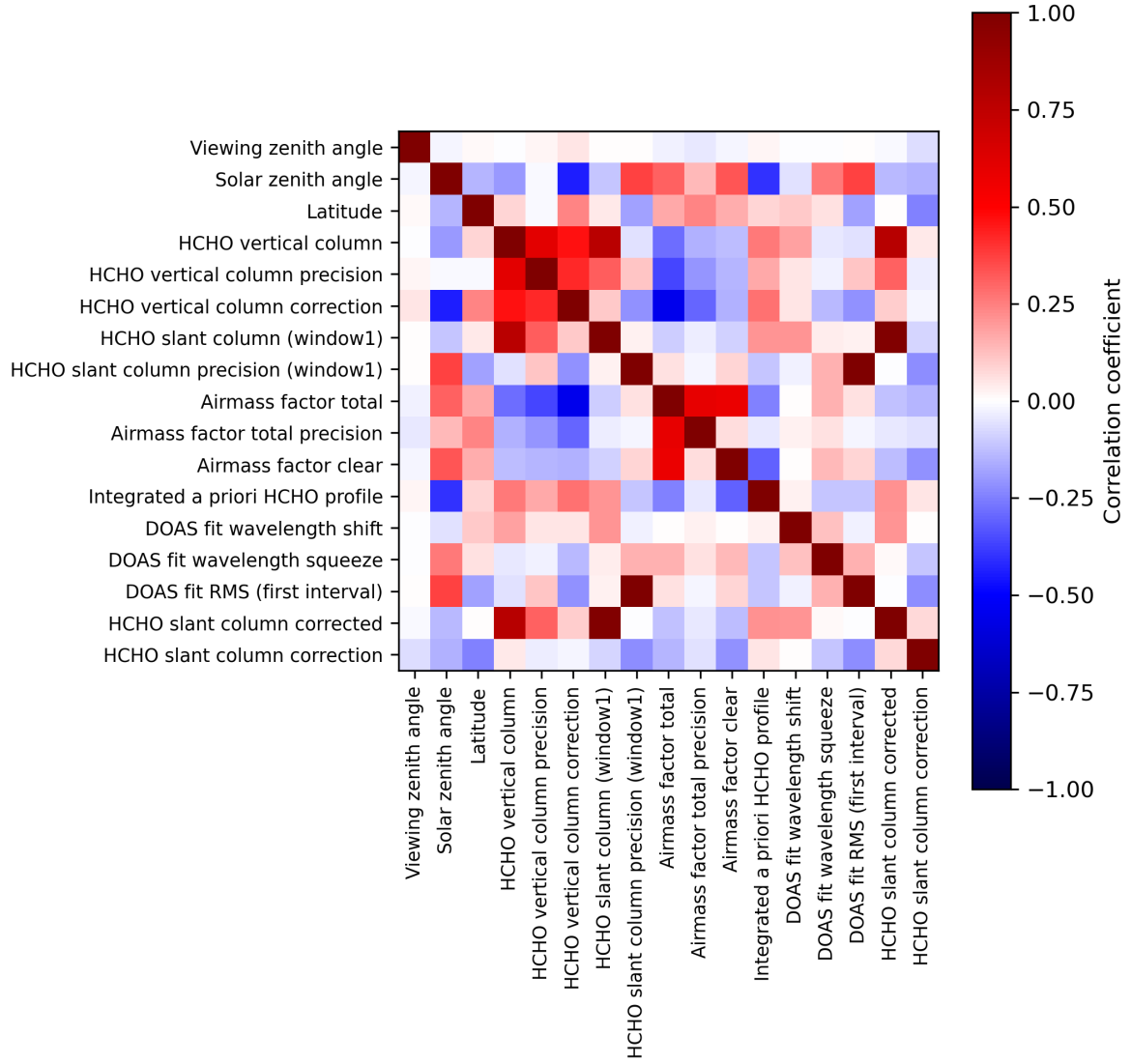
Figure 2: Map of correlation matrix for 2023-08-14 to 2023-08-16.
