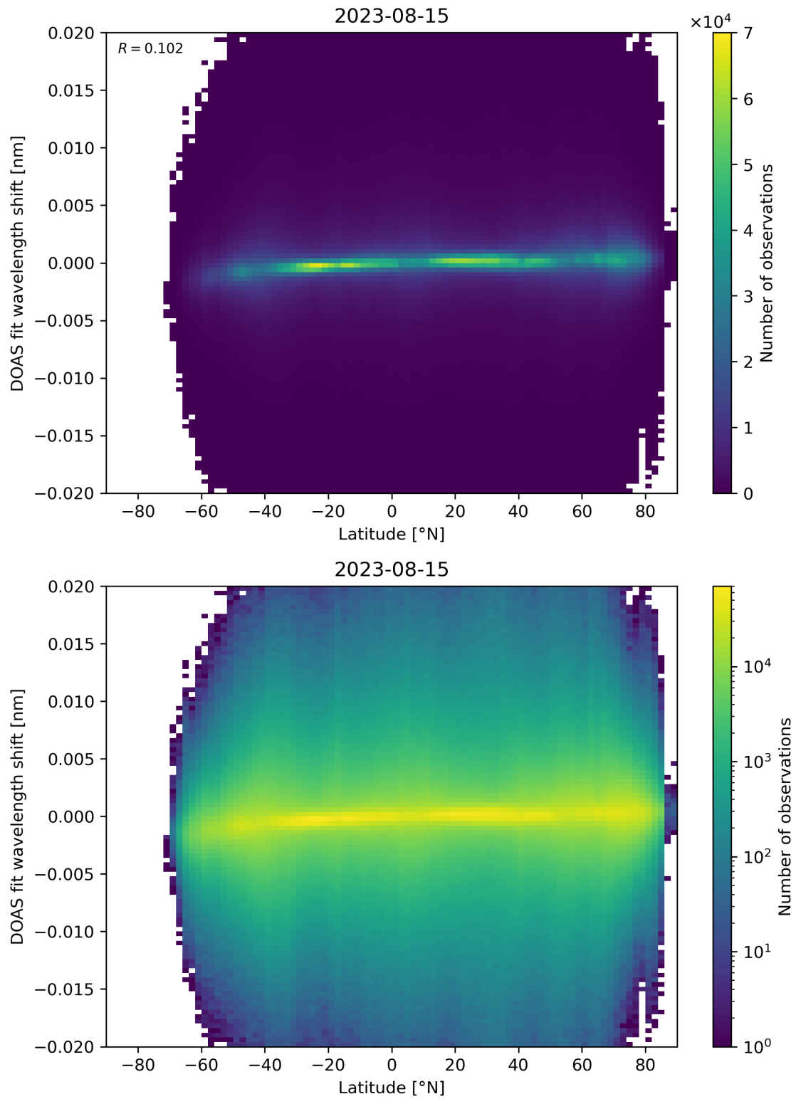
Figure 154: Scatter density plot of “Latitude” against “DOAS fit wavelength shift” for 2023-08-14 to 2023-08-16.
