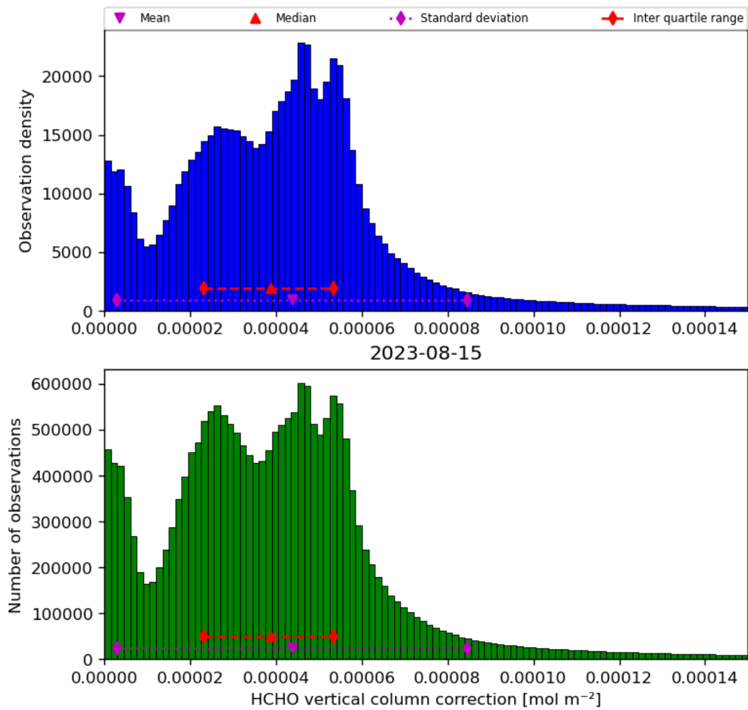
Figure 37: Histogram of “HCHO vertical column correction” for 2023-08-14 to 2023-08-16
