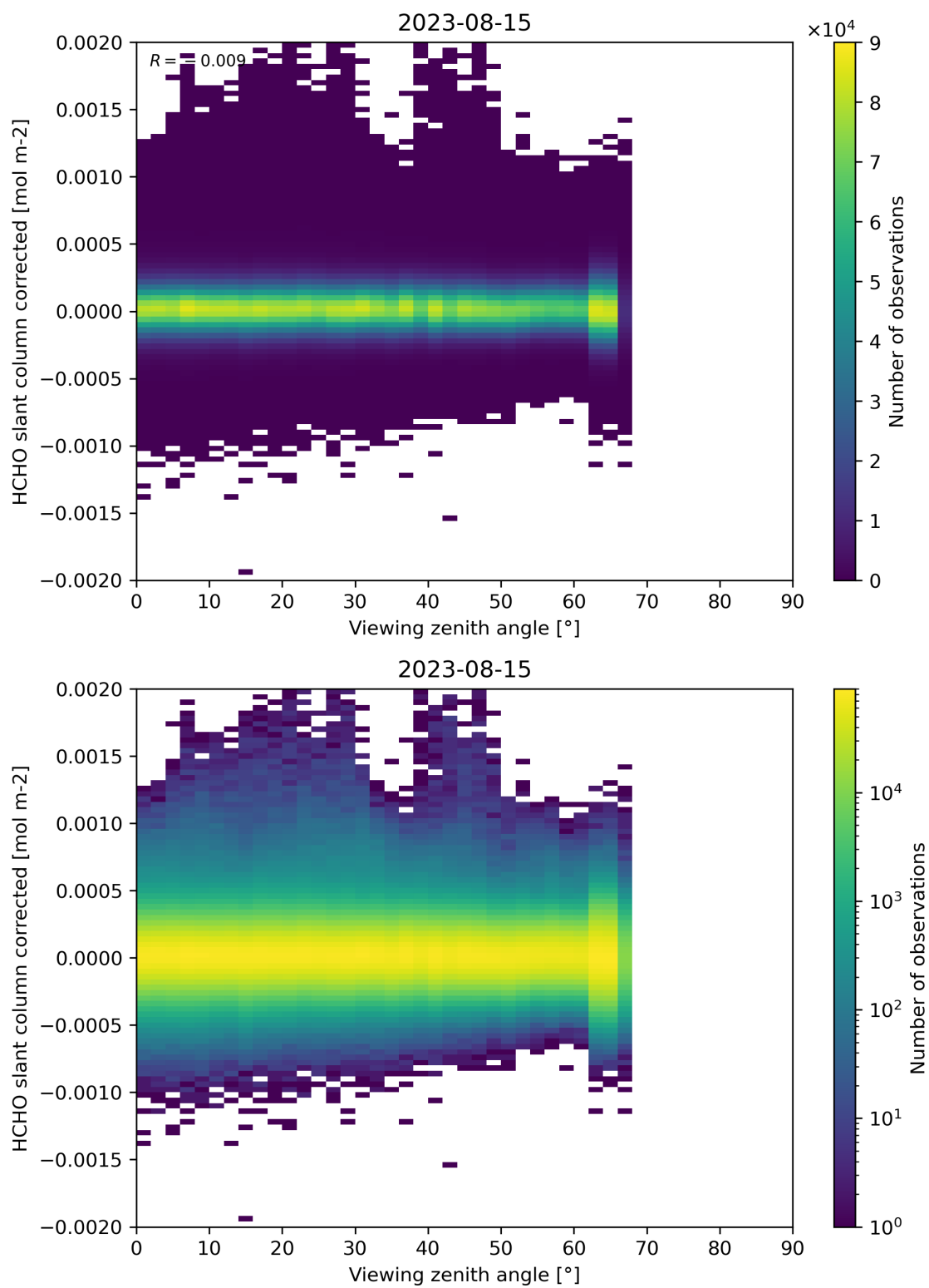
Figure 186: Scatter density plot of “Viewing zenith angle” against “HCHO slant column corrected” for 2023-08-14 to 2023-08-16.
