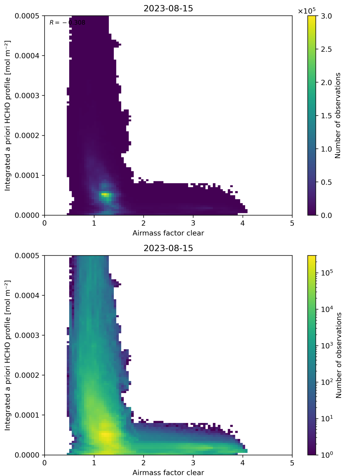
Figure 76: Scatter density plot of “Airmass factor clear” against “Integrated a priori HCHO profile” for 2023-08-14 to 2023-08-16.
