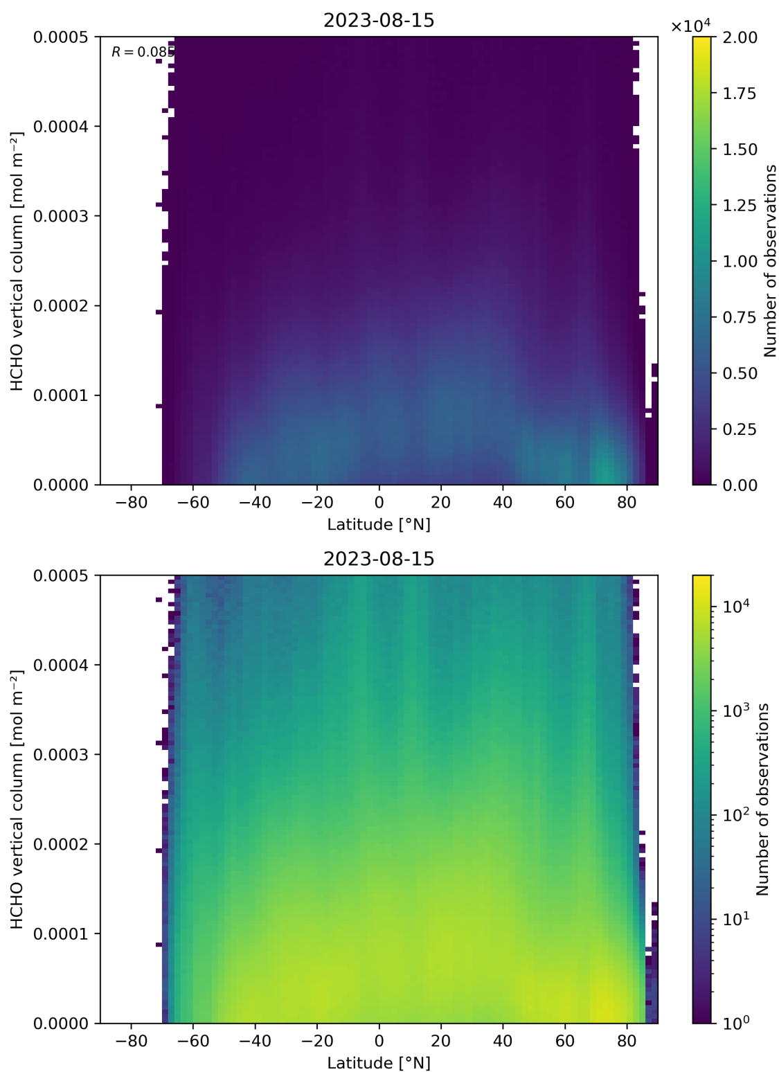
Figure 163: Scatter density plot of “Latitude” against “HCHO vertical column” for 2023-08-14 to 2023-08-16.
