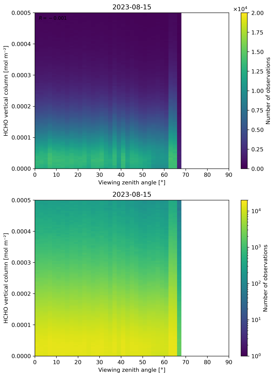
Figure 192: Scatter density plot of “Viewing zenith angle” against “HCHO vertical column” for 2023-08-14 to 2023-08-16.
