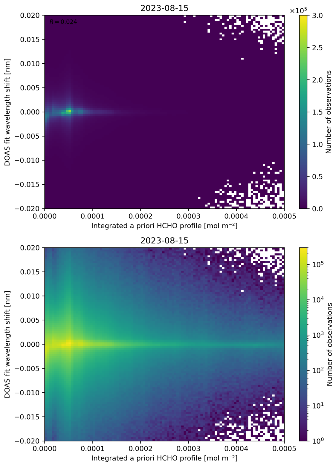
Figure 149: Scatter density plot of “Integrated a priori HCHO profile” against “DOAS fit wavelength shift” for 2023-08-14 to 2023-08-16.
