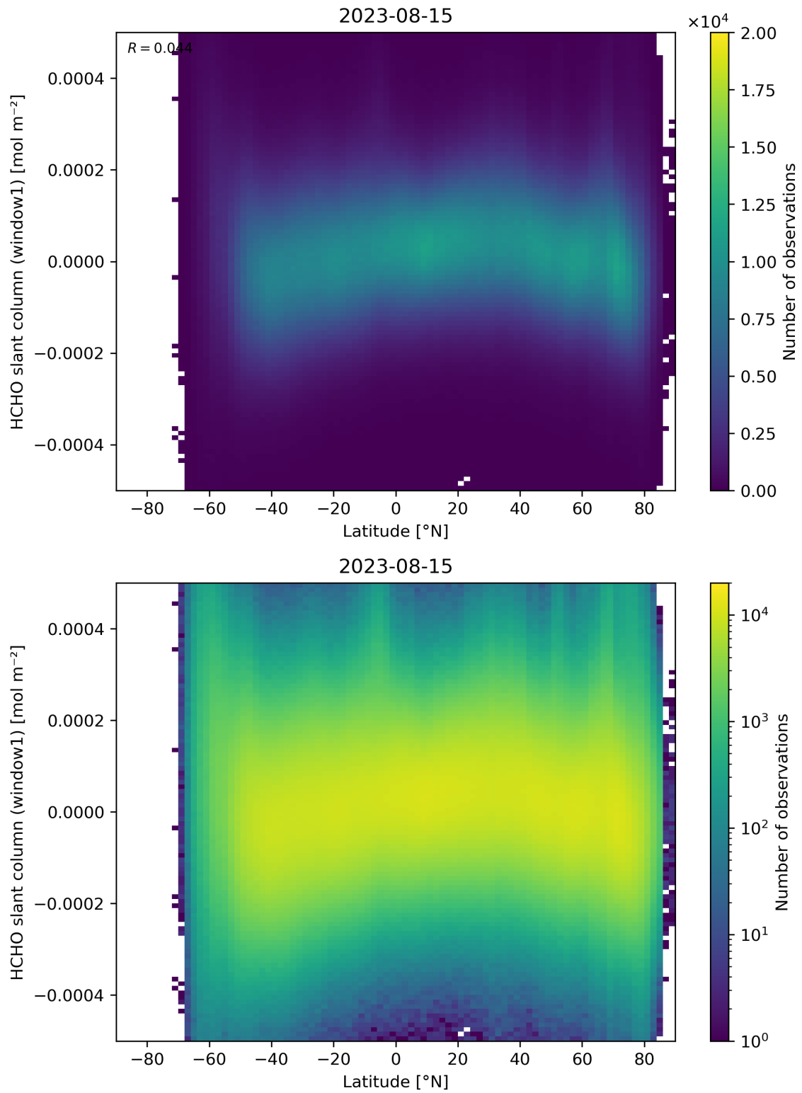
Figure 159: Scatter density plot of “Latitude” against “HCHO slant column (window1)” for 2023-08-14 to 2023-08-16.
