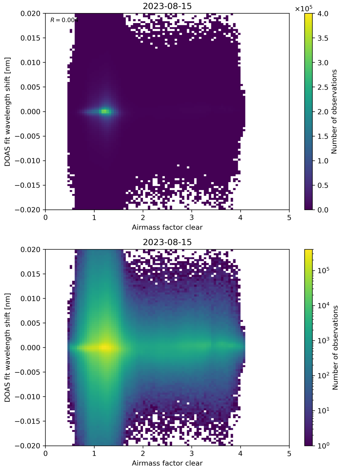
Figure 72: Scatter density plot of “Airmass factor clear” against “DOAS fit wavelength shift” for 2023-08-14 to 2023-08-16.
