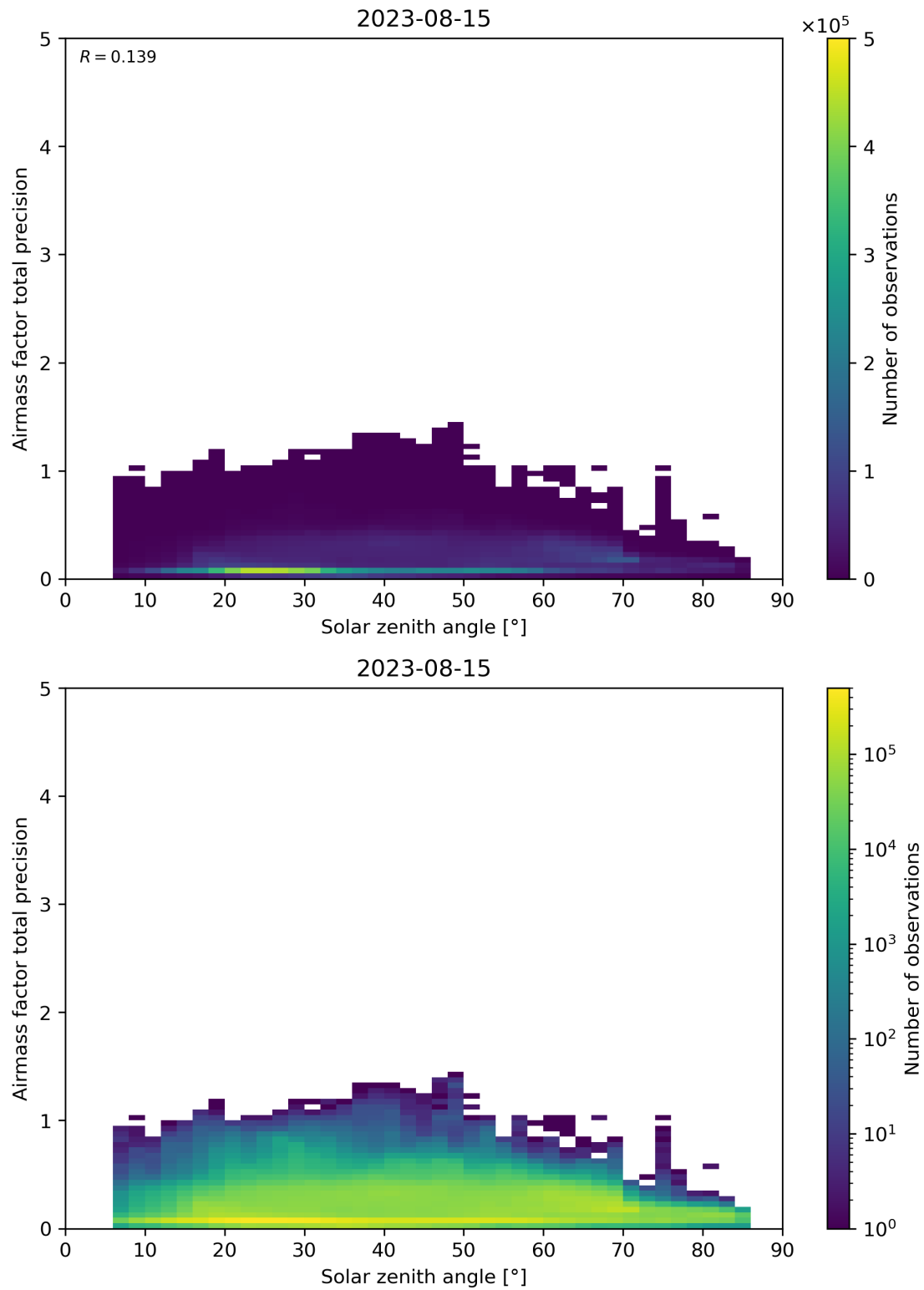
Figure 176: Scatter density plot of “Solar zenith angle” against “Airmass factor total precision” for 2023-08-14 to 2023-08-16.
