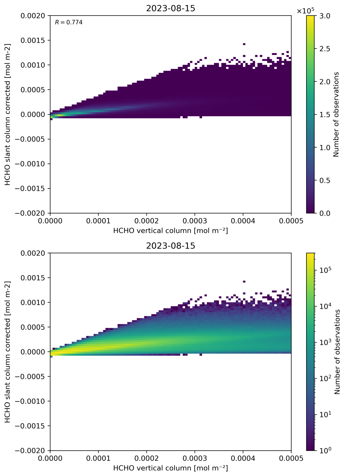
Figure 127: Scatter density plot of “HCHO vertical column” against “HCHO slant column corrected” for 2023-08-14 to 2023-08-16.
