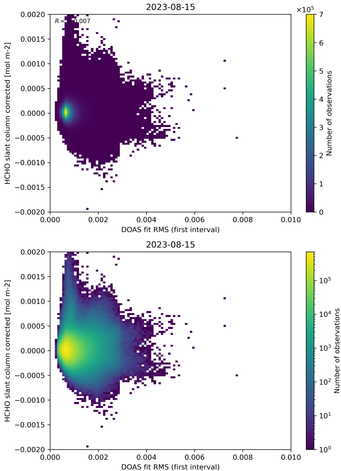
Figure 62: Scatter density plot of “DOAS fit RMS (first interval)” against “HCHO slant column corrected” for 2023-08-14 to 2023-08-16.
