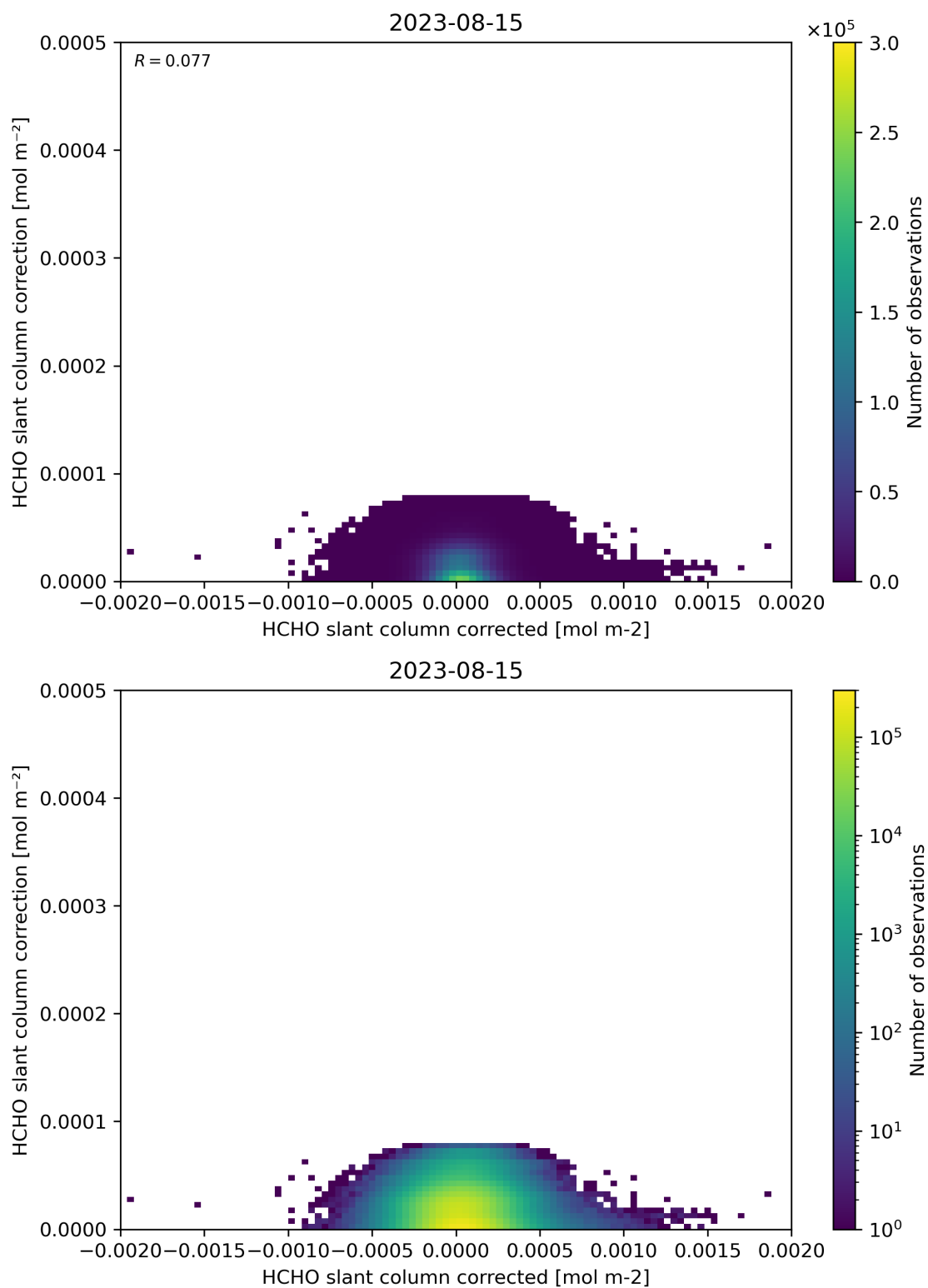
Figure 77: Scatter density plot of “HCHO slant column corrected” against “HCHO slant column correction” for 2023-08-14 to 2023-08-16.
