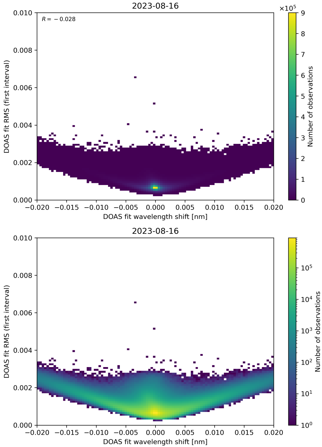
Figure 64: Scatter density plot of “DOAS fit wavelength shift” against “DOAS fit RMS (first interval)” for 2023-08-15 to 2023-08-17.
