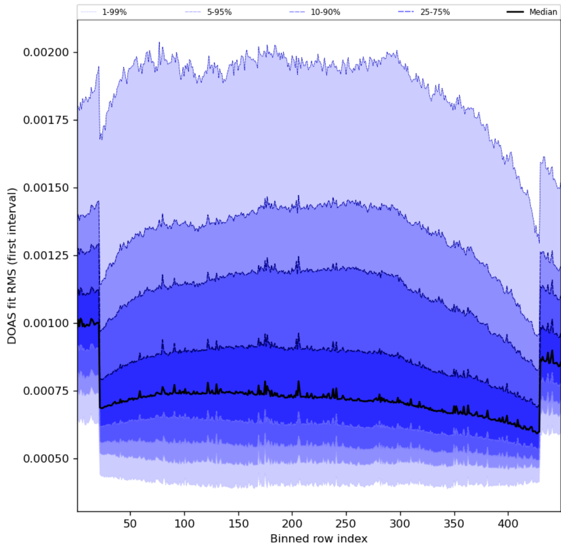
Figure 60: Along track statistics of “DOAS fit RMS (first interval)” for 2023-08-15 to 2023-08-17
