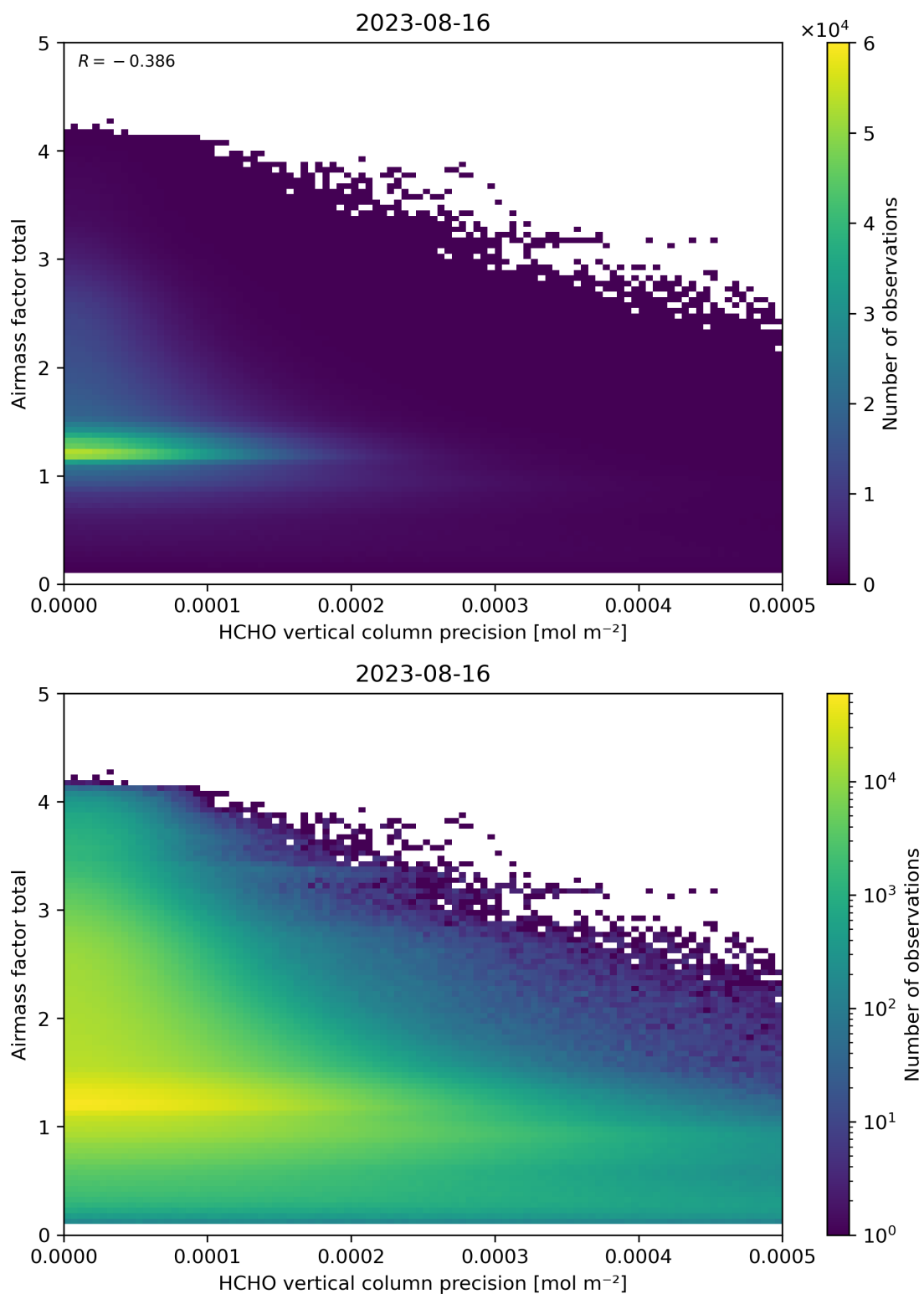
Figure 144: Scatter density plot of “HCHO vertical column precision” against “Airmass factor total” for 2023-08-15 to 2023-08-17.
