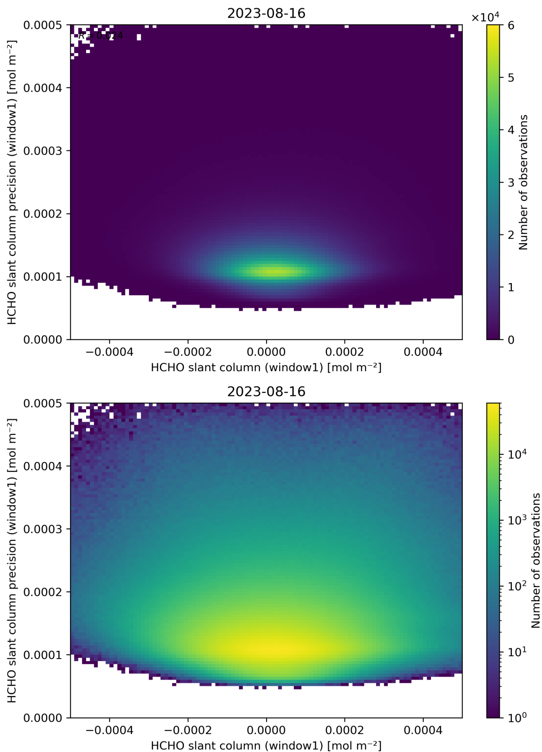
Figure 84: Scatter density plot of “HCHO slant column (window1)” against “HCHO slant column precision (window1)” for 2023-08-15 to 2023-08-17.
