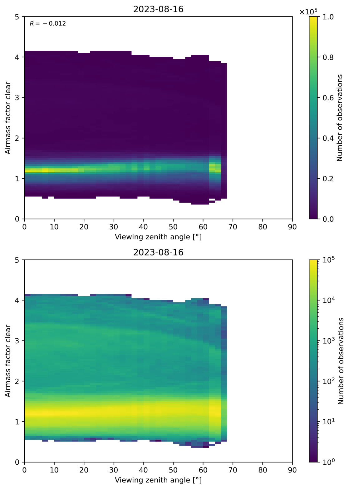
Figure 185: Scatter density plot of “Viewing zenith angle” against “Airmass factor clear” for 2023-08-15 to 2023-08-17.
