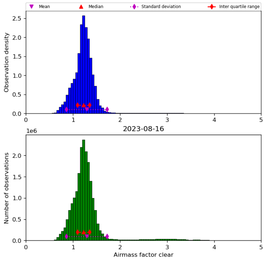
Figure 42: Histogram of “Airmass factor clear” for 2023-08-15 to 2023-08-17
