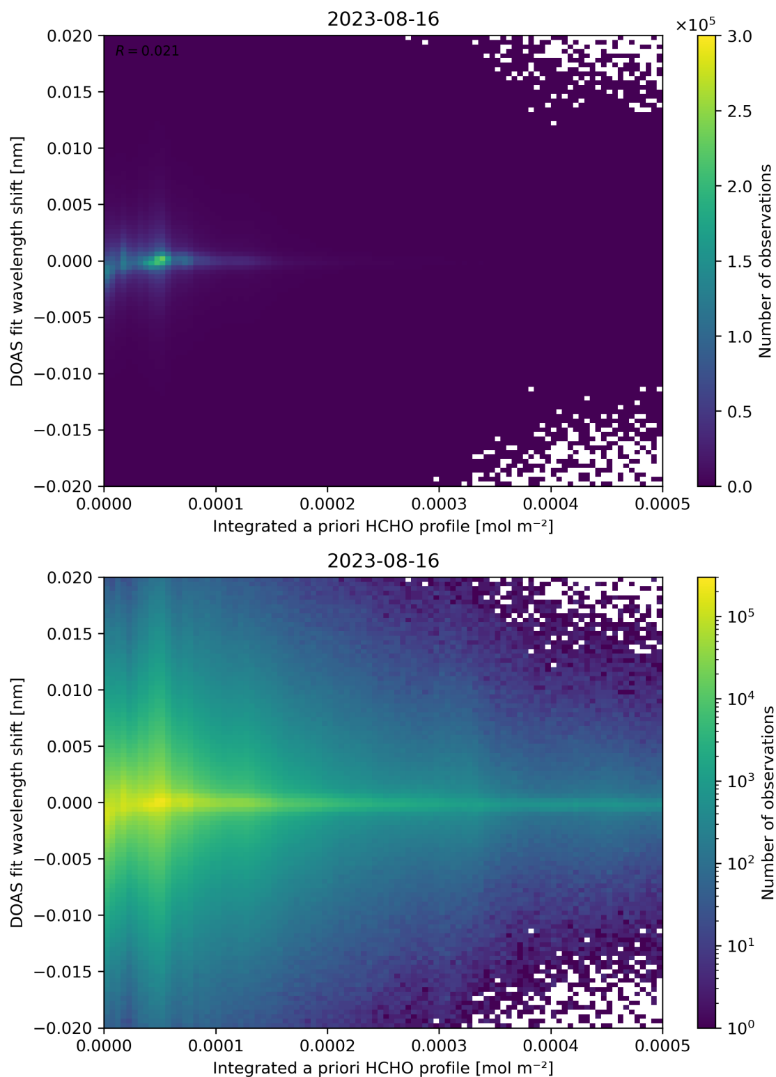
Figure 149: Scatter density plot of “Integrated a priori HCHO profile” against “DOAS fit wavelength shift” for 2023-08-15 to 2023-08-17.
