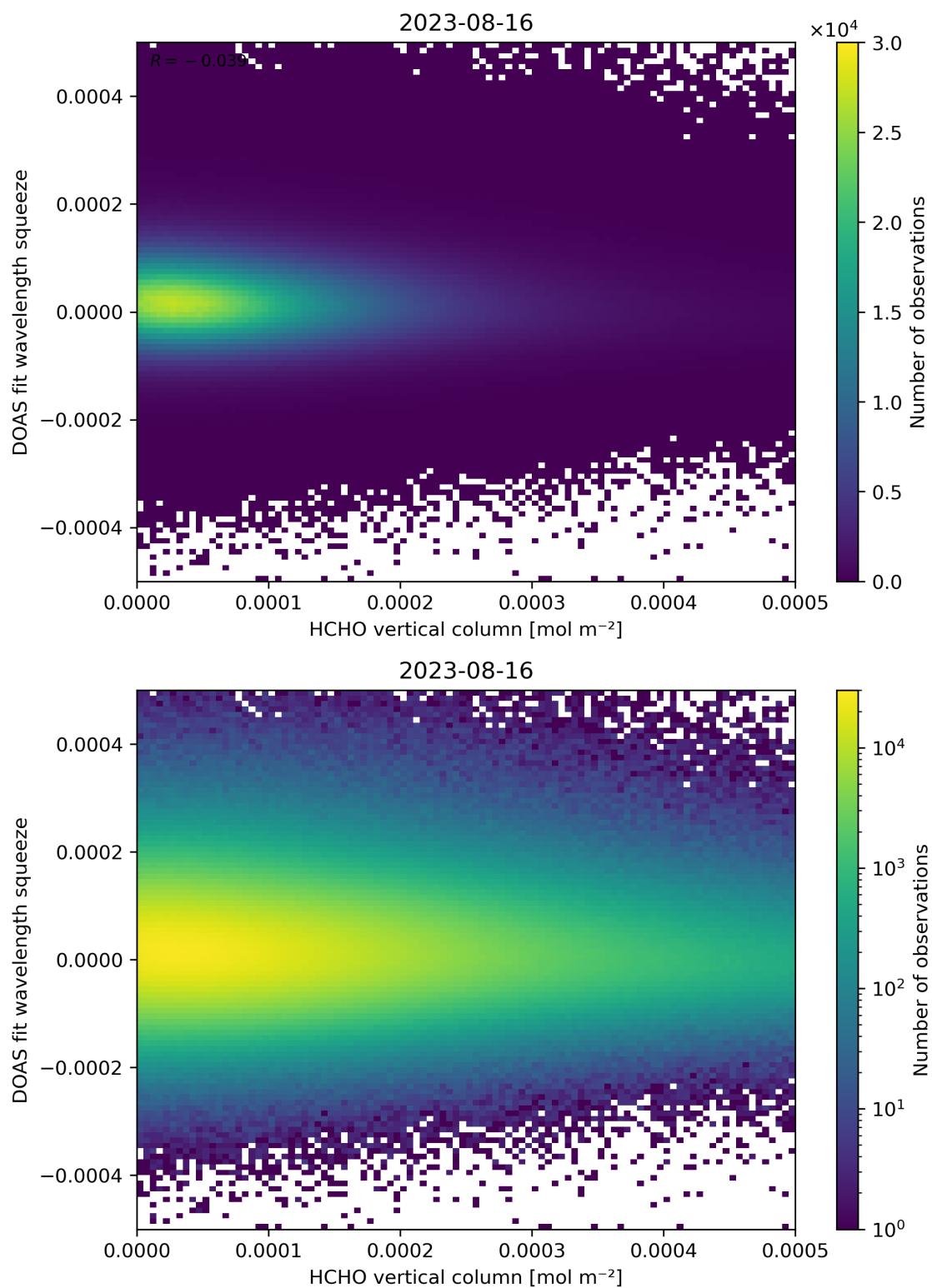
Figure 125: Scatter density plot of “HCHO vertical column” against “DOAS fit wavelength squeeze” for 2023-08-15 to 2023-08-17.
