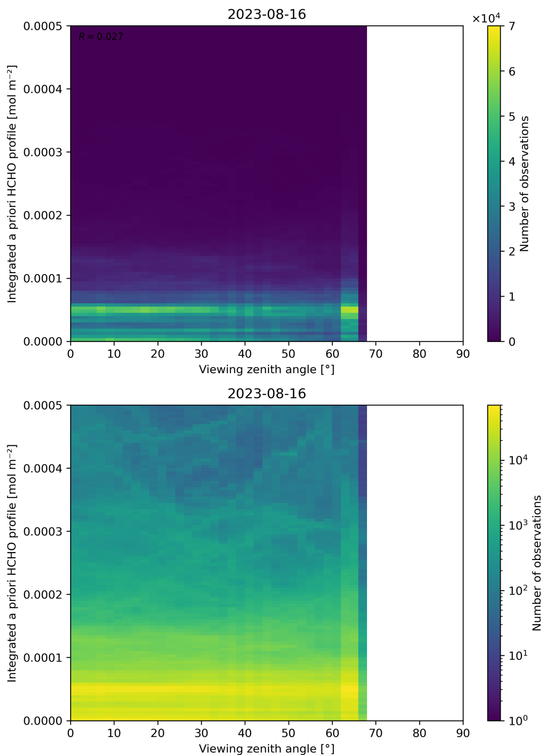
Figure 195: Scatter density plot of “Viewing zenith angle” against “Integrated a priori HCHO profile” for 2023-08-15 to 2023-08-17.
