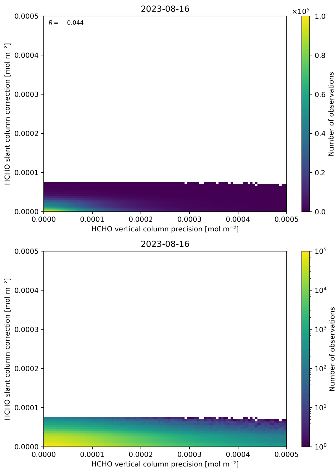
Figure 141: Scatter density plot of “HCHO vertical column precision” against “HCHO slant column correction” for 2023-08-15 to 2023-08-17.
