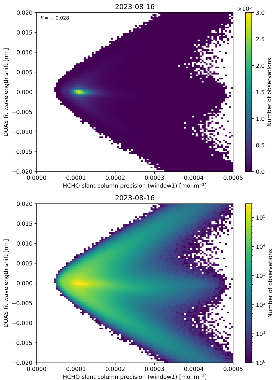
Figure 89: Scatter density plot of “HCHO slant column precision (window1)” against “DOAS fit wavelength shift” for 2023-08-15 to 2023-08-17.
