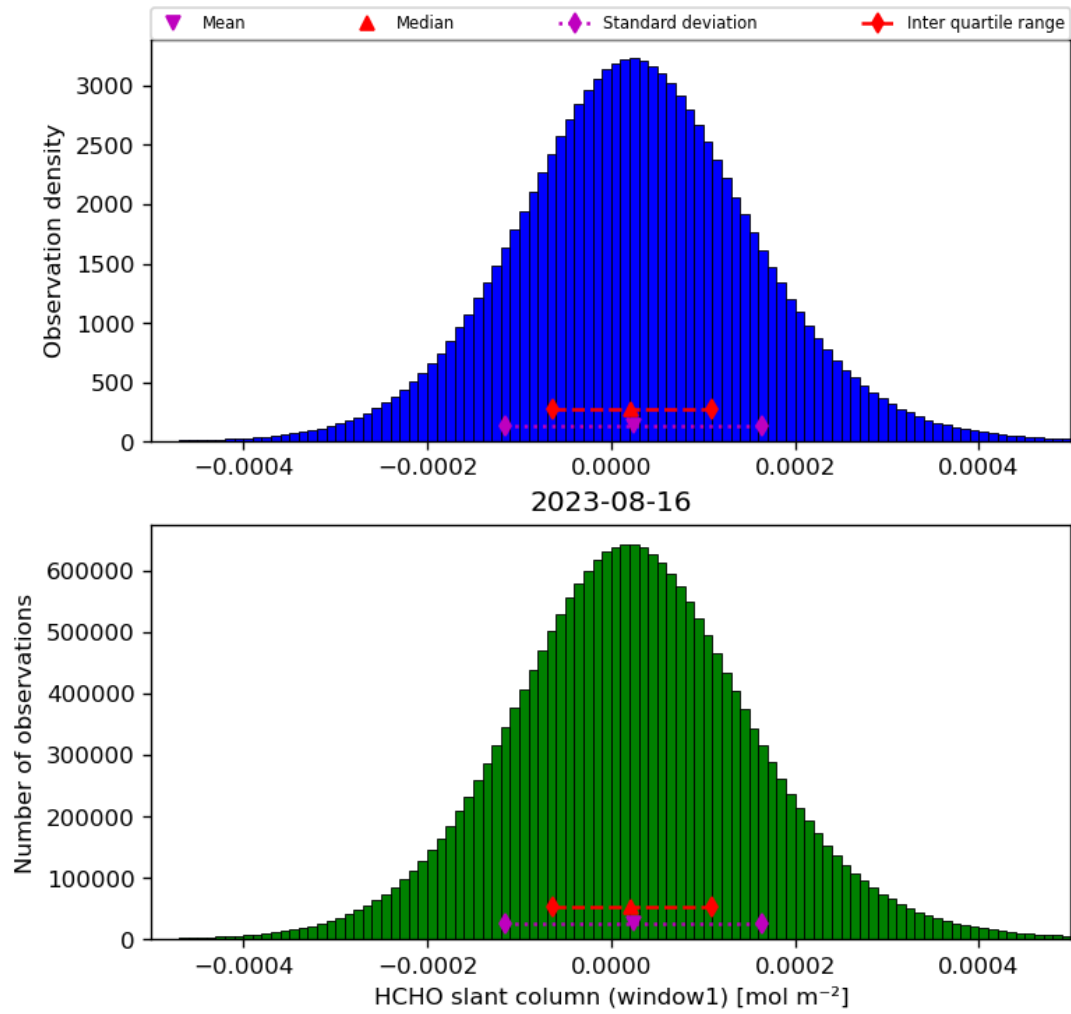
Figure 38: Histogram of “HCHO slant column (window1)” for 2023-08-15 to 2023-08-17
