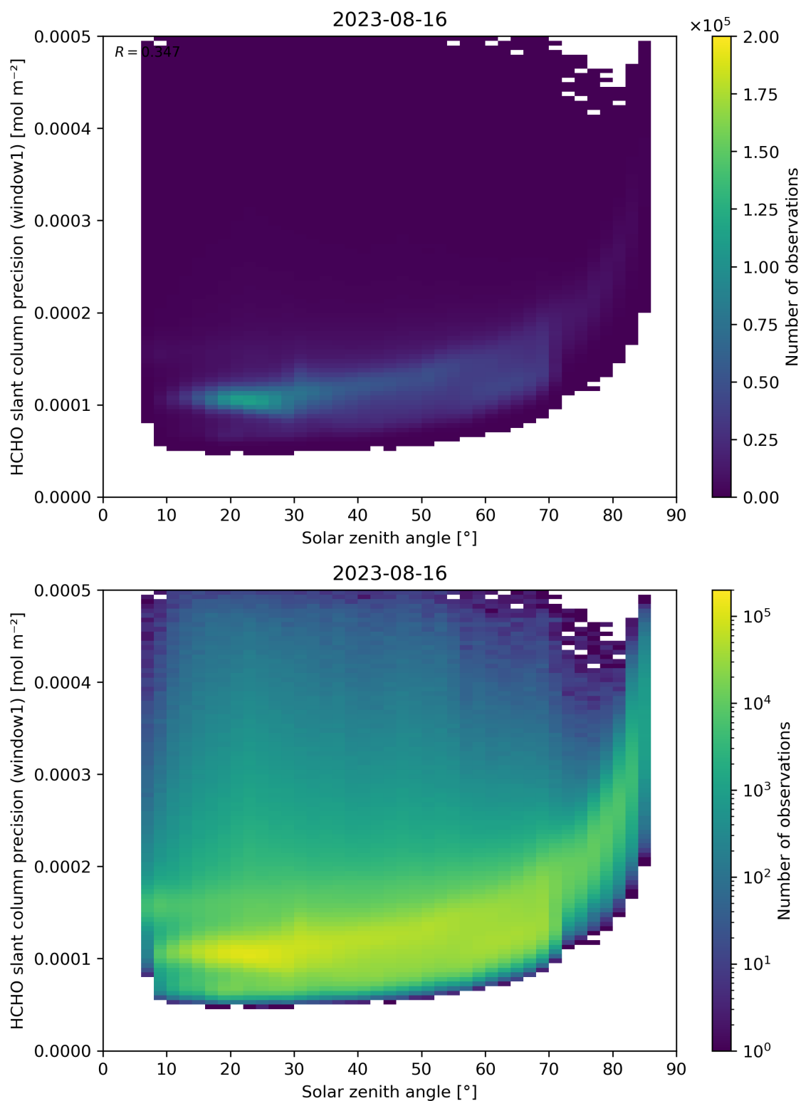
Figure 174: Scatter density plot of “Solar zenith angle” against “HCHO slant column precision (window1)” for 2023-08-15 to 2023-08-17.
