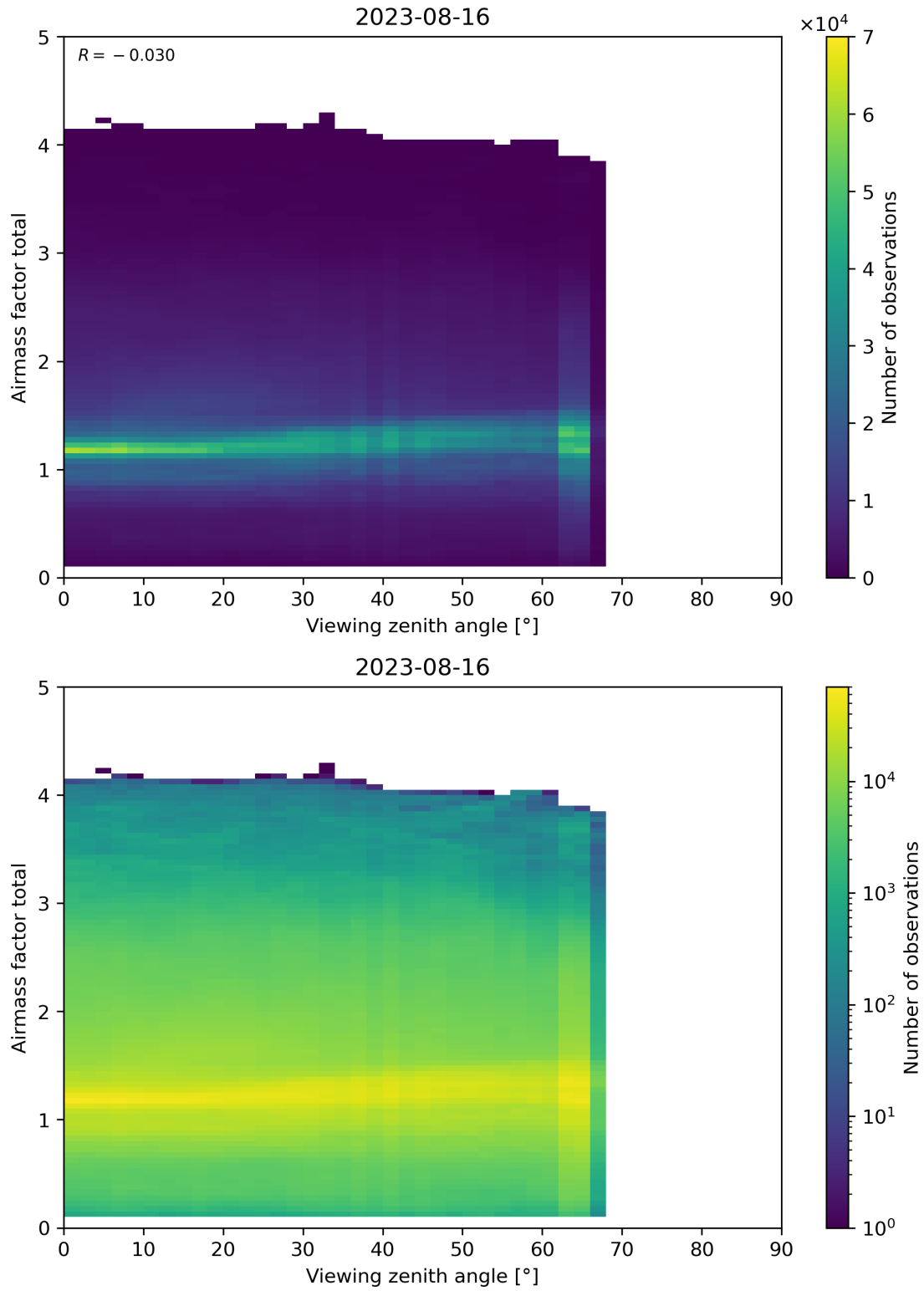
Figure 190: Scatter density plot of “Viewing zenith angle” against “Airmass factor total” for 2023-08-15 to 2023-08-17.
