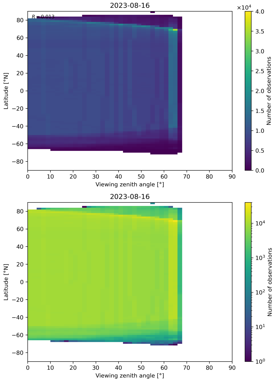
Figure 196: Scatter density plot of “Viewing zenith angle” against “Latitude” for 2023-08-15 to 2023-08-17.
