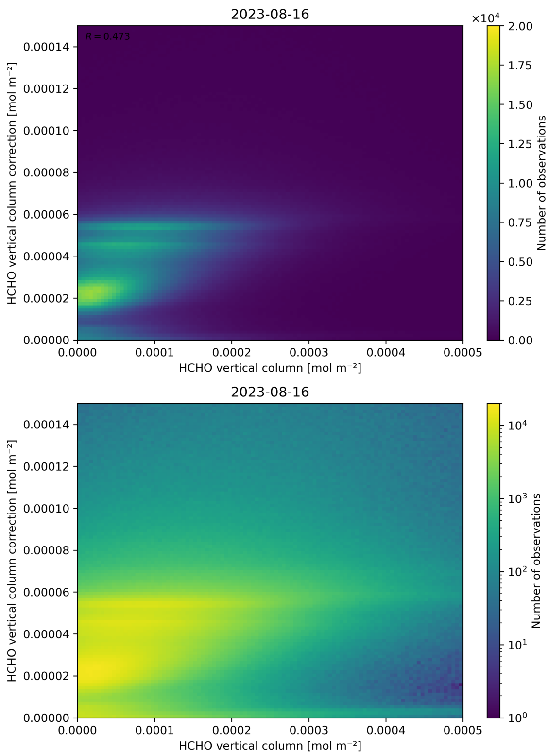
Figure 133: Scatter density plot of “HCHO vertical column” against “HCHO vertical column correction” for 2023-08-15 to 2023-08-17.
