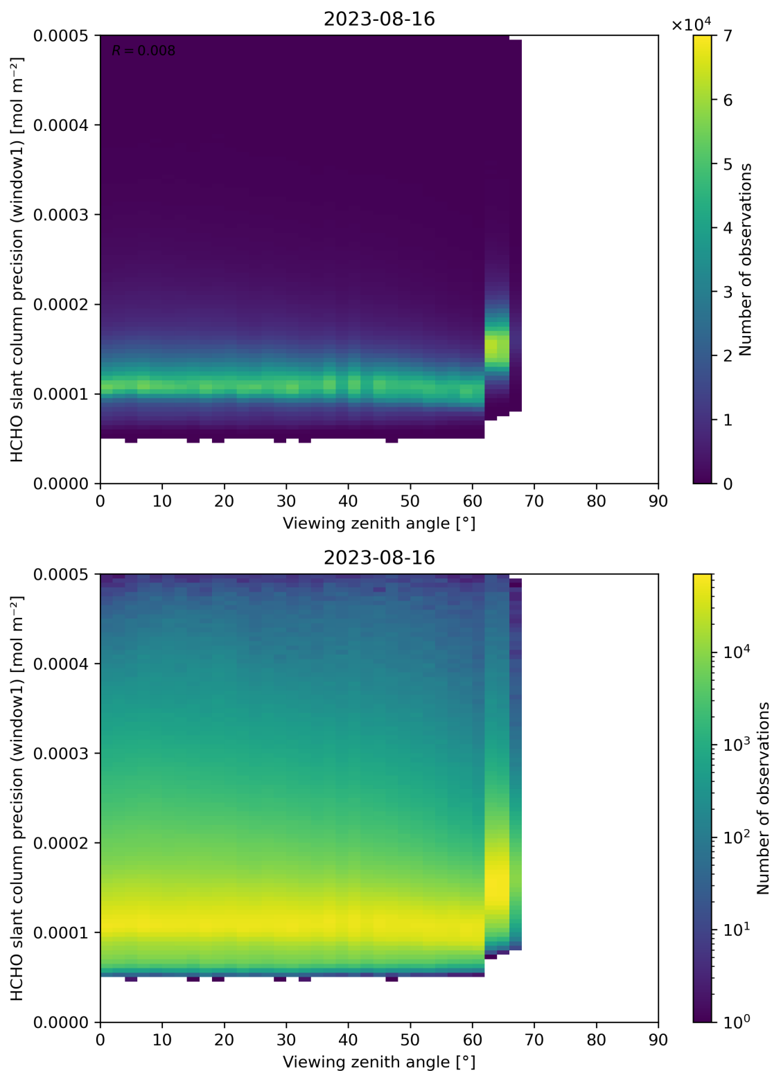
Figure 189: Scatter density plot of “Viewing zenith angle” against “HCHO slant column precision (window1)” for 2023-08-15 to 2023-08-17.
