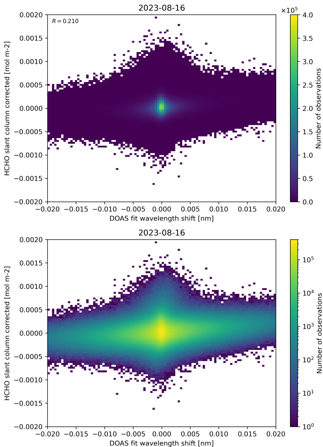
Figure 66: Scatter density plot of “DOAS fit wavelength shift” against “HCHO slant column corrected” for 2023-08-15 to 2023-08-17.
