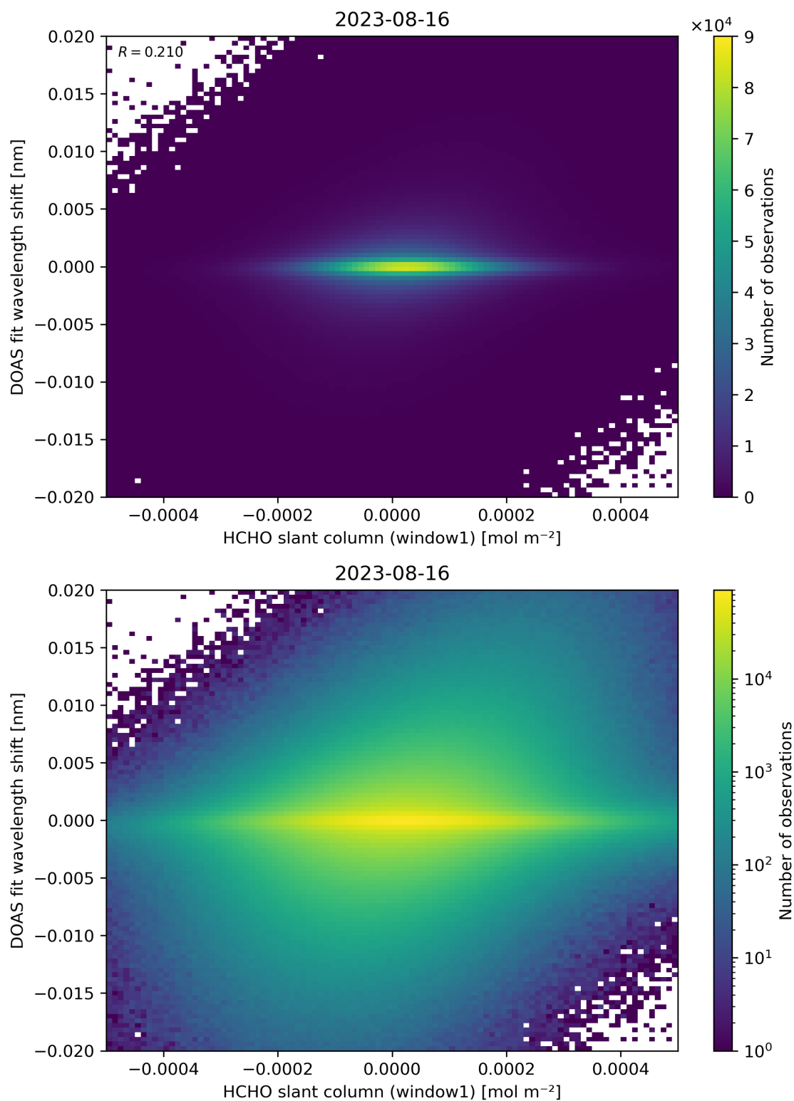
Figure 79: Scatter density plot of “HCHO slant column (window1)” against “DOAS fit wavelength shift” for 2023-08-15 to 2023-08-17.
