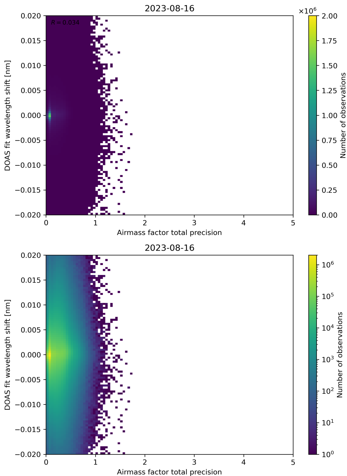
Figure 106: Scatter density plot of “Airmass factor total precision” against “DOAS fit wavelength shift” for 2023-08-15 to 2023-08-17.
