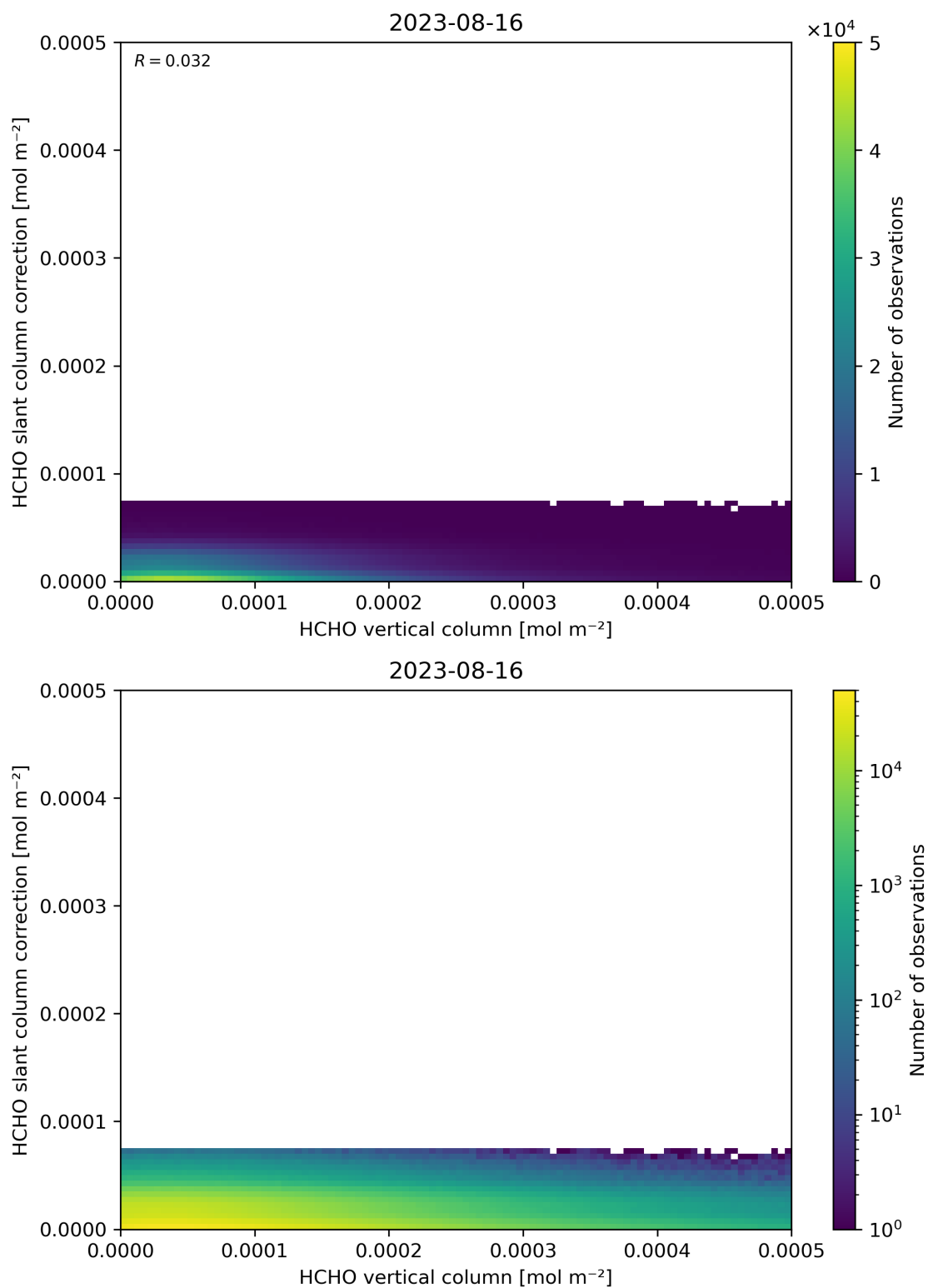
Figure 128: Scatter density plot of “HCHO vertical column” against “HCHO slant column correction” for 2023-08-15 to 2023-08-17.
