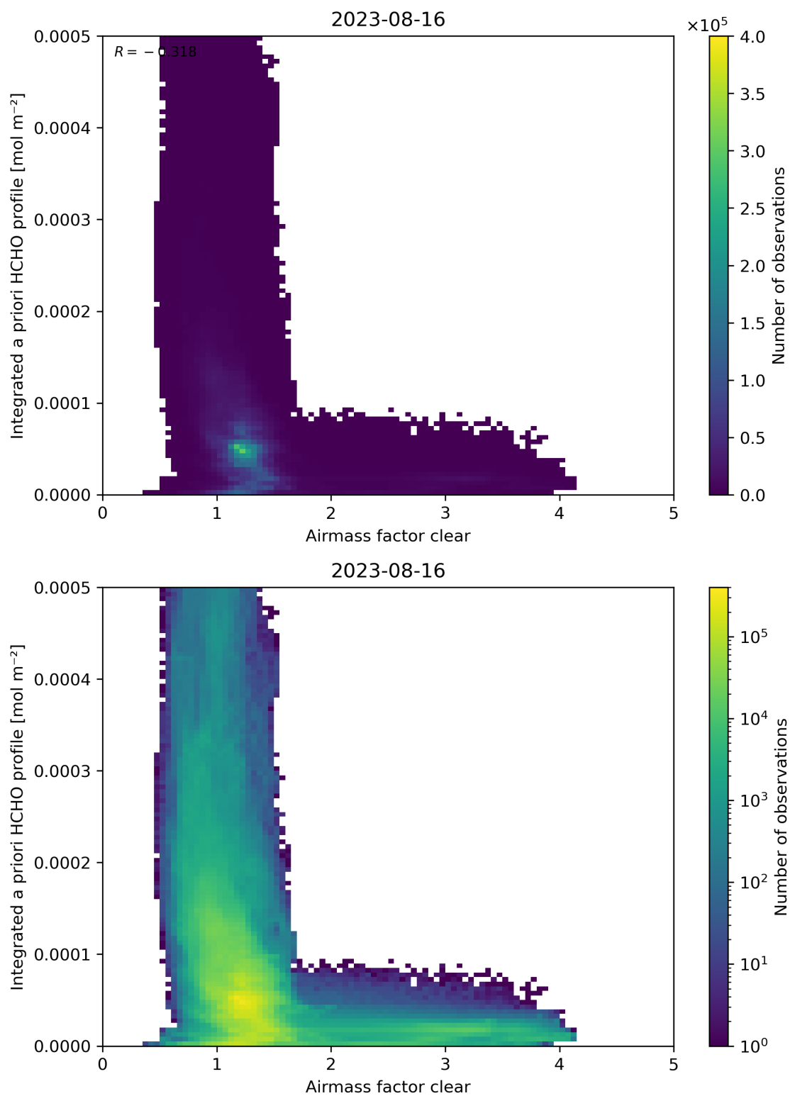
Figure 76: Scatter density plot of “Airmass factor clear” against “Integrated a priori HCHO profile” for 2023-08-15 to 2023-08-17.
