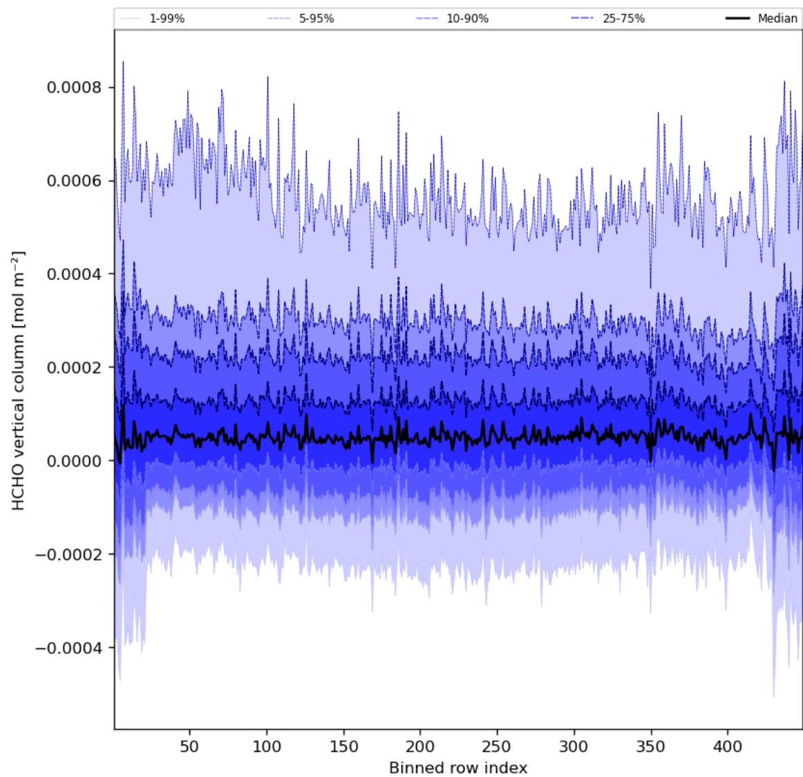
Figure 49: Along track statistics of “HCHO vertical column” for 2023-08-15 to 2023-08-17
