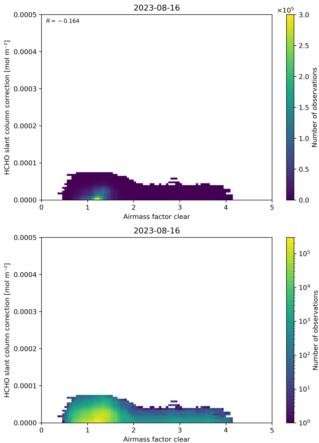
Figure 75: Scatter density plot of “Airmass factor clear” against “HCHO slant column correction” for 2023-08-15 to 2023-08-17.
