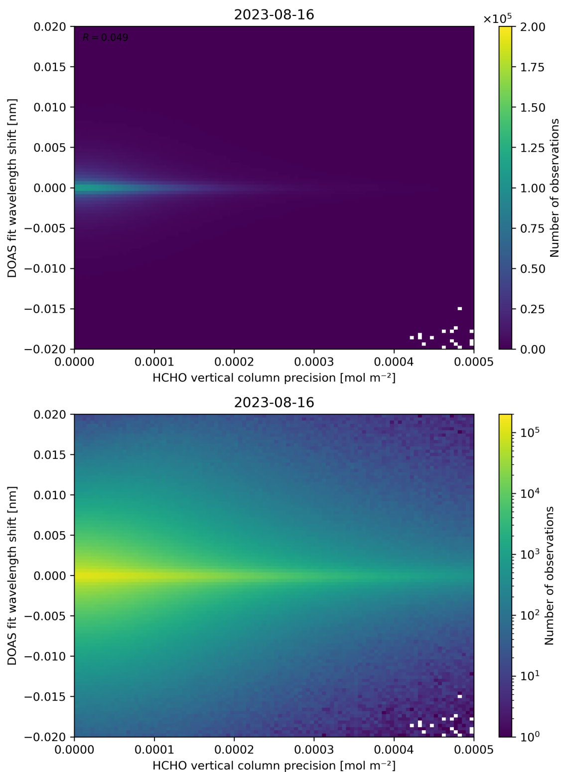
Figure 137: Scatter density plot of “HCHO vertical column precision” against “DOAS fit wavelength shift” for 2023-08-15 to 2023-08-17.
