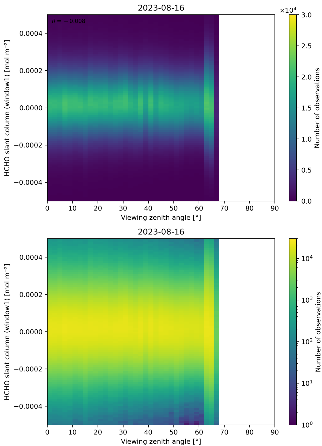
Figure 188: Scatter density plot of “Viewing zenith angle” against “HCHO slant column (window1)” for 2023-08-15 to 2023-08-17.
