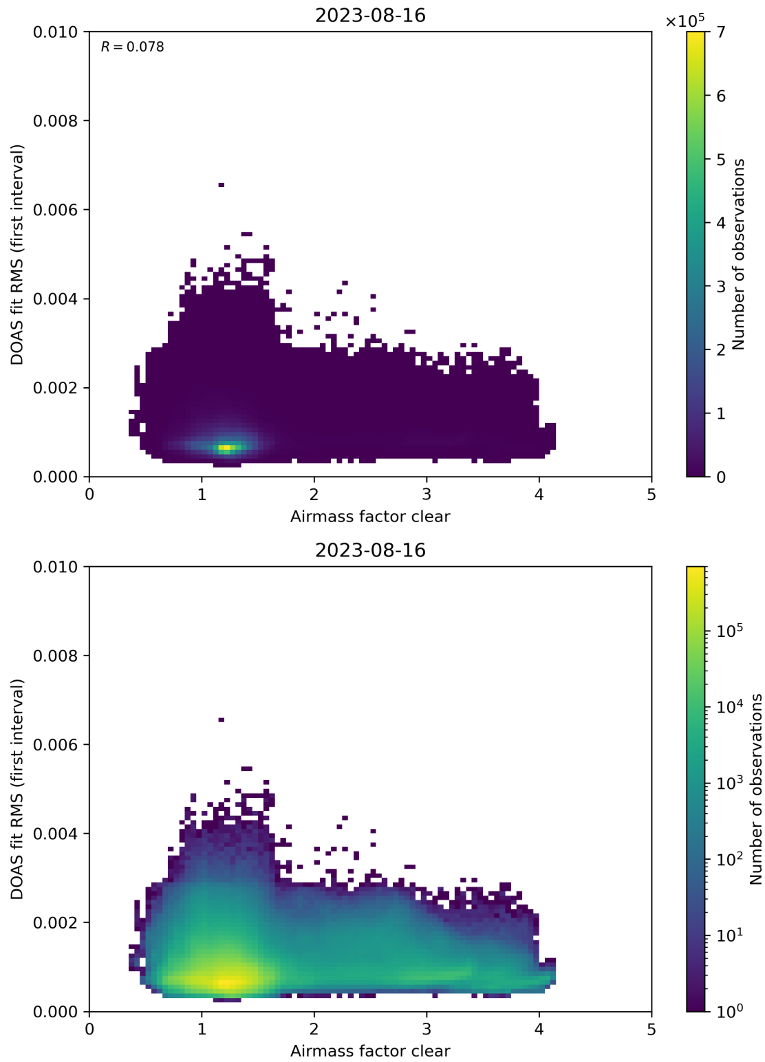
Figure 71: Scatter density plot of “Airmass factor clear” against “DOAS fit RMS (first interval)” for 2023-08-15 to 2023-08-17.
