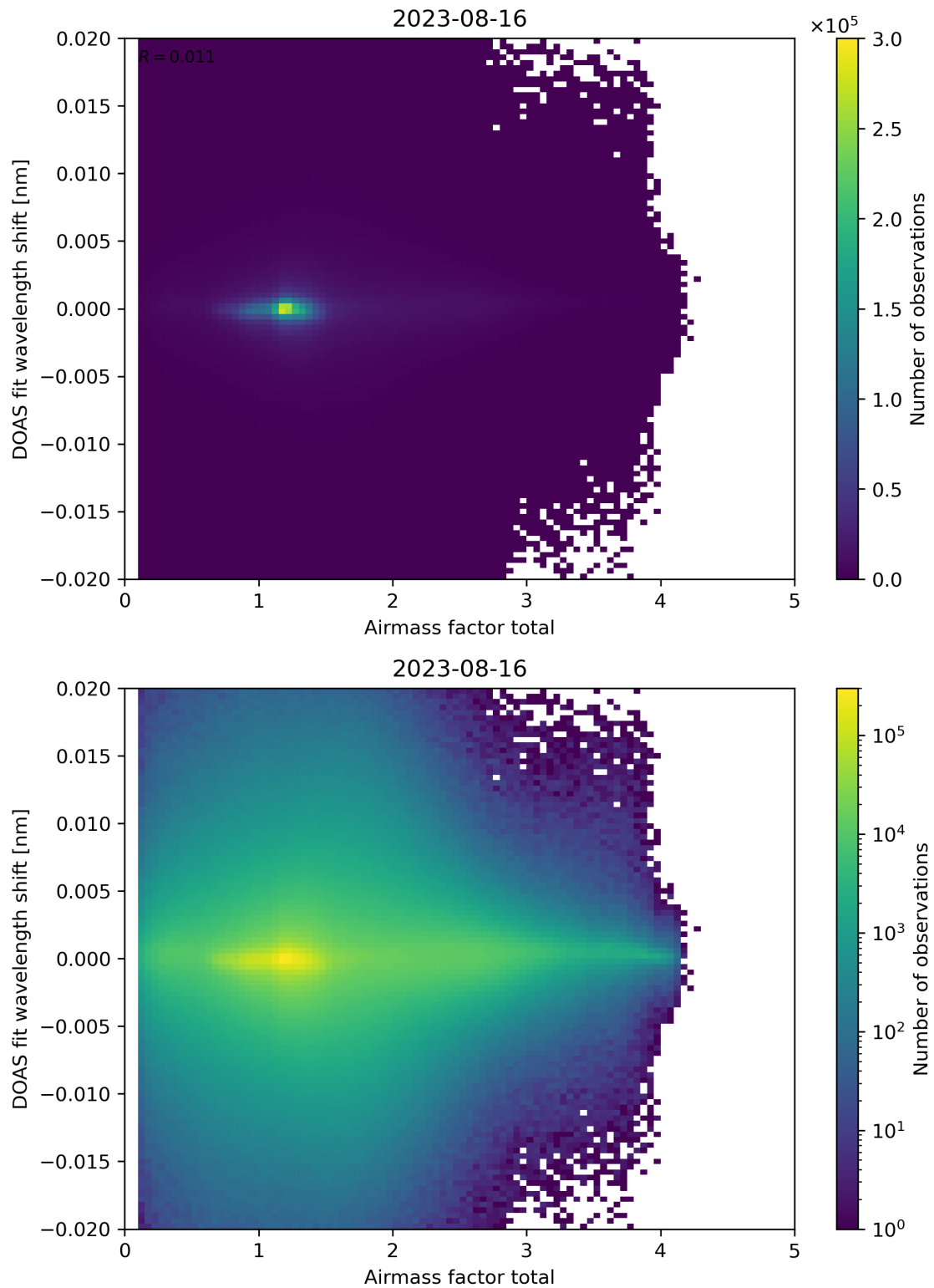
Figure 98: Scatter density plot of “Airmass factor total” against “DOAS fit wavelength shift” for 2023-08-15 to 2023-08-17.
