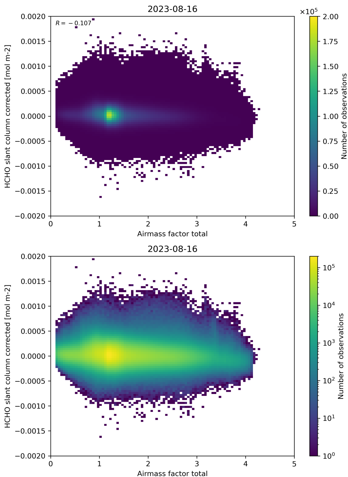
Figure 101: Scatter density plot of “Airmass factor total” against “HCHO slant column corrected” for 2023-08-15 to 2023-08-17.
