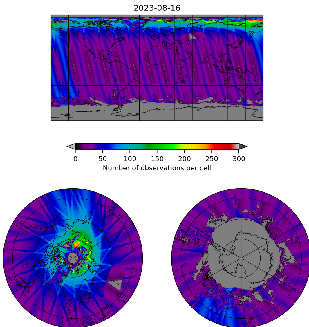
Figure 19: Map of the number of observations for 2023-08-15 to 2023-08-17
