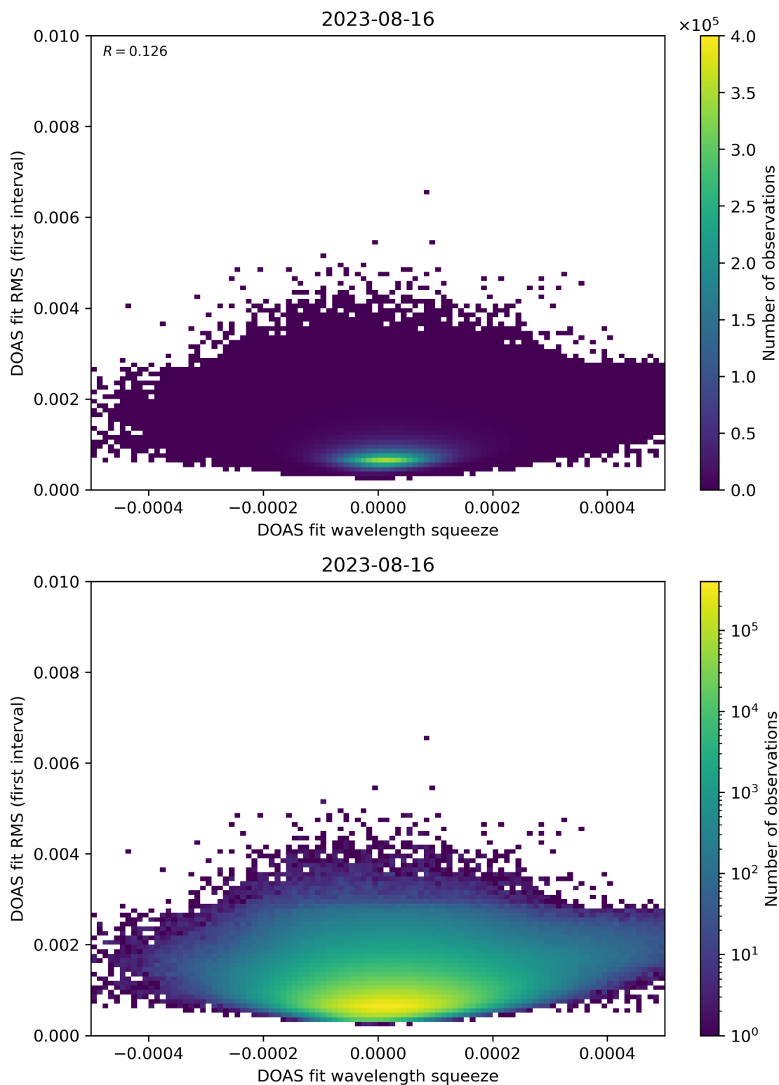
Figure 68: Scatter density plot of “DOAS fit wavelength squeeze” against “DOAS fit RMS (first interval)” for 2023-08-15 to 2023-08-17.
