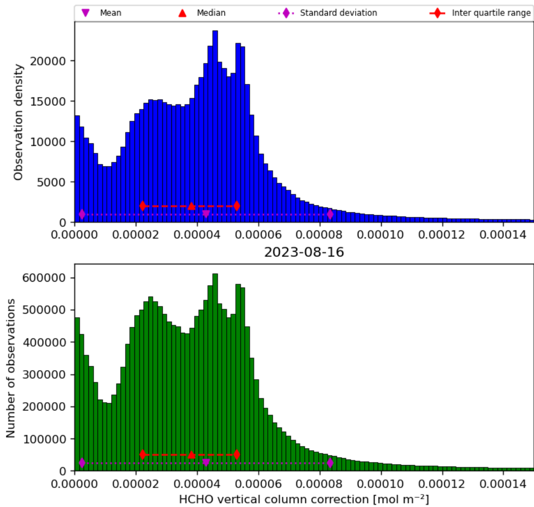
Figure 37: Histogram of “HCHO vertical column correction” for 2023-08-15 to 2023-08-17
