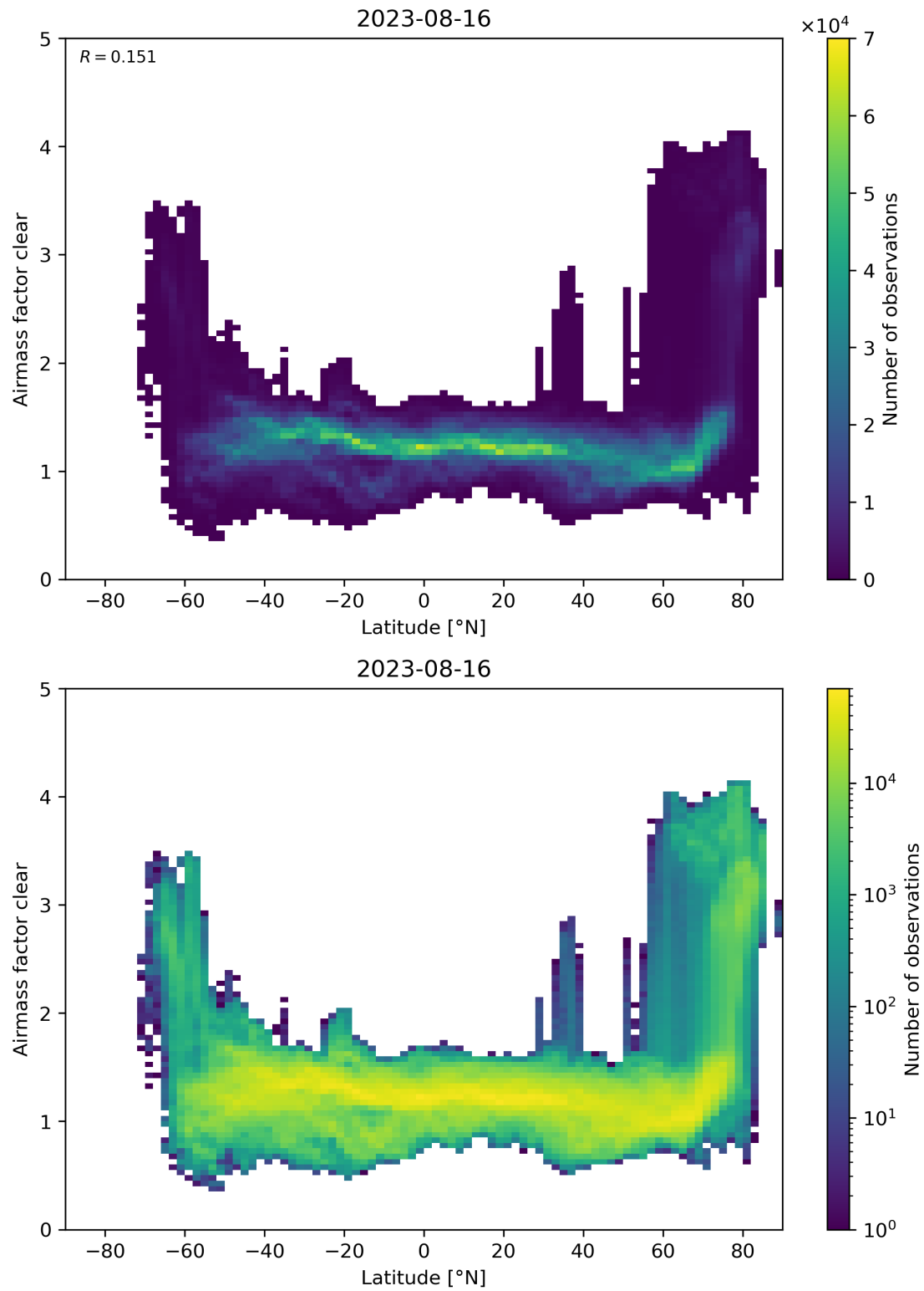
Figure 156: Scatter density plot of “Latitude” against “Airmass factor clear” for 2023-08-15 to 2023-08-17.
