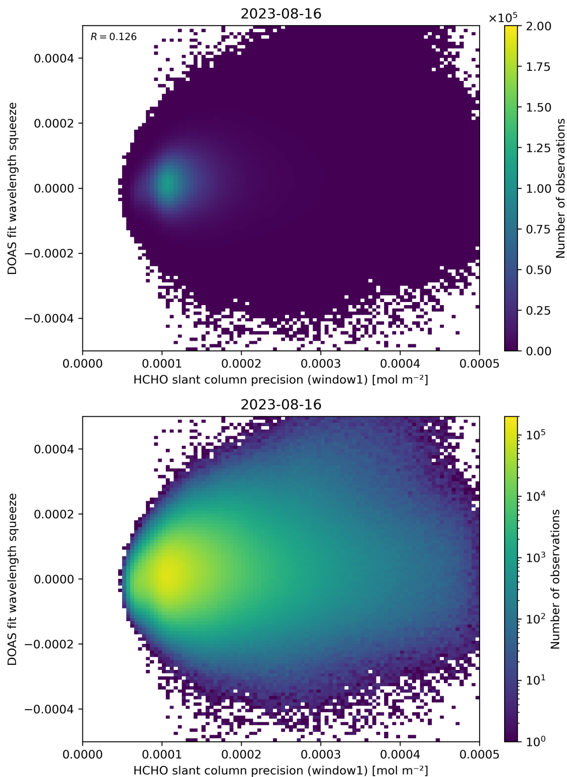
Figure 90: Scatter density plot of “HCHO slant column precision (window1)” against “DOAS fit wavelength squeeze” for 2023-08-15 to 2023-08-17.
