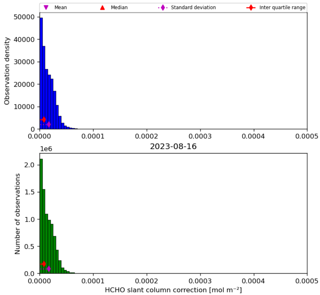
Figure 47: Histogram of “HCHO slant column correction” for 2023-08-15 to 2023-08-17
