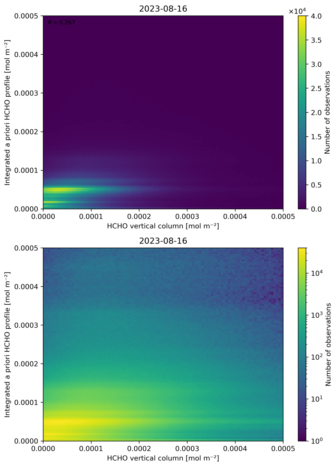
Figure 135: Scatter density plot of “HCHO vertical column” against “Integrated a priori HCHO profile” for 2023-08-15 to 2023-08-17.
