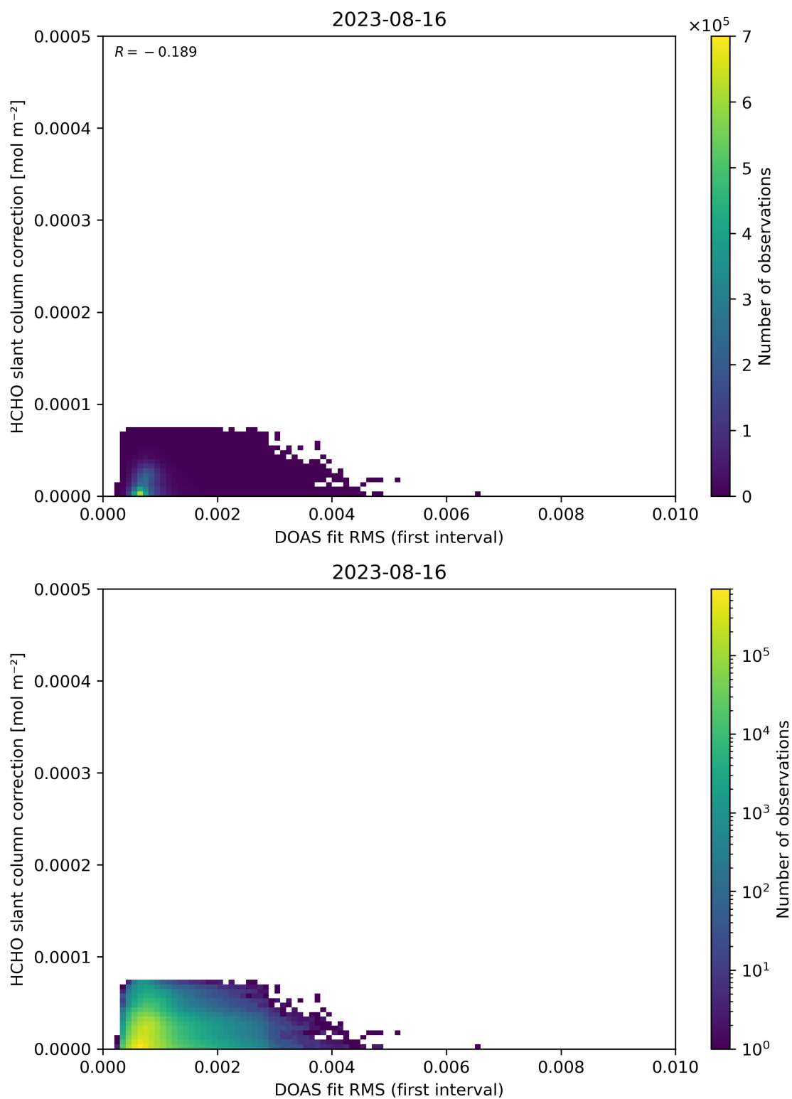
Figure 63: Scatter density plot of “DOAS fit RMS (first interval)” against “HCHO slant column correction” for 2023-08-15 to 2023-08-17.
