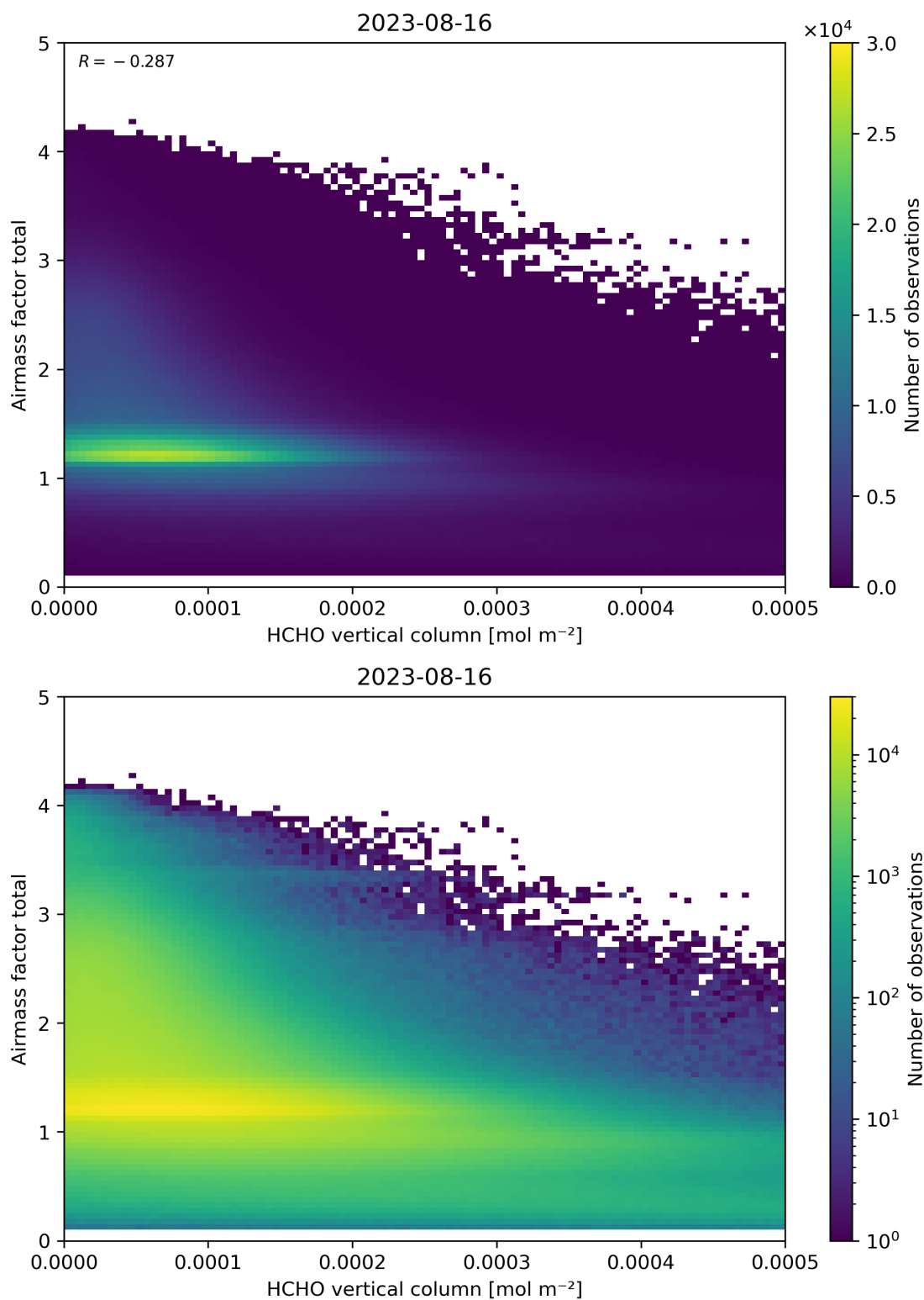
Figure 131: Scatter density plot of “HCHO vertical column” against “Airmass factor total” for 2023-08-15 to 2023-08-17.
