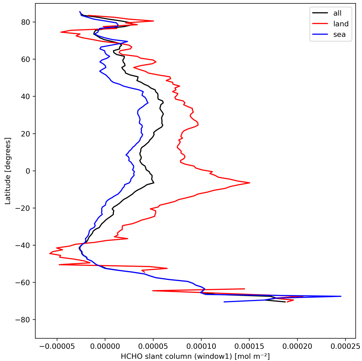
Figure 24: Zonal average of “HCHO slant column (window1)” for 2023-08-15 to 2023-08-17.
