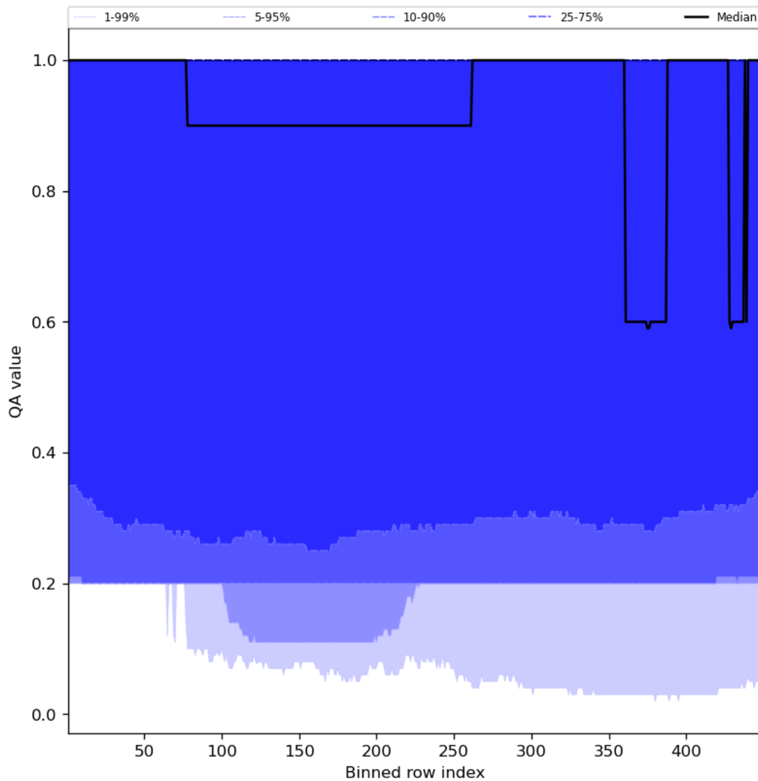
Figure 48: Along track statistics of “QA value” for 2023-08-15 to 2023-08-17
