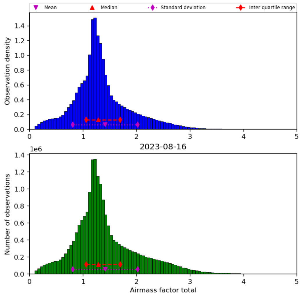
Figure 40: Histogram of “Airmass factor total” for 2023-08-15 to 2023-08-17
