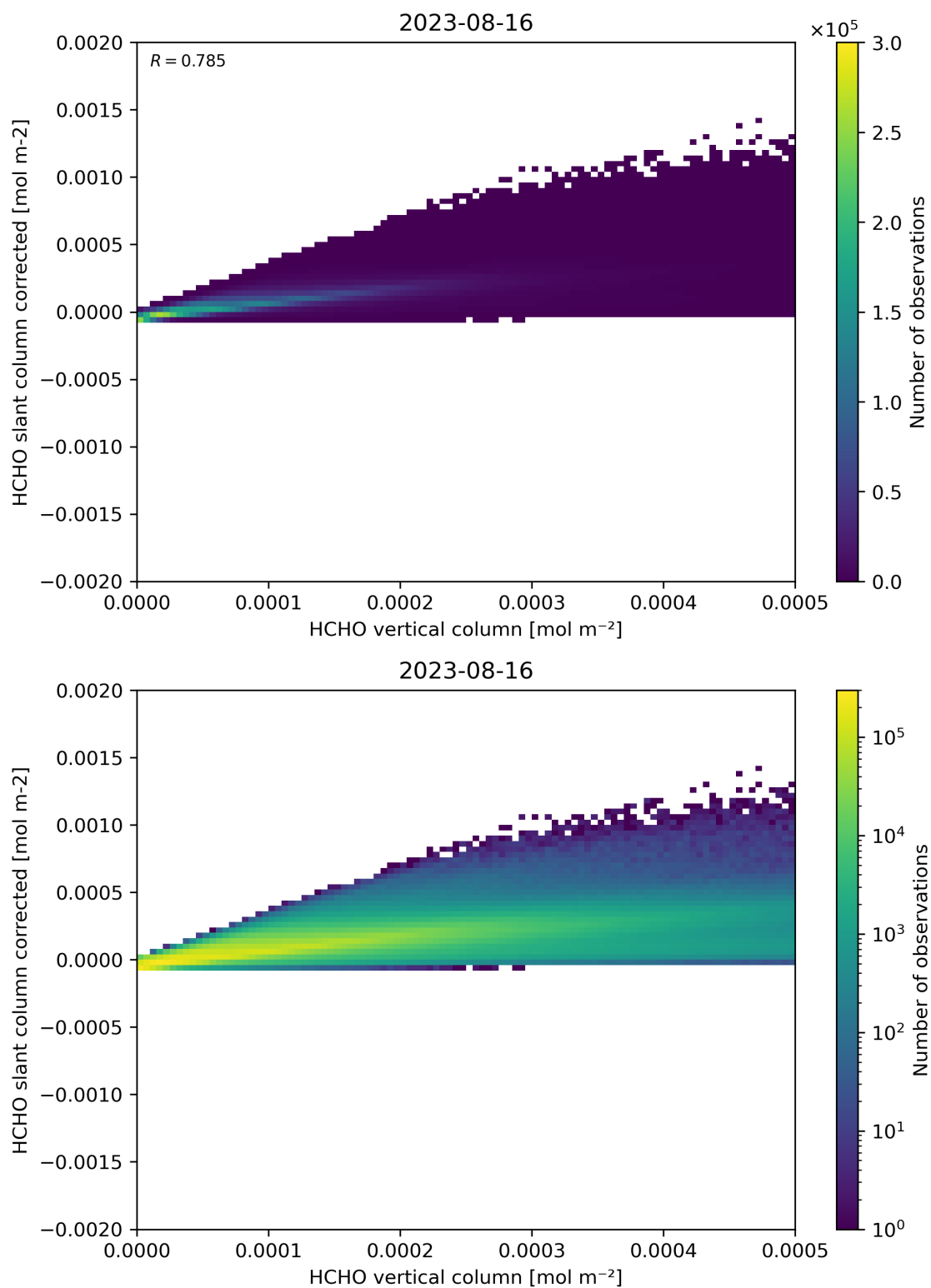
Figure 127: Scatter density plot of “HCHO vertical column” against “HCHO slant column corrected” for 2023-08-15 to 2023-08-17.
