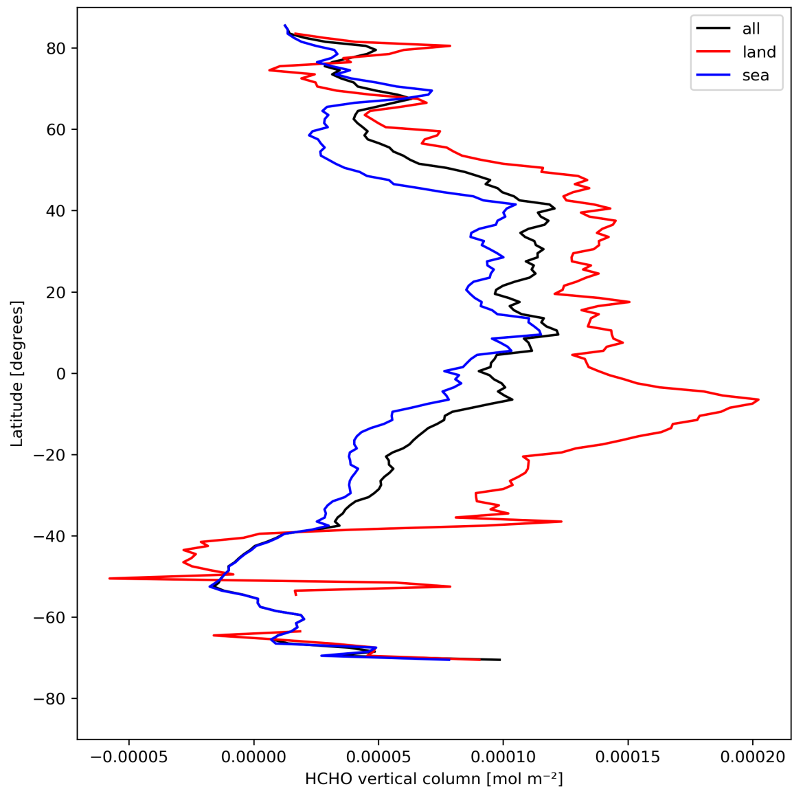
Figure 21: Zonal average of “HCHO vertical column” for 2023-08-15 to 2023-08-17.
