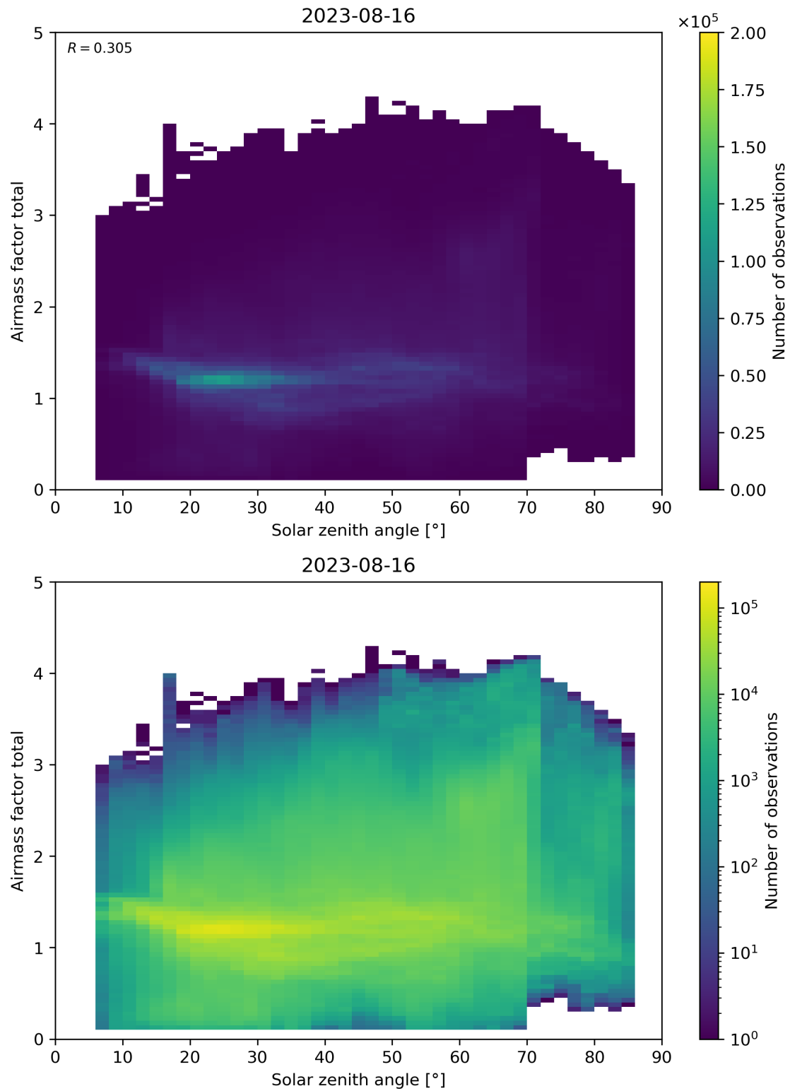
Figure 175: Scatter density plot of “Solar zenith angle” against “Airmass factor total” for 2023-08-15 to 2023-08-17.
