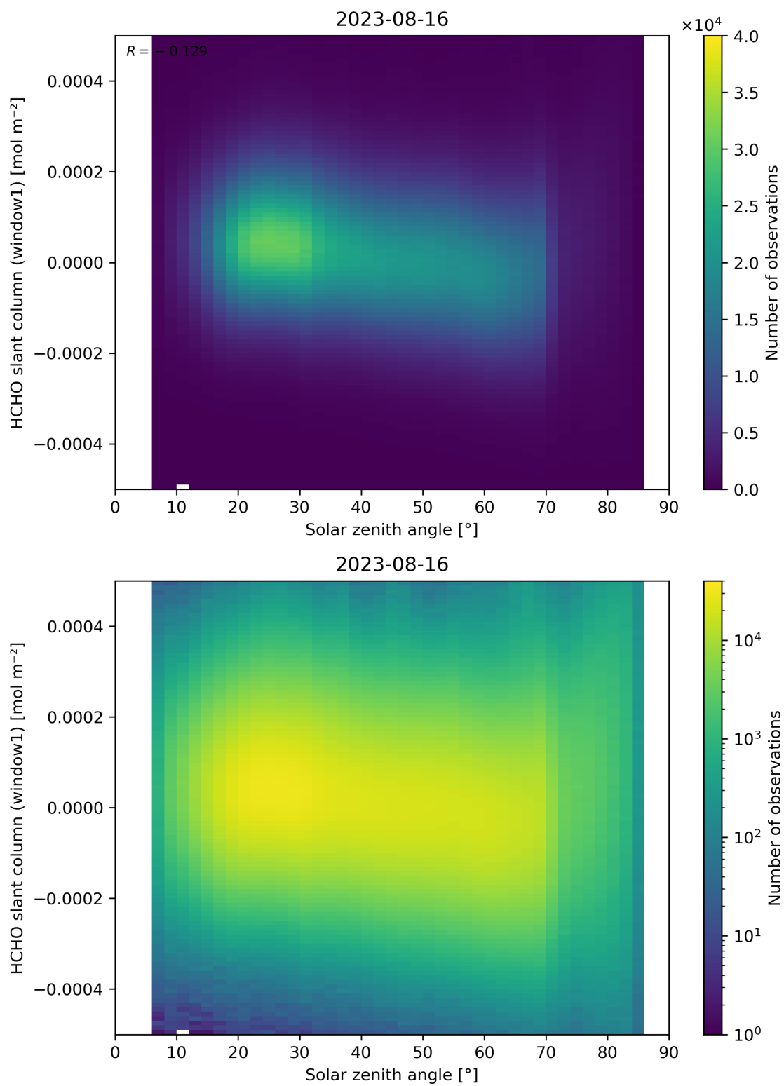
Figure 173: Scatter density plot of “Solar zenith angle” against “HCHO slant column (window1)” for 2023-08-15 to 2023-08-17.
