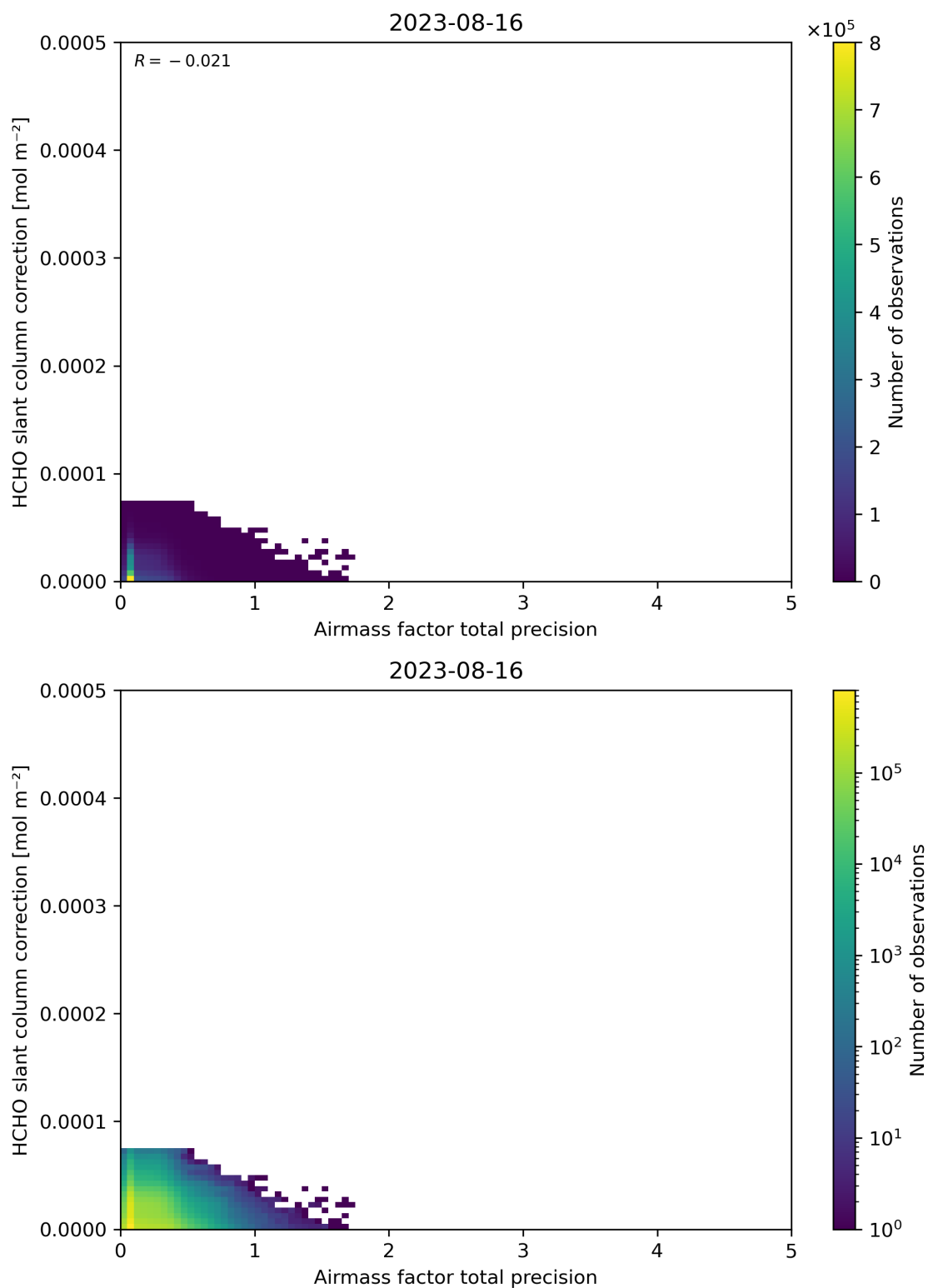
Figure 110: Scatter density plot of “Airmass factor total precision” against “HCHO slant column correction” for 2023-08-15 to 2023-08-17.
