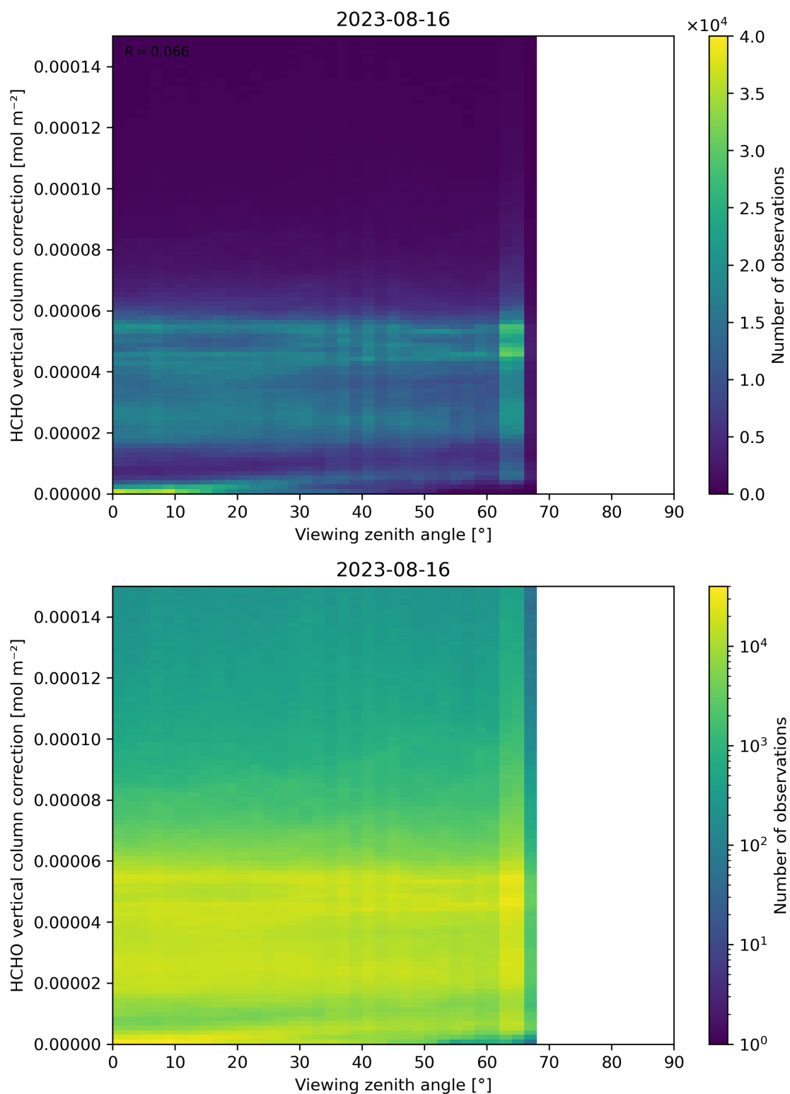
Figure 193: Scatter density plot of “Viewing zenith angle” against “HCHO vertical column correction” for 2023-08-15 to 2023-08-17.
