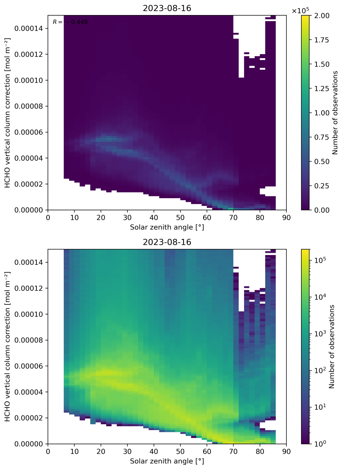
Figure 178: Scatter density plot of “Solar zenith angle” against “HCHO vertical column correction” for 2023-08-15 to 2023-08-17.
