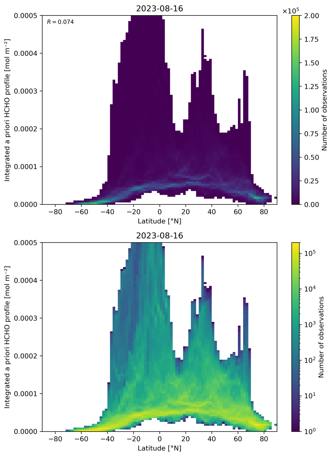
Figure 166: Scatter density plot of “Latitude” against “Integrated a priori HCHO profile” for 2023-08-15 to 2023-08-17.
