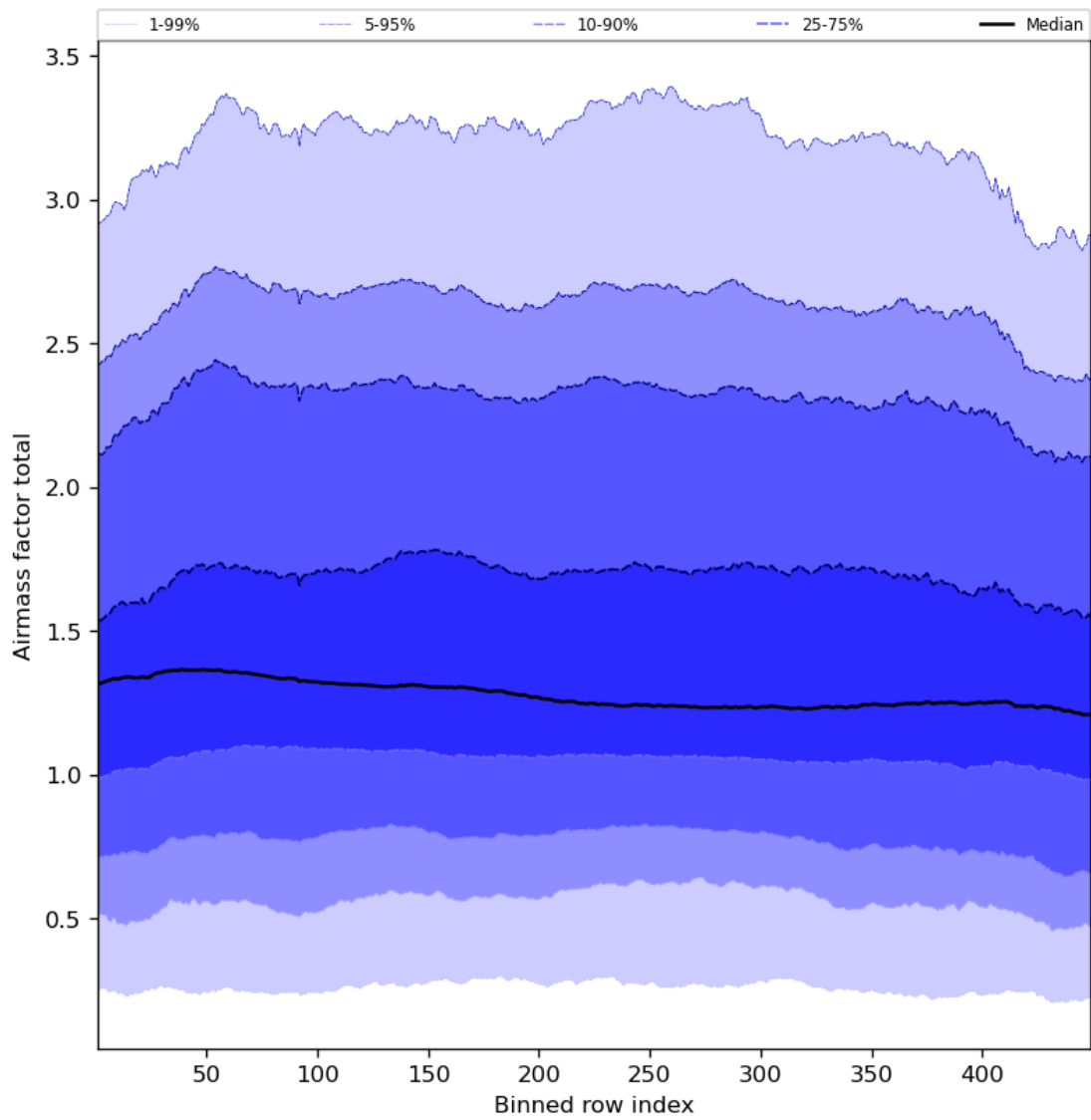
Figure 54: Along track statistics of “Airmass factor total” for 2023-08-15 to 2023-08-17
