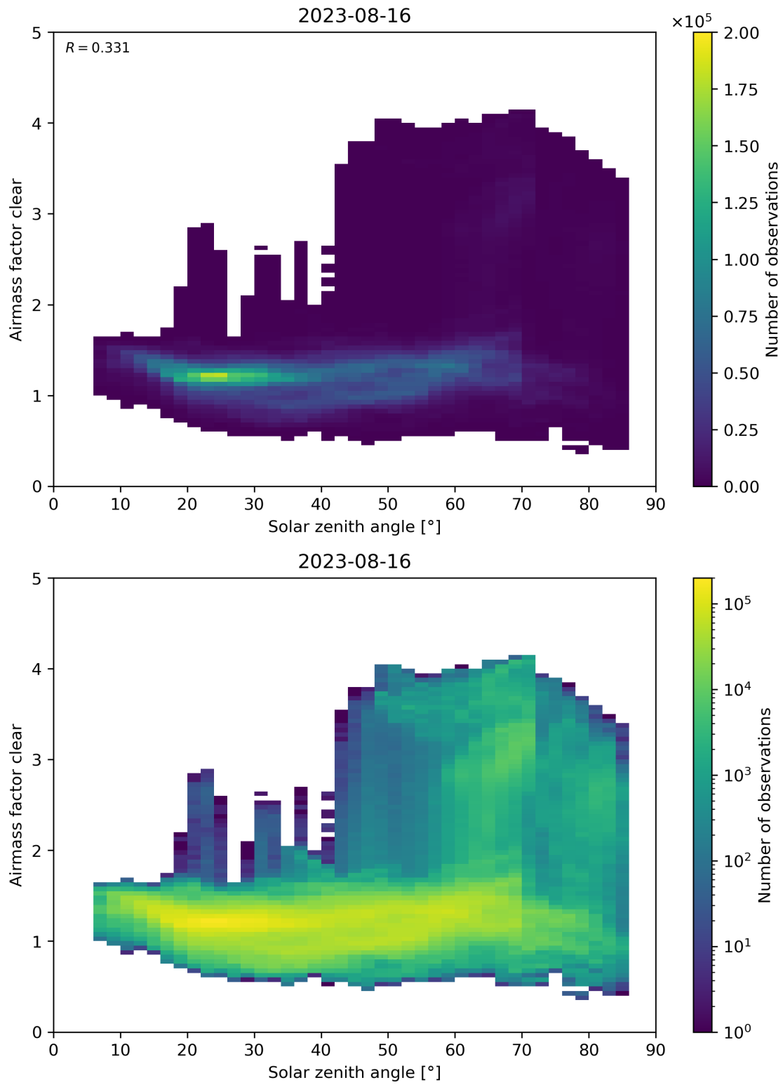
Figure 170: Scatter density plot of “Solar zenith angle” against “Airmass factor clear” for 2023-08-15 to 2023-08-17.
