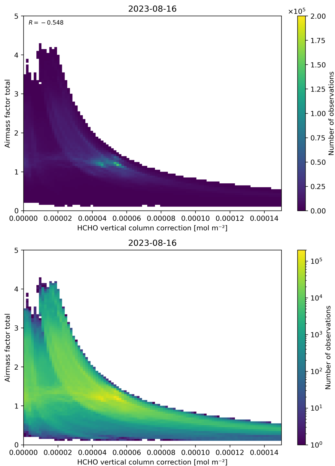
Figure 120: Scatter density plot of “HCHO vertical column correction” against “Airmass factor total” for 2023-08-15 to 2023-08-17.
