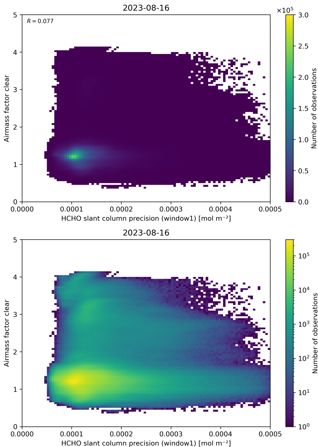
Figure 91: Scatter density plot of “HCHO slant column precision (window1)” against “Airmass factor clear” for 2023-08-15 to 2023-08-17.
