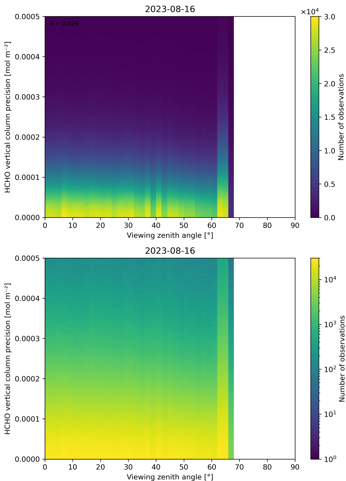
Figure 194: Scatter density plot of “Viewing zenith angle” against “HCHO vertical column precision” for 2023-08-15 to 2023-08-17.
