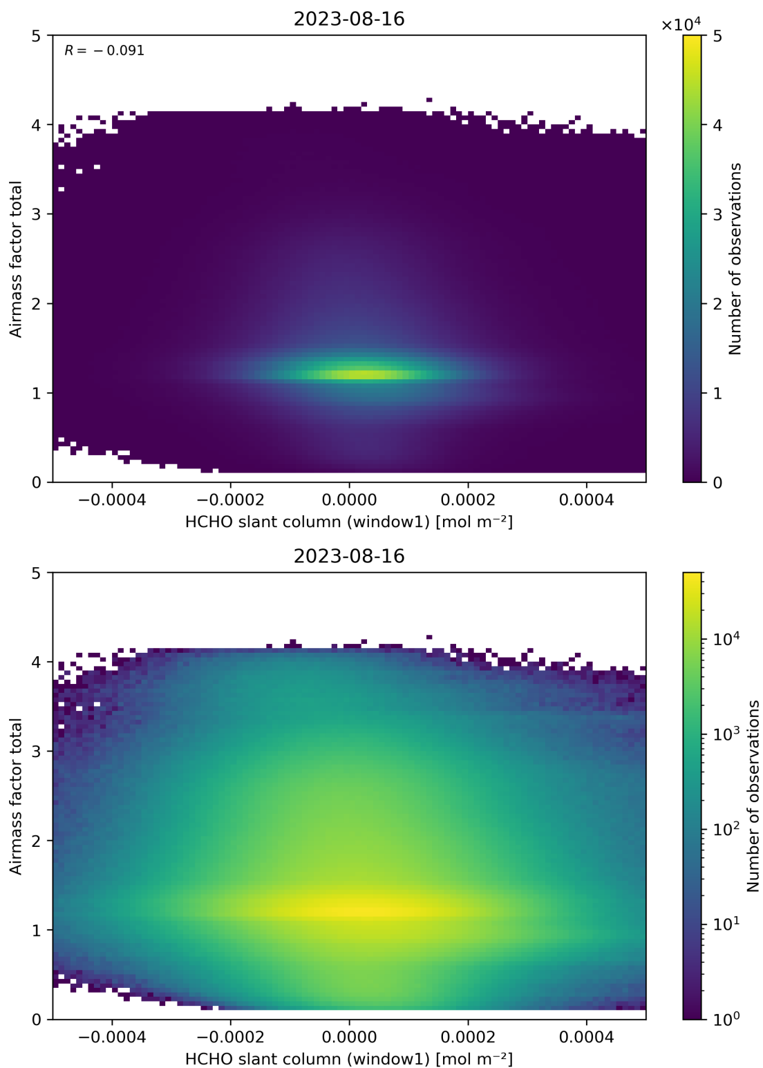
Figure 85: Scatter density plot of “HCHO slant column (window1)” against “Airmass factor total” for 2023-08-15 to 2023-08-17.
