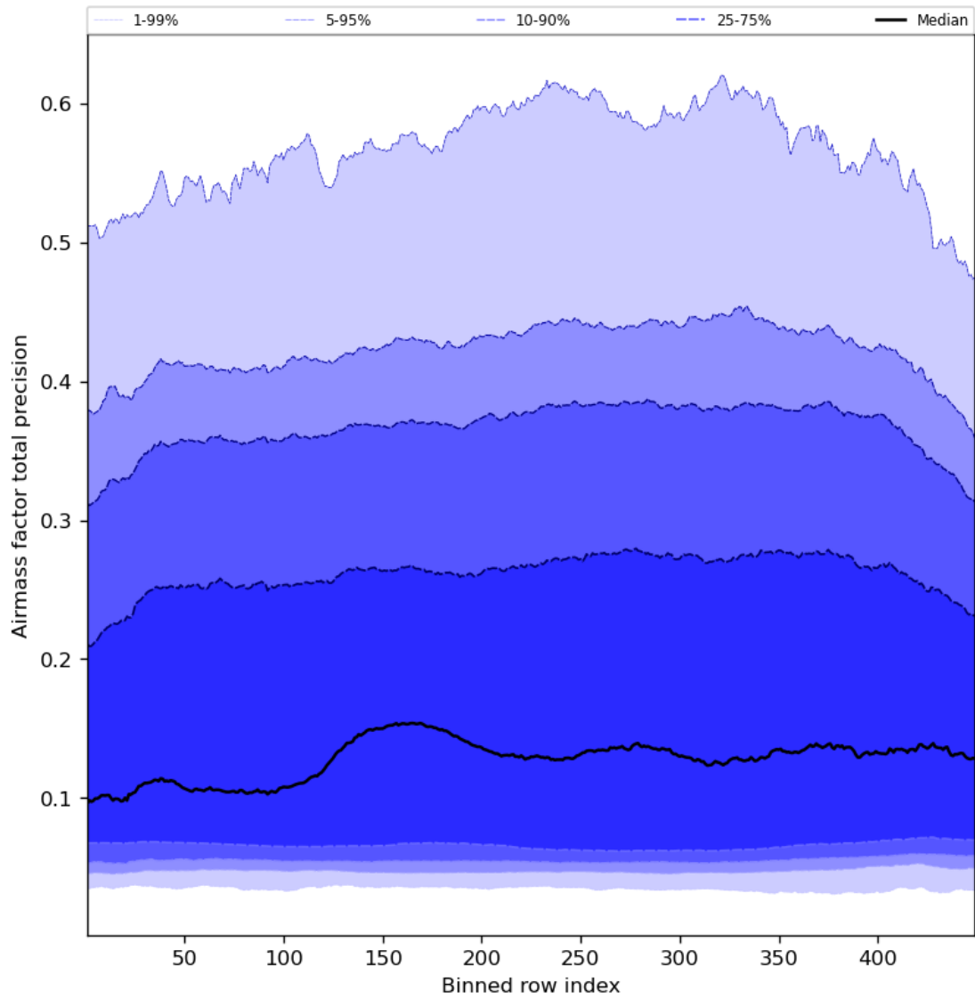
Figure 55: Along track statistics of “Airmass factor total precision” for 2023-08-15 to 2023-08-17
