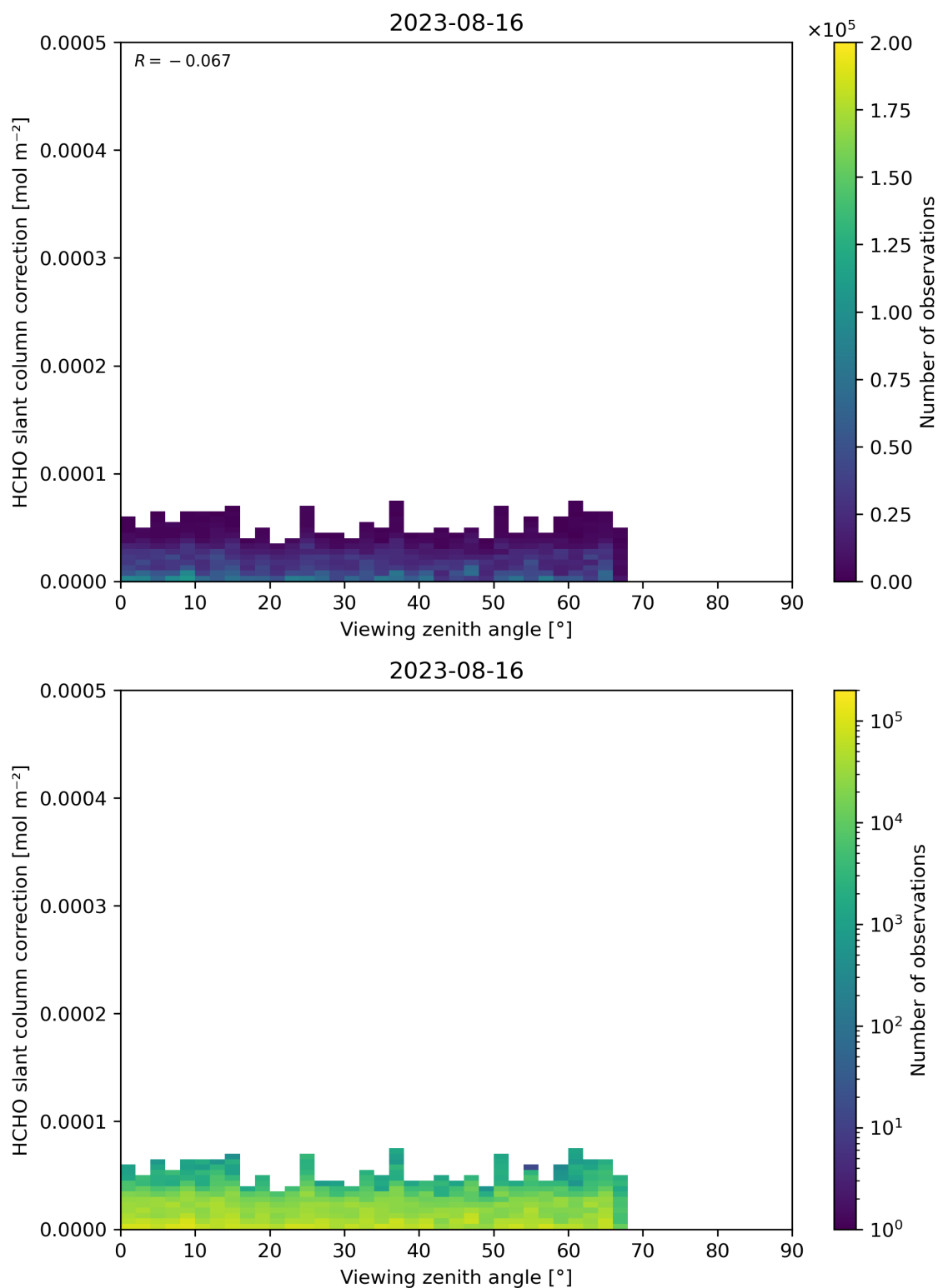
Figure 187: Scatter density plot of “Viewing zenith angle” against “HCHO slant column correction” for 2023-08-15 to 2023-08-17.
