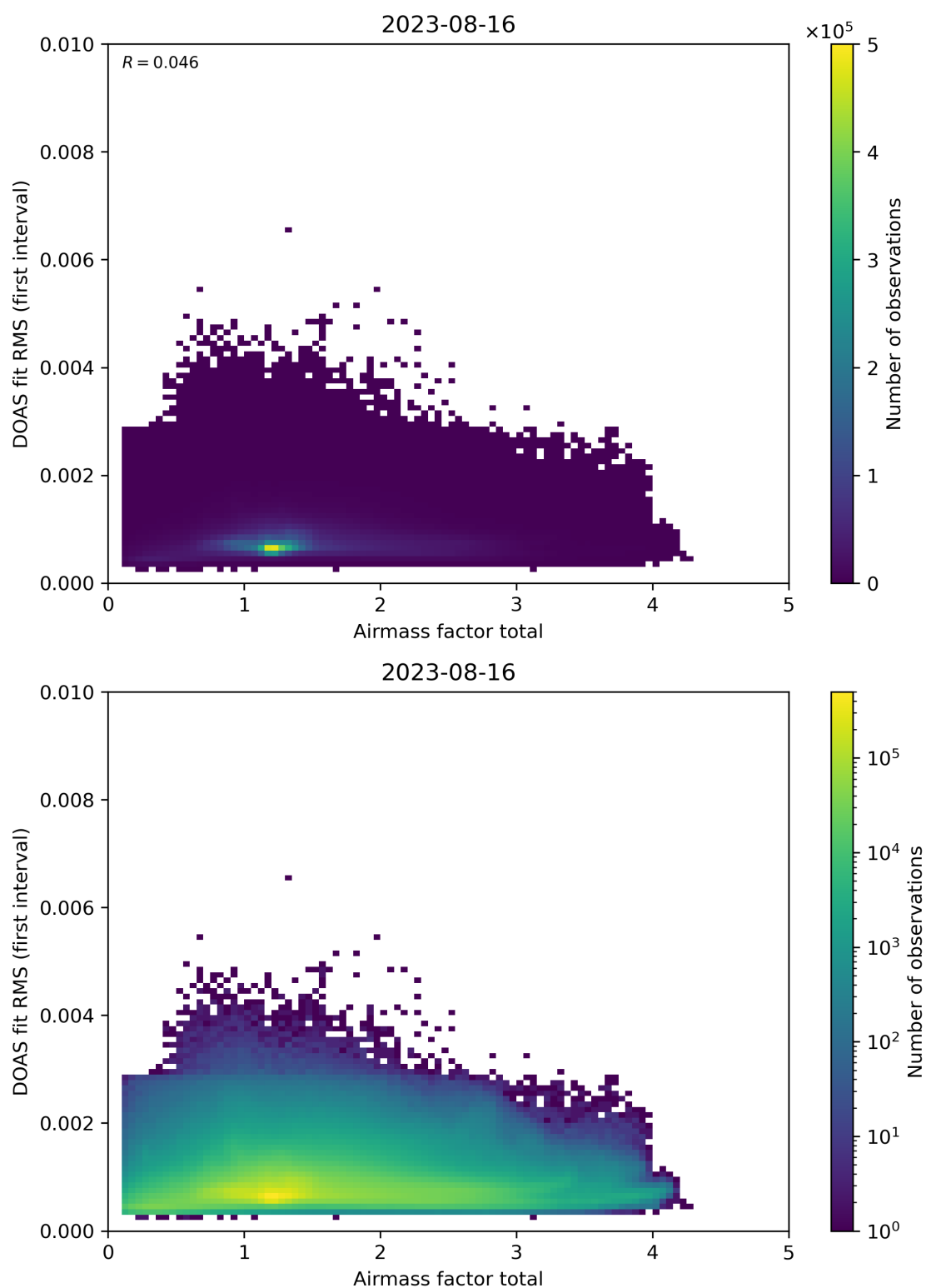
Figure 97: Scatter density plot of “Airmass factor total” against “DOAS fit RMS (first interval)” for 2023-08-15 to 2023-08-17.
