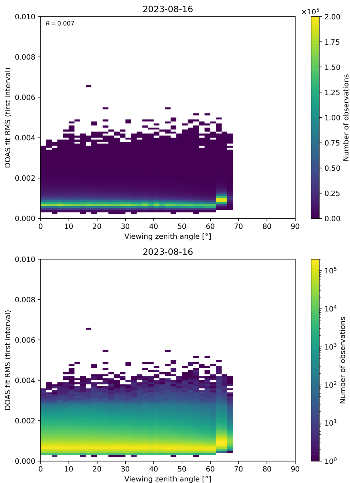
Figure 182: Scatter density plot of “Viewing zenith angle” against “DOAS fit RMS (first interval)” for 2023-08-15 to 2023-08-17.
