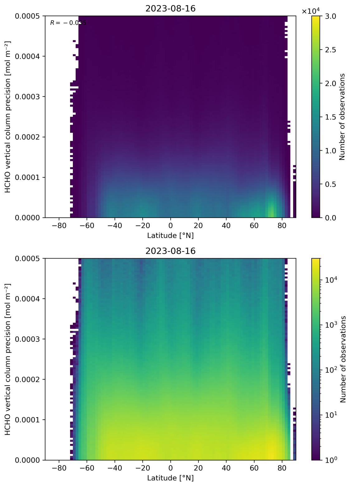
Figure 165: Scatter density plot of “Latitude” against “HCHO vertical column precision” for 2023-08-15 to 2023-08-17.
