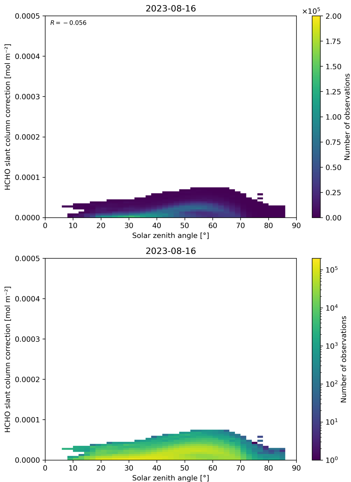
Figure 172: Scatter density plot of “Solar zenith angle” against “HCHO slant column correction” for 2023-08-15 to 2023-08-17.
