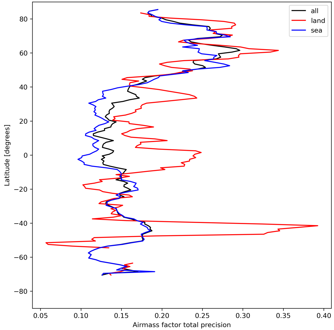
Figure 27: Zonal average of “Airmass factor total precision” for 2023-08-15 to 2023-08-17.
