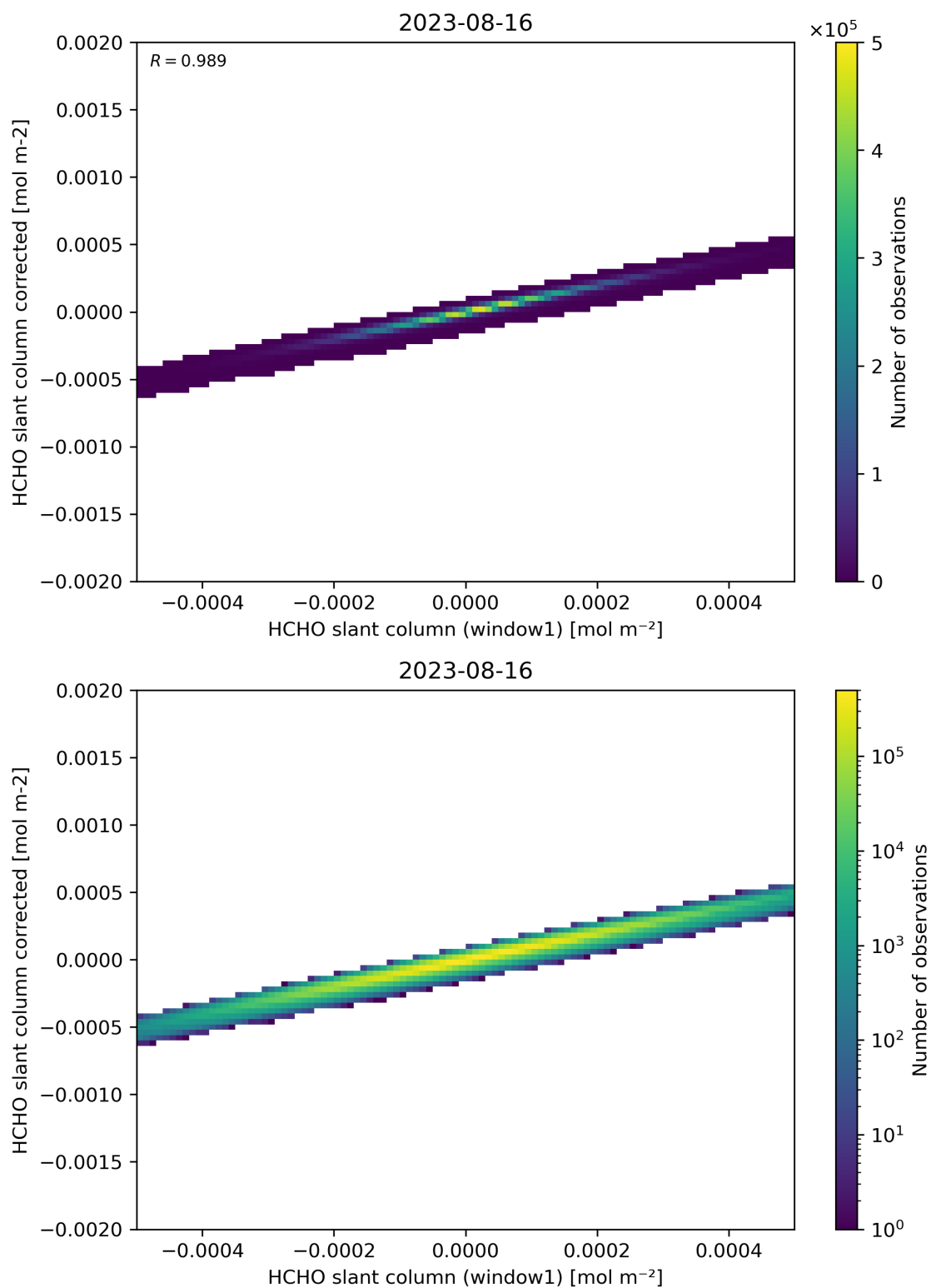
Figure 82: Scatter density plot of “HCHO slant column (window1)” against “HCHO slant column corrected” for 2023-08-15 to 2023-08-17.
