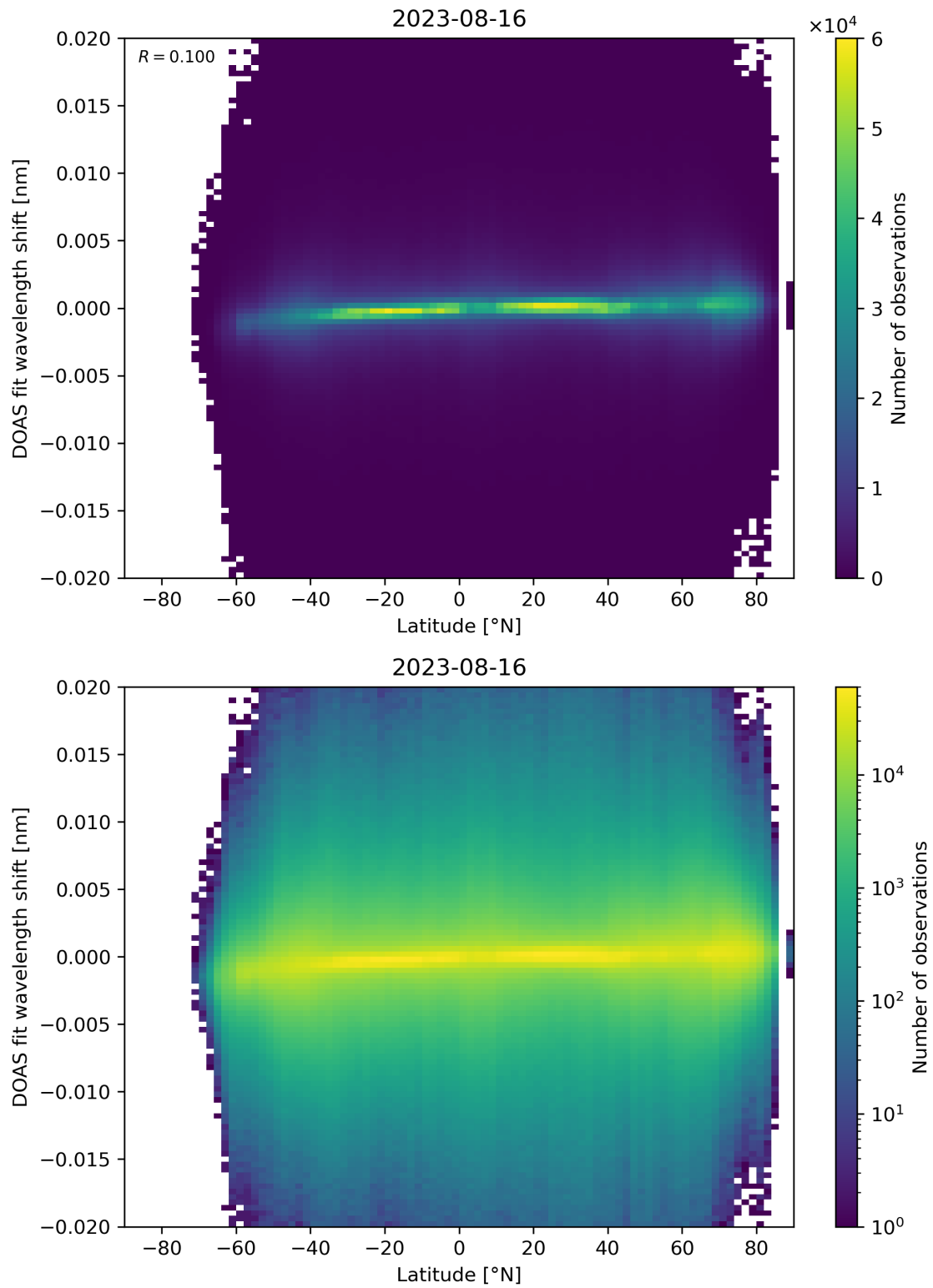
Figure 154: Scatter density plot of “Latitude” against “DOAS fit wavelength shift” for 2023-08-15 to 2023-08-17.
