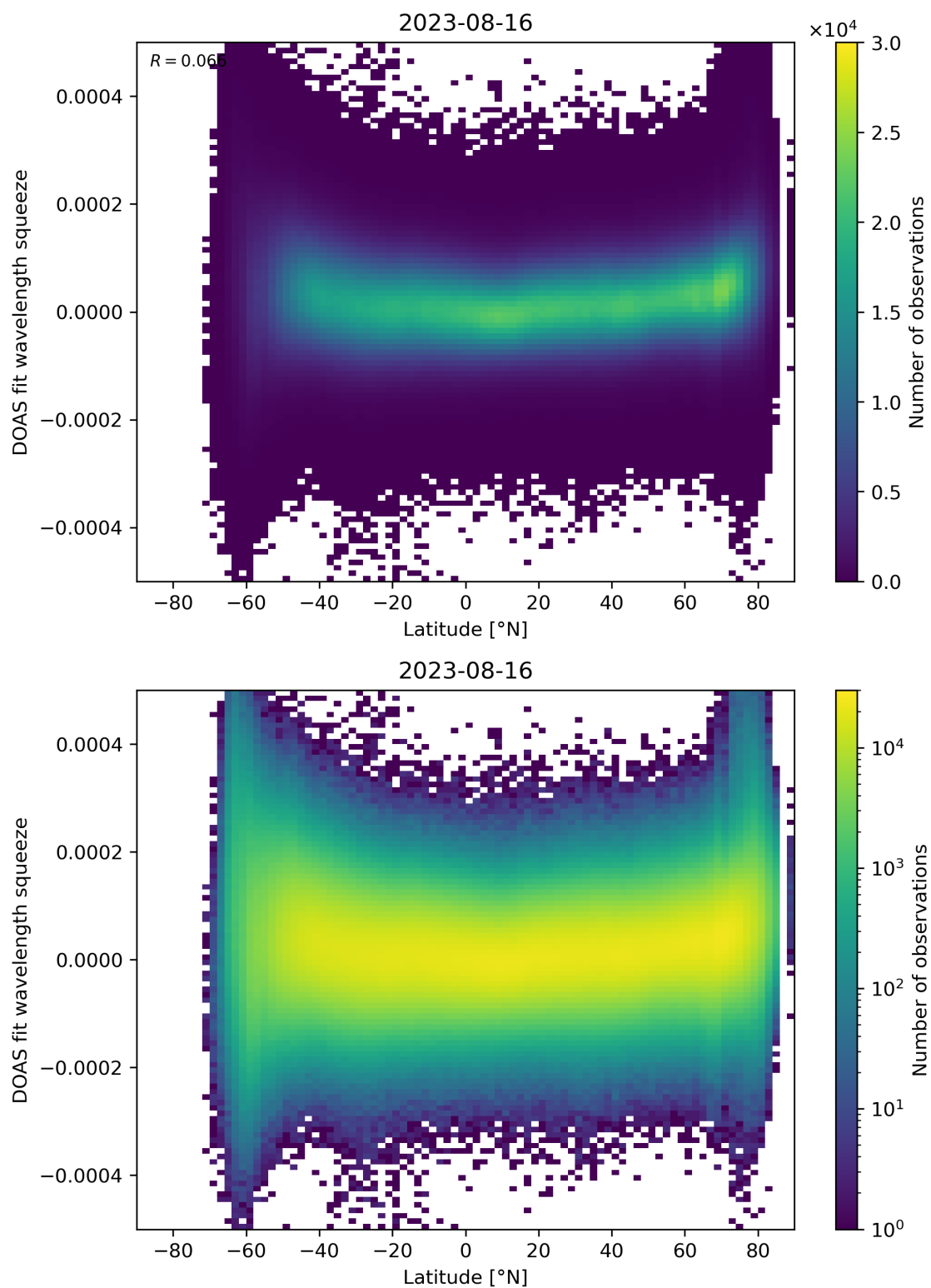
Figure 155: Scatter density plot of “Latitude” against “DOAS fit wavelength squeeze” for 2023-08-15 to 2023-08-17.
