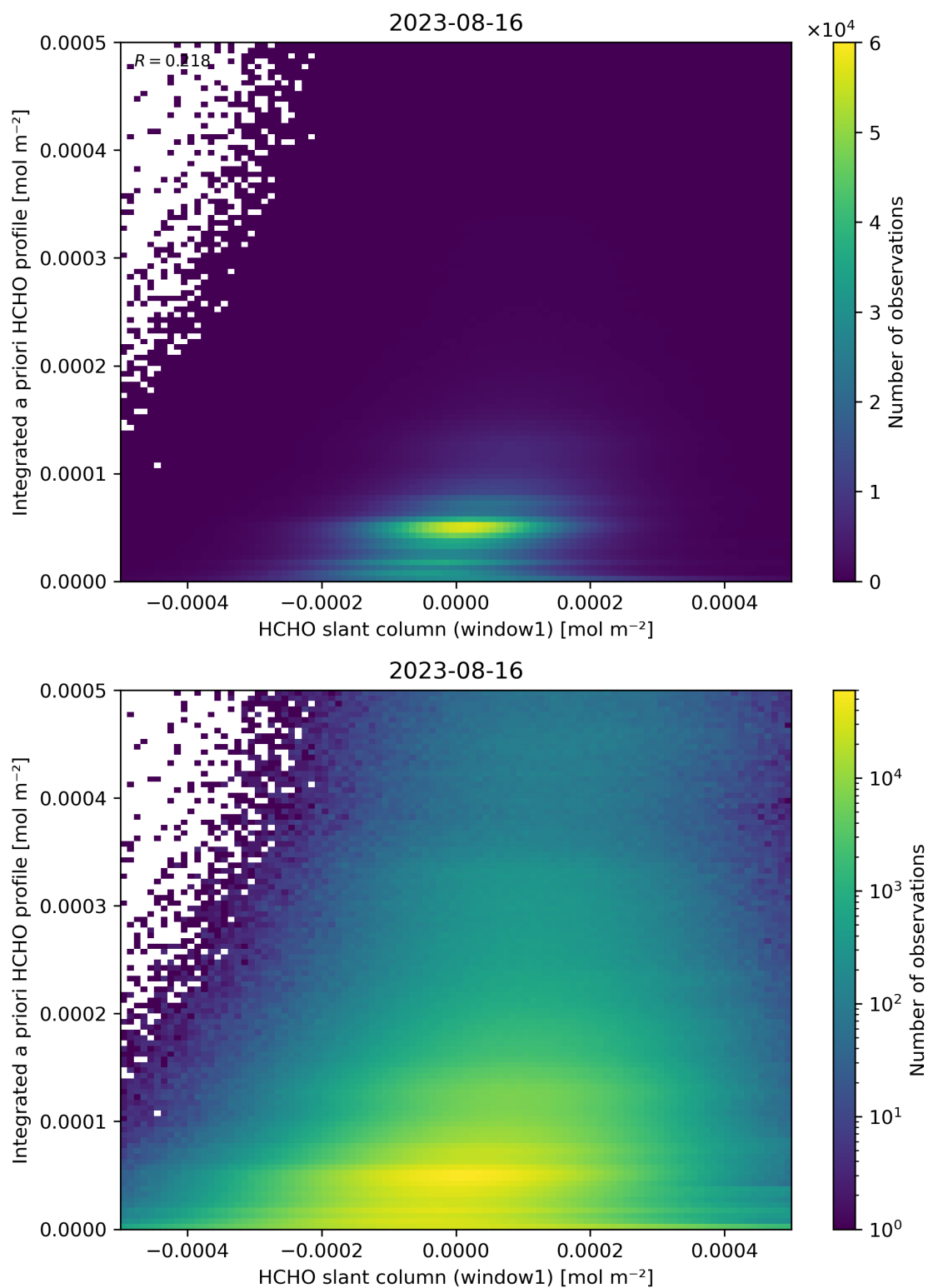
Figure 87: Scatter density plot of “HCHO slant column (window1)” against “Integrated a priori HCHO profile” for 2023-08-15 to 2023-08-17.
