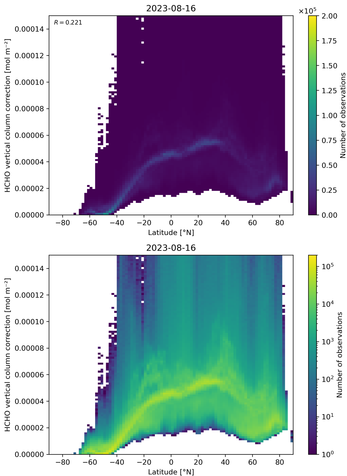
Figure 164: Scatter density plot of “Latitude” against “HCHO vertical column correction” for 2023-08-15 to 2023-08-17.
