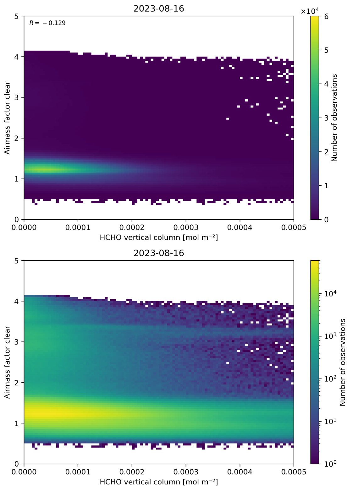
Figure 126: Scatter density plot of “HCHO vertical column” against “Airmass factor clear” for 2023-08-15 to 2023-08-17.
