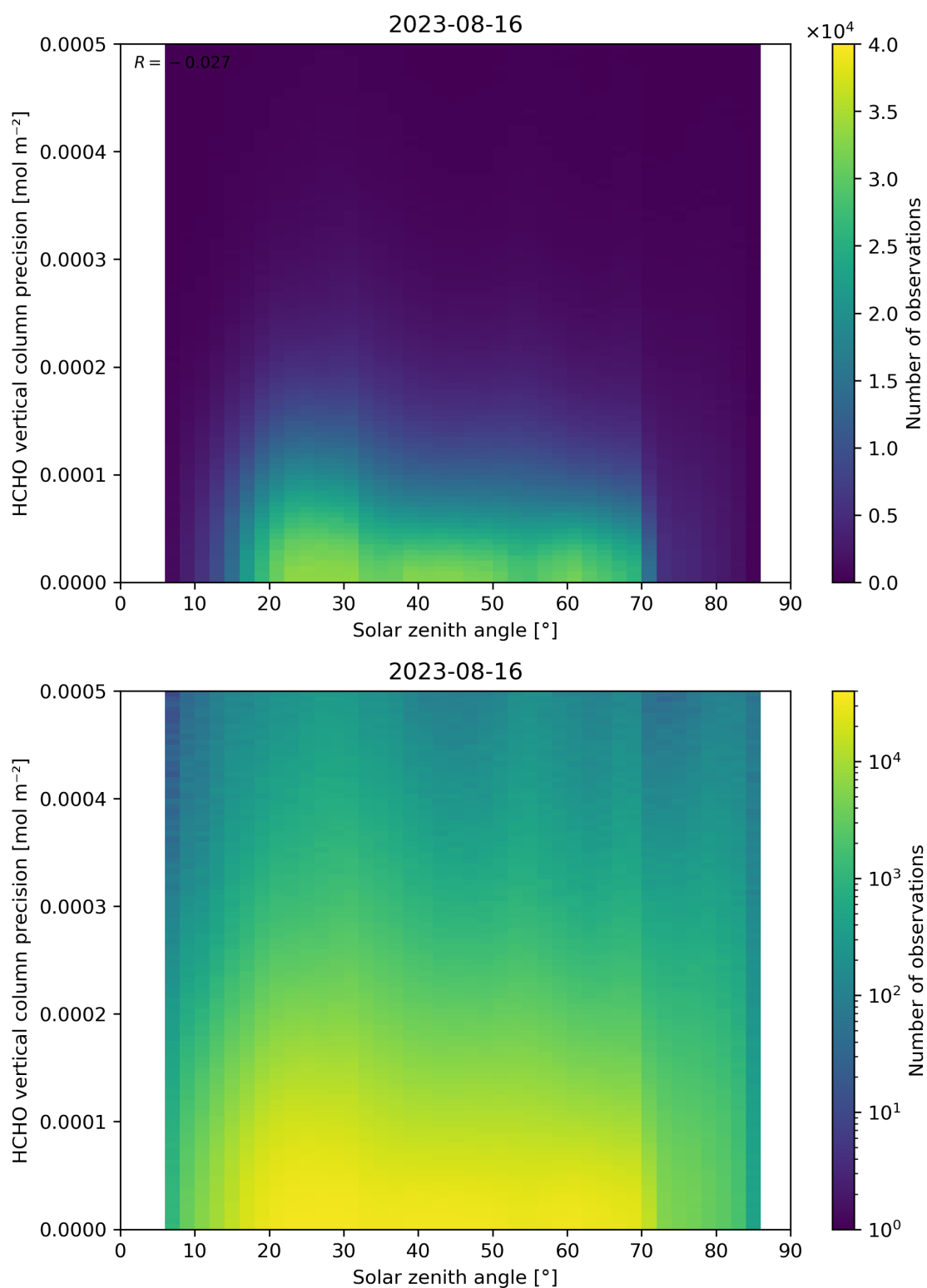
Figure 179: Scatter density plot of “Solar zenith angle” against “HCHO vertical column precision” for 2023-08-15 to 2023-08-17.
