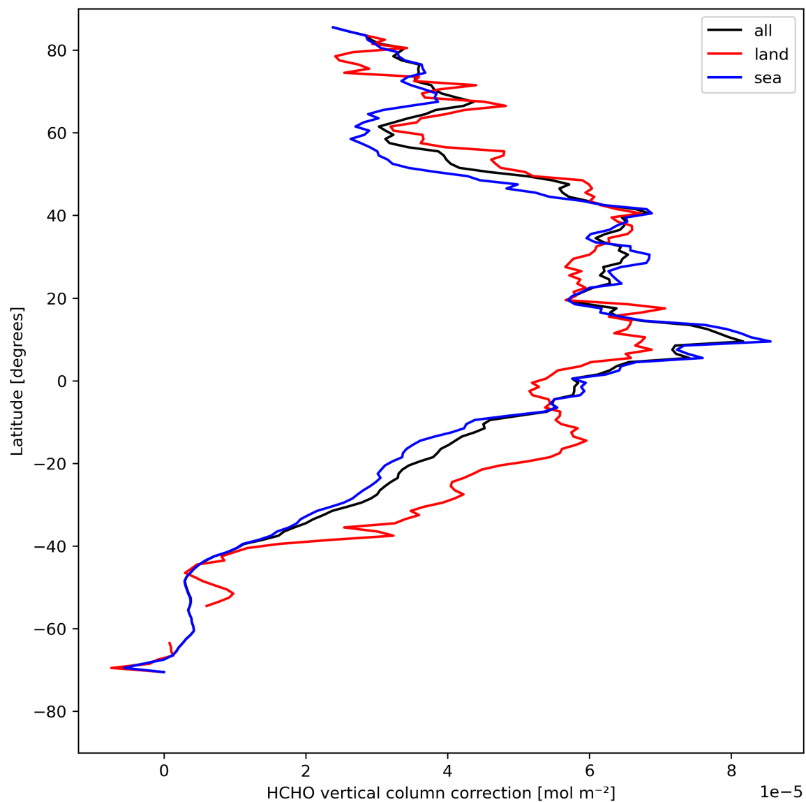
Figure 23: Zonal average of “HCHO vertical column correction” for 2023-08-15 to 2023-08-17.
