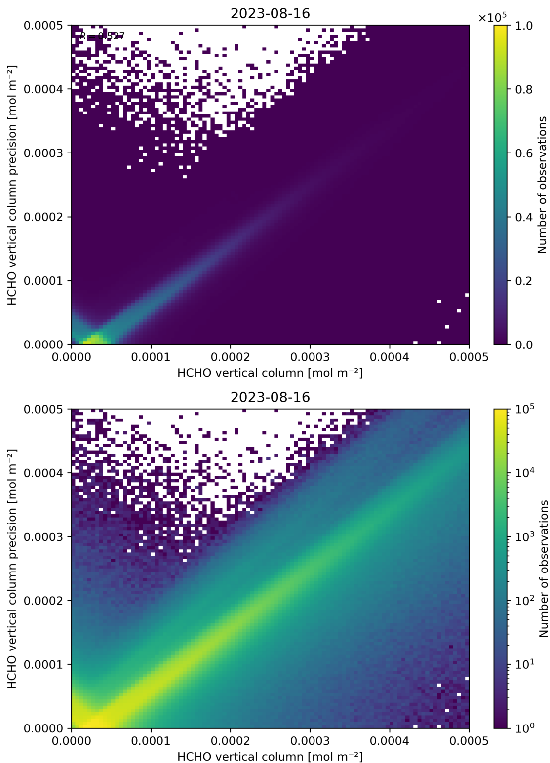
Figure 134: Scatter density plot of “HCHO vertical column” against “HCHO vertical column precision” for 2023-08-15 to 2023-08-17.
