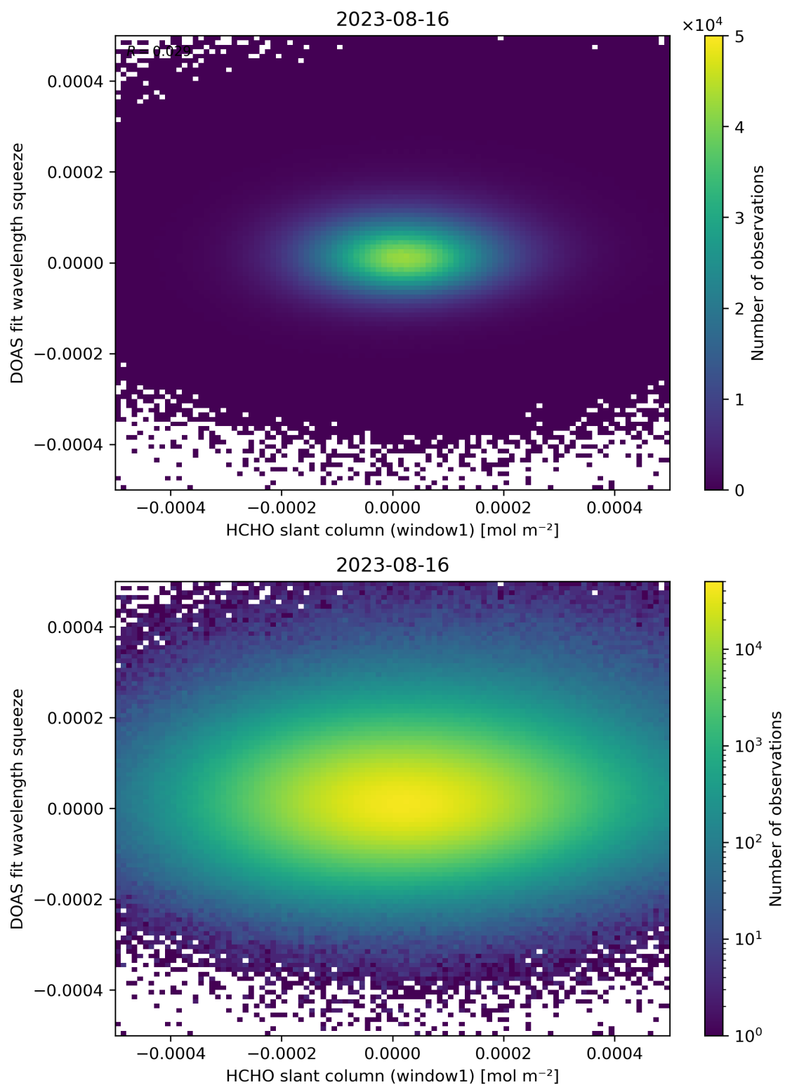
Figure 80: Scatter density plot of “HCHO slant column (window1)” against “DOAS fit wavelength squeeze” for 2023-08-15 to 2023-08-17.
