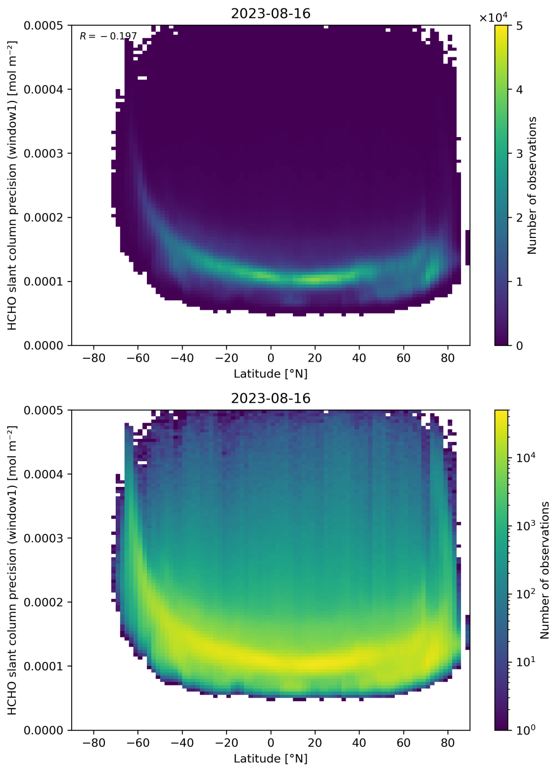
Figure 160: Scatter density plot of “Latitude” against “HCHO slant column precision (window1)” for 2023-08-15 to 2023-08-17.
