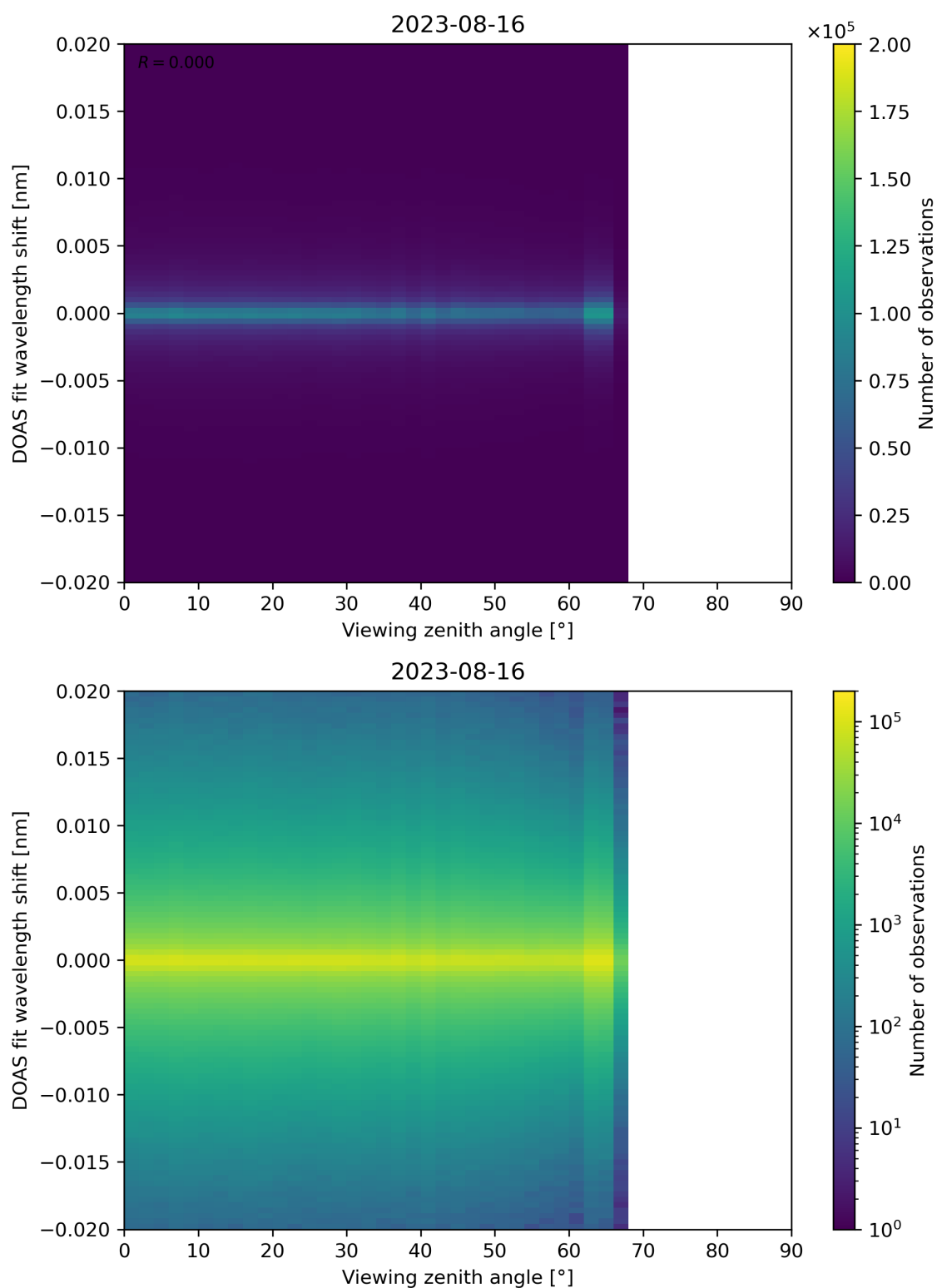
Figure 183: Scatter density plot of “Viewing zenith angle” against “DOAS fit wavelength shift” for 2023-08-15 to 2023-08-17.
