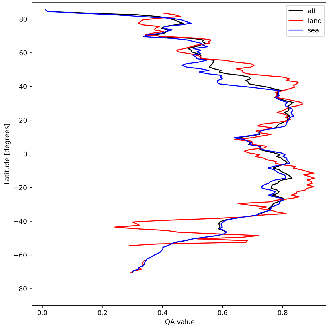
Figure 20: Zonal average of “QA value” for 2023-08-15 to 2023-08-17.
