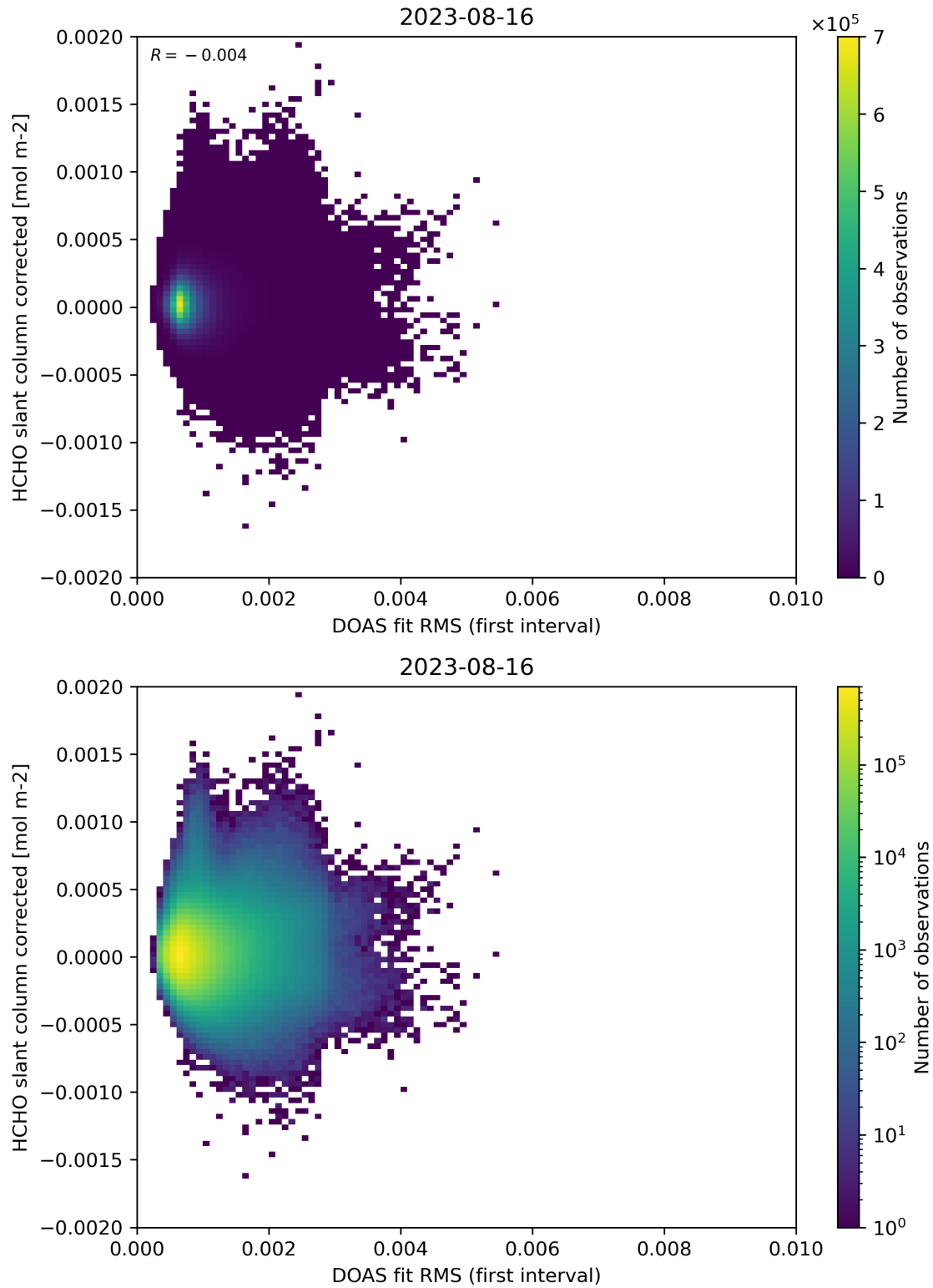
Figure 62: Scatter density plot of “DOAS fit RMS (first interval)” against “HCHO slant column corrected” for 2023-08-15 to 2023-08-17.
