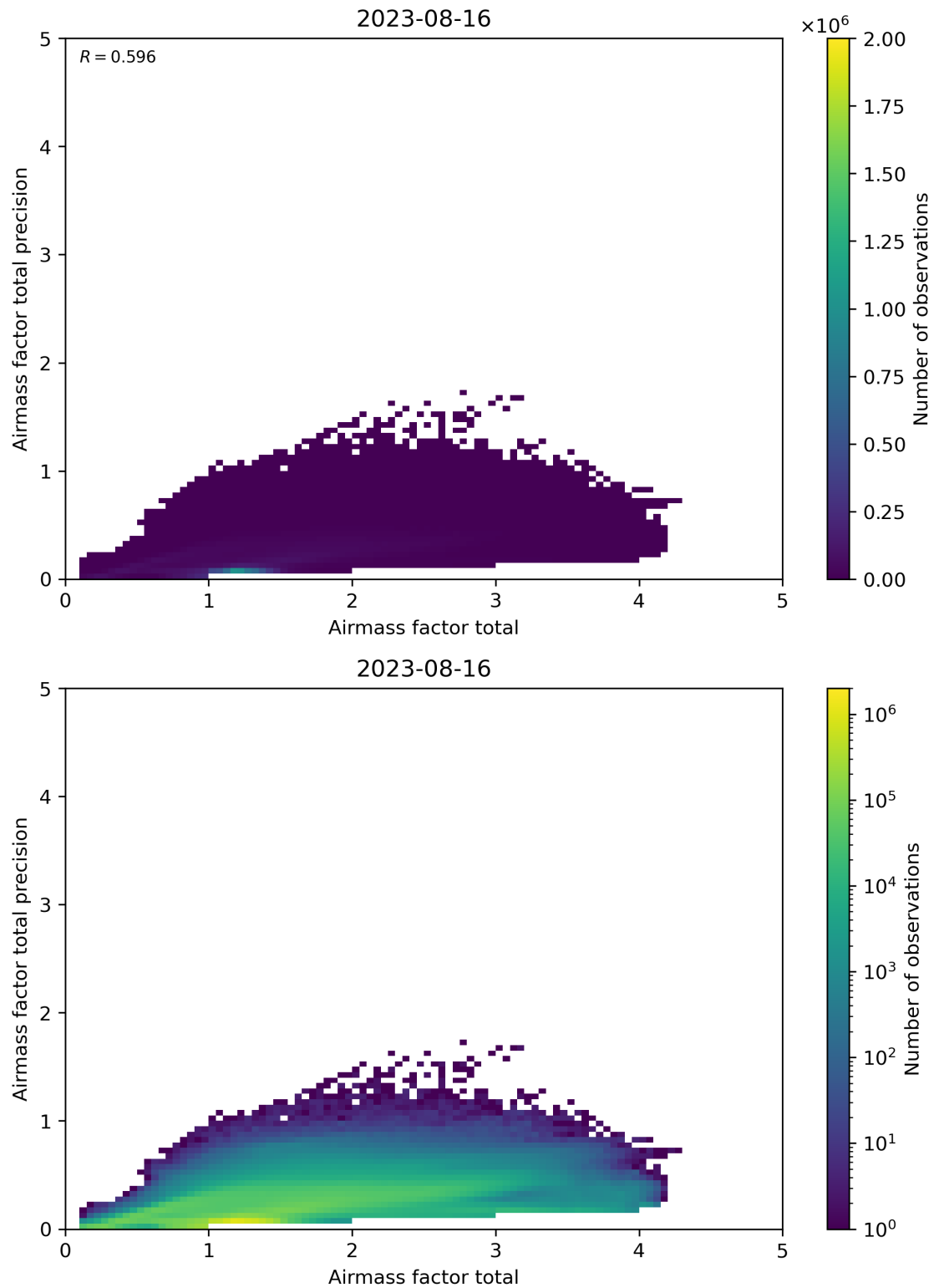
Figure 103: Scatter density plot of “Airmass factor total” against “Airmass factor total precision” for 2023-08-15 to 2023-08-17.
