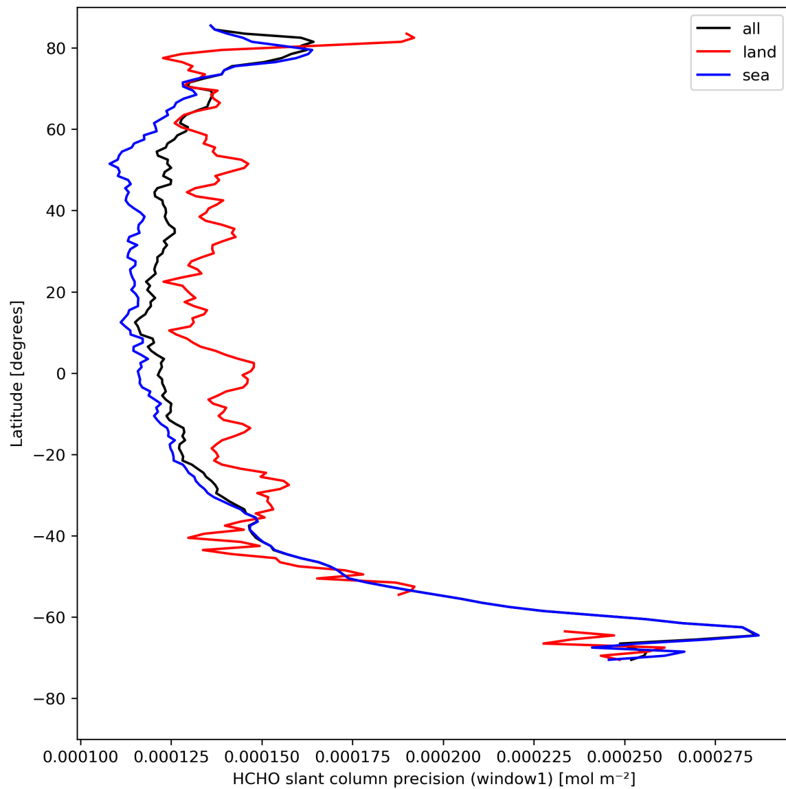
Figure 25: Zonal average of “HCHO slant column precision (window1)” for 2023-08-15 to 2023-08-17.
