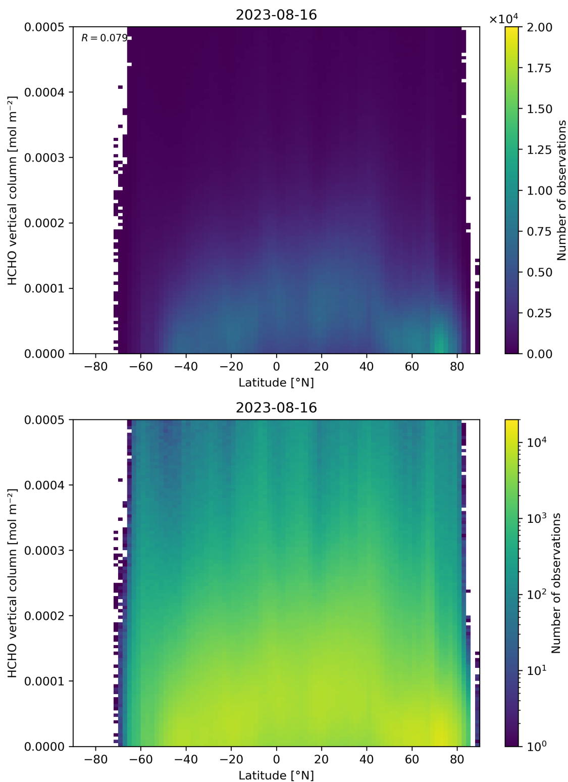
Figure 163: Scatter density plot of “Latitude” against “HCHO vertical column” for 2023-08-15 to 2023-08-17.
