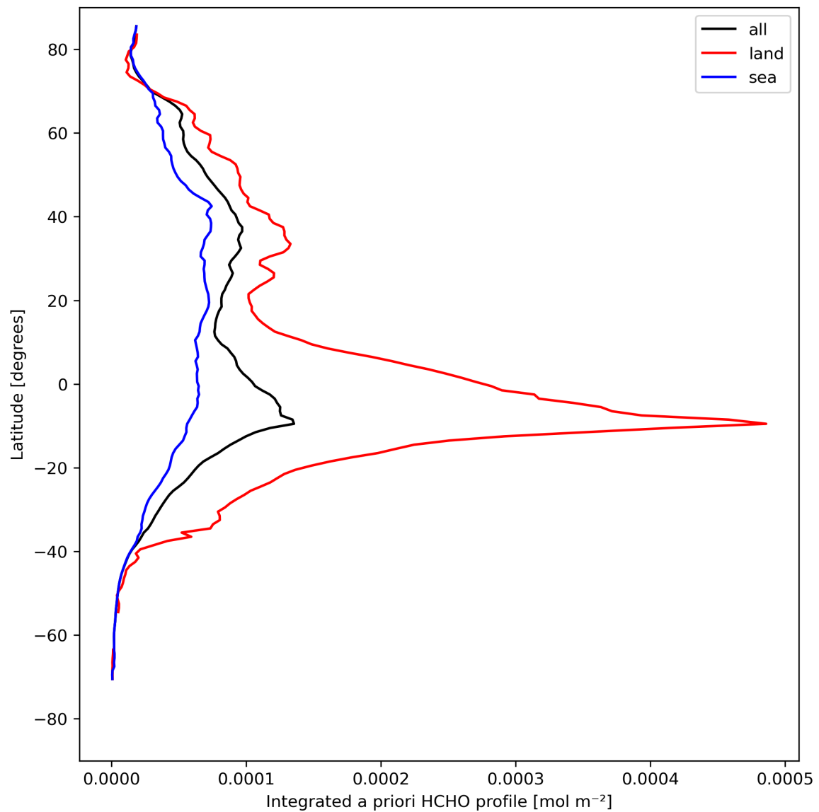
Figure 29: Zonal average of “Integrated a priori HCHO profile” for 2023-08-15 to 2023-08-17.
