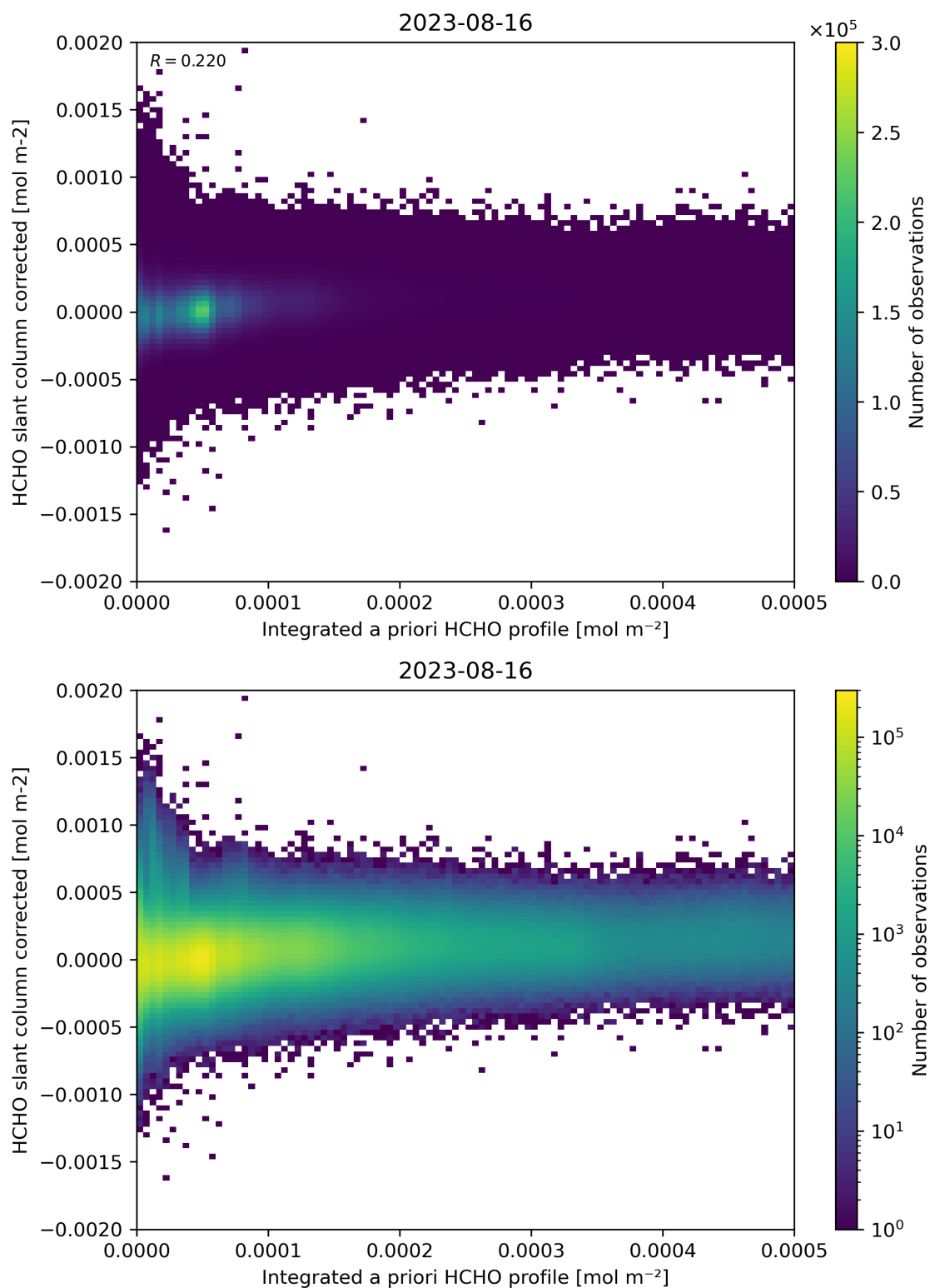
Figure 151: Scatter density plot of “Integrated a priori HCHO profile” against “HCHO slant column corrected” for 2023-08-15 to 2023-08-17.
