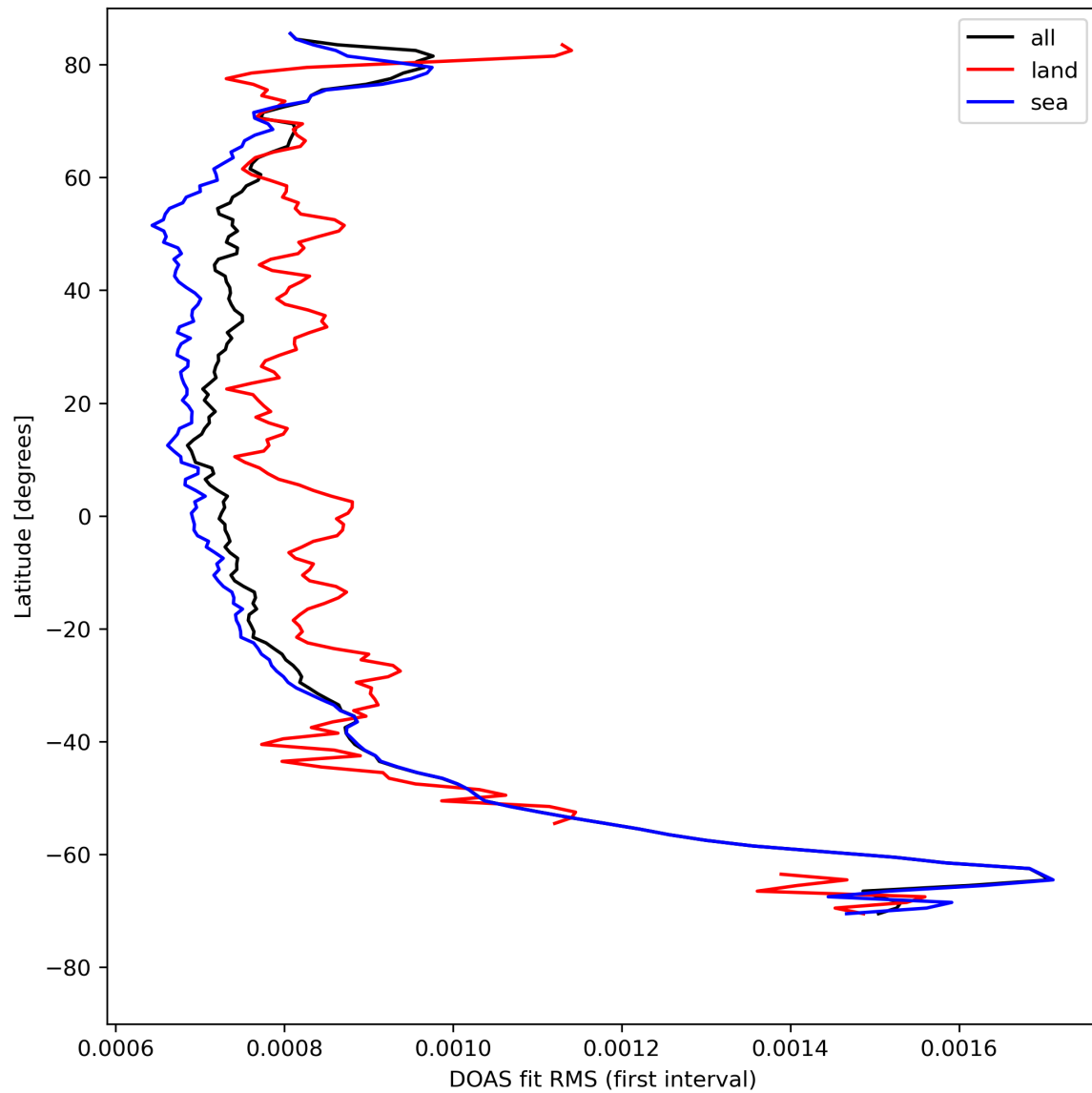
Figure 32: Zonal average of "DOAS fit RMS (first interval)" for 2023-08-15 to 2023-08-17.
