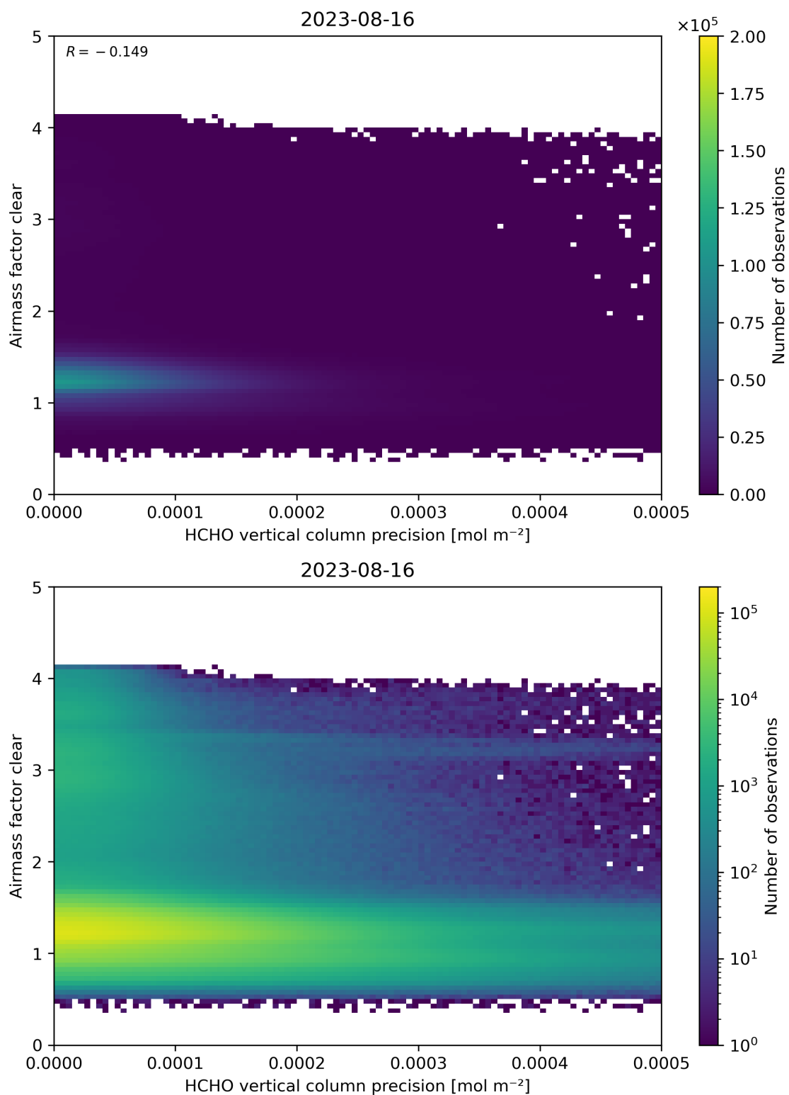
Figure 139: Scatter density plot of “HCHO vertical column precision” against “Airmass factor clear” for 2023-08-15 to 2023-08-17.
