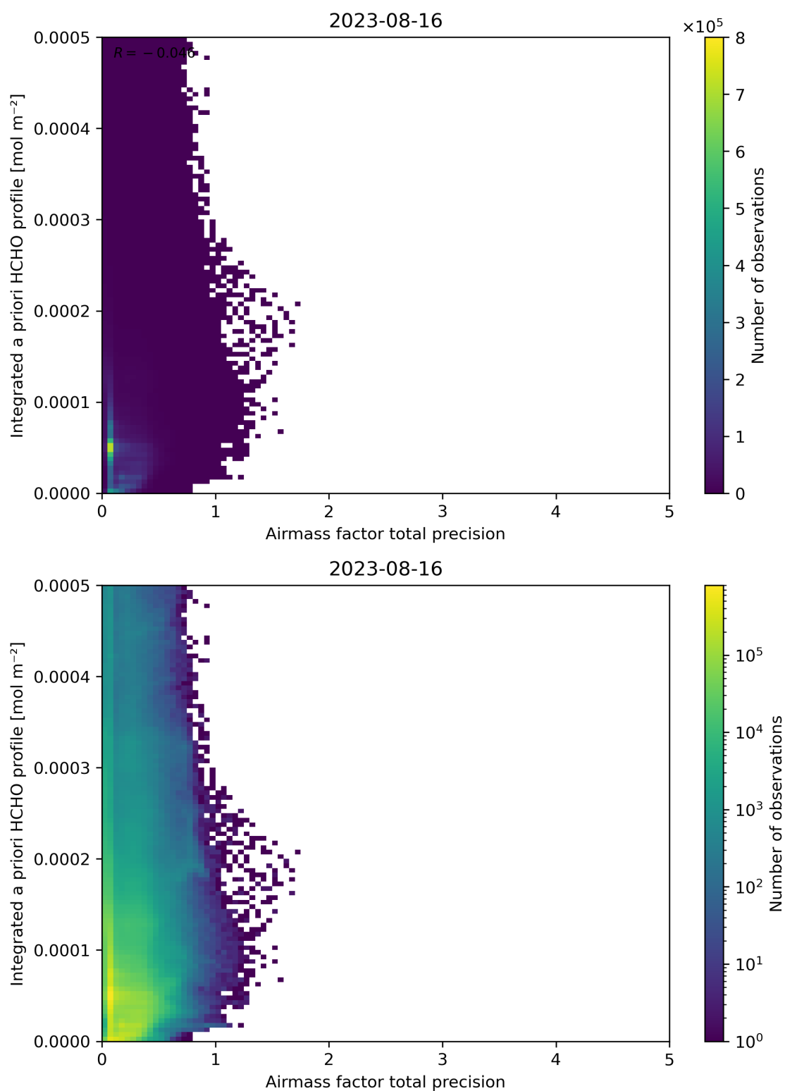
Figure 111: Scatter density plot of “Airmass factor total precision” against “Integrated a priori HCHO profile” for 2023-08-15 to 2023-08-17.
