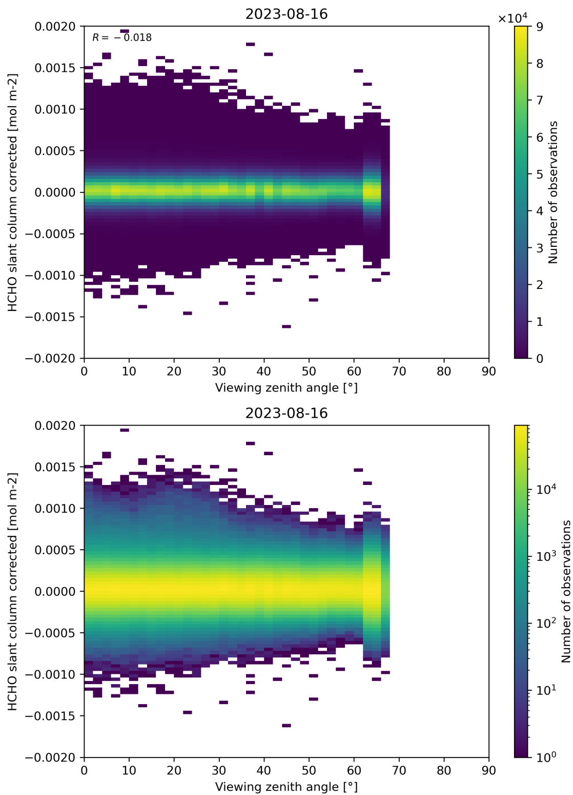
Figure 186: Scatter density plot of “Viewing zenith angle” against “HCHO slant column corrected” for 2023-08-15 to 2023-08-17.
