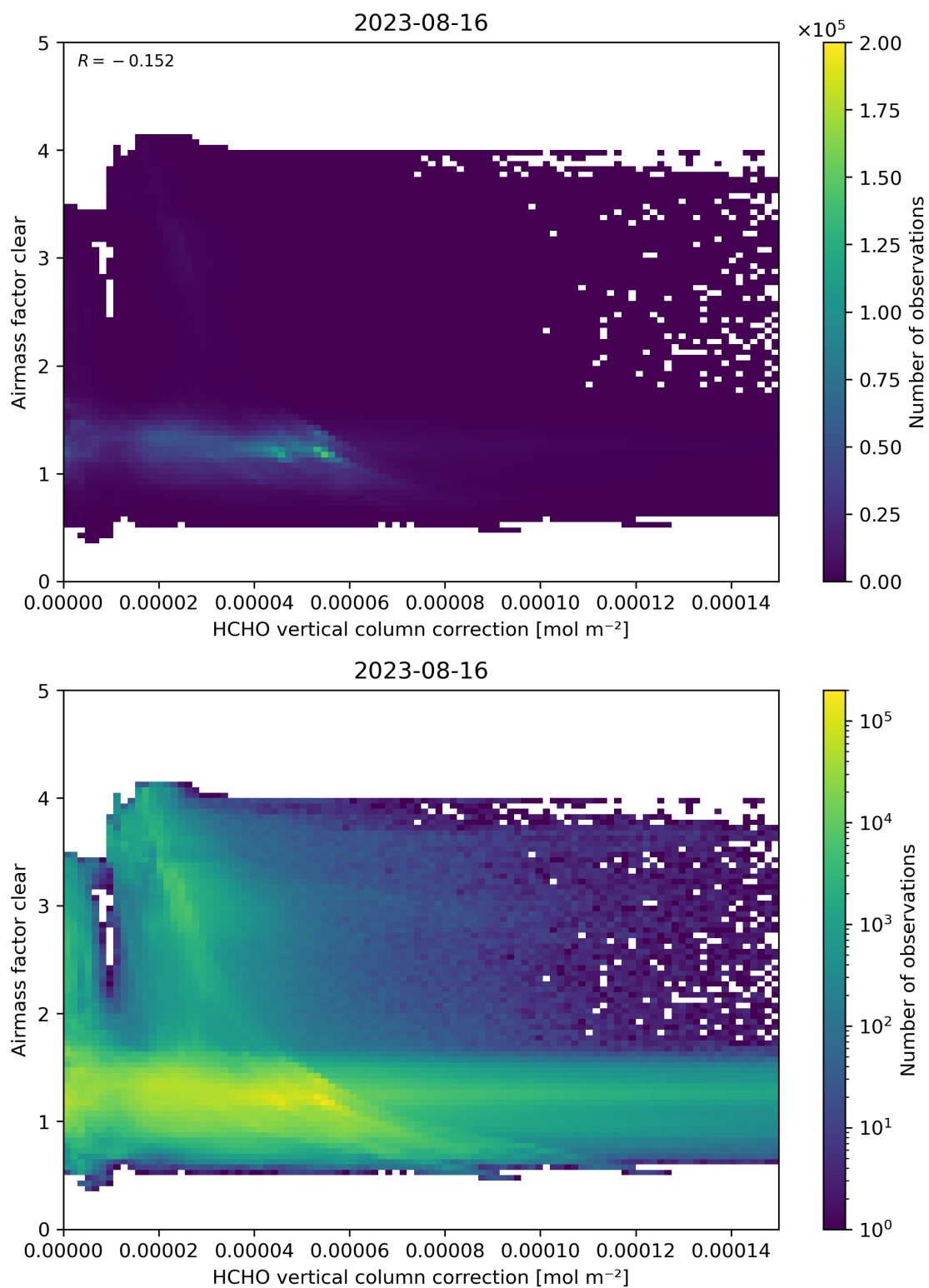
Figure 115: Scatter density plot of “HCHO vertical column correction” against “Airmass factor clear” for 2023-08-15 to 2023-08-17.
