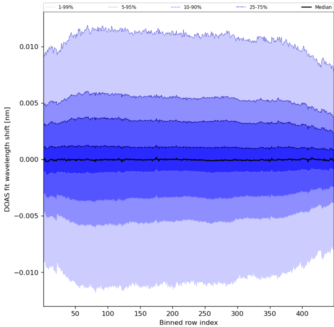
Figure 58: Along track statistics of “DOAS fit wavelength shift” for 2023-08-15 to 2023-08-17
