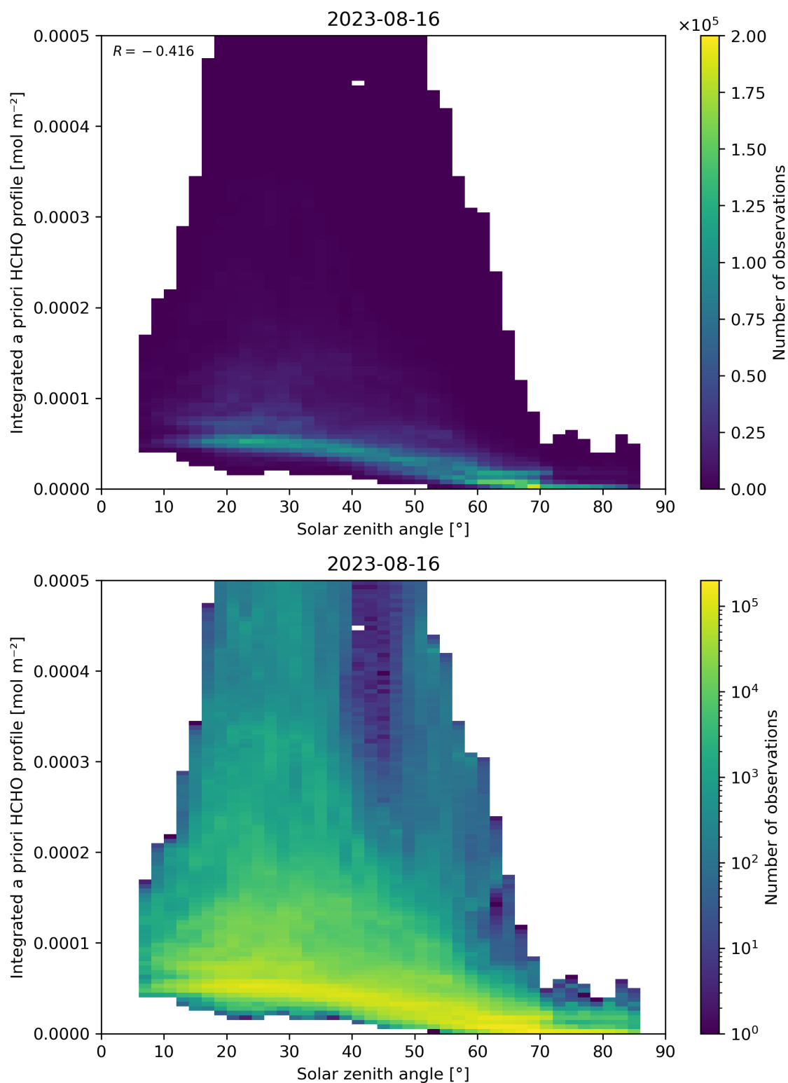
Figure 180: Scatter density plot of “Solar zenith angle” against “Integrated a priori HCHO profile” for 2023-08-15 to 2023-08-17.
