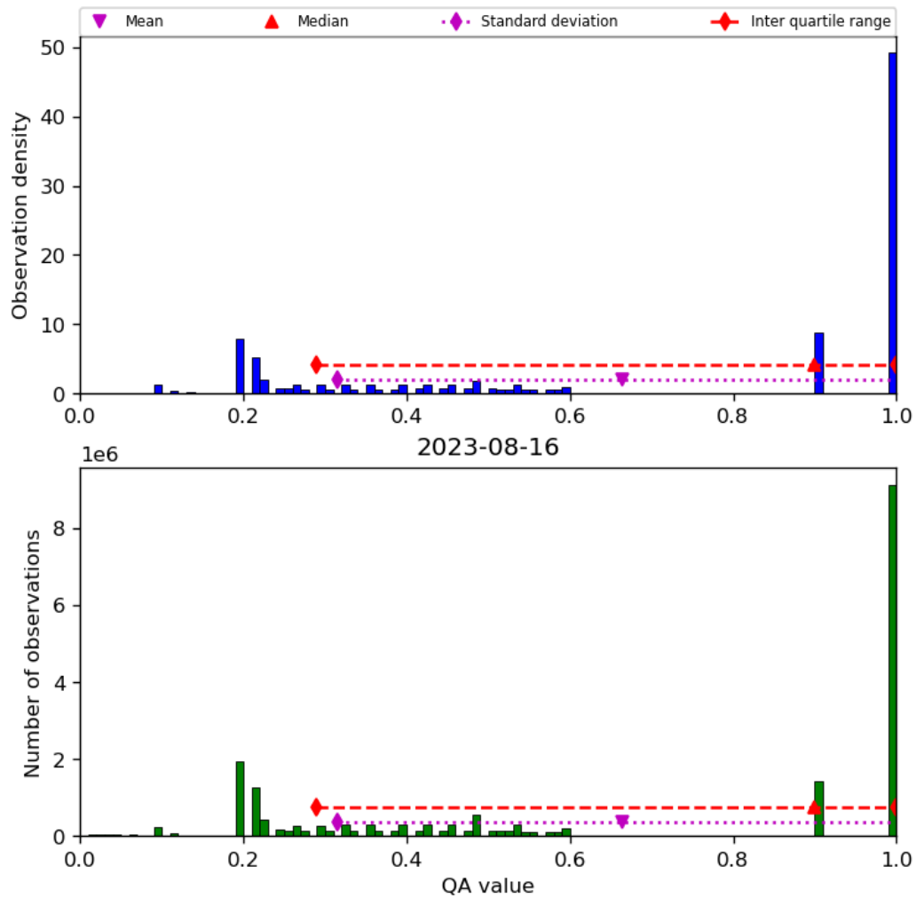
Figure 34: Histogram of “QA value” for 2023-08-15 to 2023-08-17
