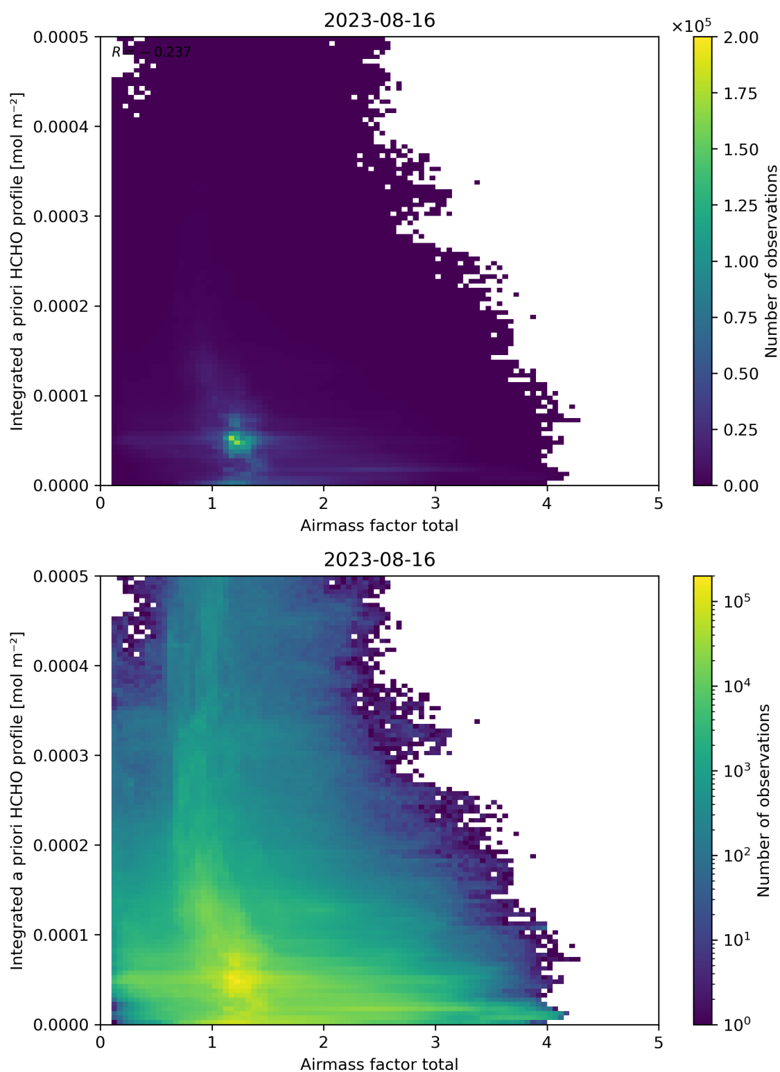
Figure 104: Scatter density plot of “Airmass factor total” against “Integrated a priori HCHO profile” for 2023-08-15 to 2023-08-17.
