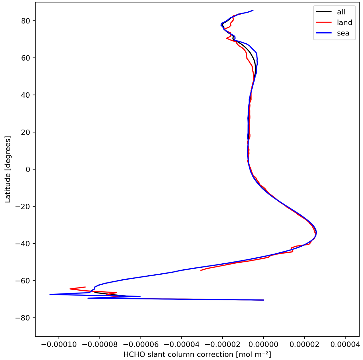
Figure 33: Zonal average of "HCHO slant column correction" for 2023-08-15 to 2023-08-17.
