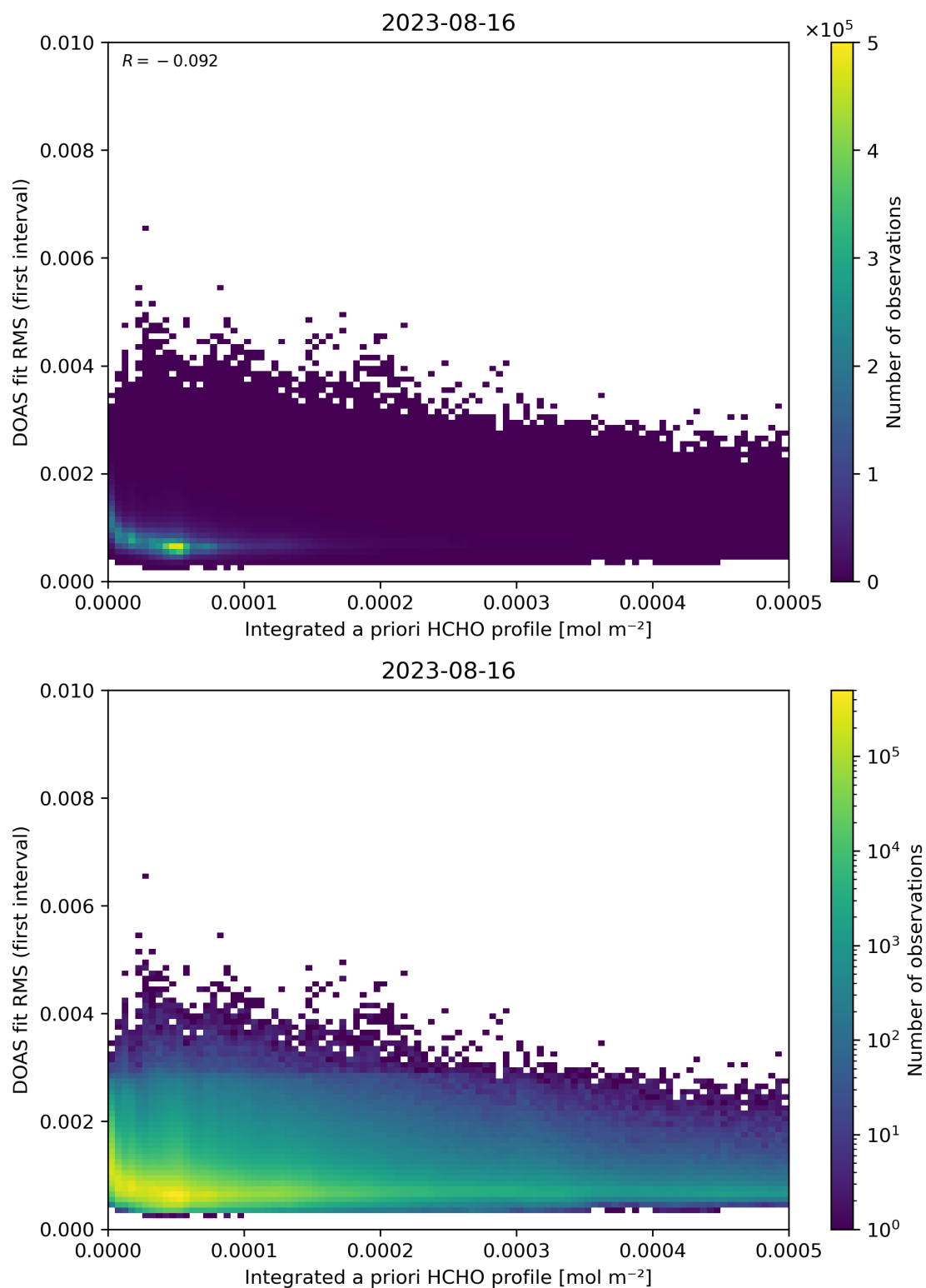
Figure 148: Scatter density plot of “Integrated a priori HCHO profile” against “DOAS fit RMS (first interval)” for 2023-08-15 to 2023-08-17.
