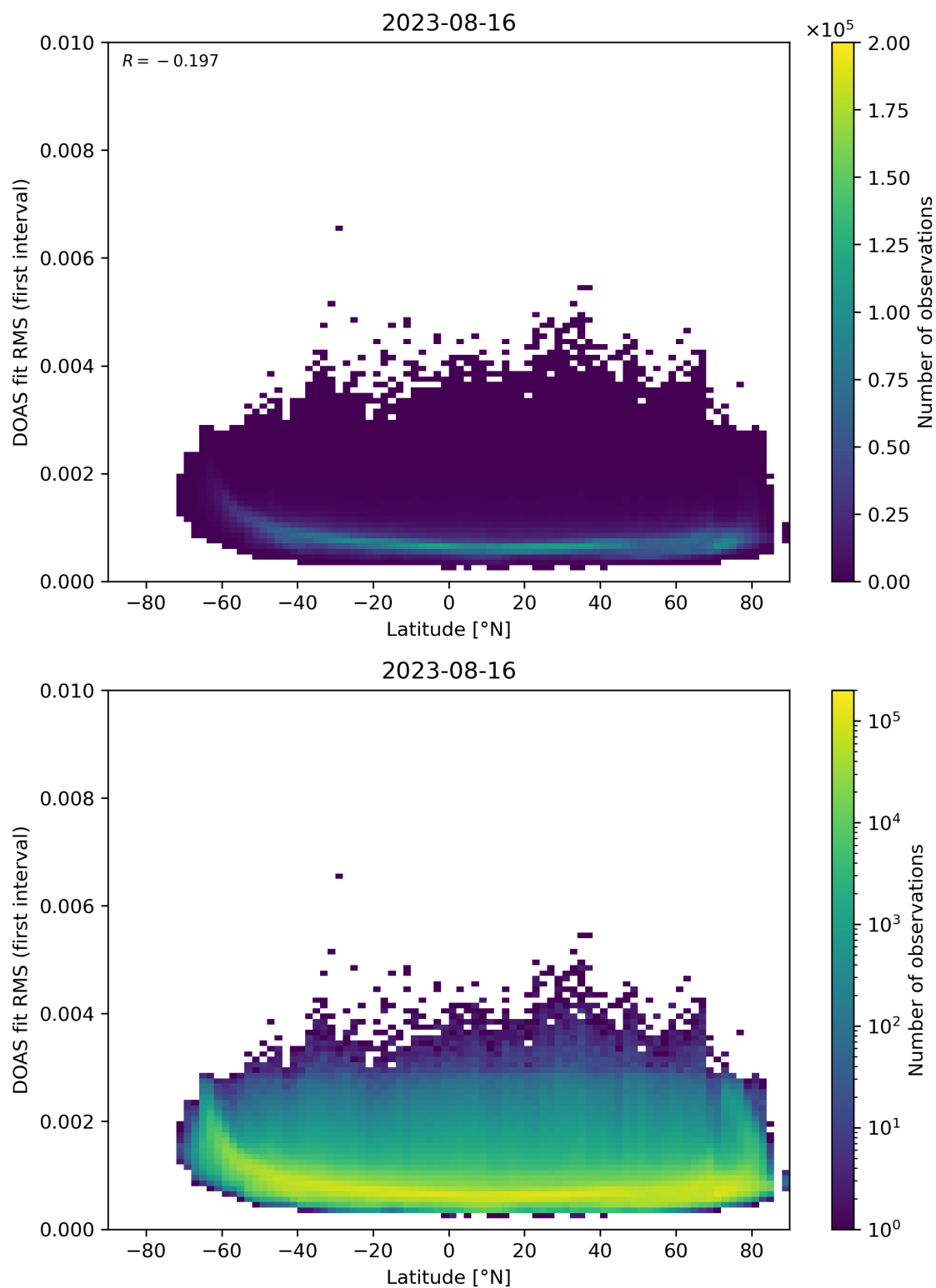
Figure 153: Scatter density plot of “Latitude” against “DOAS fit RMS (first interval)” for 2023-08-15 to 2023-08-17.
