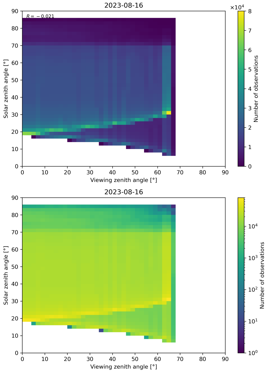
Figure 197: Scatter density plot of “Viewing zenith angle” against “Solar zenith angle” for 2023-08-15 to 2023-08-17.
