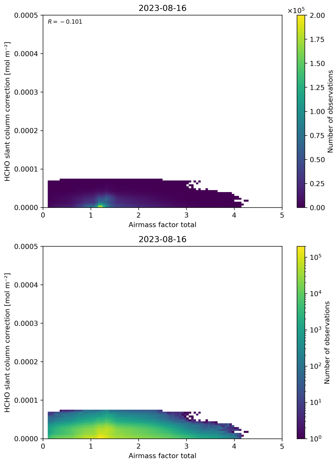
Figure 102: Scatter density plot of “Airmass factor total” against “HCHO slant column correction” for 2023-08-15 to 2023-08-17.
