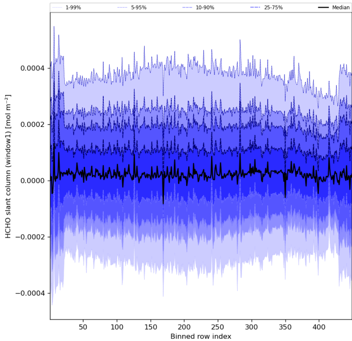
Figure 52: Along track statistics of “HCHO slant column (window1)” for 2023-08-15 to 2023-08-17
