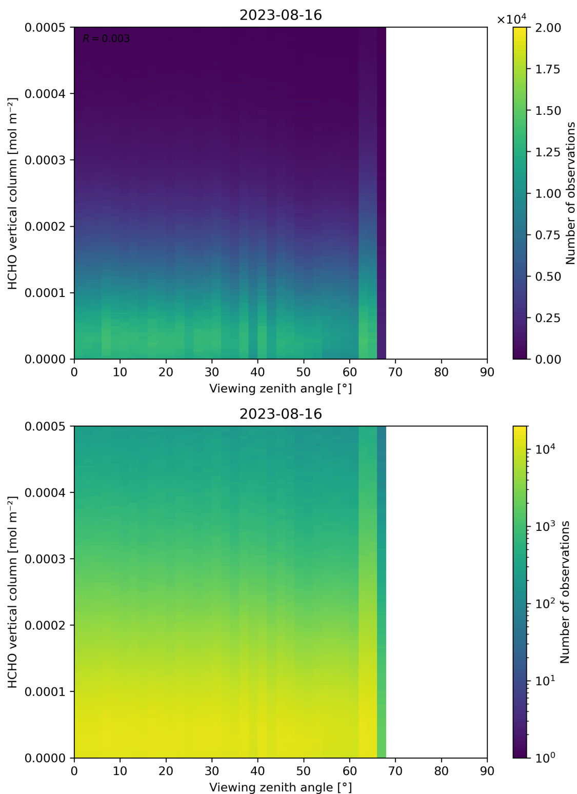
Figure 192: Scatter density plot of “Viewing zenith angle” against “HCHO vertical column” for 2023-08-15 to 2023-08-17.
