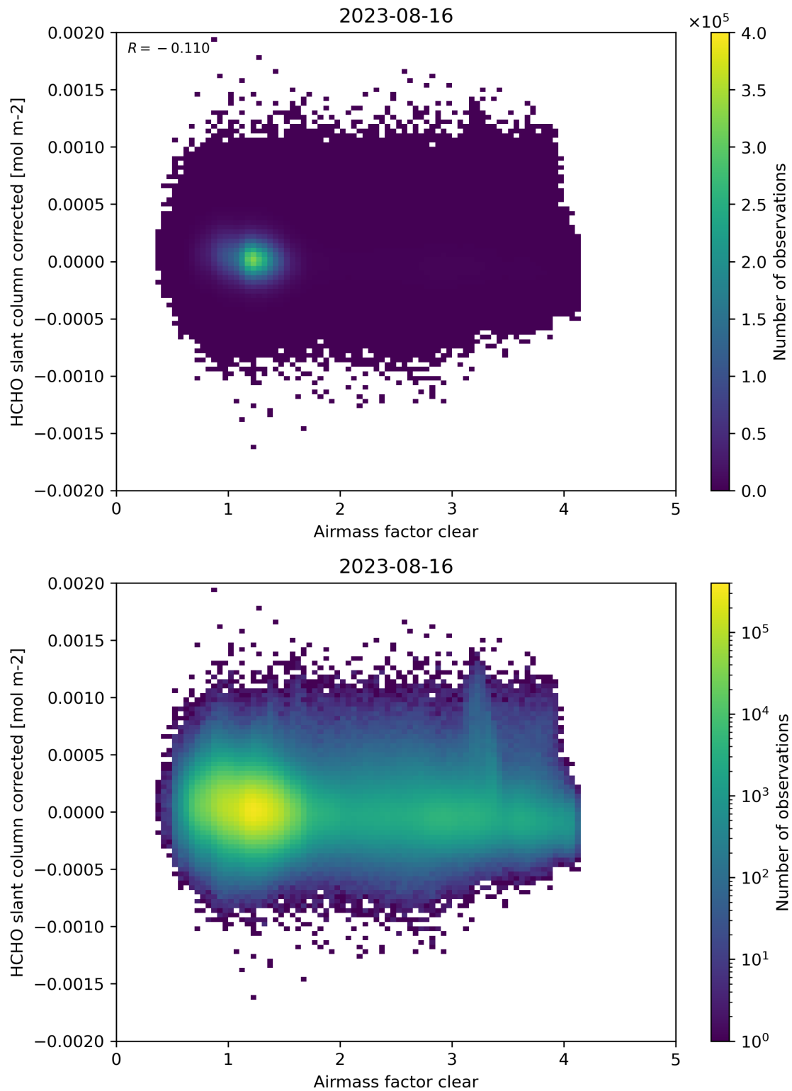
Figure 74: Scatter density plot of “Airmass factor clear” against “HCHO slant column corrected” for 2023-08-15 to 2023-08-17.
