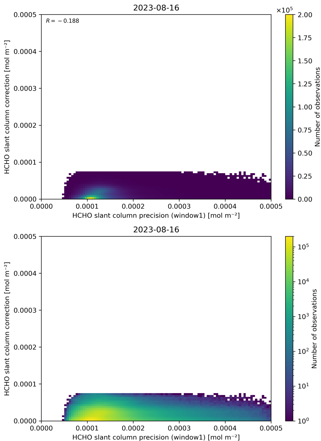
Figure 93: Scatter density plot of “HCHO slant column precision (window1)” against “HCHO slant column correction” for 2023-08-15 to 2023-08-17.
