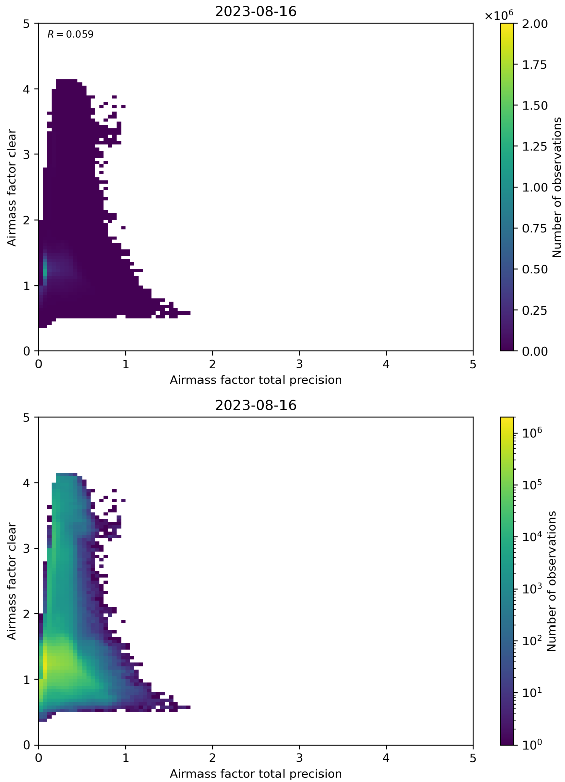
Figure 108: Scatter density plot of “Airmass factor total precision” against “Airmass factor clear” for 2023-08-15 to 2023-08-17.
