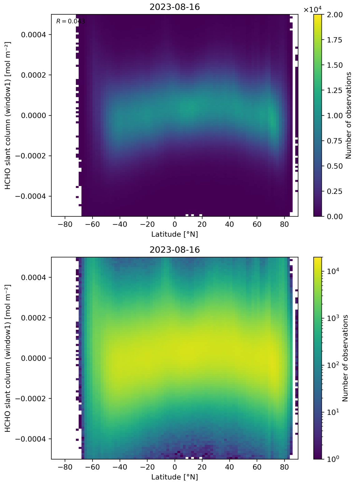
Figure 159: Scatter density plot of “Latitude” against “HCHO slant column (window1)” for 2023-08-15 to 2023-08-17.
