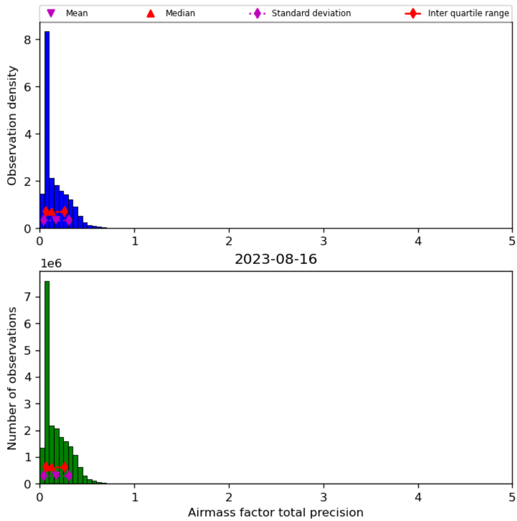
Figure 41: Histogram of “Airmass factor total precision” for 2023-08-15 to 2023-08-17
