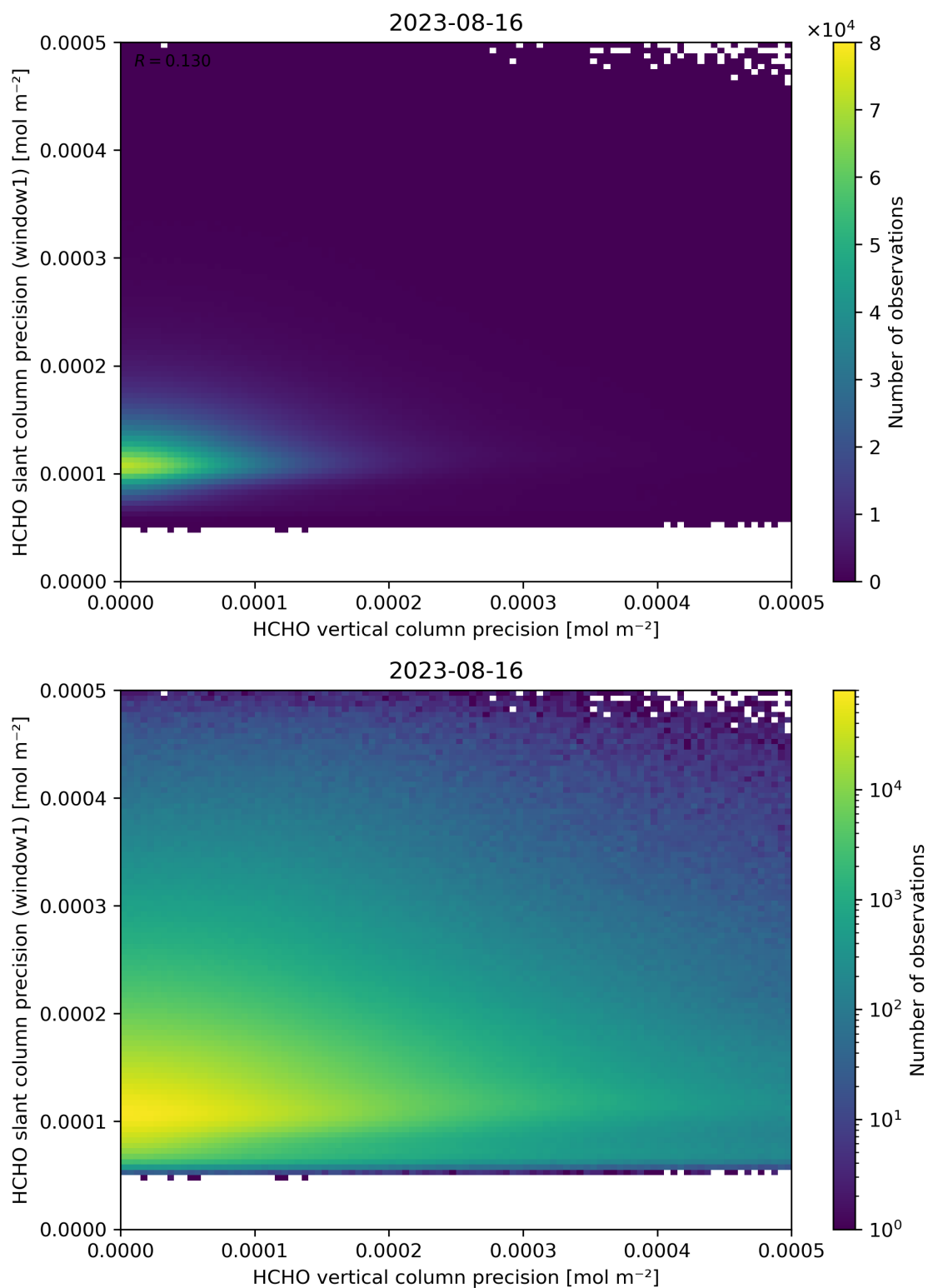
Figure 143: Scatter density plot of “HCHO vertical column precision” against “HCHO slant column precision (window1)” for 2023-08-15 to 2023-08-17.
