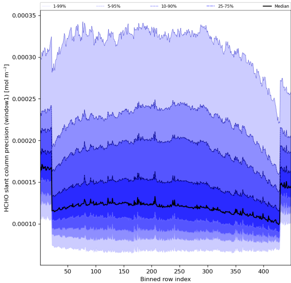
Figure 53: Along track statistics of “HCHO slant column precision (window1)” for 2023-08-15 to 2023-08-17
