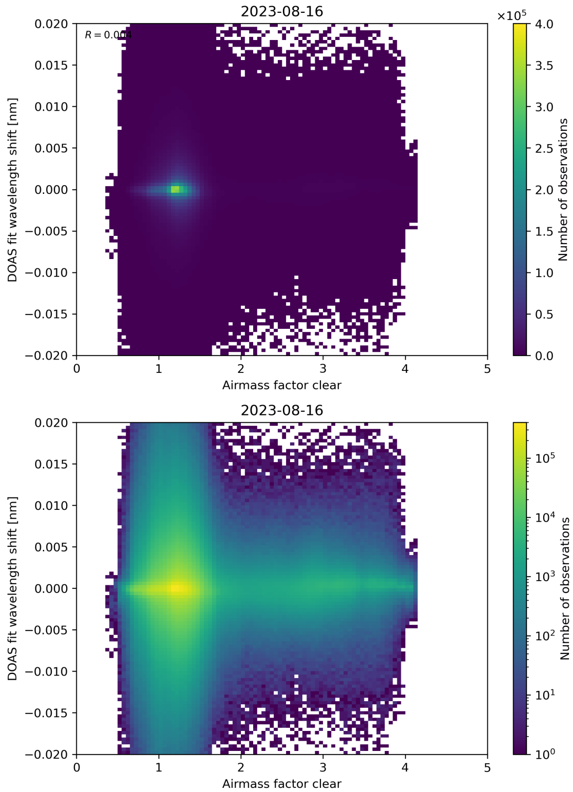
Figure 72: Scatter density plot of “Airmass factor clear” against “DOAS fit wavelength shift” for 2023-08-15 to 2023-08-17.
