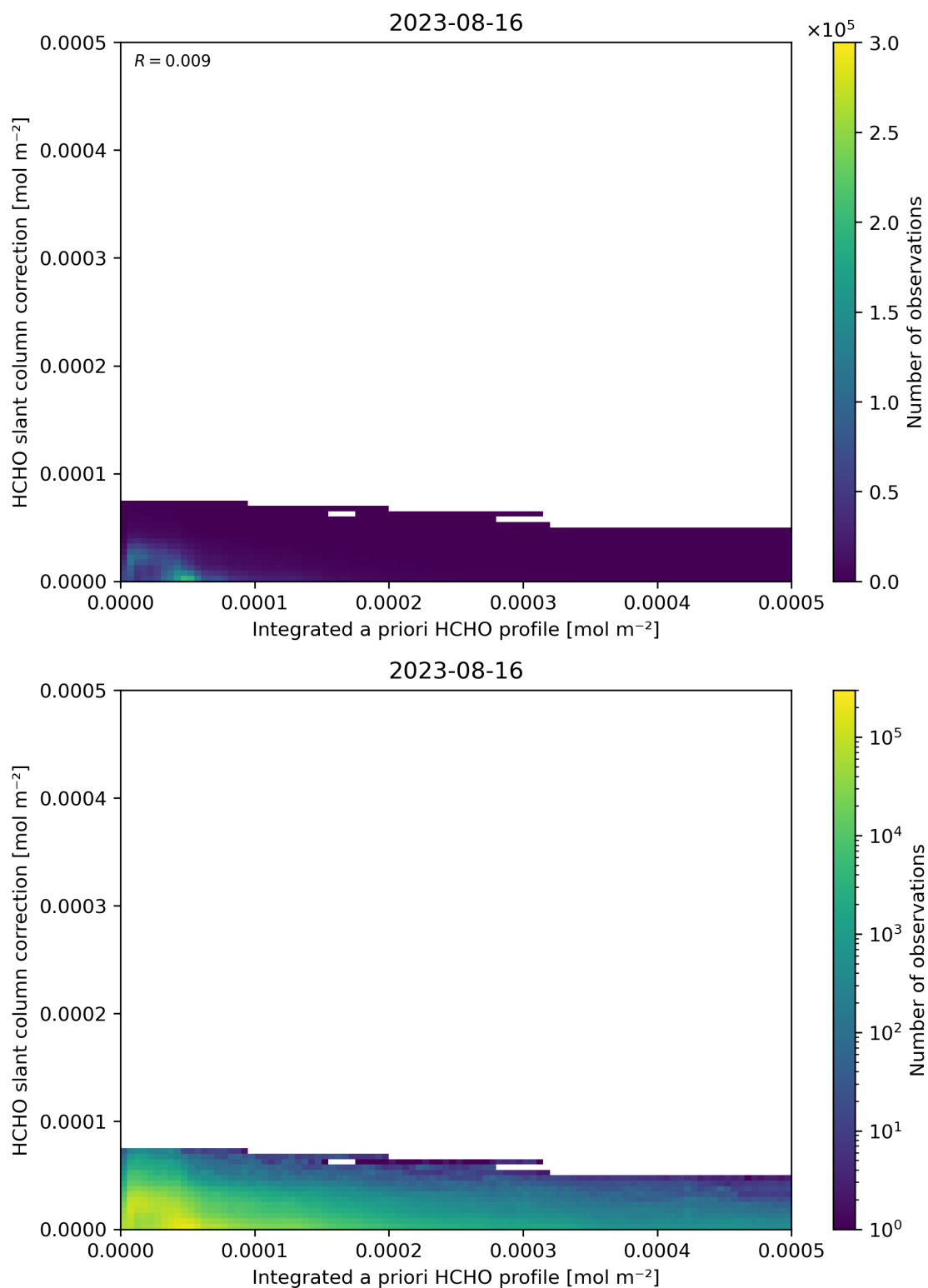
Figure 152: Scatter density plot of “Integrated a priori HCHO profile” against “HCHO slant column correction” for 2023-08-15 to 2023-08-17.
