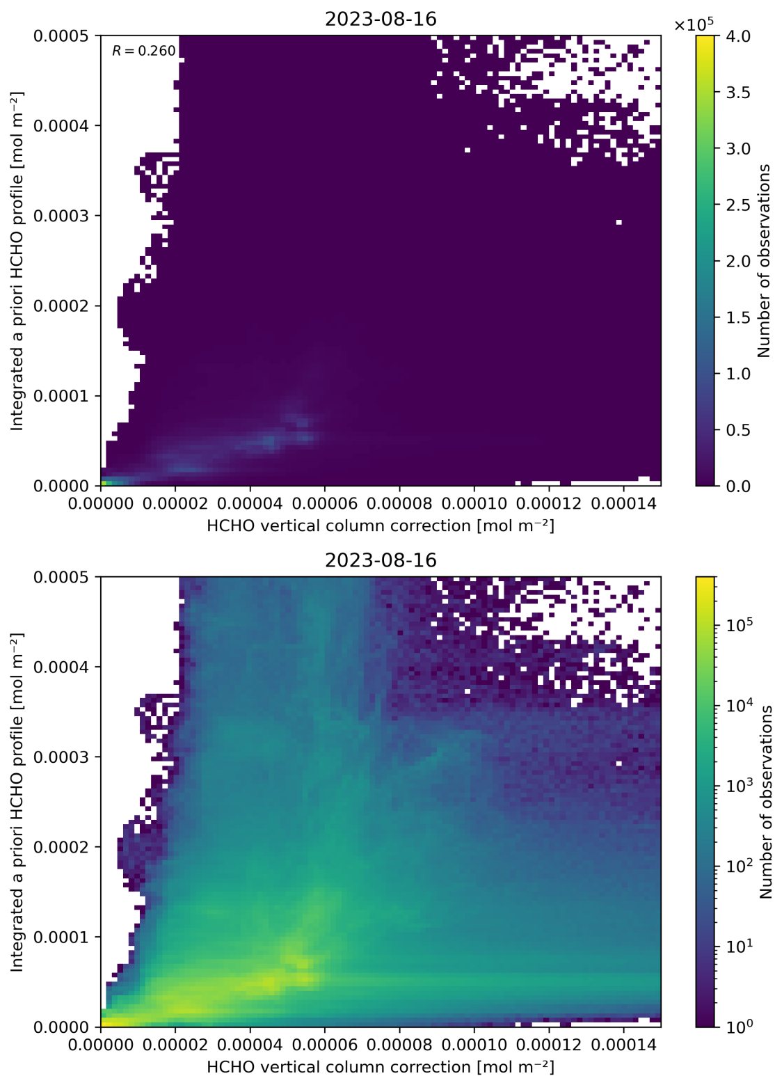
Figure 122: Scatter density plot of “HCHO vertical column correction” against “Integrated a priori HCHO profile” for 2023-08-15 to 2023-08-17.
