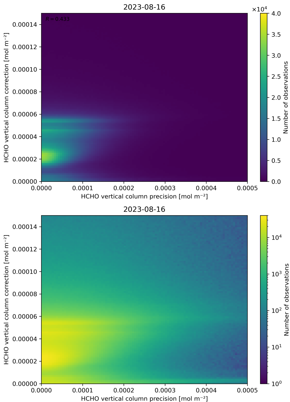
Figure 146: Scatter density plot of “HCHO vertical column precision” against “HCHO vertical column correction” for 2023-08-15 to 2023-08-17.
