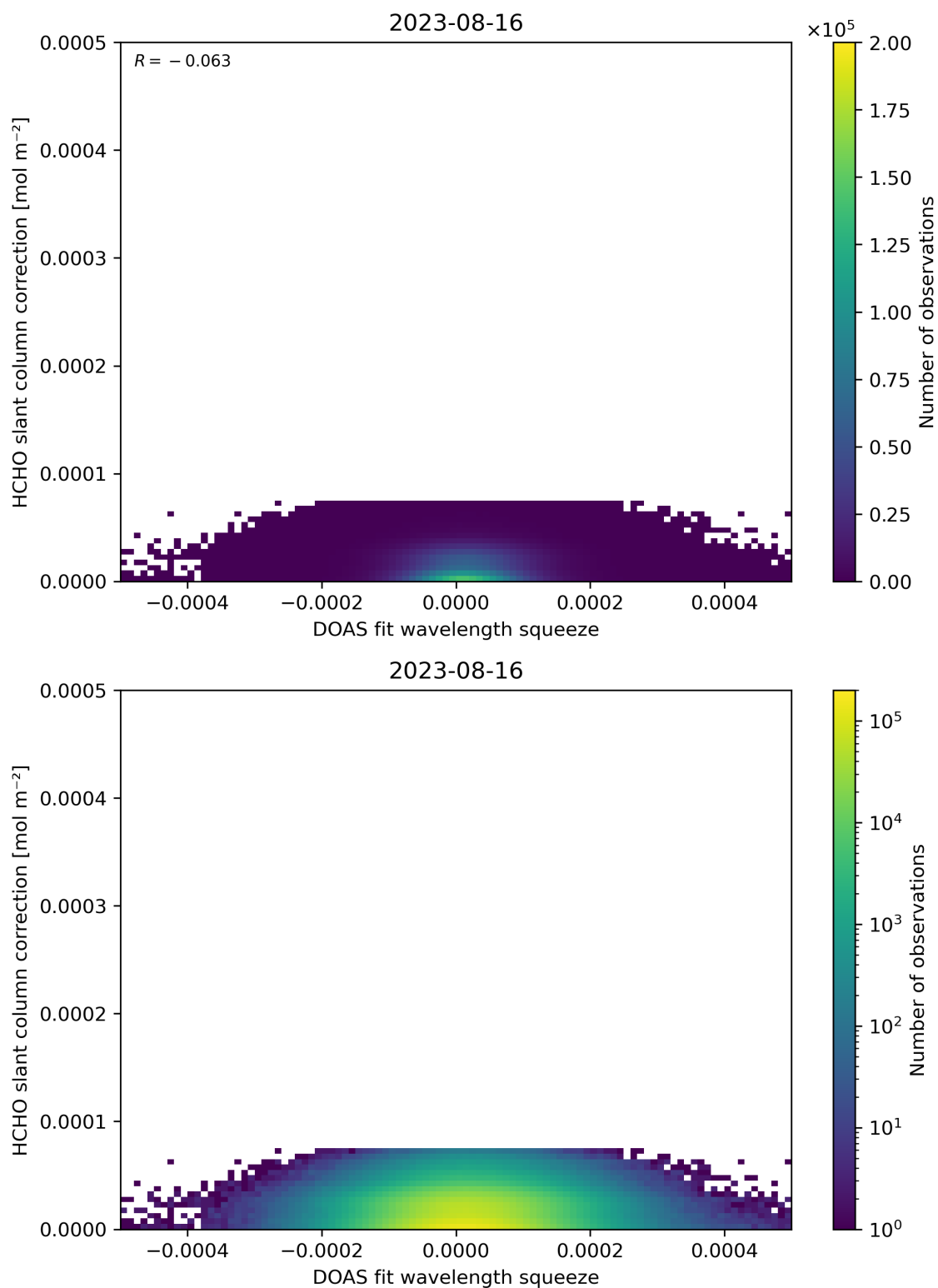
Figure 70: Scatter density plot of “DOAS fit wavelength squeeze” against “HCHO slant column correction” for 2023-08-15 to 2023-08-17.
