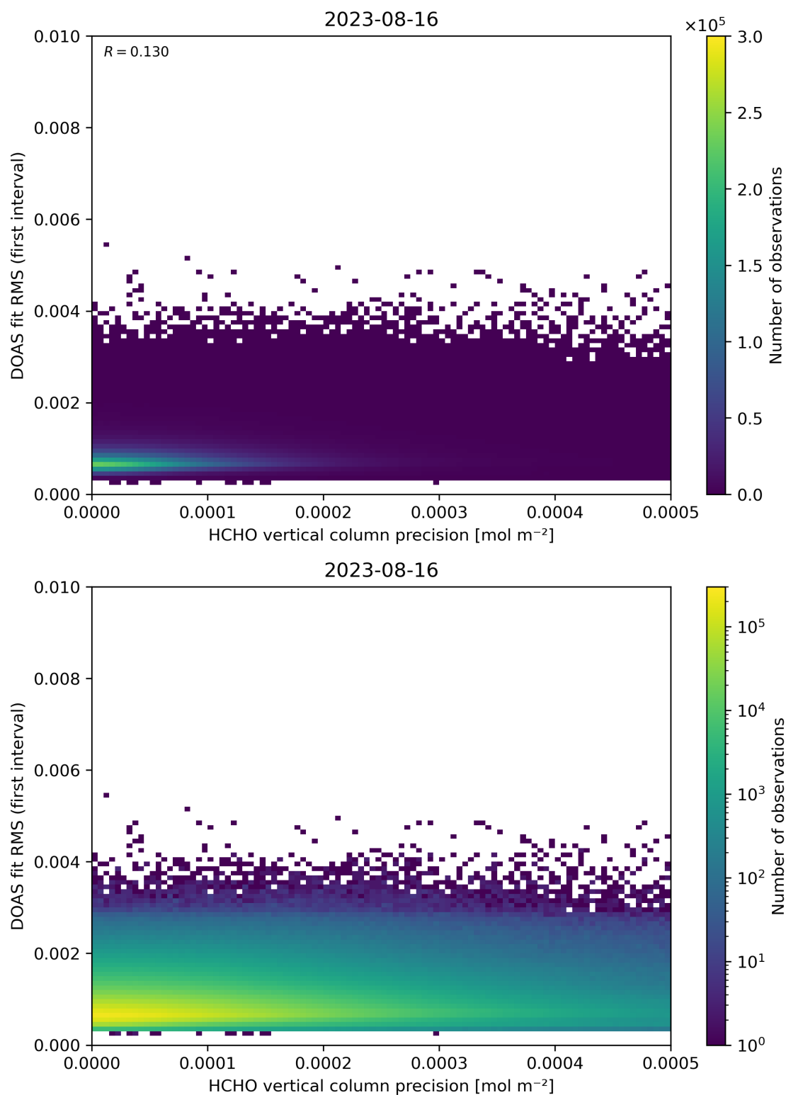
Figure 136: Scatter density plot of “HCHO vertical column precision” against “DOAS fit RMS (first interval)” for 2023-08-15 to 2023-08-17.
