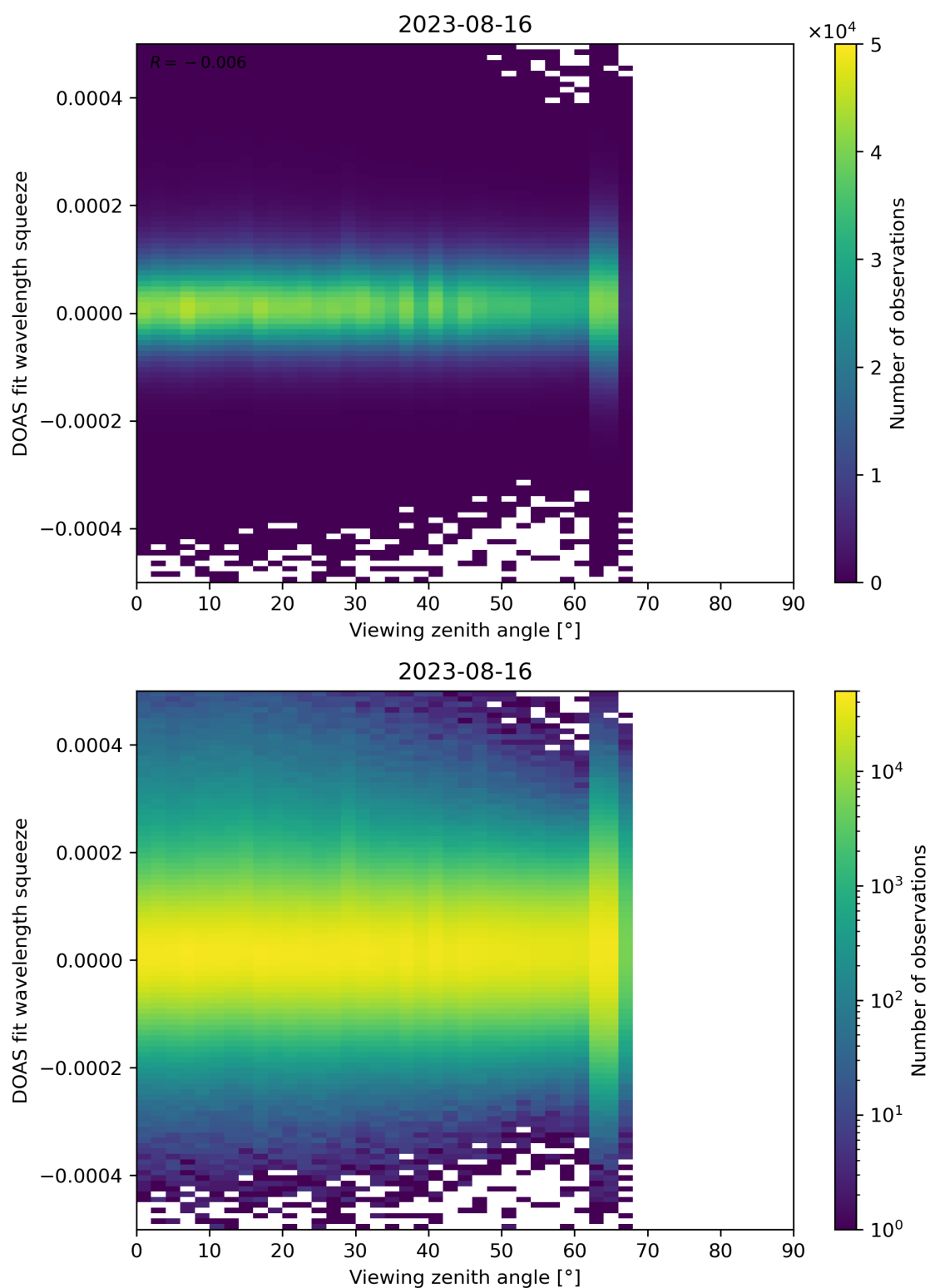
Figure 184: Scatter density plot of “Viewing zenith angle” against “DOAS fit wavelength squeeze” for 2023-08-15 to 2023-08-17.
