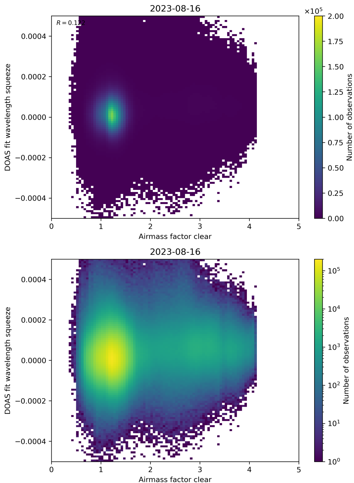
Figure 73: Scatter density plot of “Airmass factor clear” against “DOAS fit wavelength squeeze” for 2023-08-15 to 2023-08-17.
