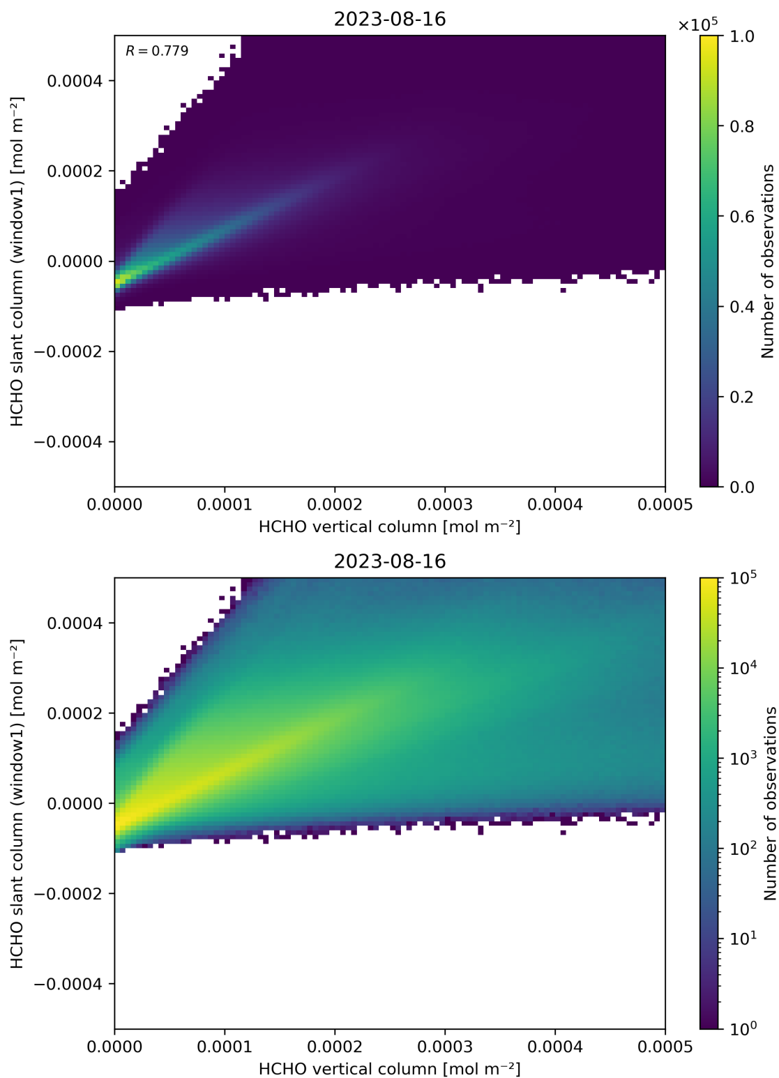
Figure 129: Scatter density plot of “HCHO vertical column” against “HCHO slant column (window1)” for 2023-08-15 to 2023-08-17.
