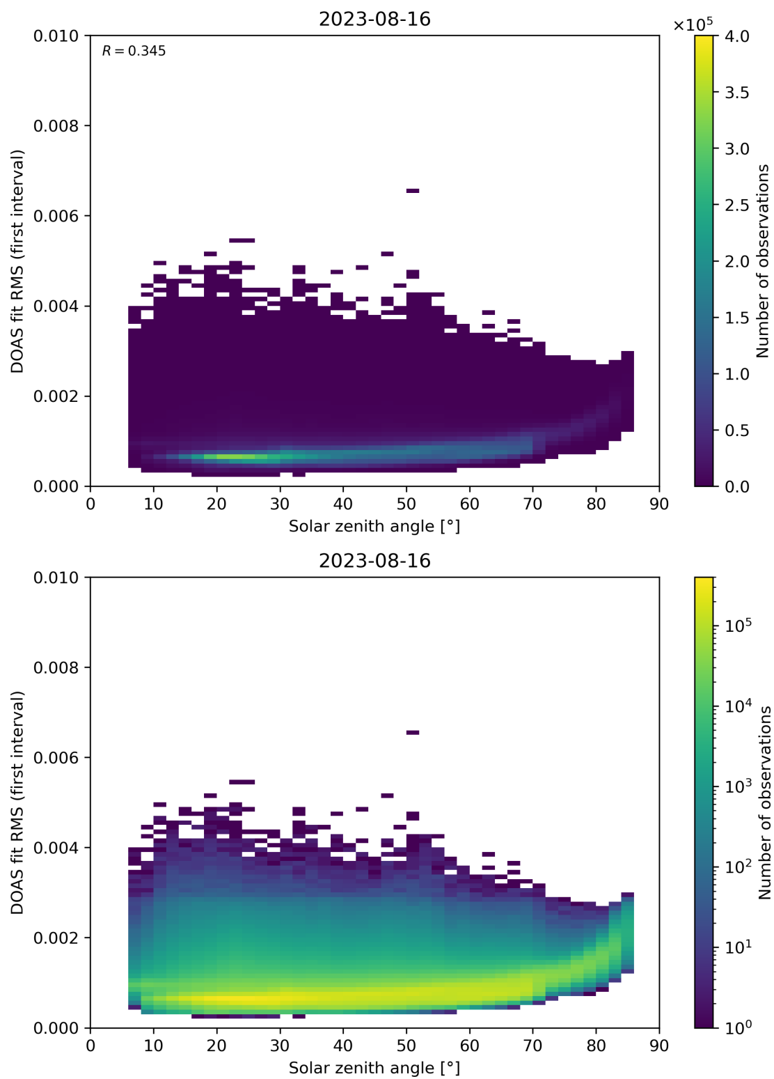
Figure 167: Scatter density plot of “Solar zenith angle” against “DOAS fit RMS (first interval)” for 2023-08-15 to 2023-08-17.
