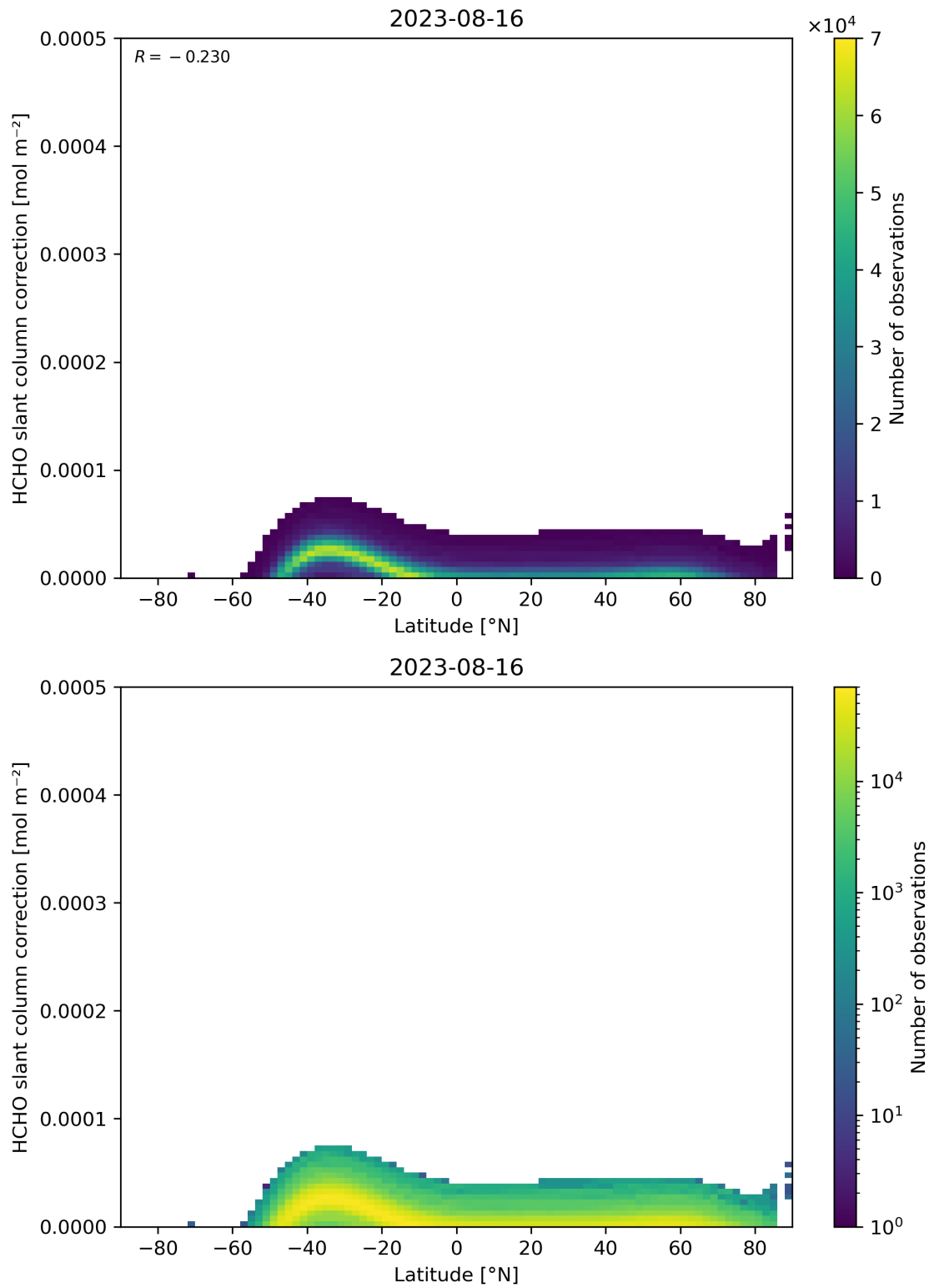
Figure 158: Scatter density plot of “Latitude” against “HCHO slant column correction” for 2023-08-15 to 2023-08-17.
