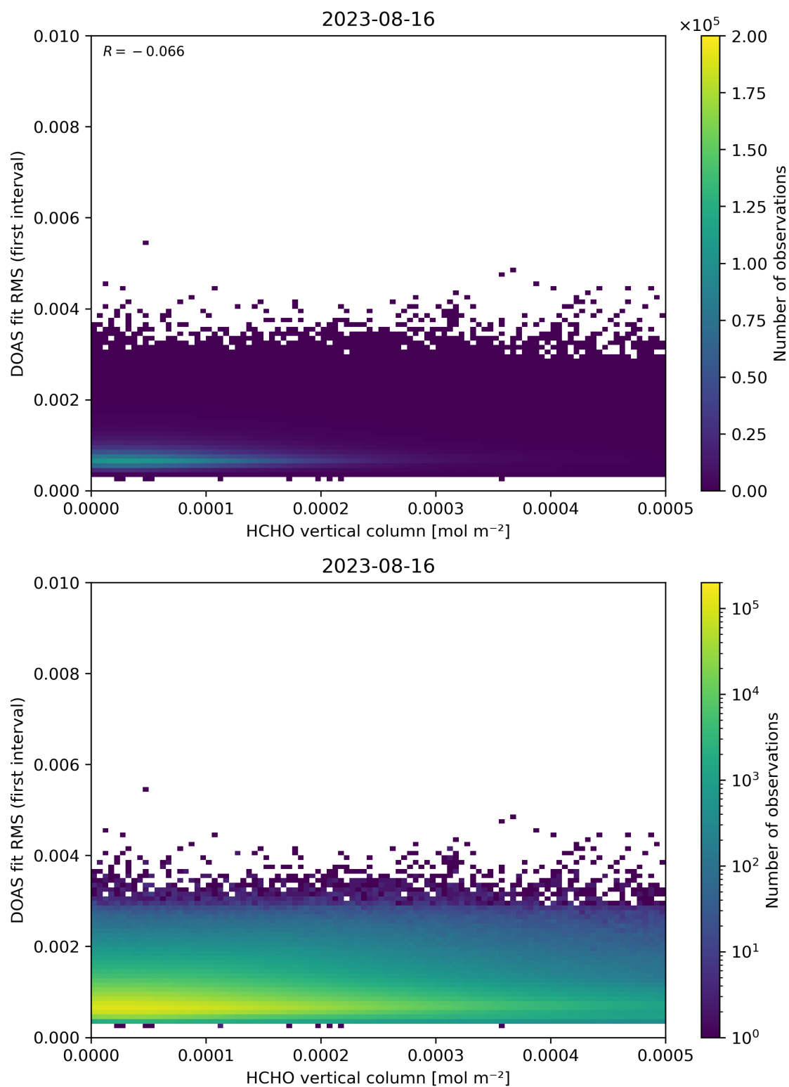
Figure 123: Scatter density plot of “HCHO vertical column” against “DOAS fit RMS (first interval)” for 2023-08-15 to 2023-08-17.
