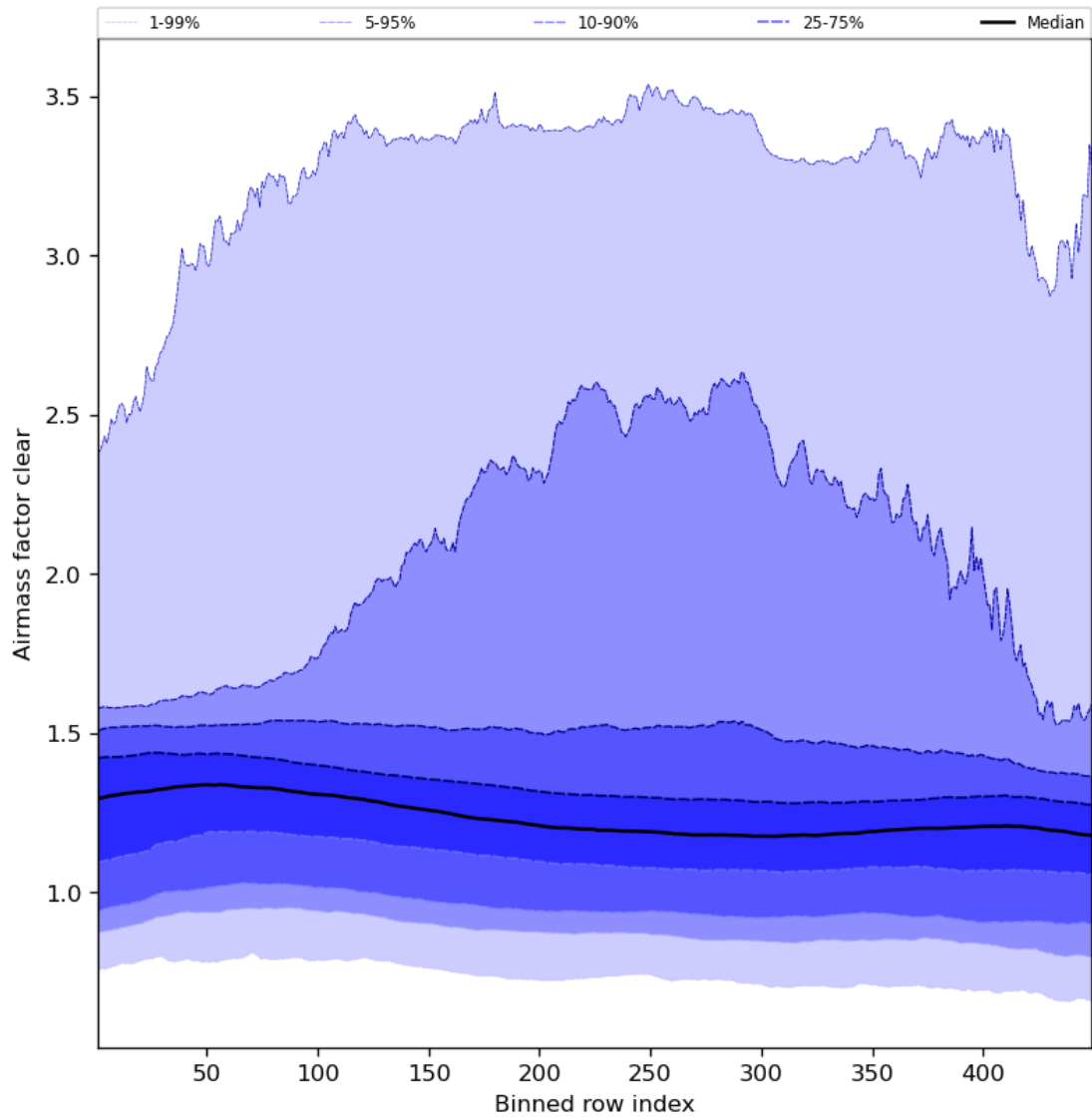
Figure 56: Along track statistics of “Airmass factor clear” for 2023-08-15 to 2023-08-17
