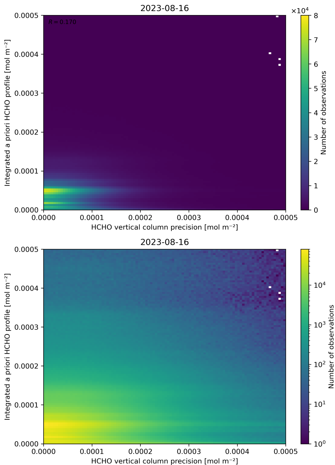
Figure 147: Scatter density plot of “HCHO vertical column precision” against “Integrated a priori HCHO profile” for 2023-08-15 to 2023-08-17.
