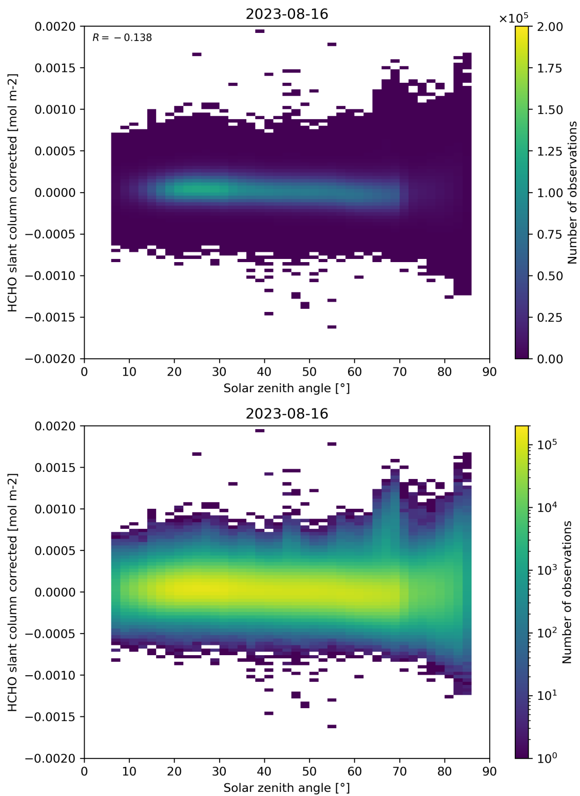
Figure 171: Scatter density plot of “Solar zenith angle” against “HCHO slant column corrected” for 2023-08-15 to 2023-08-17.
