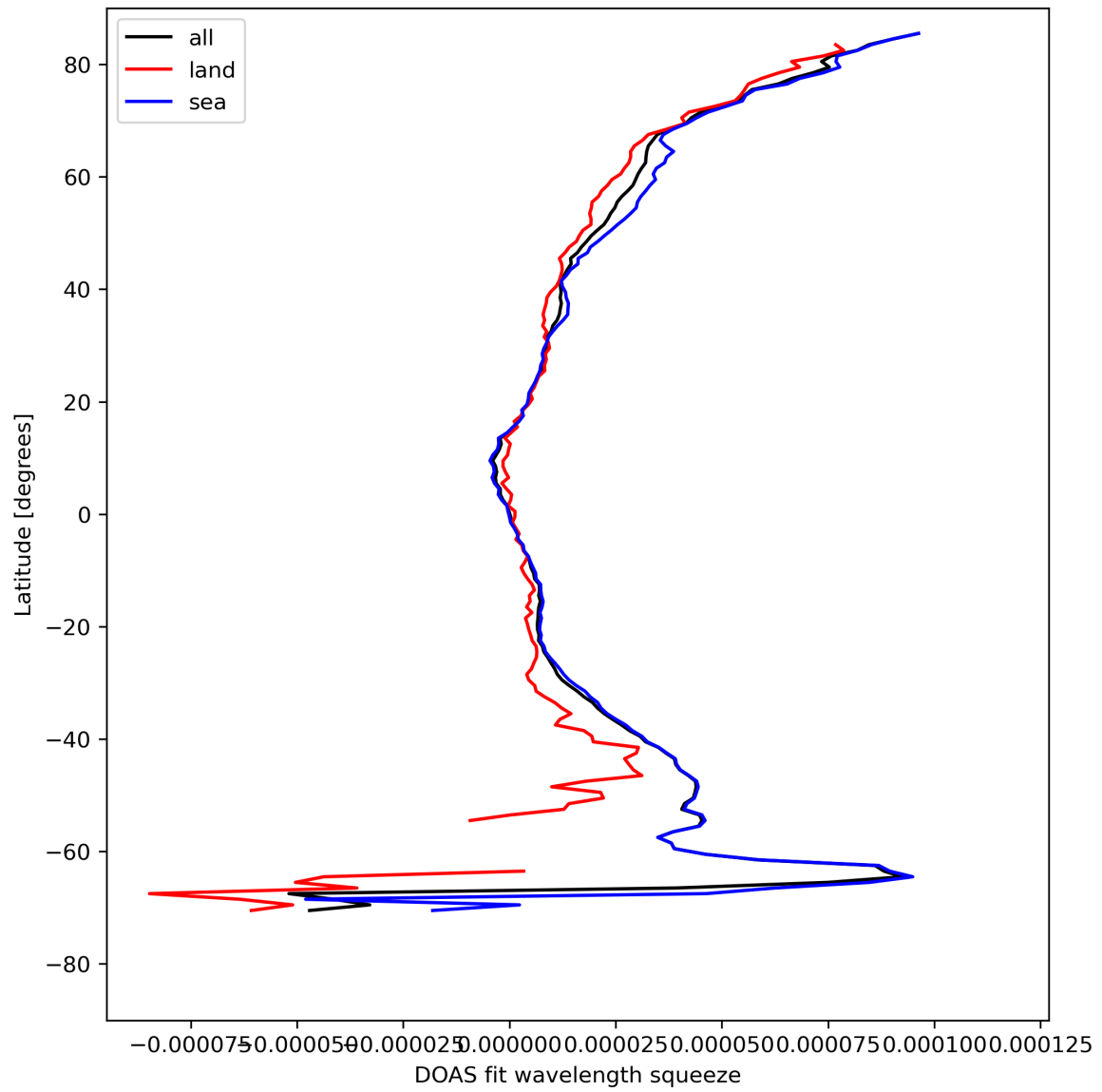
Figure 31: Zonal average of “DOAS fit wavelength squeeze” for 2023-08-15 to 2023-08-17.
