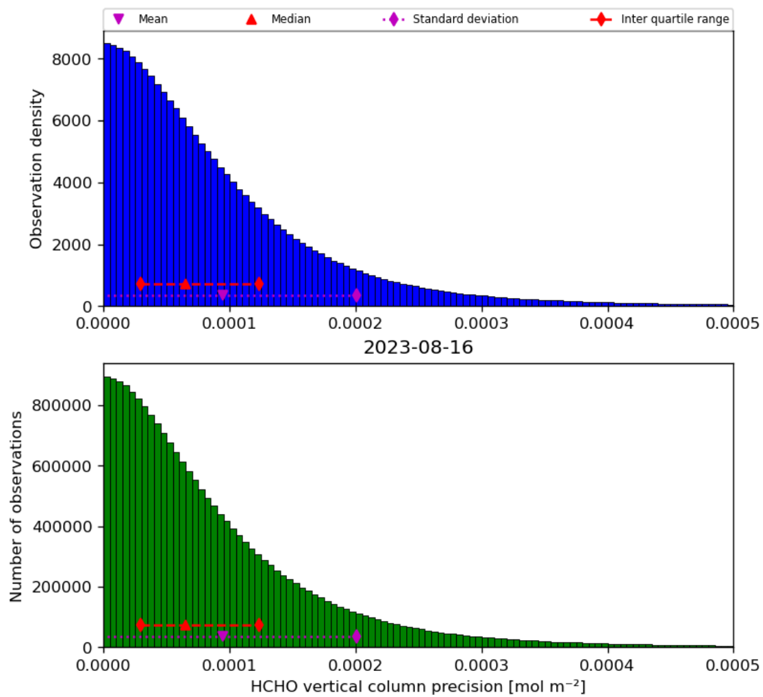
Figure 36: Histogram of “HCHO vertical column precision” for 2023-08-15 to 2023-08-17
