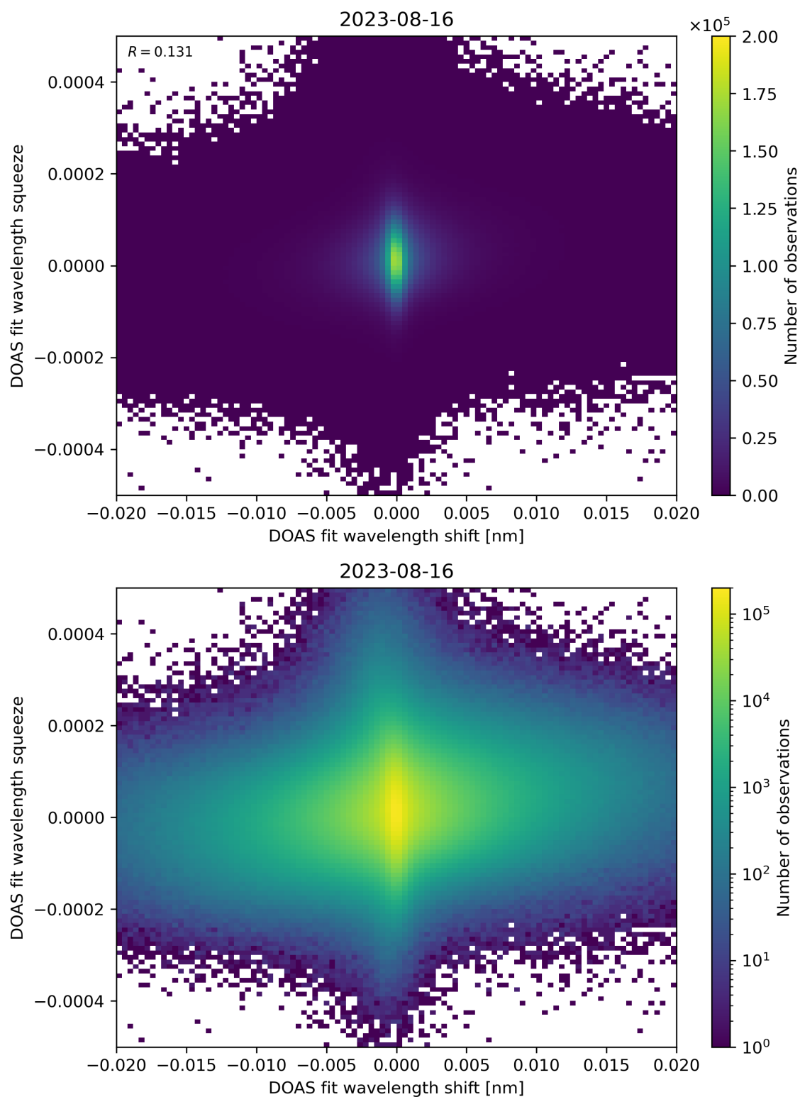
Figure 65: Scatter density plot of “DOAS fit wavelength shift” against “DOAS fit wavelength squeeze” for 2023-08-15 to 2023-08-17.
