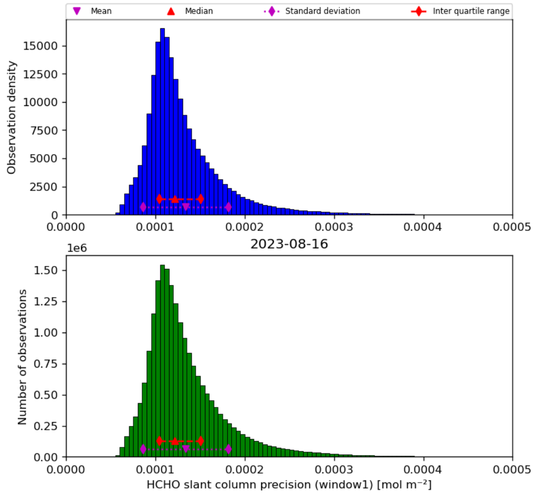
Figure 39: Histogram of “HCHO slant column precision (window1)” for 2023-08-15 to 2023-08-17
