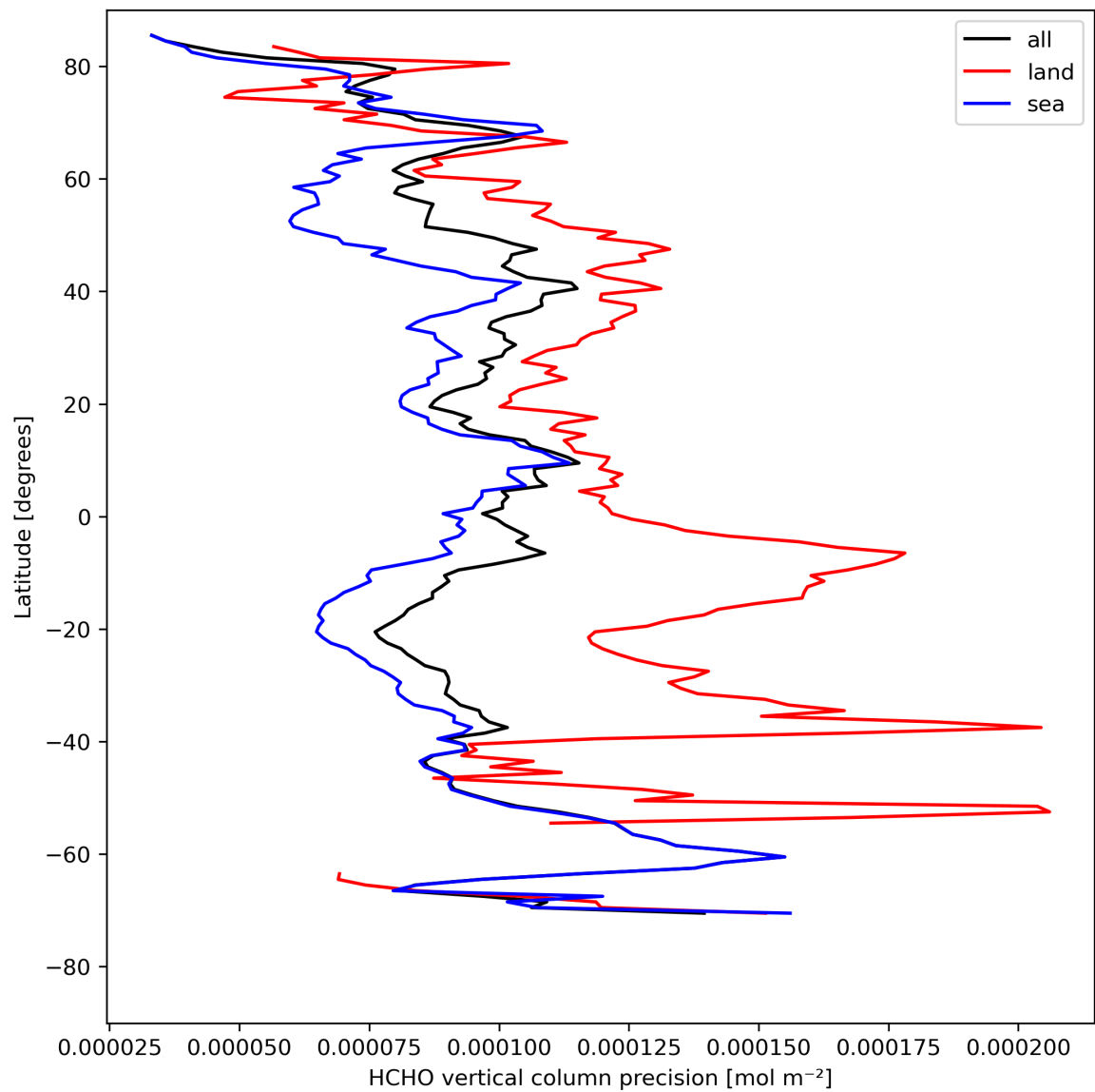
Figure 22: Zonal average of “HCHO vertical column precision” for 2023-08-15 to 2023-08-17.
