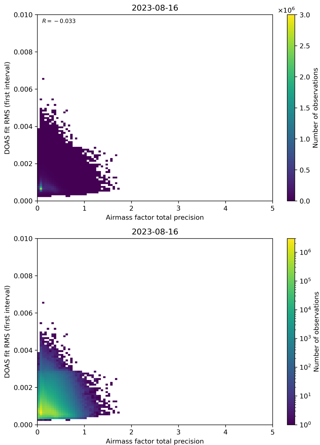
Figure 105: Scatter density plot of “Airmass factor total precision” against “DOAS fit RMS (first interval)” for 2023-08-15 to 2023-08-17.
