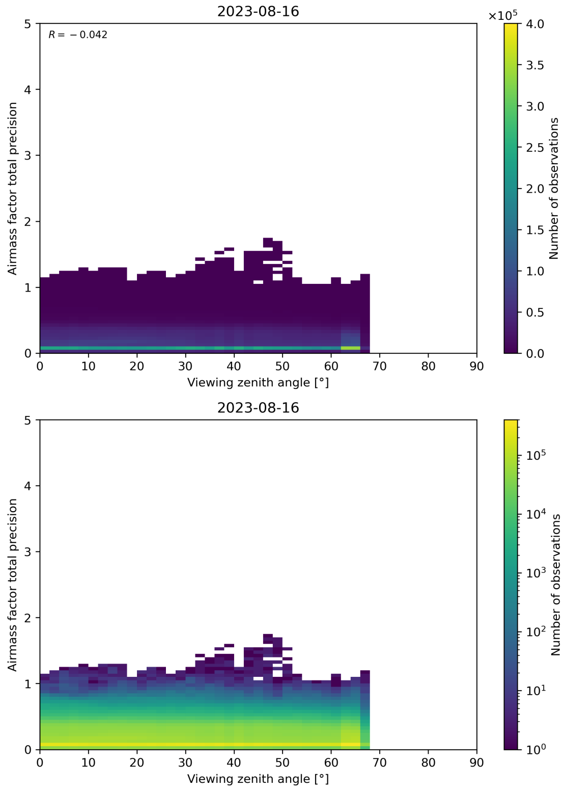
Figure 191: Scatter density plot of “Viewing zenith angle” against “Airmass factor total precision” for 2023-08-15 to 2023-08-17.
