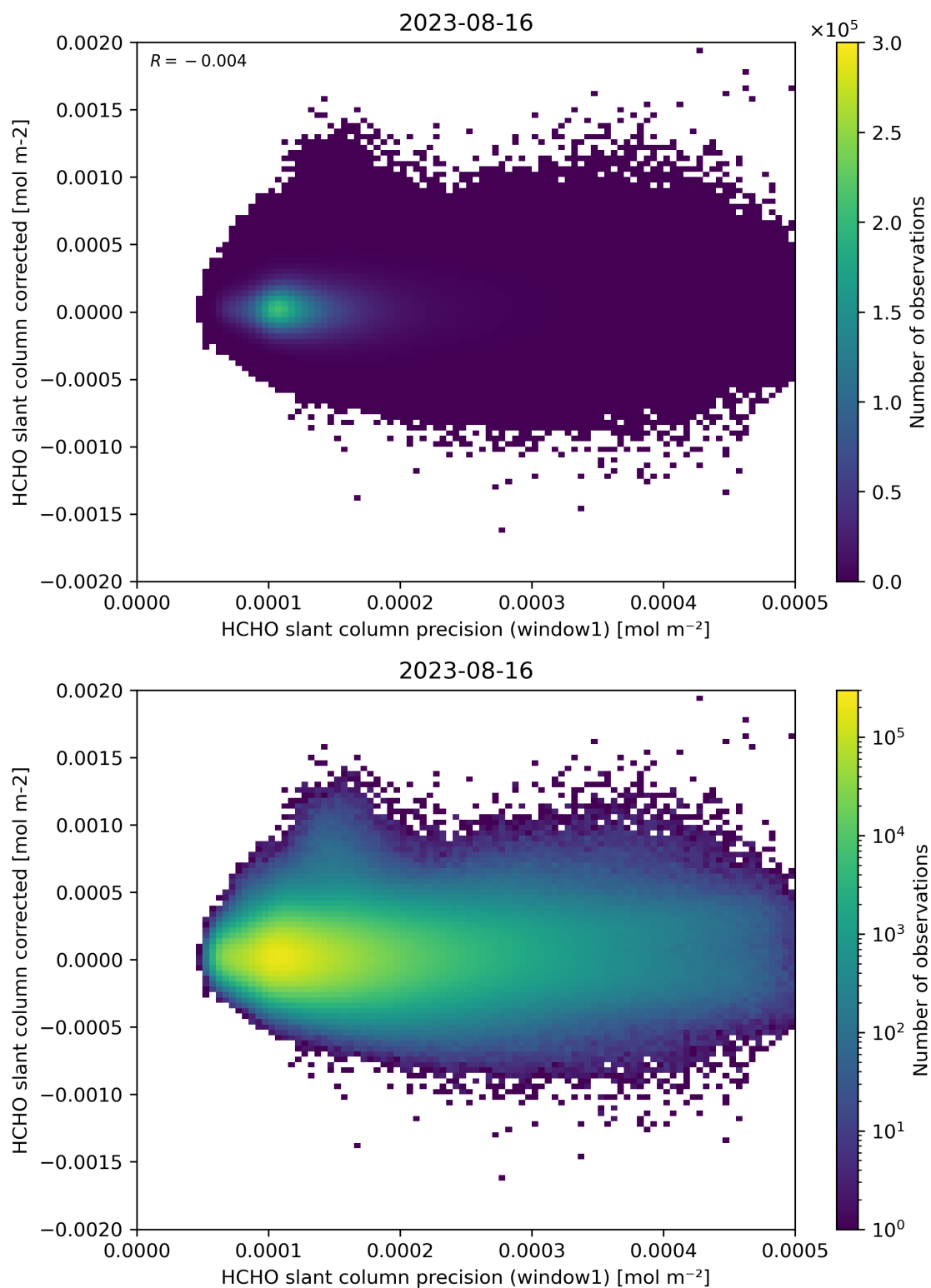
Figure 92: Scatter density plot of “HCHO slant column precision (window1)” against “HCHO slant column corrected” for 2023-08-15 to 2023-08-17.
