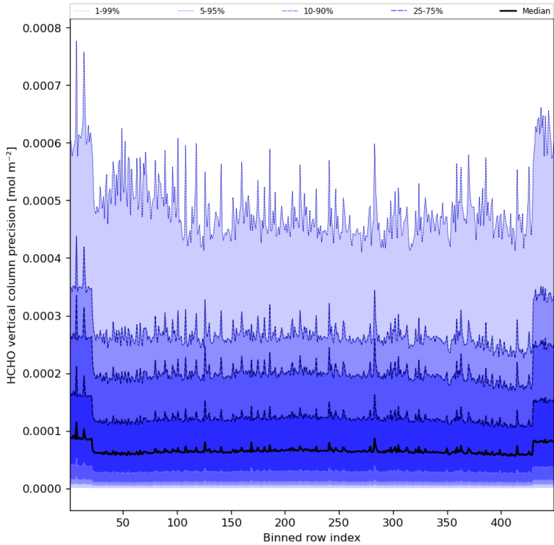
Figure 50: Along track statistics of “HCHO vertical column precision” for 2023-08-15 to 2023-08-17
