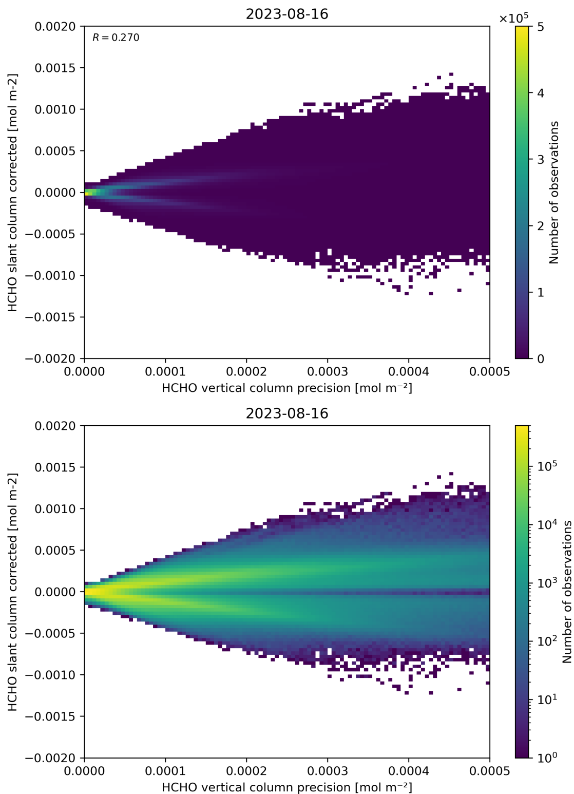
Figure 140: Scatter density plot of “HCHO vertical column precision” against “HCHO slant column corrected” for 2023-08-15 to 2023-08-17.
