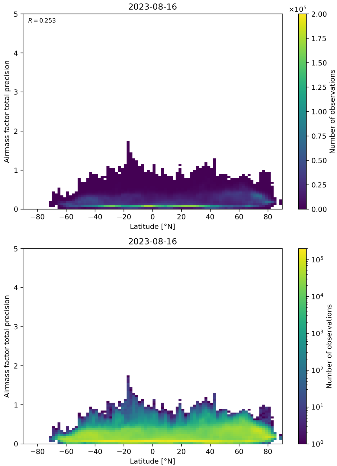
Figure 162: Scatter density plot of “Latitude” against “Airmass factor total precision” for 2023-08-15 to 2023-08-17.
