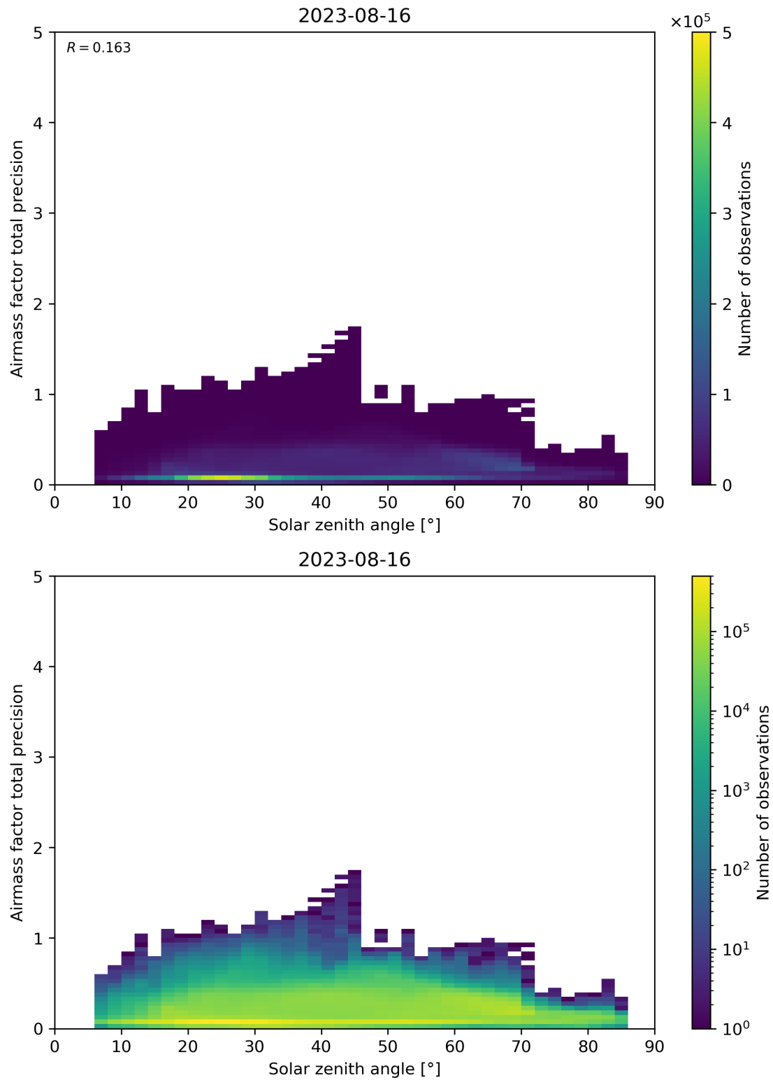
Figure 176: Scatter density plot of “Solar zenith angle” against “Airmass factor total precision” for 2023-08-15 to 2023-08-17.
