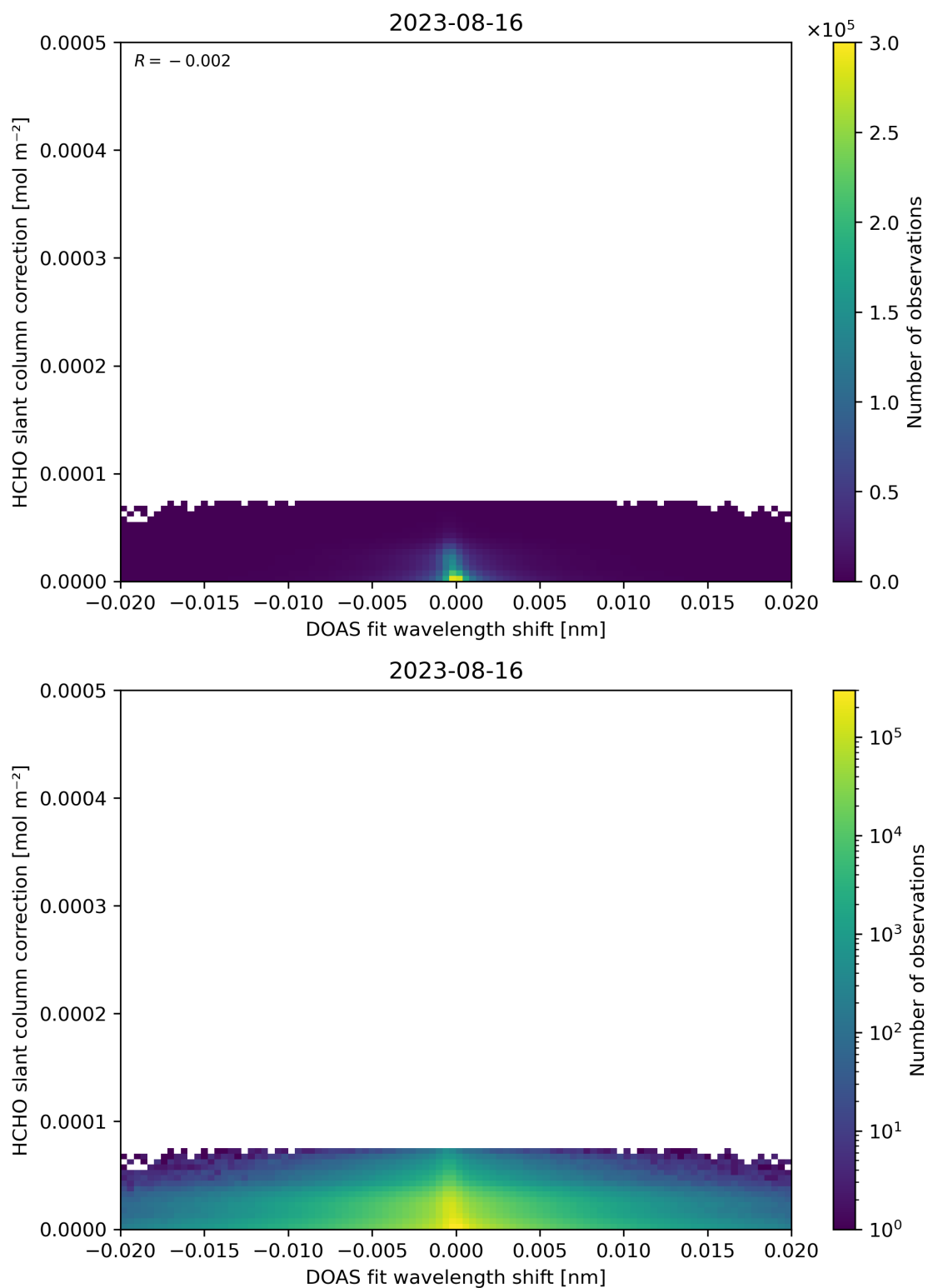
Figure 67: Scatter density plot of “DOAS fit wavelength shift” against “HCHO slant column correction” for 2023-08-15 to 2023-08-17.
