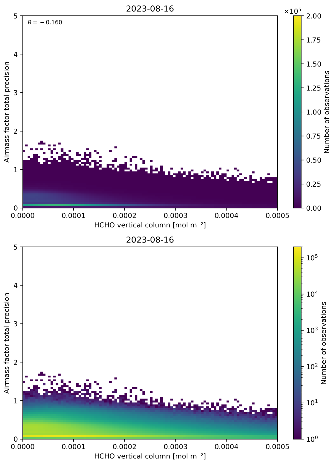
Figure 132: Scatter density plot of “HCHO vertical column” against “Airmass factor total precision” for 2023-08-15 to 2023-08-17.
