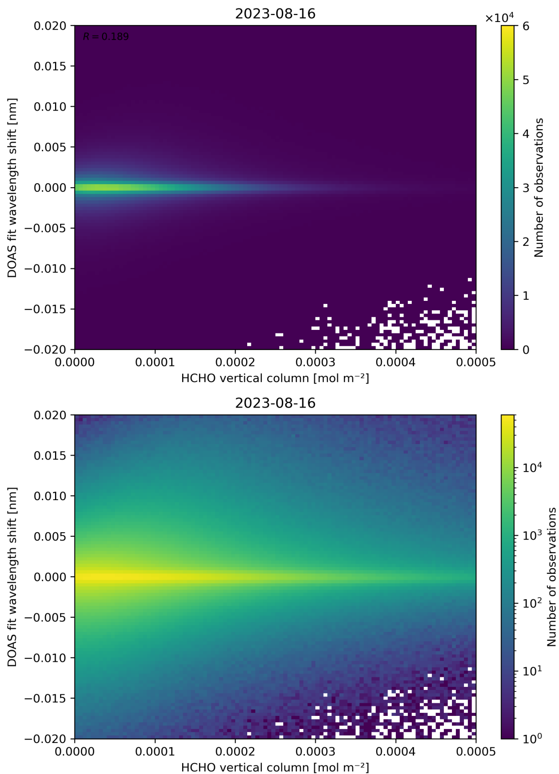
Figure 124: Scatter density plot of “HCHO vertical column” against “DOAS fit wavelength shift” for 2023-08-15 to 2023-08-17.
