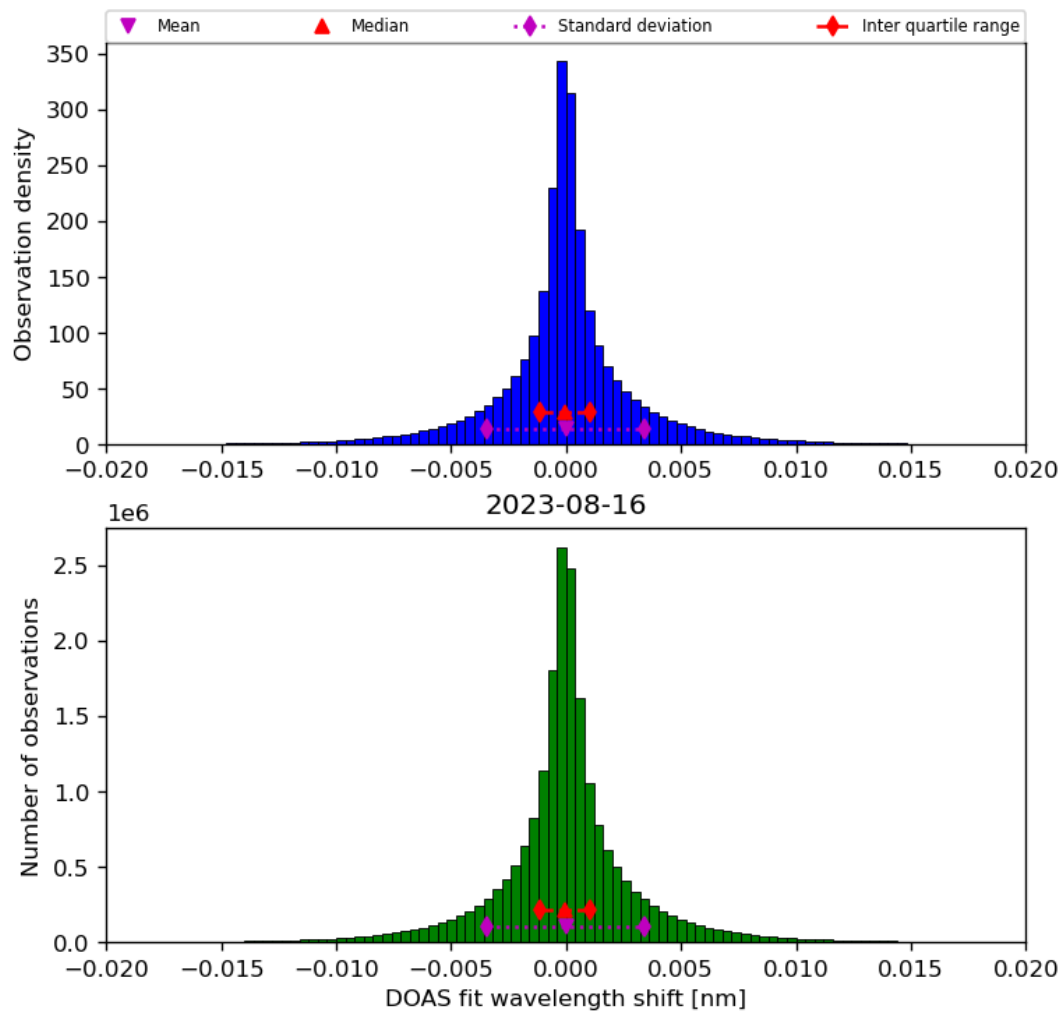
Figure 44: Histogram of “DOAS fit wavelength shift” for 2023-08-15 to 2023-08-17
