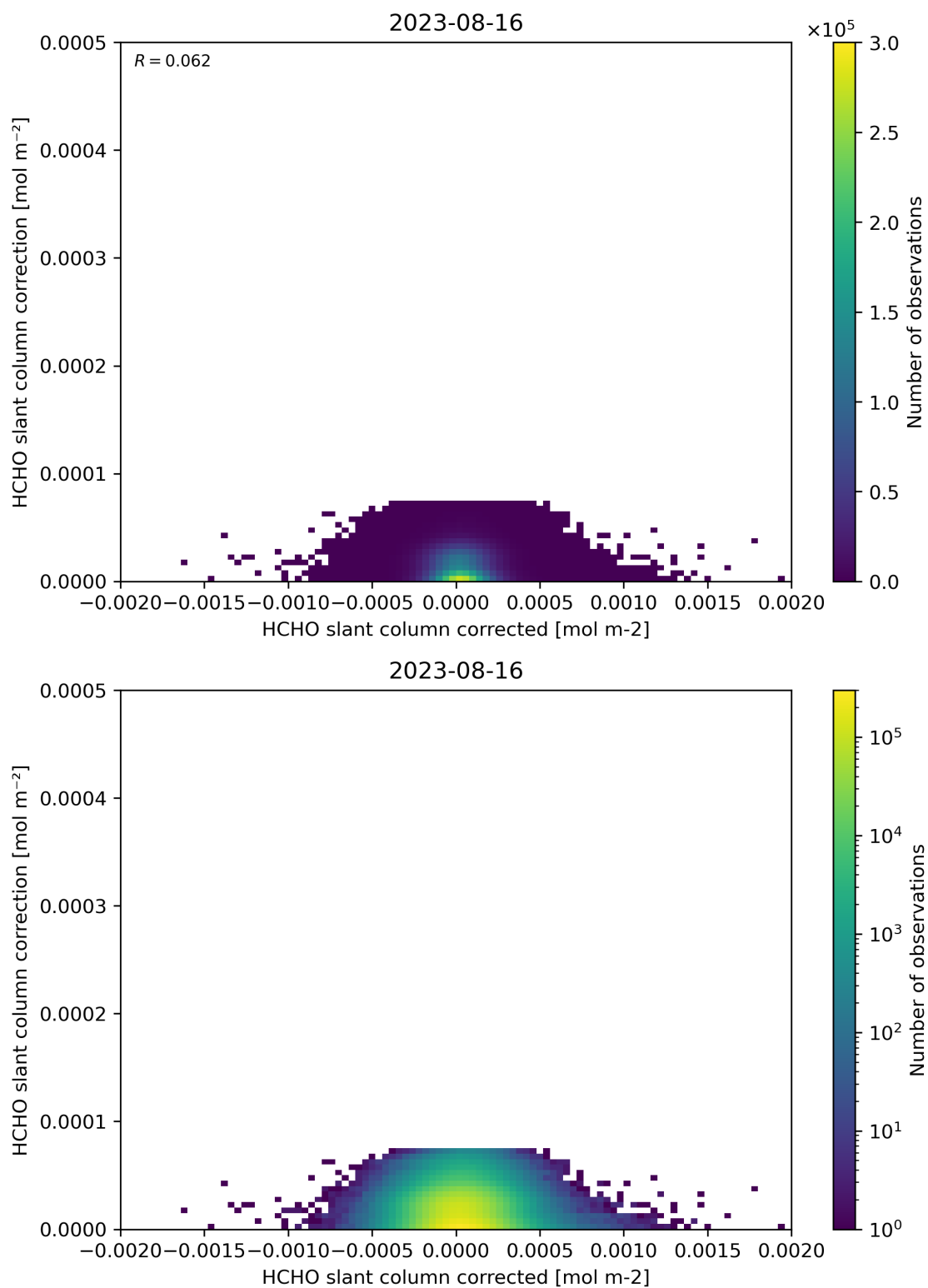
Figure 77: Scatter density plot of “HCHO slant column corrected” against “HCHO slant column correction” for 2023-08-15 to 2023-08-17.
