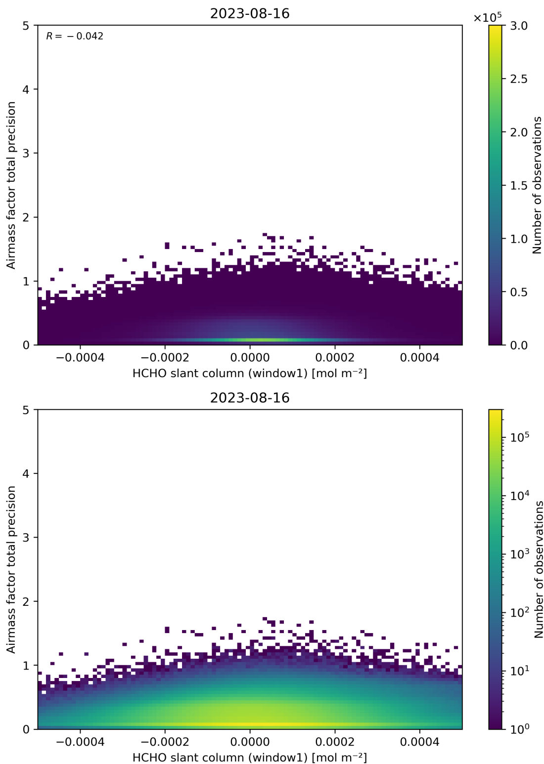
Figure 86: Scatter density plot of “HCHO slant column (window1)” against “Airmass factor total precision” for 2023-08-15 to 2023-08-17.
