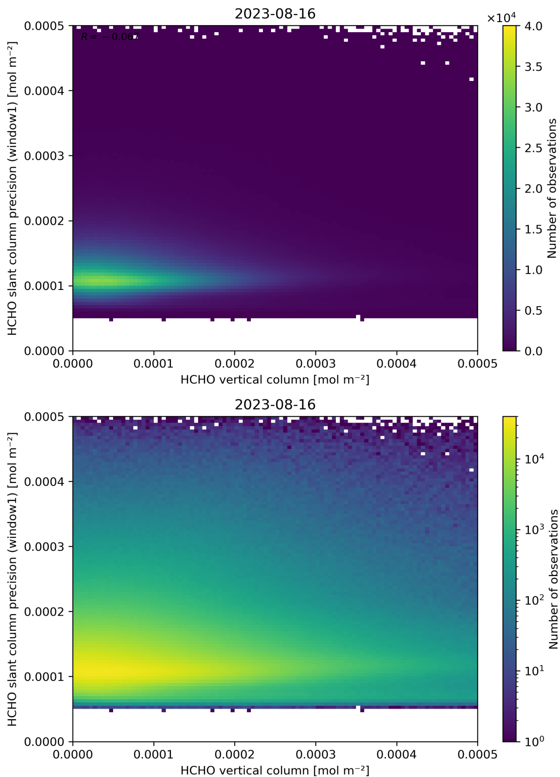
Figure 130: Scatter density plot of “HCHO vertical column” against “HCHO slant column precision (window1)” for 2023-08-15 to 2023-08-17.
