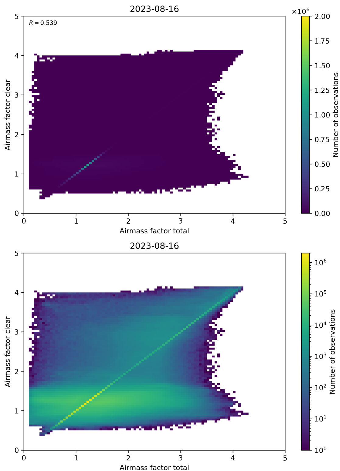
Figure 100: Scatter density plot of “Airmass factor total” against “Airmass factor clear” for 2023-08-15 to 2023-08-17.
