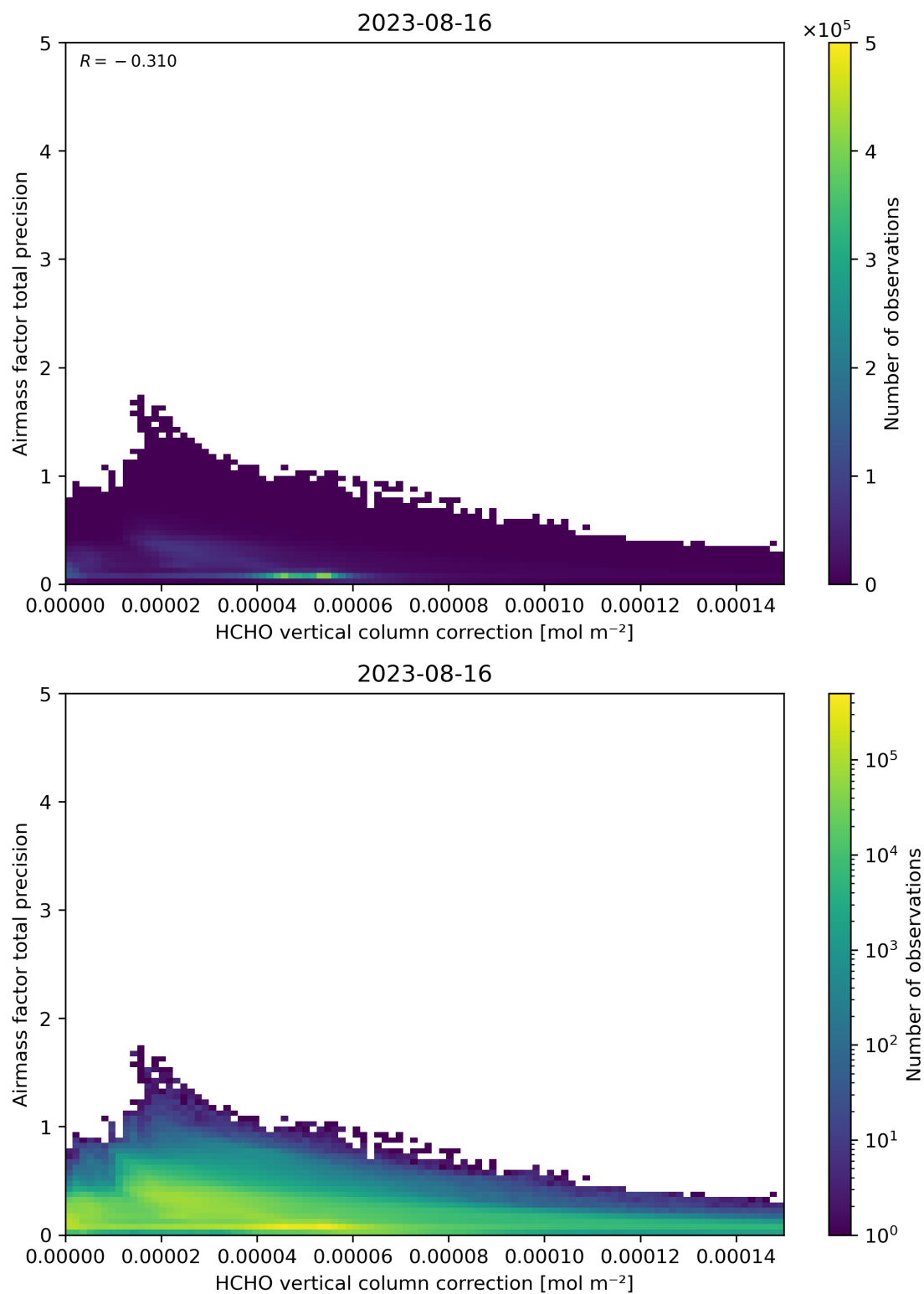
Figure 121: Scatter density plot of “HCHO vertical column correction” against “Airmass factor total precision” for 2023-08-15 to 2023-08-17.
