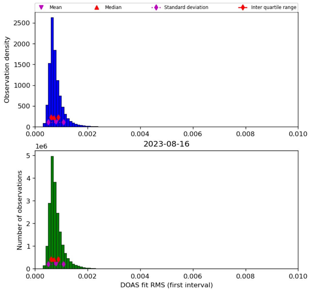
Figure 46: Histogram of “DOAS fit RMS (first interval)” for 2023-08-15 to 2023-08-17
