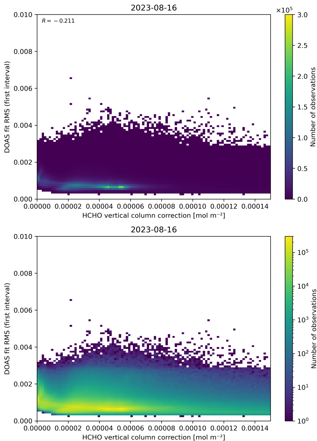
Figure 112: Scatter density plot of “HCHO vertical column correction” against “DOAS fit RMS (first interval)” for 2023-08-15 to 2023-08-17.
