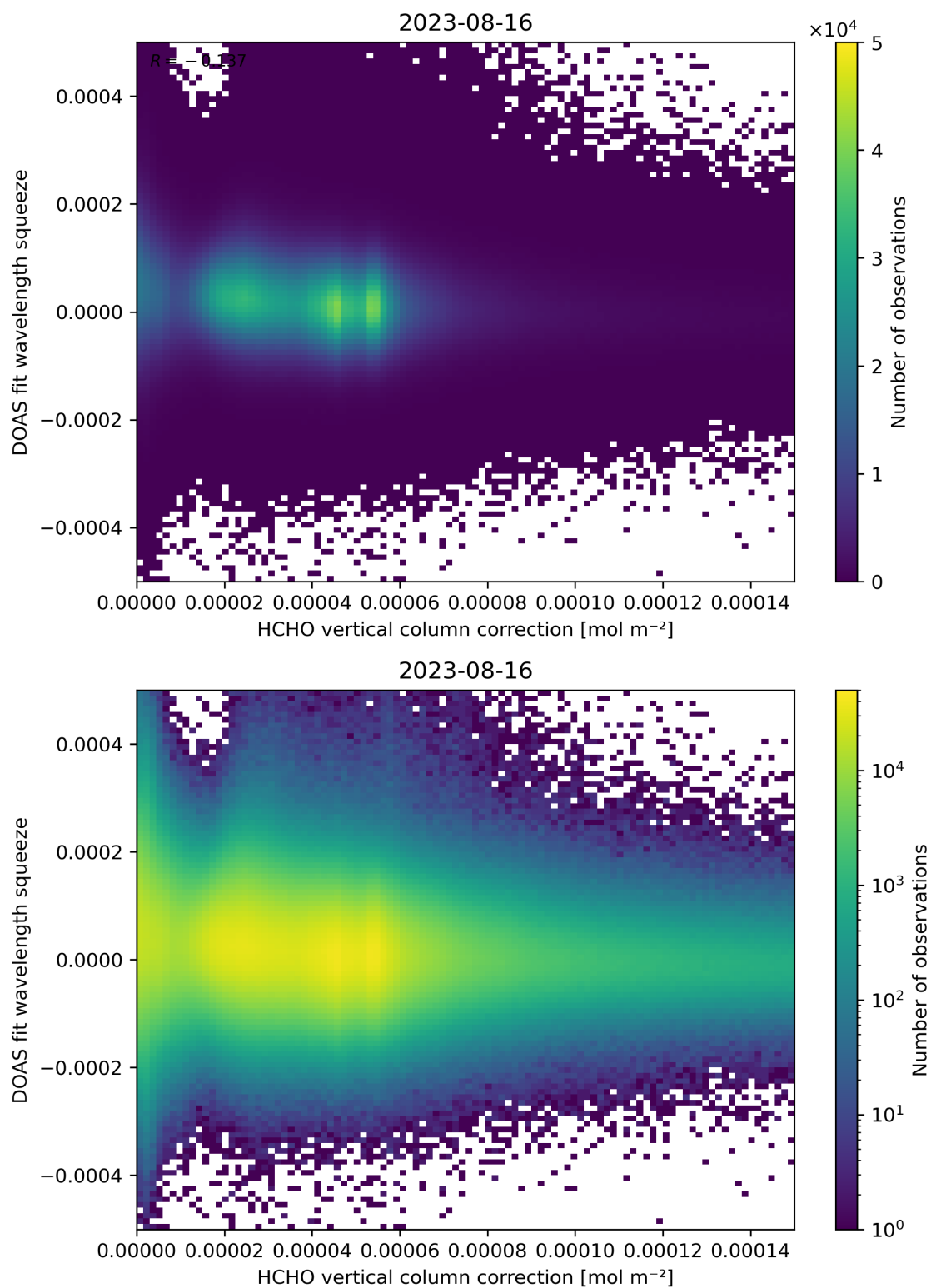
Figure 114: Scatter density plot of “HCHO vertical column correction” against “DOAS fit wavelength squeeze” for 2023-08-15 to 2023-08-17.
