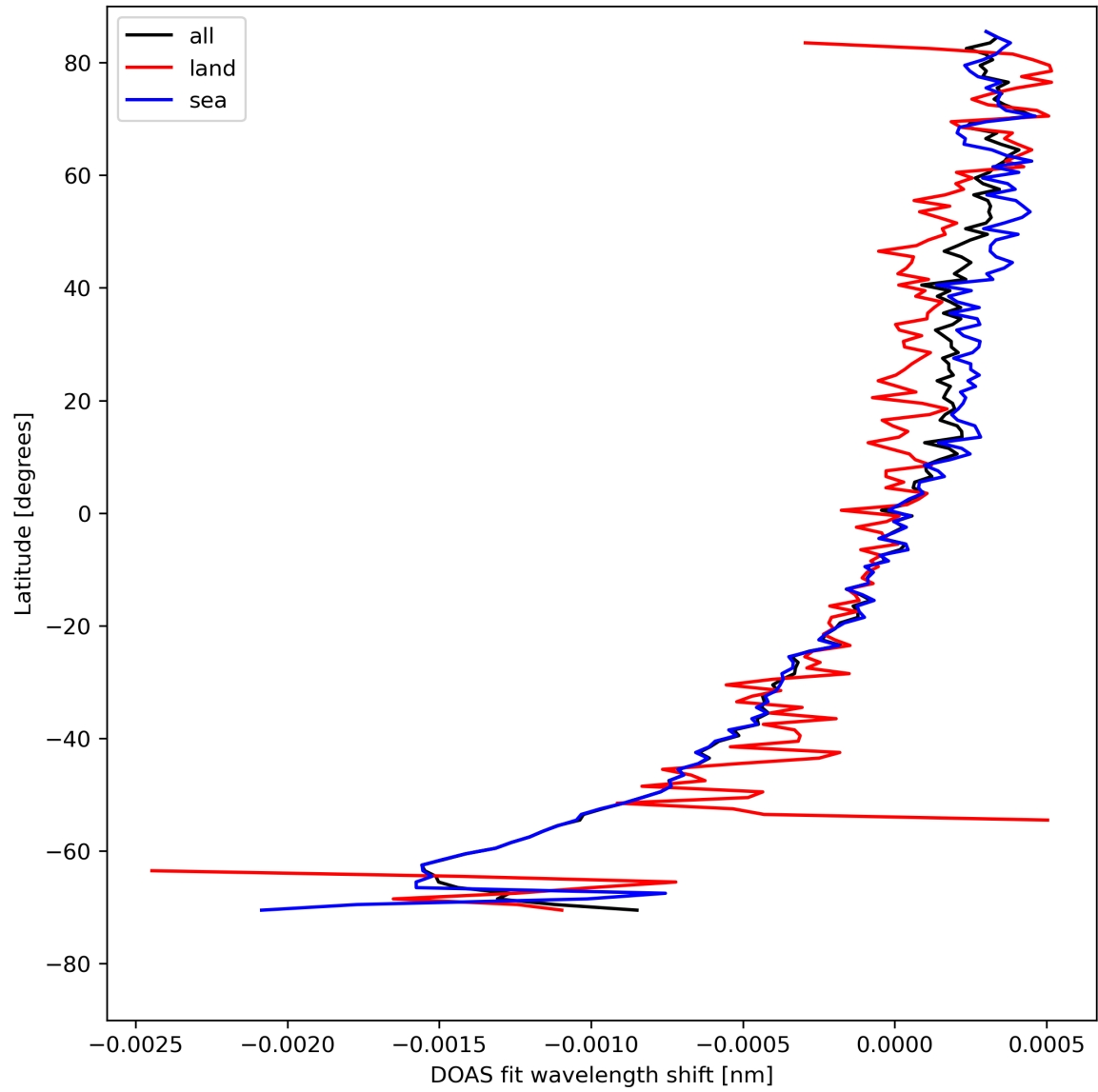
Figure 30: Zonal average of “DOAS fit wavelength shift” for 2023-08-15 to 2023-08-17.
