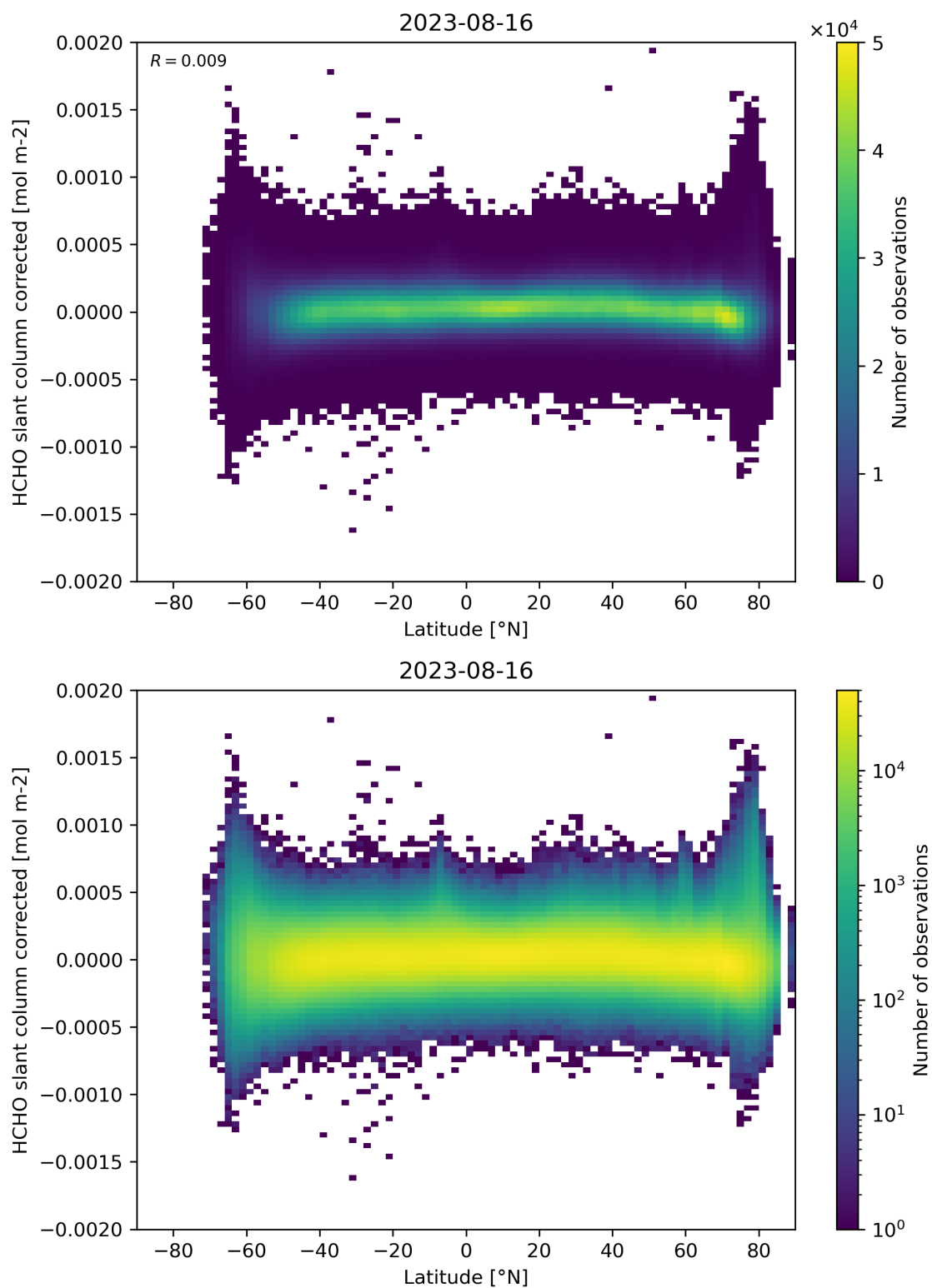
Figure 157: Scatter density plot of “Latitude” against “HCHO slant column corrected” for 2023-08-15 to 2023-08-17.
