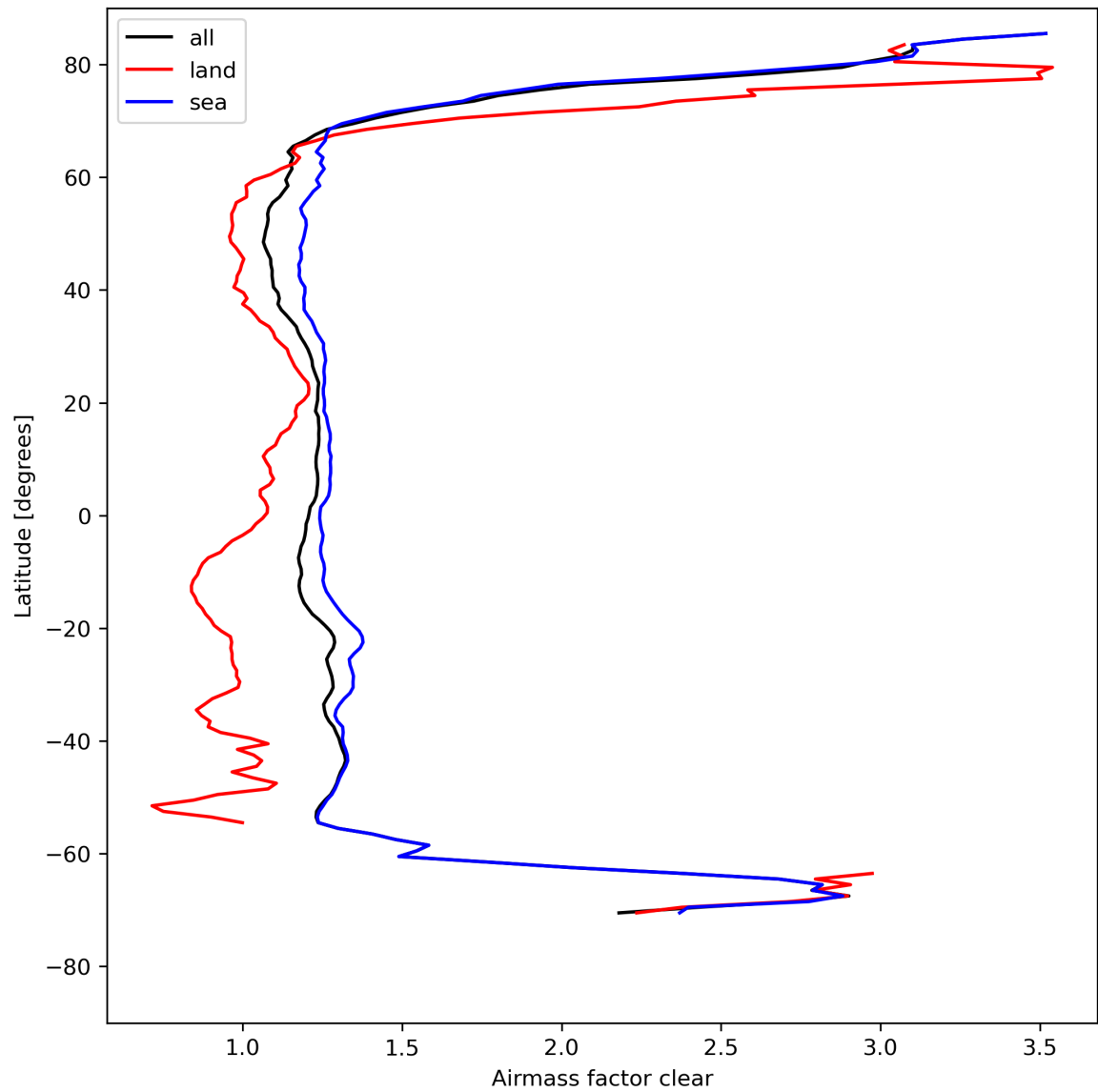
Figure 28: Zonal average of “Airmass factor clear” for 2023-08-15 to 2023-08-17.
