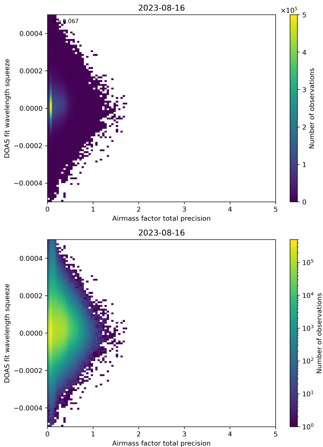
Figure 107: Scatter density plot of “Airmass factor total precision” against “DOAS fit wavelength squeeze” for 2023-08-15 to 2023-08-17.
