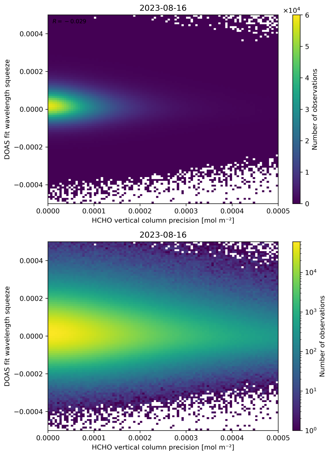
Figure 138: Scatter density plot of “HCHO vertical column precision” against “DOAS fit wavelength squeeze” for 2023-08-15 to 2023-08-17.
