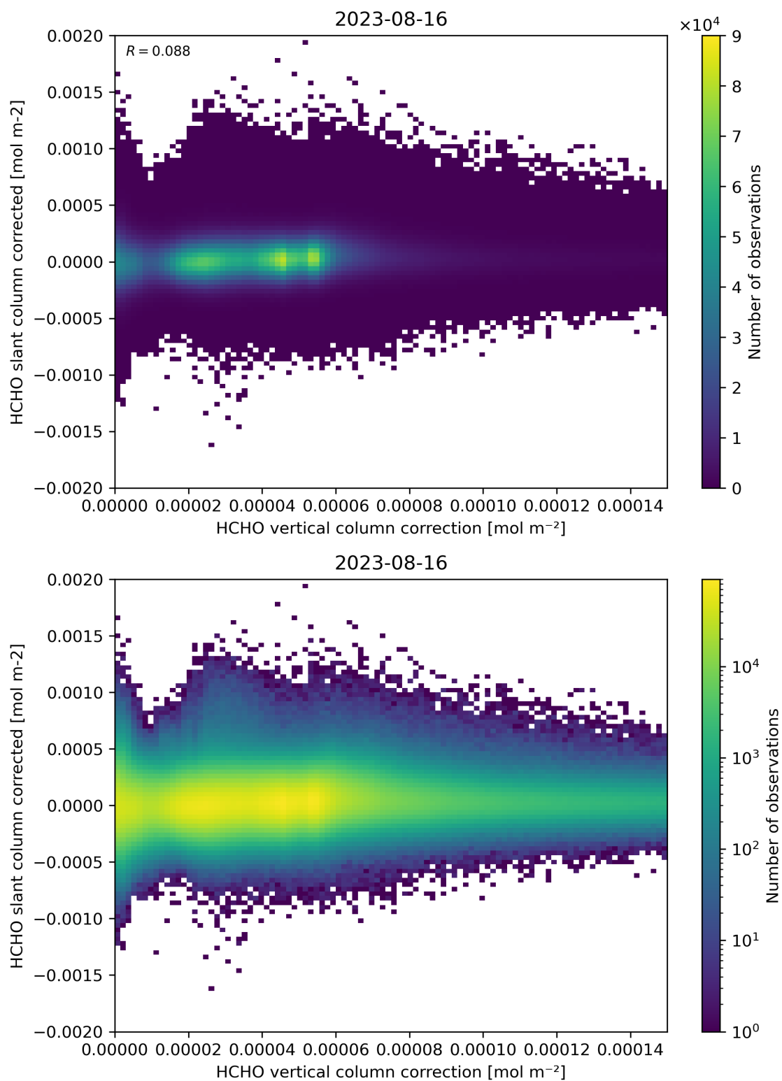
Figure 116: Scatter density plot of “HCHO vertical column correction” against “HCHO slant column corrected” for 2023-08-15 to 2023-08-17.
