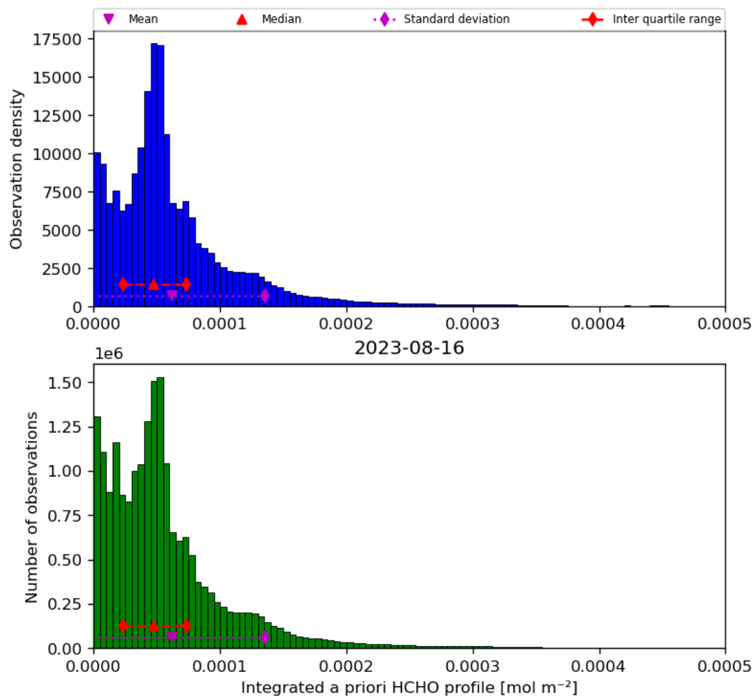
Figure 43: Histogram of “Integrated a priori HCHO profile” for 2023-08-15 to 2023-08-17
