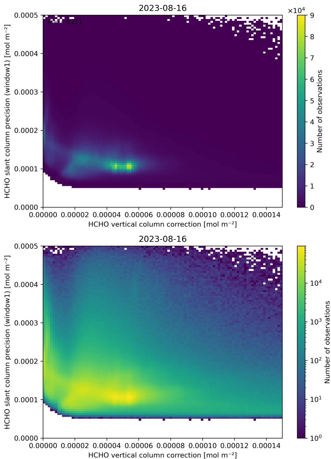
Figure 119: Scatter density plot of “HCHO vertical column correction” against “HCHO slant column precision (window1)” for 2023-08-15 to 2023-08-17.
