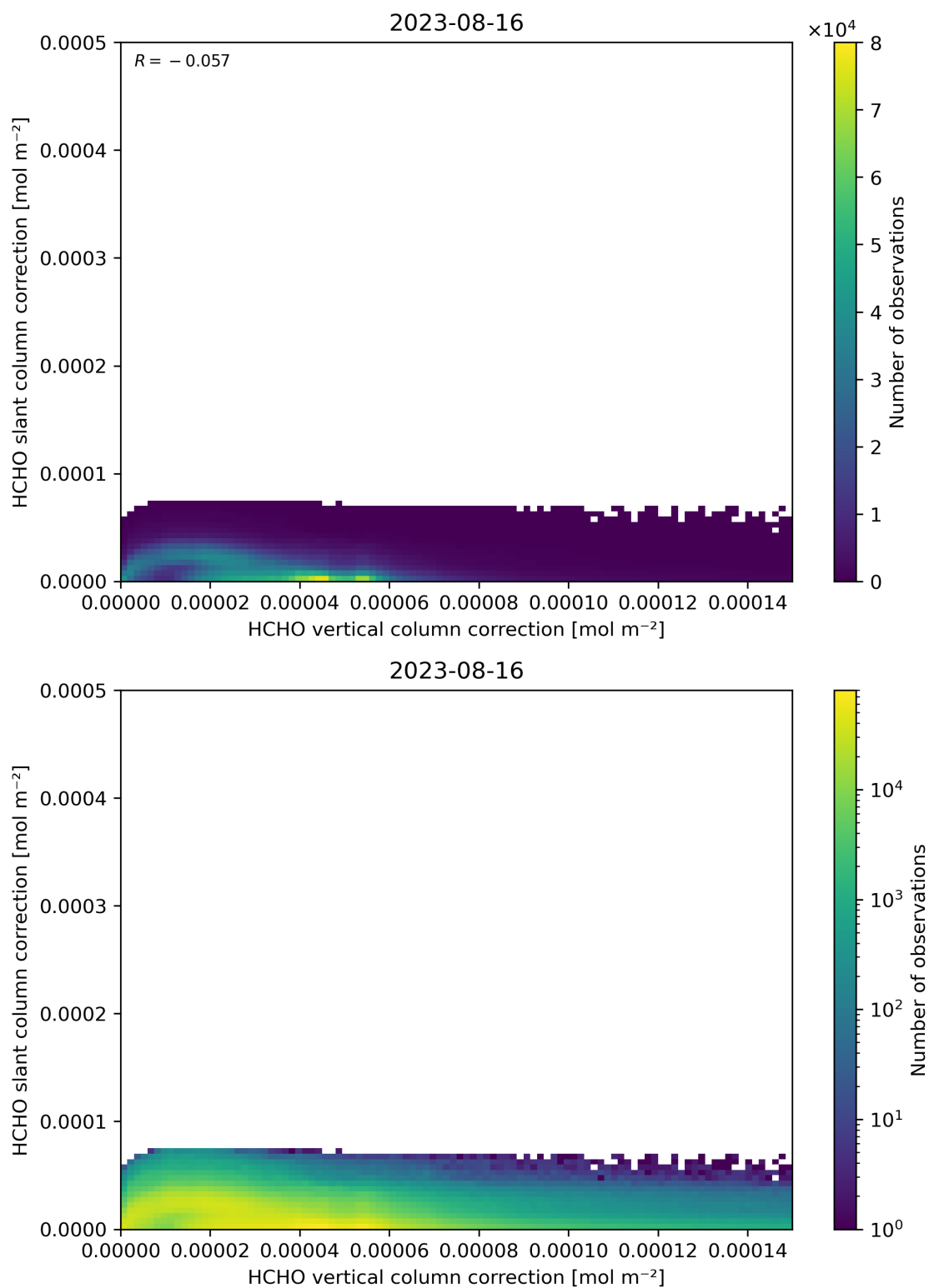
Figure 117: Scatter density plot of “HCHO vertical column correction” against “HCHO slant column correction” for 2023-08-15 to 2023-08-17.
