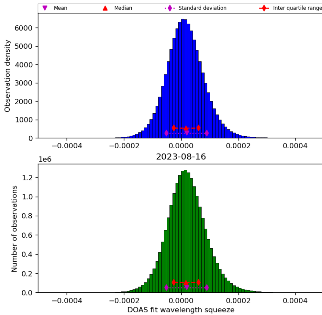
Figure 45: Histogram of “DOAS fit wavelength squeeze” for 2023-08-15 to 2023-08-17
