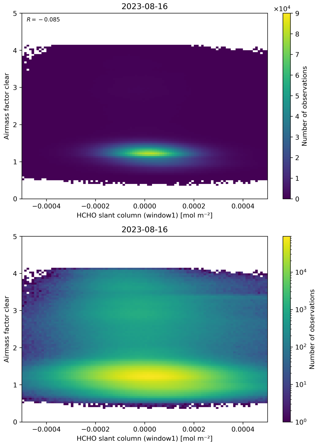
Figure 81: Scatter density plot of “HCHO slant column (window1)” against “Airmass factor clear” for 2023-08-15 to 2023-08-17.
