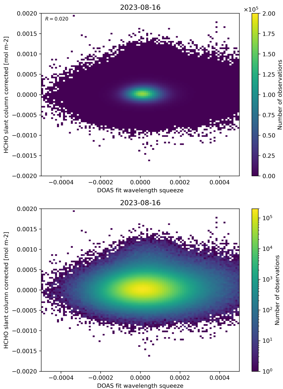
Figure 69: Scatter density plot of “DOAS fit wavelength squeeze” against “HCHO slant column corrected” for 2023-08-15 to 2023-08-17.
