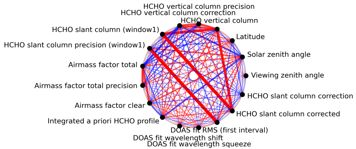
Figure 1: Map of correlation graph for 2023-08-15 to 2023-08-17.
