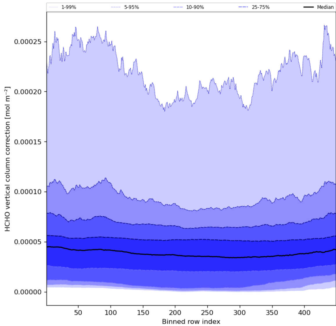
Figure 51: Along track statistics of “HCHO vertical column correction” for 2023-08-15 to 2023-08-17
