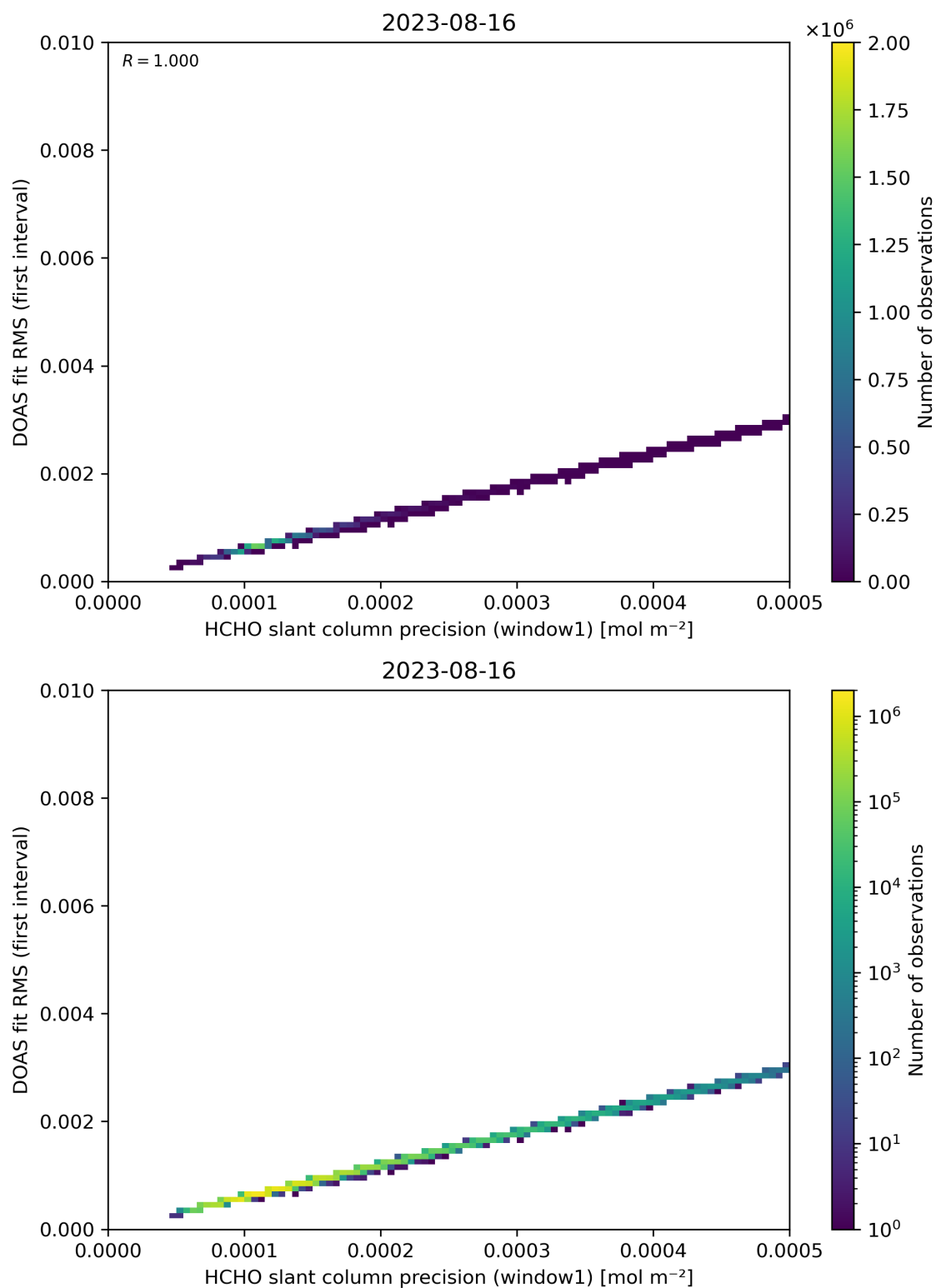
Figure 88: Scatter density plot of “HCHO slant column precision (window1)” against “DOAS fit RMS (first interval)” for 2023-08-15 to 2023-08-17.
