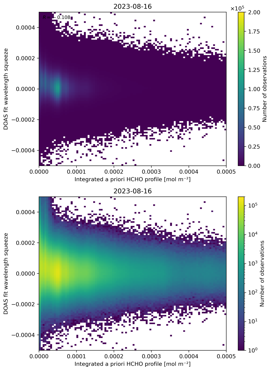
Figure 150: Scatter density plot of “Integrated a priori HCHO profile” against “DOAS fit wavelength squeeze” for 2023-08-15 to 2023-08-17.
