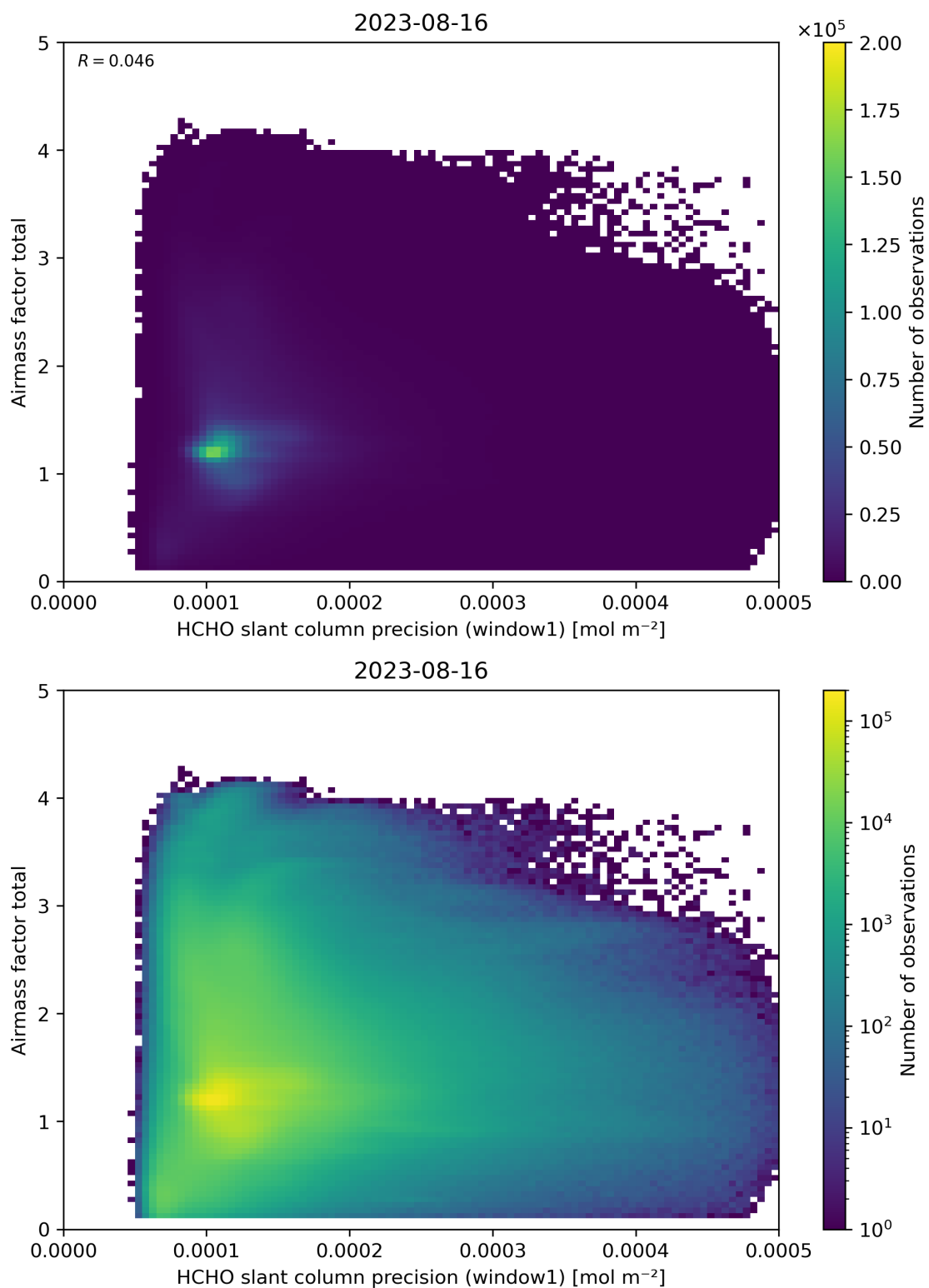
Figure 94: Scatter density plot of “HCHO slant column precision (window1)” against “Airmass factor total” for 2023-08-15 to 2023-08-17.
