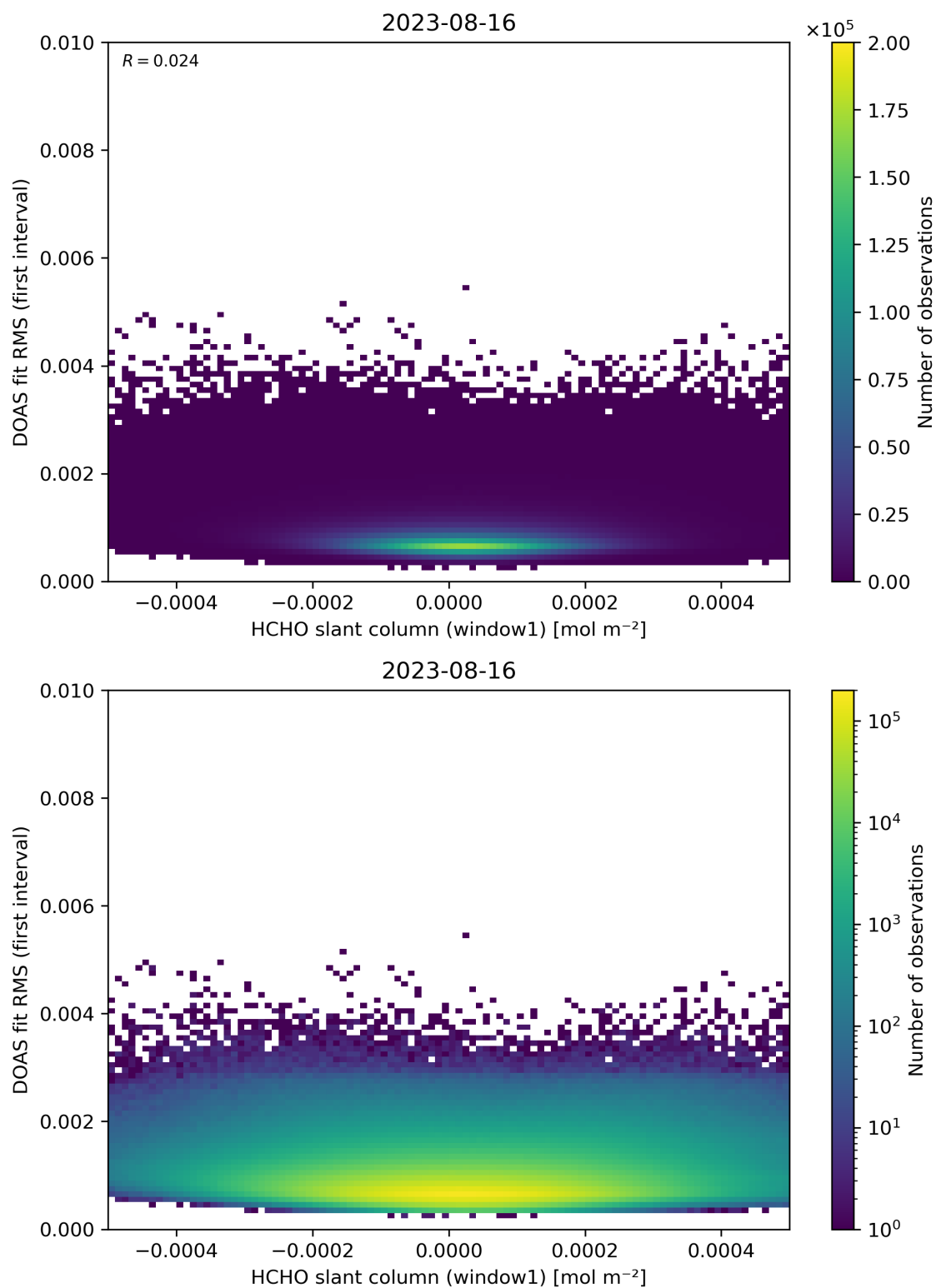
Figure 78: Scatter density plot of “HCHO slant column (window1)” against “DOAS fit RMS (first interval)” for 2023-08-15 to 2023-08-17.
