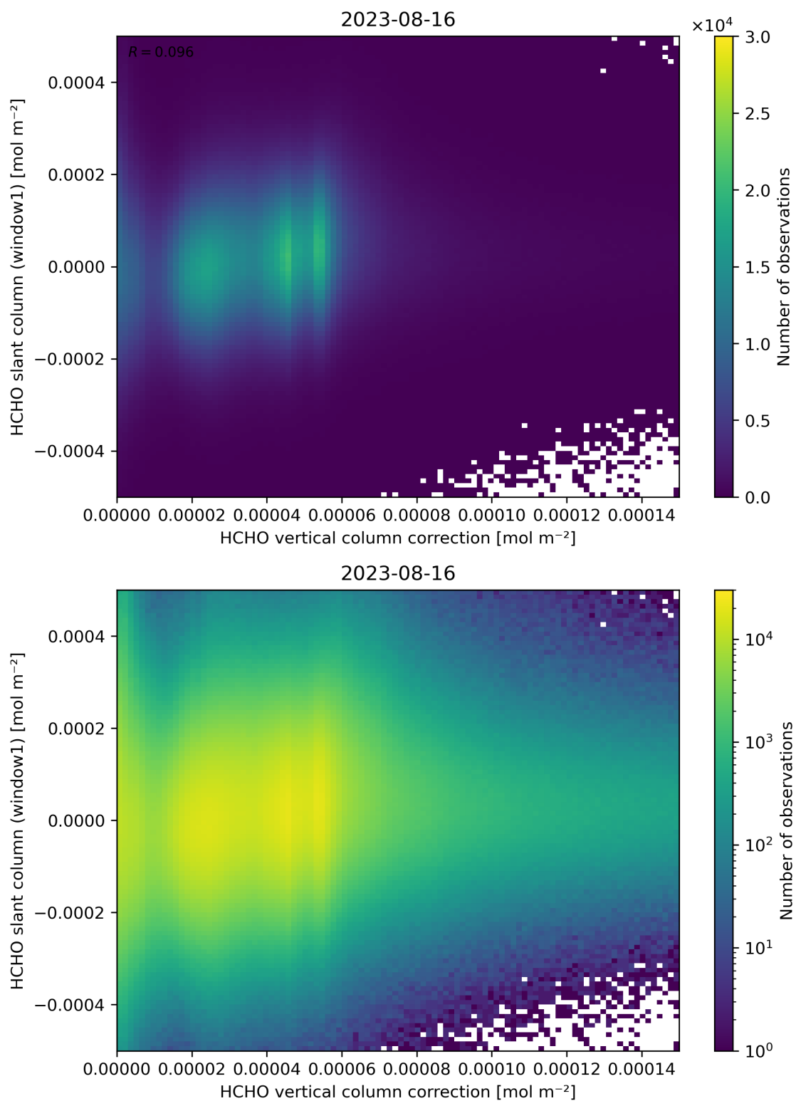
Figure 118: Scatter density plot of “HCHO vertical column correction” against “HCHO slant column (window1)” for 2023-08-15 to 2023-08-17.
