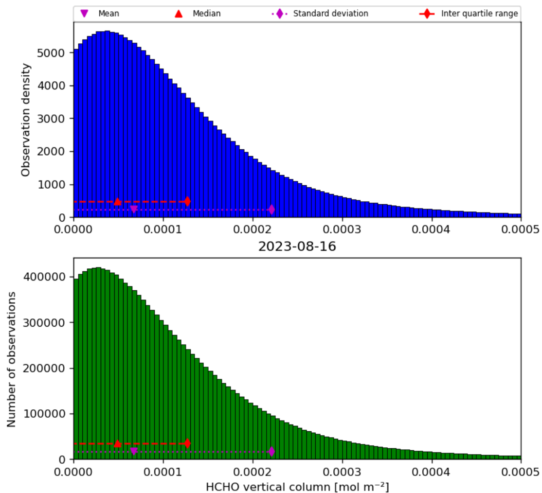
Figure 35: Histogram of “HCHO vertical column” for 2023-08-15 to 2023-08-17
