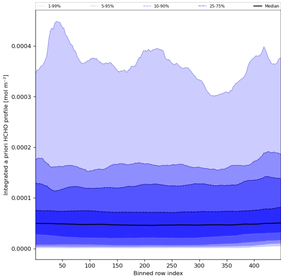
Figure 57: Along track statistics of “Integrated a priori HCHO profile” for 2023-08-15 to 2023-08-17
