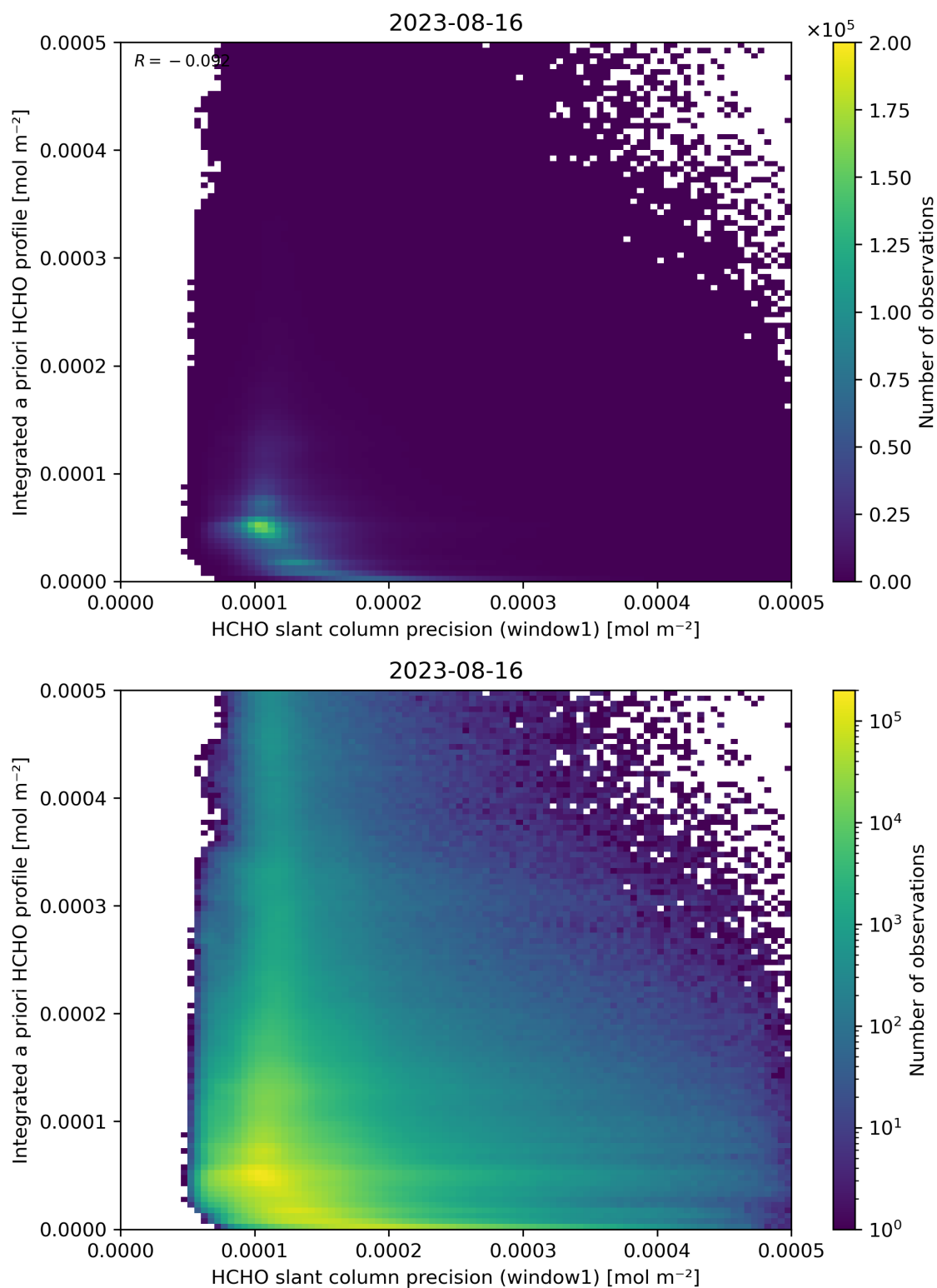
Figure 96: Scatter density plot of “HCHO slant column precision (window1)” against “Integrated a priori HCHO profile” for 2023-08-15 to 2023-08-17.
