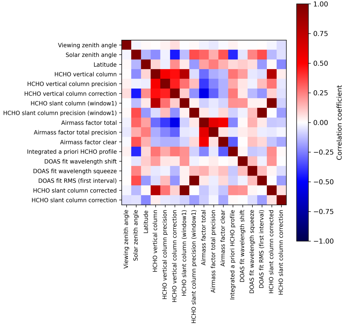
Figure 2: Map of correlation matrix for 2023-08-15 to 2023-08-17.
