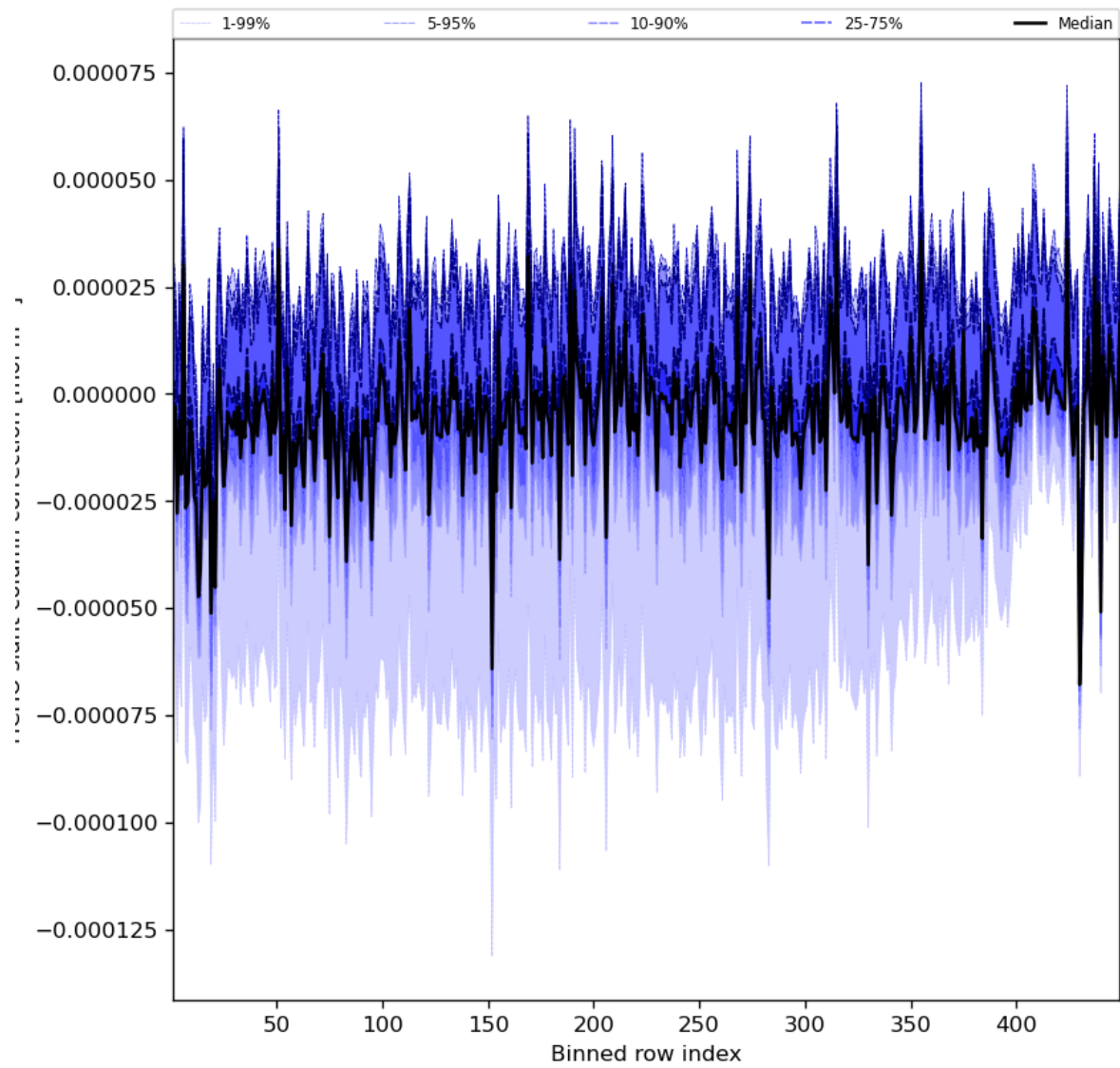
Figure 61: Along track statistics of “HCHO slant column correction” for 2023-08-15 to 2023-08-17
