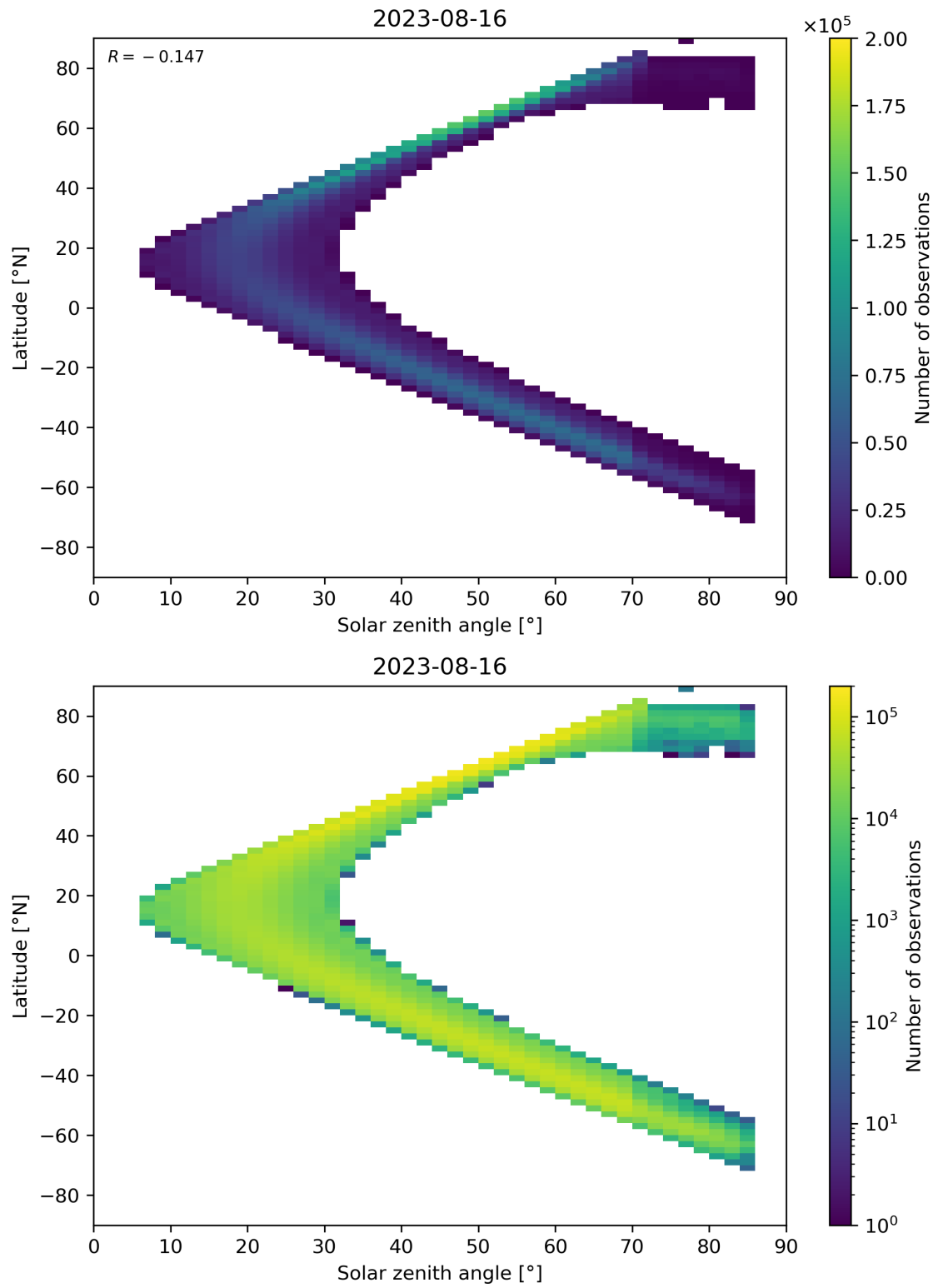
Figure 181: Scatter density plot of “Solar zenith angle” against “Latitude” for 2023-08-15 to 2023-08-17.
