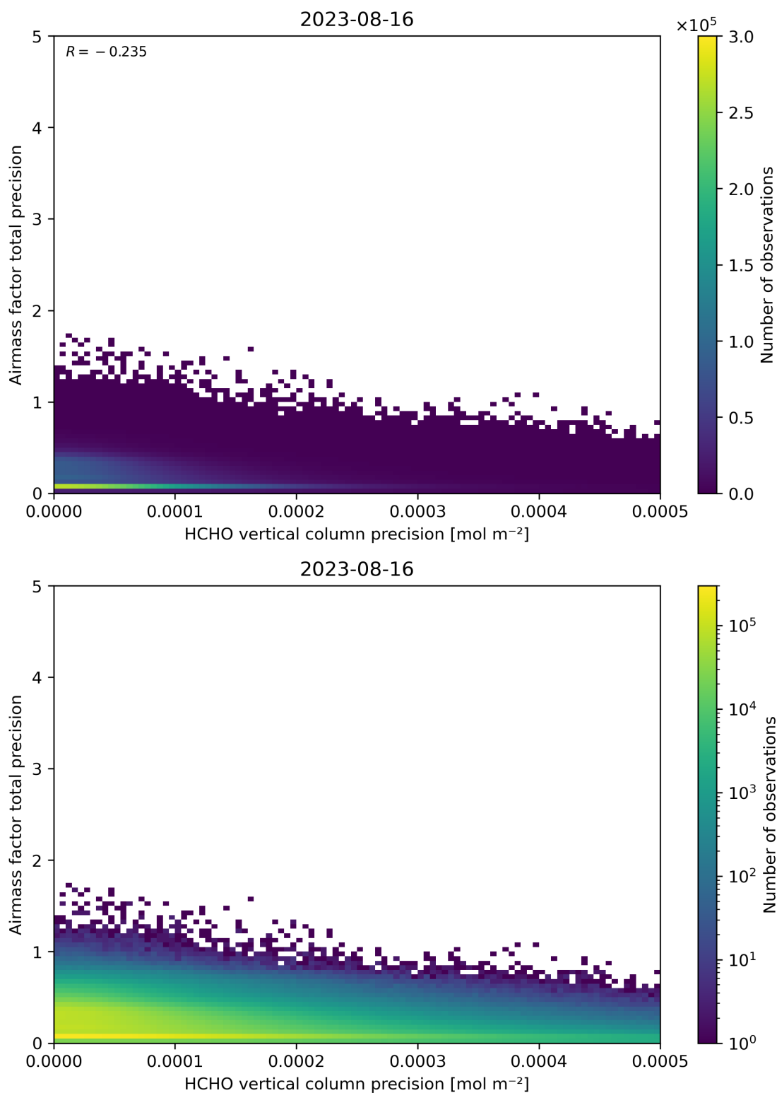
Figure 145: Scatter density plot of “HCHO vertical column precision” against “Airmass factor total precision” for 2023-08-15 to 2023-08-17.
