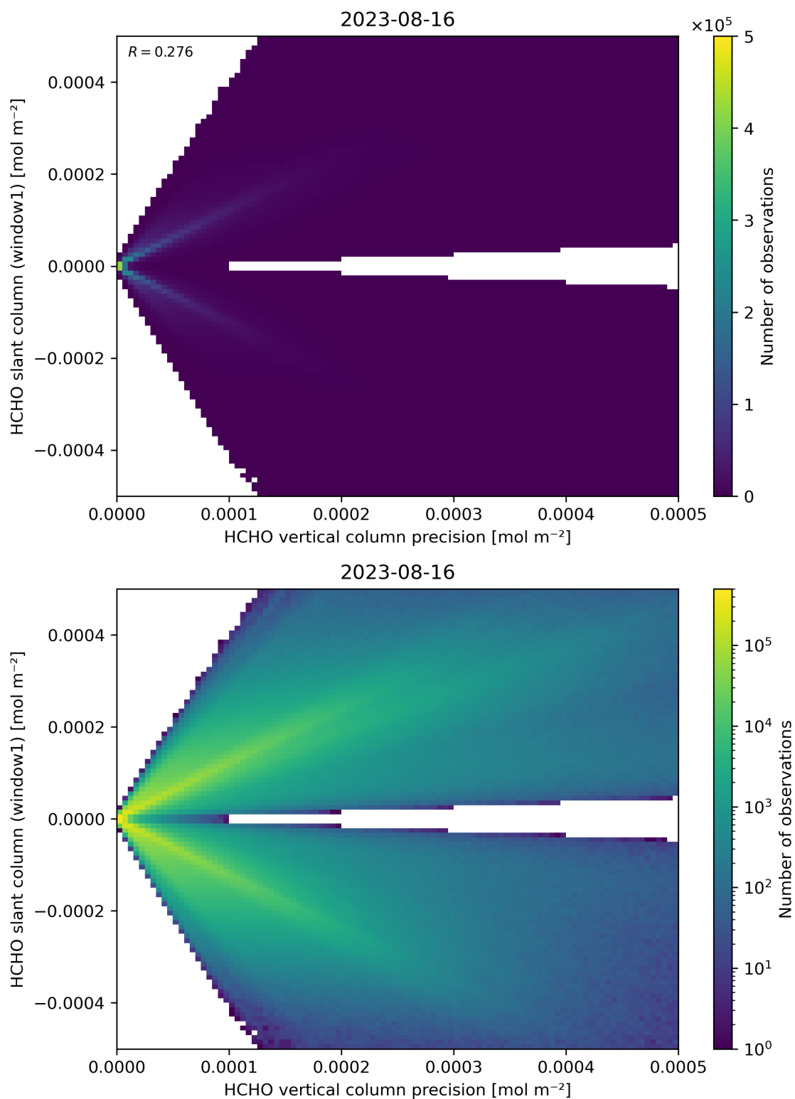
Figure 142: Scatter density plot of “HCHO vertical column precision” against “HCHO slant column (window1)” for 2023-08-15 to 2023-08-17.
