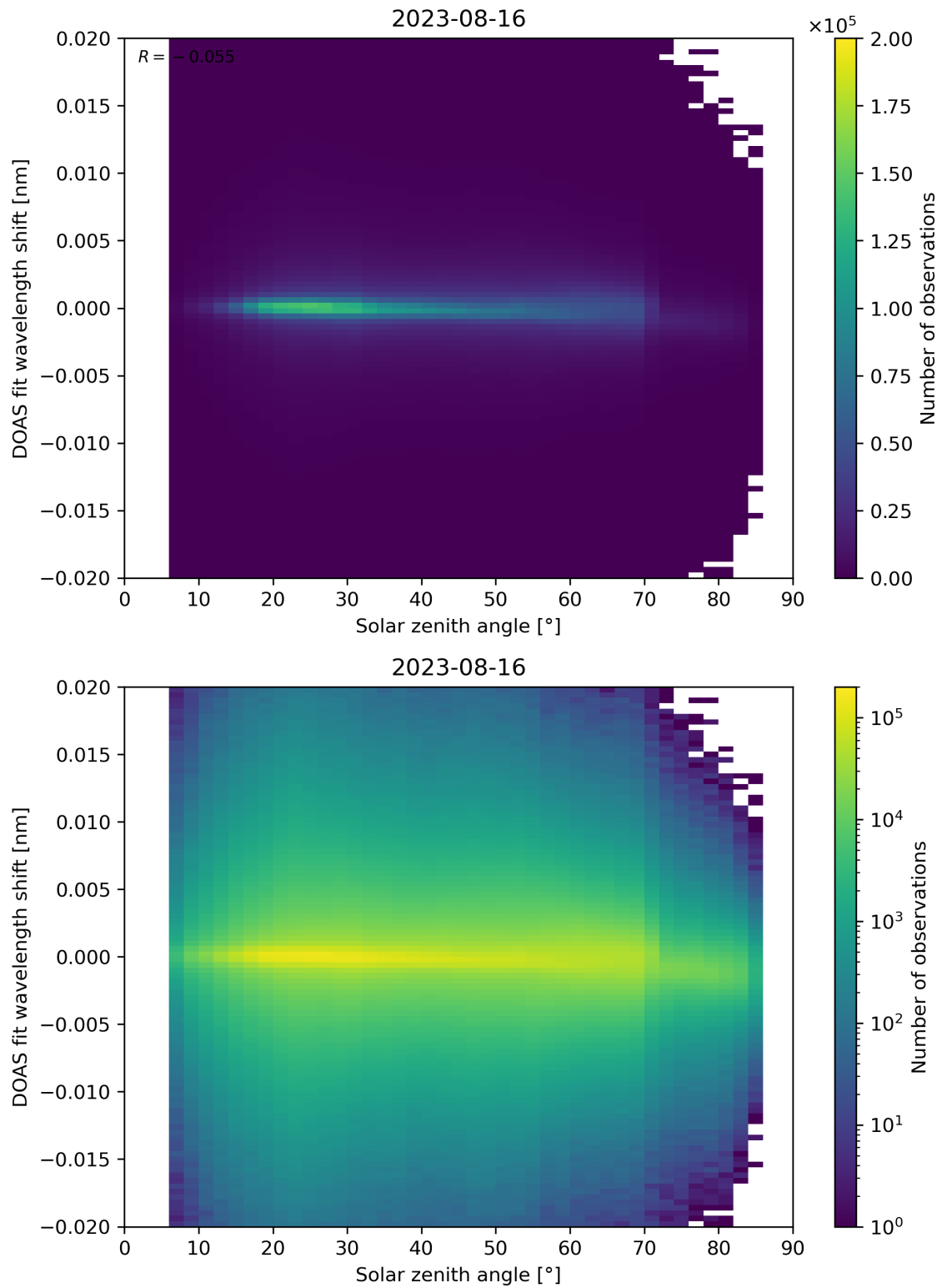
Figure 168: Scatter density plot of “Solar zenith angle” against “DOAS fit wavelength shift” for 2023-08-15 to 2023-08-17.
