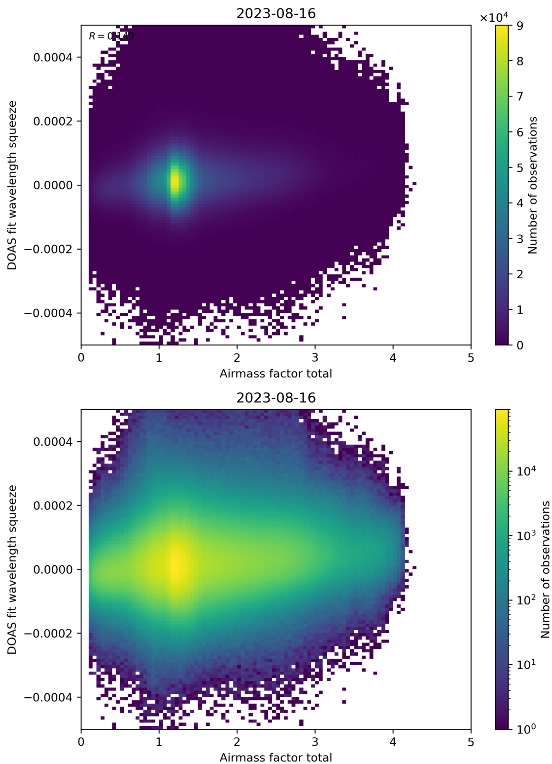
Figure 99: Scatter density plot of “Airmass factor total” against “DOAS fit wavelength squeeze” for 2023-08-15 to 2023-08-17.
