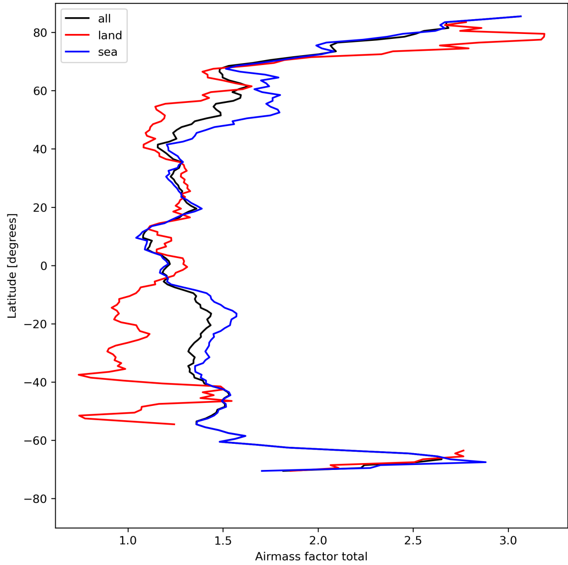
Figure 26: Zonal average of “Airmass factor total” for 2023-08-15 to 2023-08-17.
