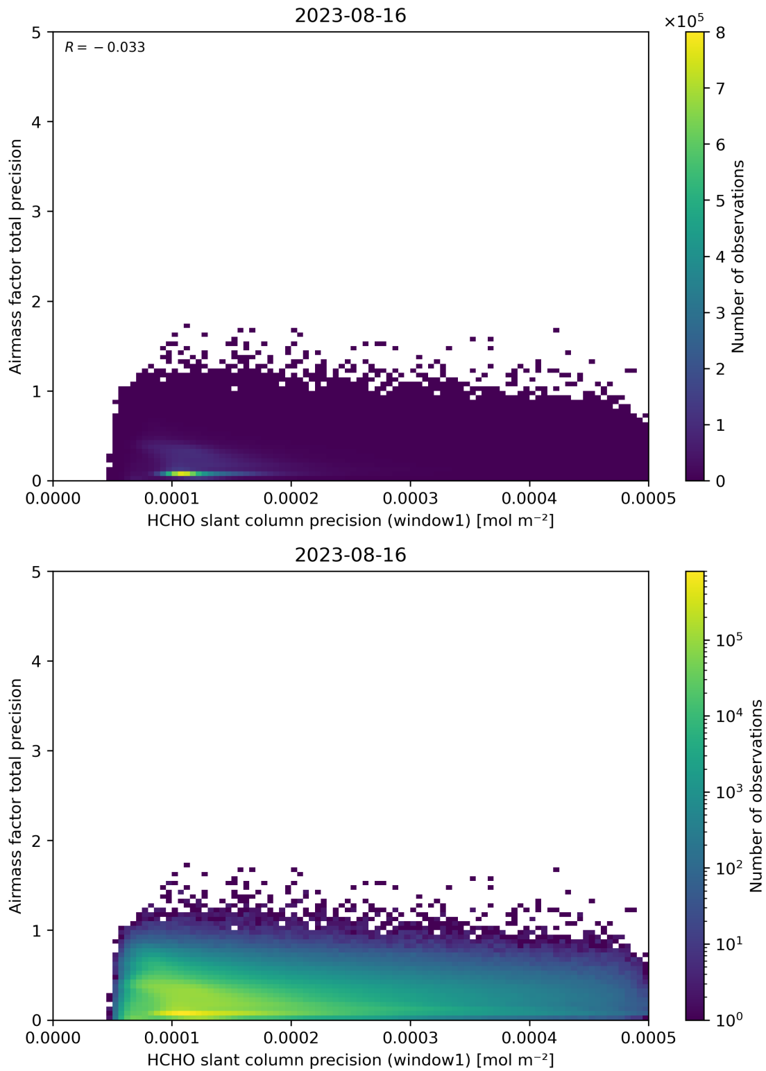
Figure 95: Scatter density plot of “HCHO slant column precision (window1)” against “Airmass factor total precision” for 2023-08-15 to 2023-08-17.
