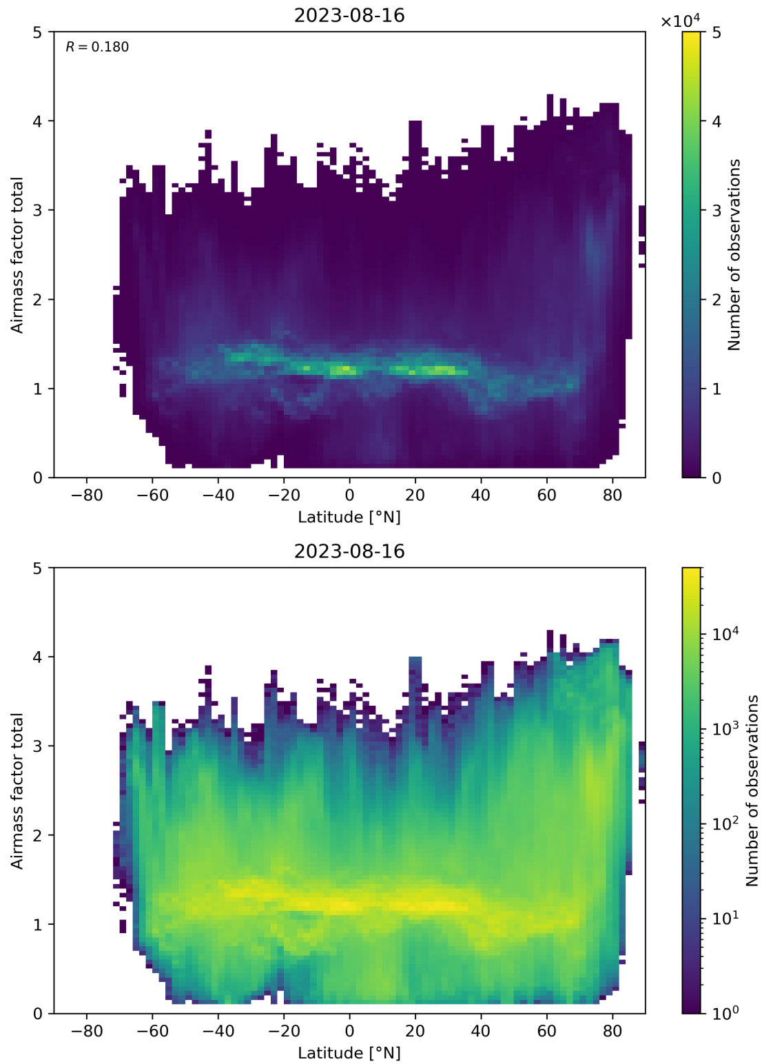
Figure 161: Scatter density plot of “Latitude” against “Airmass factor total” for 2023-08-15 to 2023-08-17.
