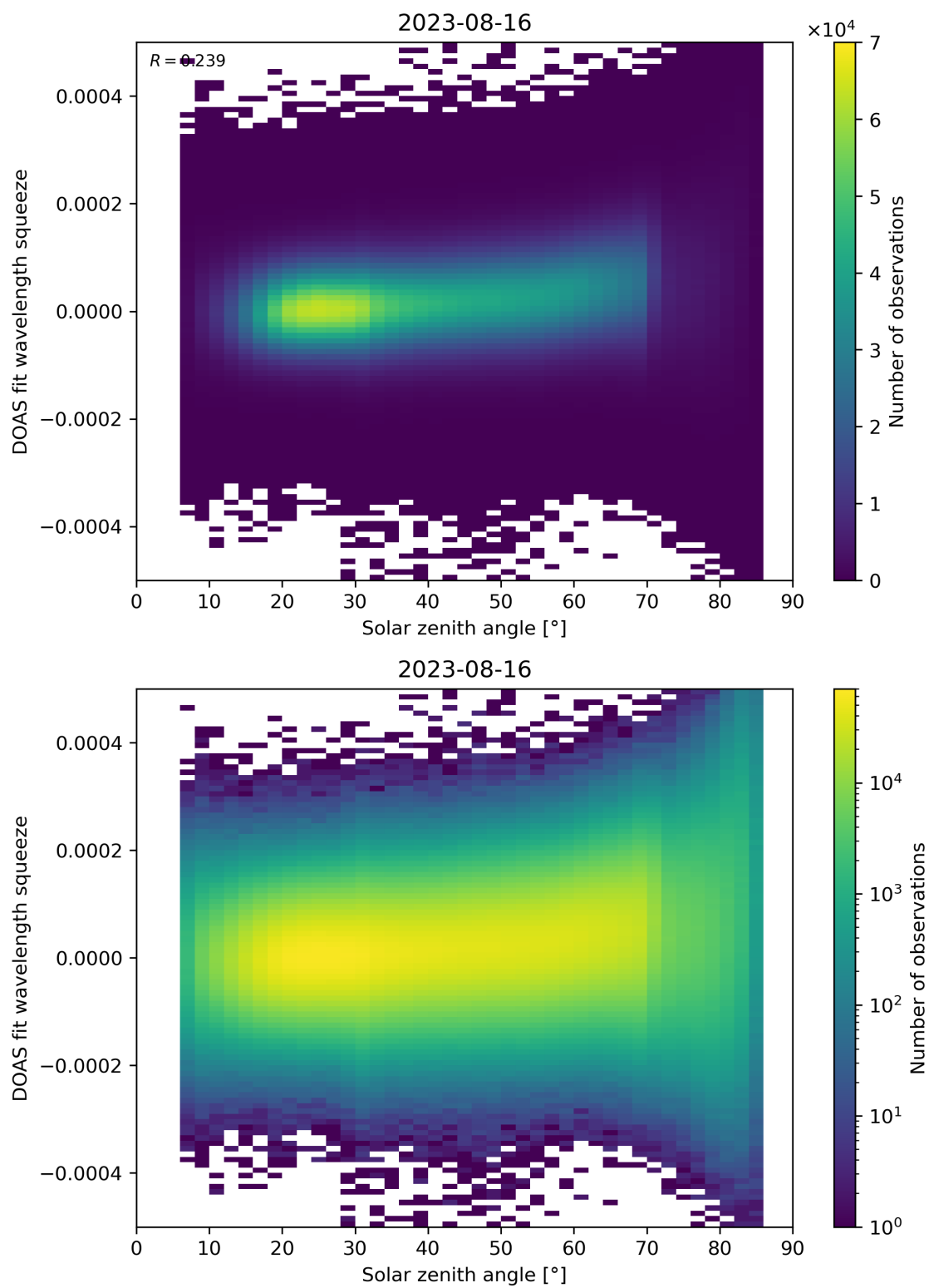
Figure 169: Scatter density plot of “Solar zenith angle” against “DOAS fit wavelength squeeze” for 2023-08-15 to 2023-08-17.
