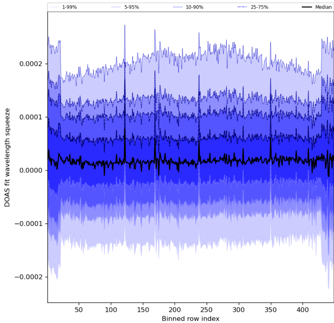
Figure 59: Along track statistics of “DOAS fit wavelength squeeze” for 2023-08-15 to 2023-08-17
