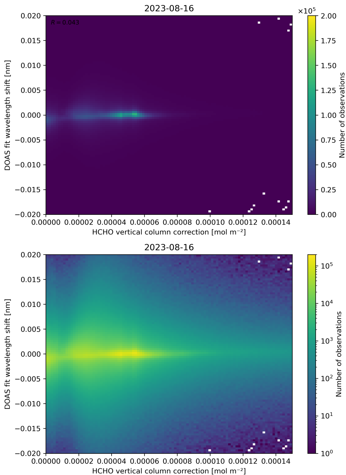
Figure 113: Scatter density plot of “HCHO vertical column correction” against “DOAS fit wavelength shift” for 2023-08-15 to 2023-08-17.
