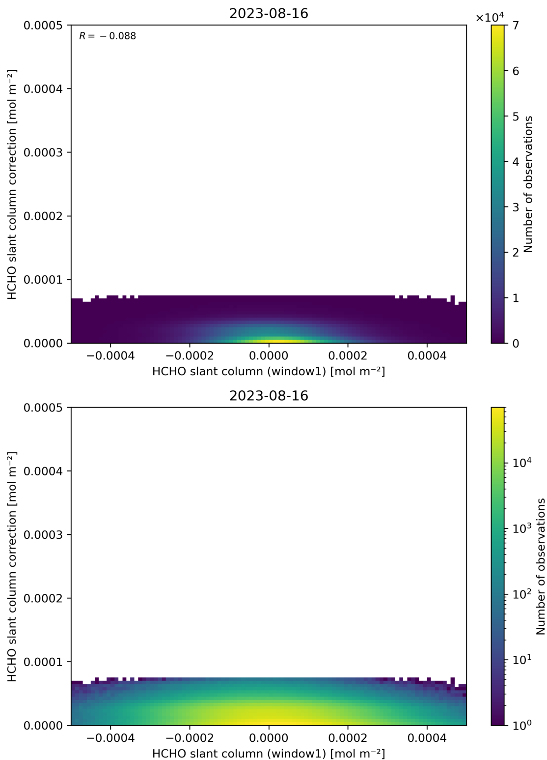
Figure 83: Scatter density plot of “HCHO slant column (window1)” against “HCHO slant column correction” for 2023-08-15 to 2023-08-17.
