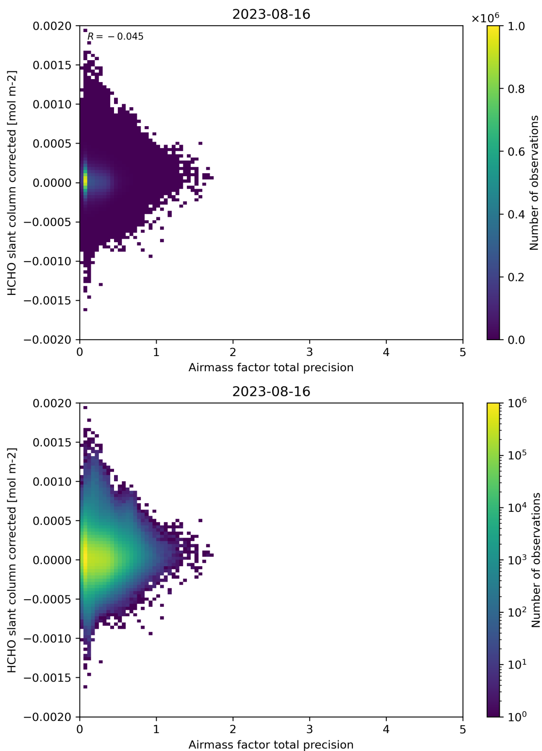
Figure 109: Scatter density plot of “Airmass factor total precision” against “HCHO slant column corrected” for 2023-08-15 to 2023-08-17.
