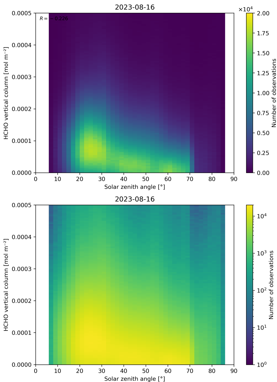
Figure 177: Scatter density plot of “Solar zenith angle” against “HCHO vertical column” for 2023-08-15 to 2023-08-17.
