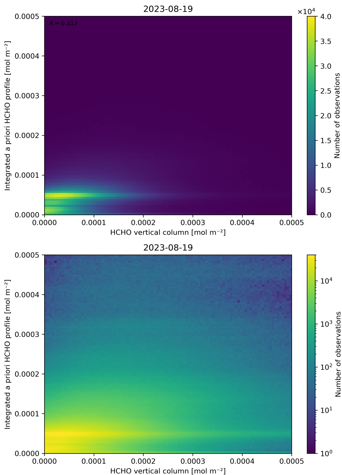
Figure 135: Scatter density plot of “HCHO vertical column” against “Integrated a priori HCHO profile” for 2023-08-18 to 2023-08-20.
