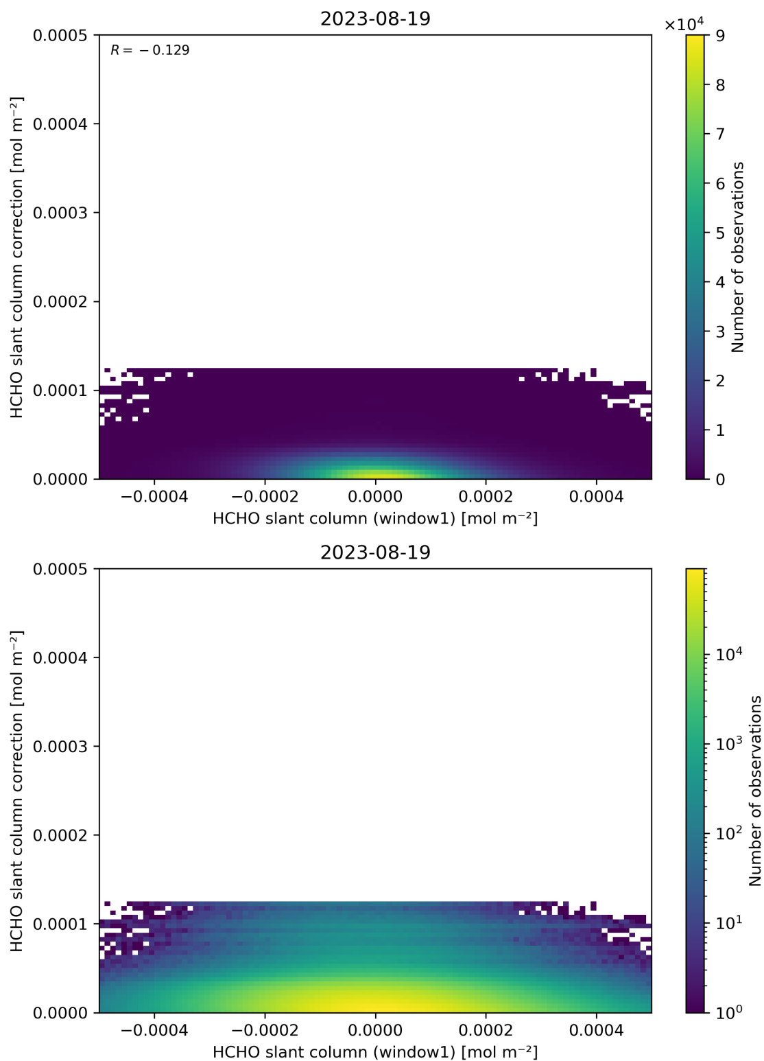
Figure 83: Scatter density plot of “HCHO slant column (window1)” against “HCHO slant column correction” for 2023-08-18 to 2023-08-20.
