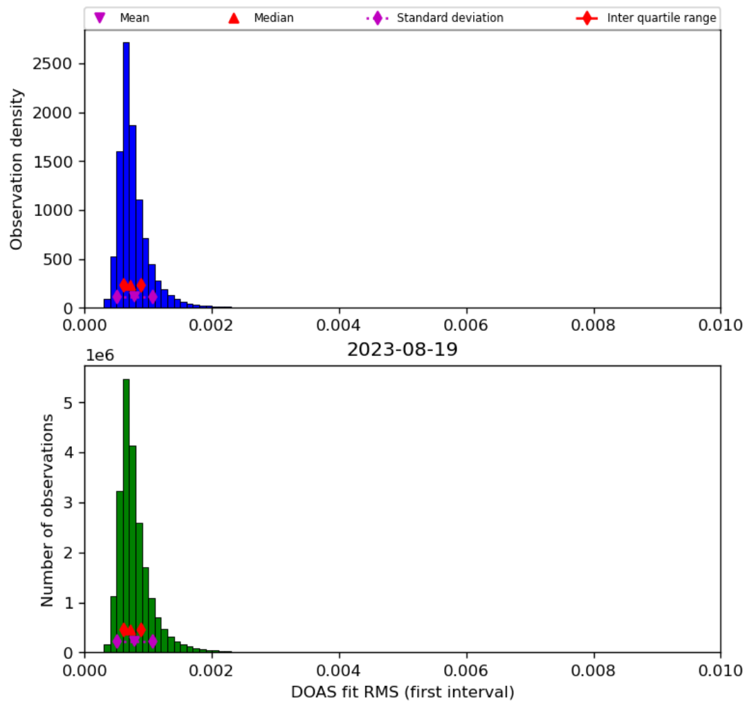
Figure 46: Histogram of “DOAS fit RMS (first interval)” for 2023-08-18 to 2023-08-20
