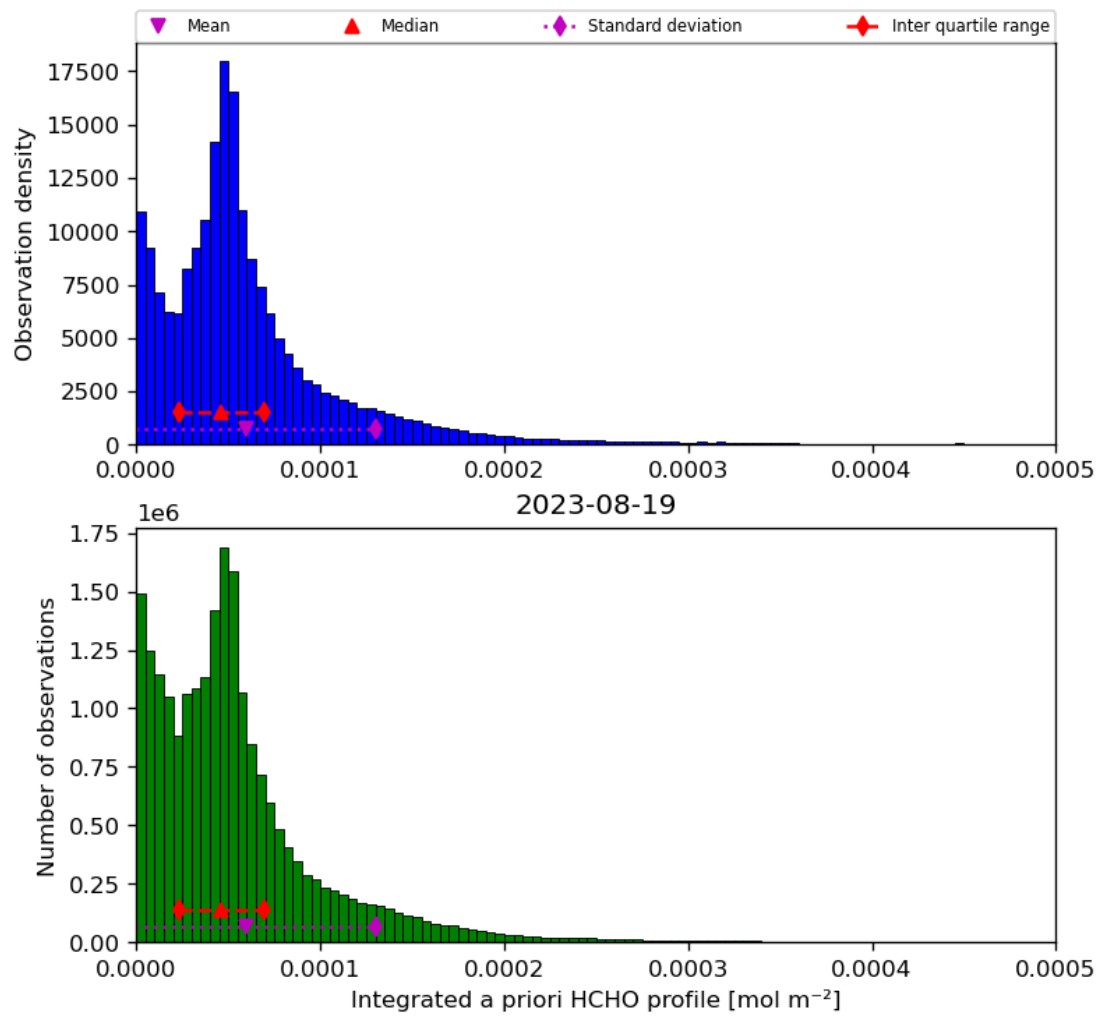
Figure 43: Histogram of “Integrated a priori HCHO profile” for 2023-08-18 to 2023-08-20
