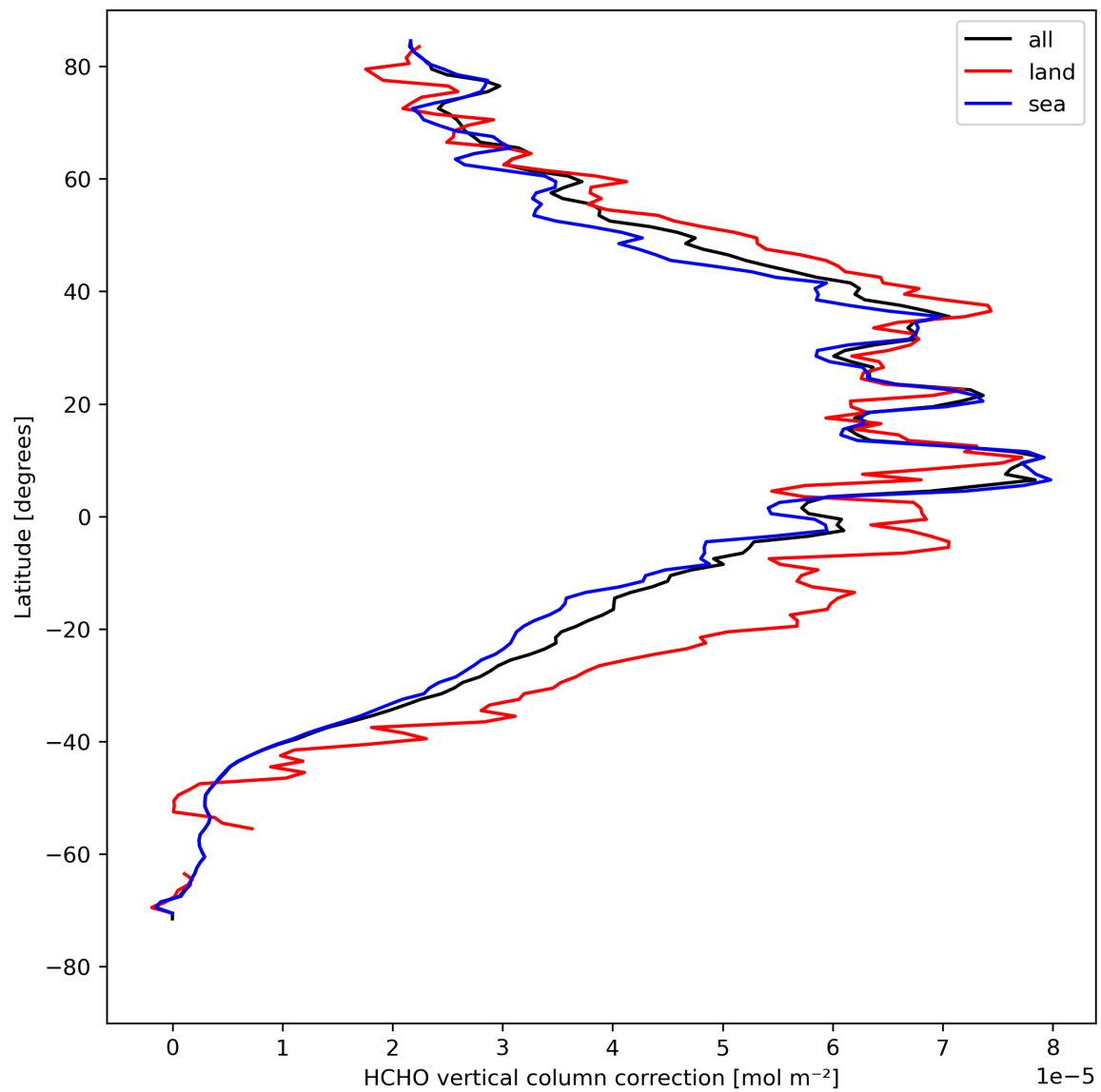
Figure 23: Zonal average of “HCHO vertical column correction” for 2023-08-18 to 2023-08-20.
