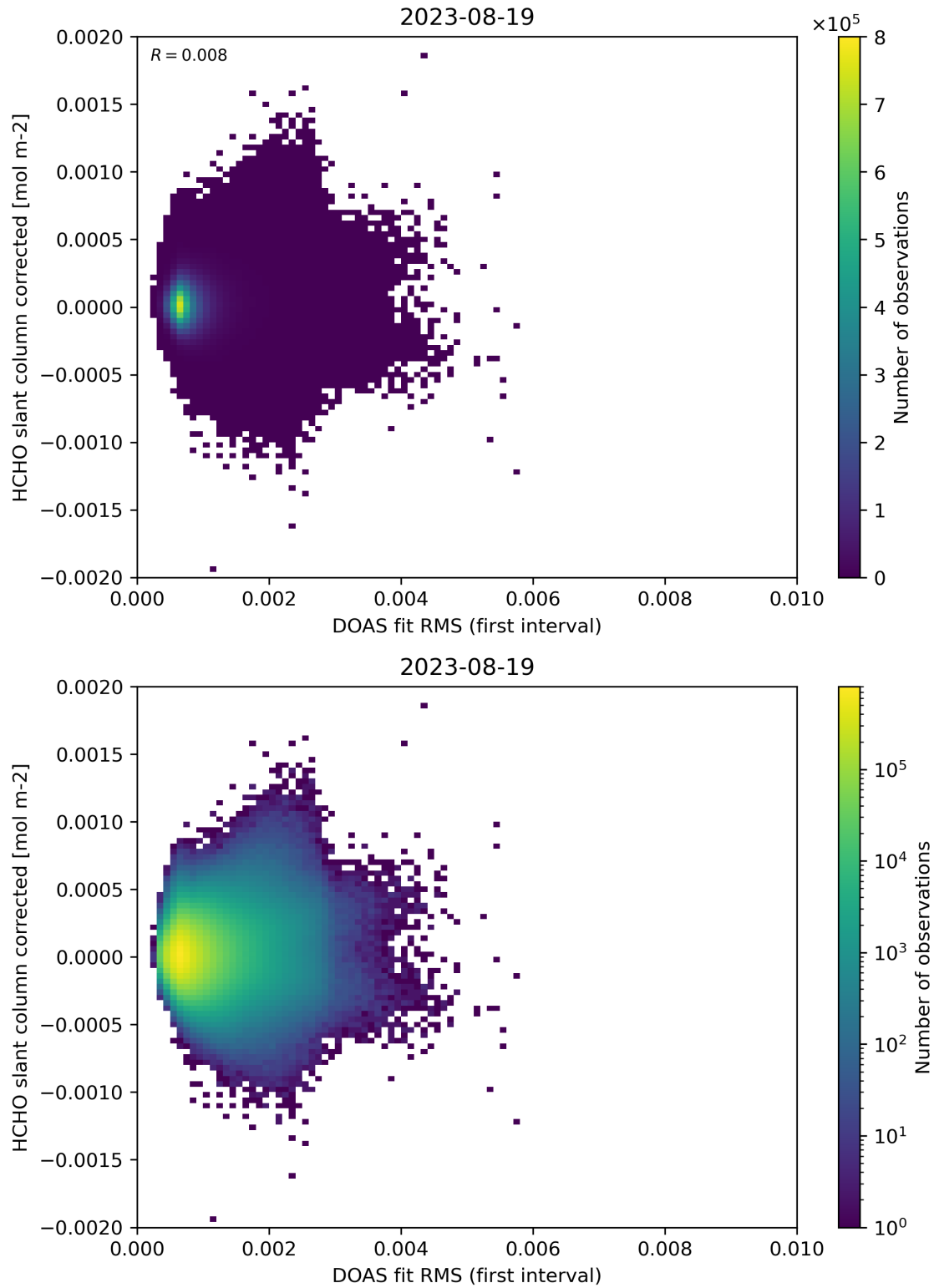
Figure 62: Scatter density plot of “DOAS fit RMS (first interval)” against “HCHO slant column corrected” for 2023-08-18 to 2023-08-20.
