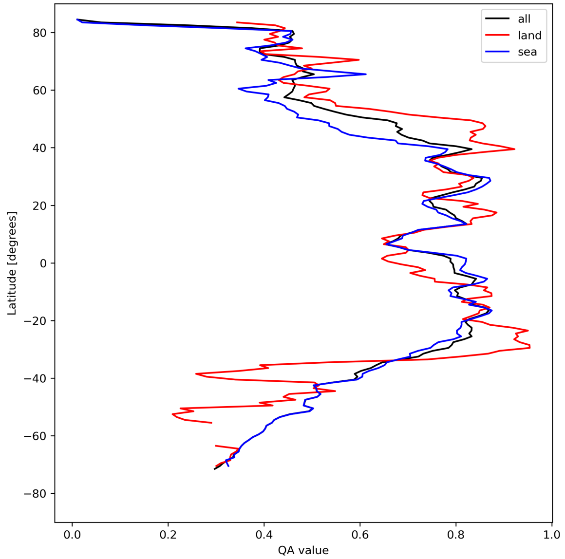
Figure 20: Zonal average of “QA value” for 2023-08-18 to 2023-08-20.
