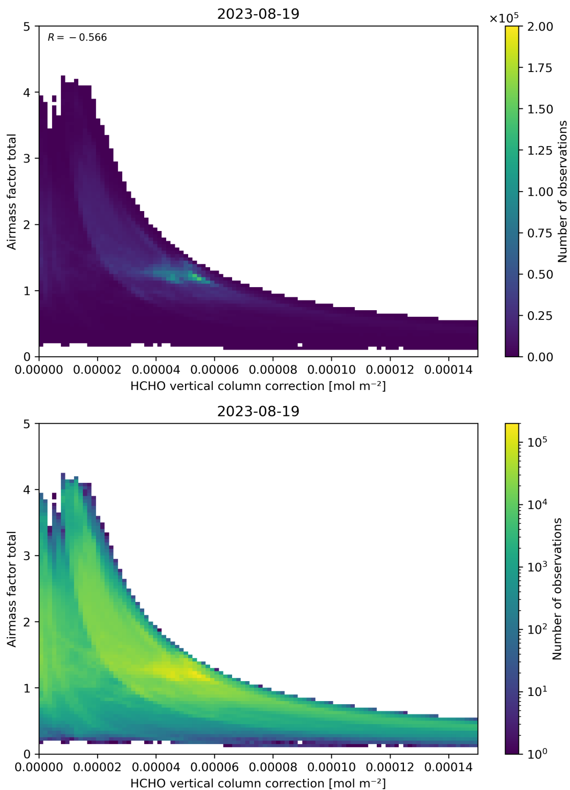
Figure 120: Scatter density plot of “HCHO vertical column correction” against “Airmass factor total” for 2023-08-18 to 2023-08-20.
