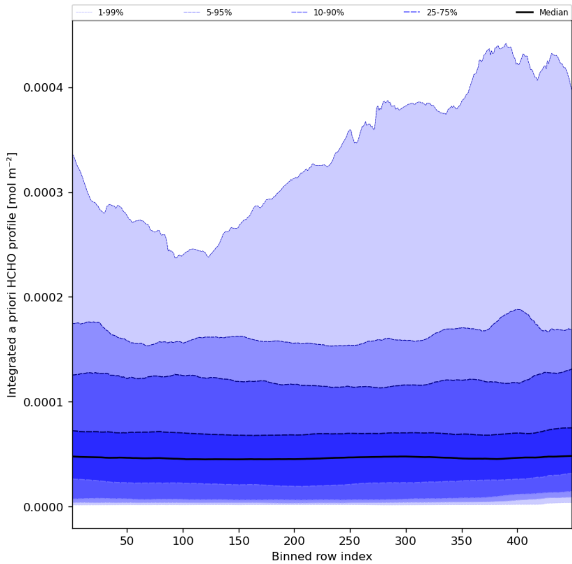
Figure 57: Along track statistics of “Integrated a priori HCHO profile” for 2023-08-18 to 2023-08-20
