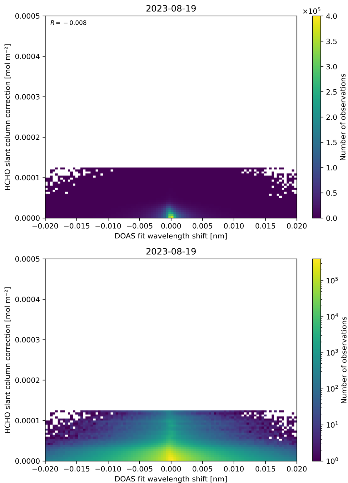
Figure 67: Scatter density plot of “DOAS fit wavelength shift” against “HCHO slant column correction” for 2023-08-18 to 2023-08-20.
