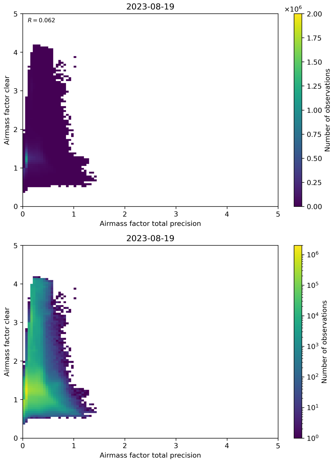
Figure 108: Scatter density plot of “Airmass factor total precision” against “Airmass factor clear” for 2023-08-18 to 2023-08-20.
