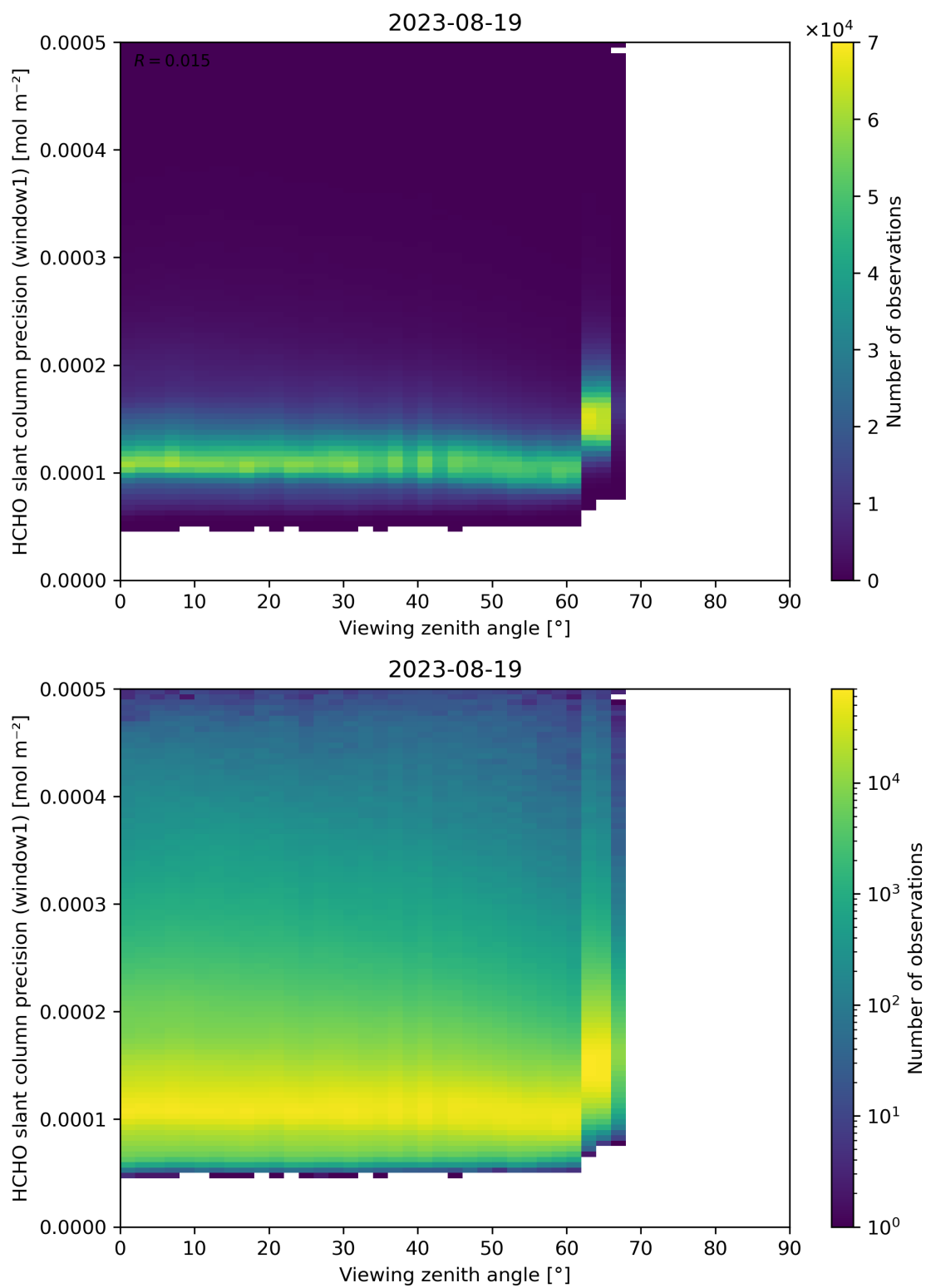
Figure 189: Scatter density plot of “Viewing zenith angle” against “HCHO slant column precision (window1)” for 2023-08-18 to 2023-08-20.
