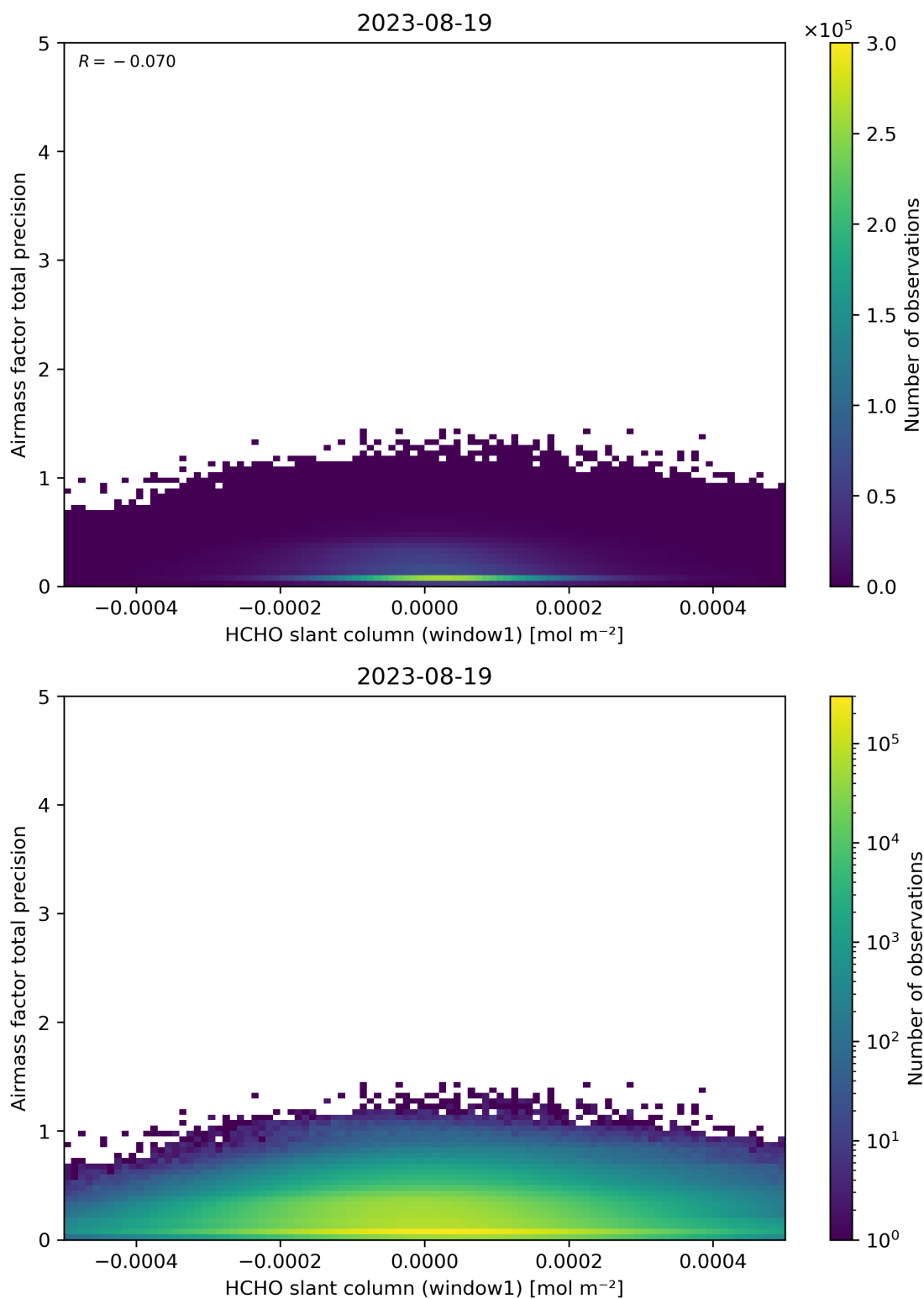
Figure 86: Scatter density plot of “HCHO slant column (window1)” against “Airmass factor total precision” for 2023-08-18 to 2023-08-20.
