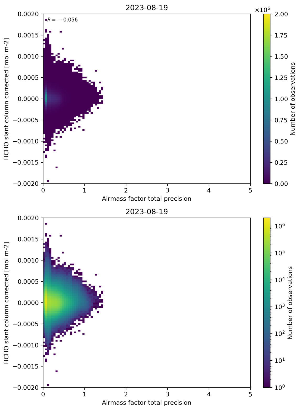
Figure 109: Scatter density plot of “Airmass factor total precision” against “HCHO slant column corrected” for 2023-08-18 to 2023-08-20.
