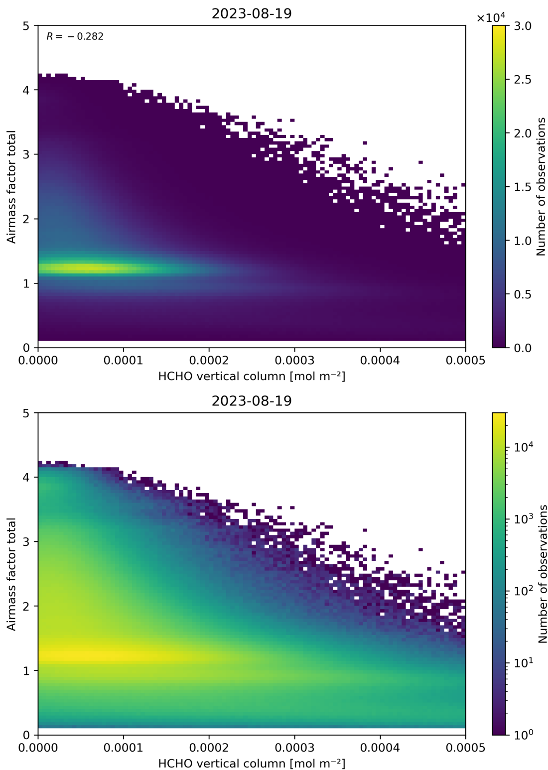
Figure 131: Scatter density plot of “HCHO vertical column” against “Airmass factor total” for 2023-08-18 to 2023-08-20.
