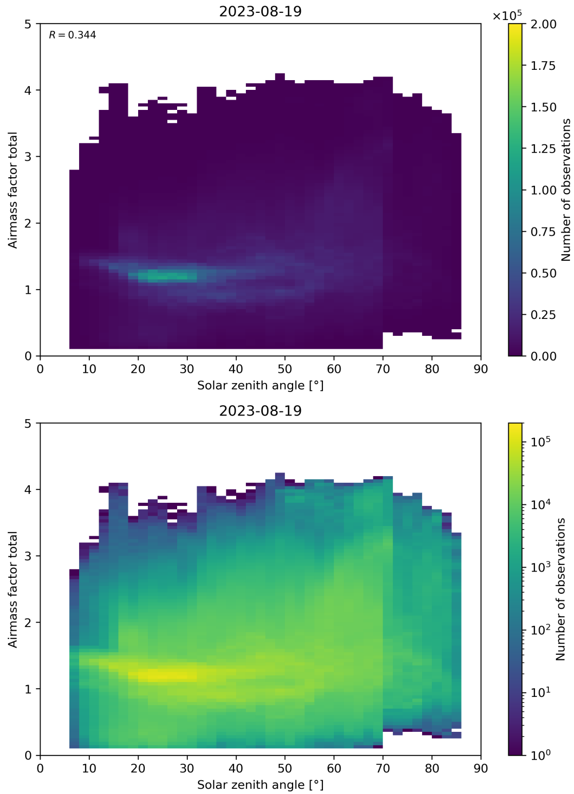
Figure 175: Scatter density plot of “Solar zenith angle” against “Airmass factor total” for 2023-08-18 to 2023-08-20.
