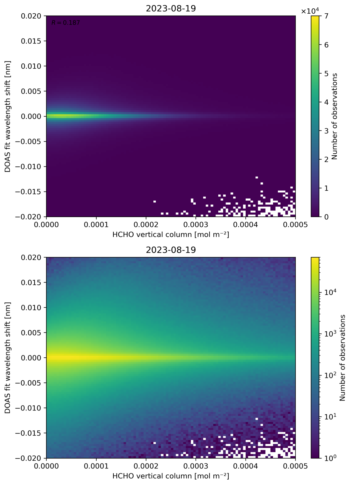
Figure 124: Scatter density plot of “HCHO vertical column” against “DOAS fit wavelength shift” for 2023-08-18 to 2023-08-20.
