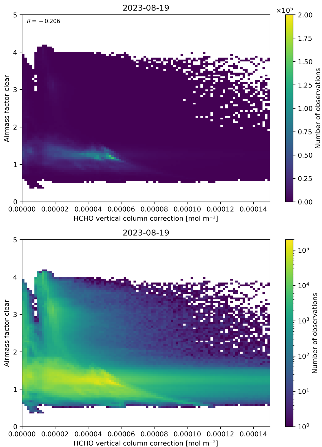
Figure 115: Scatter density plot of “HCHO vertical column correction” against “Airmass factor clear” for 2023-08-18 to 2023-08-20.
