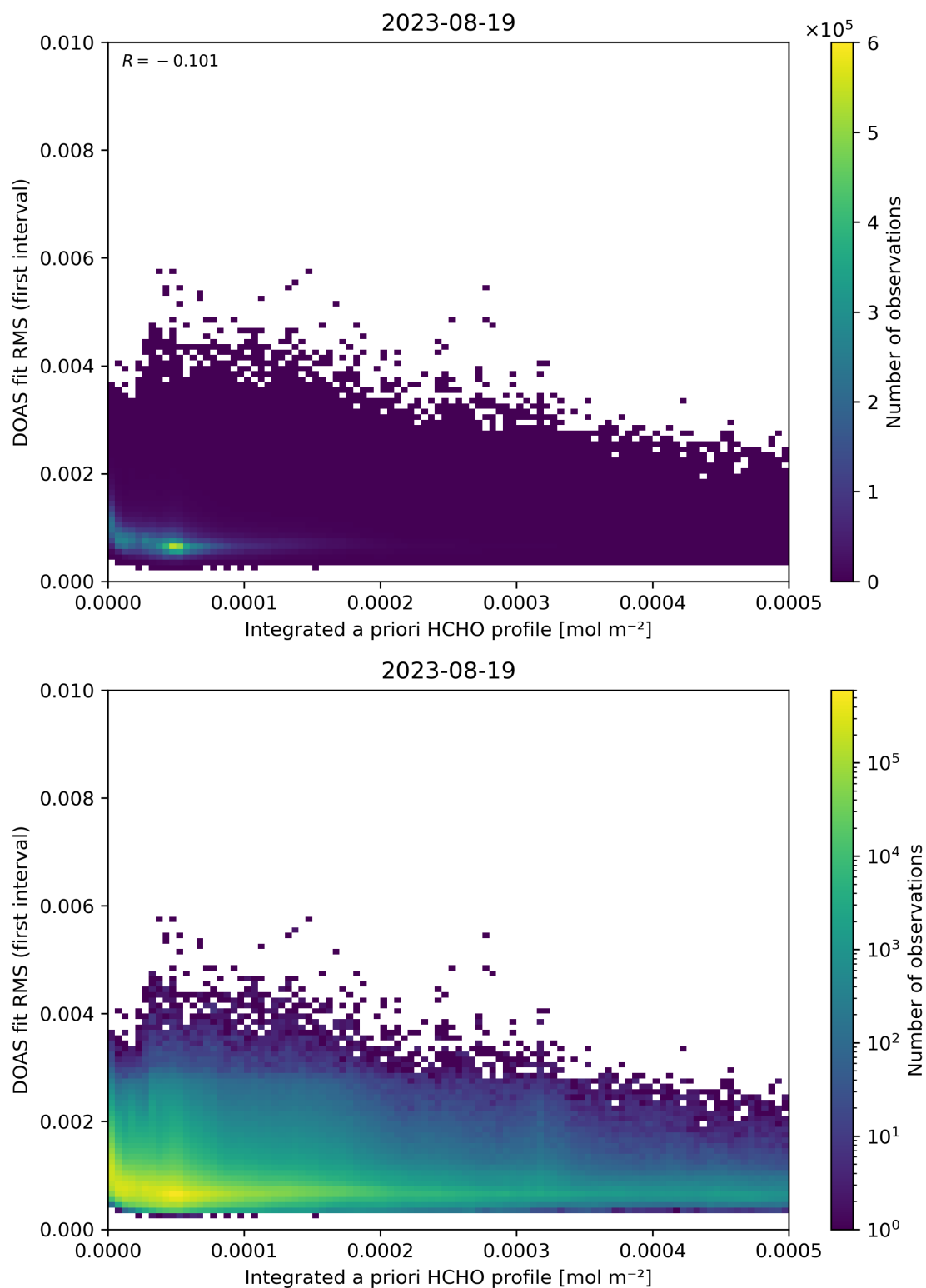
Figure 148: Scatter density plot of “Integrated a priori HCHO profile” against “DOAS fit RMS (first interval)” for 2023-08-18 to 2023-08-20.
