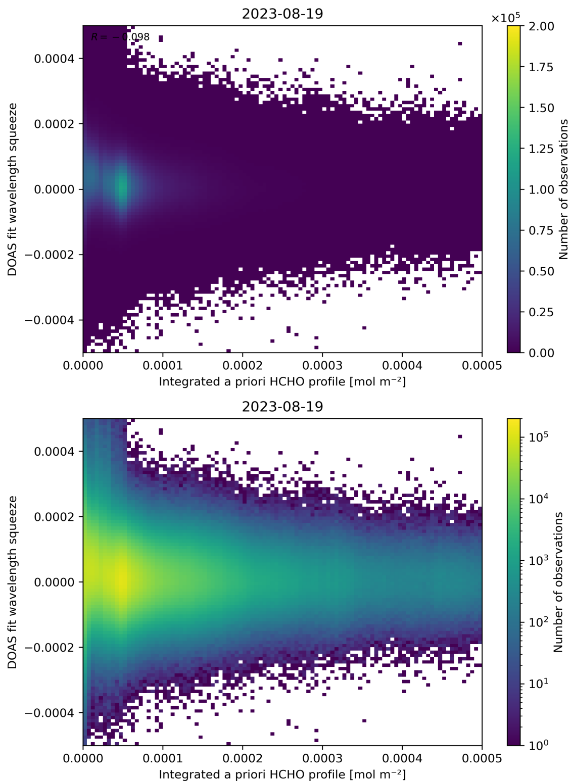
Figure 150: Scatter density plot of “Integrated a priori HCHO profile” against “DOAS fit wavelength squeeze” for 2023-08-18 to 2023-08-20.
