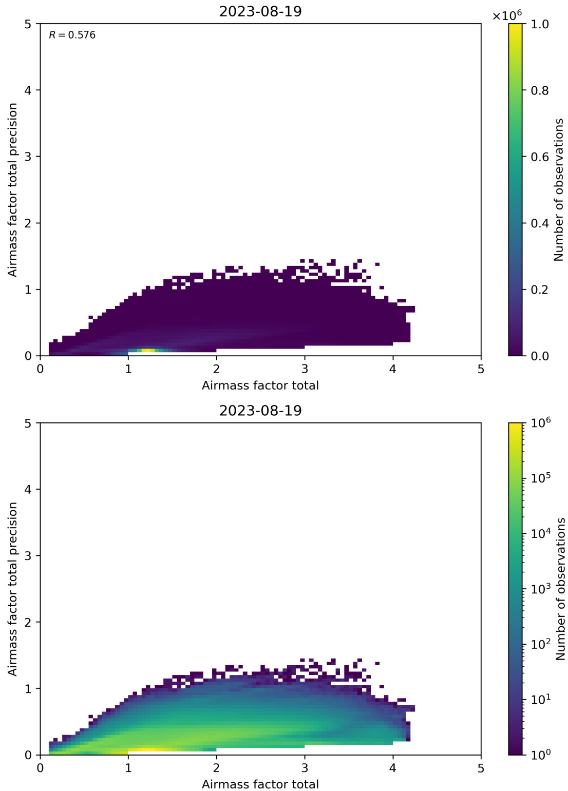
Figure 103: Scatter density plot of “Airmass factor total” against “Airmass factor total precision” for 2023-08-18 to 2023-08-20.
