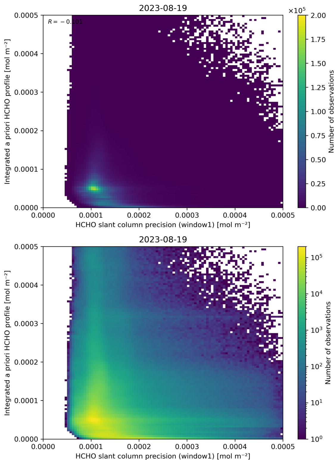
Figure 96: Scatter density plot of “HCHO slant column precision (window1)” against “Integrated a priori HCHO profile” for 2023-08-18 to 2023-08-20.
