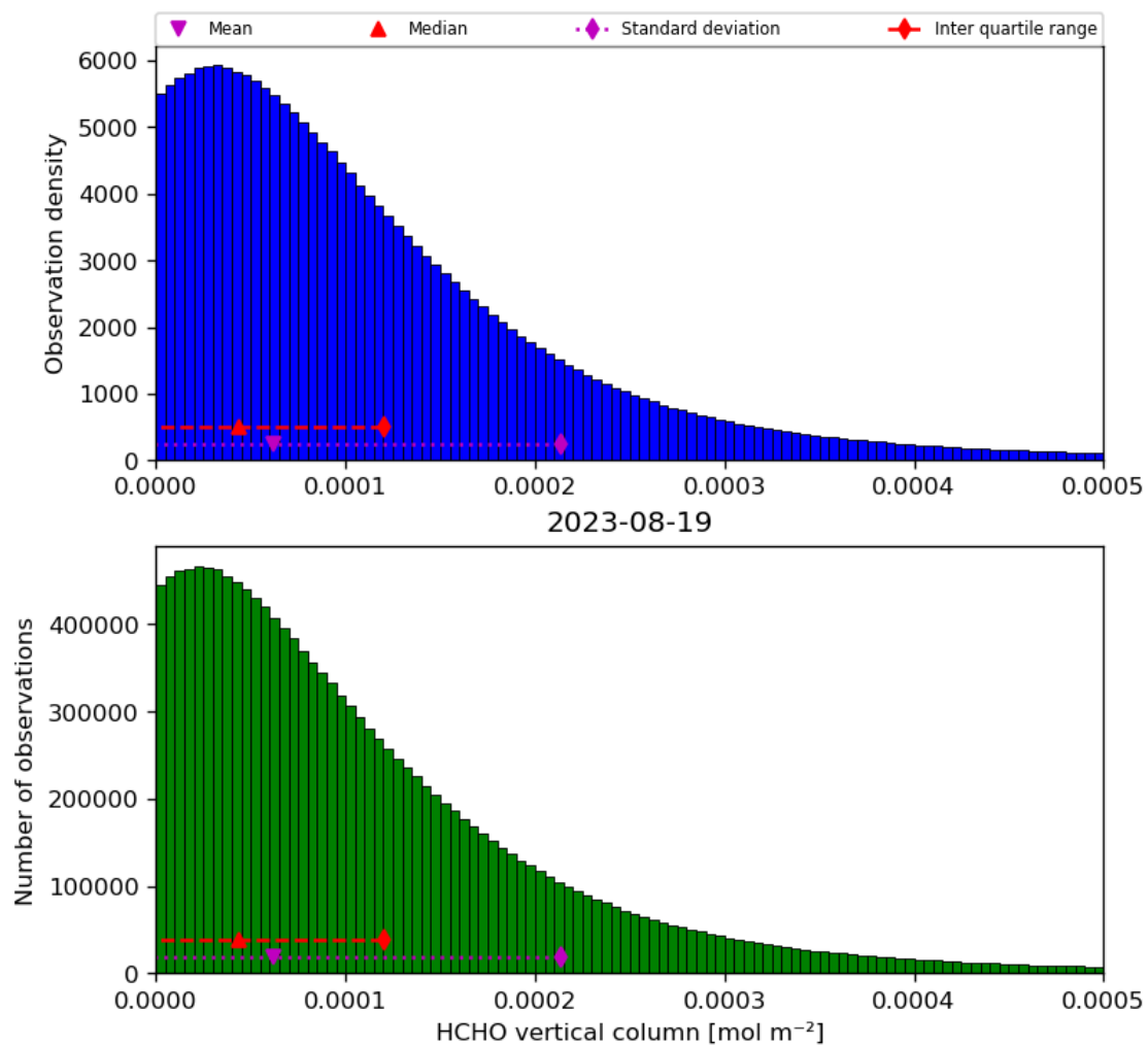
Figure 35: Histogram of “HCHO vertical column” for 2023-08-18 to 2023-08-20
