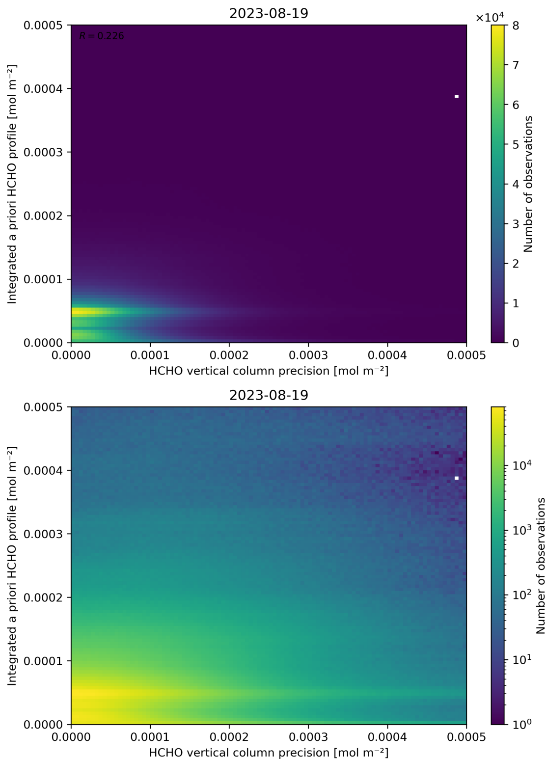
Figure 147: Scatter density plot of “HCHO vertical column precision” against “Integrated a priori HCHO profile” for 2023-08-18 to 2023-08-20.
