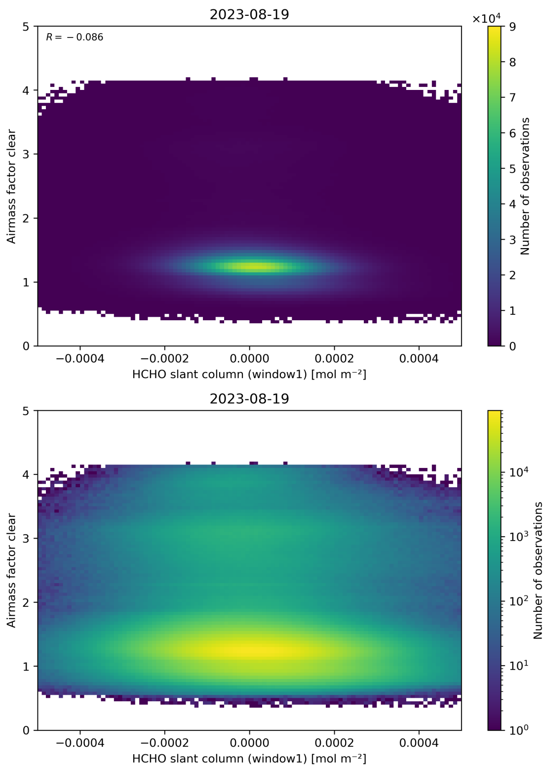
Figure 81: Scatter density plot of “HCHO slant column (window1)” against “Airmass factor clear” for 2023-08-18 to 2023-08-20.
