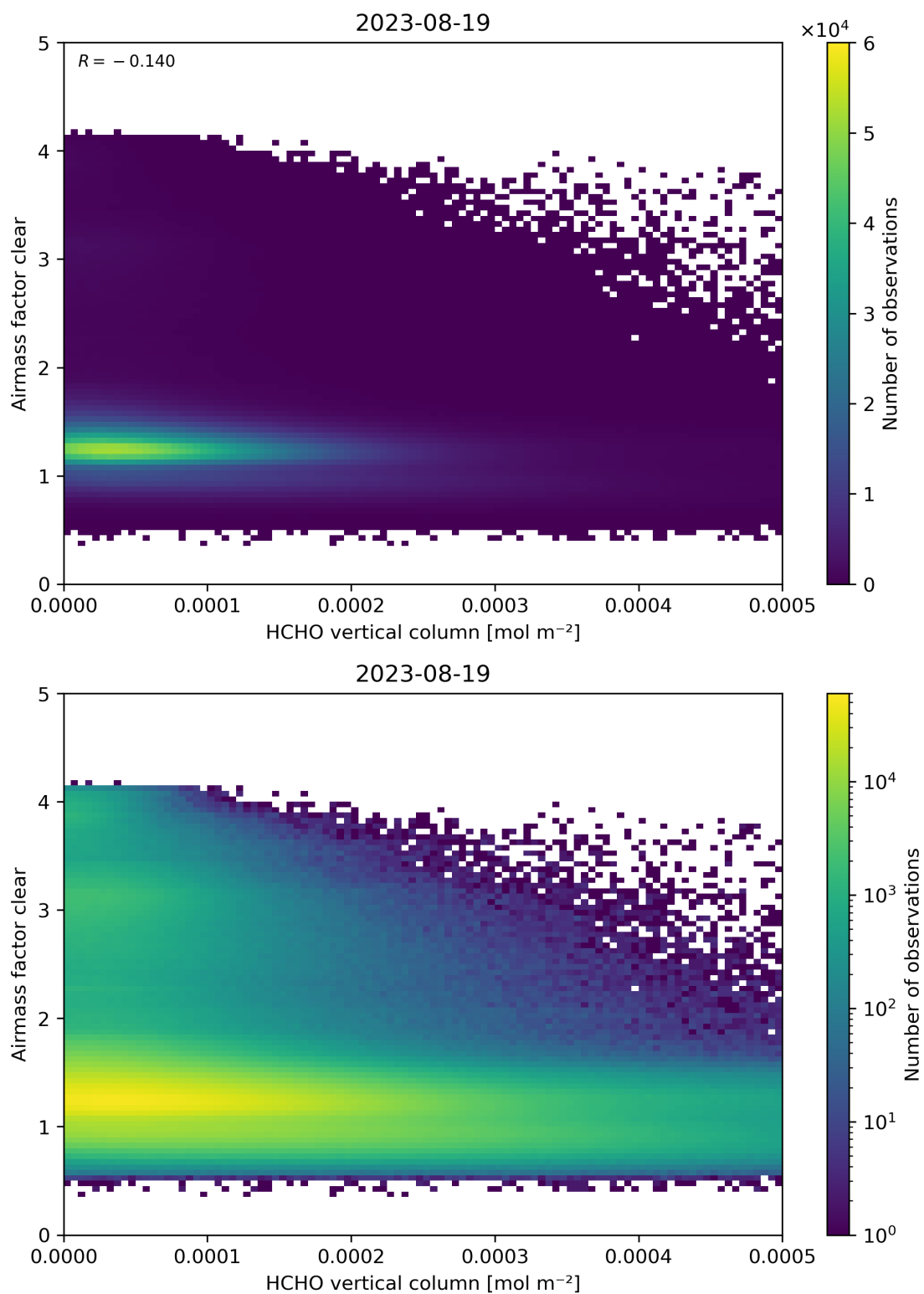
Figure 126: Scatter density plot of “HCHO vertical column” against “Airmass factor clear” for 2023-08-18 to 2023-08-20.
