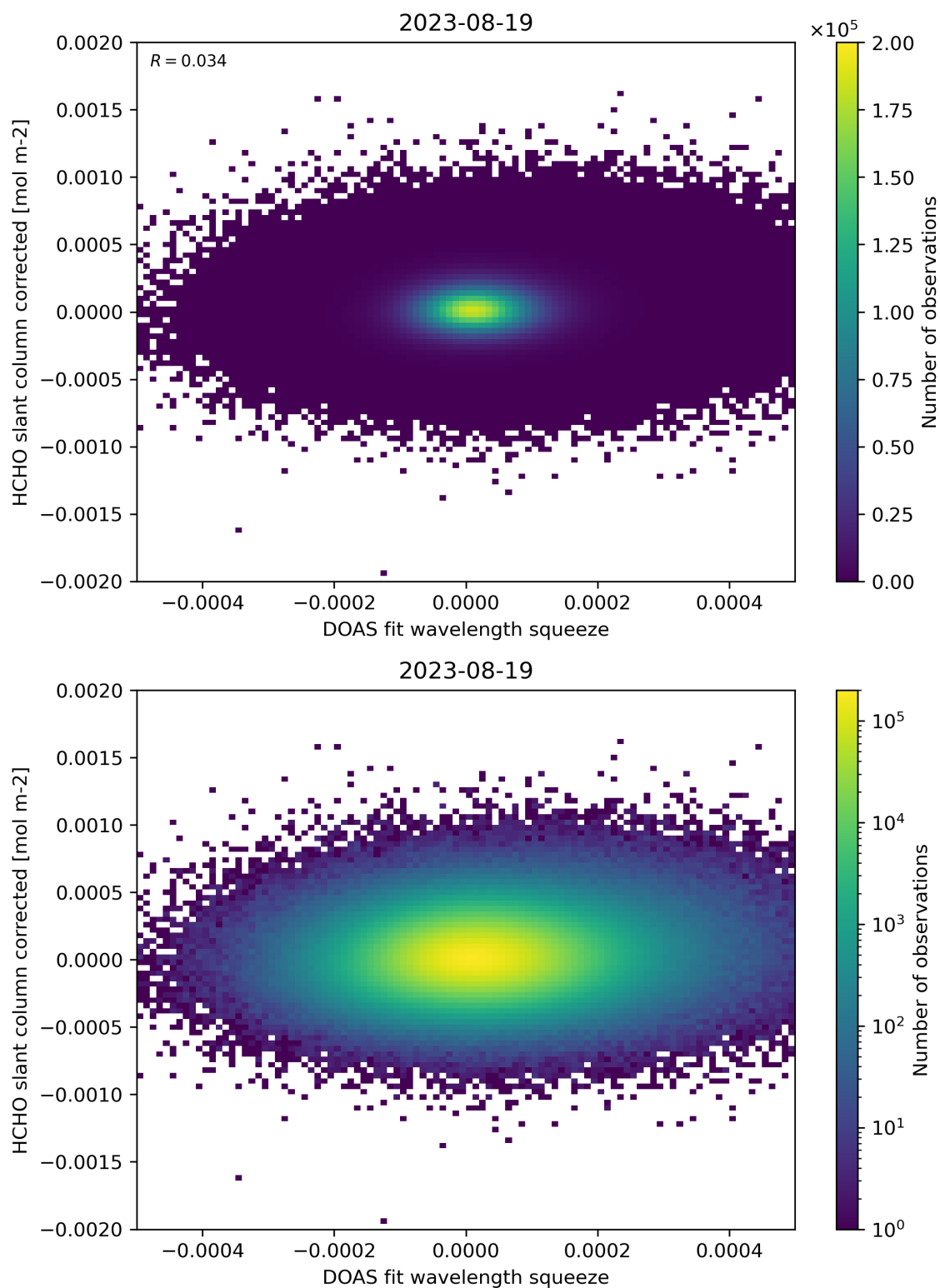
Figure 69: Scatter density plot of “DOAS fit wavelength squeeze” against “HCHO slant column corrected” for 2023-08-18 to 2023-08-20.
