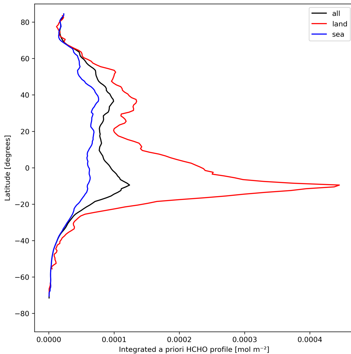
Figure 29: Zonal average of “Integrated a priori HCHO profile” for 2023-08-18 to 2023-08-20.
