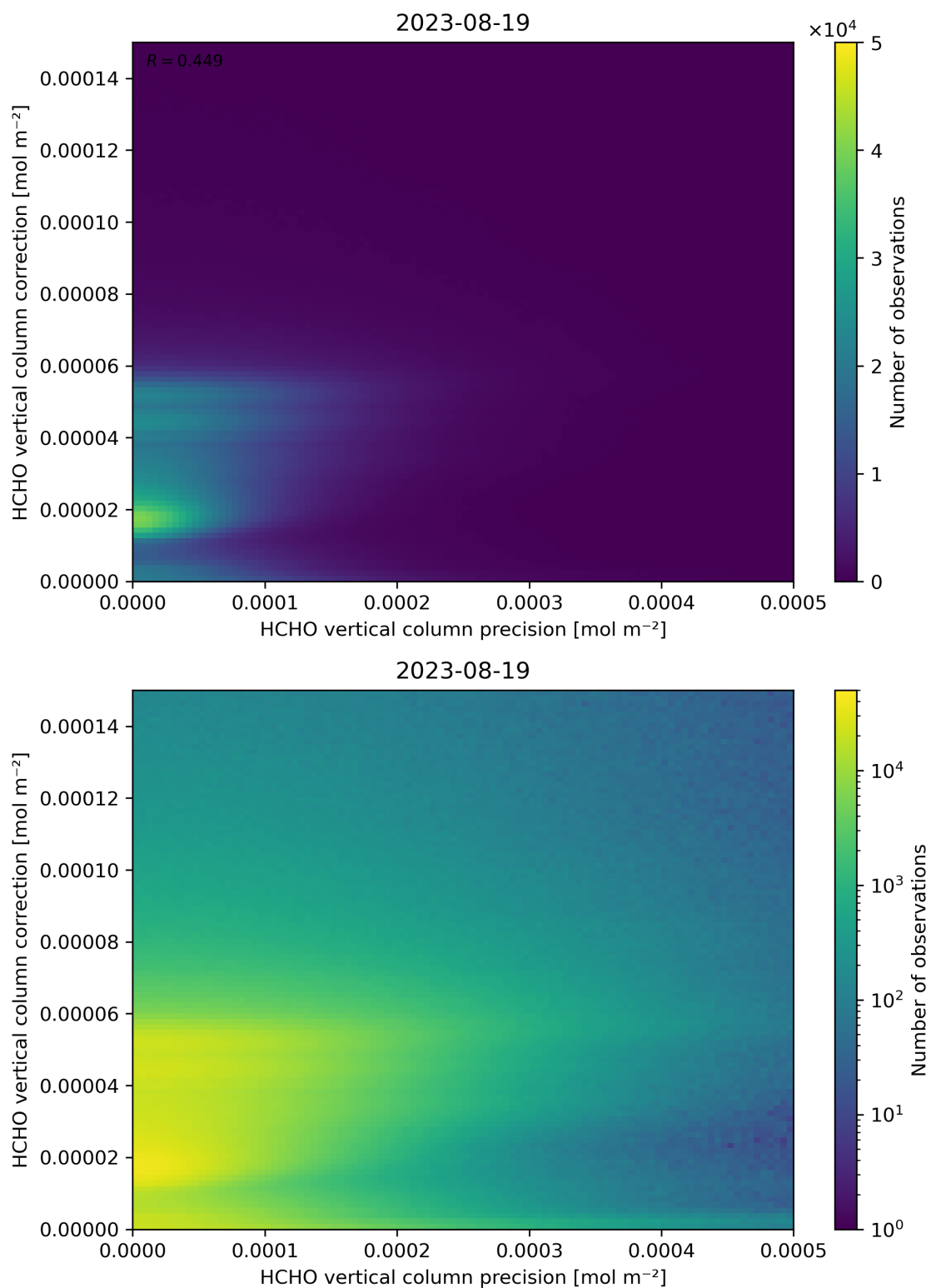
Figure 146: Scatter density plot of “HCHO vertical column precision” against “HCHO vertical column correction” for 2023-08-18 to 2023-08-20.
