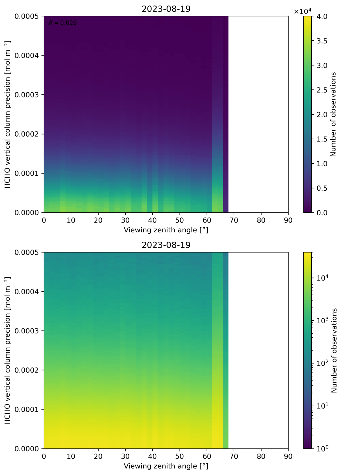
Figure 194: Scatter density plot of “Viewing zenith angle” against “HCHO vertical column precision” for 2023-08-18 to 2023-08-20.
