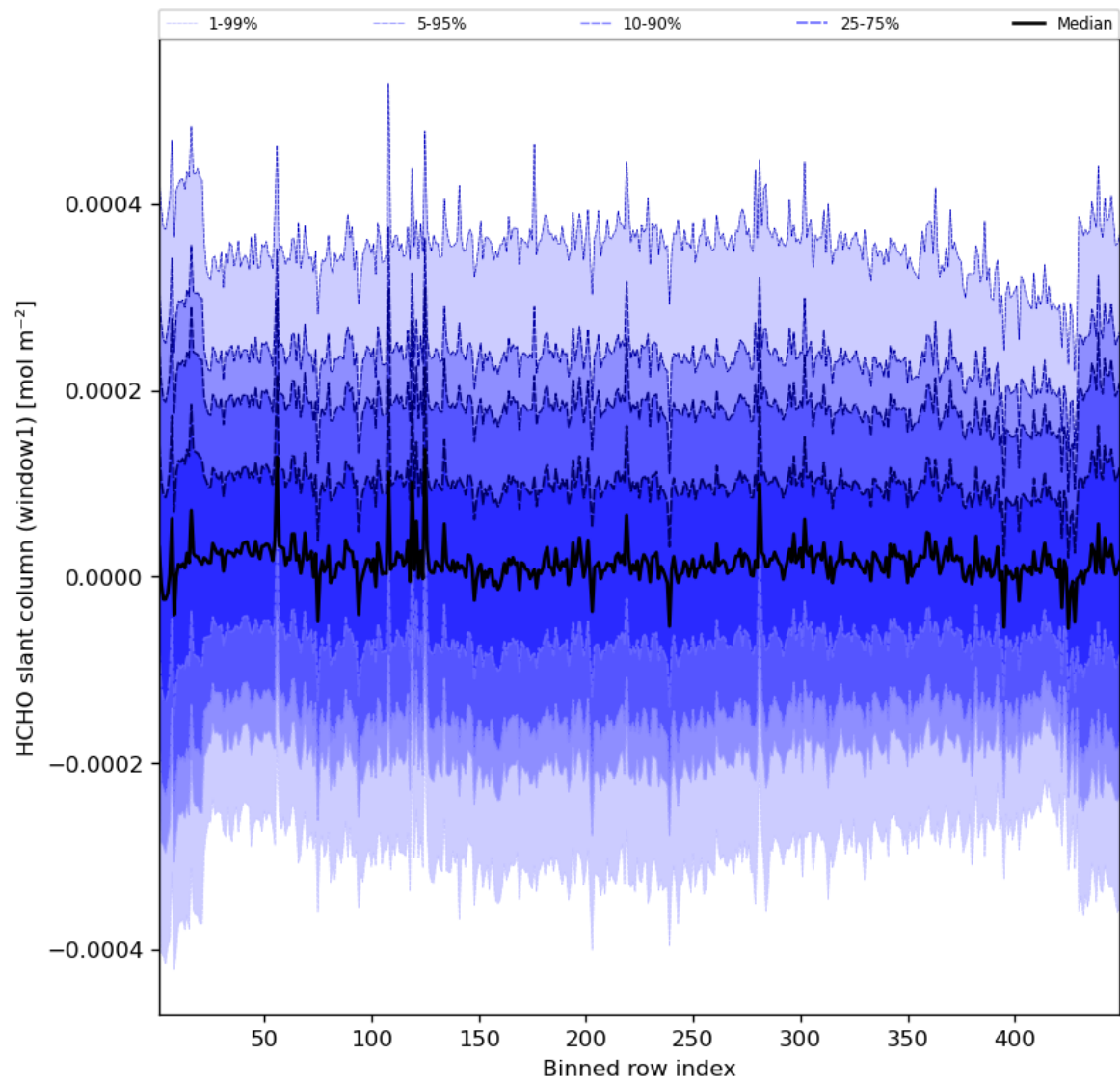
Figure 52: Along track statistics of “HCHO slant column (window1)” for 2023-08-18 to 2023-08-20
