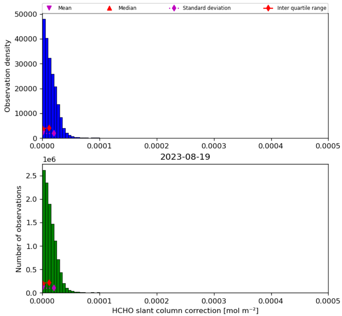
Figure 47: Histogram of “HCHO slant column correction” for 2023-08-18 to 2023-08-20
