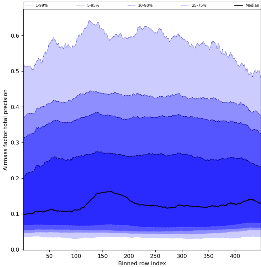
Figure 55: Along track statistics of “Airmass factor total precision” for 2023-08-18 to 2023-08-20
