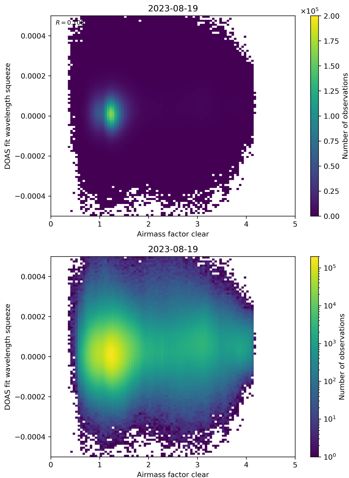
Figure 73: Scatter density plot of “Airmass factor clear” against “DOAS fit wavelength squeeze” for 2023-08-18 to 2023-08-20.
