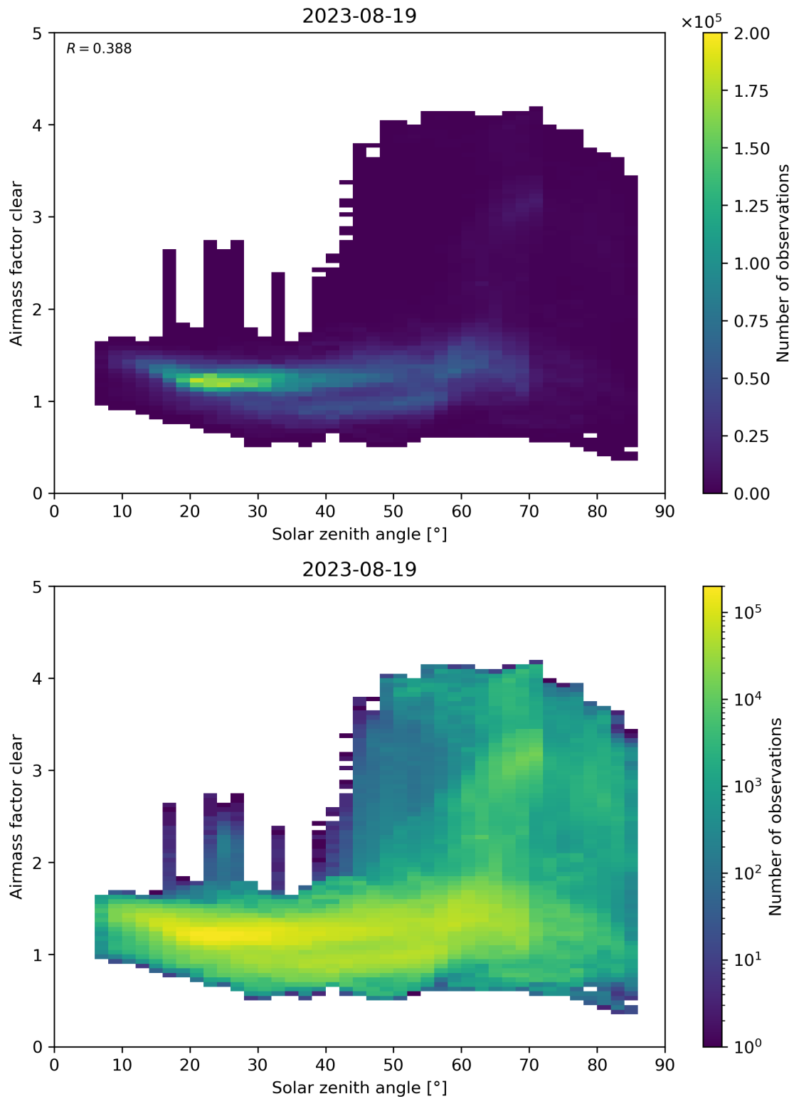
Figure 170: Scatter density plot of “Solar zenith angle” against “Airmass factor clear” for 2023-08-18 to 2023-08-20.
