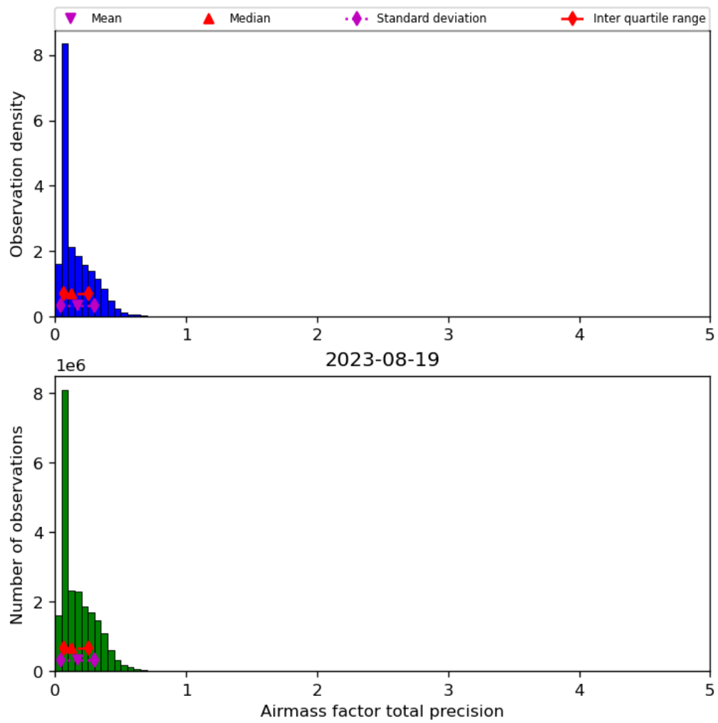
Figure 41: Histogram of “Airmass factor total precision” for 2023-08-18 to 2023-08-20
