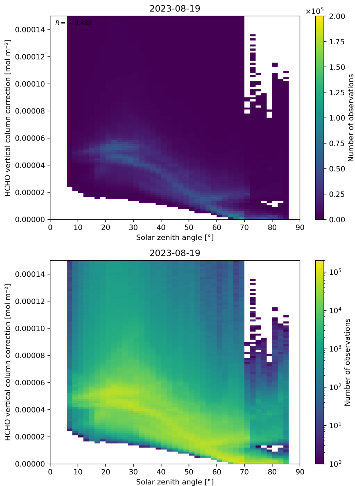
Figure 178: Scatter density plot of “Solar zenith angle” against “HCHO vertical column correction” for 2023-08-18 to 2023-08-20.
