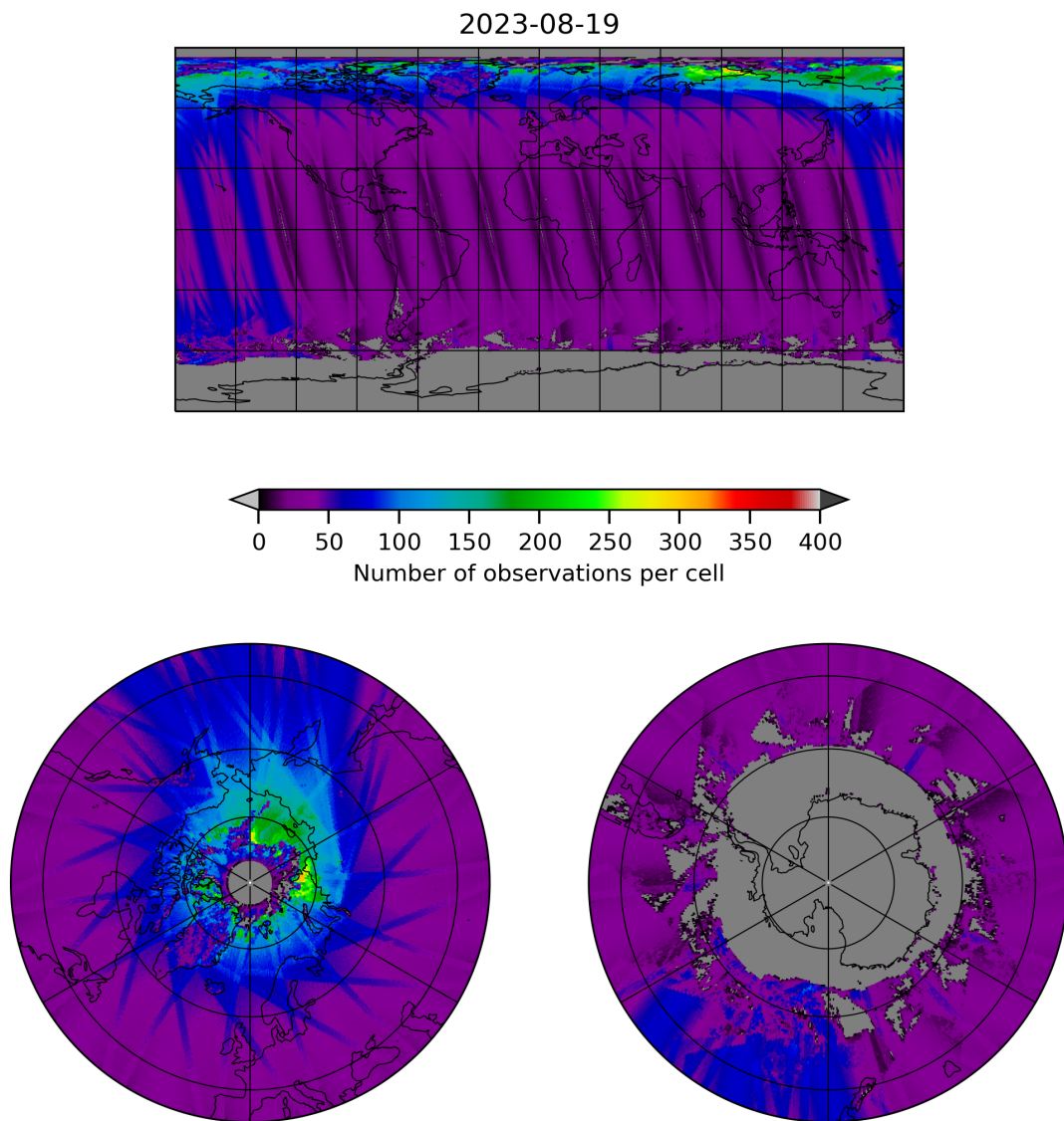
Figure 19: Map of the number of observations for 2023-08-18 to 2023-08-20
