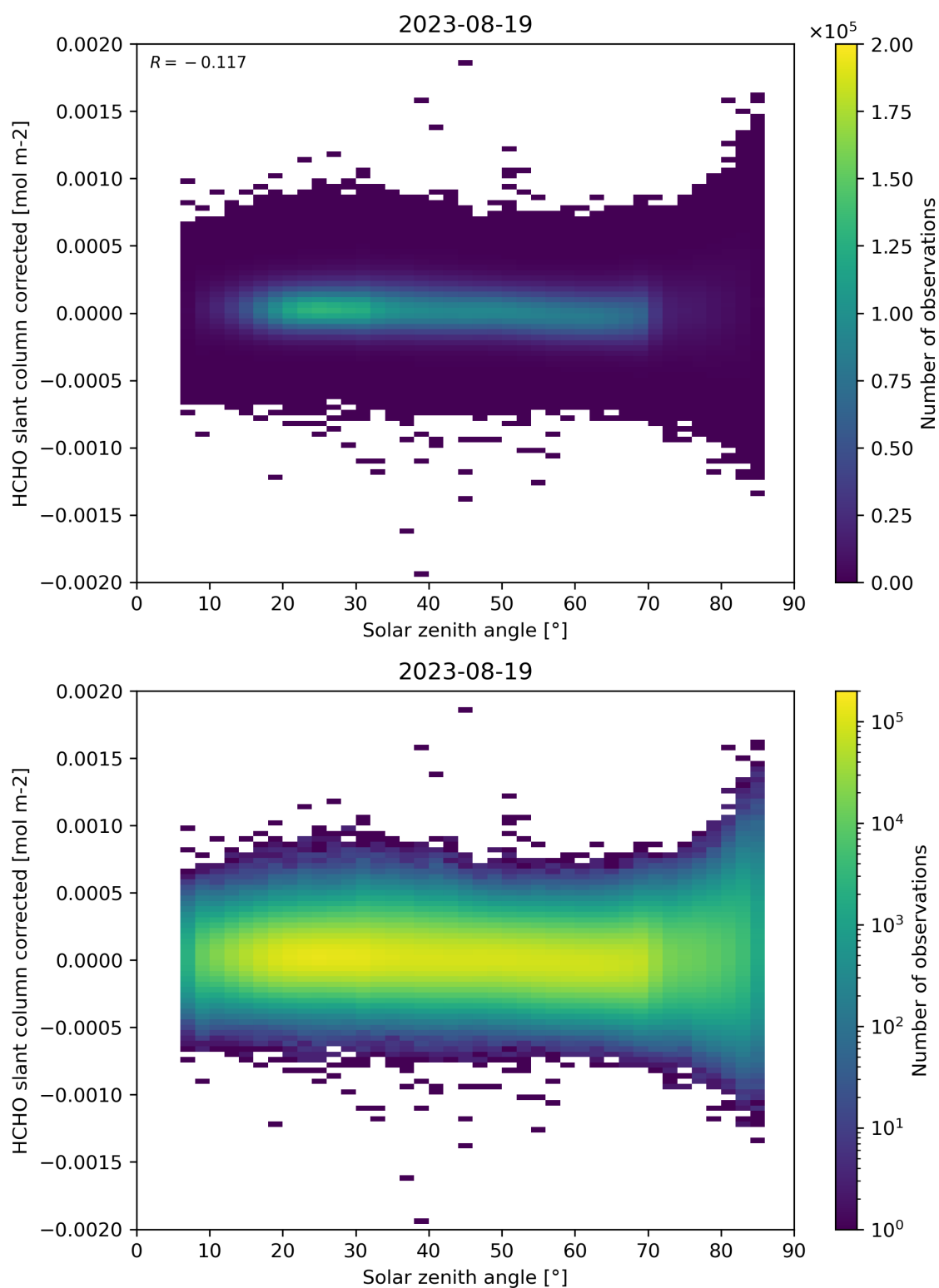
Figure 171: Scatter density plot of “Solar zenith angle” against “HCHO slant column corrected” for 2023-08-18 to 2023-08-20.
