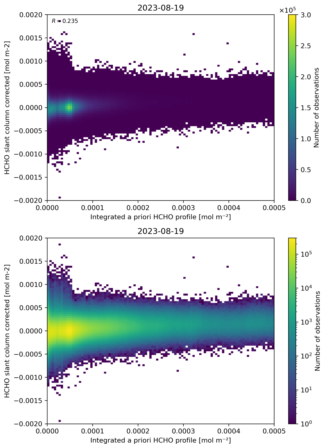
Figure 151: Scatter density plot of “Integrated a priori HCHO profile” against “HCHO slant column corrected” for 2023-08-18 to 2023-08-20.
