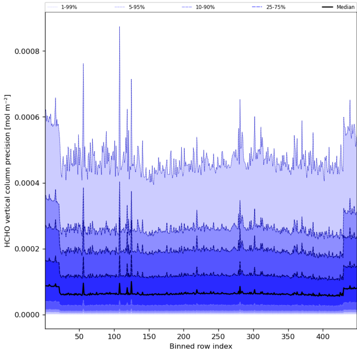
Figure 50: Along track statistics of "HCHO vertical column precision" for 2023-08-18 to 2023-08-20
