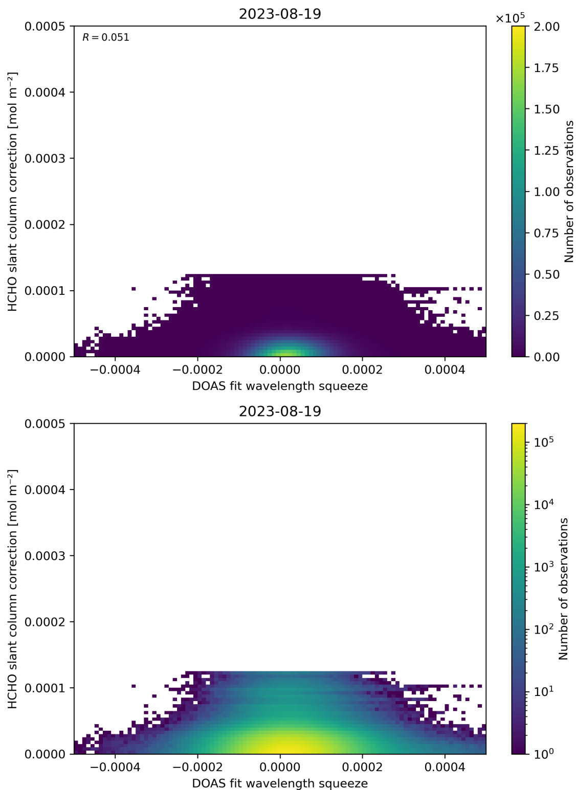
Figure 70: Scatter density plot of “DOAS fit wavelength squeeze” against “HCHO slant column correction” for 2023-08-18 to 2023-08-20.
