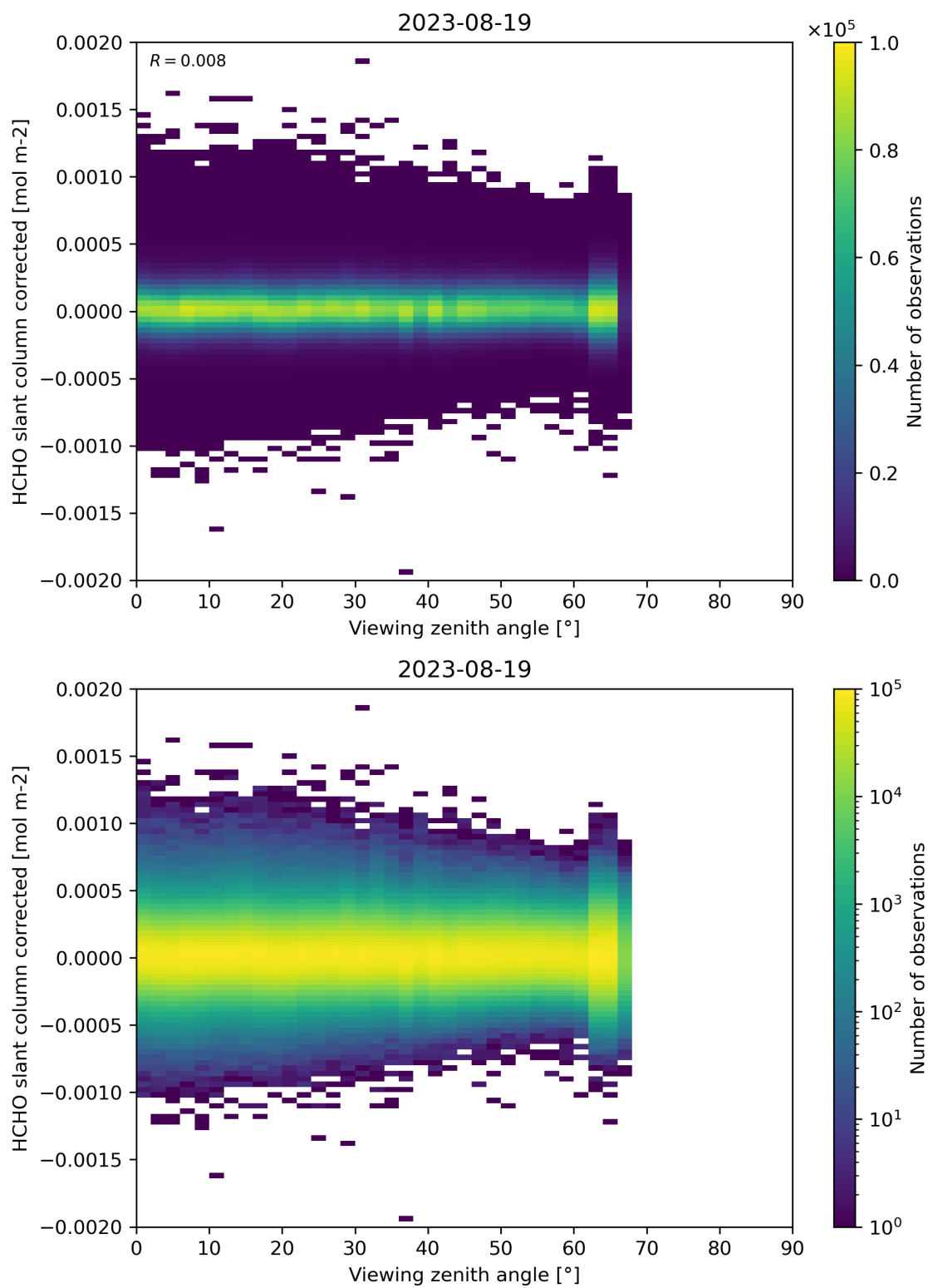
Figure 186: Scatter density plot of “Viewing zenith angle” against “HCHO slant column corrected” for 2023-08-18 to 2023-08-20.
