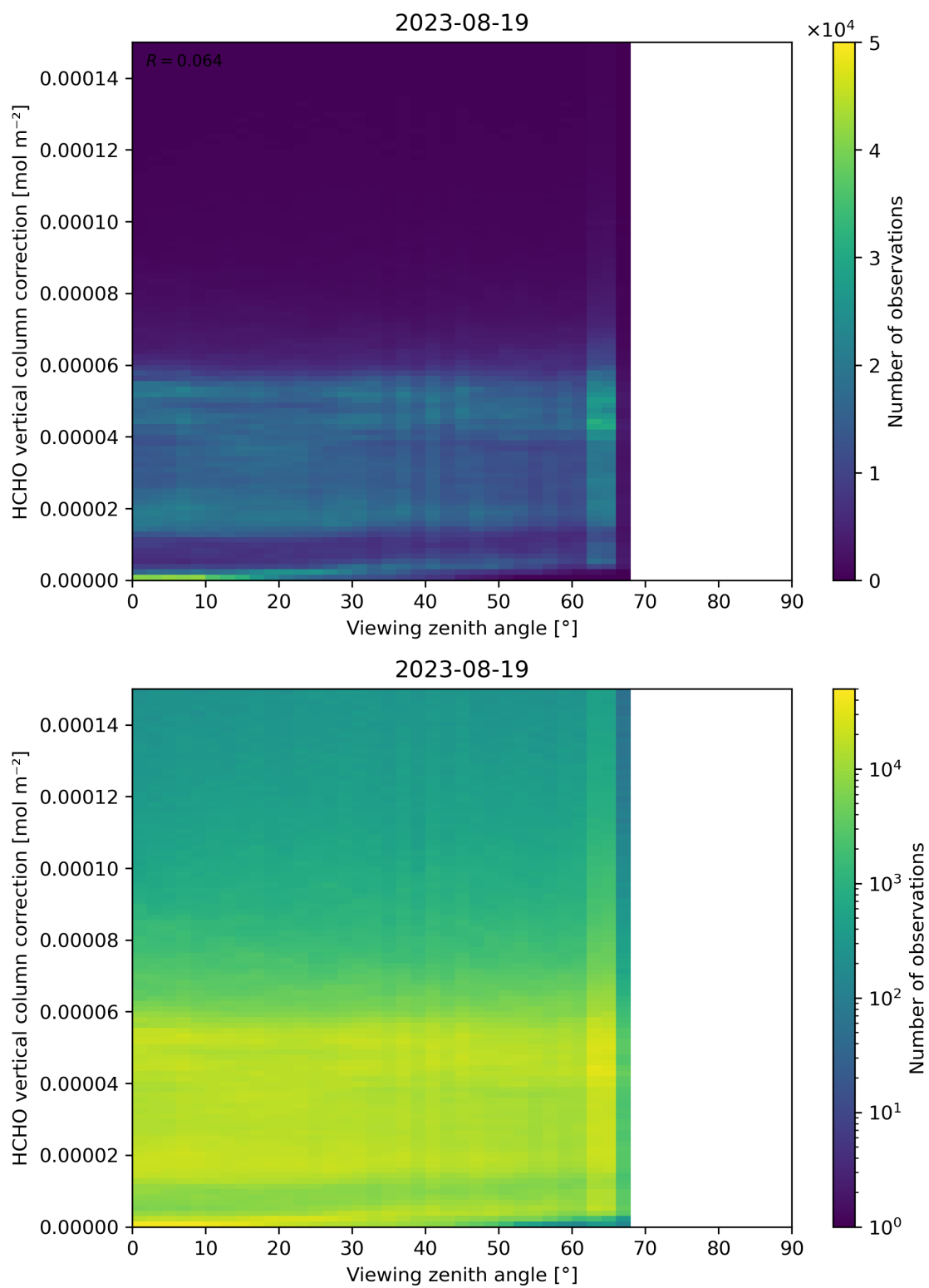
Figure 193: Scatter density plot of “Viewing zenith angle” against “HCHO vertical column correction” for 2023-08-18 to 2023-08-20.
