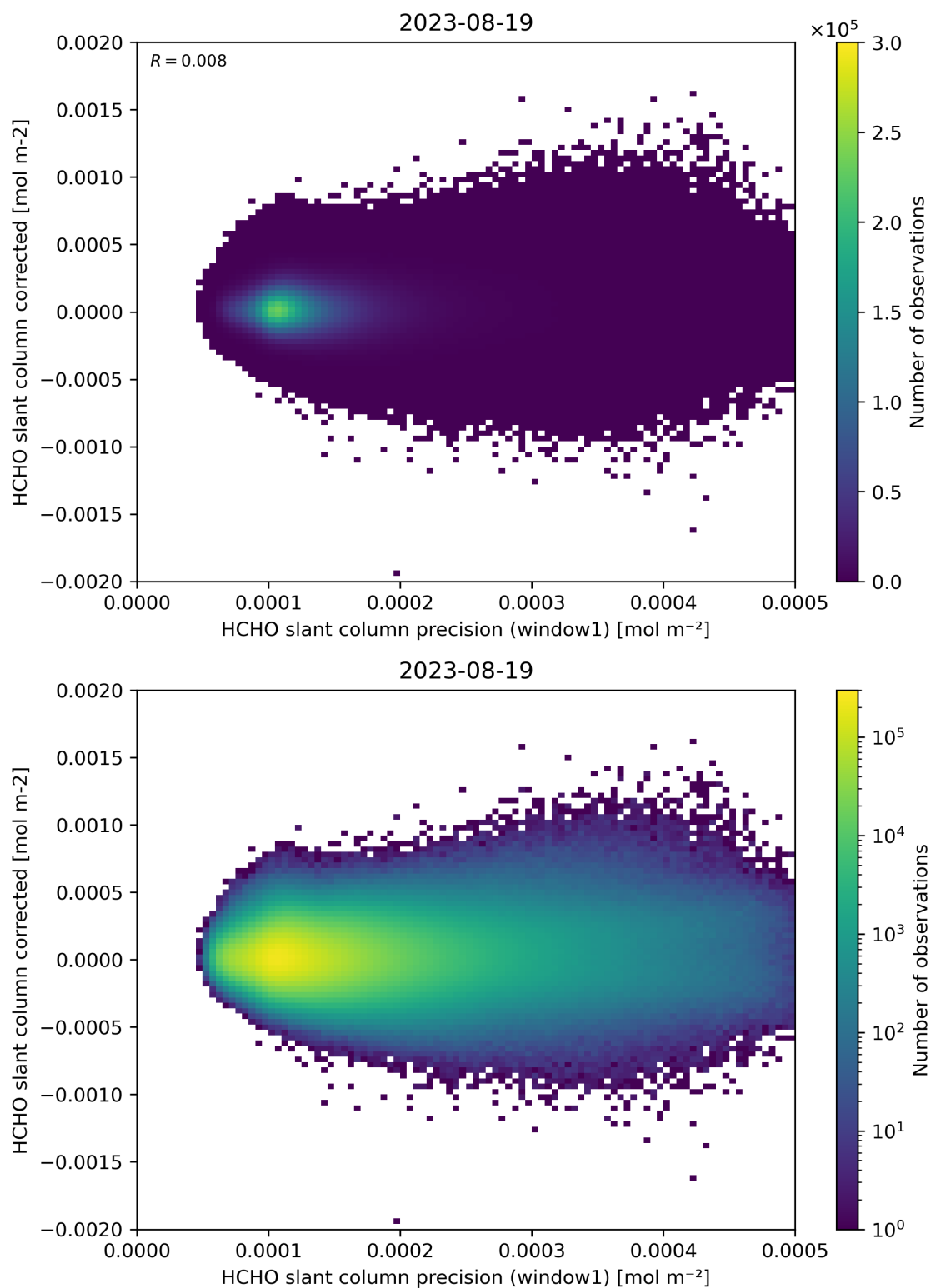
Figure 92: Scatter density plot of “HCHO slant column precision (window1)” against “HCHO slant column corrected” for 2023-08-18 to 2023-08-20.
