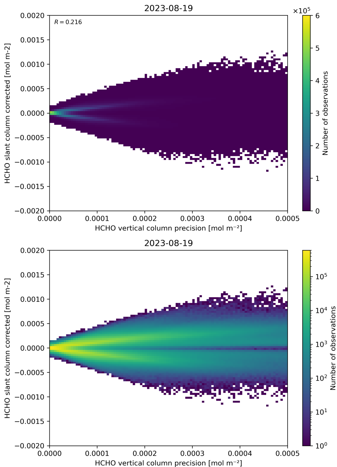
Figure 140: Scatter density plot of “HCHO vertical column precision” against “HCHO slant column corrected” for 2023-08-18 to 2023-08-20.
