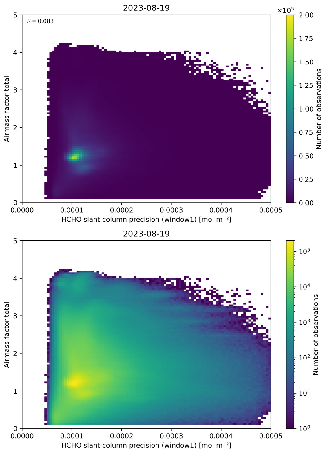
Figure 94: Scatter density plot of “HCHO slant column precision (window1)” against “Airmass factor total” for 2023-08-18 to 2023-08-20.
