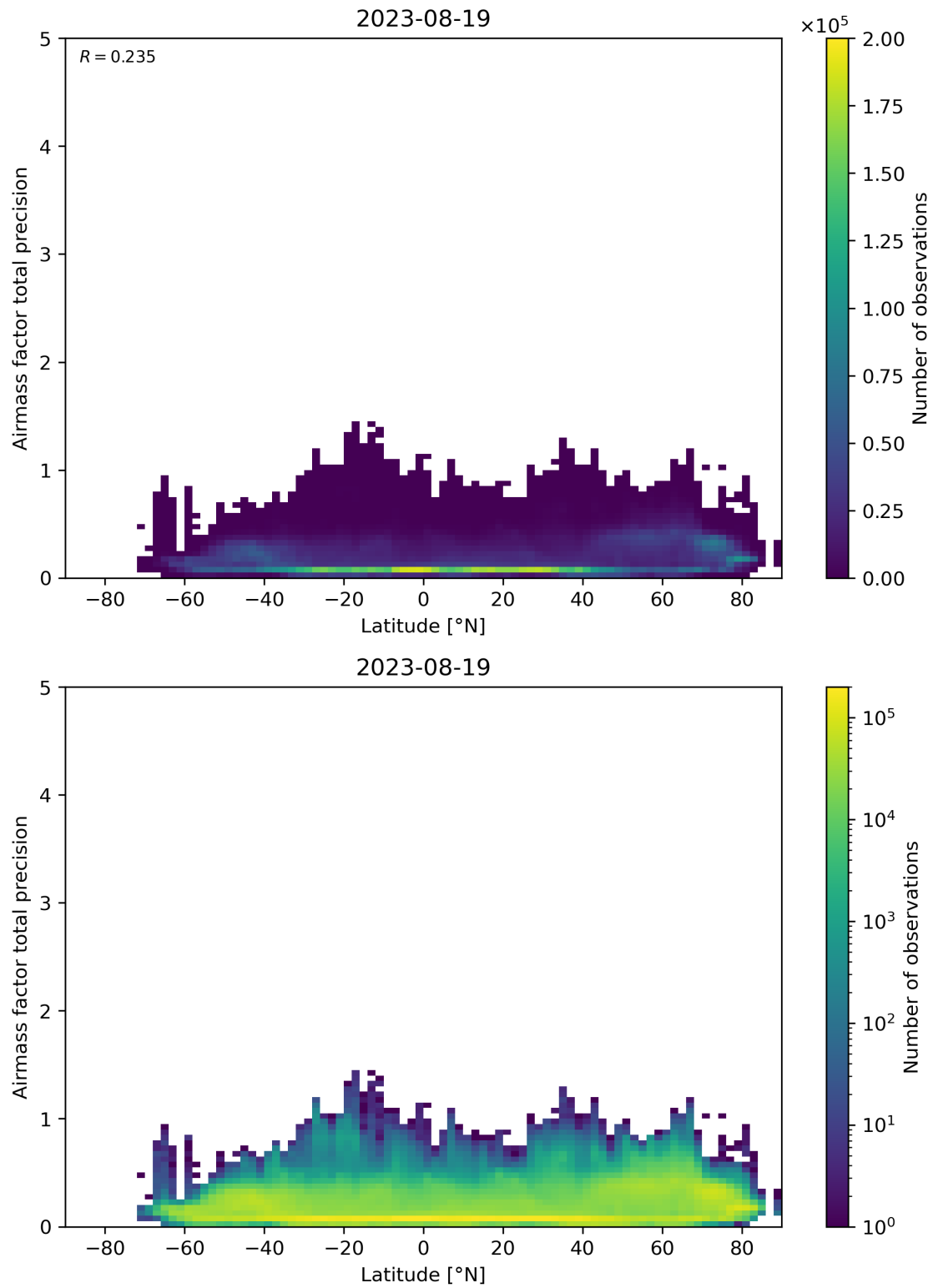
Figure 162: Scatter density plot of “Latitude” against “Airmass factor total precision” for 2023-08-18 to 2023-08-20.
