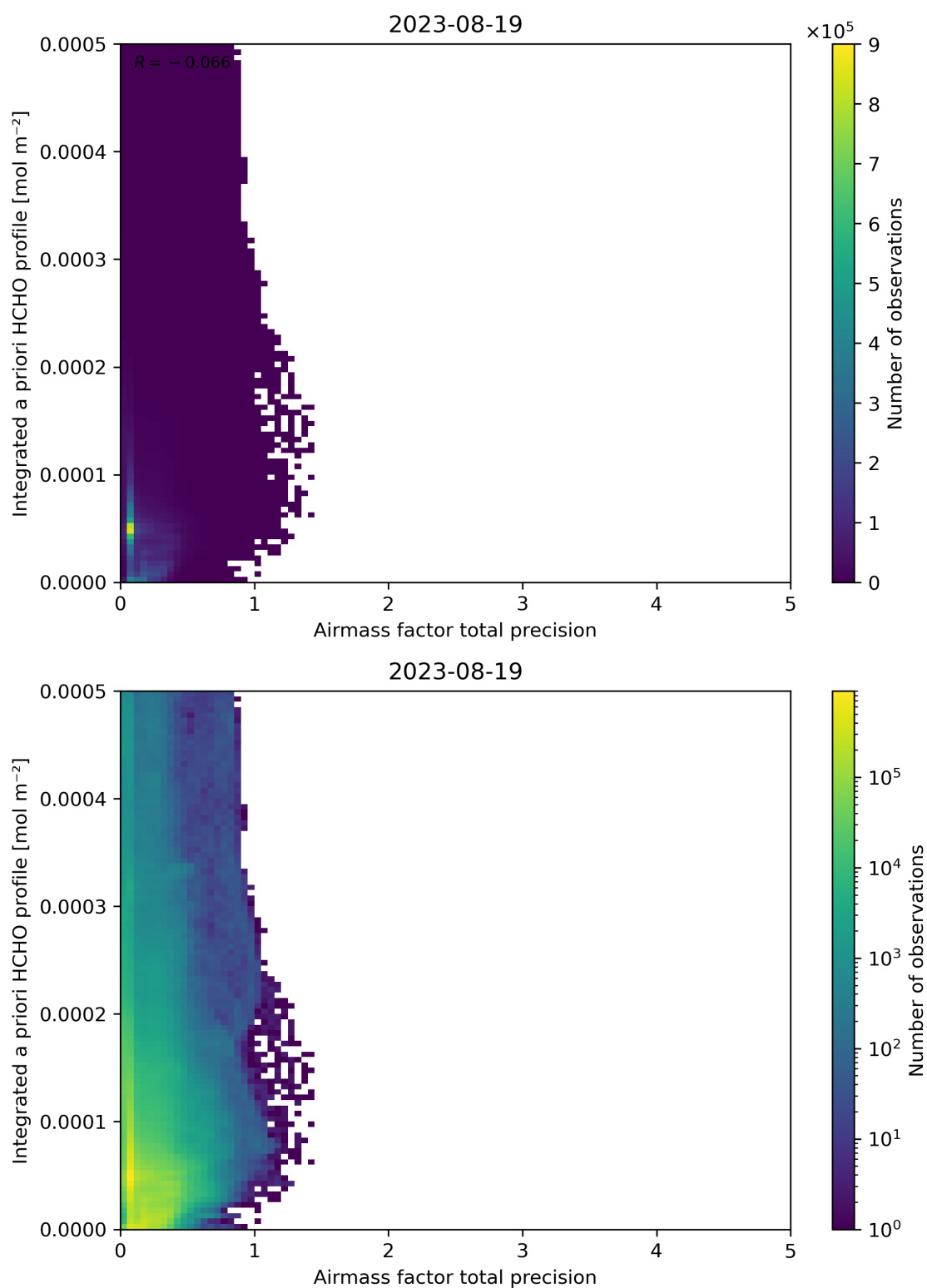
Figure 111: Scatter density plot of “Airmass factor total precision” against “Integrated a priori HCHO profile” for 2023-08-18 to 2023-08-20.
