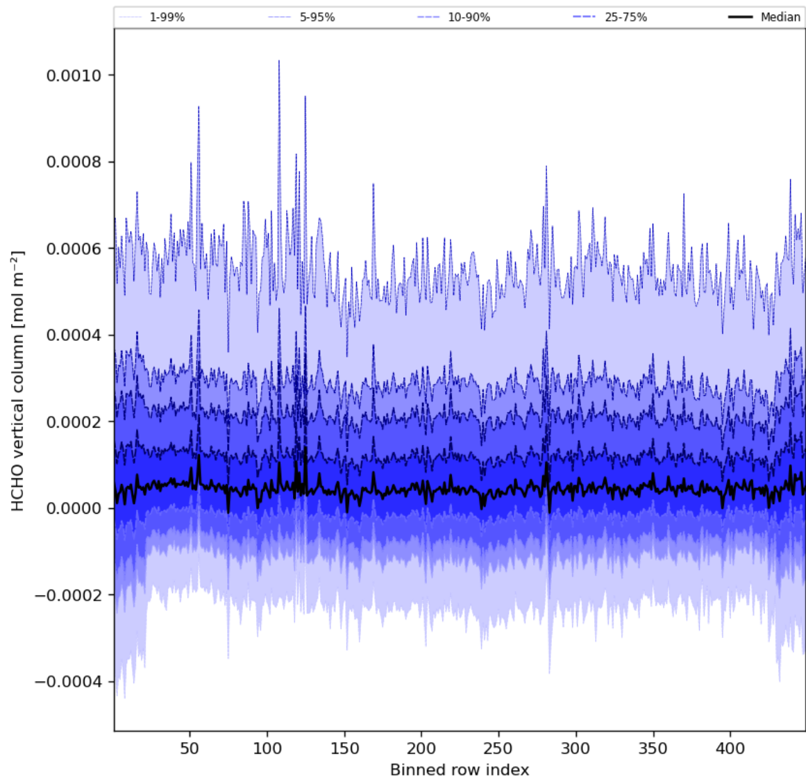
Figure 49: Along track statistics of “HCHO vertical column” for 2023-08-18 to 2023-08-20
