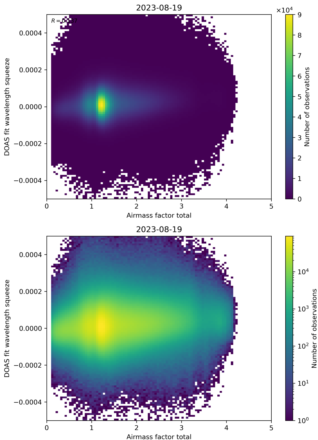
Figure 99: Scatter density plot of “Airmass factor total” against “DOAS fit wavelength squeeze” for 2023-08-18 to 2023-08-20.
