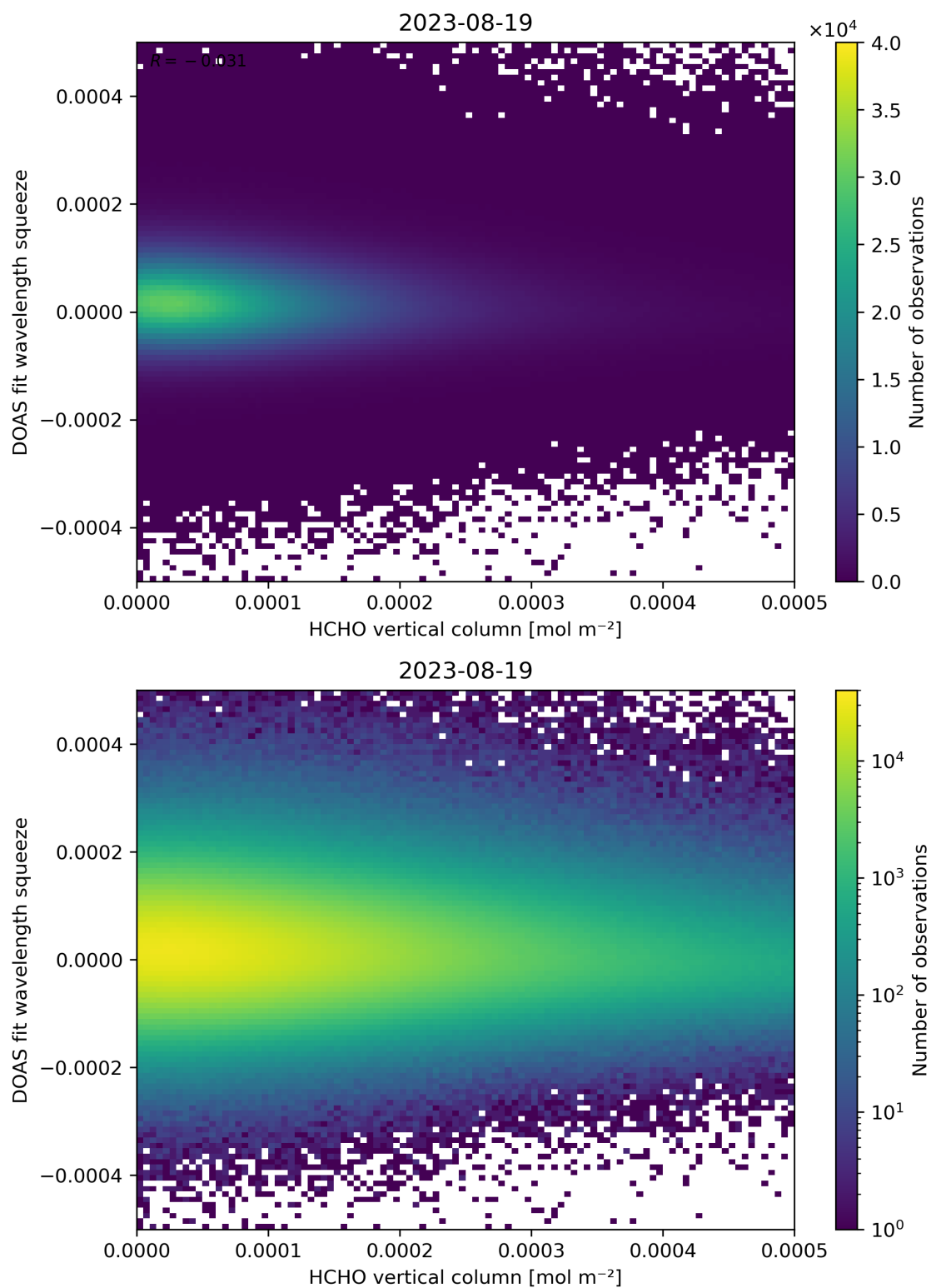
Figure 125: Scatter density plot of “HCHO vertical column” against “DOAS fit wavelength squeeze” for 2023-08-18 to 2023-08-20.
