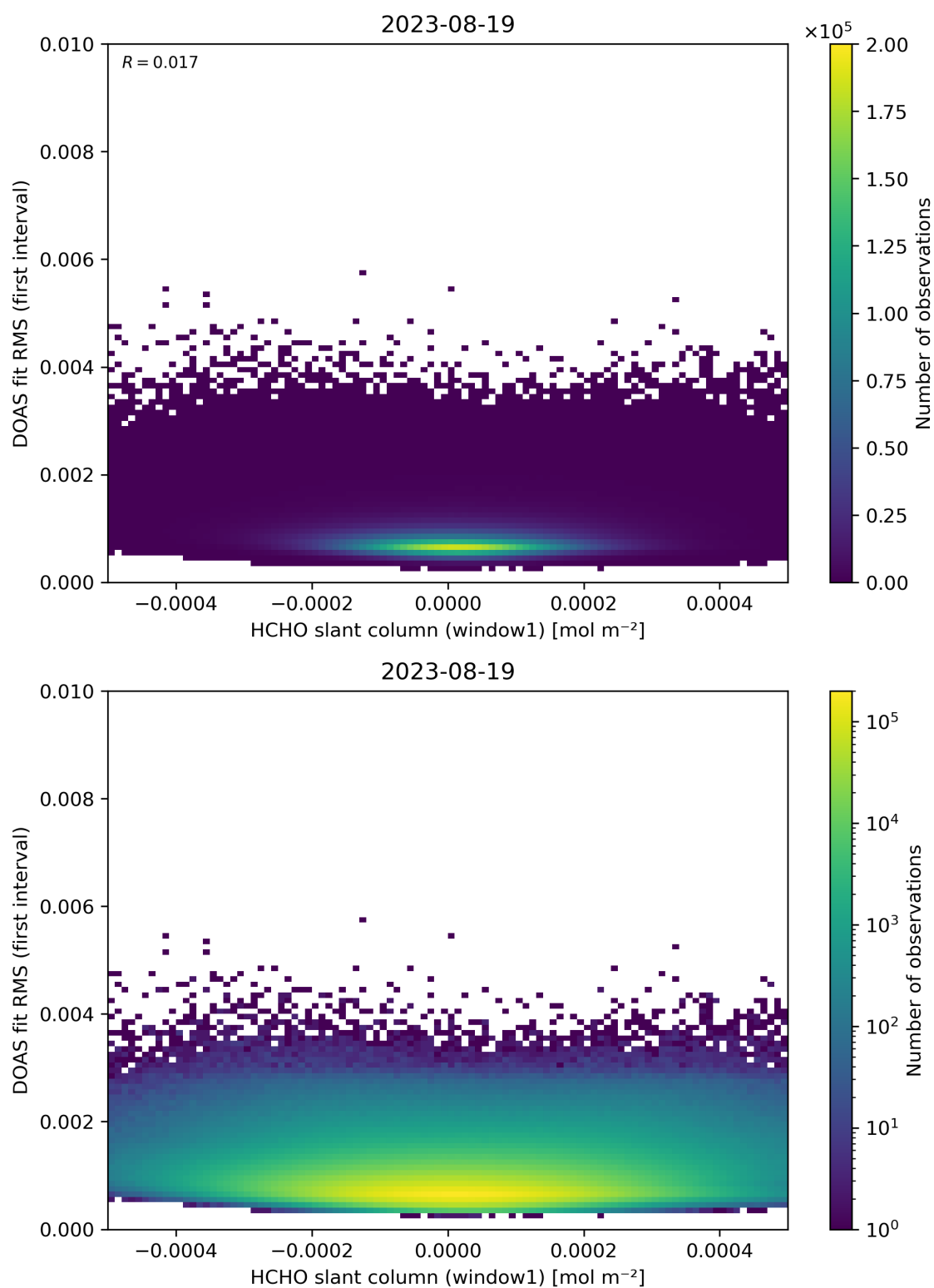
Figure 78: Scatter density plot of “HCHO slant column (window1)” against “DOAS fit RMS (first interval)” for 2023-08-18 to 2023-08-20.
