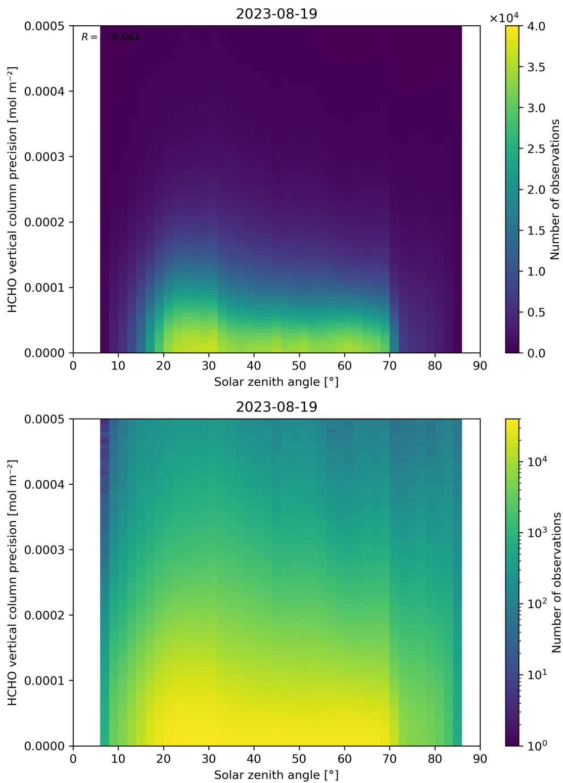
Figure 179: Scatter density plot of “Solar zenith angle” against “HCHO vertical column precision” for 2023-08-18 to 2023-08-20.
