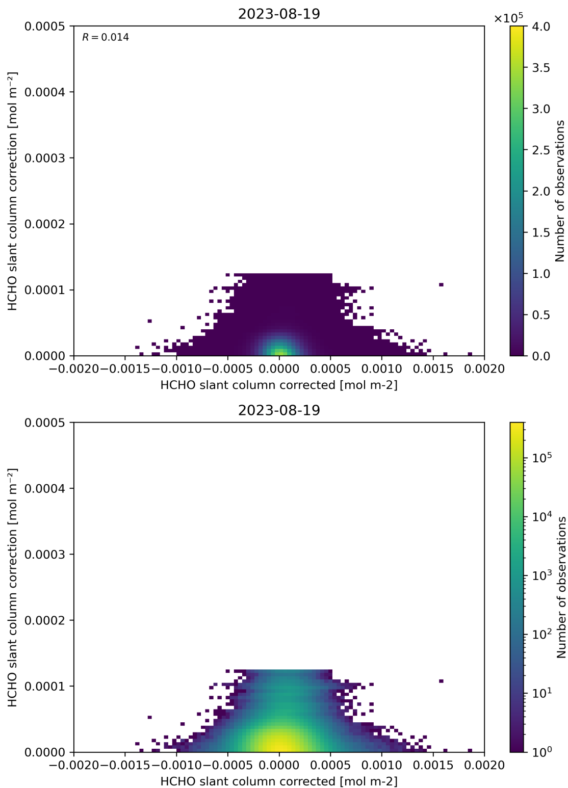
Figure 77: Scatter density plot of “HCHO slant column corrected” against “HCHO slant column correction” for 2023-08-18 to 2023-08-20.
