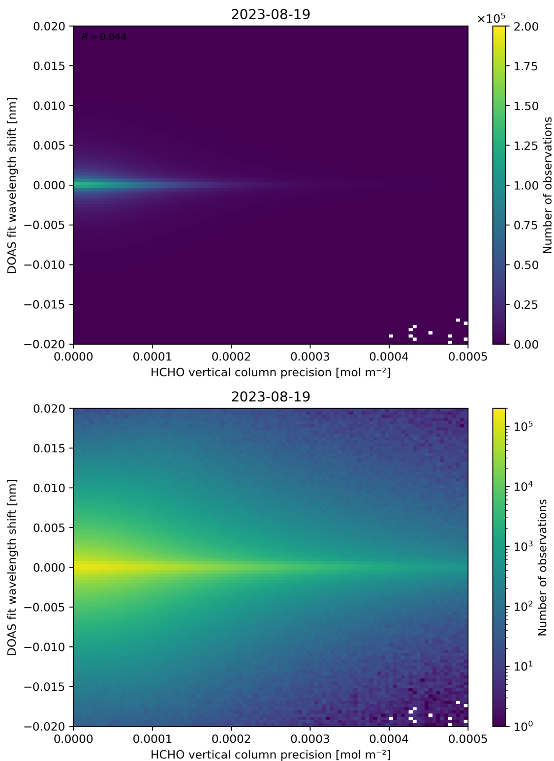
Figure 137: Scatter density plot of “HCHO vertical column precision” against “DOAS fit wavelength shift” for 2023-08-18 to 2023-08-20.
