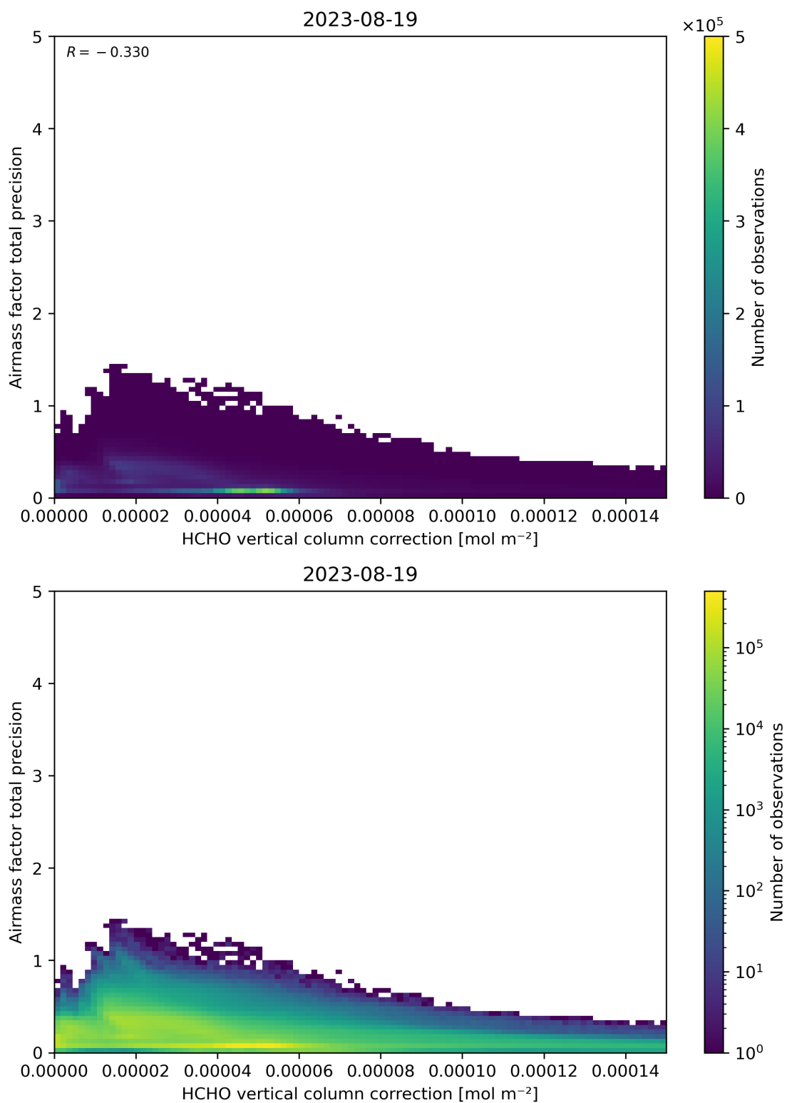
Figure 121: Scatter density plot of “HCHO vertical column correction” against “Airmass factor total precision” for 2023-08-18 to 2023-08-20.
