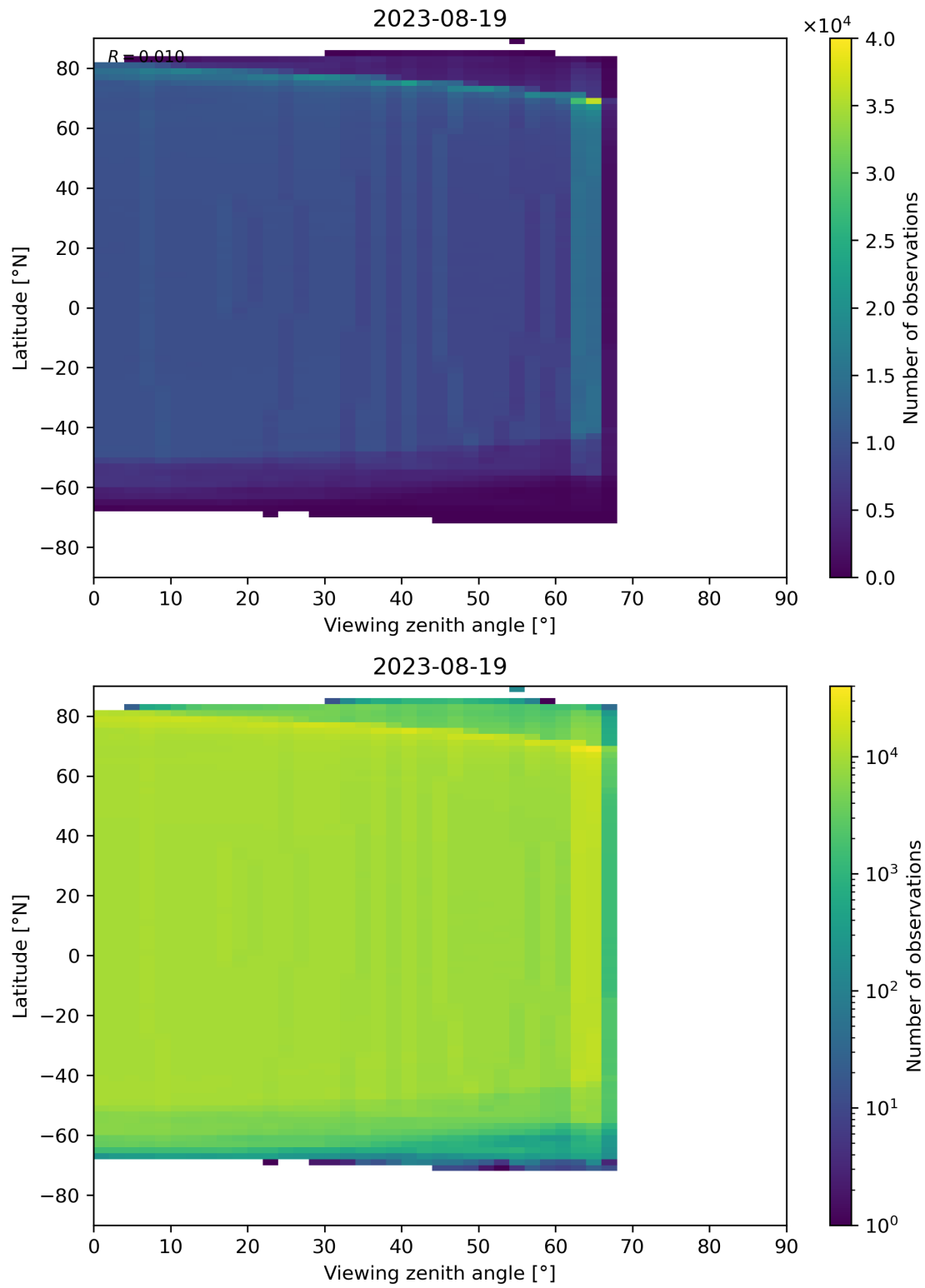
Figure 196: Scatter density plot of “Viewing zenith angle” against “Latitude” for 2023-08-18 to 2023-08-20.
