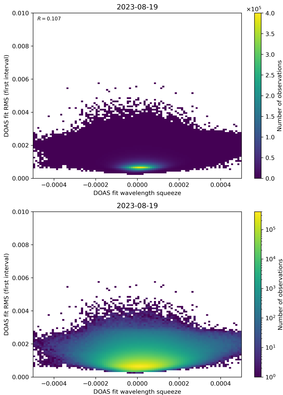
Figure 68: Scatter density plot of “DOAS fit wavelength squeeze” against “DOAS fit RMS (first interval)” for 2023-08-18 to 2023-08-20.
