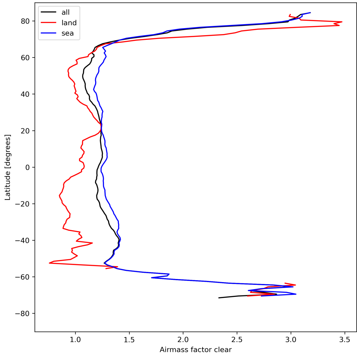
Figure 28: Zonal average of “Airmass factor clear” for 2023-08-18 to 2023-08-20.
