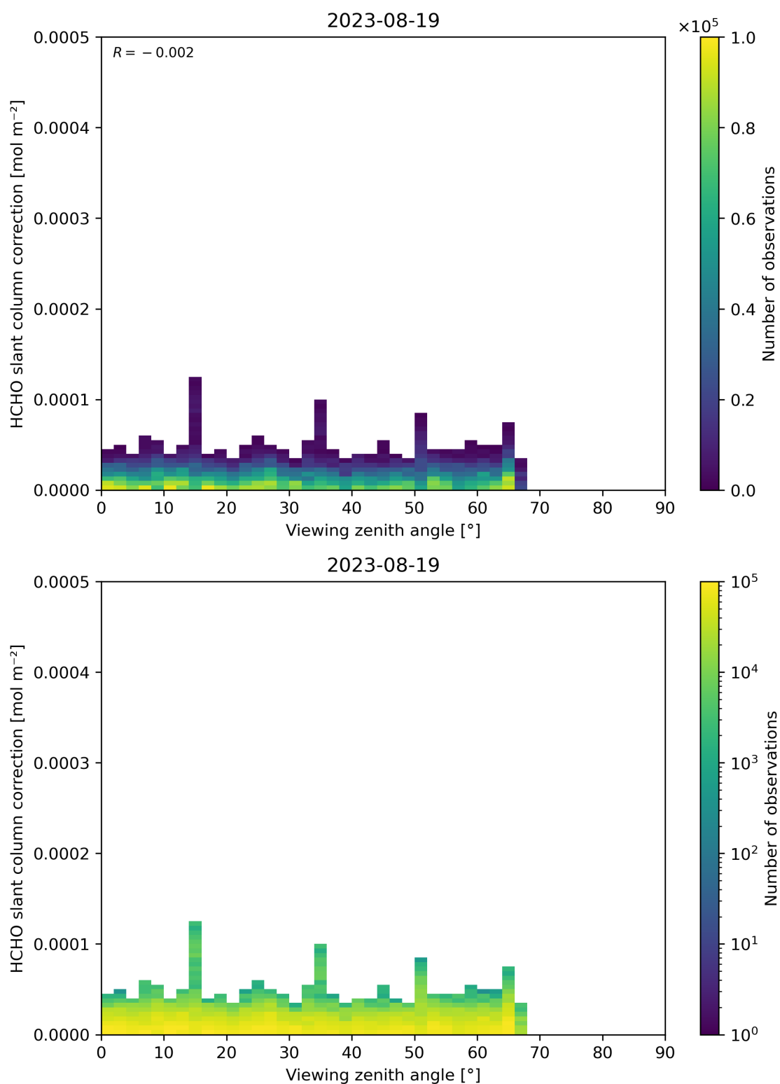
Figure 187: Scatter density plot of “Viewing zenith angle” against “HCHO slant column correction” for 2023-08-18 to 2023-08-20.
