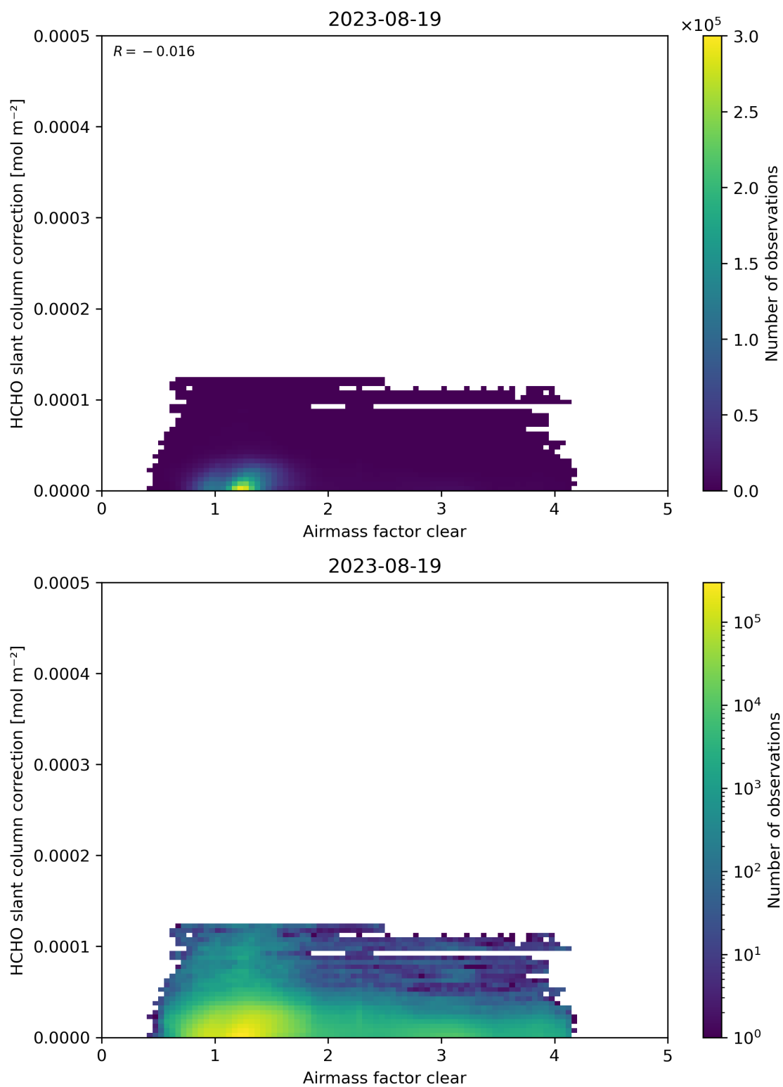
Figure 75: Scatter density plot of “Airmass factor clear” against “HCHO slant column correction” for 2023-08-18 to 2023-08-20.
