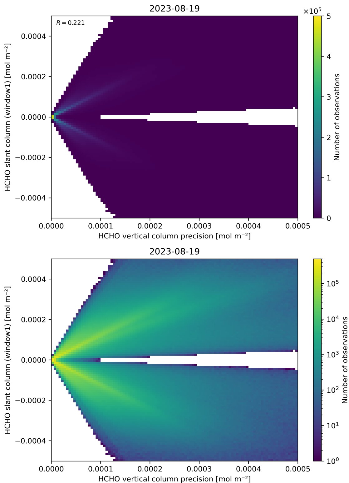
Figure 142: Scatter density plot of “HCHO vertical column precision” against “HCHO slant column (window1)” for 2023-08-18 to 2023-08-20.
