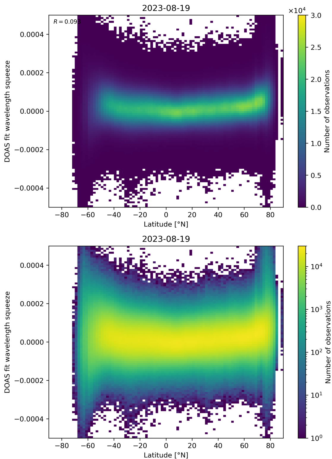
Figure 155: Scatter density plot of “Latitude” against “DOAS fit wavelength squeeze” for 2023-08-18 to 2023-08-20.
