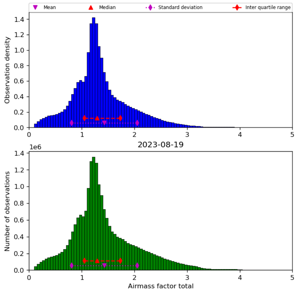
Figure 40: Histogram of “Airmass factor total” for 2023-08-18 to 2023-08-20
