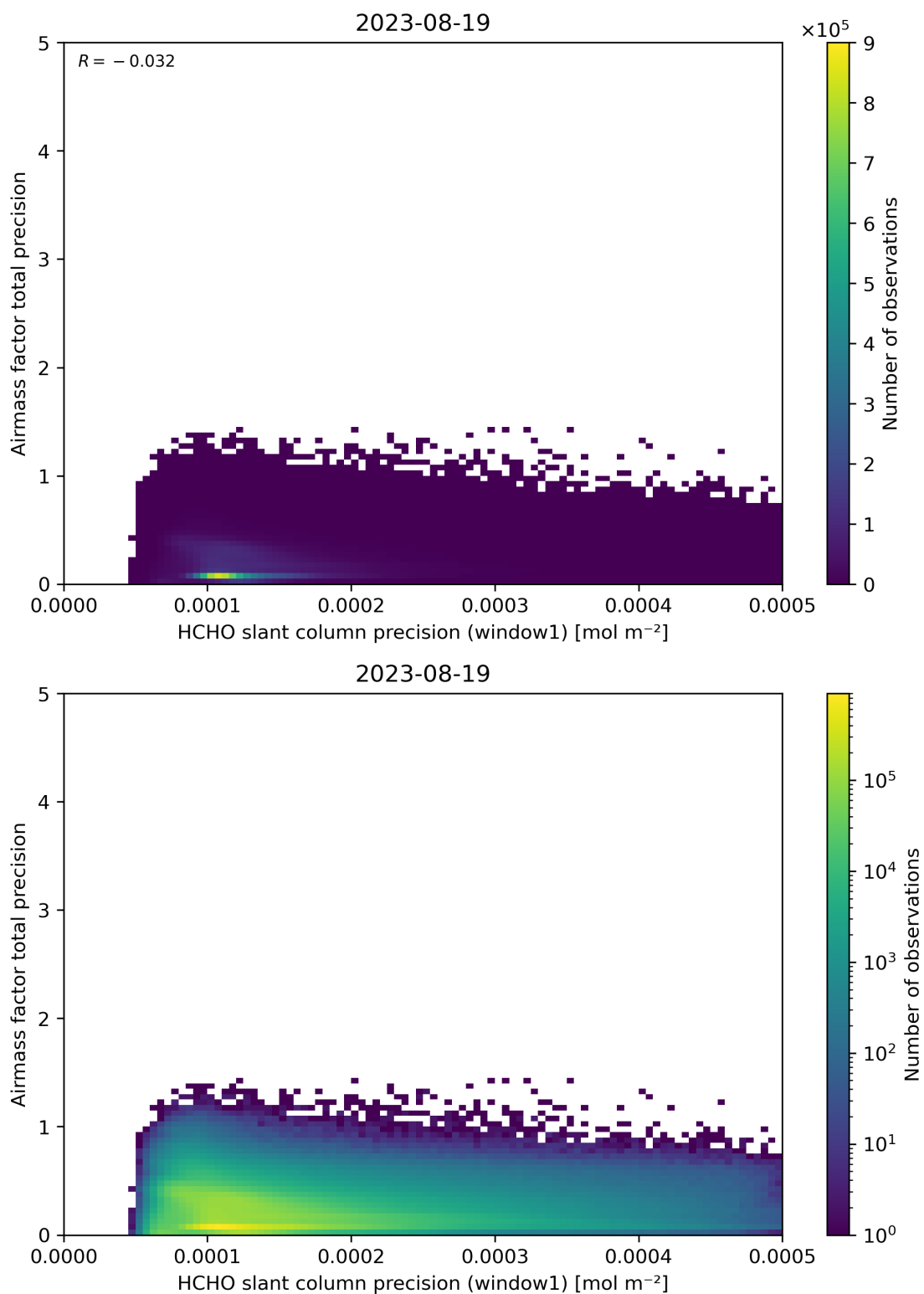
Figure 95: Scatter density plot of “HCHO slant column precision (window1)” against “Airmass factor total precision” for 2023-08-18 to 2023-08-20.
