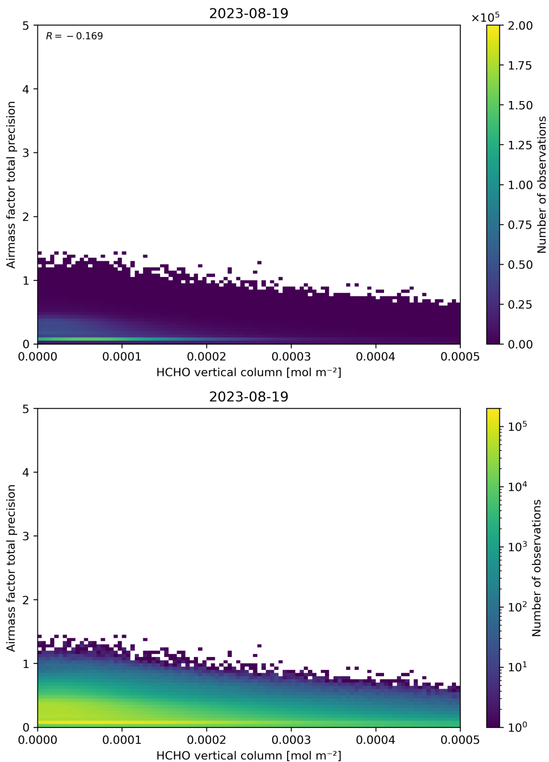
Figure 132: Scatter density plot of “HCHO vertical column” against “Airmass factor total precision” for 2023-08-18 to 2023-08-20.
