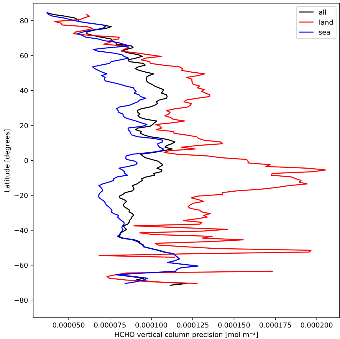
Figure 22: Zonal average of “HCHO vertical column precision” for 2023-08-18 to 2023-08-20.
