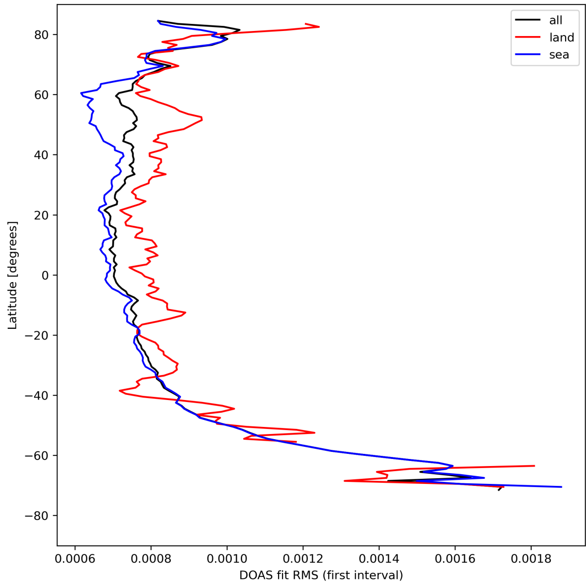
Figure 32: Zonal average of “DOAS fit RMS (first interval)” for 2023-08-18 to 2023-08-20.
