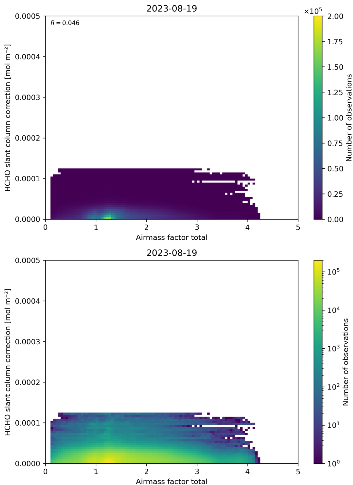
Figure 102: Scatter density plot of “Airmass factor total” against “HCHO slant column correction” for 2023-08-18 to 2023-08-20.
