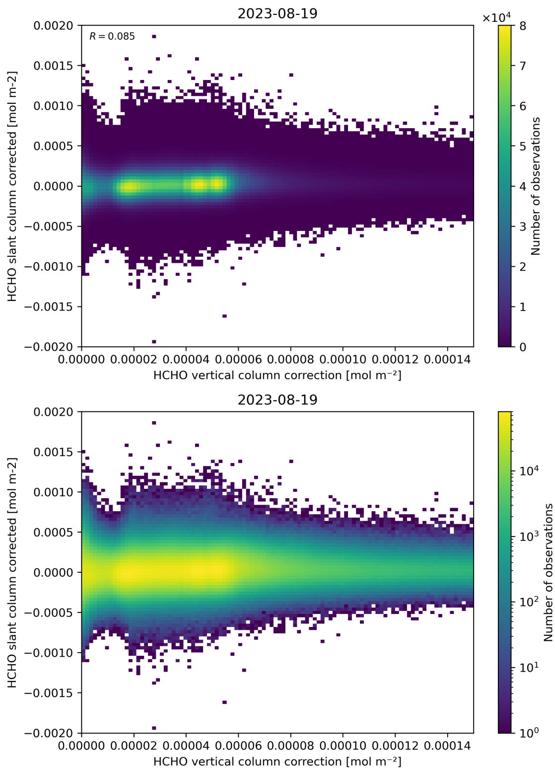
Figure 116: Scatter density plot of “HCHO vertical column correction” against “HCHO slant column corrected” for 2023-08-18 to 2023-08-20.
