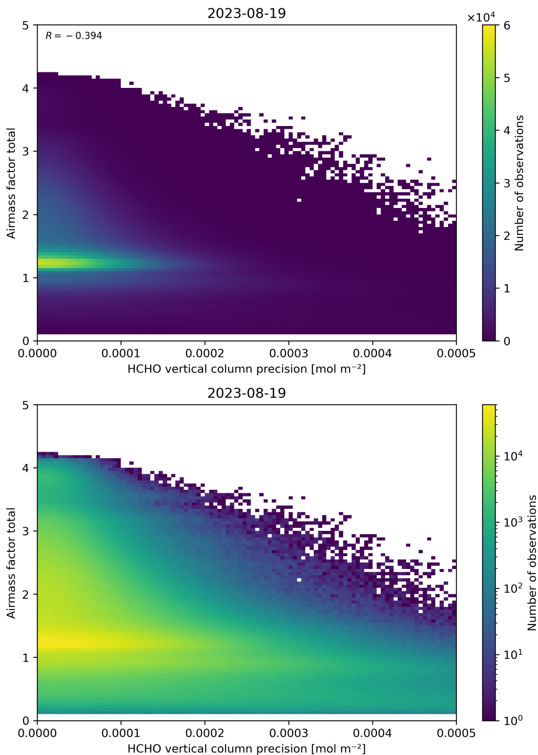
Figure 144: Scatter density plot of “HCHO vertical column precision” against “Airmass factor total” for 2023-08-18 to 2023-08-20.
