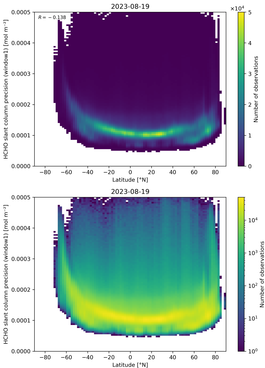
Figure 160: Scatter density plot of “Latitude” against “HCHO slant column precision (window1)” for 2023-08-18 to 2023-08-20.
