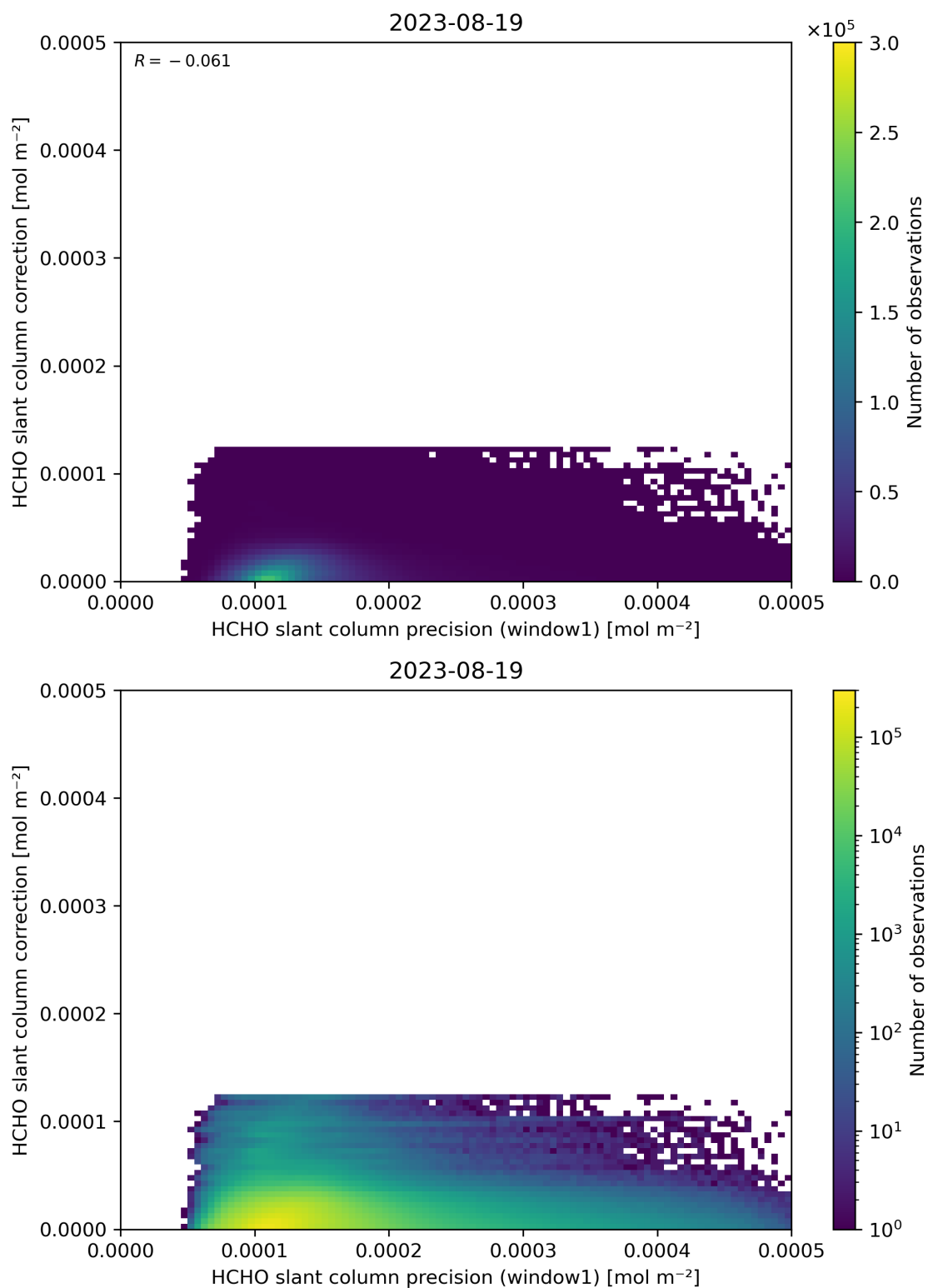
Figure 93: Scatter density plot of “HCHO slant column precision (window1)” against “HCHO slant column correction” for 2023-08-18 to 2023-08-20.
