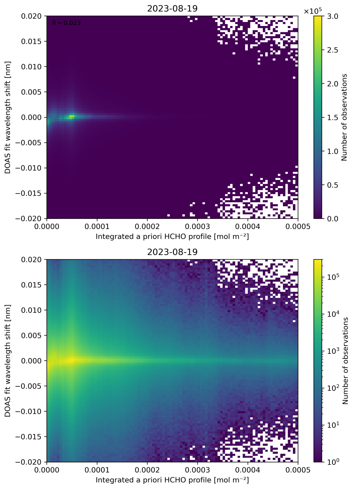
Figure 149: Scatter density plot of “Integrated a priori HCHO profile” against “DOAS fit wavelength shift” for 2023-08-18 to 2023-08-20.
