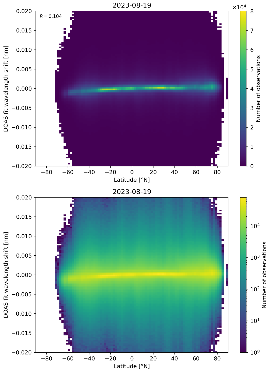
Figure 154: Scatter density plot of “Latitude” against “DOAS fit wavelength shift” for 2023-08-18 to 2023-08-20.
