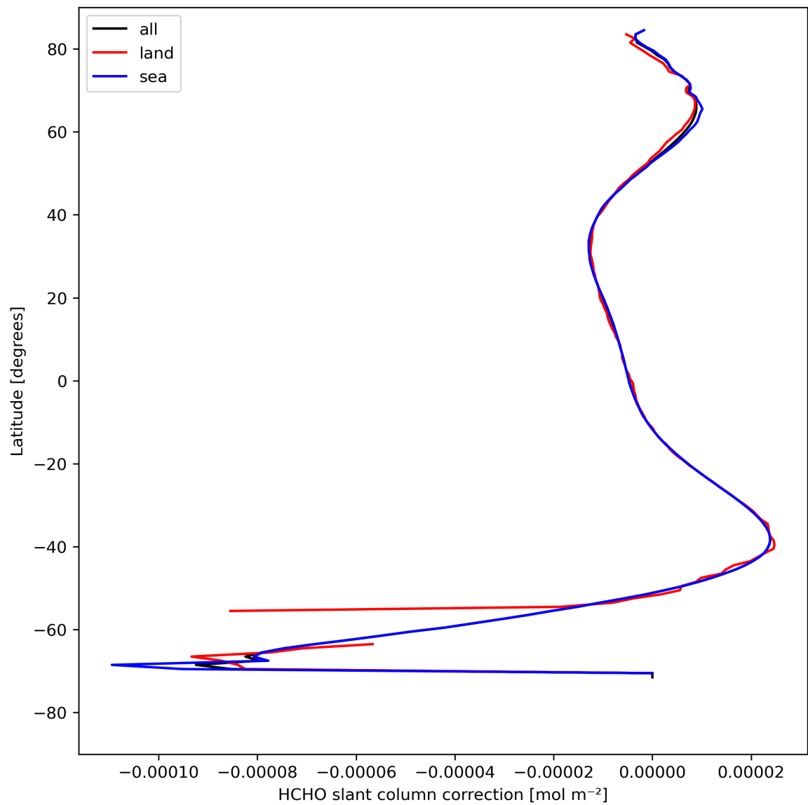
Figure 33: Zonal average of “HCHO slant column correction” for 2023-08-18 to 2023-08-20.
