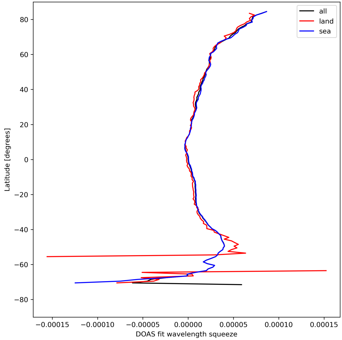
Figure 31: Zonal average of “DOAS fit wavelength squeeze” for 2023-08-18 to 2023-08-20.
