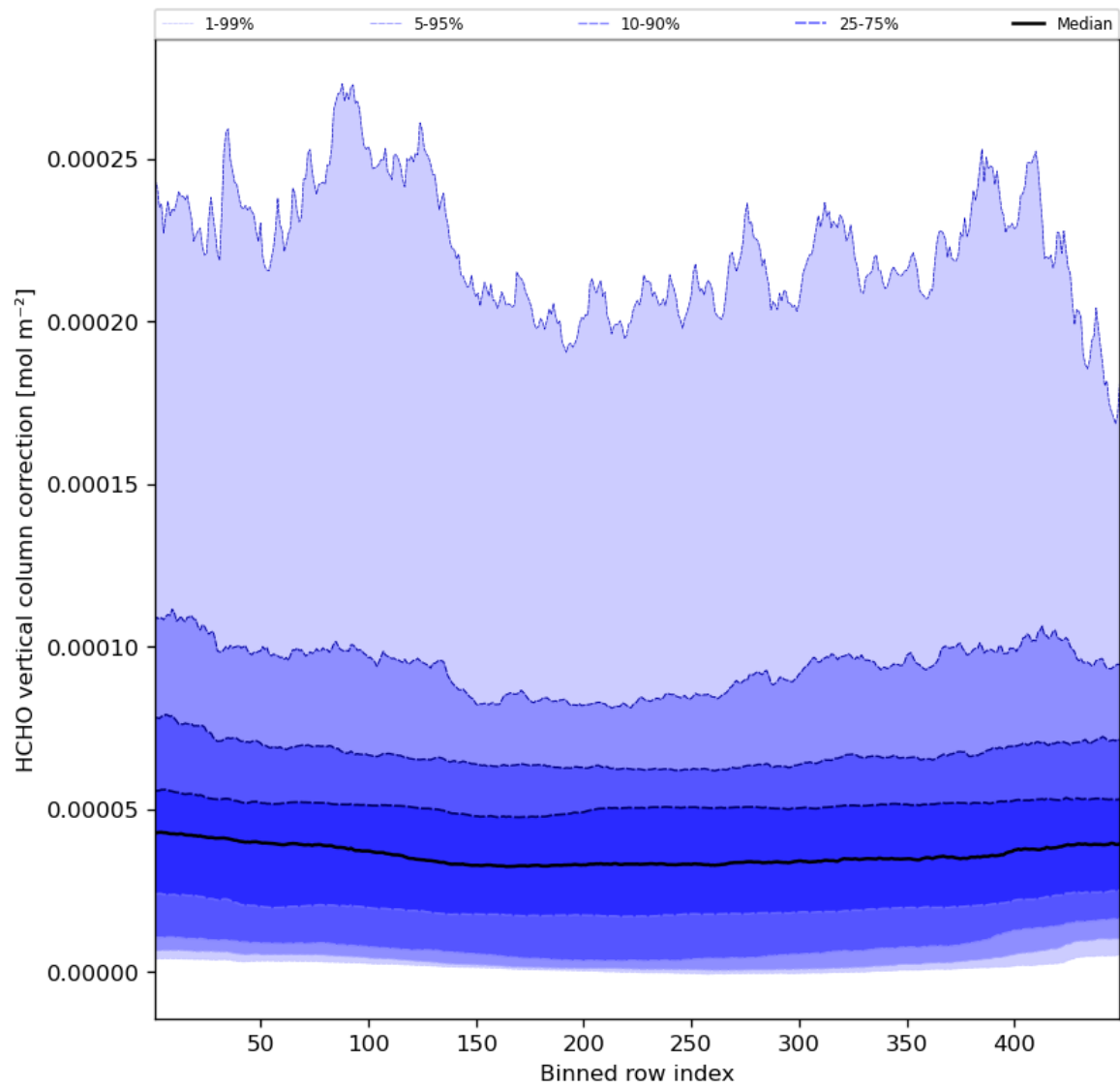
Figure 51: Along track statistics of “HCHO vertical column correction” for 2023-08-18 to 2023-08-20
