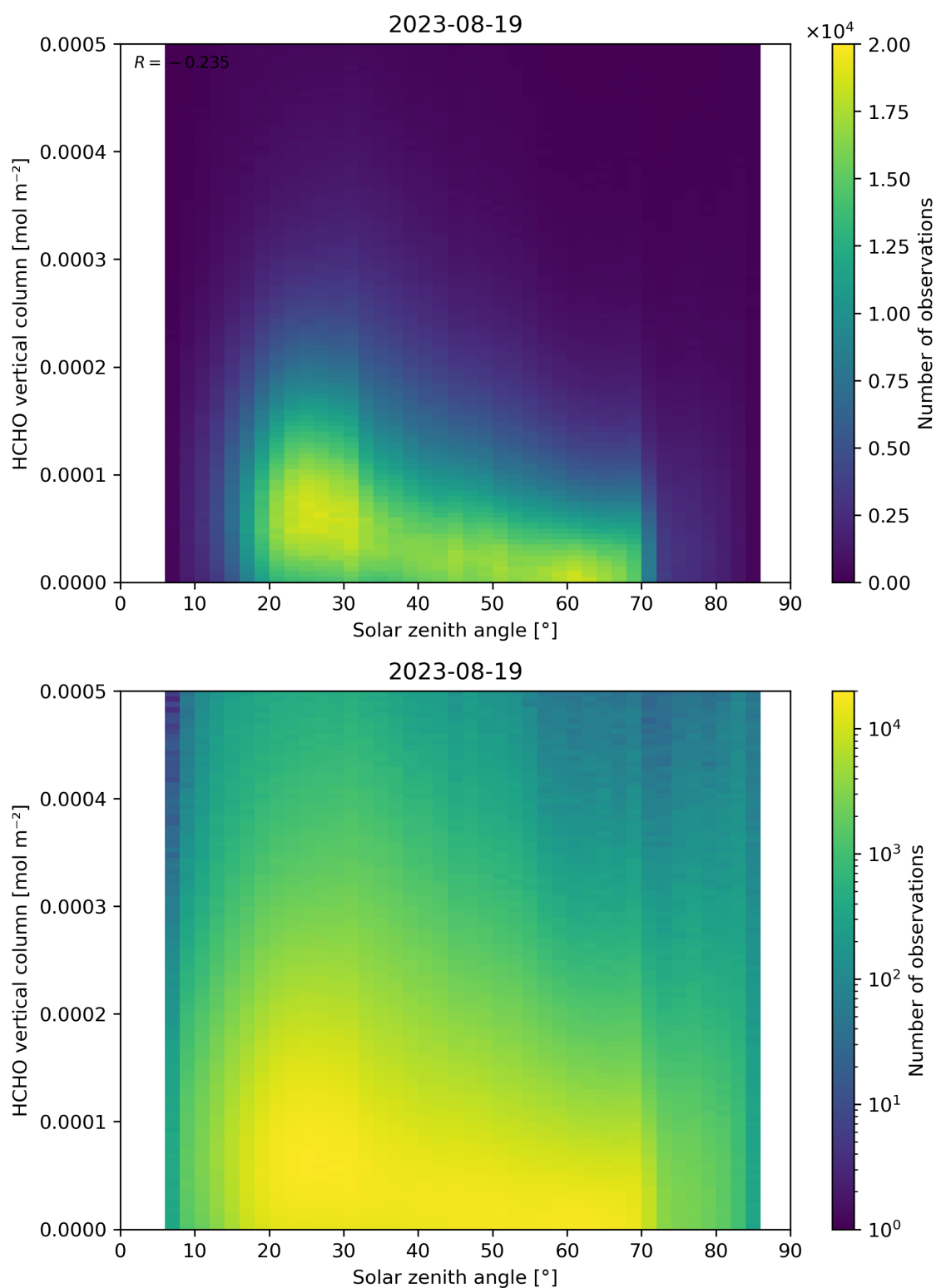
Figure 177: Scatter density plot of “Solar zenith angle” against “HCHO vertical column” for 2023-08-18 to 2023-08-20.
