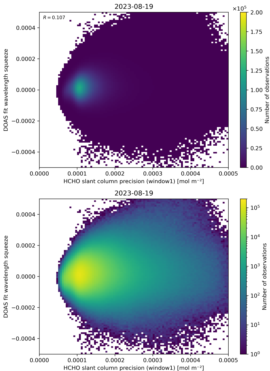
Figure 90: Scatter density plot of “HCHO slant column precision (window1)” against “DOAS fit wavelength squeeze” for 2023-08-18 to 2023-08-20.
