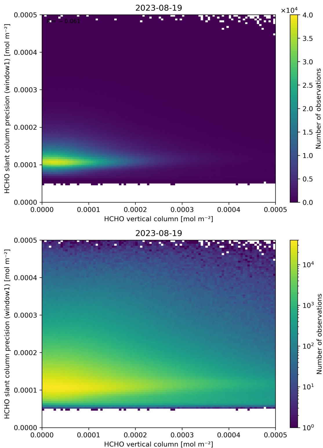
Figure 130: Scatter density plot of “HCHO vertical column” against “HCHO slant column precision (window1)” for 2023-08-18 to 2023-08-20.
