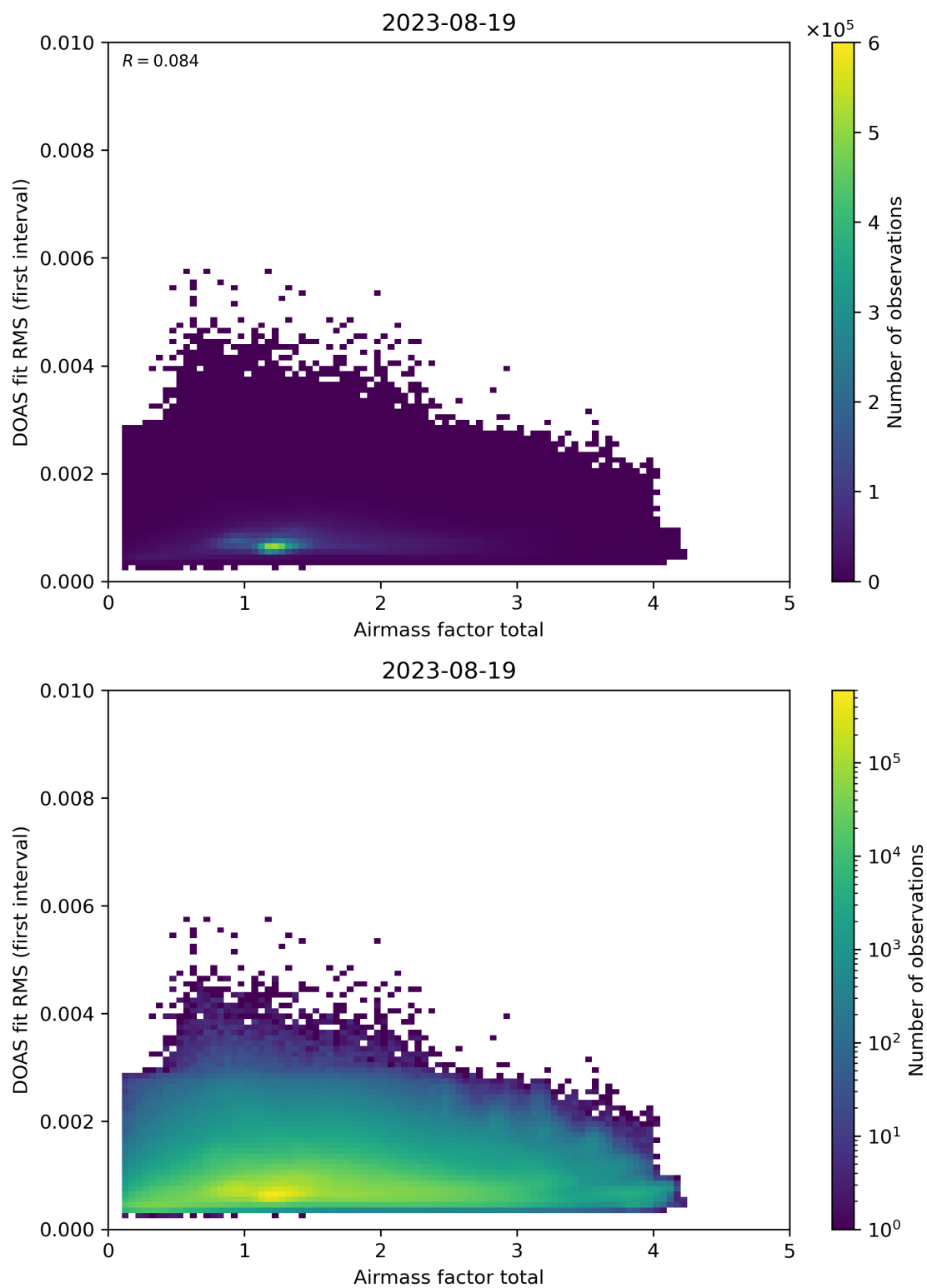
Figure 97: Scatter density plot of “Airmass factor total” against “DOAS fit RMS (first interval)” for 2023-08-18 to 2023-08-20.
