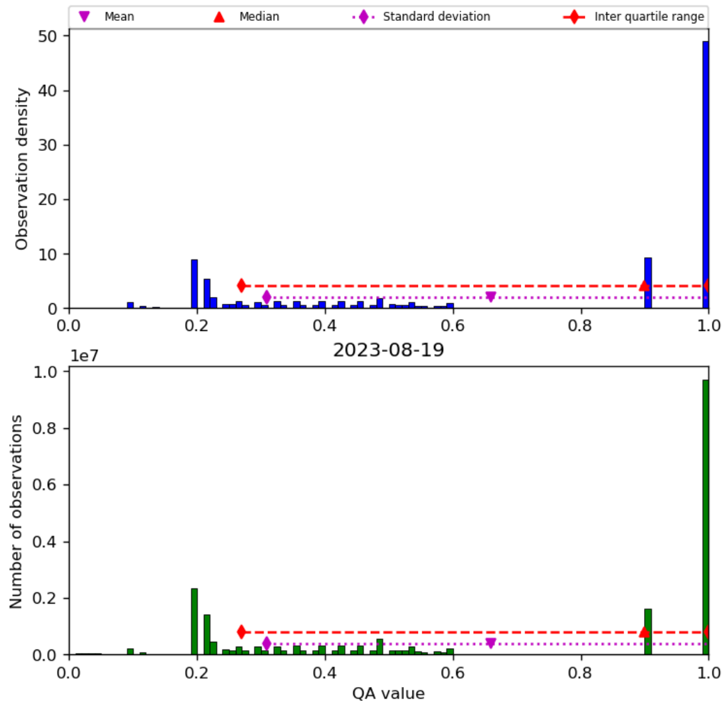
Figure 34: Histogram of “QA value” for 2023-08-18 to 2023-08-20
