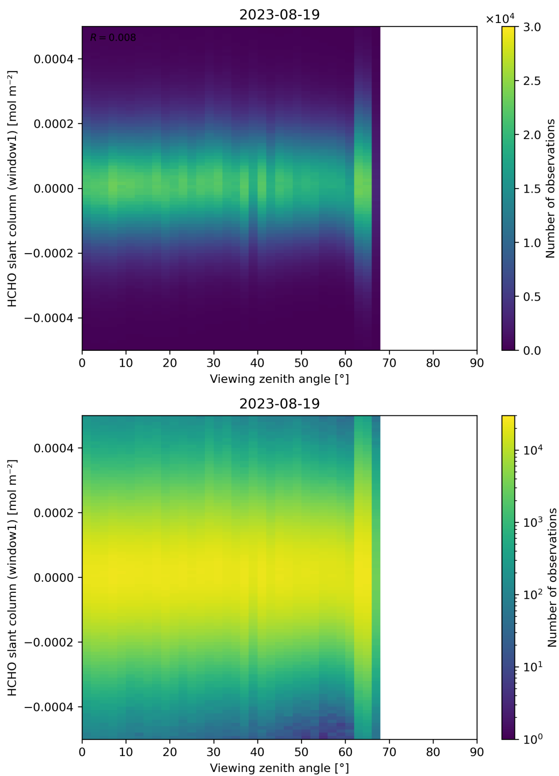
Figure 188: Scatter density plot of “Viewing zenith angle” against “HCHO slant column (window1)” for 2023-08-18 to 2023-08-20.
