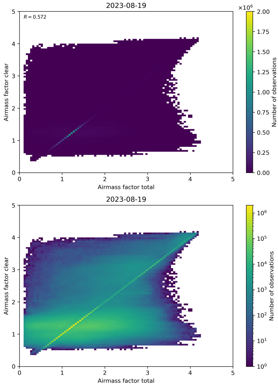
Figure 100: Scatter density plot of “Airmass factor total” against “Airmass factor clear” for 2023-08-18 to 2023-08-20.
