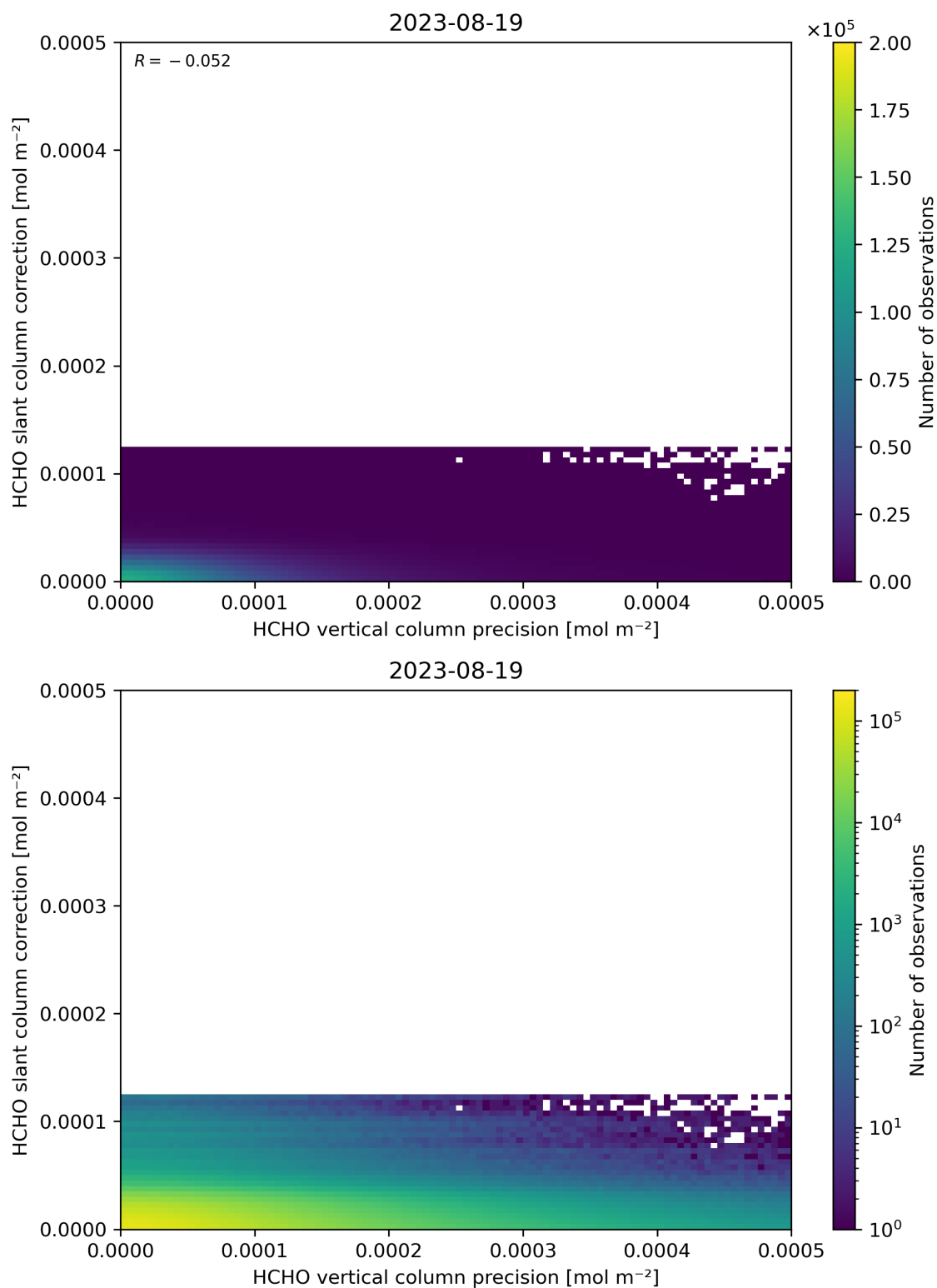
Figure 141: Scatter density plot of “HCHO vertical column precision” against “HCHO slant column correction” for 2023-08-18 to 2023-08-20.
