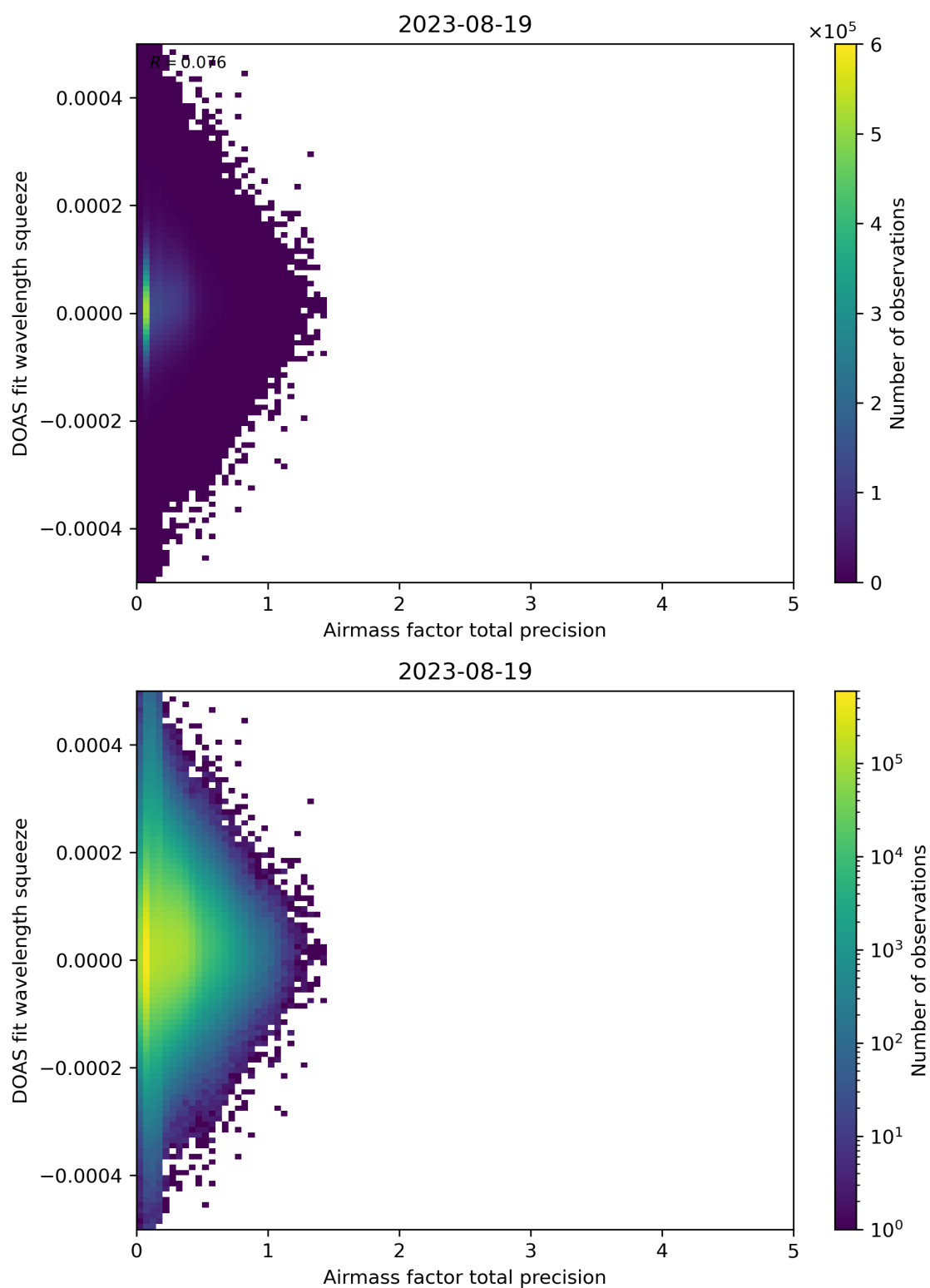
Figure 107: Scatter density plot of “Airmass factor total precision” against “DOAS fit wavelength squeeze” for 2023-08-18 to 2023-08-20.
