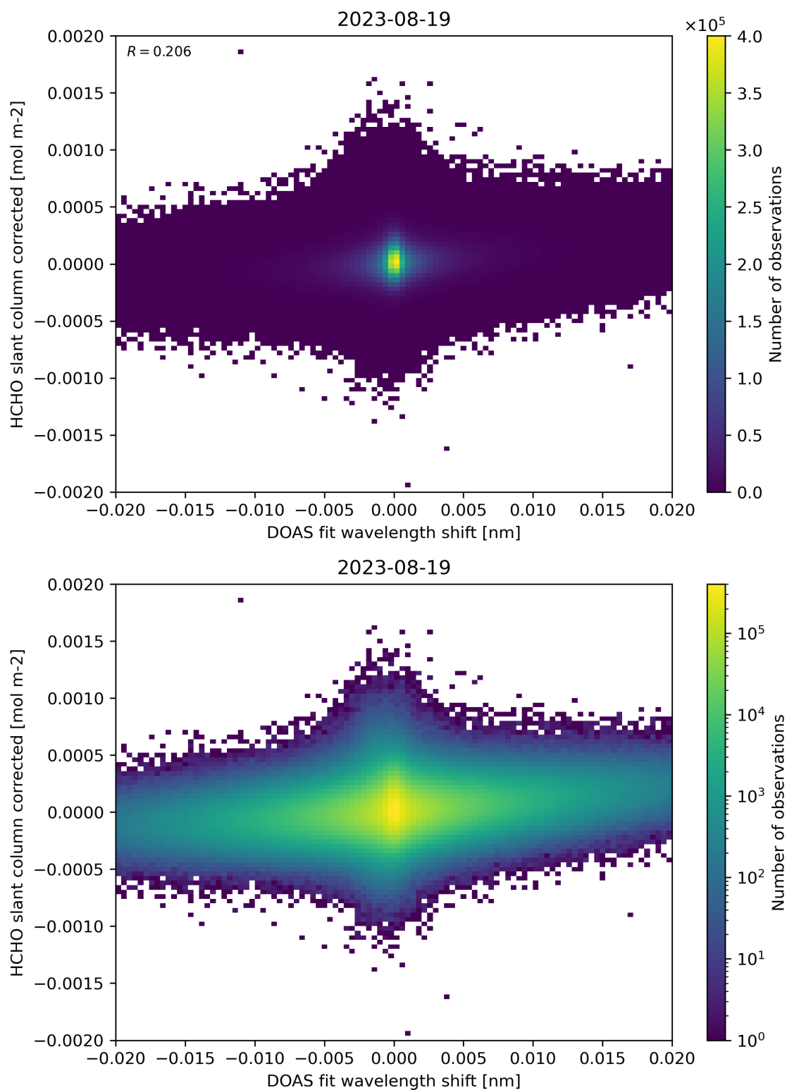
Figure 66: Scatter density plot of “DOAS fit wavelength shift” against “HCHO slant column corrected” for 2023-08-18 to 2023-08-20.
