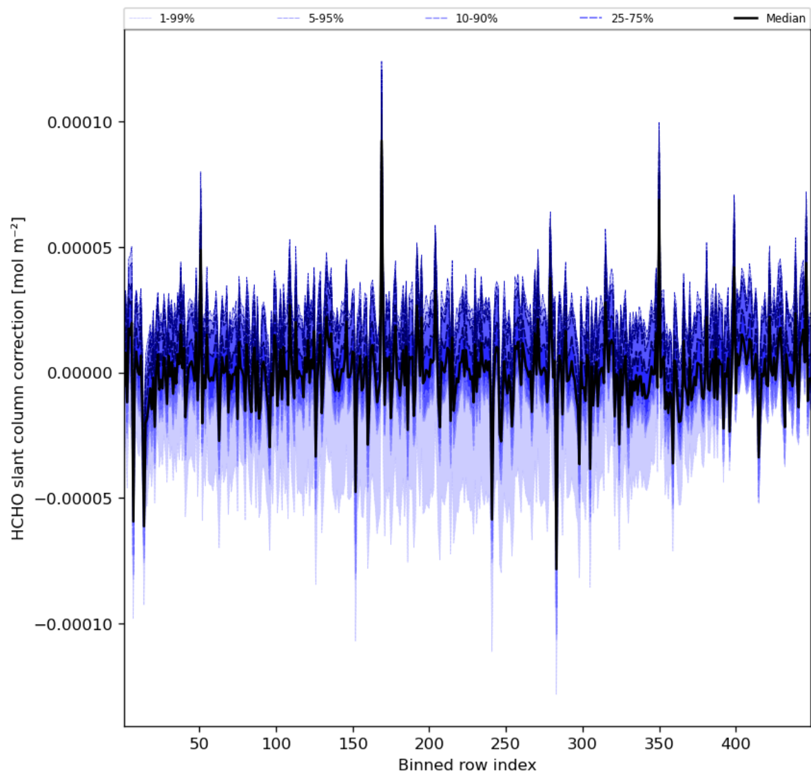
Figure 61: Along track statistics of “HCHO slant column correction” for 2023-08-18 to 2023-08-20
