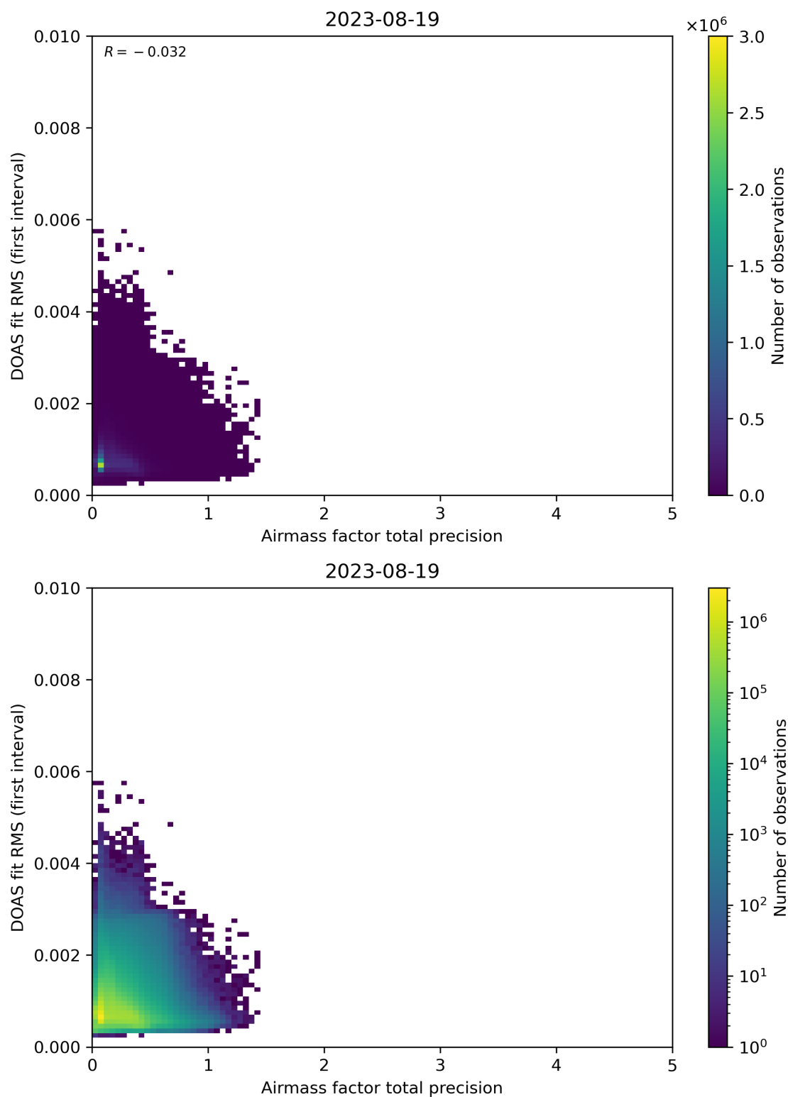
Figure 105: Scatter density plot of “Airmass factor total precision” against “DOAS fit RMS (first interval)” for 2023-08-18 to 2023-08-20.
