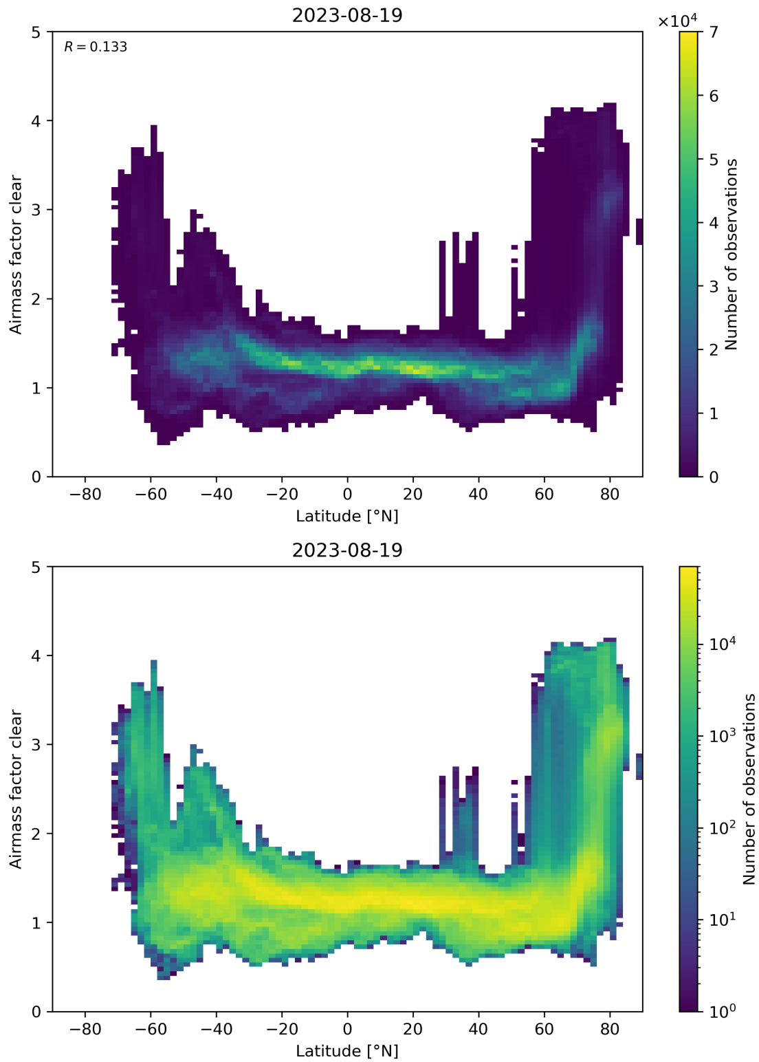
Figure 156: Scatter density plot of “Latitude” against “Airmass factor clear” for 2023-08-18 to 2023-08-20.
