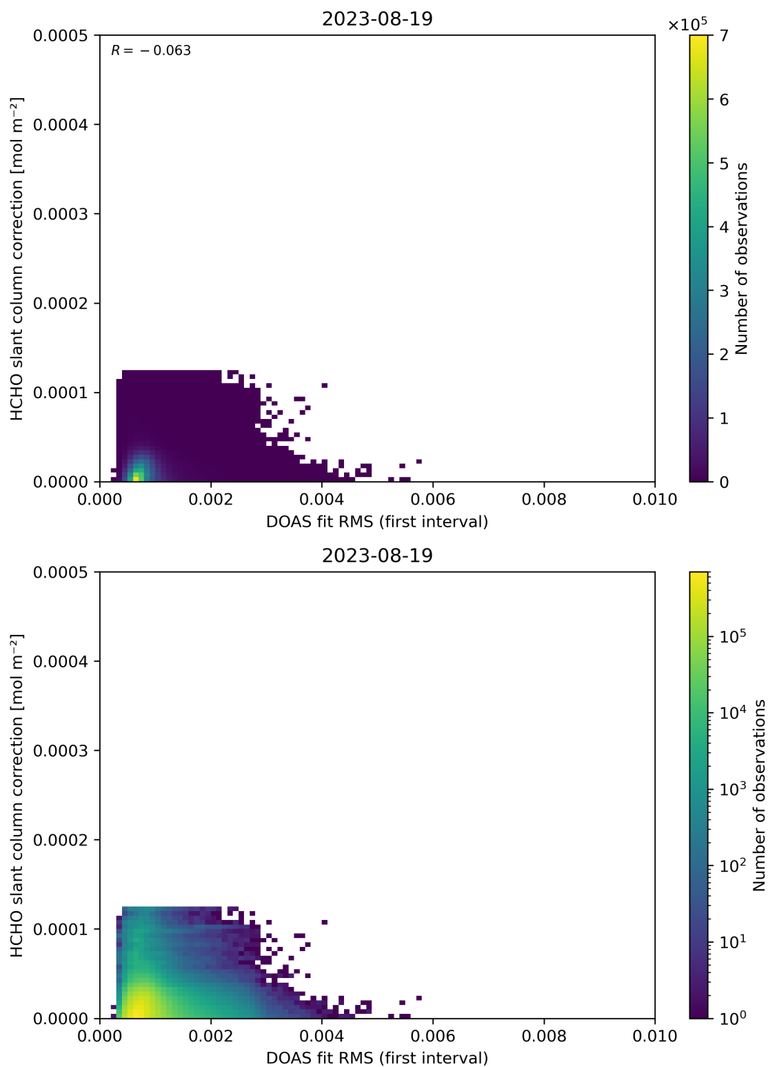
Figure 63: Scatter density plot of “DOAS fit RMS (first interval)” against “HCHO slant column correction” for 2023-08-18 to 2023-08-20.
