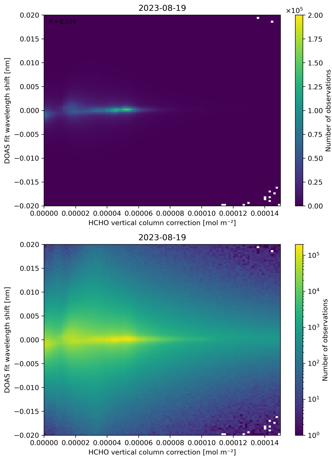
Figure 113: Scatter density plot of “HCHO vertical column correction” against “DOAS fit wavelength shift” for 2023-08-18 to 2023-08-20.
