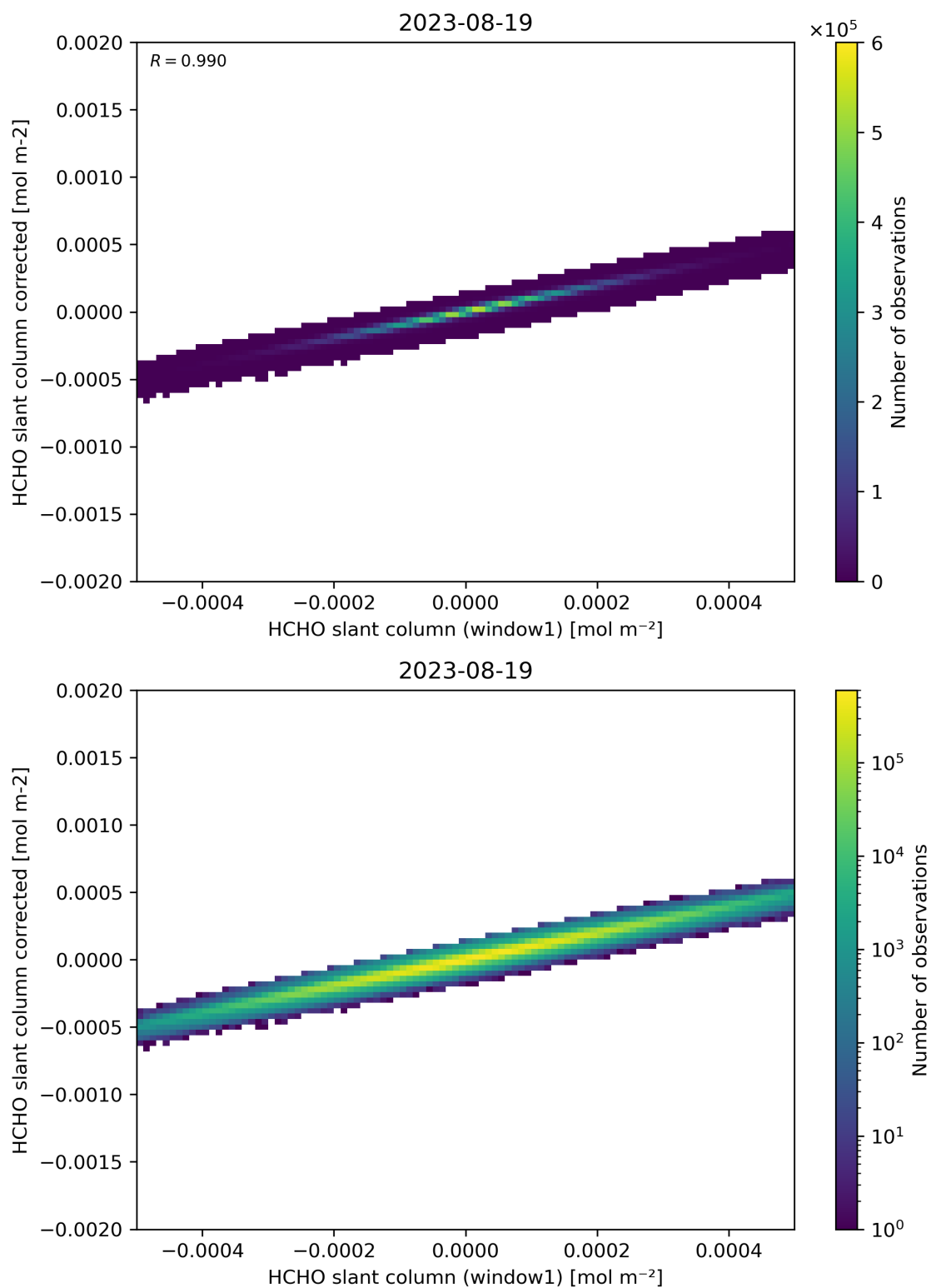
Figure 82: Scatter density plot of “HCHO slant column (window1)” against “HCHO slant column corrected” for 2023-08-18 to 2023-08-20.
