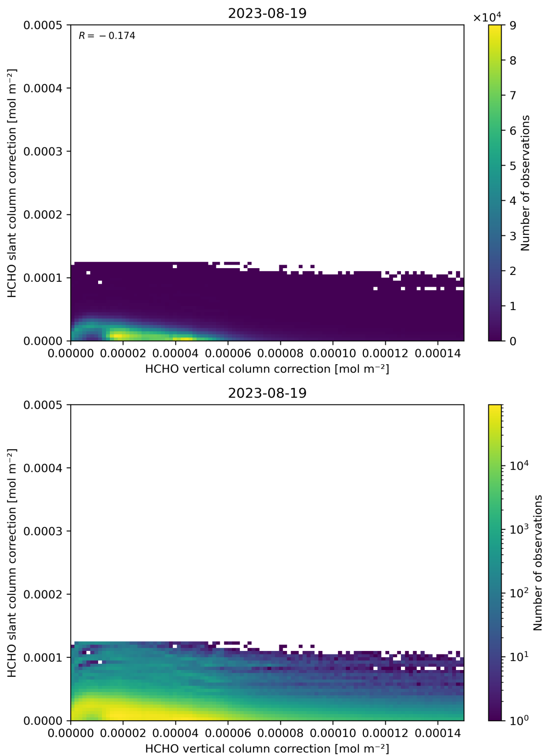
Figure 117: Scatter density plot of “HCHO vertical column correction” against “HCHO slant column correction” for 2023-08-18 to 2023-08-20.
