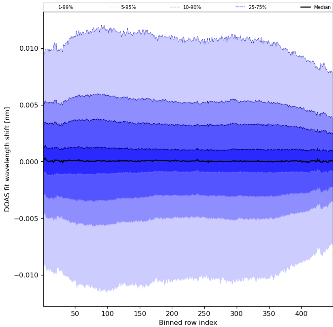
Figure 58: Along track statistics of “DOAS fit wavelength shift” for 2023-08-18 to 2023-08-20
