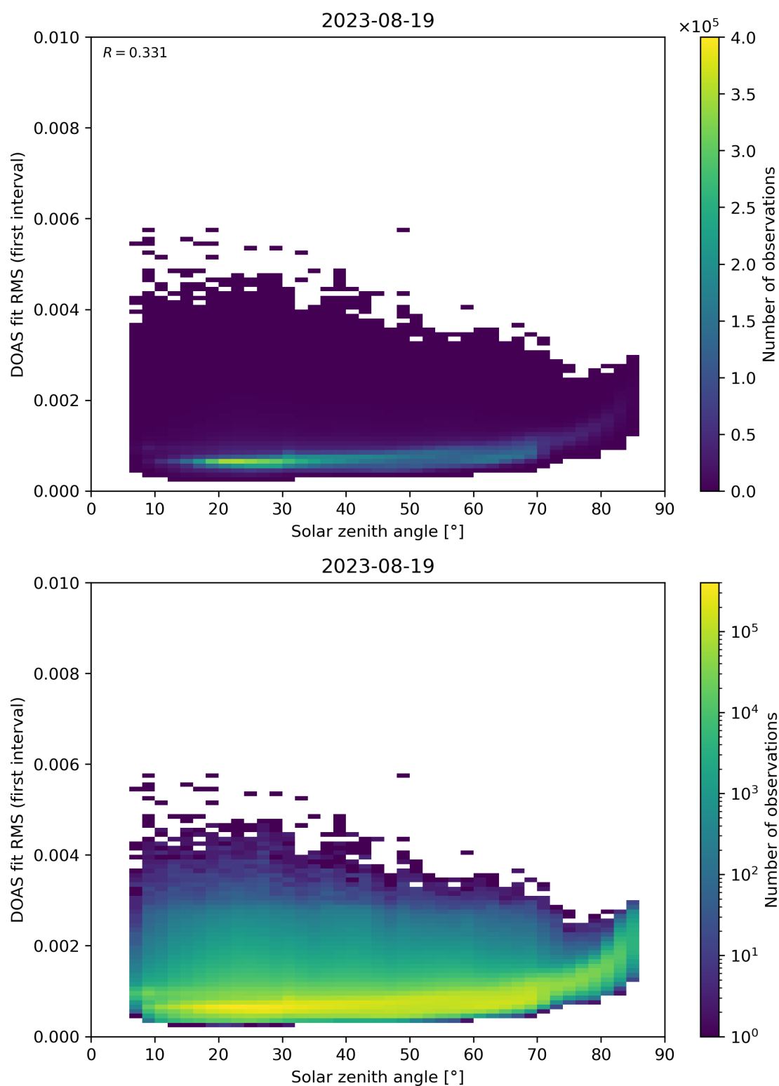
Figure 167: Scatter density plot of “Solar zenith angle” against “DOAS fit RMS (first interval)” for 2023-08-18 to 2023-08-20.
