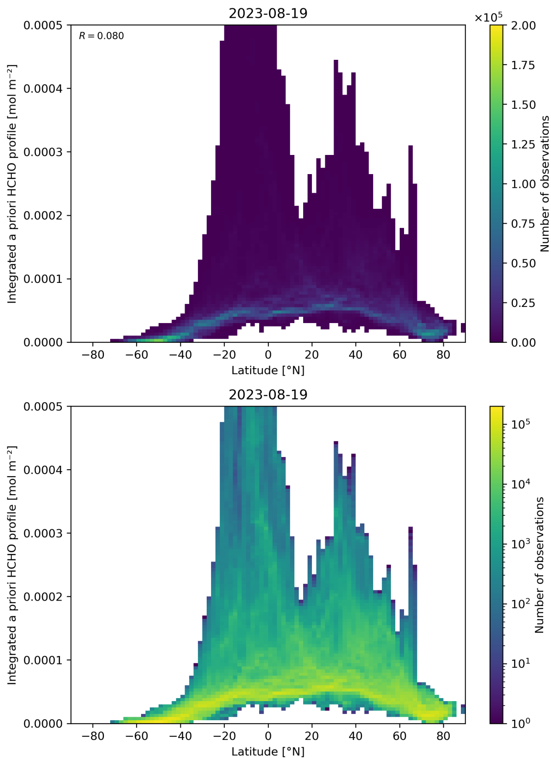
Figure 166: Scatter density plot of “Latitude” against “Integrated a priori HCHO profile” for 2023-08-18 to 2023-08-20.
