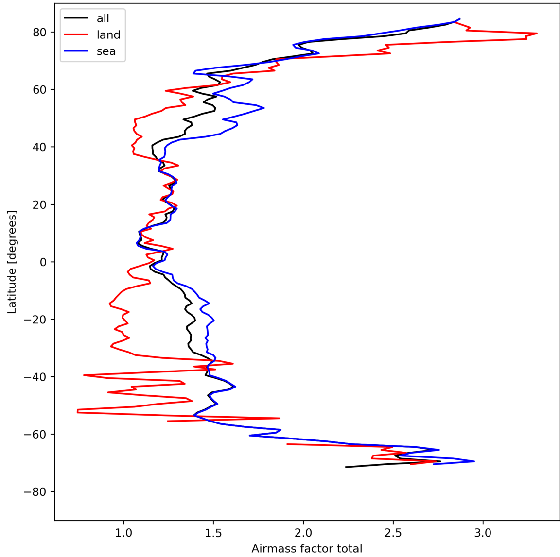
Figure 26: Zonal average of “Airmass factor total” for 2023-08-18 to 2023-08-20.
