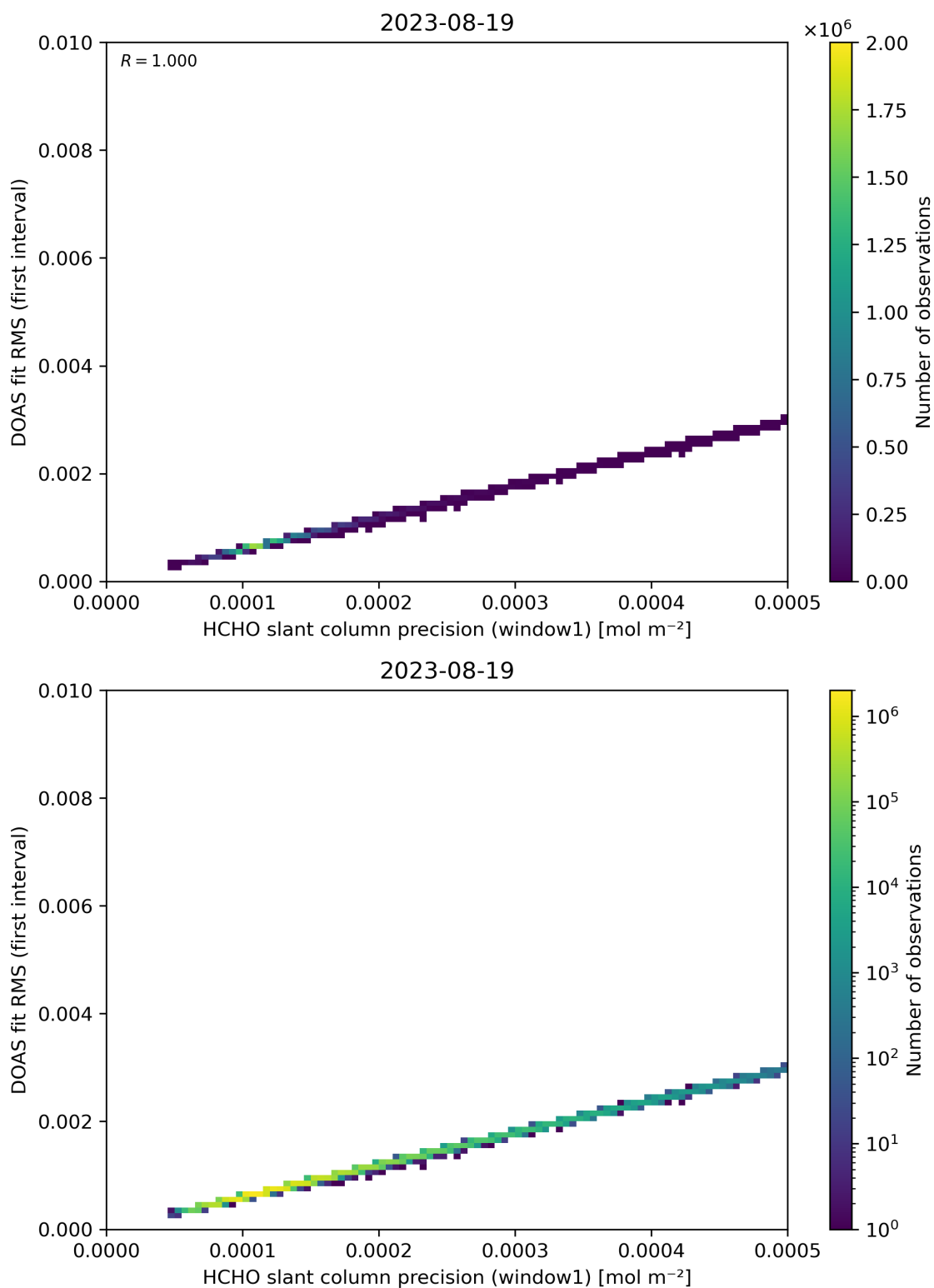
Figure 88: Scatter density plot of “HCHO slant column precision (window1)” against “DOAS fit RMS (first interval)” for 2023-08-18 to 2023-08-20.
