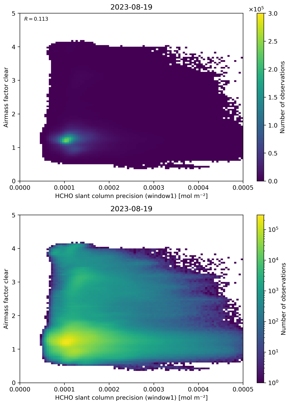
Figure 91: Scatter density plot of “HCHO slant column precision (window1)” against “Airmass factor clear” for 2023-08-18 to 2023-08-20.
