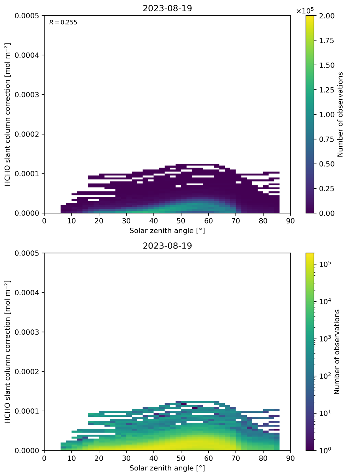
Figure 172: Scatter density plot of “Solar zenith angle” against “HCHO slant column correction” for 2023-08-18 to 2023-08-20.
