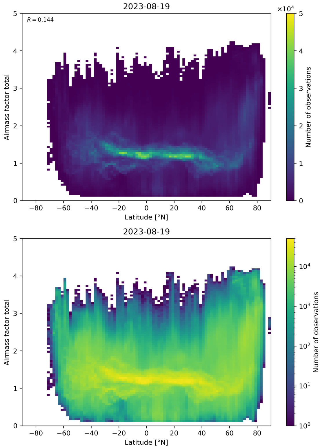
Figure 161: Scatter density plot of “Latitude” against “Airmass factor total” for 2023-08-18 to 2023-08-20.
