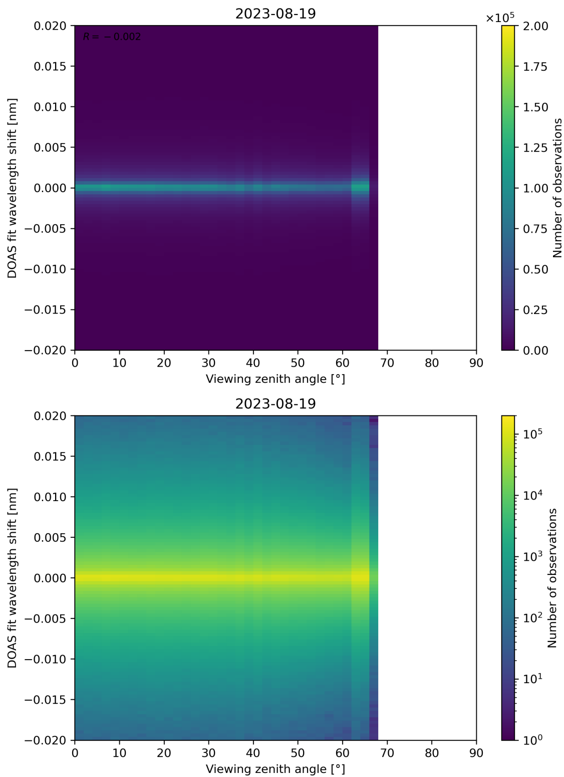
Figure 183: Scatter density plot of “Viewing zenith angle” against “DOAS fit wavelength shift” for 2023-08-18 to 2023-08-20.
