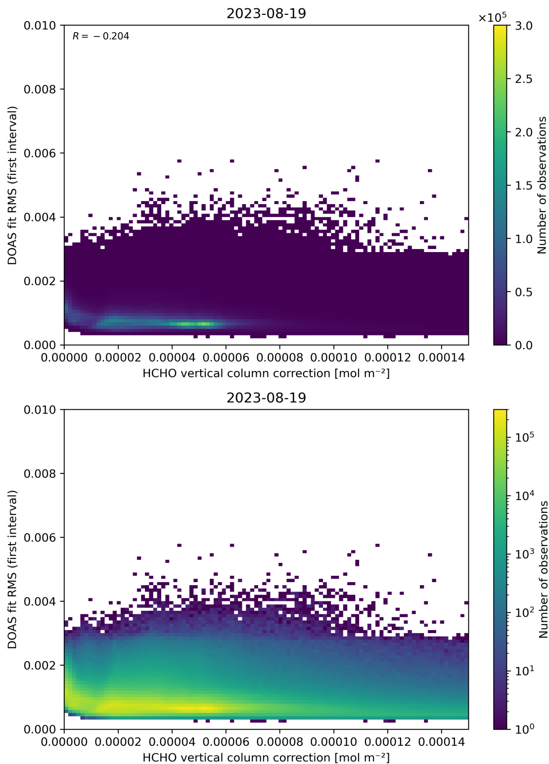
Figure 112: Scatter density plot of “HCHO vertical column correction” against “DOAS fit RMS (first interval)” for 2023-08-18 to 2023-08-20.
