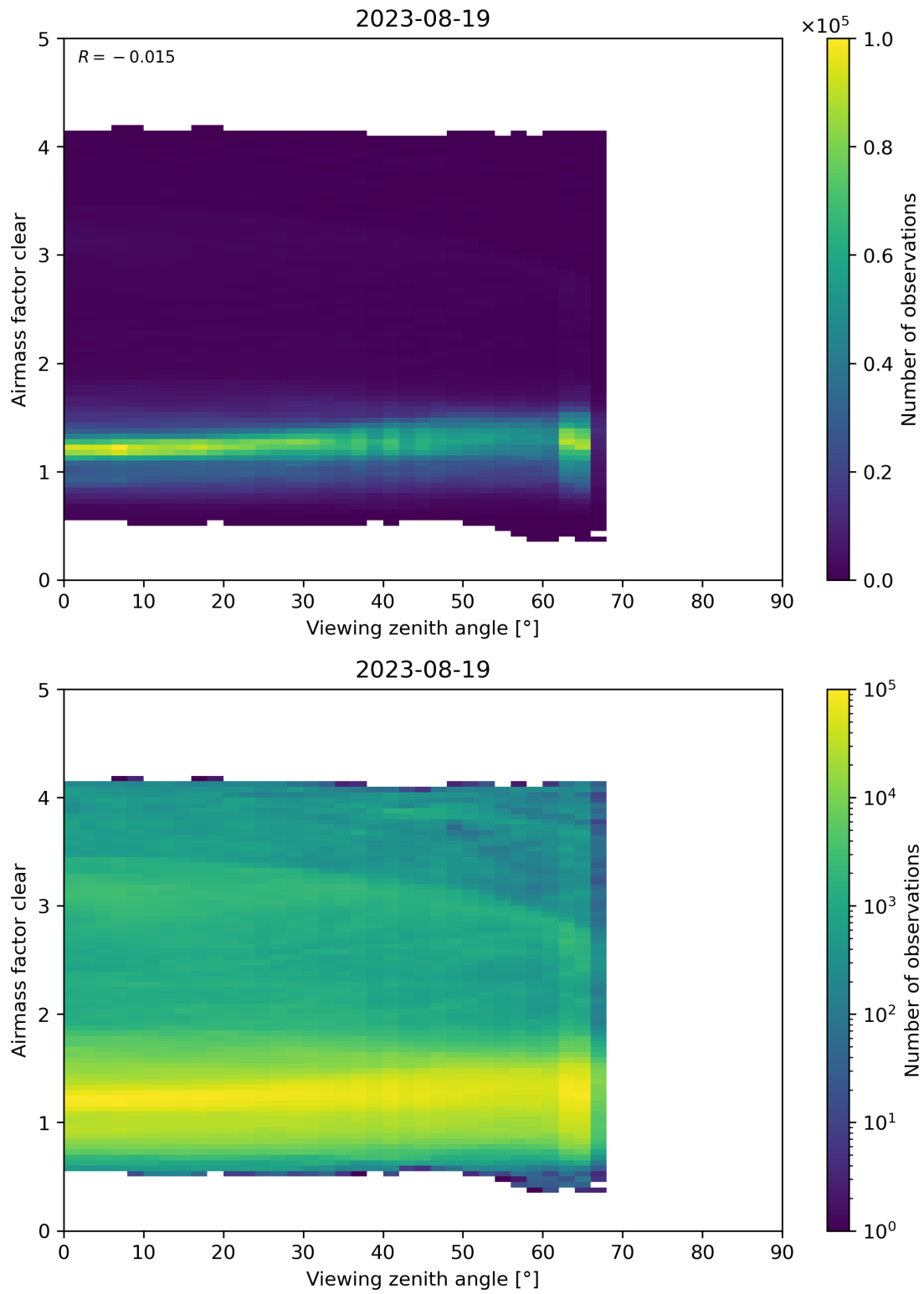
Figure 185: Scatter density plot of “Viewing zenith angle” against “Airmass factor clear” for 2023-08-18 to 2023-08-20.
