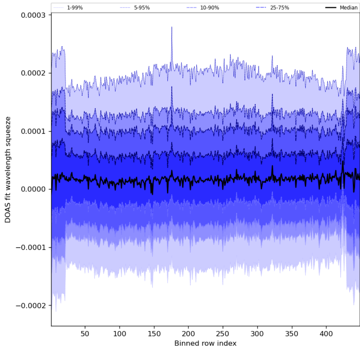
Figure 59: Along track statistics of “DOAS fit wavelength squeeze” for 2023-08-18 to 2023-08-20
