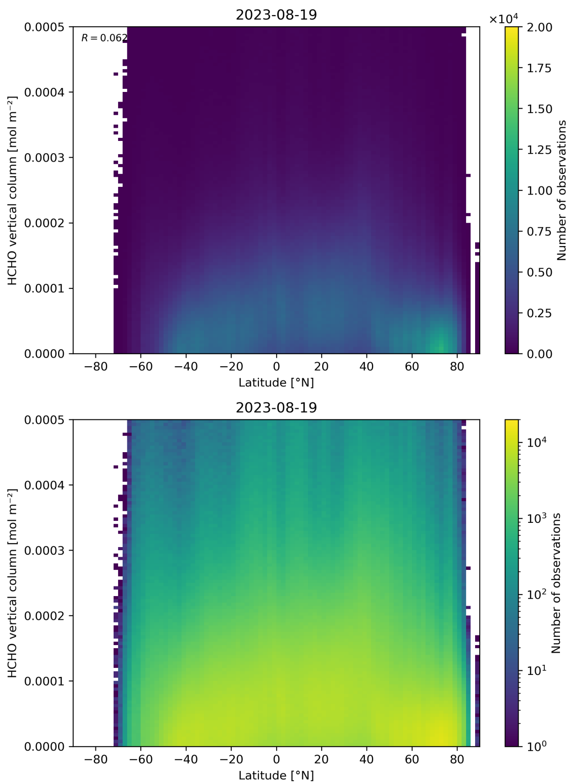
Figure 163: Scatter density plot of “Latitude” against “HCHO vertical column” for 2023-08-18 to 2023-08-20.
