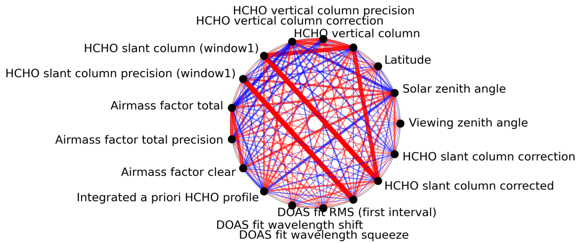
Figure 1: Map of correlation graph for 2023-08-18 to 2023-08-20.
