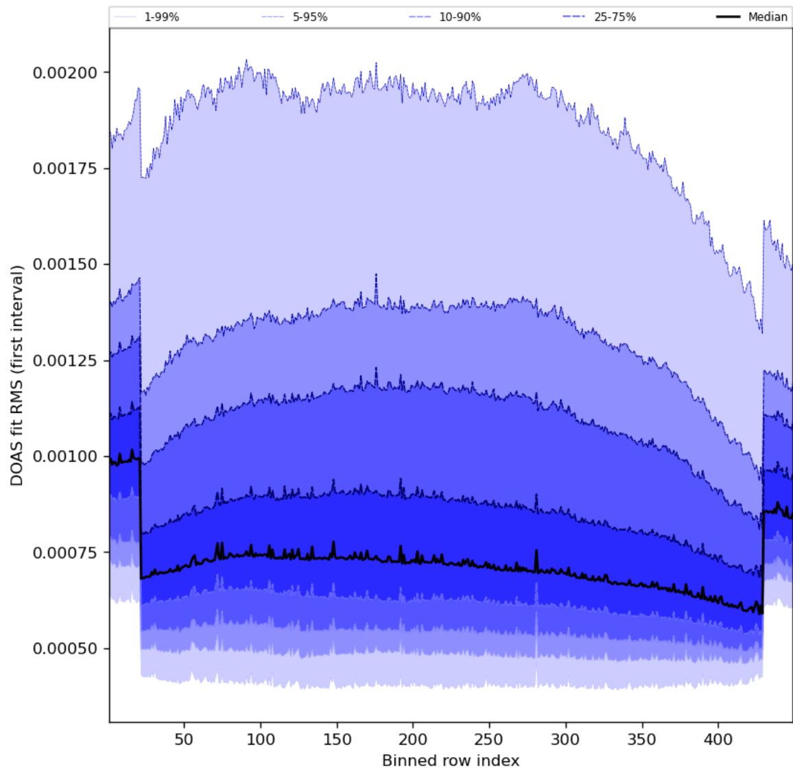
Figure 60: Along track statistics of “DOAS fit RMS (first interval)” for 2023-08-18 to 2023-08-20
