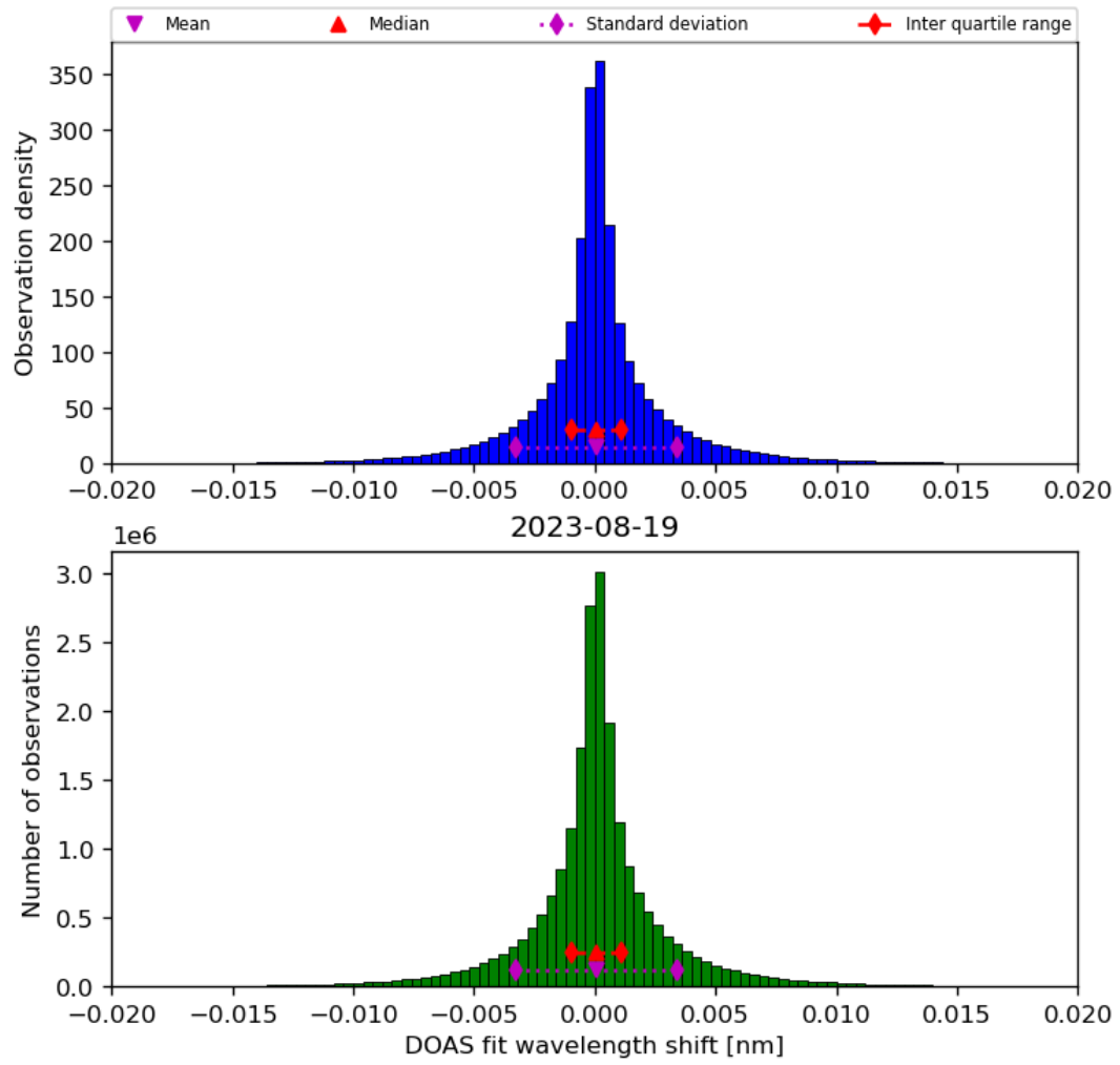
Figure 44: Histogram of “DOAS fit wavelength shift” for 2023-08-18 to 2023-08-20
