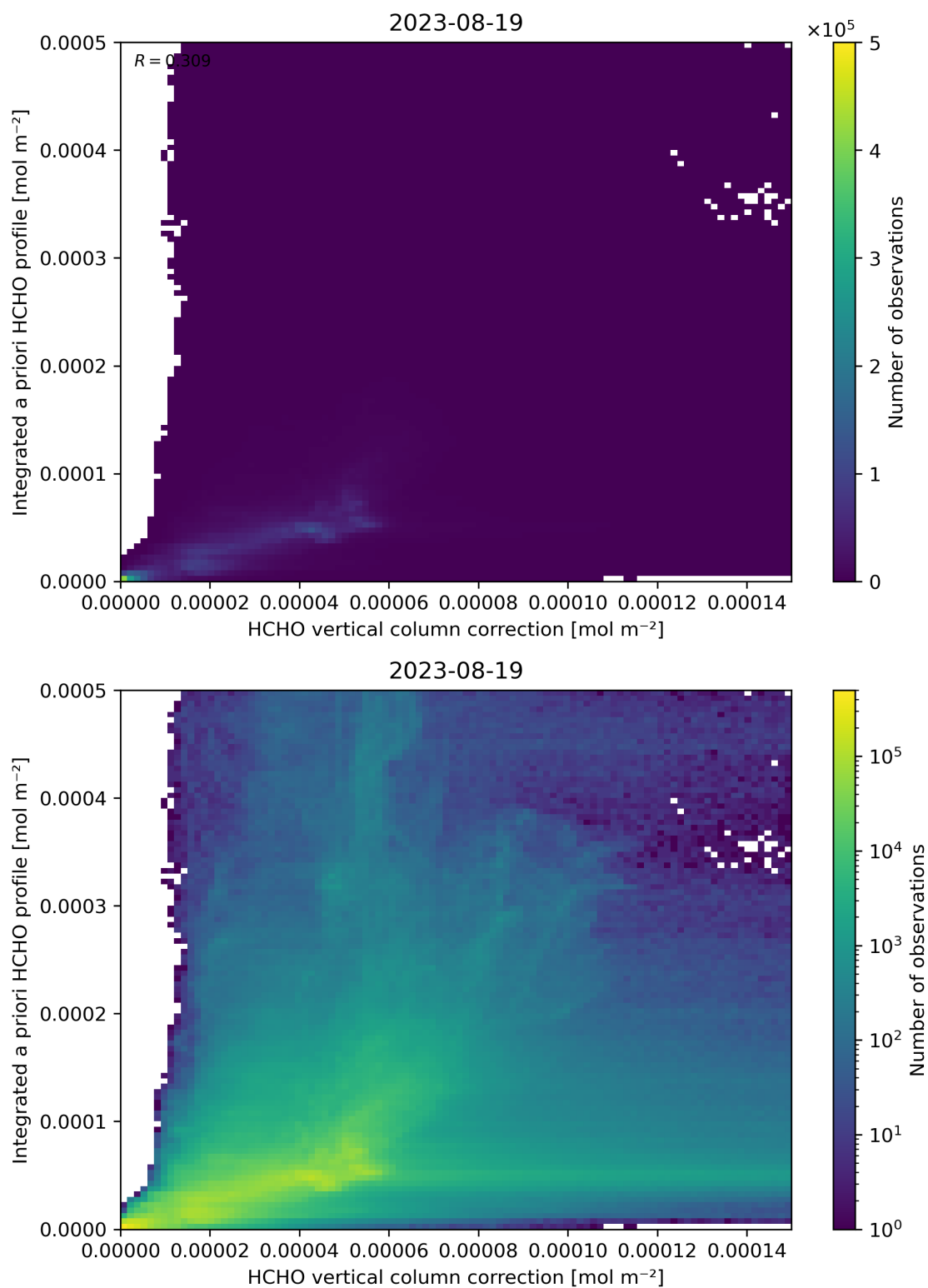
Figure 122: Scatter density plot of “HCHO vertical column correction” against “Integrated a priori HCHO profile” for 2023-08-18 to 2023-08-20.
