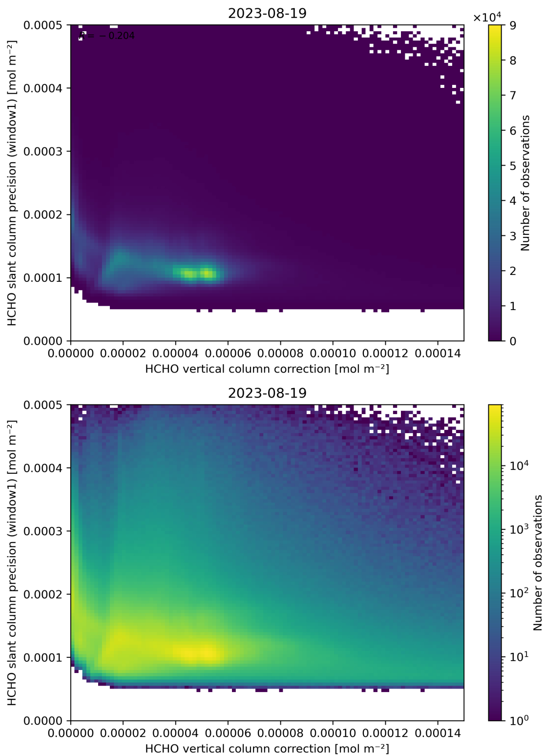
Figure 119: Scatter density plot of “HCHO vertical column correction” against “HCHO slant column precision (window1)” for 2023-08-18 to 2023-08-20.
