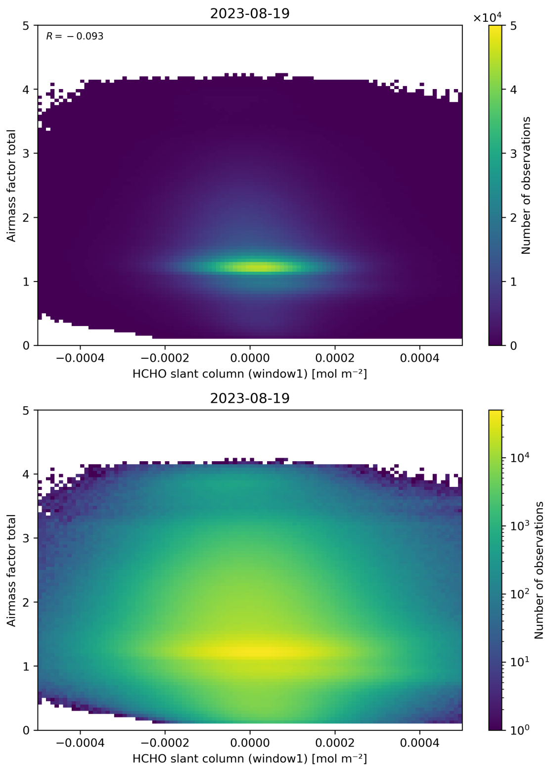
Figure 85: Scatter density plot of “HCHO slant column (window1)” against “Airmass factor total” for 2023-08-18 to 2023-08-20.
