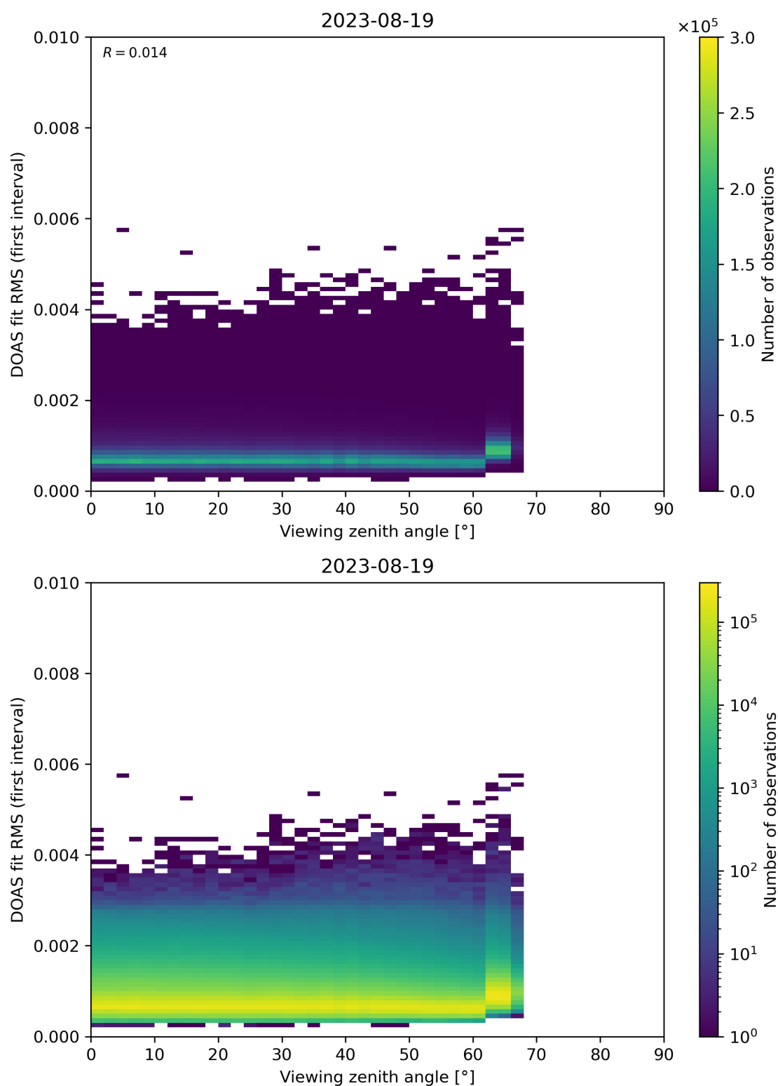
Figure 182: Scatter density plot of “Viewing zenith angle” against “DOAS fit RMS (first interval)” for 2023-08-18 to 2023-08-20.
