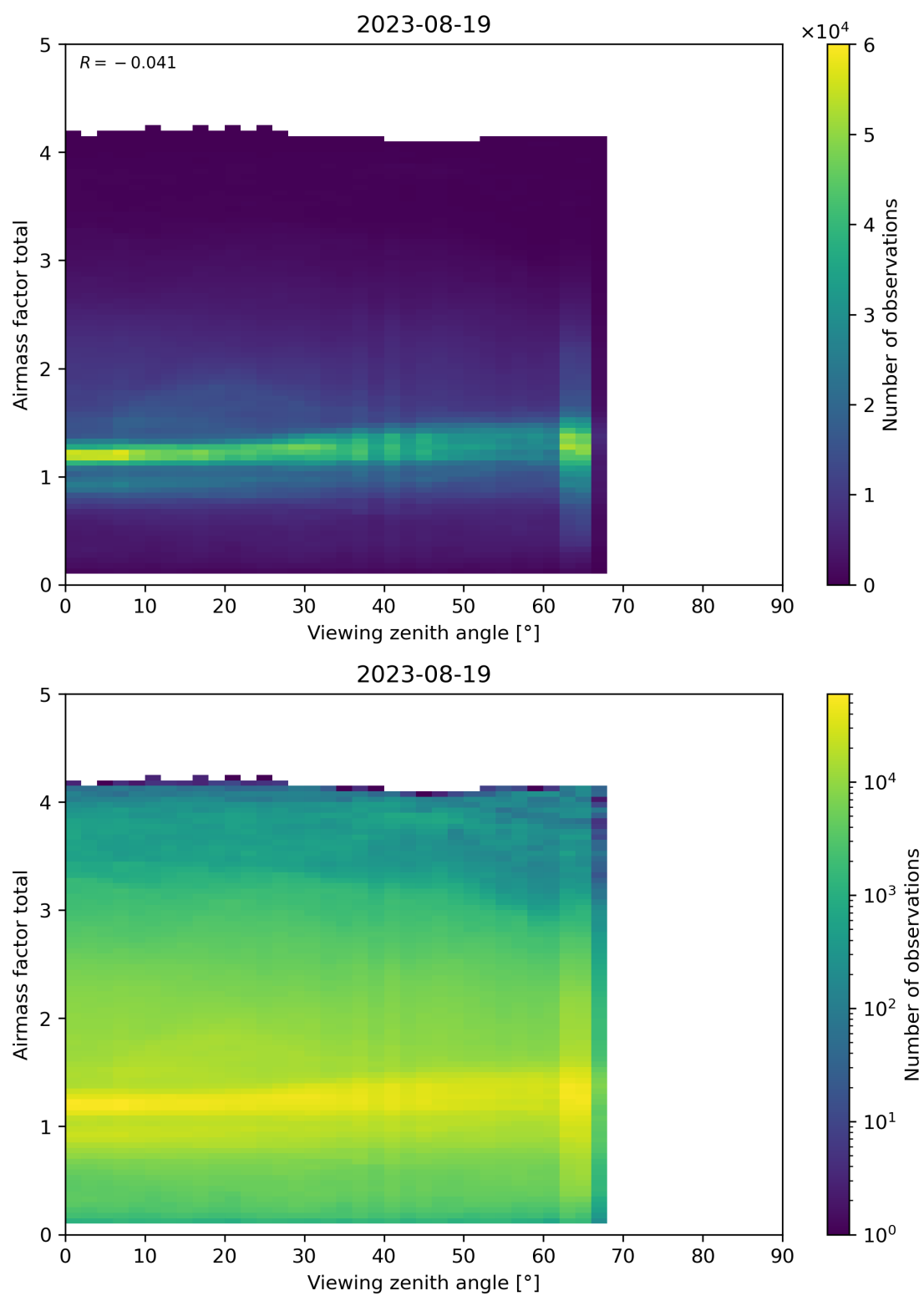
Figure 190: Scatter density plot of “Viewing zenith angle” against “Airmass factor total” for 2023-08-18 to 2023-08-20.
