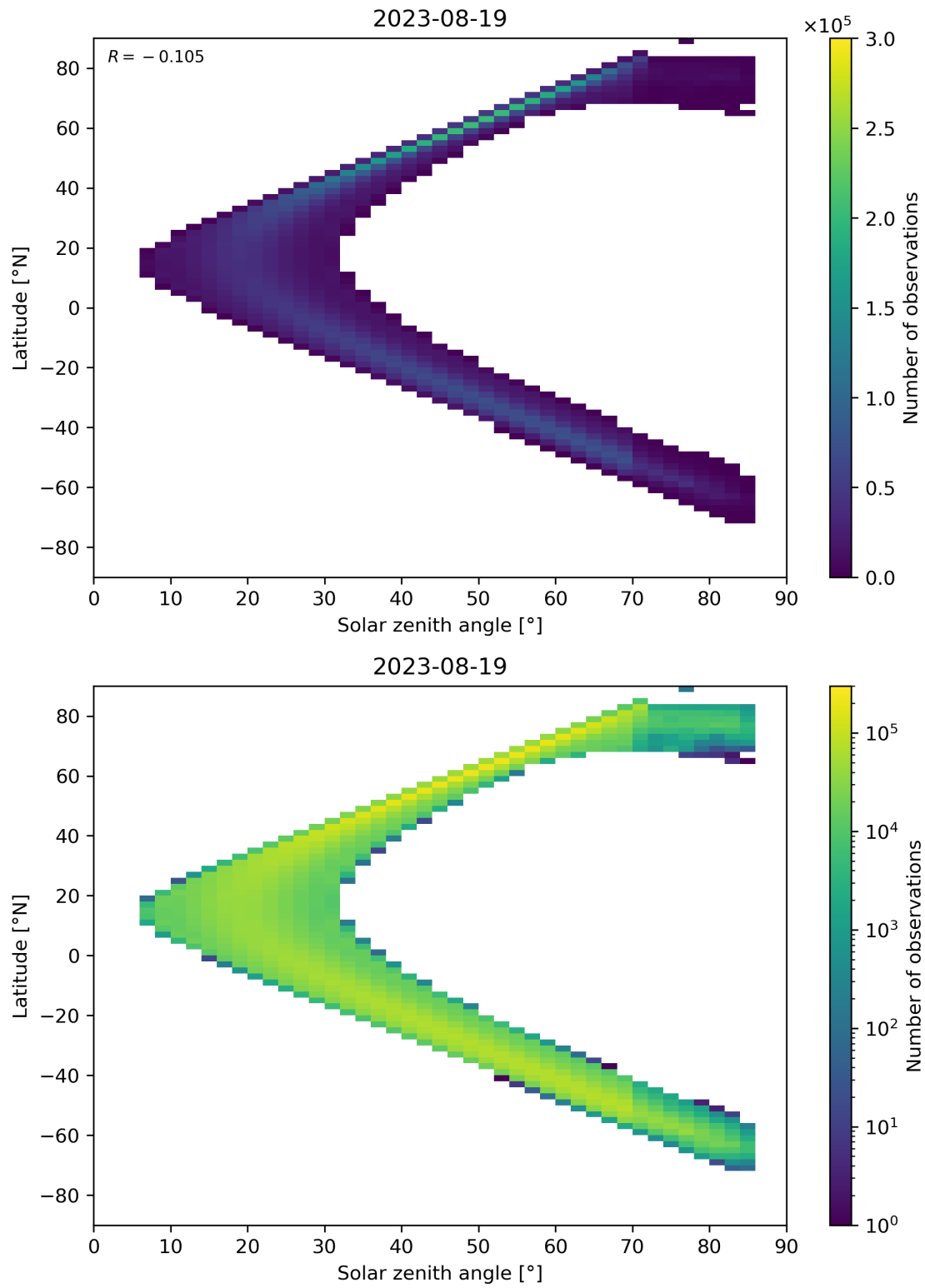
Figure 181: Scatter density plot of “Solar zenith angle” against “Latitude” for 2023-08-18 to 2023-08-20.
