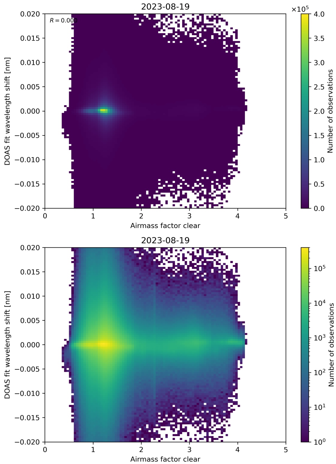
Figure 72: Scatter density plot of “Airmass factor clear” against “DOAS fit wavelength shift” for 2023-08-18 to 2023-08-20.
