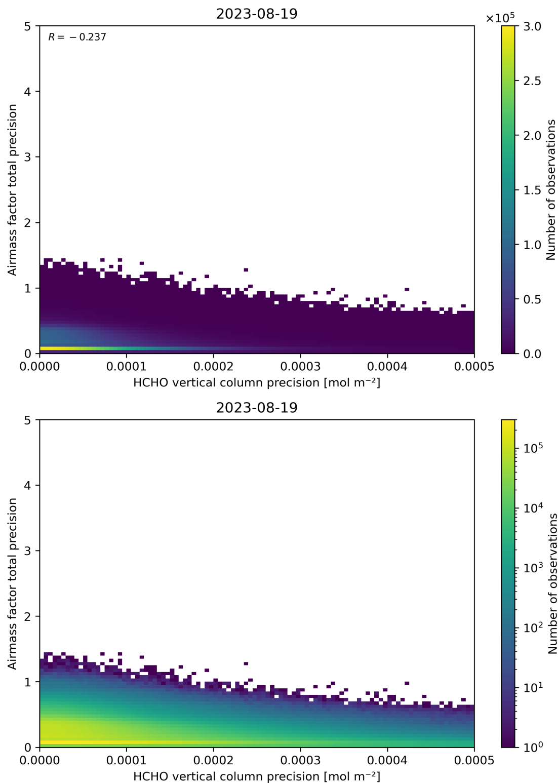
Figure 145: Scatter density plot of “HCHO vertical column precision” against “Airmass factor total precision” for 2023-08-18 to 2023-08-20.
