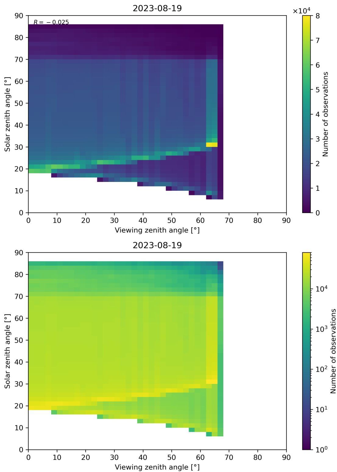
Figure 197: Scatter density plot of “Viewing zenith angle” against “Solar zenith angle” for 2023-08-18 to 2023-08-20.
