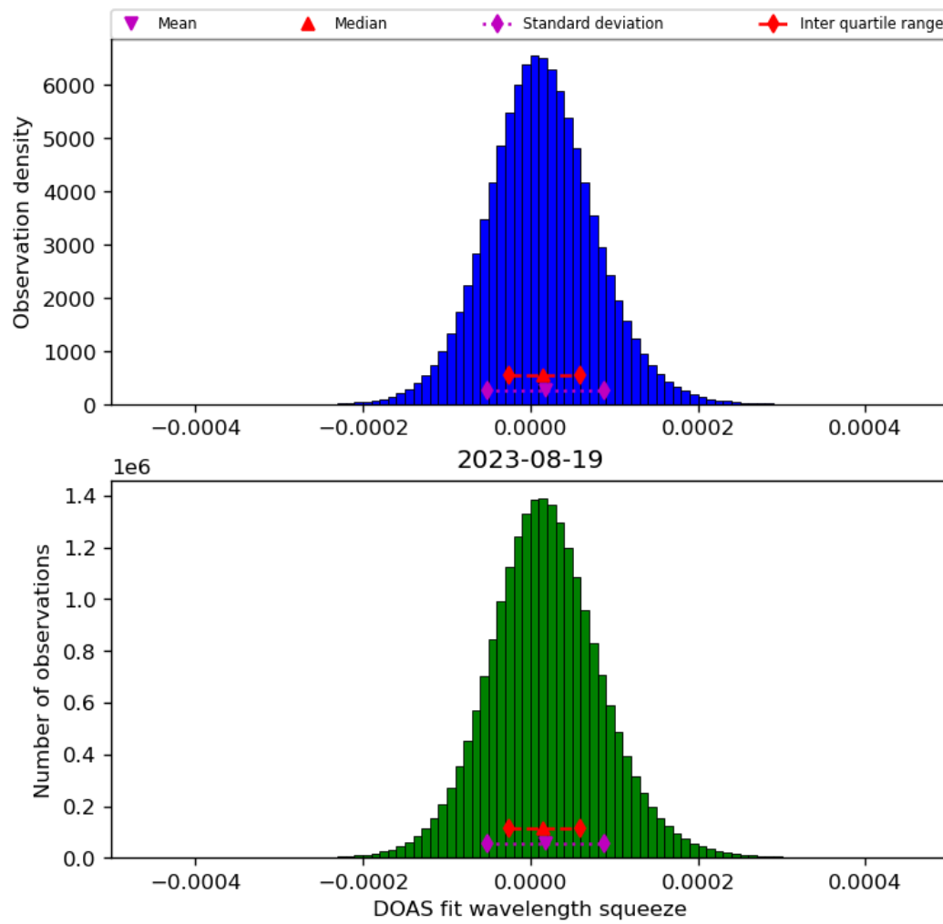
Figure 45: Histogram of “DOAS fit wavelength squeeze” for 2023-08-18 to 2023-08-20
