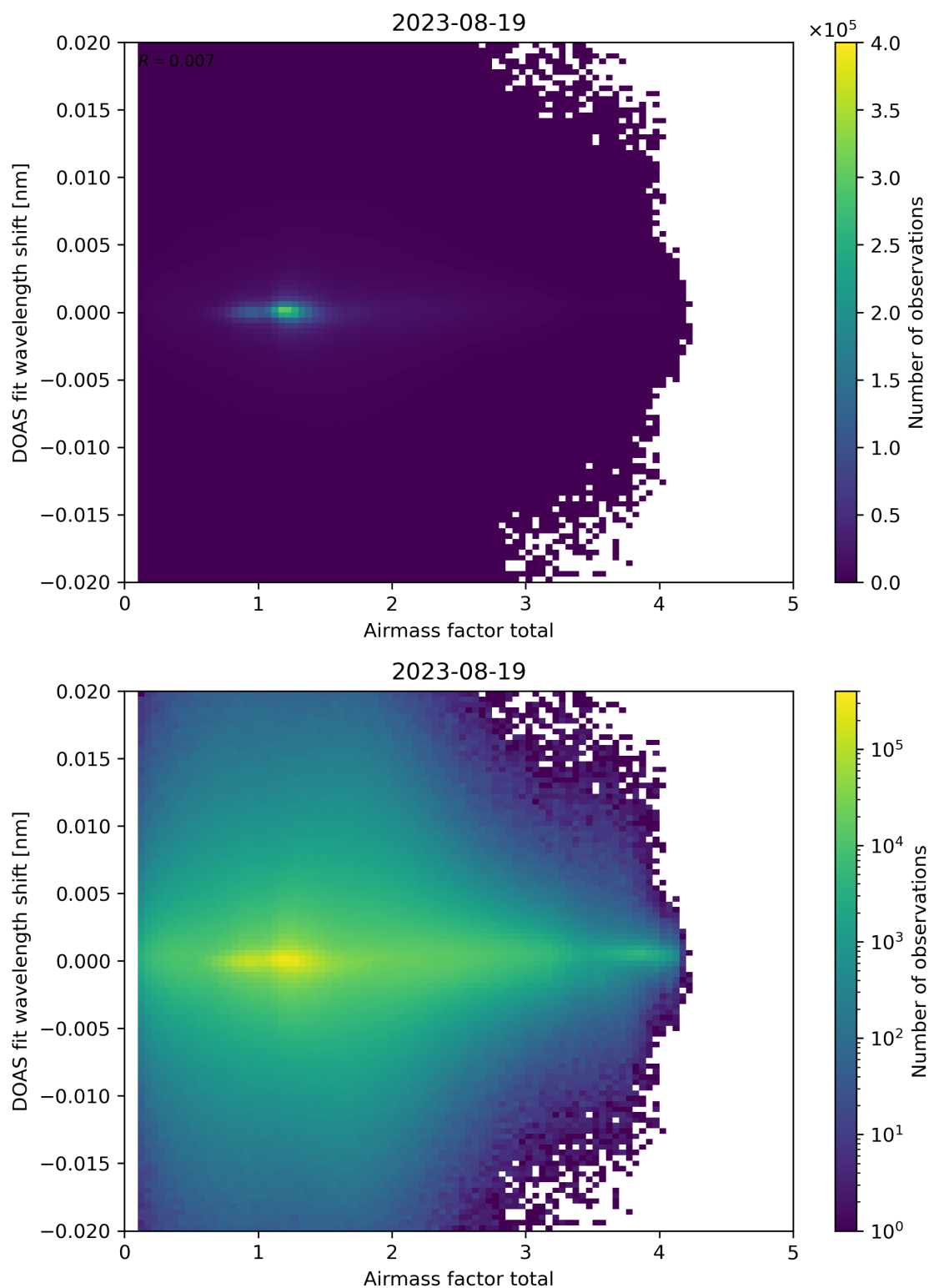
Figure 98: Scatter density plot of “Airmass factor total” against “DOAS fit wavelength shift” for 2023-08-18 to 2023-08-20.
