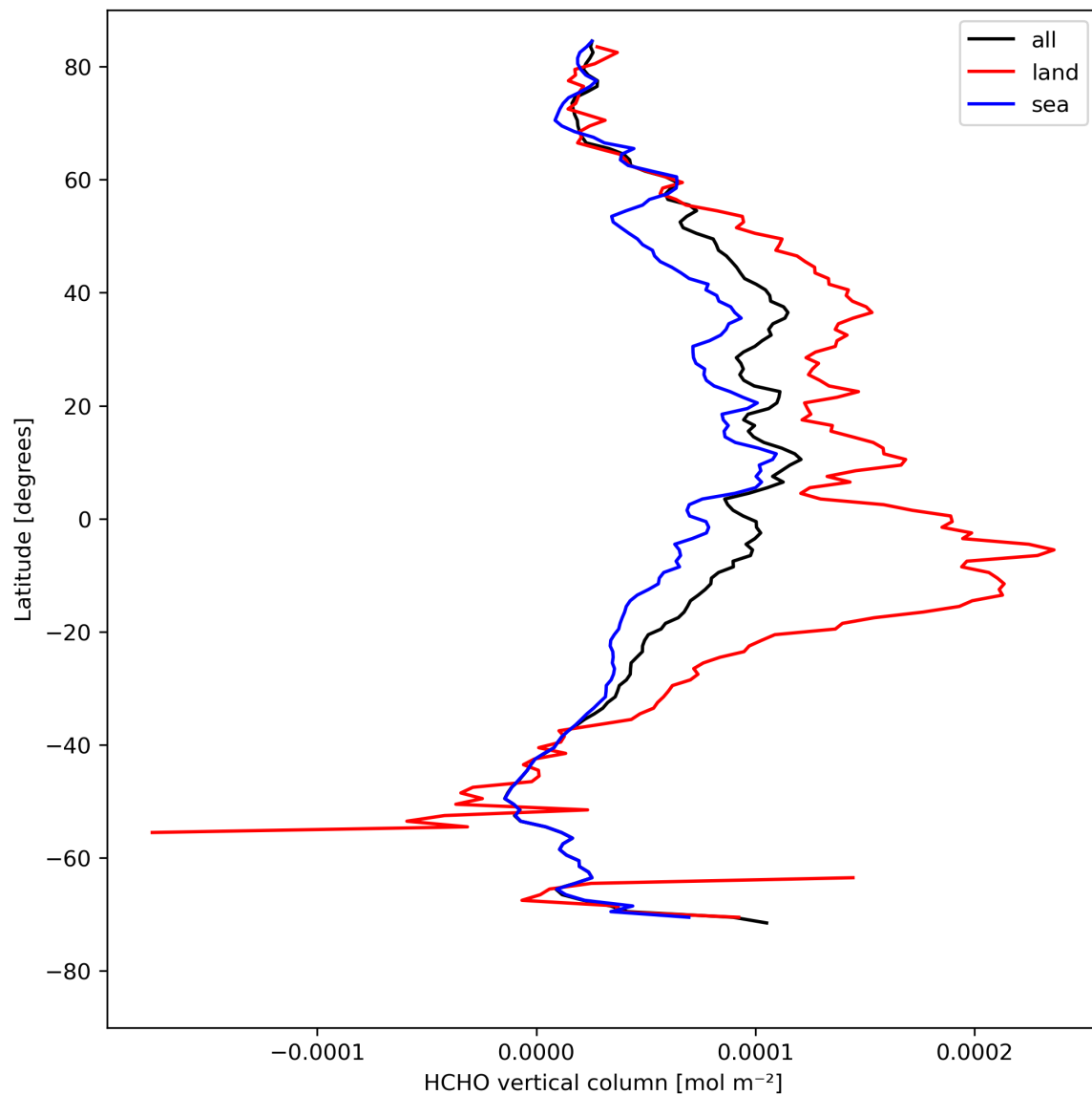
Figure 21: Zonal average of “HCHO vertical column” for 2023-08-18 to 2023-08-20.
