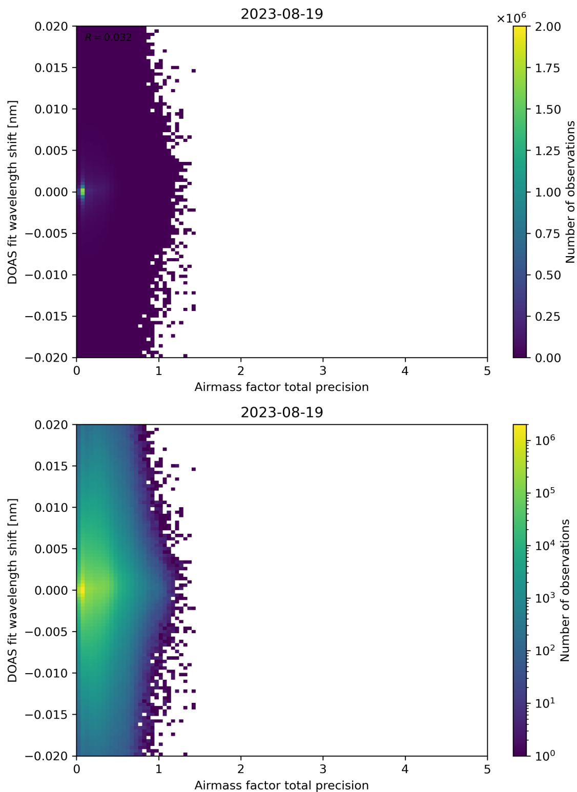
Figure 106: Scatter density plot of “Airmass factor total precision” against “DOAS fit wavelength shift” for 2023-08-18 to 2023-08-20.
