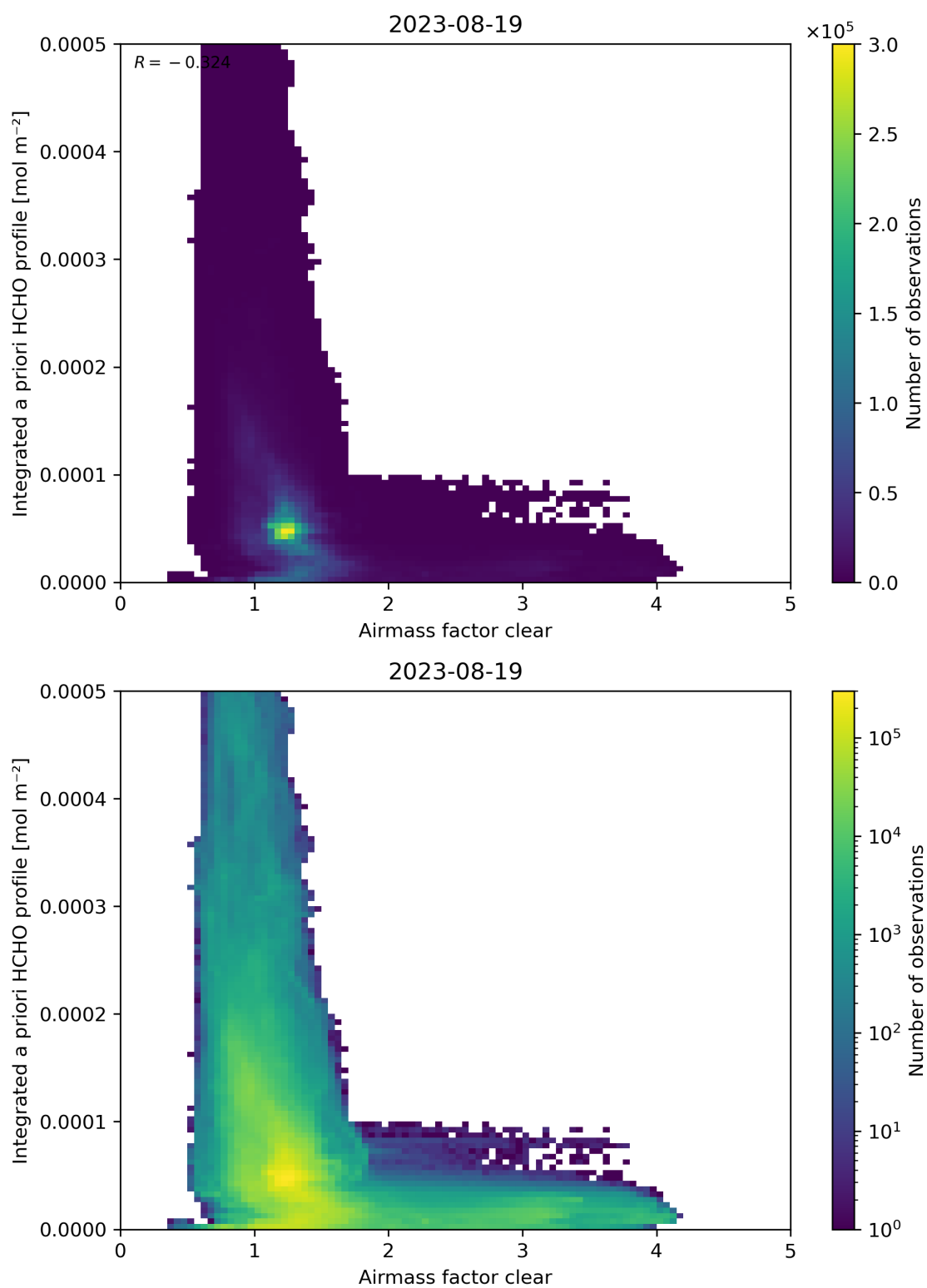
Figure 76: Scatter density plot of “Airmass factor clear” against “Integrated a priori HCHO profile” for 2023-08-18 to 2023-08-20.
