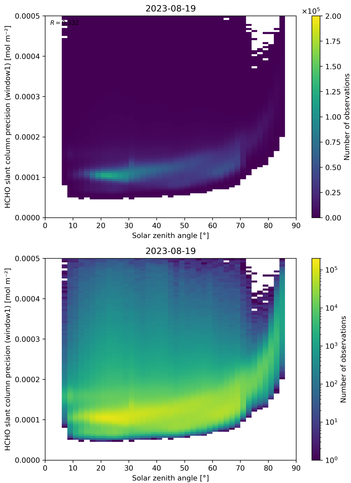
Figure 174: Scatter density plot of “Solar zenith angle” against “HCHO slant column precision (window1)” for 2023-08-18 to 2023-08-20.
