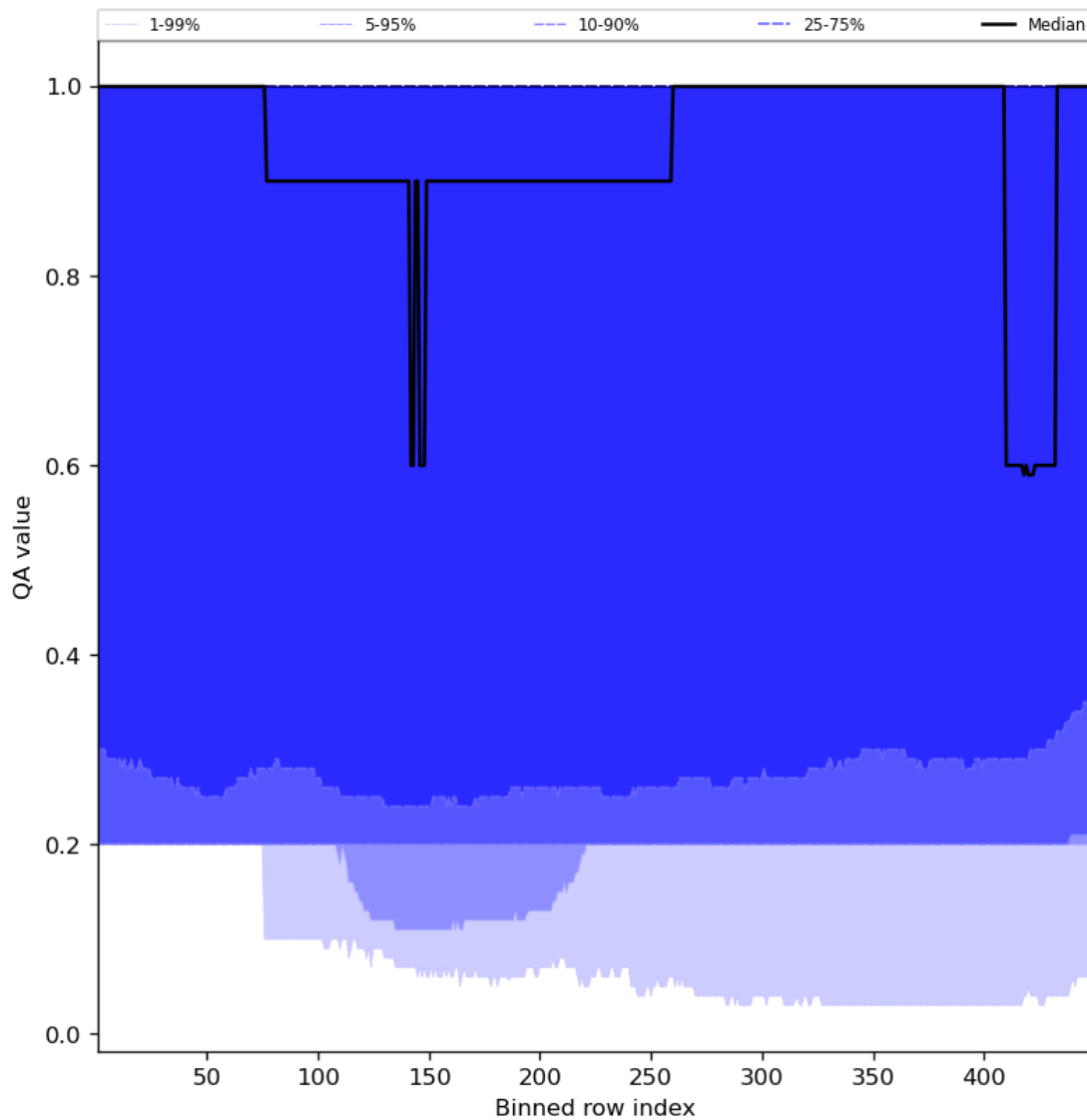
Figure 48: Along track statistics of “QA value” for 2023-08-18 to 2023-08-20
