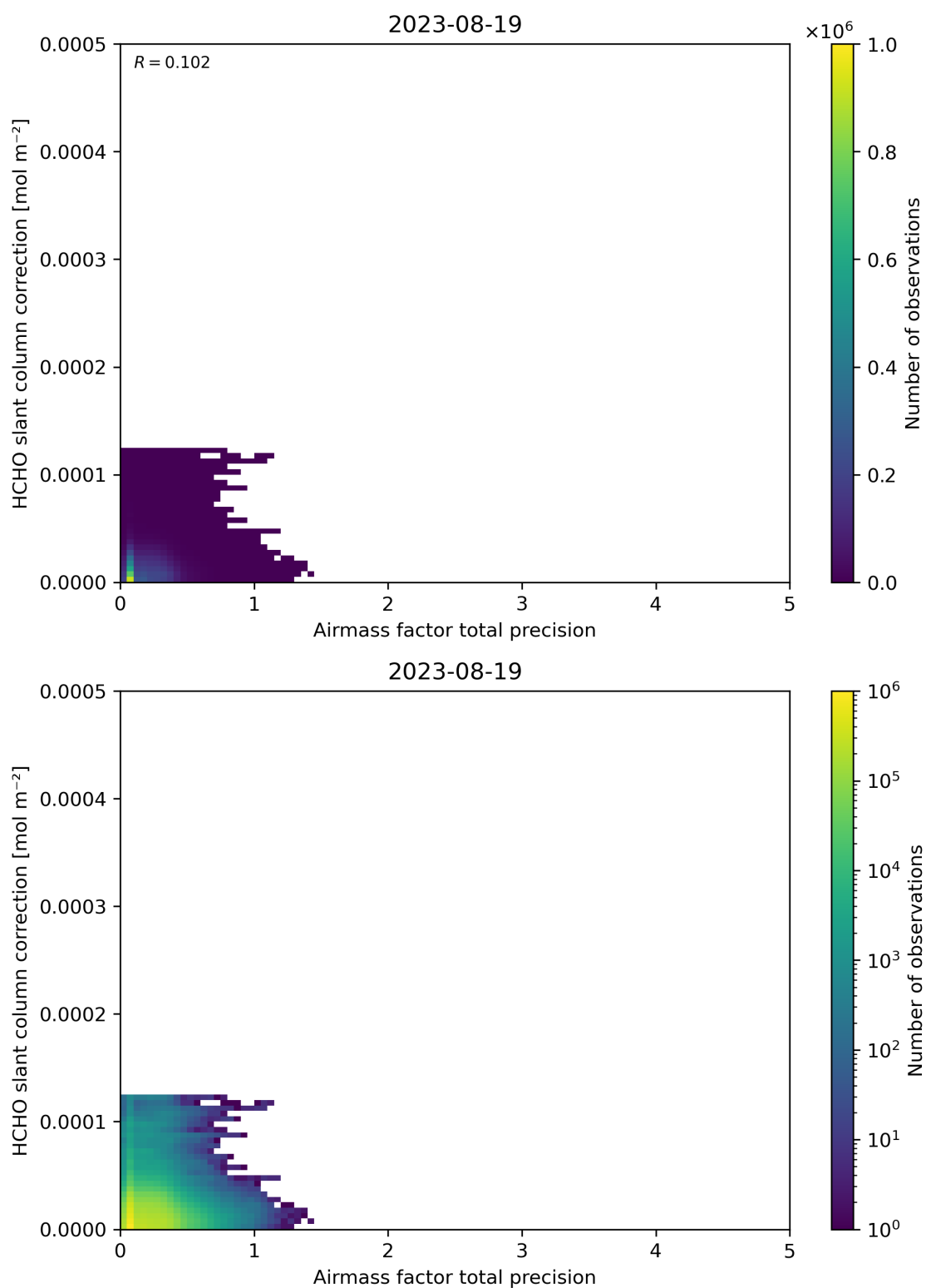
Figure 110: Scatter density plot of “Airmass factor total precision” against “HCHO slant column correction” for 2023-08-18 to 2023-08-20.
