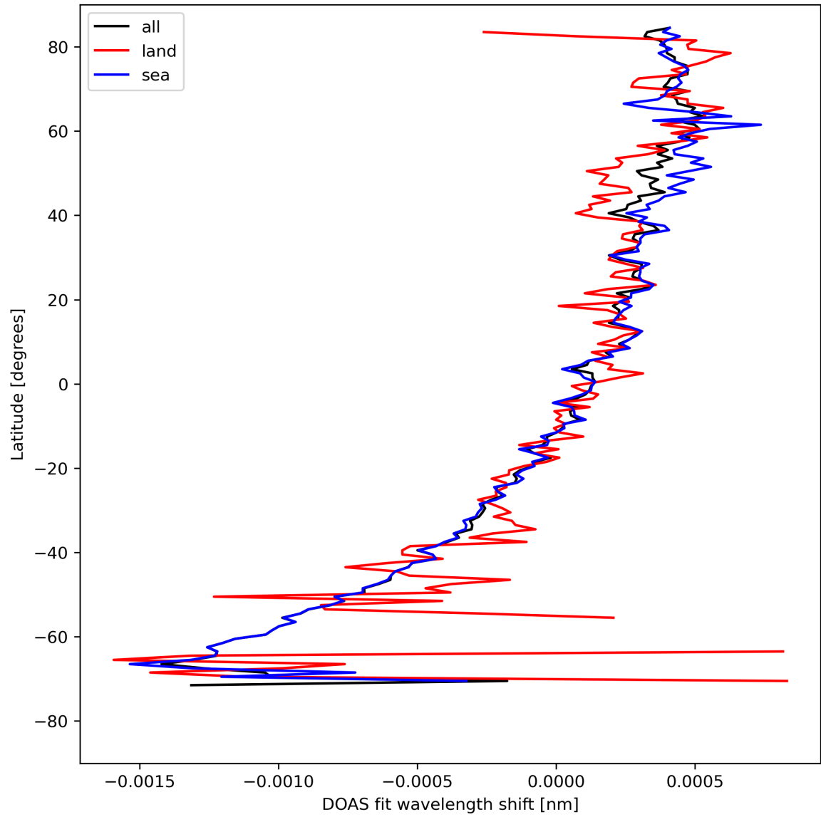
Figure 30: Zonal average of “DOAS fit wavelength shift” for 2023-08-18 to 2023-08-20.
