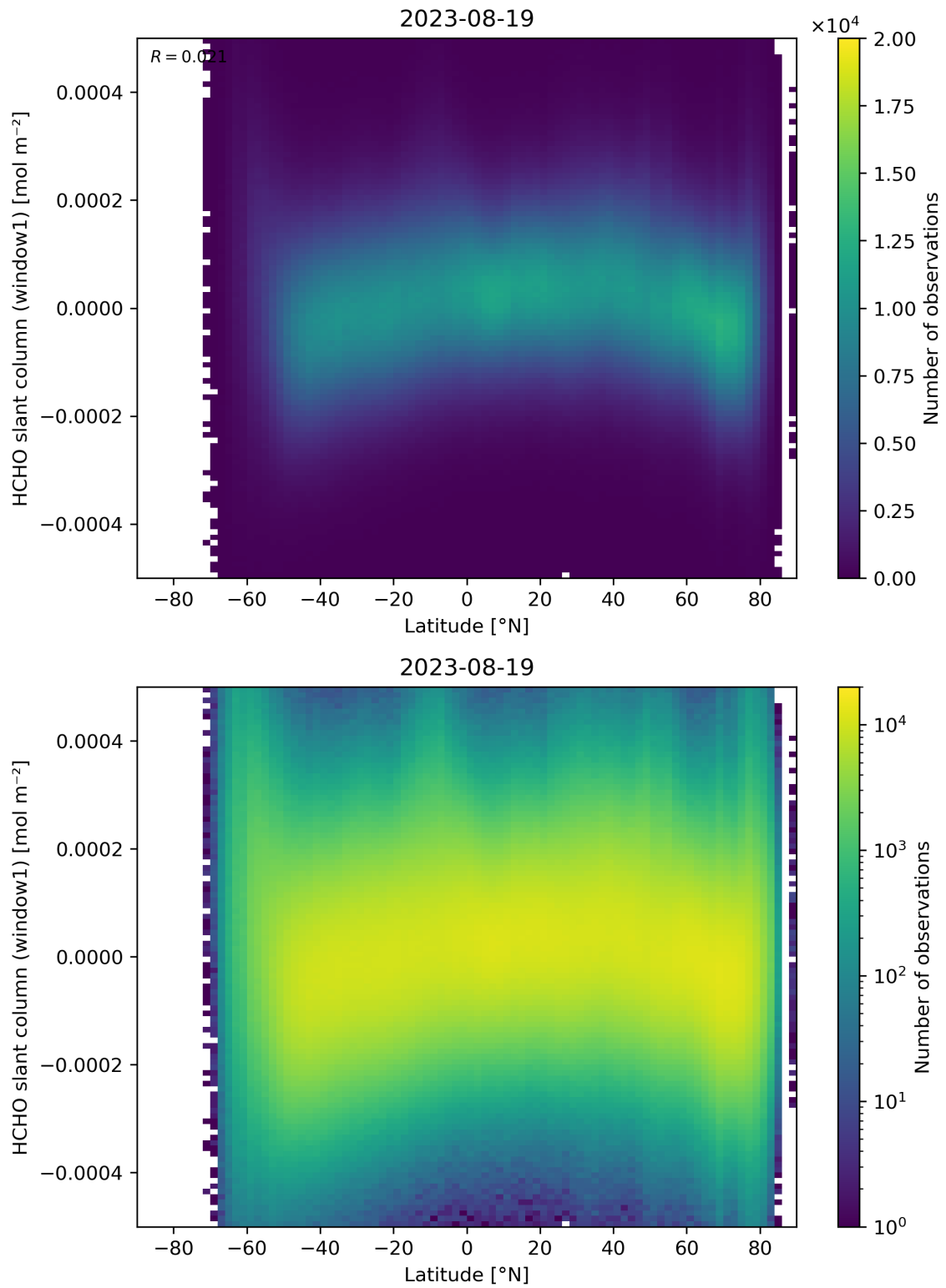
Figure 159: Scatter density plot of “Latitude” against “HCHO slant column (window1)” for 2023-08-18 to 2023-08-20.
