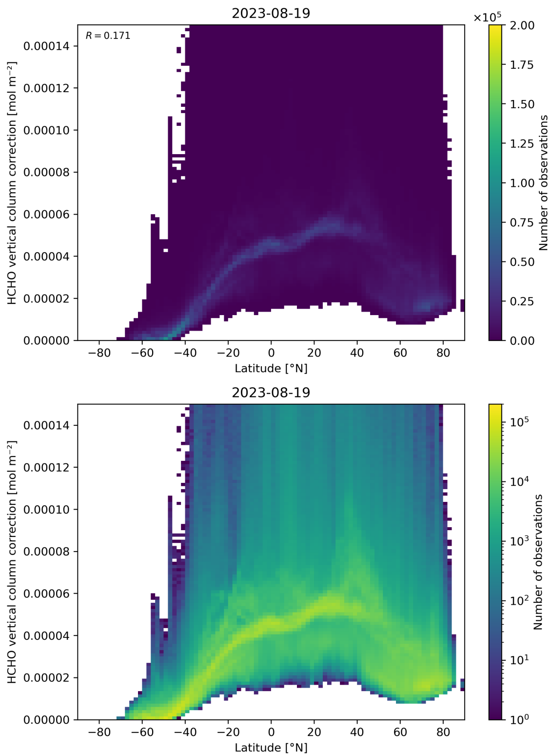
Figure 164: Scatter density plot of “Latitude” against “HCHO vertical column correction” for 2023-08-18 to 2023-08-20.
