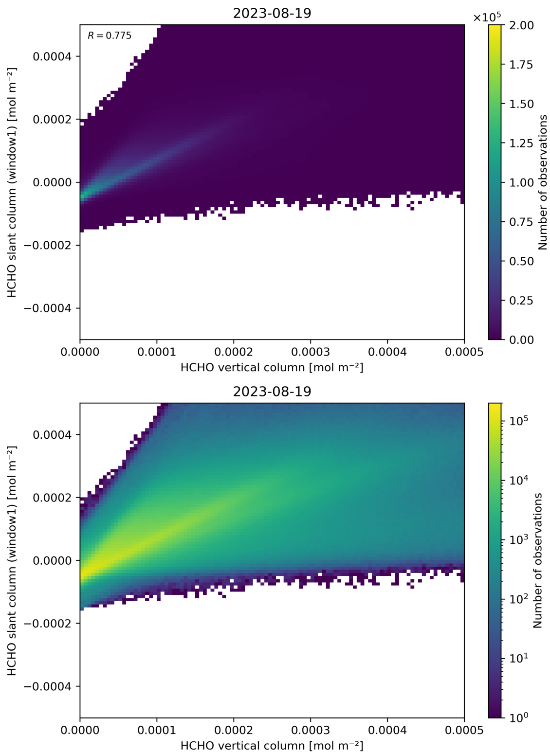
Figure 129: Scatter density plot of “HCHO vertical column” against “HCHO slant column (window1)” for 2023-08-18 to 2023-08-20.
