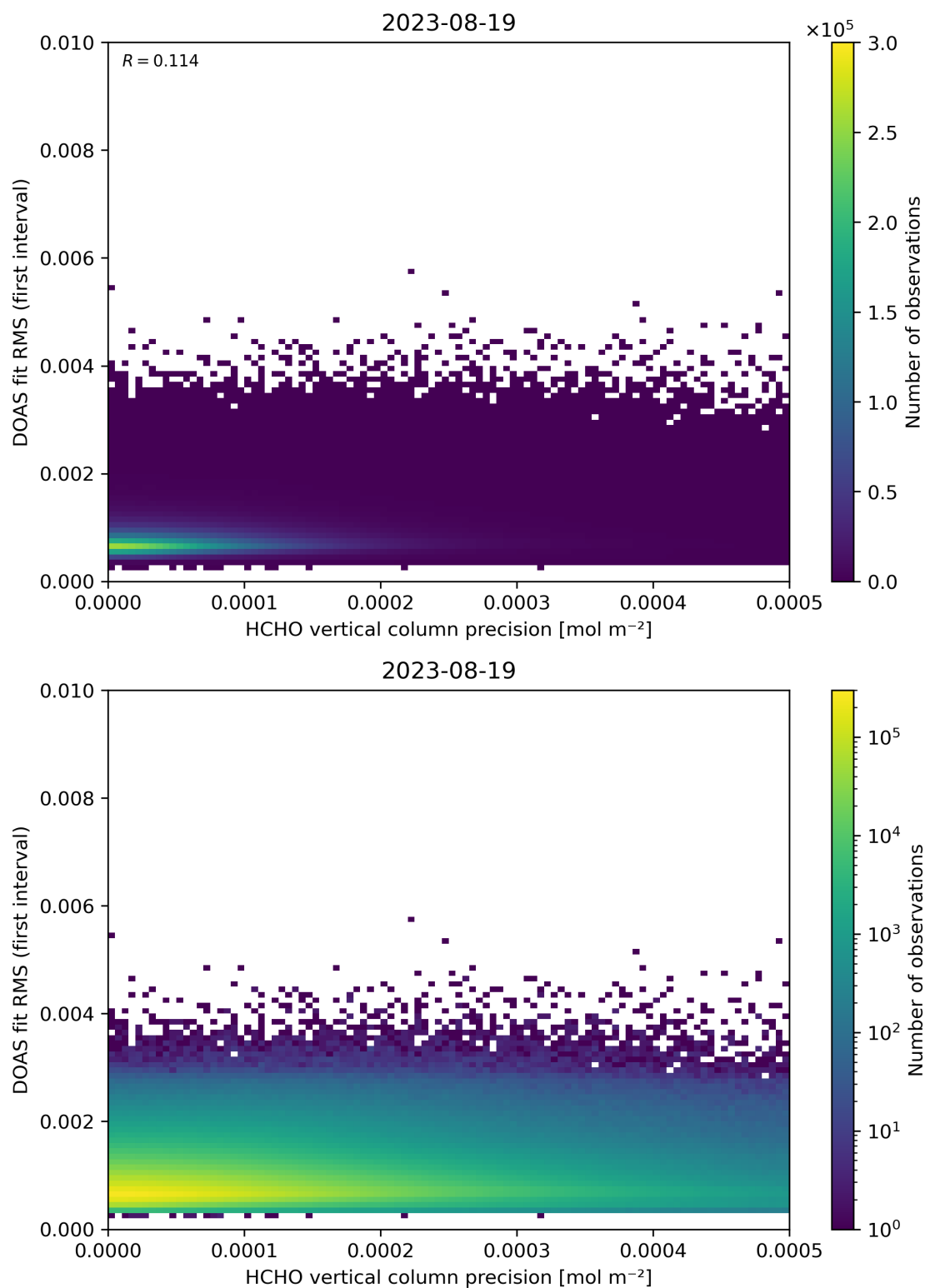
Figure 136: Scatter density plot of “HCHO vertical column precision” against “DOAS fit RMS (first interval)” for 2023-08-18 to 2023-08-20.
