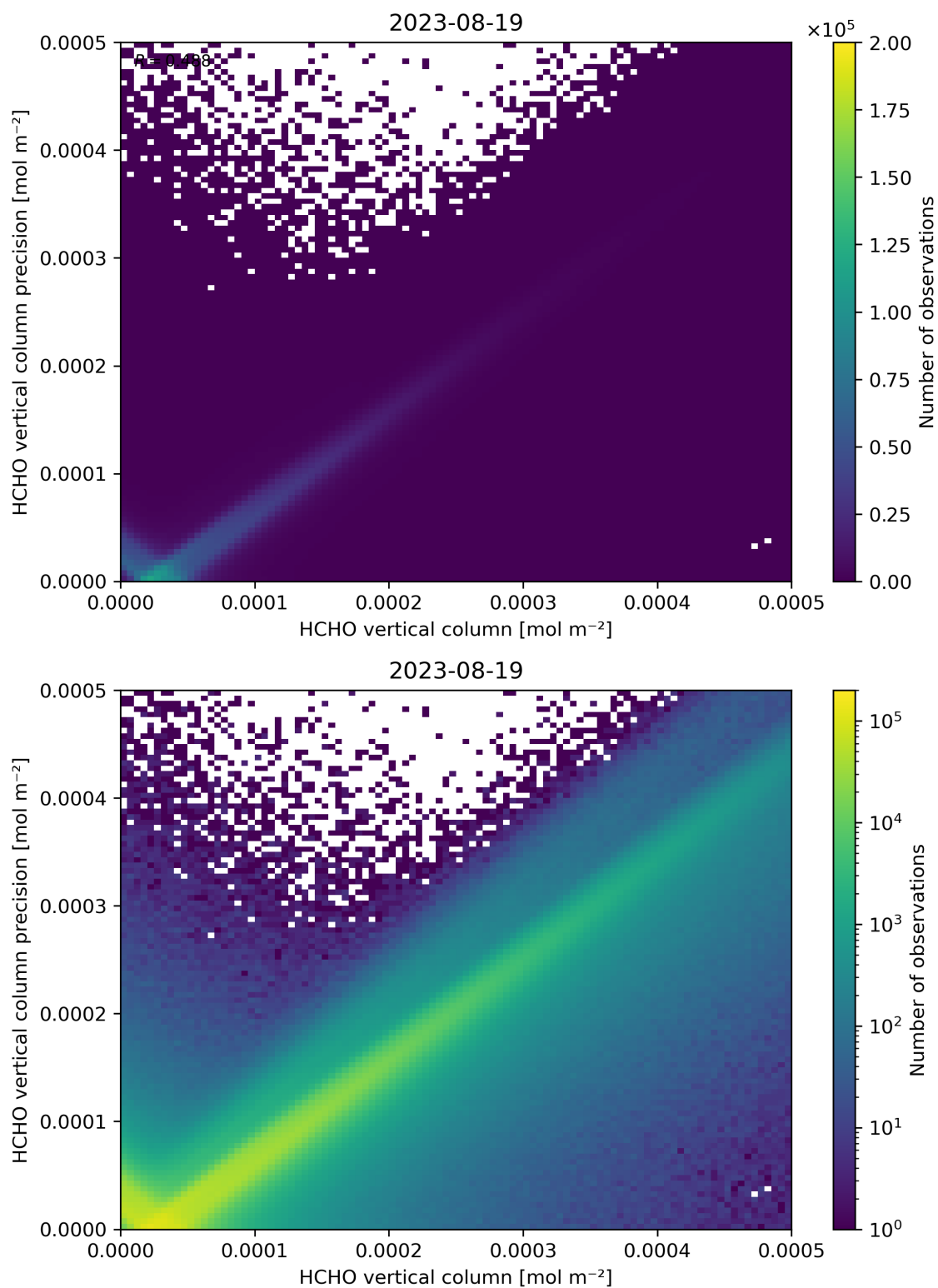
Figure 134: Scatter density plot of “HCHO vertical column” against “HCHO vertical column precision” for 2023-08-18 to 2023-08-20.
