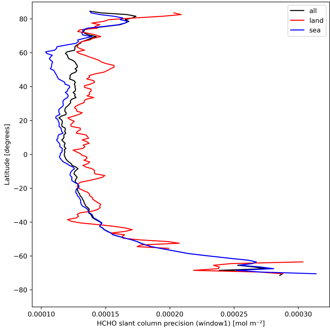
Figure 25: Zonal average of “HCHO slant column precision (window1)” for 2023-08-18 to 2023-08-20.
