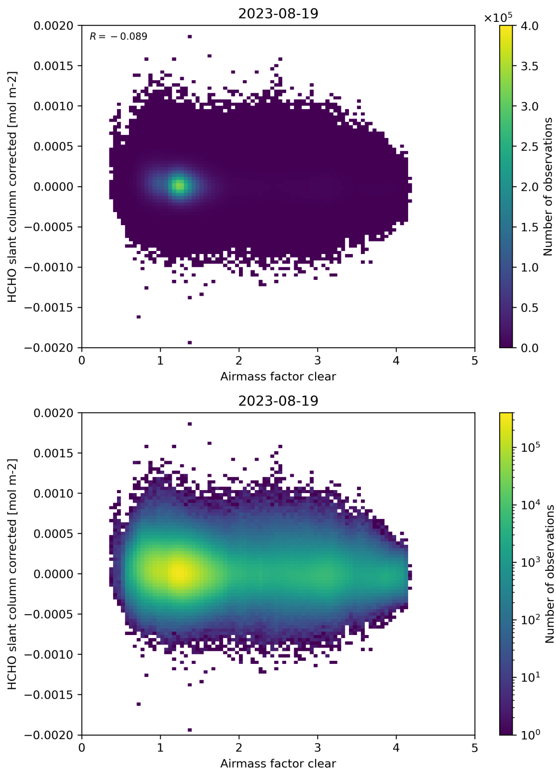
Figure 74: Scatter density plot of “Airmass factor clear” against “HCHO slant column corrected” for 2023-08-18 to 2023-08-20.
