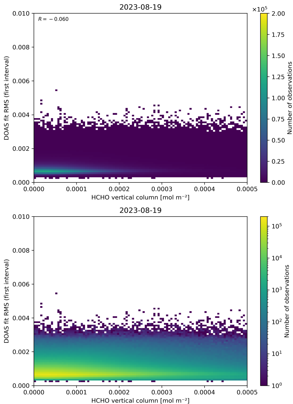
Figure 123: Scatter density plot of “HCHO vertical column” against “DOAS fit RMS (first interval)” for 2023-08-18 to 2023-08-20.
