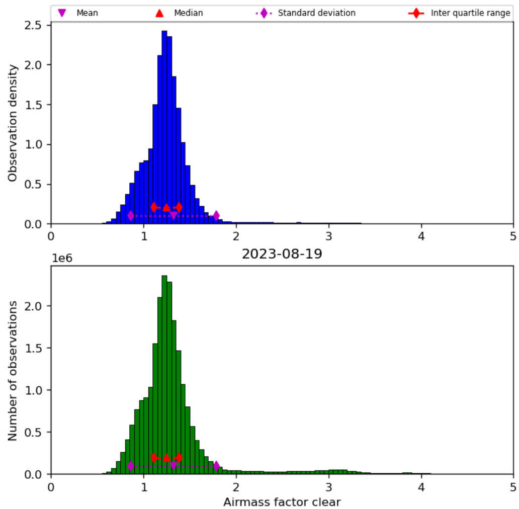
Figure 42: Histogram of “Airmass factor clear” for 2023-08-18 to 2023-08-20
