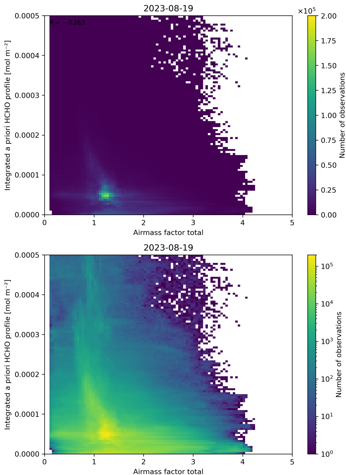
Figure 104: Scatter density plot of “Airmass factor total” against “Integrated a priori HCHO profile” for 2023-08-18 to 2023-08-20.
