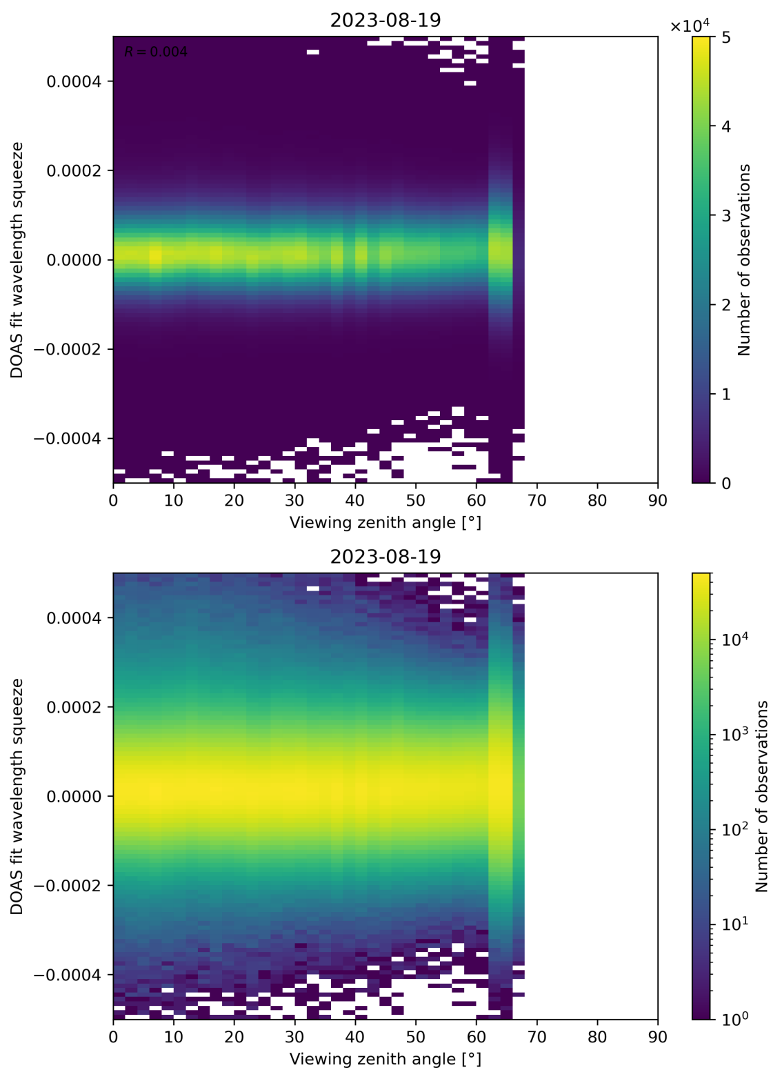
Figure 184: Scatter density plot of “Viewing zenith angle” against “DOAS fit wavelength squeeze” for 2023-08-18 to 2023-08-20.
