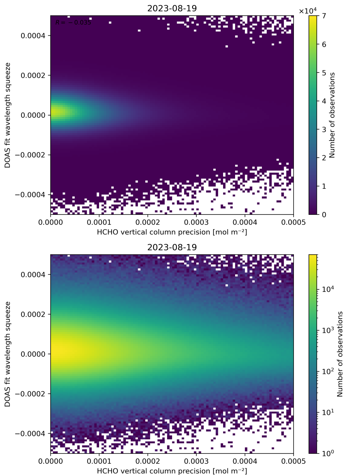
Figure 138: Scatter density plot of “HCHO vertical column precision” against “DOAS fit wavelength squeeze” for 2023-08-18 to 2023-08-20.
