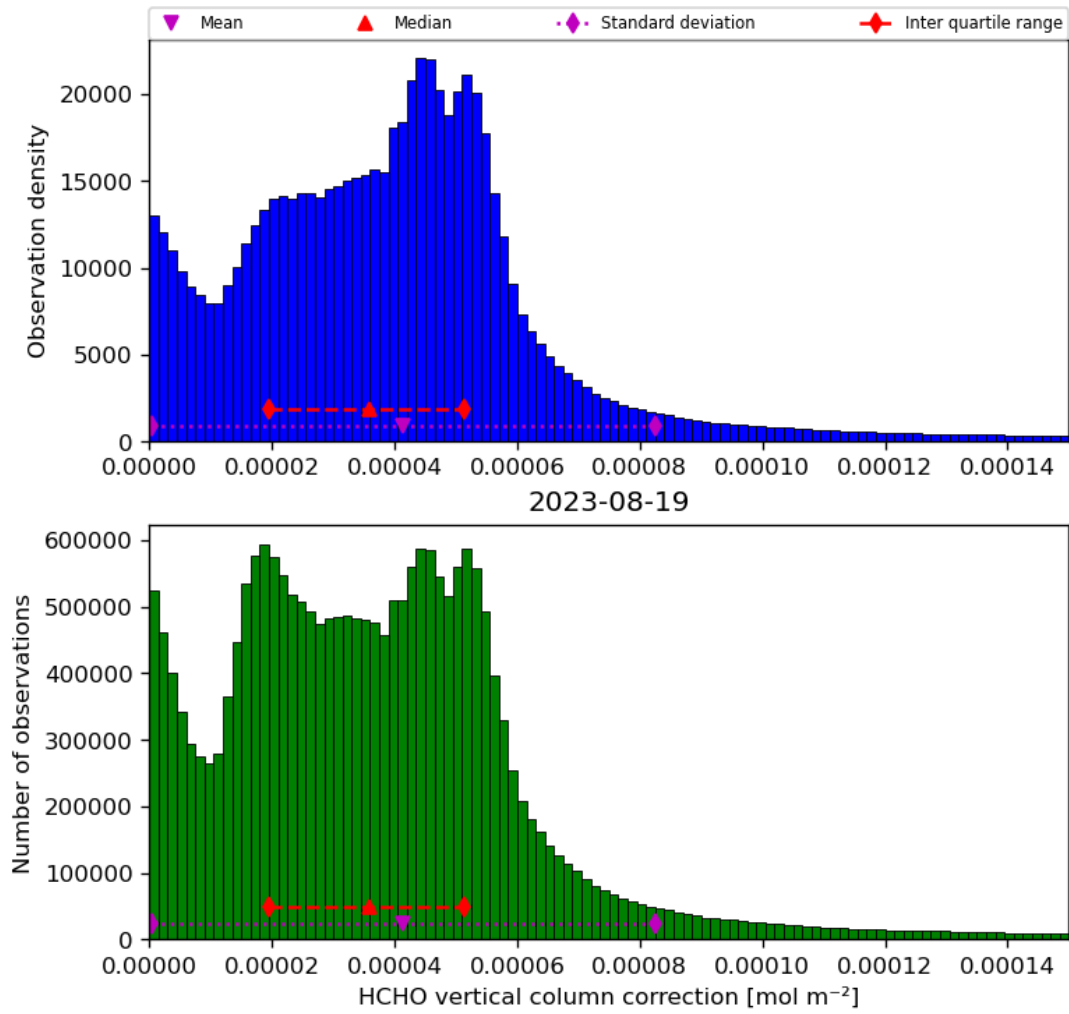
Figure 37: Histogram of “HCHO vertical column correction” for 2023-08-18 to 2023-08-20
