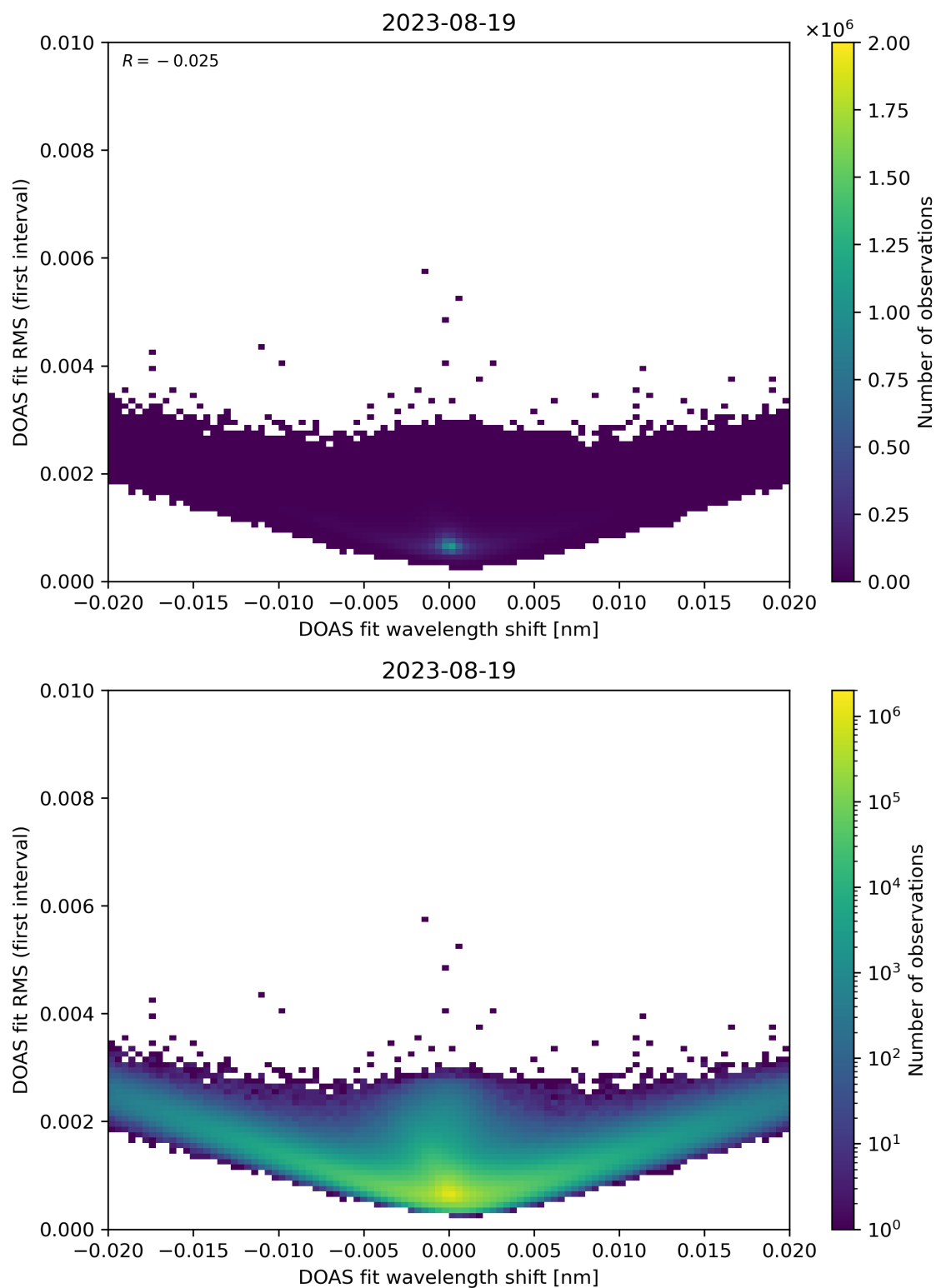
Figure 64: Scatter density plot of “DOAS fit wavelength shift” against “DOAS fit RMS (first interval)” for 2023-08-18 to 2023-08-20.
