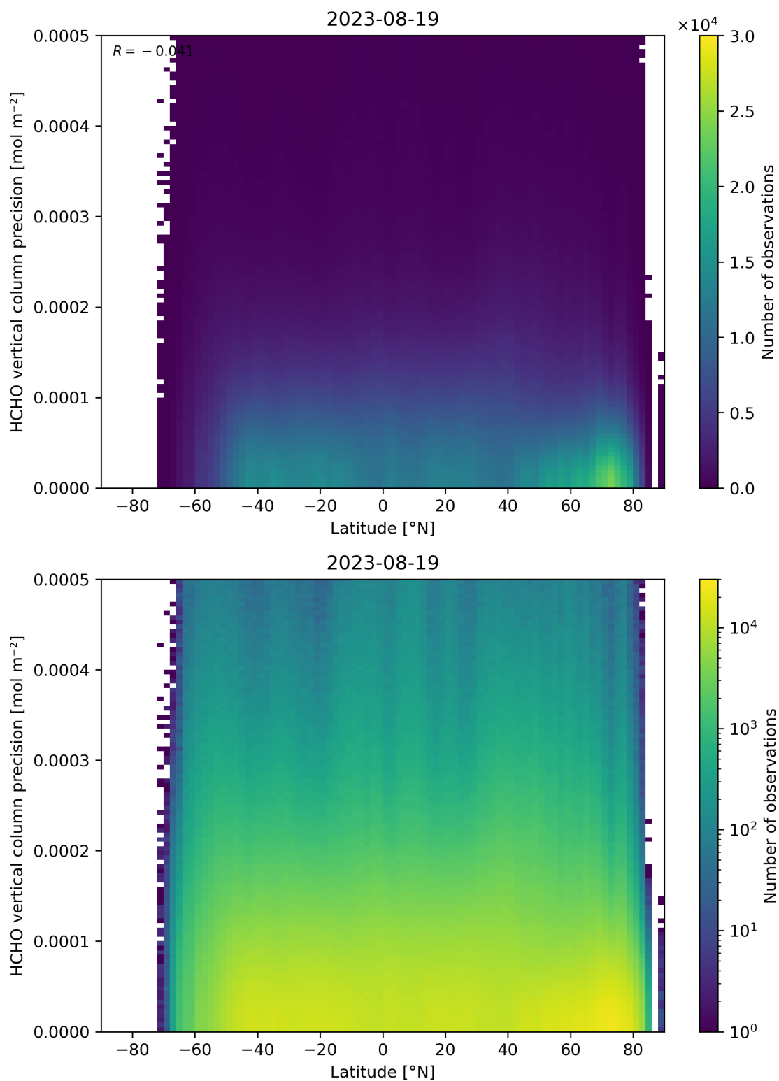
Figure 165: Scatter density plot of “Latitude” against “HCHO vertical column precision” for 2023-08-18 to 2023-08-20.
