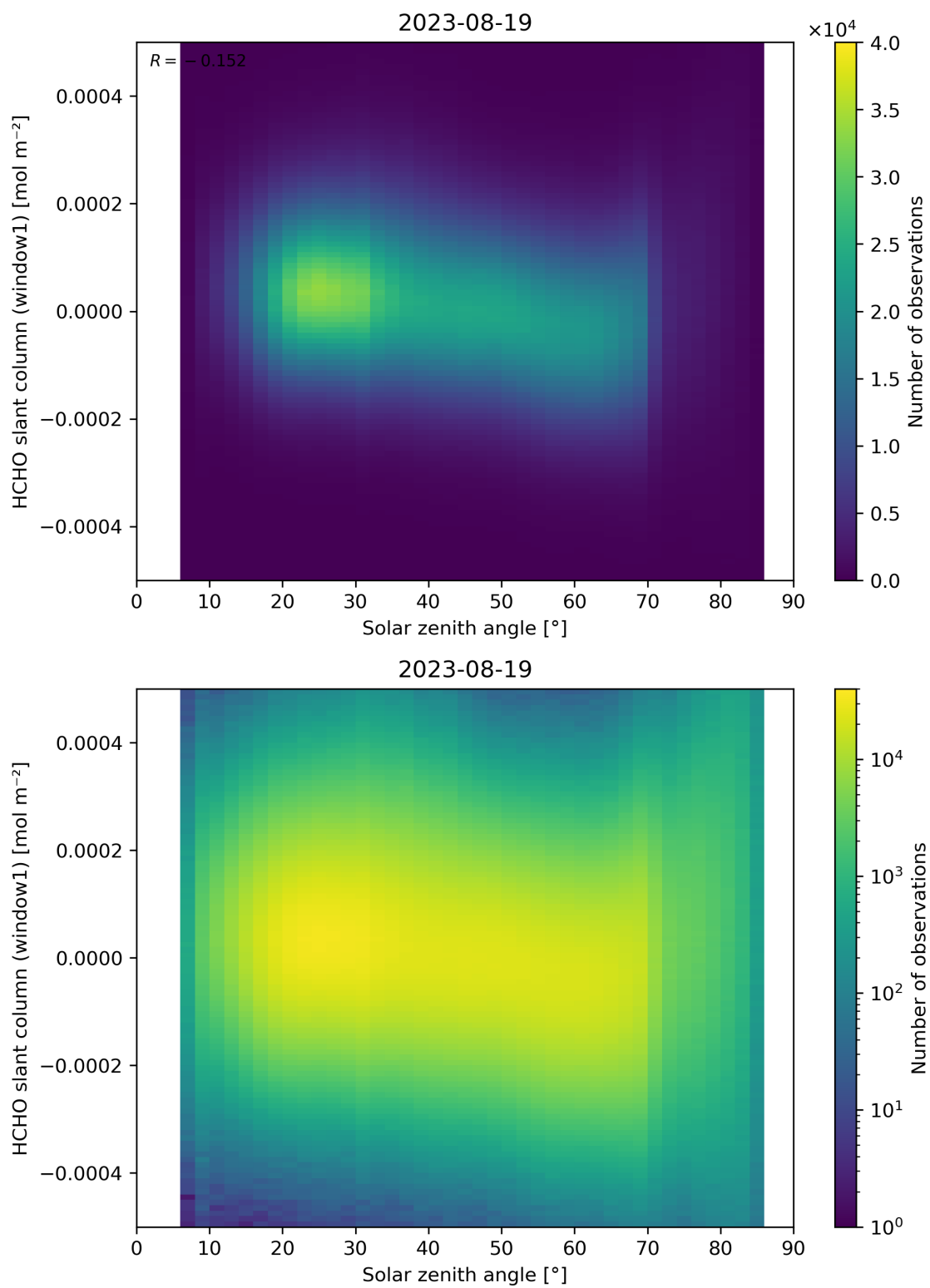
Figure 173: Scatter density plot of “Solar zenith angle” against “HCHO slant column (window1)” for 2023-08-18 to 2023-08-20.
