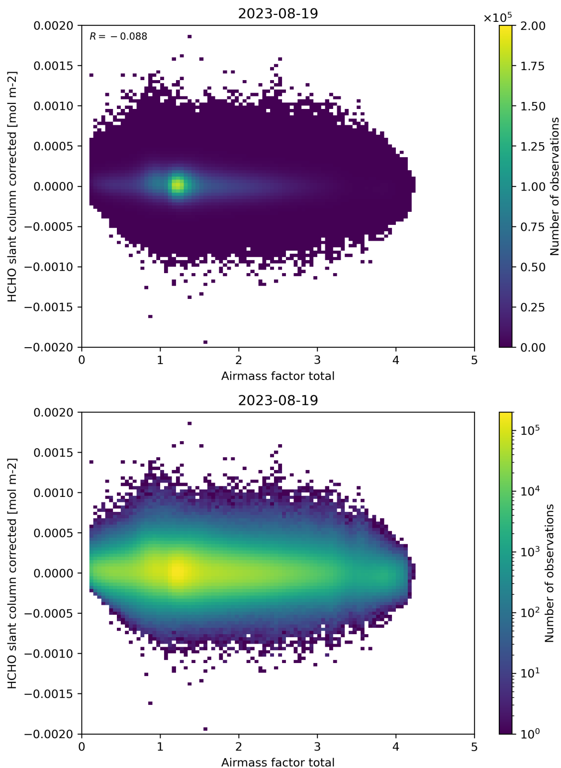
Figure 101: Scatter density plot of “Airmass factor total” against “HCHO slant column corrected” for 2023-08-18 to 2023-08-20.
