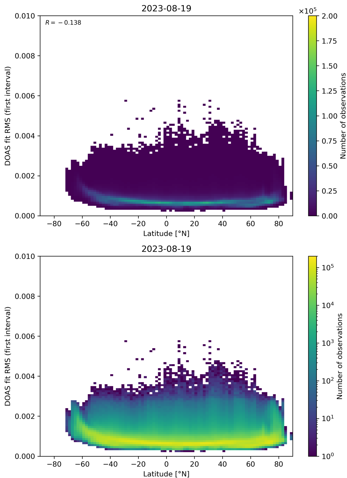
Figure 153: Scatter density plot of “Latitude” against “DOAS fit RMS (first interval)” for 2023-08-18 to 2023-08-20.
