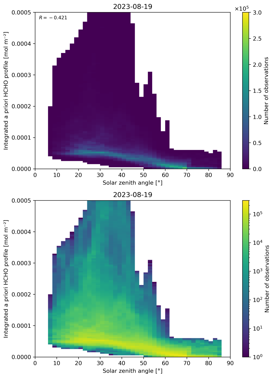
Figure 180: Scatter density plot of “Solar zenith angle” against “Integrated a priori HCHO profile” for 2023-08-18 to 2023-08-20.
