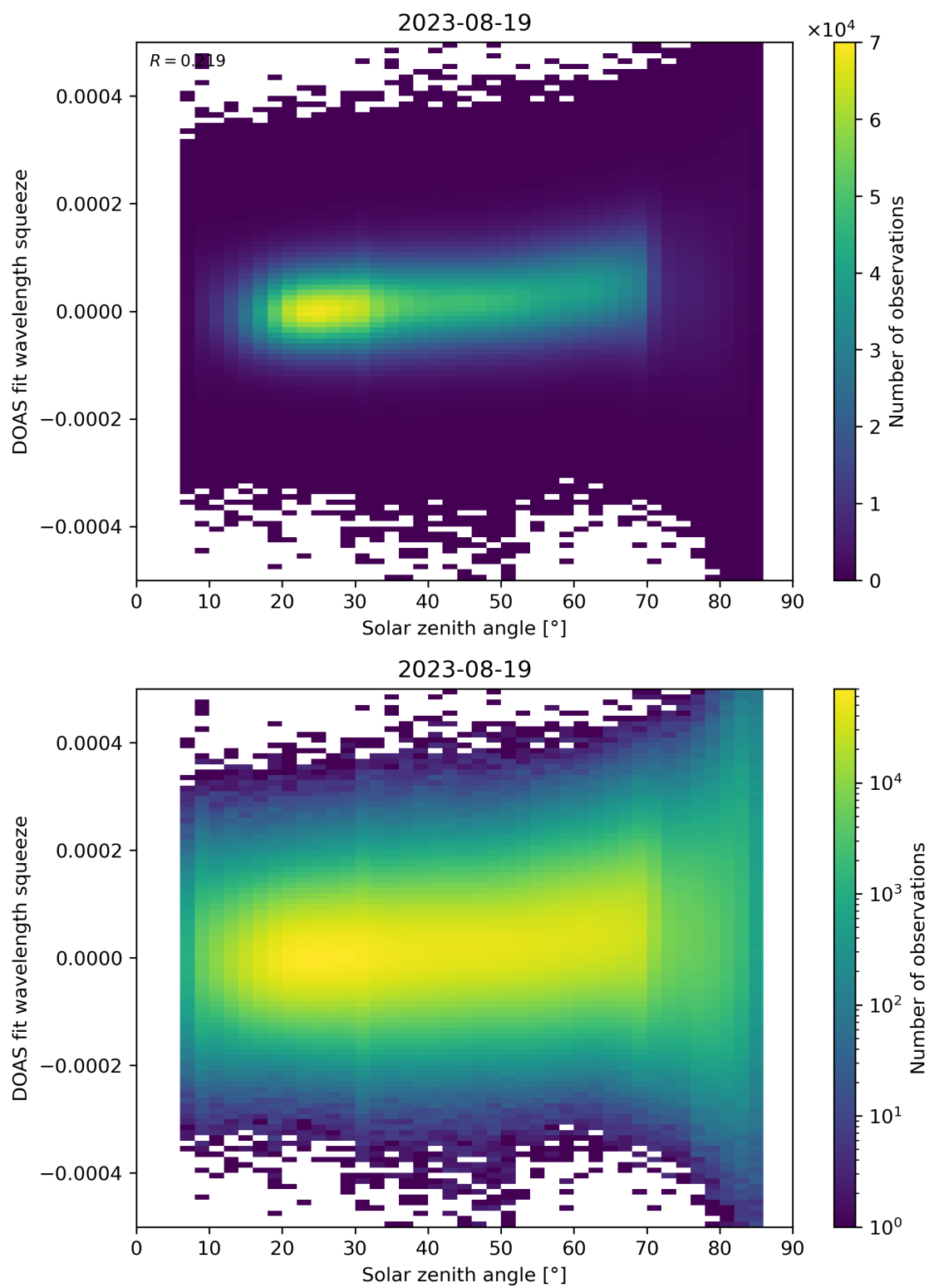
Figure 169: Scatter density plot of “Solar zenith angle” against “DOAS fit wavelength squeeze” for 2023-08-18 to 2023-08-20.
