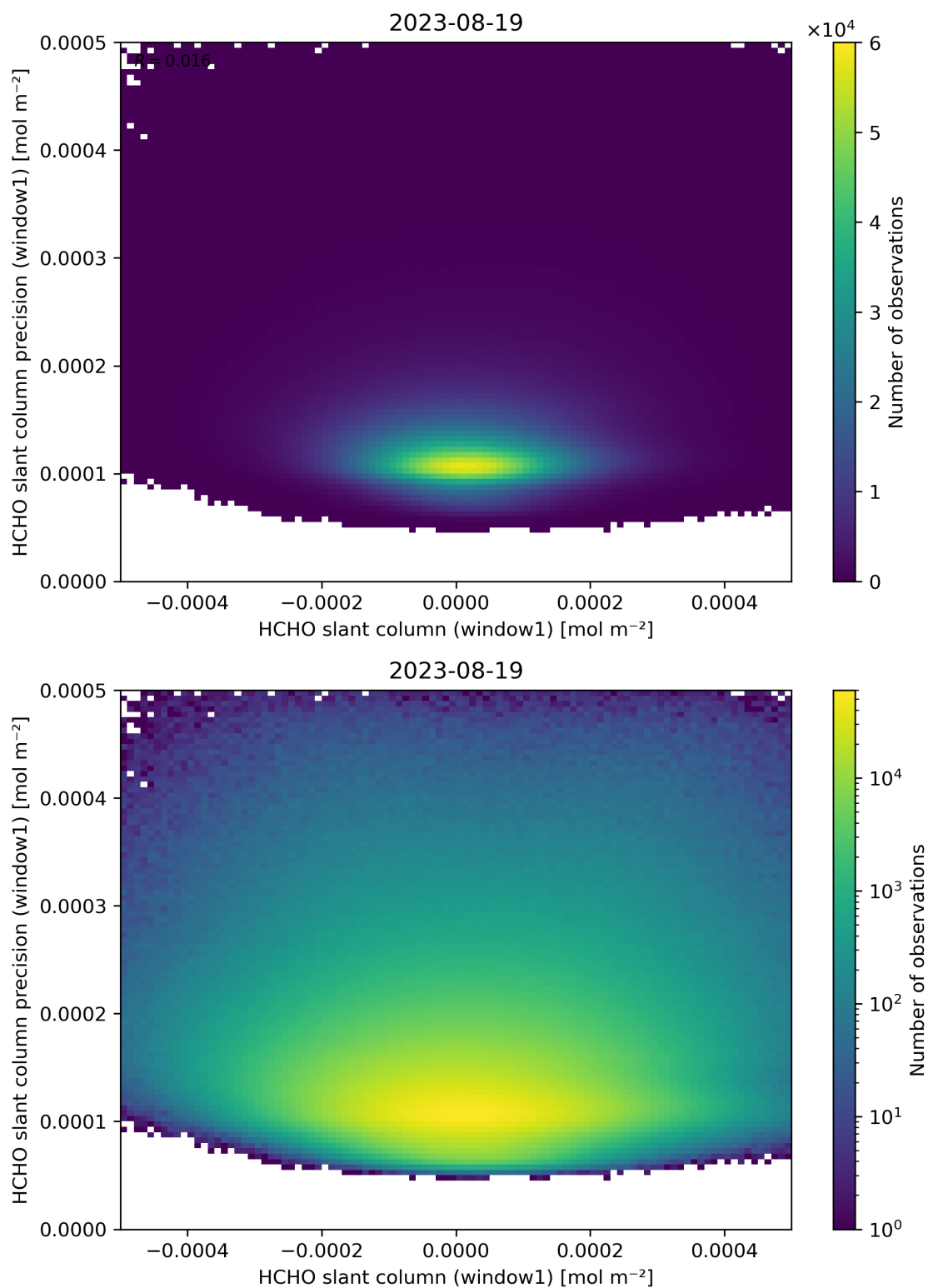
Figure 84: Scatter density plot of “HCHO slant column (window1)” against “HCHO slant column precision (window1)” for 2023-08-18 to 2023-08-20.
