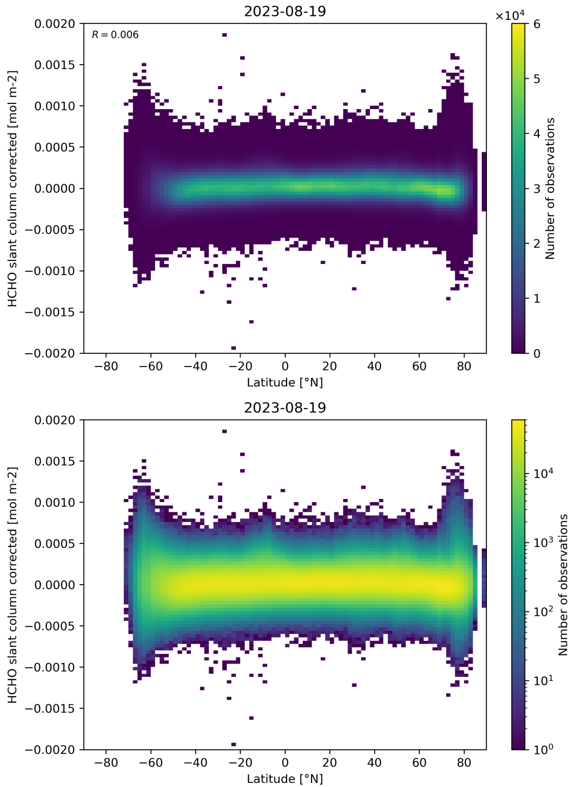
Figure 157: Scatter density plot of “Latitude” against “HCHO slant column corrected” for 2023-08-18 to 2023-08-20.
