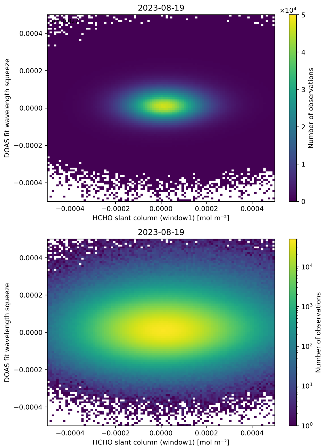
Figure 80: Scatter density plot of “HCHO slant column (window1)” against “DOAS fit wavelength squeeze” for 2023-08-18 to 2023-08-20.
