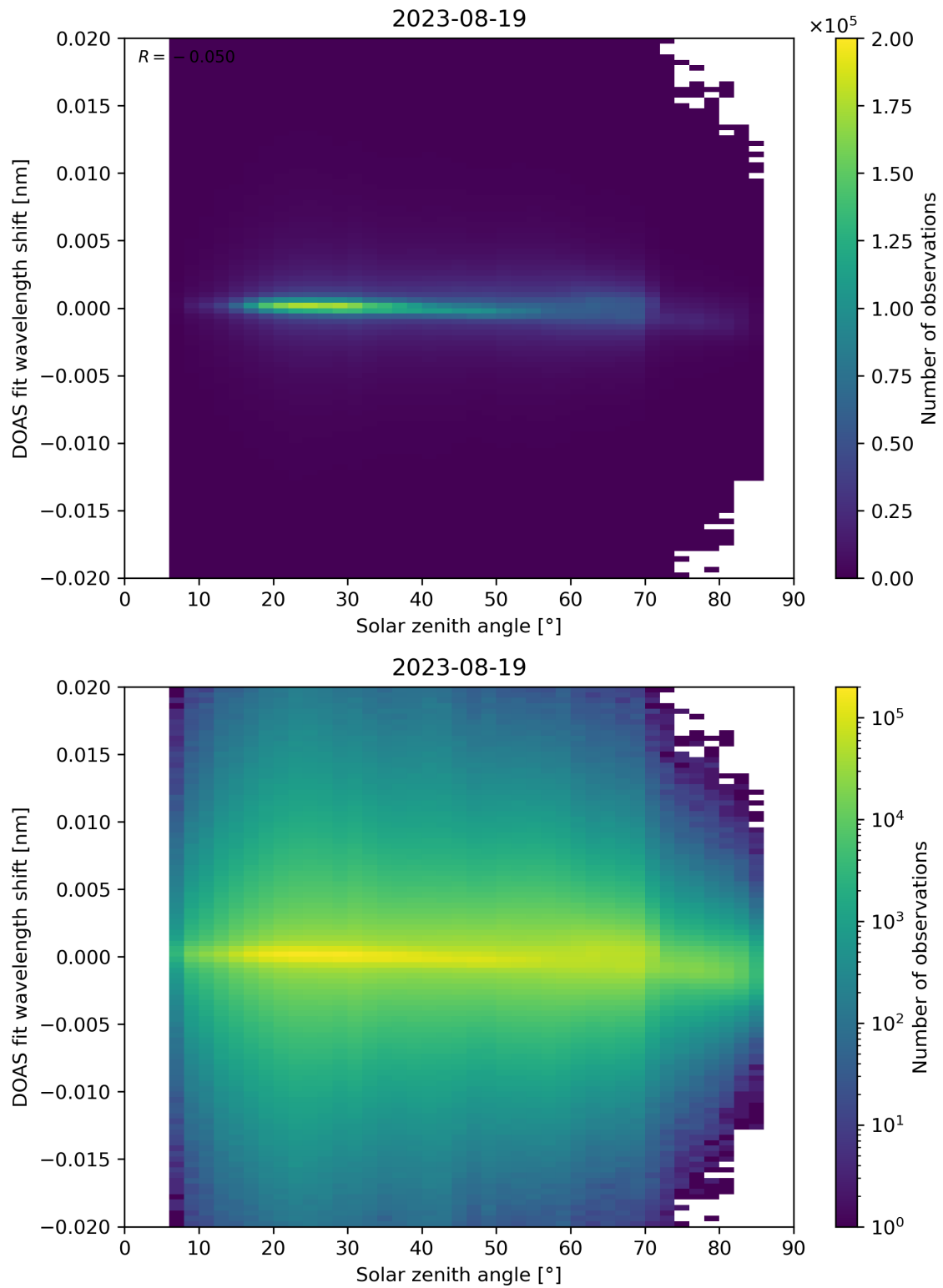
Figure 168: Scatter density plot of “Solar zenith angle” against “DOAS fit wavelength shift” for 2023-08-18 to 2023-08-20.
