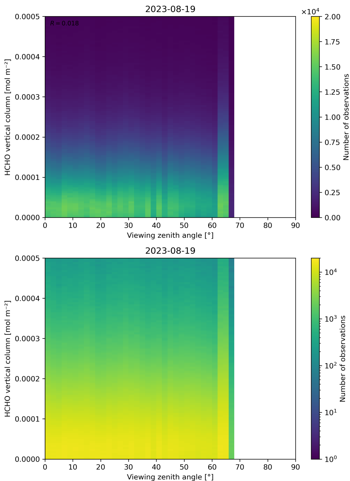
Figure 192: Scatter density plot of “Viewing zenith angle” against “HCHO vertical column” for 2023-08-18 to 2023-08-20.
