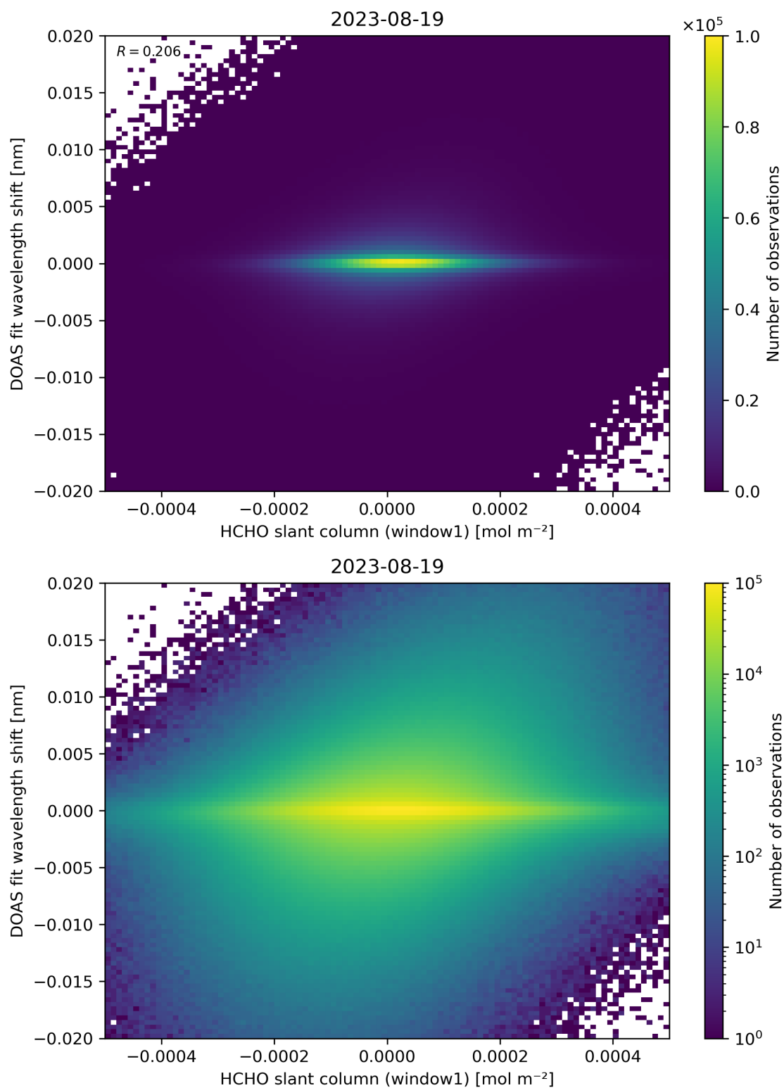
Figure 79: Scatter density plot of “HCHO slant column (window1)” against “DOAS fit wavelength shift” for 2023-08-18 to 2023-08-20.
