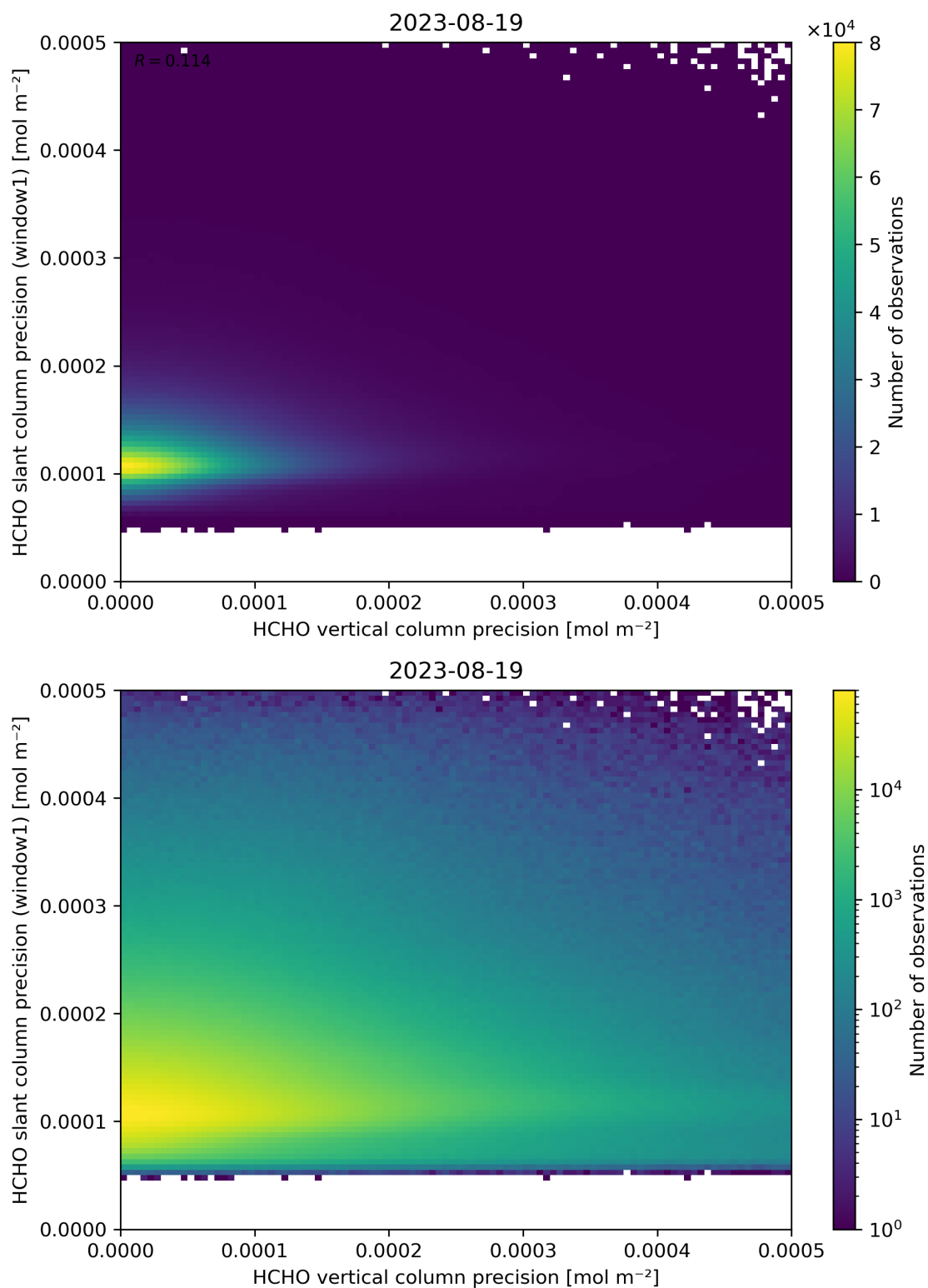
Figure 143: Scatter density plot of “HCHO vertical column precision” against “HCHO slant column precision (window1)” for 2023-08-18 to 2023-08-20.
