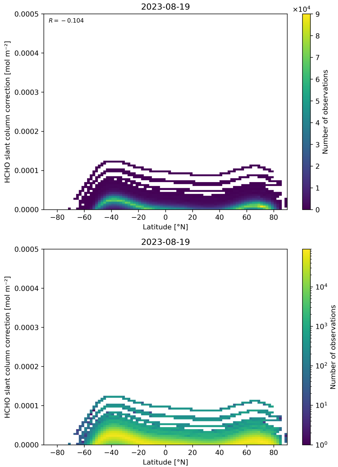
Figure 158: Scatter density plot of “Latitude” against “HCHO slant column correction” for 2023-08-18 to 2023-08-20.
