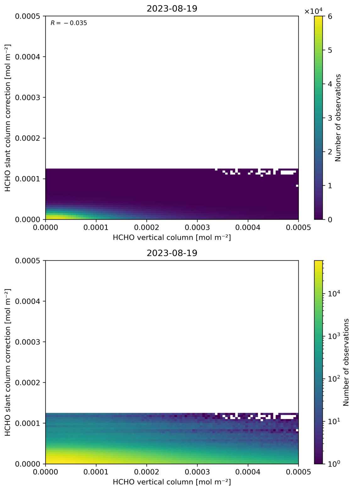
Figure 128: Scatter density plot of “HCHO vertical column” against “HCHO slant column correction” for 2023-08-18 to 2023-08-20.
