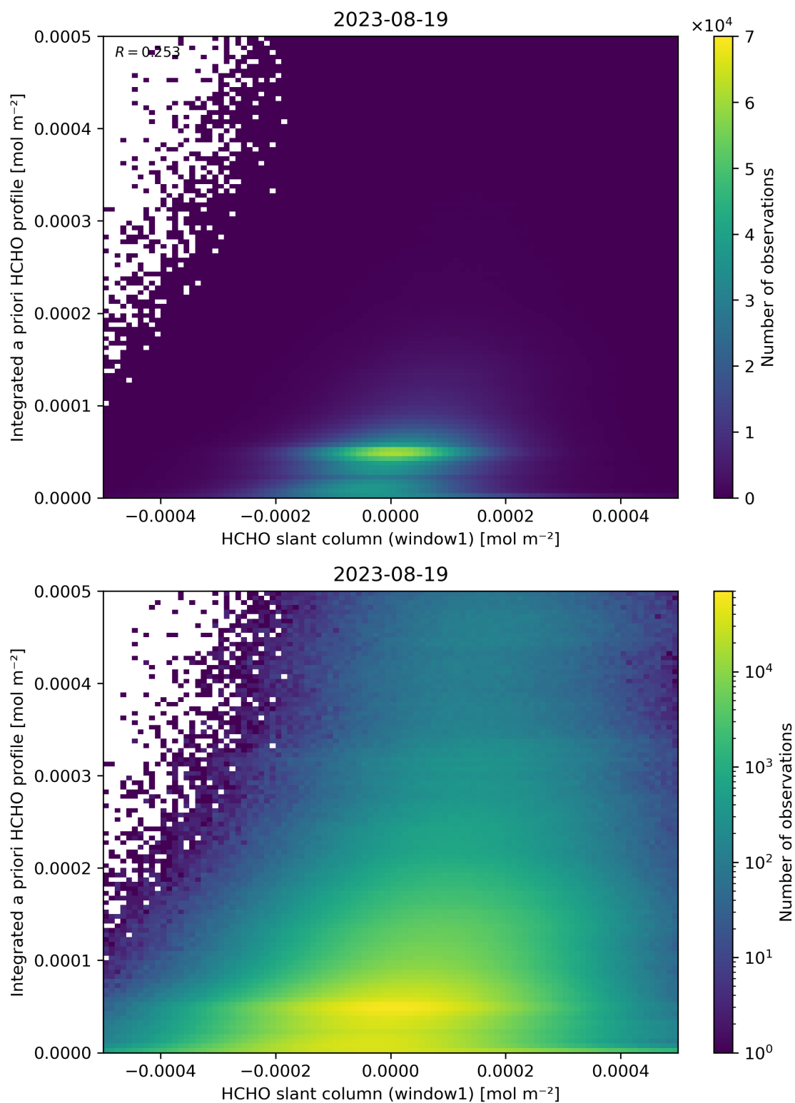
Figure 87: Scatter density plot of “HCHO slant column (window1)” against “Integrated a priori HCHO profile” for 2023-08-18 to 2023-08-20.
