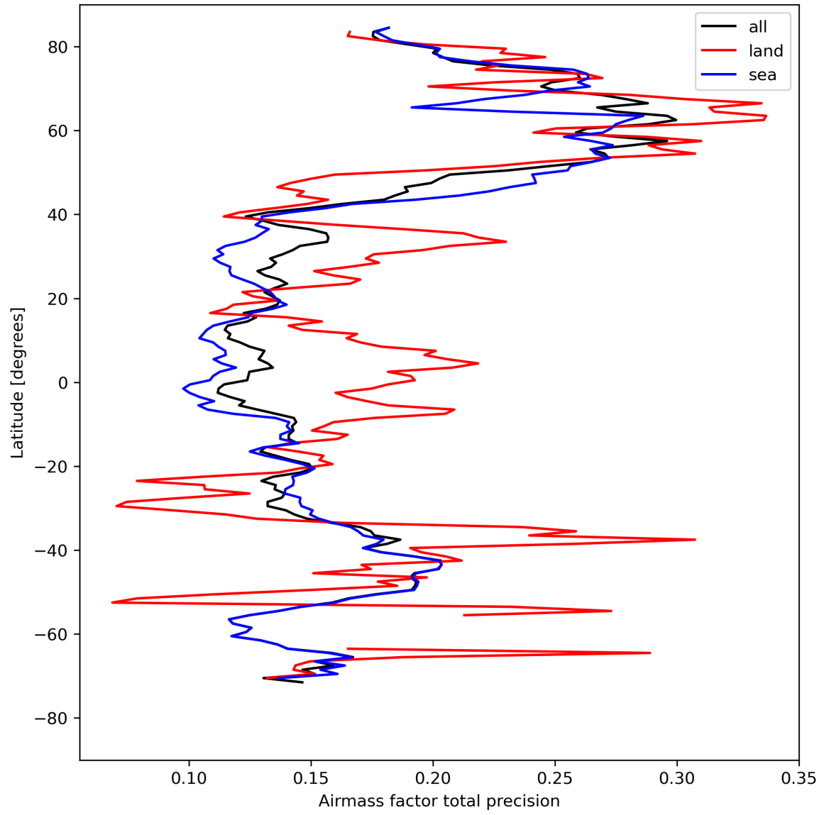
Figure 27: Zonal average of “Airmass factor total precision” for 2023-08-18 to 2023-08-20.
