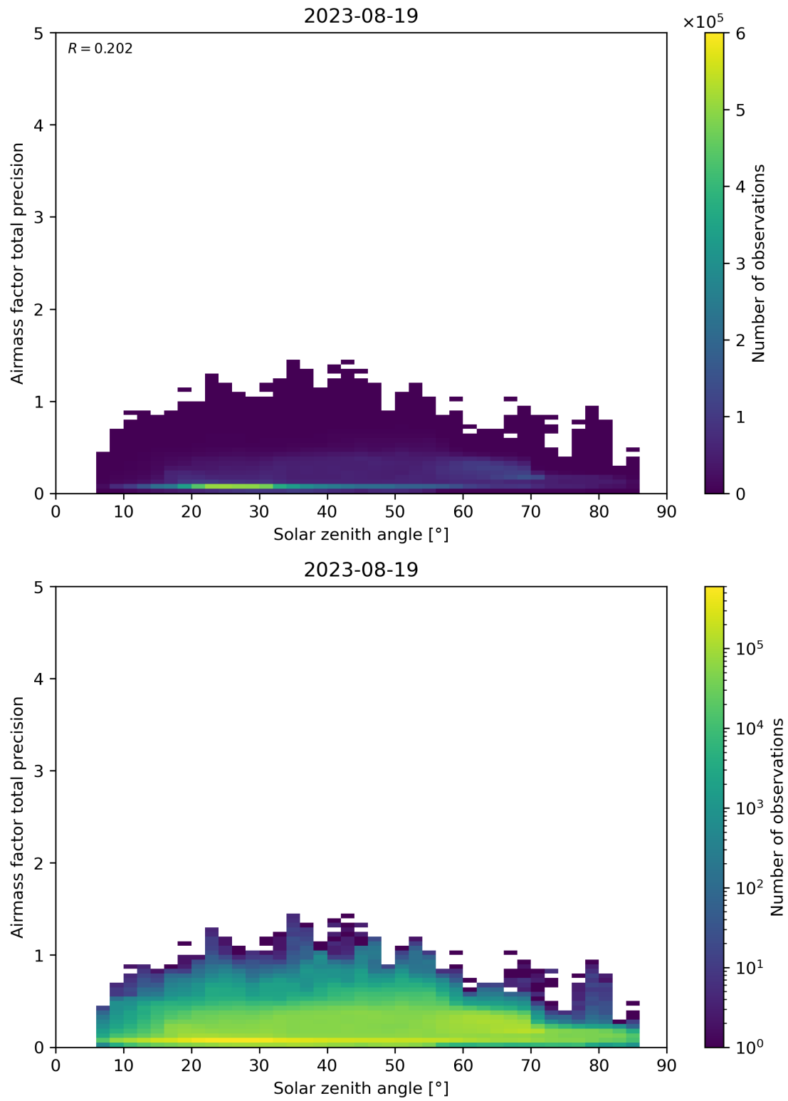
Figure 176: Scatter density plot of “Solar zenith angle” against “Airmass factor total precision” for 2023-08-18 to 2023-08-20.
