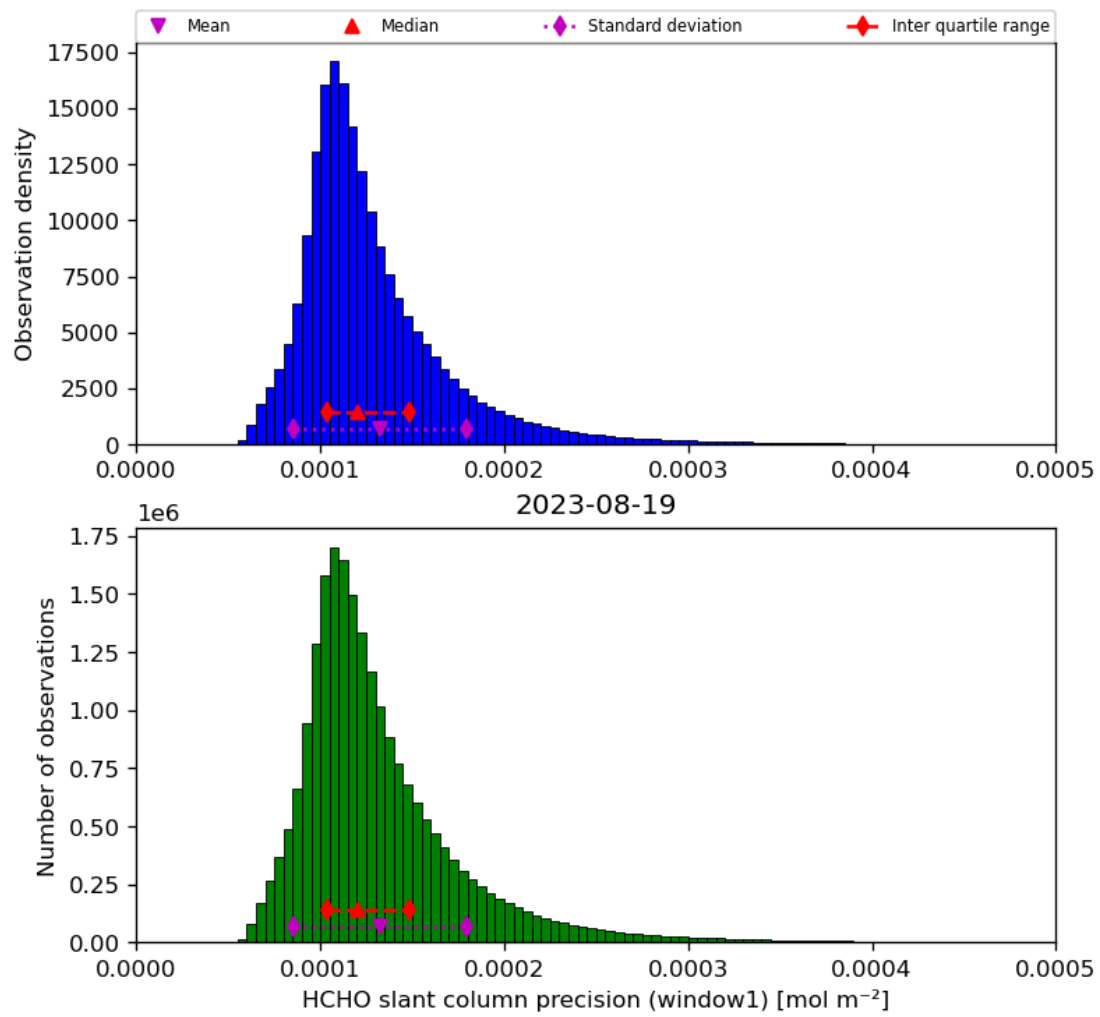
Figure 39: Histogram of “HCHO slant column precision (window1)” for 2023-08-18 to 2023-08-20
