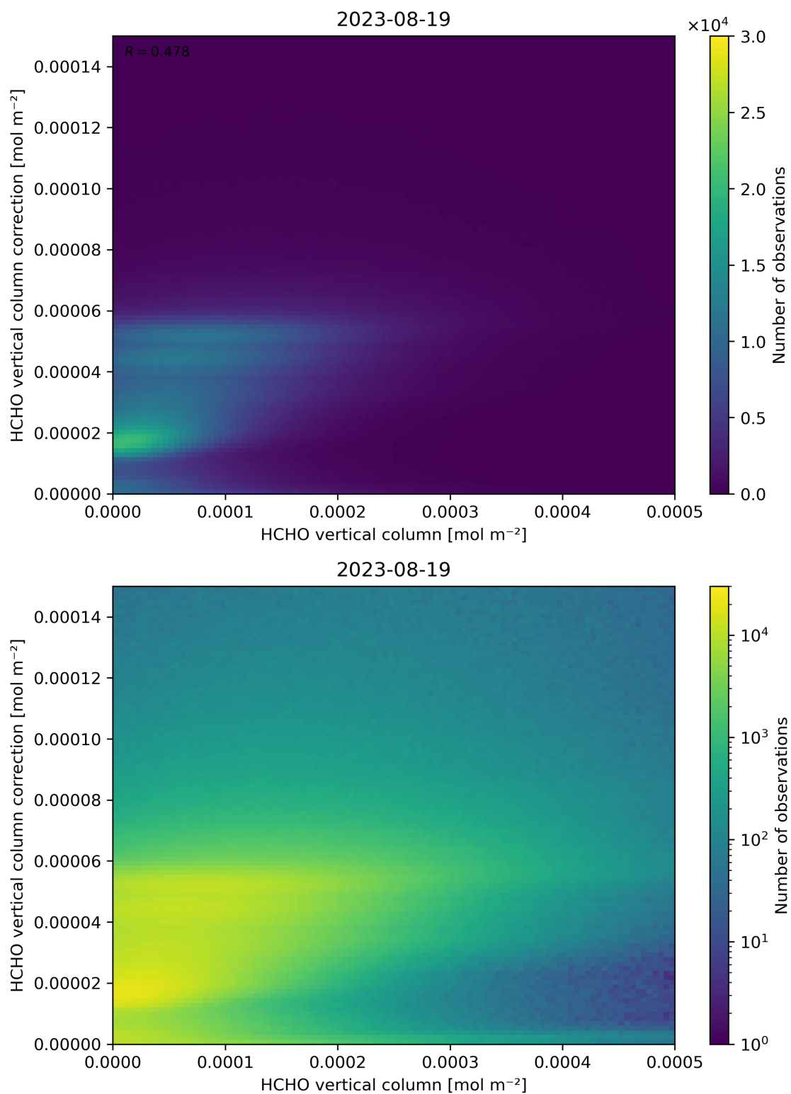
Figure 133: Scatter density plot of “HCHO vertical column” against “HCHO vertical column correction” for 2023-08-18 to 2023-08-20.
