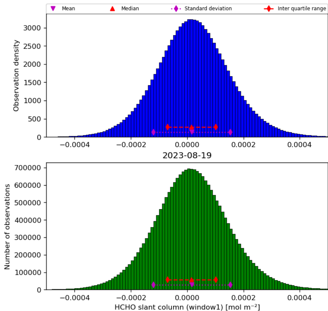
Figure 38: Histogram of “HCHO slant column (window1)” for 2023-08-18 to 2023-08-20
