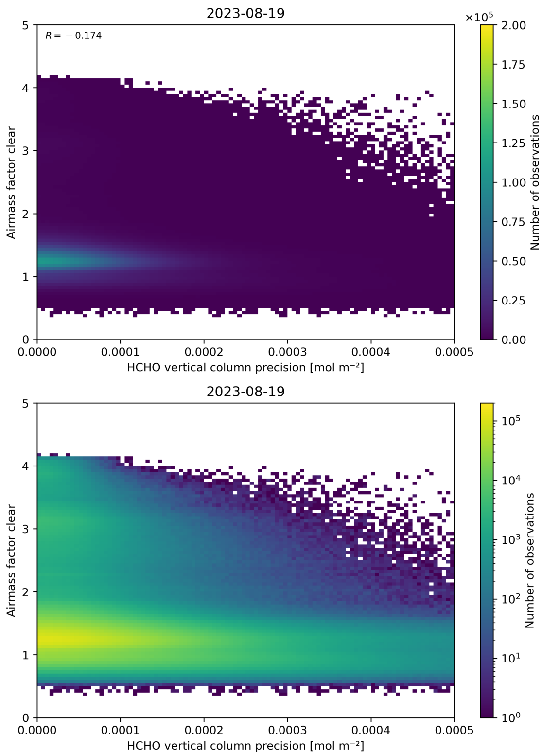
Figure 139: Scatter density plot of “HCHO vertical column precision” against “Airmass factor clear” for 2023-08-18 to 2023-08-20.
