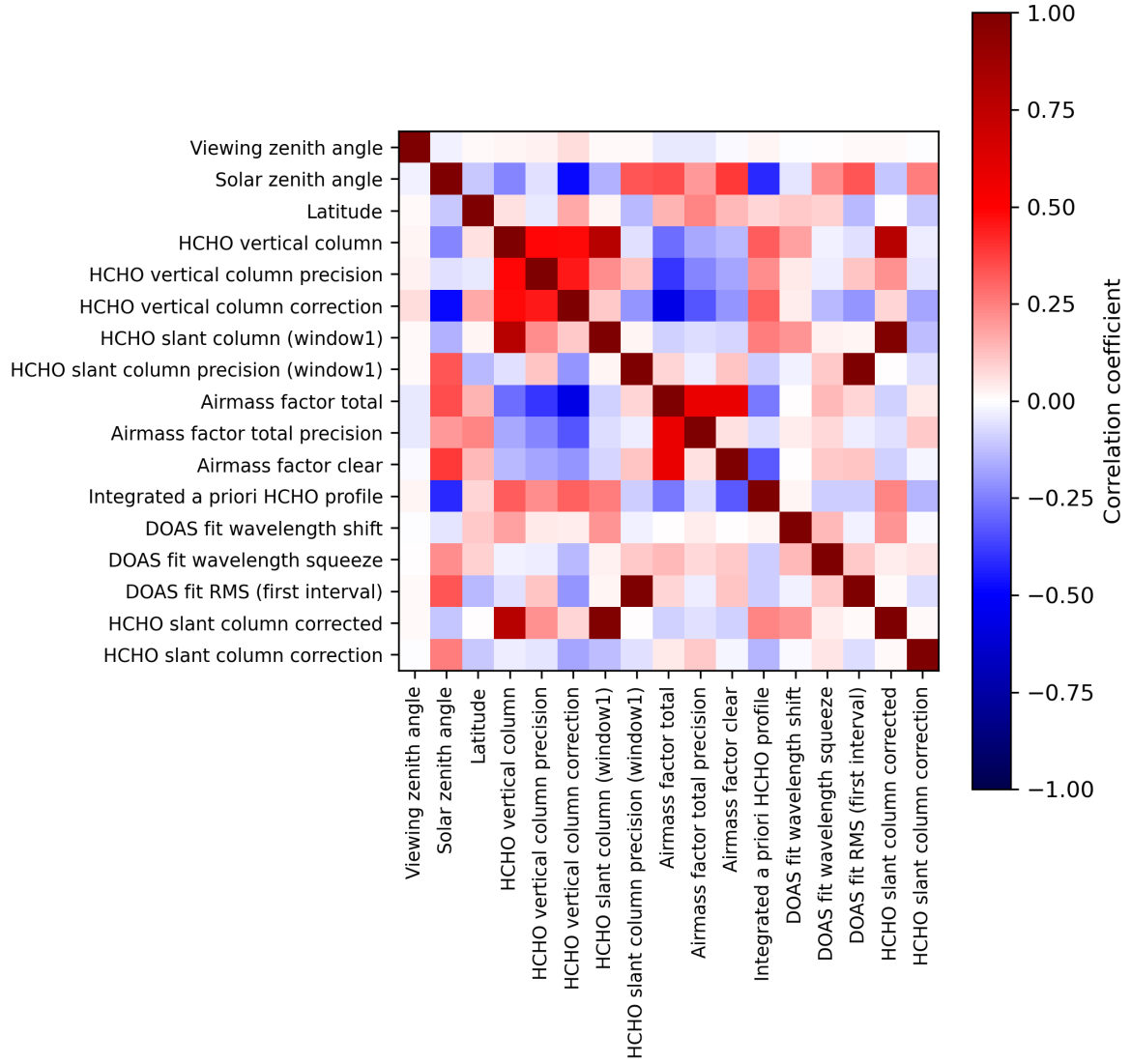
Figure 2: Map of correlation matrix for 2023-08-18 to 2023-08-20.
