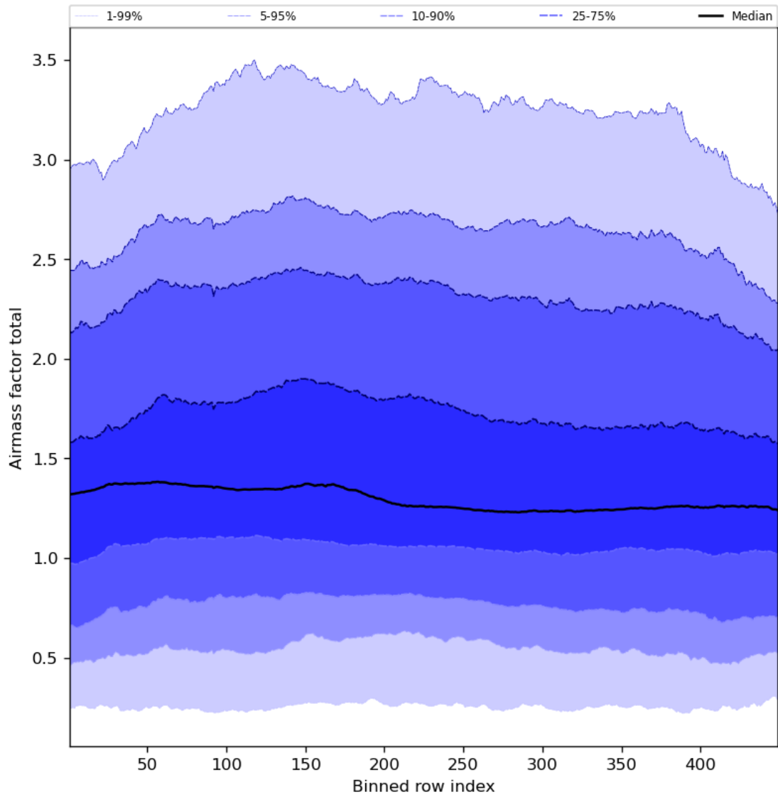
Figure 54: Along track statistics of “Airmass factor total” for 2023-08-18 to 2023-08-20
