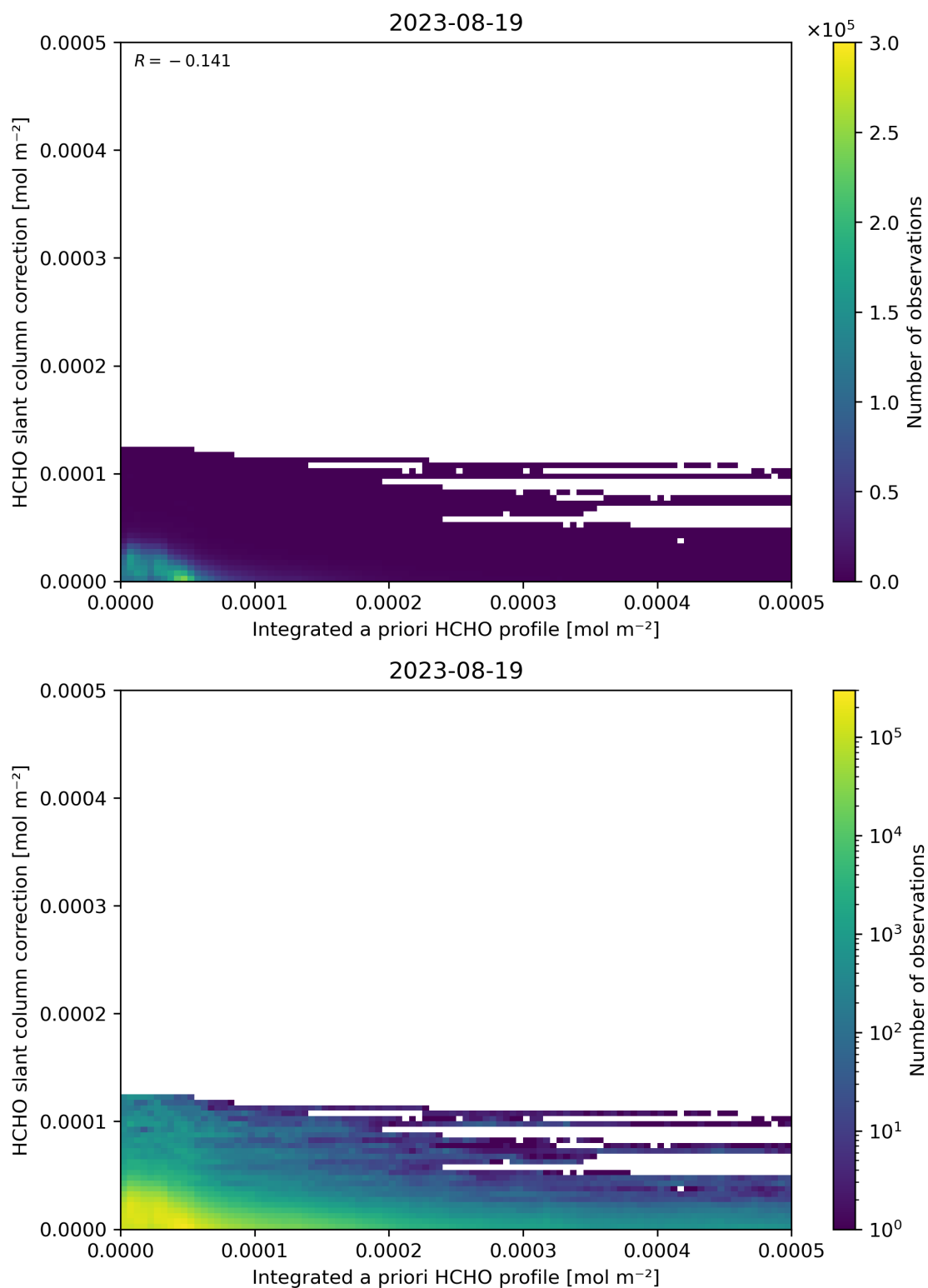
Figure 152: Scatter density plot of “Integrated a priori HCHO profile” against “HCHO slant column correction” for 2023-08-18 to 2023-08-20.
