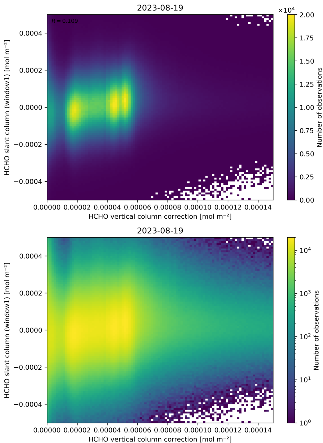
Figure 118: Scatter density plot of “HCHO vertical column correction” against “HCHO slant column (window1)” for 2023-08-18 to 2023-08-20.
