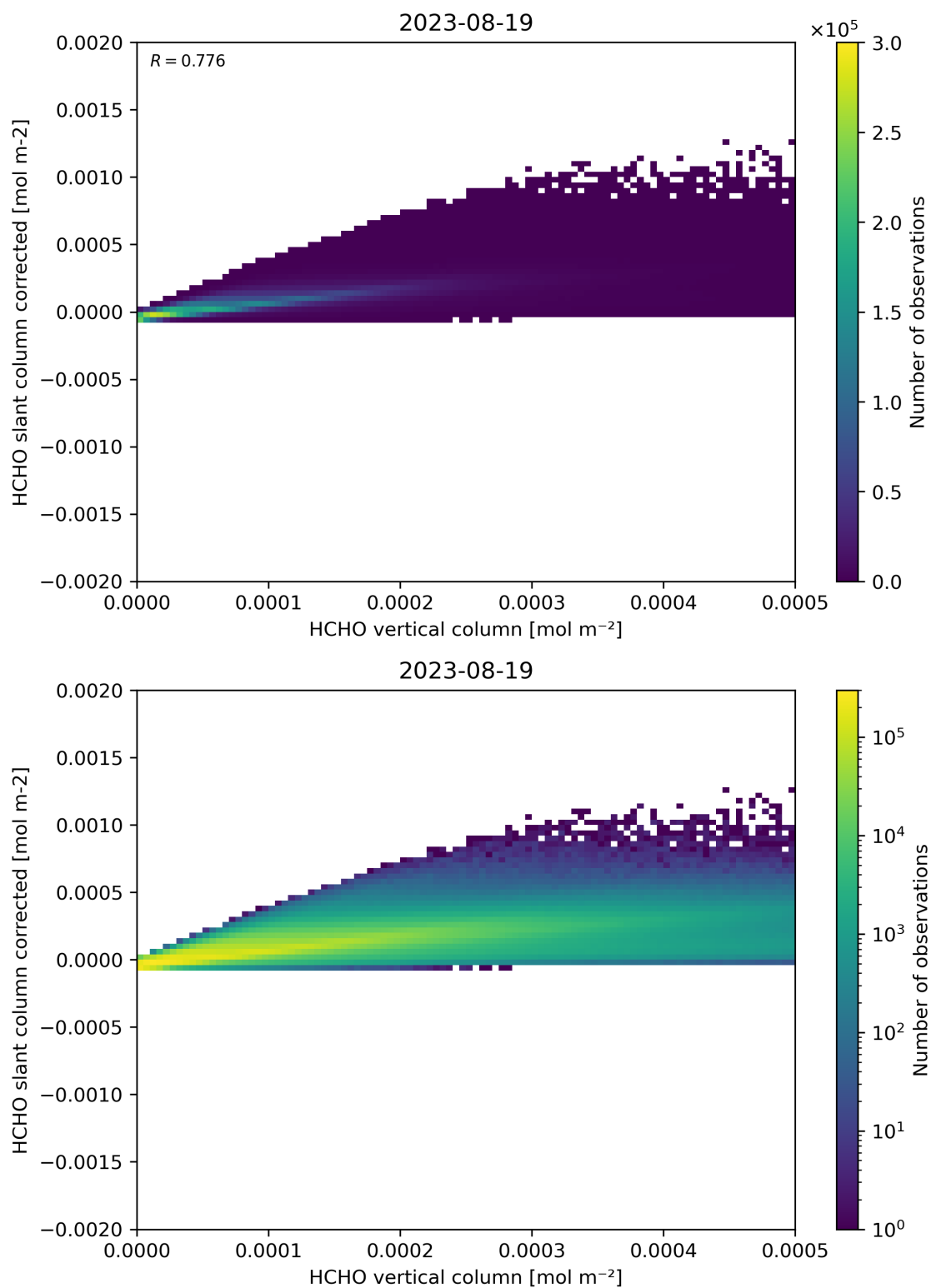
Figure 127: Scatter density plot of “HCHO vertical column” against “HCHO slant column corrected” for 2023-08-18 to 2023-08-20.
