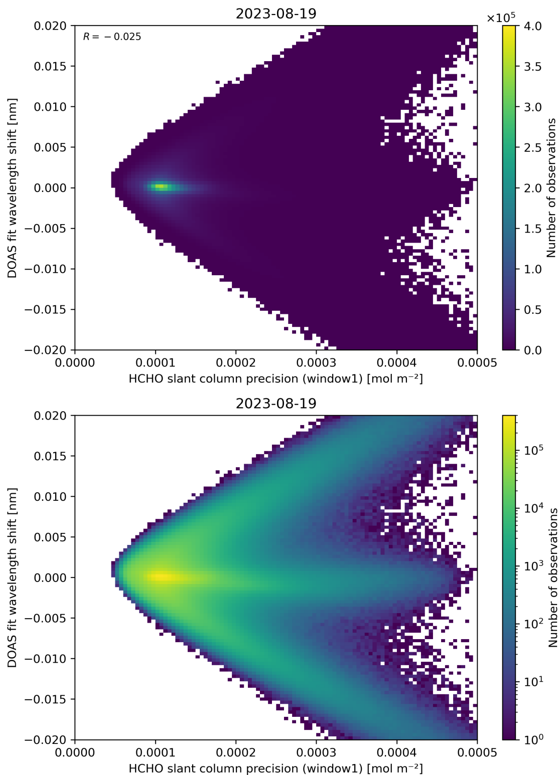
Figure 89: Scatter density plot of “HCHO slant column precision (window1)” against “DOAS fit wavelength shift” for 2023-08-18 to 2023-08-20.
