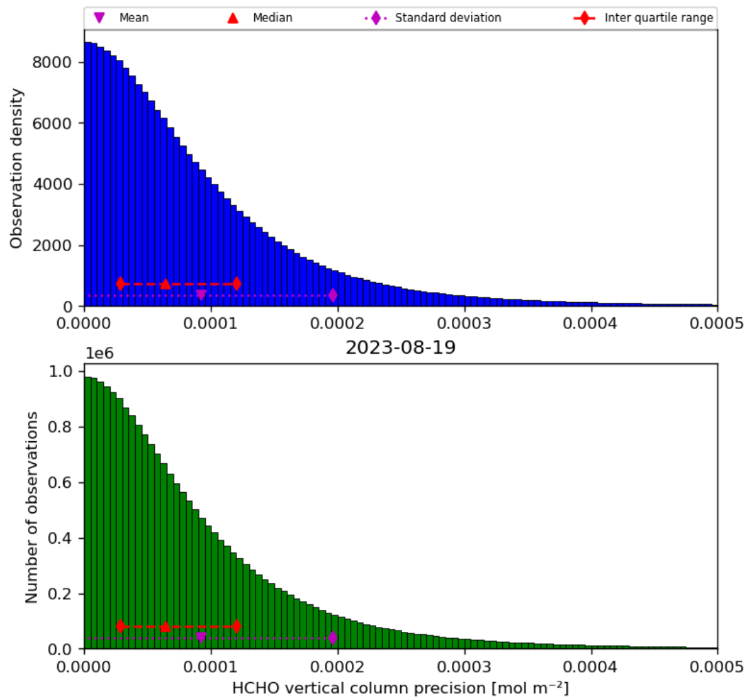
Figure 36: Histogram of “HCHO vertical column precision” for 2023-08-18 to 2023-08-20
