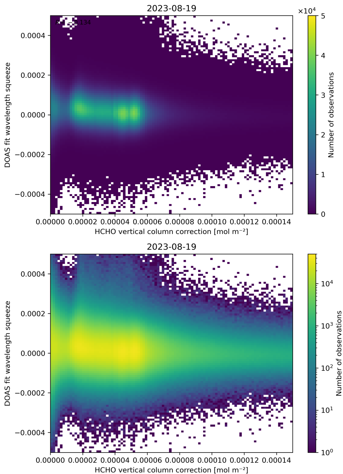
Figure 114: Scatter density plot of “HCHO vertical column correction” against “DOAS fit wavelength squeeze” for 2023-08-18 to 2023-08-20.
