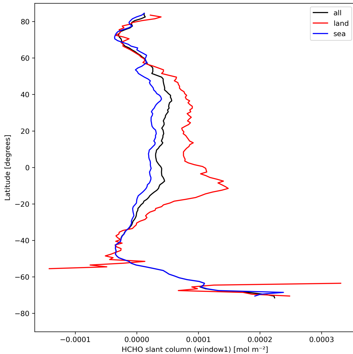
Figure 24: Zonal average of “HCHO slant column (window1)” for 2023-08-18 to 2023-08-20.
