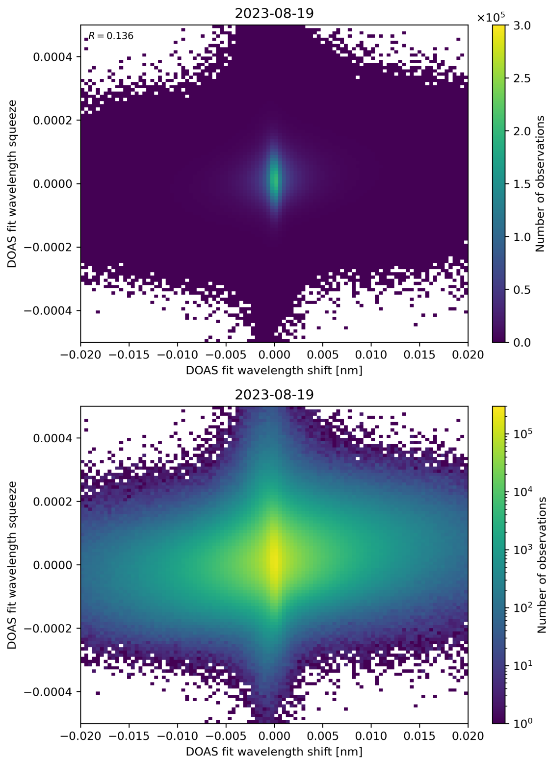
Figure 65: Scatter density plot of “DOAS fit wavelength shift” against “DOAS fit wavelength squeeze” for 2023-08-18 to 2023-08-20.
