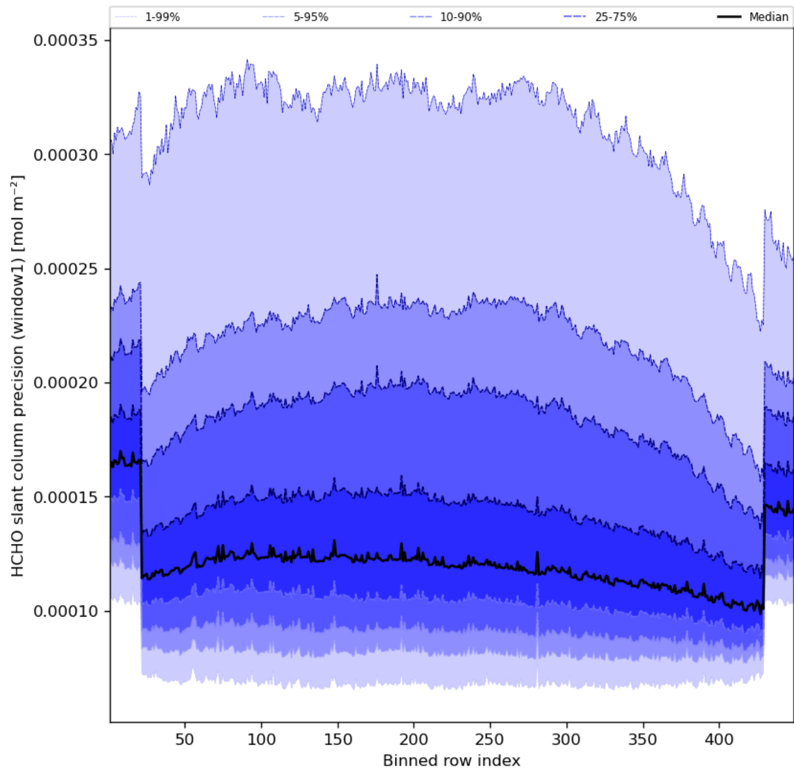
Figure 53: Along track statistics of “HCHO slant column precision (window1)” for 2023-08-18 to 2023-08-20
