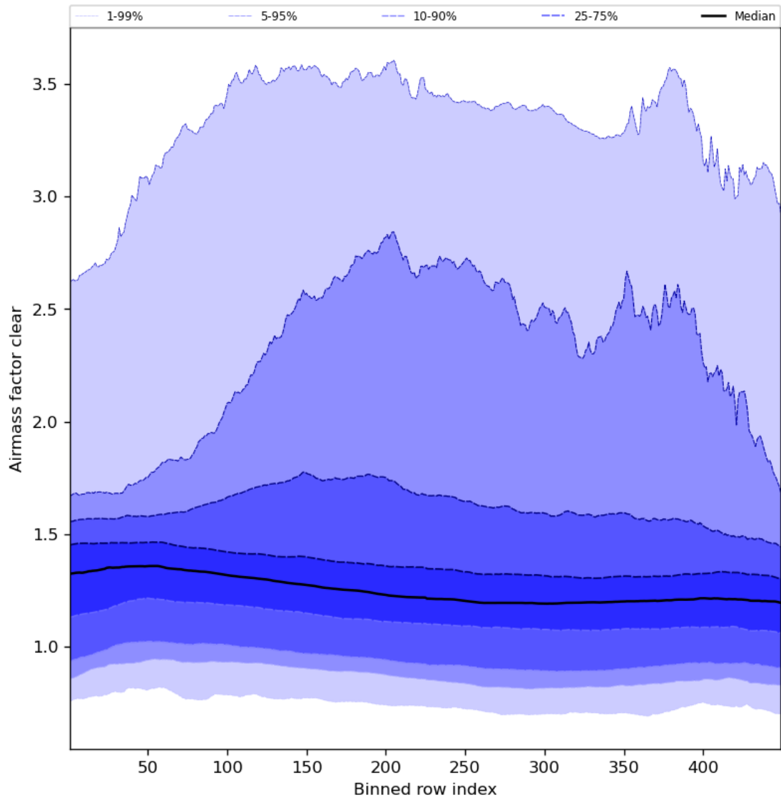
Figure 56: Along track statistics of “Airmass factor clear” for 2023-08-18 to 2023-08-20
