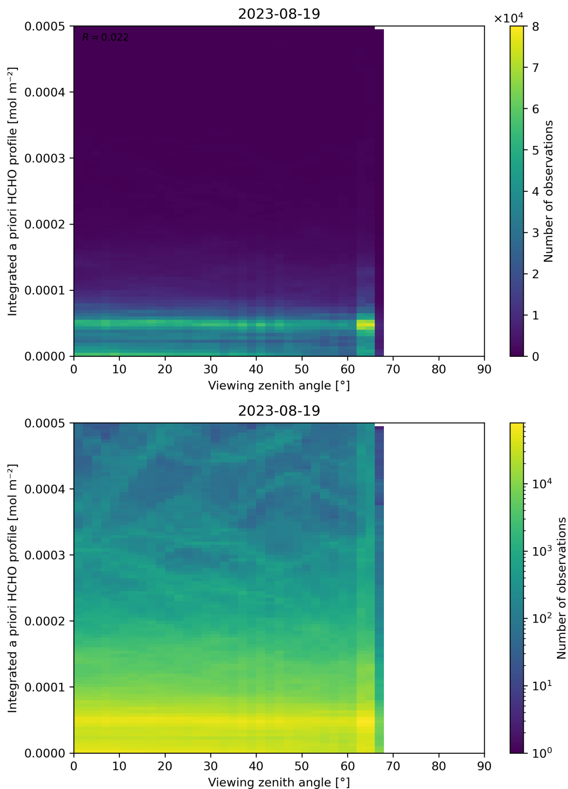
Figure 195: Scatter density plot of “Viewing zenith angle” against “Integrated a priori HCHO profile” for 2023-08-18 to 2023-08-20.
