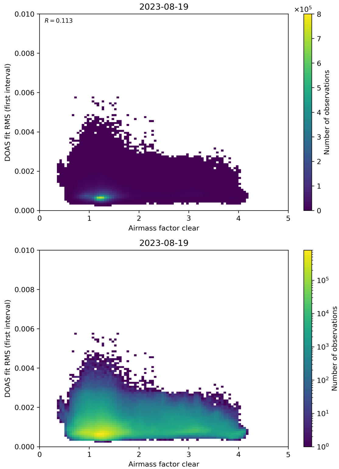
Figure 71: Scatter density plot of “Airmass factor clear” against “DOAS fit RMS (first interval)” for 2023-08-18 to 2023-08-20.
