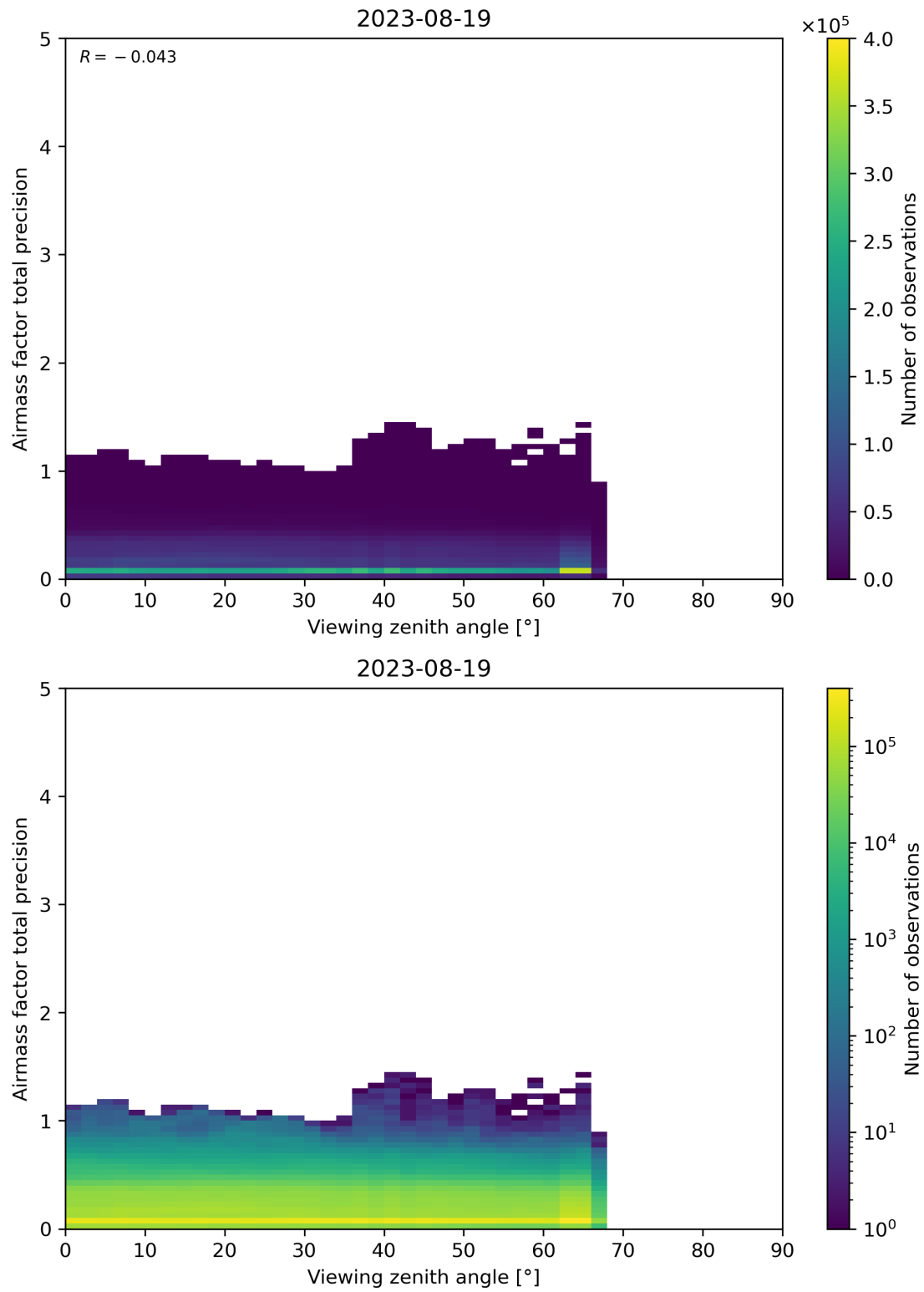
Figure 191: Scatter density plot of “Viewing zenith angle” against “Airmass factor total precision” for 2023-08-18 to 2023-08-20.
