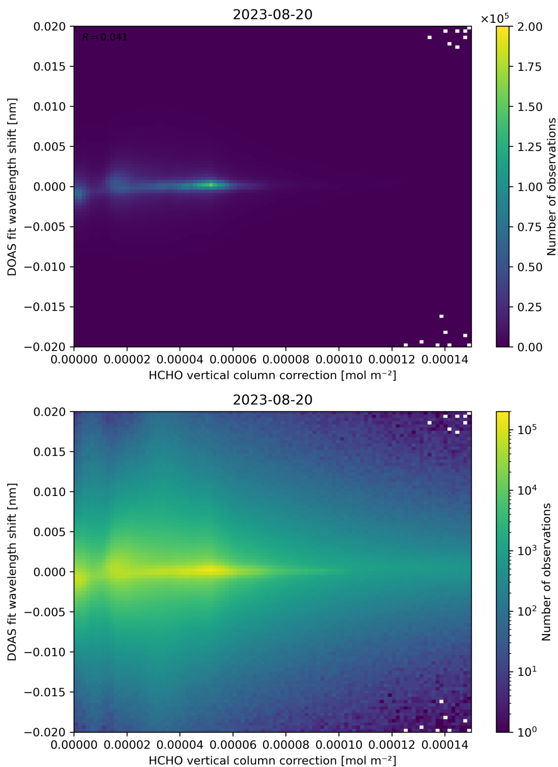
Figure 113: Scatter density plot of “HCHO vertical column correction” against “DOAS fit wavelength shift” for 2023-08-20 to 2023-08-21.
