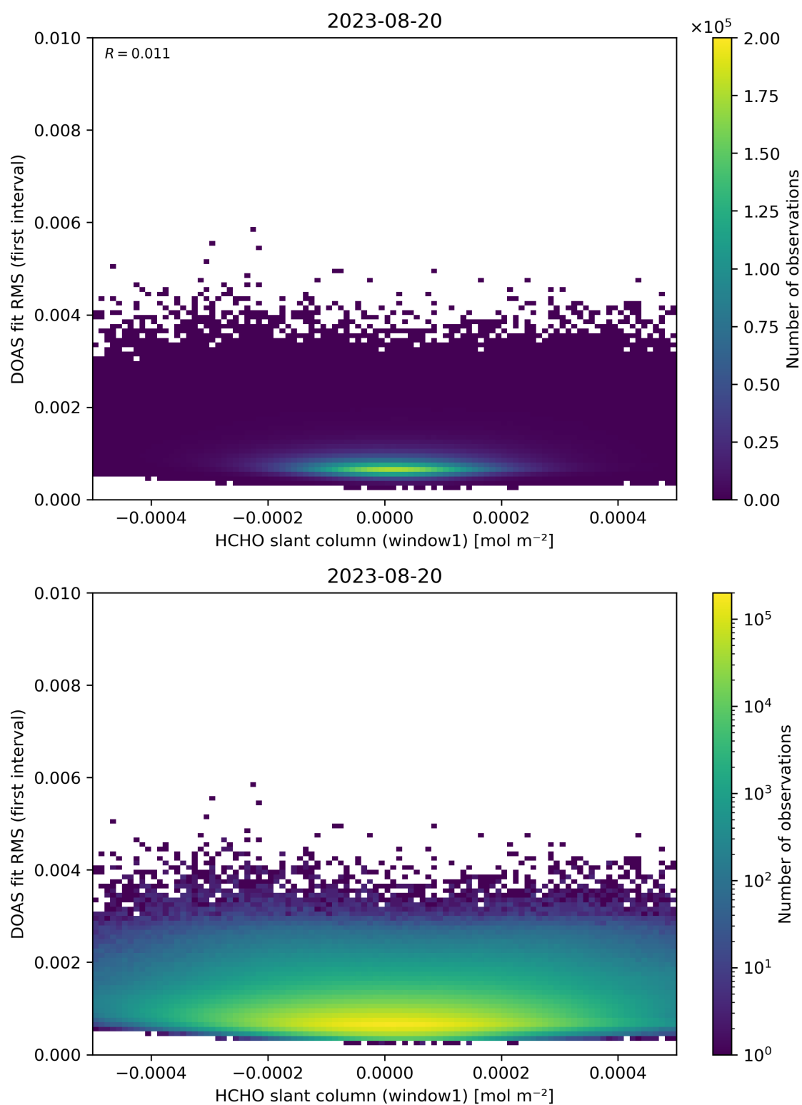
Figure 78: Scatter density plot of “HCHO slant column (window1)” against “DOAS fit RMS (first interval)” for 2023-08-20 to 2023-08-21.
