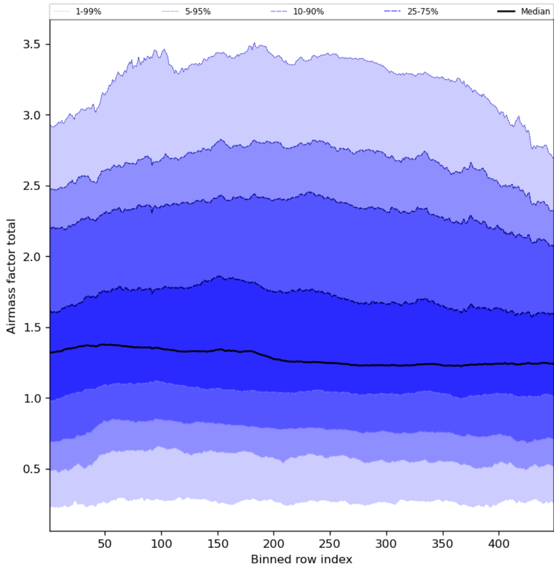
Figure 54: Along track statistics of “Airmass factor total” for 2023-08-20 to 2023-08-21
