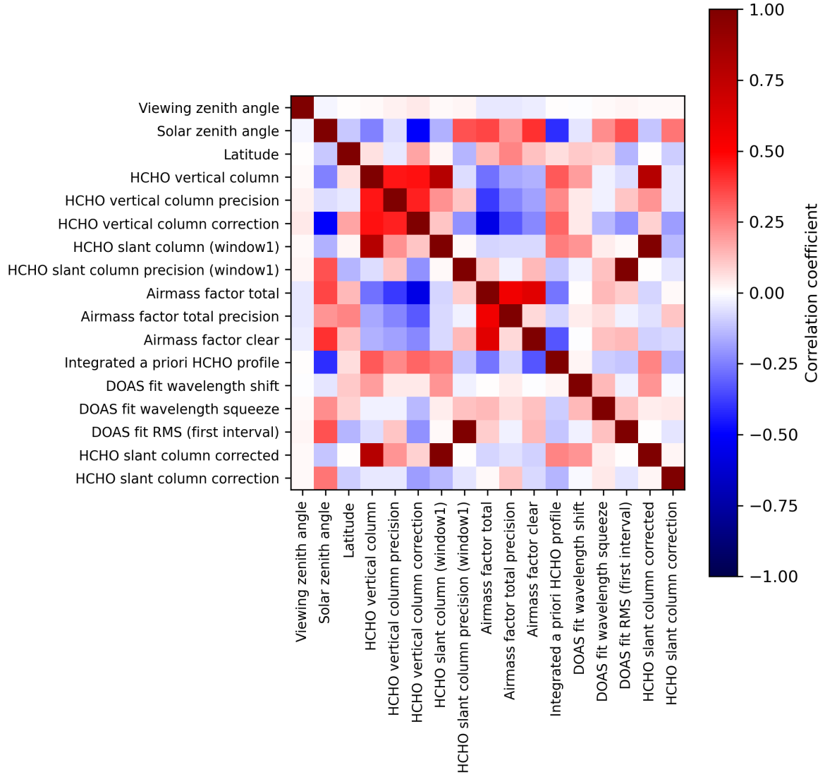
Figure 2: Map of correlation matrix for 2023-08-20 to 2023-08-21.
