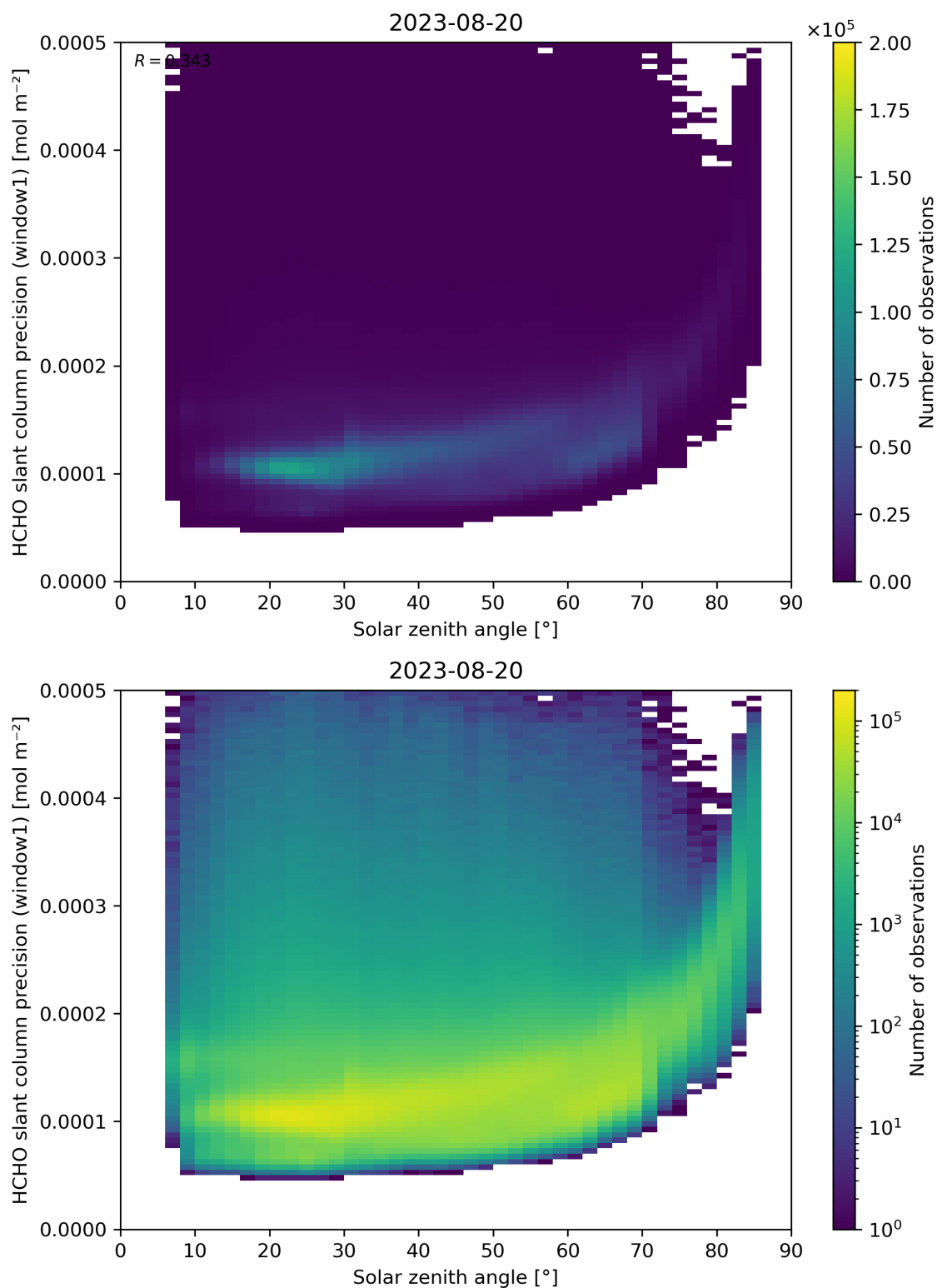
Figure 174: Scatter density plot of “Solar zenith angle” against “HCHO slant column precision (window1)” for 2023-08-20 to 2023-08-21.
