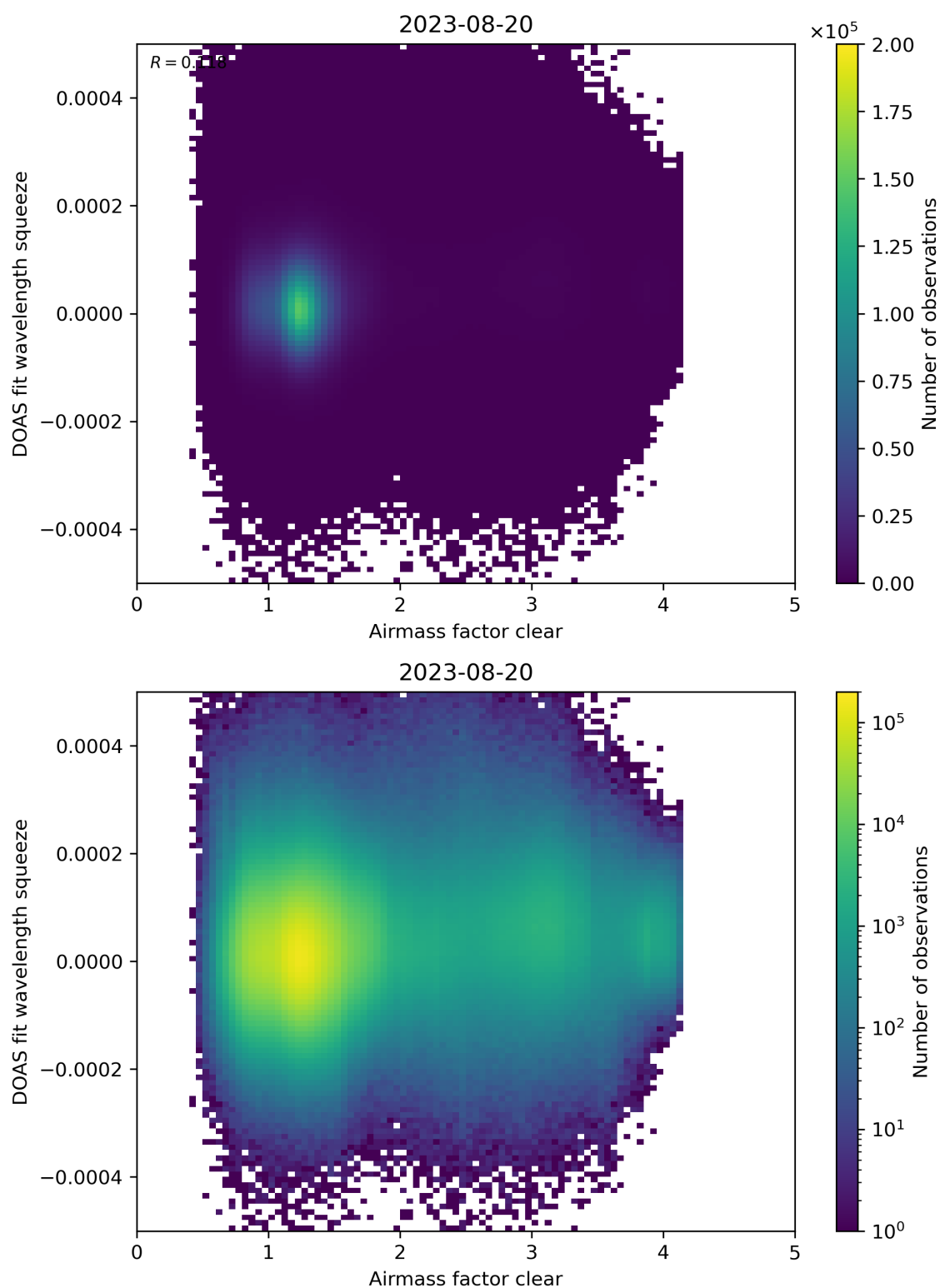
Figure 73: Scatter density plot of “Airmass factor clear” against “DOAS fit wavelength squeeze” for 2023-08-20 to 2023-08-21.
