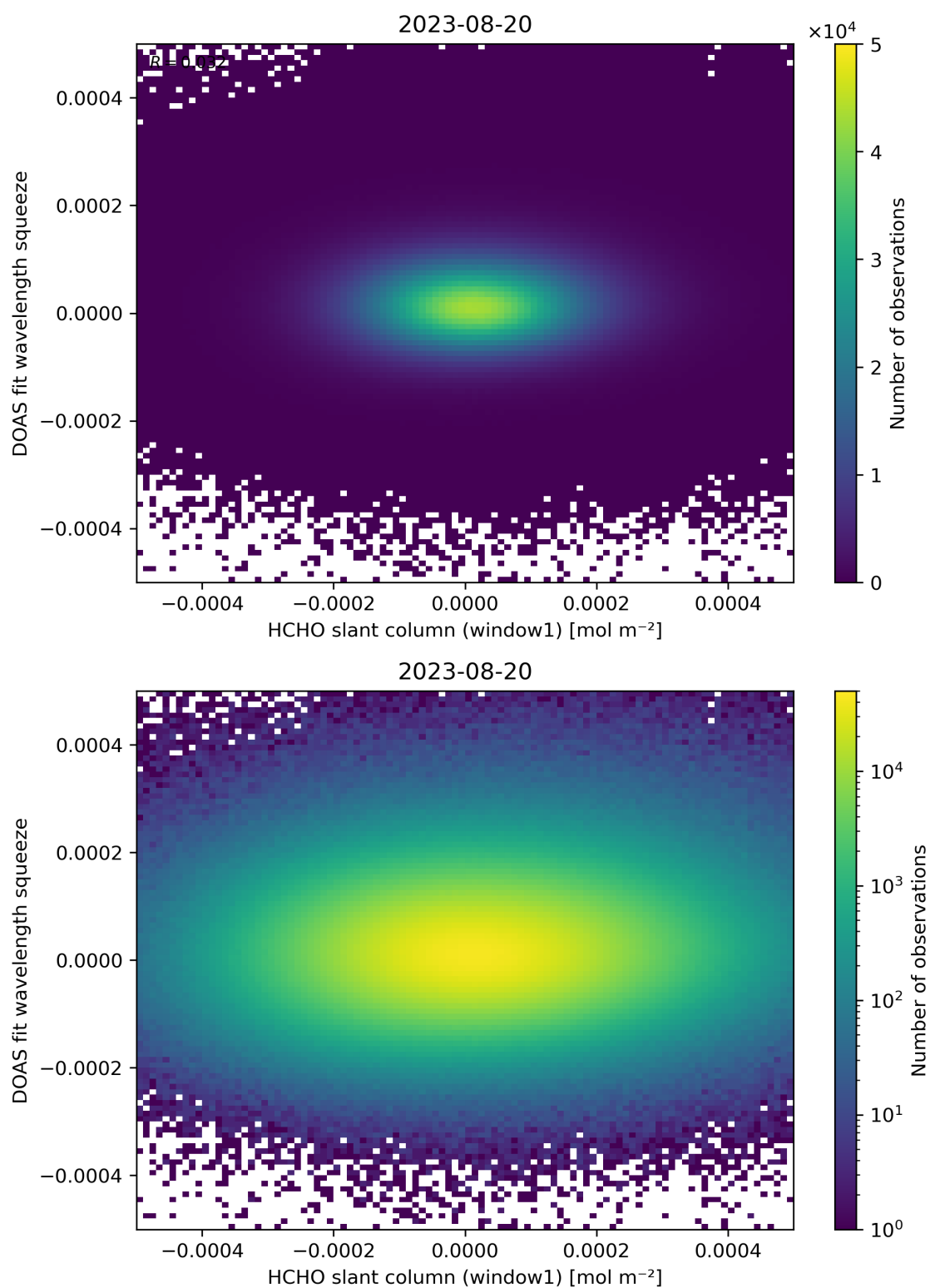
Figure 80: Scatter density plot of “HCHO slant column (window1)” against “DOAS fit wavelength squeeze” for 2023-08-20 to 2023-08-21.
