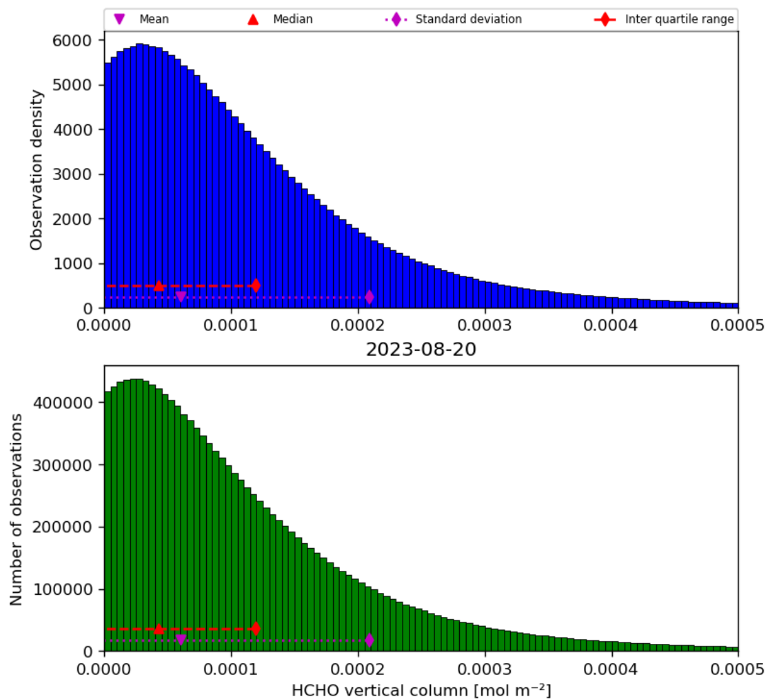
Figure 35: Histogram of “HCHO vertical column” for 2023-08-20 to 2023-08-21
