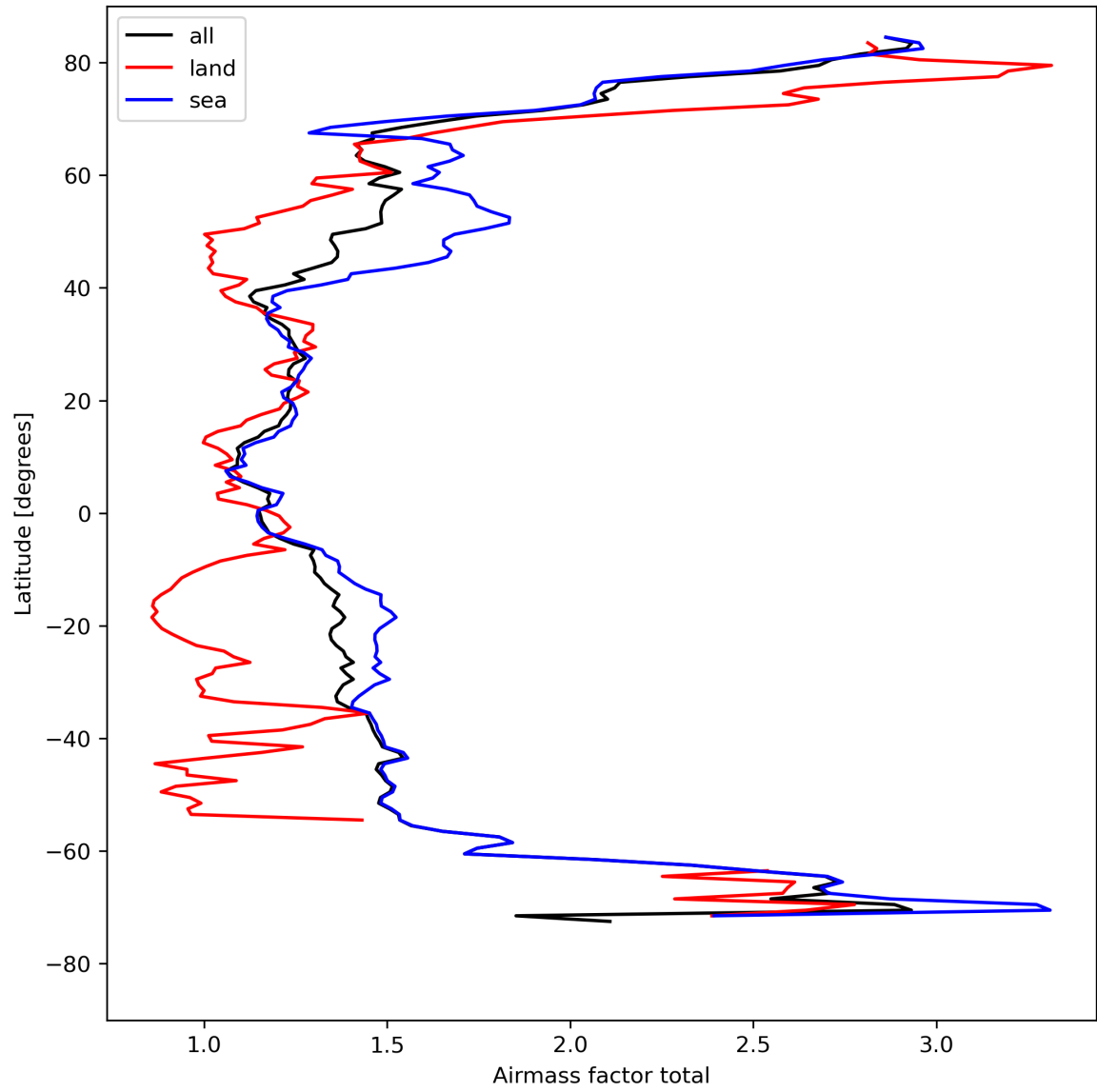
Figure 26: Zonal average of “Airmass factor total” for 2023-08-20 to 2023-08-21.
