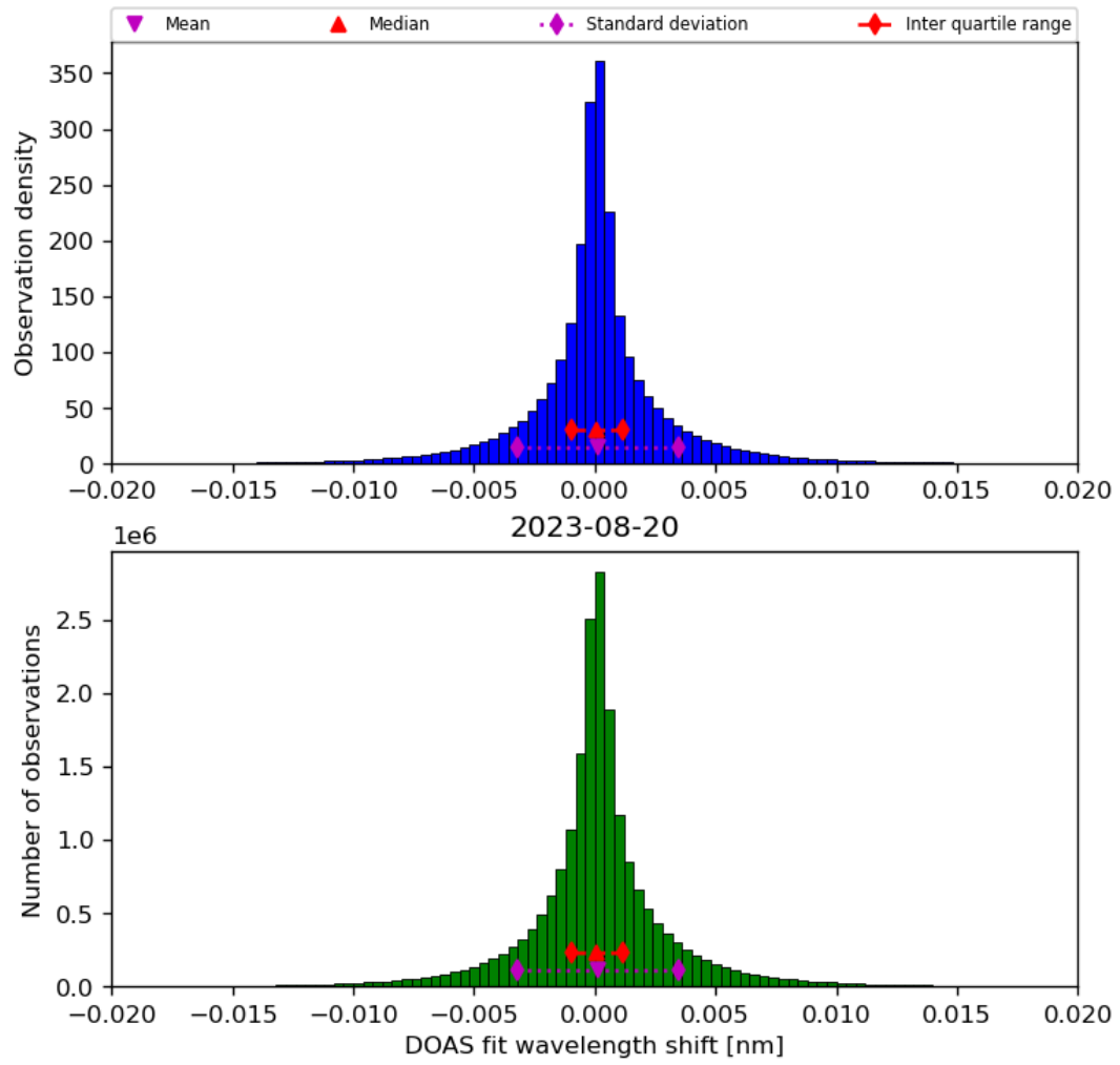
Figure 44: Histogram of “DOAS fit wavelength shift” for 2023-08-20 to 2023-08-21
