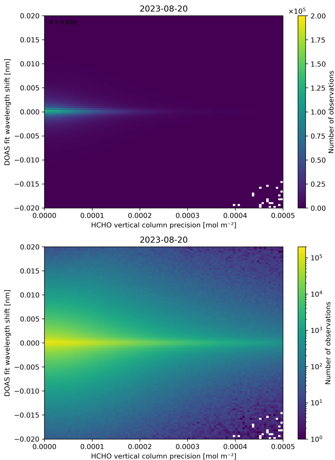
Figure 137: Scatter density plot of “HCHO vertical column precision” against “DOAS fit wavelength shift” for 2023-08-20 to 2023-08-21.
