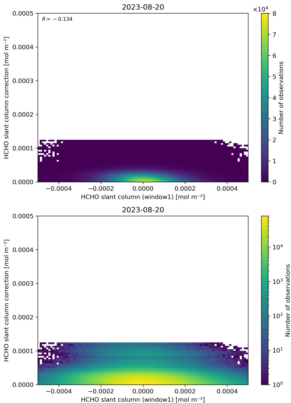
Figure 83: Scatter density plot of “HCHO slant column (window1)” against “HCHO slant column correction” for 2023-08-20 to 2023-08-21.
