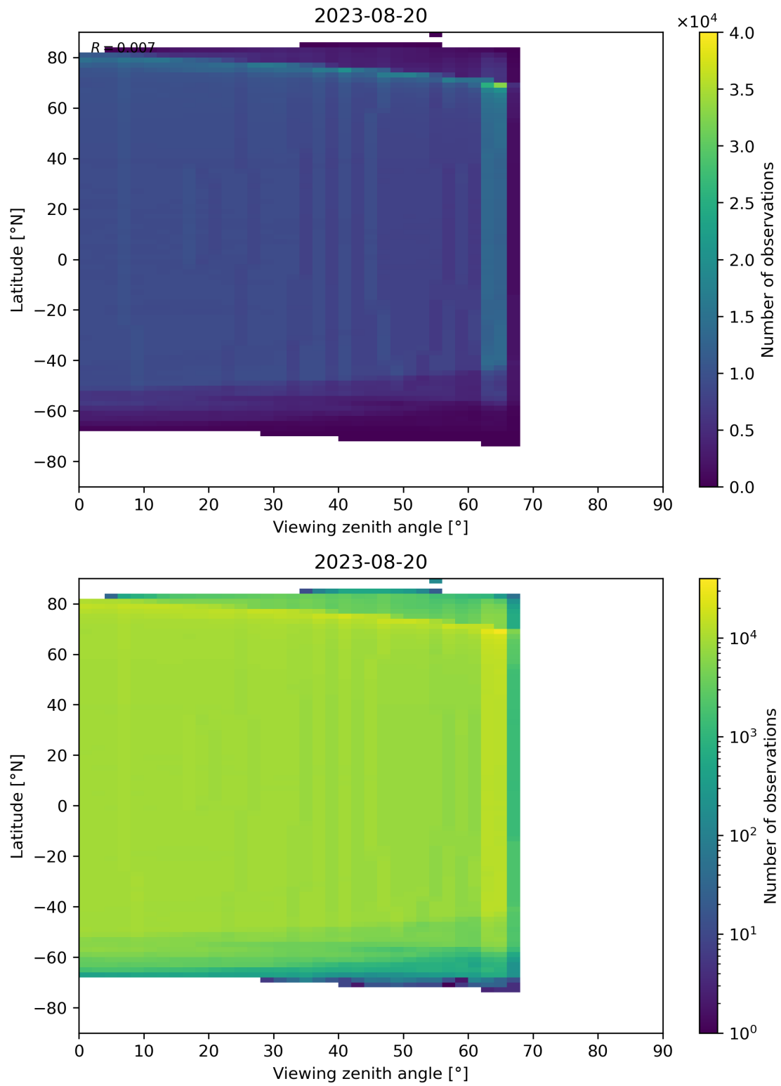
Figure 196: Scatter density plot of “Viewing zenith angle” against “Latitude” for 2023-08-20 to 2023-08-21.
