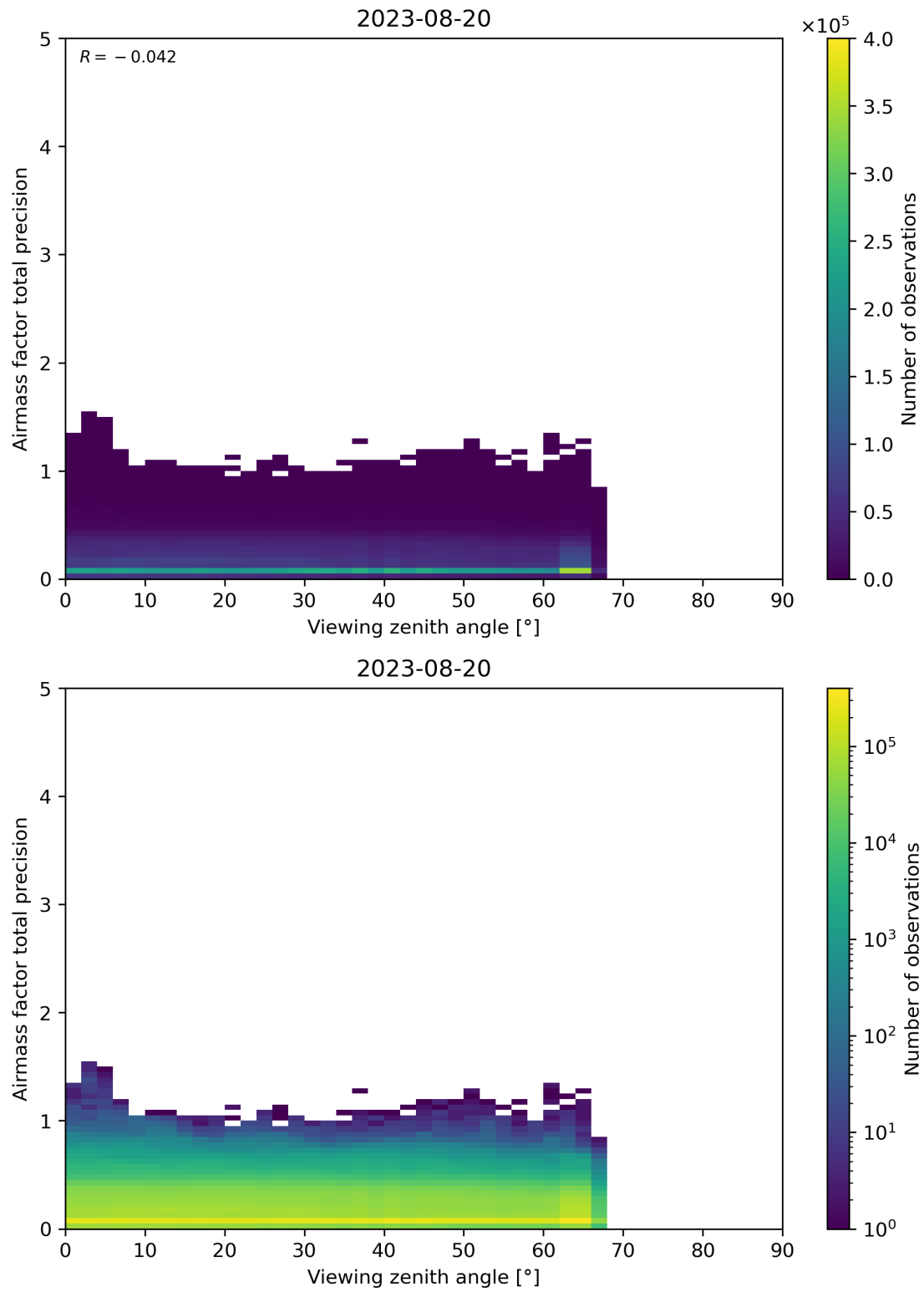
Figure 191: Scatter density plot of “Viewing zenith angle” against “Airmass factor total precision” for 2023-08-20 to 2023-08-21.
