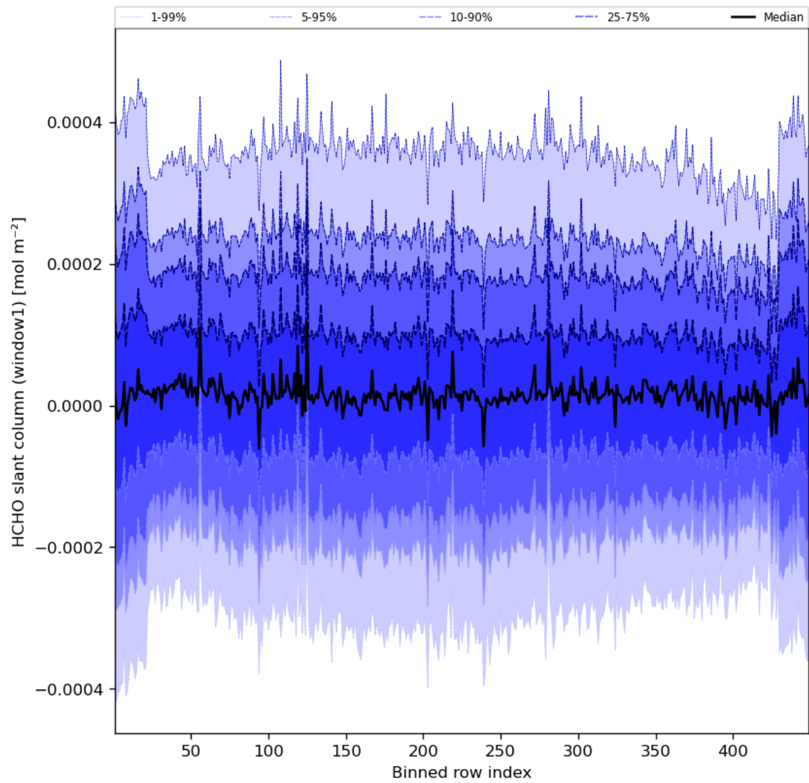
Figure 52: Along track statistics of “HCHO slant column (window1)” for 2023-08-20 to 2023-08-21
