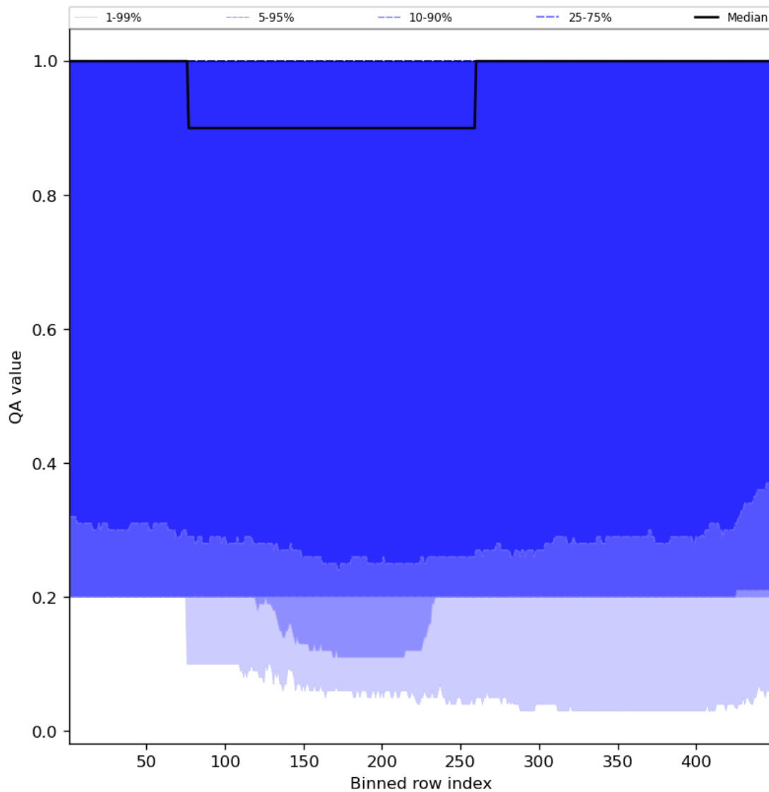
Figure 48: Along track statistics of “QA value” for 2023-08-20 to 2023-08-21
