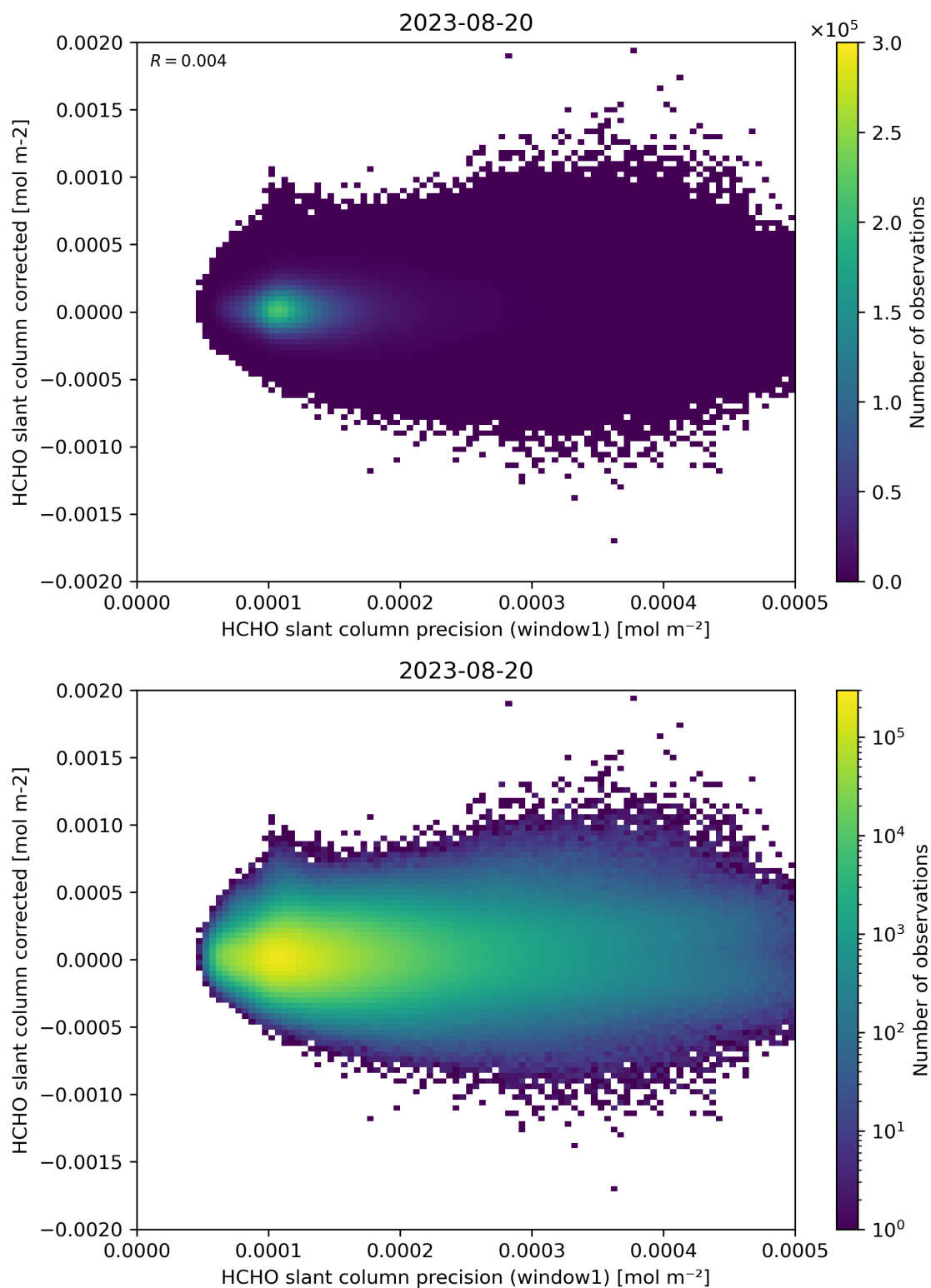
Figure 92: Scatter density plot of “HCHO slant column precision (window1)” against “HCHO slant column corrected” for 2023-08-20 to 2023-08-21.
