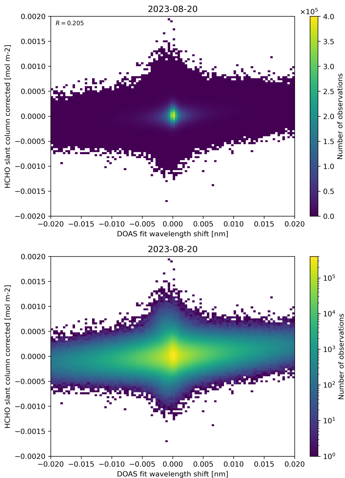
Figure 66: Scatter density plot of “DOAS fit wavelength shift” against “HCHO slant column corrected” for 2023-08-20 to 2023-08-21.
