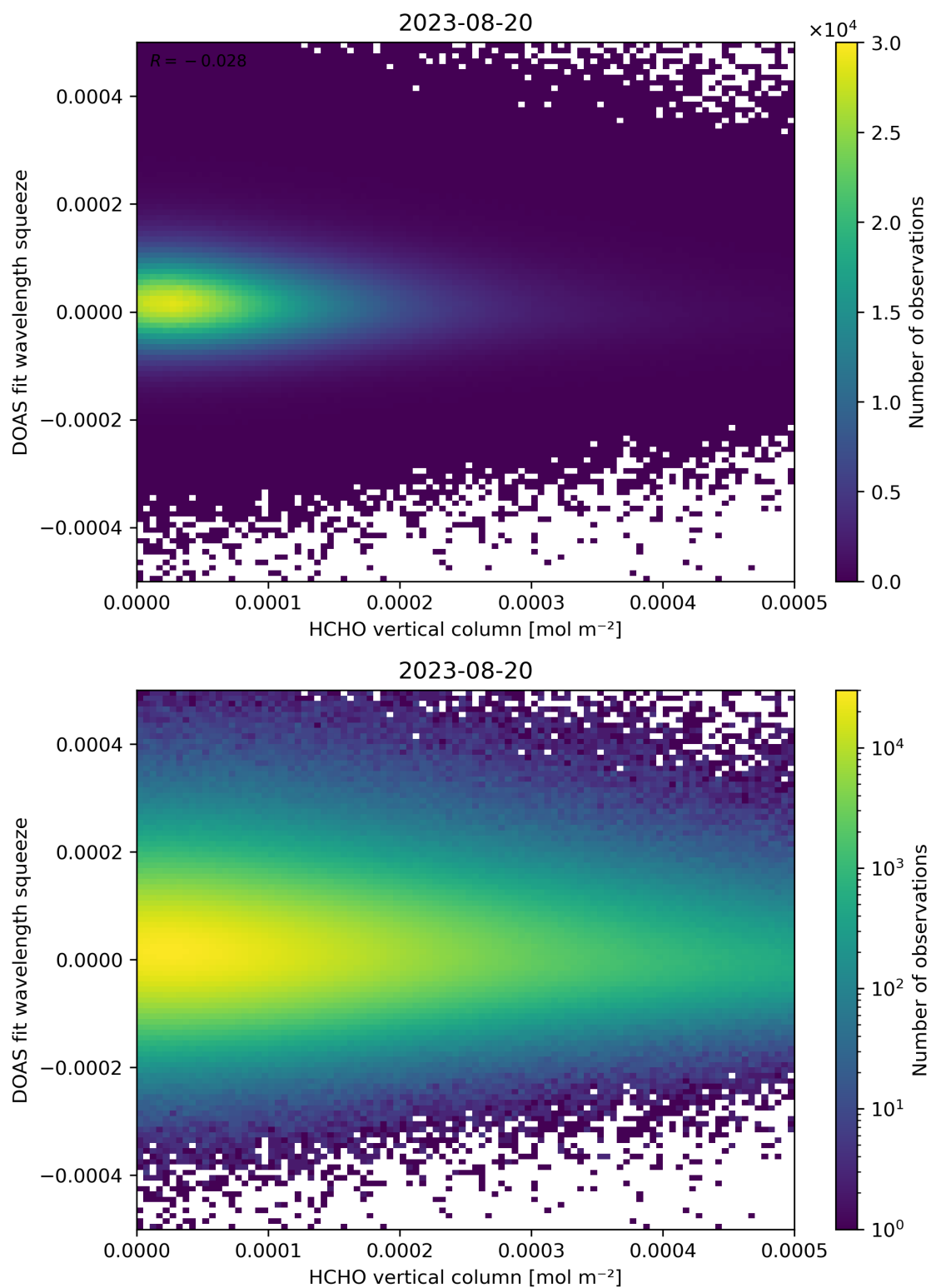
Figure 125: Scatter density plot of “HCHO vertical column” against “DOAS fit wavelength squeeze” for 2023-08-20 to 2023-08-21.
