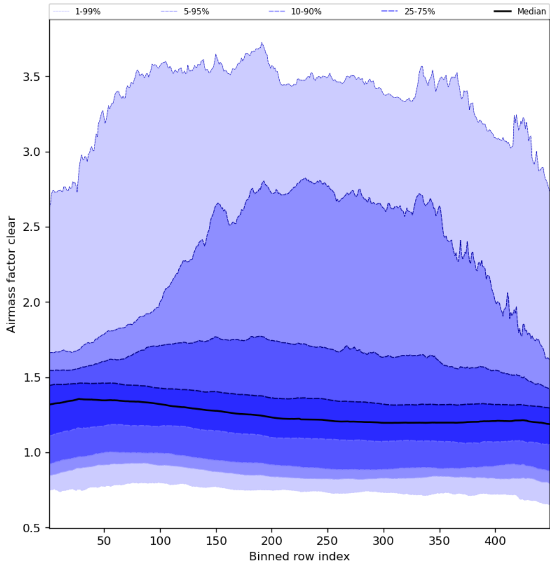
Figure 56: Along track statistics of “Airmass factor clear” for 2023-08-20 to 2023-08-21
