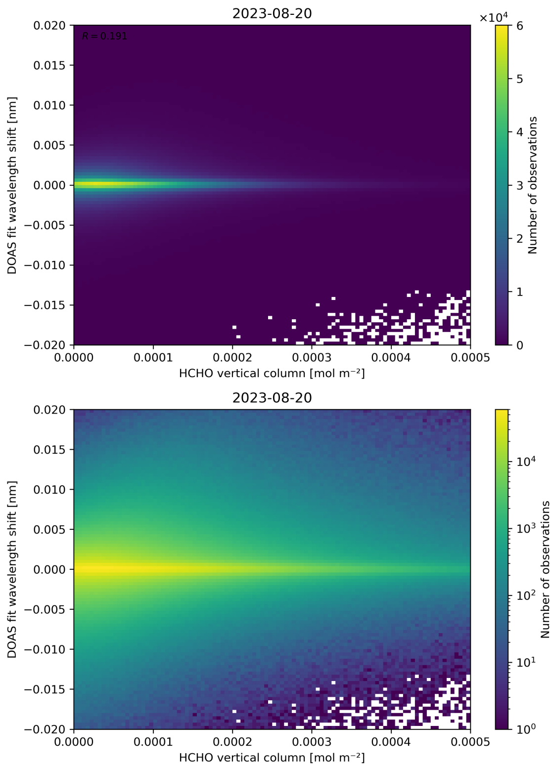
Figure 124: Scatter density plot of “HCHO vertical column” against “DOAS fit wavelength shift” for 2023-08-20 to 2023-08-21.
