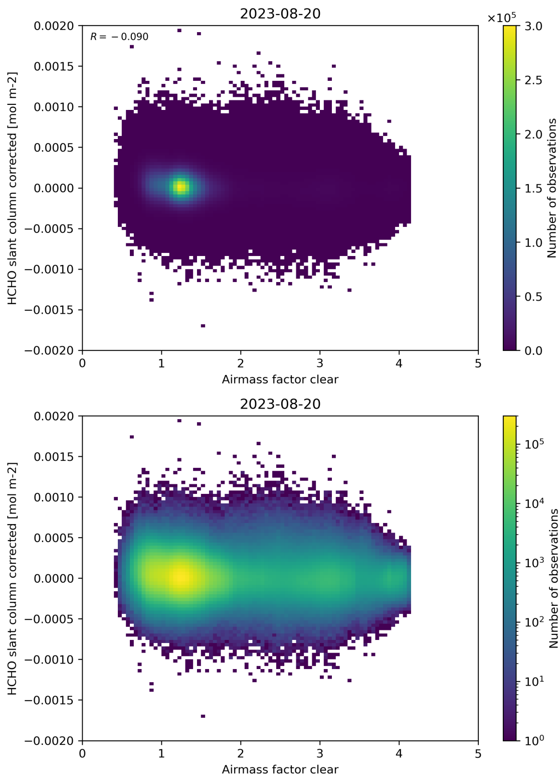
Figure 74: Scatter density plot of “Airmass factor clear” against “HCHO slant column corrected” for 2023-08-20 to 2023-08-21.
