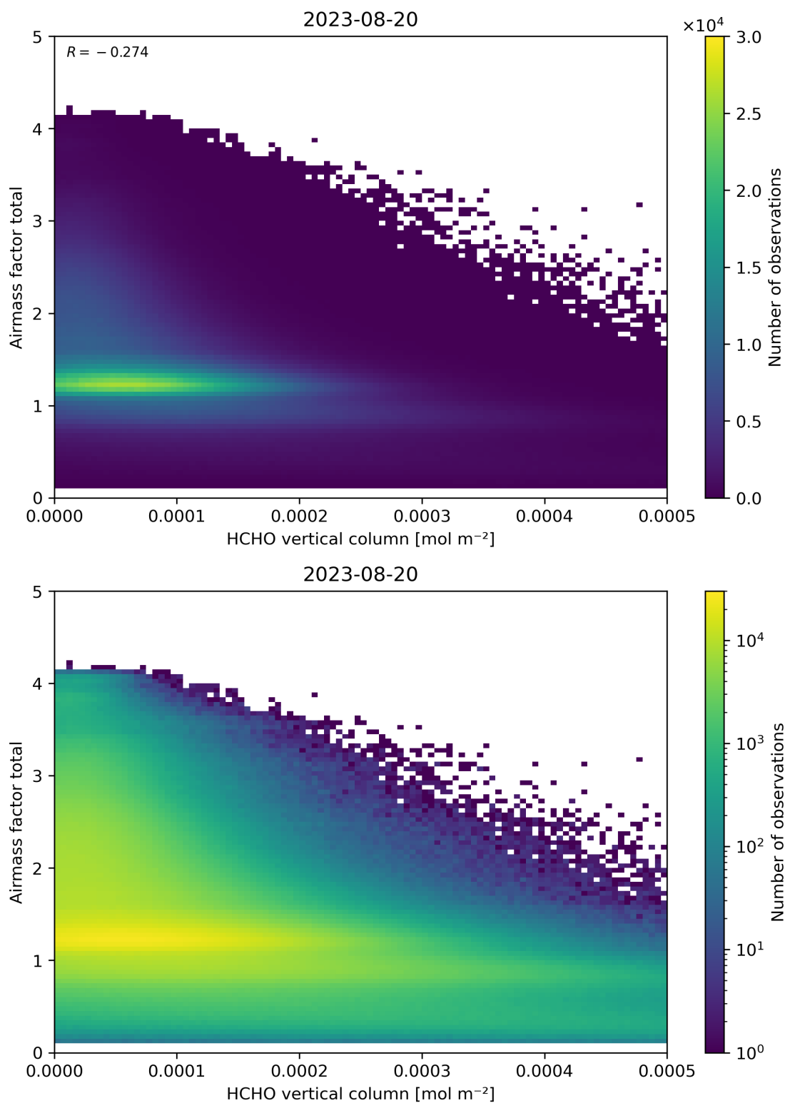
Figure 131: Scatter density plot of “HCHO vertical column” against “Airmass factor total” for 2023-08-20 to 2023-08-21.
