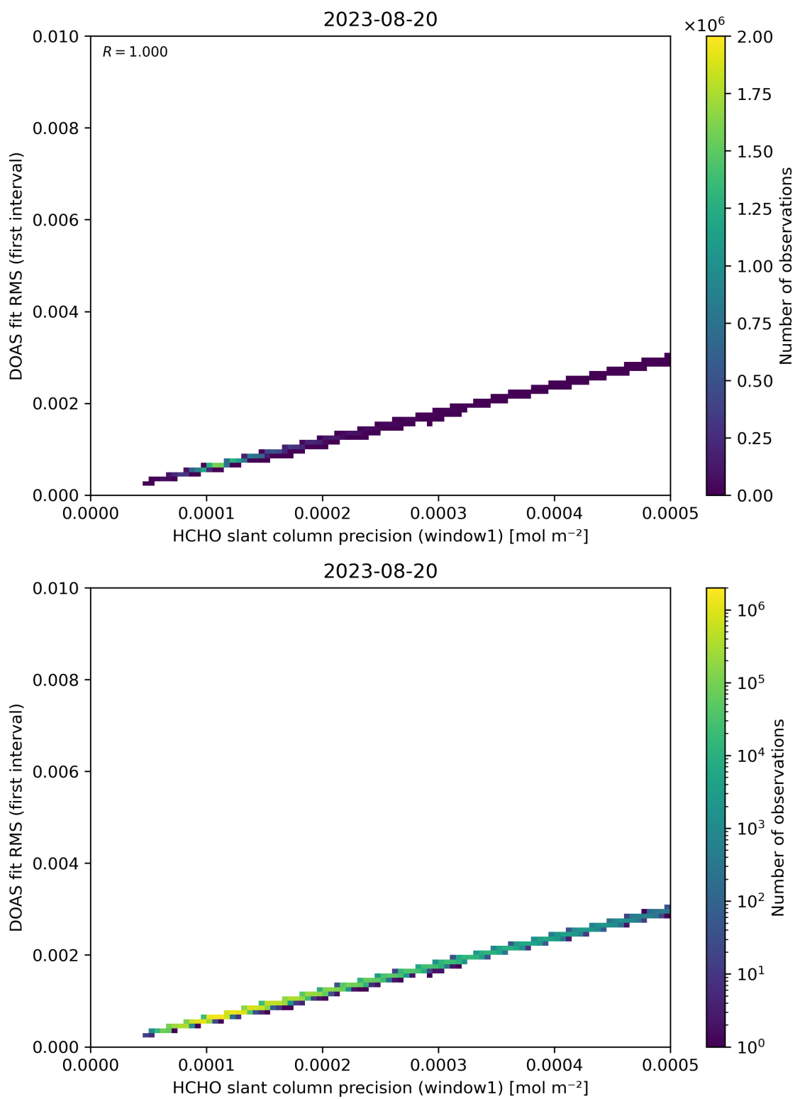
Figure 88: Scatter density plot of “HCHO slant column precision (window1)” against “DOAS fit RMS (first interval)” for 2023-08-20 to 2023-08-21.
