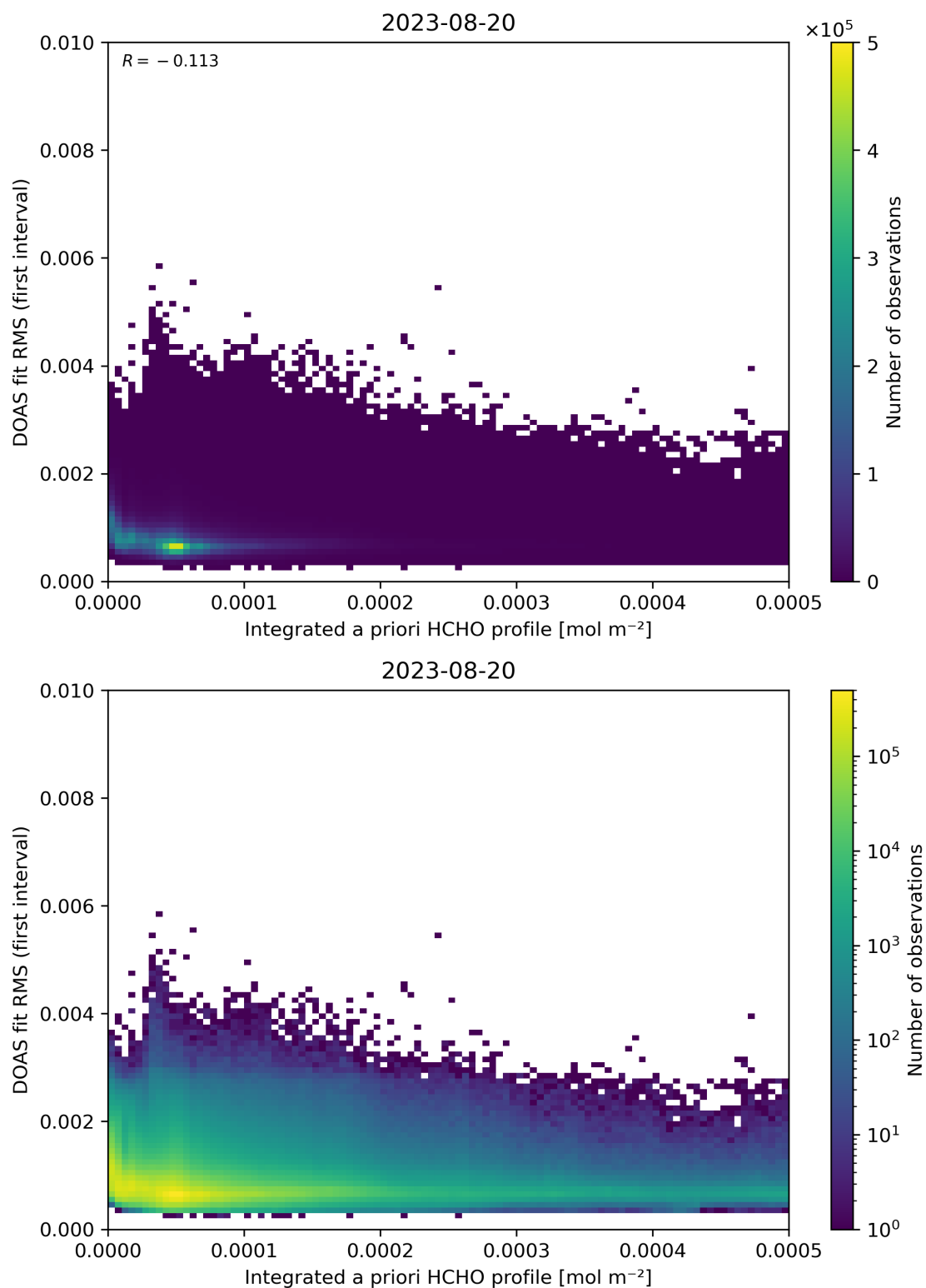
Figure 148: Scatter density plot of “Integrated a priori HCHO profile” against “DOAS fit RMS (first interval)” for 2023-08-20 to 2023-08-21.
