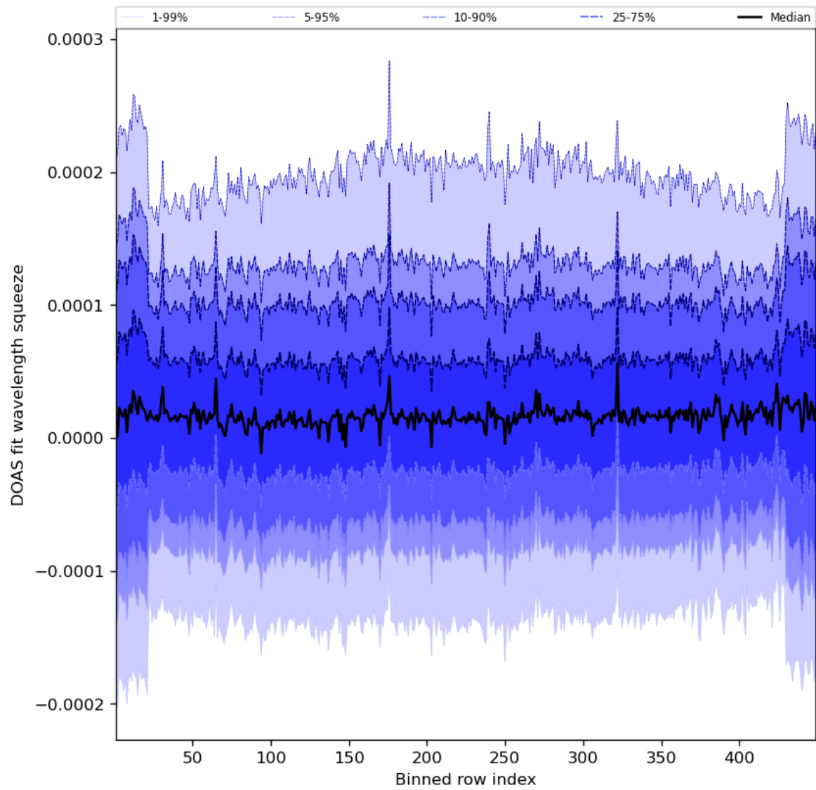
Figure 59: Along track statistics of “DOAS fit wavelength squeeze” for 2023-08-20 to 2023-08-21
