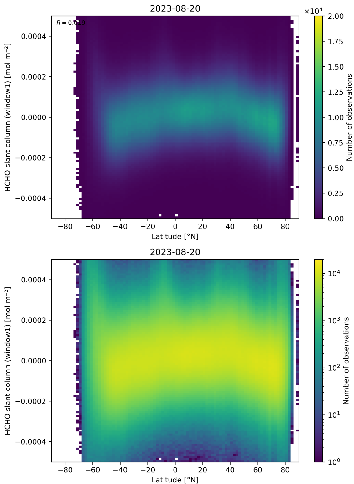
Figure 159: Scatter density plot of “Latitude” against “HCHO slant column (window1)” for 2023-08-20 to 2023-08-21.
