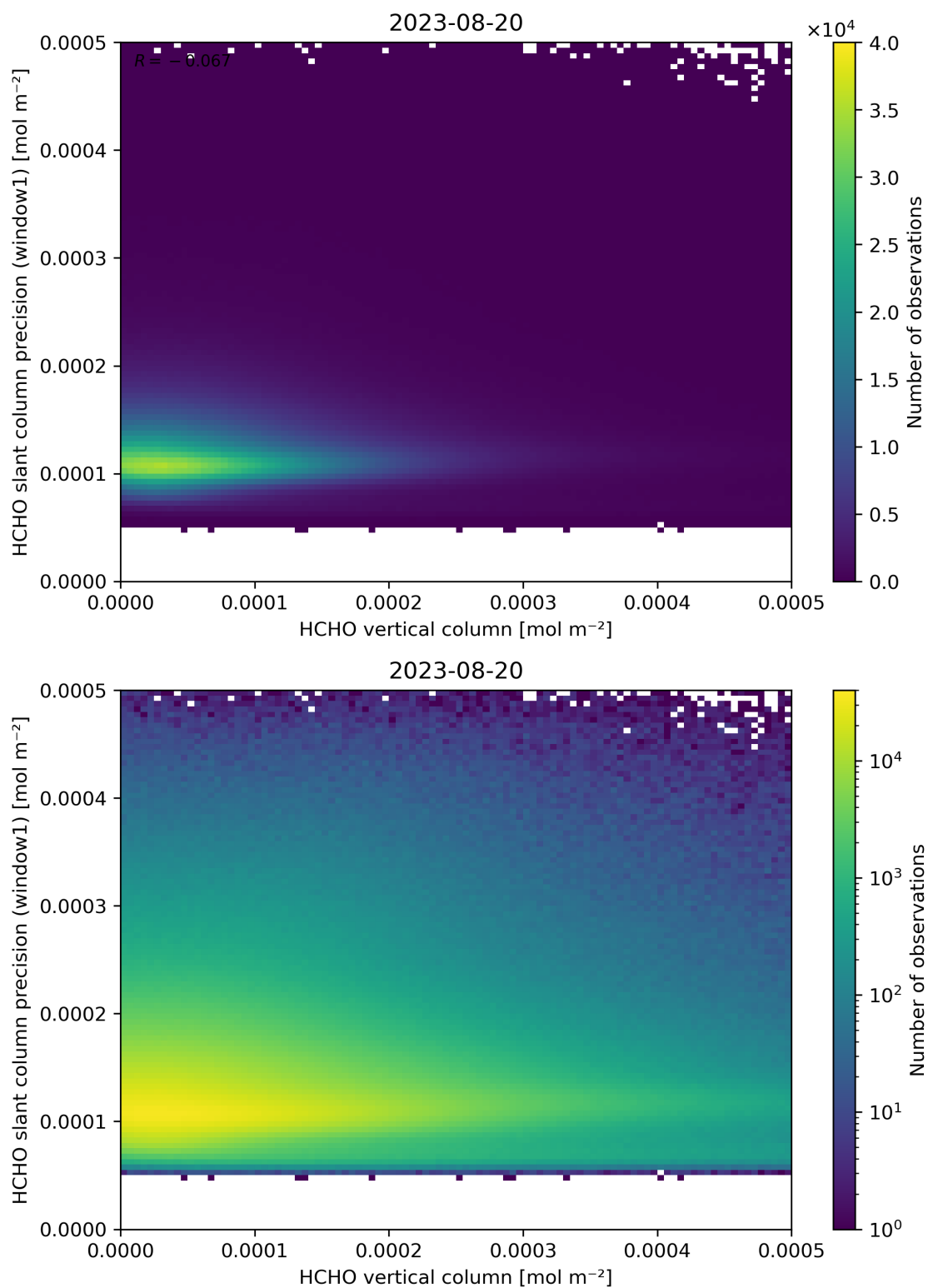
Figure 130: Scatter density plot of “HCHO vertical column” against “HCHO slant column precision (window1)” for 2023-08-20 to 2023-08-21.
