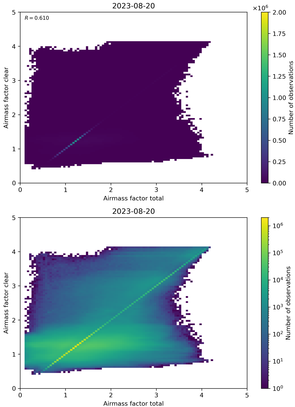
Figure 100: Scatter density plot of “Airmass factor total” against “Airmass factor clear” for 2023-08-20 to 2023-08-21.
