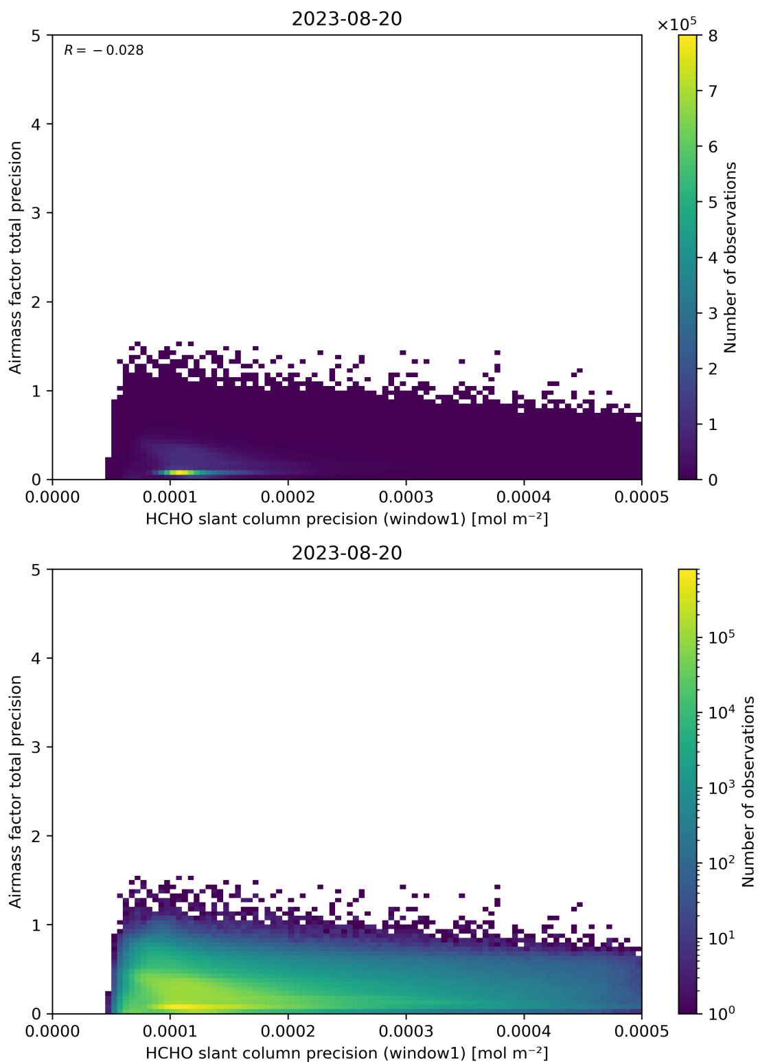
Figure 95: Scatter density plot of “HCHO slant column precision (window1)” against “Airmass factor total precision” for 2023-08-20 to 2023-08-21.
