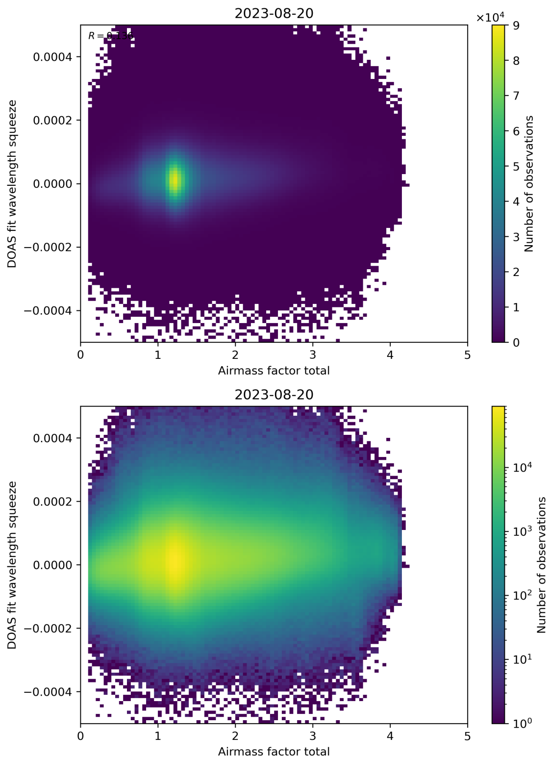
Figure 99: Scatter density plot of “Airmass factor total” against “DOAS fit wavelength squeeze” for 2023-08-20 to 2023-08-21.
