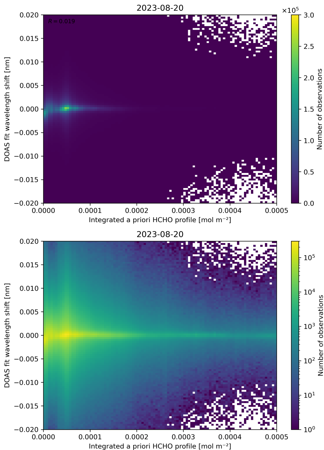
Figure 149: Scatter density plot of “Integrated a priori HCHO profile” against “DOAS fit wavelength shift” for 2023-08-20 to 2023-08-21.
