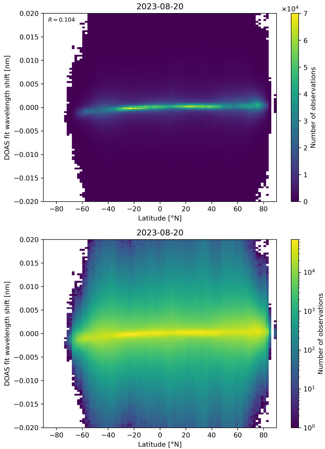
Figure 154: Scatter density plot of “Latitude” against “DOAS fit wavelength shift” for 2023-08-20 to 2023-08-21.
