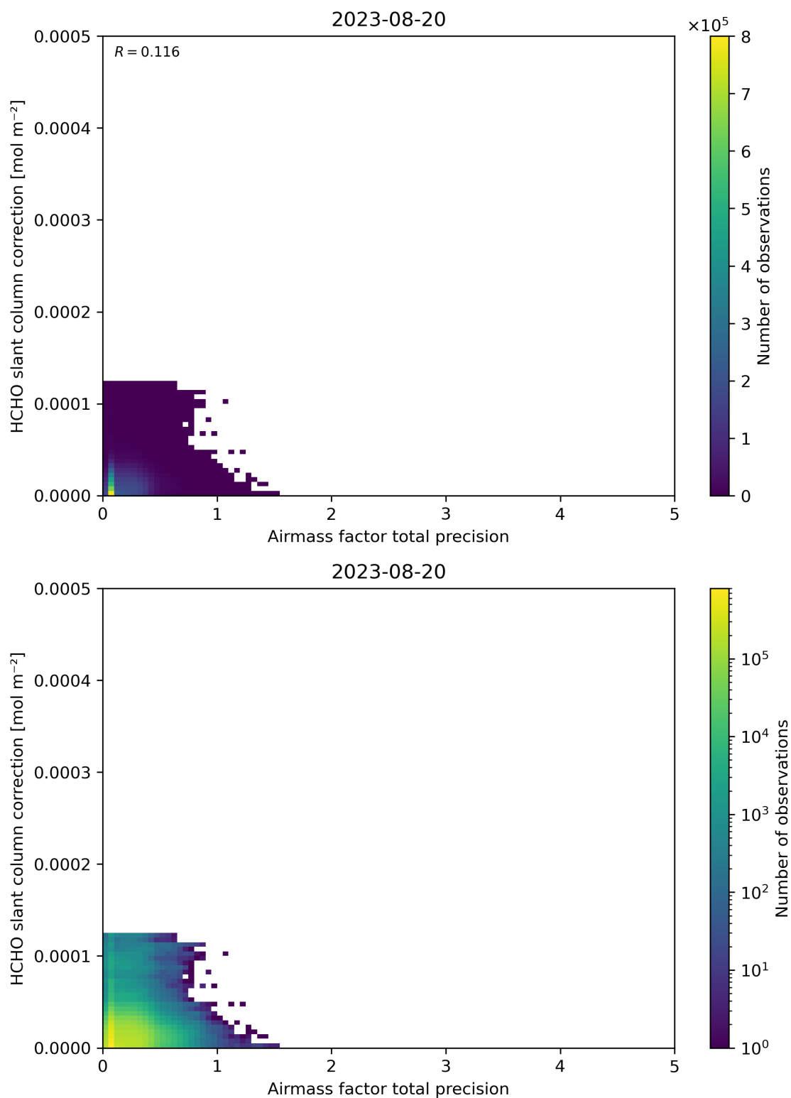
Figure 110: Scatter density plot of “Airmass factor total precision” against “HCHO slant column correction” for 2023-08-20 to 2023-08-21.
