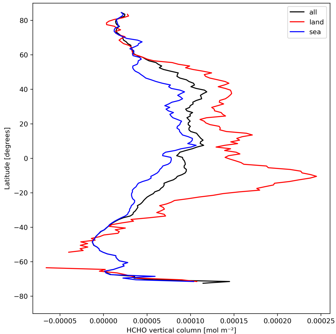
Figure 21: Zonal average of “HCHO vertical column” for 2023-08-20 to 2023-08-21.
