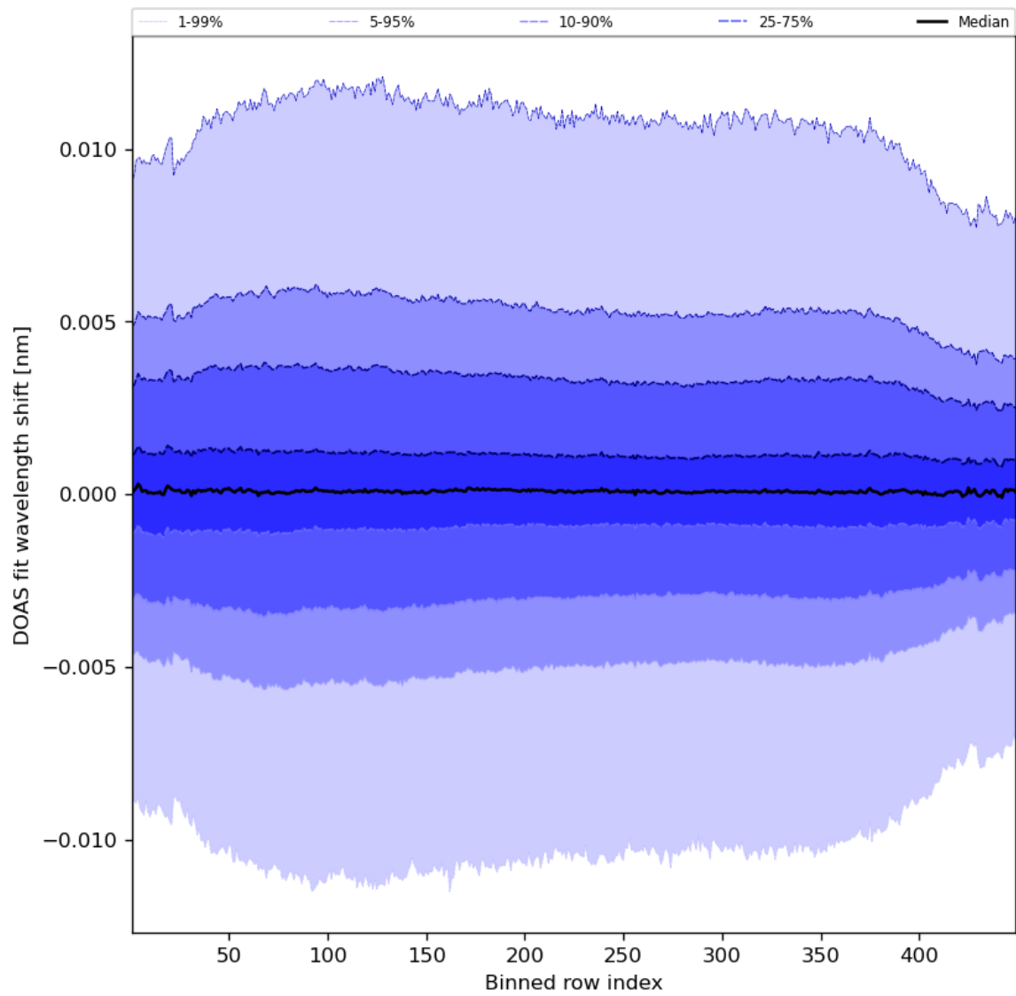
Figure 58: Along track statistics of “DOAS fit wavelength shift” for 2023-08-20 to 2023-08-21
