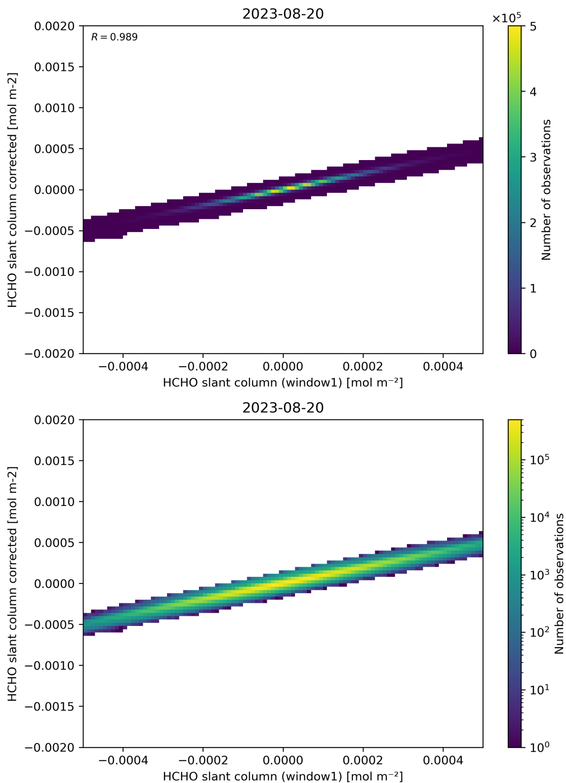
Figure 82: Scatter density plot of “HCHO slant column (window1)” against “HCHO slant column corrected” for 2023-08-20 to 2023-08-21.
