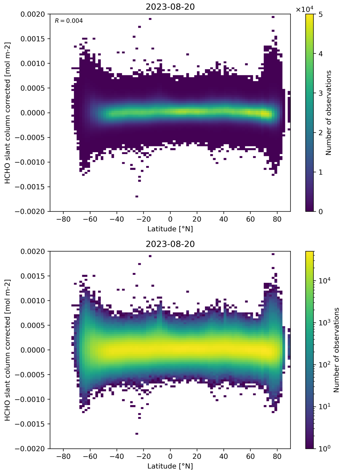
Figure 157: Scatter density plot of “Latitude” against “HCHO slant column corrected” for 2023-08-20 to 2023-08-21.
