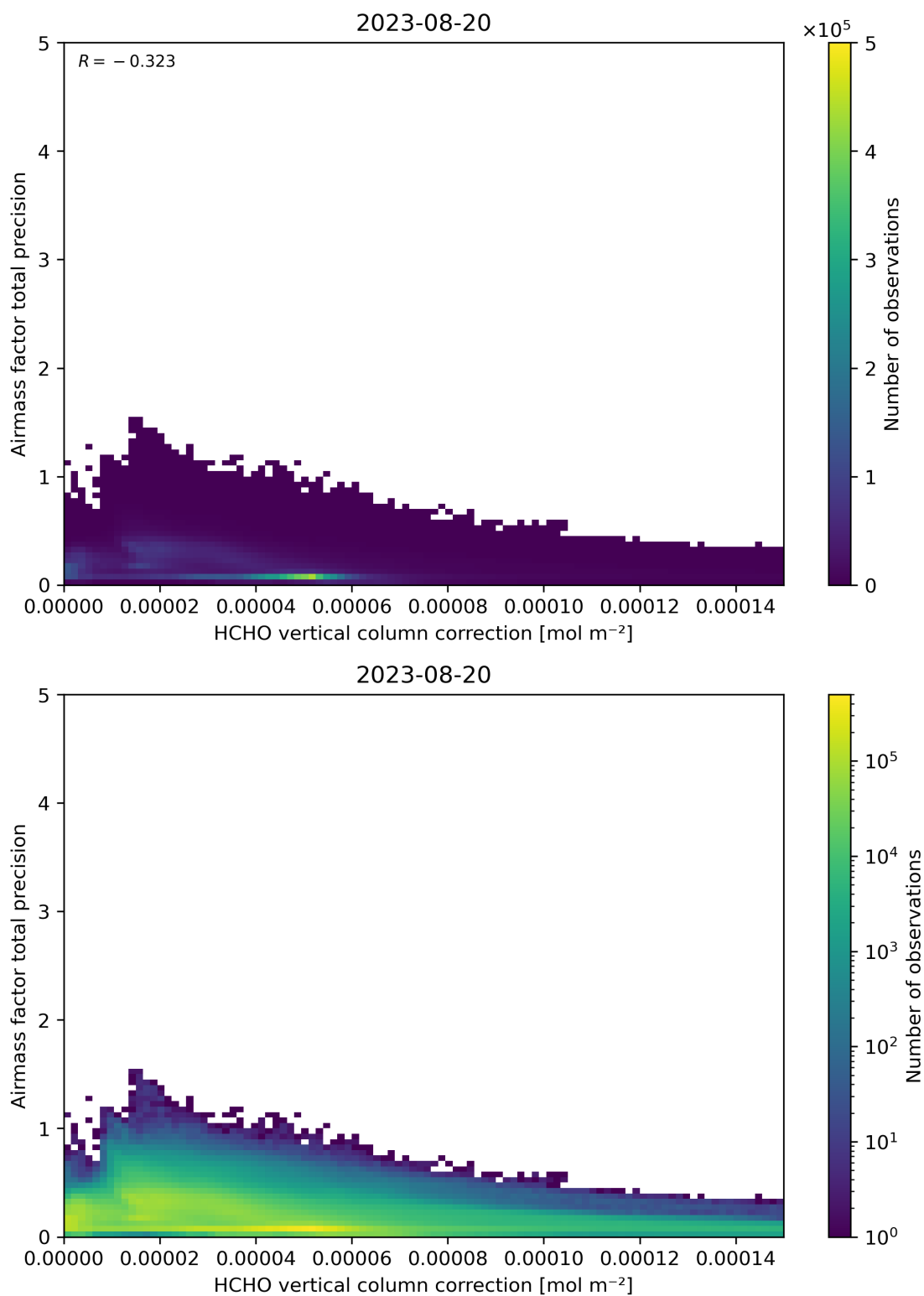
Figure 121: Scatter density plot of “HCHO vertical column correction” against “Airmass factor total precision” for 2023-08-20 to 2023-08-21.
