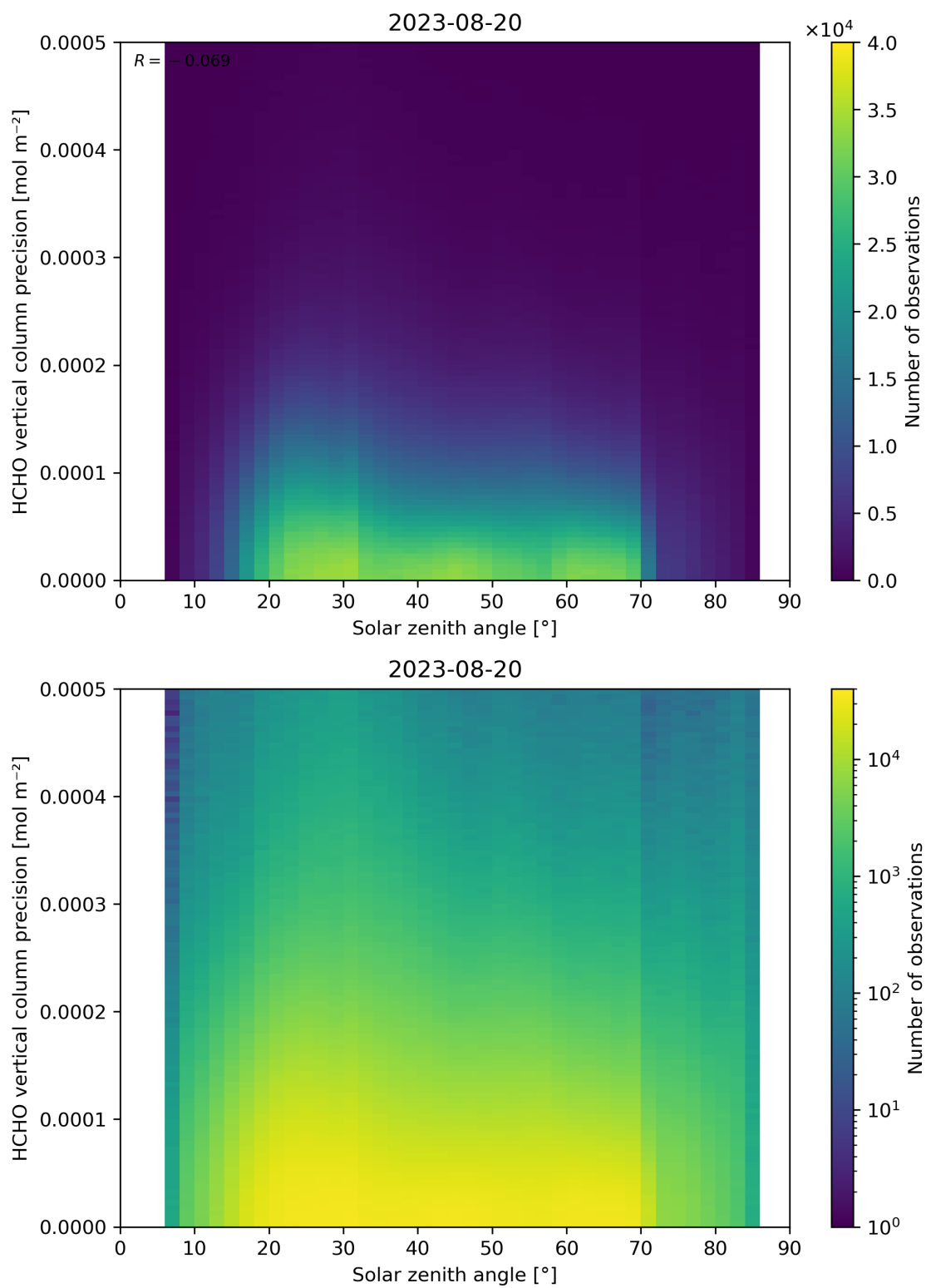
Figure 179: Scatter density plot of “Solar zenith angle” against “HCHO vertical column precision” for 2023-08-20 to 2023-08-21.
