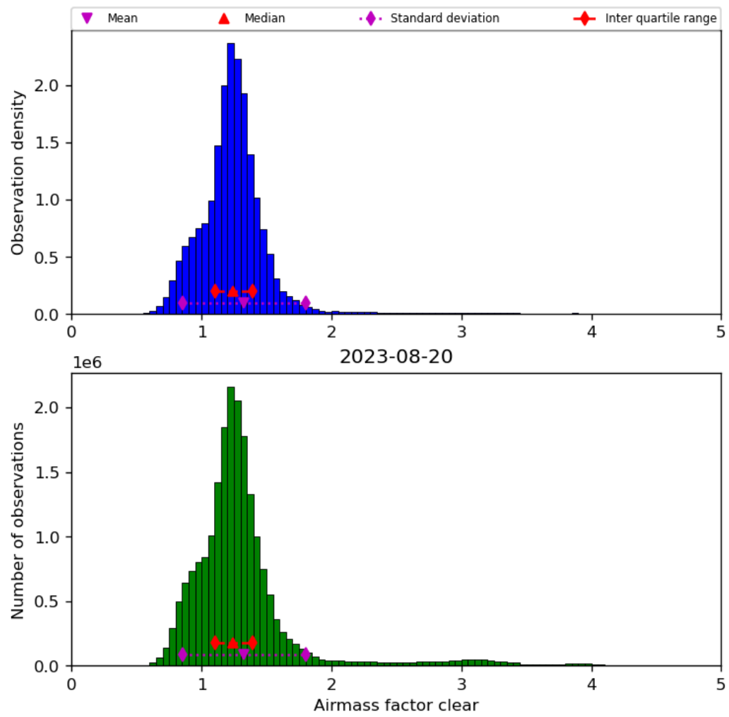
Figure 42: Histogram of “Airmass factor clear” for 2023-08-20 to 2023-08-21
