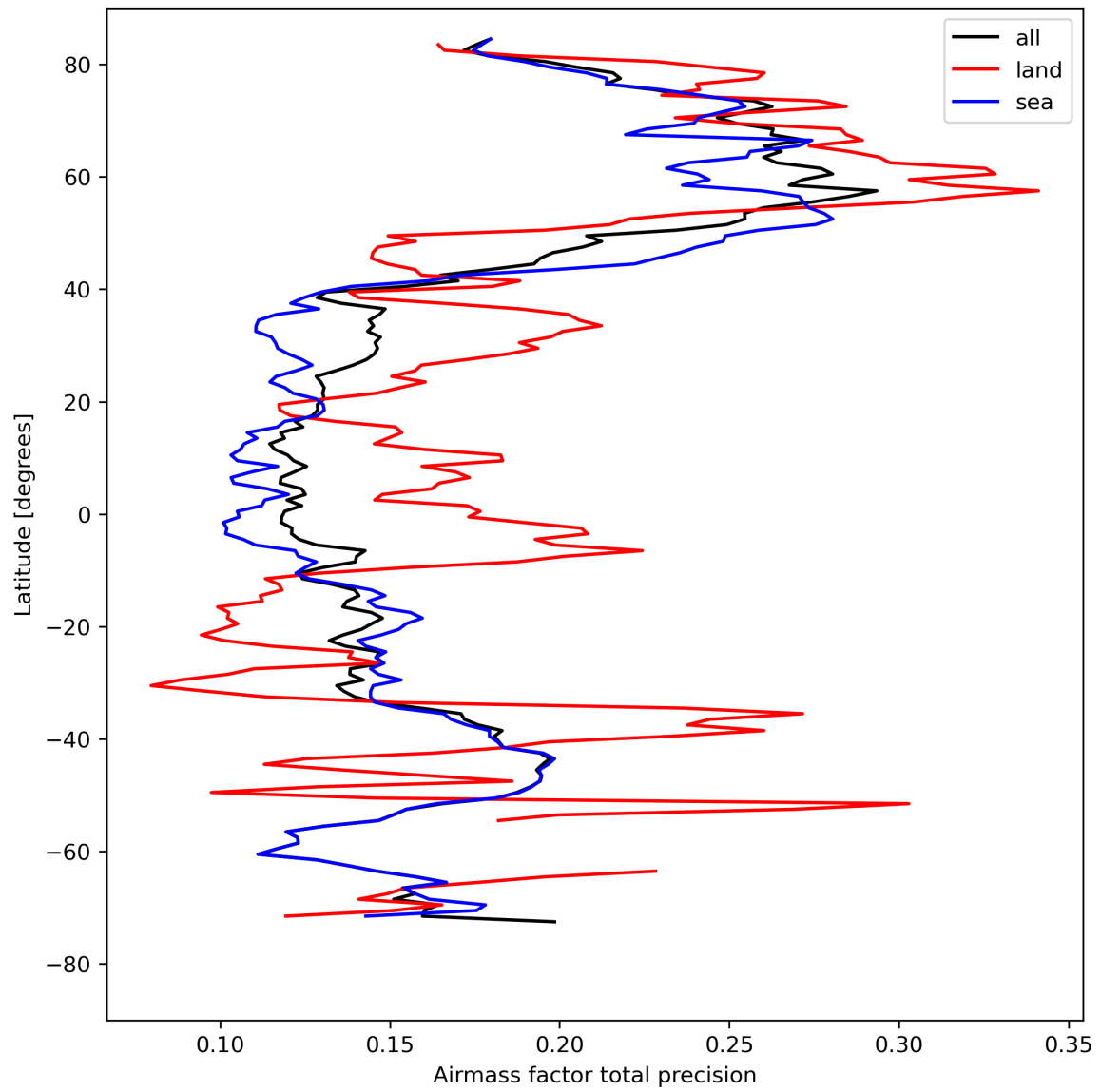
Figure 27: Zonal average of “Airmass factor total precision” for 2023-08-20 to 2023-08-21.
