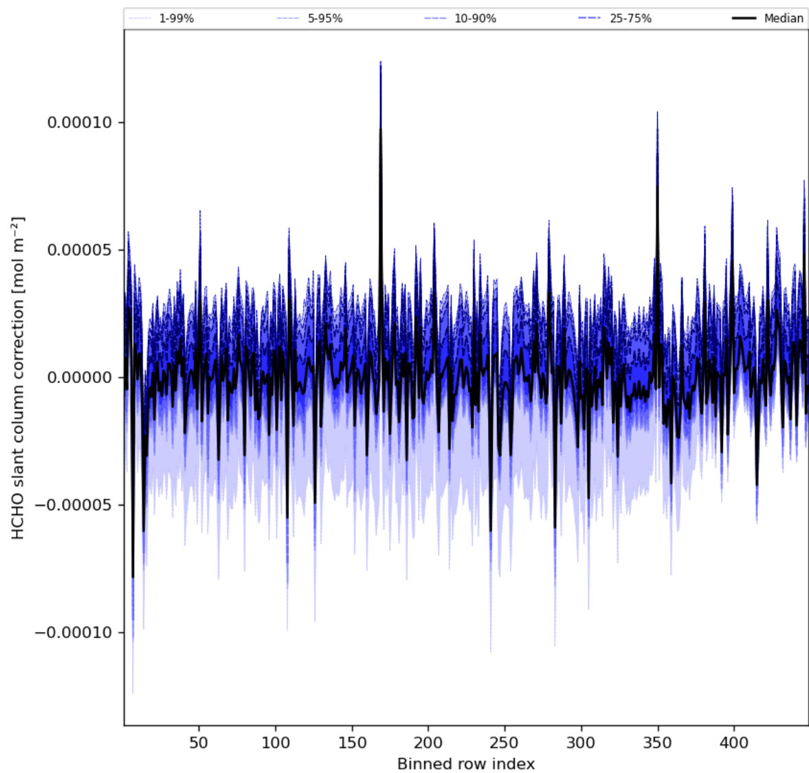
Figure 61: Along track statistics of “HCHO slant column correction” for 2023-08-20 to 2023-08-21
