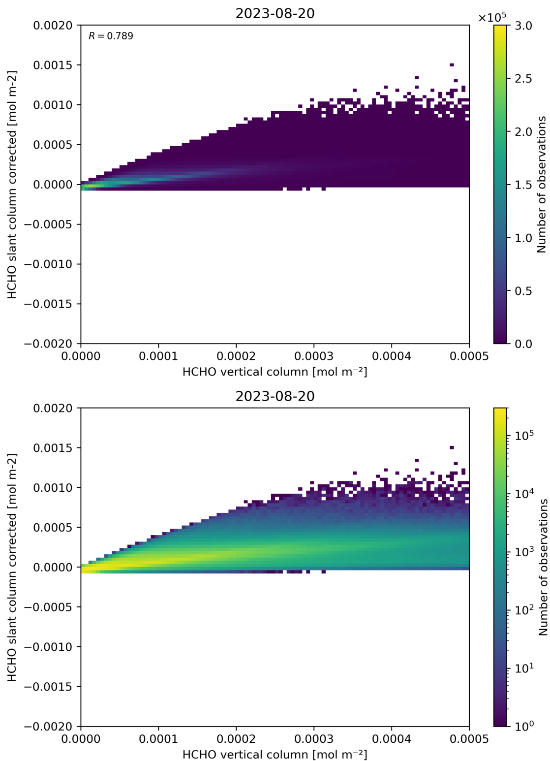
Figure 127: Scatter density plot of “HCHO vertical column” against “HCHO slant column corrected” for 2023-08-20 to 2023-08-21.
