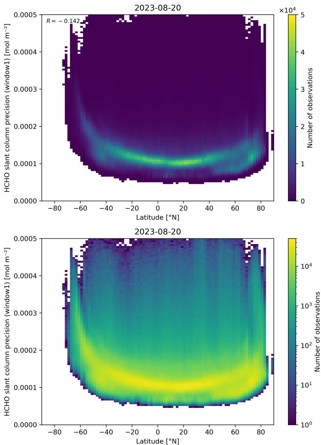
Figure 160: Scatter density plot of “Latitude” against “HCHO slant column precision (window1)” for 2023-08-20 to 2023-08-21.
