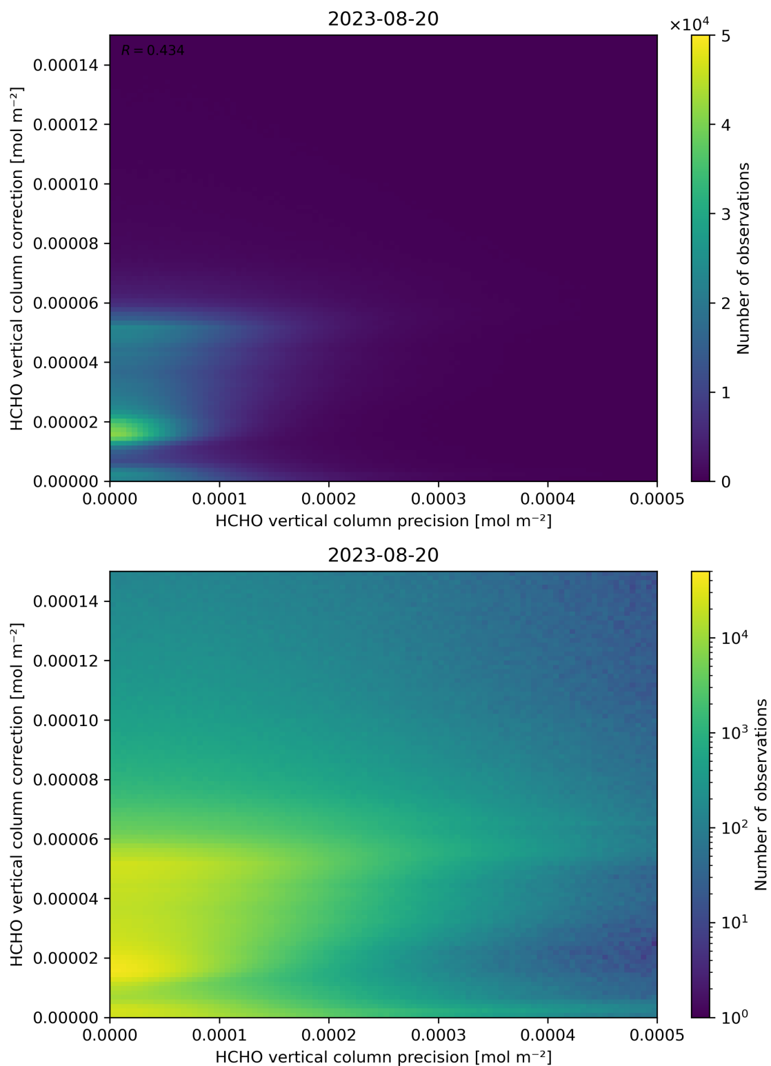
Figure 146: Scatter density plot of “HCHO vertical column precision” against “HCHO vertical column correction” for 2023-08-20 to 2023-08-21.
