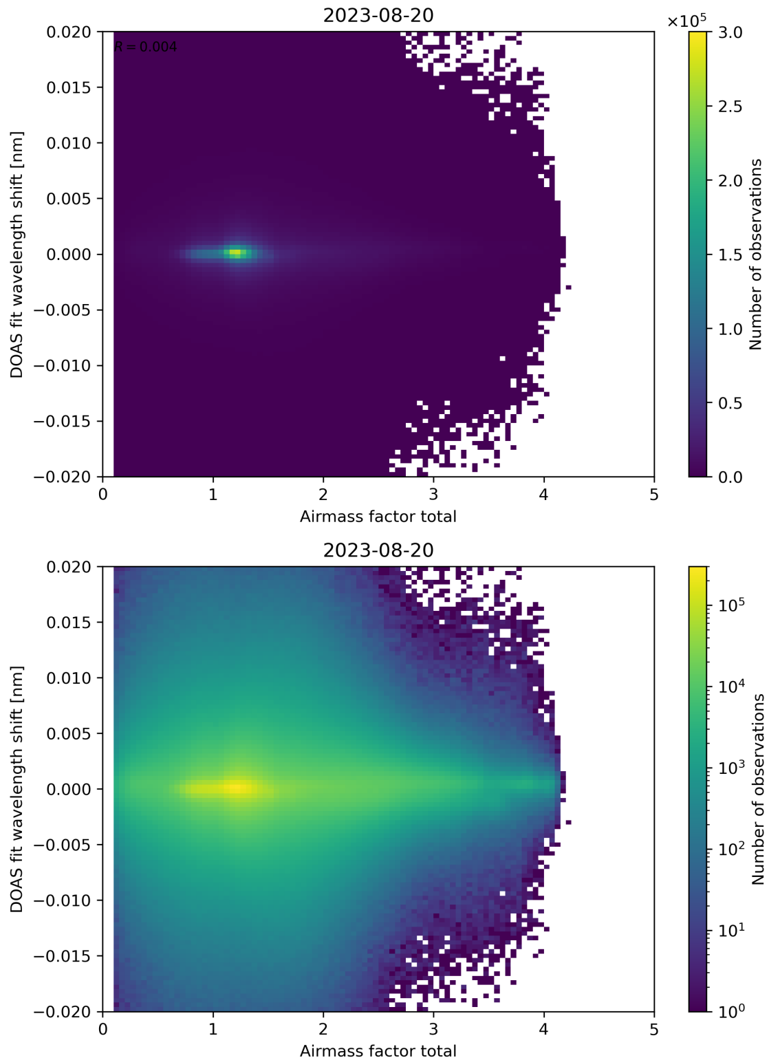
Figure 98: Scatter density plot of “Airmass factor total” against “DOAS fit wavelength shift” for 2023-08-20 to 2023-08-21.
