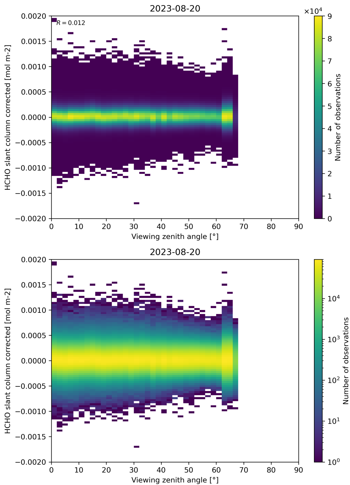
Figure 186: Scatter density plot of “Viewing zenith angle” against “HCHO slant column corrected” for 2023-08-20 to 2023-08-21.
