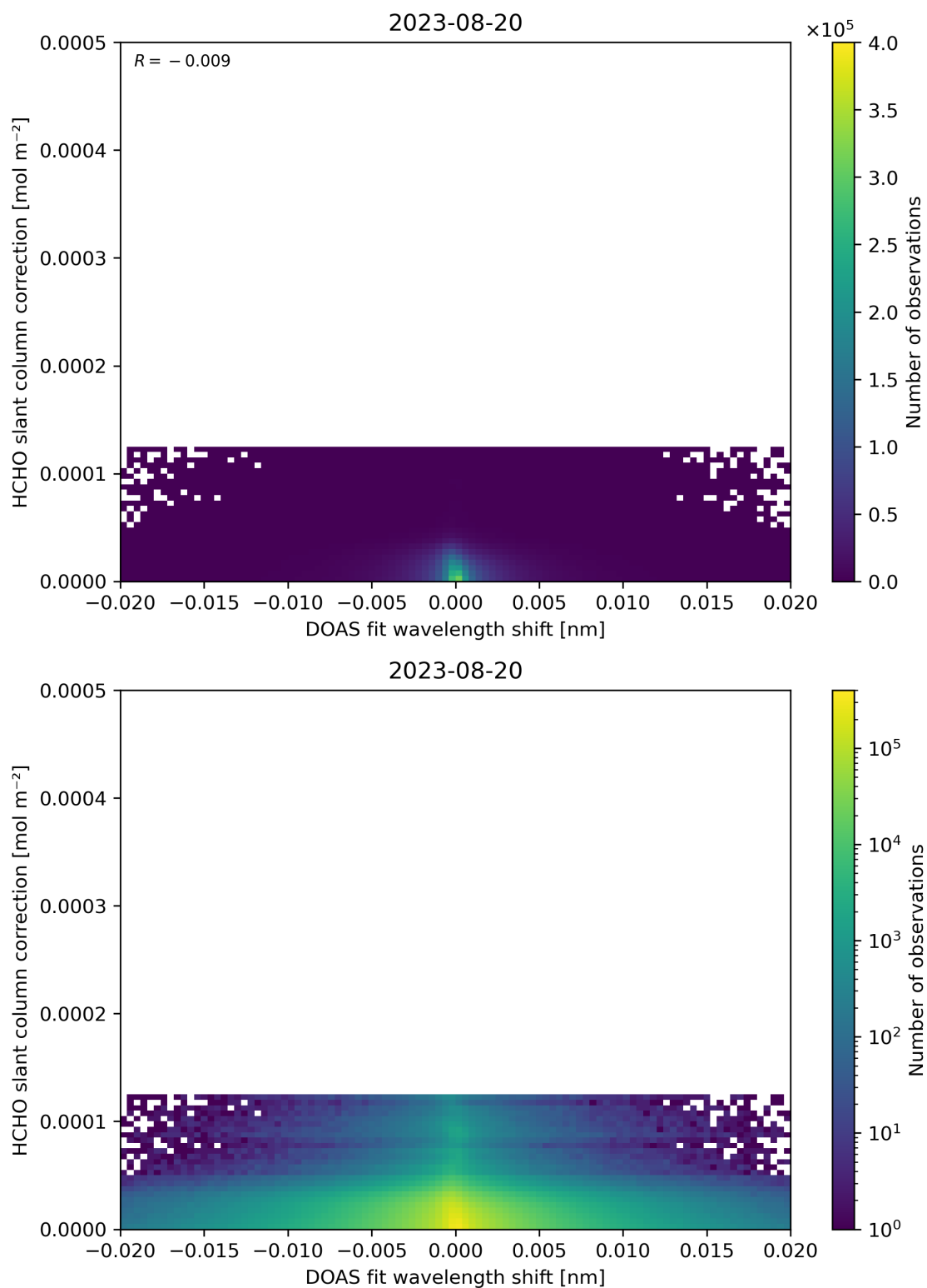
Figure 67: Scatter density plot of “DOAS fit wavelength shift” against “HCHO slant column correction” for 2023-08-20 to 2023-08-21.
