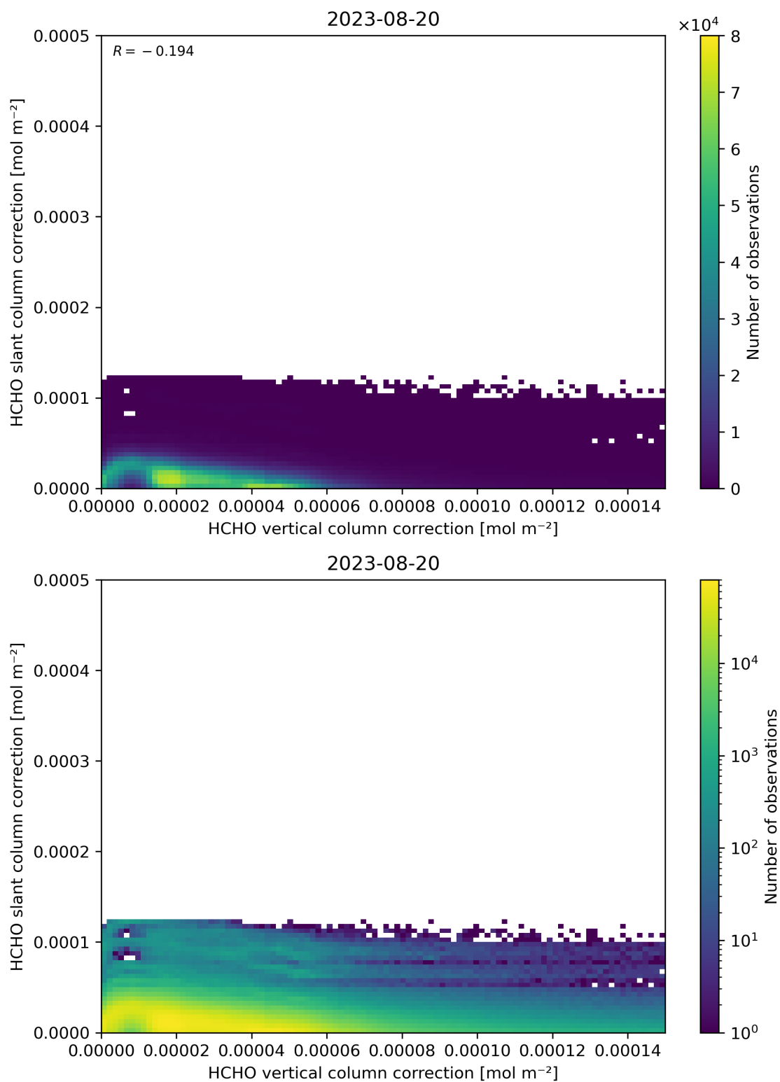
Figure 117: Scatter density plot of “HCHO vertical column correction” against “HCHO slant column correction” for 2023-08-20 to 2023-08-21.
