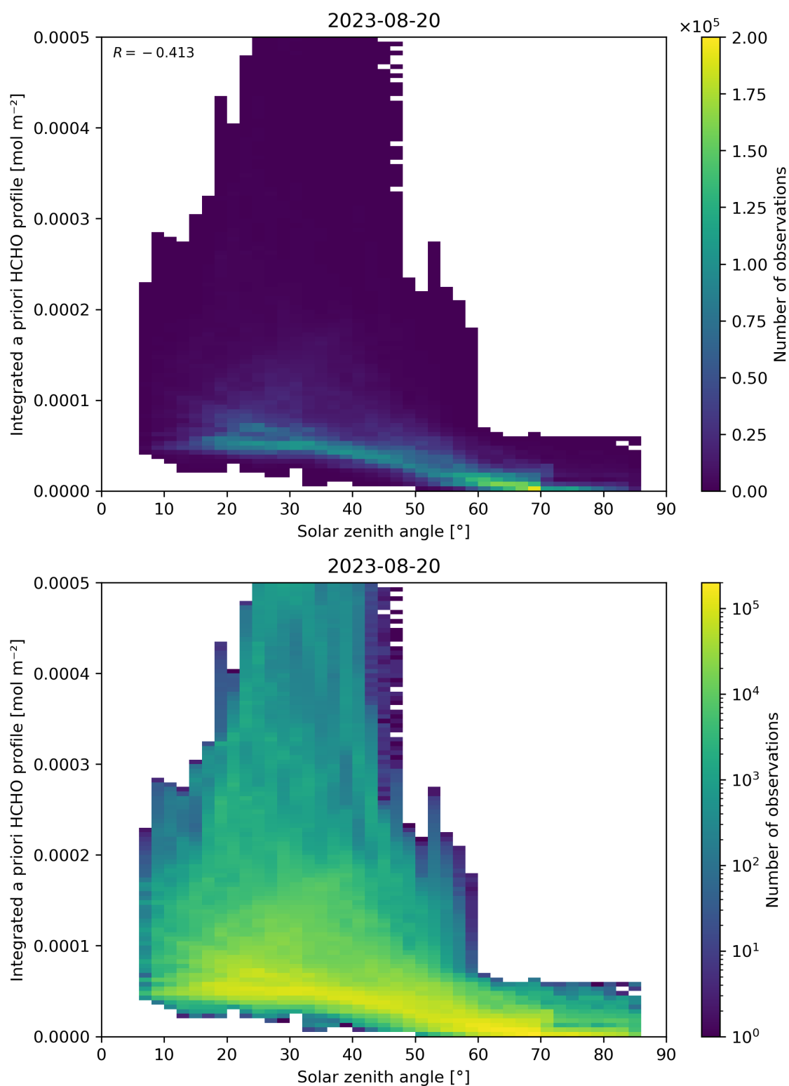
Figure 180: Scatter density plot of “Solar zenith angle” against “Integrated a priori HCHO profile” for 2023-08-20 to 2023-08-21.
