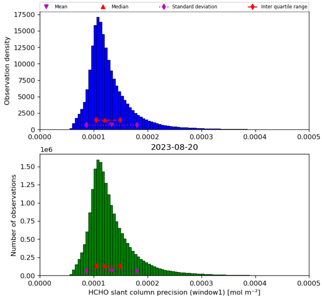
Figure 39: Histogram of “HCHO slant column precision (window1)” for 2023-08-20 to 2023-08-21
