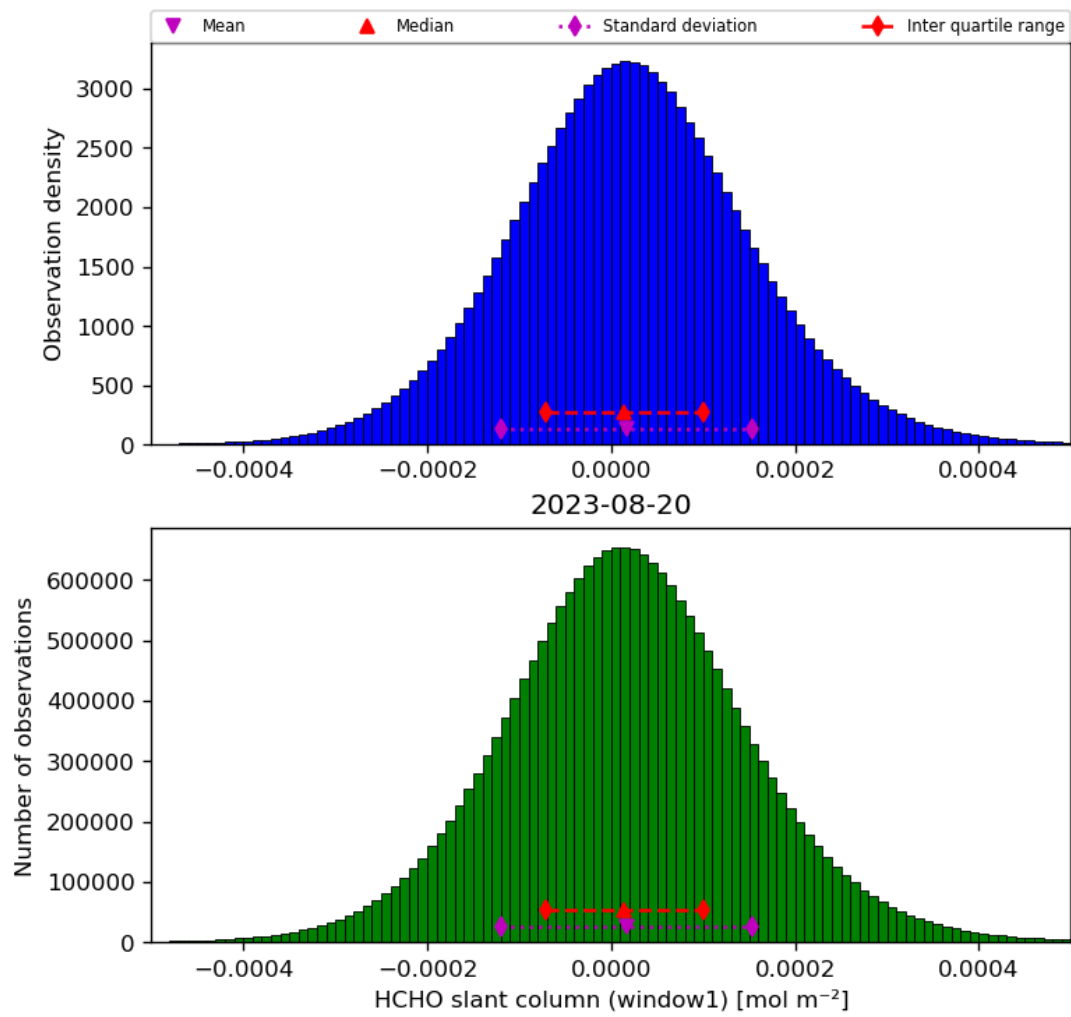
Figure 38: Histogram of “HCHO slant column (window1)” for 2023-08-20 to 2023-08-21
