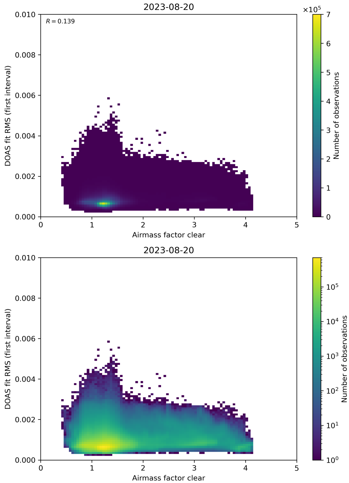
Figure 71: Scatter density plot of “Airmass factor clear” against “DOAS fit RMS (first interval)” for 2023-08-20 to 2023-08-21.
