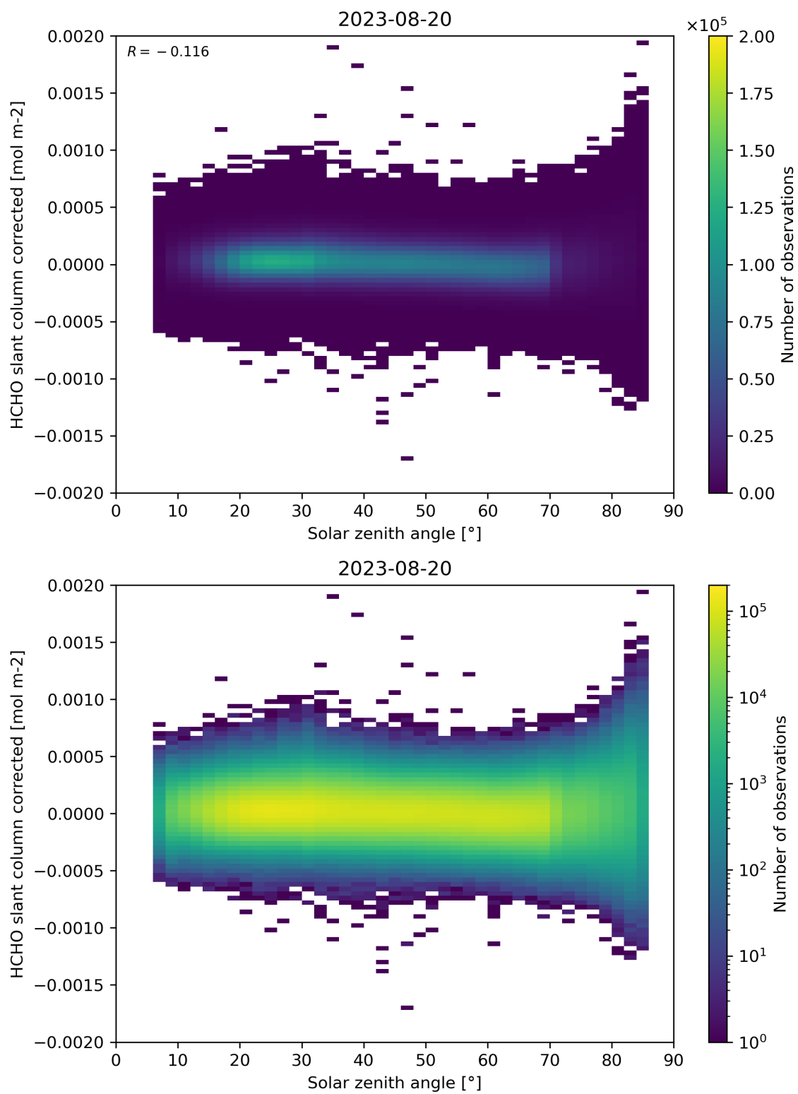
Figure 171: Scatter density plot of “Solar zenith angle” against “HCHO slant column corrected” for 2023-08-20 to 2023-08-21.
