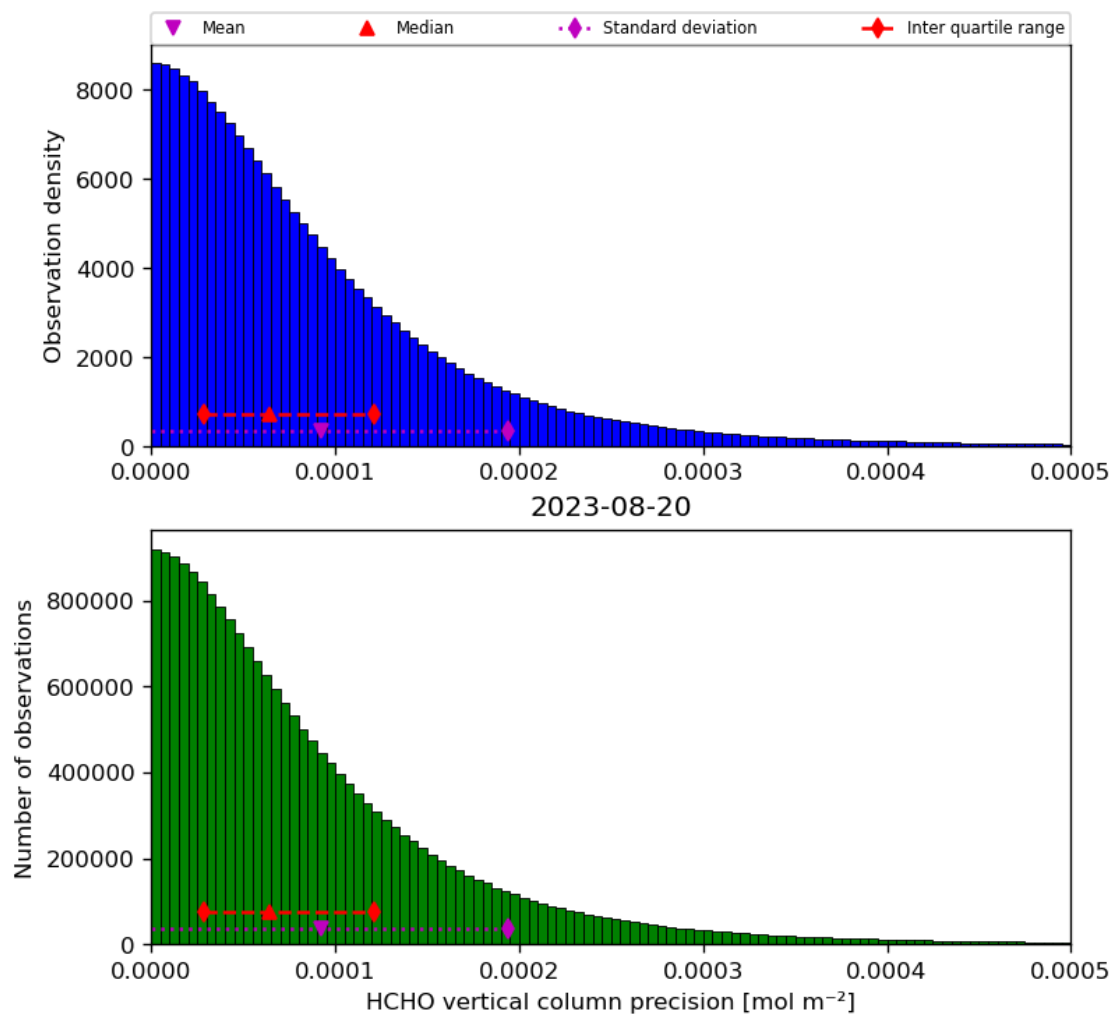
Figure 36: Histogram of “HCHO vertical column precision” for 2023-08-20 to 2023-08-21
