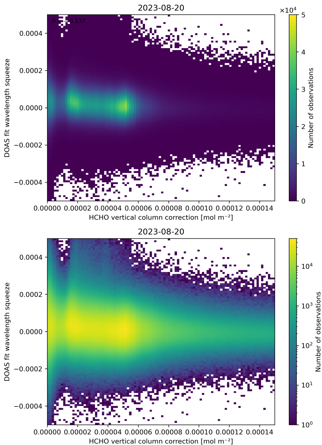
Figure 114: Scatter density plot of “HCHO vertical column correction” against “DOAS fit wavelength squeeze” for 2023-08-20 to 2023-08-21.
