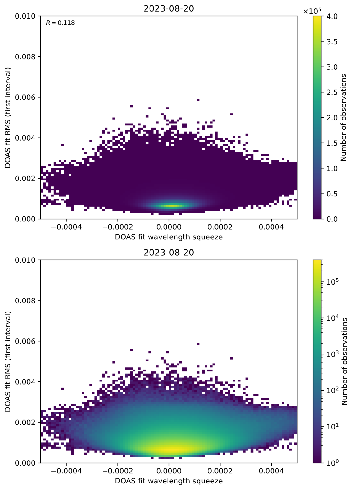
Figure 68: Scatter density plot of “DOAS fit wavelength squeeze” against “DOAS fit RMS (first interval)” for 2023-08-20 to 2023-08-21.
