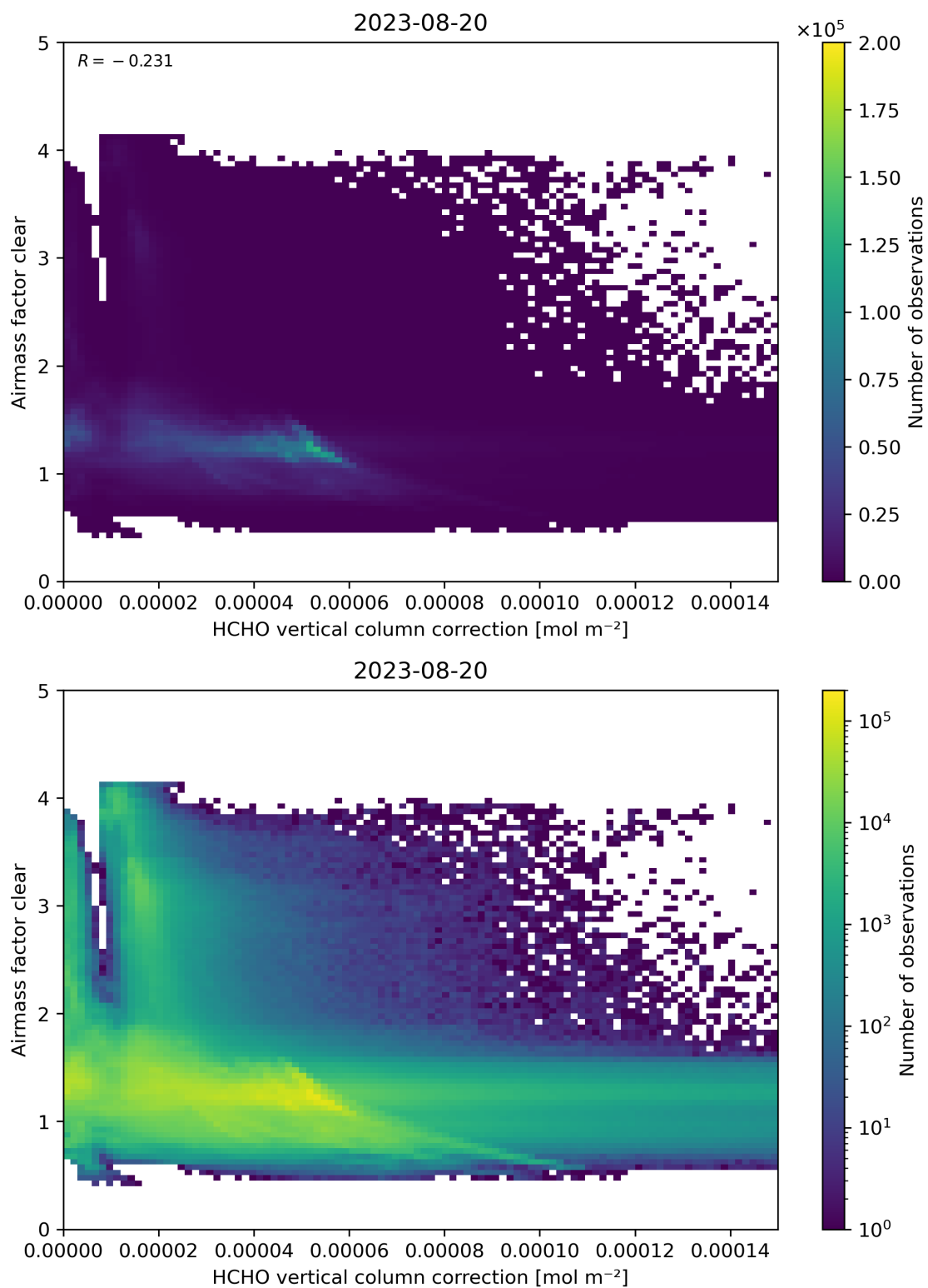
Figure 115: Scatter density plot of “HCHO vertical column correction” against “Airmass factor clear” for 2023-08-20 to 2023-08-21.
