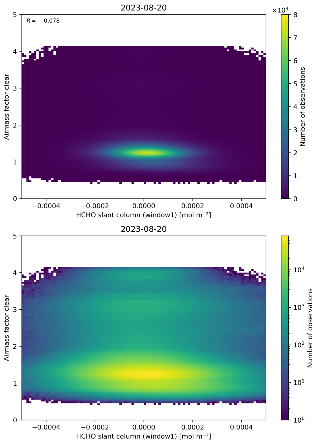
Figure 81: Scatter density plot of “HCHO slant column (window1)” against “Airmass factor clear” for 2023-08-20 to 2023-08-21.
