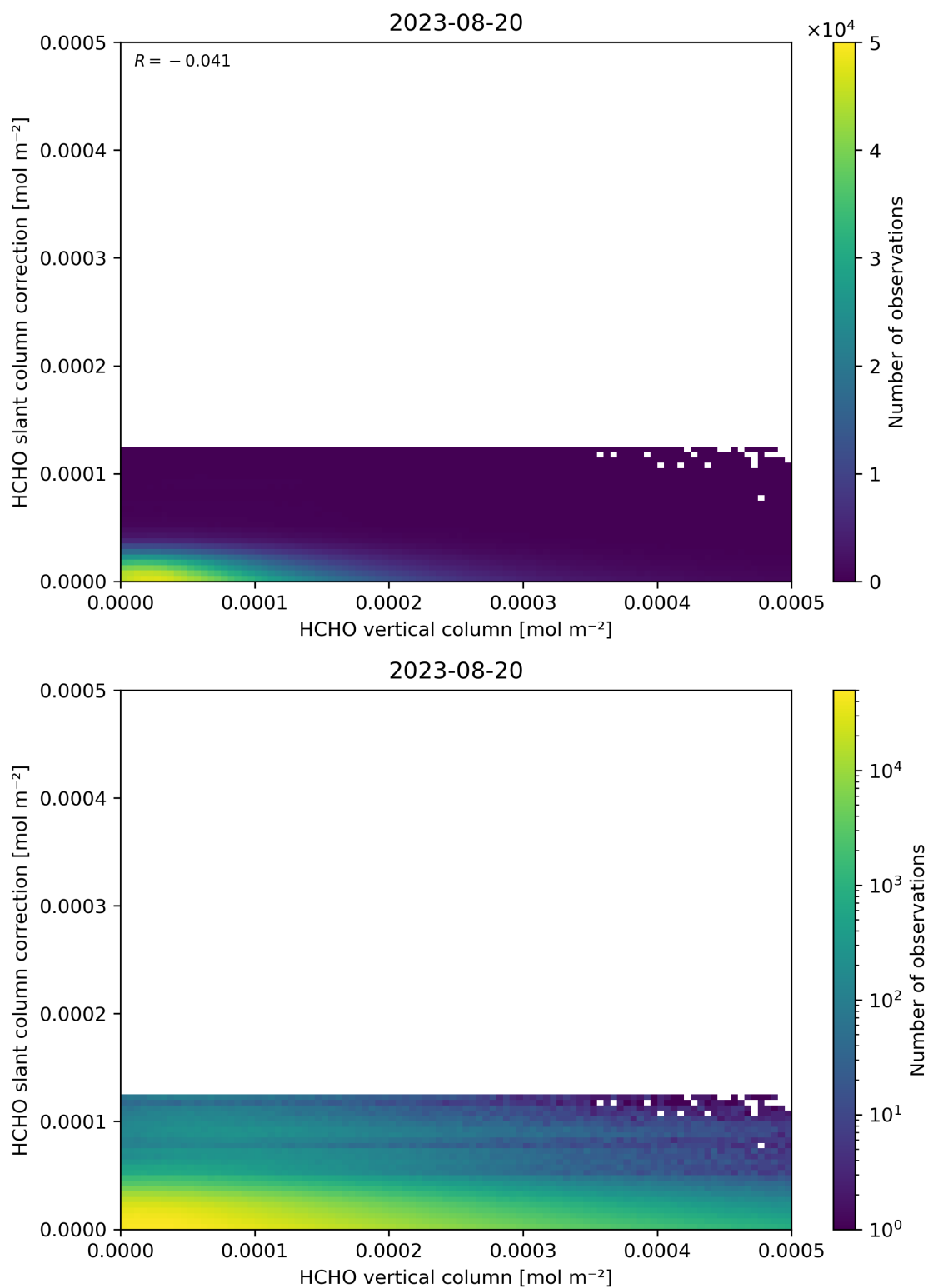
Figure 128: Scatter density plot of “HCHO vertical column” against “HCHO slant column correction” for 2023-08-20 to 2023-08-21.
