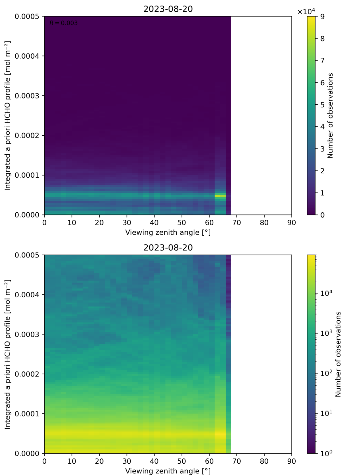
Figure 195: Scatter density plot of “Viewing zenith angle” against “Integrated a priori HCHO profile” for 2023-08-20 to 2023-08-21.
