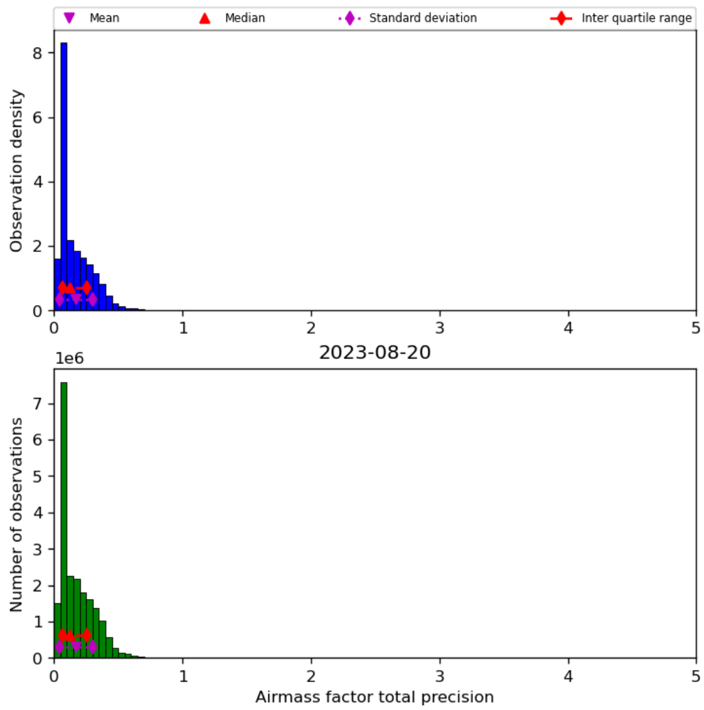
Figure 41: Histogram of “Airmass factor total precision” for 2023-08-20 to 2023-08-21
