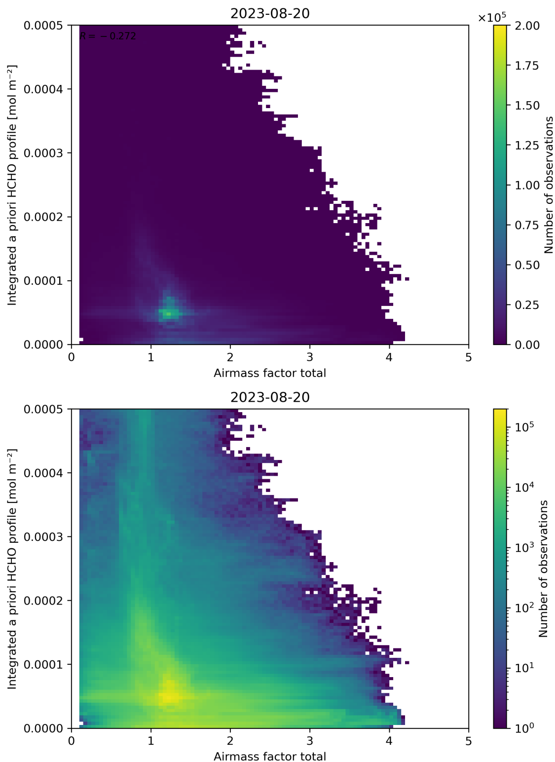
Figure 104: Scatter density plot of “Airmass factor total” against “Integrated a priori HCHO profile” for 2023-08-20 to 2023-08-21.
