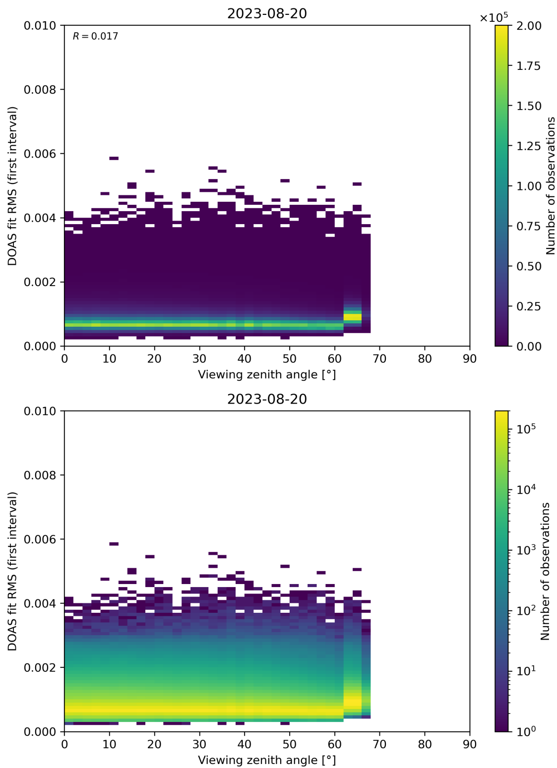
Figure 182: Scatter density plot of “Viewing zenith angle” against “DOAS fit RMS (first interval)” for 2023-08-20 to 2023-08-21.
