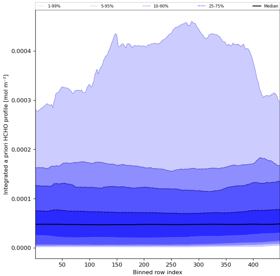
Figure 57: Along track statistics of “Integrated a priori HCHO profile” for 2023-08-20 to 2023-08-21
