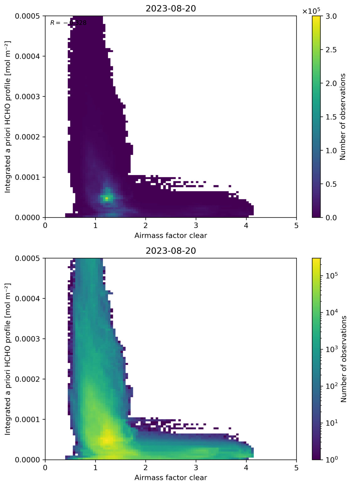
Figure 76: Scatter density plot of “Airmass factor clear” against “Integrated a priori HCHO profile” for 2023-08-20 to 2023-08-21.
