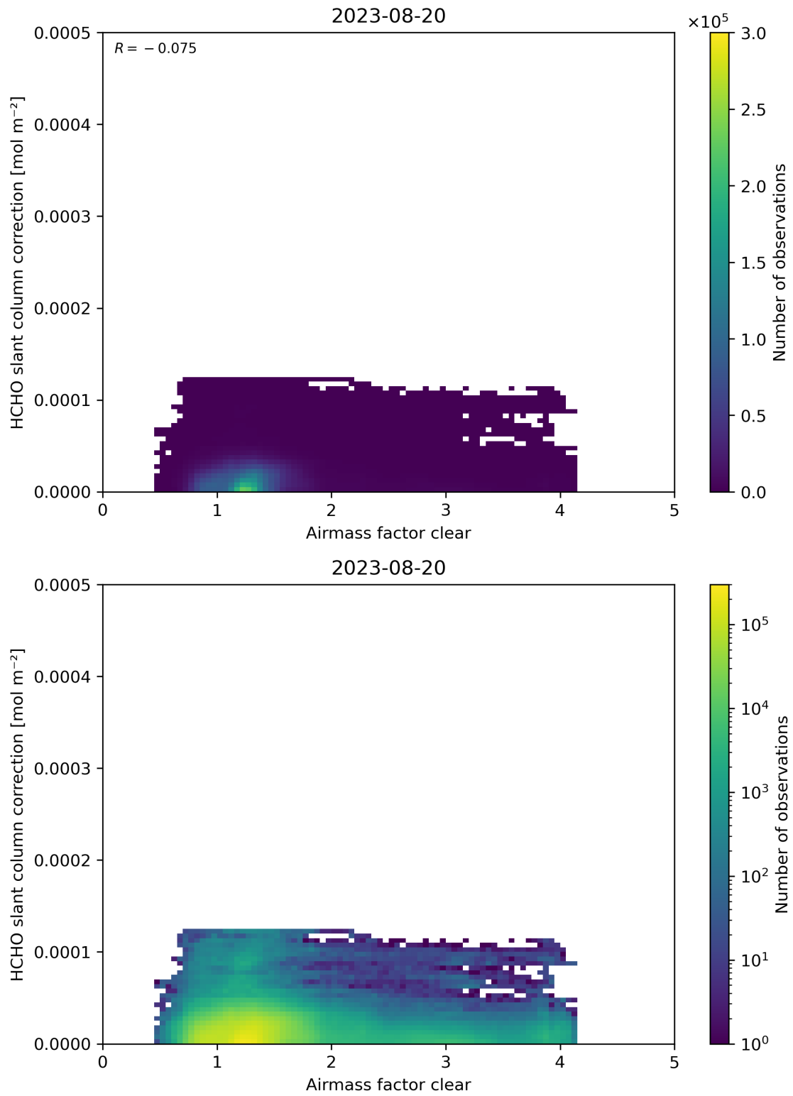
Figure 75: Scatter density plot of “Airmass factor clear” against “HCHO slant column correction” for 2023-08-20 to 2023-08-21.
