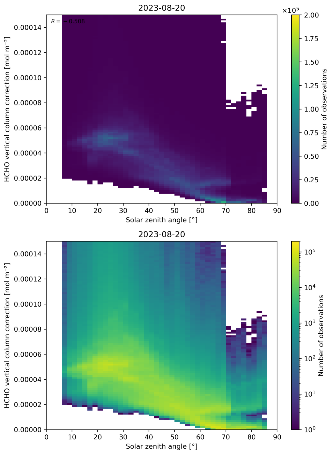
Figure 178: Scatter density plot of “Solar zenith angle” against “HCHO vertical column correction” for 2023-08-20 to 2023-08-21.
