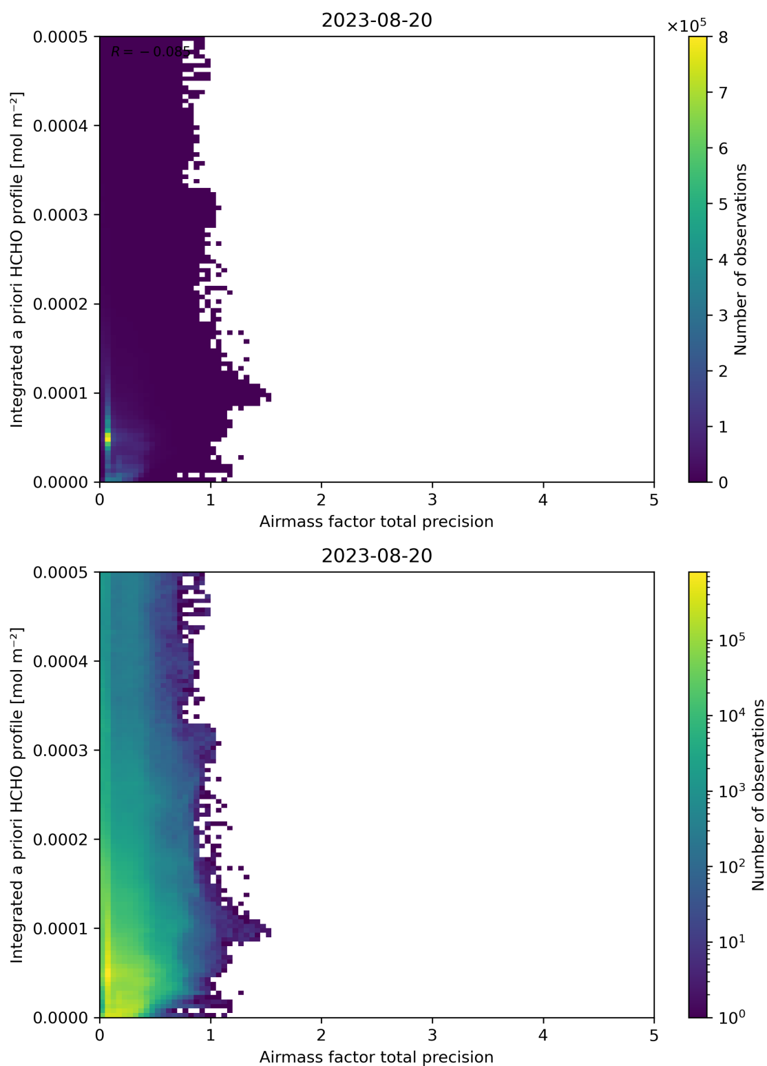
Figure 111: Scatter density plot of “Airmass factor total precision” against “Integrated a priori HCHO profile” for 2023-08-20 to 2023-08-21.
