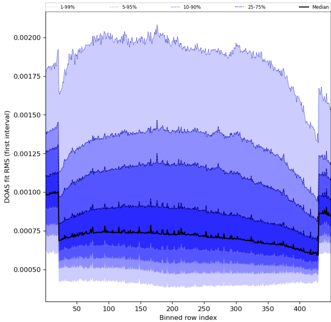
Figure 60: Along track statistics of “DOAS fit RMS (first interval)” for 2023-08-20 to 2023-08-21
