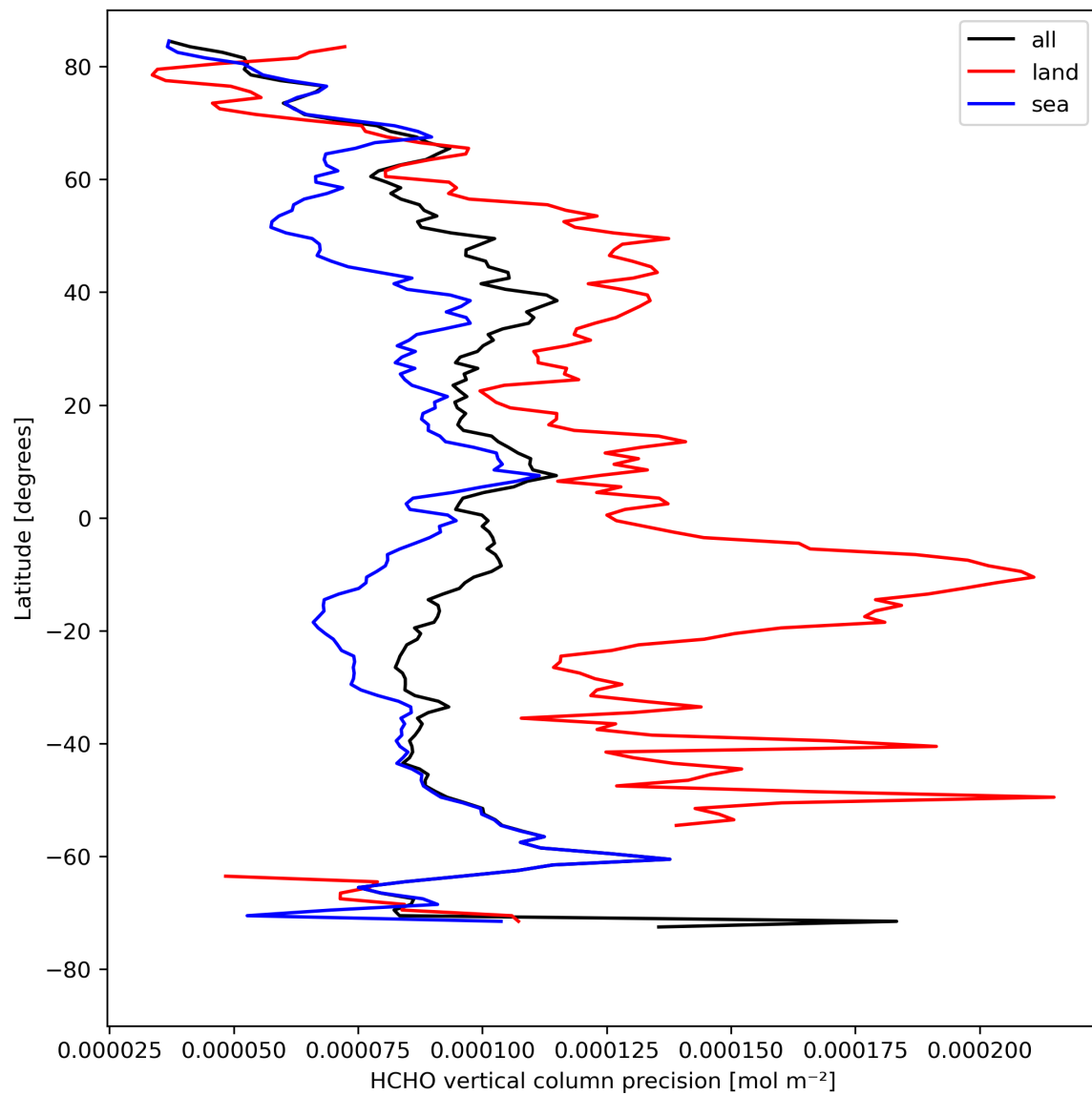
Figure 22: Zonal average of “HCHO vertical column precision” for 2023-08-20 to 2023-08-21.
