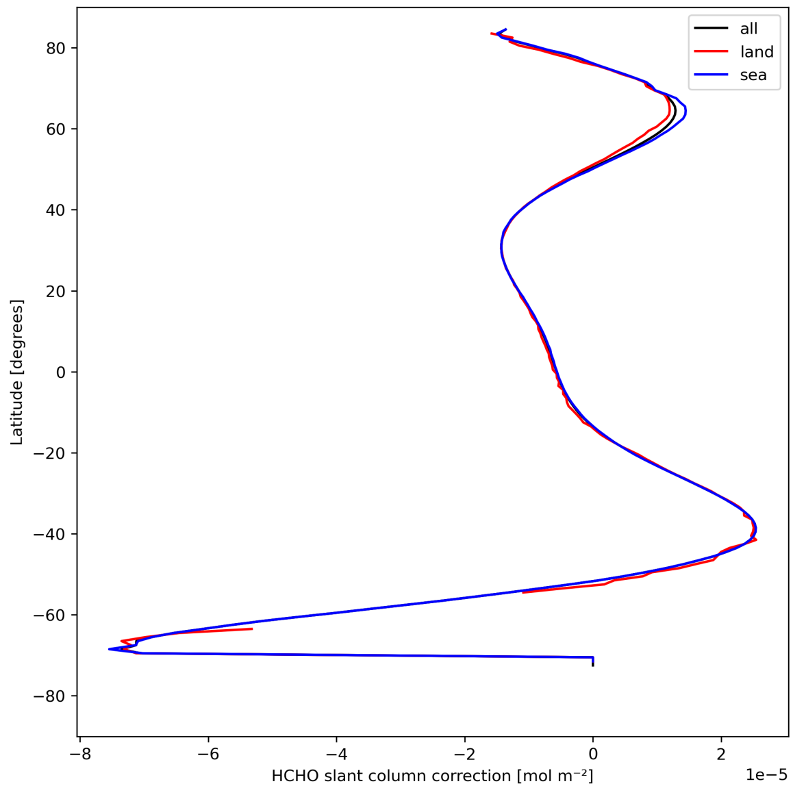
Figure 33: Zonal average of “HCHO slant column correction” for 2023-08-20 to 2023-08-21.
