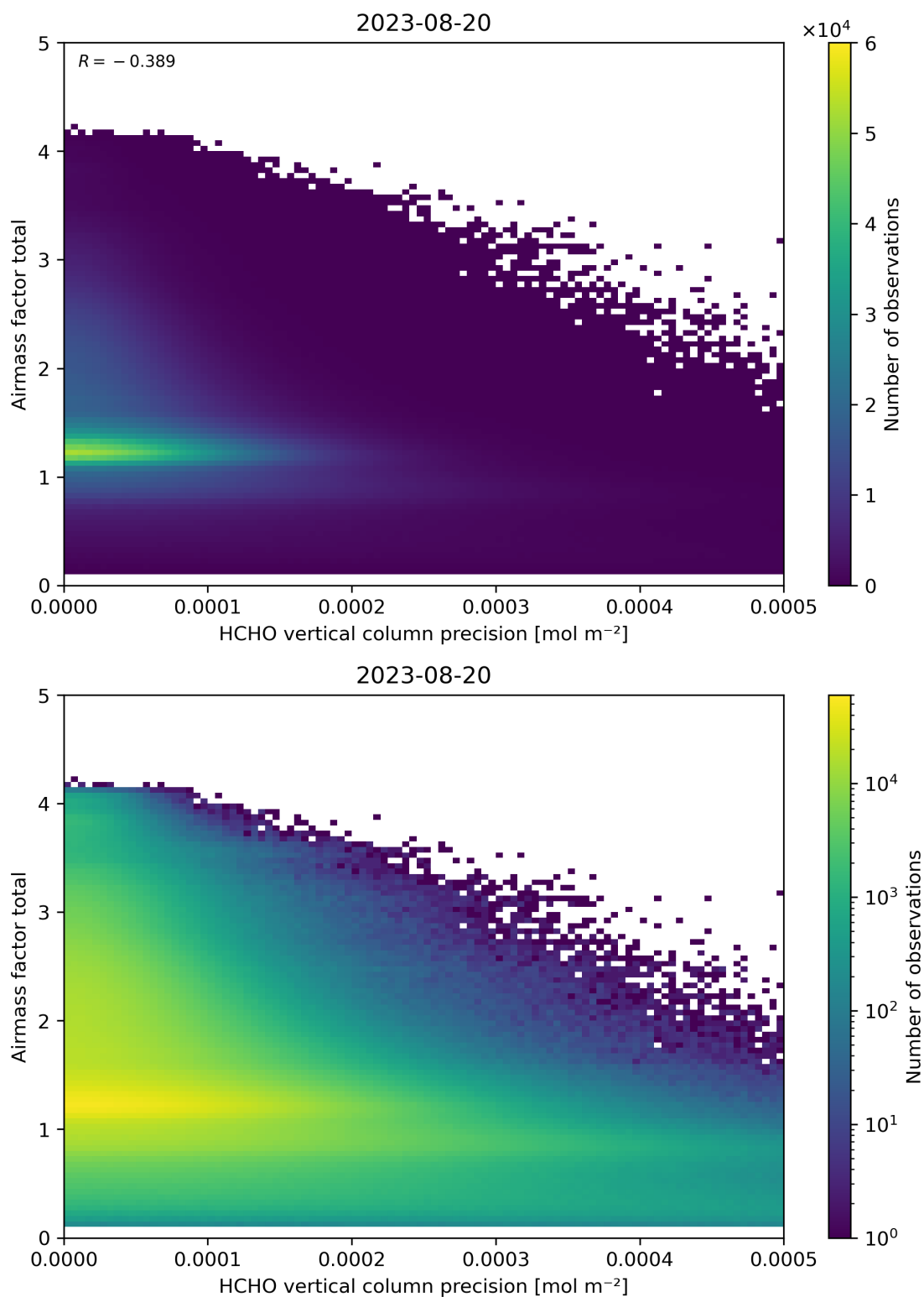
Figure 144: Scatter density plot of “HCHO vertical column precision” against “Airmass factor total” for 2023-08-20 to 2023-08-21.
