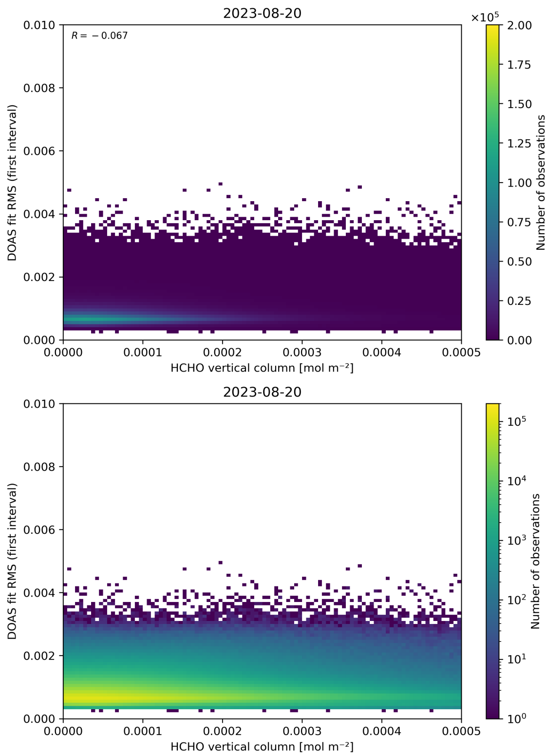
Figure 123: Scatter density plot of “HCHO vertical column” against “DOAS fit RMS (first interval)” for 2023-08-20 to 2023-08-21.
