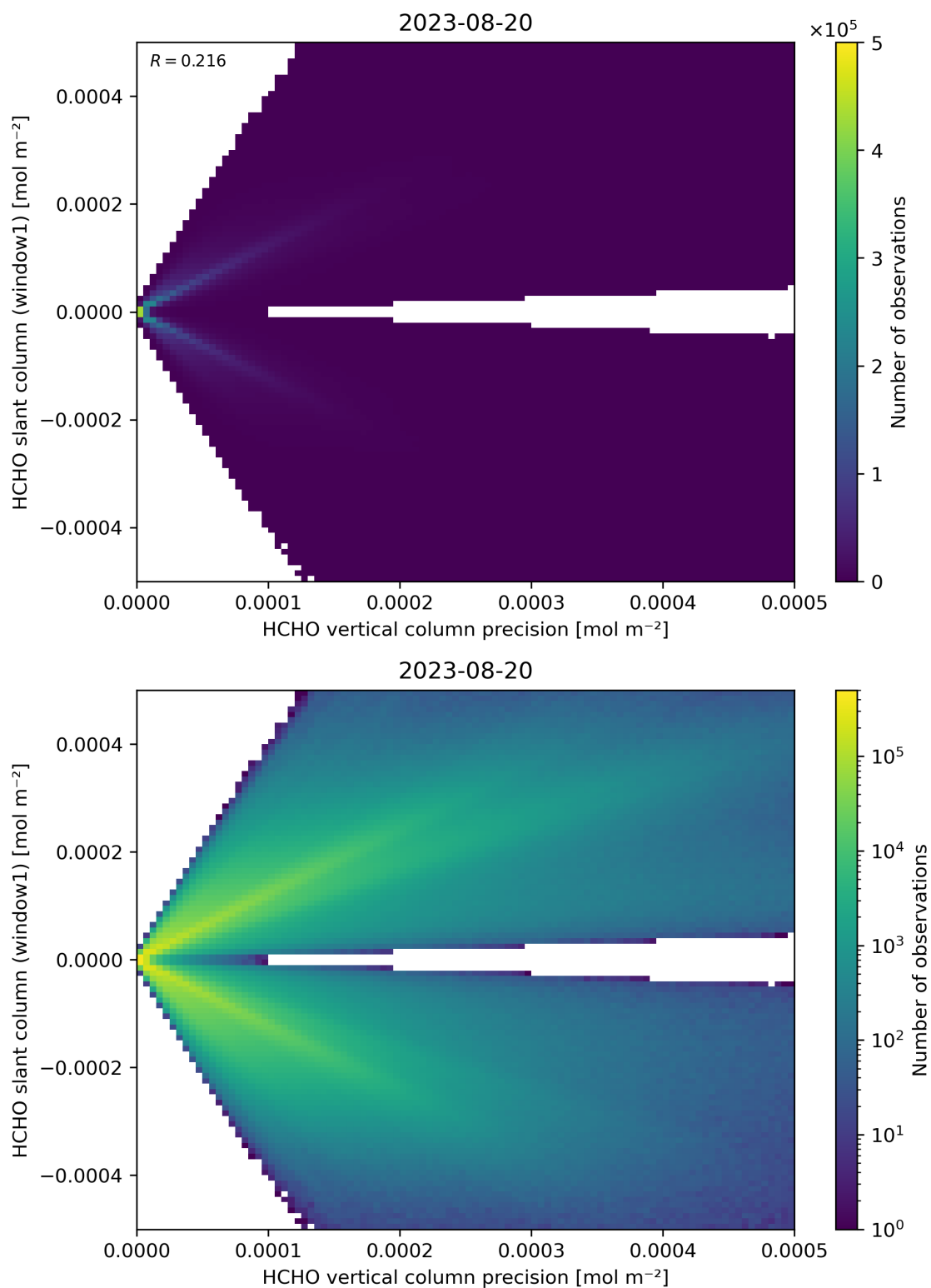
Figure 142: Scatter density plot of “HCHO vertical column precision” against “HCHO slant column (window1)” for 2023-08-20 to 2023-08-21.
