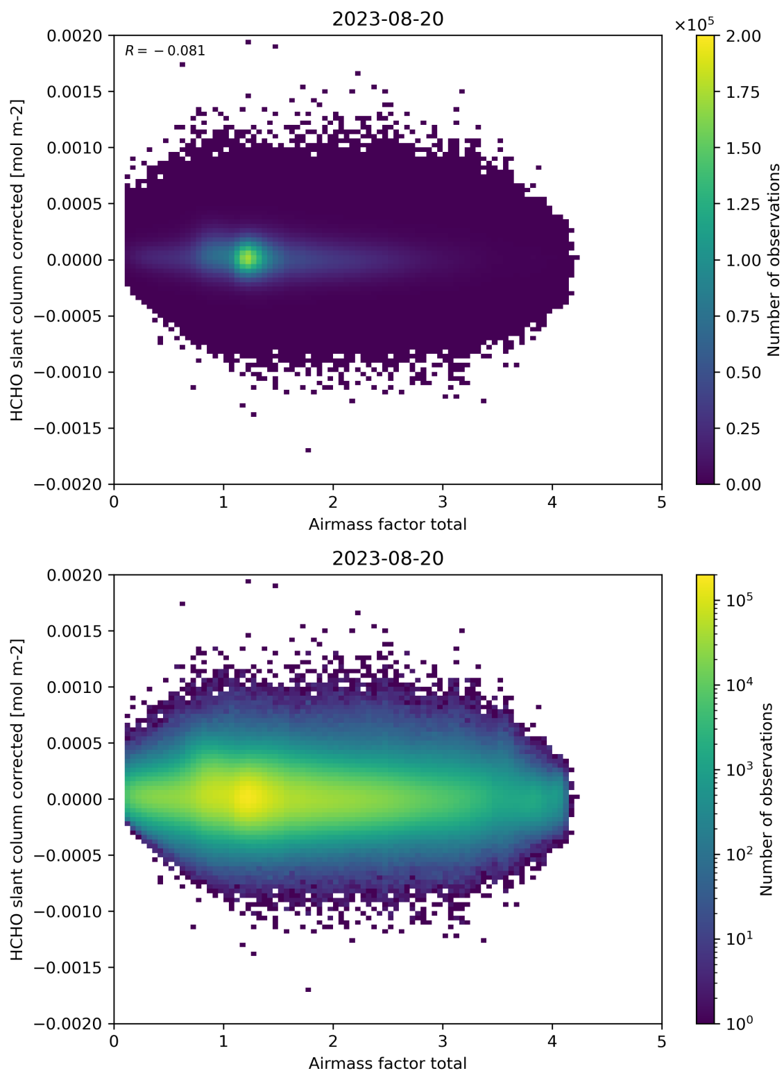
Figure 101: Scatter density plot of “Airmass factor total” against “HCHO slant column corrected” for 2023-08-20 to 2023-08-21.
