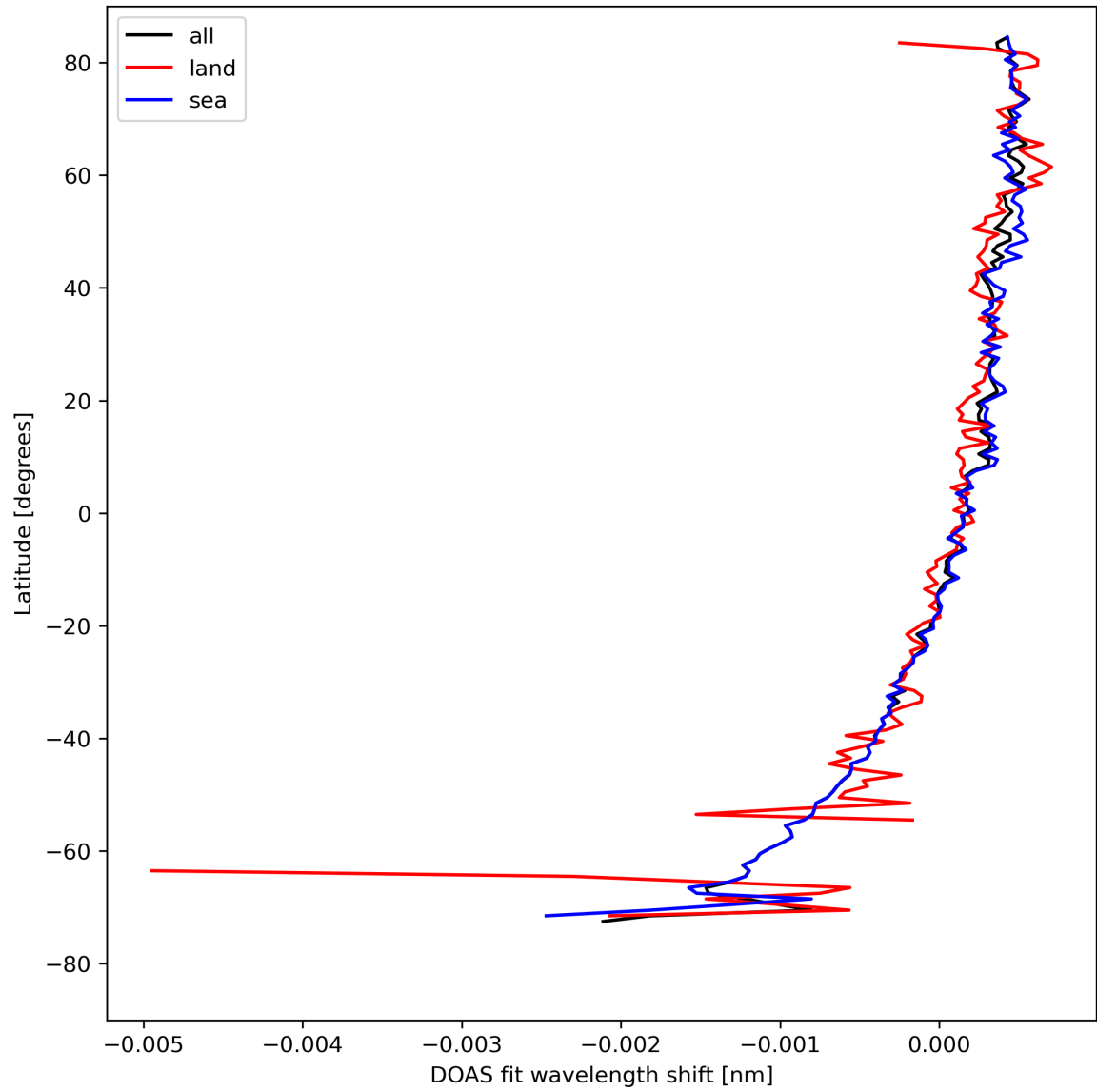
Figure 30: Zonal average of “DOAS fit wavelength shift” for 2023-08-20 to 2023-08-21.
