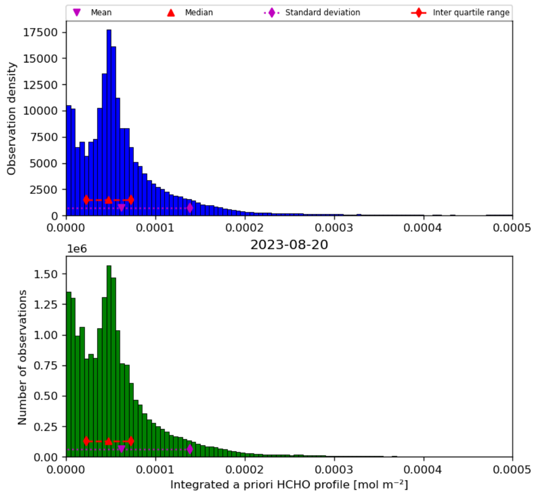
Figure 43: Histogram of “Integrated a priori HCHO profile” for 2023-08-20 to 2023-08-21
