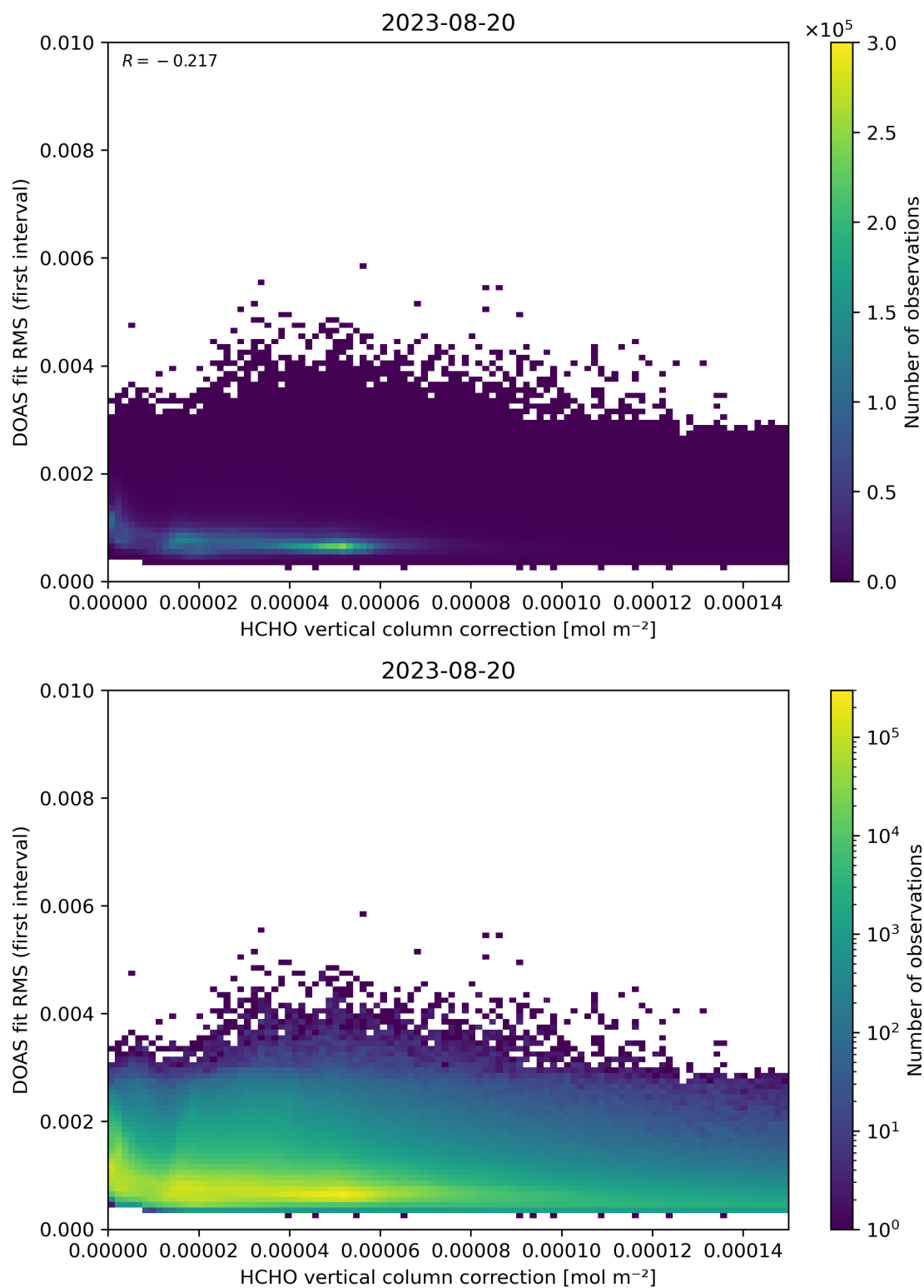
Figure 112: Scatter density plot of “HCHO vertical column correction” against “DOAS fit RMS (first interval)” for 2023-08-20 to 2023-08-21.
