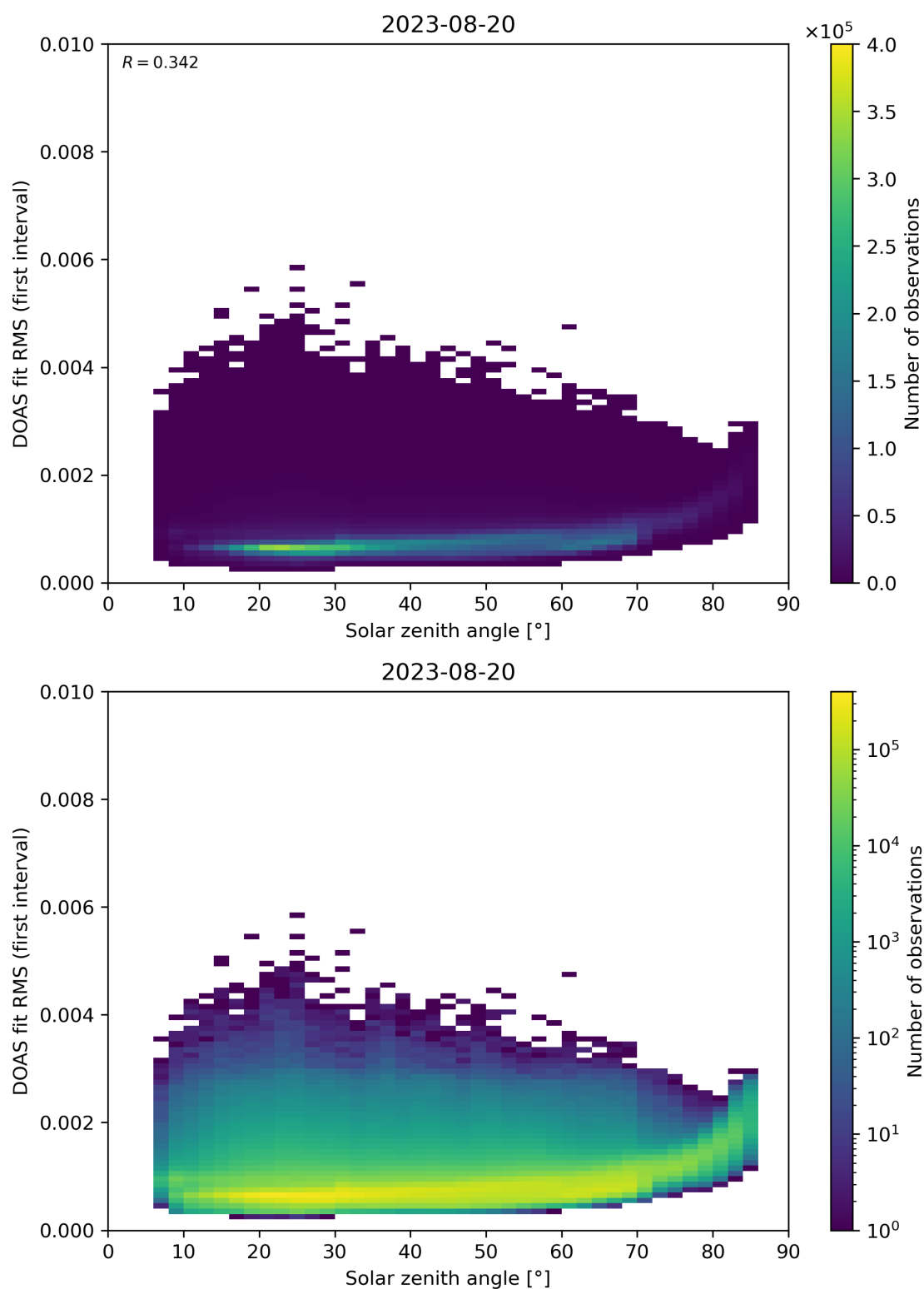
Figure 167: Scatter density plot of “Solar zenith angle” against “DOAS fit RMS (first interval)” for 2023-08-20 to 2023-08-21.
