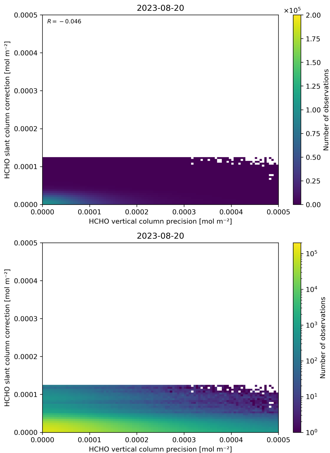
Figure 141: Scatter density plot of “HCHO vertical column precision” against “HCHO slant column correction” for 2023-08-20 to 2023-08-21.
