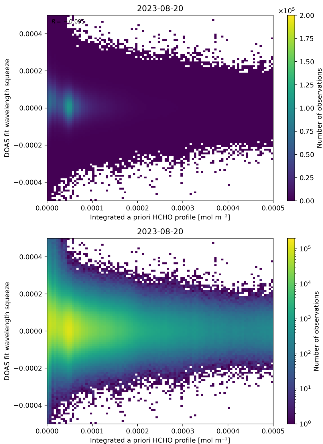
Figure 150: Scatter density plot of “Integrated a priori HCHO profile” against “DOAS fit wavelength squeeze” for 2023-08-20 to 2023-08-21.
