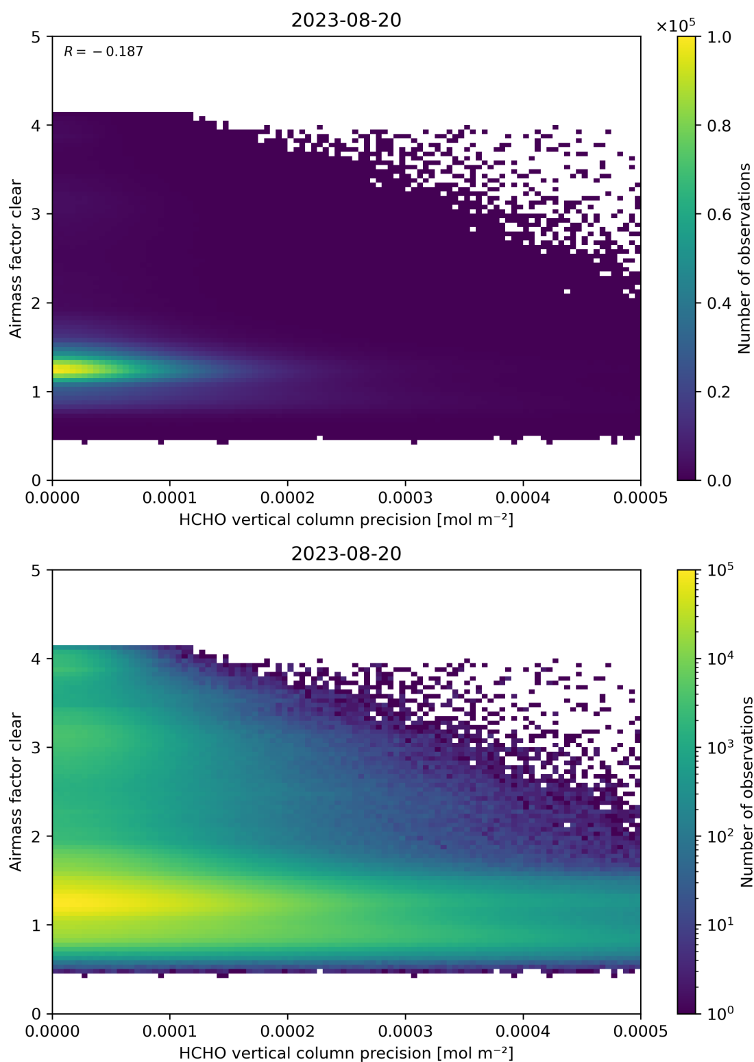
Figure 139: Scatter density plot of “HCHO vertical column precision” against “Airmass factor clear” for 2023-08-20 to 2023-08-21.
