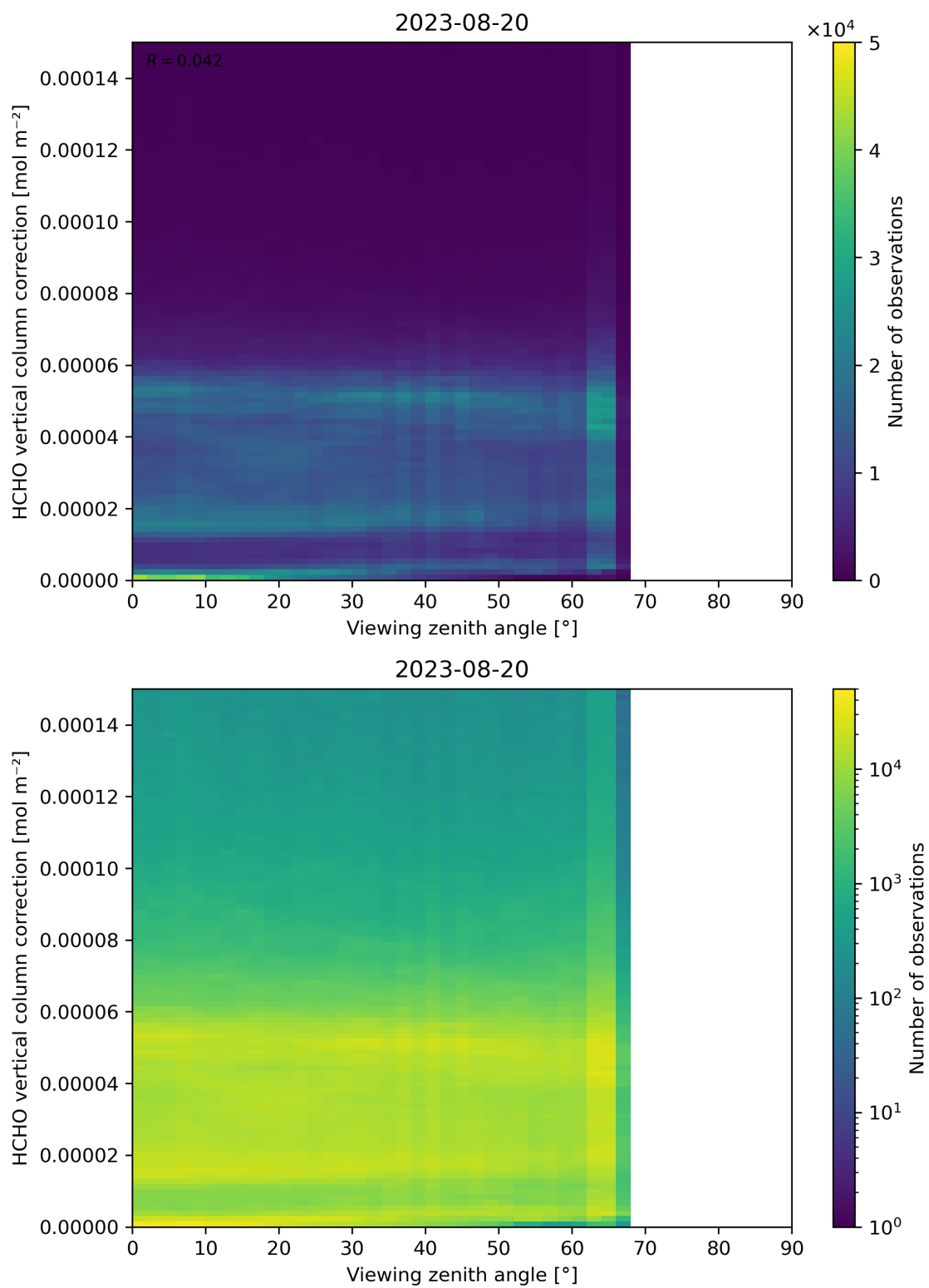
Figure 193: Scatter density plot of “Viewing zenith angle” against “HCHO vertical column correction” for 2023-08-20 to 2023-08-21.
