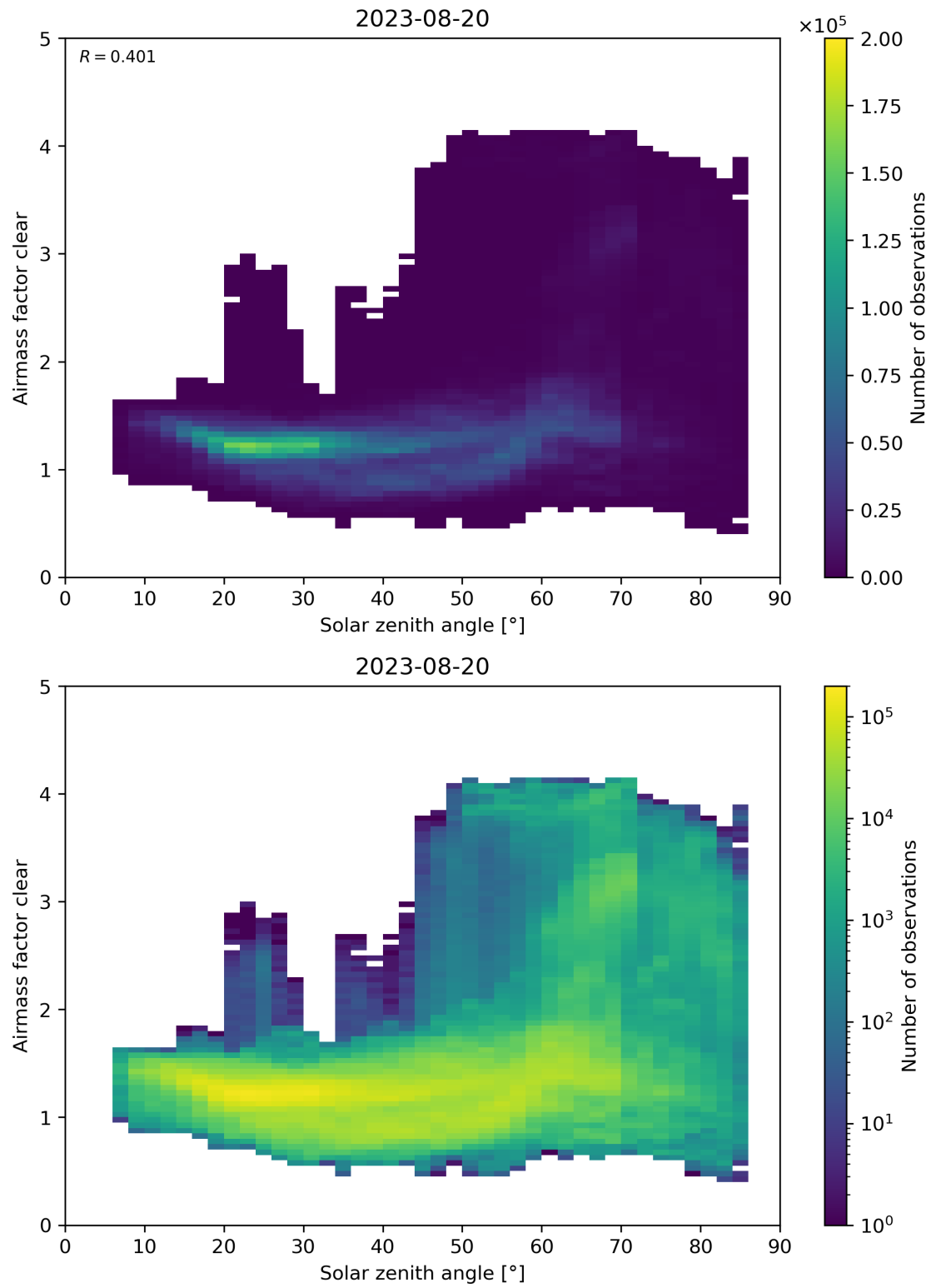
Figure 170: Scatter density plot of “Solar zenith angle” against “Airmass factor clear” for 2023-08-20 to 2023-08-21.
