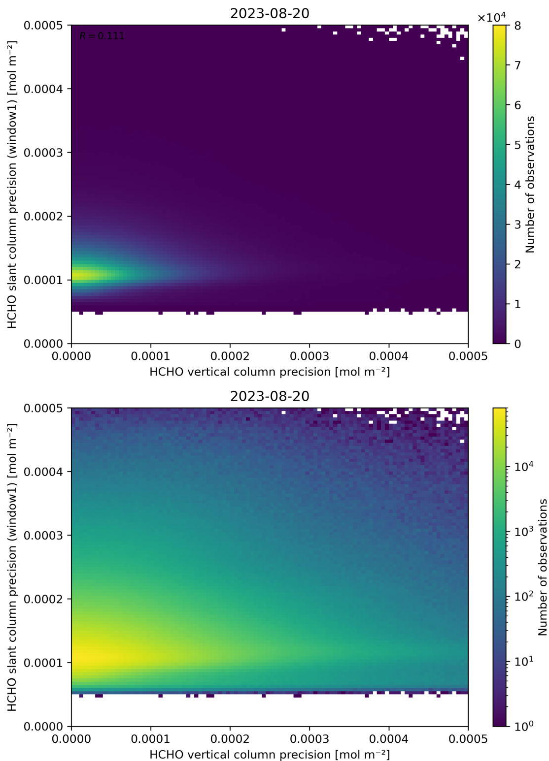
Figure 143: Scatter density plot of “HCHO vertical column precision” against “HCHO slant column precision (window1)” for 2023-08-20 to 2023-08-21.
