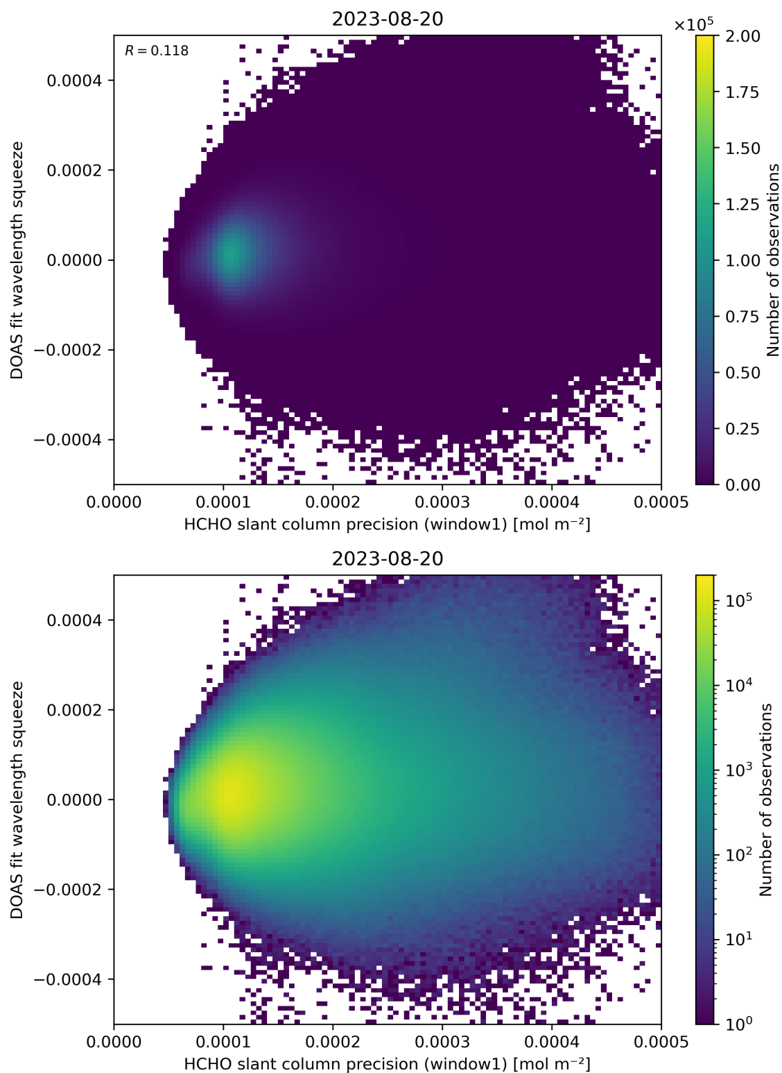
Figure 90: Scatter density plot of “HCHO slant column precision (window1)” against “DOAS fit wavelength squeeze” for 2023-08-20 to 2023-08-21.
