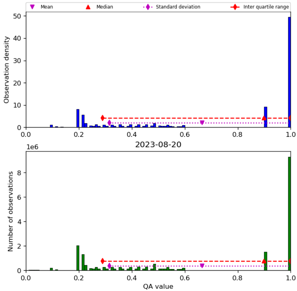
Figure 34: Histogram of “QA value” for 2023-08-20 to 2023-08-21
