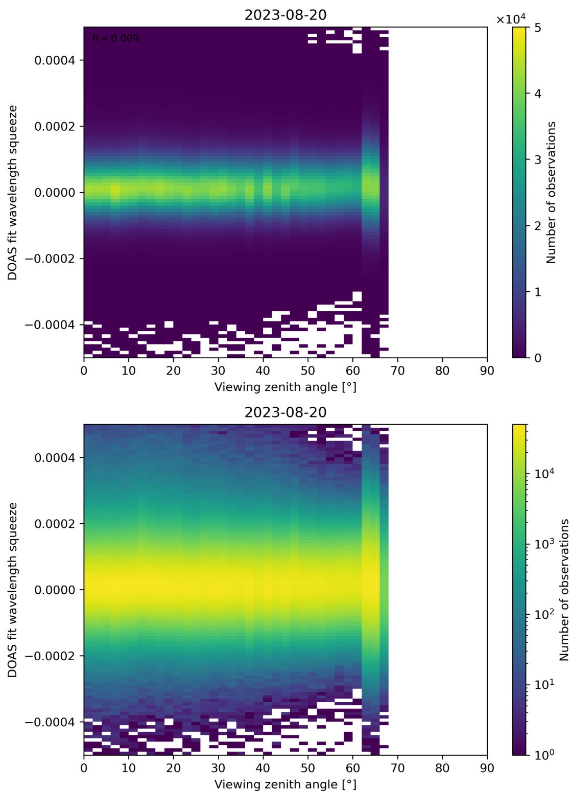
Figure 184: Scatter density plot of “Viewing zenith angle” against “DOAS fit wavelength squeeze” for 2023-08-20 to 2023-08-21.
