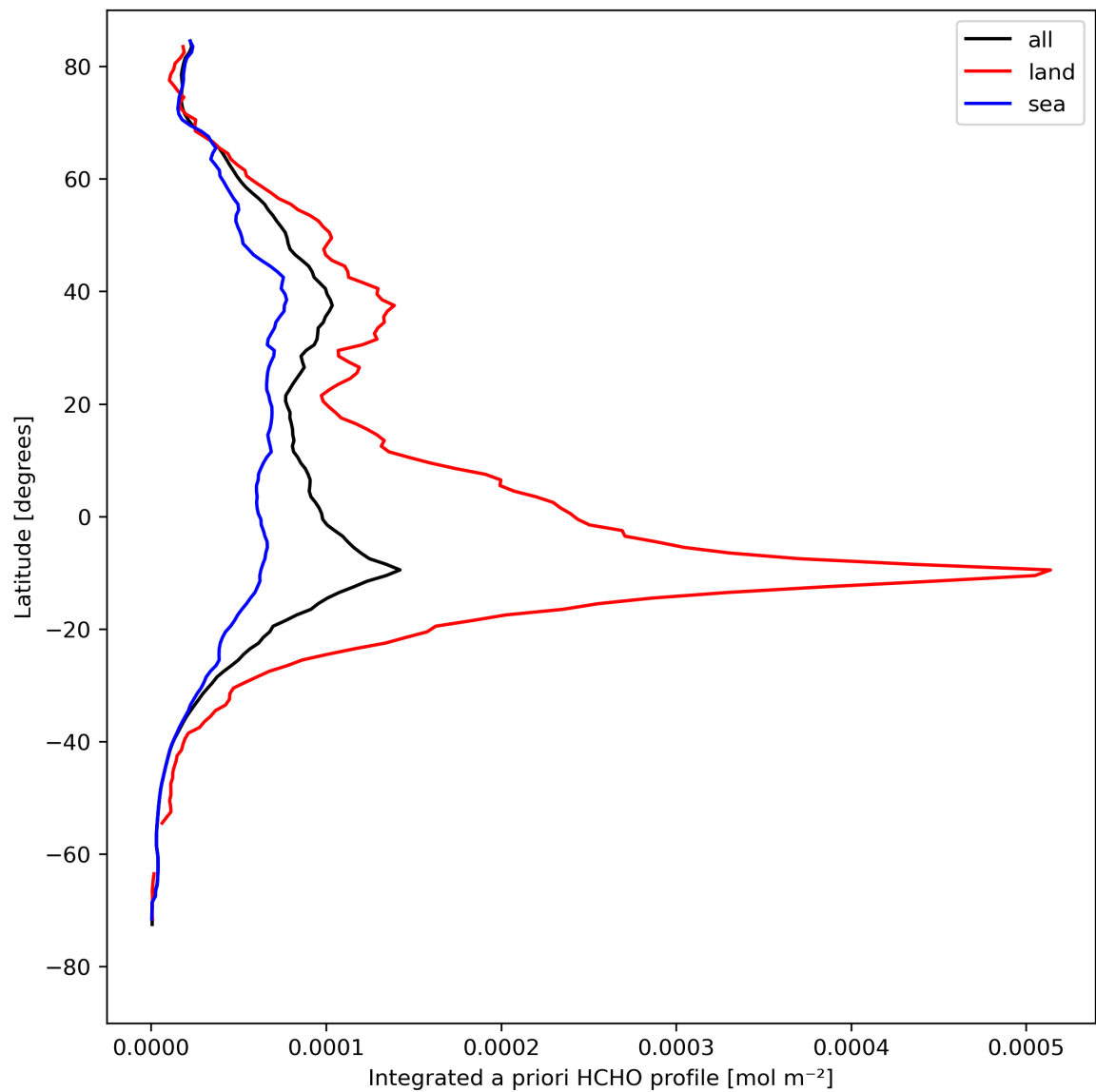
Figure 29: Zonal average of “Integrated a priori HCHO profile” for 2023-08-20 to 2023-08-21.
