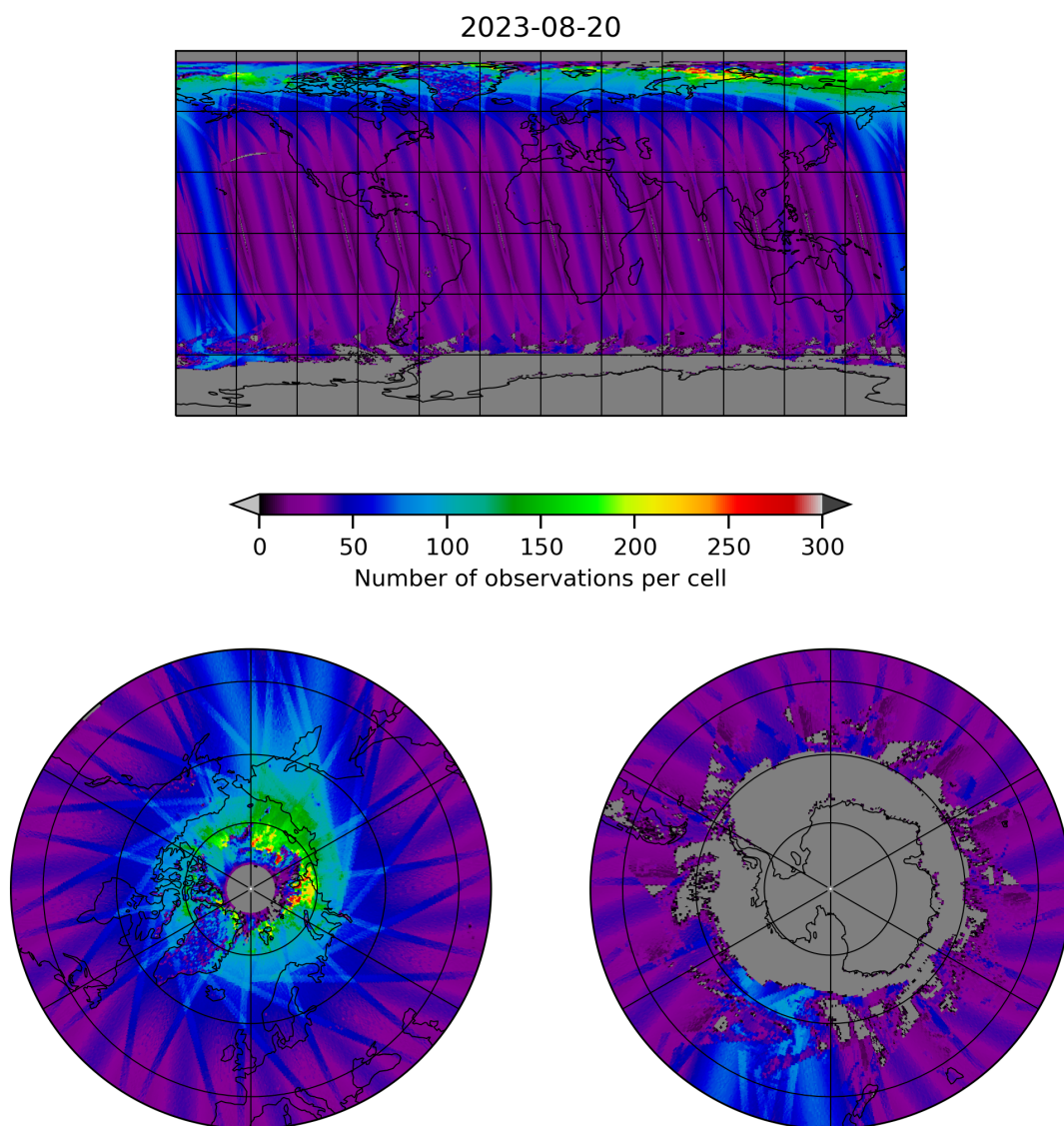
Figure 19: Map of the number of observations for 2023-08-20 to 2023-08-21
