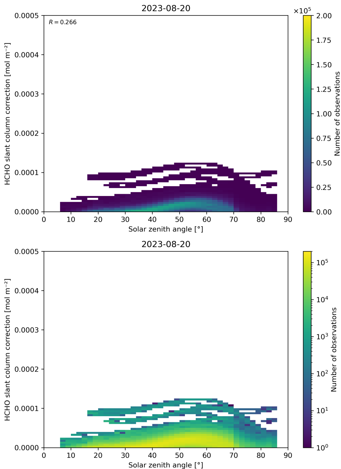
Figure 172: Scatter density plot of “Solar zenith angle” against “HCHO slant column correction” for 2023-08-20 to 2023-08-21.
