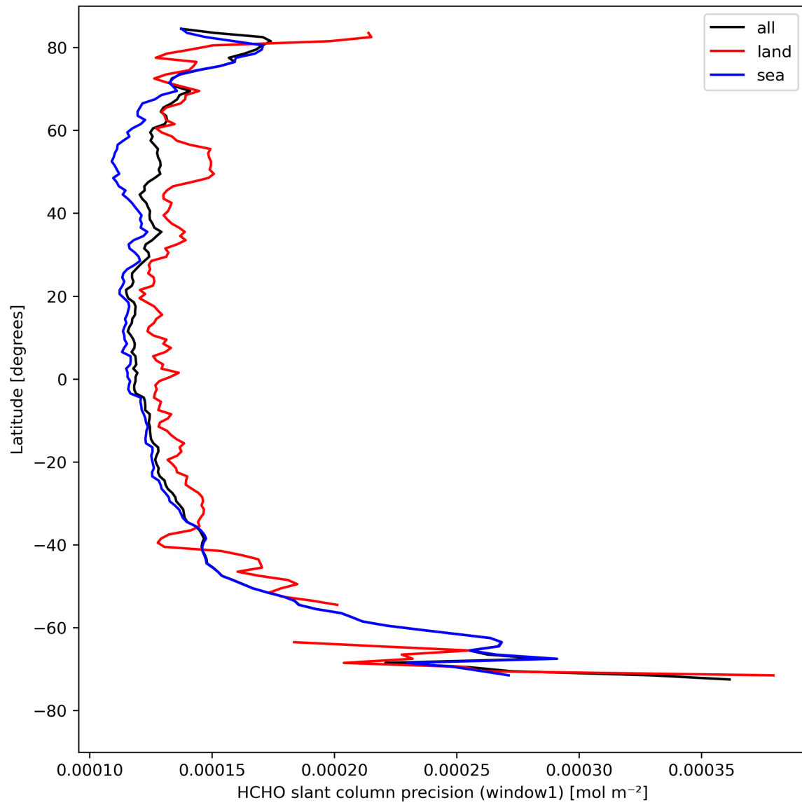
Figure 25: Zonal average of “HCHO slant column precision (window1)” for 2023-08-20 to 2023-08-21.
