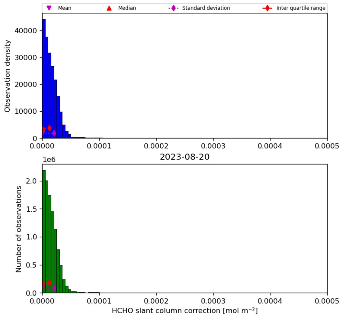
Figure 47: Histogram of “HCHO slant column correction” for 2023-08-20 to 2023-08-21
