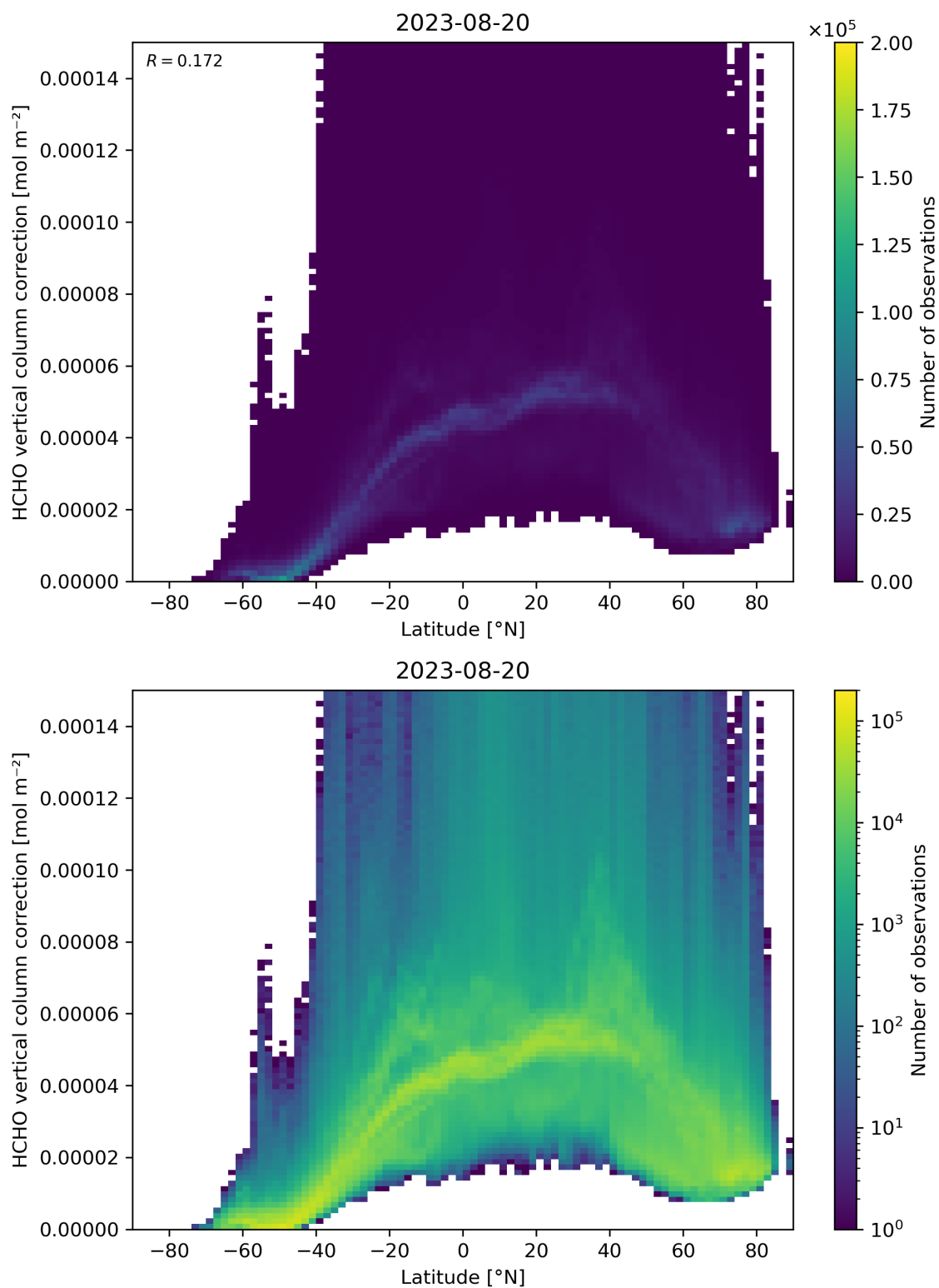
Figure 164: Scatter density plot of “Latitude” against “HCHO vertical column correction” for 2023-08-20 to 2023-08-21.
