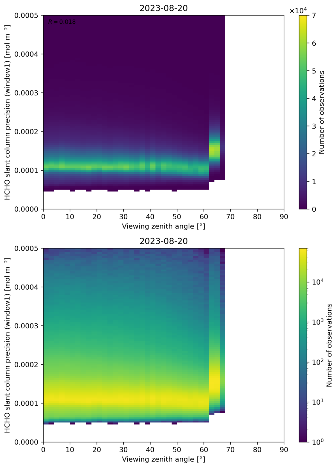
Figure 189: Scatter density plot of “Viewing zenith angle” against “HCHO slant column precision (window1)” for 2023-08-20 to 2023-08-21.
