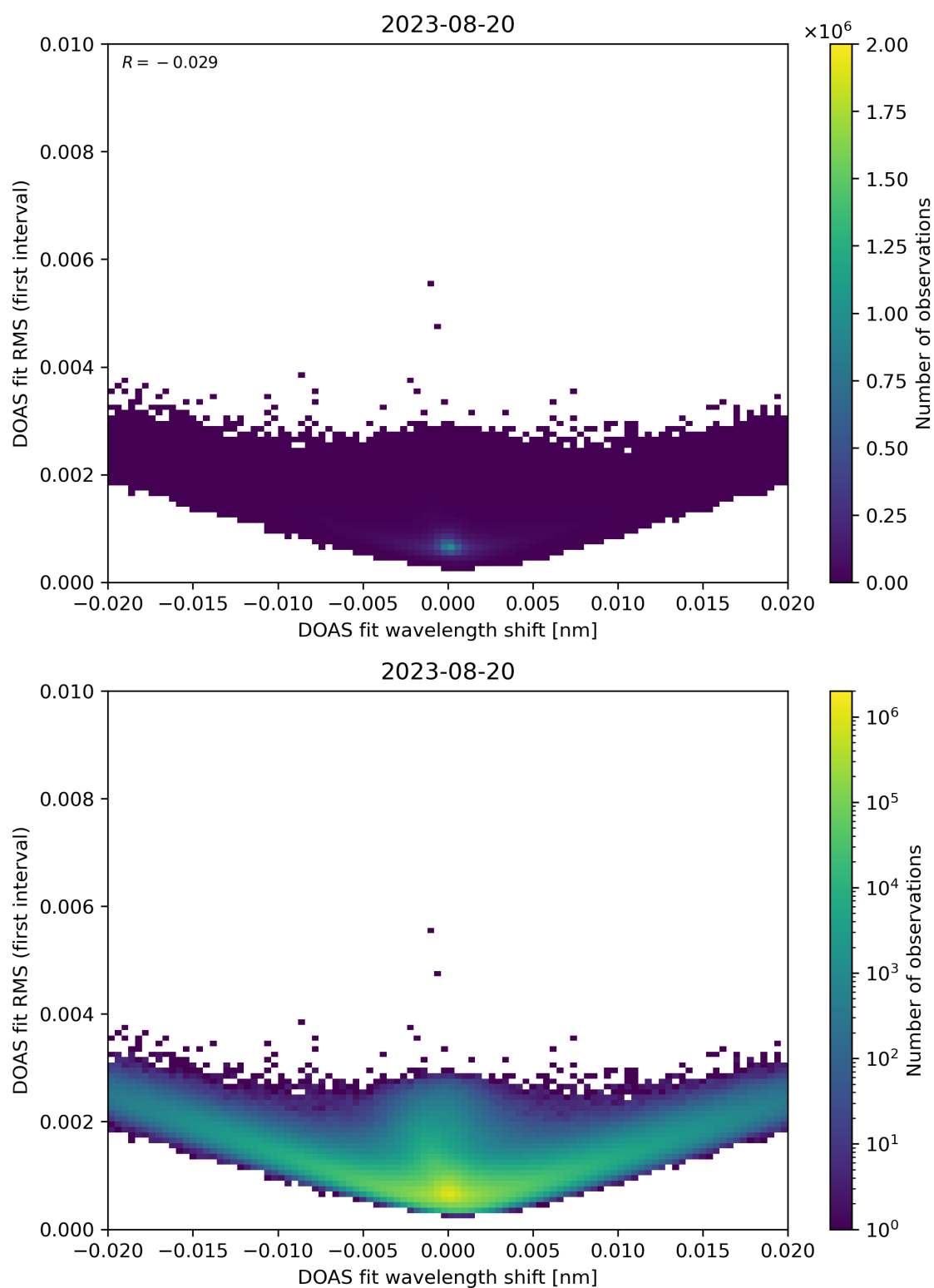
Figure 64: Scatter density plot of “DOAS fit wavelength shift” against “DOAS fit RMS (first interval)” for 2023-08-20 to 2023-08-21.
