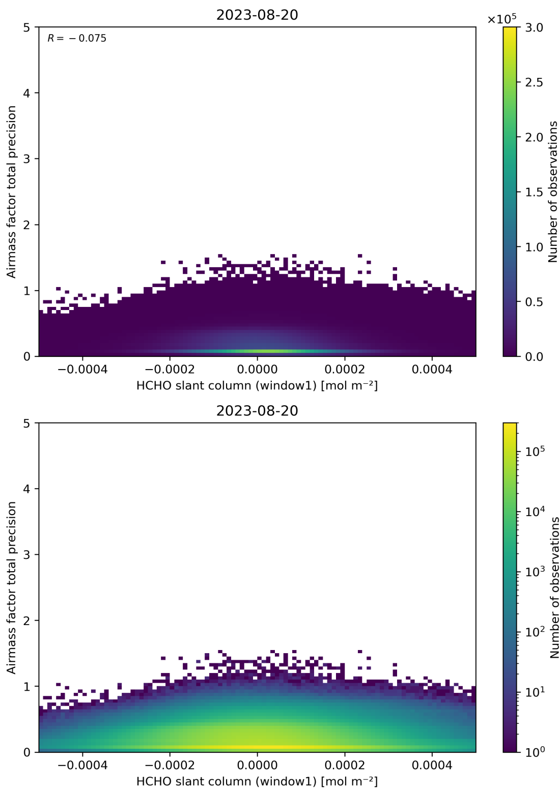
Figure 86: Scatter density plot of “HCHO slant column (window1)” against “Airmass factor total precision” for 2023-08-20 to 2023-08-21.
