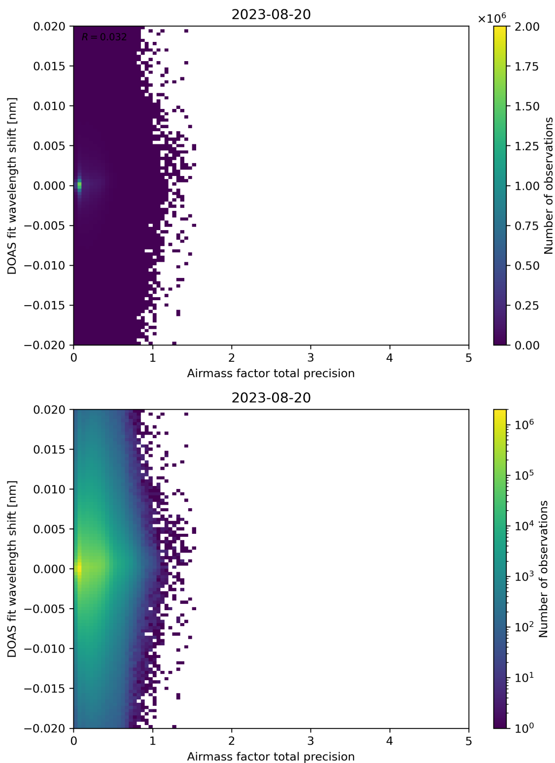
Figure 106: Scatter density plot of “Airmass factor total precision” against “DOAS fit wavelength shift” for 2023-08-20 to 2023-08-21.
