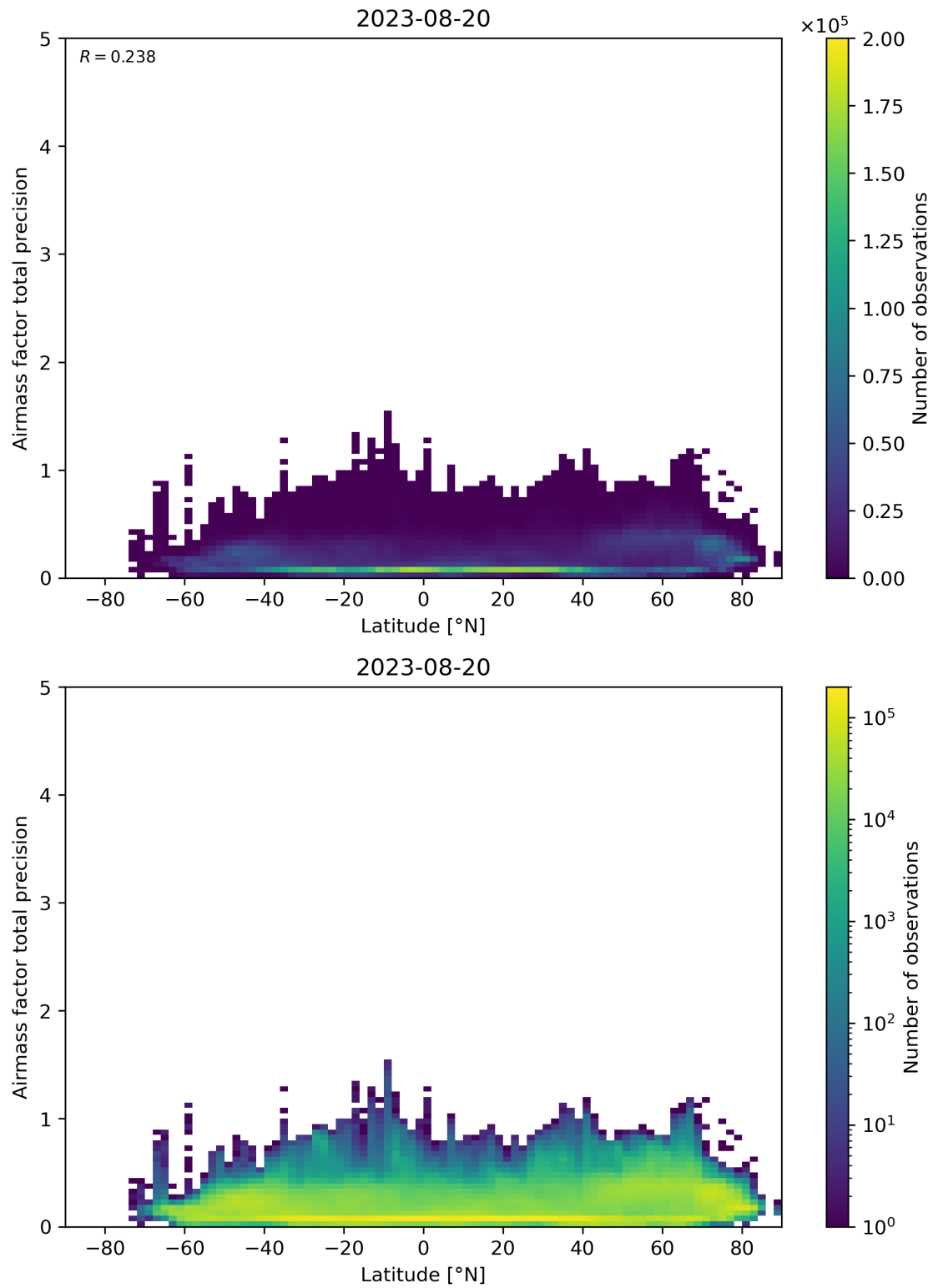
Figure 162: Scatter density plot of “Latitude” against “Airmass factor total precision” for 2023-08-20 to 2023-08-21.
