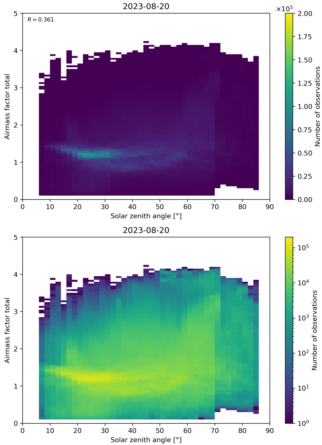
Figure 175: Scatter density plot of “Solar zenith angle” against “Airmass factor total” for 2023-08-20 to 2023-08-21.
