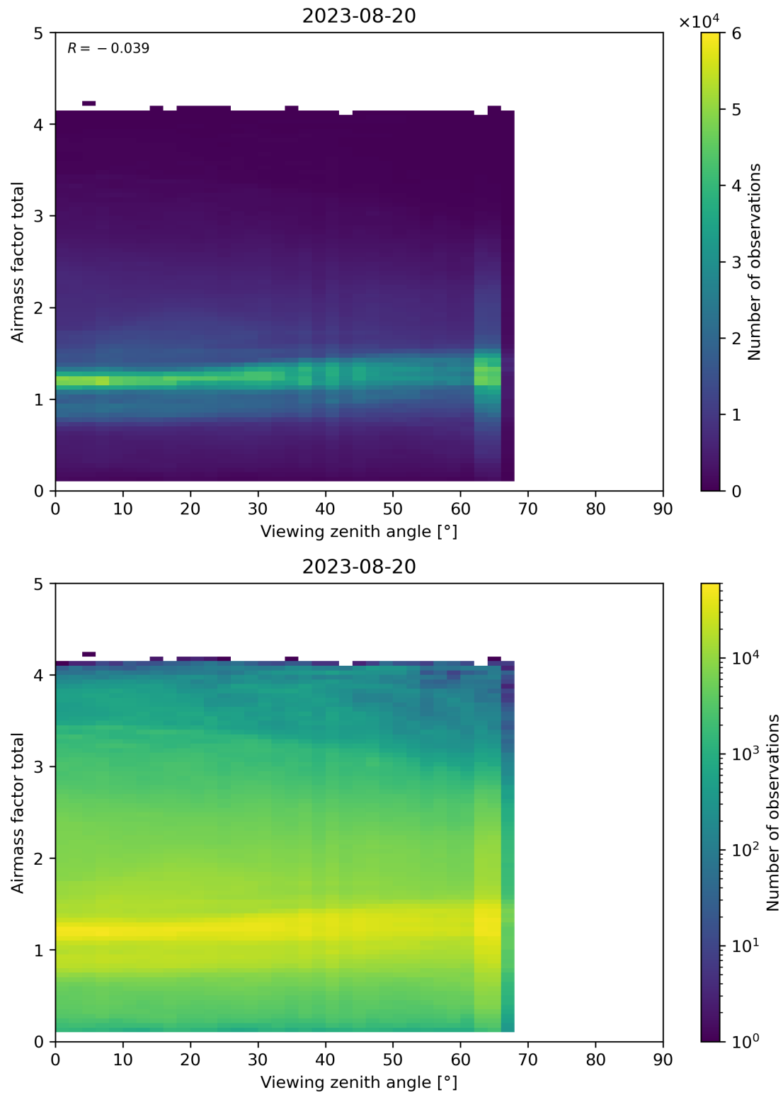
Figure 190: Scatter density plot of “Viewing zenith angle” against “Airmass factor total” for 2023-08-20 to 2023-08-21.
