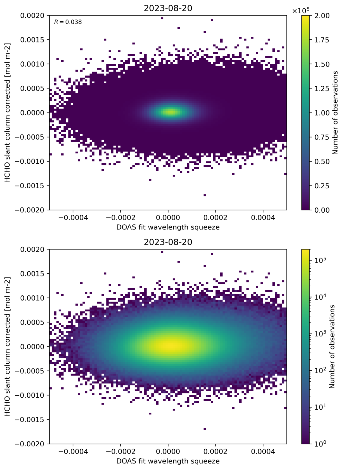
Figure 69: Scatter density plot of “DOAS fit wavelength squeeze” against “HCHO slant column corrected” for 2023-08-20 to 2023-08-21.
