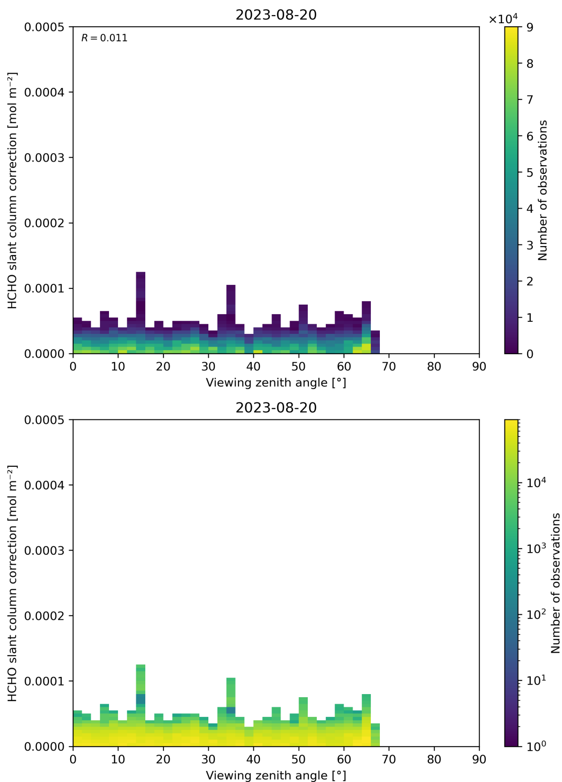
Figure 187: Scatter density plot of “Viewing zenith angle” against “HCHO slant column correction” for 2023-08-20 to 2023-08-21.
