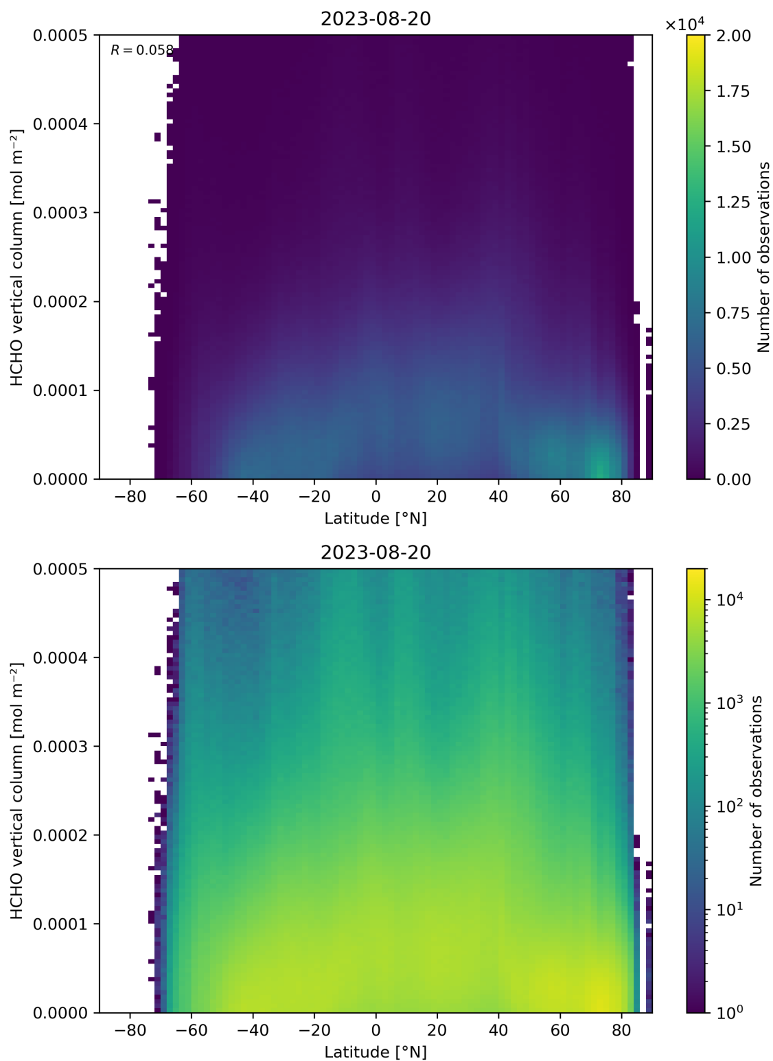
Figure 163: Scatter density plot of “Latitude” against “HCHO vertical column” for 2023-08-20 to 2023-08-21.
