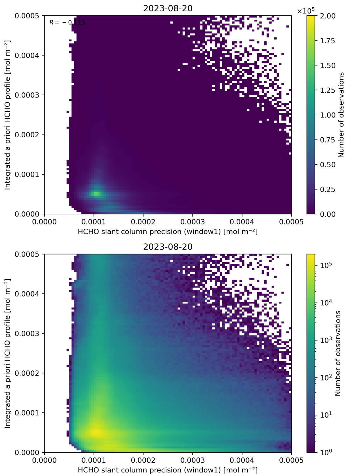
Figure 96: Scatter density plot of “HCHO slant column precision (window1)” against “Integrated a priori HCHO profile” for 2023-08-20 to 2023-08-21.
