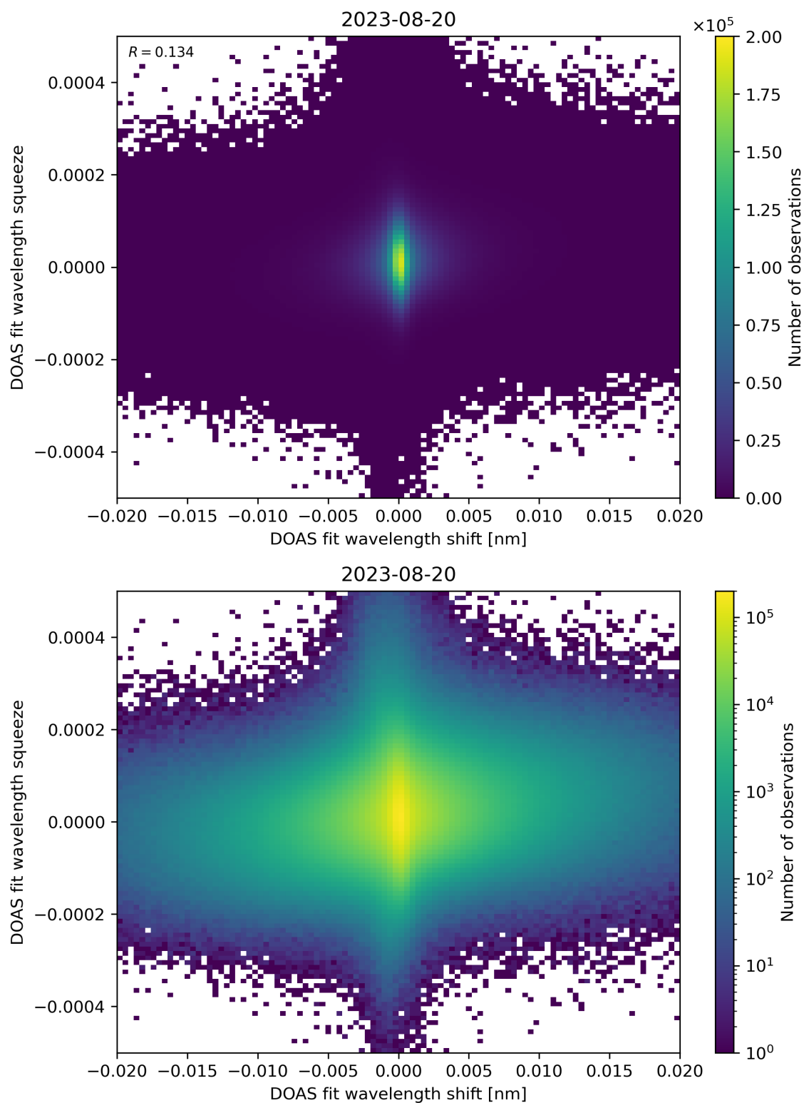
Figure 65: Scatter density plot of “DOAS fit wavelength shift” against “DOAS fit wavelength squeeze” for 2023-08-20 to 2023-08-21.
