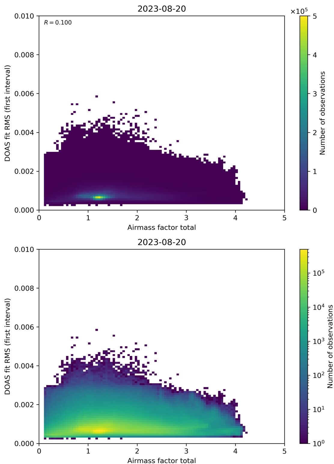
Figure 97: Scatter density plot of “Airmass factor total” against “DOAS fit RMS (first interval)” for 2023-08-20 to 2023-08-21.
