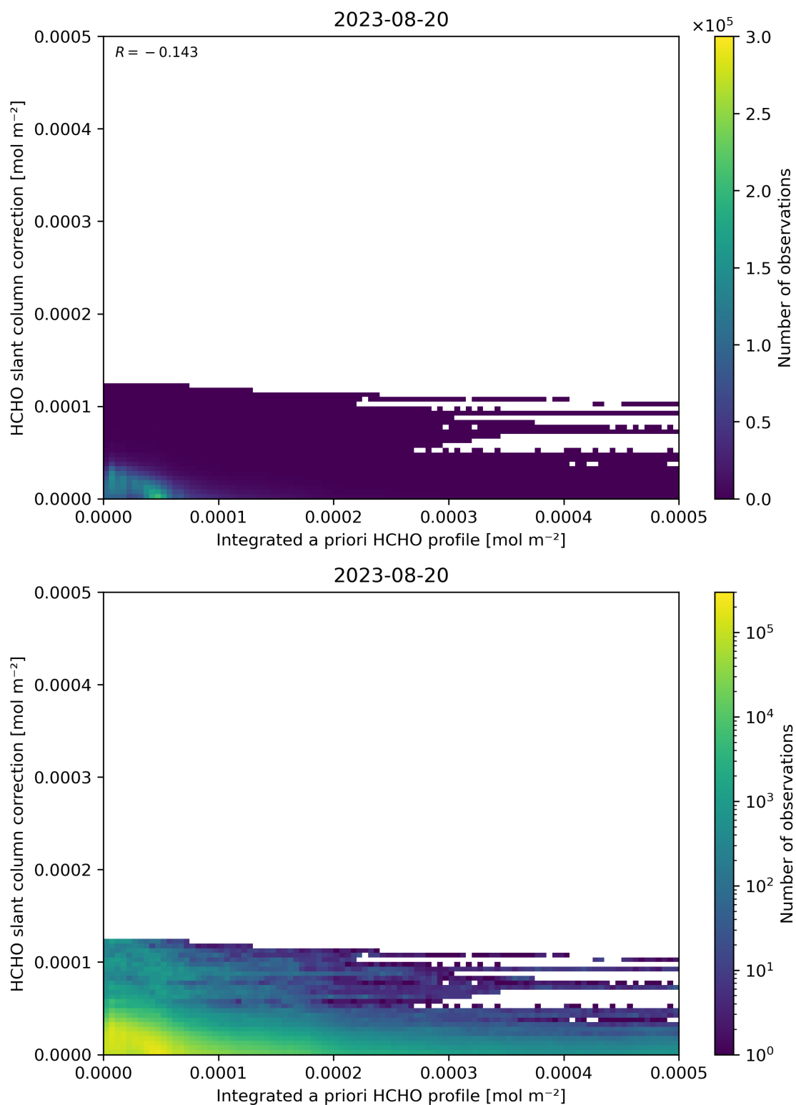
Figure 152: Scatter density plot of “Integrated a priori HCHO profile” against “HCHO slant column correction” for 2023-08-20 to 2023-08-21.
