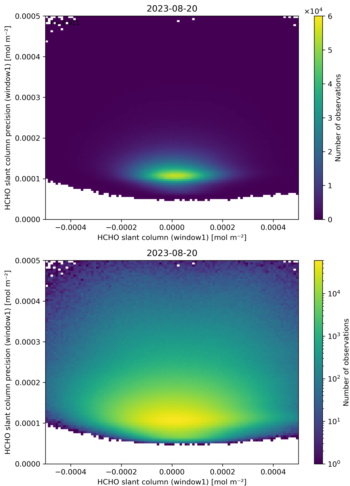
Figure 84: Scatter density plot of “HCHO slant column (window1)” against “HCHO slant column precision (window1)” for 2023-08-20 to 2023-08-21.
