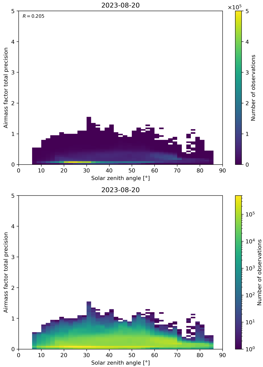
Figure 176: Scatter density plot of “Solar zenith angle” against “Airmass factor total precision” for 2023-08-20 to 2023-08-21.
