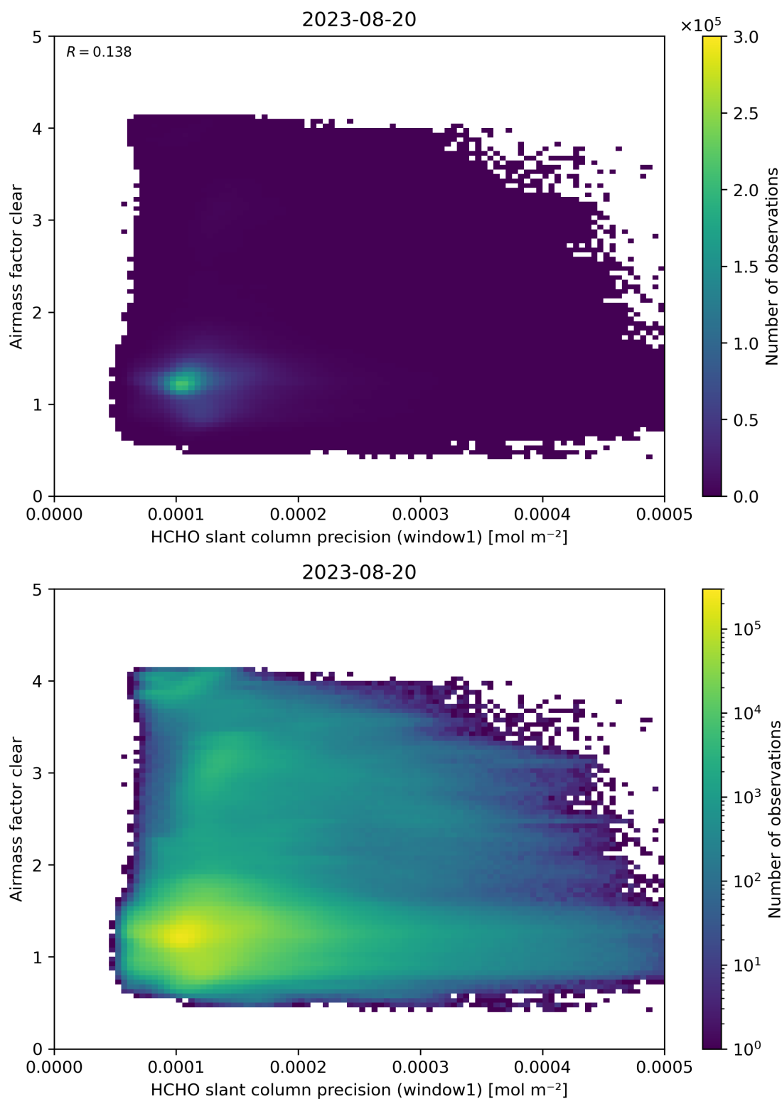
Figure 91: Scatter density plot of “HCHO slant column precision (window1)” against “Airmass factor clear” for 2023-08-20 to 2023-08-21.
