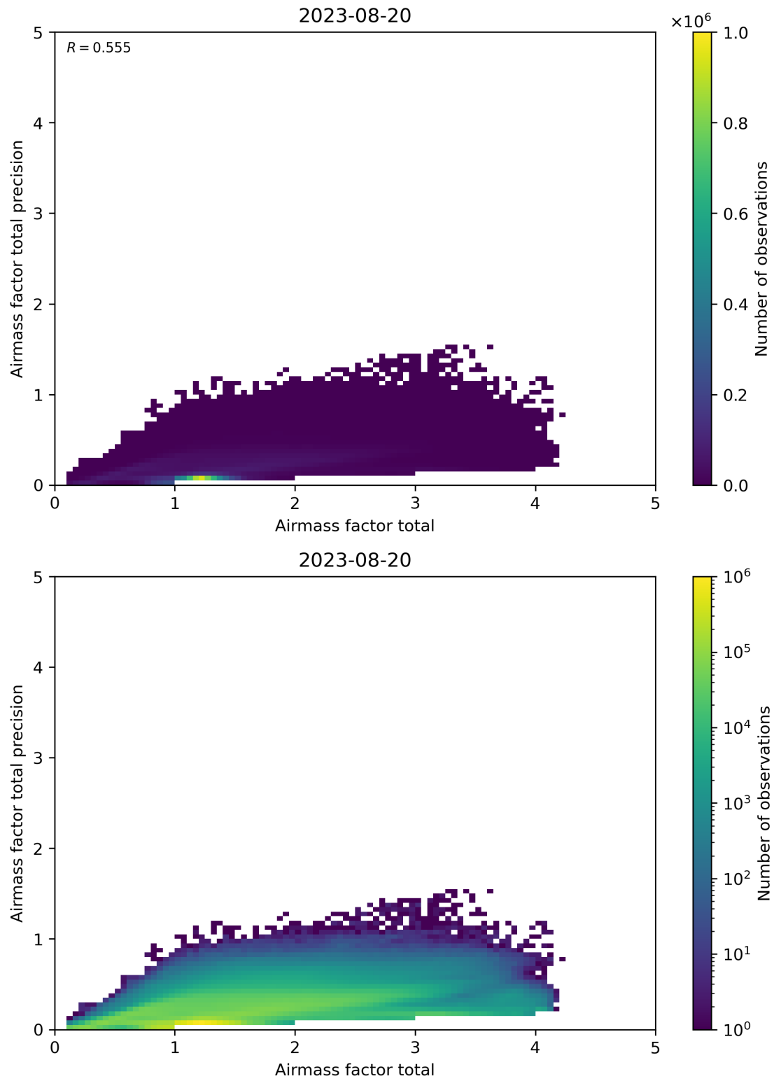
Figure 103: Scatter density plot of “Airmass factor total” against “Airmass factor total precision” for 2023-08-20 to 2023-08-21.
