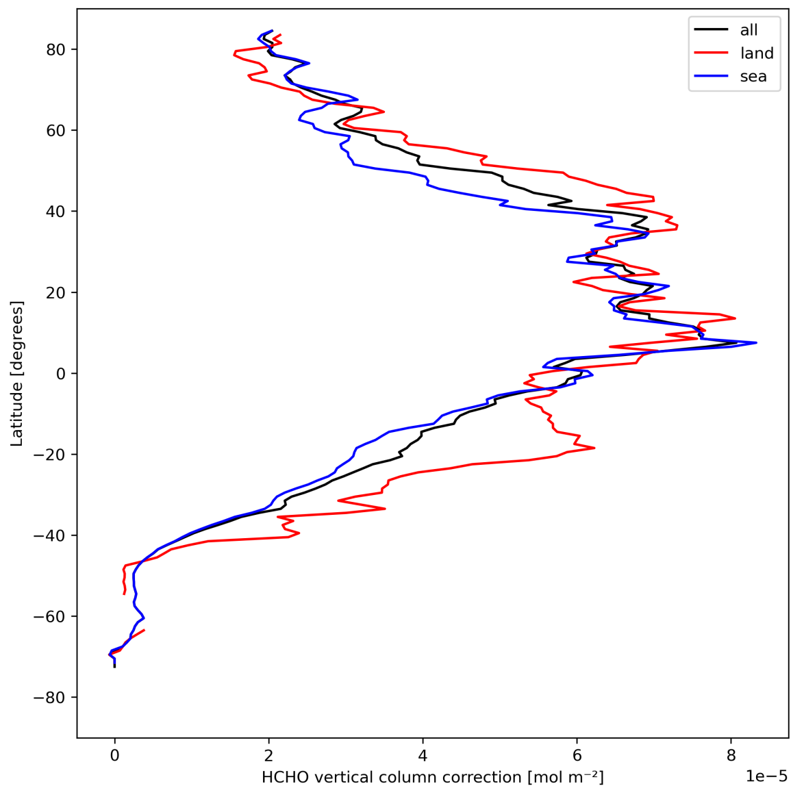
Figure 23: Zonal average of “HCHO vertical column correction” for 2023-08-20 to 2023-08-21.
