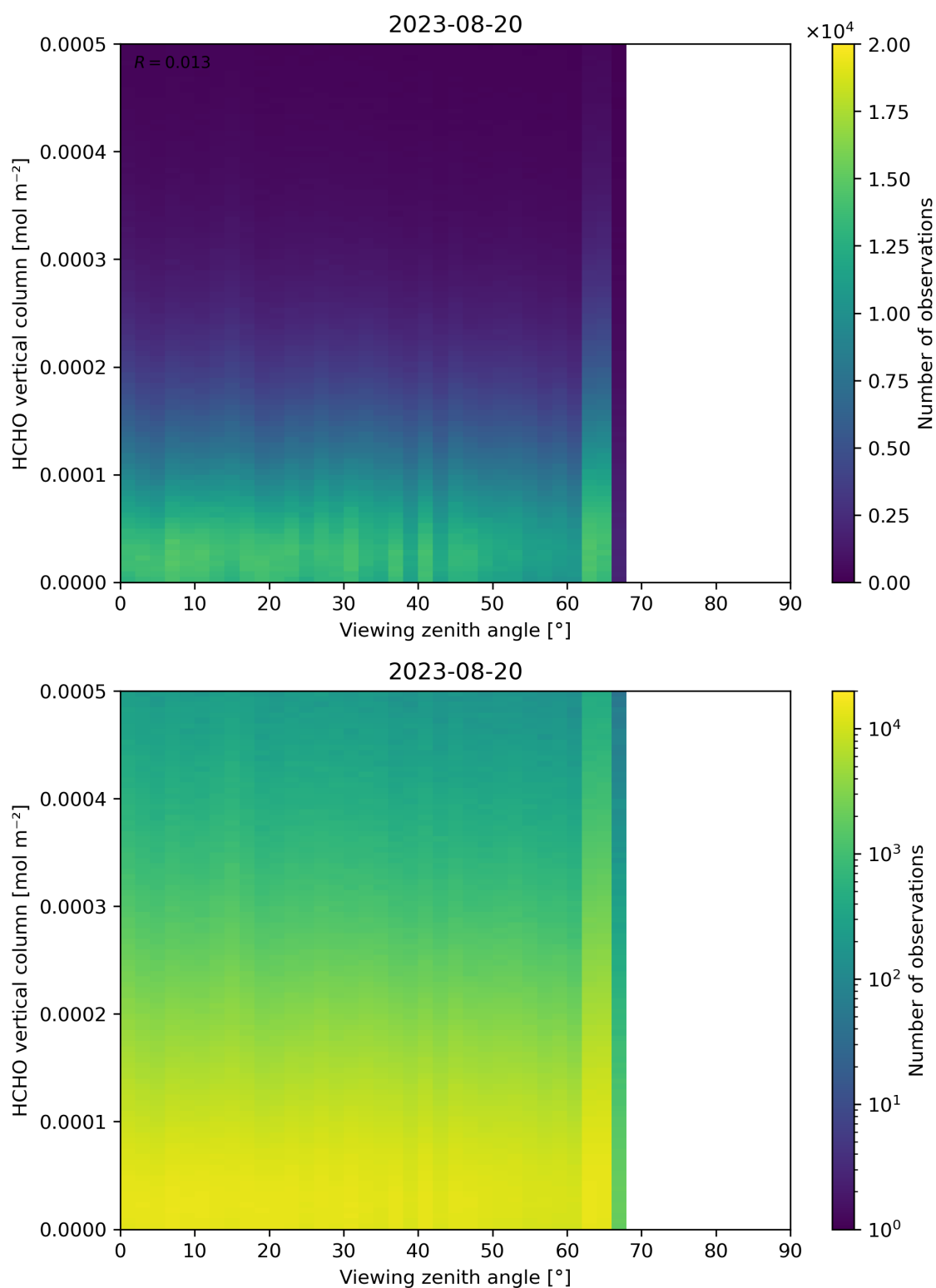
Figure 192: Scatter density plot of “Viewing zenith angle” against “HCHO vertical column” for 2023-08-20 to 2023-08-21.
