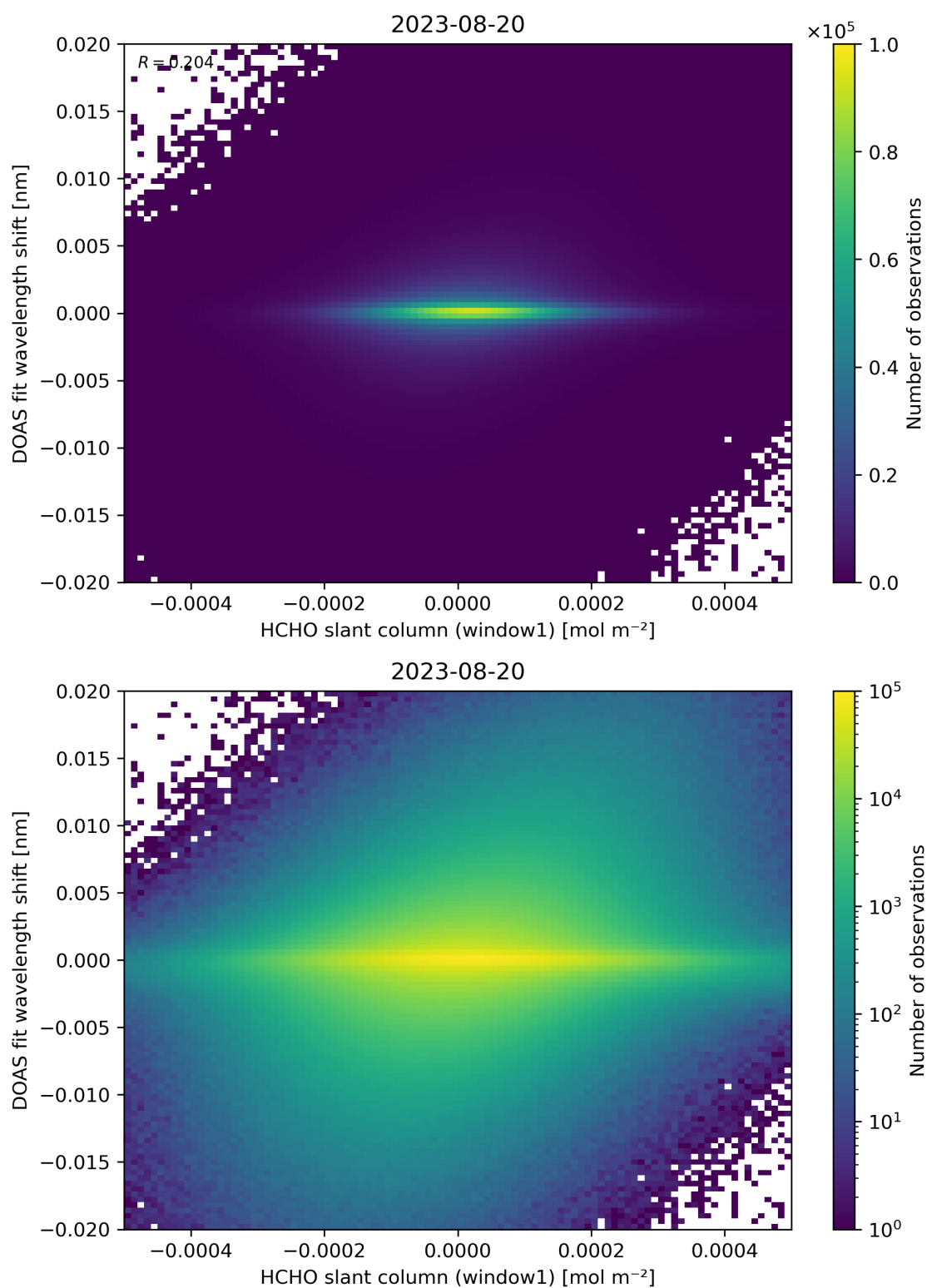
Figure 79: Scatter density plot of “HCHO slant column (window1)” against “DOAS fit wavelength shift” for 2023-08-20 to 2023-08-21.
