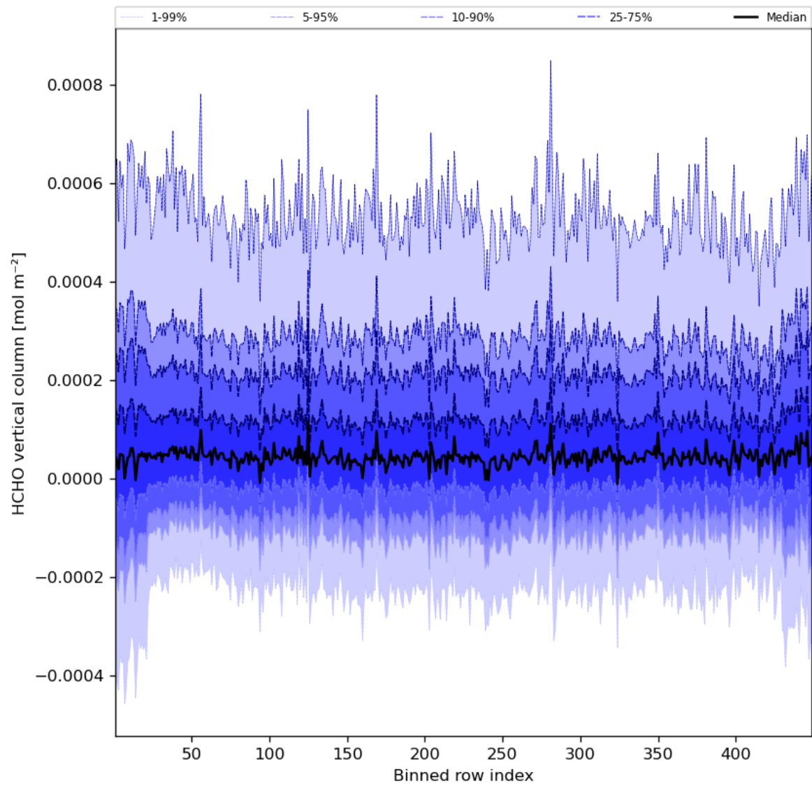
Figure 49: Along track statistics of “HCHO vertical column” for 2023-08-20 to 2023-08-21
