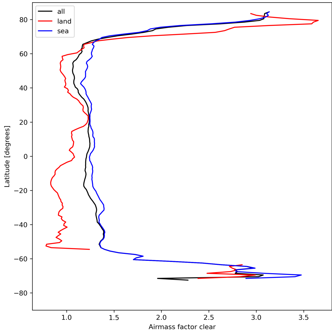
Figure 28: Zonal average of “Airmass factor clear” for 2023-08-20 to 2023-08-21.
