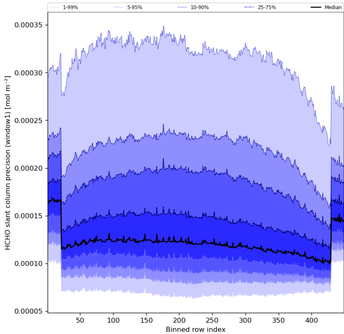
Figure 53: Along track statistics of “HCHO slant column precision (window1)” for 2023-08-20 to 2023-08-21
