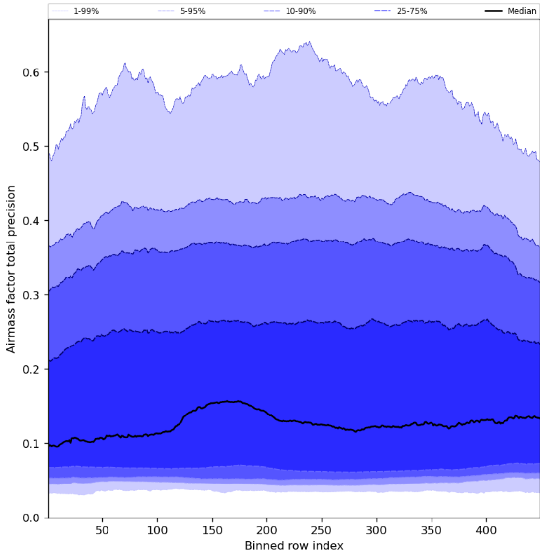
Figure 55: Along track statistics of “Airmass factor total precision” for 2023-08-20 to 2023-08-21
