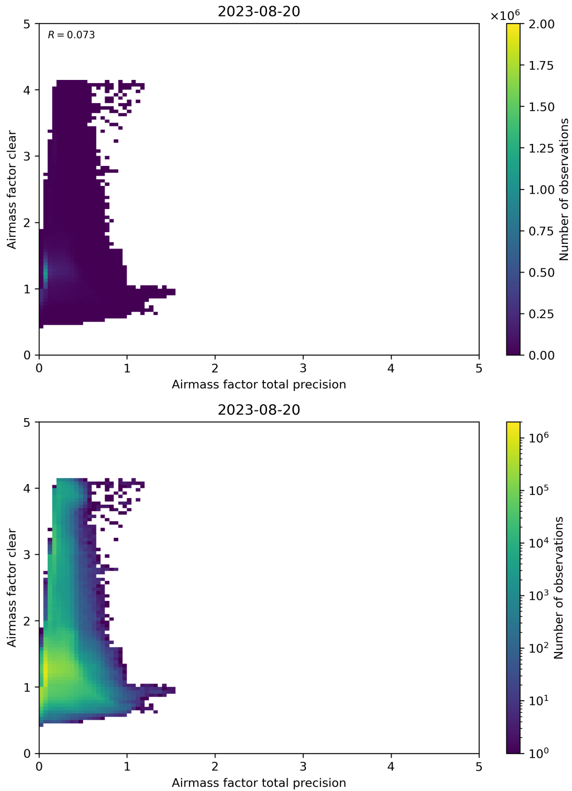
Figure 108: Scatter density plot of “Airmass factor total precision” against “Airmass factor clear” for 2023-08-20 to 2023-08-21.
