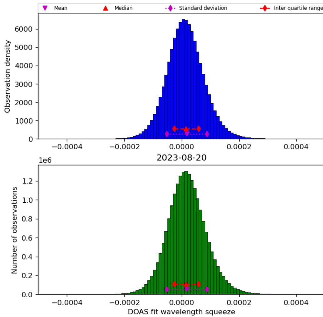
Figure 45: Histogram of “DOAS fit wavelength squeeze” for 2023-08-20 to 2023-08-21
