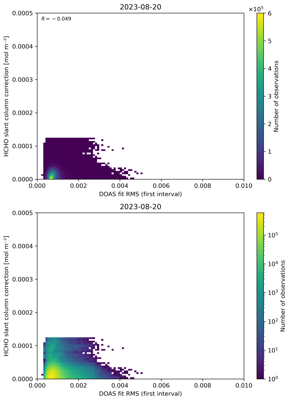
Figure 63: Scatter density plot of “DOAS fit RMS (first interval)” against “HCHO slant column correction” for 2023-08-20 to 2023-08-21.
