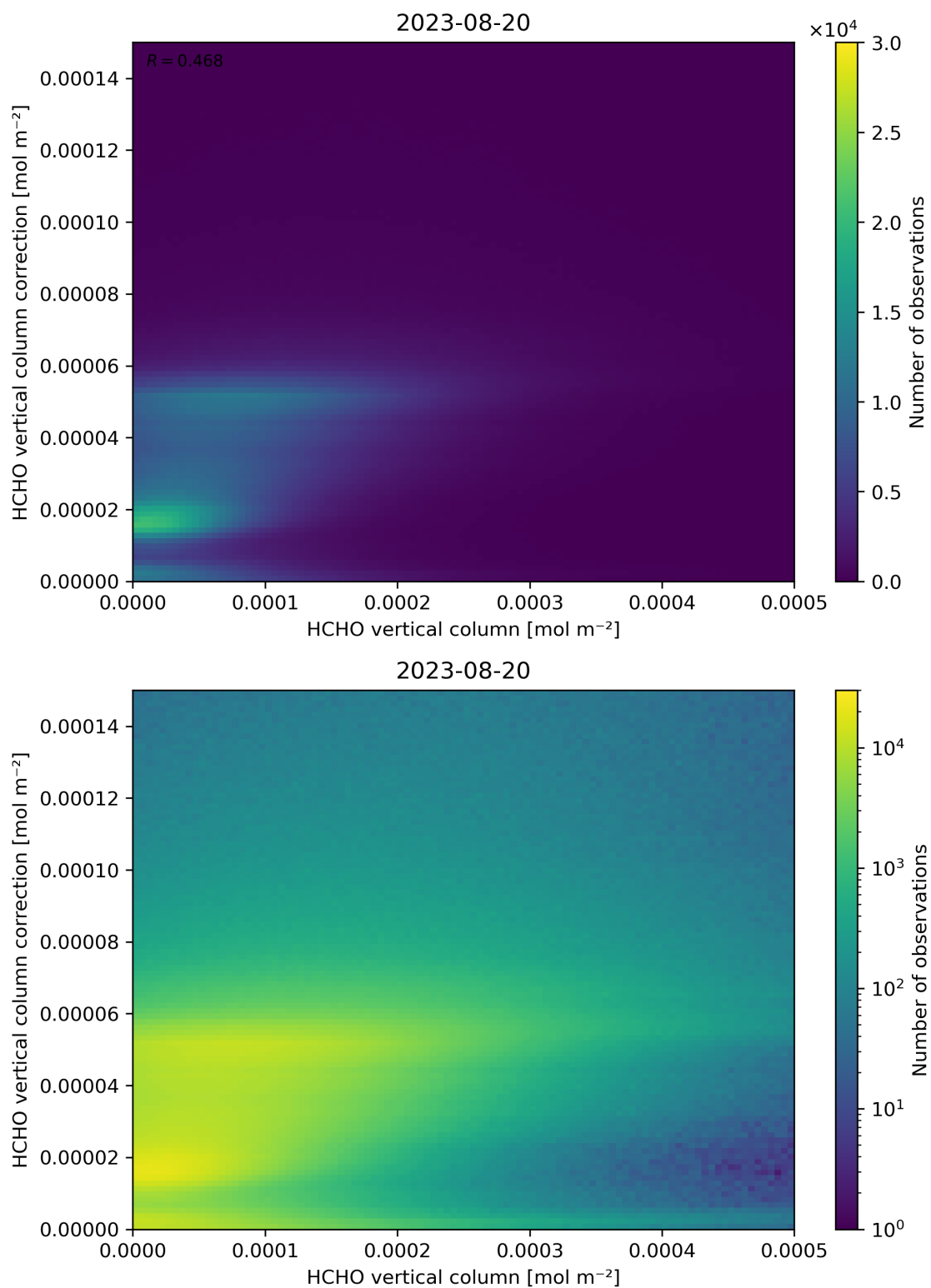
Figure 133: Scatter density plot of “HCHO vertical column” against “HCHO vertical column correction” for 2023-08-20 to 2023-08-21.
