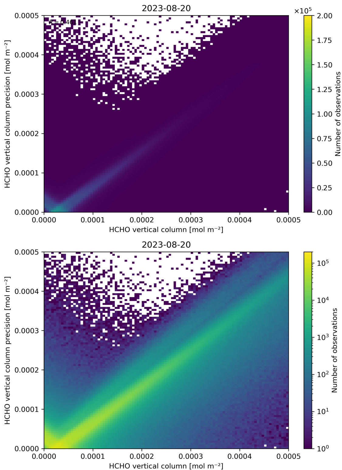
Figure 134: Scatter density plot of “HCHO vertical column” against “HCHO vertical column precision” for 2023-08-20 to 2023-08-21.
