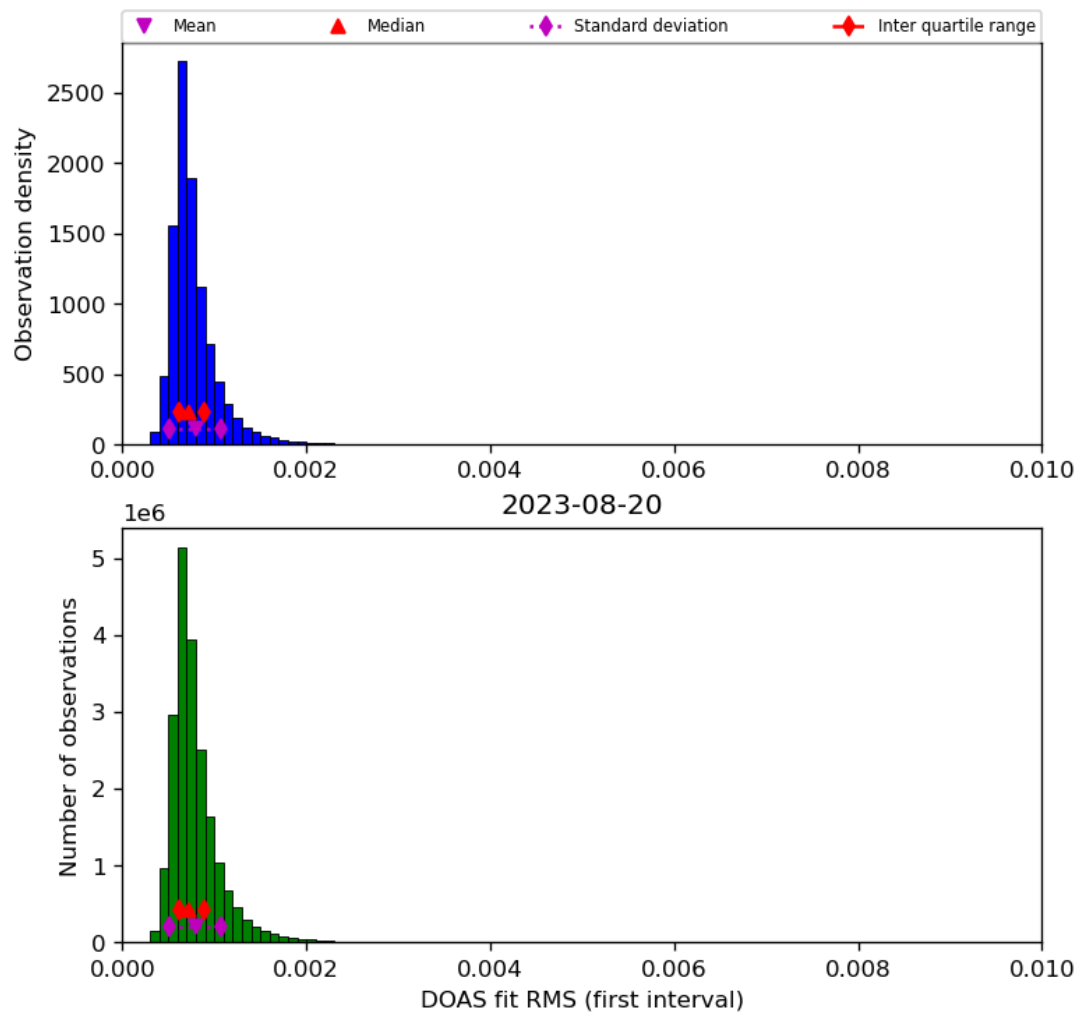
Figure 46: Histogram of “DOAS fit RMS (first interval)” for 2023-08-20 to 2023-08-21
