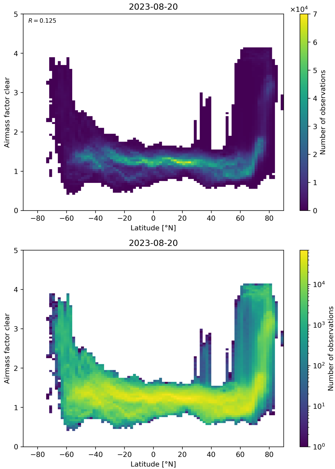
Figure 156: Scatter density plot of “Latitude” against “Airmass factor clear” for 2023-08-20 to 2023-08-21.
