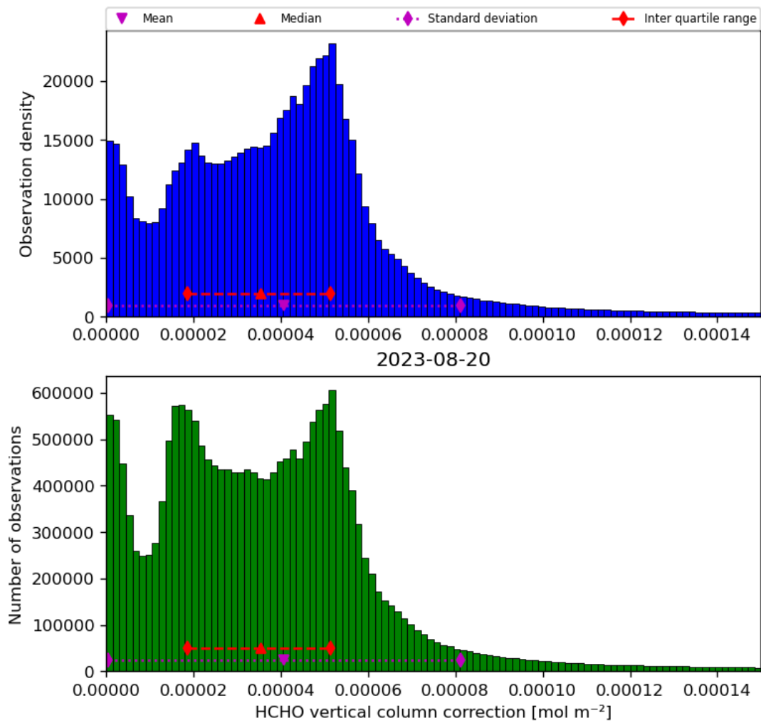
Figure 37: Histogram of “HCHO vertical column correction” for 2023-08-20 to 2023-08-21
