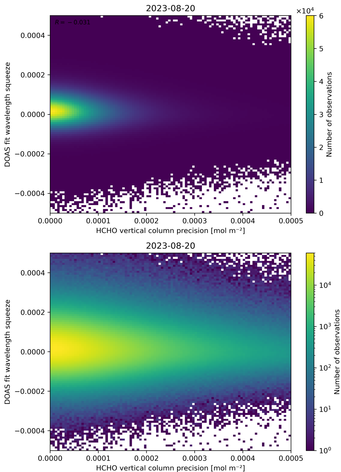
Figure 138: Scatter density plot of “HCHO vertical column precision” against “DOAS fit wavelength squeeze” for 2023-08-20 to 2023-08-21.
