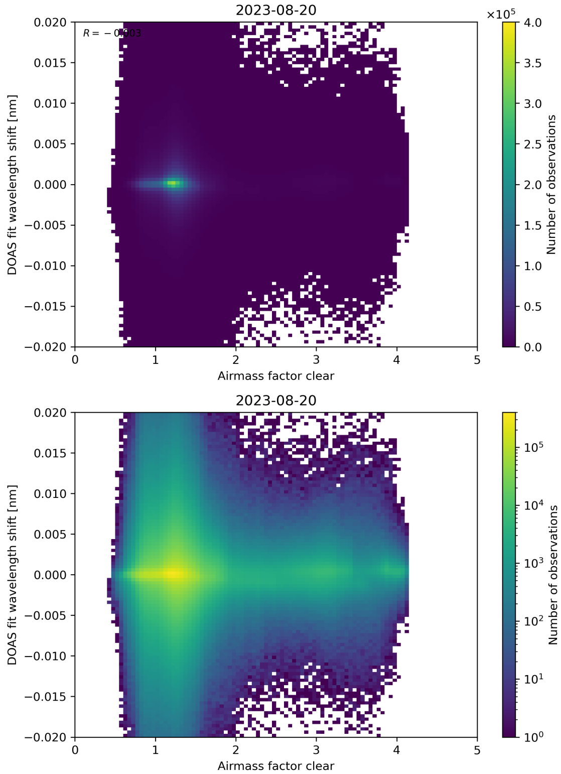
Figure 72: Scatter density plot of “Airmass factor clear” against “DOAS fit wavelength shift” for 2023-08-20 to 2023-08-21.
