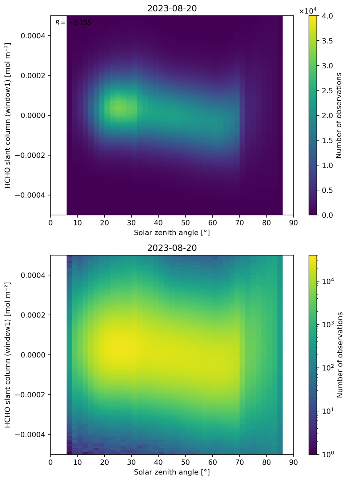
Figure 173: Scatter density plot of “Solar zenith angle” against “HCHO slant column (window1)” for 2023-08-20 to 2023-08-21.
