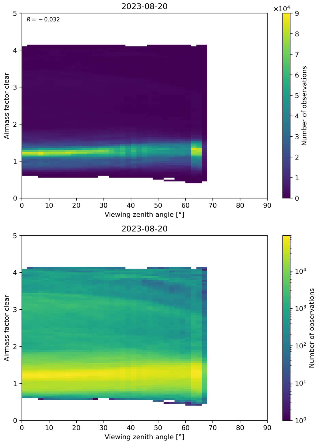
Figure 185: Scatter density plot of “Viewing zenith angle” against “Airmass factor clear” for 2023-08-20 to 2023-08-21.
