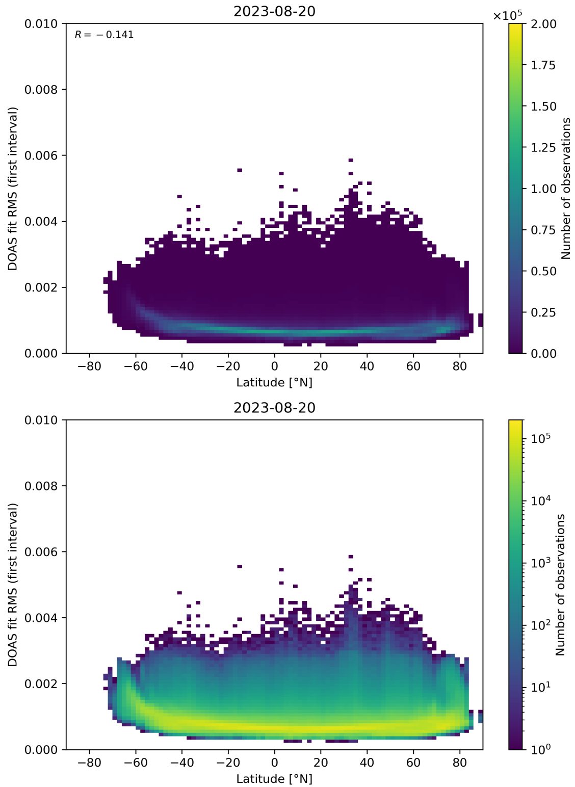
Figure 153: Scatter density plot of “Latitude” against “DOAS fit RMS (first interval)” for 2023-08-20 to 2023-08-21.
