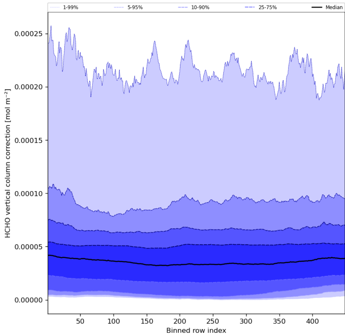
Figure 51: Along track statistics of “HCHO vertical column correction” for 2023-08-20 to 2023-08-21
