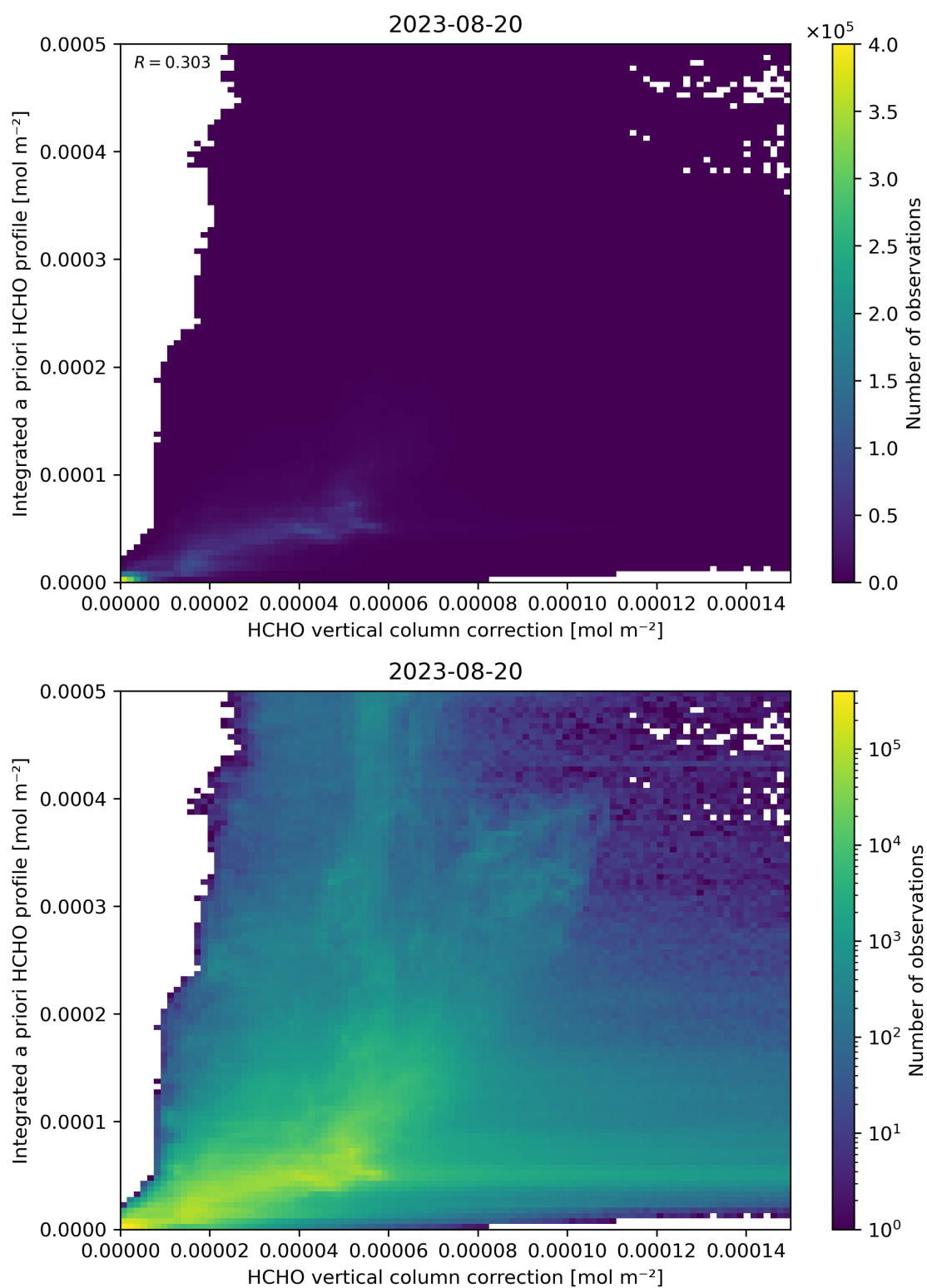
Figure 122: Scatter density plot of “HCHO vertical column correction” against “Integrated a priori HCHO profile” for 2023-08-20 to 2023-08-21.
