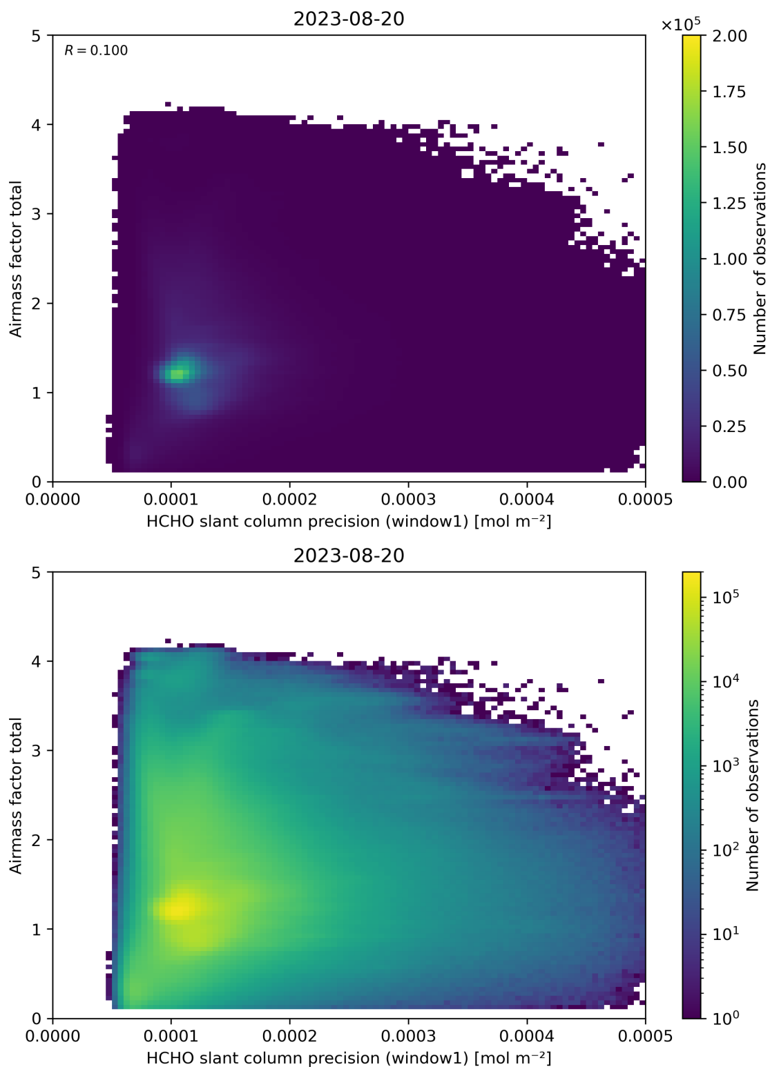
Figure 94: Scatter density plot of “HCHO slant column precision (window1)” against “Airmass factor total” for 2023-08-20 to 2023-08-21.
