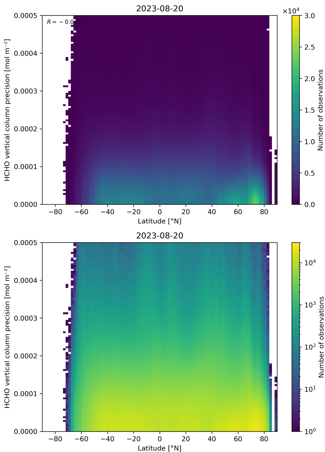
Figure 165: Scatter density plot of “Latitude” against “HCHO vertical column precision” for 2023-08-20 to 2023-08-21.
