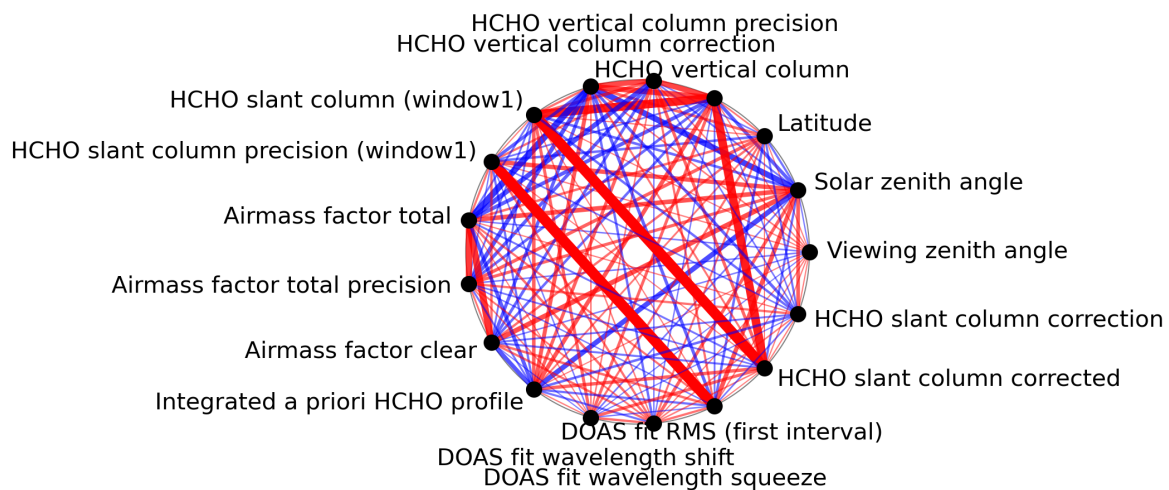
Figure 1: Map of correlation graph for 2023-08-20 to 2023-08-21.
