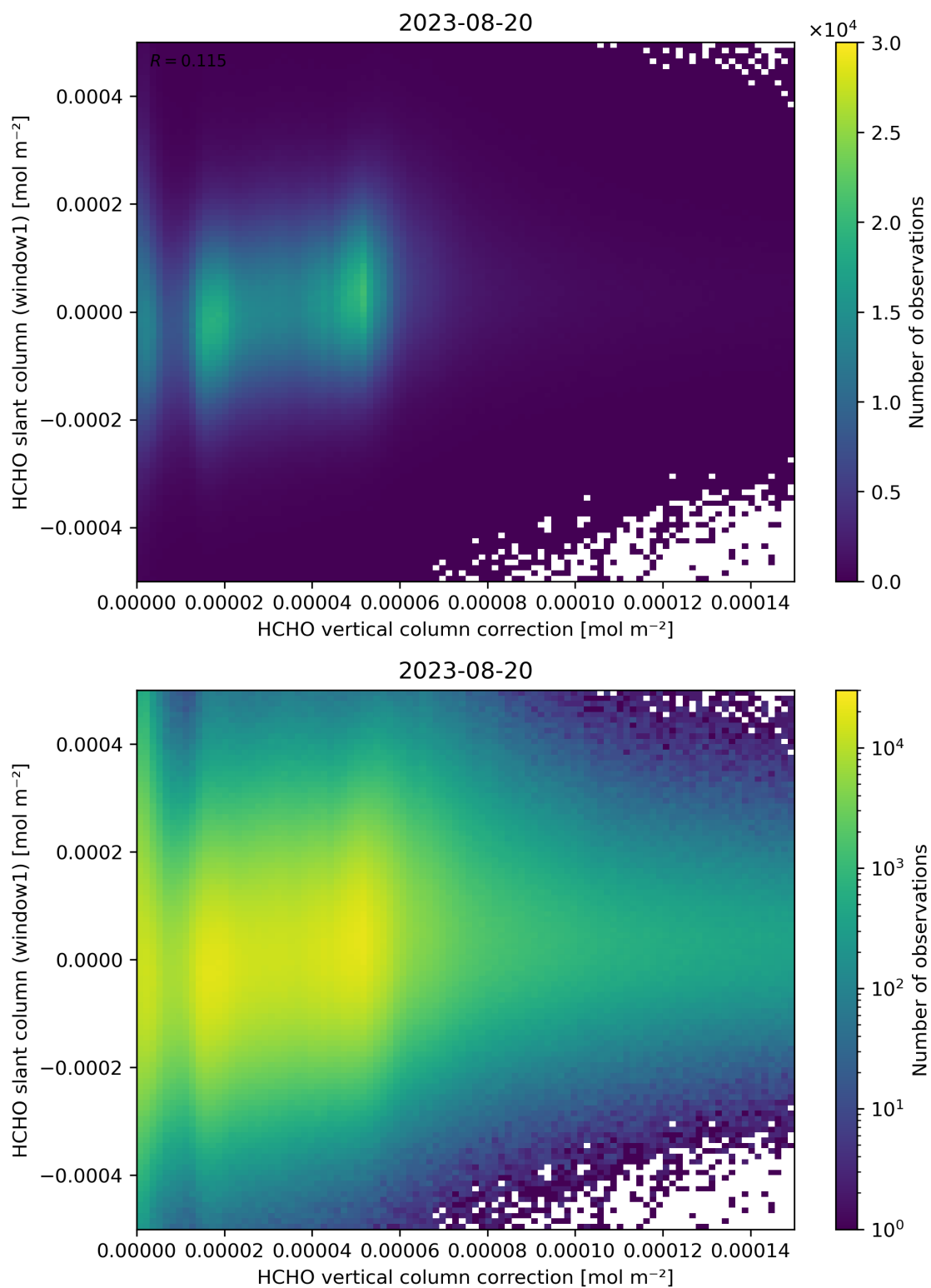
Figure 118: Scatter density plot of “HCHO vertical column correction” against “HCHO slant column (window1)” for 2023-08-20 to 2023-08-21.
