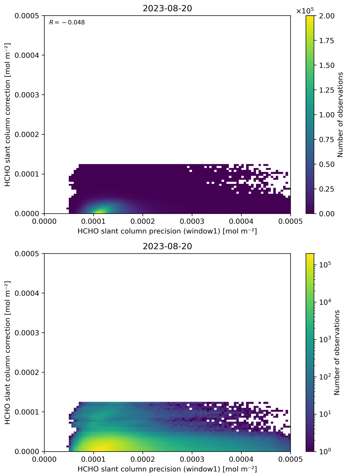
Figure 93: Scatter density plot of “HCHO slant column precision (window1)” against “HCHO slant column correction” for 2023-08-20 to 2023-08-21.
