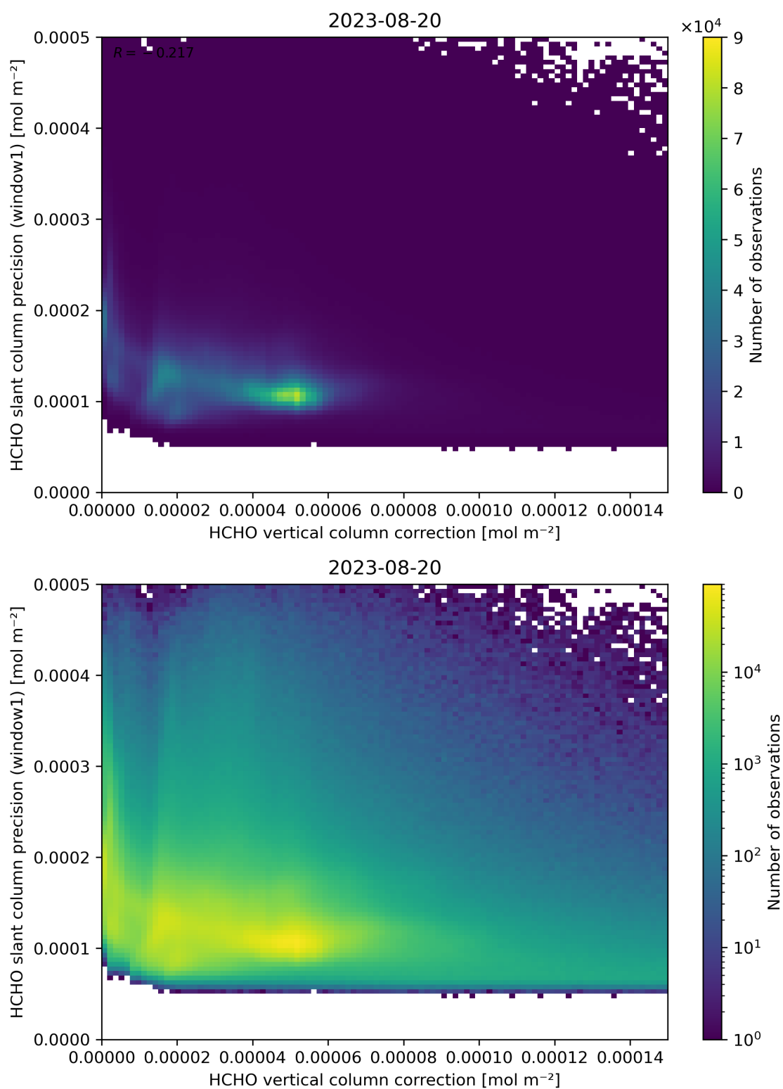
Figure 119: Scatter density plot of “HCHO vertical column correction” against “HCHO slant column precision (window1)” for 2023-08-20 to 2023-08-21.
