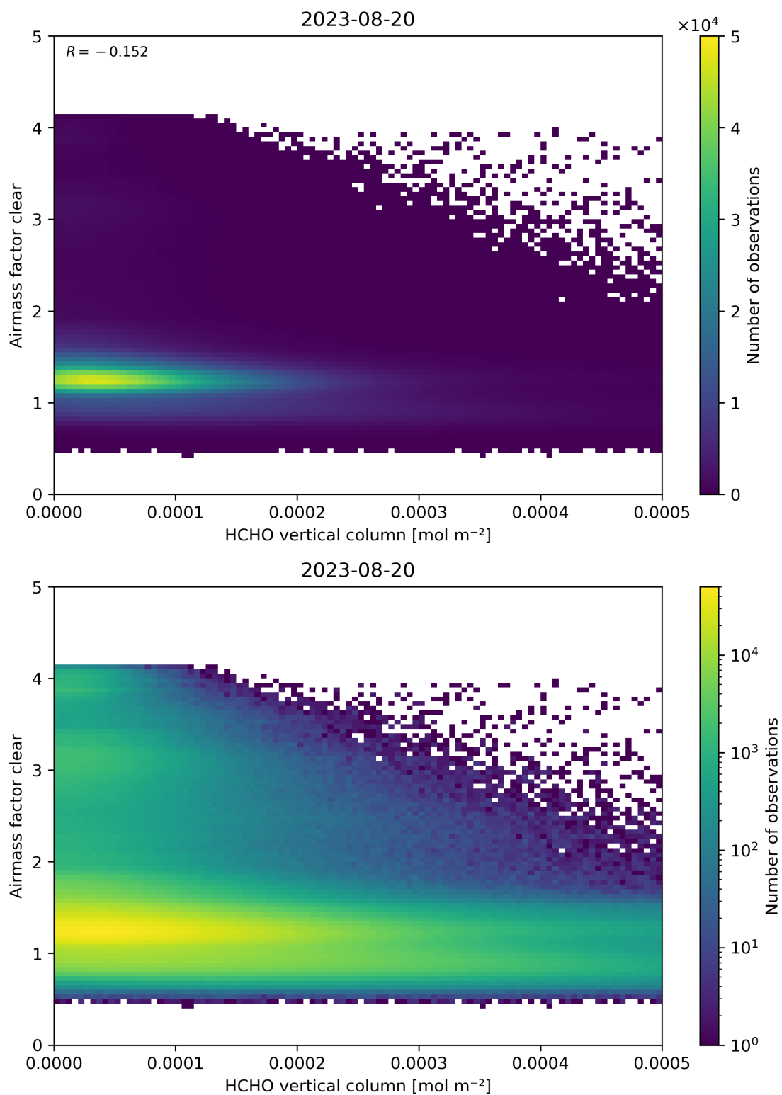
Figure 126: Scatter density plot of “HCHO vertical column” against “Airmass factor clear” for 2023-08-20 to 2023-08-21.
