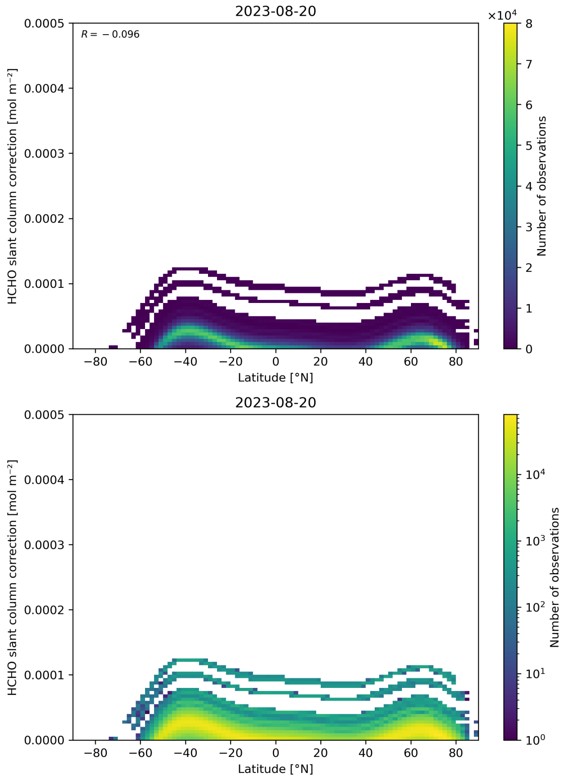
Figure 158: Scatter density plot of “Latitude” against “HCHO slant column correction” for 2023-08-20 to 2023-08-21.
