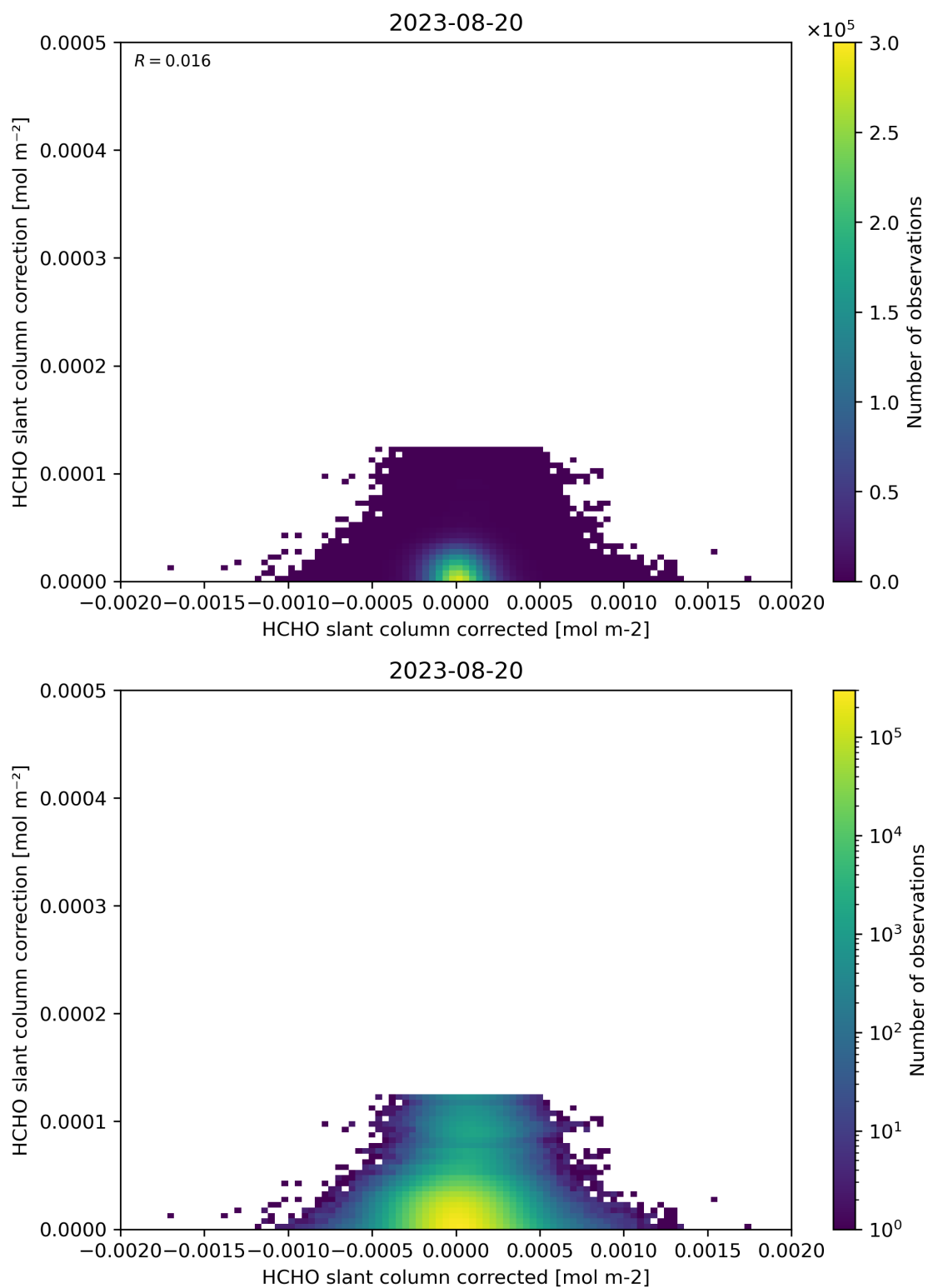
Figure 77: Scatter density plot of “HCHO slant column corrected” against “HCHO slant column correction” for 2023-08-20 to 2023-08-21.
