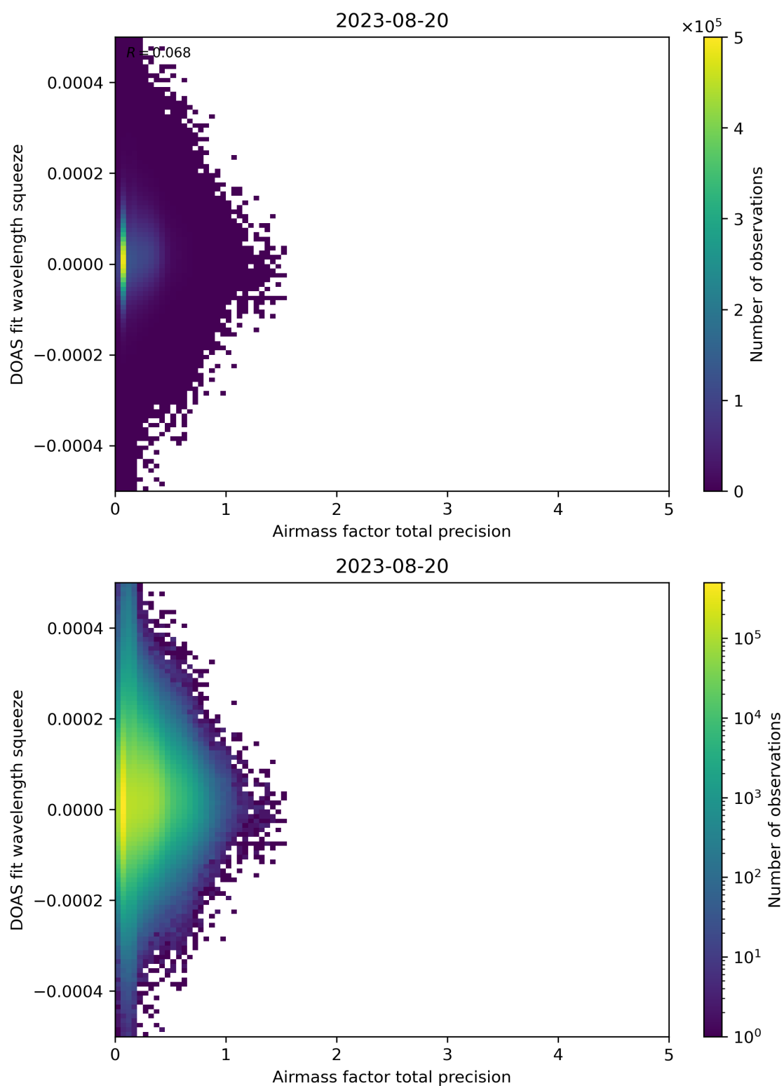
Figure 107: Scatter density plot of “Airmass factor total precision” against “DOAS fit wavelength squeeze” for 2023-08-20 to 2023-08-21.
