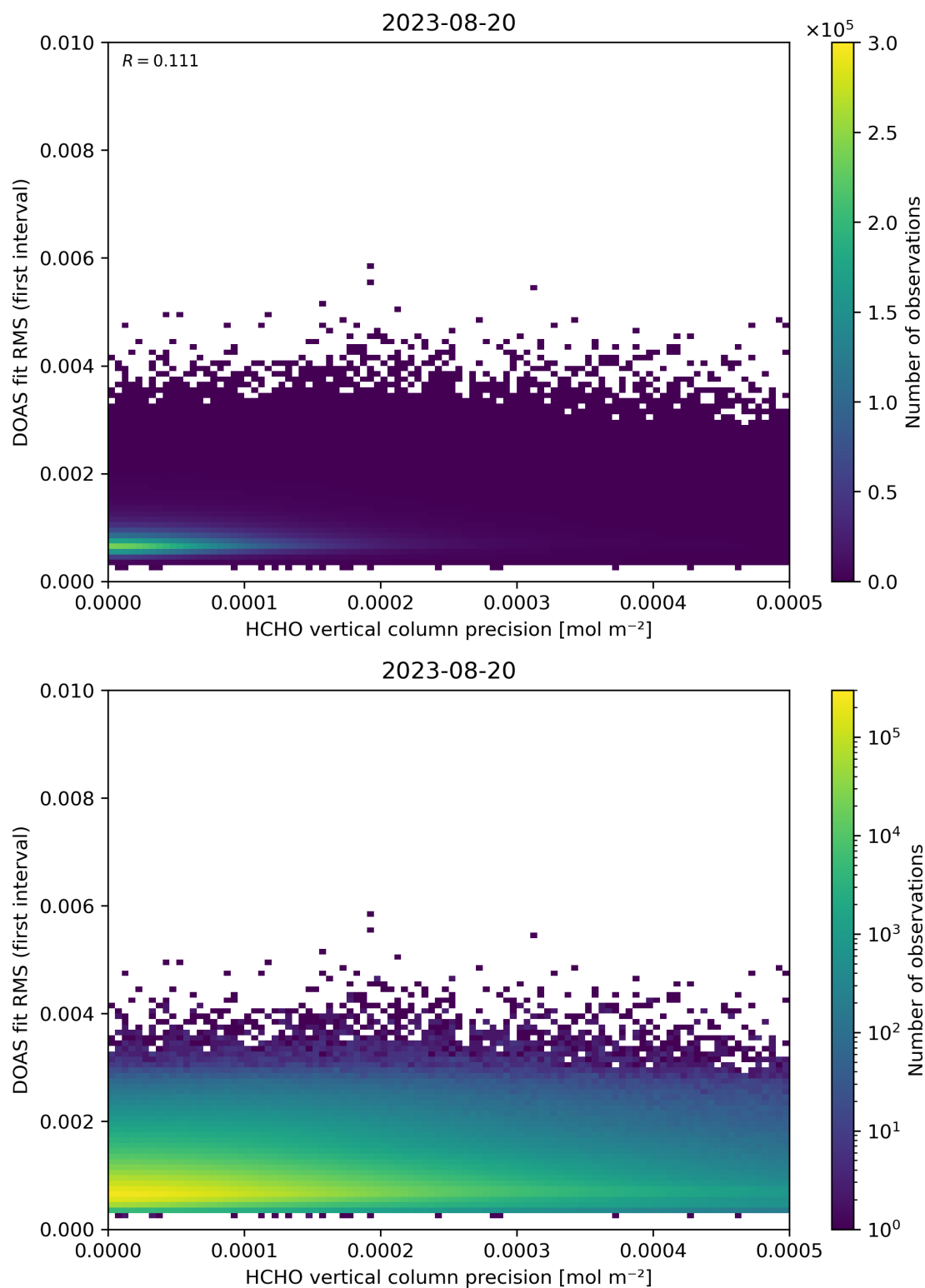
Figure 136: Scatter density plot of “HCHO vertical column precision” against “DOAS fit RMS (first interval)” for 2023-08-20 to 2023-08-21.
