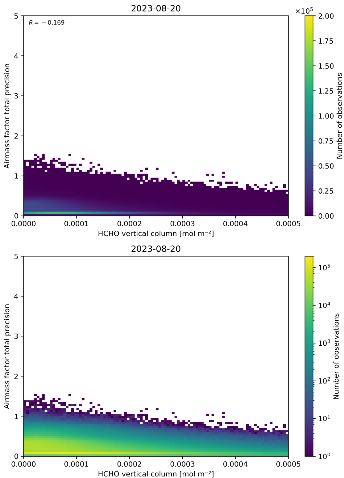
Figure 132: Scatter density plot of “HCHO vertical column” against “Airmass factor total precision” for 2023-08-20 to 2023-08-21.
