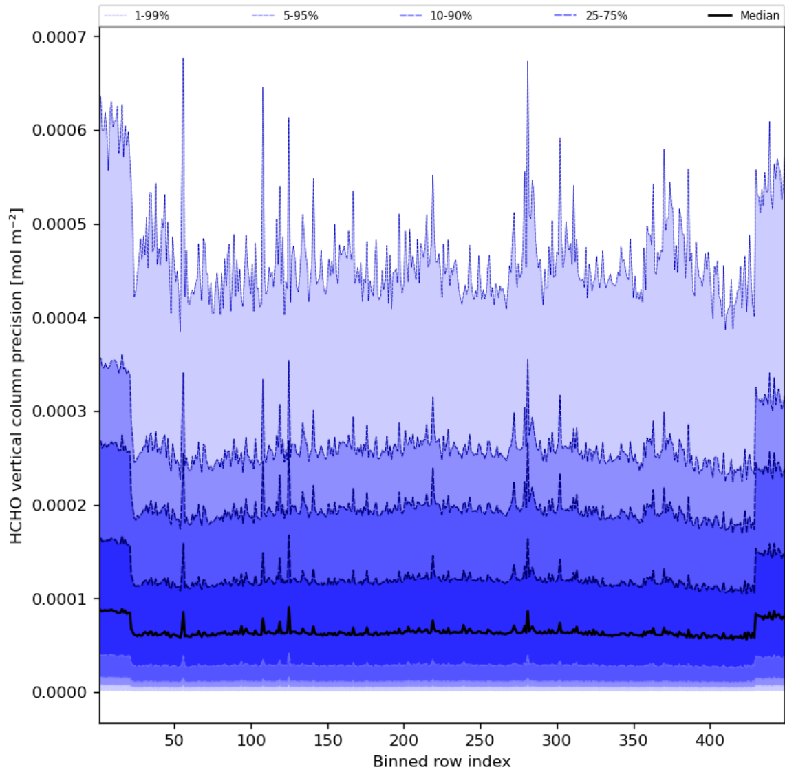
Figure 50: Along track statistics of “HCHO vertical column precision” for 2023-08-20 to 2023-08-21
