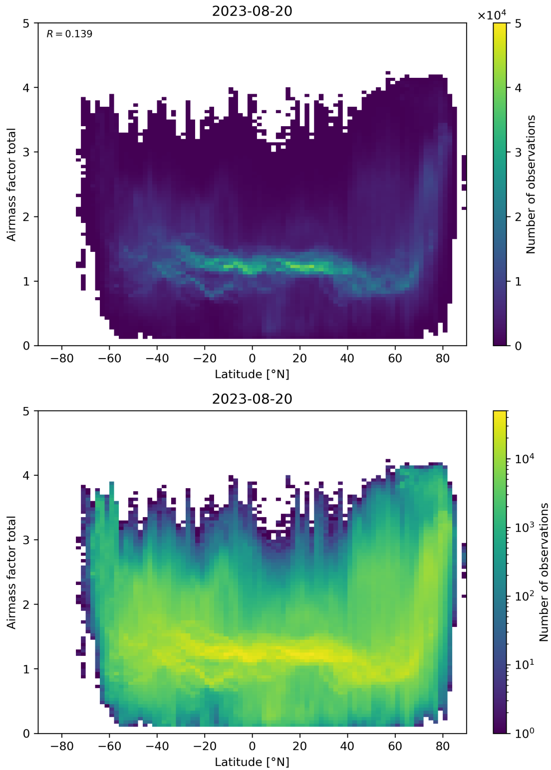
Figure 161: Scatter density plot of “Latitude” against “Airmass factor total” for 2023-08-20 to 2023-08-21.
