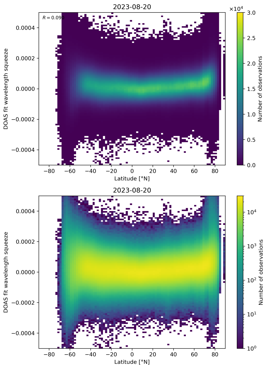
Figure 155: Scatter density plot of “Latitude” against “DOAS fit wavelength squeeze” for 2023-08-20 to 2023-08-21.
