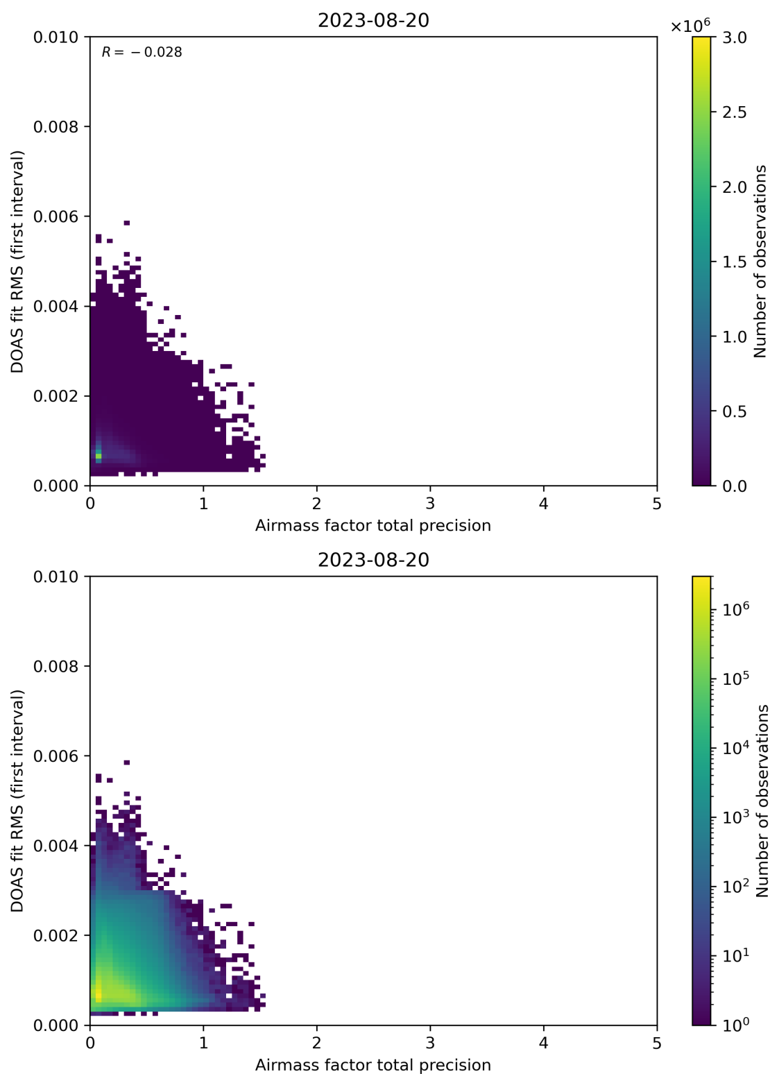
Figure 105: Scatter density plot of “Airmass factor total precision” against “DOAS fit RMS (first interval)” for 2023-08-20 to 2023-08-21.
