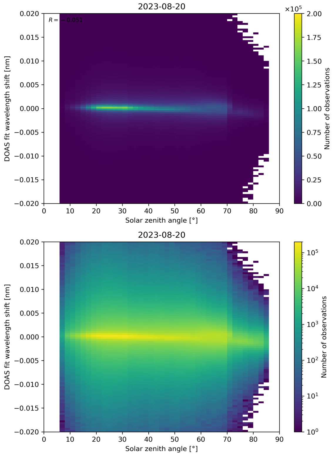
Figure 168: Scatter density plot of “Solar zenith angle” against “DOAS fit wavelength shift” for 2023-08-20 to 2023-08-21.
