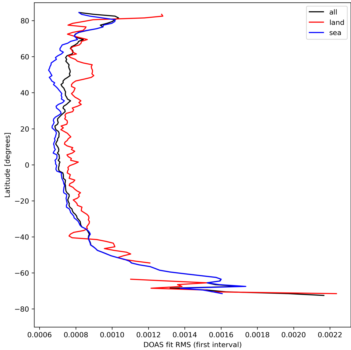
Figure 32: Zonal average of “DOAS fit RMS (first interval)” for 2023-08-20 to 2023-08-21.
