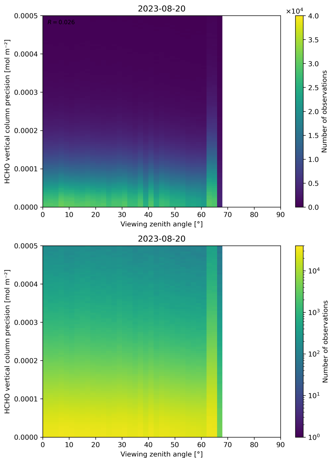
Figure 194: Scatter density plot of “Viewing zenith angle” against “HCHO vertical column precision” for 2023-08-20 to 2023-08-21.
