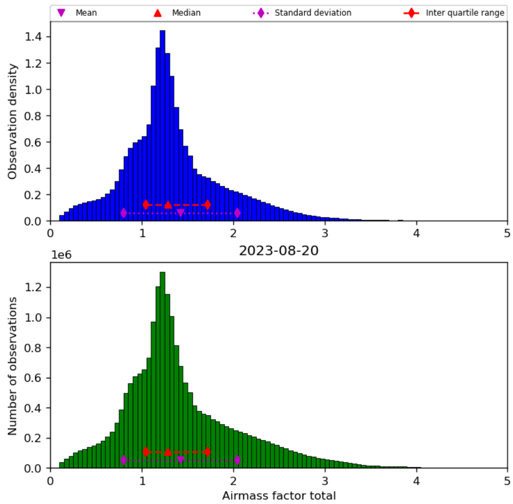
Figure 40: Histogram of “Airmass factor total” for 2023-08-20 to 2023-08-21
