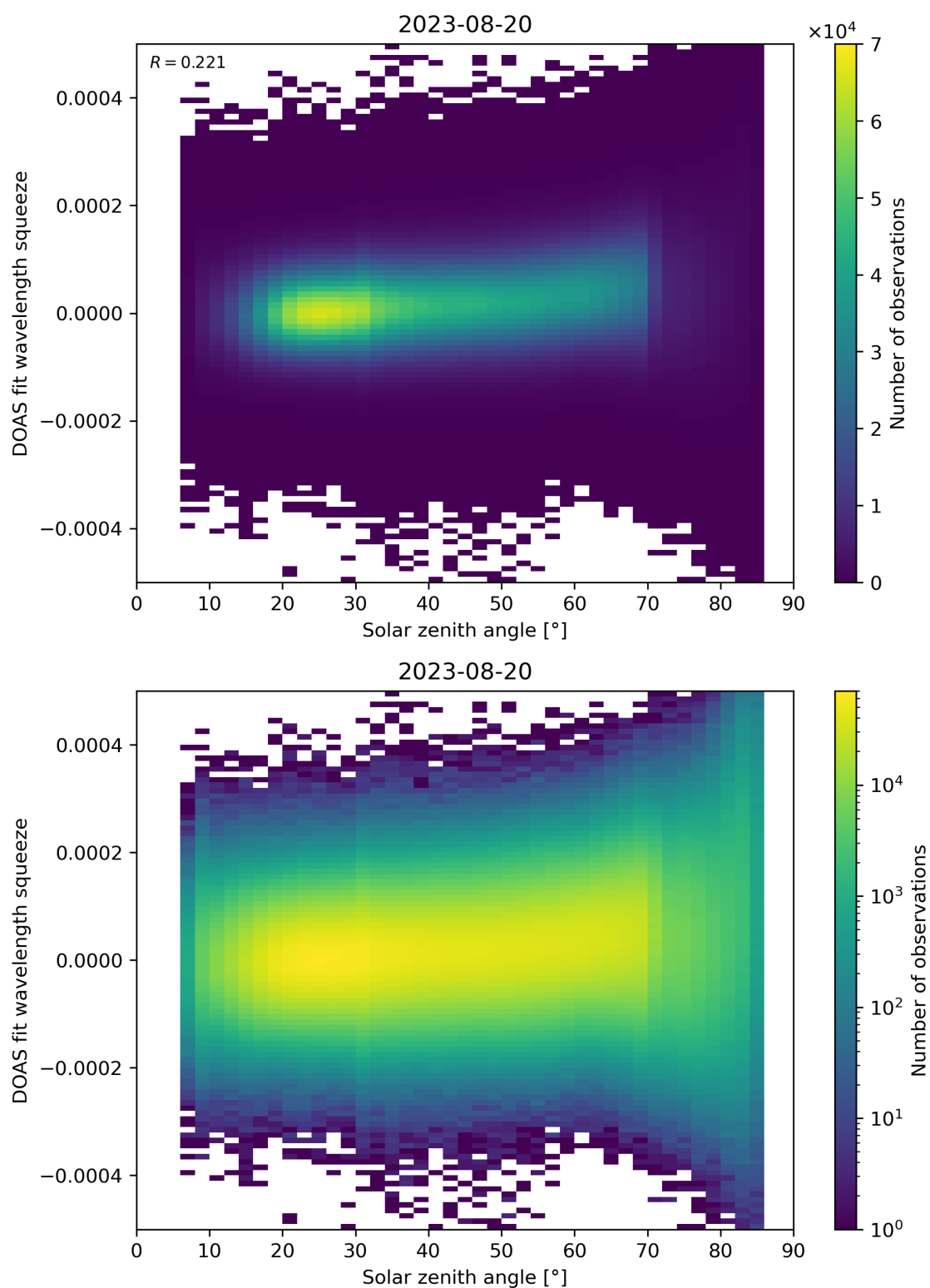
Figure 169: Scatter density plot of “Solar zenith angle” against “DOAS fit wavelength squeeze” for 2023-08-20 to 2023-08-21.
