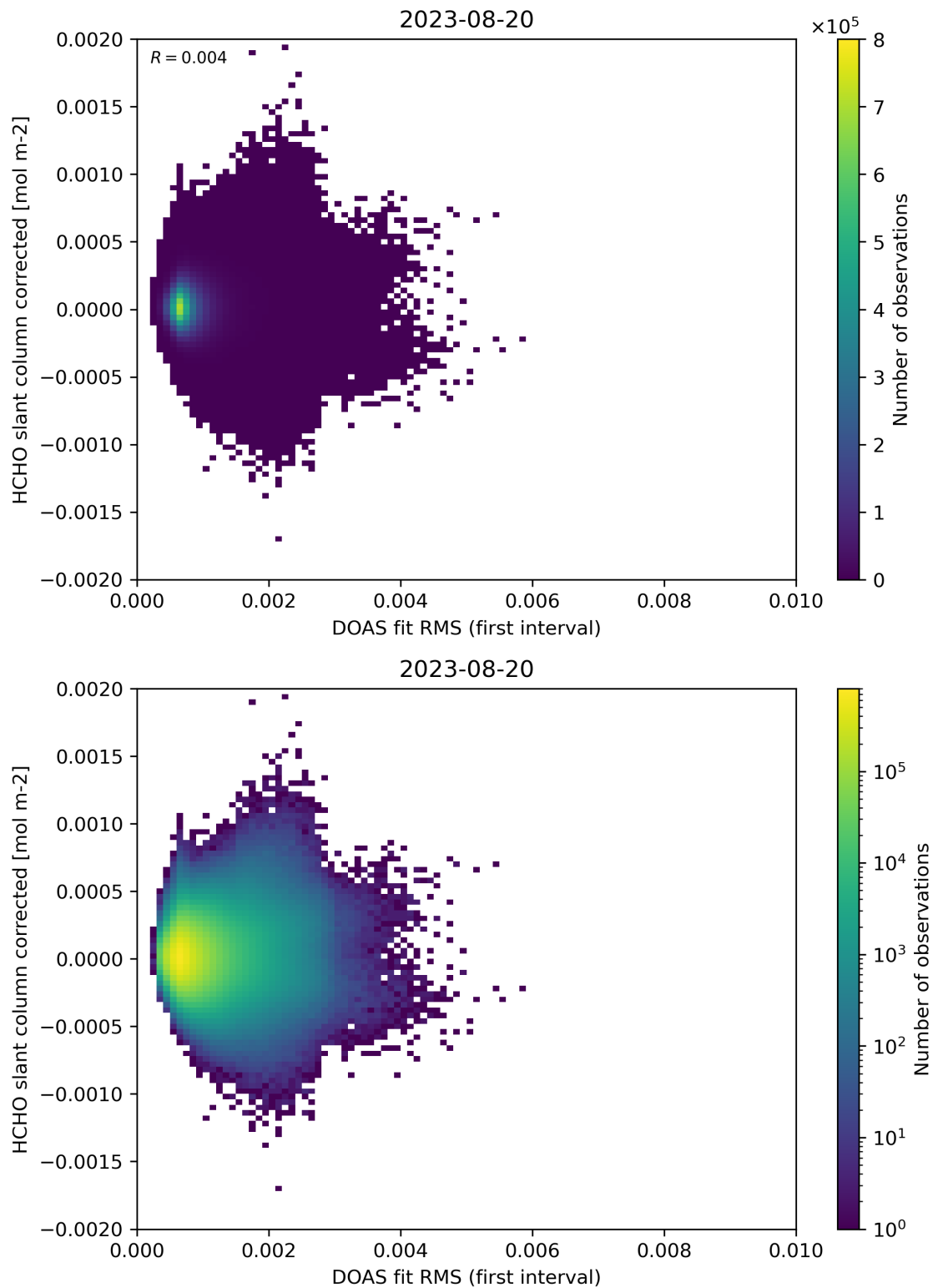
Figure 62: Scatter density plot of “DOAS fit RMS (first interval)” against “HCHO slant column corrected” for 2023-08-20 to 2023-08-21.
