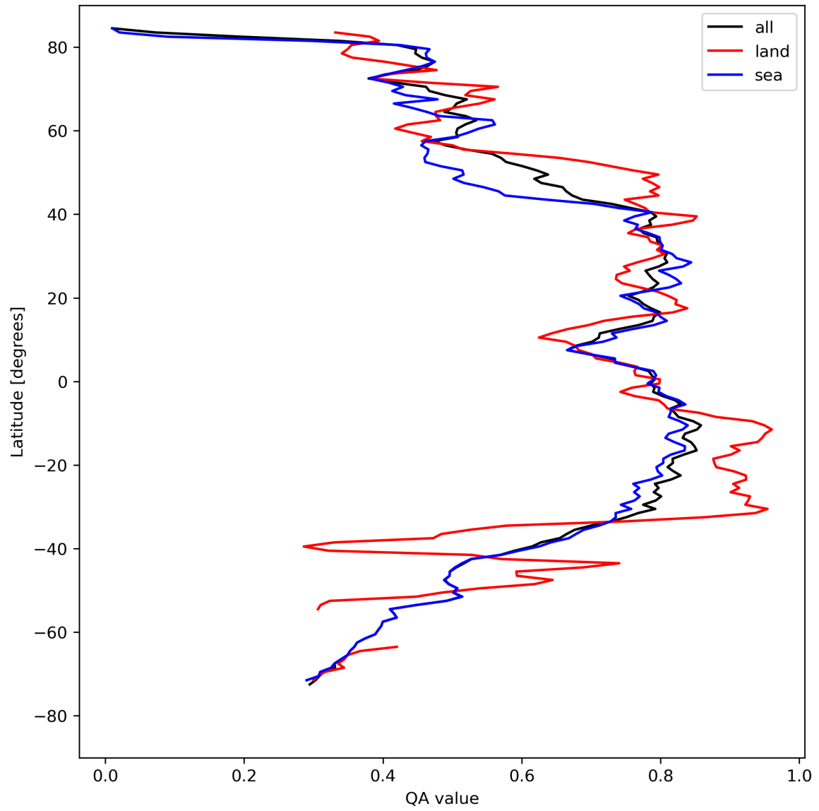
Figure 20: Zonal average of “QA value” for 2023-08-20 to 2023-08-21.
