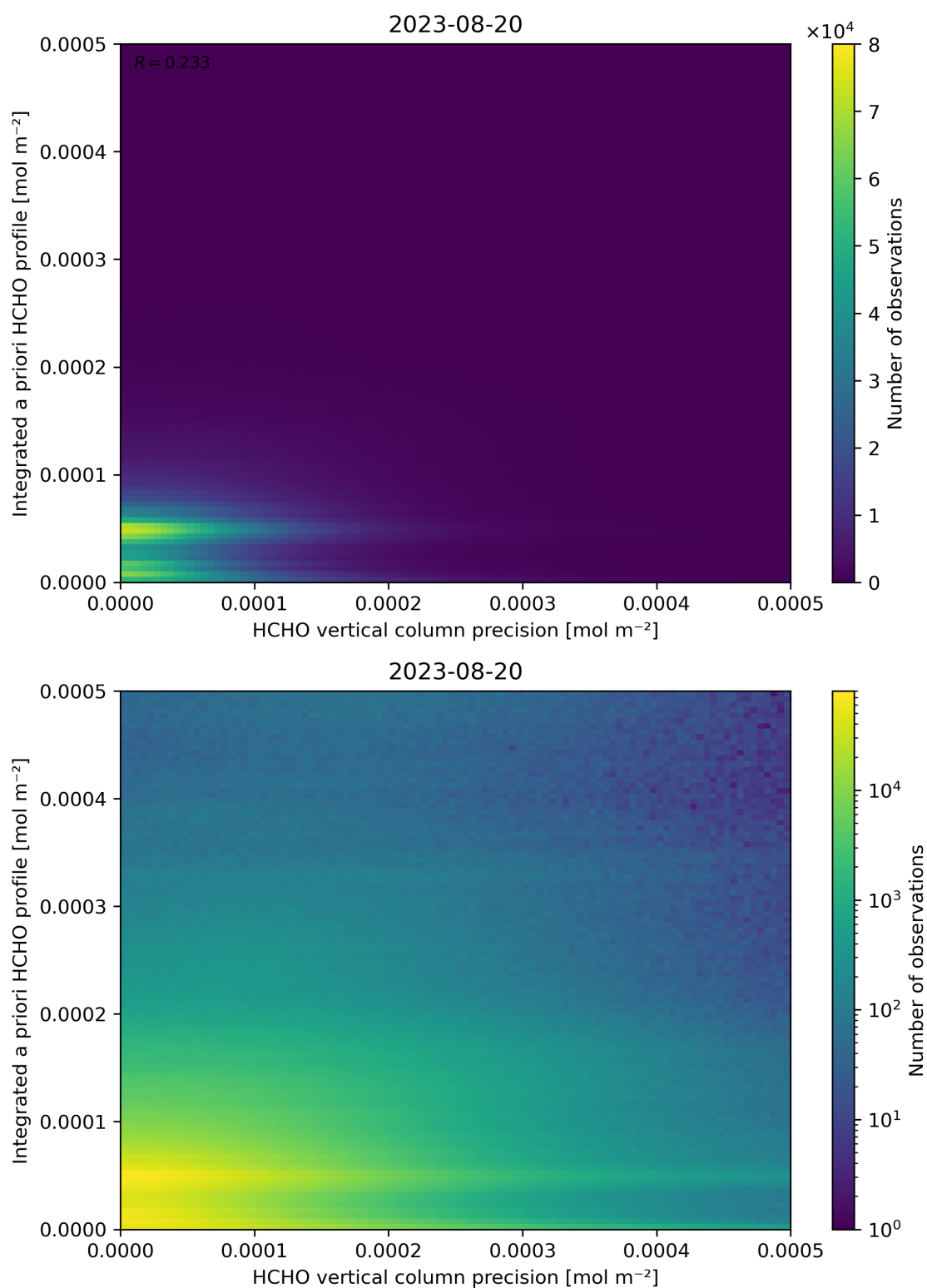
Figure 147: Scatter density plot of “HCHO vertical column precision” against “Integrated a priori HCHO profile” for 2023-08-20 to 2023-08-21.
