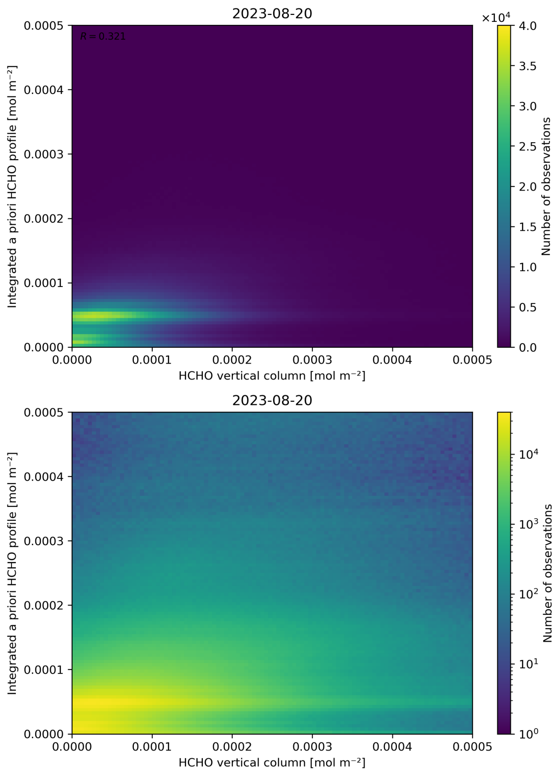
Figure 135: Scatter density plot of “HCHO vertical column” against “Integrated a priori HCHO profile” for 2023-08-20 to 2023-08-21.
