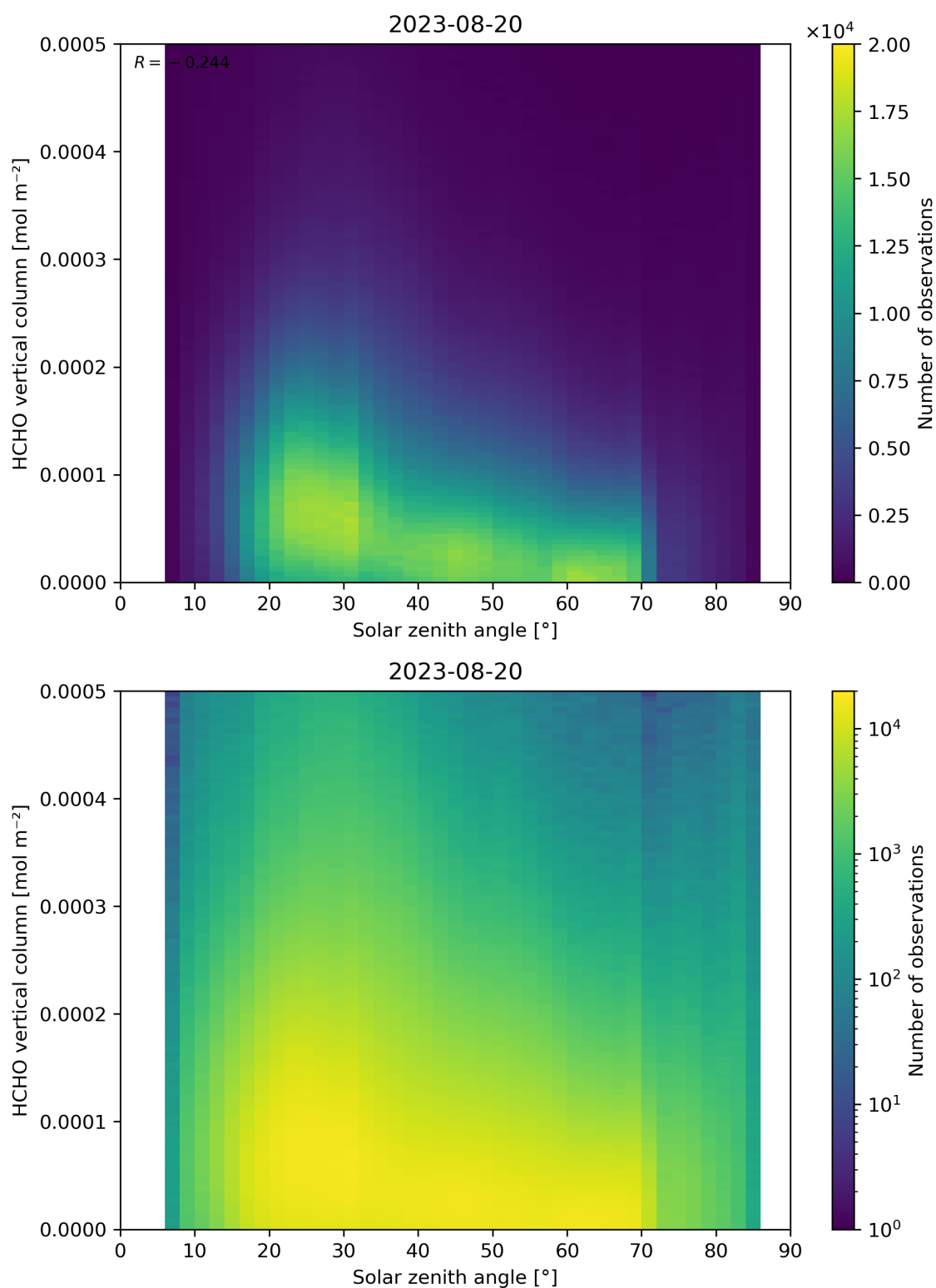
Figure 177: Scatter density plot of “Solar zenith angle” against “HCHO vertical column” for 2023-08-20 to 2023-08-21.
