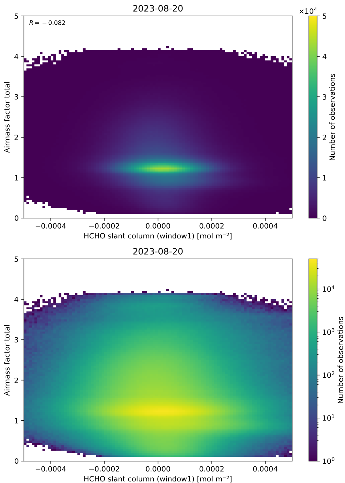
Figure 85: Scatter density plot of “HCHO slant column (window1)” against “Airmass factor total” for 2023-08-20 to 2023-08-21.
