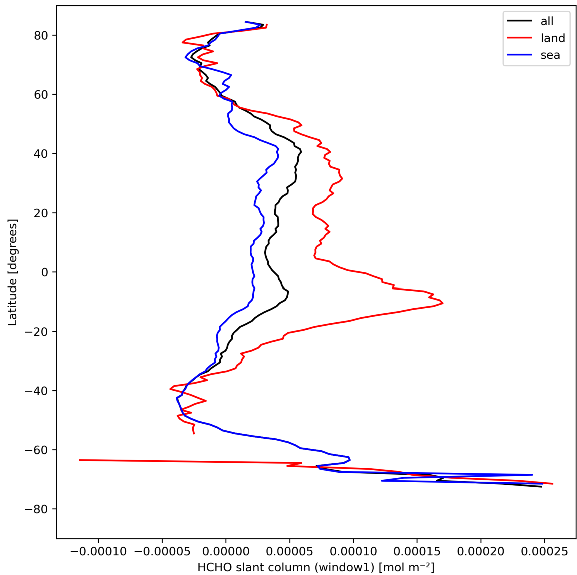
Figure 24: Zonal average of “HCHO slant column (window1)” for 2023-08-20 to 2023-08-21.
