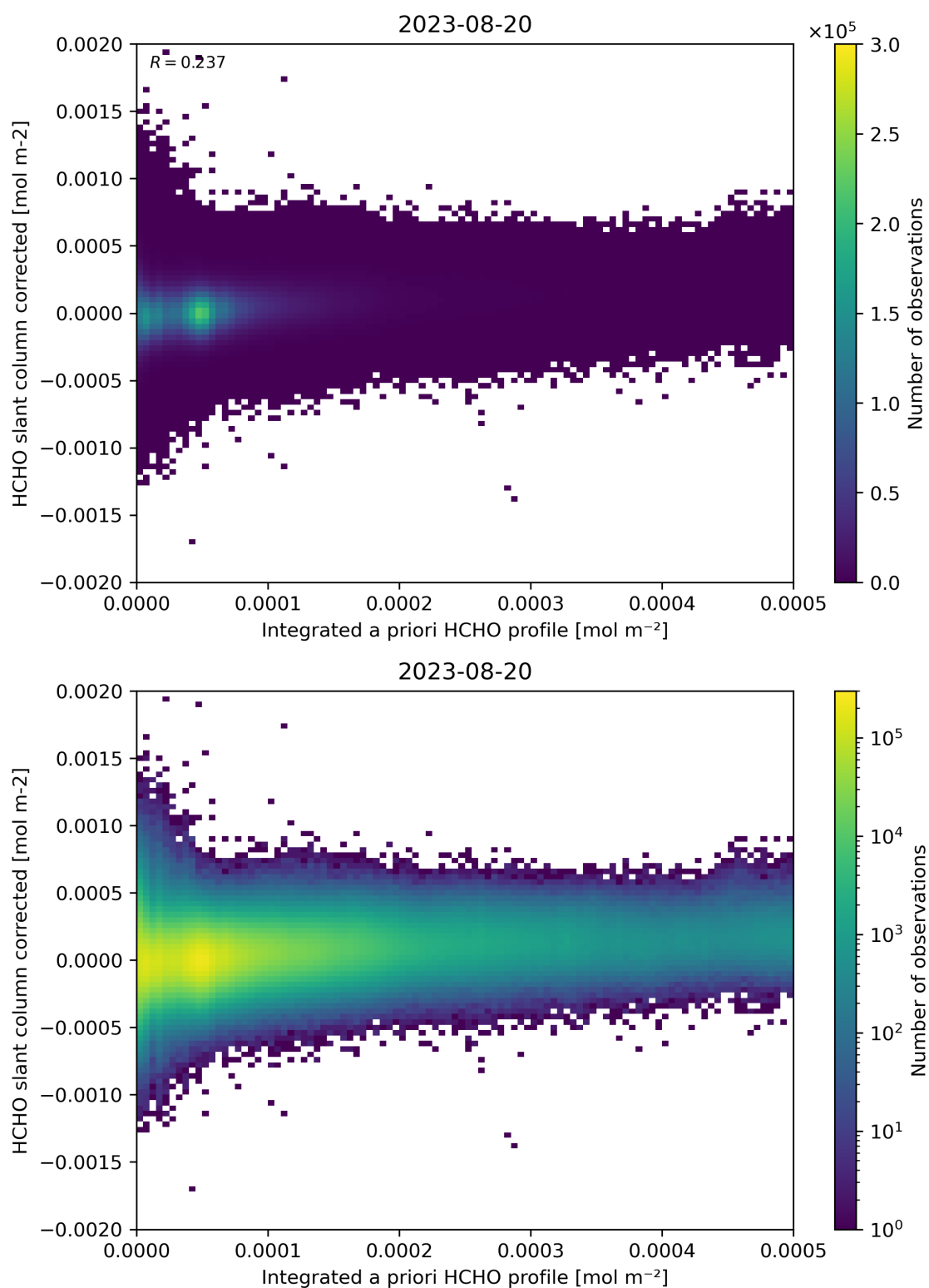
Figure 151: Scatter density plot of “Integrated a priori HCHO profile” against “HCHO slant column corrected” for 2023-08-20 to 2023-08-21.
