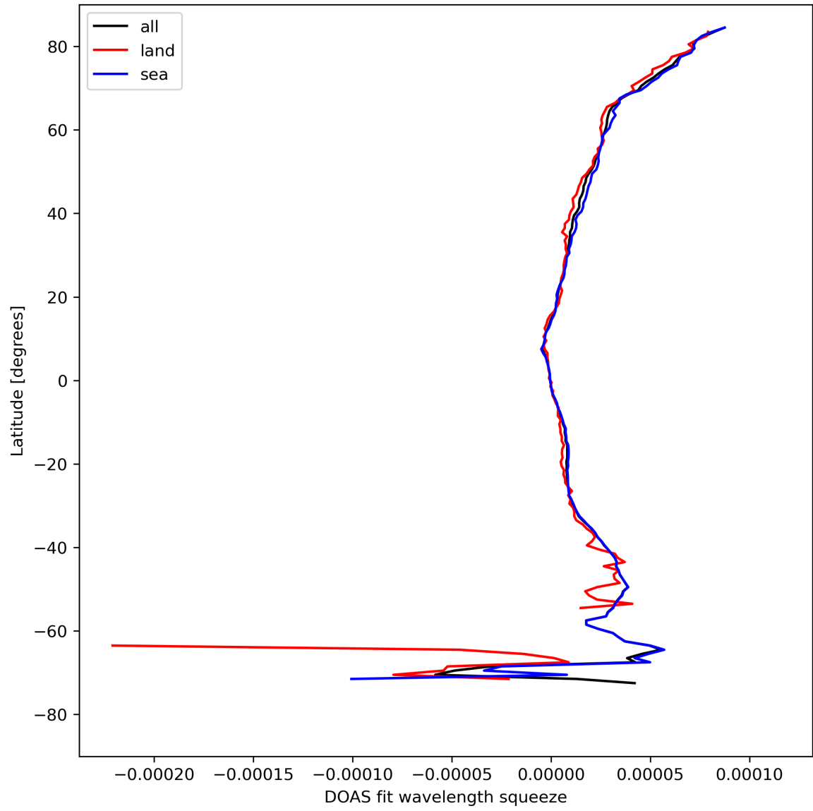
Figure 31: Zonal average of “DOAS fit wavelength squeeze” for 2023-08-20 to 2023-08-21.
