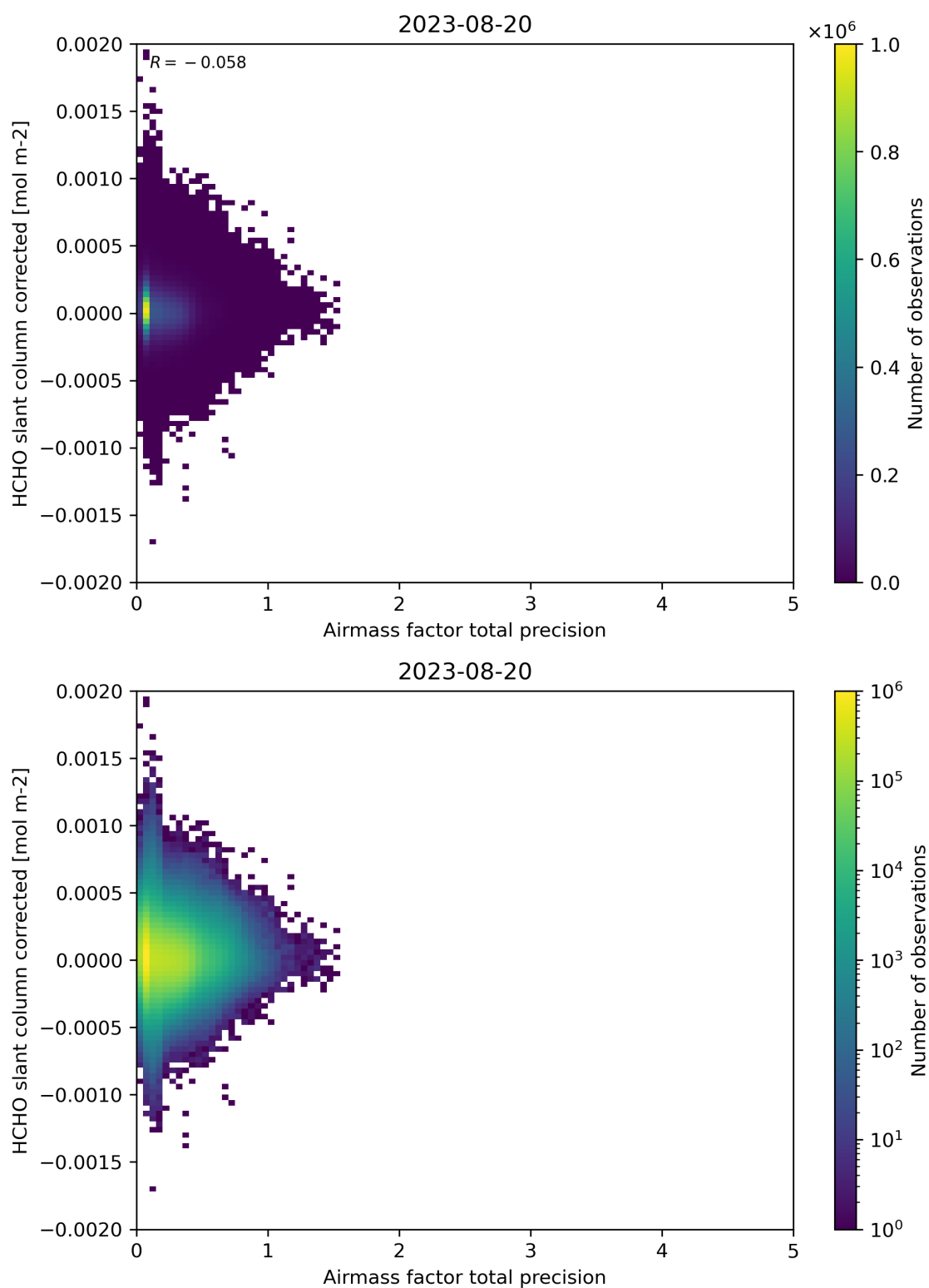
Figure 109: Scatter density plot of “Airmass factor total precision” against “HCHO slant column corrected” for 2023-08-20 to 2023-08-21.
