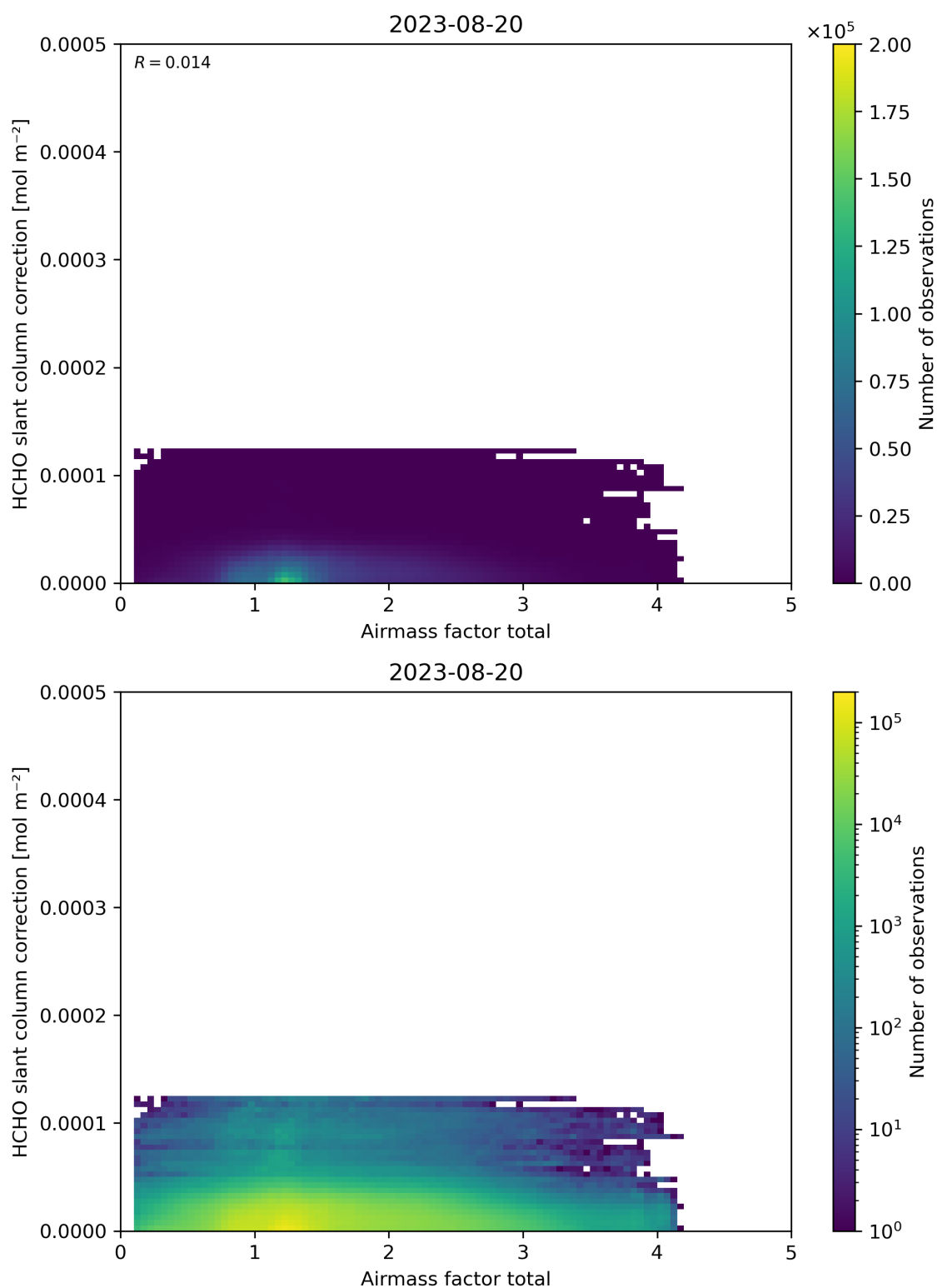
Figure 102: Scatter density plot of “Airmass factor total” against “HCHO slant column correction” for 2023-08-20 to 2023-08-21.
