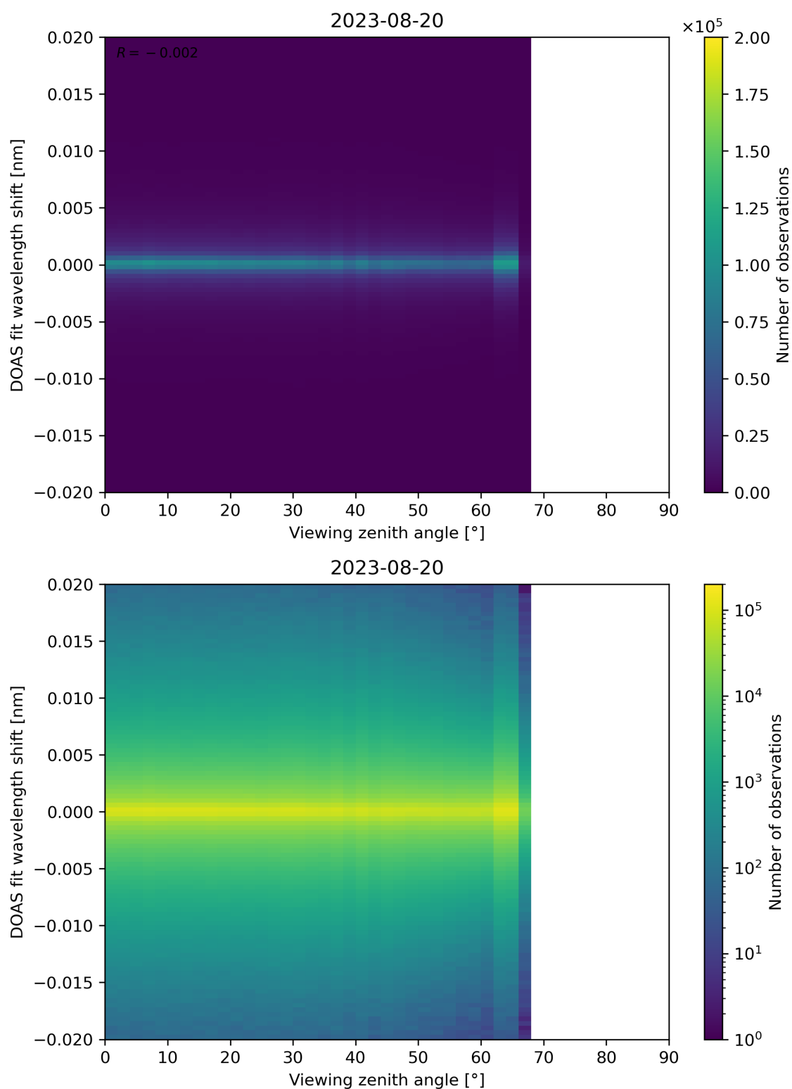
Figure 183: Scatter density plot of “Viewing zenith angle” against “DOAS fit wavelength shift” for 2023-08-20 to 2023-08-21.
