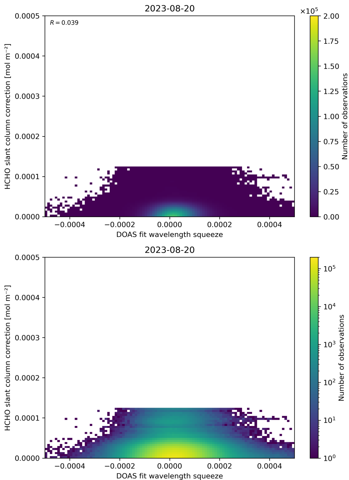
Figure 70: Scatter density plot of “DOAS fit wavelength squeeze” against “HCHO slant column correction” for 2023-08-20 to 2023-08-21.
