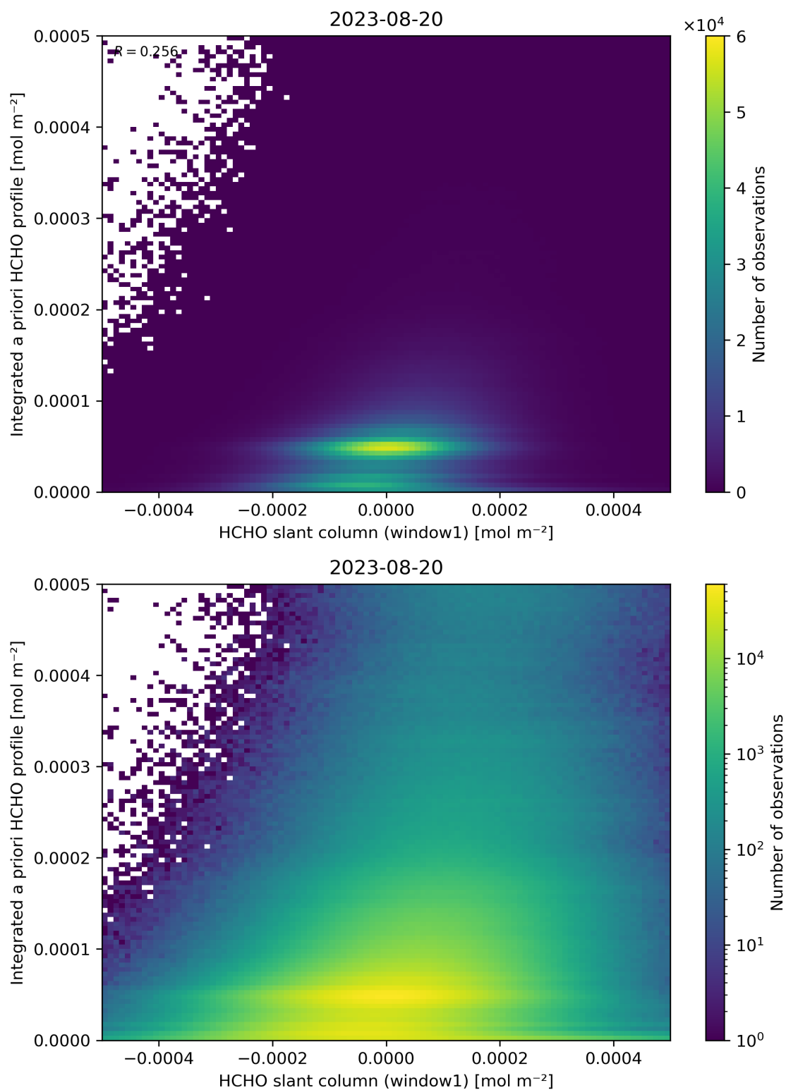
Figure 87: Scatter density plot of “HCHO slant column (window1)” against “Integrated a priori HCHO profile” for 2023-08-20 to 2023-08-21.
