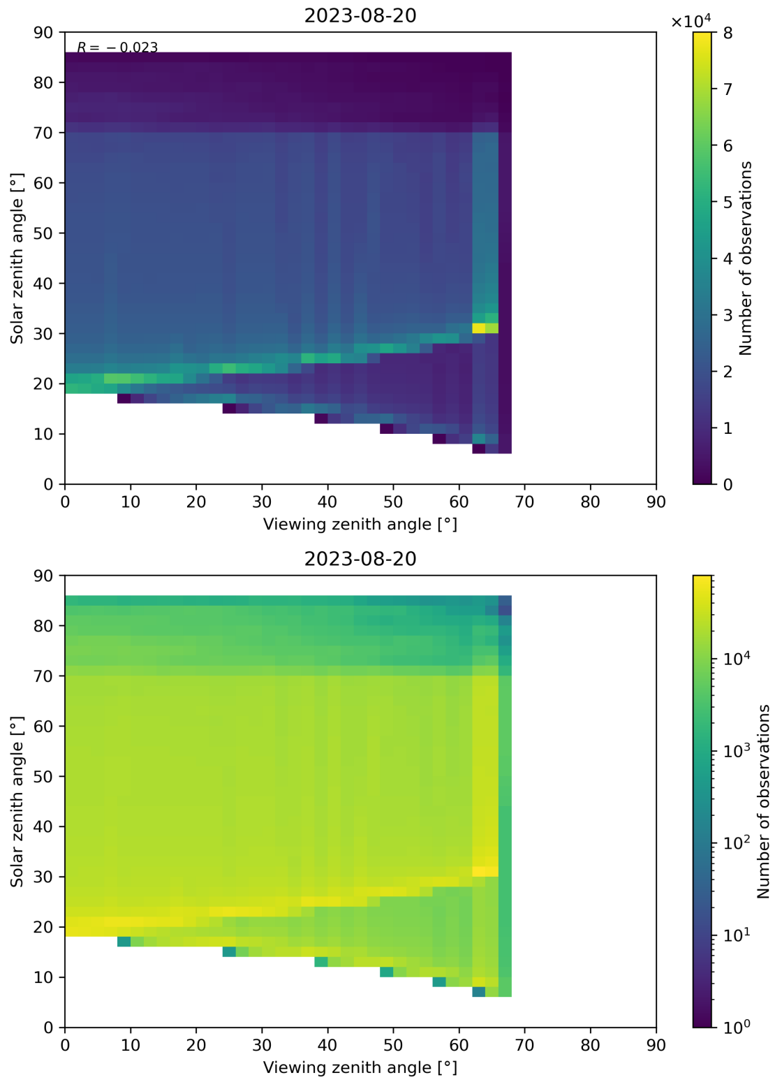
Figure 197: Scatter density plot of “Viewing zenith angle” against “Solar zenith angle” for 2023-08-20 to 2023-08-21.
