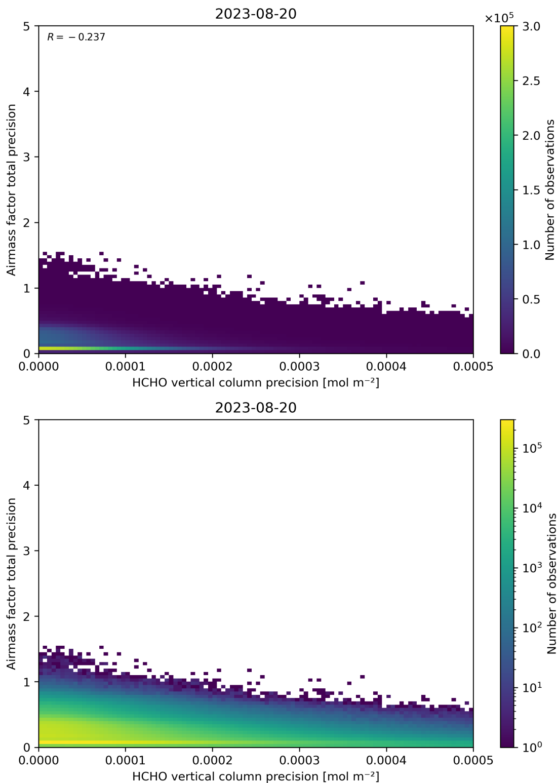
Figure 145: Scatter density plot of “HCHO vertical column precision” against “Airmass factor total precision” for 2023-08-20 to 2023-08-21.
