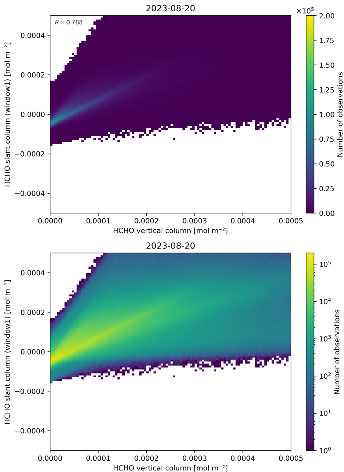
Figure 129: Scatter density plot of “HCHO vertical column” against “HCHO slant column (window1)” for 2023-08-20 to 2023-08-21.
