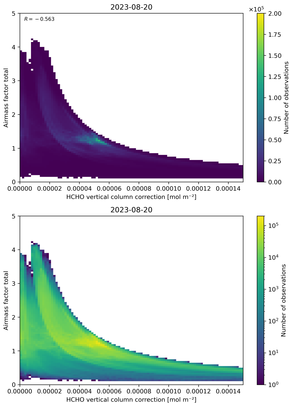
Figure 120: Scatter density plot of “HCHO vertical column correction” against “Airmass factor total” for 2023-08-20 to 2023-08-21.
