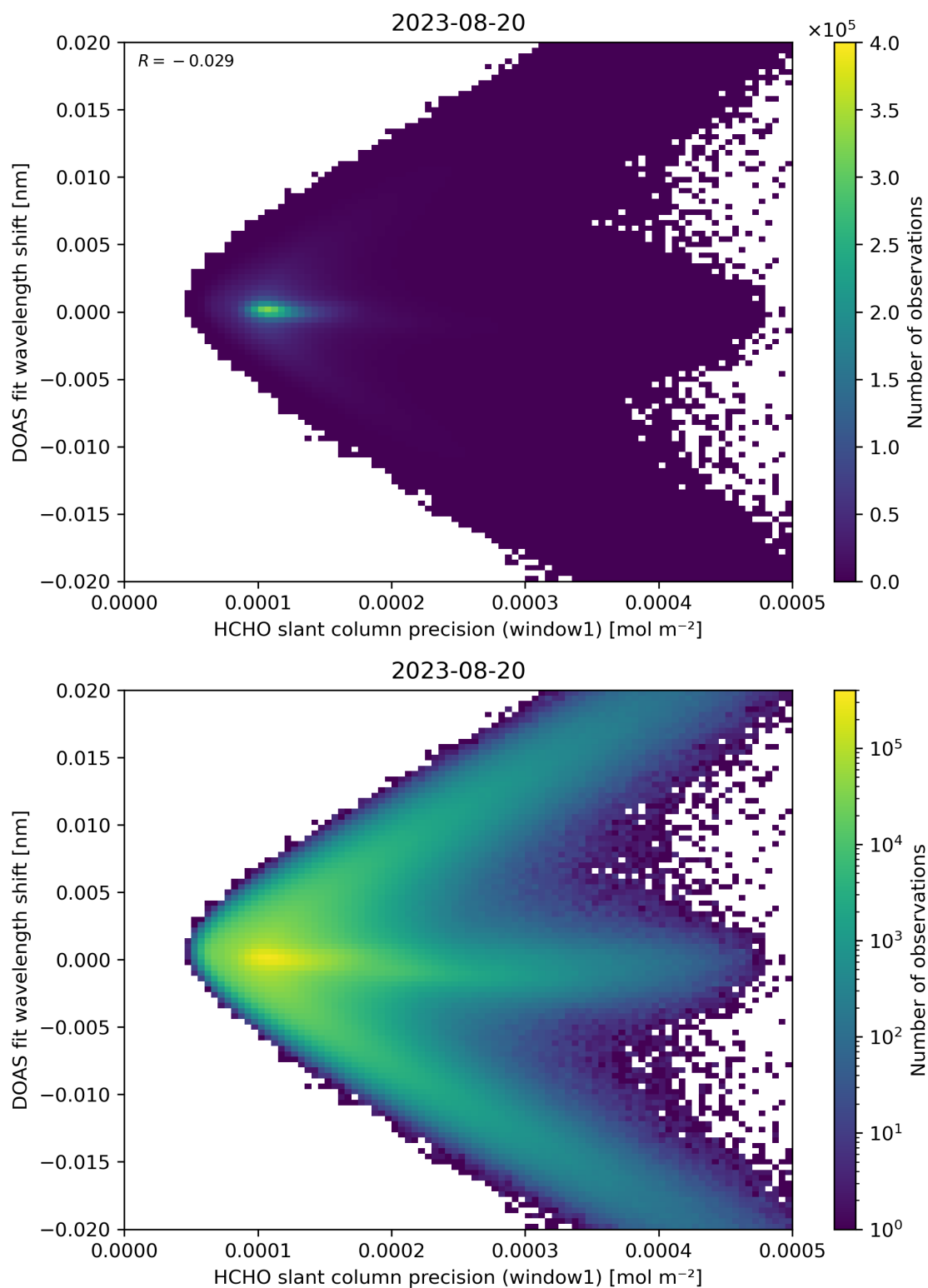
Figure 89: Scatter density plot of “HCHO slant column precision (window1)” against “DOAS fit wavelength shift” for 2023-08-20 to 2023-08-21.
