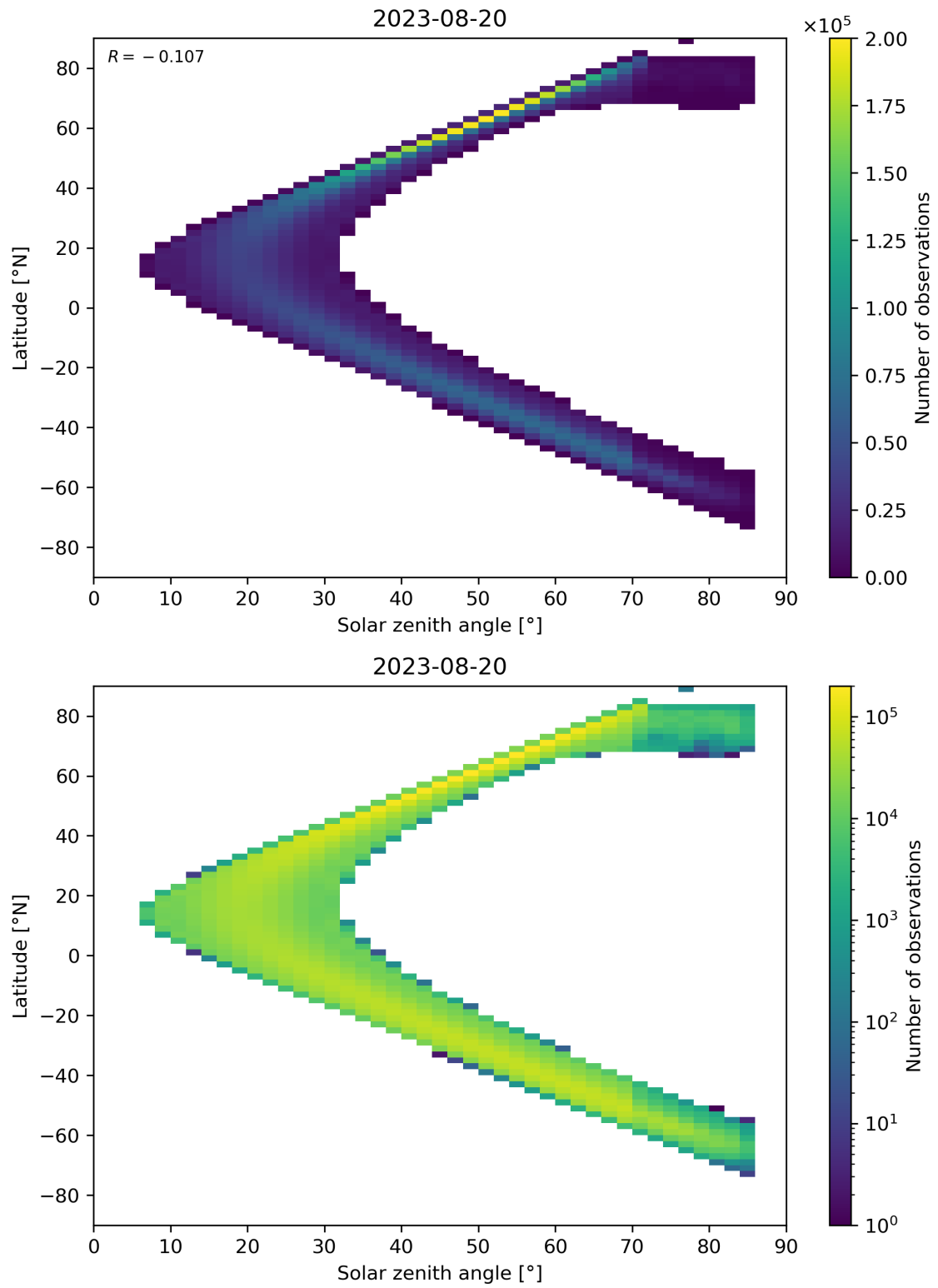
Figure 181: Scatter density plot of “Solar zenith angle” against “Latitude” for 2023-08-20 to 2023-08-21.
