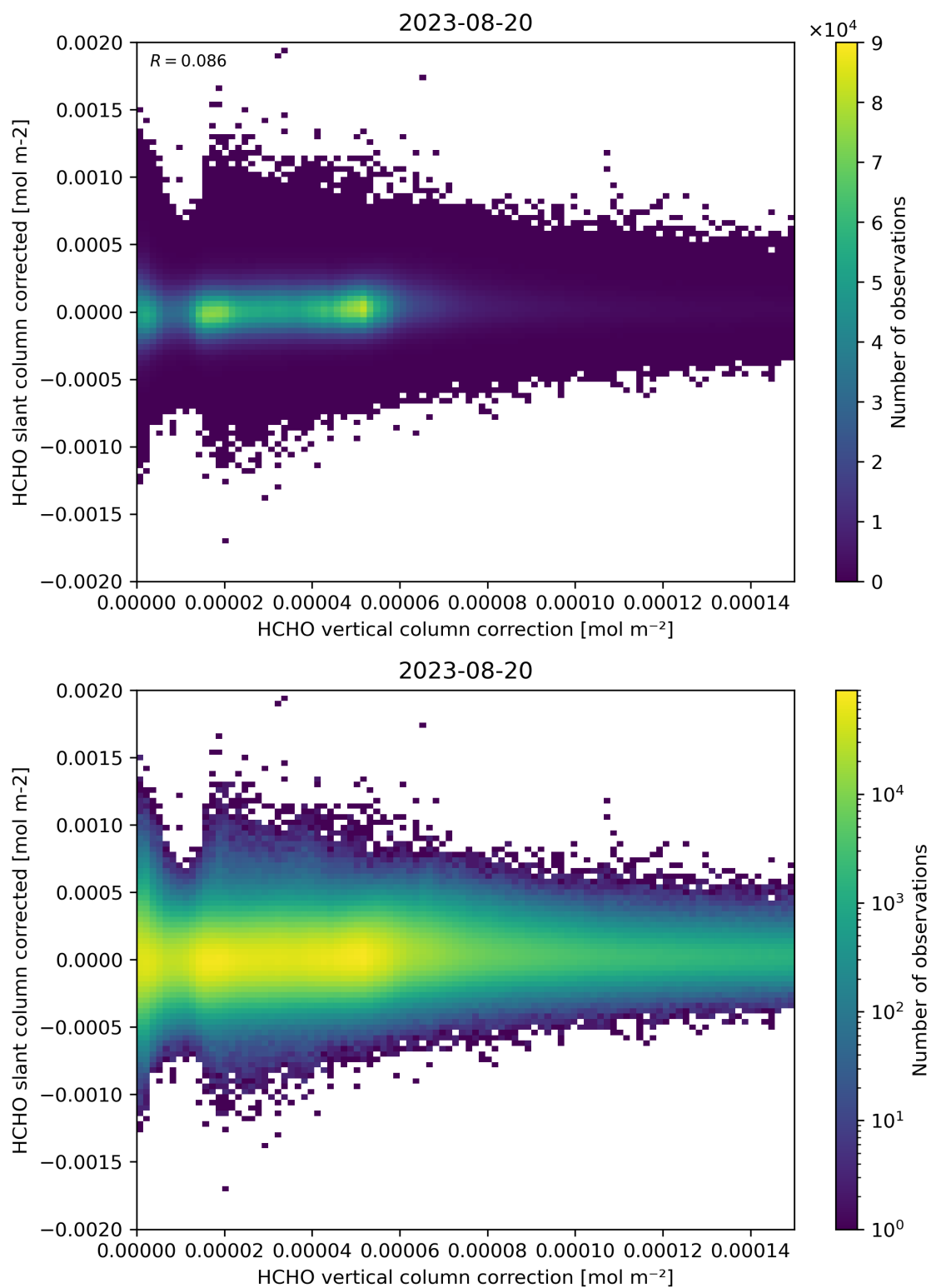
Figure 116: Scatter density plot of “HCHO vertical column correction” against “HCHO slant column corrected” for 2023-08-20 to 2023-08-21.
