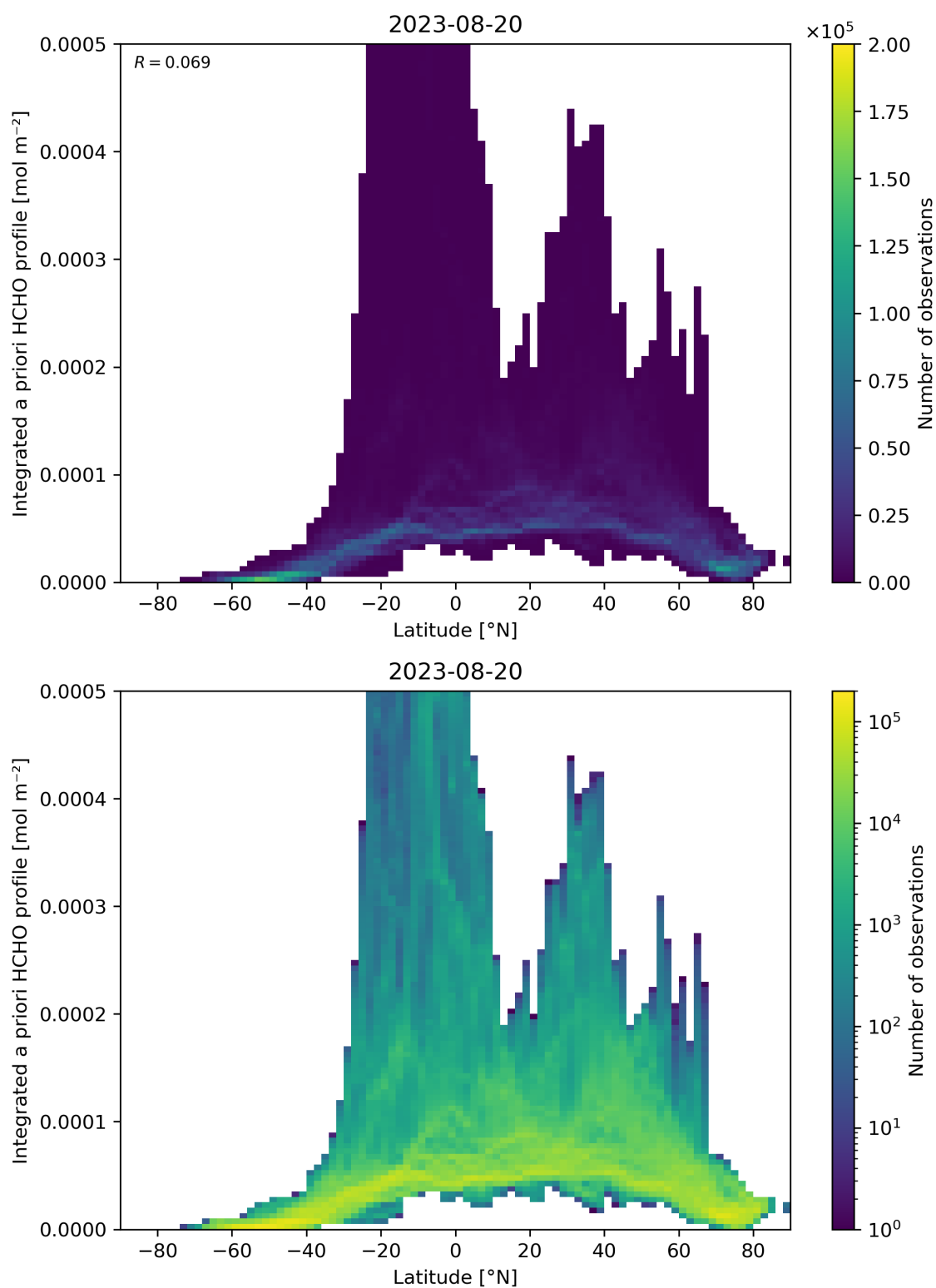
Figure 166: Scatter density plot of “Latitude” against “Integrated a priori HCHO profile” for 2023-08-20 to 2023-08-21.
