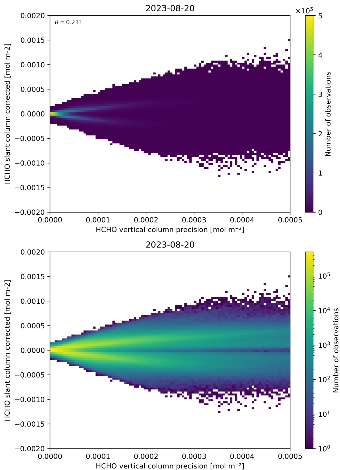
Figure 140: Scatter density plot of “HCHO vertical column precision” against “HCHO slant column corrected” for 2023-08-20 to 2023-08-21.
