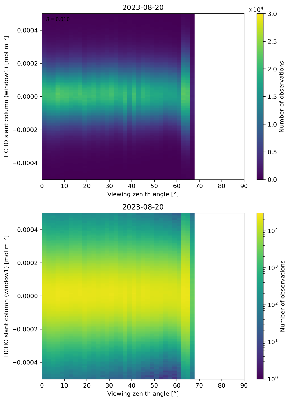
Figure 188: Scatter density plot of “Viewing zenith angle” against “HCHO slant column (window1)” for 2023-08-20 to 2023-08-21.
