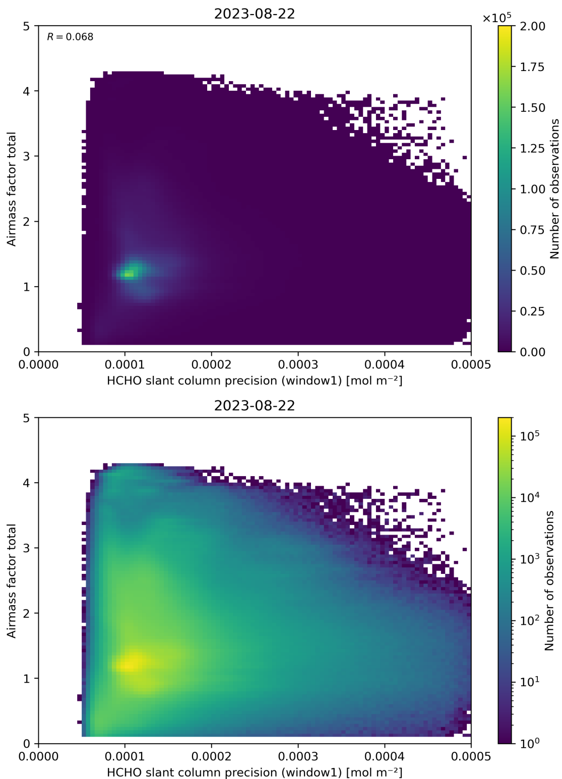
Figure 94: Scatter density plot of “HCHO slant column precision (window1)” against “Airmass factor total” for 2023-08-21 to 2023-08-23.
