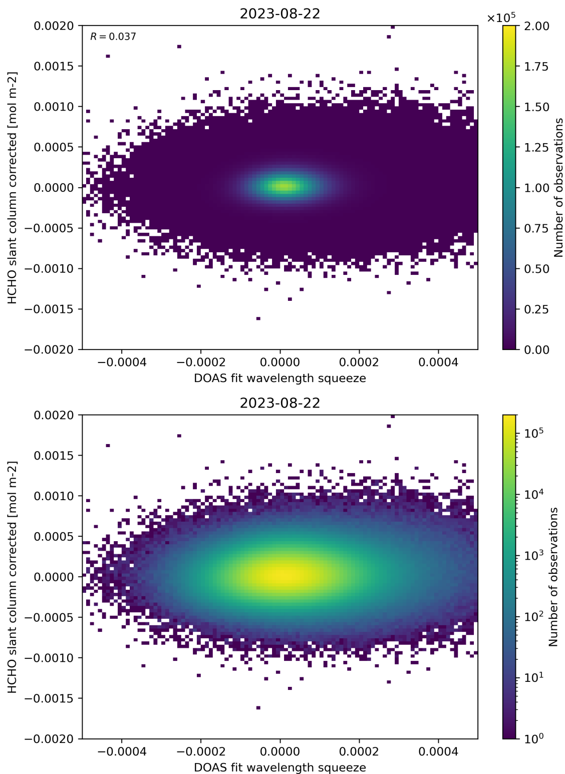
Figure 69: Scatter density plot of “DOAS fit wavelength squeeze” against “HCHO slant column corrected” for 2023-08-21 to 2023-08-23.
