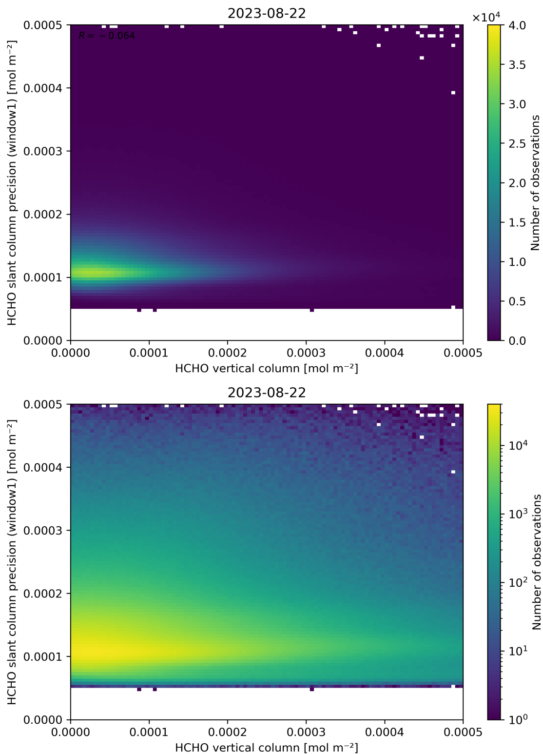
Figure 130: Scatter density plot of “HCHO vertical column” against “HCHO slant column precision (window1)” for 2023-08-21 to 2023-08-23.
