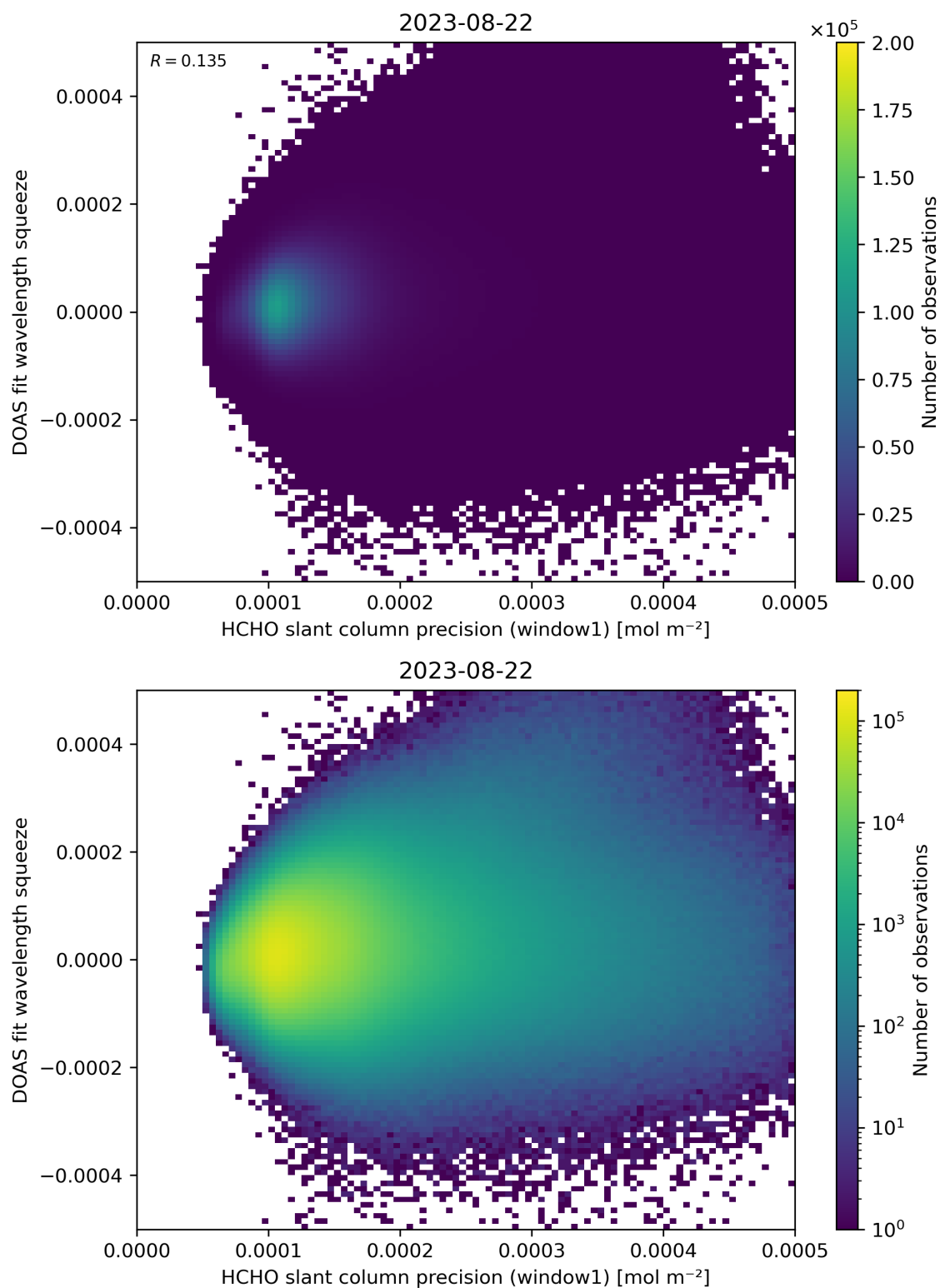
Figure 90: Scatter density plot of “HCHO slant column precision (window1)” against “DOAS fit wavelength squeeze” for 2023-08-21 to 2023-08-23.
