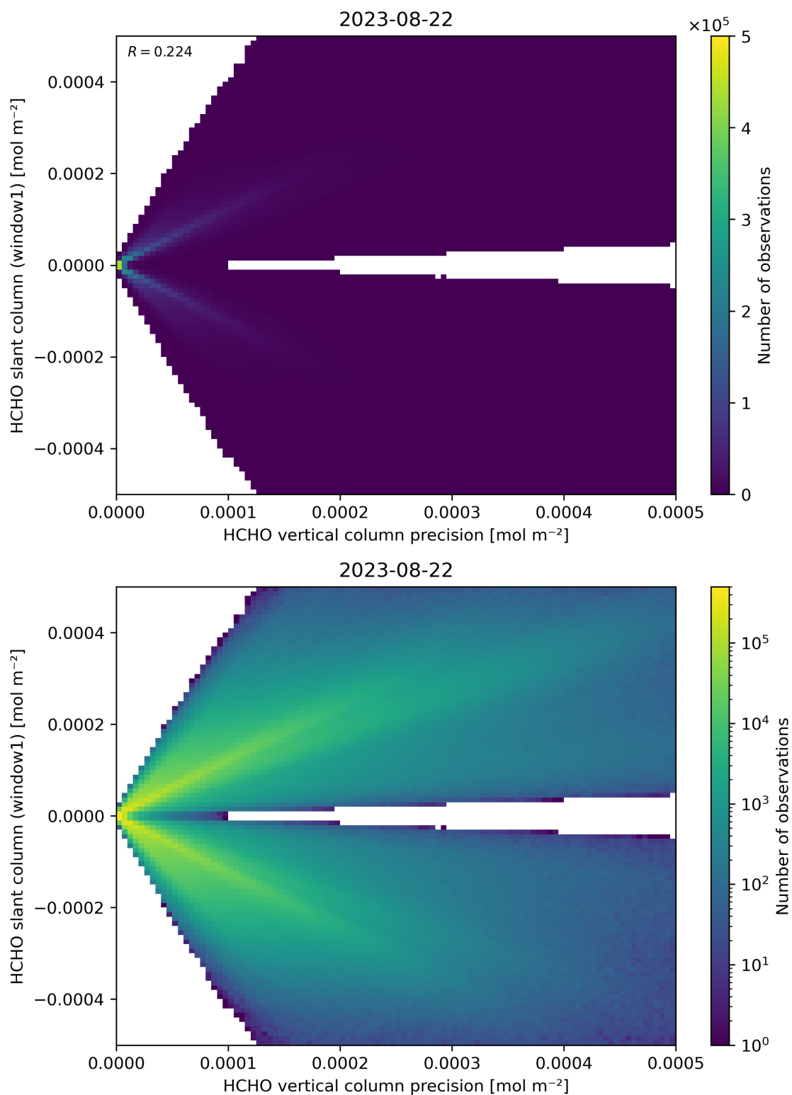
Figure 142: Scatter density plot of “HCHO vertical column precision” against “HCHO slant column (window1)” for 2023-08-21 to 2023-08-23.
