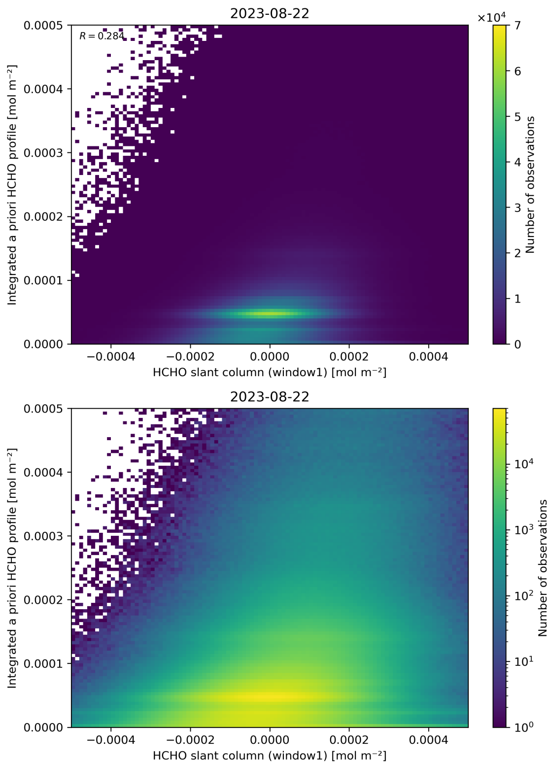
Figure 87: Scatter density plot of “HCHO slant column (window1)” against “Integrated a priori HCHO profile” for 2023-08-21 to 2023-08-23.
