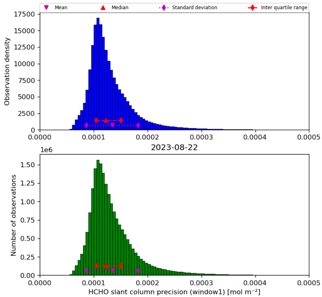
Figure 39: Histogram of “HCHO slant column precision (window1)” for 2023-08-21 to 2023-08-23
