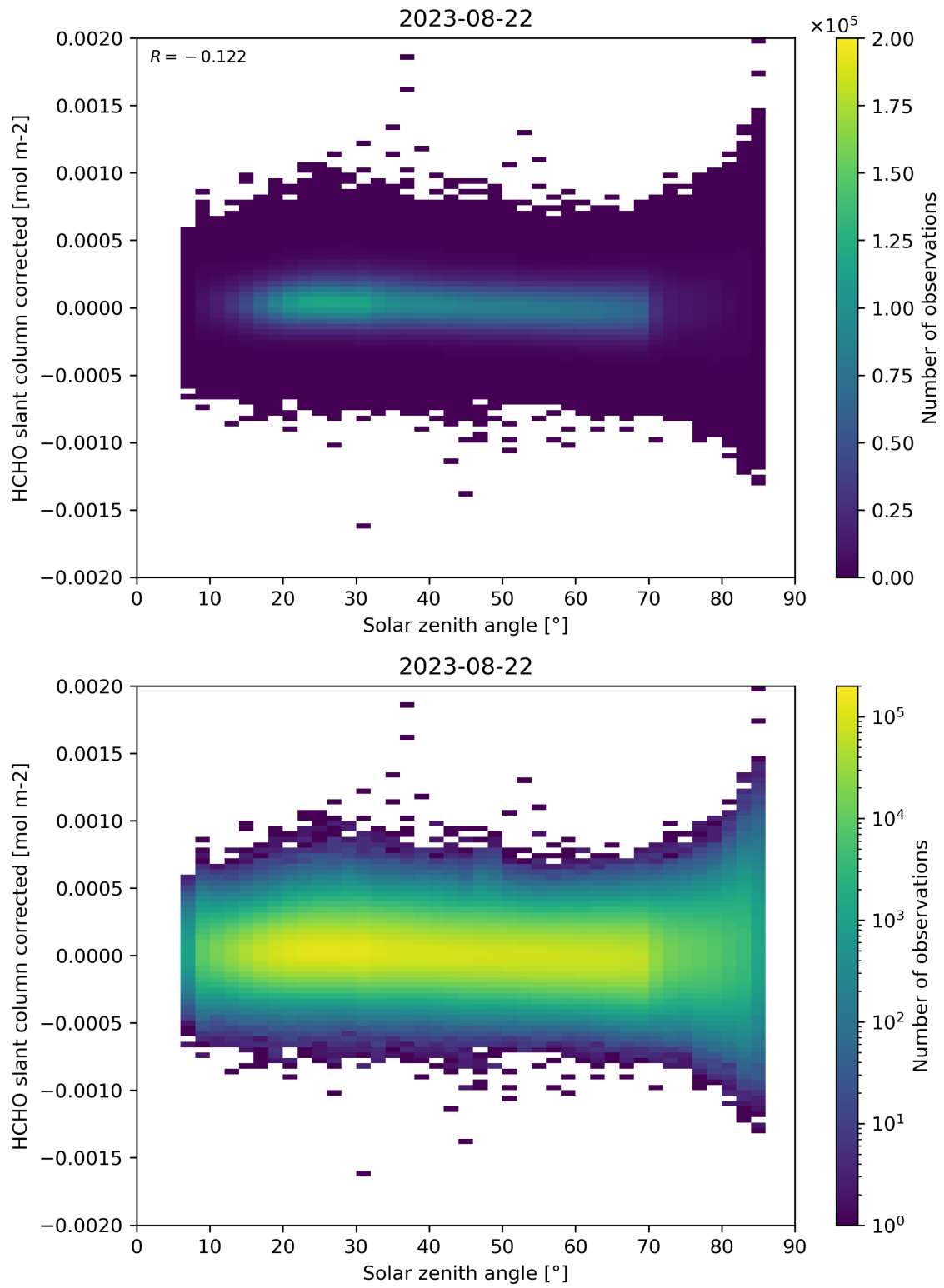
Figure 171: Scatter density plot of “Solar zenith angle” against “HCHO slant column corrected” for 2023-08-21 to 2023-08-23.
