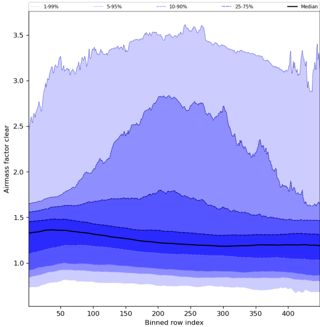
Figure 56: Along track statistics of “Airmass factor clear” for 2023-08-21 to 2023-08-23
