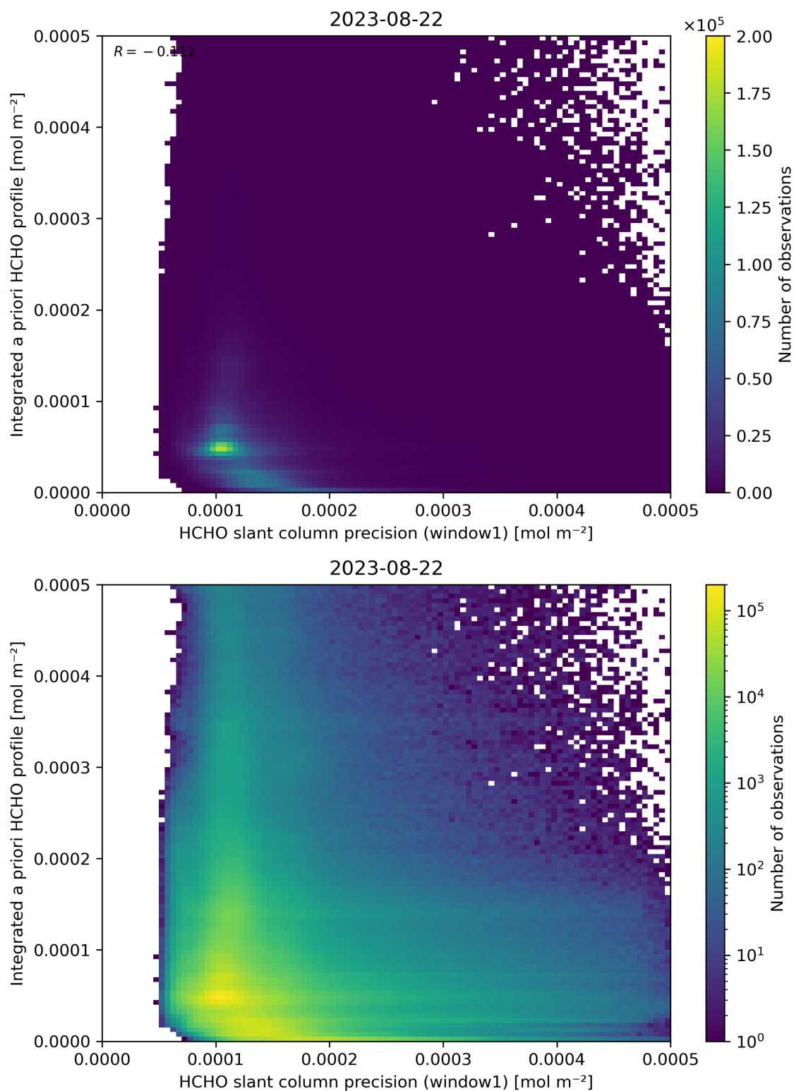
Figure 96: Scatter density plot of “HCHO slant column precision (window1)” against “Integrated a priori HCHO profile” for 2023-08-21 to 2023-08-23.
