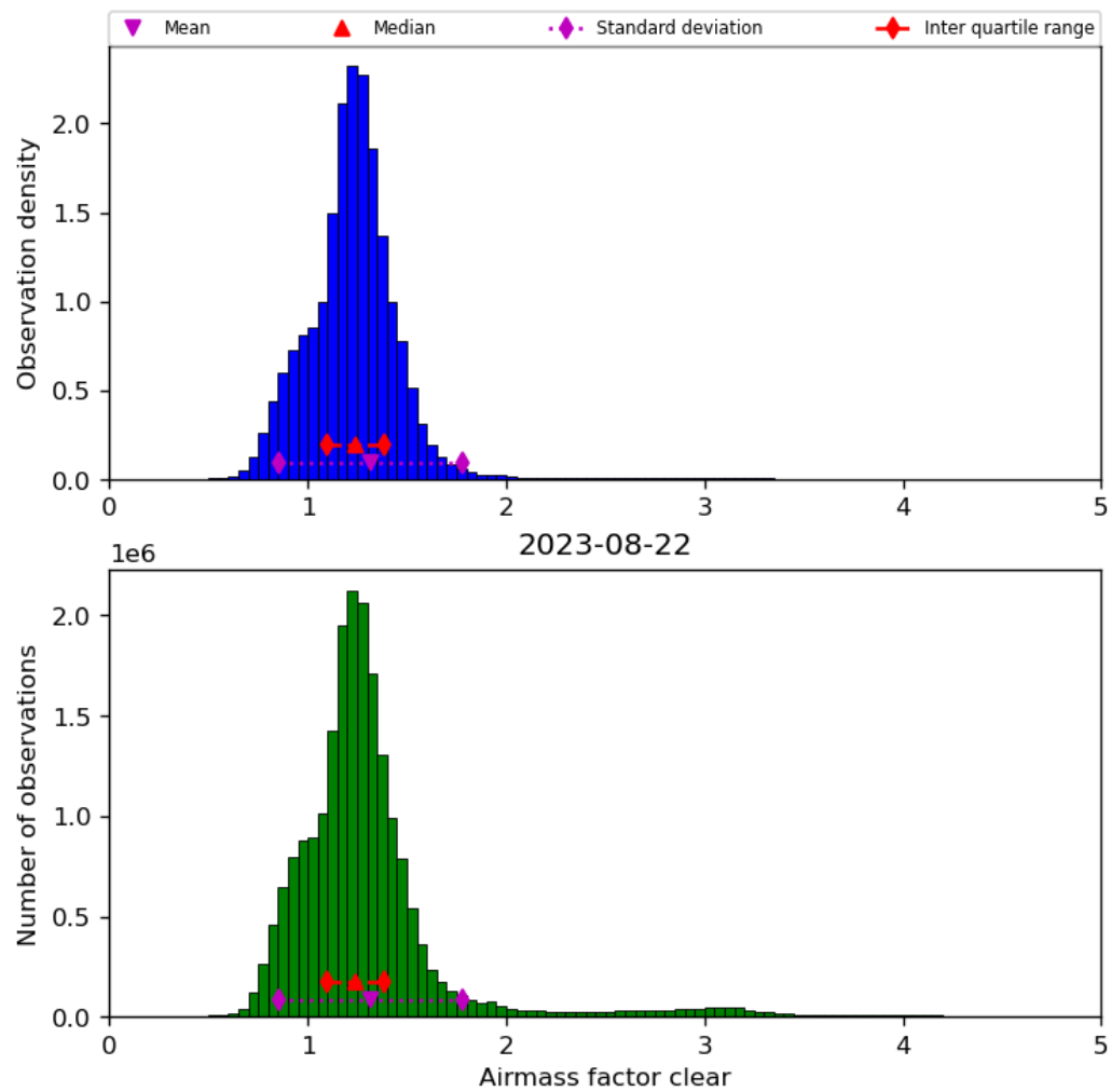
Figure 42: Histogram of “Airmass factor clear” for 2023-08-21 to 2023-08-23
