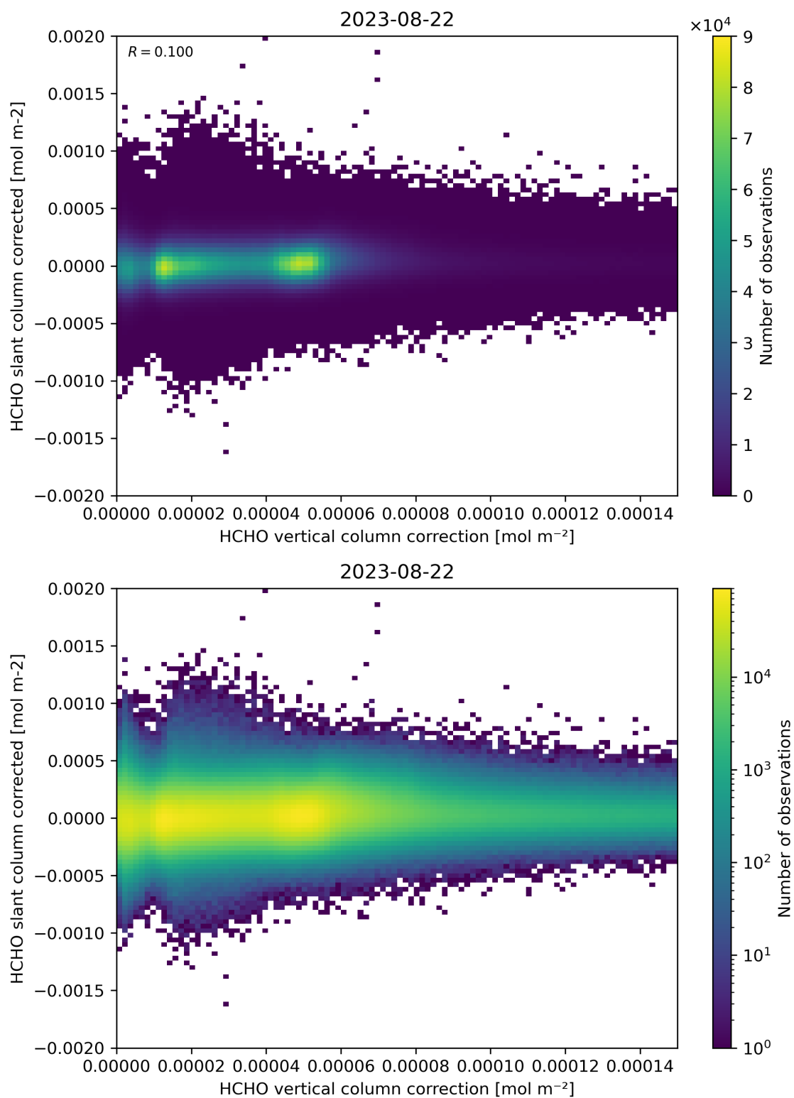
Figure 116: Scatter density plot of “HCHO vertical column correction” against “HCHO slant column corrected” for 2023-08-21 to 2023-08-23.
