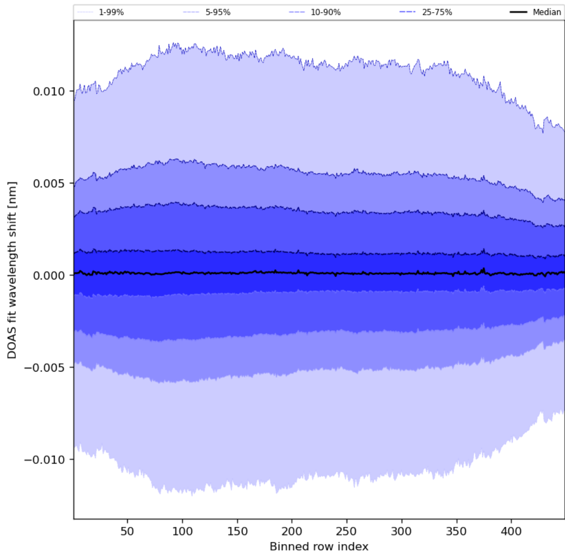
Figure 58: Along track statistics of “DOAS fit wavelength shift” for 2023-08-21 to 2023-08-23
