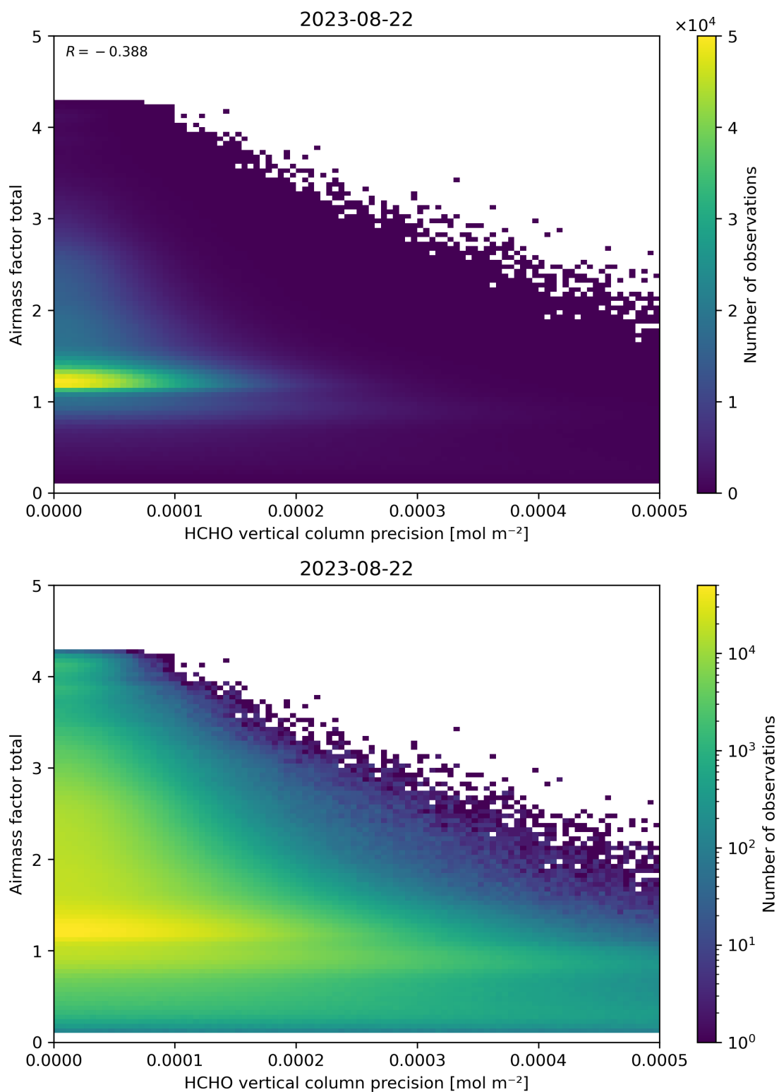
Figure 144: Scatter density plot of “HCHO vertical column precision” against “Airmass factor total” for 2023-08-21 to 2023-08-23.
