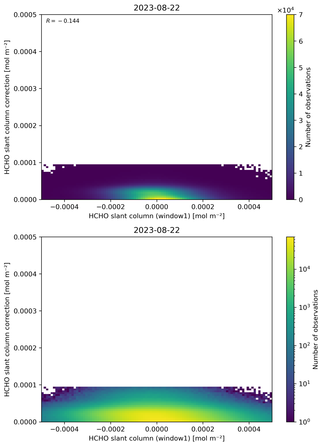
Figure 83: Scatter density plot of “HCHO slant column (window1)” against “HCHO slant column correction” for 2023-08-21 to 2023-08-23.
