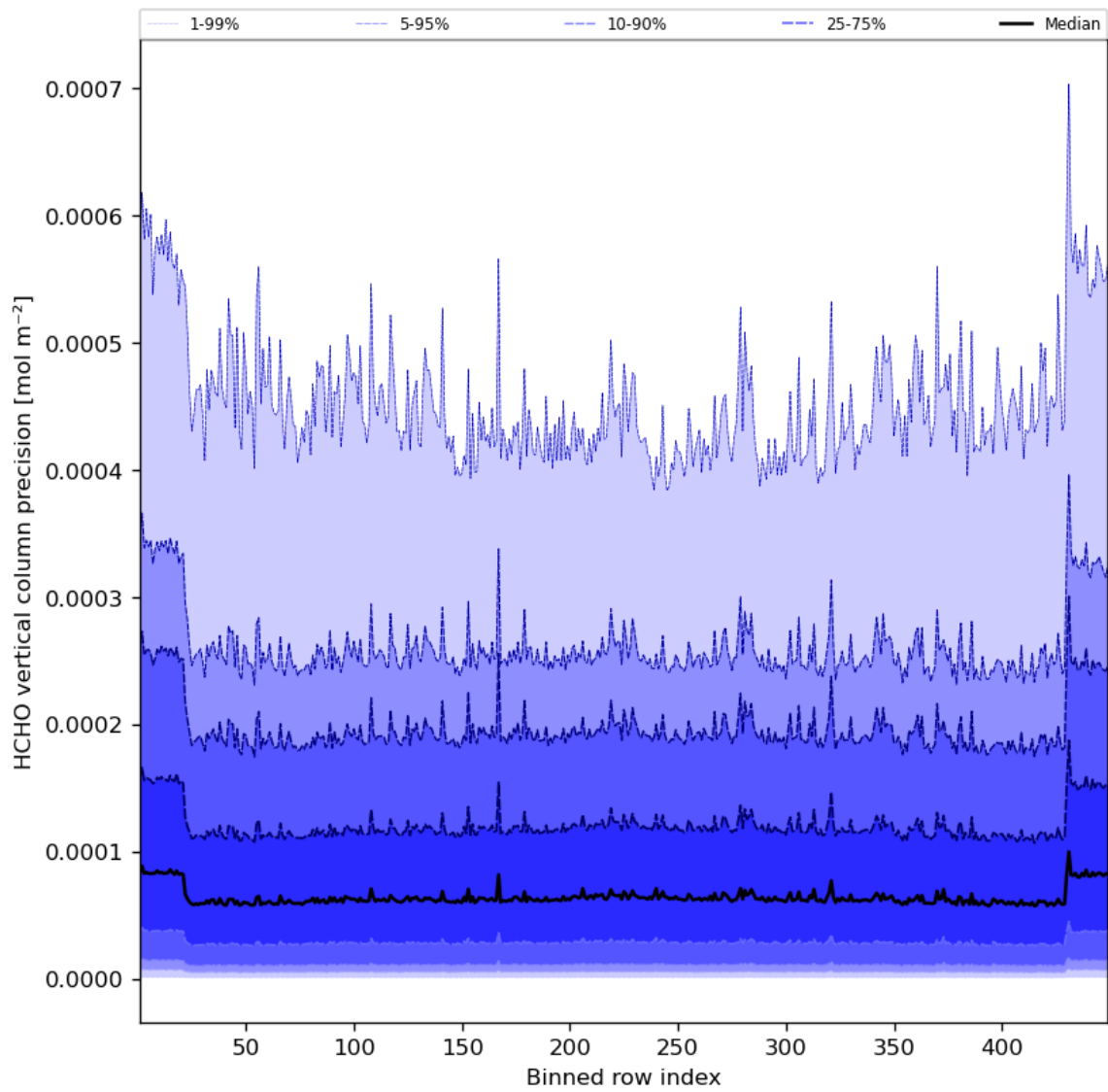
Figure 50: Along track statistics of “HCHO vertical column precision” for 2023-08-21 to 2023-08-23
