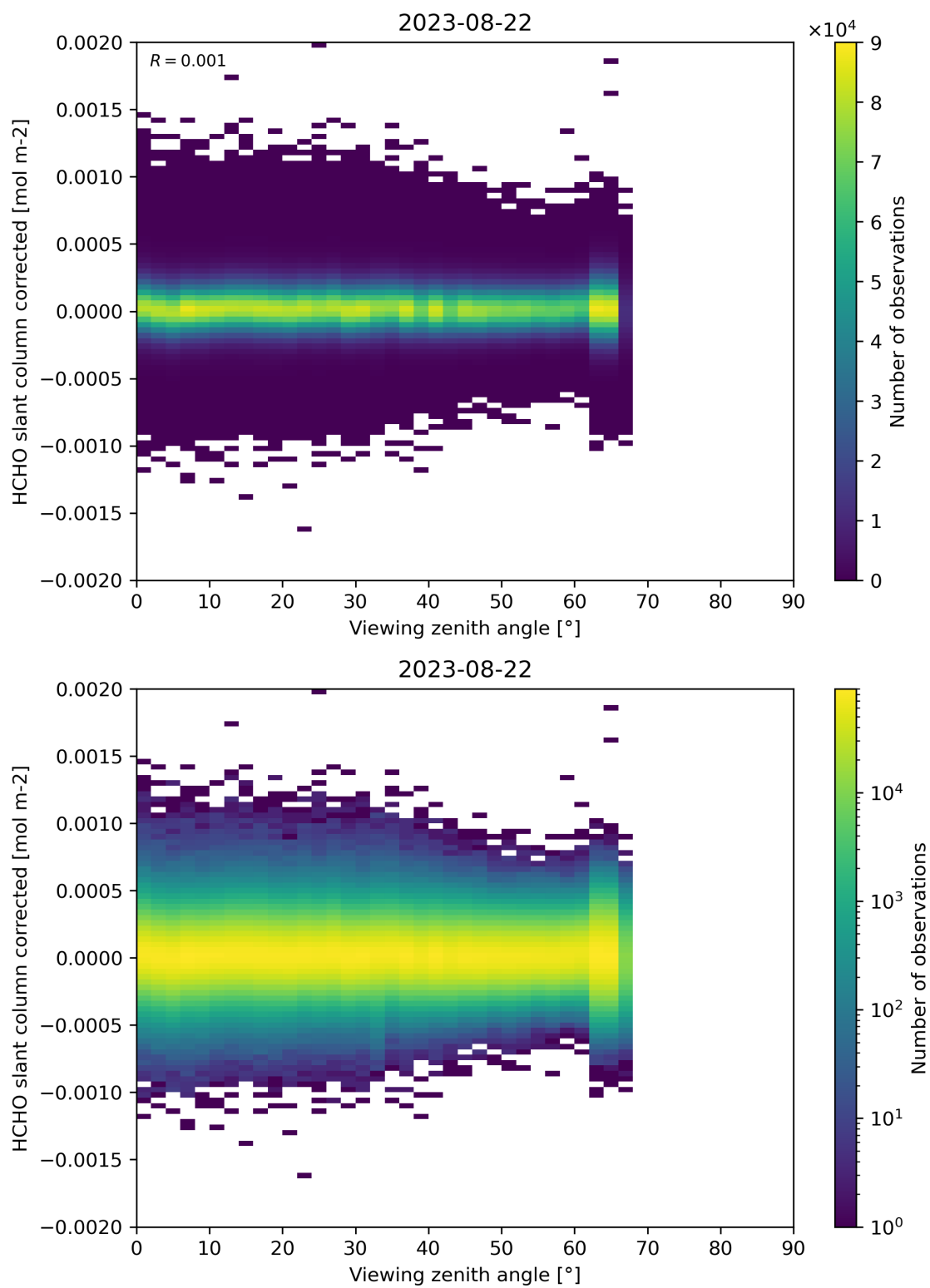
Figure 186: Scatter density plot of “Viewing zenith angle” against “HCHO slant column corrected” for 2023-08-21 to 2023-08-23.
