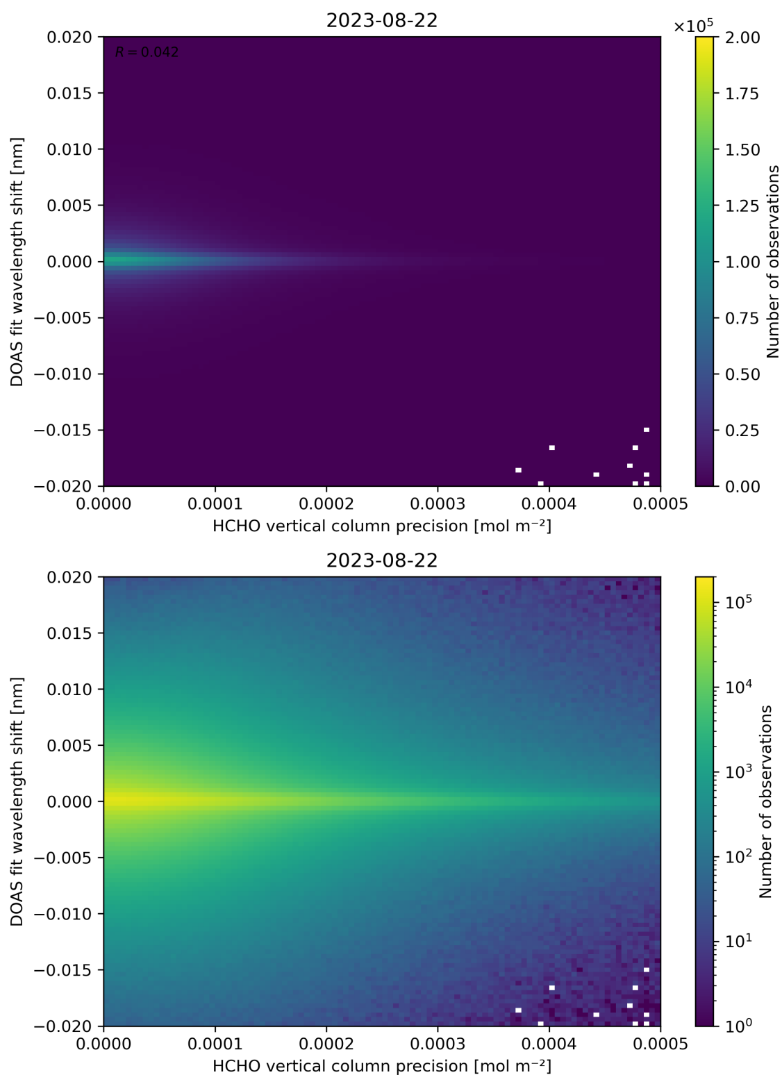
Figure 137: Scatter density plot of “HCHO vertical column precision” against “DOAS fit wavelength shift” for 2023-08-21 to 2023-08-23.
