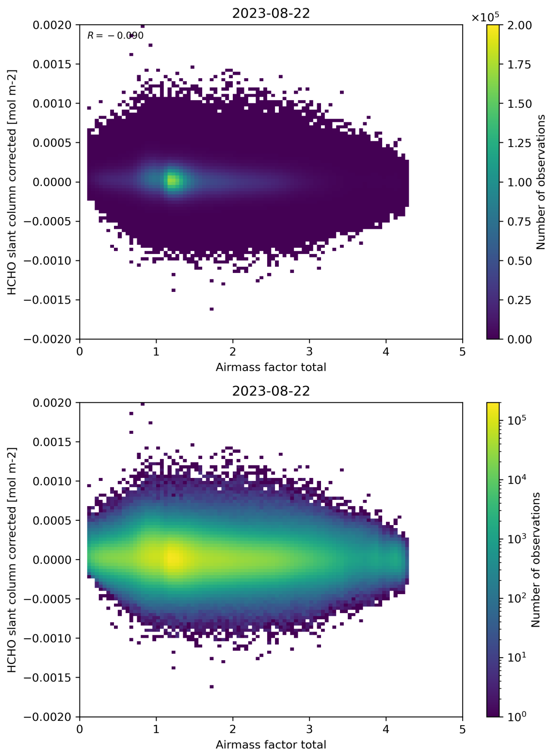
Figure 101: Scatter density plot of “Airmass factor total” against “HCHO slant column corrected” for 2023-08-21 to 2023-08-23.
