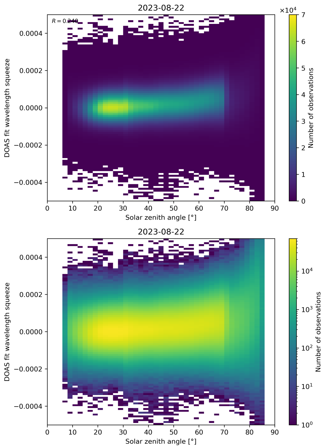
Figure 169: Scatter density plot of “Solar zenith angle” against “DOAS fit wavelength squeeze” for 2023-08-21 to 2023-08-23.
