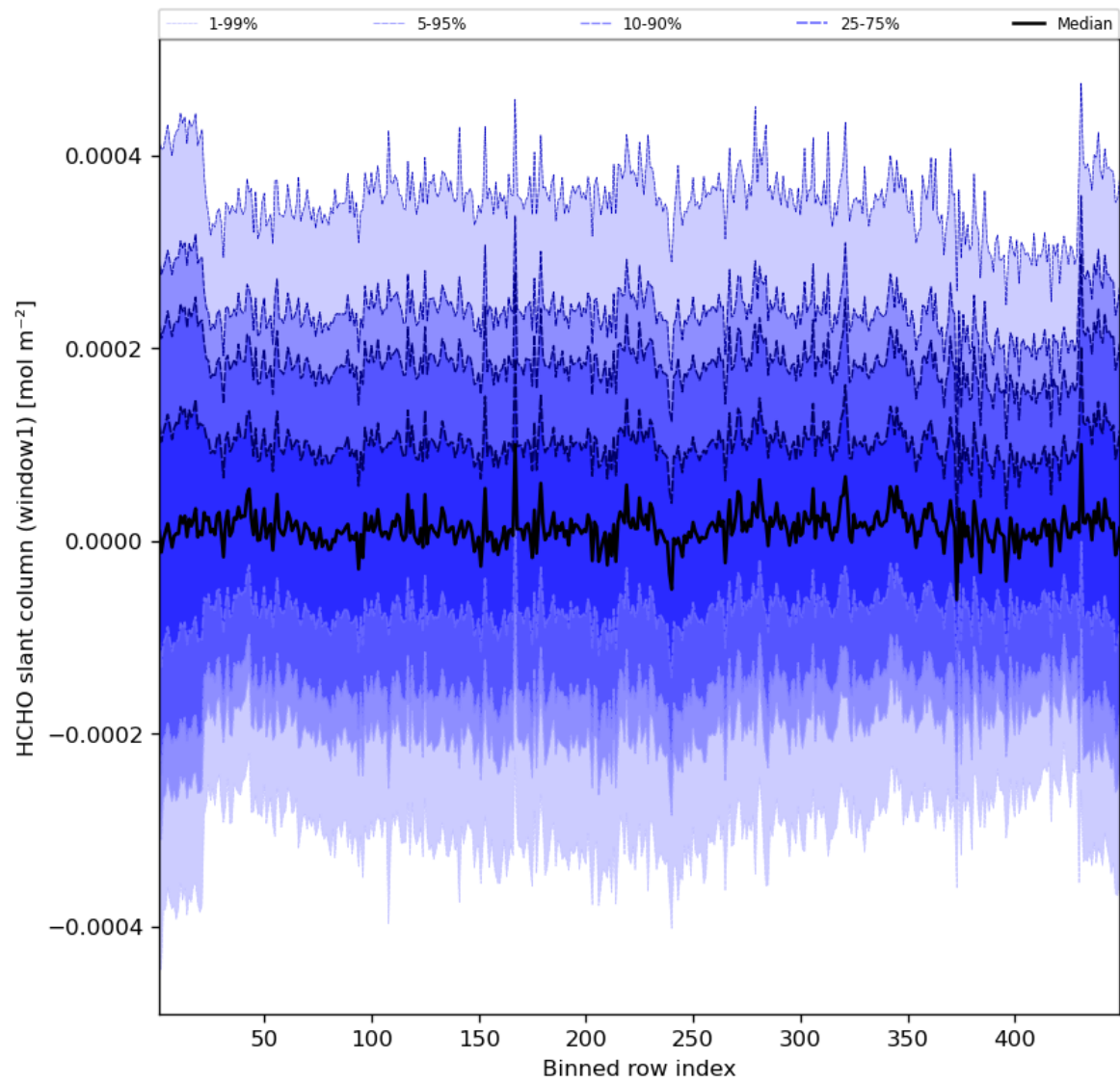
Figure 52: Along track statistics of “HCHO slant column (window1)” for 2023-08-21 to 2023-08-23
