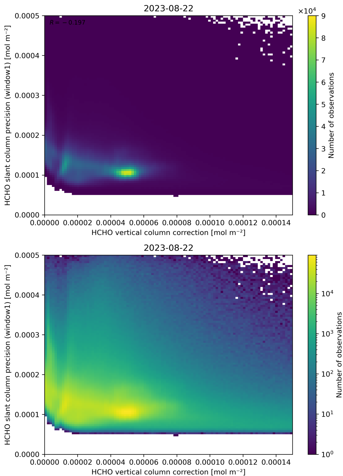
Figure 119: Scatter density plot of “HCHO vertical column correction” against “HCHO slant column precision (window1)” for 2023-08-21 to 2023-08-23.
