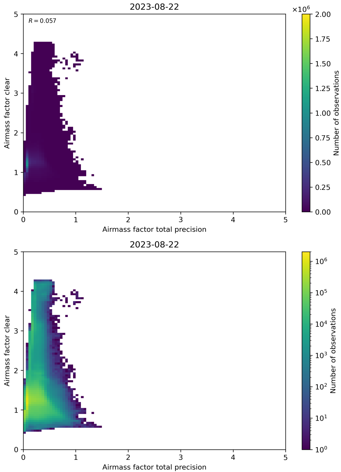
Figure 108: Scatter density plot of “Airmass factor total precision” against “Airmass factor clear” for 2023-08-21 to 2023-08-23.
