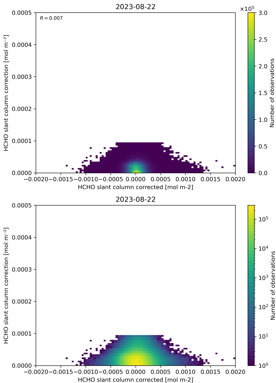
Figure 77: Scatter density plot of “HCHO slant column corrected” against “HCHO slant column correction” for 2023-08-21 to 2023-08-23.
