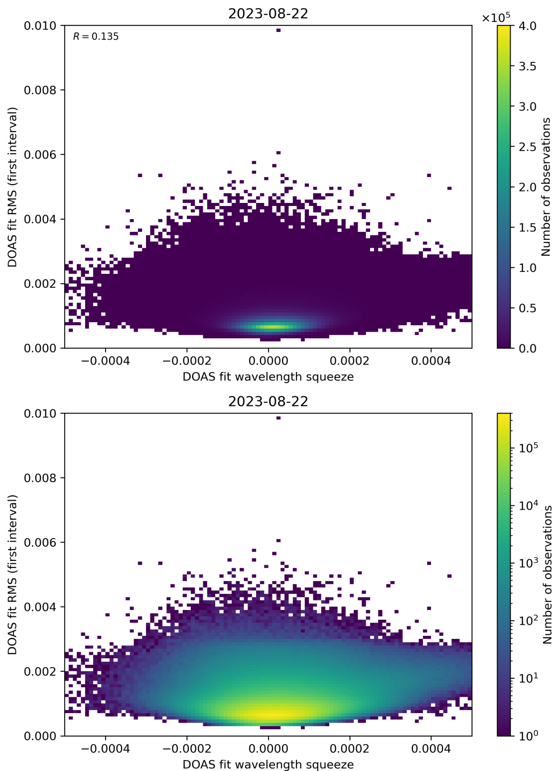
Figure 68: Scatter density plot of “DOAS fit wavelength squeeze” against “DOAS fit RMS (first interval)” for 2023-08-21 to 2023-08-23.
