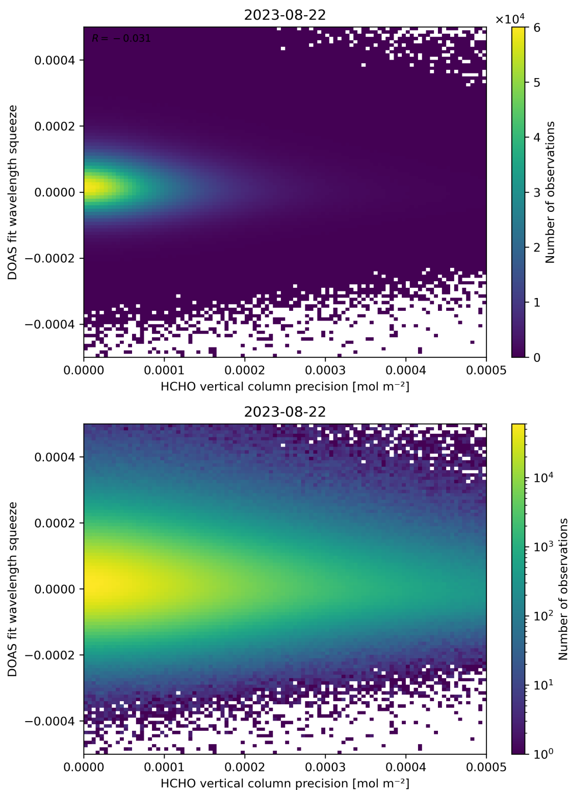
Figure 138: Scatter density plot of “HCHO vertical column precision” against “DOAS fit wavelength squeeze” for 2023-08-21 to 2023-08-23.
