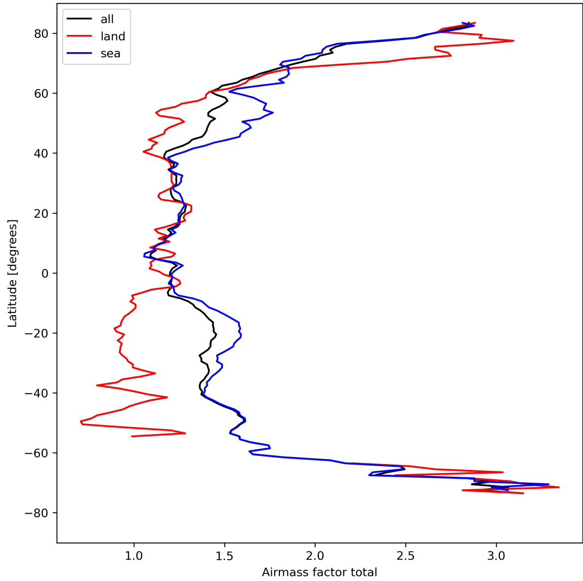
Figure 26: Zonal average of “Airmass factor total” for 2023-08-21 to 2023-08-23.
