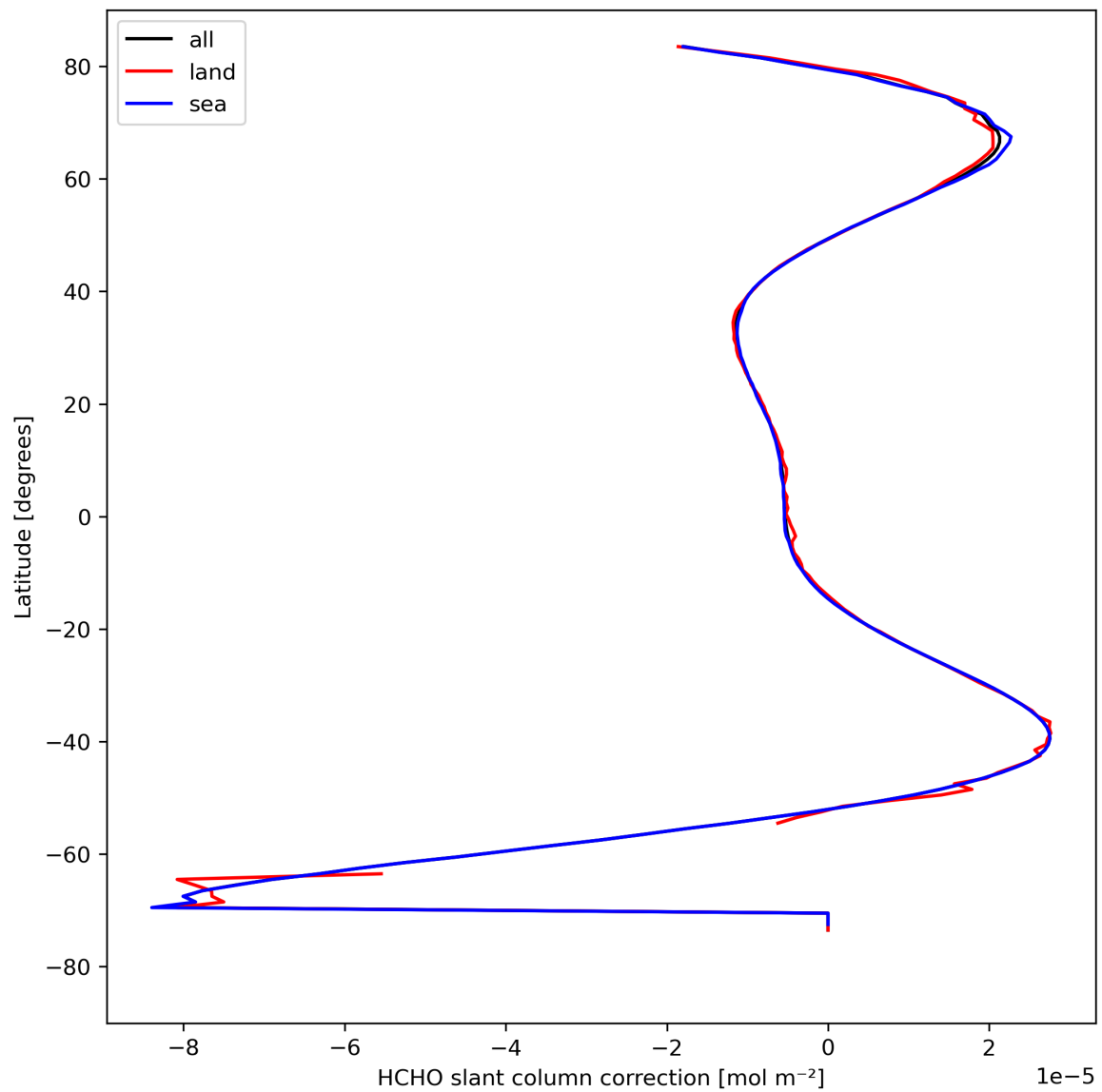
Figure 33: Zonal average of “HCHO slant column correction” for 2023-08-21 to 2023-08-23.
