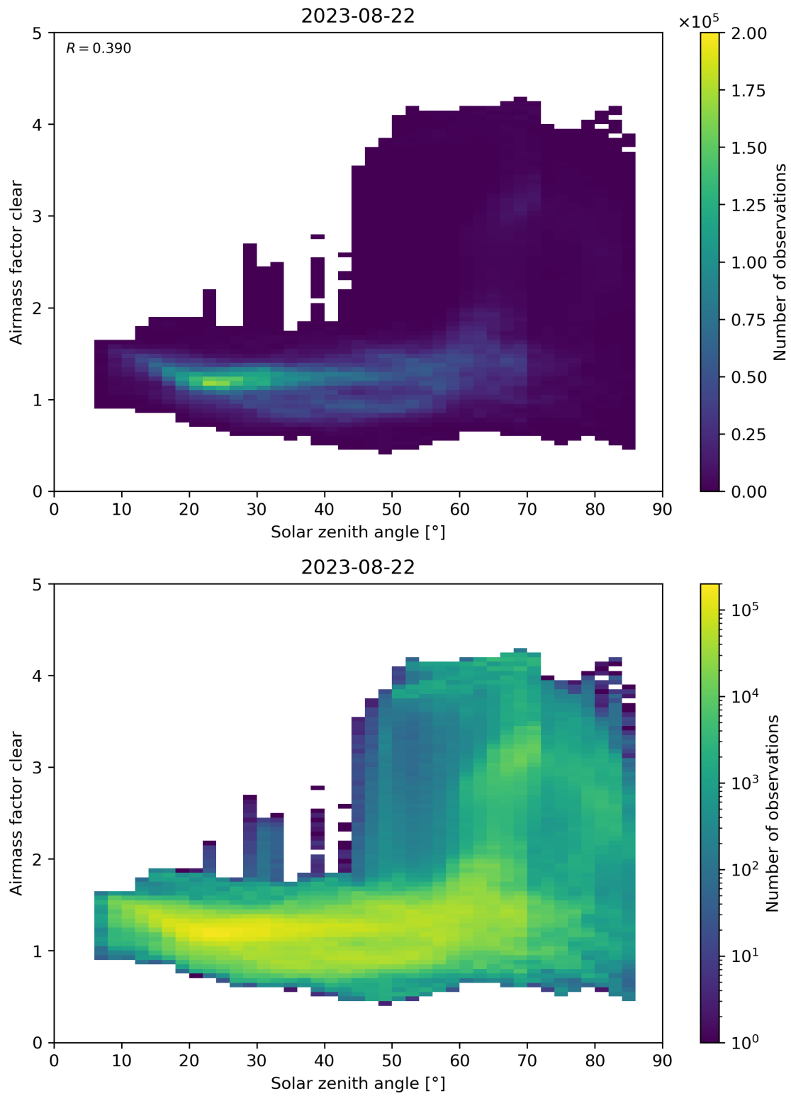
Figure 170: Scatter density plot of “Solar zenith angle” against “Airmass factor clear” for 2023-08-21 to 2023-08-23.
