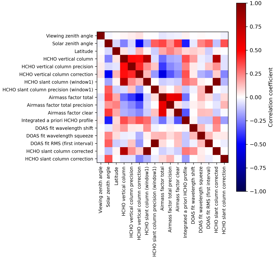
Figure 2: Map of correlation matrix for 2023-08-21 to 2023-08-23.
