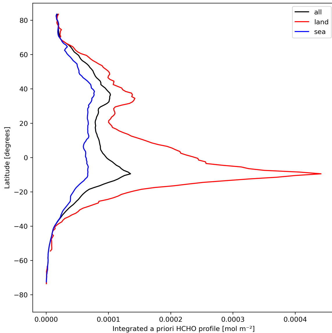
Figure 29: Zonal average of “Integrated a priori HCHO profile” for 2023-08-21 to 2023-08-23.
