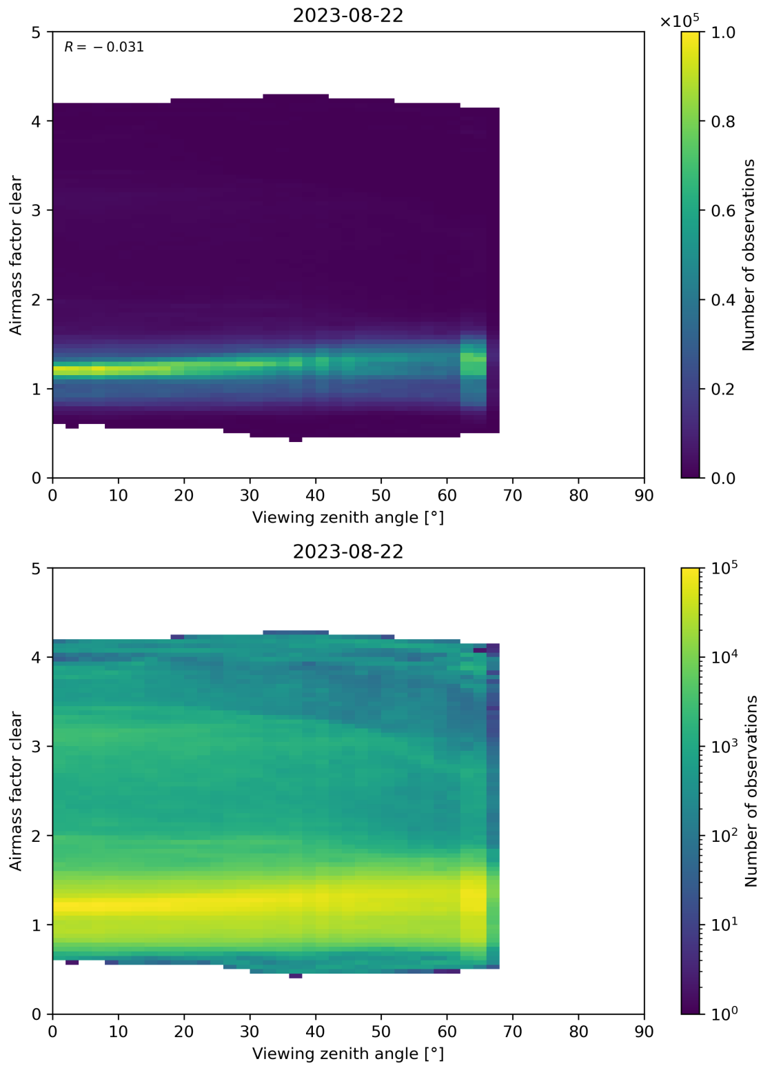
Figure 185: Scatter density plot of “Viewing zenith angle” against “Airmass factor clear” for 2023-08-21 to 2023-08-23.
