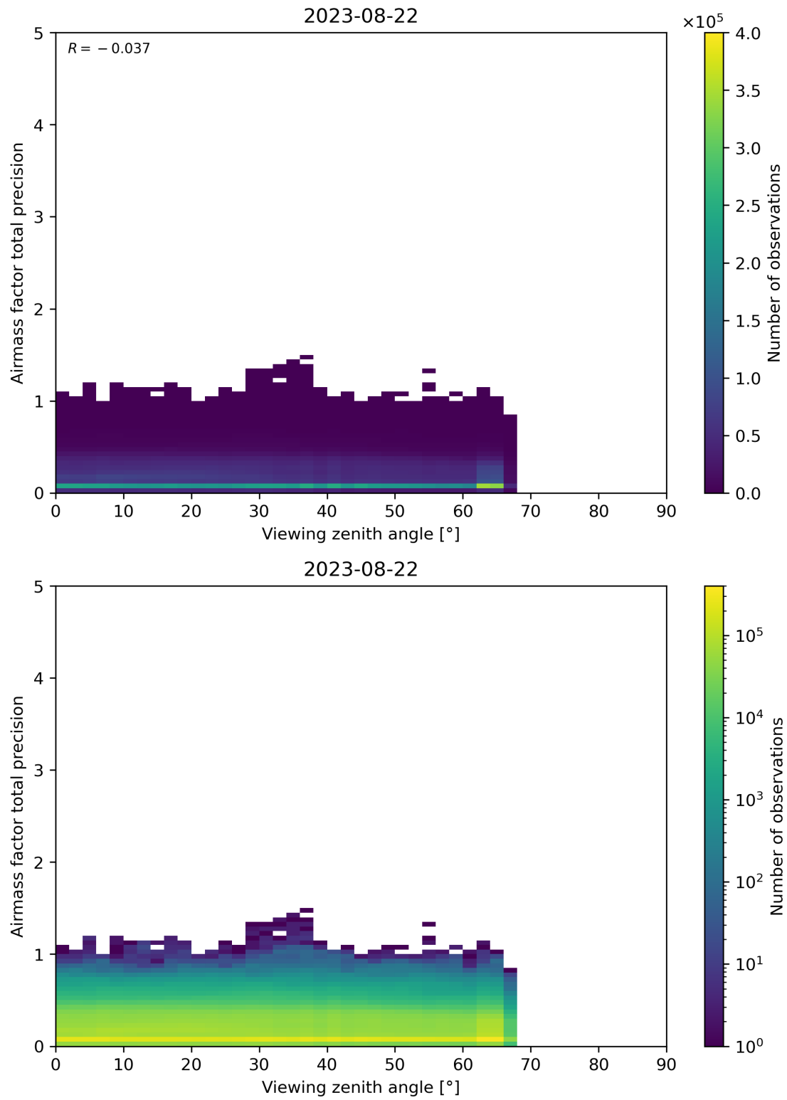
Figure 191: Scatter density plot of “Viewing zenith angle” against “Airmass factor total precision” for 2023-08-21 to 2023-08-23.
