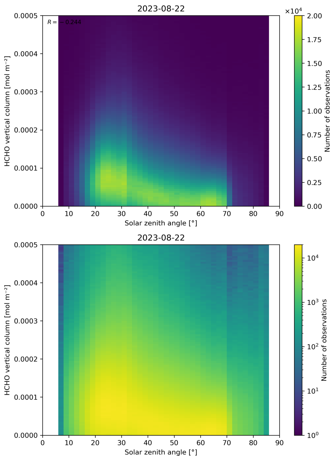
Figure 177: Scatter density plot of “Solar zenith angle” against “HCHO vertical column” for 2023-08-21 to 2023-08-23.
