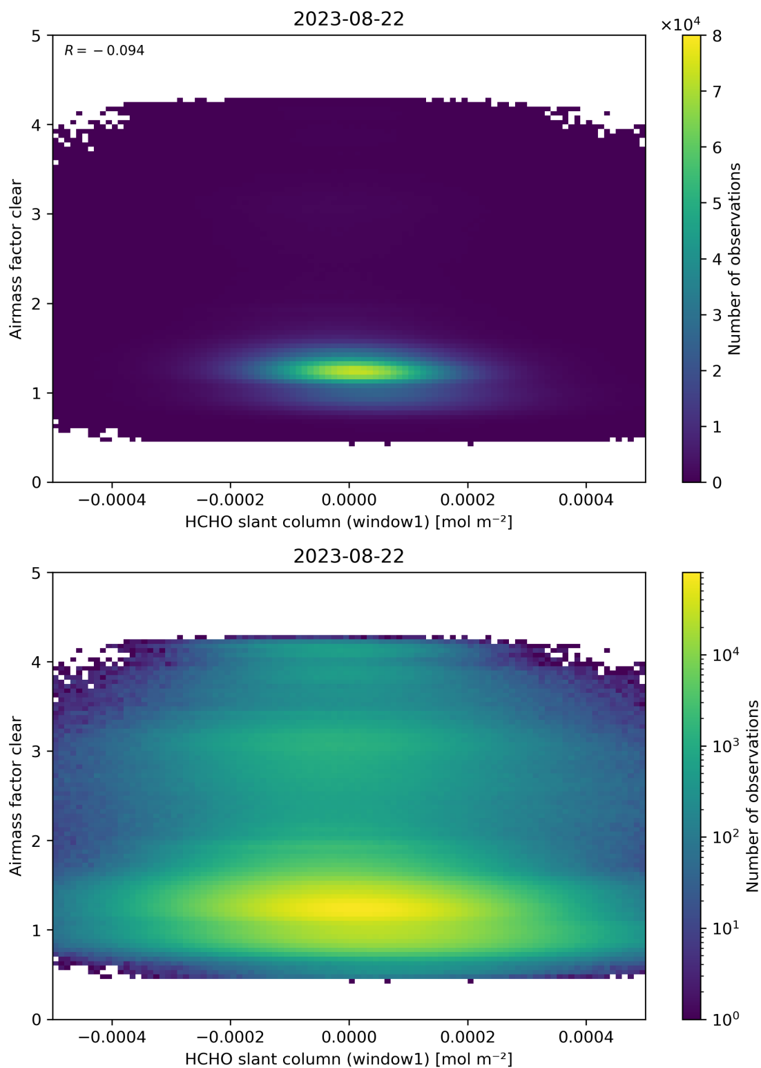
Figure 81: Scatter density plot of “HCHO slant column (window1)” against “Airmass factor clear” for 2023-08-21 to 2023-08-23.
