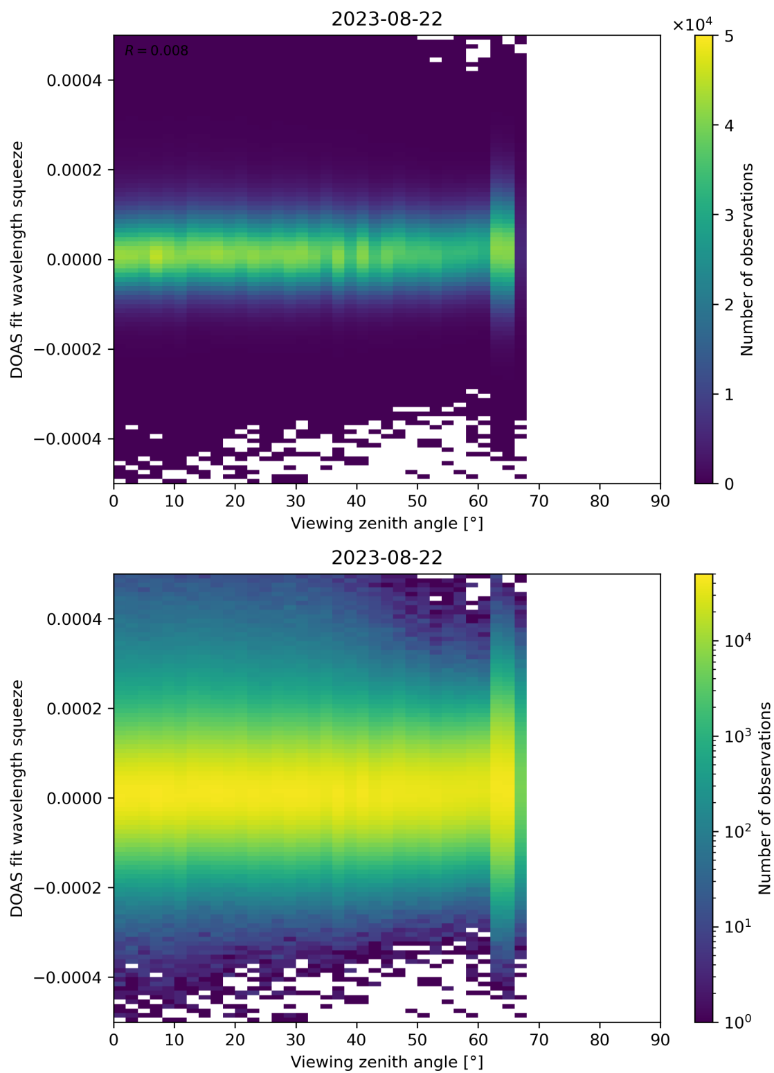
Figure 184: Scatter density plot of “Viewing zenith angle” against “DOAS fit wavelength squeeze” for 2023-08-21 to 2023-08-23.
