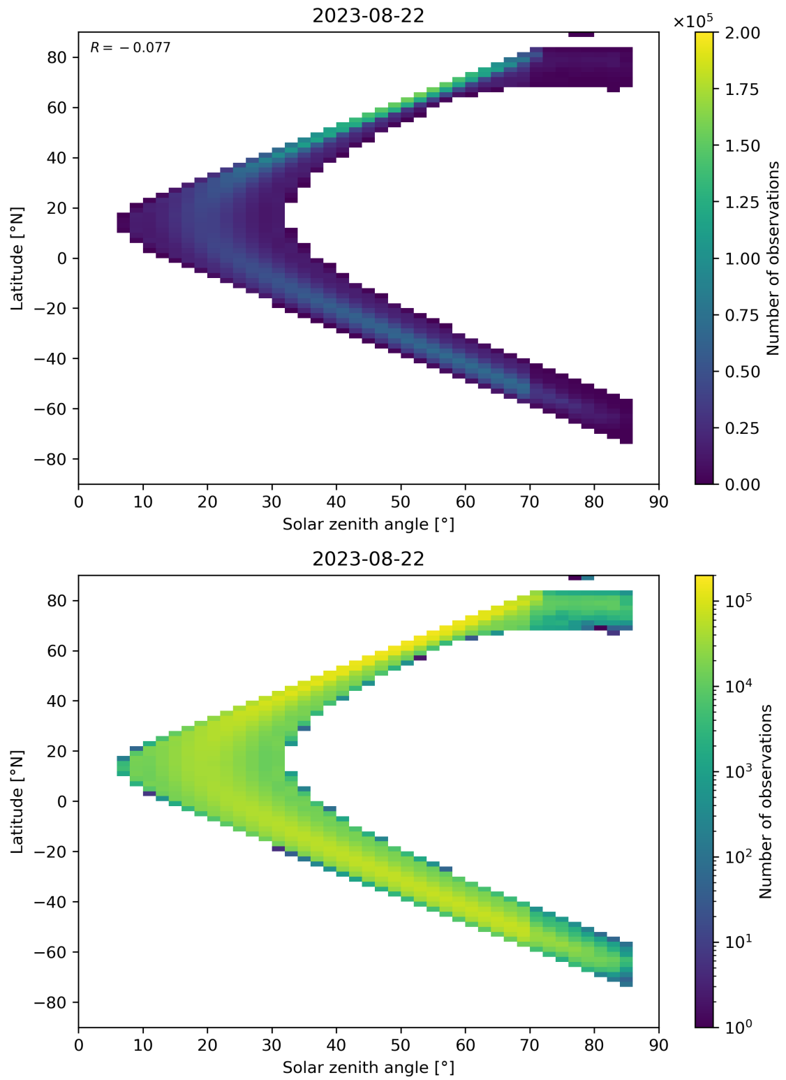
Figure 181: Scatter density plot of “Solar zenith angle” against “Latitude” for 2023-08-21 to 2023-08-23.
