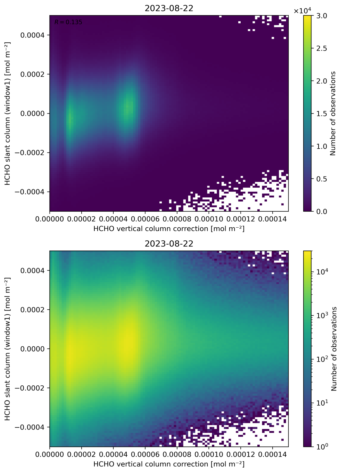
Figure 118: Scatter density plot of “HCHO vertical column correction” against “HCHO slant column (window1)” for 2023-08-21 to 2023-08-23.
