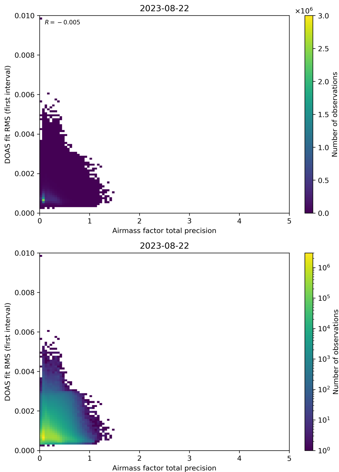
Figure 105: Scatter density plot of “Airmass factor total precision” against “DOAS fit RMS (first interval)” for 2023-08-21 to 2023-08-23.
