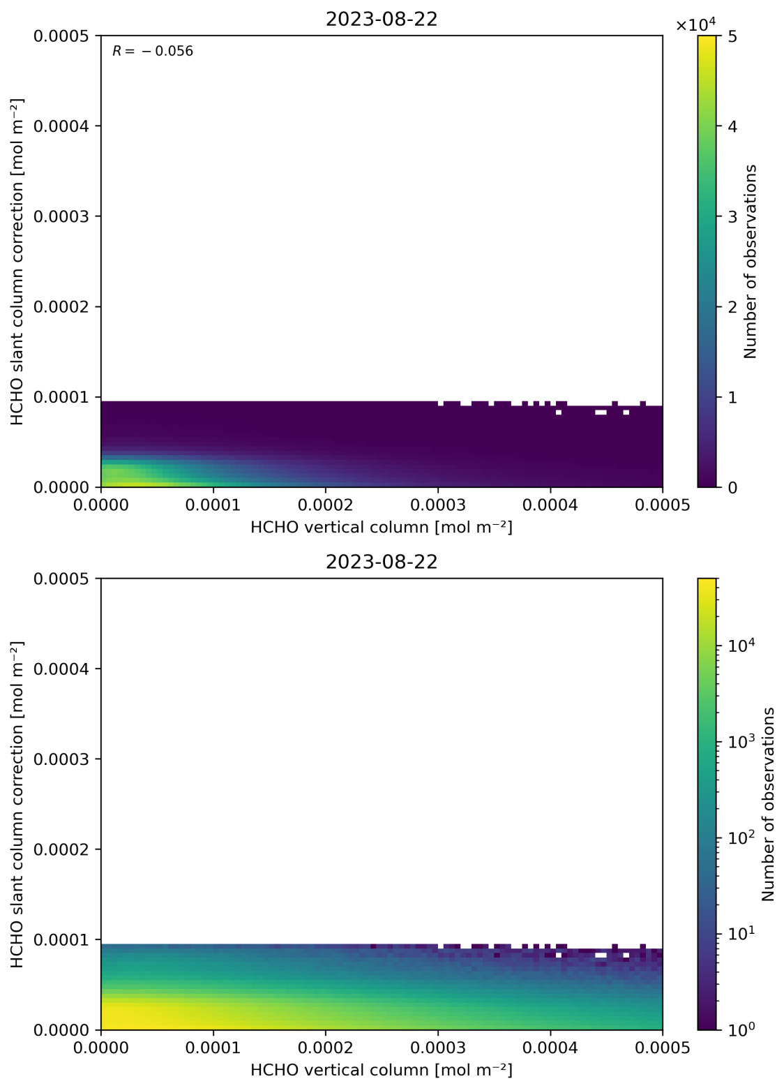
Figure 128: Scatter density plot of “HCHO vertical column” against “HCHO slant column correction” for 2023-08-21 to 2023-08-23.
