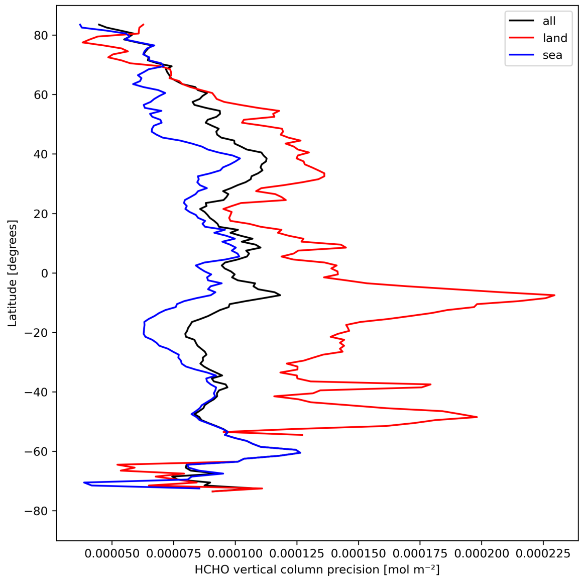
Figure 22: Zonal average of “HCHO vertical column precision” for 2023-08-21 to 2023-08-23.
