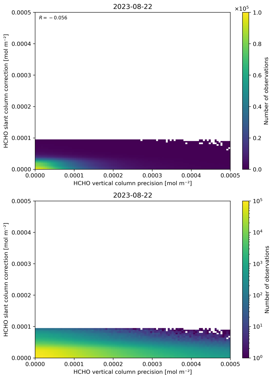
Figure 141: Scatter density plot of “HCHO vertical column precision” against “HCHO slant column correction” for 2023-08-21 to 2023-08-23.
