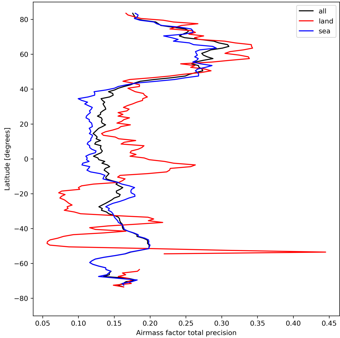
Figure 27: Zonal average of “Airmass factor total precision” for 2023-08-21 to 2023-08-23.
