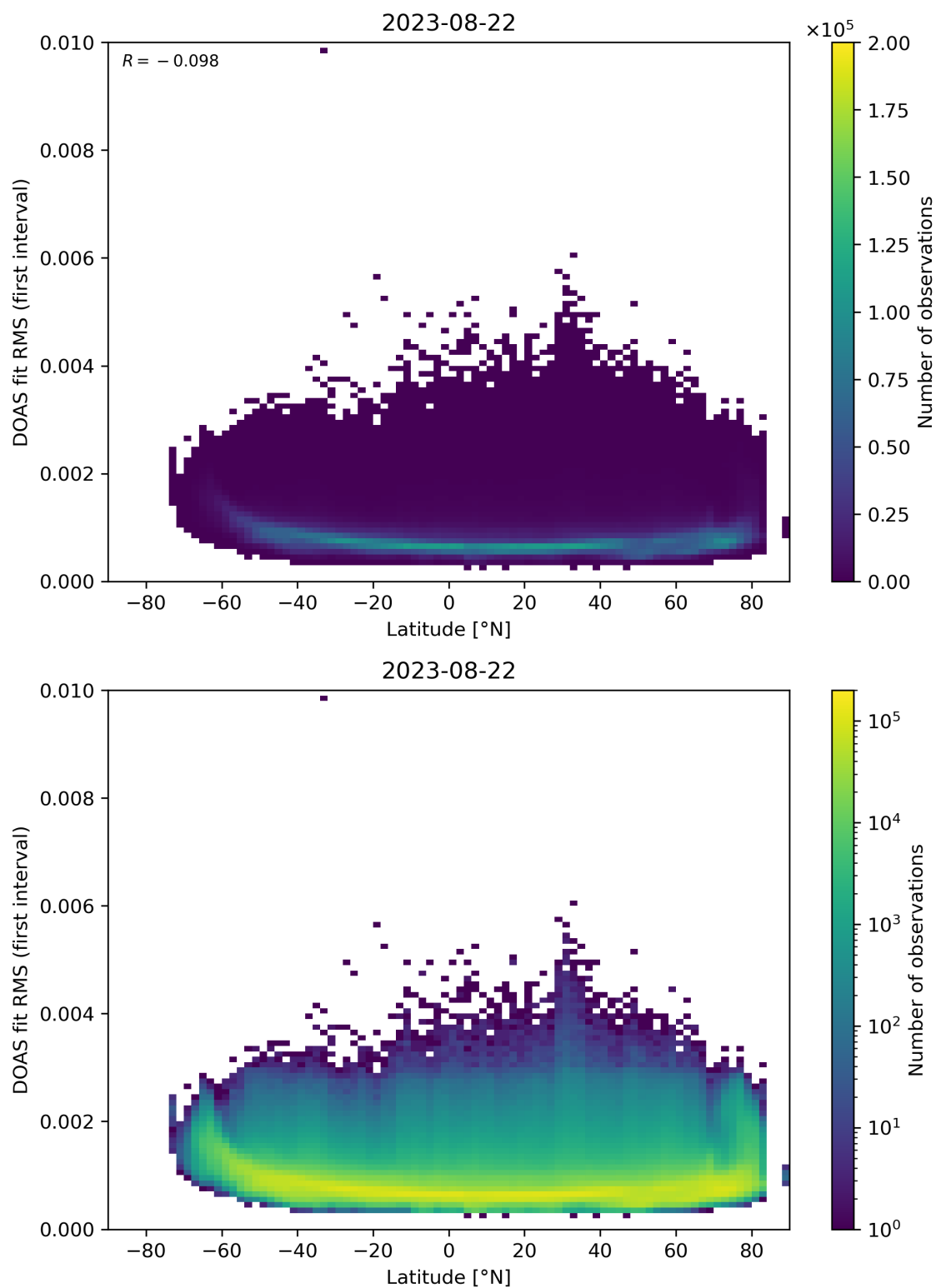
Figure 153: Scatter density plot of “Latitude” against “DOAS fit RMS (first interval)” for 2023-08-21 to 2023-08-23.
