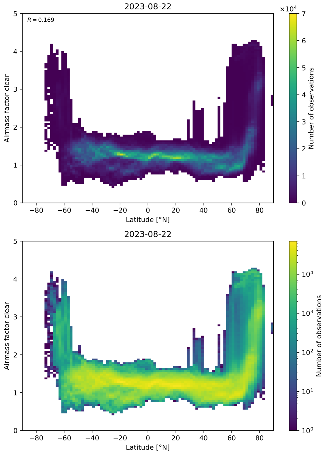
Figure 156: Scatter density plot of “Latitude” against “Airmass factor clear” for 2023-08-21 to 2023-08-23.
