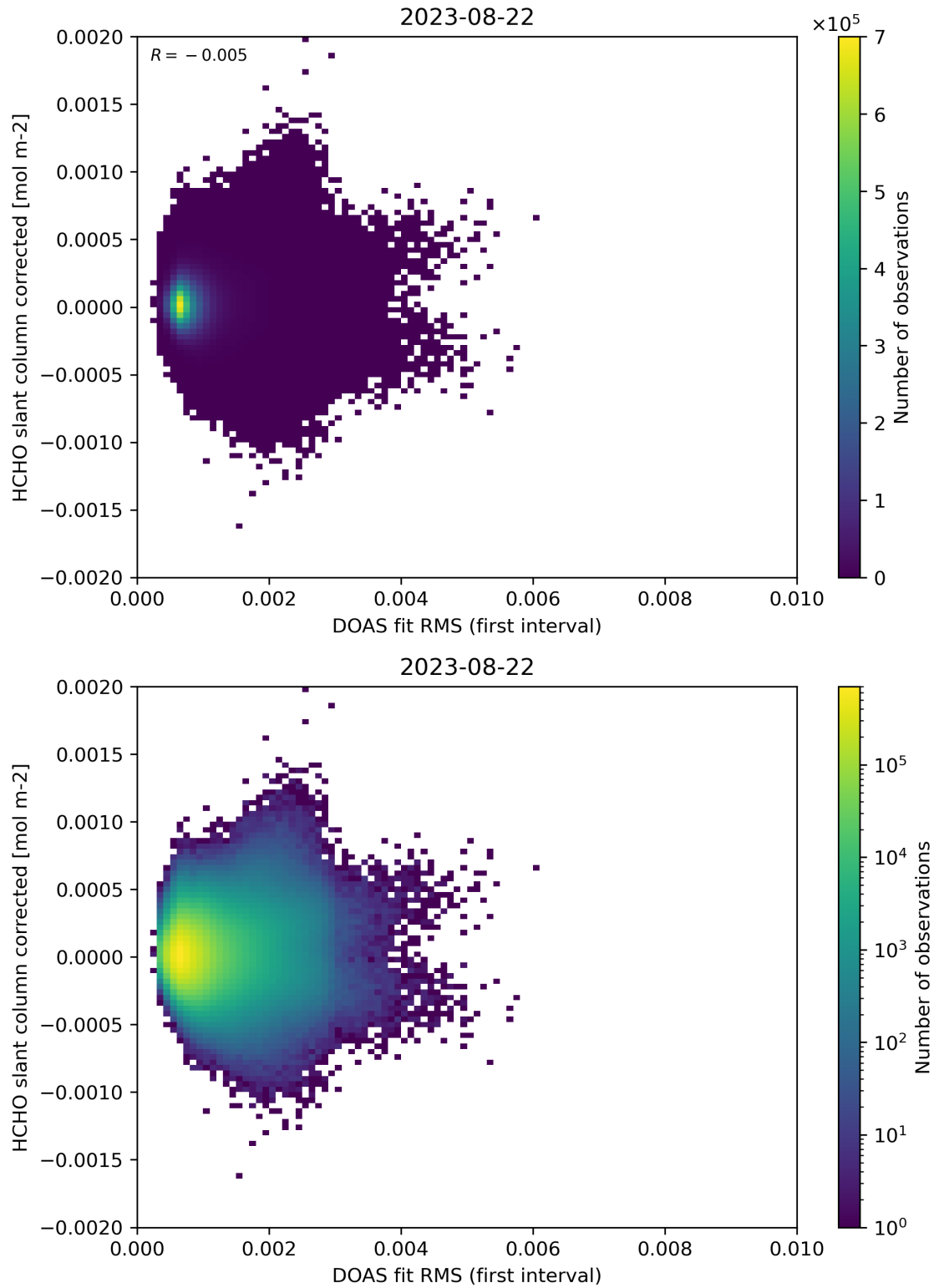
Figure 62: Scatter density plot of “DOAS fit RMS (first interval)” against “HCHO slant column corrected” for 2023-08-21 to 2023-08-23.
