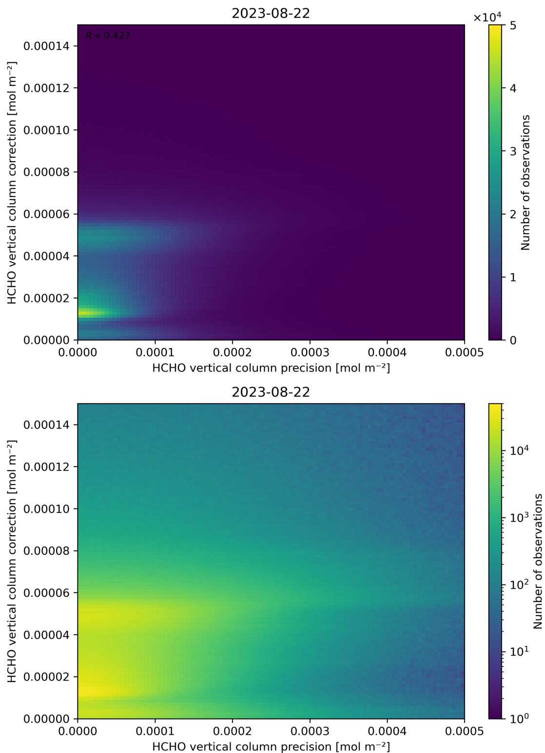
Figure 146: Scatter density plot of “HCHO vertical column precision” against “HCHO vertical column correction” for 2023-08-21 to 2023-08-23.
