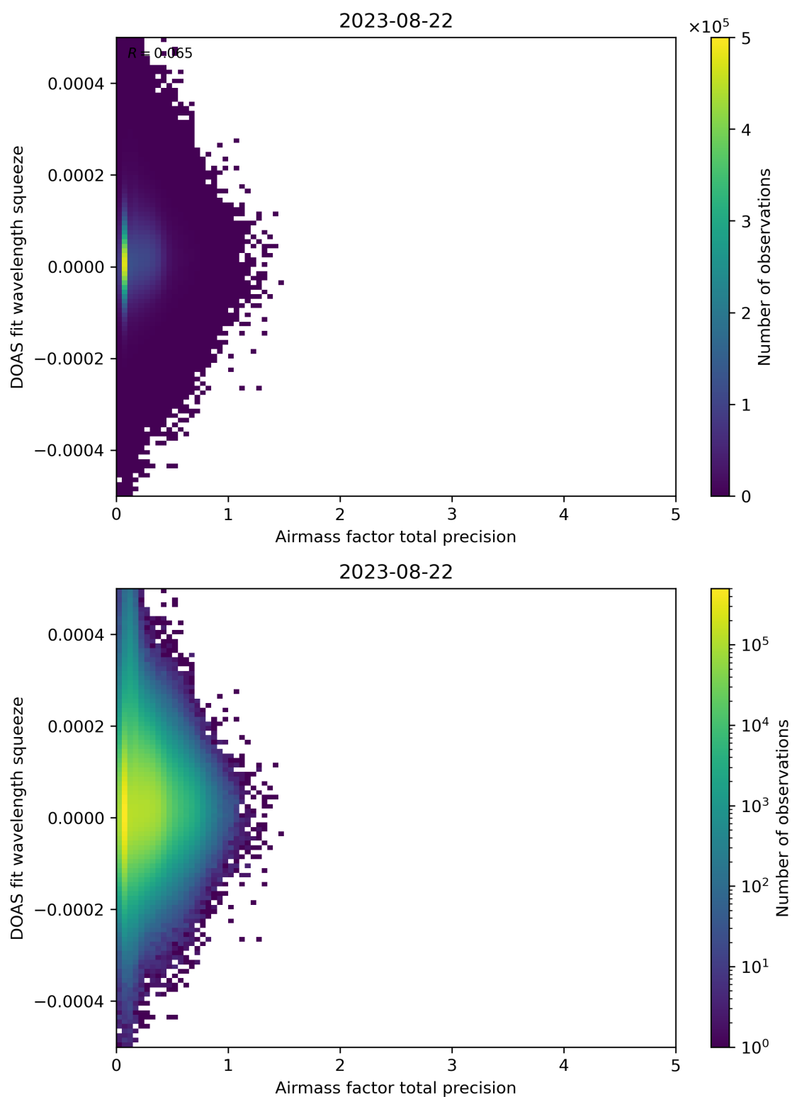
Figure 107: Scatter density plot of “Airmass factor total precision” against “DOAS fit wavelength squeeze” for 2023-08-21 to 2023-08-23.
