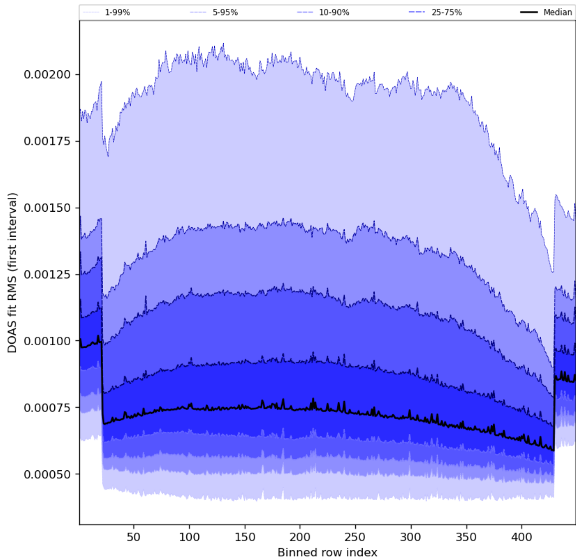
Figure 60: Along track statistics of “DOAS fit RMS (first interval)” for 2023-08-21 to 2023-08-23
