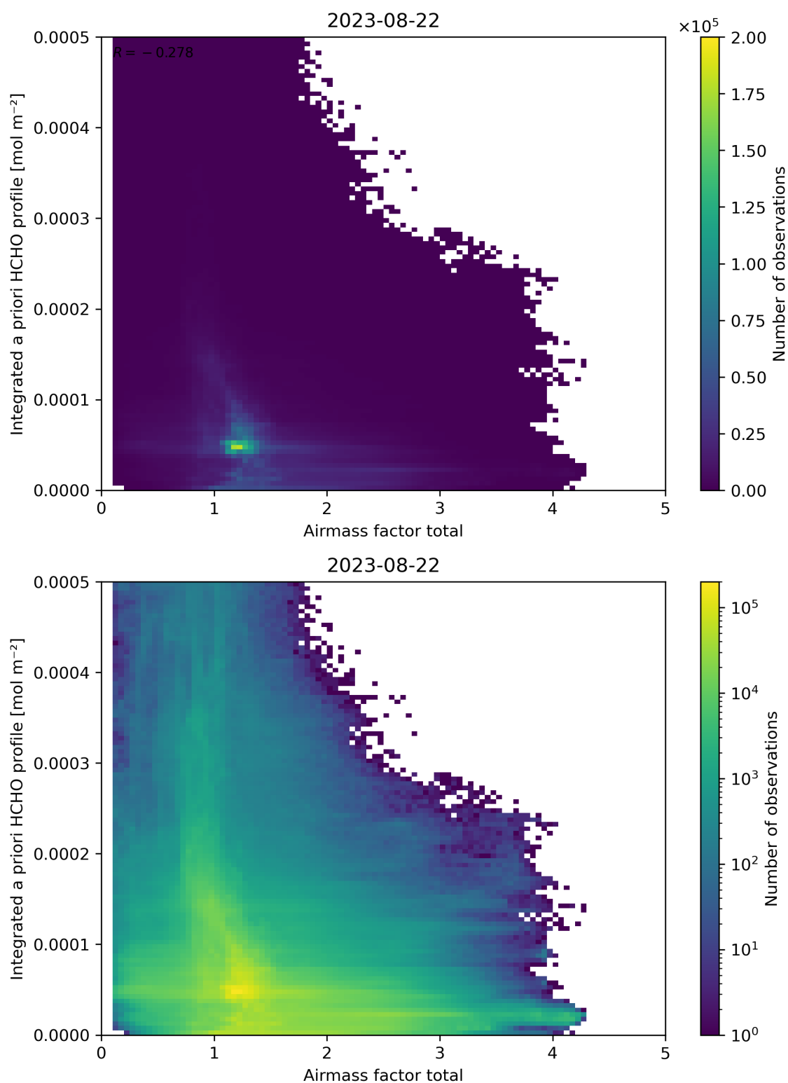
Figure 104: Scatter density plot of “Airmass factor total” against “Integrated a priori HCHO profile” for 2023-08-21 to 2023-08-23.
