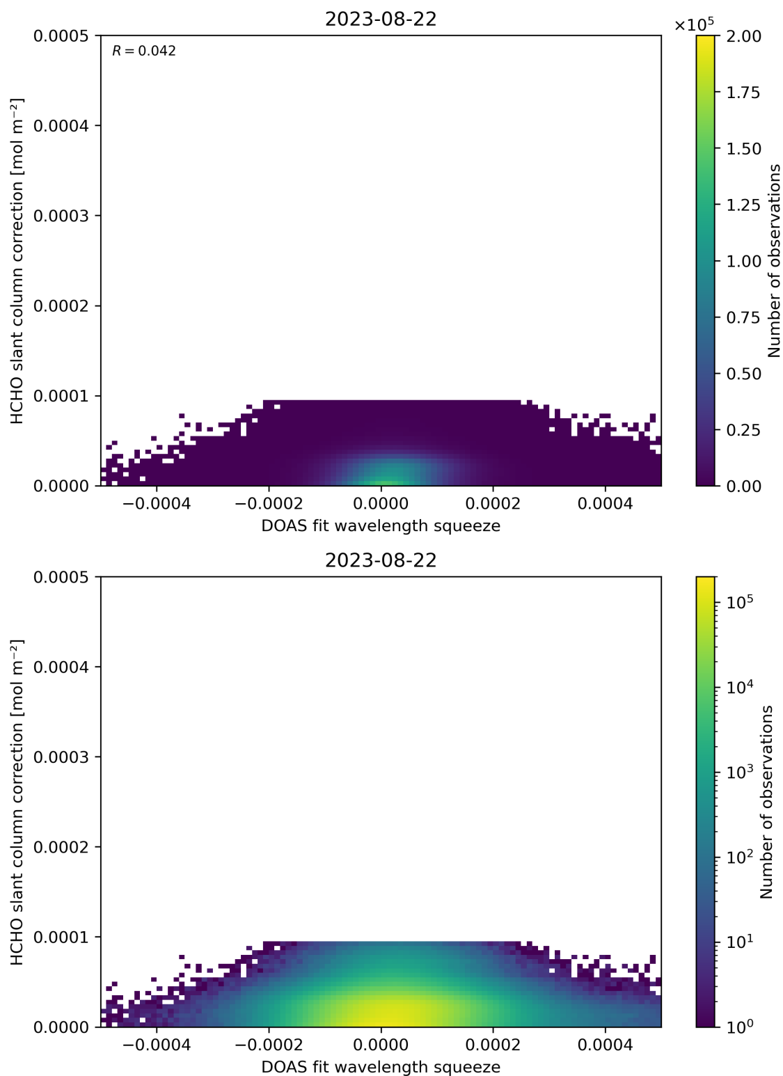
Figure 70: Scatter density plot of “DOAS fit wavelength squeeze” against “HCHO slant column correction” for 2023-08-21 to 2023-08-23.
