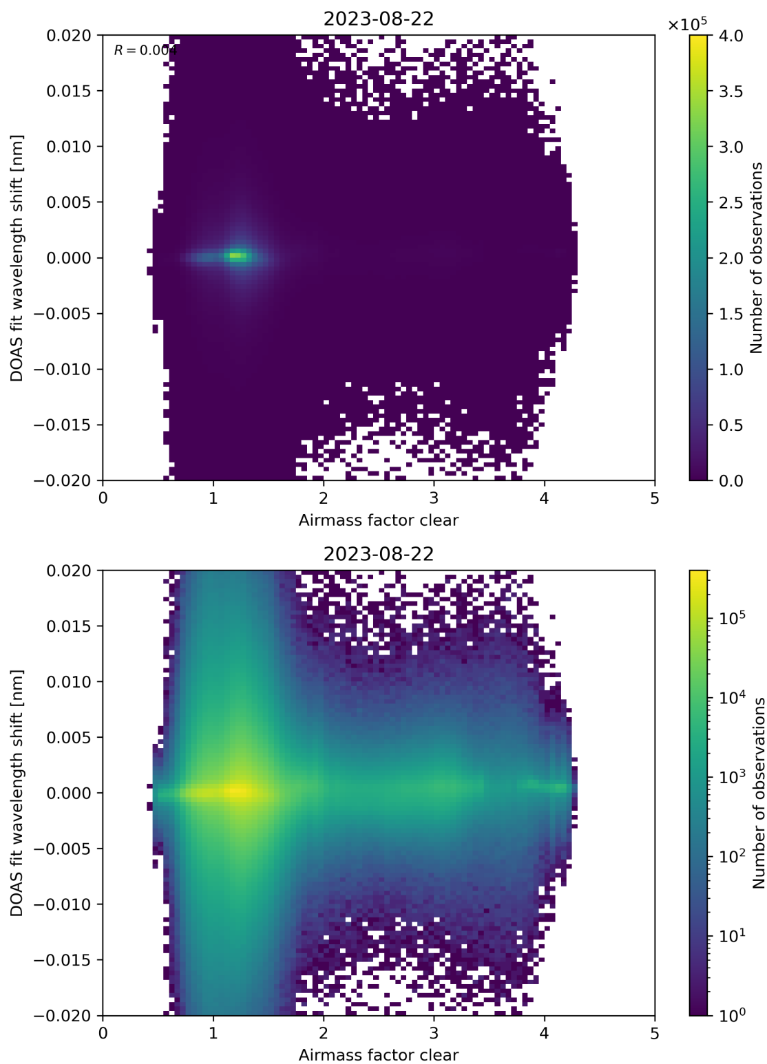
Figure 72: Scatter density plot of “Airmass factor clear” against “DOAS fit wavelength shift” for 2023-08-21 to 2023-08-23.
