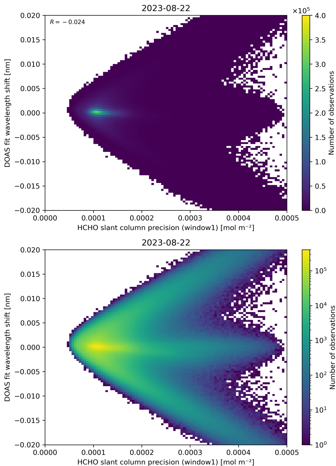
Figure 89: Scatter density plot of “HCHO slant column precision (window1)” against “DOAS fit wavelength shift” for 2023-08-21 to 2023-08-23.
