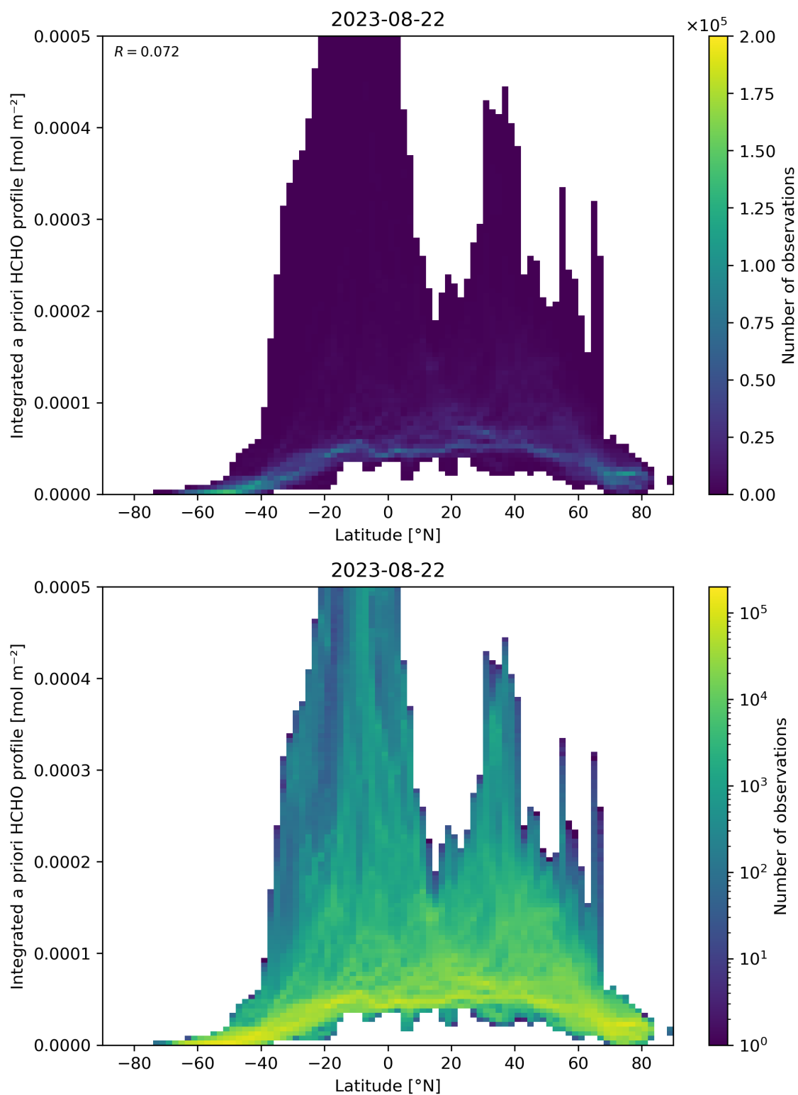
Figure 166: Scatter density plot of “Latitude” against “Integrated a priori HCHO profile” for 2023-08-21 to 2023-08-23.
