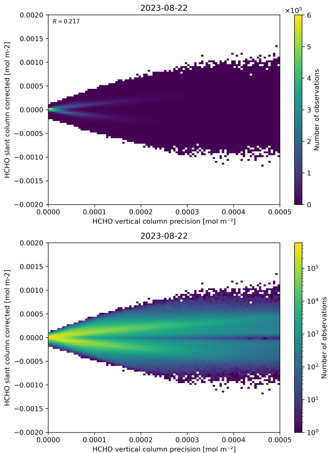
Figure 140: Scatter density plot of “HCHO vertical column precision” against “HCHO slant column corrected” for 2023-08-21 to 2023-08-23.
