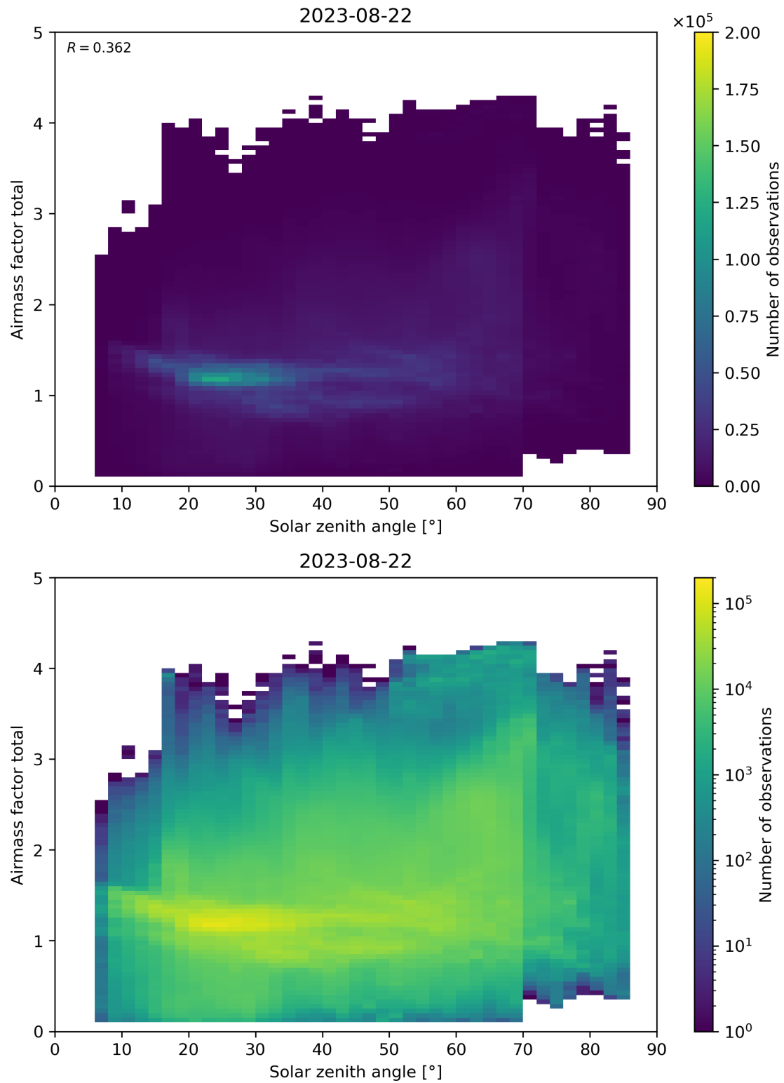
Figure 175: Scatter density plot of “Solar zenith angle” against “Airmass factor total” for 2023-08-21 to 2023-08-23.
