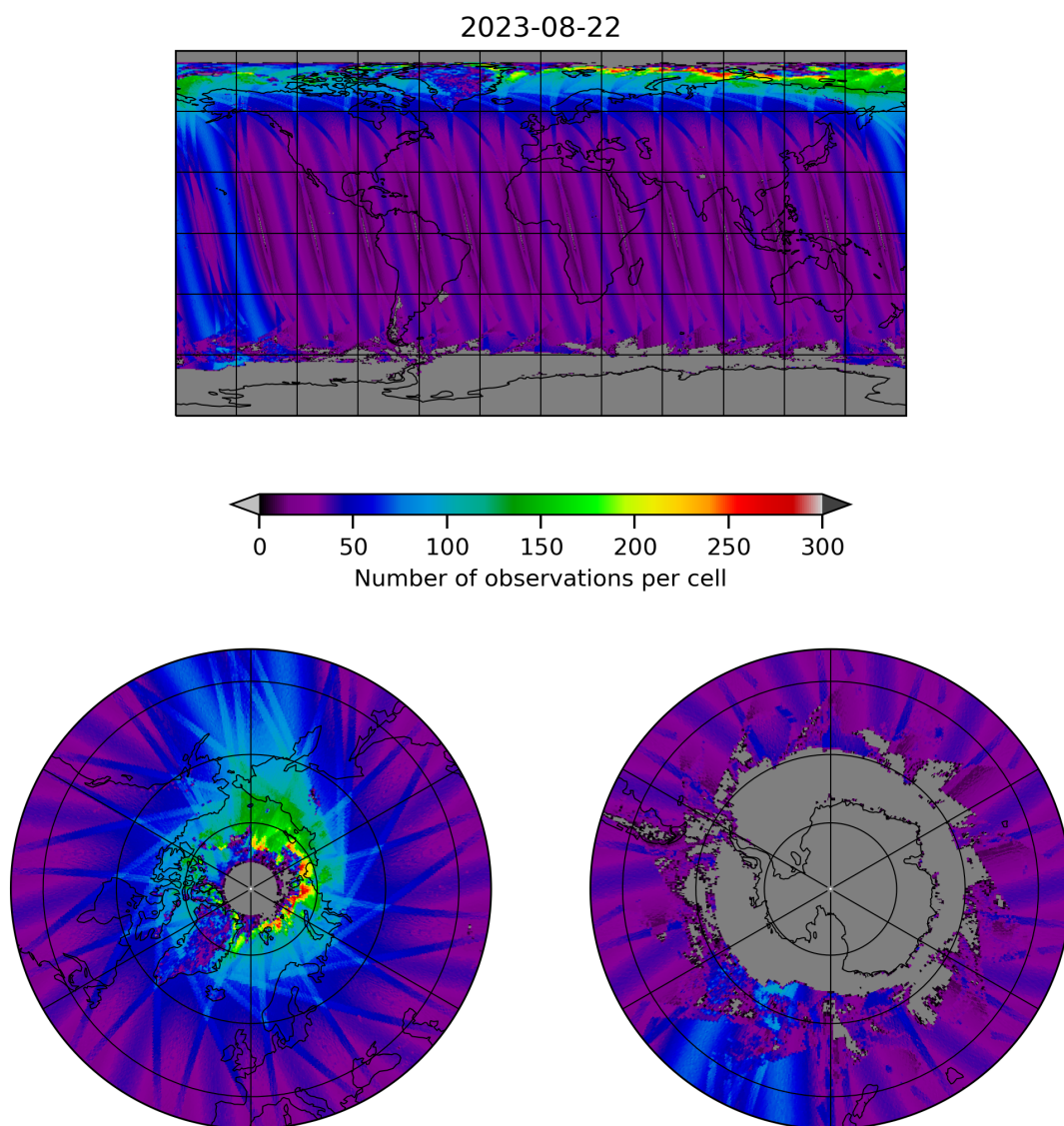
Figure 19: Map of the number of observations for 2023-08-21 to 2023-08-23
