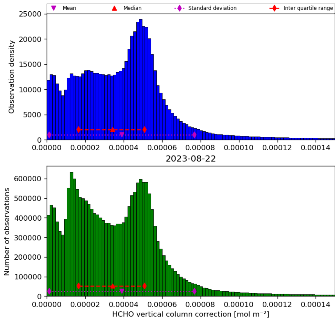
Figure 37: Histogram of “HCHO vertical column correction” for 2023-08-21 to 2023-08-23
