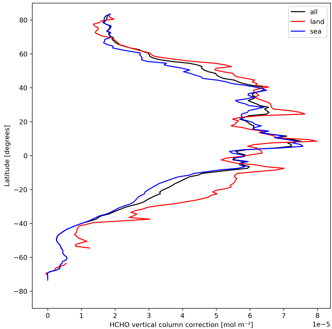
Figure 23: Zonal average of “HCHO vertical column correction” for 2023-08-21 to 2023-08-23.
