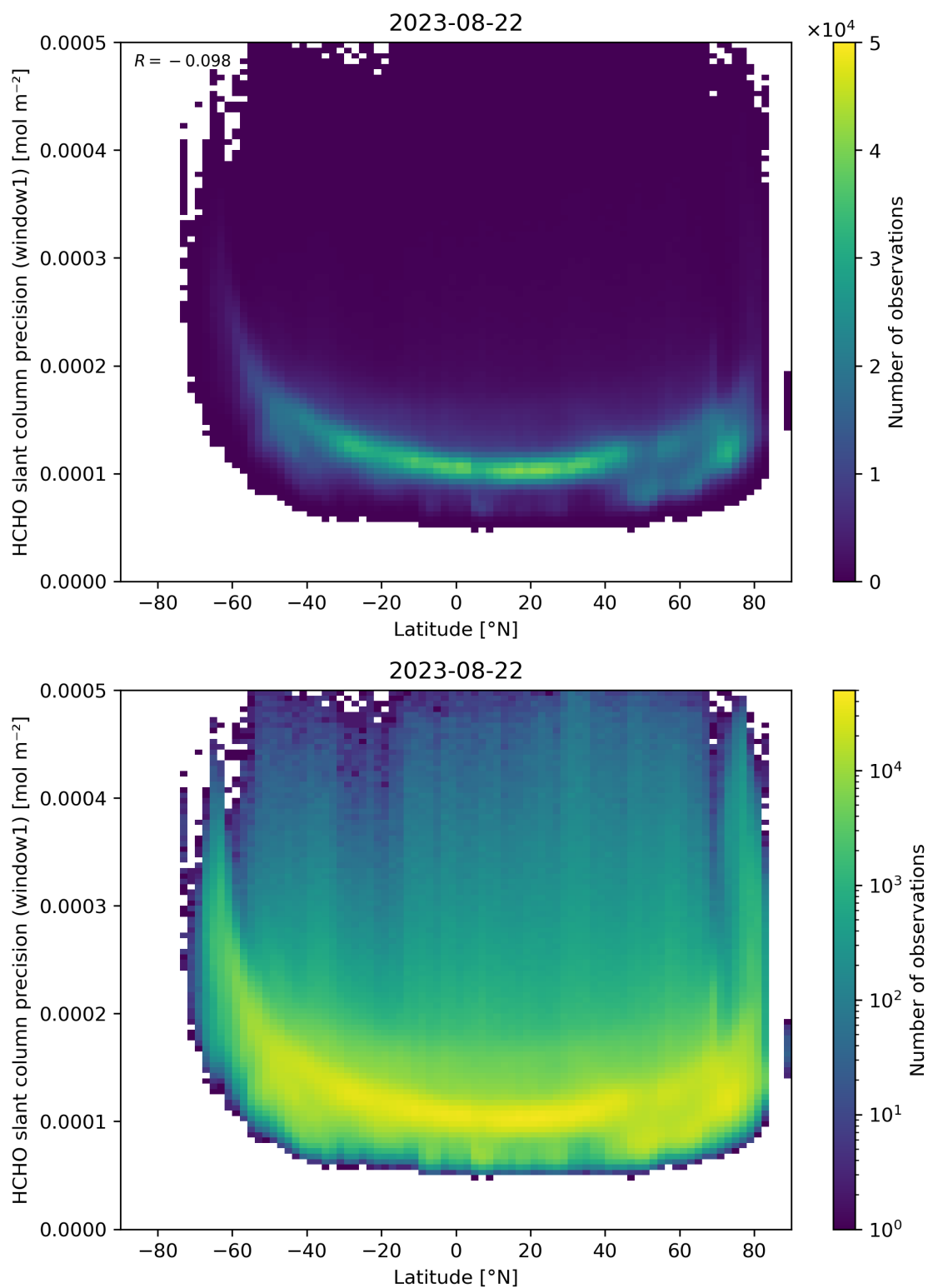
Figure 160: Scatter density plot of “Latitude” against “HCHO slant column precision (window1)” for 2023-08-21 to 2023-08-23.
