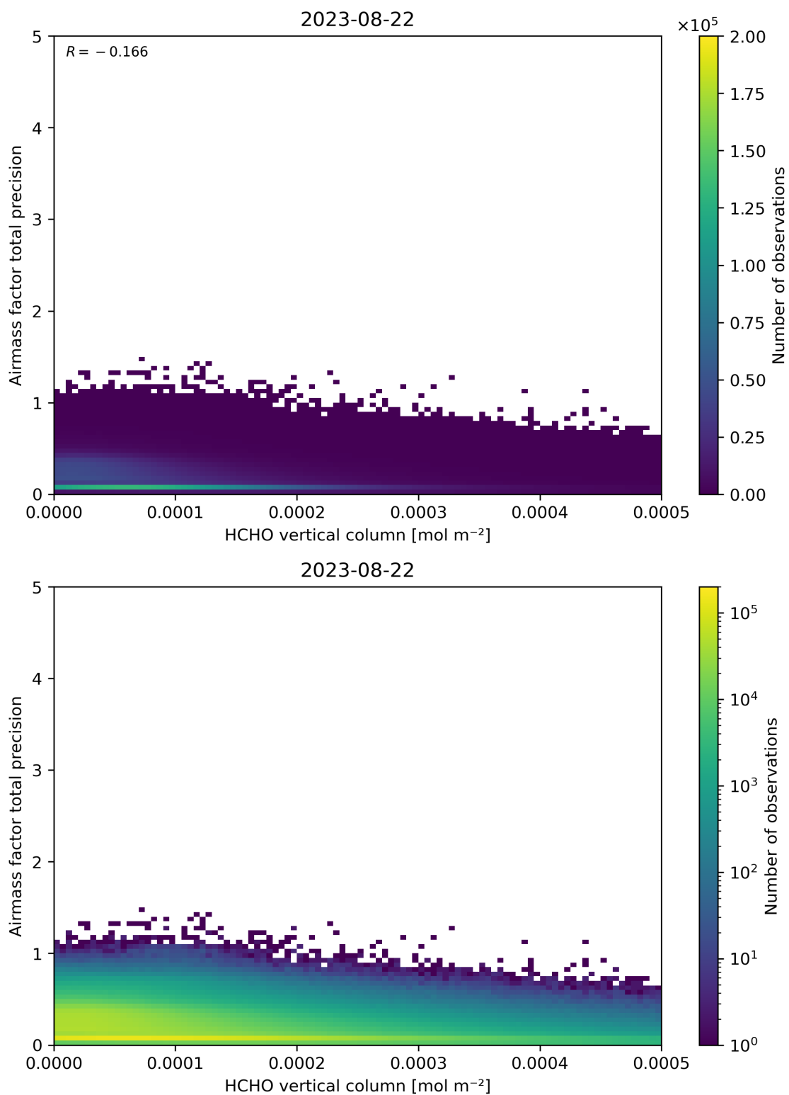
Figure 132: Scatter density plot of “HCHO vertical column” against “Airmass factor total precision” for 2023-08-21 to 2023-08-23.
