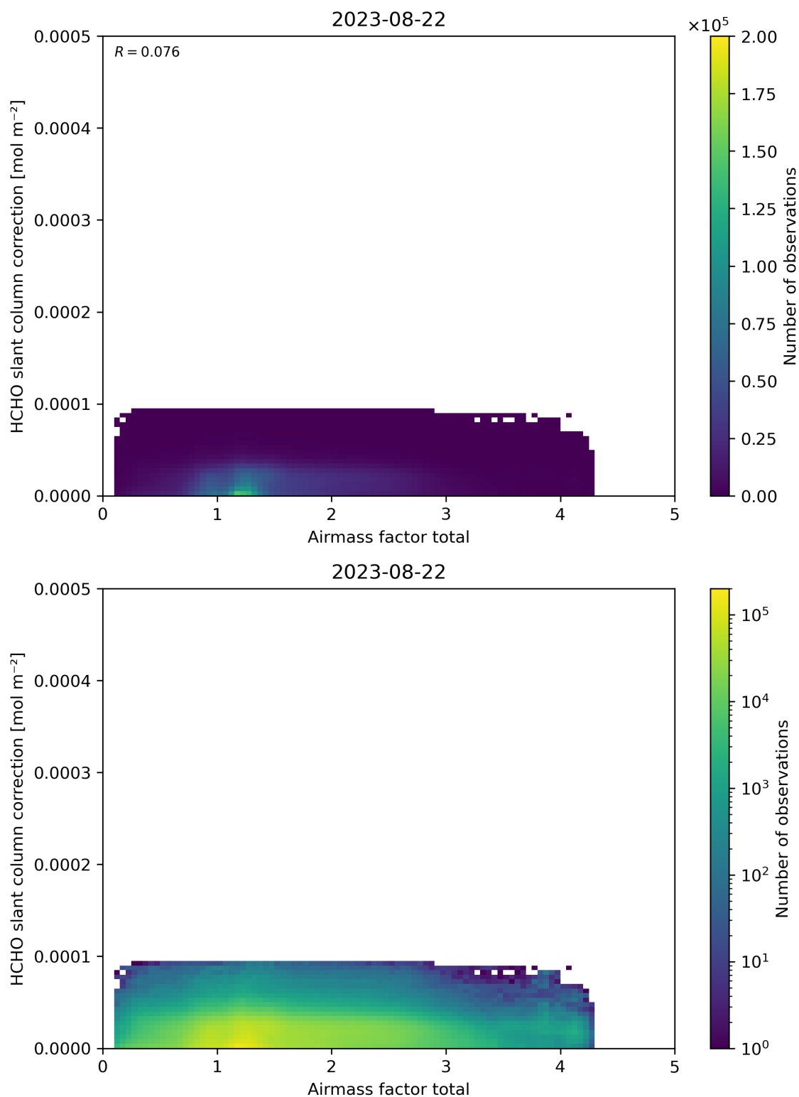
Figure 102: Scatter density plot of “Airmass factor total” against “HCHO slant column correction” for 2023-08-21 to 2023-08-23.
