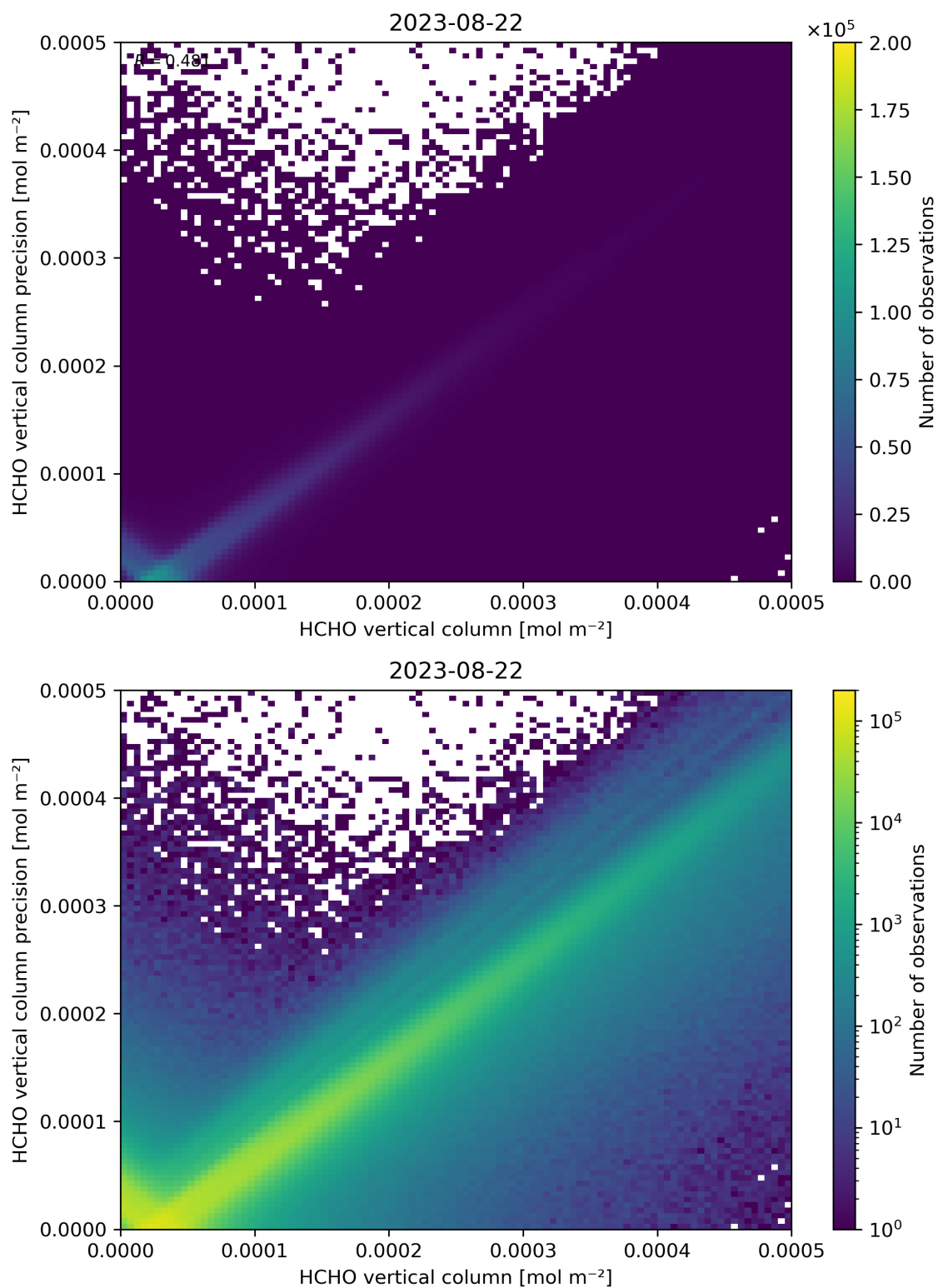
Figure 134: Scatter density plot of “HCHO vertical column” against “HCHO vertical column precision” for 2023-08-21 to 2023-08-23.
