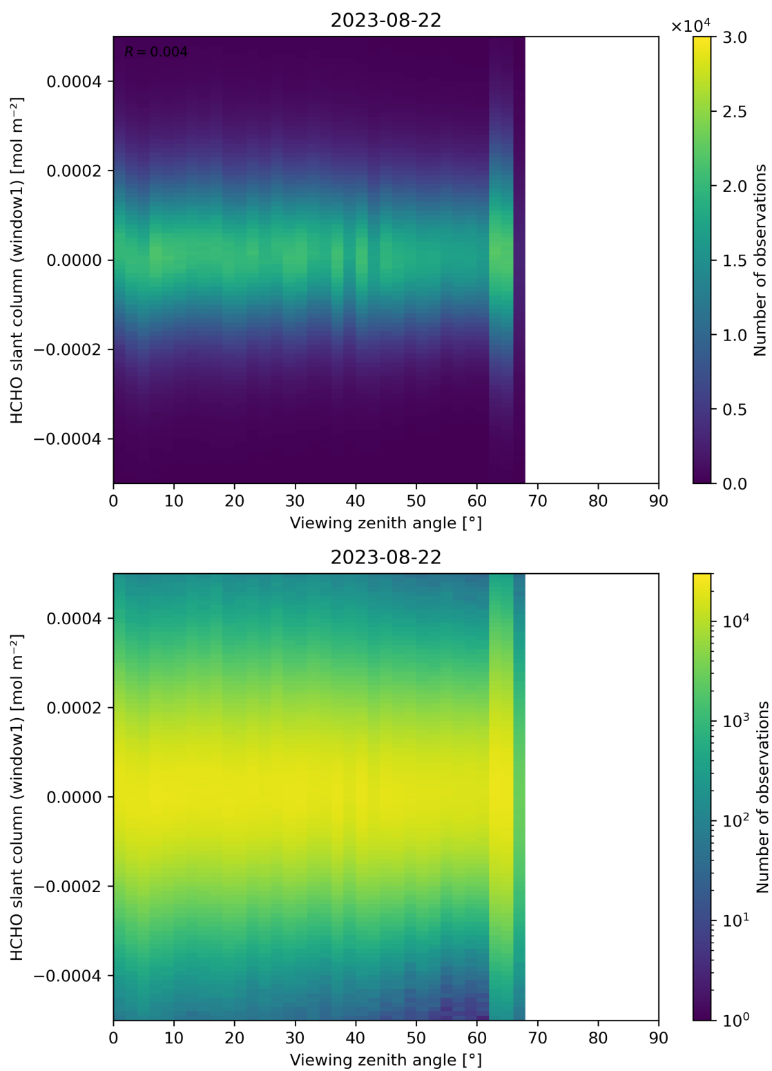
Figure 188: Scatter density plot of “Viewing zenith angle” against “HCHO slant column (window1)” for 2023-08-21 to 2023-08-23.
