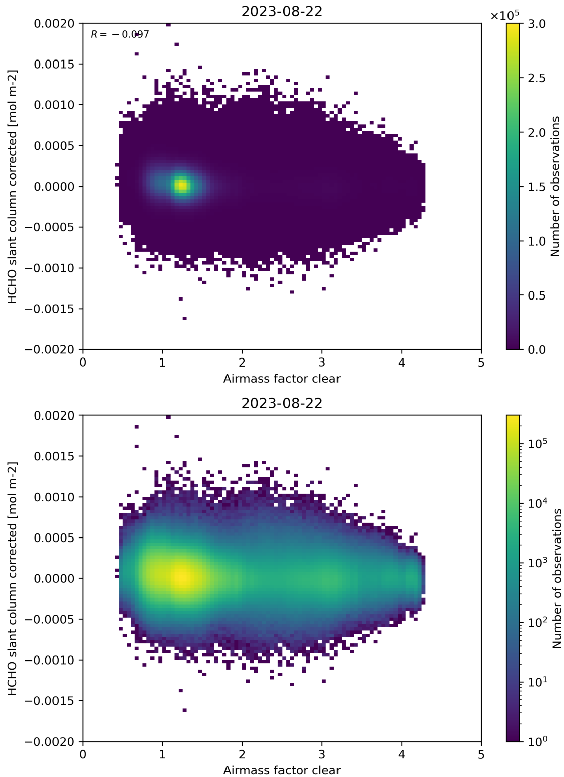
Figure 74: Scatter density plot of “Airmass factor clear” against “HCHO slant column corrected” for 2023-08-21 to 2023-08-23.
