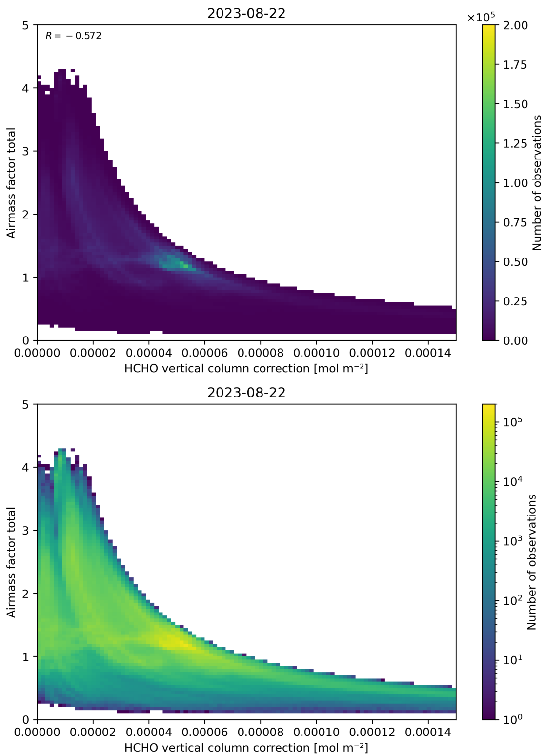
Figure 120: Scatter density plot of “HCHO vertical column correction” against “Airmass factor total” for 2023-08-21 to 2023-08-23.
