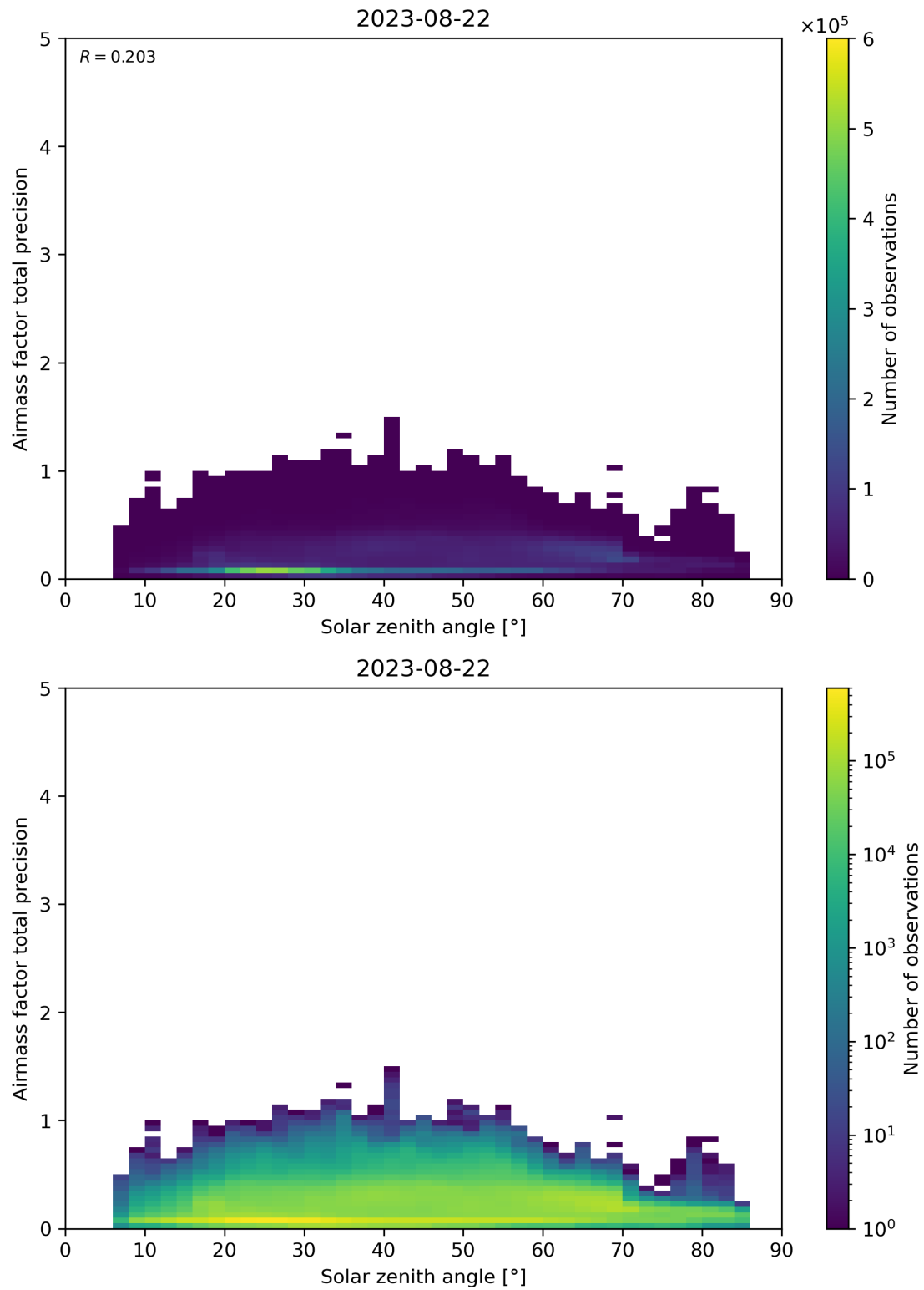
Figure 176: Scatter density plot of “Solar zenith angle” against “Airmass factor total precision” for 2023-08-21 to 2023-08-23.
