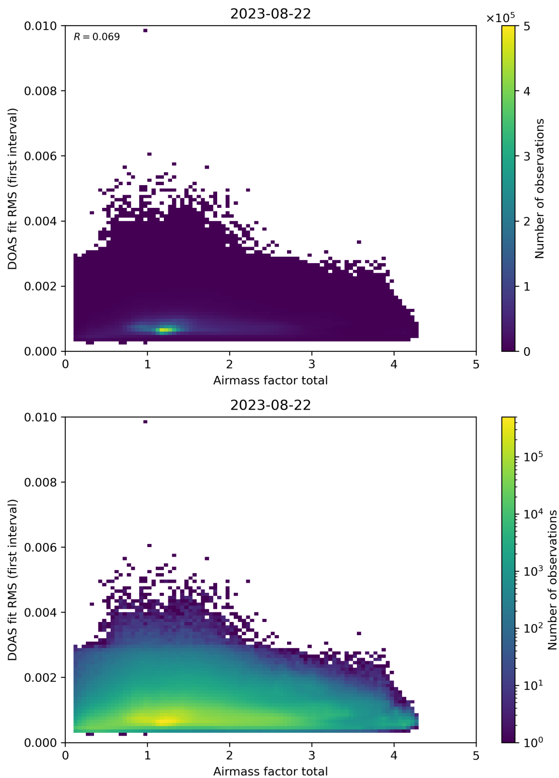
Figure 97: Scatter density plot of “Airmass factor total” against “DOAS fit RMS (first interval)” for 2023-08-21 to 2023-08-23.
