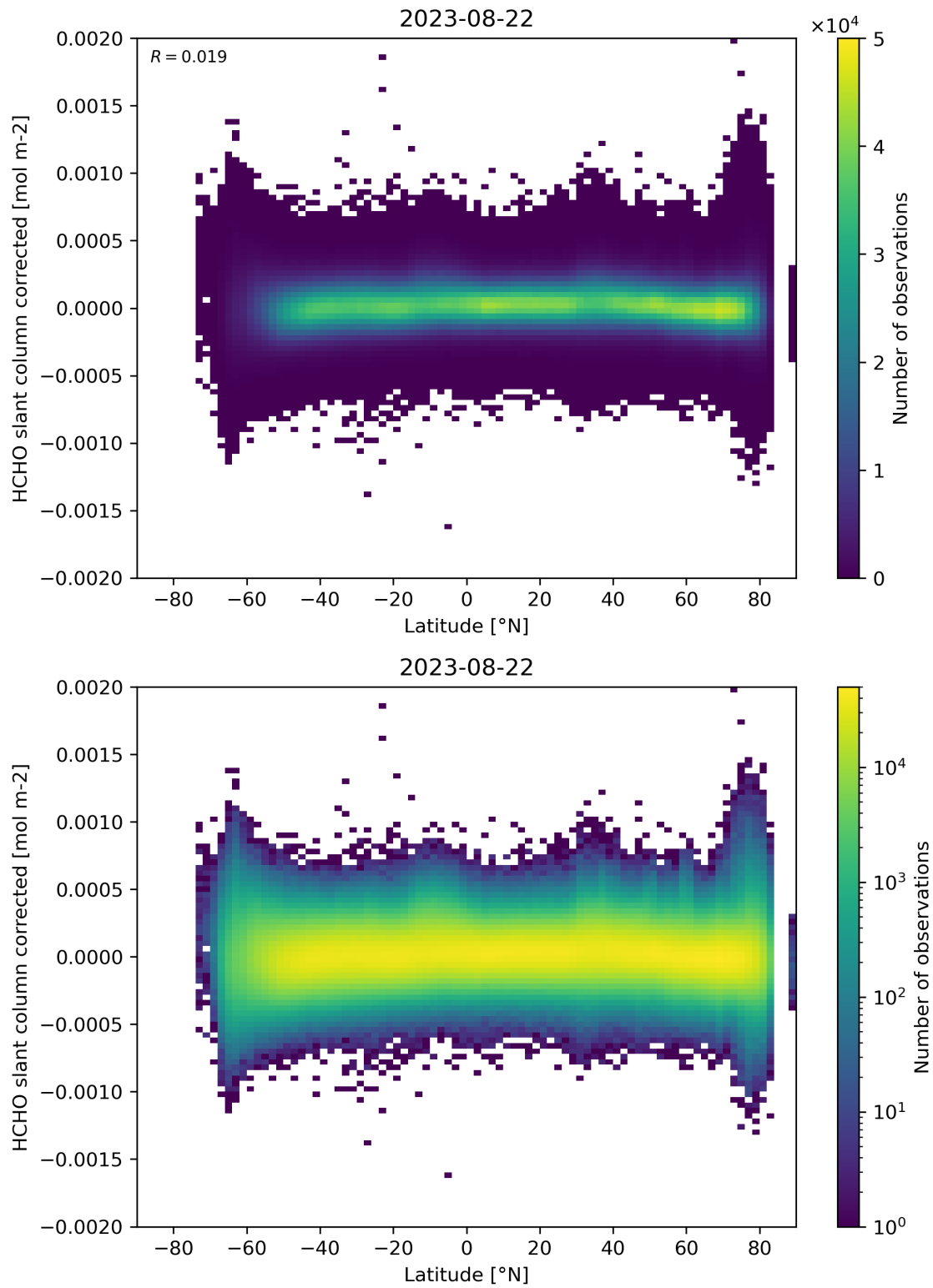
Figure 157: Scatter density plot of “Latitude” against “HCHO slant column corrected” for 2023-08-21 to 2023-08-23.
