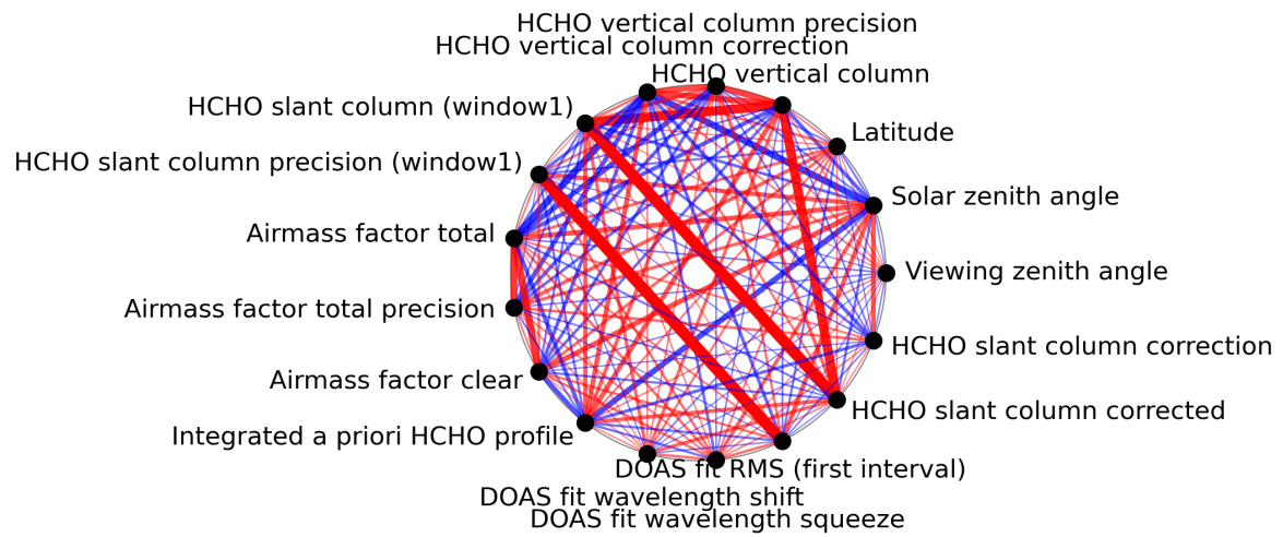
Figure 1: Map of correlation graph for 2023-08-21 to 2023-08-23.
