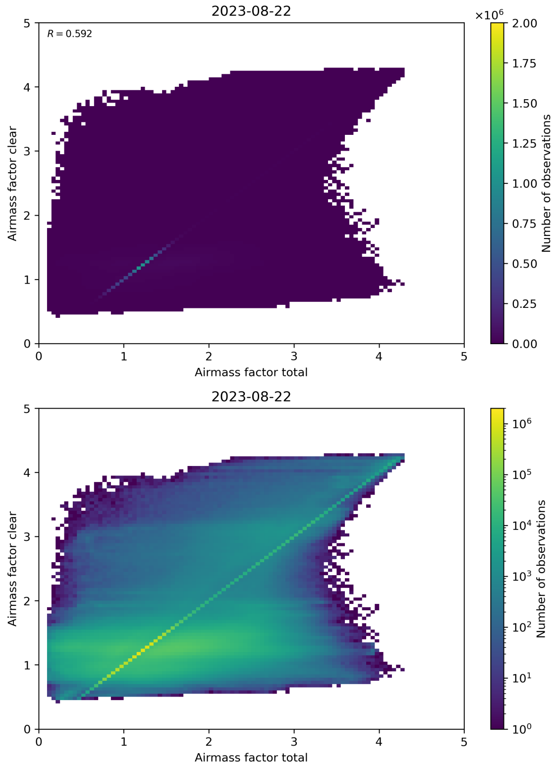
Figure 100: Scatter density plot of “Airmass factor total” against “Airmass factor clear” for 2023-08-21 to 2023-08-23.
