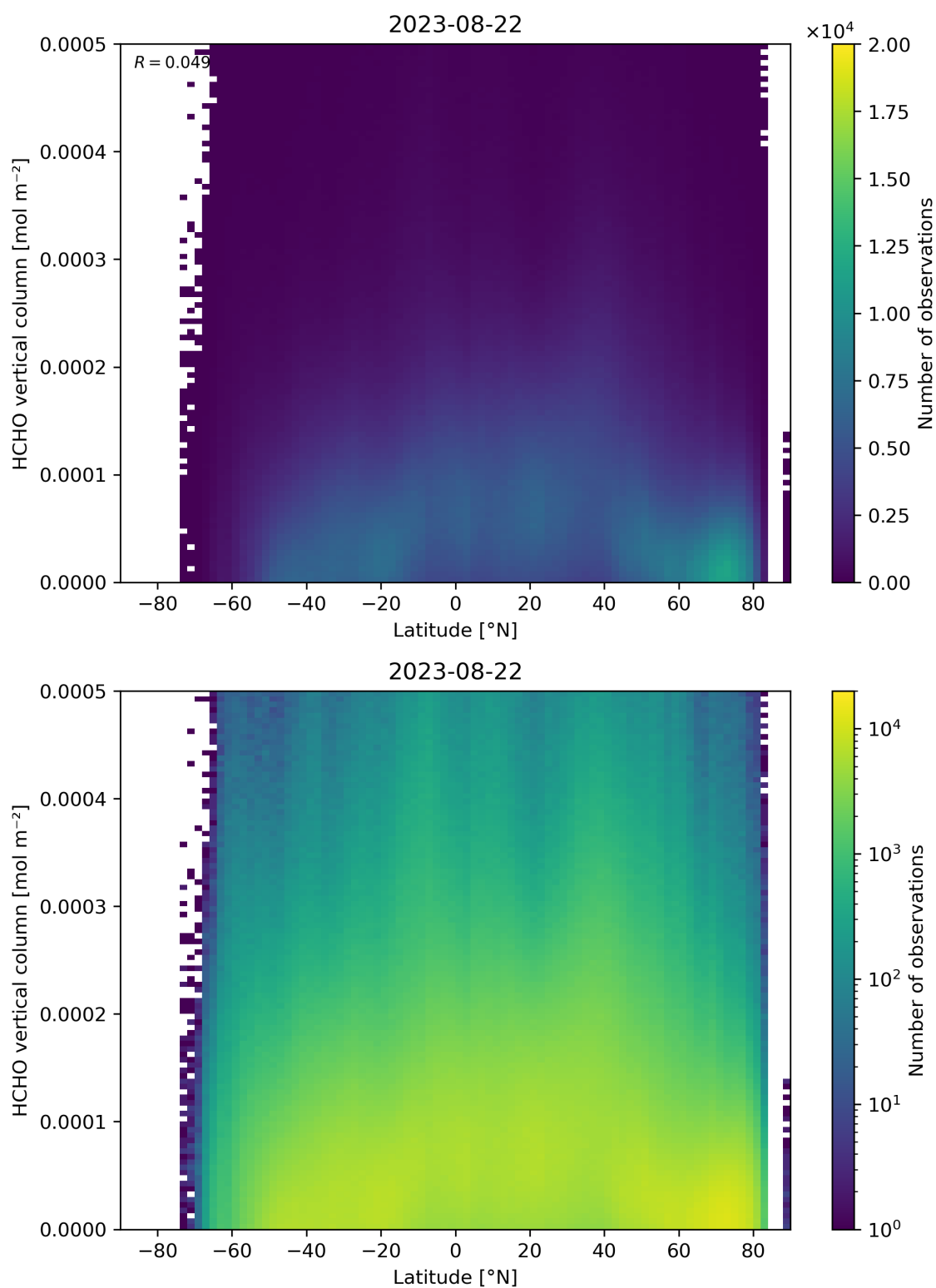
Figure 163: Scatter density plot of “Latitude” against “HCHO vertical column” for 2023-08-21 to 2023-08-23.
