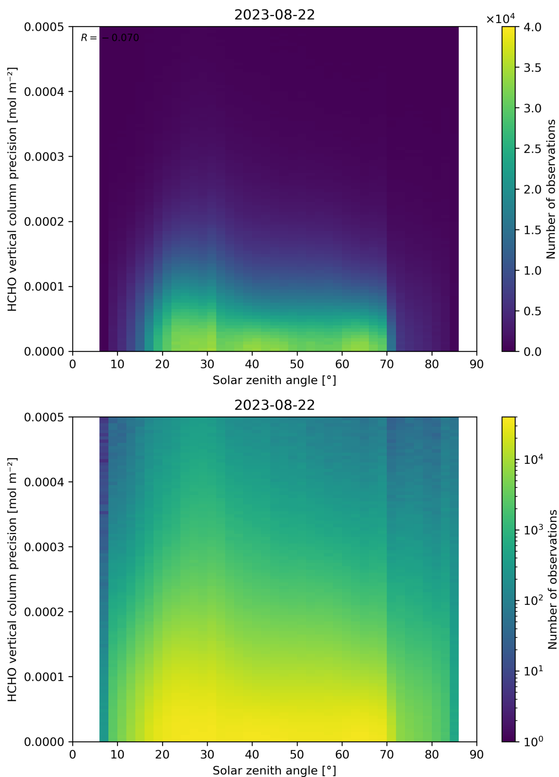
Figure 179: Scatter density plot of “Solar zenith angle” against “HCHO vertical column precision” for 2023-08-21 to 2023-08-23.
