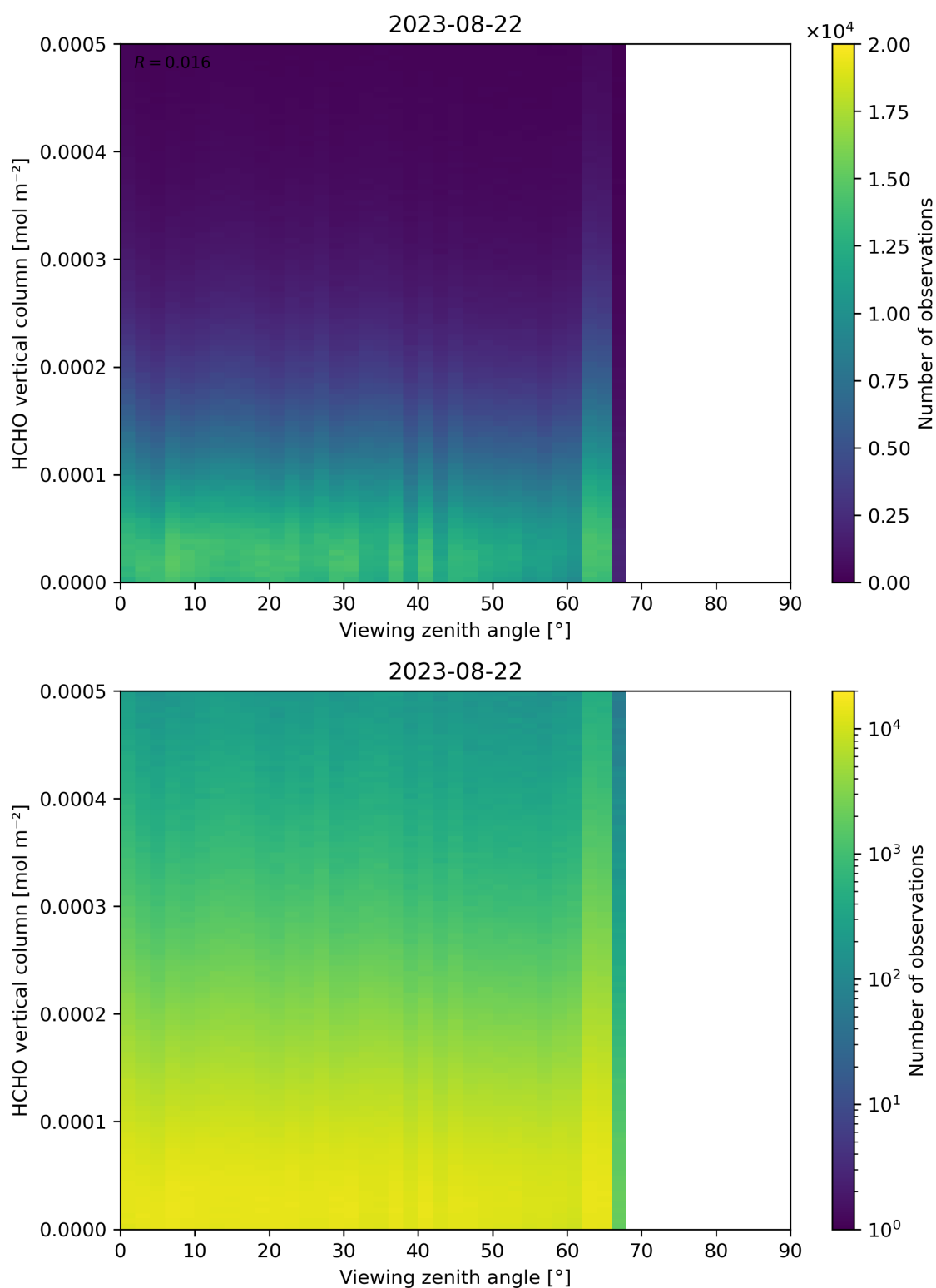
Figure 192: Scatter density plot of “Viewing zenith angle” against “HCHO vertical column” for 2023-08-21 to 2023-08-23.
