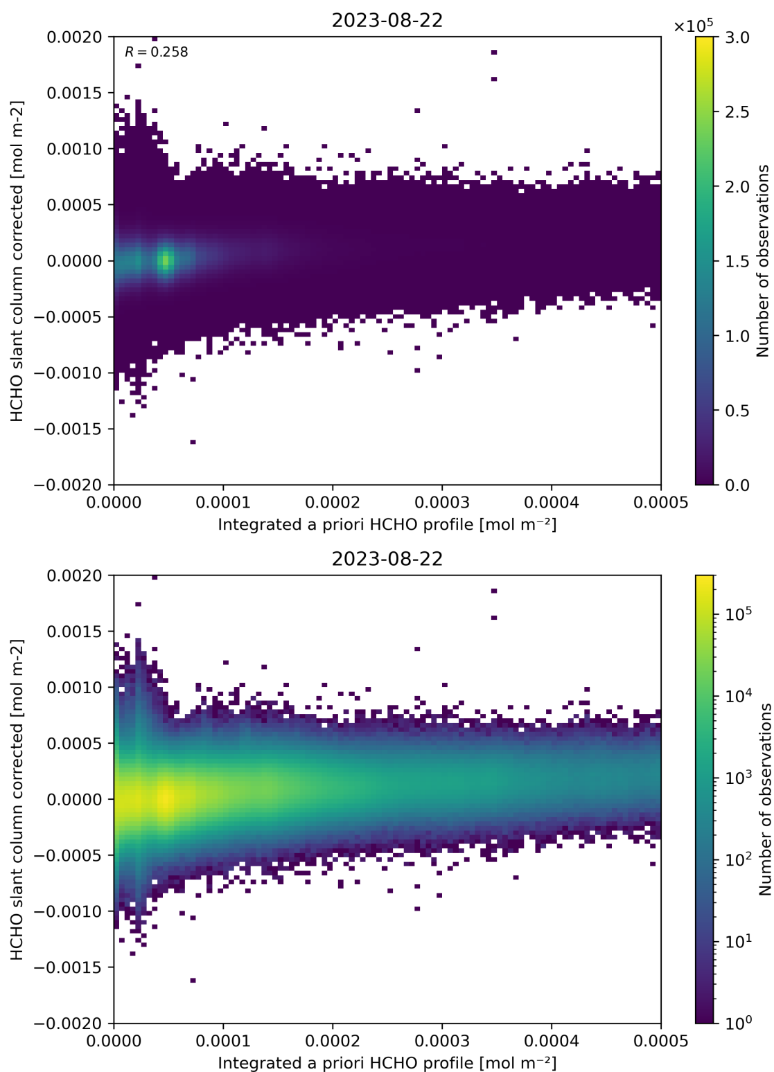
Figure 151: Scatter density plot of “Integrated a priori HCHO profile” against “HCHO slant column corrected” for 2023-08-21 to 2023-08-23.
