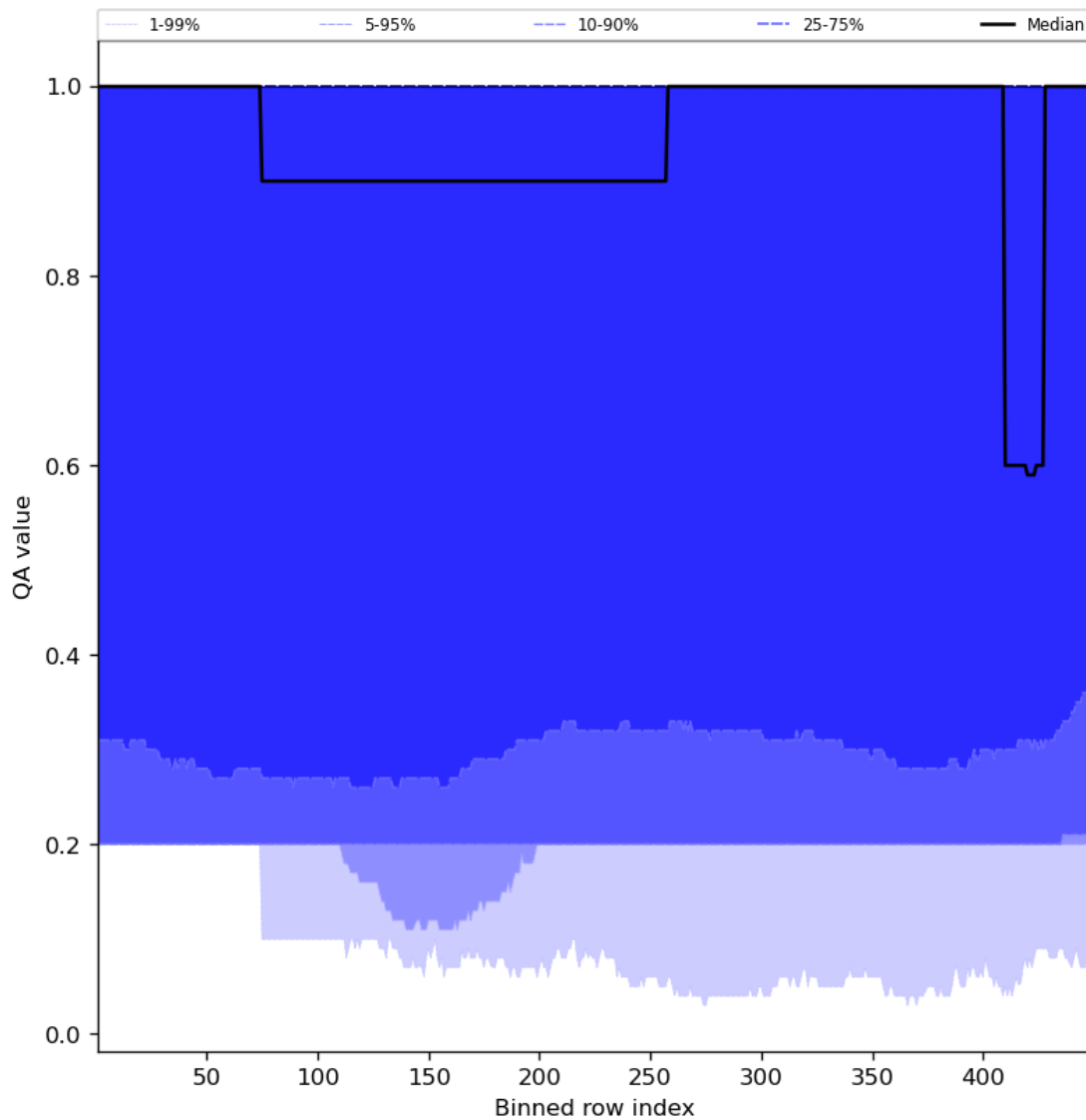
Figure 48: Along track statistics of “QA value” for 2023-08-21 to 2023-08-23
