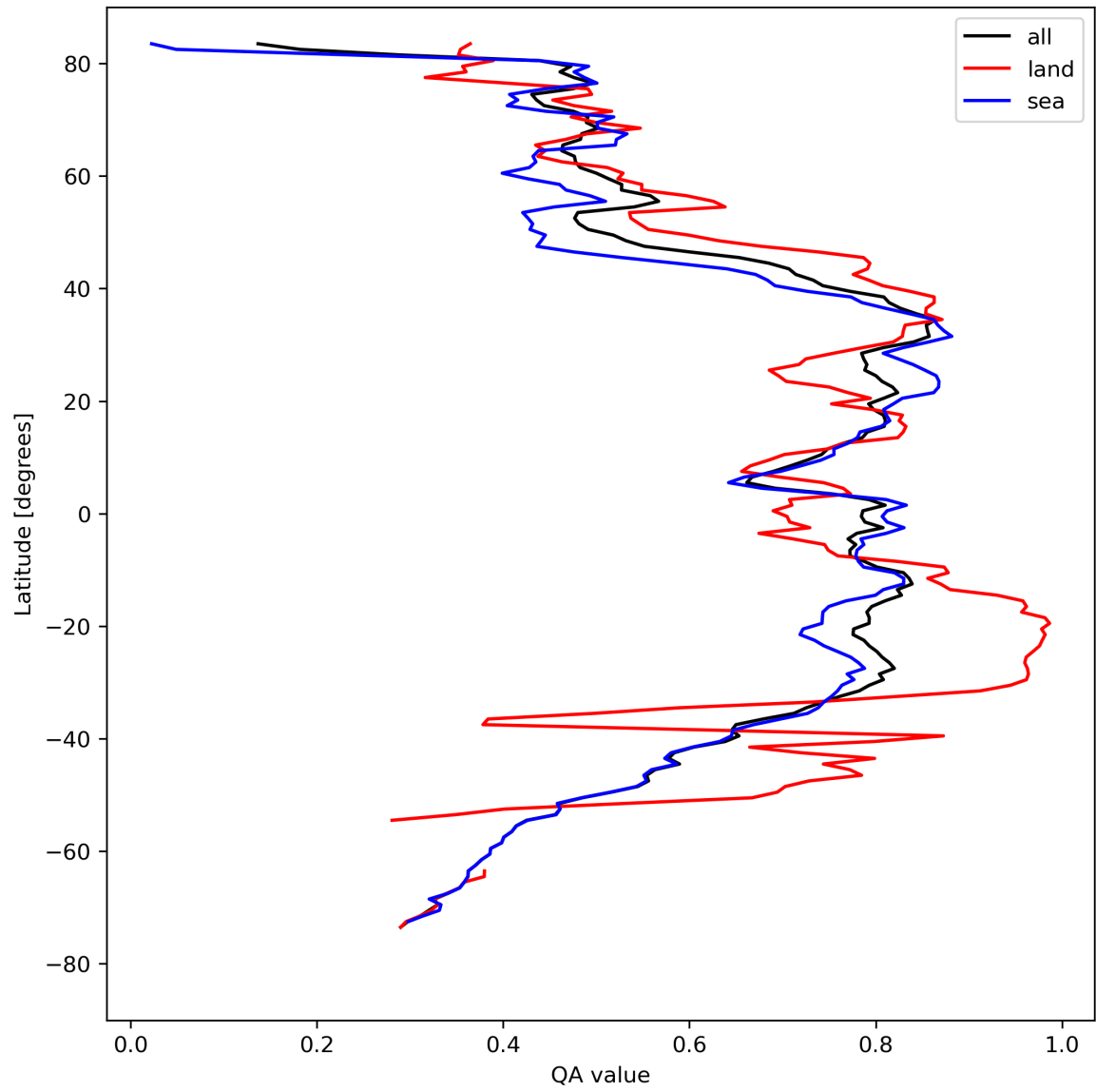
Figure 20: Zonal average of “QA value” for 2023-08-21 to 2023-08-23.
