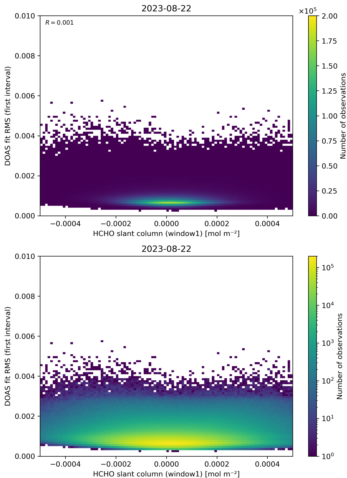
Figure 78: Scatter density plot of “HCHO slant column (window1)” against “DOAS fit RMS (first interval)” for 2023-08-21 to 2023-08-23.
