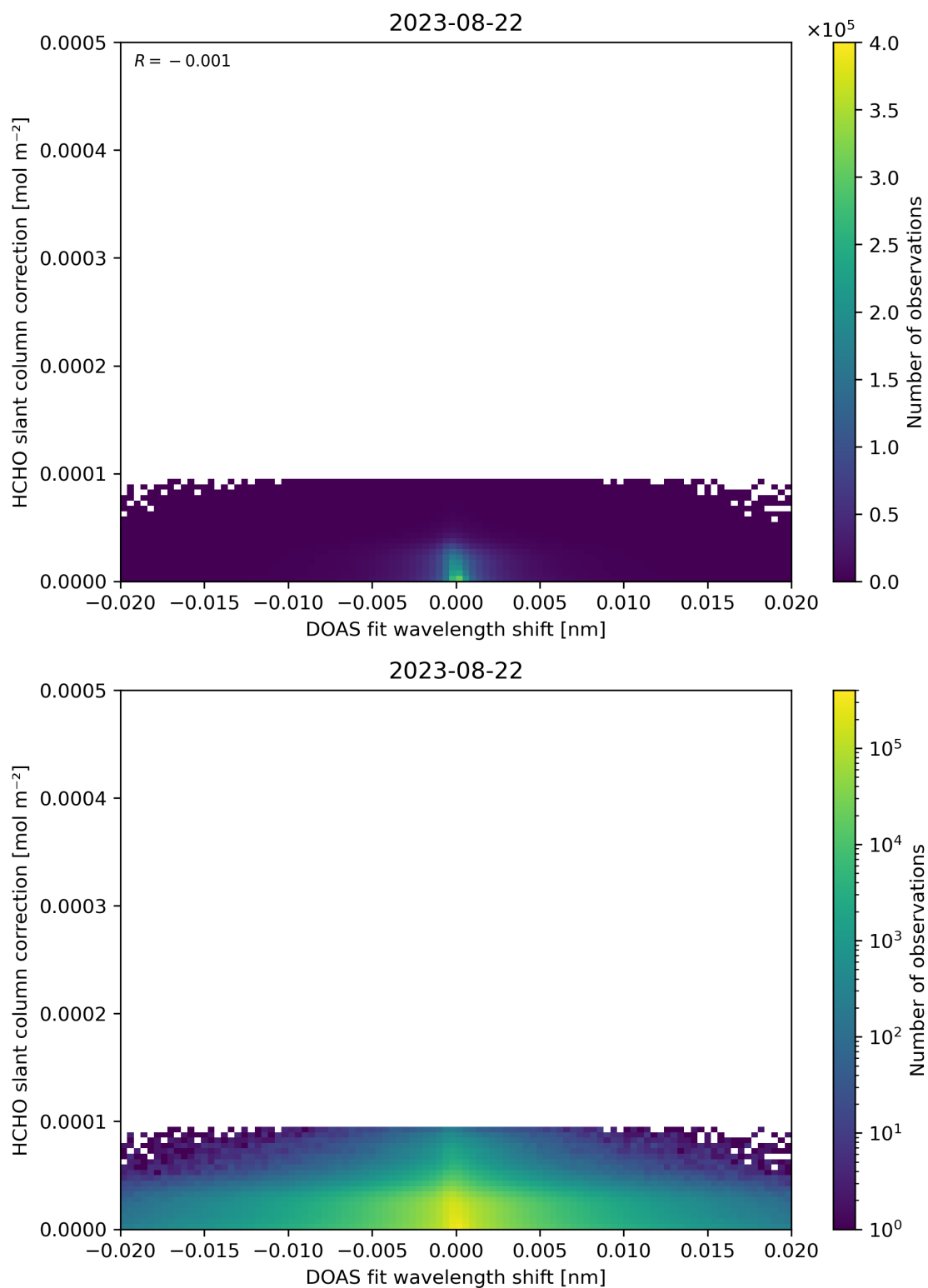
Figure 67: Scatter density plot of “DOAS fit wavelength shift” against “HCHO slant column correction” for 2023-08-21 to 2023-08-23.
