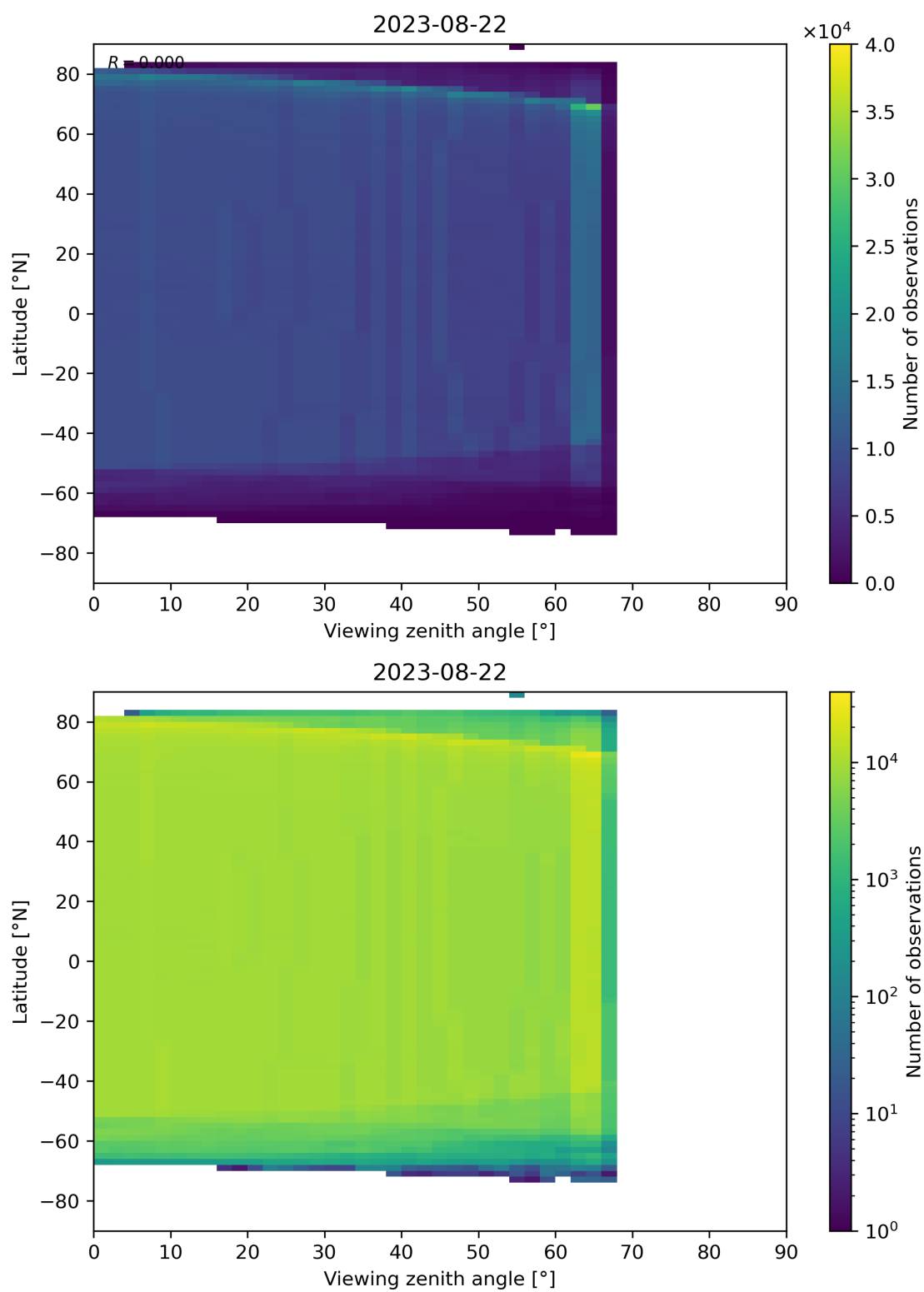
Figure 196: Scatter density plot of “Viewing zenith angle” against “Latitude” for 2023-08-21 to 2023-08-23.
