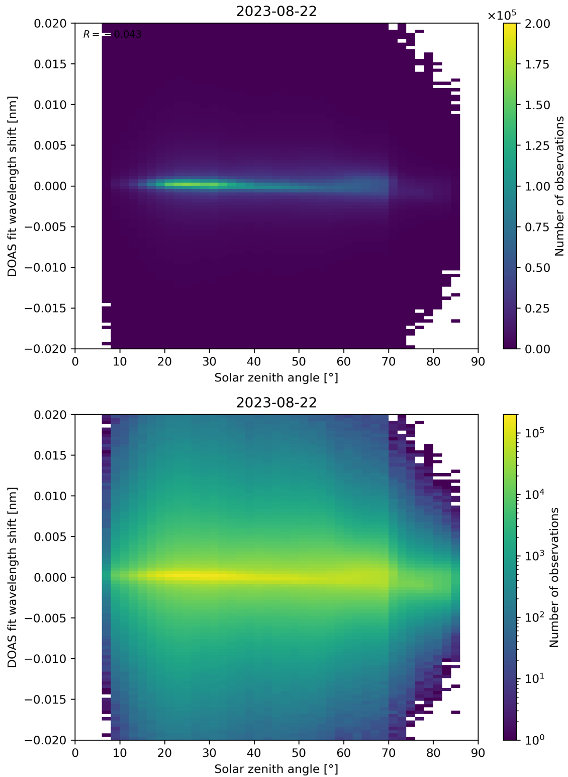
Figure 168: Scatter density plot of “Solar zenith angle” against “DOAS fit wavelength shift” for 2023-08-21 to 2023-08-23.
