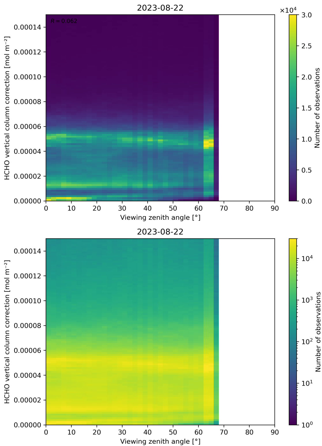
Figure 193: Scatter density plot of “Viewing zenith angle” against “HCHO vertical column correction” for 2023-08-21 to 2023-08-23.
