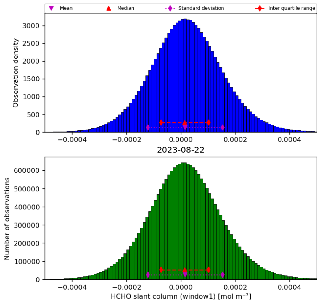
Figure 38: Histogram of “HCHO slant column (window1)” for 2023-08-21 to 2023-08-23
