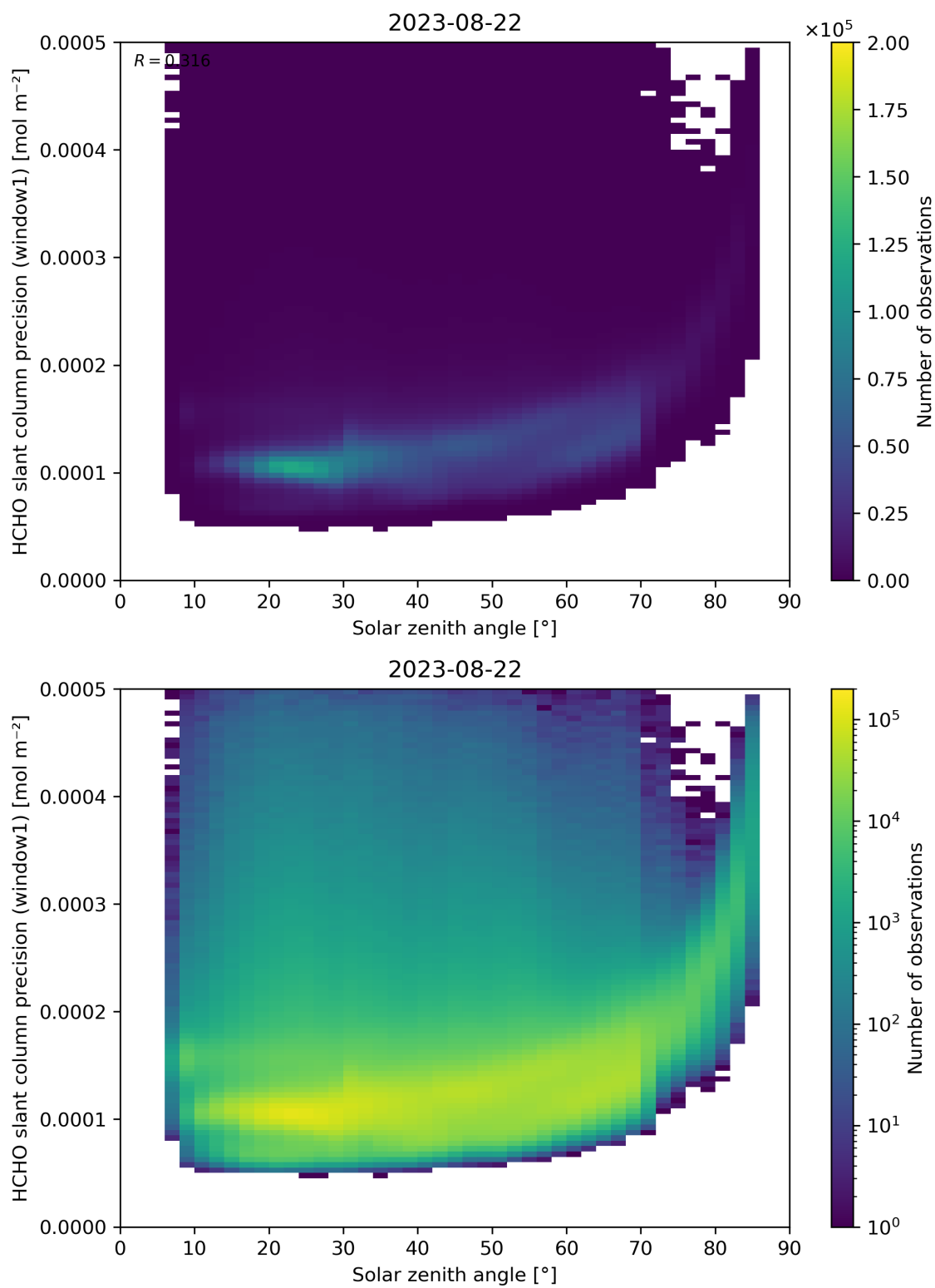
Figure 174: Scatter density plot of “Solar zenith angle” against “HCHO slant column precision (window1)” for 2023-08-21 to 2023-08-23.
