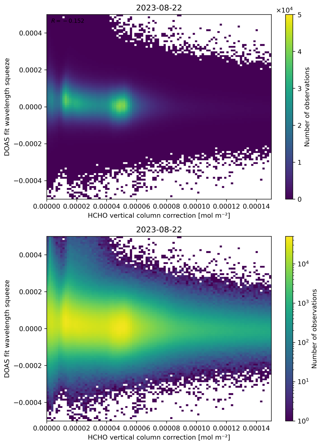
Figure 114: Scatter density plot of “HCHO vertical column correction” against “DOAS fit wavelength squeeze” for 2023-08-21 to 2023-08-23.
