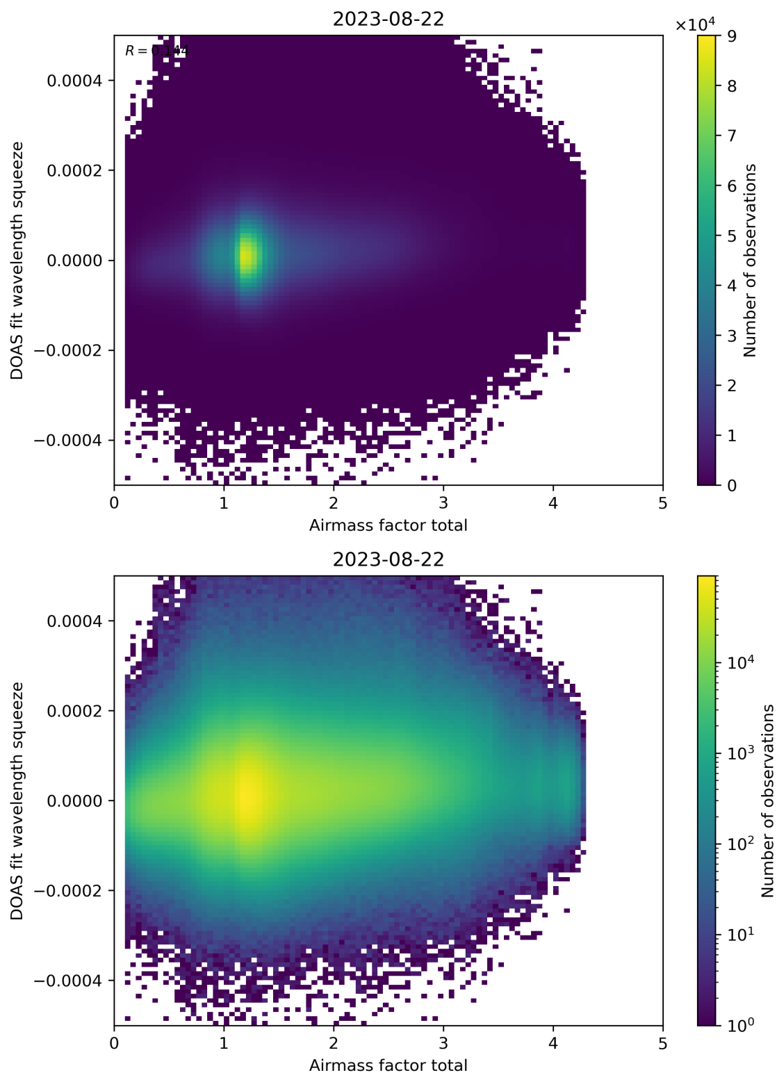
Figure 99: Scatter density plot of “Airmass factor total” against “DOAS fit wavelength squeeze” for 2023-08-21 to 2023-08-23.
