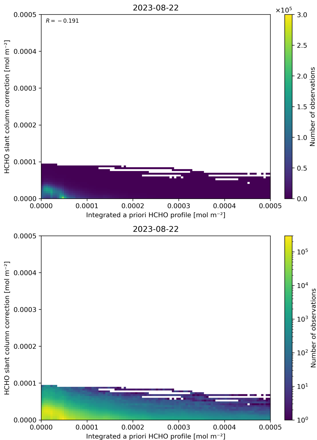
Figure 152: Scatter density plot of “Integrated a priori HCHO profile” against “HCHO slant column correction” for 2023-08-21 to 2023-08-23.
