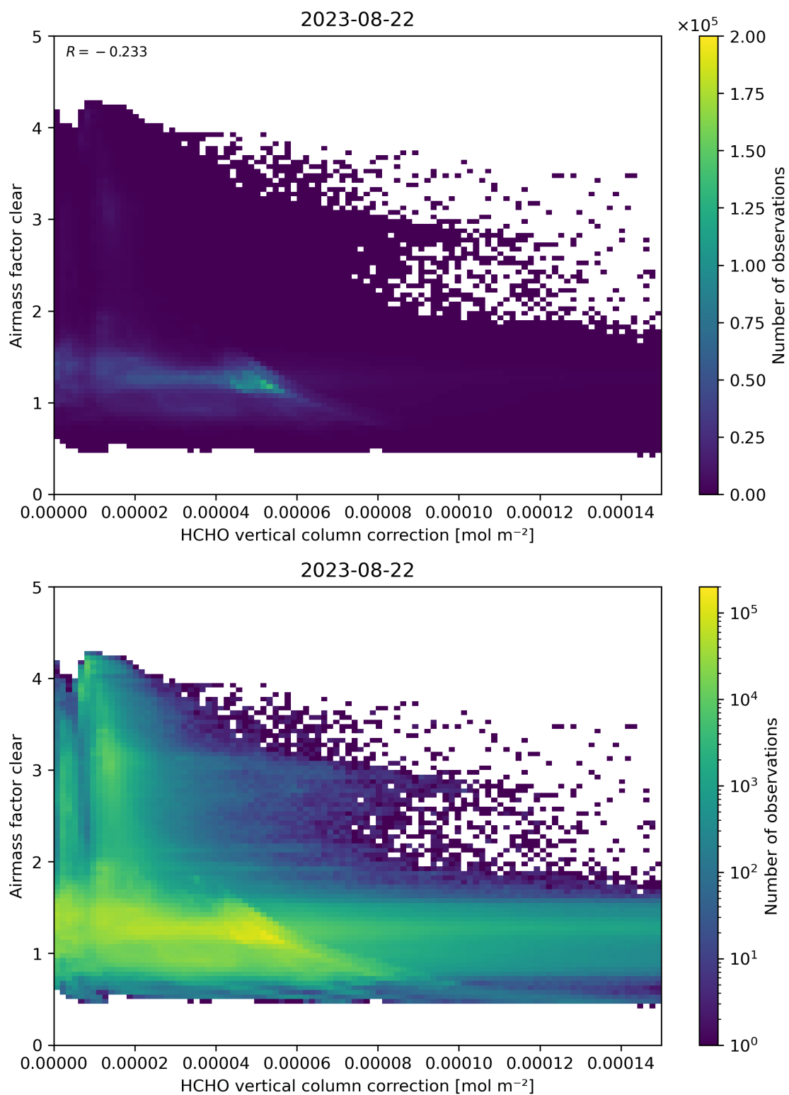
Figure 115: Scatter density plot of “HCHO vertical column correction” against “Airmass factor clear” for 2023-08-21 to 2023-08-23.
