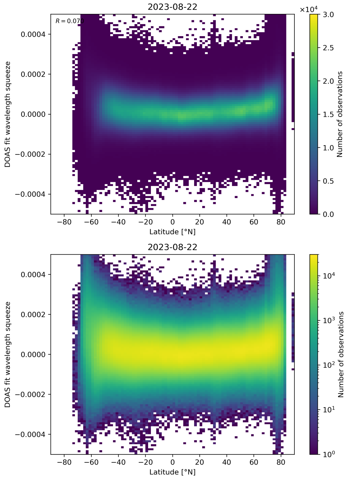
Figure 155: Scatter density plot of “Latitude” against “DOAS fit wavelength squeeze” for 2023-08-21 to 2023-08-23.
