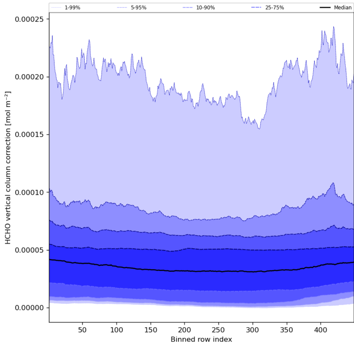
Figure 51: Along track statistics of “HCHO vertical column correction” for 2023-08-21 to 2023-08-23
