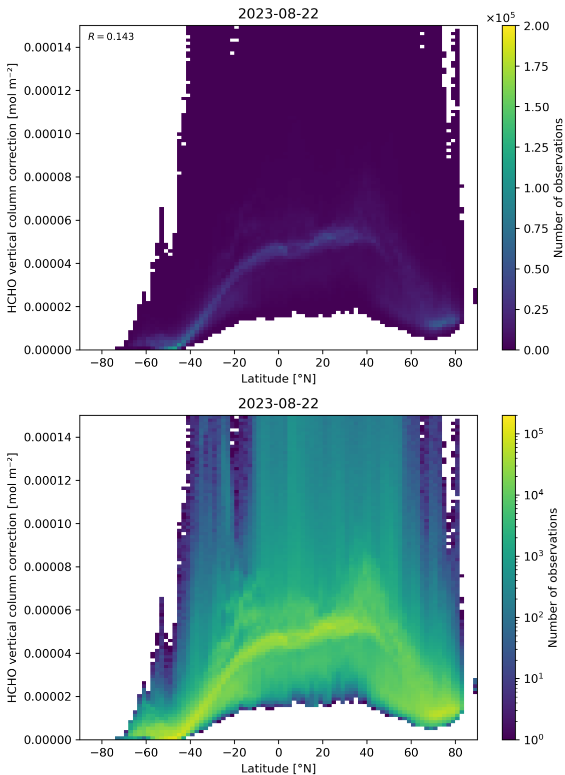
Figure 164: Scatter density plot of “Latitude” against “HCHO vertical column correction” for 2023-08-21 to 2023-08-23.
