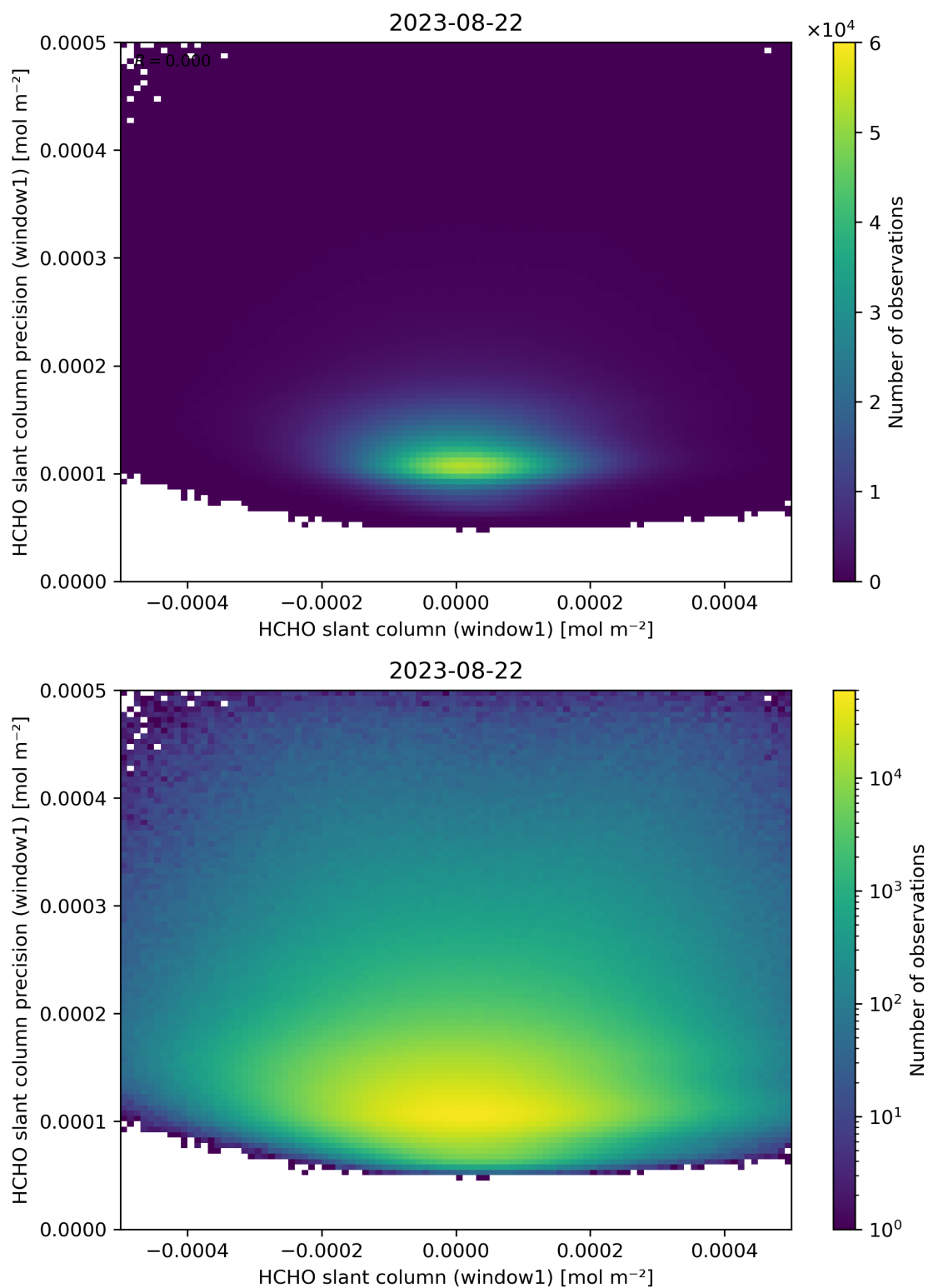
Figure 84: Scatter density plot of “HCHO slant column (window1)” against “HCHO slant column precision (window1)” for 2023-08-21 to 2023-08-23.
