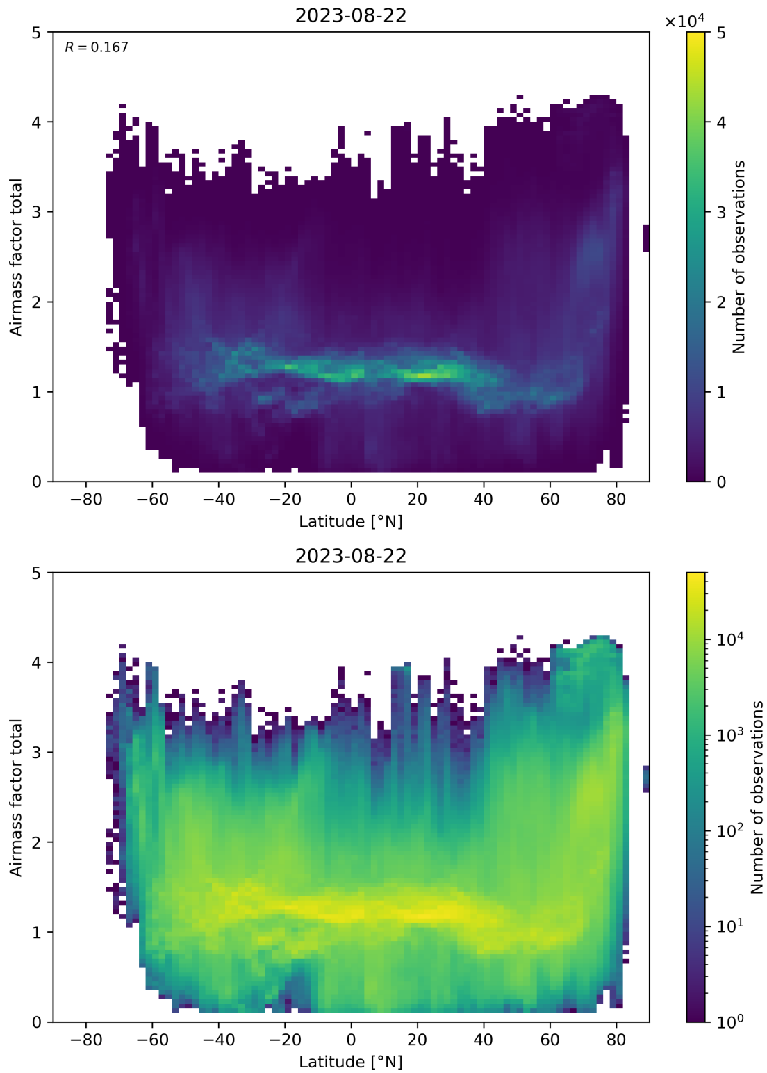
Figure 161: Scatter density plot of “Latitude” against “Airmass factor total” for 2023-08-21 to 2023-08-23.
