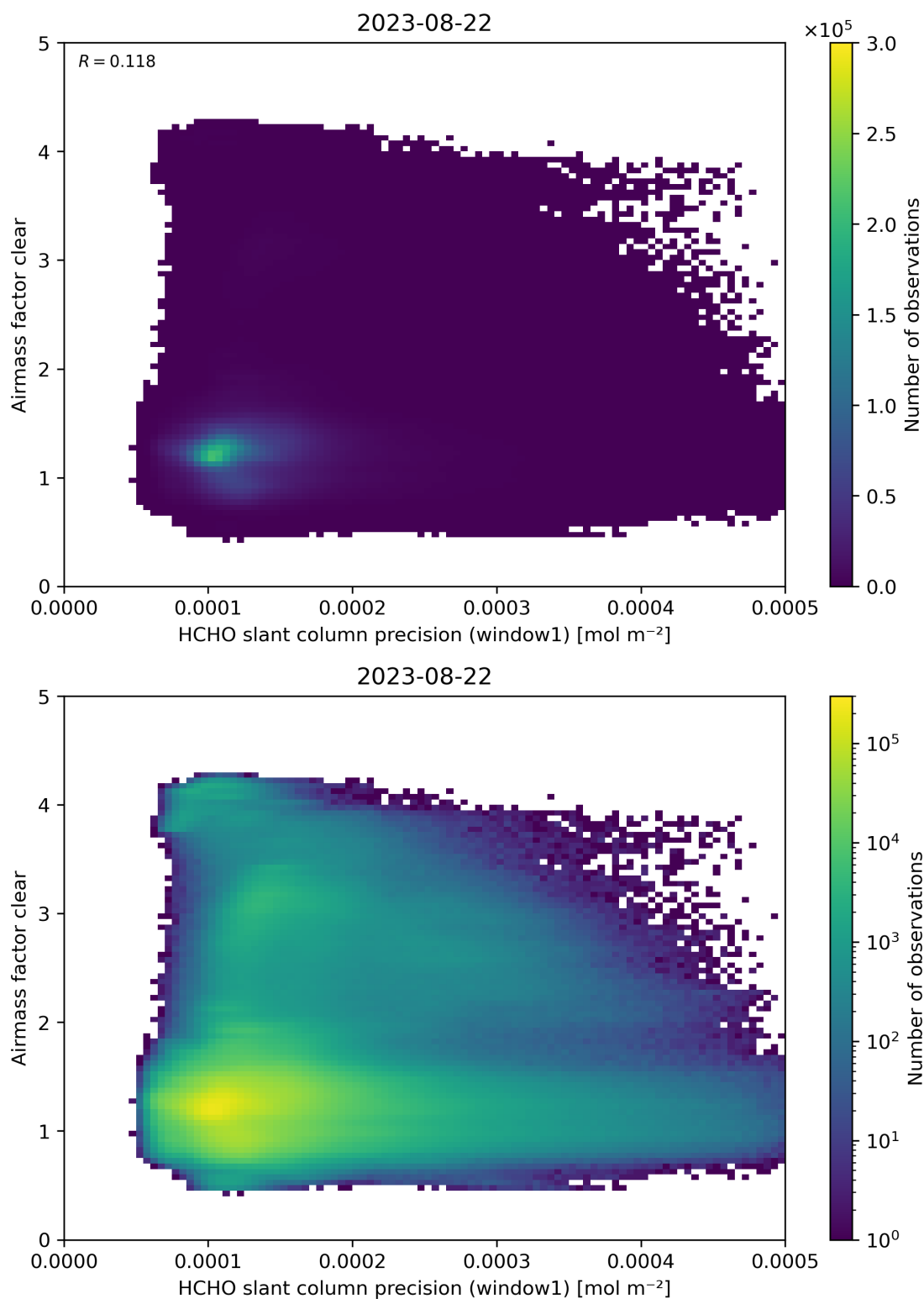
Figure 91: Scatter density plot of “HCHO slant column precision (window1)” against “Airmass factor clear” for 2023-08-21 to 2023-08-23.
