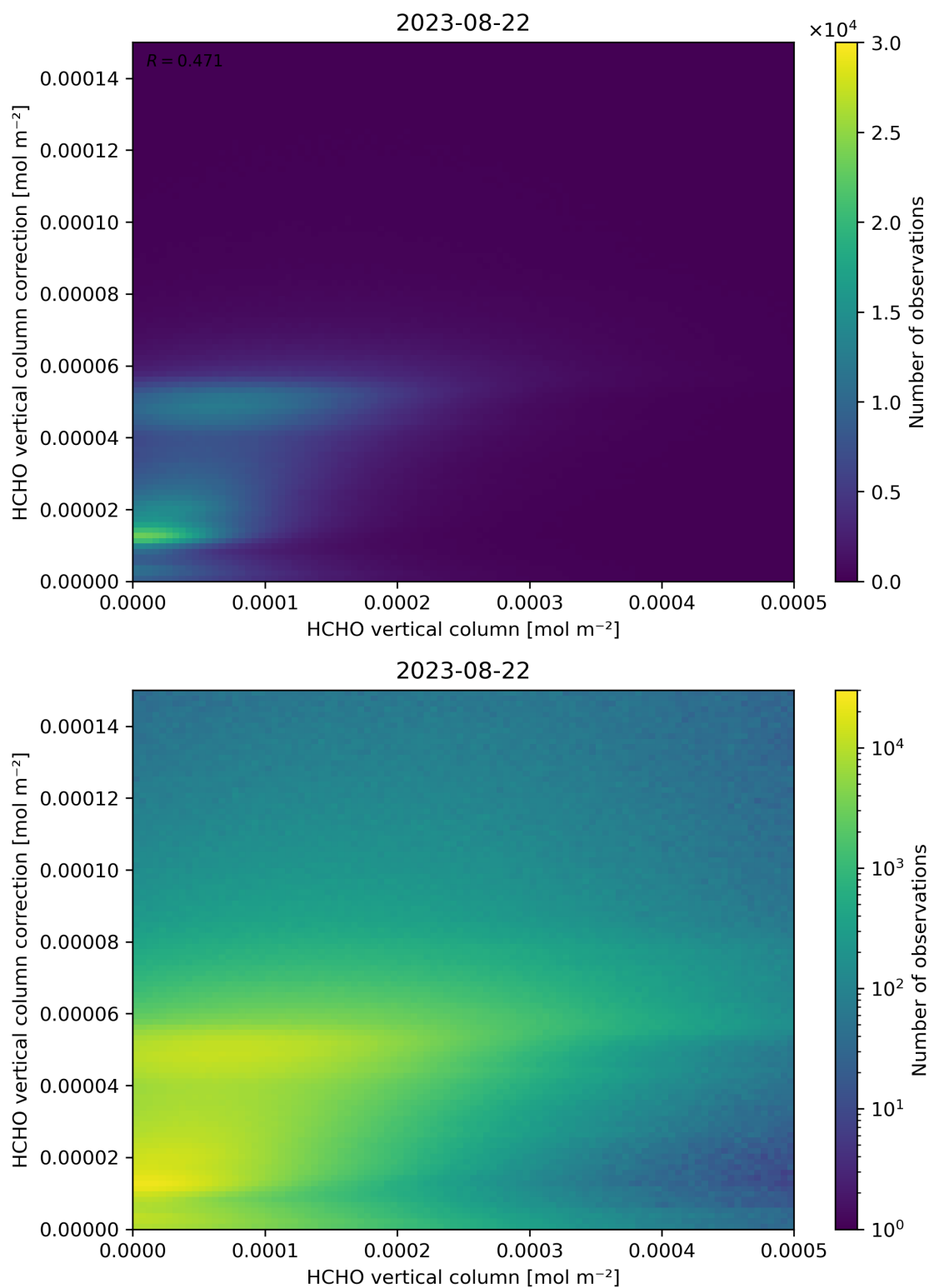
Figure 133: Scatter density plot of “HCHO vertical column” against “HCHO vertical column correction” for 2023-08-21 to 2023-08-23.
