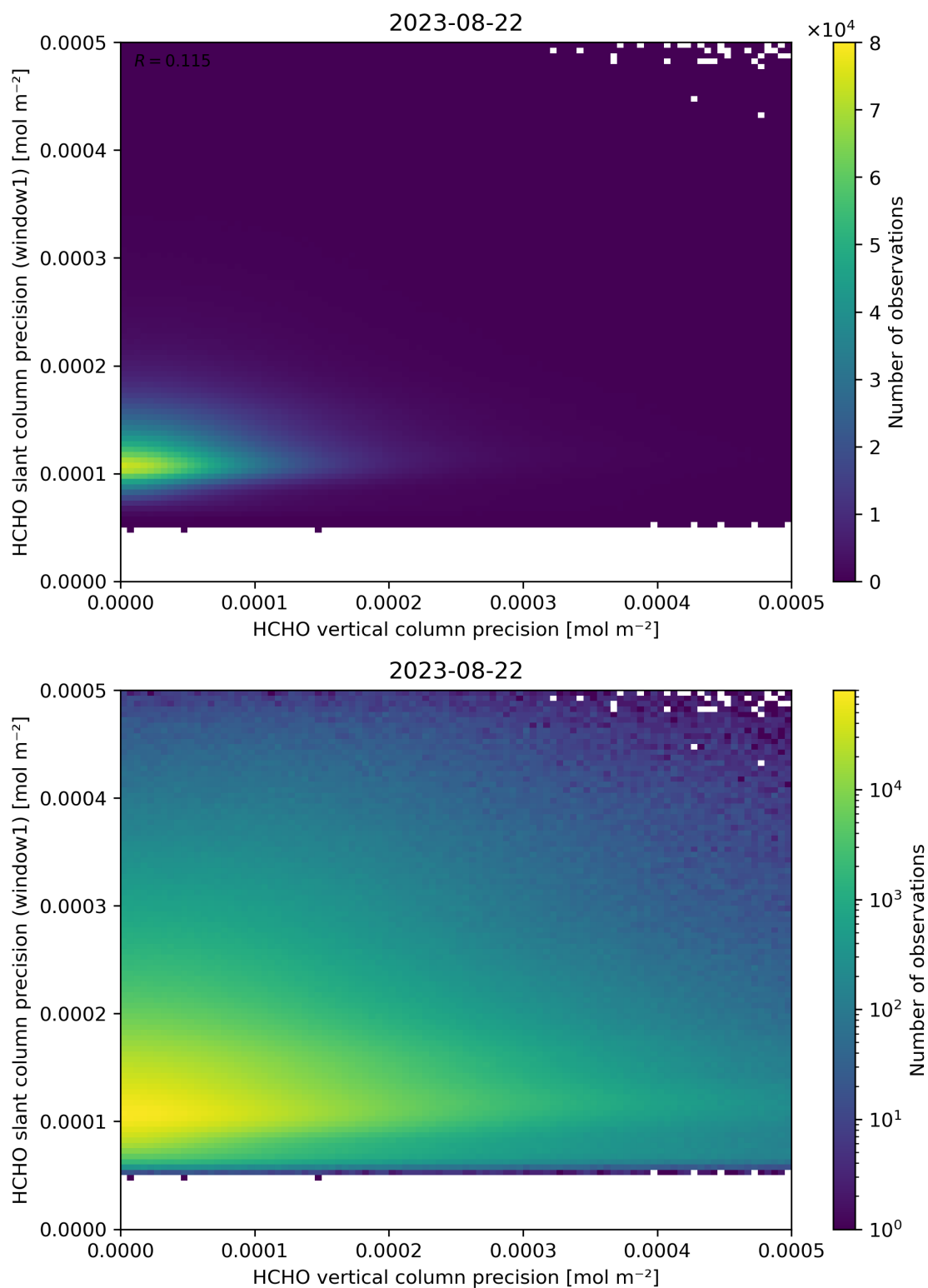
Figure 143: Scatter density plot of “HCHO vertical column precision” against “HCHO slant column precision (window1)” for 2023-08-21 to 2023-08-23.
