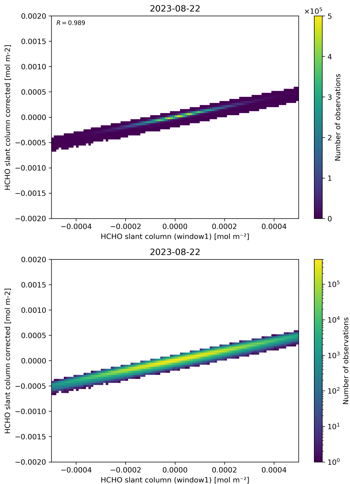
Figure 82: Scatter density plot of “HCHO slant column (window1)” against “HCHO slant column corrected” for 2023-08-21 to 2023-08-23.
