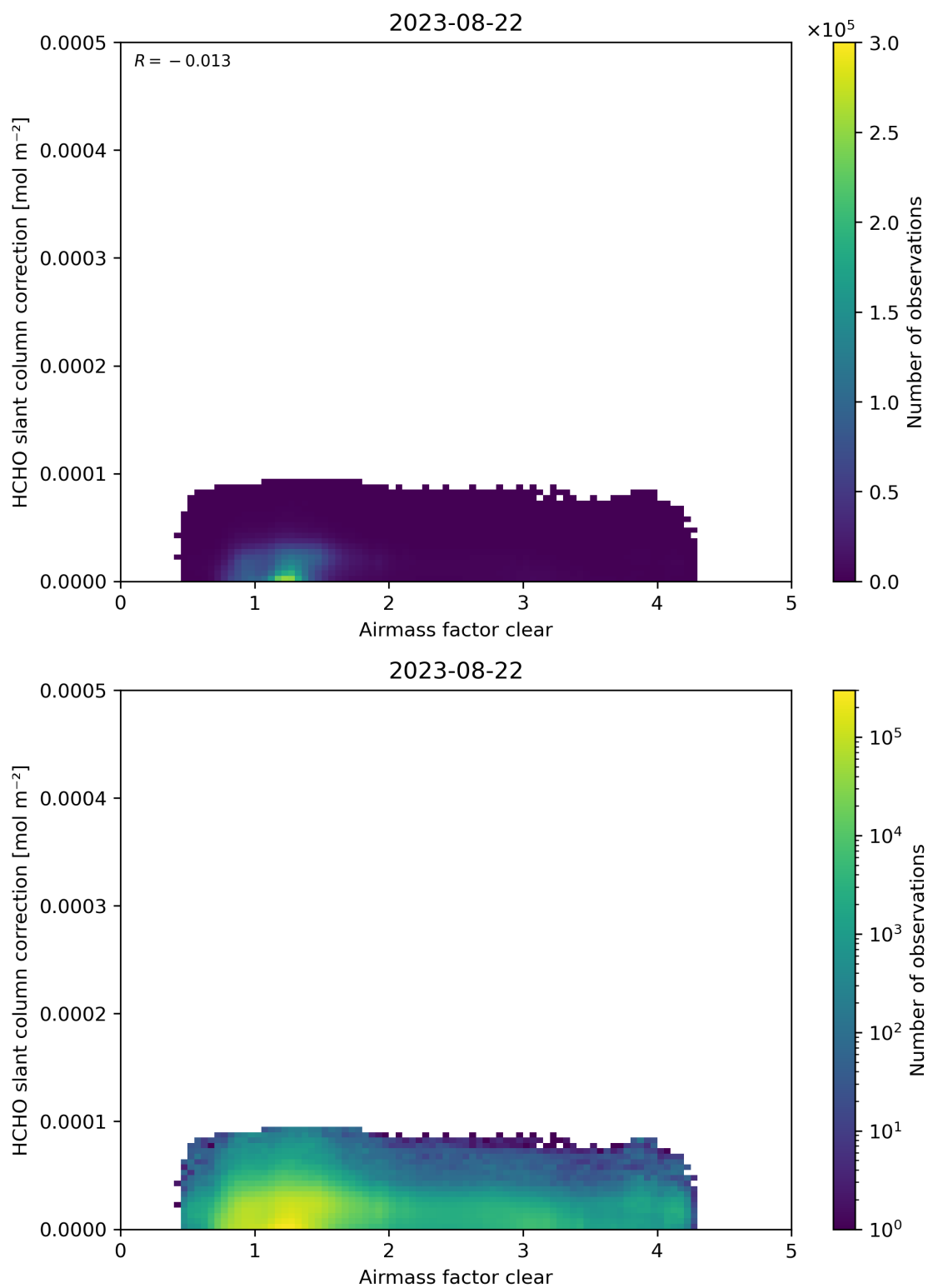
Figure 75: Scatter density plot of “Airmass factor clear” against “HCHO slant column correction” for 2023-08-21 to 2023-08-23.
