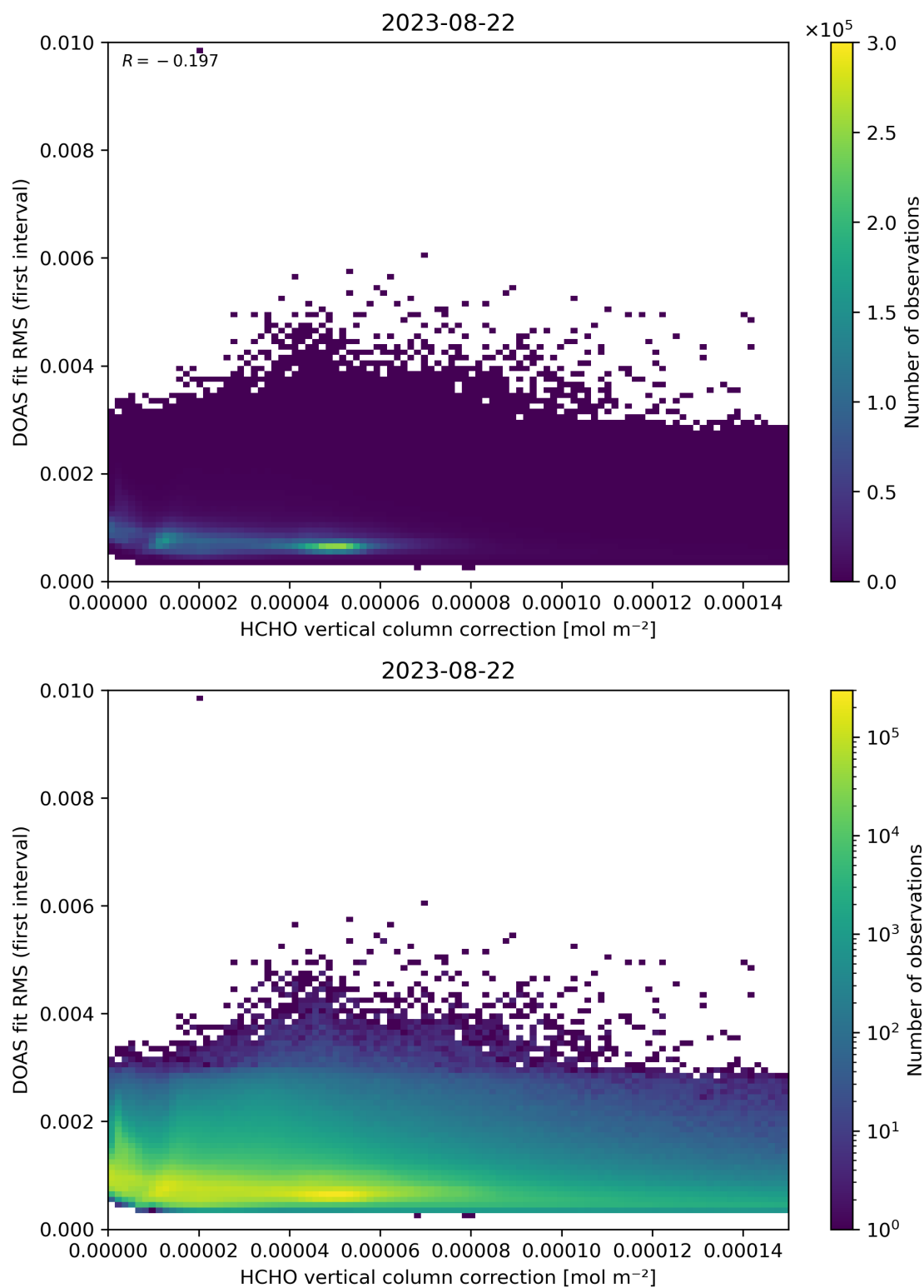
Figure 112: Scatter density plot of “HCHO vertical column correction” against “DOAS fit RMS (first interval)” for 2023-08-21 to 2023-08-23.
