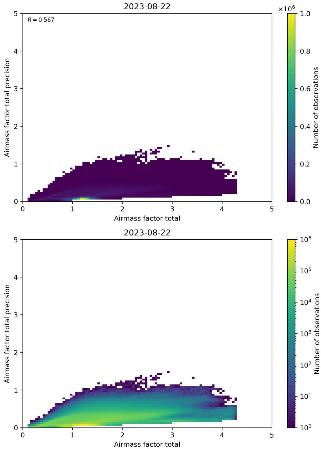
Figure 103: Scatter density plot of “Airmass factor total” against “Airmass factor total precision” for 2023-08-21 to 2023-08-23.
