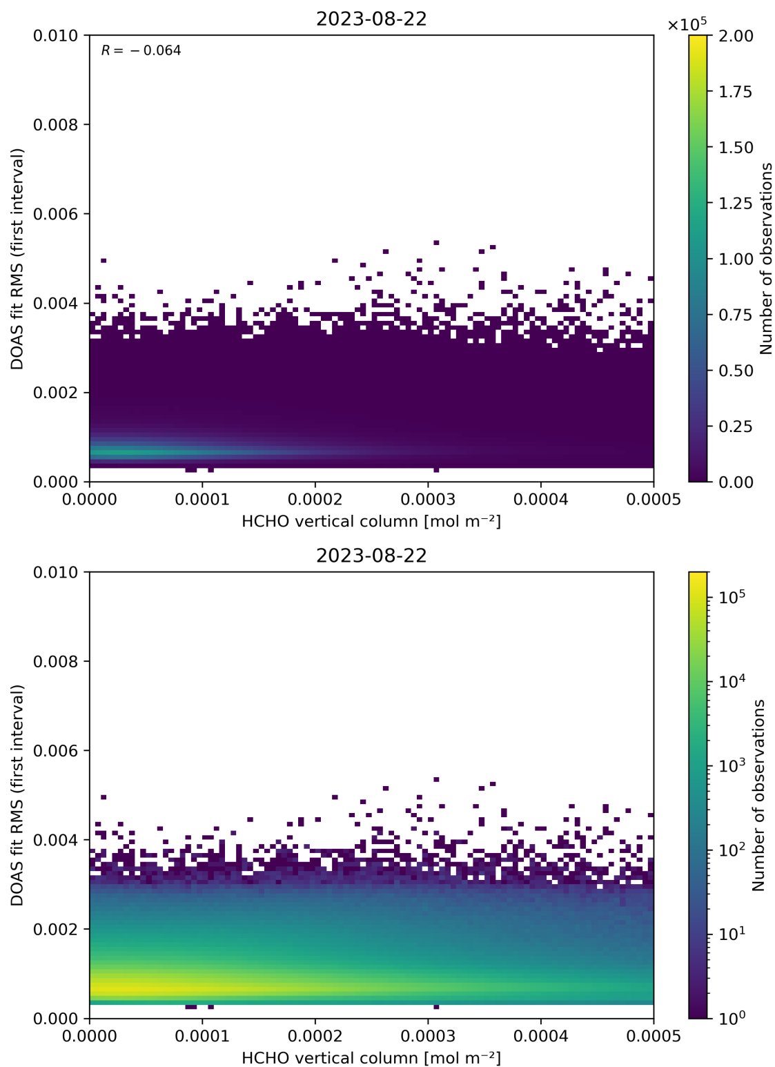
Figure 123: Scatter density plot of “HCHO vertical column” against “DOAS fit RMS (first interval)” for 2023-08-21 to 2023-08-23.
