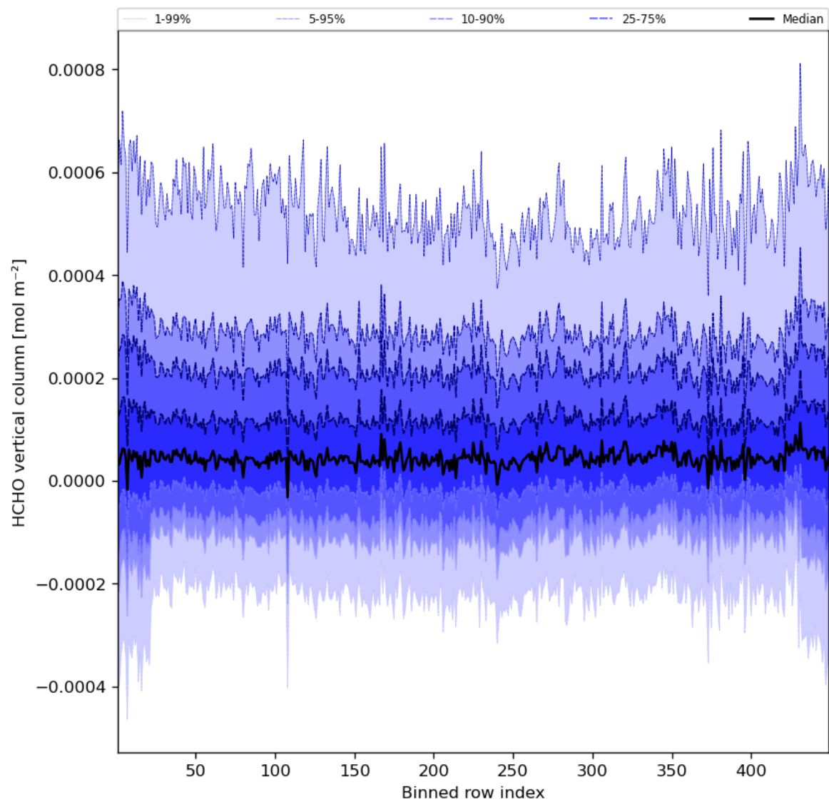
Figure 49: Along track statistics of “HCHO vertical column” for 2023-08-21 to 2023-08-23
