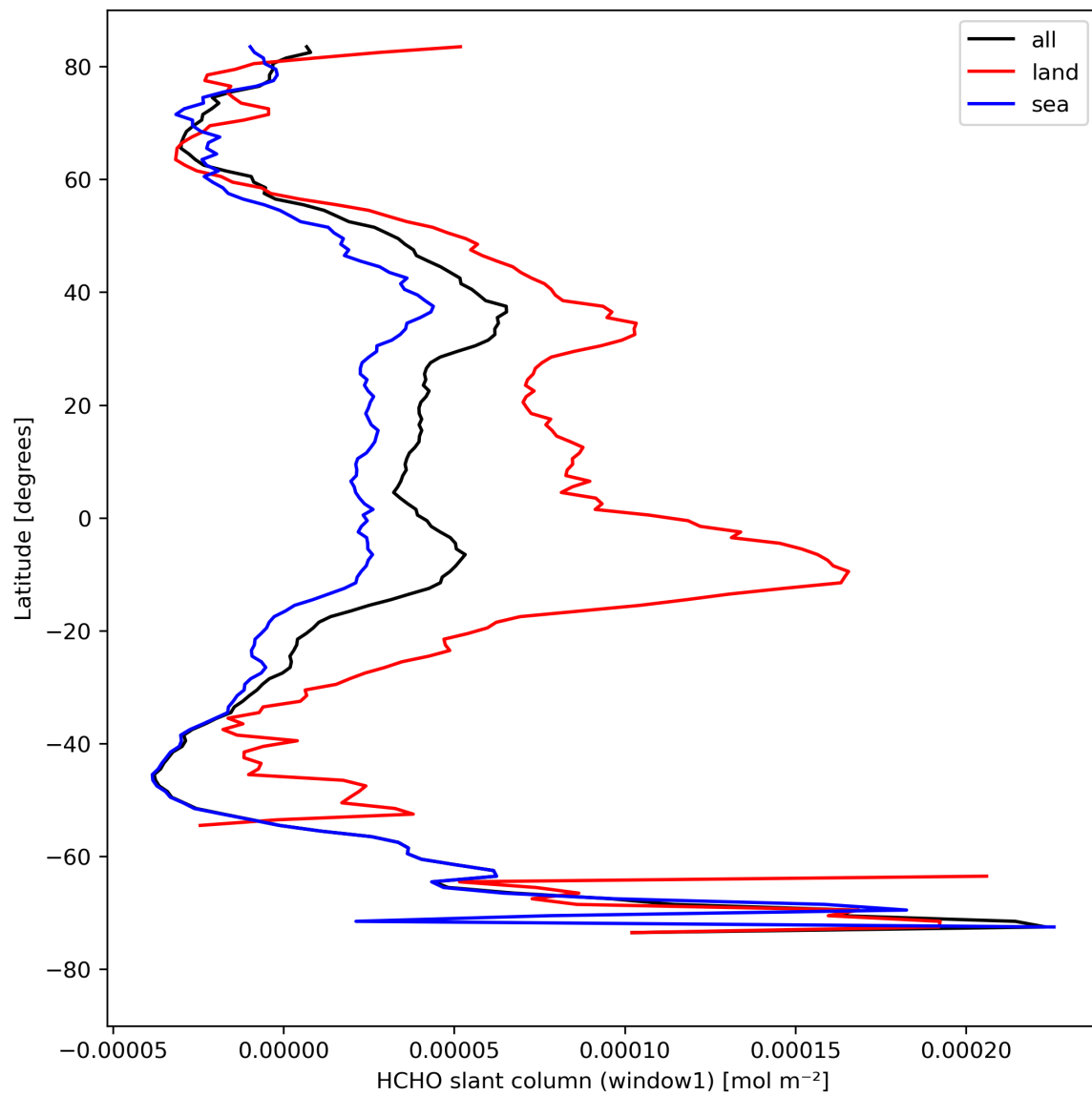
Figure 24: Zonal average of “HCHO slant column (window1)” for 2023-08-21 to 2023-08-23.
