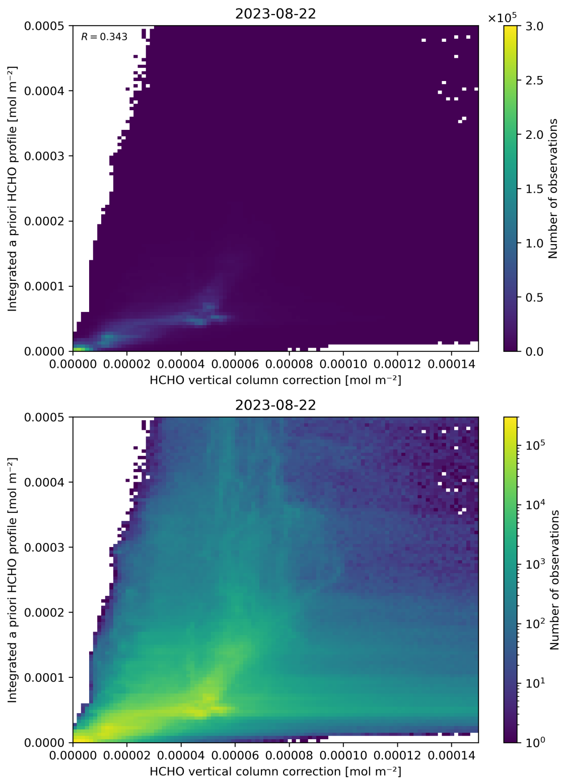
Figure 122: Scatter density plot of “HCHO vertical column correction” against “Integrated a priori HCHO profile” for 2023-08-21 to 2023-08-23.
