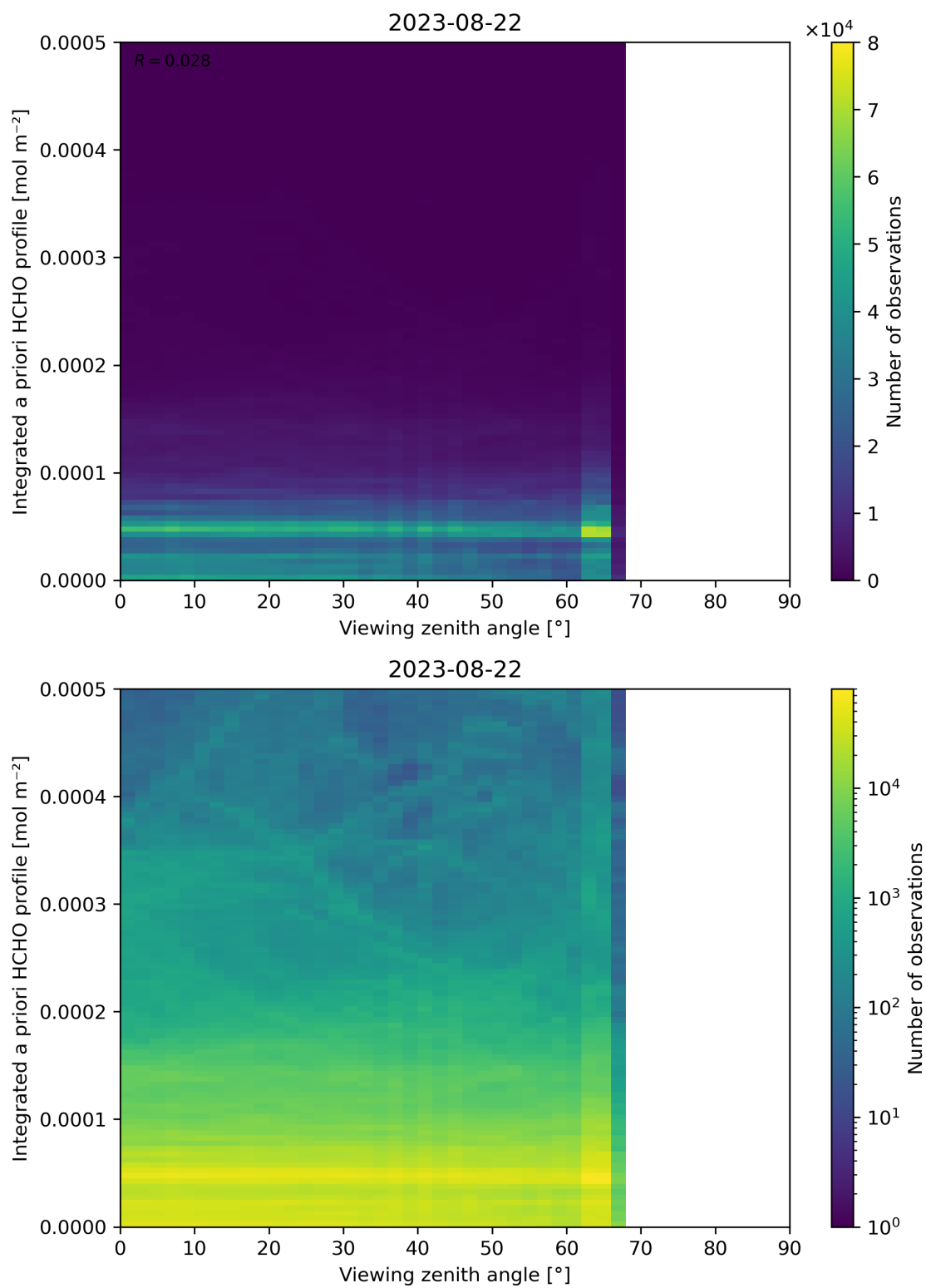
Figure 195: Scatter density plot of “Viewing zenith angle” against “Integrated a priori HCHO profile” for 2023-08-21 to 2023-08-23.
