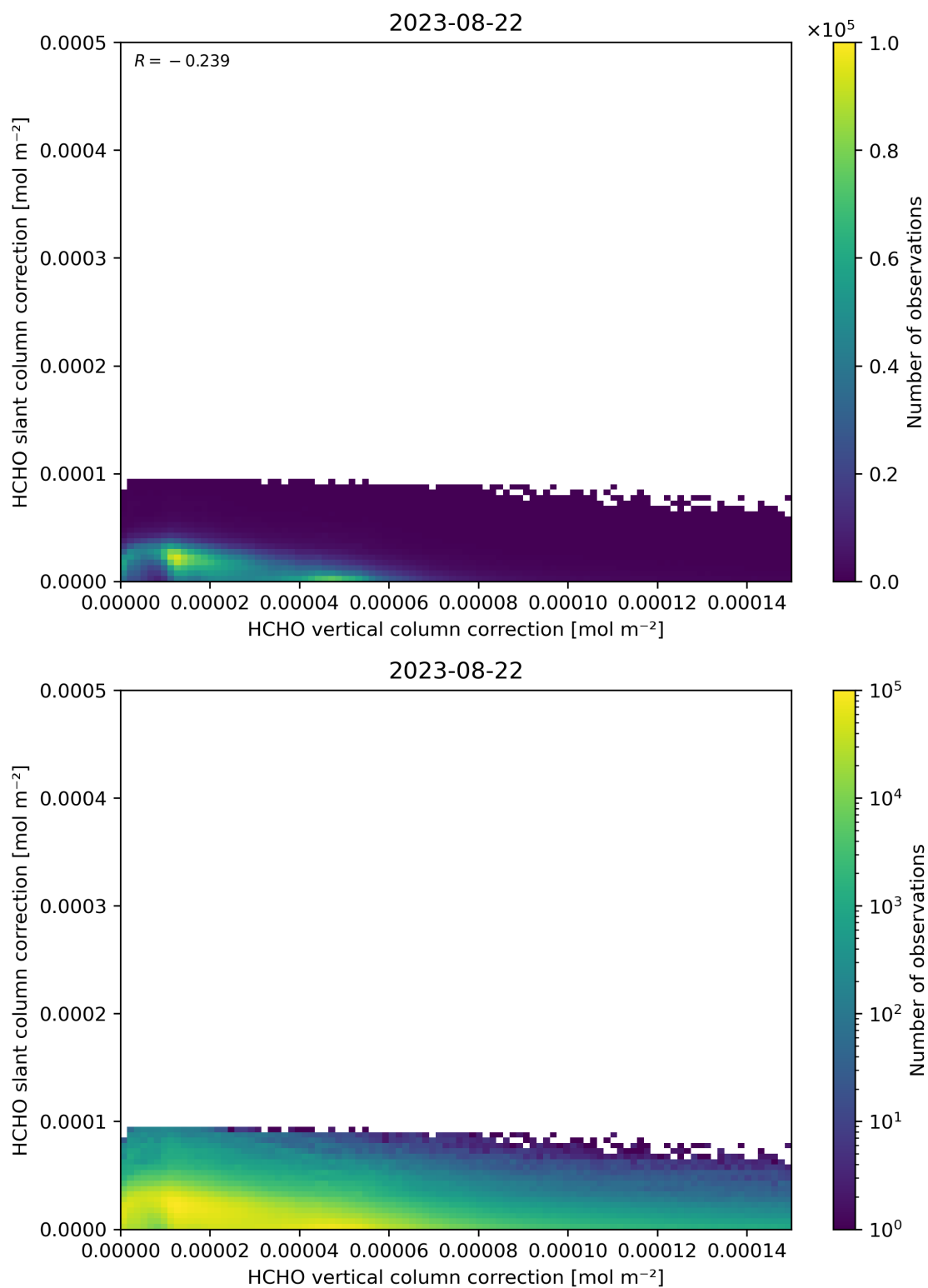
Figure 117: Scatter density plot of “HCHO vertical column correction” against “HCHO slant column correction” for 2023-08-21 to 2023-08-23.
