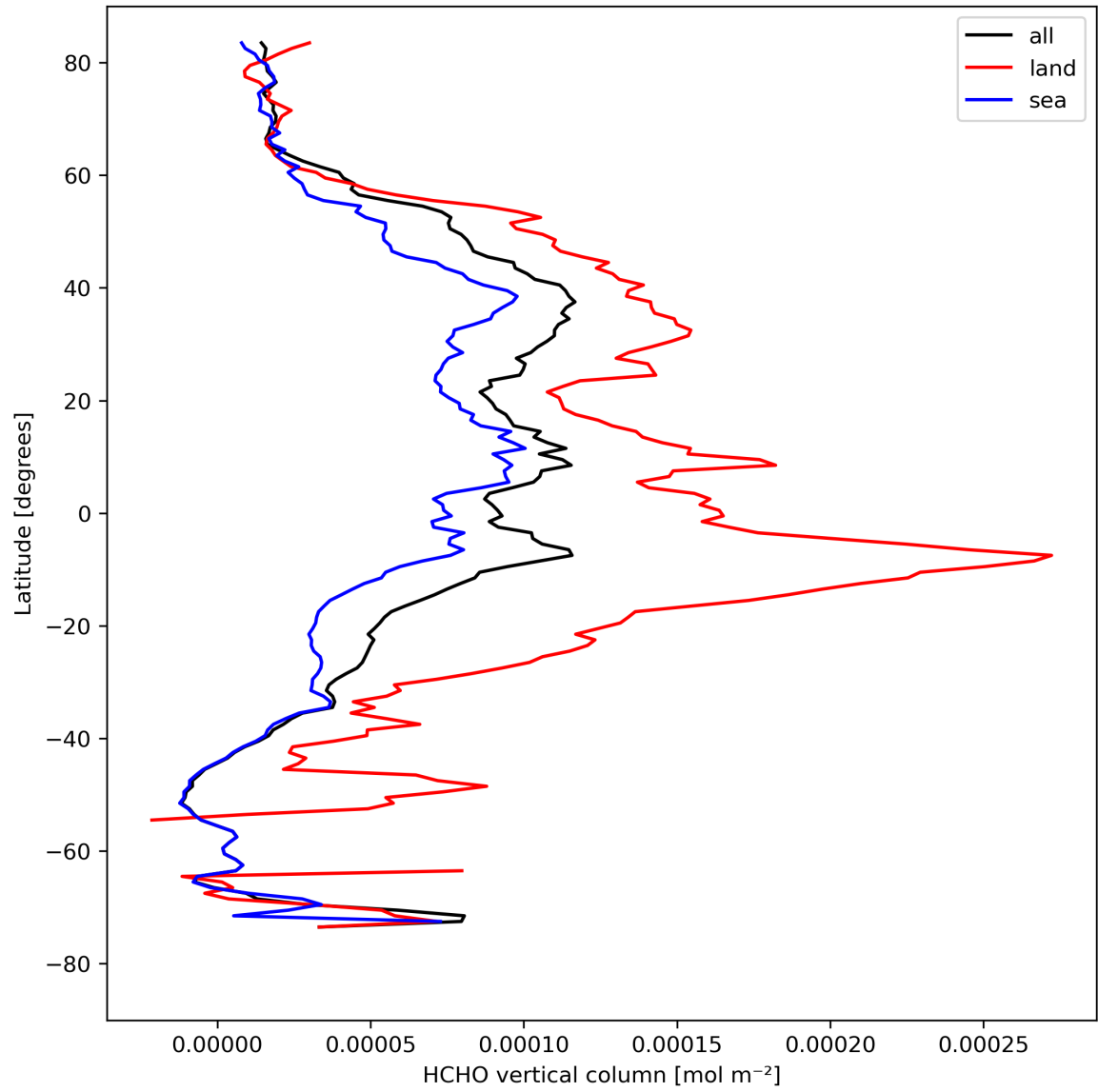
Figure 21: Zonal average of “HCHO vertical column” for 2023-08-21 to 2023-08-23.
