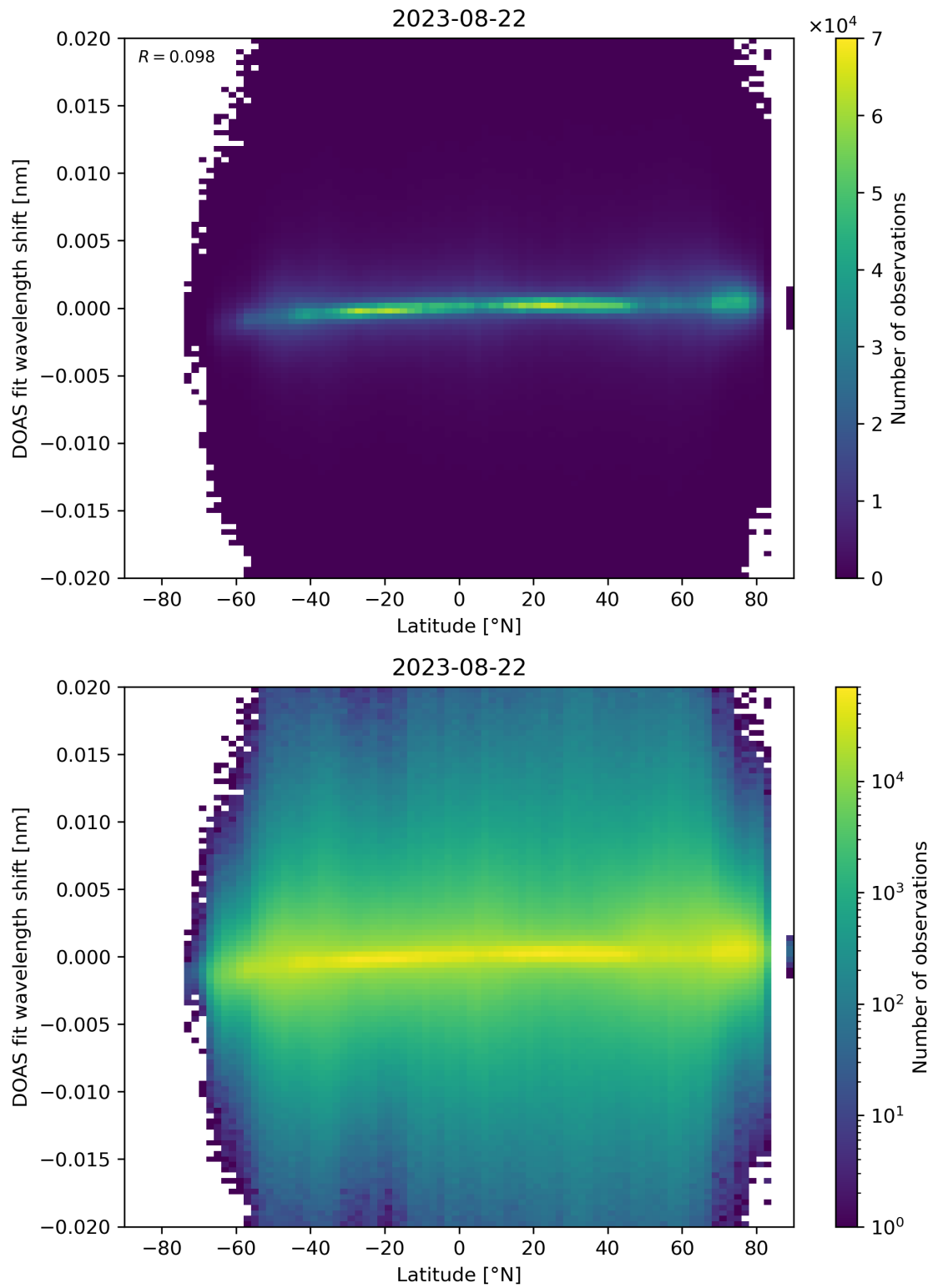
Figure 154: Scatter density plot of “Latitude” against “DOAS fit wavelength shift” for 2023-08-21 to 2023-08-23.
