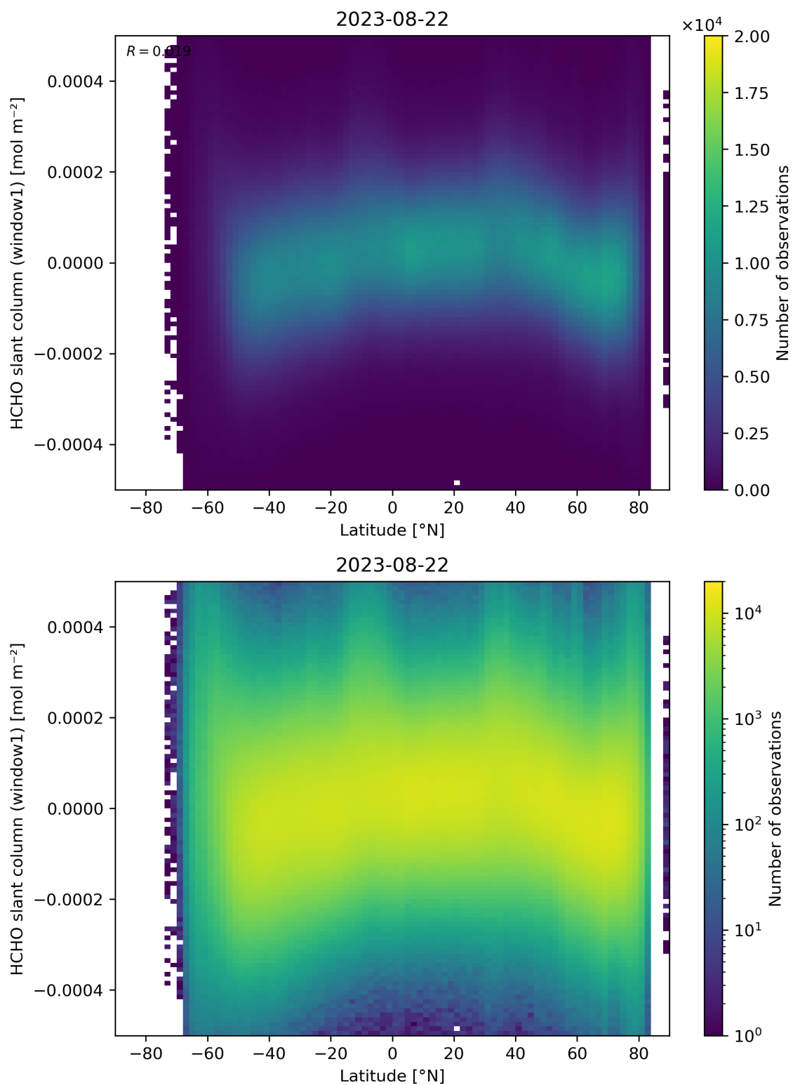
Figure 159: Scatter density plot of “Latitude” against “HCHO slant column (window1)” for 2023-08-21 to 2023-08-23.
