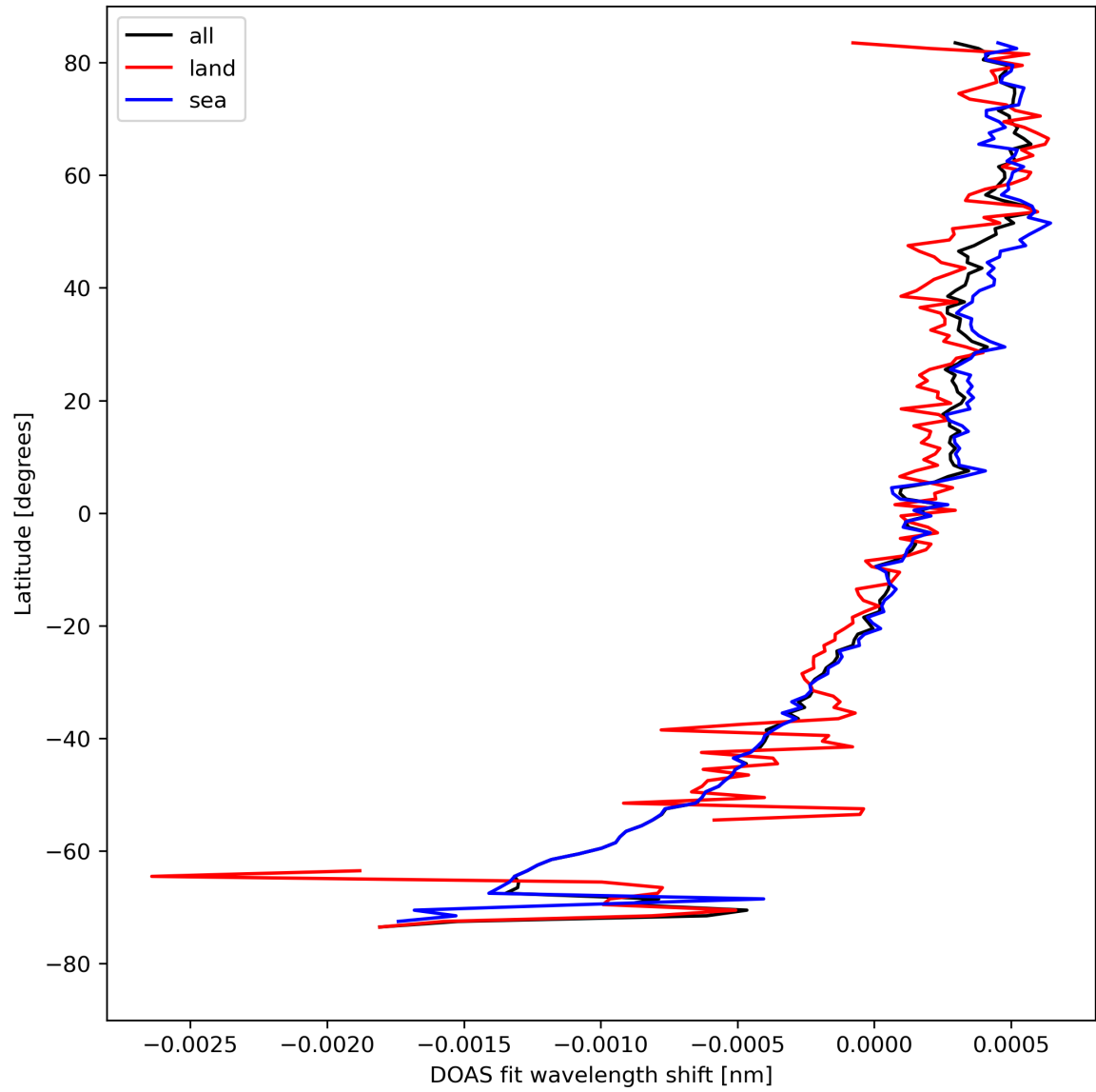
Figure 30: Zonal average of “DOAS fit wavelength shift” for 2023-08-21 to 2023-08-23.
