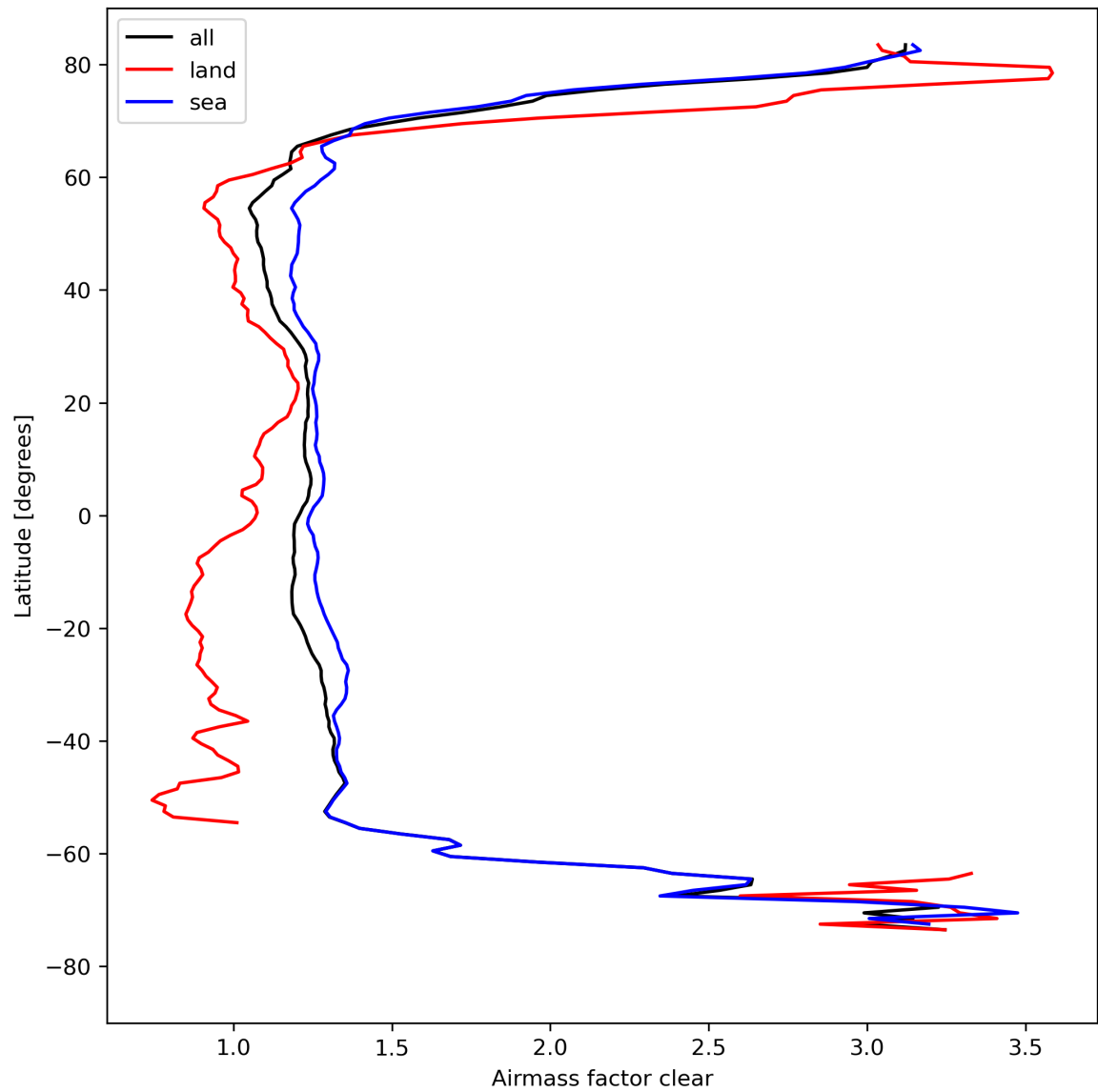
Figure 28: Zonal average of “Airmass factor clear” for 2023-08-21 to 2023-08-23.
