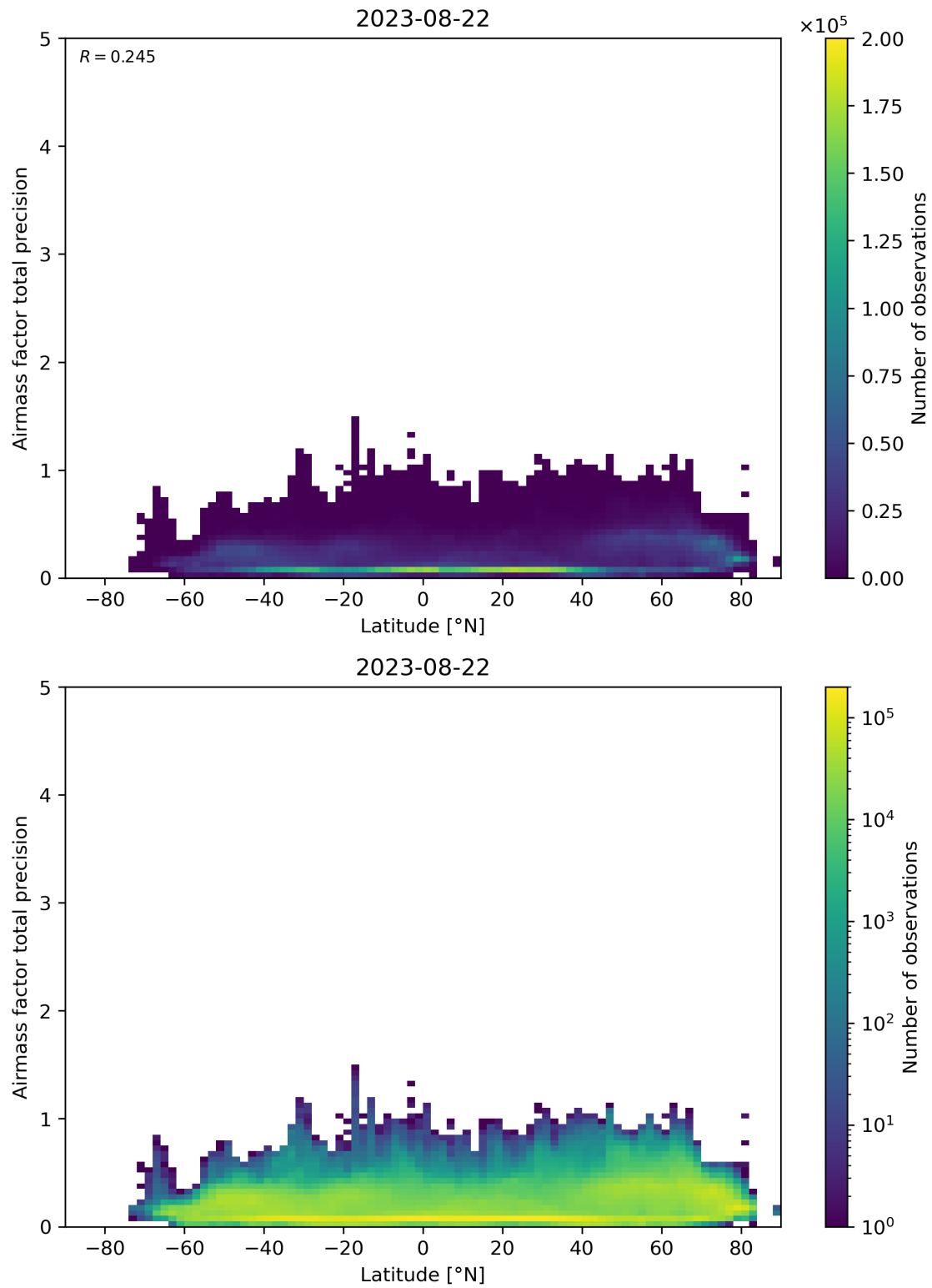
Figure 162: Scatter density plot of “Latitude” against “Airmass factor total precision” for 2023-08-21 to 2023-08-23.
