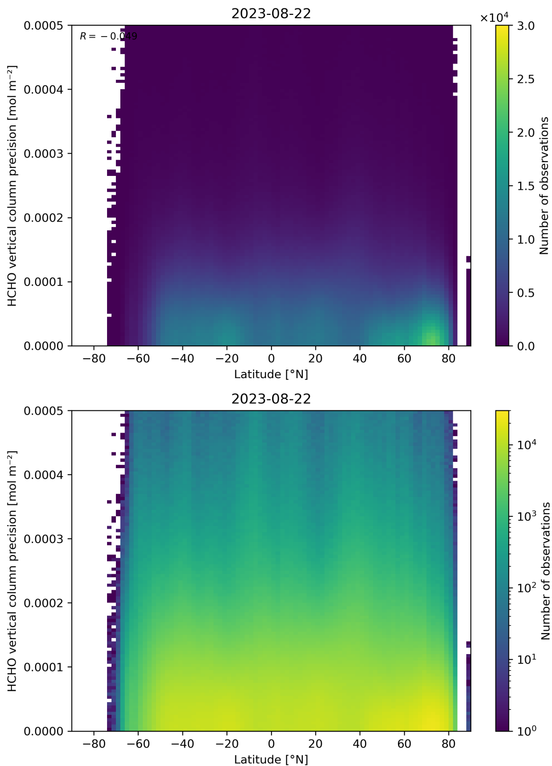
Figure 165: Scatter density plot of “Latitude” against “HCHO vertical column precision” for 2023-08-21 to 2023-08-23.
