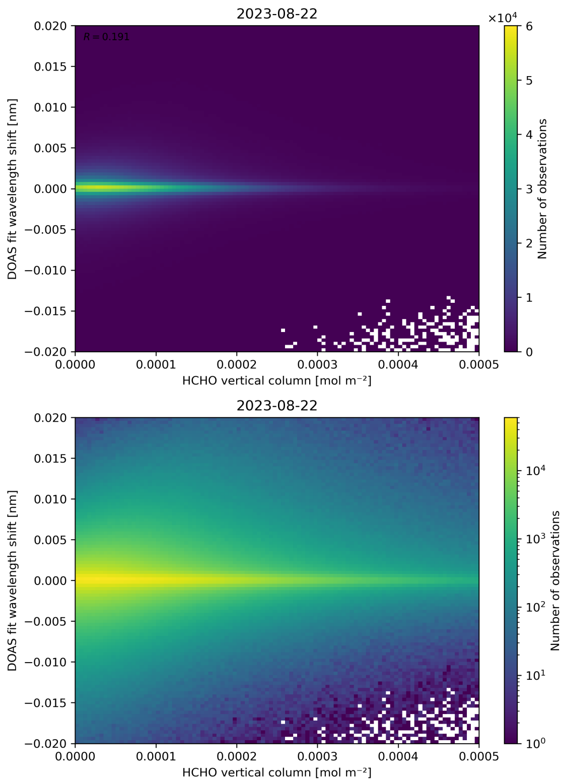
Figure 124: Scatter density plot of “HCHO vertical column” against “DOAS fit wavelength shift” for 2023-08-21 to 2023-08-23.
