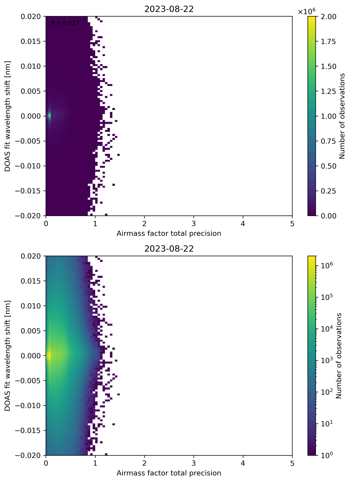
Figure 106: Scatter density plot of “Airmass factor total precision” against “DOAS fit wavelength shift” for 2023-08-21 to 2023-08-23.
