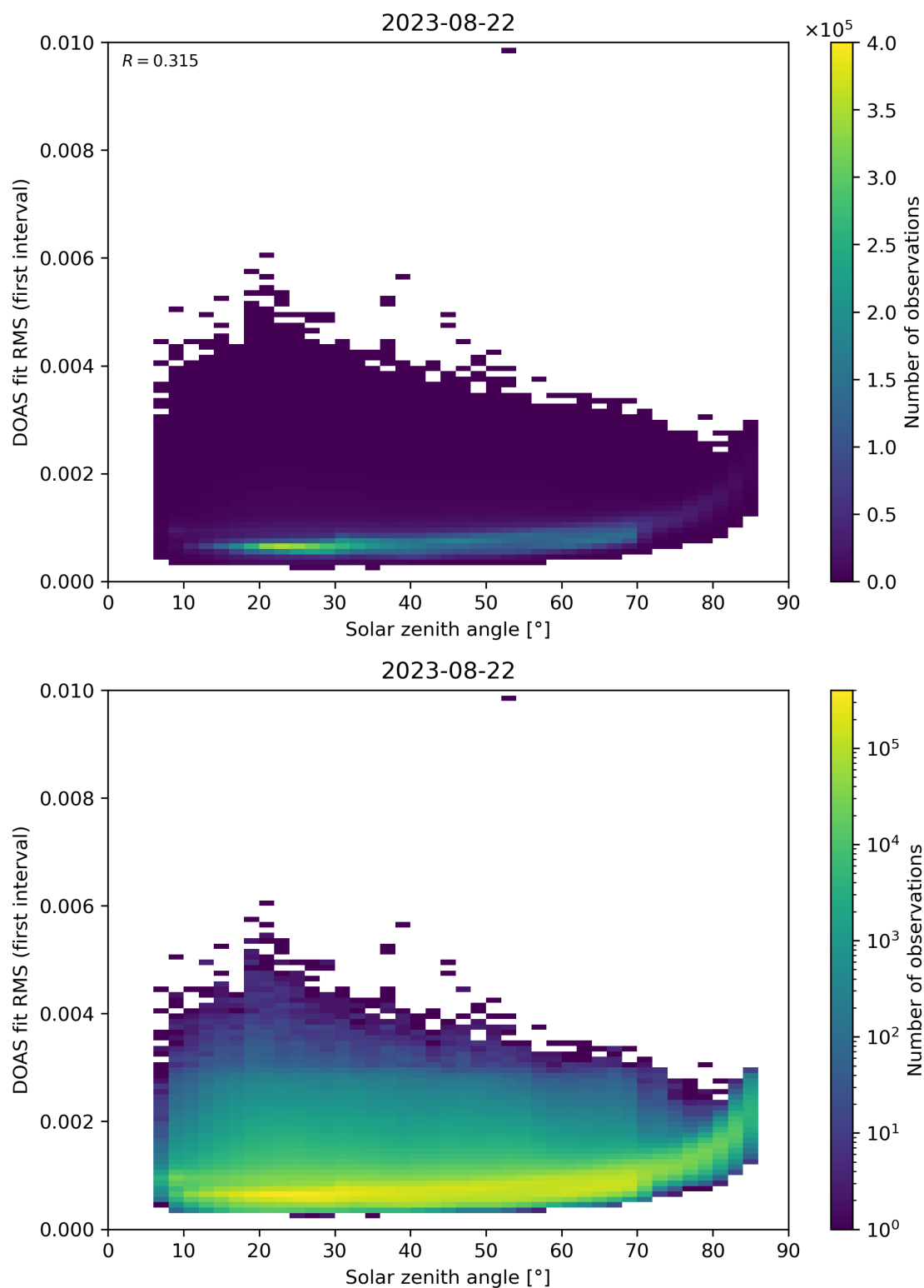
Figure 167: Scatter density plot of “Solar zenith angle” against “DOAS fit RMS (first interval)” for 2023-08-21 to 2023-08-23.
