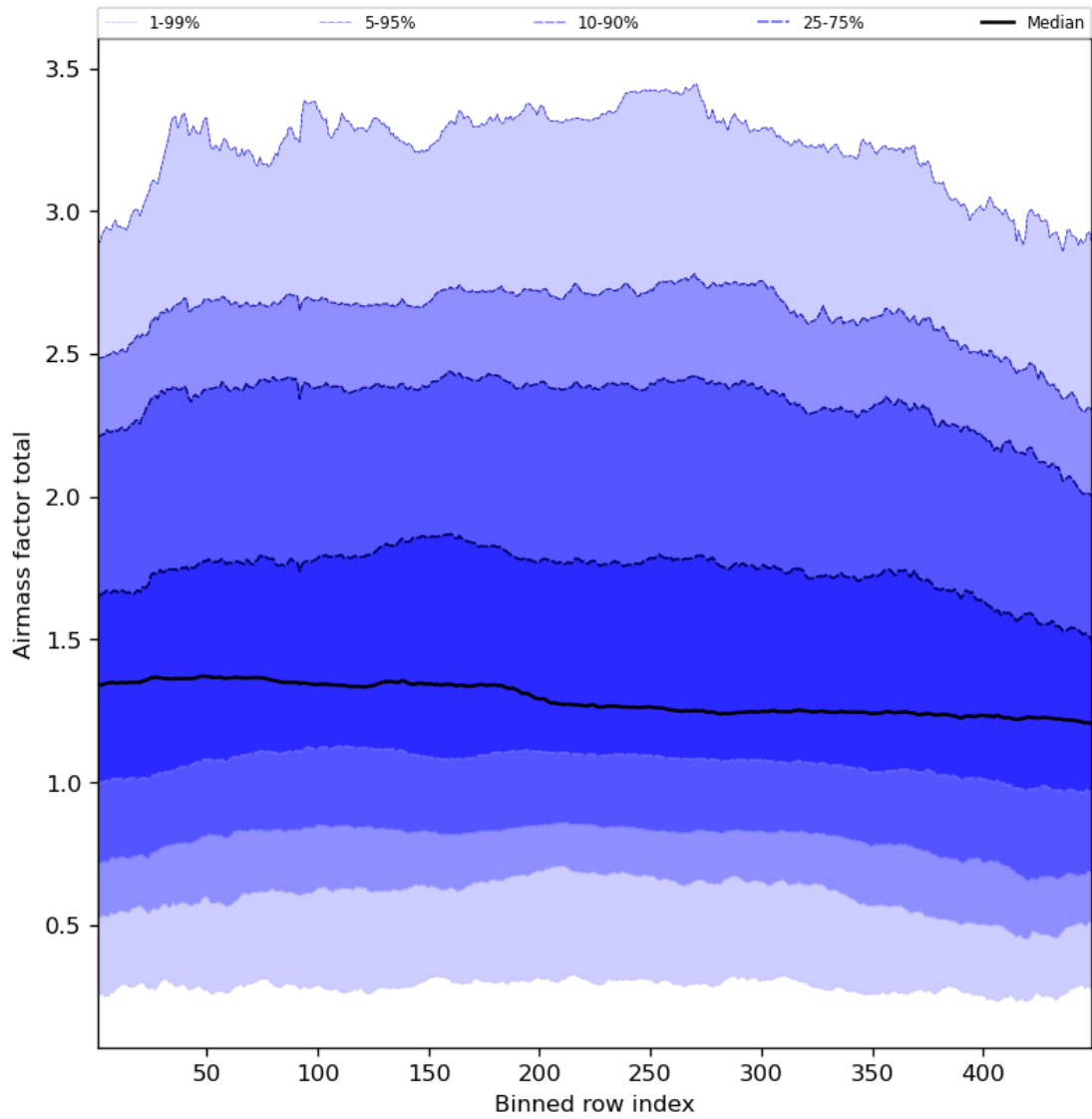
Figure 54: Along track statistics of “Airmass factor total” for 2023-08-21 to 2023-08-23
