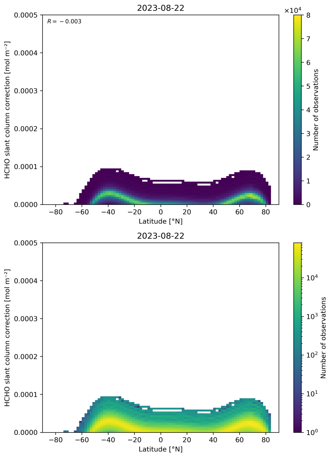
Figure 158: Scatter density plot of “Latitude” against “HCHO slant column correction” for 2023-08-21 to 2023-08-23.
