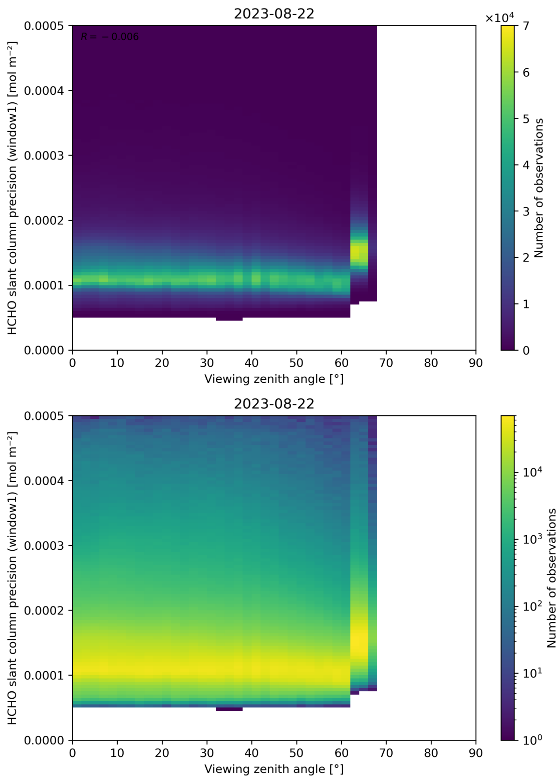
Figure 189: Scatter density plot of “Viewing zenith angle” against “HCHO slant column precision (window1)” for 2023-08-21 to 2023-08-23.
