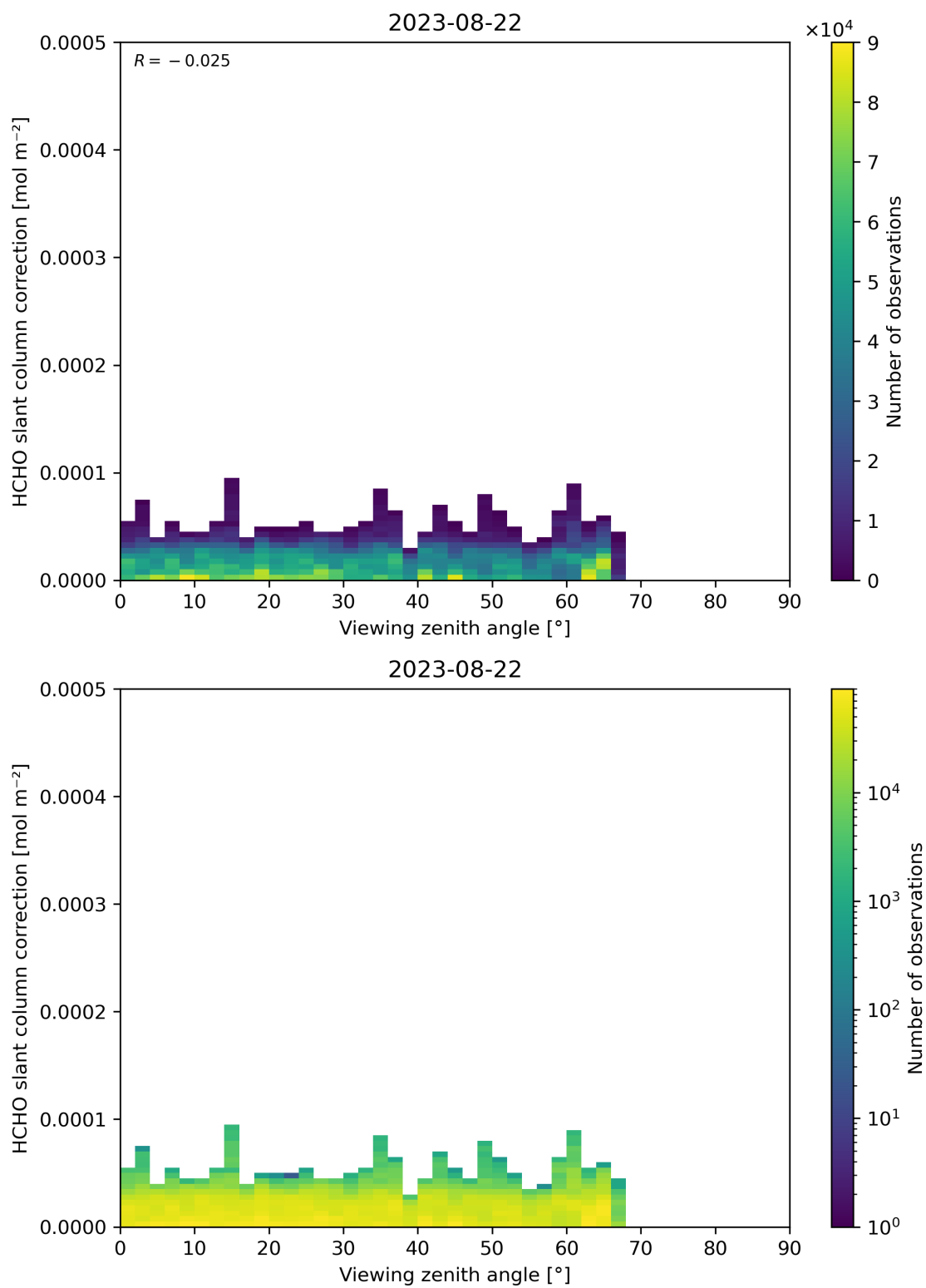
Figure 187: Scatter density plot of “Viewing zenith angle” against “HCHO slant column correction” for 2023-08-21 to 2023-08-23.
