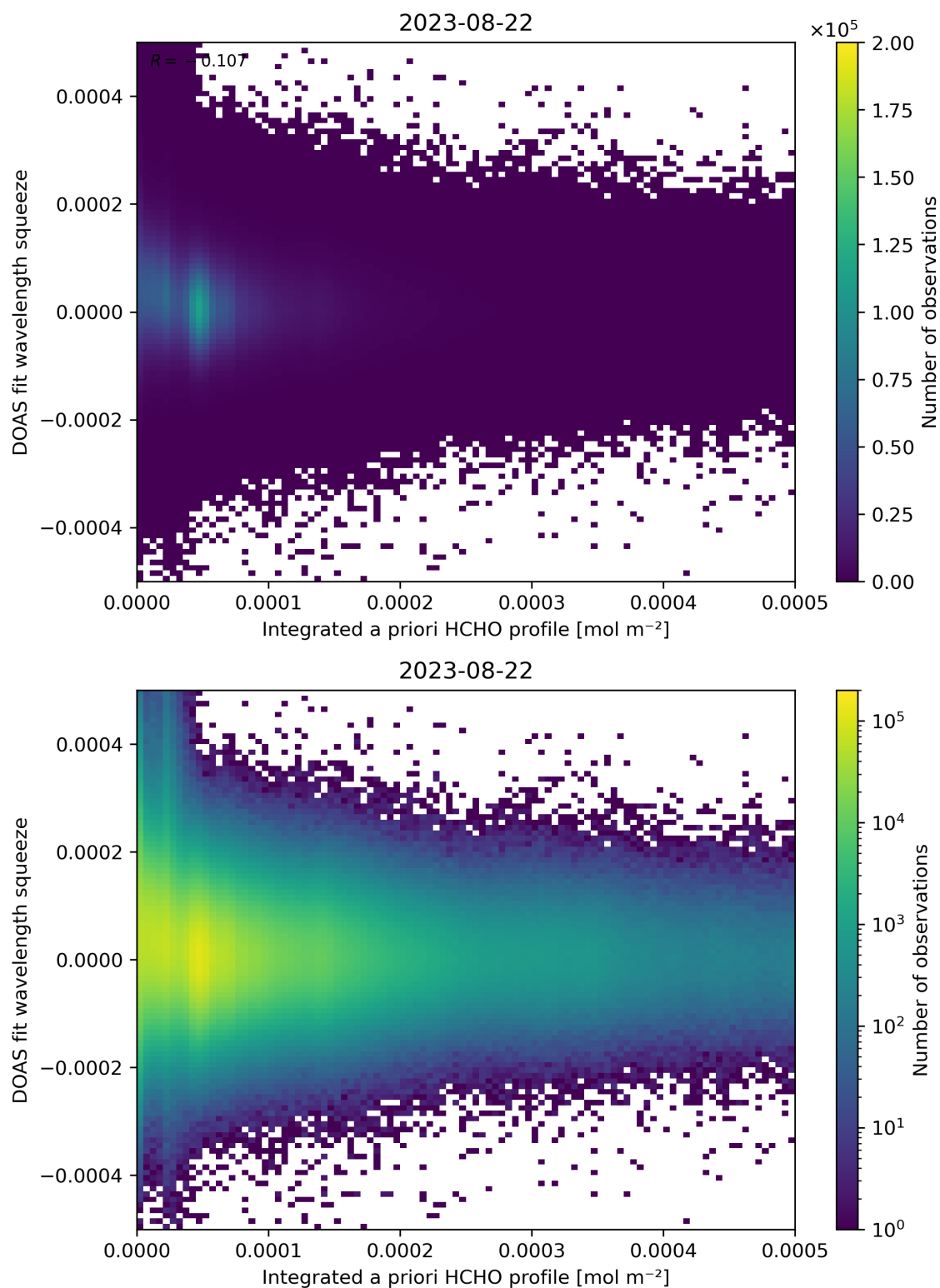
Figure 150: Scatter density plot of “Integrated a priori HCHO profile” against “DOAS fit wavelength squeeze” for 2023-08-21 to 2023-08-23.
