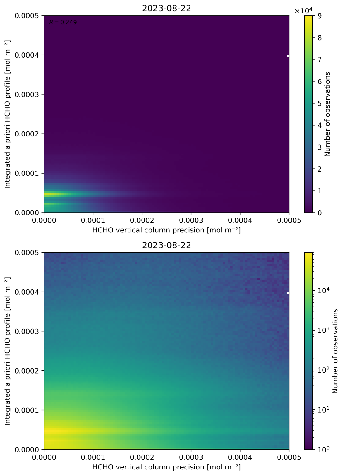
Figure 147: Scatter density plot of “HCHO vertical column precision” against “Integrated a priori HCHO profile” for 2023-08-21 to 2023-08-23.
