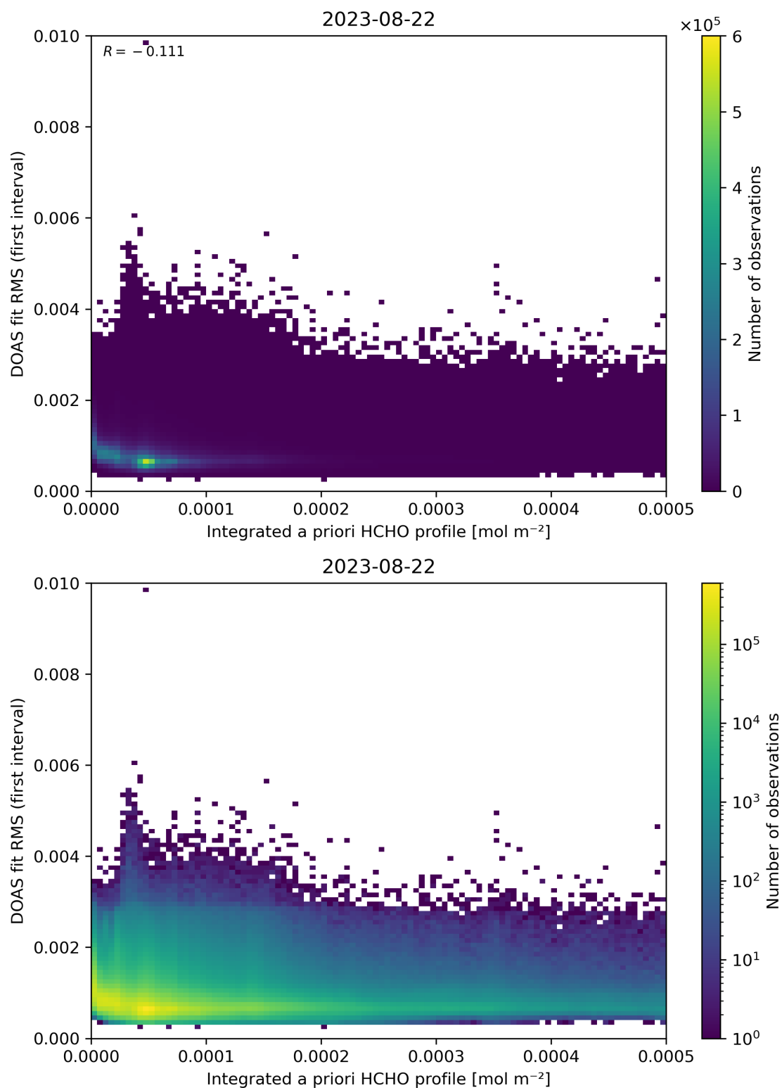
Figure 148: Scatter density plot of “Integrated a priori HCHO profile” against “DOAS fit RMS (first interval)” for 2023-08-21 to 2023-08-23.
