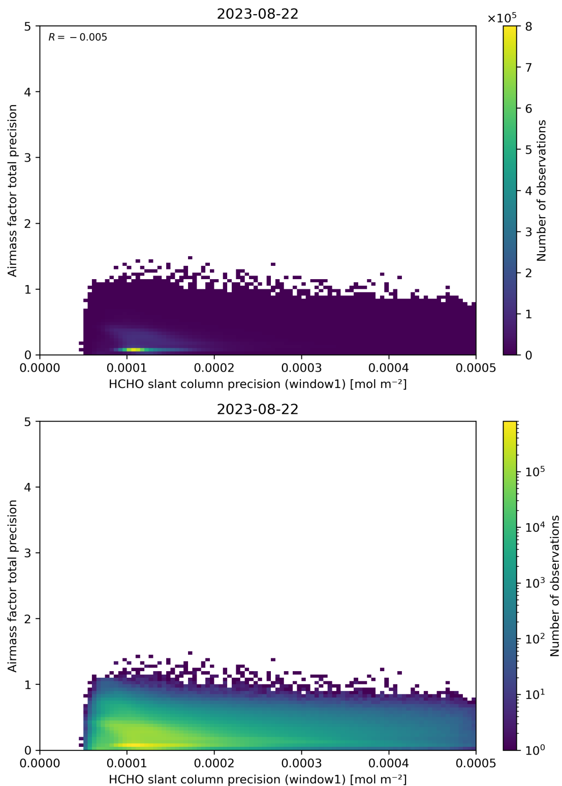
Figure 95: Scatter density plot of “HCHO slant column precision (window1)” against “Airmass factor total precision” for 2023-08-21 to 2023-08-23.
