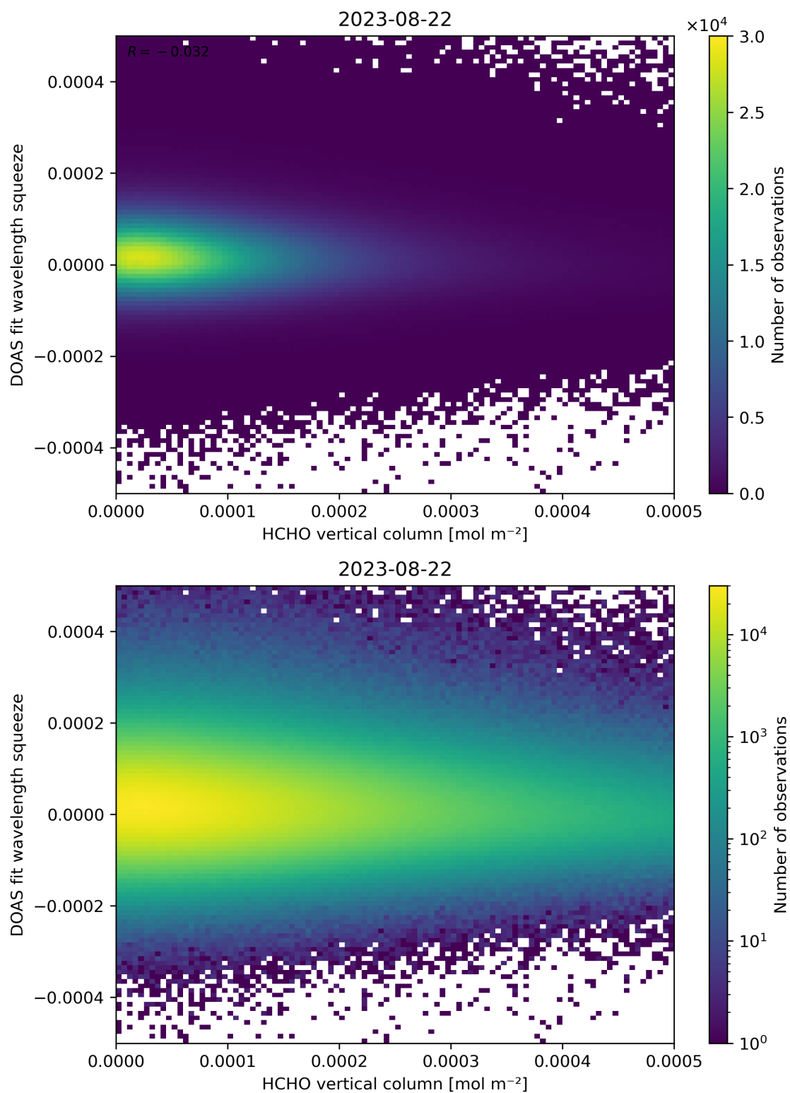
Figure 125: Scatter density plot of “HCHO vertical column” against “DOAS fit wavelength squeeze” for 2023-08-21 to 2023-08-23.
