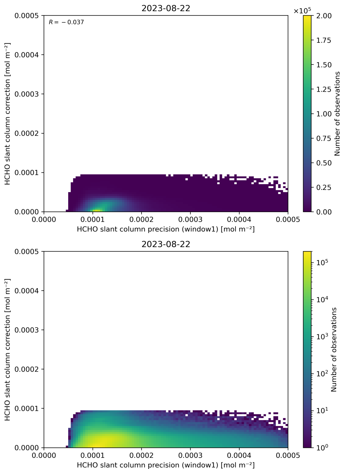
Figure 93: Scatter density plot of “HCHO slant column precision (window1)” against “HCHO slant column correction” for 2023-08-21 to 2023-08-23.
