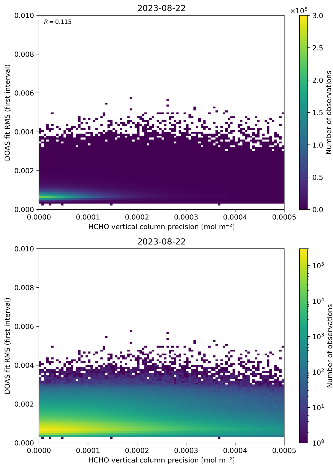
Figure 136: Scatter density plot of “HCHO vertical column precision” against “DOAS fit RMS (first interval)” for 2023-08-21 to 2023-08-23.
