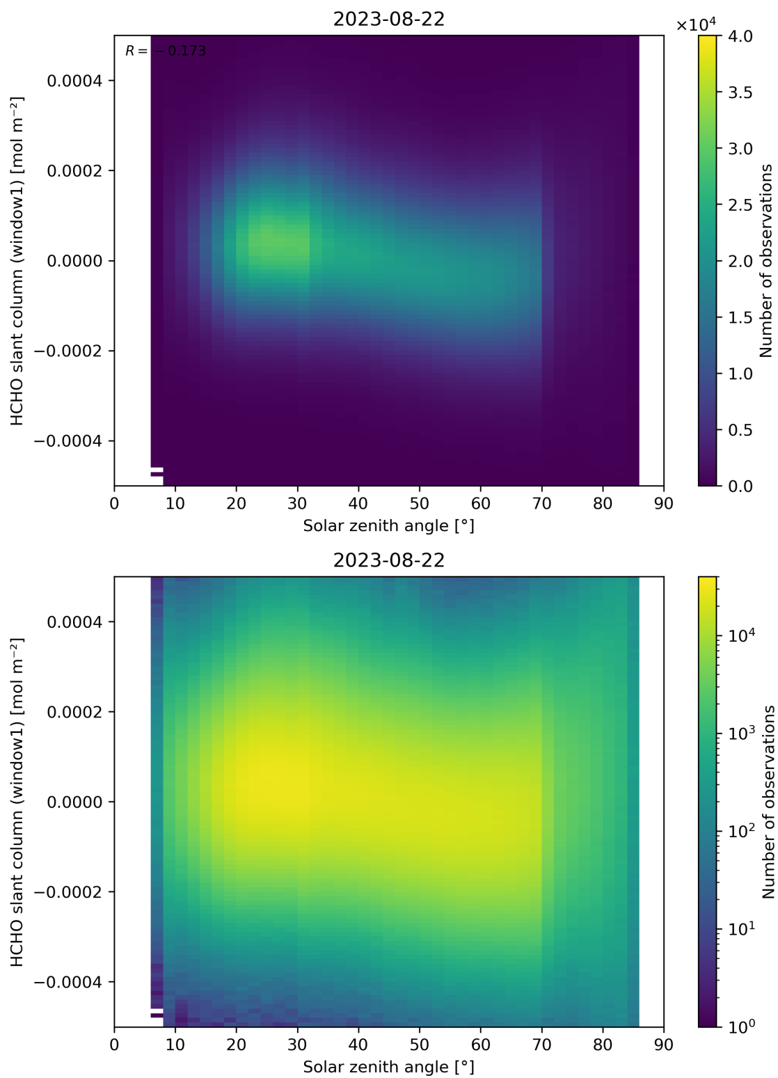
Figure 173: Scatter density plot of “Solar zenith angle” against “HCHO slant column (window1)” for 2023-08-21 to 2023-08-23.
