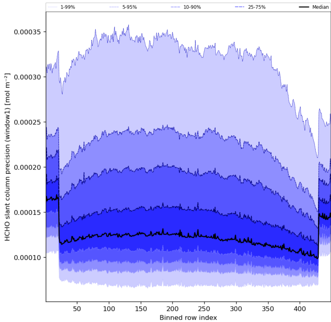
Figure 53: Along track statistics of “HCHO slant column precision (window1)” for 2023-08-21 to 2023-08-23
