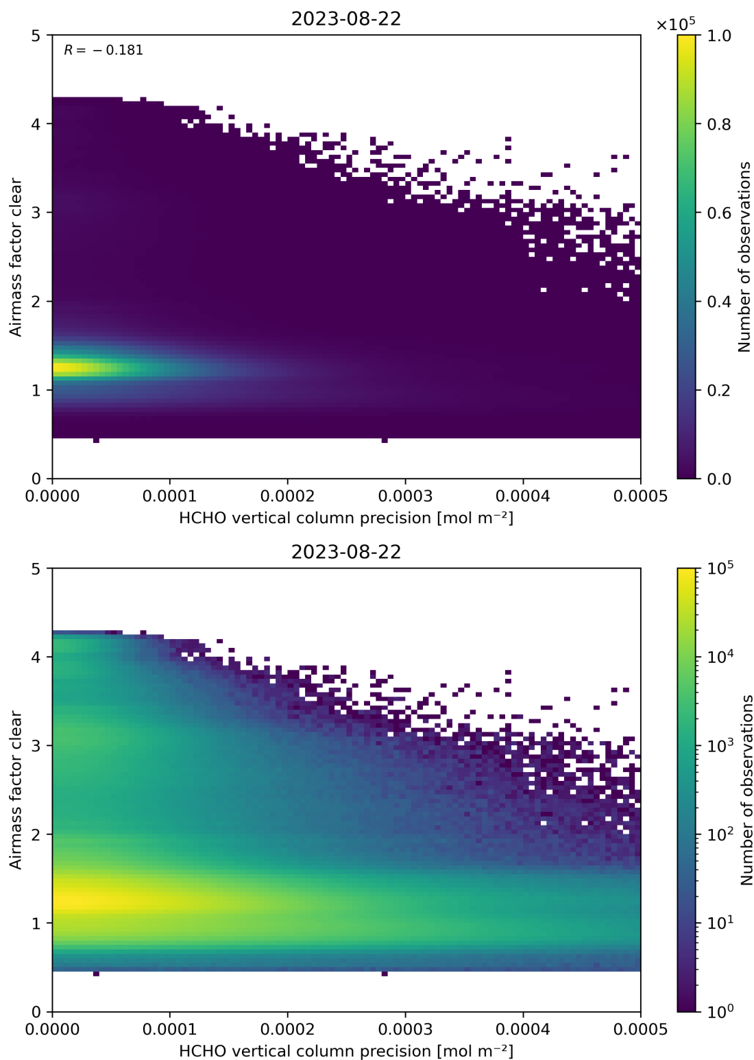
Figure 139: Scatter density plot of “HCHO vertical column precision” against “Airmass factor clear” for 2023-08-21 to 2023-08-23.
