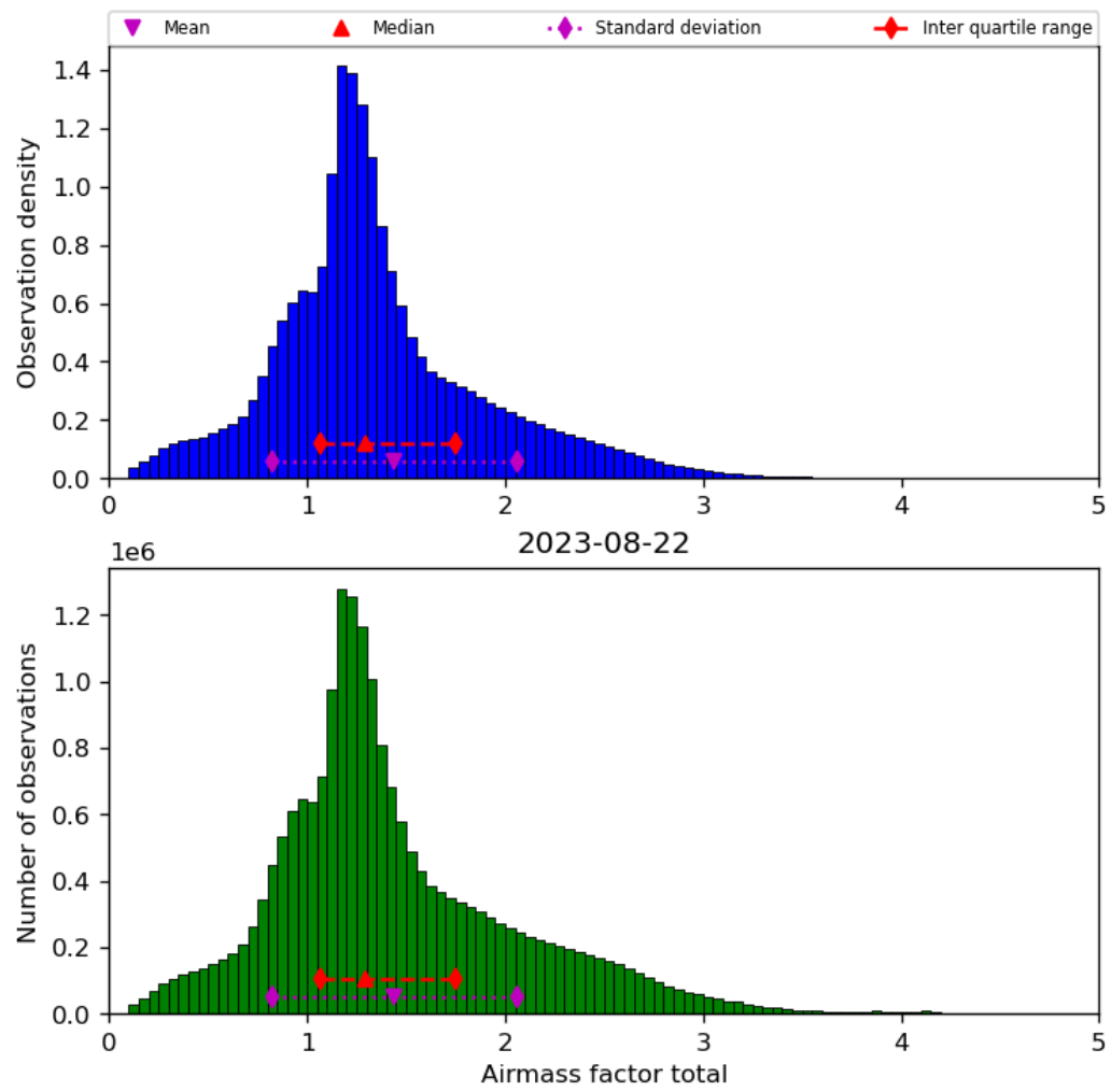
Figure 40: Histogram of “Airmass factor total” for 2023-08-21 to 2023-08-23
