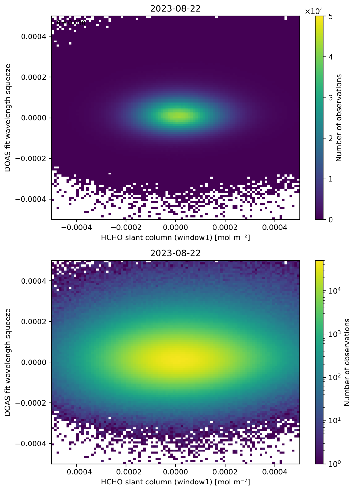
Figure 80: Scatter density plot of “HCHO slant column (window1)” against “DOAS fit wavelength squeeze” for 2023-08-21 to 2023-08-23.
