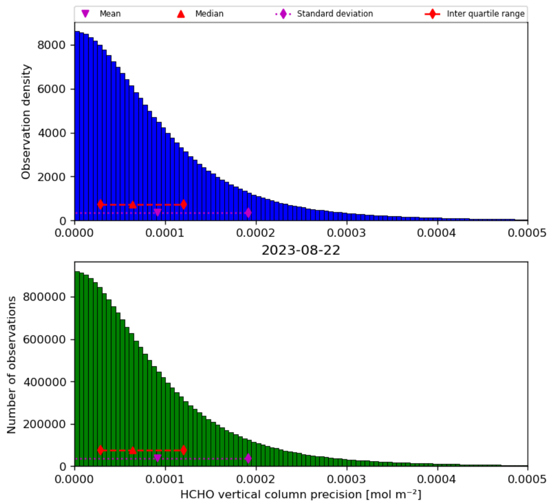
Figure 36: Histogram of “HCHO vertical column precision” for 2023-08-21 to 2023-08-23
