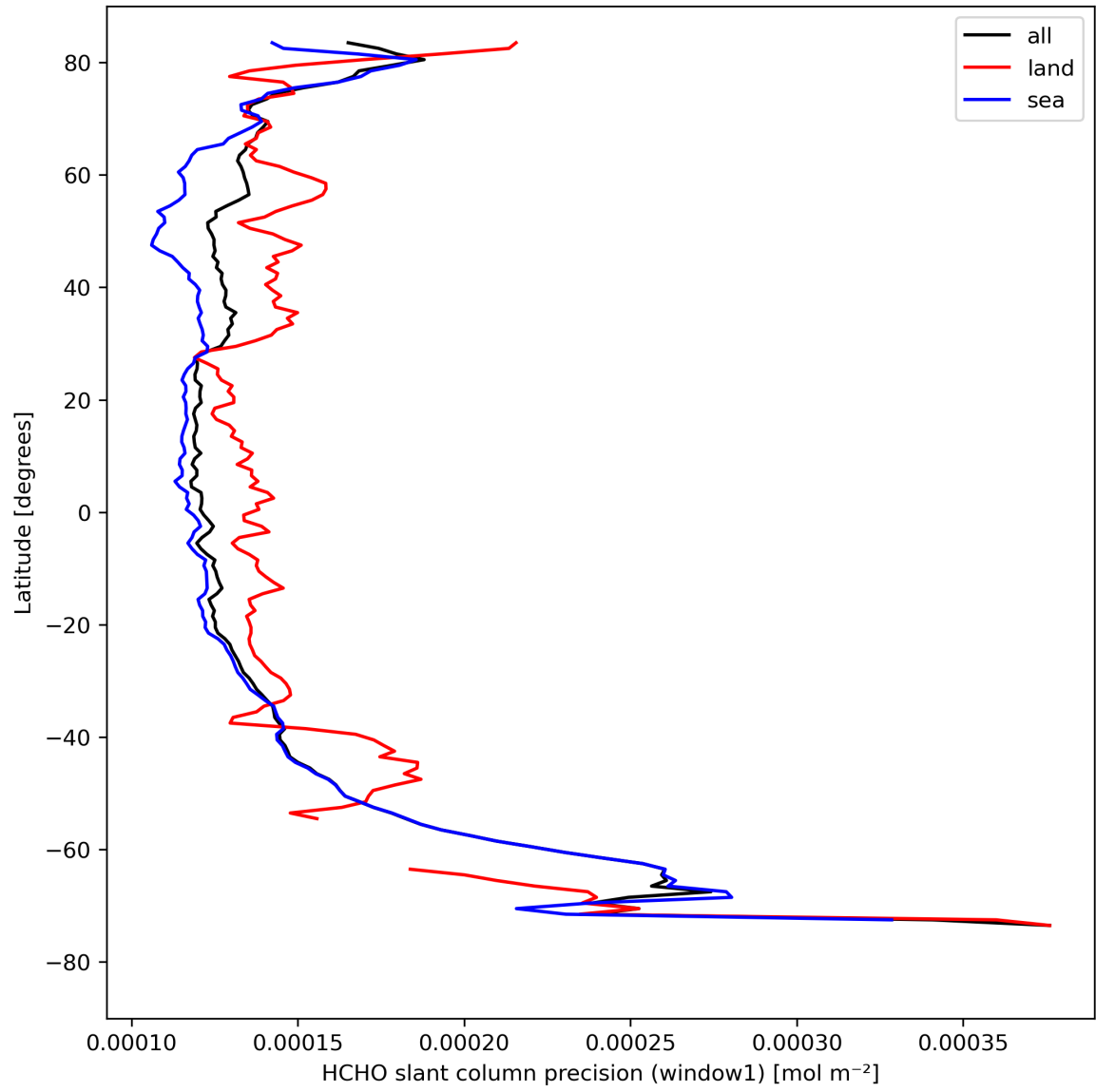
Figure 25: Zonal average of “HCHO slant column precision (window1)” for 2023-08-21 to 2023-08-23.
