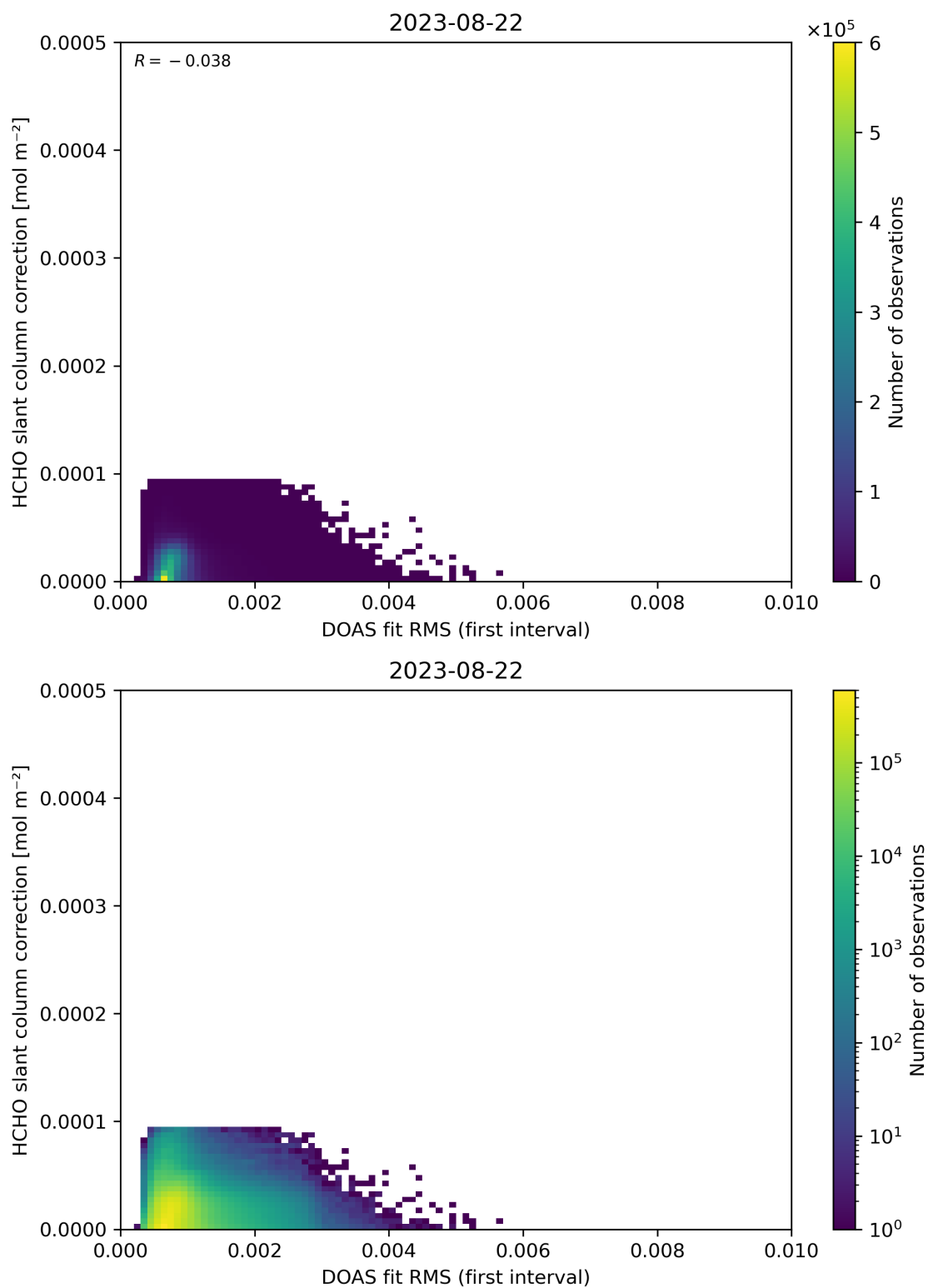
Figure 63: Scatter density plot of “DOAS fit RMS (first interval)” against “HCHO slant column correction” for 2023-08-21 to 2023-08-23.
