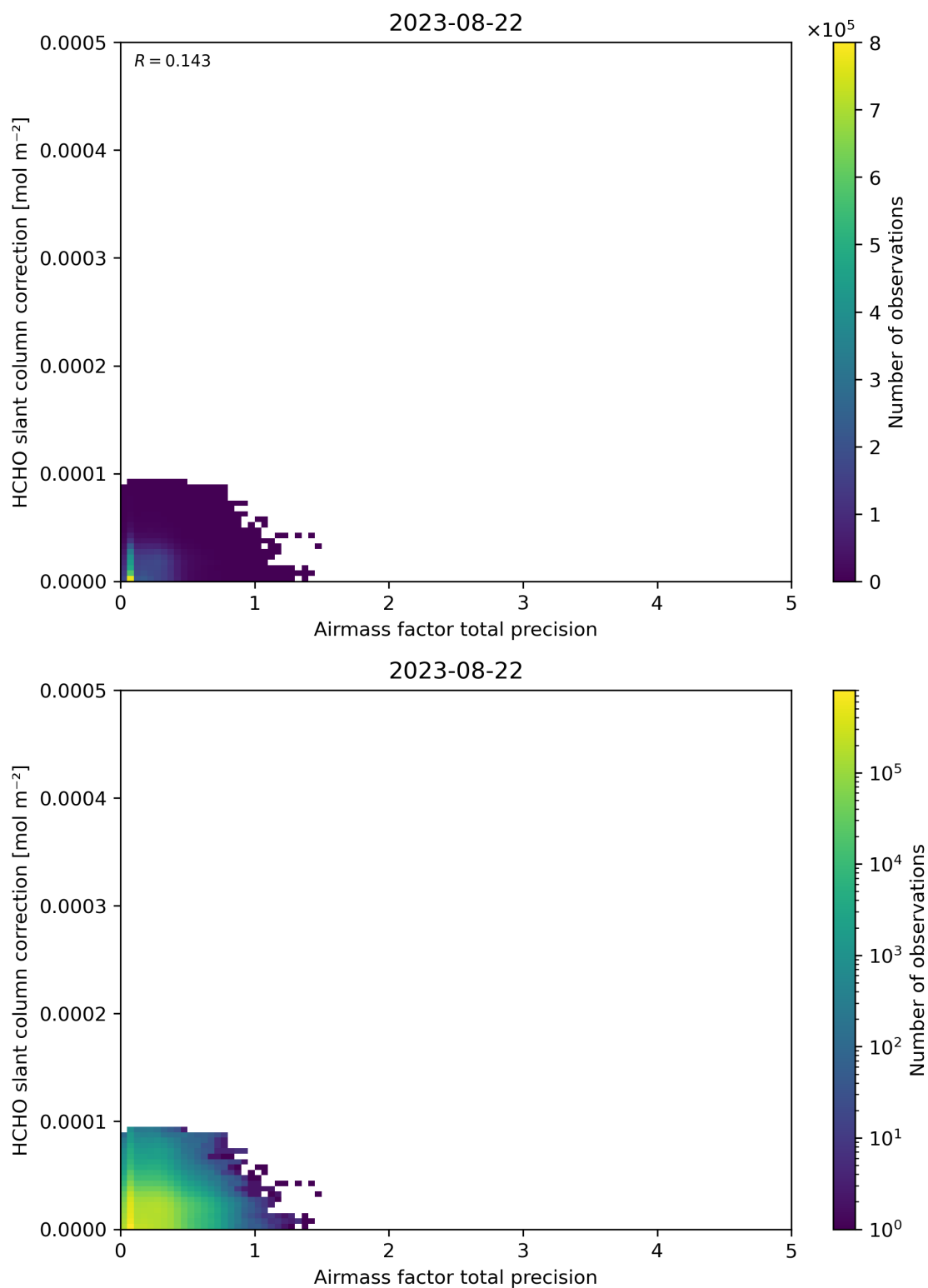
Figure 110: Scatter density plot of “Airmass factor total precision” against “HCHO slant column correction” for 2023-08-21 to 2023-08-23.
