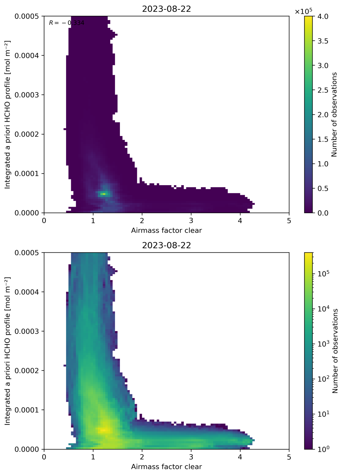
Figure 76: Scatter density plot of “Airmass factor clear” against “Integrated a priori HCHO profile” for 2023-08-21 to 2023-08-23.
