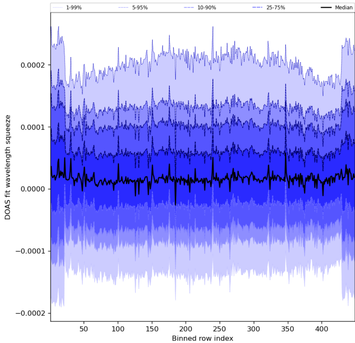
Figure 59: Along track statistics of “DOAS fit wavelength squeeze” for 2023-08-21 to 2023-08-23
