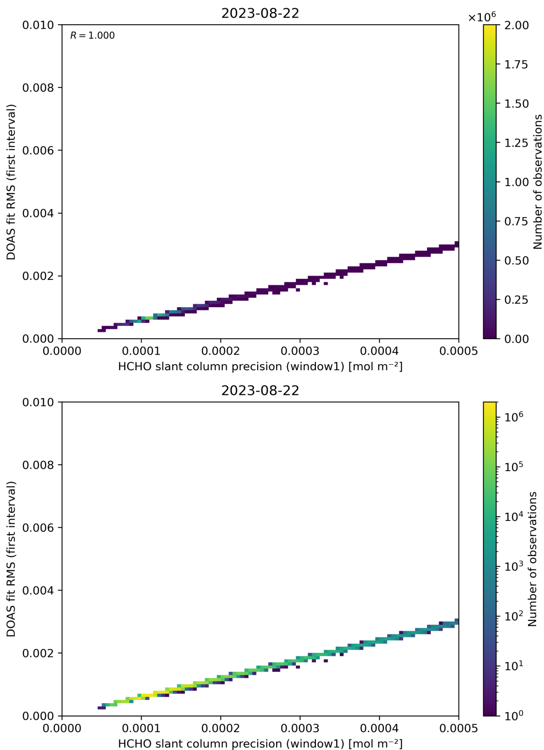
Figure 88: Scatter density plot of “HCHO slant column precision (window1)” against “DOAS fit RMS (first interval)” for 2023-08-21 to 2023-08-23.
