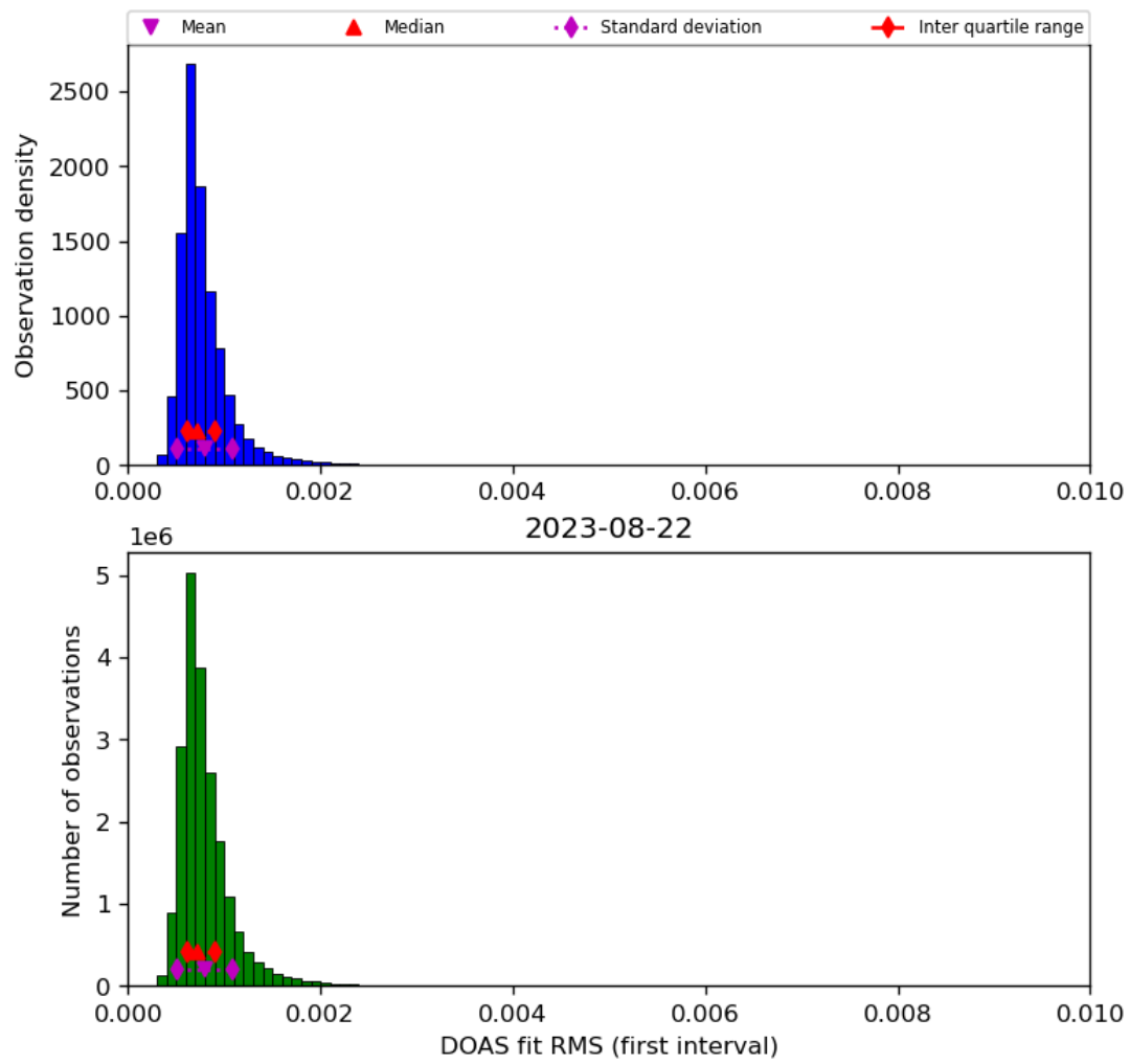
Figure 46: Histogram of “DOAS fit RMS (first interval)” for 2023-08-21 to 2023-08-23
