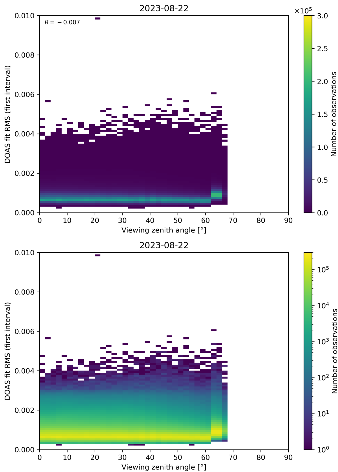
Figure 182: Scatter density plot of “Viewing zenith angle” against “DOAS fit RMS (first interval)” for 2023-08-21 to 2023-08-23.
