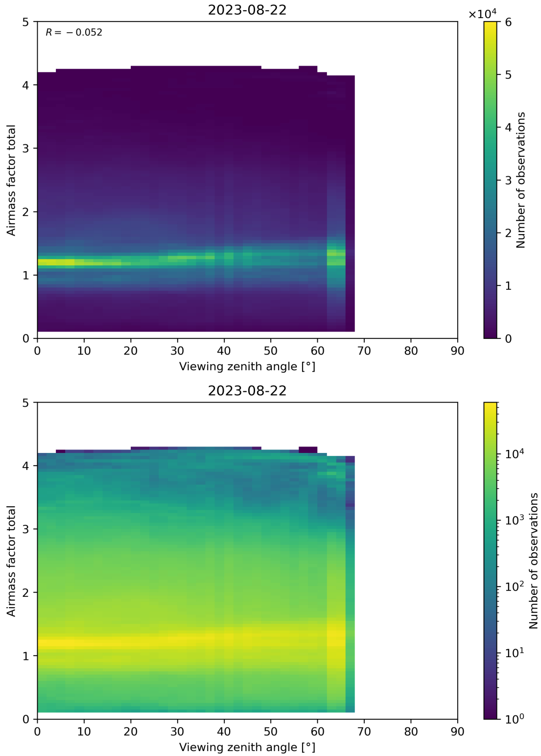
Figure 190: Scatter density plot of “Viewing zenith angle” against “Airmass factor total” for 2023-08-21 to 2023-08-23.
