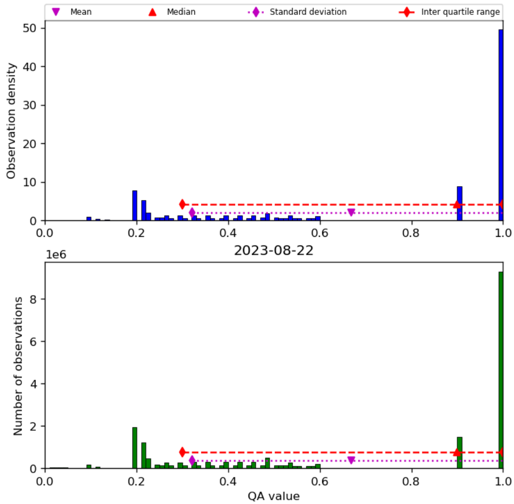
Figure 34: Histogram of “QA value” for 2023-08-21 to 2023-08-23
