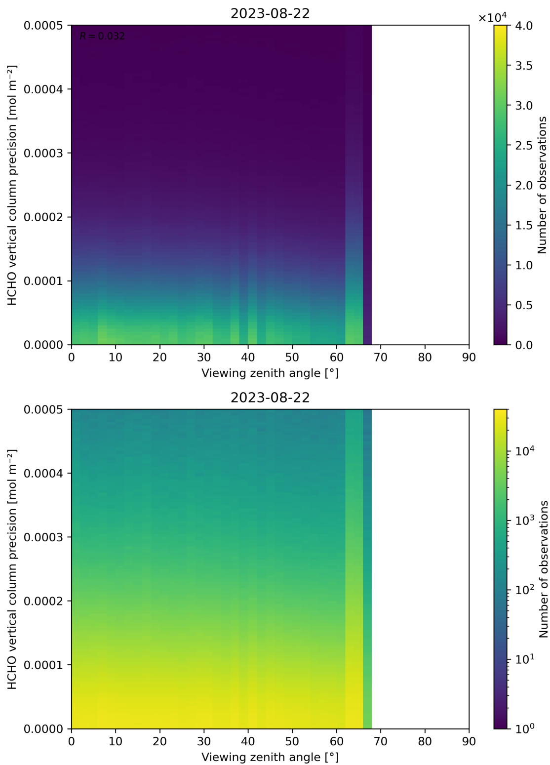
Figure 194: Scatter density plot of “Viewing zenith angle” against “HCHO vertical column precision” for 2023-08-21 to 2023-08-23.
