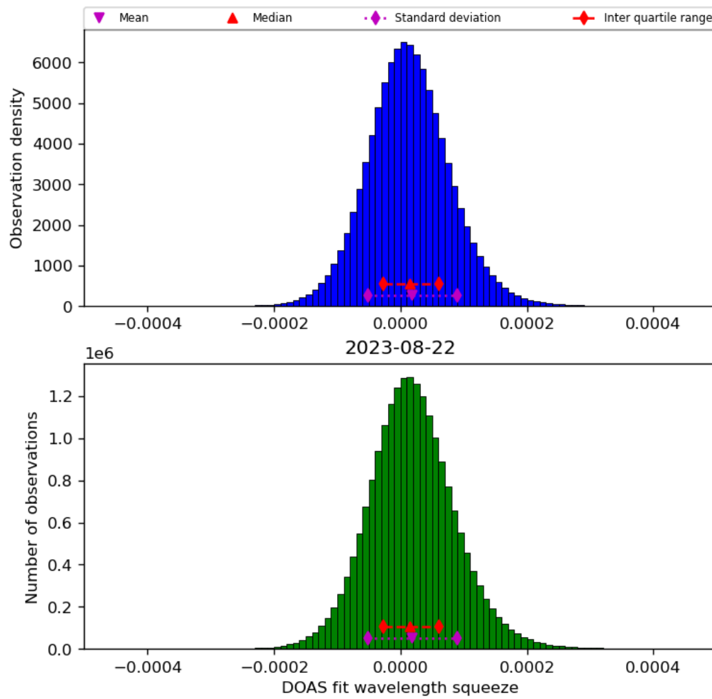
Figure 45: Histogram of “DOAS fit wavelength squeeze” for 2023-08-21 to 2023-08-23
