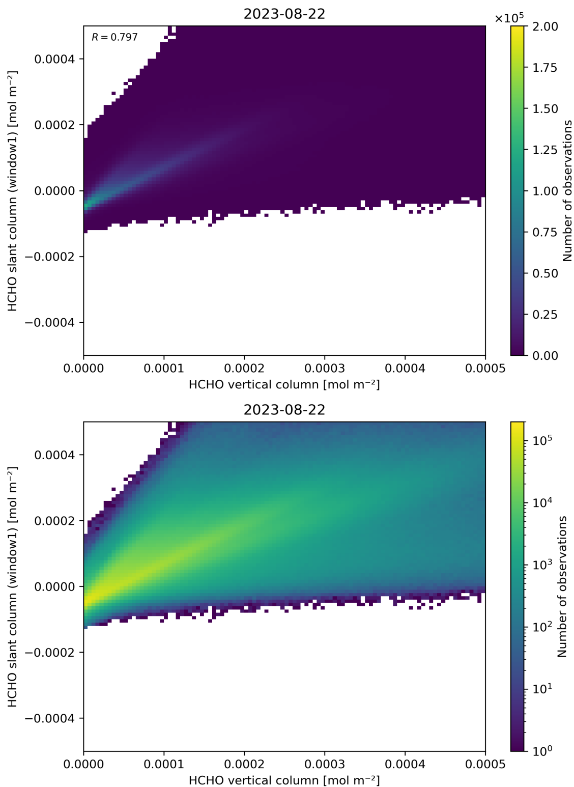
Figure 129: Scatter density plot of “HCHO vertical column” against “HCHO slant column (window1)” for 2023-08-21 to 2023-08-23.
