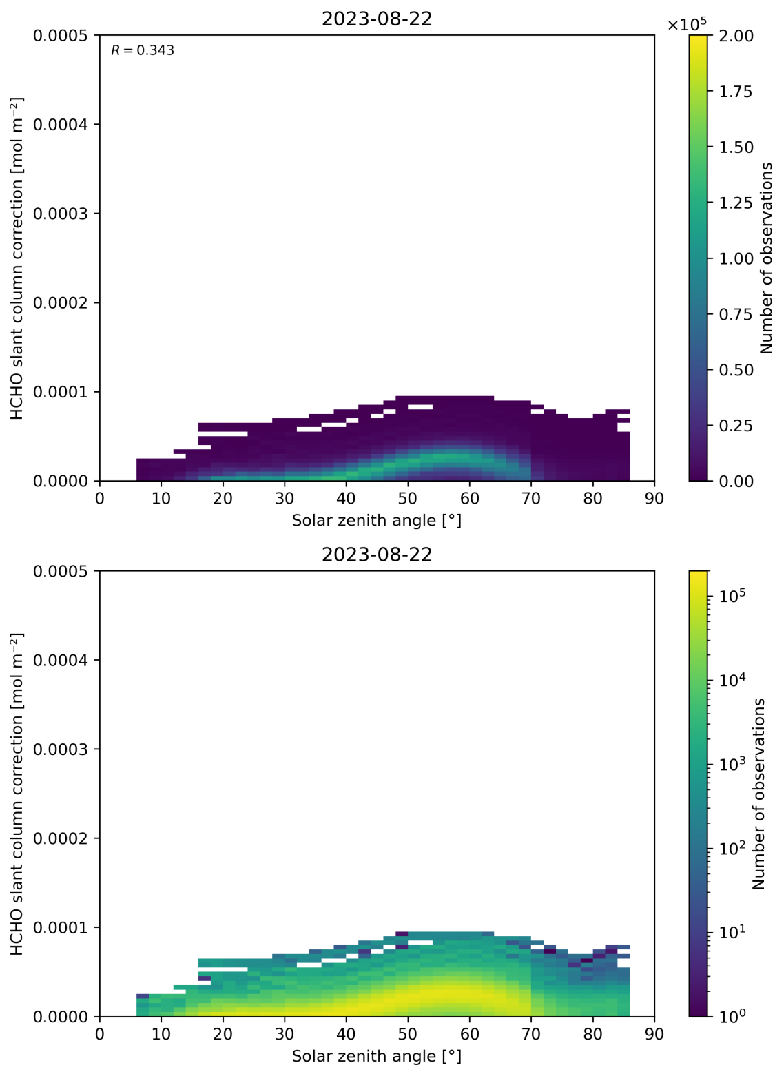
Figure 172: Scatter density plot of “Solar zenith angle” against “HCHO slant column correction” for 2023-08-21 to 2023-08-23.
