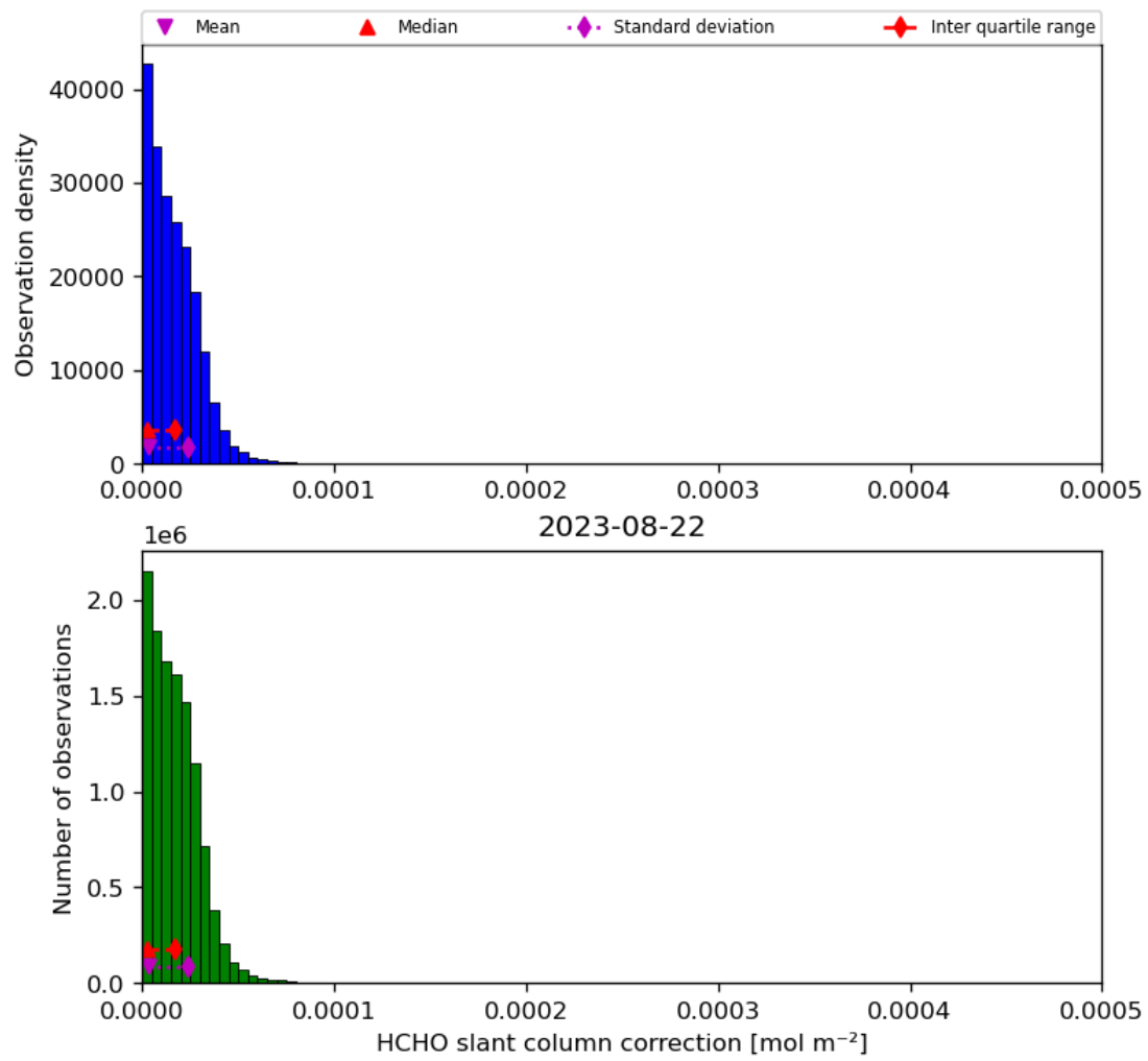
Figure 47: Histogram of “HCHO slant column correction” for 2023-08-21 to 2023-08-23
