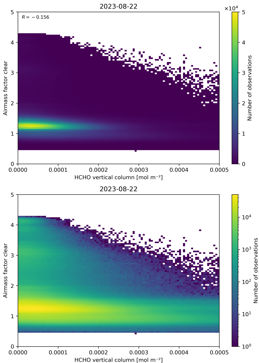
Figure 126: Scatter density plot of “HCHO vertical column” against “Airmass factor clear” for 2023-08-21 to 2023-08-23.
