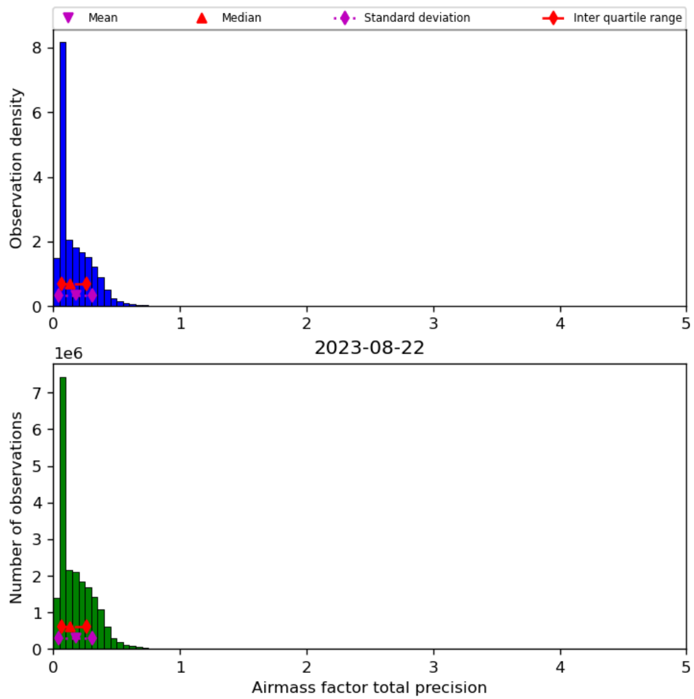
Figure 41: Histogram of “Airmass factor total precision” for 2023-08-21 to 2023-08-23
