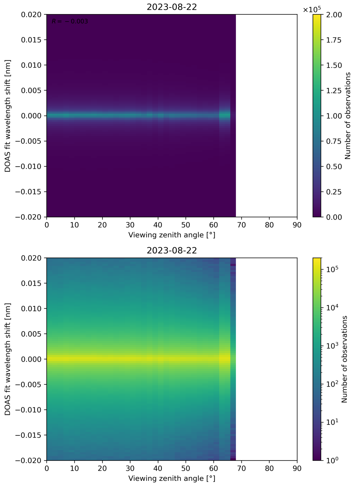
Figure 183: Scatter density plot of “Viewing zenith angle” against “DOAS fit wavelength shift” for 2023-08-21 to 2023-08-23.
