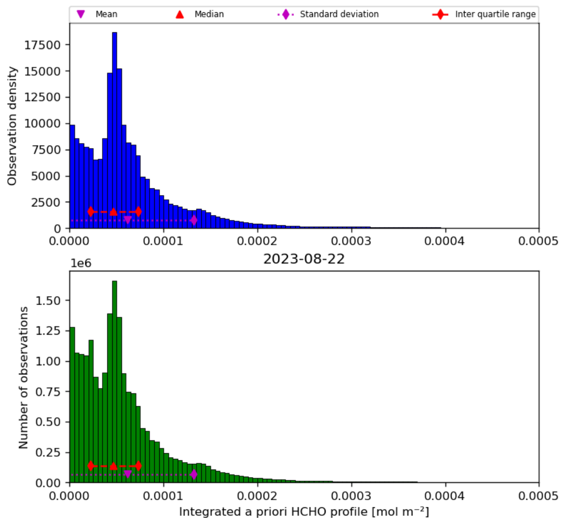
Figure 43: Histogram of “Integrated a priori HCHO profile” for 2023-08-21 to 2023-08-23
