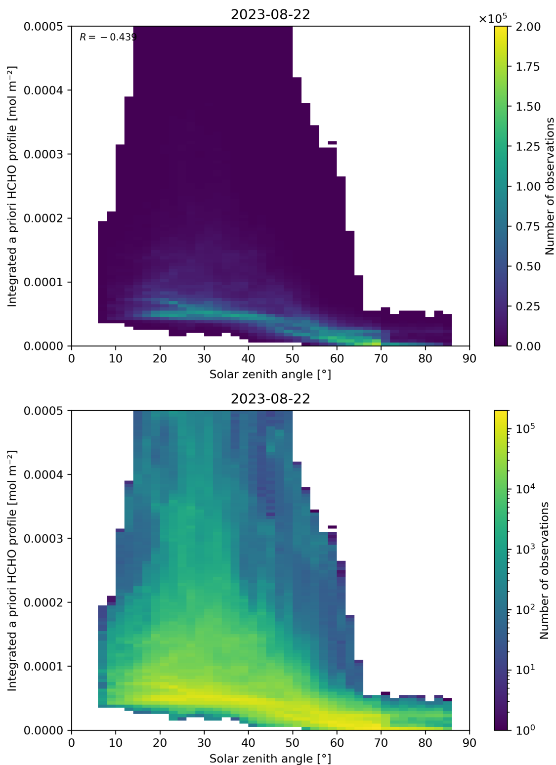
Figure 180: Scatter density plot of “Solar zenith angle” against “Integrated a priori HCHO profile” for 2023-08-21 to 2023-08-23.
