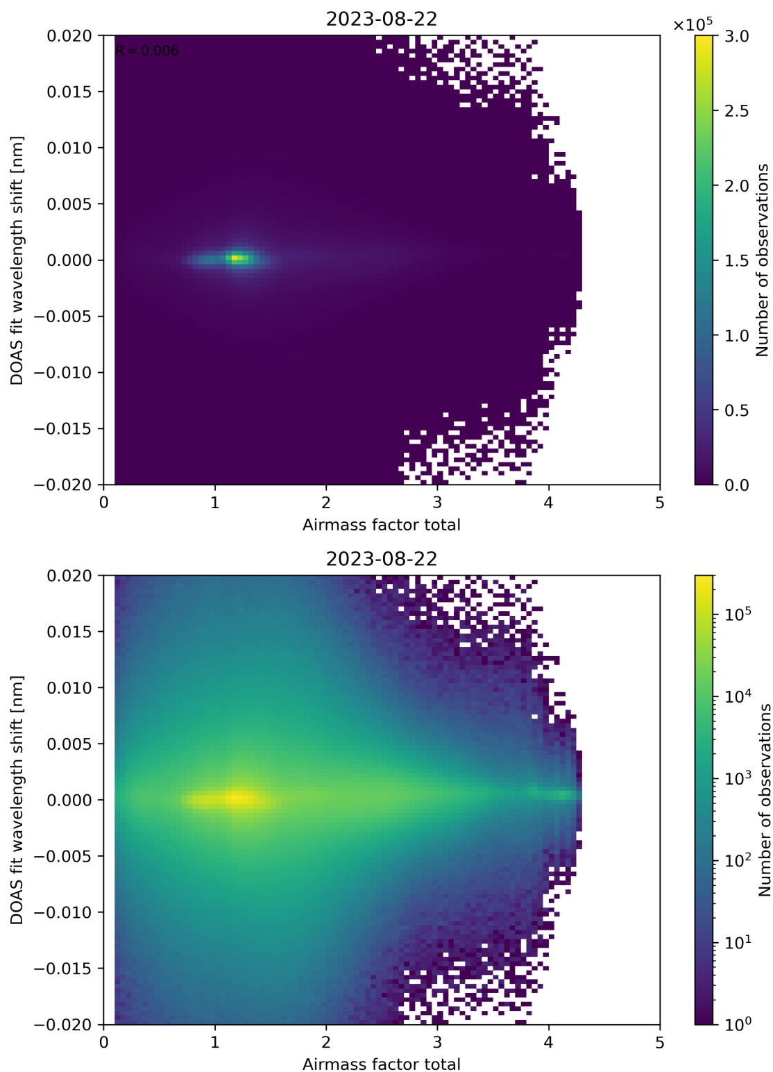
Figure 98: Scatter density plot of “Airmass factor total” against “DOAS fit wavelength shift” for 2023-08-21 to 2023-08-23.
