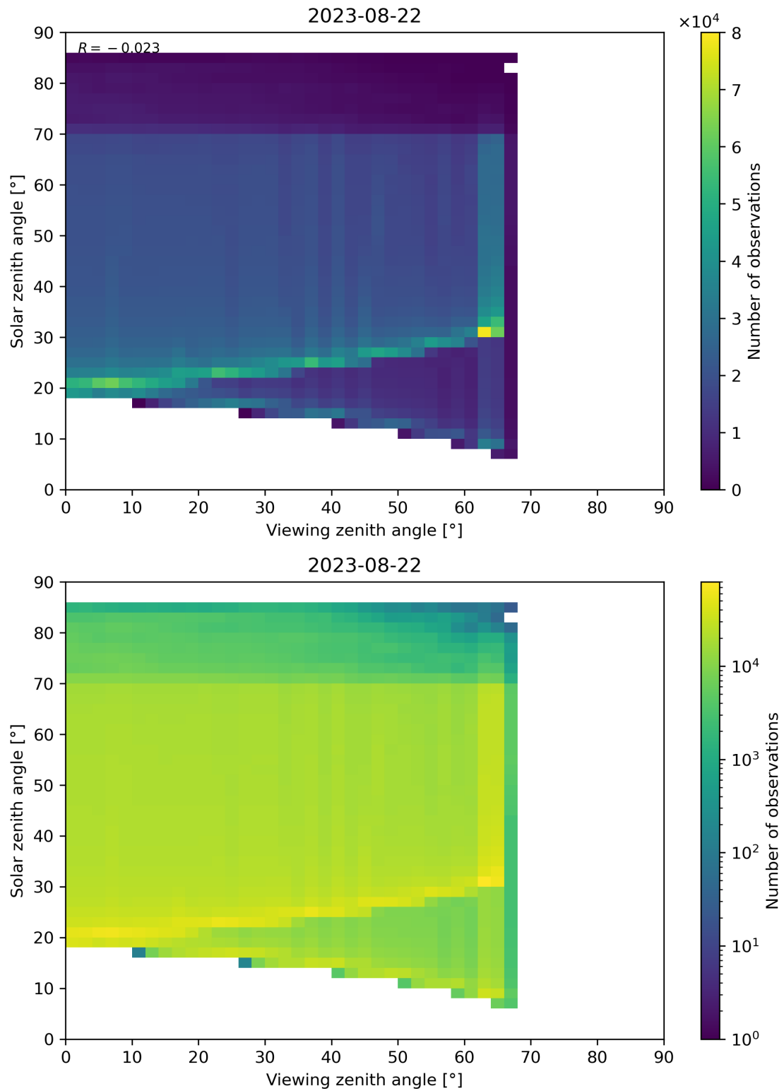
Figure 197: Scatter density plot of “Viewing zenith angle” against “Solar zenith angle” for 2023-08-21 to 2023-08-23.
