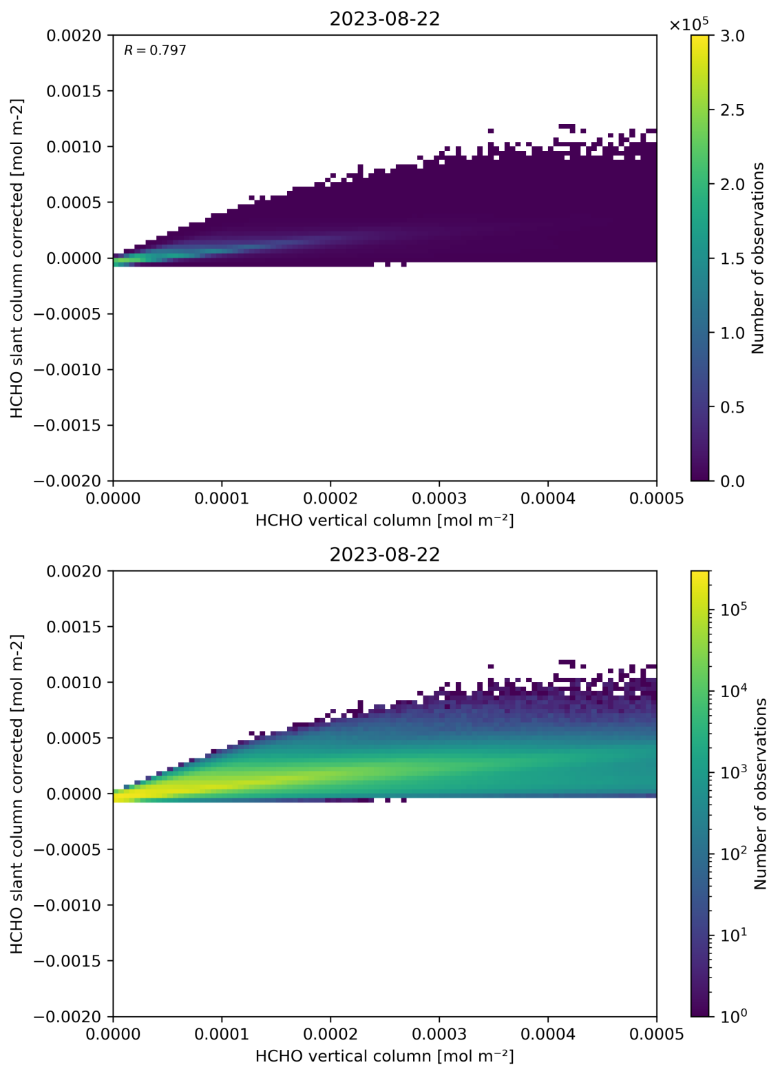
Figure 127: Scatter density plot of “HCHO vertical column” against “HCHO slant column corrected” for 2023-08-21 to 2023-08-23.
