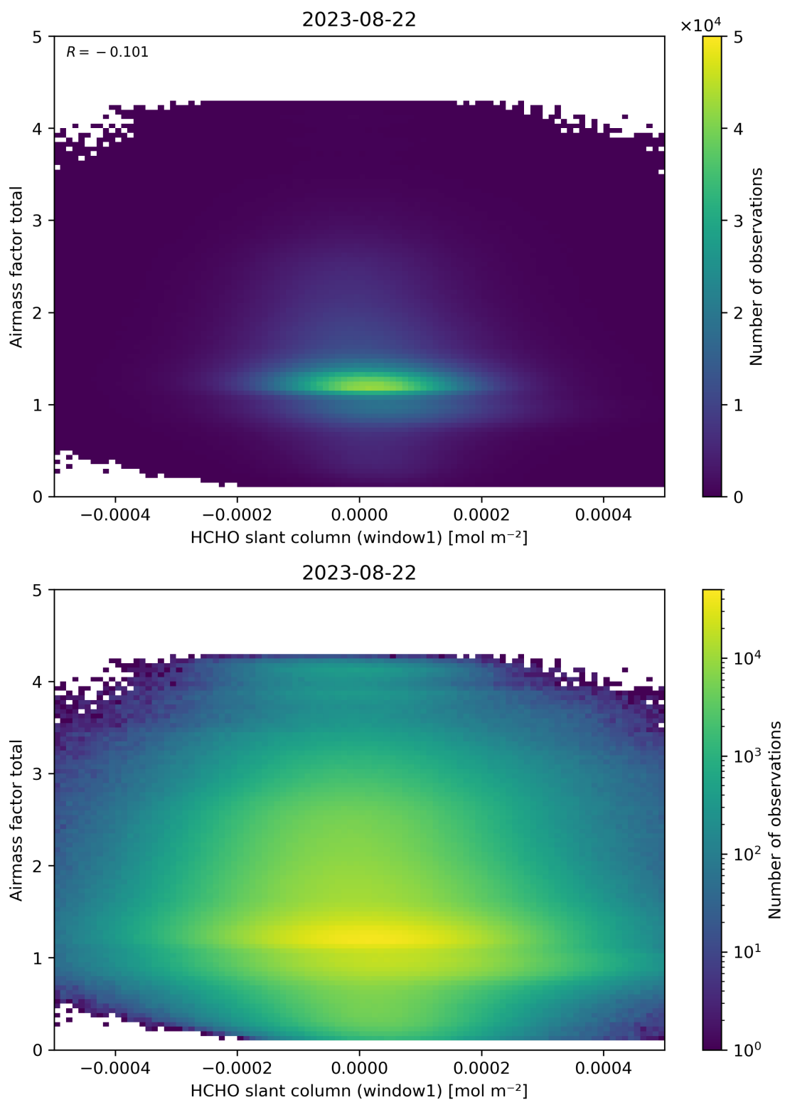
Figure 85: Scatter density plot of “HCHO slant column (window1)” against “Airmass factor total” for 2023-08-21 to 2023-08-23.
