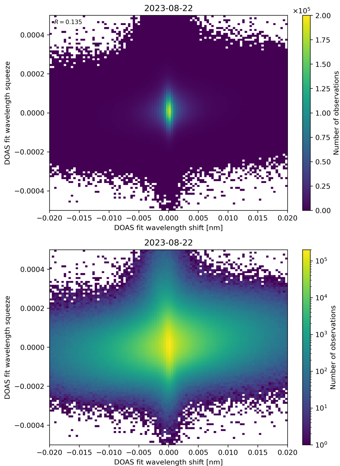
Figure 65: Scatter density plot of “DOAS fit wavelength shift” against “DOAS fit wavelength squeeze” for 2023-08-21 to 2023-08-23.
