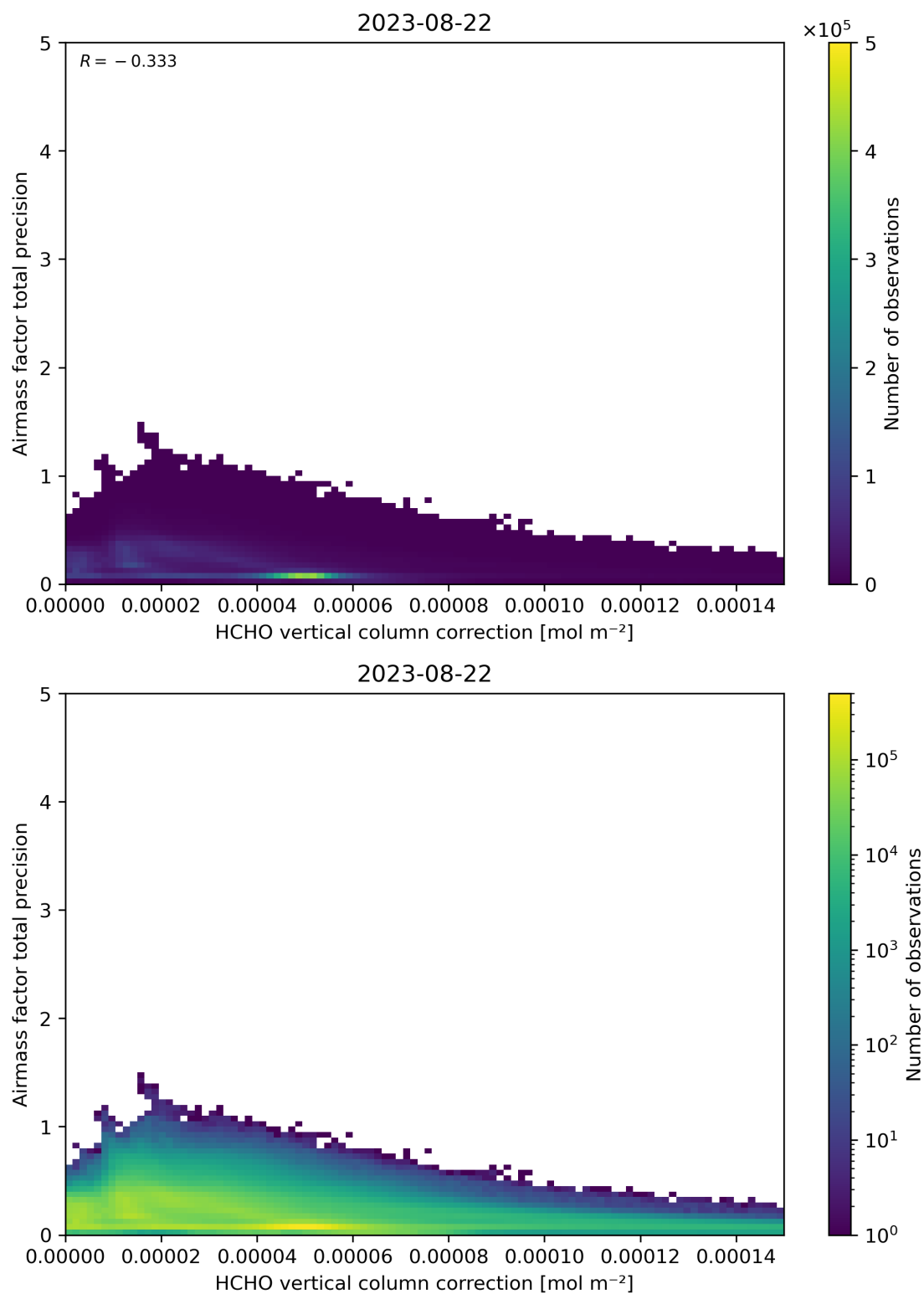
Figure 121: Scatter density plot of “HCHO vertical column correction” against “Airmass factor total precision” for 2023-08-21 to 2023-08-23.
