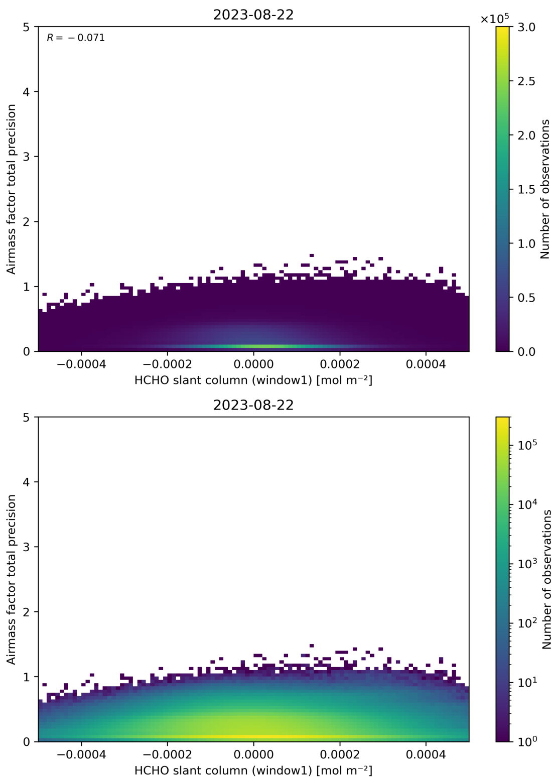
Figure 86: Scatter density plot of “HCHO slant column (window1)” against “Airmass factor total precision” for 2023-08-21 to 2023-08-23.
