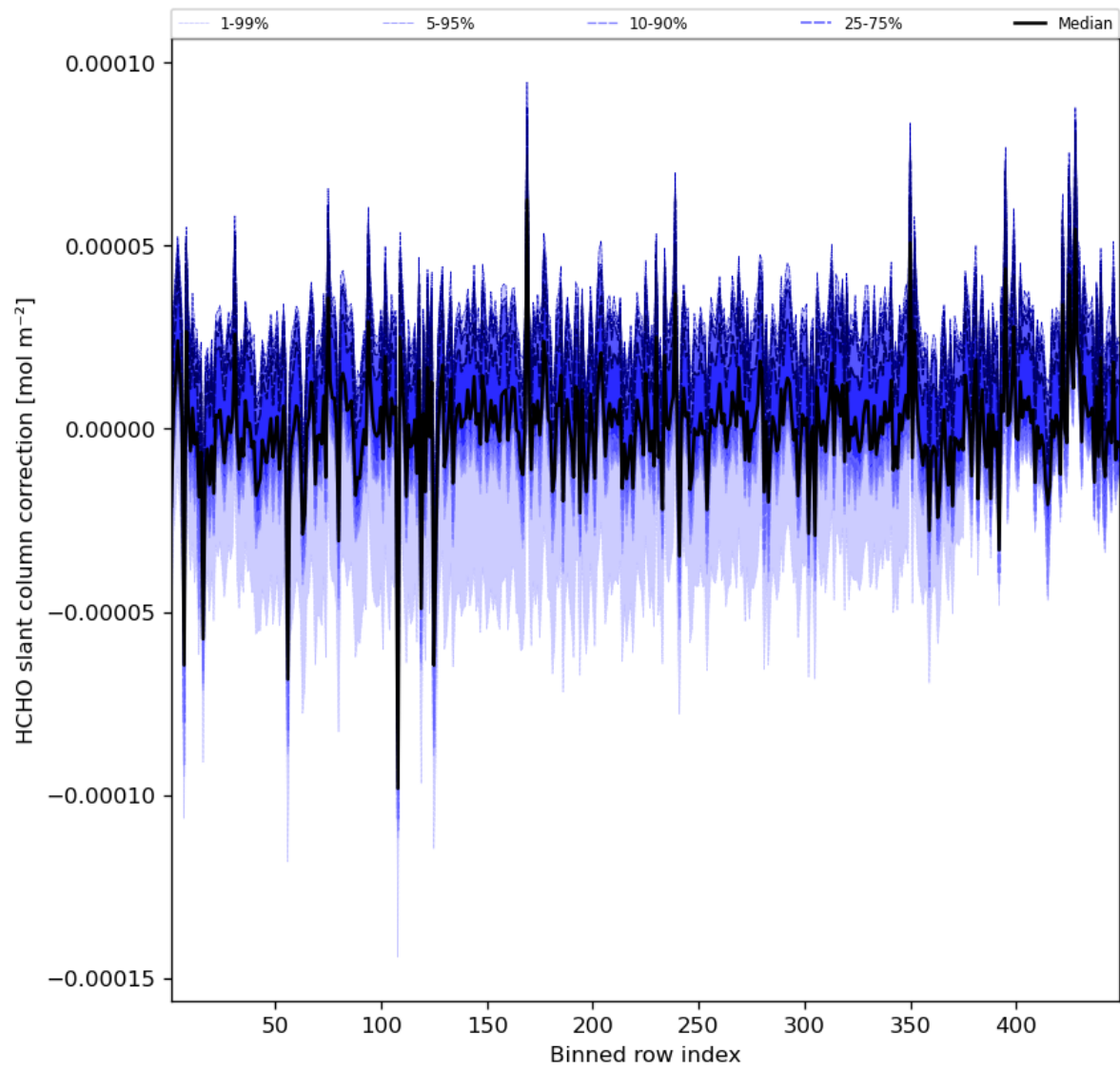
Figure 61: Along track statistics of “HCHO slant column correction” for 2023-08-21 to 2023-08-23
