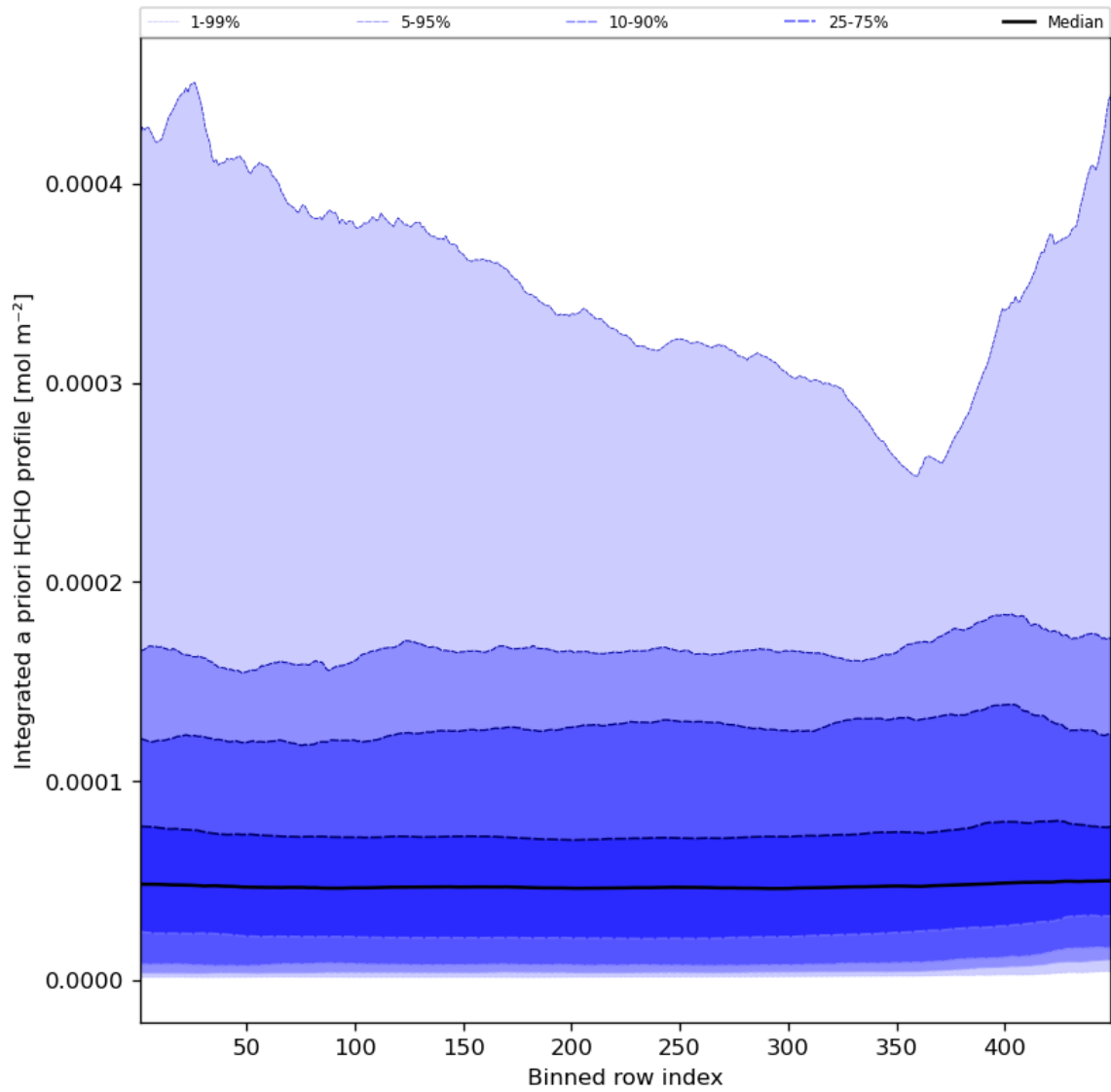
Figure 57: Along track statistics of “Integrated a priori HCHO profile” for 2023-08-21 to 2023-08-23
