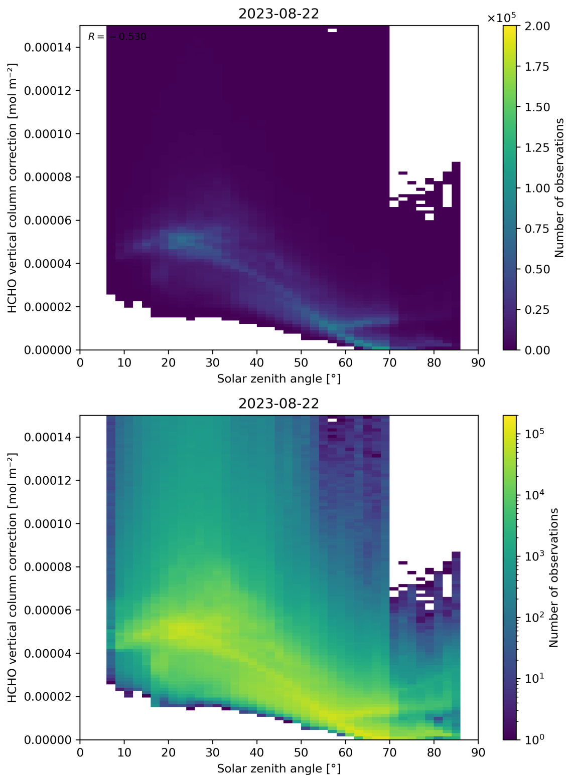
Figure 178: Scatter density plot of “Solar zenith angle” against “HCHO vertical column correction” for 2023-08-21 to 2023-08-23.
