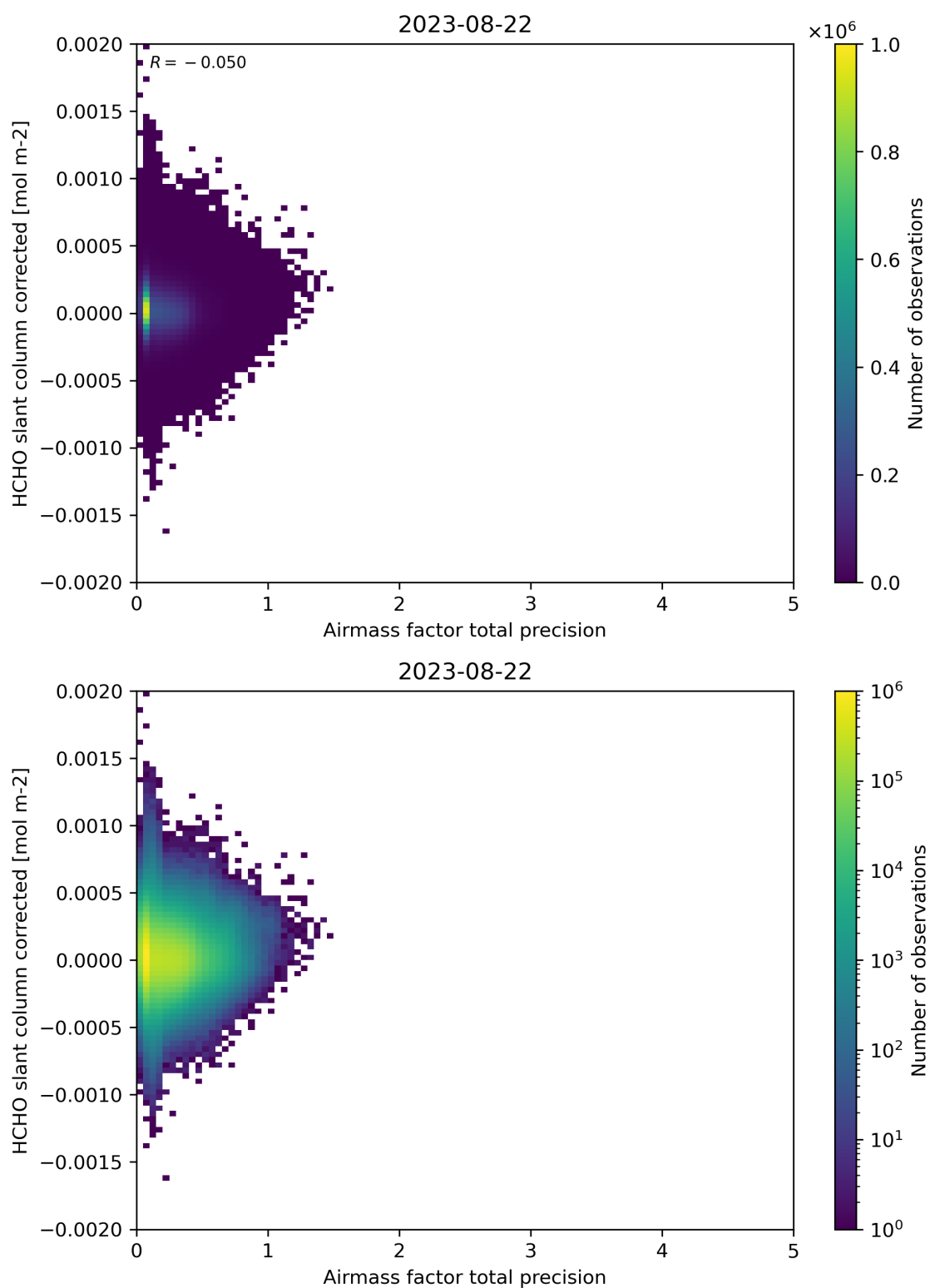
Figure 109: Scatter density plot of “Airmass factor total precision” against “HCHO slant column corrected” for 2023-08-21 to 2023-08-23.
