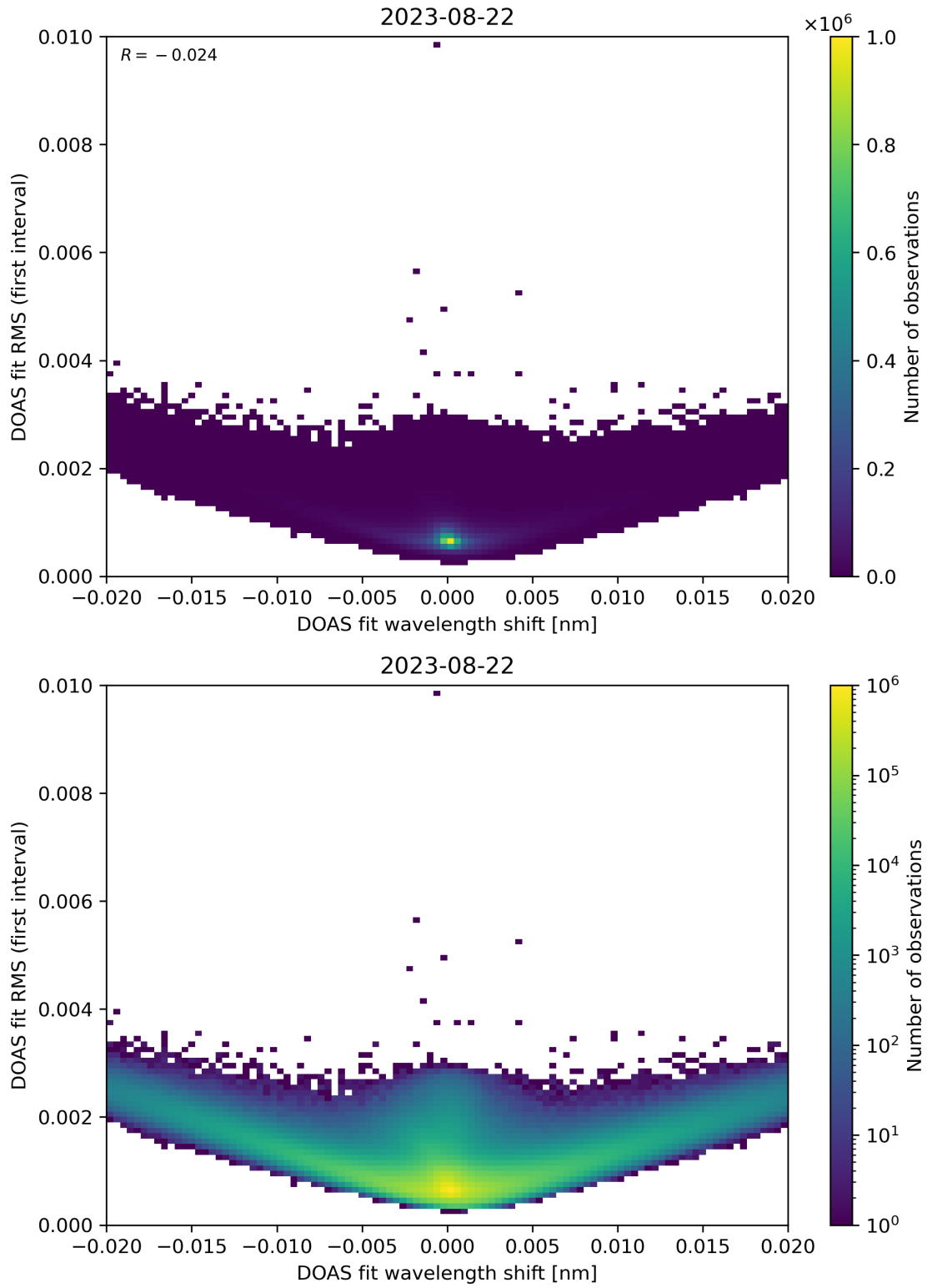
Figure 64: Scatter density plot of “DOAS fit wavelength shift” against “DOAS fit RMS (first interval)” for 2023-08-21 to 2023-08-23.
