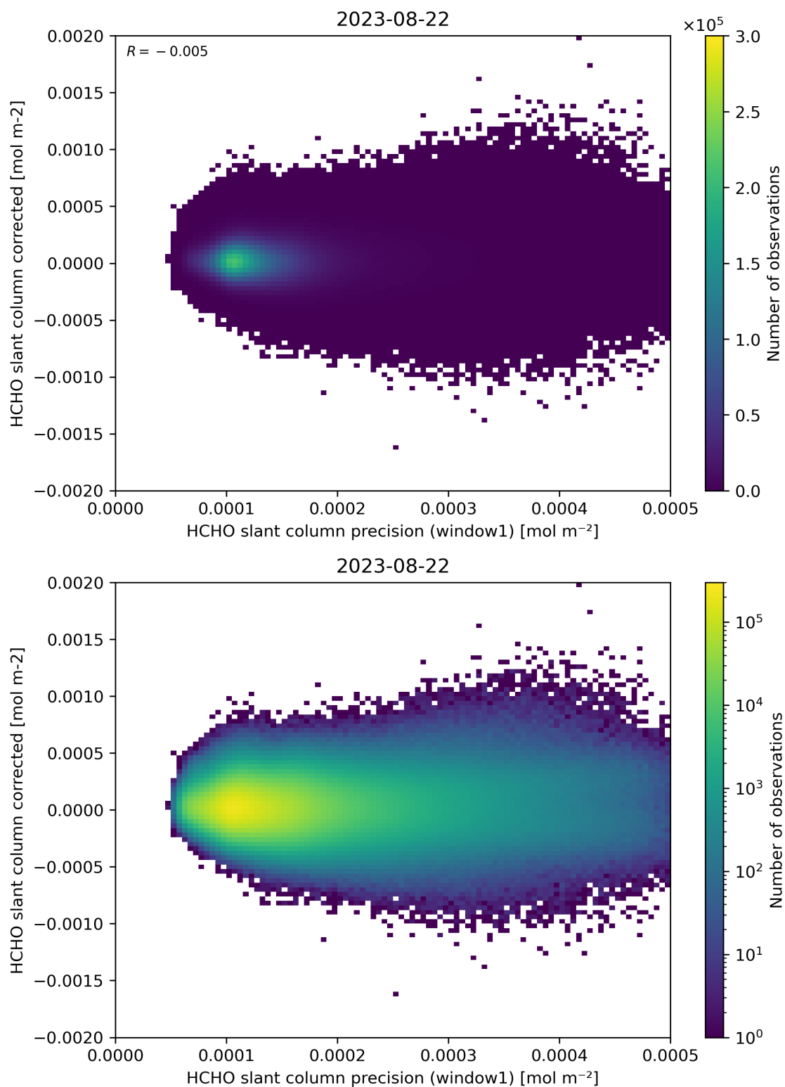
Figure 92: Scatter density plot of “HCHO slant column precision (window1)” against “HCHO slant column corrected” for 2023-08-21 to 2023-08-23.
