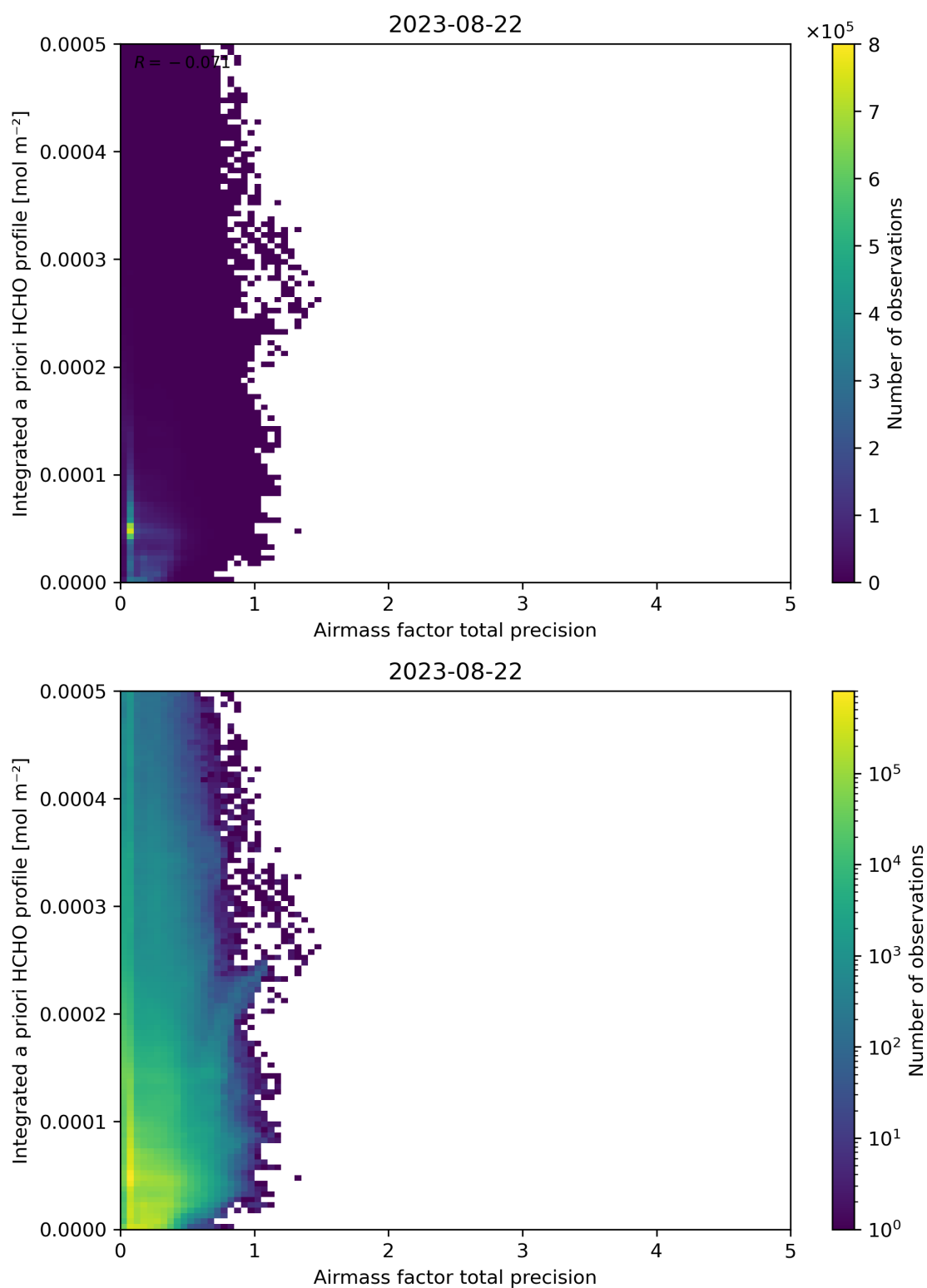
Figure 111: Scatter density plot of “Airmass factor total precision” against “Integrated a priori HCHO profile” for 2023-08-21 to 2023-08-23.
