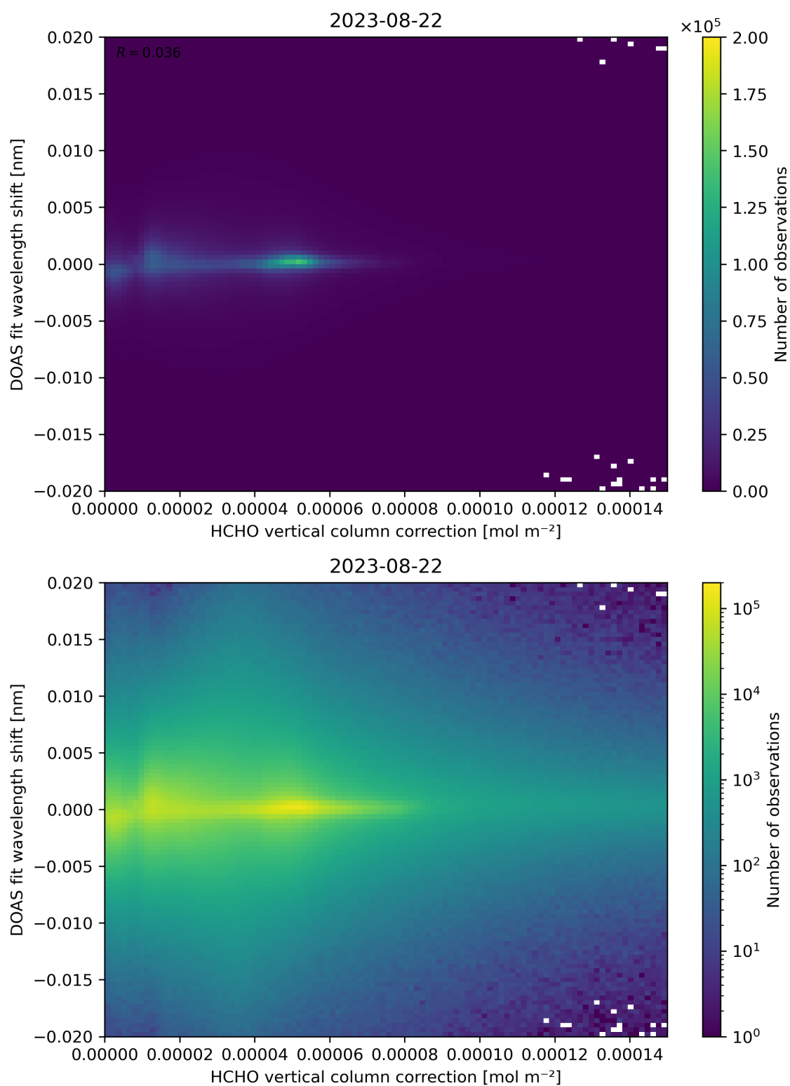
Figure 113: Scatter density plot of “HCHO vertical column correction” against “DOAS fit wavelength shift” for 2023-08-21 to 2023-08-23.
