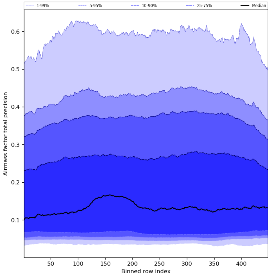
Figure 55: Along track statistics of “Airmass factor total precision” for 2023-08-21 to 2023-08-23
