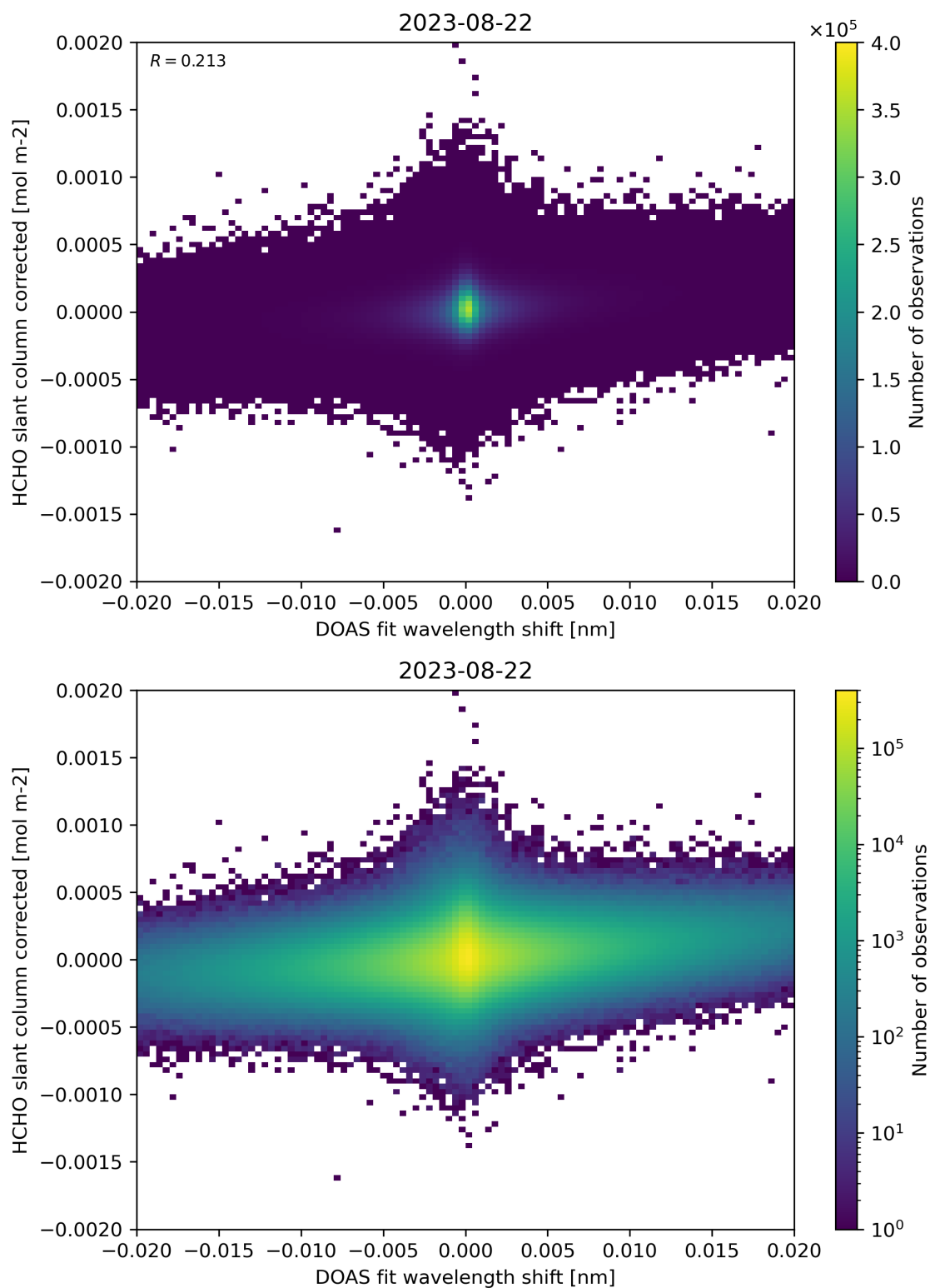
Figure 66: Scatter density plot of “DOAS fit wavelength shift” against “HCHO slant column corrected” for 2023-08-21 to 2023-08-23.
