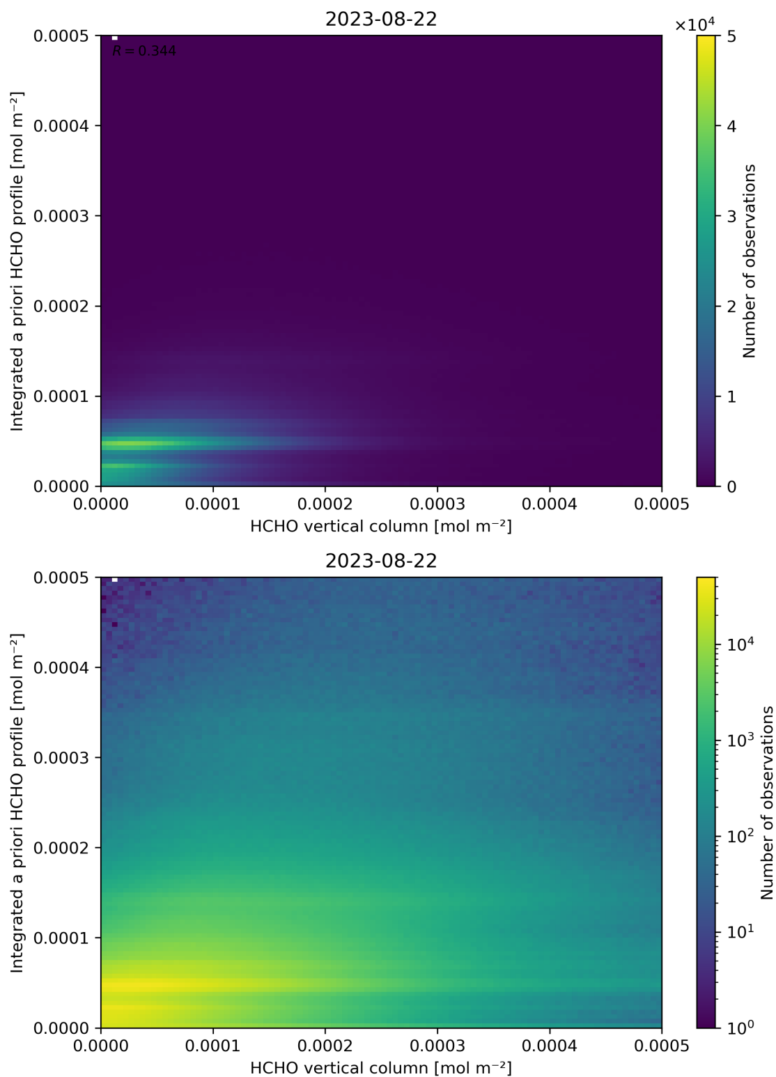
Figure 135: Scatter density plot of “HCHO vertical column” against “Integrated a priori HCHO profile” for 2023-08-21 to 2023-08-23.
