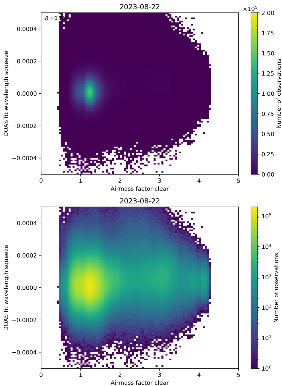
Figure 73: Scatter density plot of “Airmass factor clear” against “DOAS fit wavelength squeeze” for 2023-08-21 to 2023-08-23.
