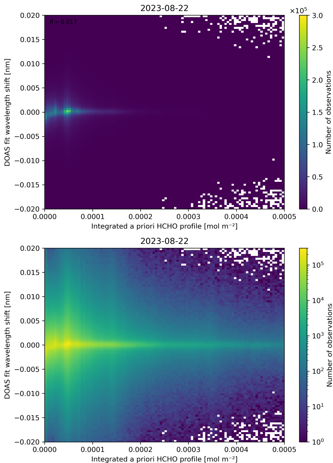
Figure 149: Scatter density plot of “Integrated a priori HCHO profile” against “DOAS fit wavelength shift” for 2023-08-21 to 2023-08-23.
