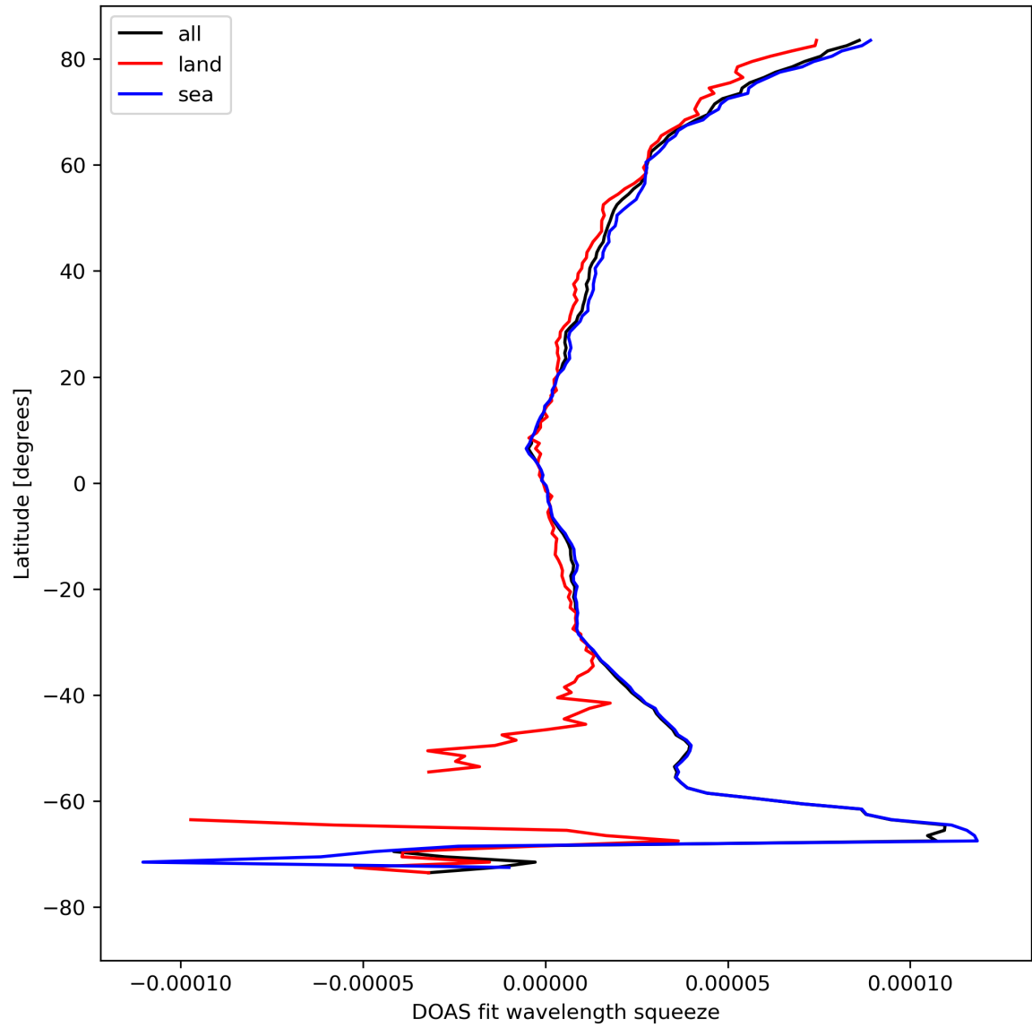
Figure 31: Zonal average of “DOAS fit wavelength squeeze” for 2023-08-21 to 2023-08-23.
