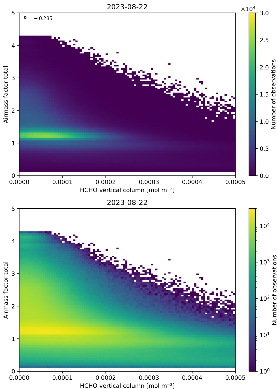
Figure 131: Scatter density plot of “HCHO vertical column” against “Airmass factor total” for 2023-08-21 to 2023-08-23.
