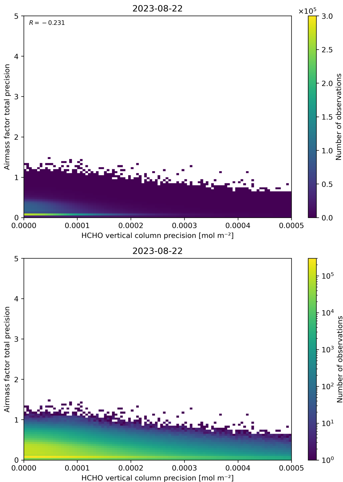
Figure 145: Scatter density plot of “HCHO vertical column precision” against “Airmass factor total precision” for 2023-08-21 to 2023-08-23.
