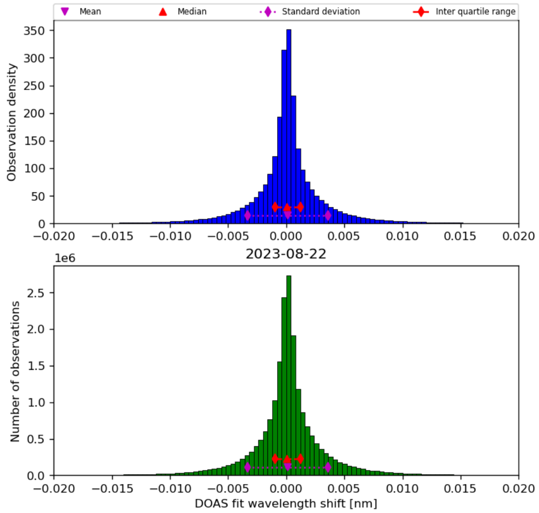
Figure 44: Histogram of “DOAS fit wavelength shift” for 2023-08-21 to 2023-08-23
