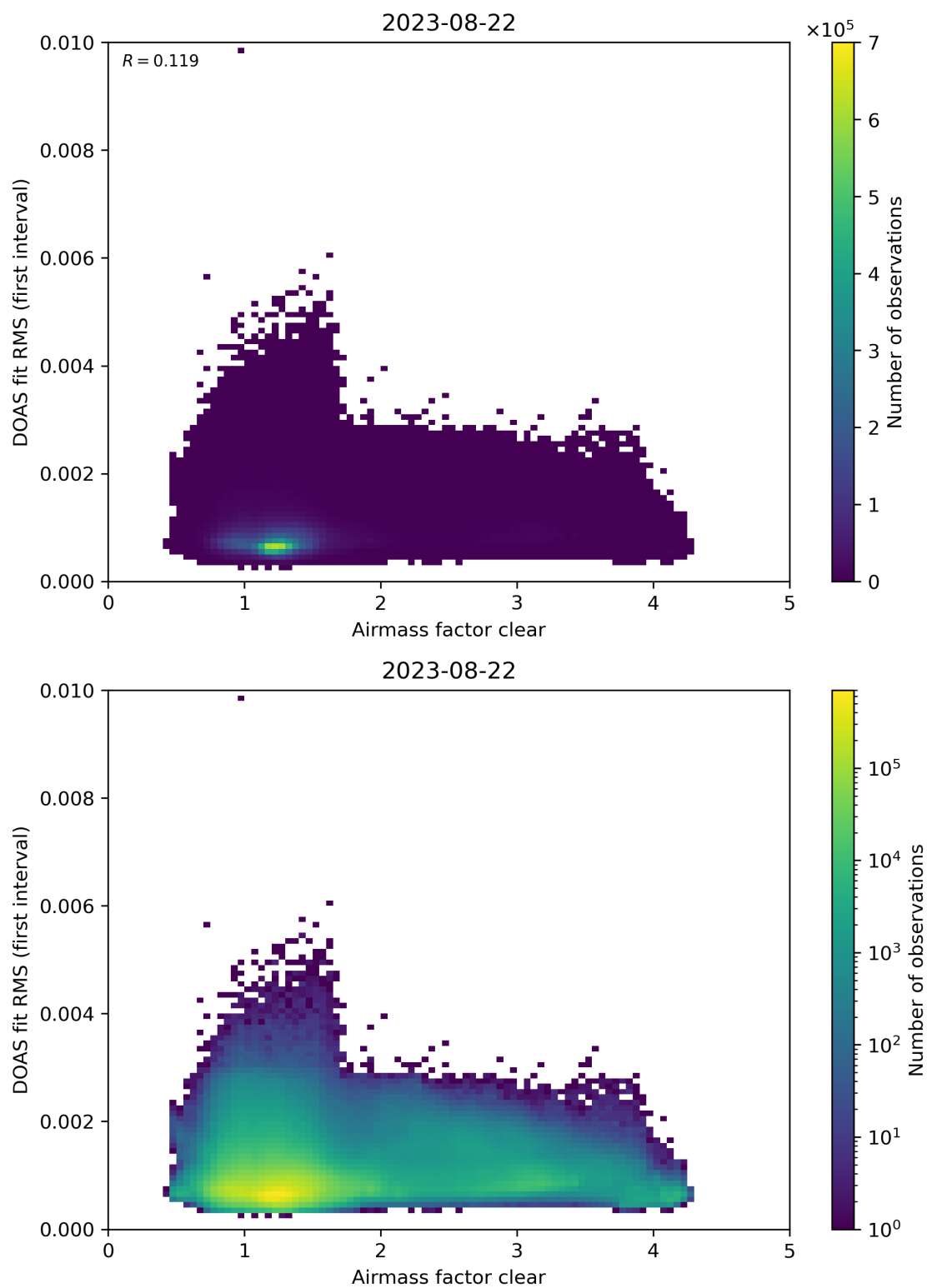
Figure 71: Scatter density plot of “Airmass factor clear” against “DOAS fit RMS (first interval)” for 2023-08-21 to 2023-08-23.
