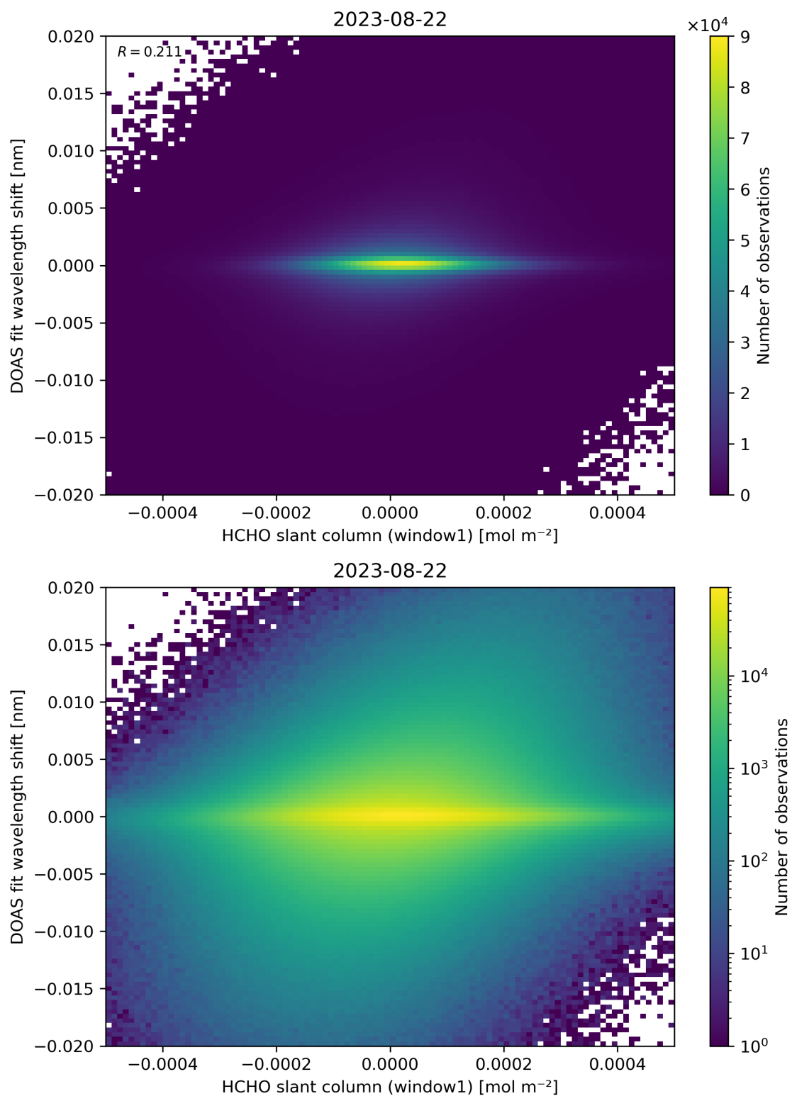
Figure 79: Scatter density plot of “HCHO slant column (window1)” against “DOAS fit wavelength shift” for 2023-08-21 to 2023-08-23.
