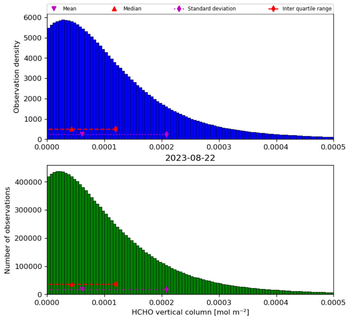
Figure 35: Histogram of “HCHO vertical column” for 2023-08-21 to 2023-08-23
