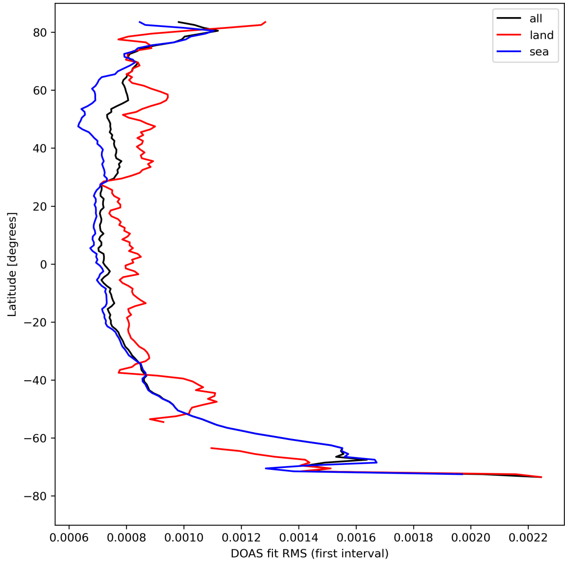
Figure 32: Zonal average of “DOAS fit RMS (first interval)” for 2023-08-21 to 2023-08-23.
