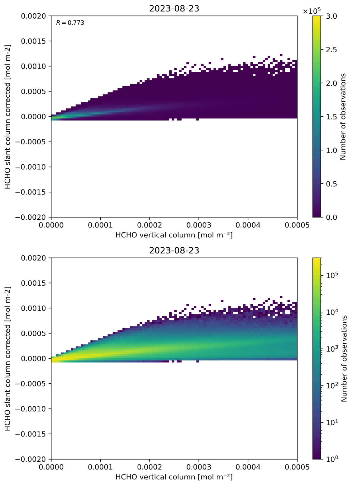
Figure 127: Scatter density plot of “HCHO vertical column” against “HCHO slant column corrected” for 2023-08-22 to 2023-08-24.
