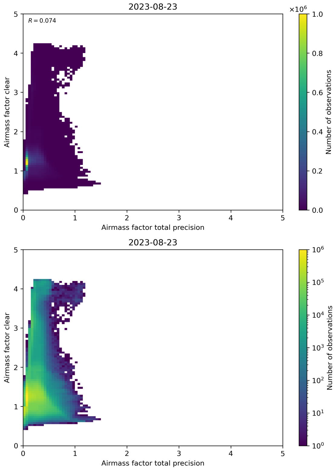
Figure 108: Scatter density plot of “Airmass factor total precision” against “Airmass factor clear” for 2023-08-22 to 2023-08-24.
