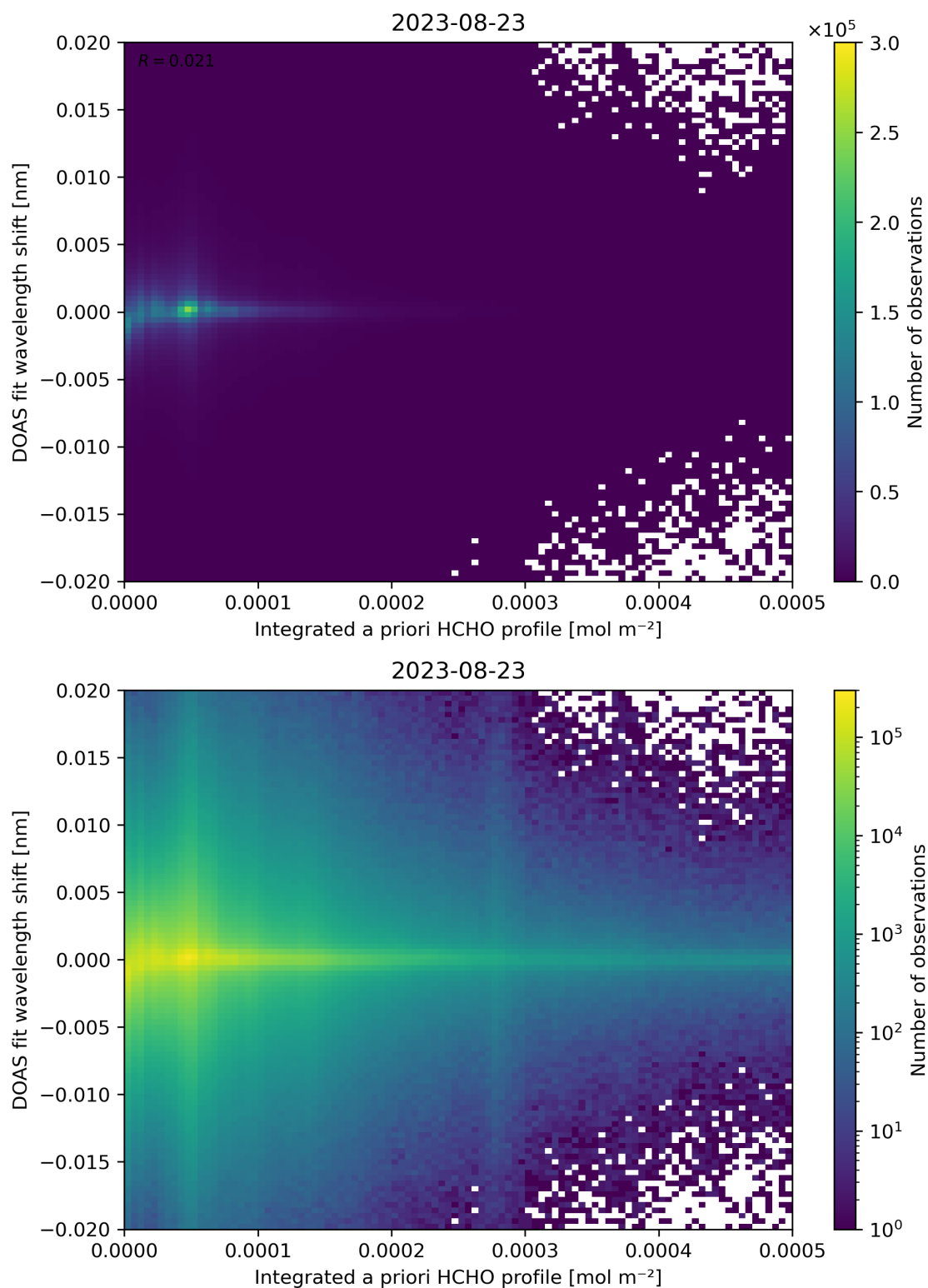
Figure 149: Scatter density plot of “Integrated a priori HCHO profile” against “DOAS fit wavelength shift” for 2023-08-22 to 2023-08-24.
