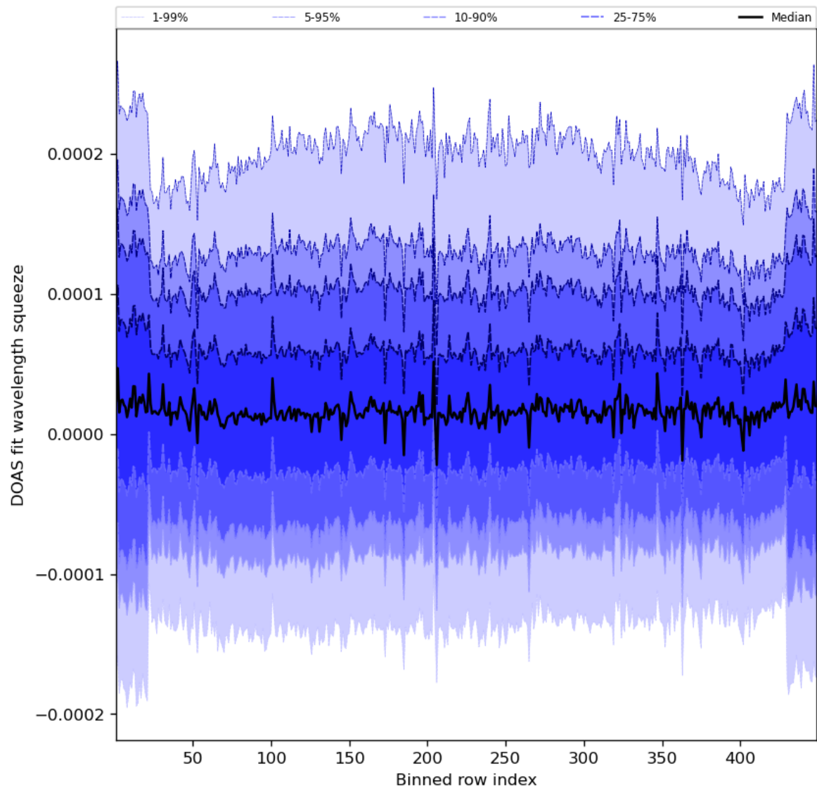
Figure 59: Along track statistics of “DOAS fit wavelength squeeze” for 2023-08-22 to 2023-08-24
