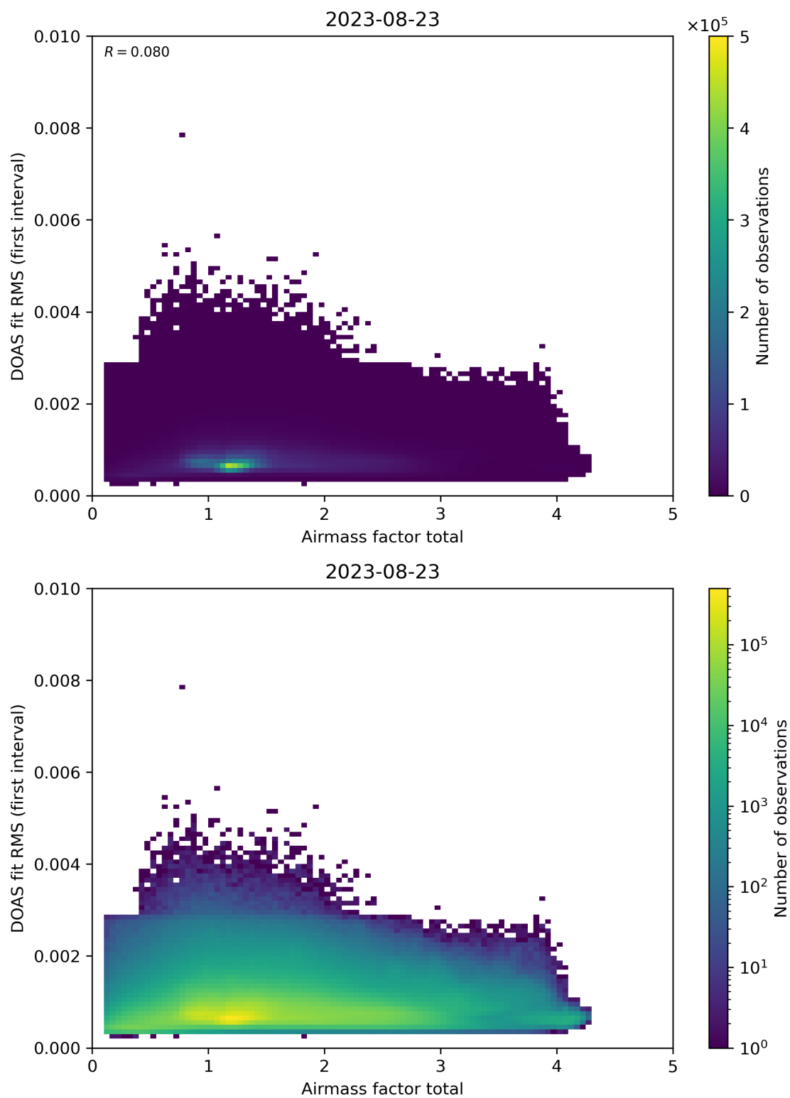
Figure 97: Scatter density plot of “Airmass factor total” against “DOAS fit RMS (first interval)” for 2023-08-22 to 2023-08-24.
