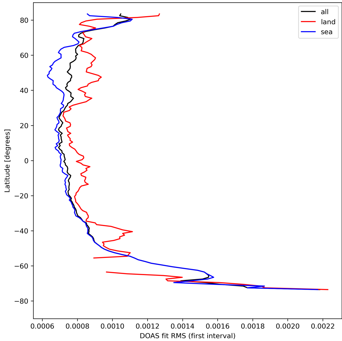
Figure 32: Zonal average of "DOAS fit RMS (first interval)" for 2023-08-22 to 2023-08-24.
