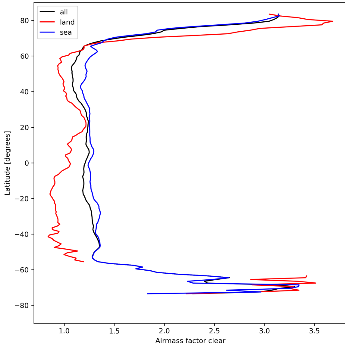
Figure 28: Zonal average of “Airmass factor clear” for 2023-08-22 to 2023-08-24.
