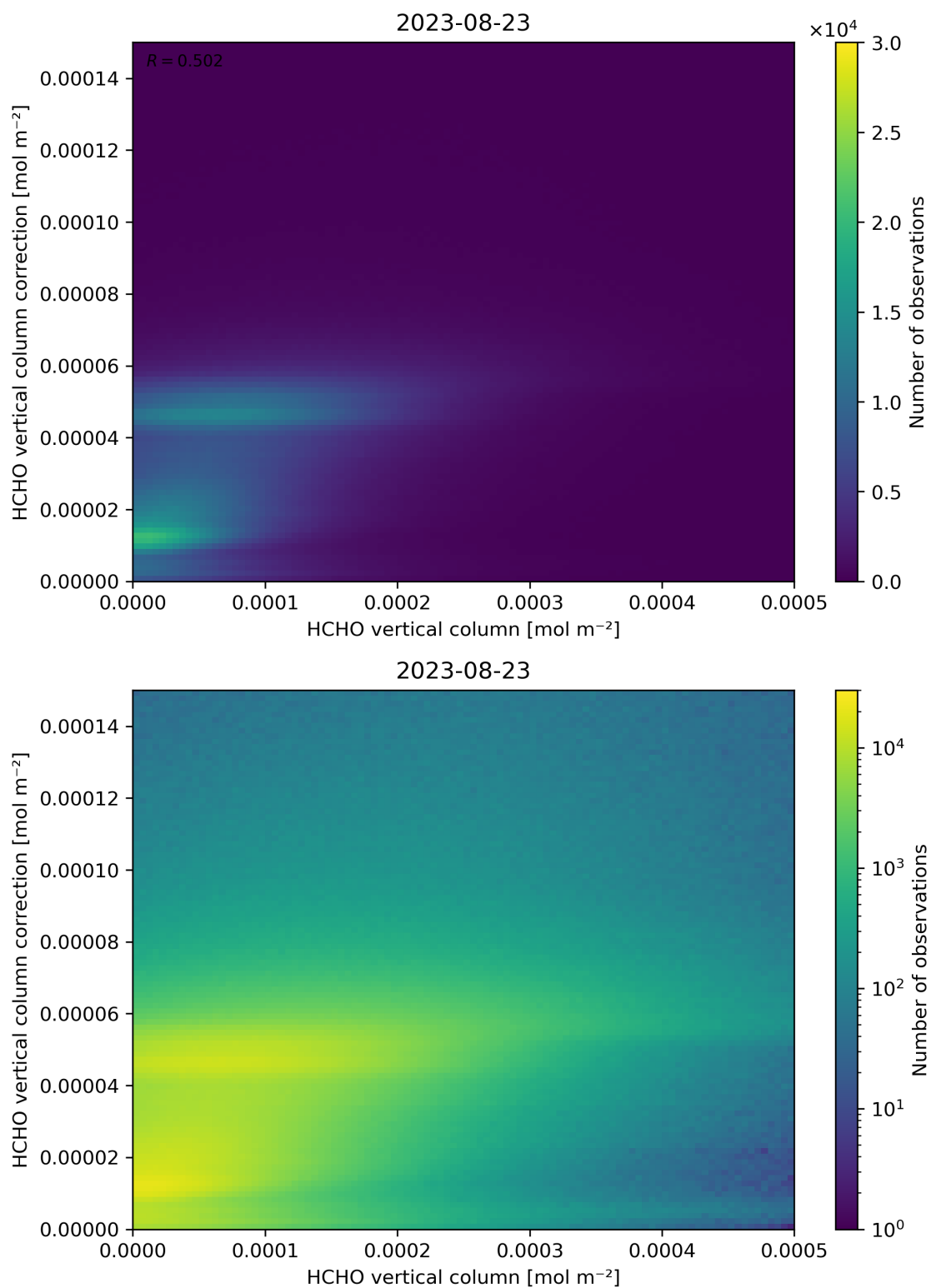
Figure 133: Scatter density plot of “HCHO vertical column” against “HCHO vertical column correction” for 2023-08-22 to 2023-08-24.
