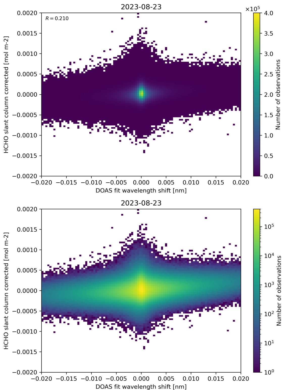
Figure 66: Scatter density plot of “DOAS fit wavelength shift” against “HCHO slant column corrected” for 2023-08-22 to 2023-08-24.
