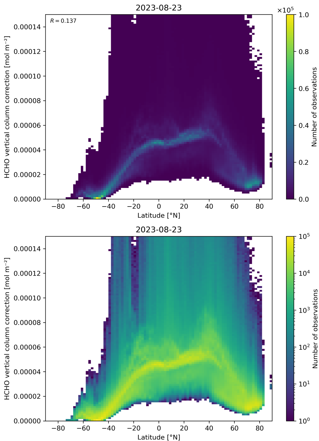
Figure 164: Scatter density plot of “Latitude” against “HCHO vertical column correction” for 2023-08-22 to 2023-08-24.
