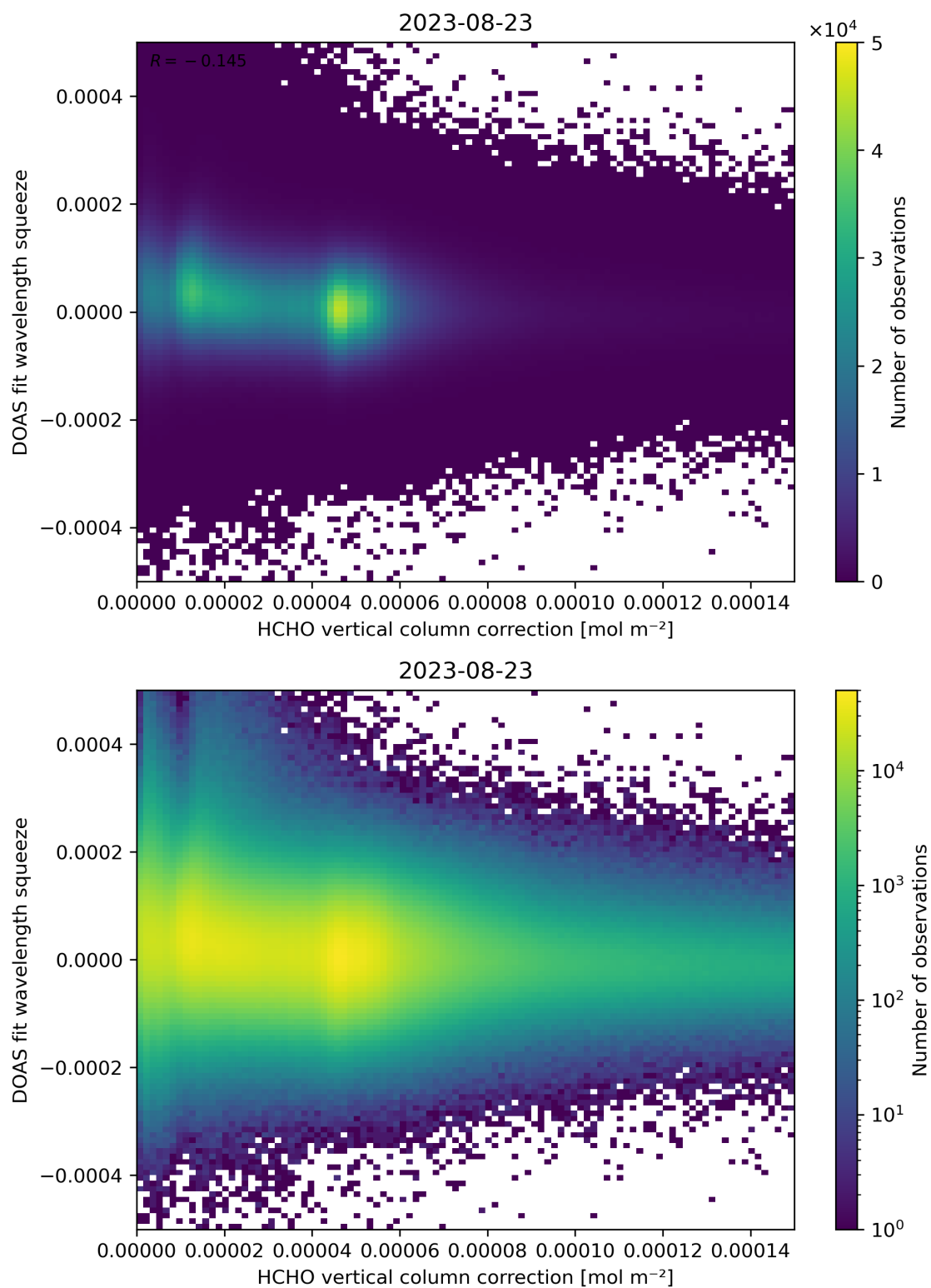
Figure 114: Scatter density plot of “HCHO vertical column correction” against “DOAS fit wavelength squeeze” for 2023-08-22 to 2023-08-24.
