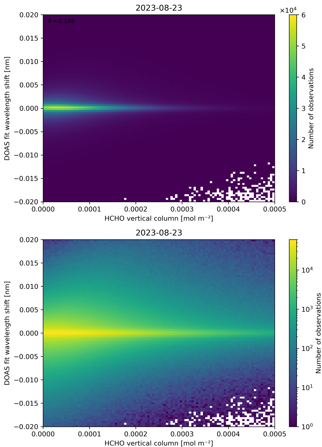
Figure 124: Scatter density plot of “HCHO vertical column” against “DOAS fit wavelength shift” for 2023-08-22 to 2023-08-24.
