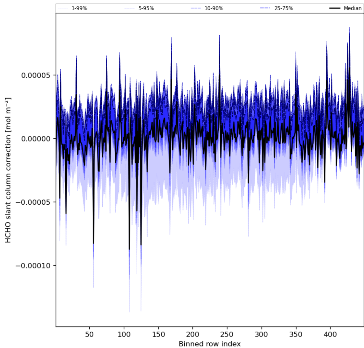
Figure 61: Along track statistics of “HCHO slant column correction” for 2023-08-22 to 2023-08-24
