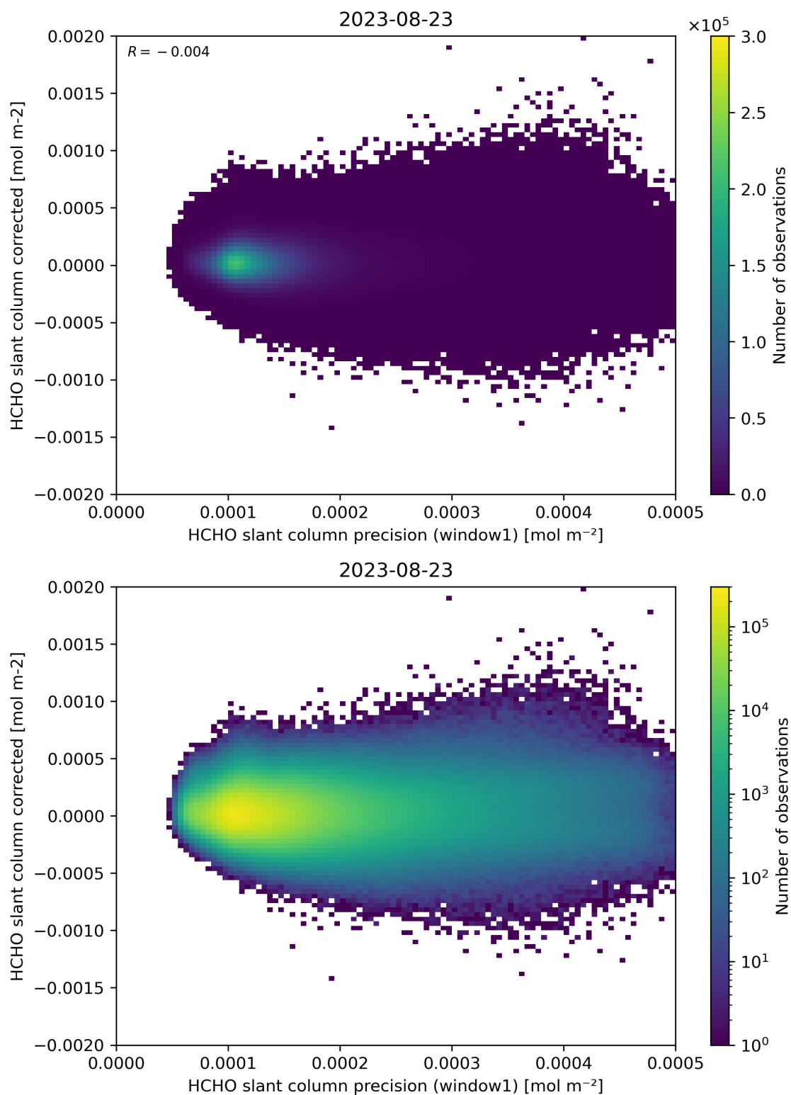
Figure 92: Scatter density plot of “HCHO slant column precision (window1)” against “HCHO slant column corrected” for 2023-08-22 to 2023-08-24.
