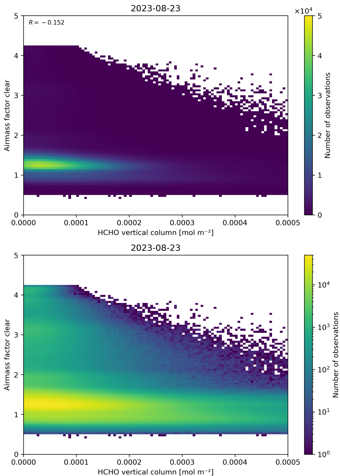
Figure 126: Scatter density plot of “HCHO vertical column” against “Airmass factor clear” for 2023-08-22 to 2023-08-24.
