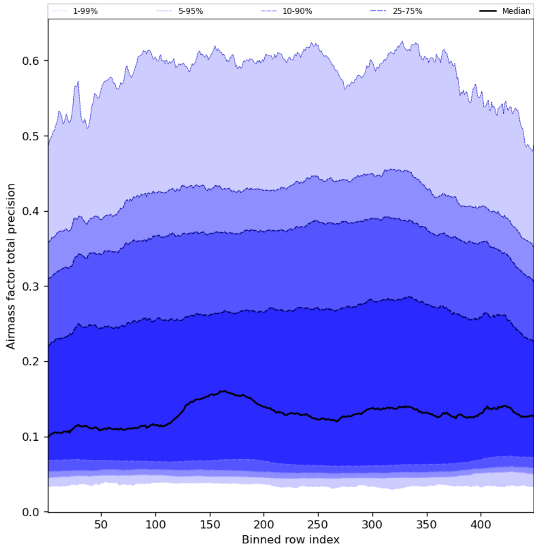
Figure 55: Along track statistics of “Airmass factor total precision” for 2023-08-22 to 2023-08-24
