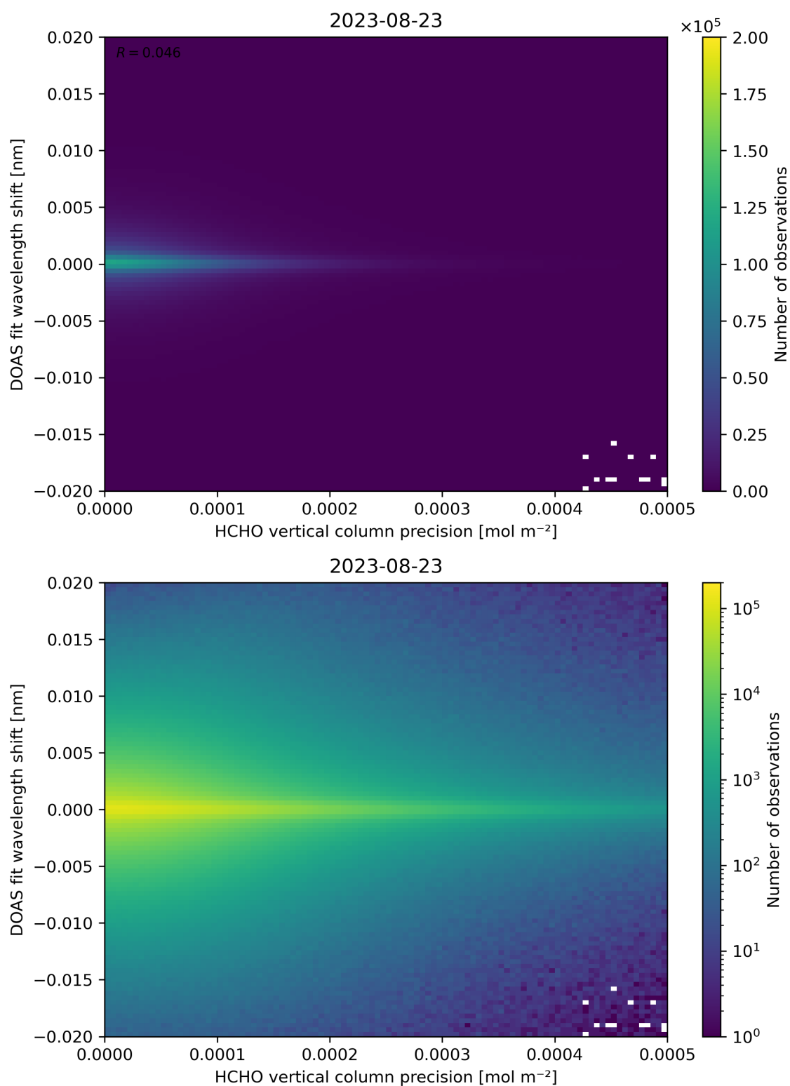
Figure 137: Scatter density plot of “HCHO vertical column precision” against “DOAS fit wavelength shift” for 2023-08-22 to 2023-08-24.
