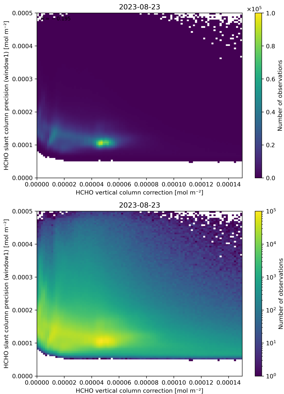
Figure 119: Scatter density plot of “HCHO vertical column correction” against “HCHO slant column precision (window1)” for 2023-08-22 to 2023-08-24.
