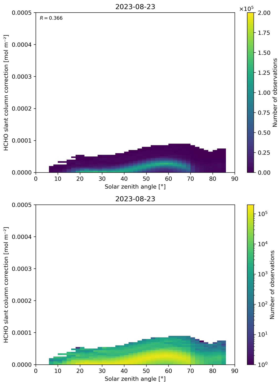
Figure 172: Scatter density plot of “Solar zenith angle” against “HCHO slant column correction” for 2023-08-22 to 2023-08-24.
