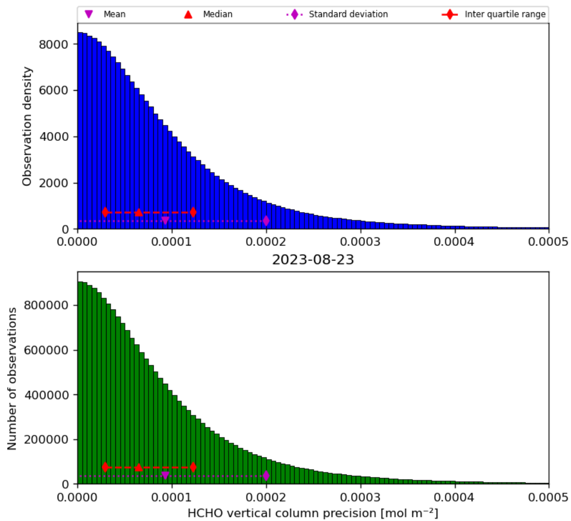
Figure 36: Histogram of “HCHO vertical column precision” for 2023-08-22 to 2023-08-24
