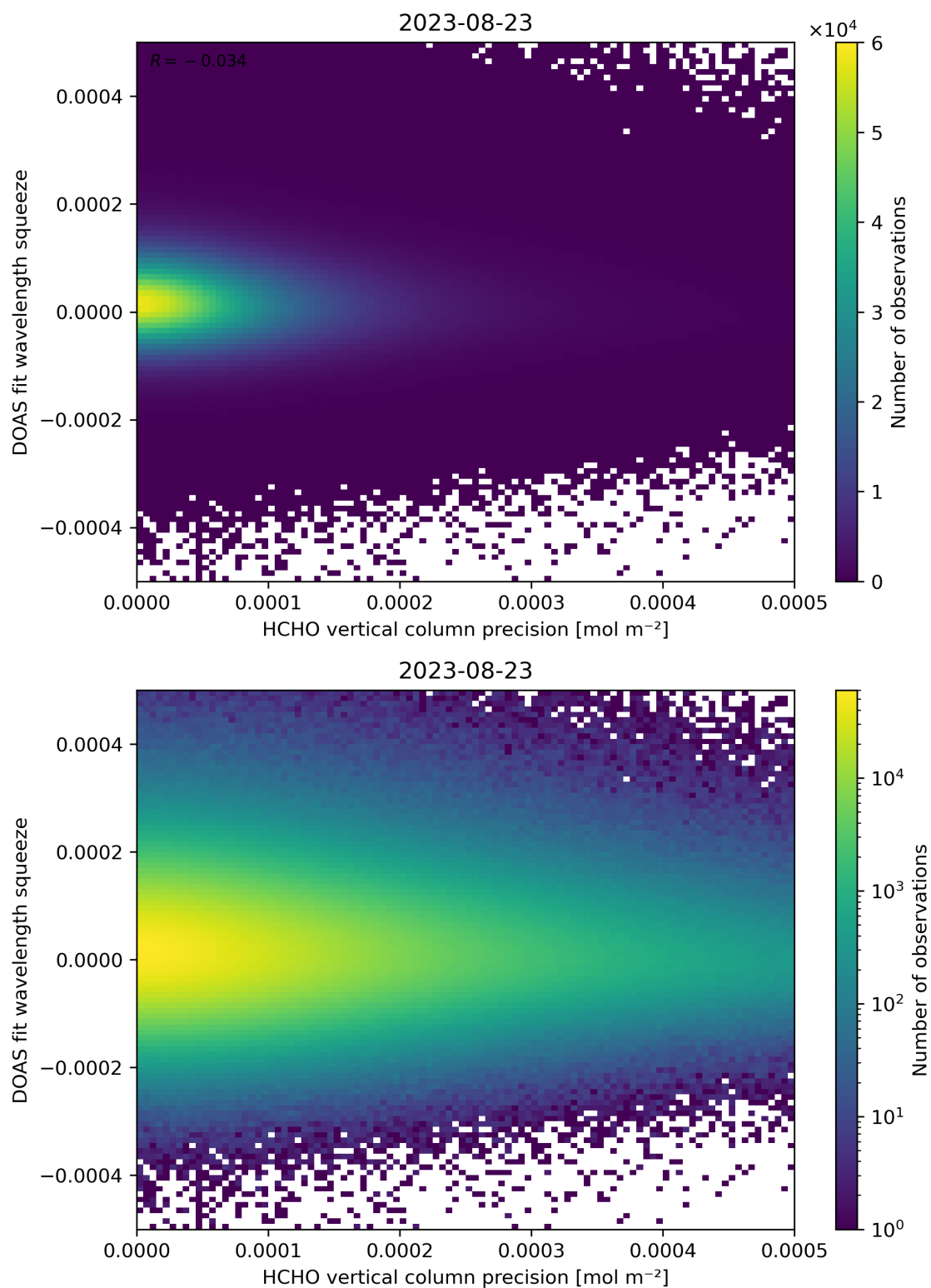
Figure 138: Scatter density plot of “HCHO vertical column precision” against “DOAS fit wavelength squeeze” for 2023-08-22 to 2023-08-24.
