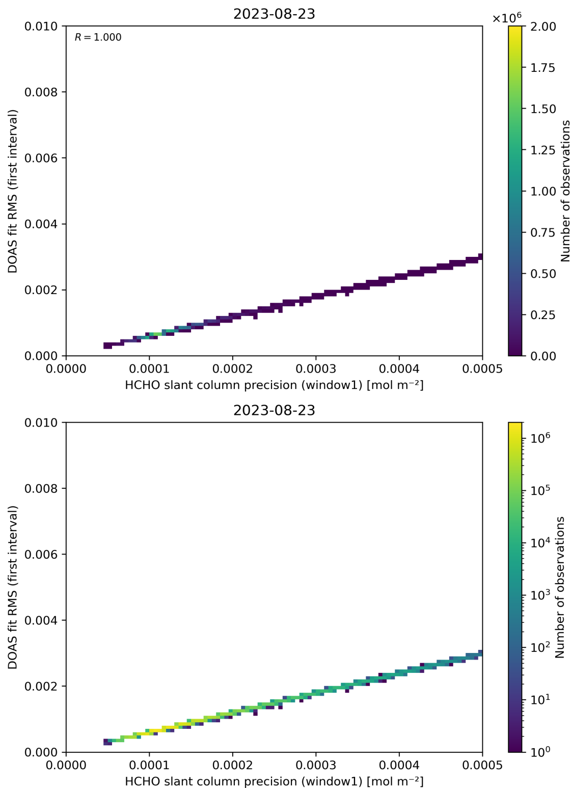
Figure 88: Scatter density plot of “HCHO slant column precision (window1)” against “DOAS fit RMS (first interval)” for 2023-08-22 to 2023-08-24.
