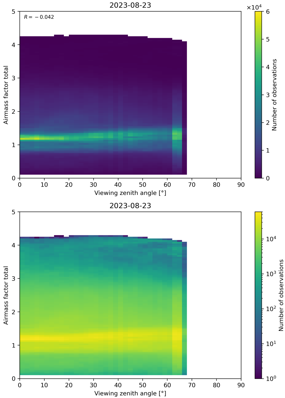
Figure 190: Scatter density plot of “Viewing zenith angle” against “Airmass factor total” for 2023-08-22 to 2023-08-24.
