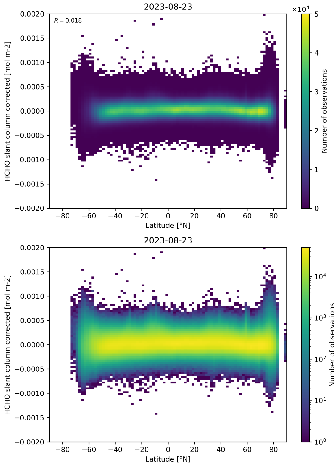
Figure 157: Scatter density plot of “Latitude” against “HCHO slant column corrected” for 2023-08-22 to 2023-08-24.
