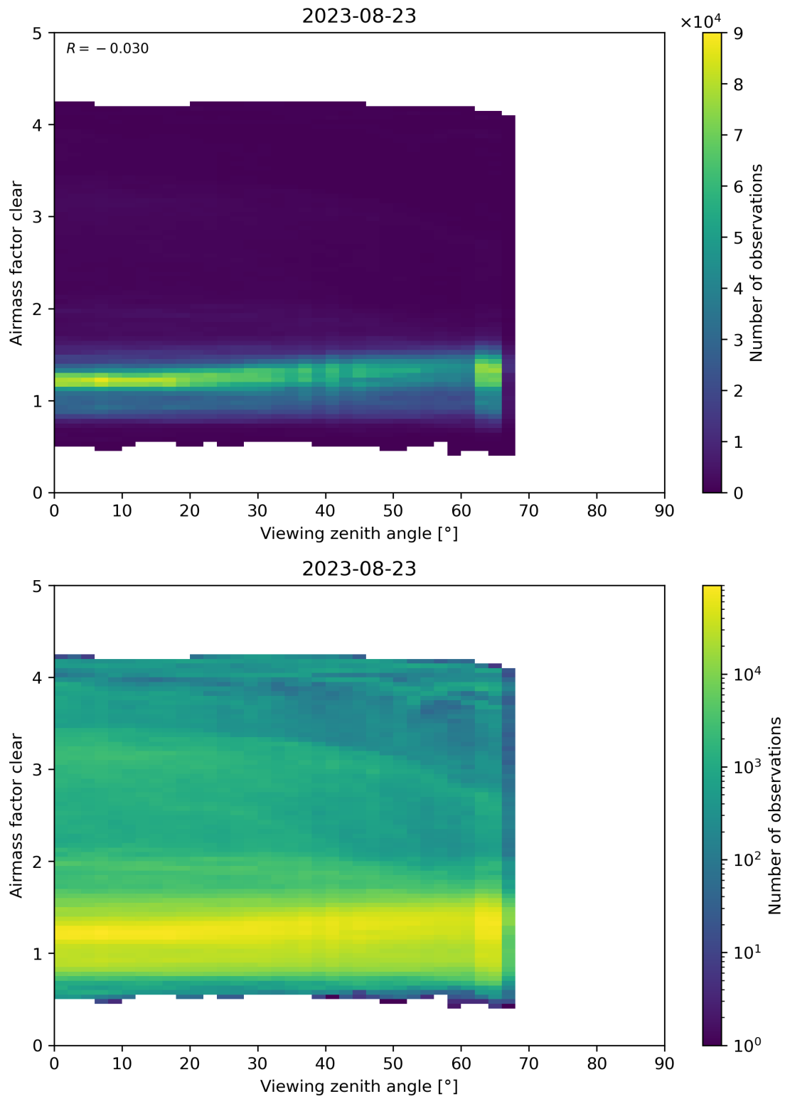
Figure 185: Scatter density plot of “Viewing zenith angle” against “Airmass factor clear” for 2023-08-22 to 2023-08-24.
