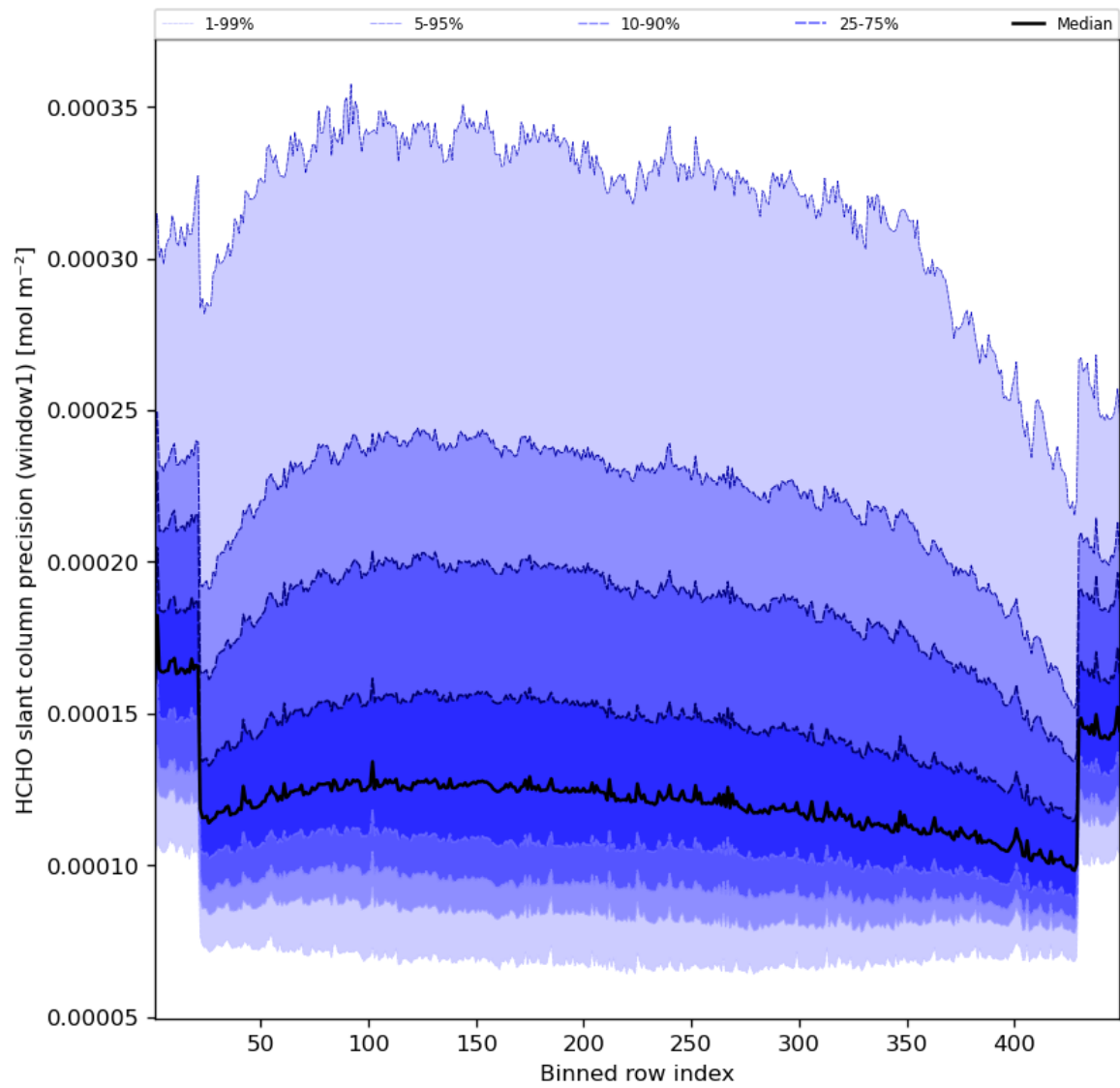
Figure 53: Along track statistics of "HCHO slant column precision (window1)" for 2023-08-22 to 2023-08-24
