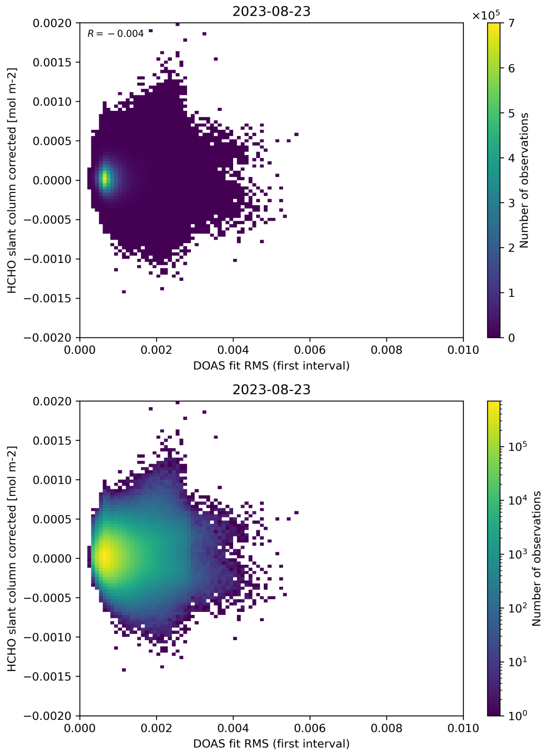
Figure 62: Scatter density plot of “DOAS fit RMS (first interval)” against “HCHO slant column corrected” for 2023-08-22 to 2023-08-24.
