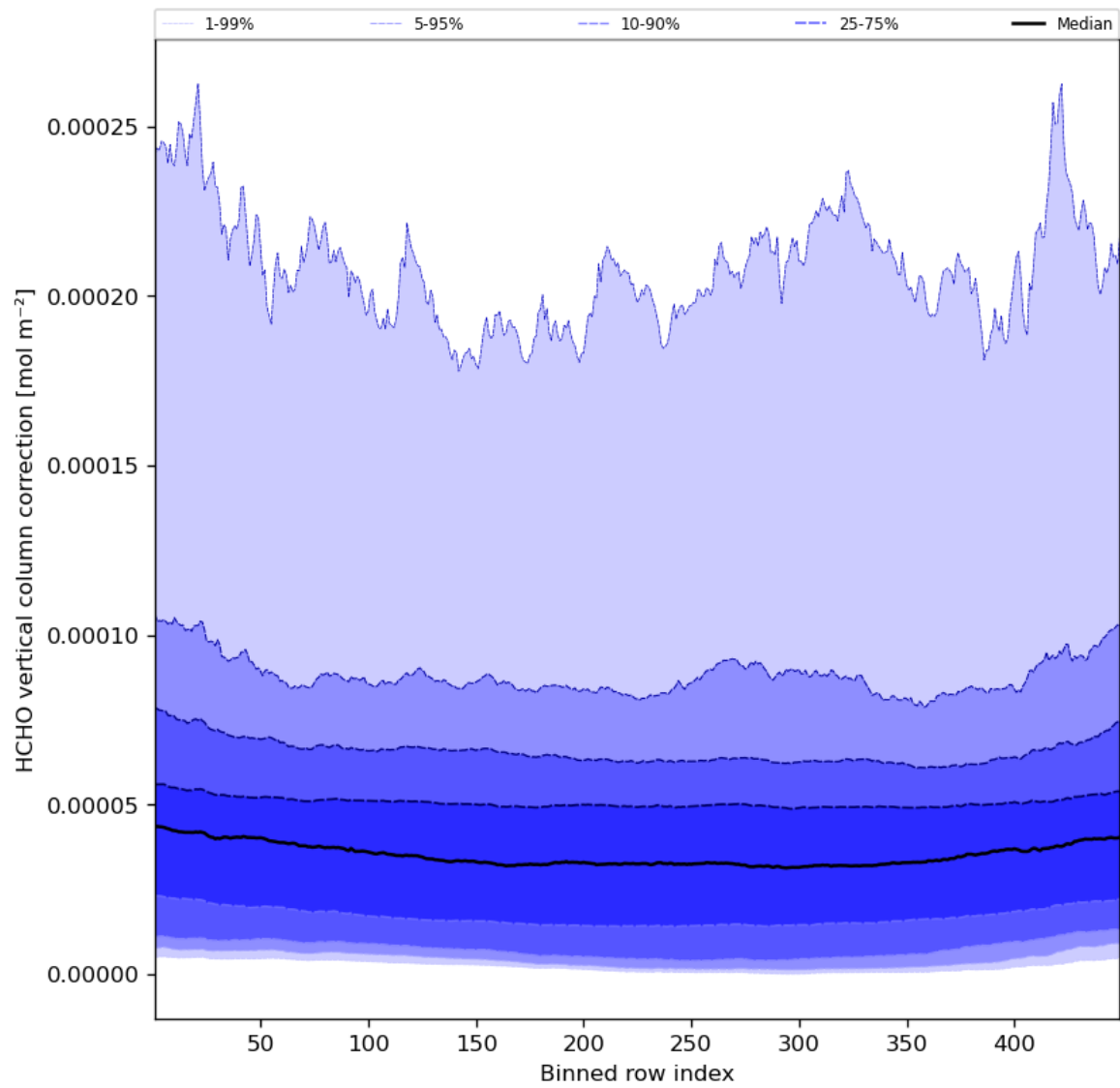
Figure 51: Along track statistics of “HCHO vertical column correction” for 2023-08-22 to 2023-08-24
