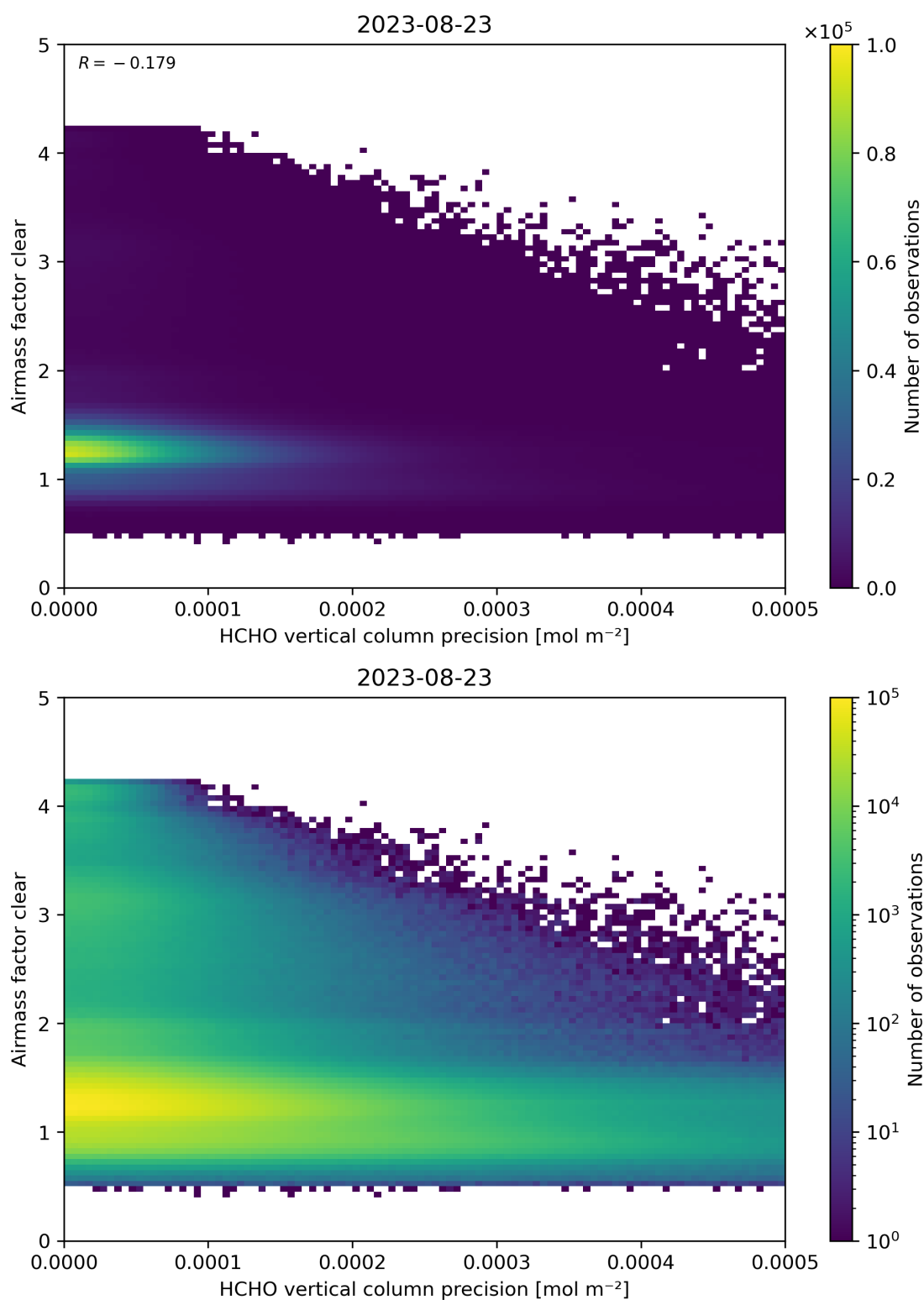
Figure 139: Scatter density plot of “HCHO vertical column precision” against “Airmass factor clear” for 2023-08-22 to 2023-08-24.
