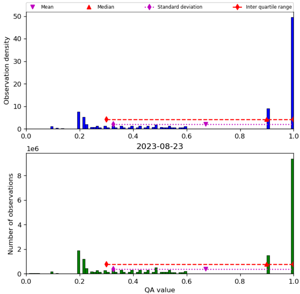
Figure 34: Histogram of “QA value” for 2023-08-22 to 2023-08-24
