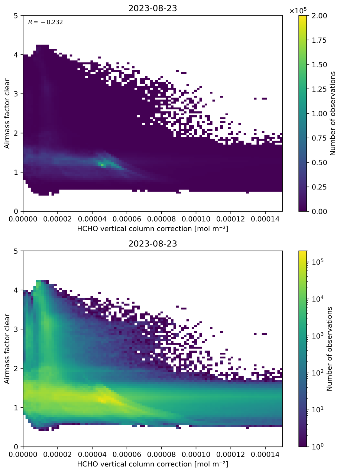
Figure 115: Scatter density plot of “HCHO vertical column correction” against “Airmass factor clear” for 2023-08-22 to 2023-08-24.
