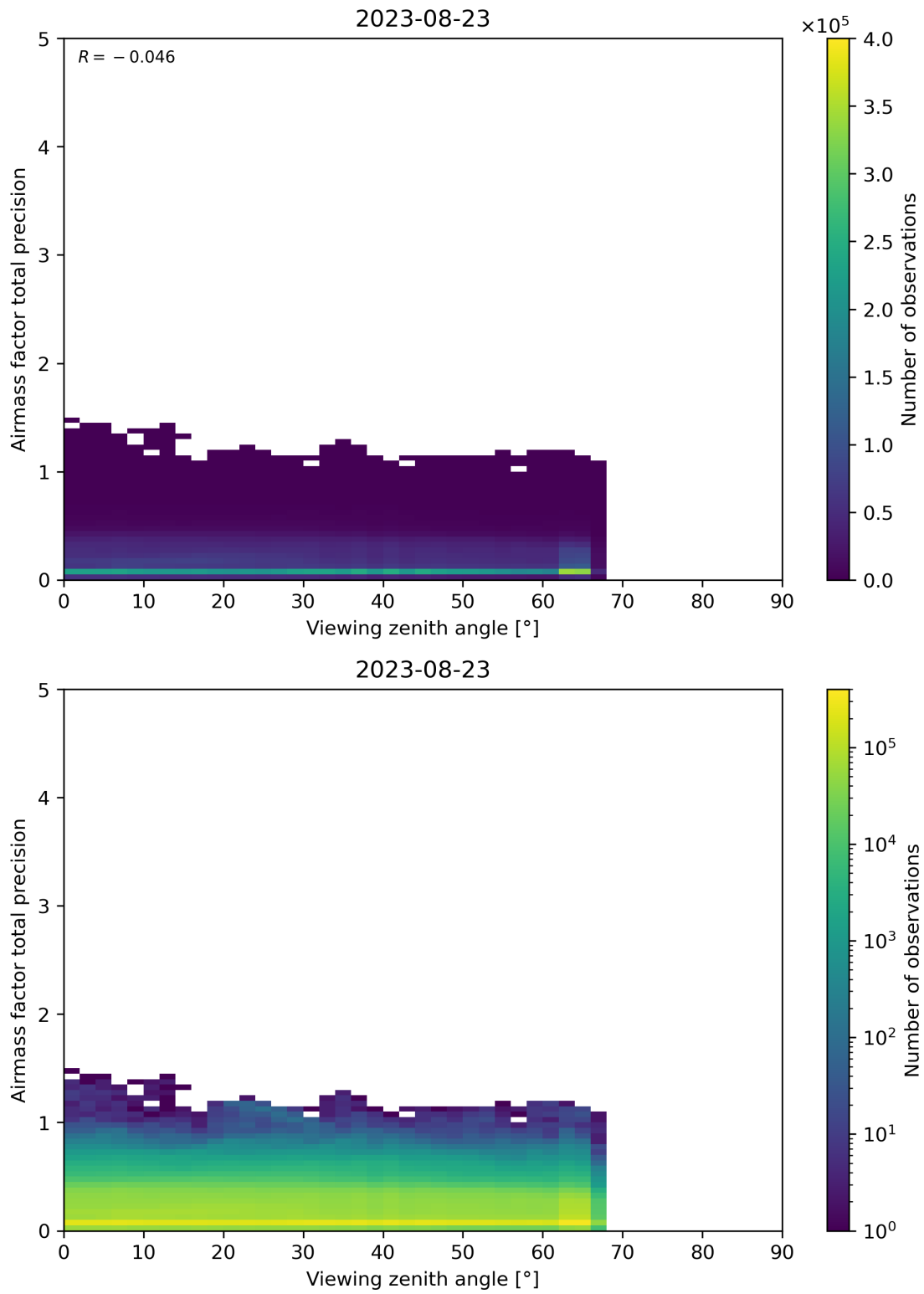
Figure 191: Scatter density plot of “Viewing zenith angle” against “Airmass factor total precision” for 2023-08-22 to 2023-08-24.
