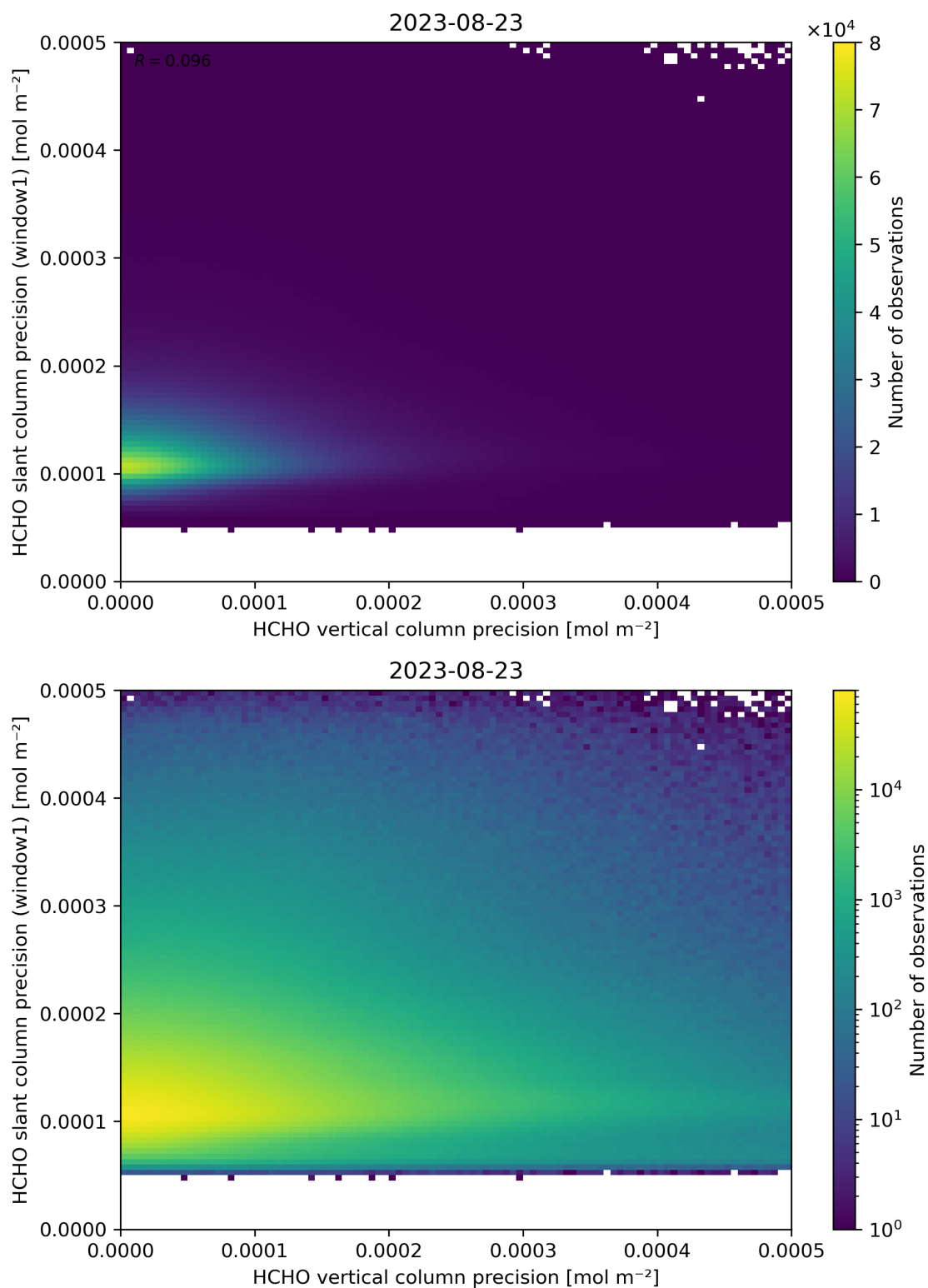
Figure 143: Scatter density plot of “HCHO vertical column precision” against “HCHO slant column precision (window1)” for 2023-08-22 to 2023-08-24.
