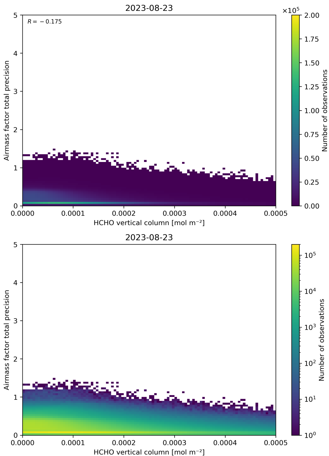
Figure 132: Scatter density plot of “HCHO vertical column” against “Airmass factor total precision” for 2023-08-22 to 2023-08-24.
