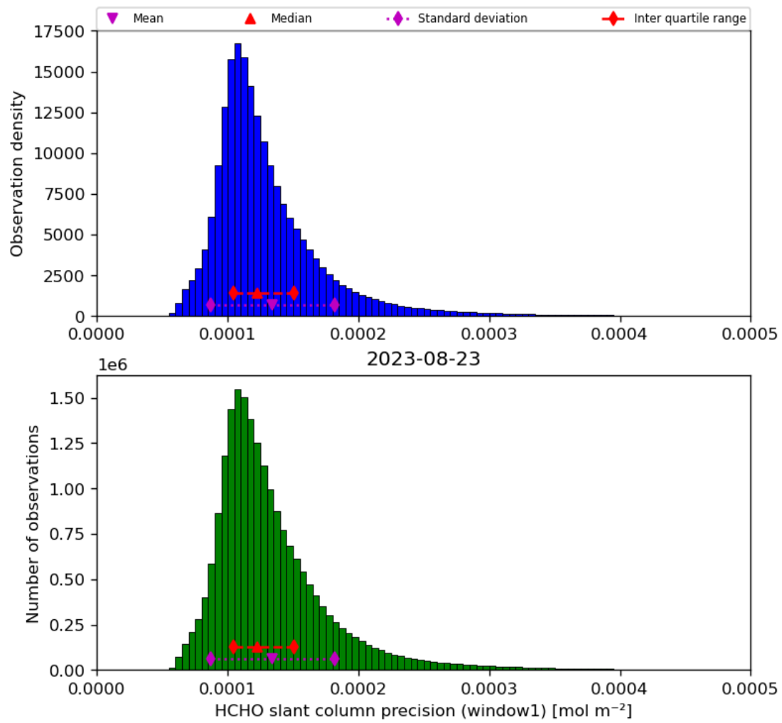
Figure 39: Histogram of “HCHO slant column precision (window1)” for 2023-08-22 to 2023-08-24
