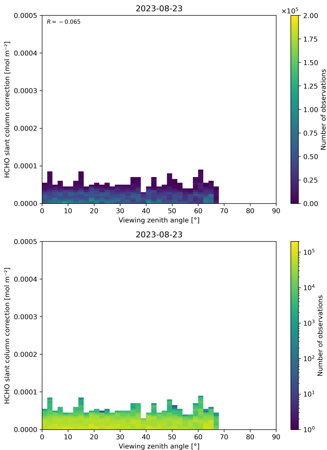
Figure 187: Scatter density plot of “Viewing zenith angle” against “HCHO slant column correction” for 2023-08-22 to 2023-08-24.
