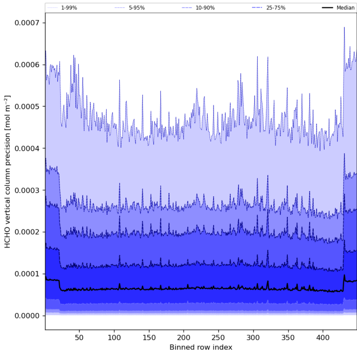
Figure 50: Along track statistics of “HCHO vertical column precision” for 2023-08-22 to 2023-08-24
