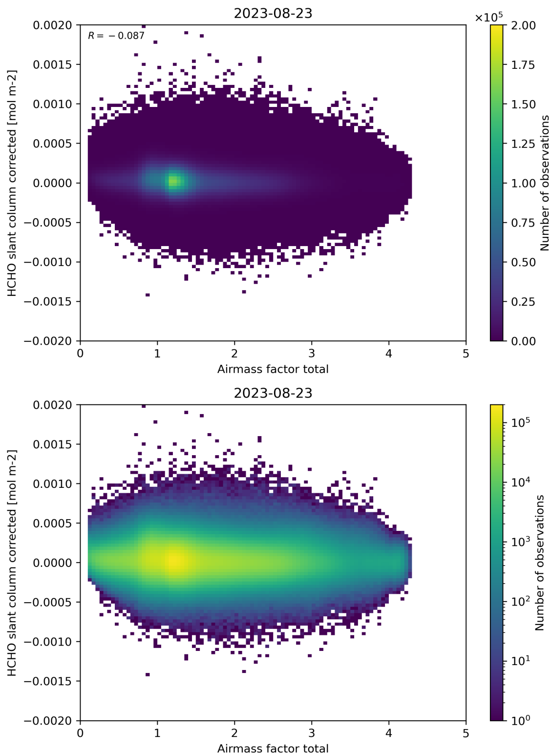
Figure 101: Scatter density plot of “Airmass factor total” against “HCHO slant column corrected” for 2023-08-22 to 2023-08-24.
