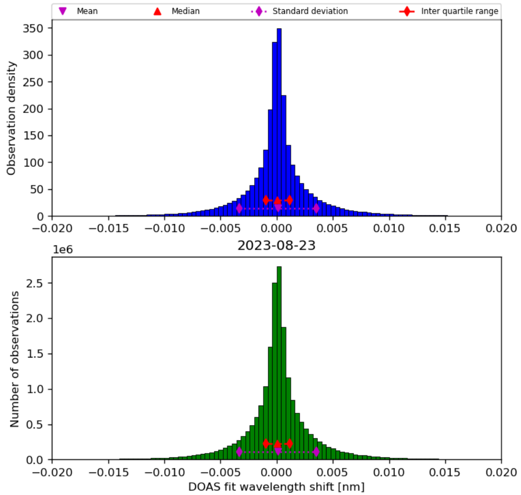
Figure 44: Histogram of “DOAS fit wavelength shift” for 2023-08-22 to 2023-08-24
