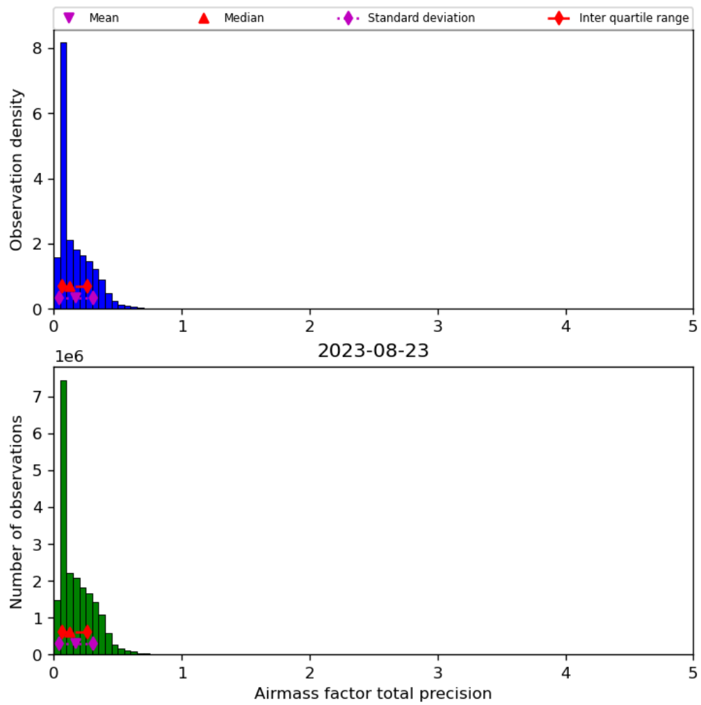
Figure 41: Histogram of “Airmass factor total precision” for 2023-08-22 to 2023-08-24
