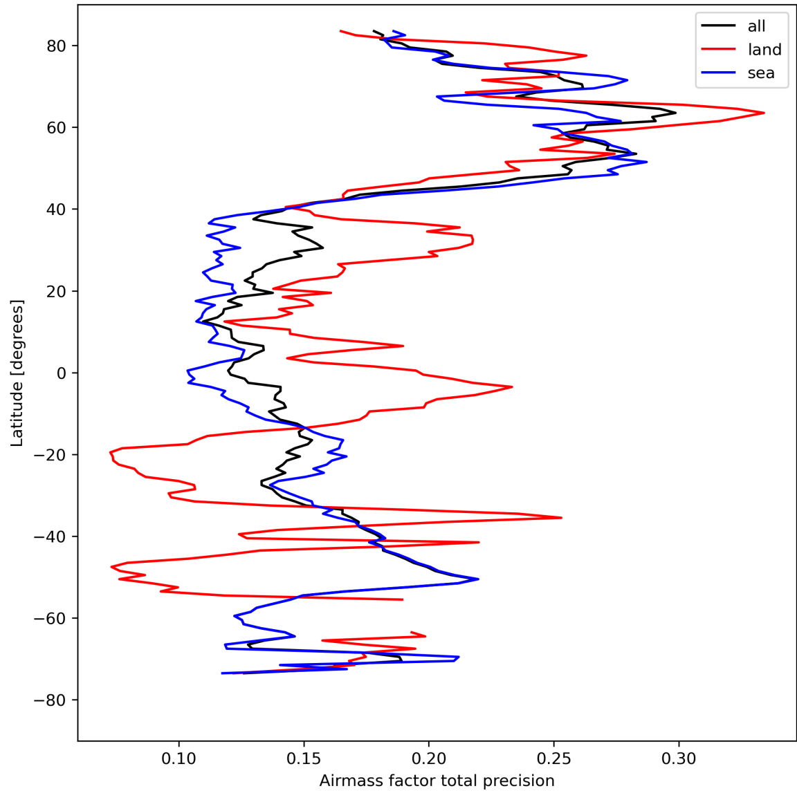
Figure 27: Zonal average of “Airmass factor total precision” for 2023-08-22 to 2023-08-24.
