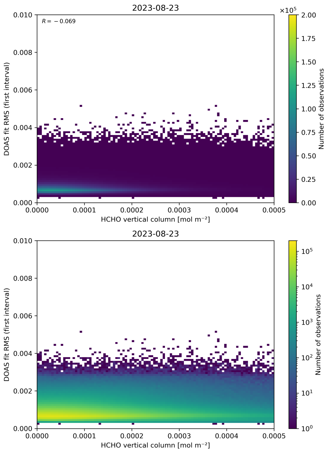
Figure 123: Scatter density plot of “HCHO vertical column” against “DOAS fit RMS (first interval)” for 2023-08-22 to 2023-08-24.
