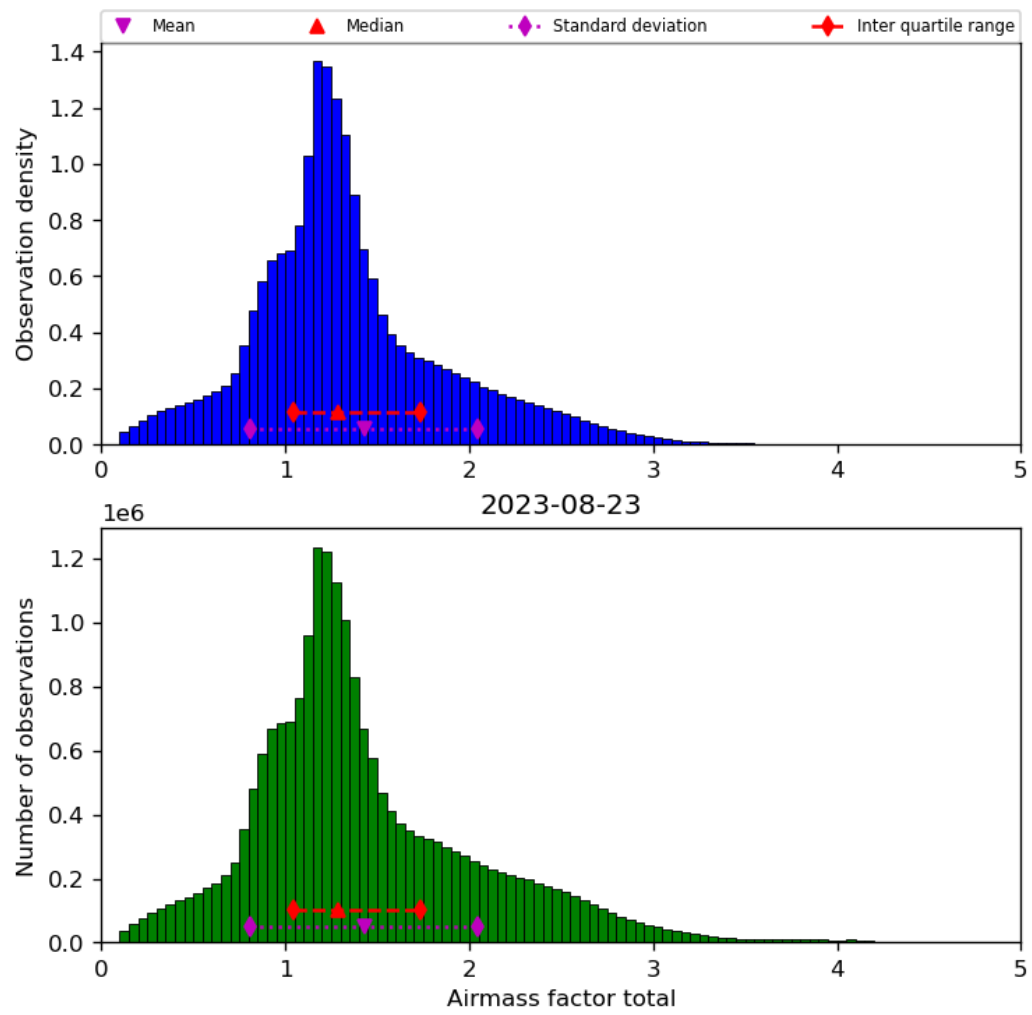
Figure 40: Histogram of “Airmass factor total” for 2023-08-22 to 2023-08-24
