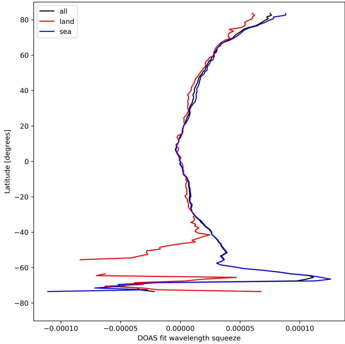
Figure 31: Zonal average of “DOAS fit wavelength squeeze” for 2023-08-22 to 2023-08-24.
