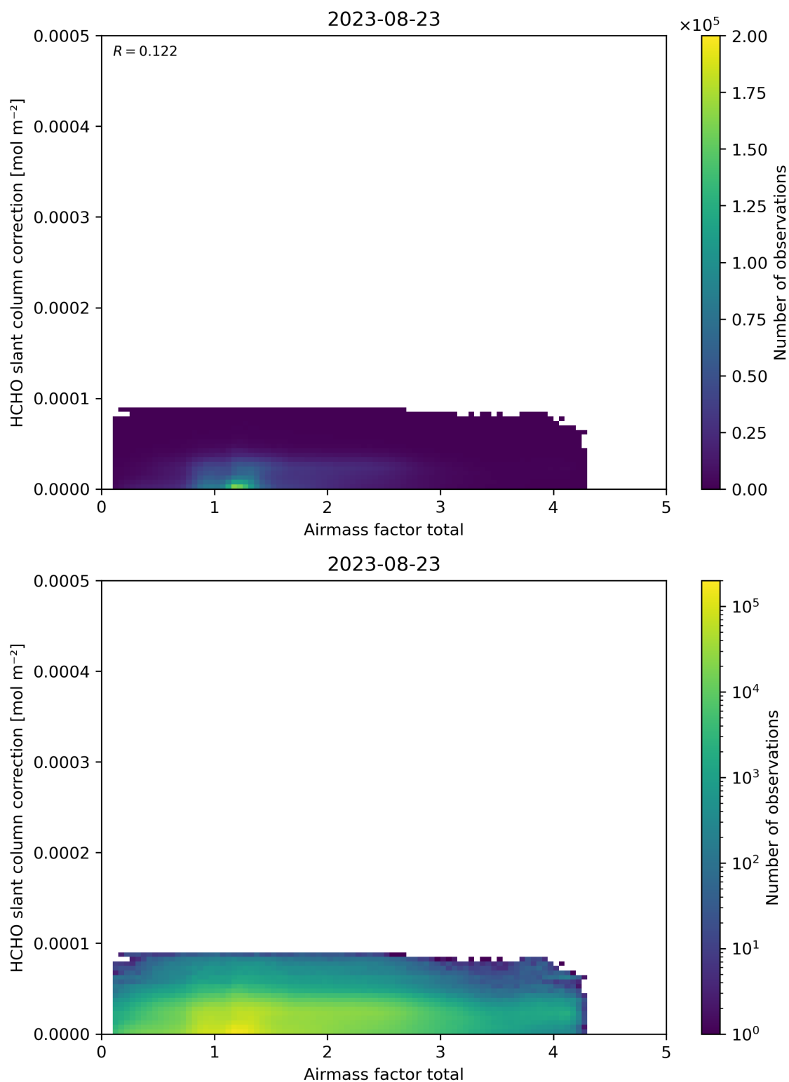
Figure 102: Scatter density plot of “Airmass factor total” against “HCHO slant column correction” for 2023-08-22 to 2023-08-24.
