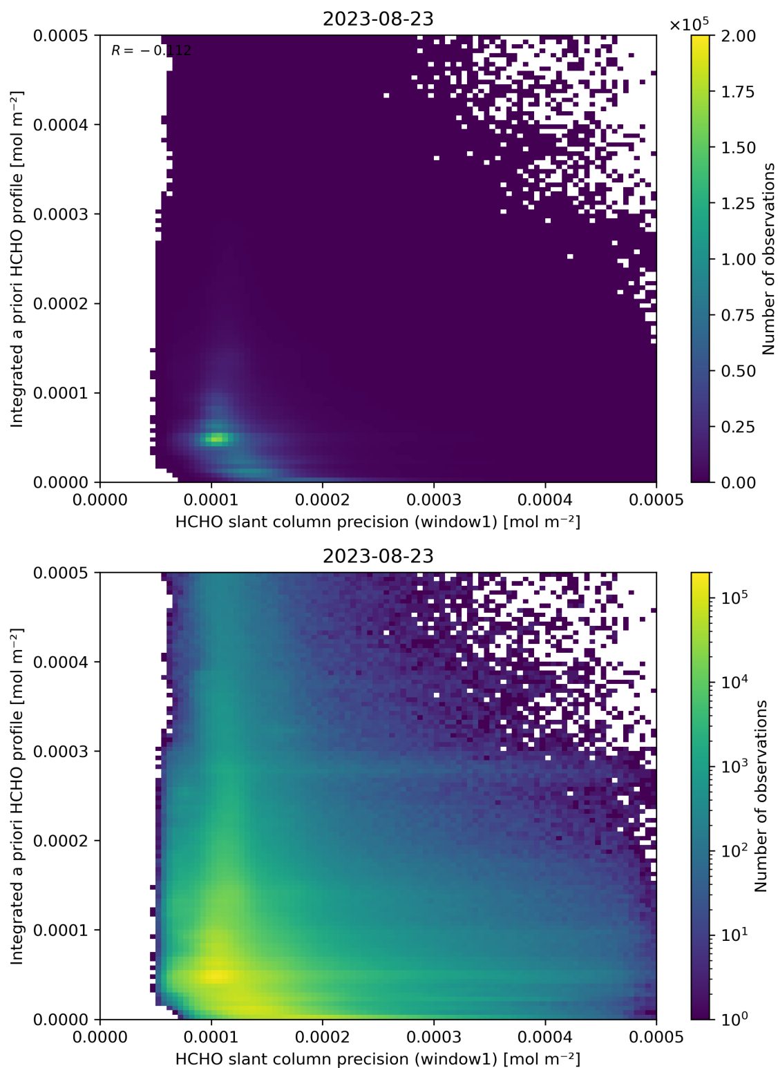
Figure 96: Scatter density plot of “HCHO slant column precision (window1)” against “Integrated a priori HCHO profile” for 2023-08-22 to 2023-08-24.
