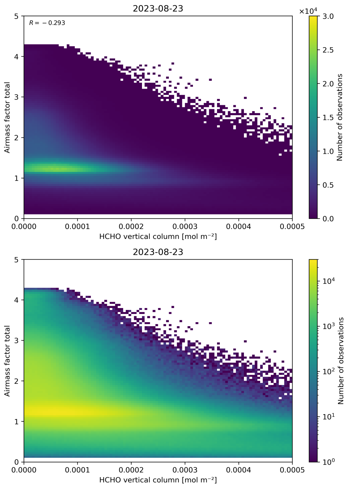
Figure 131: Scatter density plot of “HCHO vertical column” against “Airmass factor total” for 2023-08-22 to 2023-08-24.
