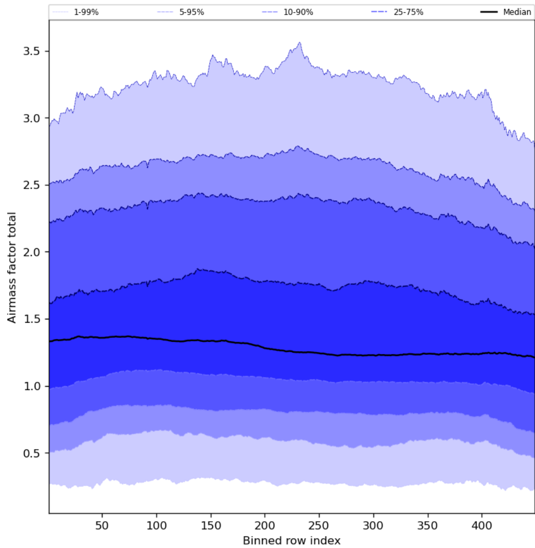
Figure 54: Along track statistics of “Airmass factor total” for 2023-08-22 to 2023-08-24
