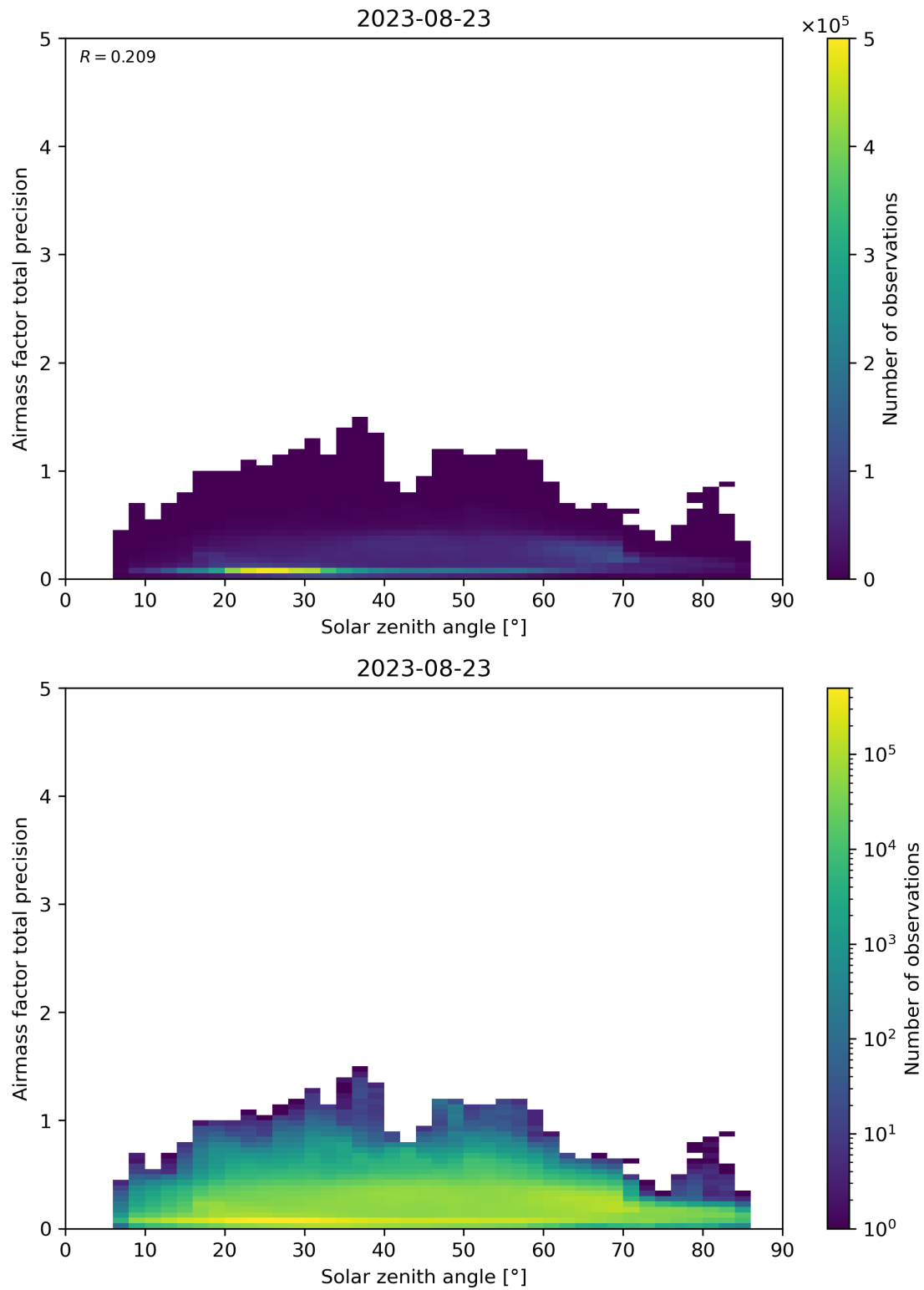
Figure 176: Scatter density plot of “Solar zenith angle” against “Airmass factor total precision” for 2023-08-22 to 2023-08-24.
