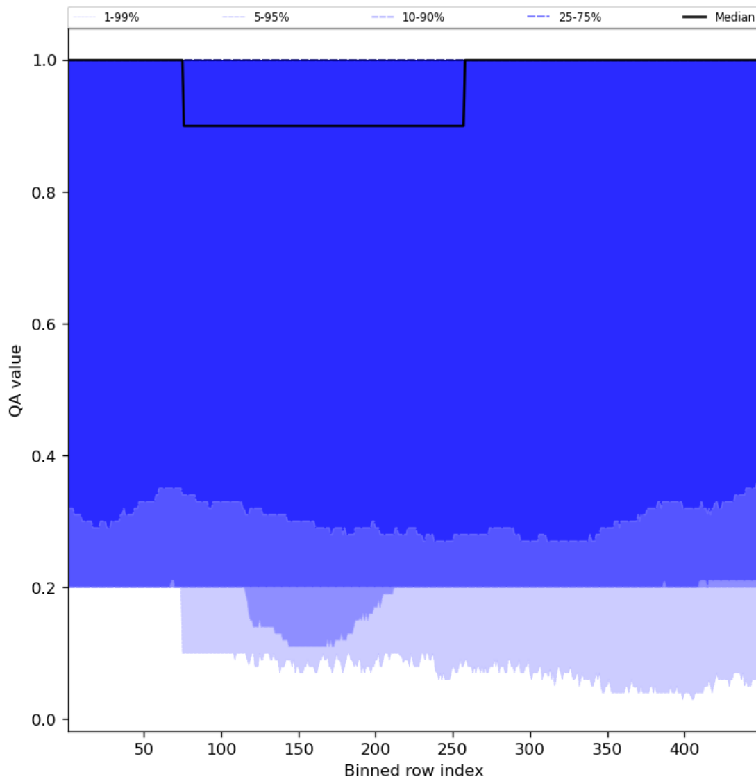
Figure 48: Along track statistics of “QA value” for 2023-08-22 to 2023-08-24
