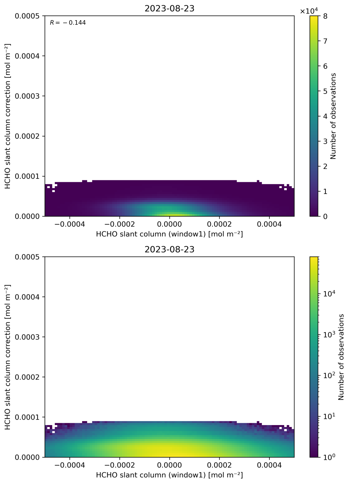
Figure 83: Scatter density plot of “HCHO slant column (window1)” against “HCHO slant column correction” for 2023-08-22 to 2023-08-24.
