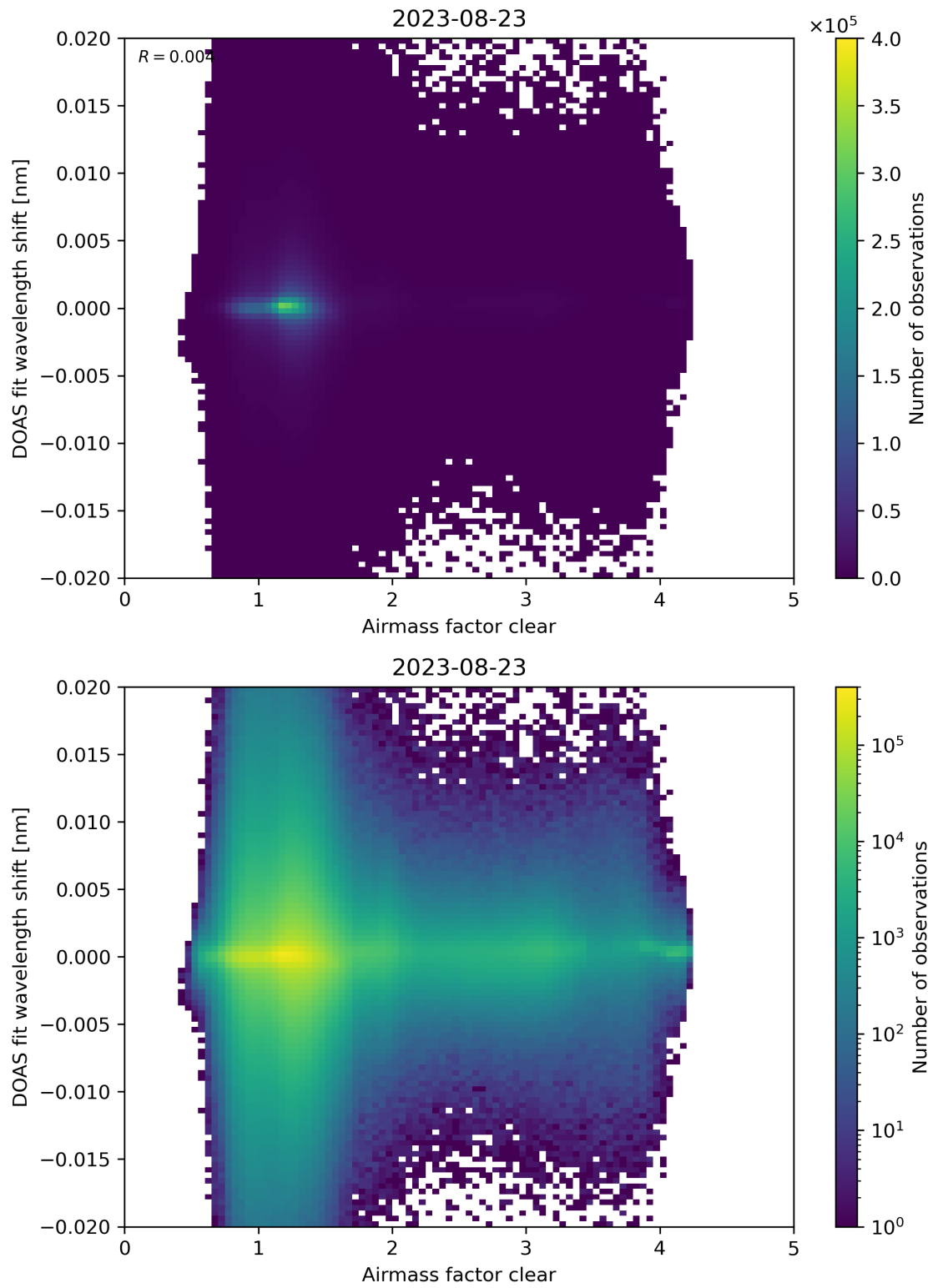
Figure 72: Scatter density plot of “Airmass factor clear” against “DOAS fit wavelength shift” for 2023-08-22 to 2023-08-24.
