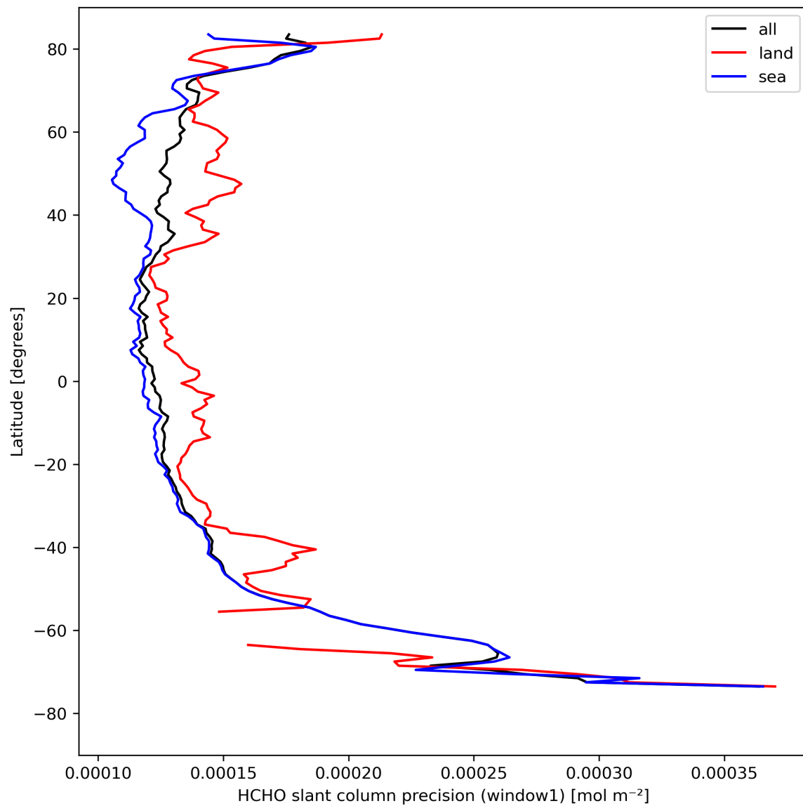
Figure 25: Zonal average of “HCHO slant column precision (window1)” for 2023-08-22 to 2023-08-24.
