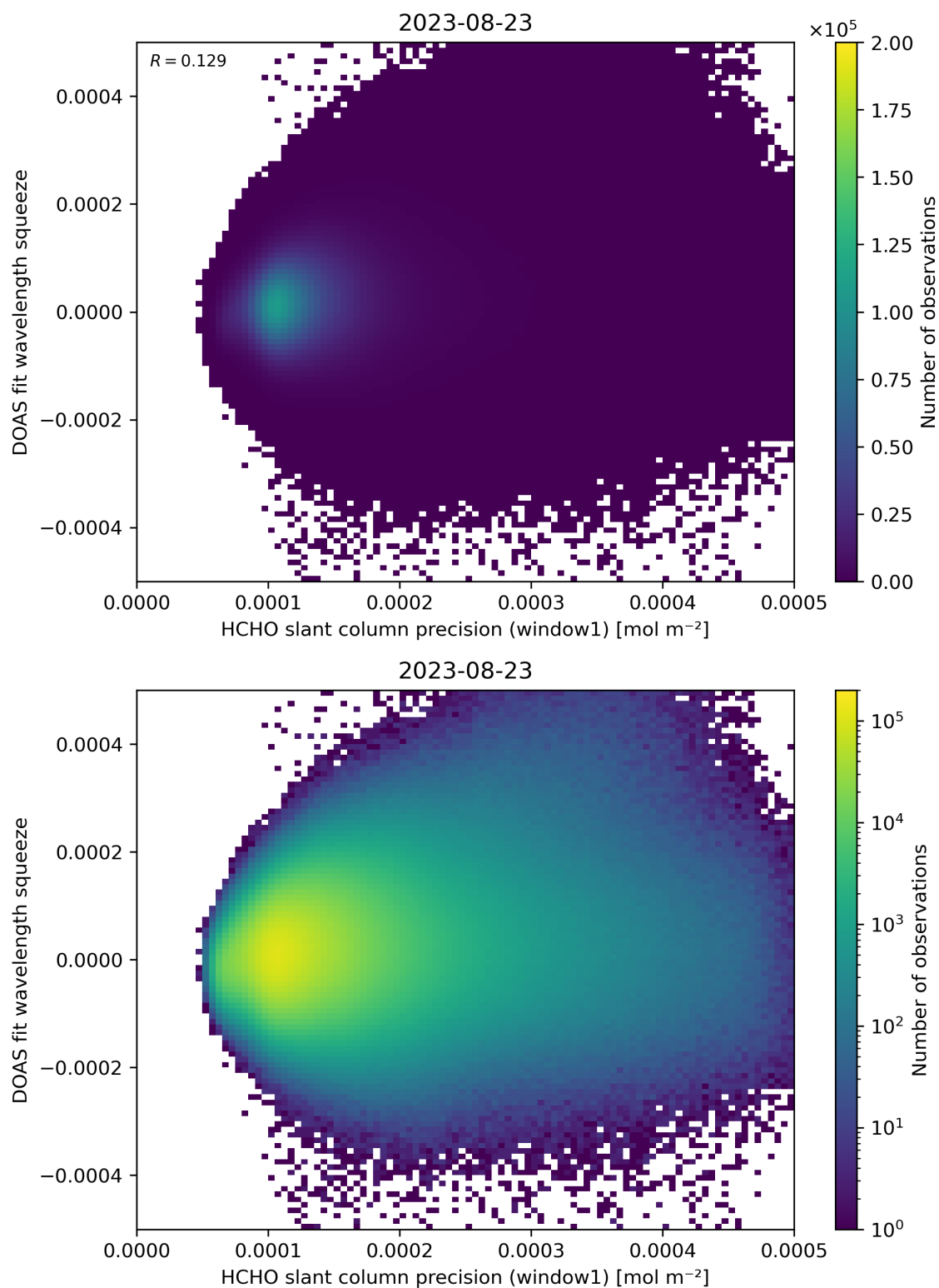
Figure 90: Scatter density plot of “HCHO slant column precision (window1)” against “DOAS fit wavelength squeeze” for 2023-08-22 to 2023-08-24.
