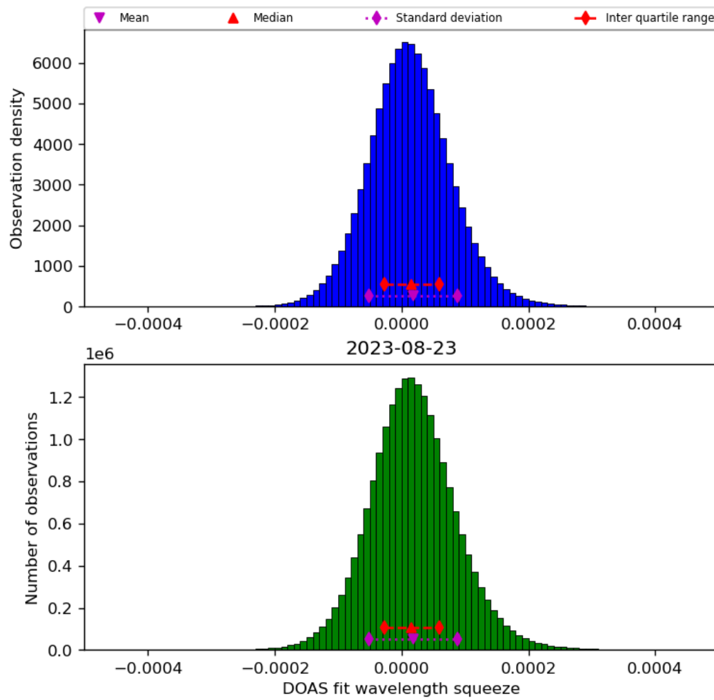
Figure 45: Histogram of “DOAS fit wavelength squeeze” for 2023-08-22 to 2023-08-24
