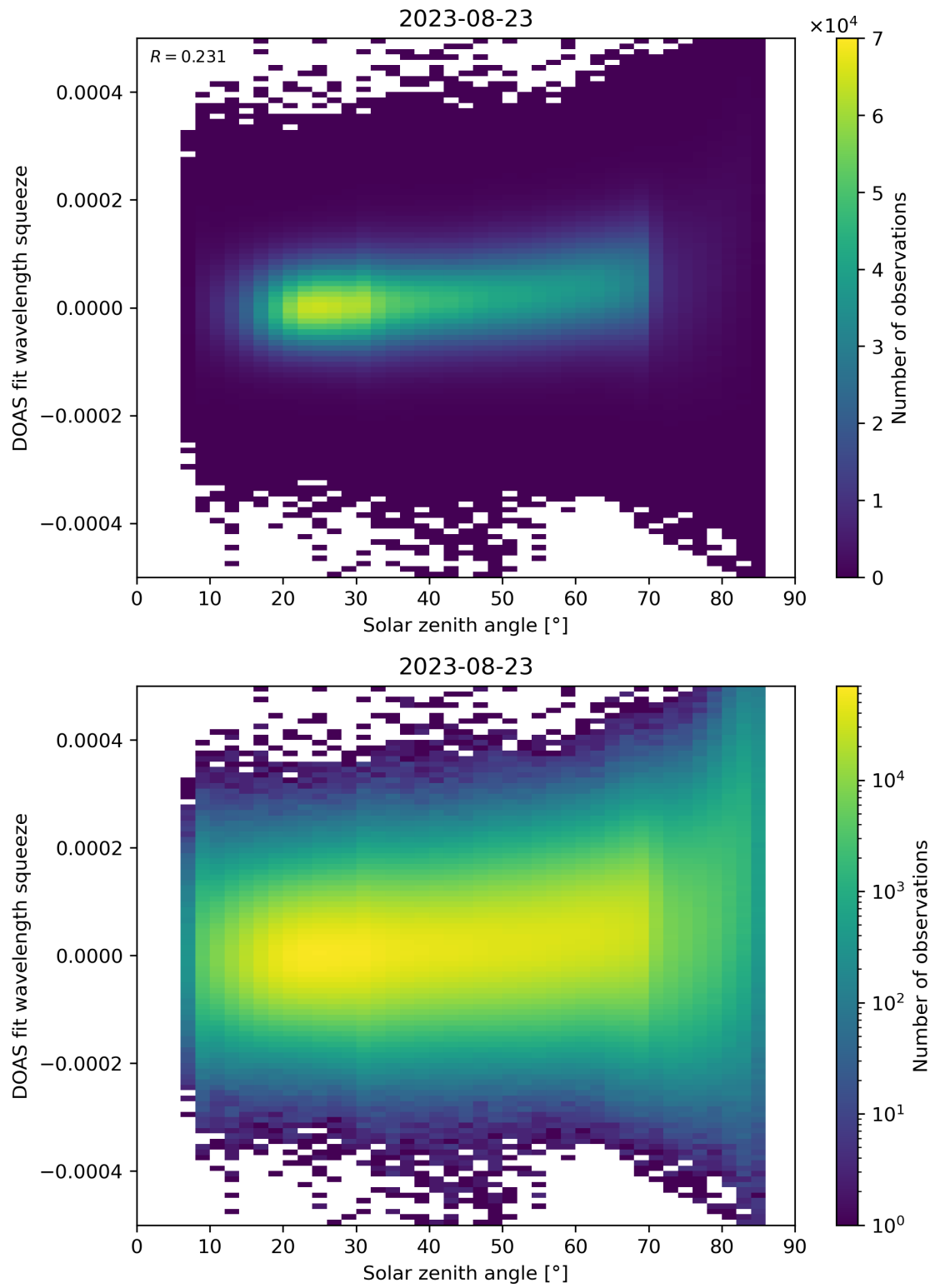
Figure 169: Scatter density plot of “Solar zenith angle” against “DOAS fit wavelength squeeze” for 2023-08-22 to 2023-08-24.
