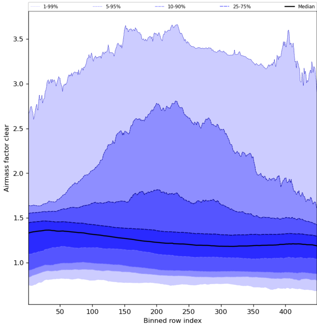
Figure 56: Along track statistics of “Airmass factor clear” for 2023-08-22 to 2023-08-24
