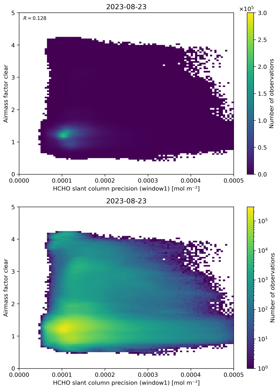
Figure 91: Scatter density plot of “HCHO slant column precision (window1)” against “Airmass factor clear” for 2023-08-22 to 2023-08-24.
