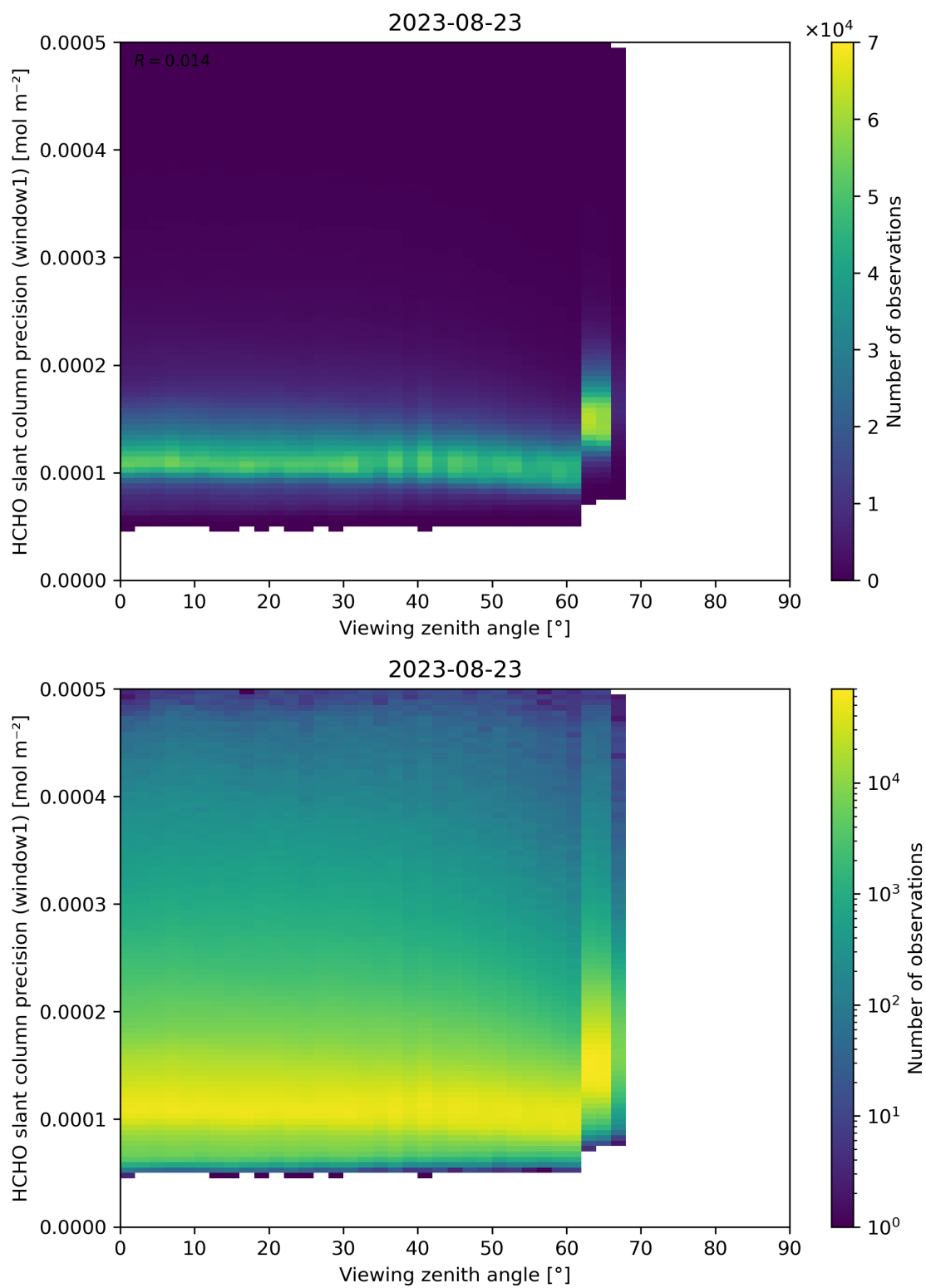
Figure 189: Scatter density plot of “Viewing zenith angle” against “HCHO slant column precision (window1)” for 2023-08-22 to 2023-08-24.
