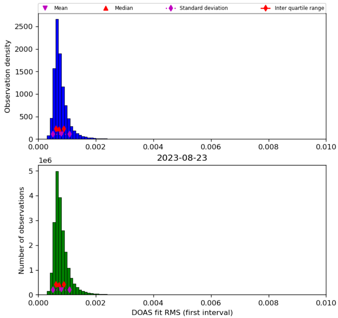
Figure 46: Histogram of “DOAS fit RMS (first interval)” for 2023-08-22 to 2023-08-24
