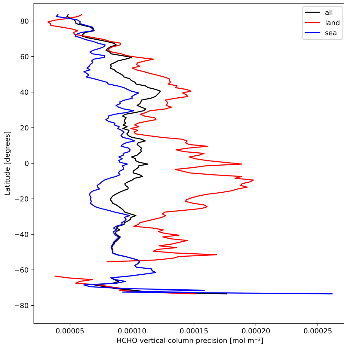
Figure 22: Zonal average of “HCHO vertical column precision” for 2023-08-22 to 2023-08-24.
