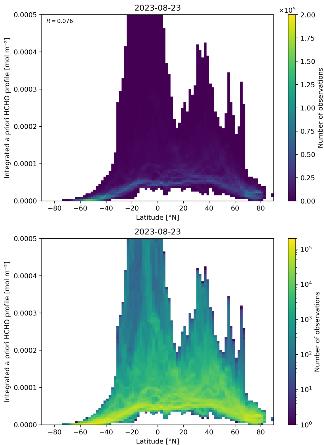
Figure 166: Scatter density plot of “Latitude” against “Integrated a priori HCHO profile” for 2023-08-22 to 2023-08-24.
