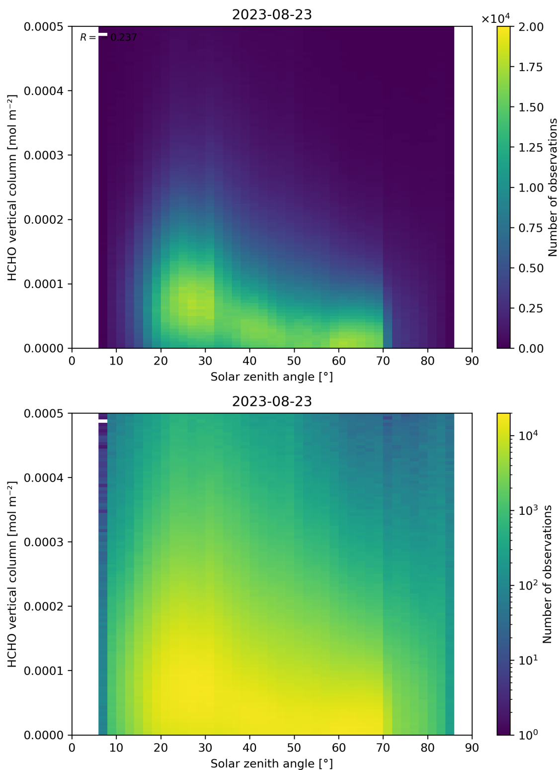
Figure 177: Scatter density plot of “Solar zenith angle” against “HCHO vertical column” for 2023-08-22 to 2023-08-24.
