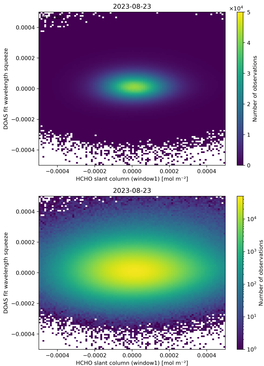
Figure 80: Scatter density plot of “HCHO slant column (window1)” against “DOAS fit wavelength squeeze” for 2023-08-22 to 2023-08-24.
