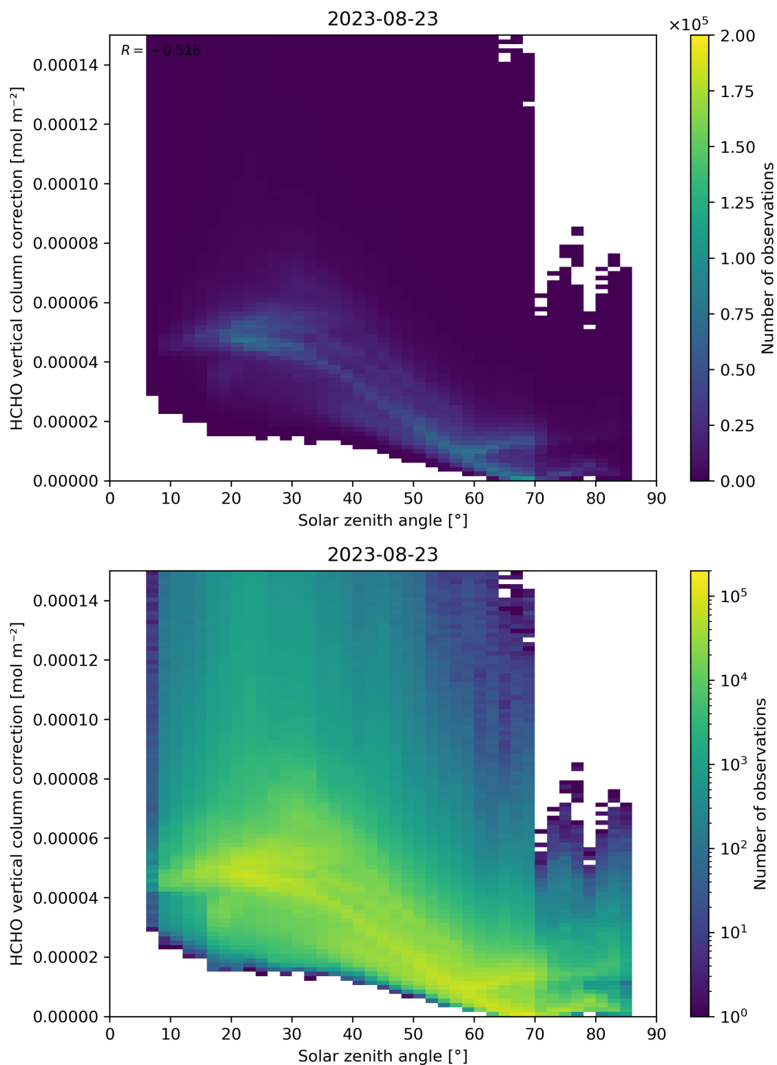
Figure 178: Scatter density plot of “Solar zenith angle” against “HCHO vertical column correction” for 2023-08-22 to 2023-08-24.
