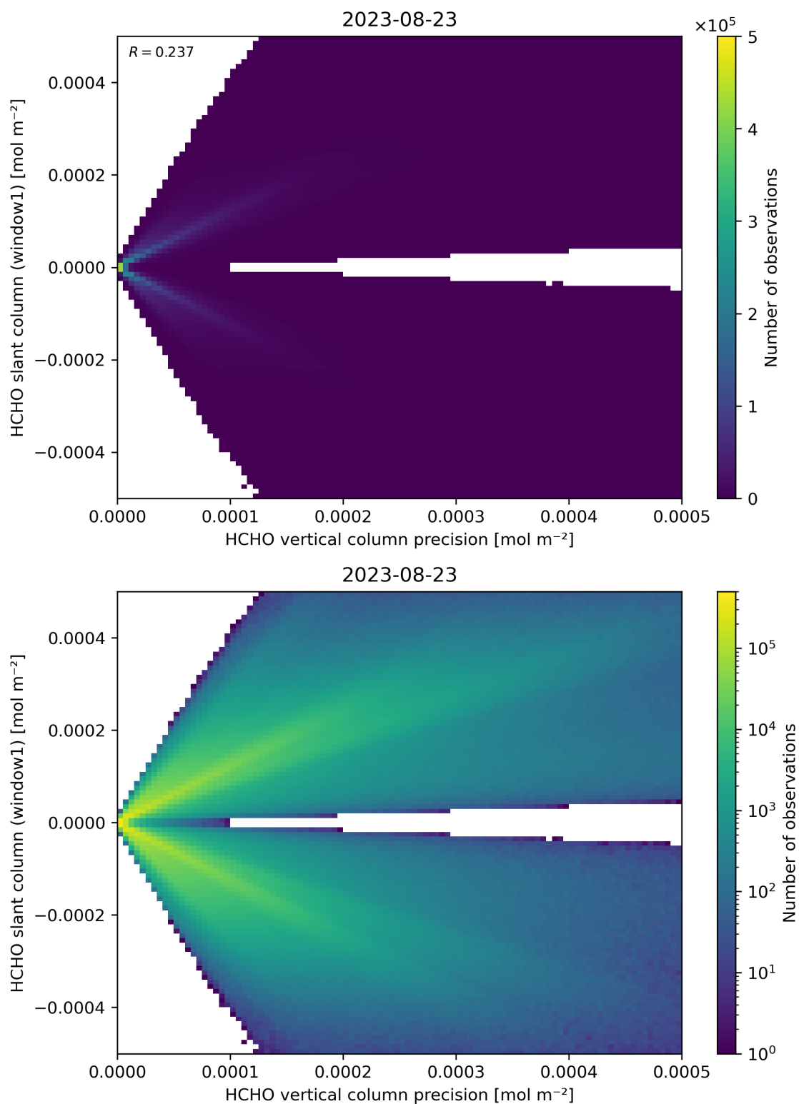
Figure 142: Scatter density plot of “HCHO vertical column precision” against “HCHO slant column (window1)” for 2023-08-22 to 2023-08-24.
