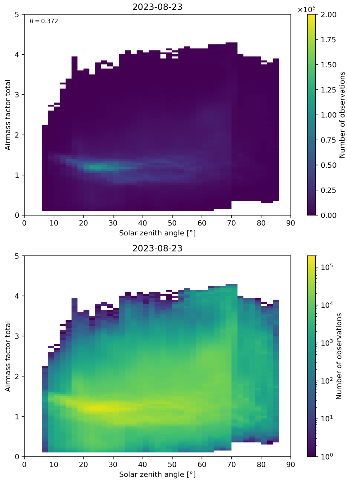
Figure 175: Scatter density plot of “Solar zenith angle” against “Airmass factor total” for 2023-08-22 to 2023-08-24.
