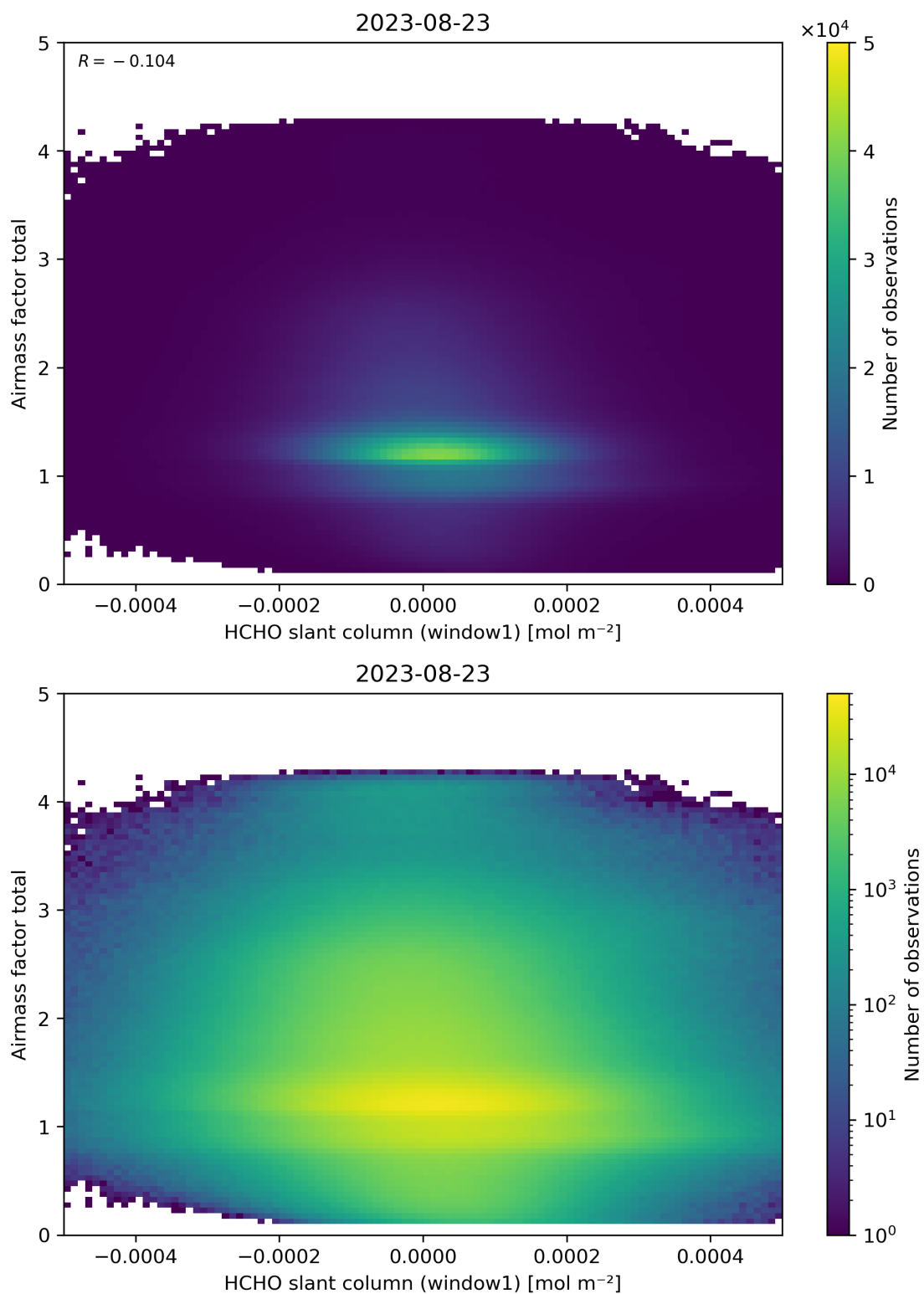
Figure 85: Scatter density plot of “HCHO slant column (window1)” against “Airmass factor total” for 2023-08-22 to 2023-08-24.
