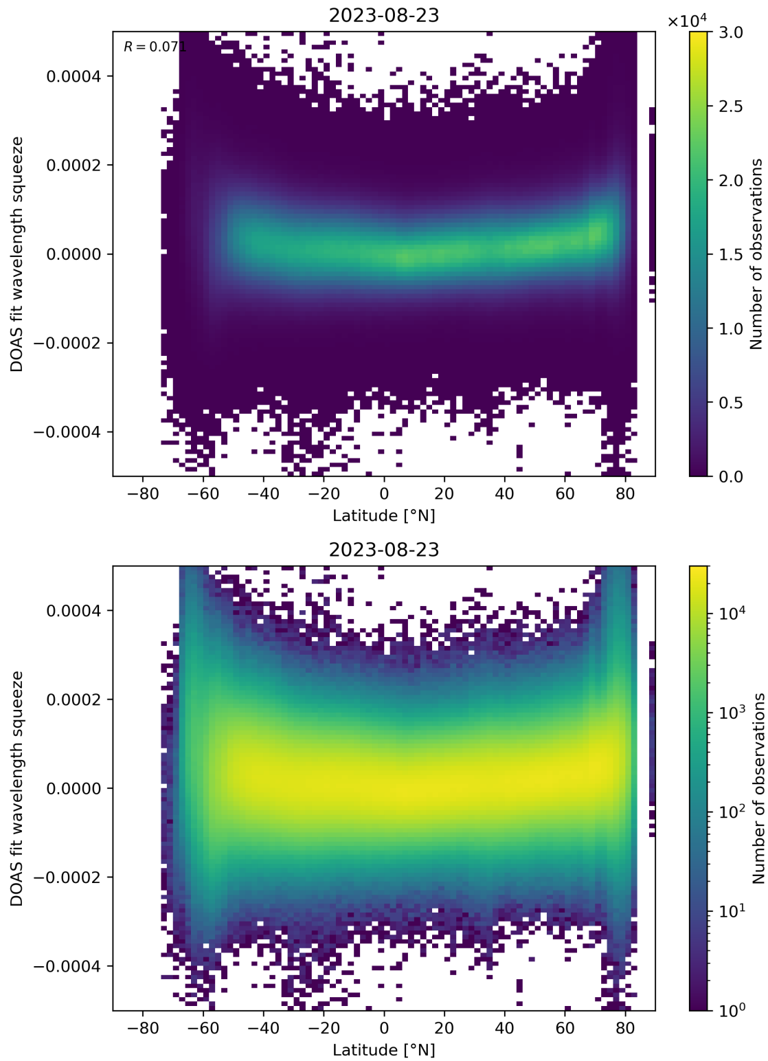
Figure 155: Scatter density plot of “Latitude” against “DOAS fit wavelength squeeze” for 2023-08-22 to 2023-08-24.
