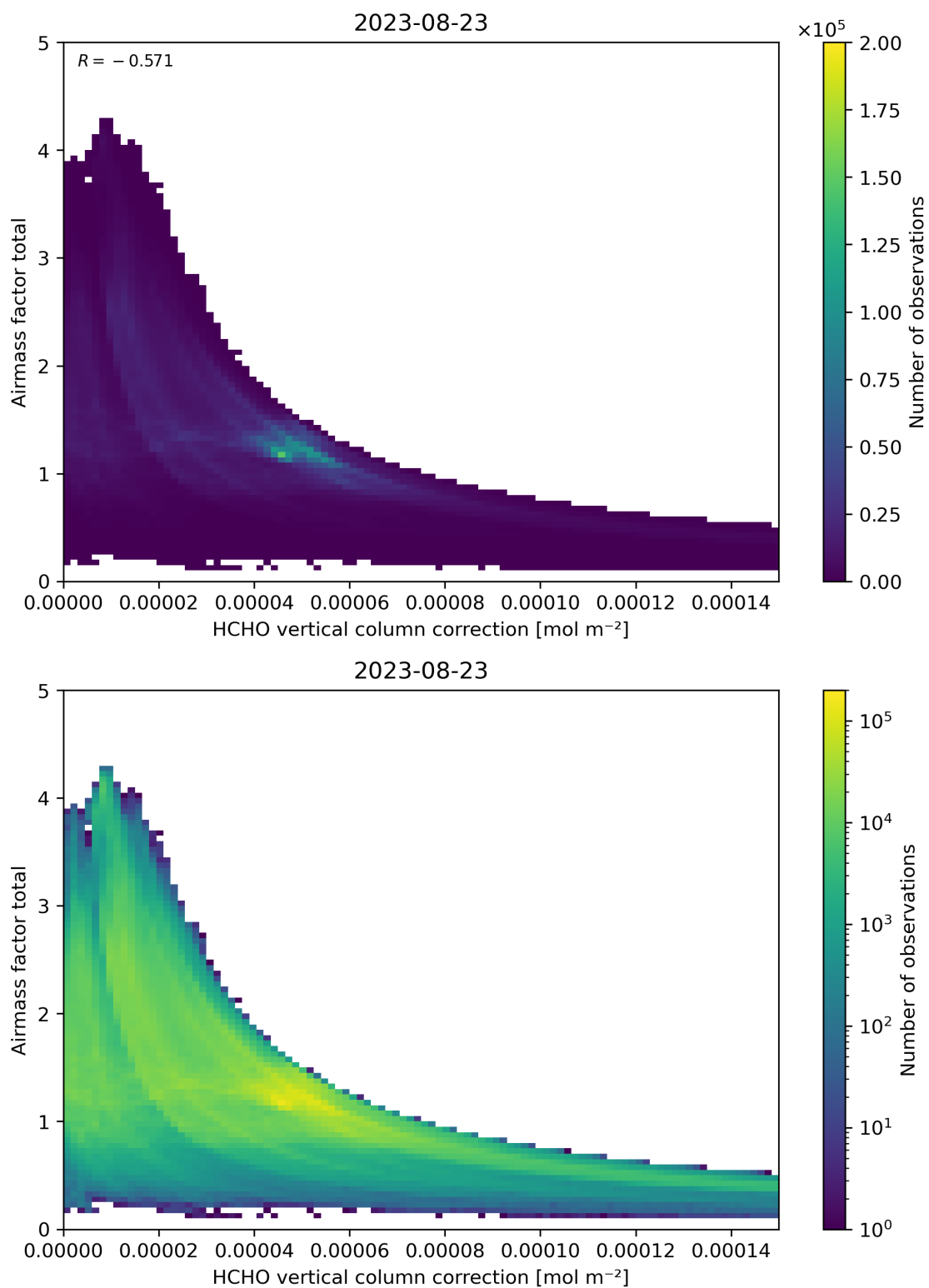
Figure 120: Scatter density plot of “HCHO vertical column correction” against “Airmass factor total” for 2023-08-22 to 2023-08-24.
