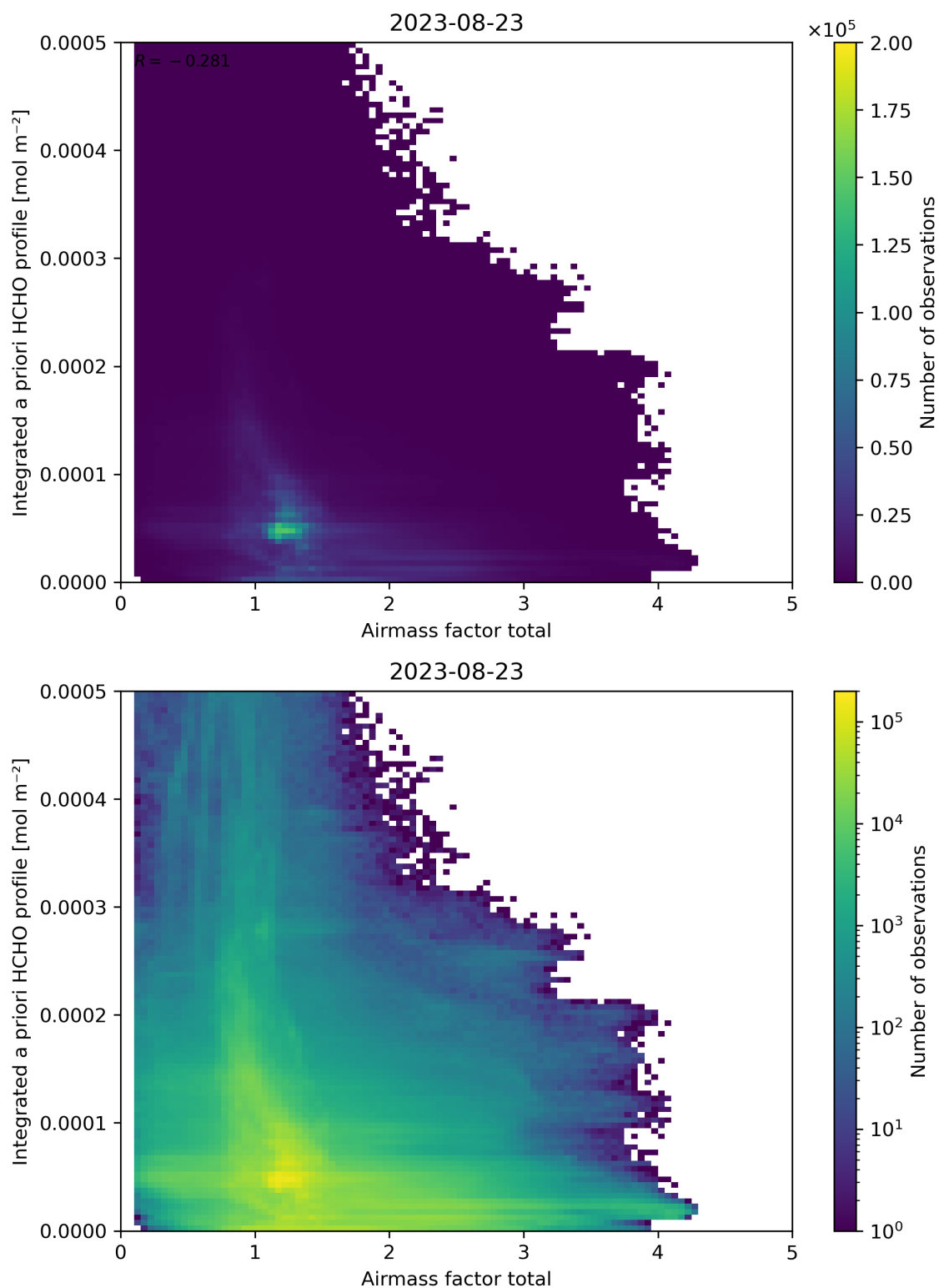
Figure 104: Scatter density plot of “Airmass factor total” against “Integrated a priori HCHO profile” for 2023-08-22 to 2023-08-24.
