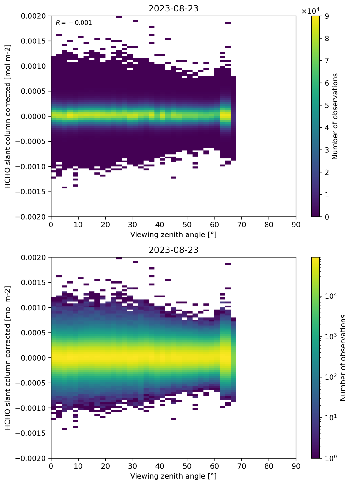
Figure 186: Scatter density plot of “Viewing zenith angle” against “HCHO slant column corrected” for 2023-08-22 to 2023-08-24.
