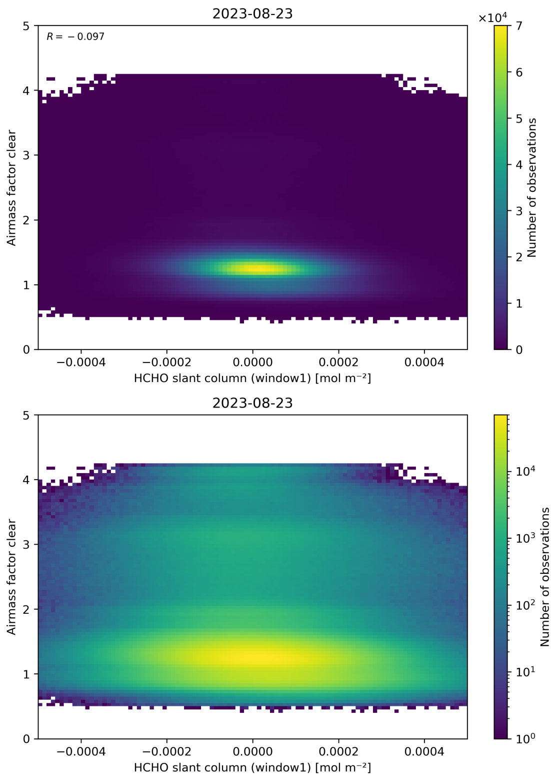
Figure 81: Scatter density plot of “HCHO slant column (window1)” against “Airmass factor clear” for 2023-08-22 to 2023-08-24.
