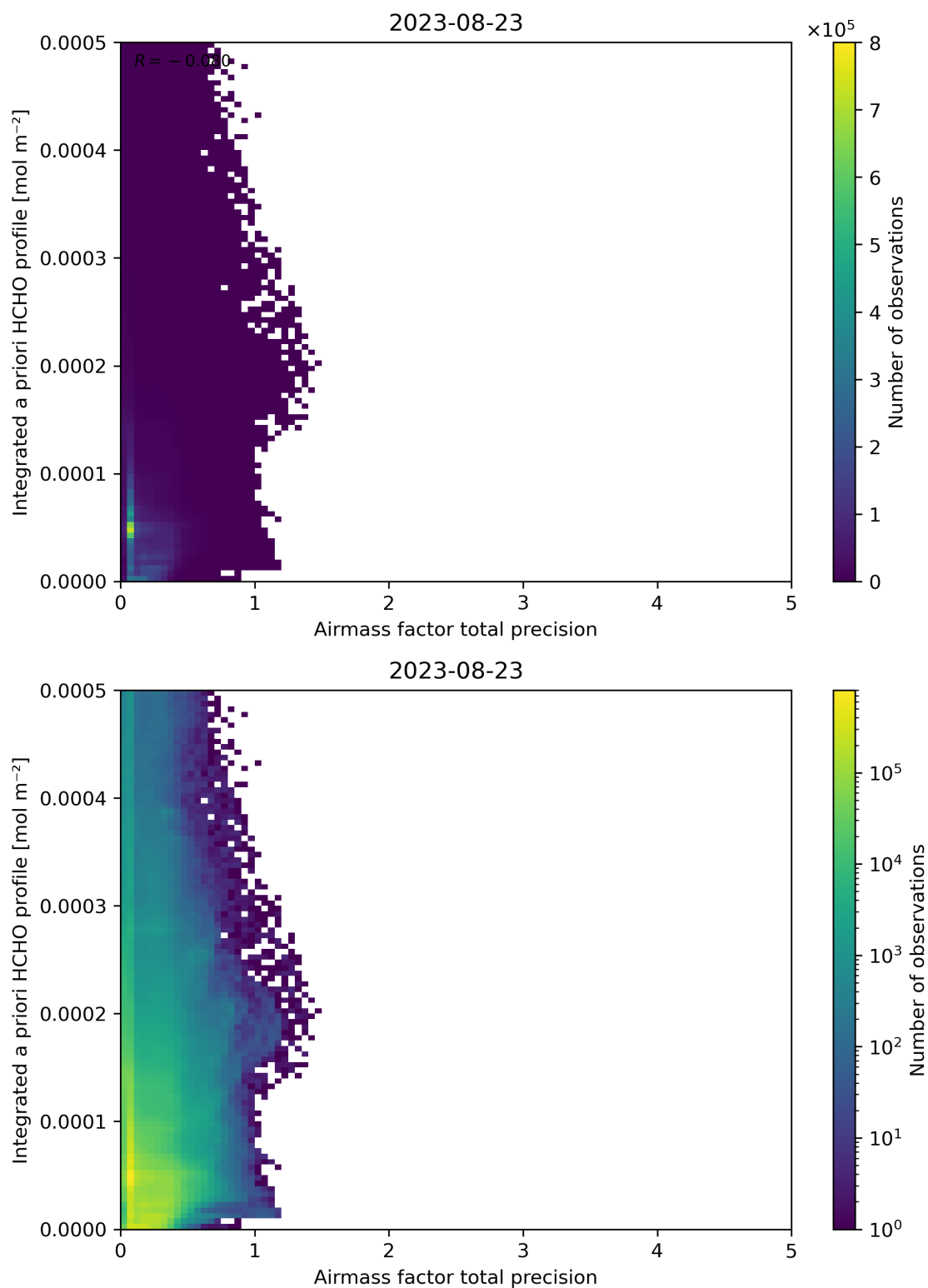
Figure 111: Scatter density plot of “Airmass factor total precision” against “Integrated a priori HCHO profile” for 2023-08-22 to 2023-08-24.
