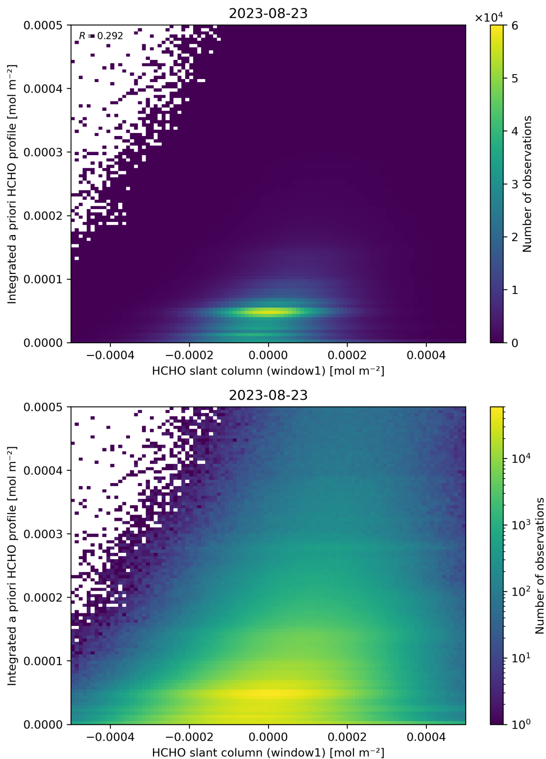
Figure 87: Scatter density plot of “HCHO slant column (window1)” against “Integrated a priori HCHO profile” for 2023-08-22 to 2023-08-24.
