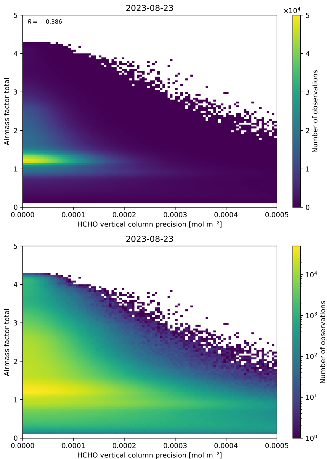
Figure 144: Scatter density plot of “HCHO vertical column precision” against “Airmass factor total” for 2023-08-22 to 2023-08-24.
