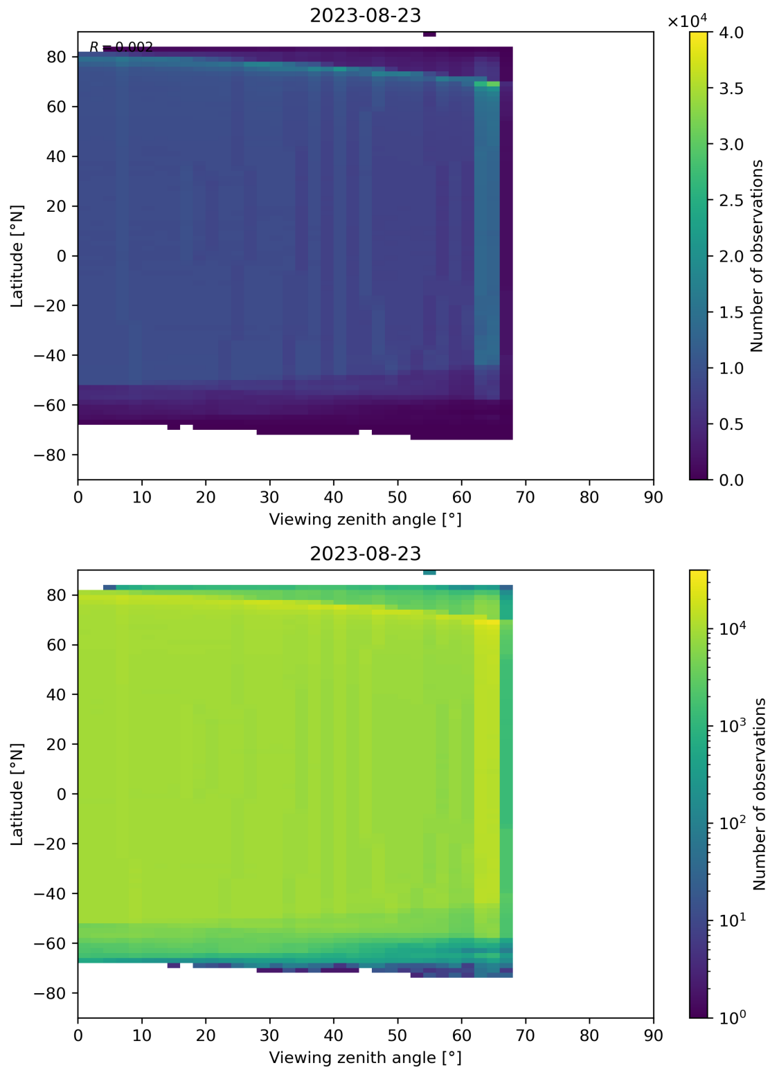
Figure 196: Scatter density plot of “Viewing zenith angle” against “Latitude” for 2023-08-22 to 2023-08-24.
