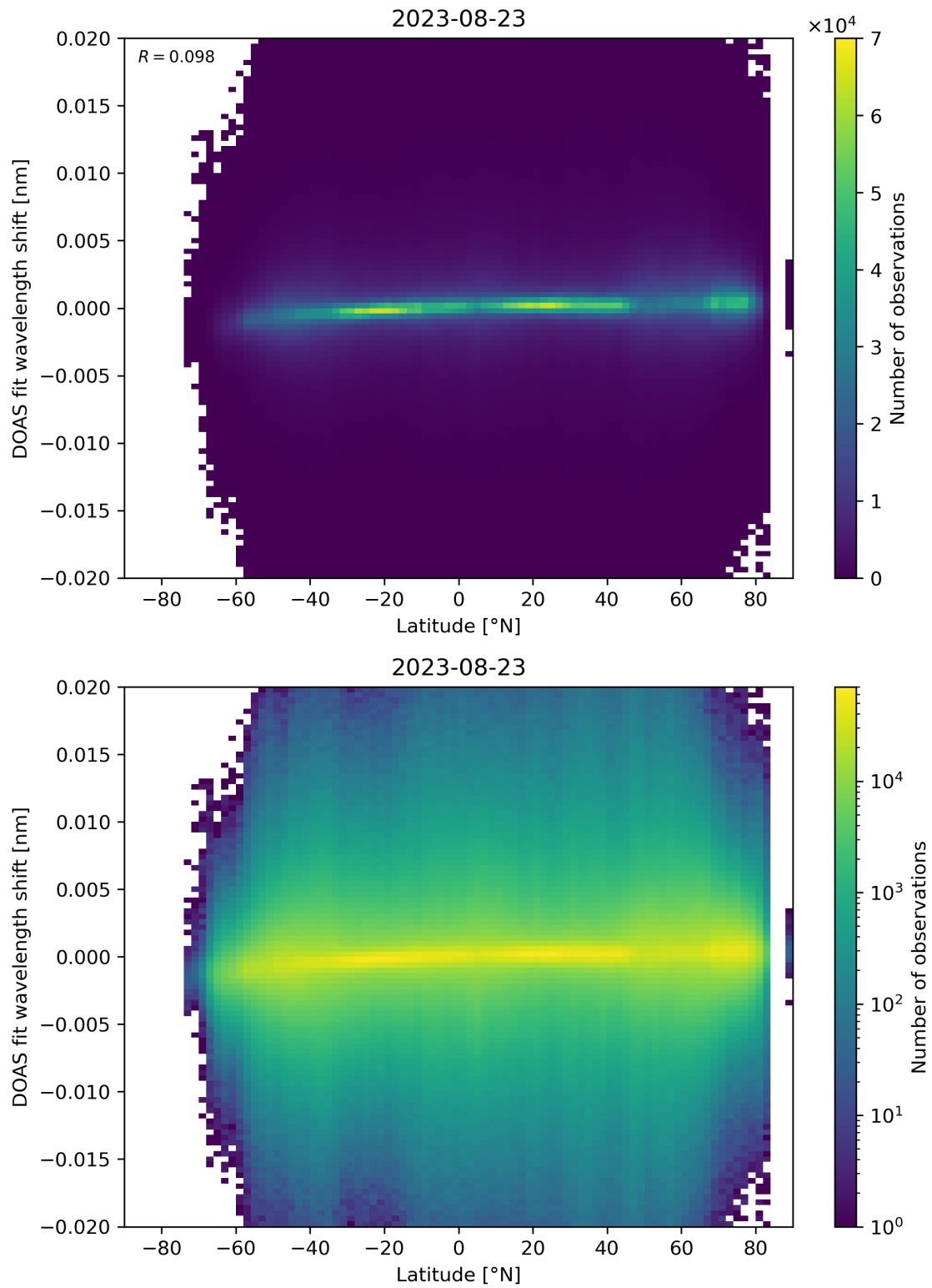
Figure 154: Scatter density plot of “Latitude” against “DOAS fit wavelength shift” for 2023-08-22 to 2023-08-24.
