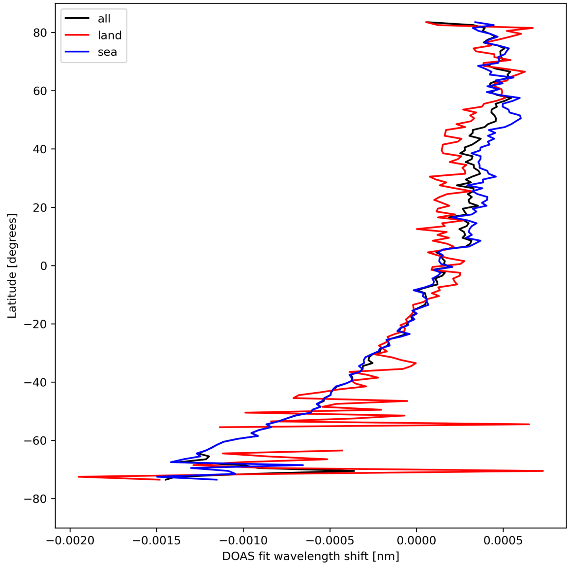
Figure 30: Zonal average of “DOAS fit wavelength shift” for 2023-08-22 to 2023-08-24.
