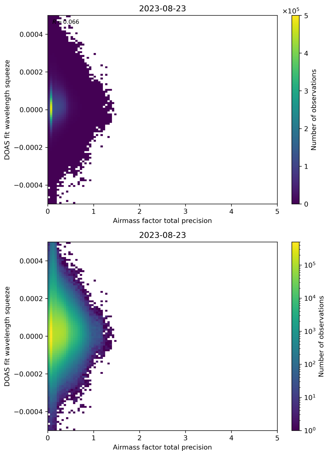
Figure 107: Scatter density plot of “Airmass factor total precision” against “DOAS fit wavelength squeeze” for 2023-08-22 to 2023-08-24.
