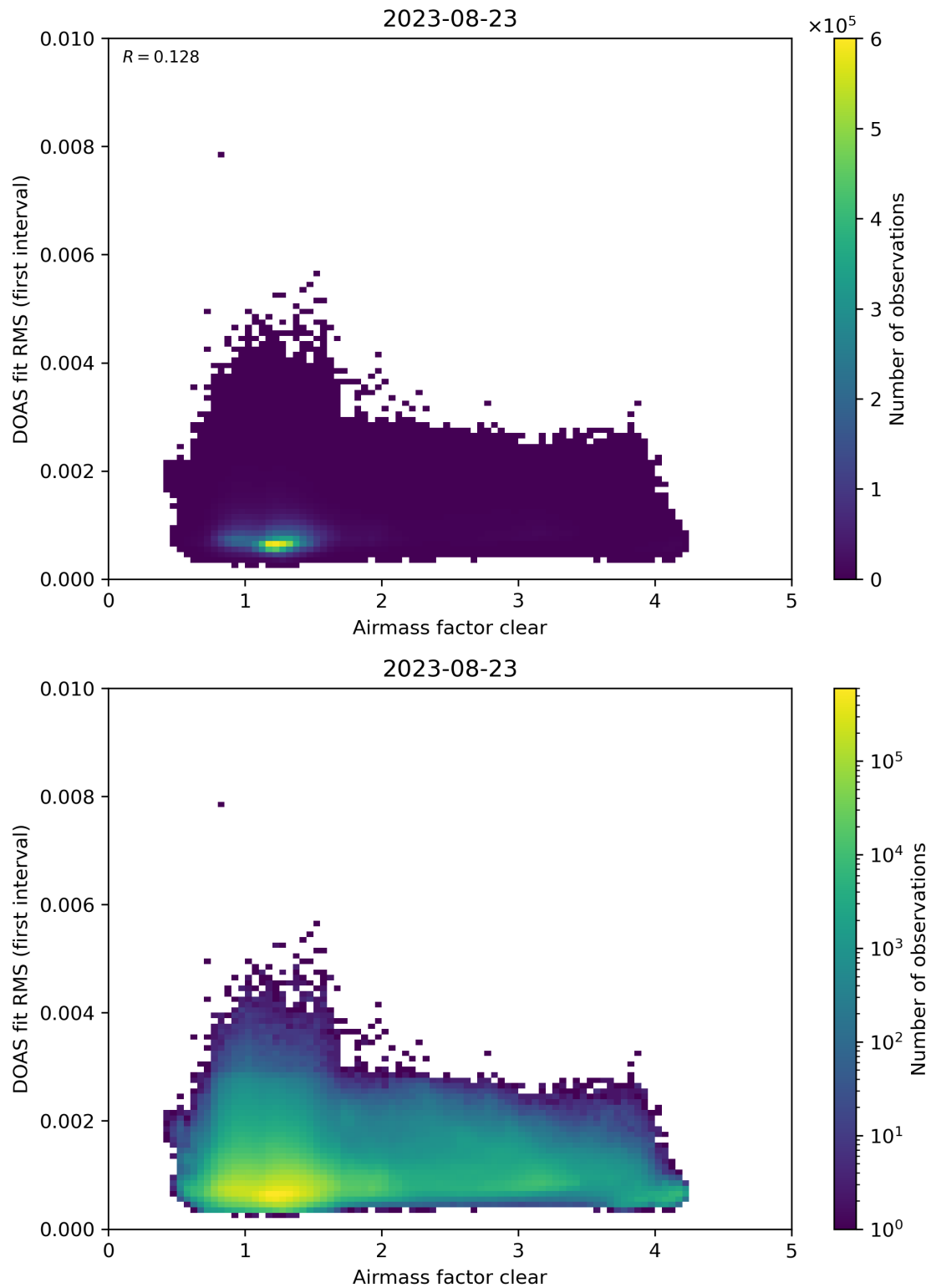
Figure 71: Scatter density plot of “Airmass factor clear” against “DOAS fit RMS (first interval)” for 2023-08-22 to 2023-08-24.
