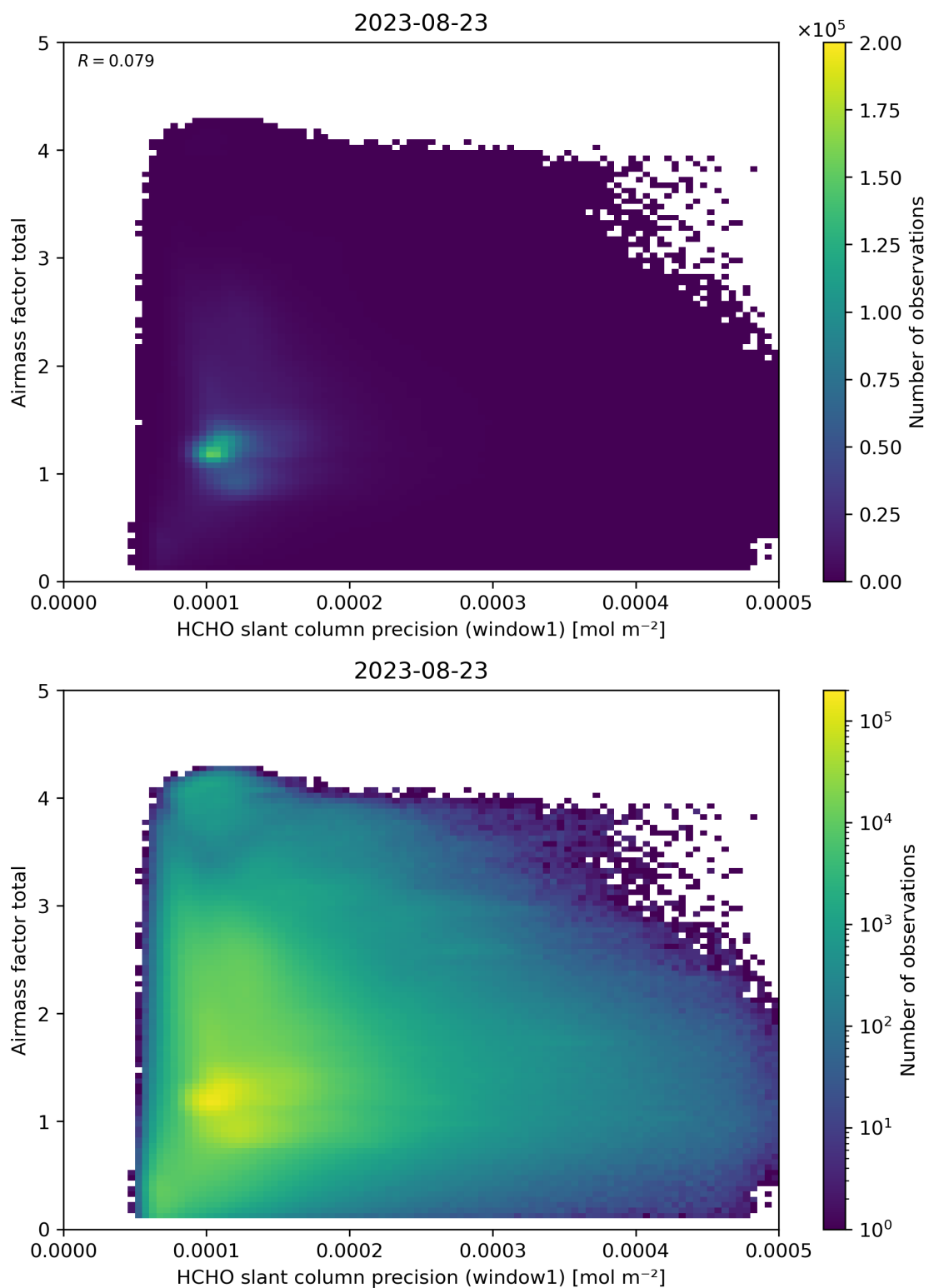
Figure 94: Scatter density plot of “HCHO slant column precision (window1)” against “Airmass factor total” for 2023-08-22 to 2023-08-24.
