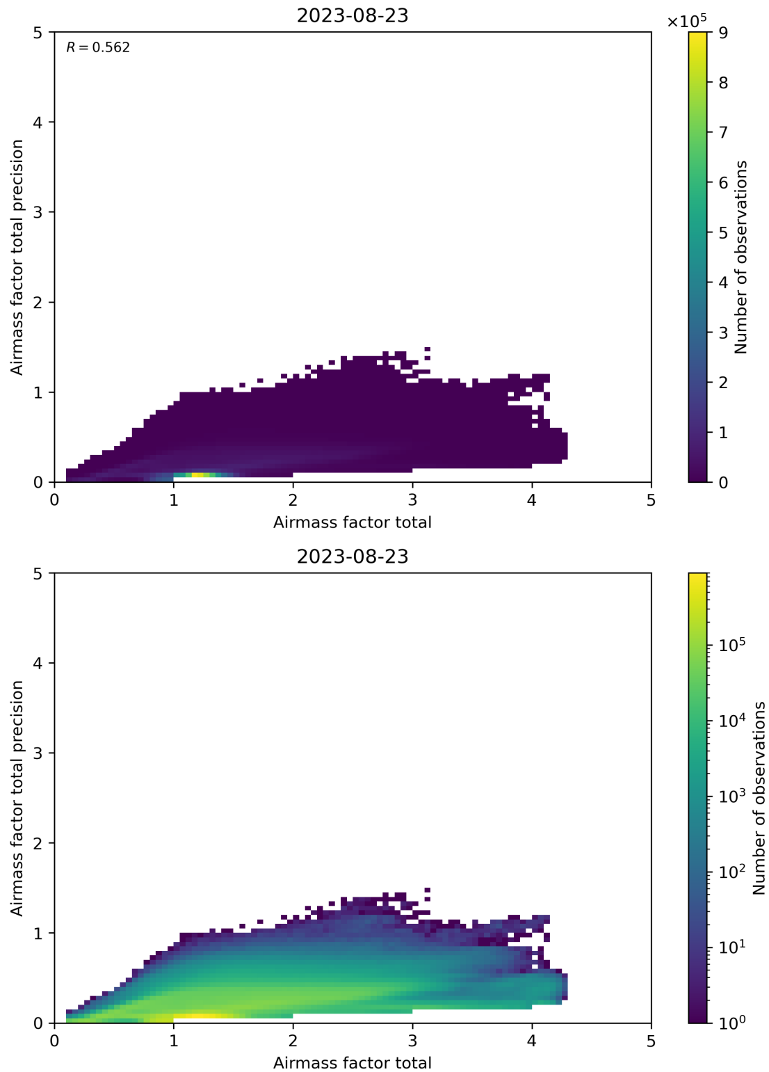
Figure 103: Scatter density plot of “Airmass factor total” against “Airmass factor total precision” for 2023-08-22 to 2023-08-24.
