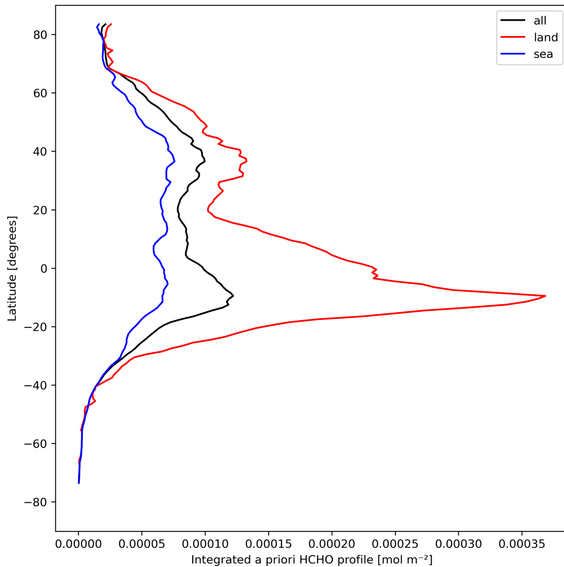
Figure 29: Zonal average of “Integrated a priori HCHO profile” for 2023-08-22 to 2023-08-24.
