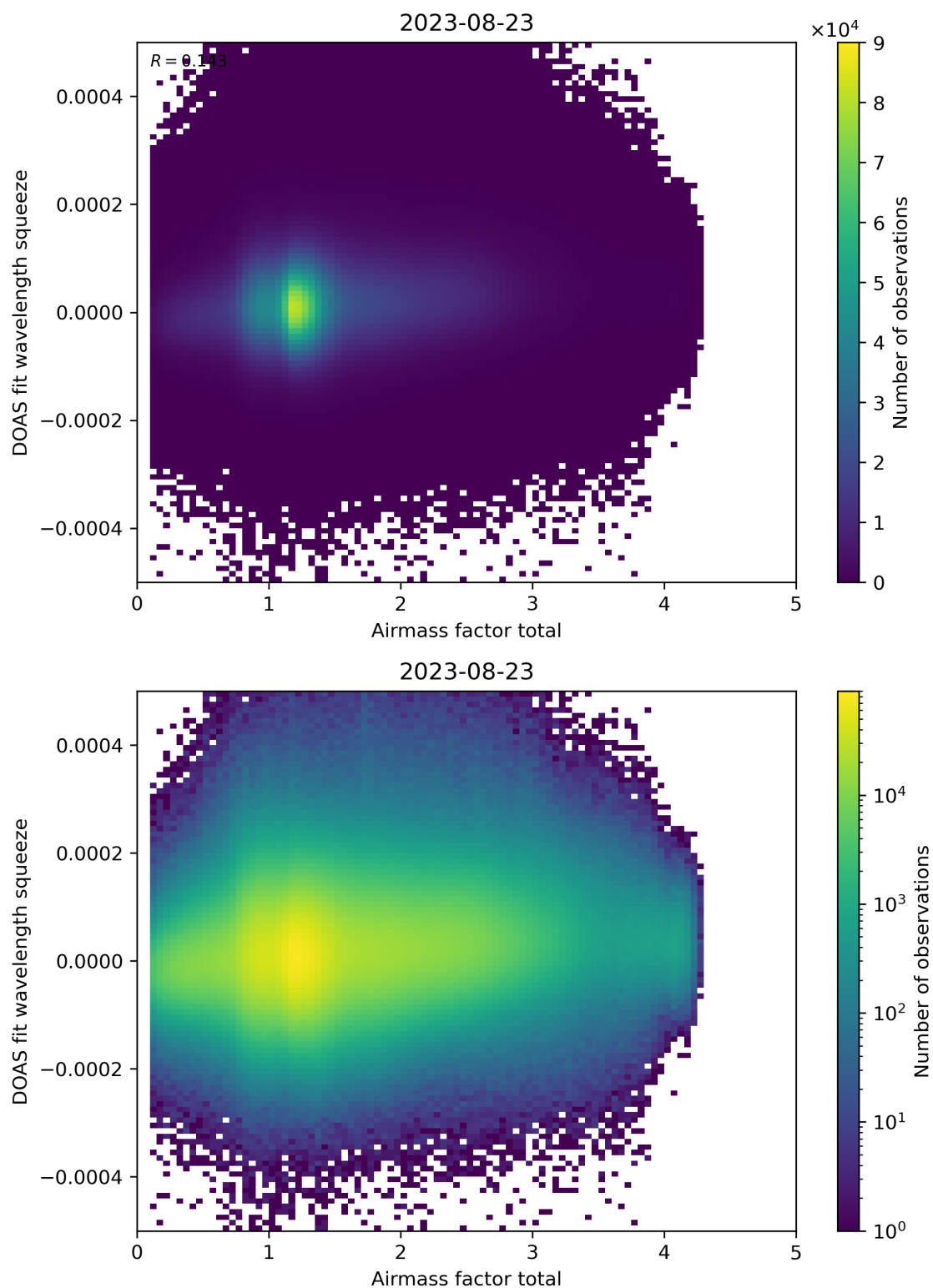
Figure 99: Scatter density plot of “Airmass factor total” against “DOAS fit wavelength squeeze” for 2023-08-22 to 2023-08-24.
