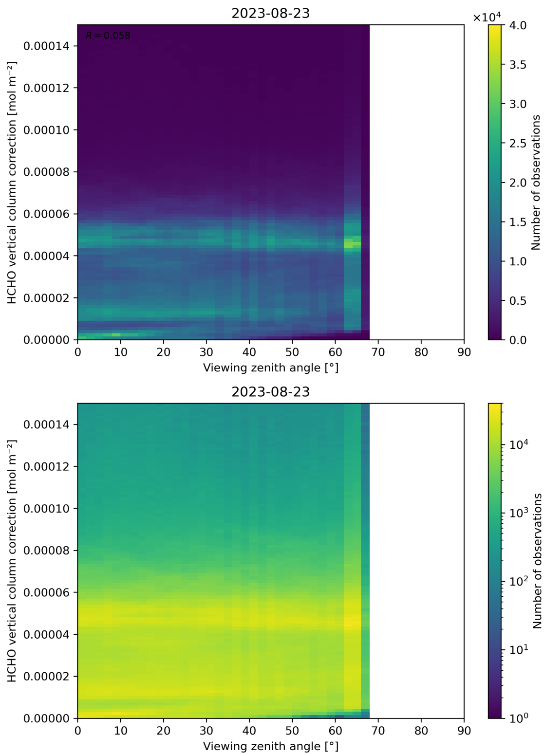
Figure 193: Scatter density plot of “Viewing zenith angle” against “HCHO vertical column correction” for 2023-08-22 to 2023-08-24.
