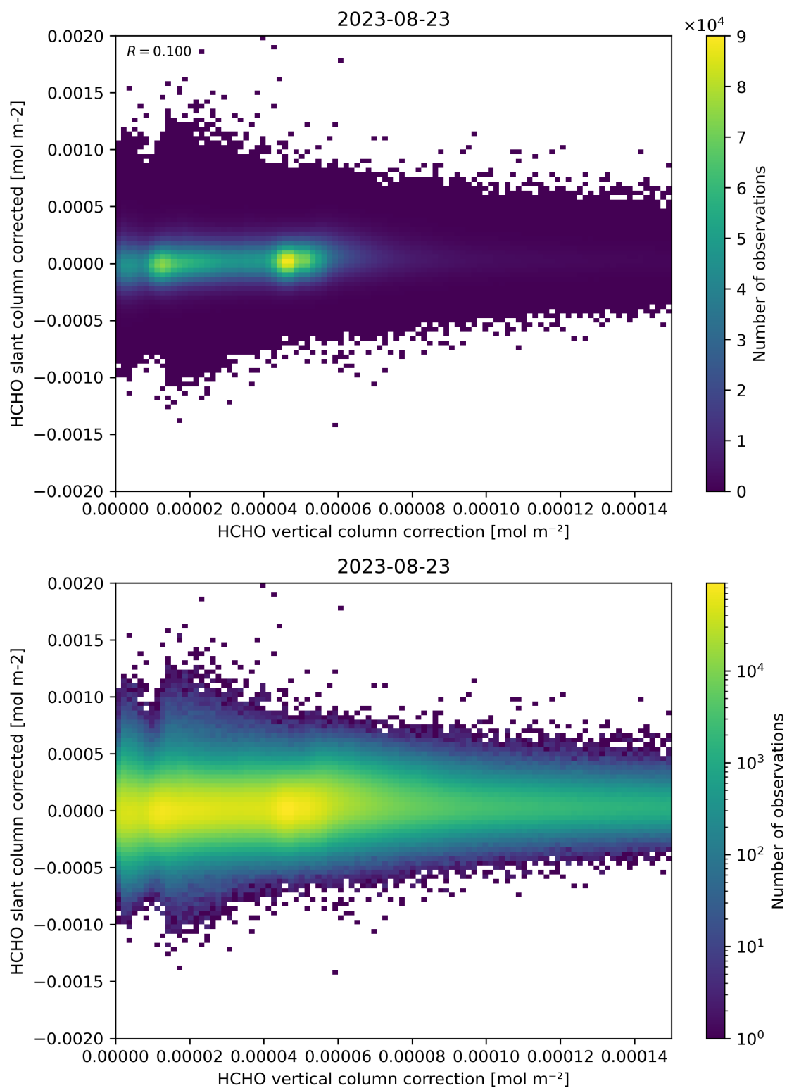
Figure 116: Scatter density plot of “HCHO vertical column correction” against “HCHO slant column corrected” for 2023-08-22 to 2023-08-24.
