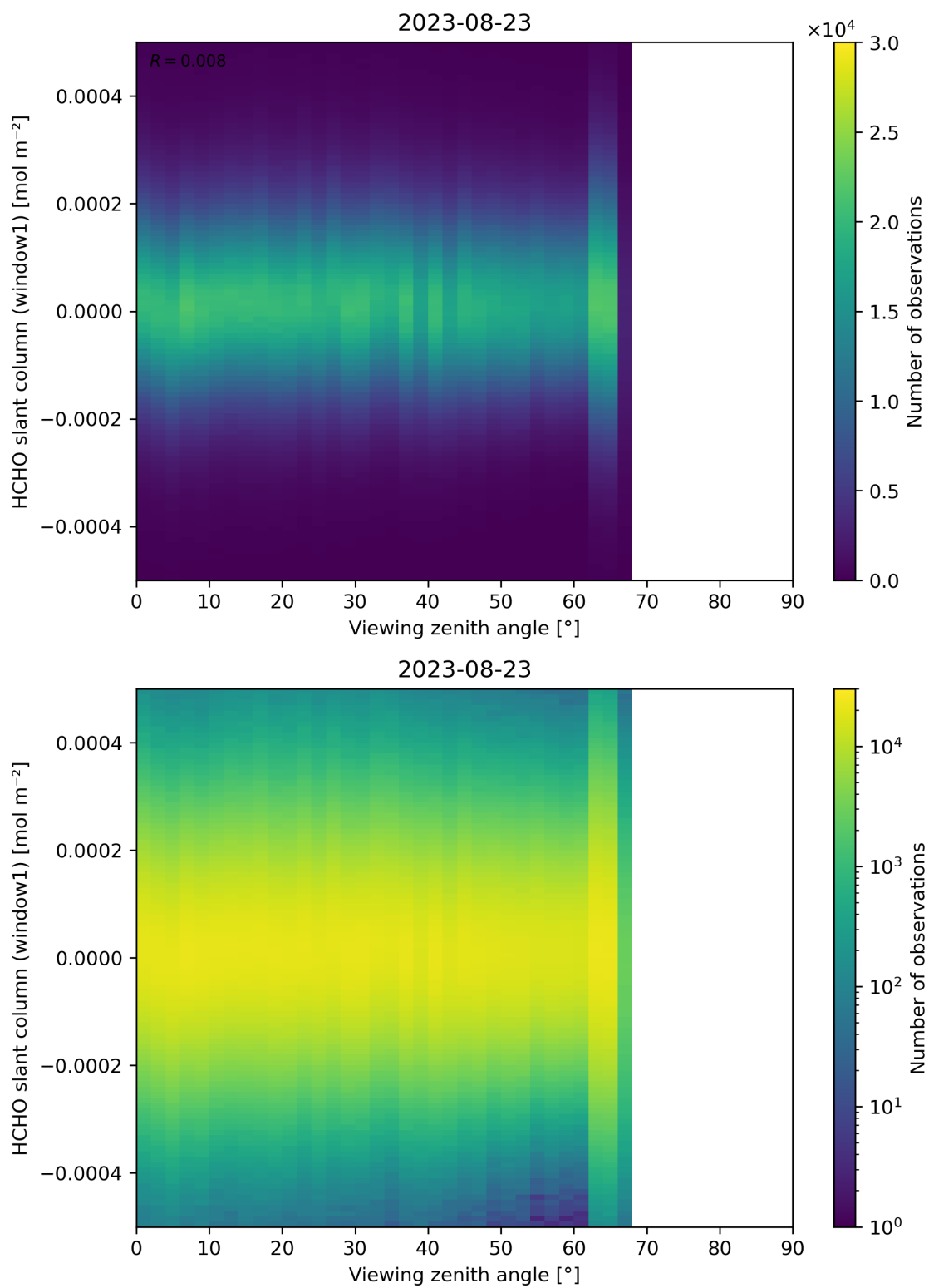
Figure 188: Scatter density plot of “Viewing zenith angle” against “HCHO slant column (window1)” for 2023-08-22 to 2023-08-24.
