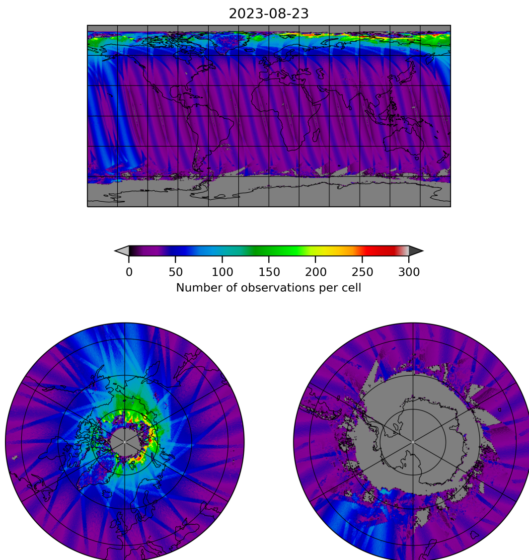
Figure 19: Map of the number of observations for 2023-08-22 to 2023-08-24
