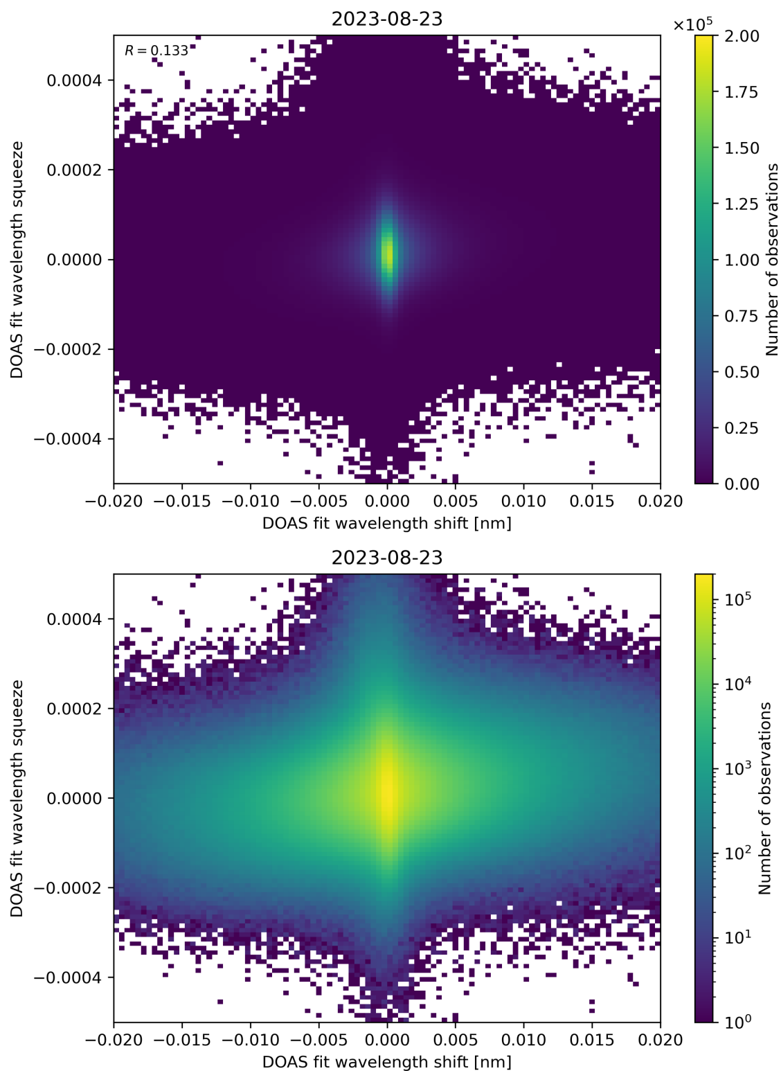
Figure 65: Scatter density plot of “DOAS fit wavelength shift” against “DOAS fit wavelength squeeze” for 2023-08-22 to 2023-08-24.
