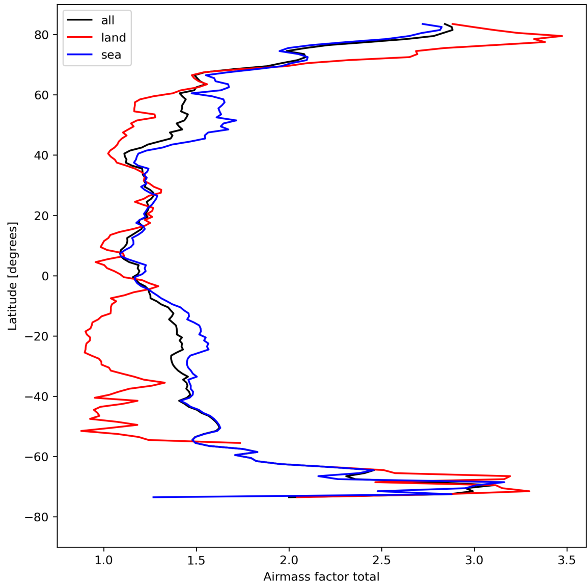
Figure 26: Zonal average of “Airmass factor total” for 2023-08-22 to 2023-08-24.
