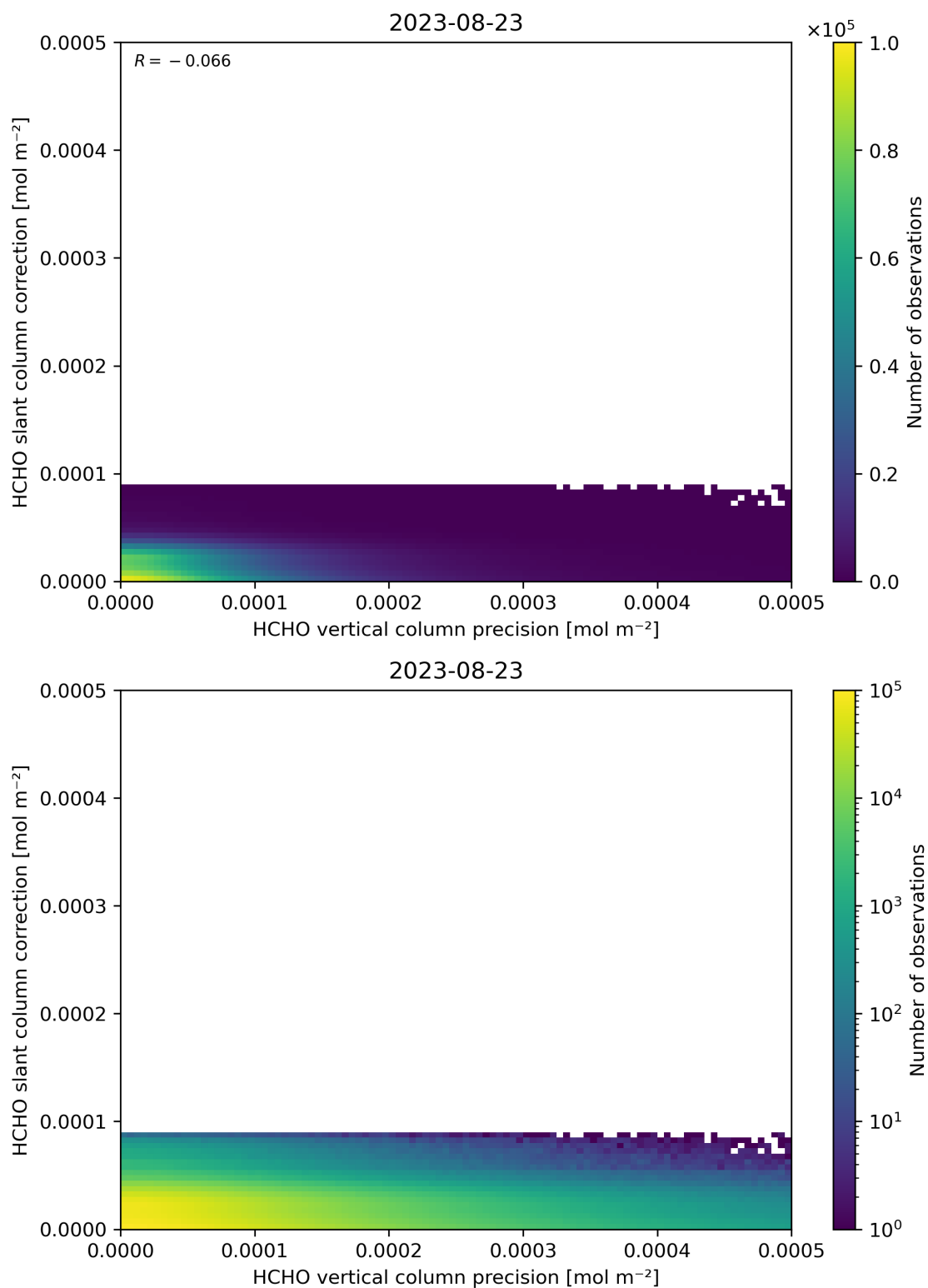
Figure 141: Scatter density plot of “HCHO vertical column precision” against “HCHO slant column correction” for 2023-08-22 to 2023-08-24.
