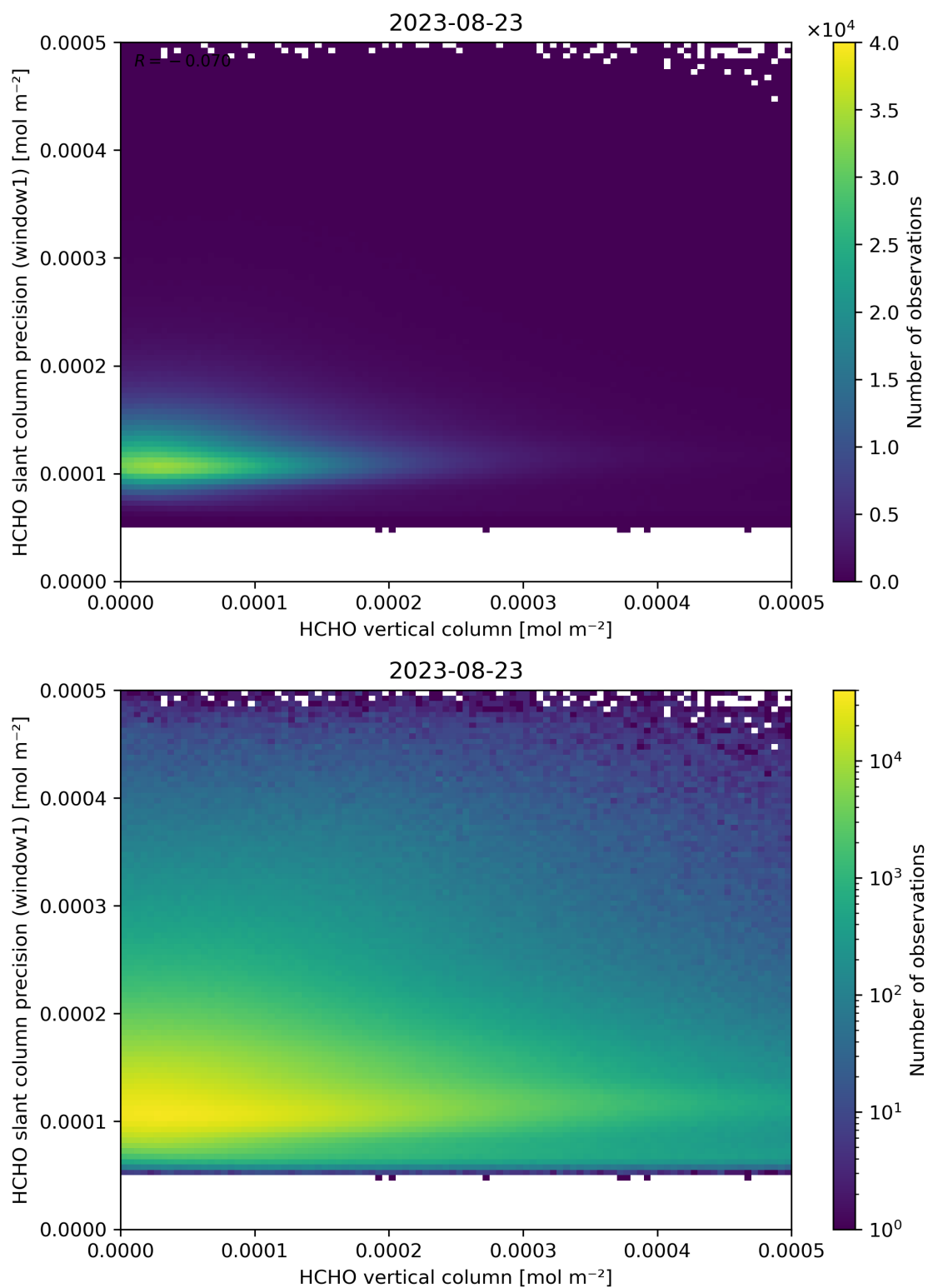
Figure 130: Scatter density plot of “HCHO vertical column” against “HCHO slant column precision (window1)” for 2023-08-22 to 2023-08-24.
