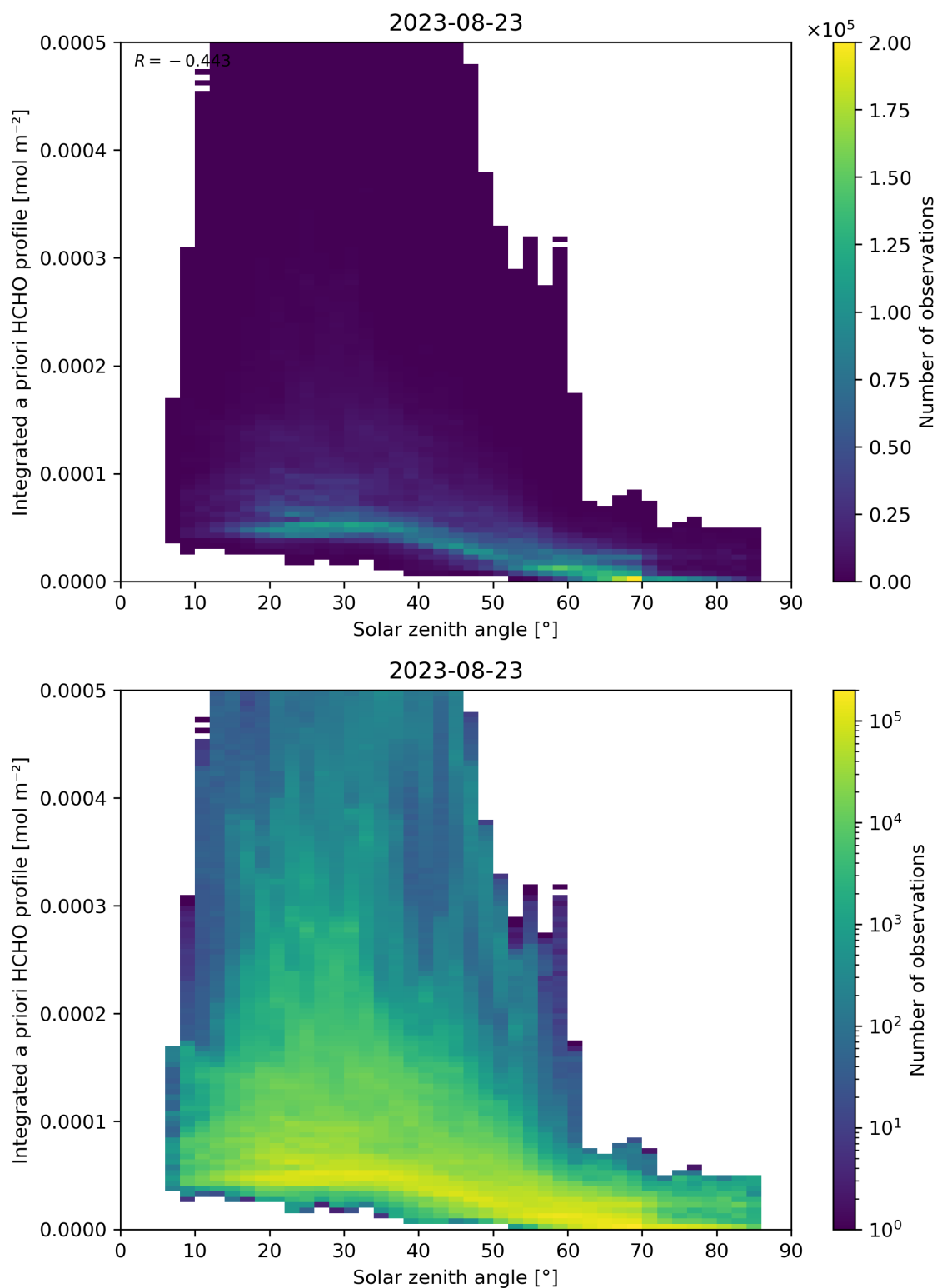
Figure 180: Scatter density plot of “Solar zenith angle” against “Integrated a priori HCHO profile” for 2023-08-22 to 2023-08-24.
