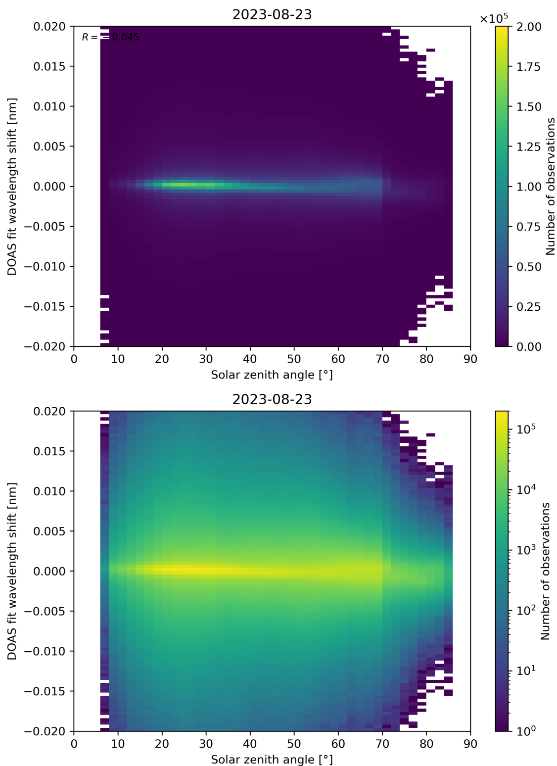
Figure 168: Scatter density plot of “Solar zenith angle” against “DOAS fit wavelength shift” for 2023-08-22 to 2023-08-24.
