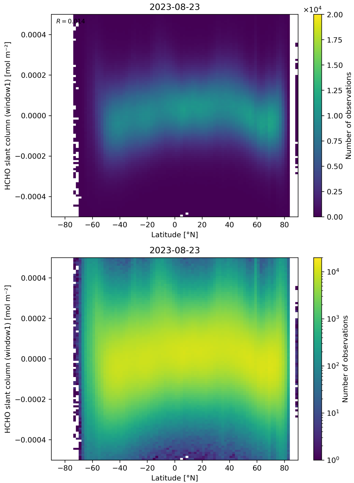
Figure 159: Scatter density plot of “Latitude” against “HCHO slant column (window1)” for 2023-08-22 to 2023-08-24.
