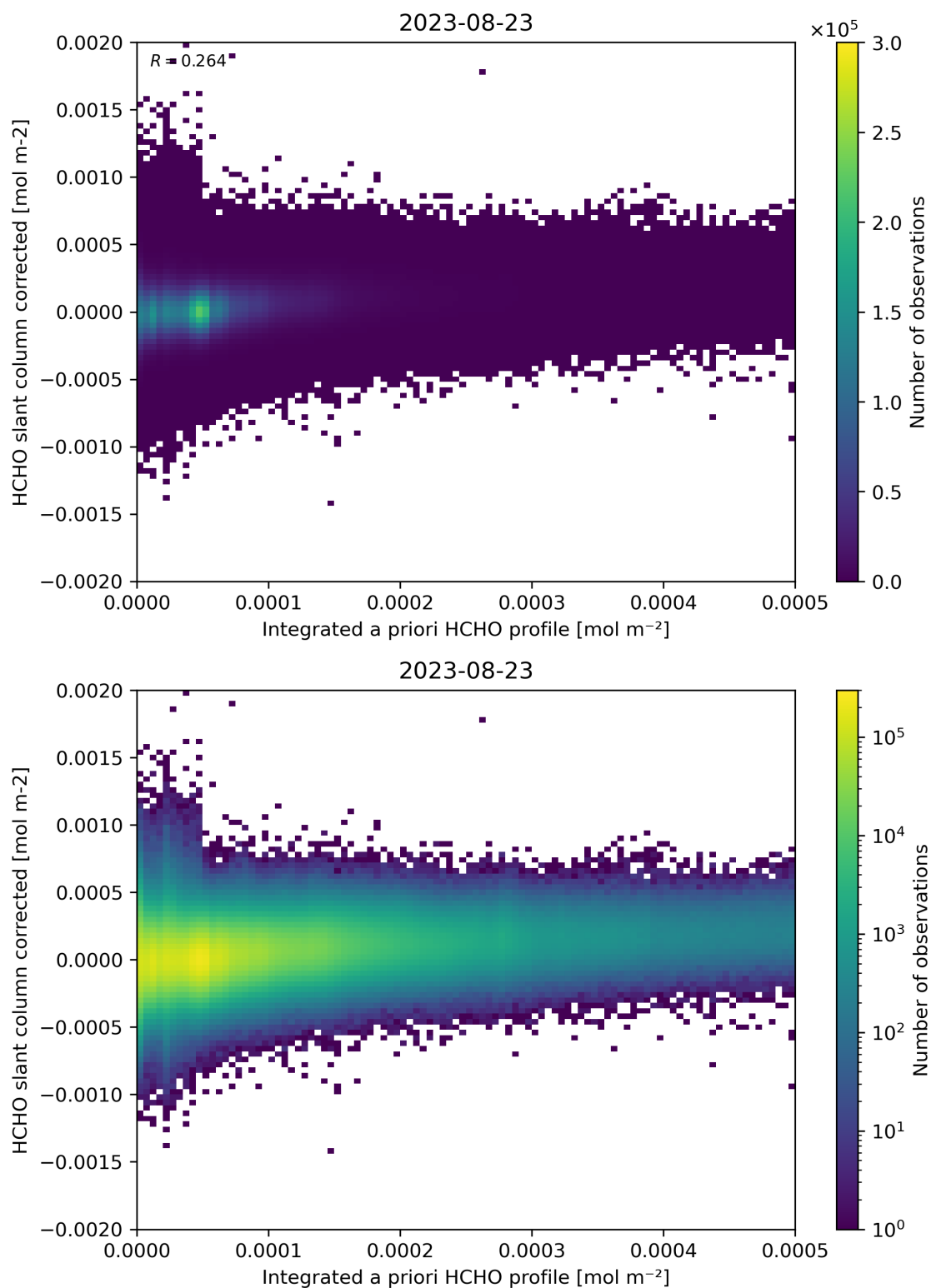
Figure 151: Scatter density plot of “Integrated a priori HCHO profile” against “HCHO slant column corrected” for 2023-08-22 to 2023-08-24.
