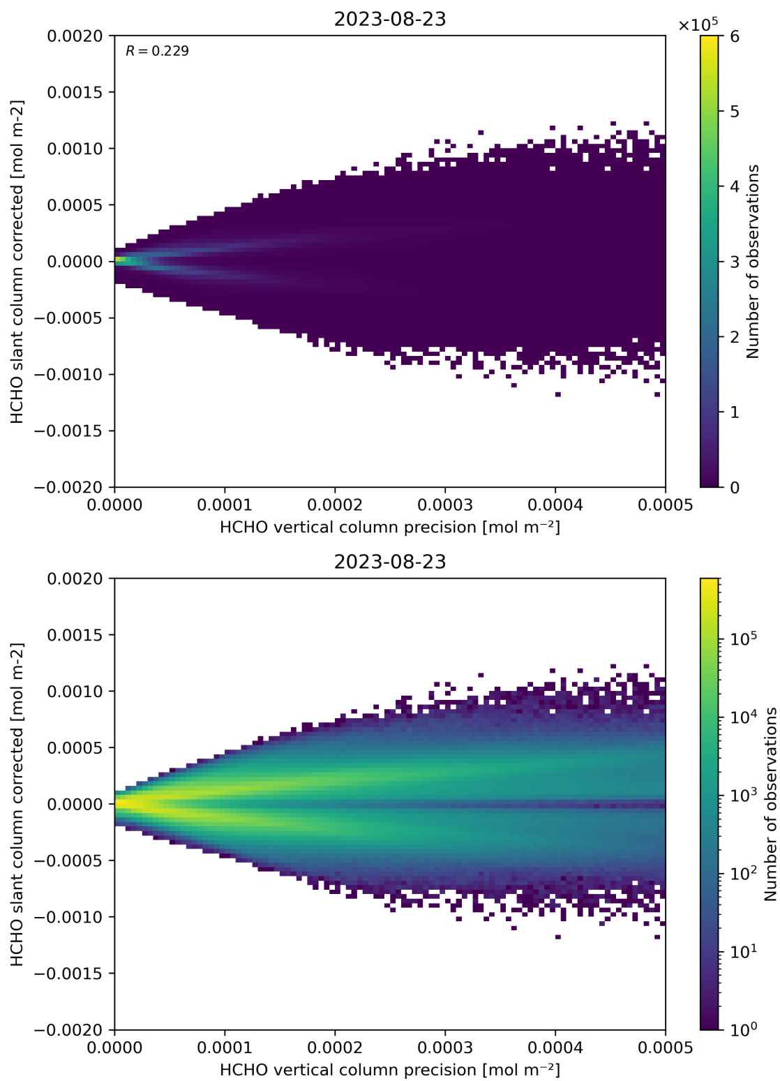
Figure 140: Scatter density plot of “HCHO vertical column precision” against “HCHO slant column corrected” for 2023-08-22 to 2023-08-24.
