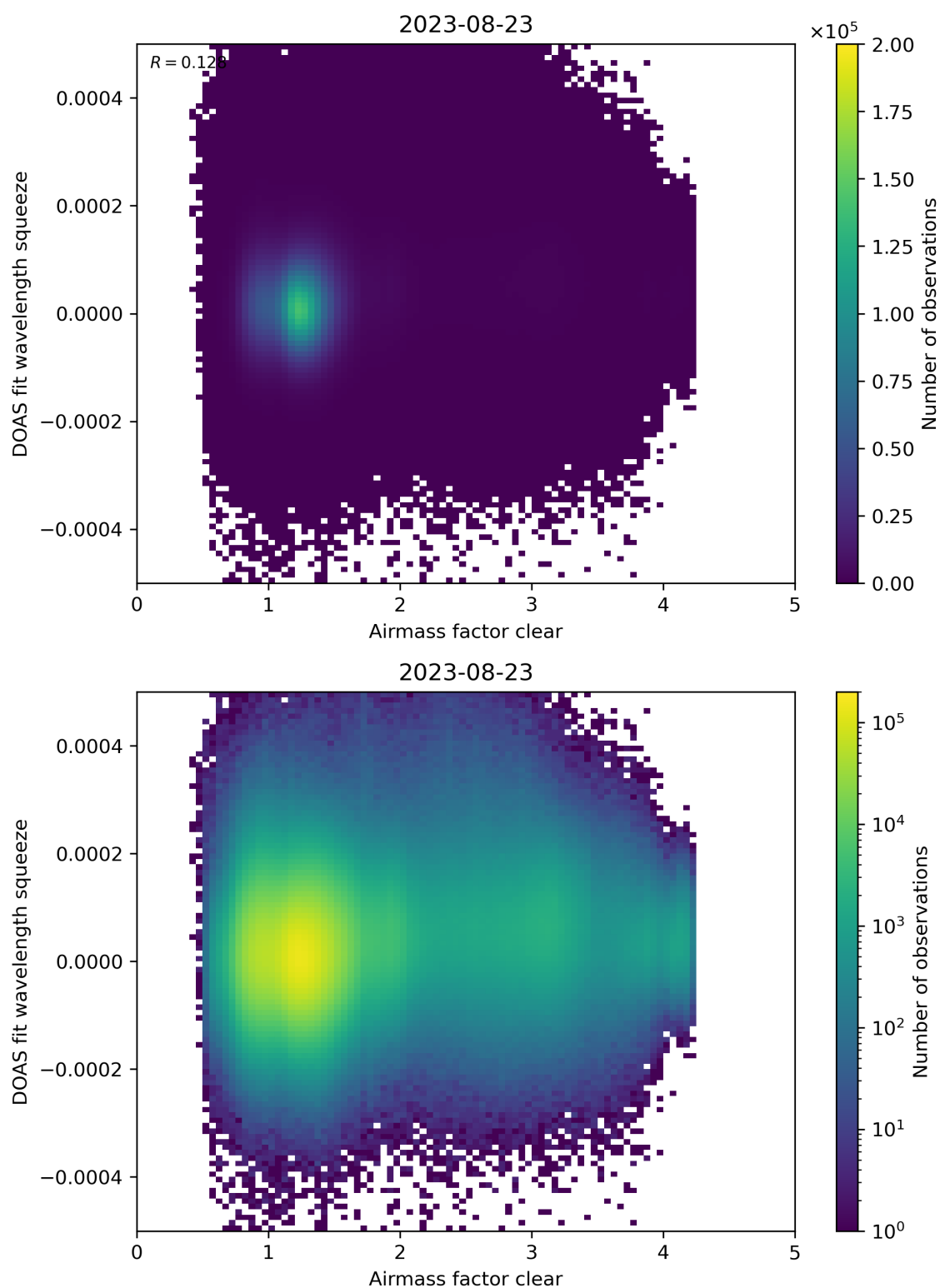
Figure 73: Scatter density plot of “Airmass factor clear” against “DOAS fit wavelength squeeze” for 2023-08-22 to 2023-08-24.
