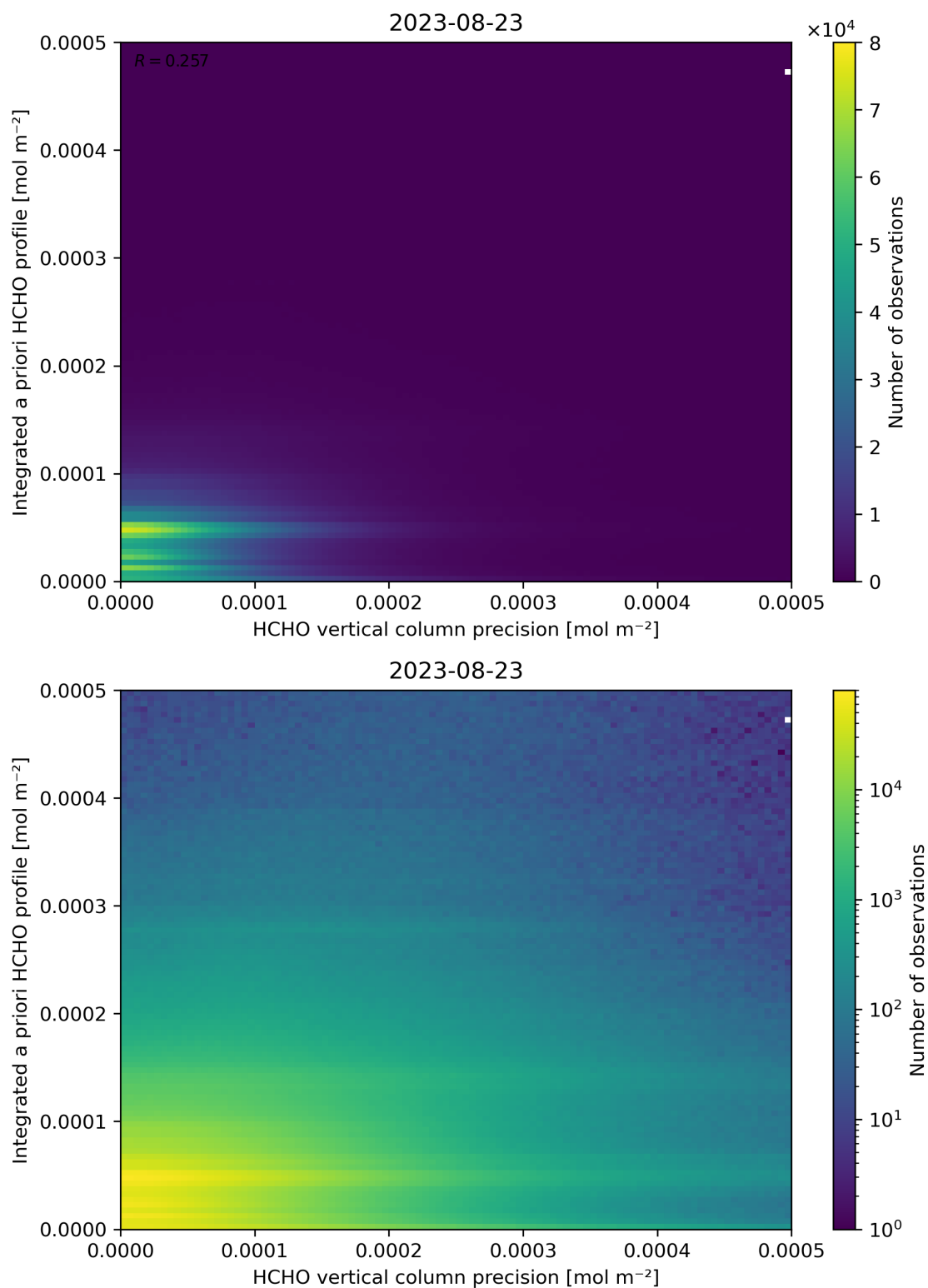
Figure 147: Scatter density plot of “HCHO vertical column precision” against “Integrated a priori HCHO profile” for 2023-08-22 to 2023-08-24.
