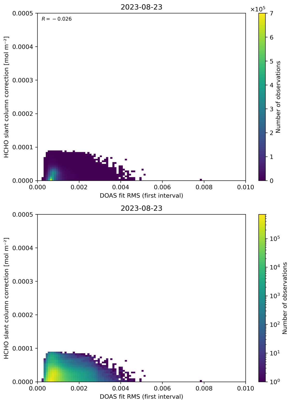
Figure 63: Scatter density plot of “DOAS fit RMS (first interval)” against “HCHO slant column correction” for 2023-08-22 to 2023-08-24.
