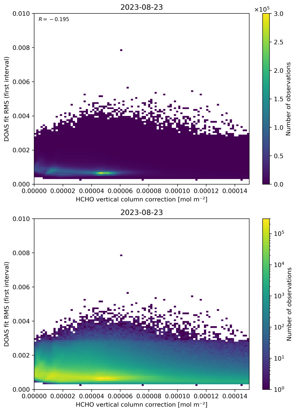
Figure 112: Scatter density plot of “HCHO vertical column correction” against “DOAS fit RMS (first interval)” for 2023-08-22 to 2023-08-24.
