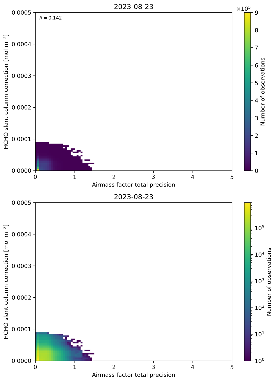
Figure 110: Scatter density plot of “Airmass factor total precision” against “HCHO slant column correction” for 2023-08-22 to 2023-08-24.
