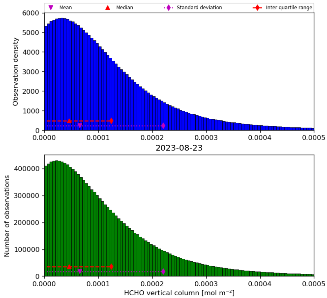
Figure 35: Histogram of “HCHO vertical column” for 2023-08-22 to 2023-08-24
