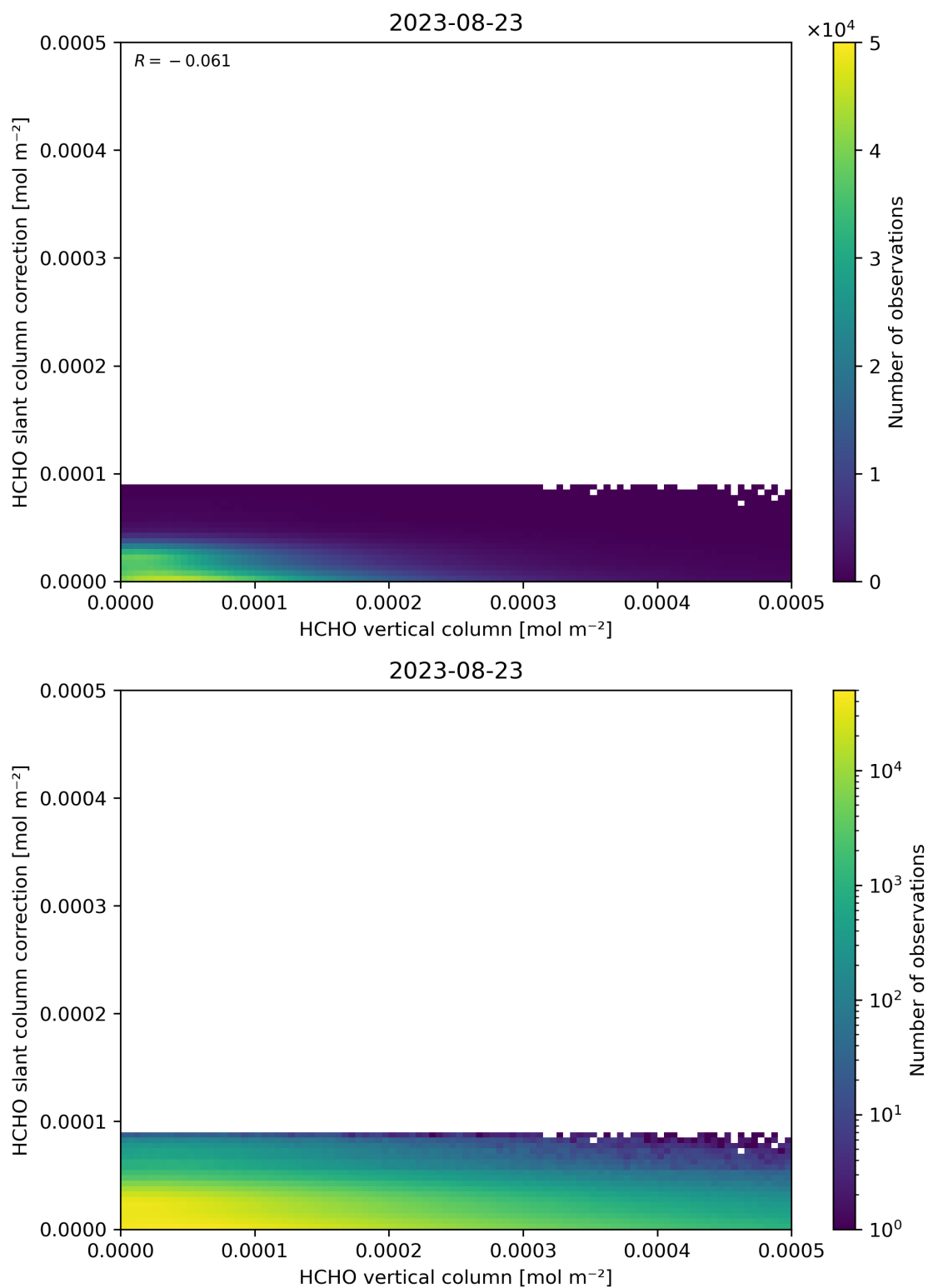
Figure 128: Scatter density plot of “HCHO vertical column” against “HCHO slant column correction” for 2023-08-22 to 2023-08-24.
