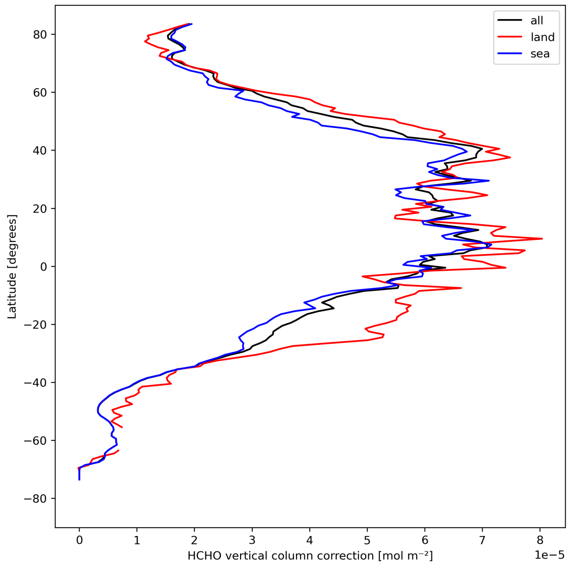
Figure 23: Zonal average of “HCHO vertical column correction” for 2023-08-22 to 2023-08-24.
