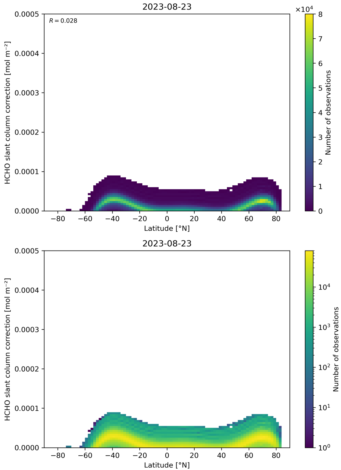
Figure 158: Scatter density plot of “Latitude” against “HCHO slant column correction” for 2023-08-22 to 2023-08-24.
