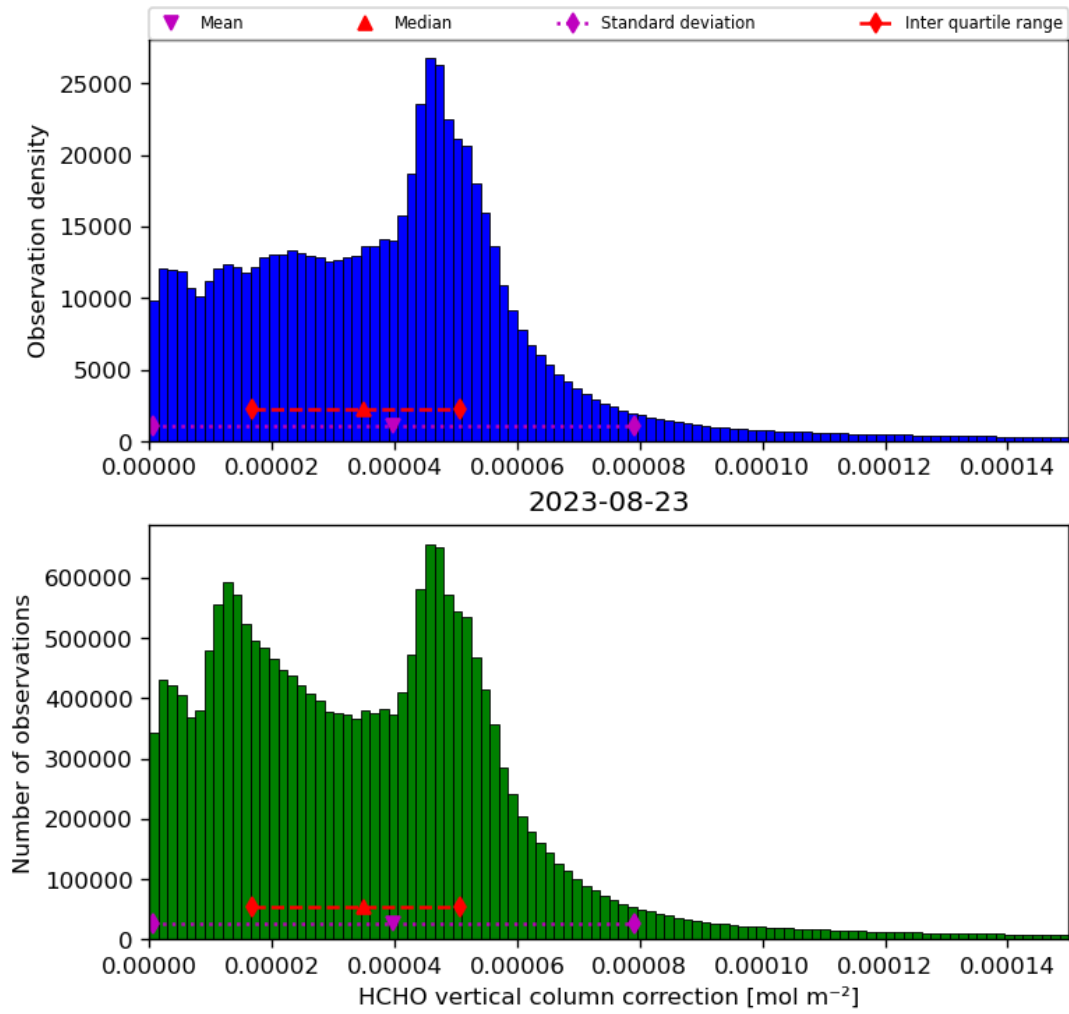
Figure 37: Histogram of “HCHO vertical column correction” for 2023-08-22 to 2023-08-24
