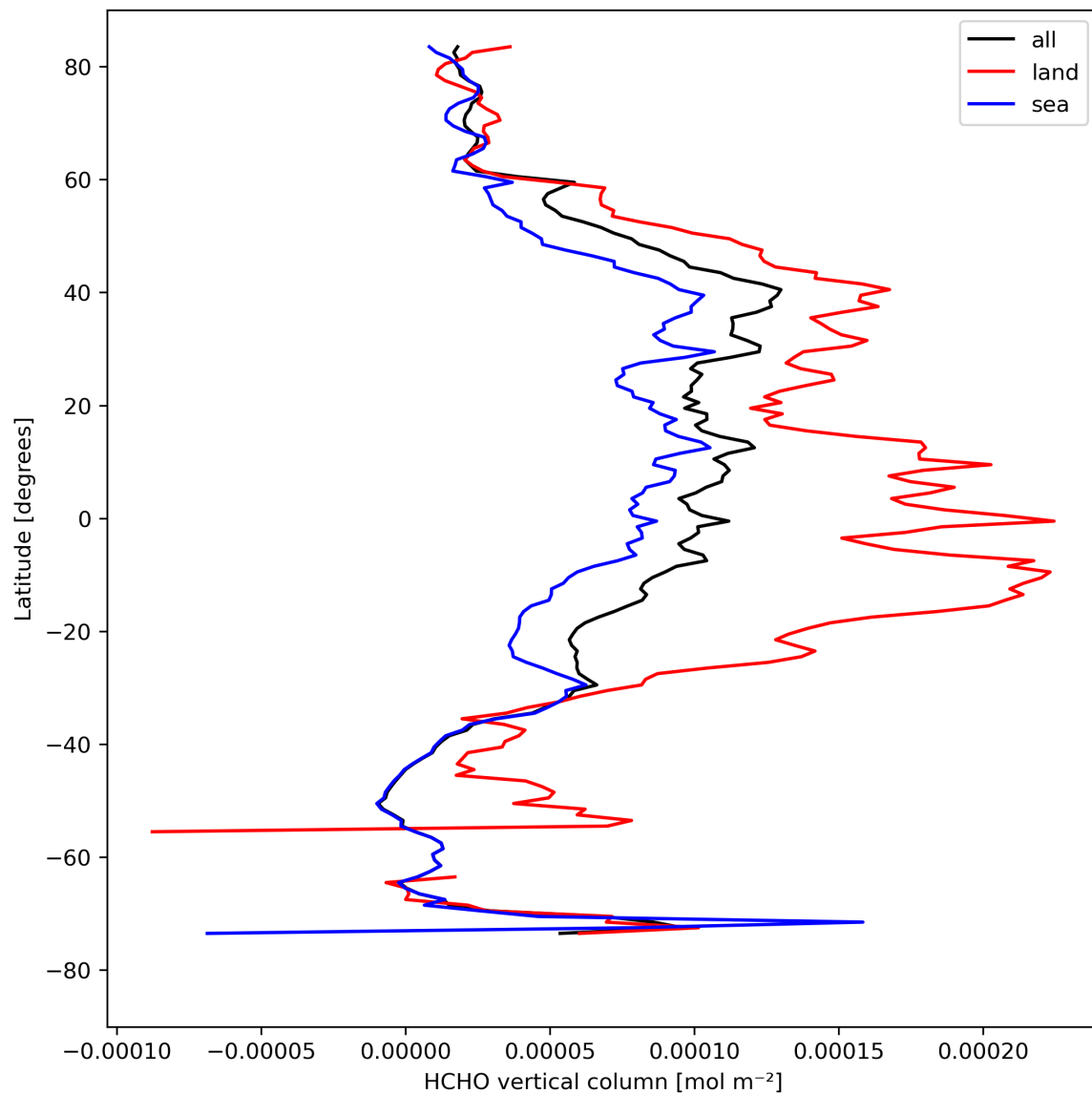
Figure 21: Zonal average of “HCHO vertical column” for 2023-08-22 to 2023-08-24.
