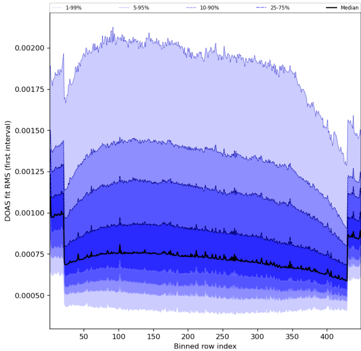
Figure 60: Along track statistics of “DOAS fit RMS (first interval)” for 2023-08-22 to 2023-08-24
