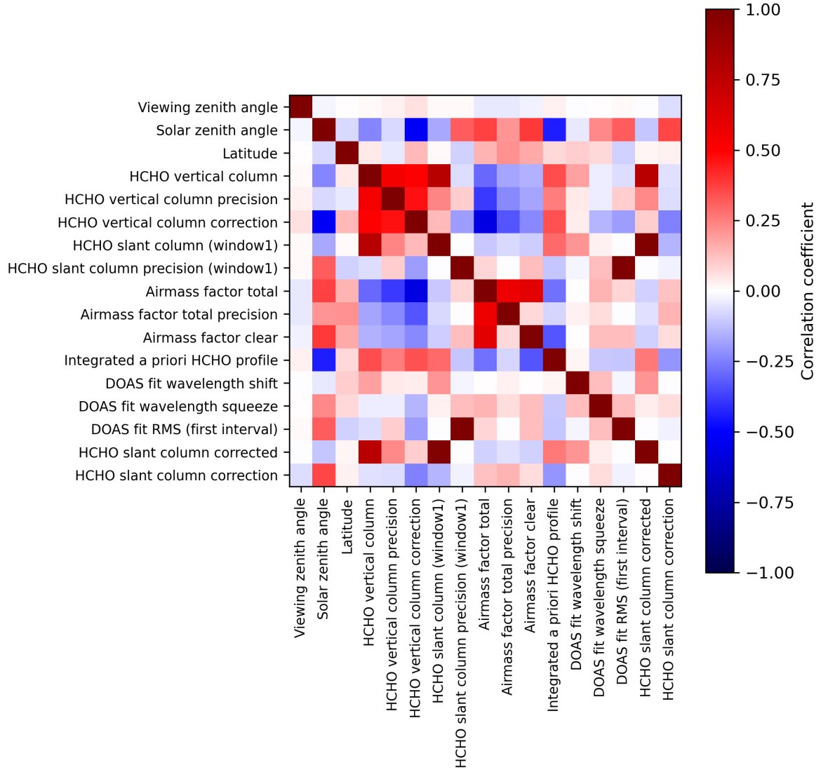
Figure 2: Map of correlation matrix for 2023-08-22 to 2023-08-24.
