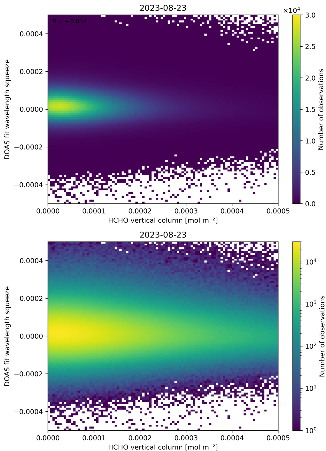
Figure 125: Scatter density plot of “HCHO vertical column” against “DOAS fit wavelength squeeze” for 2023-08-22 to 2023-08-24.
