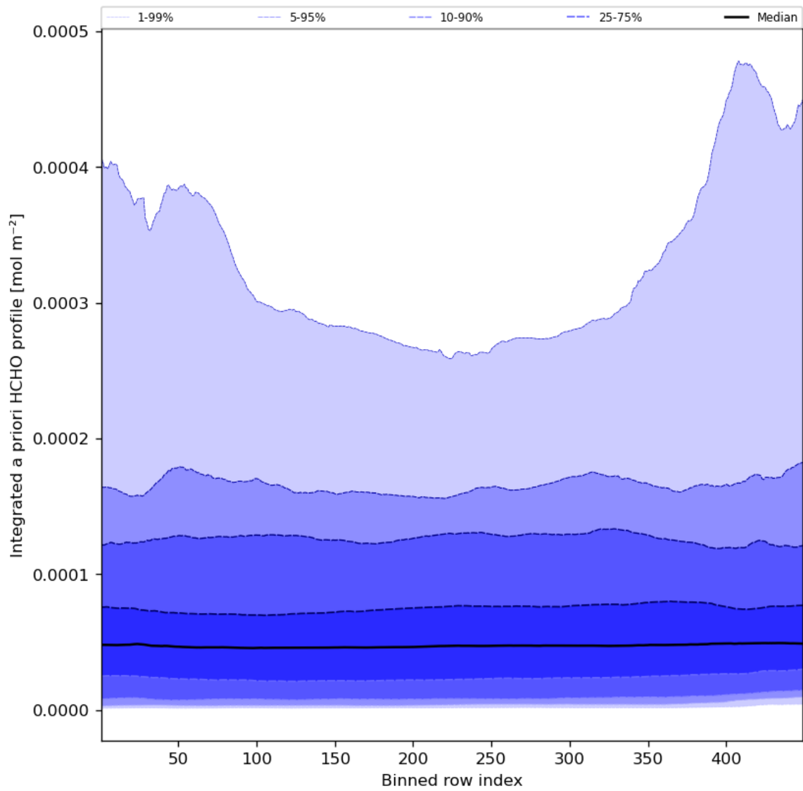
Figure 57: Along track statistics of “Integrated a priori HCHO profile” for 2023-08-22 to 2023-08-24
