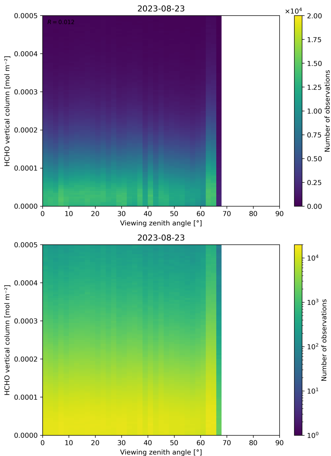
Figure 192: Scatter density plot of “Viewing zenith angle” against “HCHO vertical column” for 2023-08-22 to 2023-08-24.
