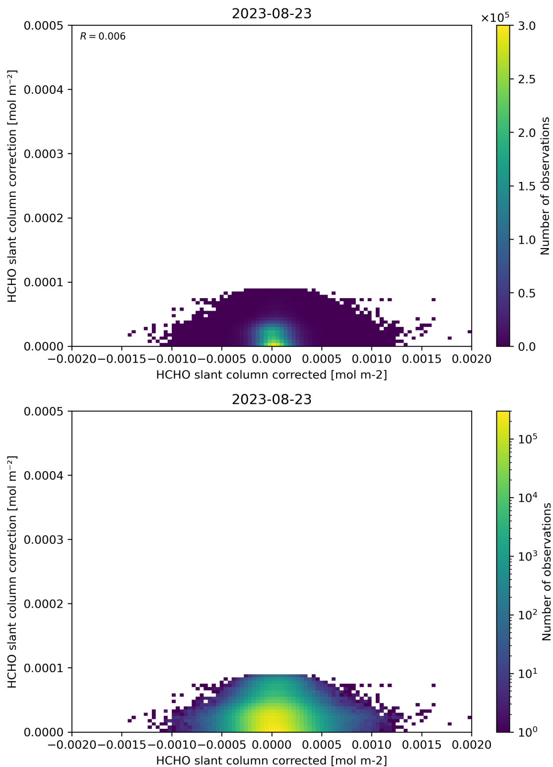
Figure 77: Scatter density plot of “HCHO slant column corrected” against “HCHO slant column correction” for 2023-08-22 to 2023-08-24.
