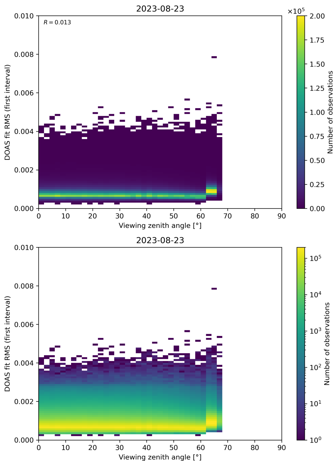
Figure 182: Scatter density plot of “Viewing zenith angle” against “DOAS fit RMS (first interval)” for 2023-08-22 to 2023-08-24.
