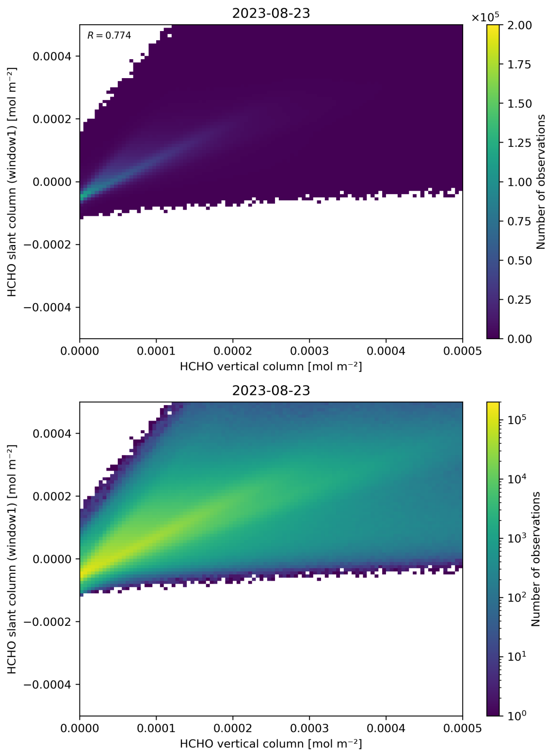
Figure 129: Scatter density plot of “HCHO vertical column” against “HCHO slant column (window1)” for 2023-08-22 to 2023-08-24.
