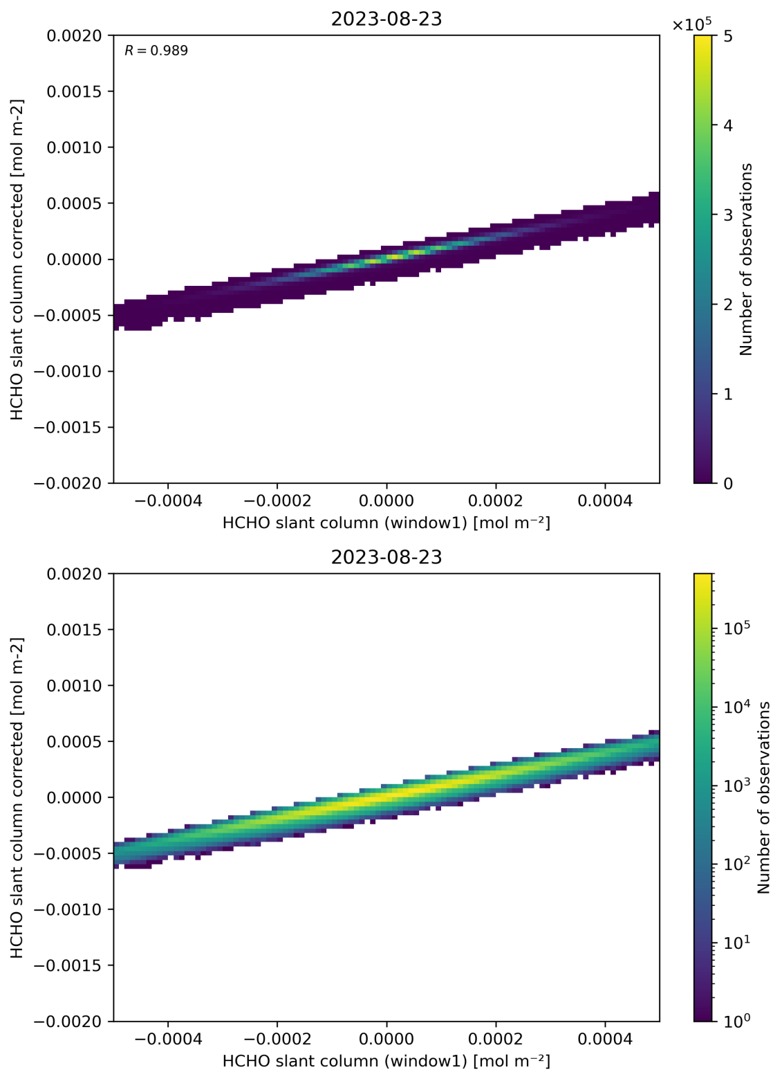
Figure 82: Scatter density plot of “HCHO slant column (window1)” against “HCHO slant column corrected” for 2023-08-22 to 2023-08-24.
