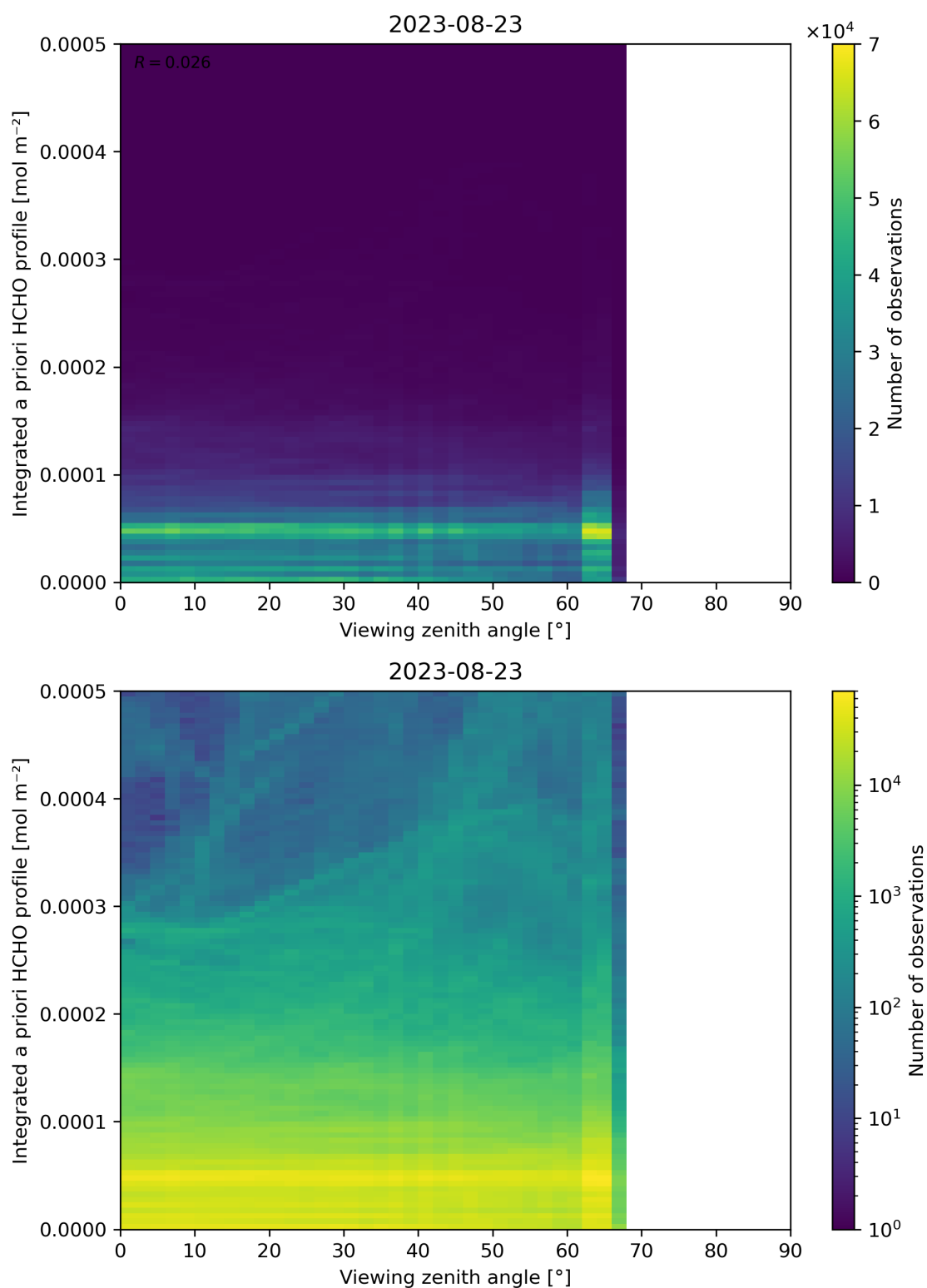
Figure 195: Scatter density plot of “Viewing zenith angle” against “Integrated a priori HCHO profile” for 2023-08-22 to 2023-08-24.
