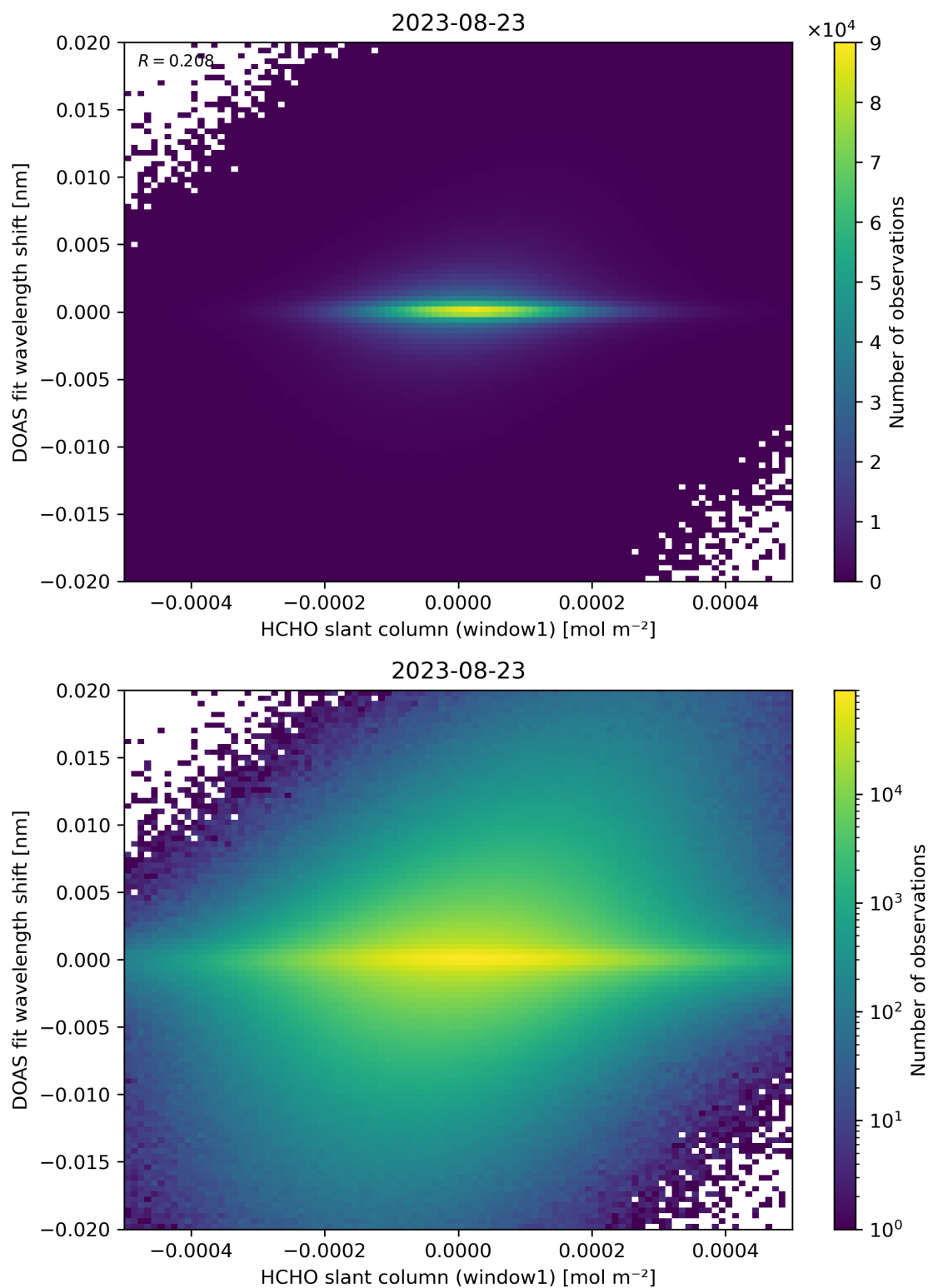
Figure 79: Scatter density plot of “HCHO slant column (window1)” against “DOAS fit wavelength shift” for 2023-08-22 to 2023-08-24.
