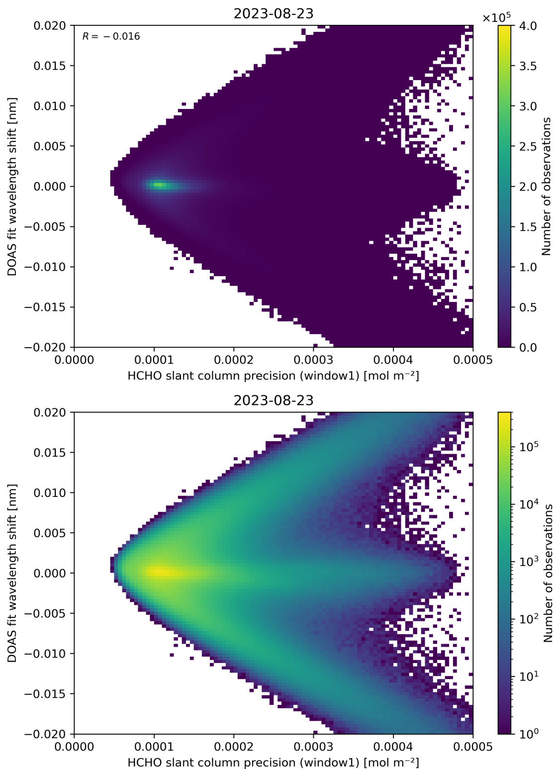
Figure 89: Scatter density plot of “HCHO slant column precision (window1)” against “DOAS fit wavelength shift” for 2023-08-22 to 2023-08-24.
