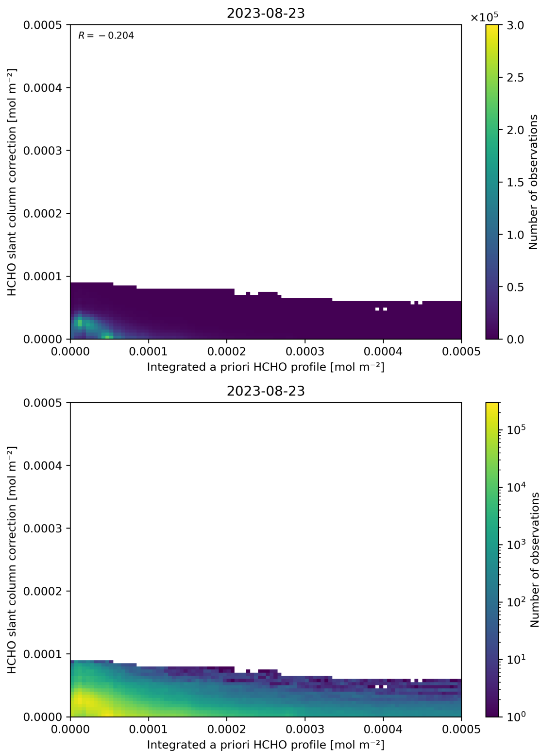
Figure 152: Scatter density plot of “Integrated a priori HCHO profile” against “HCHO slant column correction” for 2023-08-22 to 2023-08-24.
