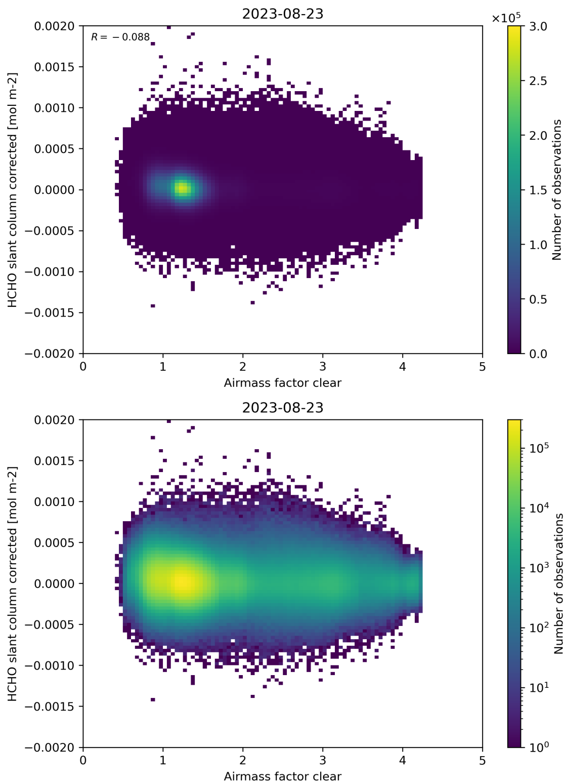
Figure 74: Scatter density plot of “Airmass factor clear” against “HCHO slant column corrected” for 2023-08-22 to 2023-08-24.
