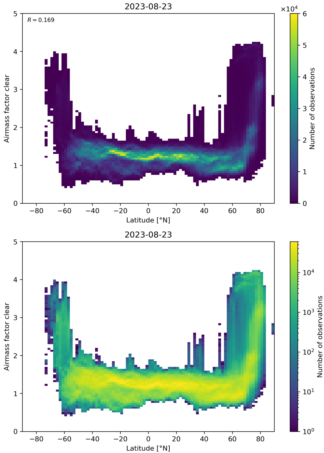
Figure 156: Scatter density plot of “Latitude” against “Airmass factor clear” for 2023-08-22 to 2023-08-24.
