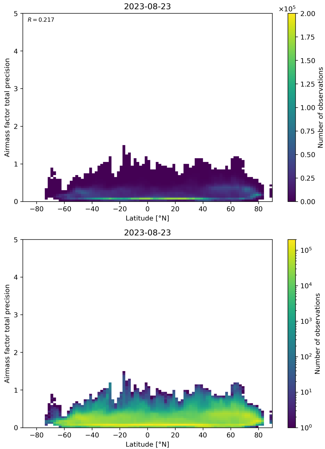
Figure 162: Scatter density plot of “Latitude” against “Airmass factor total precision” for 2023-08-22 to 2023-08-24.
