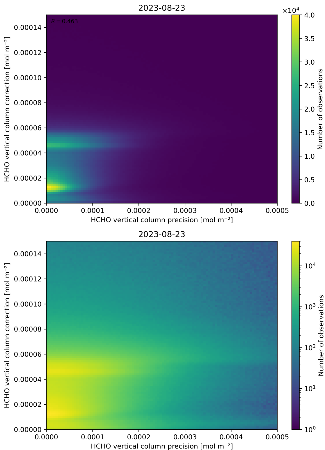
Figure 146: Scatter density plot of “HCHO vertical column precision” against “HCHO vertical column correction” for 2023-08-22 to 2023-08-24.
