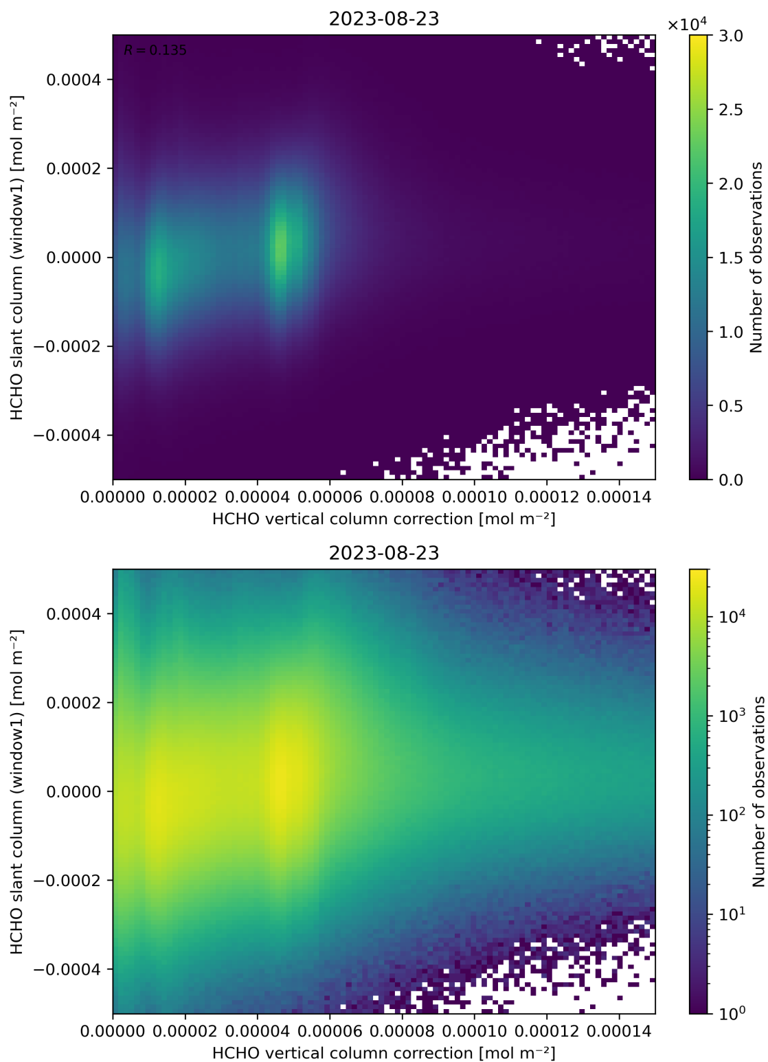
Figure 118: Scatter density plot of “HCHO vertical column correction” against “HCHO slant column (window1)” for 2023-08-22 to 2023-08-24.
