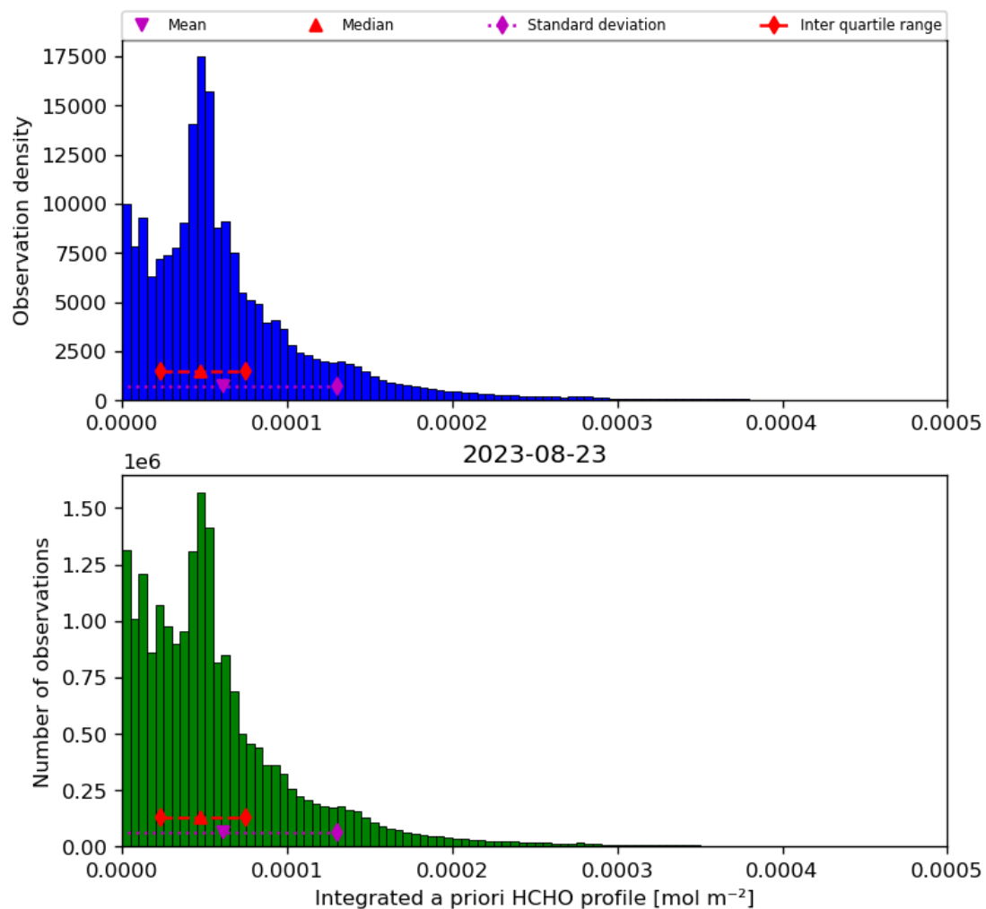
Figure 43: Histogram of “Integrated a priori HCHO profile” for 2023-08-22 to 2023-08-24
