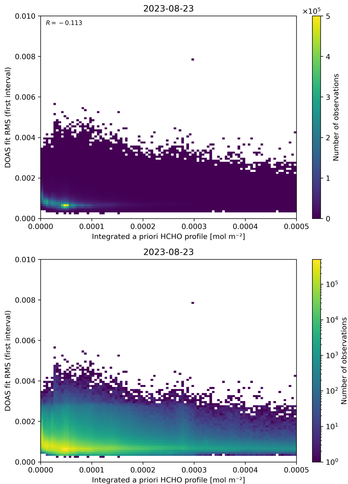
Figure 148: Scatter density plot of “Integrated a priori HCHO profile” against “DOAS fit RMS (first interval)” for 2023-08-22 to 2023-08-24.
