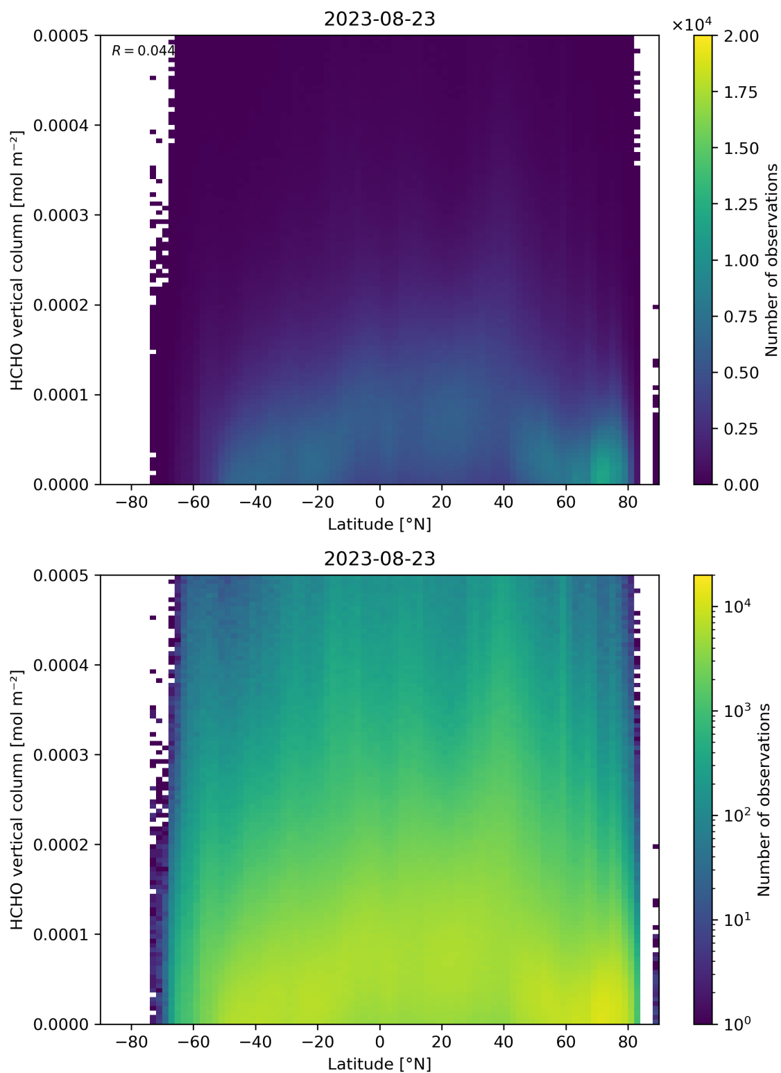
Figure 163: Scatter density plot of “Latitude” against “HCHO vertical column” for 2023-08-22 to 2023-08-24.
