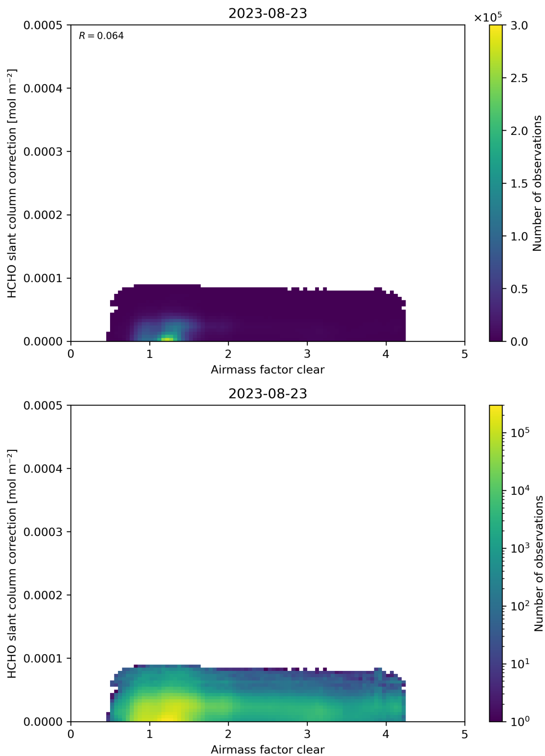
Figure 75: Scatter density plot of “Airmass factor clear” against “HCHO slant column correction” for 2023-08-22 to 2023-08-24.
