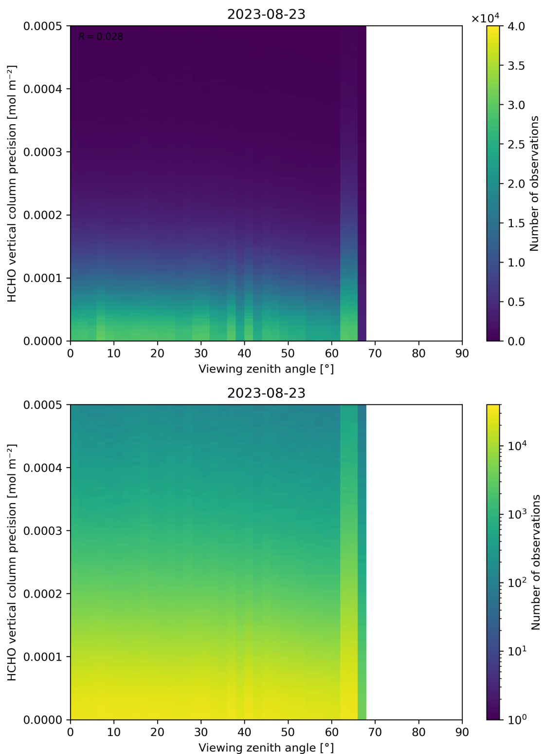
Figure 194: Scatter density plot of “Viewing zenith angle” against “HCHO vertical column precision” for 2023-08-22 to 2023-08-24.
