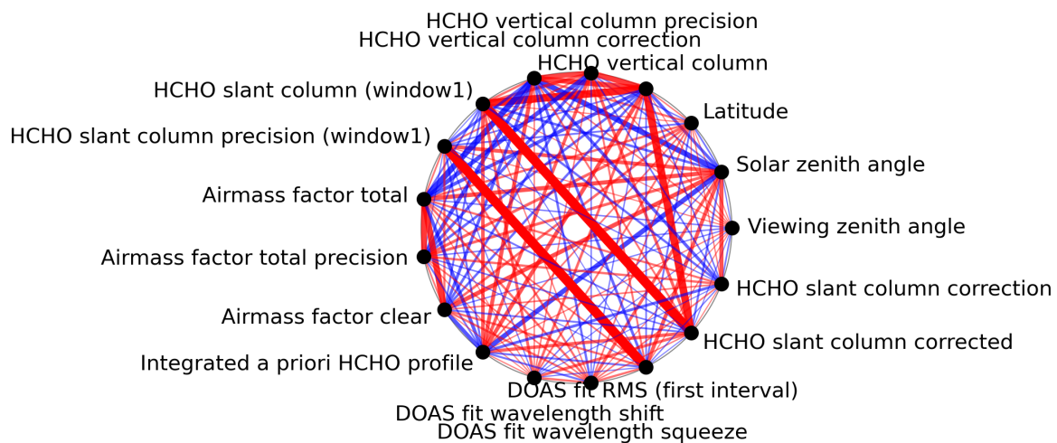
Figure 1: Map of correlation graph for 2023-08-22 to 2023-08-24.
