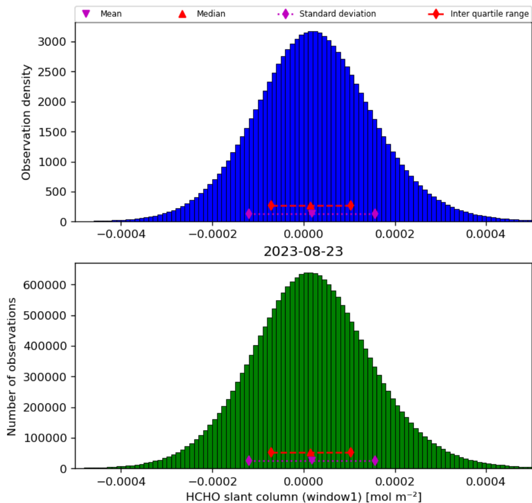
Figure 38: Histogram of “HCHO slant column (window1)” for 2023-08-22 to 2023-08-24
