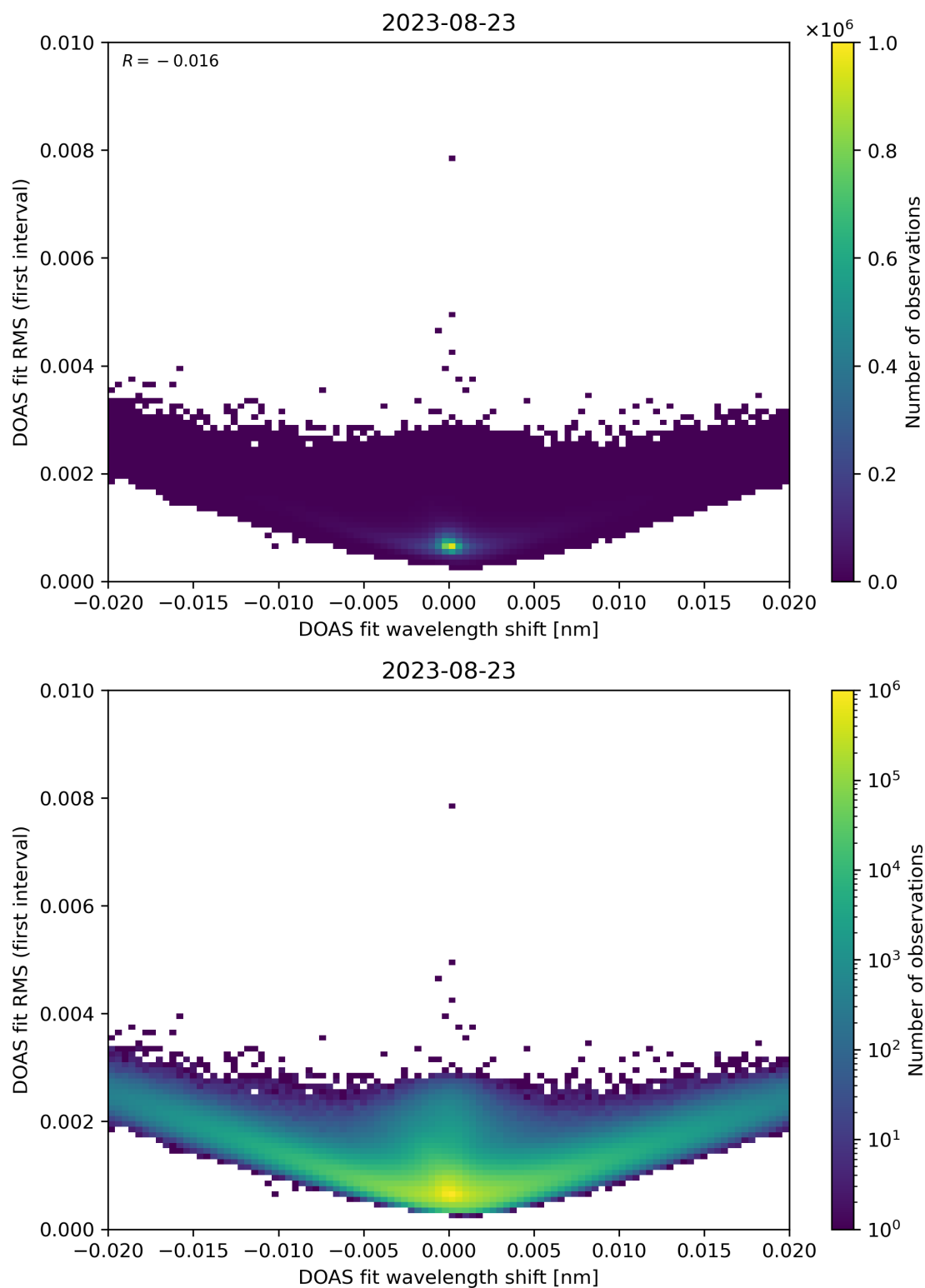
Figure 64: Scatter density plot of “DOAS fit wavelength shift” against “DOAS fit RMS (first interval)” for 2023-08-22 to 2023-08-24.
