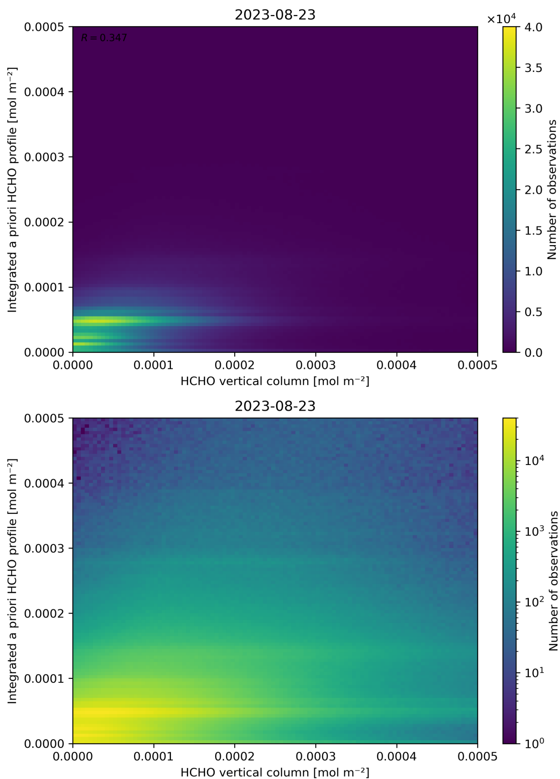
Figure 135: Scatter density plot of “HCHO vertical column” against “Integrated a priori HCHO profile” for 2023-08-22 to 2023-08-24.
