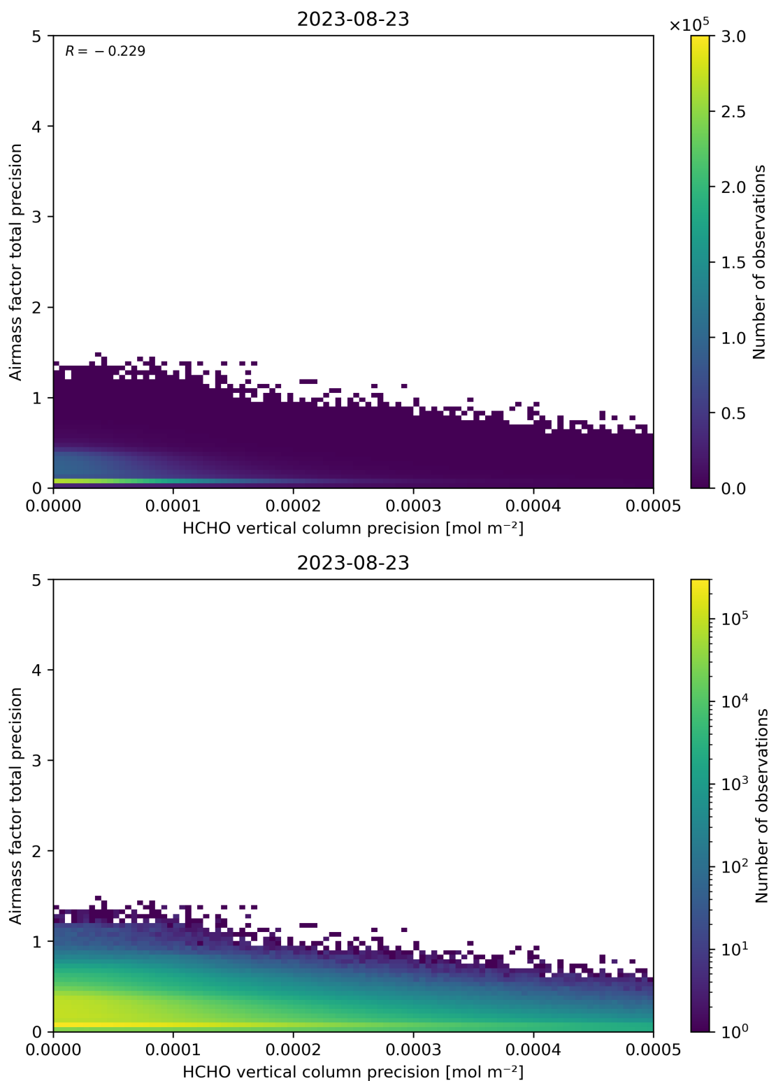
Figure 145: Scatter density plot of “HCHO vertical column precision” against “Airmass factor total precision” for 2023-08-22 to 2023-08-24.
