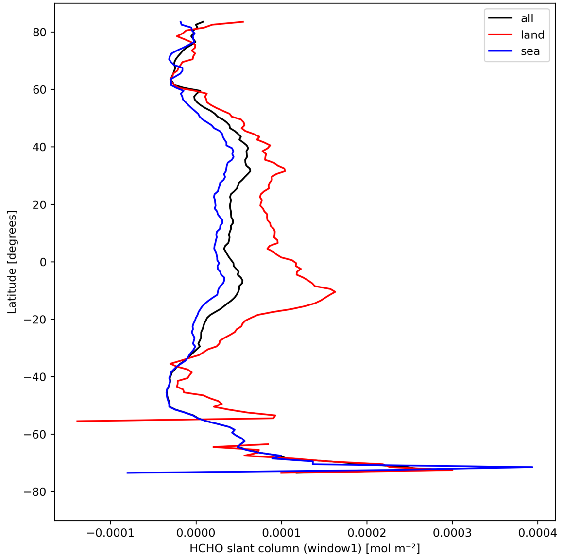
Figure 24: Zonal average of “HCHO slant column (window1)” for 2023-08-22 to 2023-08-24.
