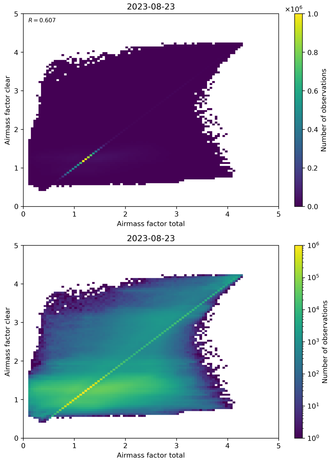
Figure 100: Scatter density plot of “Airmass factor total” against “Airmass factor clear” for 2023-08-22 to 2023-08-24.
