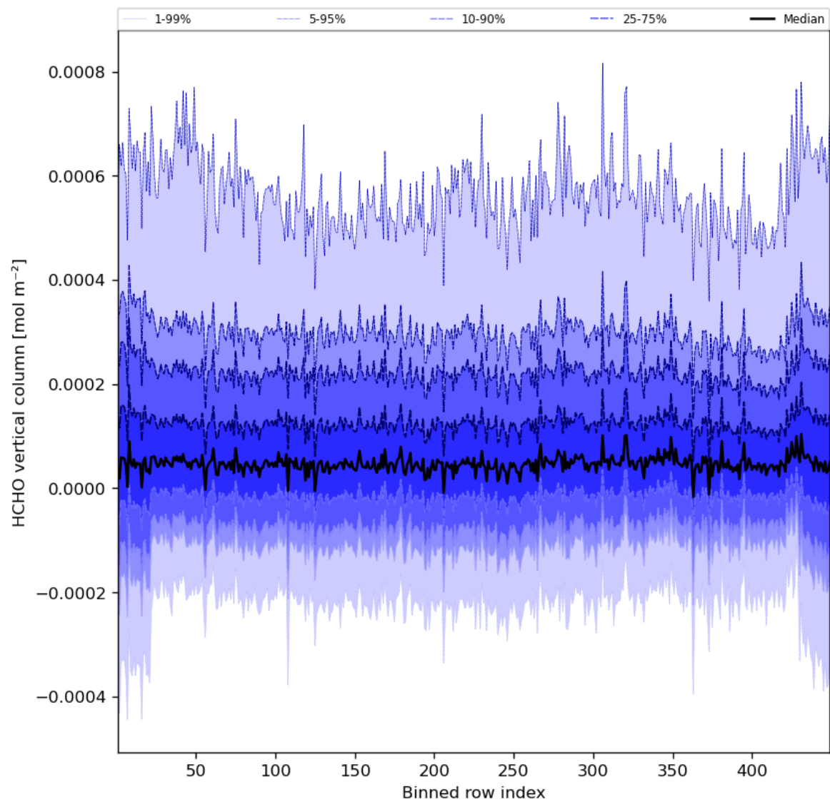
Figure 49: Along track statistics of “HCHO vertical column” for 2023-08-22 to 2023-08-24
