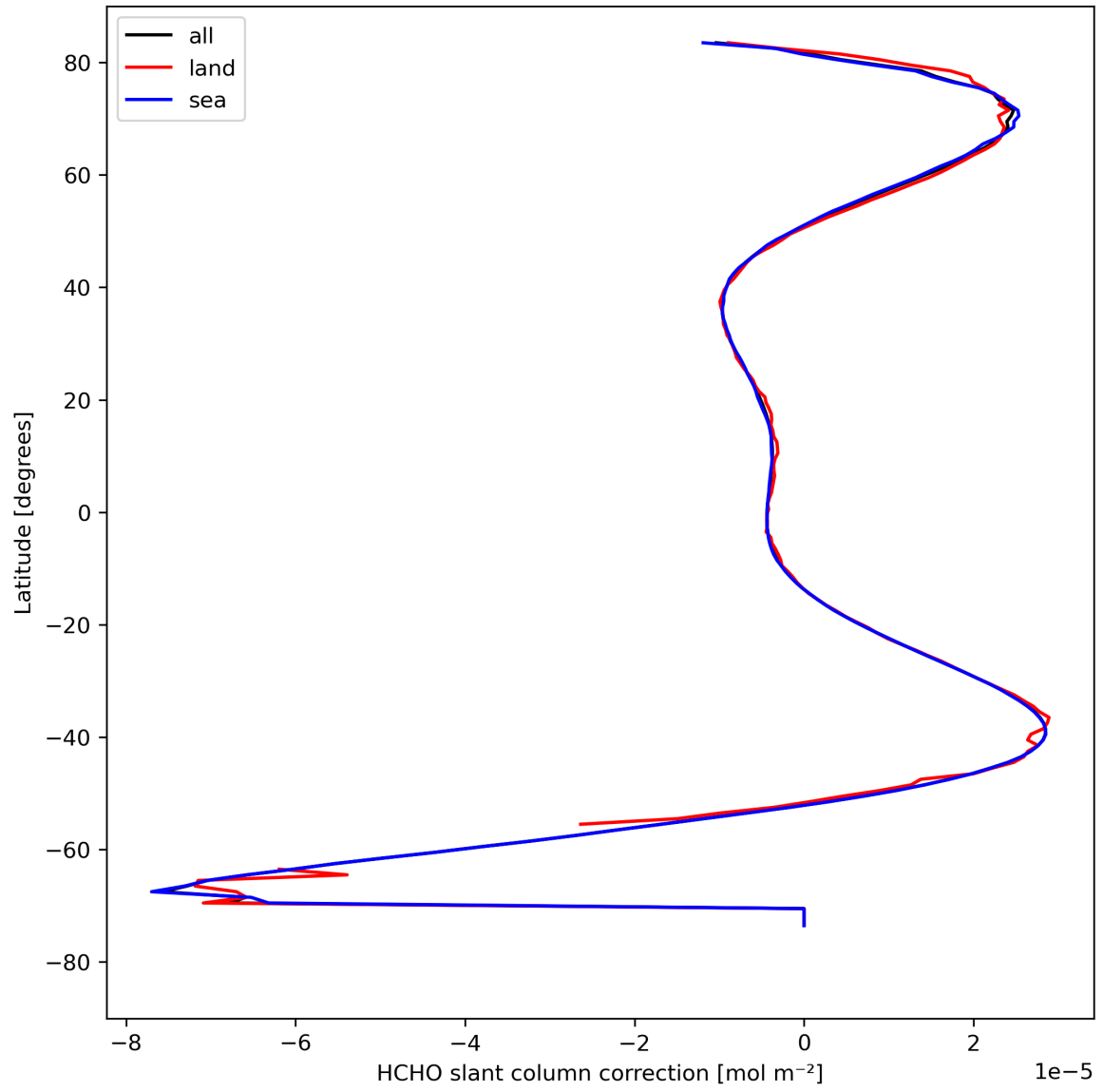
Figure 33: Zonal average of “HCHO slant column correction” for 2023-08-22 to 2023-08-24.
