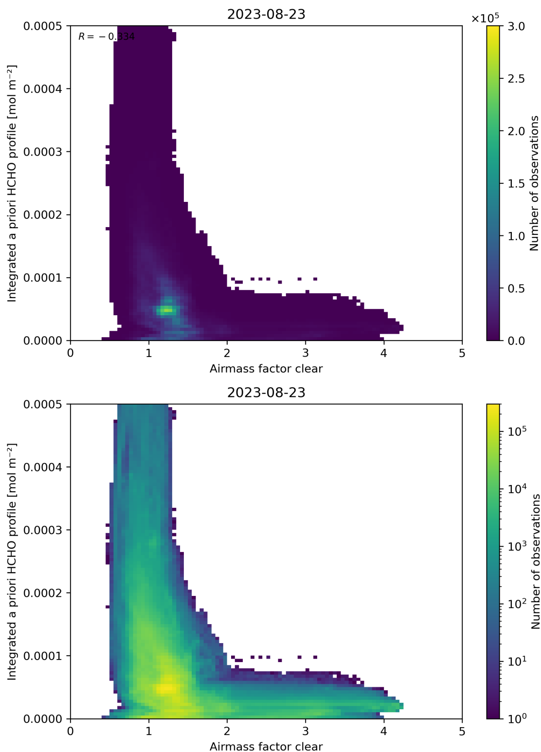
Figure 76: Scatter density plot of “Airmass factor clear” against “Integrated a priori HCHO profile” for 2023-08-22 to 2023-08-24.
