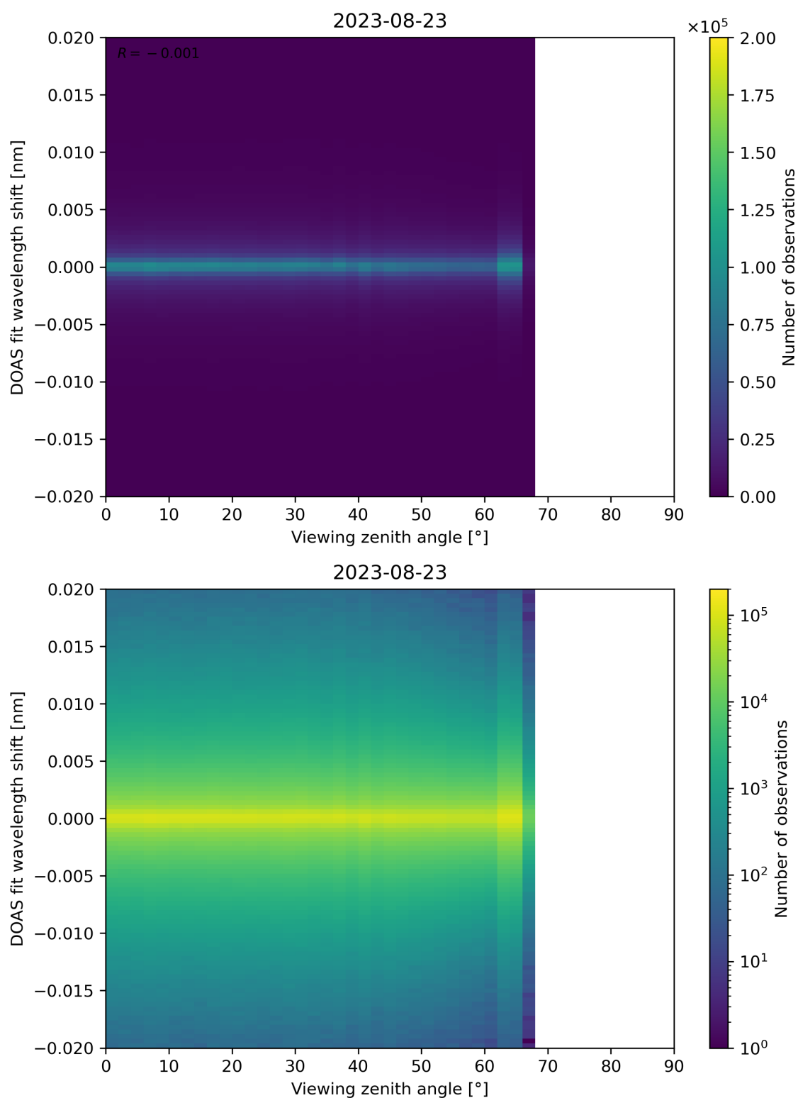
Figure 183: Scatter density plot of “Viewing zenith angle” against “DOAS fit wavelength shift” for 2023-08-22 to 2023-08-24.
