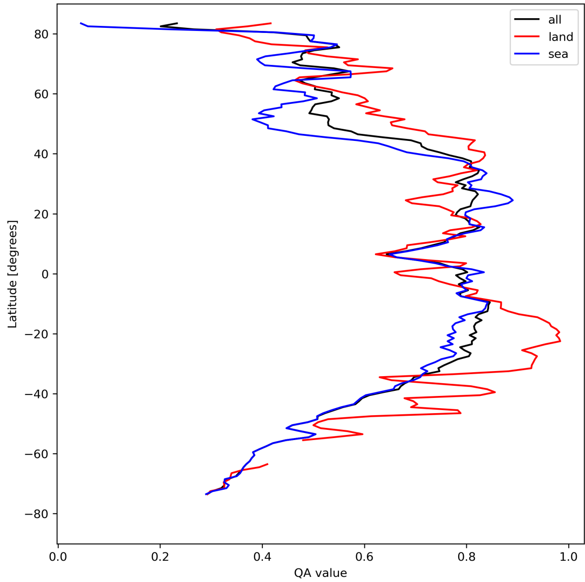
Figure 20: Zonal average of “QA value” for 2023-08-22 to 2023-08-24.
