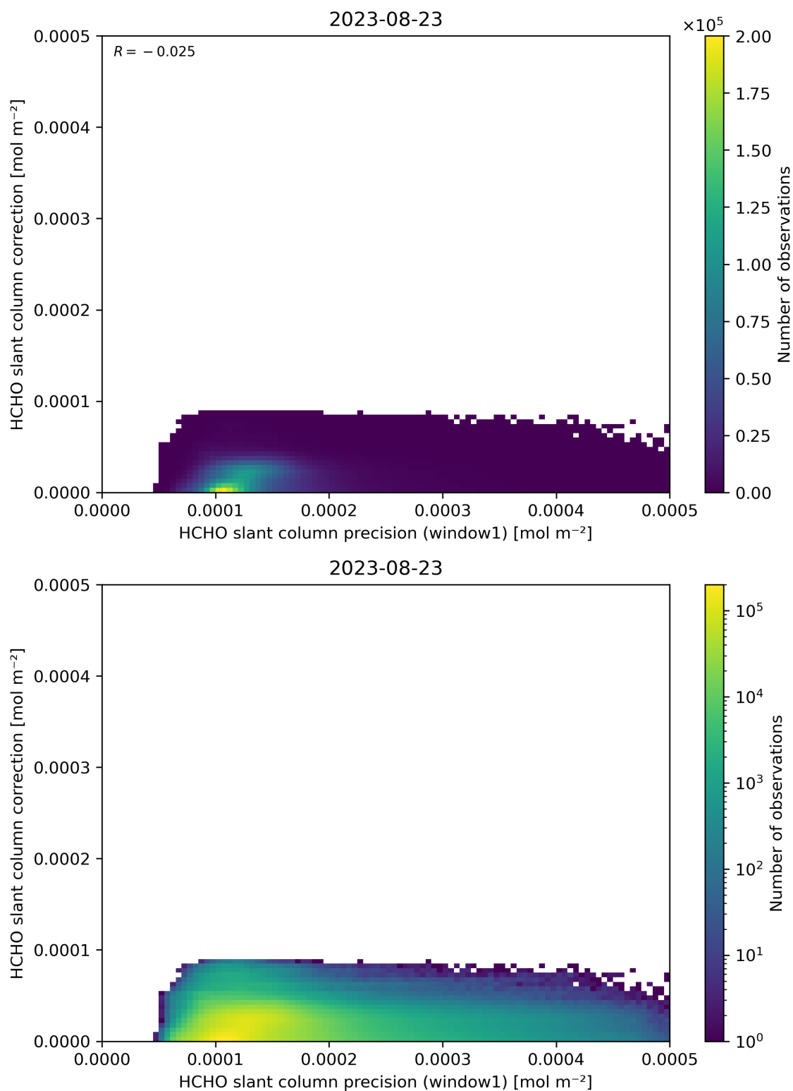
Figure 93: Scatter density plot of “HCHO slant column precision (window1)” against “HCHO slant column correction” for 2023-08-22 to 2023-08-24.
