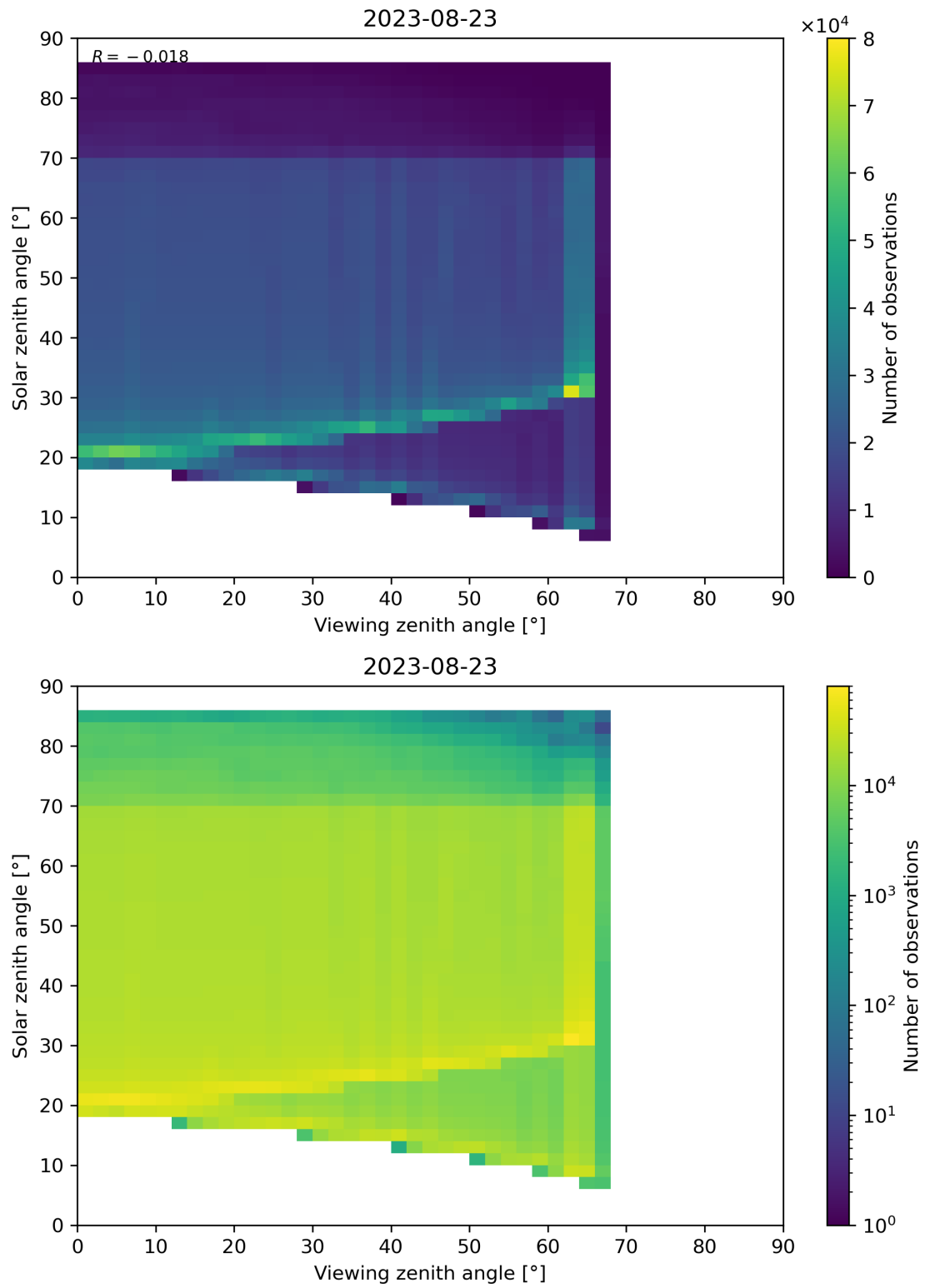
Figure 197: Scatter density plot of “Viewing zenith angle” against “Solar zenith angle” for 2023-08-22 to 2023-08-24.
