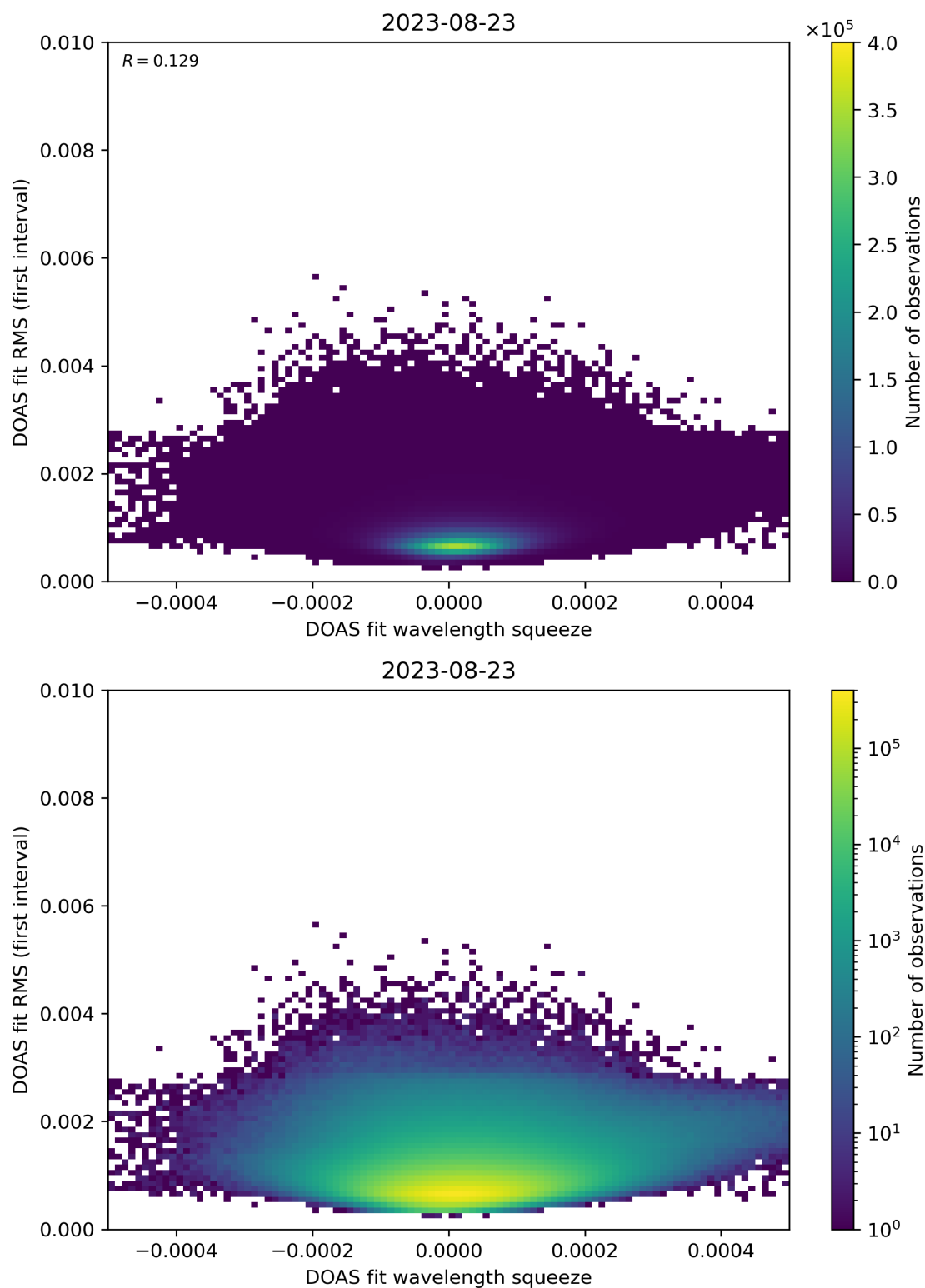
Figure 68: Scatter density plot of “DOAS fit wavelength squeeze” against “DOAS fit RMS (first interval)” for 2023-08-22 to 2023-08-24.
