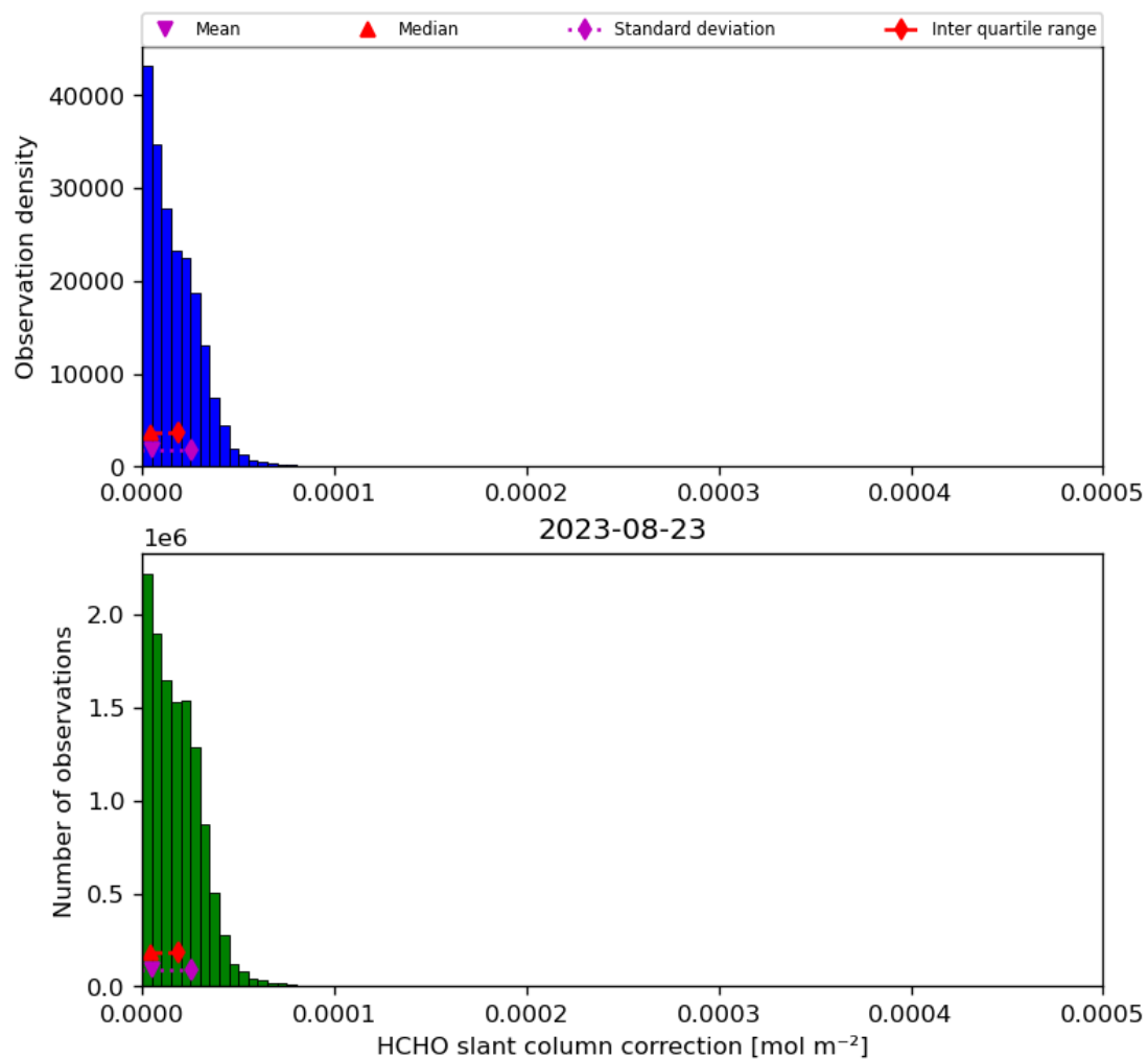
Figure 47: Histogram of “HCHO slant column correction” for 2023-08-22 to 2023-08-24
