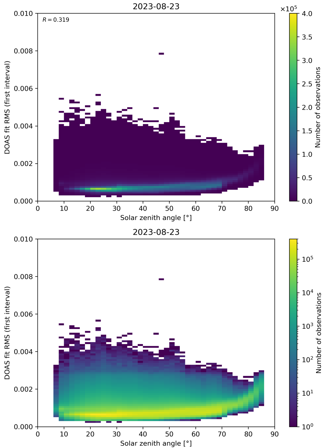
Figure 167: Scatter density plot of “Solar zenith angle” against “DOAS fit RMS (first interval)” for 2023-08-22 to 2023-08-24.
