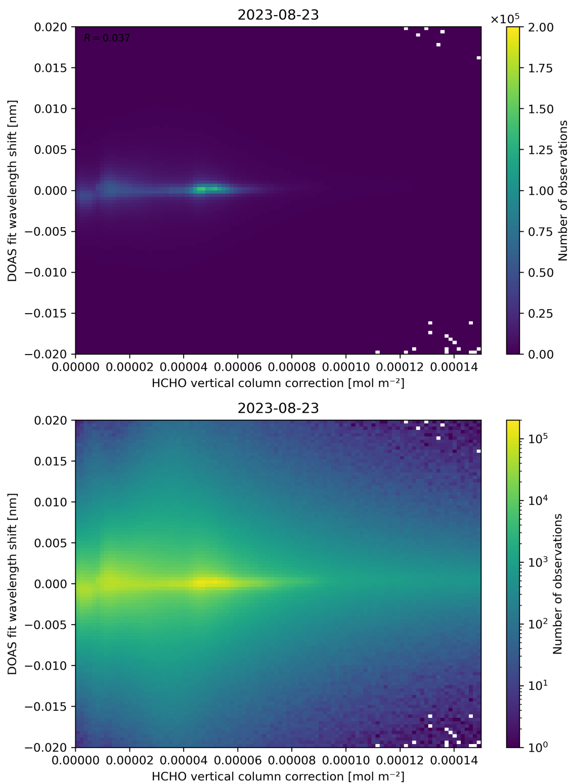
Figure 113: Scatter density plot of “HCHO vertical column correction” against “DOAS fit wavelength shift” for 2023-08-22 to 2023-08-24.
