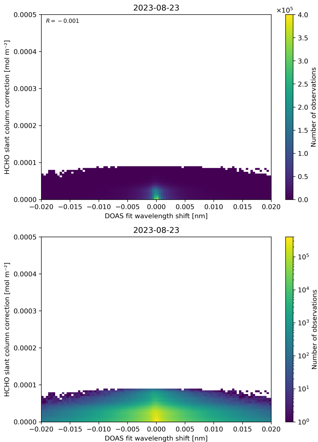
Figure 67: Scatter density plot of “DOAS fit wavelength shift” against “HCHO slant column correction” for 2023-08-22 to 2023-08-24.
