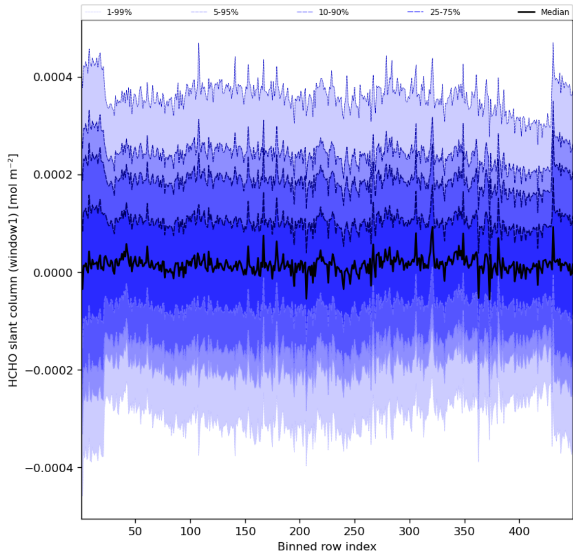
Figure 52: Along track statistics of “HCHO slant column (window1)” for 2023-08-22 to 2023-08-24
