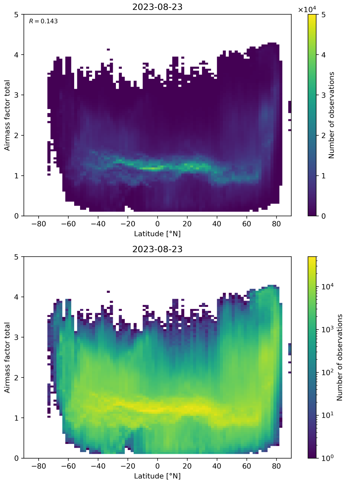
Figure 161: Scatter density plot of “Latitude” against “Airmass factor total” for 2023-08-22 to 2023-08-24.
