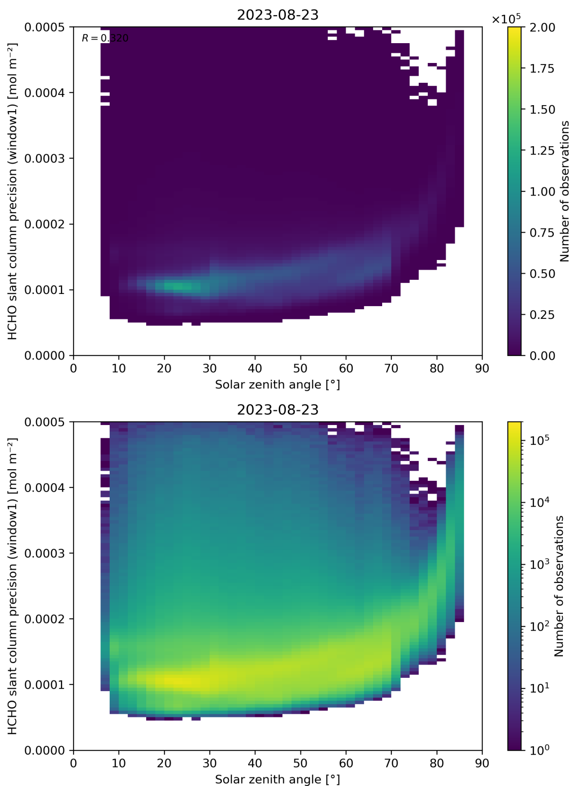
Figure 174: Scatter density plot of “Solar zenith angle” against “HCHO slant column precision (window1)” for 2023-08-22 to 2023-08-24.
