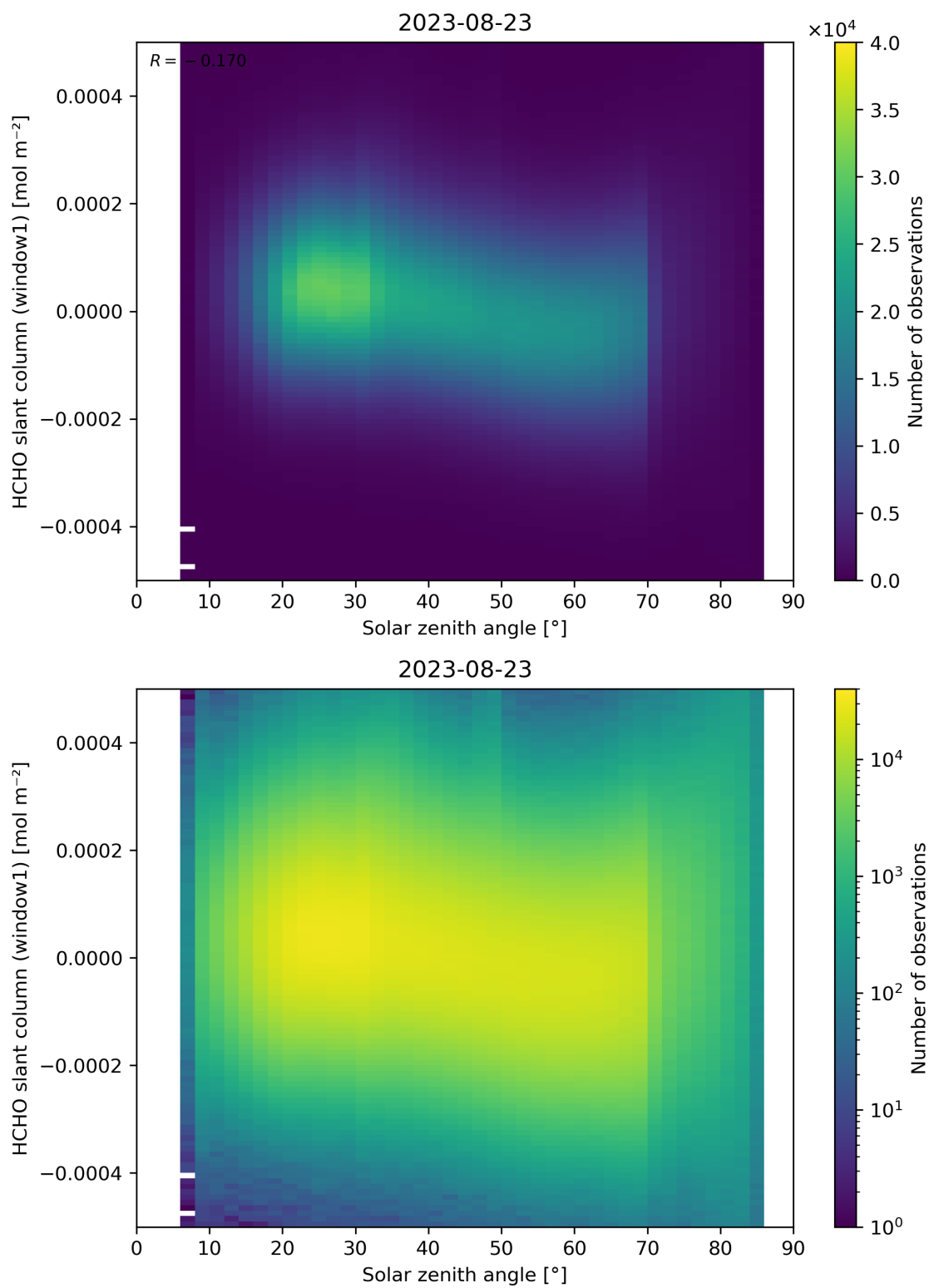
Figure 173: Scatter density plot of “Solar zenith angle” against “HCHO slant column (window1)” for 2023-08-22 to 2023-08-24.
