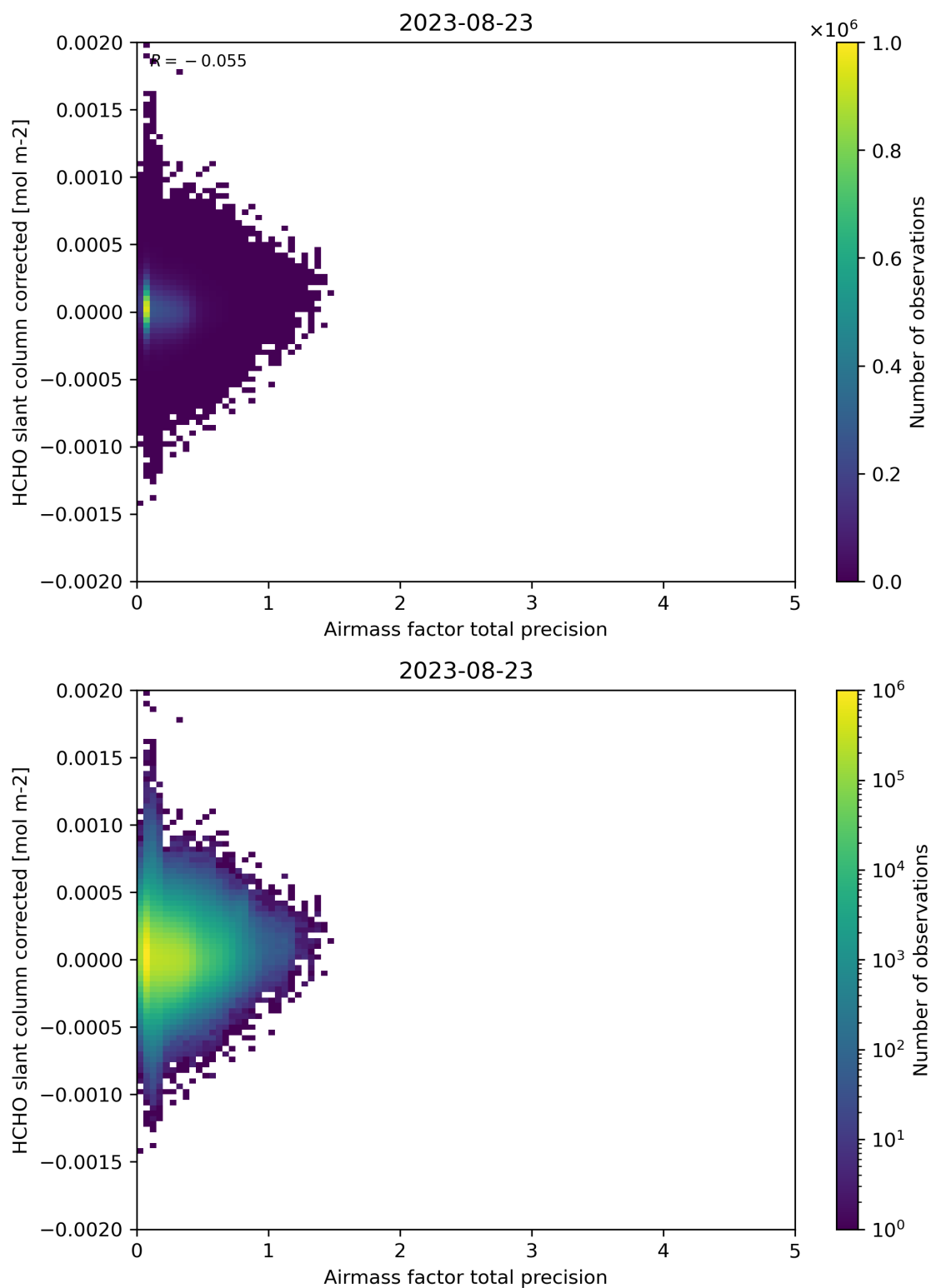
Figure 109: Scatter density plot of “Airmass factor total precision” against “HCHO slant column corrected” for 2023-08-22 to 2023-08-24.
