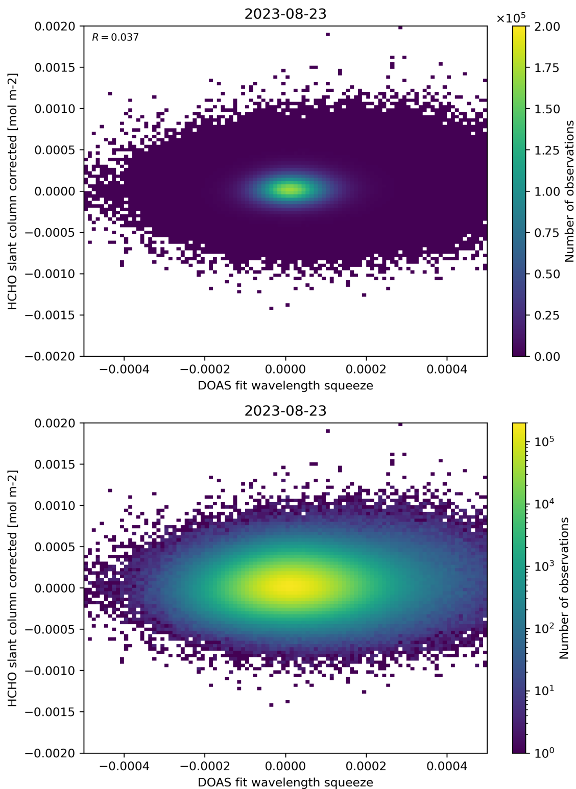
Figure 69: Scatter density plot of “DOAS fit wavelength squeeze” against “HCHO slant column corrected” for 2023-08-22 to 2023-08-24.
