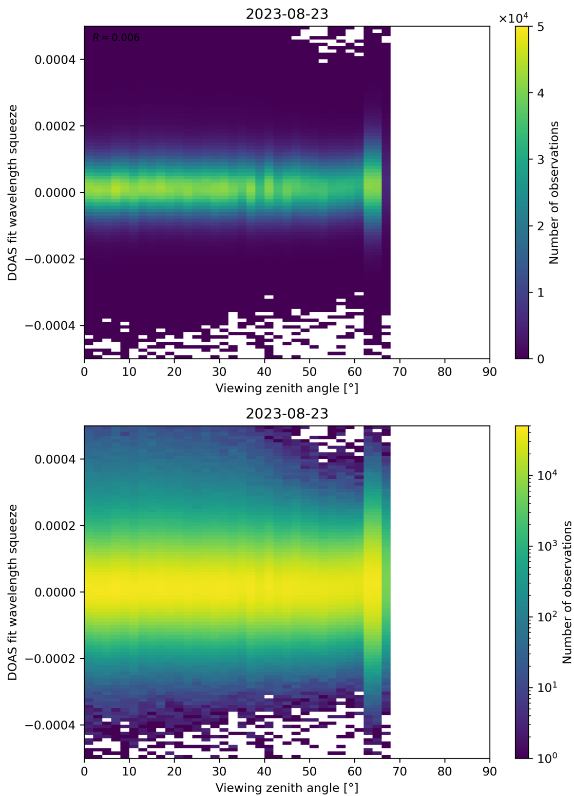
Figure 184: Scatter density plot of “Viewing zenith angle” against “DOAS fit wavelength squeeze” for 2023-08-22 to 2023-08-24.
