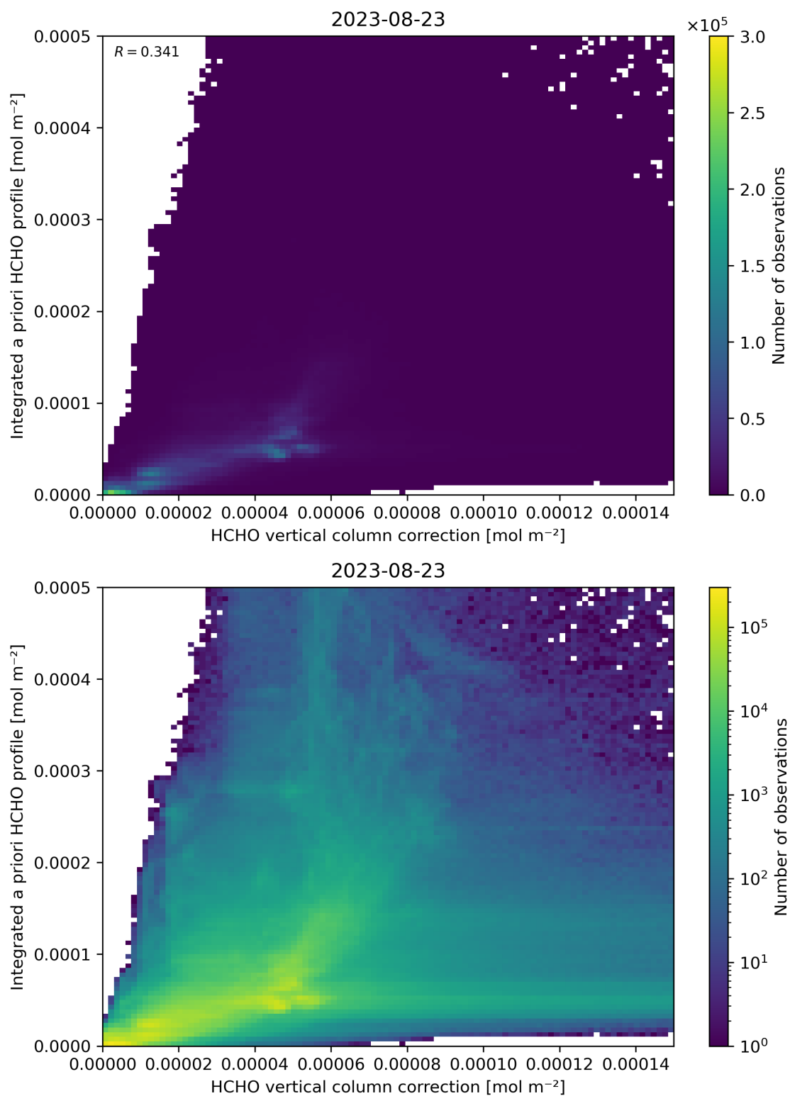
Figure 122: Scatter density plot of “HCHO vertical column correction” against “Integrated a priori HCHO profile” for 2023-08-22 to 2023-08-24.
