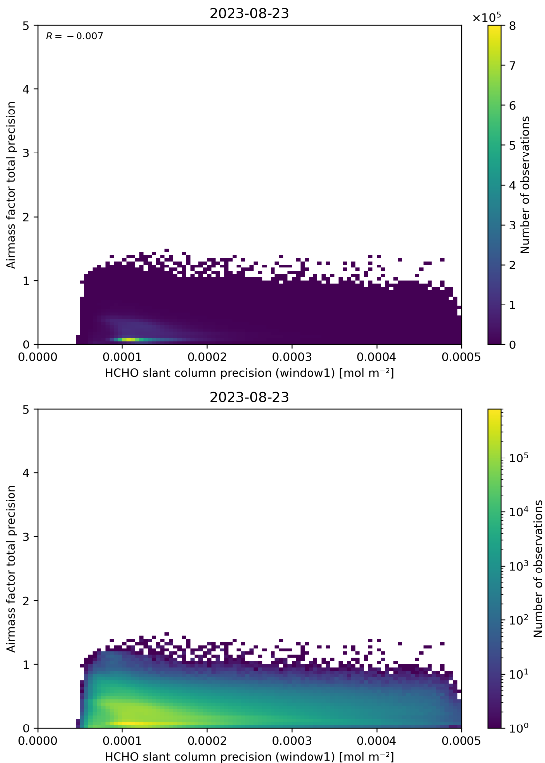
Figure 95: Scatter density plot of “HCHO slant column precision (window1)” against “Airmass factor total precision” for 2023-08-22 to 2023-08-24.
