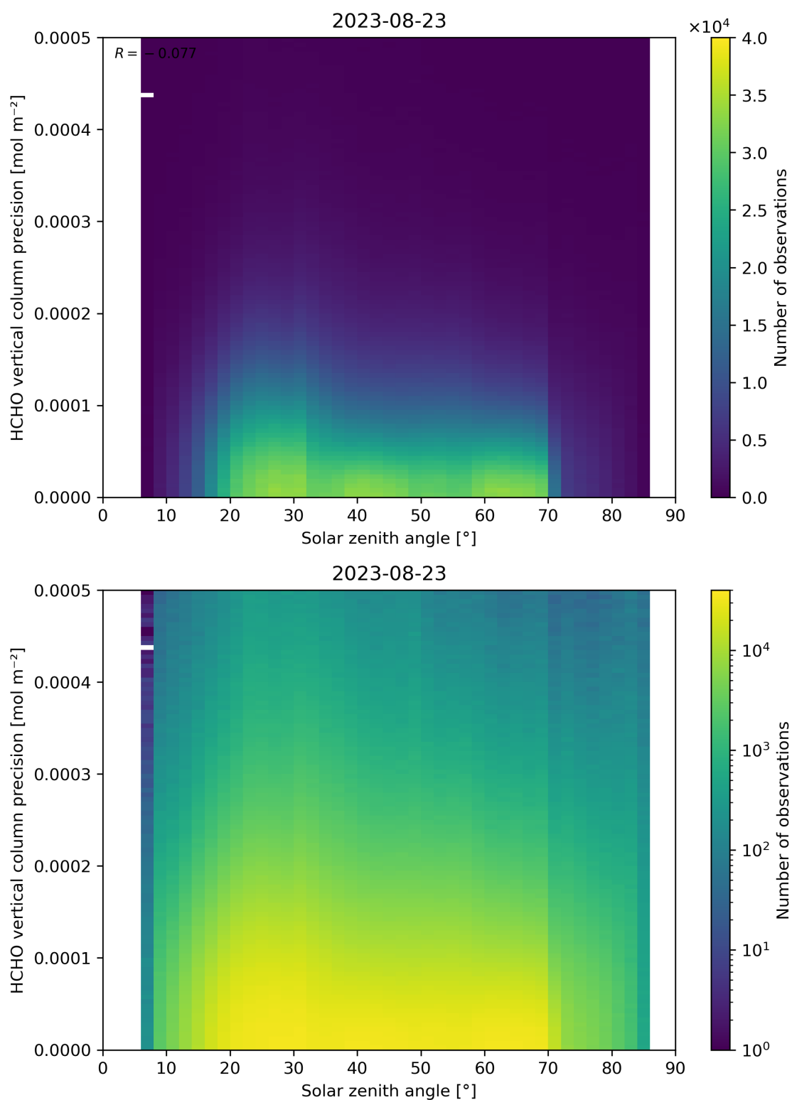
Figure 179: Scatter density plot of “Solar zenith angle” against “HCHO vertical column precision” for 2023-08-22 to 2023-08-24.
