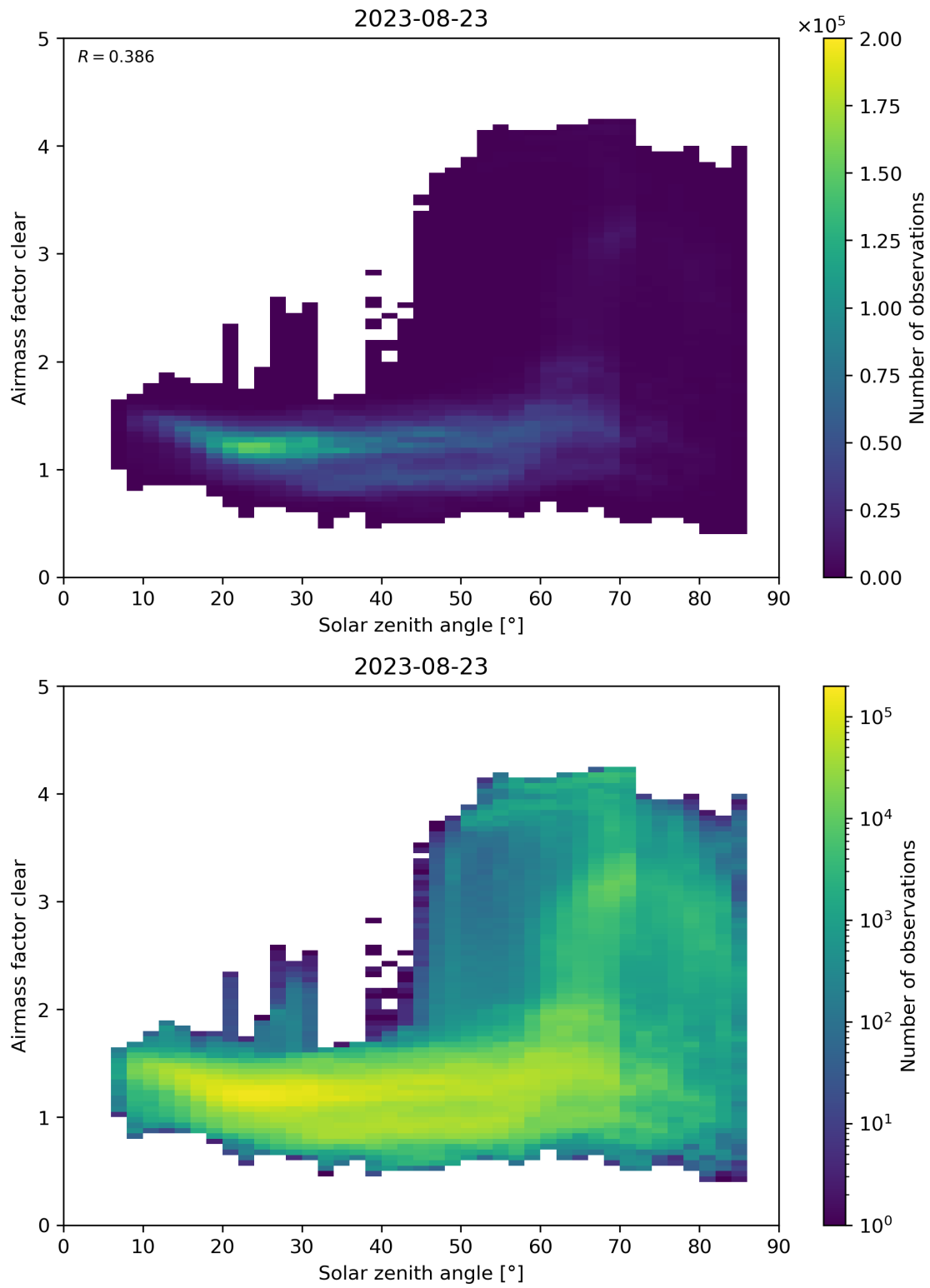
Figure 170: Scatter density plot of “Solar zenith angle” against “Airmass factor clear” for 2023-08-22 to 2023-08-24.
