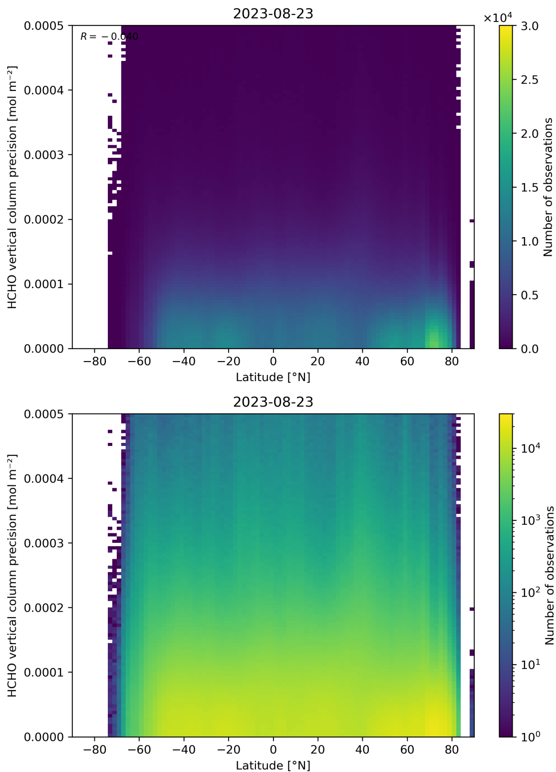
Figure 165: Scatter density plot of “Latitude” against “HCHO vertical column precision” for 2023-08-22 to 2023-08-24.
