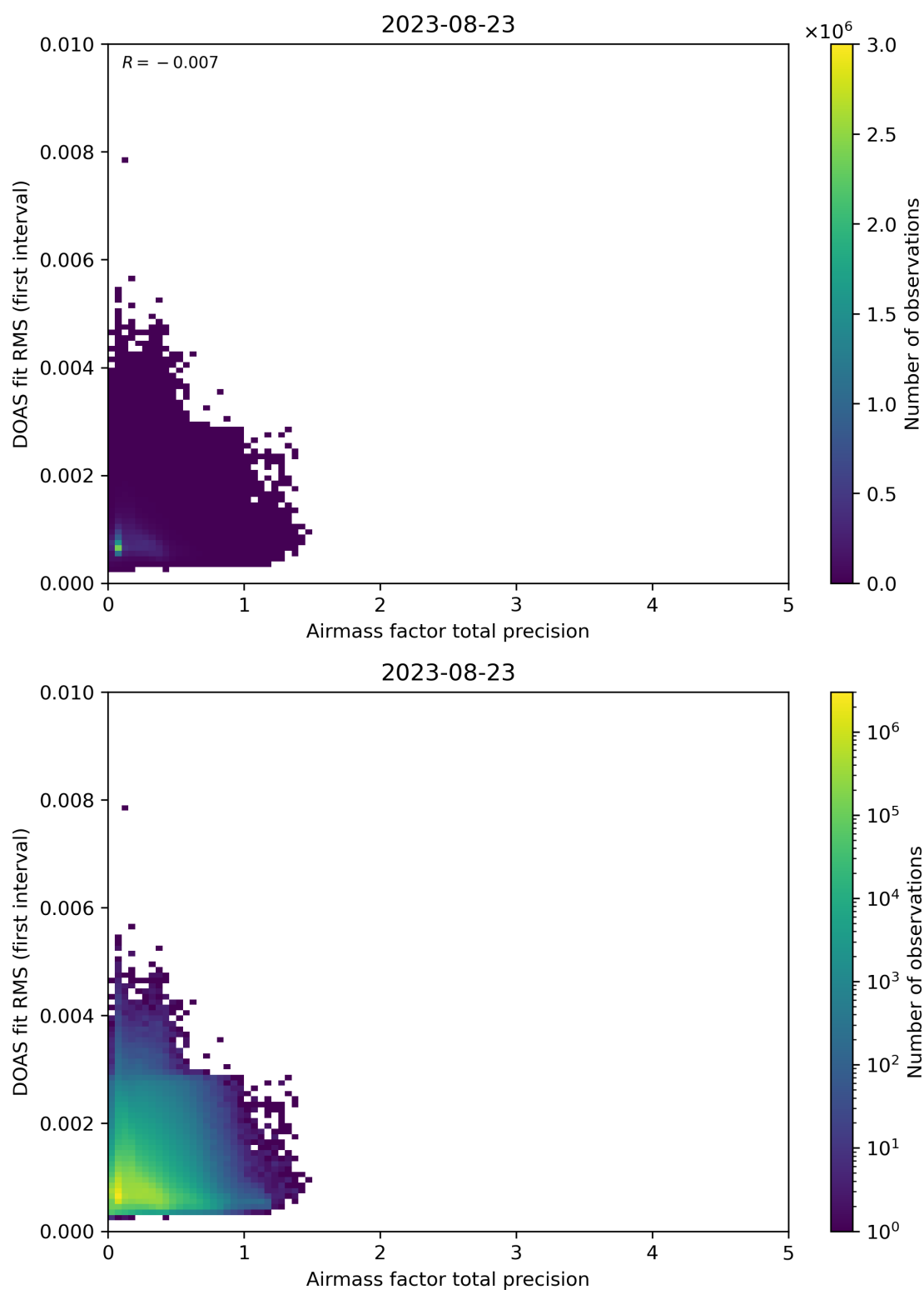
Figure 105: Scatter density plot of “Airmass factor total precision” against “DOAS fit RMS (first interval)” for 2023-08-22 to 2023-08-24.
