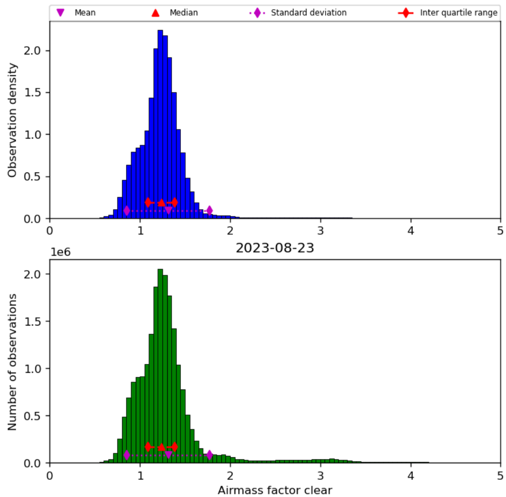
Figure 42: Histogram of “Airmass factor clear” for 2023-08-22 to 2023-08-24
