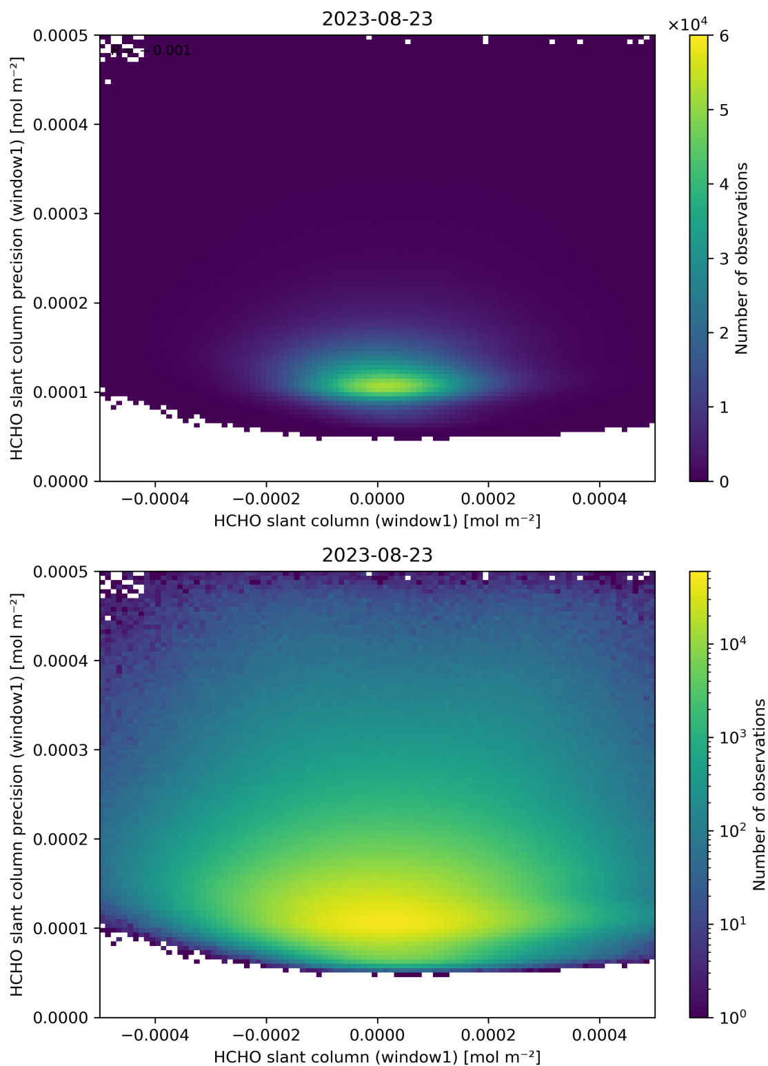
Figure 84: Scatter density plot of “HCHO slant column (window1)” against “HCHO slant column precision (window1)” for 2023-08-22 to 2023-08-24.
