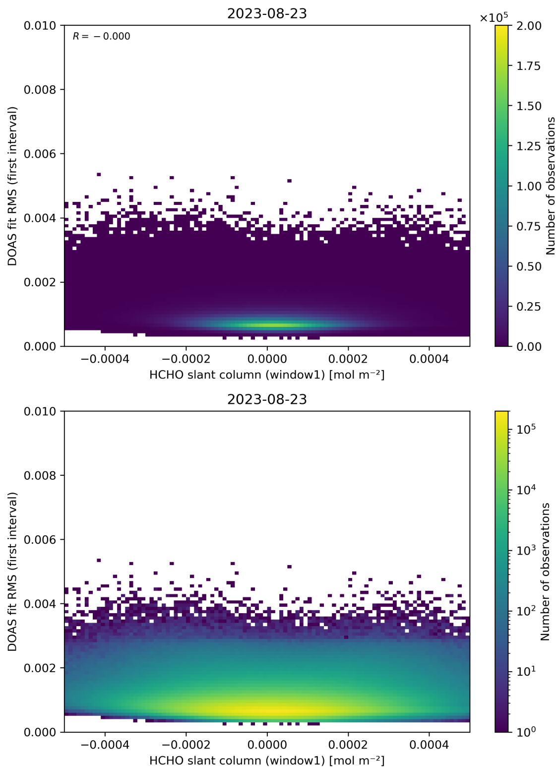
Figure 78: Scatter density plot of “HCHO slant column (window1)” against “DOAS fit RMS (first interval)” for 2023-08-22 to 2023-08-24.
