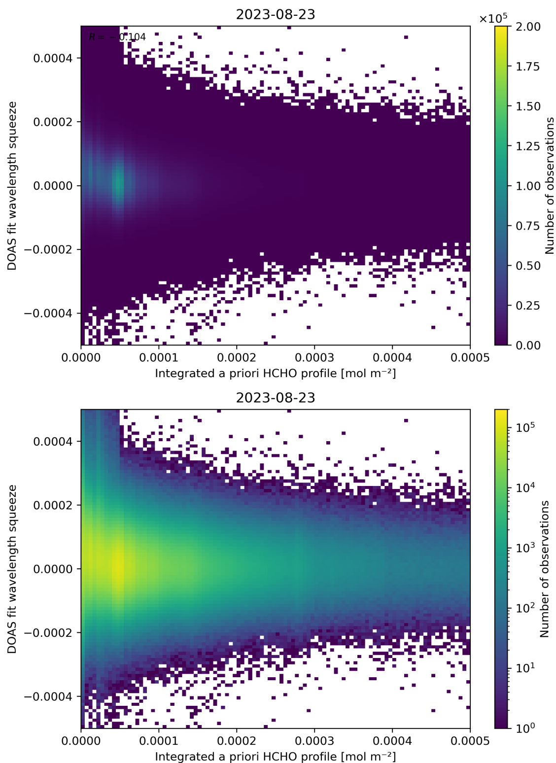
Figure 150: Scatter density plot of “Integrated a priori HCHO profile” against “DOAS fit wavelength squeeze” for 2023-08-22 to 2023-08-24.
