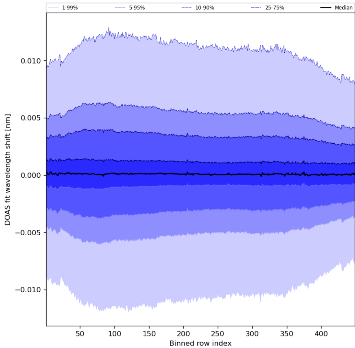
Figure 58: Along track statistics of “DOAS fit wavelength shift” for 2023-08-22 to 2023-08-24
