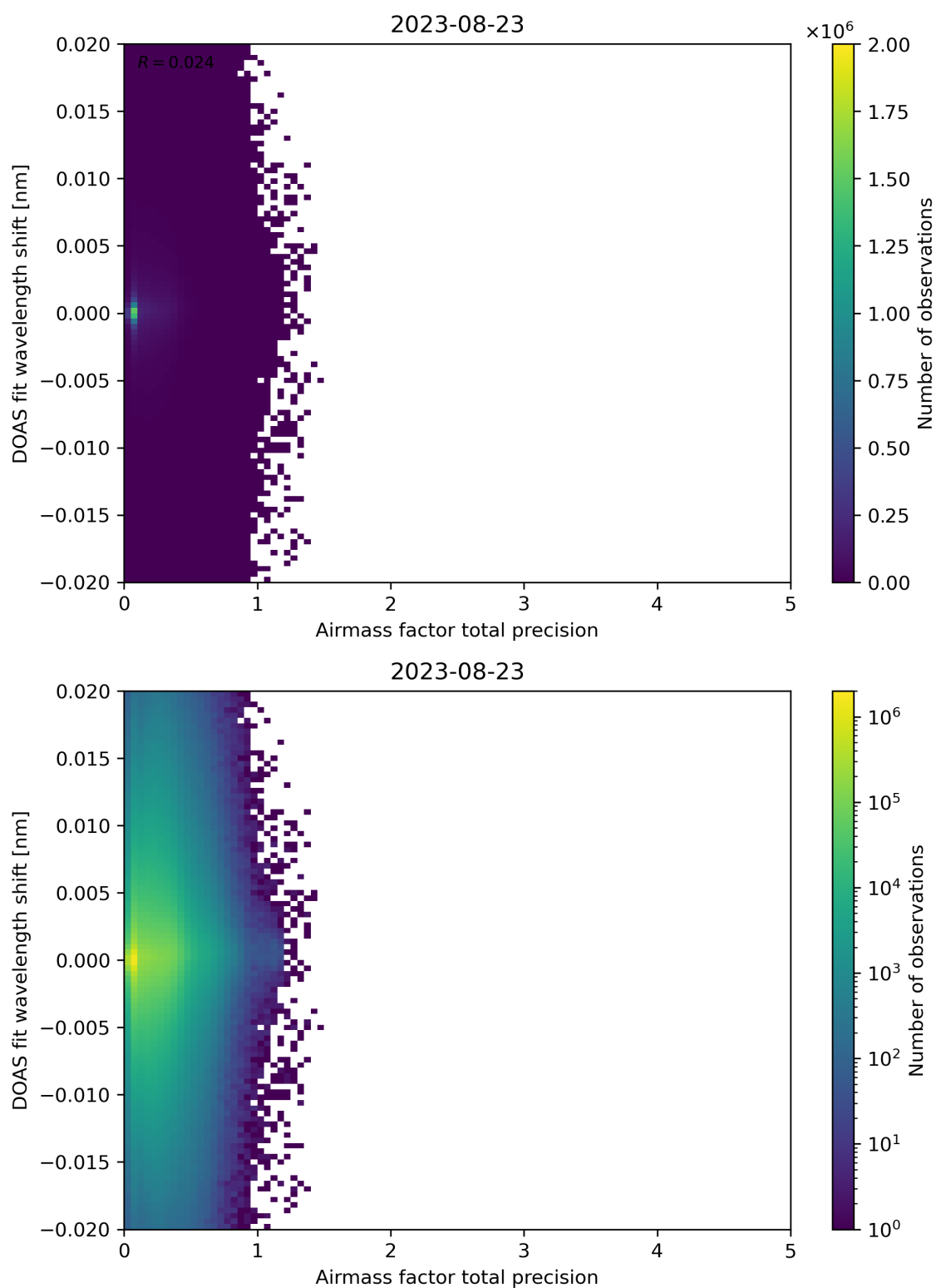
Figure 106: Scatter density plot of “Airmass factor total precision” against “DOAS fit wavelength shift” for 2023-08-22 to 2023-08-24.
