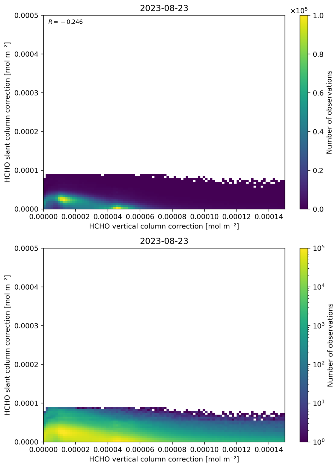
Figure 117: Scatter density plot of “HCHO vertical column correction” against “HCHO slant column correction” for 2023-08-22 to 2023-08-24.
