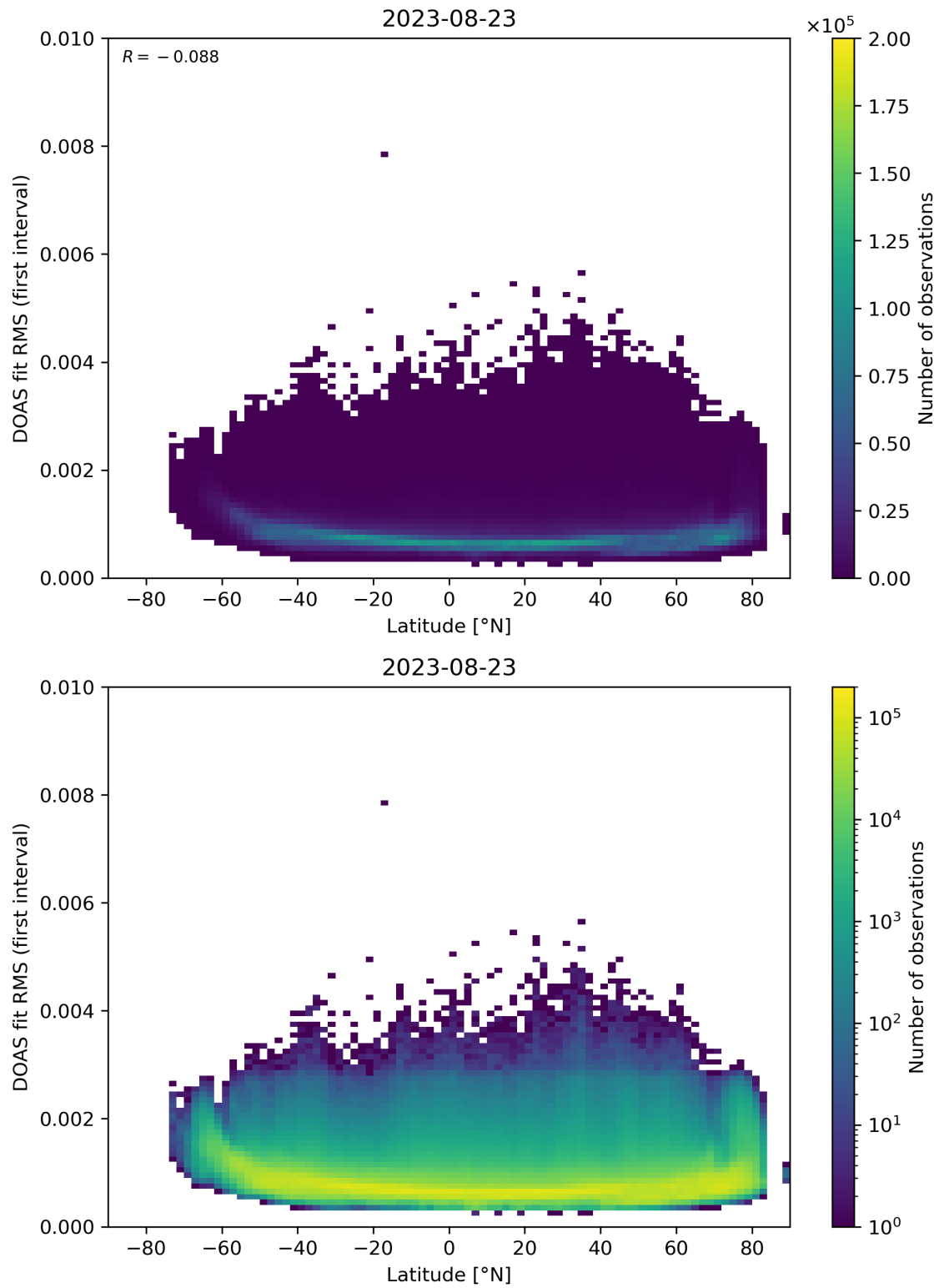
Figure 153: Scatter density plot of “Latitude” against “DOAS fit RMS (first interval)” for 2023-08-22 to 2023-08-24.
