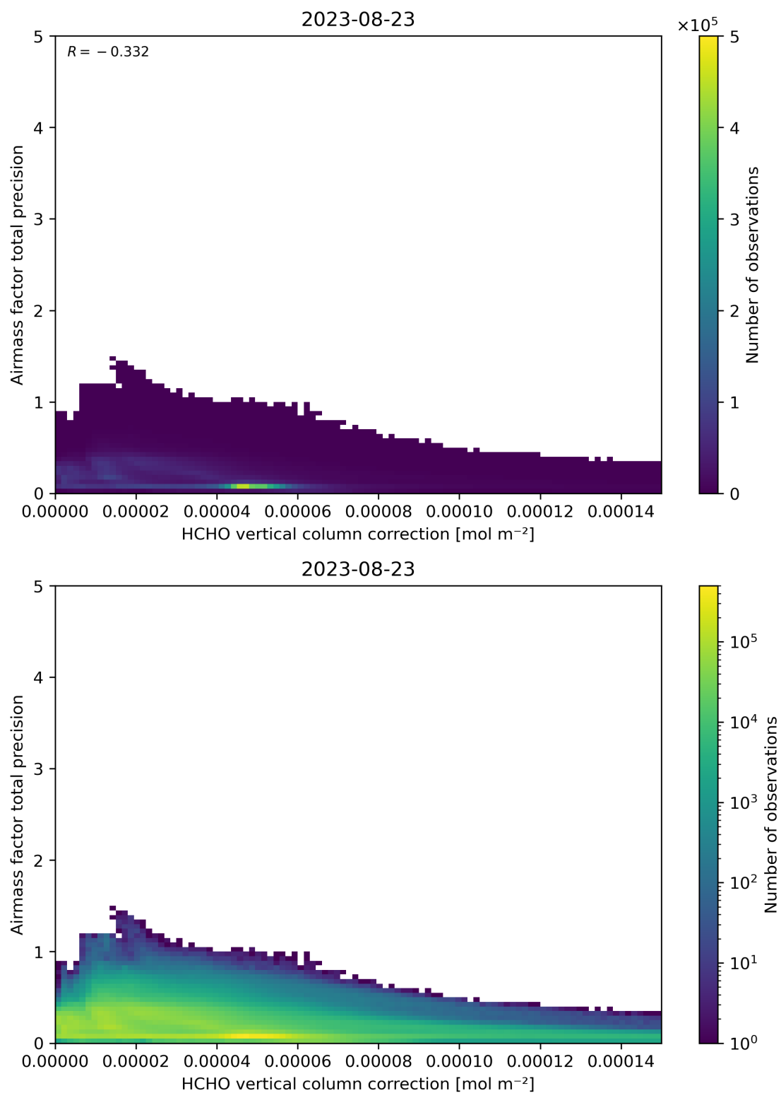
Figure 121: Scatter density plot of “HCHO vertical column correction” against “Airmass factor total precision” for 2023-08-22 to 2023-08-24.
