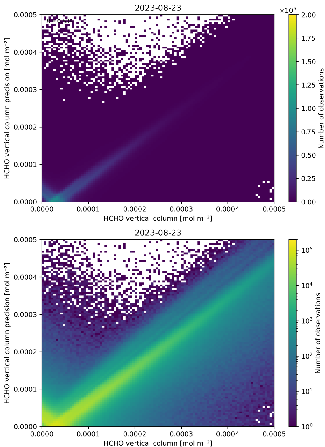
Figure 134: Scatter density plot of “HCHO vertical column” against “HCHO vertical column precision” for 2023-08-22 to 2023-08-24.
