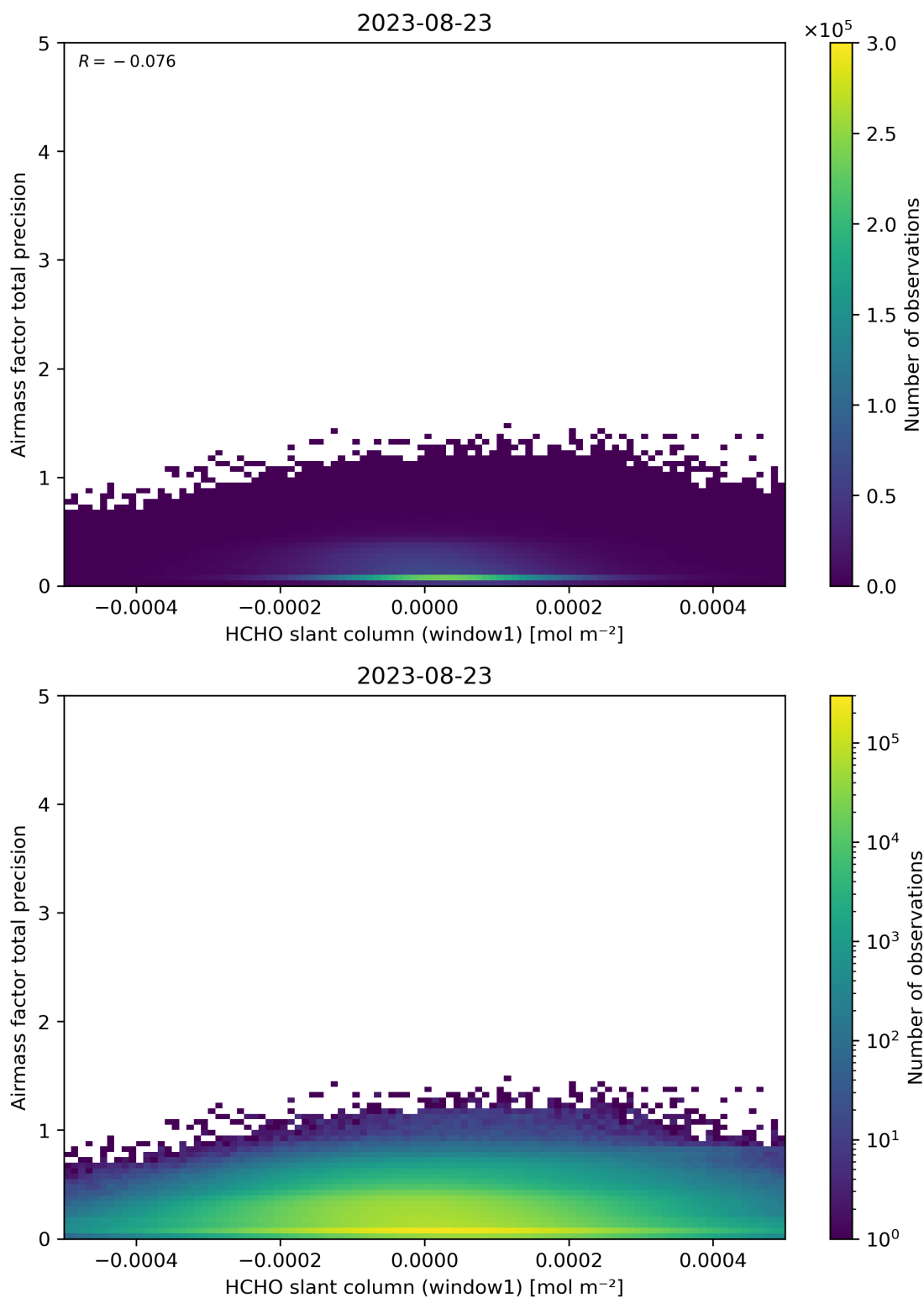
Figure 86: Scatter density plot of “HCHO slant column (window1)” against “Airmass factor total precision” for 2023-08-22 to 2023-08-24.
