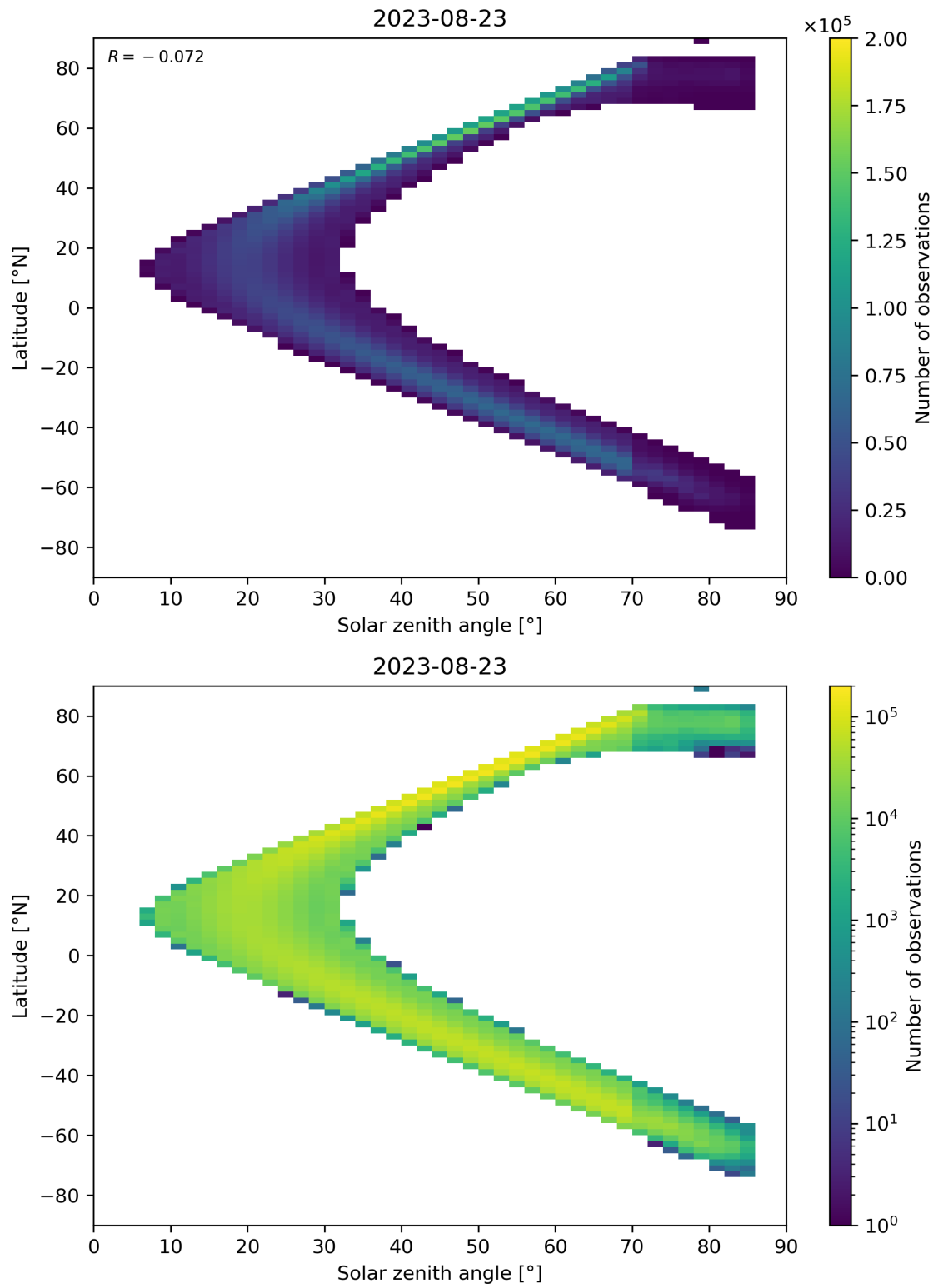
Figure 181: Scatter density plot of “Solar zenith angle” against “Latitude” for 2023-08-22 to 2023-08-24.
