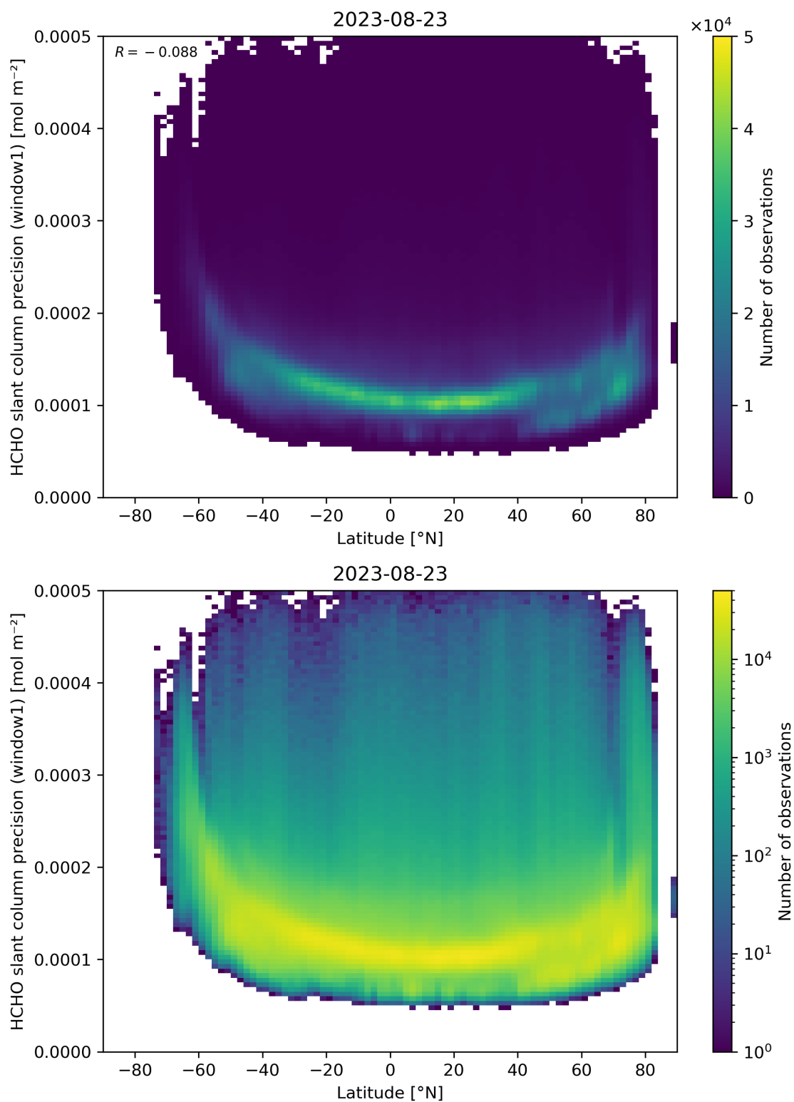
Figure 160: Scatter density plot of “Latitude” against “HCHO slant column precision (window1)” for 2023-08-22 to 2023-08-24.
