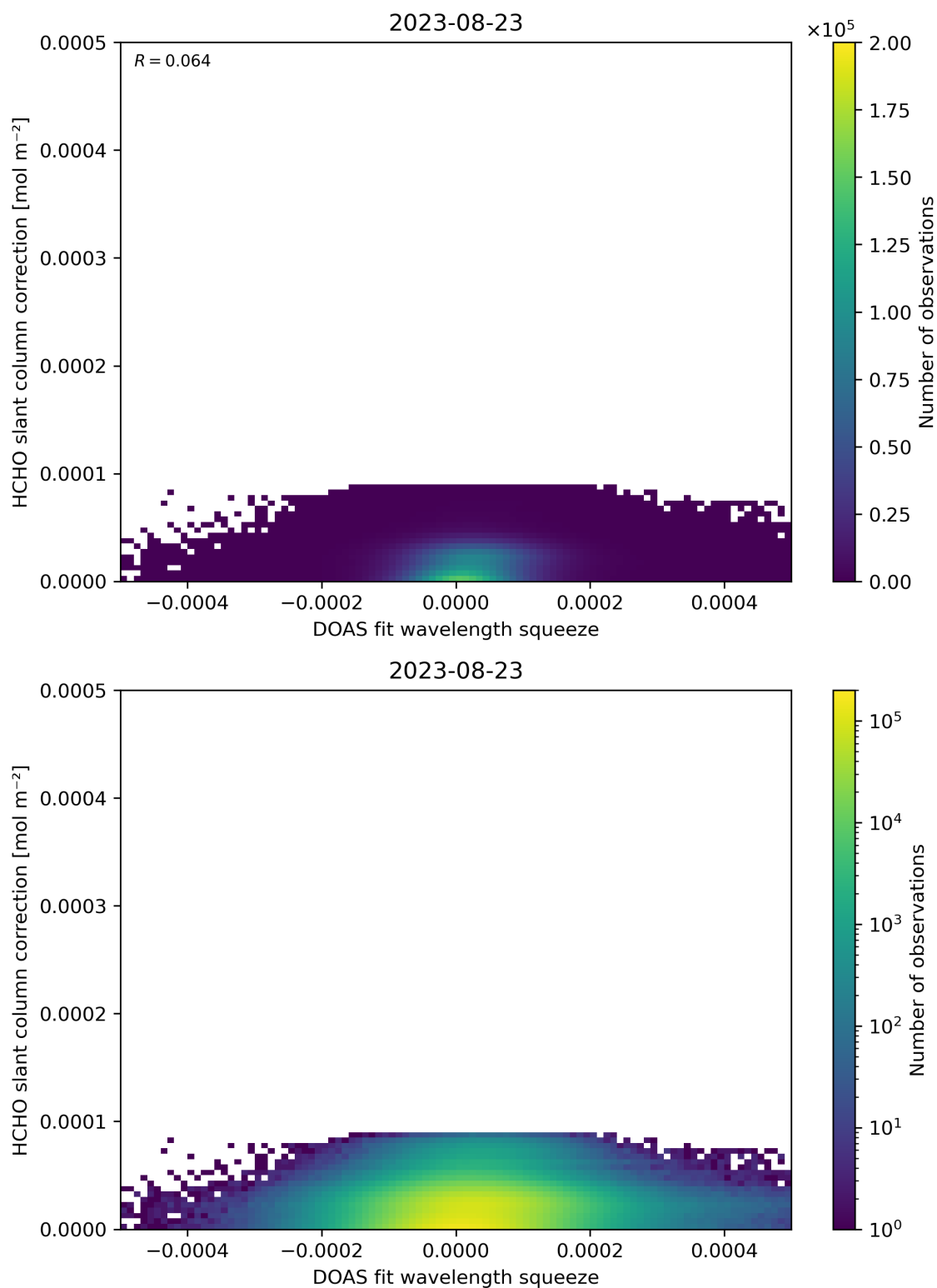
Figure 70: Scatter density plot of “DOAS fit wavelength squeeze” against “HCHO slant column correction” for 2023-08-22 to 2023-08-24.
