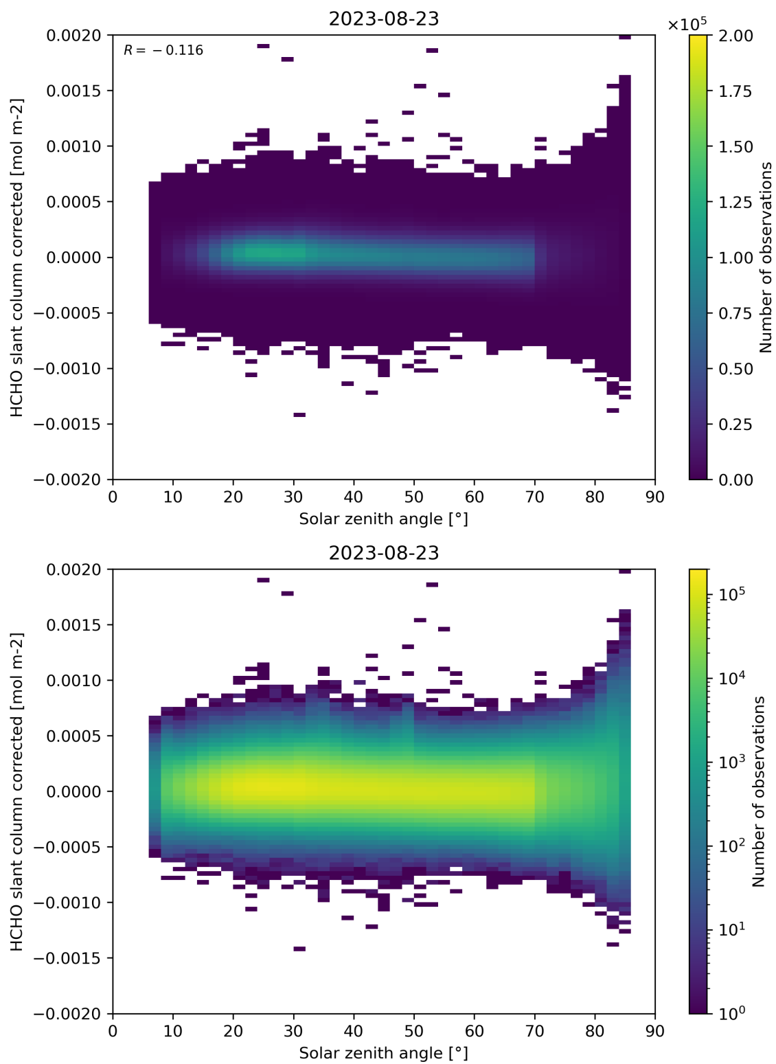
Figure 171: Scatter density plot of “Solar zenith angle” against “HCHO slant column corrected” for 2023-08-22 to 2023-08-24.
