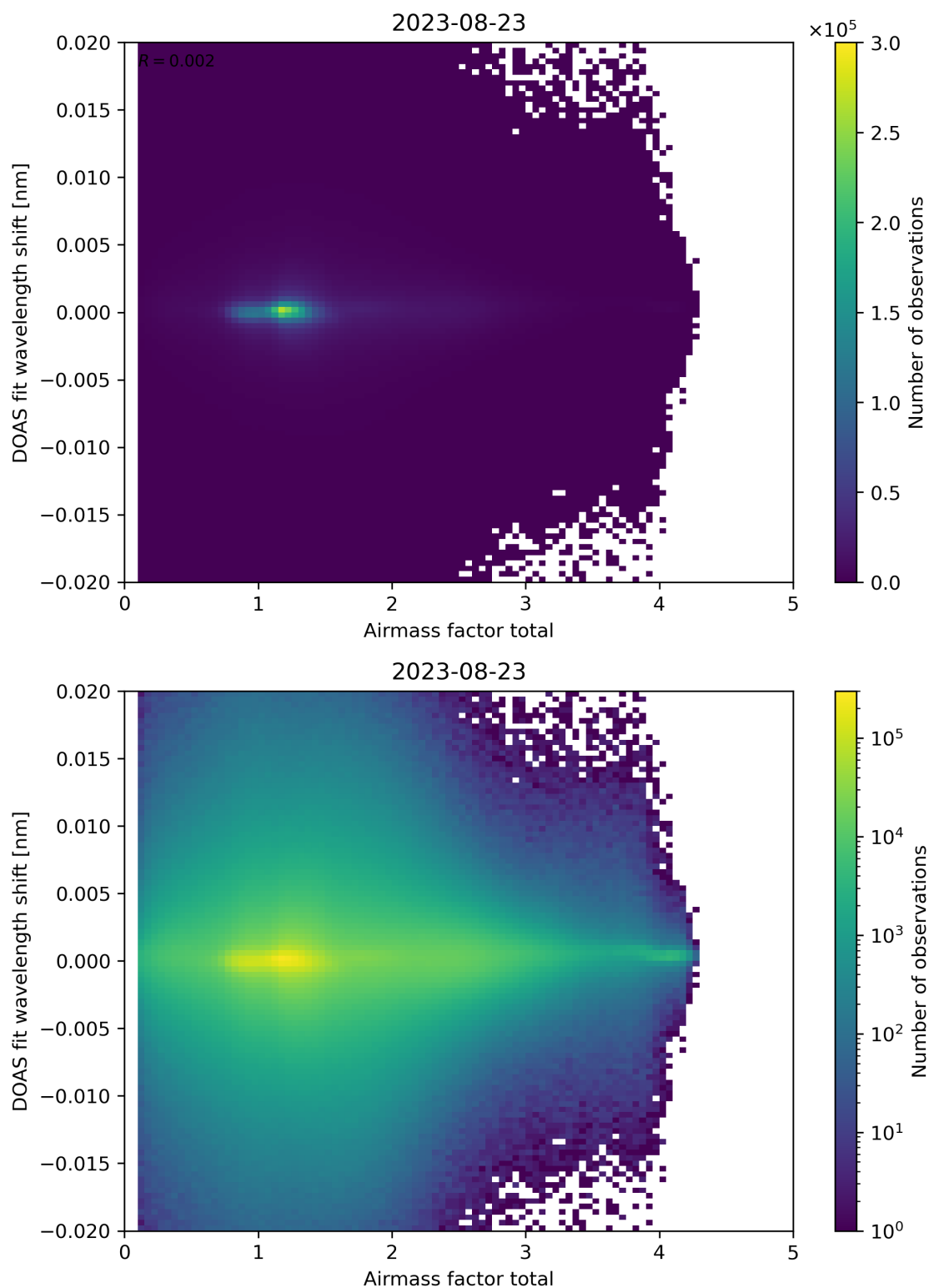
Figure 98: Scatter density plot of “Airmass factor total” against “DOAS fit wavelength shift” for 2023-08-22 to 2023-08-24.
