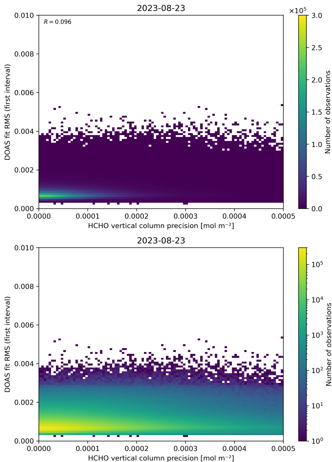
Figure 136: Scatter density plot of “HCHO vertical column precision” against “DOAS fit RMS (first interval)” for 2023-08-22 to 2023-08-24.
