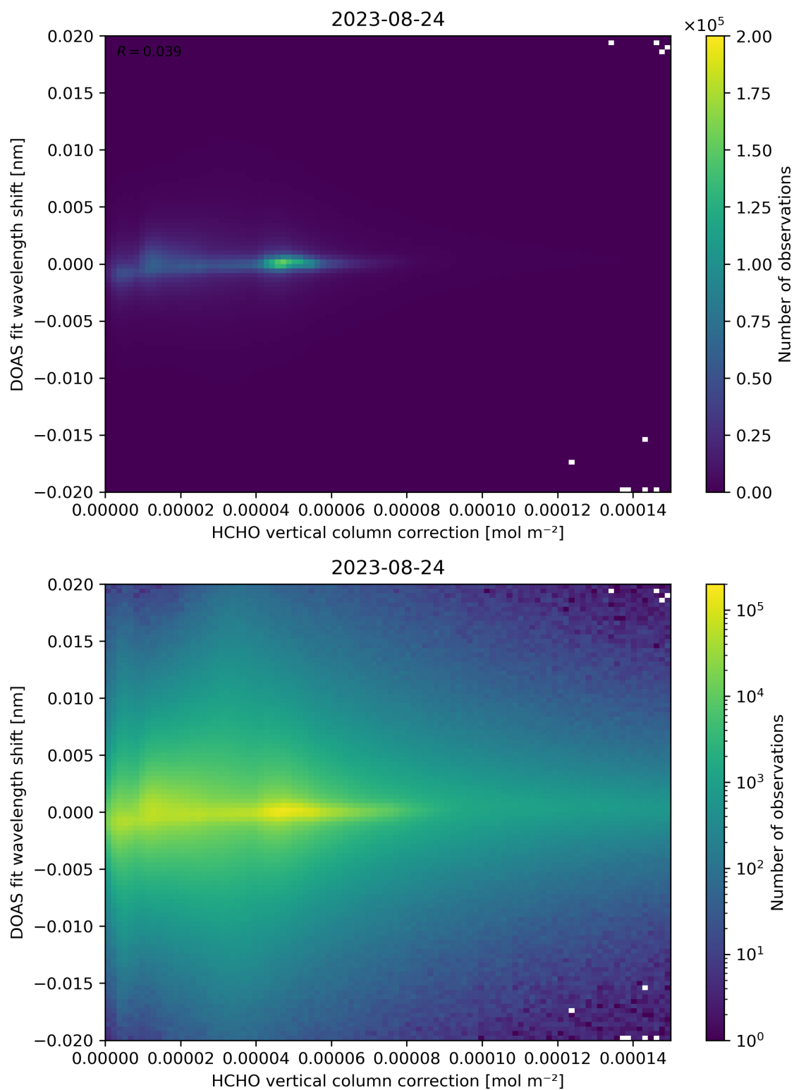
Figure 113: Scatter density plot of “HCHO vertical column correction” against “DOAS fit wavelength shift” for 2023-08-23 to 2023-08-25.
