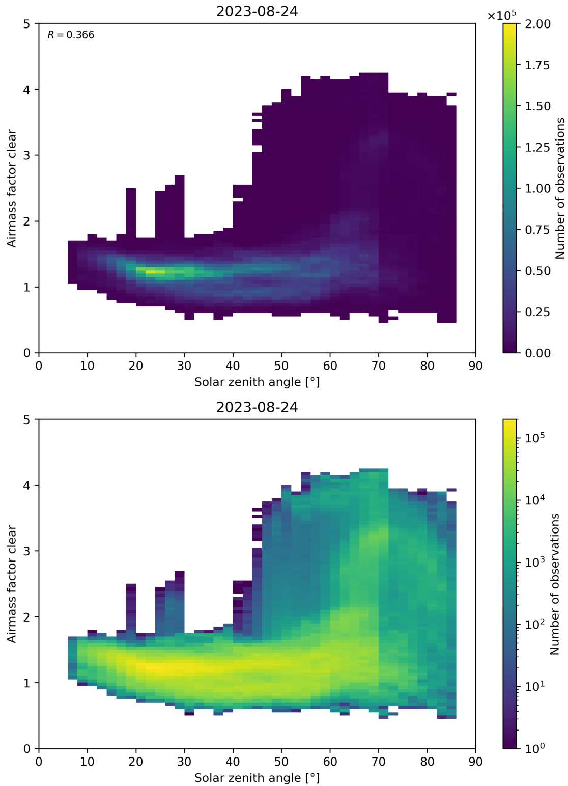
Figure 170: Scatter density plot of “Solar zenith angle” against “Airmass factor clear” for 2023-08-23 to 2023-08-25.
