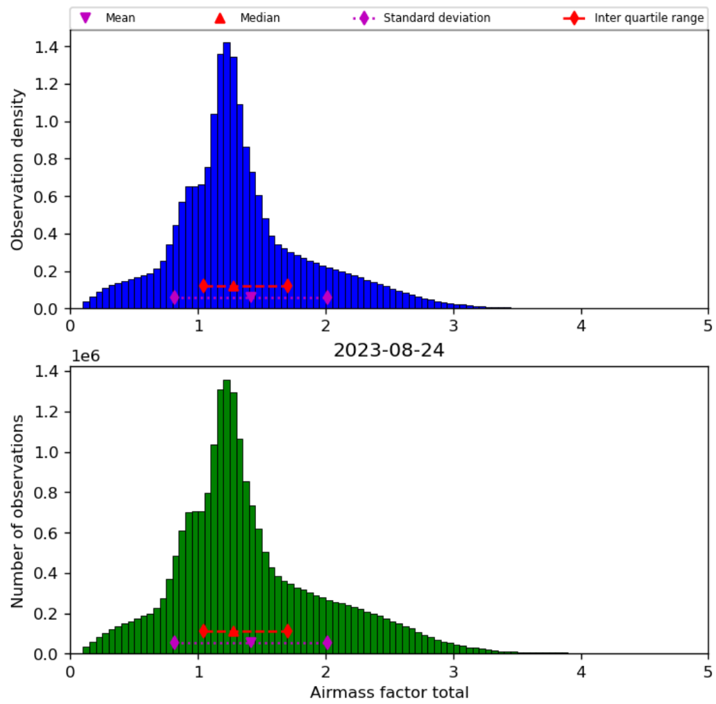
Figure 40: Histogram of “Airmass factor total” for 2023-08-23 to 2023-08-25
