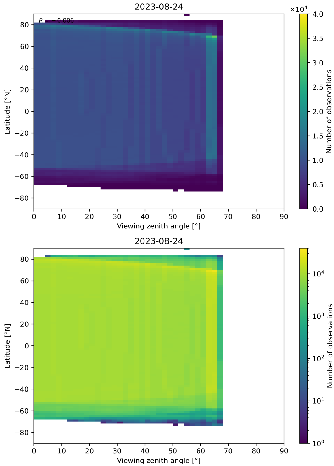
Figure 196: Scatter density plot of “Viewing zenith angle” against “Latitude” for 2023-08-23 to 2023-08-25.
