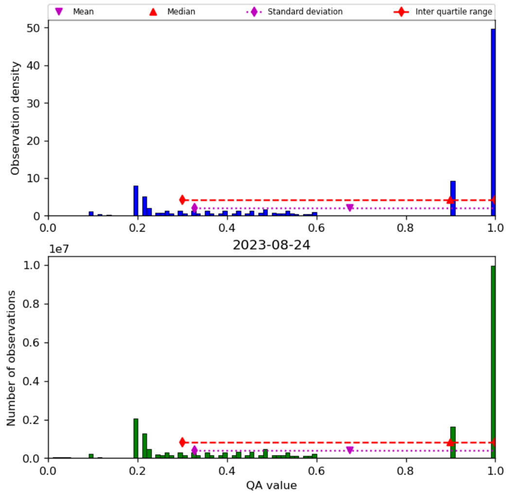
Figure 34: Histogram of “QA value” for 2023-08-23 to 2023-08-25
