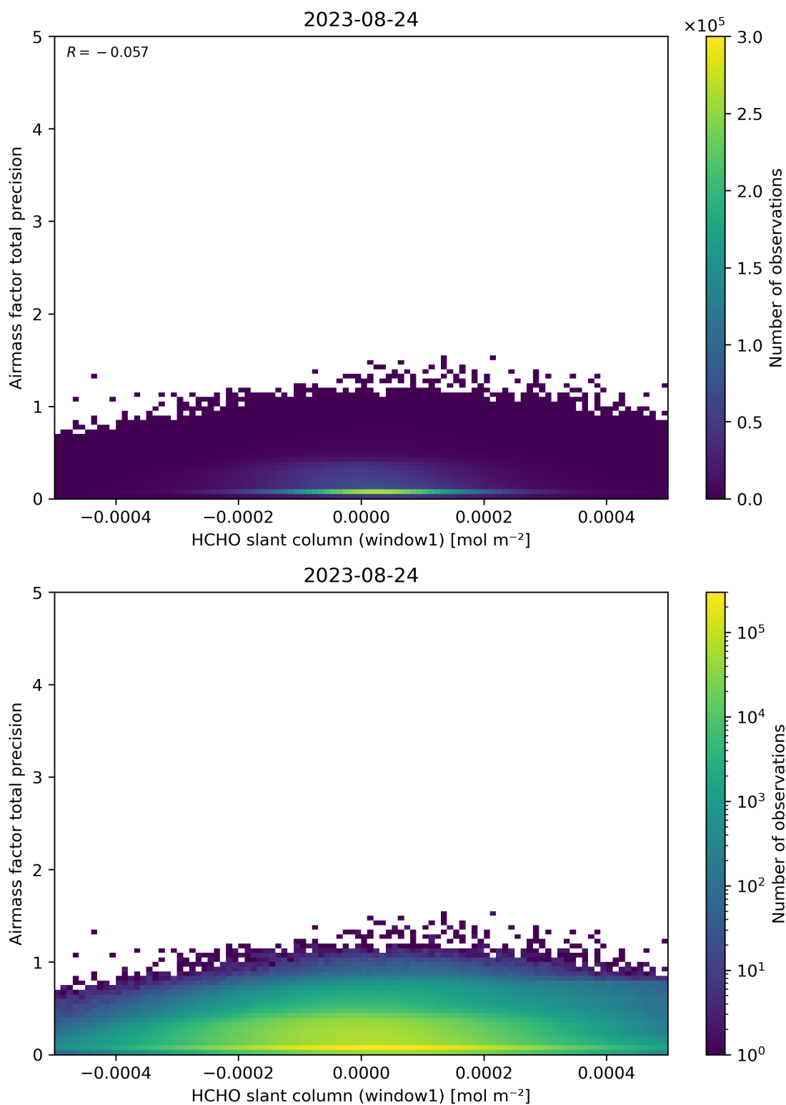
Figure 86: Scatter density plot of “HCHO slant column (window1)” against “Airmass factor total precision” for 2023-08-23 to 2023-08-25.
