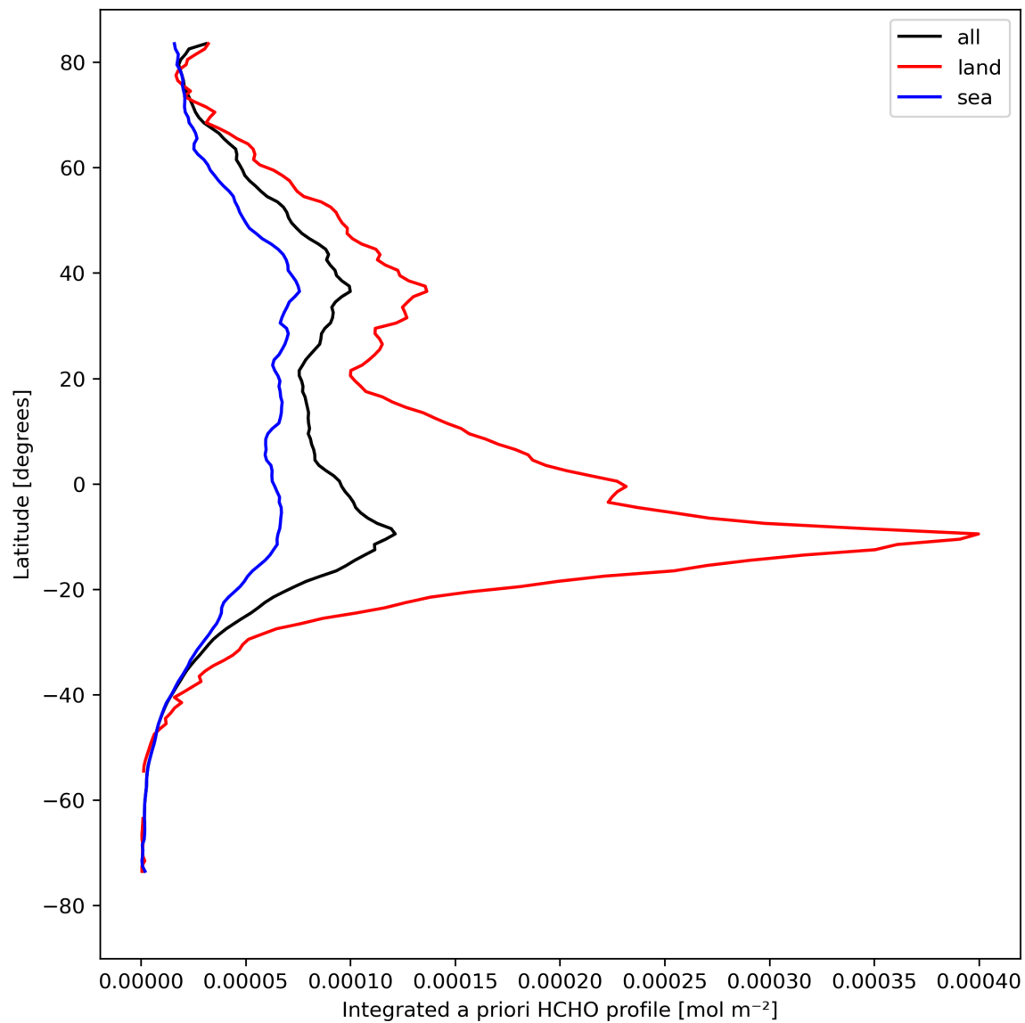
Figure 29: Zonal average of “Integrated a priori HCHO profile” for 2023-08-23 to 2023-08-25.
