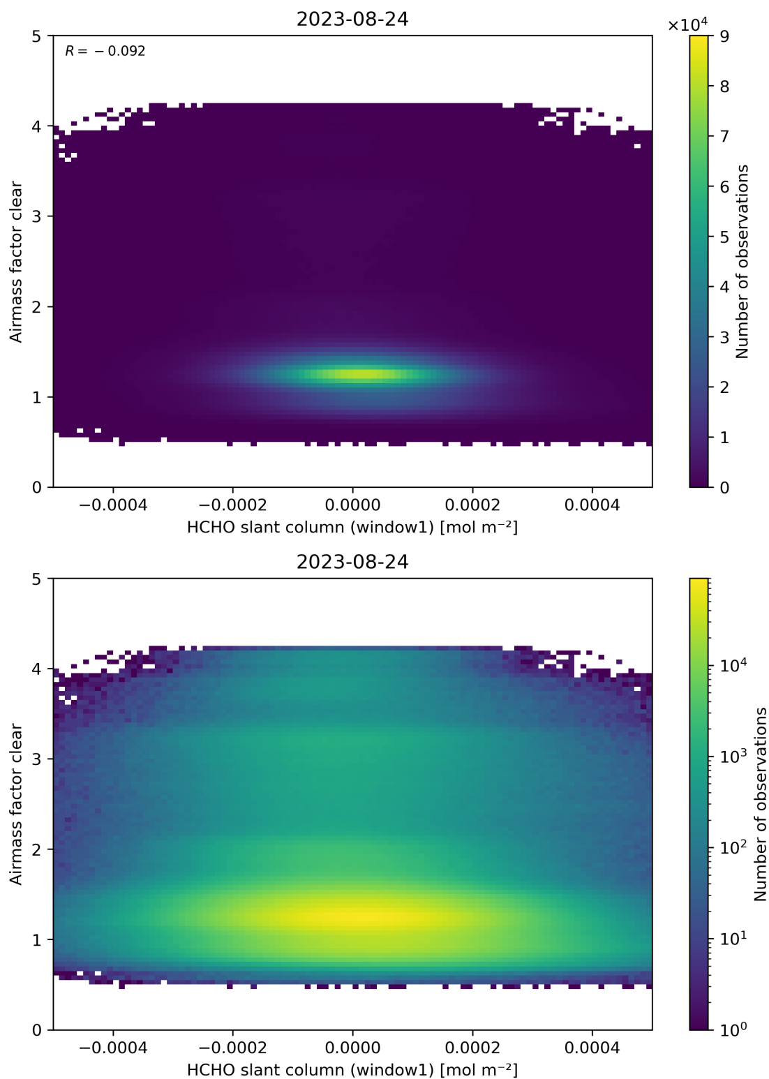
Figure 81: Scatter density plot of “HCHO slant column (window1)” against “Airmass factor clear” for 2023-08-23 to 2023-08-25.
