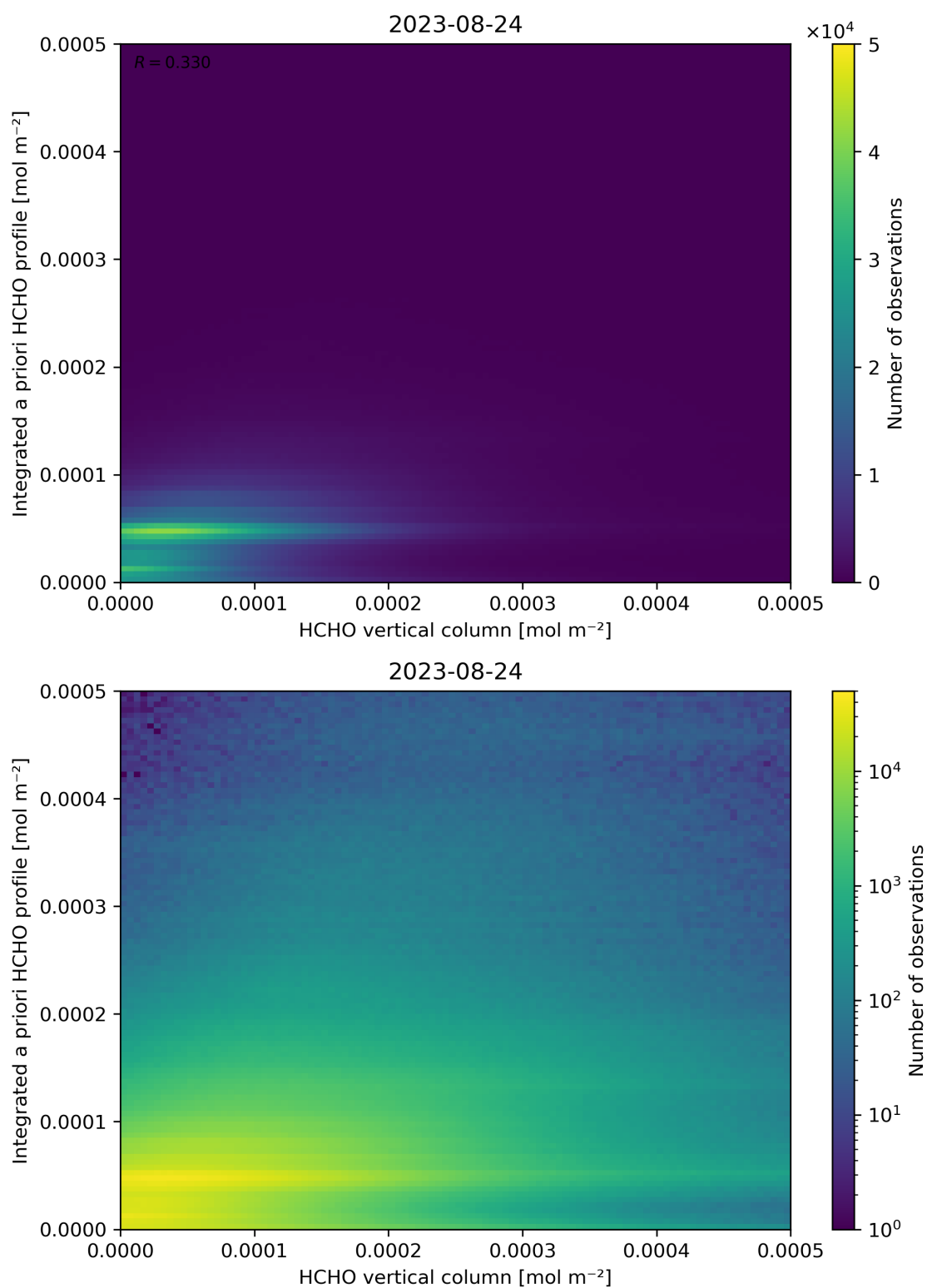
Figure 135: Scatter density plot of “HCHO vertical column” against “Integrated a priori HCHO profile” for 2023-08-23 to 2023-08-25.
