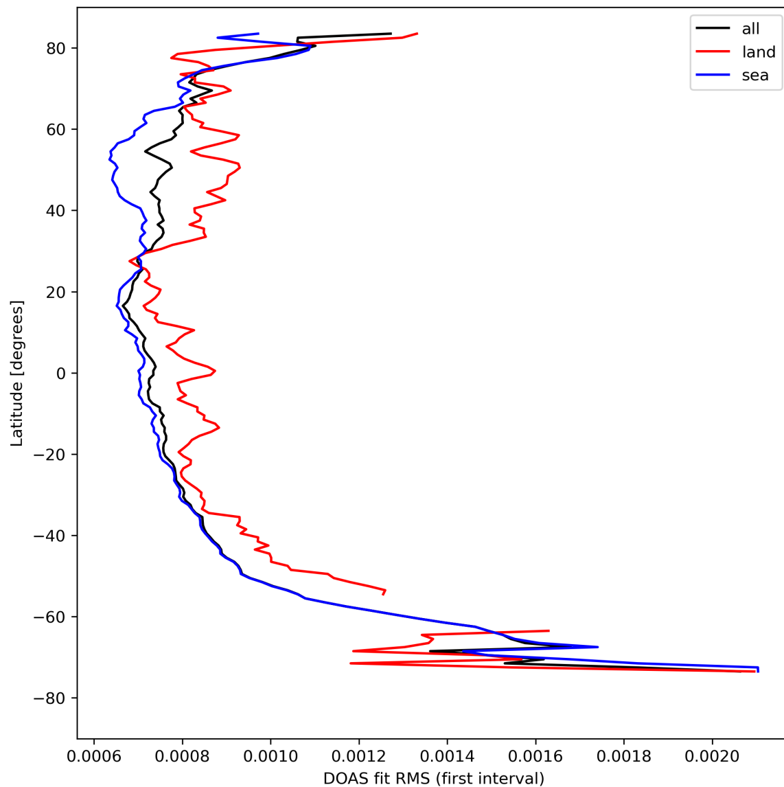
Figure 32: Zonal average of “DOAS fit RMS (first interval)” for 2023-08-23 to 2023-08-25.
