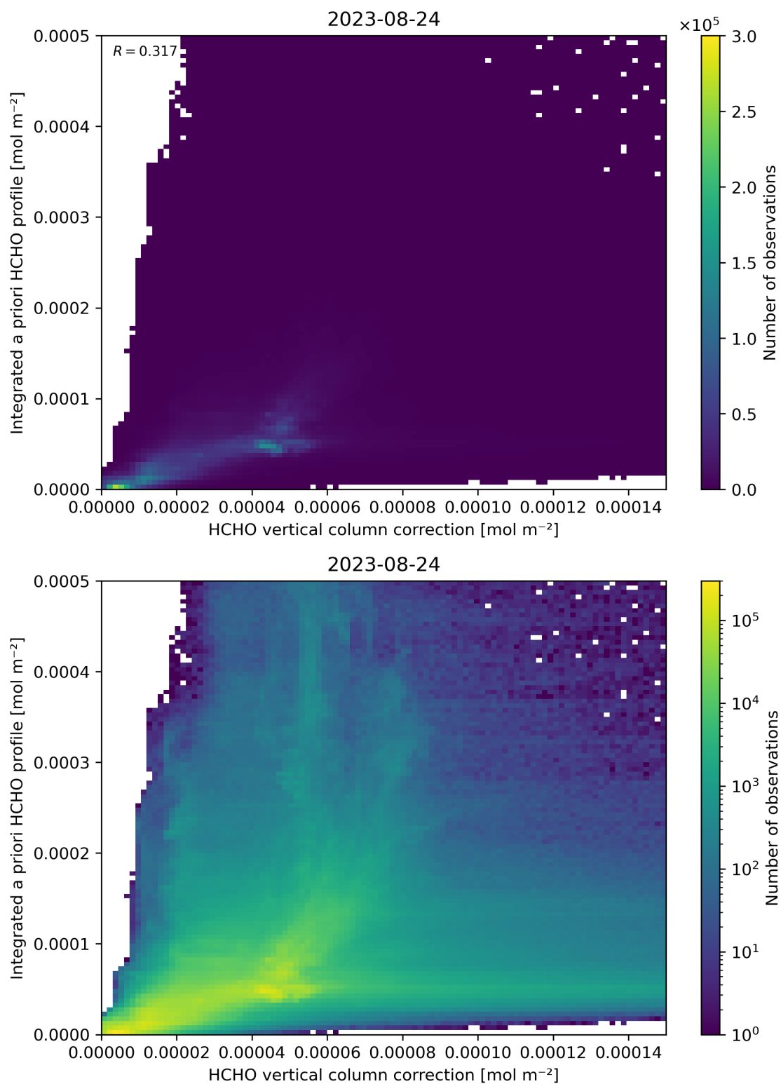
Figure 122: Scatter density plot of “HCHO vertical column correction” against “Integrated a priori HCHO profile” for 2023-08-23 to 2023-08-25.
