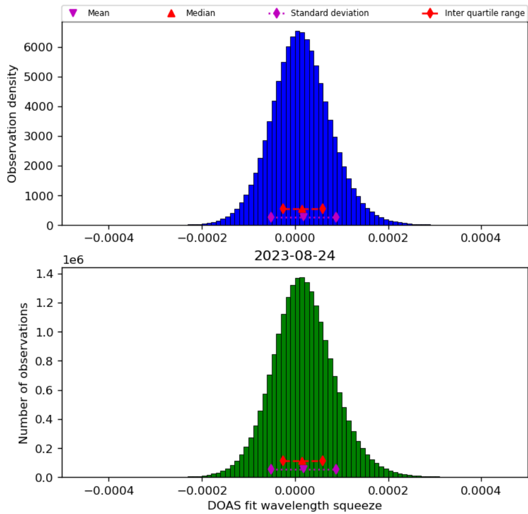
Figure 45: Histogram of “DOAS fit wavelength squeeze” for 2023-08-23 to 2023-08-25
