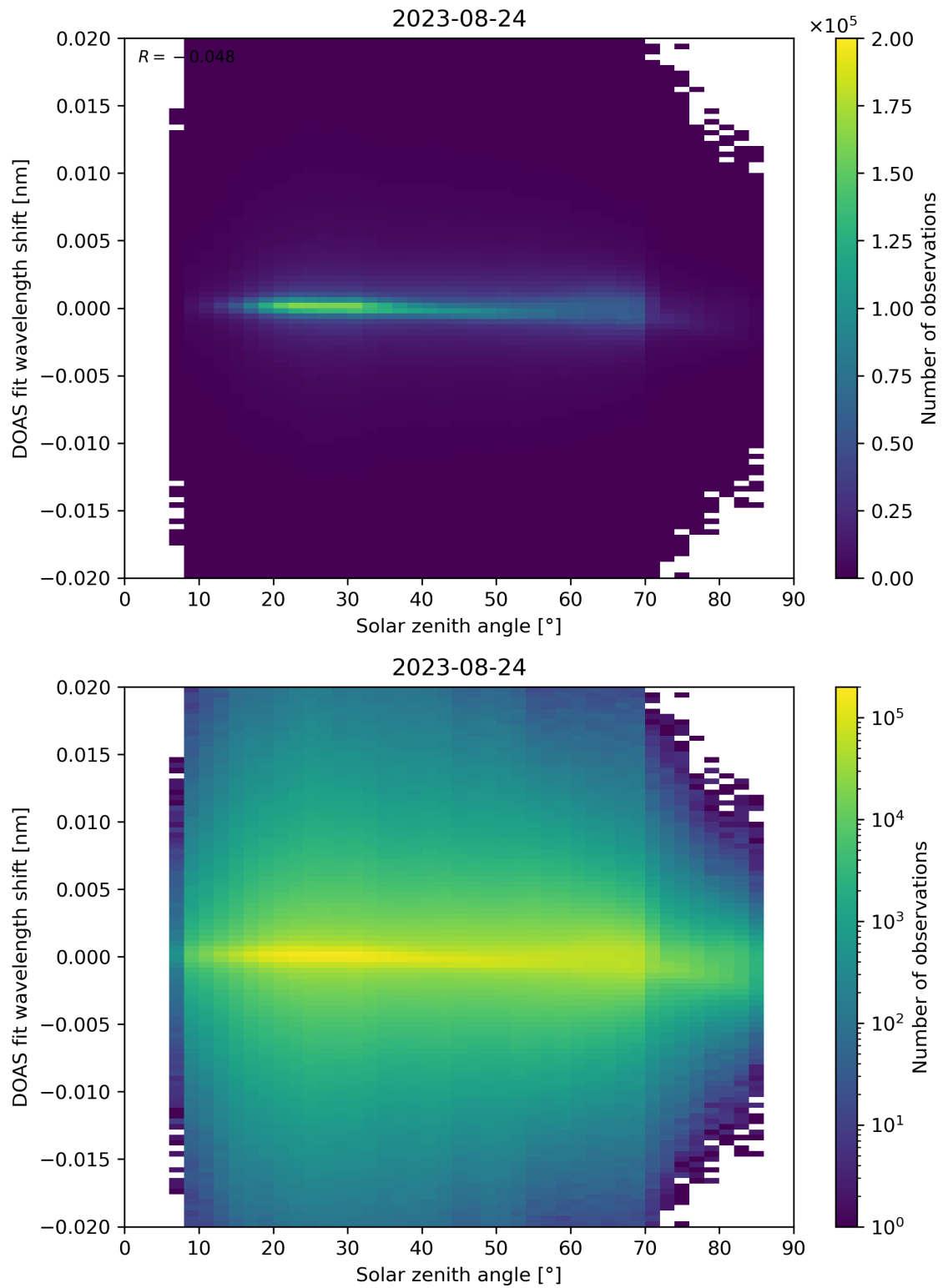
Figure 168: Scatter density plot of “Solar zenith angle” against “DOAS fit wavelength shift” for 2023-08-23 to 2023-08-25.
