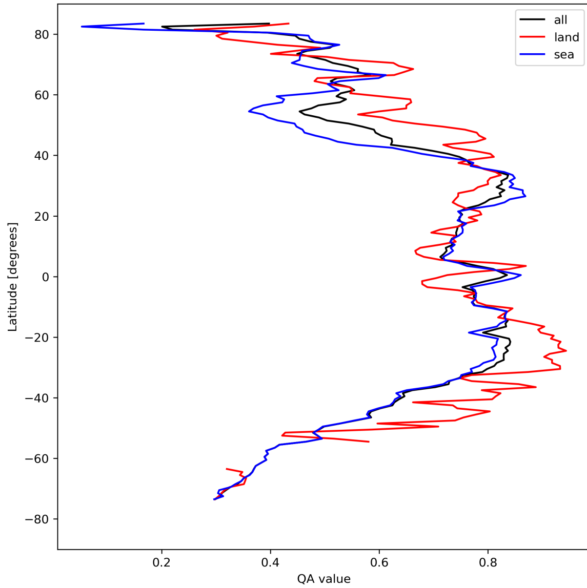
Figure 20: Zonal average of “QA value” for 2023-08-23 to 2023-08-25.
