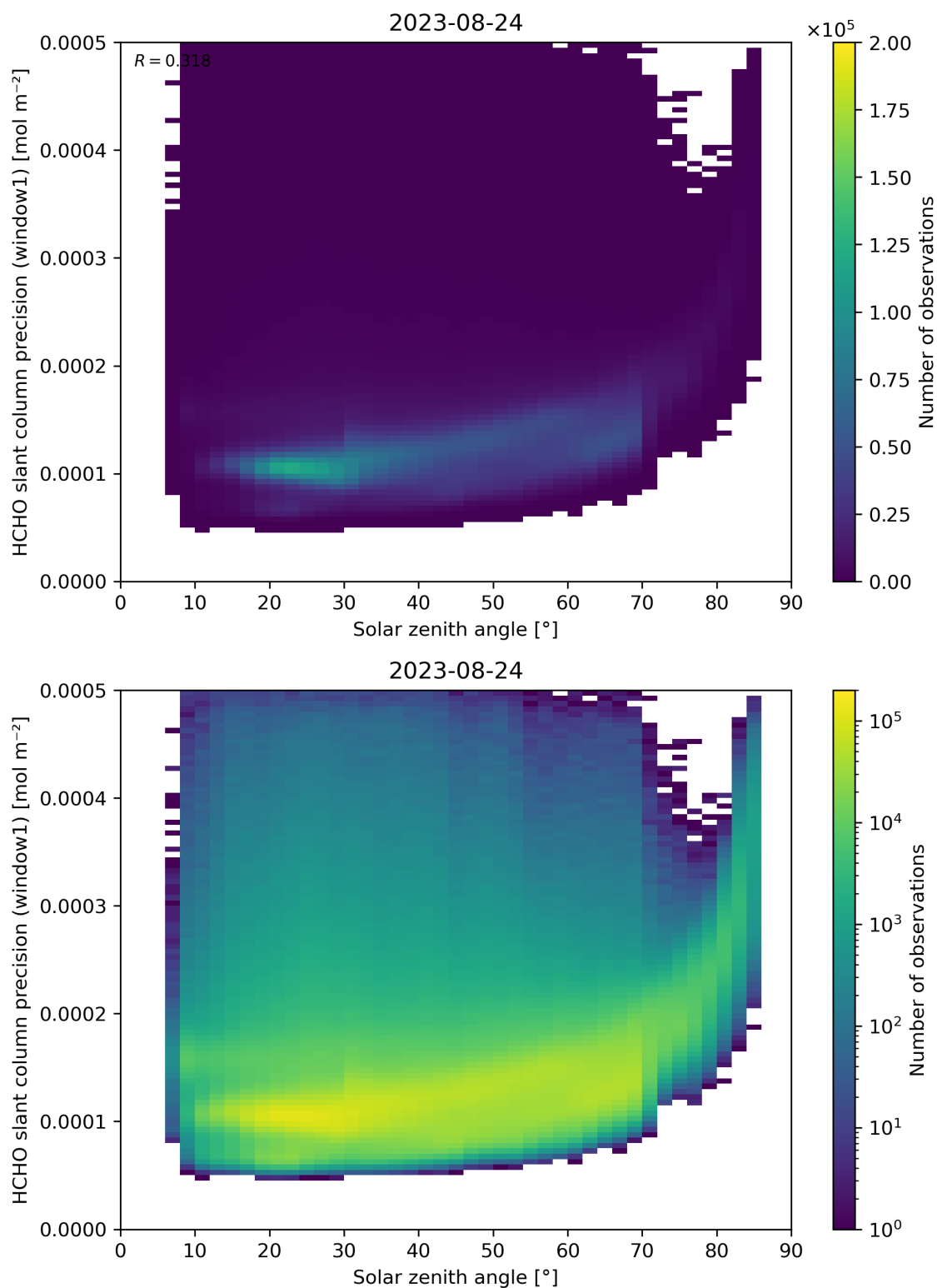
Figure 174: Scatter density plot of “Solar zenith angle” against “HCHO slant column precision (window1)” for 2023-08-23 to 2023-08-25.
