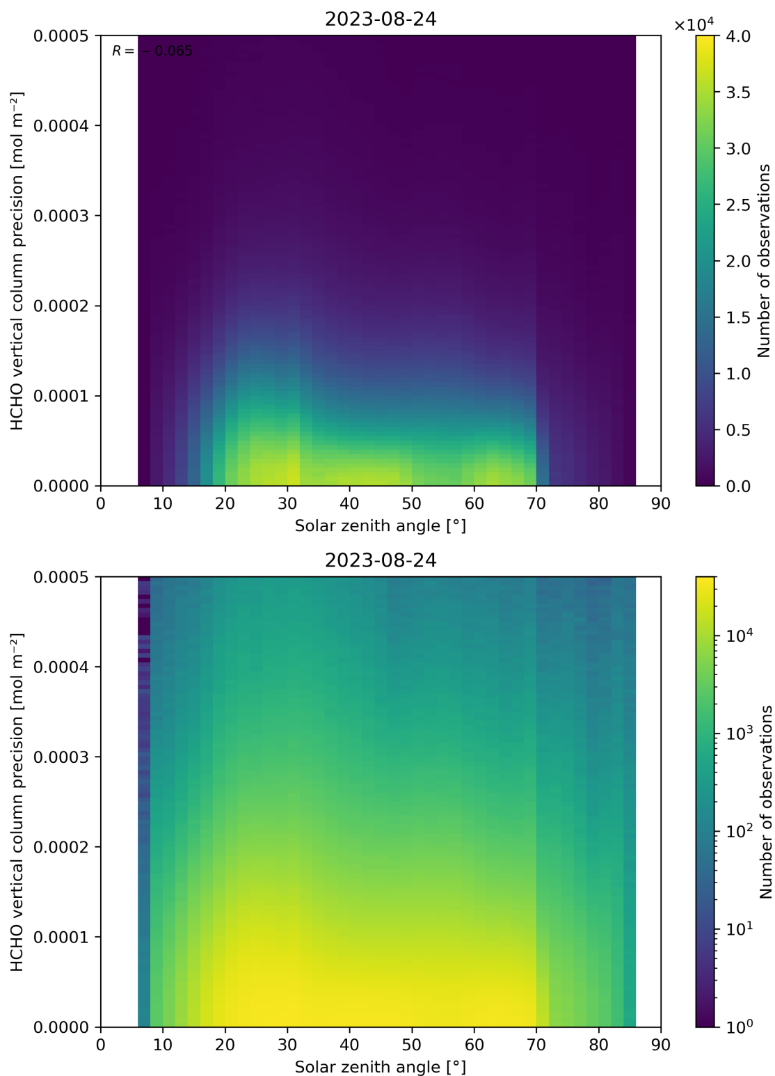
Figure 179: Scatter density plot of “Solar zenith angle” against “HCHO vertical column precision” for 2023-08-23 to 2023-08-25.
