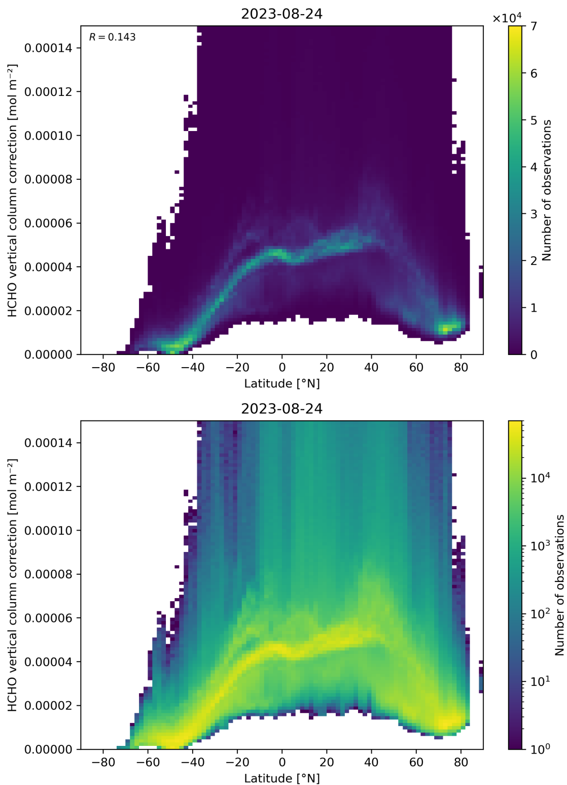
Figure 164: Scatter density plot of “Latitude” against “HCHO vertical column correction” for 2023-08-23 to 2023-08-25.
