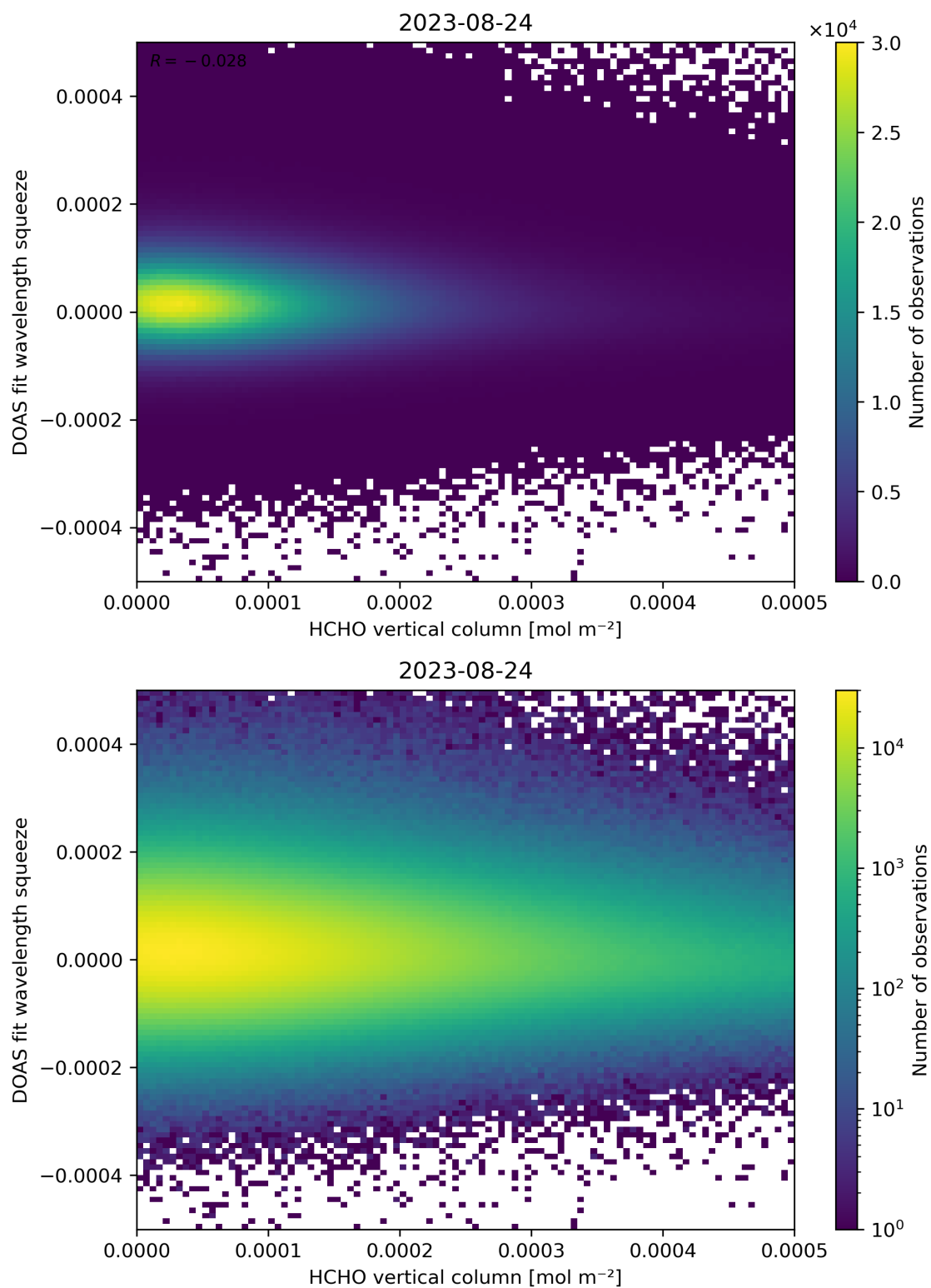
Figure 125: Scatter density plot of “HCHO vertical column” against “DOAS fit wavelength squeeze” for 2023-08-23 to 2023-08-25.
