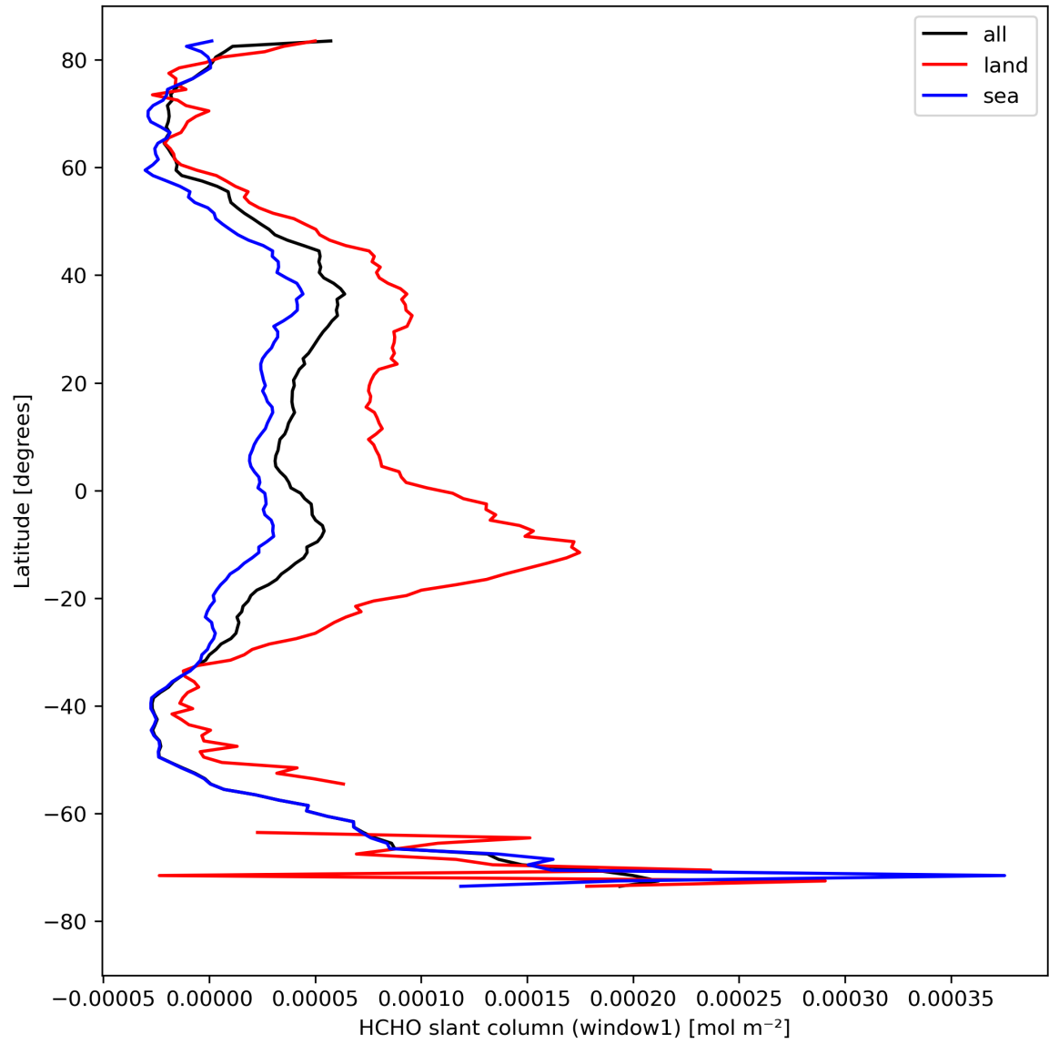
Figure 24: Zonal average of “HCHO slant column (window1)” for 2023-08-23 to 2023-08-25.
