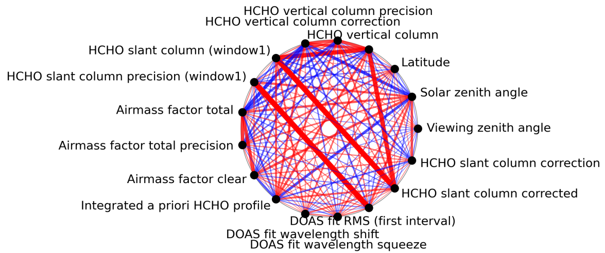
Figure 1: Map of correlation graph for 2023-08-23 to 2023-08-25.
