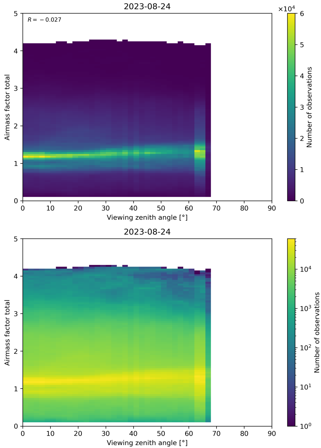
Figure 190: Scatter density plot of “Viewing zenith angle” against “Airmass factor total” for 2023-08-23 to 2023-08-25.
