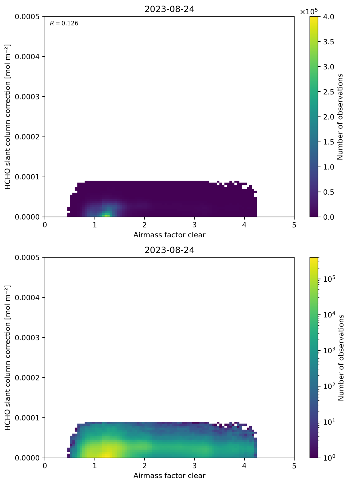
Figure 75: Scatter density plot of “Airmass factor clear” against “HCHO slant column correction” for 2023-08-23 to 2023-08-25.
