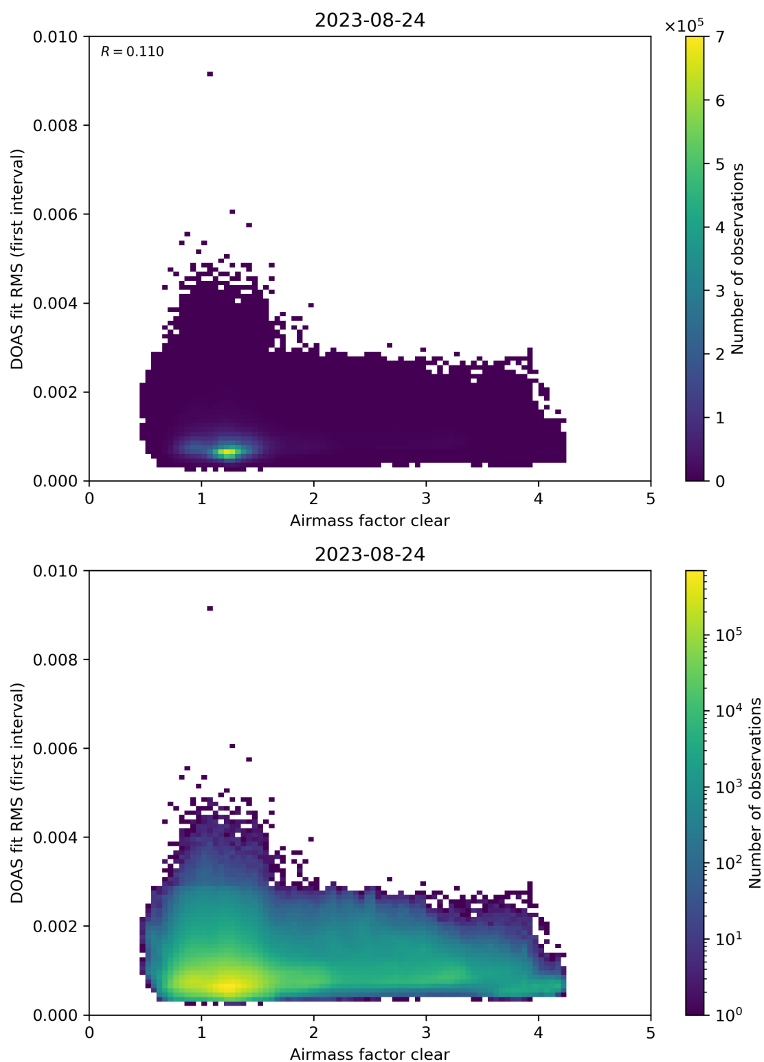
Figure 71: Scatter density plot of “Airmass factor clear” against “DOAS fit RMS (first interval)” for 2023-08-23 to 2023-08-25.
