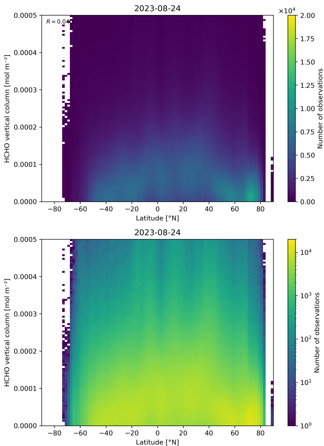
Figure 163: Scatter density plot of “Latitude” against “HCHO vertical column” for 2023-08-23 to 2023-08-25.
