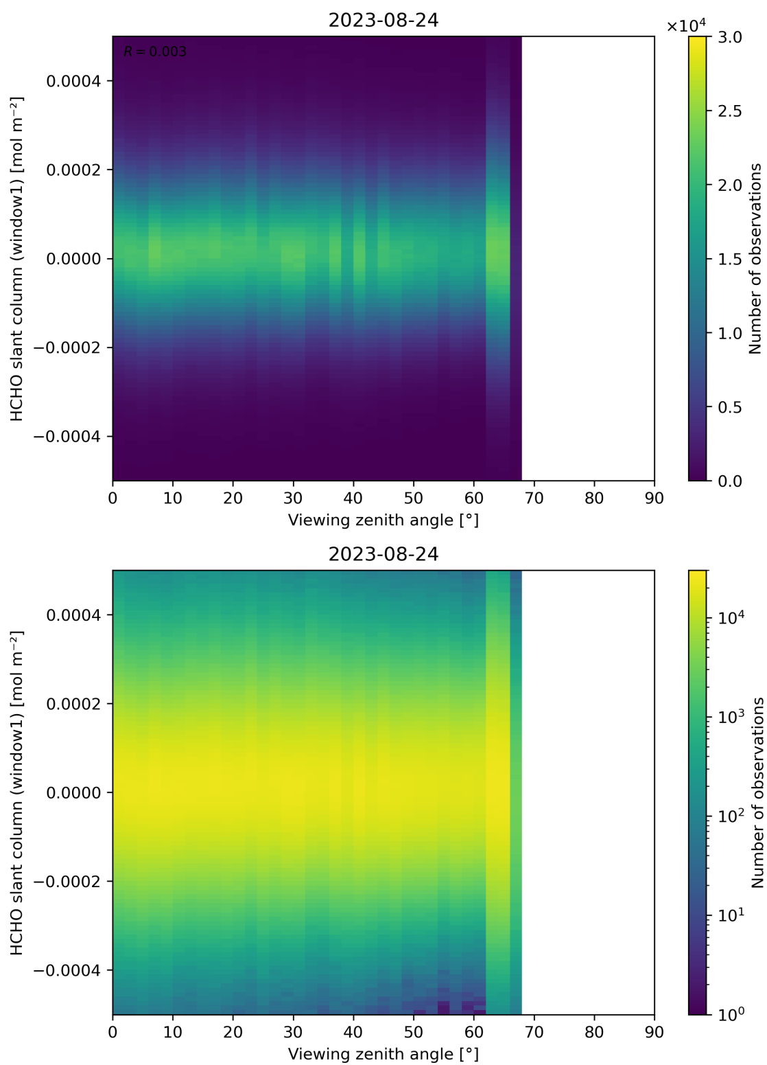
Figure 188: Scatter density plot of “Viewing zenith angle” against “HCHO slant column (window1)” for 2023-08-23 to 2023-08-25.
