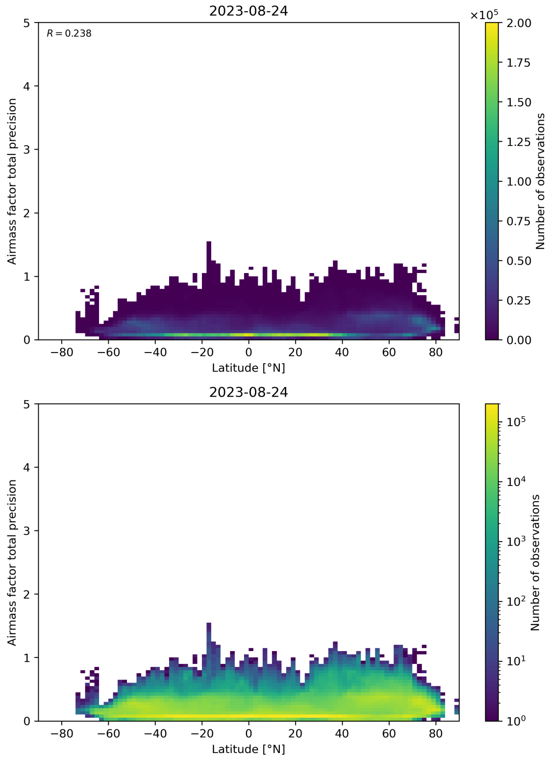
Figure 162: Scatter density plot of “Latitude” against “Airmass factor total precision” for 2023-08-23 to 2023-08-25.
