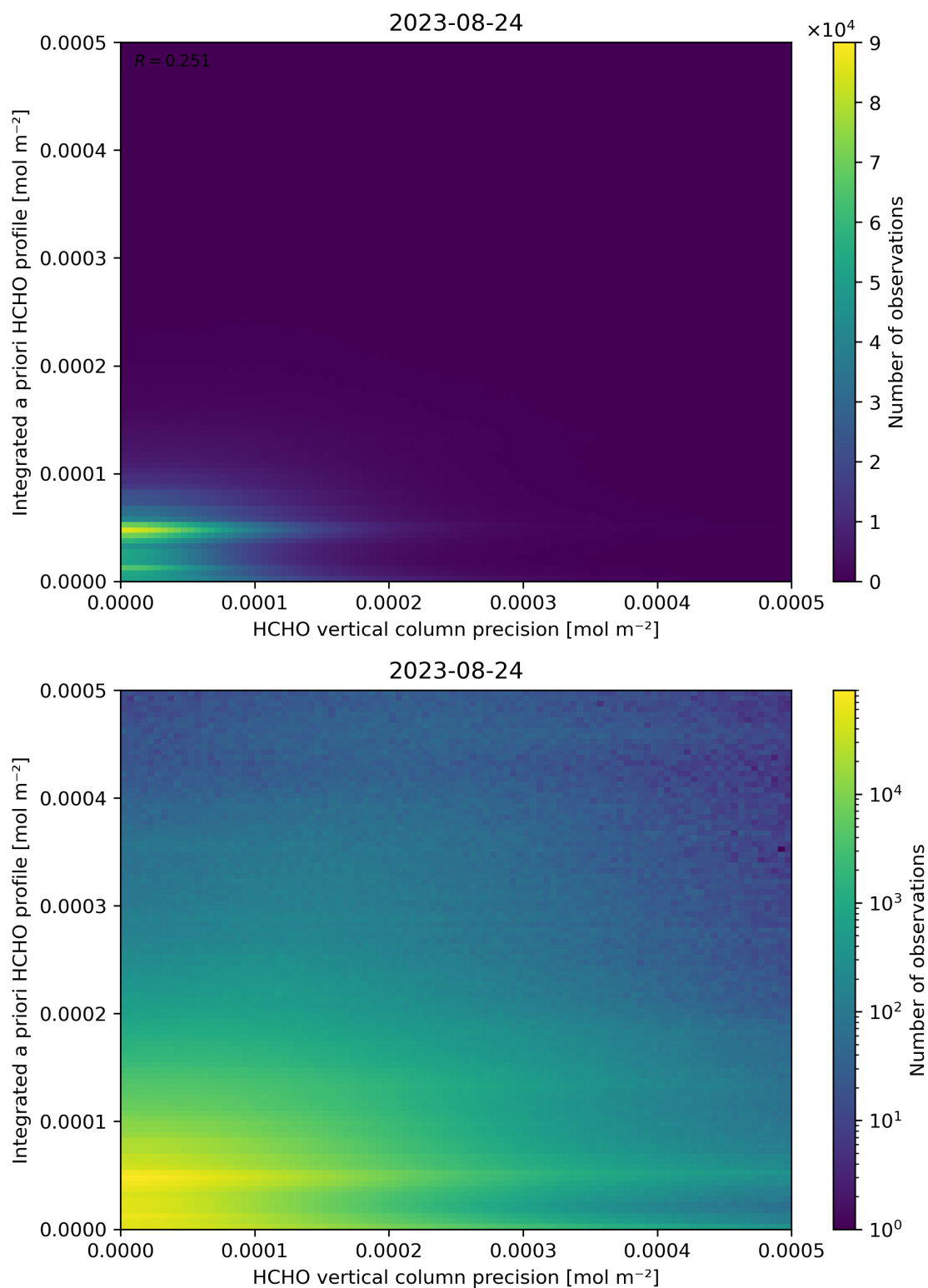
Figure 147: Scatter density plot of “HCHO vertical column precision” against “Integrated a priori HCHO profile” for 2023-08-23 to 2023-08-25.
