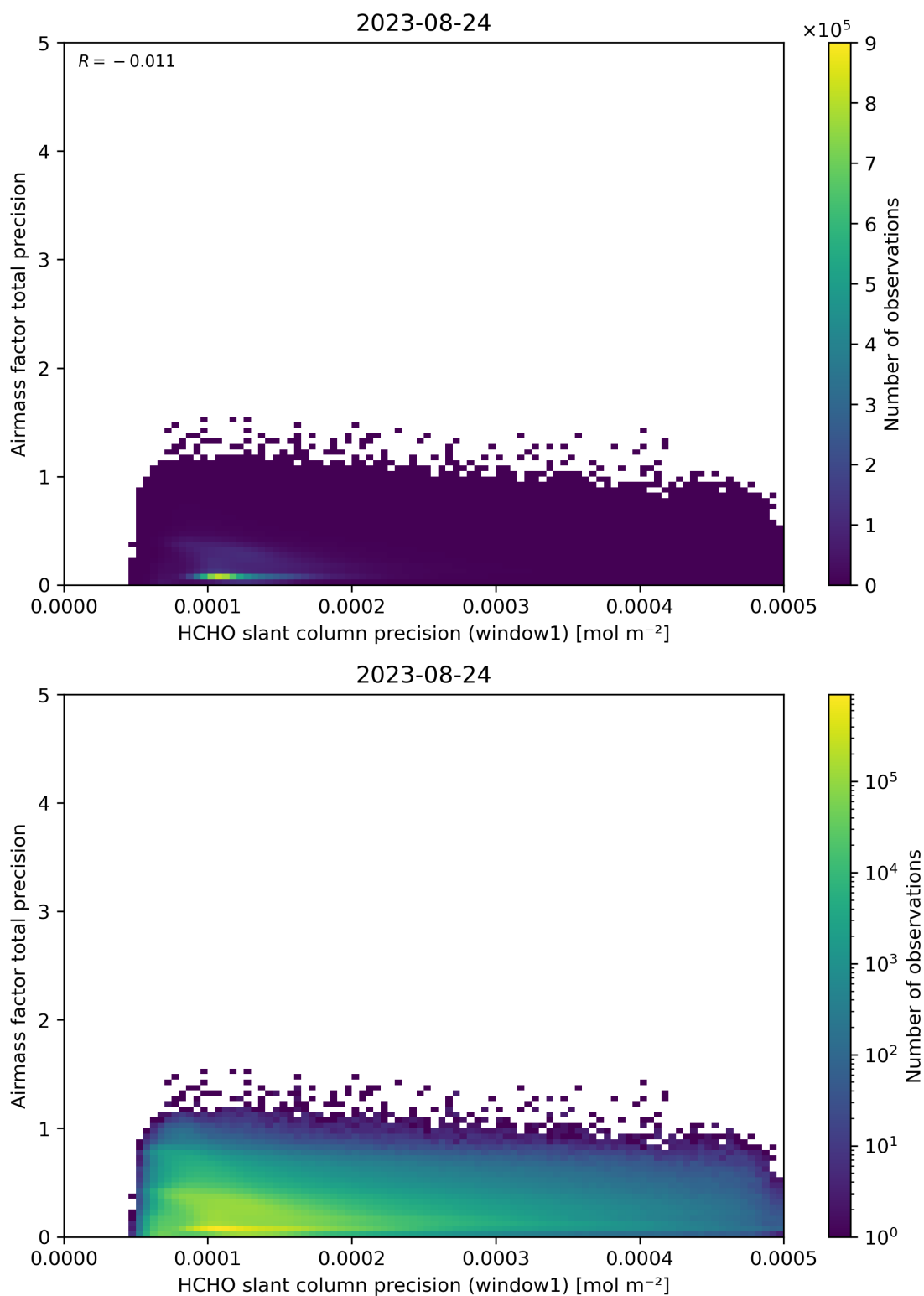
Figure 95: Scatter density plot of “HCHO slant column precision (window1)” against “Airmass factor total precision” for 2023-08-23 to 2023-08-25.
