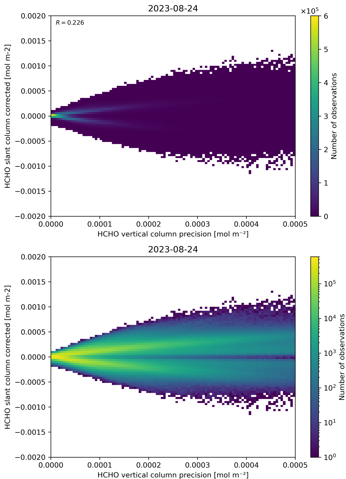
Figure 140: Scatter density plot of “HCHO vertical column precision” against “HCHO slant column corrected” for 2023-08-23 to 2023-08-25.
