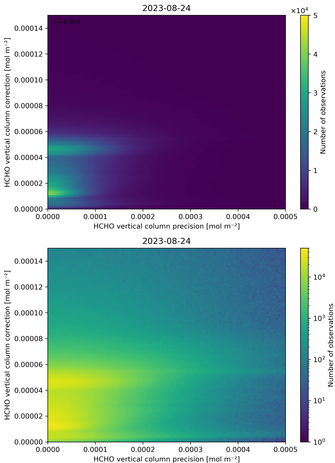
Figure 146: Scatter density plot of “HCHO vertical column precision” against “HCHO vertical column correction” for 2023-08-23 to 2023-08-25.
