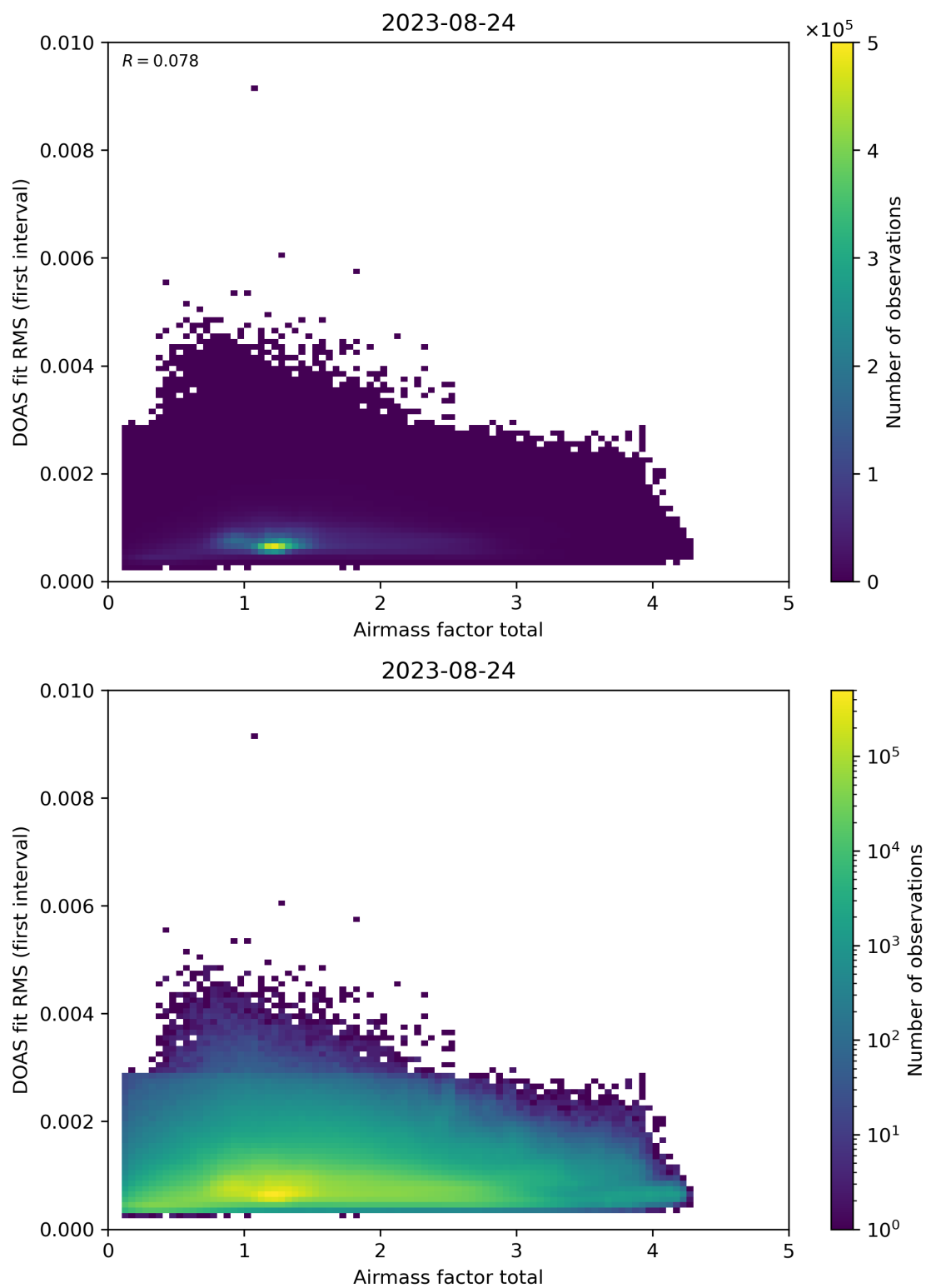
Figure 97: Scatter density plot of “Airmass factor total” against “DOAS fit RMS (first interval)” for 2023-08-23 to 2023-08-25.
