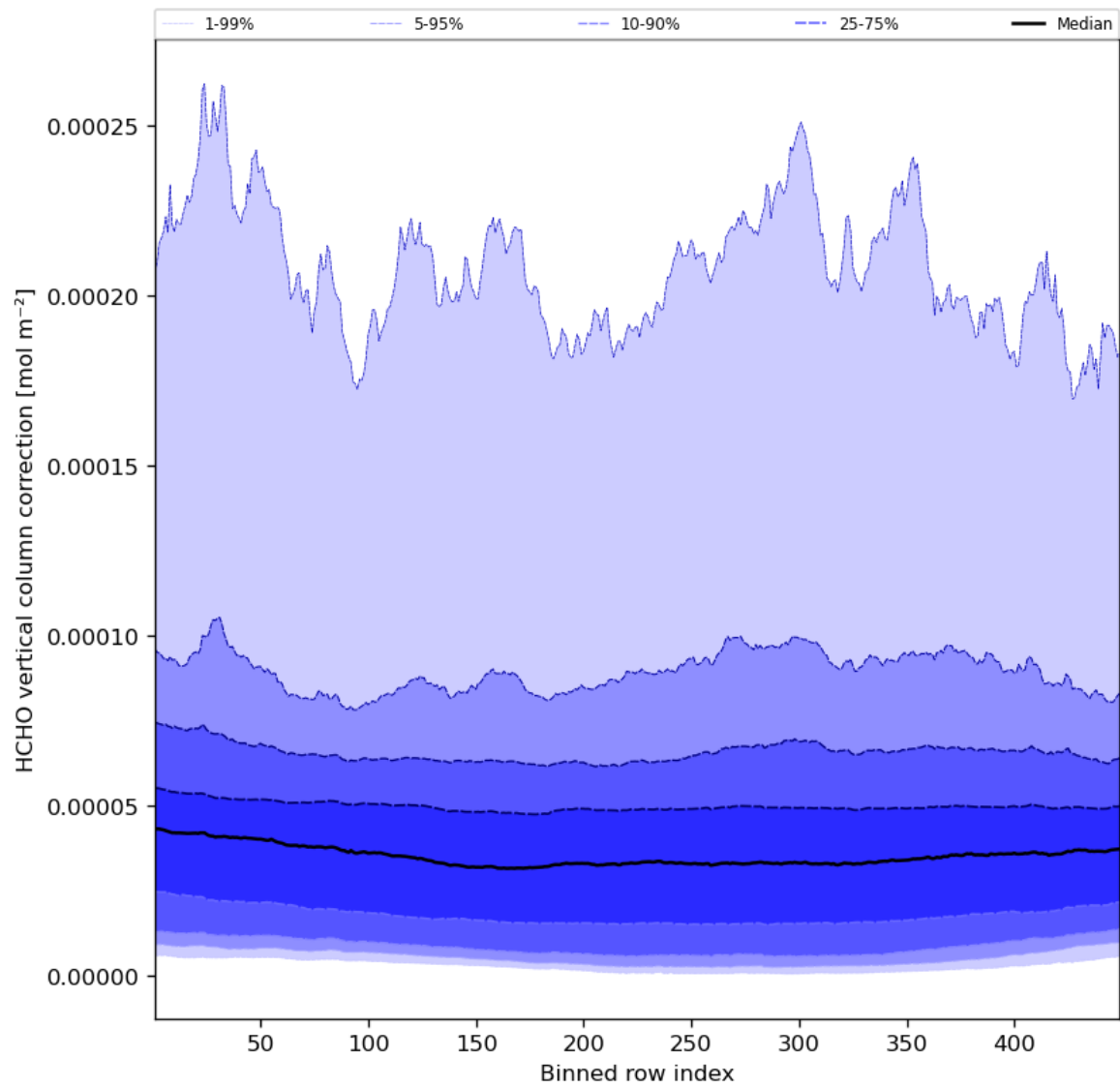
Figure 51: Along track statistics of “HCHO vertical column correction” for 2023-08-23 to 2023-08-25
