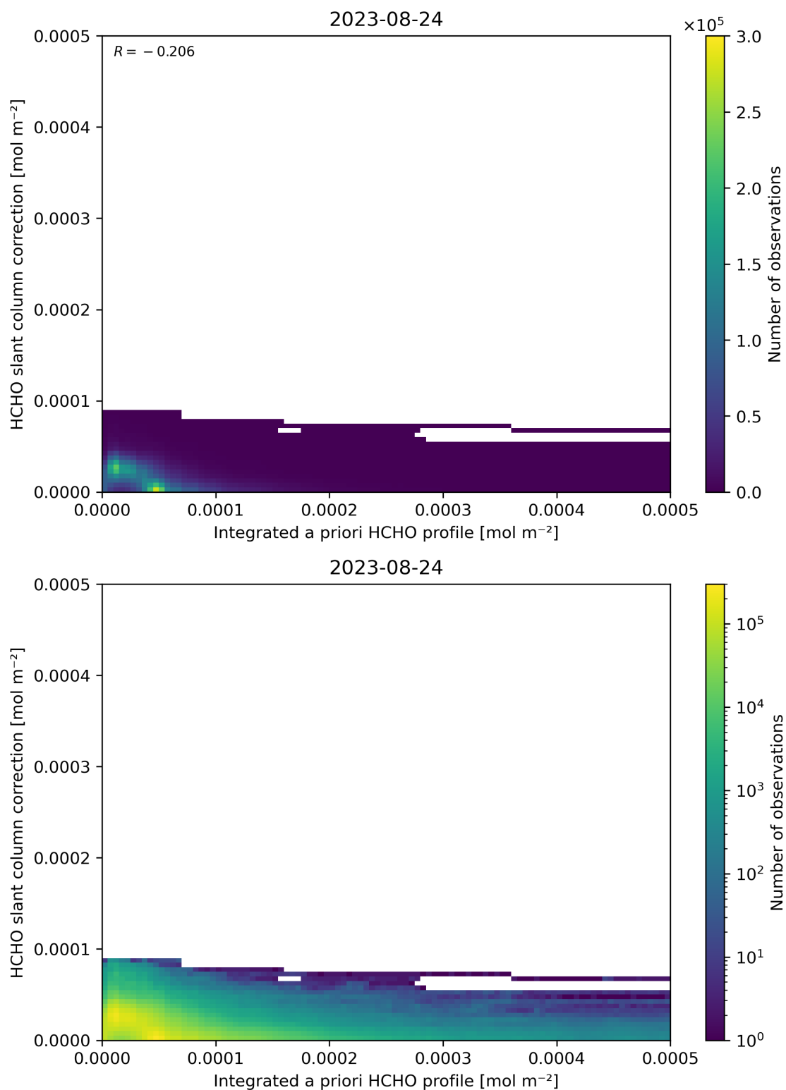
Figure 152: Scatter density plot of “Integrated a priori HCHO profile” against “HCHO slant column correction” for 2023-08-23 to 2023-08-25.
