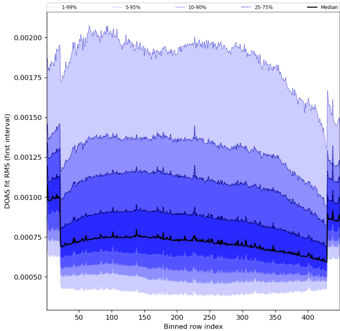
Figure 60: Along track statistics of “DOAS fit RMS (first interval)” for 2023-08-23 to 2023-08-25
