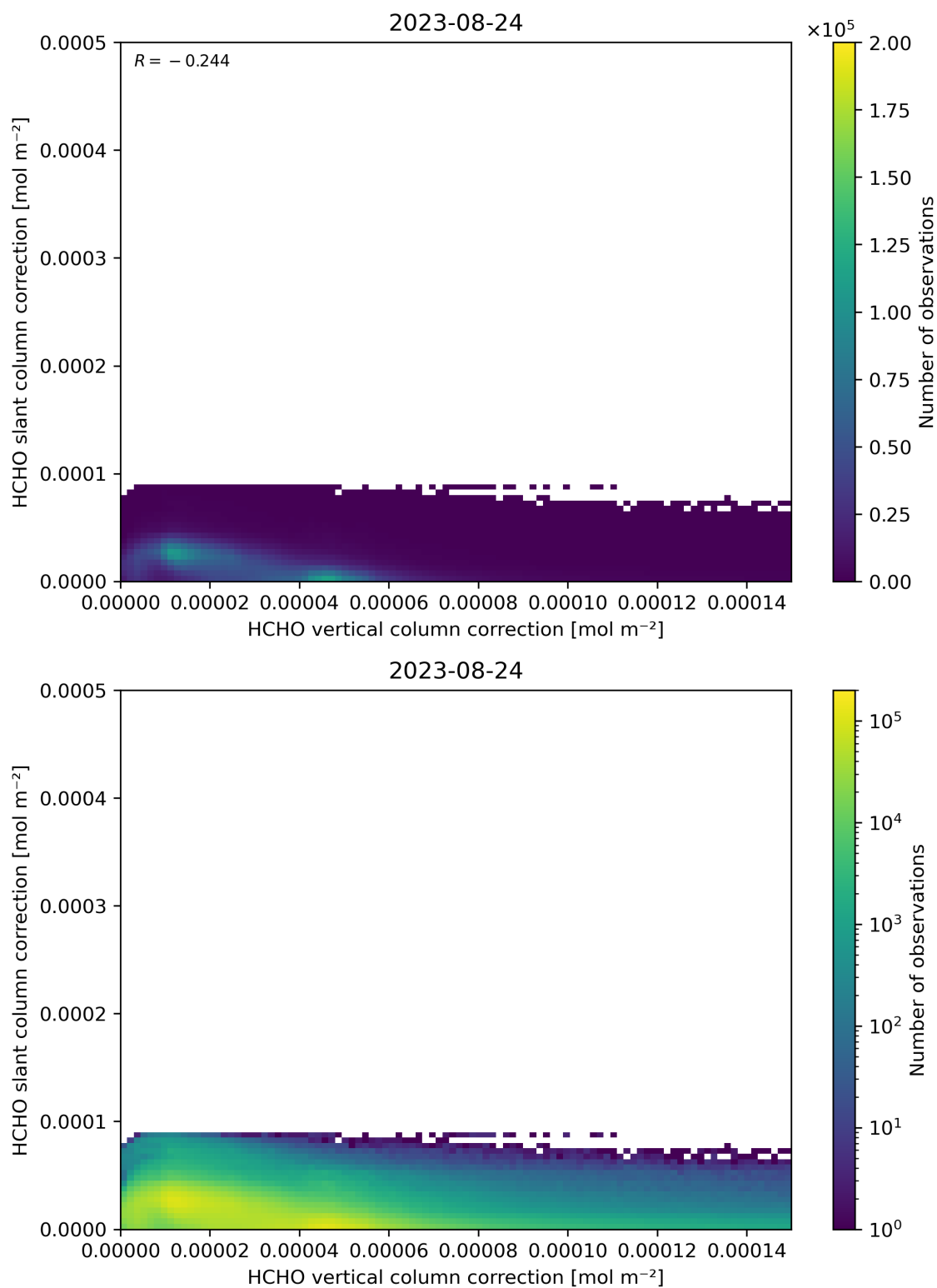
Figure 117: Scatter density plot of “HCHO vertical column correction” against “HCHO slant column correction” for 2023-08-23 to 2023-08-25.
