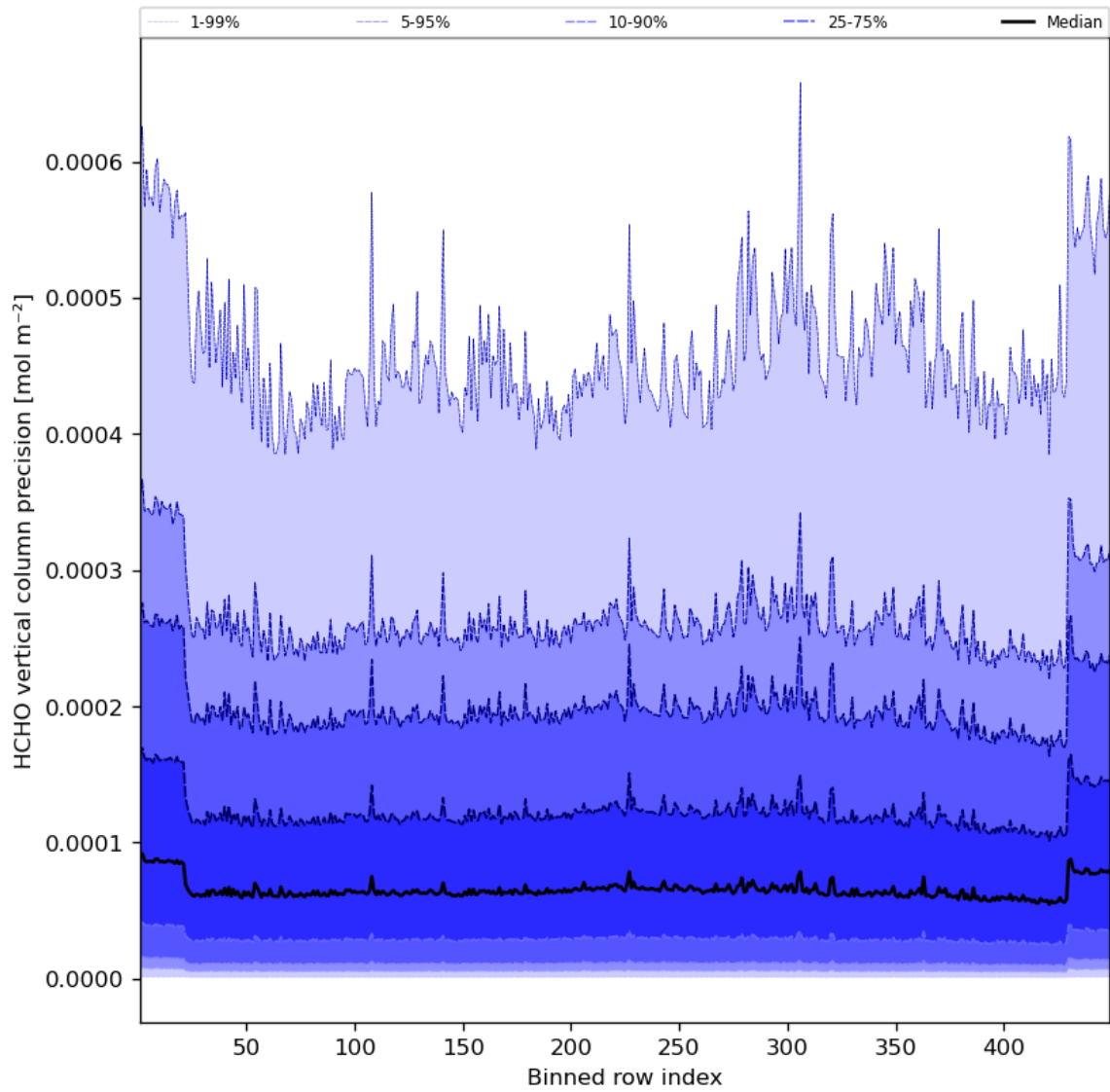
Figure 50: Along track statistics of “HCHO vertical column precision” for 2023-08-23 to 2023-08-25
