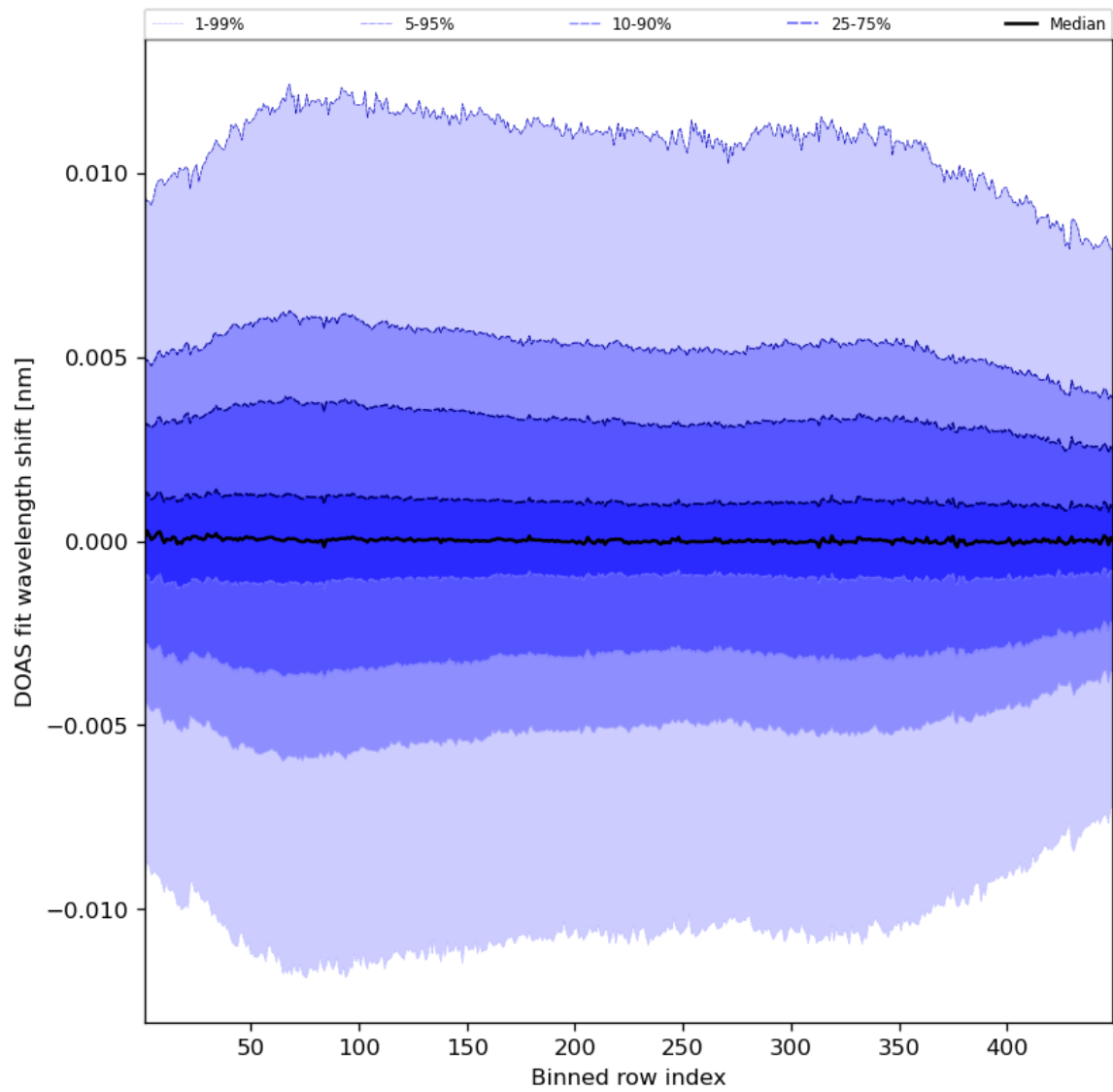
Figure 58: Along track statistics of “DOAS fit wavelength shift” for 2023-08-23 to 2023-08-25
