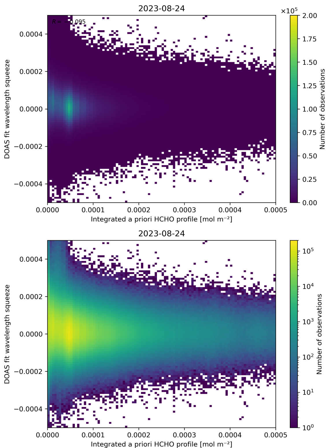
Figure 150: Scatter density plot of “Integrated a priori HCHO profile” against “DOAS fit wavelength squeeze” for 2023-08-23 to 2023-08-25.
