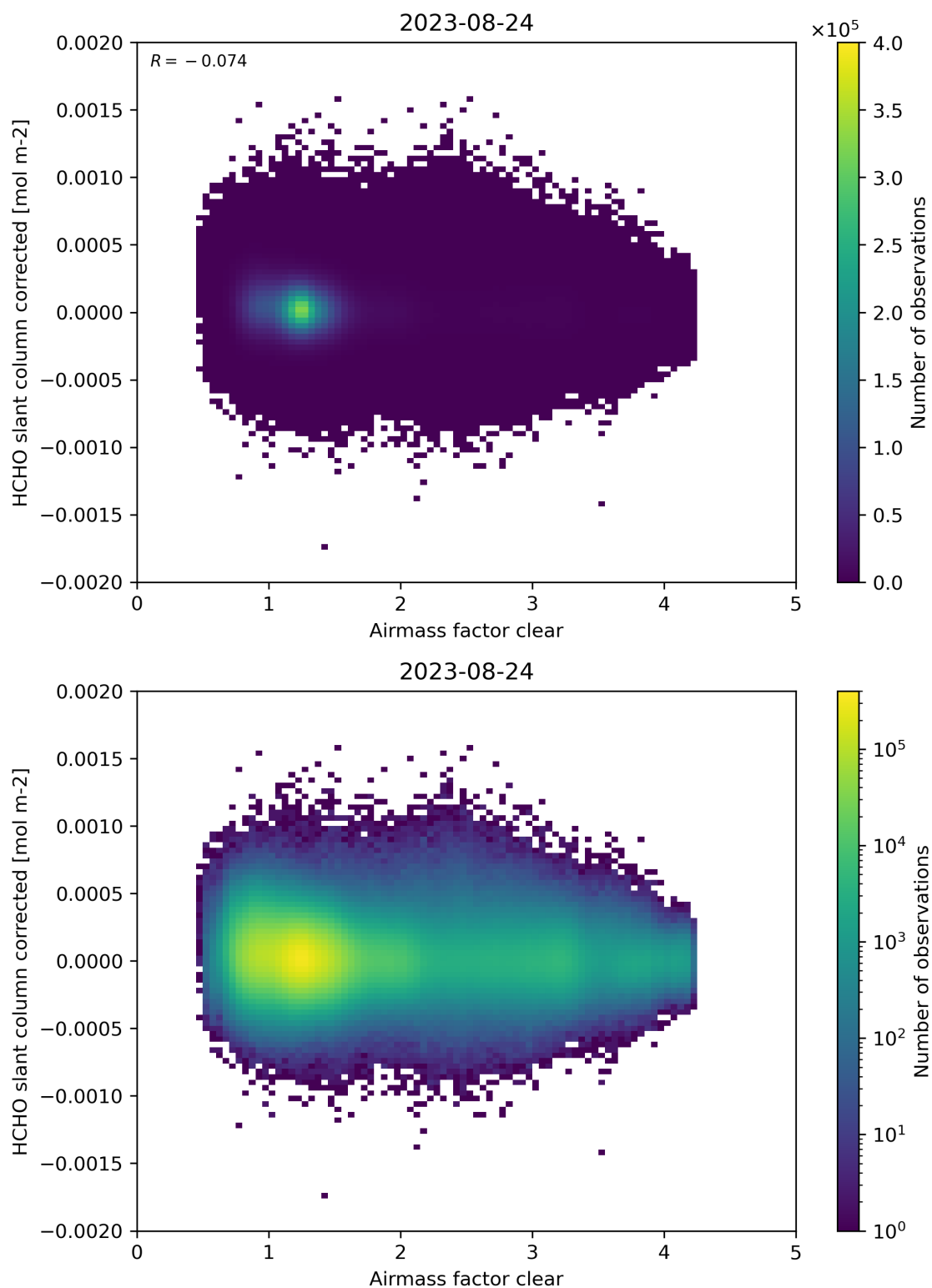
Figure 74: Scatter density plot of “Airmass factor clear” against “HCHO slant column corrected” for 2023-08-23 to 2023-08-25.
