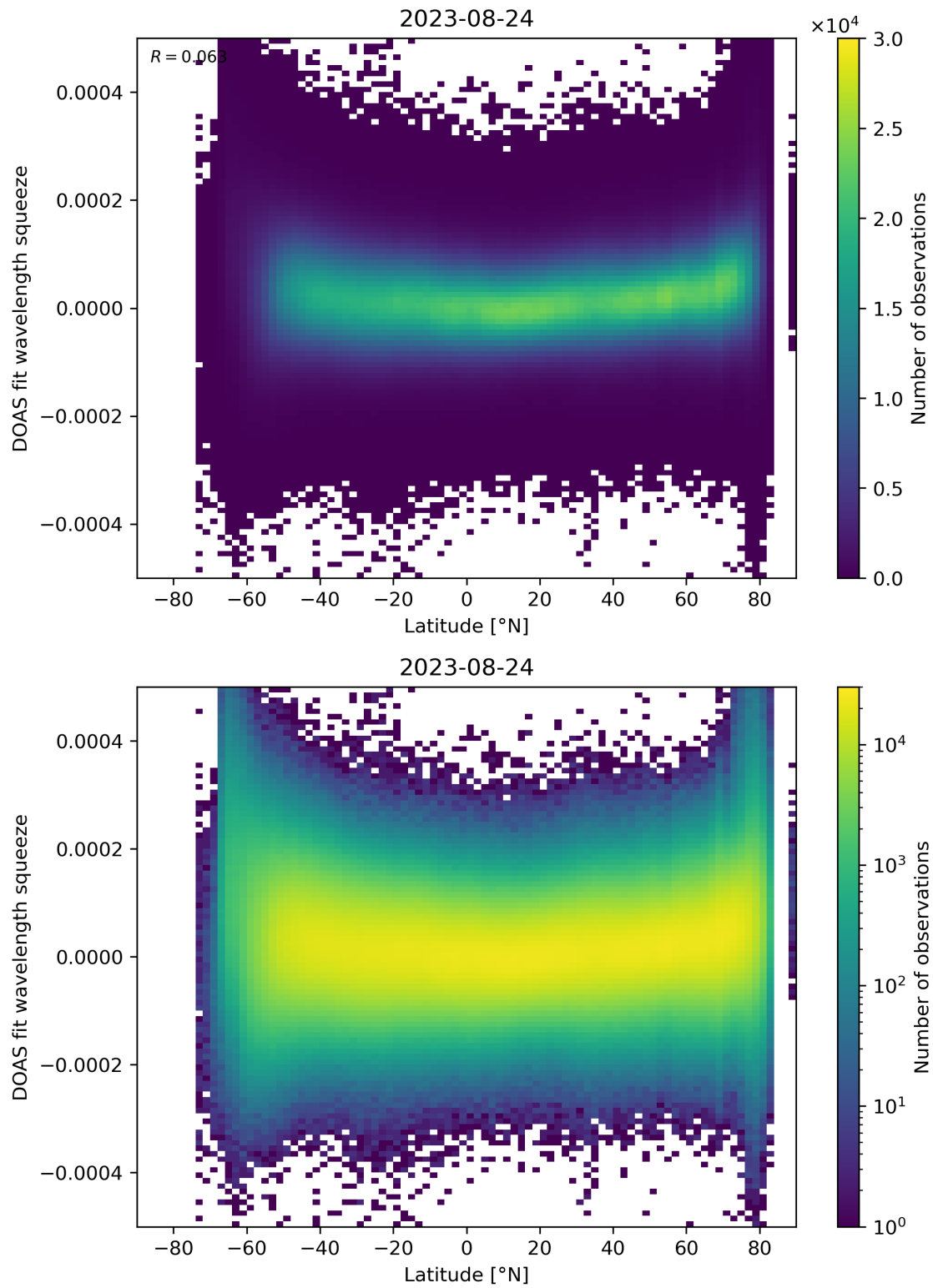
Figure 155: Scatter density plot of “Latitude” against “DOAS fit wavelength squeeze” for 2023-08-23 to 2023-08-25.
