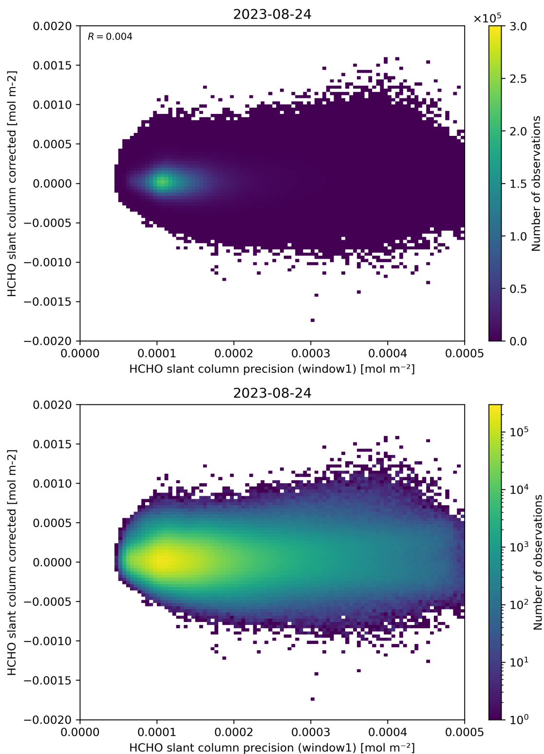
Figure 92: Scatter density plot of “HCHO slant column precision (window1)” against “HCHO slant column corrected” for 2023-08-23 to 2023-08-25.
