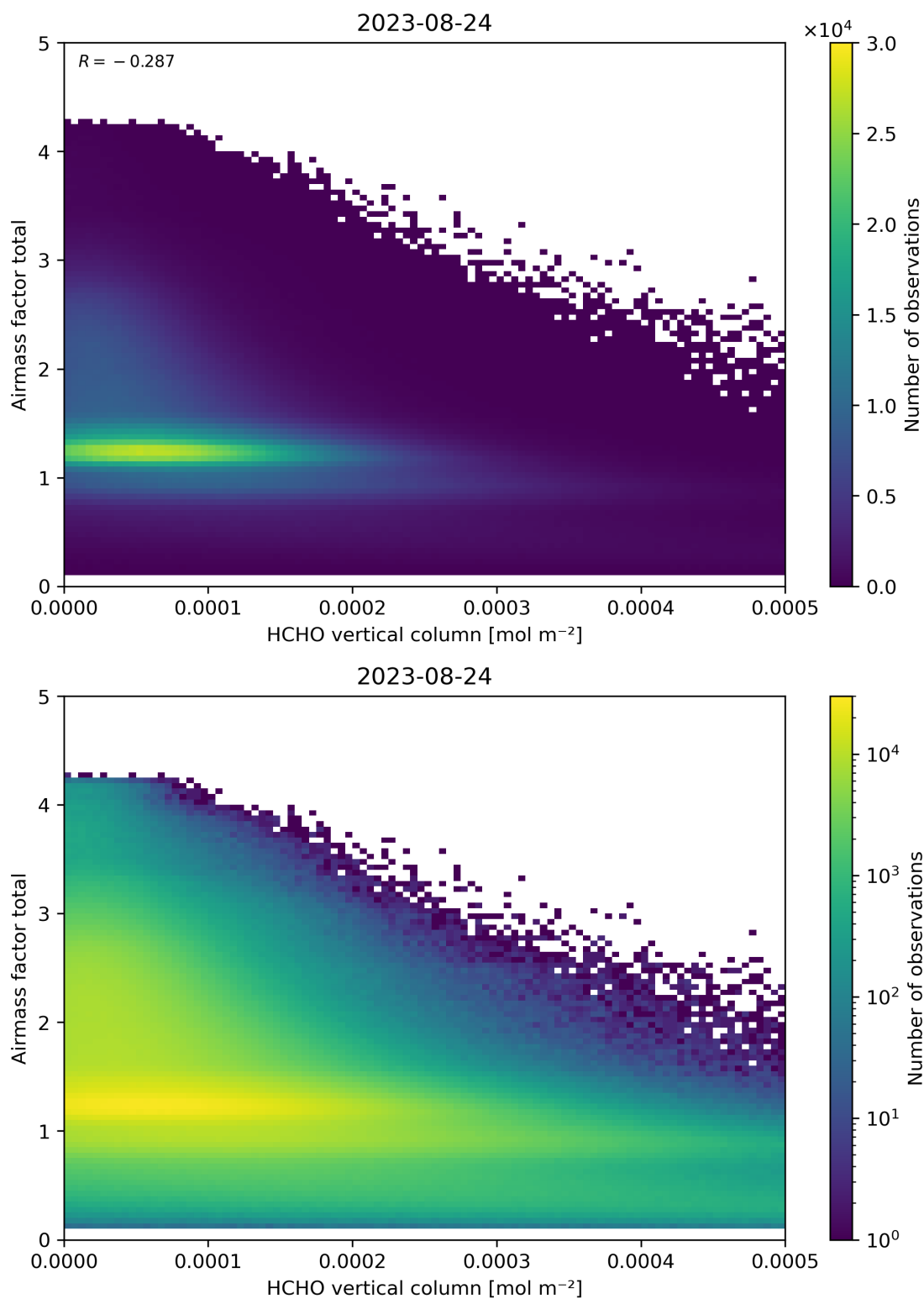
Figure 131: Scatter density plot of “HCHO vertical column” against “Airmass factor total” for 2023-08-23 to 2023-08-25.
