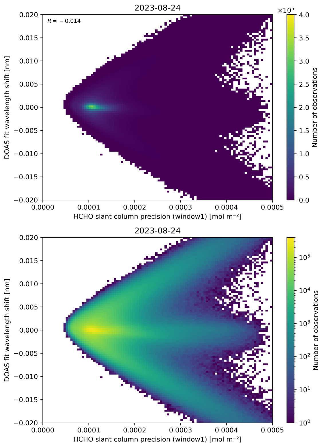
Figure 89: Scatter density plot of “HCHO slant column precision (window1)” against “DOAS fit wavelength shift” for 2023-08-23 to 2023-08-25.
