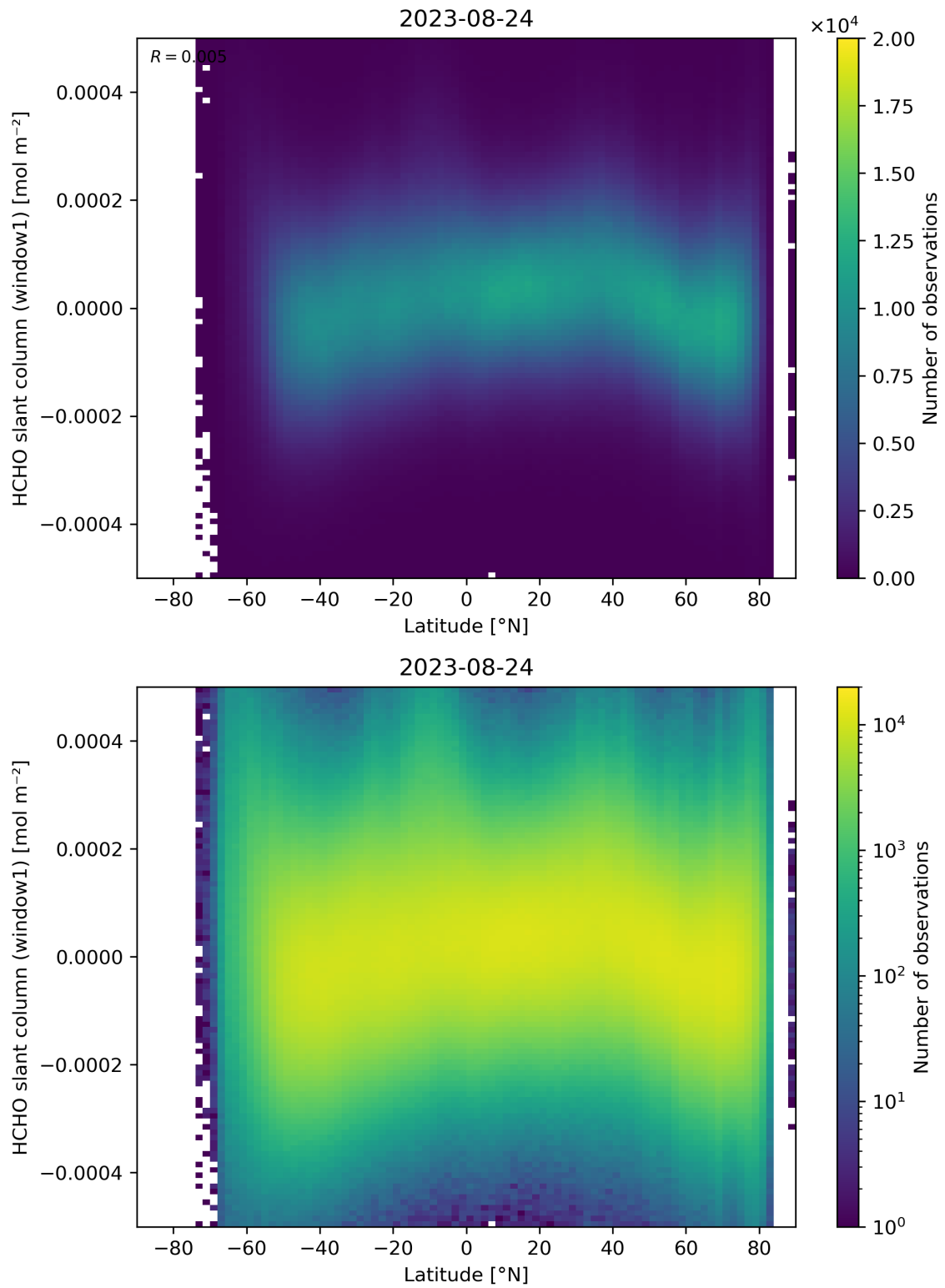
Figure 159: Scatter density plot of “Latitude” against “HCHO slant column (window1)” for 2023-08-23 to 2023-08-25.
