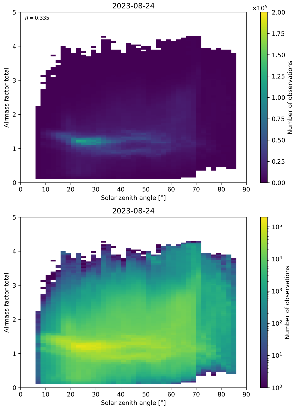
Figure 175: Scatter density plot of “Solar zenith angle” against “Airmass factor total” for 2023-08-23 to 2023-08-25.
