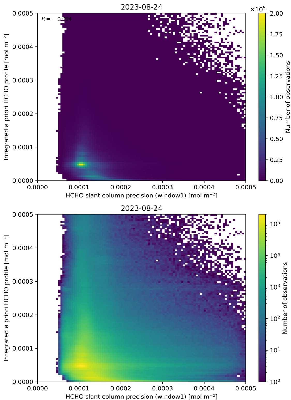
Figure 96: Scatter density plot of “HCHO slant column precision (window1)” against “Integrated a priori HCHO profile” for 2023-08-23 to 2023-08-25.
