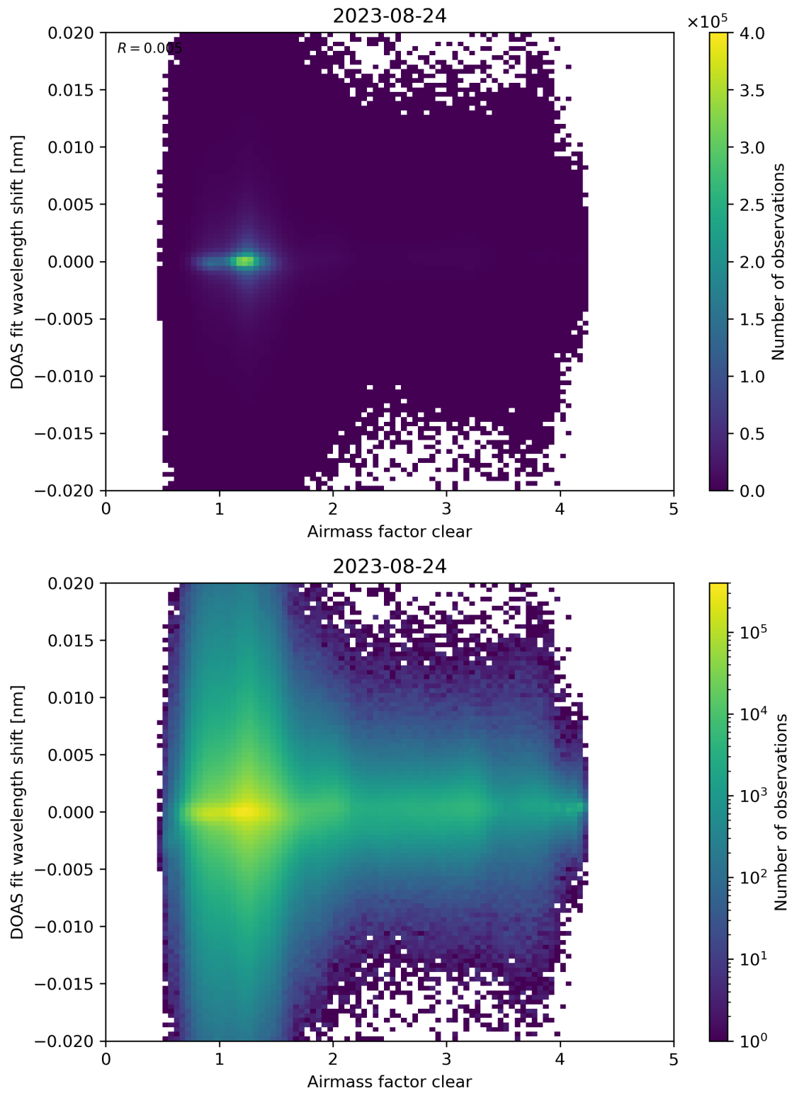
Figure 72: Scatter density plot of “Airmass factor clear” against “DOAS fit wavelength shift” for 2023-08-23 to 2023-08-25.
