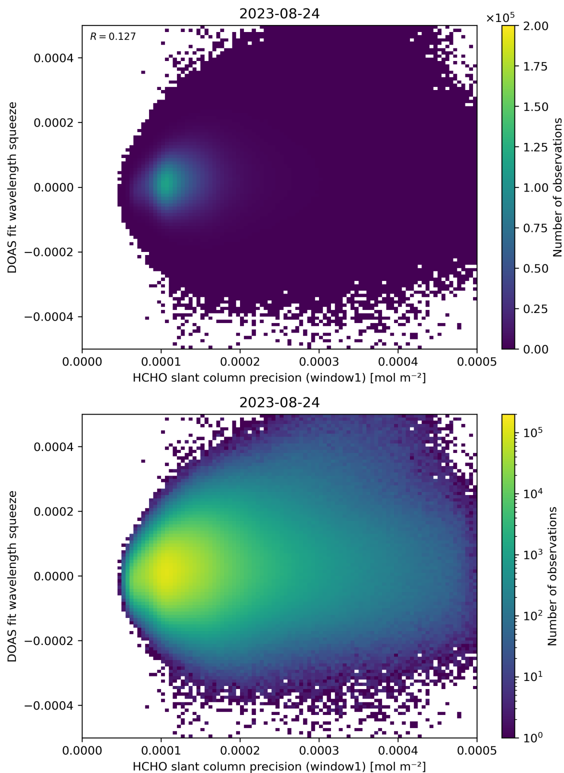
Figure 90: Scatter density plot of “HCHO slant column precision (window1)” against “DOAS fit wavelength squeeze” for 2023-08-23 to 2023-08-25.
