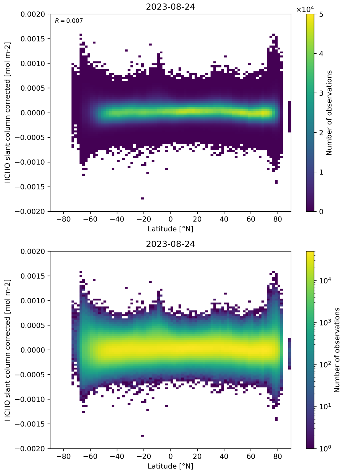
Figure 157: Scatter density plot of “Latitude” against “HCHO slant column corrected” for 2023-08-23 to 2023-08-25.
