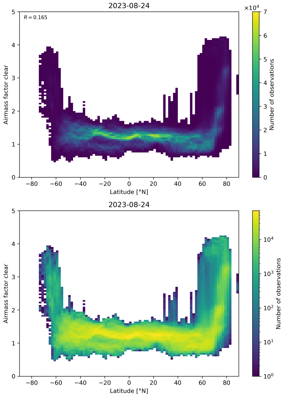
Figure 156: Scatter density plot of “Latitude” against “Airmass factor clear” for 2023-08-23 to 2023-08-25.
