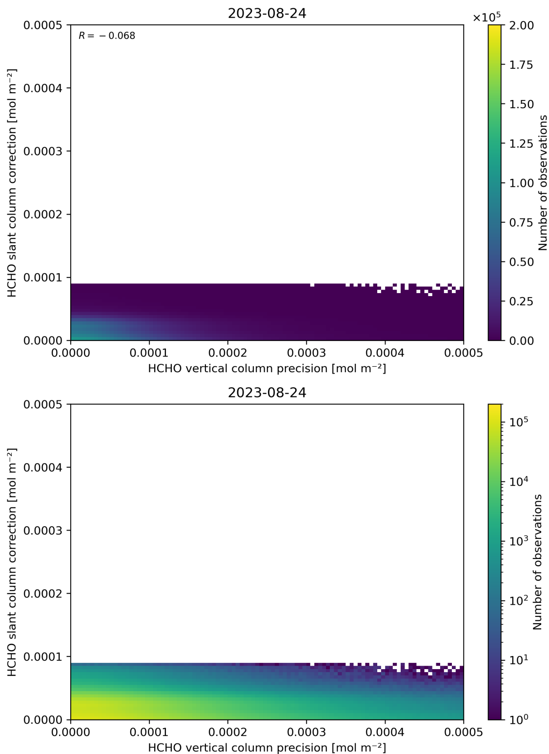
Figure 141: Scatter density plot of “HCHO vertical column precision” against “HCHO slant column correction” for 2023-08-23 to 2023-08-25.
