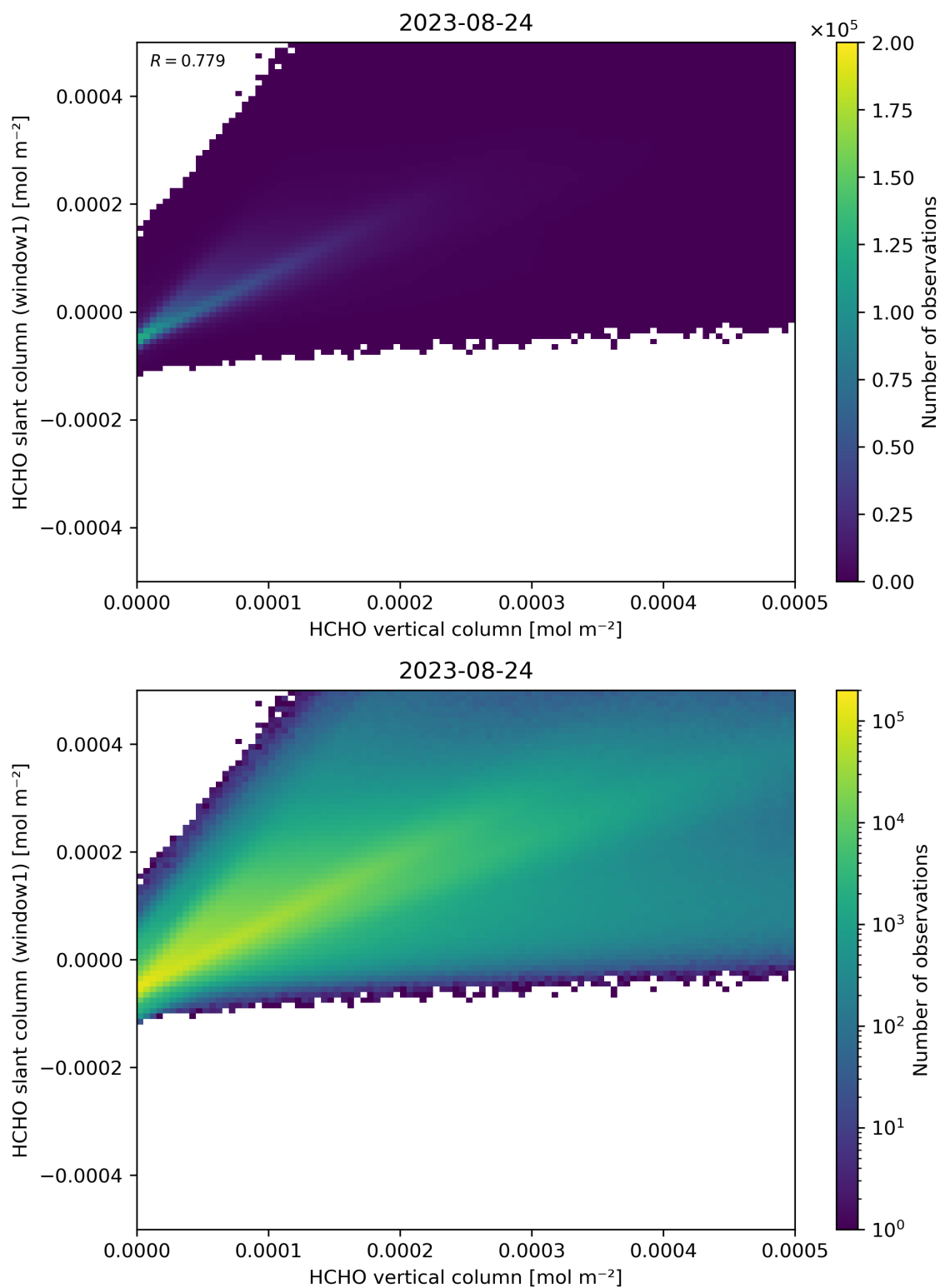
Figure 129: Scatter density plot of “HCHO vertical column” against “HCHO slant column (window1)” for 2023-08-23 to 2023-08-25.
