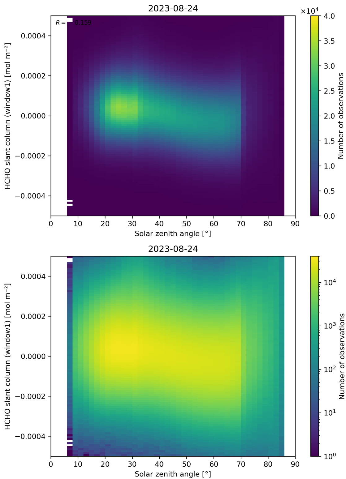
Figure 173: Scatter density plot of “Solar zenith angle” against “HCHO slant column (window1)” for 2023-08-23 to 2023-08-25.
