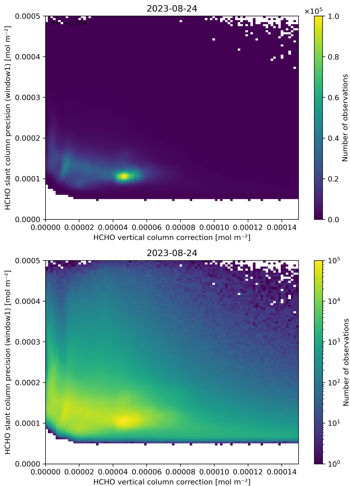
Figure 119: Scatter density plot of “HCHO vertical column correction” against “HCHO slant column precision (window1)” for 2023-08-23 to 2023-08-25.
