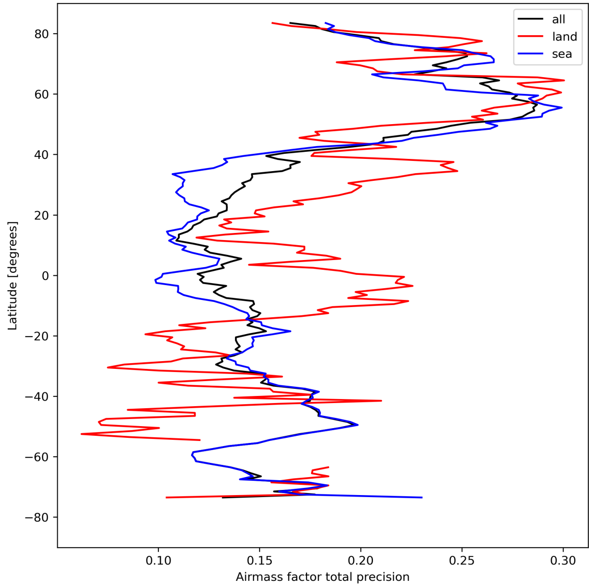
Figure 27: Zonal average of “Airmass factor total precision” for 2023-08-23 to 2023-08-25.
