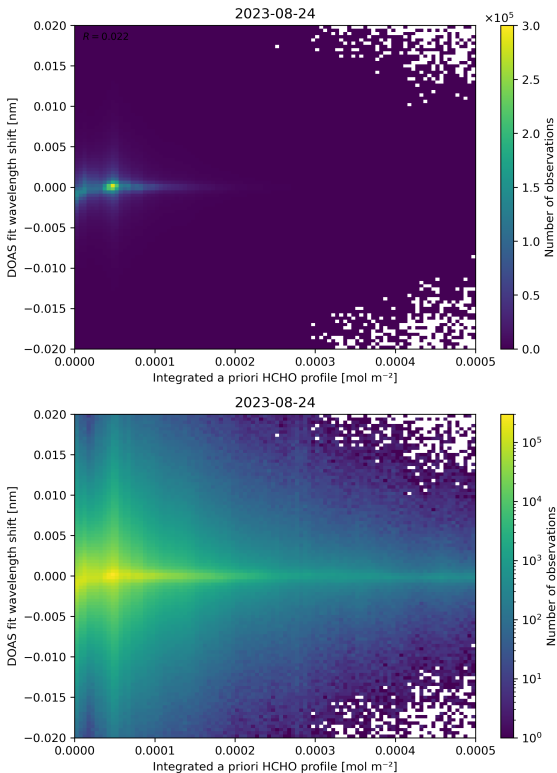
Figure 149: Scatter density plot of “Integrated a priori HCHO profile” against “DOAS fit wavelength shift” for 2023-08-23 to 2023-08-25.
