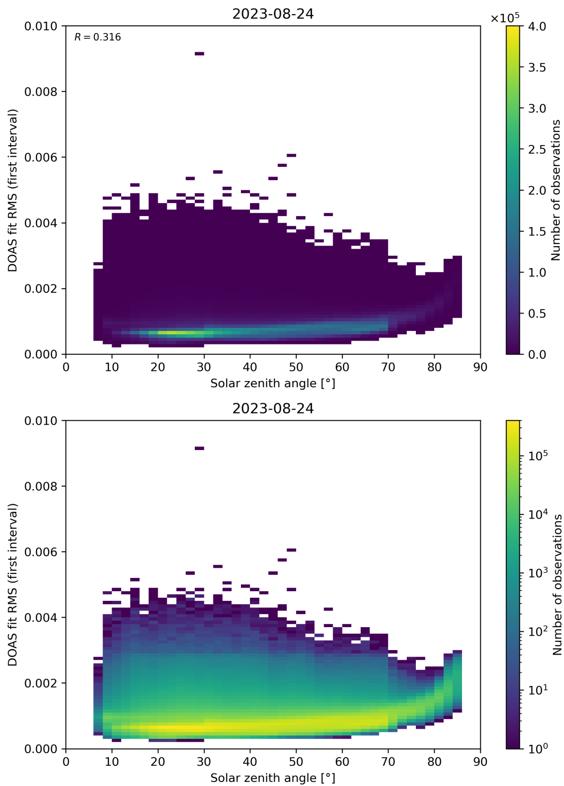
Figure 167: Scatter density plot of “Solar zenith angle” against “DOAS fit RMS (first interval)” for 2023-08-23 to 2023-08-25.
