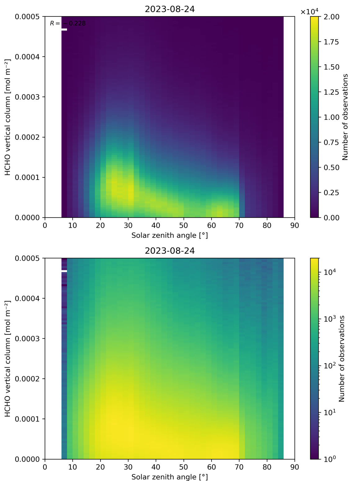
Figure 177: Scatter density plot of “Solar zenith angle” against “HCHO vertical column” for 2023-08-23 to 2023-08-25.
