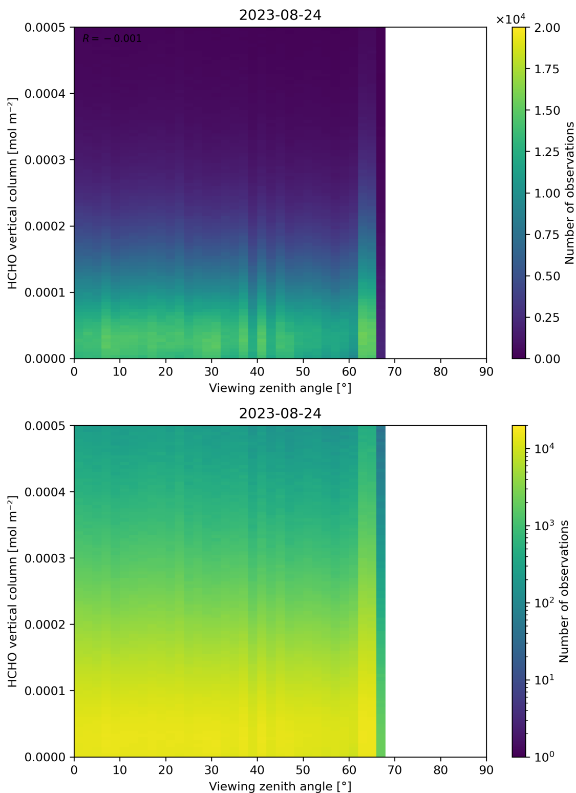
Figure 192: Scatter density plot of “Viewing zenith angle” against “HCHO vertical column” for 2023-08-23 to 2023-08-25.
