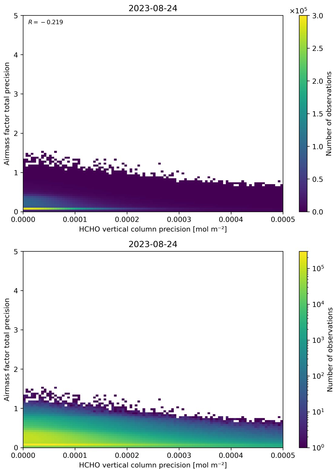
Figure 145: Scatter density plot of “HCHO vertical column precision” against “Airmass factor total precision” for 2023-08-23 to 2023-08-25.
