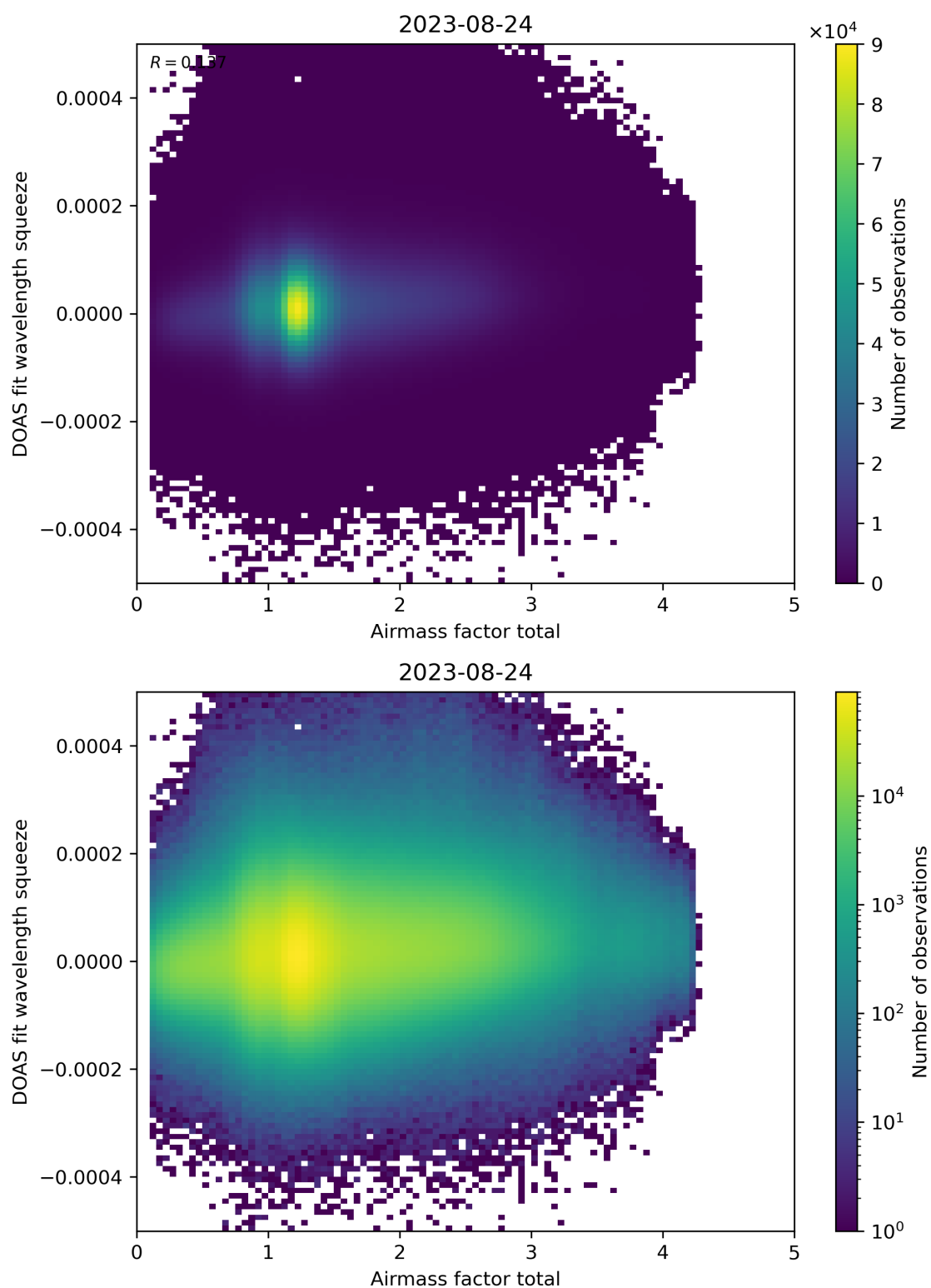
Figure 99: Scatter density plot of “Airmass factor total” against “DOAS fit wavelength squeeze” for 2023-08-23 to 2023-08-25.
