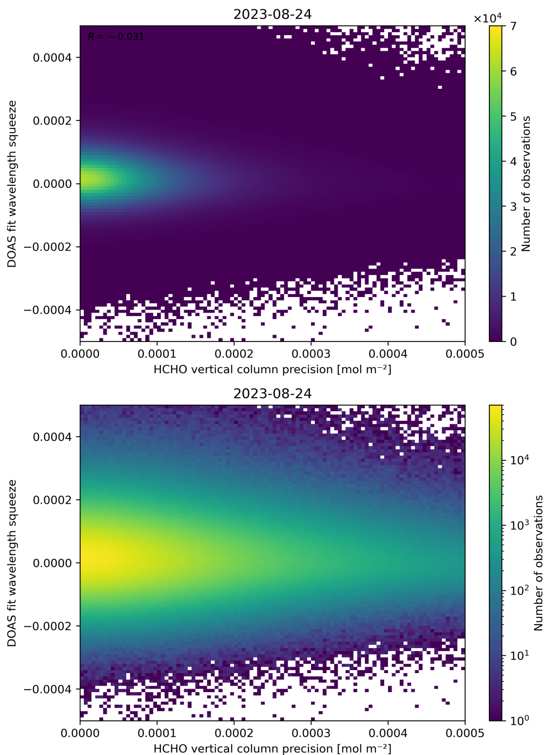
Figure 138: Scatter density plot of “HCHO vertical column precision” against “DOAS fit wavelength squeeze” for 2023-08-23 to 2023-08-25.
