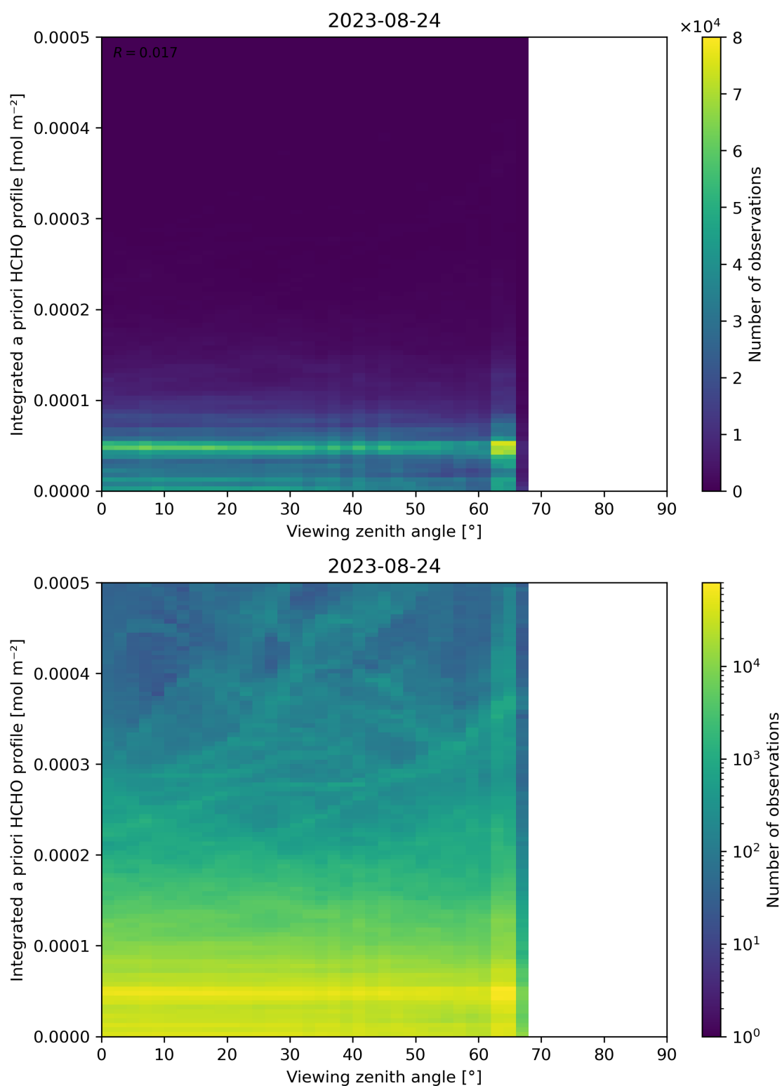
Figure 195: Scatter density plot of “Viewing zenith angle” against “Integrated a priori HCHO profile” for 2023-08-23 to 2023-08-25.
