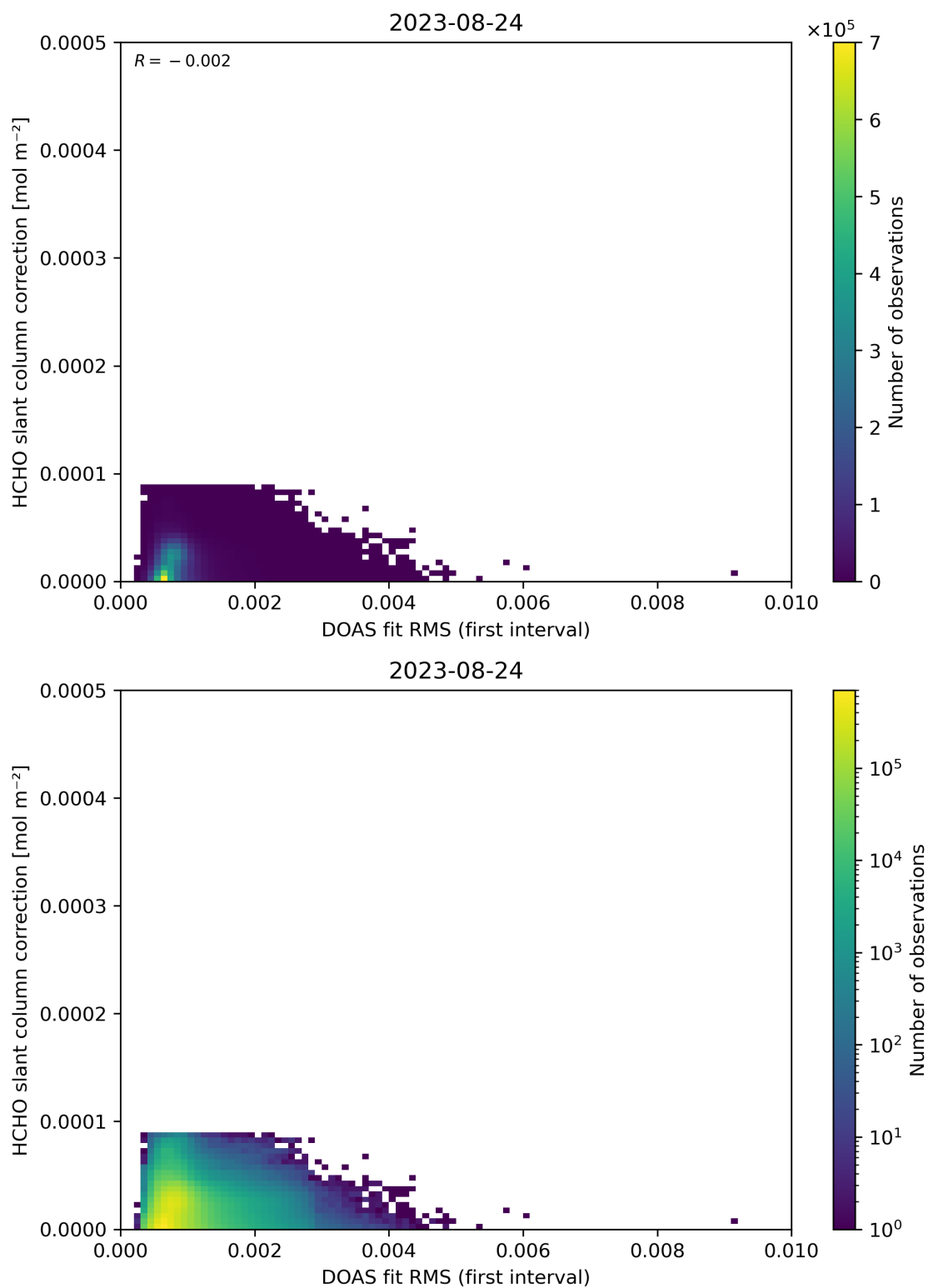
Figure 63: Scatter density plot of “DOAS fit RMS (first interval)” against “HCHO slant column correction” for 2023-08-23 to 2023-08-25.
