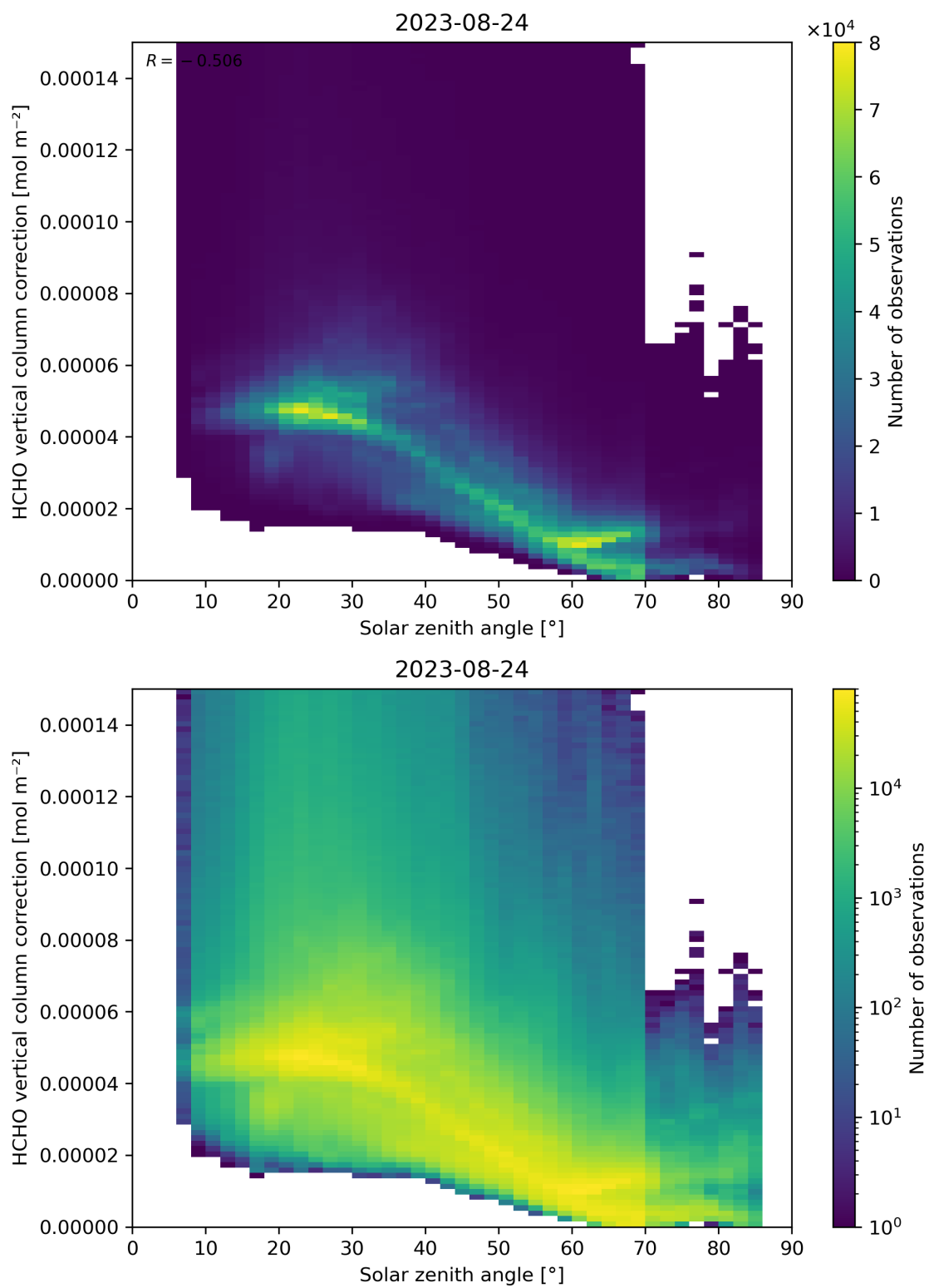
Figure 178: Scatter density plot of “Solar zenith angle” against “HCHO vertical column correction” for 2023-08-23 to 2023-08-25.
