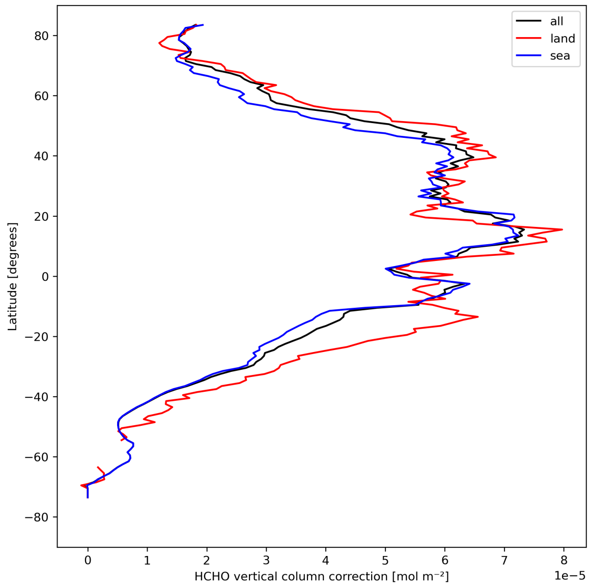
Figure 23: Zonal average of “HCHO vertical column correction” for 2023-08-23 to 2023-08-25.
