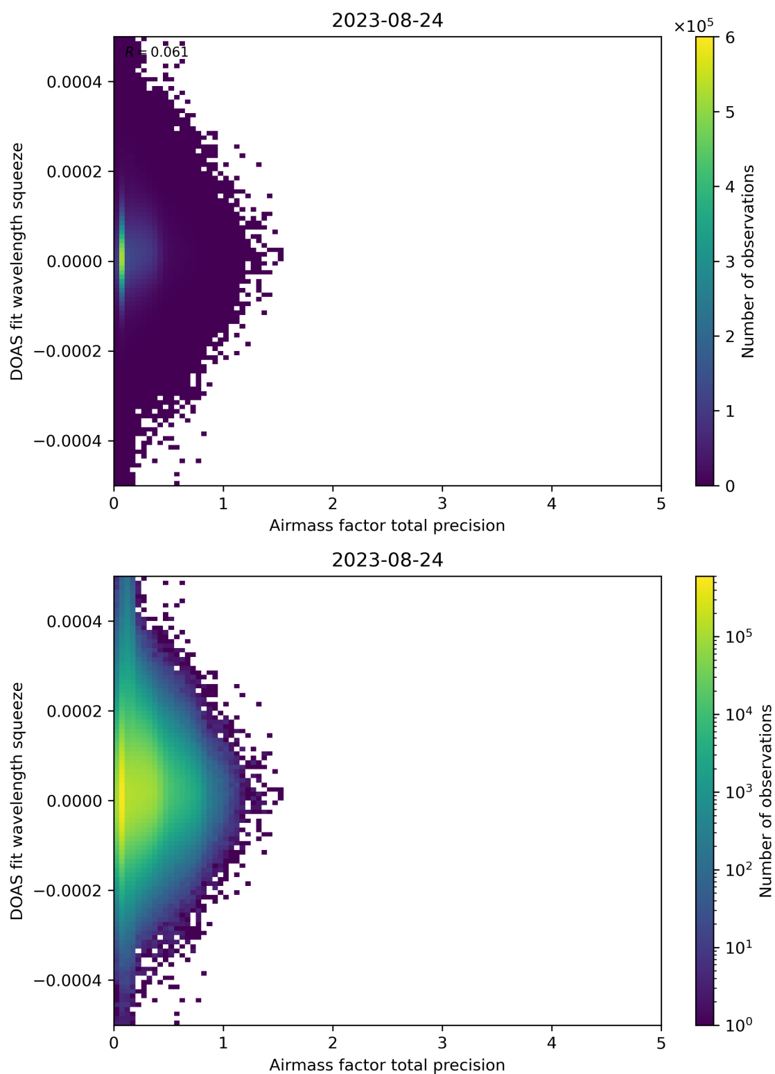
Figure 107: Scatter density plot of “Airmass factor total precision” against “DOAS fit wavelength squeeze” for 2023-08-23 to 2023-08-25.
