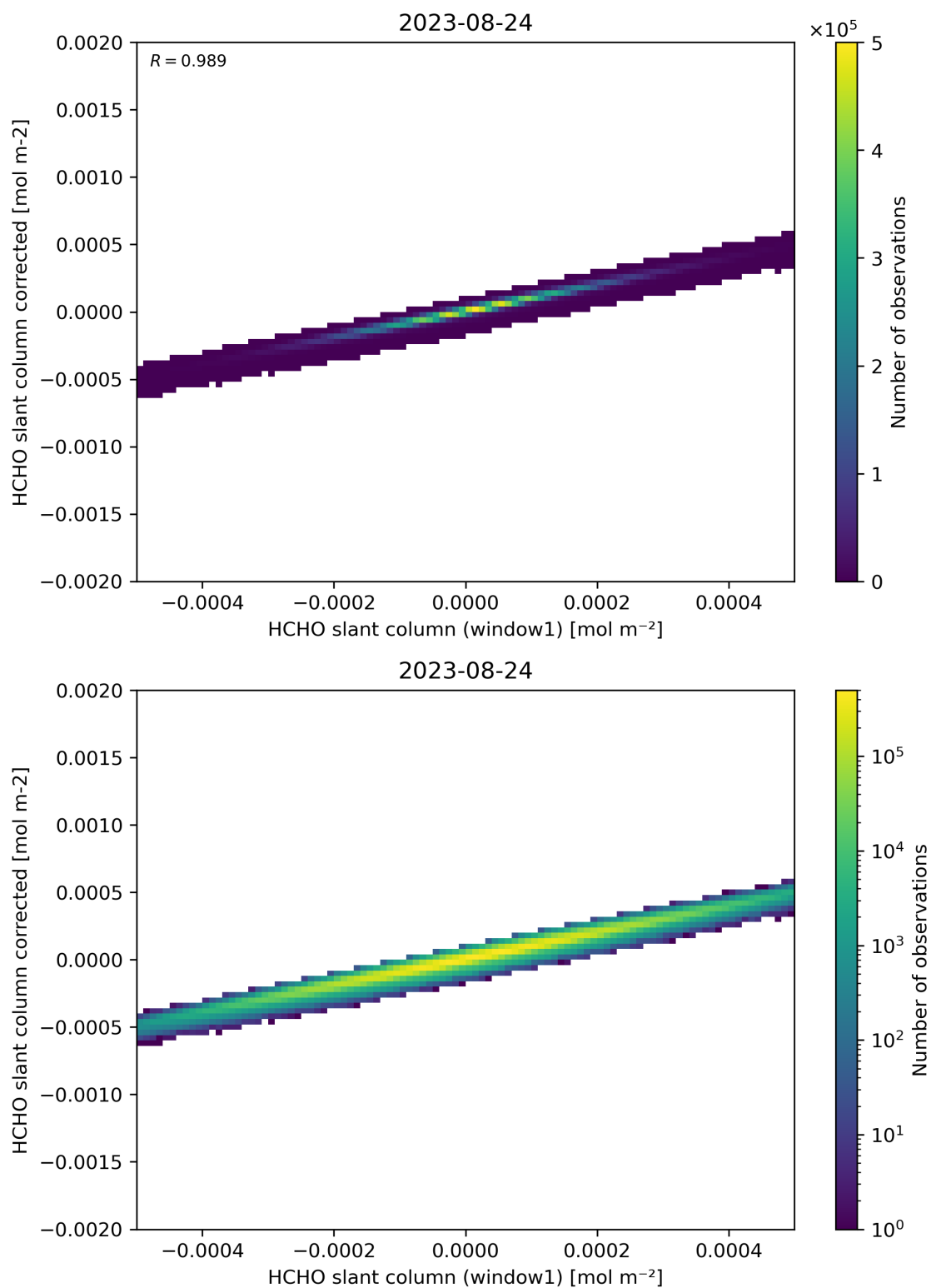
Figure 82: Scatter density plot of “HCHO slant column (window1)” against “HCHO slant column corrected” for 2023-08-23 to 2023-08-25.
