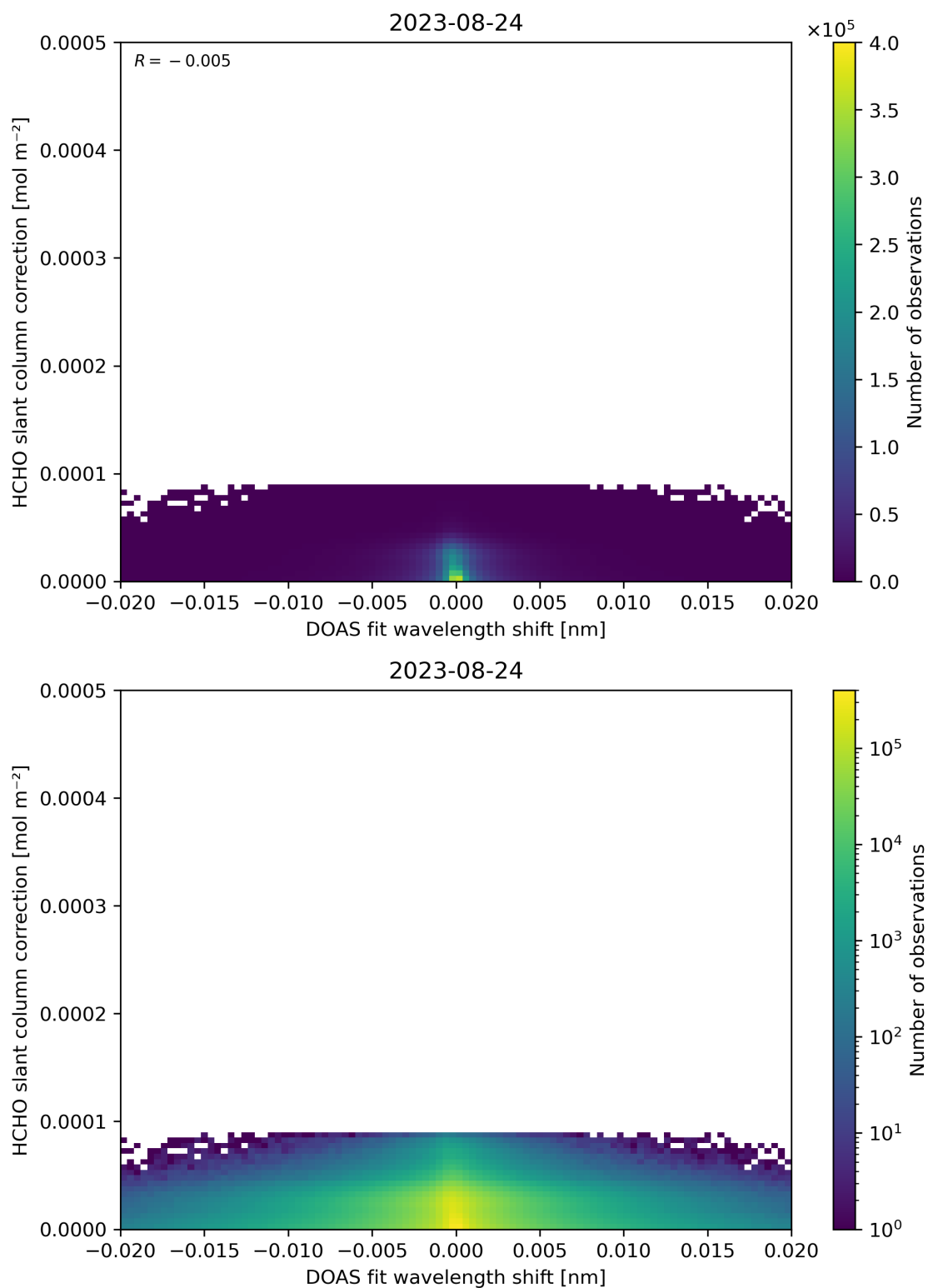
Figure 67: Scatter density plot of “DOAS fit wavelength shift” against “HCHO slant column correction” for 2023-08-23 to 2023-08-25.
