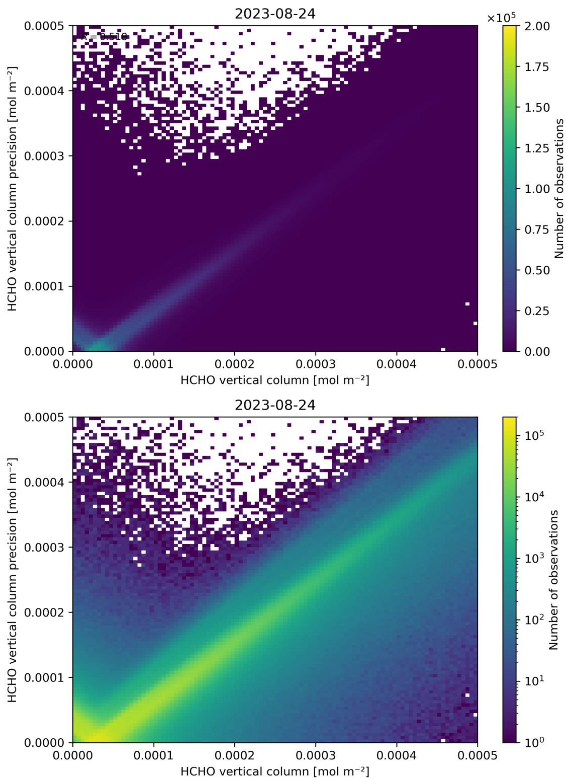
Figure 134: Scatter density plot of “HCHO vertical column” against “HCHO vertical column precision” for 2023-08-23 to 2023-08-25.
