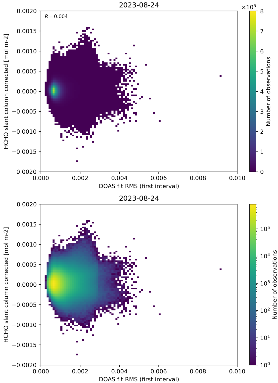
Figure 62: Scatter density plot of “DOAS fit RMS (first interval)” against “HCHO slant column corrected” for 2023-08-23 to 2023-08-25.
