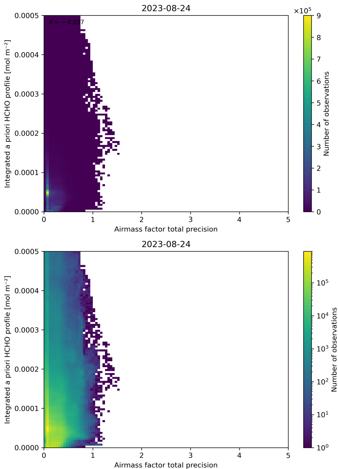
Figure 111: Scatter density plot of “Airmass factor total precision” against “Integrated a priori HCHO profile” for 2023-08-23 to 2023-08-25.
