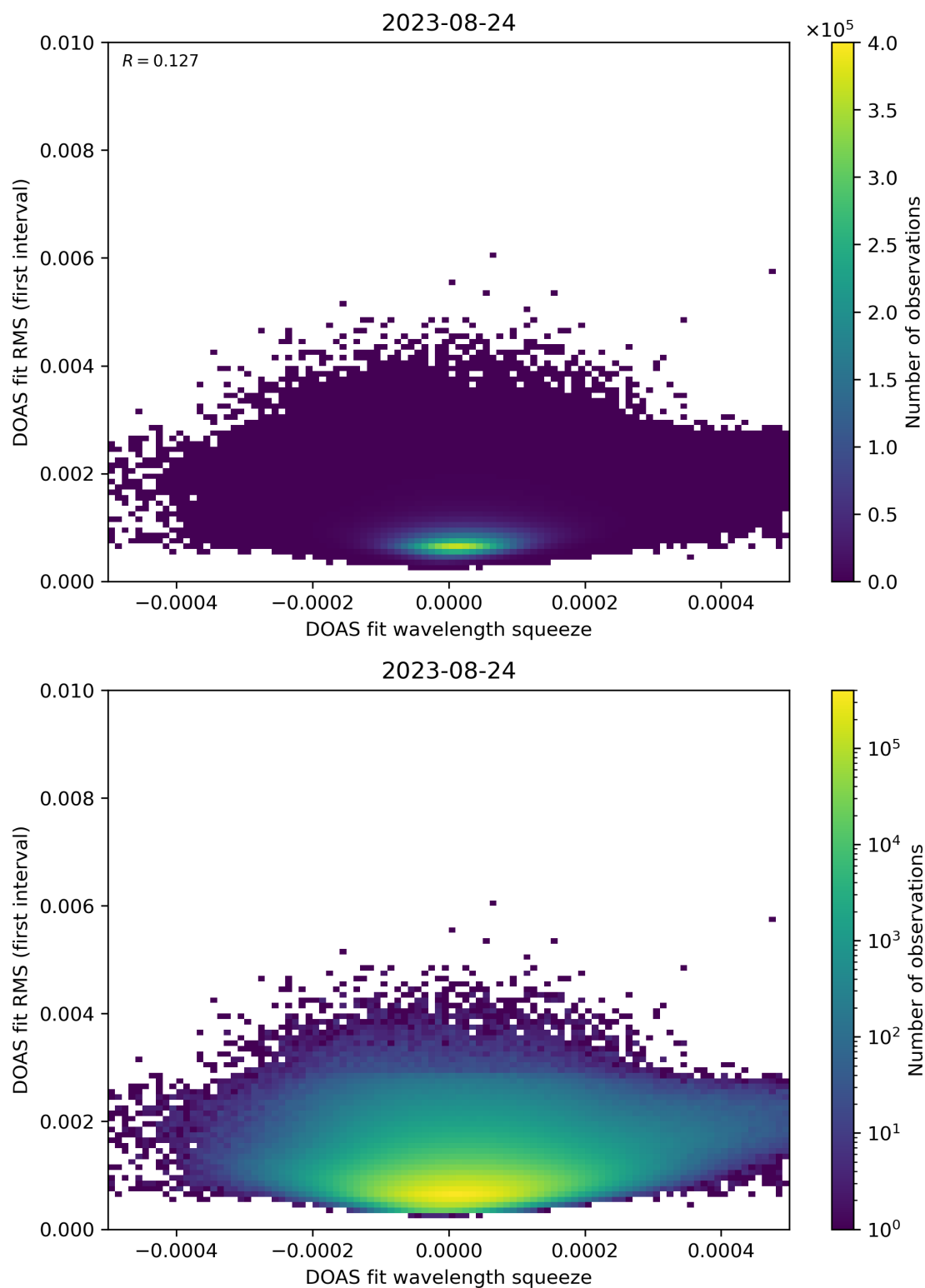
Figure 68: Scatter density plot of “DOAS fit wavelength squeeze” against “DOAS fit RMS (first interval)” for 2023-08-23 to 2023-08-25.
