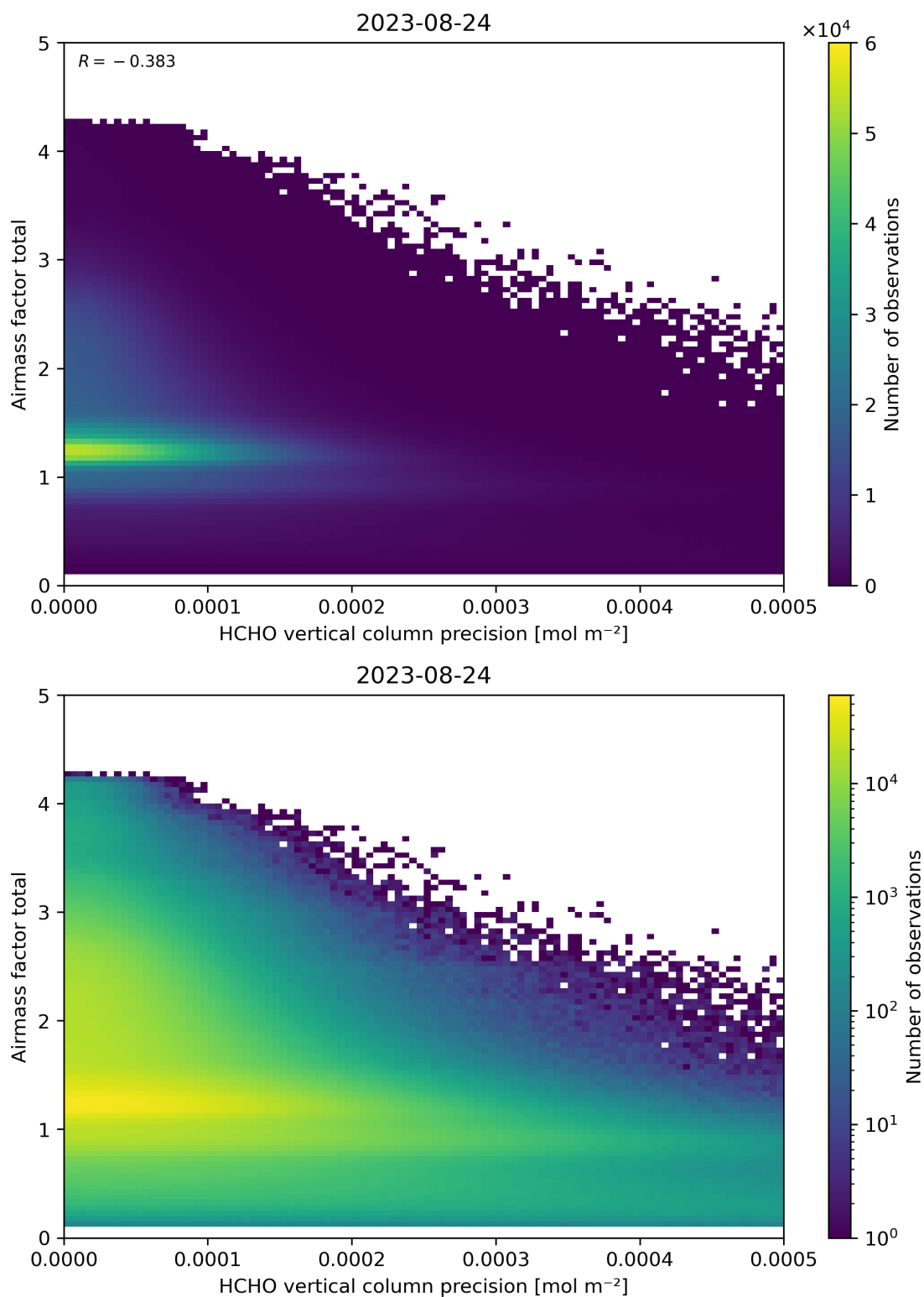
Figure 144: Scatter density plot of “HCHO vertical column precision” against “Airmass factor total” for 2023-08-23 to 2023-08-25.
