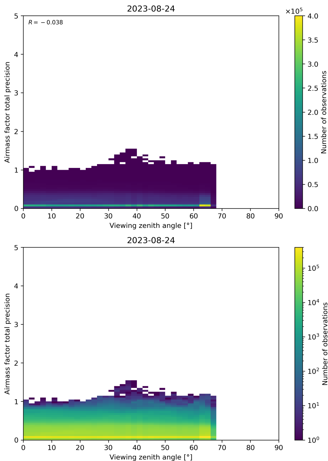
Figure 191: Scatter density plot of “Viewing zenith angle” against “Airmass factor total precision” for 2023-08-23 to 2023-08-25.
