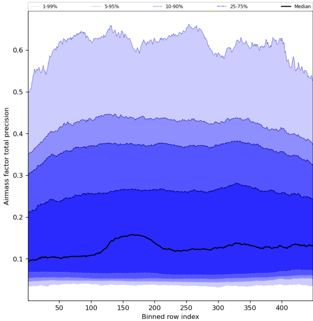
Figure 55: Along track statistics of “Airmass factor total precision” for 2023-08-23 to 2023-08-25
