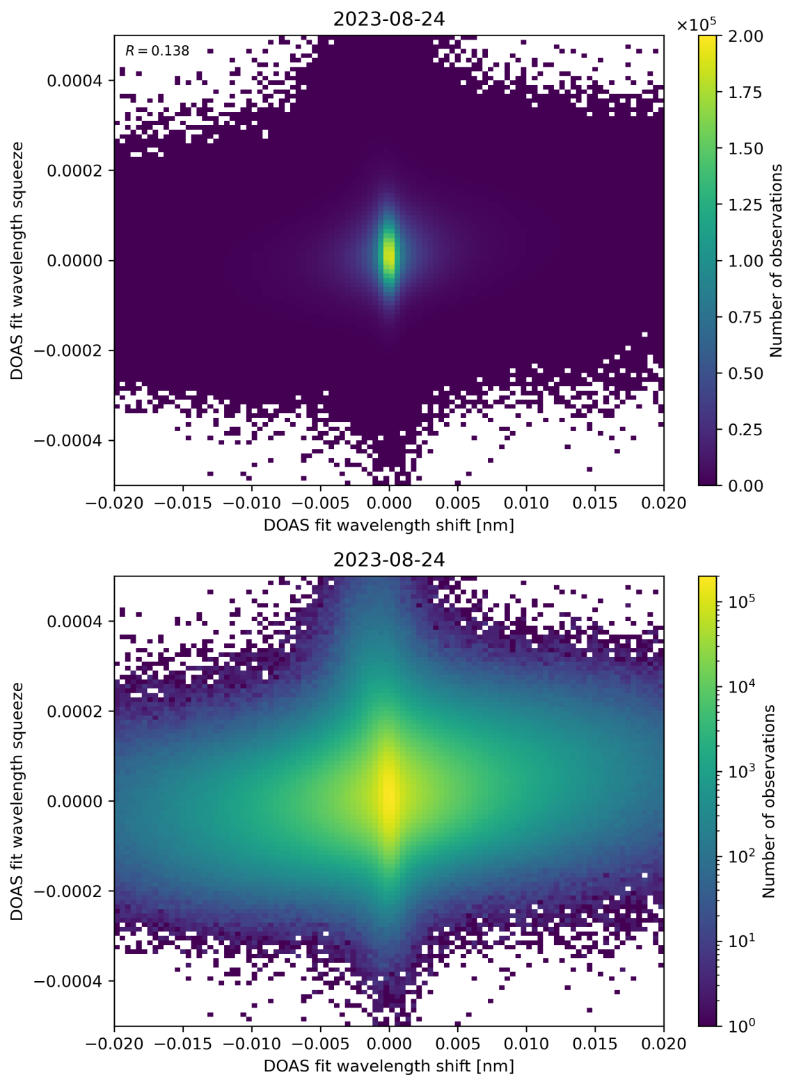
Figure 65: Scatter density plot of “DOAS fit wavelength shift” against “DOAS fit wavelength squeeze” for 2023-08-23 to 2023-08-25.
