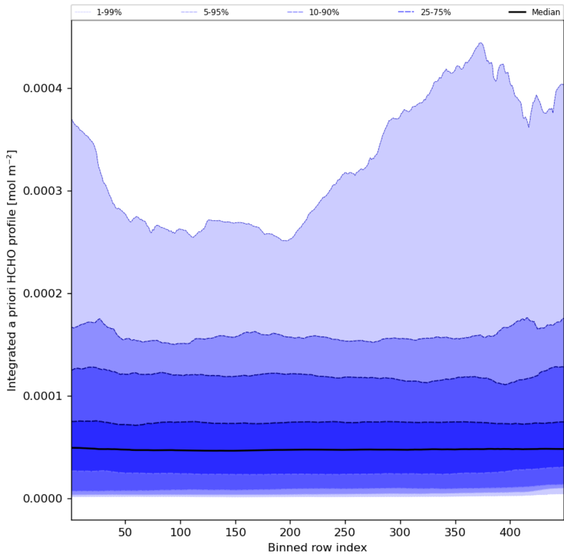
Figure 57: Along track statistics of “Integrated a priori HCHO profile” for 2023-08-23 to 2023-08-25
