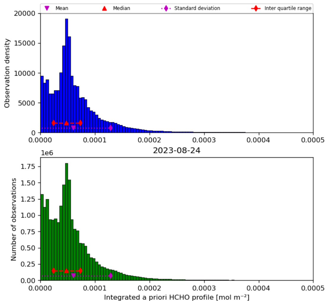
Figure 43: Histogram of “Integrated a priori HCHO profile” for 2023-08-23 to 2023-08-25
