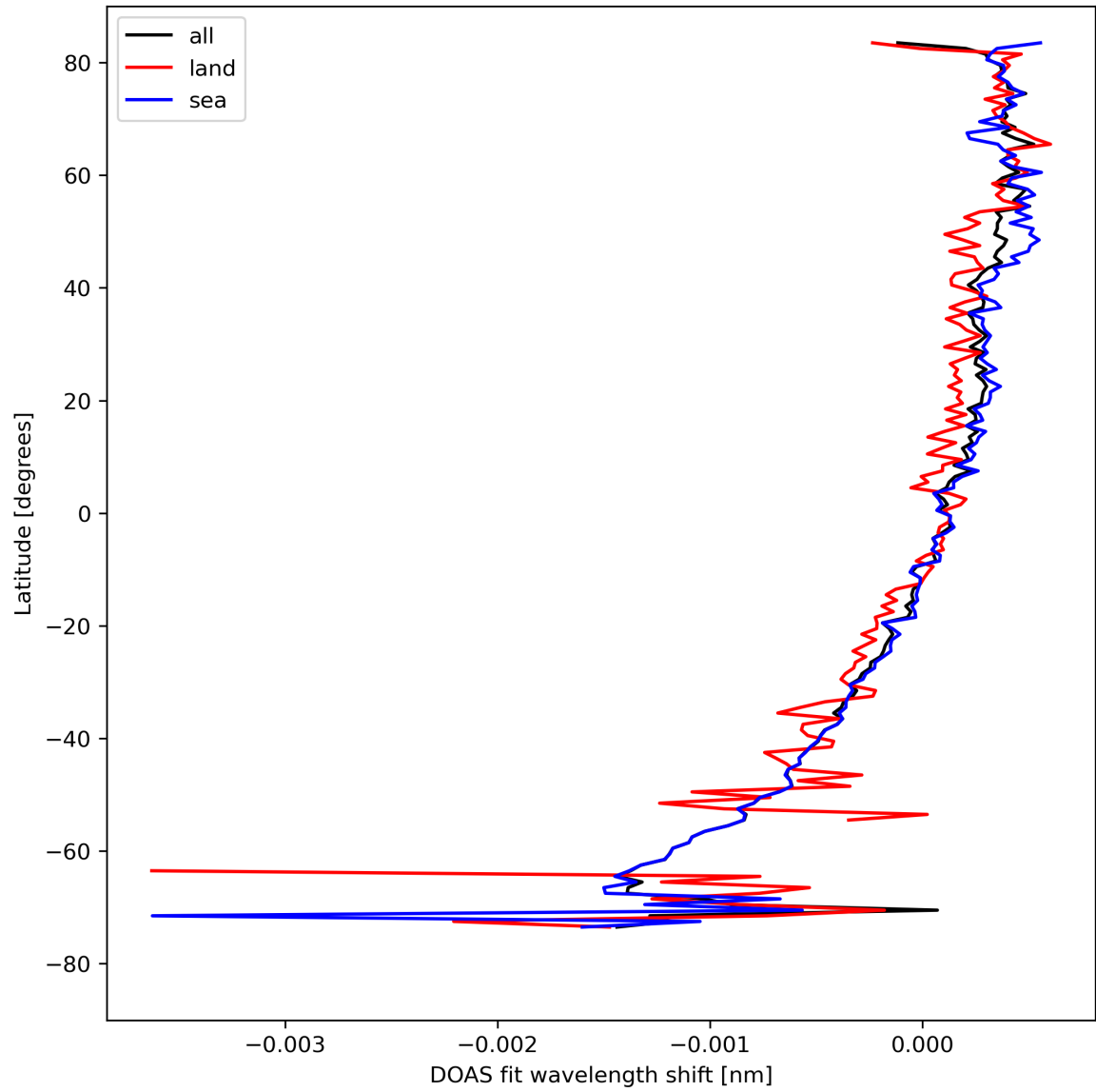
Figure 30: Zonal average of “DOAS fit wavelength shift” for 2023-08-23 to 2023-08-25.
