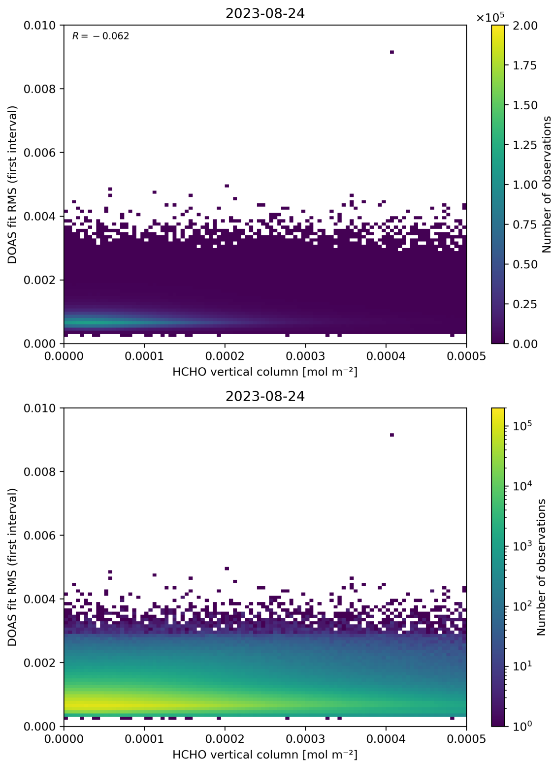
Figure 123: Scatter density plot of “HCHO vertical column” against “DOAS fit RMS (first interval)” for 2023-08-23 to 2023-08-25.
