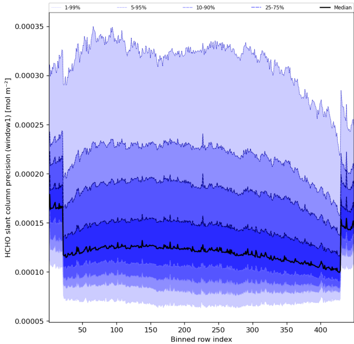
Figure 53: Along track statistics of “HCHO slant column precision (window1)” for 2023-08-23 to 2023-08-25
