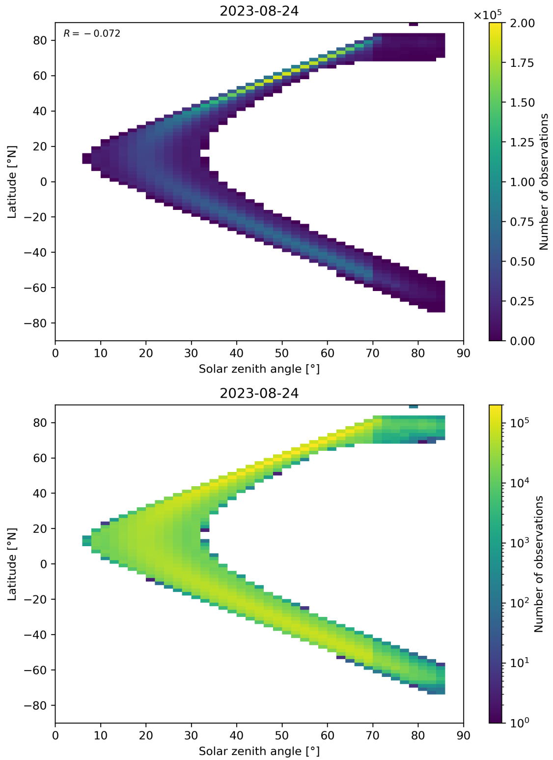
Figure 181: Scatter density plot of “Solar zenith angle” against “Latitude” for 2023-08-23 to 2023-08-25.
