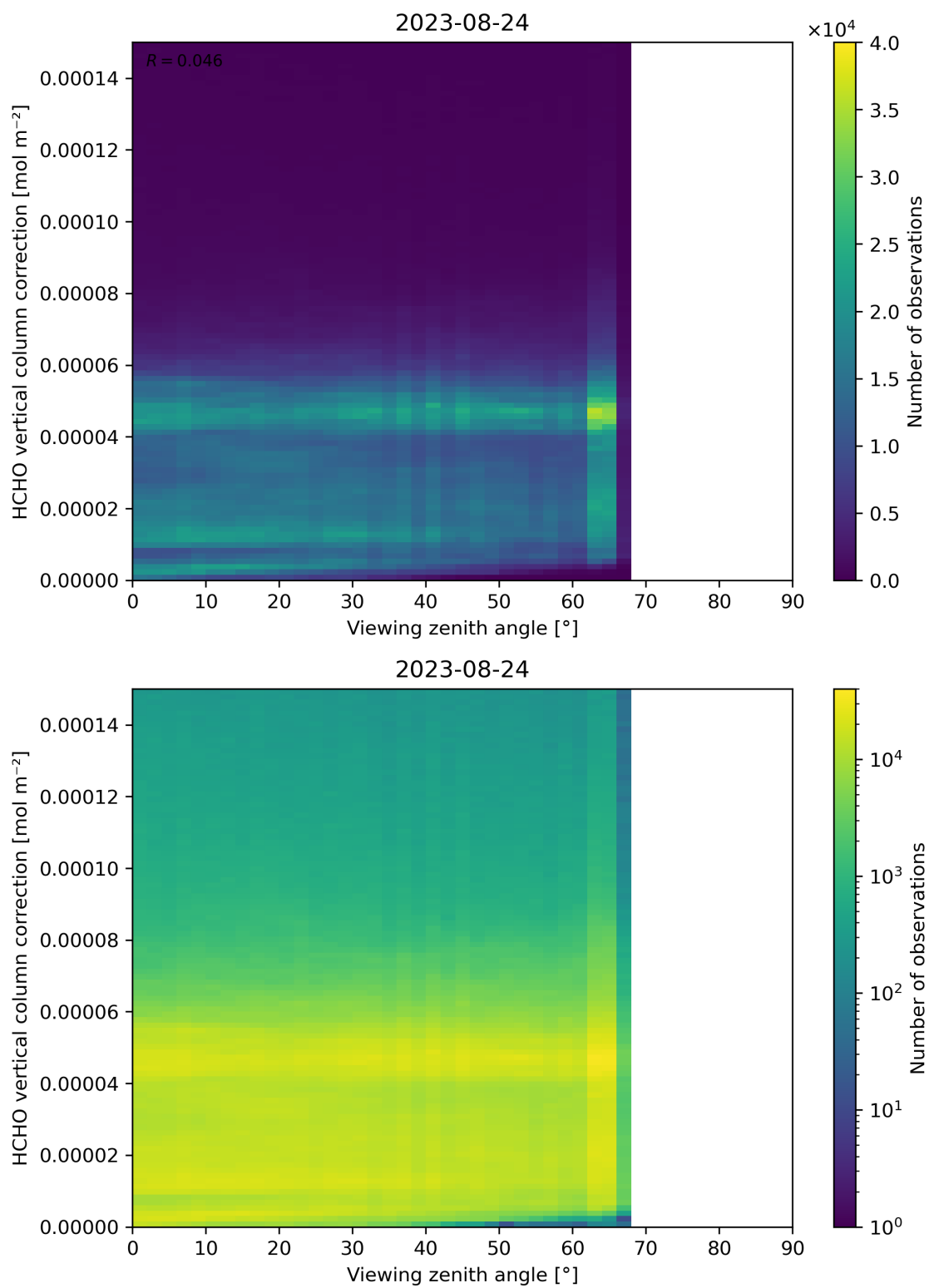
Figure 193: Scatter density plot of “Viewing zenith angle” against “HCHO vertical column correction” for 2023-08-23 to 2023-08-25.
