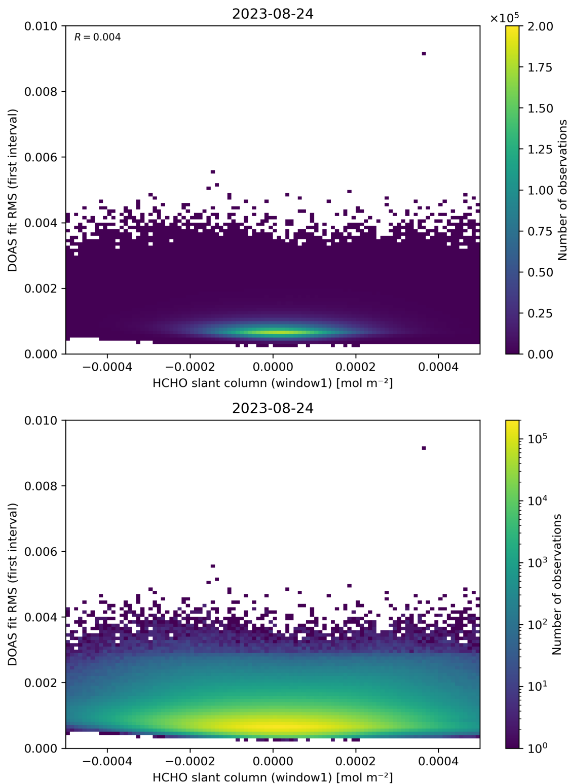
Figure 78: Scatter density plot of “HCHO slant column (window1)” against “DOAS fit RMS (first interval)” for 2023-08-23 to 2023-08-25.
