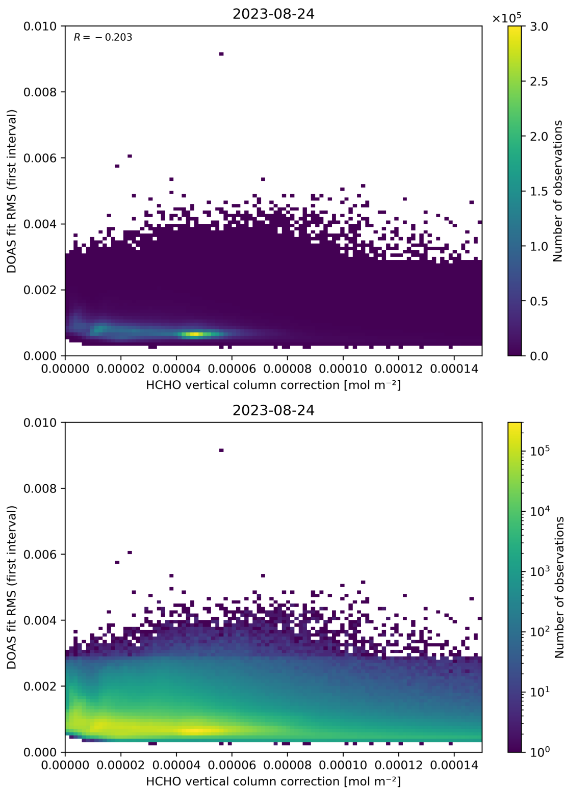
Figure 112: Scatter density plot of “HCHO vertical column correction” against “DOAS fit RMS (first interval)” for 2023-08-23 to 2023-08-25.
