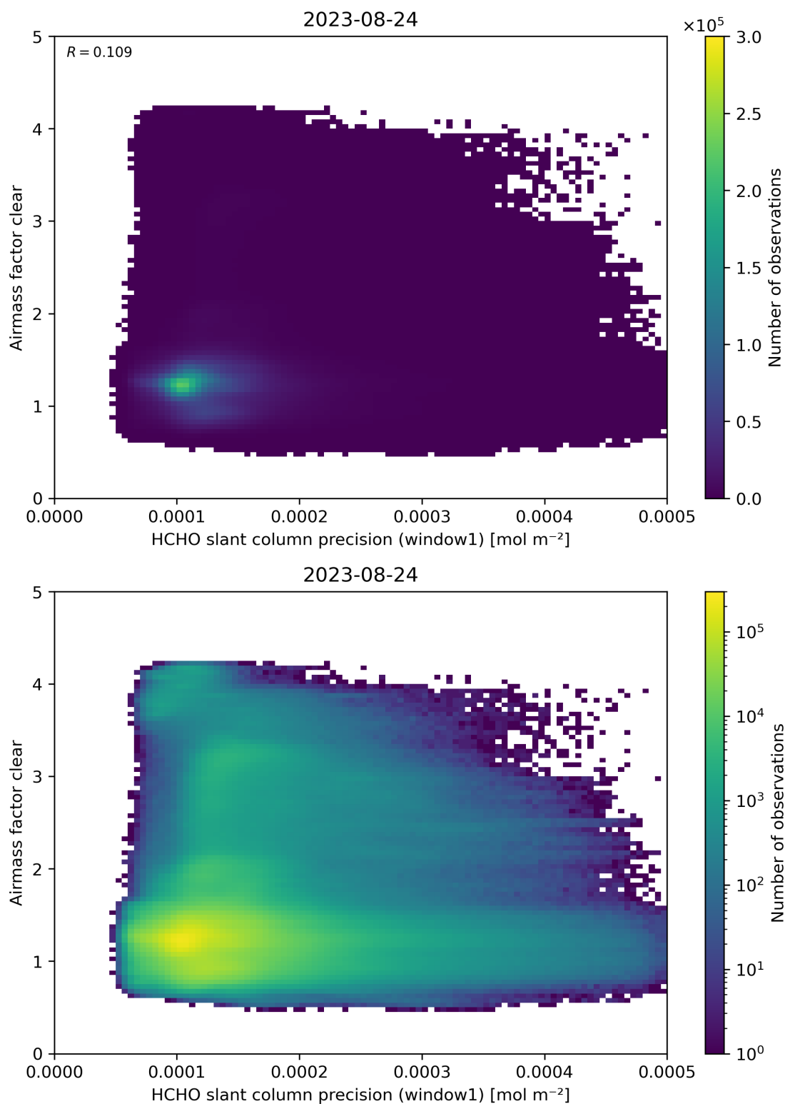
Figure 91: Scatter density plot of “HCHO slant column precision (window1)” against “Airmass factor clear” for 2023-08-23 to 2023-08-25.
