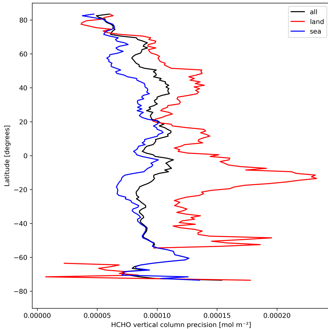
Figure 22: Zonal average of “HCHO vertical column precision” for 2023-08-23 to 2023-08-25.
