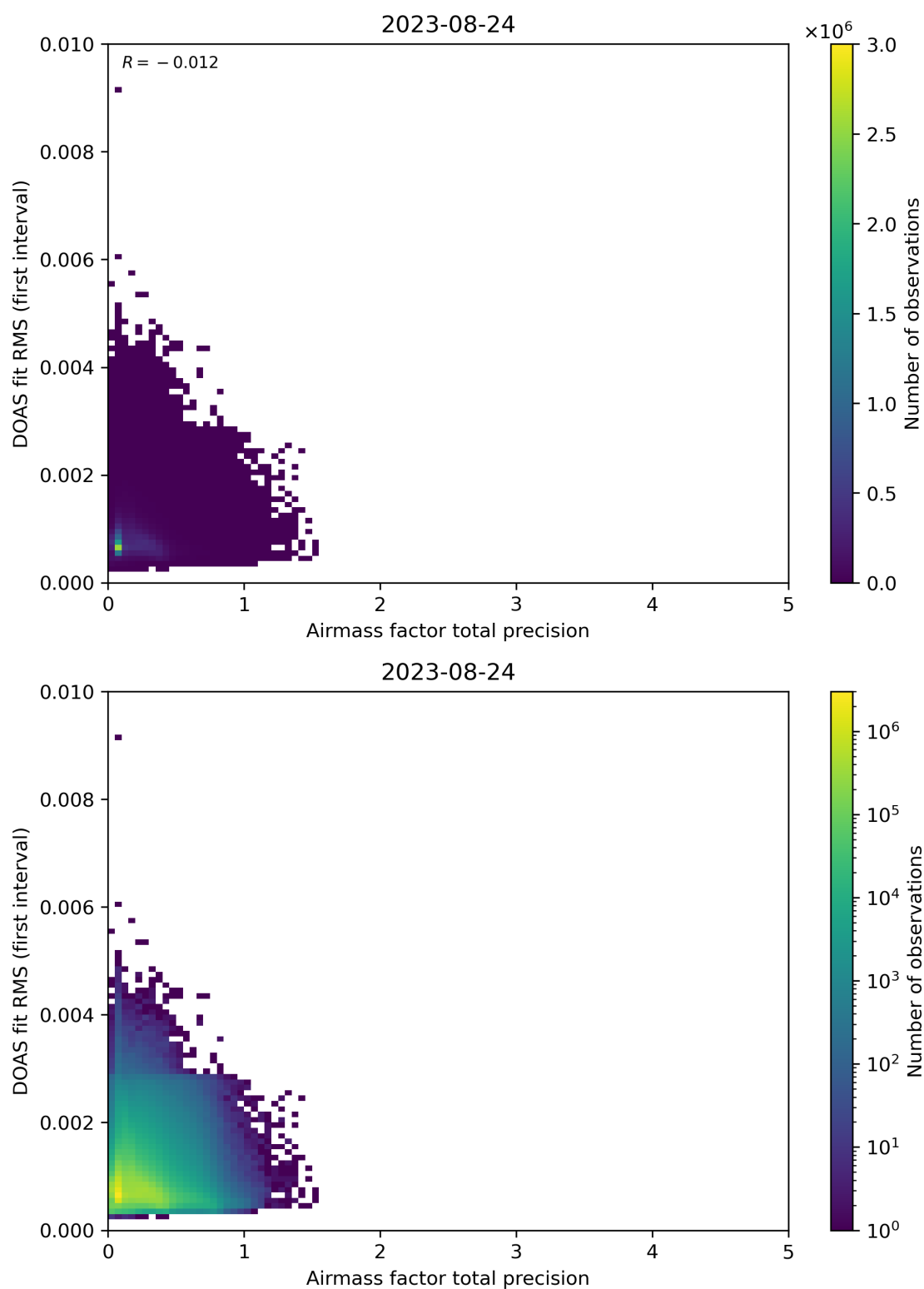
Figure 105: Scatter density plot of “Airmass factor total precision” against “DOAS fit RMS (first interval)” for 2023-08-23 to 2023-08-25.
