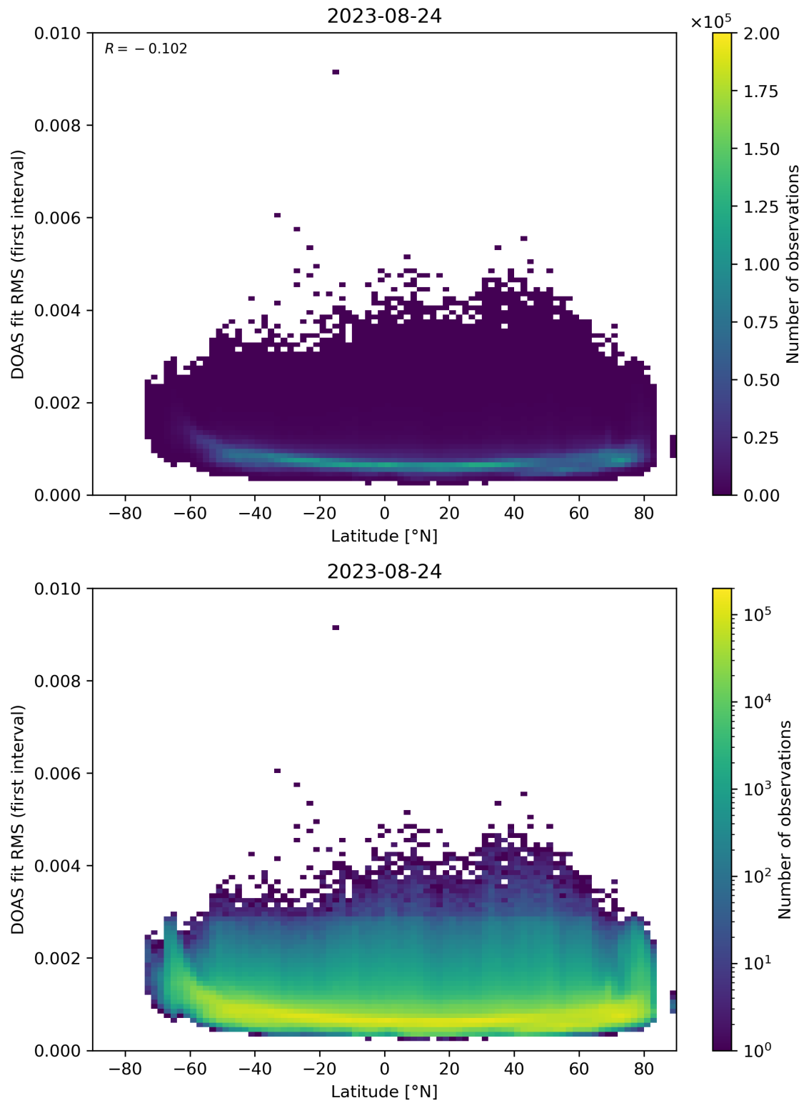
Figure 153: Scatter density plot of “Latitude” against “DOAS fit RMS (first interval)” for 2023-08-23 to 2023-08-25.
