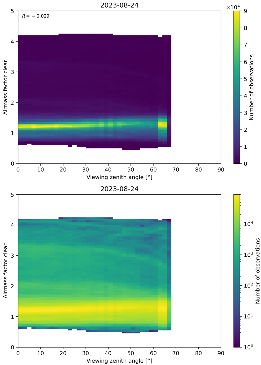
Figure 185: Scatter density plot of “Viewing zenith angle” against “Airmass factor clear” for 2023-08-23 to 2023-08-25.
