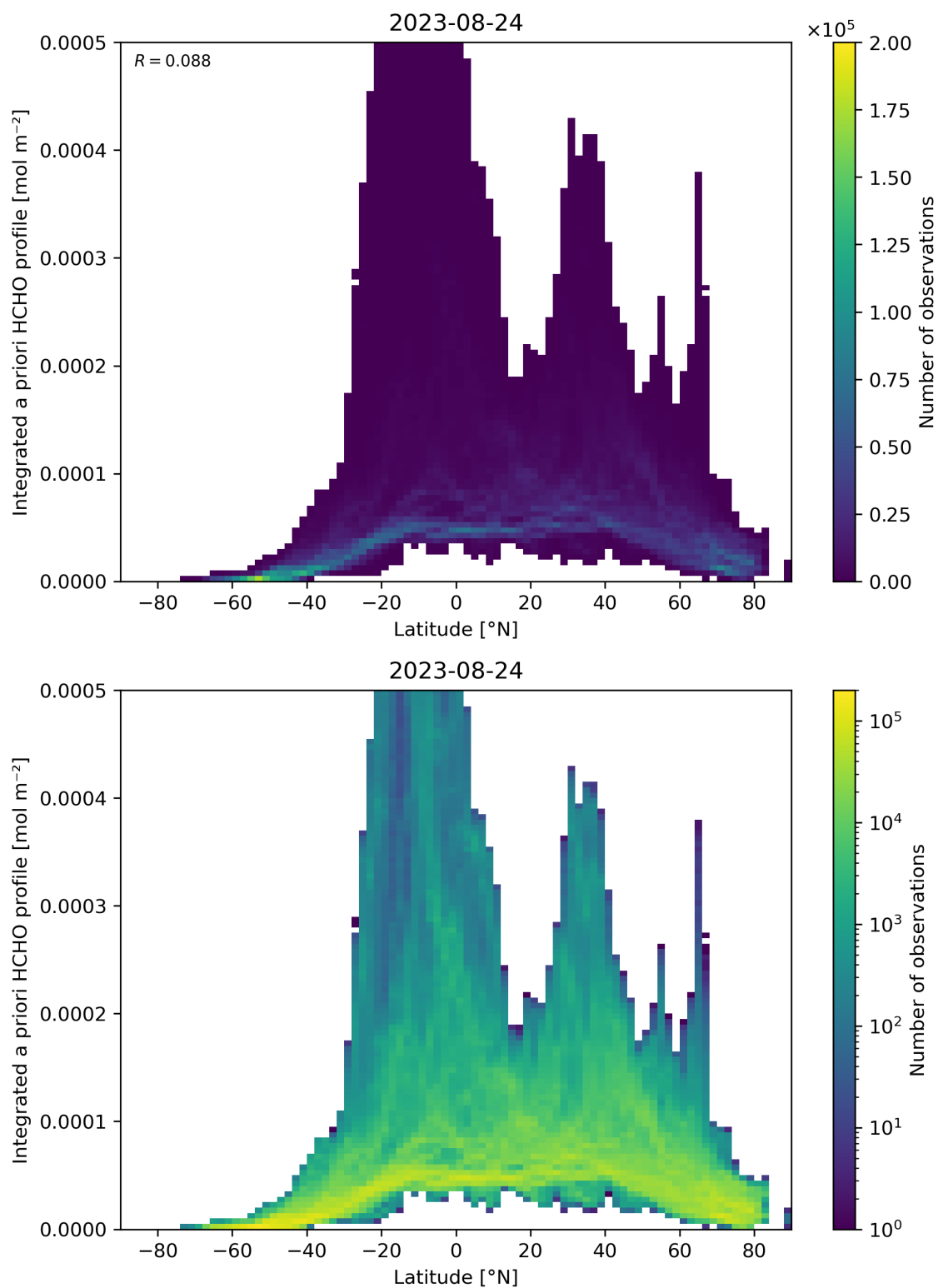
Figure 166: Scatter density plot of “Latitude” against “Integrated a priori HCHO profile” for 2023-08-23 to 2023-08-25.
