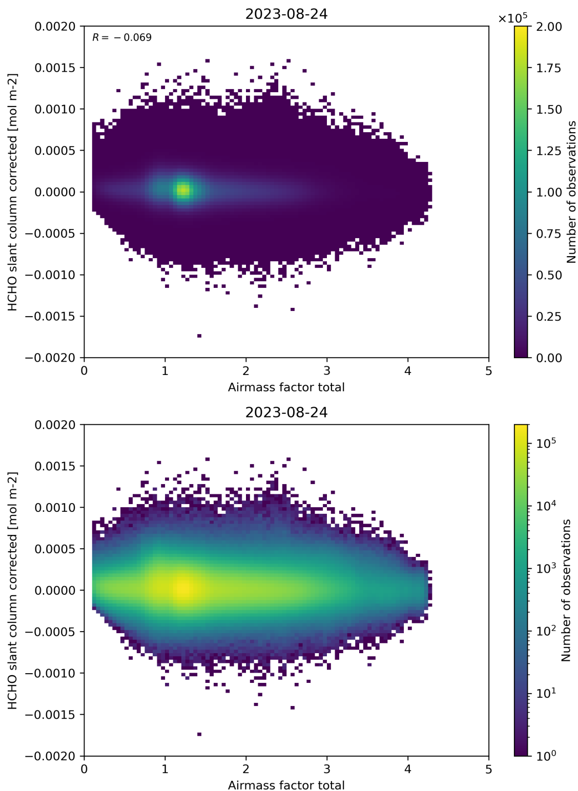
Figure 101: Scatter density plot of “Airmass factor total” against “HCHO slant column corrected” for 2023-08-23 to 2023-08-25.
