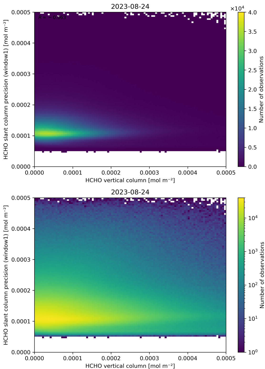
Figure 130: Scatter density plot of “HCHO vertical column” against “HCHO slant column precision (window1)” for 2023-08-23 to 2023-08-25.
