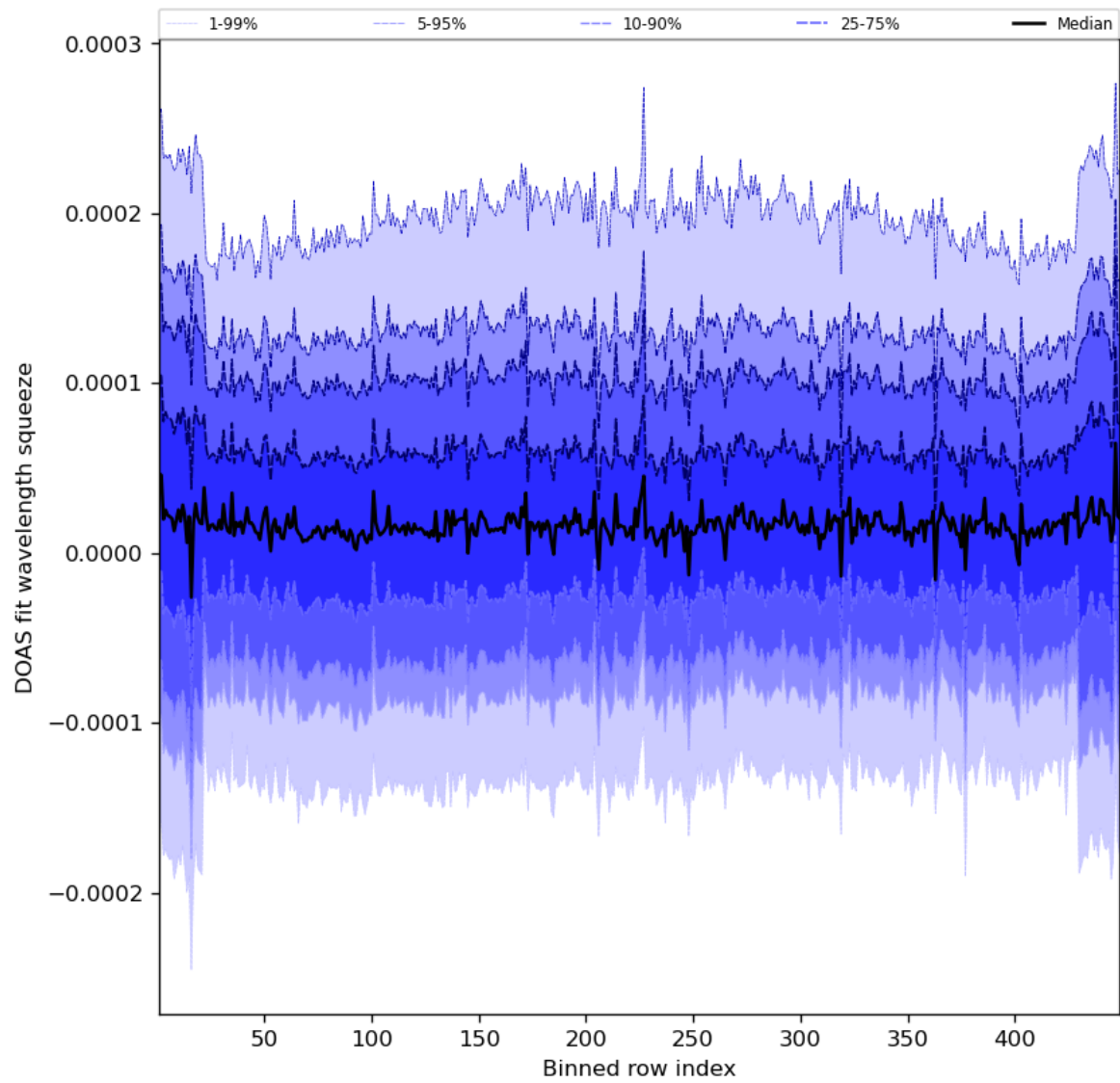
Figure 59: Along track statistics of “DOAS fit wavelength squeeze” for 2023-08-23 to 2023-08-25
