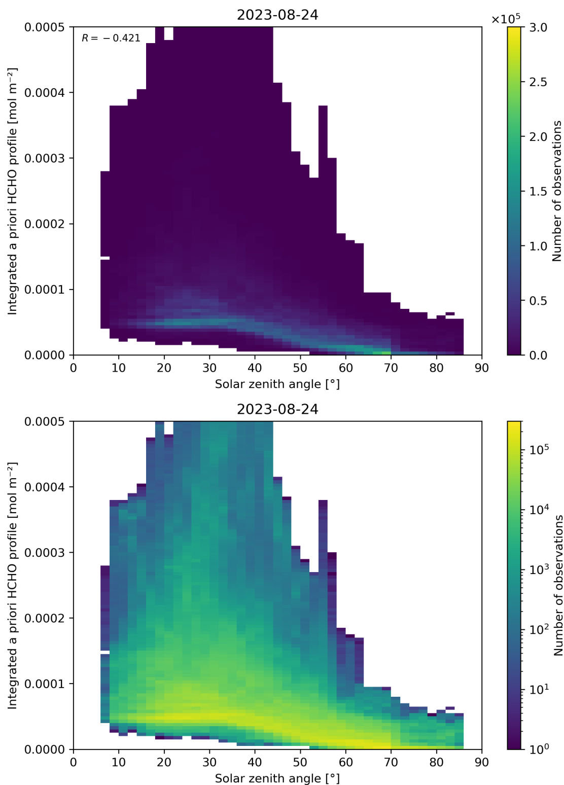
Figure 180: Scatter density plot of “Solar zenith angle” against “Integrated a priori HCHO profile” for 2023-08-23 to 2023-08-25.
