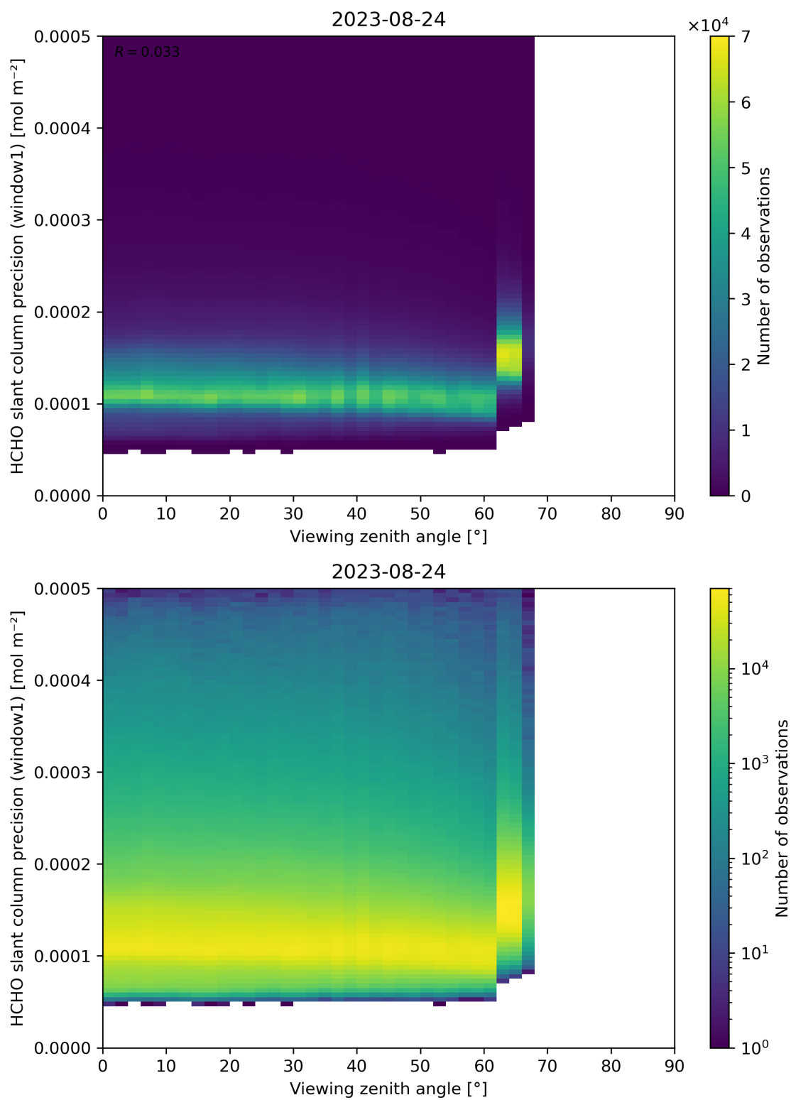
Figure 189: Scatter density plot of “Viewing zenith angle” against “HCHO slant column precision (window1)” for 2023-08-23 to 2023-08-25.
