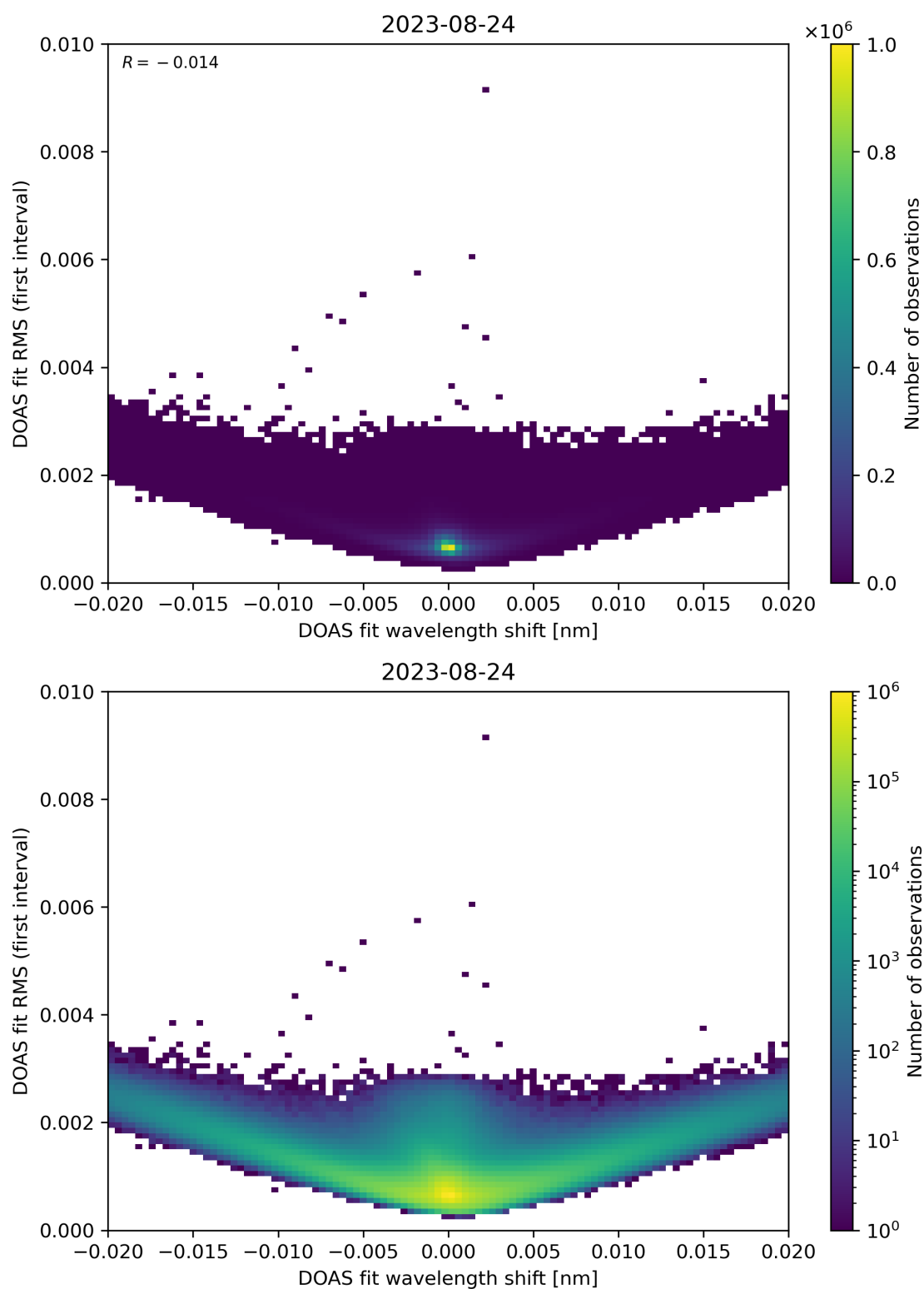
Figure 64: Scatter density plot of “DOAS fit wavelength shift” against “DOAS fit RMS (first interval)” for 2023-08-23 to 2023-08-25.
