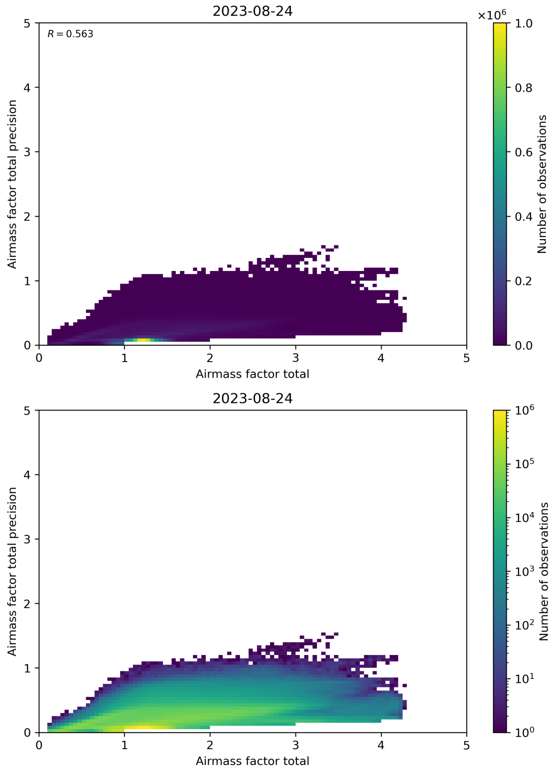
Figure 103: Scatter density plot of “Airmass factor total” against “Airmass factor total precision” for 2023-08-23 to 2023-08-25.
