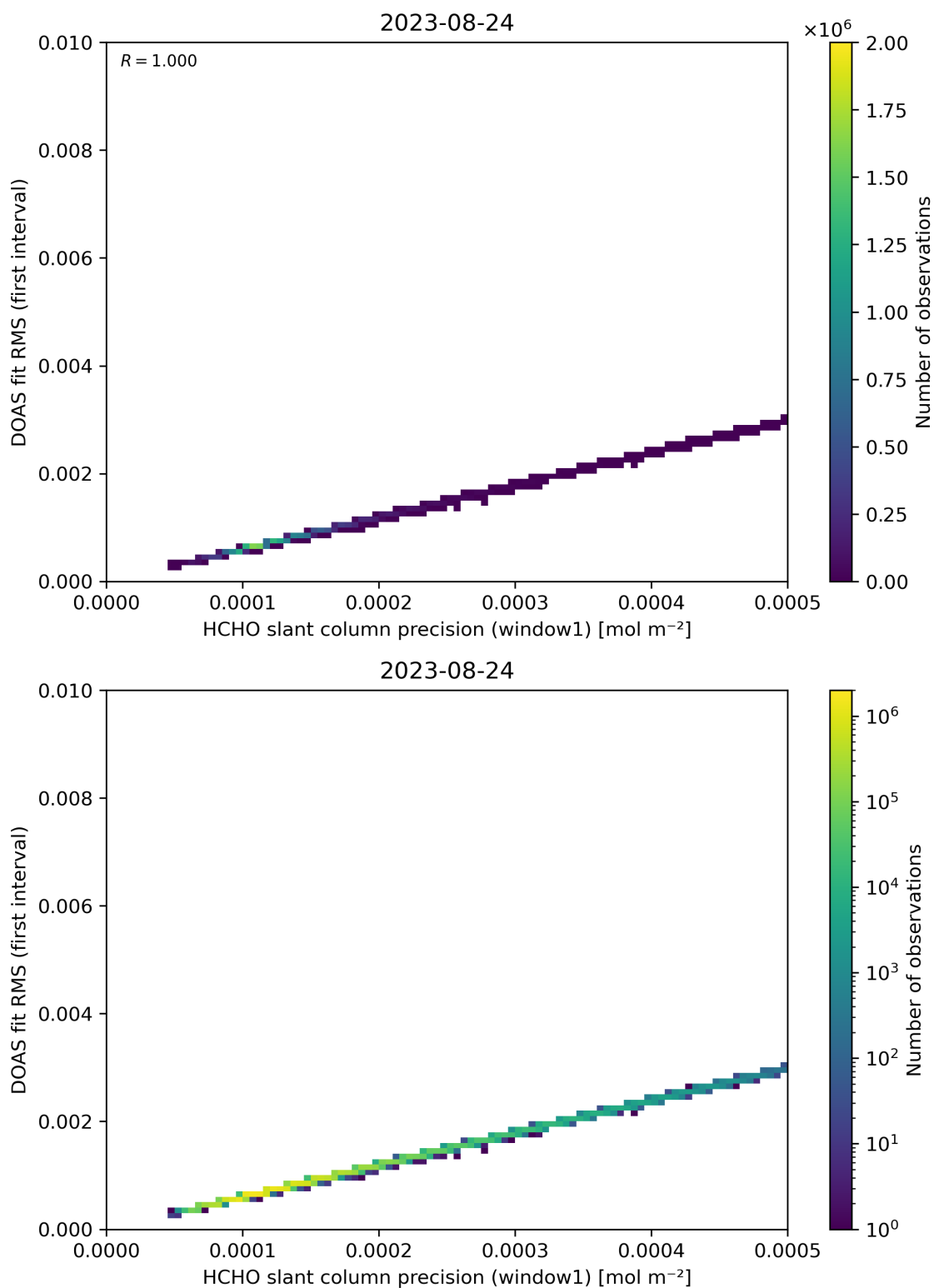
Figure 88: Scatter density plot of “HCHO slant column precision (window1)” against “DOAS fit RMS (first interval)” for 2023-08-23 to 2023-08-25.
