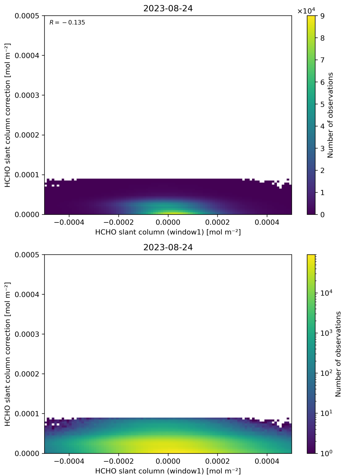
Figure 83: Scatter density plot of “HCHO slant column (window1)” against “HCHO slant column correction” for 2023-08-23 to 2023-08-25.
