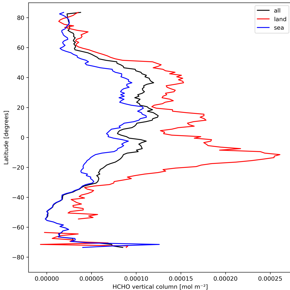
Figure 21: Zonal average of “HCHO vertical column” for 2023-08-23 to 2023-08-25.
