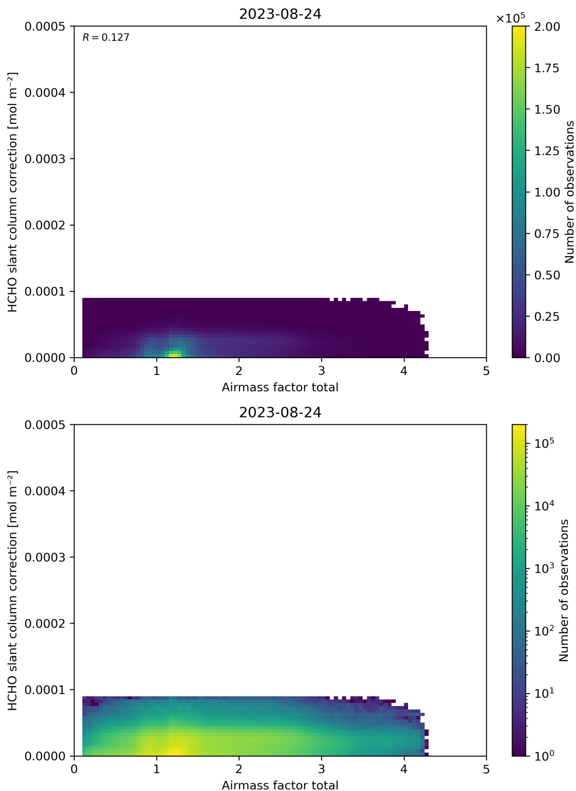
Figure 102: Scatter density plot of “Airmass factor total” against “HCHO slant column correction” for 2023-08-23 to 2023-08-25.
