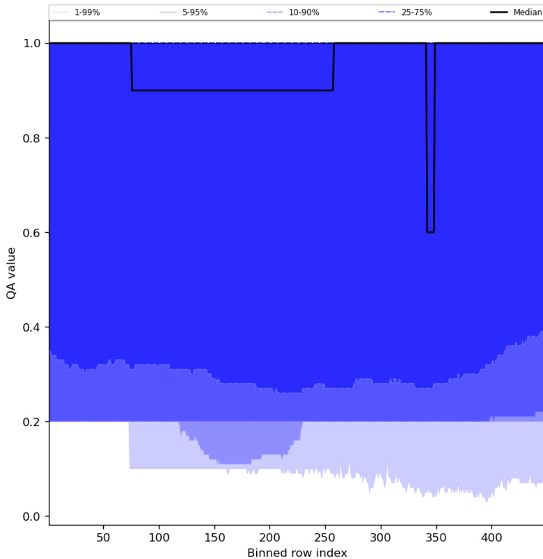
Figure 48: Along track statistics of “QA value” for 2023-08-23 to 2023-08-25
