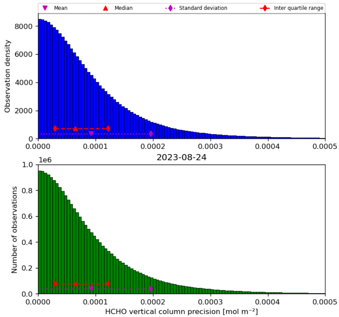
Figure 36: Histogram of “HCHO vertical column precision” for 2023-08-23 to 2023-08-25
