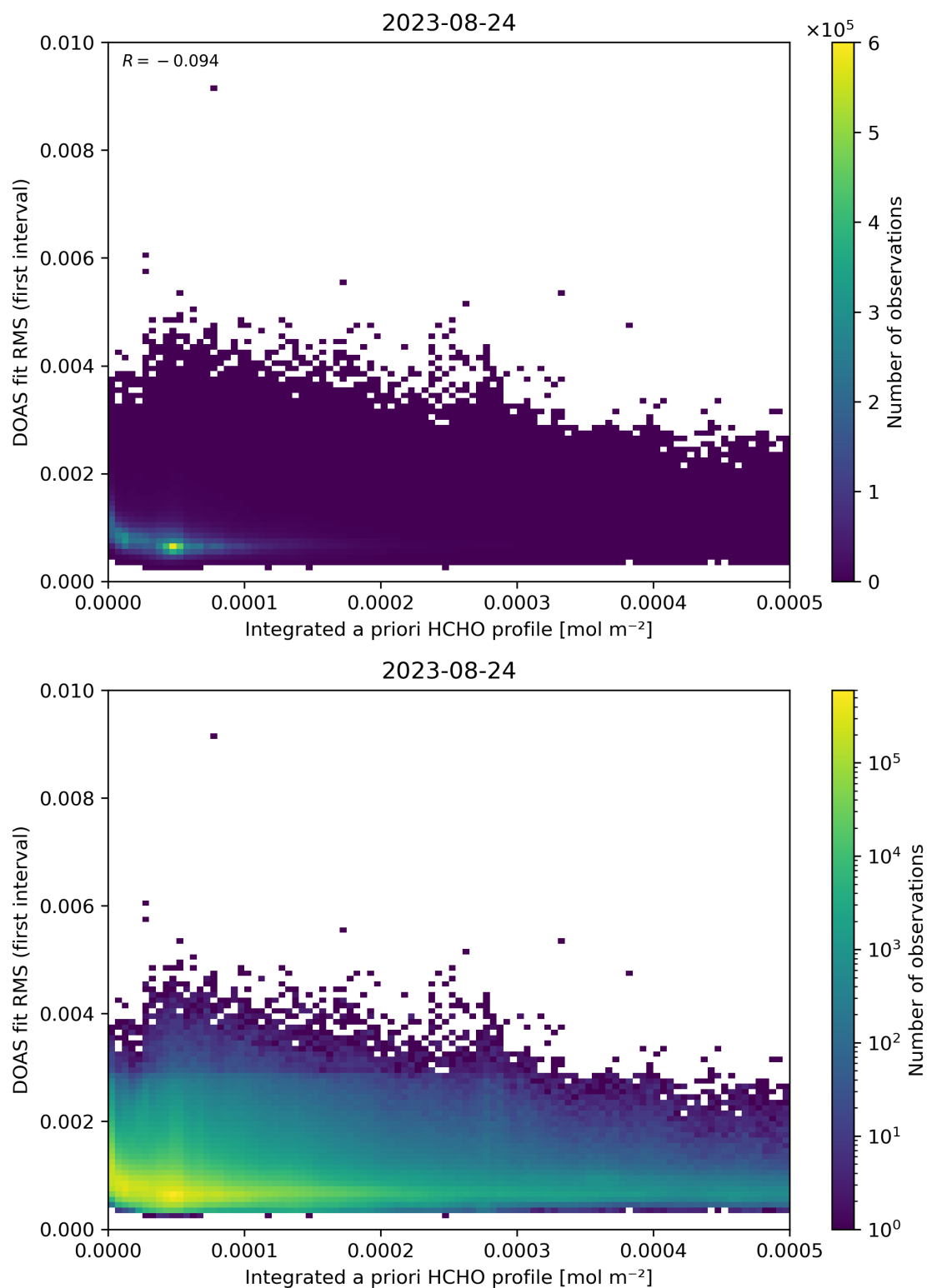
Figure 148: Scatter density plot of “Integrated a priori HCHO profile” against “DOAS fit RMS (first interval)” for 2023-08-23 to 2023-08-25.
