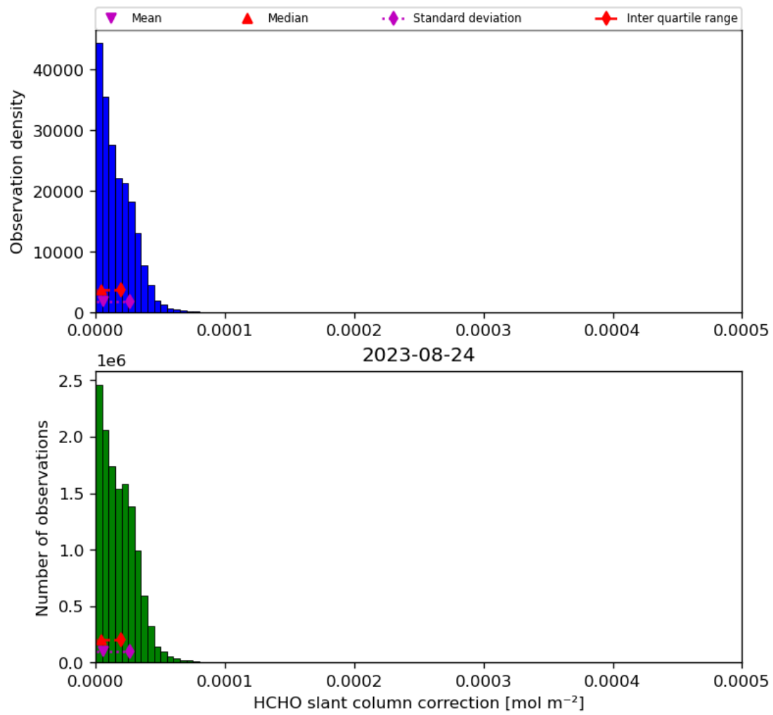
Figure 47: Histogram of “HCHO slant column correction” for 2023-08-23 to 2023-08-25
