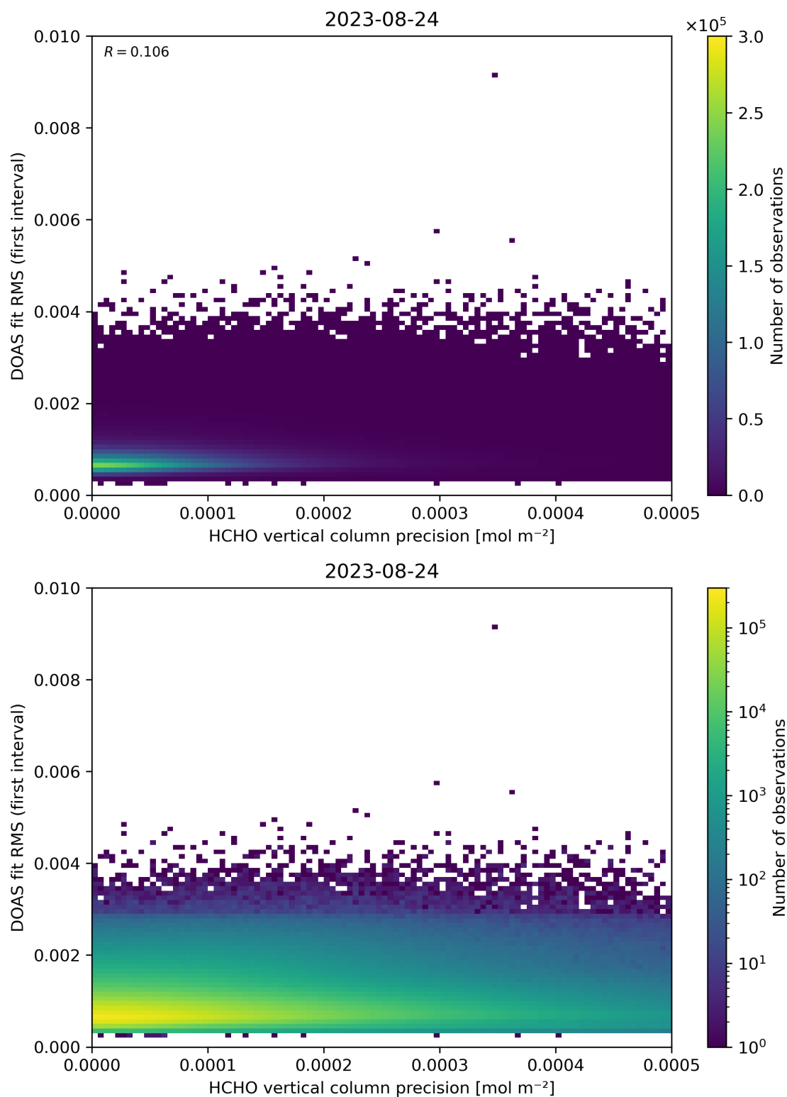
Figure 136: Scatter density plot of “HCHO vertical column precision” against “DOAS fit RMS (first interval)” for 2023-08-23 to 2023-08-25.
