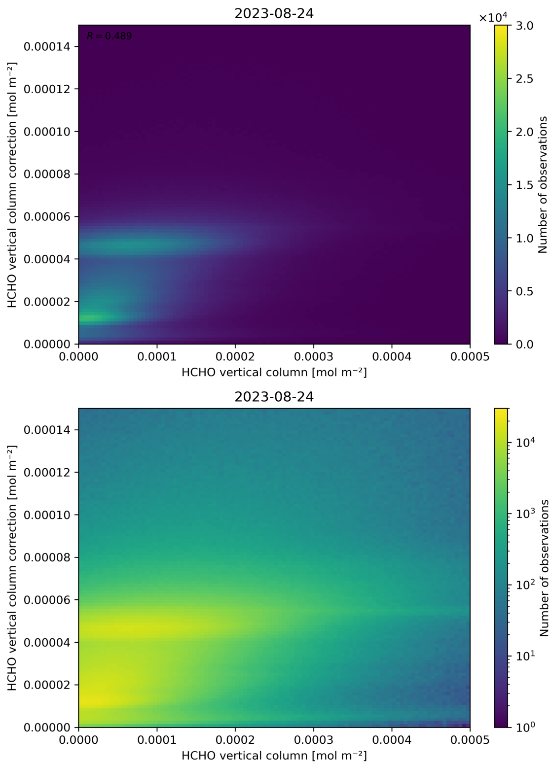
Figure 133: Scatter density plot of “HCHO vertical column” against “HCHO vertical column correction” for 2023-08-23 to 2023-08-25.
