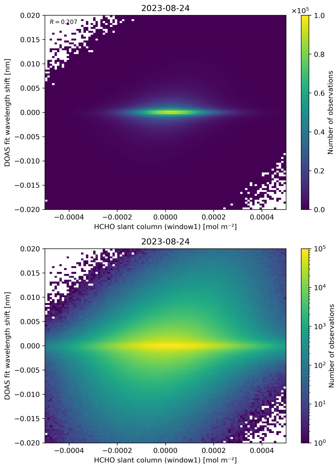
Figure 79: Scatter density plot of “HCHO slant column (window1)” against “DOAS fit wavelength shift” for 2023-08-23 to 2023-08-25.
