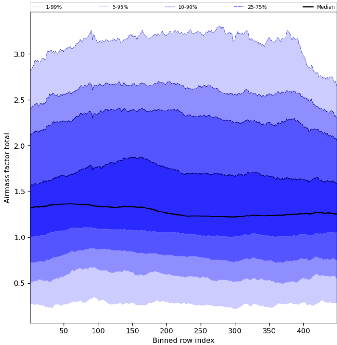
Figure 54: Along track statistics of “Airmass factor total” for 2023-08-23 to 2023-08-25
