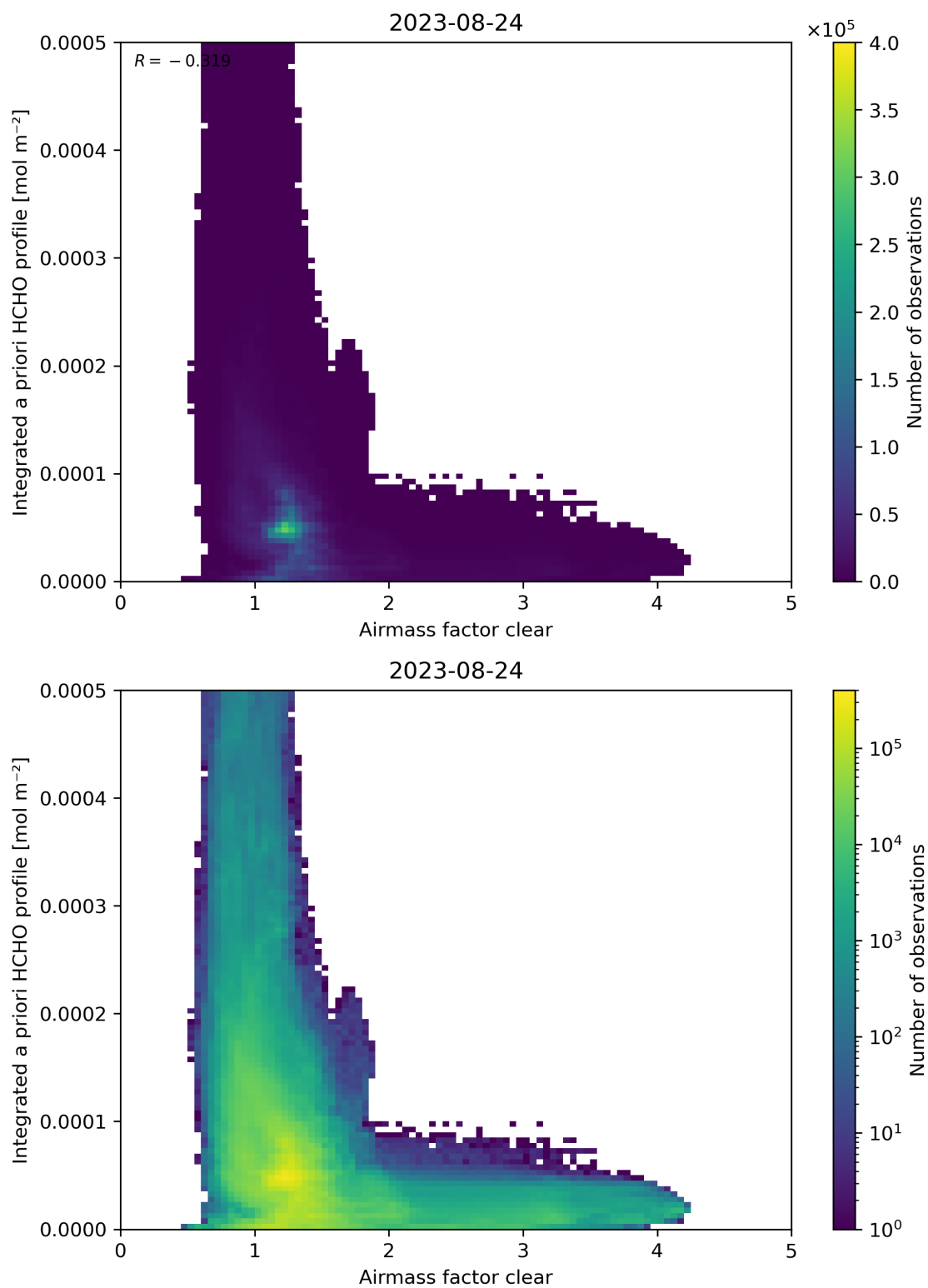
Figure 76: Scatter density plot of “Airmass factor clear” against “Integrated a priori HCHO profile” for 2023-08-23 to 2023-08-25.
