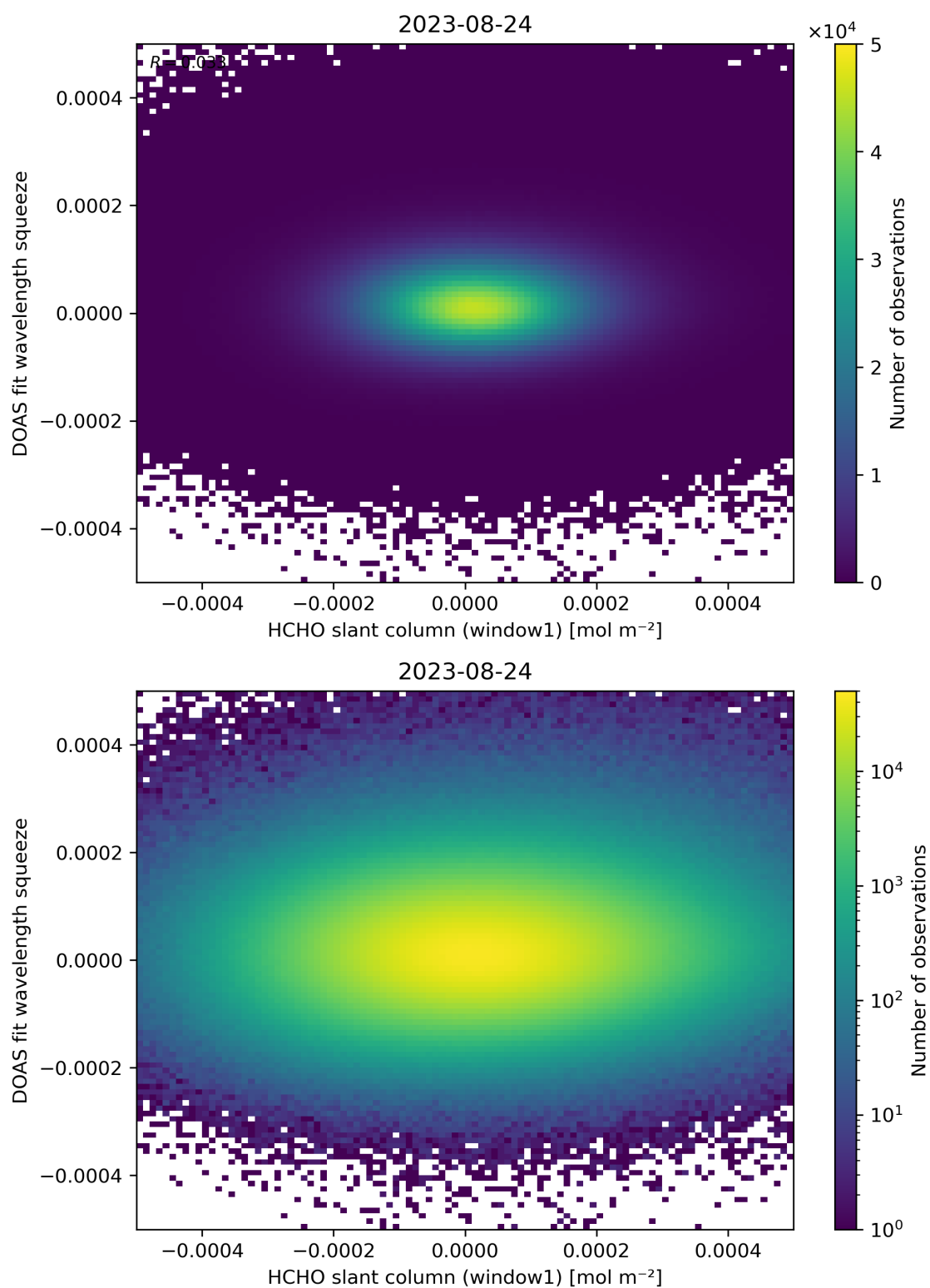
Figure 80: Scatter density plot of “HCHO slant column (window1)” against “DOAS fit wavelength squeeze” for 2023-08-23 to 2023-08-25.
