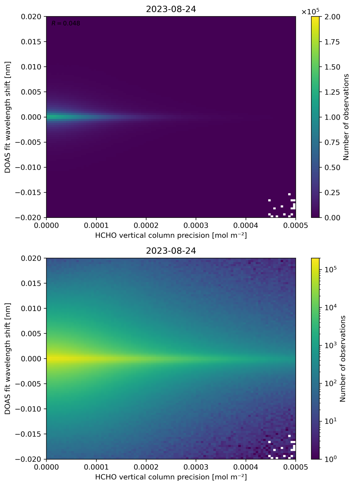
Figure 137: Scatter density plot of “HCHO vertical column precision” against “DOAS fit wavelength shift” for 2023-08-23 to 2023-08-25.
