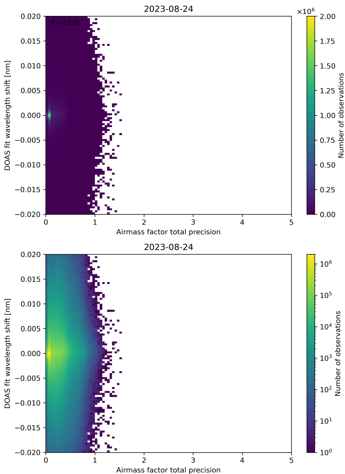
Figure 106: Scatter density plot of “Airmass factor total precision” against “DOAS fit wavelength shift” for 2023-08-23 to 2023-08-25.
