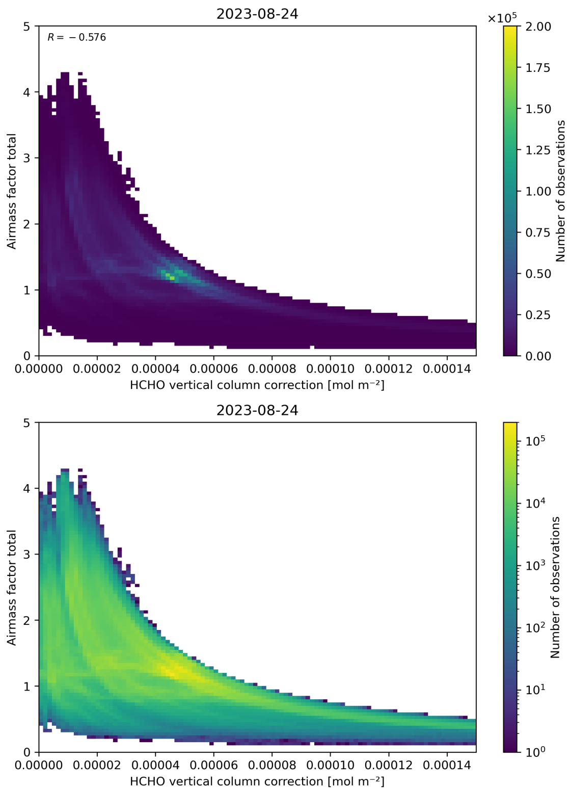
Figure 120: Scatter density plot of “HCHO vertical column correction” against “Airmass factor total” for 2023-08-23 to 2023-08-25.
