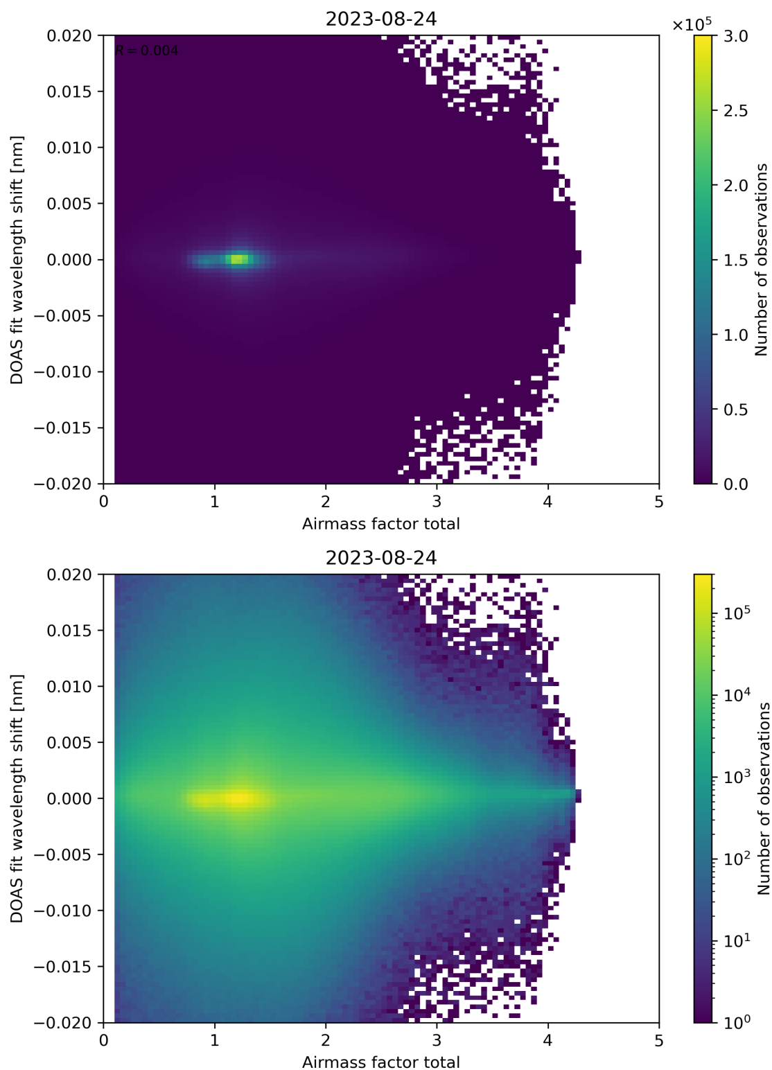
Figure 98: Scatter density plot of “Airmass factor total” against “DOAS fit wavelength shift” for 2023-08-23 to 2023-08-25.
