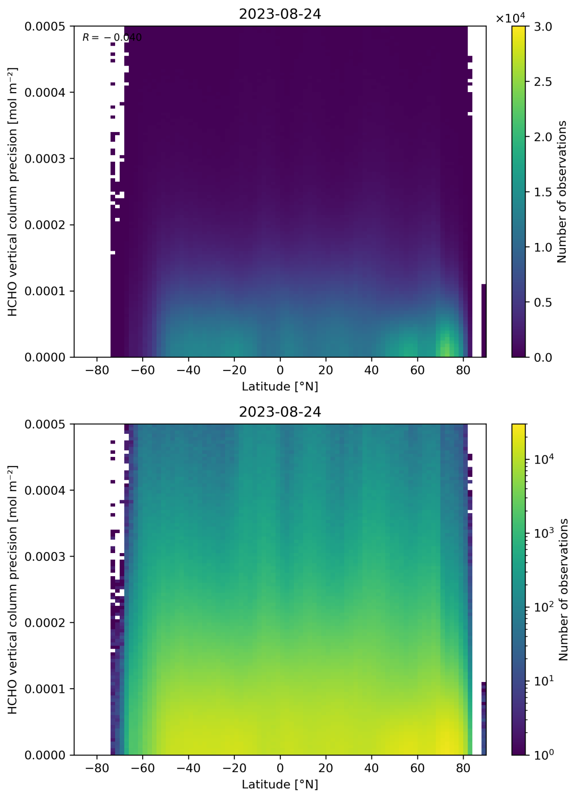
Figure 165: Scatter density plot of “Latitude” against “HCHO vertical column precision” for 2023-08-23 to 2023-08-25.
