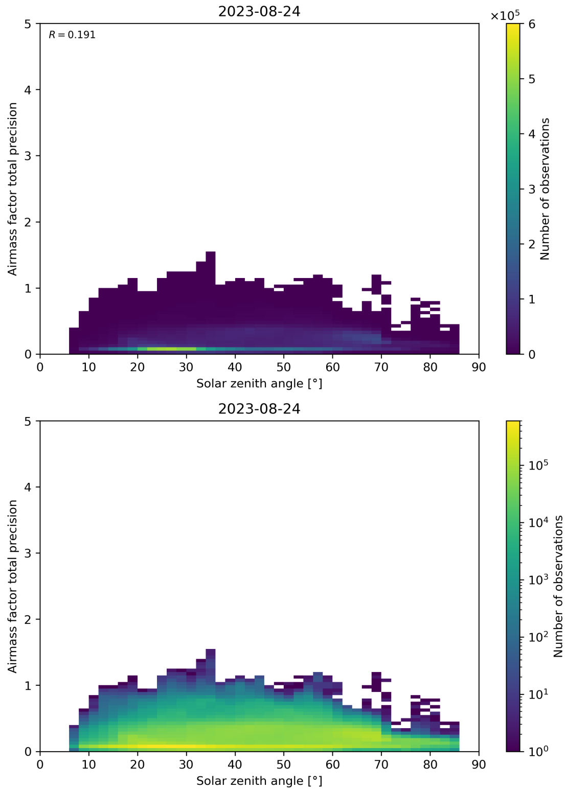
Figure 176: Scatter density plot of “Solar zenith angle” against “Airmass factor total precision” for 2023-08-23 to 2023-08-25.
