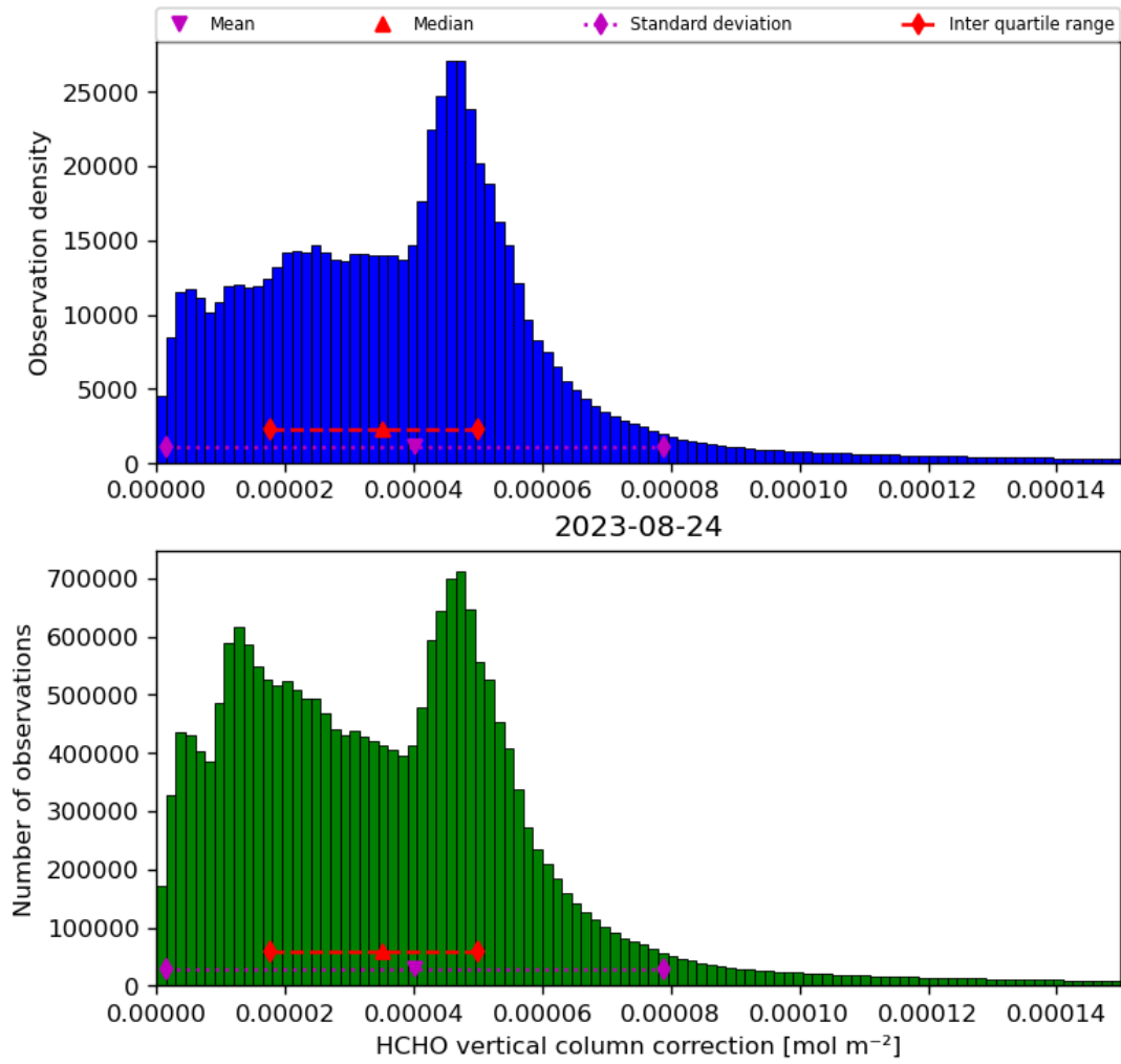
Figure 37: Histogram of “HCHO vertical column correction” for 2023-08-23 to 2023-08-25
