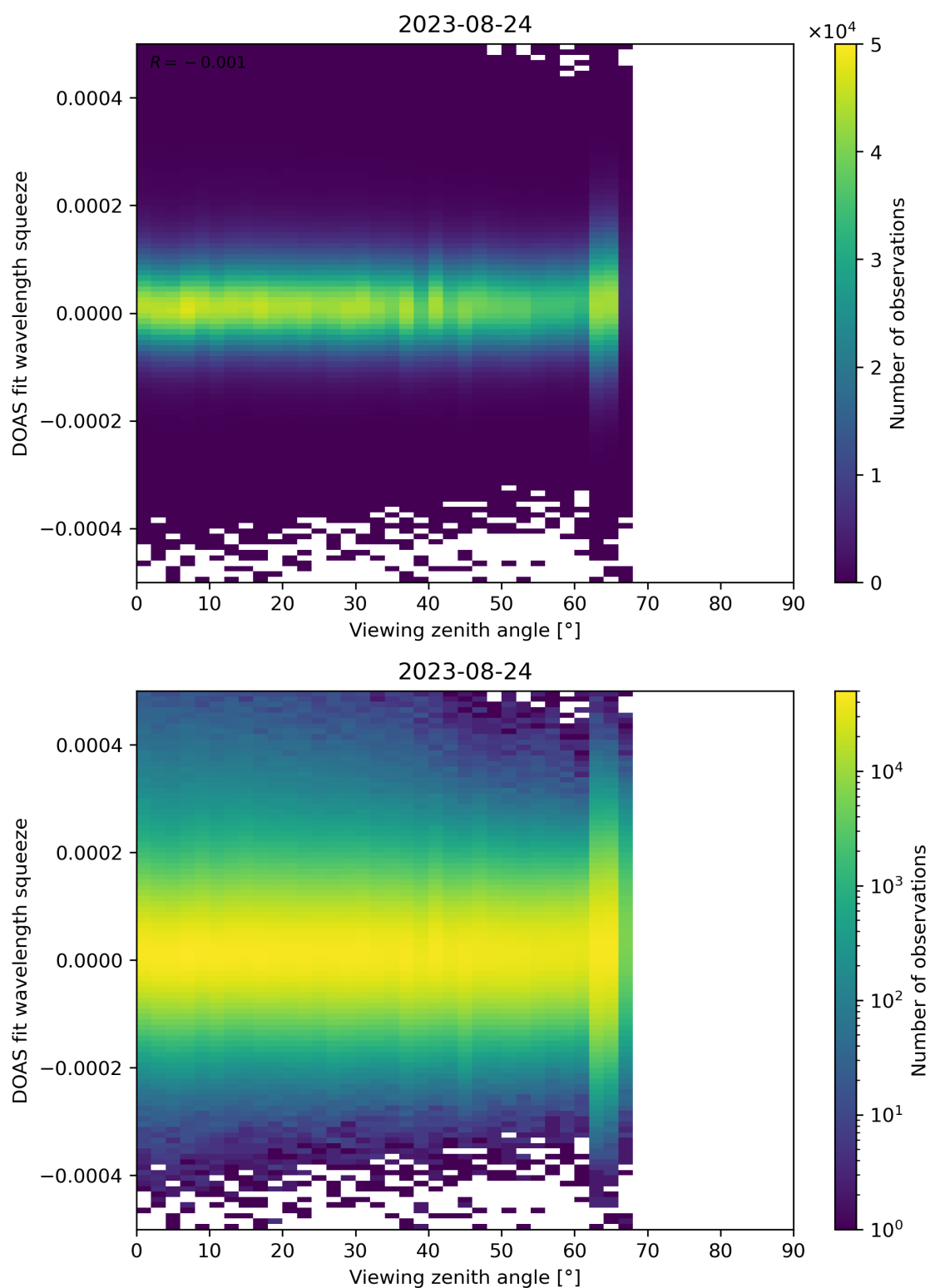
Figure 184: Scatter density plot of “Viewing zenith angle” against “DOAS fit wavelength squeeze” for 2023-08-23 to 2023-08-25.
