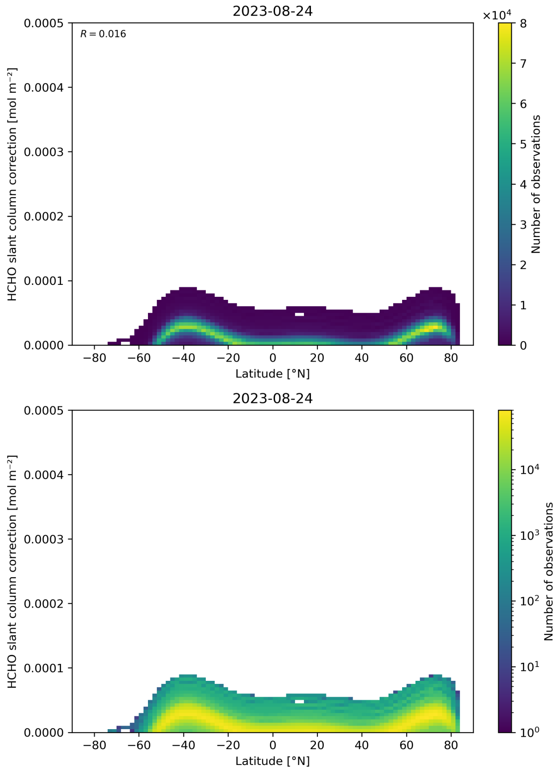
Figure 158: Scatter density plot of “Latitude” against “HCHO slant column correction” for 2023-08-23 to 2023-08-25.
