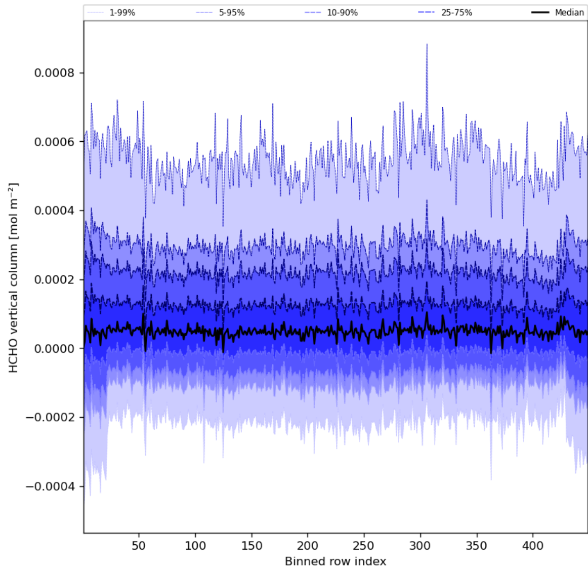
Figure 49: Along track statistics of “HCHO vertical column” for 2023-08-23 to 2023-08-25
