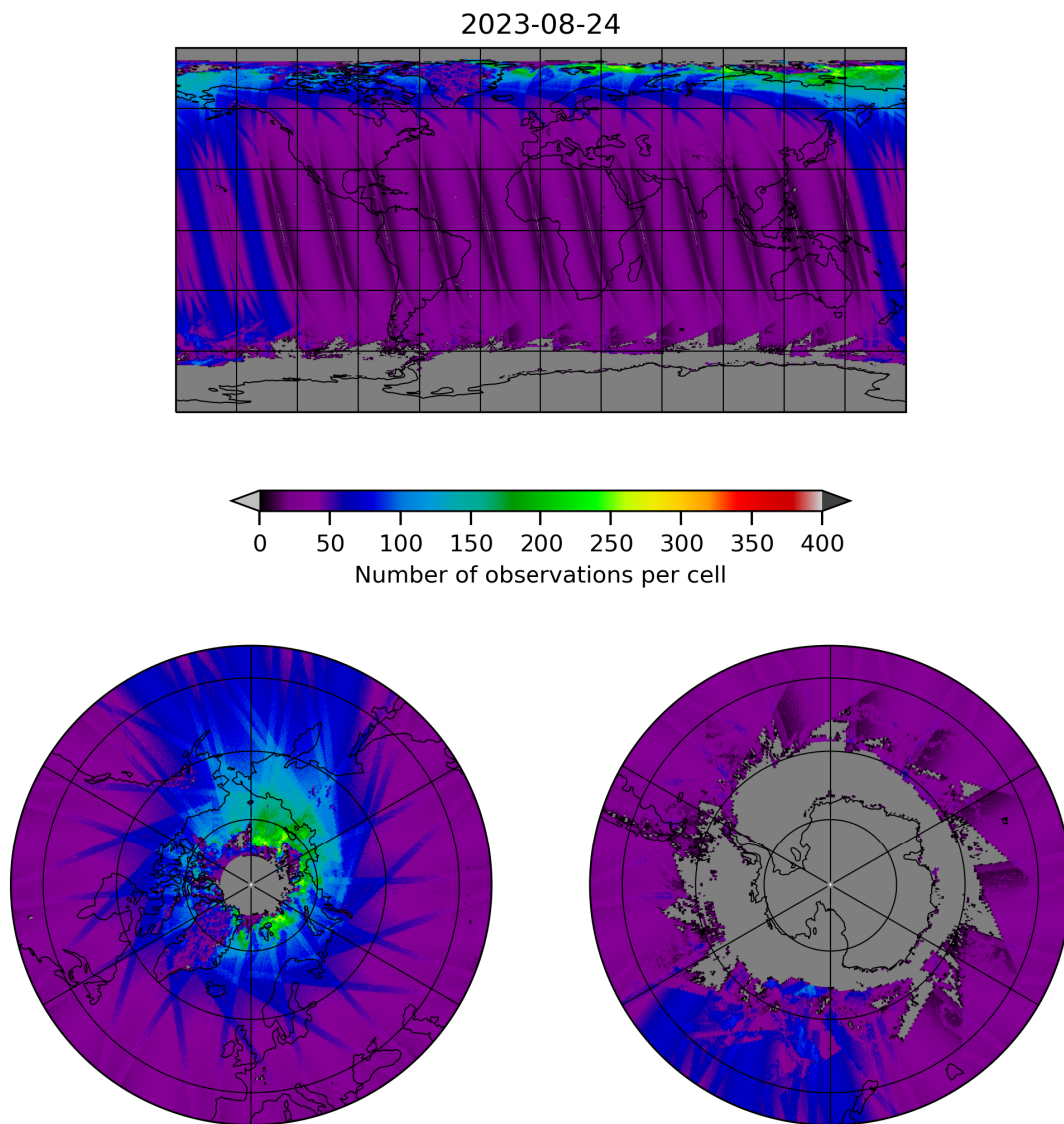
Figure 19: Map of the number of observations for 2023-08-23 to 2023-08-25
