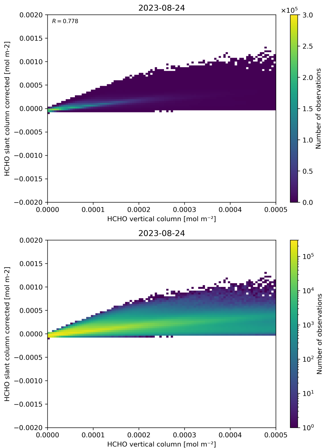
Figure 127: Scatter density plot of “HCHO vertical column” against “HCHO slant column corrected” for 2023-08-23 to 2023-08-25.
