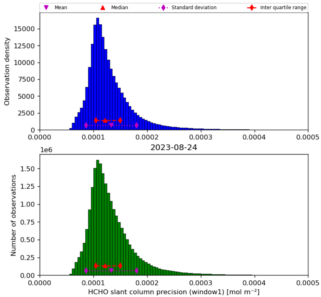
Figure 39: Histogram of “HCHO slant column precision (window1)” for 2023-08-23 to 2023-08-25
