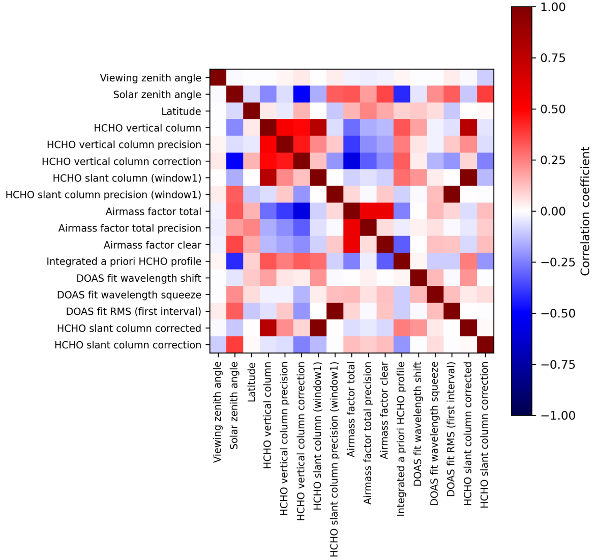
Figure 2: Map of correlation matrix for 2023-08-23 to 2023-08-25.
