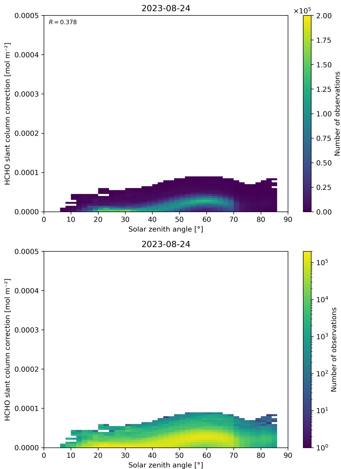
Figure 172: Scatter density plot of “Solar zenith angle” against “HCHO slant column correction” for 2023-08-23 to 2023-08-25.
