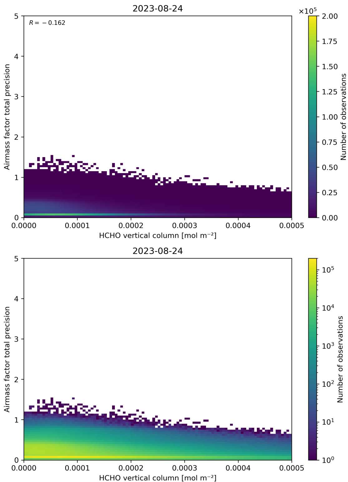
Figure 132: Scatter density plot of “HCHO vertical column” against “Airmass factor total precision” for 2023-08-23 to 2023-08-25.
