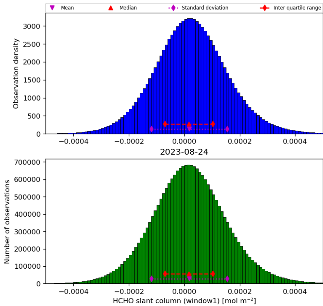
Figure 38: Histogram of “HCHO slant column (window1)” for 2023-08-23 to 2023-08-25
