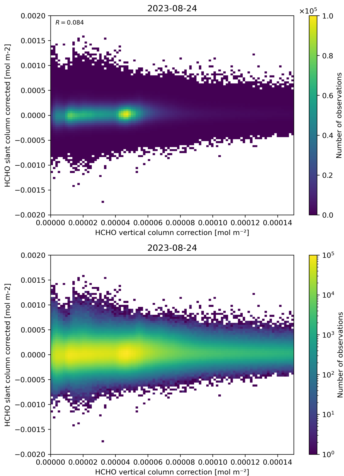
Figure 116: Scatter density plot of “HCHO vertical column correction” against “HCHO slant column corrected” for 2023-08-23 to 2023-08-25.
