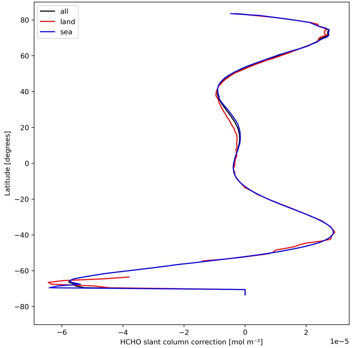
Figure 33: Zonal average of “HCHO slant column correction” for 2023-08-23 to 2023-08-25.
