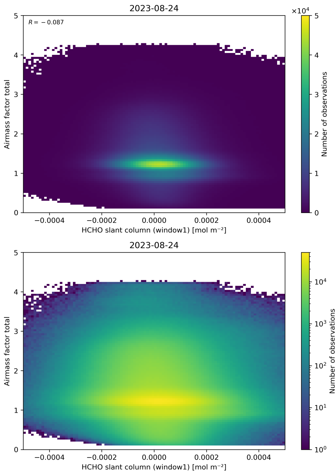
Figure 85: Scatter density plot of “HCHO slant column (window1)” against “Airmass factor total” for 2023-08-23 to 2023-08-25.
