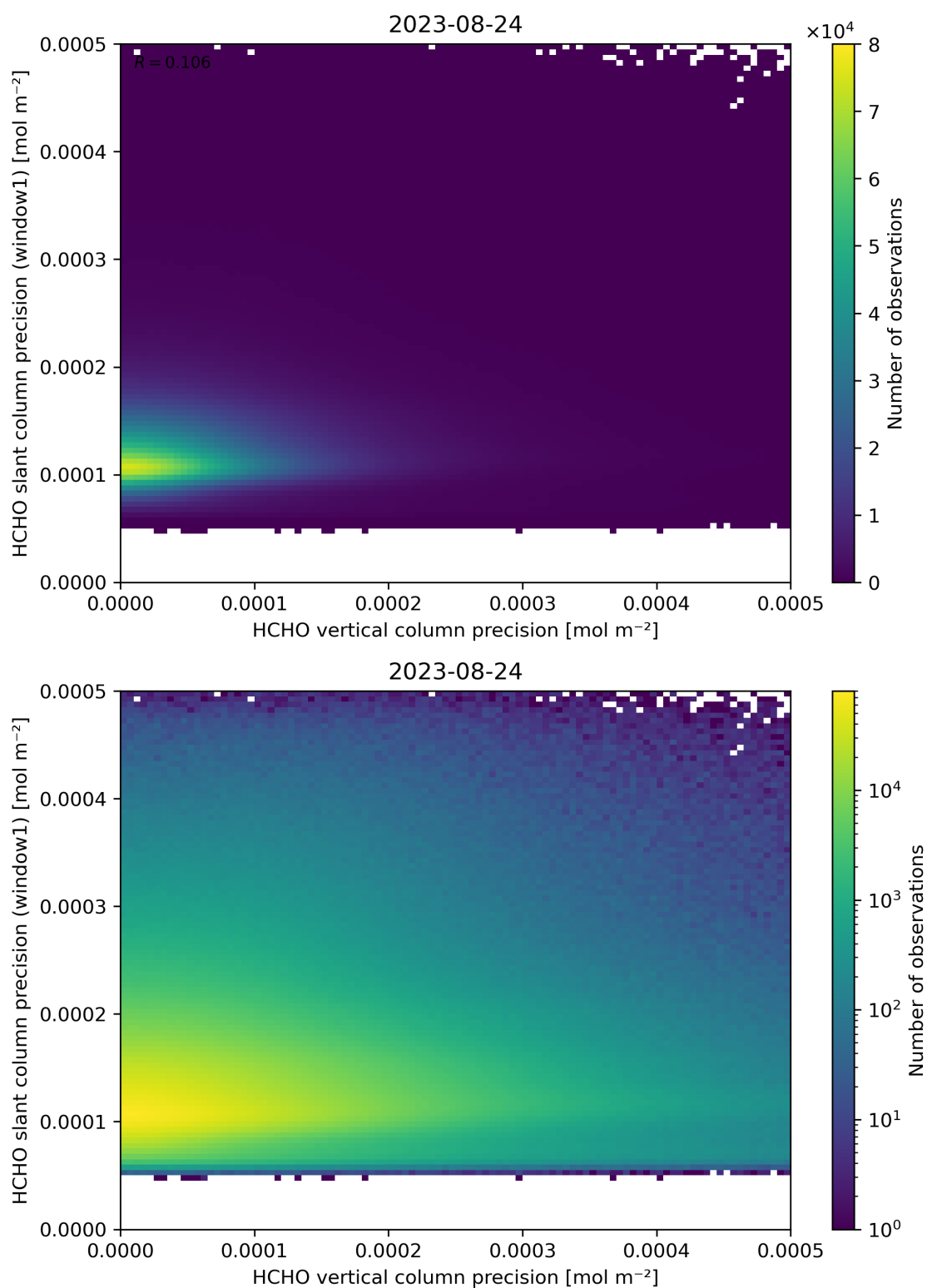
Figure 143: Scatter density plot of “HCHO vertical column precision” against “HCHO slant column precision (window1)” for 2023-08-23 to 2023-08-25.
