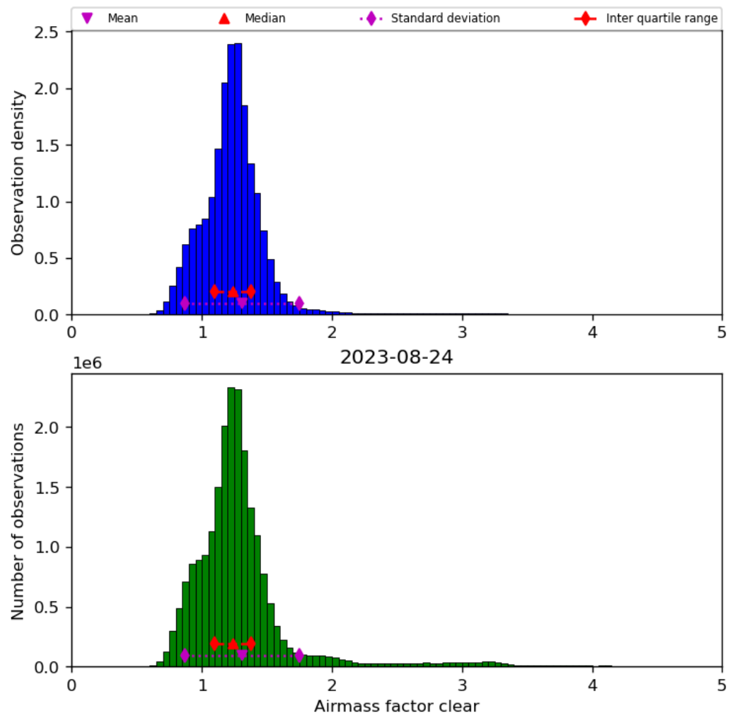
Figure 42: Histogram of “Airmass factor clear” for 2023-08-23 to 2023-08-25
