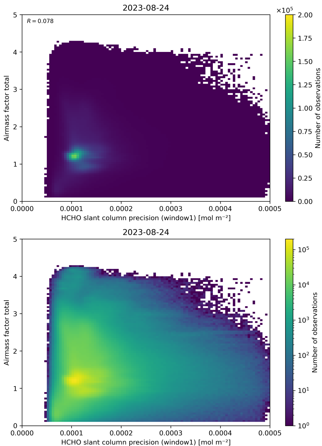
Figure 94: Scatter density plot of “HCHO slant column precision (window1)” against “Airmass factor total” for 2023-08-23 to 2023-08-25.
