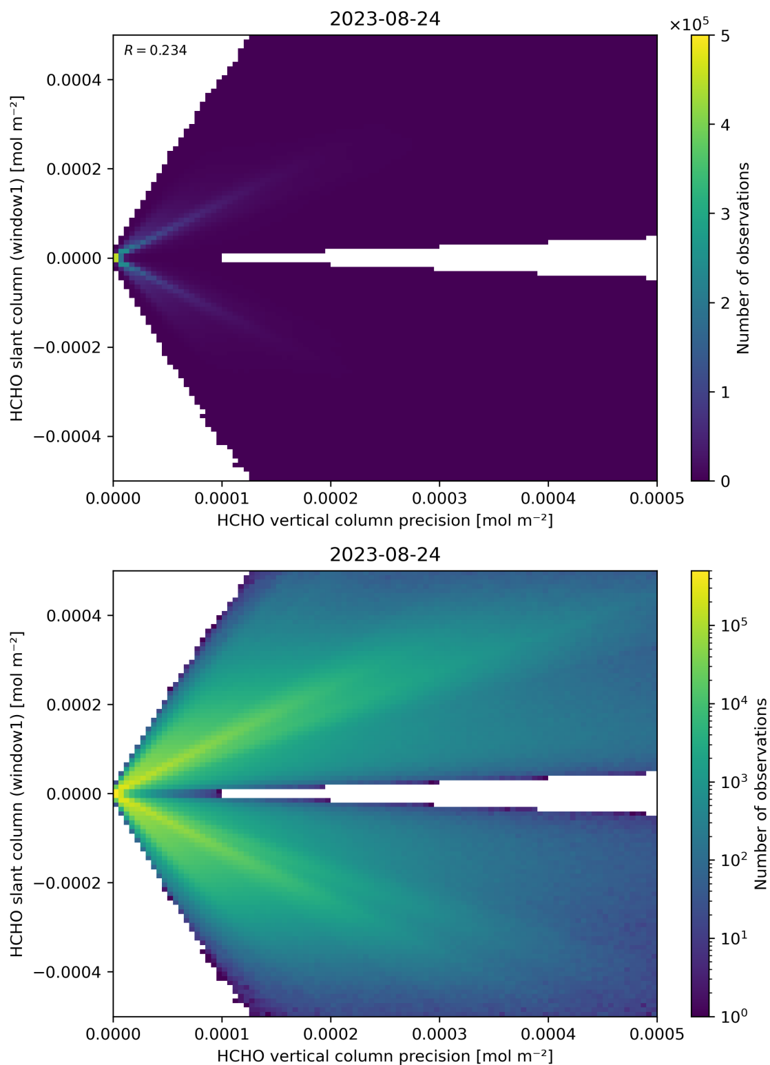
Figure 142: Scatter density plot of “HCHO vertical column precision” against “HCHO slant column (window1)” for 2023-08-23 to 2023-08-25.
