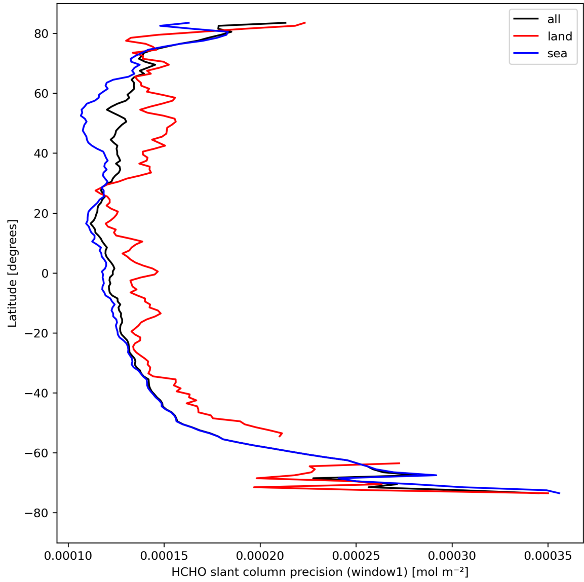
Figure 25: Zonal average of “HCHO slant column precision (window1)” for 2023-08-23 to 2023-08-25.
