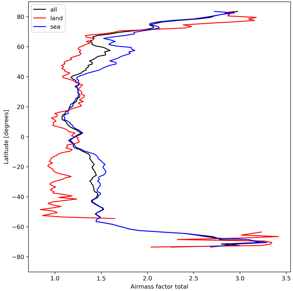
Figure 26: Zonal average of “Airmass factor total” for 2023-08-23 to 2023-08-25.
