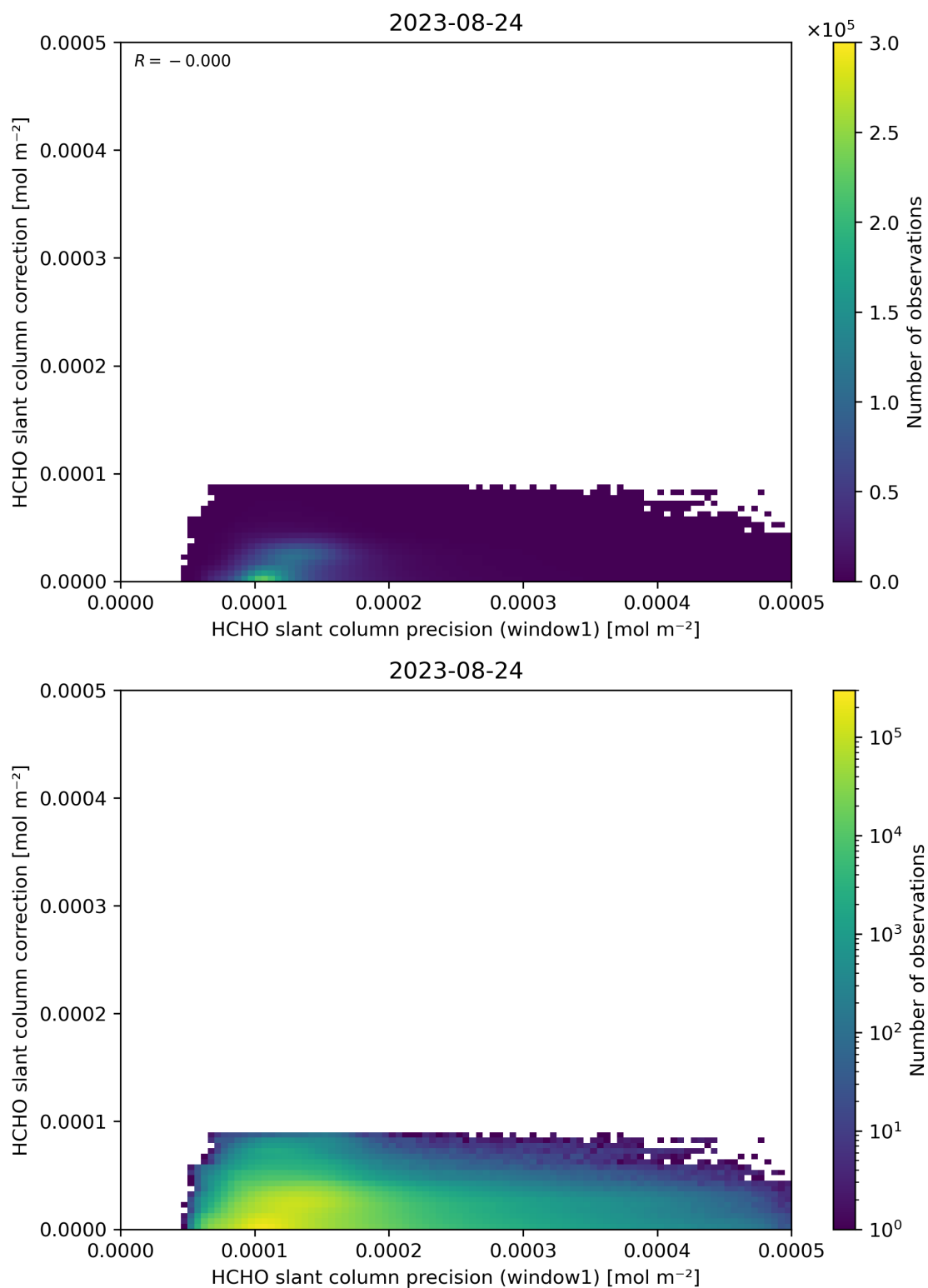
Figure 93: Scatter density plot of “HCHO slant column precision (window1)” against “HCHO slant column correction” for 2023-08-23 to 2023-08-25.
