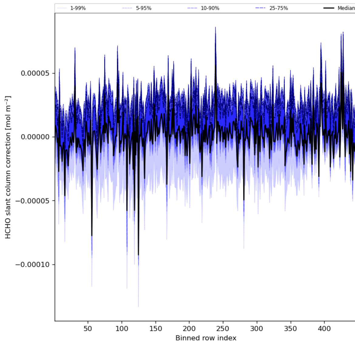
Figure 61: Along track statistics of “HCHO slant column correction” for 2023-08-23 to 2023-08-25
