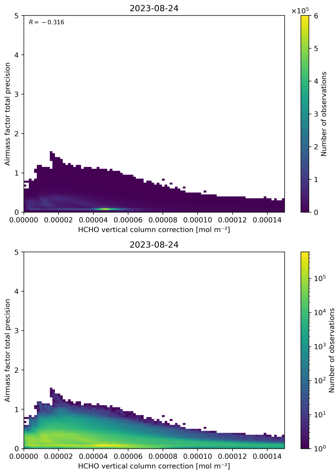
Figure 121: Scatter density plot of “HCHO vertical column correction” against “Airmass factor total precision” for 2023-08-23 to 2023-08-25.
