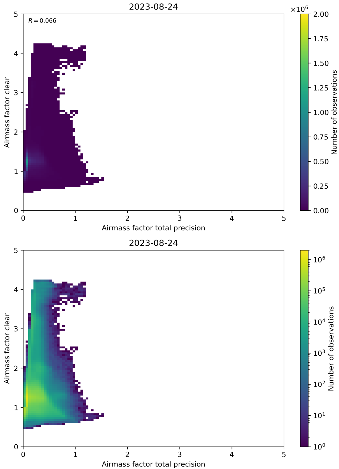
Figure 108: Scatter density plot of “Airmass factor total precision” against “Airmass factor clear” for 2023-08-23 to 2023-08-25.
