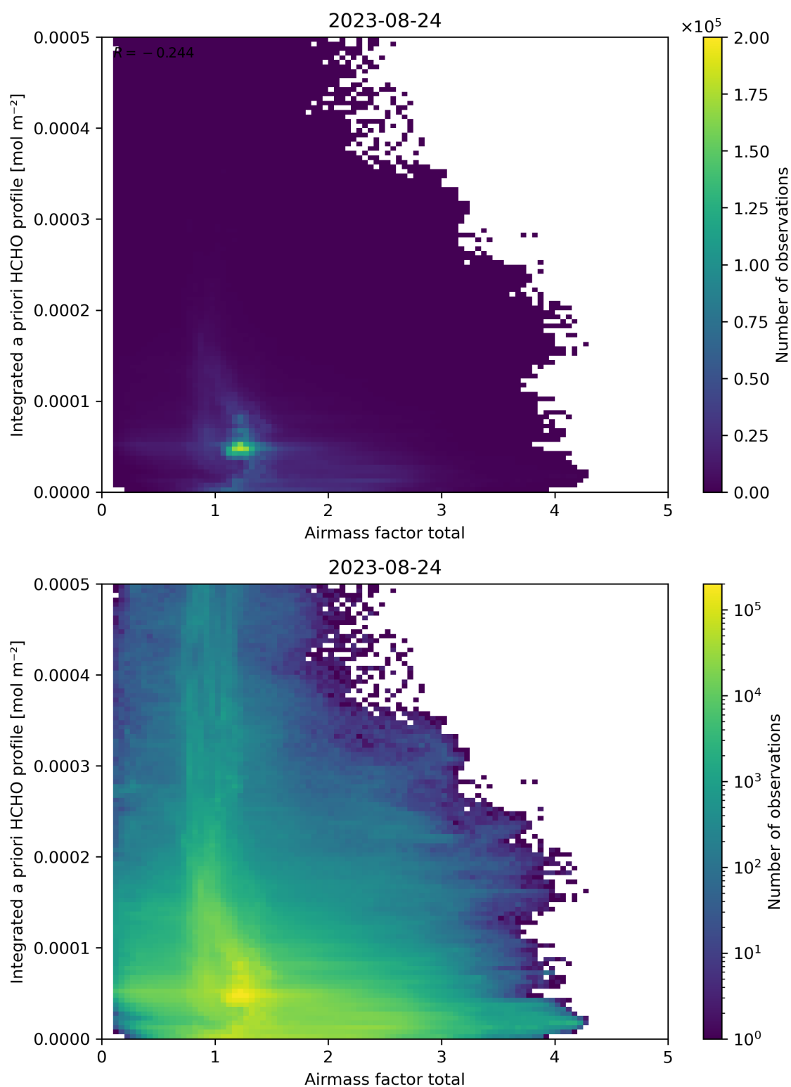
Figure 104: Scatter density plot of “Airmass factor total” against “Integrated a priori HCHO profile” for 2023-08-23 to 2023-08-25.
