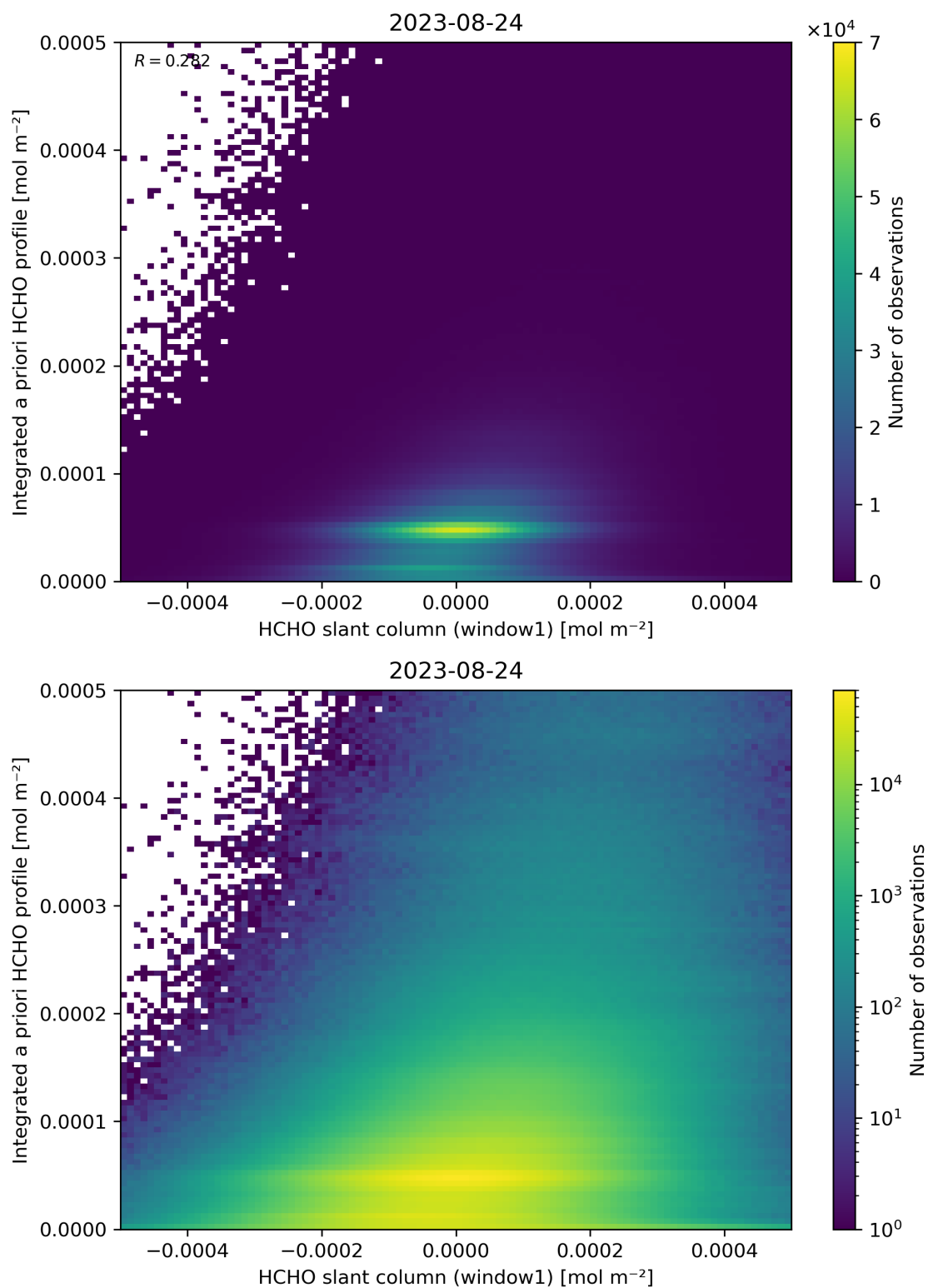
Figure 87: Scatter density plot of “HCHO slant column (window1)” against “Integrated a priori HCHO profile” for 2023-08-23 to 2023-08-25.
