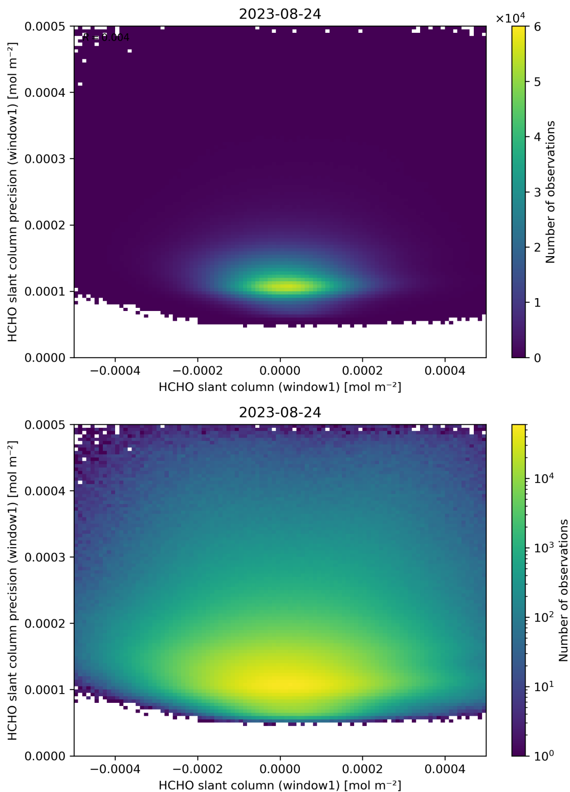
Figure 84: Scatter density plot of “HCHO slant column (window1)” against “HCHO slant column precision (window1)” for 2023-08-23 to 2023-08-25.
