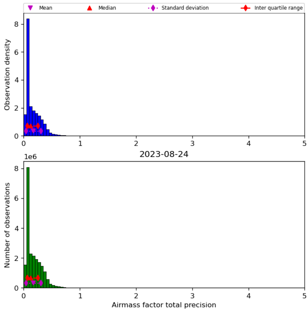
Figure 41: Histogram of “Airmass factor total precision” for 2023-08-23 to 2023-08-25
