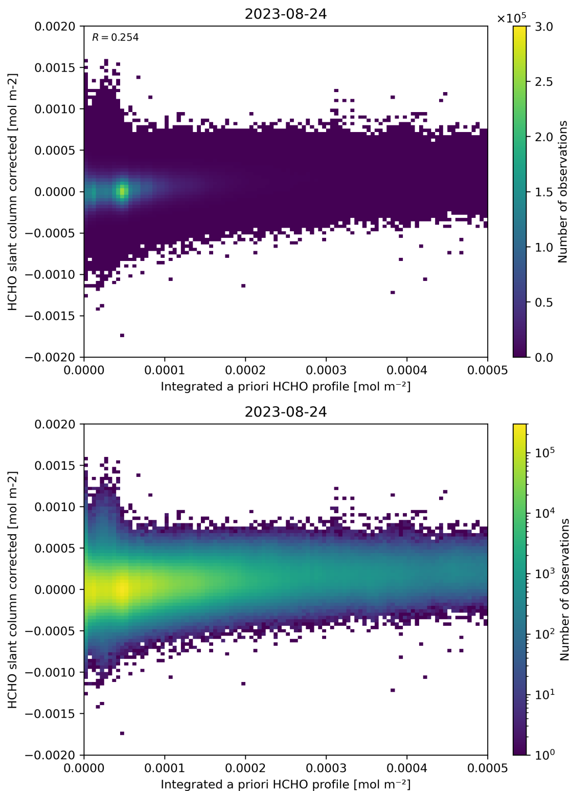
Figure 151: Scatter density plot of “Integrated a priori HCHO profile” against “HCHO slant column corrected” for 2023-08-23 to 2023-08-25.
