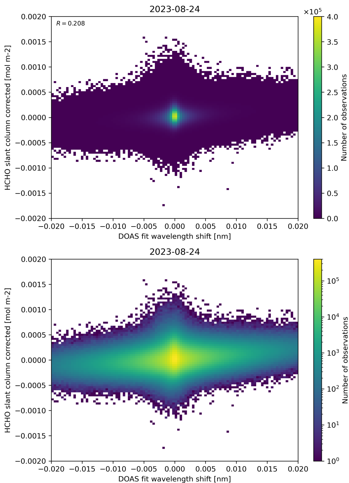
Figure 66: Scatter density plot of “DOAS fit wavelength shift” against “HCHO slant column corrected” for 2023-08-23 to 2023-08-25.
