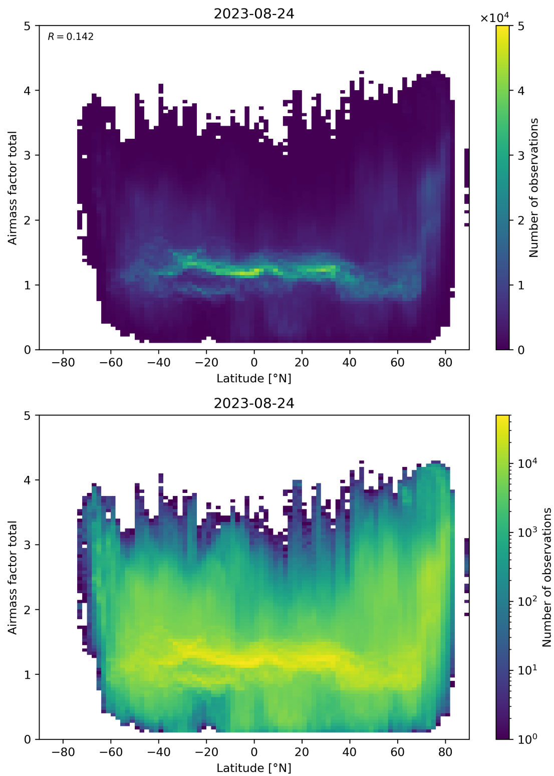
Figure 161: Scatter density plot of “Latitude” against “Airmass factor total” for 2023-08-23 to 2023-08-25.
