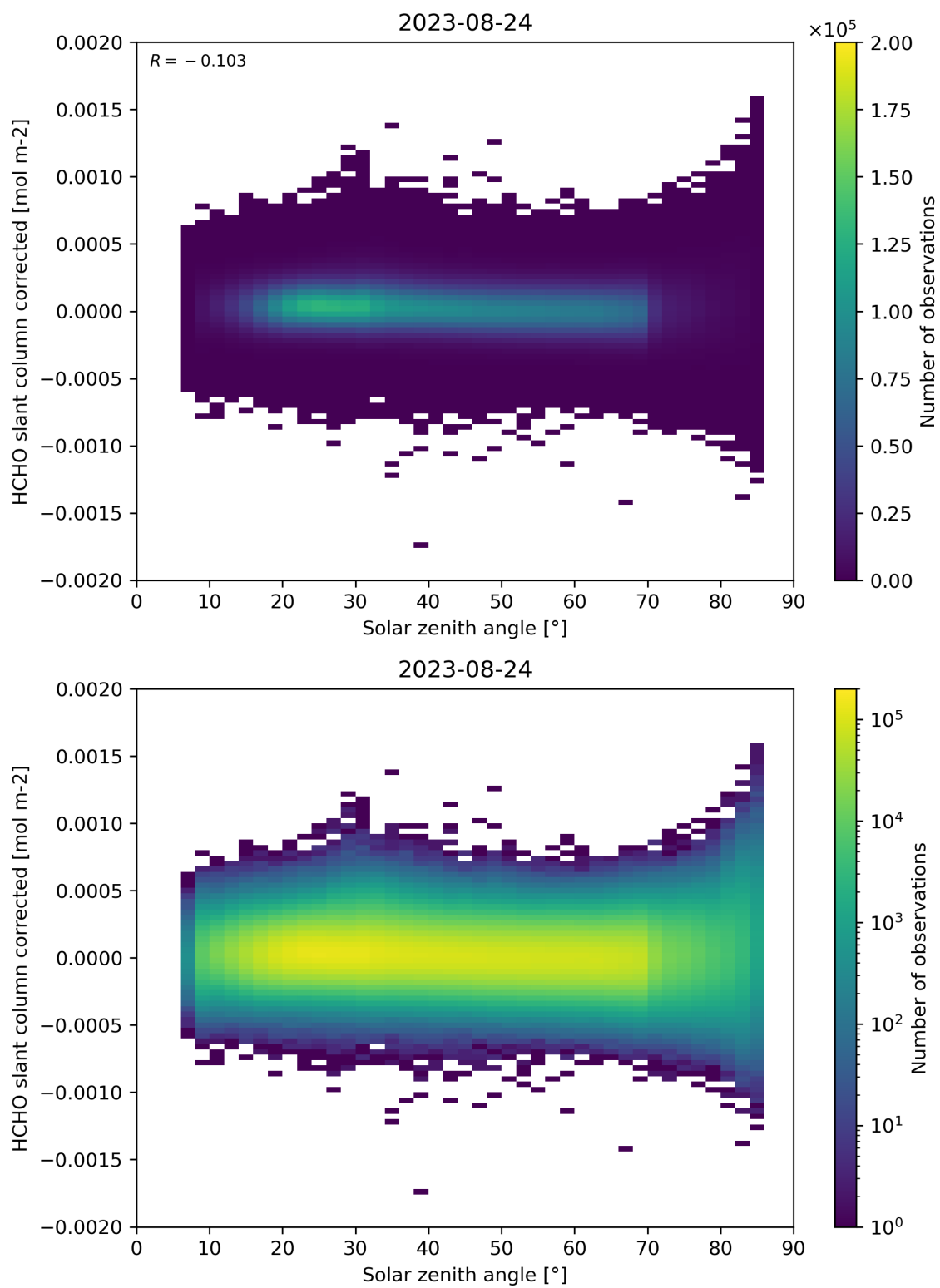
Figure 171: Scatter density plot of “Solar zenith angle” against “HCHO slant column corrected” for 2023-08-23 to 2023-08-25.
