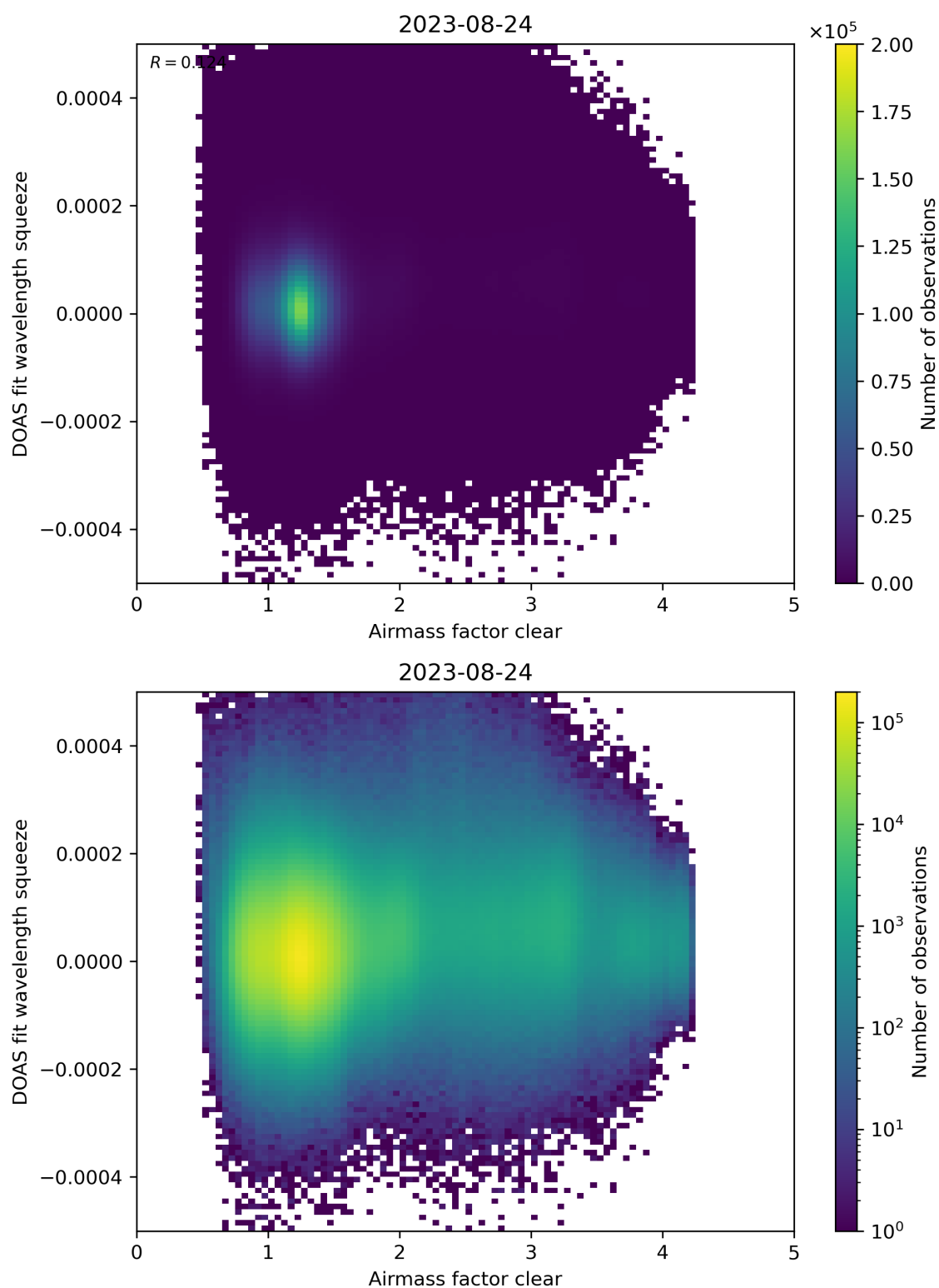
Figure 73: Scatter density plot of “Airmass factor clear” against “DOAS fit wavelength squeeze” for 2023-08-23 to 2023-08-25.
