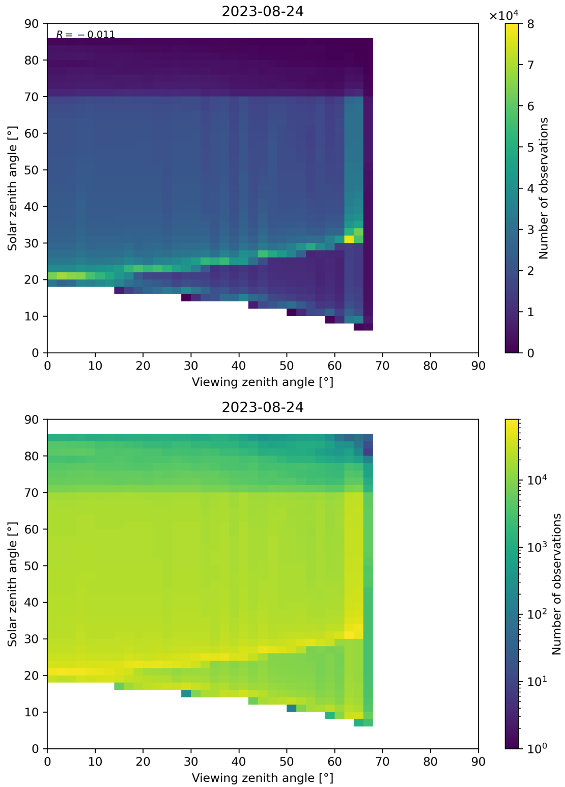
Figure 197: Scatter density plot of “Viewing zenith angle” against “Solar zenith angle” for 2023-08-23 to 2023-08-25.
