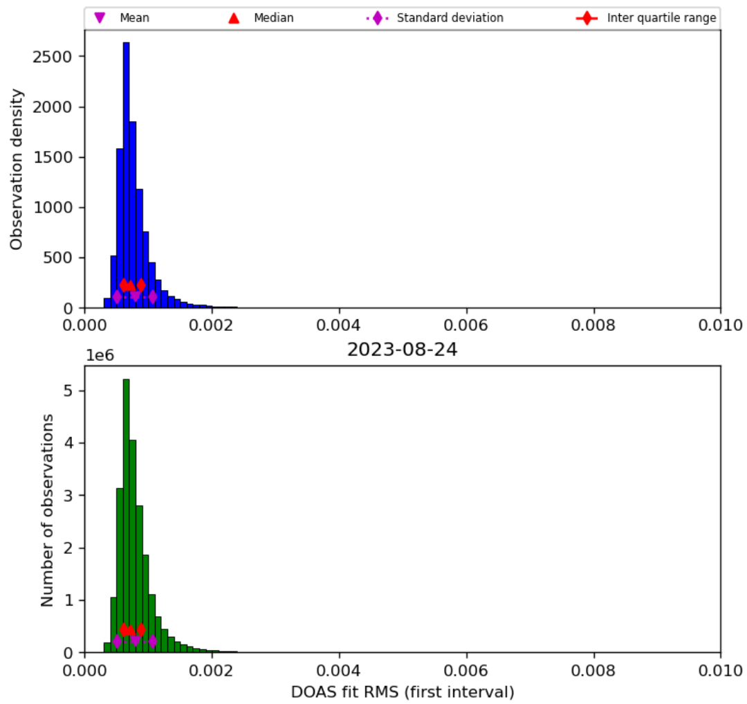
Figure 46: Histogram of “DOAS fit RMS (first interval)” for 2023-08-23 to 2023-08-25
