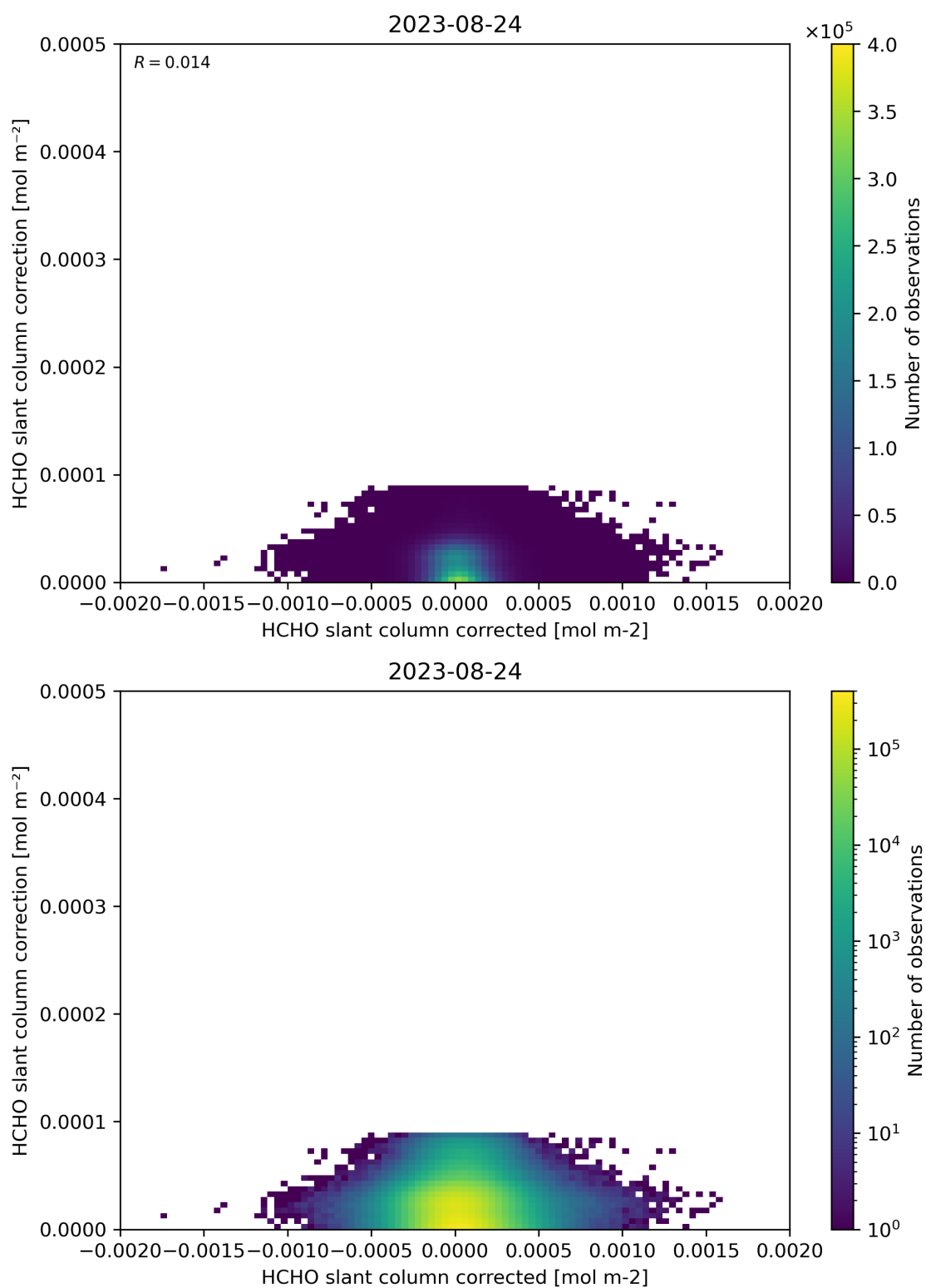
Figure 77: Scatter density plot of “HCHO slant column corrected” against “HCHO slant column correction” for 2023-08-23 to 2023-08-25.
