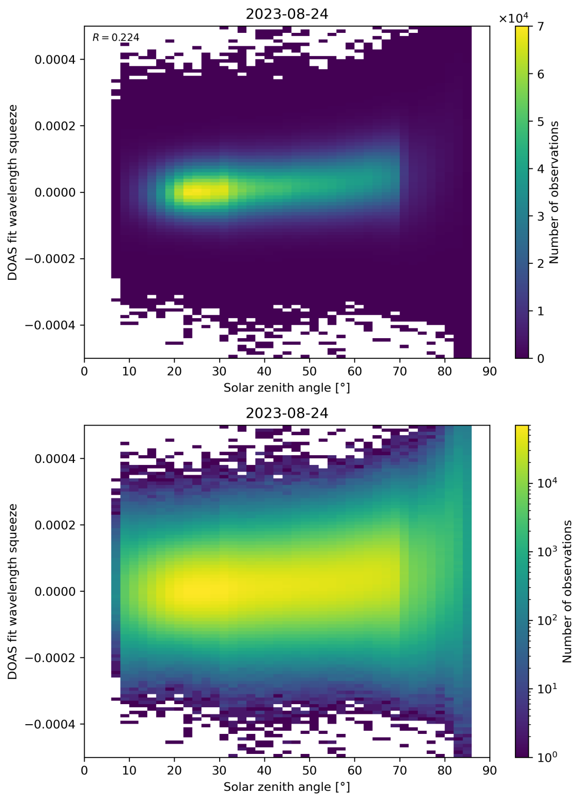
Figure 169: Scatter density plot of “Solar zenith angle” against “DOAS fit wavelength squeeze” for 2023-08-23 to 2023-08-25.
