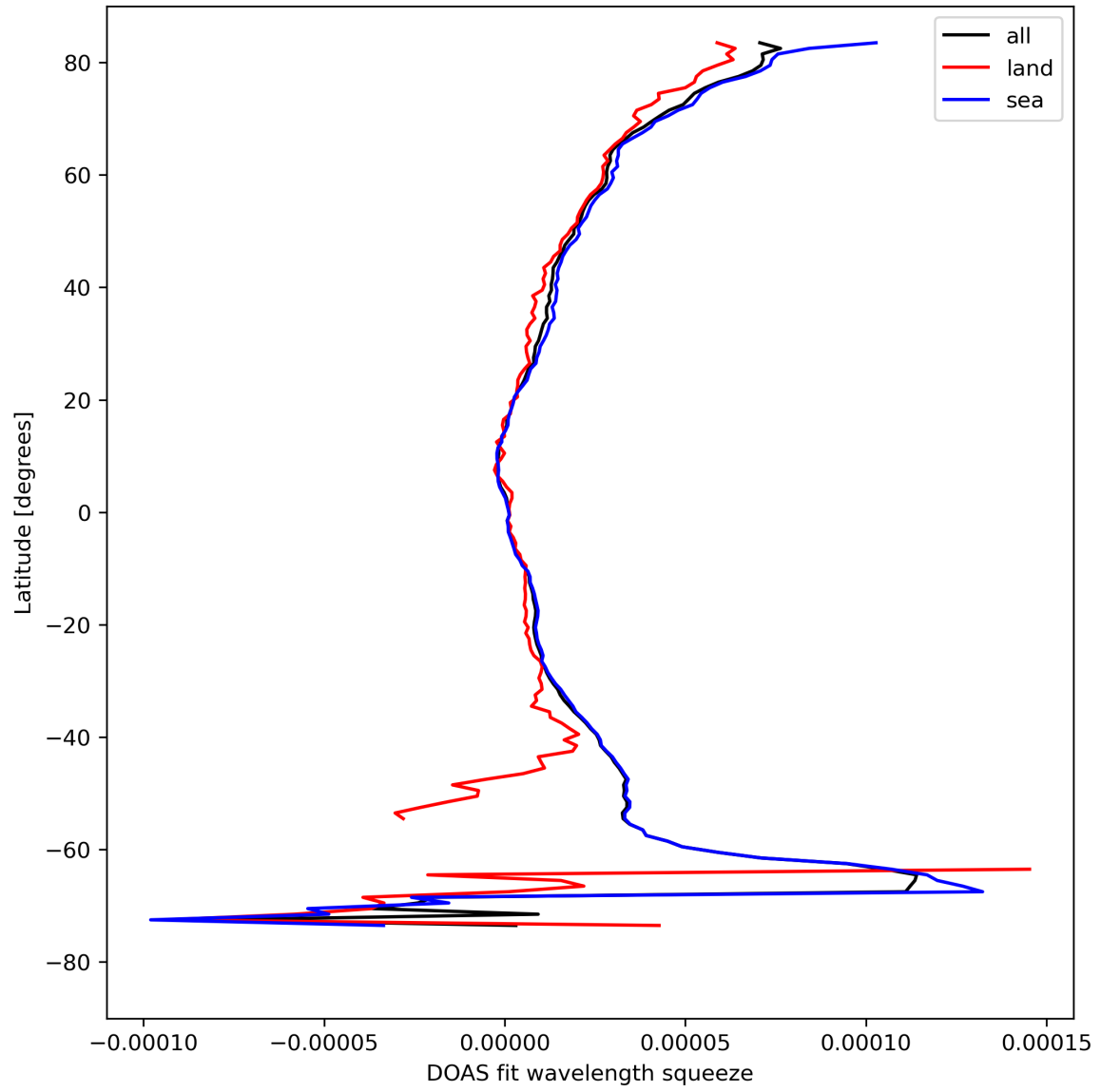
Figure 31: Zonal average of “DOAS fit wavelength squeeze” for 2023-08-23 to 2023-08-25.
