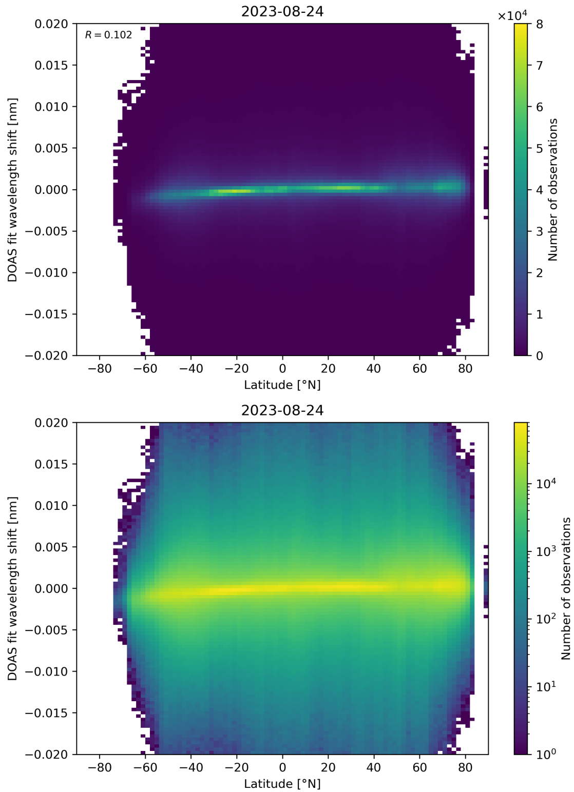
Figure 154: Scatter density plot of “Latitude” against “DOAS fit wavelength shift” for 2023-08-23 to 2023-08-25.
