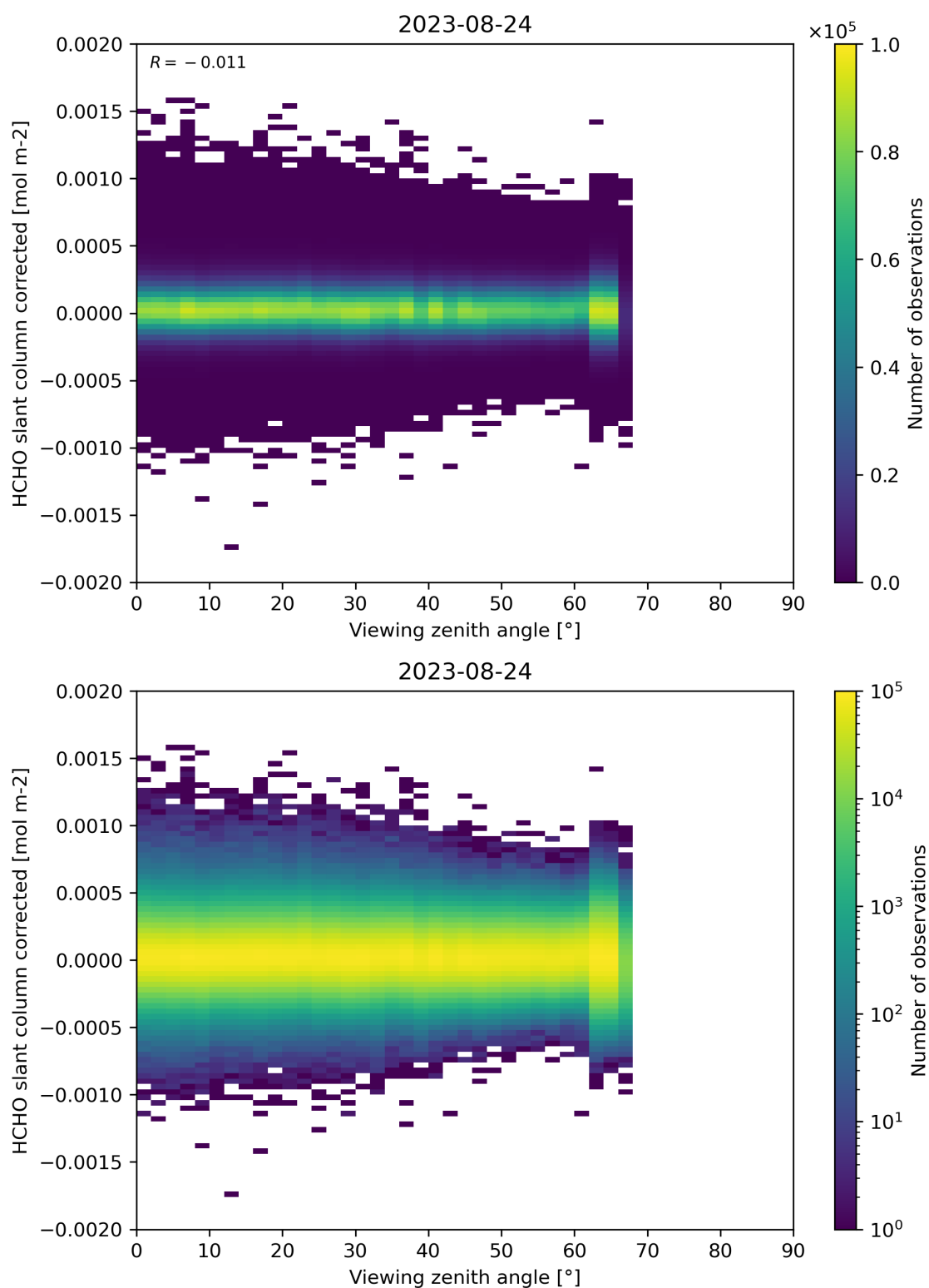
Figure 186: Scatter density plot of “Viewing zenith angle” against “HCHO slant column corrected” for 2023-08-23 to 2023-08-25.
