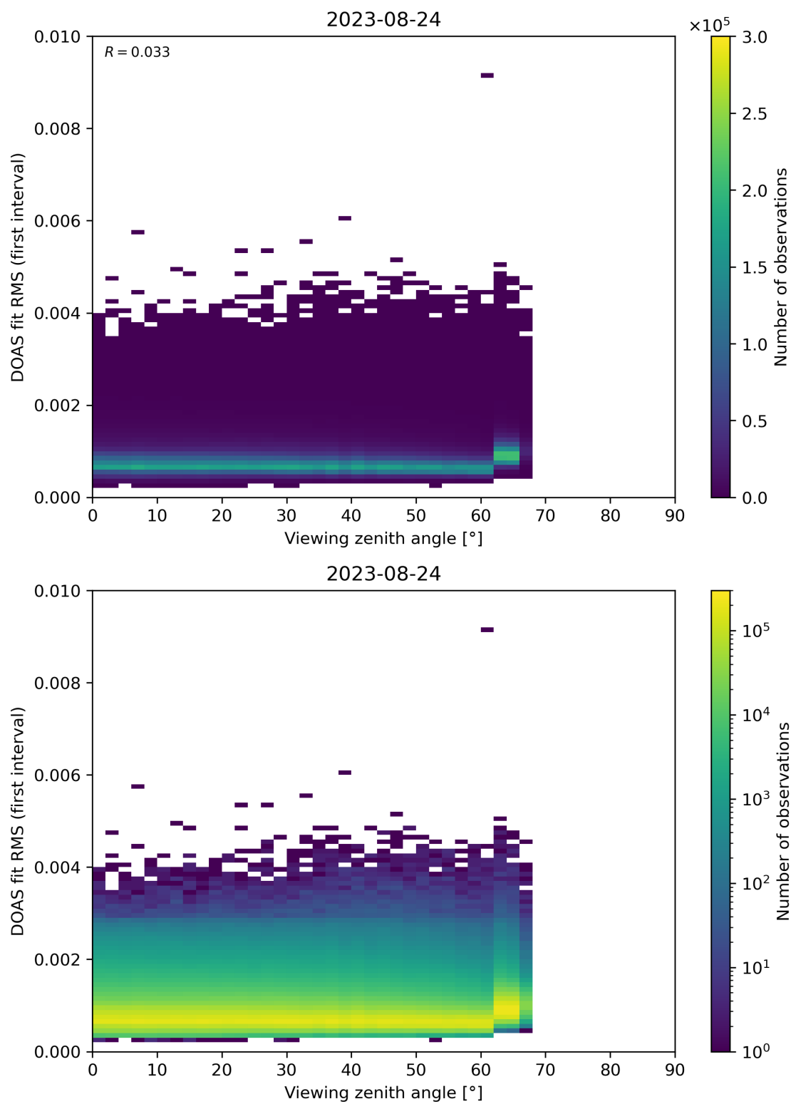
Figure 182: Scatter density plot of “Viewing zenith angle” against “DOAS fit RMS (first interval)” for 2023-08-23 to 2023-08-25.
