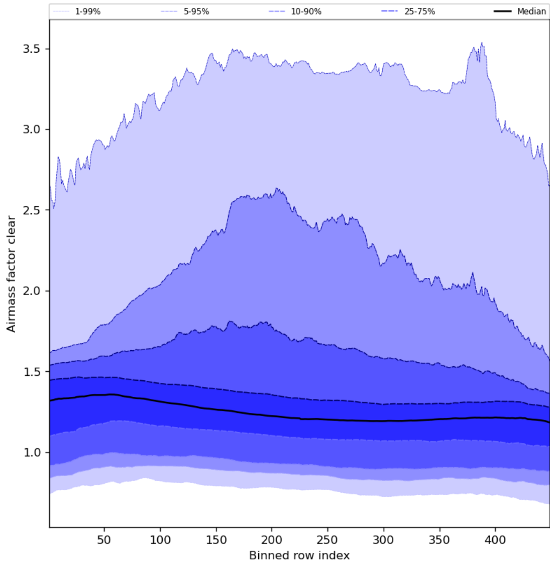
Figure 56: Along track statistics of “Airmass factor clear” for 2023-08-23 to 2023-08-25
