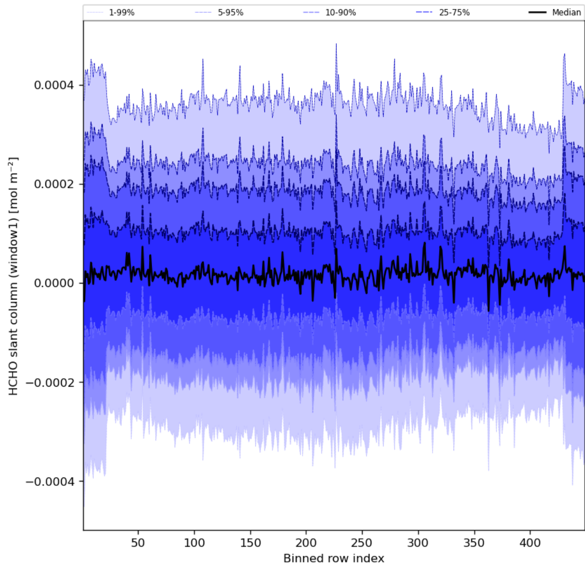
Figure 52: Along track statistics of “HCHO slant column (window1)” for 2023-08-23 to 2023-08-25
