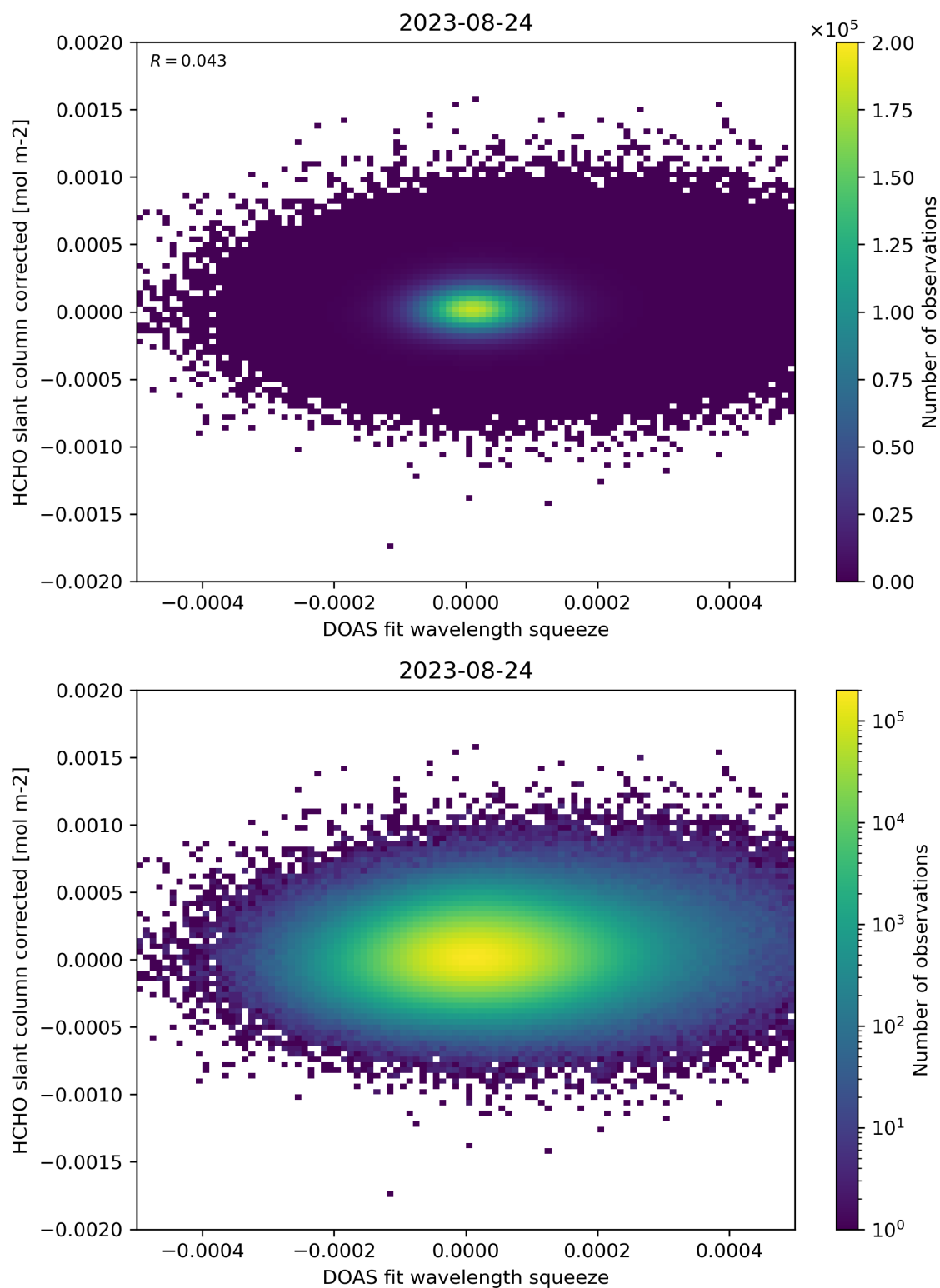
Figure 69: Scatter density plot of “DOAS fit wavelength squeeze” against “HCHO slant column corrected” for 2023-08-23 to 2023-08-25.
