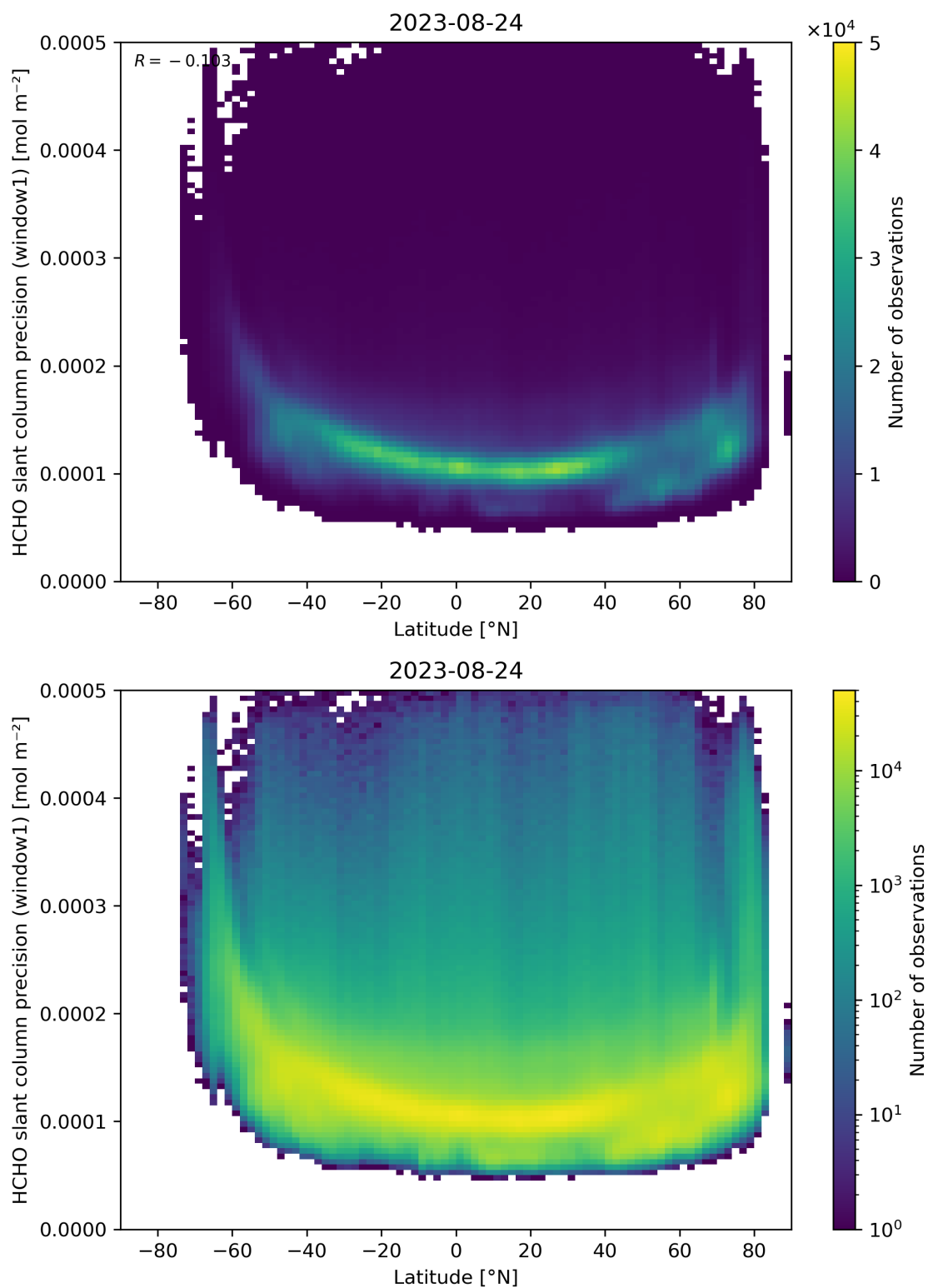
Figure 160: Scatter density plot of “Latitude” against “HCHO slant column precision (window1)” for 2023-08-23 to 2023-08-25.
