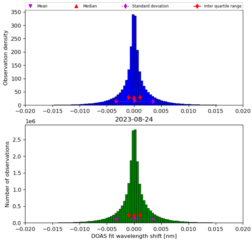
Figure 44: Histogram of “DOAS fit wavelength shift” for 2023-08-23 to 2023-08-25
