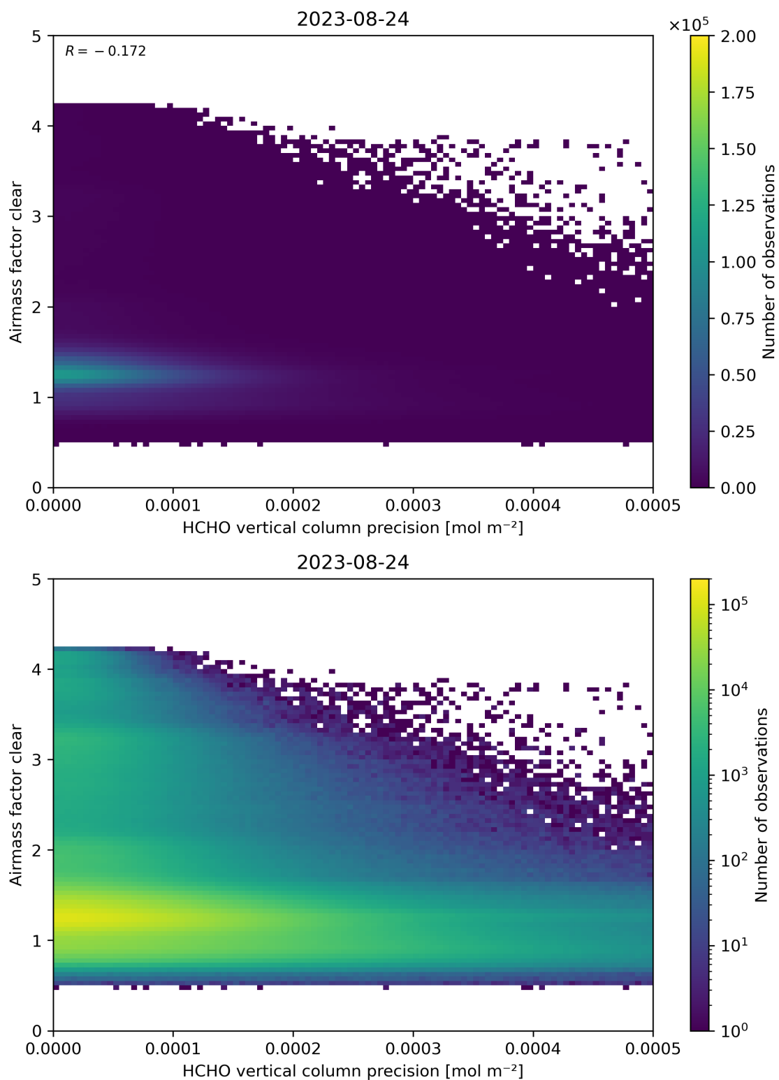
Figure 139: Scatter density plot of “HCHO vertical column precision” against “Airmass factor clear” for 2023-08-23 to 2023-08-25.
