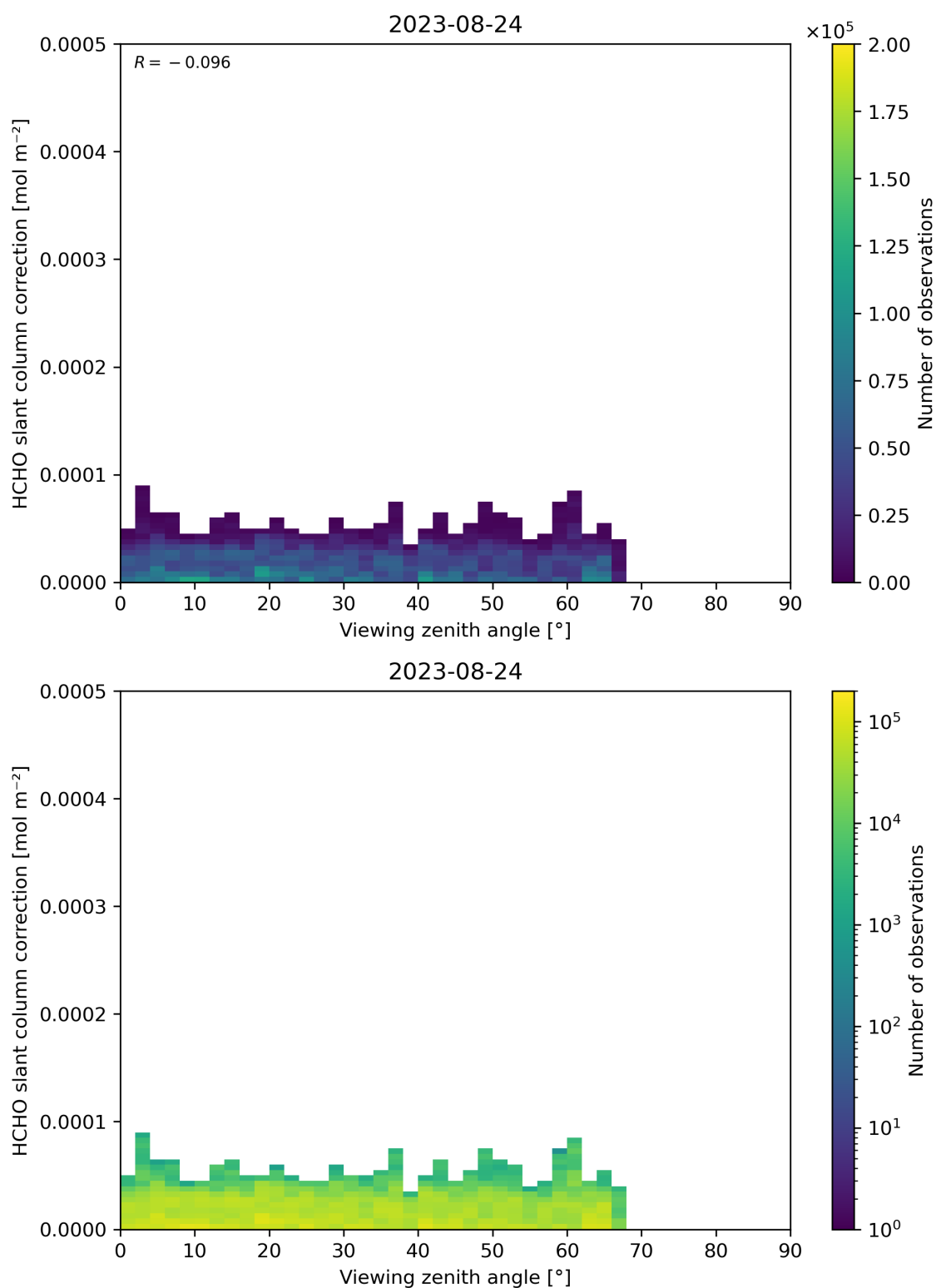
Figure 187: Scatter density plot of “Viewing zenith angle” against “HCHO slant column correction” for 2023-08-23 to 2023-08-25.
