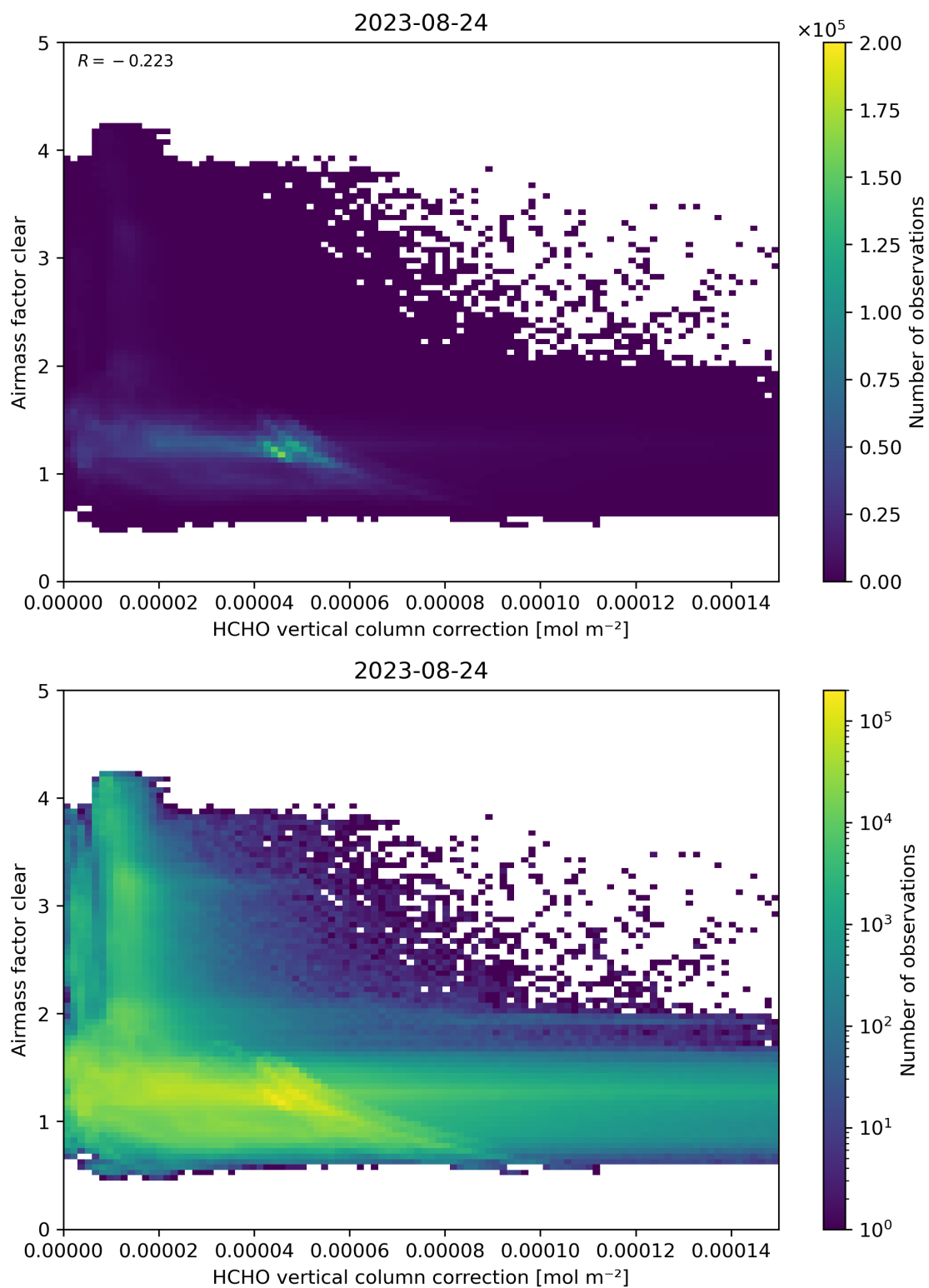
Figure 115: Scatter density plot of “HCHO vertical column correction” against “Airmass factor clear” for 2023-08-23 to 2023-08-25.
