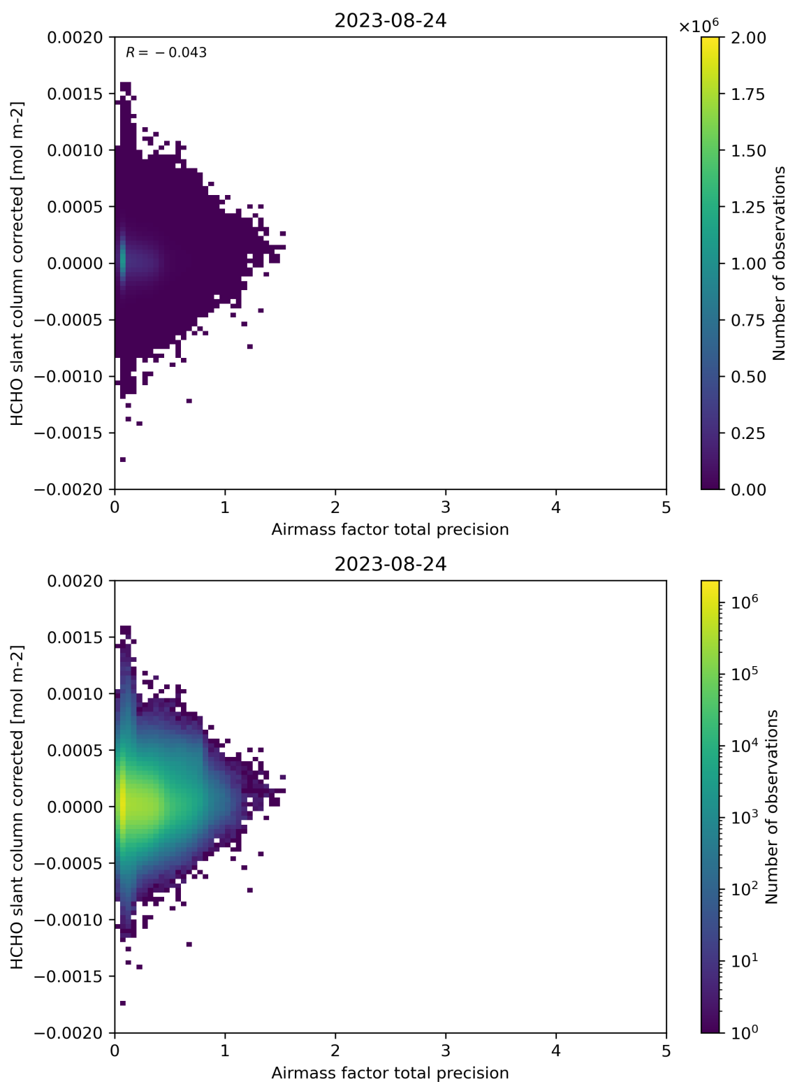
Figure 109: Scatter density plot of “Airmass factor total precision” against “HCHO slant column corrected” for 2023-08-23 to 2023-08-25.
