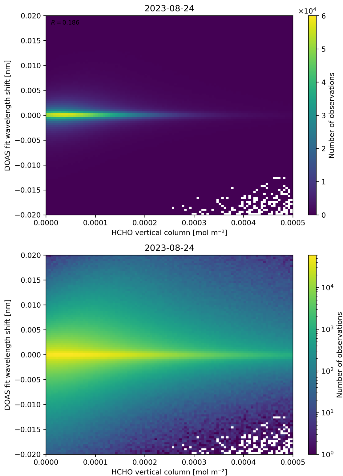
Figure 124: Scatter density plot of “HCHO vertical column” against “DOAS fit wavelength shift” for 2023-08-23 to 2023-08-25.
