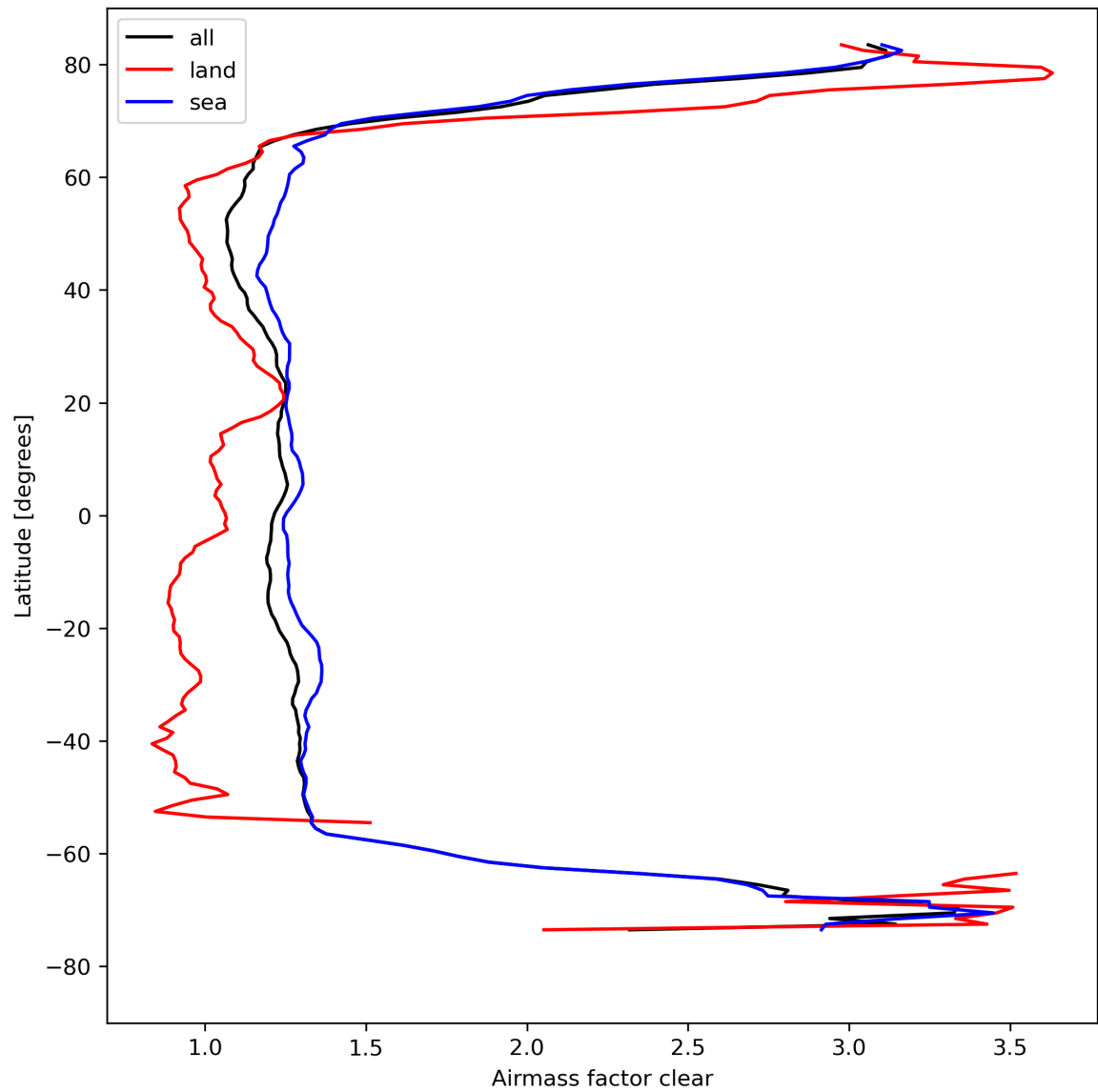
Figure 28: Zonal average of “Airmass factor clear” for 2023-08-23 to 2023-08-25.
