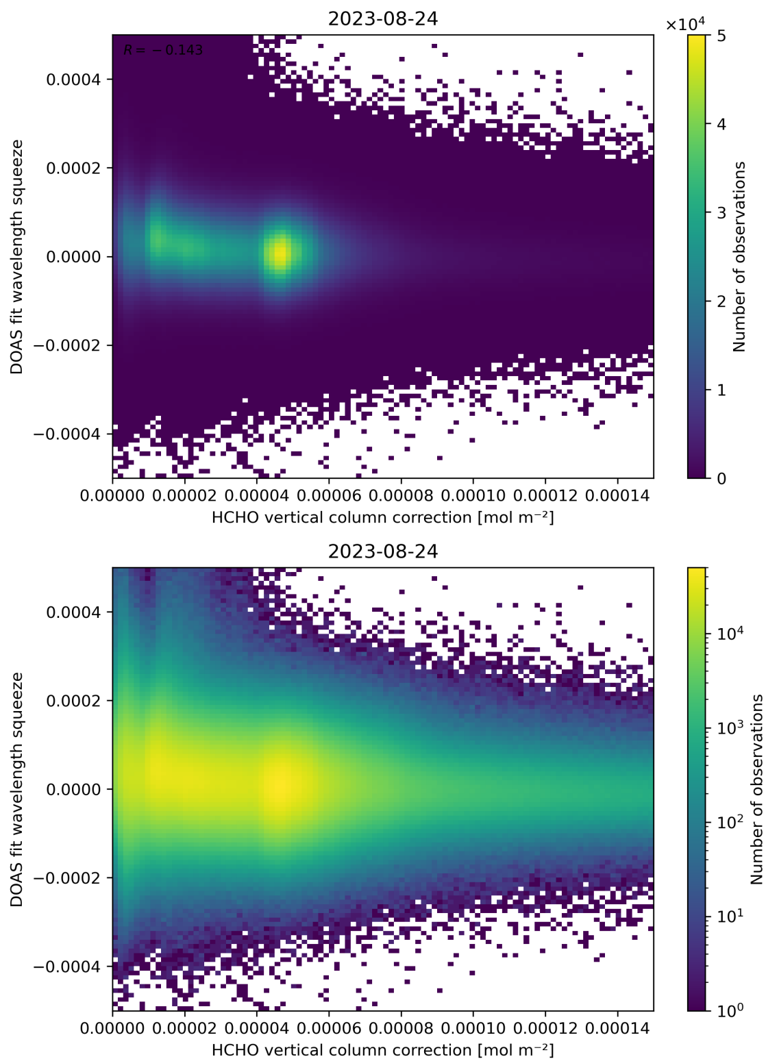
Figure 114: Scatter density plot of “HCHO vertical column correction” against “DOAS fit wavelength squeeze” for 2023-08-23 to 2023-08-25.
