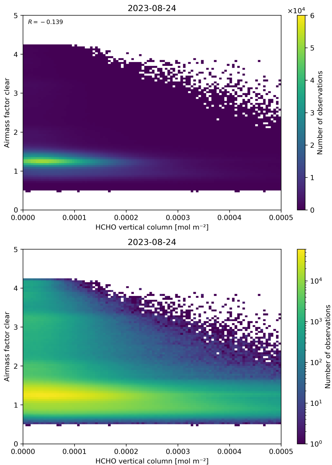
Figure 126: Scatter density plot of “HCHO vertical column” against “Airmass factor clear” for 2023-08-23 to 2023-08-25.
