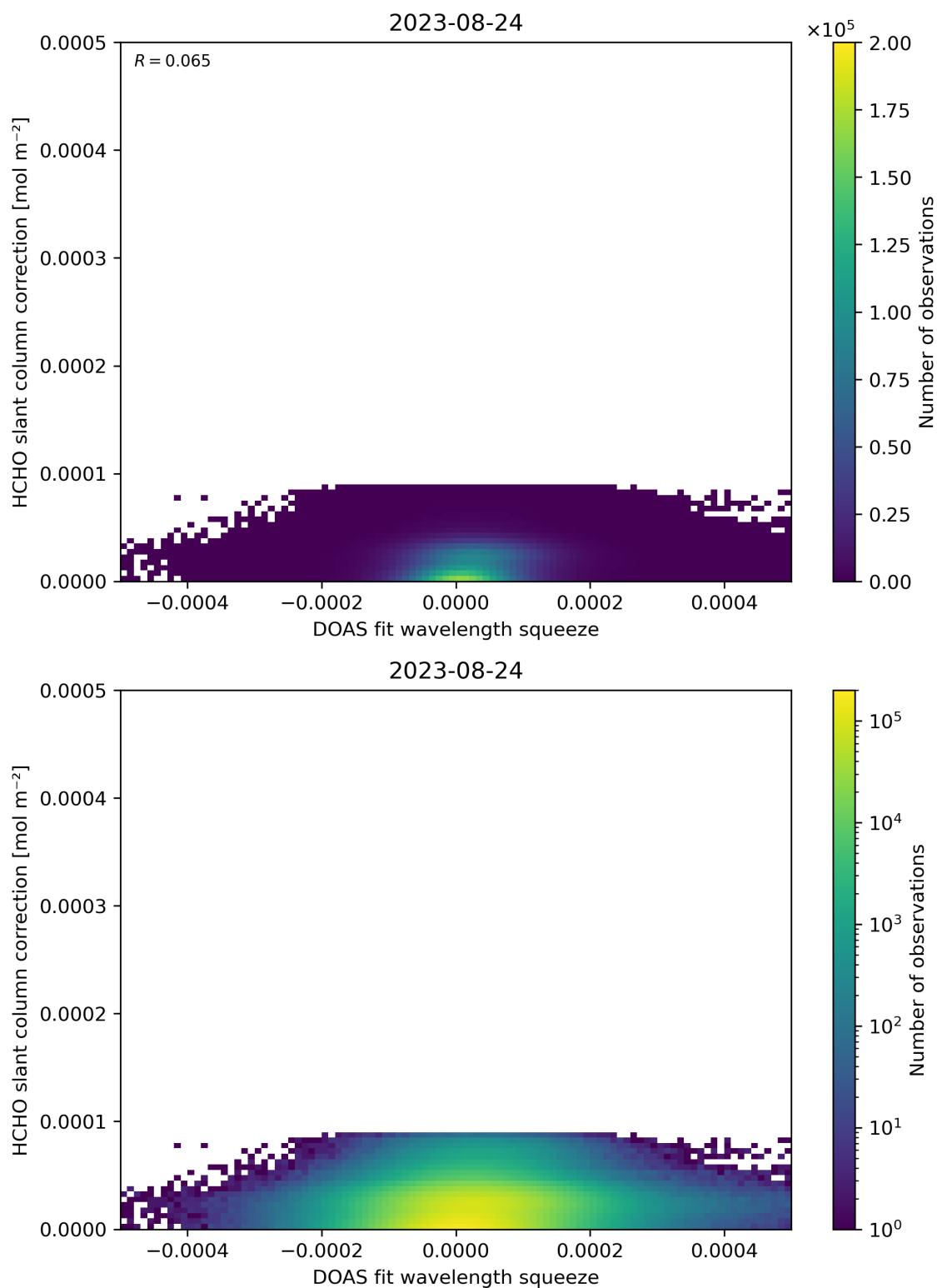
Figure 70: Scatter density plot of “DOAS fit wavelength squeeze” against “HCHO slant column correction” for 2023-08-23 to 2023-08-25.
