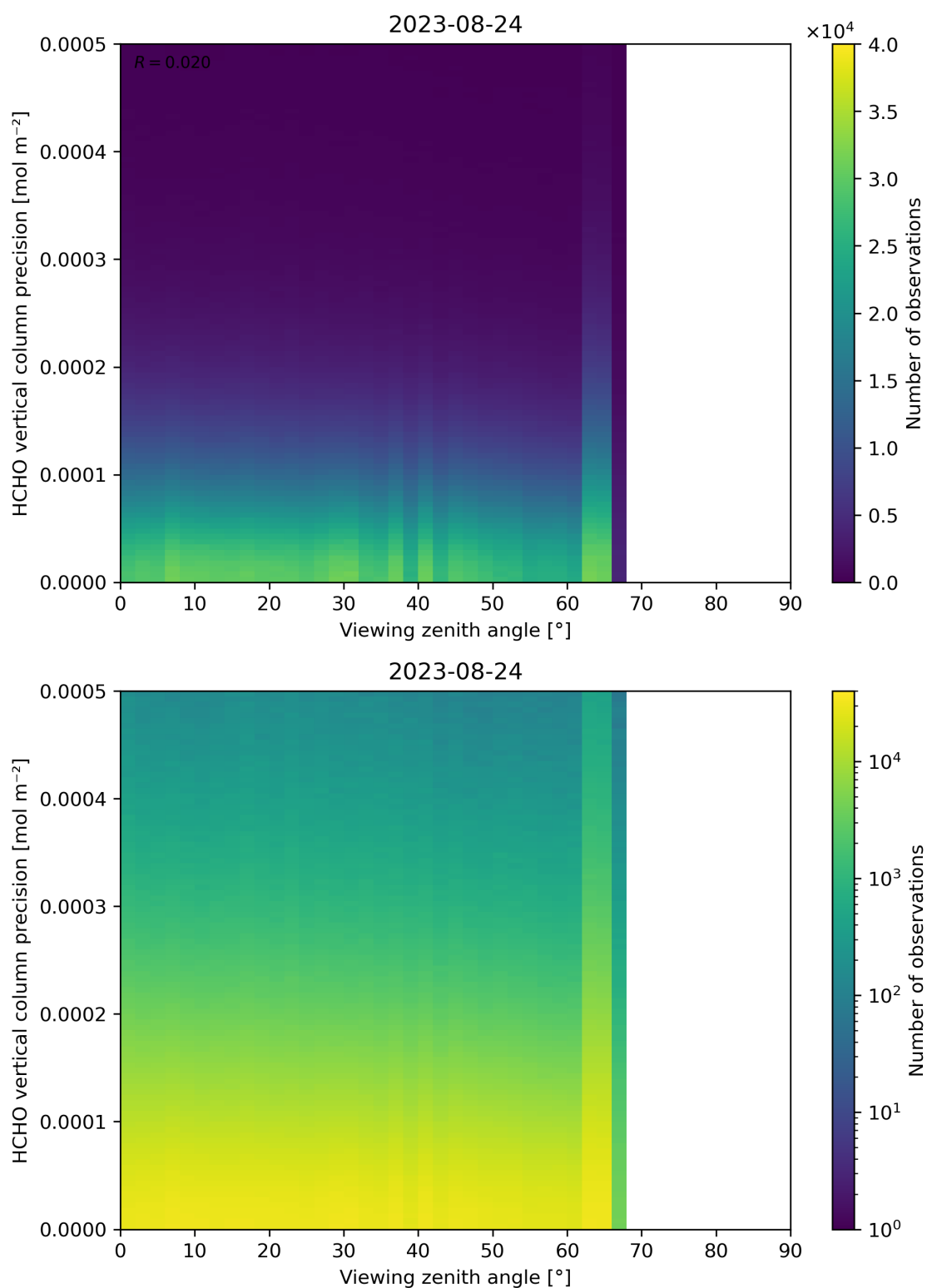
Figure 194: Scatter density plot of “Viewing zenith angle” against “HCHO vertical column precision” for 2023-08-23 to 2023-08-25.
