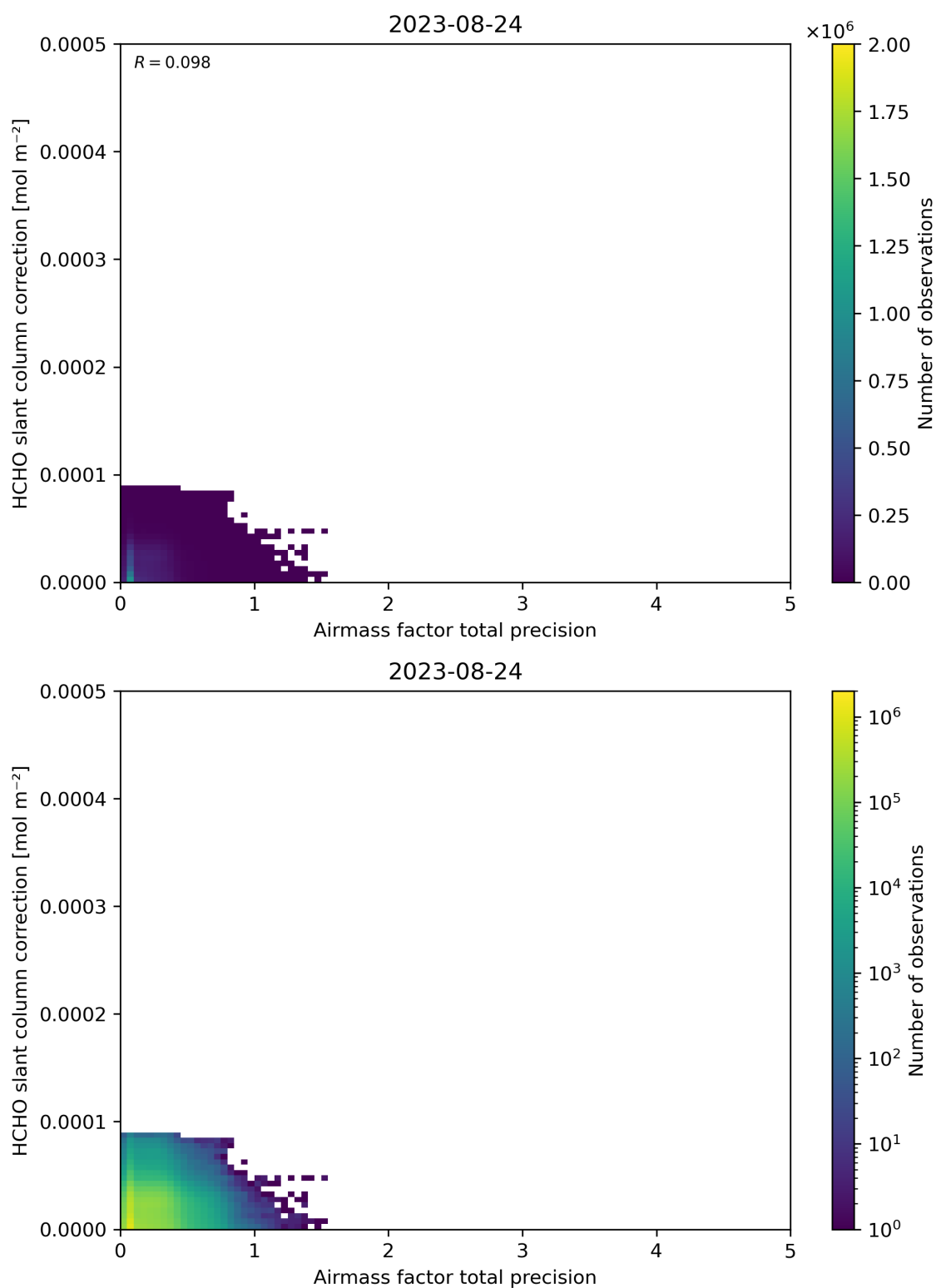
Figure 110: Scatter density plot of “Airmass factor total precision” against “HCHO slant column correction” for 2023-08-23 to 2023-08-25.
