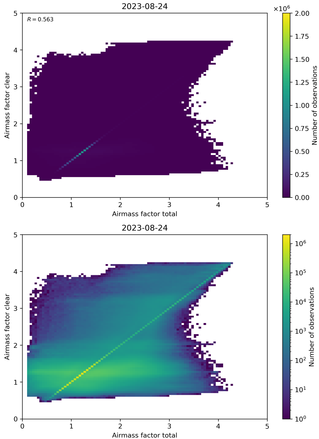
Figure 100: Scatter density plot of “Airmass factor total” against “Airmass factor clear” for 2023-08-23 to 2023-08-25.
