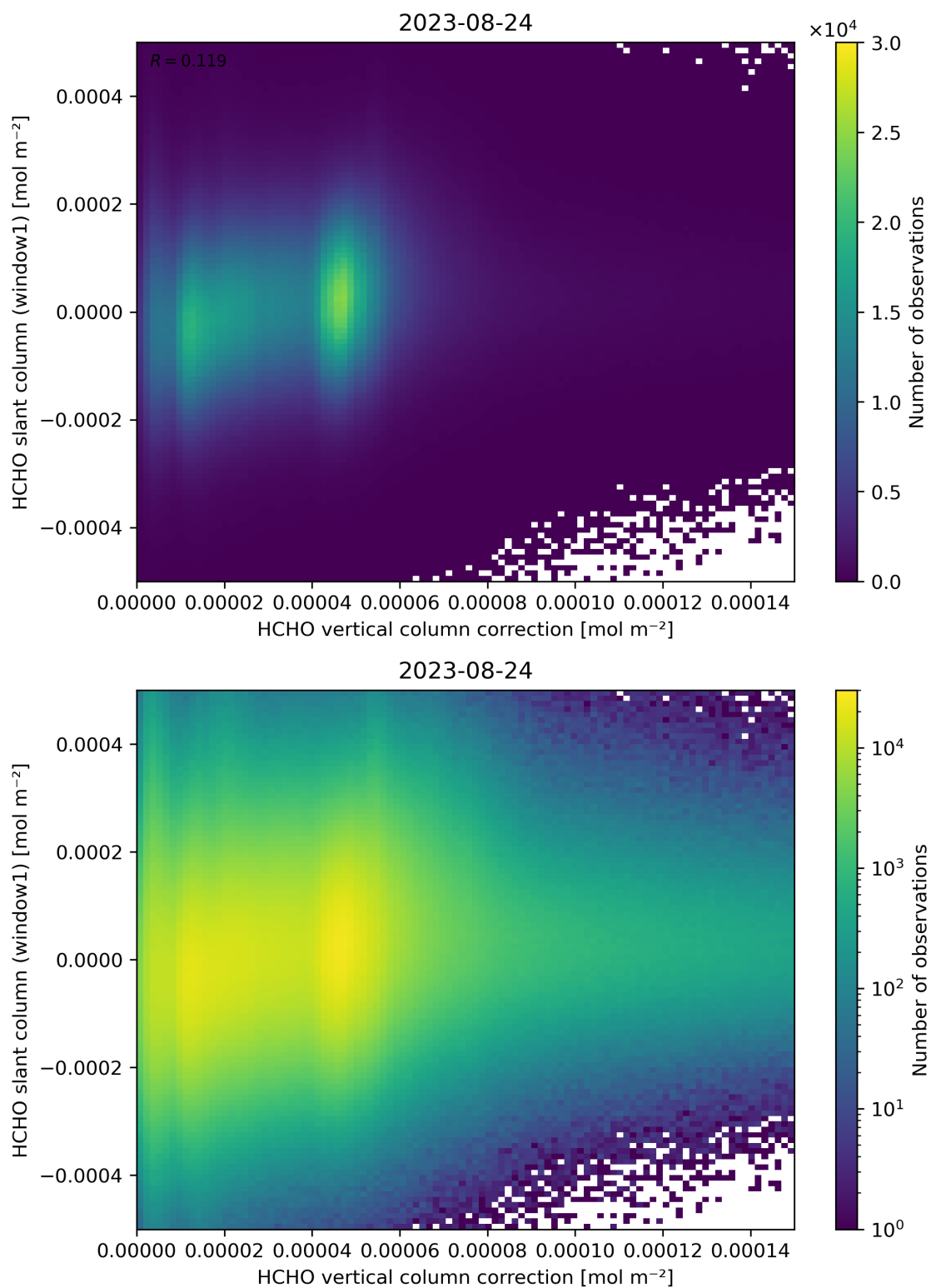
Figure 118: Scatter density plot of “HCHO vertical column correction” against “HCHO slant column (window1)” for 2023-08-23 to 2023-08-25.
