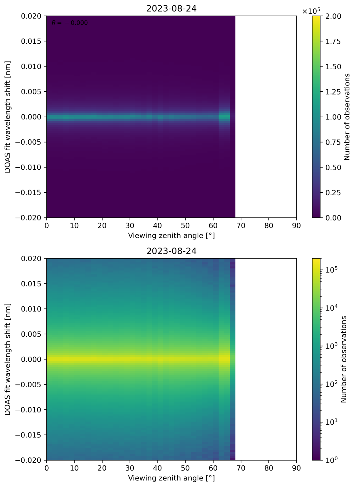
Figure 183: Scatter density plot of “Viewing zenith angle” against “DOAS fit wavelength shift” for 2023-08-23 to 2023-08-25.
