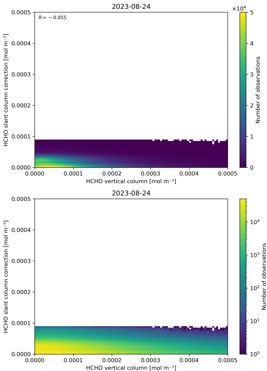
Figure 128: Scatter density plot of “HCHO vertical column” against “HCHO slant column correction” for 2023-08-23 to 2023-08-25.
