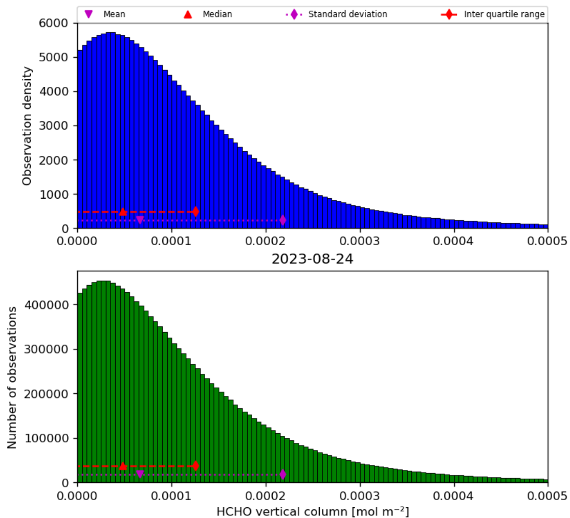
Figure 35: Histogram of “HCHO vertical column” for 2023-08-23 to 2023-08-25
