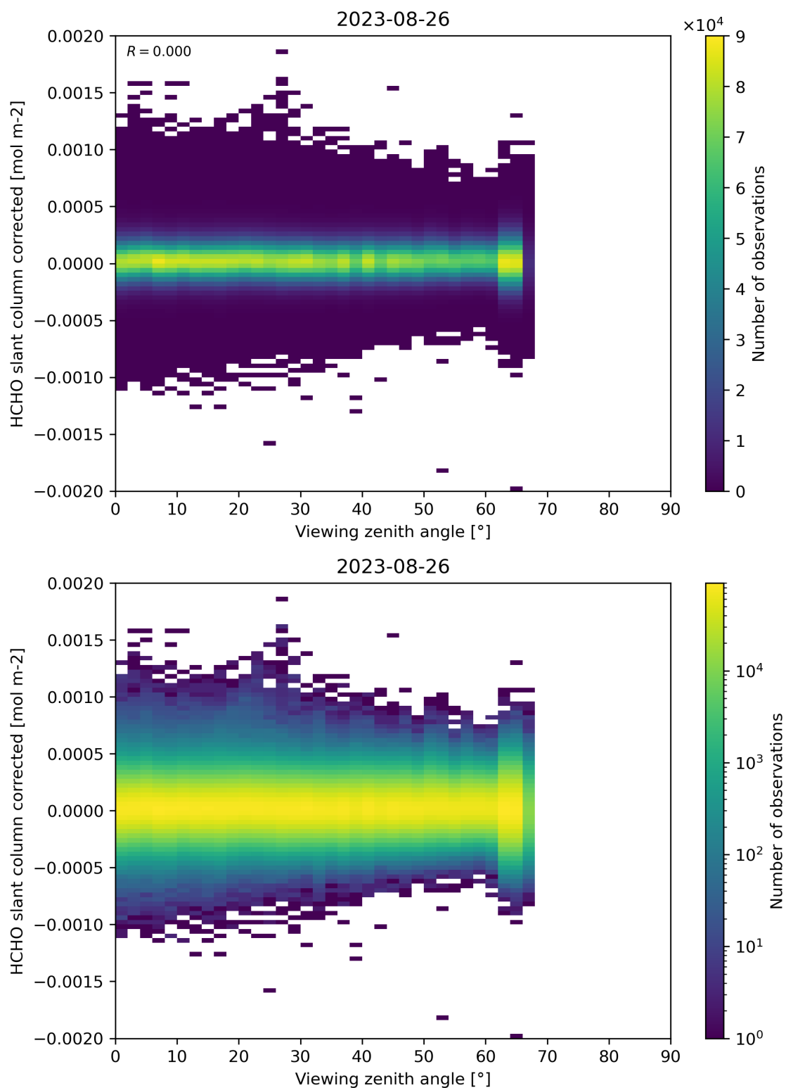
Figure 186: Scatter density plot of “Viewing zenith angle” against “HCHO slant column corrected” for 2023-08-25 to 2023-08-27.
