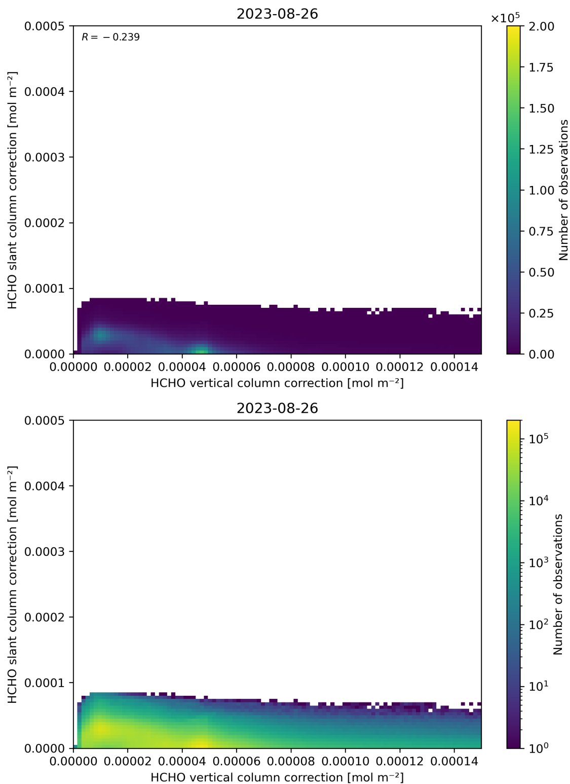
Figure 117: Scatter density plot of “HCHO vertical column correction” against “HCHO slant column correction” for 2023-08-25 to 2023-08-27.
