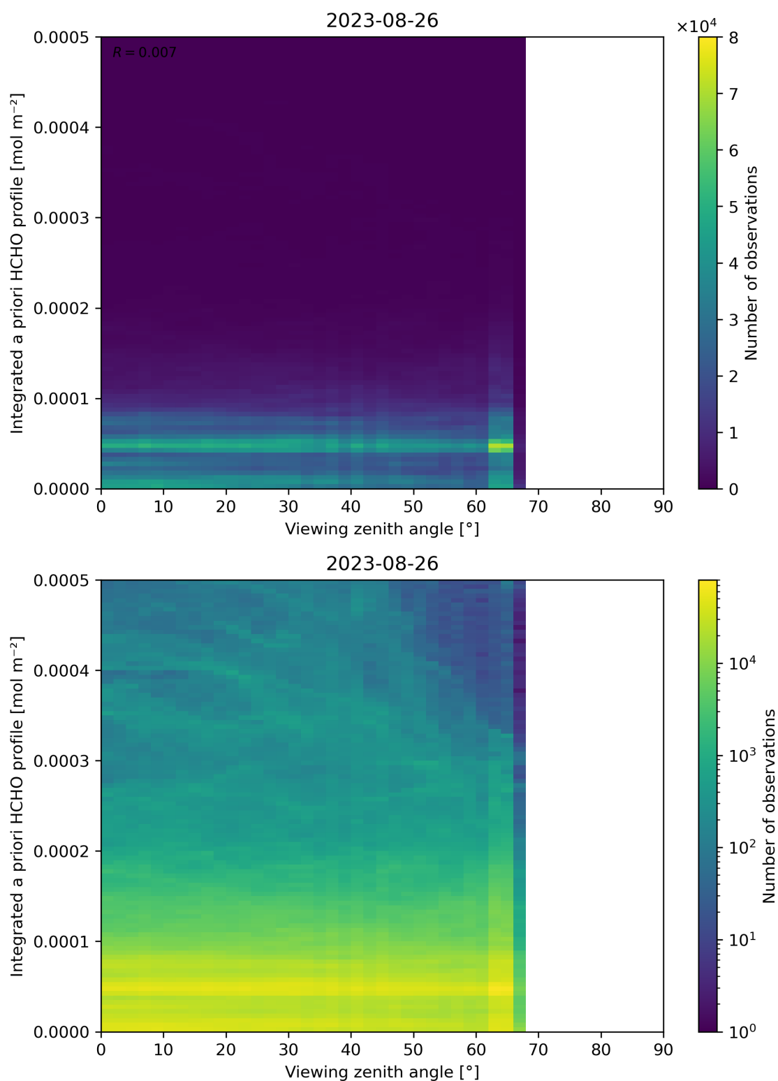
Figure 195: Scatter density plot of “Viewing zenith angle” against “Integrated a priori HCHO profile” for 2023-08-25 to 2023-08-27.
