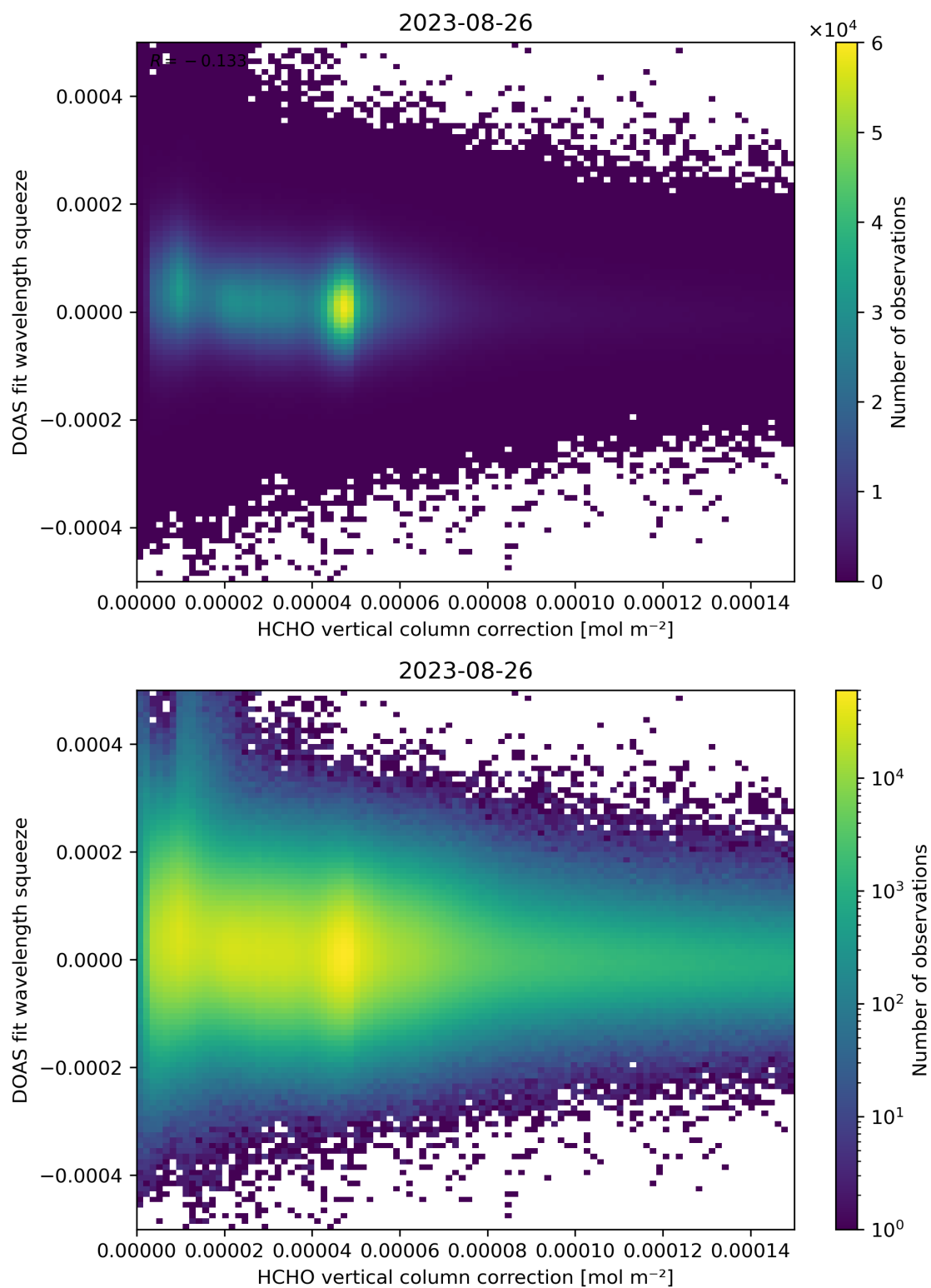
Figure 114: Scatter density plot of “HCHO vertical column correction” against “DOAS fit wavelength squeeze” for 2023-08-25 to 2023-08-27.
