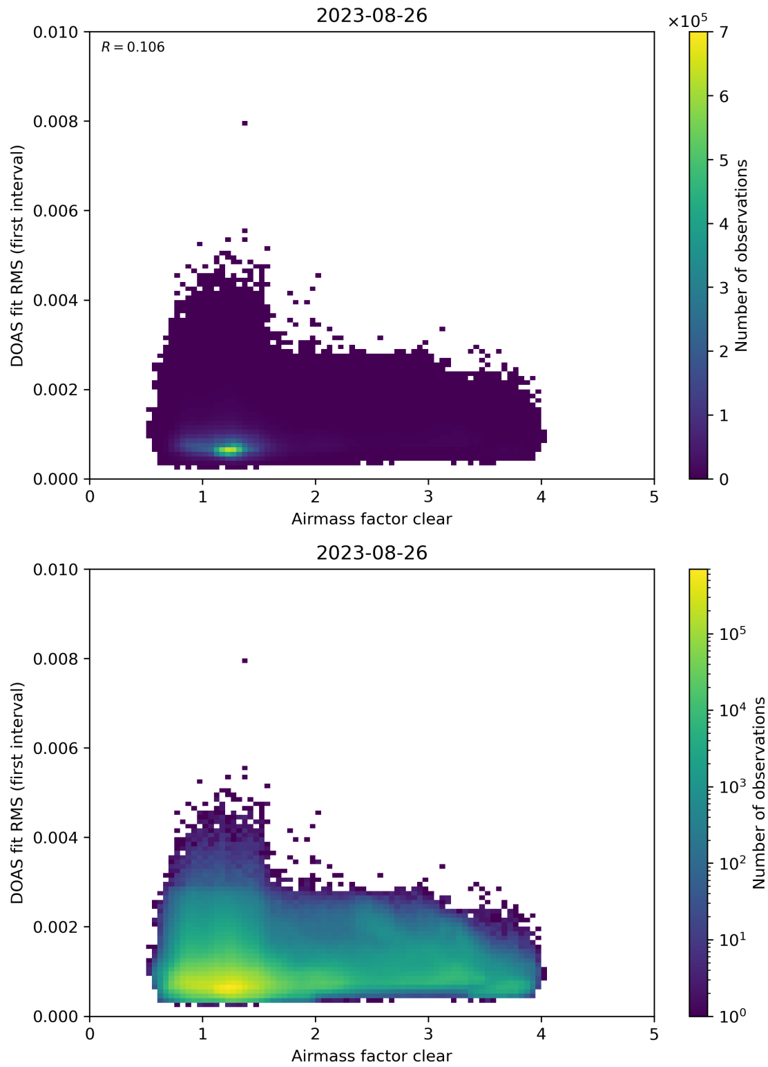
Figure 71: Scatter density plot of “Airmass factor clear” against “DOAS fit RMS (first interval)” for 2023-08-25 to 2023-08-27.
