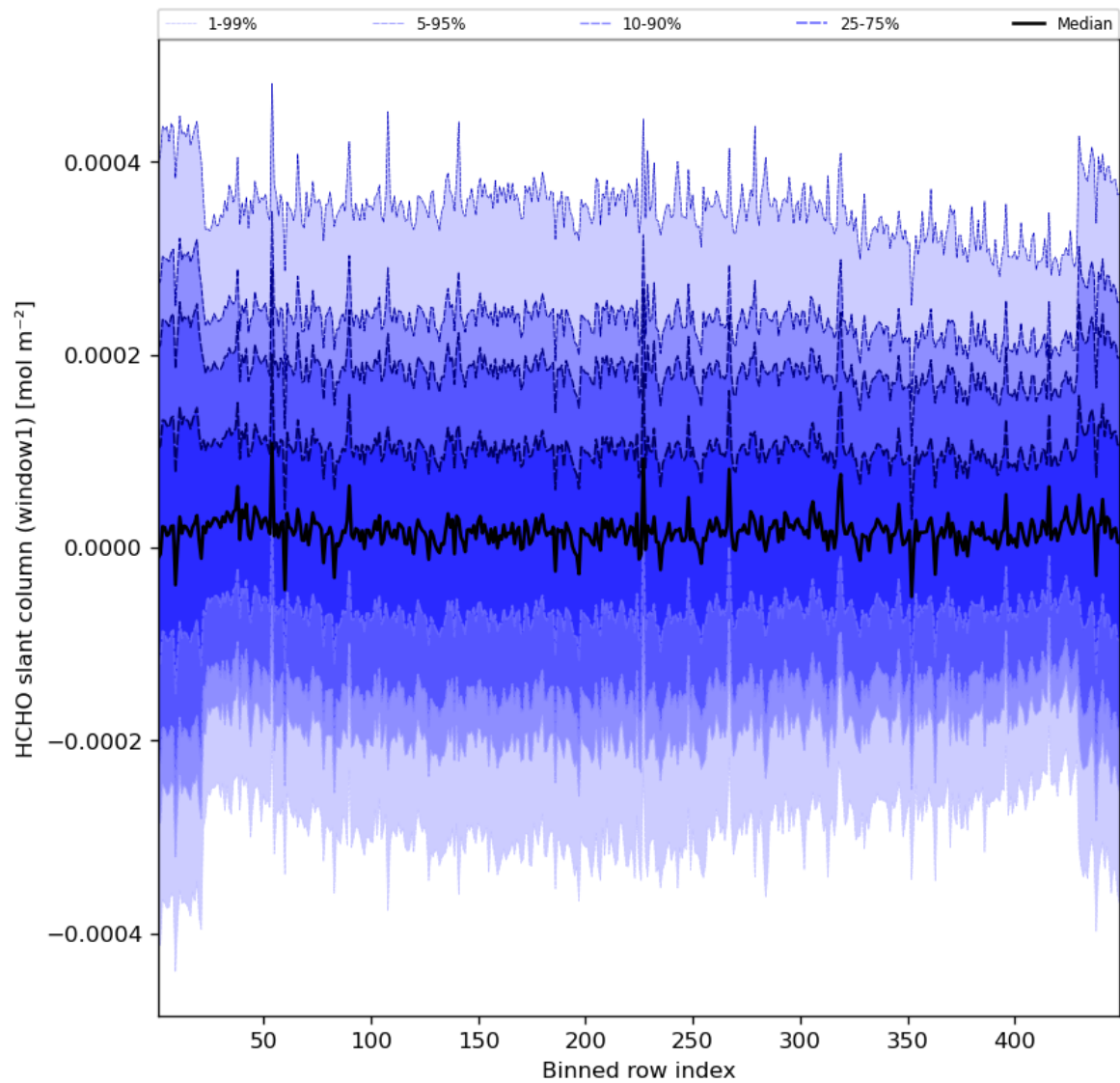
Figure 52: Along track statistics of “HCHO slant column (window1)” for 2023-08-25 to 2023-08-27
