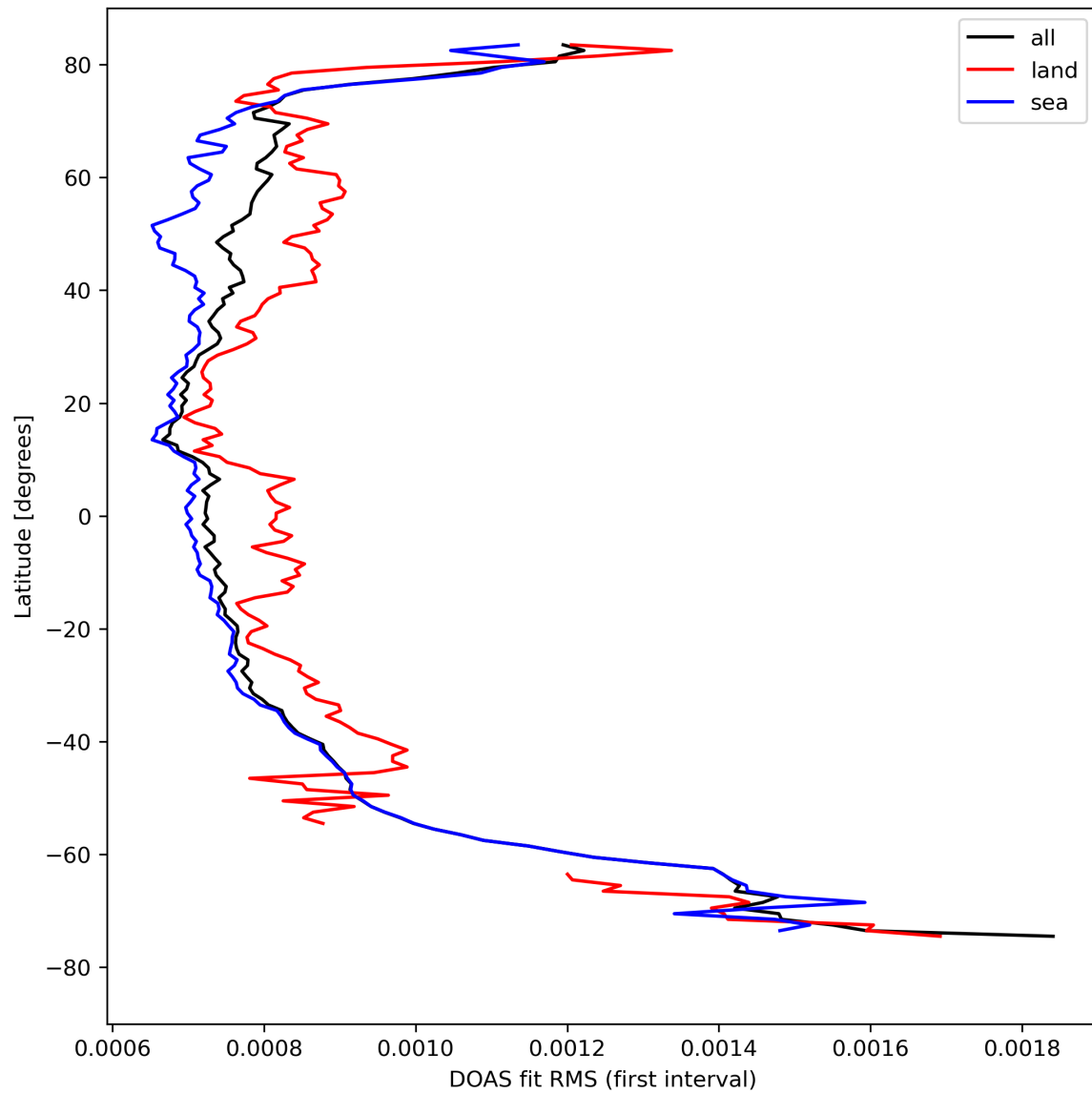
Figure 32: Zonal average of “DOAS fit RMS (first interval)” for 2023-08-25 to 2023-08-27.
