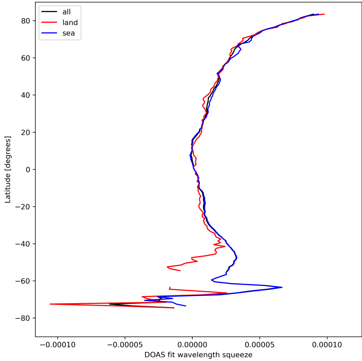
Figure 31: Zonal average of “DOAS fit wavelength squeeze” for 2023-08-25 to 2023-08-27.
