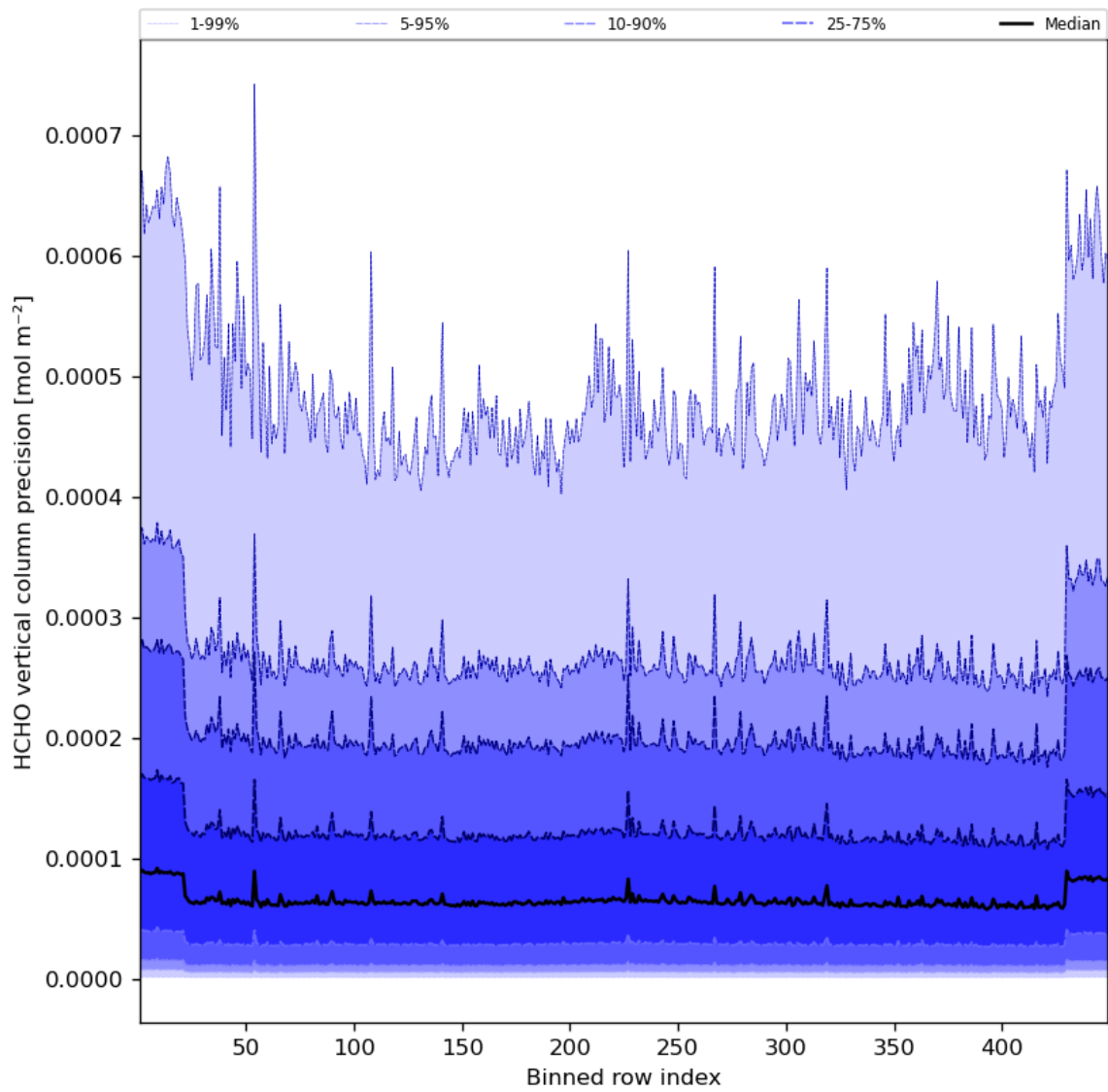
Figure 50: Along track statistics of “HCHO vertical column precision” for 2023-08-25 to 2023-08-27
