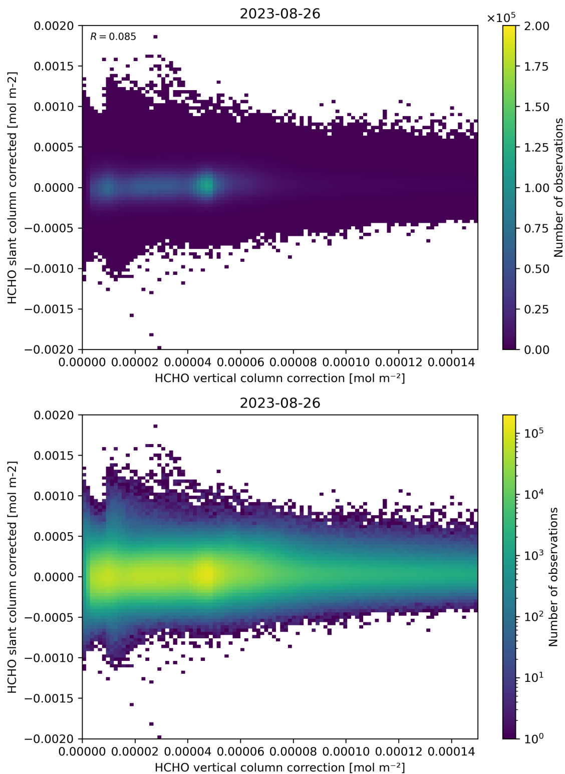
Figure 116: Scatter density plot of “HCHO vertical column correction” against “HCHO slant column corrected” for 2023-08-25 to 2023-08-27.
