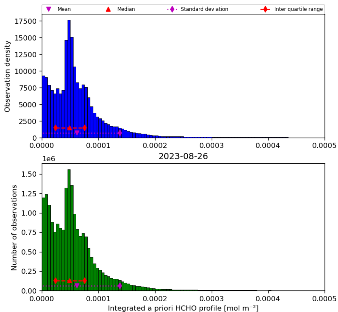
Figure 43: Histogram of “Integrated a priori HCHO profile” for 2023-08-25 to 2023-08-27
