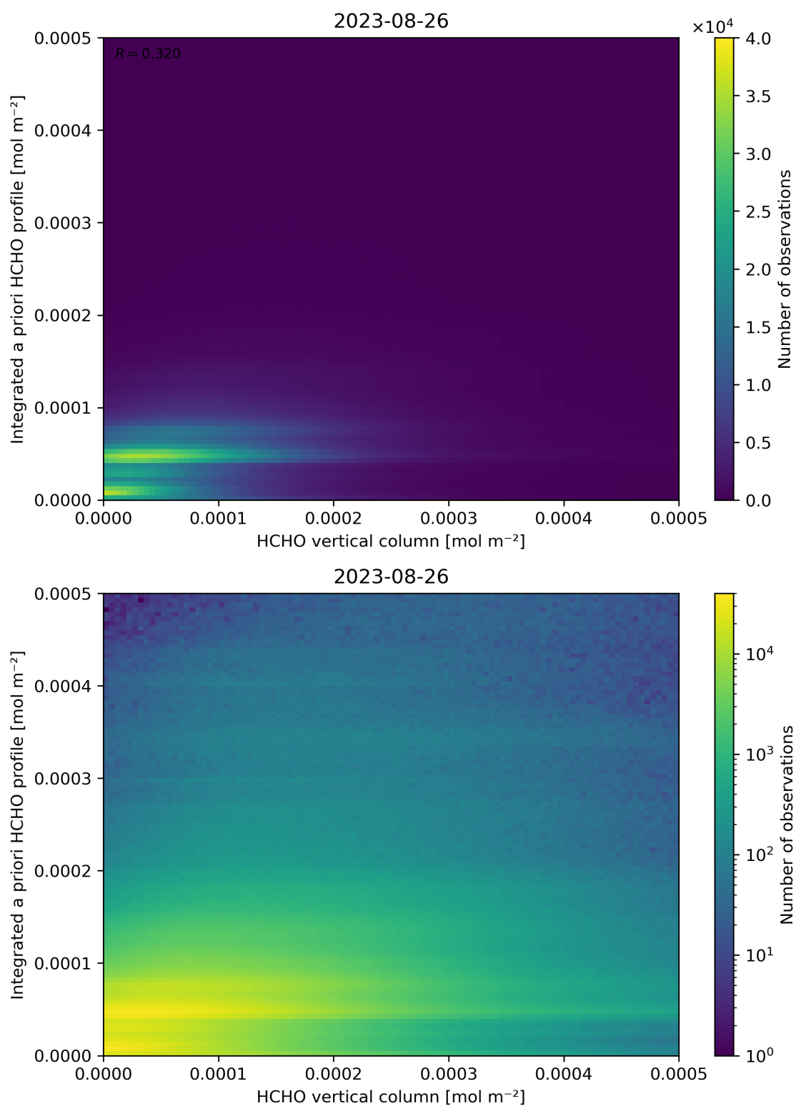
Figure 135: Scatter density plot of “HCHO vertical column” against “Integrated a priori HCHO profile” for 2023-08-25 to 2023-08-27.
