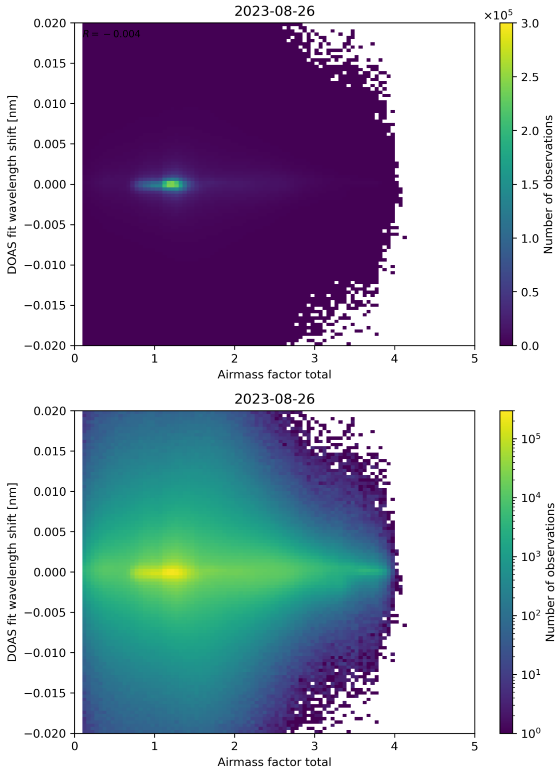
Figure 98: Scatter density plot of “Airmass factor total” against “DOAS fit wavelength shift” for 2023-08-25 to 2023-08-27.
