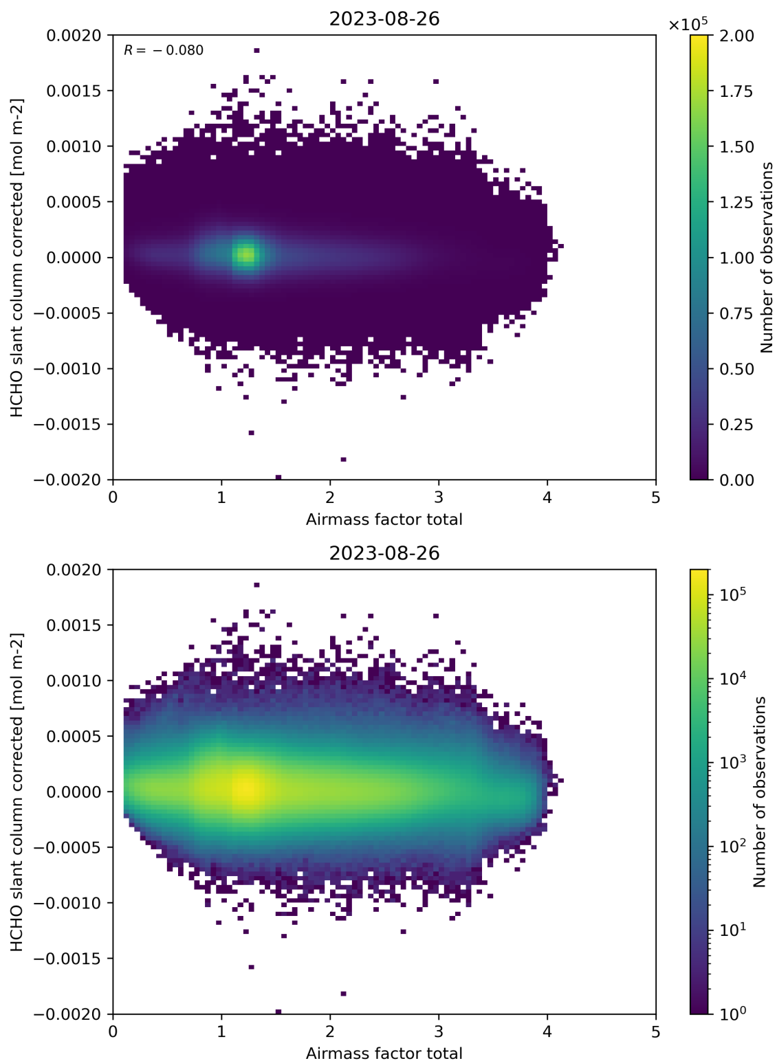
Figure 101: Scatter density plot of “Airmass factor total” against “HCHO slant column corrected” for 2023-08-25 to 2023-08-27.
