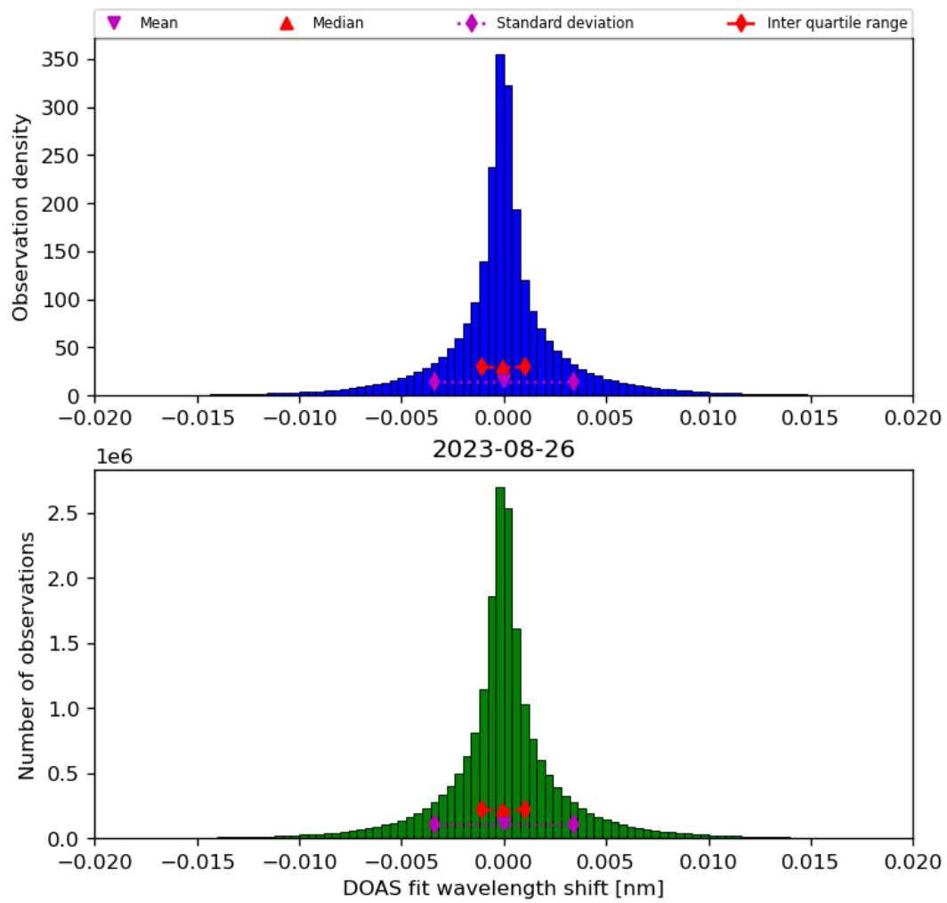
Figure 44: Histogram of “DOAS fit wavelength shift” for 2023-08-25 to 2023-08-27
