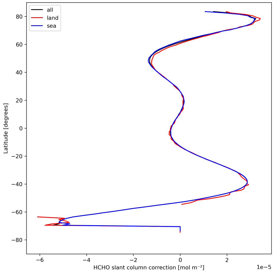
Figure 33: Zonal average of “HCHO slant column correction” for 2023-08-25 to 2023-08-27.
