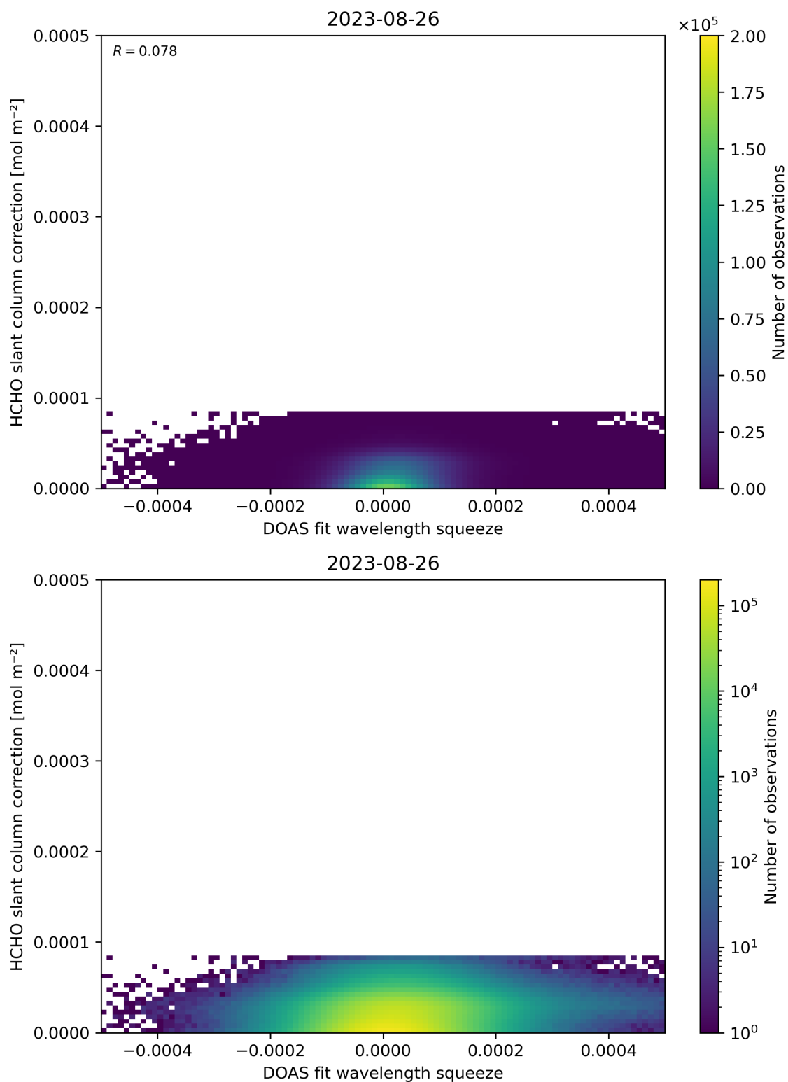
Figure 70: Scatter density plot of “DOAS fit wavelength squeeze” against “HCHO slant column correction” for 2023-08-25 to 2023-08-27.
