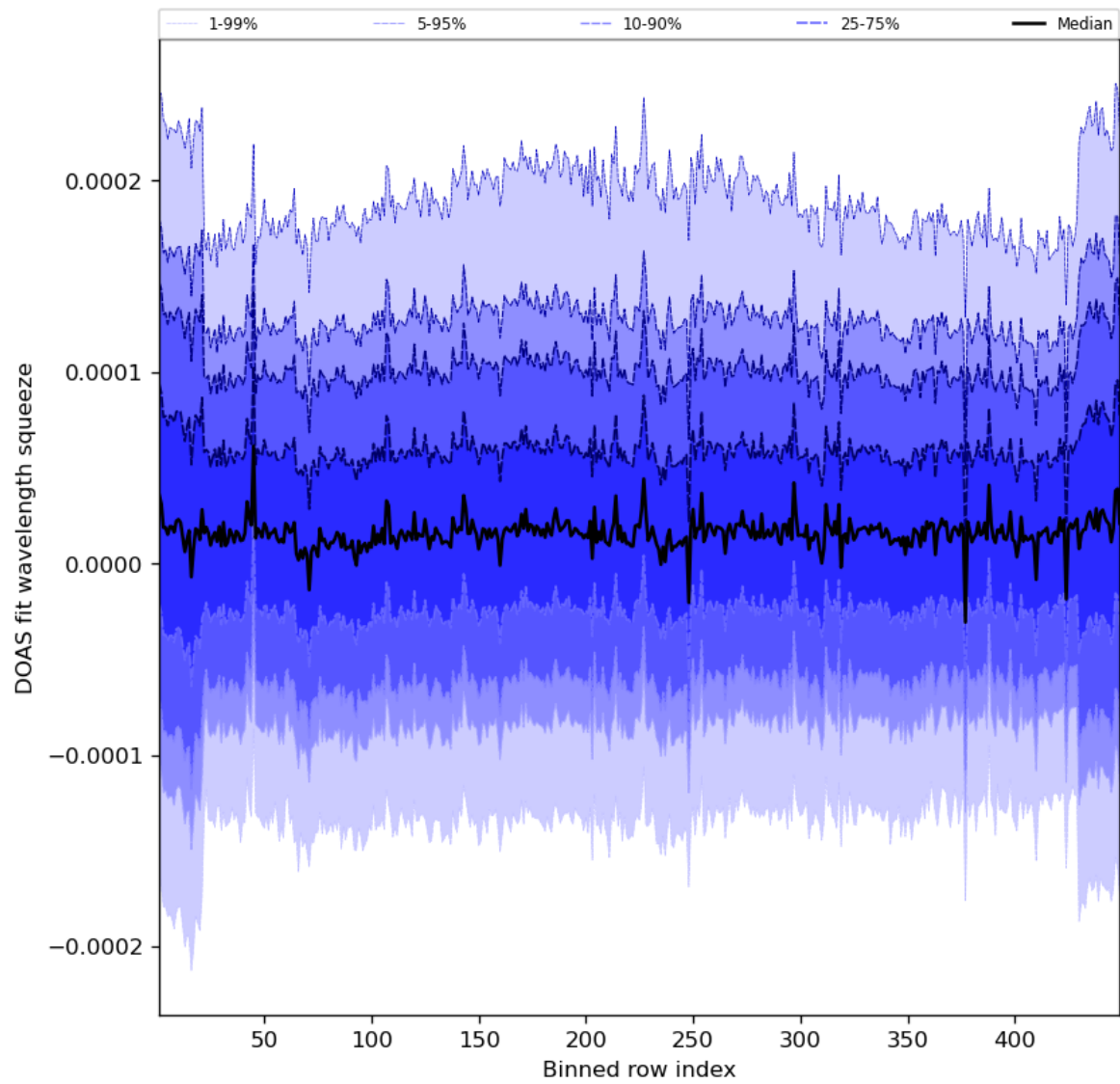
Figure 59: Along track statistics of “DOAS fit wavelength squeeze” for 2023-08-25 to 2023-08-27
