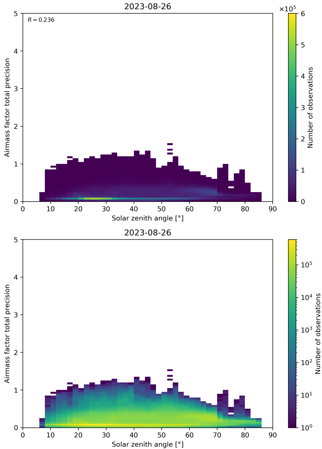
Figure 176: Scatter density plot of “Solar zenith angle” against “Airmass factor total precision” for 2023-08-25 to 2023-08-27.
