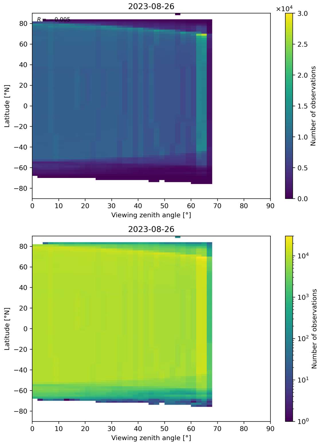
Figure 196: Scatter density plot of “Viewing zenith angle” against “Latitude” for 2023-08-25 to 2023-08-27.
