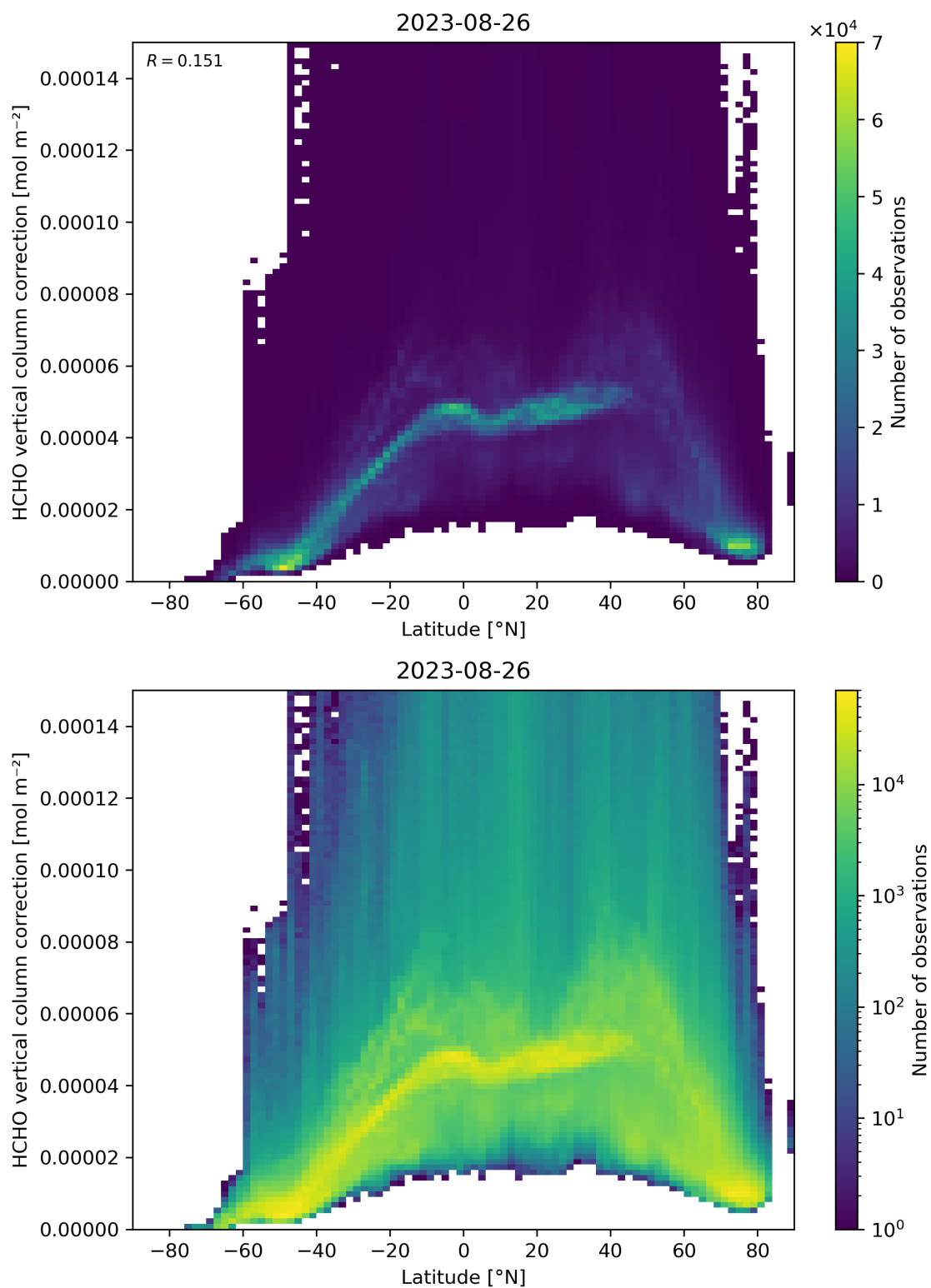
Figure 164: Scatter density plot of “Latitude” against “HCHO vertical column correction” for 2023-08-25 to 2023-08-27.
