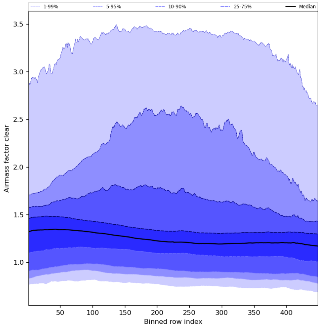
Figure 56: Along track statistics of “Airmass factor clear” for 2023-08-25 to 2023-08-27
