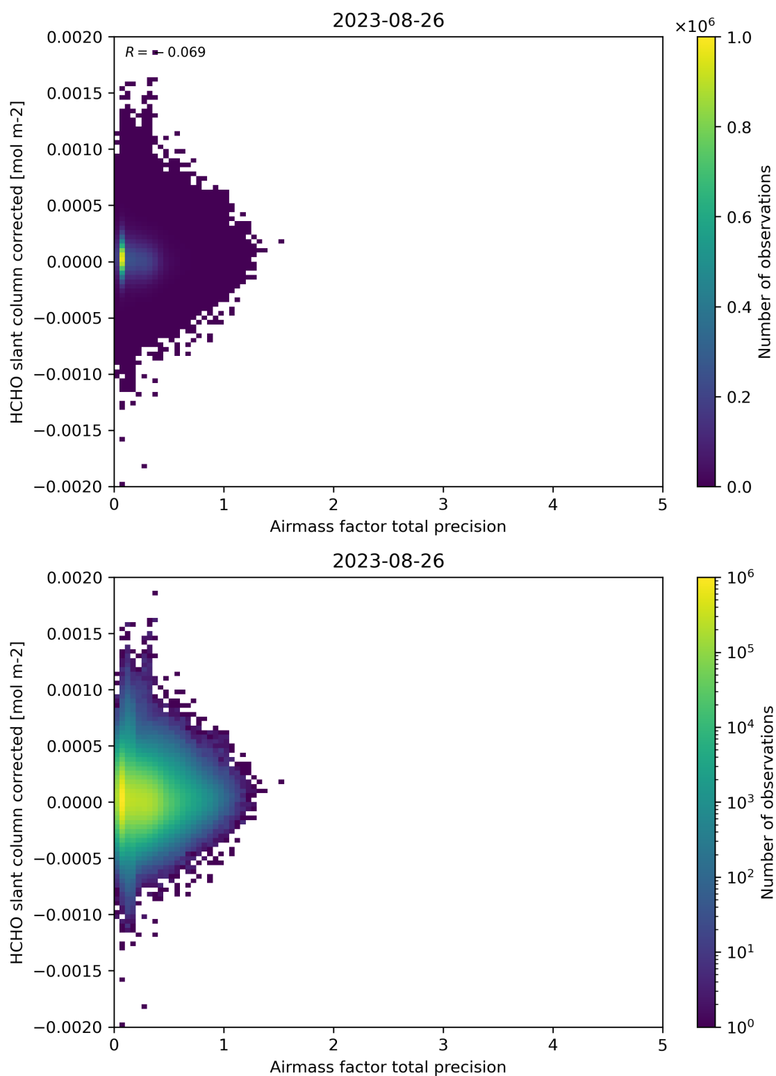
Figure 109: Scatter density plot of “Airmass factor total precision” against “HCHO slant column corrected” for 2023-08-25 to 2023-08-27.
