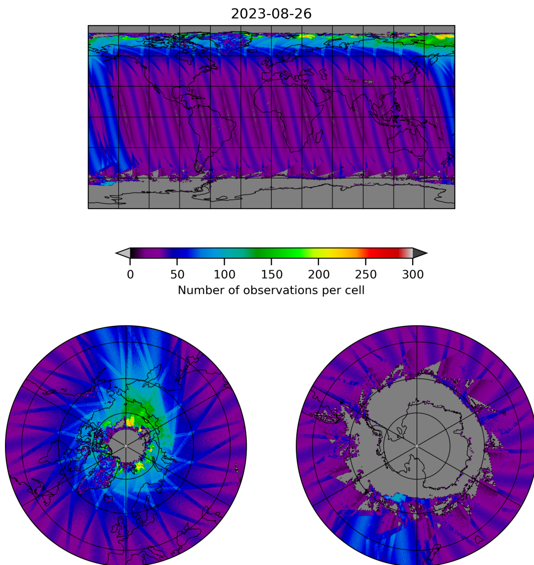
Figure 19: Map of the number of observations for 2023-08-25 to 2023-08-27
