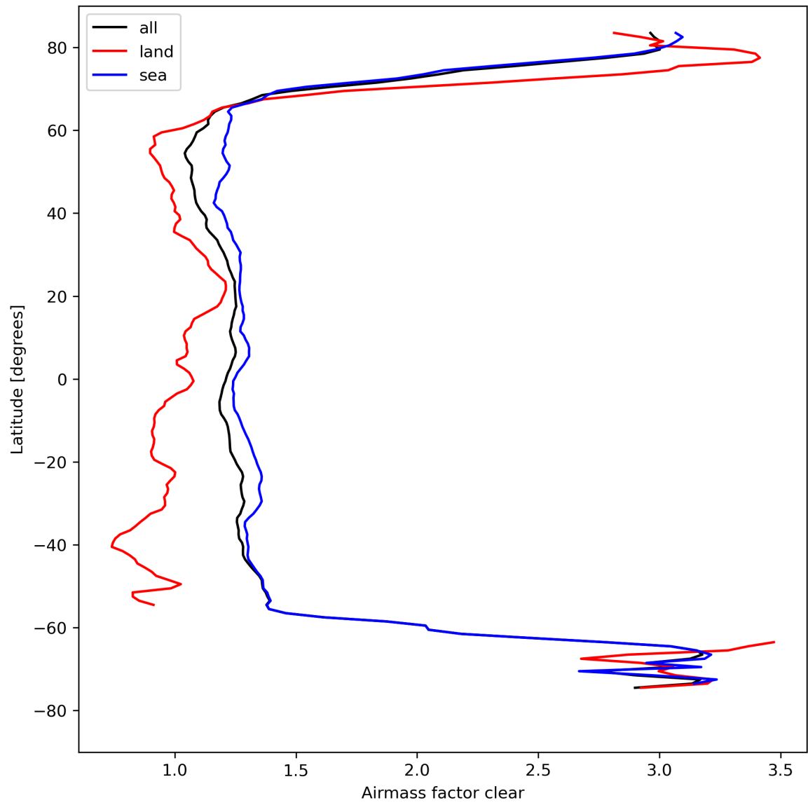
Figure 28: Zonal average of “Airmass factor clear” for 2023-08-25 to 2023-08-27.
