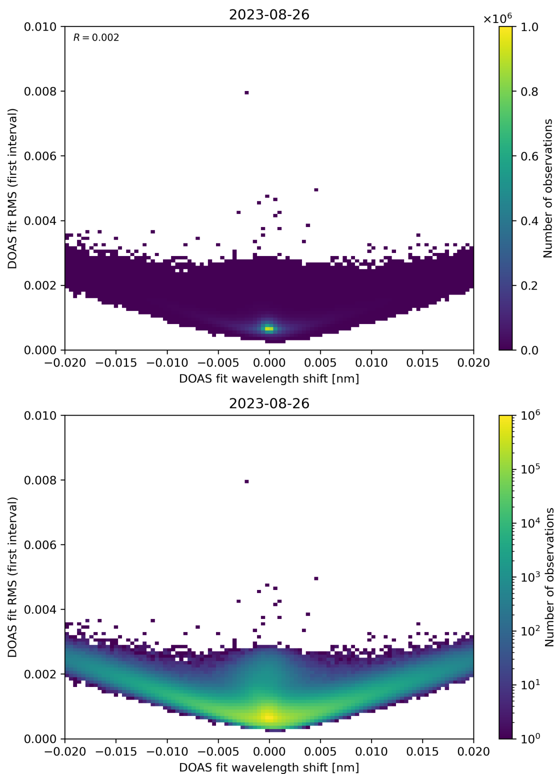
Figure 64: Scatter density plot of “DOAS fit wavelength shift” against “DOAS fit RMS (first interval)” for 2023-08-25 to 2023-08-27.
