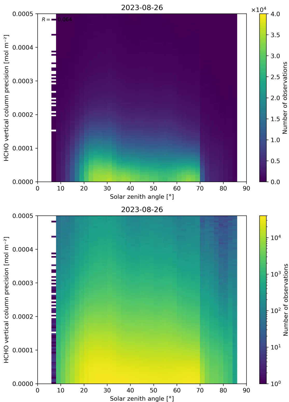
Figure 179: Scatter density plot of “Solar zenith angle” against “HCHO vertical column precision” for 2023-08-25 to 2023-08-27.
