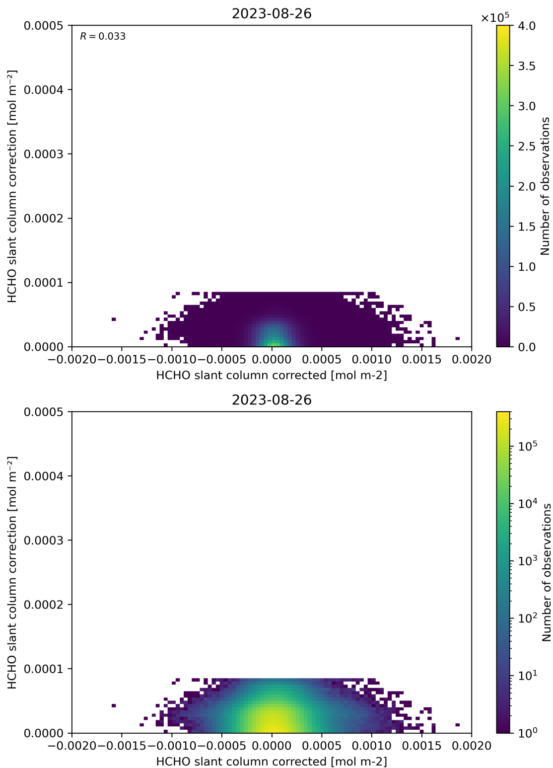
Figure 77: Scatter density plot of “HCHO slant column corrected” against “HCHO slant column correction” for 2023-08-25 to 2023-08-27.
