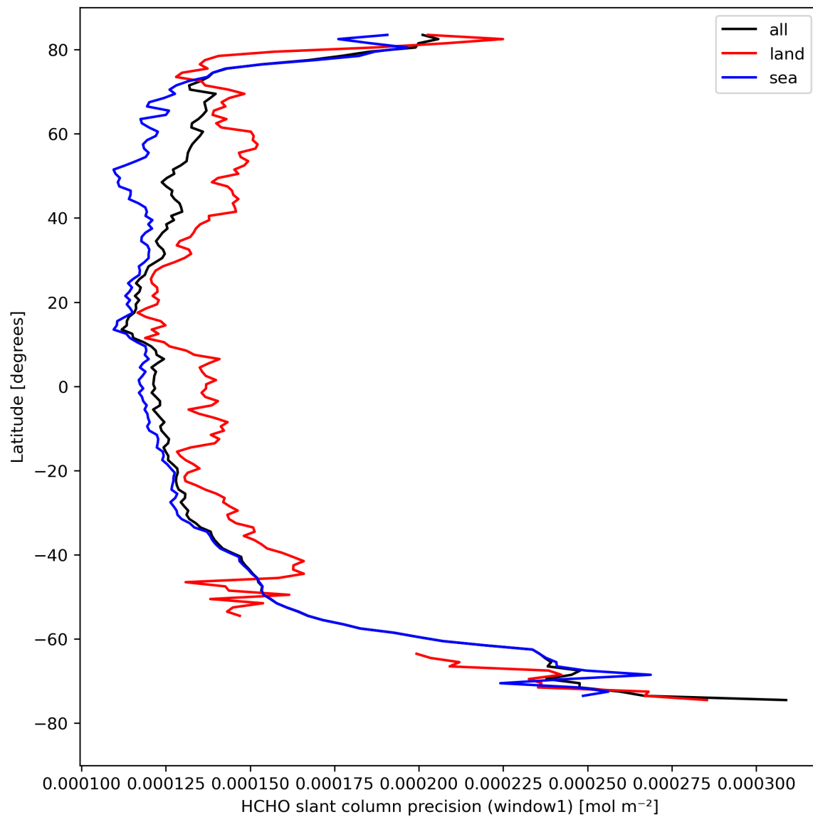
Figure 25: Zonal average of "HCHO slant column precision (window1)" for 2023-08-25 to 2023-08-27.
