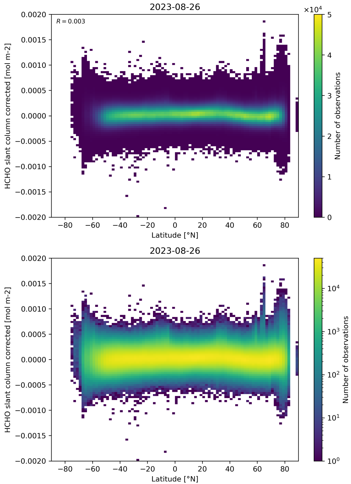
Figure 157: Scatter density plot of “Latitude” against “HCHO slant column corrected” for 2023-08-25 to 2023-08-27.
