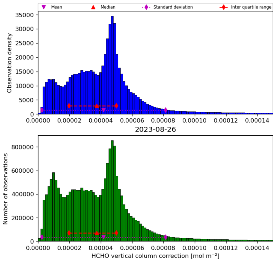
Figure 37: Histogram of “HCHO vertical column correction” for 2023-08-25 to 2023-08-27
