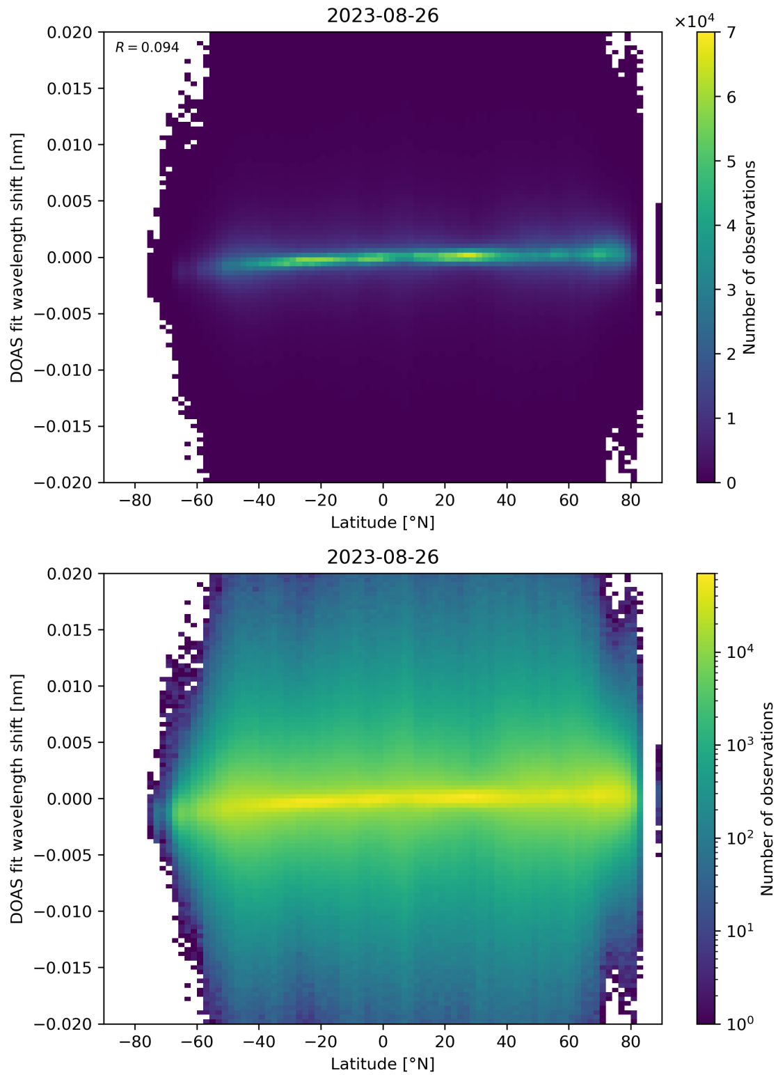
Figure 154: Scatter density plot of “Latitude” against “DOAS fit wavelength shift” for 2023-08-25 to 2023-08-27.
