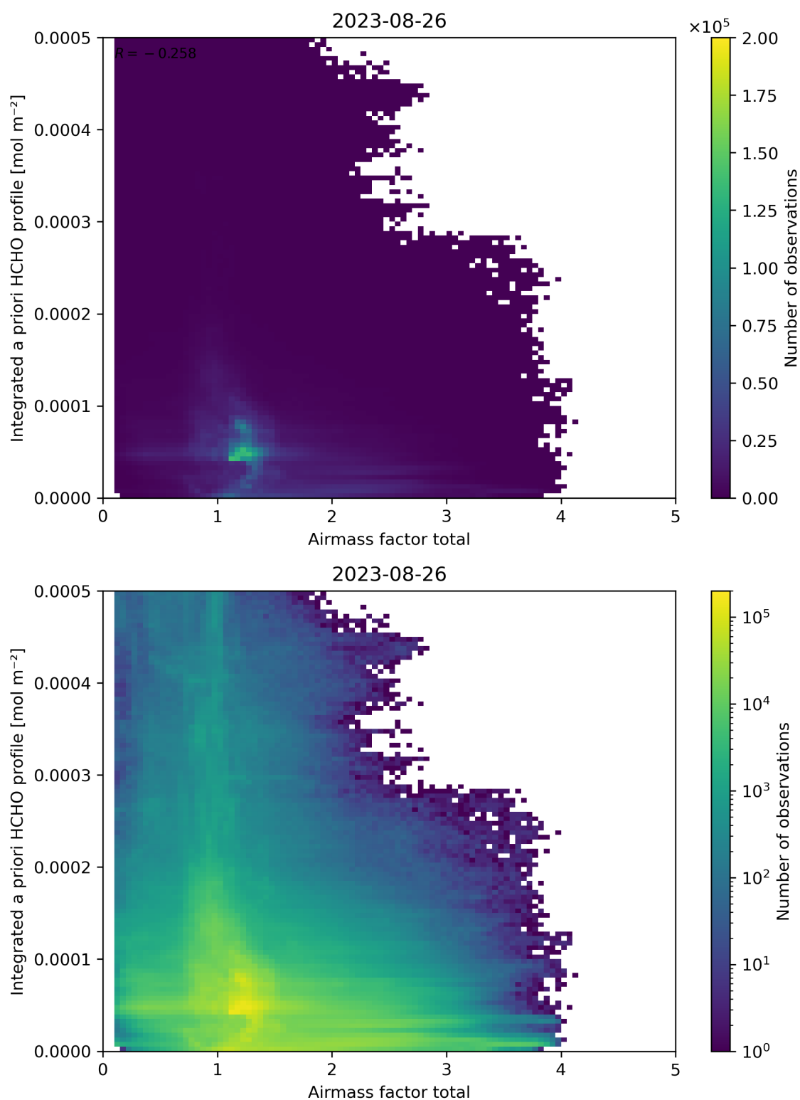
Figure 104: Scatter density plot of “Airmass factor total” against “Integrated a priori HCHO profile” for 2023-08-25 to 2023-08-27.
