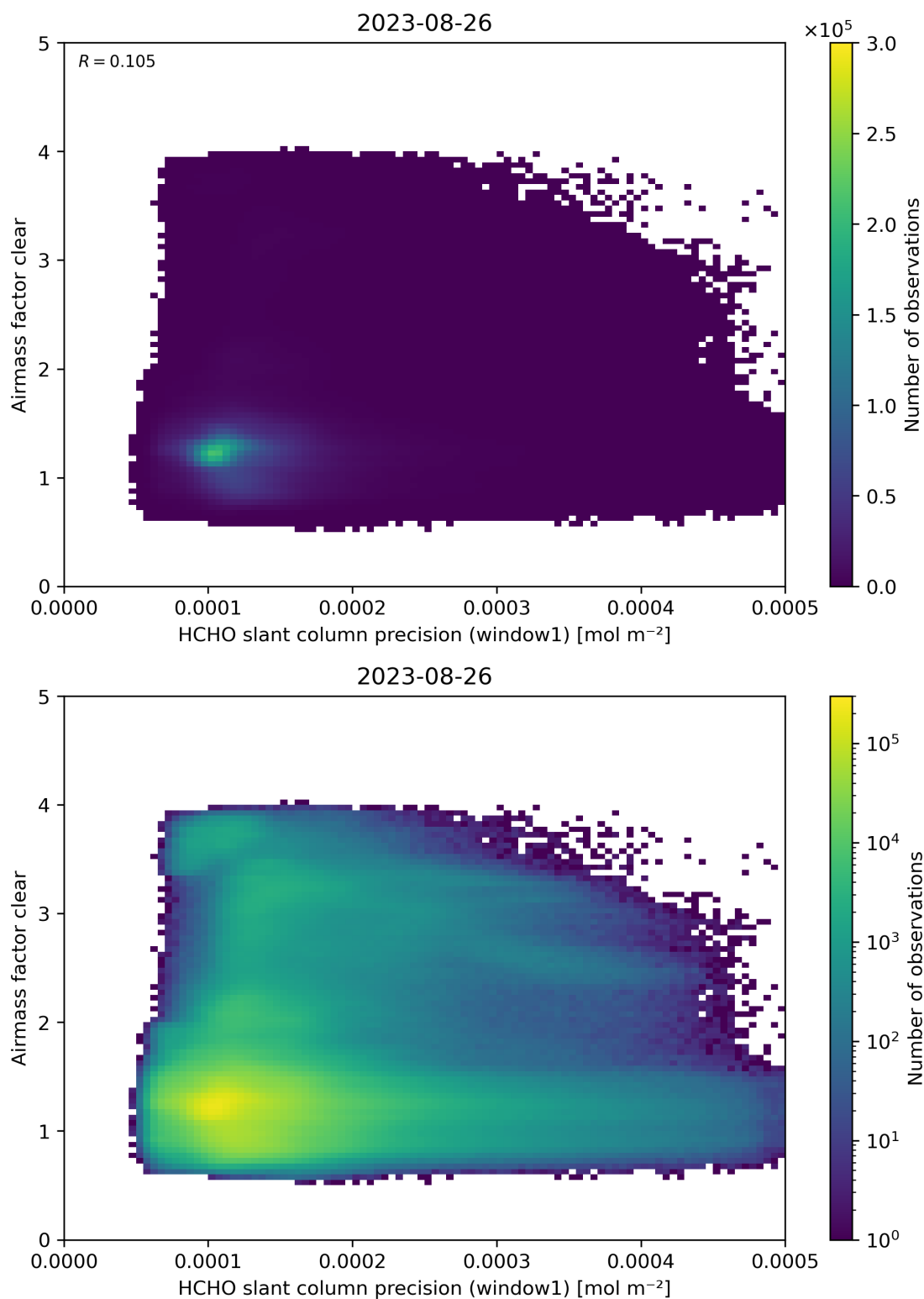
Figure 91: Scatter density plot of “HCHO slant column precision (window1)” against “Airmass factor clear” for 2023-08-25 to 2023-08-27.
