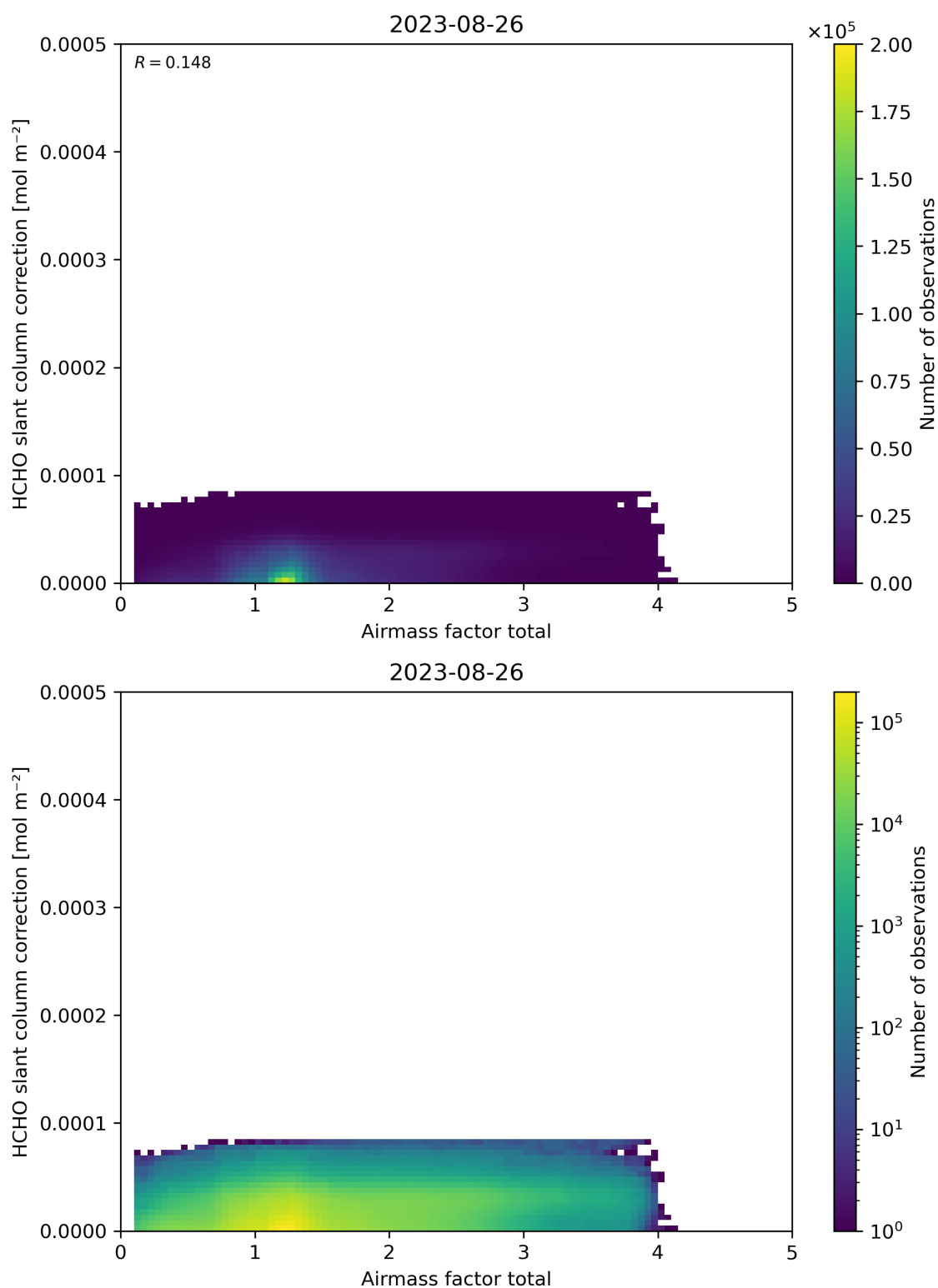
Figure 102: Scatter density plot of “Airmass factor total” against “HCHO slant column correction” for 2023-08-25 to 2023-08-27.
