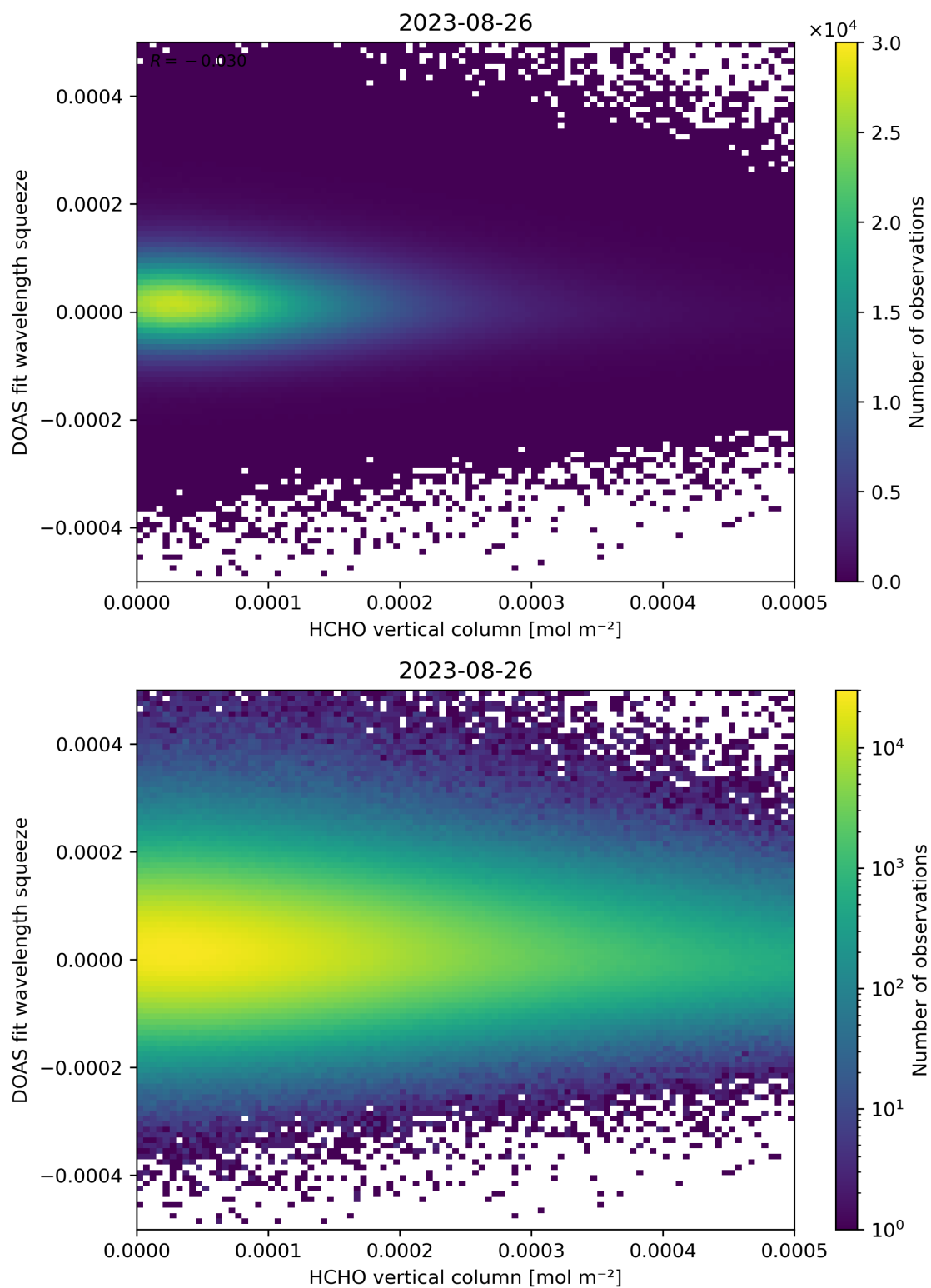
Figure 125: Scatter density plot of “HCHO vertical column” against “DOAS fit wavelength squeeze” for 2023-08-25 to 2023-08-27.
