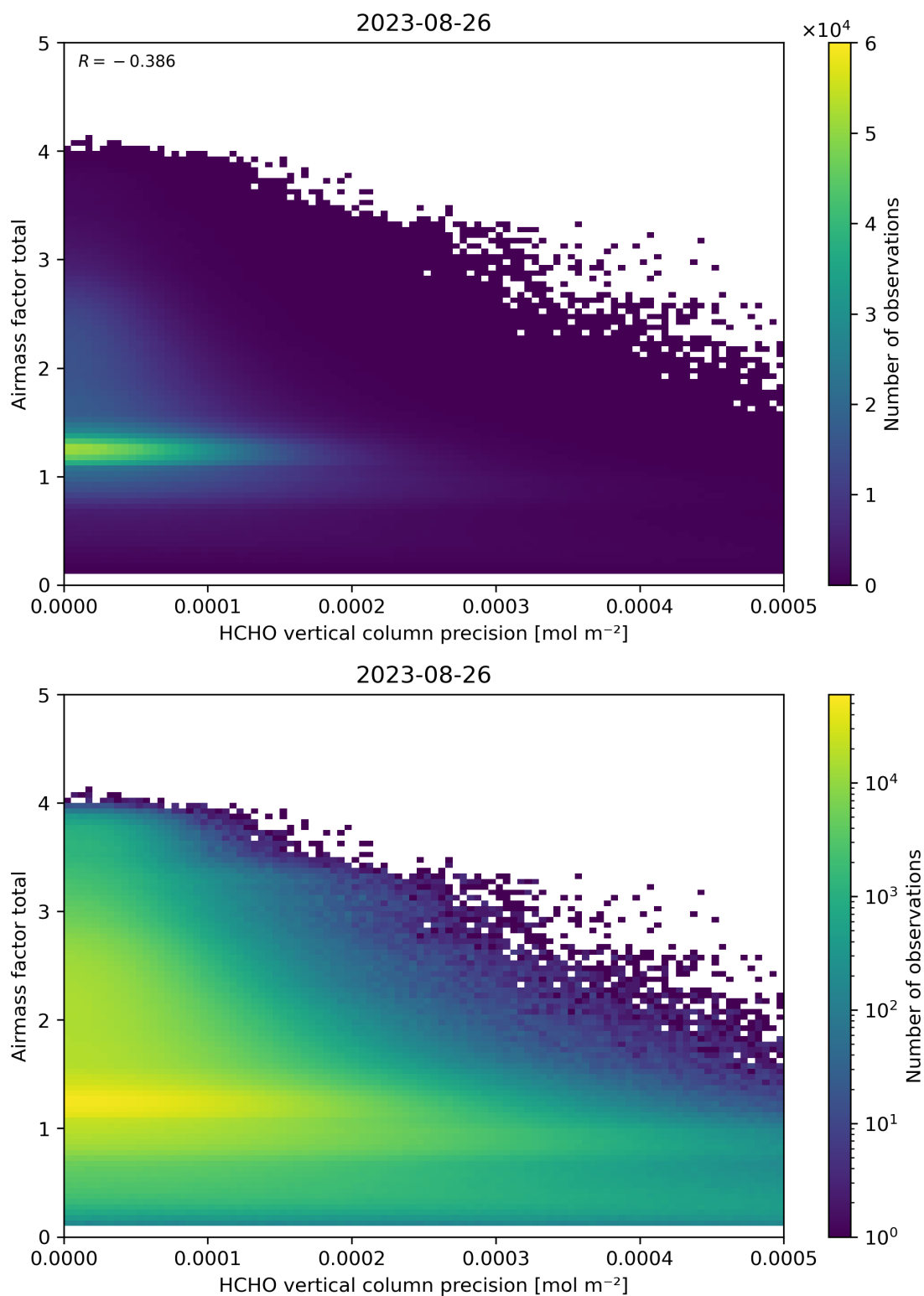
Figure 144: Scatter density plot of “HCHO vertical column precision” against “Airmass factor total” for 2023-08-25 to 2023-08-27.
