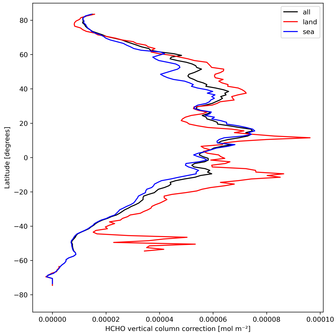
Figure 23: Zonal average of “HCHO vertical column correction” for 2023-08-25 to 2023-08-27.
