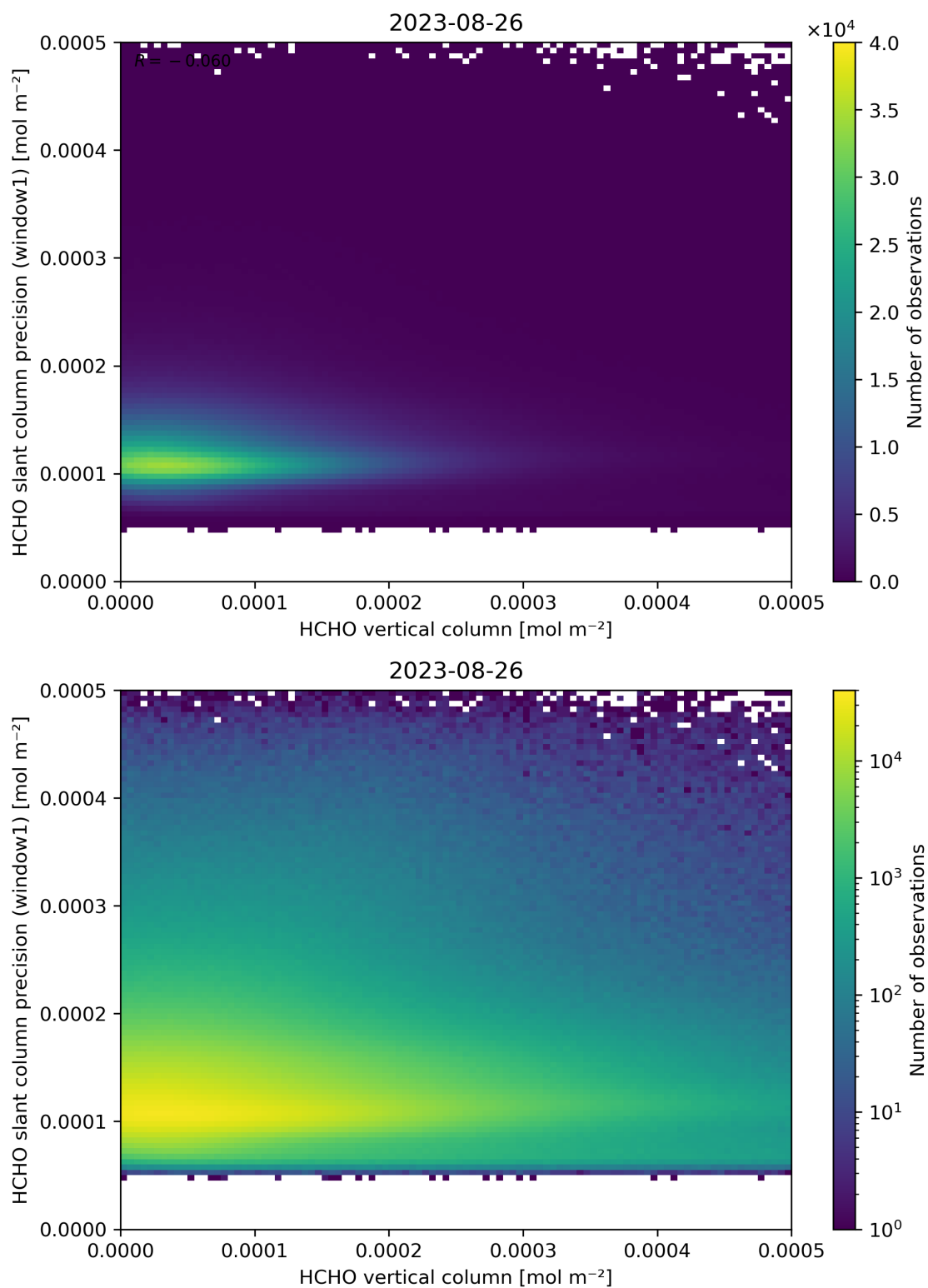
Figure 130: Scatter density plot of “HCHO vertical column” against “HCHO slant column precision (window1)” for 2023-08-25 to 2023-08-27.
