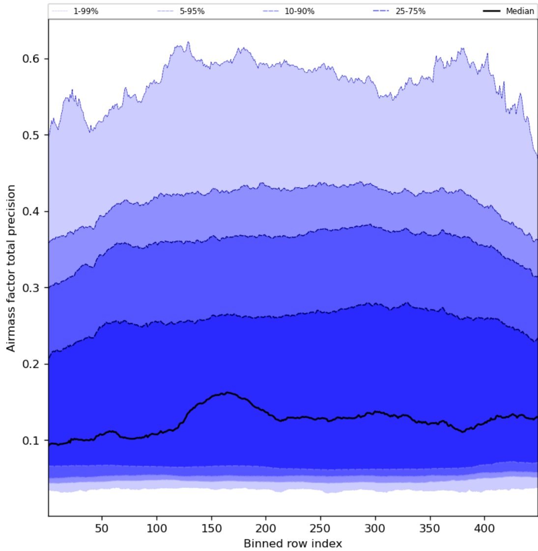
Figure 55: Along track statistics of “Airmass factor total precision” for 2023-08-25 to 2023-08-27
