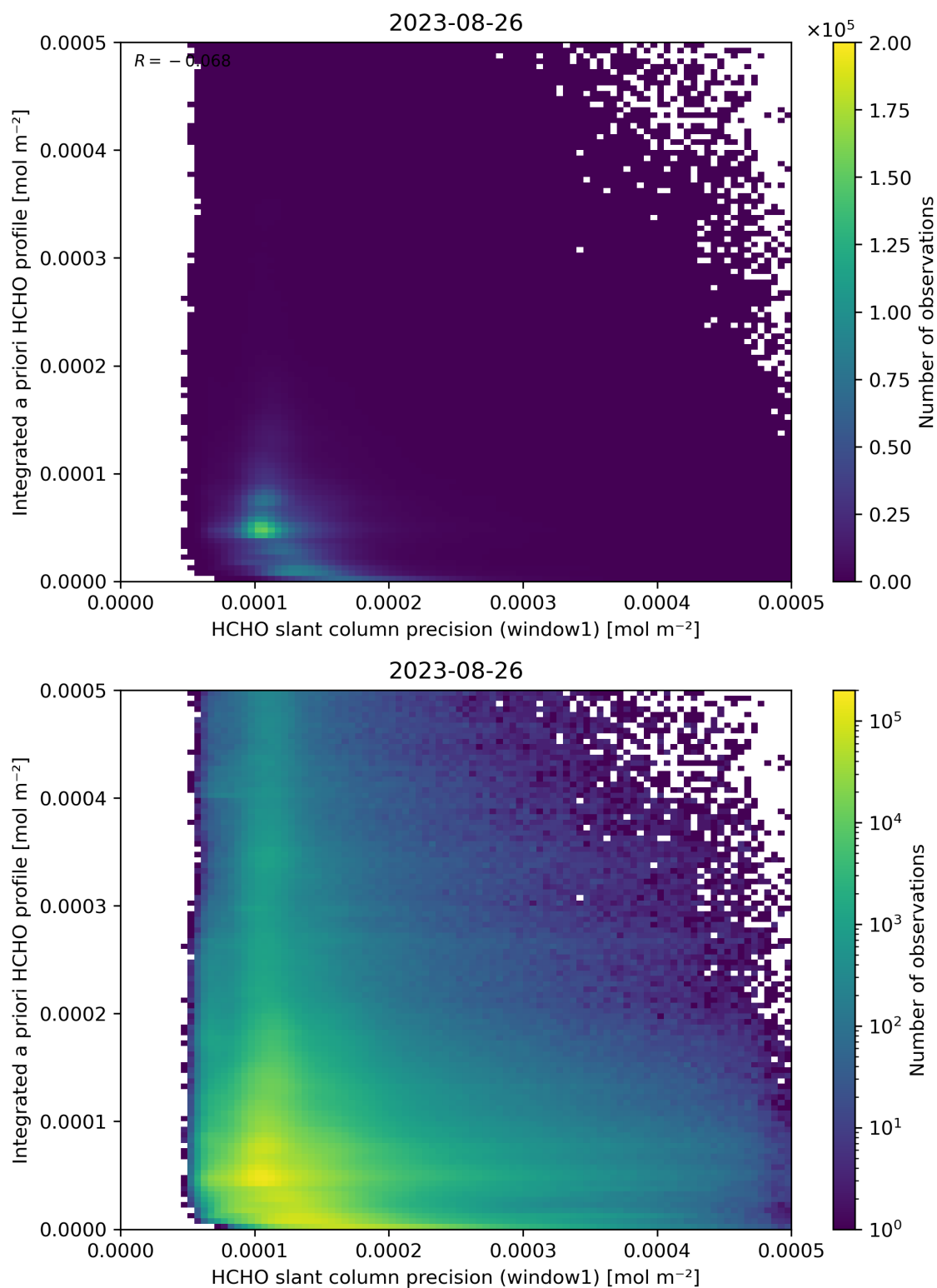
Figure 96: Scatter density plot of “HCHO slant column precision (window1)” against “Integrated a priori HCHO profile” for 2023-08-25 to 2023-08-27.
