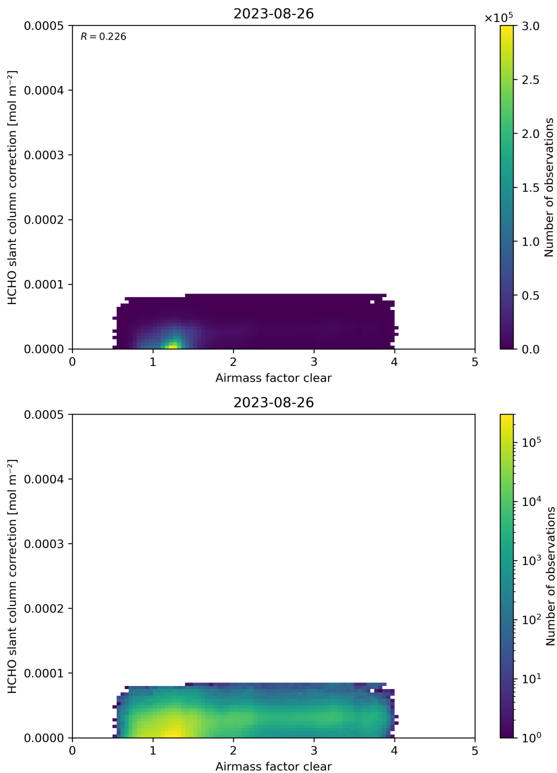
Figure 75: Scatter density plot of “Airmass factor clear” against “HCHO slant column correction” for 2023-08-25 to 2023-08-27.
