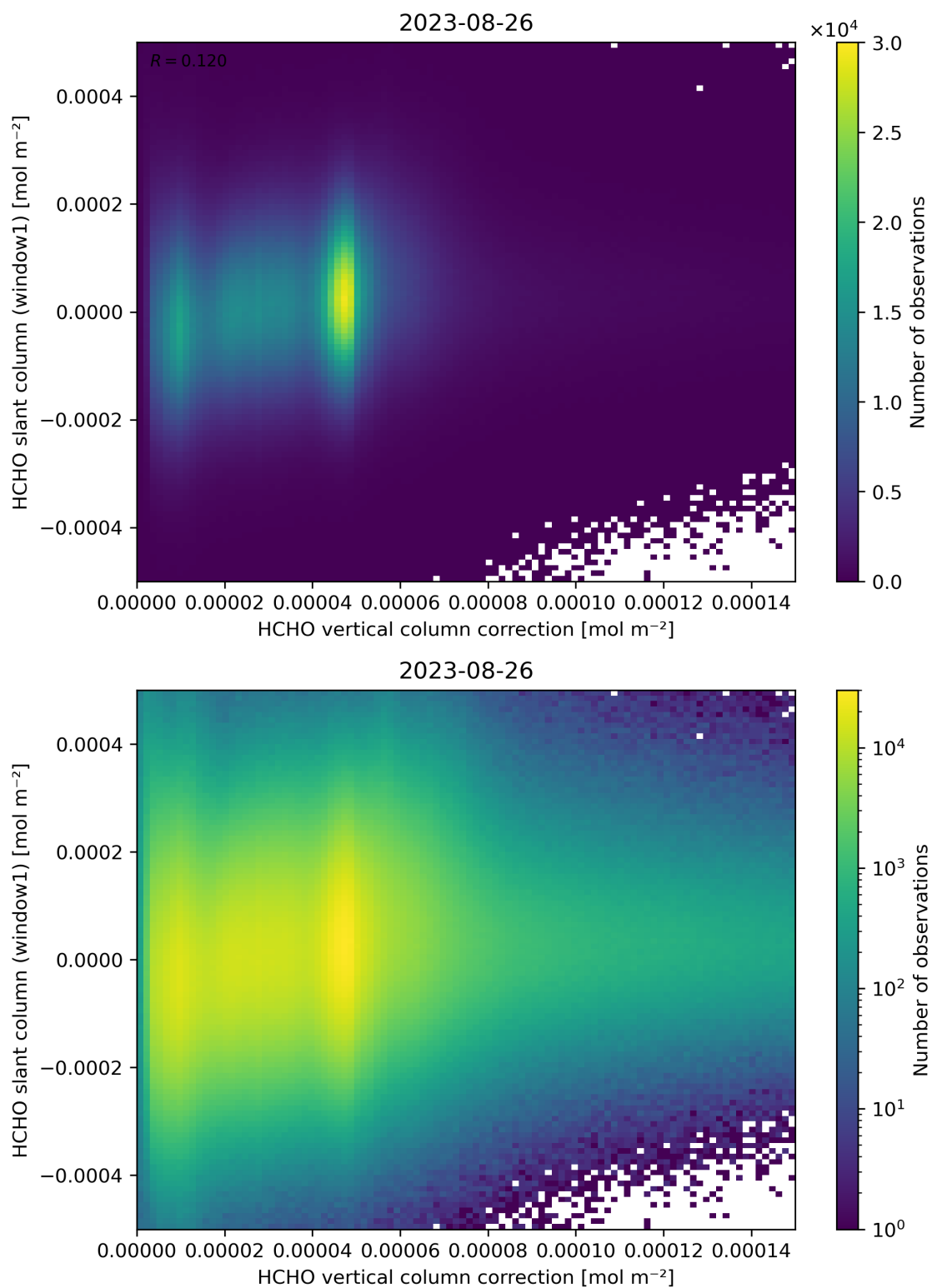
Figure 118: Scatter density plot of “HCHO vertical column correction” against “HCHO slant column (window1)” for 2023-08-25 to 2023-08-27.
