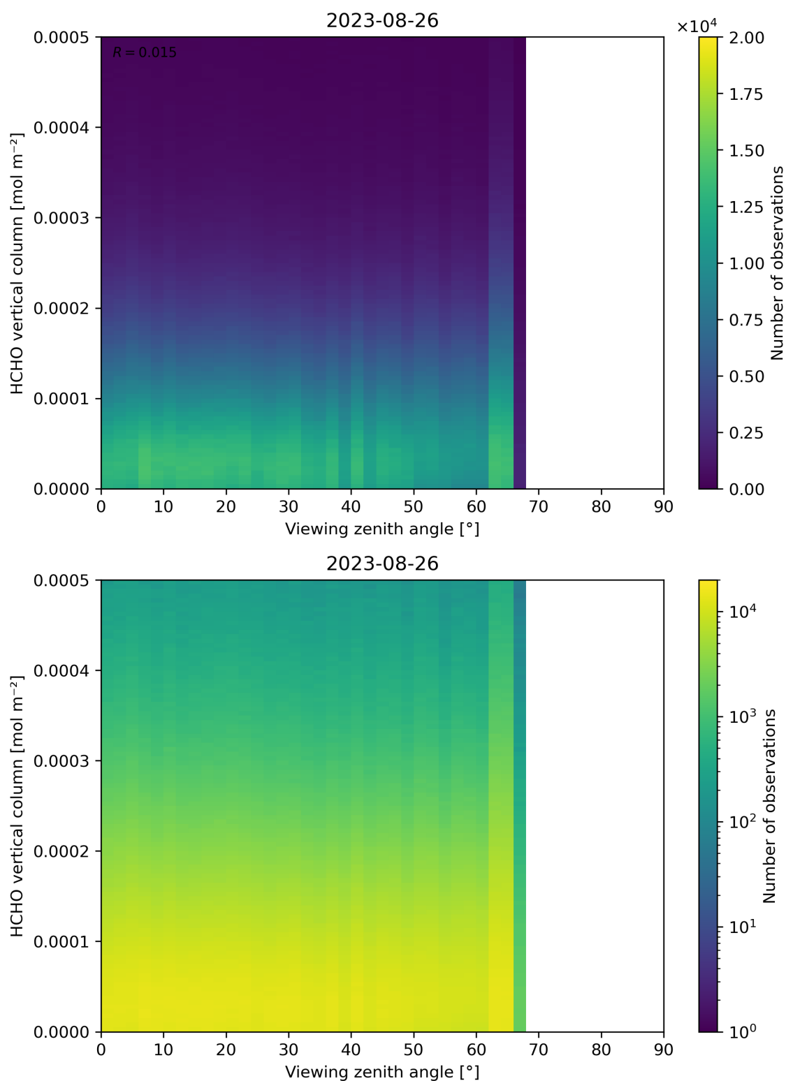
Figure 192: Scatter density plot of “Viewing zenith angle” against “HCHO vertical column” for 2023-08-25 to 2023-08-27.
