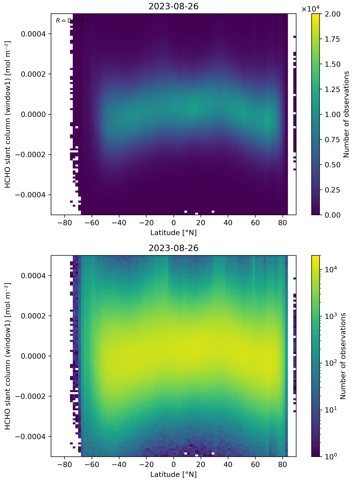
Figure 159: Scatter density plot of “Latitude” against “HCHO slant column (window1)” for 2023-08-25 to 2023-08-27.
