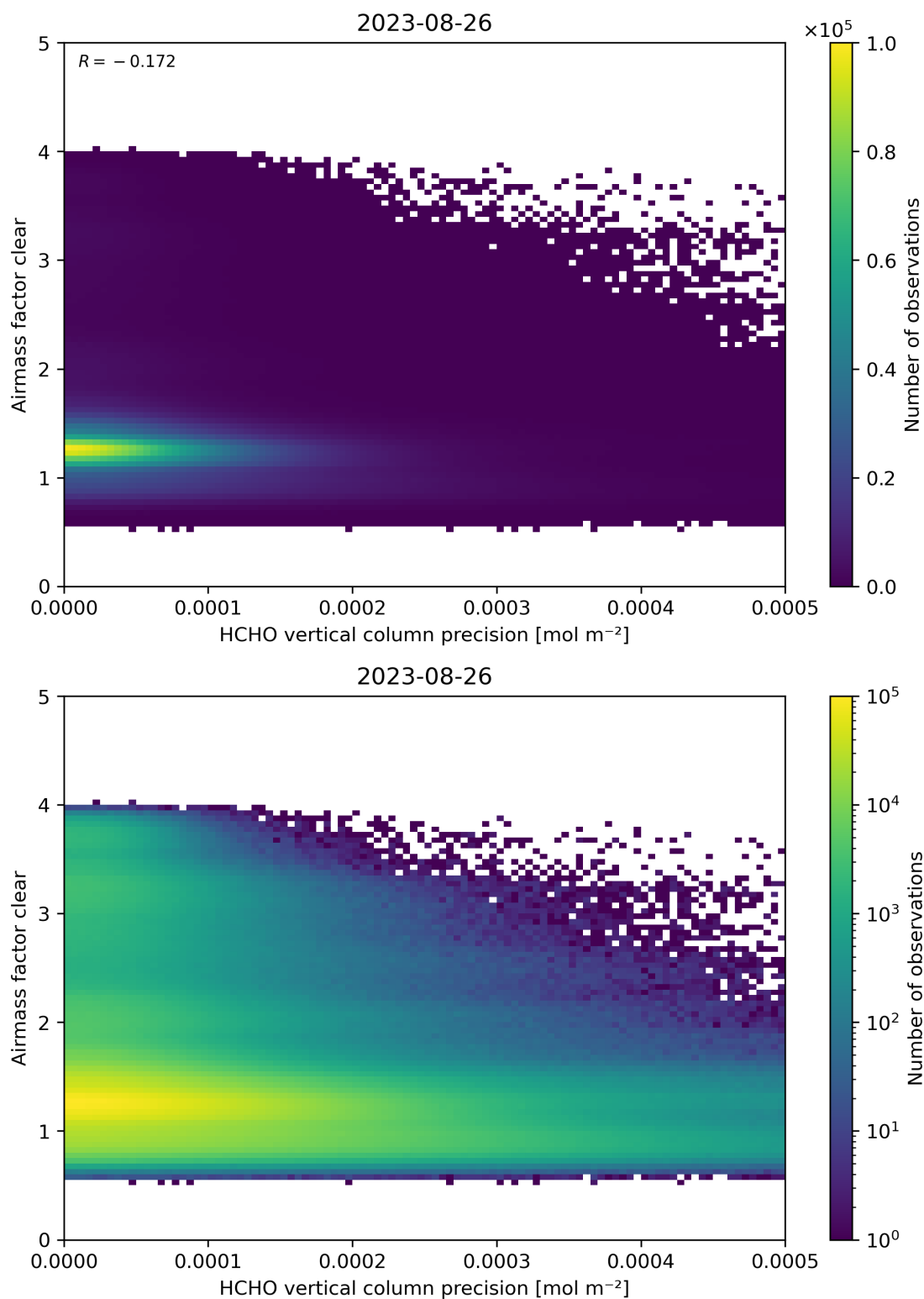
Figure 139: Scatter density plot of “HCHO vertical column precision” against “Airmass factor clear” for 2023-08-25 to 2023-08-27.
