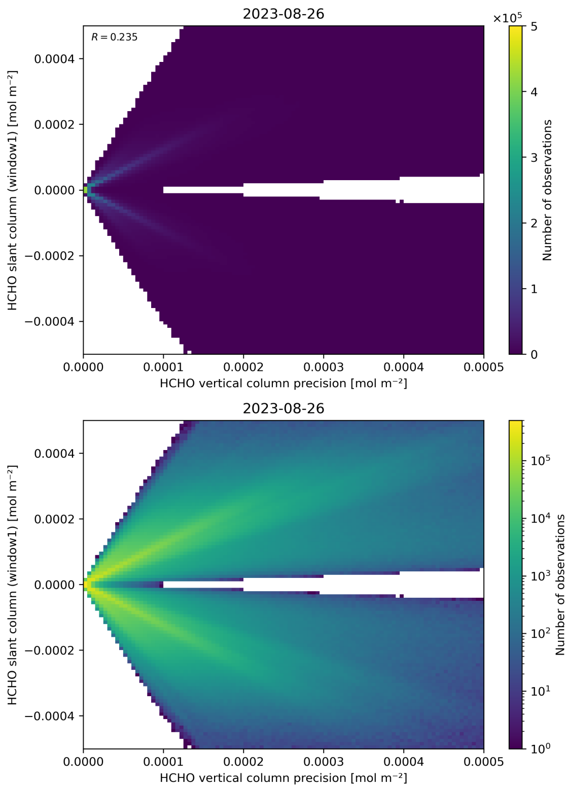
Figure 142: Scatter density plot of “HCHO vertical column precision” against “HCHO slant column (window1)” for 2023-08-25 to 2023-08-27.
