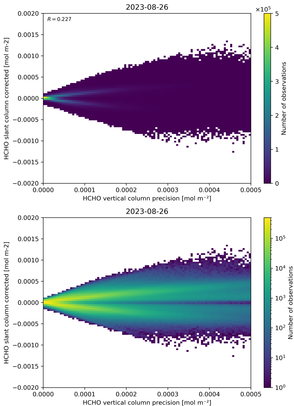
Figure 140: Scatter density plot of “HCHO vertical column precision” against “HCHO slant column corrected” for 2023-08-25 to 2023-08-27.
