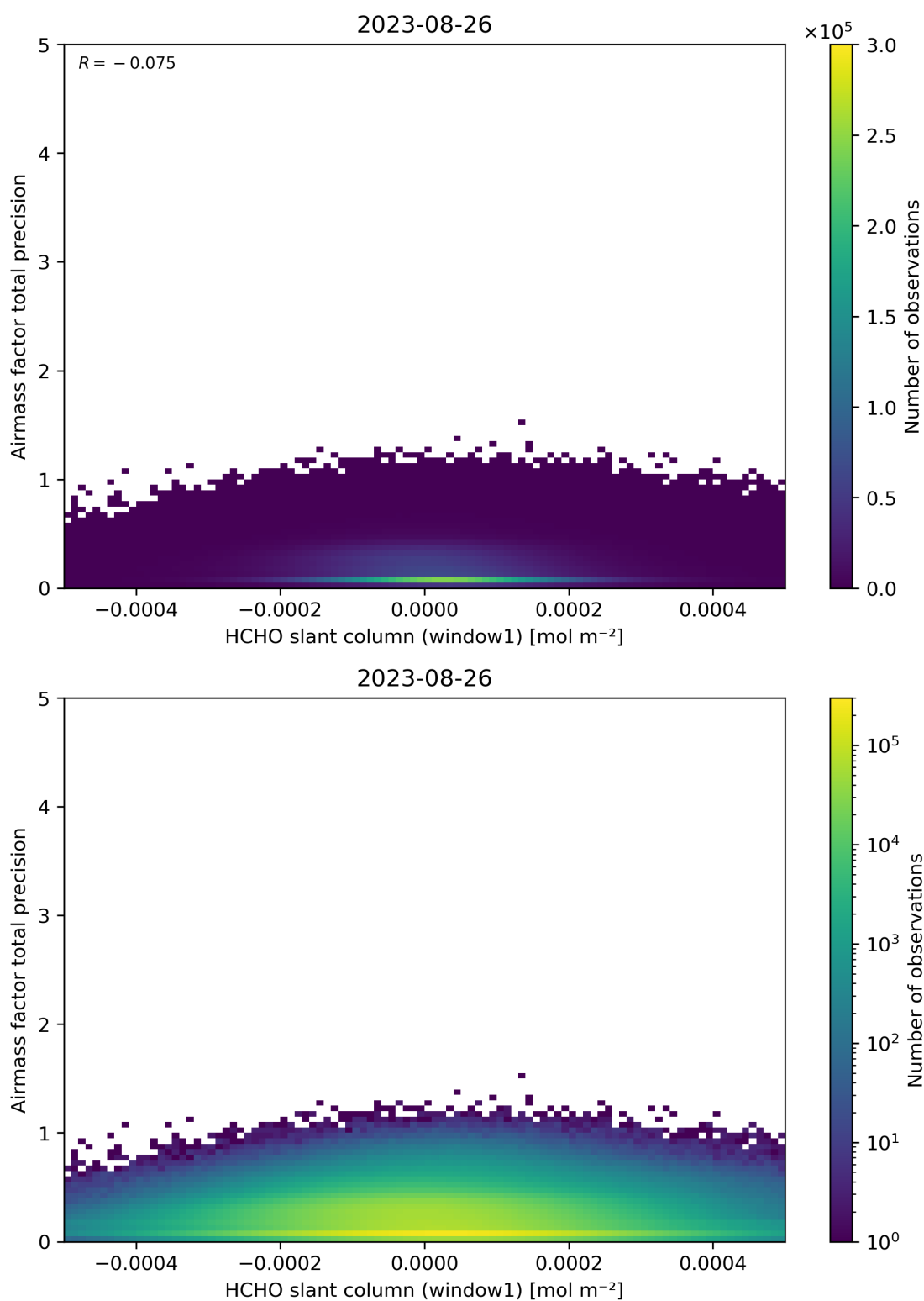
Figure 86: Scatter density plot of “HCHO slant column (window1)” against “Airmass factor total precision” for 2023-08-25 to 2023-08-27.
