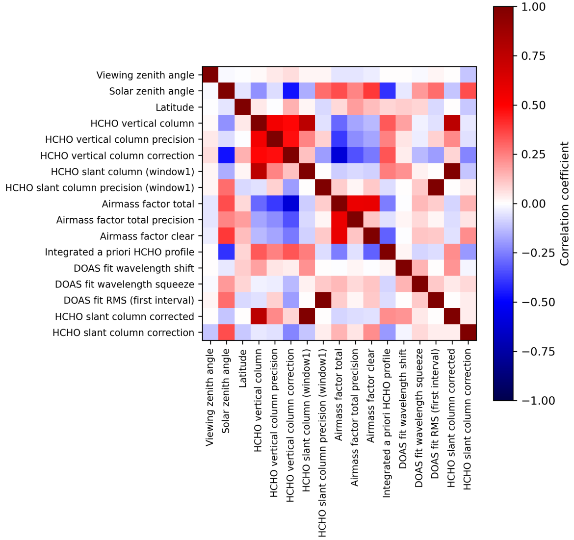
Figure 2: Map of correlation matrix for 2023-08-25 to 2023-08-27.
