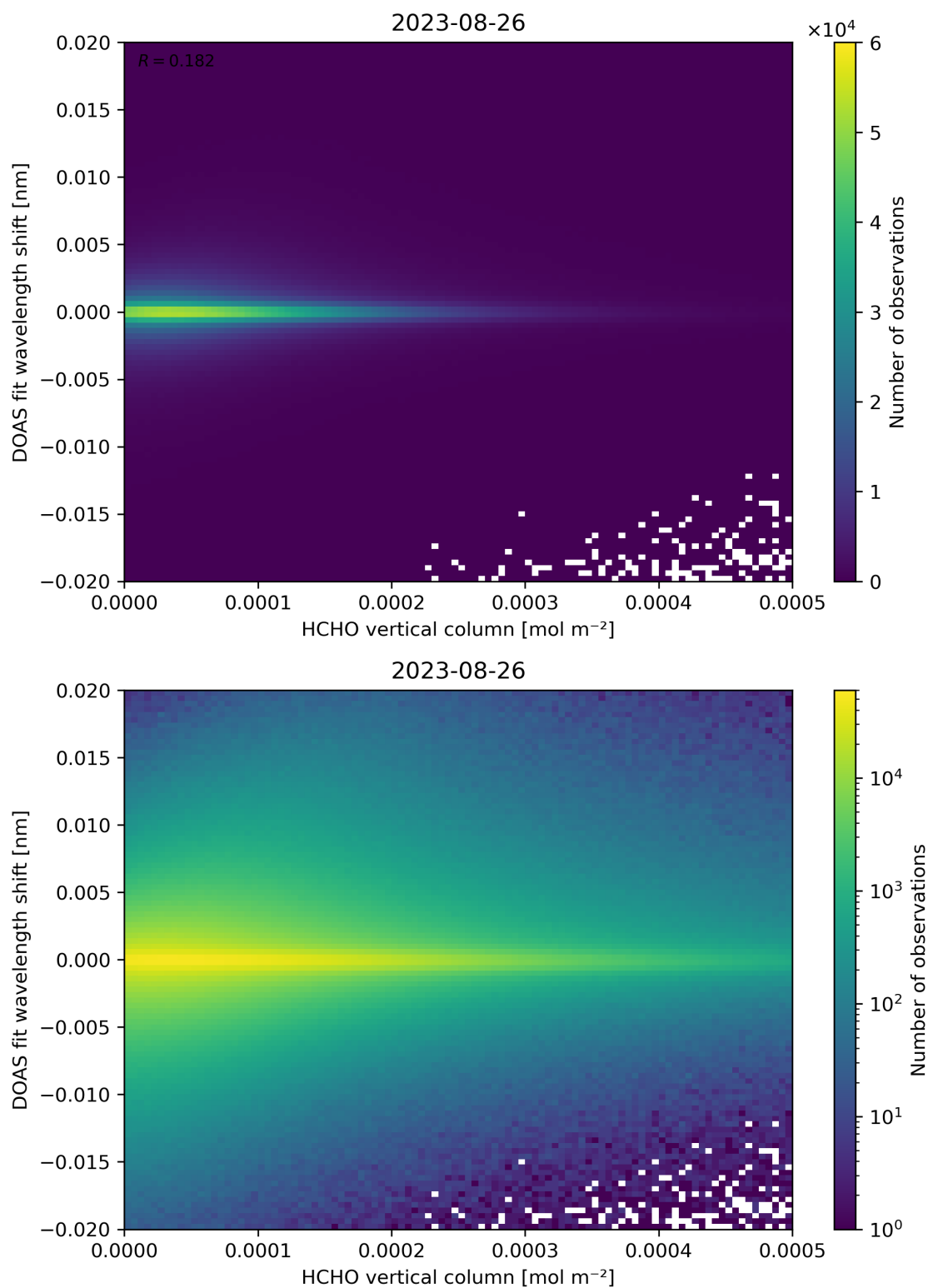
Figure 124: Scatter density plot of “HCHO vertical column” against “DOAS fit wavelength shift” for 2023-08-25 to 2023-08-27.
