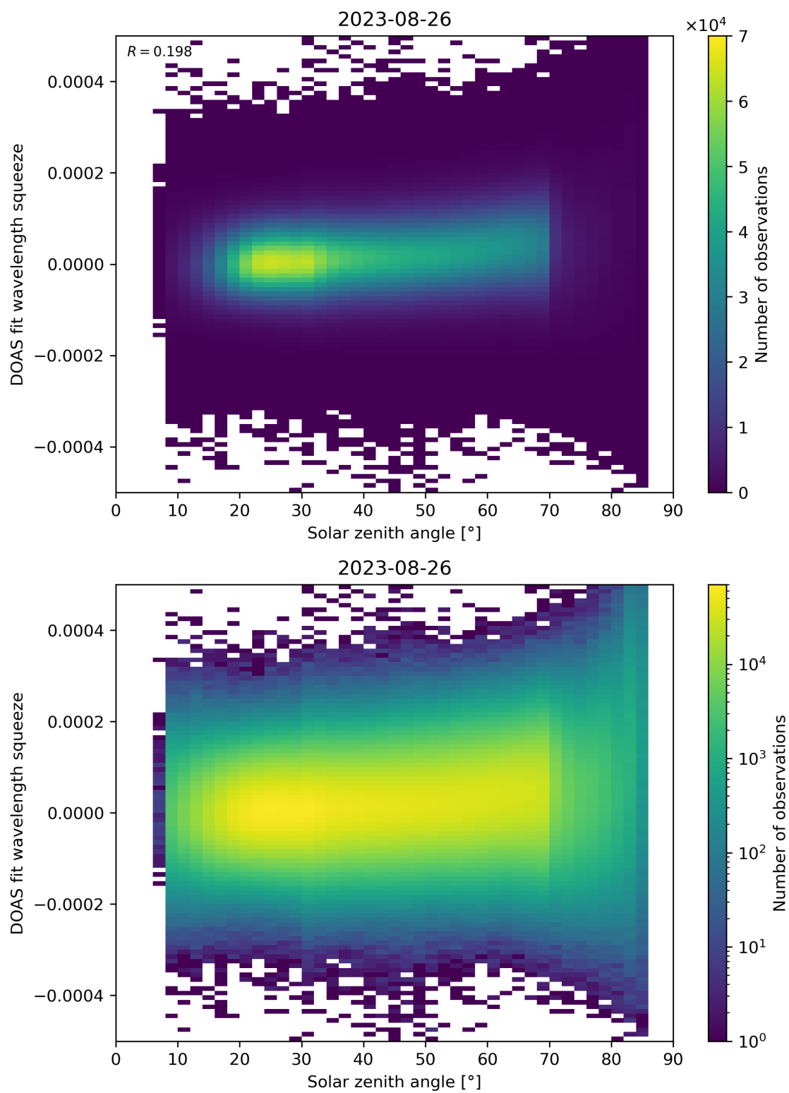
Figure 169: Scatter density plot of “Solar zenith angle” against “DOAS fit wavelength squeeze” for 2023-08-25 to 2023-08-27.
