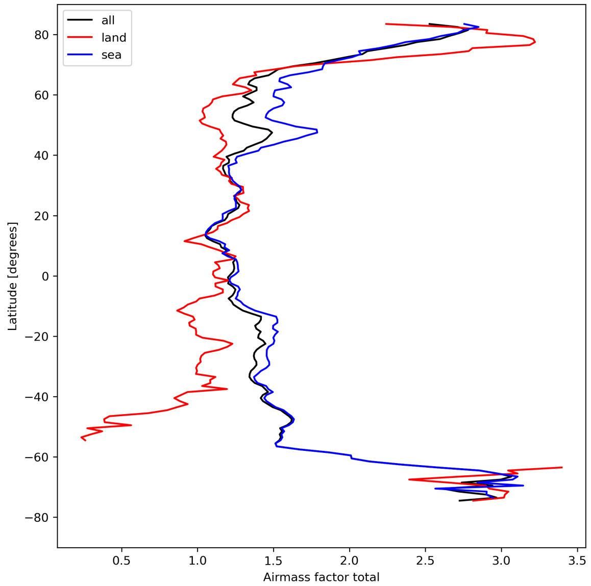
Figure 26: Zonal average of “Airmass factor total” for 2023-08-25 to 2023-08-27.
