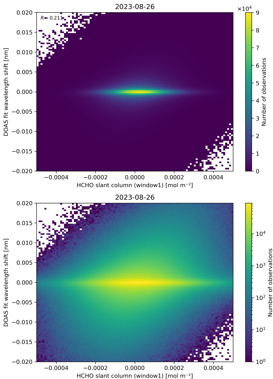
Figure 79: Scatter density plot of “HCHO slant column (window1)” against “DOAS fit wavelength shift” for 2023-08-25 to 2023-08-27.
