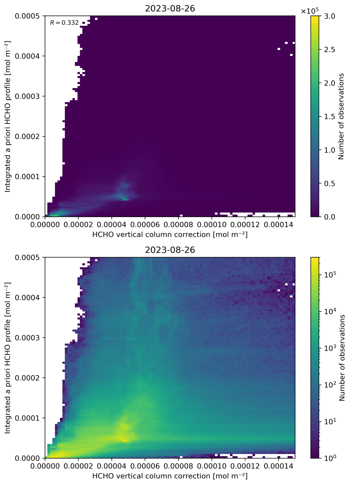
Figure 122: Scatter density plot of “HCHO vertical column correction” against “Integrated a priori HCHO profile” for 2023-08-25 to 2023-08-27.
