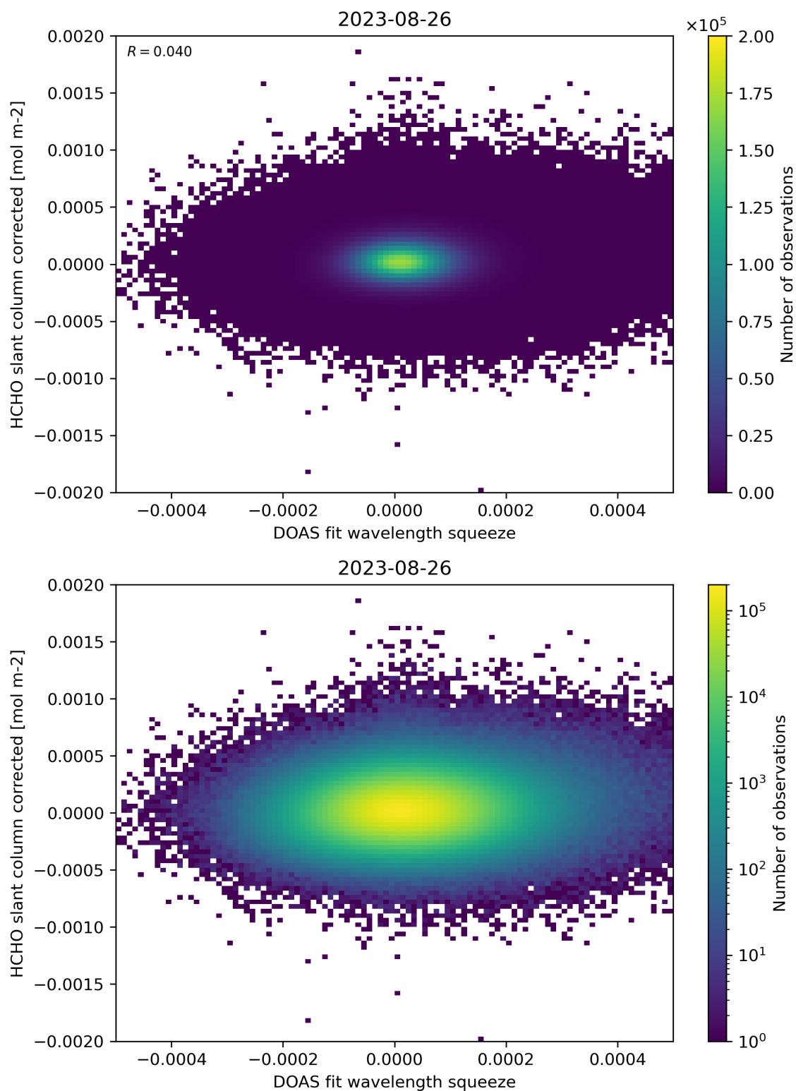
Figure 69: Scatter density plot of “DOAS fit wavelength squeeze” against “HCHO slant column corrected” for 2023-08-25 to 2023-08-27.
