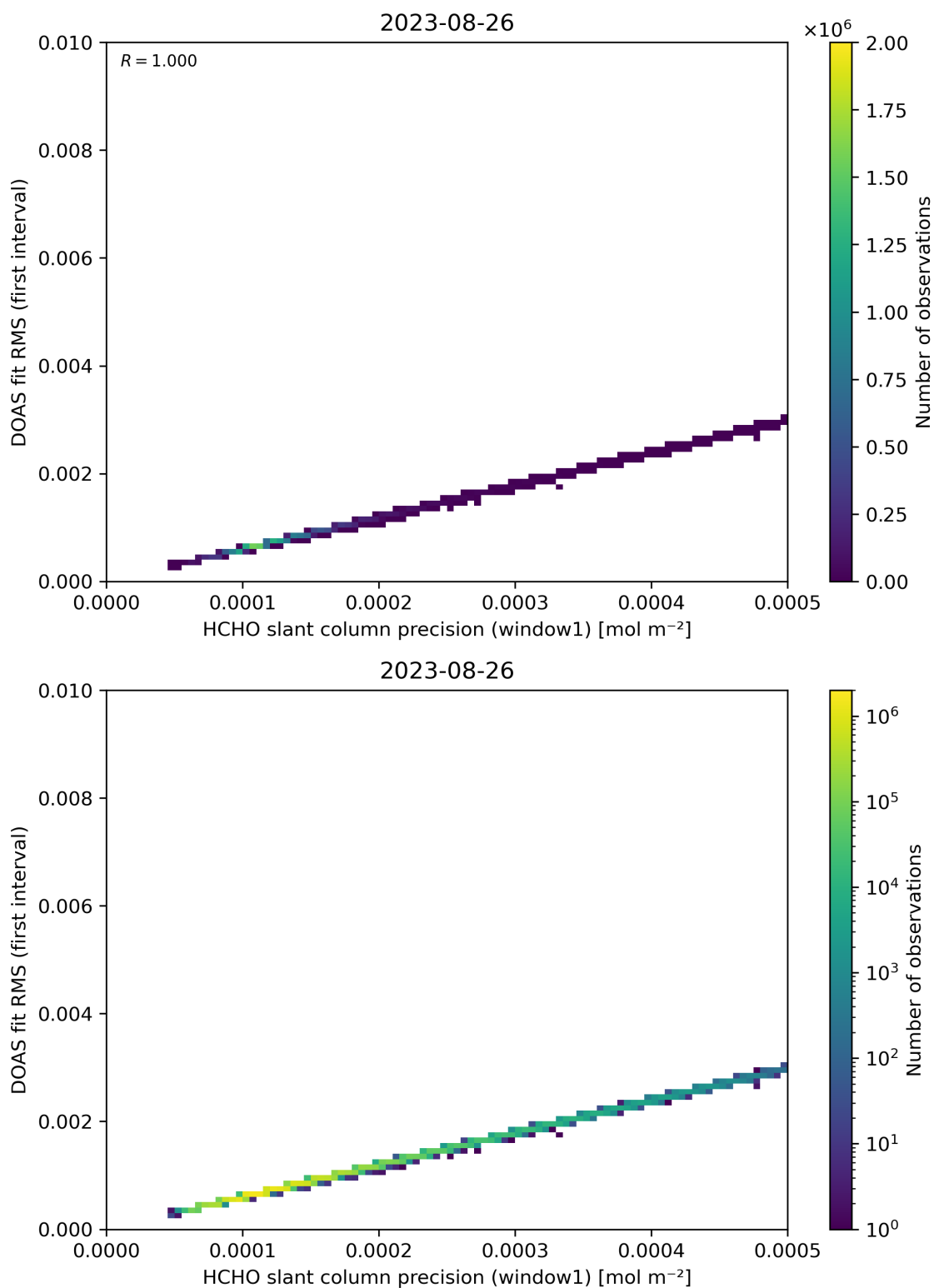
Figure 88: Scatter density plot of “HCHO slant column precision (window1)” against “DOAS fit RMS (first interval)” for 2023-08-25 to 2023-08-27.
