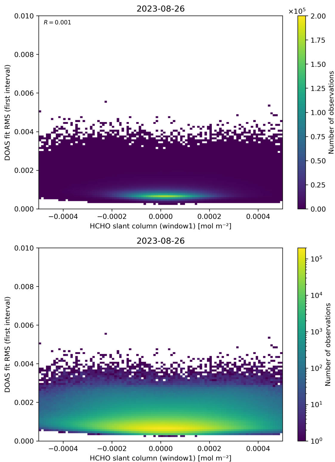
Figure 78: Scatter density plot of “HCHO slant column (window1)” against “DOAS fit RMS (first interval)” for 2023-08-25 to 2023-08-27.
