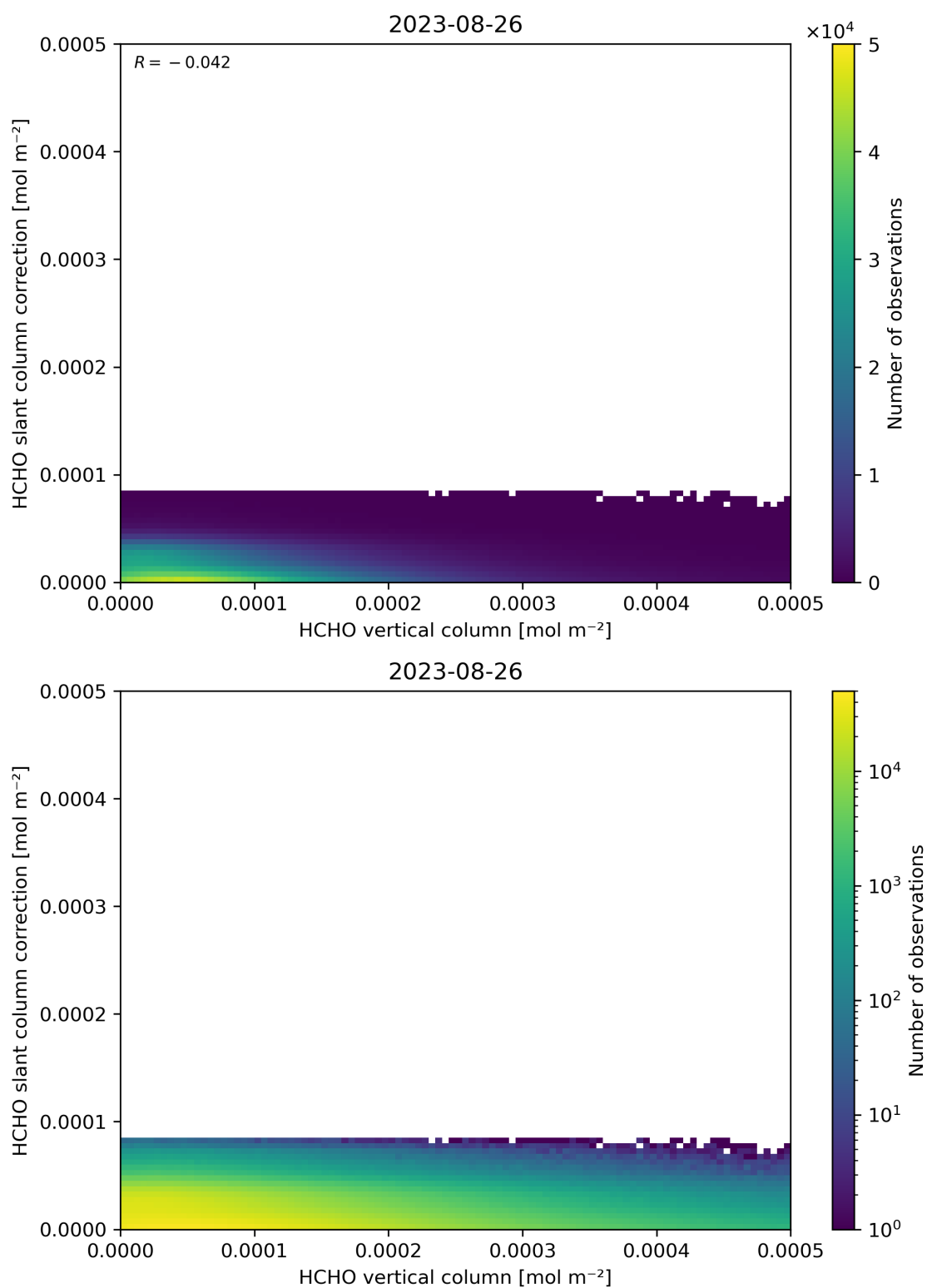
Figure 128: Scatter density plot of “HCHO vertical column” against “HCHO slant column correction” for 2023-08-25 to 2023-08-27.
