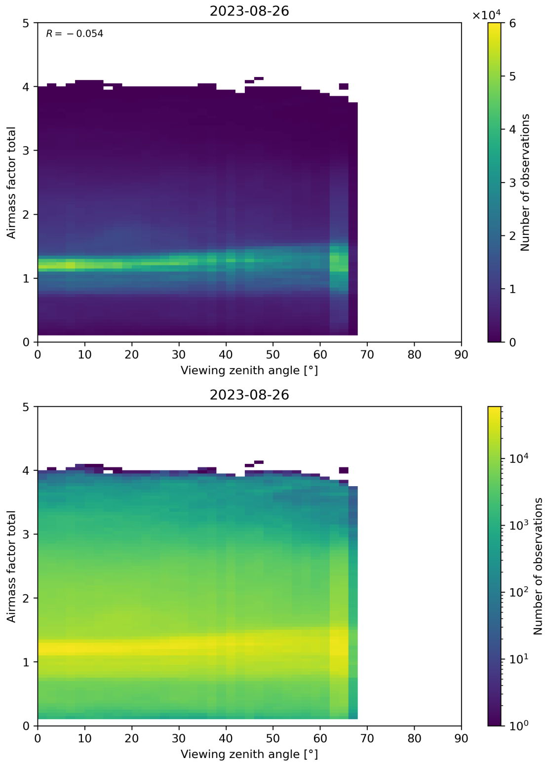
Figure 190: Scatter density plot of “Viewing zenith angle” against “Airmass factor total” for 2023-08-25 to 2023-08-27.
