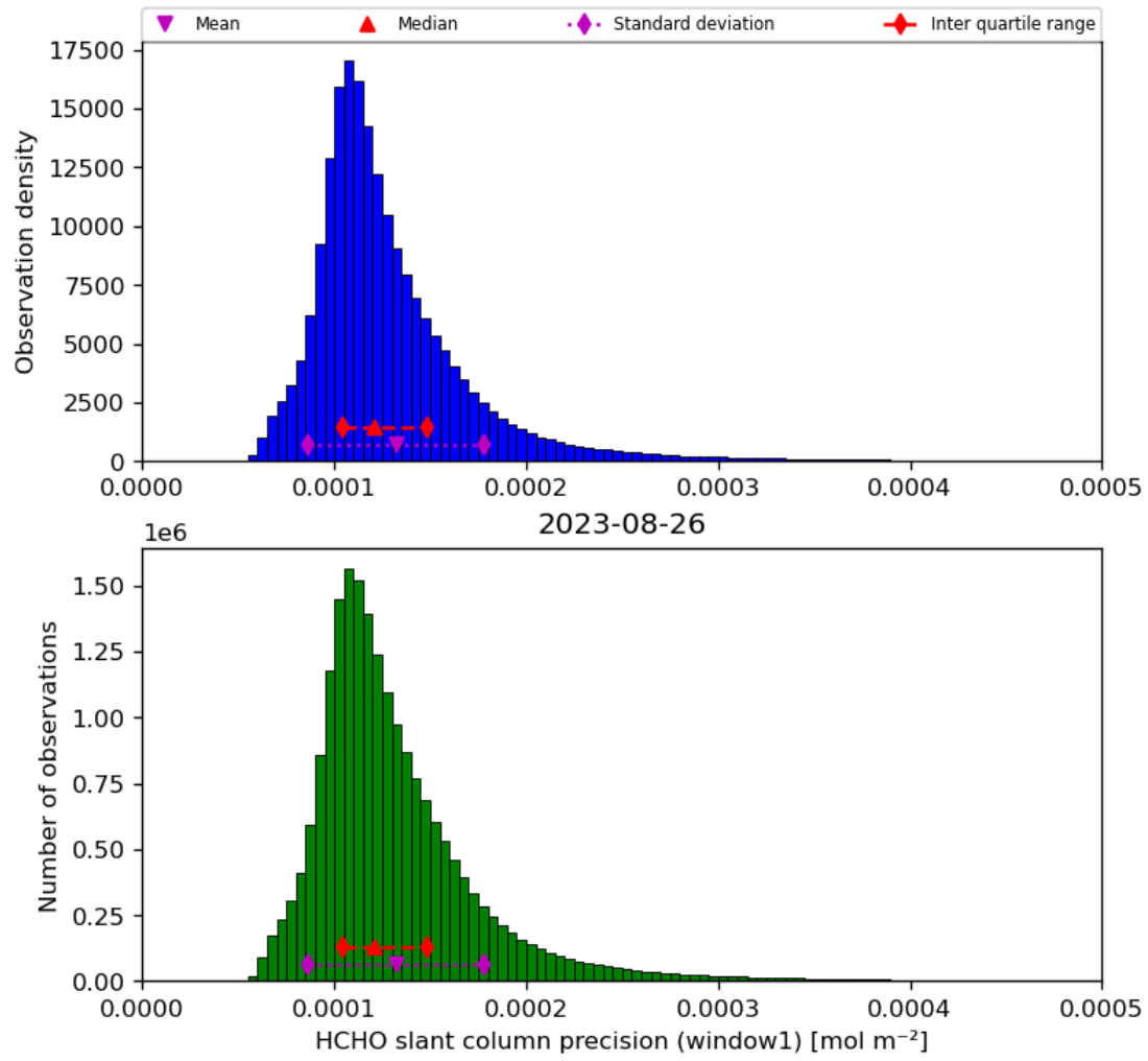
Figure 39: Histogram of “HCHO slant column precision (window1)” for 2023-08-25 to 2023-08-27
