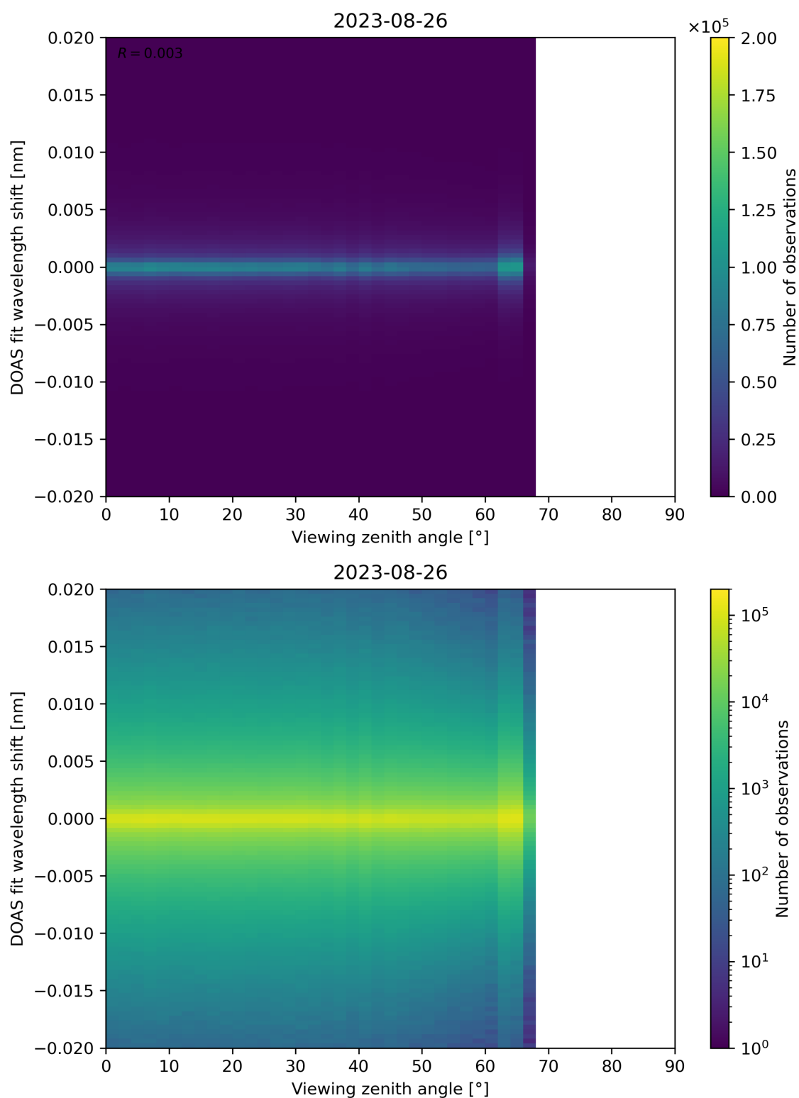
Figure 183: Scatter density plot of “Viewing zenith angle” against “DOAS fit wavelength shift” for 2023-08-25 to 2023-08-27.
