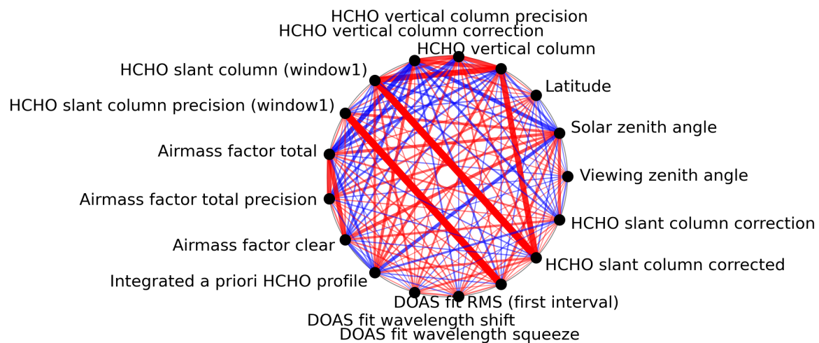
Figure 1: Map of correlation graph for 2023-08-25 to 2023-08-27.
