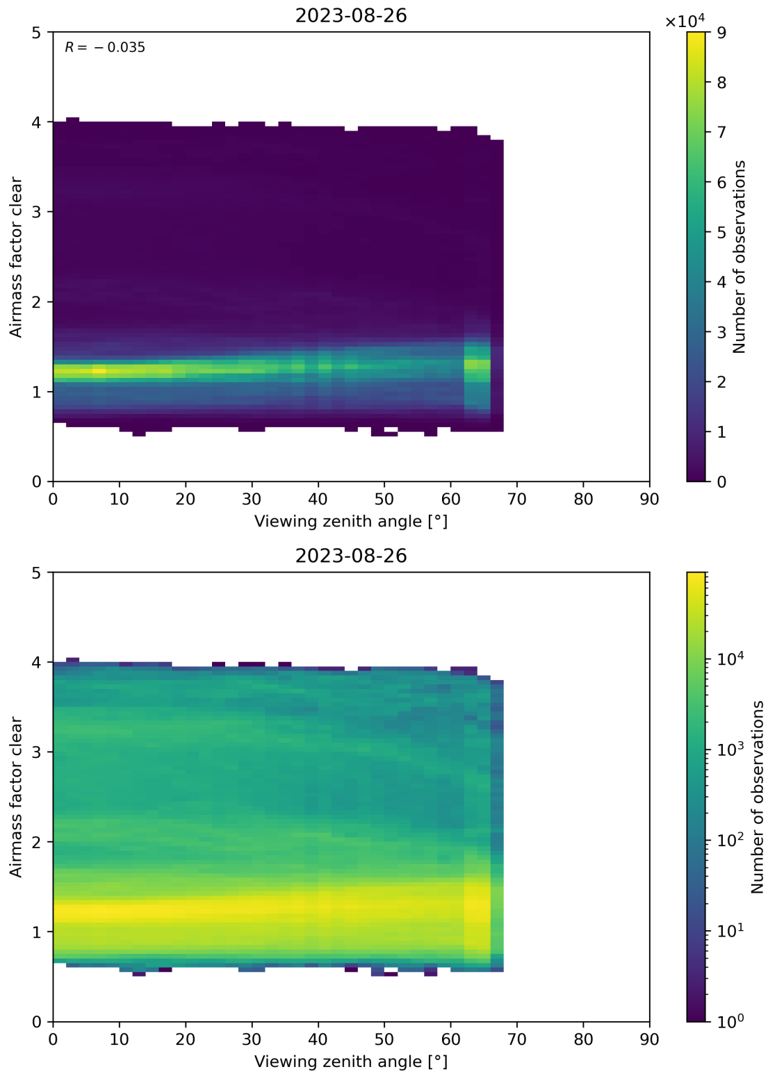
Figure 185: Scatter density plot of “Viewing zenith angle” against “Airmass factor clear” for 2023-08-25 to 2023-08-27.
