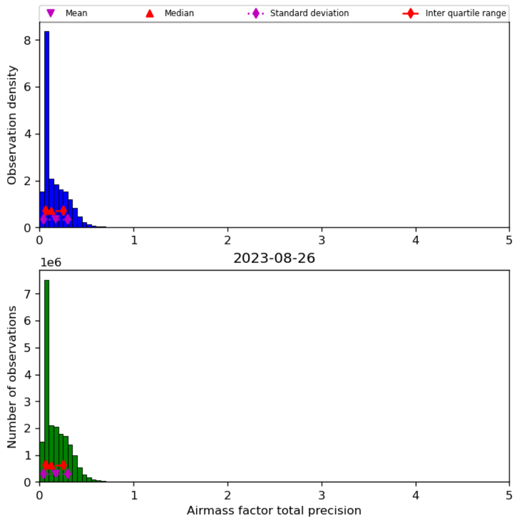
Figure 41: Histogram of “Airmass factor total precision” for 2023-08-25 to 2023-08-27
