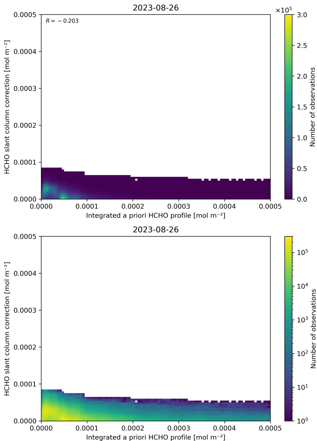
Figure 152: Scatter density plot of “Integrated a priori HCHO profile” against “HCHO slant column correction” for 2023-08-25 to 2023-08-27.
