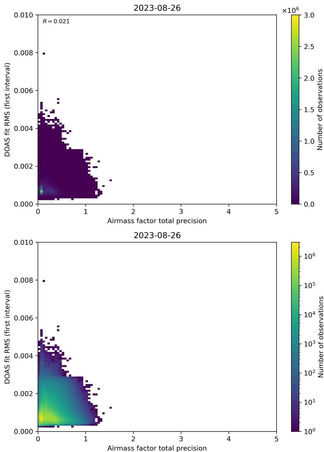
Figure 105: Scatter density plot of “Airmass factor total precision” against “DOAS fit RMS (first interval)” for 2023-08-25 to 2023-08-27.
