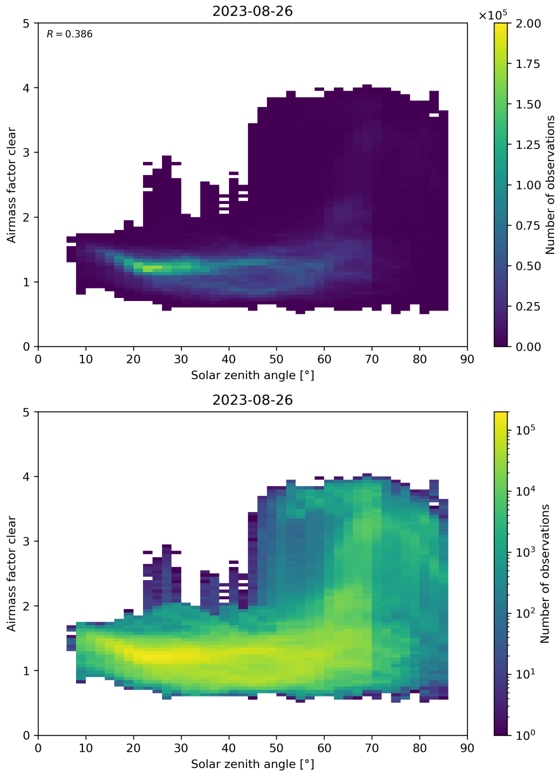
Figure 170: Scatter density plot of “Solar zenith angle” against “Airmass factor clear” for 2023-08-25 to 2023-08-27.
