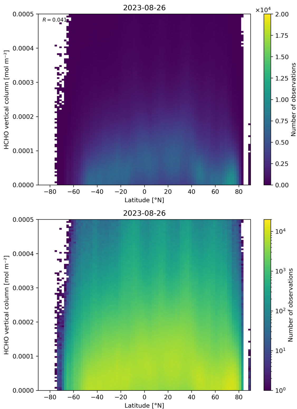
Figure 163: Scatter density plot of “Latitude” against “HCHO vertical column” for 2023-08-25 to 2023-08-27.
