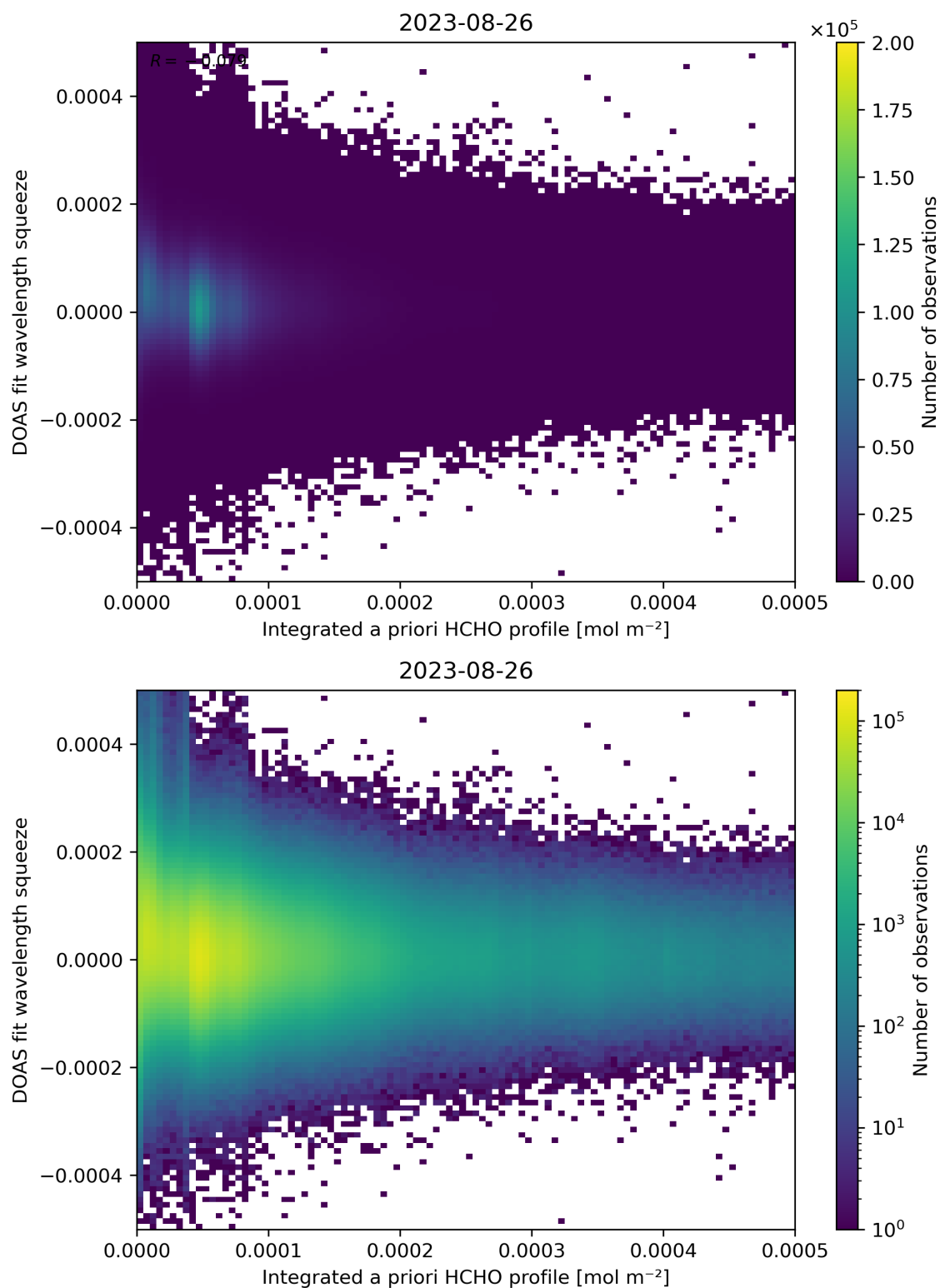
Figure 150: Scatter density plot of “Integrated a priori HCHO profile” against “DOAS fit wavelength squeeze” for 2023-08-25 to 2023-08-27.
