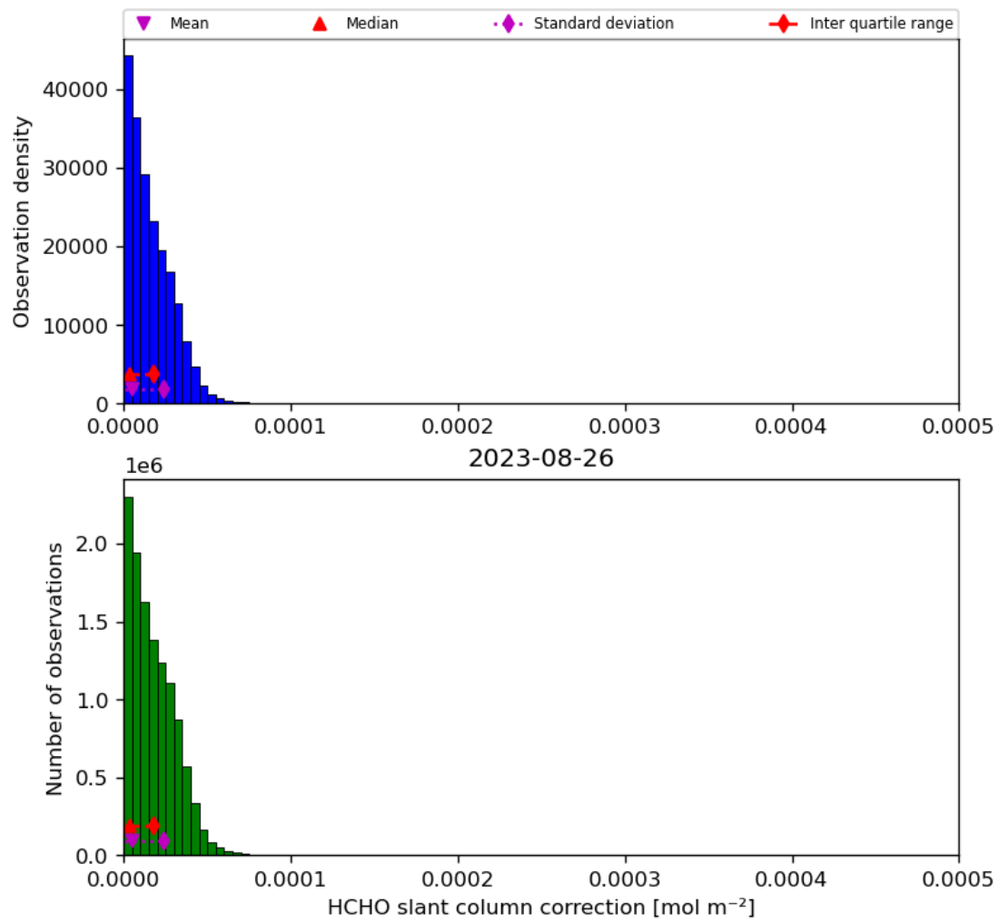
Figure 47: Histogram of “HCHO slant column correction” for 2023-08-25 to 2023-08-27
