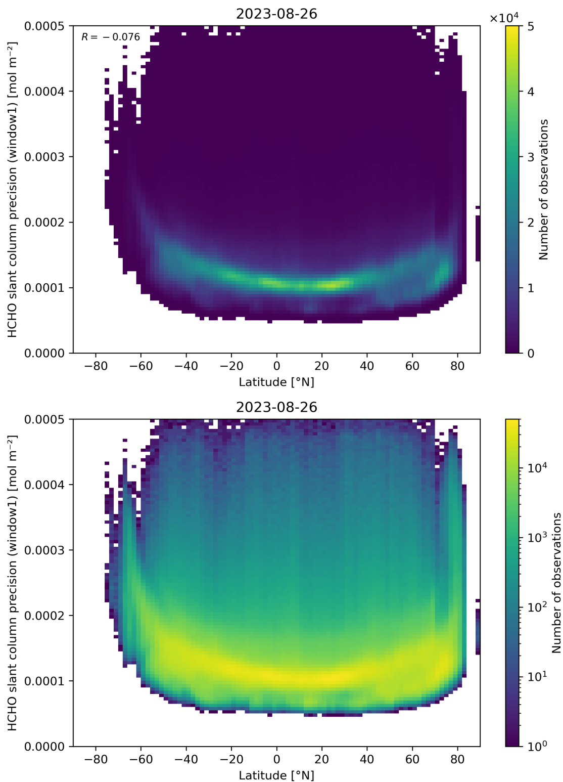
Figure 160: Scatter density plot of “Latitude” against “HCHO slant column precision (window1)” for 2023-08-25 to 2023-08-27.
