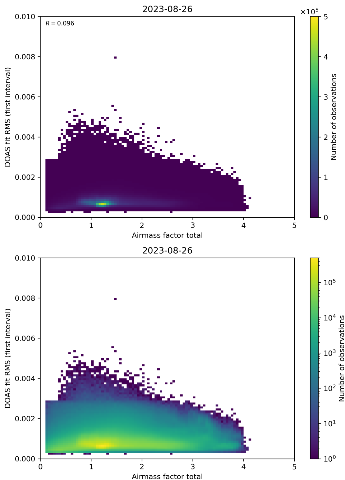
Figure 97: Scatter density plot of “Airmass factor total” against “DOAS fit RMS (first interval)” for 2023-08-25 to 2023-08-27.
