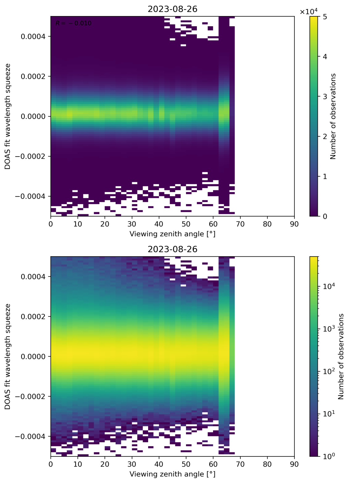
Figure 184: Scatter density plot of “Viewing zenith angle” against “DOAS fit wavelength squeeze” for 2023-08-25 to 2023-08-27.
