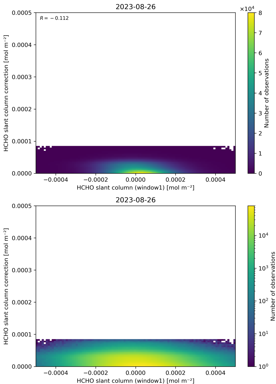
Figure 83: Scatter density plot of “HCHO slant column (window1)” against “HCHO slant column correction” for 2023-08-25 to 2023-08-27.
