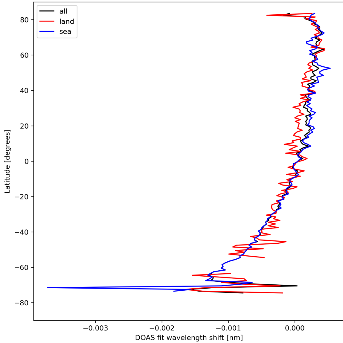
Figure 30: Zonal average of “DOAS fit wavelength shift” for 2023-08-25 to 2023-08-27.
