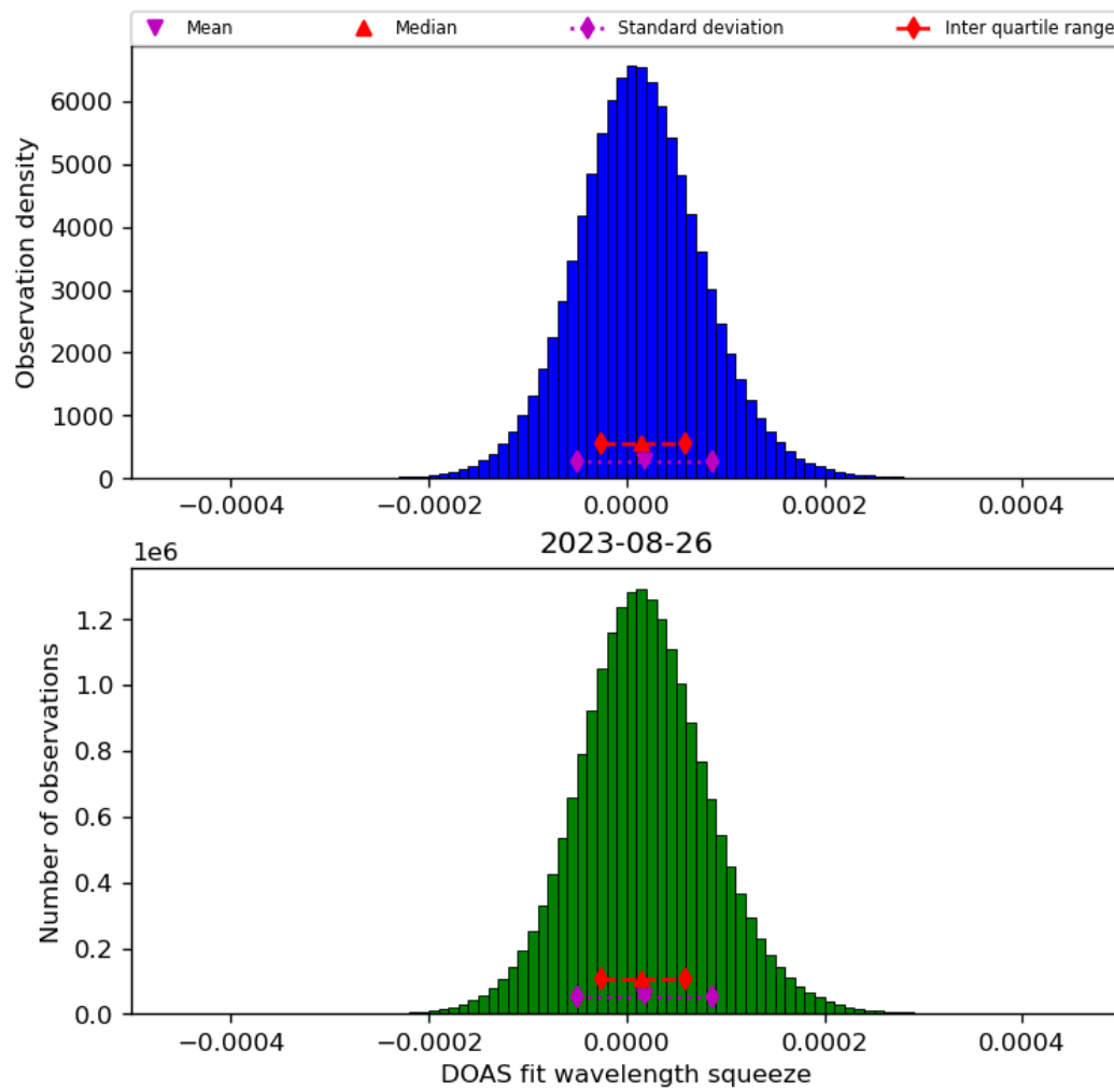
Figure 45: Histogram of “DOAS fit wavelength squeeze” for 2023-08-25 to 2023-08-27
