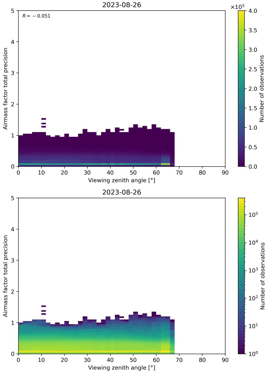
Figure 191: Scatter density plot of “Viewing zenith angle” against “Airmass factor total precision” for 2023-08-25 to 2023-08-27.
