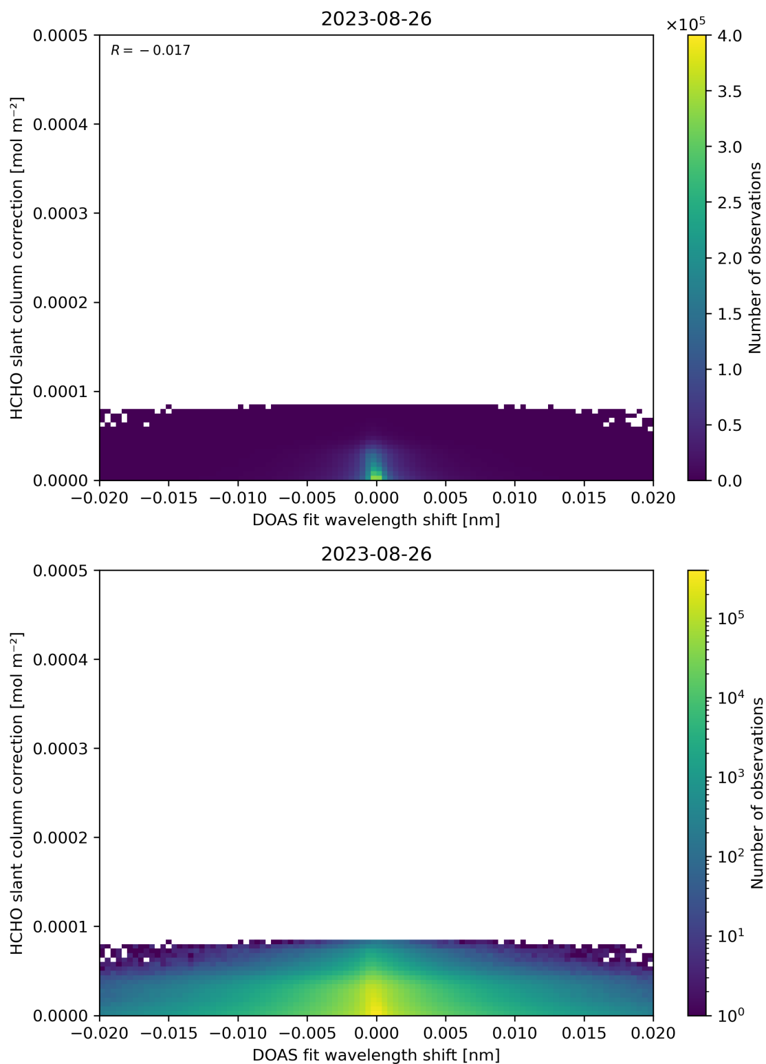
Figure 67: Scatter density plot of “DOAS fit wavelength shift” against “HCHO slant column correction” for 2023-08-25 to 2023-08-27.
