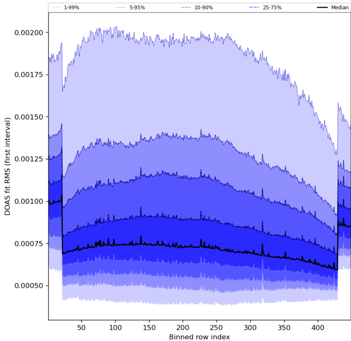
Figure 60: Along track statistics of “DOAS fit RMS (first interval)” for 2023-08-25 to 2023-08-27
