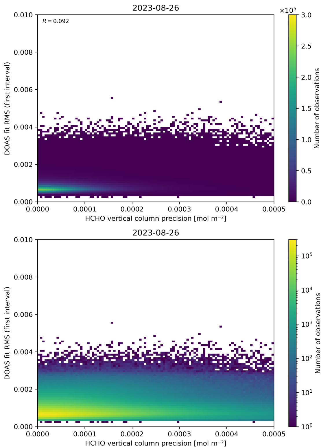
Figure 136: Scatter density plot of “HCHO vertical column precision” against “DOAS fit RMS (first interval)” for 2023-08-25 to 2023-08-27.
