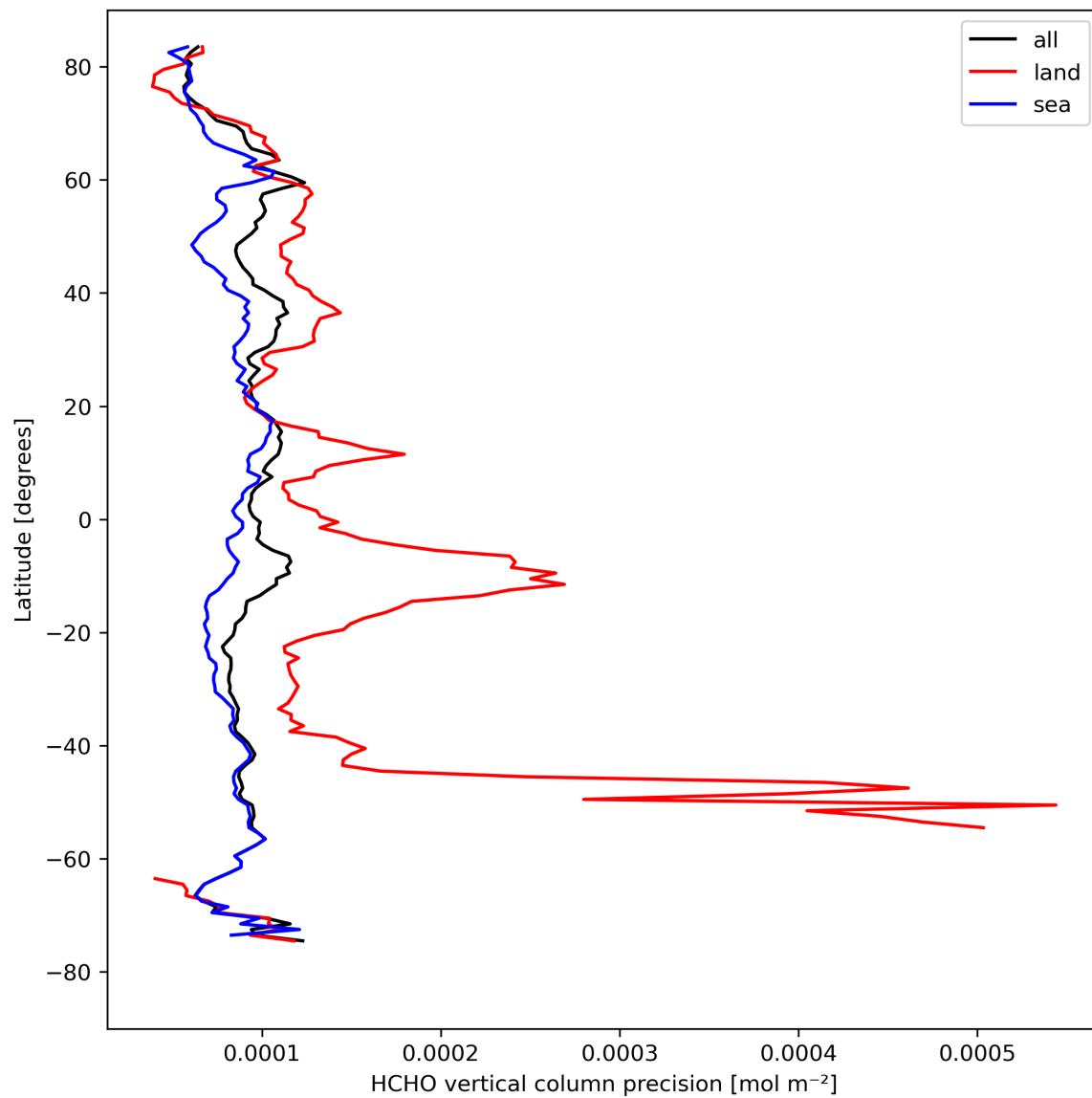
Figure 22: Zonal average of “HCHO vertical column precision” for 2023-08-25 to 2023-08-27.
