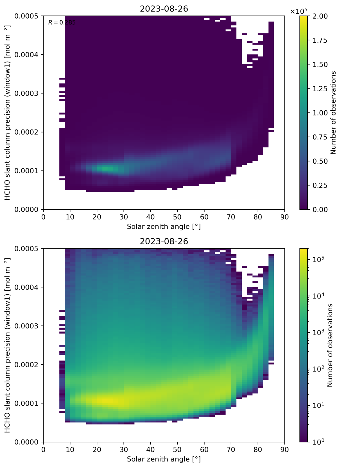
Figure 174: Scatter density plot of “Solar zenith angle” against “HCHO slant column precision (window1)” for 2023-08-25 to 2023-08-27.
