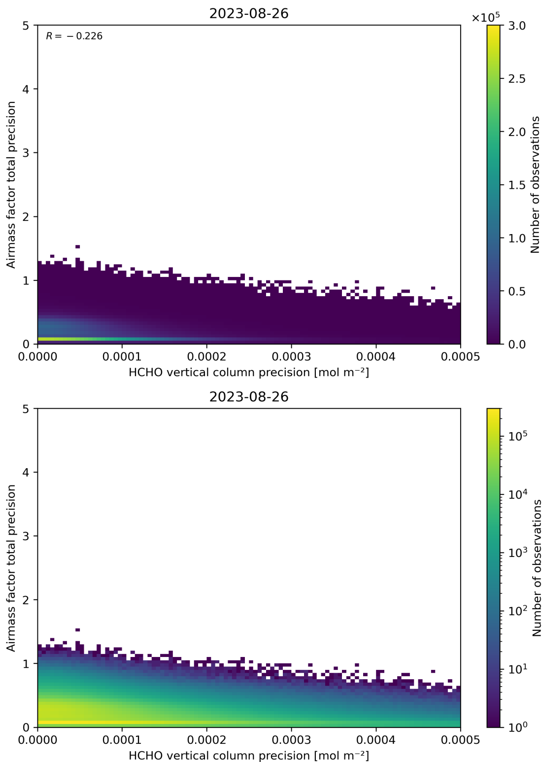
Figure 145: Scatter density plot of “HCHO vertical column precision” against “Airmass factor total precision” for 2023-08-25 to 2023-08-27.
