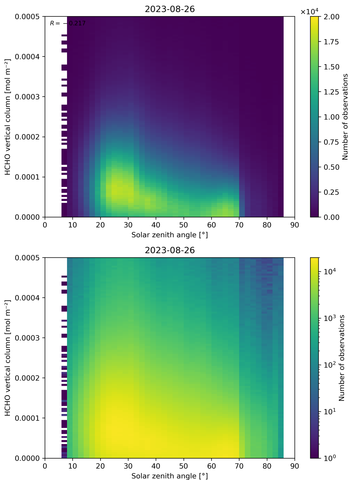
Figure 177: Scatter density plot of “Solar zenith angle” against “HCHO vertical column” for 2023-08-25 to 2023-08-27.
