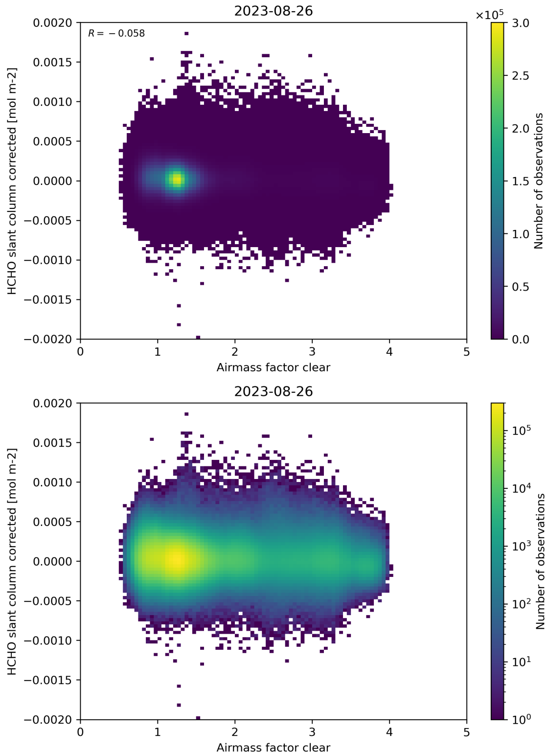
Figure 74: Scatter density plot of “Airmass factor clear” against “HCHO slant column corrected” for 2023-08-25 to 2023-08-27.
