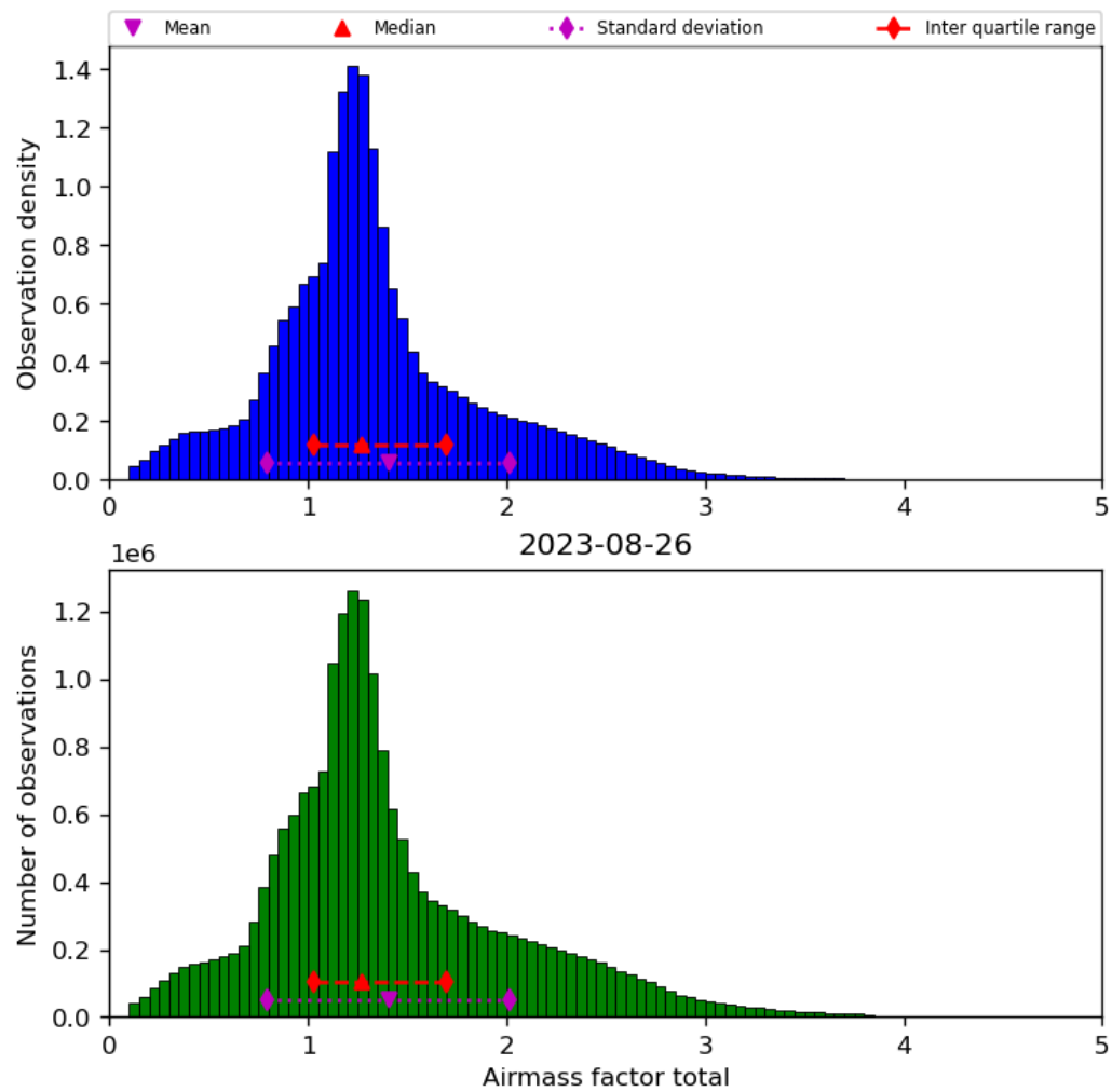
Figure 40: Histogram of “Airmass factor total” for 2023-08-25 to 2023-08-27
