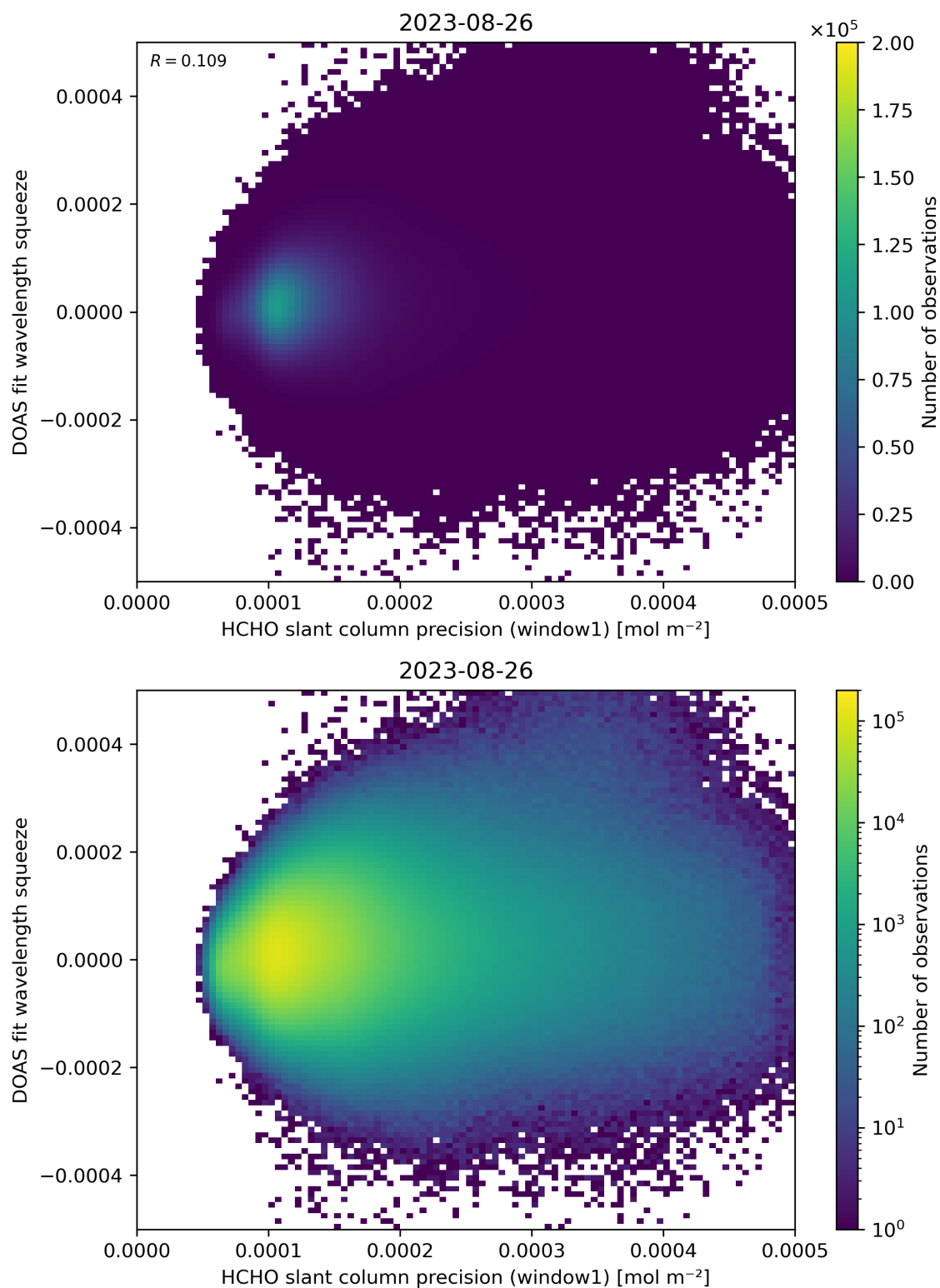
Figure 90: Scatter density plot of “HCHO slant column precision (window1)” against “DOAS fit wavelength squeeze” for 2023-08-25 to 2023-08-27.
