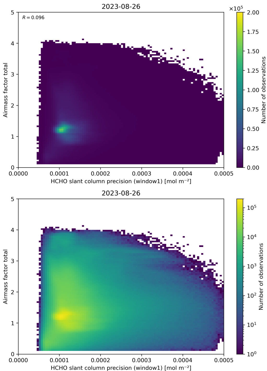
Figure 94: Scatter density plot of “HCHO slant column precision (window1)” against “Airmass factor total” for 2023-08-25 to 2023-08-27.
