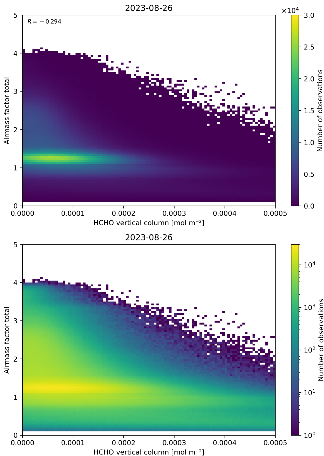
Figure 131: Scatter density plot of “HCHO vertical column” against “Airmass factor total” for 2023-08-25 to 2023-08-27.
