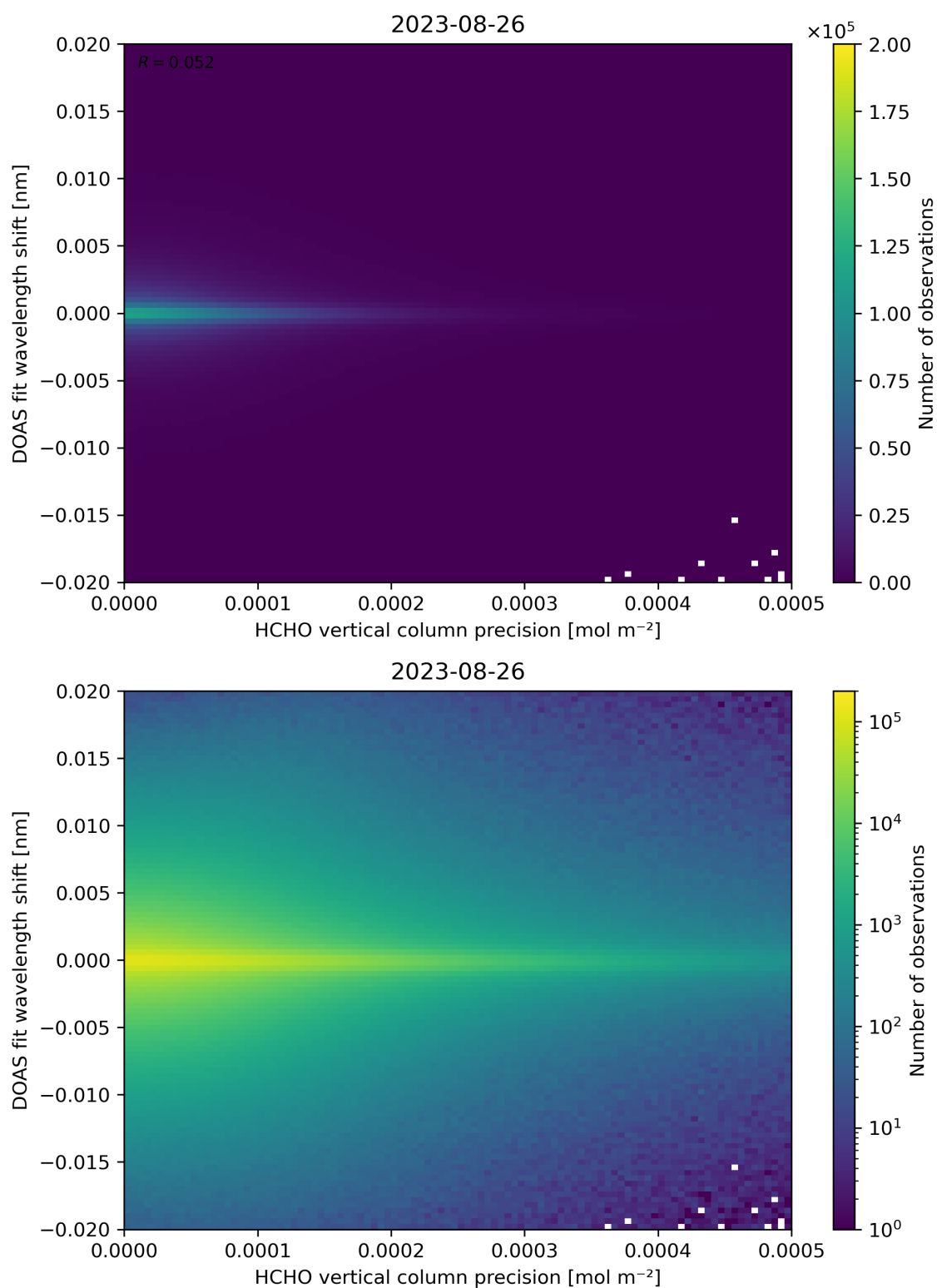
Figure 137: Scatter density plot of “HCHO vertical column precision” against “DOAS fit wavelength shift” for 2023-08-25 to 2023-08-27.
