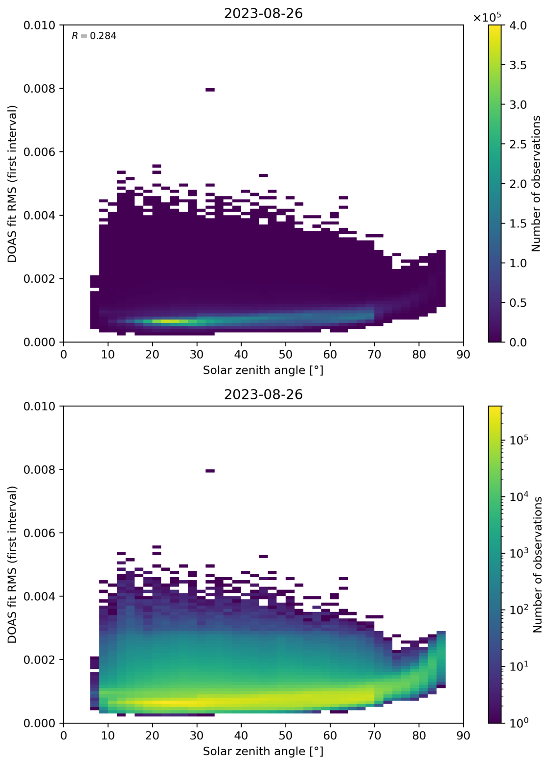
Figure 167: Scatter density plot of “Solar zenith angle” against “DOAS fit RMS (first interval)” for 2023-08-25 to 2023-08-27.
