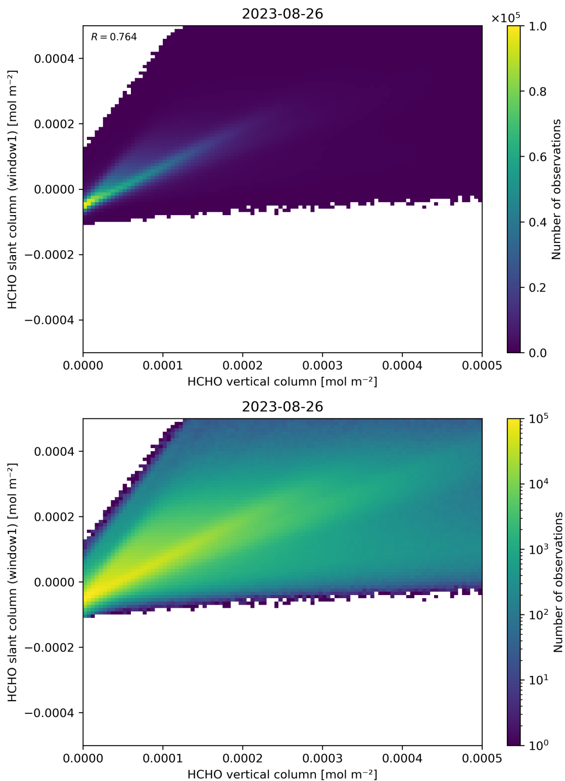
Figure 129: Scatter density plot of “HCHO vertical column” against “HCHO slant column (window1)” for 2023-08-25 to 2023-08-27.
