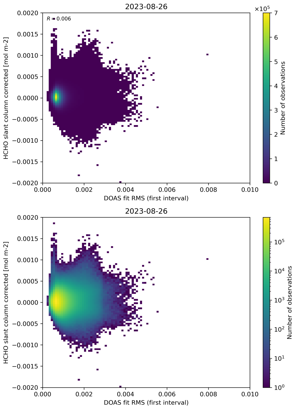
Figure 62: Scatter density plot of “DOAS fit RMS (first interval)” against “HCHO slant column corrected” for 2023-08-25 to 2023-08-27.
