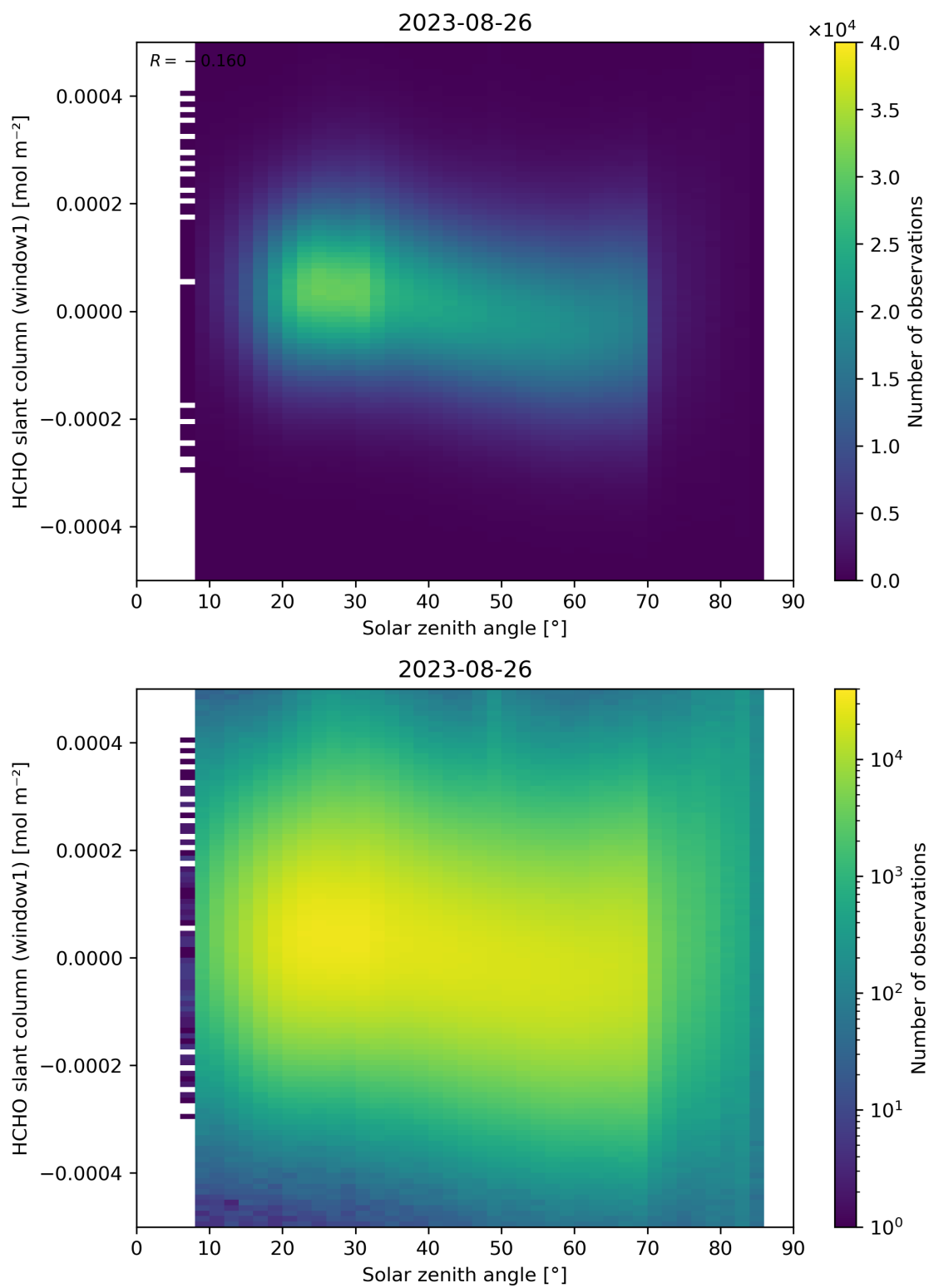
Figure 173: Scatter density plot of “Solar zenith angle” against “HCHO slant column (window1)” for 2023-08-25 to 2023-08-27.
