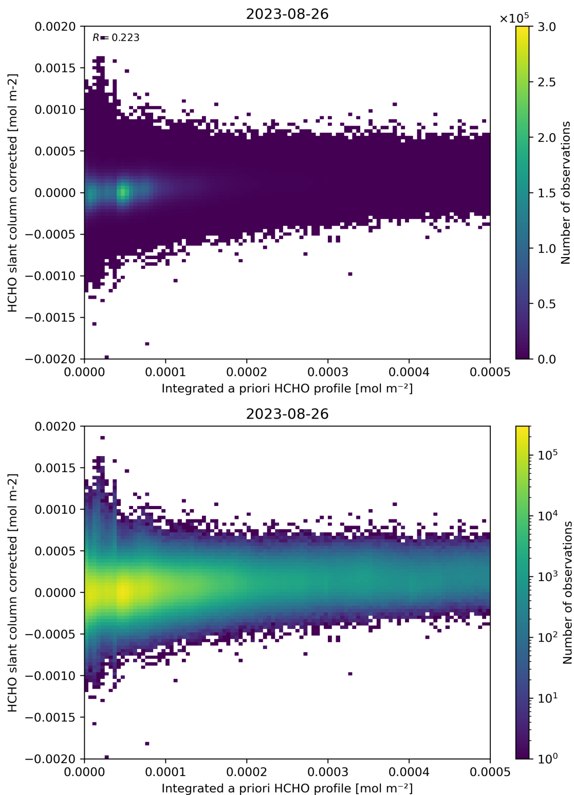
Figure 151: Scatter density plot of “Integrated a priori HCHO profile” against “HCHO slant column corrected” for 2023-08-25 to 2023-08-27.
