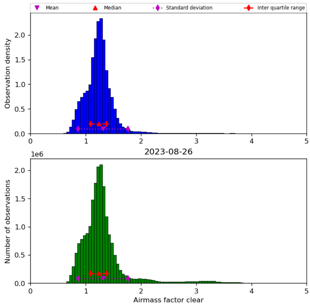
Figure 42: Histogram of “Airmass factor clear” for 2023-08-25 to 2023-08-27
