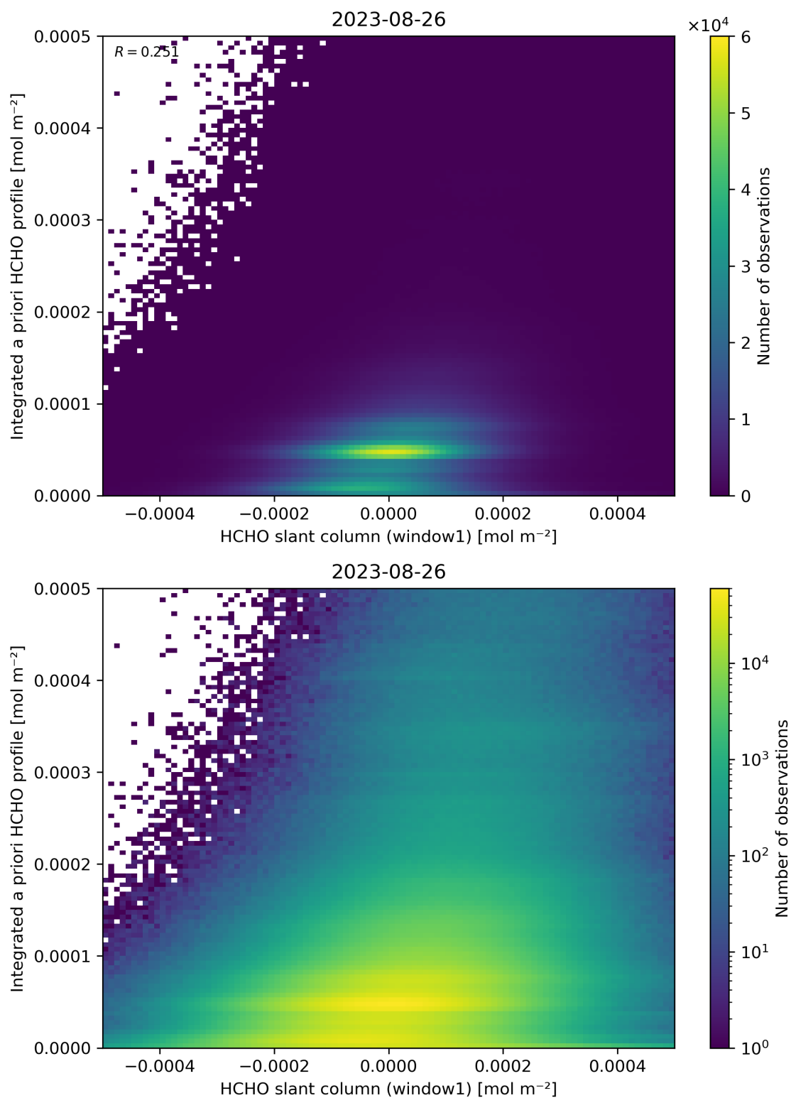
Figure 87: Scatter density plot of “HCHO slant column (window1)” against “Integrated a priori HCHO profile” for 2023-08-25 to 2023-08-27.
