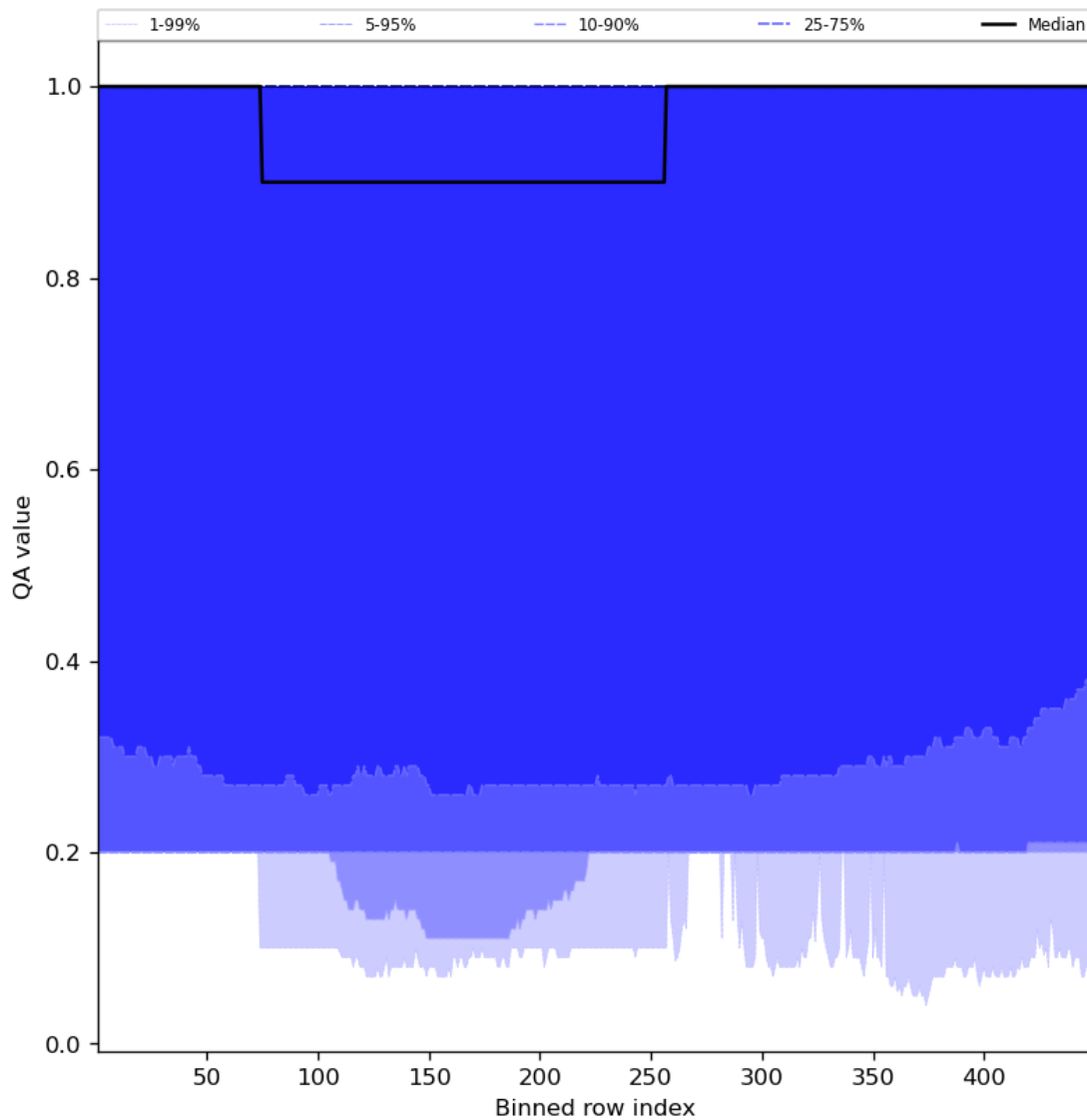
Figure 48: Along track statistics of “QA value” for 2023-08-25 to 2023-08-27
