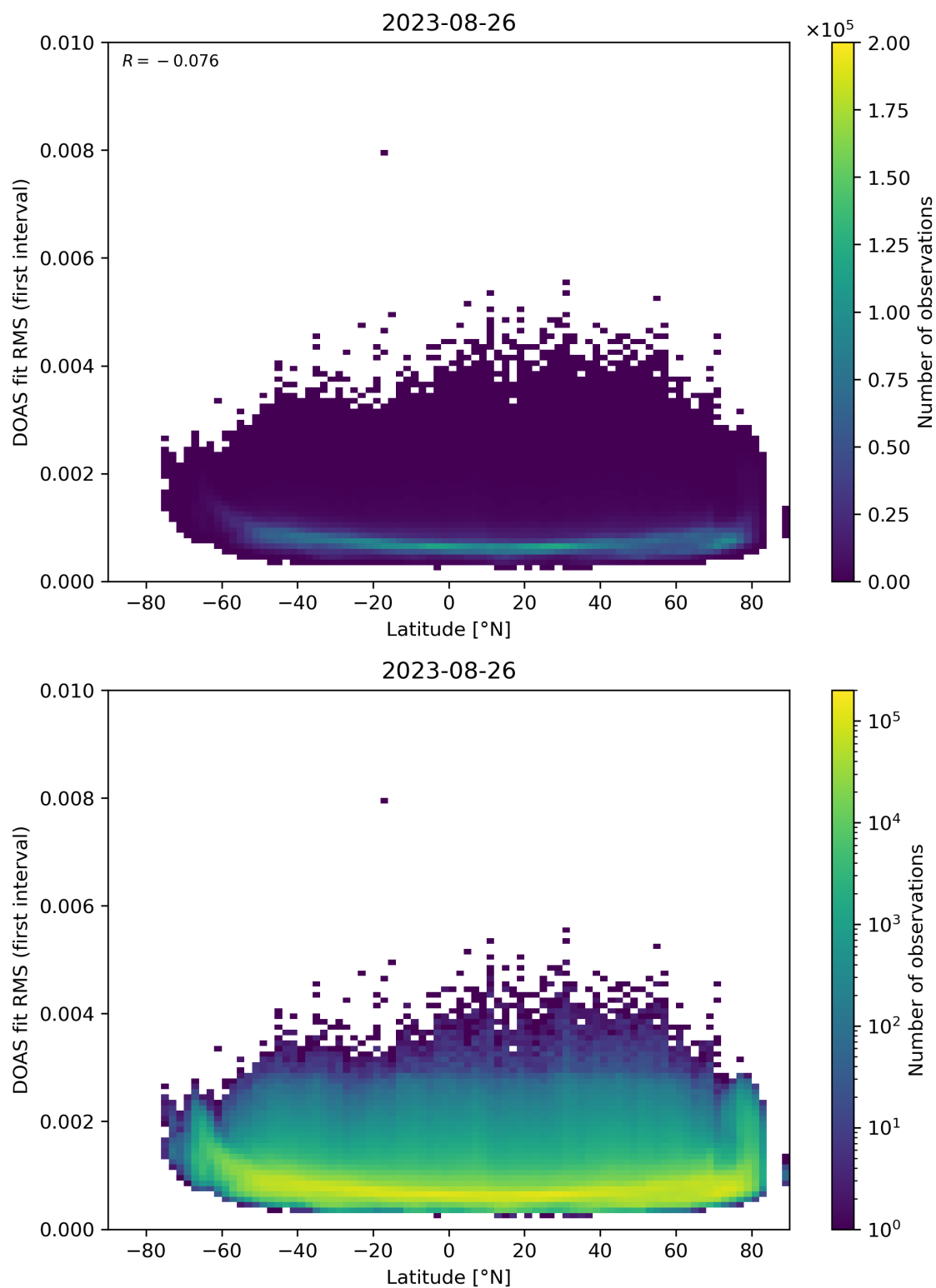
Figure 153: Scatter density plot of “Latitude” against “DOAS fit RMS (first interval)” for 2023-08-25 to 2023-08-27.
