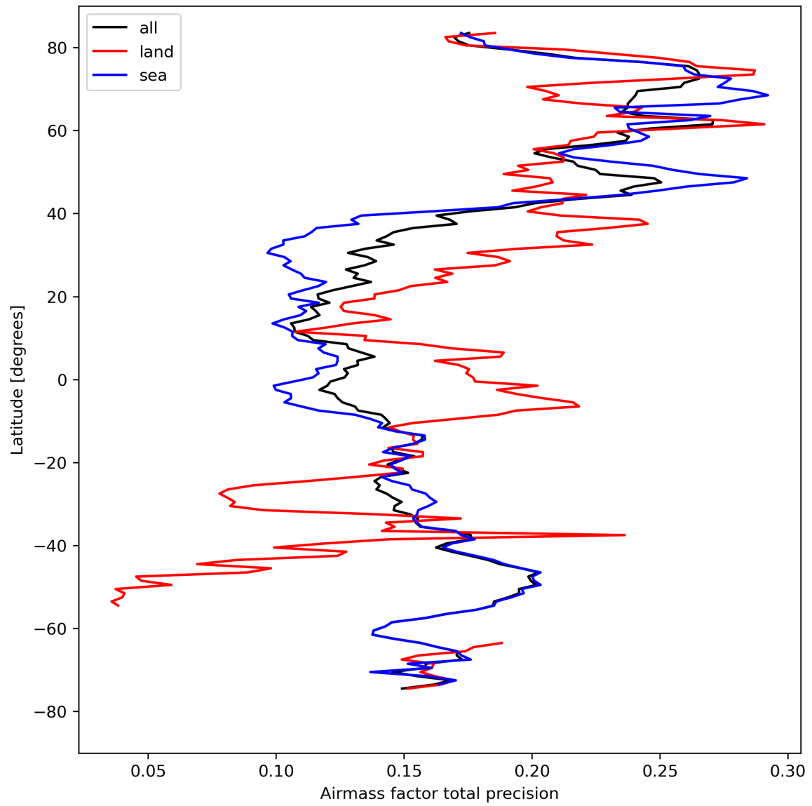
Figure 27: Zonal average of “Airmass factor total precision” for 2023-08-25 to 2023-08-27.
