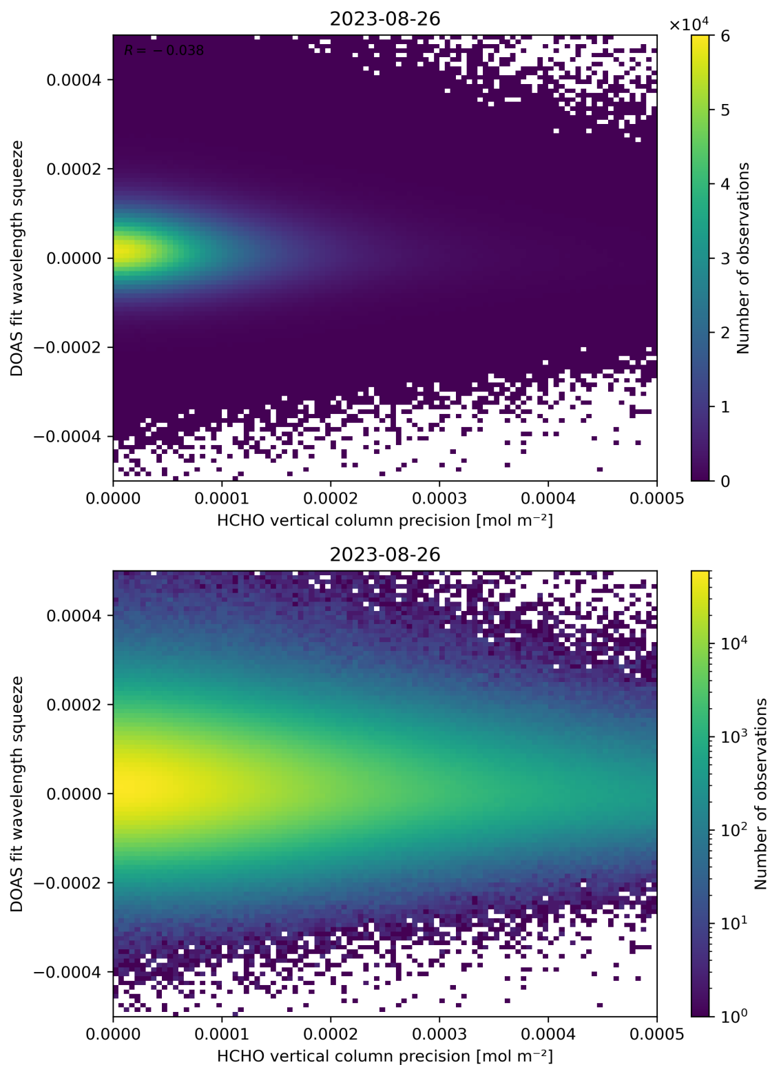
Figure 138: Scatter density plot of “HCHO vertical column precision” against “DOAS fit wavelength squeeze” for 2023-08-25 to 2023-08-27.
