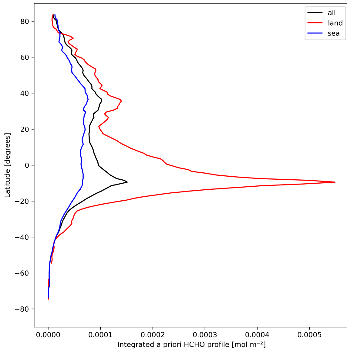
Figure 29: Zonal average of “Integrated a priori HCHO profile” for 2023-08-25 to 2023-08-27.
