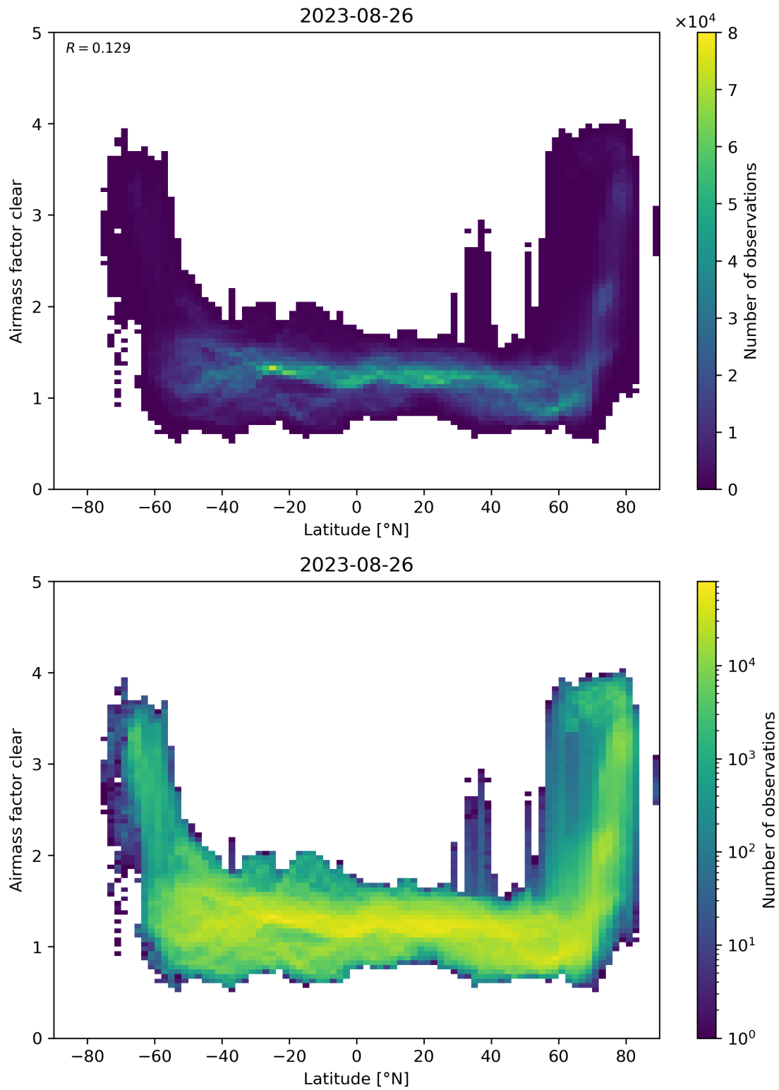
Figure 156: Scatter density plot of “Latitude” against “Airmass factor clear” for 2023-08-25 to 2023-08-27.
