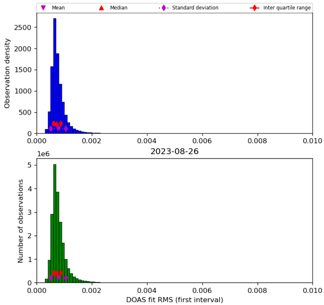
Figure 46: Histogram of “DOAS fit RMS (first interval)” for 2023-08-25 to 2023-08-27
