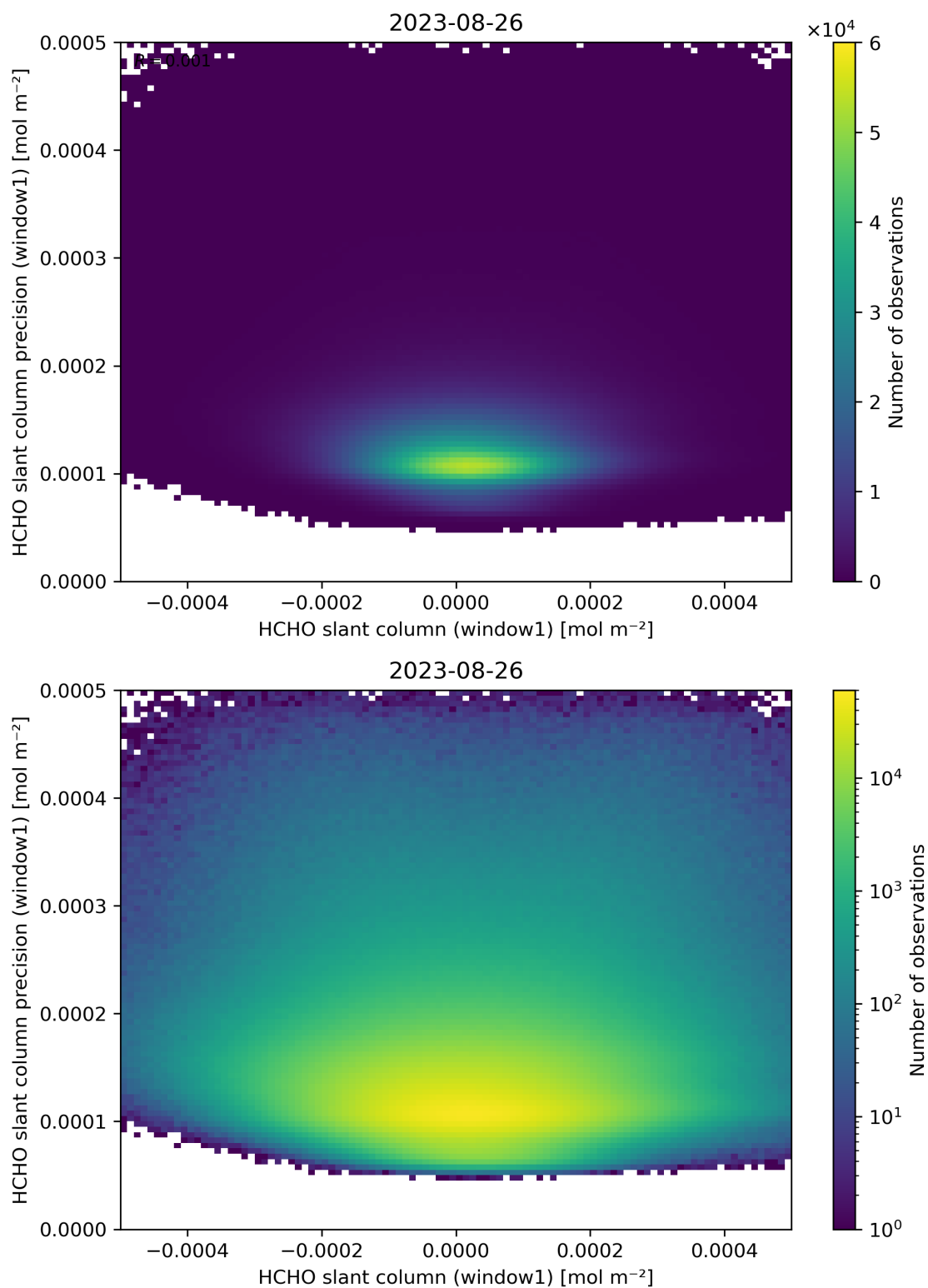
Figure 84: Scatter density plot of “HCHO slant column (window1)” against “HCHO slant column precision (window1)” for 2023-08-25 to 2023-08-27.
