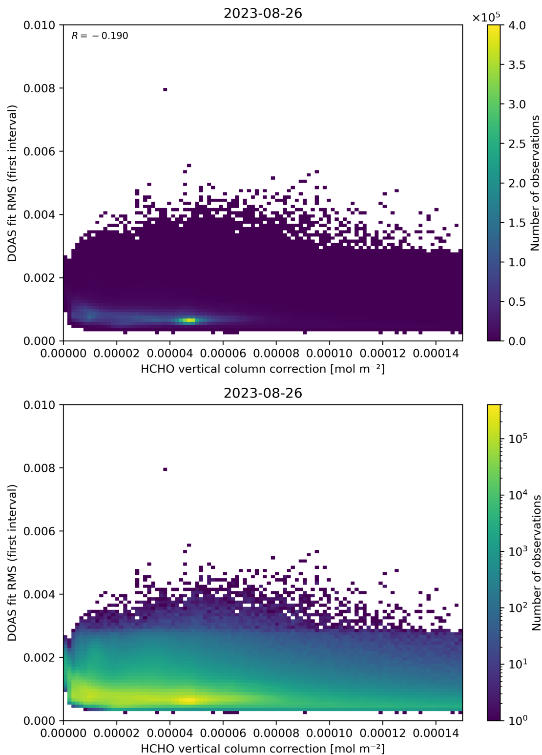
Figure 112: Scatter density plot of “HCHO vertical column correction” against “DOAS fit RMS (first interval)” for 2023-08-25 to 2023-08-27.
