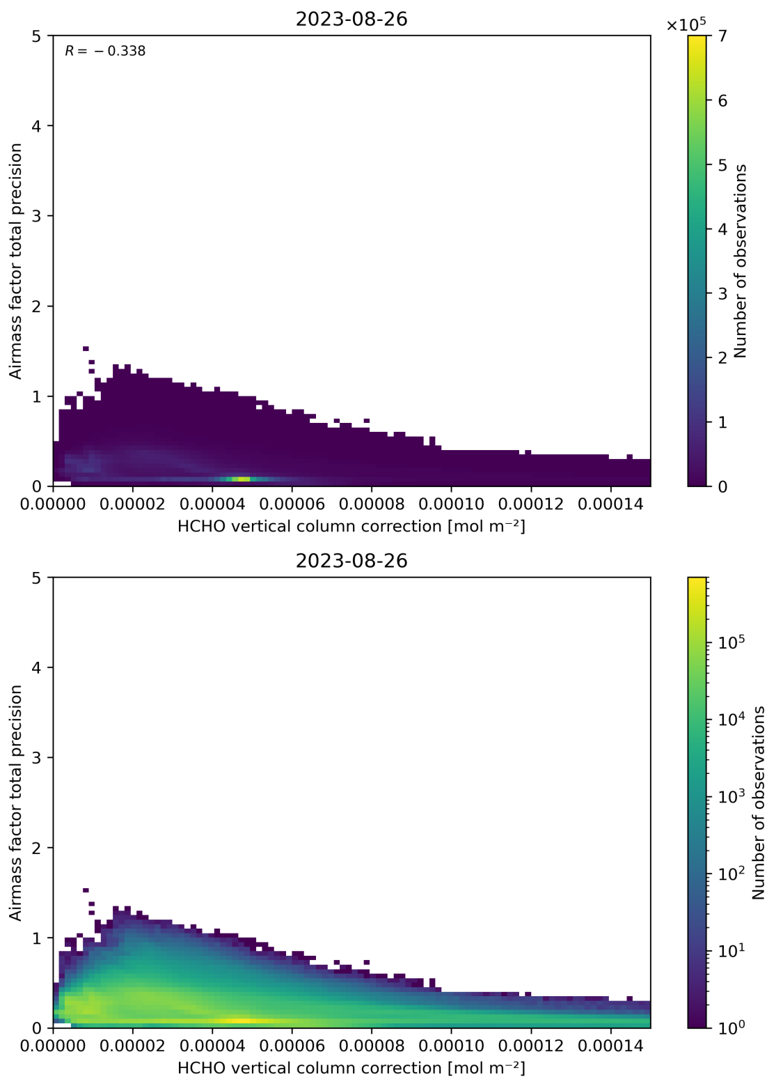
Figure 121: Scatter density plot of “HCHO vertical column correction” against “Airmass factor total precision” for 2023-08-25 to 2023-08-27.
