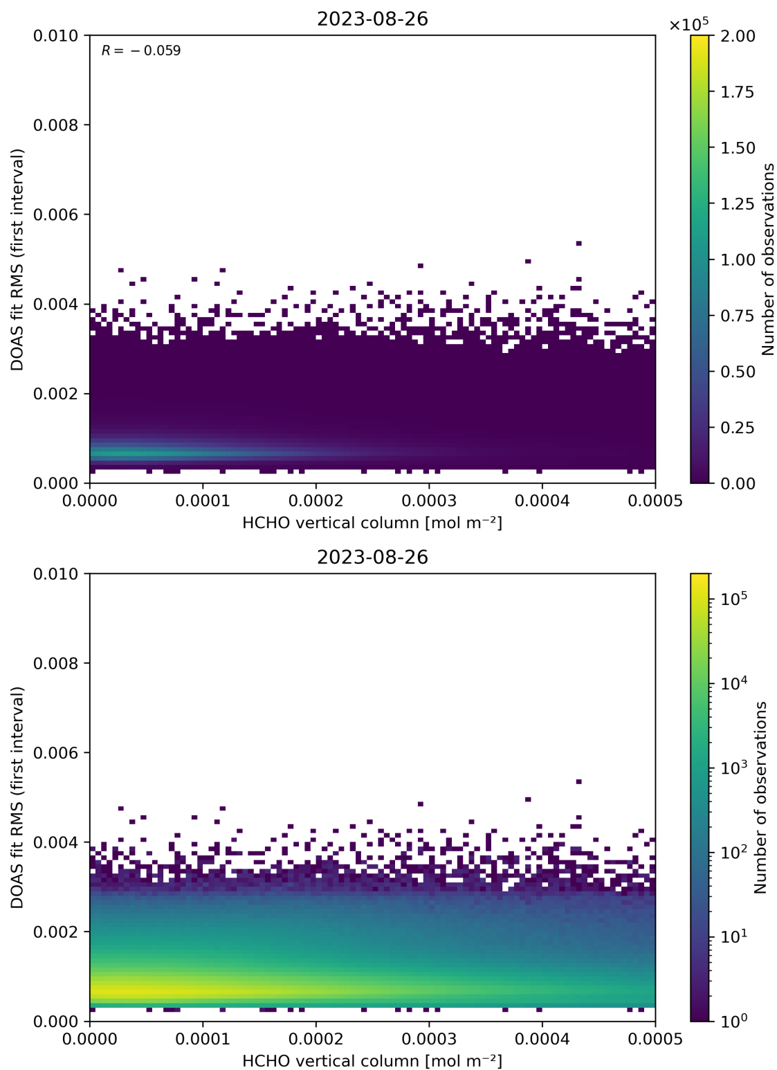
Figure 123: Scatter density plot of “HCHO vertical column” against “DOAS fit RMS (first interval)” for 2023-08-25 to 2023-08-27.
