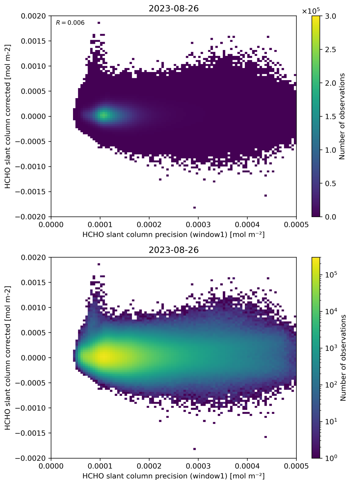
Figure 92: Scatter density plot of “HCHO slant column precision (window1)” against “HCHO slant column corrected” for 2023-08-25 to 2023-08-27.
