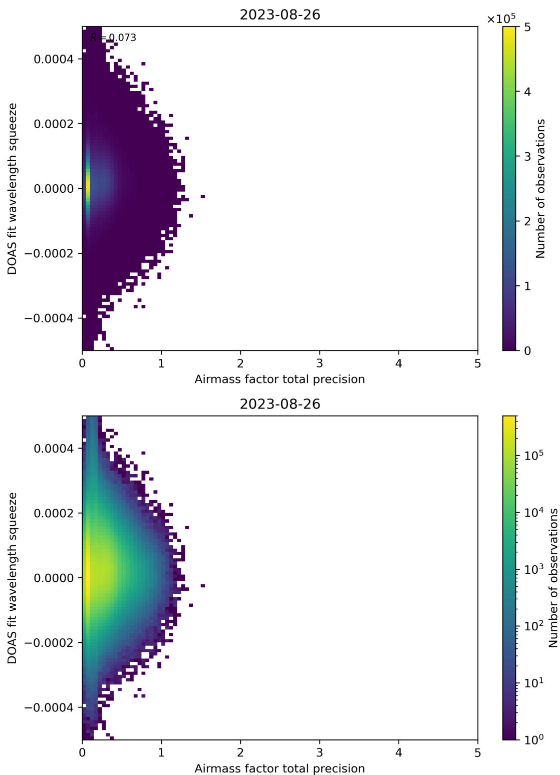
Figure 107: Scatter density plot of “Airmass factor total precision” against “DOAS fit wavelength squeeze” for 2023-08-25 to 2023-08-27.
