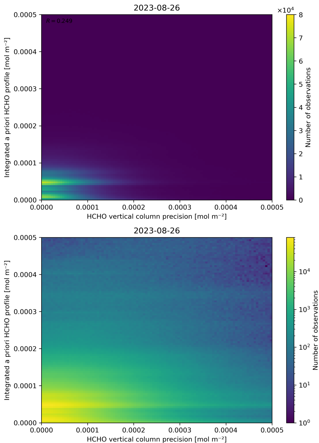
Figure 147: Scatter density plot of “HCHO vertical column precision” against “Integrated a priori HCHO profile” for 2023-08-25 to 2023-08-27.
