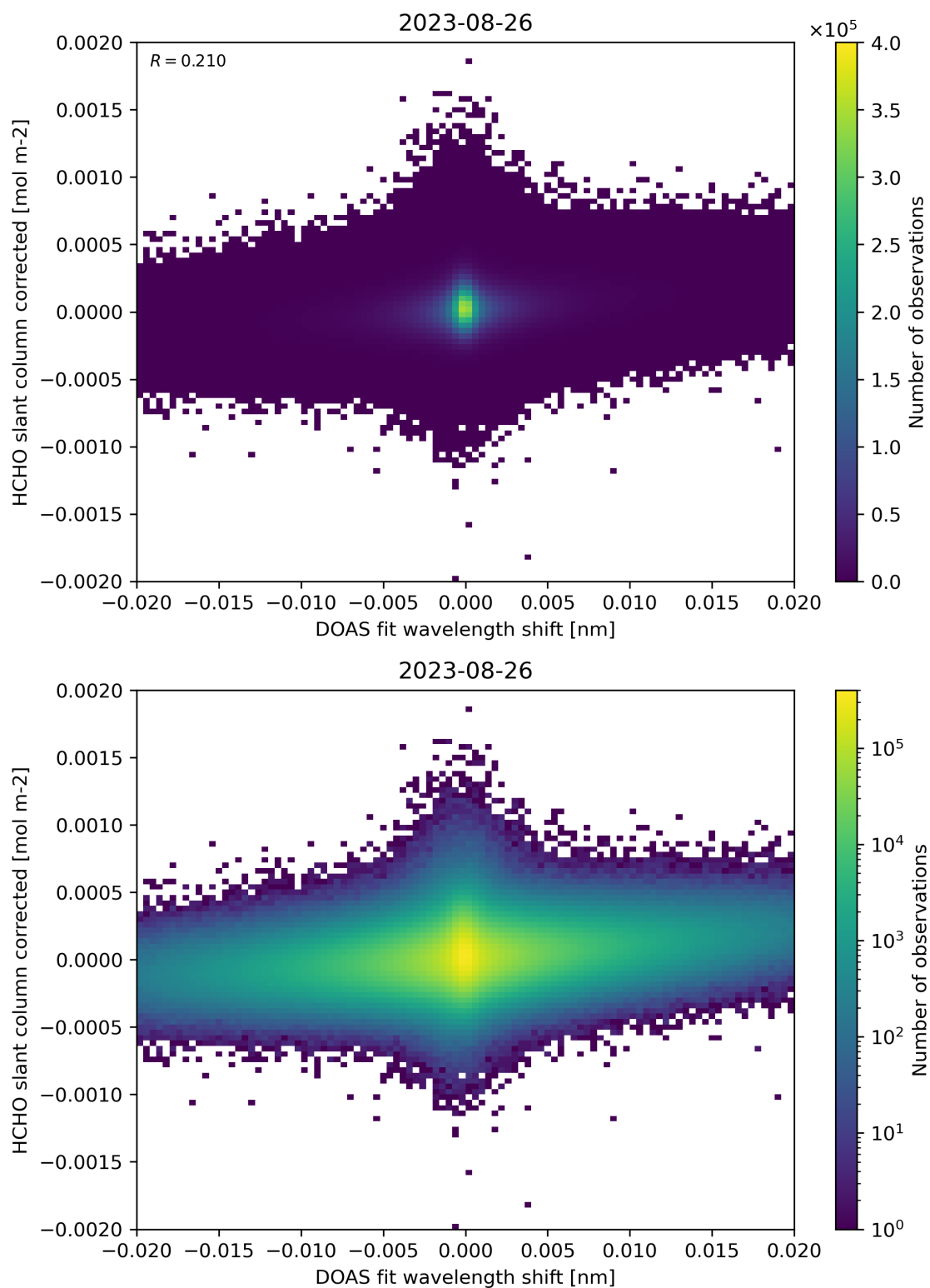
Figure 66: Scatter density plot of “DOAS fit wavelength shift” against “HCHO slant column corrected” for 2023-08-25 to 2023-08-27.
