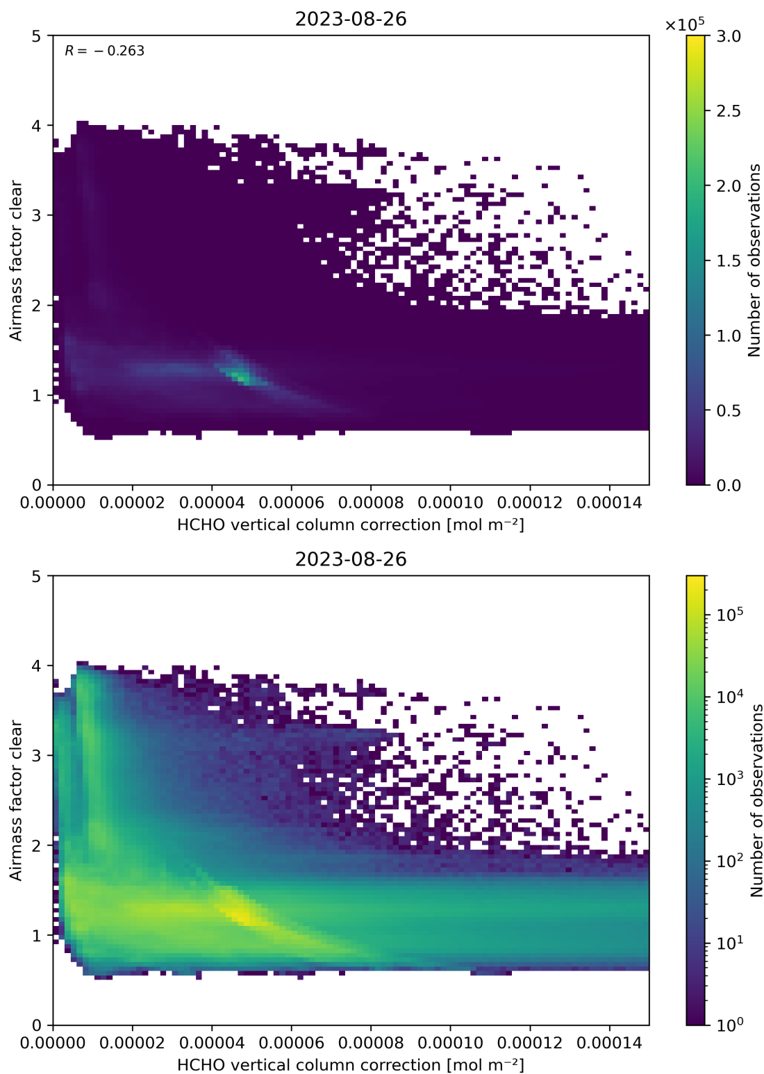
Figure 115: Scatter density plot of “HCHO vertical column correction” against “Airmass factor clear” for 2023-08-25 to 2023-08-27.
