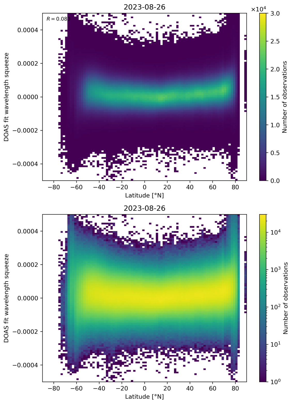
Figure 155: Scatter density plot of “Latitude” against “DOAS fit wavelength squeeze” for 2023-08-25 to 2023-08-27.
