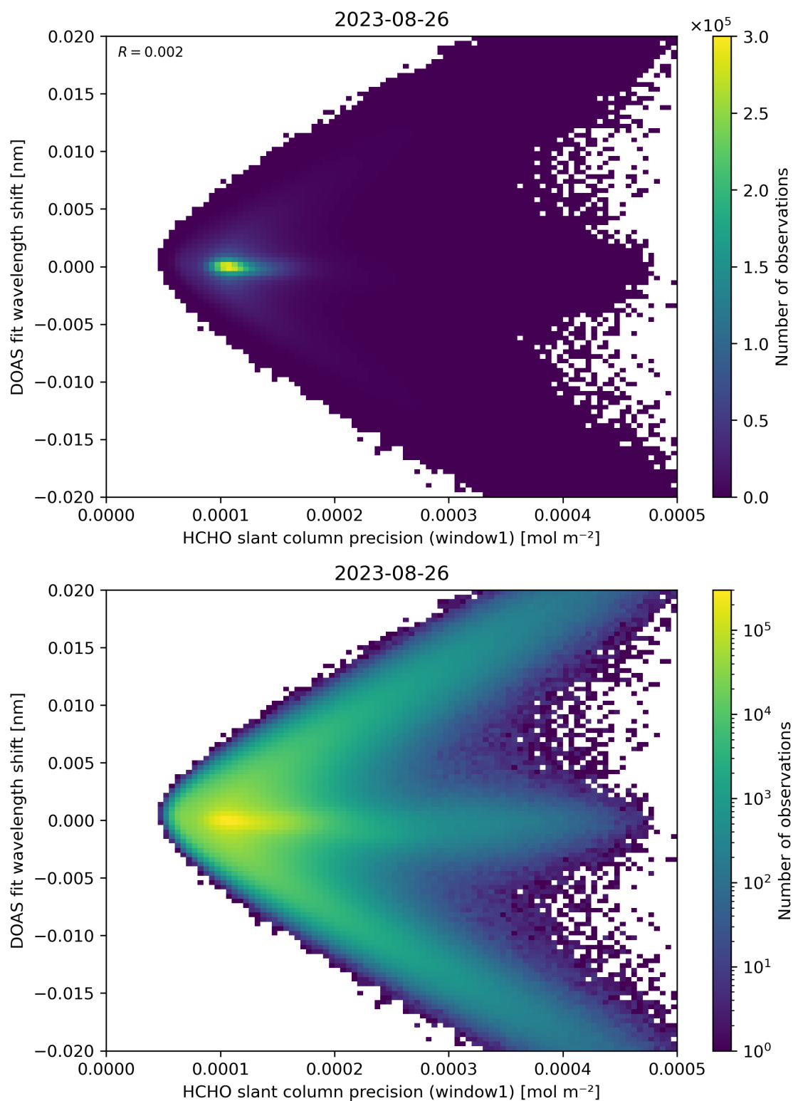
Figure 89: Scatter density plot of “HCHO slant column precision (window1)” against “DOAS fit wavelength shift” for 2023-08-25 to 2023-08-27.
