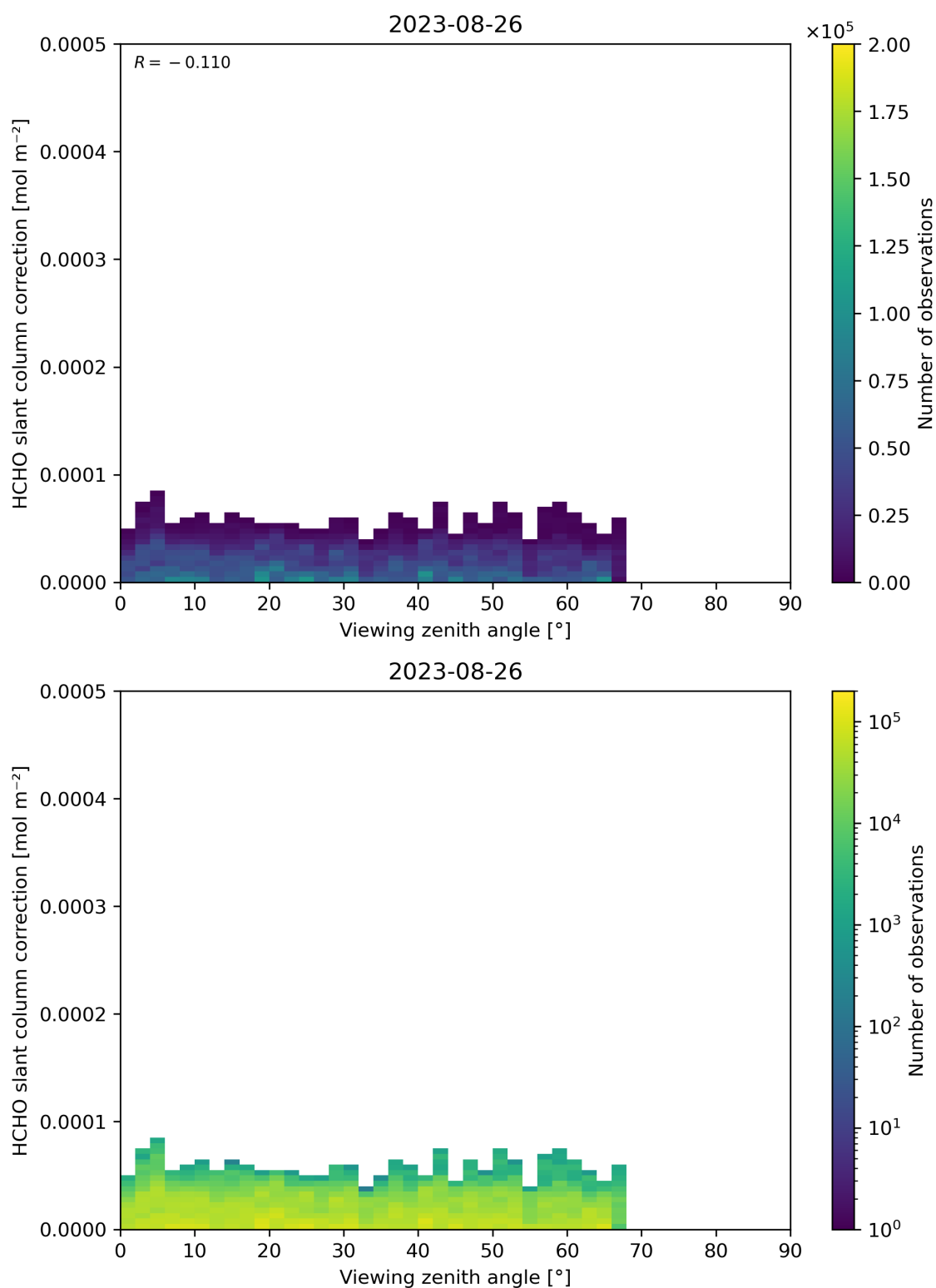
Figure 187: Scatter density plot of “Viewing zenith angle” against “HCHO slant column correction” for 2023-08-25 to 2023-08-27.
