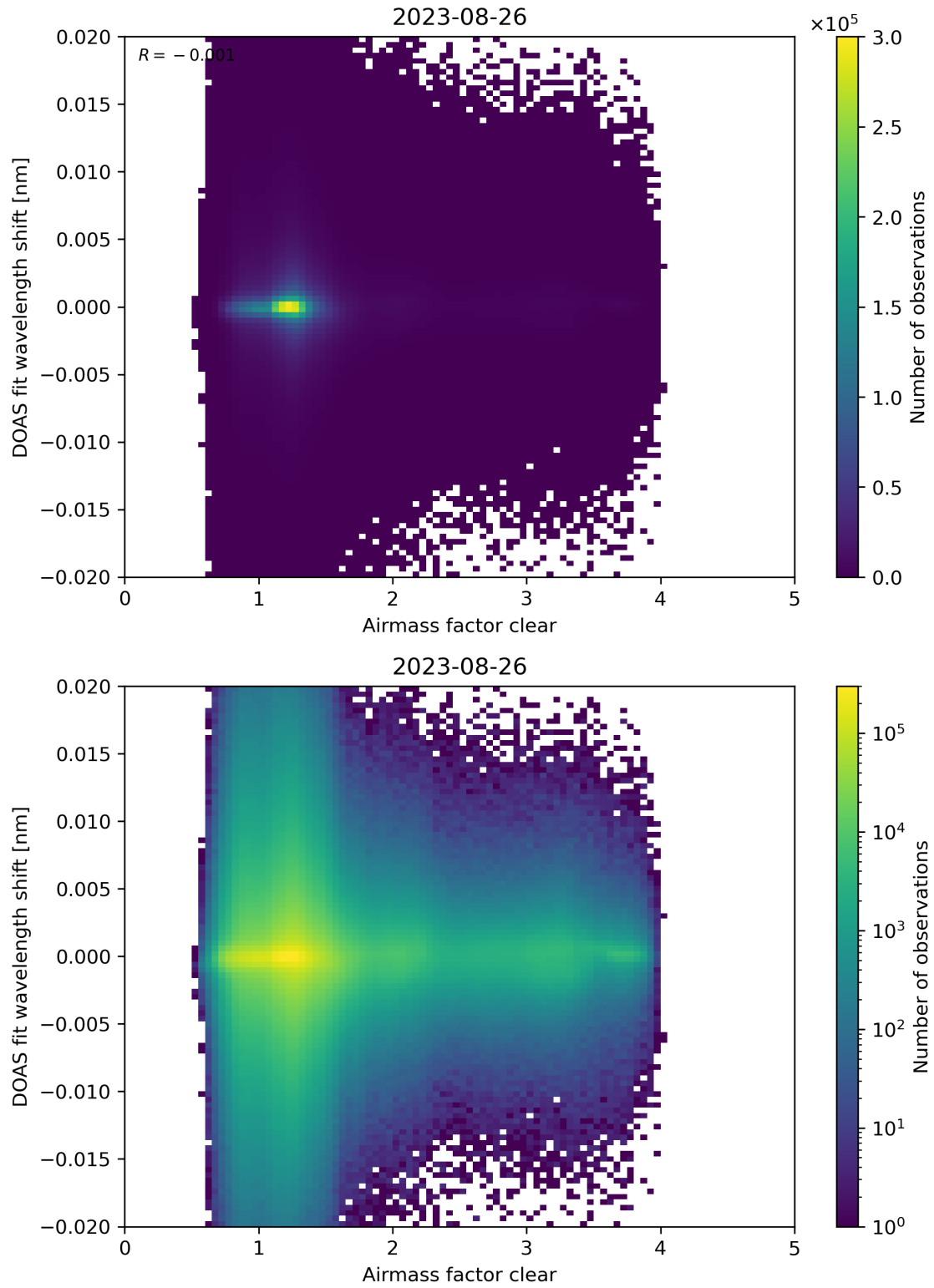
Figure 72: Scatter density plot of “Airmass factor clear” against “DOAS fit wavelength shift” for 2023-08-25 to 2023-08-27.
