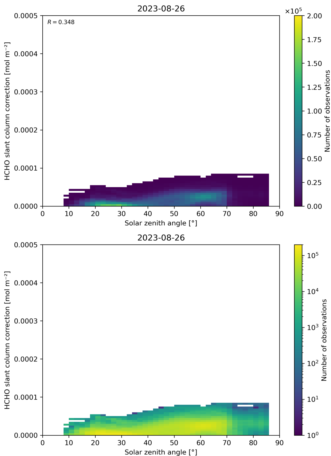
Figure 172: Scatter density plot of “Solar zenith angle” against “HCHO slant column correction” for 2023-08-25 to 2023-08-27.
