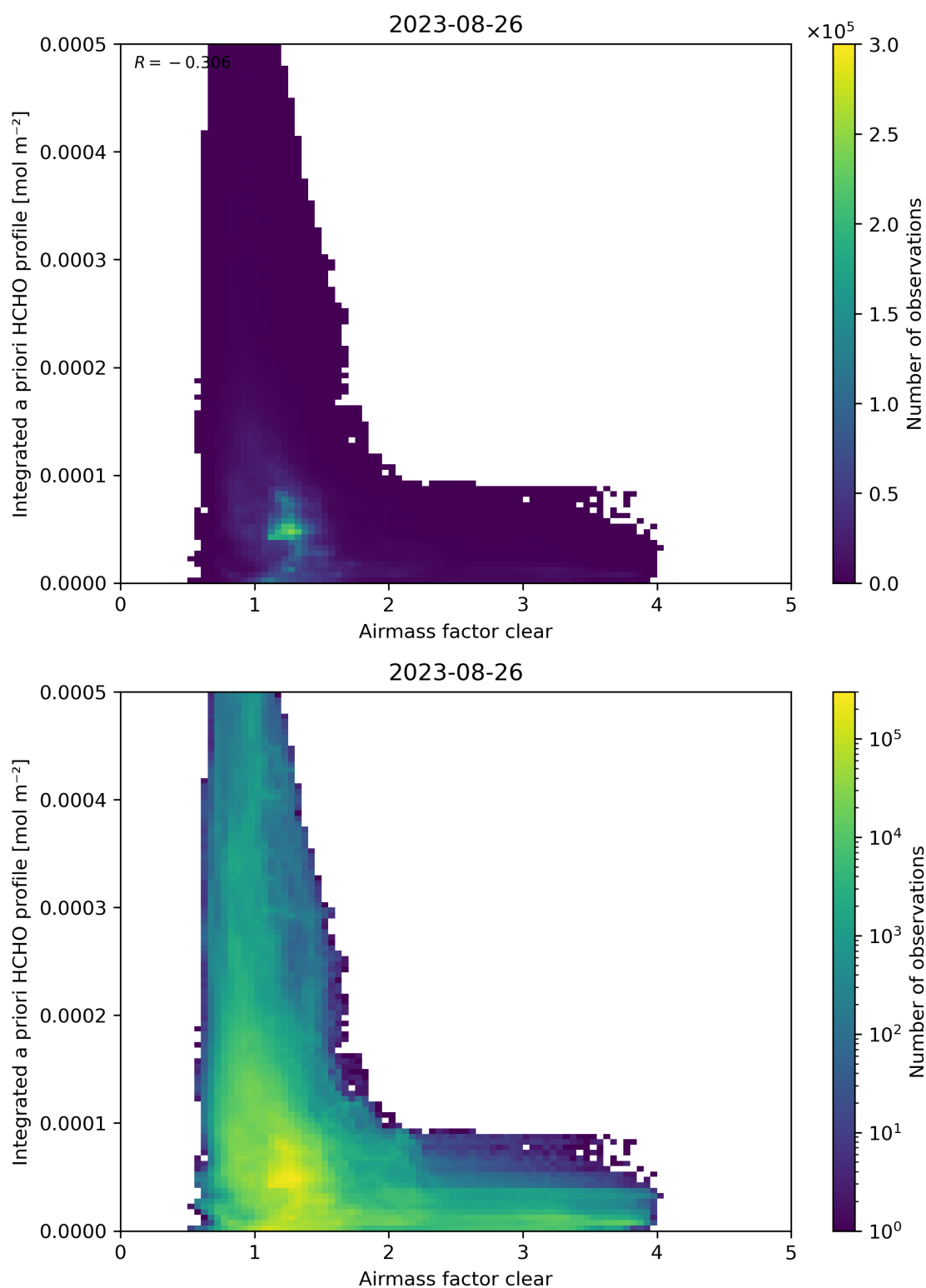
Figure 76: Scatter density plot of “Airmass factor clear” against “Integrated a priori HCHO profile” for 2023-08-25 to 2023-08-27.
