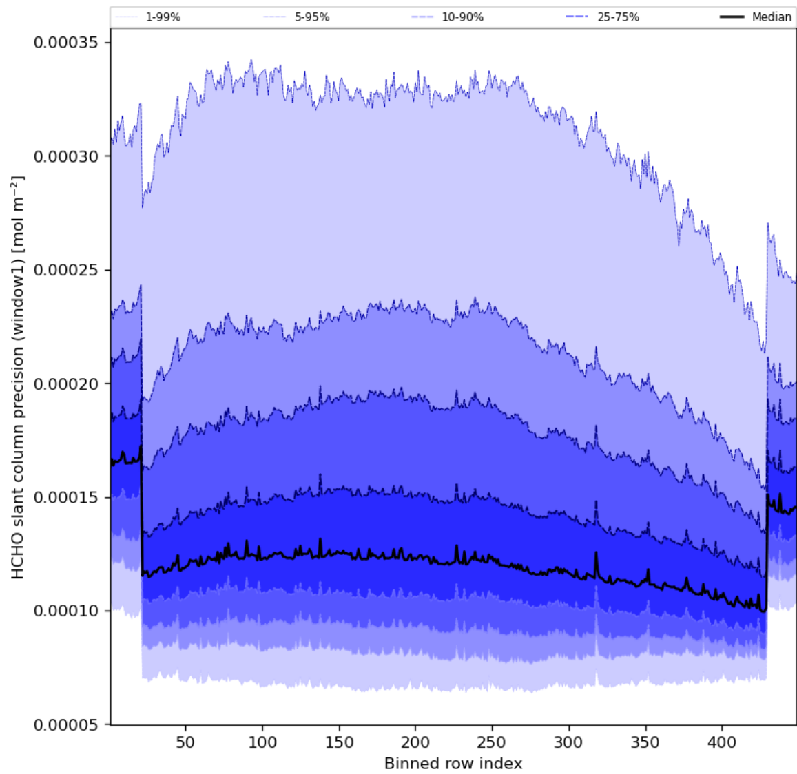
Figure 53: Along track statistics of “HCHO slant column precision (window1)” for 2023-08-25 to 2023-08-27
