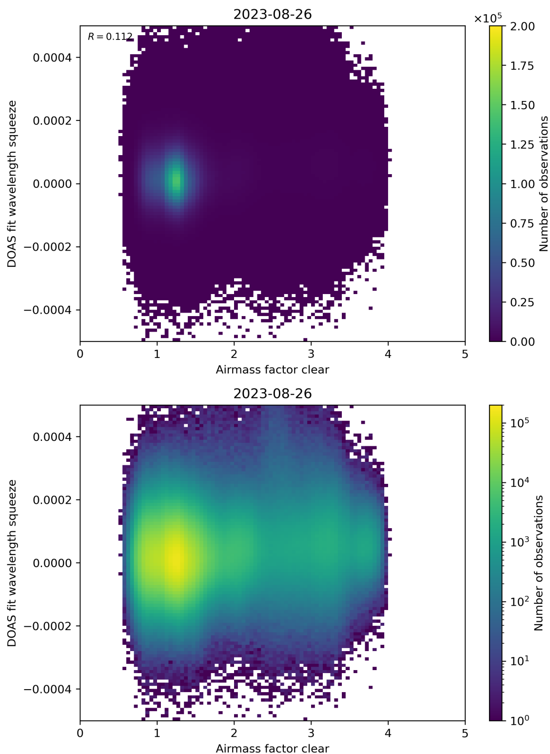
Figure 73: Scatter density plot of “Airmass factor clear” against “DOAS fit wavelength squeeze” for 2023-08-25 to 2023-08-27.
