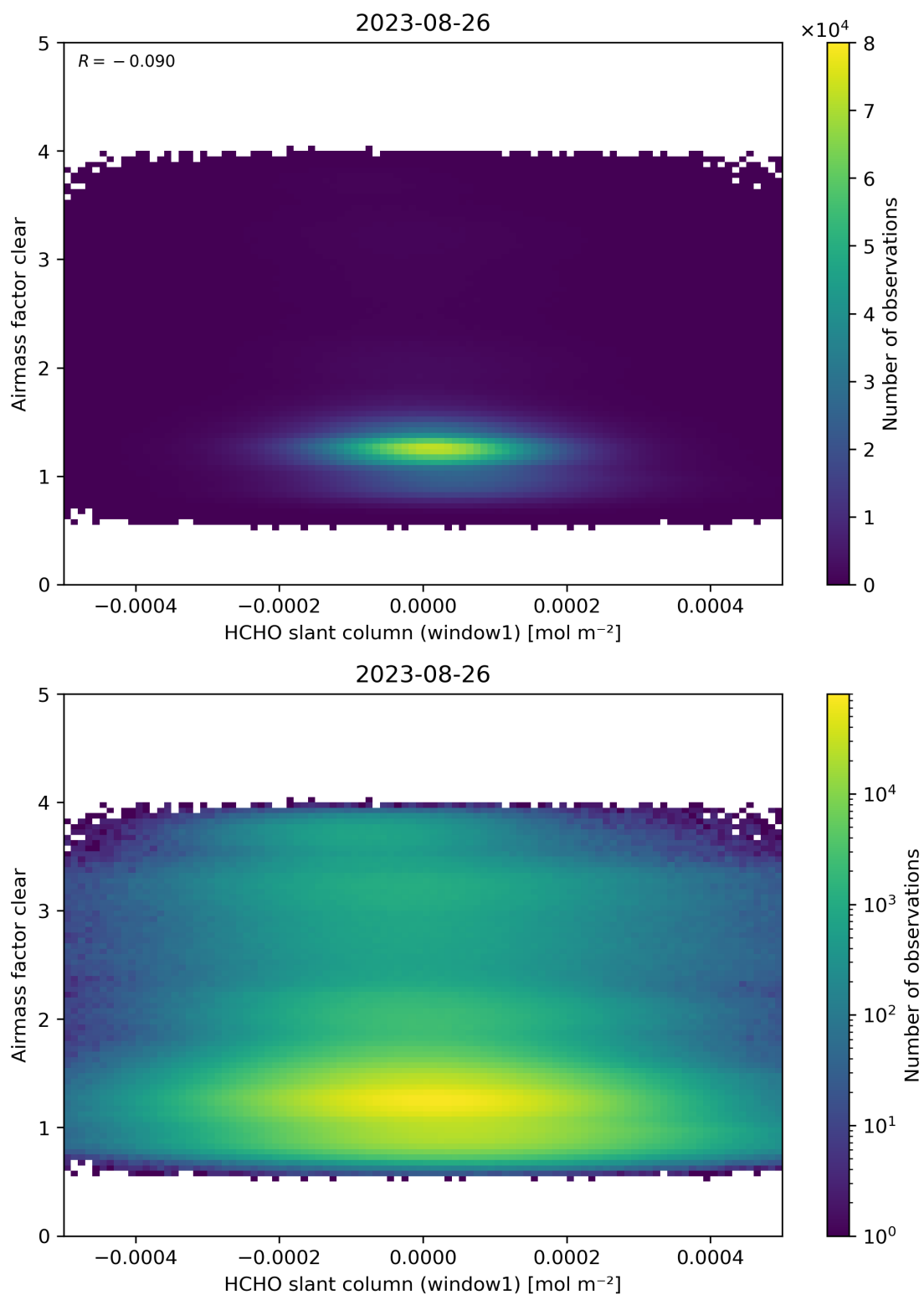
Figure 81: Scatter density plot of “HCHO slant column (window1)” against “Airmass factor clear” for 2023-08-25 to 2023-08-27.
