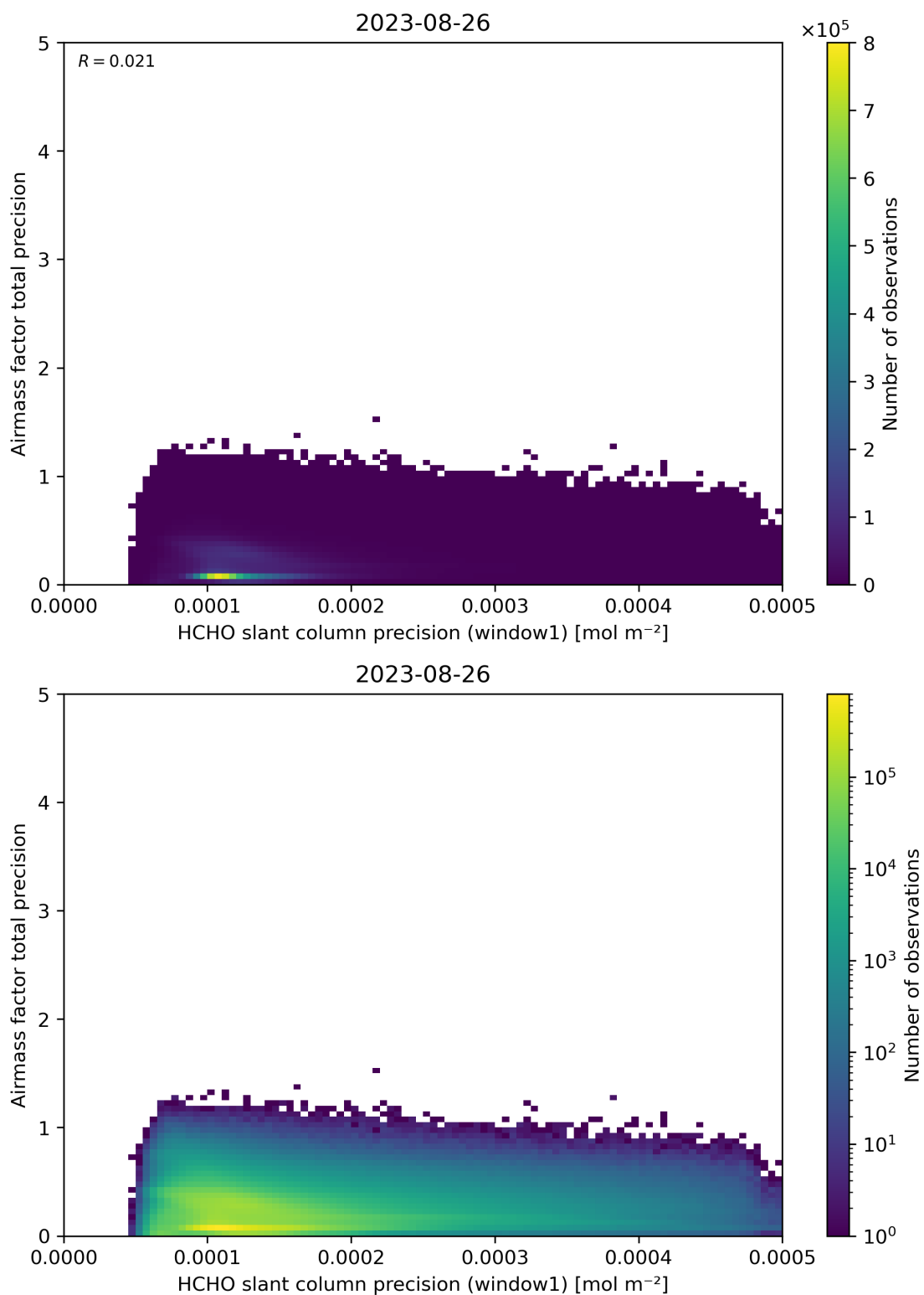
Figure 95: Scatter density plot of “HCHO slant column precision (window1)” against “Airmass factor total precision” for 2023-08-25 to 2023-08-27.
