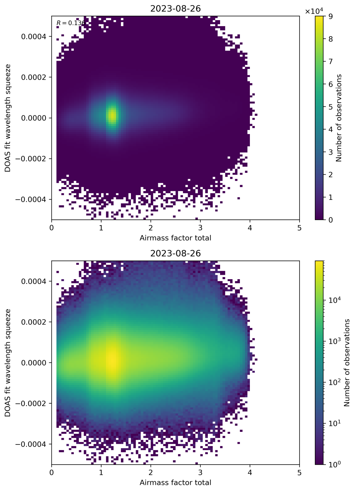
Figure 99: Scatter density plot of “Airmass factor total” against “DOAS fit wavelength squeeze” for 2023-08-25 to 2023-08-27.
