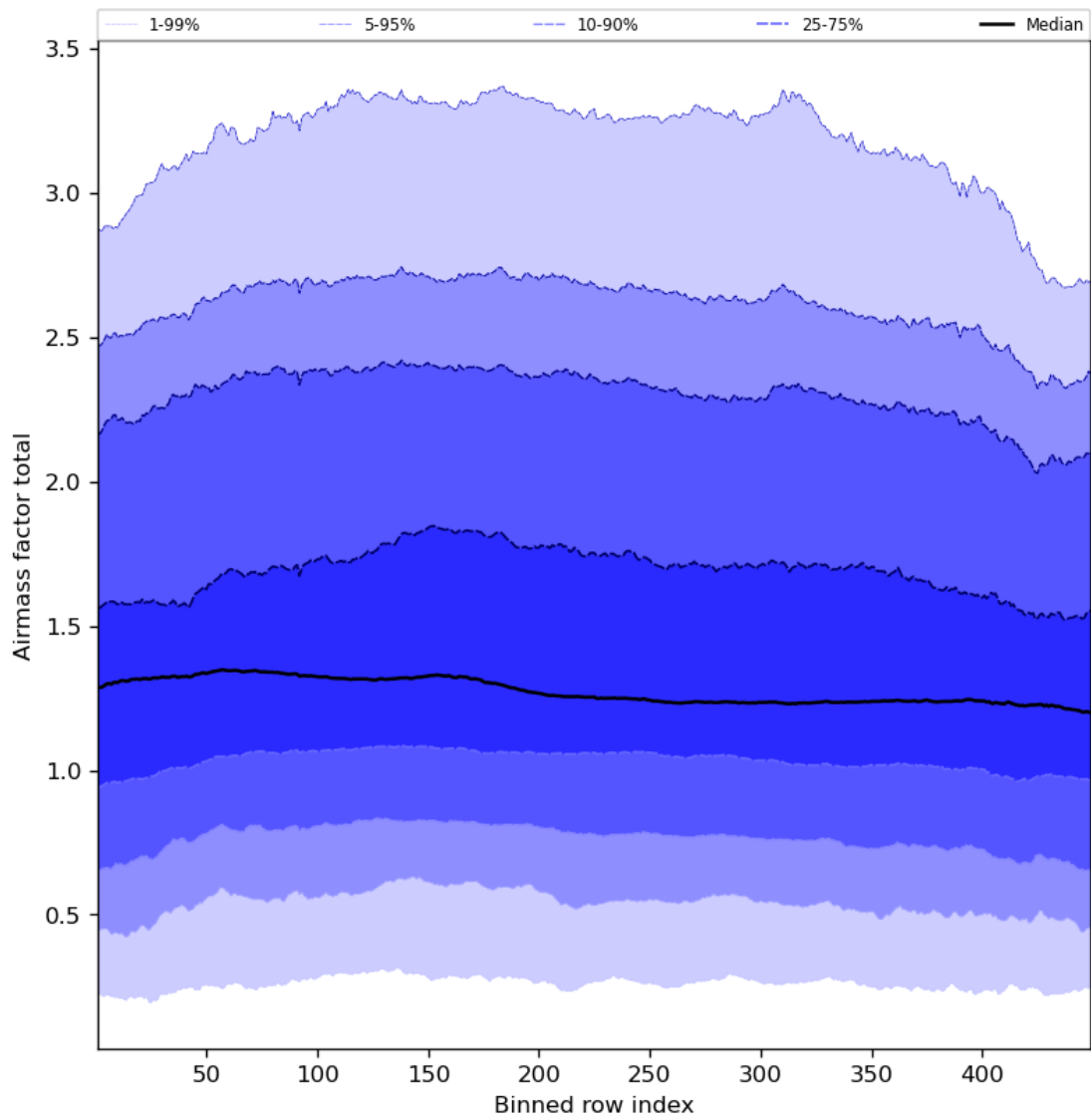
Figure 54: Along track statistics of “Airmass factor total” for 2023-08-25 to 2023-08-27
