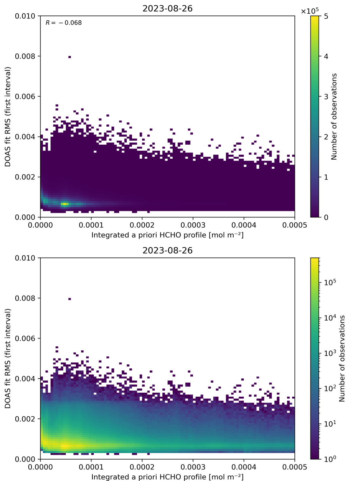
Figure 148: Scatter density plot of “Integrated a priori HCHO profile” against “DOAS fit RMS (first interval)” for 2023-08-25 to 2023-08-27.
