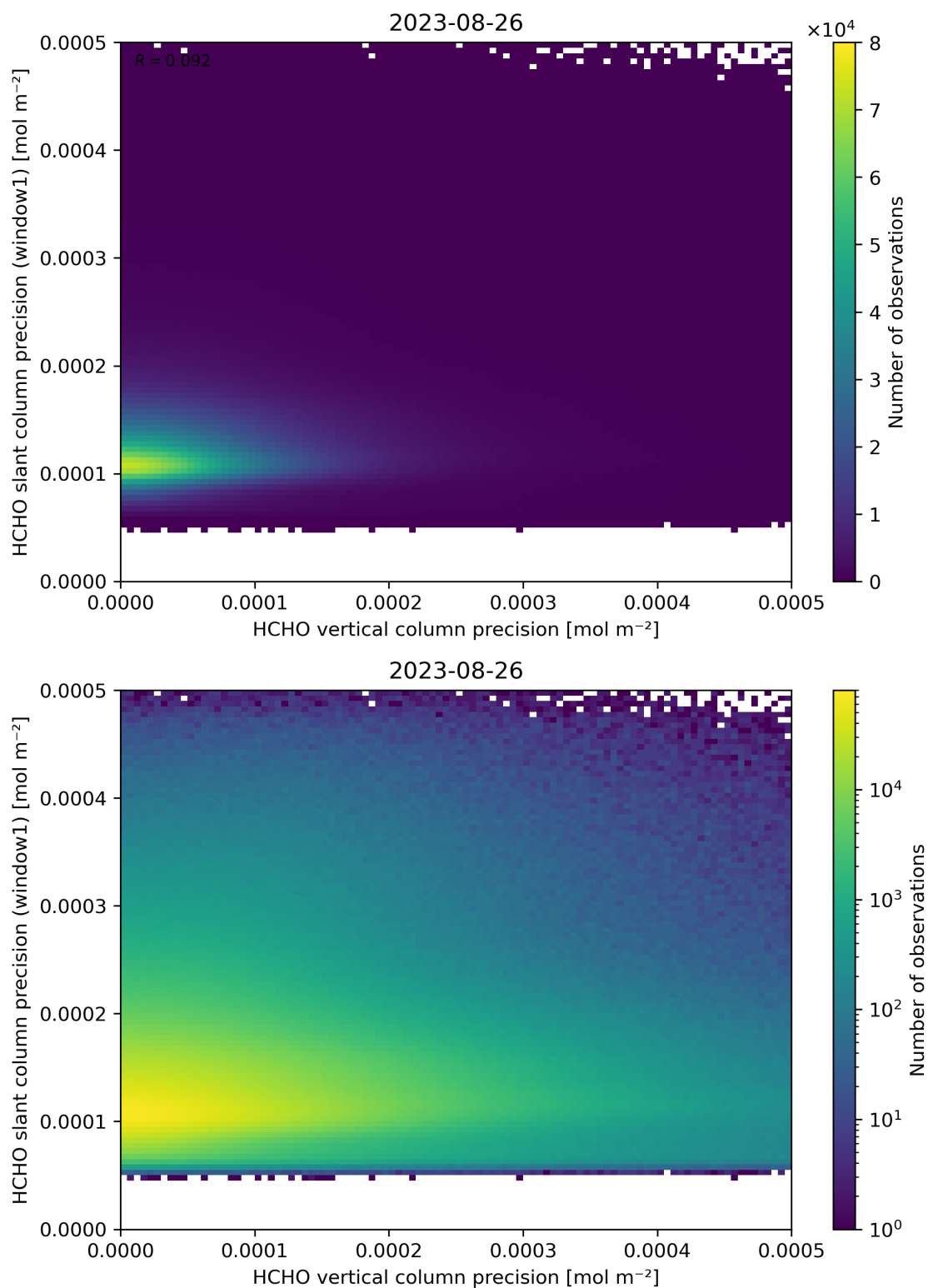
Figure 143: Scatter density plot of “HCHO vertical column precision” against “HCHO slant column precision (window1)” for 2023-08-25 to 2023-08-27.
