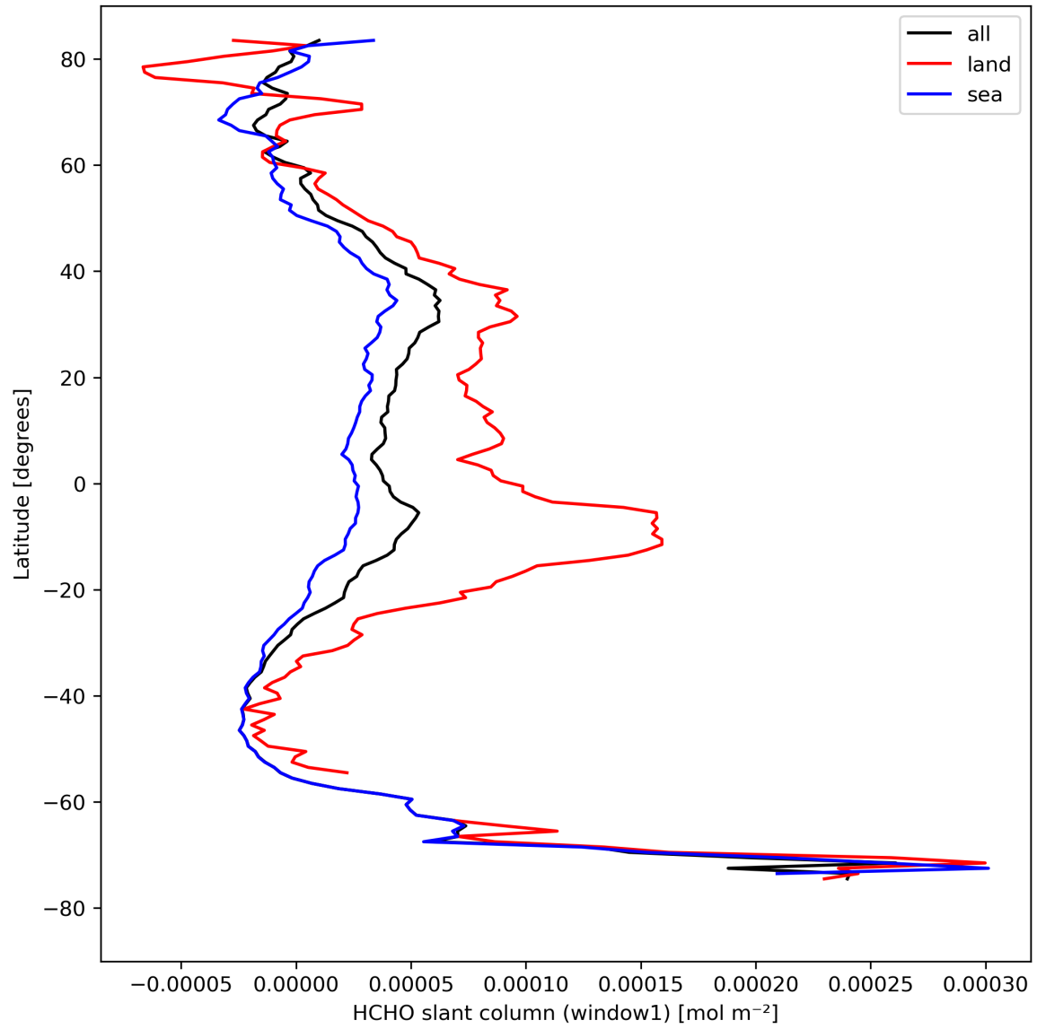
Figure 24: Zonal average of “HCHO slant column (window1)” for 2023-08-25 to 2023-08-27.
