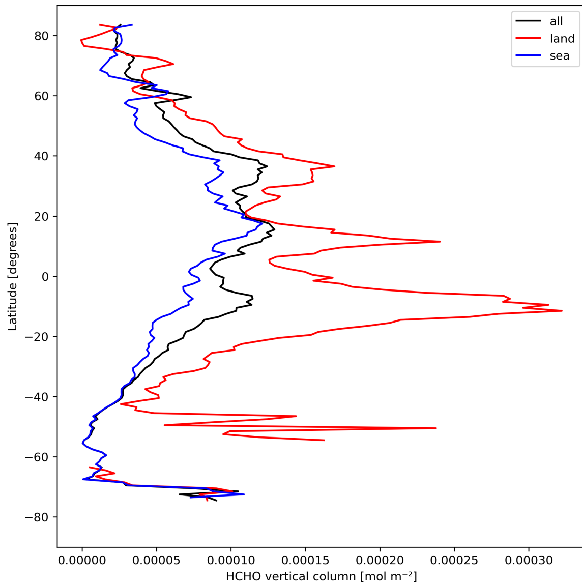
Figure 21: Zonal average of “HCHO vertical column” for 2023-08-25 to 2023-08-27.
