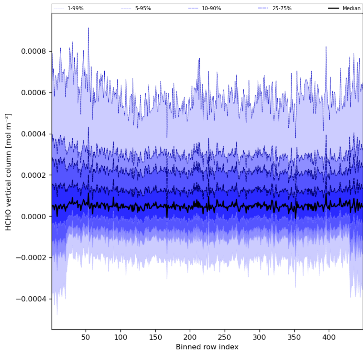
Figure 49: Along track statistics of “HCHO vertical column” for 2023-08-25 to 2023-08-27
