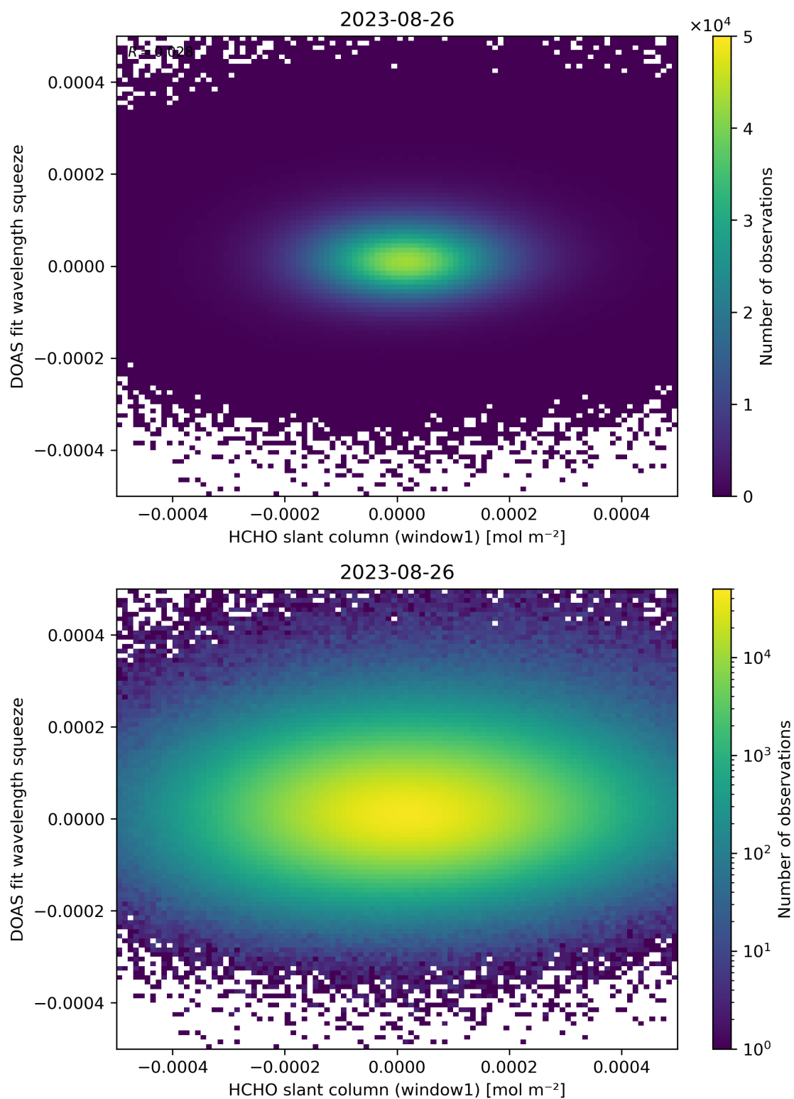
Figure 80: Scatter density plot of “HCHO slant column (window1)” against “DOAS fit wavelength squeeze” for 2023-08-25 to 2023-08-27.
