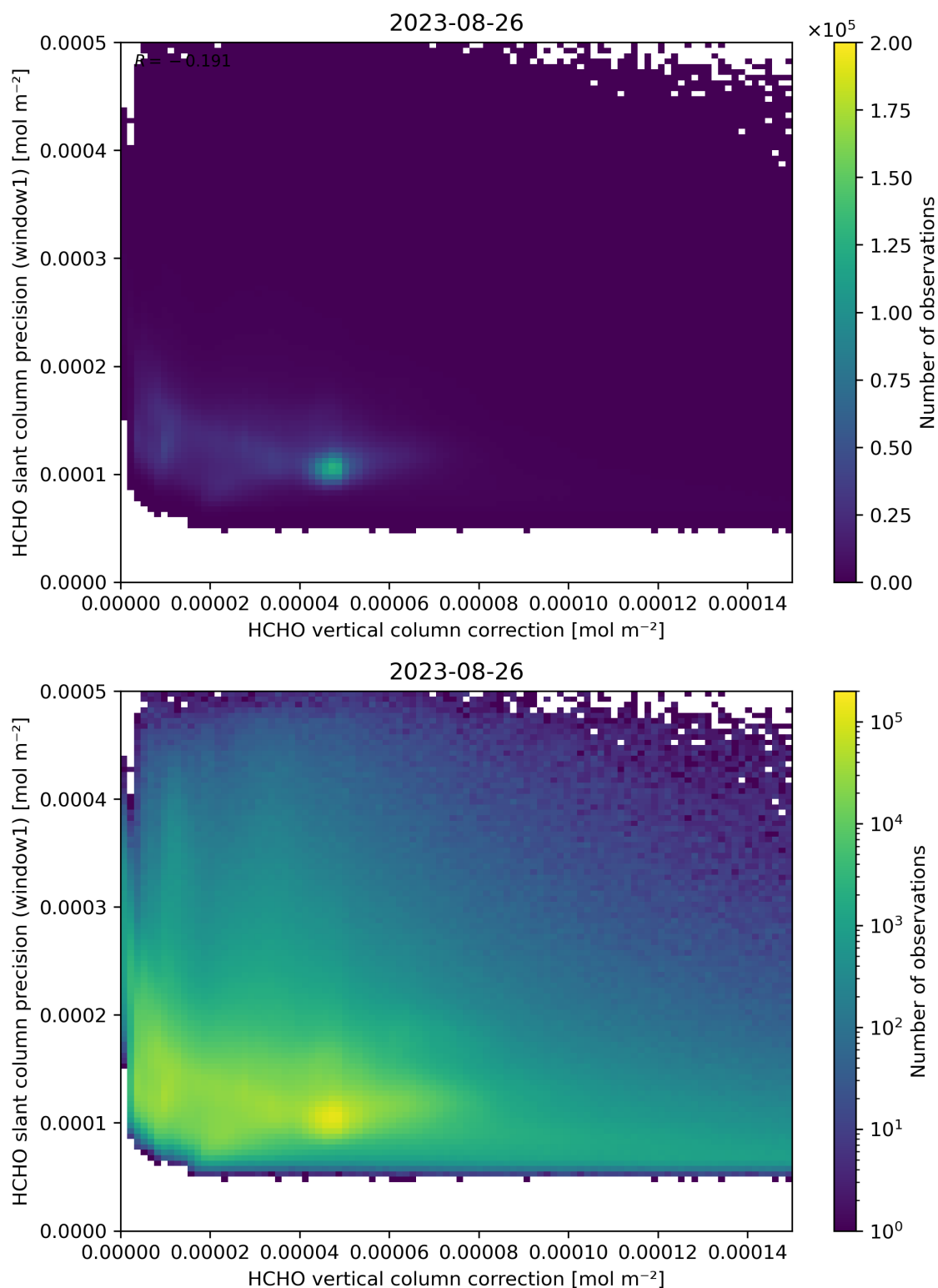
Figure 119: Scatter density plot of “HCHO vertical column correction” against “HCHO slant column precision (window1)” for 2023-08-25 to 2023-08-27.
