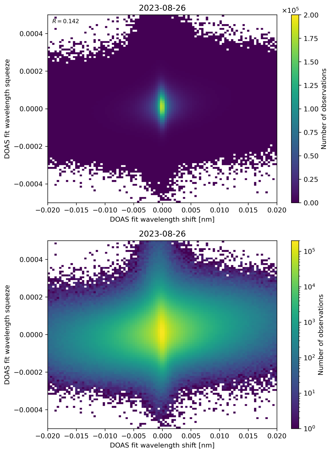
Figure 65: Scatter density plot of “DOAS fit wavelength shift” against “DOAS fit wavelength squeeze” for 2023-08-25 to 2023-08-27.
