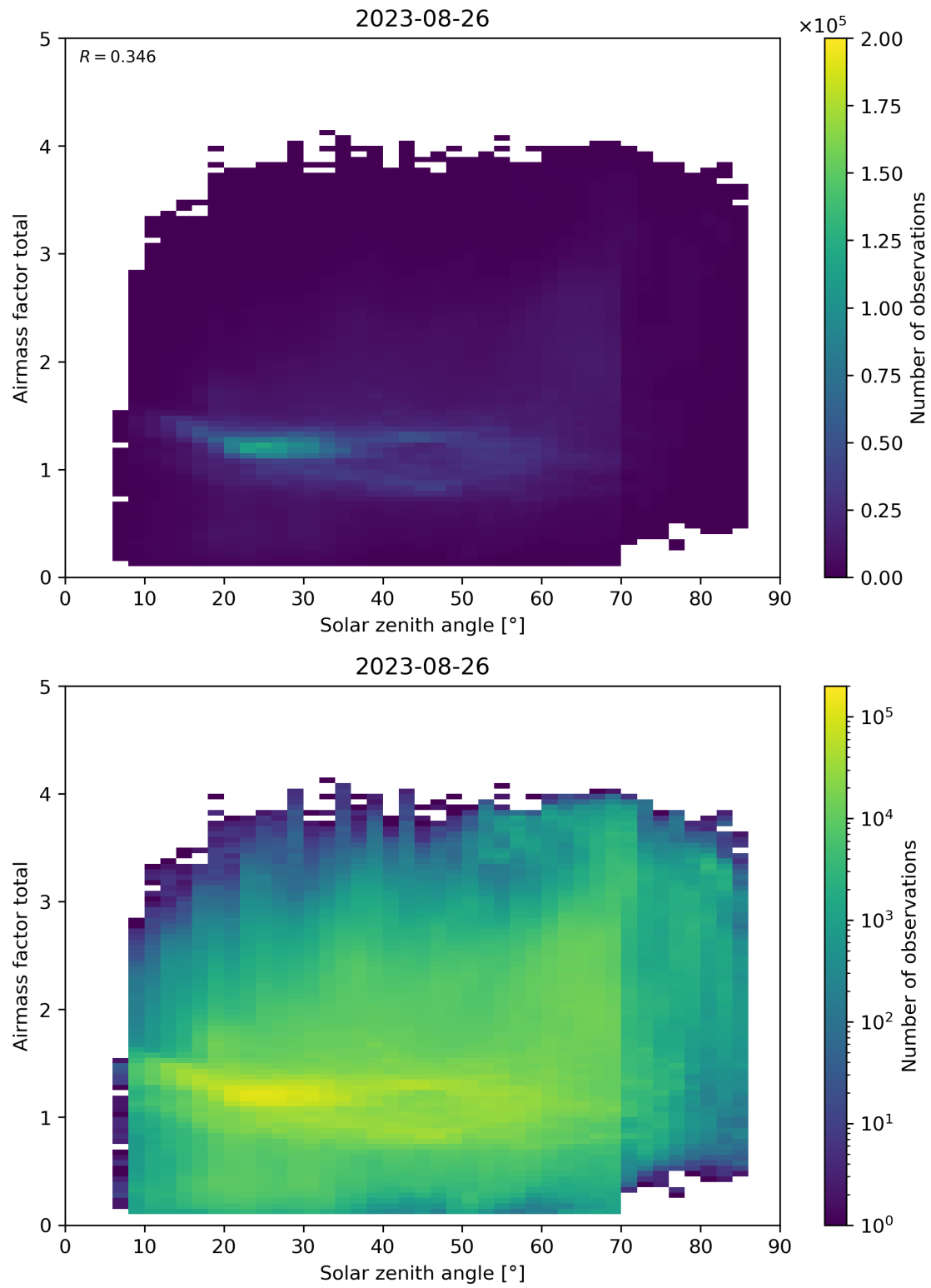
Figure 175: Scatter density plot of “Solar zenith angle” against “Airmass factor total” for 2023-08-25 to 2023-08-27.
