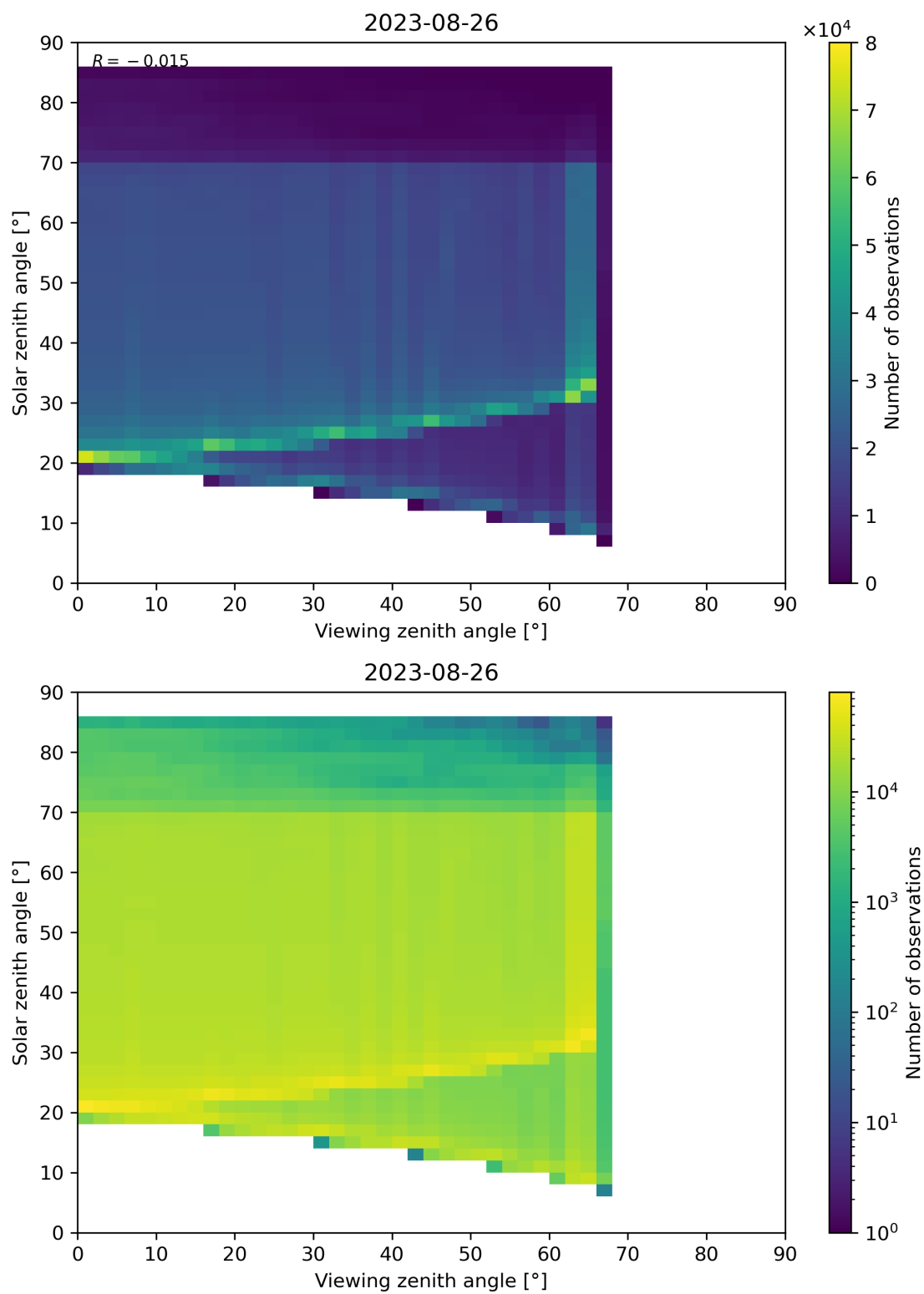
Figure 197: Scatter density plot of “Viewing zenith angle” against “Solar zenith angle” for 2023-08-25 to 2023-08-27.
