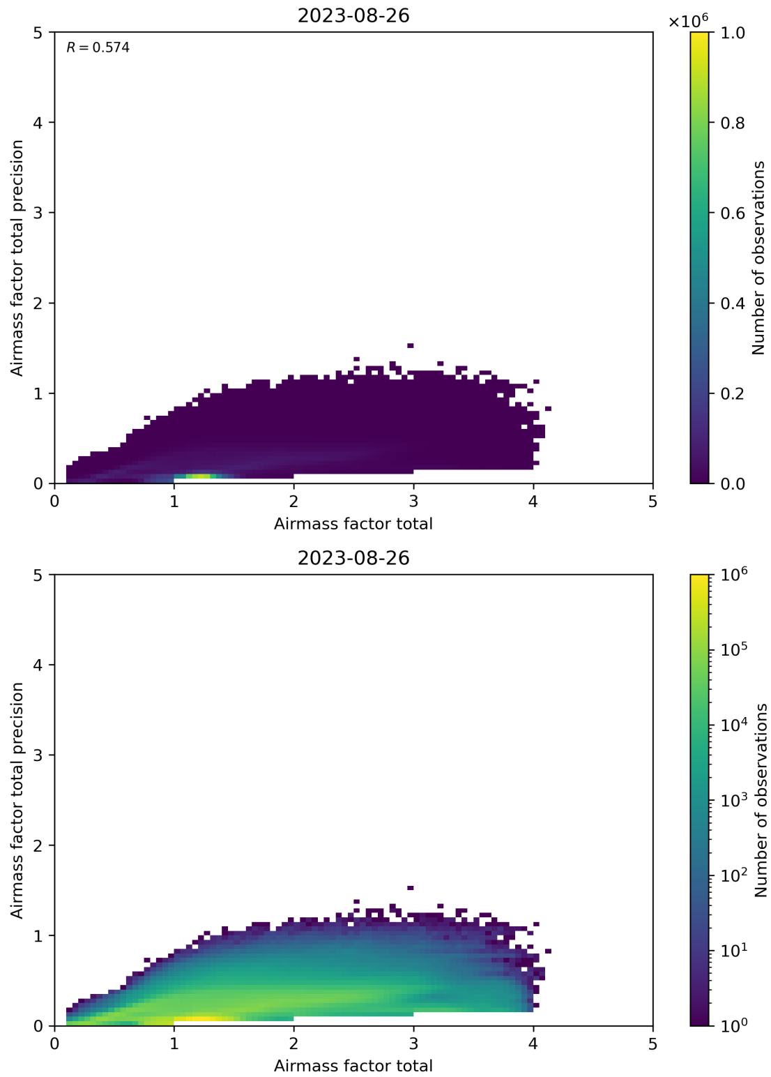
Figure 103: Scatter density plot of “Airmass factor total” against “Airmass factor total precision” for 2023-08-25 to 2023-08-27.
