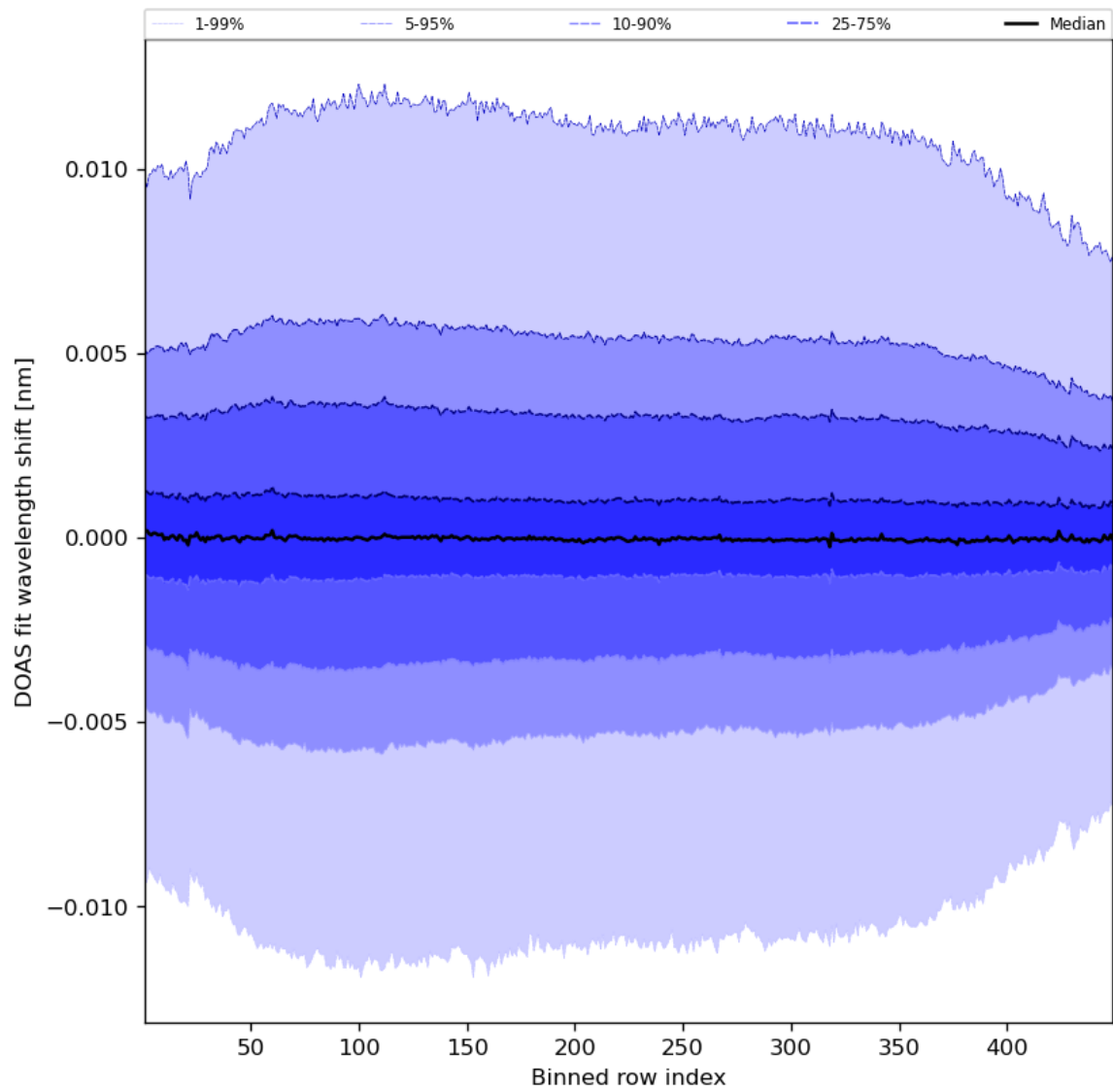
Figure 58: Along track statistics of “DOAS fit wavelength shift” for 2023-08-25 to 2023-08-27
