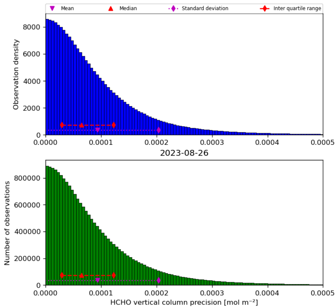
Figure 36: Histogram of “HCHO vertical column precision” for 2023-08-25 to 2023-08-27
