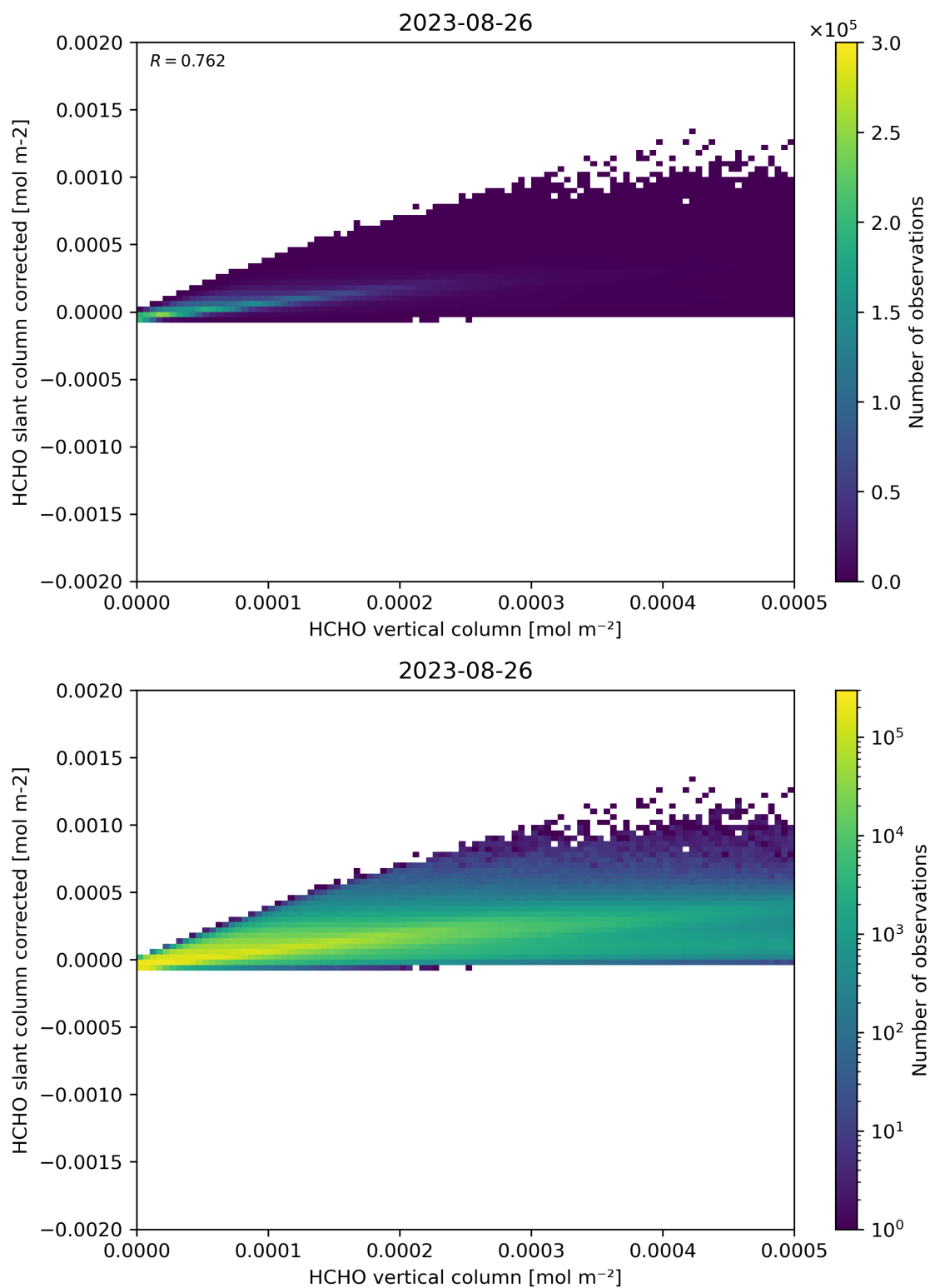
Figure 127: Scatter density plot of “HCHO vertical column” against “HCHO slant column corrected” for 2023-08-25 to 2023-08-27.
