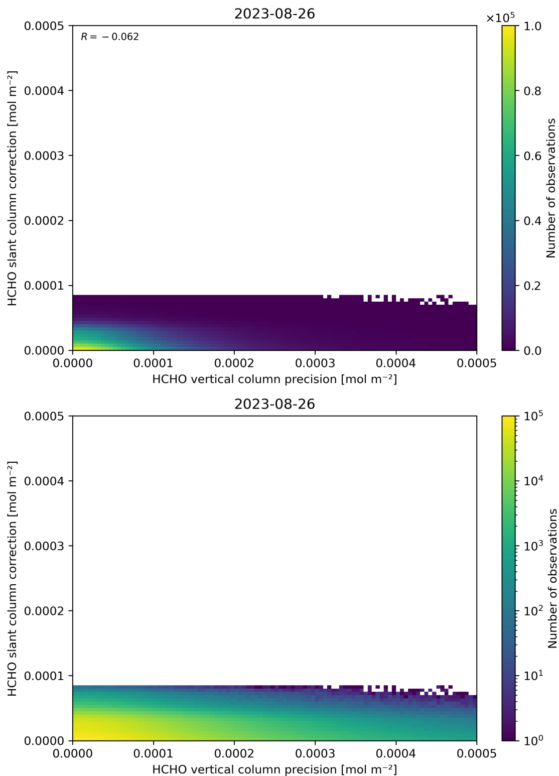
Figure 141: Scatter density plot of “HCHO vertical column precision” against “HCHO slant column correction” for 2023-08-25 to 2023-08-27.
