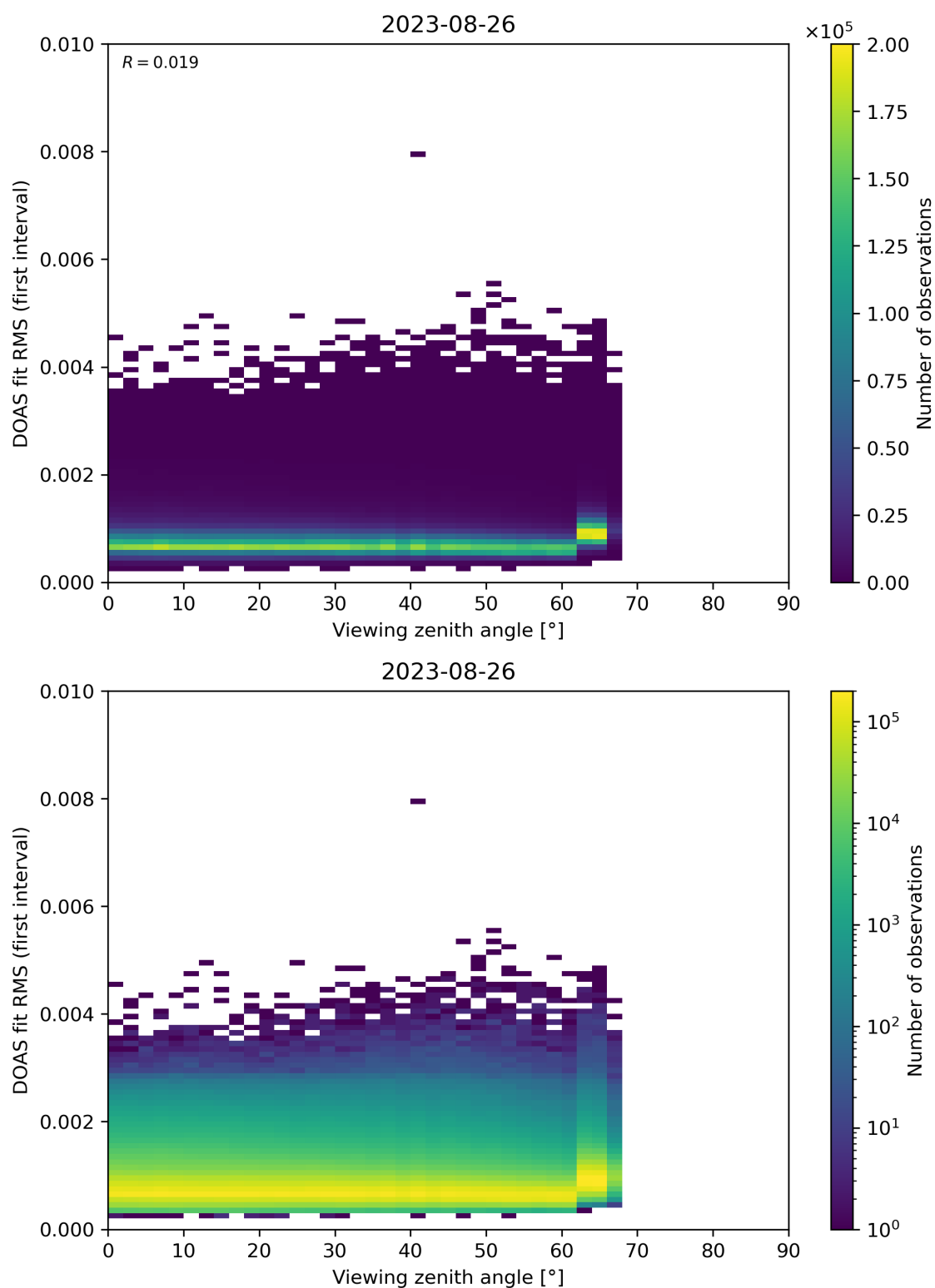
Figure 182: Scatter density plot of “Viewing zenith angle” against “DOAS fit RMS (first interval)” for 2023-08-25 to 2023-08-27.
