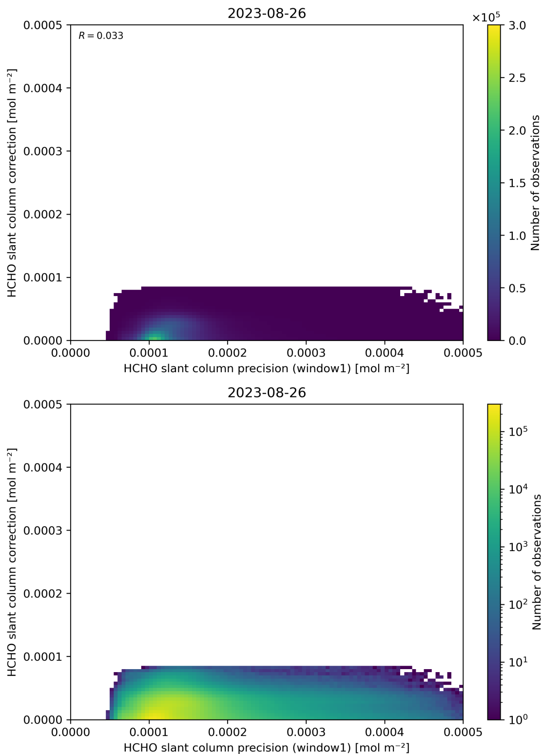
Figure 93: Scatter density plot of “HCHO slant column precision (window1)” against “HCHO slant column correction” for 2023-08-25 to 2023-08-27.
