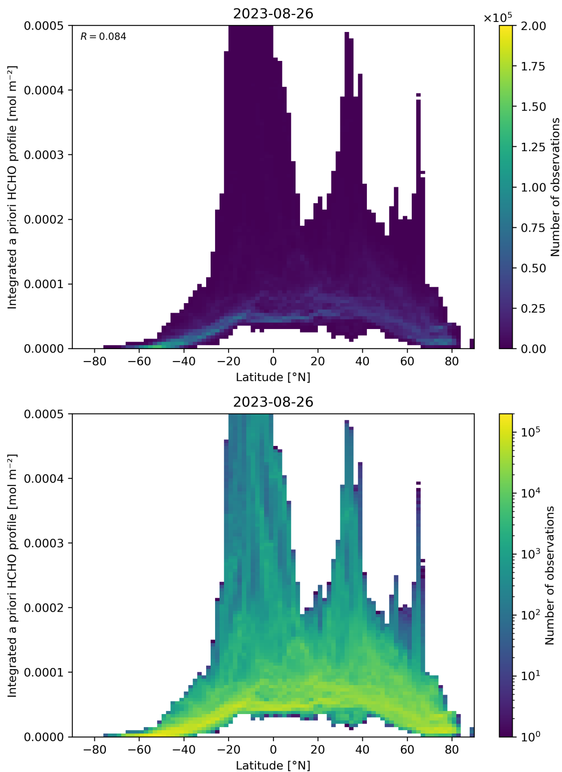
Figure 166: Scatter density plot of “Latitude” against “Integrated a priori HCHO profile” for 2023-08-25 to 2023-08-27.
