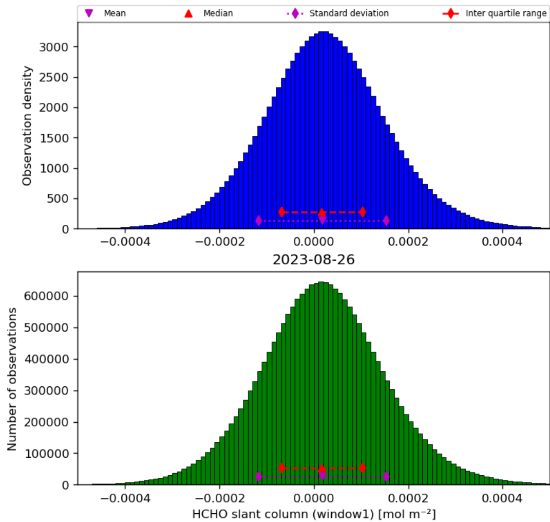
Figure 38: Histogram of “HCHO slant column (window1)” for 2023-08-25 to 2023-08-27
