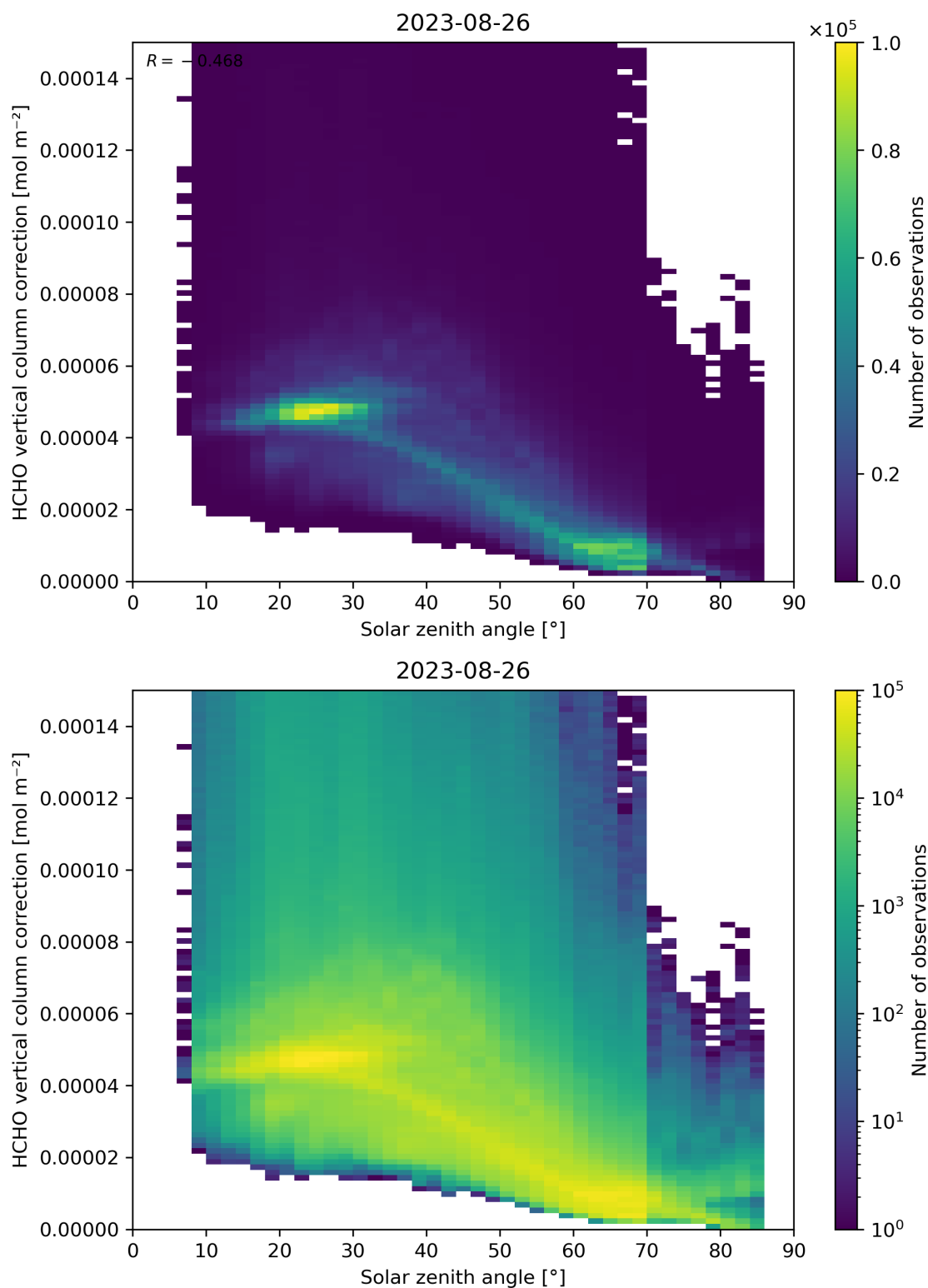
Figure 178: Scatter density plot of “Solar zenith angle” against “HCHO vertical column correction” for 2023-08-25 to 2023-08-27.
