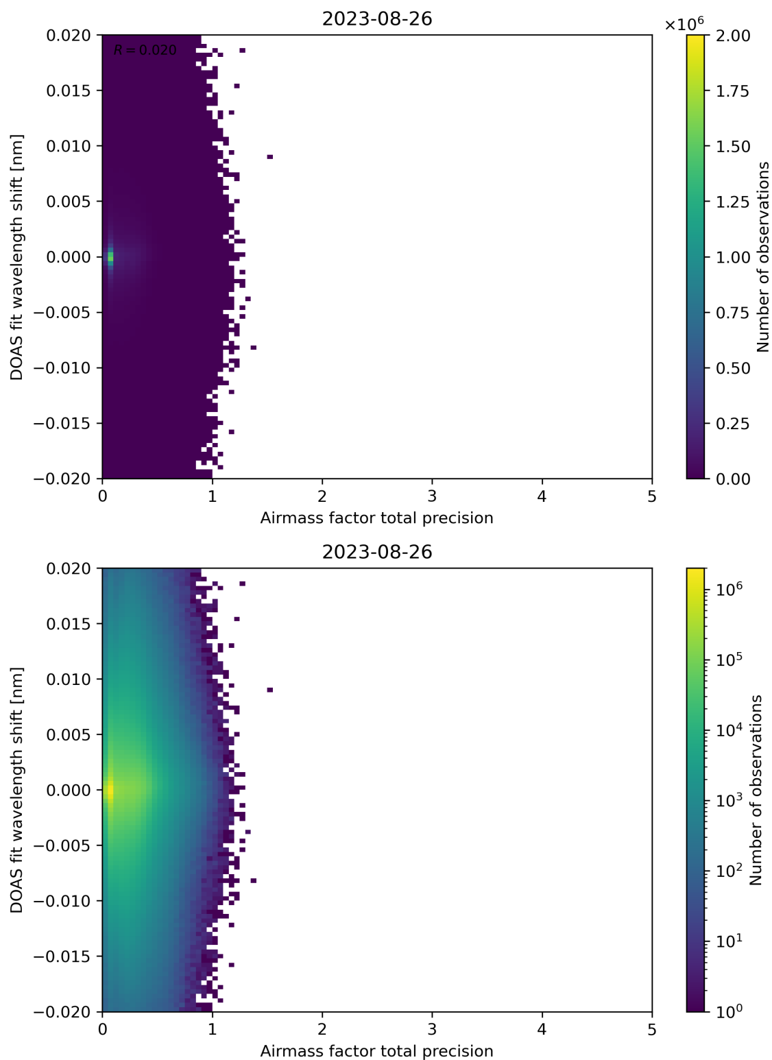
Figure 106: Scatter density plot of “Airmass factor total precision” against “DOAS fit wavelength shift” for 2023-08-25 to 2023-08-27.
