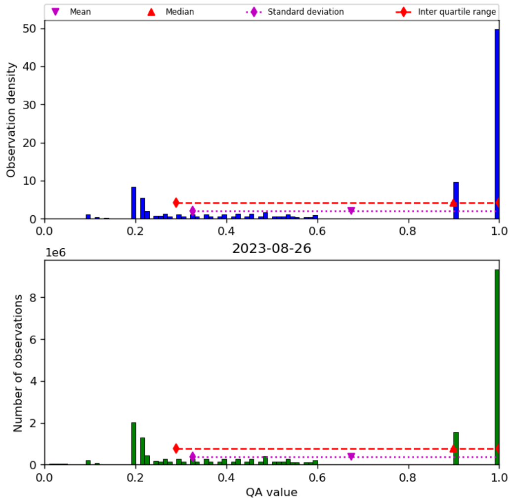
Figure 34: Histogram of “QA value” for 2023-08-25 to 2023-08-27
