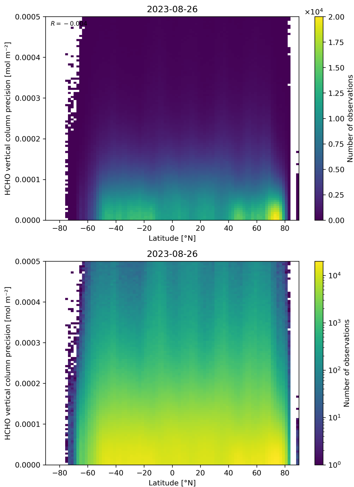
Figure 165: Scatter density plot of “Latitude” against “HCHO vertical column precision” for 2023-08-25 to 2023-08-27.
