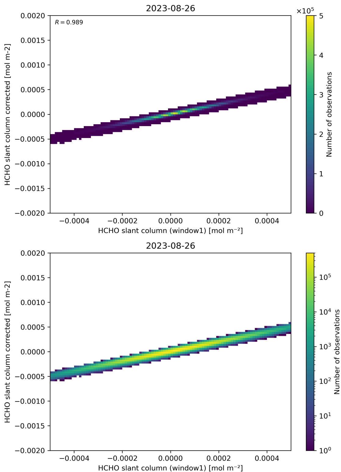
Figure 82: Scatter density plot of “HCHO slant column (window1)” against “HCHO slant column corrected” for 2023-08-25 to 2023-08-27.
