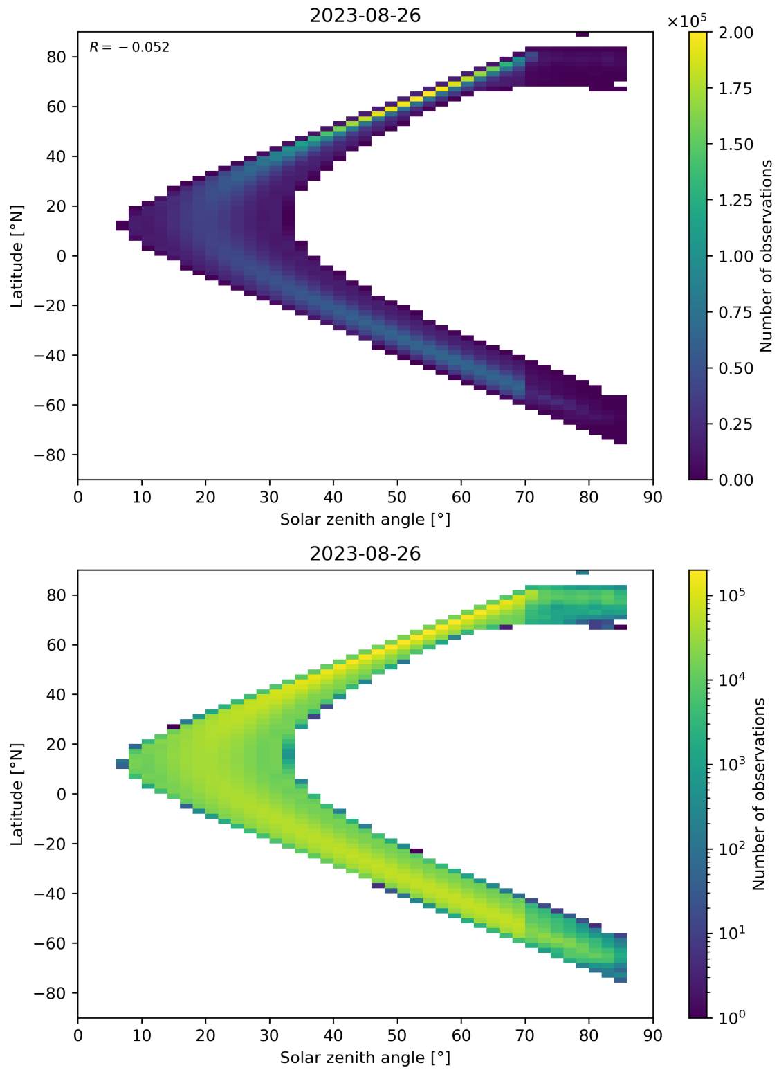
Figure 181: Scatter density plot of “Solar zenith angle” against “Latitude” for 2023-08-25 to 2023-08-27.
