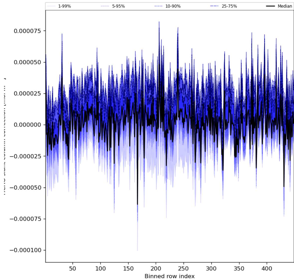
Figure 61: Along track statistics of “HCHO slant column correction” for 2023-08-25 to 2023-08-27
