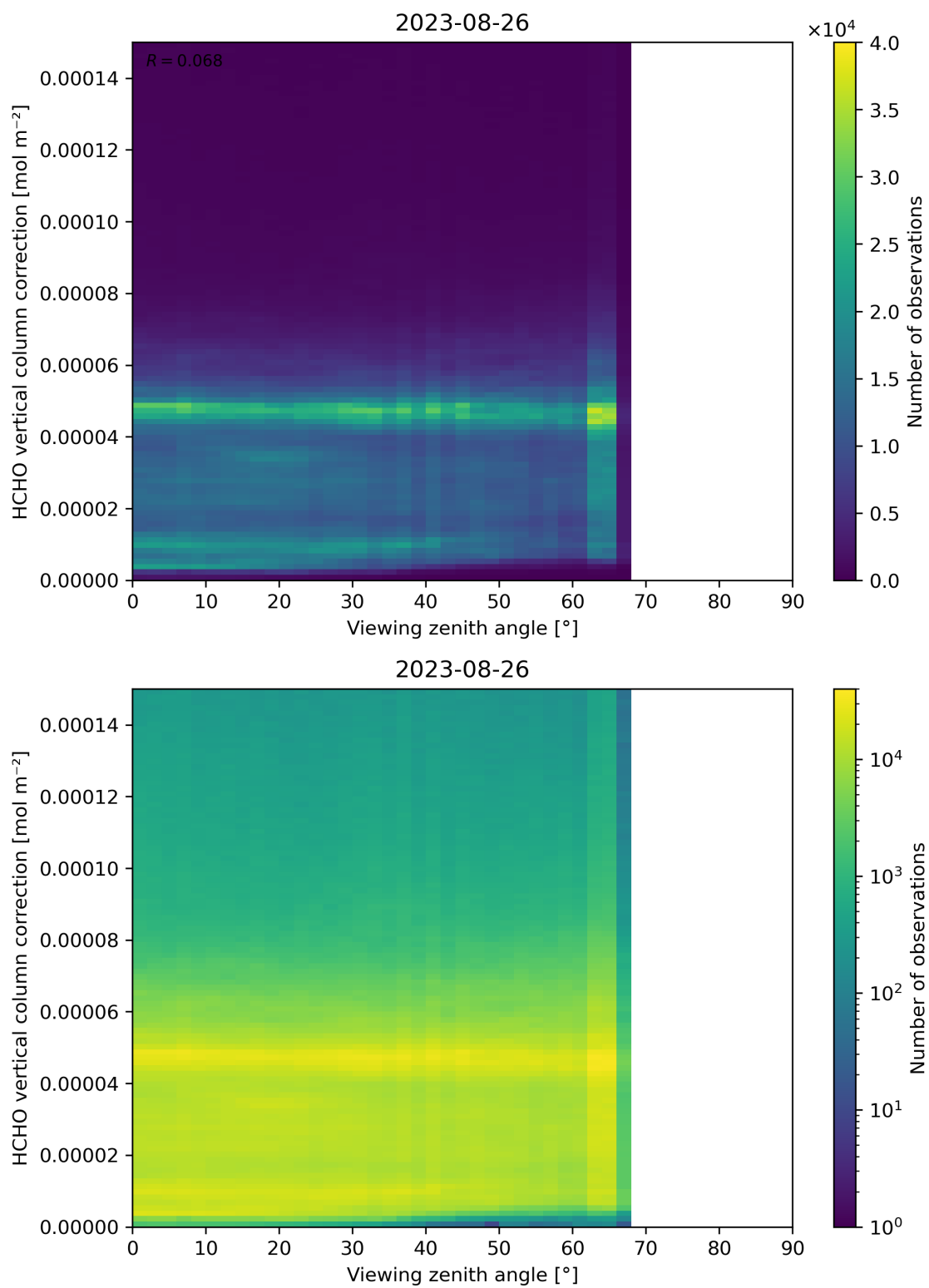
Figure 193: Scatter density plot of “Viewing zenith angle” against “HCHO vertical column correction” for 2023-08-25 to 2023-08-27.
