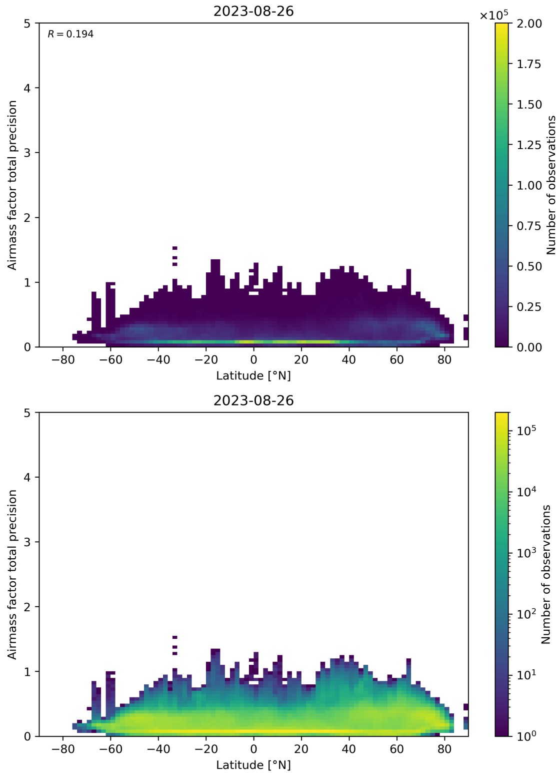
Figure 162: Scatter density plot of “Latitude” against “Airmass factor total precision” for 2023-08-25 to 2023-08-27.
