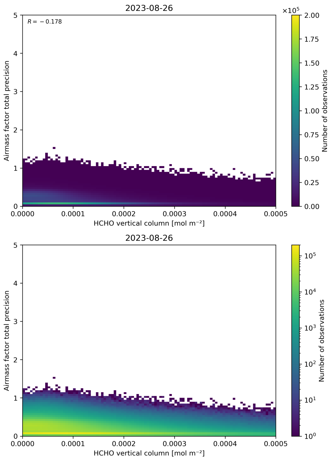
Figure 132: Scatter density plot of “HCHO vertical column” against “Airmass factor total precision” for 2023-08-25 to 2023-08-27.
