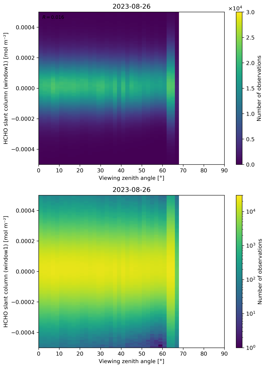
Figure 188: Scatter density plot of “Viewing zenith angle” against “HCHO slant column (window1)” for 2023-08-25 to 2023-08-27.
