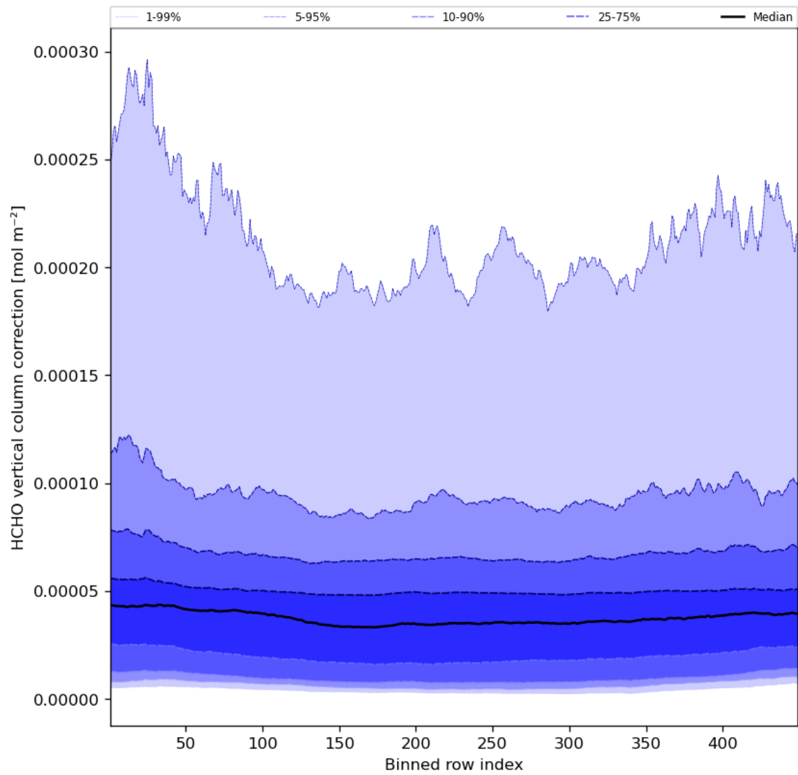
Figure 51: Along track statistics of “HCHO vertical column correction” for 2023-08-25 to 2023-08-27
