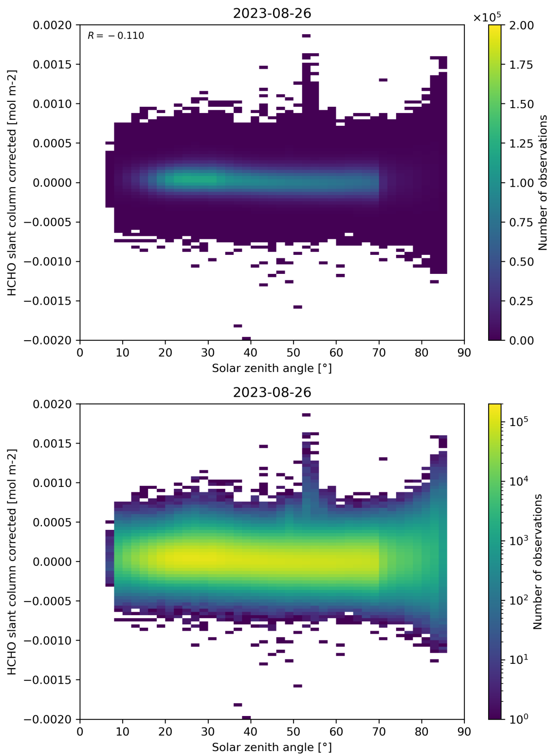
Figure 171: Scatter density plot of “Solar zenith angle” against “HCHO slant column corrected” for 2023-08-25 to 2023-08-27.
