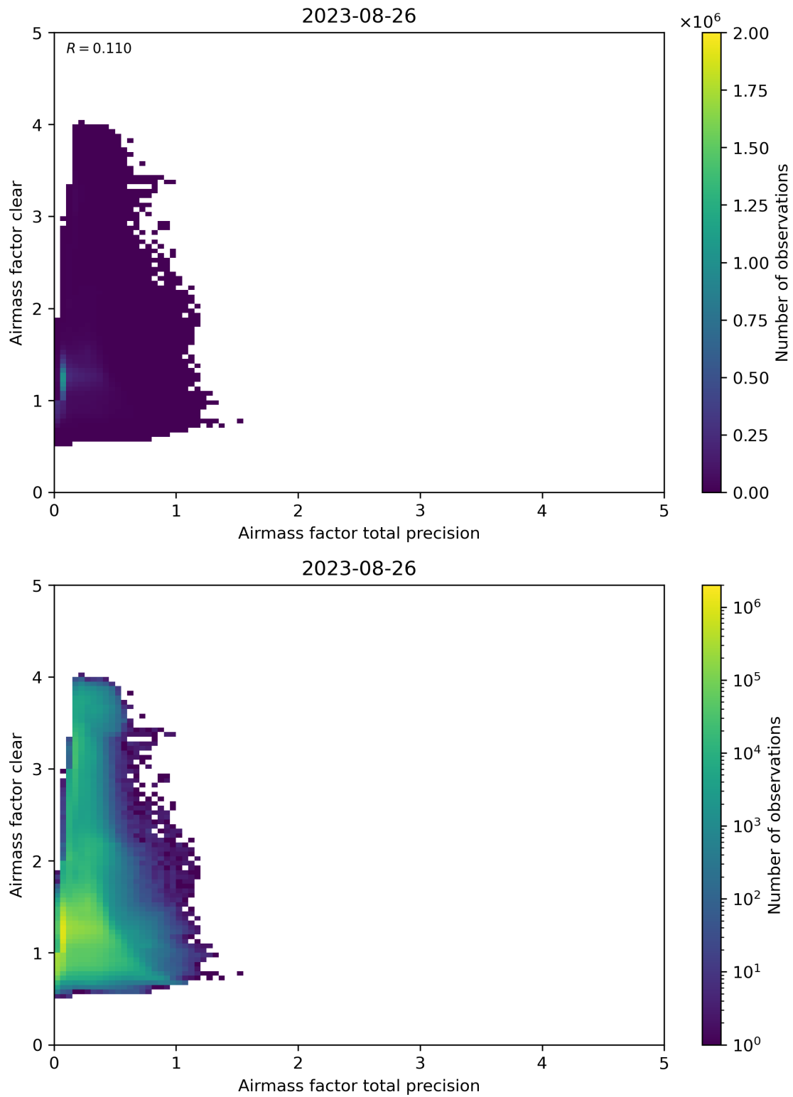
Figure 108: Scatter density plot of “Airmass factor total precision” against “Airmass factor clear” for 2023-08-25 to 2023-08-27.
