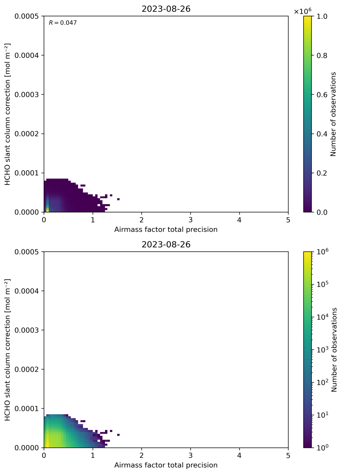
Figure 110: Scatter density plot of “Airmass factor total precision” against “HCHO slant column correction” for 2023-08-25 to 2023-08-27.
