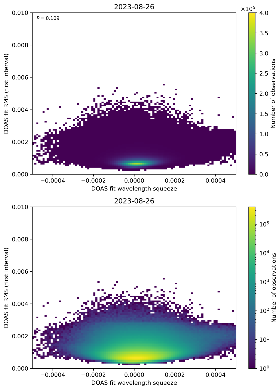
Figure 68: Scatter density plot of “DOAS fit wavelength squeeze” against “DOAS fit RMS (first interval)” for 2023-08-25 to 2023-08-27.
