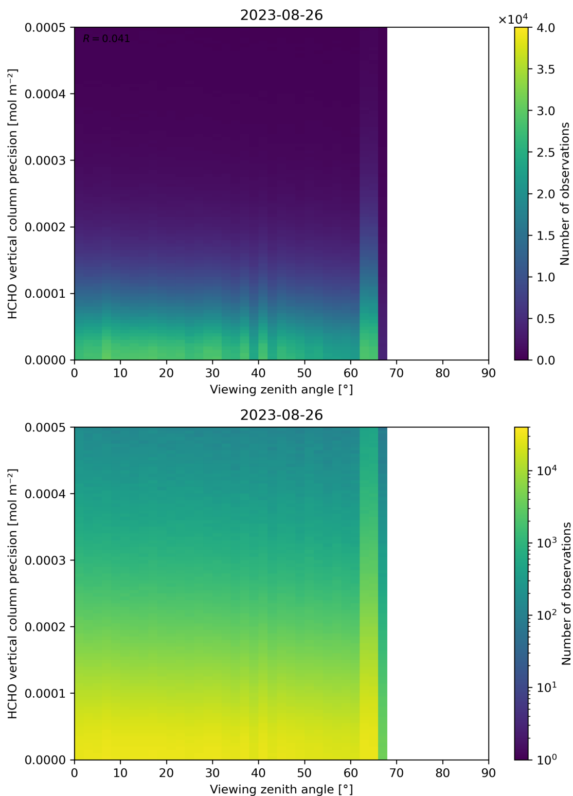
Figure 194: Scatter density plot of “Viewing zenith angle” against “HCHO vertical column precision” for 2023-08-25 to 2023-08-27.
