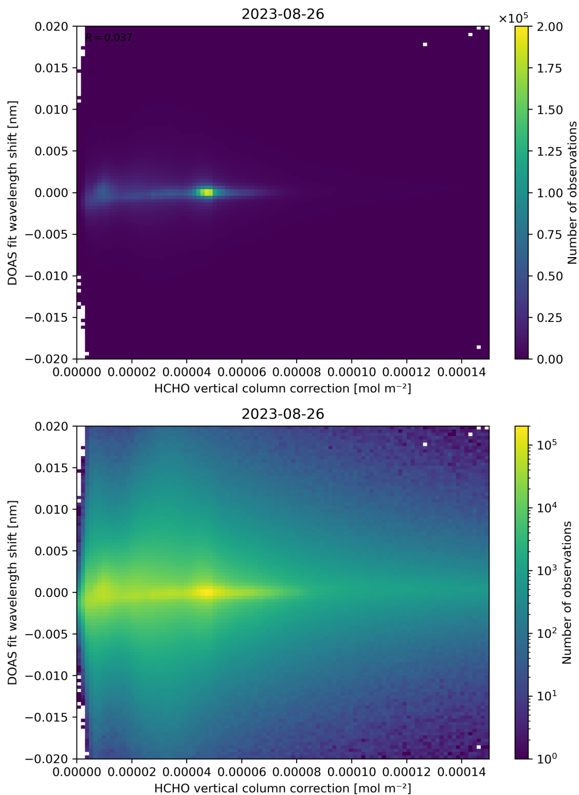
Figure 113: Scatter density plot of “HCHO vertical column correction” against “DOAS fit wavelength shift” for 2023-08-25 to 2023-08-27.
