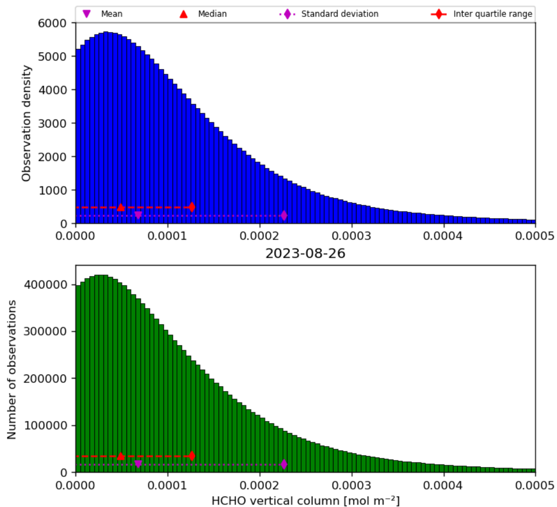
Figure 35: Histogram of “HCHO vertical column” for 2023-08-25 to 2023-08-27
