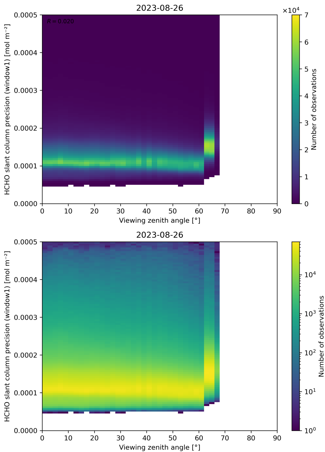
Figure 189: Scatter density plot of “Viewing zenith angle” against “HCHO slant column precision (window1)” for 2023-08-25 to 2023-08-27.
