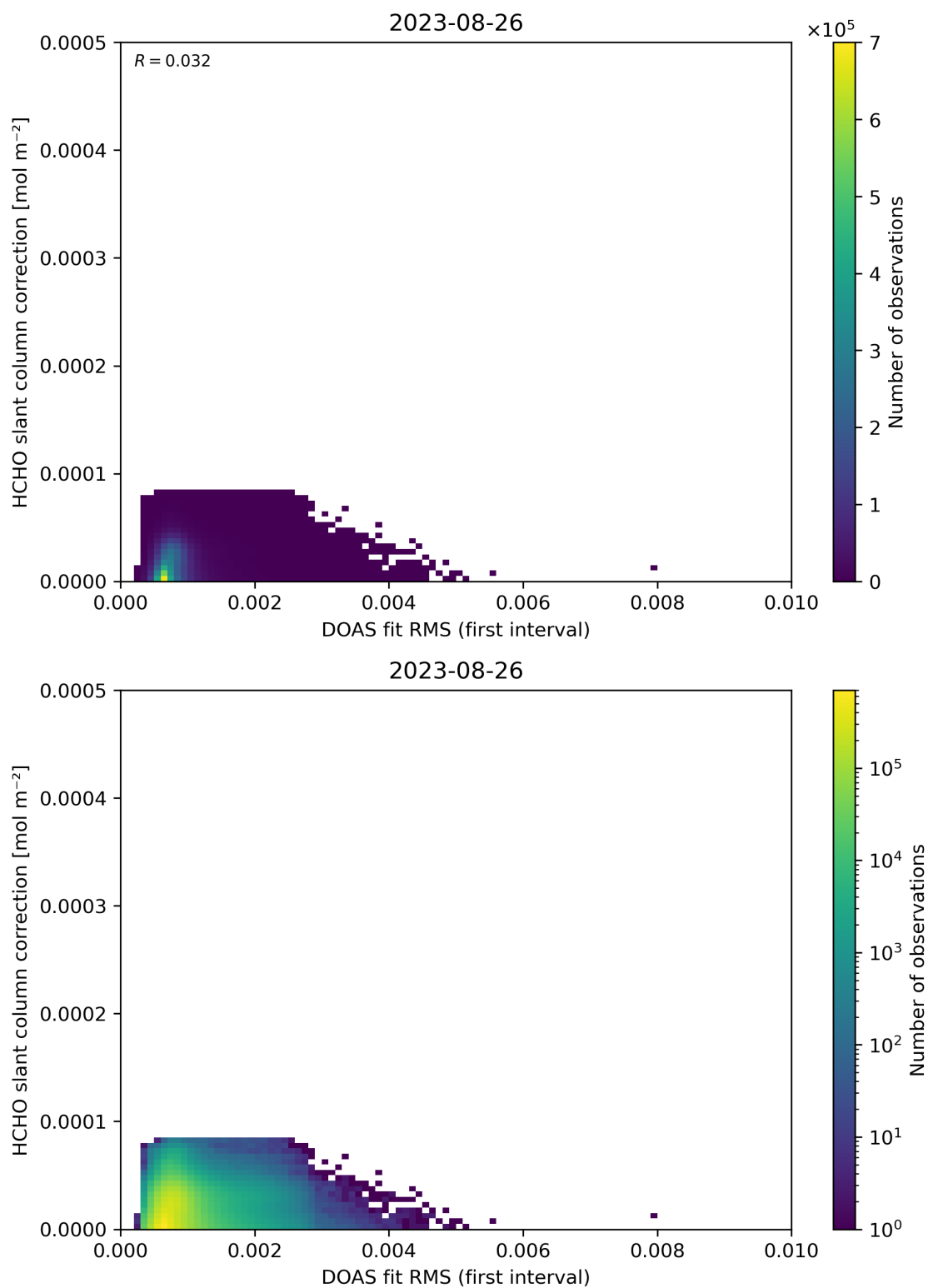
Figure 63: Scatter density plot of “DOAS fit RMS (first interval)” against “HCHO slant column correction” for 2023-08-25 to 2023-08-27.
