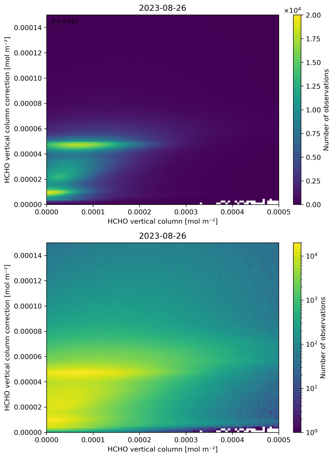
Figure 133: Scatter density plot of “HCHO vertical column” against “HCHO vertical column correction” for 2023-08-25 to 2023-08-27.
