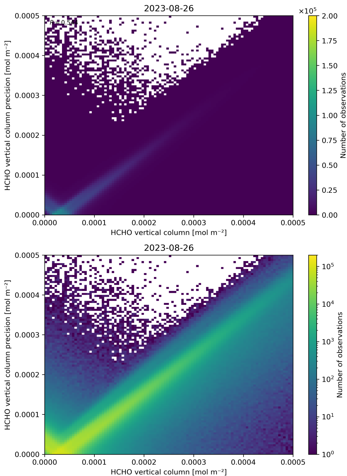
Figure 134: Scatter density plot of “HCHO vertical column” against “HCHO vertical column precision” for 2023-08-25 to 2023-08-27.
