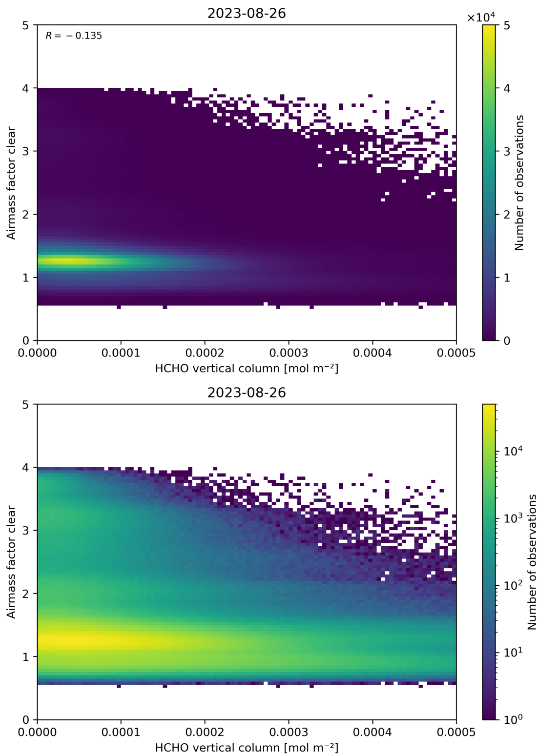
Figure 126: Scatter density plot of “HCHO vertical column” against “Airmass factor clear” for 2023-08-25 to 2023-08-27.
