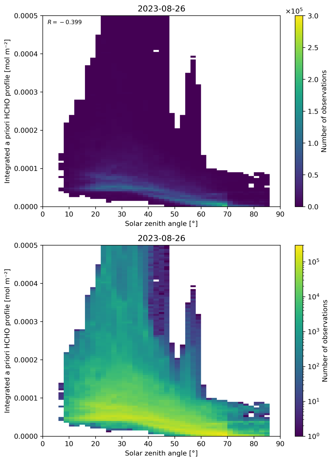
Figure 180: Scatter density plot of “Solar zenith angle” against “Integrated a priori HCHO profile” for 2023-08-25 to 2023-08-27.
