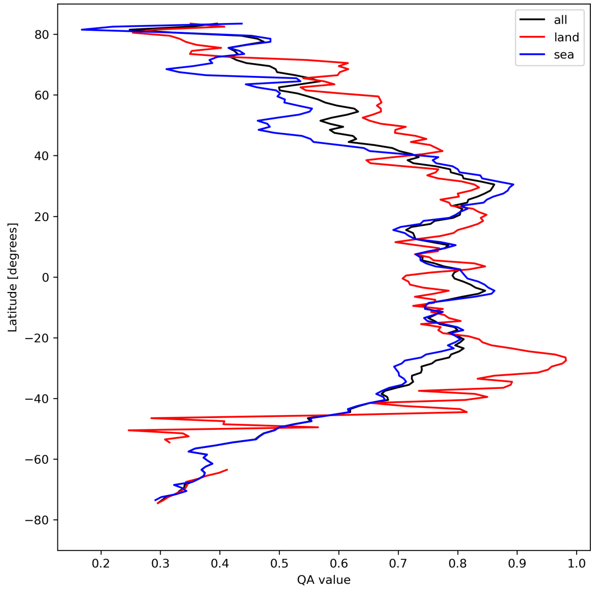
Figure 20: Zonal average of “QA value” for 2023-08-25 to 2023-08-27.
