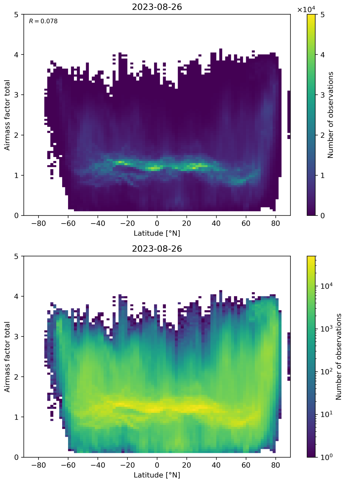
Figure 161: Scatter density plot of “Latitude” against “Airmass factor total” for 2023-08-25 to 2023-08-27.
