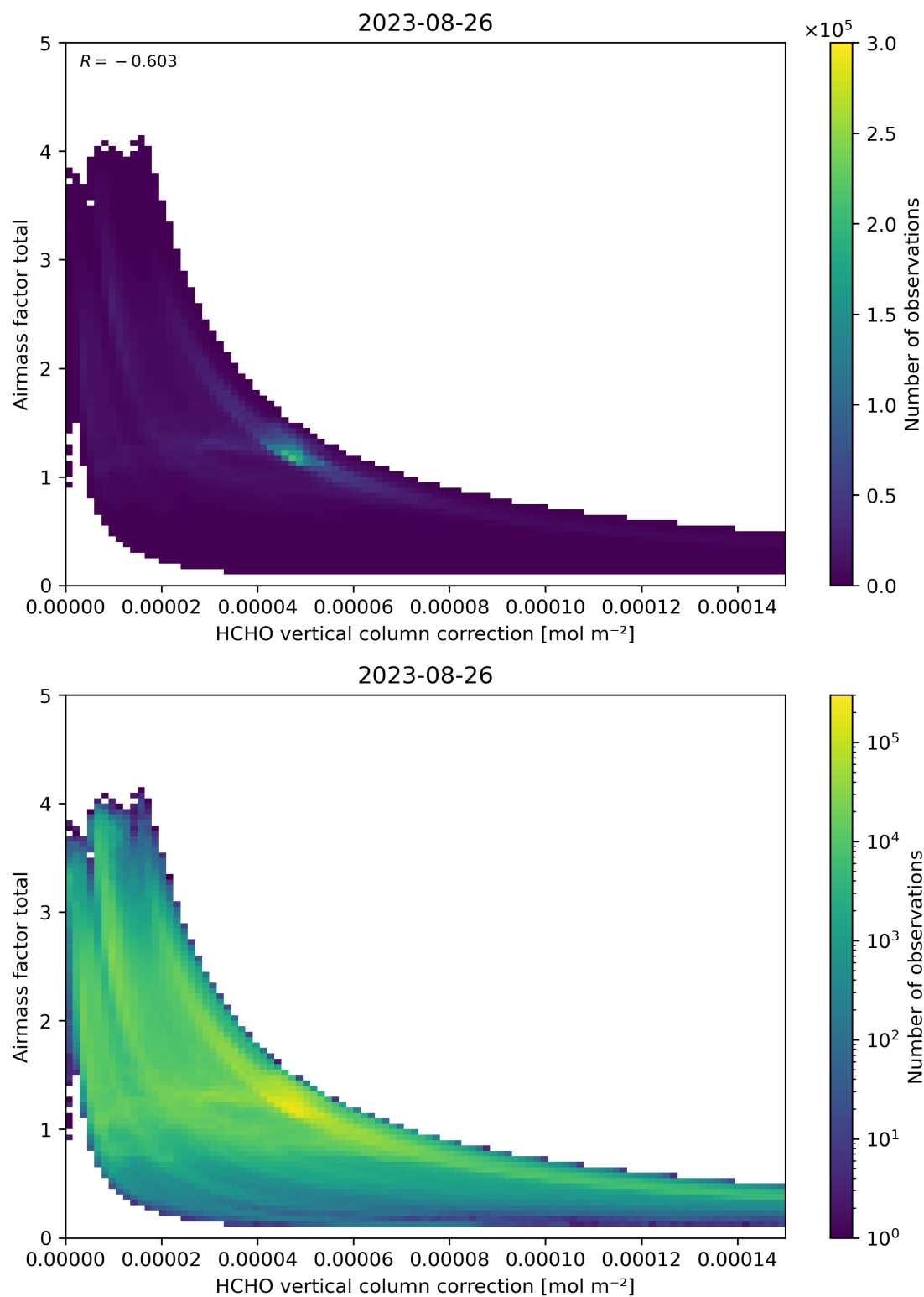
Figure 120: Scatter density plot of “HCHO vertical column correction” against “Airmass factor total” for 2023-08-25 to 2023-08-27.
