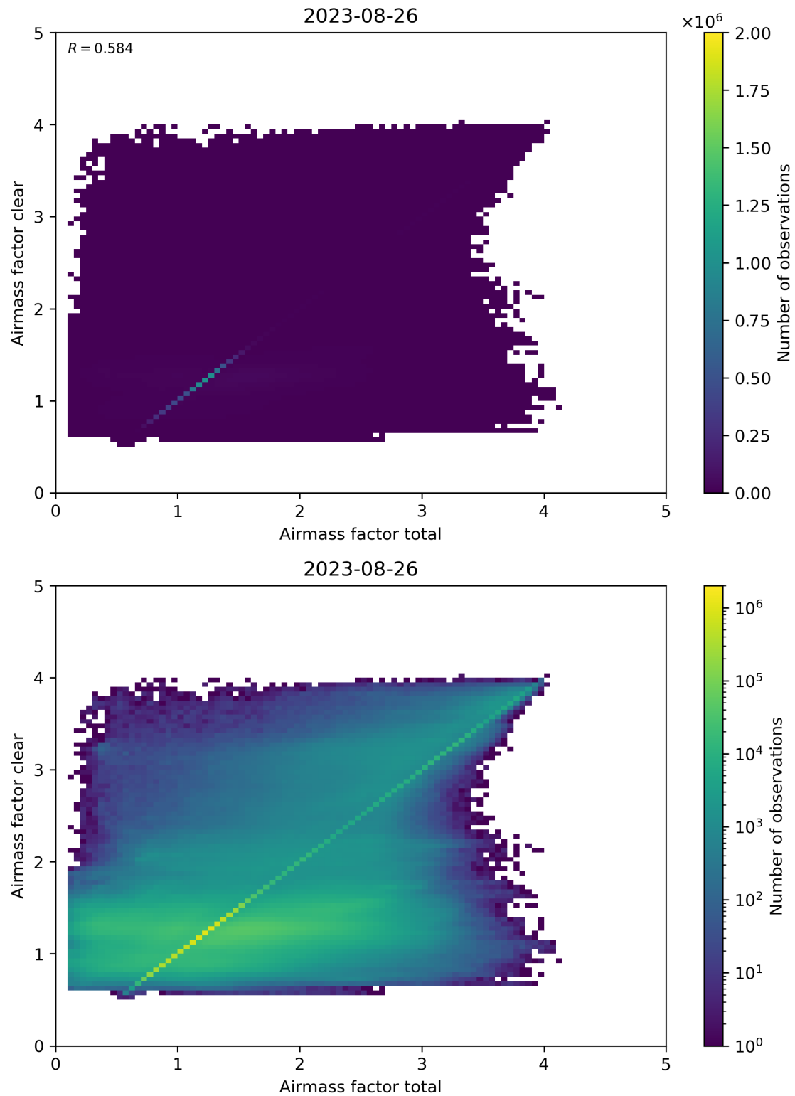
Figure 100: Scatter density plot of “Airmass factor total” against “Airmass factor clear” for 2023-08-25 to 2023-08-27.
