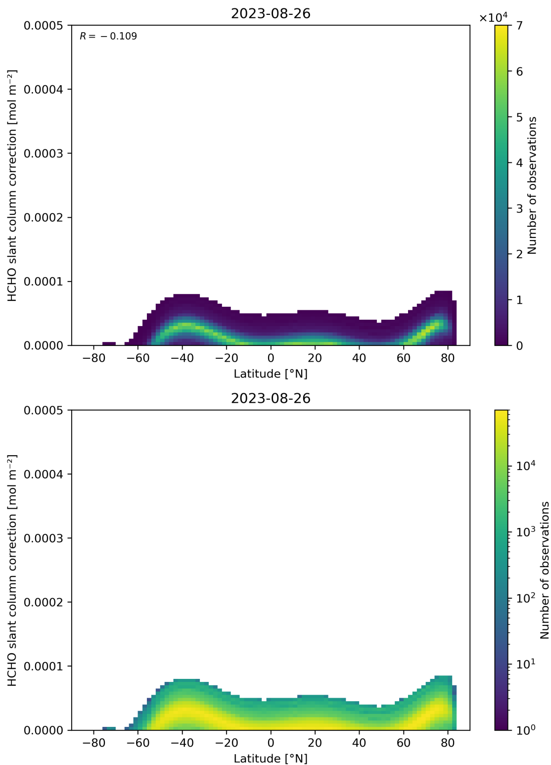
Figure 158: Scatter density plot of “Latitude” against “HCHO slant column correction” for 2023-08-25 to 2023-08-27.
