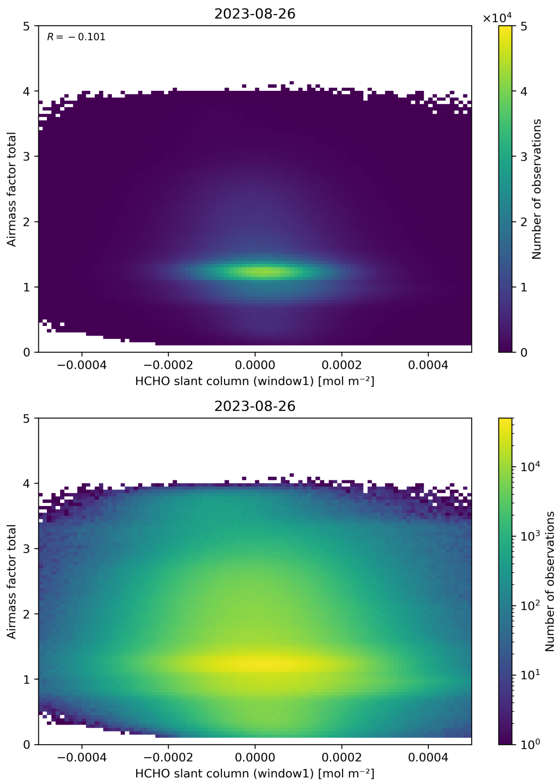
Figure 85: Scatter density plot of “HCHO slant column (window1)” against “Airmass factor total” for 2023-08-25 to 2023-08-27.
