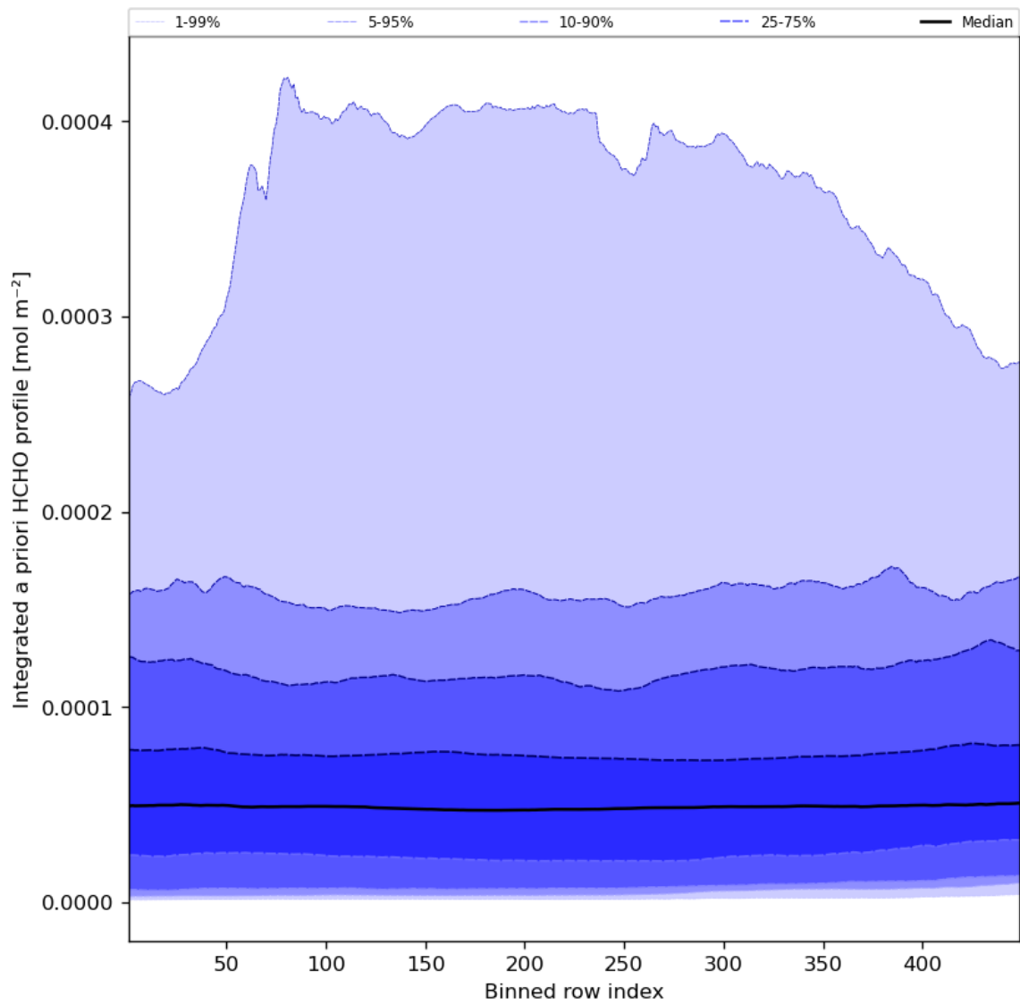
Figure 57: Along track statistics of “Integrated a priori HCHO profile” for 2023-08-25 to 2023-08-27
