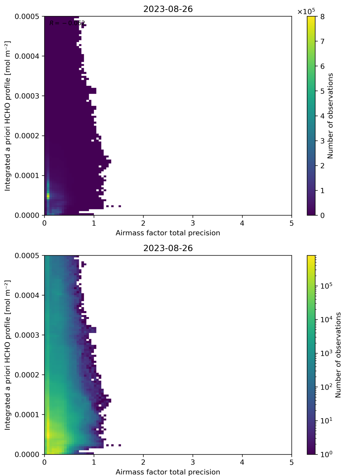
Figure 111: Scatter density plot of “Airmass factor total precision” against “Integrated a priori HCHO profile” for 2023-08-25 to 2023-08-27.
