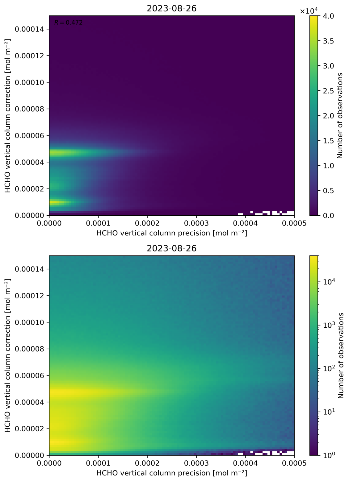
Figure 146: Scatter density plot of “HCHO vertical column precision” against “HCHO vertical column correction” for 2023-08-25 to 2023-08-27.
