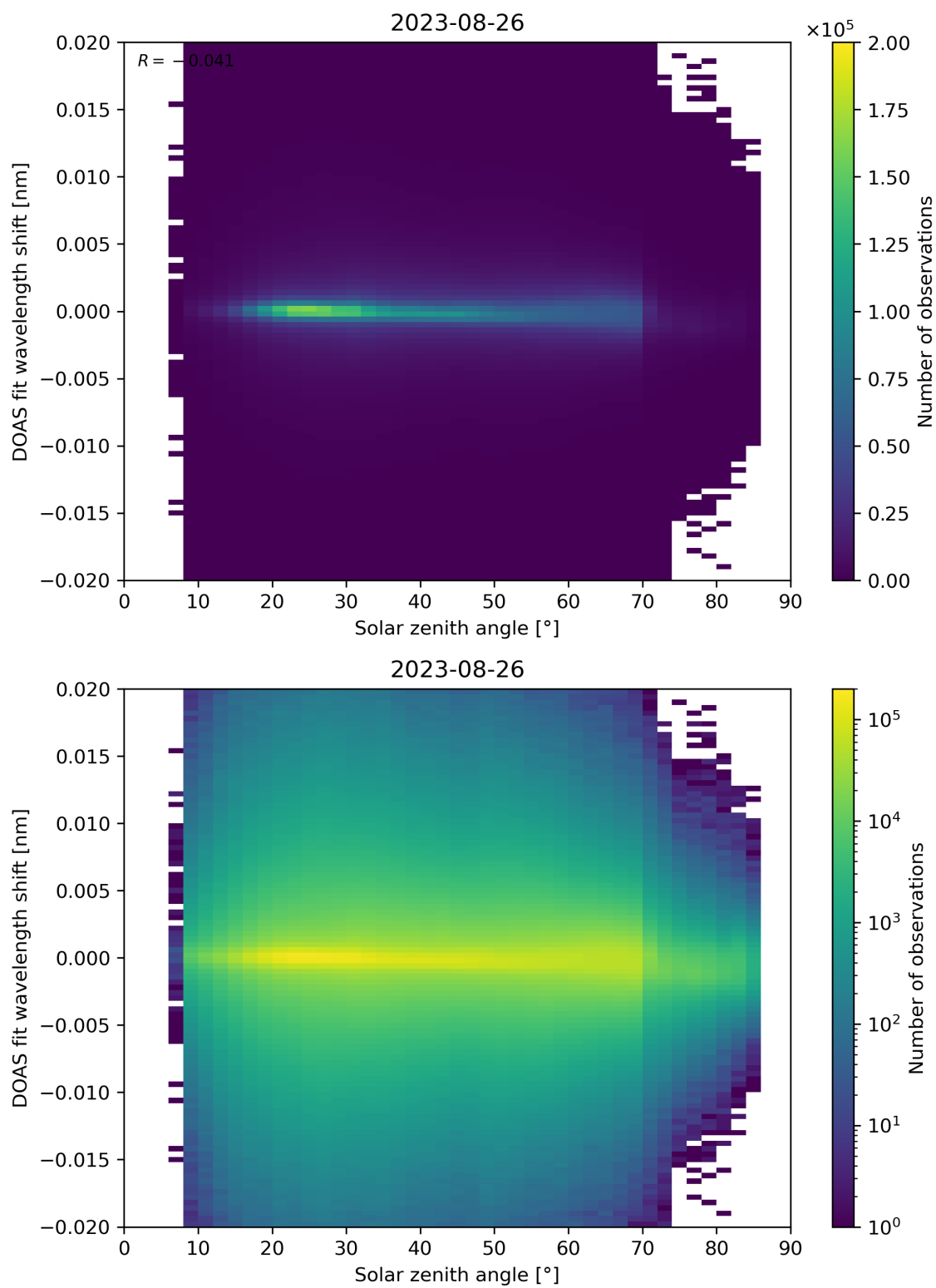
Figure 168: Scatter density plot of “Solar zenith angle” against “DOAS fit wavelength shift” for 2023-08-25 to 2023-08-27.
