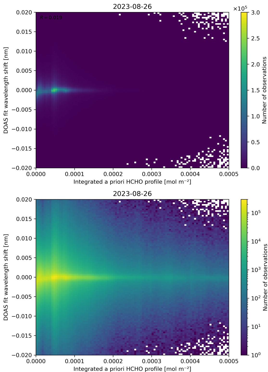
Figure 149: Scatter density plot of “Integrated a priori HCHO profile” against “DOAS fit wavelength shift” for 2023-08-25 to 2023-08-27.
