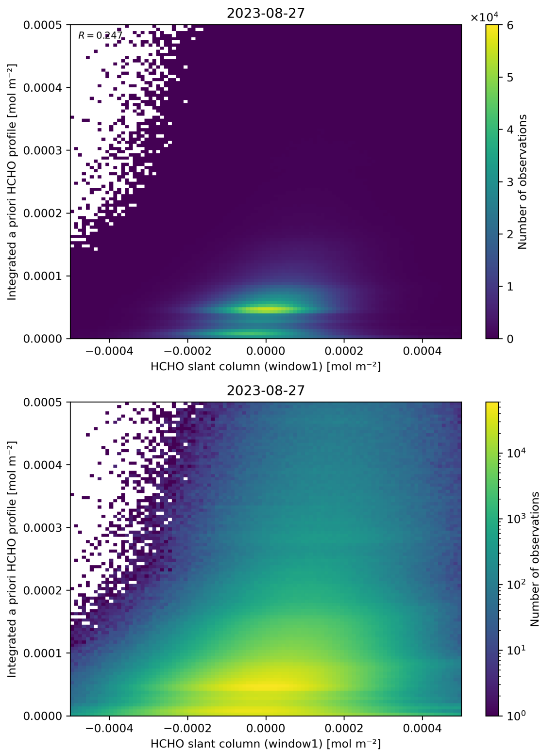
Figure 87: Scatter density plot of “HCHO slant column (window1)” against “Integrated a priori HCHO profile” for 2023-08-26 to 2023-08-28.
