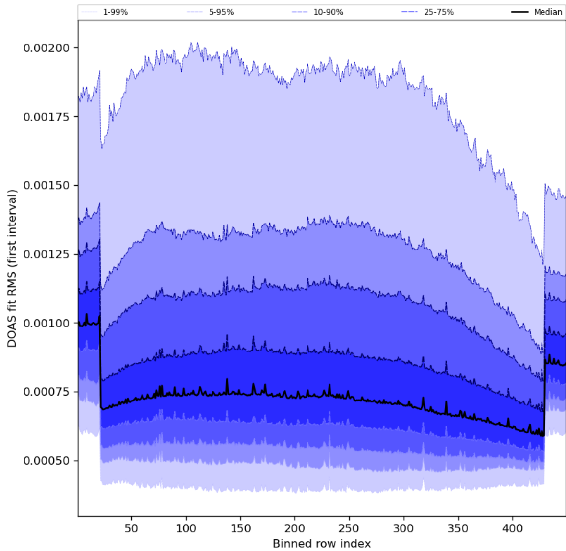
Figure 60: Along track statistics of “DOAS fit RMS (first interval)” for 2023-08-26 to 2023-08-28
