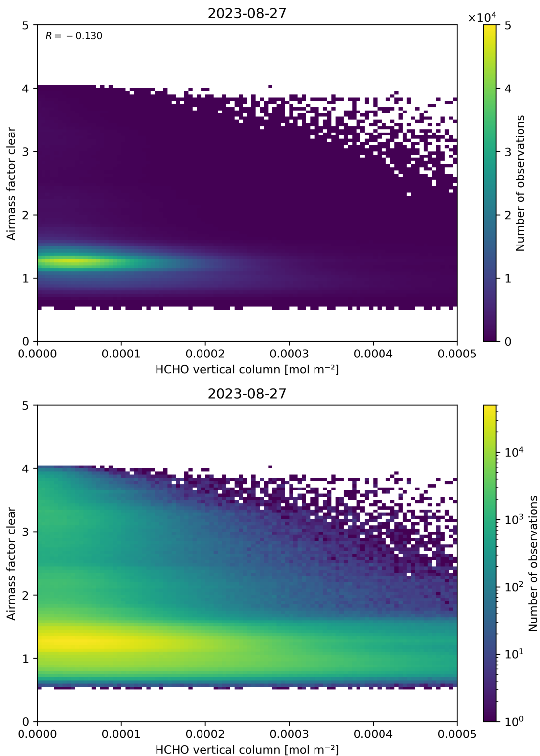
Figure 126: Scatter density plot of “HCHO vertical column” against “Airmass factor clear” for 2023-08-26 to 2023-08-28.
