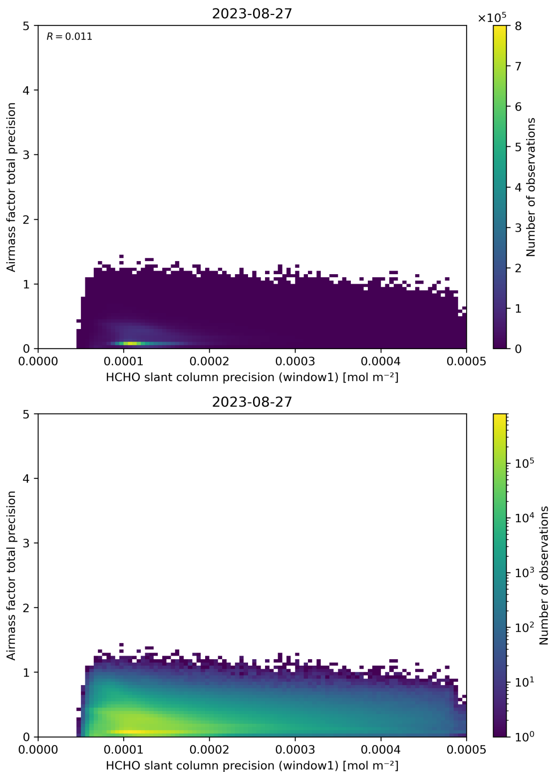
Figure 95: Scatter density plot of “HCHO slant column precision (window1)” against “Airmass factor total precision” for 2023-08-26 to 2023-08-28.
