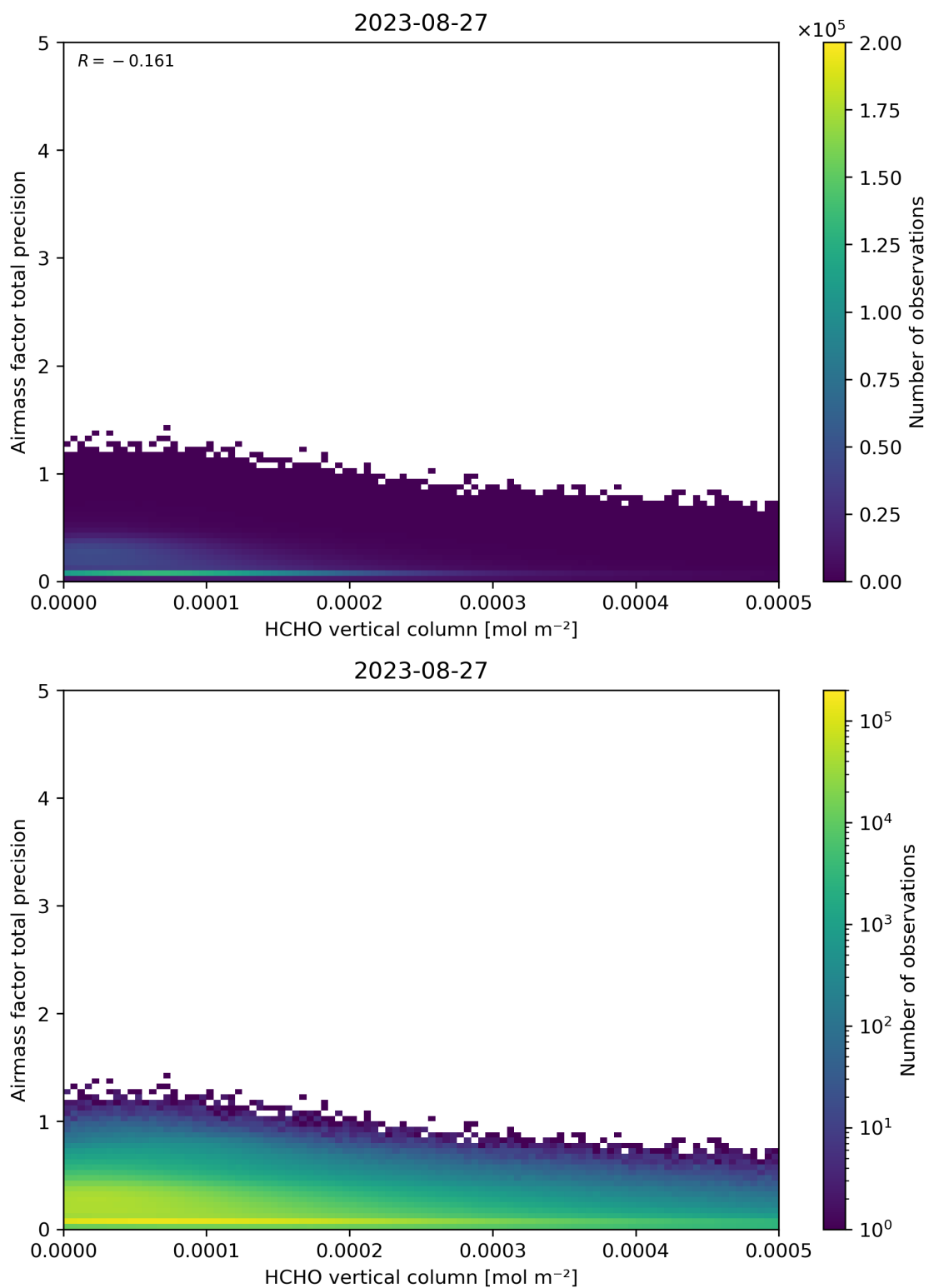
Figure 132: Scatter density plot of “HCHO vertical column” against “Airmass factor total precision” for 2023-08-26 to 2023-08-28.
