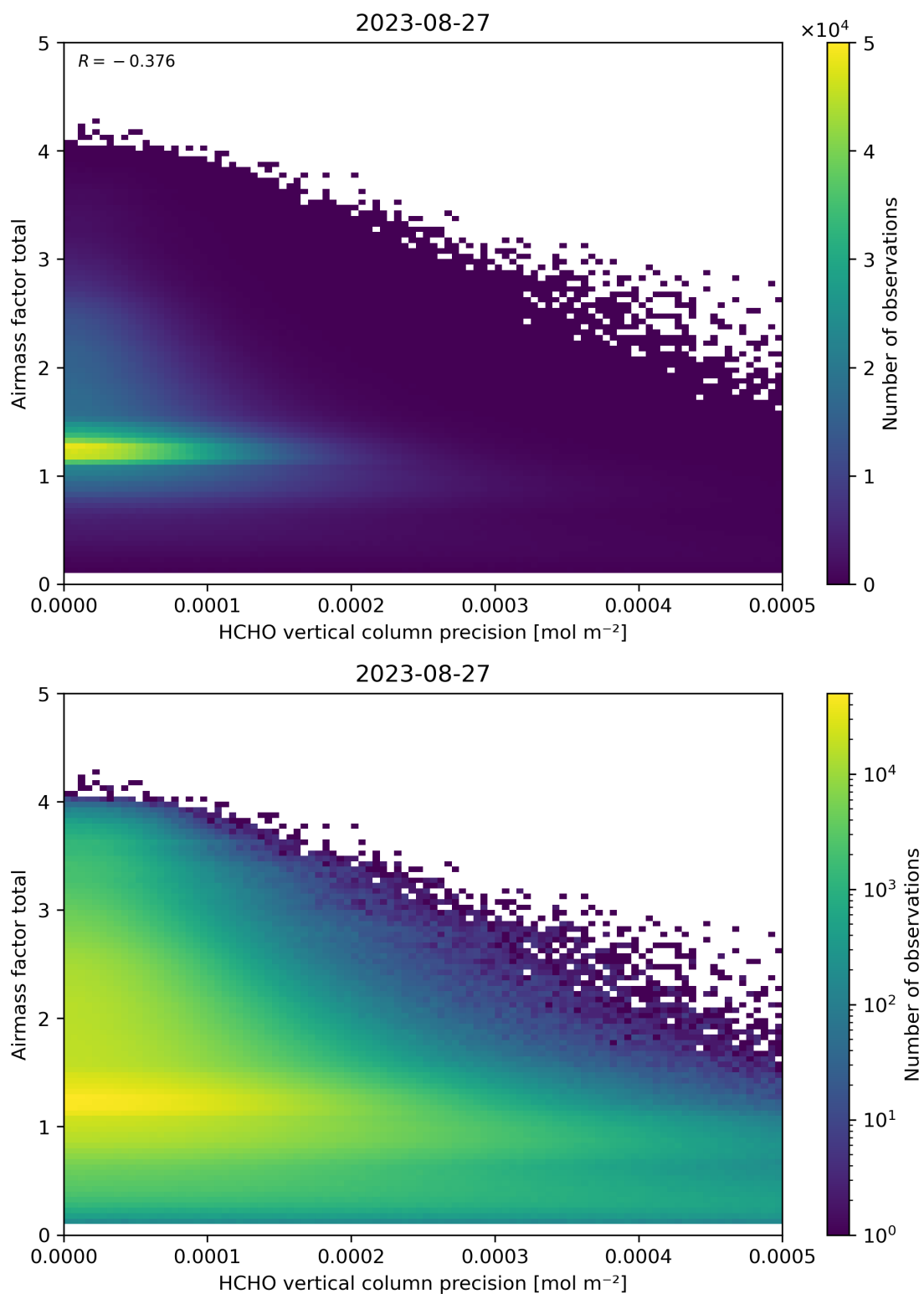
Figure 144: Scatter density plot of “HCHO vertical column precision” against “Airmass factor total” for 2023-08-26 to 2023-08-28.
