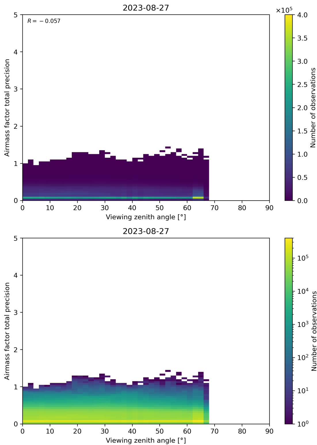
Figure 191: Scatter density plot of “Viewing zenith angle” against “Airmass factor total precision” for 2023-08-26 to 2023-08-28.
