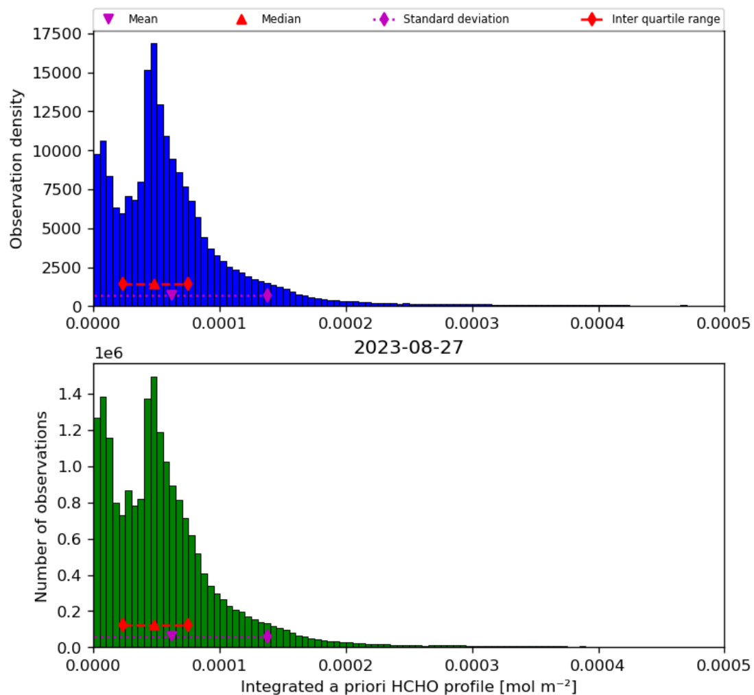
Figure 43: Histogram of “Integrated a priori HCHO profile” for 2023-08-26 to 2023-08-28
