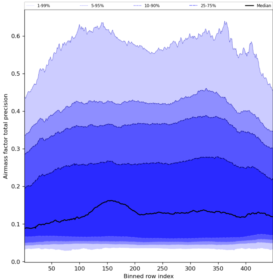
Figure 55: Along track statistics of “Airmass factor total precision” for 2023-08-26 to 2023-08-28
