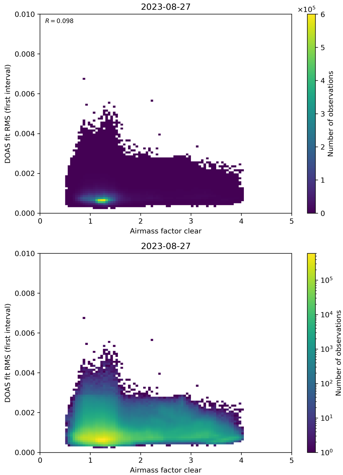
Figure 71: Scatter density plot of “Airmass factor clear” against “DOAS fit RMS (first interval)” for 2023-08-26 to 2023-08-28.
