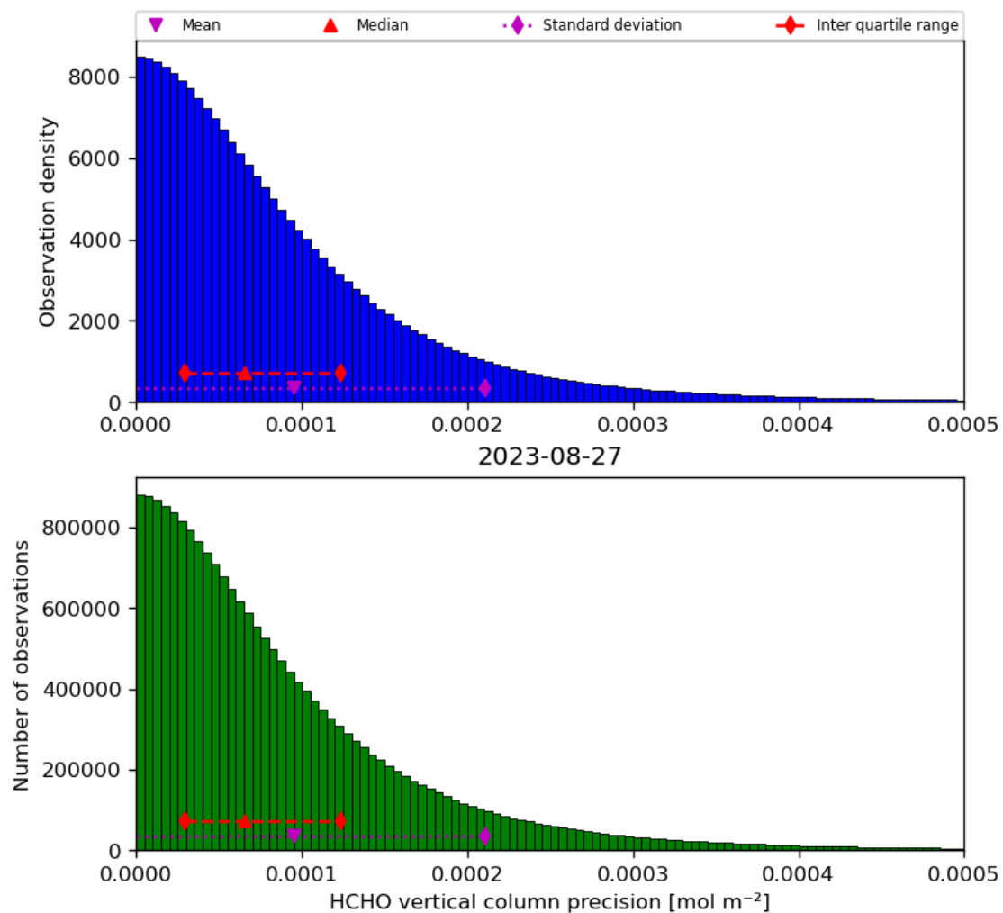
Figure 36: Histogram of “HCHO vertical column precision” for 2023-08-26 to 2023-08-28
