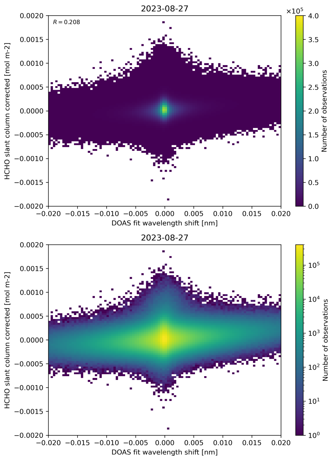
Figure 66: Scatter density plot of “DOAS fit wavelength shift” against “HCHO slant column corrected” for 2023-08-26 to 2023-08-28.
