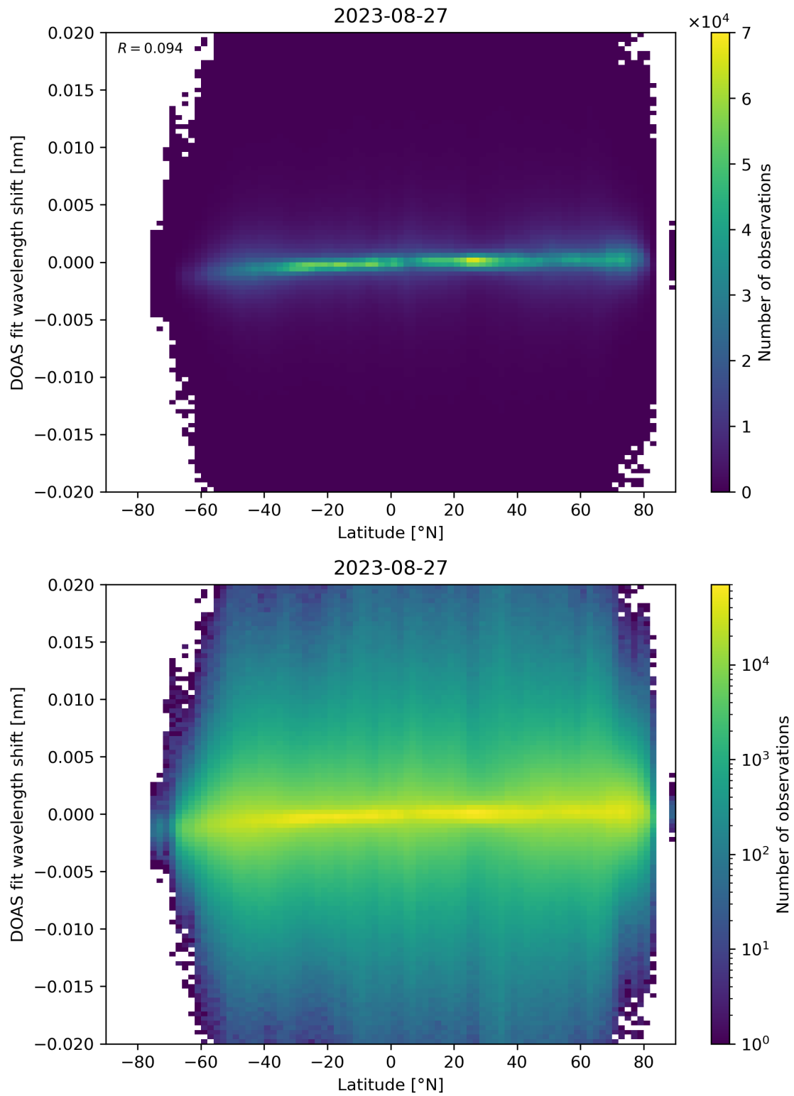
Figure 154: Scatter density plot of “Latitude” against “DOAS fit wavelength shift” for 2023-08-26 to 2023-08-28.
