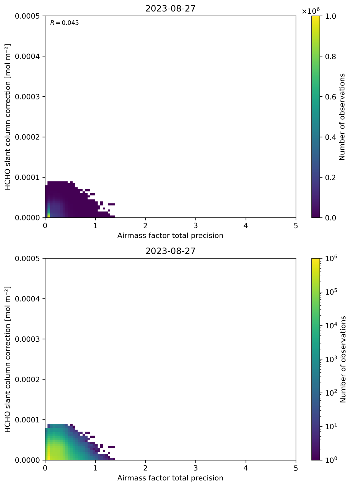
Figure 110: Scatter density plot of “Airmass factor total precision” against “HCHO slant column correction” for 2023-08-26 to 2023-08-28.
