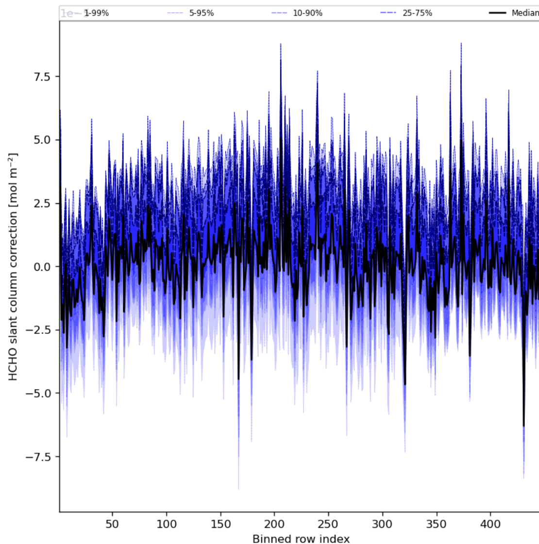
Figure 61: Along track statistics of “HCHO slant column correction” for 2023-08-26 to 2023-08-28
