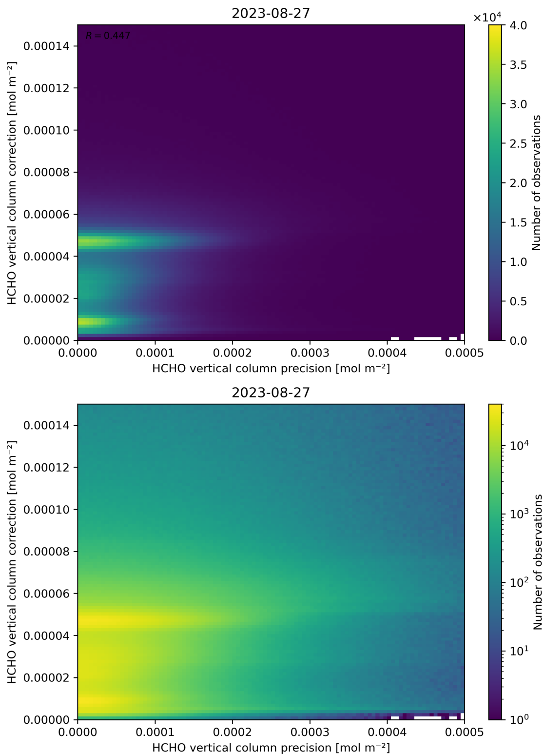
Figure 146: Scatter density plot of “HCHO vertical column precision” against “HCHO vertical column correction” for 2023-08-26 to 2023-08-28.
