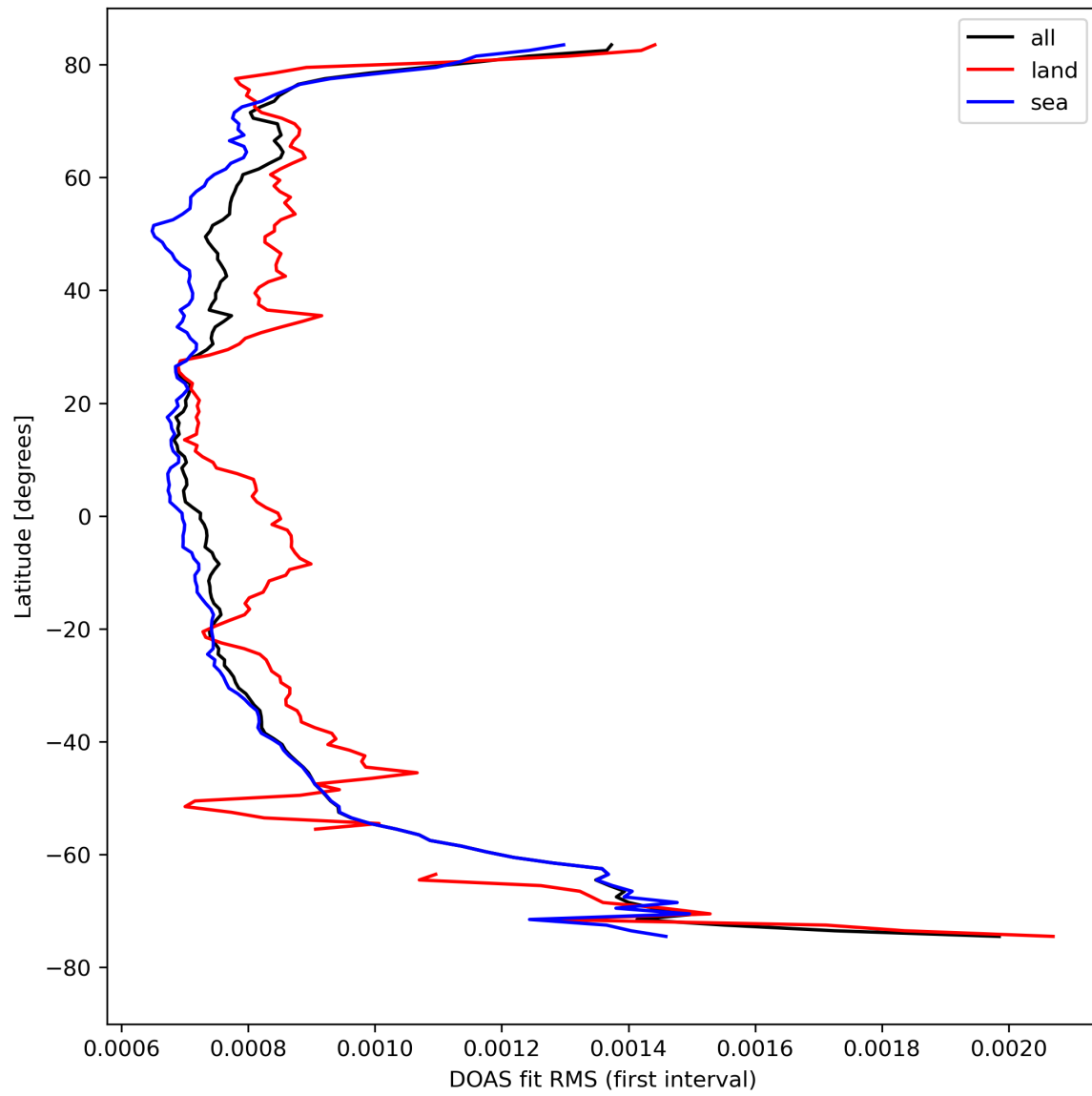
Figure 32: Zonal average of "DOAS fit RMS (first interval)" for 2023-08-26 to 2023-08-28.
