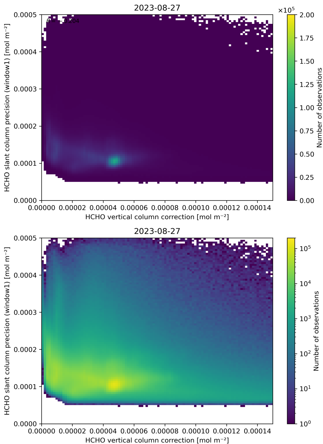
Figure 119: Scatter density plot of “HCHO vertical column correction” against “HCHO slant column precision (window1)” for 2023-08-26 to 2023-08-28.
