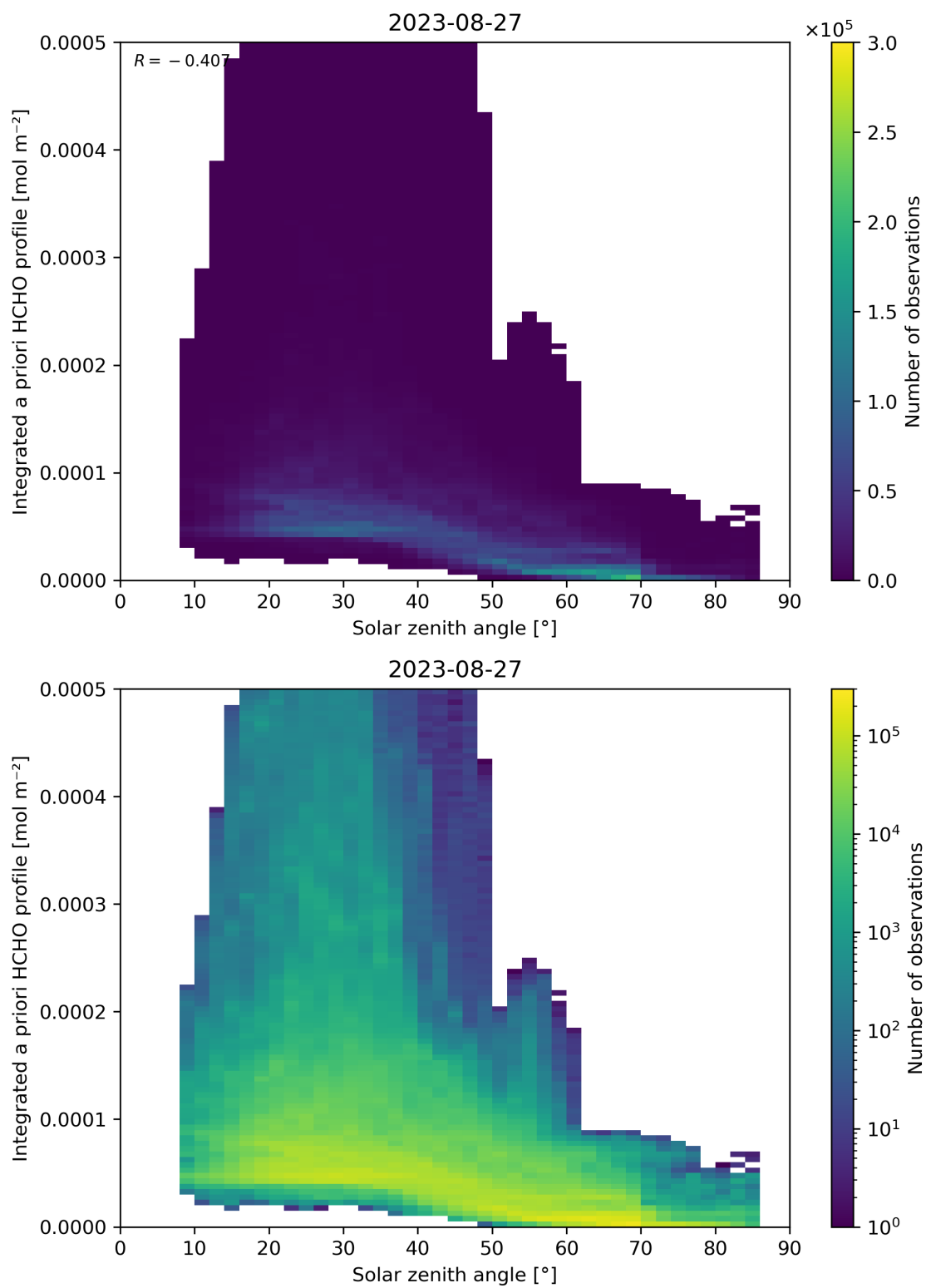
Figure 180: Scatter density plot of “Solar zenith angle” against “Integrated a priori HCHO profile” for 2023-08-26 to 2023-08-28.
