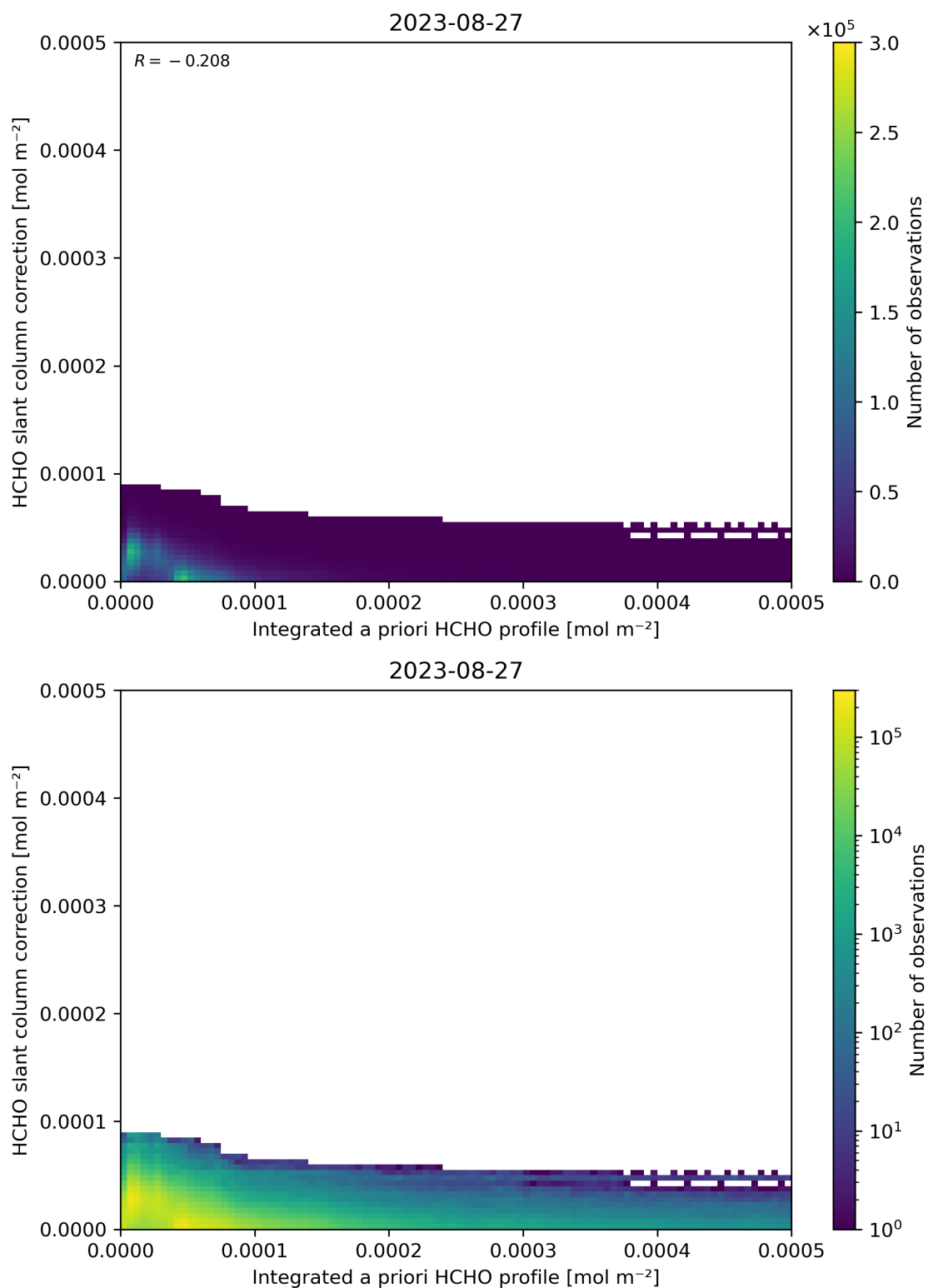
Figure 152: Scatter density plot of “Integrated a priori HCHO profile” against “HCHO slant column correction” for 2023-08-26 to 2023-08-28.
