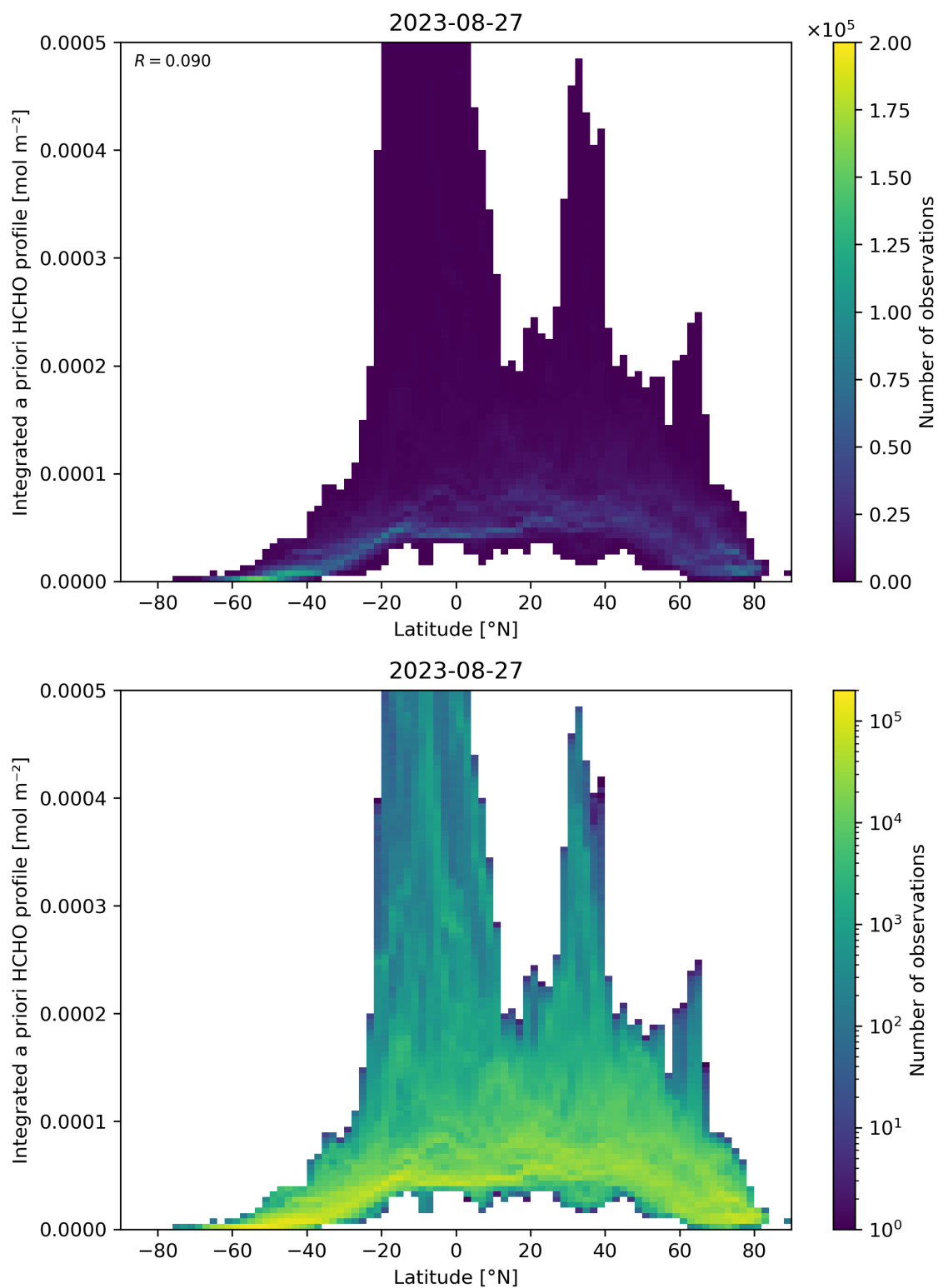
Figure 166: Scatter density plot of “Latitude” against “Integrated a priori HCHO profile” for 2023-08-26 to 2023-08-28.
