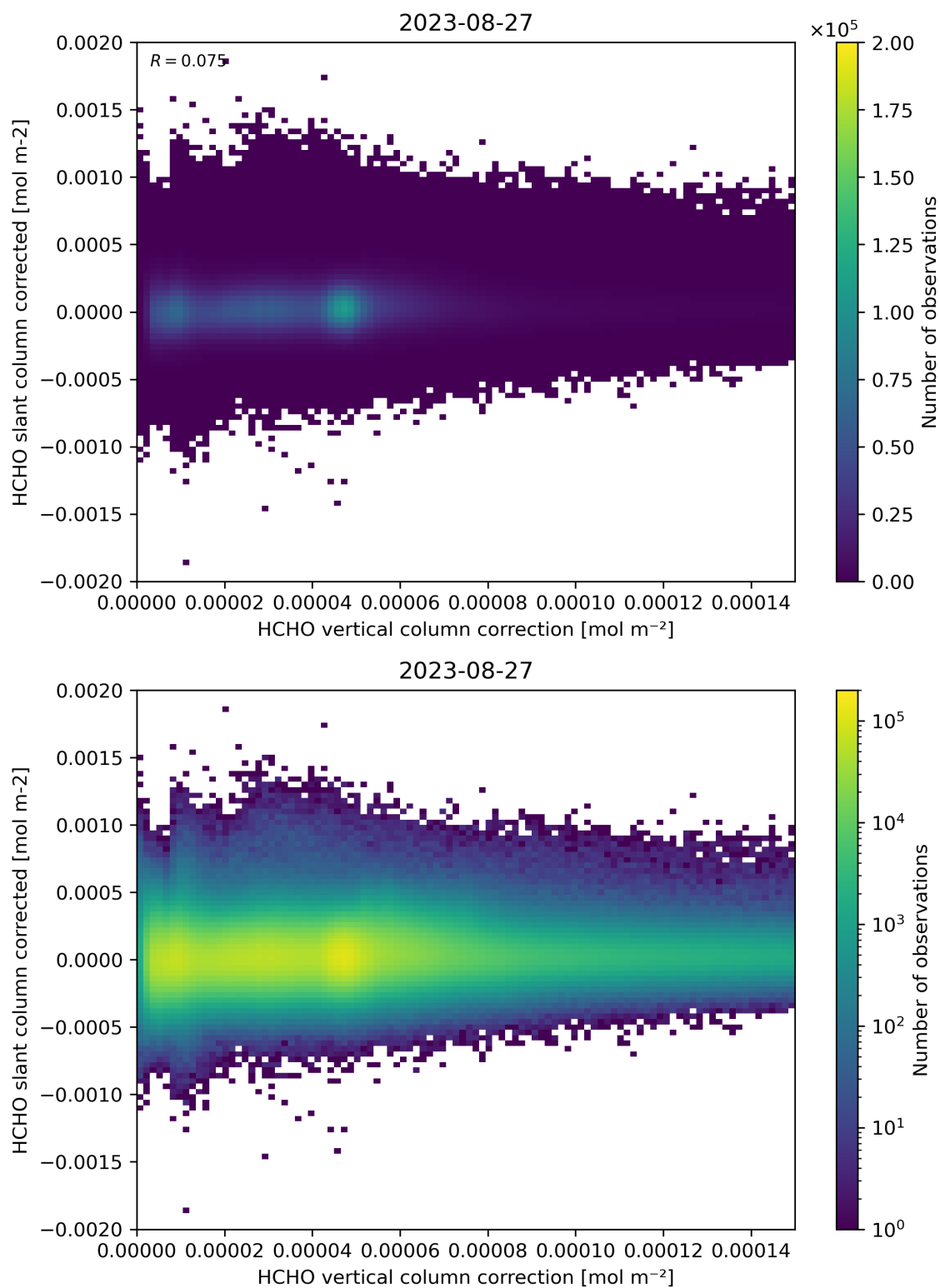
Figure 116: Scatter density plot of “HCHO vertical column correction” against “HCHO slant column corrected” for 2023-08-26 to 2023-08-28.
