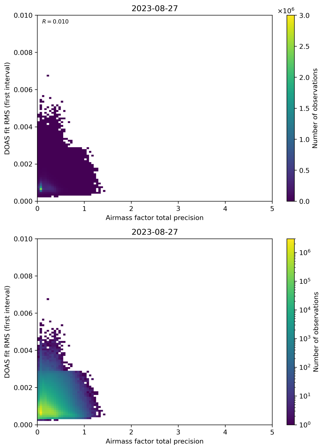
Figure 105: Scatter density plot of “Airmass factor total precision” against “DOAS fit RMS (first interval)” for 2023-08-26 to 2023-08-28.
