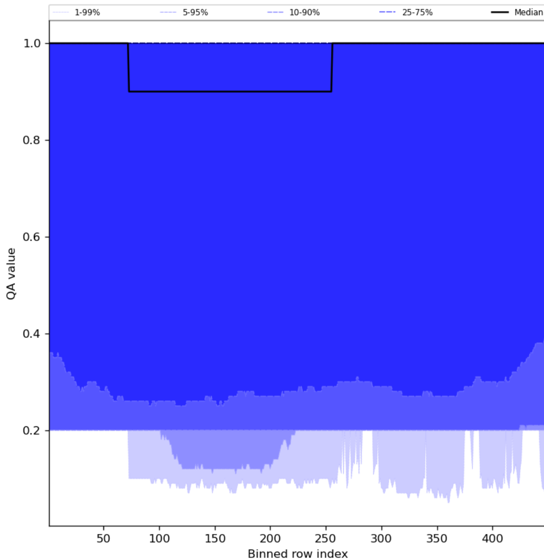
Figure 48: Along track statistics of “QA value” for 2023-08-26 to 2023-08-28
