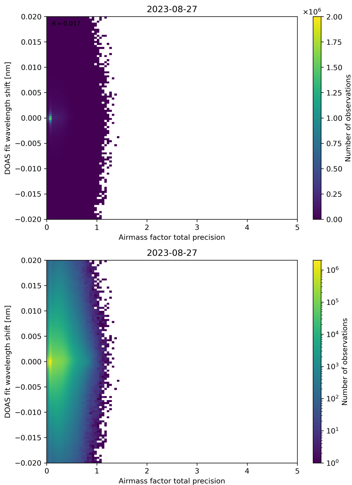
Figure 106: Scatter density plot of “Airmass factor total precision” against “DOAS fit wavelength shift” for 2023-08-26 to 2023-08-28.
