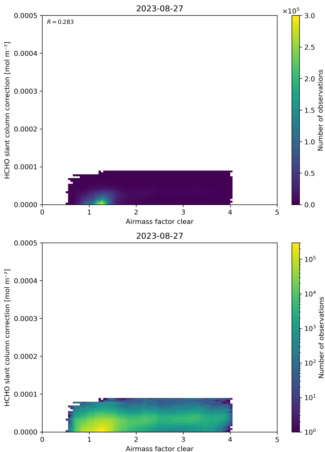
Figure 75: Scatter density plot of “Airmass factor clear” against “HCHO slant column correction” for 2023-08-26 to 2023-08-28.
