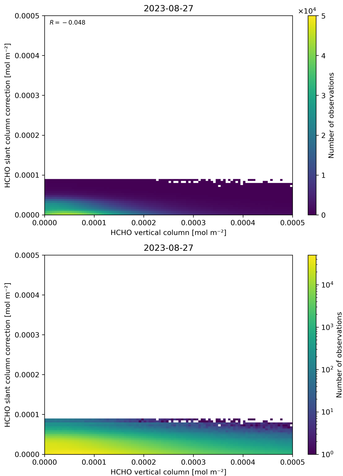
Figure 128: Scatter density plot of “HCHO vertical column” against “HCHO slant column correction” for 2023-08-26 to 2023-08-28.
