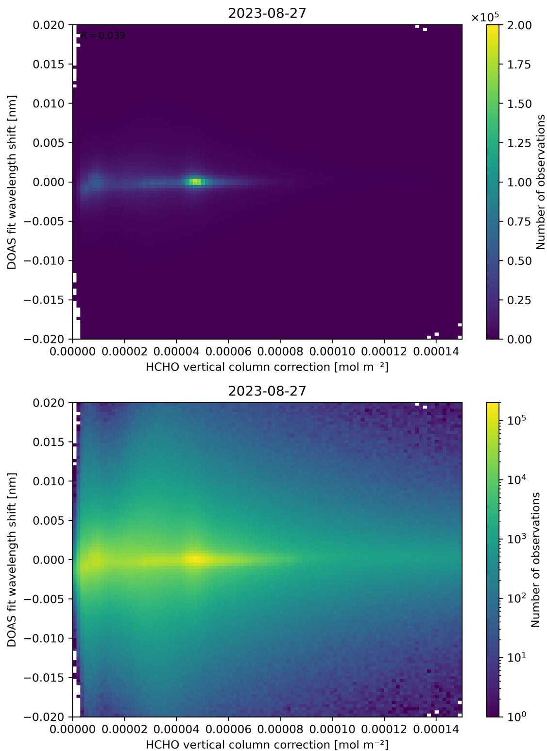
Figure 113: Scatter density plot of “HCHO vertical column correction” against “DOAS fit wavelength shift” for 2023-08-26 to 2023-08-28.
