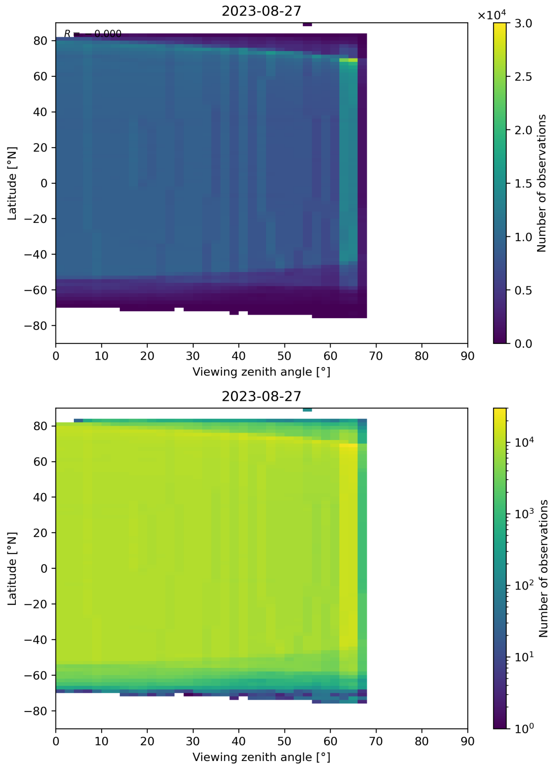
Figure 196: Scatter density plot of “Viewing zenith angle” against “Latitude” for 2023-08-26 to 2023-08-28.
