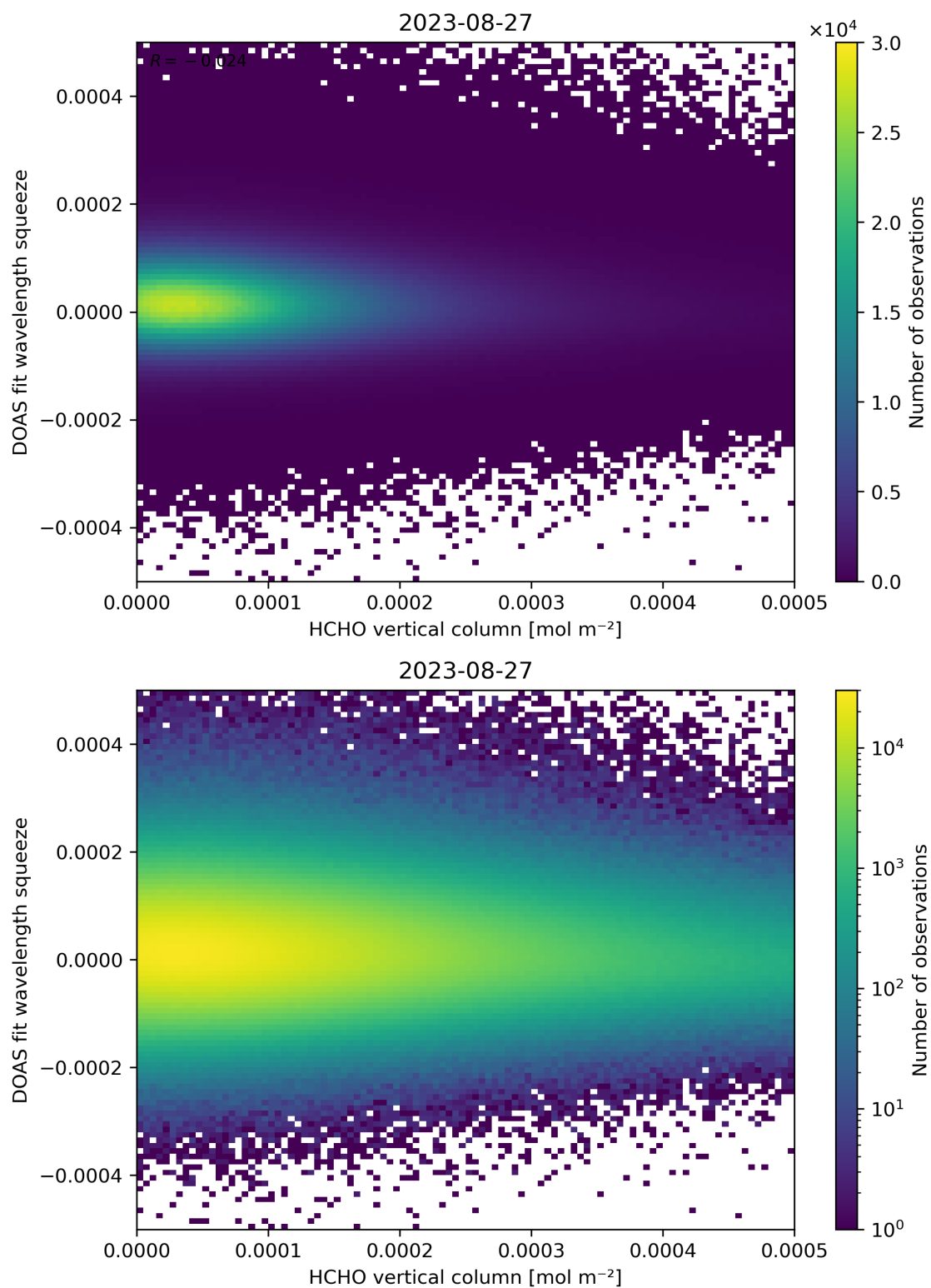
Figure 125: Scatter density plot of “HCHO vertical column” against “DOAS fit wavelength squeeze” for 2023-08-26 to 2023-08-28.
