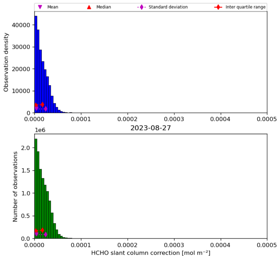
Figure 47: Histogram of “HCHO slant column correction” for 2023-08-26 to 2023-08-28
