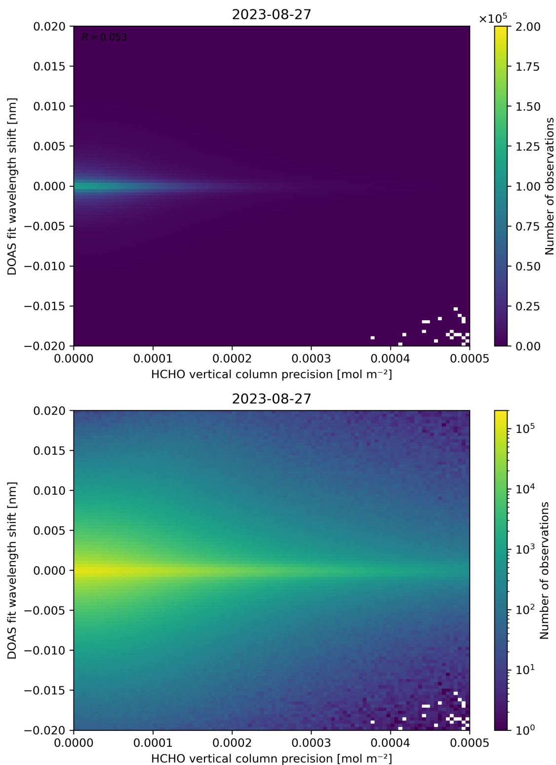
Figure 137: Scatter density plot of “HCHO vertical column precision” against “DOAS fit wavelength shift” for 2023-08-26 to 2023-08-28.
