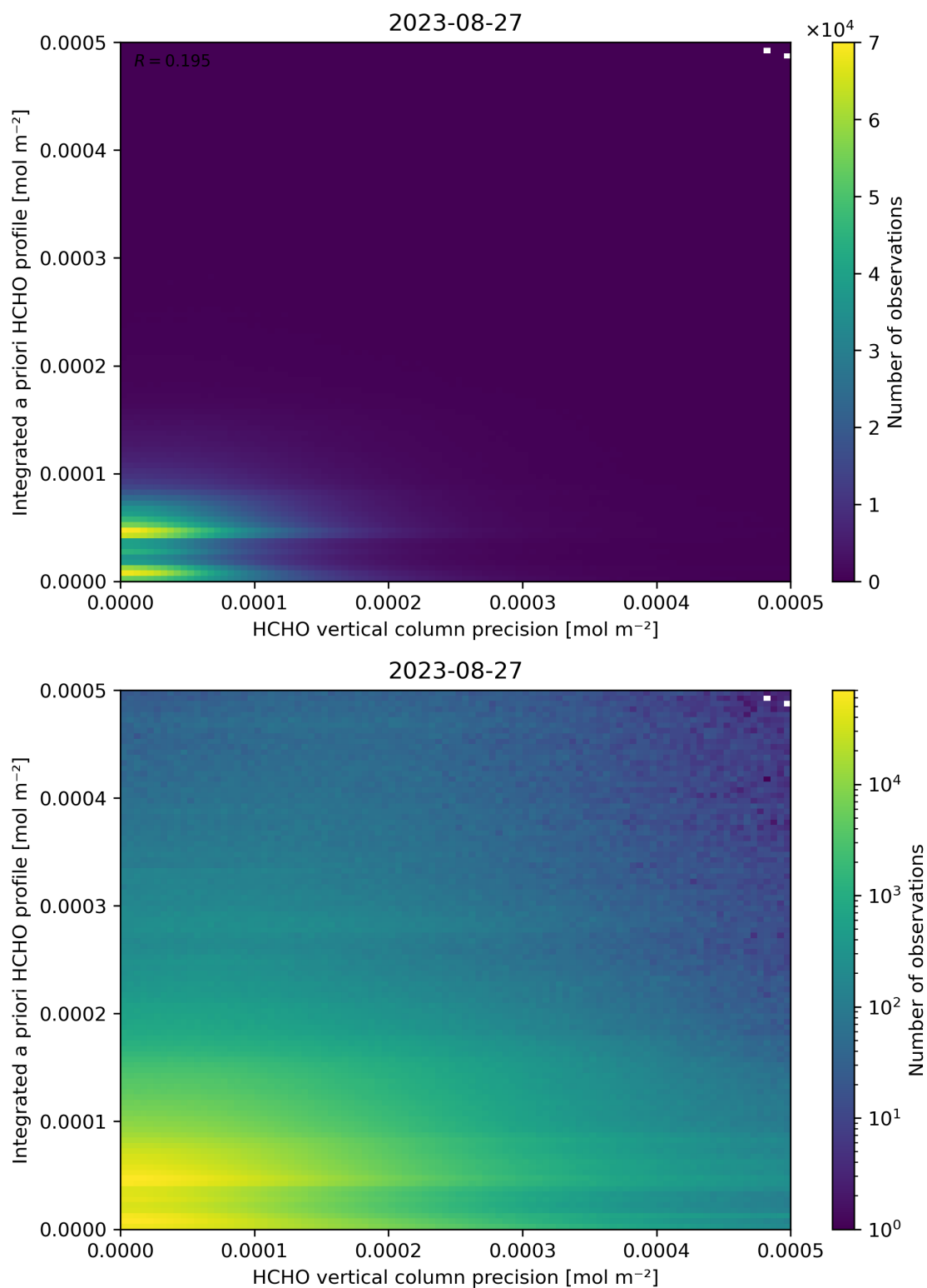
Figure 147: Scatter density plot of “HCHO vertical column precision” against “Integrated a priori HCHO profile” for 2023-08-26 to 2023-08-28.
