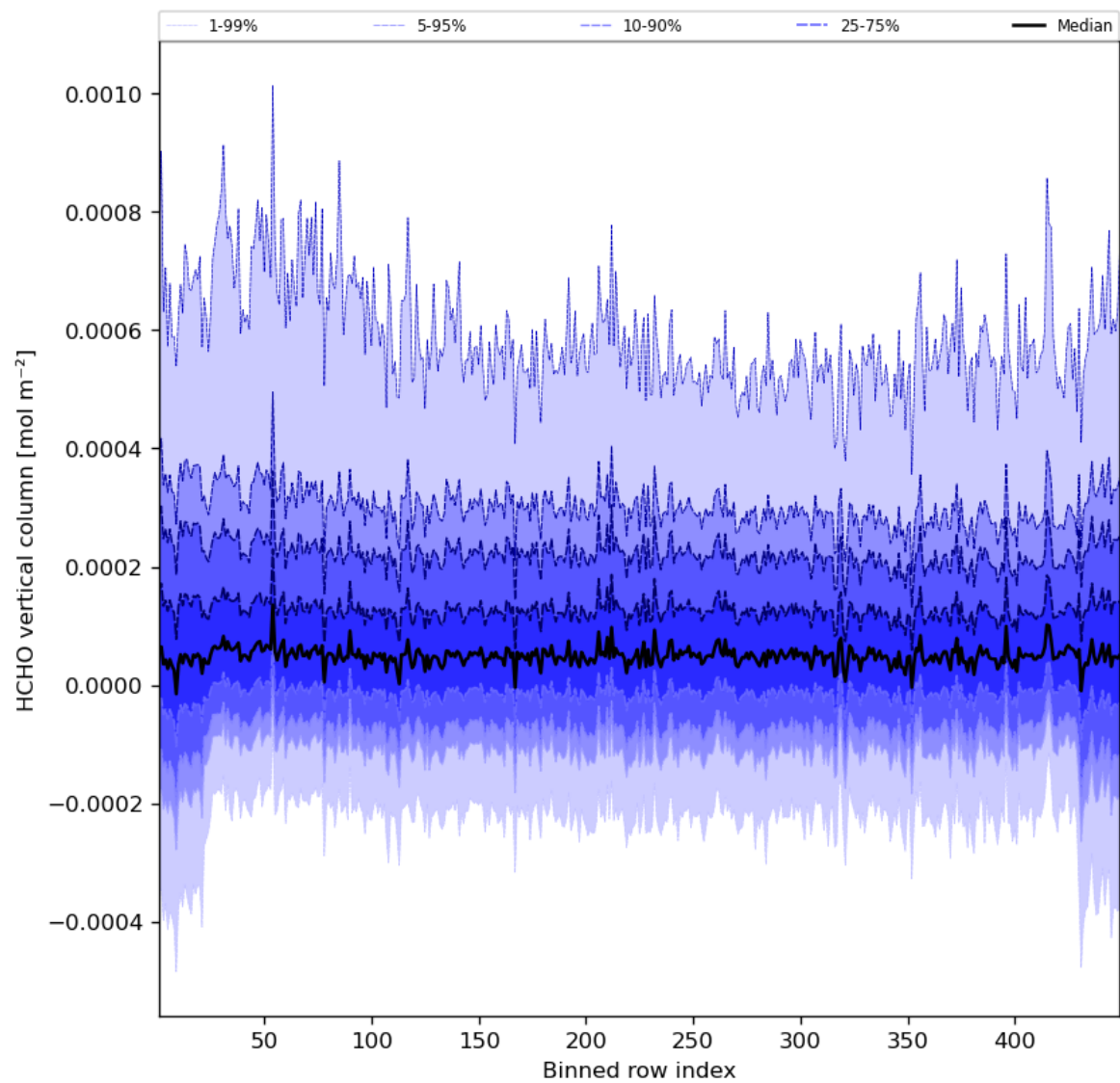
Figure 49: Along track statistics of “HCHO vertical column” for 2023-08-26 to 2023-08-28
