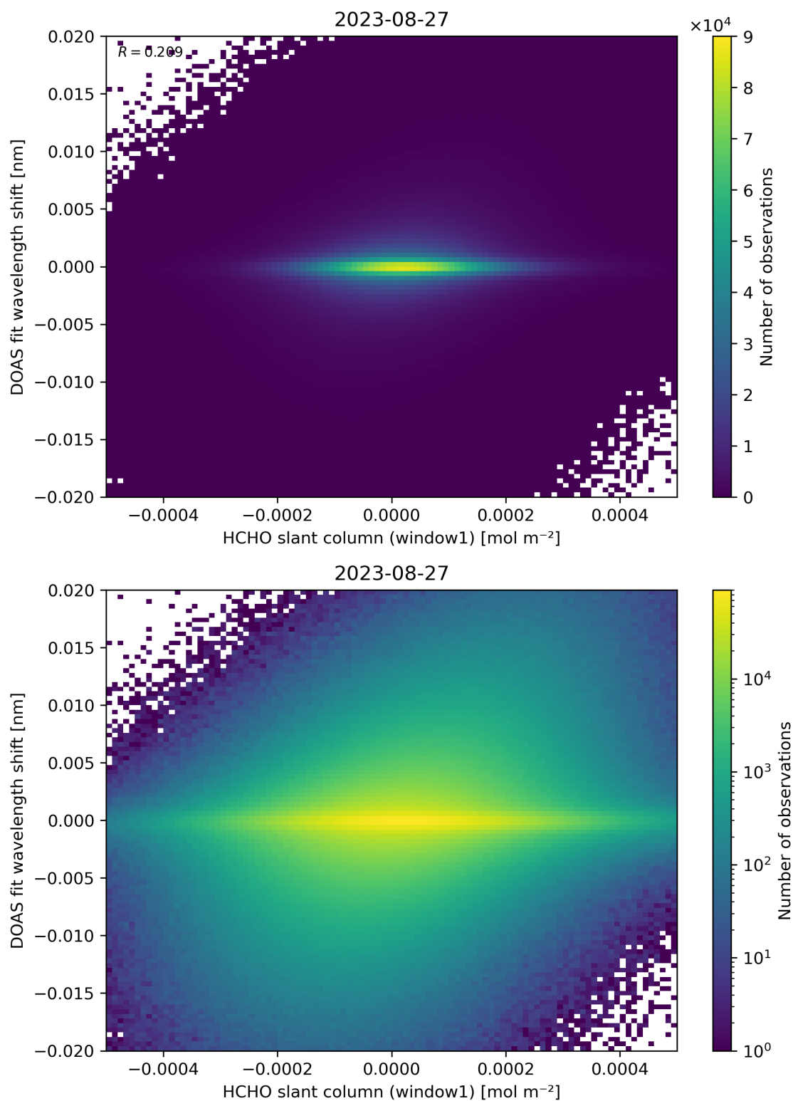
Figure 79: Scatter density plot of “HCHO slant column (window1)” against “DOAS fit wavelength shift” for 2023-08-26 to 2023-08-28.
