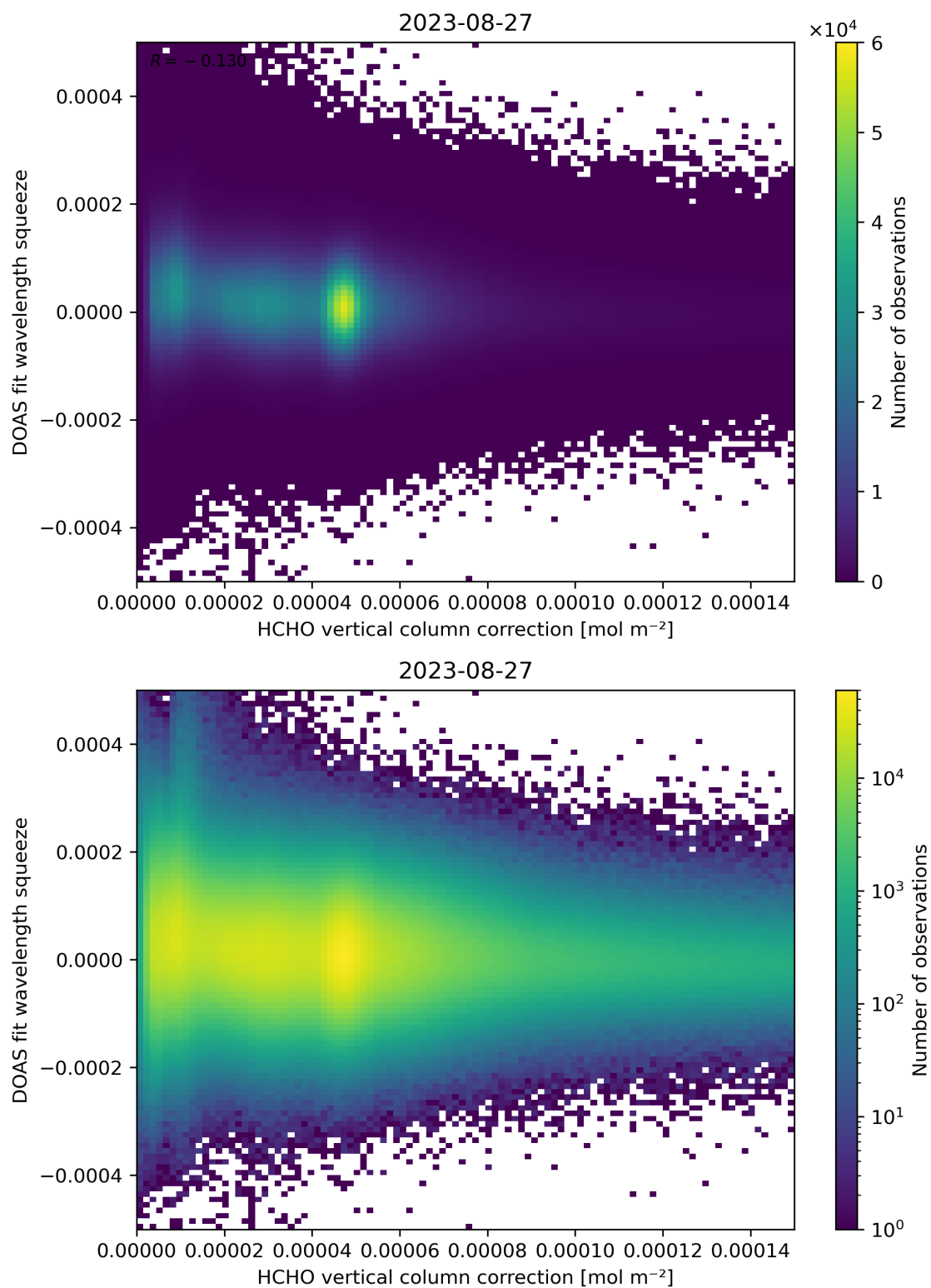
Figure 114: Scatter density plot of “HCHO vertical column correction” against “DOAS fit wavelength squeeze” for 2023-08-26 to 2023-08-28.
