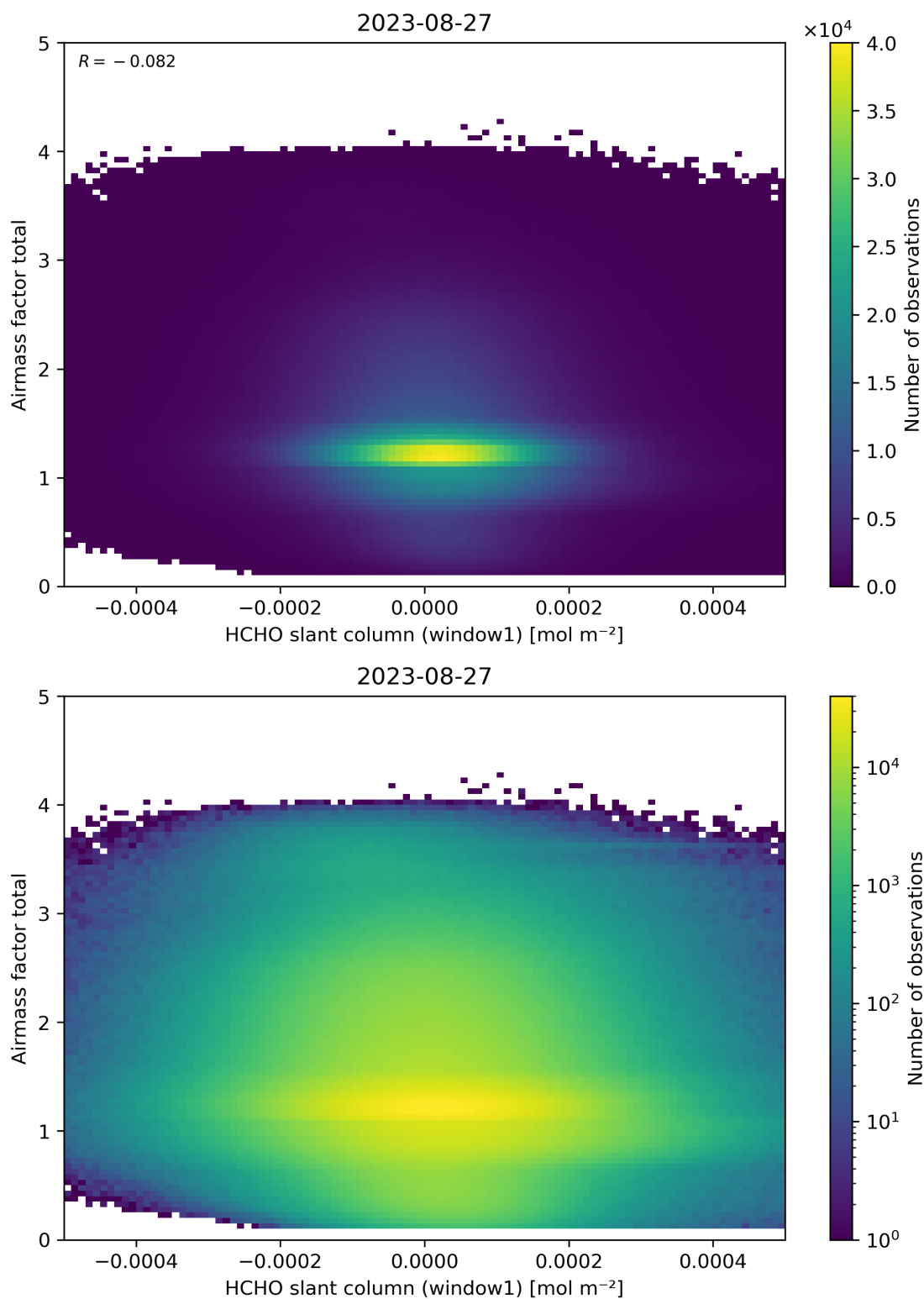
Figure 85: Scatter density plot of “HCHO slant column (window1)” against “Airmass factor total” for 2023-08-26 to 2023-08-28.
