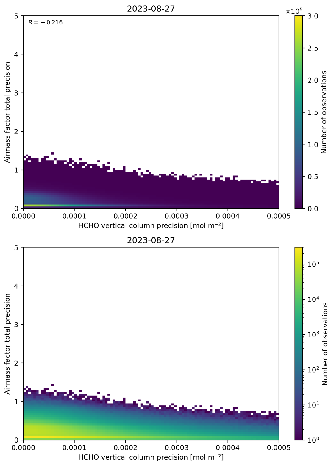
Figure 145: Scatter density plot of “HCHO vertical column precision” against “Airmass factor total precision” for 2023-08-26 to 2023-08-28.
