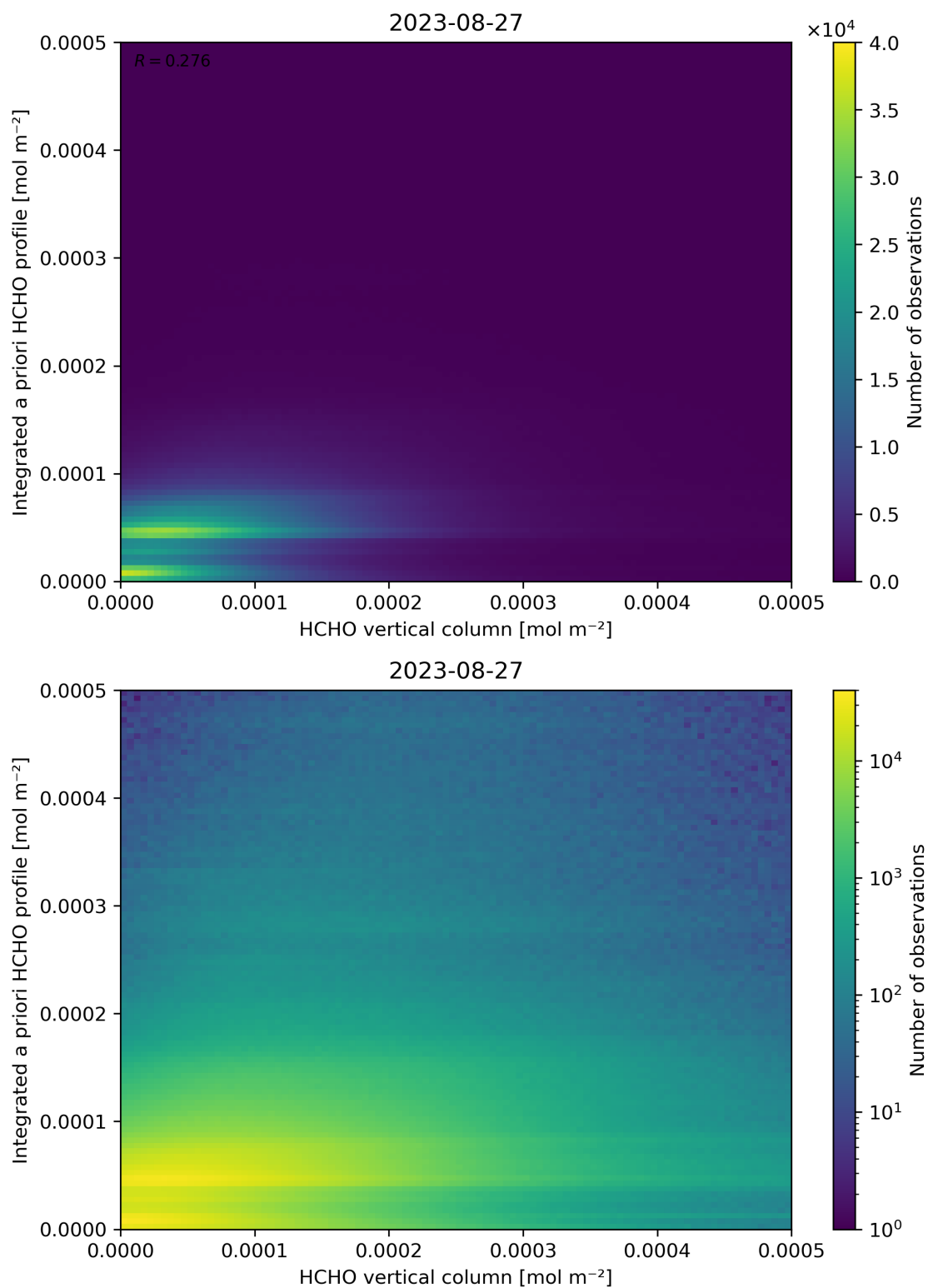
Figure 135: Scatter density plot of “HCHO vertical column” against “Integrated a priori HCHO profile” for 2023-08-26 to 2023-08-28.
