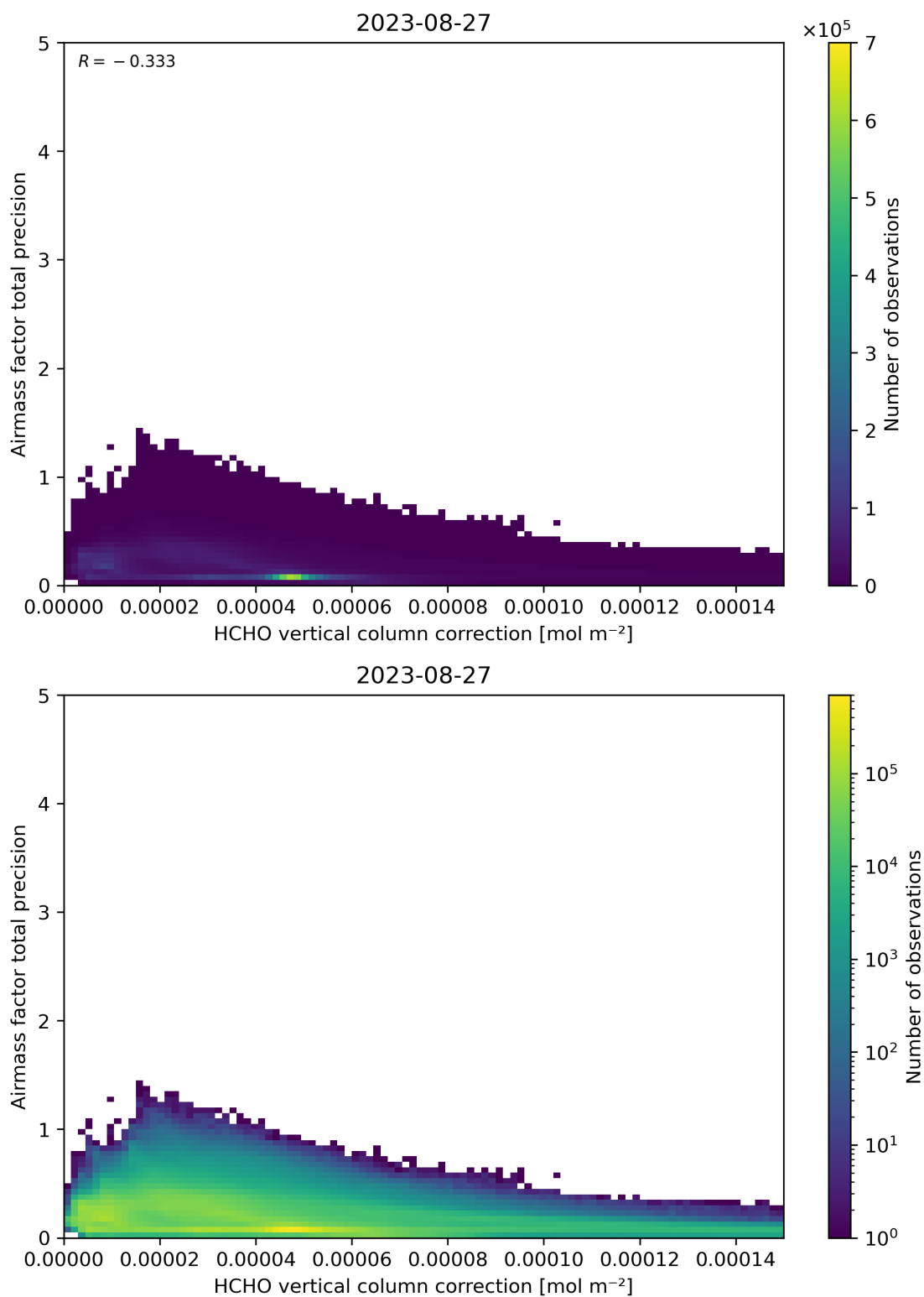
Figure 121: Scatter density plot of “HCHO vertical column correction” against “Airmass factor total precision” for 2023-08-26 to 2023-08-28.
