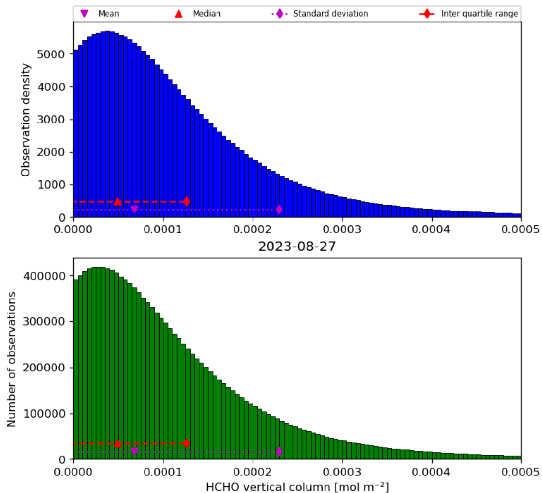
Figure 35: Histogram of “HCHO vertical column” for 2023-08-26 to 2023-08-28
