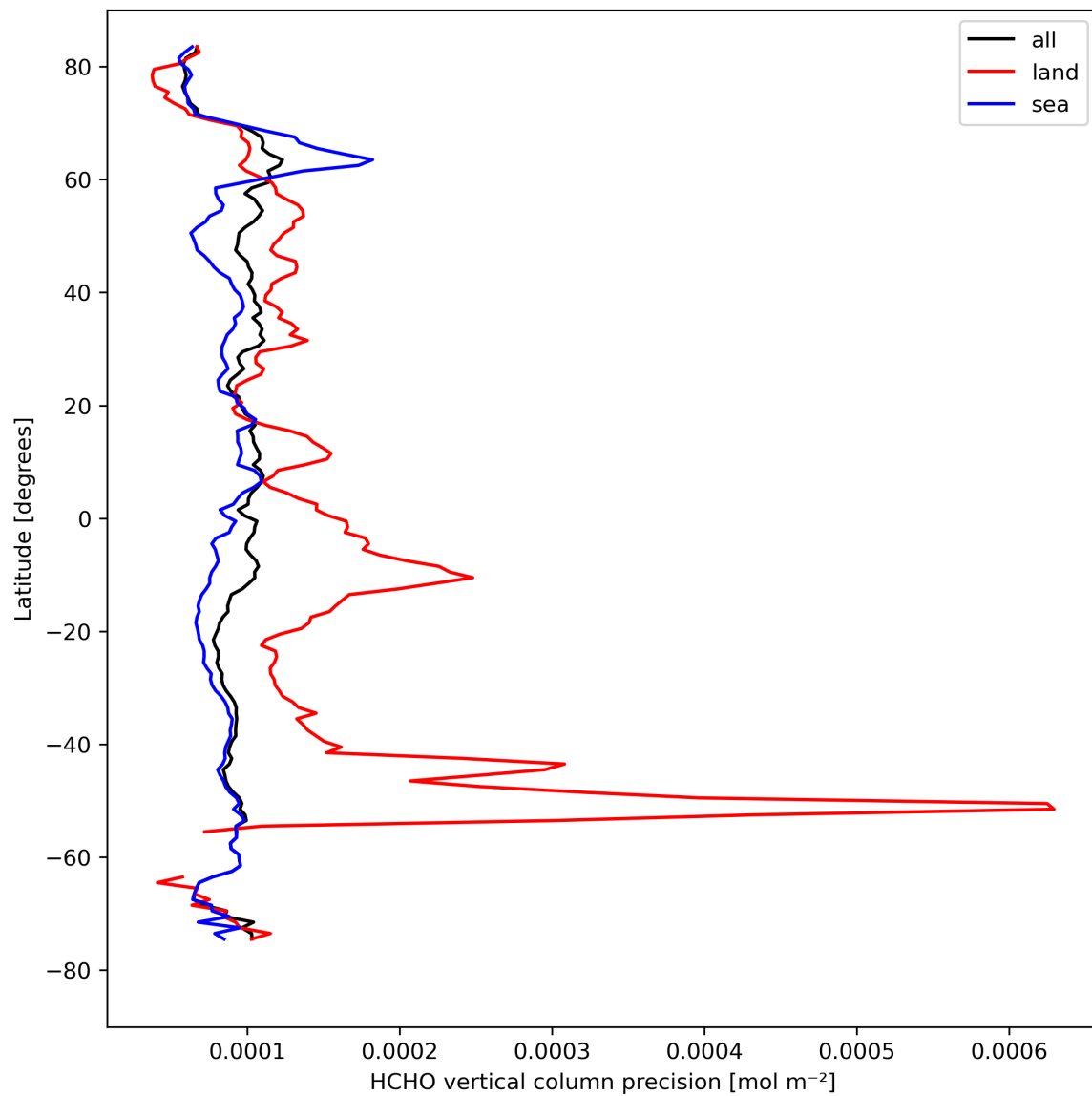
Figure 22: Zonal average of “HCHO vertical column precision” for 2023-08-26 to 2023-08-28.
