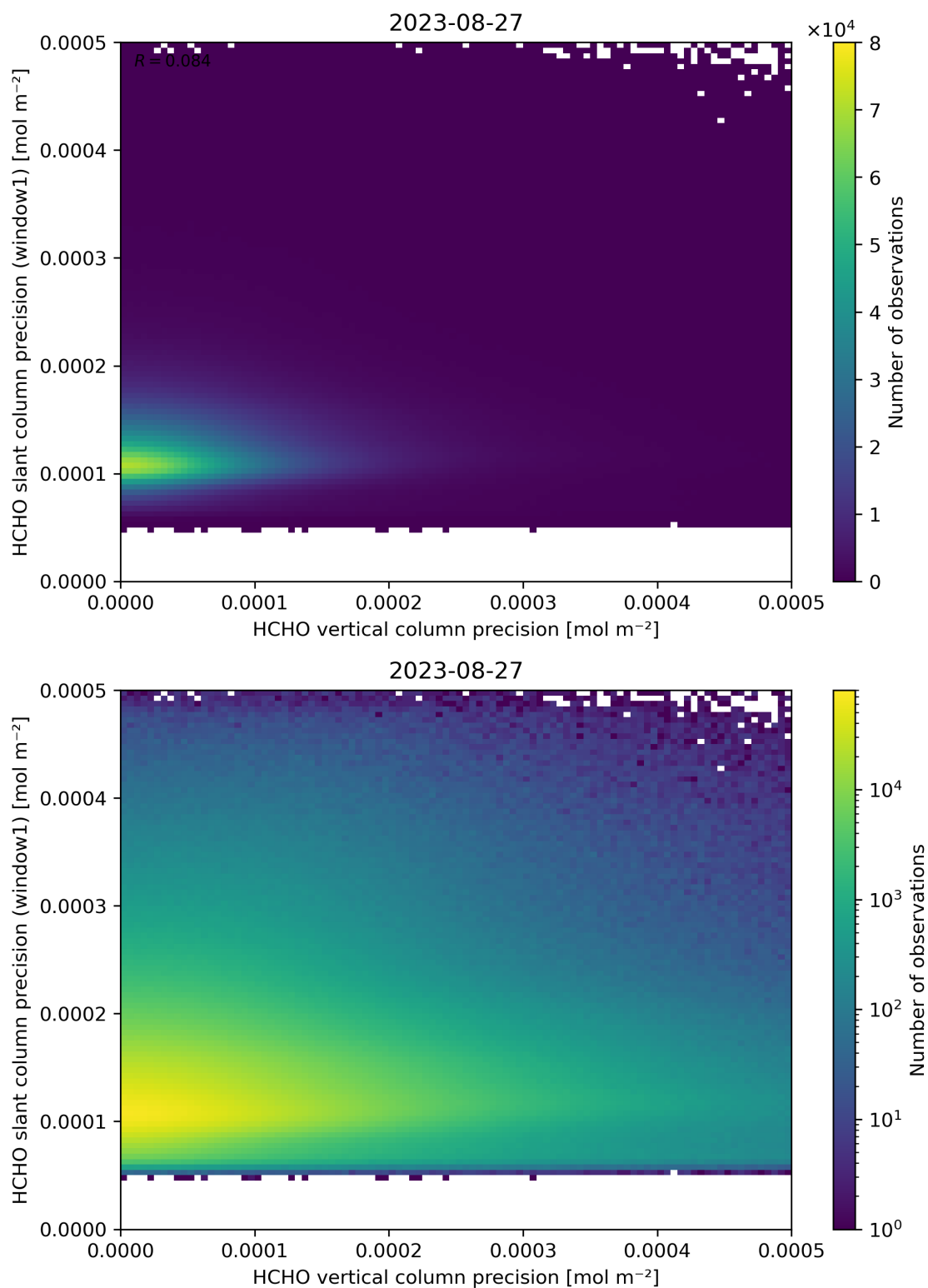
Figure 143: Scatter density plot of “HCHO vertical column precision” against “HCHO slant column precision (window1)” for 2023-08-26 to 2023-08-28.
