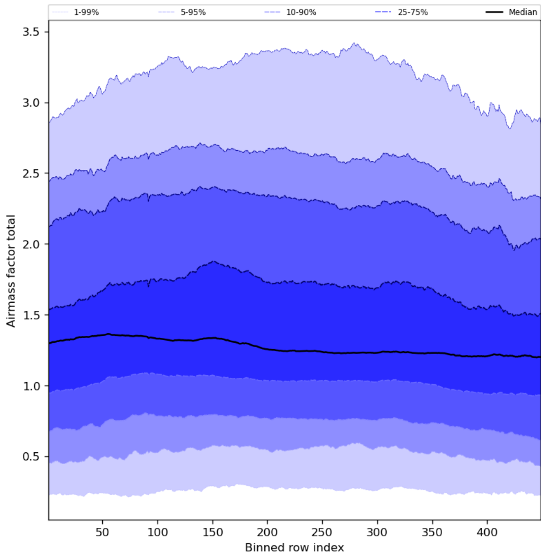
Figure 54: Along track statistics of “Airmass factor total” for 2023-08-26 to 2023-08-28
