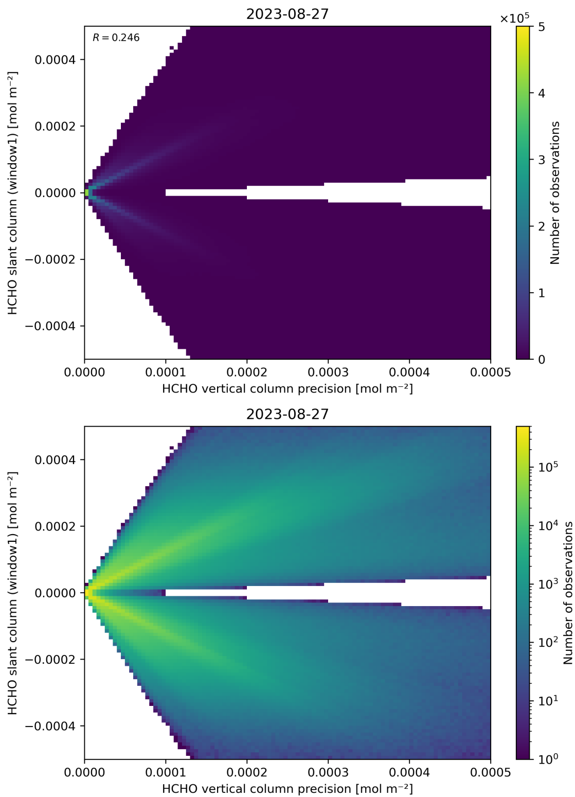
Figure 142: Scatter density plot of “HCHO vertical column precision” against “HCHO slant column (window1)” for 2023-08-26 to 2023-08-28.
