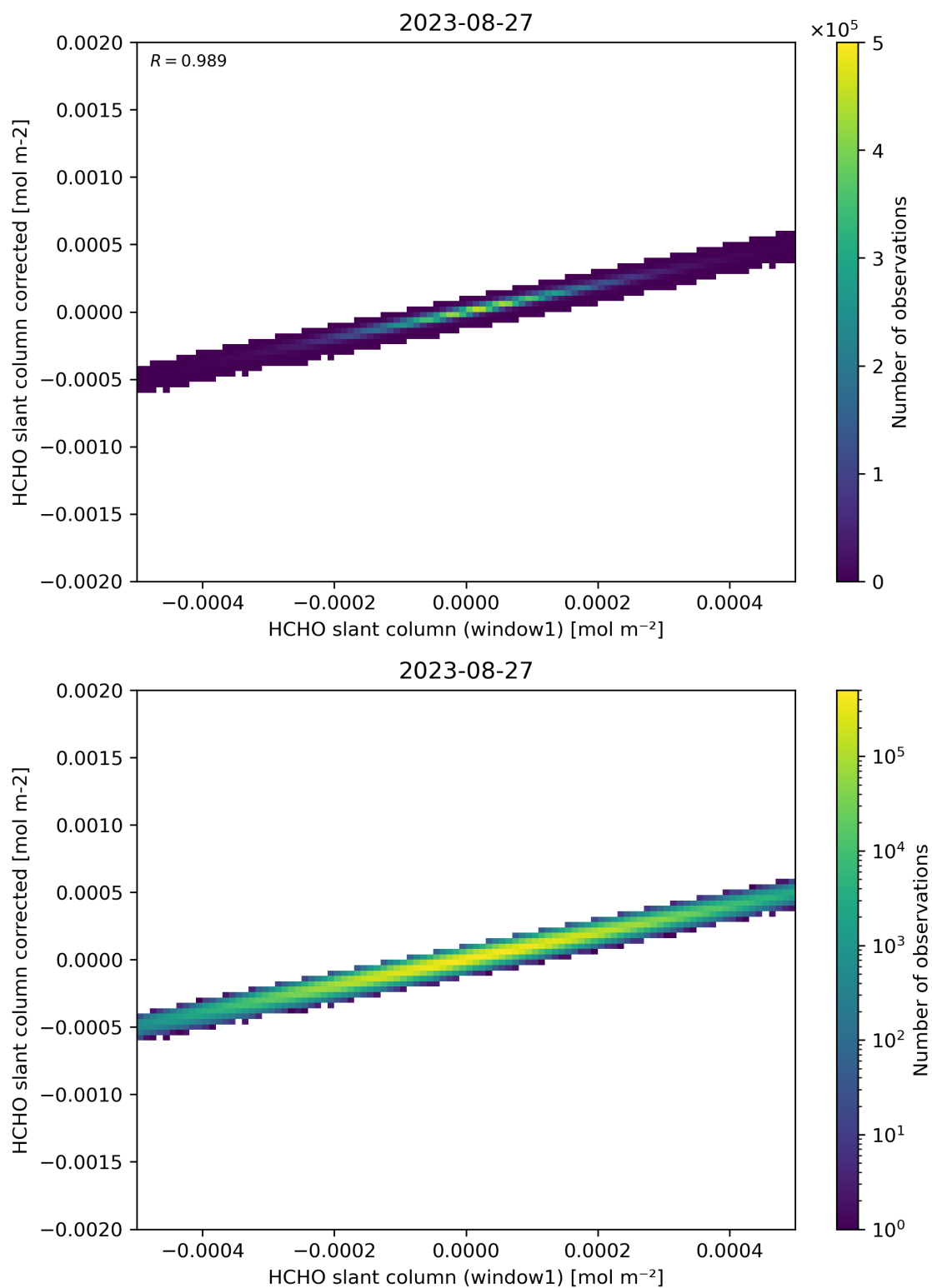
Figure 82: Scatter density plot of “HCHO slant column (window1)” against “HCHO slant column corrected” for 2023-08-26 to 2023-08-28.
