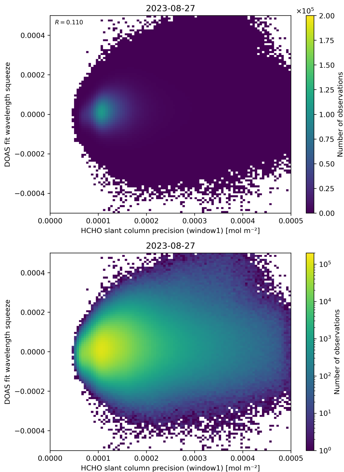
Figure 90: Scatter density plot of “HCHO slant column precision (window1)” against “DOAS fit wavelength squeeze” for 2023-08-26 to 2023-08-28.
