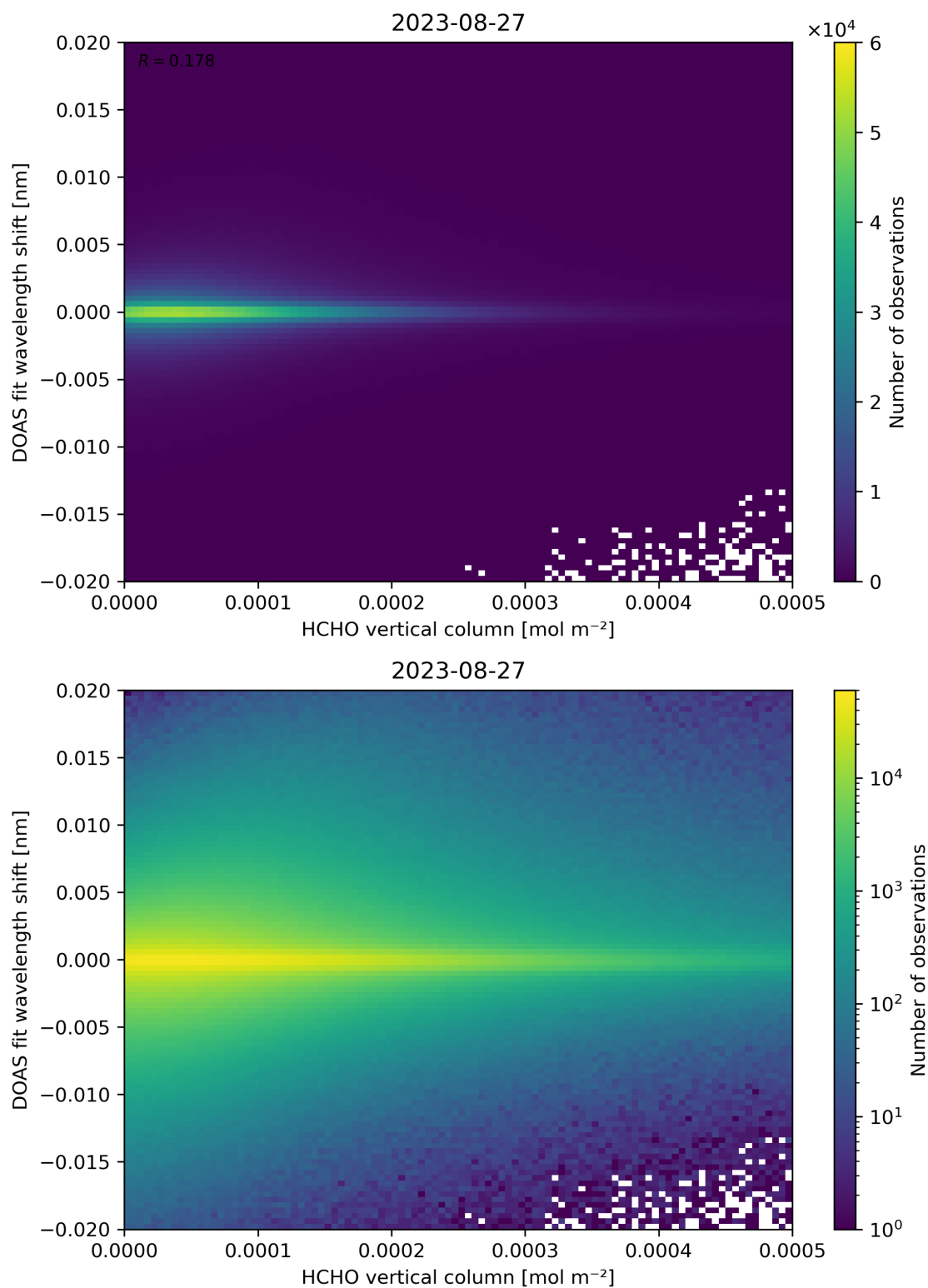
Figure 124: Scatter density plot of “HCHO vertical column” against “DOAS fit wavelength shift” for 2023-08-26 to 2023-08-28.
