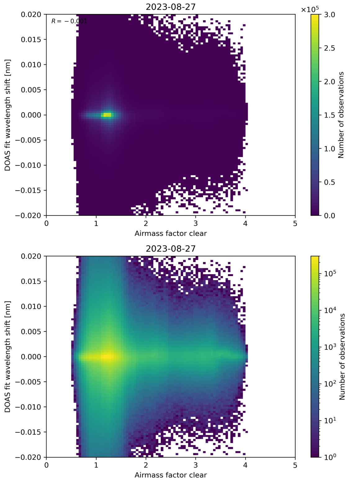
Figure 72: Scatter density plot of “Airmass factor clear” against “DOAS fit wavelength shift” for 2023-08-26 to 2023-08-28.
