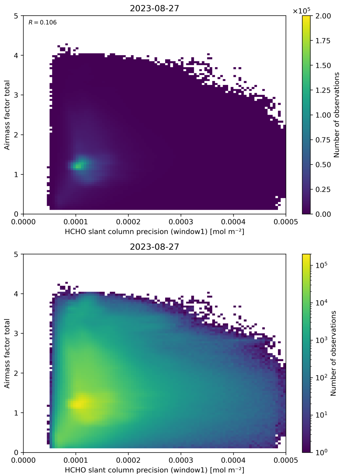
Figure 94: Scatter density plot of “HCHO slant column precision (window1)” against “Airmass factor total” for 2023-08-26 to 2023-08-28.
