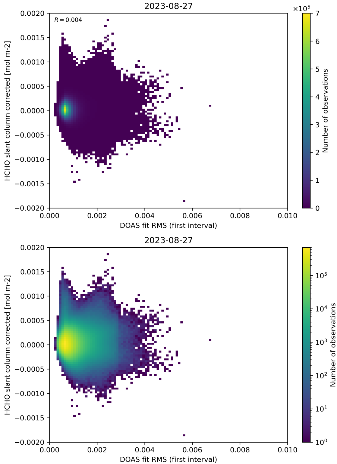
Figure 62: Scatter density plot of “DOAS fit RMS (first interval)” against “HCHO slant column corrected” for 2023-08-26 to 2023-08-28.
