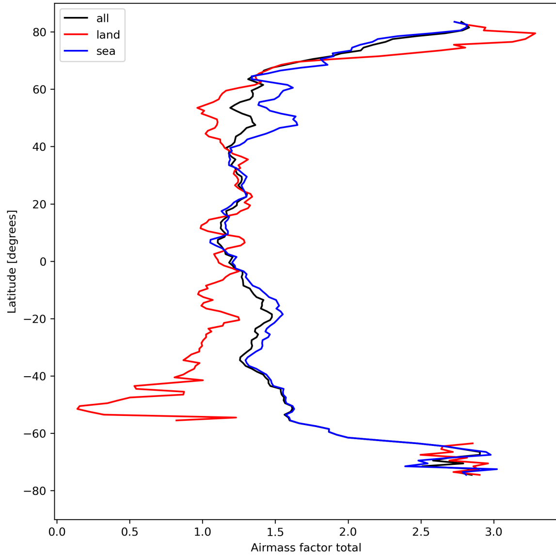
Figure 26: Zonal average of “Airmass factor total” for 2023-08-26 to 2023-08-28.
