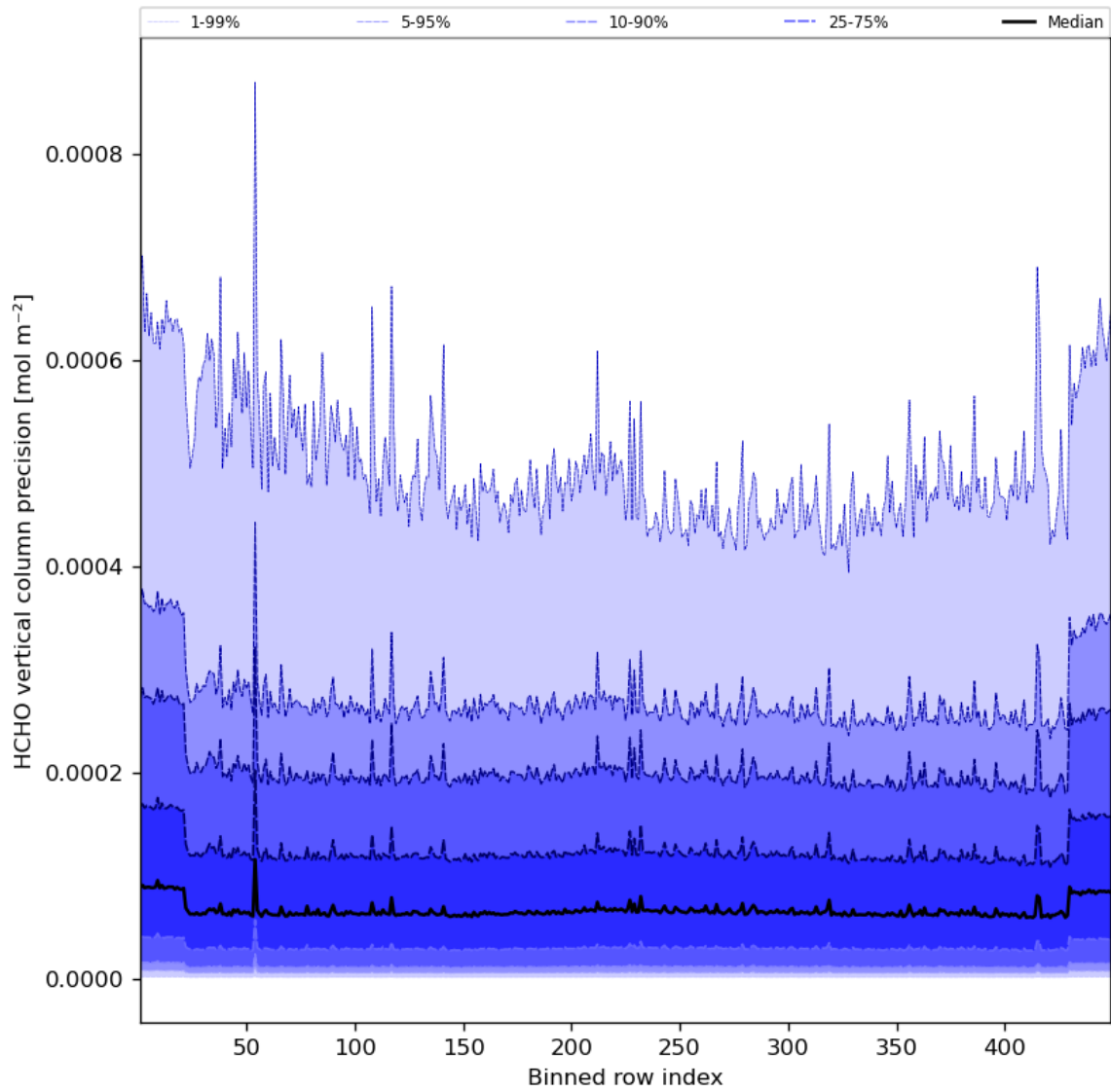
Figure 50: Along track statistics of “HCHO vertical column precision” for 2023-08-26 to 2023-08-28
