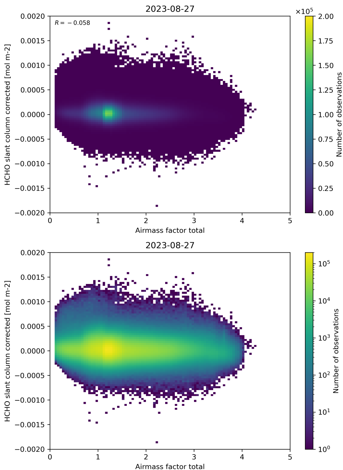
Figure 101: Scatter density plot of “Airmass factor total” against “HCHO slant column corrected” for 2023-08-26 to 2023-08-28.
