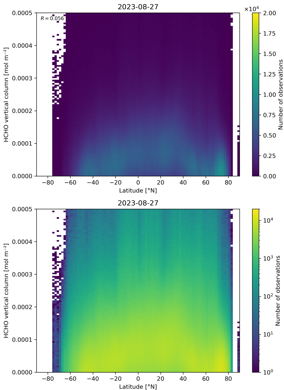
Figure 163: Scatter density plot of “Latitude” against “HCHO vertical column” for 2023-08-26 to 2023-08-28.
