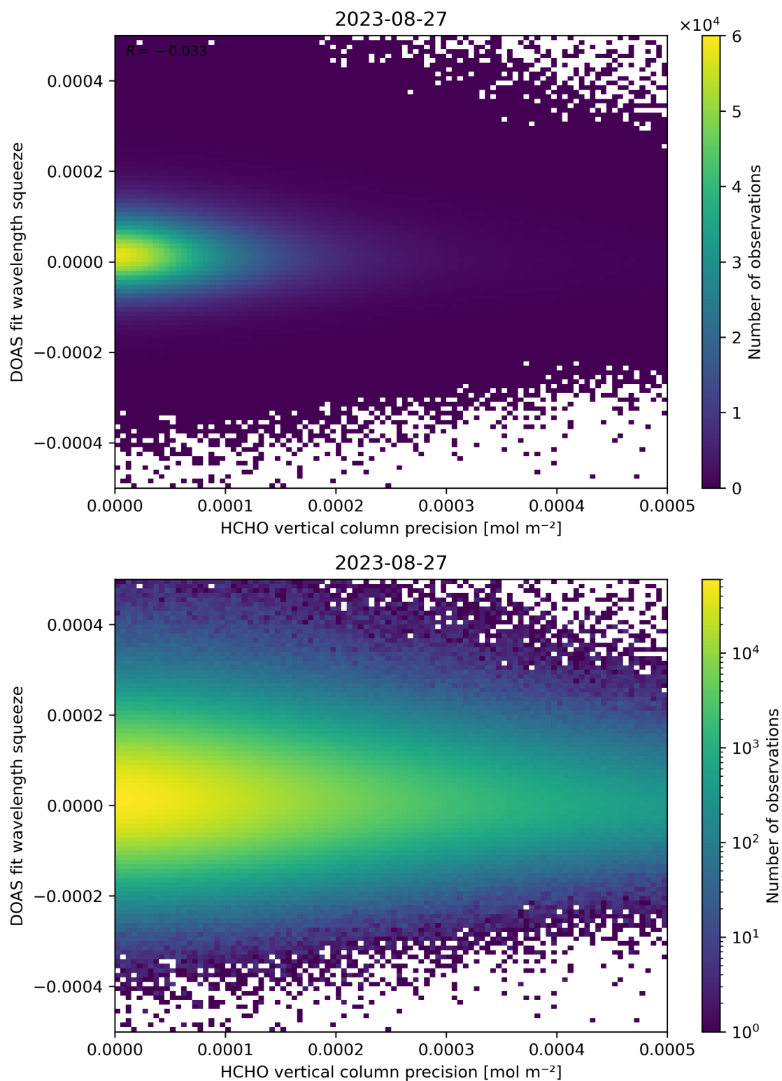
Figure 138: Scatter density plot of “HCHO vertical column precision” against “DOAS fit wavelength squeeze” for 2023-08-26 to 2023-08-28.
