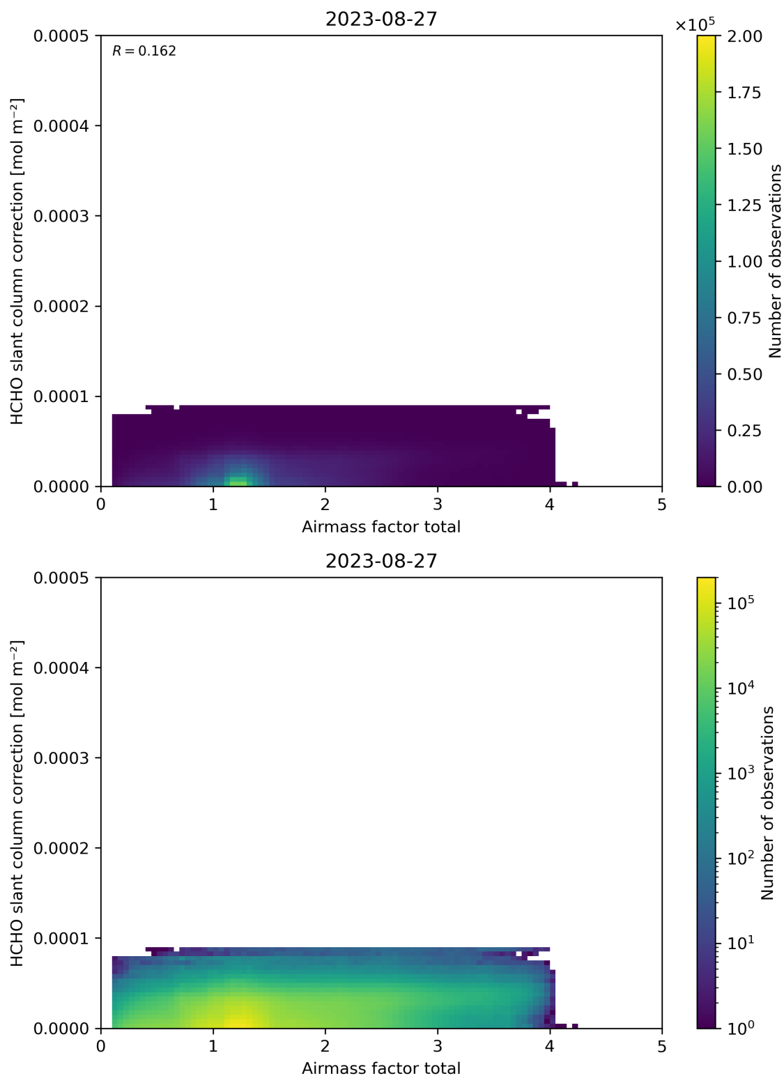
Figure 102: Scatter density plot of “Airmass factor total” against “HCHO slant column correction” for 2023-08-26 to 2023-08-28.
