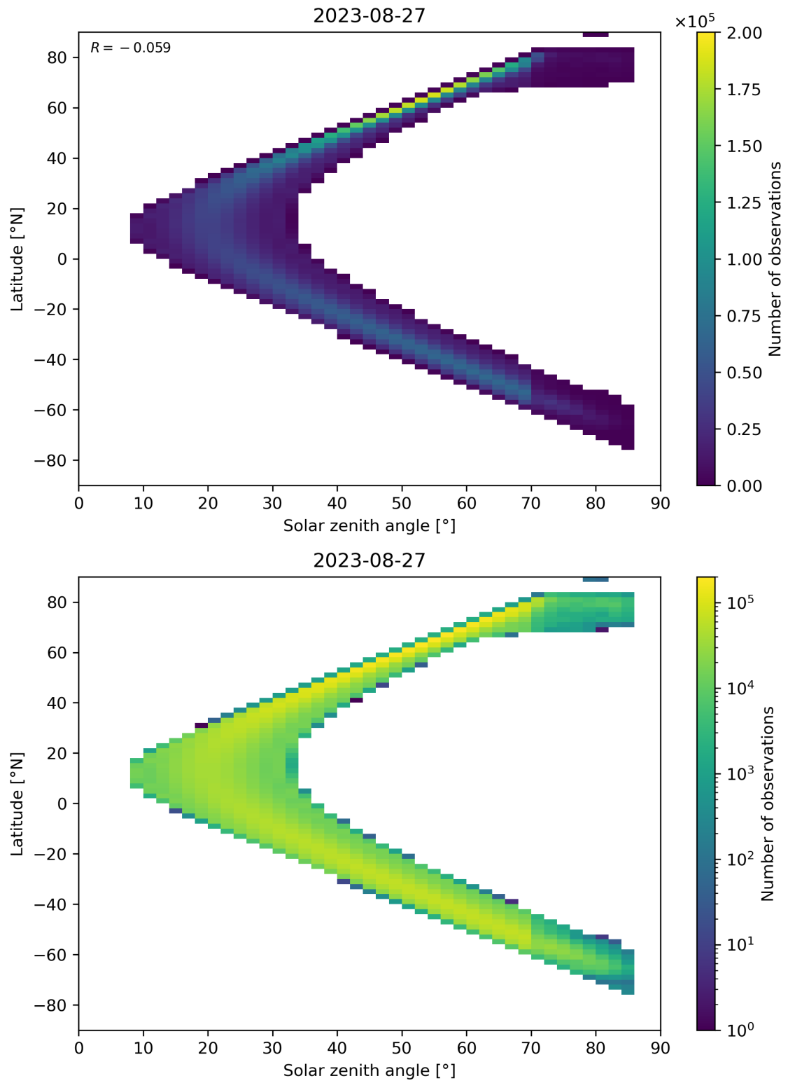
Figure 181: Scatter density plot of “Solar zenith angle” against “Latitude” for 2023-08-26 to 2023-08-28.
