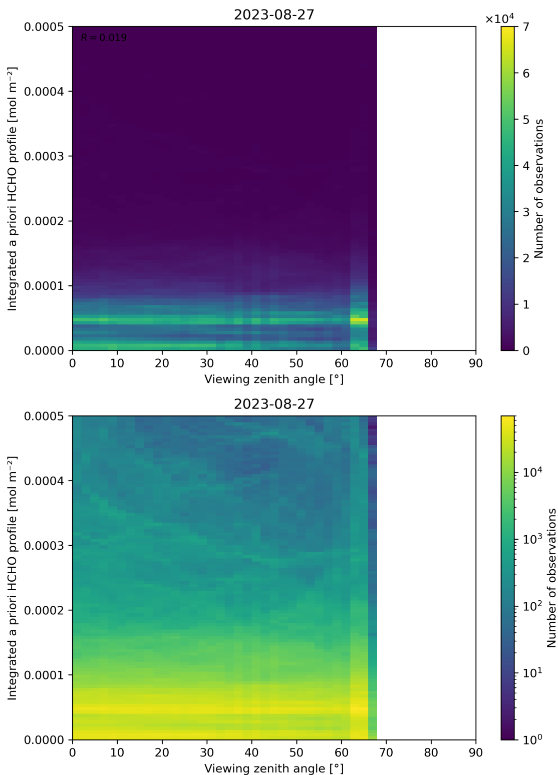
Figure 195: Scatter density plot of “Viewing zenith angle” against “Integrated a priori HCHO profile” for 2023-08-26 to 2023-08-28.
