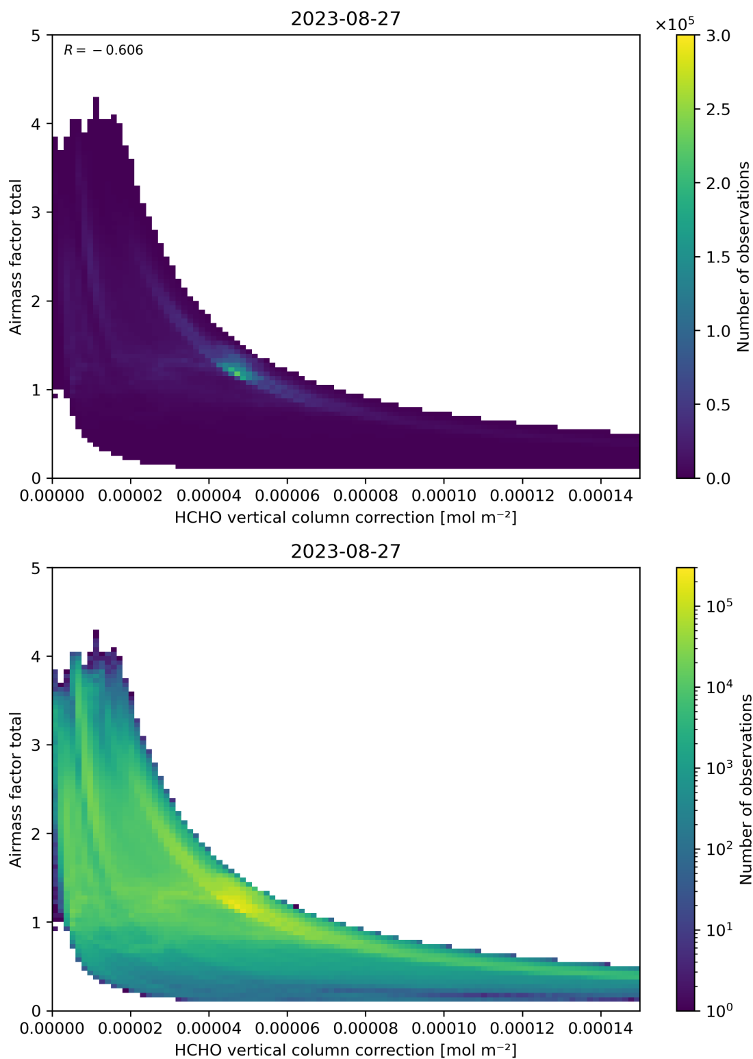
Figure 120: Scatter density plot of “HCHO vertical column correction” against “Airmass factor total” for 2023-08-26 to 2023-08-28.
