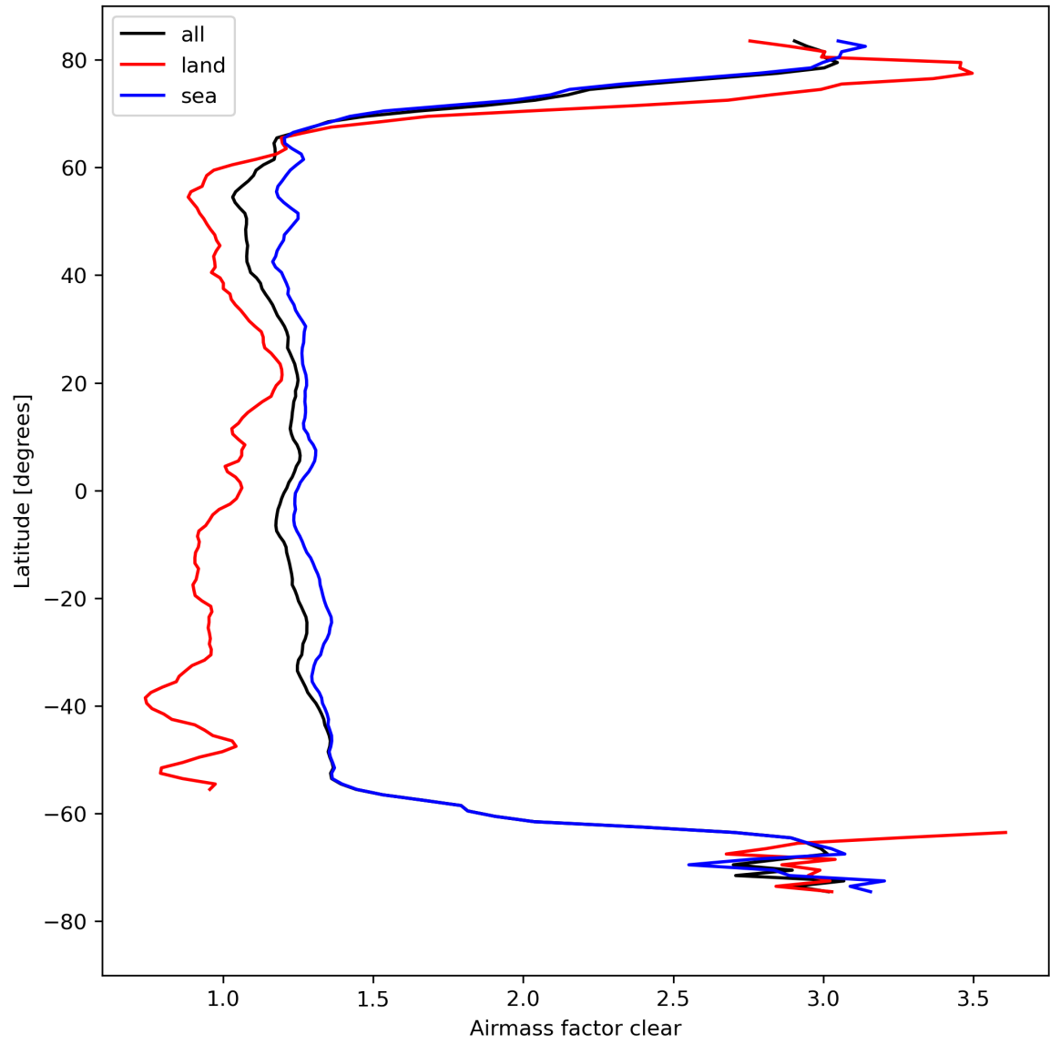
Figure 28: Zonal average of “Airmass factor clear” for 2023-08-26 to 2023-08-28.
