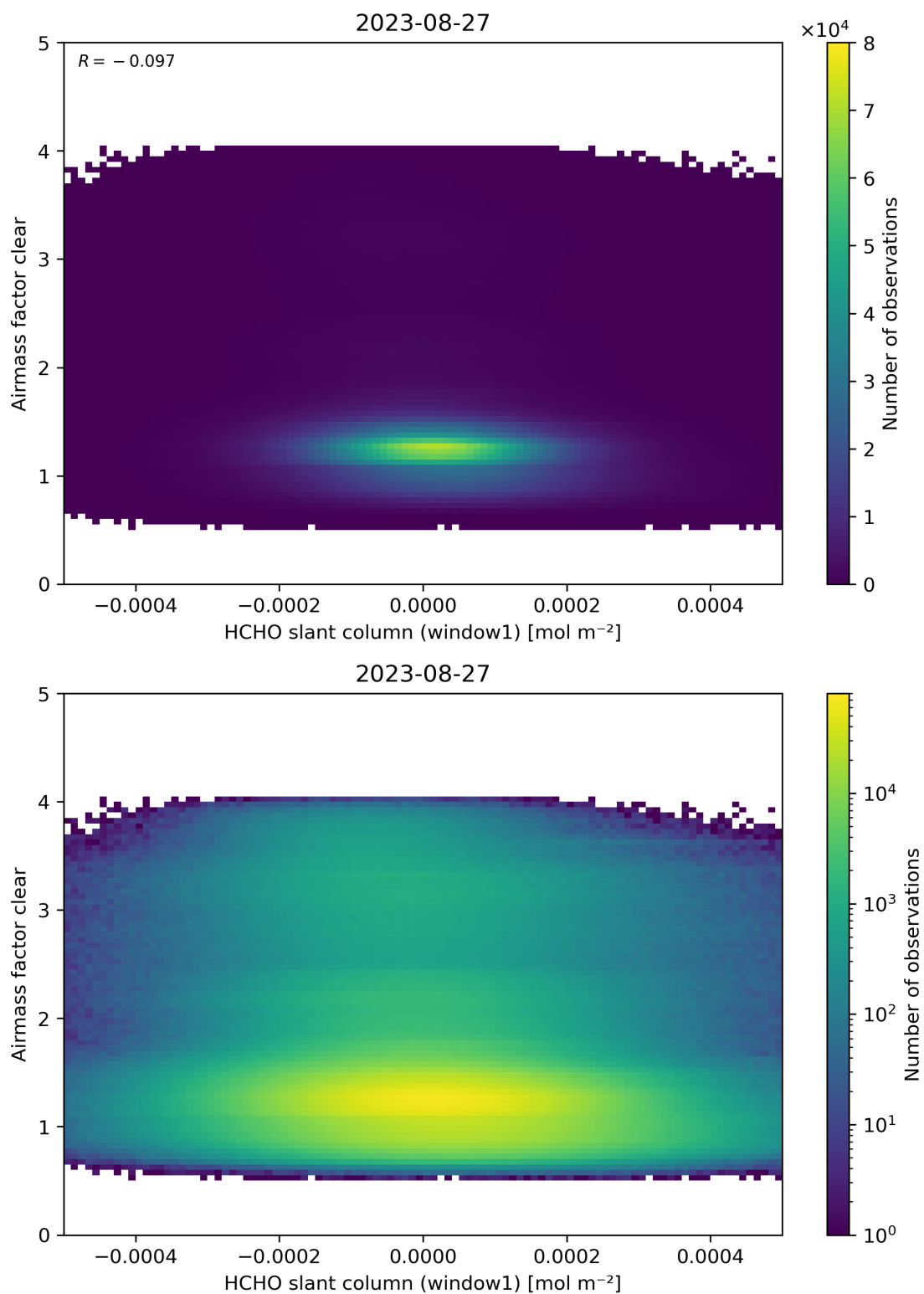
Figure 81: Scatter density plot of “HCHO slant column (window1)” against “Airmass factor clear” for 2023-08-26 to 2023-08-28.
