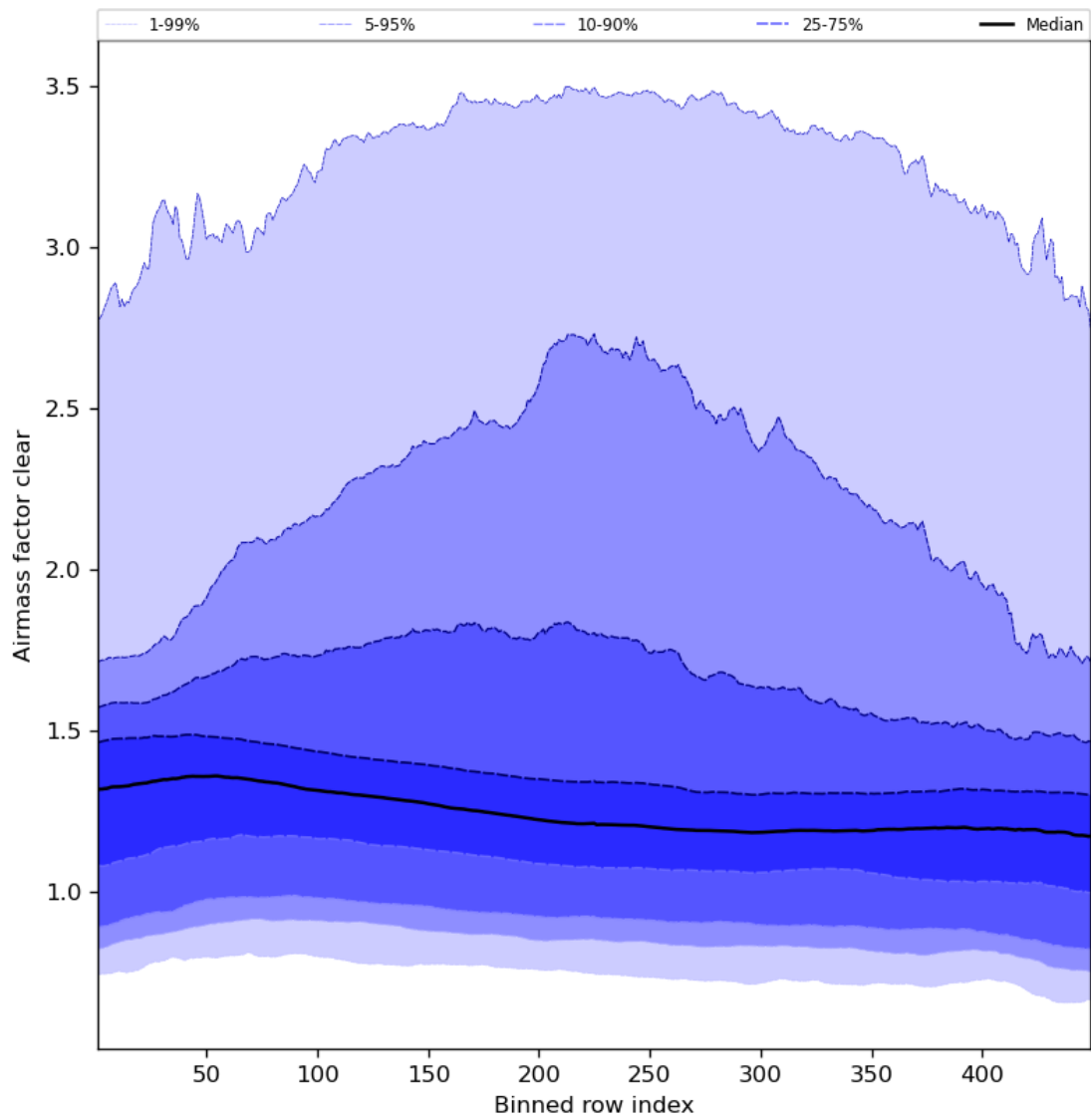
Figure 56: Along track statistics of “Airmass factor clear” for 2023-08-26 to 2023-08-28
