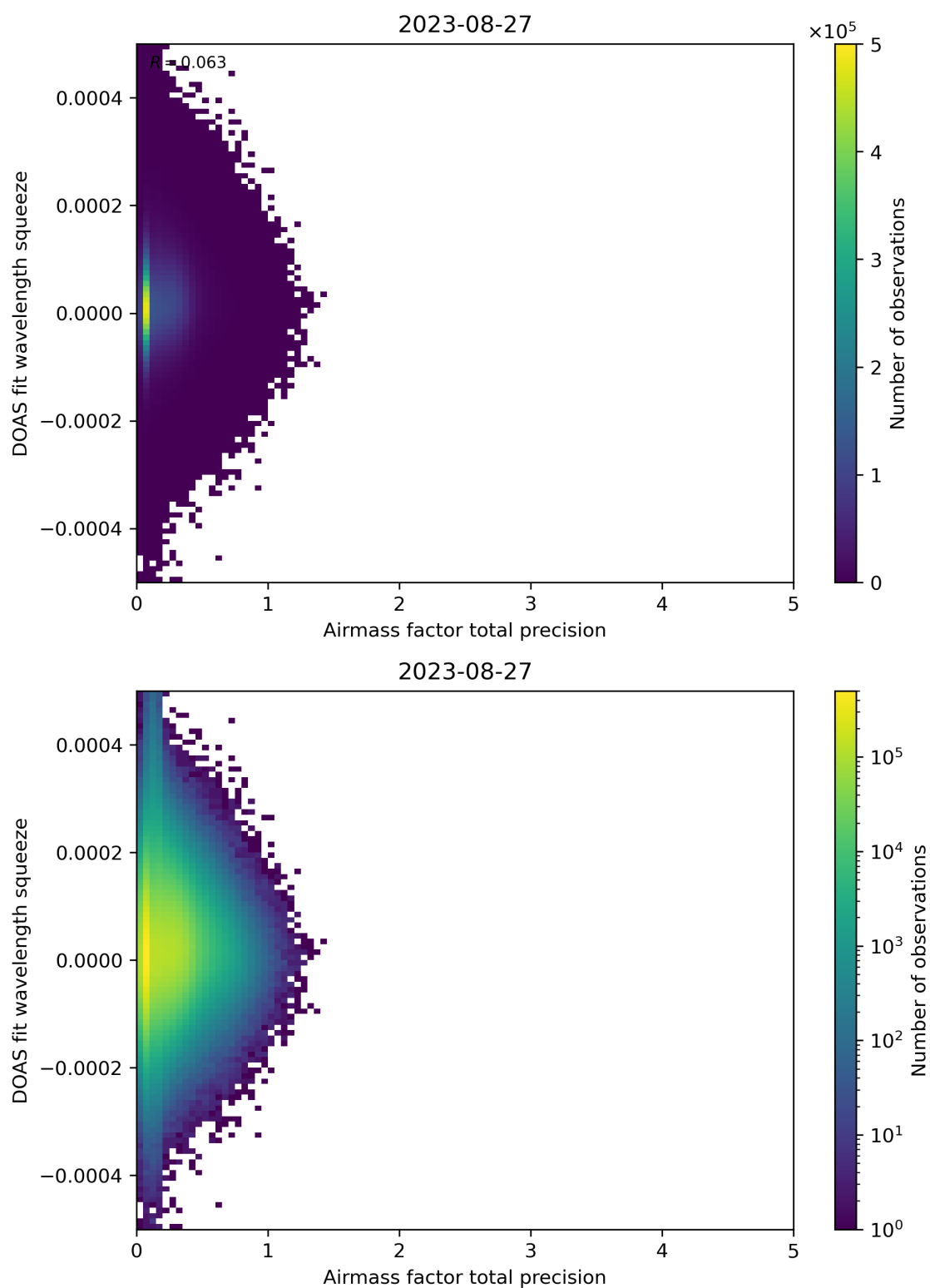
Figure 107: Scatter density plot of “Airmass factor total precision” against “DOAS fit wavelength squeeze” for 2023-08-26 to 2023-08-28.
