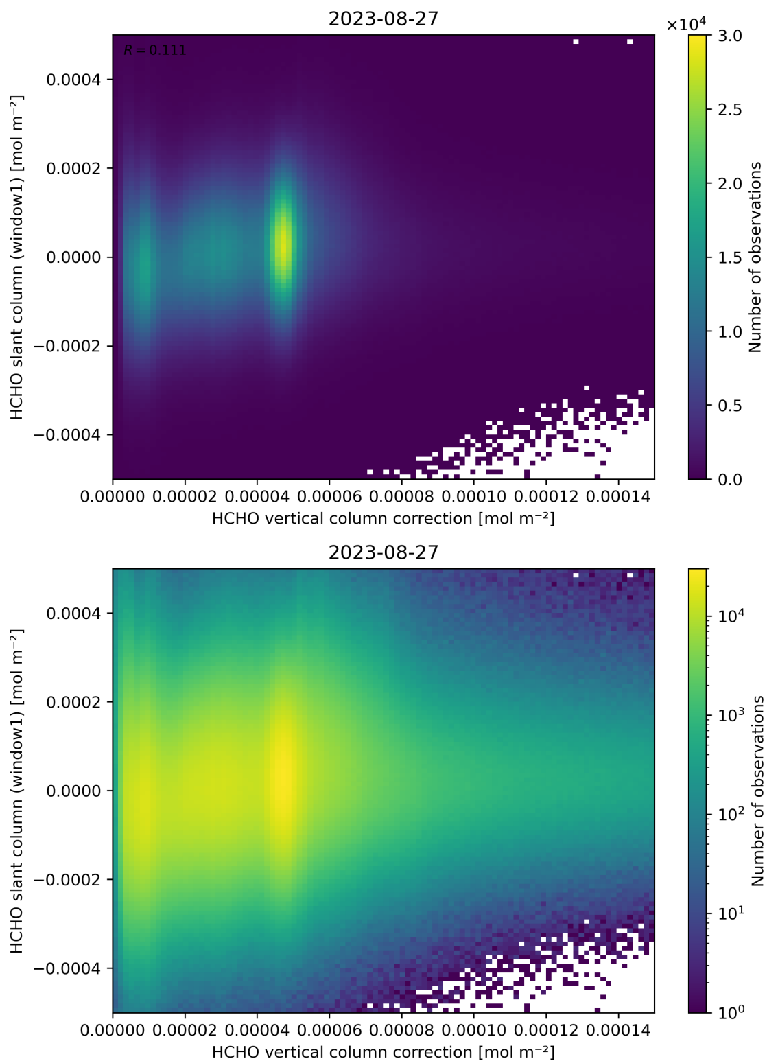
Figure 118: Scatter density plot of “HCHO vertical column correction” against “HCHO slant column (window1)” for 2023-08-26 to 2023-08-28.
