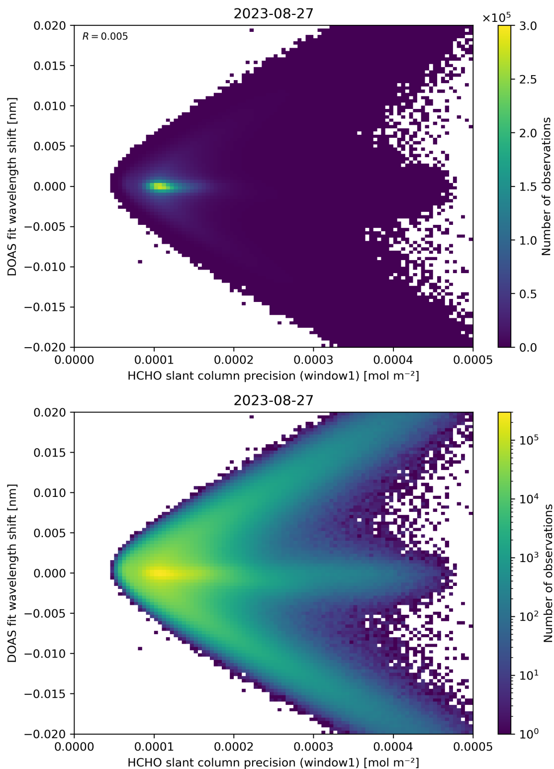
Figure 89: Scatter density plot of “HCHO slant column precision (window1)” against “DOAS fit wavelength shift” for 2023-08-26 to 2023-08-28.
