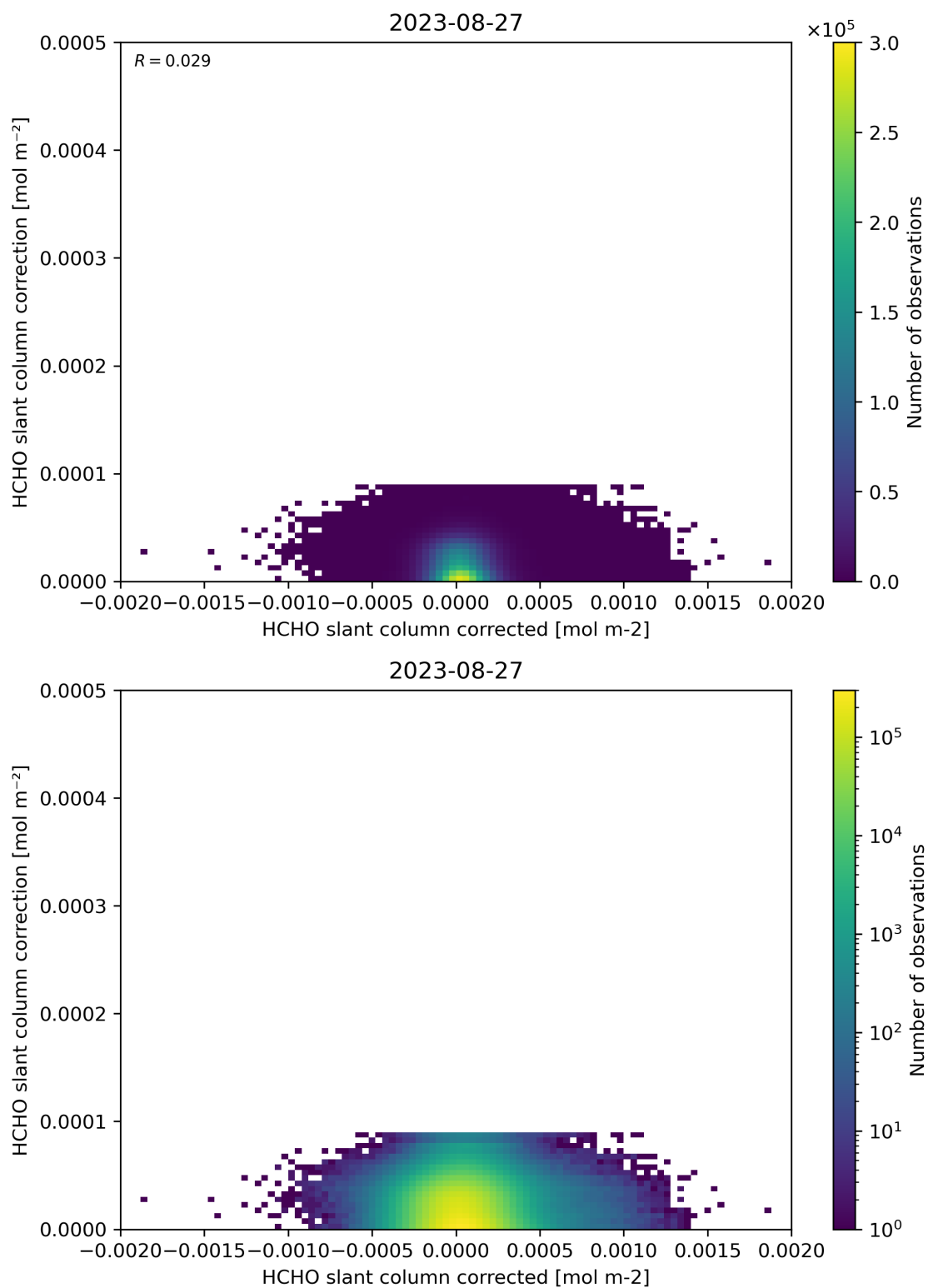
Figure 77: Scatter density plot of “HCHO slant column corrected” against “HCHO slant column correction” for 2023-08-26 to 2023-08-28.
