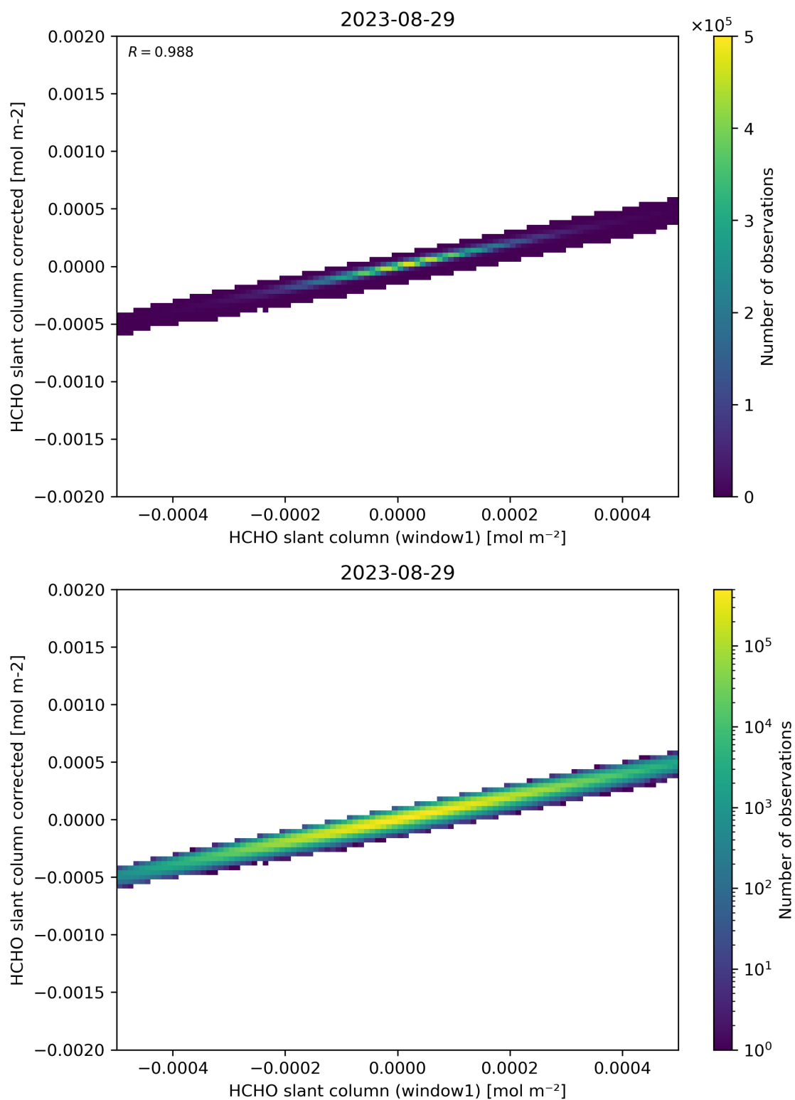
Figure 82: Scatter density plot of “HCHO slant column (window1)” against “HCHO slant column corrected” for 2023-08-28 to 2023-08-30.
