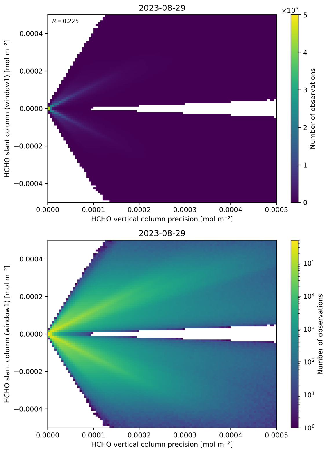
Figure 142: Scatter density plot of “HCHO vertical column precision” against “HCHO slant column (window1)” for 2023-08-28 to 2023-08-30.
