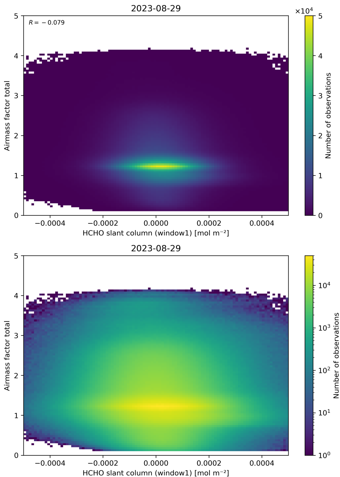
Figure 85: Scatter density plot of “HCHO slant column (window1)” against “Airmass factor total” for 2023-08-28 to 2023-08-30.
