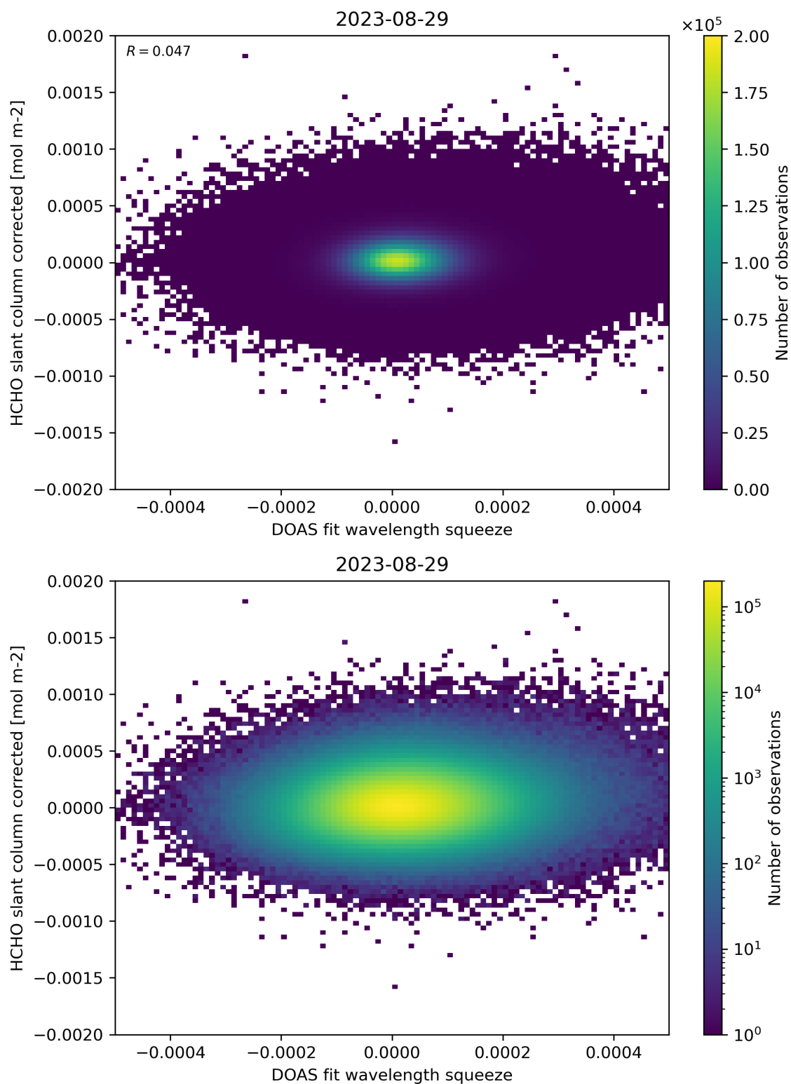
Figure 69: Scatter density plot of “DOAS fit wavelength squeeze” against “HCHO slant column corrected” for 2023-08-28 to 2023-08-30.
