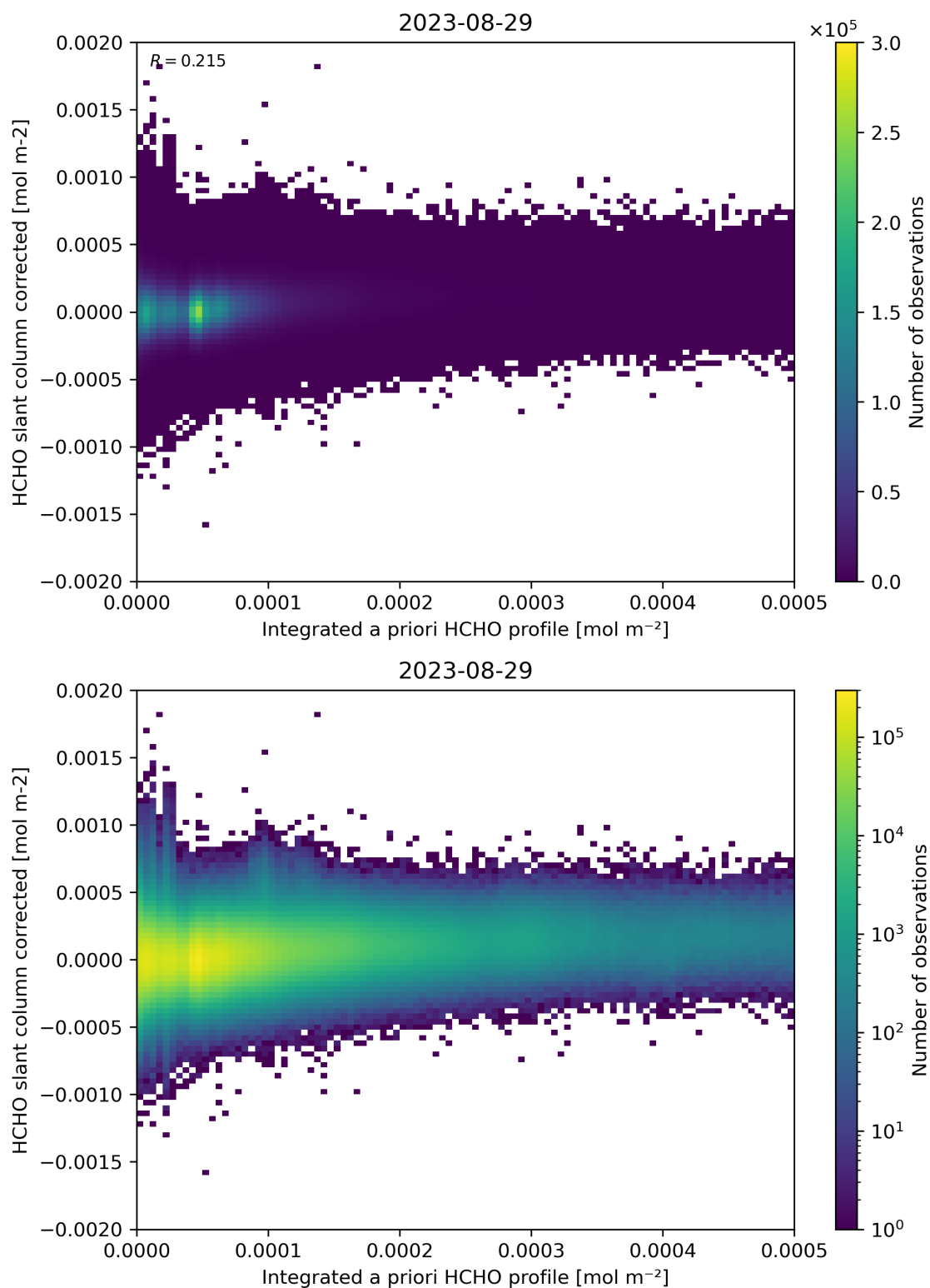
Figure 151: Scatter density plot of “Integrated a priori HCHO profile” against “HCHO slant column corrected” for 2023-08-28 to 2023-08-30.
