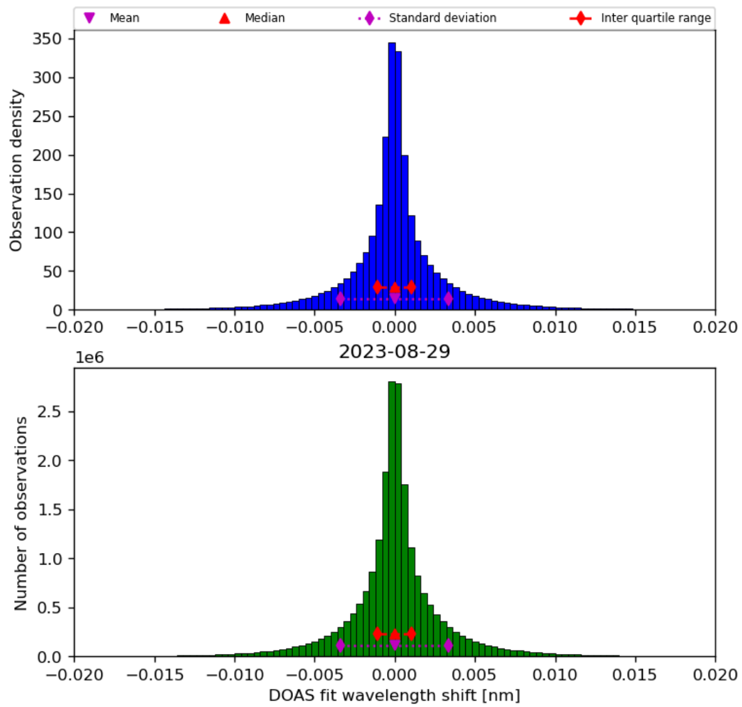
Figure 44: Histogram of “DOAS fit wavelength shift” for 2023-08-28 to 2023-08-30
