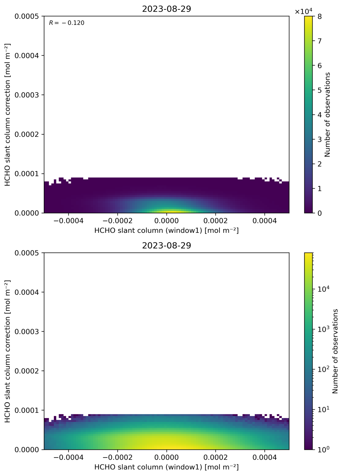
Figure 83: Scatter density plot of “HCHO slant column (window1)” against “HCHO slant column correction” for 2023-08-28 to 2023-08-30.
