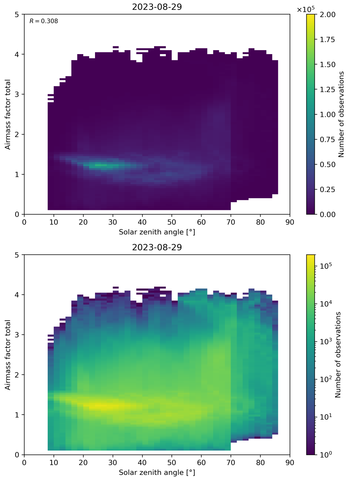
Figure 175: Scatter density plot of “Solar zenith angle” against “Airmass factor total” for 2023-08-28 to 2023-08-30.
