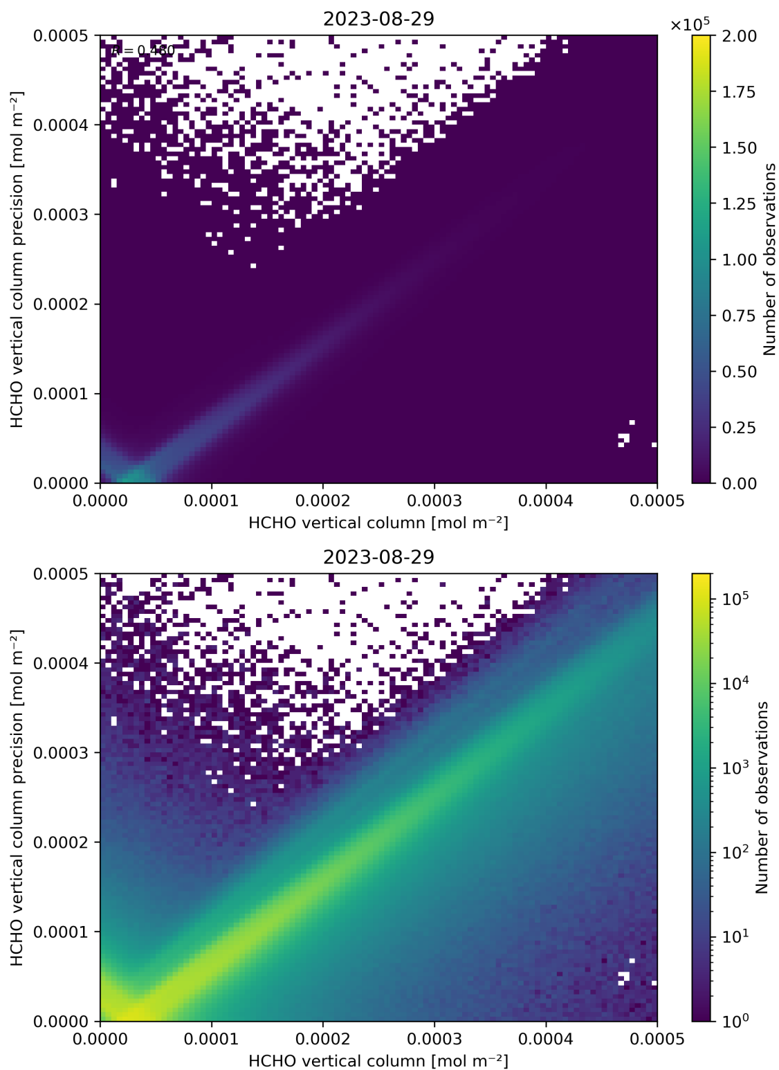
Figure 134: Scatter density plot of “HCHO vertical column” against “HCHO vertical column precision” for 2023-08-28 to 2023-08-30.
