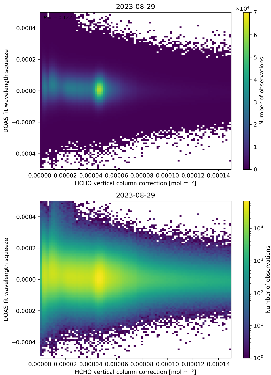
Figure 114: Scatter density plot of “HCHO vertical column correction” against “DOAS fit wavelength squeeze” for 2023-08-28 to 2023-08-30.
