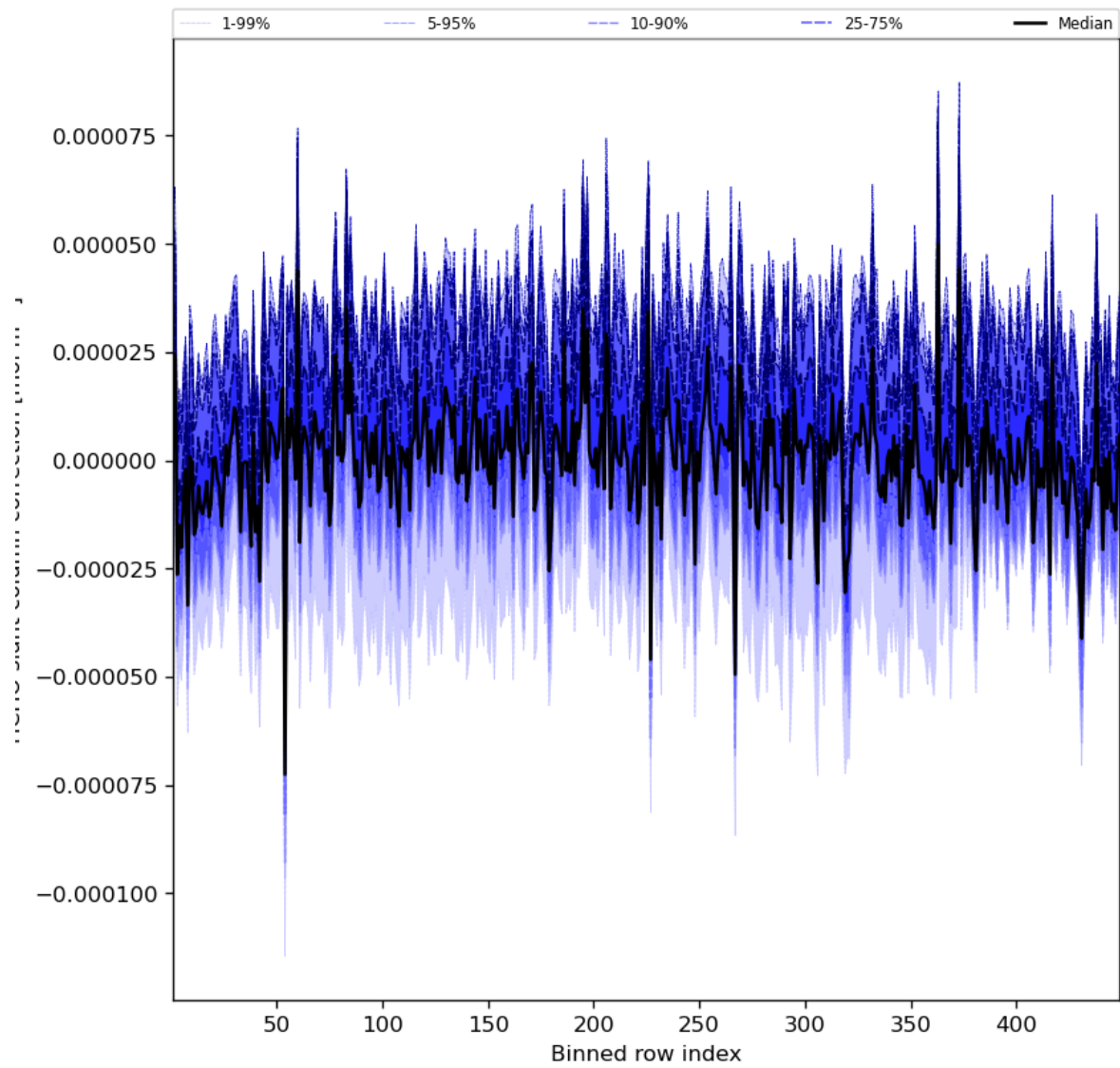
Figure 61: Along track statistics of “HCHO slant column correction” for 2023-08-28 to 2023-08-30
