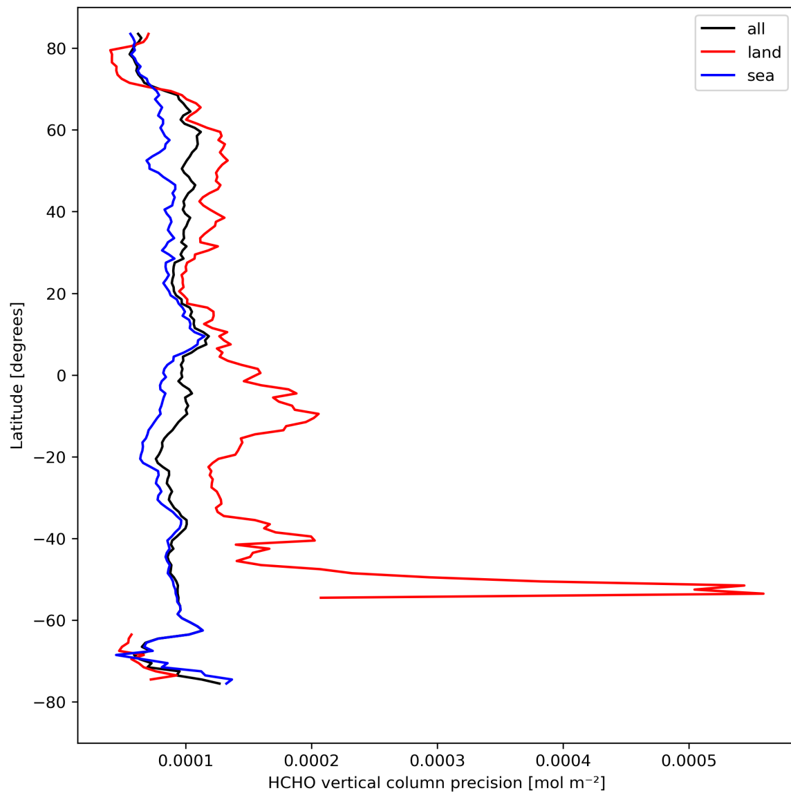
Figure 22: Zonal average of “HCHO vertical column precision” for 2023-08-28 to 2023-08-30.
