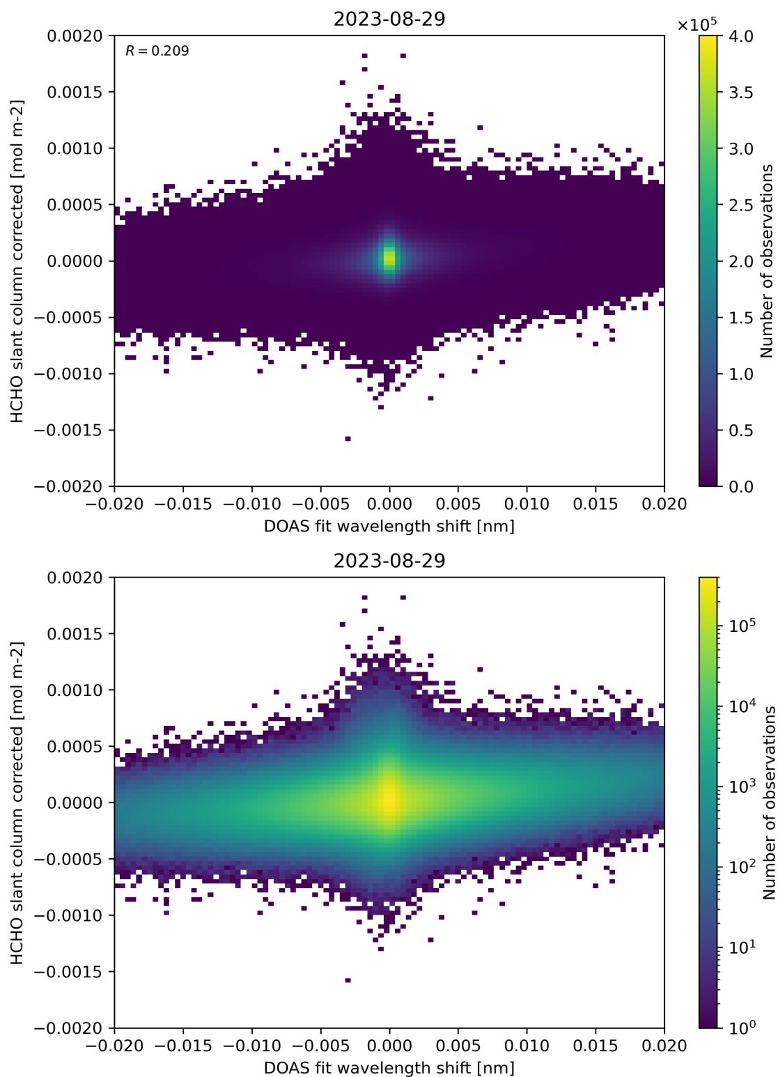
Figure 66: Scatter density plot of “DOAS fit wavelength shift” against “HCHO slant column corrected” for 2023-08-28 to 2023-08-30.
