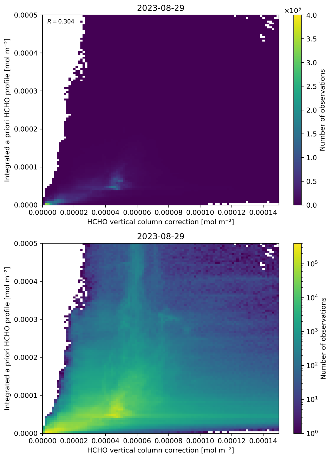
Figure 122: Scatter density plot of “HCHO vertical column correction” against “Integrated a priori HCHO profile” for 2023-08-28 to 2023-08-30.
