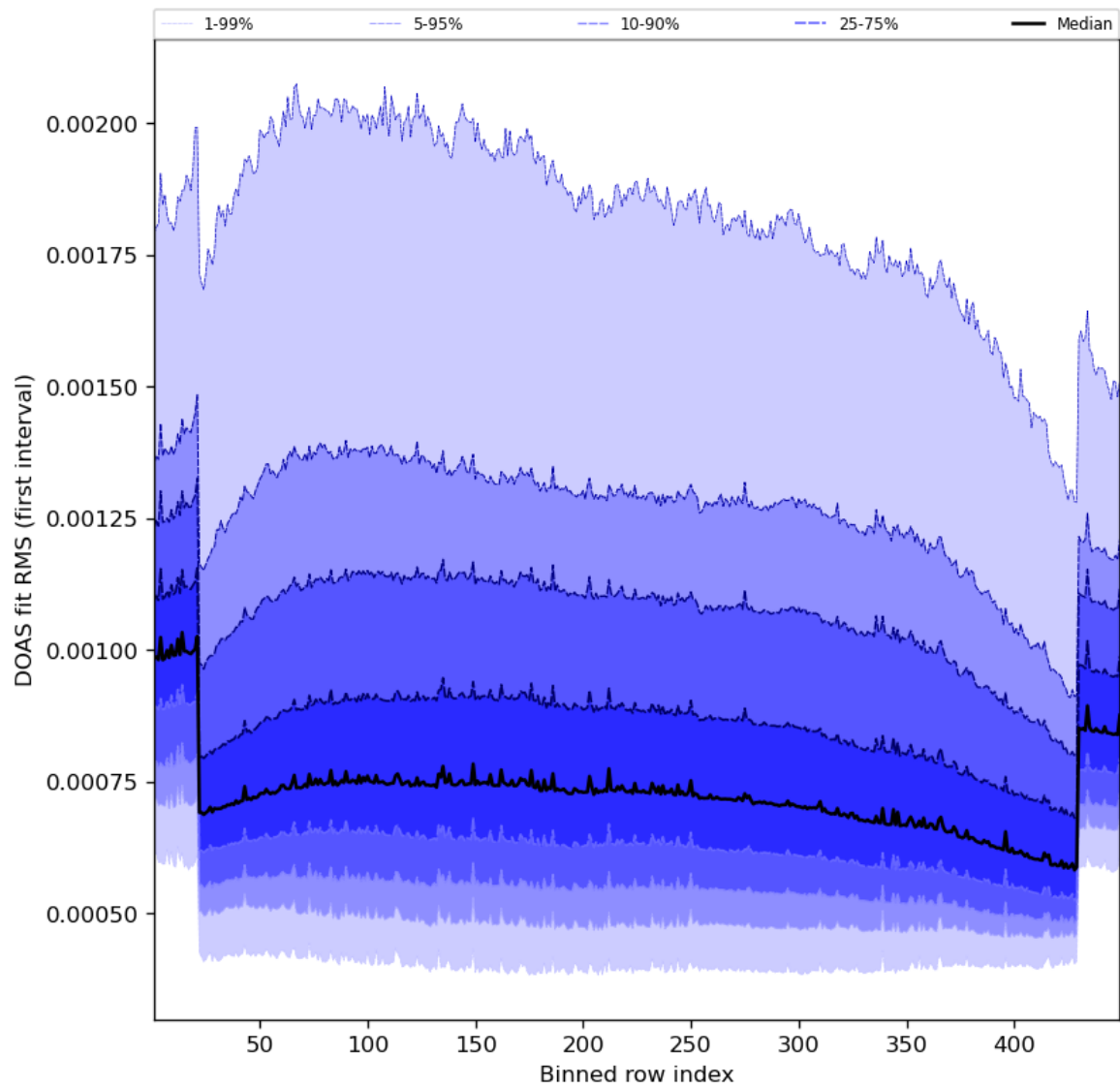
Figure 60: Along track statistics of “DOAS fit RMS (first interval)” for 2023-08-28 to 2023-08-30
