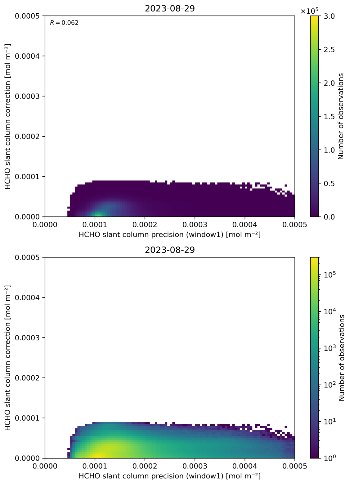
Figure 93: Scatter density plot of “HCHO slant column precision (window1)” against “HCHO slant column correction” for 2023-08-28 to 2023-08-30.
