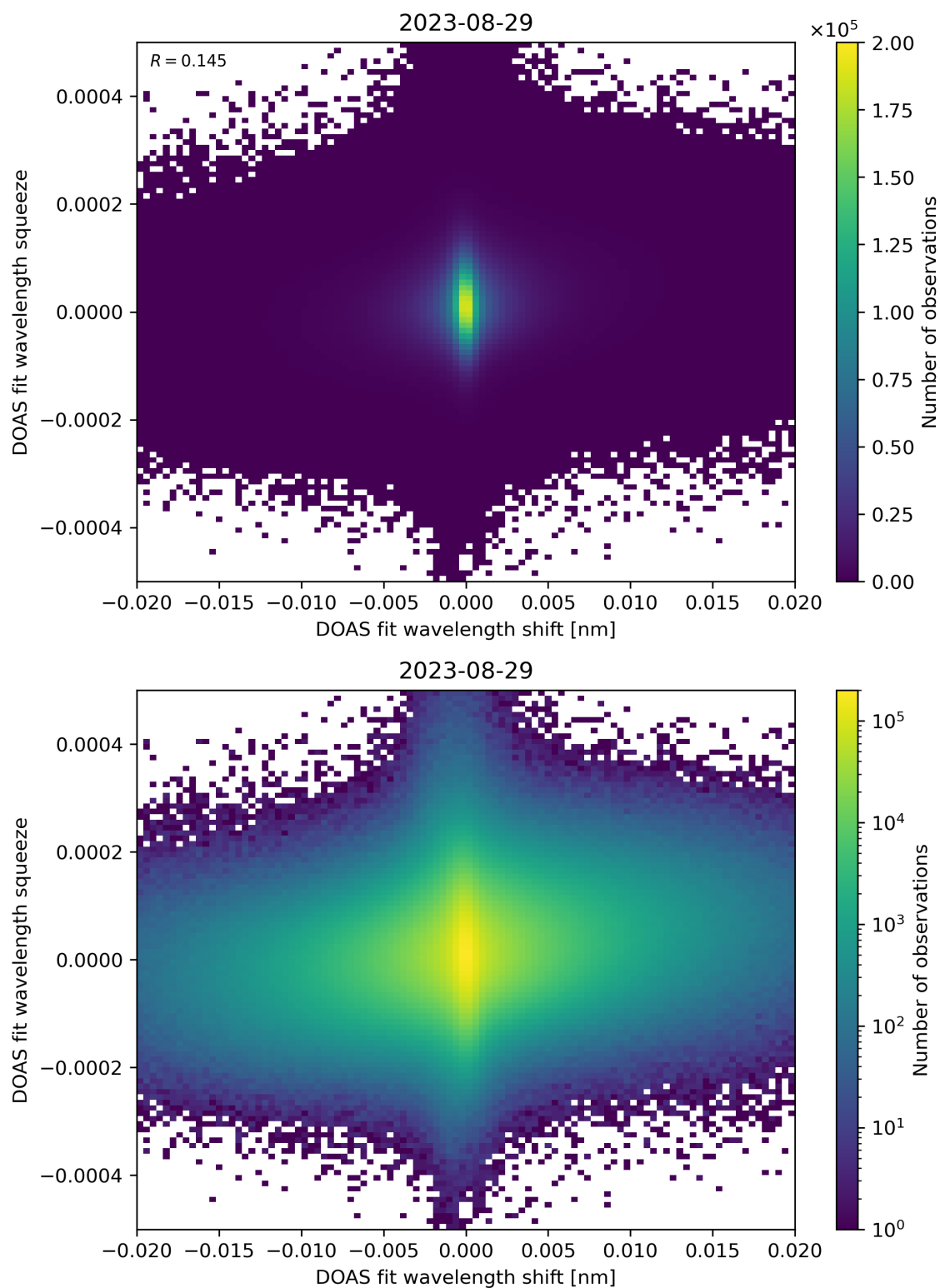
Figure 65: Scatter density plot of “DOAS fit wavelength shift” against “DOAS fit wavelength squeeze” for 2023-08-28 to 2023-08-30.
