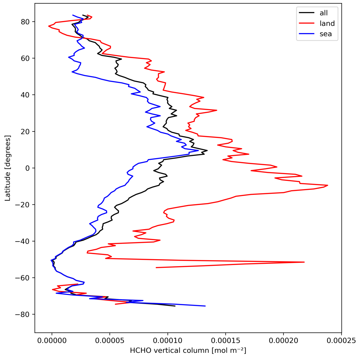
Figure 21: Zonal average of “HCHO vertical column” for 2023-08-28 to 2023-08-30.
