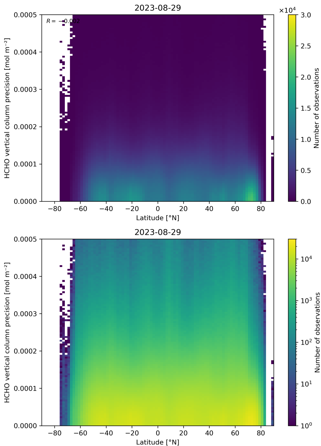
Figure 165: Scatter density plot of “Latitude” against “HCHO vertical column precision” for 2023-08-28 to 2023-08-30.
