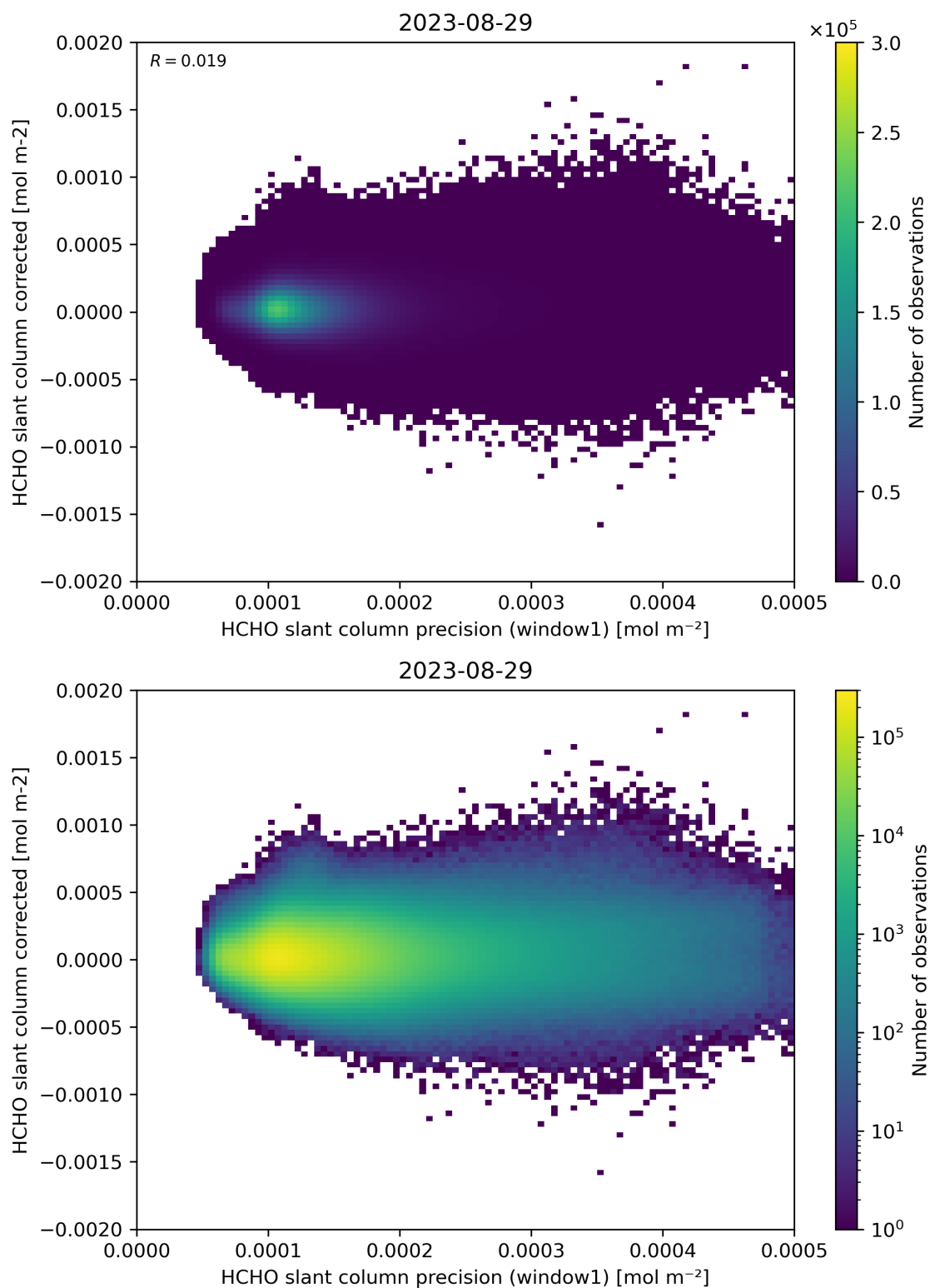
Figure 92: Scatter density plot of “HCHO slant column precision (window1)” against “HCHO slant column corrected” for 2023-08-28 to 2023-08-30.
