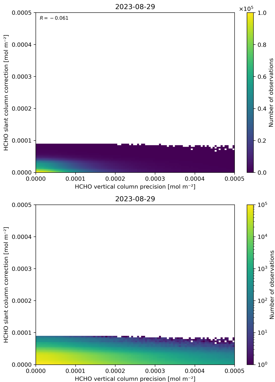
Figure 141: Scatter density plot of “HCHO vertical column precision” against “HCHO slant column correction” for 2023-08-28 to 2023-08-30.
