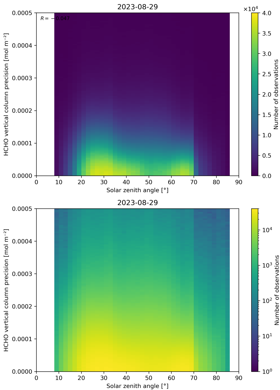
Figure 179: Scatter density plot of “Solar zenith angle” against “HCHO vertical column precision” for 2023-08-28 to 2023-08-30.
