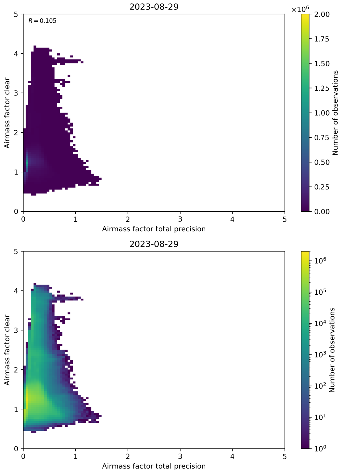
Figure 108: Scatter density plot of “Airmass factor total precision” against “Airmass factor clear” for 2023-08-28 to 2023-08-30.
