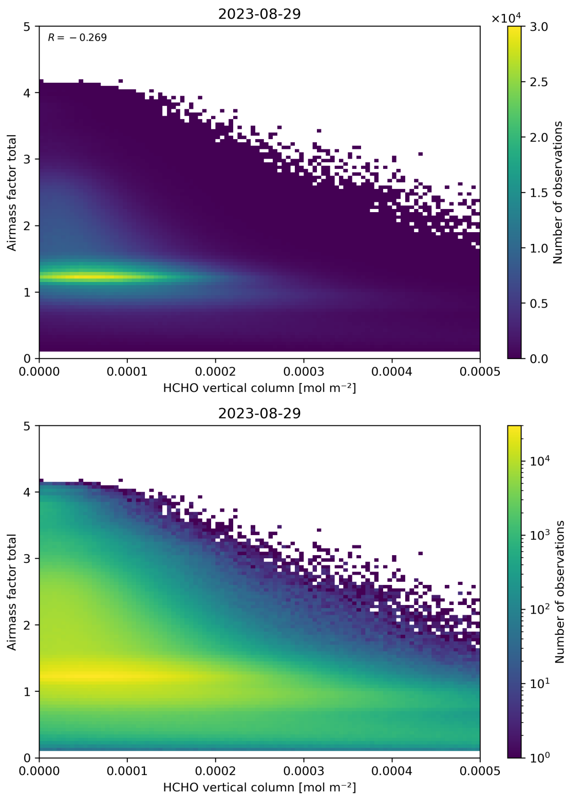
Figure 131: Scatter density plot of “HCHO vertical column” against “Airmass factor total” for 2023-08-28 to 2023-08-30.
