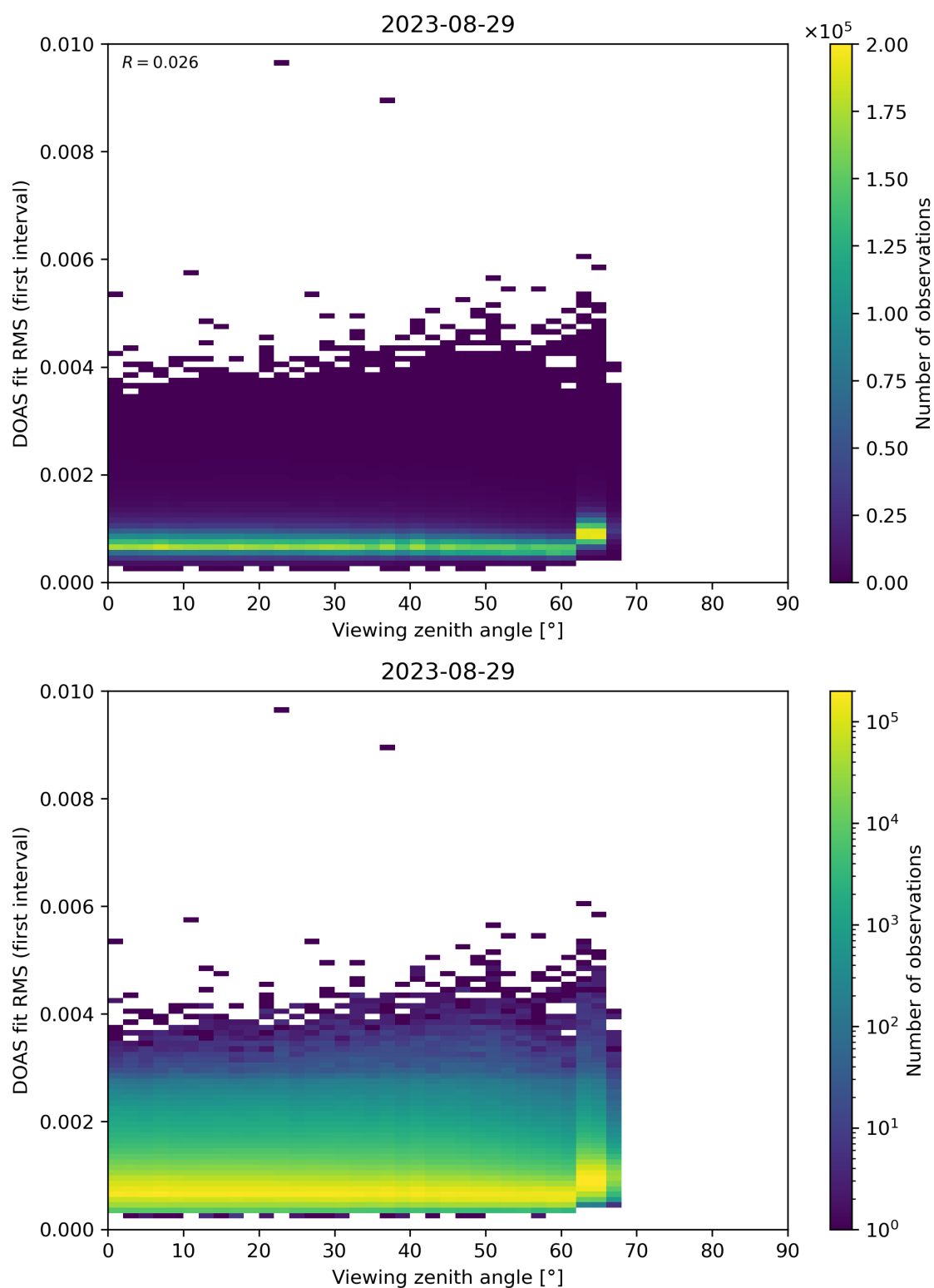
Figure 182: Scatter density plot of “Viewing zenith angle” against “DOAS fit RMS (first interval)” for 2023-08-28 to 2023-08-30.
