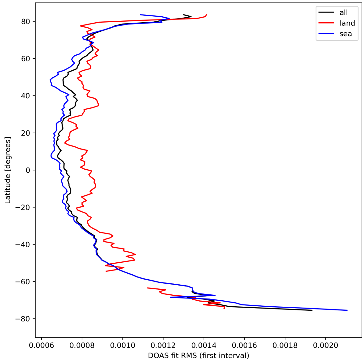
Figure 32: Zonal average of “DOAS fit RMS (first interval)” for 2023-08-28 to 2023-08-30.
