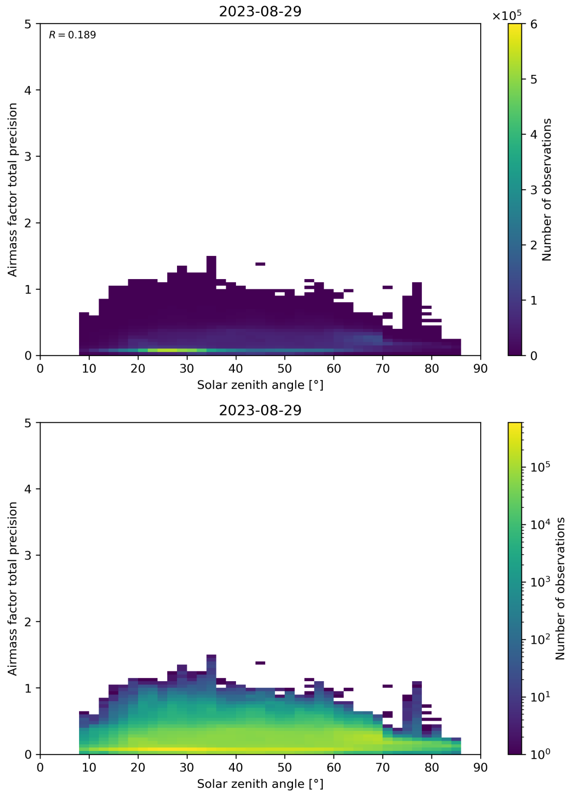
Figure 176: Scatter density plot of “Solar zenith angle” against “Airmass factor total precision” for 2023-08-28 to 2023-08-30.
