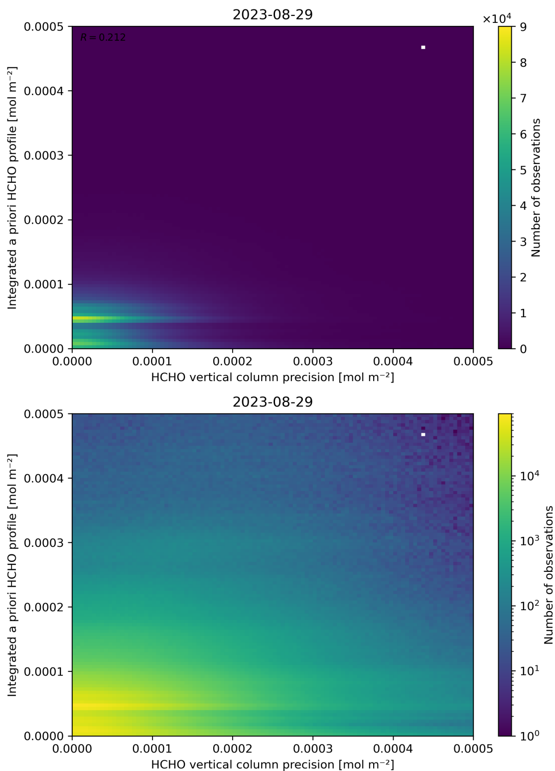
Figure 147: Scatter density plot of “HCHO vertical column precision” against “Integrated a priori HCHO profile” for 2023-08-28 to 2023-08-30.
