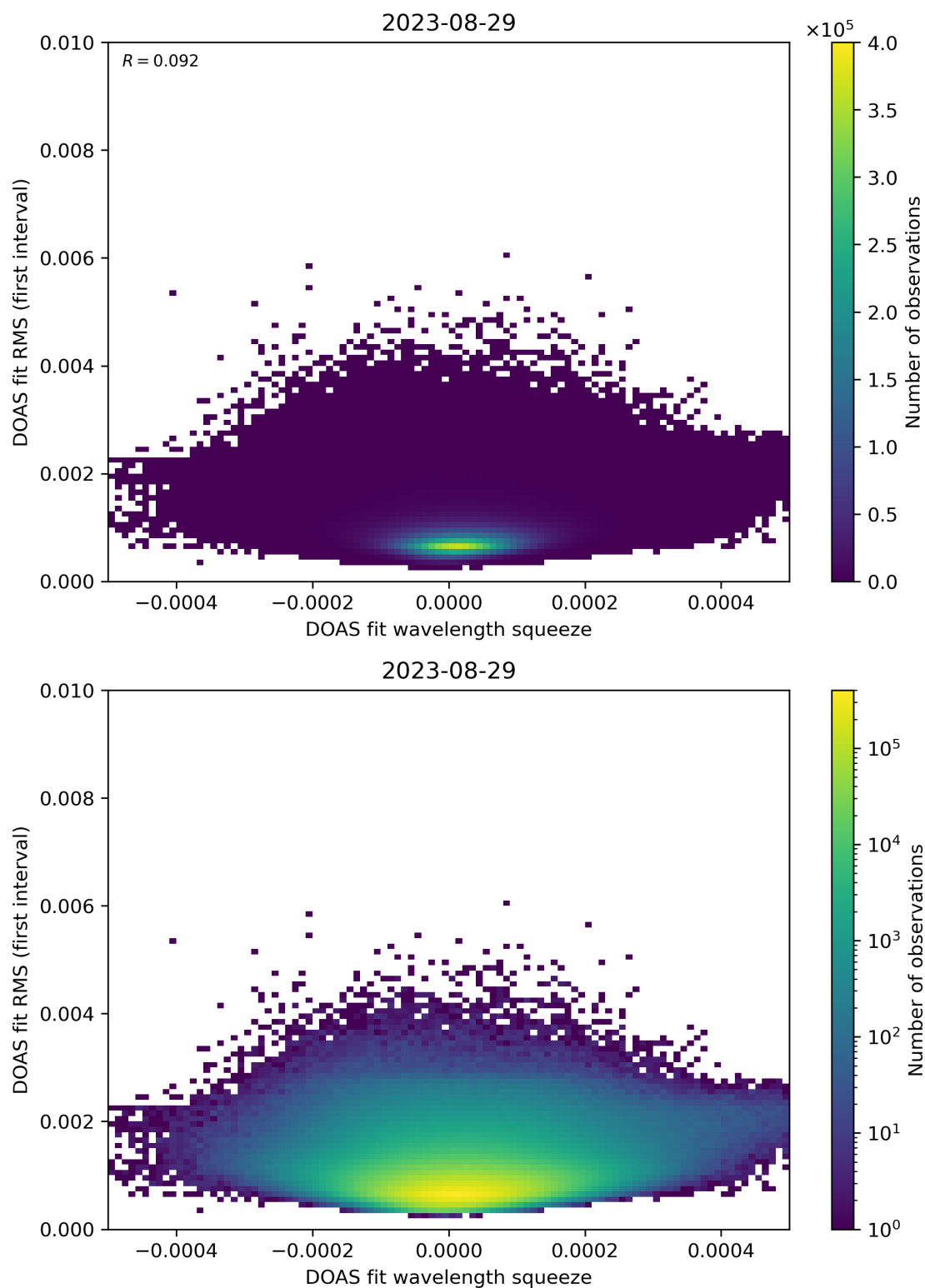
Figure 68: Scatter density plot of “DOAS fit wavelength squeeze” against “DOAS fit RMS (first interval)” for 2023-08-28 to 2023-08-30.
