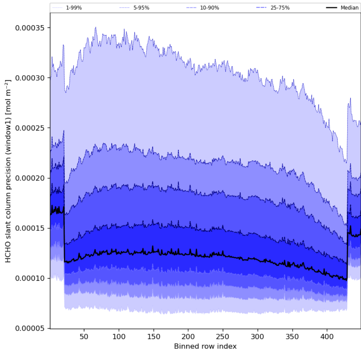
Figure 53: Along track statistics of “HCHO slant column precision (window1)” for 2023-08-28 to 2023-08-30
