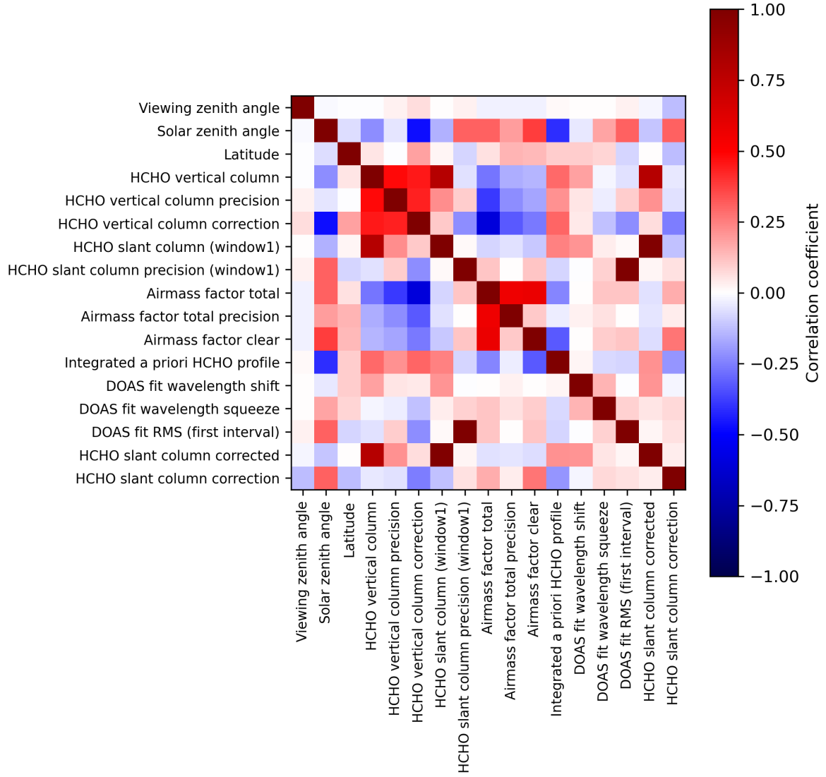
Figure 2: Map of correlation matrix for 2023-08-28 to 2023-08-30.
