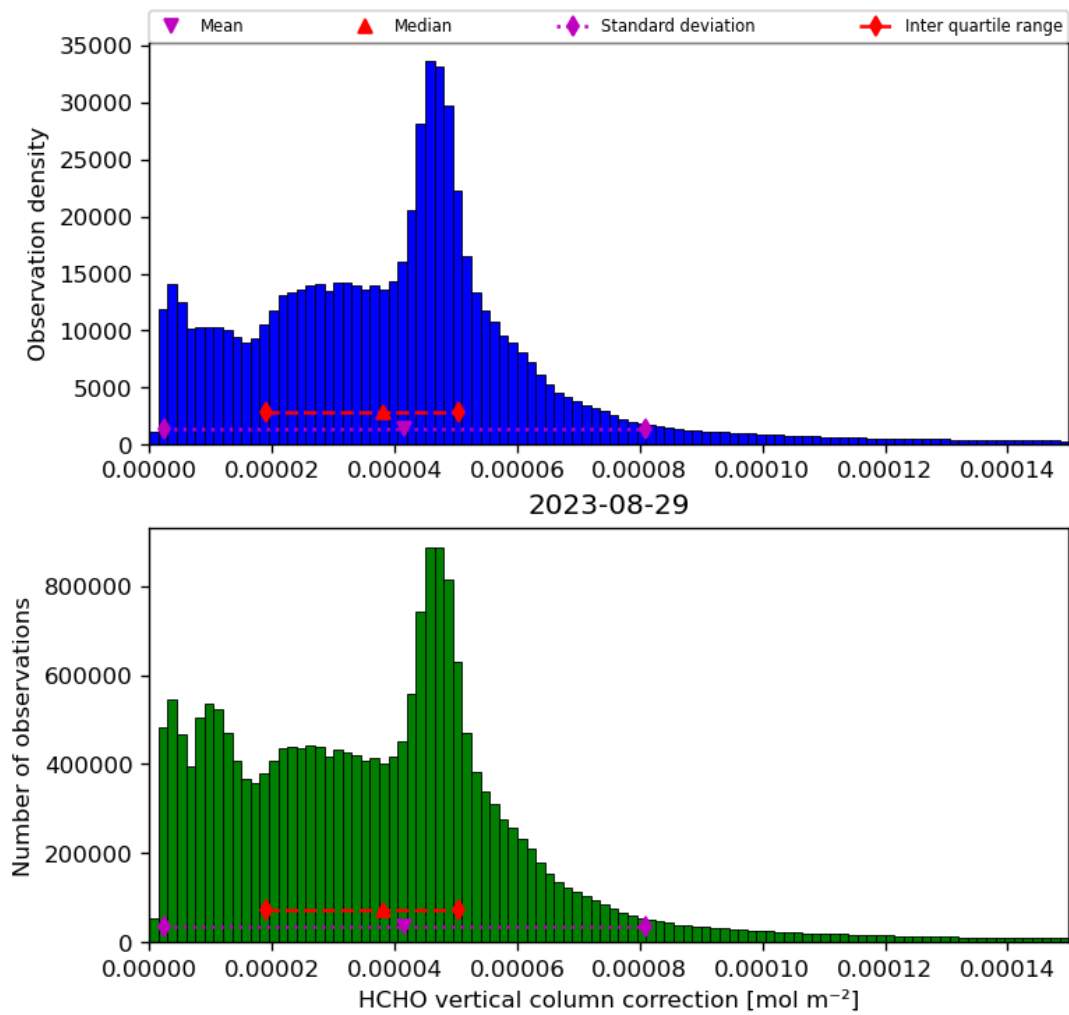
Figure 37: Histogram of “HCHO vertical column correction” for 2023-08-28 to 2023-08-30
