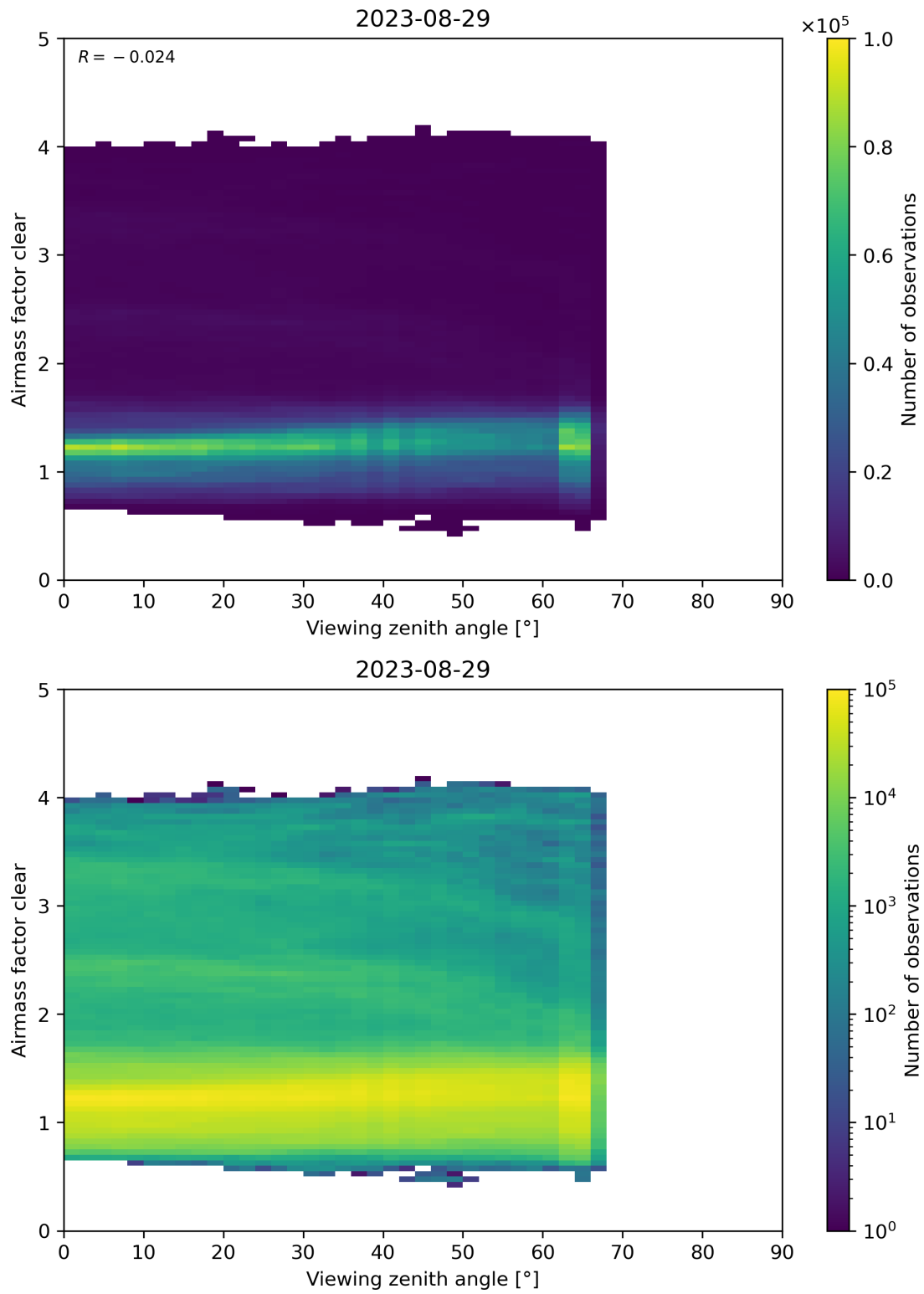
Figure 185: Scatter density plot of “Viewing zenith angle” against “Airmass factor clear” for 2023-08-28 to 2023-08-30.
