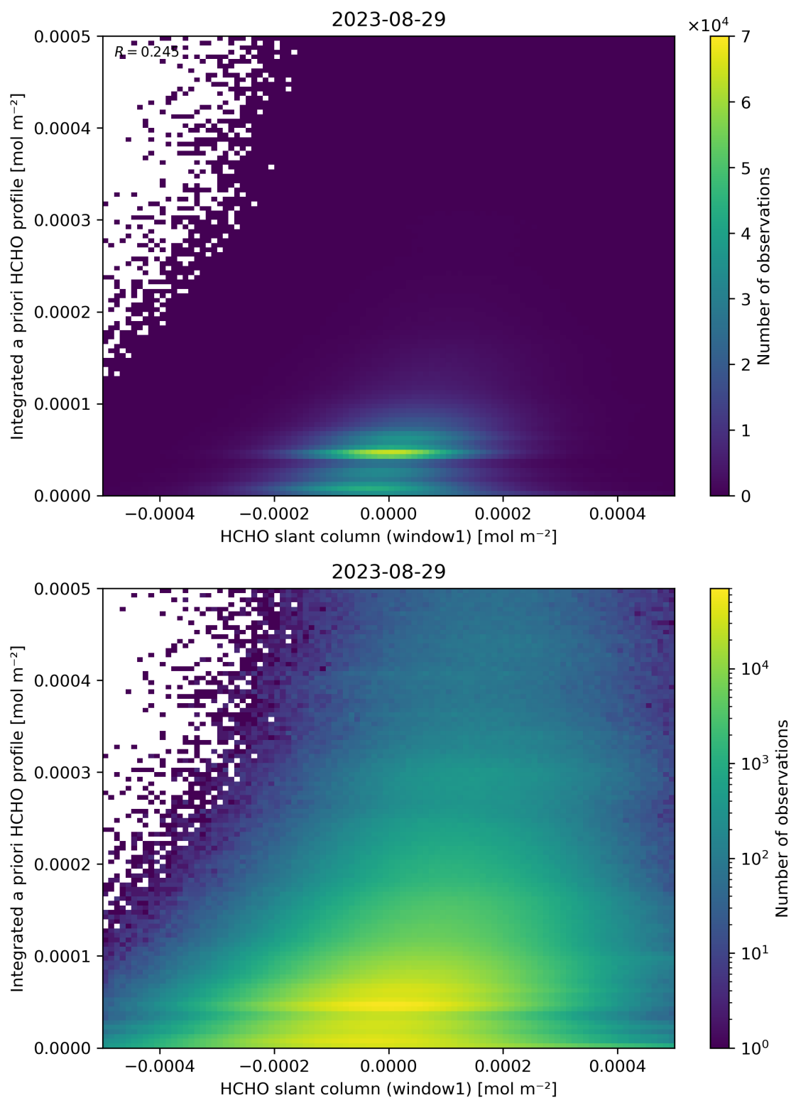
Figure 87: Scatter density plot of “HCHO slant column (window1)” against “Integrated a priori HCHO profile” for 2023-08-28 to 2023-08-30.
