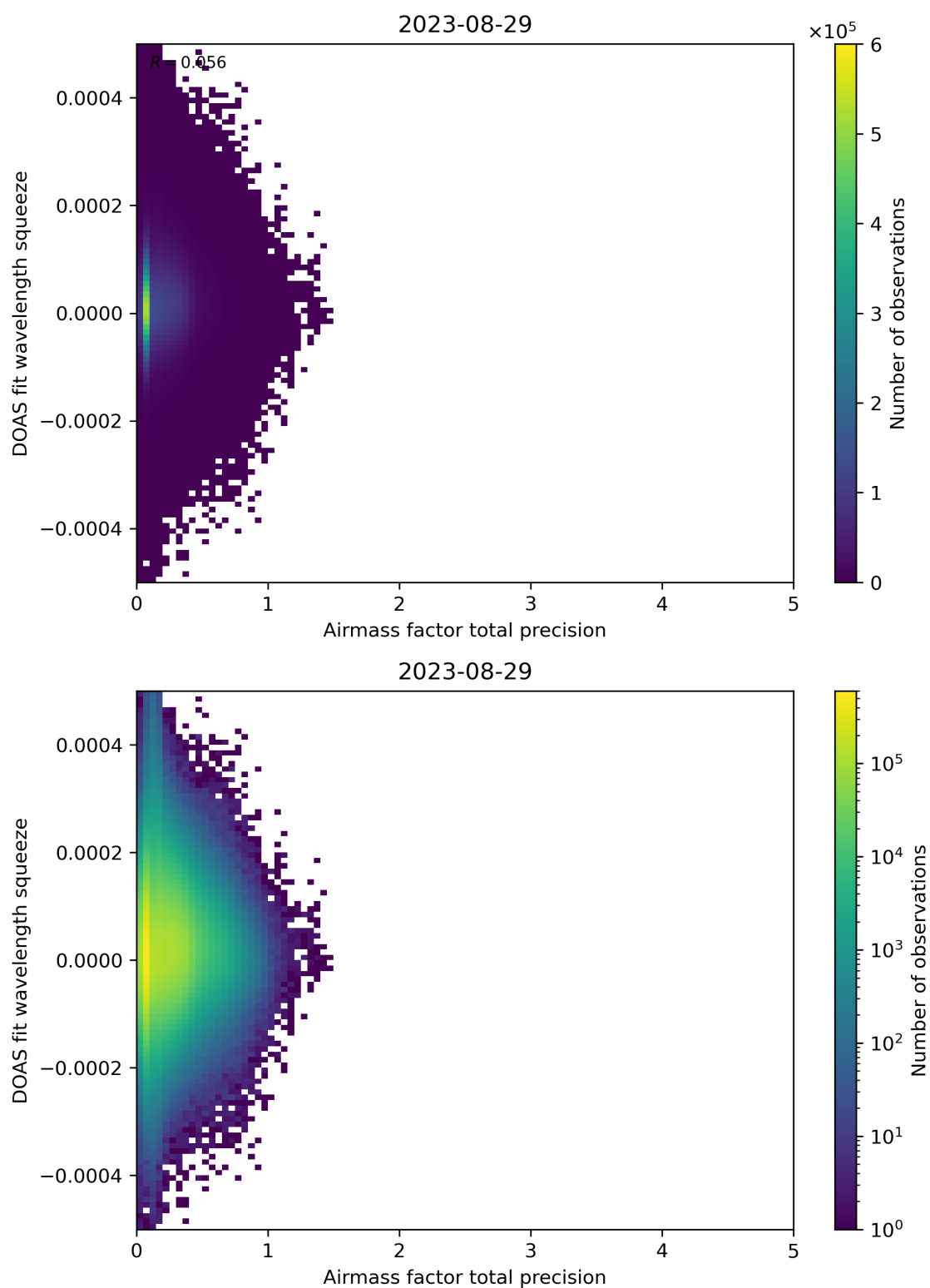
Figure 107: Scatter density plot of “Airmass factor total precision” against “DOAS fit wavelength squeeze” for 2023-08-28 to 2023-08-30.
