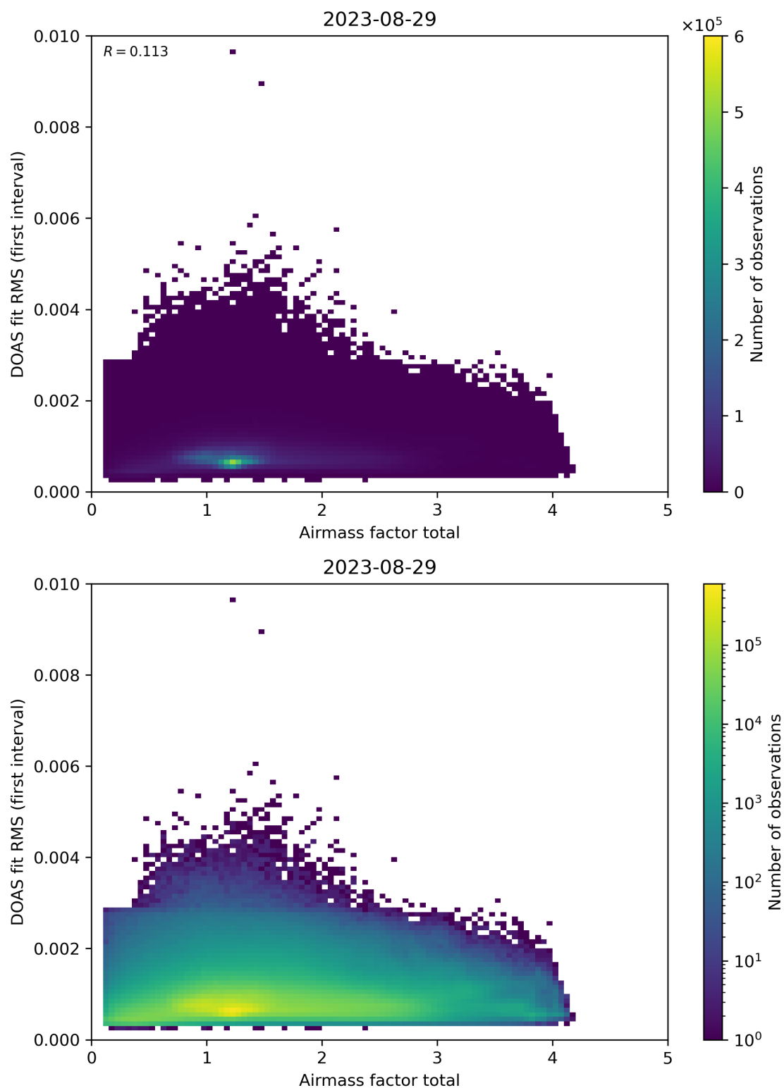
Figure 97: Scatter density plot of “Airmass factor total” against “DOAS fit RMS (first interval)” for 2023-08-28 to 2023-08-30.
