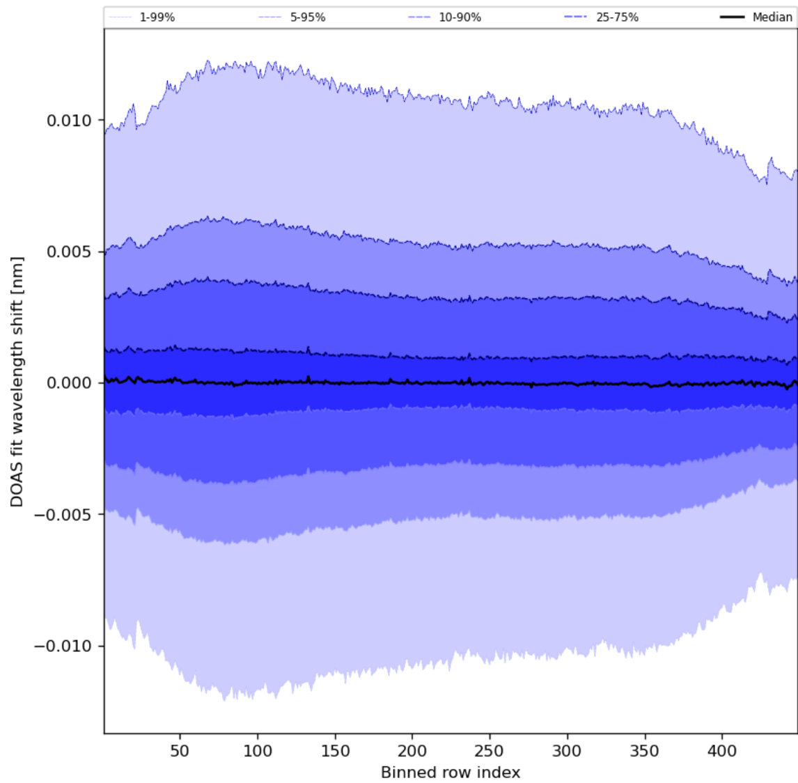
Figure 58: Along track statistics of “DOAS fit wavelength shift” for 2023-08-28 to 2023-08-30
