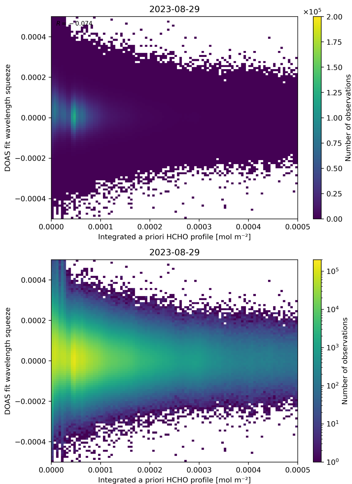
Figure 150: Scatter density plot of “Integrated a priori HCHO profile” against “DOAS fit wavelength squeeze” for 2023-08-28 to 2023-08-30.
