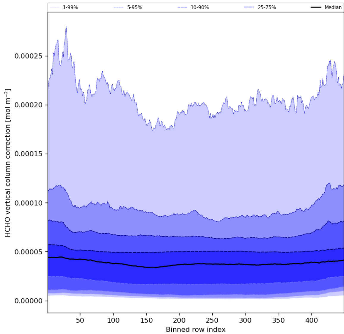
Figure 51: Along track statistics of “HCHO vertical column correction” for 2023-08-28 to 2023-08-30
