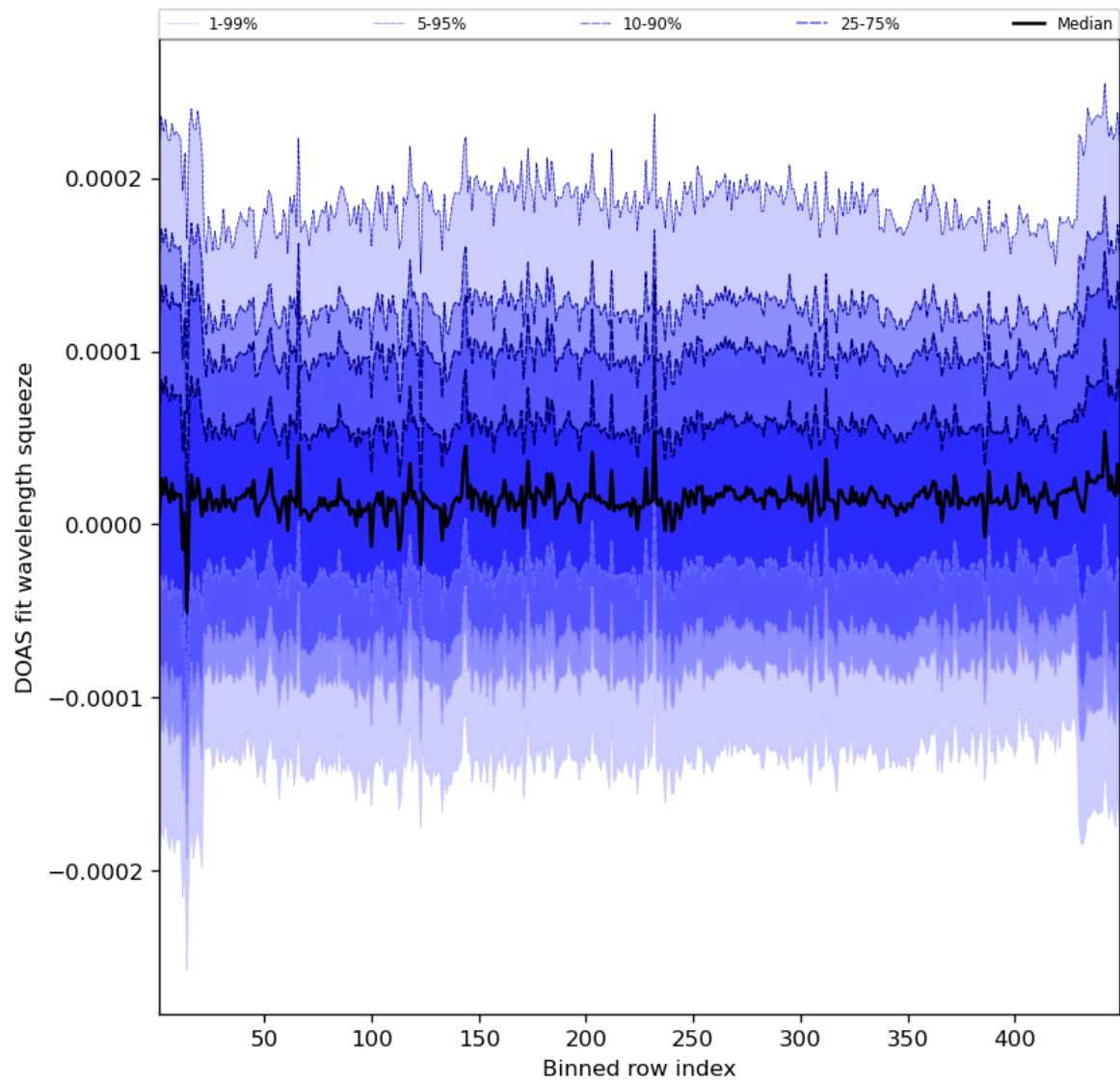
Figure 59: Along track statistics of “DOAS fit wavelength squeeze” for 2023-08-28 to 2023-08-30
