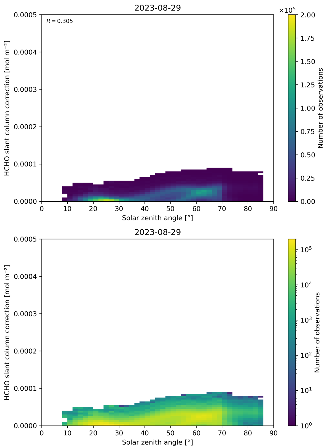
Figure 172: Scatter density plot of “Solar zenith angle” against “HCHO slant column correction” for 2023-08-28 to 2023-08-30.
