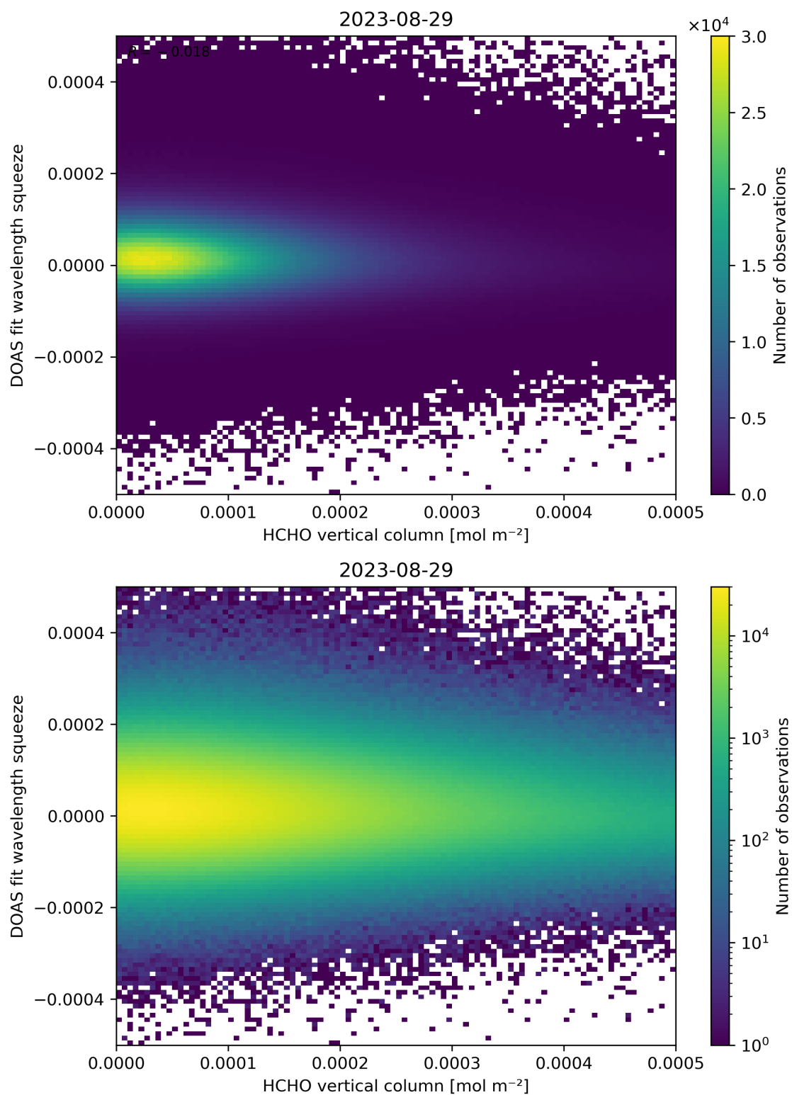
Figure 125: Scatter density plot of “HCHO vertical column” against “DOAS fit wavelength squeeze” for 2023-08-28 to 2023-08-30.
