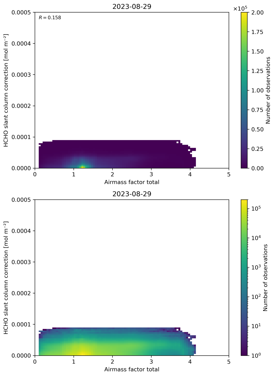
Figure 102: Scatter density plot of “Airmass factor total” against “HCHO slant column correction” for 2023-08-28 to 2023-08-30.
