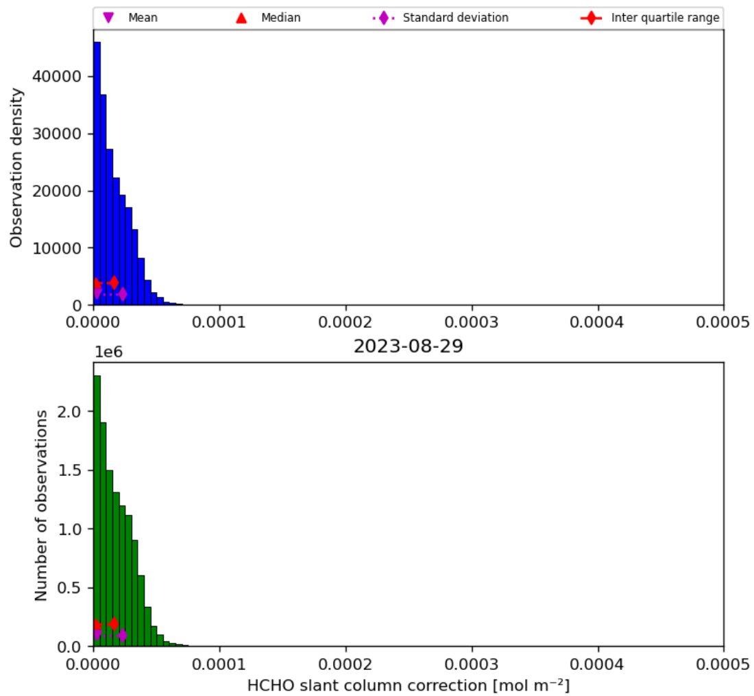
Figure 47: Histogram of “HCHO slant column correction” for 2023-08-28 to 2023-08-30
