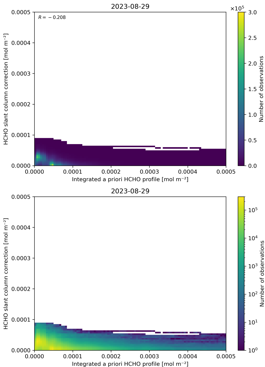
Figure 152: Scatter density plot of “Integrated a priori HCHO profile” against “HCHO slant column correction” for 2023-08-28 to 2023-08-30.
