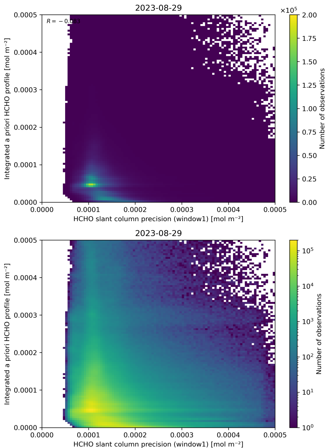
Figure 96: Scatter density plot of “HCHO slant column precision (window1)” against “Integrated a priori HCHO profile” for 2023-08-28 to 2023-08-30.
