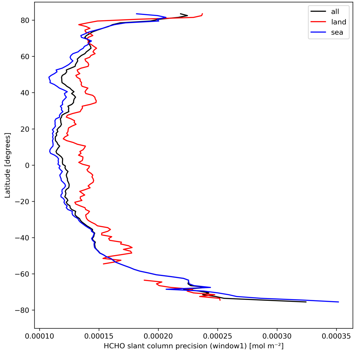
Figure 25: Zonal average of "HCHO slant column precision (window1)" for 2023-08-28 to 2023-08-30.
