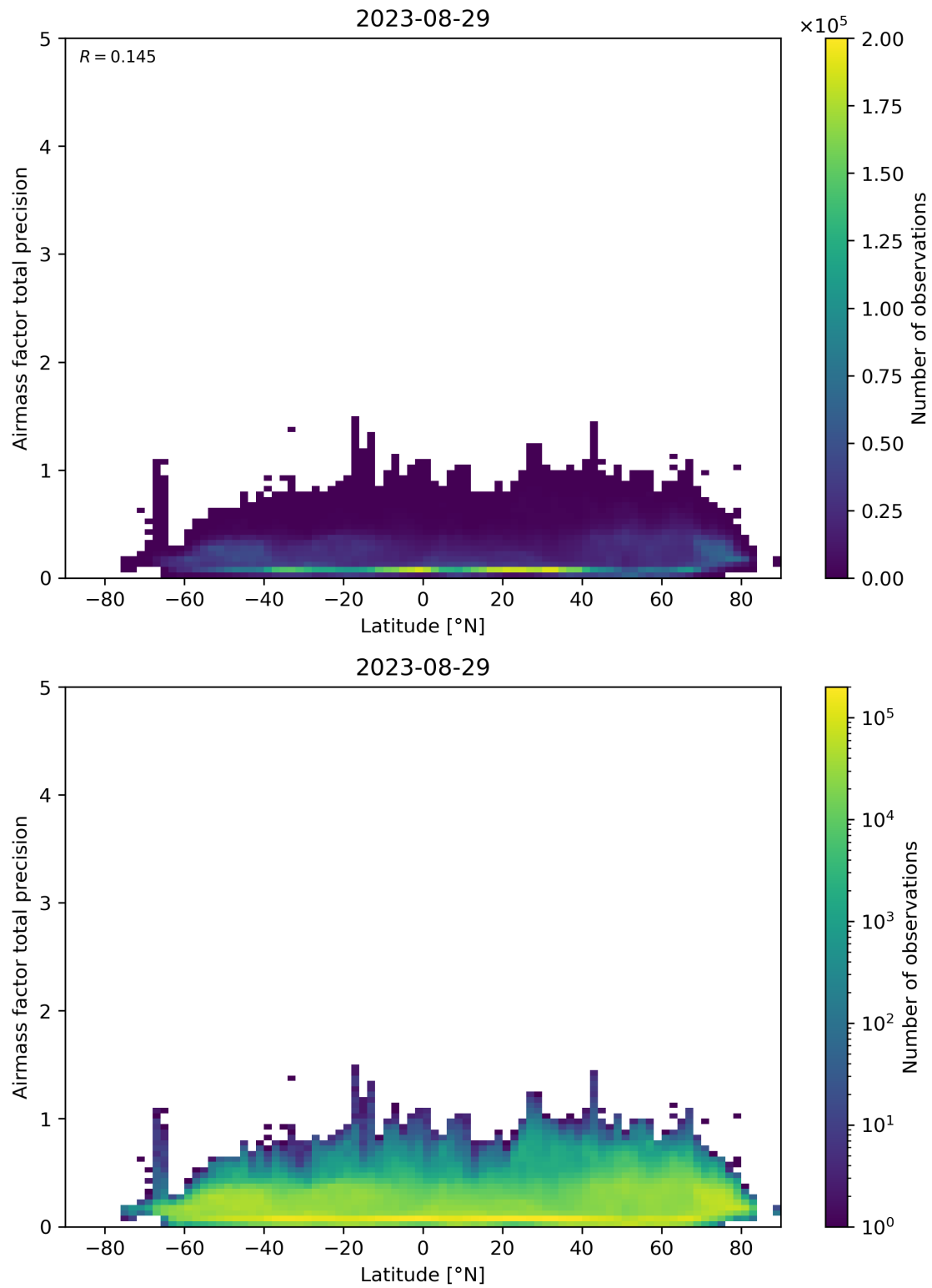
Figure 162: Scatter density plot of “Latitude” against “Airmass factor total precision” for 2023-08-28 to 2023-08-30.
