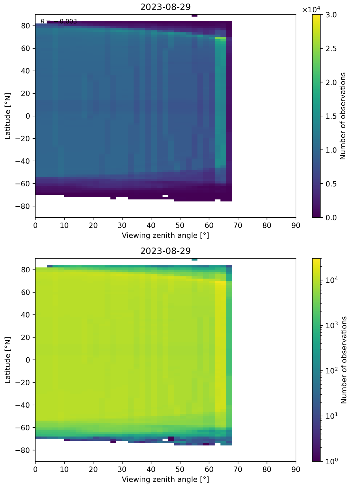
Figure 196: Scatter density plot of “Viewing zenith angle” against “Latitude” for 2023-08-28 to 2023-08-30.
