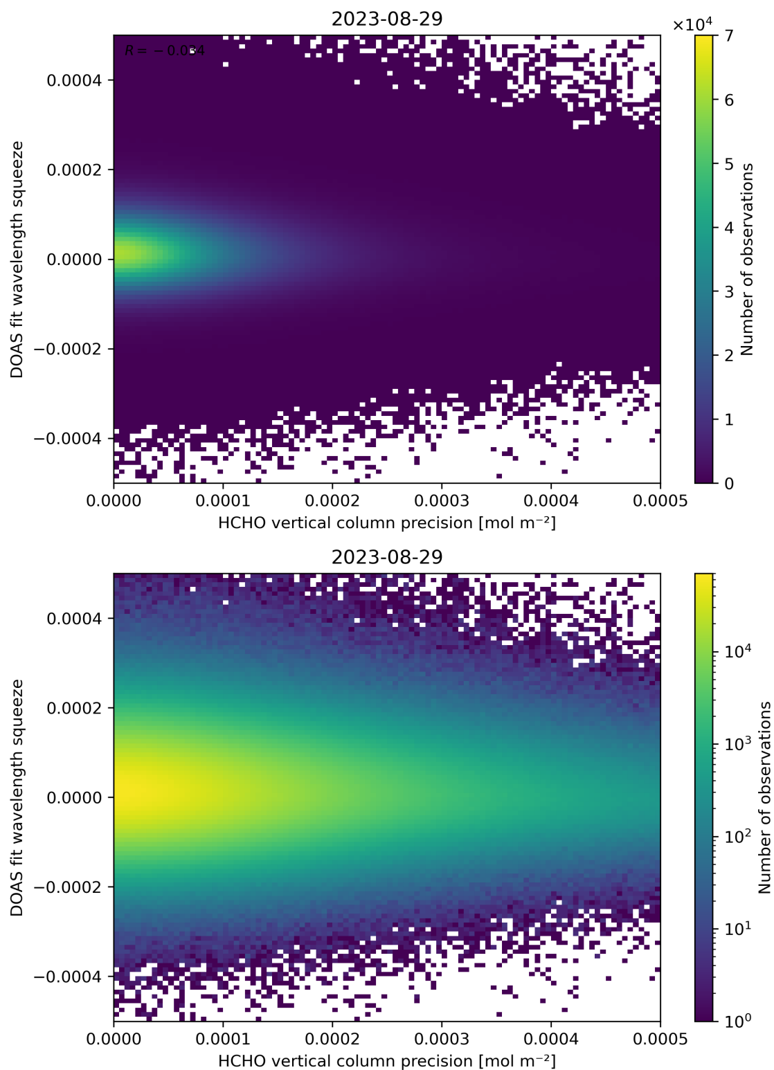
Figure 138: Scatter density plot of “HCHO vertical column precision” against “DOAS fit wavelength squeeze” for 2023-08-28 to 2023-08-30.
