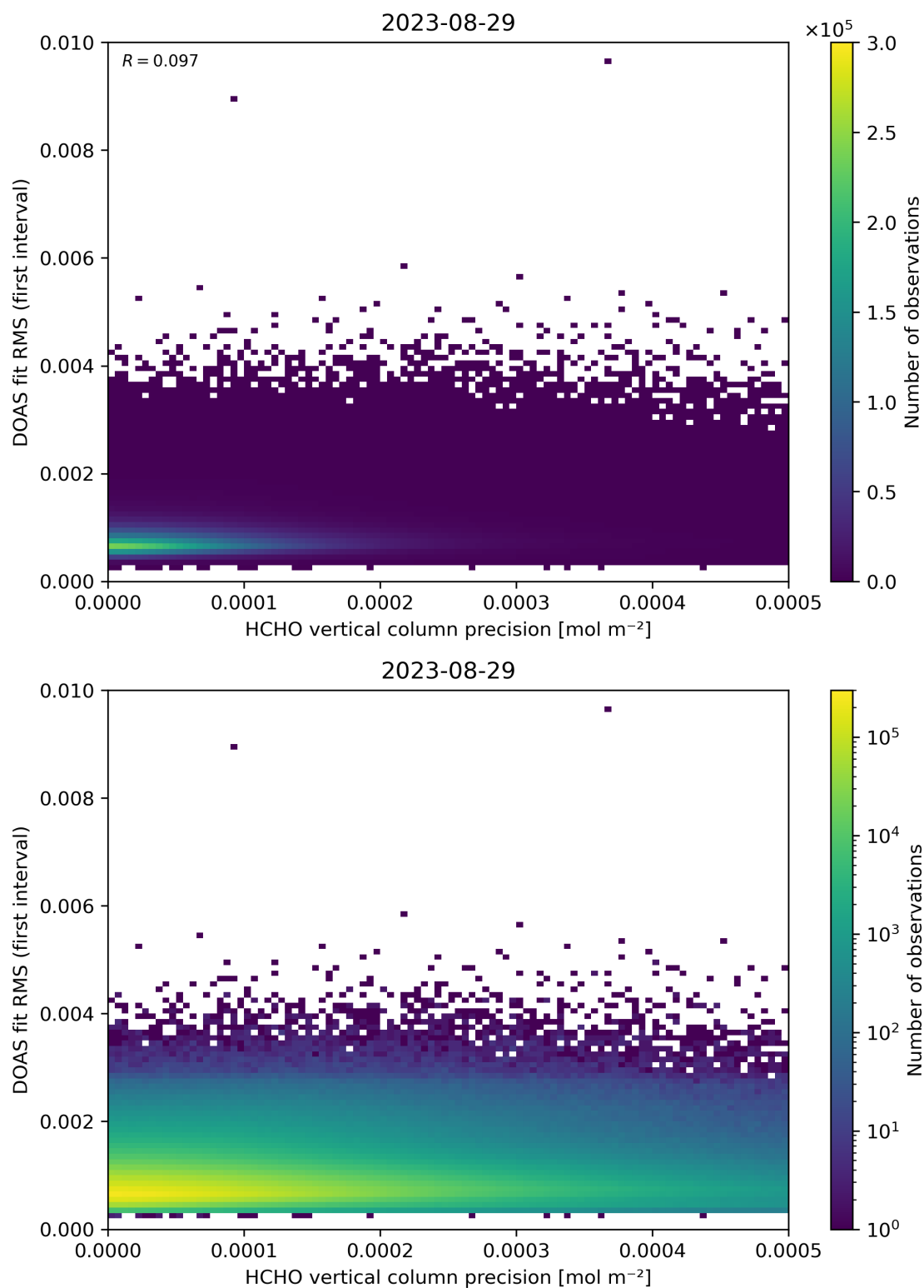
Figure 136: Scatter density plot of “HCHO vertical column precision” against “DOAS fit RMS (first interval)” for 2023-08-28 to 2023-08-30.
