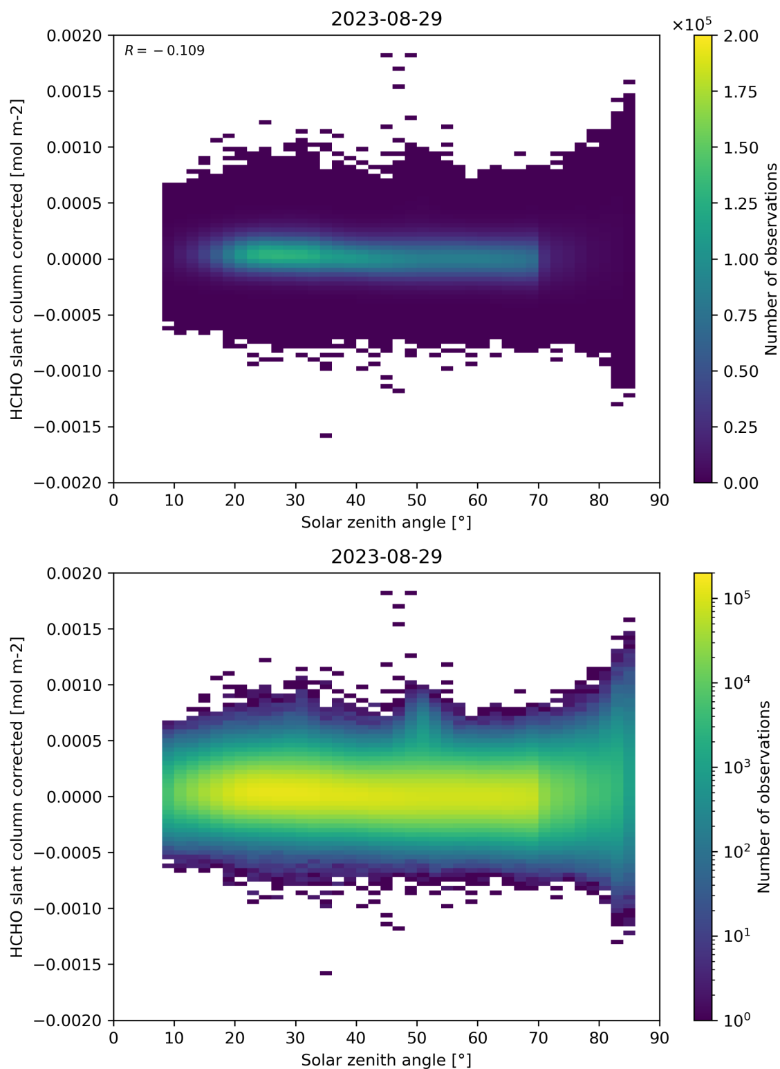
Figure 171: Scatter density plot of “Solar zenith angle” against “HCHO slant column corrected” for 2023-08-28 to 2023-08-30.
