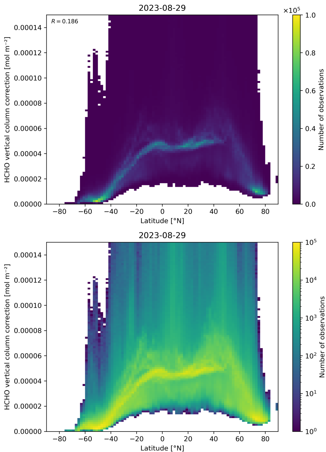
Figure 164: Scatter density plot of “Latitude” against “HCHO vertical column correction” for 2023-08-28 to 2023-08-30.
