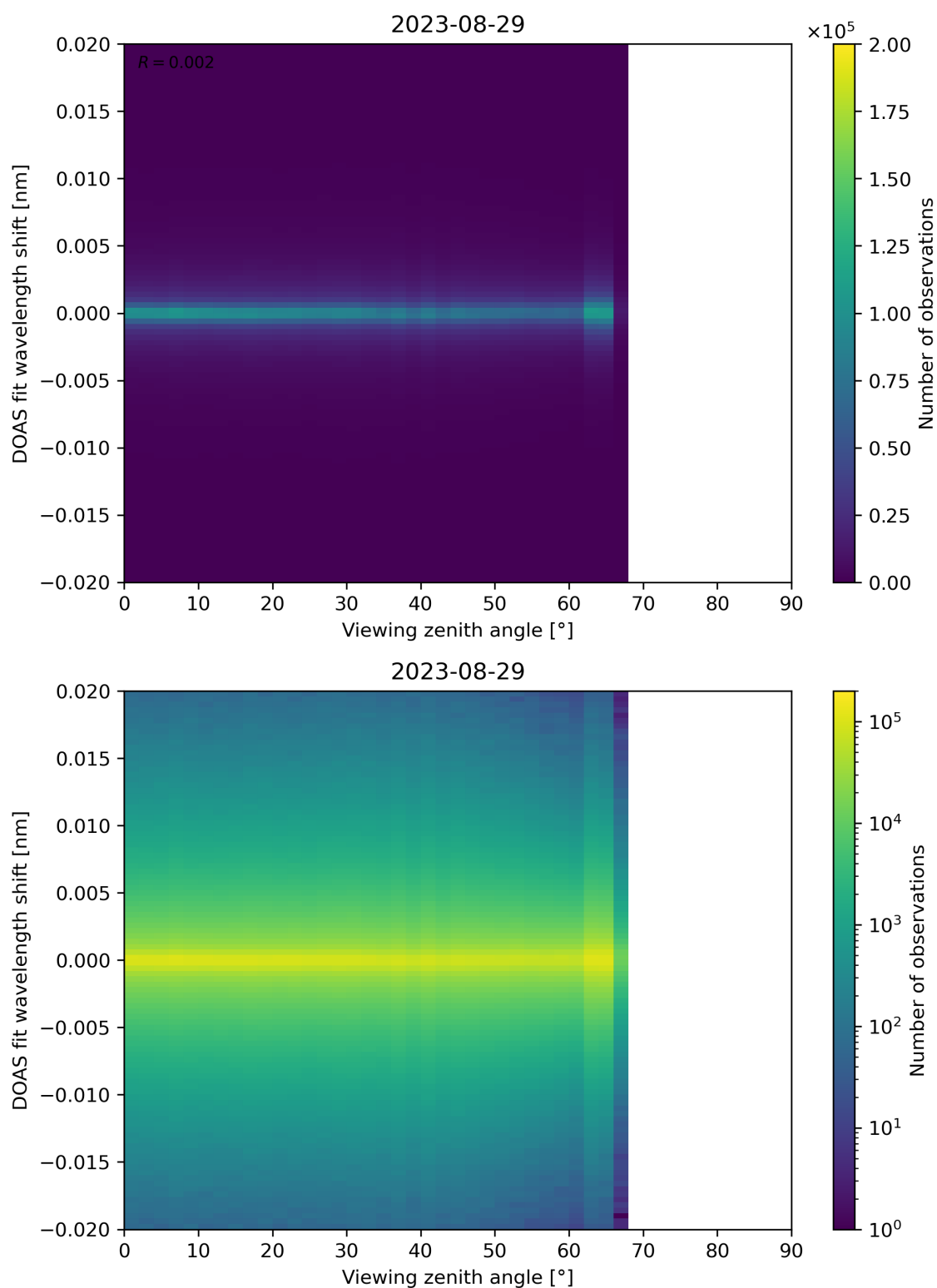
Figure 183: Scatter density plot of “Viewing zenith angle” against “DOAS fit wavelength shift” for 2023-08-28 to 2023-08-30.
