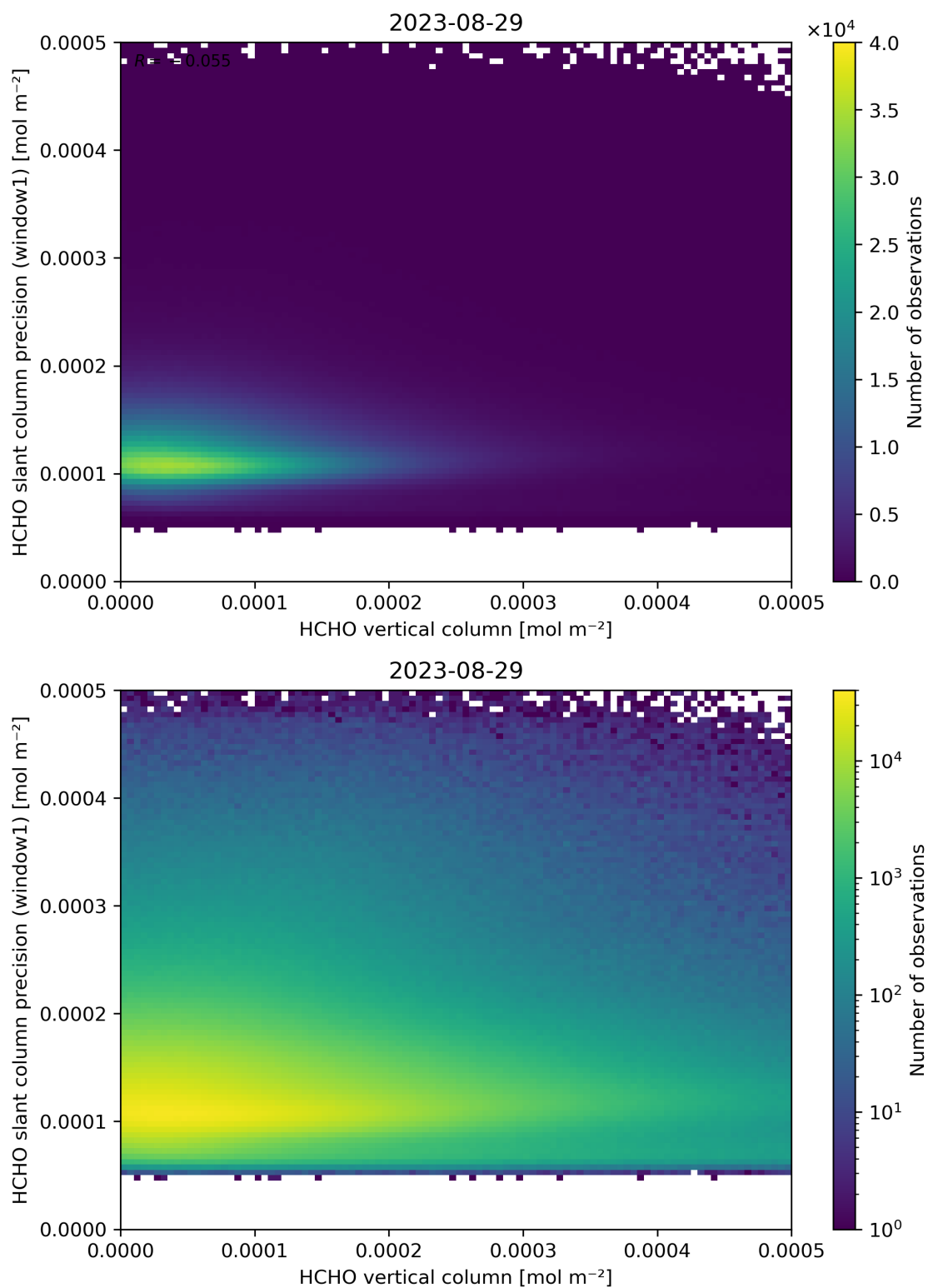
Figure 130: Scatter density plot of “HCHO vertical column” against “HCHO slant column precision (window1)” for 2023-08-28 to 2023-08-30.
