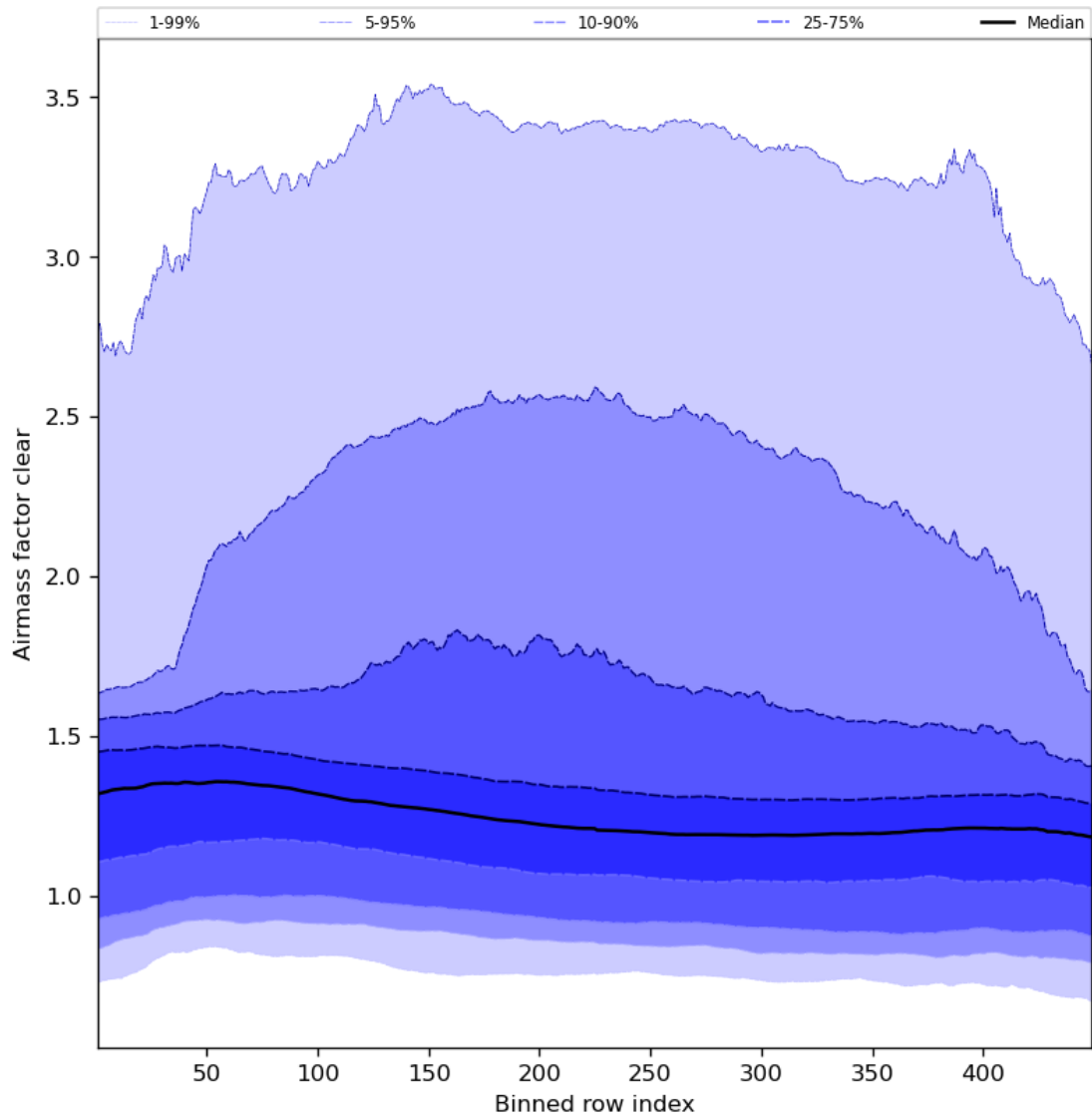
Figure 56: Along track statistics of “Airmass factor clear” for 2023-08-28 to 2023-08-30
