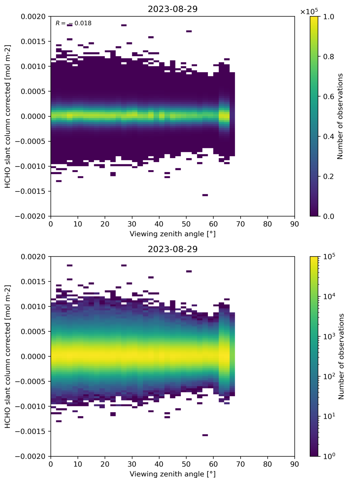
Figure 186: Scatter density plot of “Viewing zenith angle” against “HCHO slant column corrected” for 2023-08-28 to 2023-08-30.
