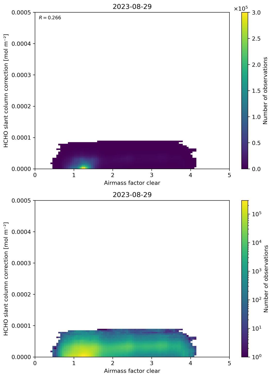
Figure 75: Scatter density plot of “Airmass factor clear” against “HCHO slant column correction” for 2023-08-28 to 2023-08-30.
