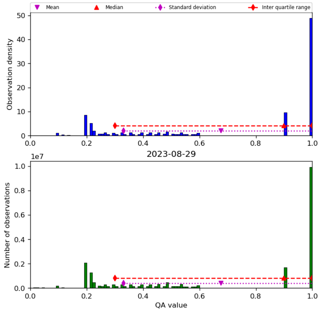
Figure 34: Histogram of “QA value” for 2023-08-28 to 2023-08-30
