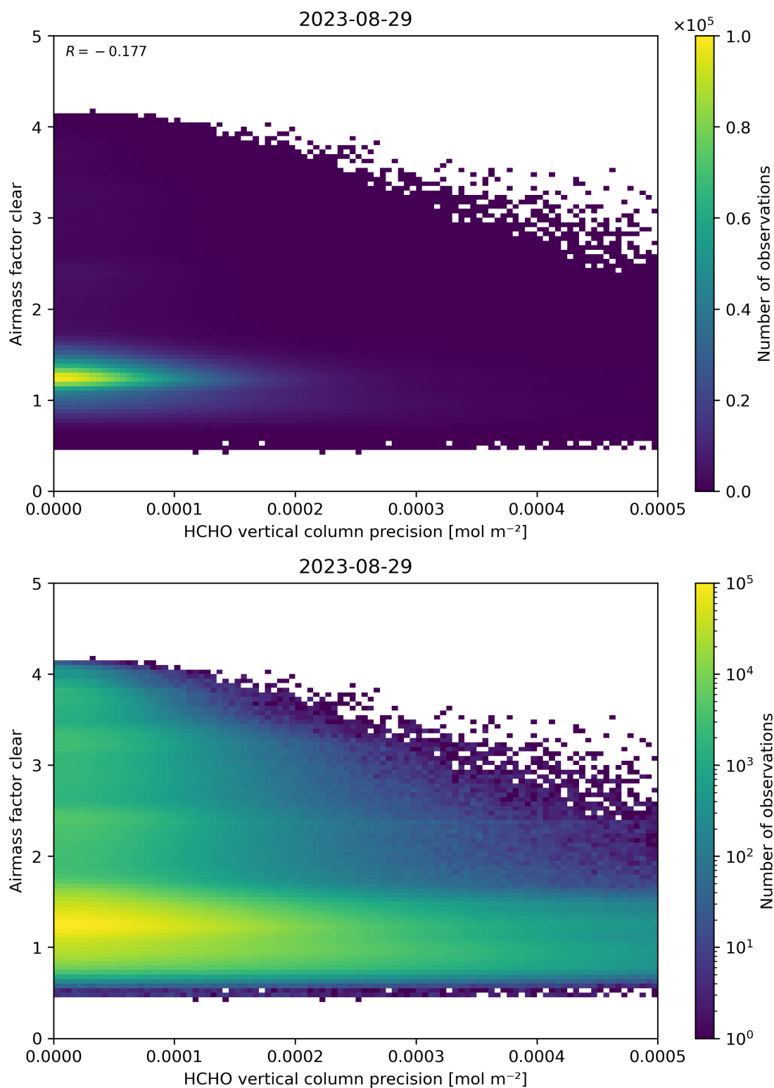
Figure 139: Scatter density plot of “HCHO vertical column precision” against “Airmass factor clear” for 2023-08-28 to 2023-08-30.
