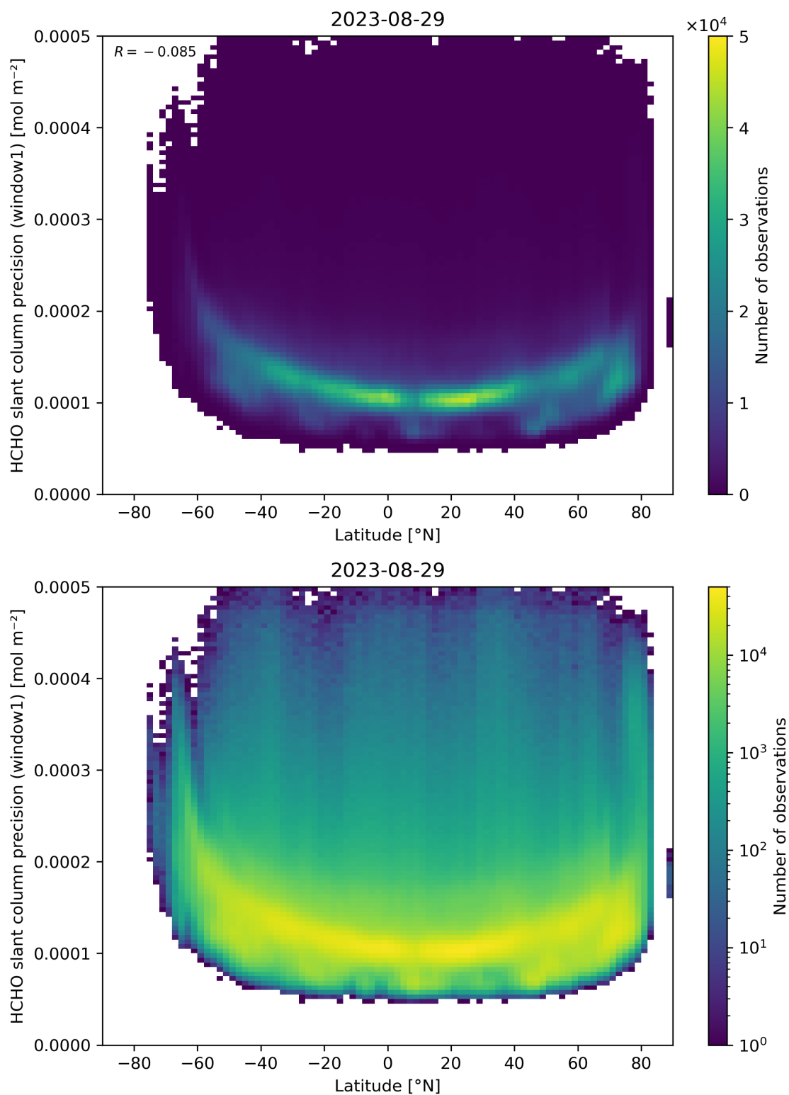
Figure 160: Scatter density plot of “Latitude” against “HCHO slant column precision (window1)” for 2023-08-28 to 2023-08-30.
