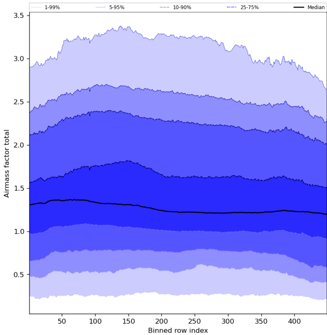
Figure 54: Along track statistics of “Airmass factor total” for 2023-08-28 to 2023-08-30
