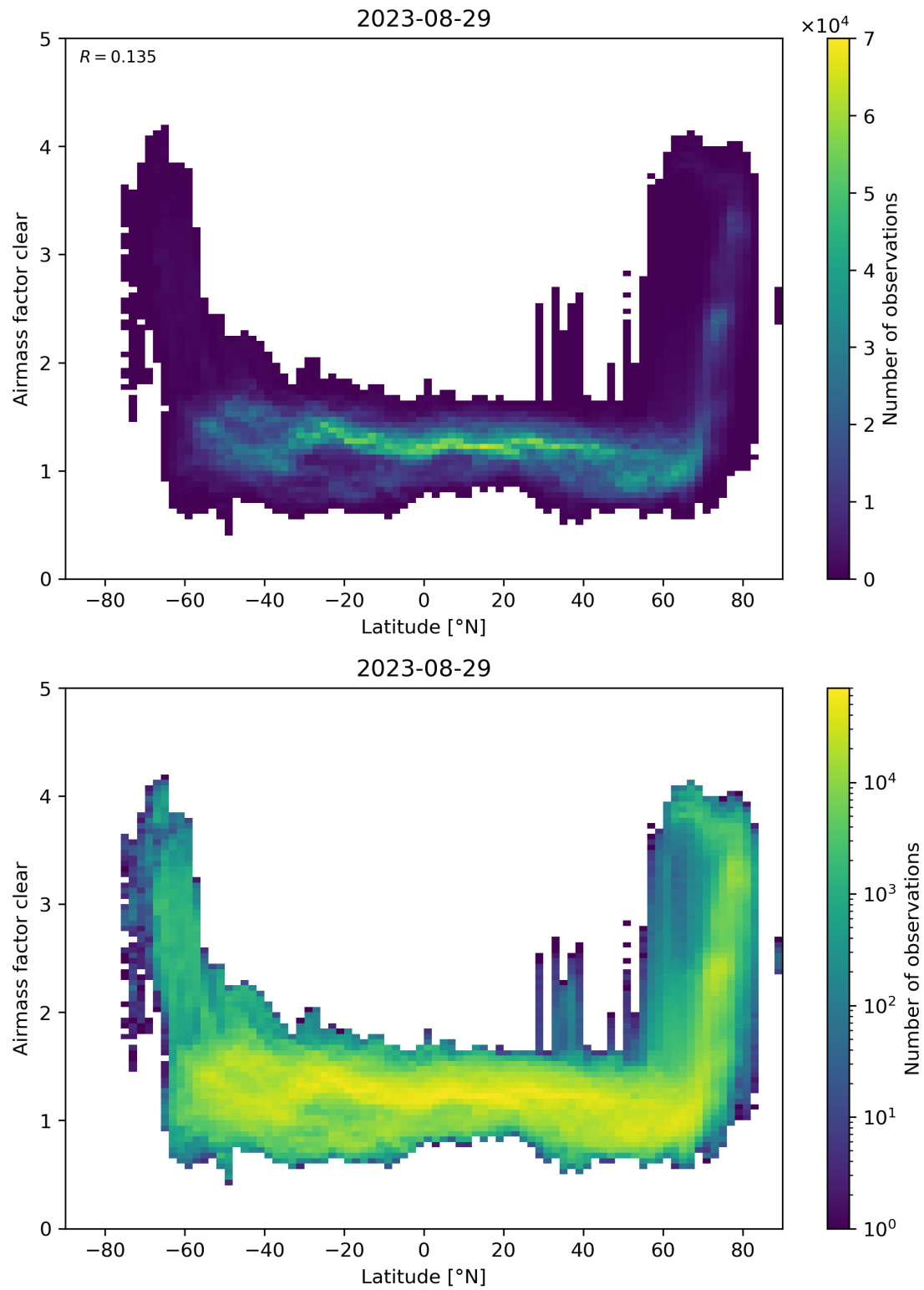
Figure 156: Scatter density plot of “Latitude” against “Airmass factor clear” for 2023-08-28 to 2023-08-30.
