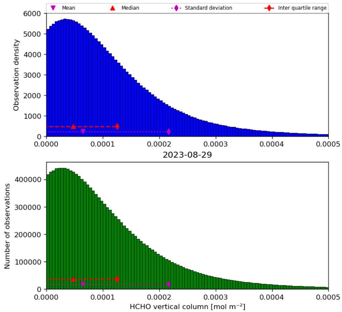
Figure 35: Histogram of “HCHO vertical column” for 2023-08-28 to 2023-08-30
