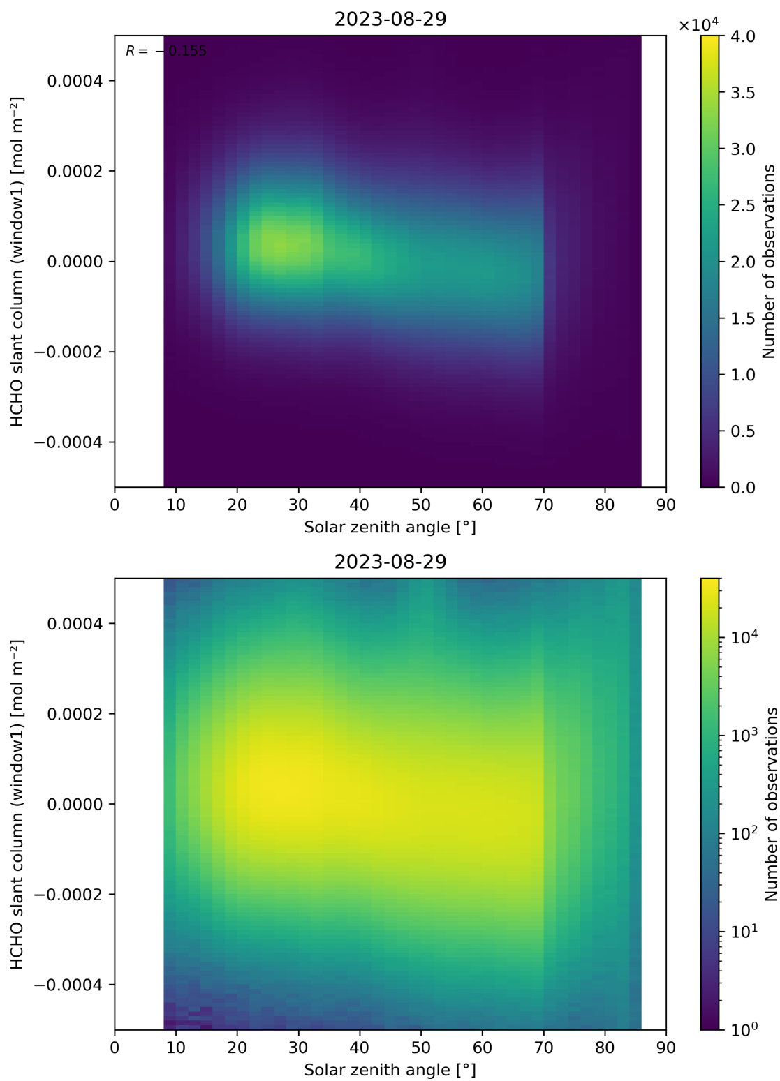
Figure 173: Scatter density plot of “Solar zenith angle” against “HCHO slant column (window1)” for 2023-08-28 to 2023-08-30.
