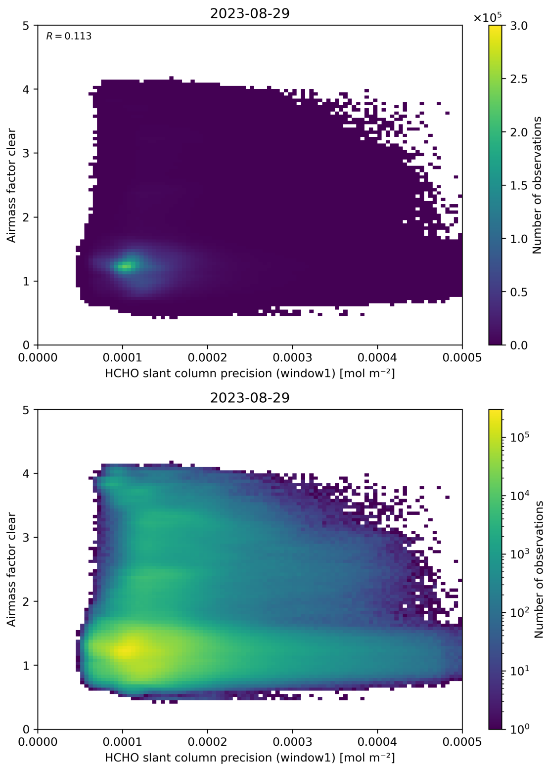
Figure 91: Scatter density plot of “HCHO slant column precision (window1)” against “Airmass factor clear” for 2023-08-28 to 2023-08-30.
