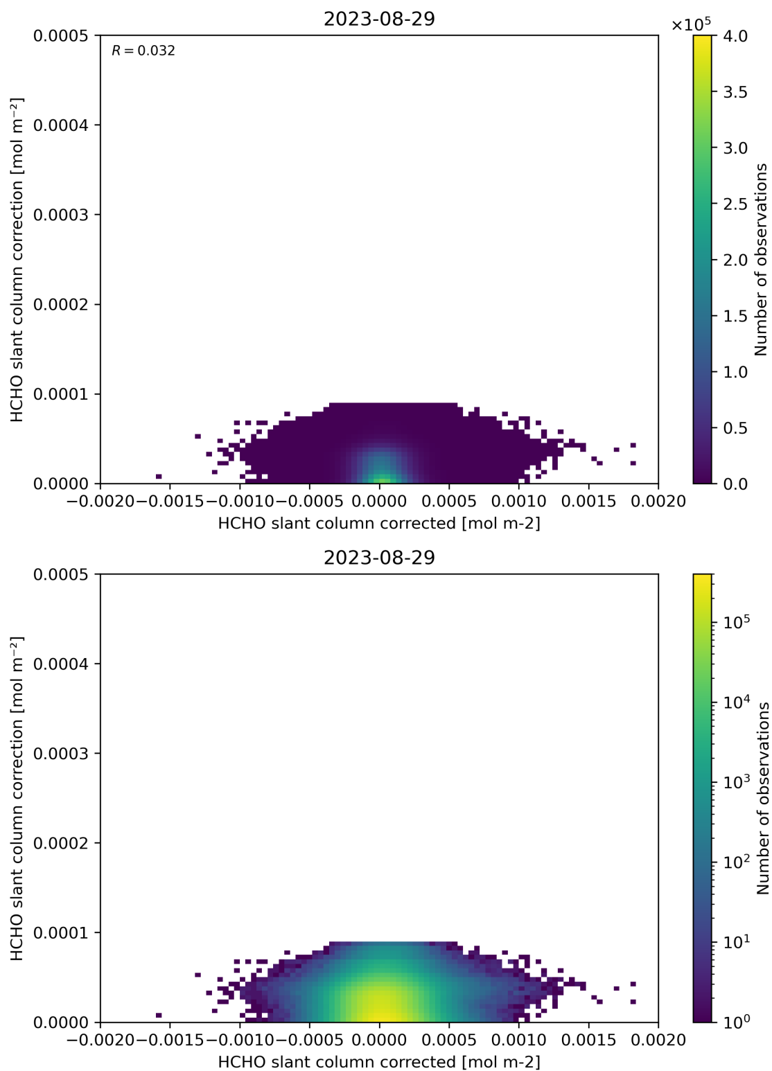
Figure 77: Scatter density plot of “HCHO slant column corrected” against “HCHO slant column correction” for 2023-08-28 to 2023-08-30.
