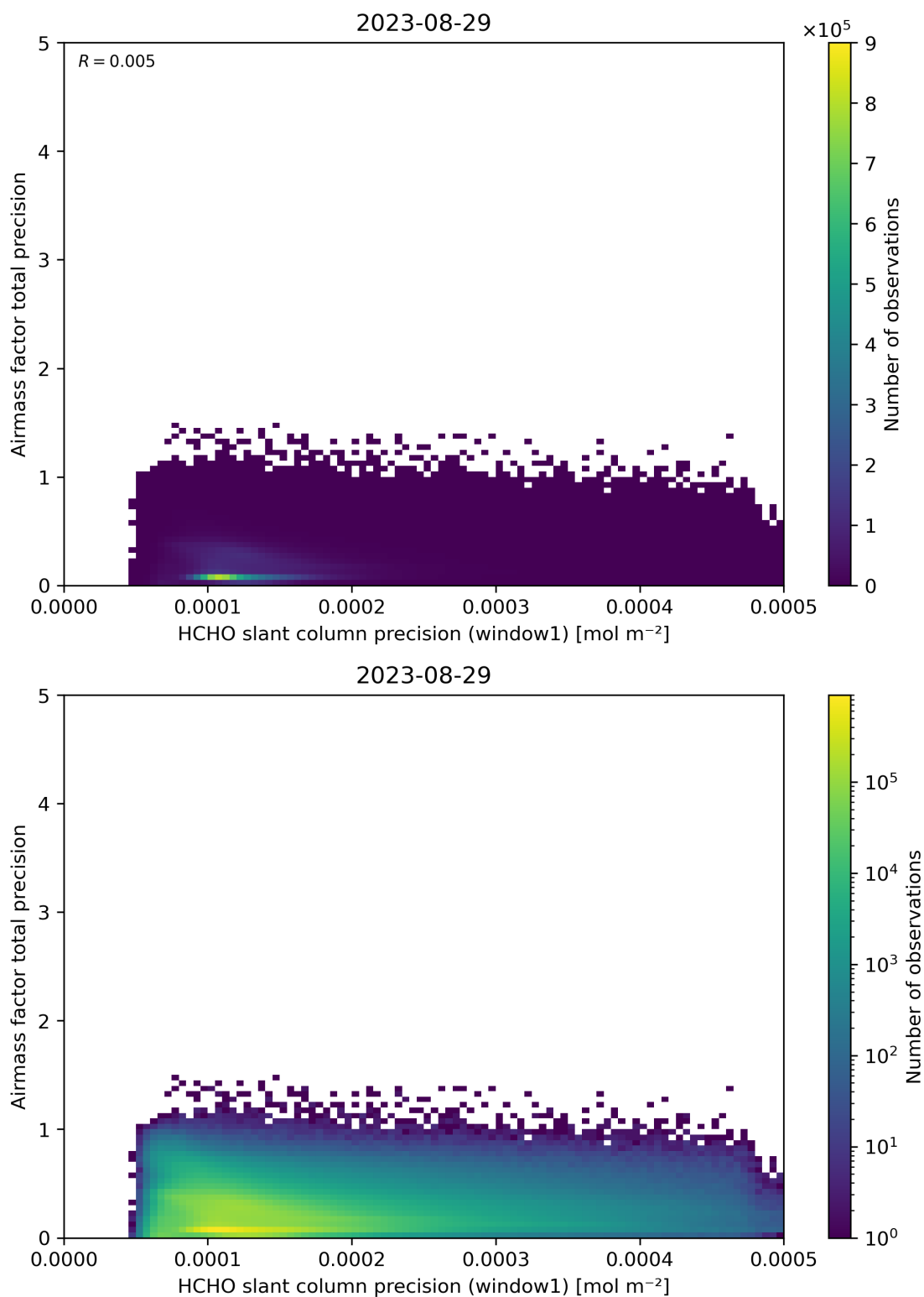
Figure 95: Scatter density plot of “HCHO slant column precision (window1)” against “Airmass factor total precision” for 2023-08-28 to 2023-08-30.
