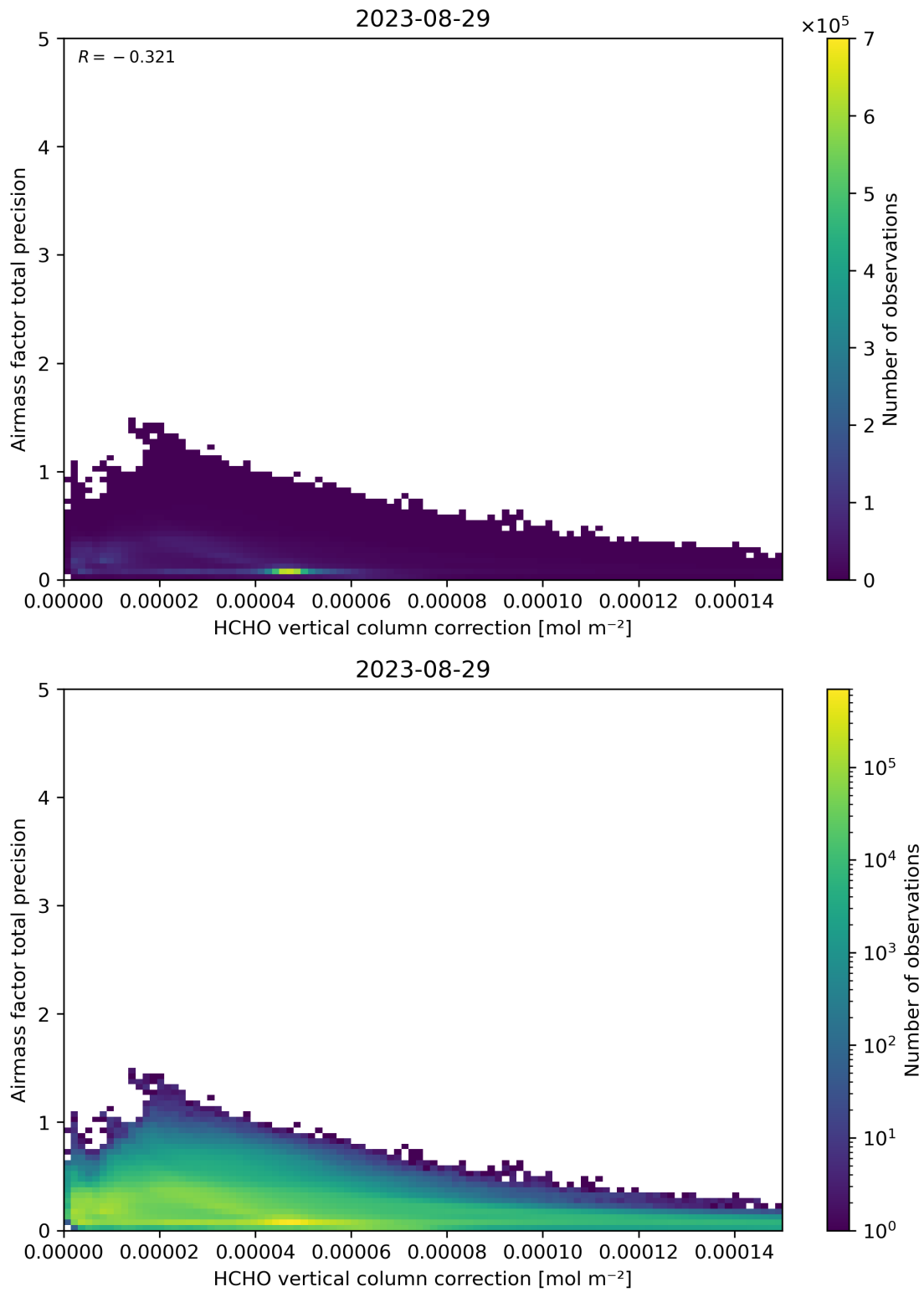
Figure 121: Scatter density plot of “HCHO vertical column correction” against “Airmass factor total precision” for 2023-08-28 to 2023-08-30.
