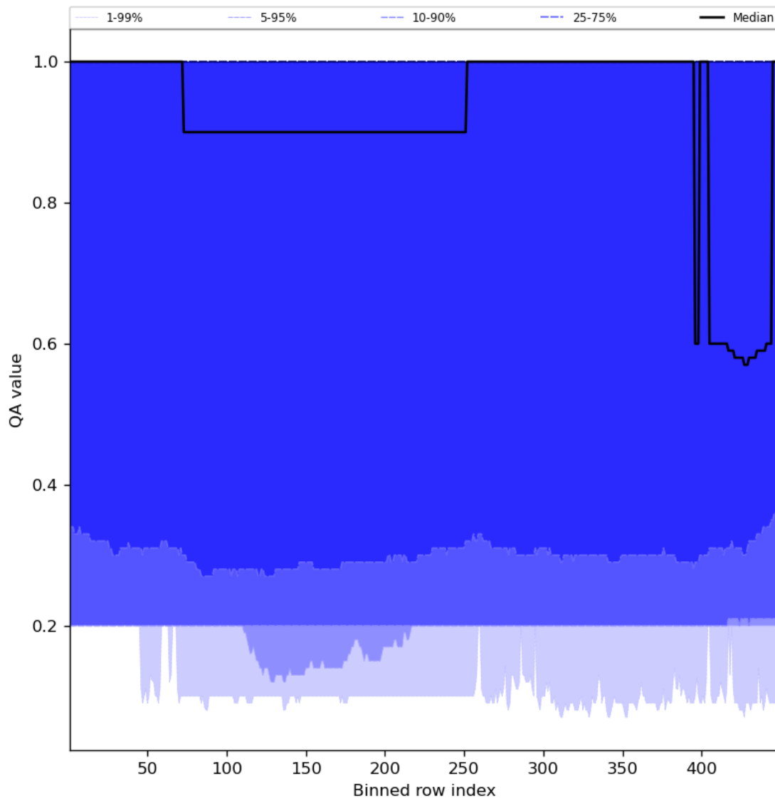
Figure 48: Along track statistics of “QA value” for 2023-08-28 to 2023-08-30
