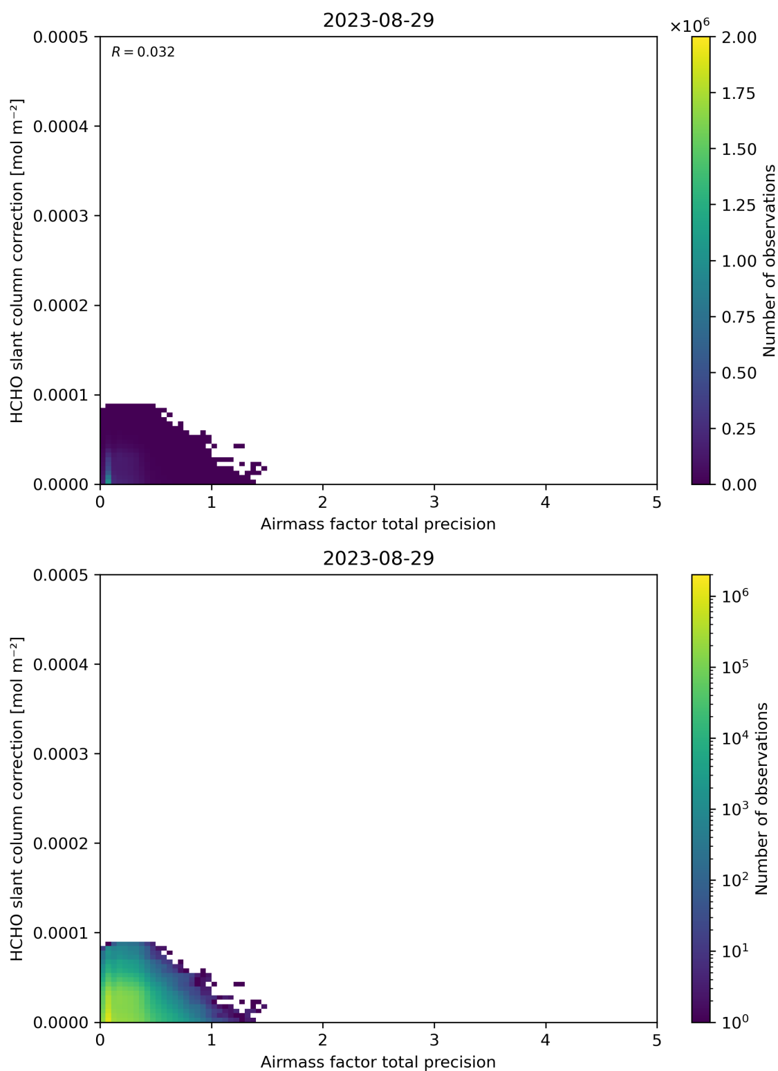
Figure 110: Scatter density plot of “Airmass factor total precision” against “HCHO slant column correction” for 2023-08-28 to 2023-08-30.
