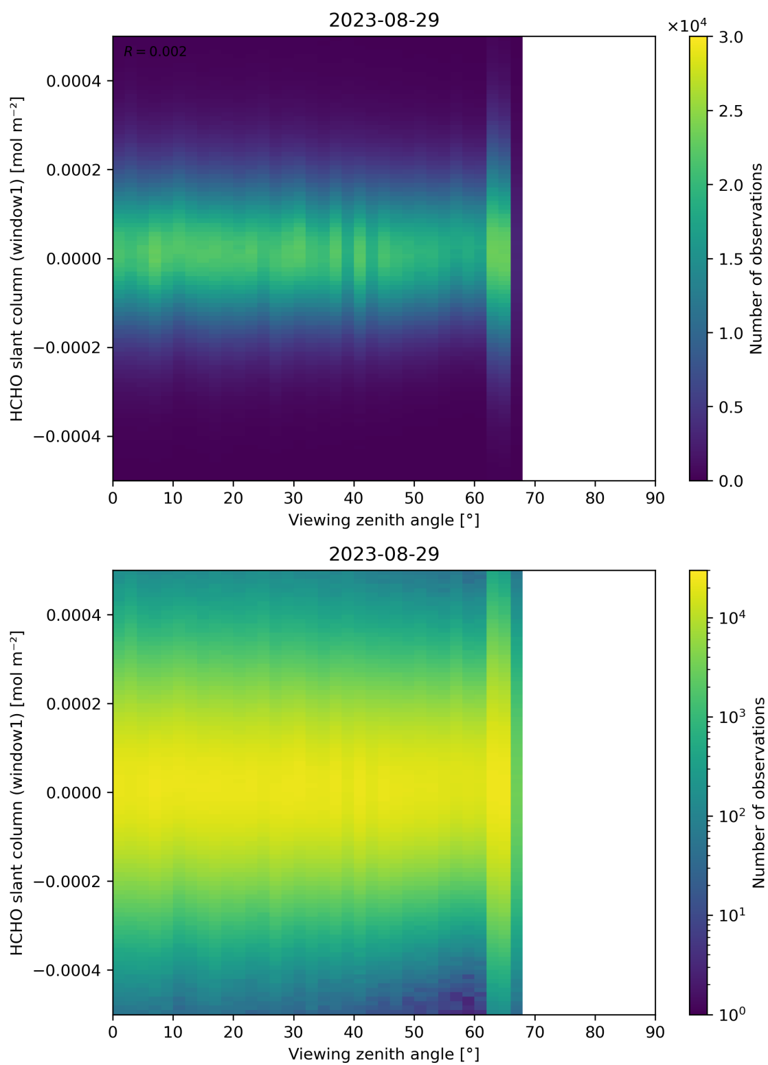
Figure 188: Scatter density plot of “Viewing zenith angle” against “HCHO slant column (window1)” for 2023-08-28 to 2023-08-30.
