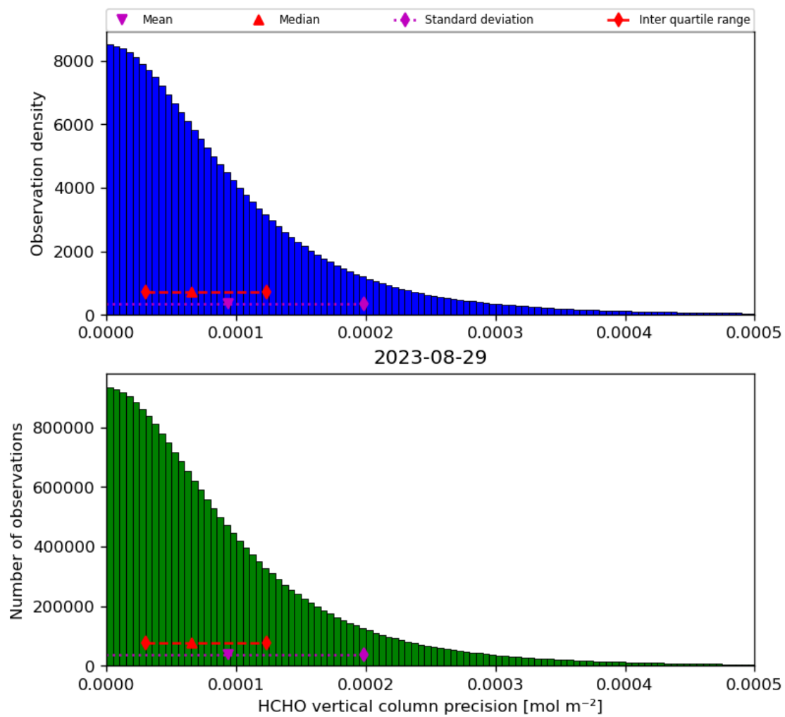
Figure 36: Histogram of “HCHO vertical column precision” for 2023-08-28 to 2023-08-30
