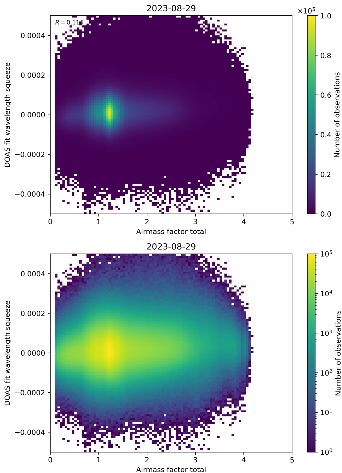
Figure 99: Scatter density plot of “Airmass factor total” against “DOAS fit wavelength squeeze” for 2023-08-28 to 2023-08-30.
