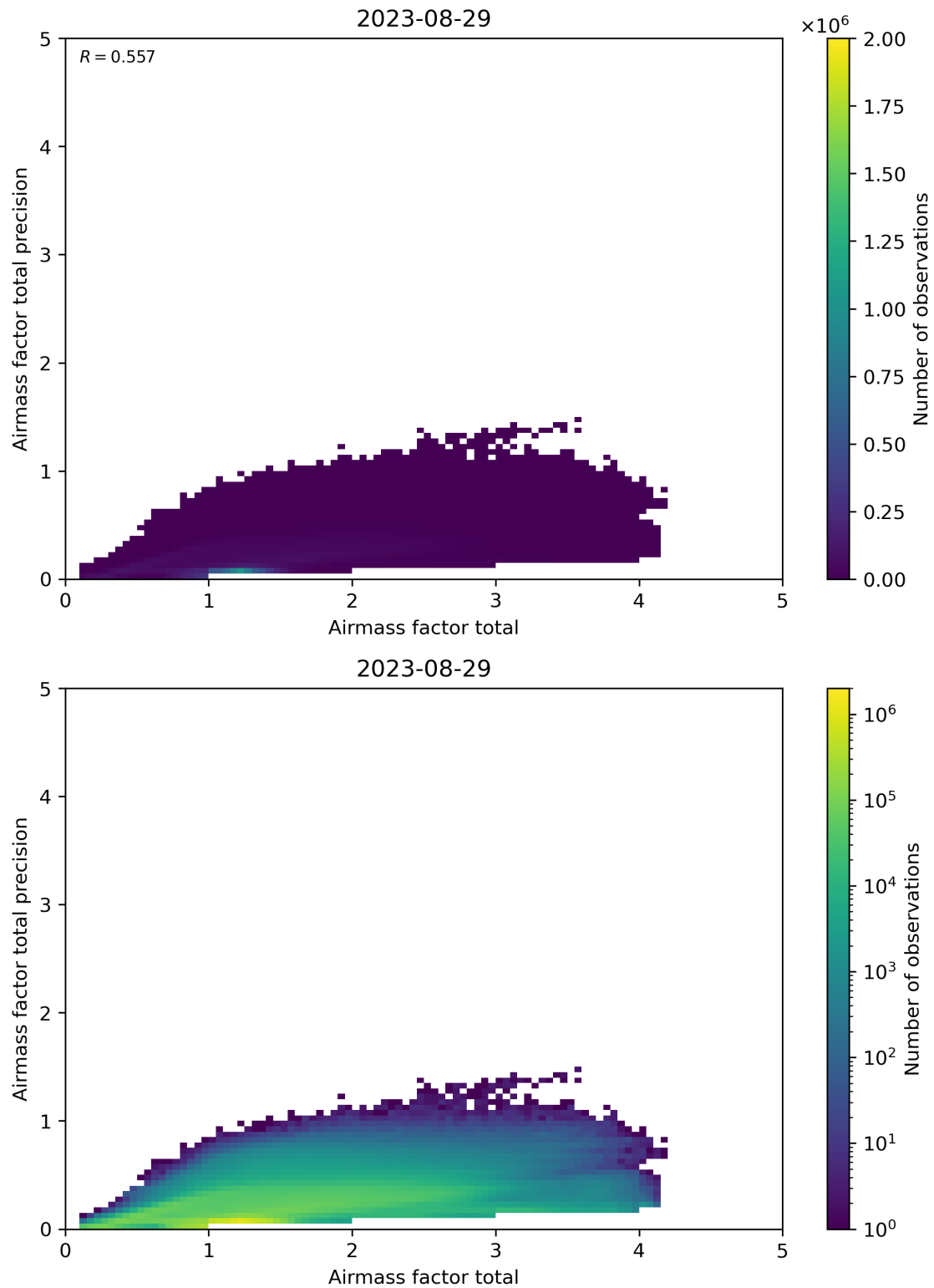
Figure 103: Scatter density plot of “Airmass factor total” against “Airmass factor total precision” for 2023-08-28 to 2023-08-30.
