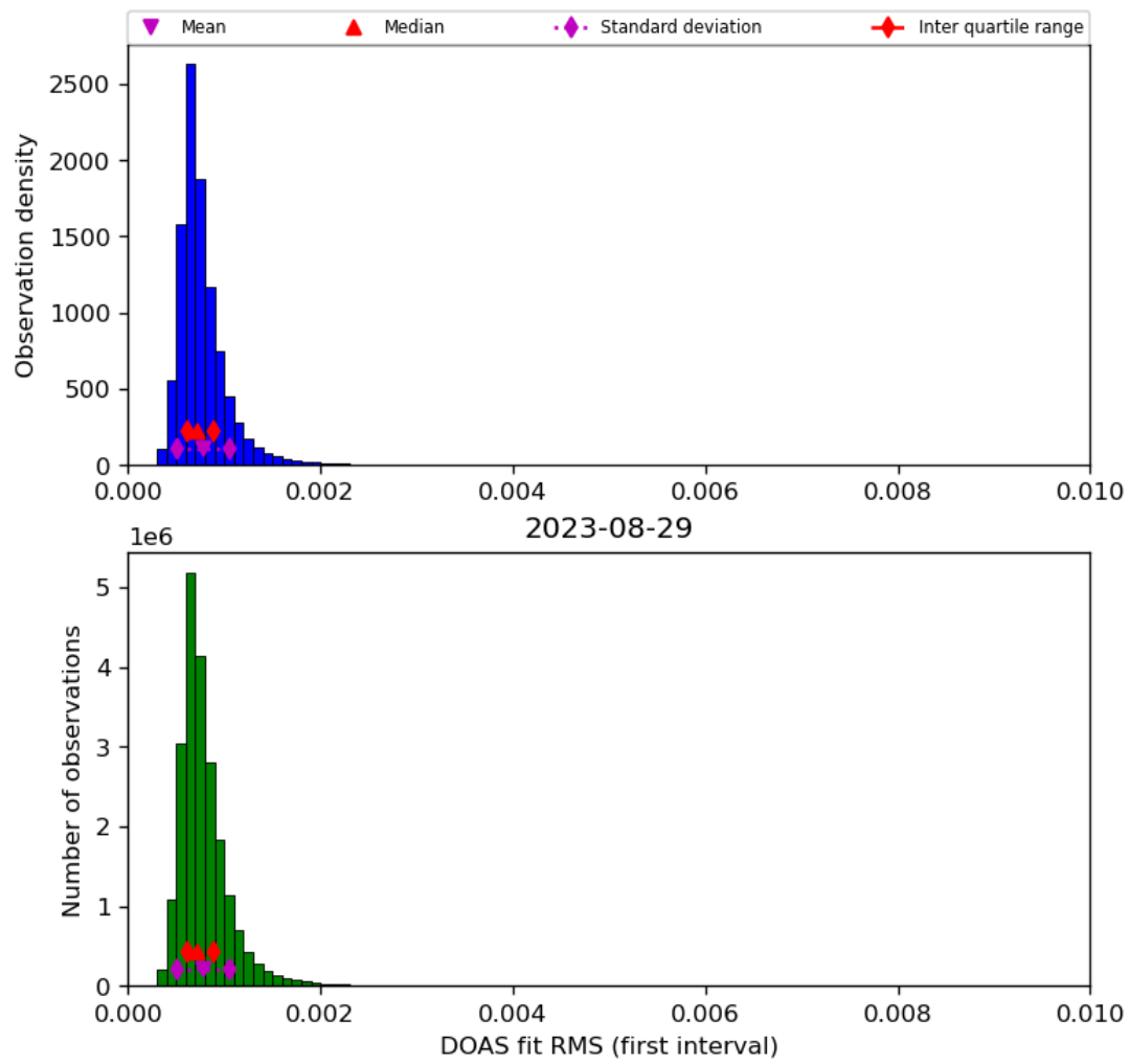
Figure 46: Histogram of “DOAS fit RMS (first interval)” for 2023-08-28 to 2023-08-30
