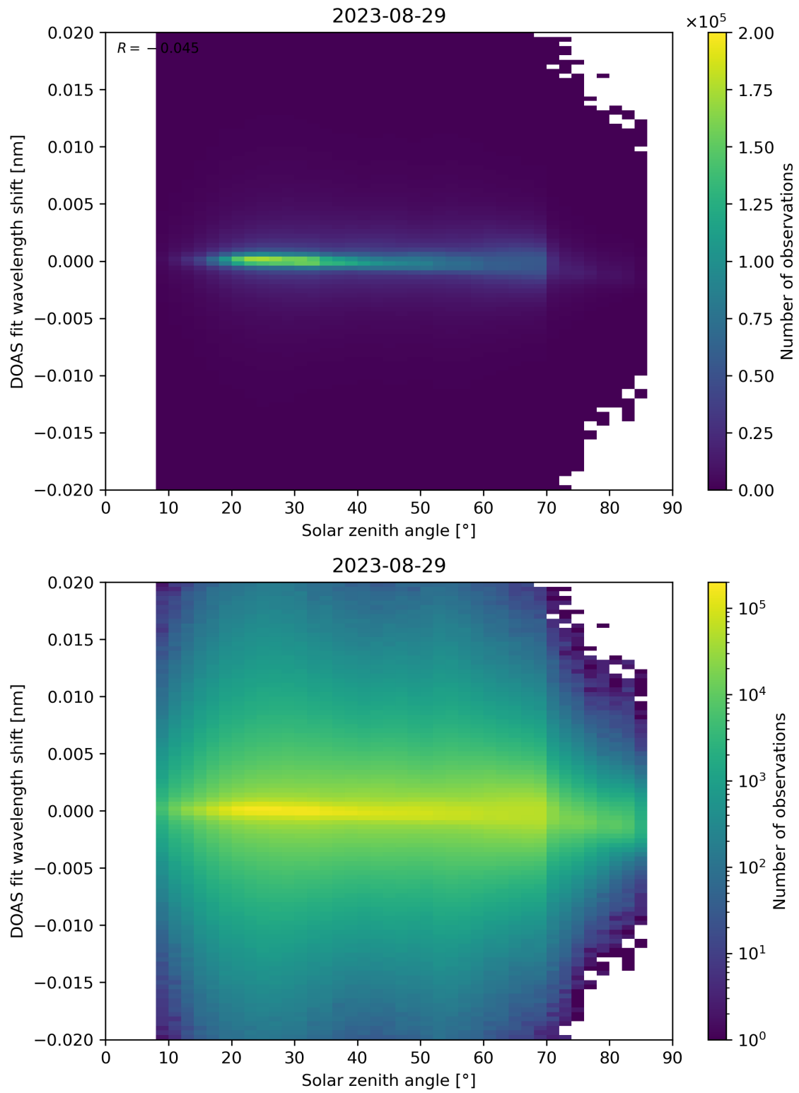
Figure 168: Scatter density plot of “Solar zenith angle” against “DOAS fit wavelength shift” for 2023-08-28 to 2023-08-30.
