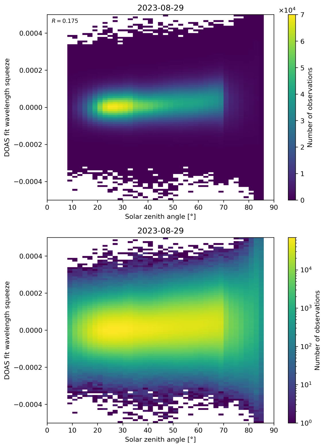
Figure 169: Scatter density plot of “Solar zenith angle” against “DOAS fit wavelength squeeze” for 2023-08-28 to 2023-08-30.
