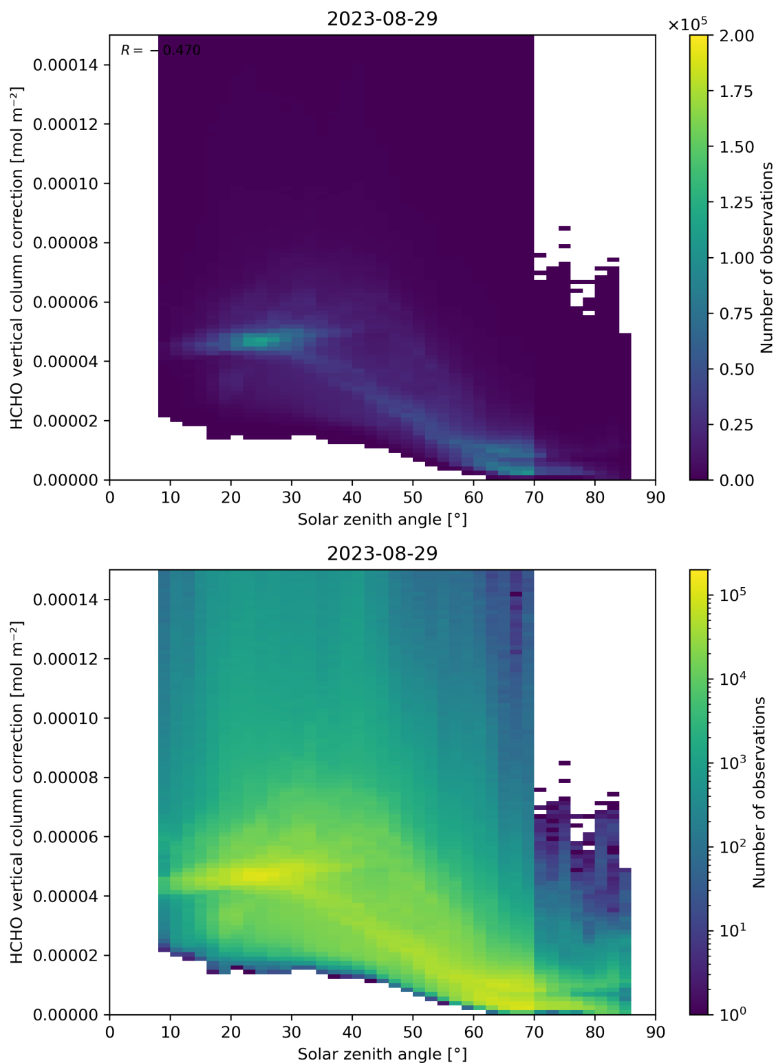
Figure 178: Scatter density plot of “Solar zenith angle” against “HCHO vertical column correction” for 2023-08-28 to 2023-08-30.
