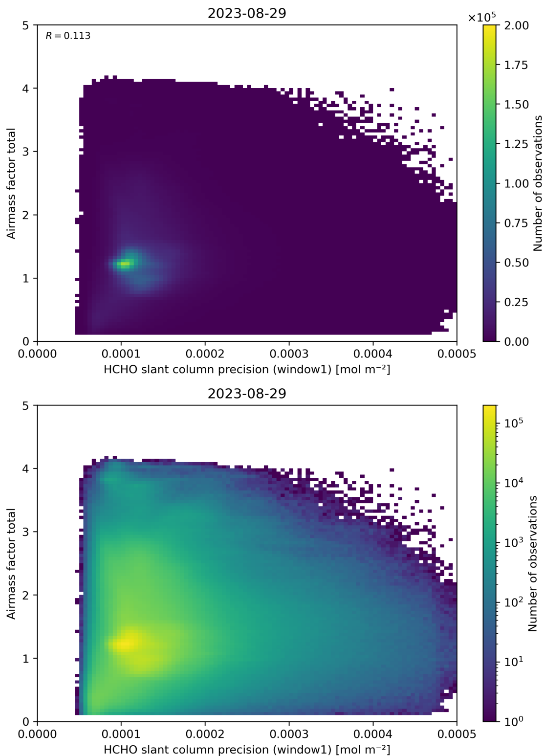
Figure 94: Scatter density plot of “HCHO slant column precision (window1)” against “Airmass factor total” for 2023-08-28 to 2023-08-30.
