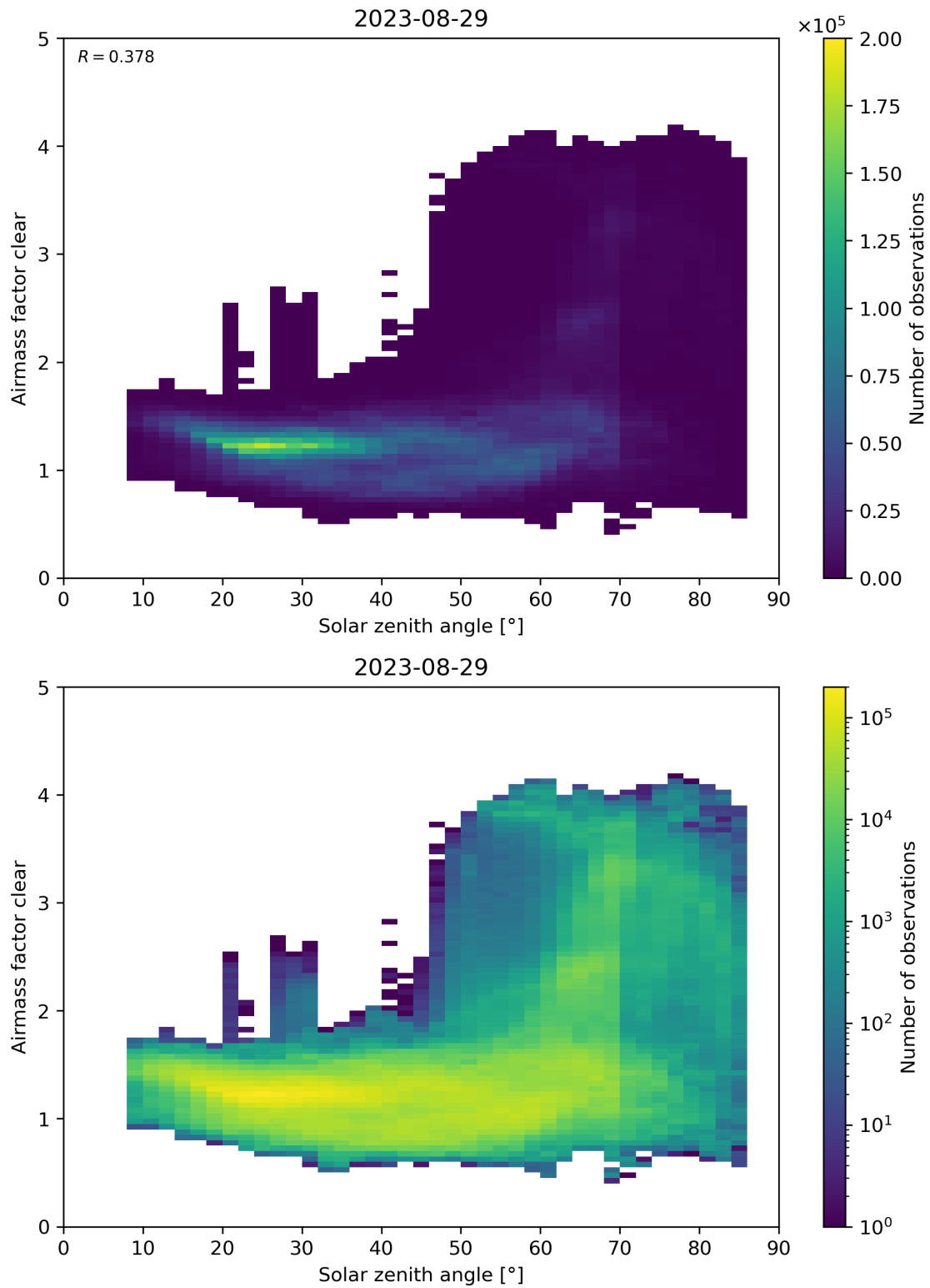
Figure 170: Scatter density plot of “Solar zenith angle” against “Airmass factor clear” for 2023-08-28 to 2023-08-30.
