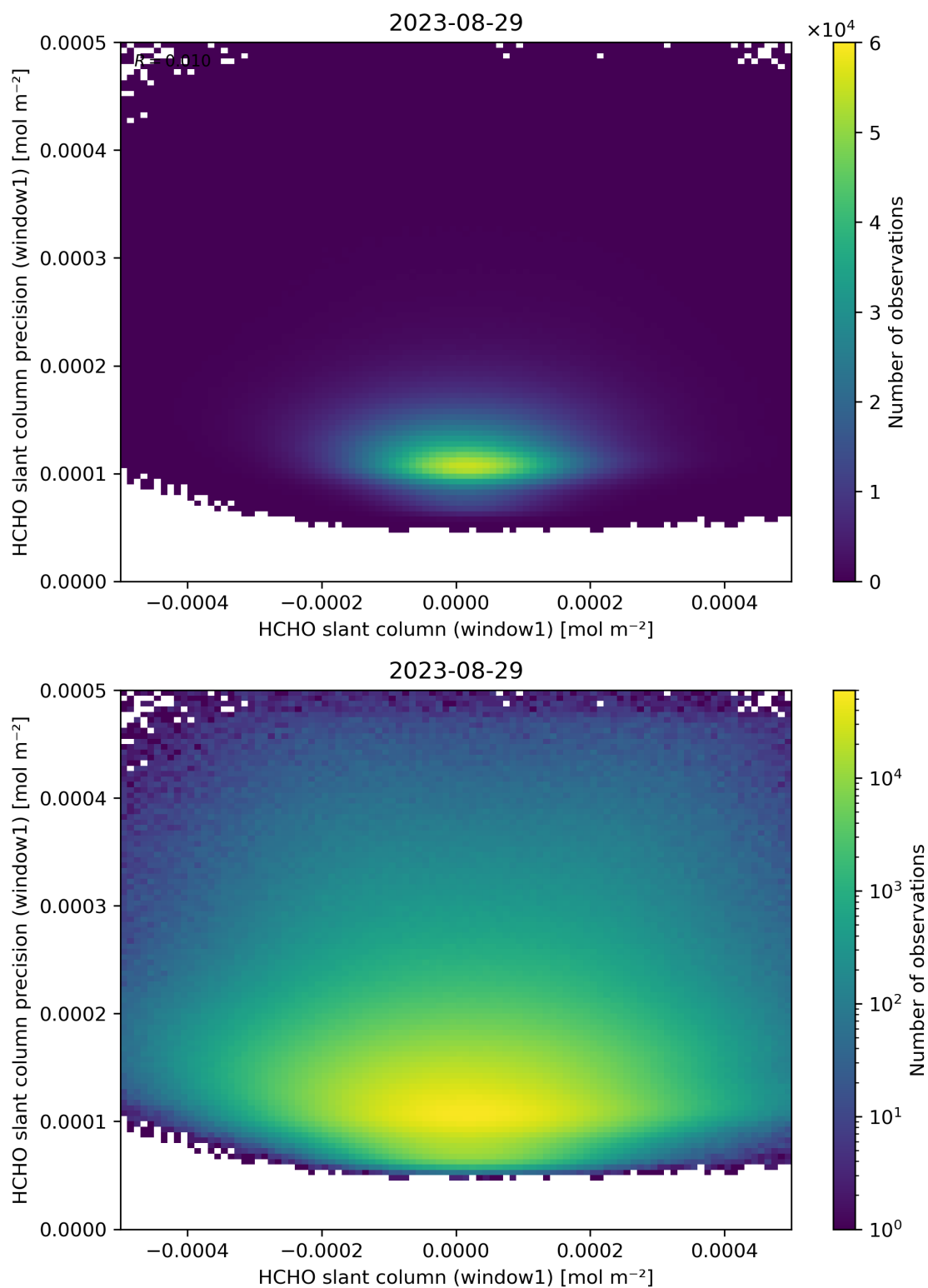
Figure 84: Scatter density plot of “HCHO slant column (window1)” against “HCHO slant column precision (window1)” for 2023-08-28 to 2023-08-30.
