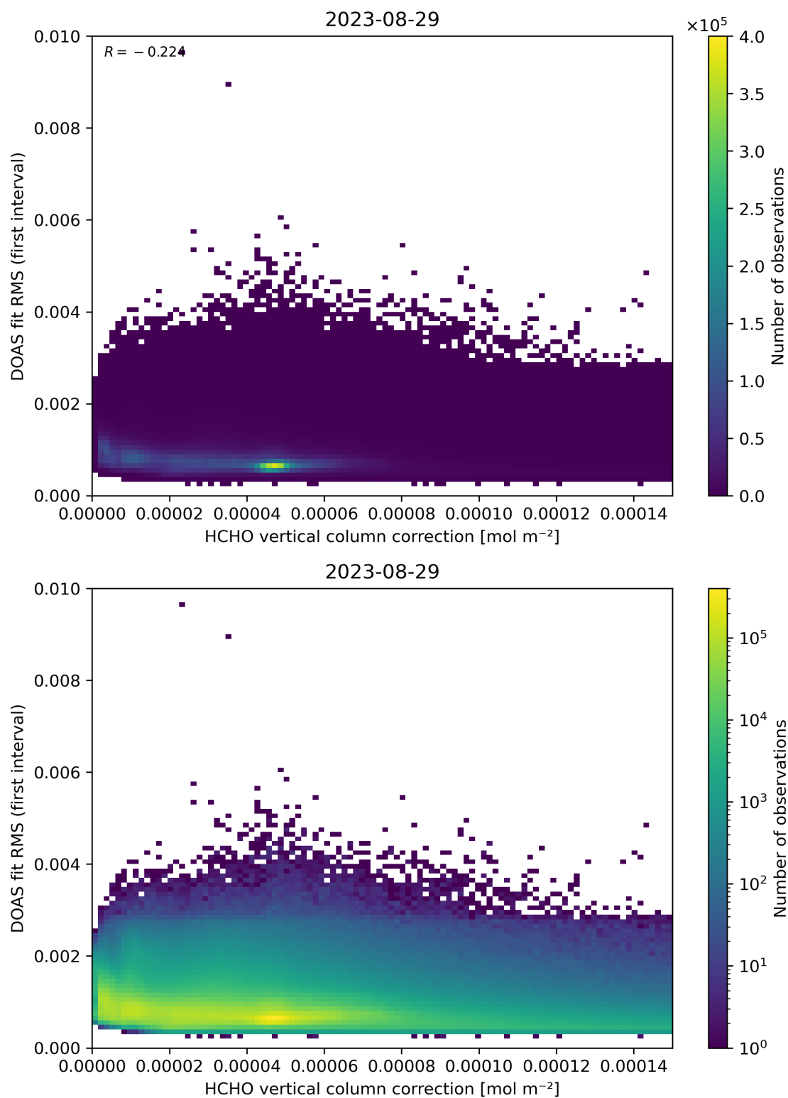
Figure 112: Scatter density plot of “HCHO vertical column correction” against “DOAS fit RMS (first interval)” for 2023-08-28 to 2023-08-30.
