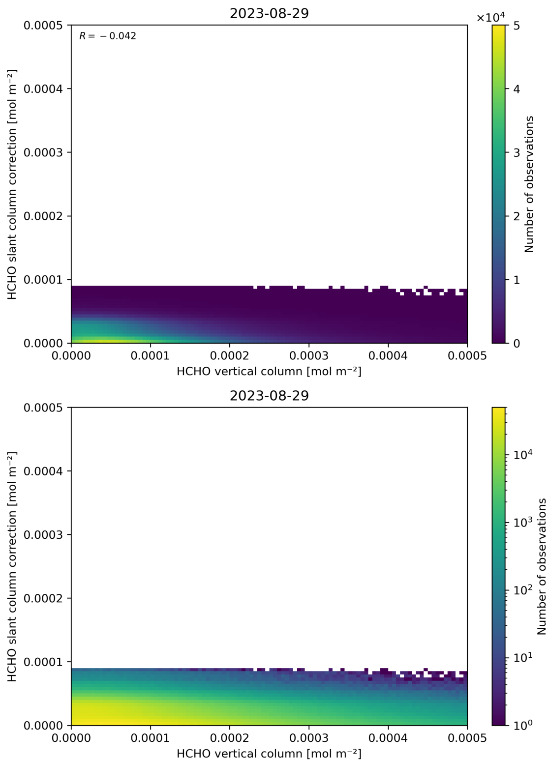
Figure 128: Scatter density plot of “HCHO vertical column” against “HCHO slant column correction” for 2023-08-28 to 2023-08-30.
