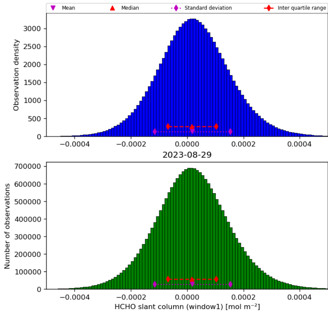
Figure 38: Histogram of “HCHO slant column (window1)” for 2023-08-28 to 2023-08-30
