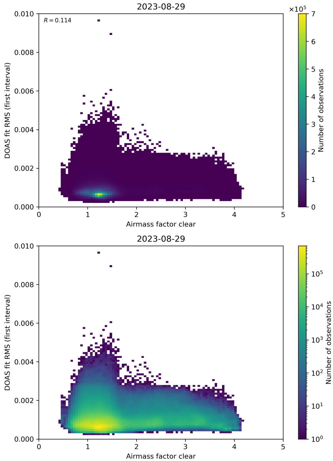
Figure 71: Scatter density plot of “Airmass factor clear” against “DOAS fit RMS (first interval)” for 2023-08-28 to 2023-08-30.
