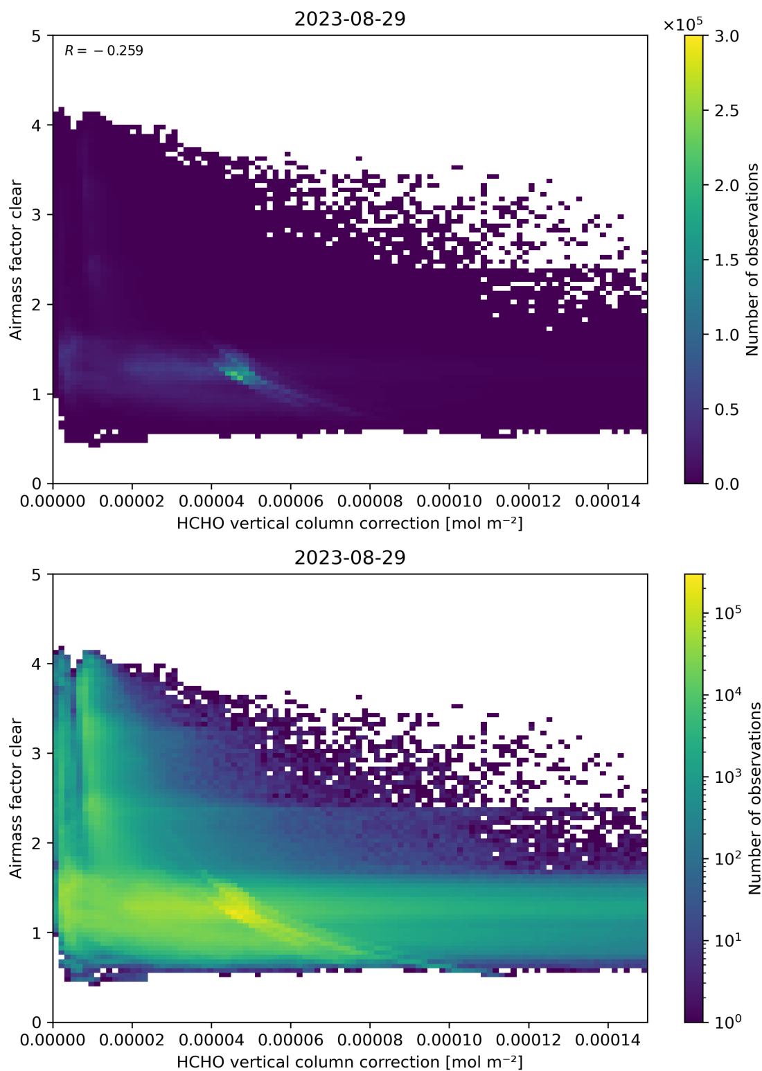
Figure 115: Scatter density plot of “HCHO vertical column correction” against “Airmass factor clear” for 2023-08-28 to 2023-08-30.
