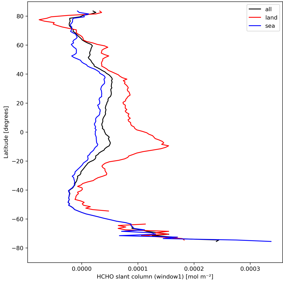
Figure 24: Zonal average of “HCHO slant column (window1)” for 2023-08-28 to 2023-08-30.
