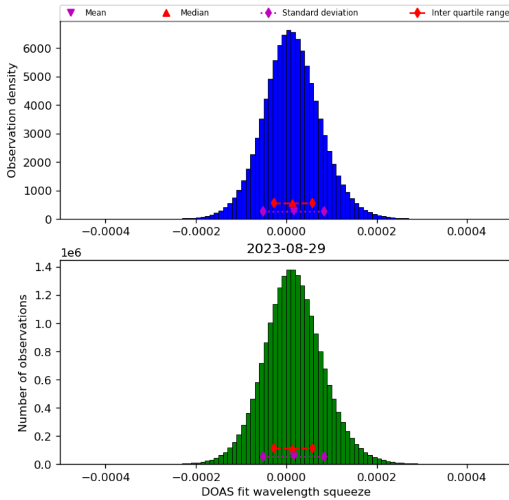
Figure 45: Histogram of “DOAS fit wavelength squeeze” for 2023-08-28 to 2023-08-30
