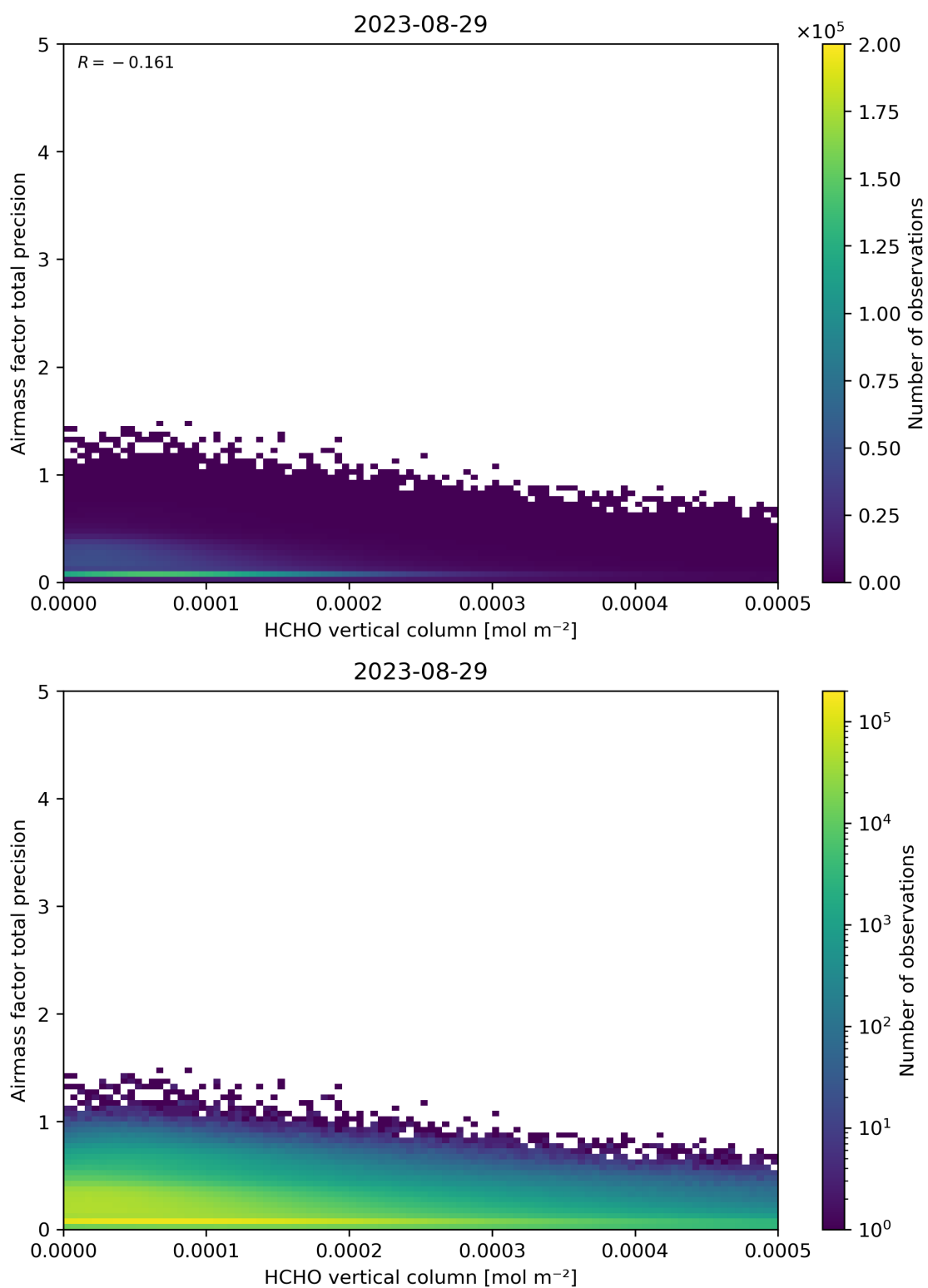
Figure 132: Scatter density plot of “HCHO vertical column” against “Airmass factor total precision” for 2023-08-28 to 2023-08-30.
