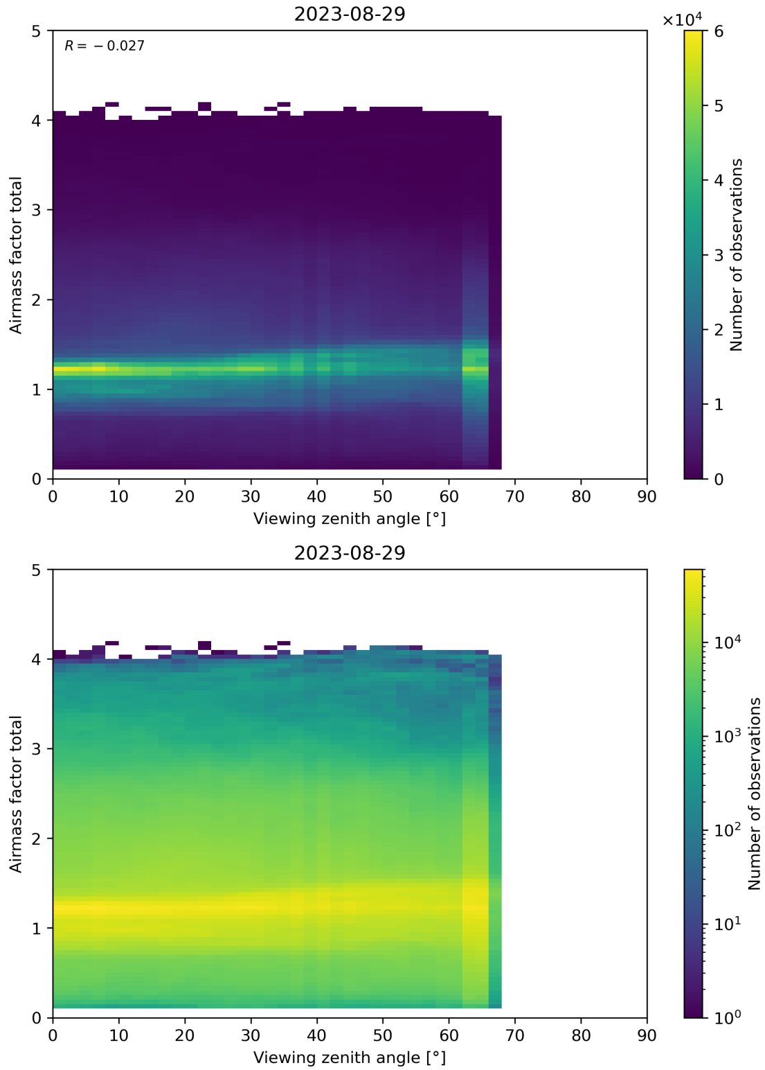
Figure 190: Scatter density plot of “Viewing zenith angle” against “Airmass factor total” for 2023-08-28 to 2023-08-30.
