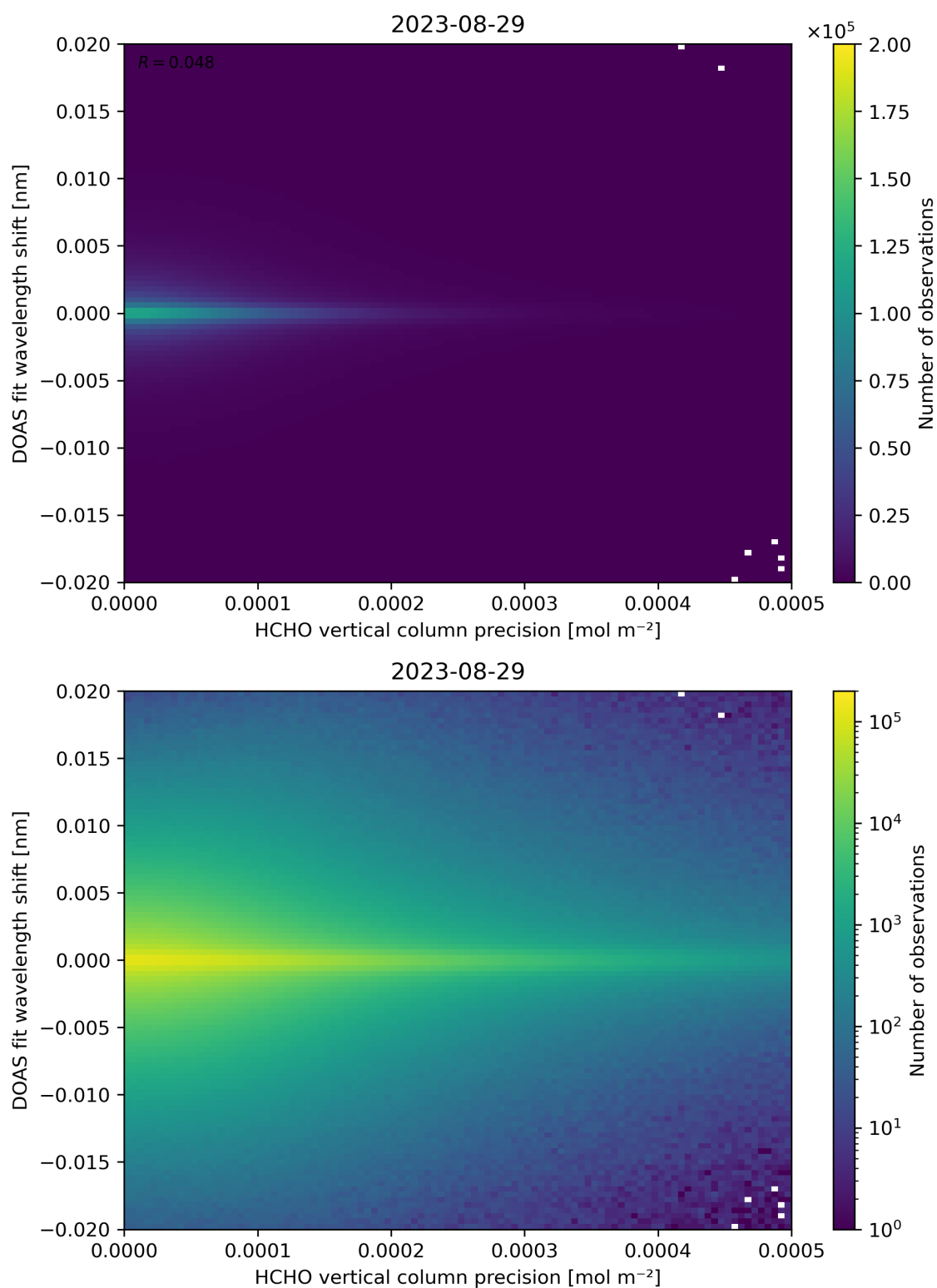
Figure 137: Scatter density plot of “HCHO vertical column precision” against “DOAS fit wavelength shift” for 2023-08-28 to 2023-08-30.
