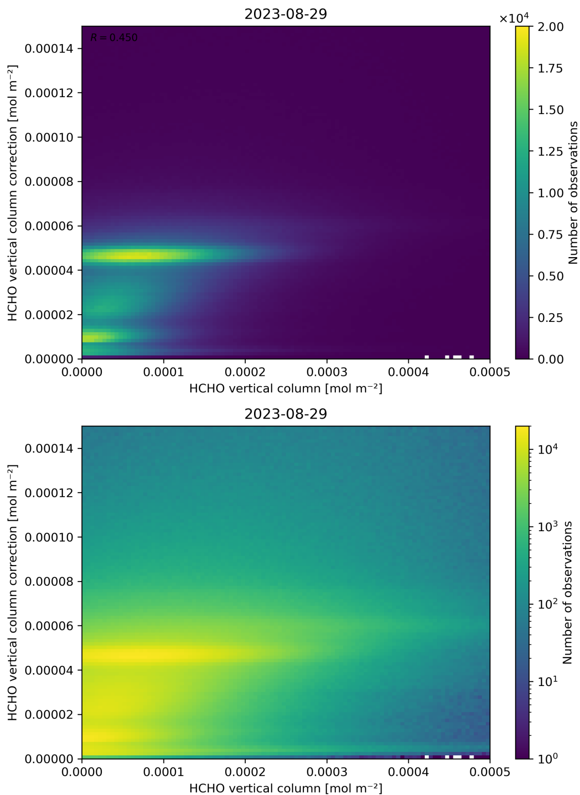
Figure 133: Scatter density plot of “HCHO vertical column” against “HCHO vertical column correction” for 2023-08-28 to 2023-08-30.
