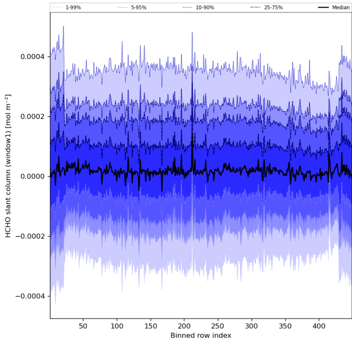
Figure 52: Along track statistics of “HCHO slant column (window1)” for 2023-08-28 to 2023-08-30
