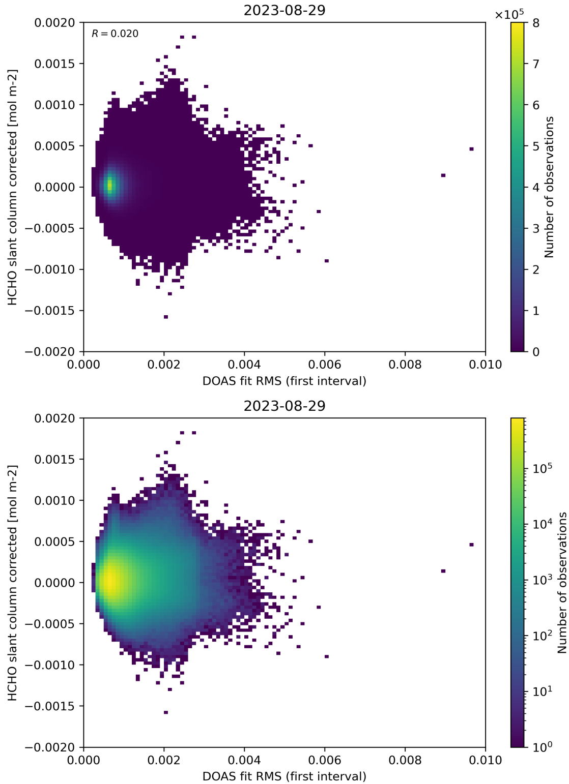
Figure 62: Scatter density plot of “DOAS fit RMS (first interval)” against “HCHO slant column corrected” for 2023-08-28 to 2023-08-30.
