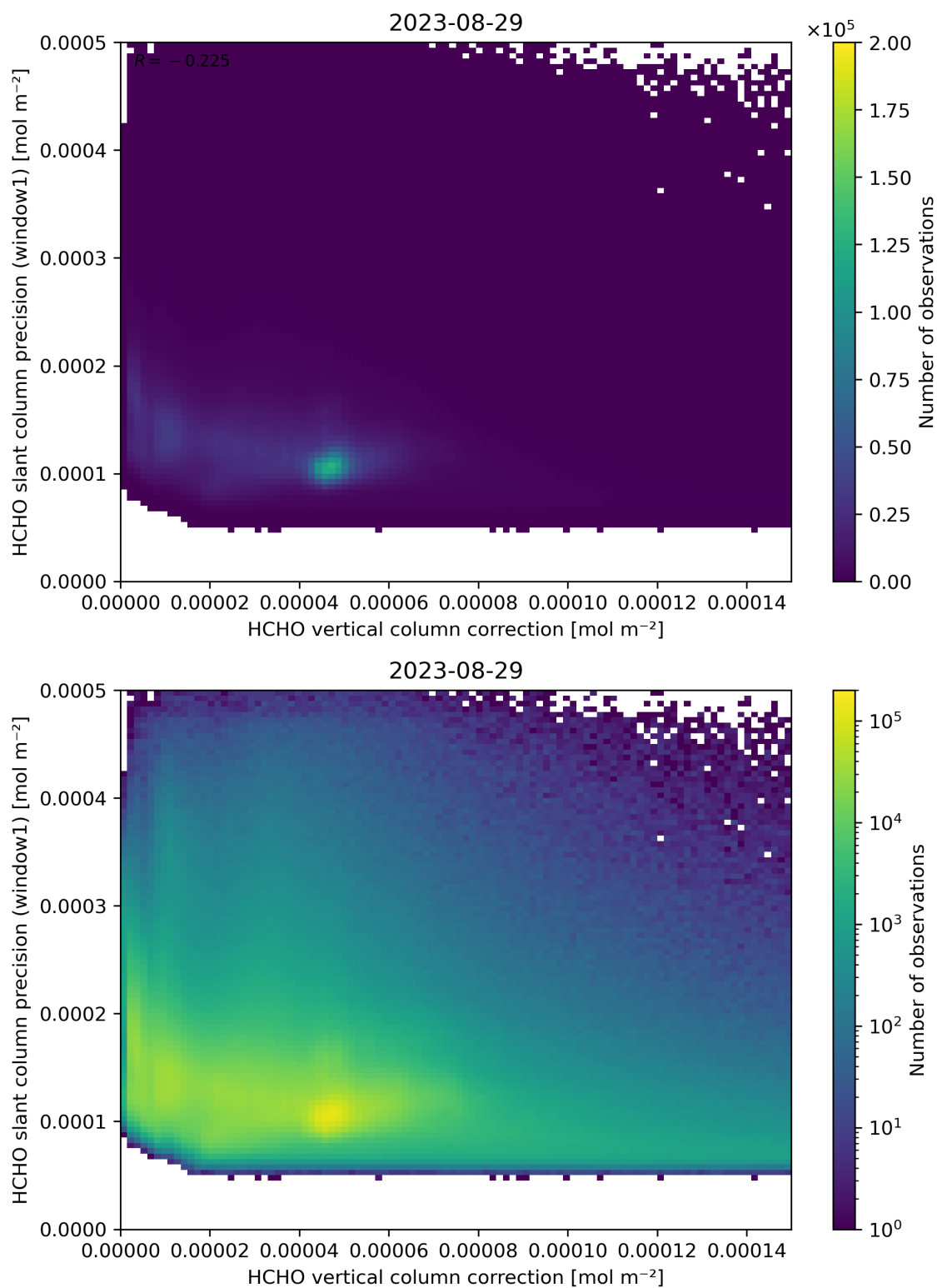
Figure 119: Scatter density plot of “HCHO vertical column correction” against “HCHO slant column precision (window1)” for 2023-08-28 to 2023-08-30.
