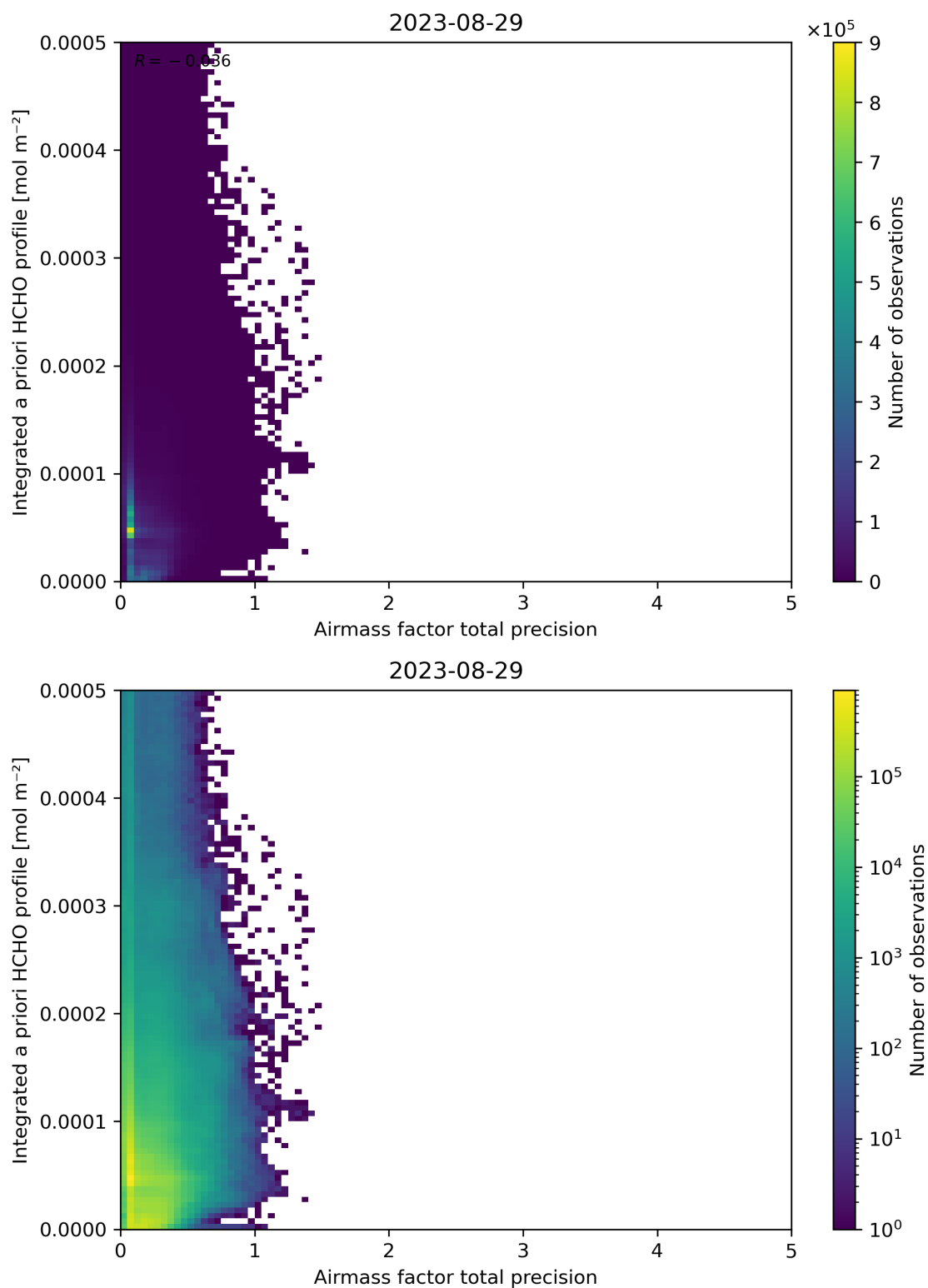
Figure 111: Scatter density plot of “Airmass factor total precision” against “Integrated a priori HCHO profile” for 2023-08-28 to 2023-08-30.
