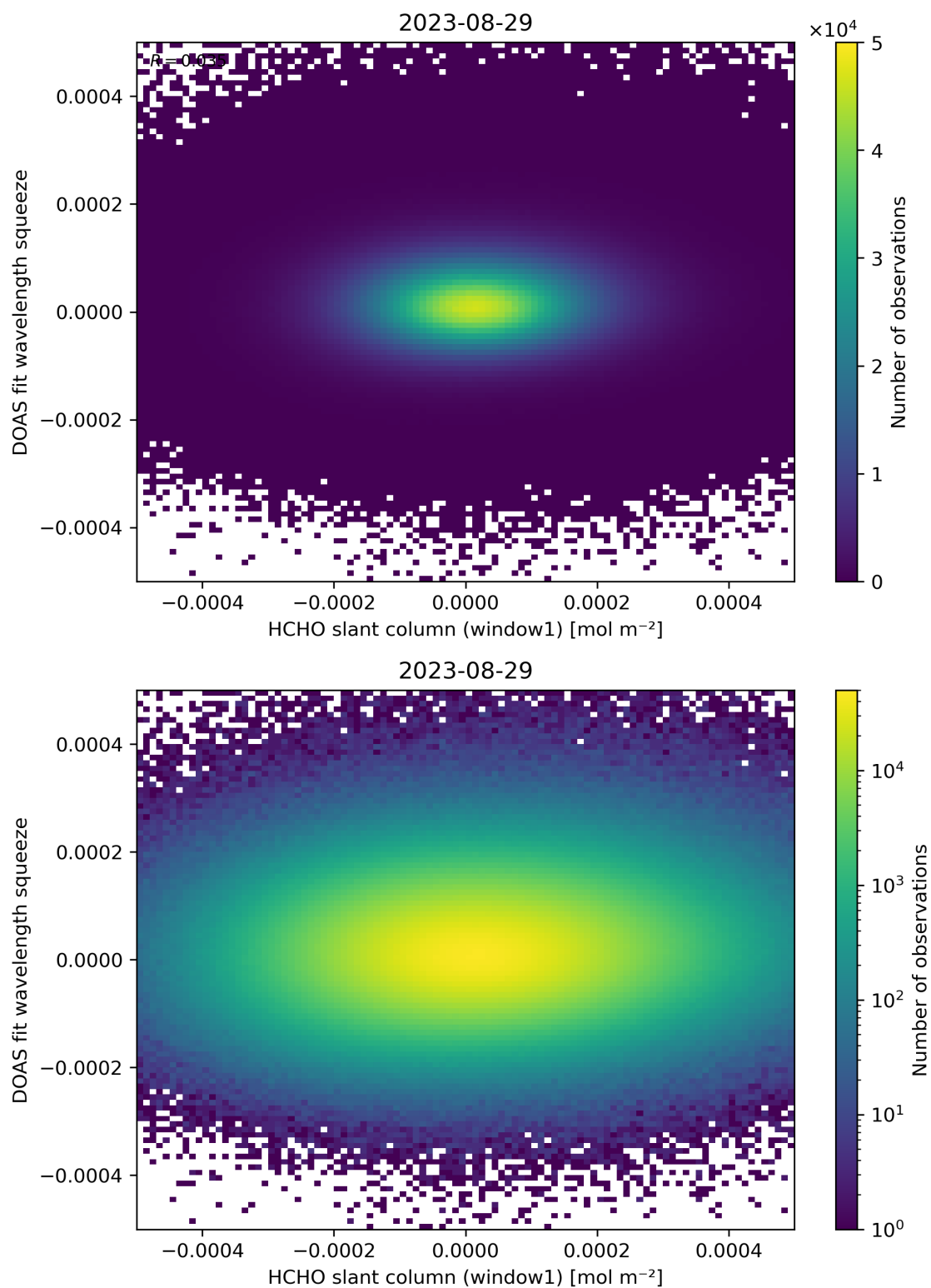
Figure 80: Scatter density plot of “HCHO slant column (window1)” against “DOAS fit wavelength squeeze” for 2023-08-28 to 2023-08-30.
