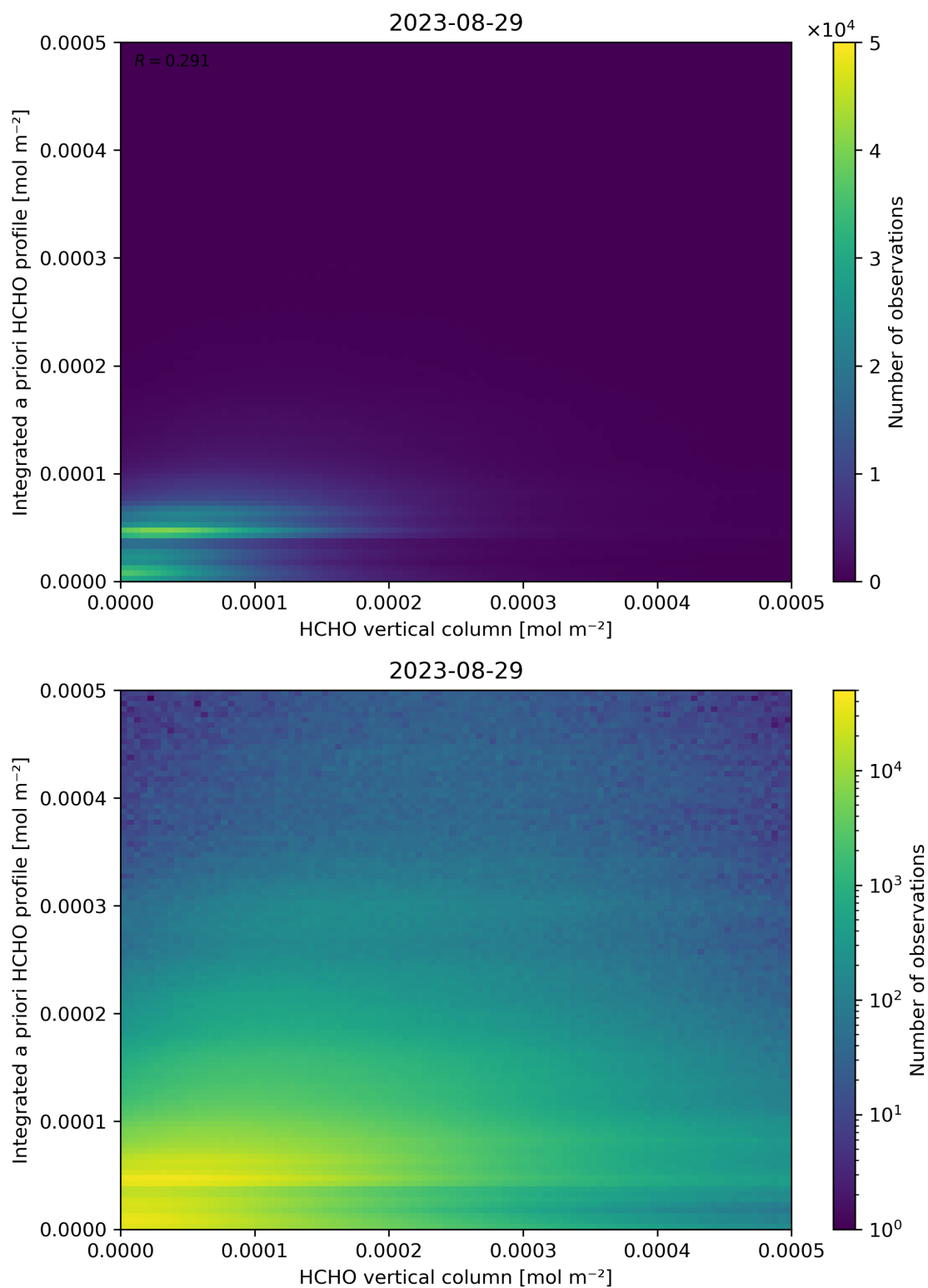
Figure 135: Scatter density plot of “HCHO vertical column” against “Integrated a priori HCHO profile” for 2023-08-28 to 2023-08-30.
