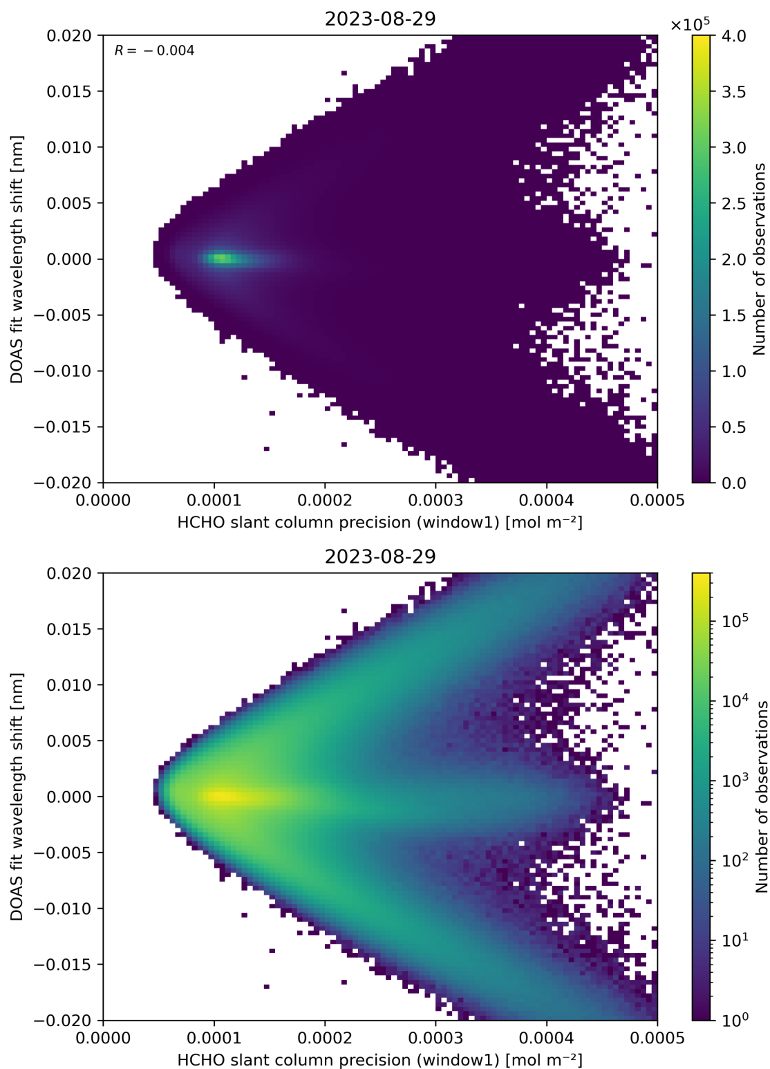
Figure 89: Scatter density plot of “HCHO slant column precision (window1)” against “DOAS fit wavelength shift” for 2023-08-28 to 2023-08-30.
