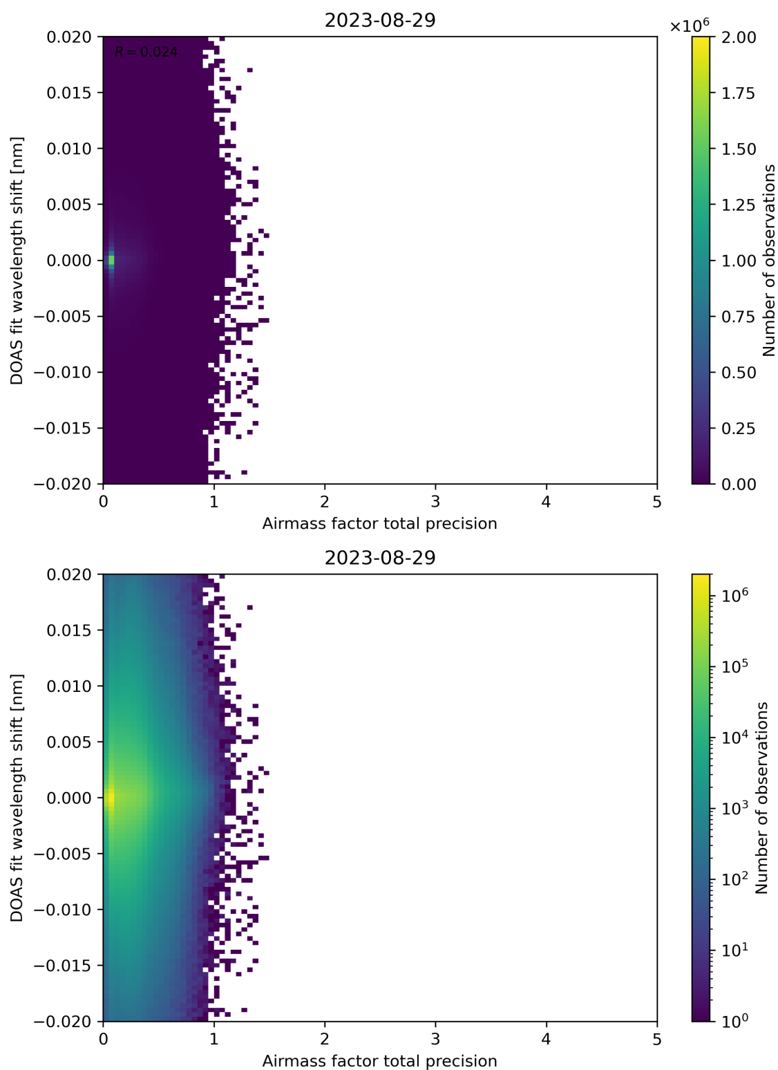
Figure 106: Scatter density plot of “Airmass factor total precision” against “DOAS fit wavelength shift” for 2023-08-28 to 2023-08-30.
