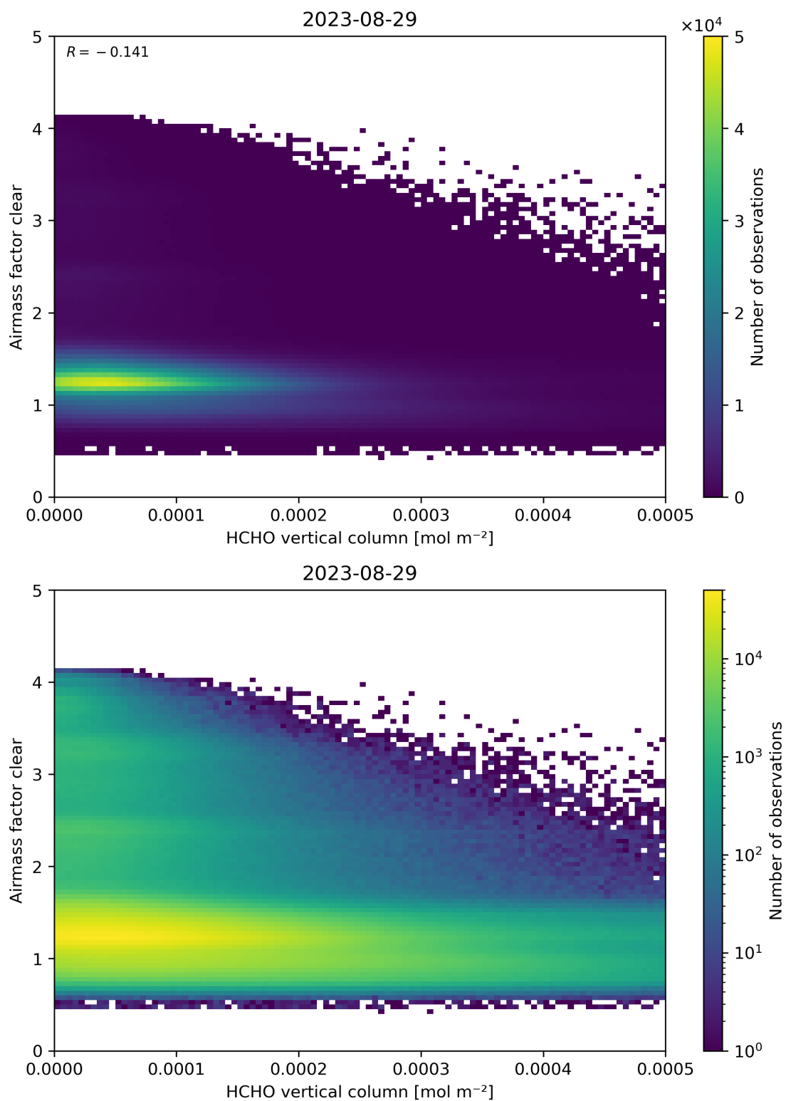
Figure 126: Scatter density plot of “HCHO vertical column” against “Airmass factor clear” for 2023-08-28 to 2023-08-30.
