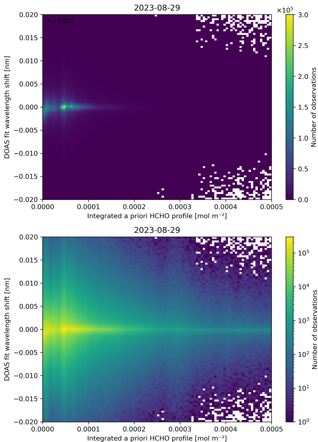
Figure 149: Scatter density plot of “Integrated a priori HCHO profile” against “DOAS fit wavelength shift” for 2023-08-28 to 2023-08-30.
