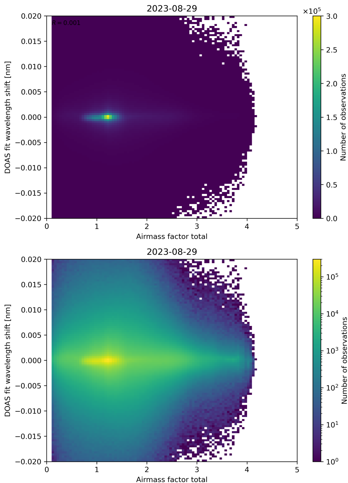
Figure 98: Scatter density plot of “Airmass factor total” against “DOAS fit wavelength shift” for 2023-08-28 to 2023-08-30.
