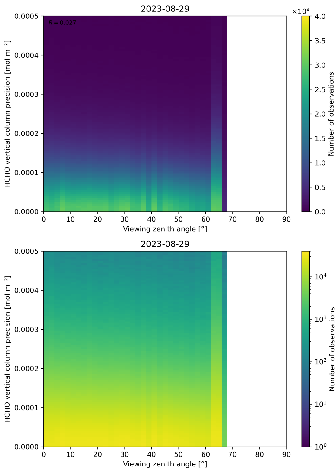
Figure 194: Scatter density plot of “Viewing zenith angle” against “HCHO vertical column precision” for 2023-08-28 to 2023-08-30.
