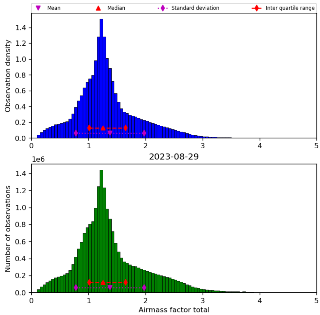
Figure 40: Histogram of “Airmass factor total” for 2023-08-28 to 2023-08-30
