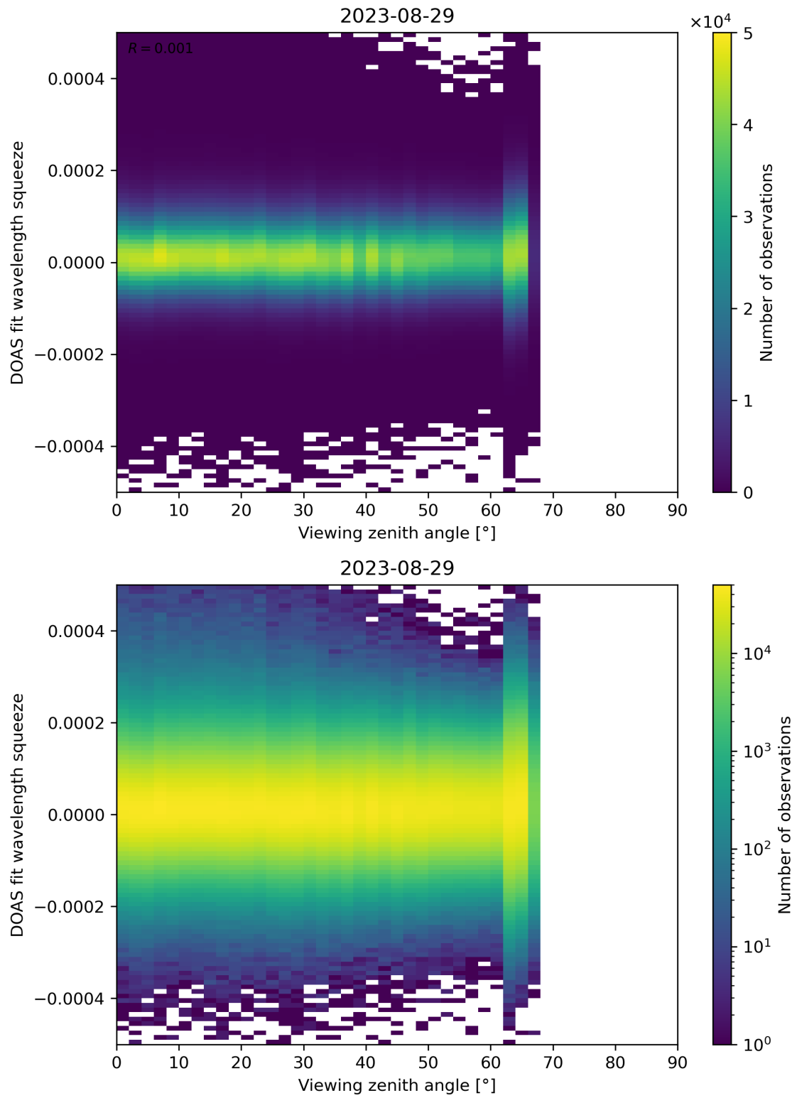
Figure 184: Scatter density plot of “Viewing zenith angle” against “DOAS fit wavelength squeeze” for 2023-08-28 to 2023-08-30.
