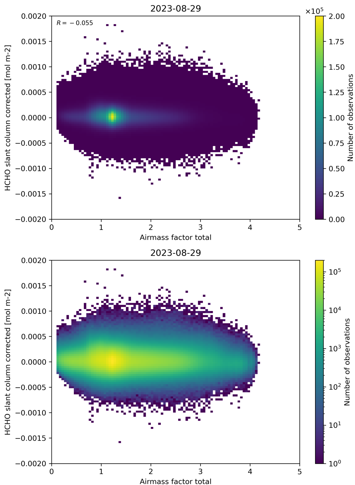
Figure 101: Scatter density plot of “Airmass factor total” against “HCHO slant column corrected” for 2023-08-28 to 2023-08-30.
