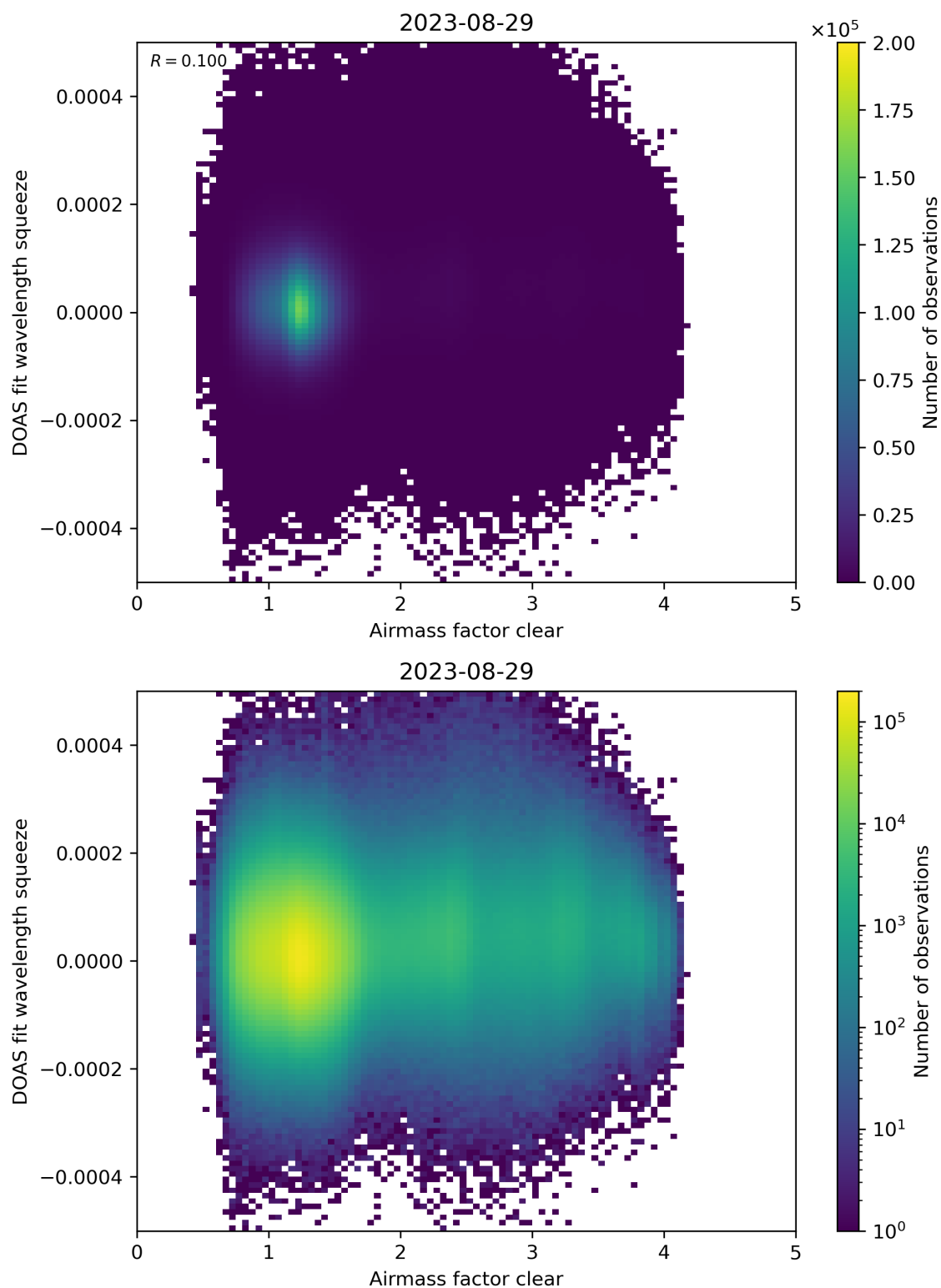
Figure 73: Scatter density plot of “Airmass factor clear” against “DOAS fit wavelength squeeze” for 2023-08-28 to 2023-08-30.
