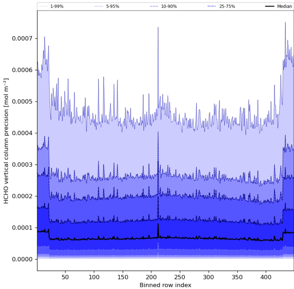
Figure 50: Along track statistics of “HCHO vertical column precision” for 2023-08-28 to 2023-08-30
