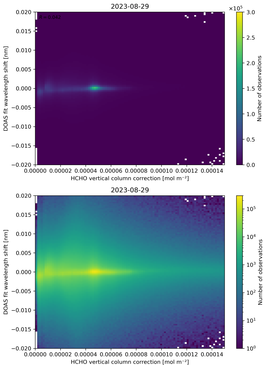
Figure 113: Scatter density plot of “HCHO vertical column correction” against “DOAS fit wavelength shift” for 2023-08-28 to 2023-08-30.
