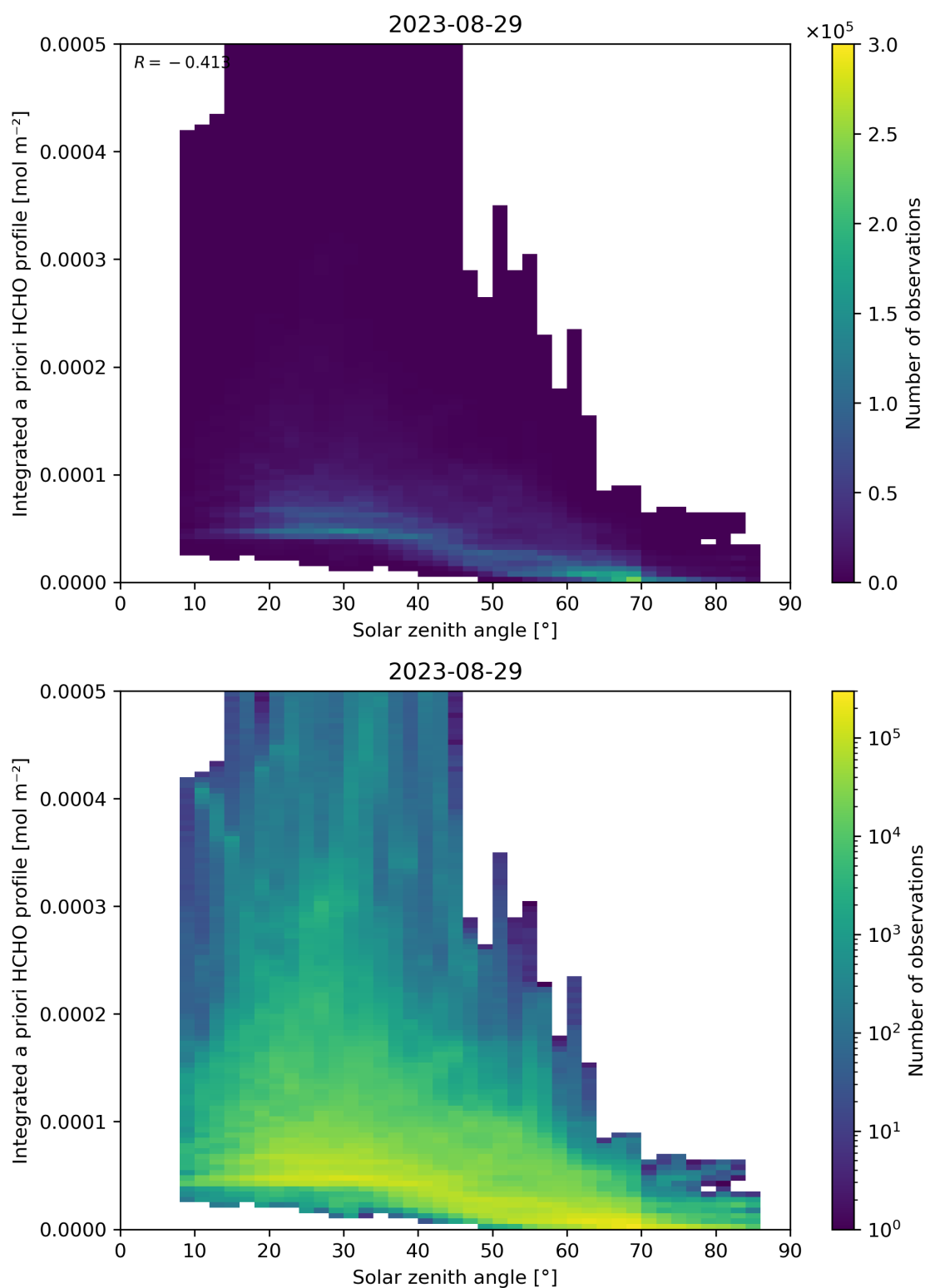
Figure 180: Scatter density plot of “Solar zenith angle” against “Integrated a priori HCHO profile” for 2023-08-28 to 2023-08-30.
