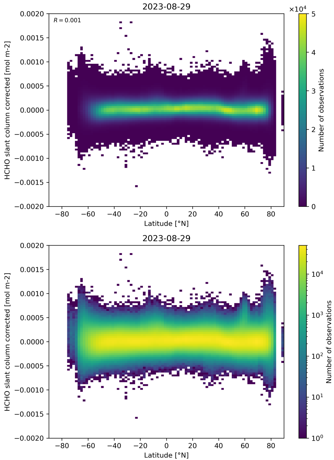
Figure 157: Scatter density plot of “Latitude” against “HCHO slant column corrected” for 2023-08-28 to 2023-08-30.
