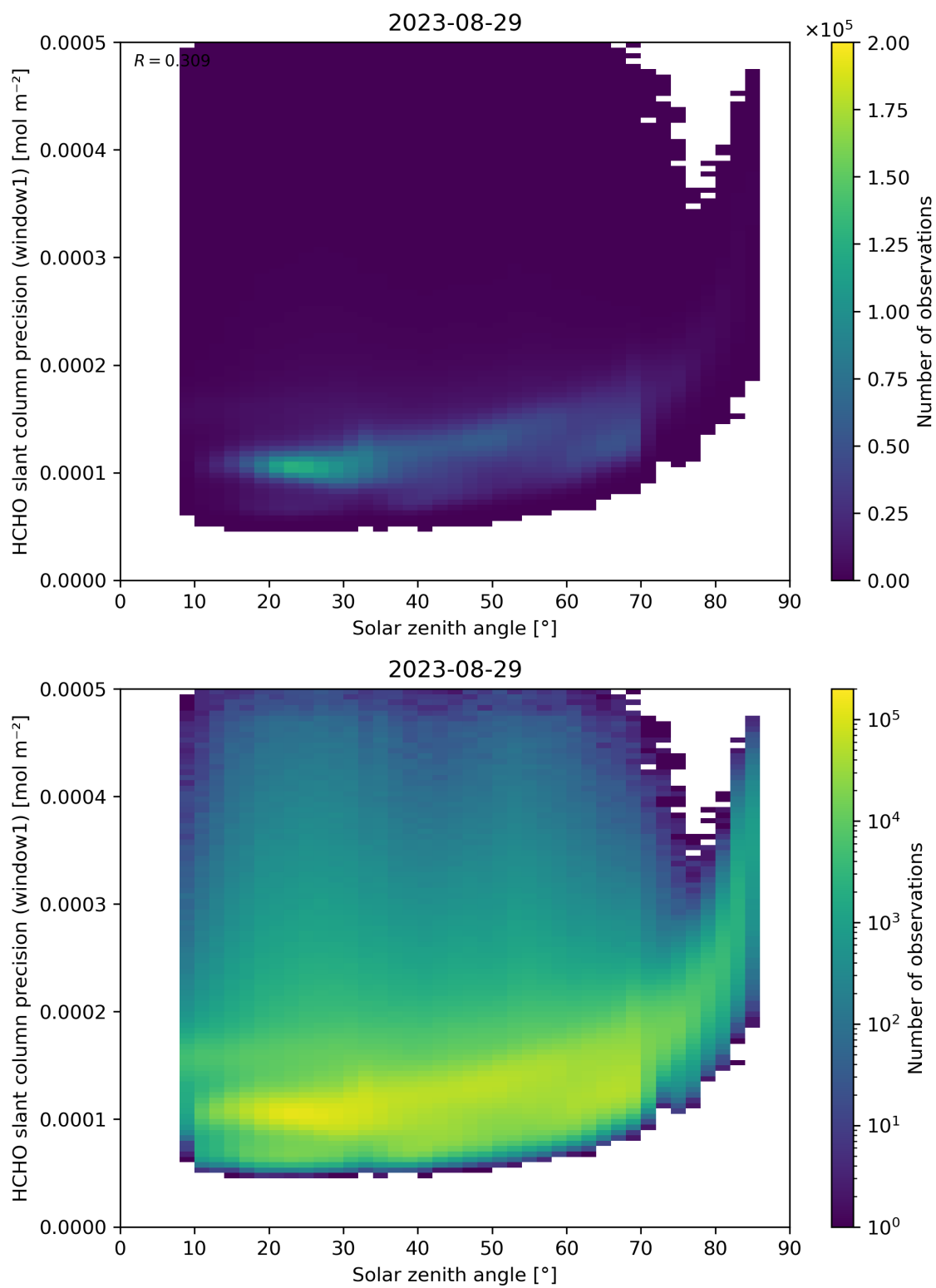
Figure 174: Scatter density plot of “Solar zenith angle” against “HCHO slant column precision (window1)” for 2023-08-28 to 2023-08-30.
