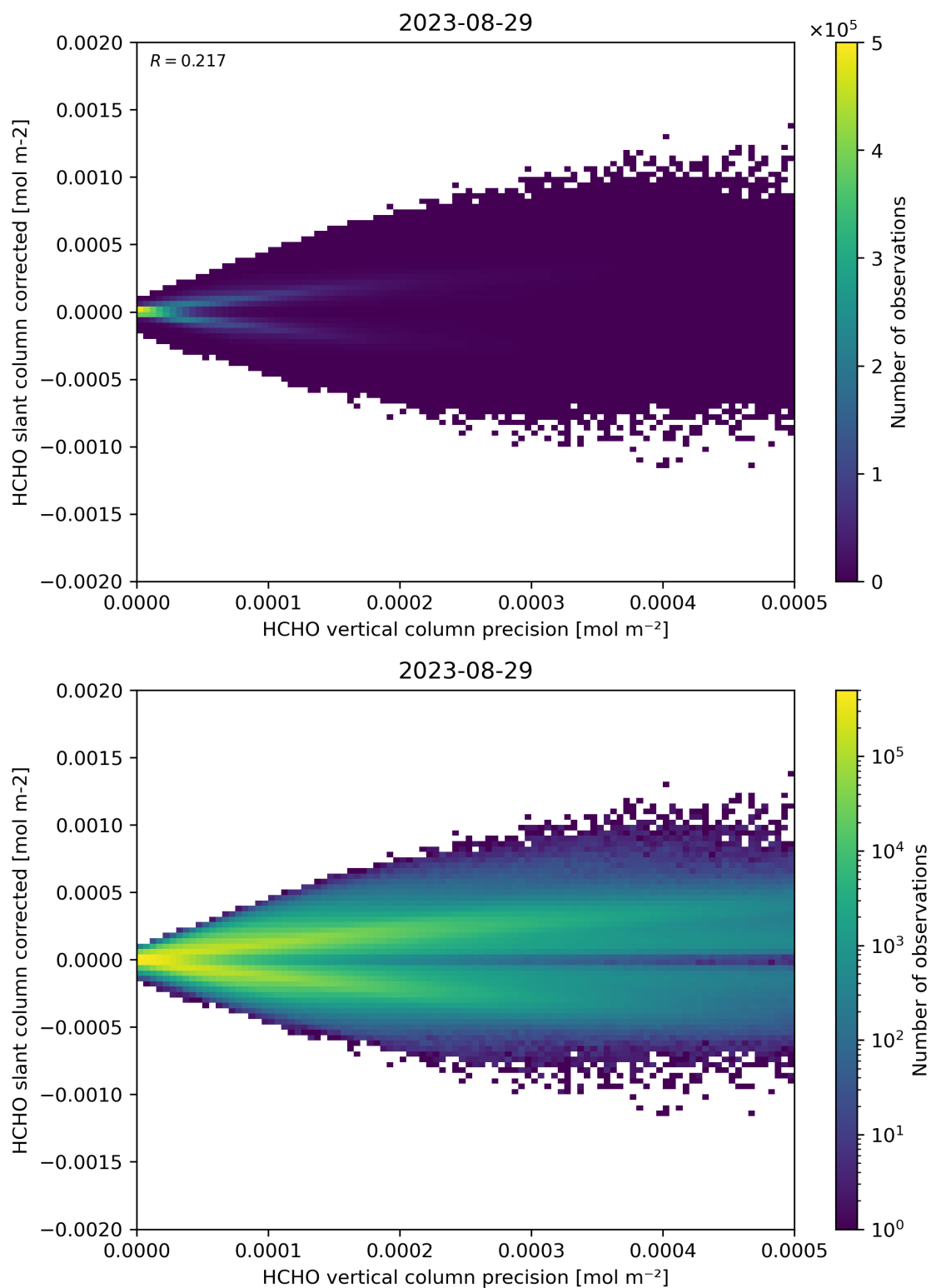
Figure 140: Scatter density plot of “HCHO vertical column precision” against “HCHO slant column corrected” for 2023-08-28 to 2023-08-30.
