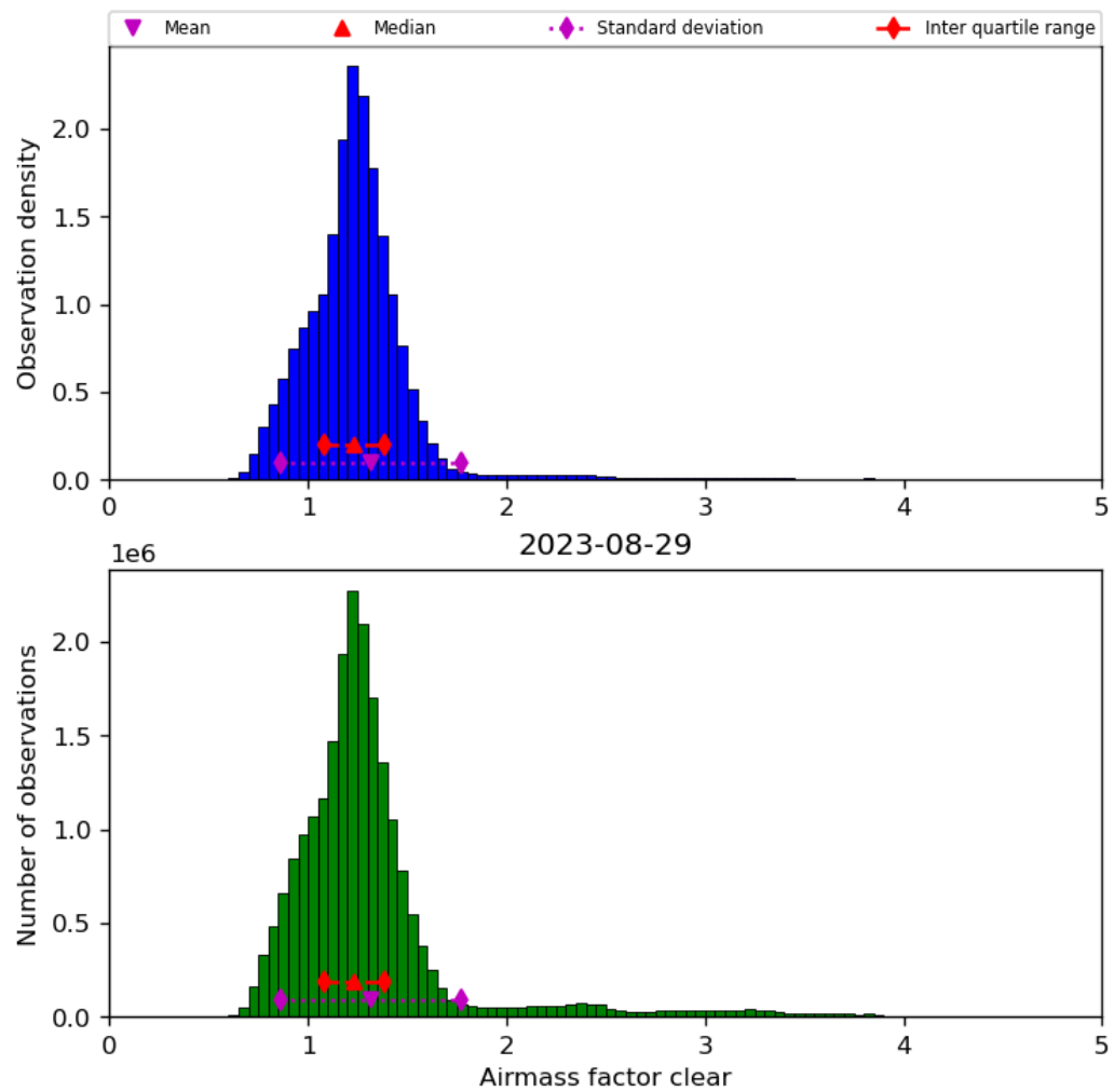
Figure 42: Histogram of “Airmass factor clear” for 2023-08-28 to 2023-08-30
