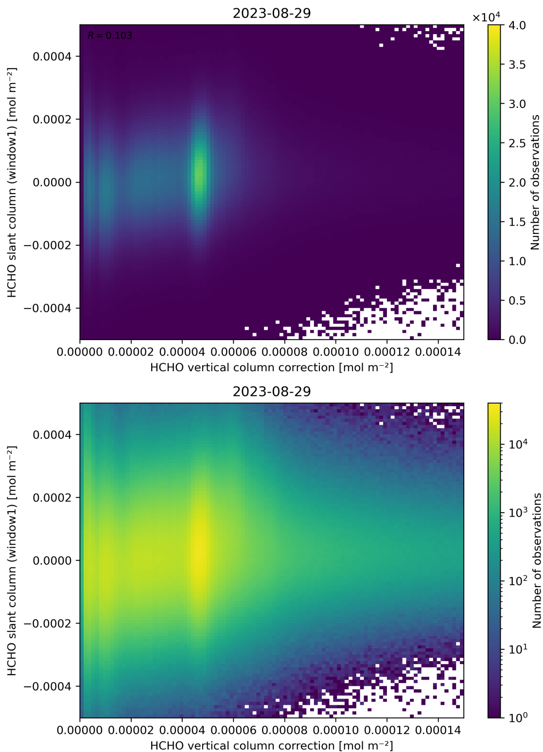
Figure 118: Scatter density plot of “HCHO vertical column correction” against “HCHO slant column (window1)” for 2023-08-28 to 2023-08-30.
