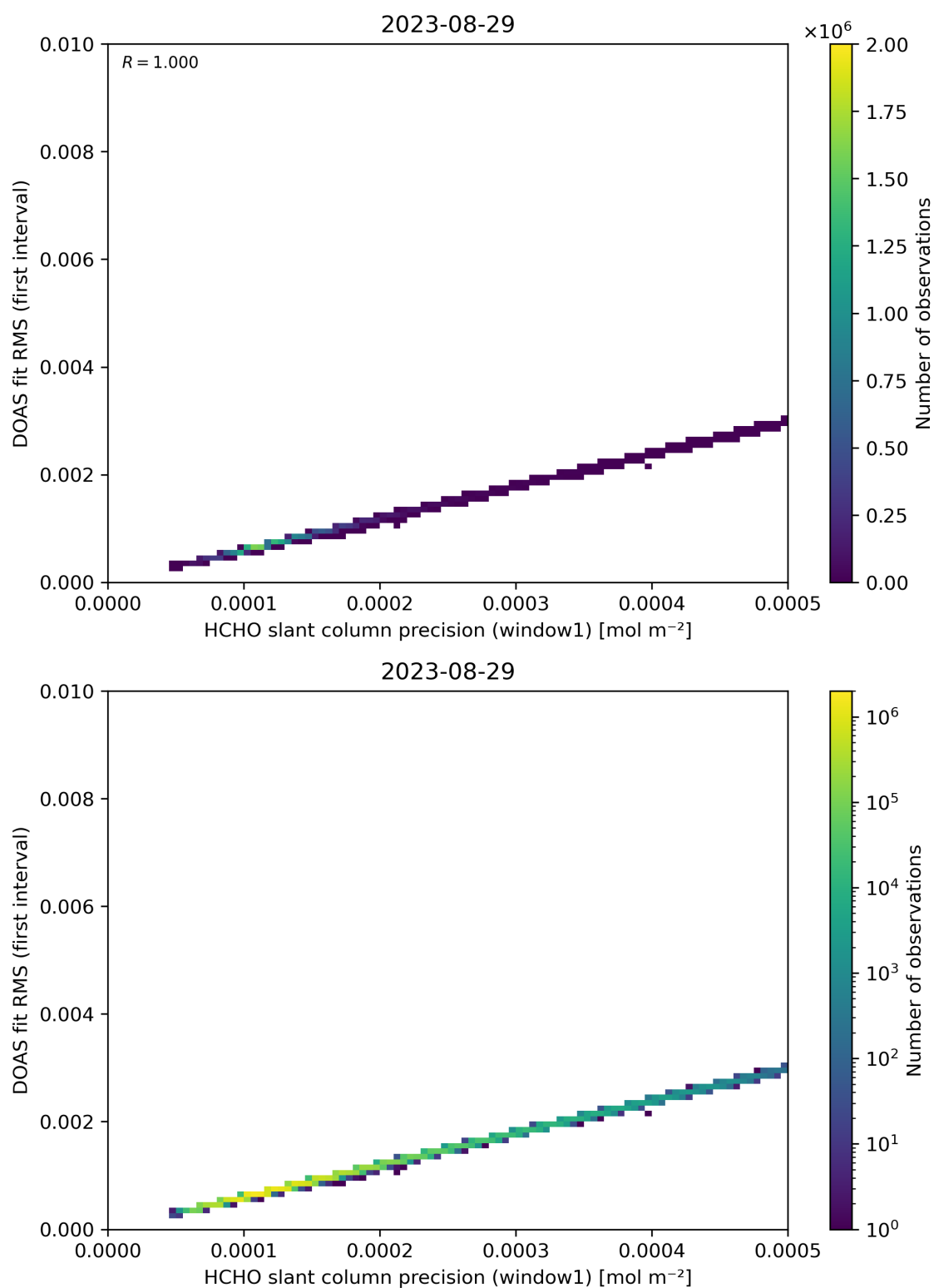
Figure 88: Scatter density plot of “HCHO slant column precision (window1)” against “DOAS fit RMS (first interval)” for 2023-08-28 to 2023-08-30.
