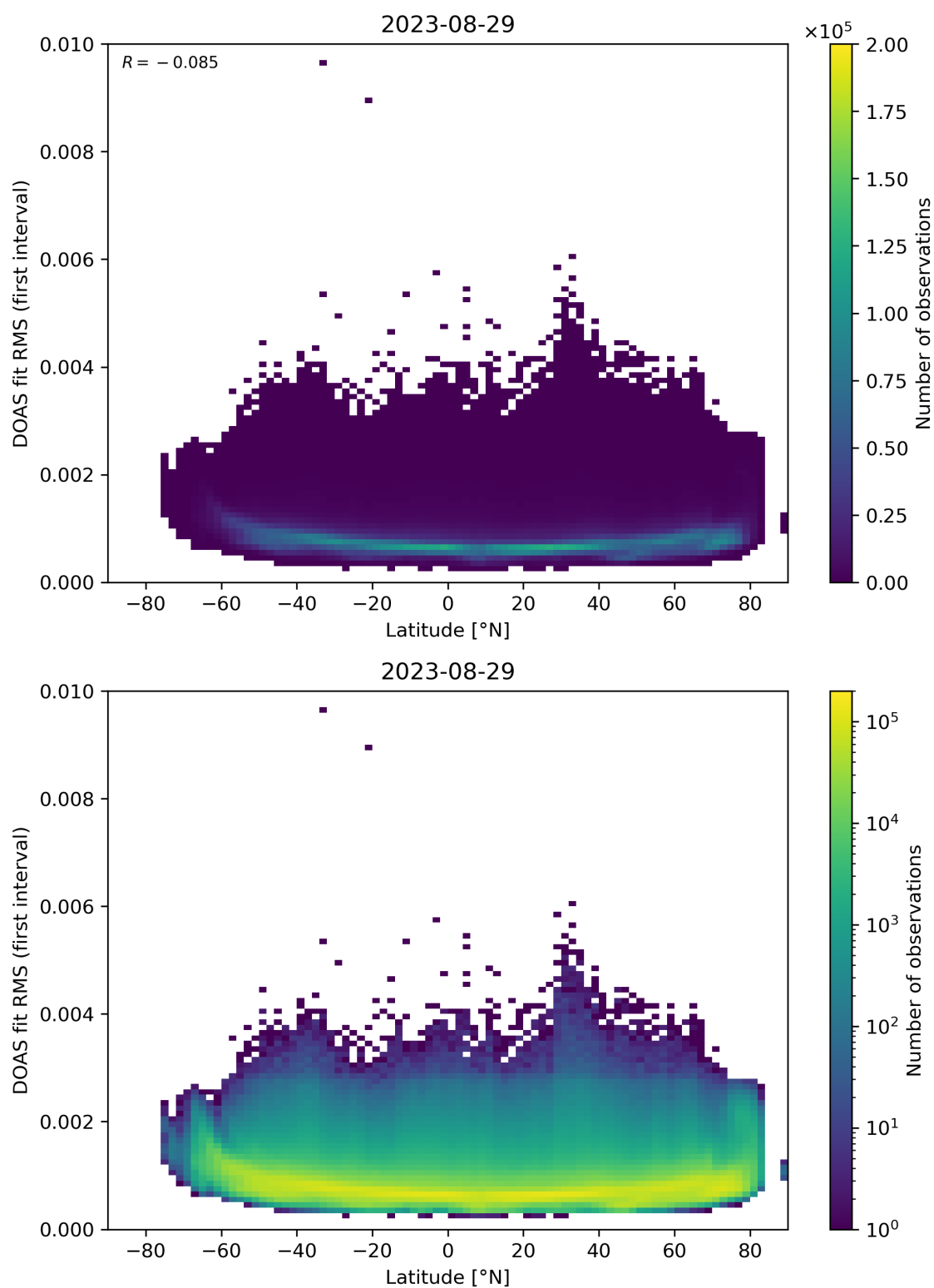
Figure 153: Scatter density plot of “Latitude” against “DOAS fit RMS (first interval)” for 2023-08-28 to 2023-08-30.
