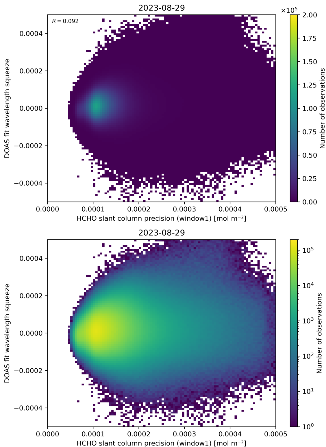
Figure 90: Scatter density plot of “HCHO slant column precision (window1)” against “DOAS fit wavelength squeeze” for 2023-08-28 to 2023-08-30.
