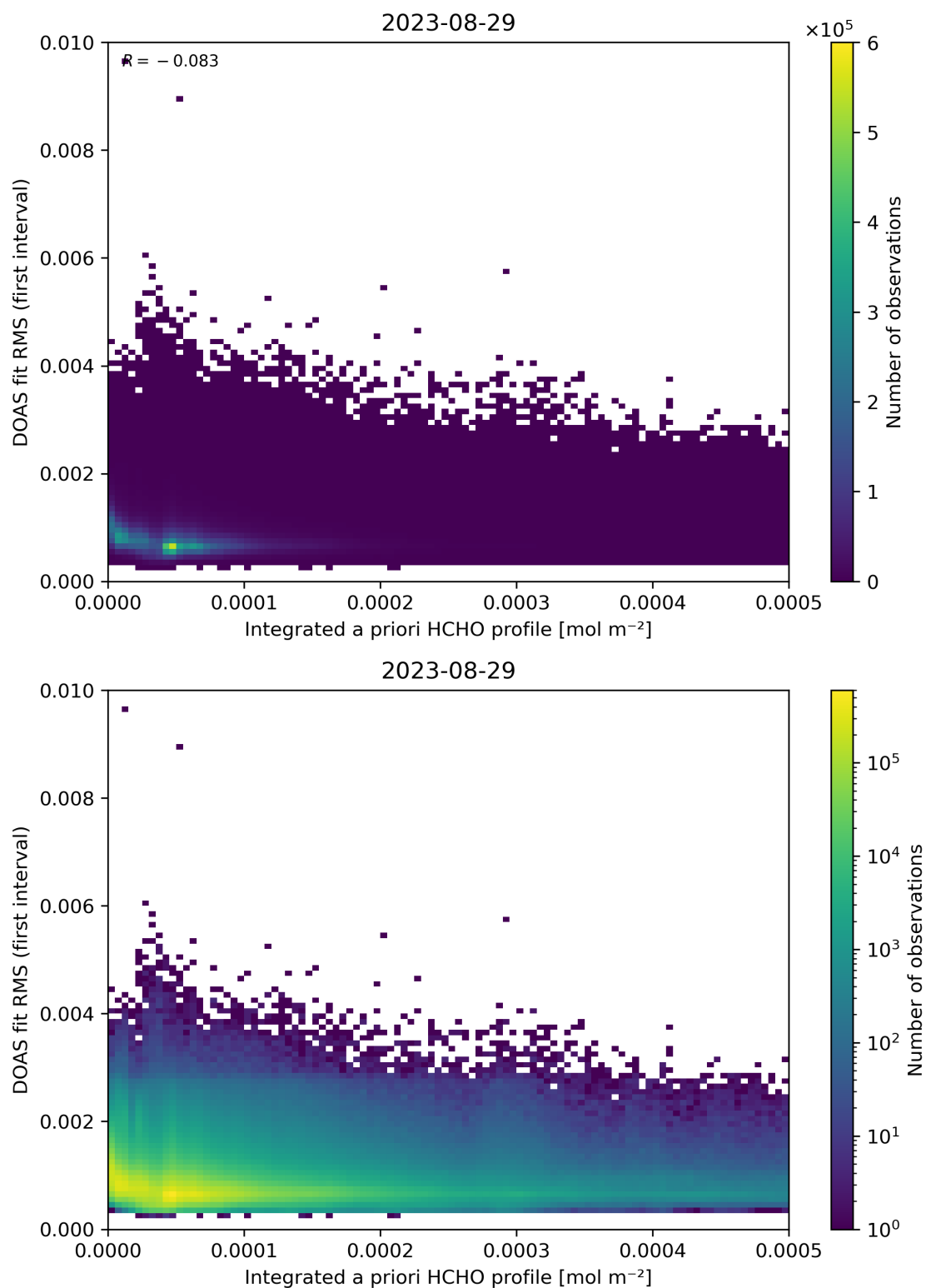
Figure 148: Scatter density plot of “Integrated a priori HCHO profile” against “DOAS fit RMS (first interval)” for 2023-08-28 to 2023-08-30.
