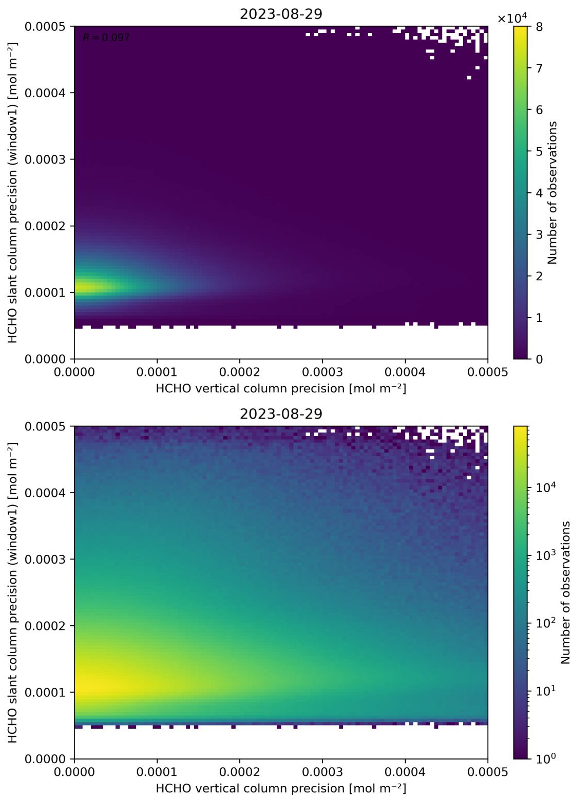
Figure 143: Scatter density plot of “HCHO vertical column precision” against “HCHO slant column precision (window1)” for 2023-08-28 to 2023-08-30.
