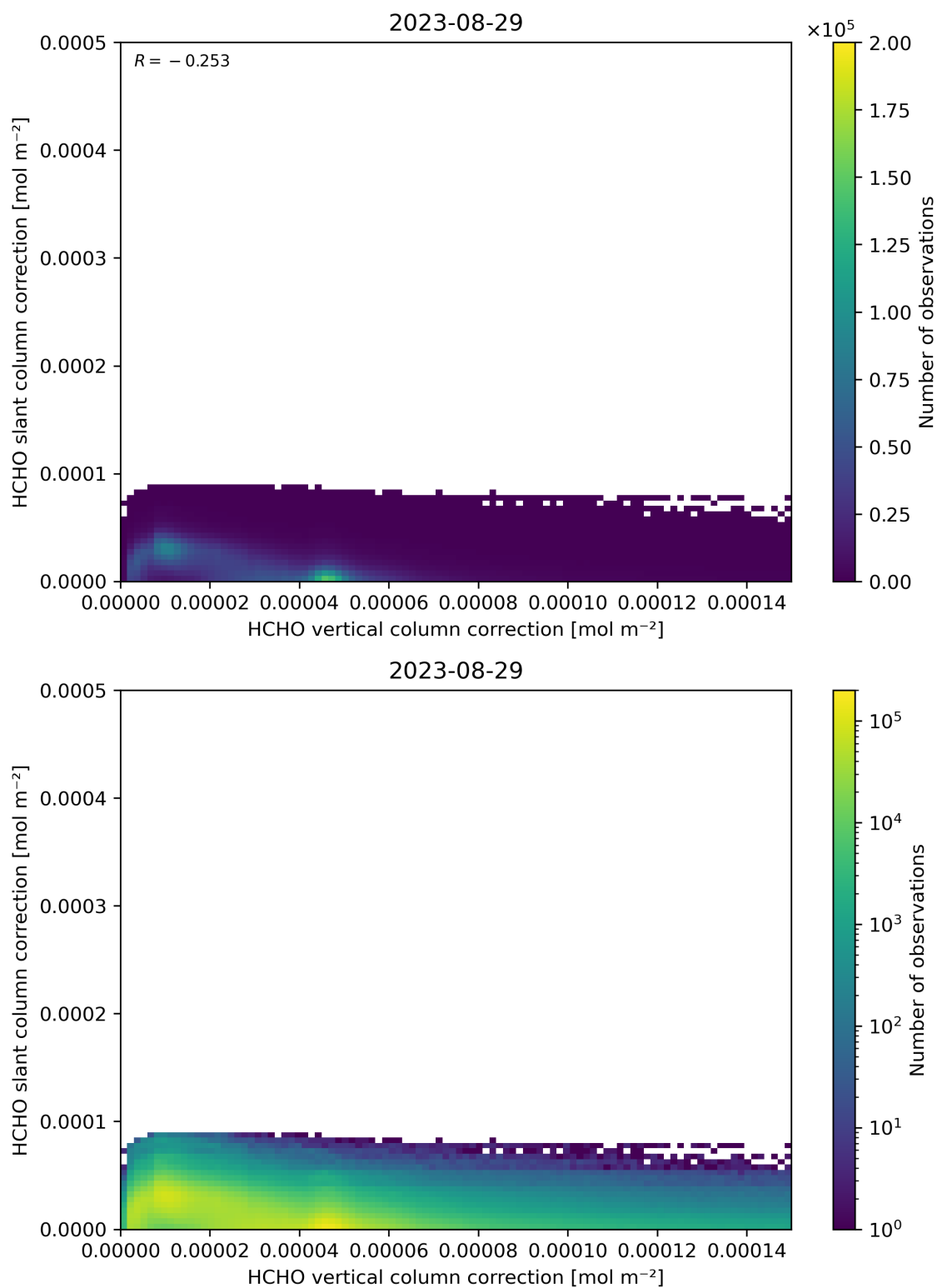
Figure 117: Scatter density plot of “HCHO vertical column correction” against “HCHO slant column correction” for 2023-08-28 to 2023-08-30.
