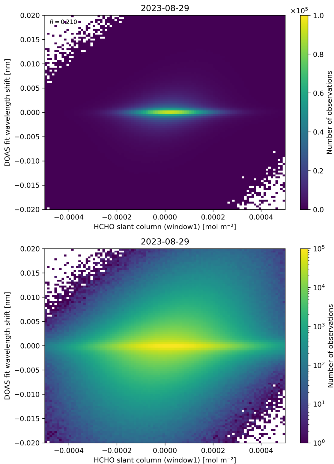
Figure 79: Scatter density plot of “HCHO slant column (window1)” against “DOAS fit wavelength shift” for 2023-08-28 to 2023-08-30.
