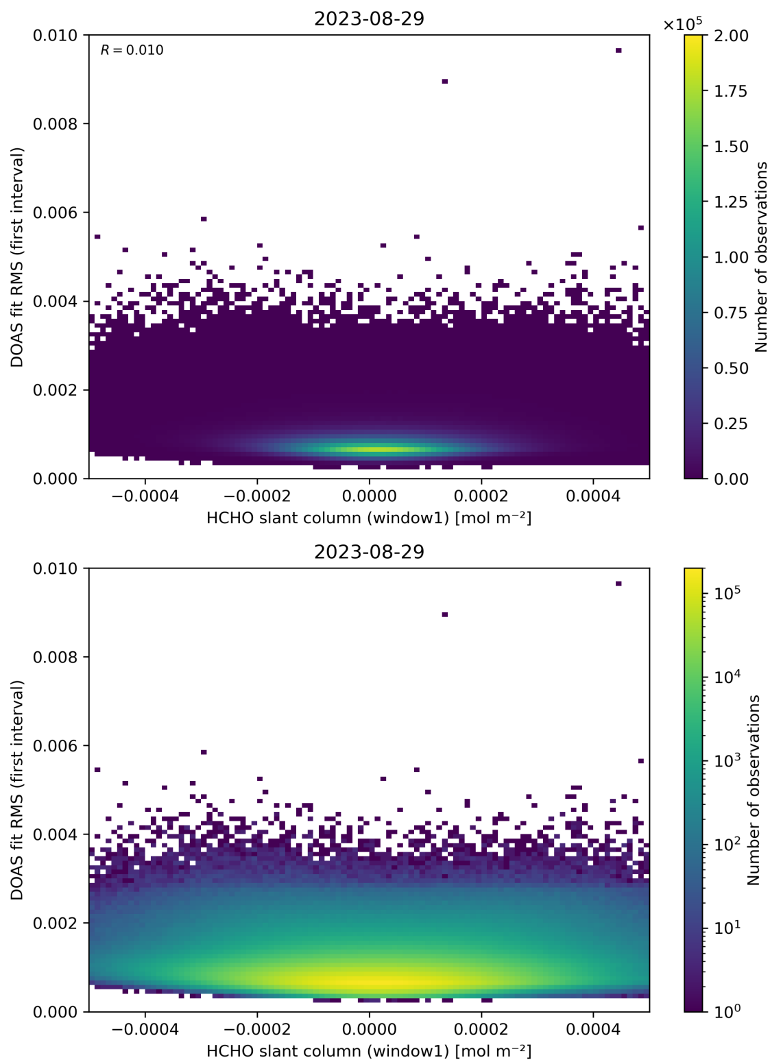
Figure 78: Scatter density plot of “HCHO slant column (window1)” against “DOAS fit RMS (first interval)” for 2023-08-28 to 2023-08-30.
