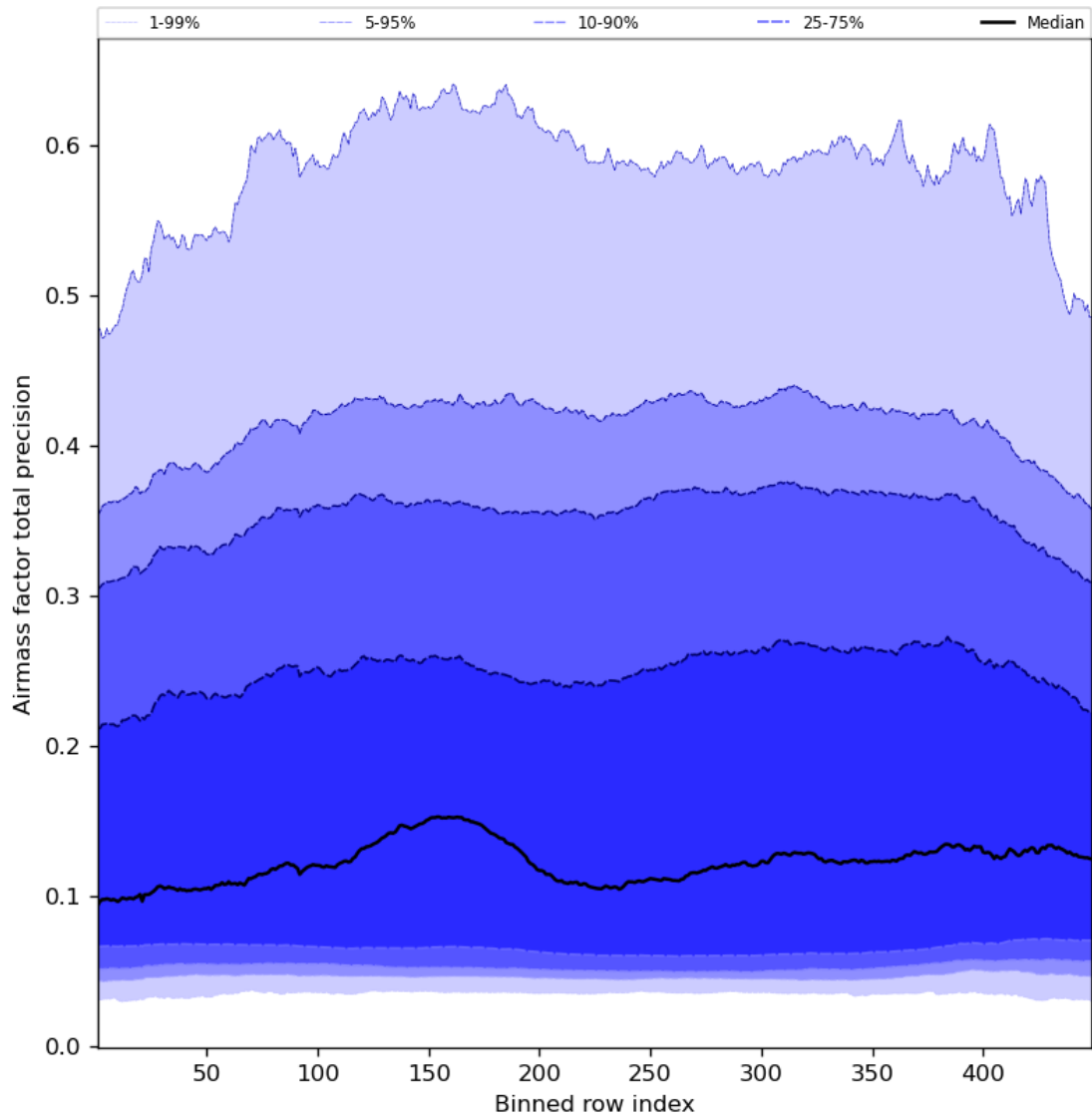
Figure 55: Along track statistics of “Airmass factor total precision” for 2023-08-28 to 2023-08-30
