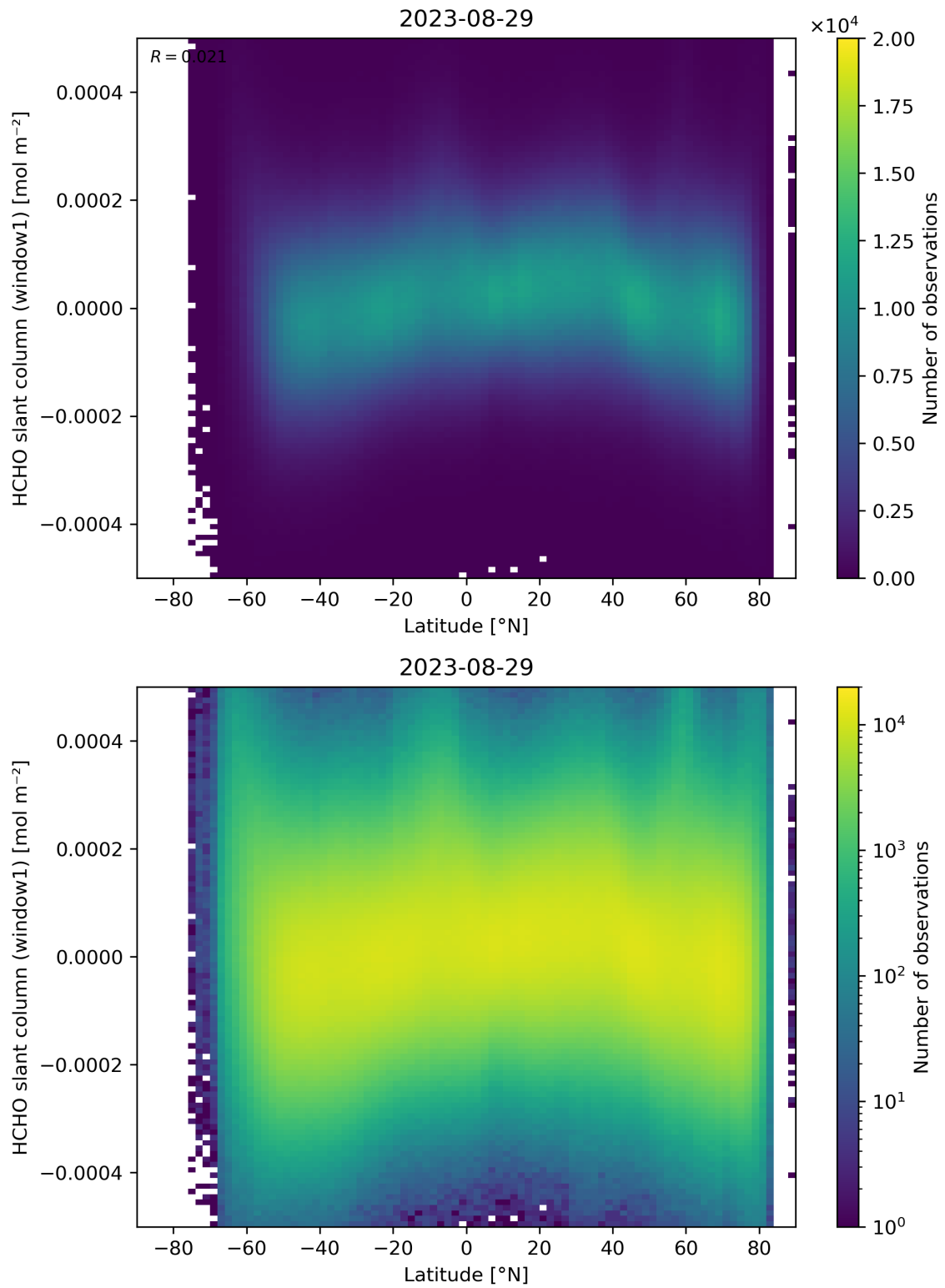
Figure 159: Scatter density plot of “Latitude” against “HCHO slant column (window1)” for 2023-08-28 to 2023-08-30.
