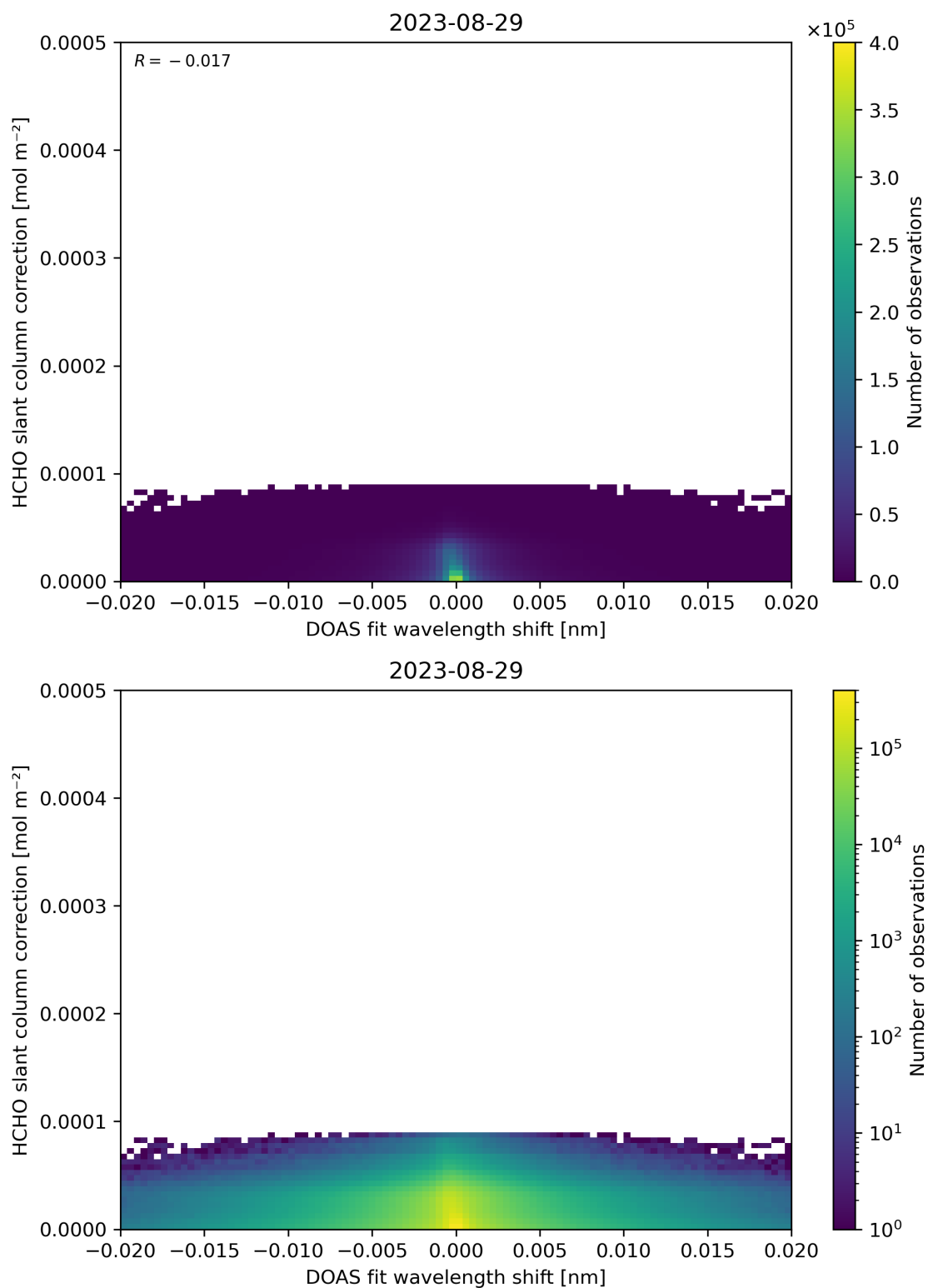
Figure 67: Scatter density plot of “DOAS fit wavelength shift” against “HCHO slant column correction” for 2023-08-28 to 2023-08-30.
