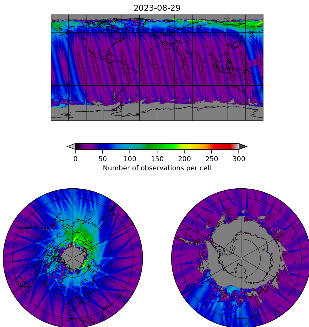
Figure 19: Map of the number of observations for 2023-08-28 to 2023-08-30
