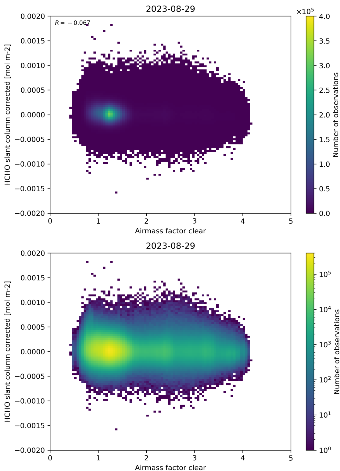
Figure 74: Scatter density plot of “Airmass factor clear” against “HCHO slant column corrected” for 2023-08-28 to 2023-08-30.
