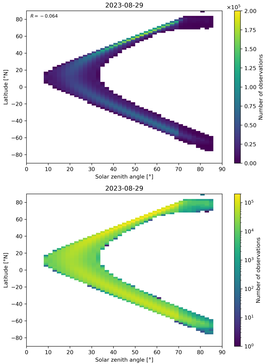
Figure 181: Scatter density plot of “Solar zenith angle” against “Latitude” for 2023-08-28 to 2023-08-30.
