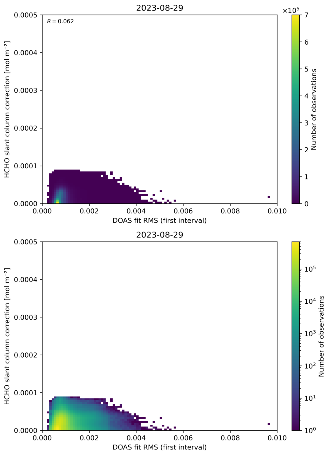
Figure 63: Scatter density plot of “DOAS fit RMS (first interval)” against “HCHO slant column correction” for 2023-08-28 to 2023-08-30.
