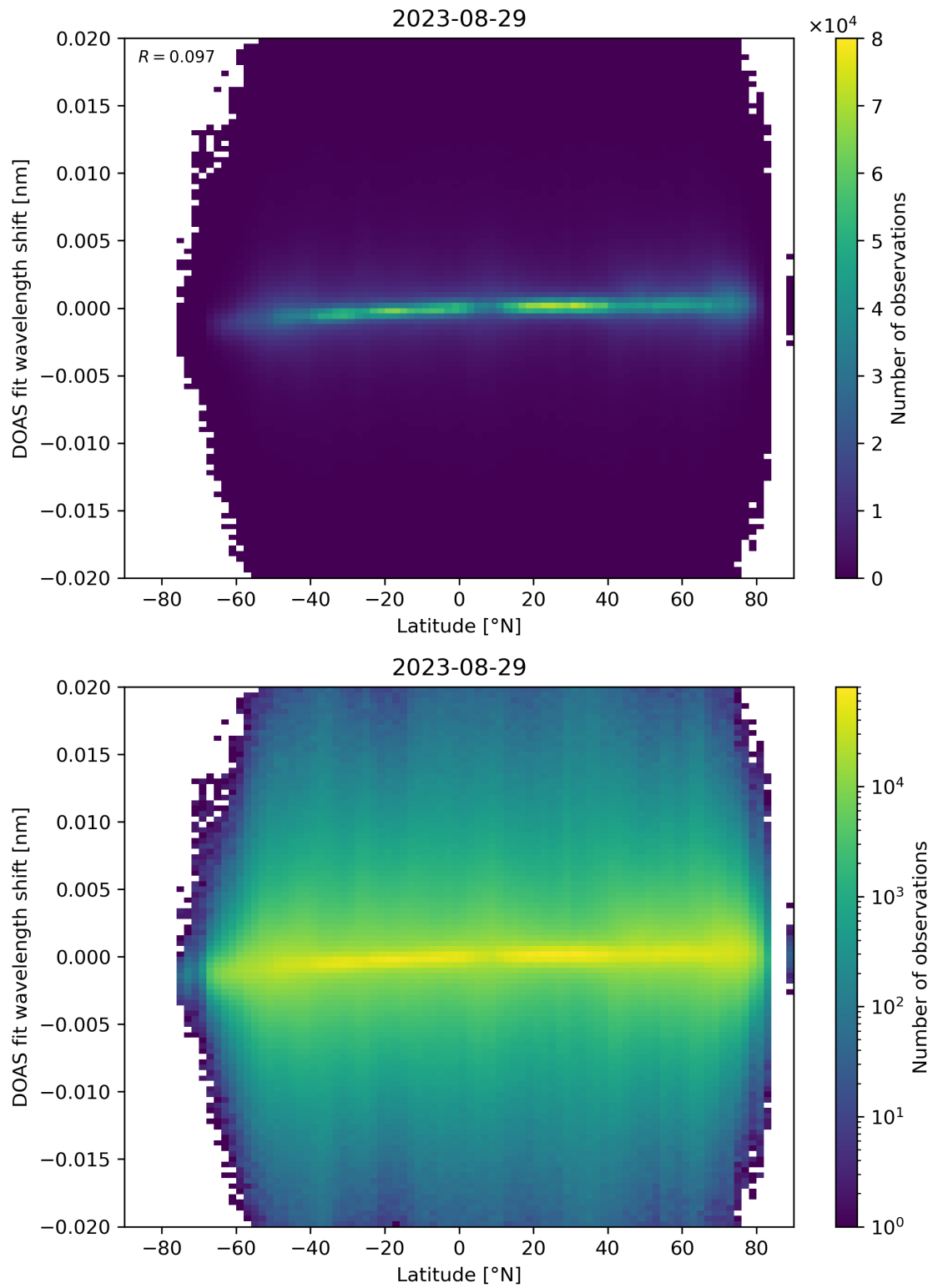
Figure 154: Scatter density plot of “Latitude” against “DOAS fit wavelength shift” for 2023-08-28 to 2023-08-30.
