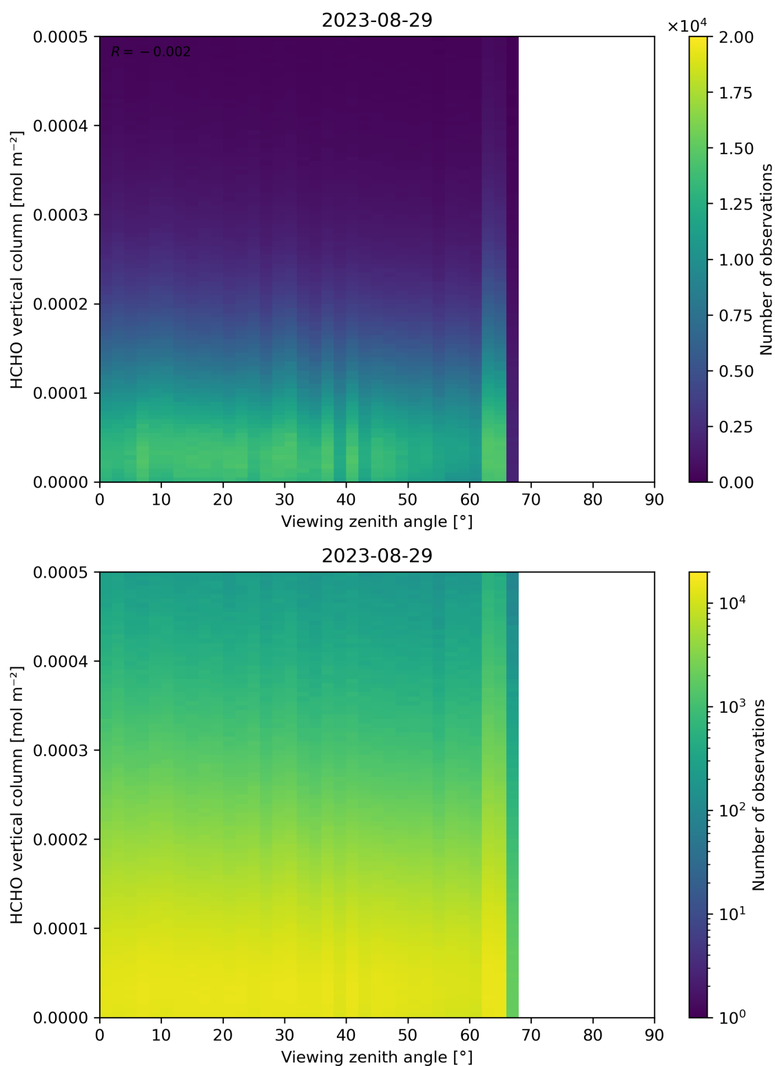
Figure 192: Scatter density plot of “Viewing zenith angle” against “HCHO vertical column” for 2023-08-28 to 2023-08-30.
