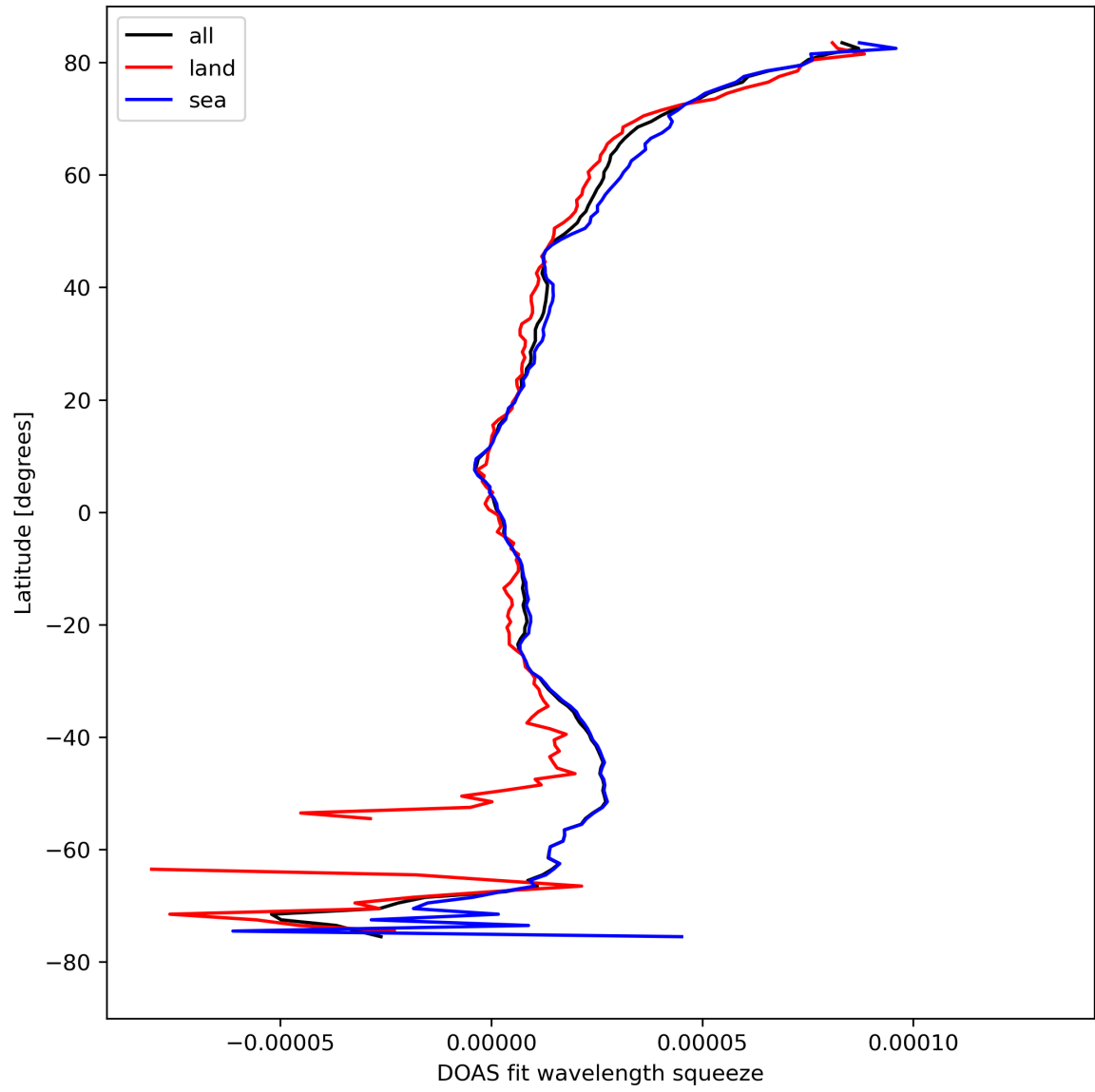
Figure 31: Zonal average of “DOAS fit wavelength squeeze” for 2023-08-28 to 2023-08-30.
