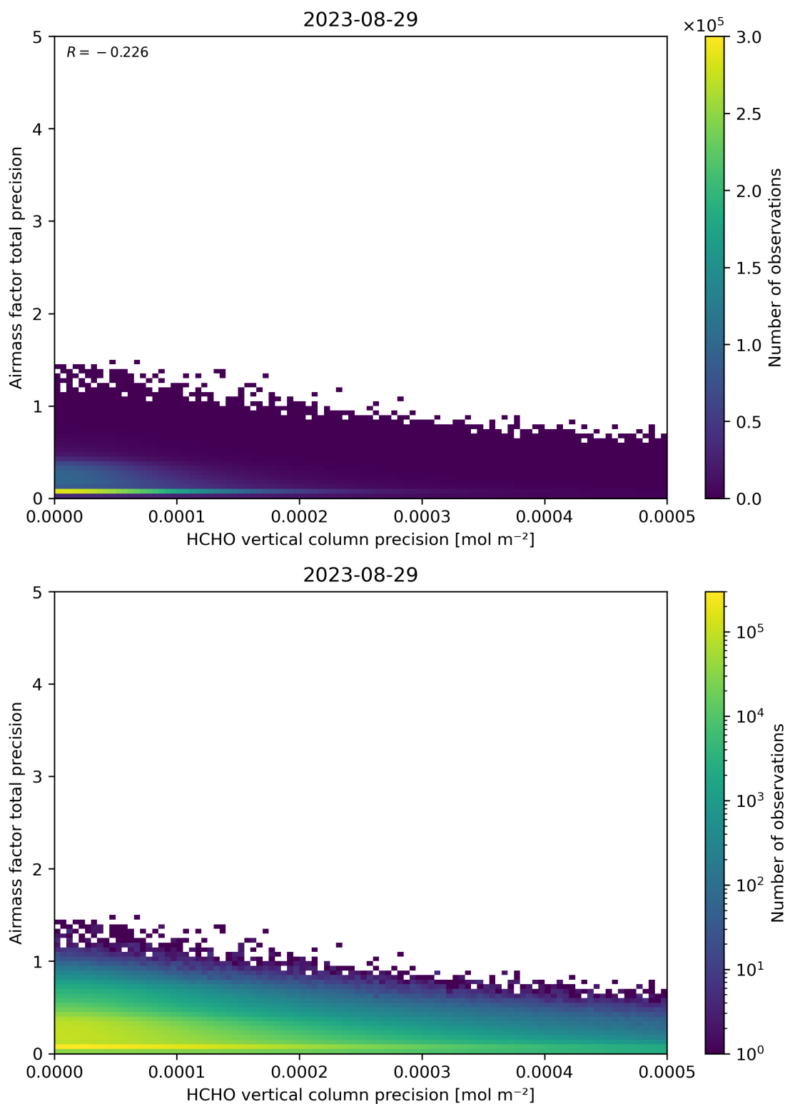
Figure 145: Scatter density plot of “HCHO vertical column precision” against “Airmass factor total precision” for 2023-08-28 to 2023-08-30.
