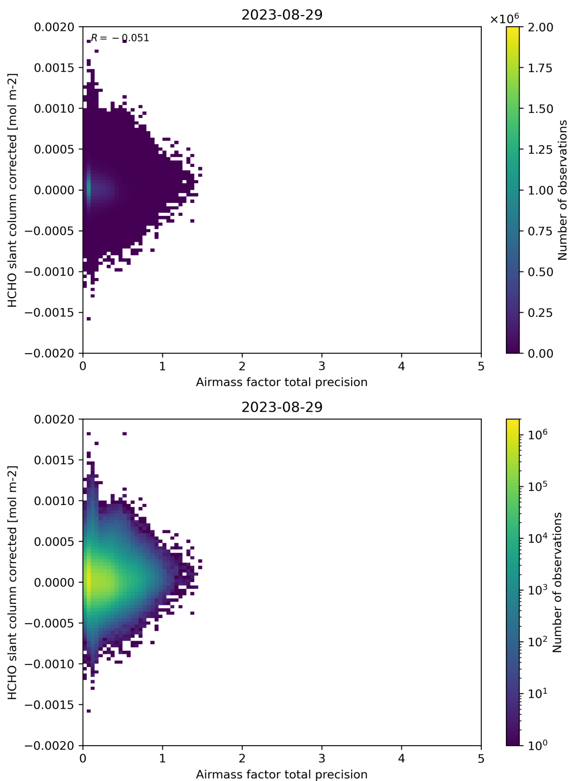
Figure 109: Scatter density plot of “Airmass factor total precision” against “HCHO slant column corrected” for 2023-08-28 to 2023-08-30.
