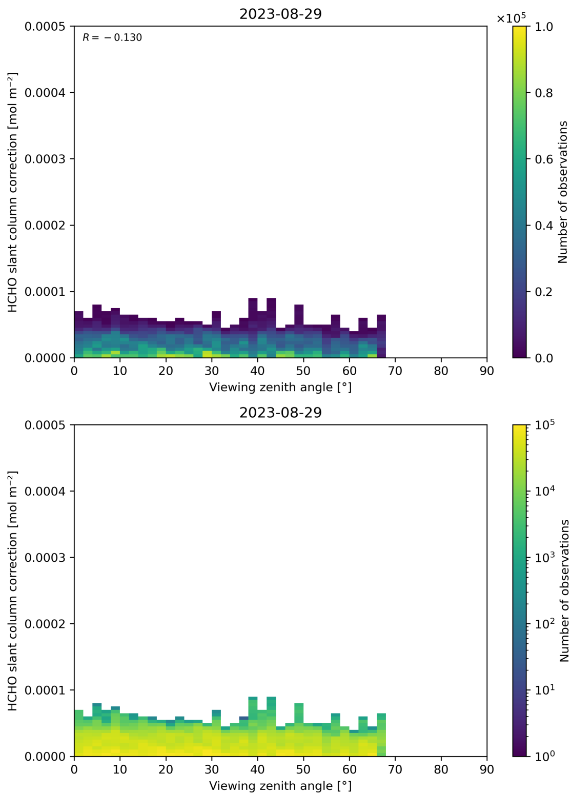
Figure 187: Scatter density plot of “Viewing zenith angle” against “HCHO slant column correction” for 2023-08-28 to 2023-08-30.
