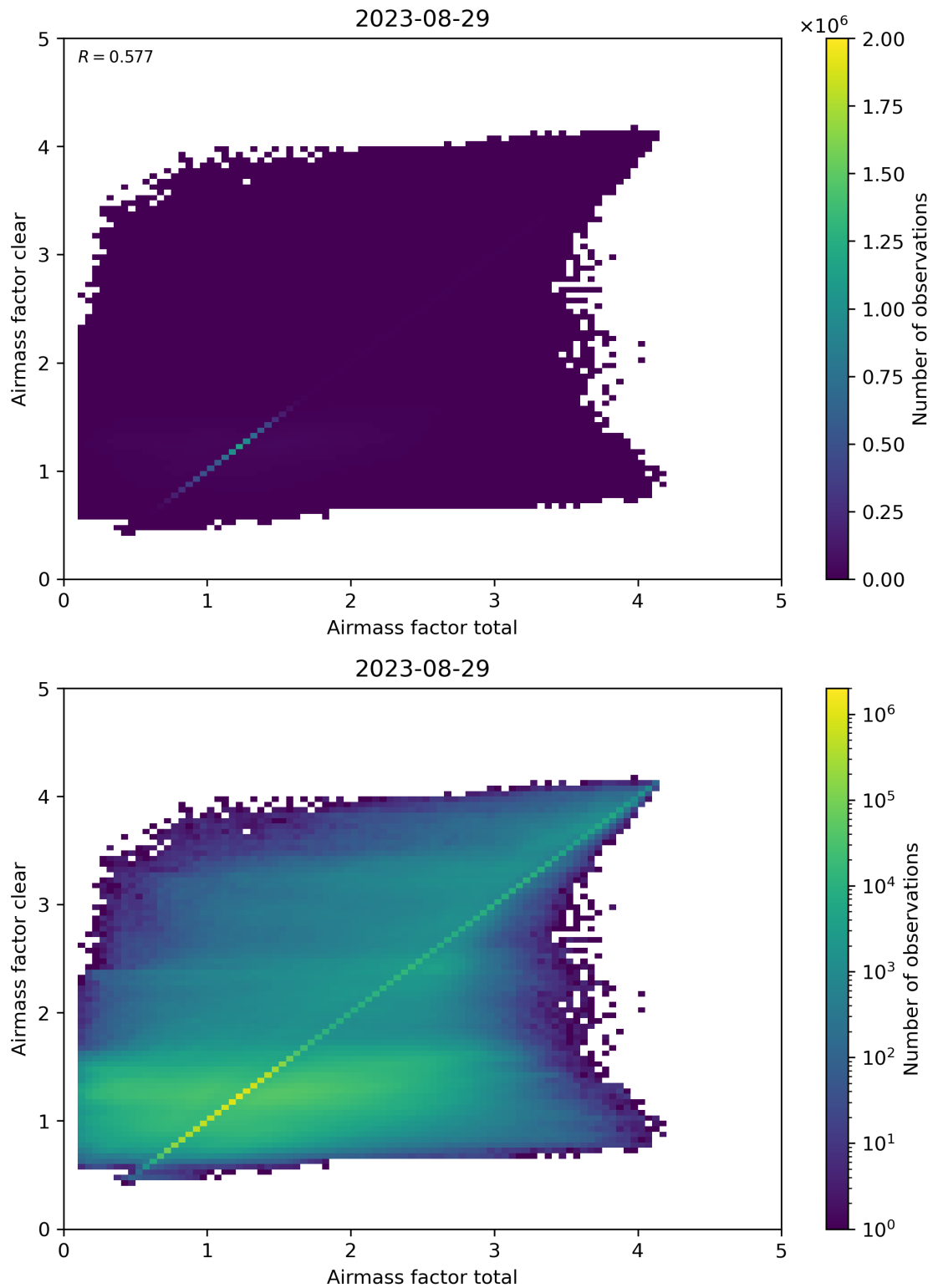
Figure 100: Scatter density plot of “Airmass factor total” against “Airmass factor clear” for 2023-08-28 to 2023-08-30.
