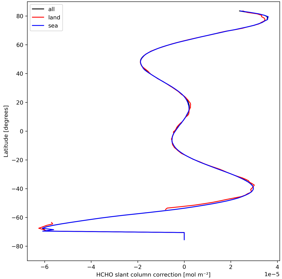
Figure 33: Zonal average of “HCHO slant column correction” for 2023-08-28 to 2023-08-30.
