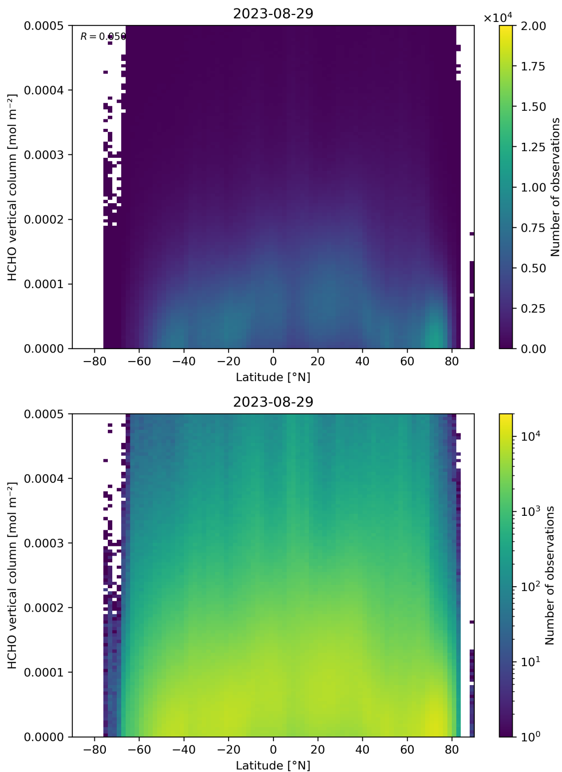
Figure 163: Scatter density plot of “Latitude” against “HCHO vertical column” for 2023-08-28 to 2023-08-30.
