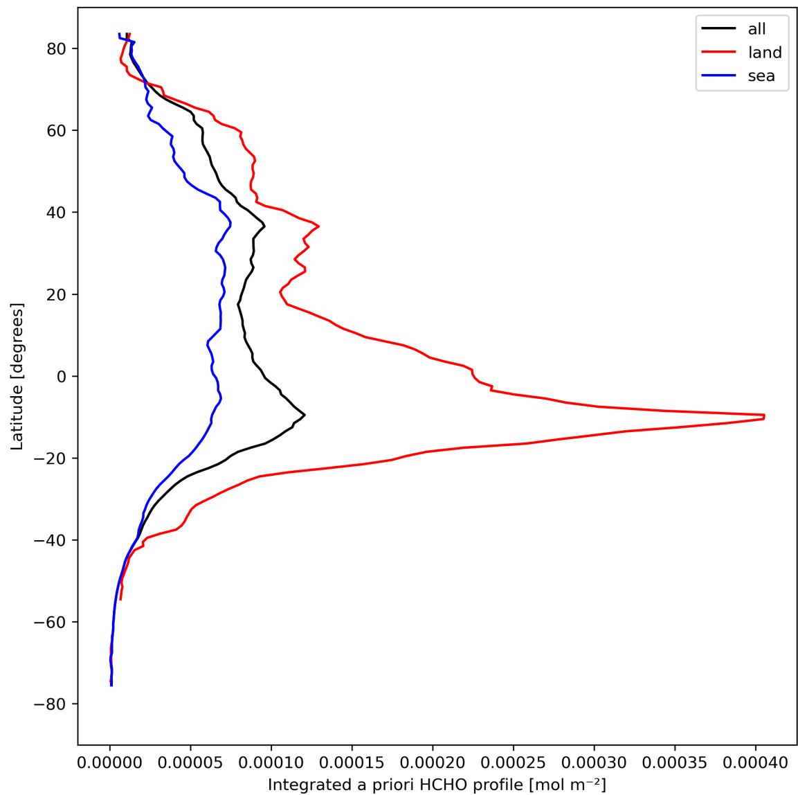
Figure 29: Zonal average of “Integrated a priori HCHO profile” for 2023-08-28 to 2023-08-30.
