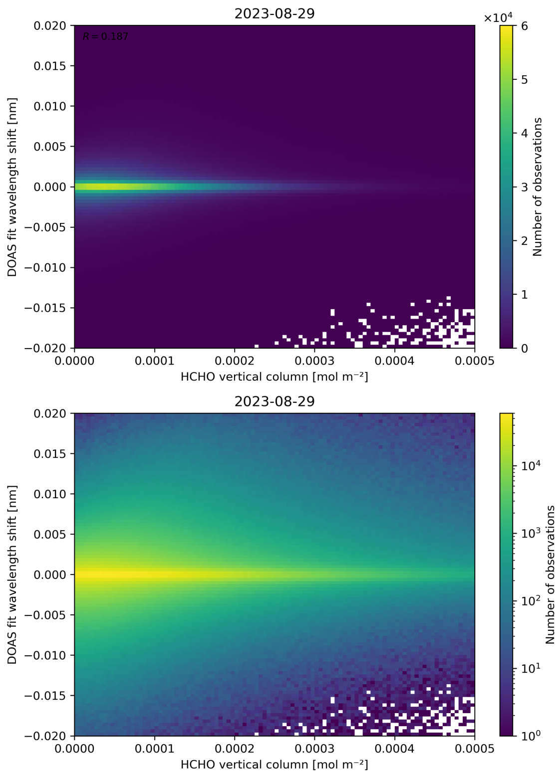
Figure 124: Scatter density plot of “HCHO vertical column” against “DOAS fit wavelength shift” for 2023-08-28 to 2023-08-30.
