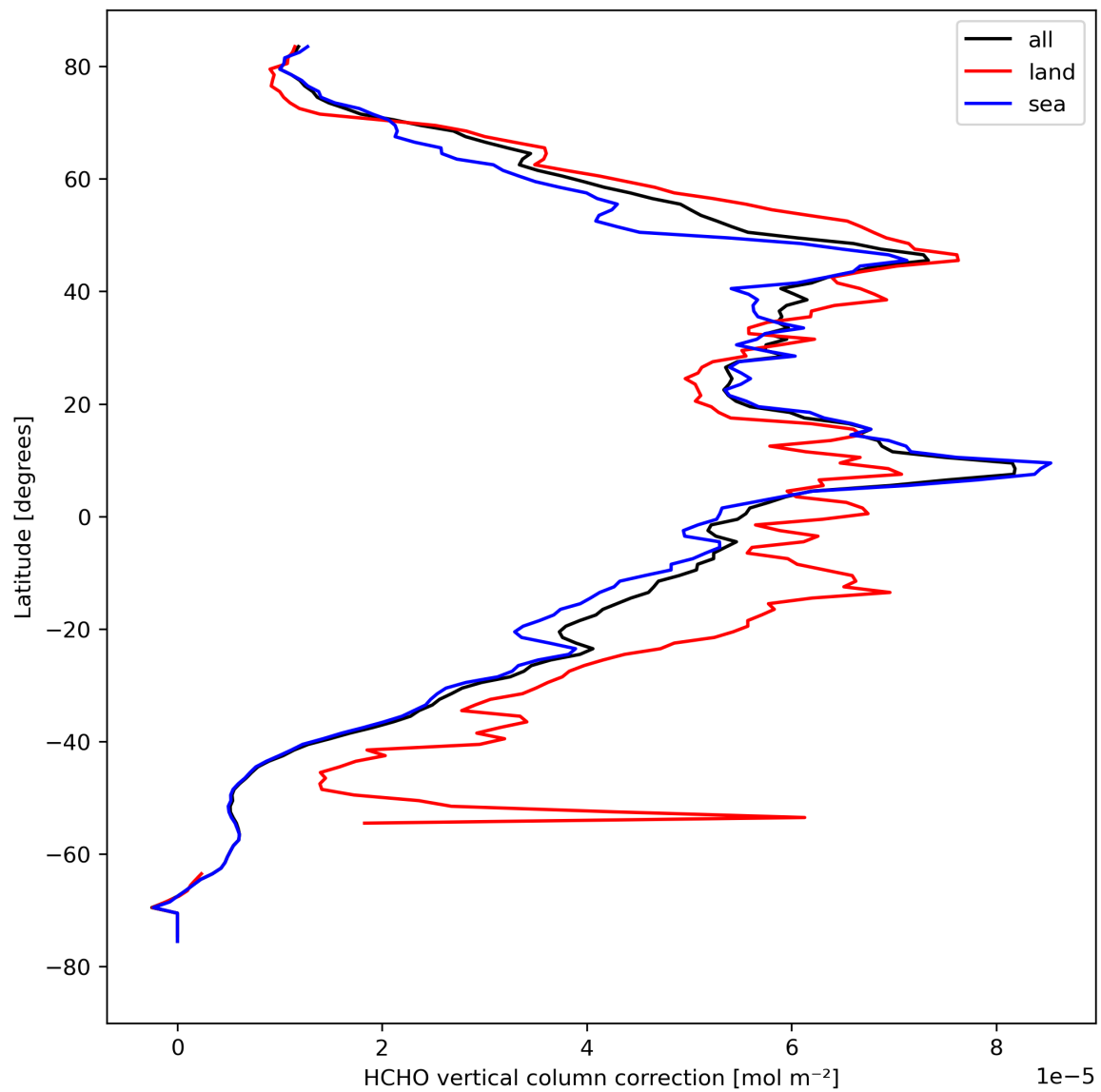
Figure 23: Zonal average of “HCHO vertical column correction” for 2023-08-28 to 2023-08-30.
