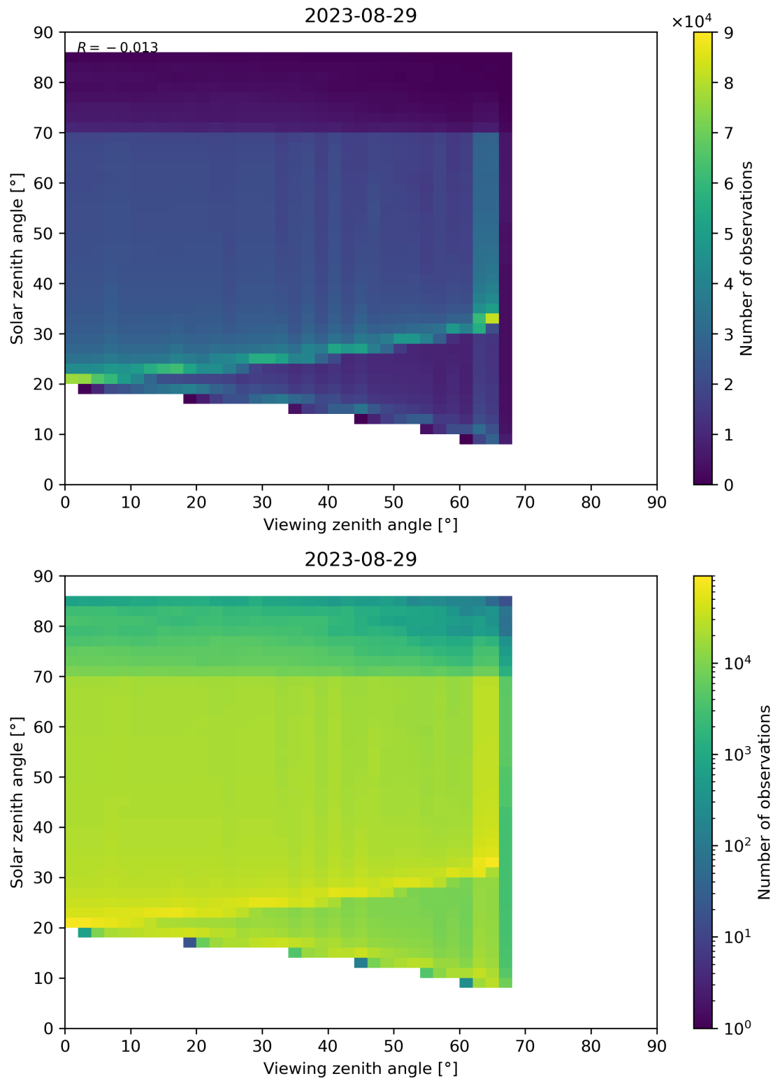
Figure 197: Scatter density plot of “Viewing zenith angle” against “Solar zenith angle” for 2023-08-28 to 2023-08-30.
