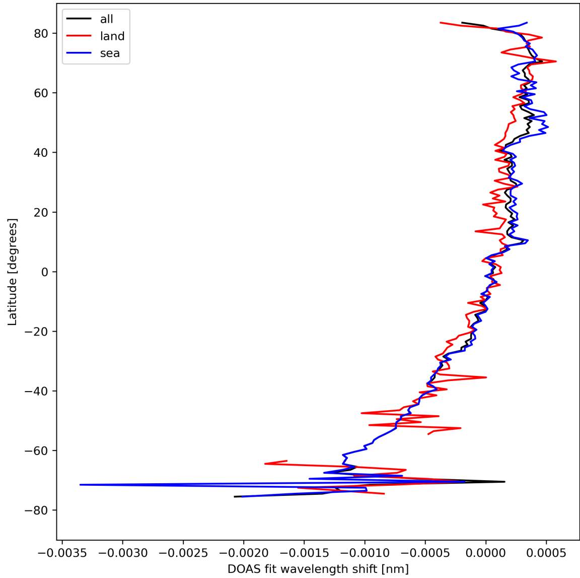
Figure 30: Zonal average of “DOAS fit wavelength shift” for 2023-08-28 to 2023-08-30.
