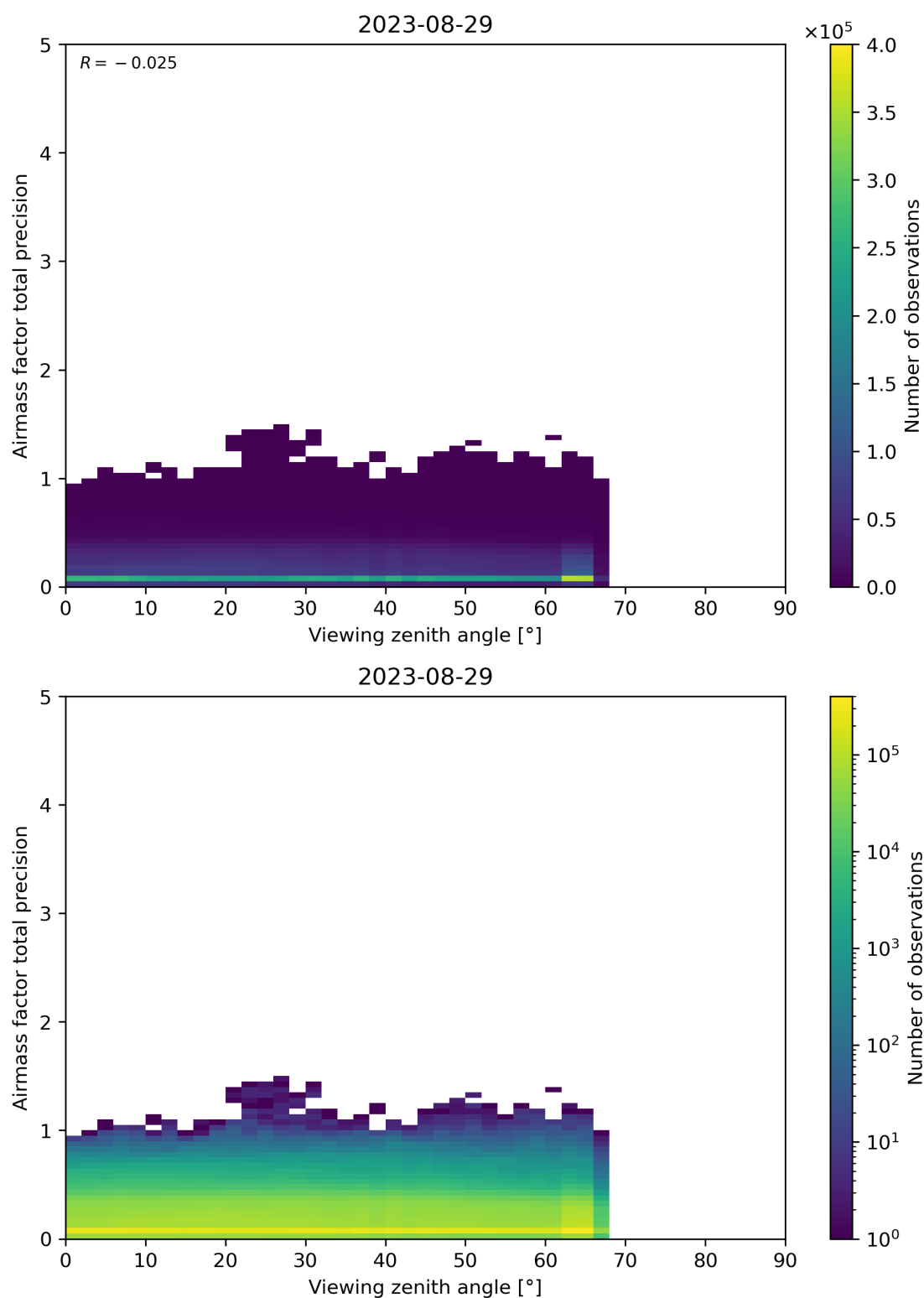
Figure 191: Scatter density plot of “Viewing zenith angle” against “Airmass factor total precision” for 2023-08-28 to 2023-08-30.
