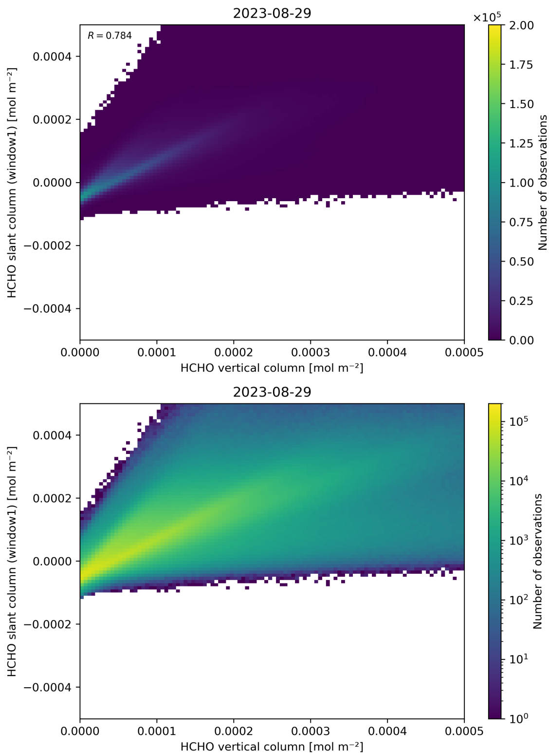
Figure 129: Scatter density plot of “HCHO vertical column” against “HCHO slant column (window1)” for 2023-08-28 to 2023-08-30.
