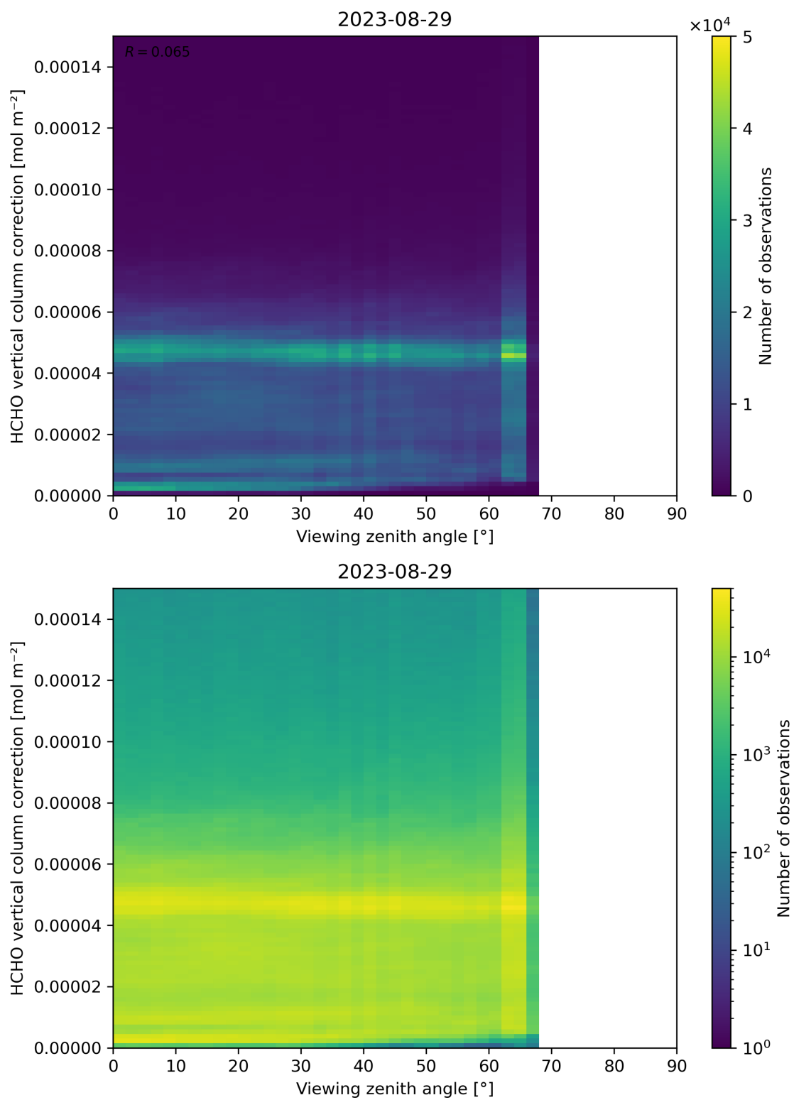
Figure 193: Scatter density plot of “Viewing zenith angle” against “HCHO vertical column correction” for 2023-08-28 to 2023-08-30.
