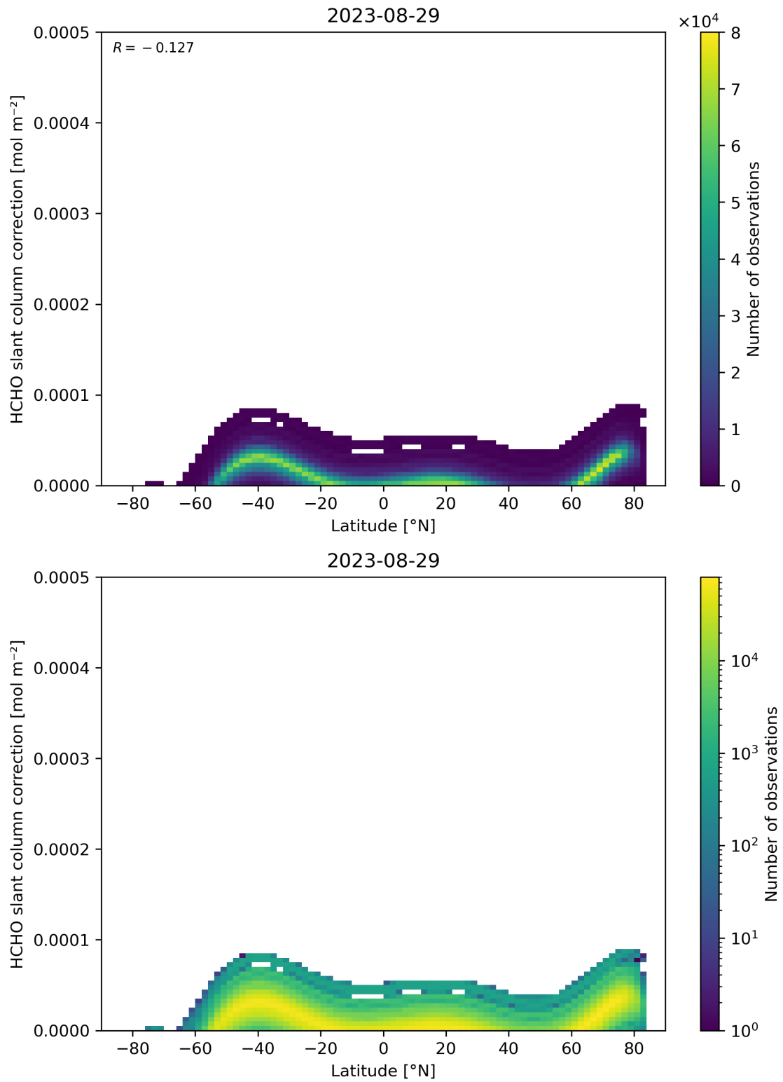
Figure 158: Scatter density plot of “Latitude” against “HCHO slant column correction” for 2023-08-28 to 2023-08-30.
