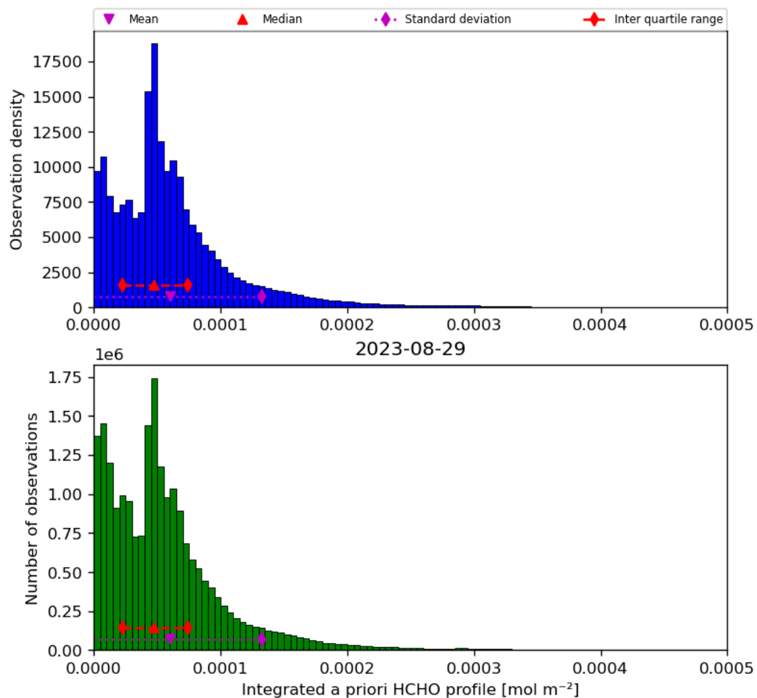
Figure 43: Histogram of “Integrated a priori HCHO profile” for 2023-08-28 to 2023-08-30
