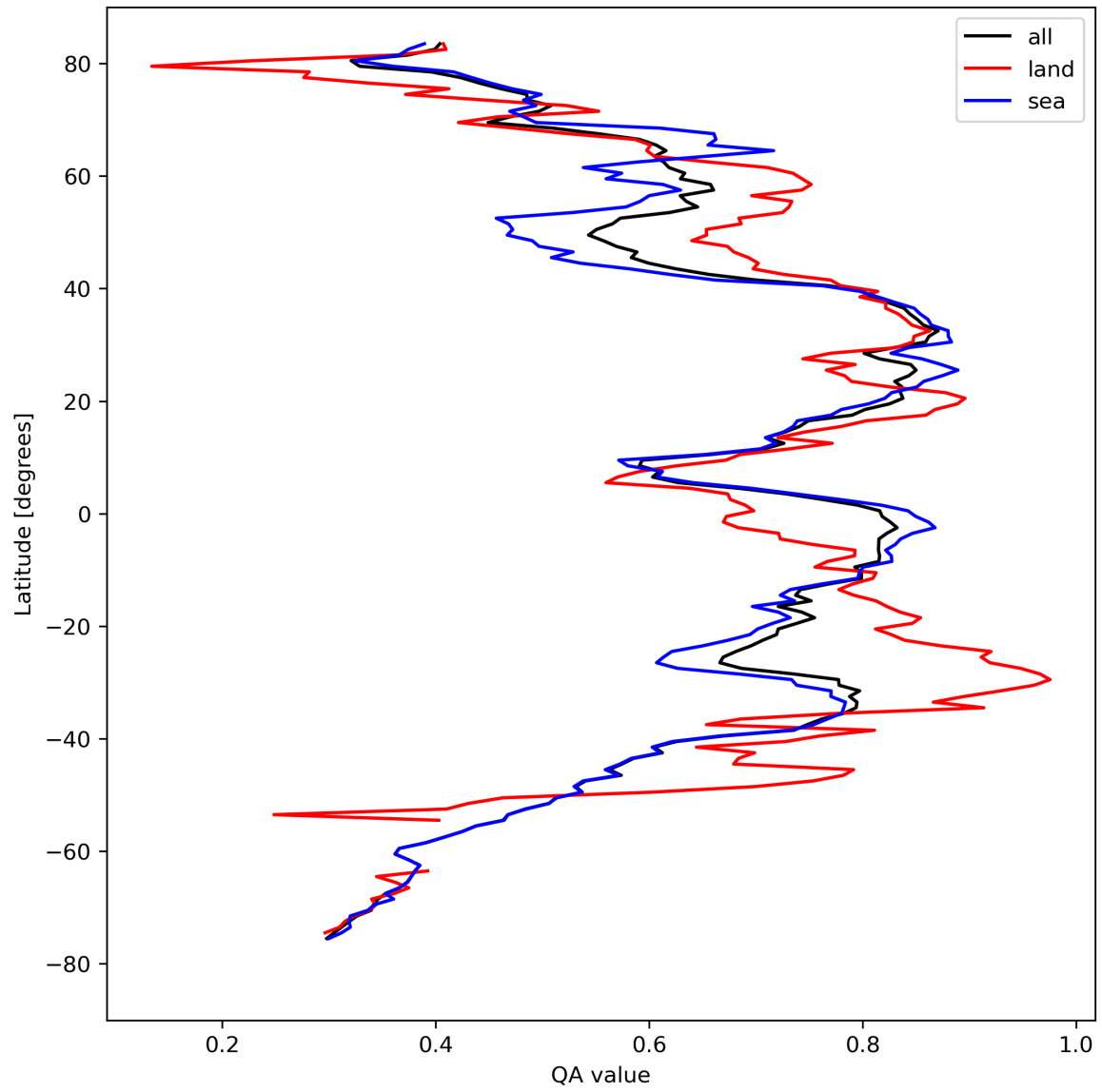
Figure 20: Zonal average of “QA value” for 2023-08-28 to 2023-08-30.
