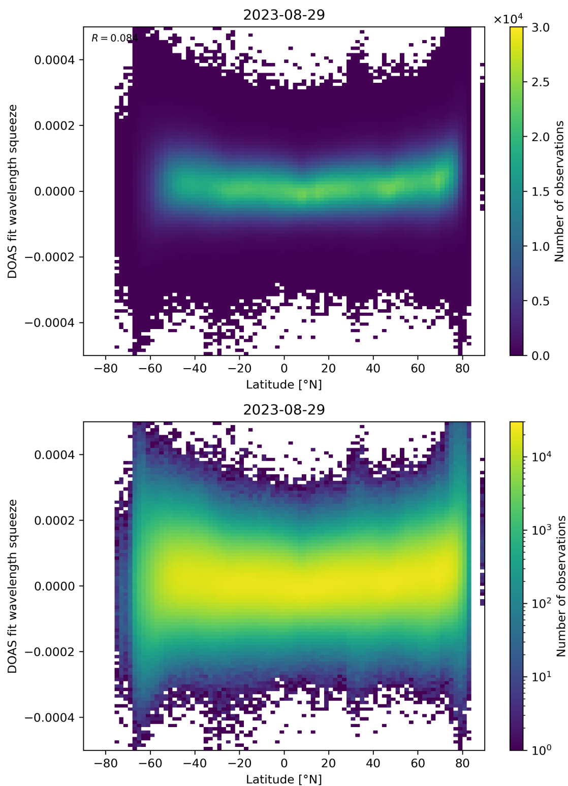
Figure 155: Scatter density plot of “Latitude” against “DOAS fit wavelength squeeze” for 2023-08-28 to 2023-08-30.
