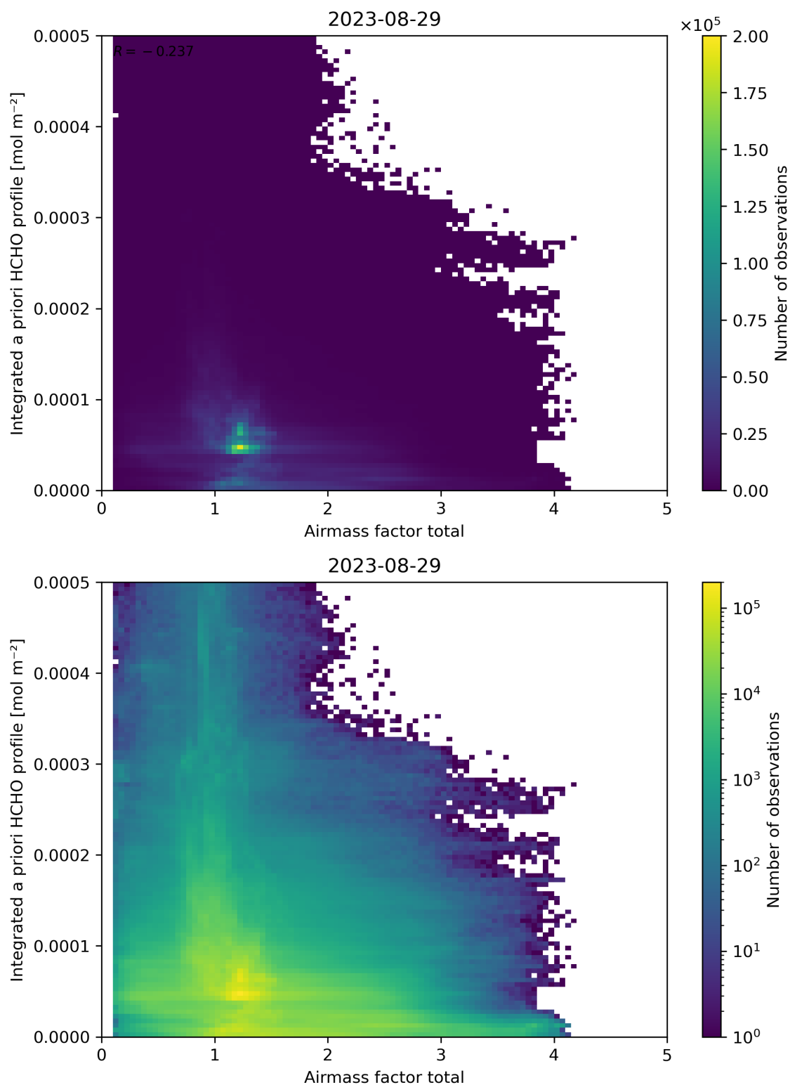
Figure 104: Scatter density plot of “Airmass factor total” against “Integrated a priori HCHO profile” for 2023-08-28 to 2023-08-30.
