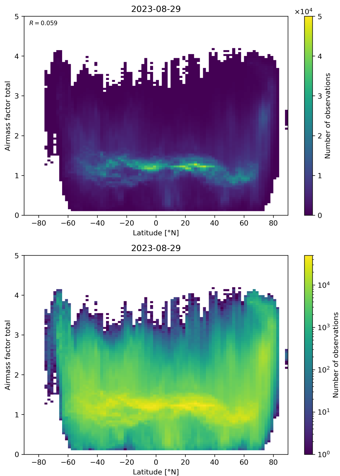
Figure 161: Scatter density plot of “Latitude” against “Airmass factor total” for 2023-08-28 to 2023-08-30.
