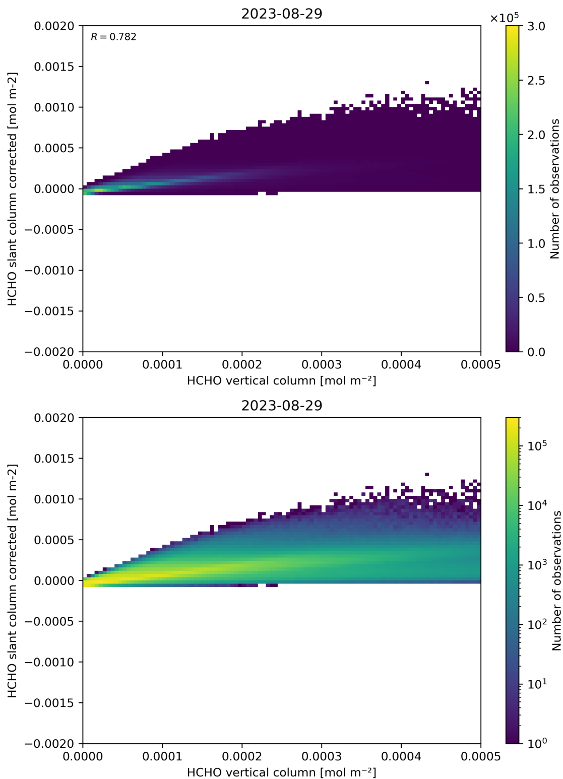
Figure 127: Scatter density plot of “HCHO vertical column” against “HCHO slant column corrected” for 2023-08-28 to 2023-08-30.
