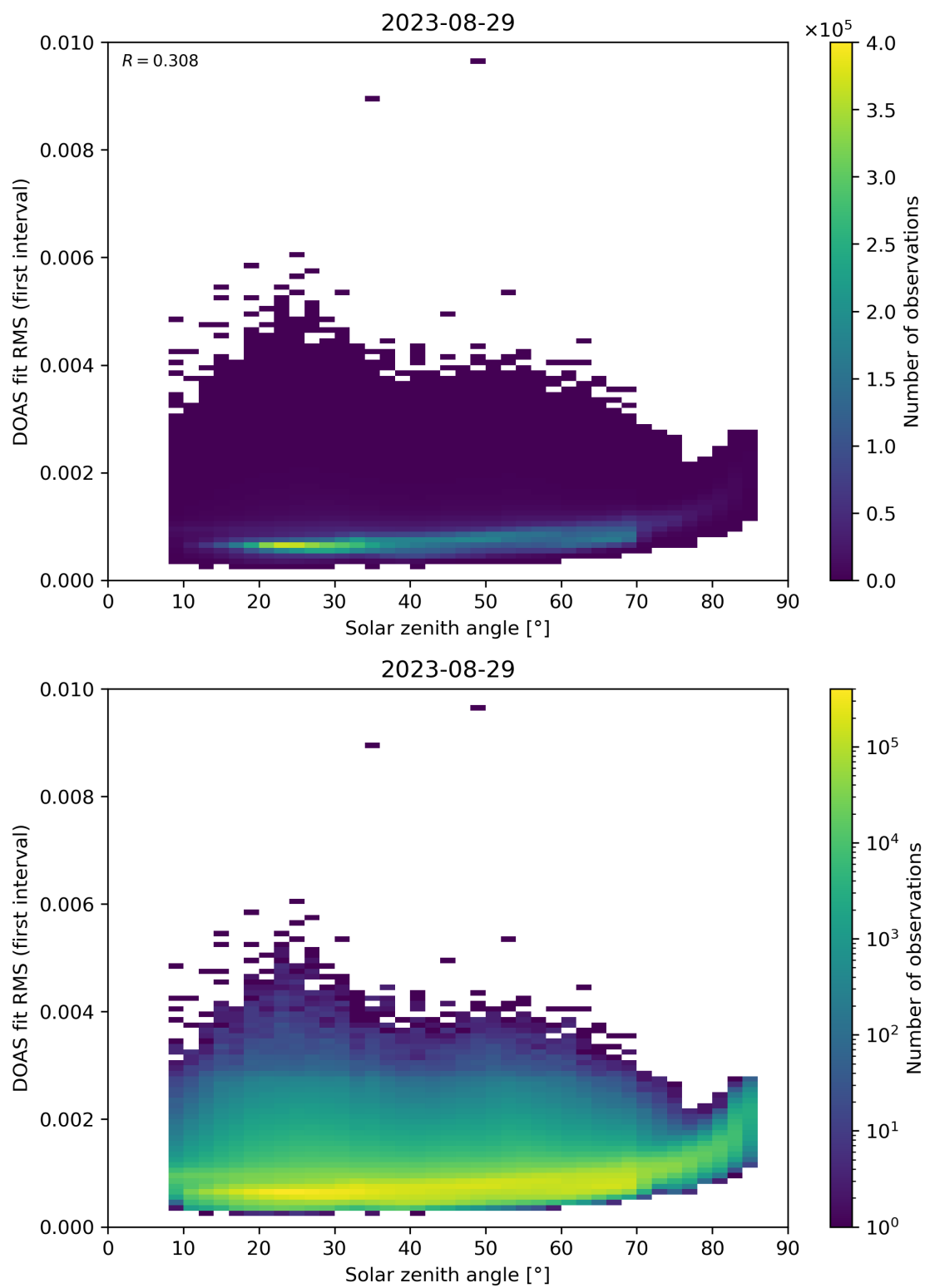
Figure 167: Scatter density plot of “Solar zenith angle” against “DOAS fit RMS (first interval)” for 2023-08-28 to 2023-08-30.
