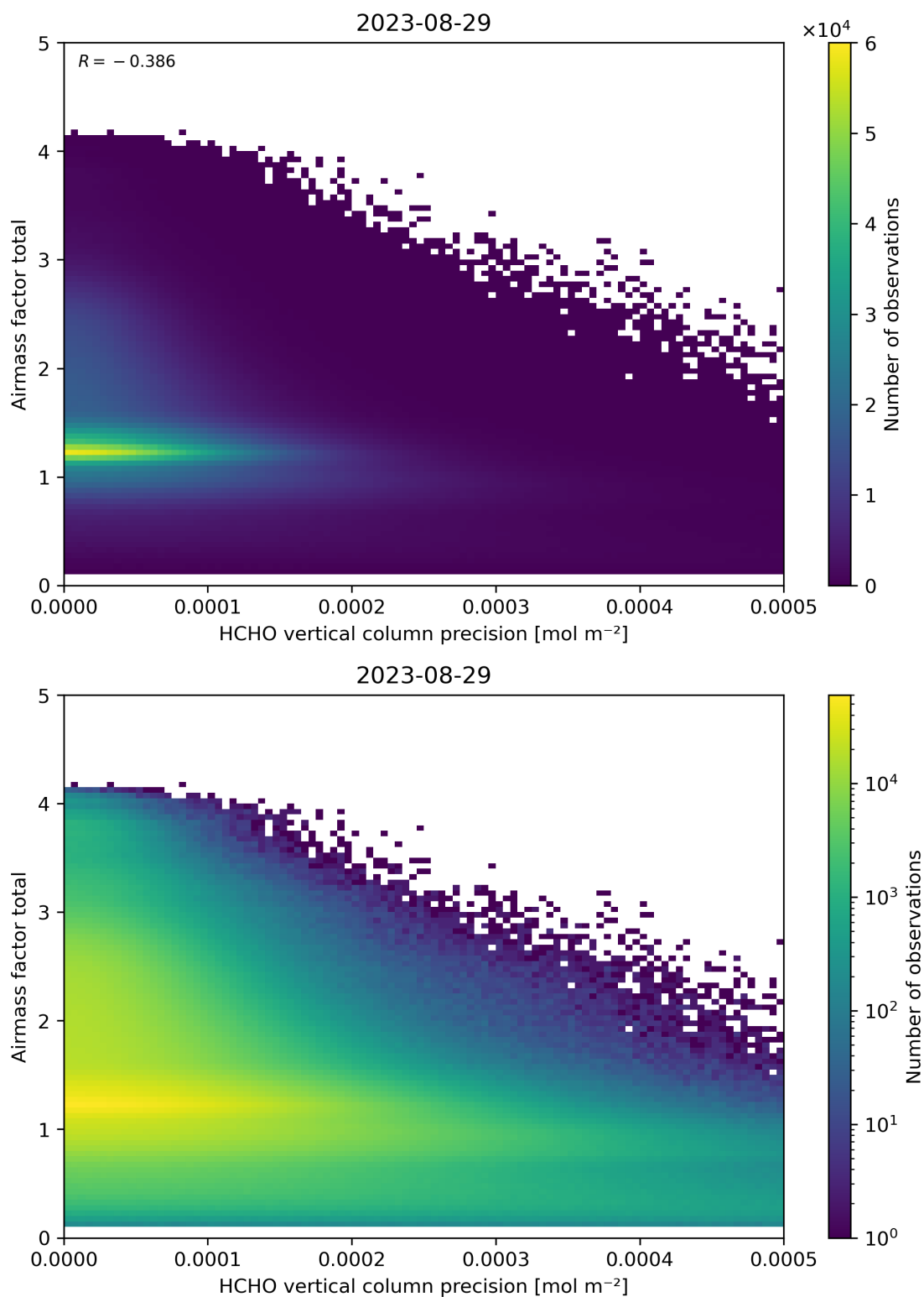
Figure 144: Scatter density plot of “HCHO vertical column precision” against “Airmass factor total” for 2023-08-28 to 2023-08-30.
