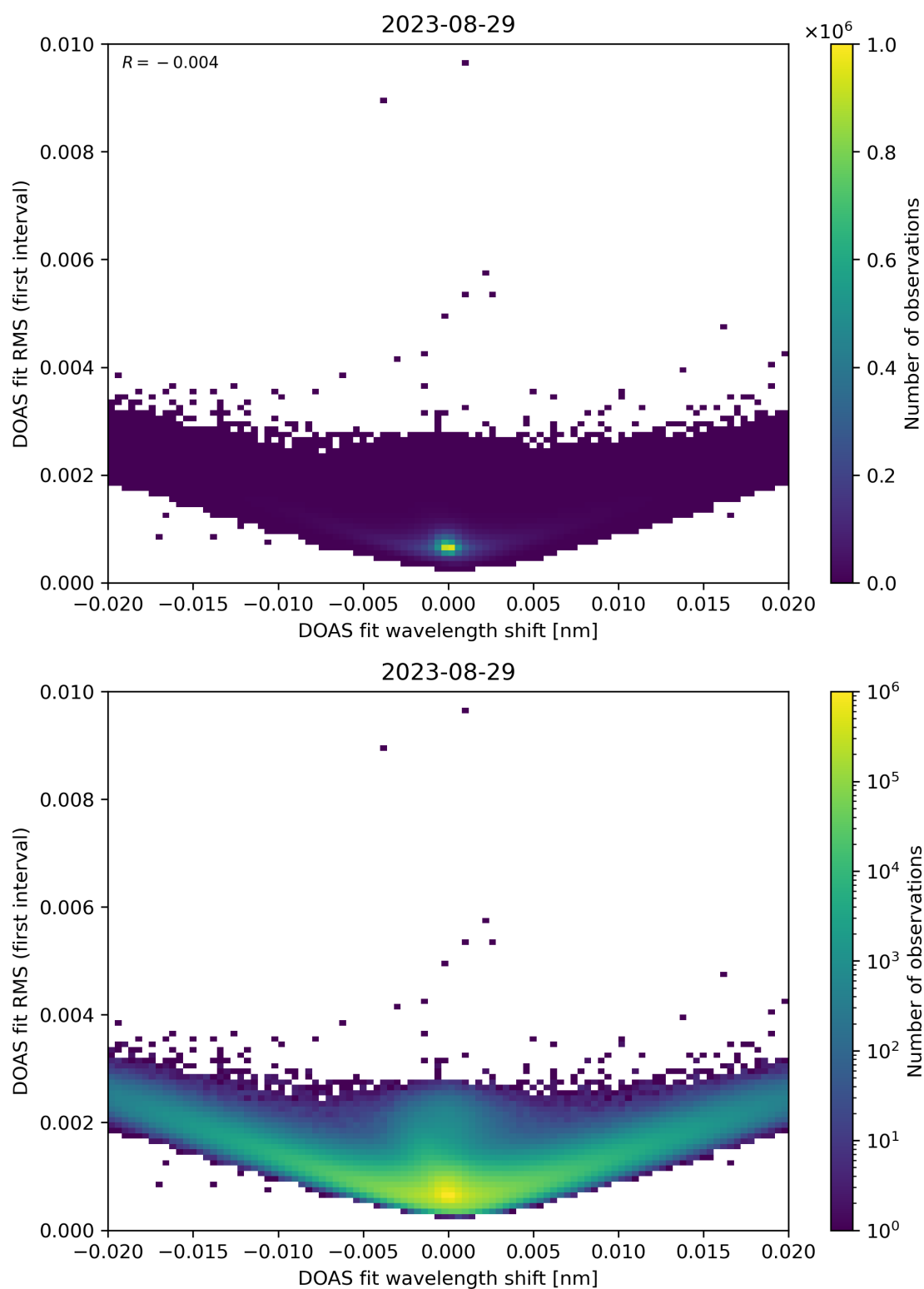
Figure 64: Scatter density plot of “DOAS fit wavelength shift” against “DOAS fit RMS (first interval)” for 2023-08-28 to 2023-08-30.
