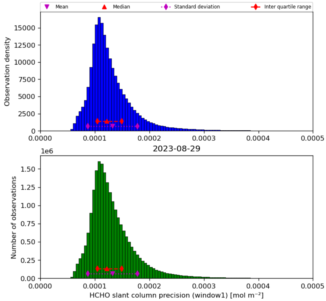
Figure 39: Histogram of “HCHO slant column precision (window1)” for 2023-08-28 to 2023-08-30
