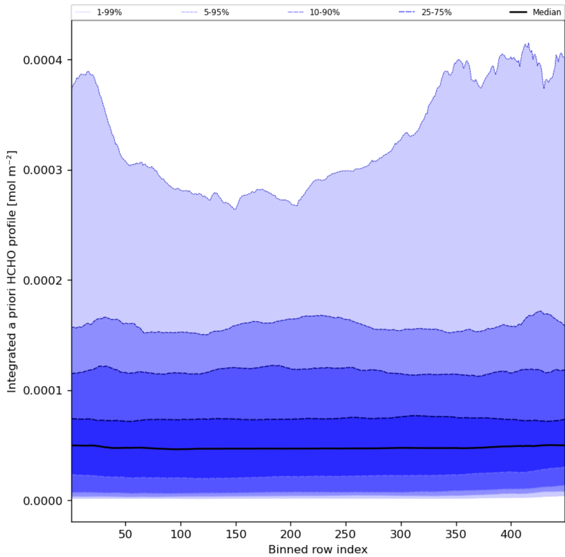
Figure 57: Along track statistics of “Integrated a priori HCHO profile” for 2023-08-28 to 2023-08-30
