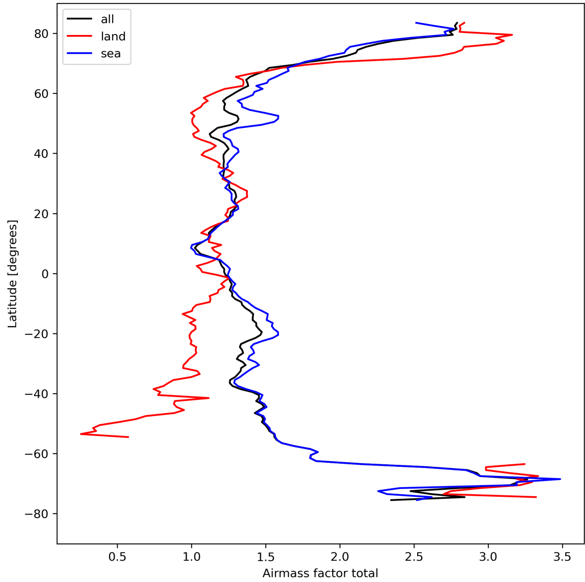
Figure 26: Zonal average of “Airmass factor total” for 2023-08-28 to 2023-08-30.
