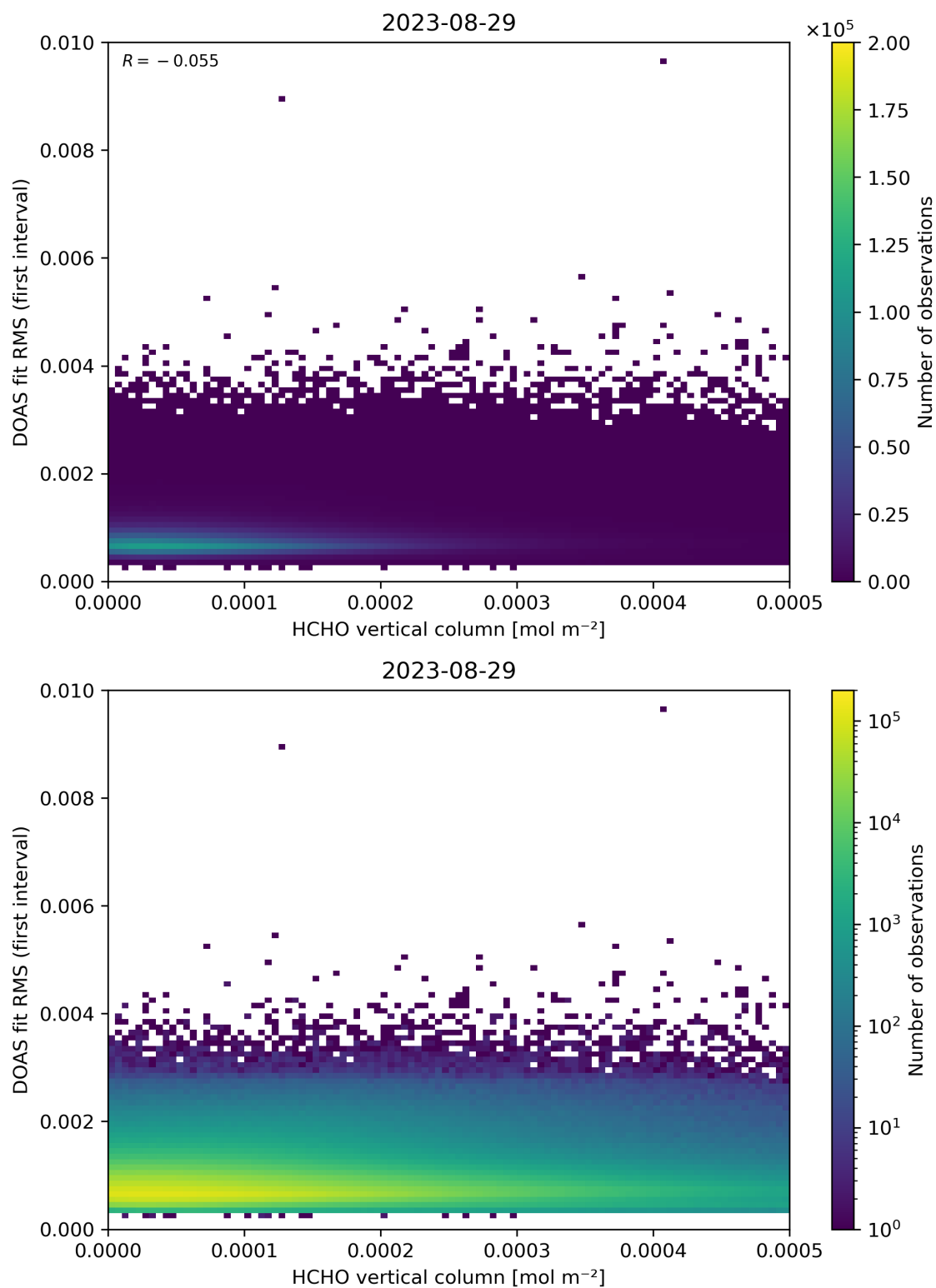
Figure 123: Scatter density plot of “HCHO vertical column” against “DOAS fit RMS (first interval)” for 2023-08-28 to 2023-08-30.
