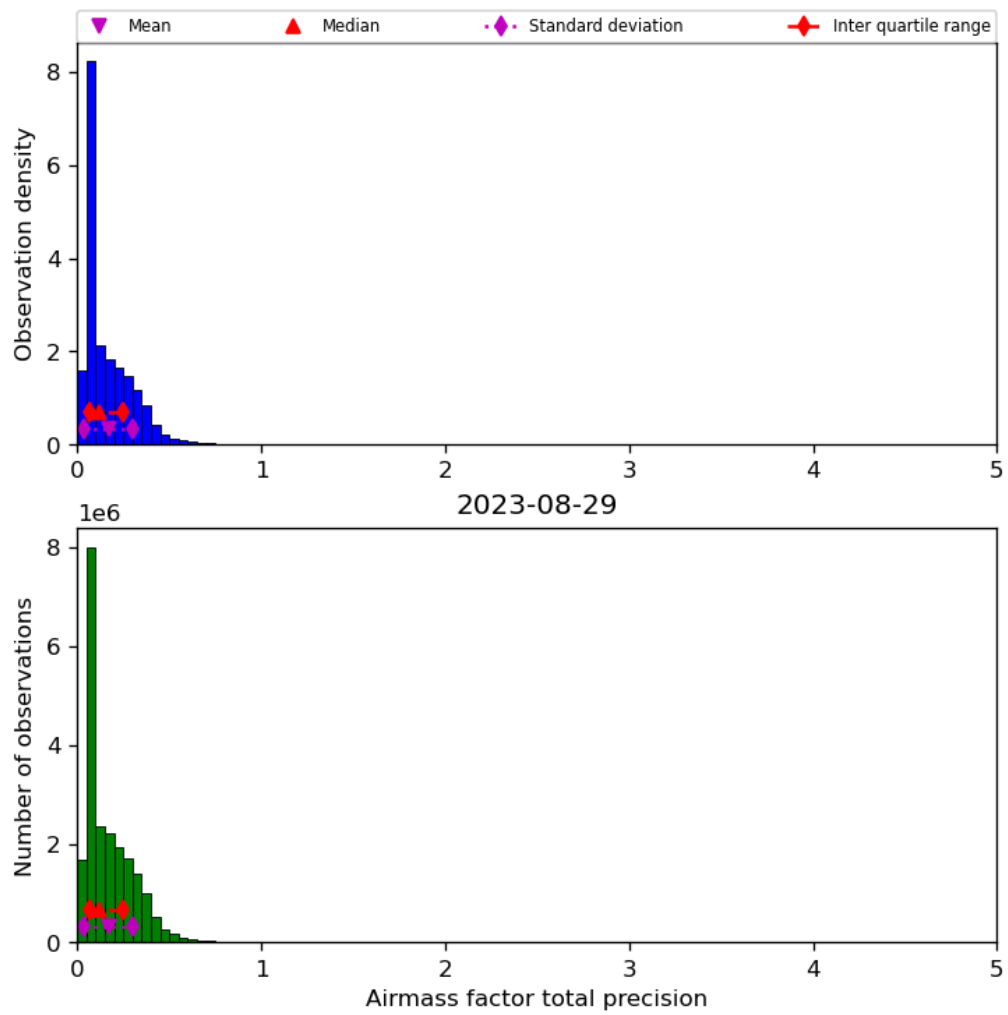
Figure 41: Histogram of “Airmass factor total precision” for 2023-08-28 to 2023-08-30
