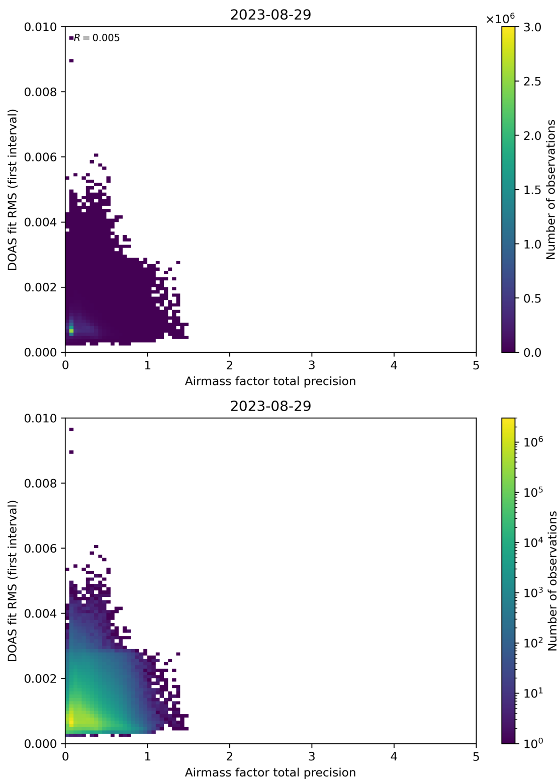
Figure 105: Scatter density plot of “Airmass factor total precision” against “DOAS fit RMS (first interval)” for 2023-08-28 to 2023-08-30.
