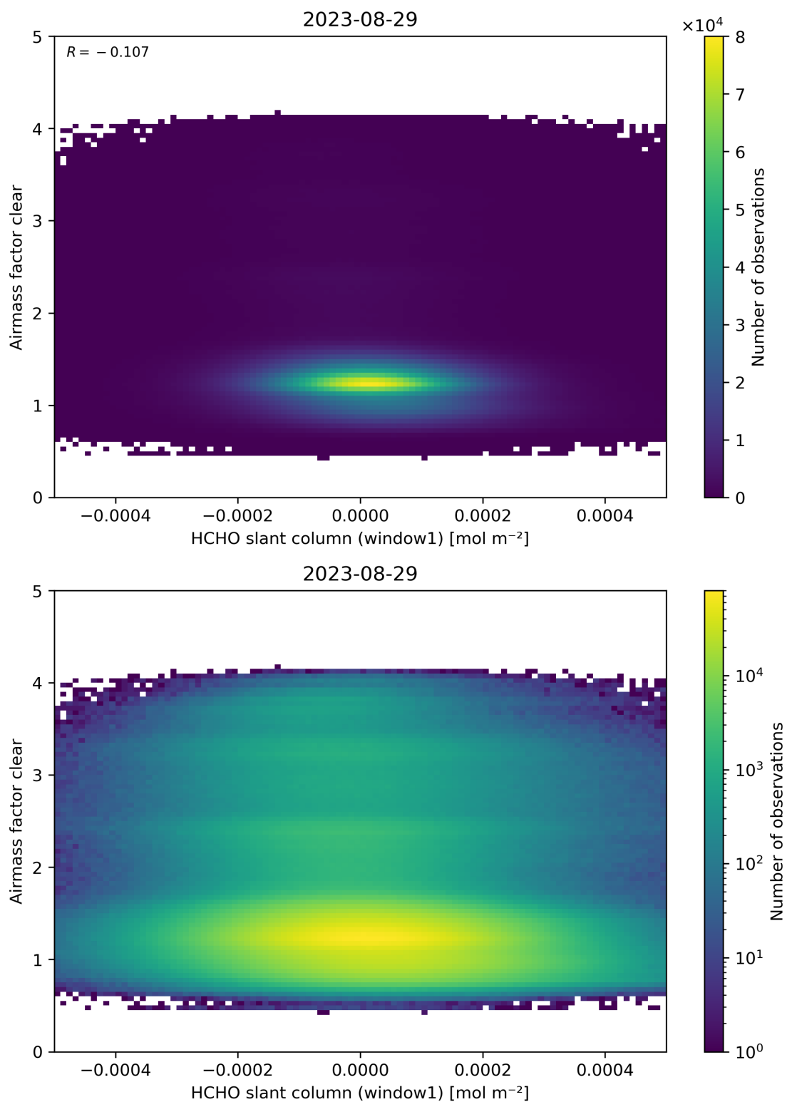
Figure 81: Scatter density plot of “HCHO slant column (window1)” against “Airmass factor clear” for 2023-08-28 to 2023-08-30.
