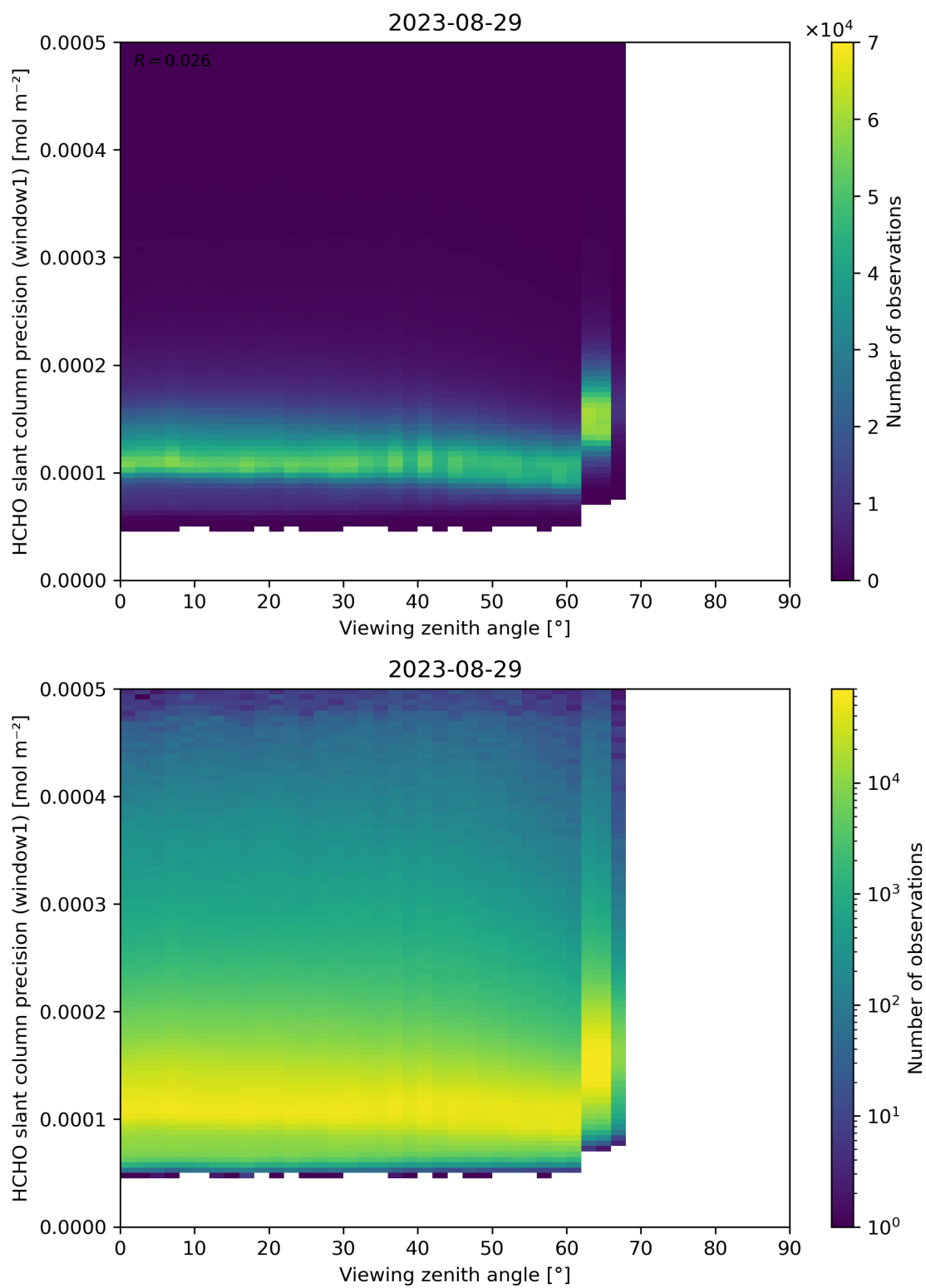
Figure 189: Scatter density plot of “Viewing zenith angle” against “HCHO slant column precision (window1)” for 2023-08-28 to 2023-08-30.
