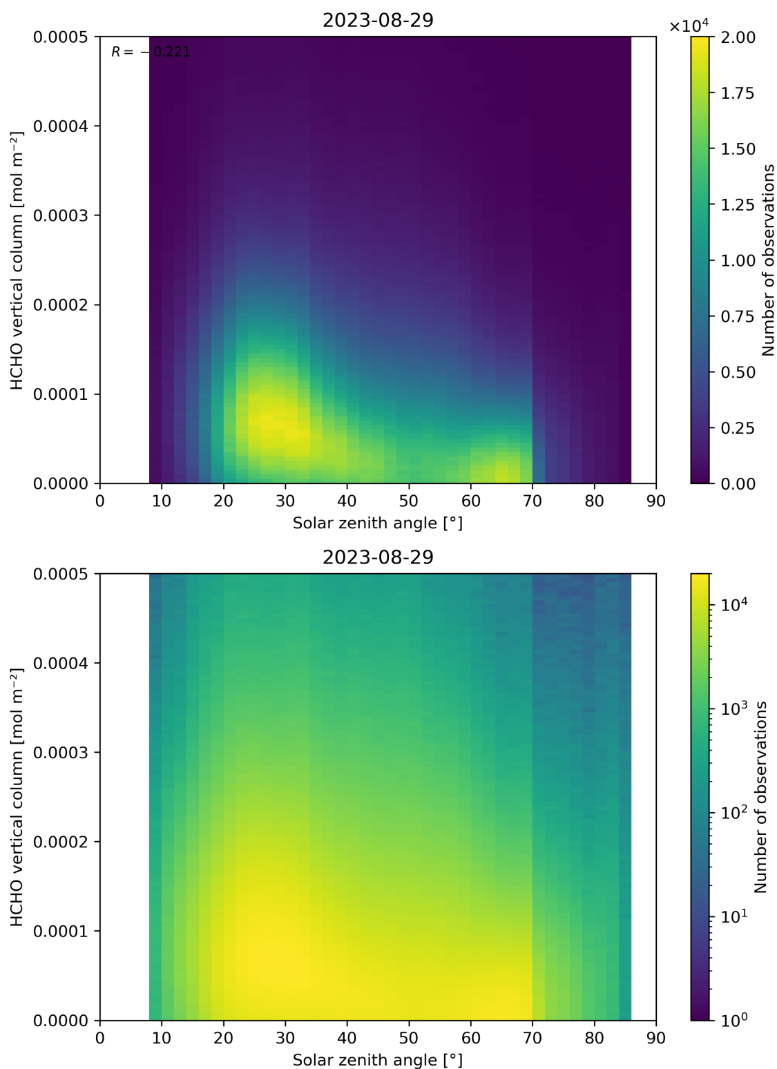
Figure 177: Scatter density plot of “Solar zenith angle” against “HCHO vertical column” for 2023-08-28 to 2023-08-30.
