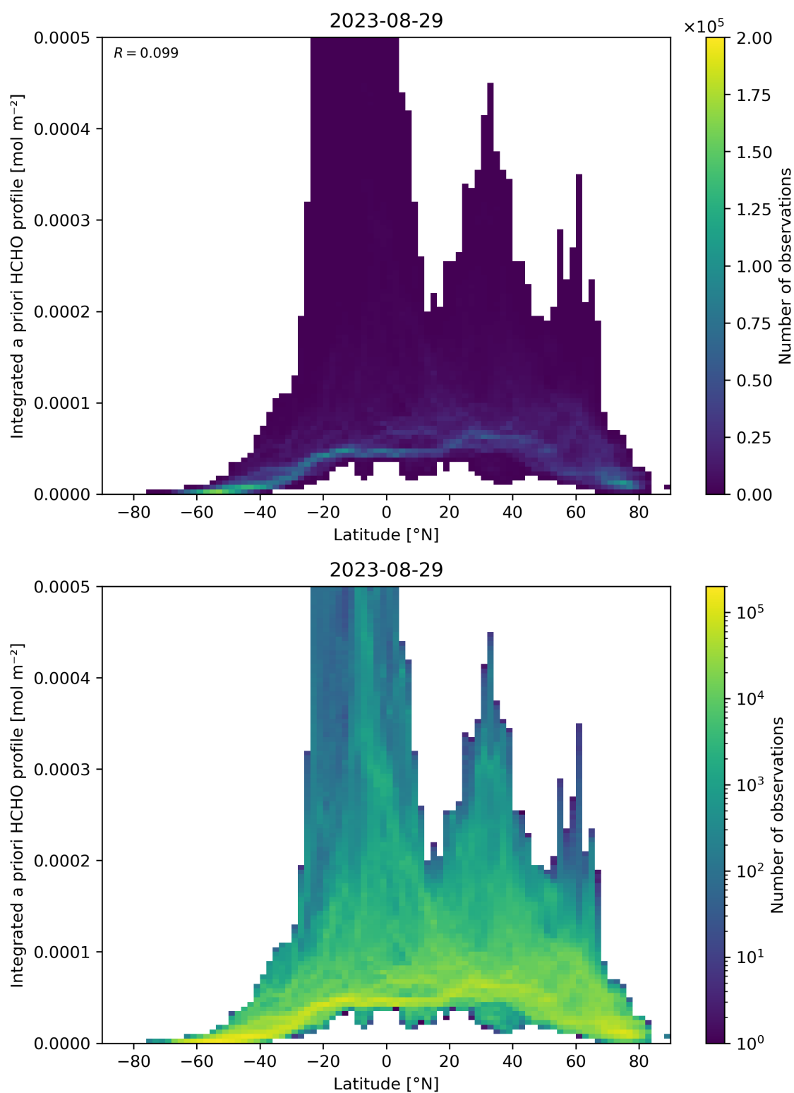
Figure 166: Scatter density plot of “Latitude” against “Integrated a priori HCHO profile” for 2023-08-28 to 2023-08-30.
