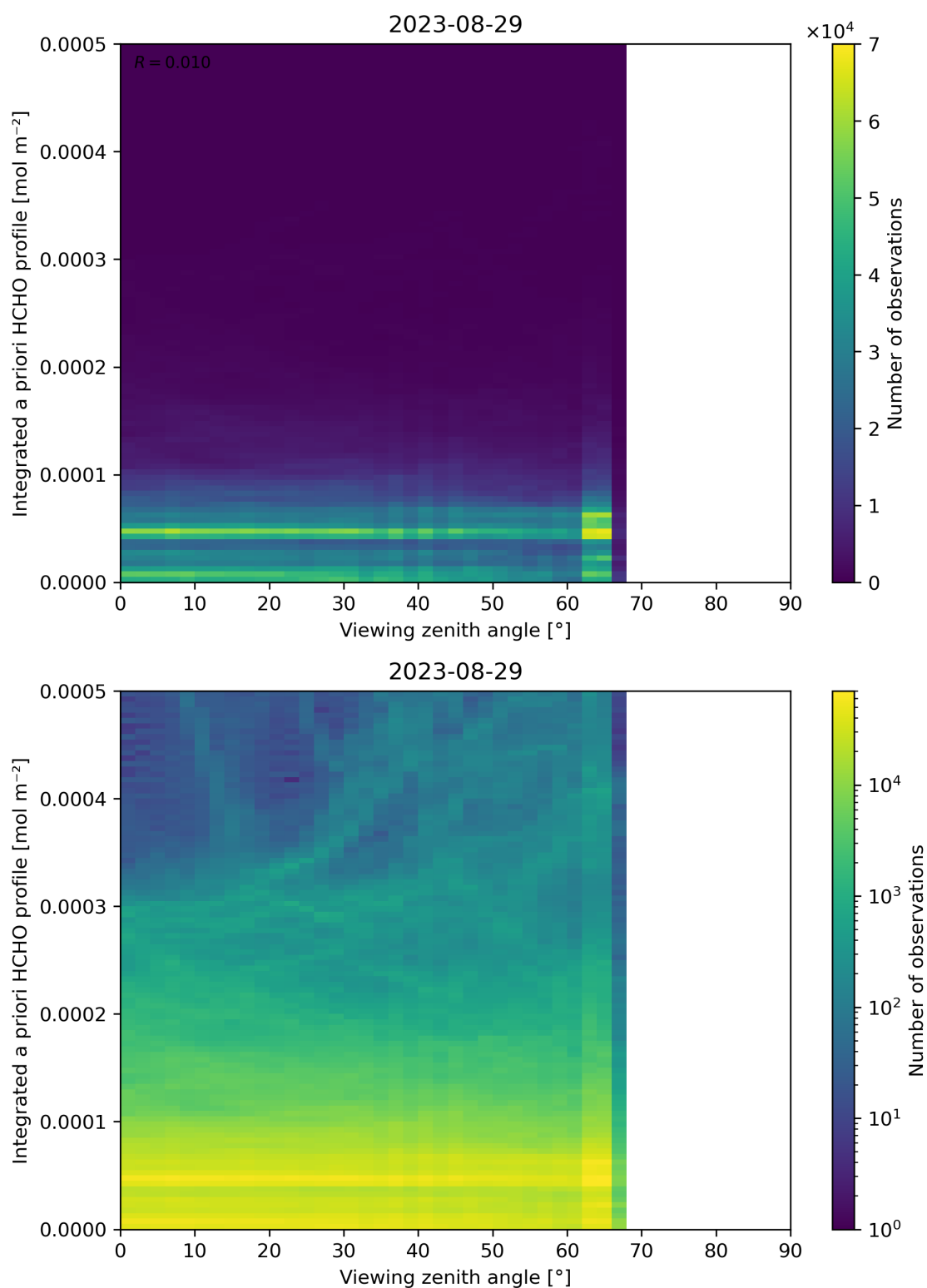
Figure 195: Scatter density plot of “Viewing zenith angle” against “Integrated a priori HCHO profile” for 2023-08-28 to 2023-08-30.
