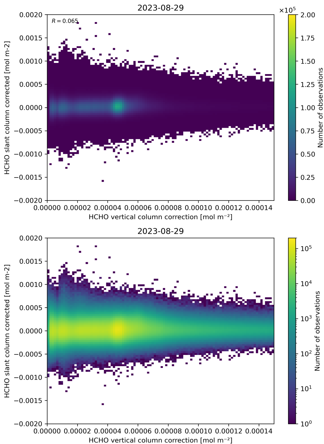
Figure 116: Scatter density plot of “HCHO vertical column correction” against “HCHO slant column corrected” for 2023-08-28 to 2023-08-30.
