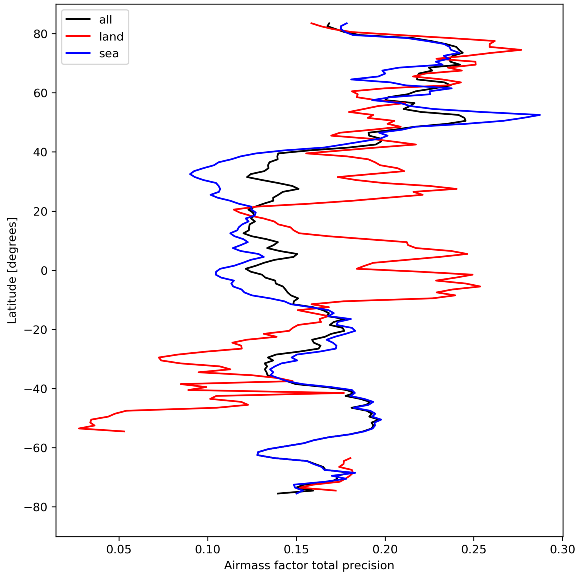
Figure 27: Zonal average of “Airmass factor total precision” for 2023-08-28 to 2023-08-30.
