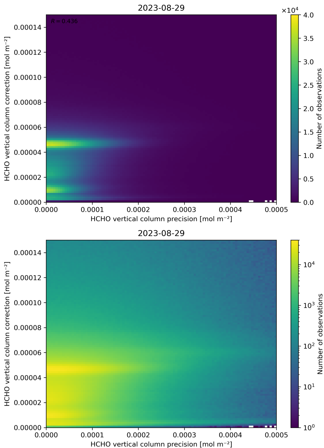
Figure 146: Scatter density plot of “HCHO vertical column precision” against “HCHO vertical column correction” for 2023-08-28 to 2023-08-30.
