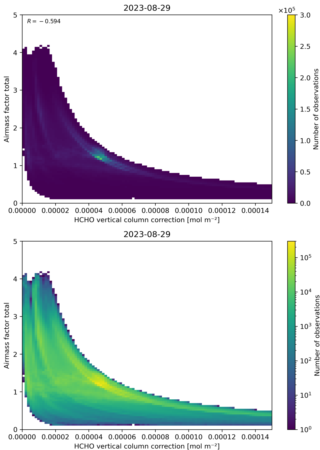
Figure 120: Scatter density plot of “HCHO vertical column correction” against “Airmass factor total” for 2023-08-28 to 2023-08-30.
