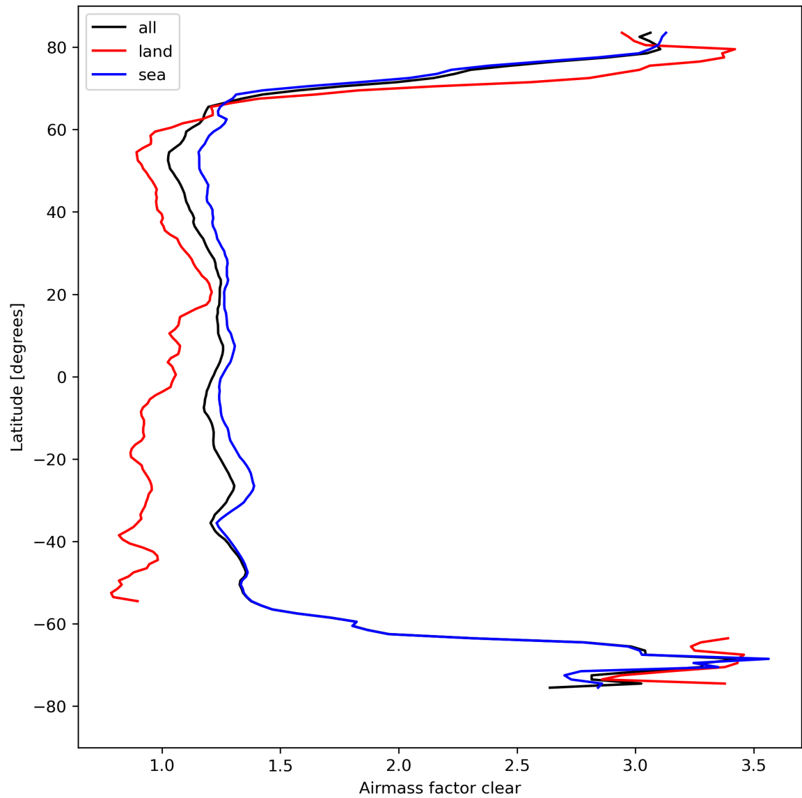
Figure 28: Zonal average of “Airmass factor clear” for 2023-08-28 to 2023-08-30.
