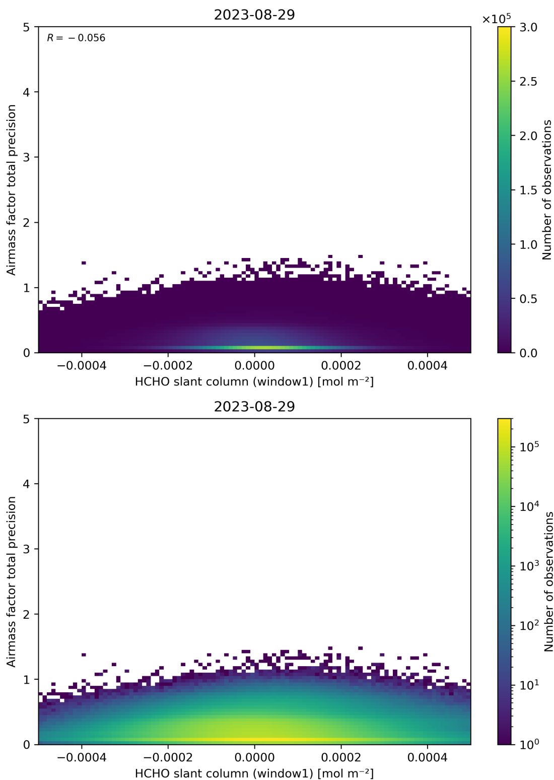
Figure 86: Scatter density plot of “HCHO slant column (window1)” against “Airmass factor total precision” for 2023-08-28 to 2023-08-30.
