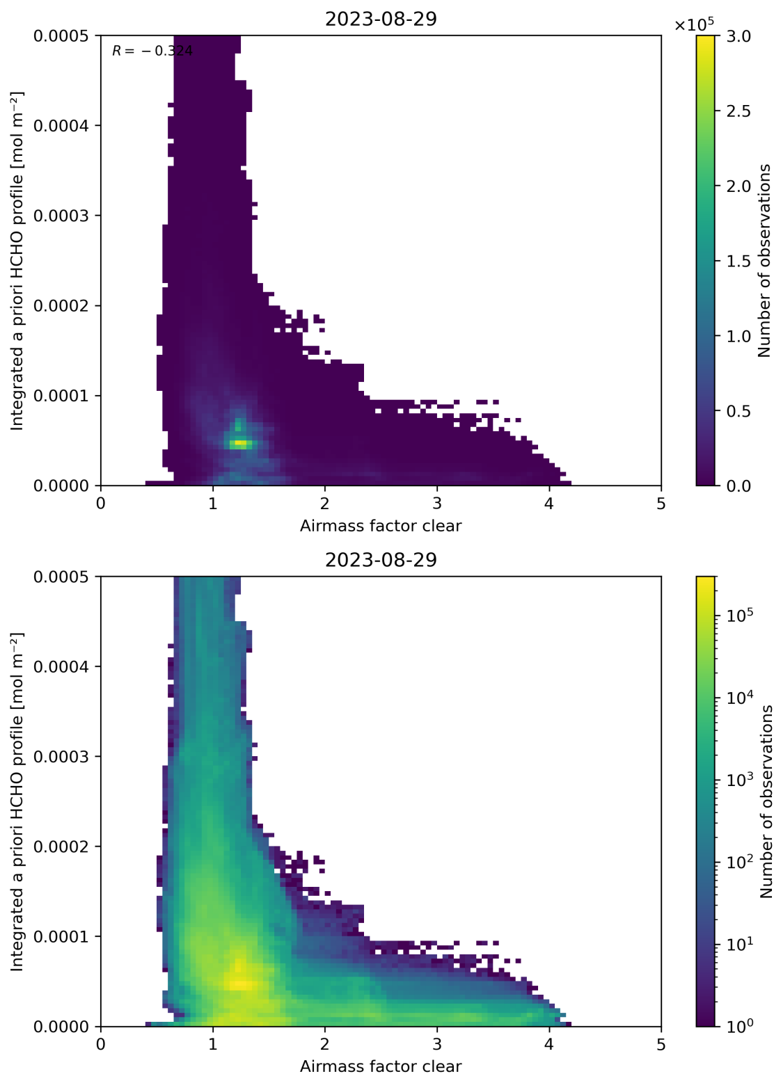
Figure 76: Scatter density plot of “Airmass factor clear” against “Integrated a priori HCHO profile” for 2023-08-28 to 2023-08-30.
