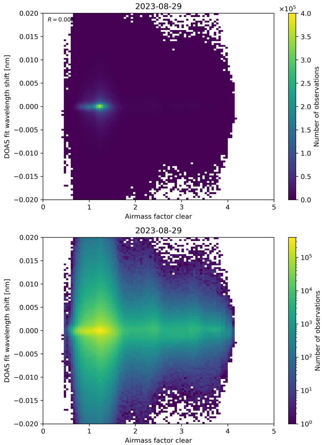
Figure 72: Scatter density plot of “Airmass factor clear” against “DOAS fit wavelength shift” for 2023-08-28 to 2023-08-30.
