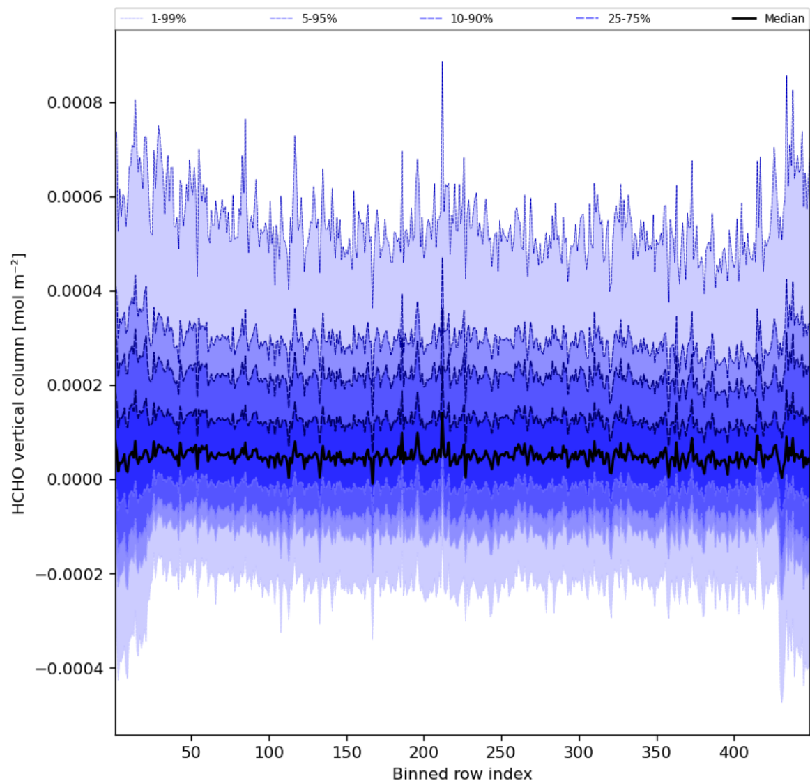
Figure 49: Along track statistics of “HCHO vertical column” for 2023-08-28 to 2023-08-30
