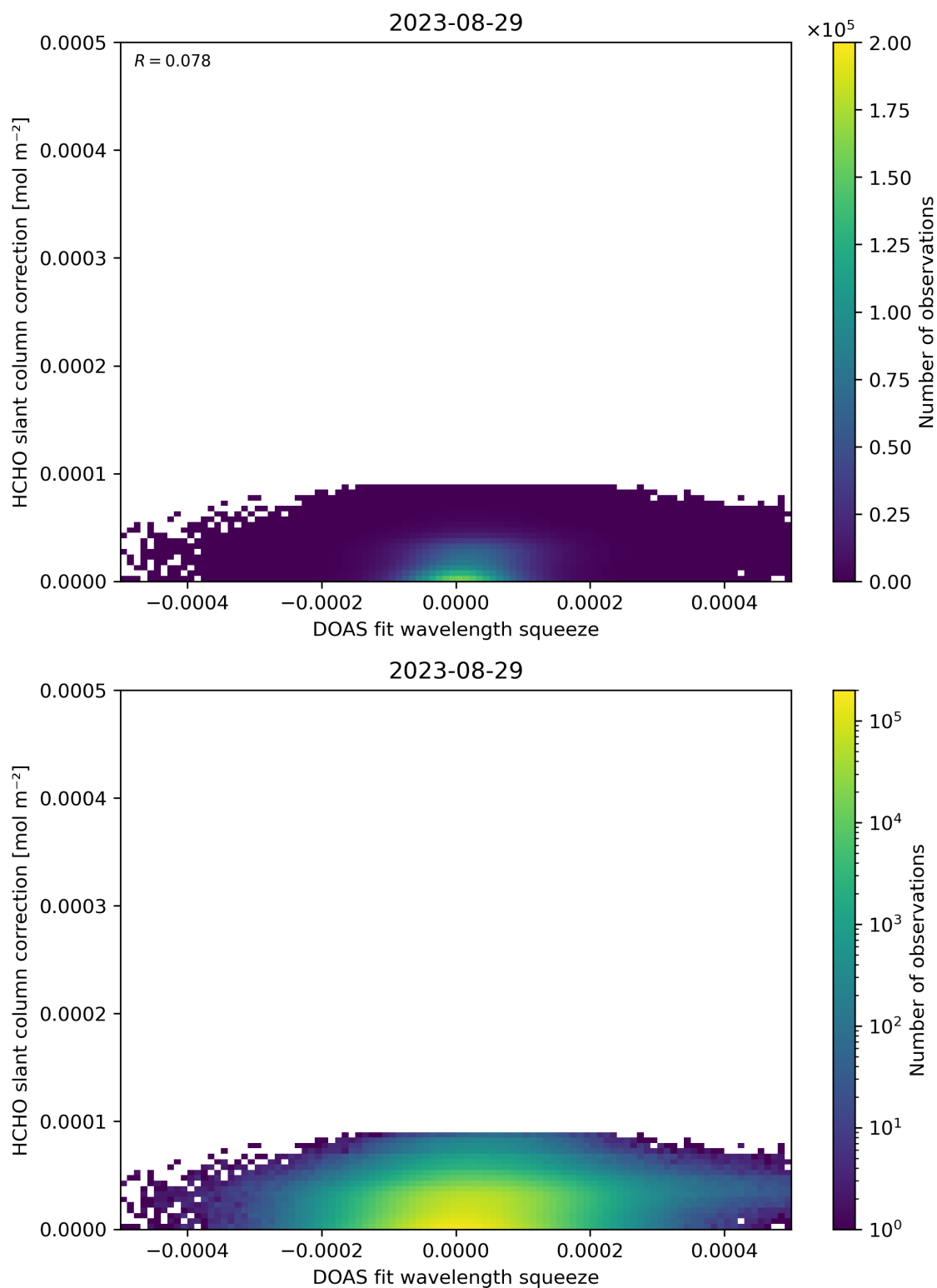
Figure 70: Scatter density plot of “DOAS fit wavelength squeeze” against “HCHO slant column correction” for 2023-08-28 to 2023-08-30.
