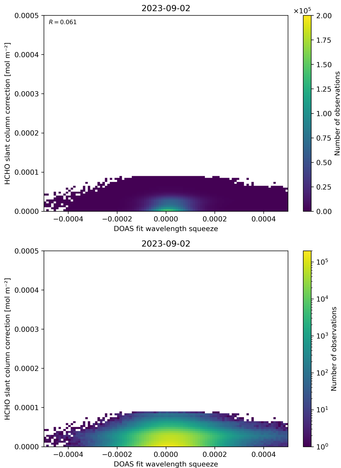
Figure 70: Scatter density plot of “DOAS fit wavelength squeeze” against “HCHO slant column correction” for 2023-09-01 to 2023-09-03.
