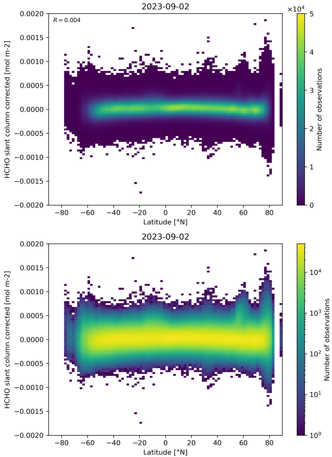
Figure 157: Scatter density plot of “Latitude” against “HCHO slant column corrected” for 2023-09-01 to 2023-09-03.
