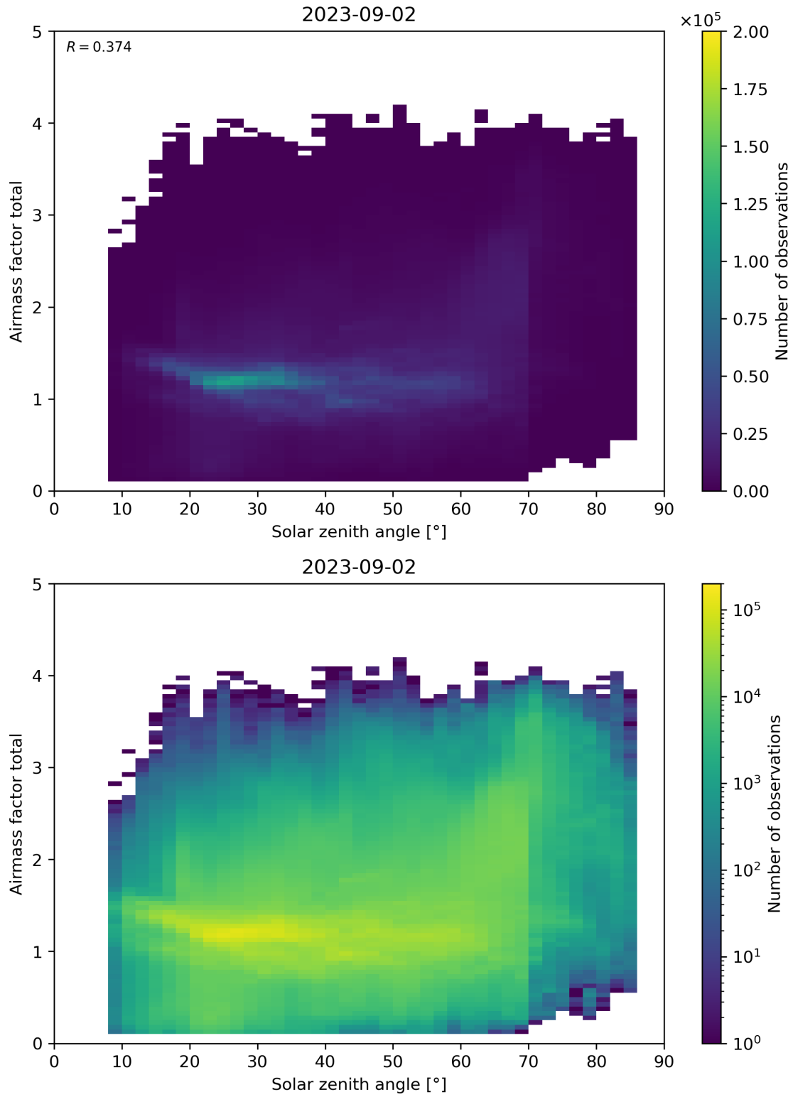
Figure 175: Scatter density plot of “Solar zenith angle” against “Airmass factor total” for 2023-09-01 to 2023-09-03.
