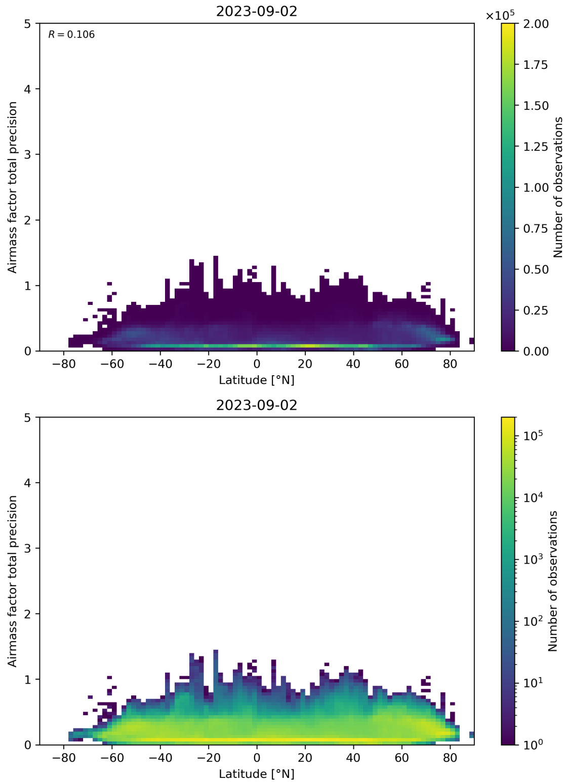
Figure 162: Scatter density plot of “Latitude” against “Airmass factor total precision” for 2023-09-01 to 2023-09-03.
