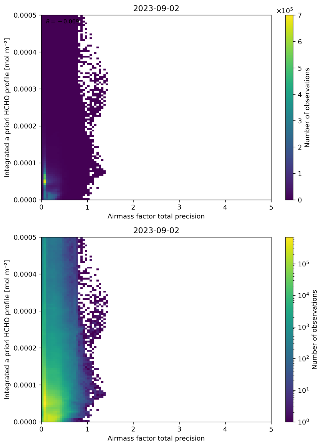
Figure 111: Scatter density plot of “Airmass factor total precision” against “Integrated a priori HCHO profile” for 2023-09-01 to 2023-09-03.
