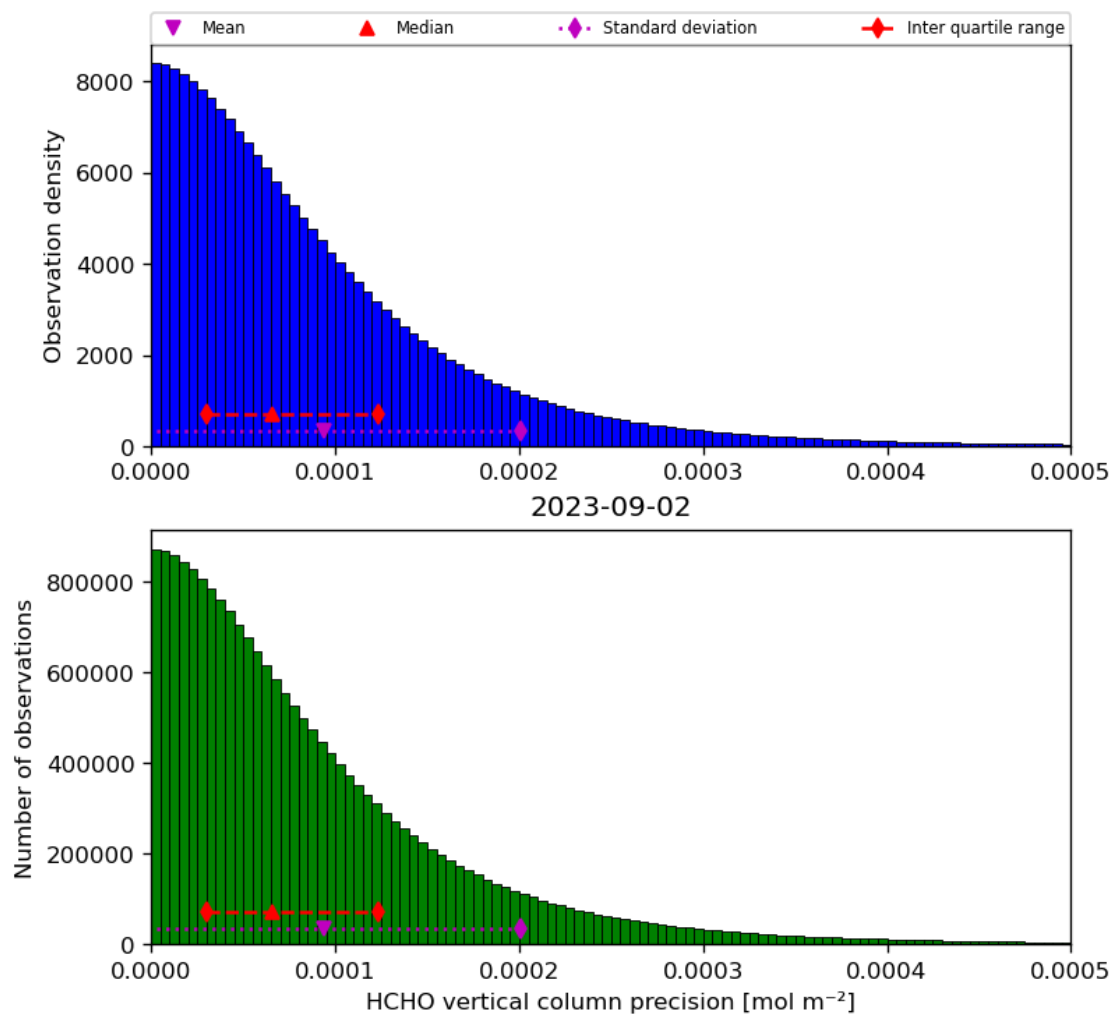
Figure 36: Histogram of “HCHO vertical column precision” for 2023-09-01 to 2023-09-03
