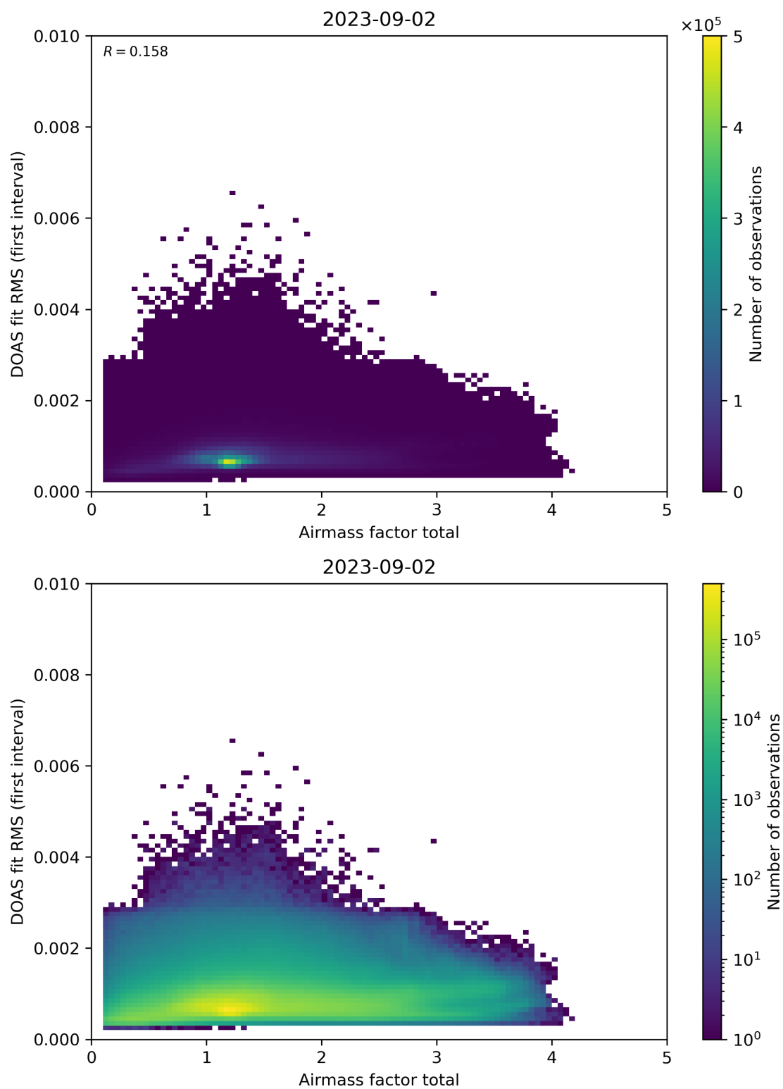
Figure 97: Scatter density plot of “Airmass factor total” against “DOAS fit RMS (first interval)” for 2023-09-01 to 2023-09-03.
