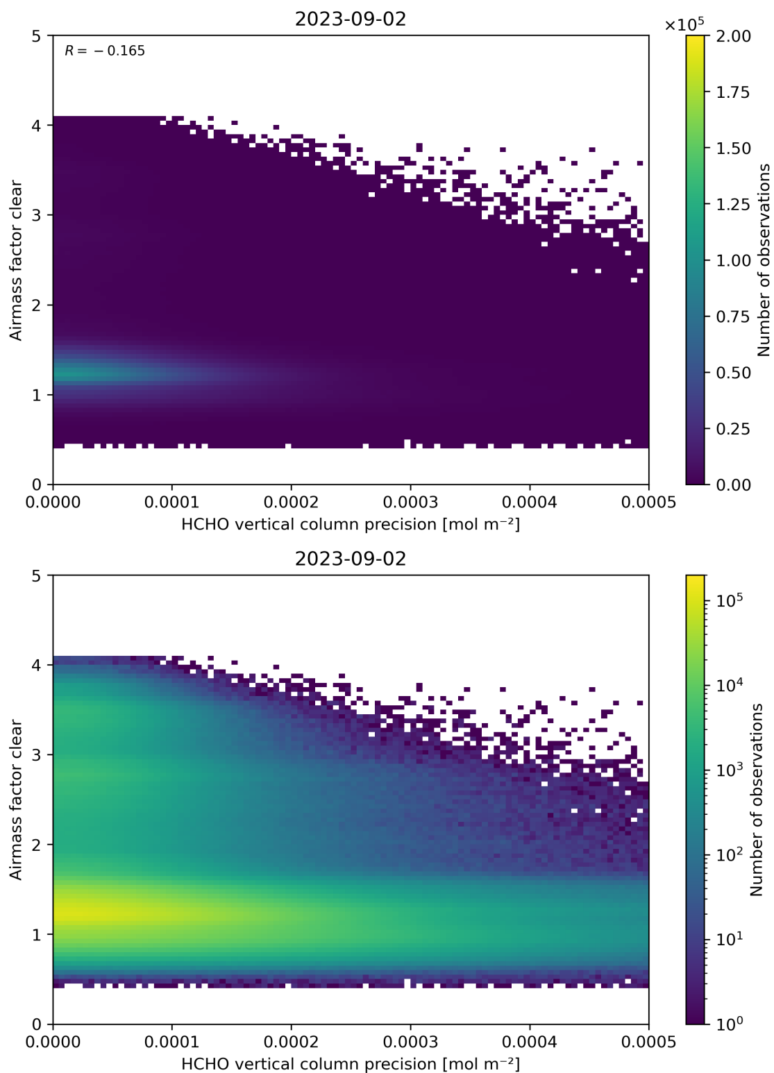
Figure 139: Scatter density plot of “HCHO vertical column precision” against “Airmass factor clear” for 2023-09-01 to 2023-09-03.
