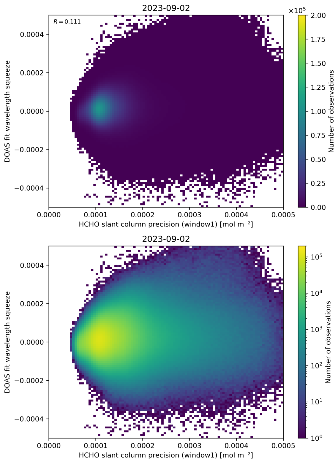
Figure 90: Scatter density plot of “HCHO slant column precision (window1)” against “DOAS fit wavelength squeeze” for 2023-09-01 to 2023-09-03.
