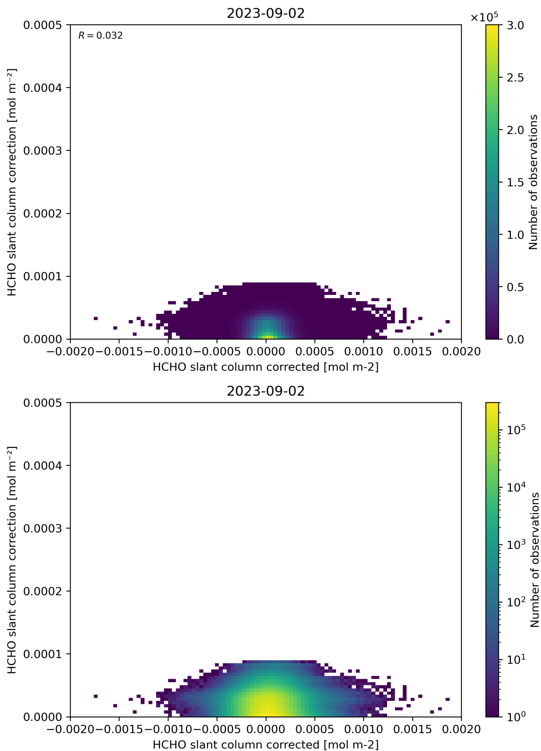
Figure 77: Scatter density plot of “HCHO slant column corrected” against “HCHO slant column correction” for 2023-09-01 to 2023-09-03.
