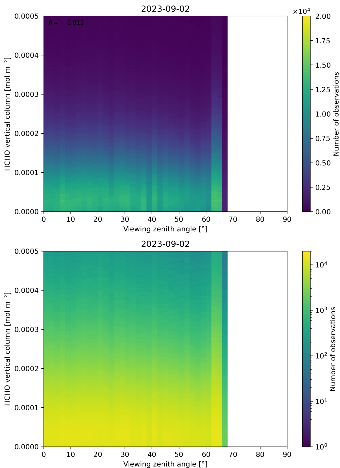
Figure 192: Scatter density plot of “Viewing zenith angle” against “HCHO vertical column” for 2023-09-01 to 2023-09-03.
