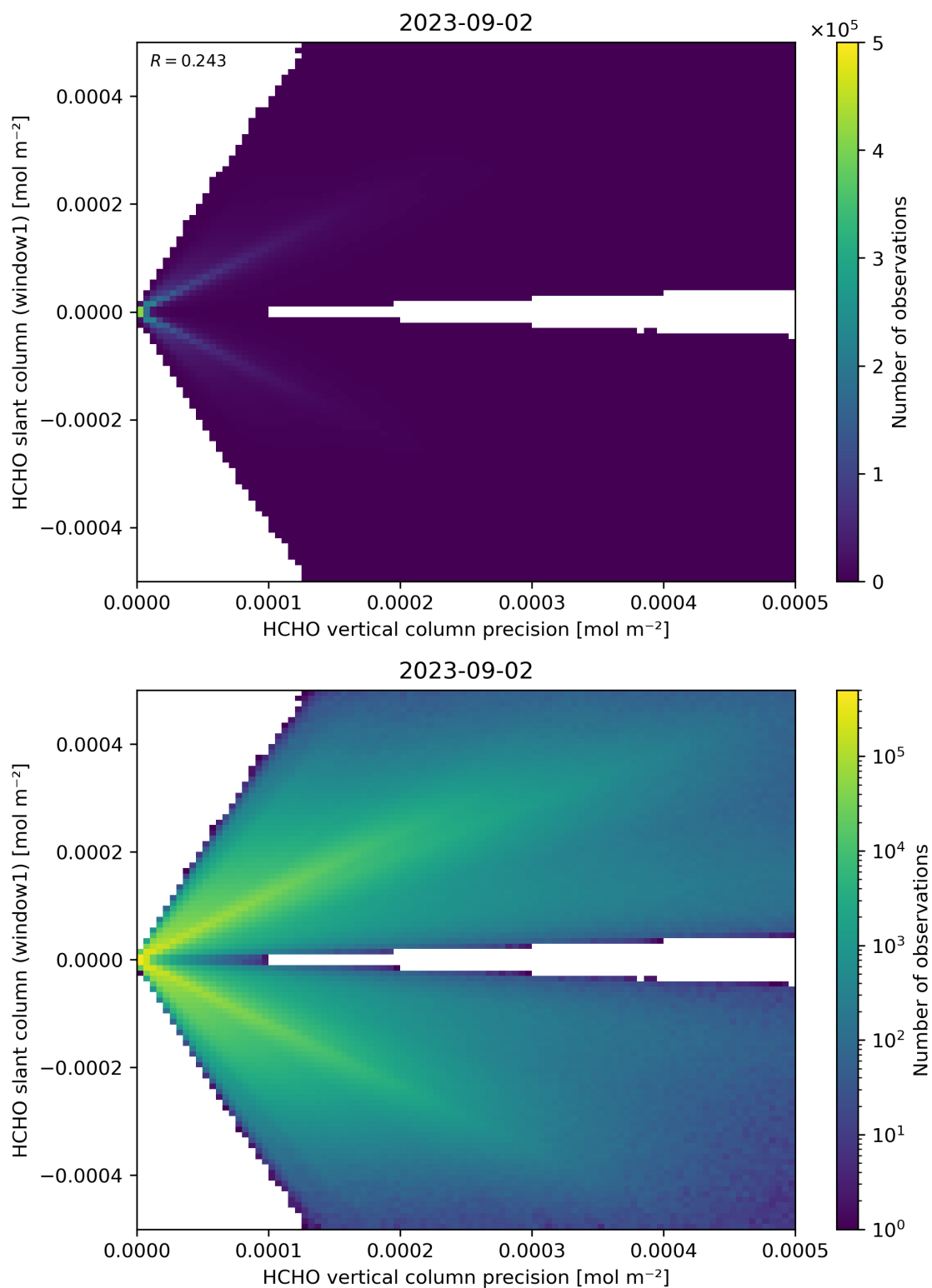
Figure 142: Scatter density plot of “HCHO vertical column precision” against “HCHO slant column (window1)” for 2023-09-01 to 2023-09-03.
