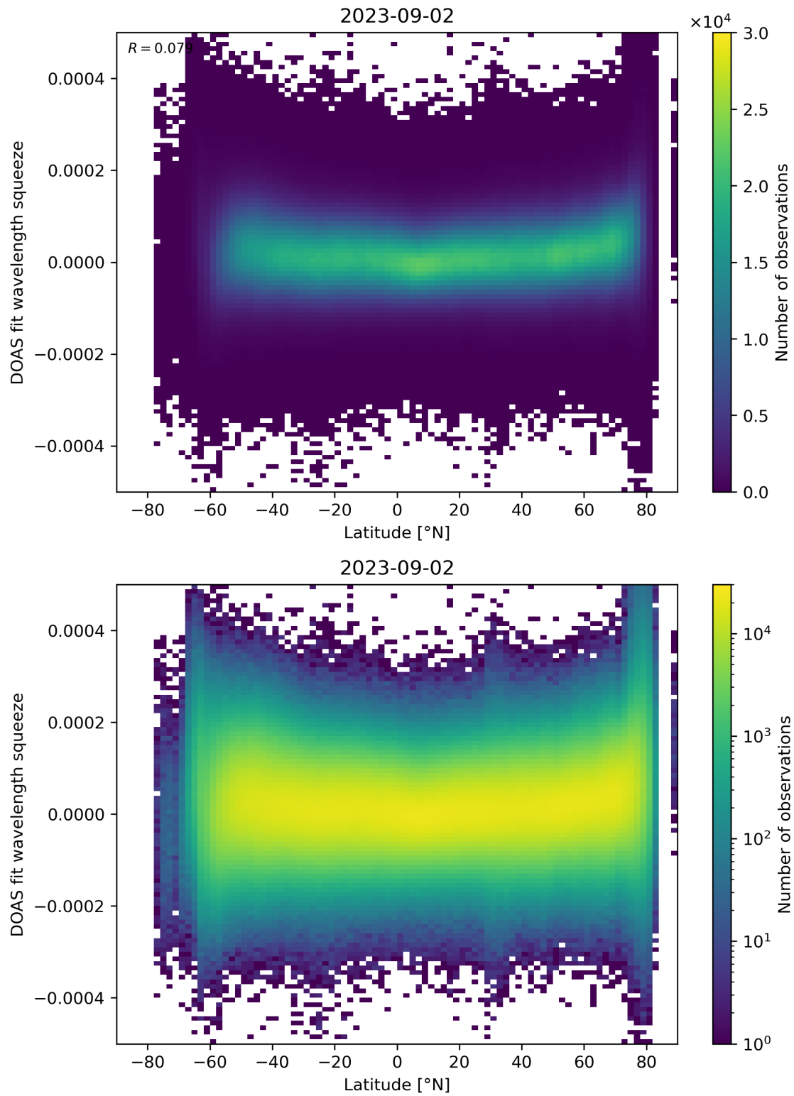
Figure 155: Scatter density plot of “Latitude” against “DOAS fit wavelength squeeze” for 2023-09-01 to 2023-09-03.
