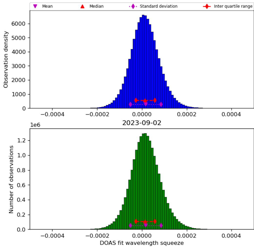
Figure 45: Histogram of “DOAS fit wavelength squeeze” for 2023-09-01 to 2023-09-03
