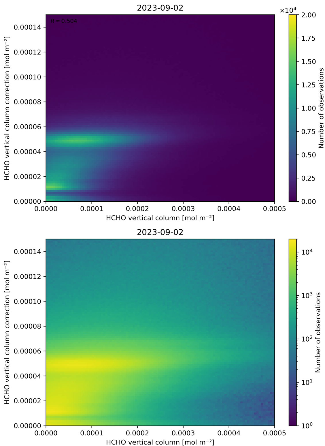
Figure 133: Scatter density plot of “HCHO vertical column” against “HCHO vertical column correction” for 2023-09-01 to 2023-09-03.
