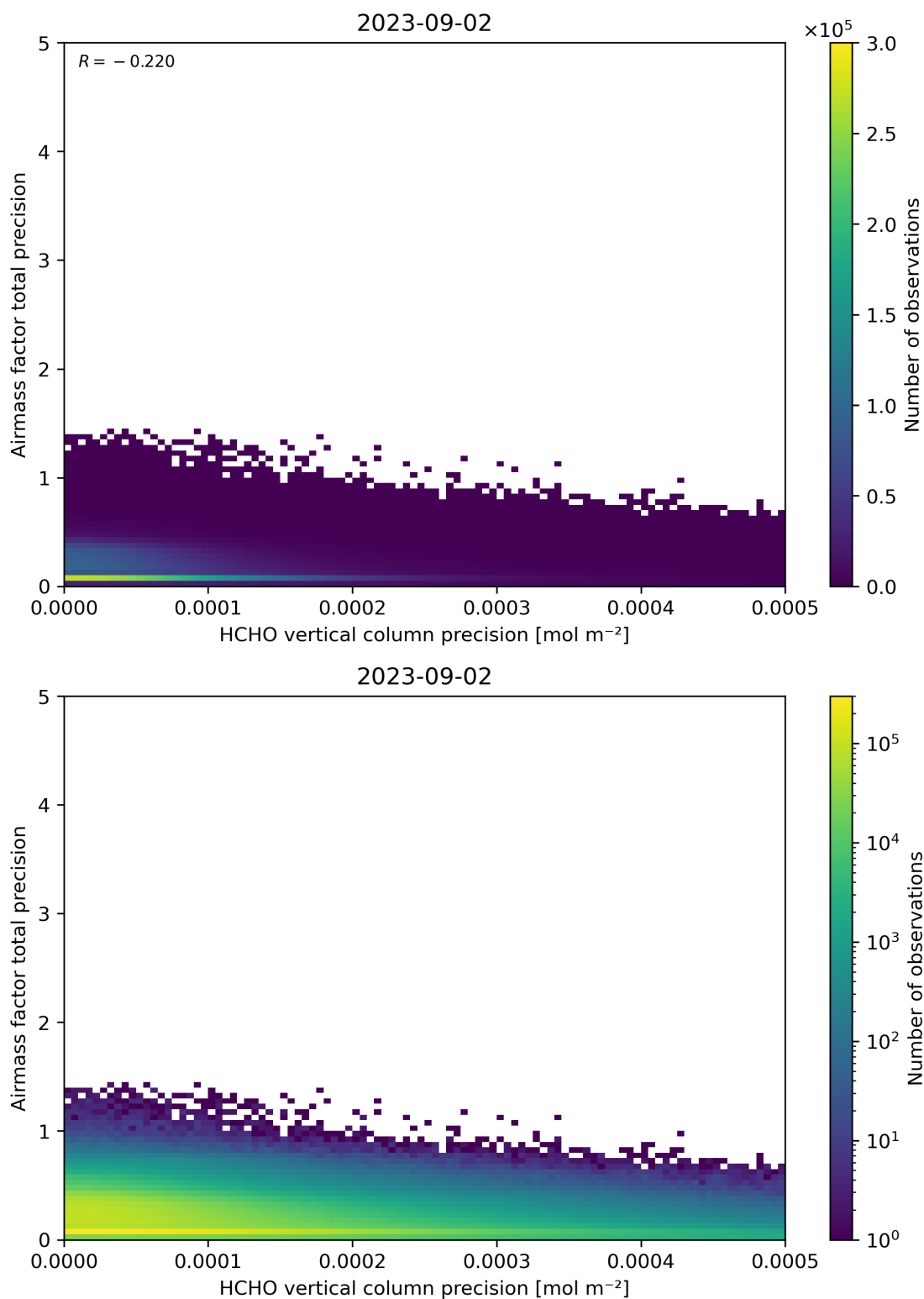
Figure 145: Scatter density plot of “HCHO vertical column precision” against “Airmass factor total precision” for 2023-09-01 to 2023-09-03.
