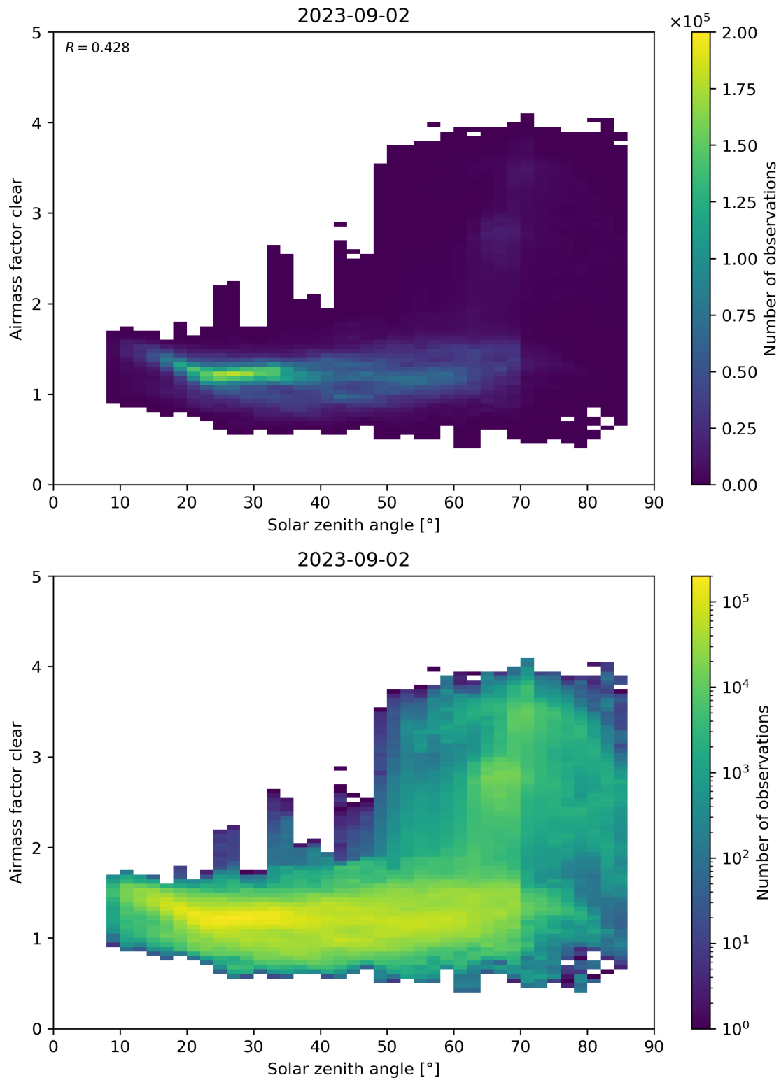
Figure 170: Scatter density plot of “Solar zenith angle” against “Airmass factor clear” for 2023-09-01 to 2023-09-03.
