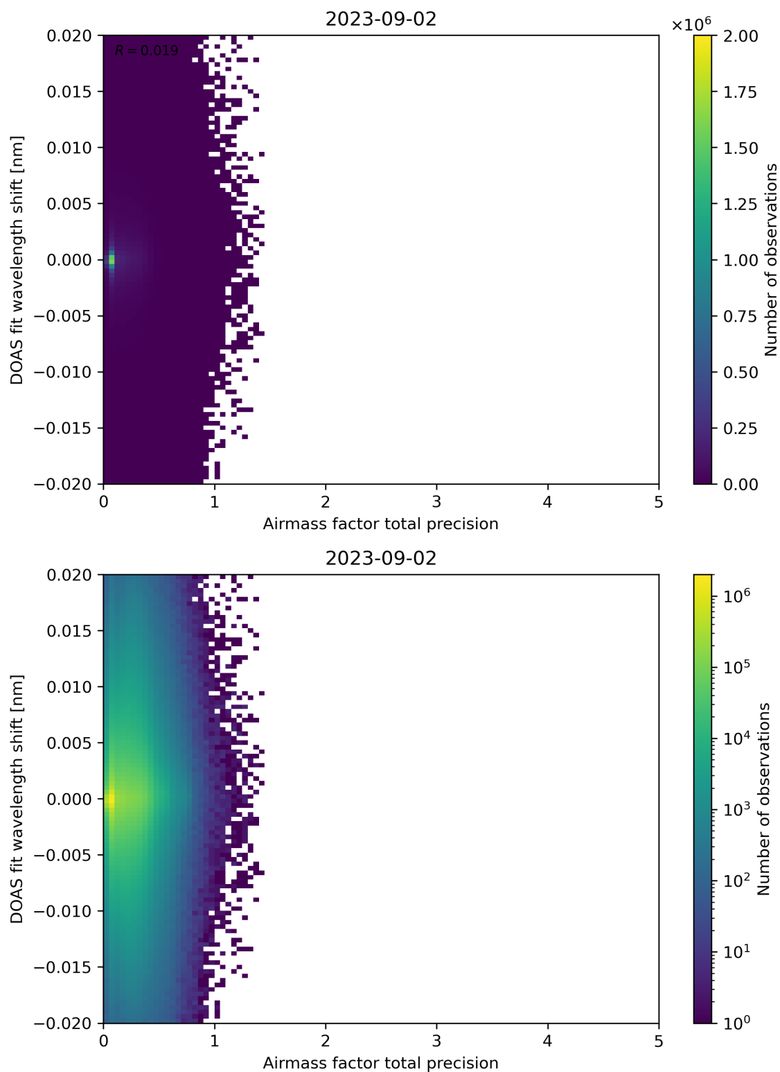
Figure 106: Scatter density plot of “Airmass factor total precision” against “DOAS fit wavelength shift” for 2023-09-01 to 2023-09-03.
