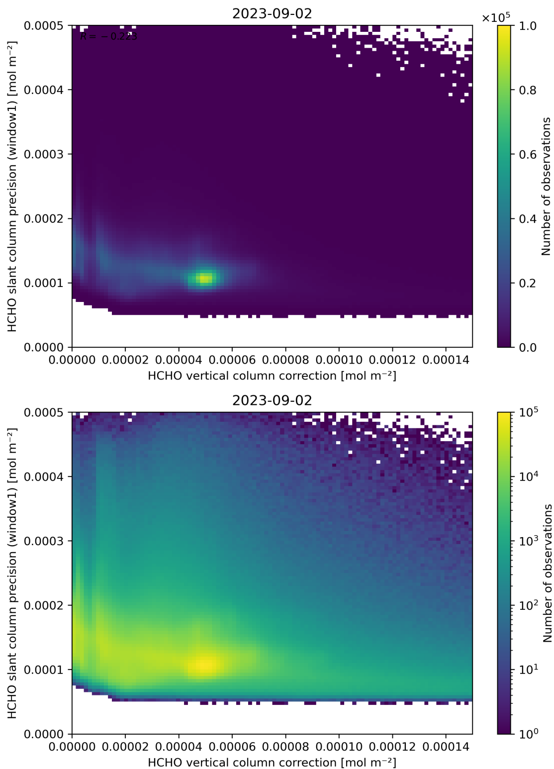
Figure 119: Scatter density plot of “HCHO vertical column correction” against “HCHO slant column precision (window1)” for 2023-09-01 to 2023-09-03.
