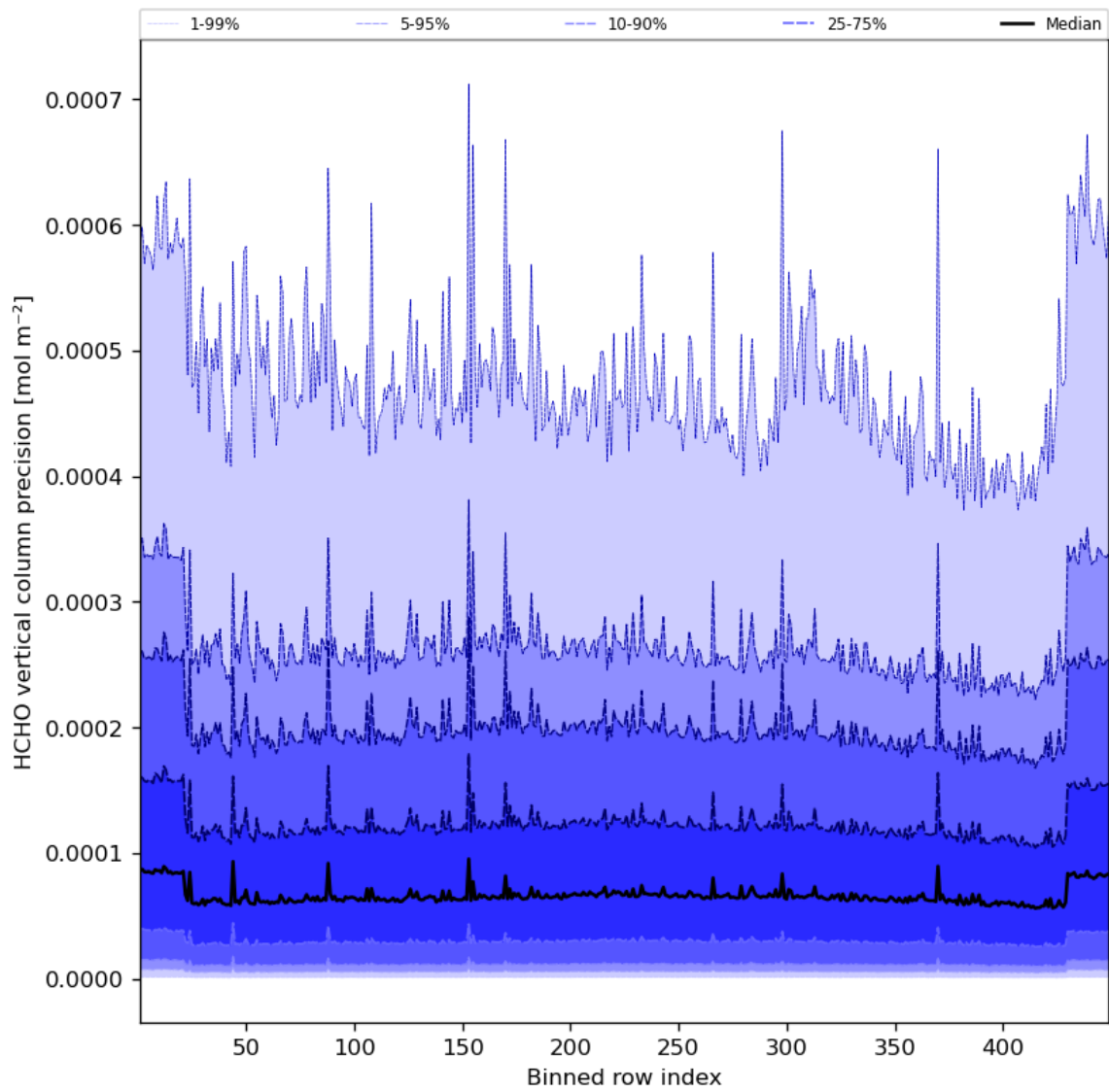
Figure 50: Along track statistics of “HCHO vertical column precision” for 2023-09-01 to 2023-09-03
