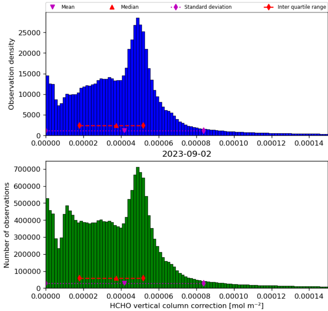
Figure 37: Histogram of “HCHO vertical column correction” for 2023-09-01 to 2023-09-03
