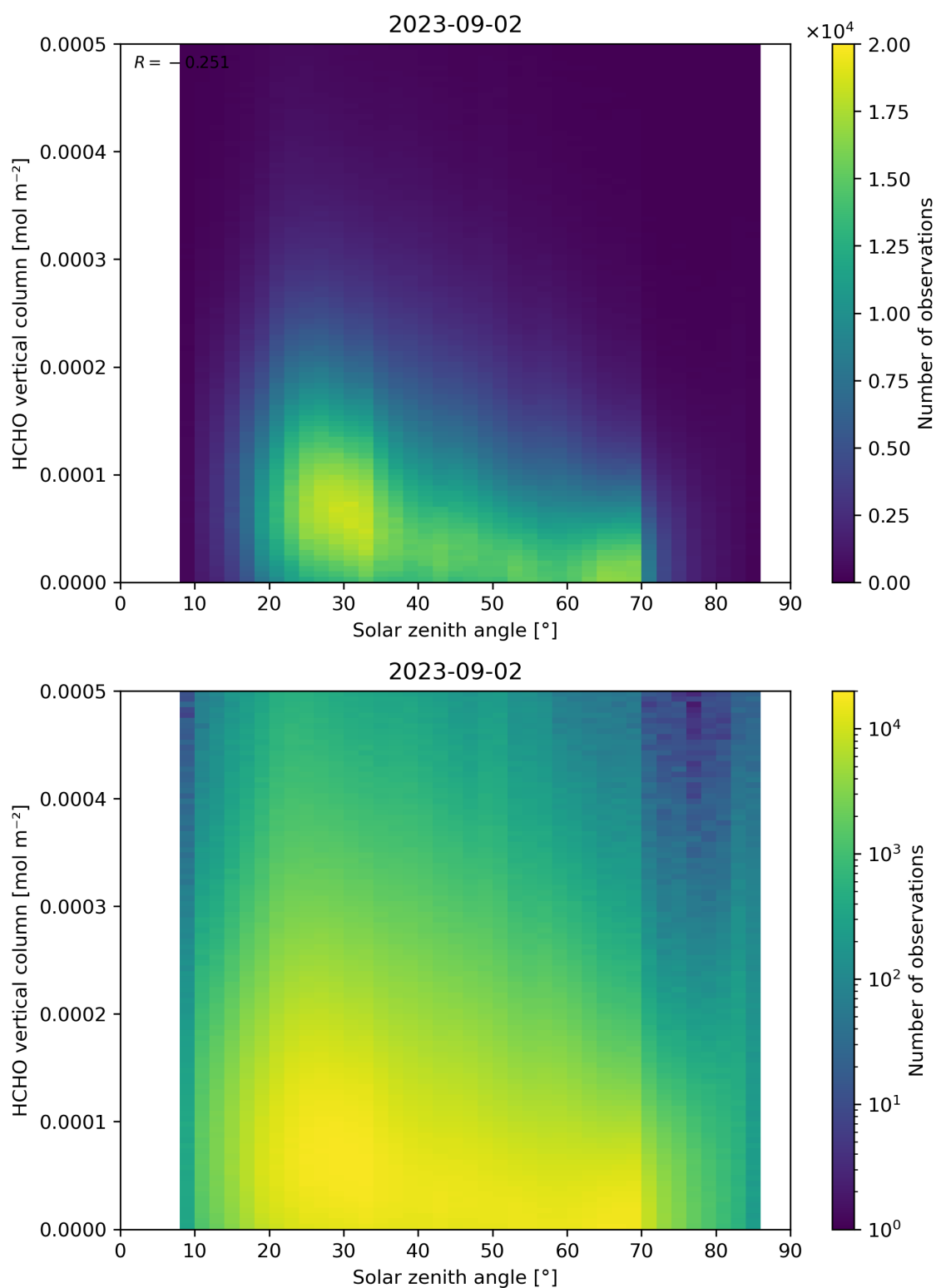
Figure 177: Scatter density plot of “Solar zenith angle” against “HCHO vertical column” for 2023-09-01 to 2023-09-03.
