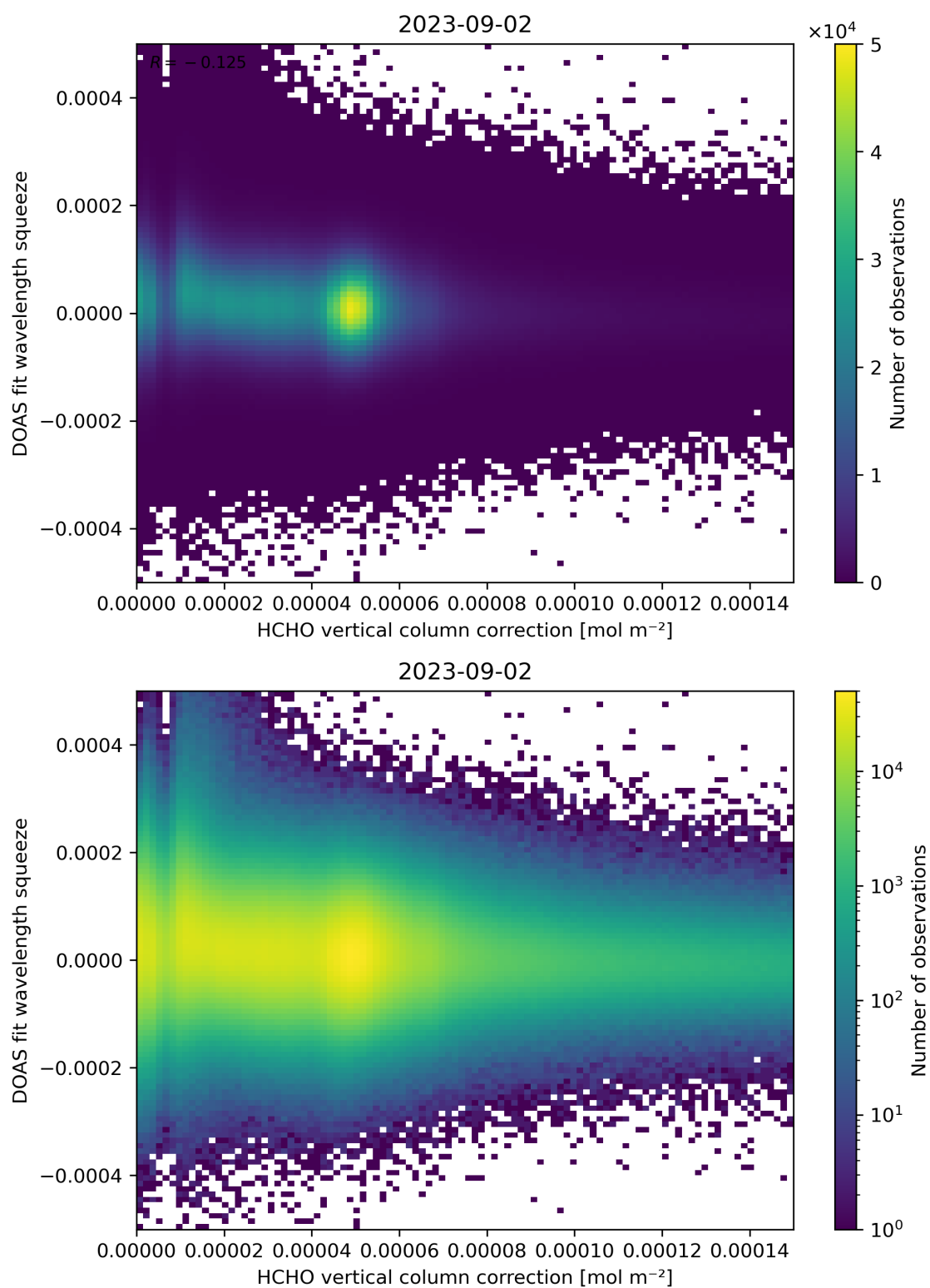
Figure 114: Scatter density plot of “HCHO vertical column correction” against “DOAS fit wavelength squeeze” for 2023-09-01 to 2023-09-03.
