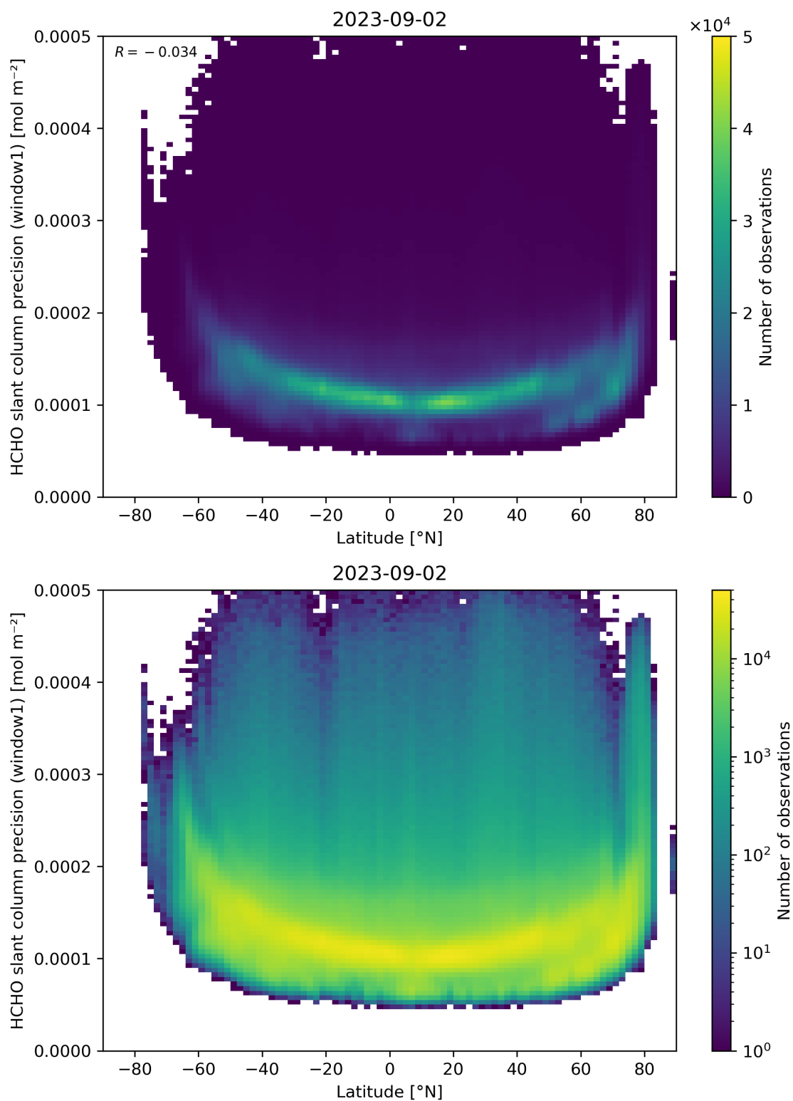
Figure 160: Scatter density plot of “Latitude” against “HCHO slant column precision (window1)” for 2023-09-01 to 2023-09-03.
