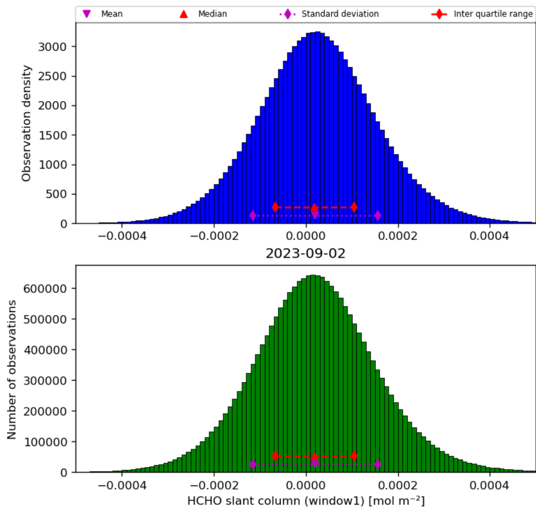
Figure 38: Histogram of “HCHO slant column (window1)” for 2023-09-01 to 2023-09-03
