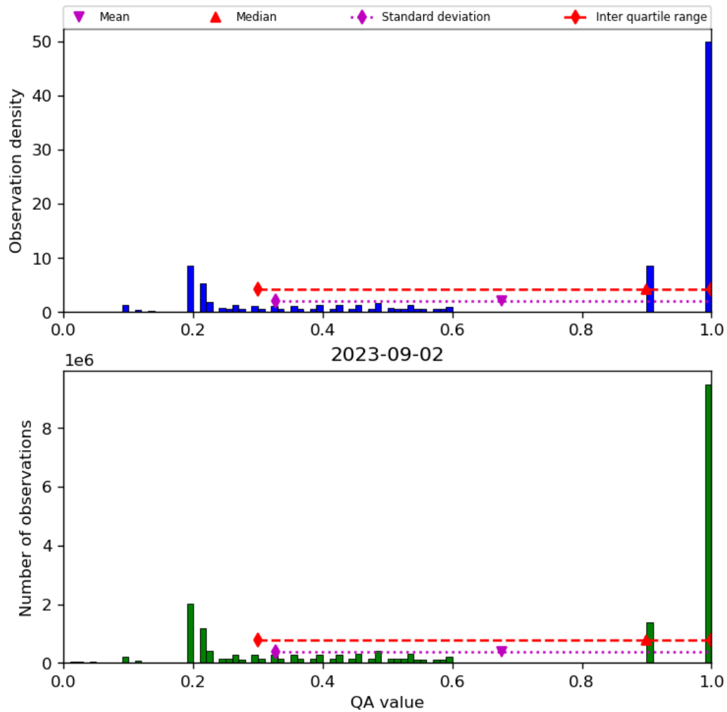
Figure 34: Histogram of “QA value” for 2023-09-01 to 2023-09-03
