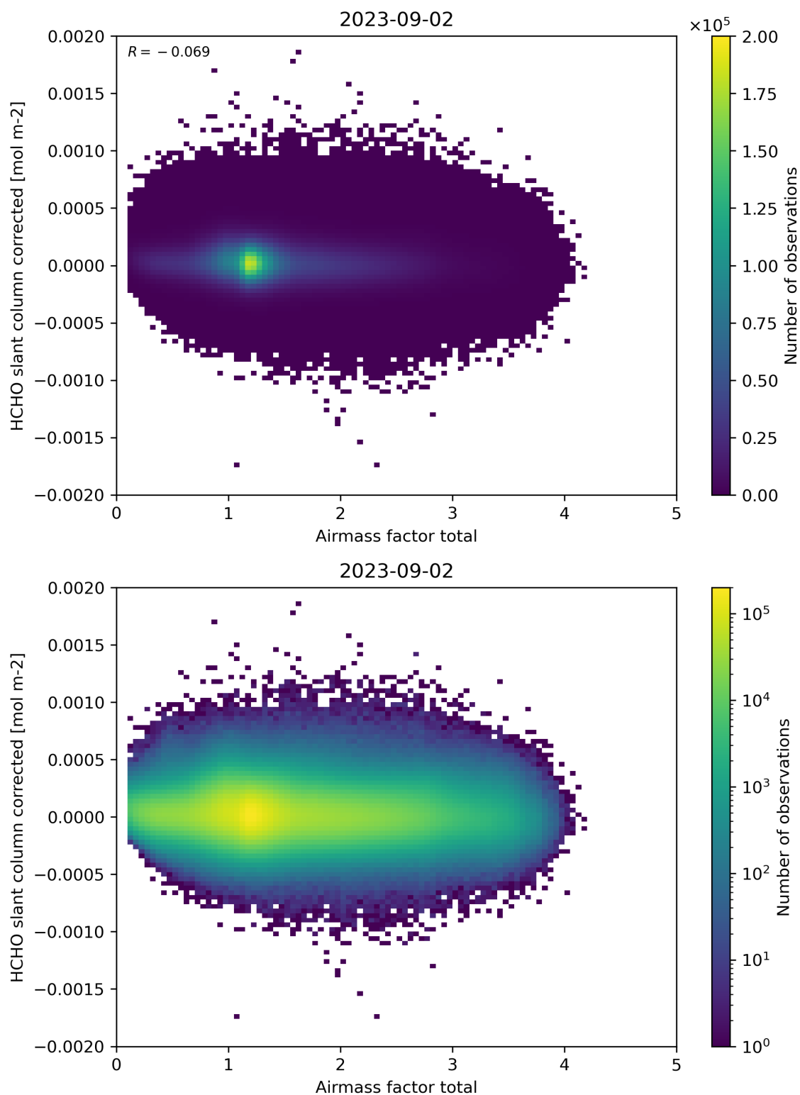
Figure 101: Scatter density plot of “Airmass factor total” against “HCHO slant column corrected” for 2023-09-01 to 2023-09-03.
