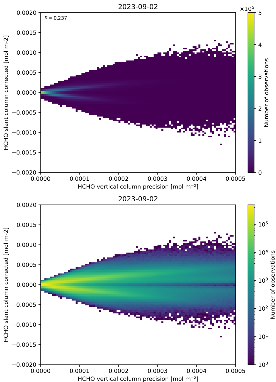
Figure 140: Scatter density plot of “HCHO vertical column precision” against “HCHO slant column corrected” for 2023-09-01 to 2023-09-03.
