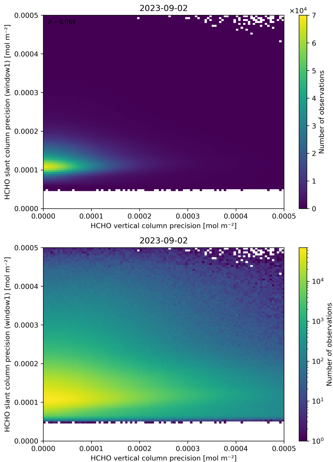
Figure 143: Scatter density plot of “HCHO vertical column precision” against “HCHO slant column precision (window1)” for 2023-09-01 to 2023-09-03.
