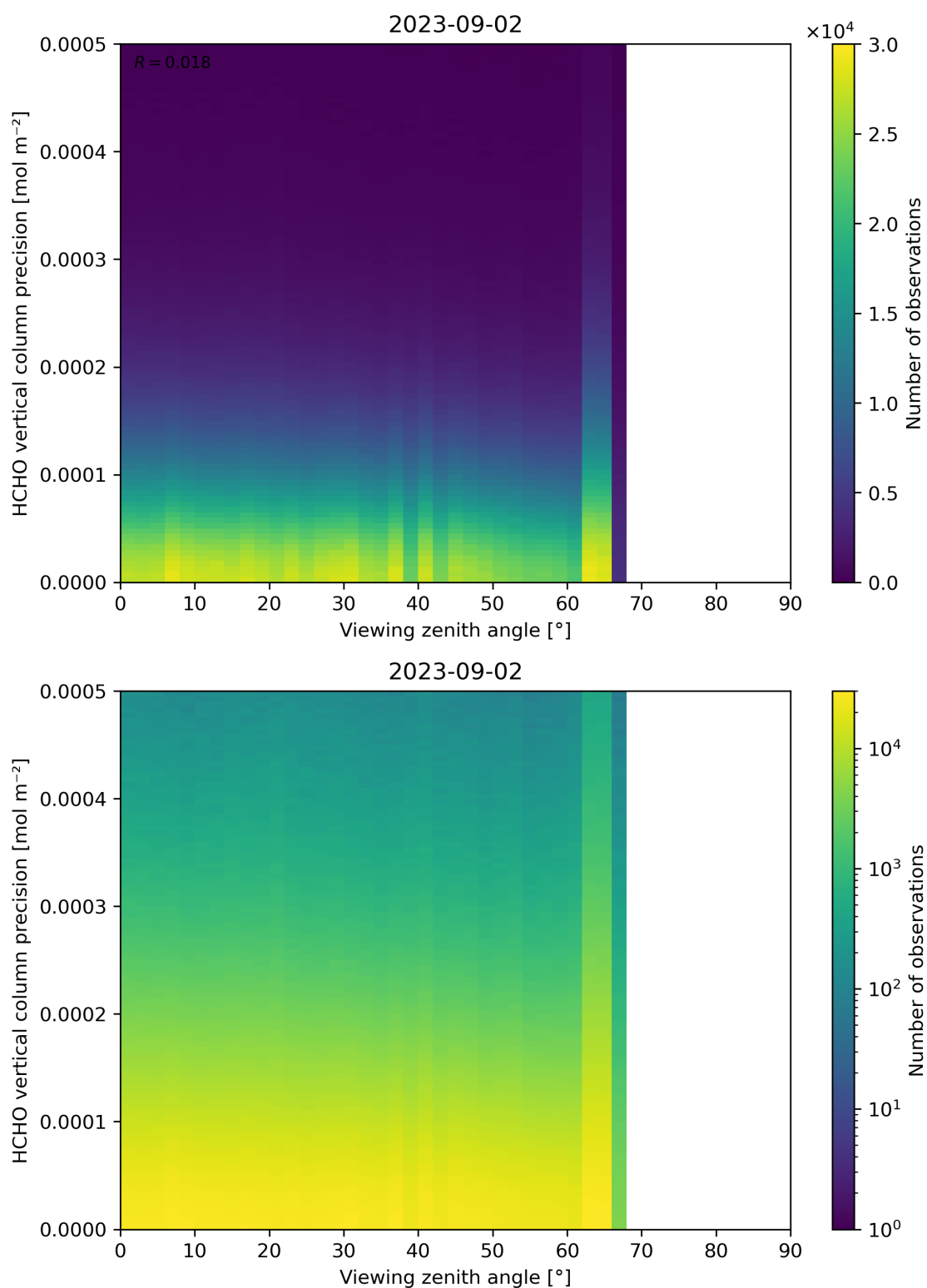
Figure 194: Scatter density plot of “Viewing zenith angle” against “HCHO vertical column precision” for 2023-09-01 to 2023-09-03.
