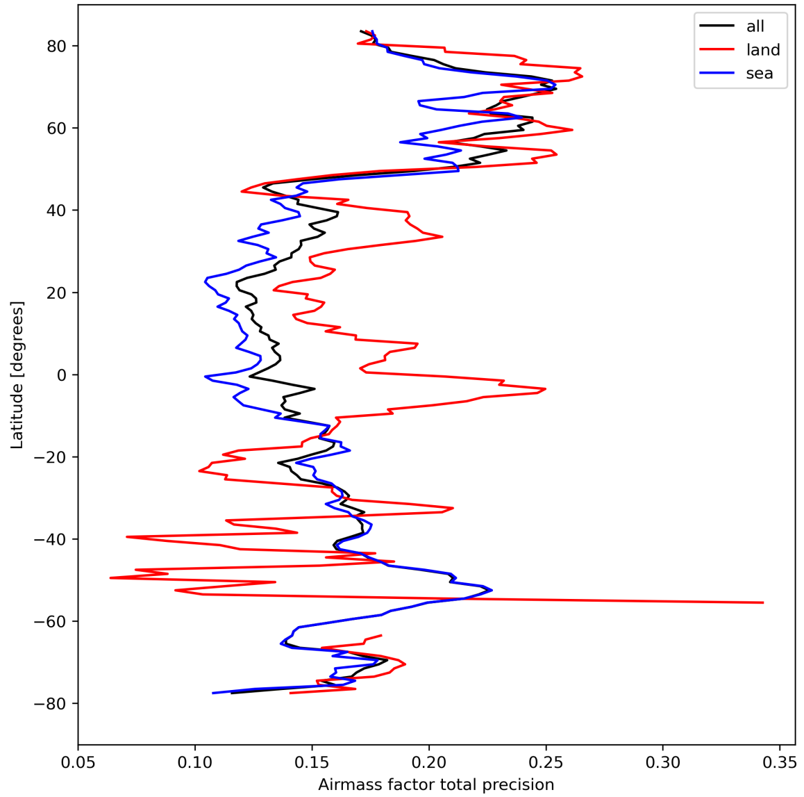
Figure 27: Zonal average of “Airmass factor total precision” for 2023-09-01 to 2023-09-03.
