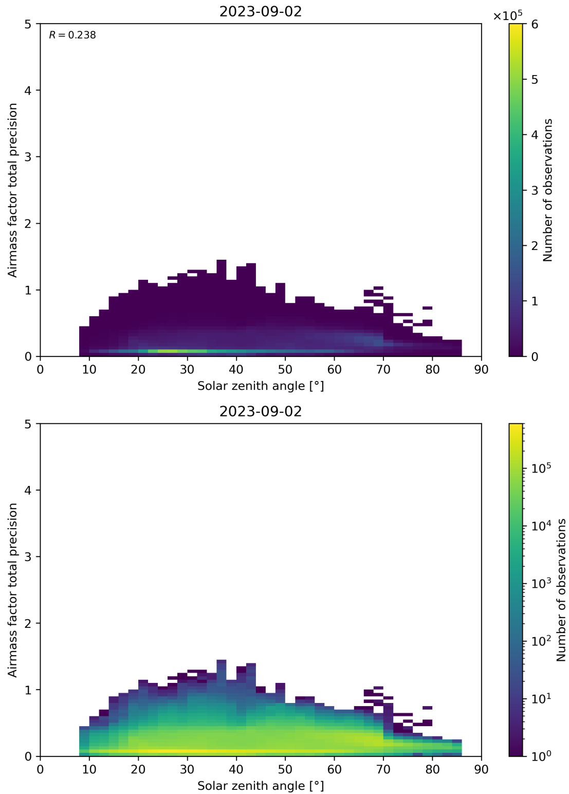
Figure 176: Scatter density plot of “Solar zenith angle” against “Airmass factor total precision” for 2023-09-01 to 2023-09-03.
