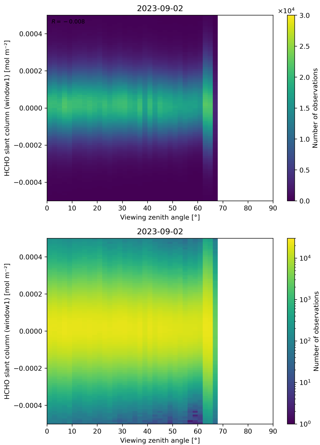
Figure 188: Scatter density plot of “Viewing zenith angle” against “HCHO slant column (window1)” for 2023-09-01 to 2023-09-03.
