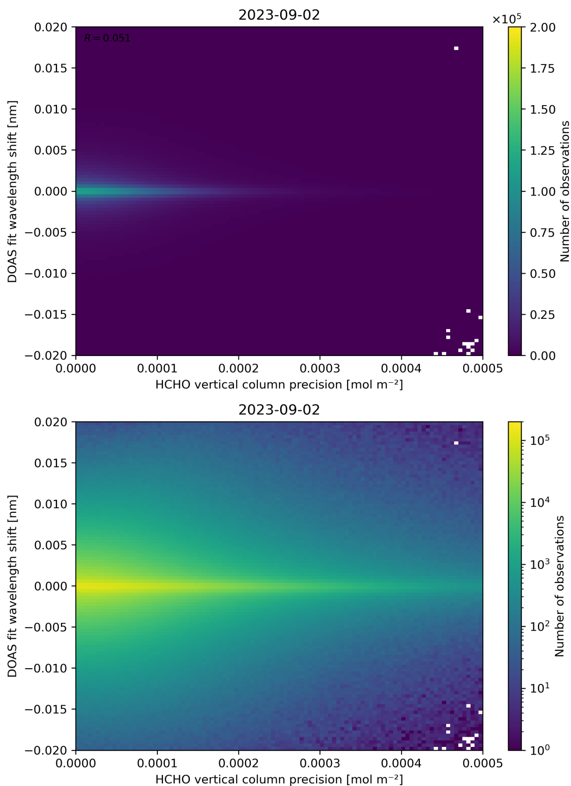
Figure 137: Scatter density plot of “HCHO vertical column precision” against “DOAS fit wavelength shift” for 2023-09-01 to 2023-09-03.
