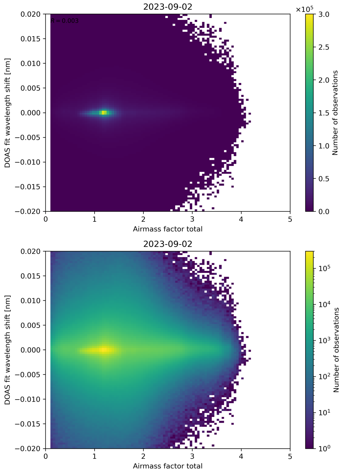
Figure 98: Scatter density plot of “Airmass factor total” against “DOAS fit wavelength shift” for 2023-09-01 to 2023-09-03.
