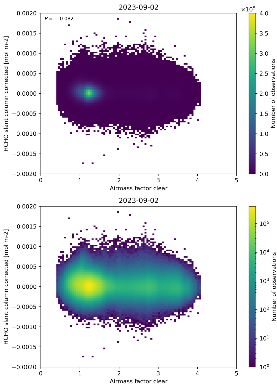
Figure 74: Scatter density plot of “Airmass factor clear” against “HCHO slant column corrected” for 2023-09-01 to 2023-09-03.
