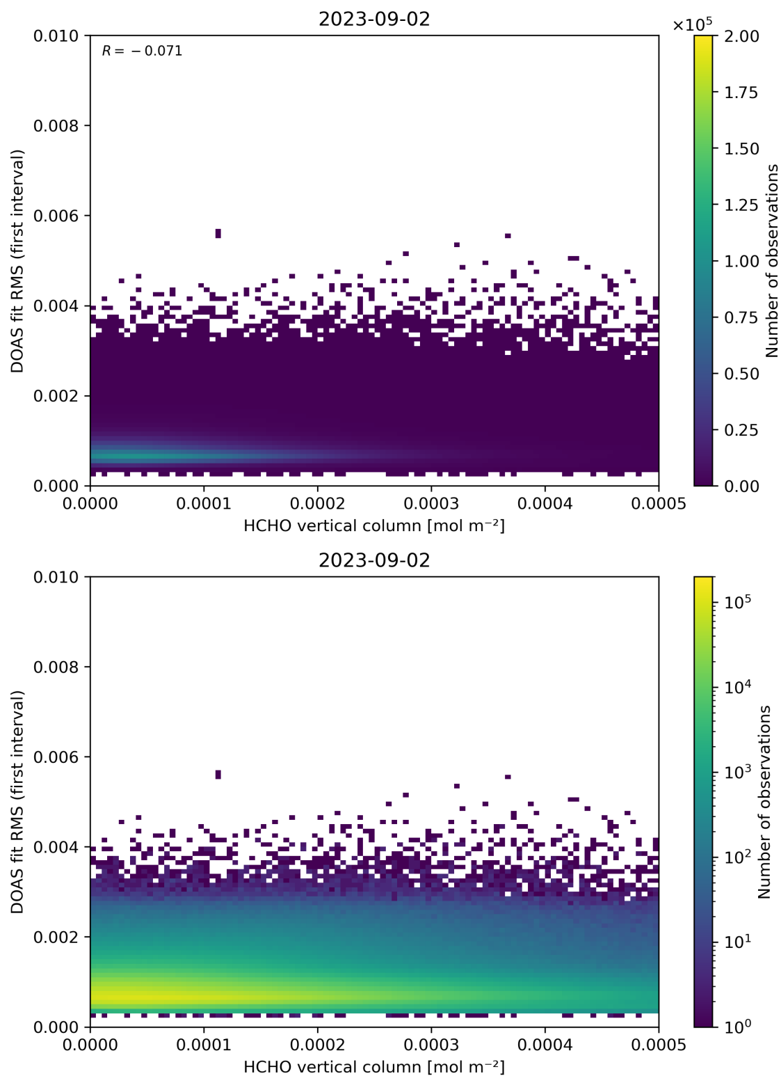
Figure 123: Scatter density plot of “HCHO vertical column” against “DOAS fit RMS (first interval)” for 2023-09-01 to 2023-09-03.
