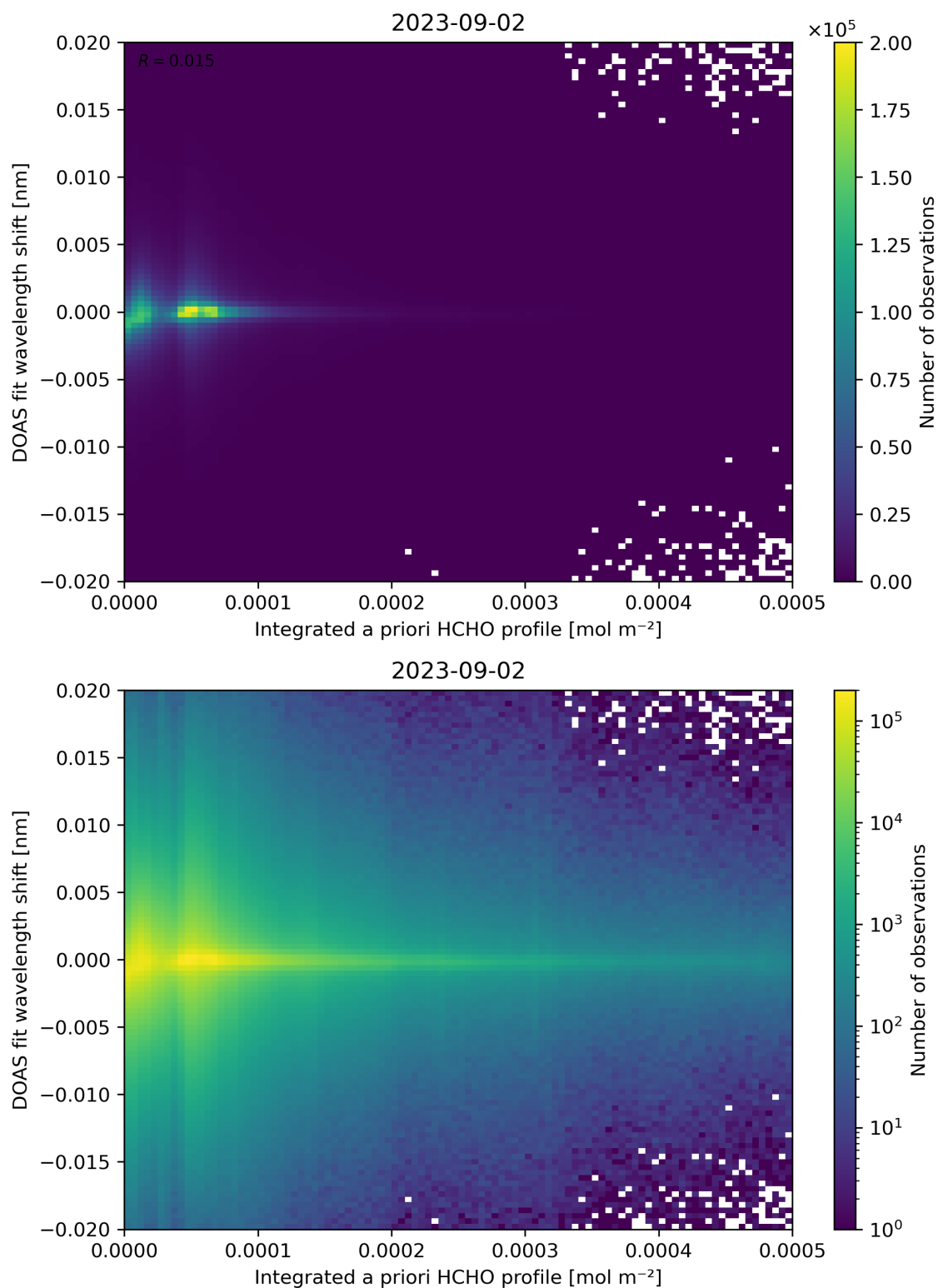
Figure 149: Scatter density plot of “Integrated a priori HCHO profile” against “DOAS fit wavelength shift” for 2023-09-01 to 2023-09-03.
