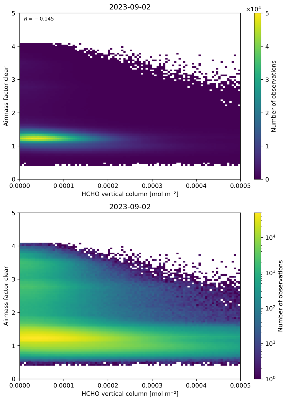
Figure 126: Scatter density plot of “HCHO vertical column” against “Airmass factor clear” for 2023-09-01 to 2023-09-03.
