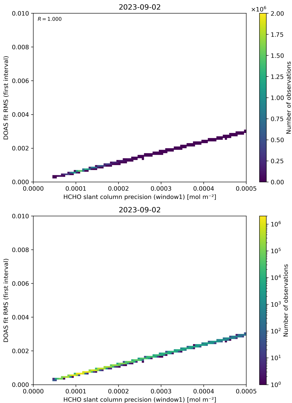
Figure 88: Scatter density plot of “HCHO slant column precision (window1)” against “DOAS fit RMS (first interval)” for 2023-09-01 to 2023-09-03.
