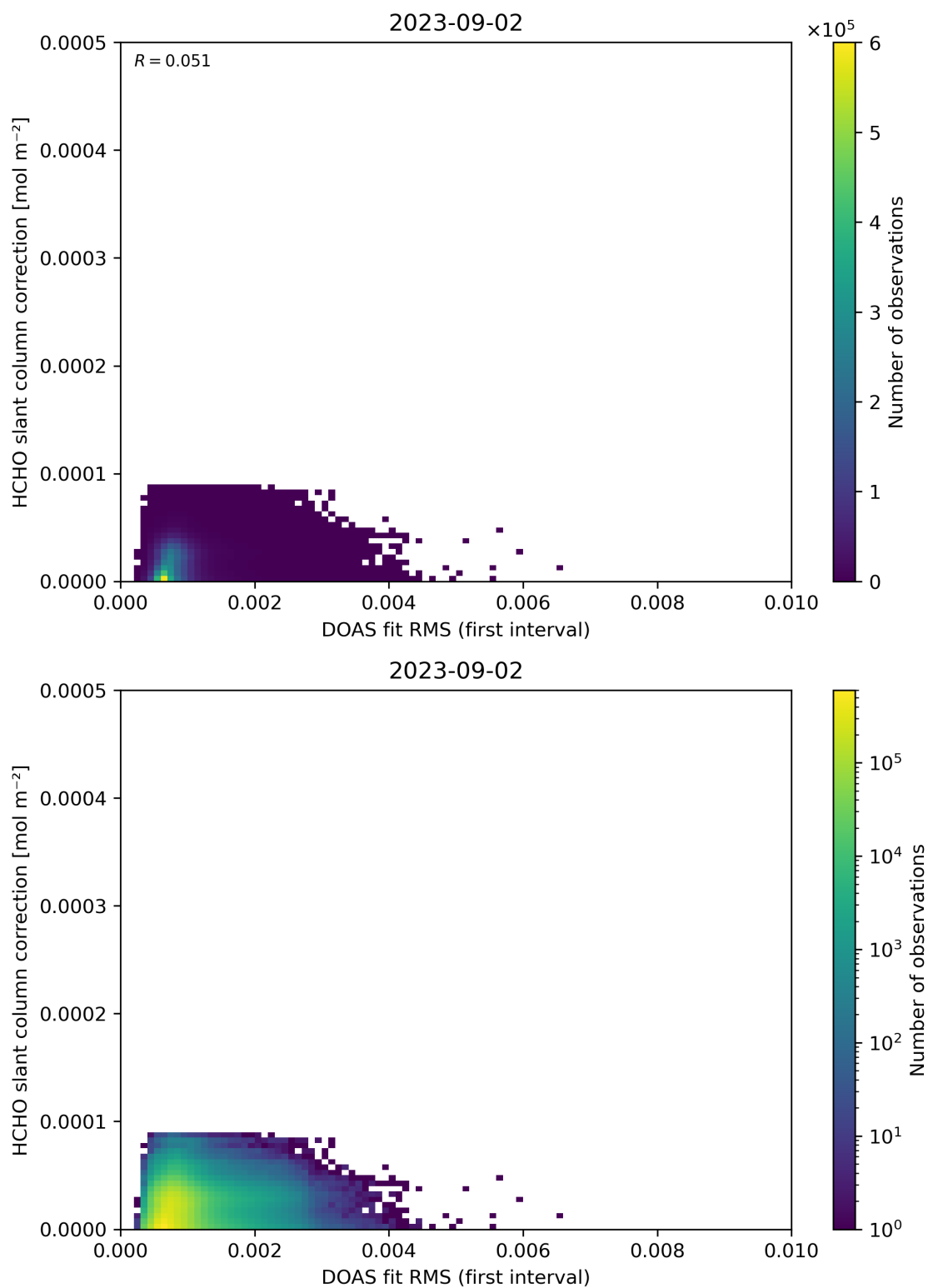
Figure 63: Scatter density plot of “DOAS fit RMS (first interval)” against “HCHO slant column correction” for 2023-09-01 to 2023-09-03.
