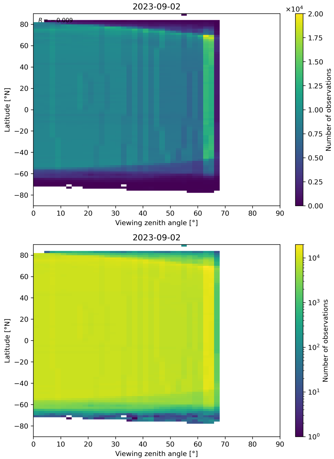
Figure 196: Scatter density plot of “Viewing zenith angle” against “Latitude” for 2023-09-01 to 2023-09-03.
