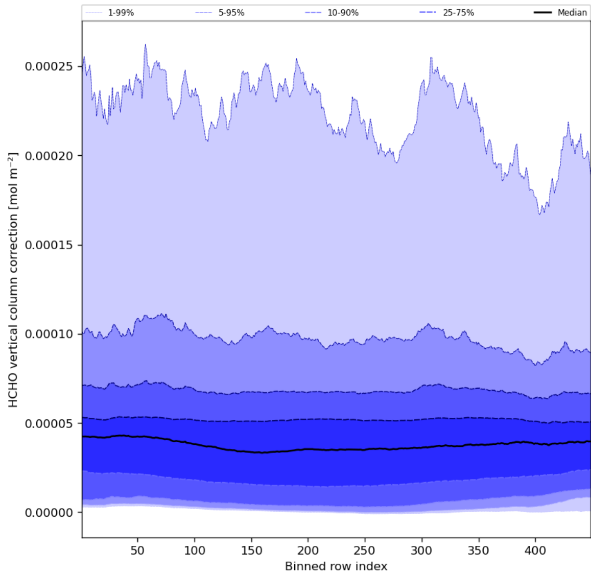
Figure 51: Along track statistics of “HCHO vertical column correction” for 2023-09-01 to 2023-09-03
