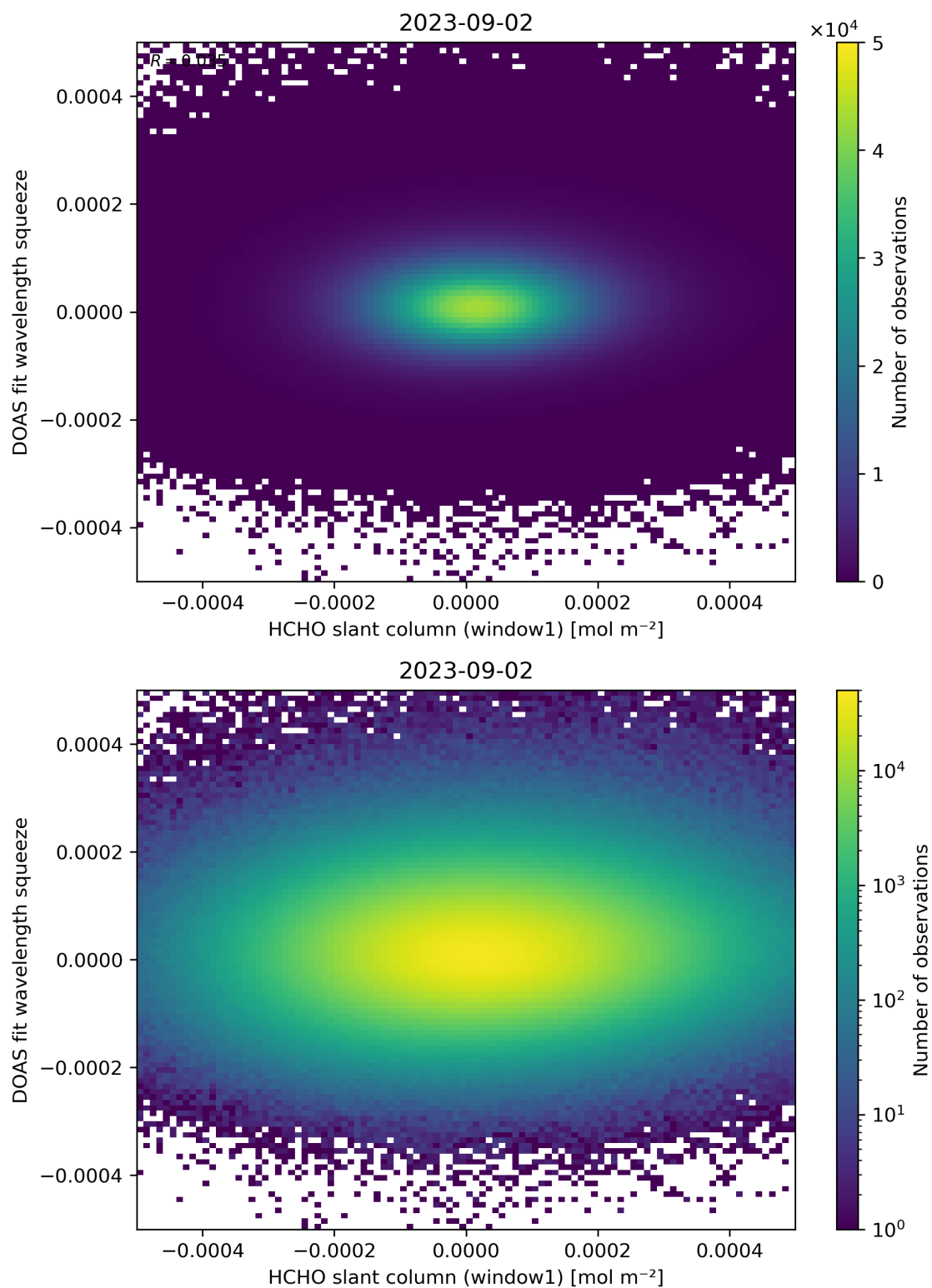
Figure 80: Scatter density plot of “HCHO slant column (window1)” against “DOAS fit wavelength squeeze” for 2023-09-01 to 2023-09-03.
