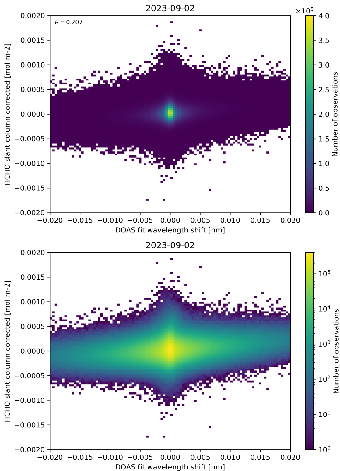
Figure 66: Scatter density plot of “DOAS fit wavelength shift” against “HCHO slant column corrected” for 2023-09-01 to 2023-09-03.
