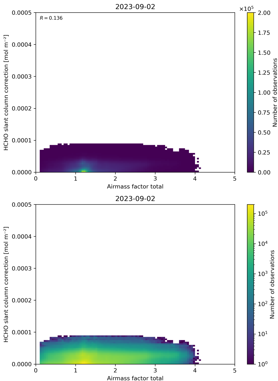
Figure 102: Scatter density plot of “Airmass factor total” against “HCHO slant column correction” for 2023-09-01 to 2023-09-03.
