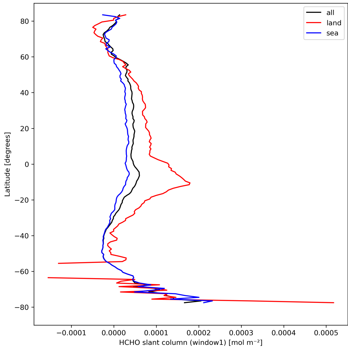
Figure 24: Zonal average of “HCHO slant column (window1)” for 2023-09-01 to 2023-09-03.
