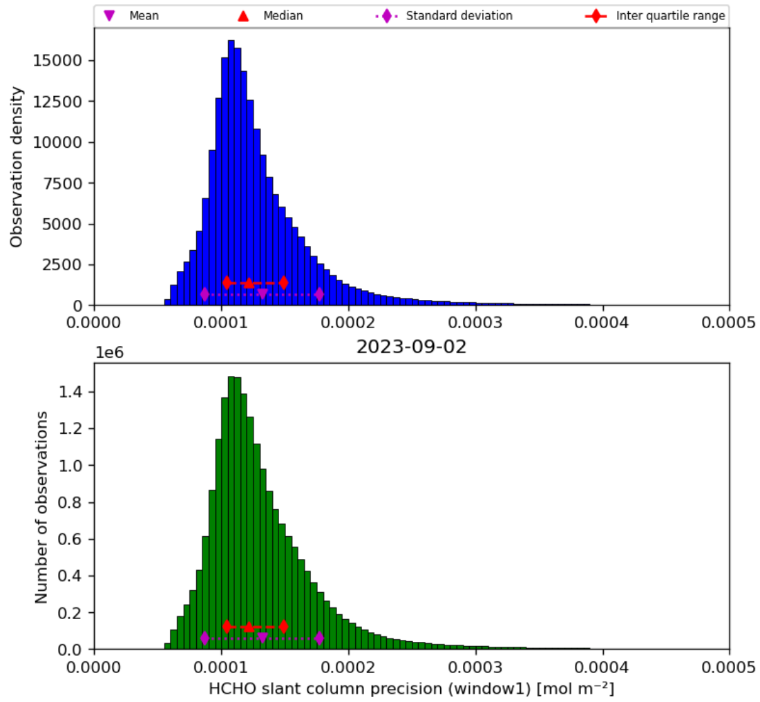
Figure 39: Histogram of “HCHO slant column precision (window1)” for 2023-09-01 to 2023-09-03
