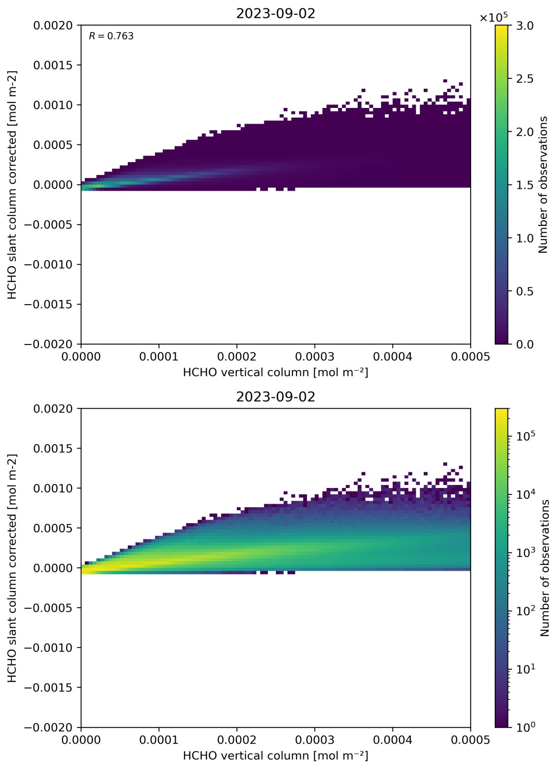
Figure 127: Scatter density plot of “HCHO vertical column” against “HCHO slant column corrected” for 2023-09-01 to 2023-09-03.
