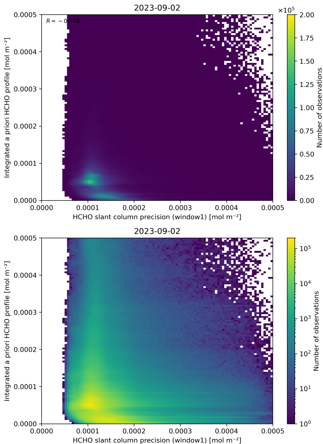
Figure 96: Scatter density plot of “HCHO slant column precision (window1)” against “Integrated a priori HCHO profile” for 2023-09-01 to 2023-09-03.
