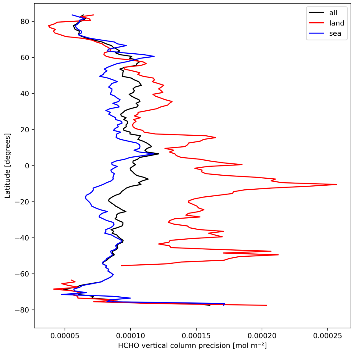
Figure 22: Zonal average of “HCHO vertical column precision” for 2023-09-01 to 2023-09-03.
