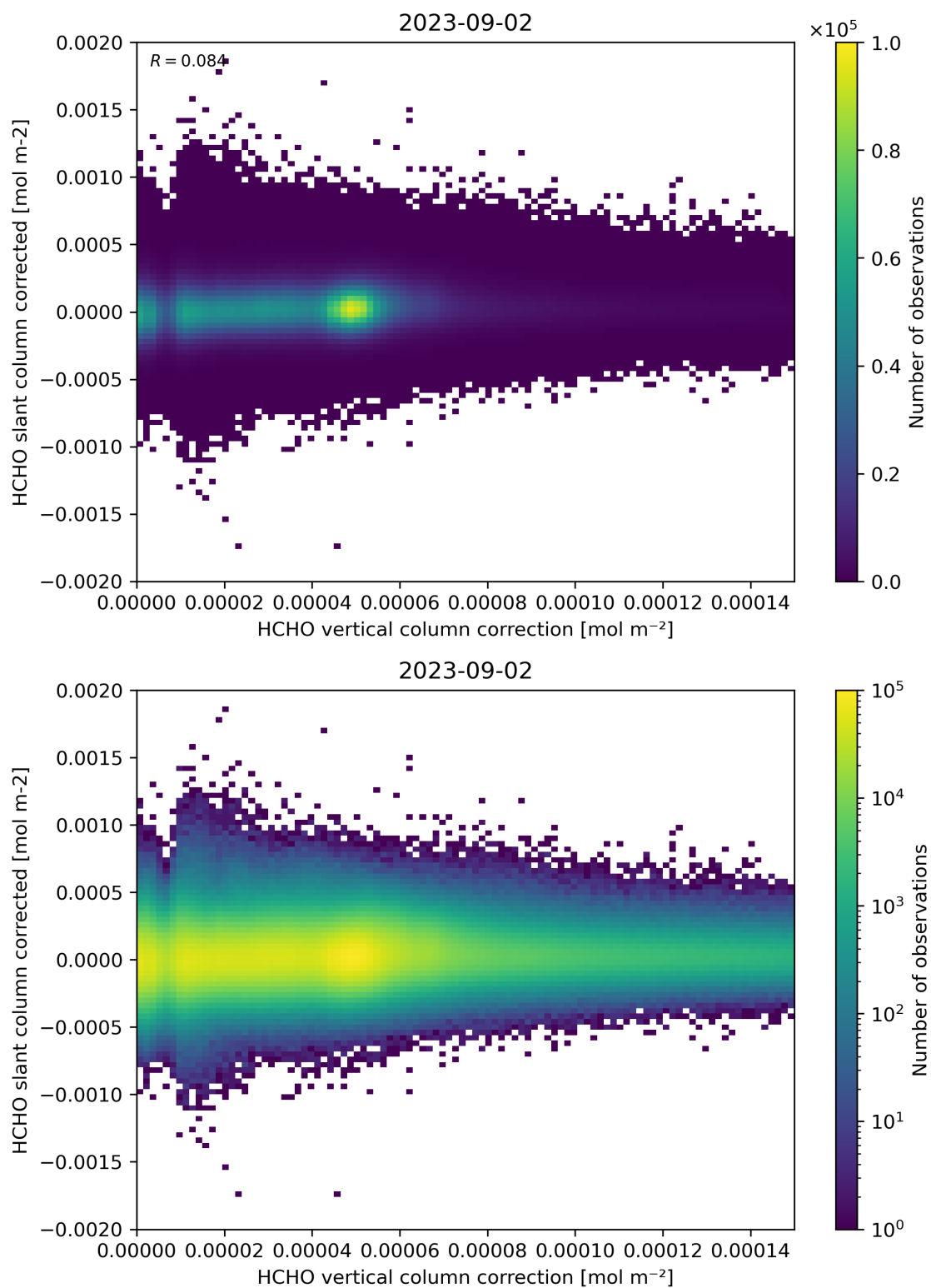
Figure 116: Scatter density plot of “HCHO vertical column correction” against “HCHO slant column corrected” for 2023-09-01 to 2023-09-03.
