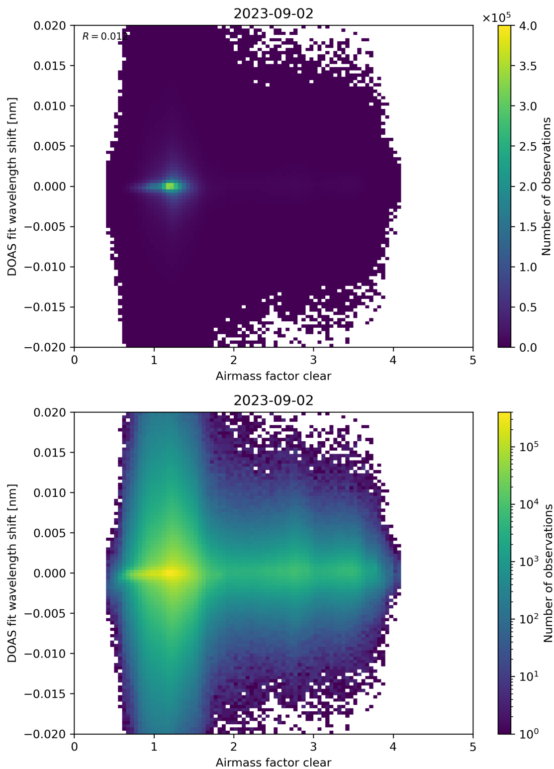
Figure 72: Scatter density plot of “Airmass factor clear” against “DOAS fit wavelength shift” for 2023-09-01 to 2023-09-03.
