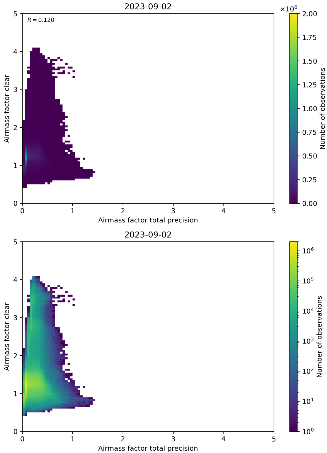
Figure 108: Scatter density plot of “Airmass factor total precision” against “Airmass factor clear” for 2023-09-01 to 2023-09-03.
