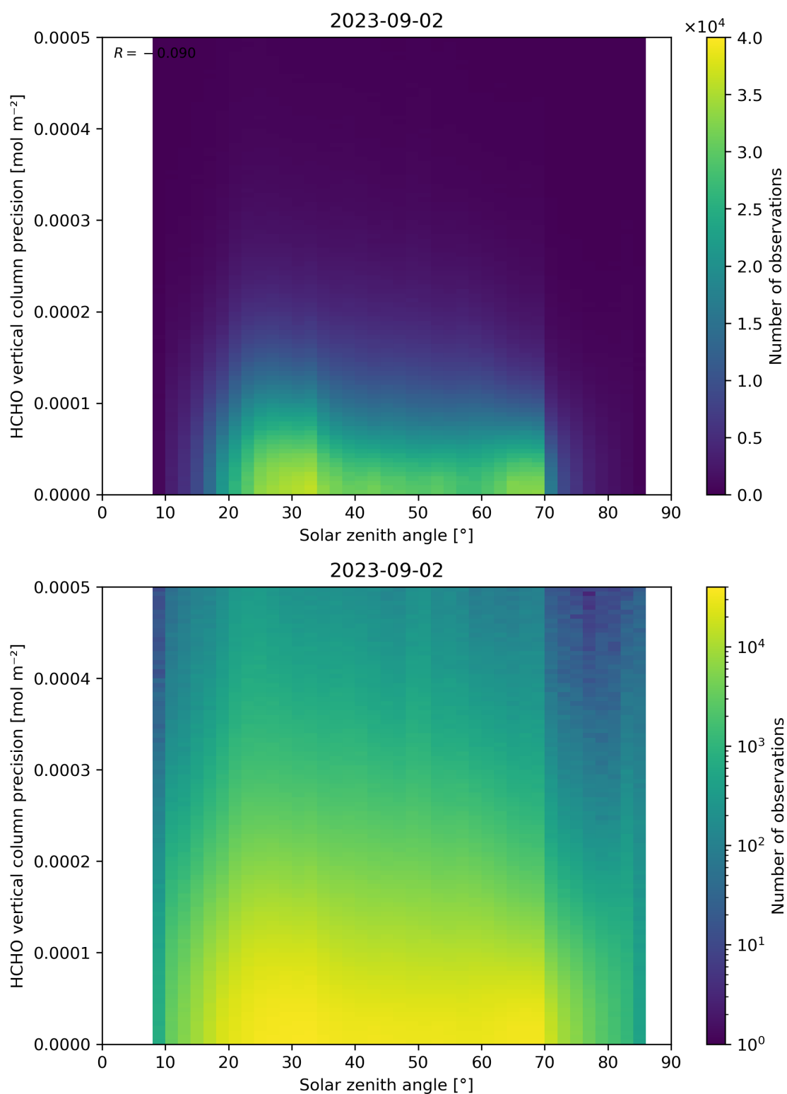
Figure 179: Scatter density plot of “Solar zenith angle” against “HCHO vertical column precision” for 2023-09-01 to 2023-09-03.
