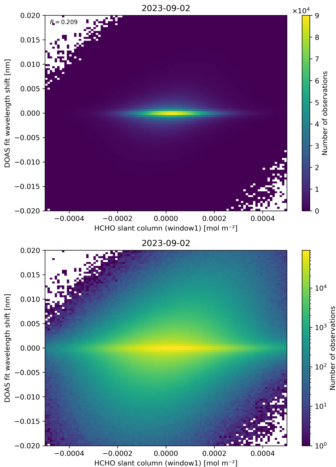
Figure 79: Scatter density plot of “HCHO slant column (window1)” against “DOAS fit wavelength shift” for 2023-09-01 to 2023-09-03.
