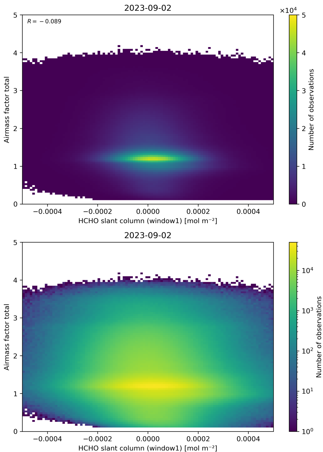
Figure 85: Scatter density plot of “HCHO slant column (window1)” against “Airmass factor total” for 2023-09-01 to 2023-09-03.
