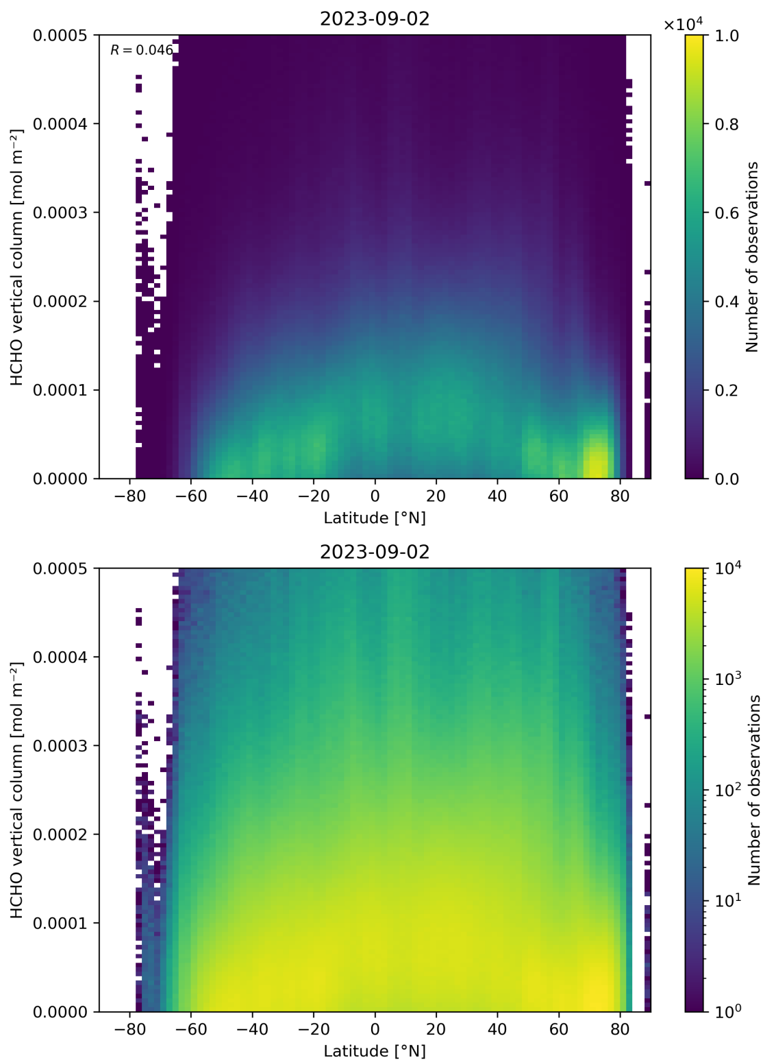
Figure 163: Scatter density plot of “Latitude” against “HCHO vertical column” for 2023-09-01 to 2023-09-03.
