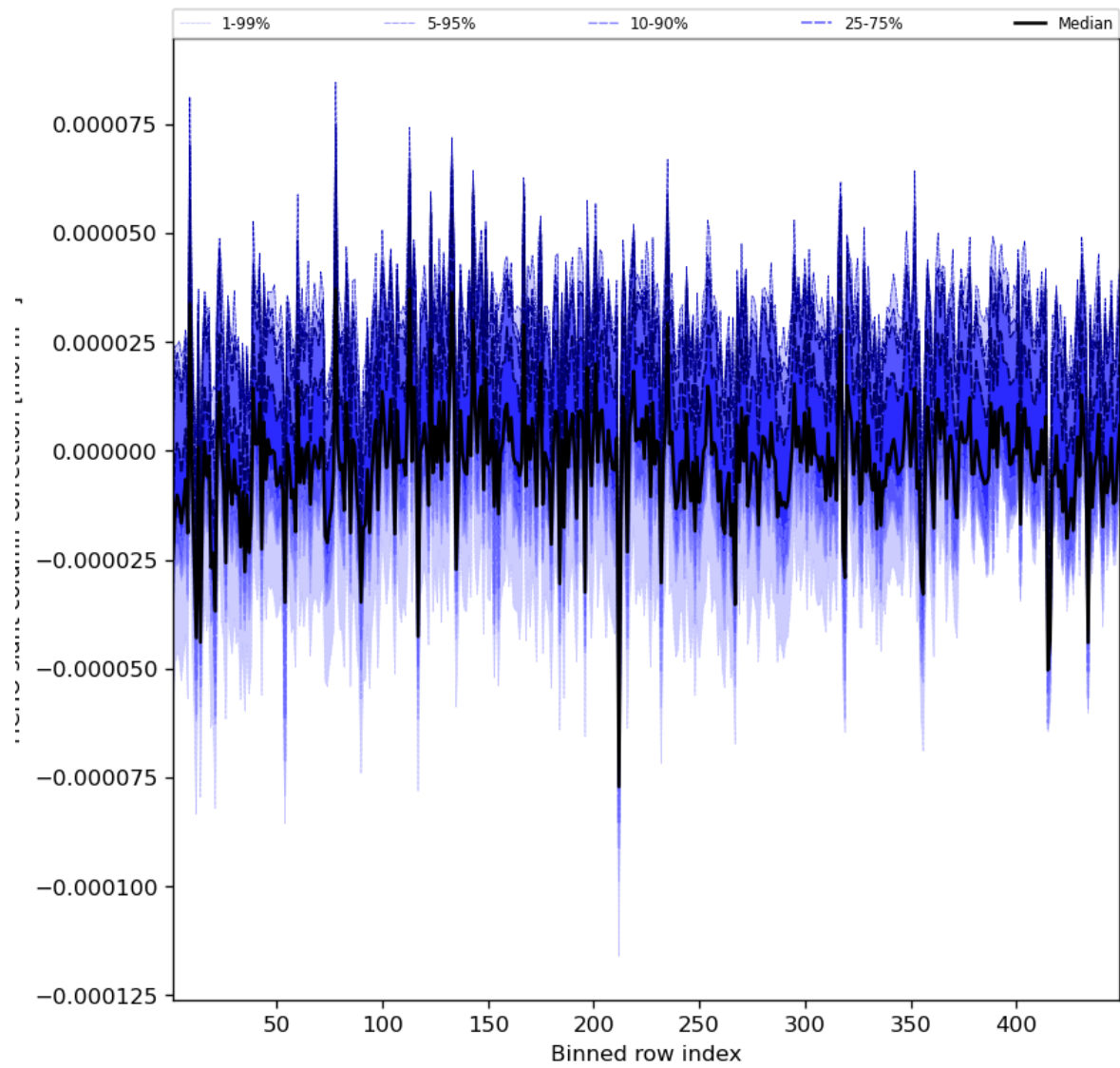
Figure 61: Along track statistics of “HCHO slant column correction” for 2023-09-01 to 2023-09-03
