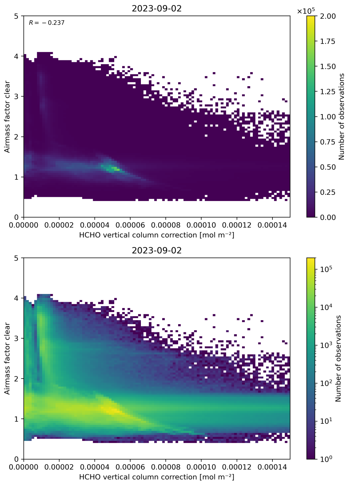
Figure 115: Scatter density plot of “HCHO vertical column correction” against “Airmass factor clear” for 2023-09-01 to 2023-09-03.
