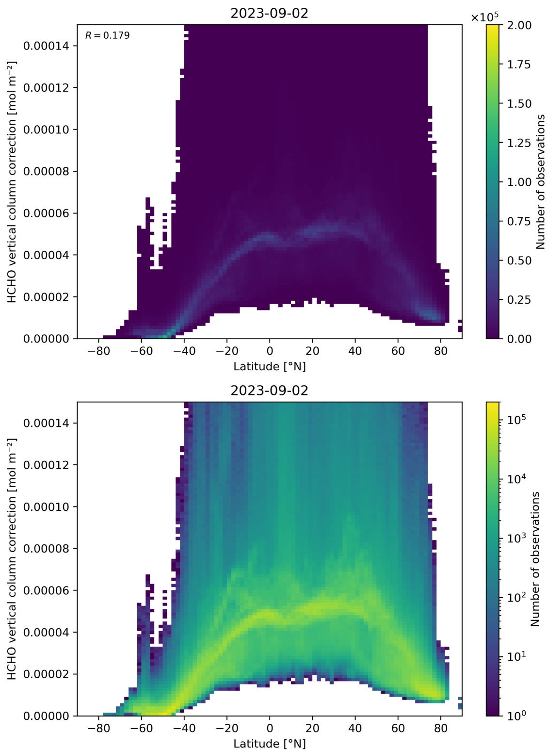
Figure 164: Scatter density plot of “Latitude” against “HCHO vertical column correction” for 2023-09-01 to 2023-09-03.
