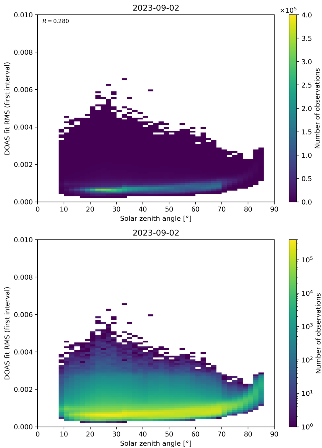
Figure 167: Scatter density plot of “Solar zenith angle” against “DOAS fit RMS (first interval)” for 2023-09-01 to 2023-09-03.
