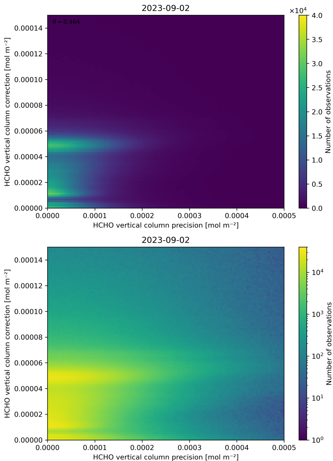
Figure 146: Scatter density plot of “HCHO vertical column precision” against “HCHO vertical column correction” for 2023-09-01 to 2023-09-03.
