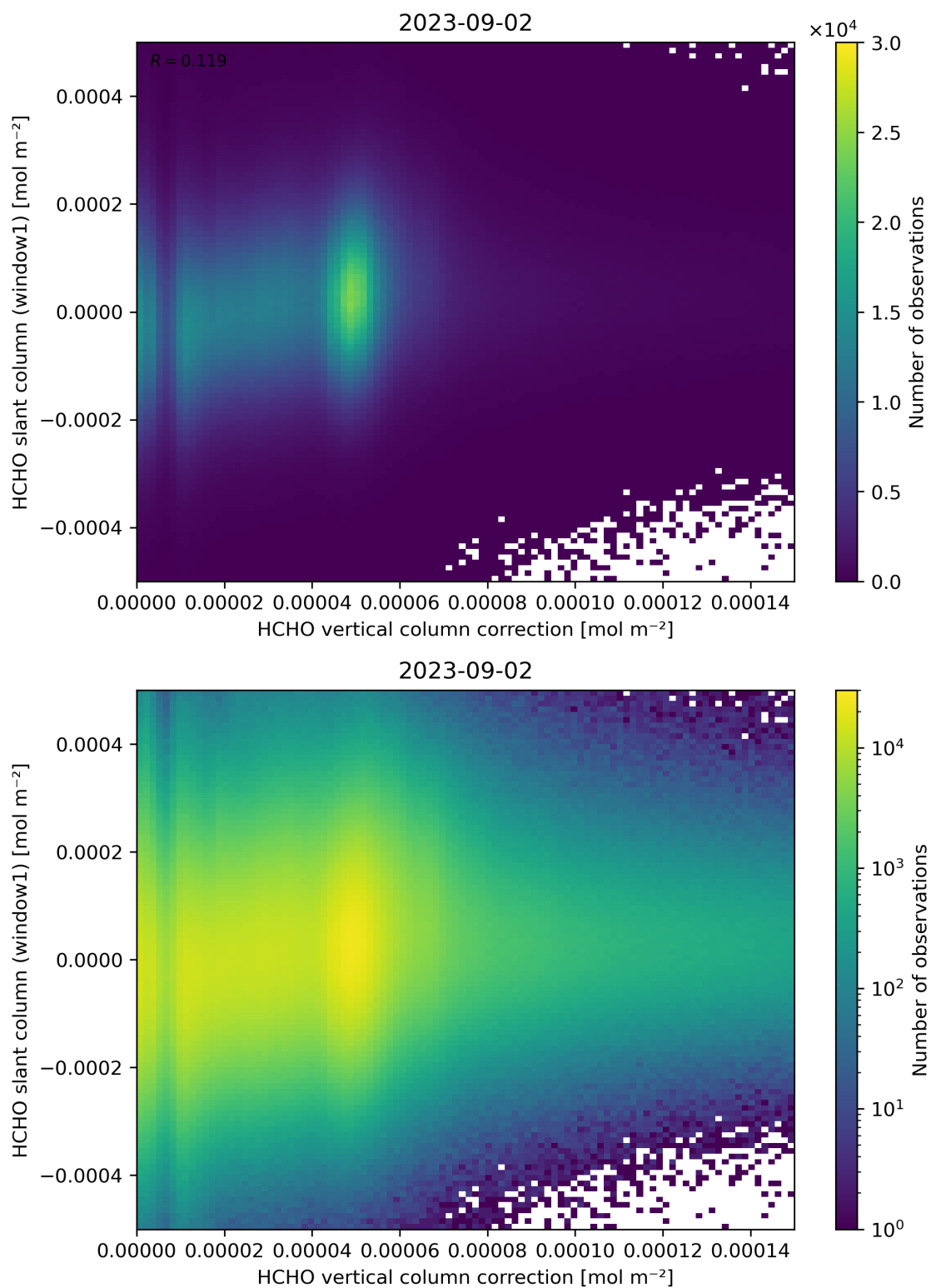
Figure 118: Scatter density plot of “HCHO vertical column correction” against “HCHO slant column (window1)” for 2023-09-01 to 2023-09-03.
