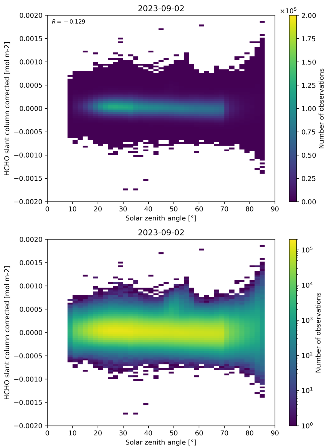
Figure 171: Scatter density plot of “Solar zenith angle” against “HCHO slant column corrected” for 2023-09-01 to 2023-09-03.
