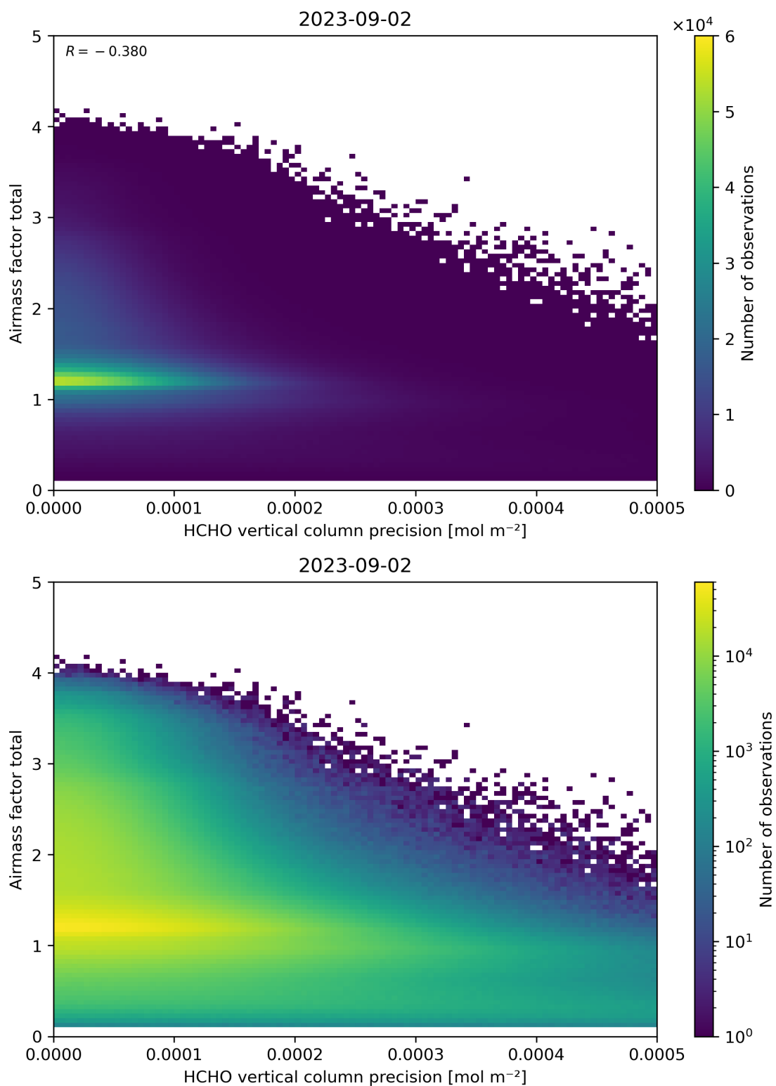
Figure 144: Scatter density plot of “HCHO vertical column precision” against “Airmass factor total” for 2023-09-01 to 2023-09-03.
