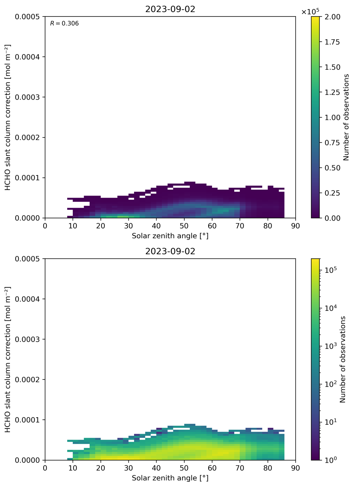
Figure 172: Scatter density plot of “Solar zenith angle” against “HCHO slant column correction” for 2023-09-01 to 2023-09-03.
