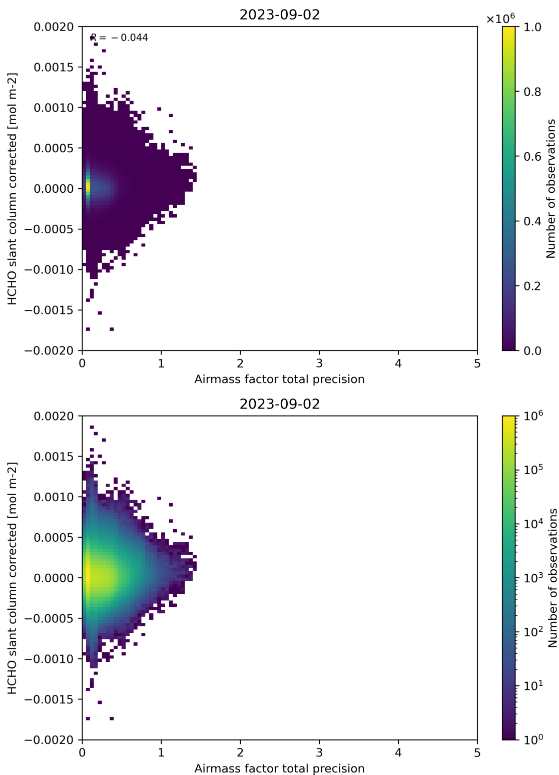
Figure 109: Scatter density plot of “Airmass factor total precision” against “HCHO slant column corrected” for 2023-09-01 to 2023-09-03.
