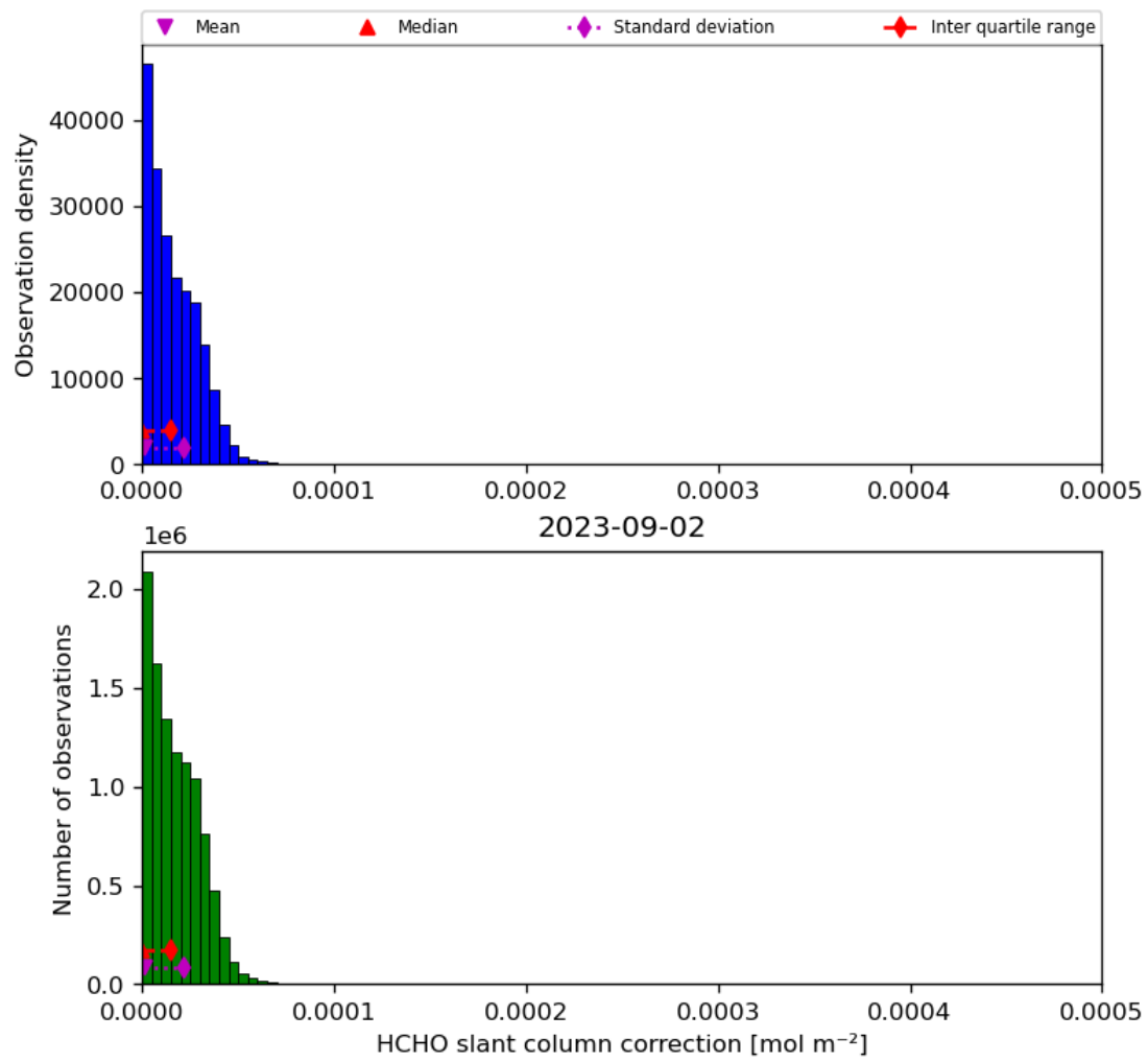
Figure 47: Histogram of “HCHO slant column correction” for 2023-09-01 to 2023-09-03
