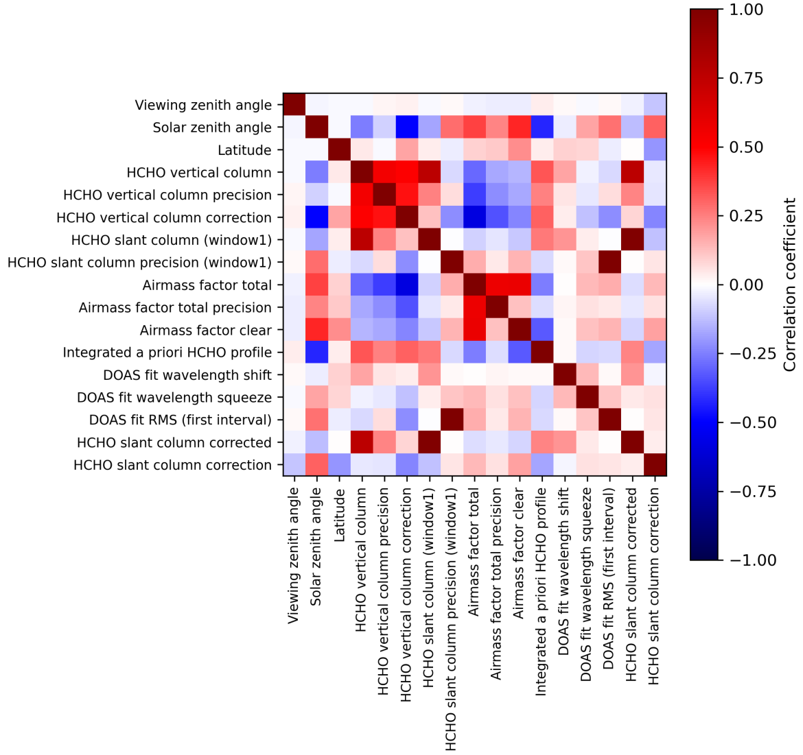
Figure 2: Map of correlation matrix for 2023-09-01 to 2023-09-03.
