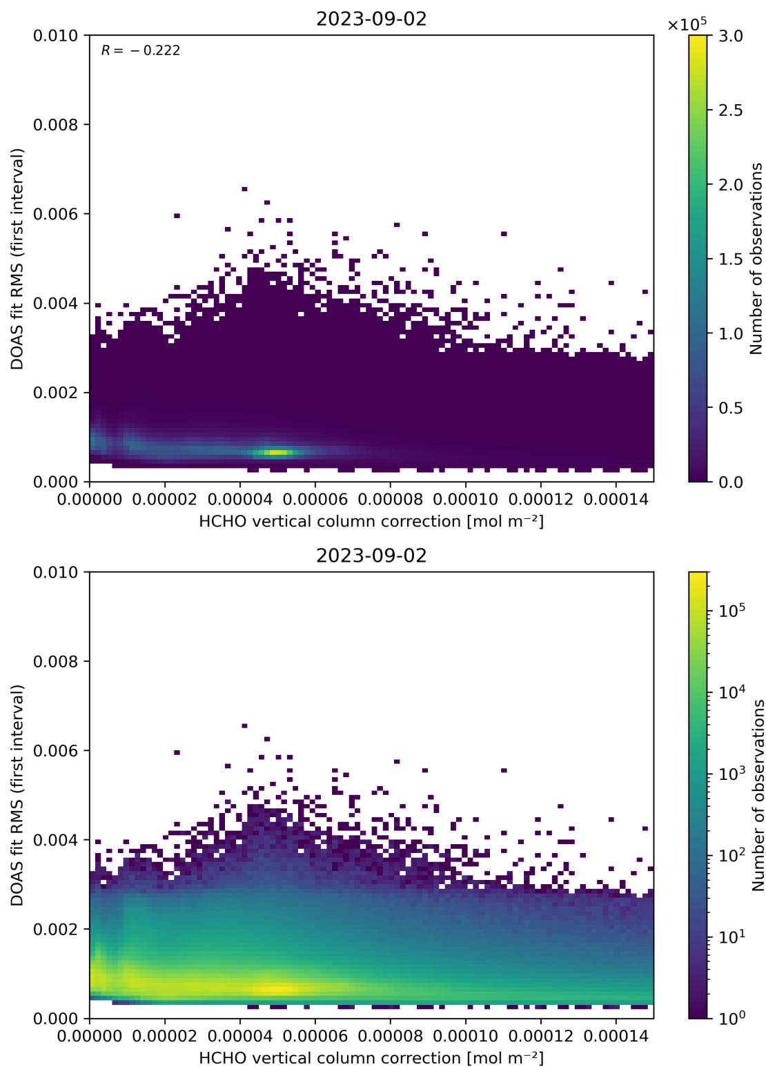
Figure 112: Scatter density plot of “HCHO vertical column correction” against “DOAS fit RMS (first interval)” for 2023-09-01 to 2023-09-03.
