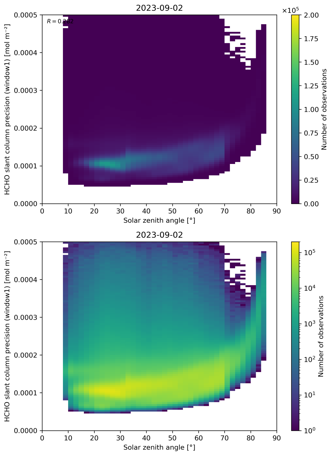
Figure 174: Scatter density plot of “Solar zenith angle” against “HCHO slant column precision (window1)” for 2023-09-01 to 2023-09-03.
