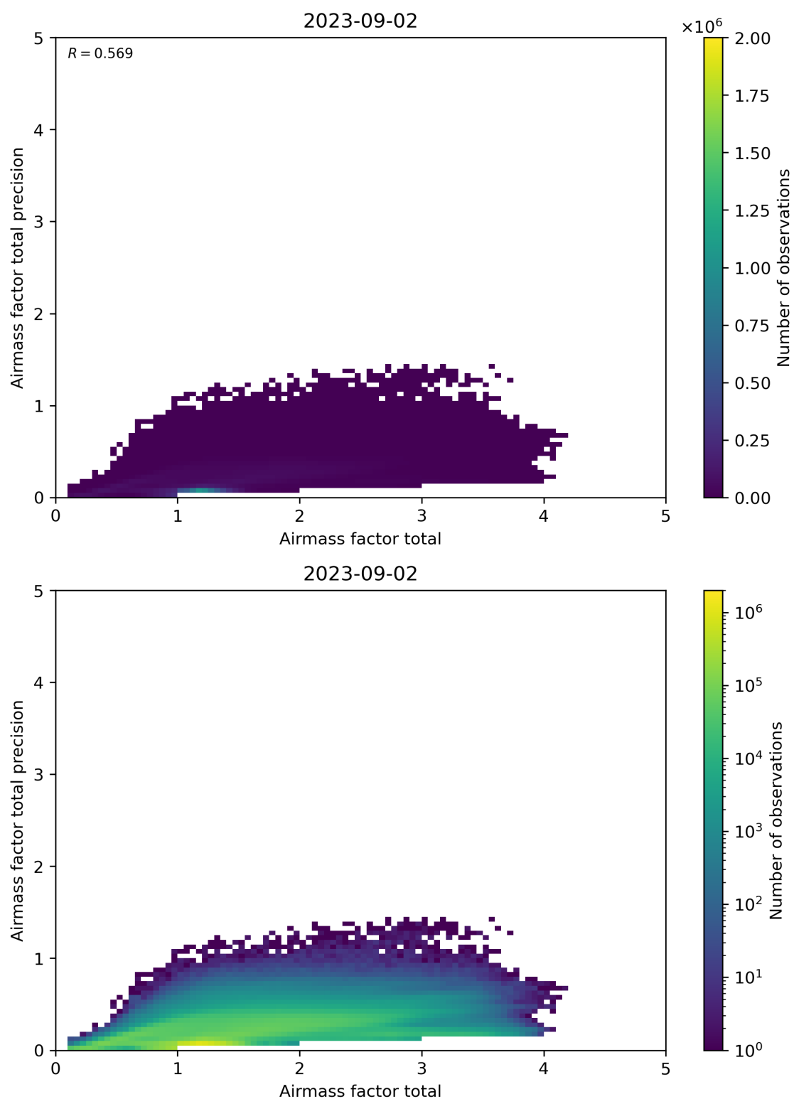
Figure 103: Scatter density plot of “Airmass factor total” against “Airmass factor total precision” for 2023-09-01 to 2023-09-03.
