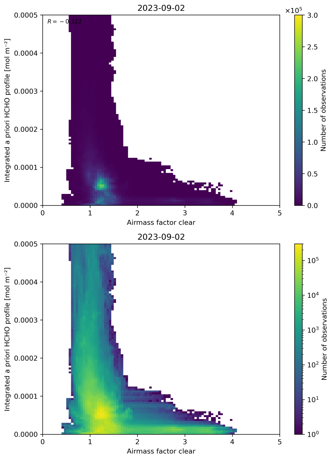
Figure 76: Scatter density plot of “Airmass factor clear” against “Integrated a priori HCHO profile” for 2023-09-01 to 2023-09-03.
