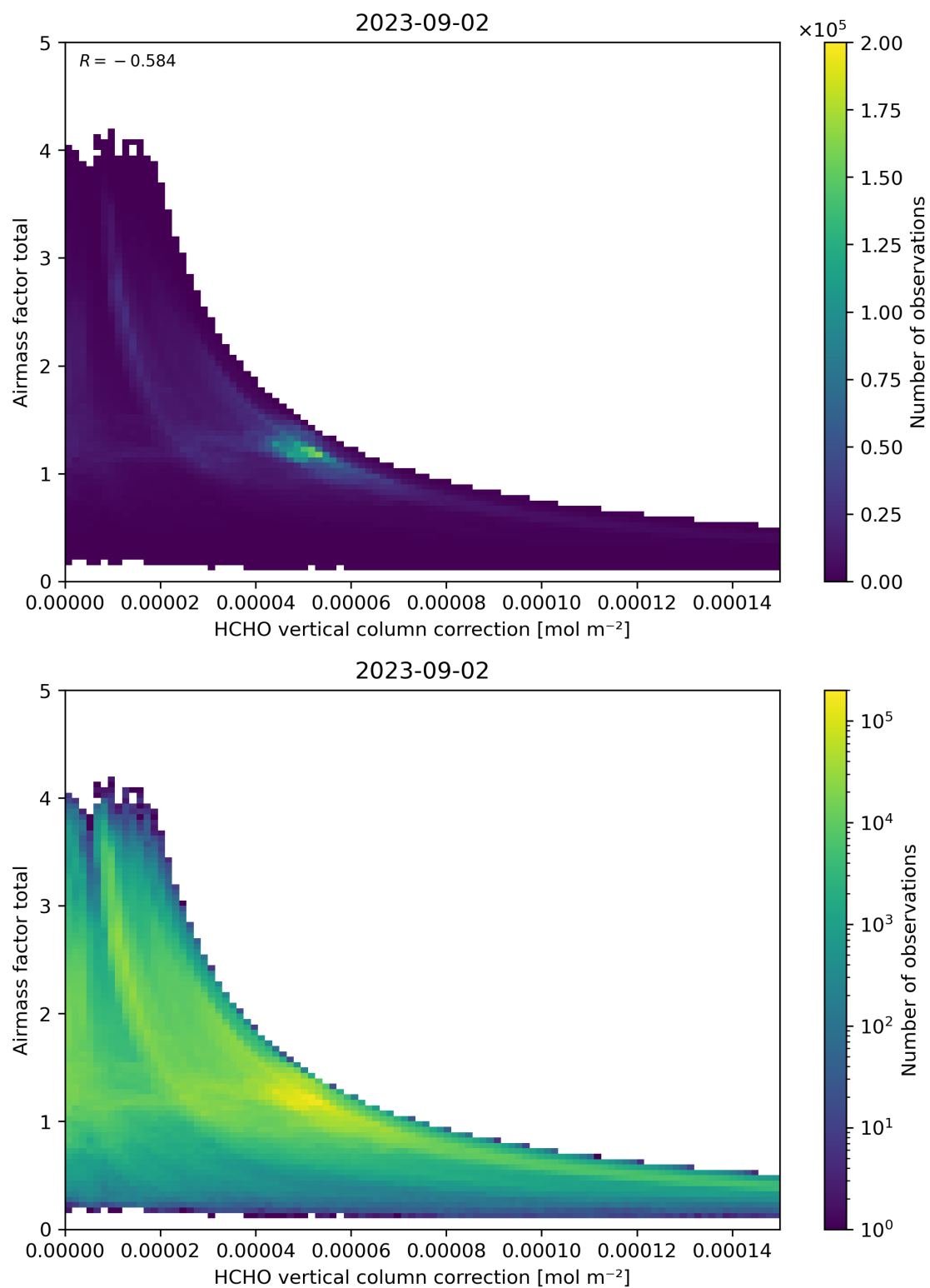
Figure 120: Scatter density plot of “HCHO vertical column correction” against “Airmass factor total” for 2023-09-01 to 2023-09-03.
