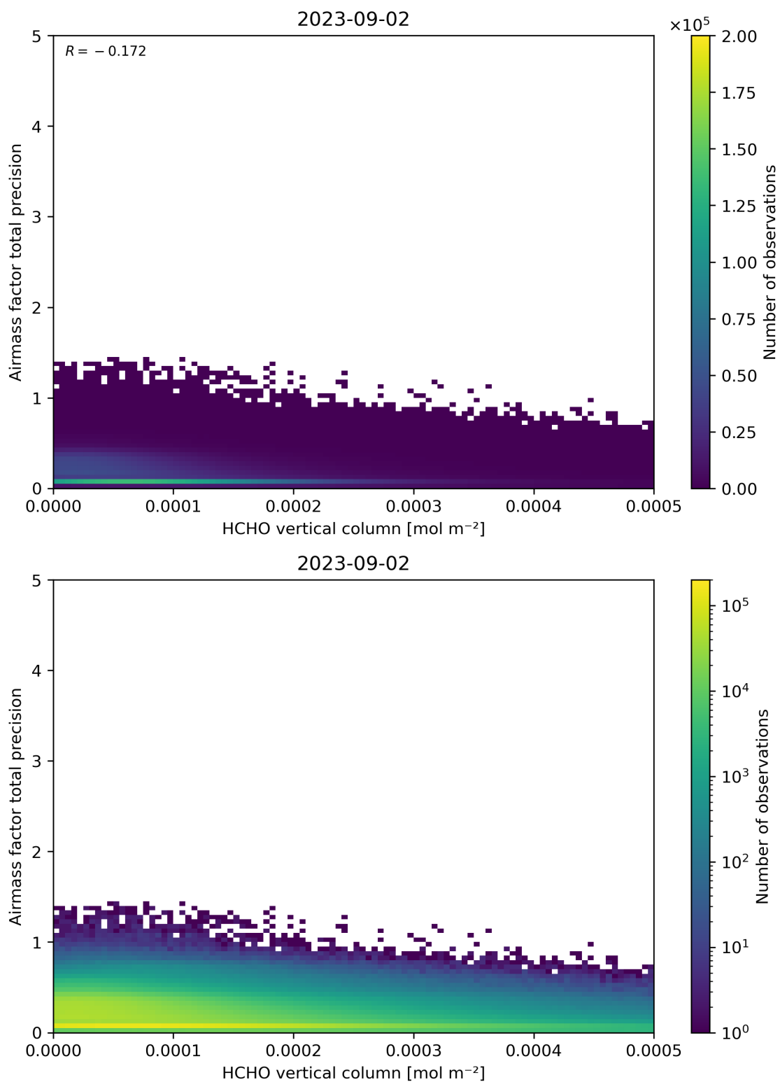
Figure 132: Scatter density plot of “HCHO vertical column” against “Airmass factor total precision” for 2023-09-01 to 2023-09-03.
