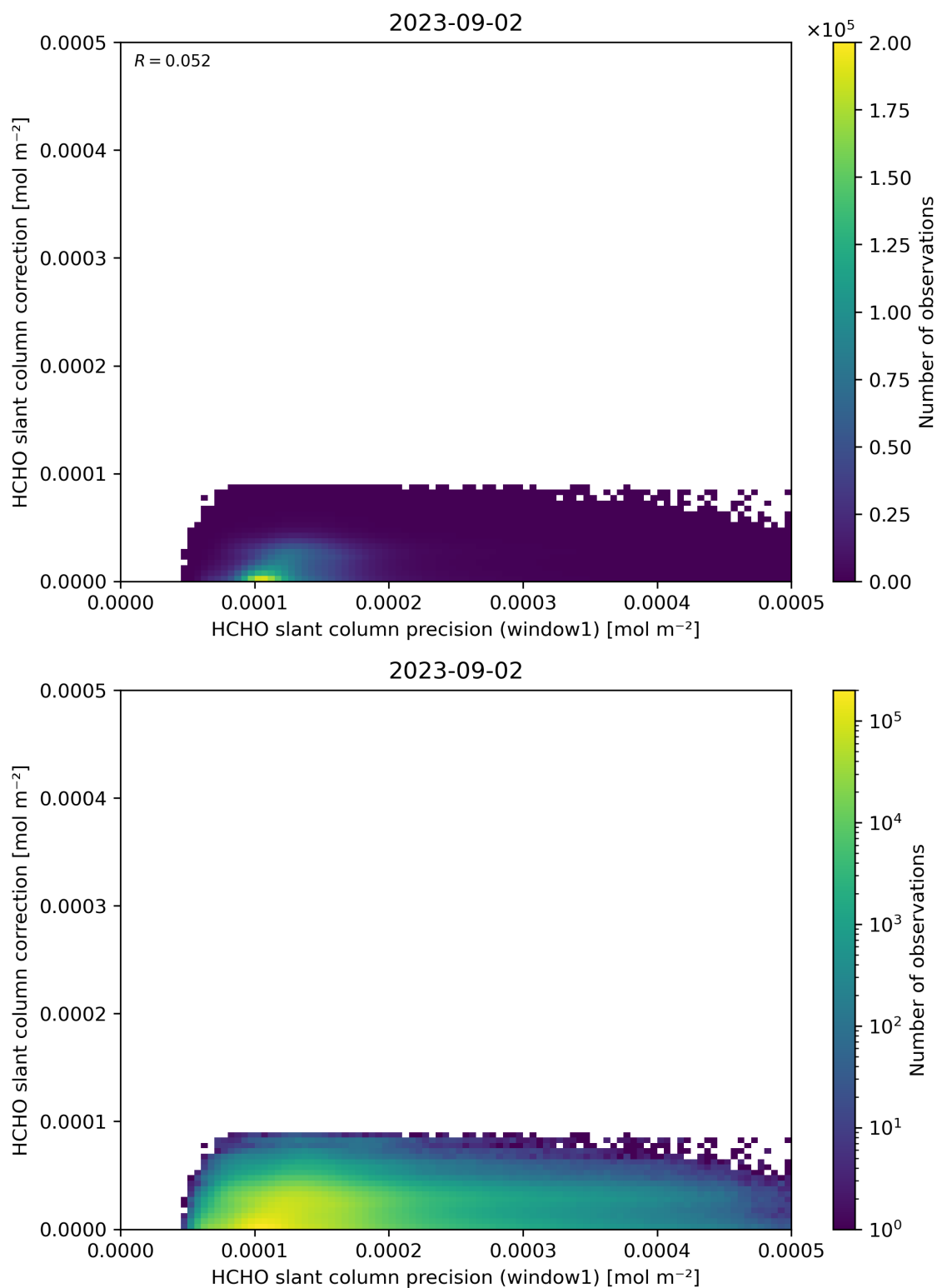
Figure 93: Scatter density plot of “HCHO slant column precision (window1)” against “HCHO slant column correction” for 2023-09-01 to 2023-09-03.
