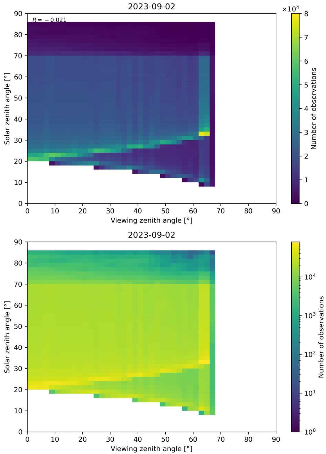
Figure 197: Scatter density plot of “Viewing zenith angle” against “Solar zenith angle” for 2023-09-01 to 2023-09-03.
