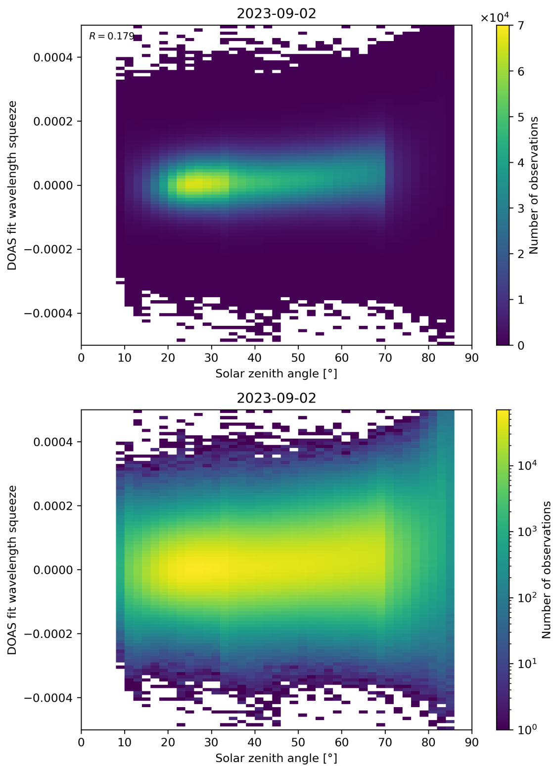
Figure 169: Scatter density plot of “Solar zenith angle” against “DOAS fit wavelength squeeze” for 2023-09-01 to 2023-09-03.
