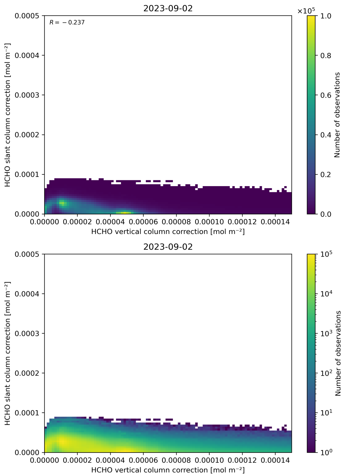
Figure 117: Scatter density plot of “HCHO vertical column correction” against “HCHO slant column correction” for 2023-09-01 to 2023-09-03.
