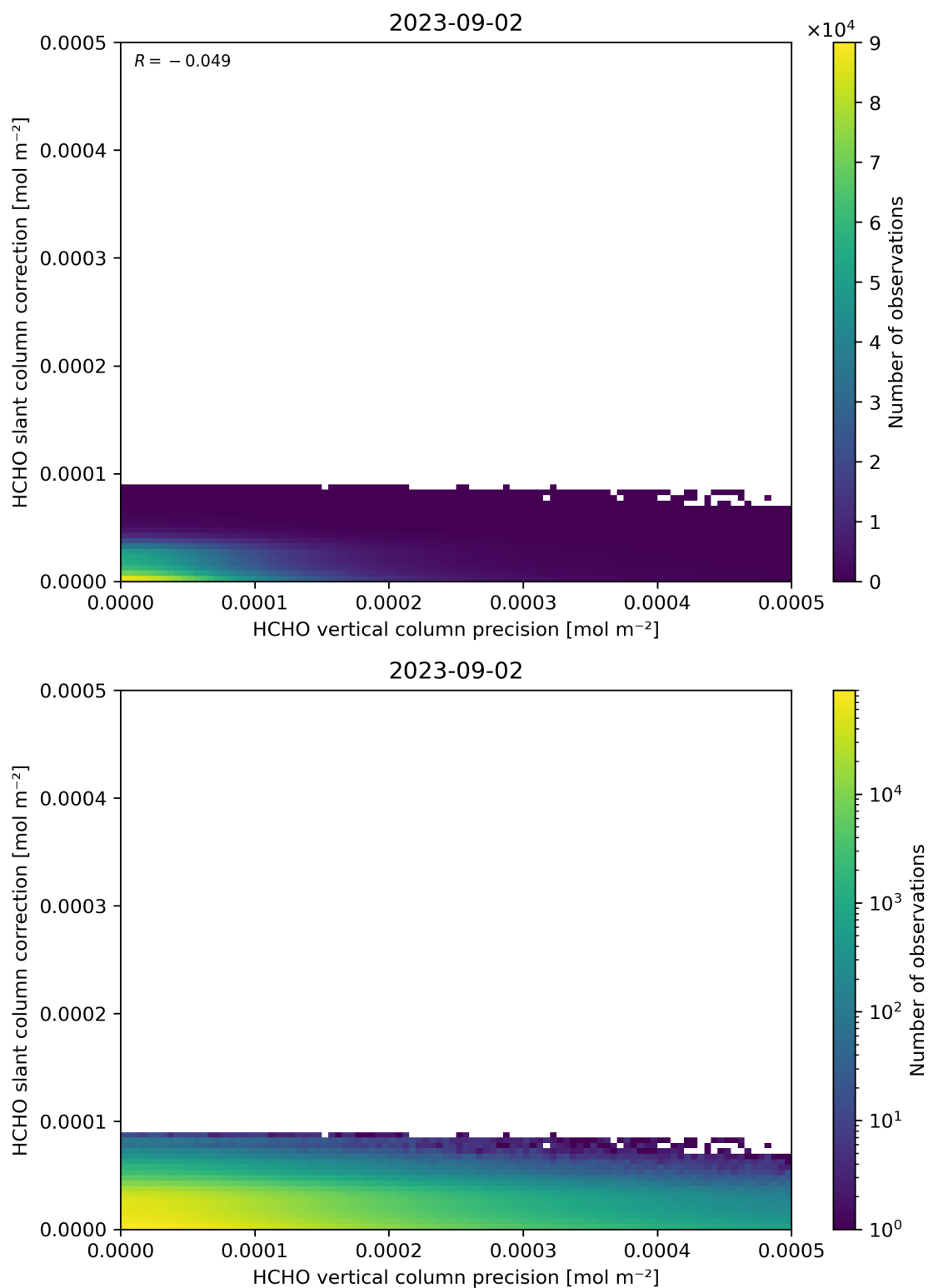
Figure 141: Scatter density plot of “HCHO vertical column precision” against “HCHO slant column correction” for 2023-09-01 to 2023-09-03.
