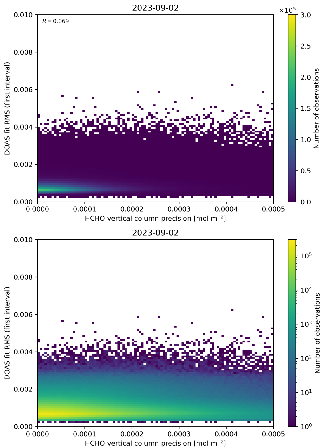
Figure 136: Scatter density plot of “HCHO vertical column precision” against “DOAS fit RMS (first interval)” for 2023-09-01 to 2023-09-03.
