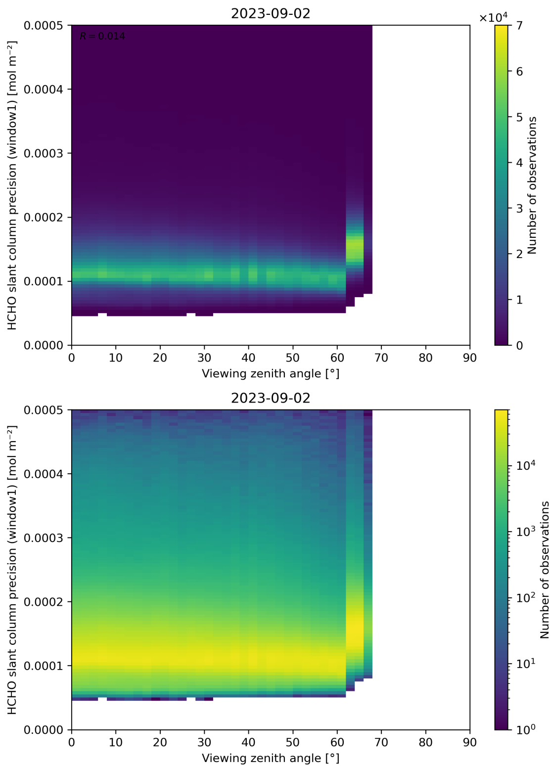
Figure 189: Scatter density plot of “Viewing zenith angle” against “HCHO slant column precision (window1)” for 2023-09-01 to 2023-09-03.
