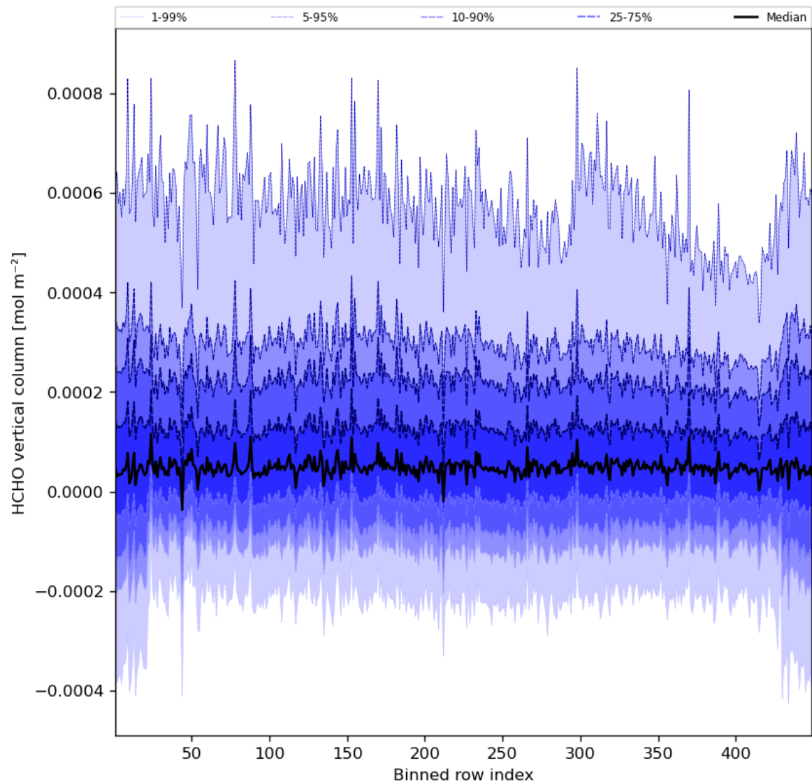
Figure 49: Along track statistics of “HCHO vertical column” for 2023-09-01 to 2023-09-03
