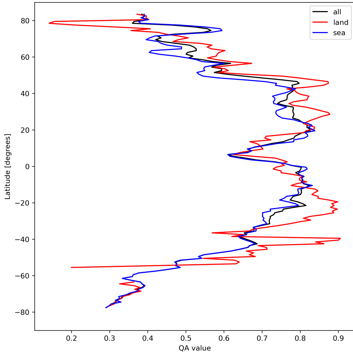
Figure 20: Zonal average of “QA value” for 2023-09-01 to 2023-09-03.
