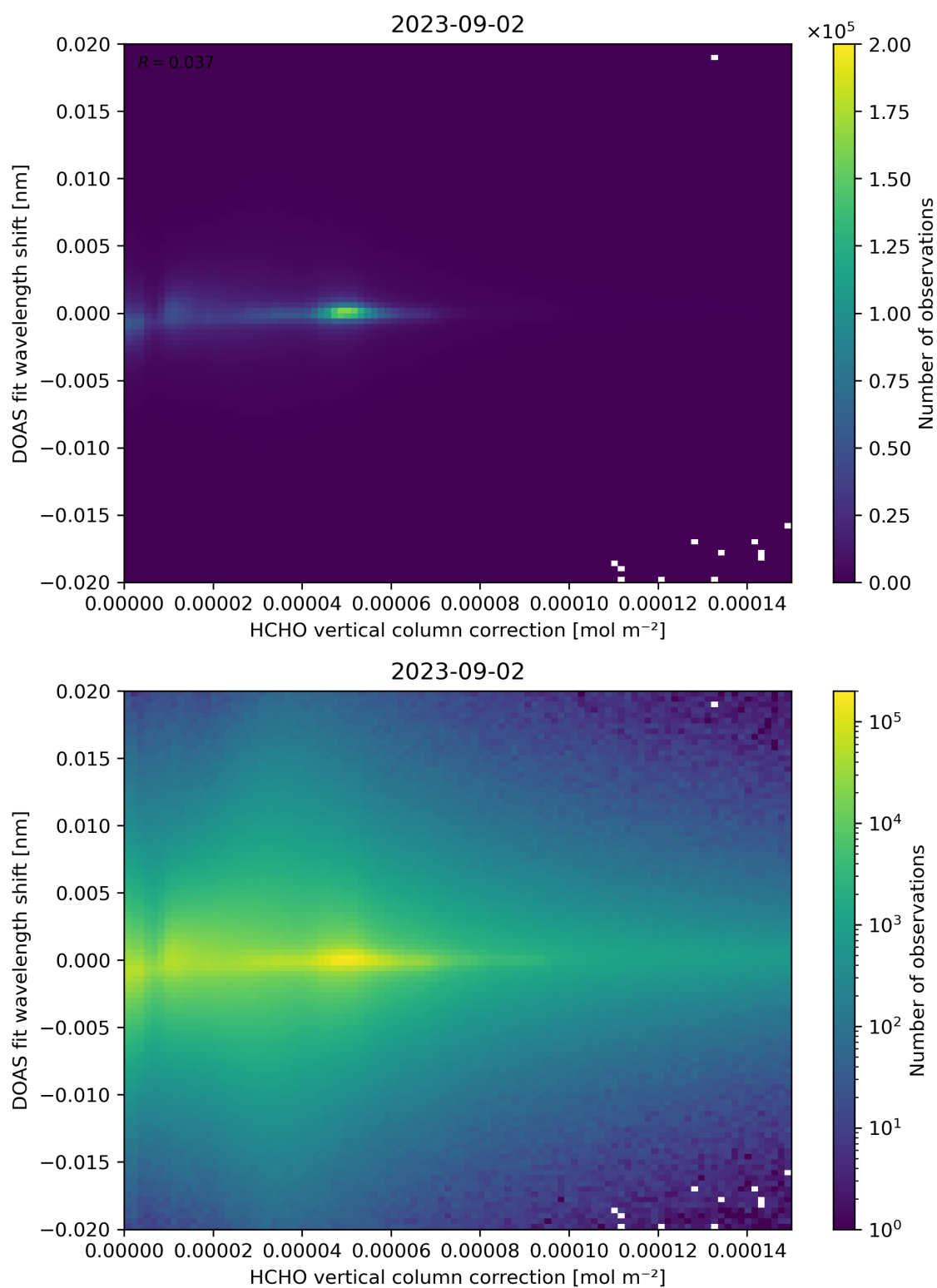
Figure 113: Scatter density plot of “HCHO vertical column correction” against “DOAS fit wavelength shift” for 2023-09-01 to 2023-09-03.
