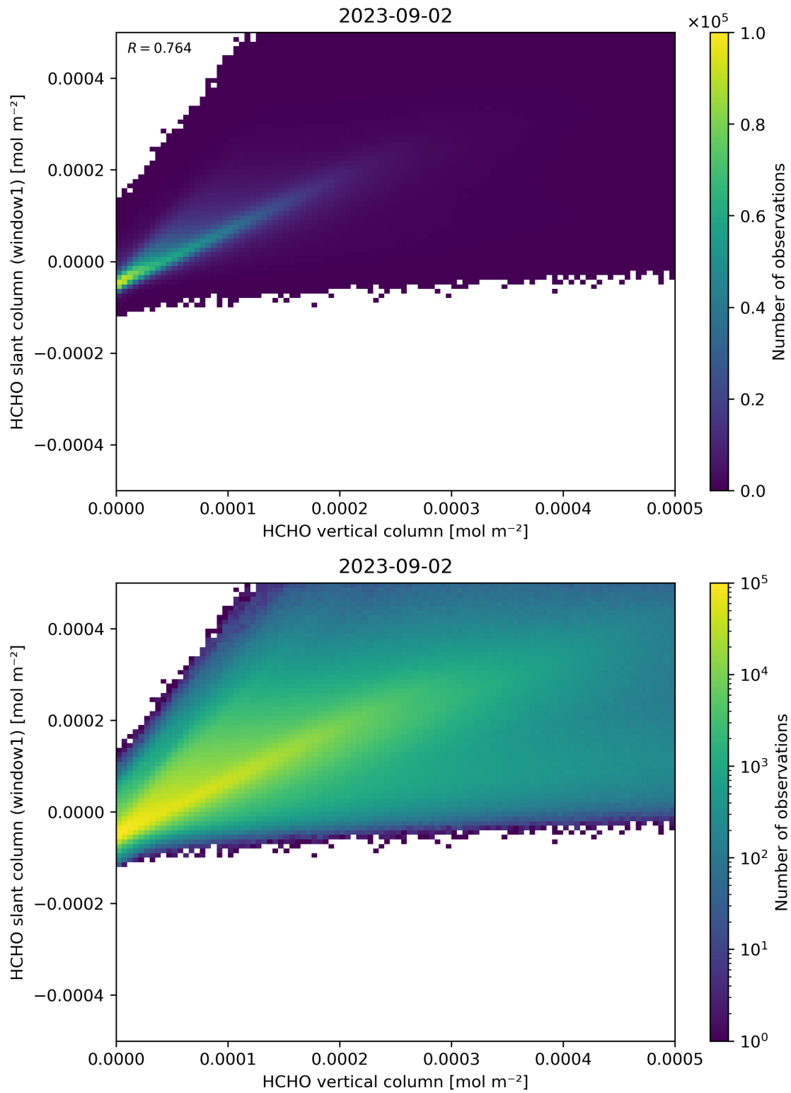
Figure 129: Scatter density plot of “HCHO vertical column” against “HCHO slant column (window1)” for 2023-09-01 to 2023-09-03.
