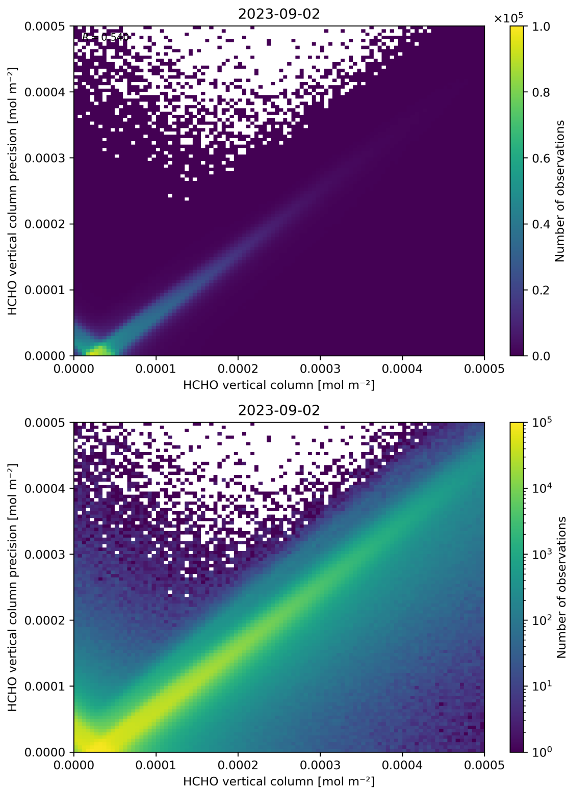
Figure 134: Scatter density plot of “HCHO vertical column” against “HCHO vertical column precision” for 2023-09-01 to 2023-09-03.
