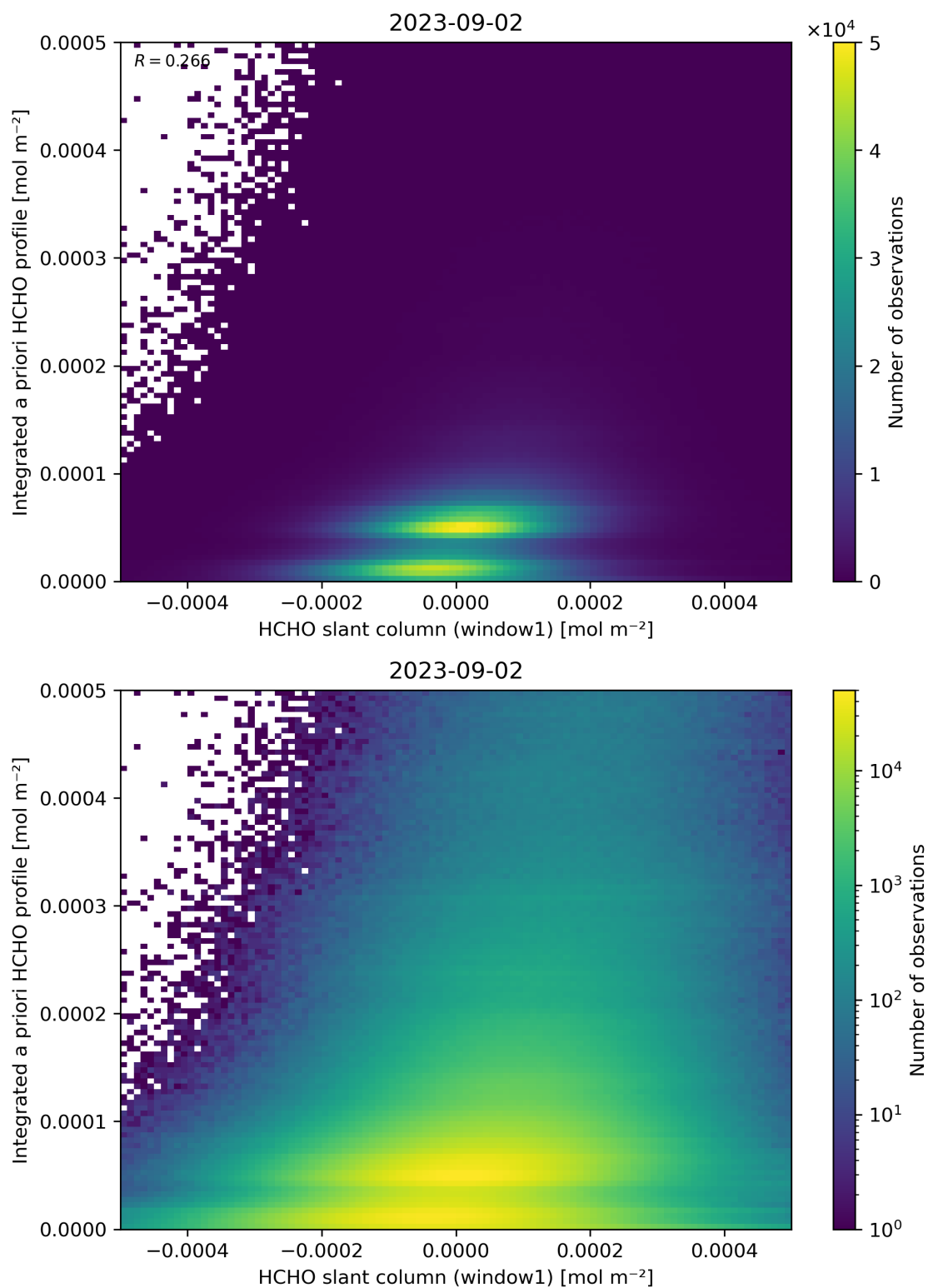
Figure 87: Scatter density plot of “HCHO slant column (window1)” against “Integrated a priori HCHO profile” for 2023-09-01 to 2023-09-03.
