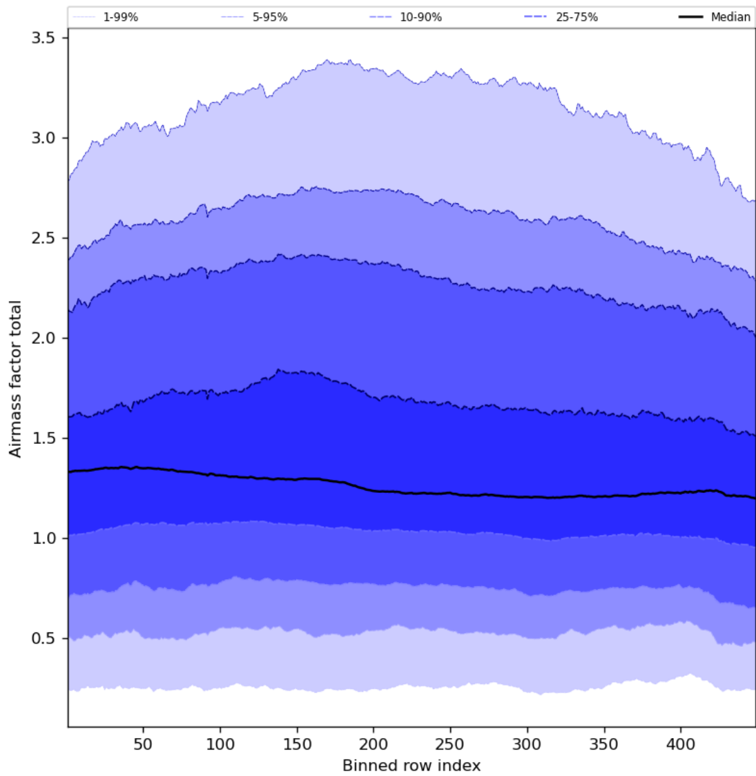
Figure 54: Along track statistics of “Airmass factor total” for 2023-09-01 to 2023-09-03
