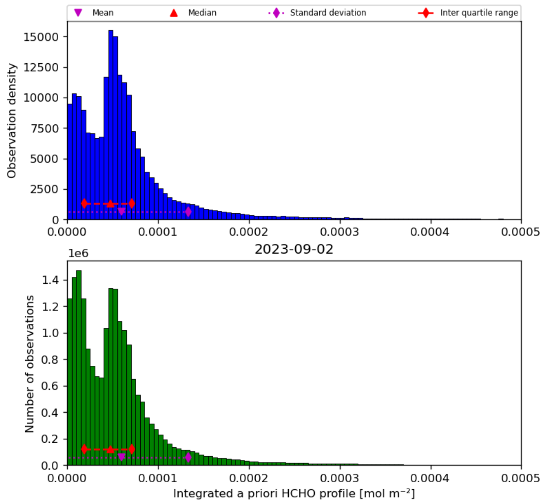
Figure 43: Histogram of “Integrated a priori HCHO profile” for 2023-09-01 to 2023-09-03
