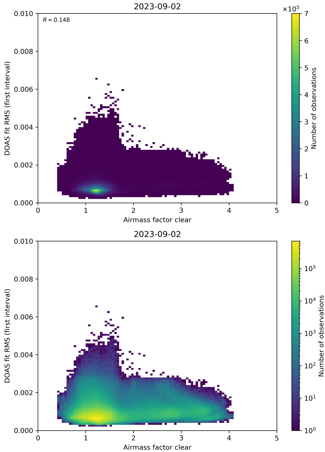
Figure 71: Scatter density plot of “Airmass factor clear” against “DOAS fit RMS (first interval)” for 2023-09-01 to 2023-09-03.
