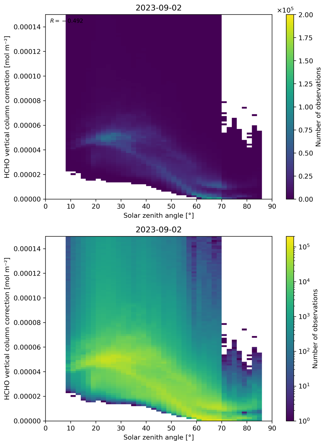
Figure 178: Scatter density plot of “Solar zenith angle” against “HCHO vertical column correction” for 2023-09-01 to 2023-09-03.
