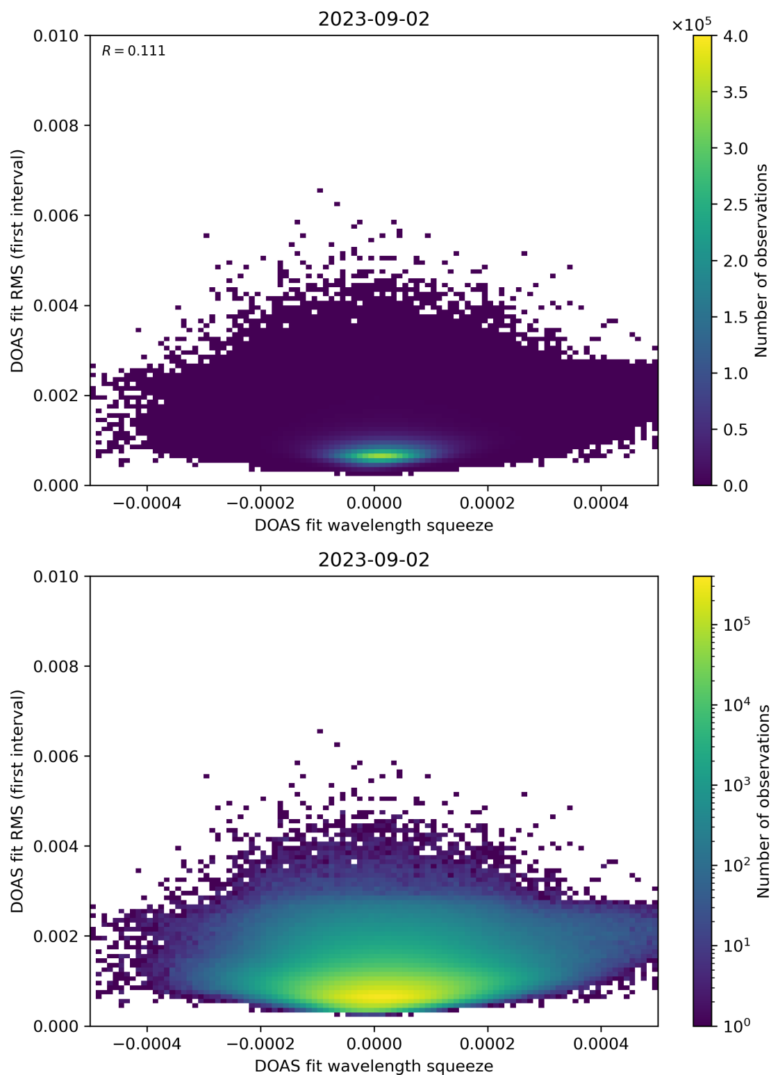
Figure 68: Scatter density plot of “DOAS fit wavelength squeeze” against “DOAS fit RMS (first interval)” for 2023-09-01 to 2023-09-03.
