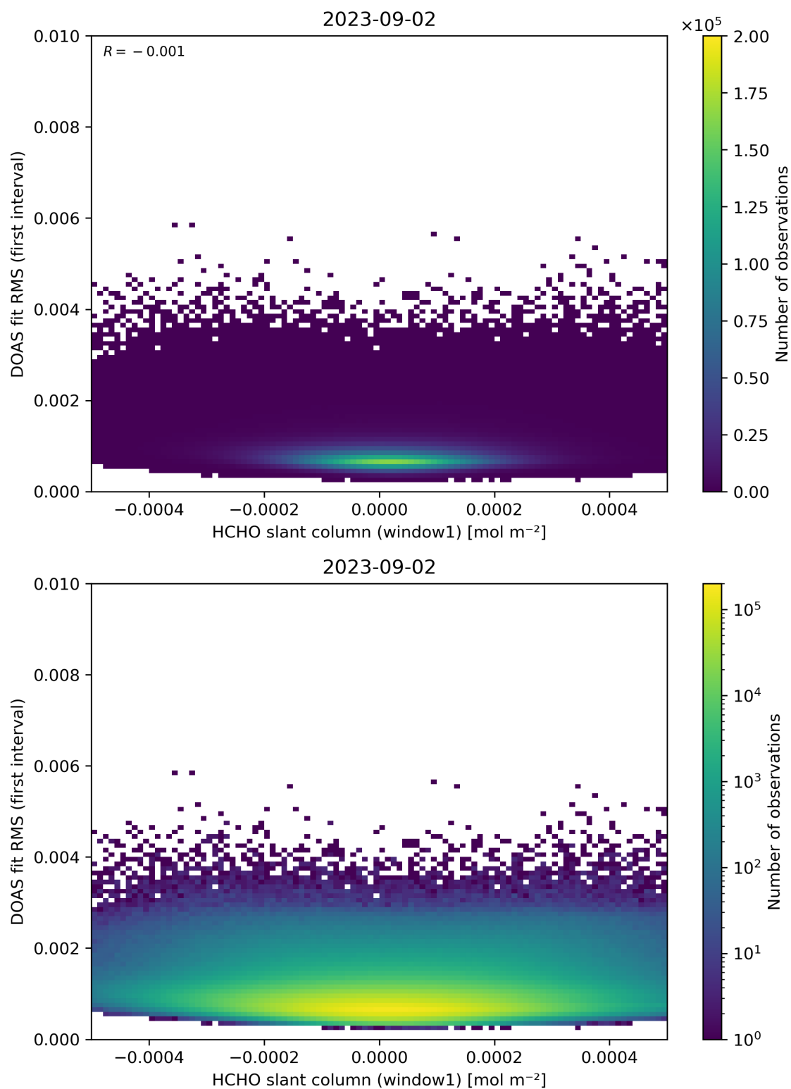
Figure 78: Scatter density plot of “HCHO slant column (window1)” against “DOAS fit RMS (first interval)” for 2023-09-01 to 2023-09-03.
