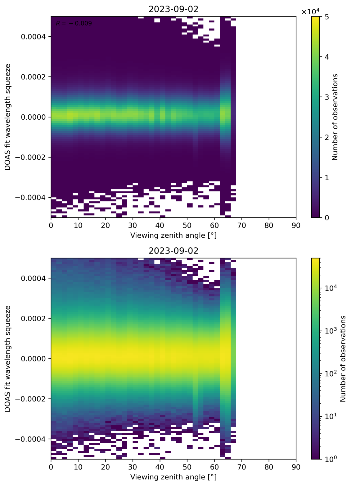
Figure 184: Scatter density plot of “Viewing zenith angle” against “DOAS fit wavelength squeeze” for 2023-09-01 to 2023-09-03.
