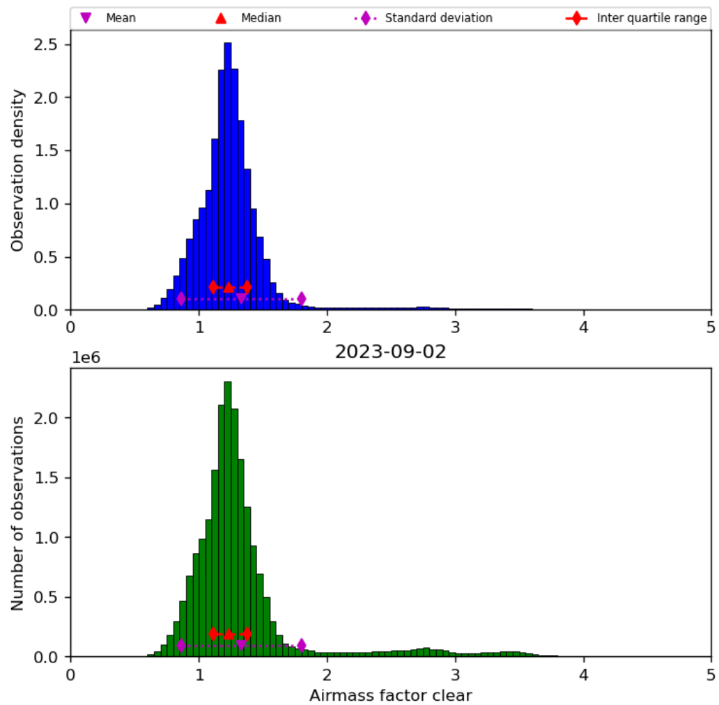
Figure 42: Histogram of “Airmass factor clear” for 2023-09-01 to 2023-09-03
