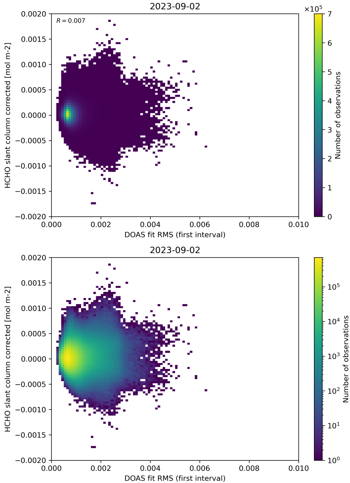
Figure 62: Scatter density plot of “DOAS fit RMS (first interval)” against “HCHO slant column corrected” for 2023-09-01 to 2023-09-03.
