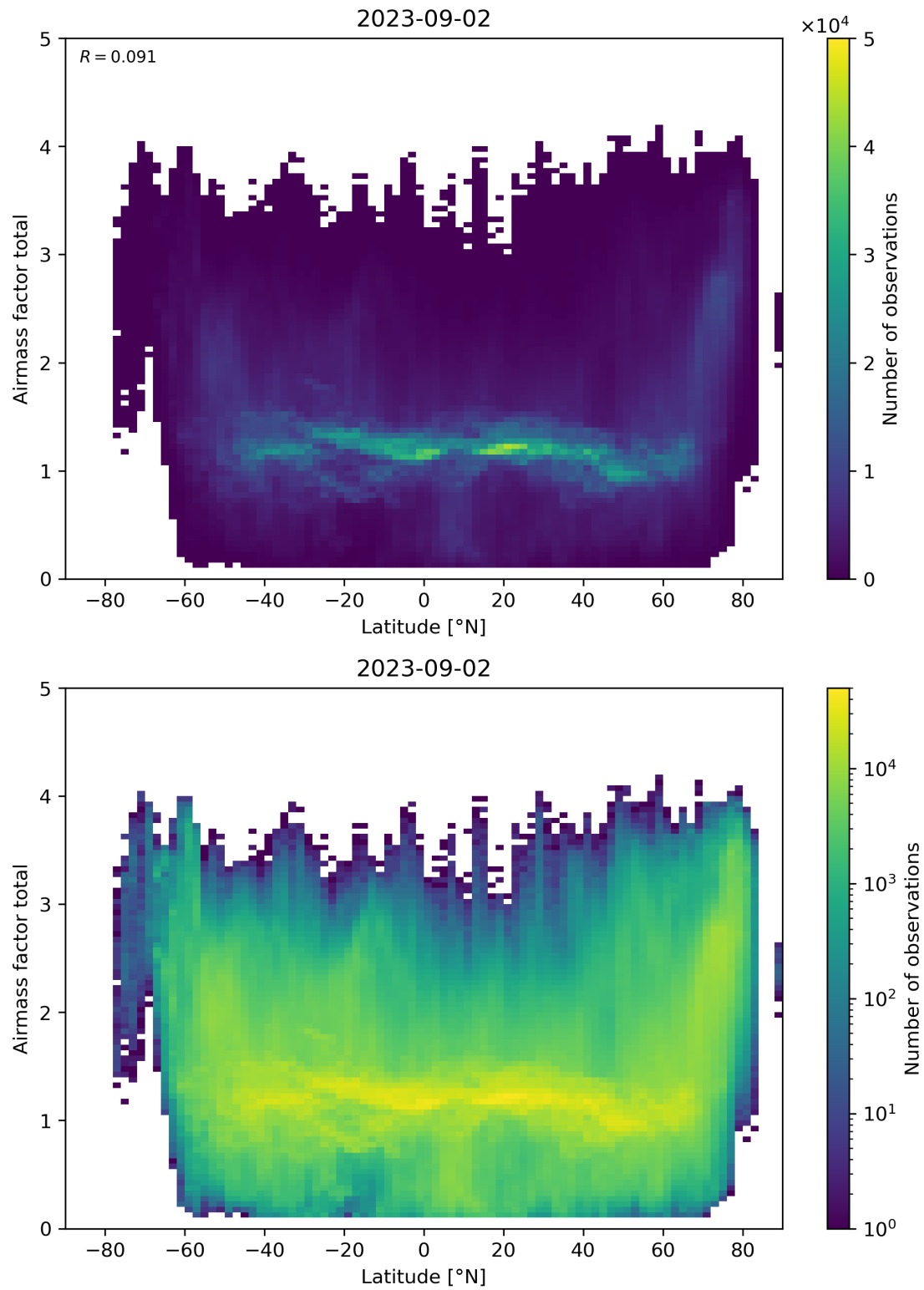
Figure 161: Scatter density plot of “Latitude” against “Airmass factor total” for 2023-09-01 to 2023-09-03.
