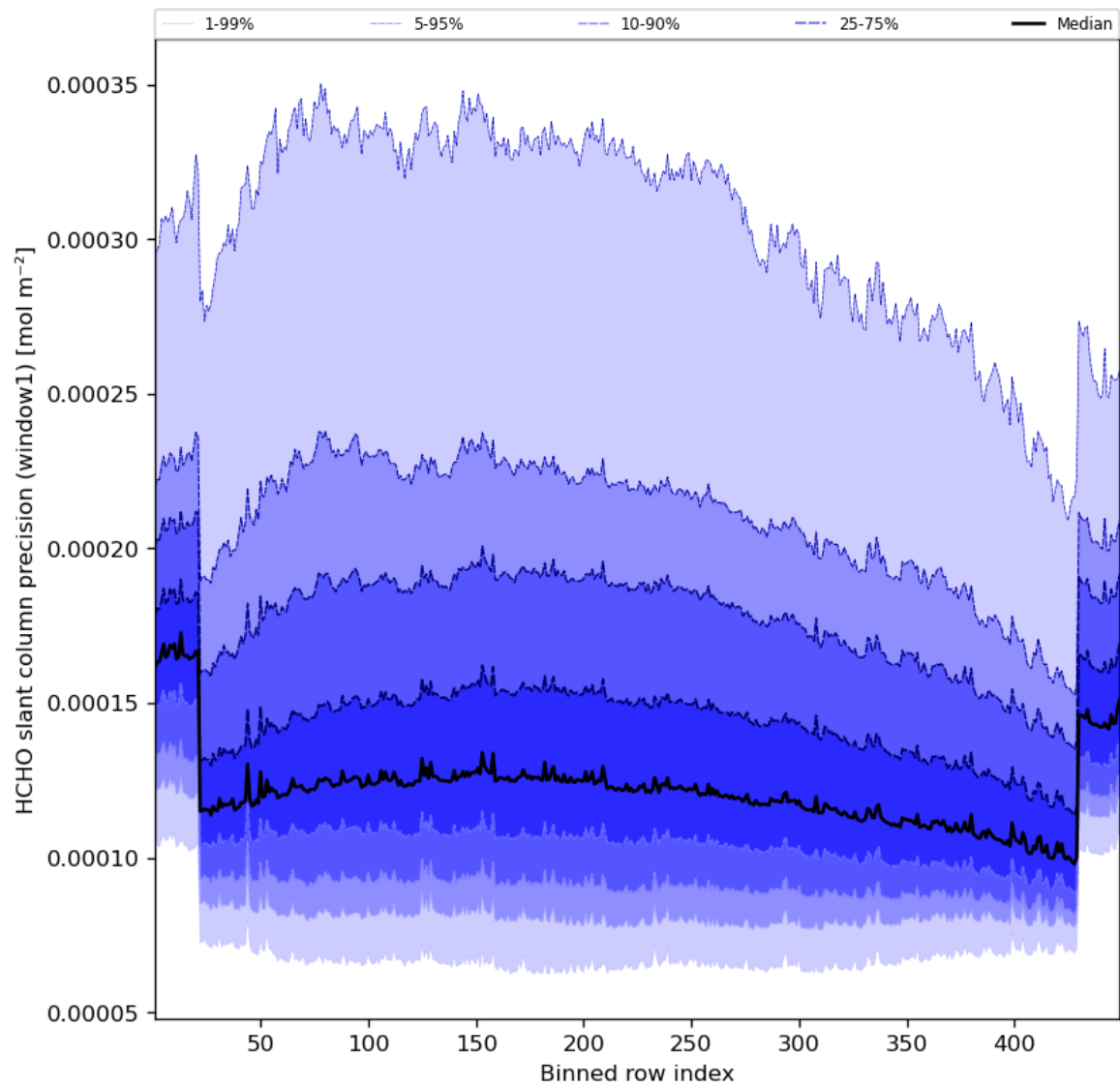
Figure 53: Along track statistics of “HCHO slant column precision (window1)” for 2023-09-01 to 2023-09-03
