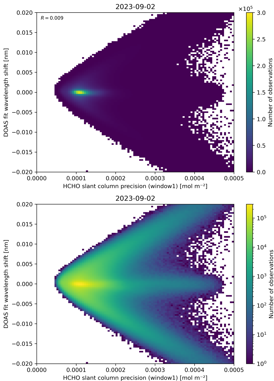
Figure 89: Scatter density plot of “HCHO slant column precision (window1)” against “DOAS fit wavelength shift” for 2023-09-01 to 2023-09-03.
