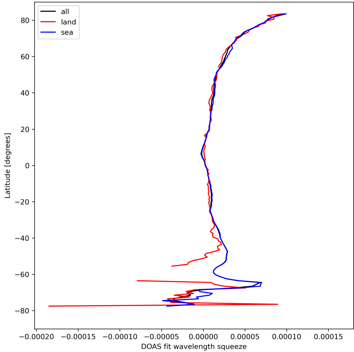
Figure 31: Zonal average of “DOAS fit wavelength squeeze” for 2023-09-01 to 2023-09-03.
