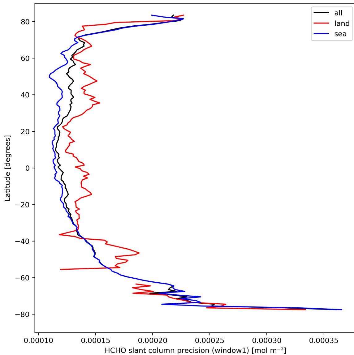
Figure 25: Zonal average of “HCHO slant column precision (window1)” for 2023-09-01 to 2023-09-03.
