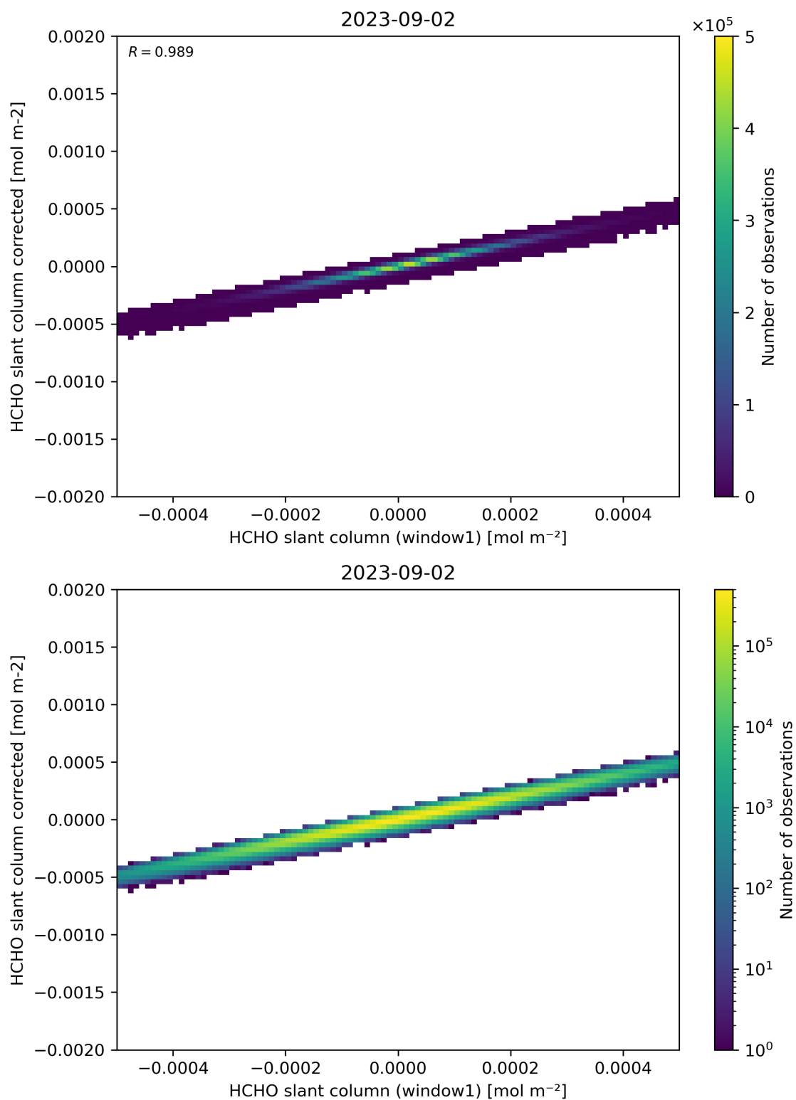
Figure 82: Scatter density plot of “HCHO slant column (window1)” against “HCHO slant column corrected” for 2023-09-01 to 2023-09-03.
