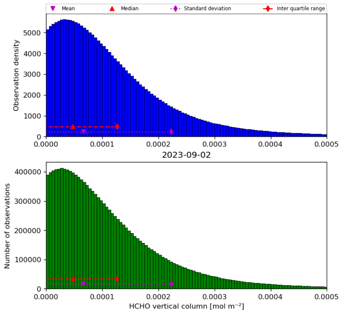
Figure 35: Histogram of “HCHO vertical column” for 2023-09-01 to 2023-09-03
