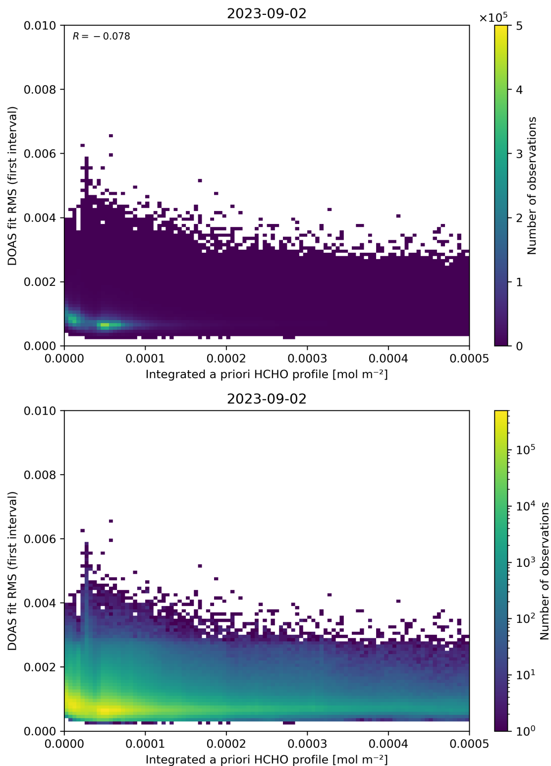
Figure 148: Scatter density plot of “Integrated a priori HCHO profile” against “DOAS fit RMS (first interval)” for 2023-09-01 to 2023-09-03.
