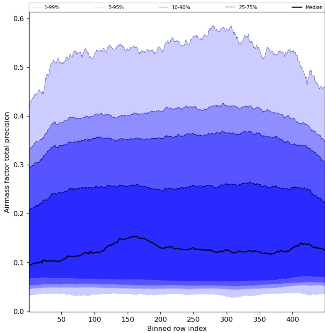
Figure 55: Along track statistics of “Airmass factor total precision” for 2023-09-01 to 2023-09-03
