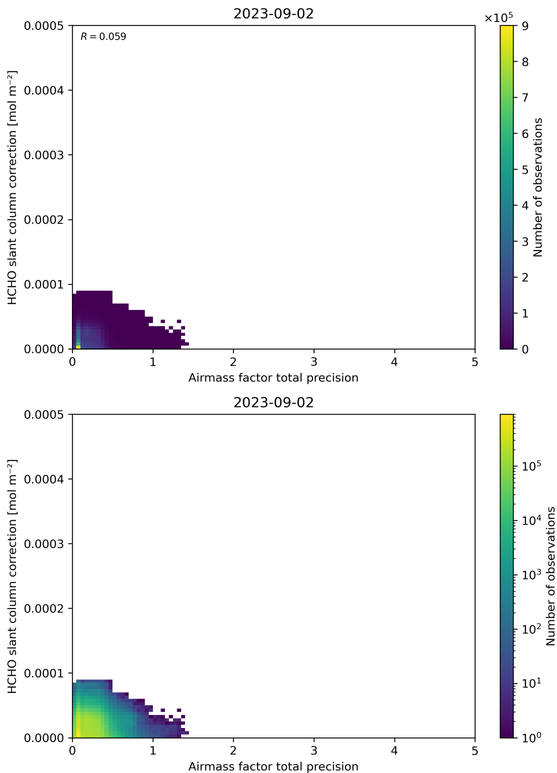
Figure 110: Scatter density plot of “Airmass factor total precision” against “HCHO slant column correction” for 2023-09-01 to 2023-09-03.
