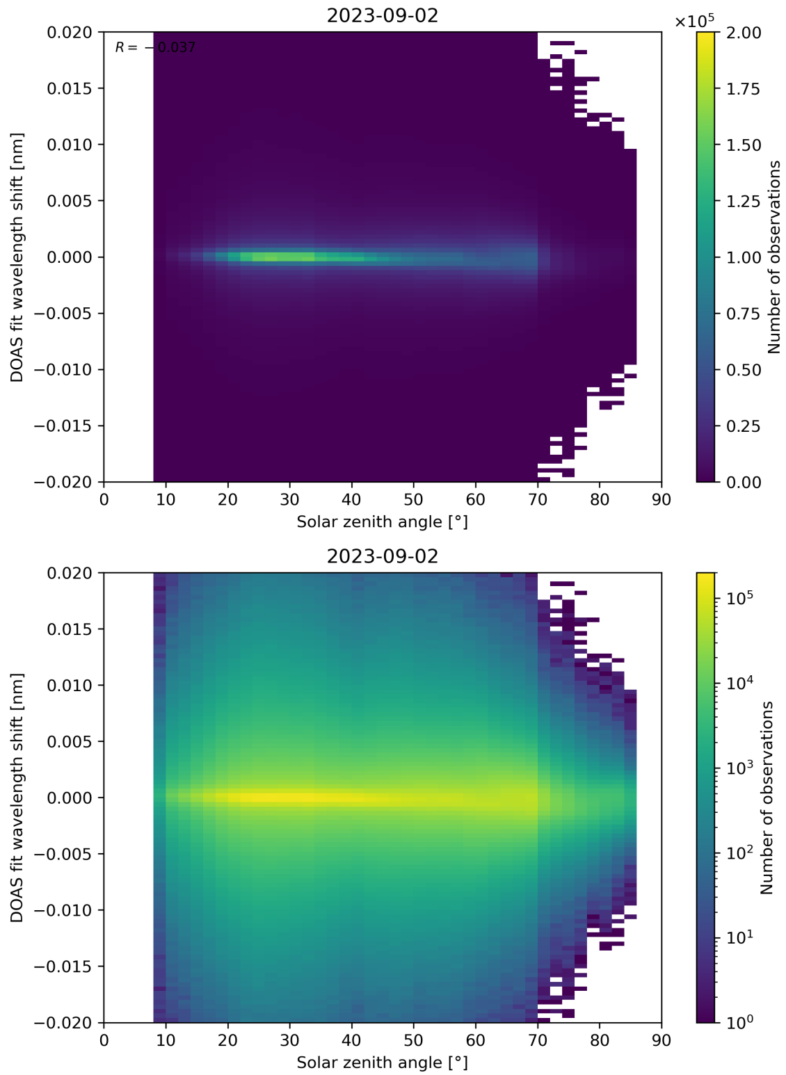
Figure 168: Scatter density plot of “Solar zenith angle” against “DOAS fit wavelength shift” for 2023-09-01 to 2023-09-03.
