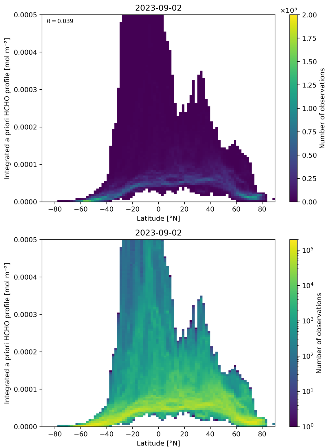
Figure 166: Scatter density plot of “Latitude” against “Integrated a priori HCHO profile” for 2023-09-01 to 2023-09-03.
