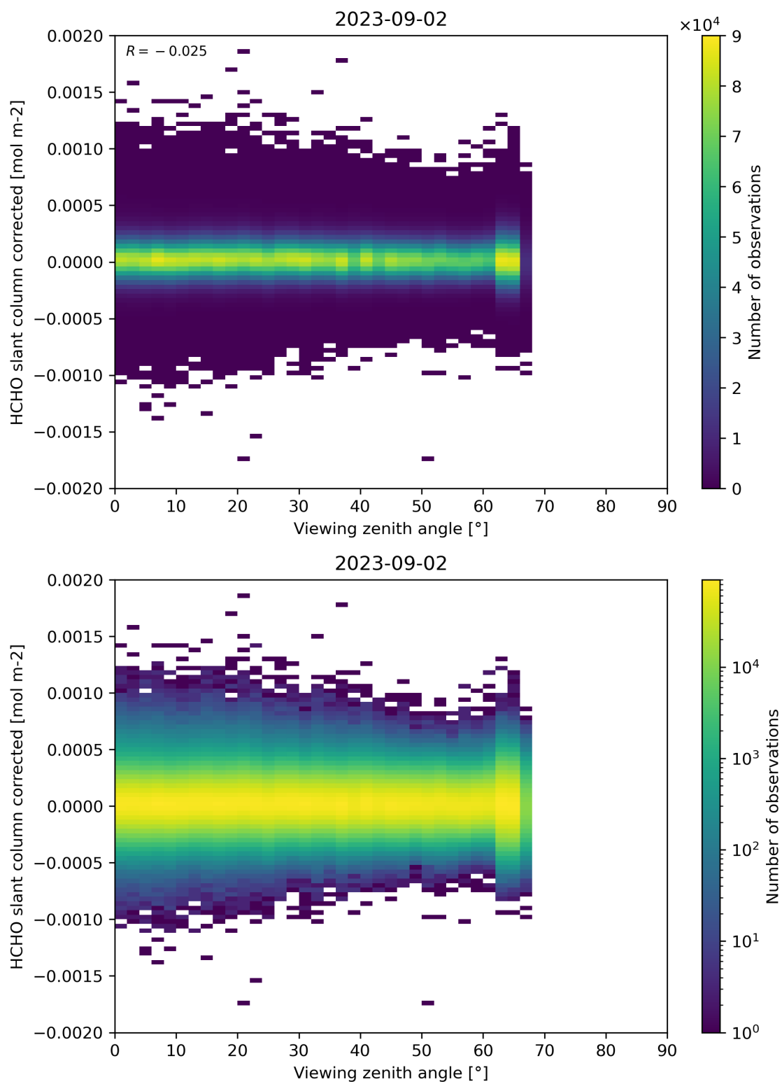
Figure 186: Scatter density plot of “Viewing zenith angle” against “HCHO slant column corrected” for 2023-09-01 to 2023-09-03.
