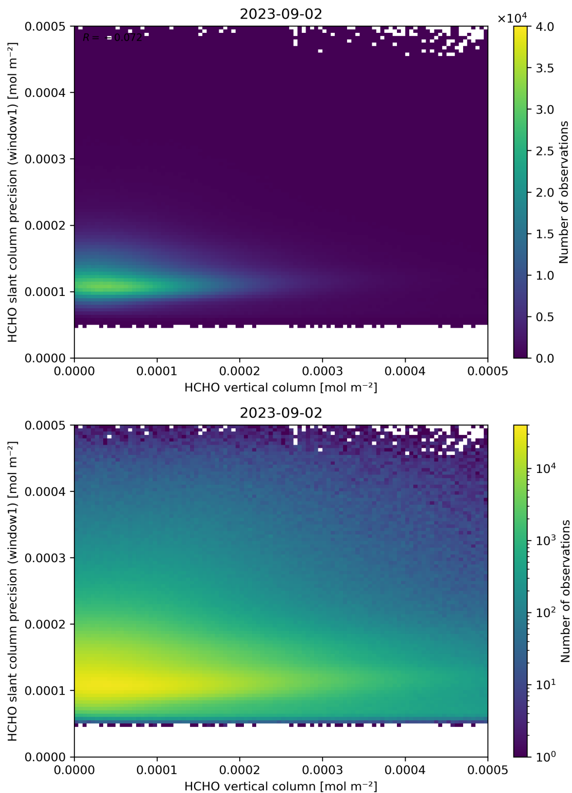
Figure 130: Scatter density plot of “HCHO vertical column” against “HCHO slant column precision (window1)” for 2023-09-01 to 2023-09-03.
