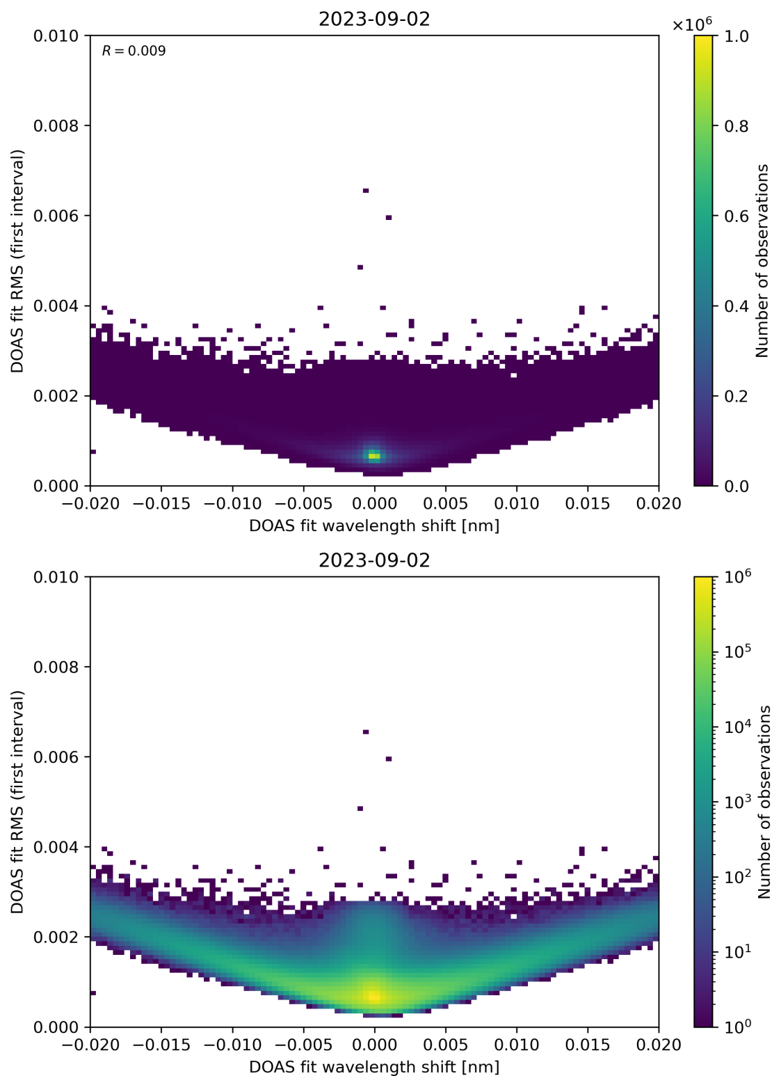
Figure 64: Scatter density plot of “DOAS fit wavelength shift” against “DOAS fit RMS (first interval)” for 2023-09-01 to 2023-09-03.
