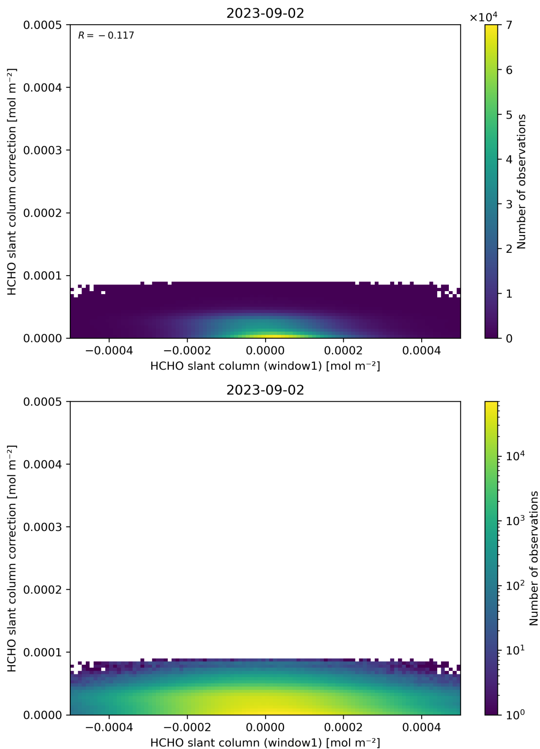
Figure 83: Scatter density plot of “HCHO slant column (window1)” against “HCHO slant column correction” for 2023-09-01 to 2023-09-03.
