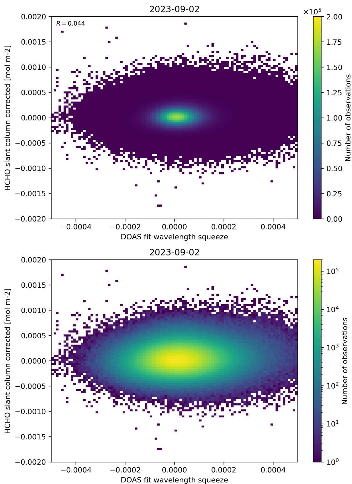
Figure 69: Scatter density plot of “DOAS fit wavelength squeeze” against “HCHO slant column corrected” for 2023-09-01 to 2023-09-03.
