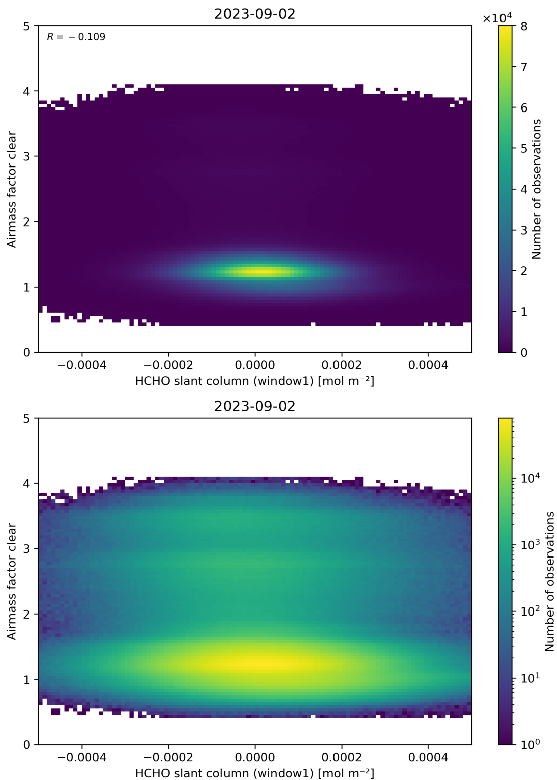
Figure 81: Scatter density plot of “HCHO slant column (window1)” against “Airmass factor clear” for 2023-09-01 to 2023-09-03.
