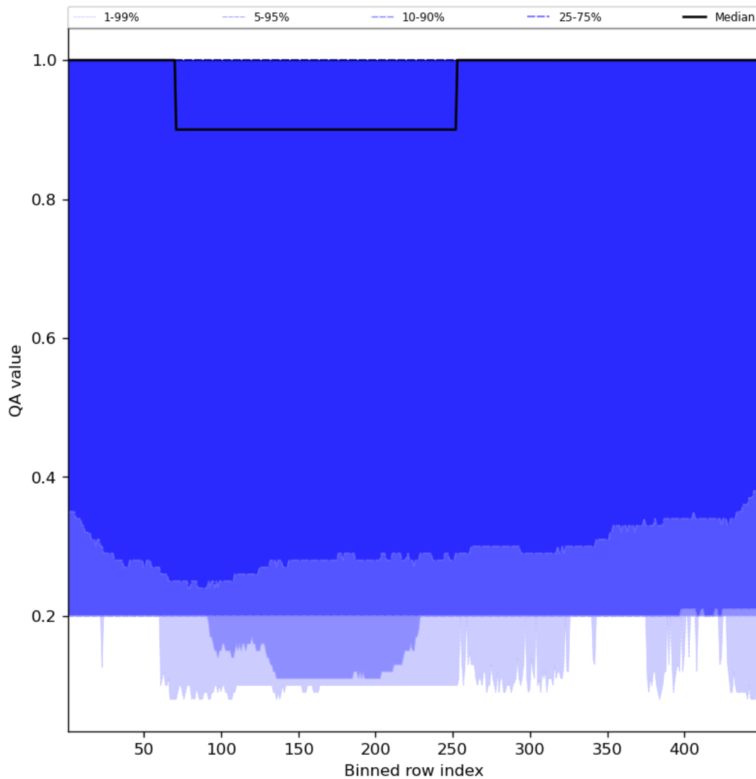
Figure 48: Along track statistics of “QA value” for 2023-09-01 to 2023-09-03
