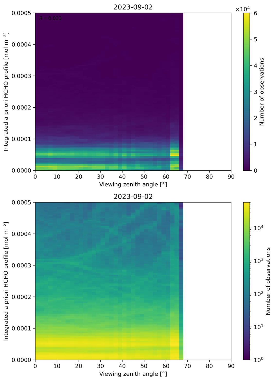
Figure 195: Scatter density plot of “Viewing zenith angle” against “Integrated a priori HCHO profile” for 2023-09-01 to 2023-09-03.
