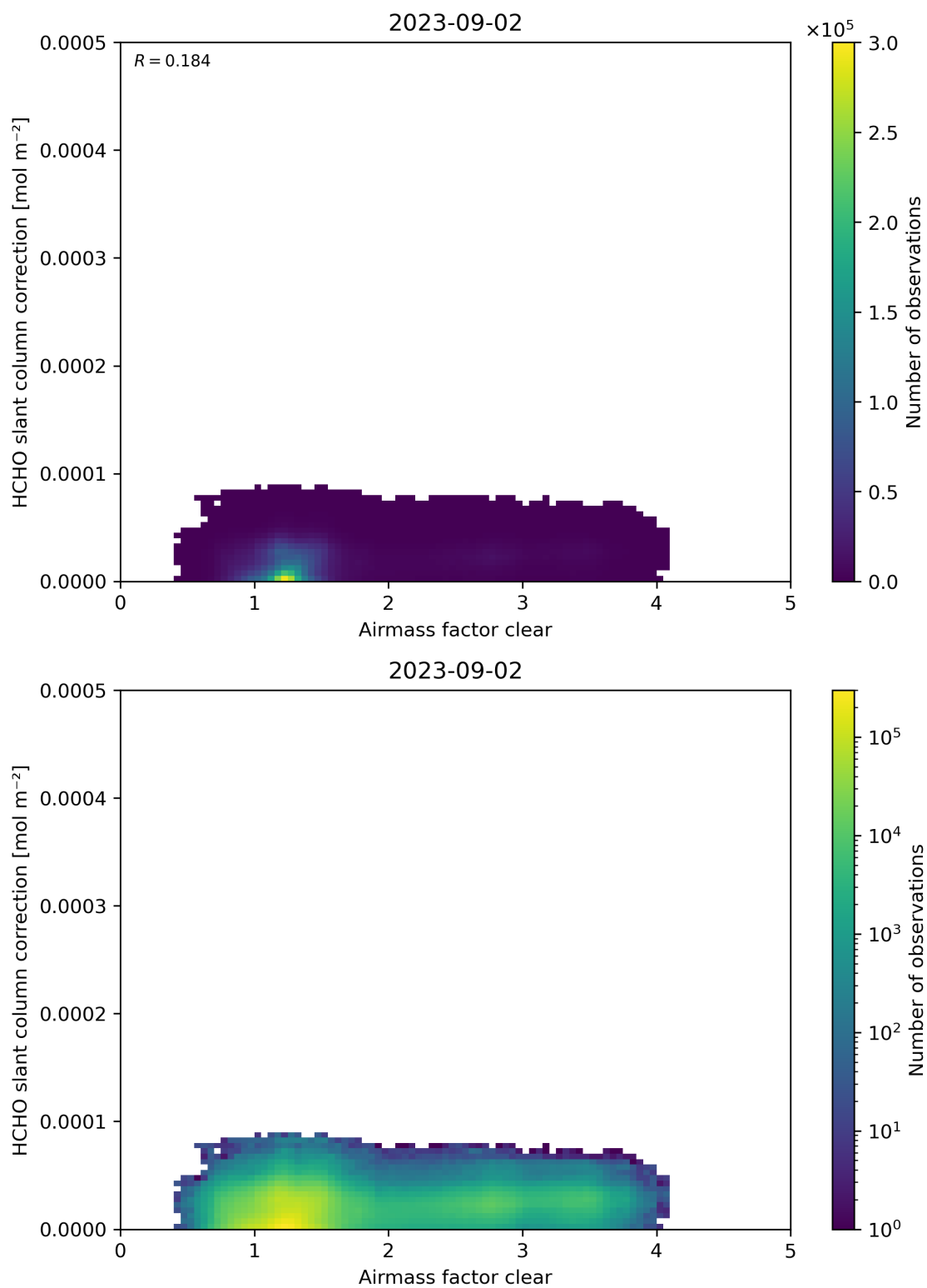
Figure 75: Scatter density plot of “Airmass factor clear” against “HCHO slant column correction” for 2023-09-01 to 2023-09-03.
