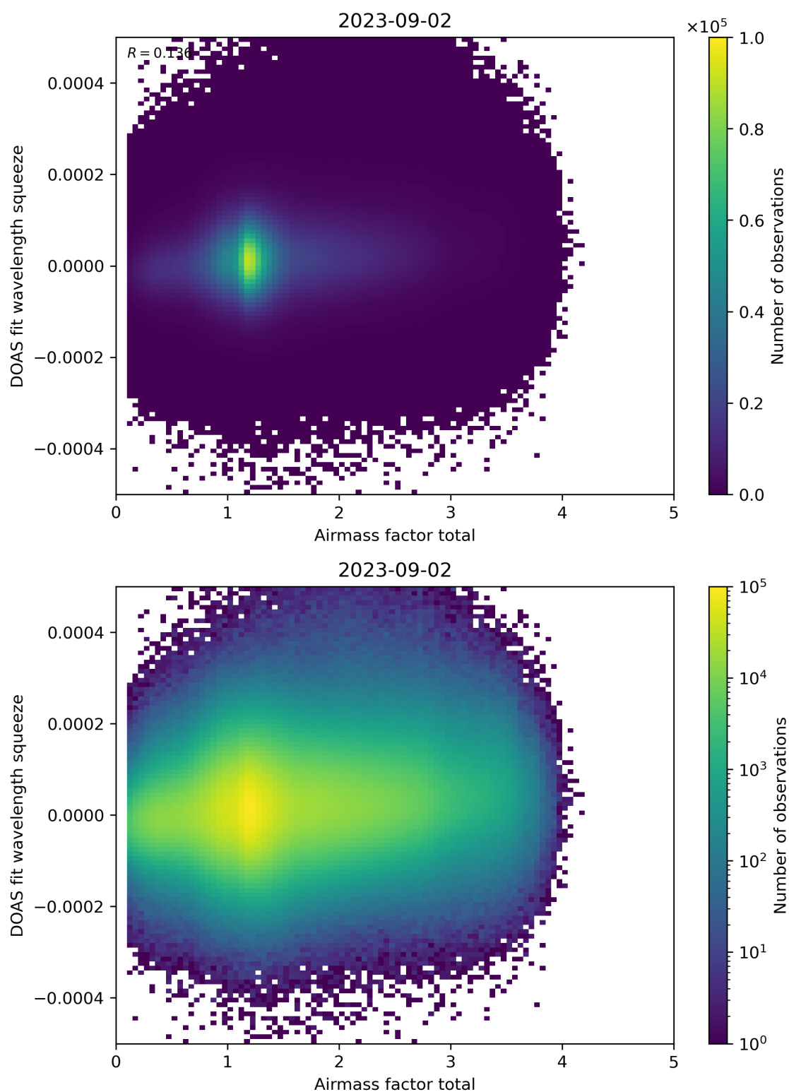
Figure 99: Scatter density plot of “Airmass factor total” against “DOAS fit wavelength squeeze” for 2023-09-01 to 2023-09-03.
