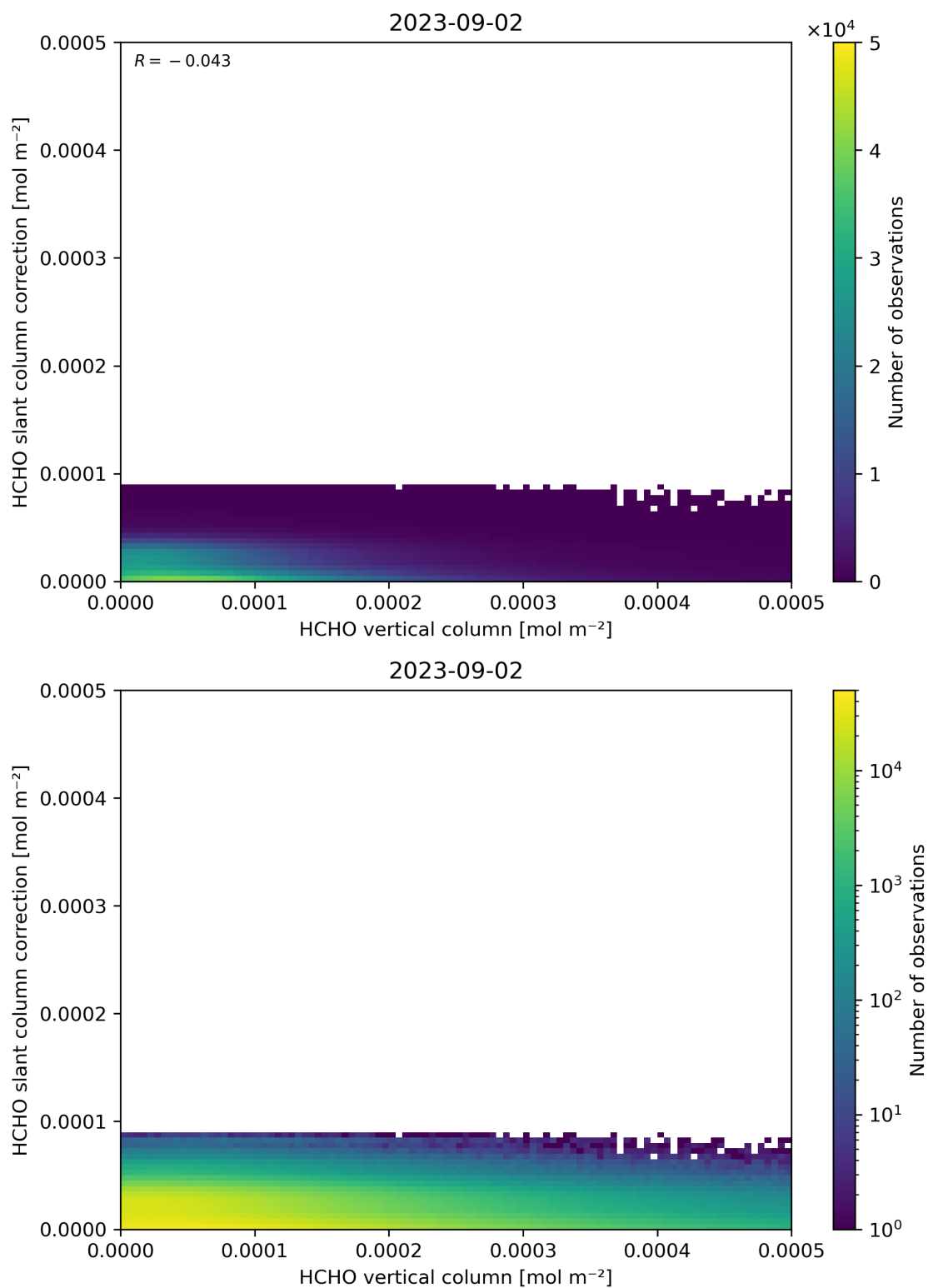
Figure 128: Scatter density plot of “HCHO vertical column” against “HCHO slant column correction” for 2023-09-01 to 2023-09-03.
