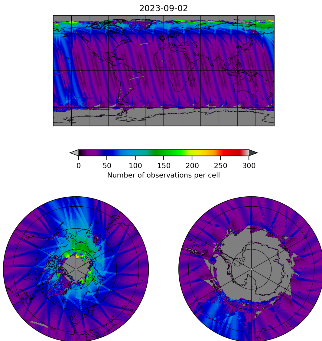
Figure 19: Map of the number of observations for 2023-09-01 to 2023-09-03
