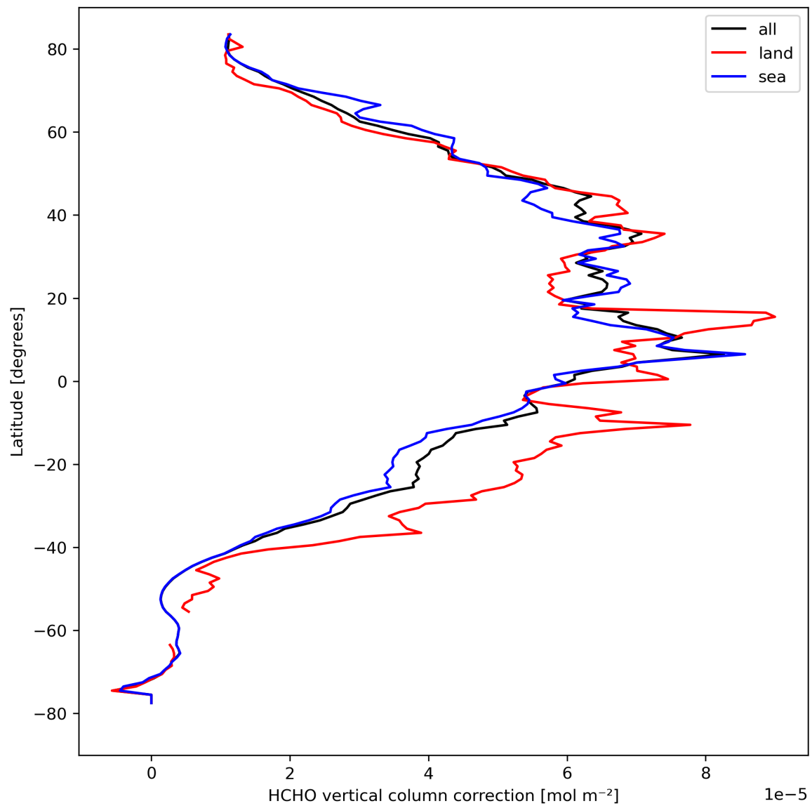
Figure 23: Zonal average of “HCHO vertical column correction” for 2023-09-01 to 2023-09-03.
