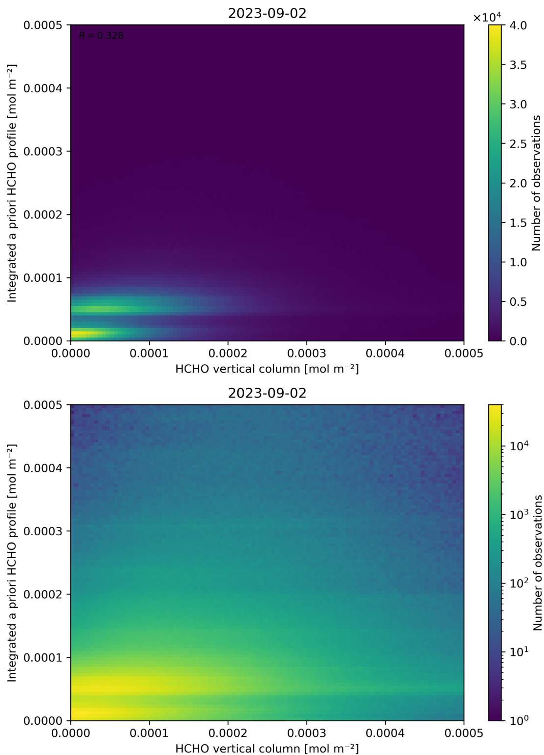
Figure 135: Scatter density plot of “HCHO vertical column” against “Integrated a priori HCHO profile” for 2023-09-01 to 2023-09-03.
