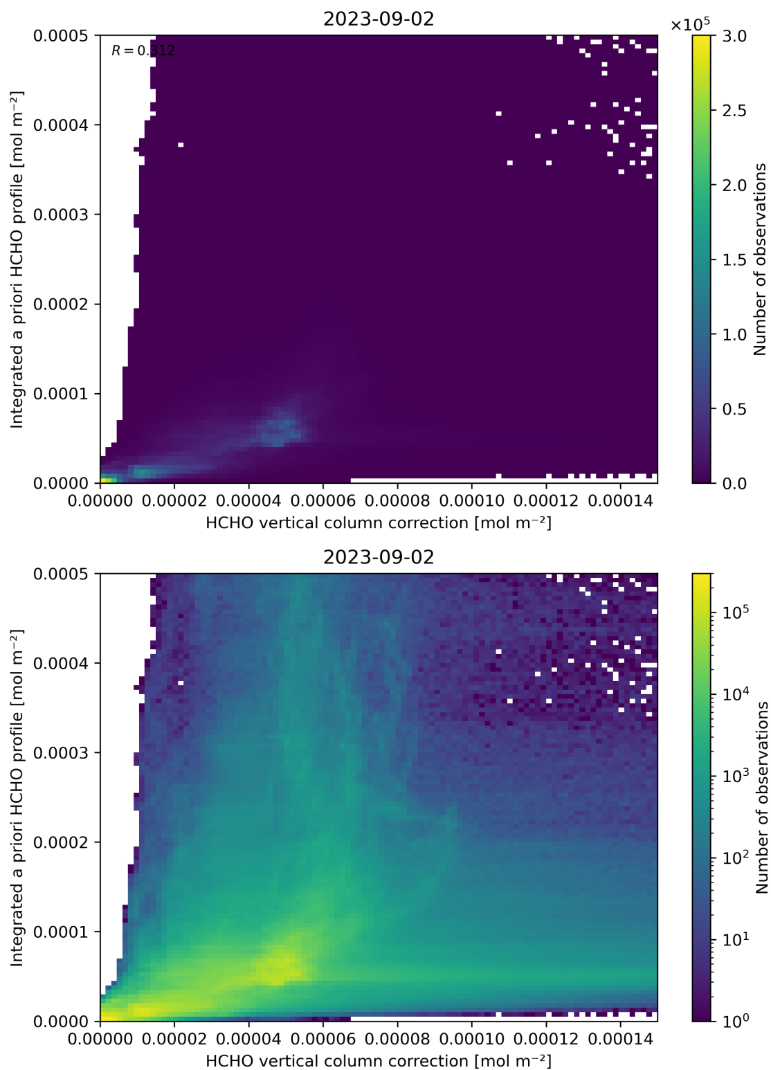
Figure 122: Scatter density plot of “HCHO vertical column correction” against “Integrated a priori HCHO profile” for 2023-09-01 to 2023-09-03.
