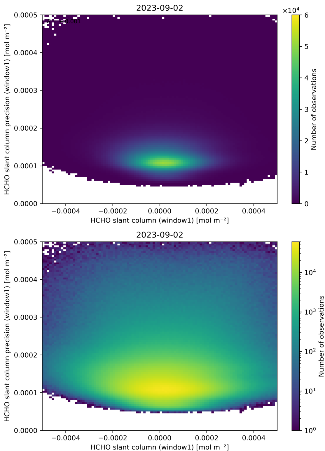
Figure 84: Scatter density plot of “HCHO slant column (window1)” against “HCHO slant column precision (window1)” for 2023-09-01 to 2023-09-03.
