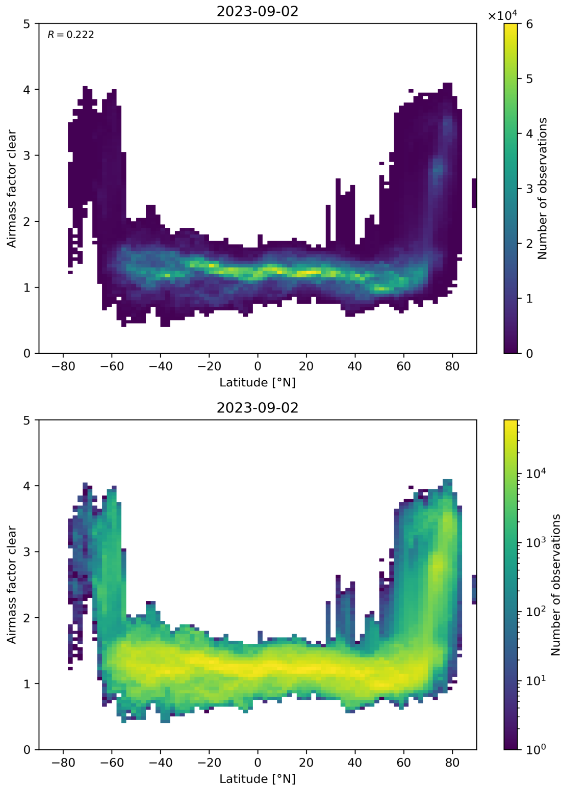
Figure 156: Scatter density plot of “Latitude” against “Airmass factor clear” for 2023-09-01 to 2023-09-03.
