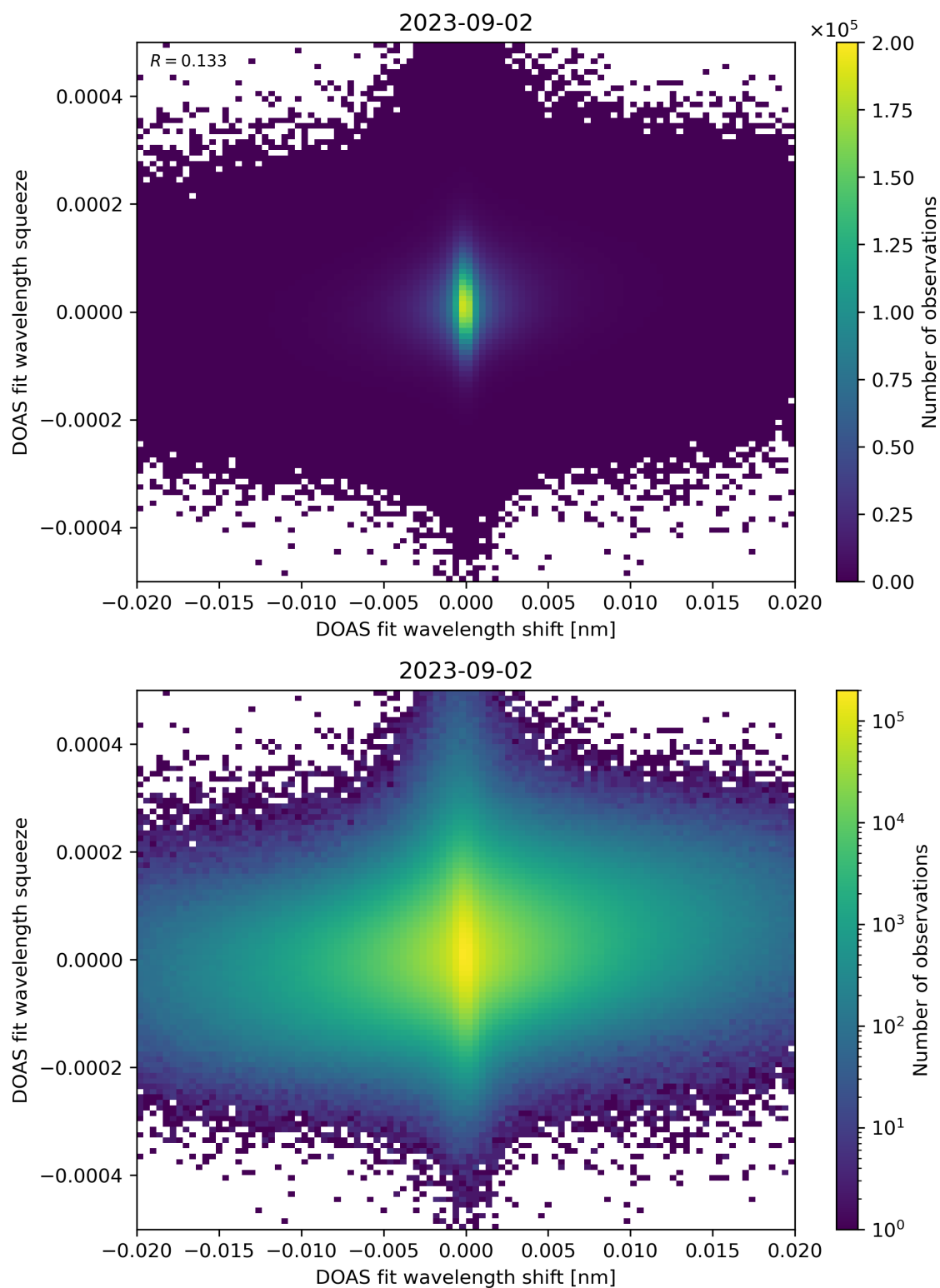
Figure 65: Scatter density plot of “DOAS fit wavelength shift” against “DOAS fit wavelength squeeze” for 2023-09-01 to 2023-09-03.
