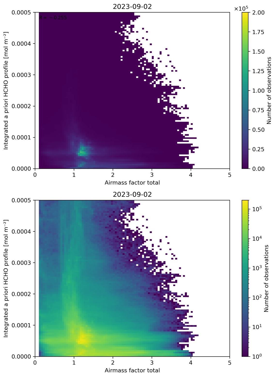
Figure 104: Scatter density plot of “Airmass factor total” against “Integrated a priori HCHO profile” for 2023-09-01 to 2023-09-03.
