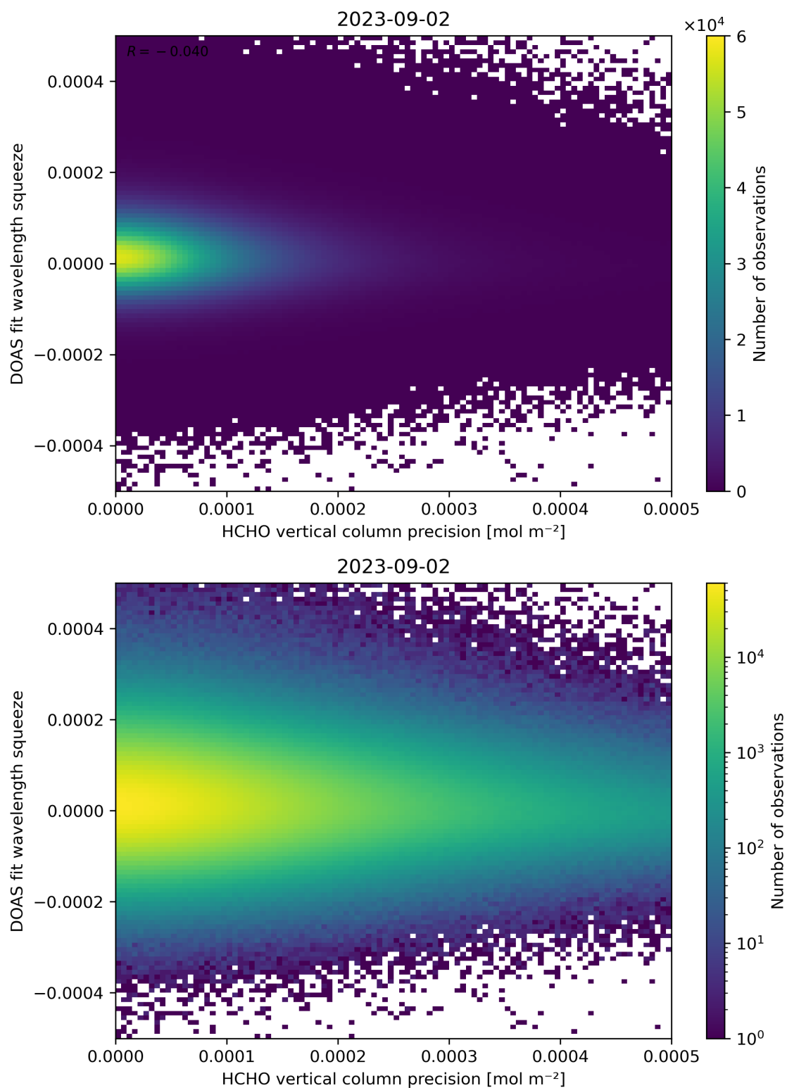
Figure 138: Scatter density plot of “HCHO vertical column precision” against “DOAS fit wavelength squeeze” for 2023-09-01 to 2023-09-03.
