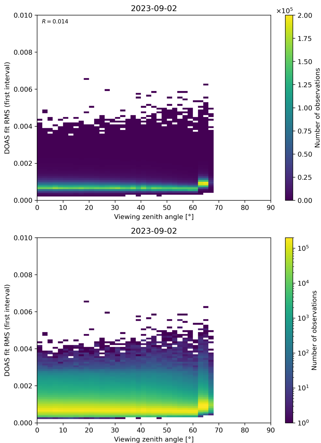
Figure 182: Scatter density plot of “Viewing zenith angle” against “DOAS fit RMS (first interval)” for 2023-09-01 to 2023-09-03.
