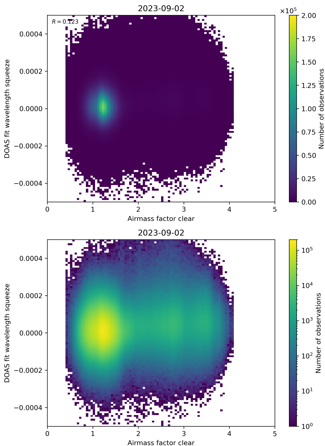
Figure 73: Scatter density plot of “Airmass factor clear” against “DOAS fit wavelength squeeze” for 2023-09-01 to 2023-09-03.
