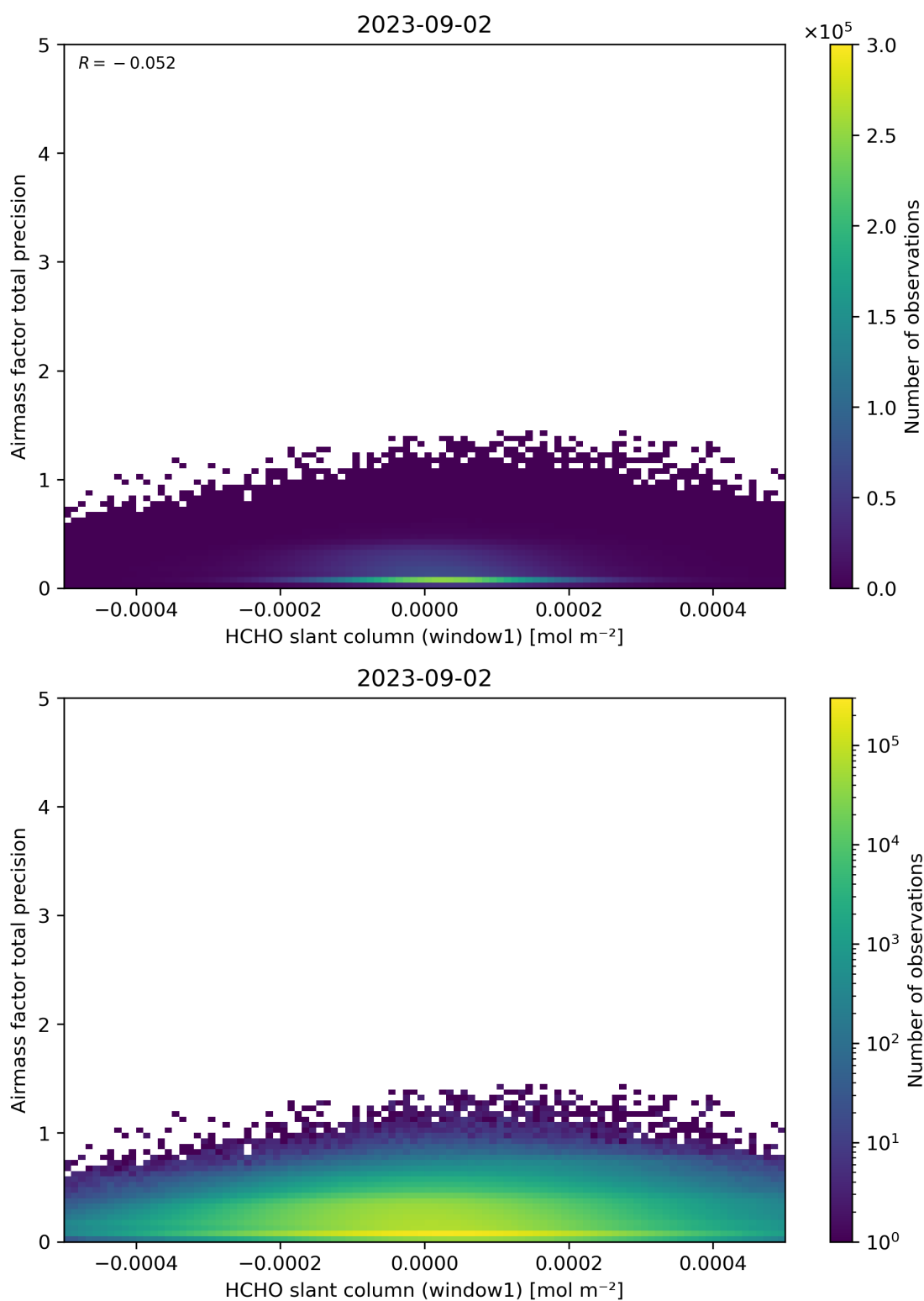
Figure 86: Scatter density plot of “HCHO slant column (window1)” against “Airmass factor total precision” for 2023-09-01 to 2023-09-03.
