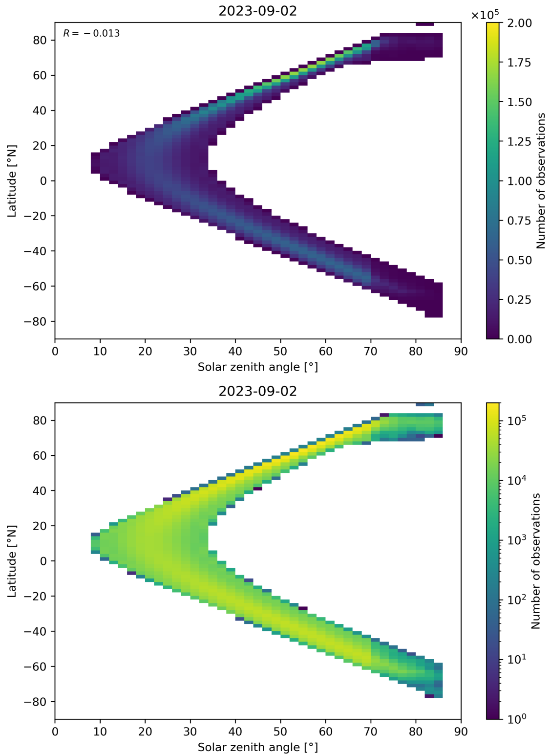
Figure 181: Scatter density plot of “Solar zenith angle” against “Latitude” for 2023-09-01 to 2023-09-03.
