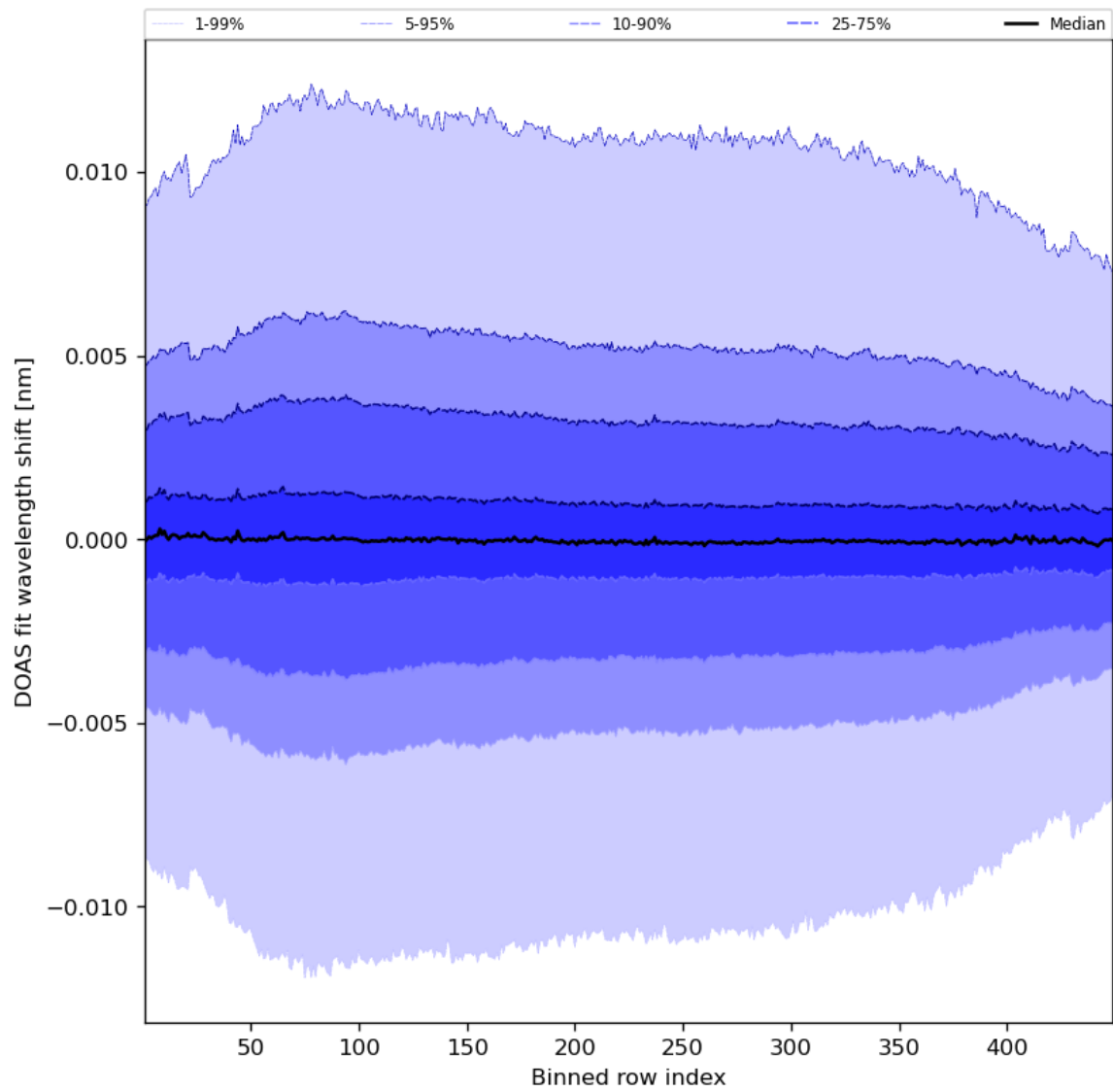
Figure 58: Along track statistics of “DOAS fit wavelength shift” for 2023-09-01 to 2023-09-03
