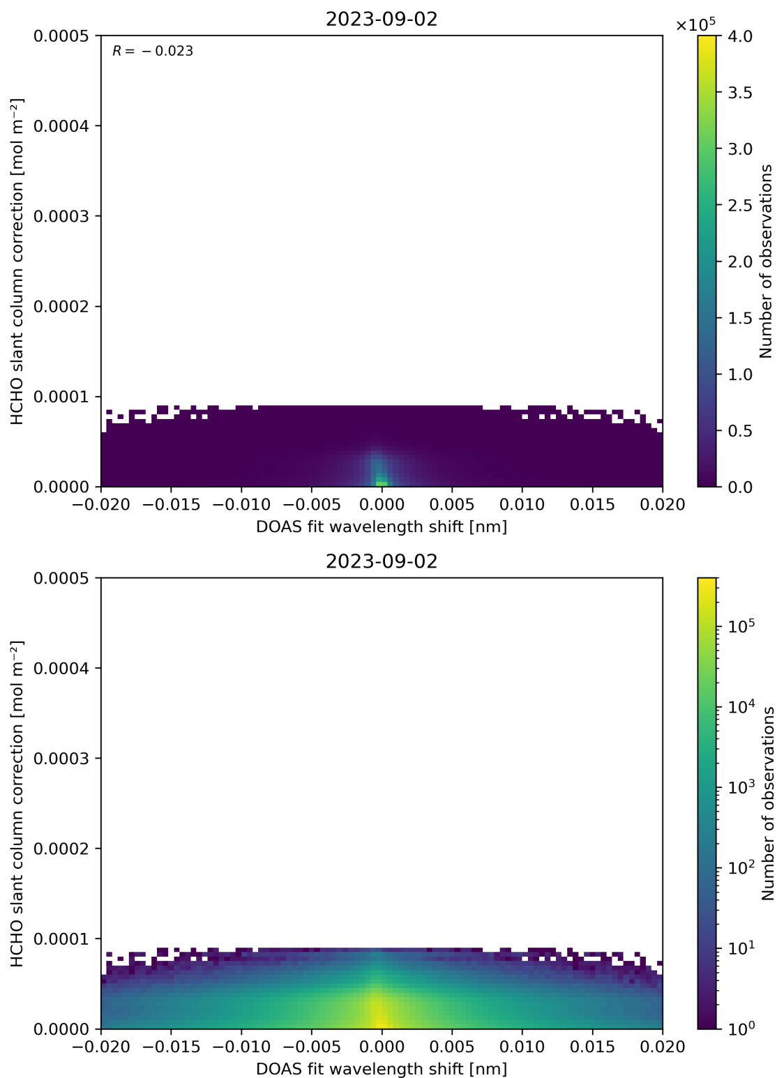
Figure 67: Scatter density plot of “DOAS fit wavelength shift” against “HCHO slant column correction” for 2023-09-01 to 2023-09-03.
