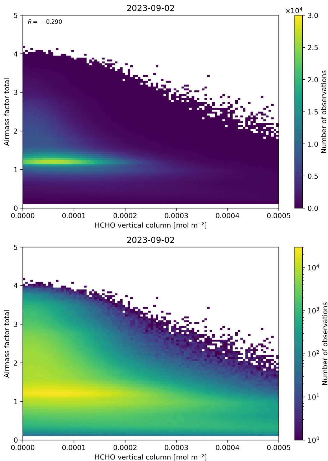
Figure 131: Scatter density plot of “HCHO vertical column” against “Airmass factor total” for 2023-09-01 to 2023-09-03.
