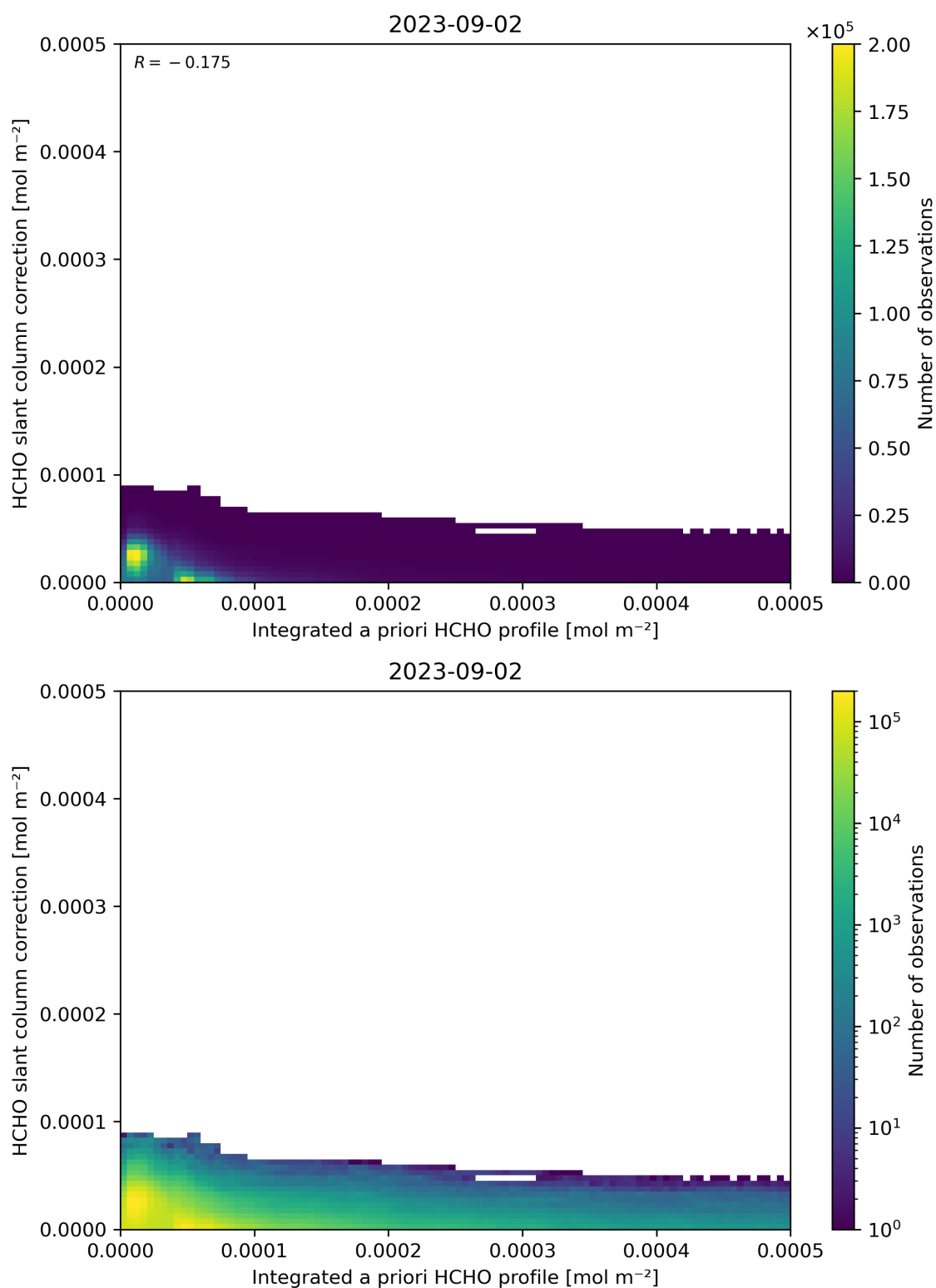
Figure 152: Scatter density plot of “Integrated a priori HCHO profile” against “HCHO slant column correction” for 2023-09-01 to 2023-09-03.
