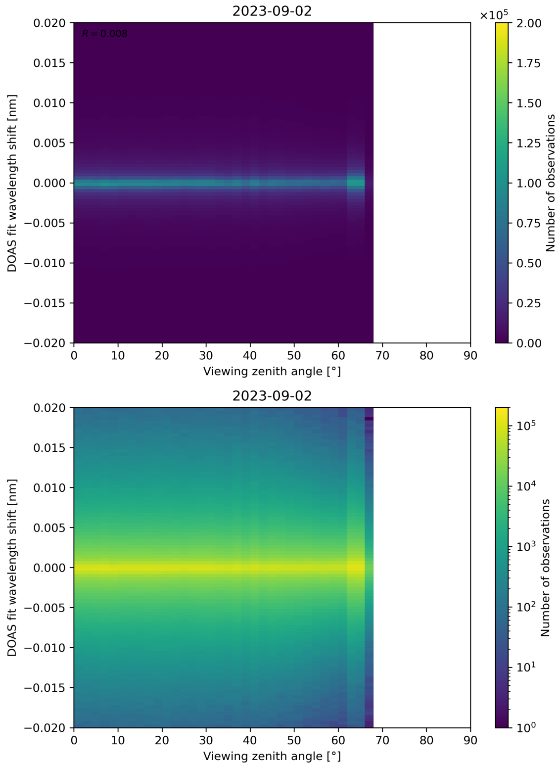
Figure 183: Scatter density plot of “Viewing zenith angle” against “DOAS fit wavelength shift” for 2023-09-01 to 2023-09-03.
