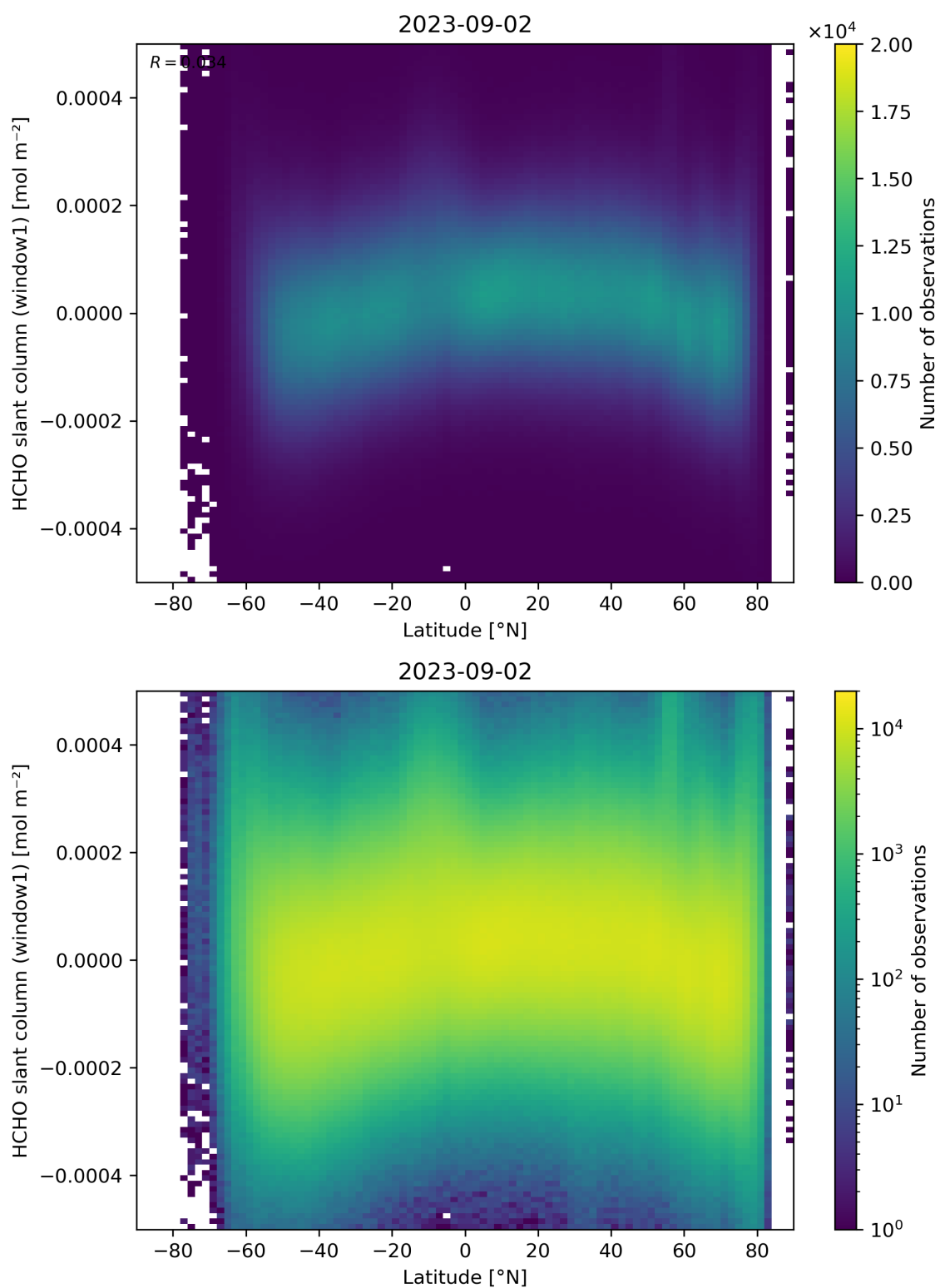
Figure 159: Scatter density plot of “Latitude” against “HCHO slant column (window1)” for 2023-09-01 to 2023-09-03.
