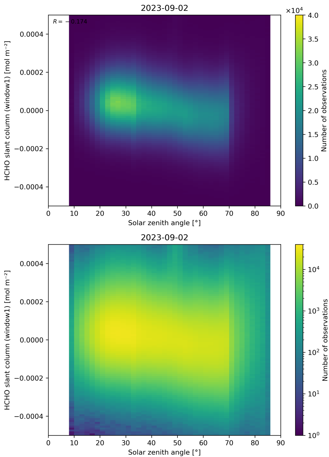
Figure 173: Scatter density plot of “Solar zenith angle” against “HCHO slant column (window1)” for 2023-09-01 to 2023-09-03.
