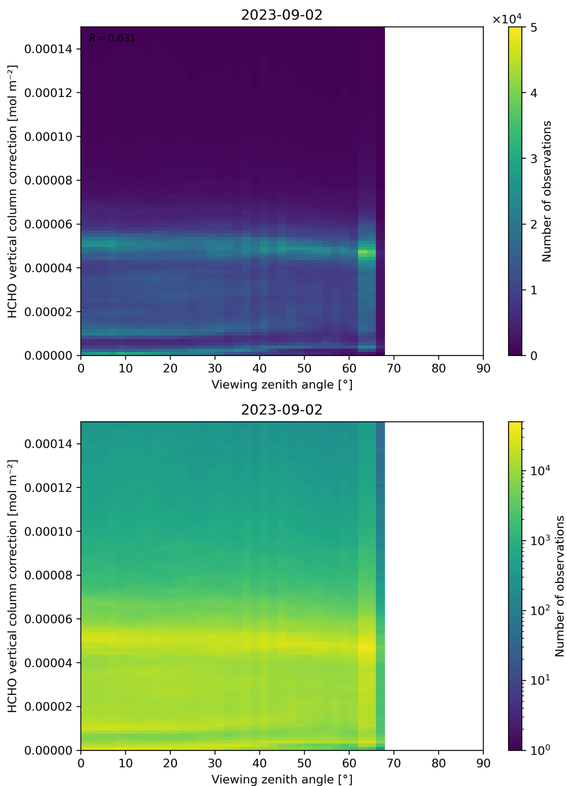
Figure 193: Scatter density plot of “Viewing zenith angle” against “HCHO vertical column correction” for 2023-09-01 to 2023-09-03.
