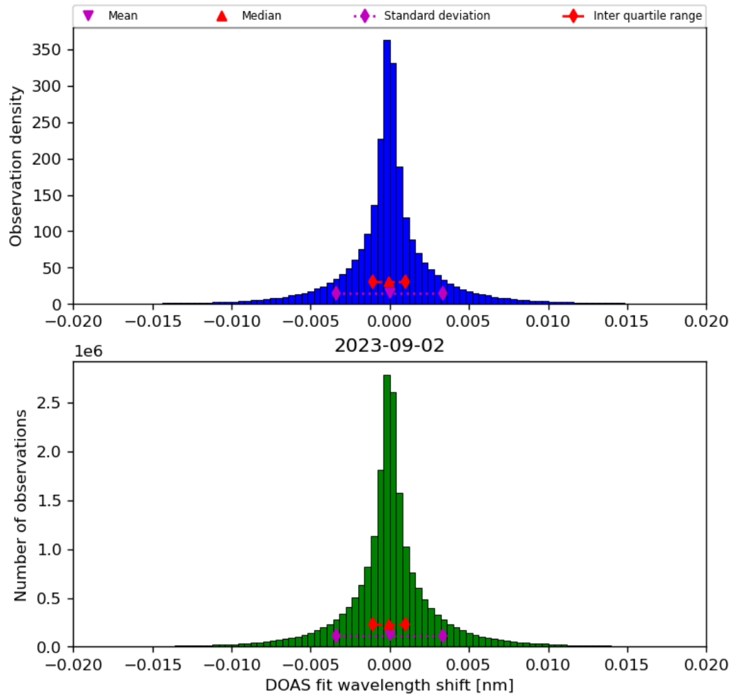
Figure 44: Histogram of “DOAS fit wavelength shift” for 2023-09-01 to 2023-09-03
