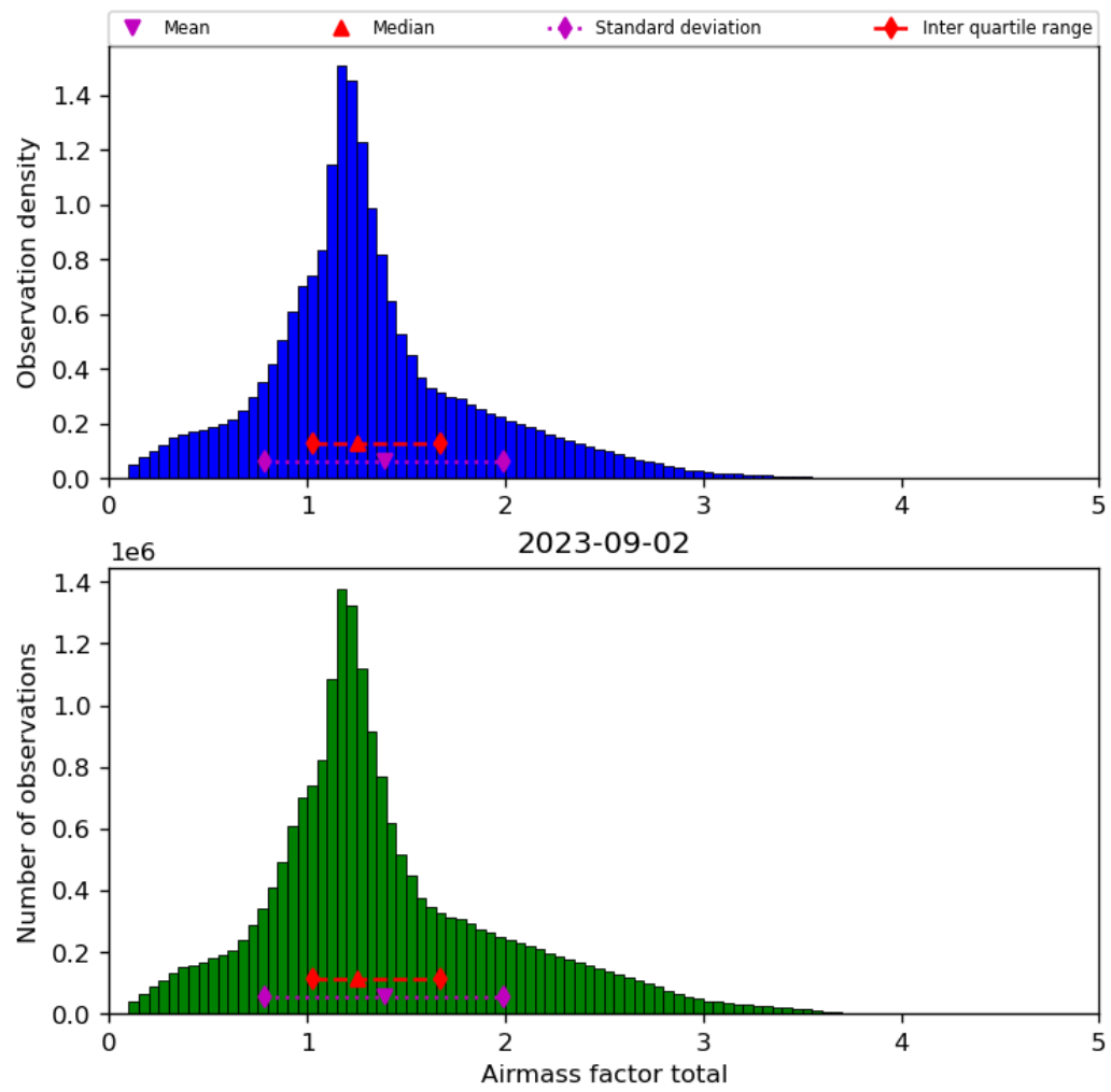
Figure 40: Histogram of “Airmass factor total” for 2023-09-01 to 2023-09-03
