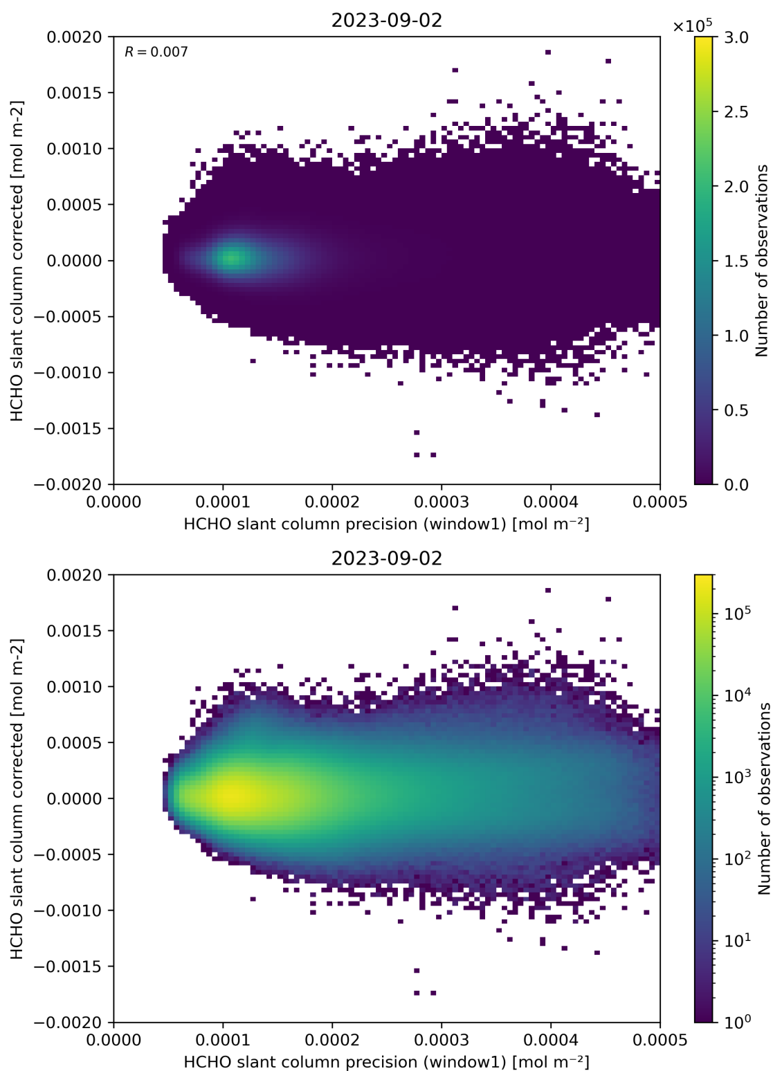
Figure 92: Scatter density plot of “HCHO slant column precision (window1)” against “HCHO slant column corrected” for 2023-09-01 to 2023-09-03.
