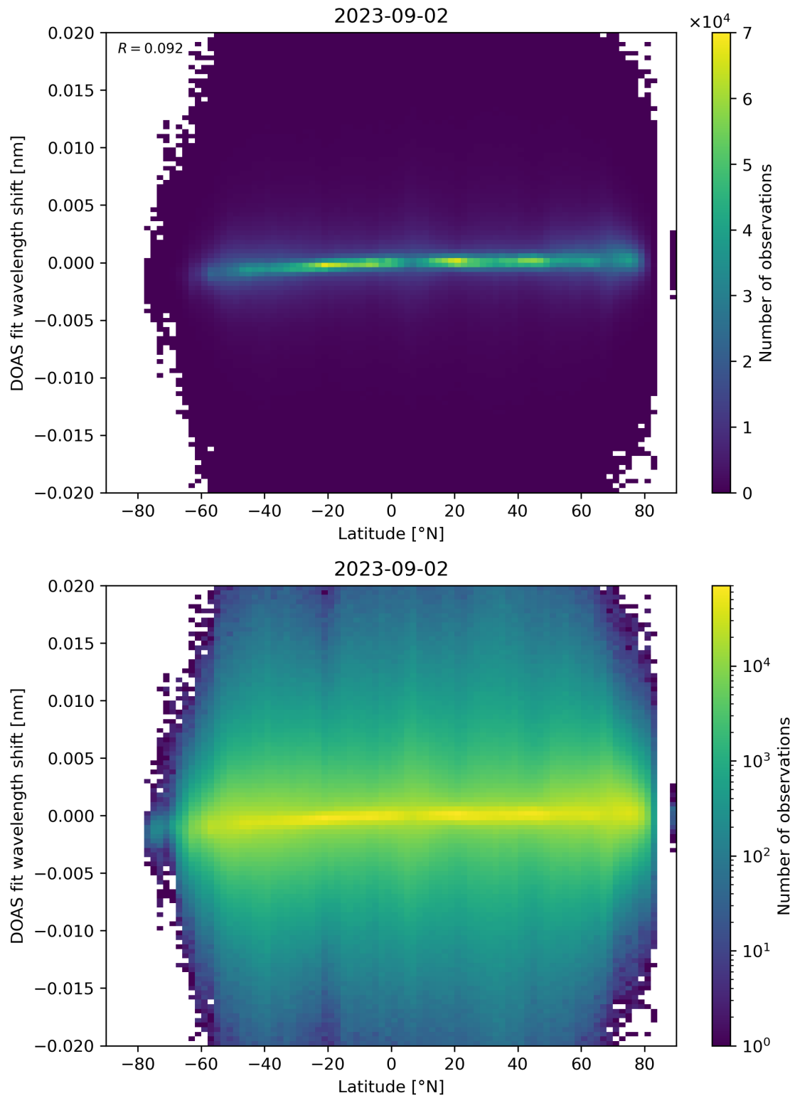
Figure 154: Scatter density plot of “Latitude” against “DOAS fit wavelength shift” for 2023-09-01 to 2023-09-03.
