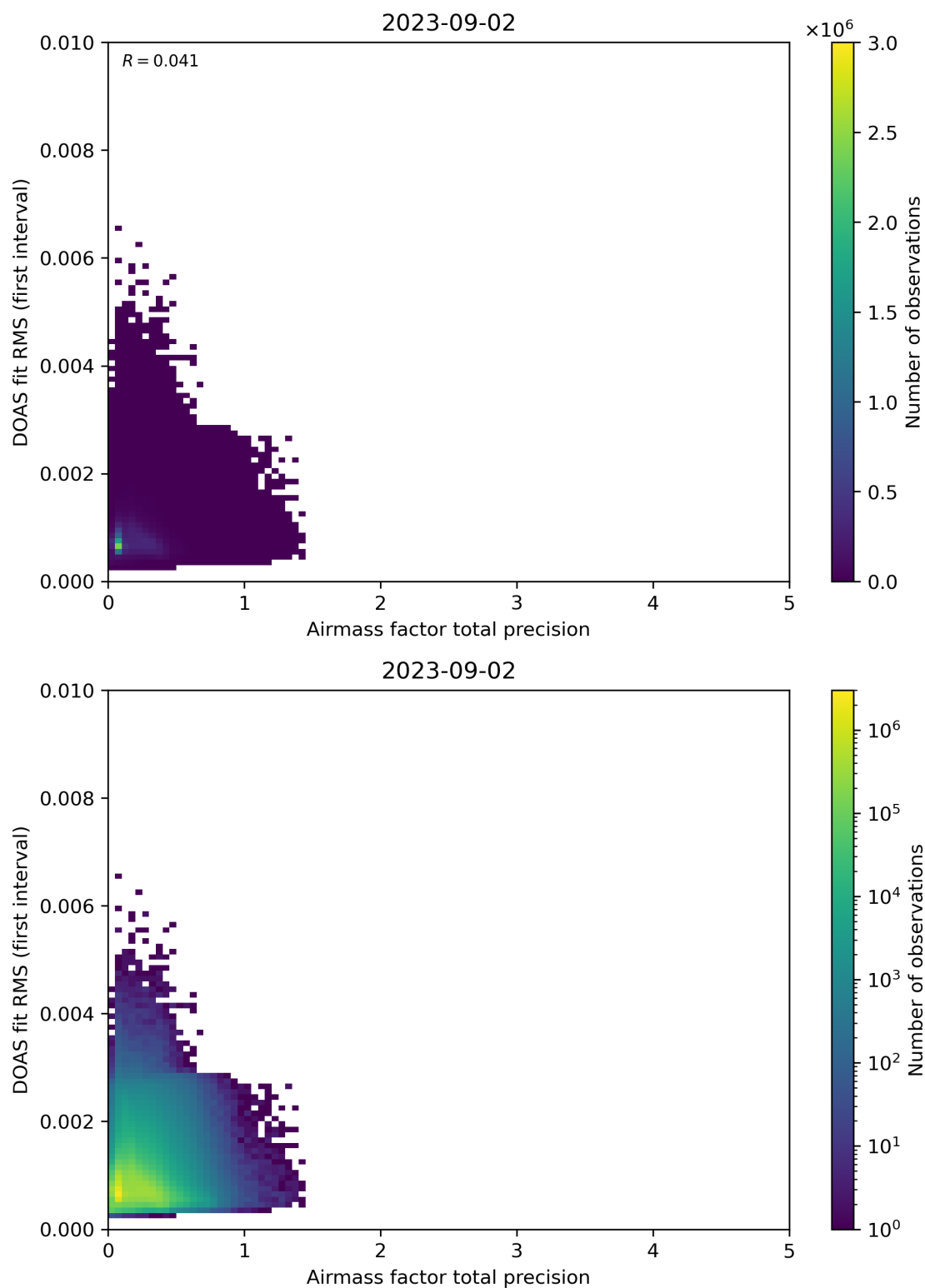
Figure 105: Scatter density plot of “Airmass factor total precision” against “DOAS fit RMS (first interval)” for 2023-09-01 to 2023-09-03.
