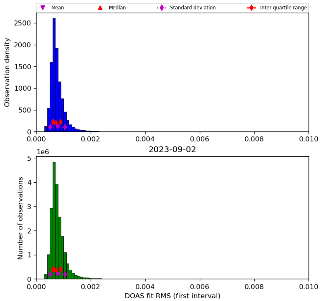
Figure 46: Histogram of “DOAS fit RMS (first interval)” for 2023-09-01 to 2023-09-03
