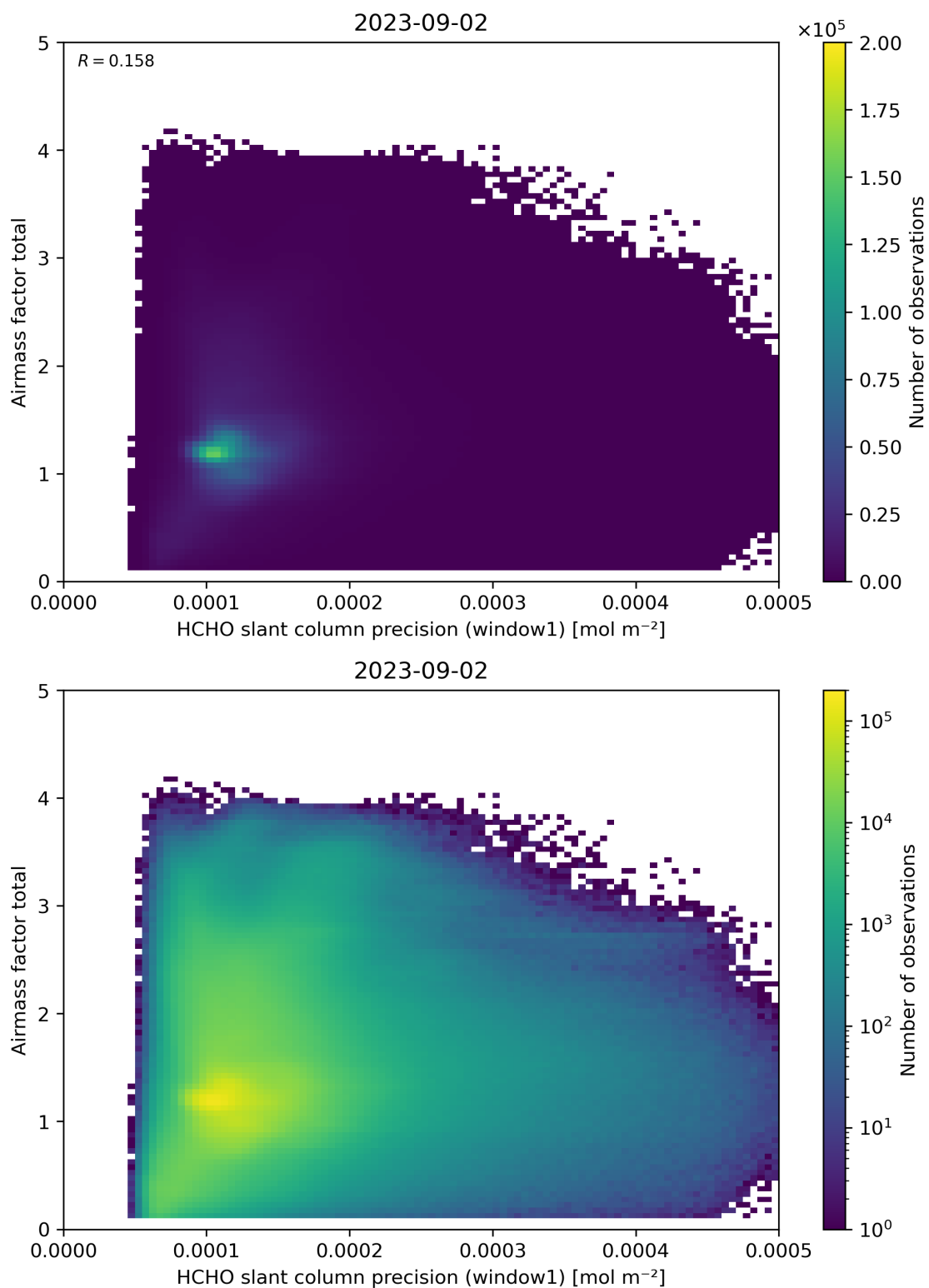
Figure 94: Scatter density plot of “HCHO slant column precision (window1)” against “Airmass factor total” for 2023-09-01 to 2023-09-03.
