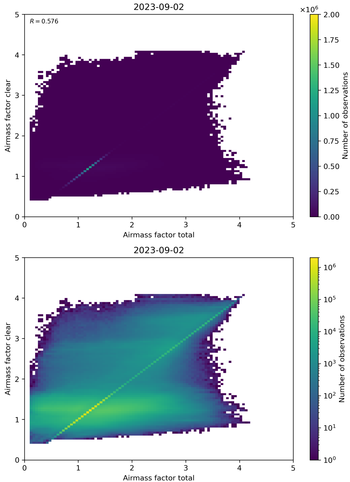
Figure 100: Scatter density plot of “Airmass factor total” against “Airmass factor clear” for 2023-09-01 to 2023-09-03.
