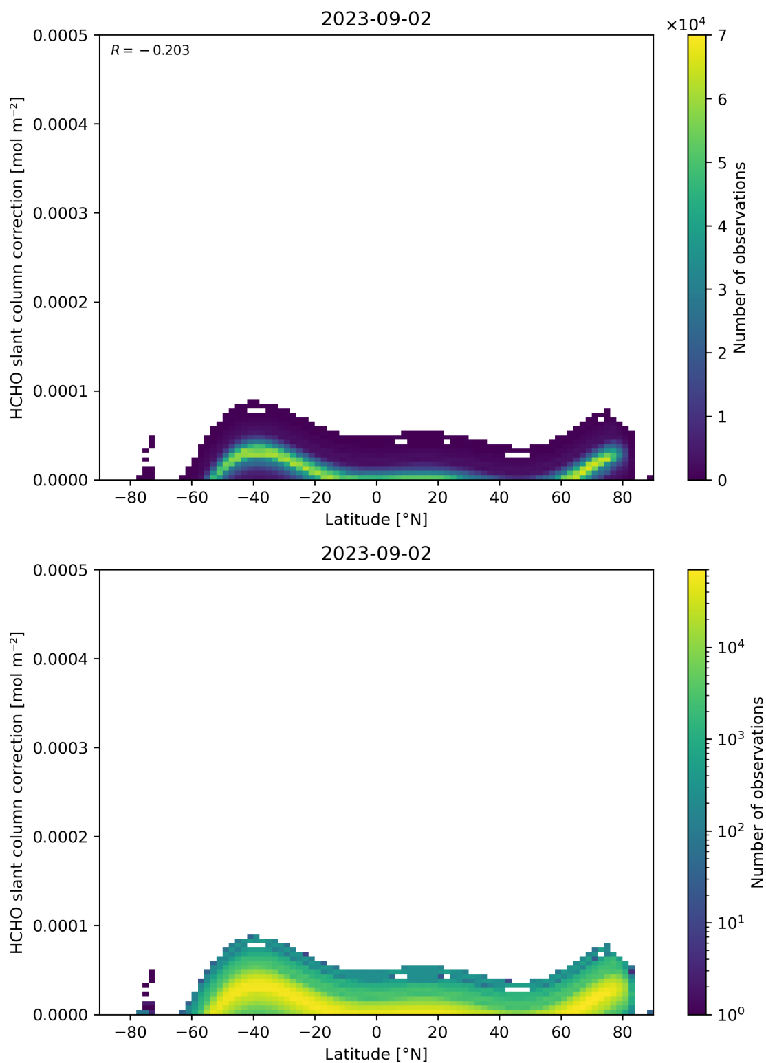
Figure 158: Scatter density plot of “Latitude” against “HCHO slant column correction” for 2023-09-01 to 2023-09-03.
