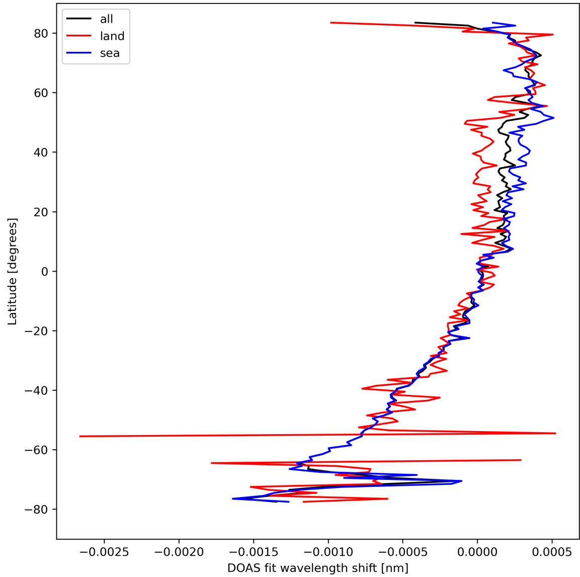
Figure 30: Zonal average of "DOAS fit wavelength shift" for 2023-09-01 to 2023-09-03.
