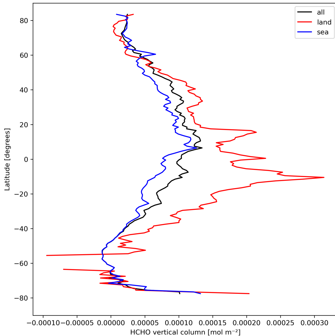
Figure 21: Zonal average of “HCHO vertical column” for 2023-09-01 to 2023-09-03.
