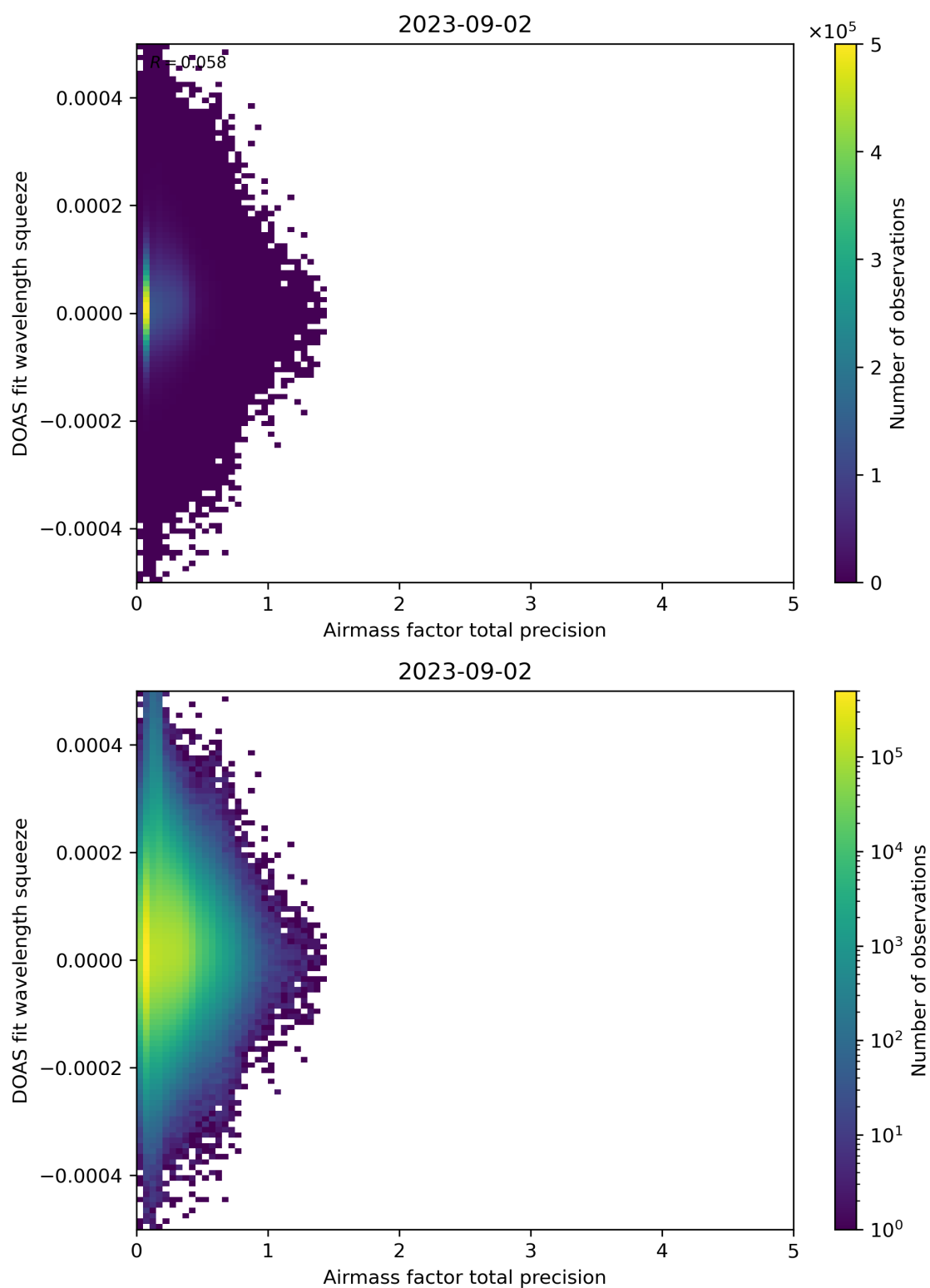
Figure 107: Scatter density plot of “Airmass factor total precision” against “DOAS fit wavelength squeeze” for 2023-09-01 to 2023-09-03.
