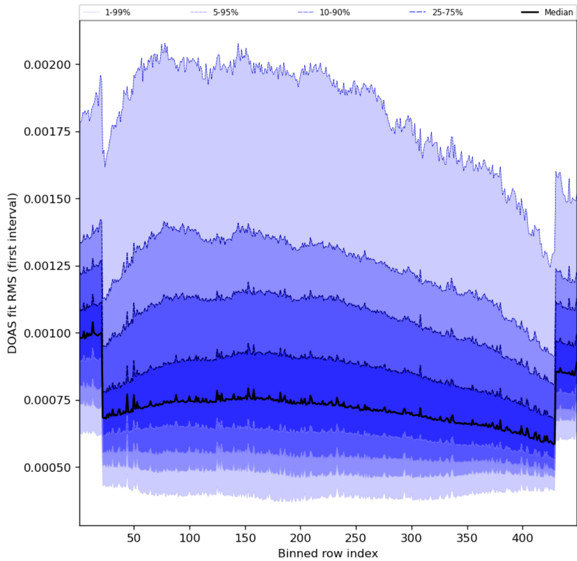
Figure 60: Along track statistics of “DOAS fit RMS (first interval)” for 2023-09-01 to 2023-09-03
