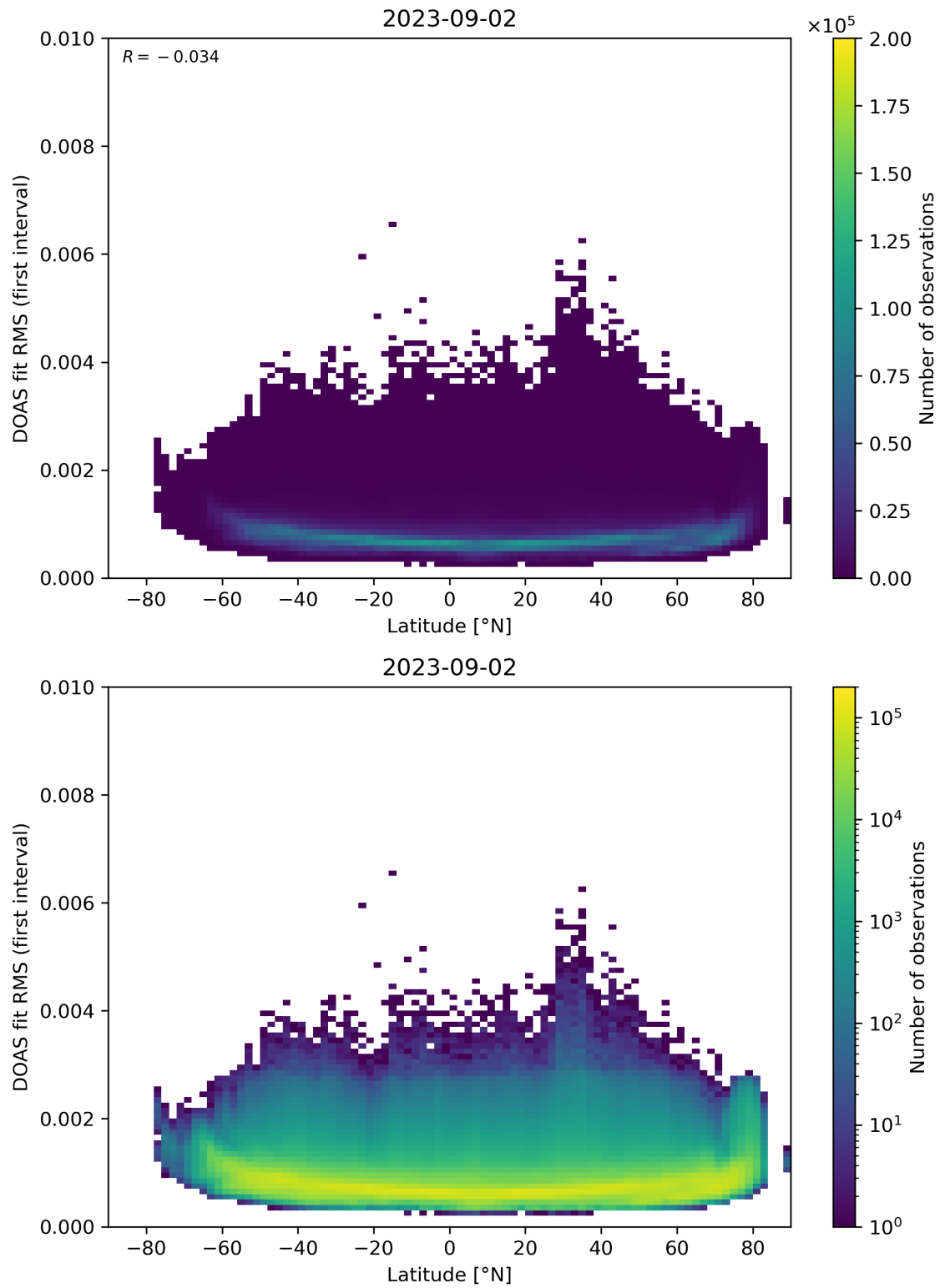
Figure 153: Scatter density plot of “Latitude” against “DOAS fit RMS (first interval)” for 2023-09-01 to 2023-09-03.
