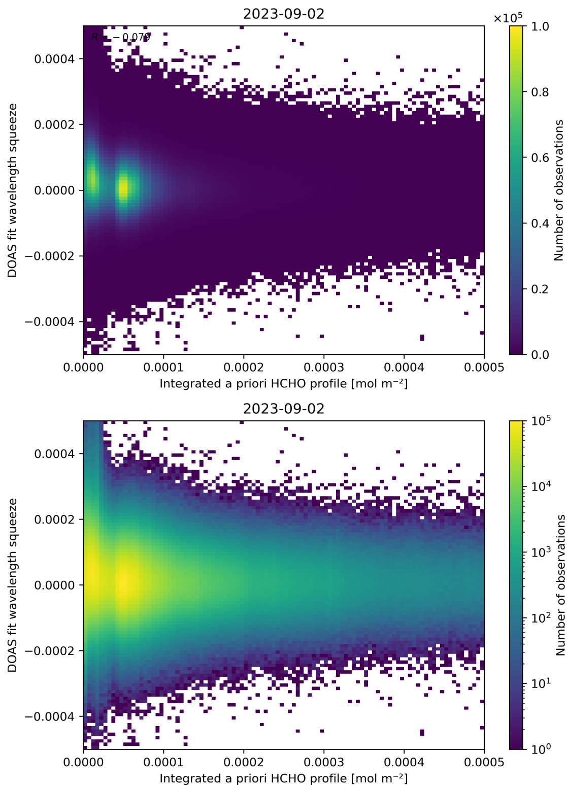
Figure 150: Scatter density plot of “Integrated a priori HCHO profile” against “DOAS fit wavelength squeeze” for 2023-09-01 to 2023-09-03.
