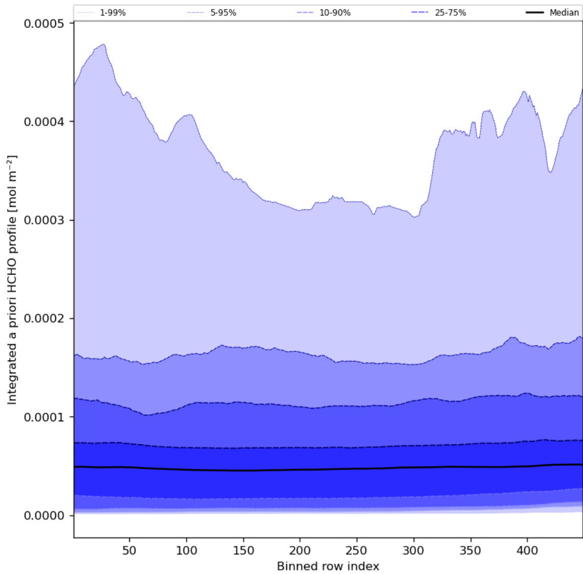
Figure 57: Along track statistics of “Integrated a priori HCHO profile” for 2023-09-01 to 2023-09-03
