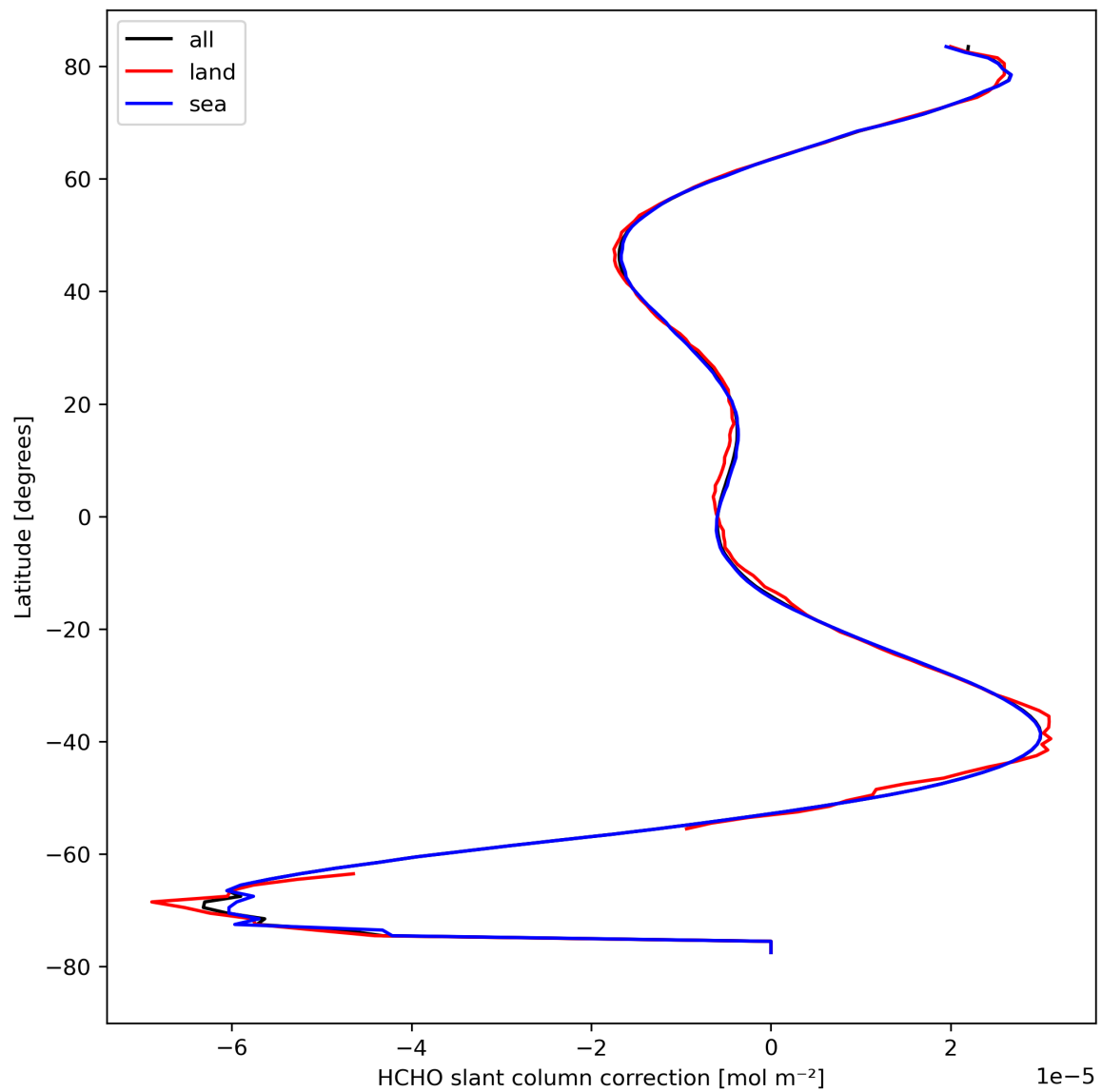
Figure 33: Zonal average of “HCHO slant column correction” for 2023-09-01 to 2023-09-03.
