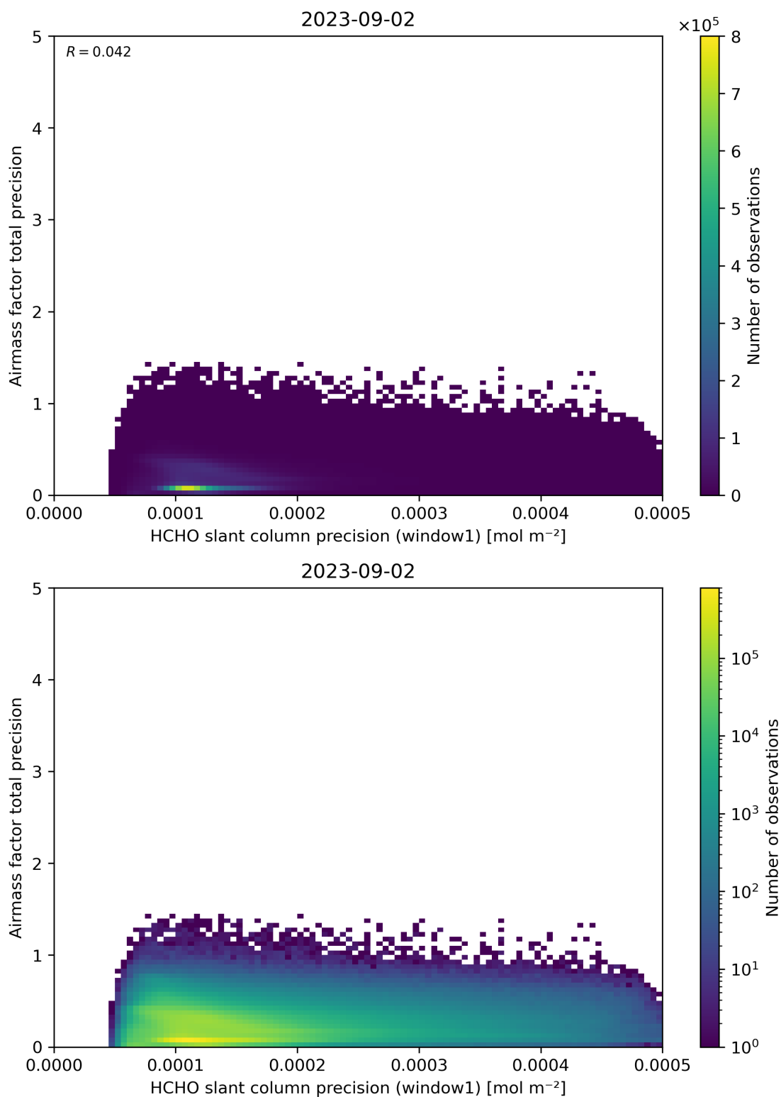
Figure 95: Scatter density plot of “HCHO slant column precision (window1)” against “Airmass factor total precision” for 2023-09-01 to 2023-09-03.
