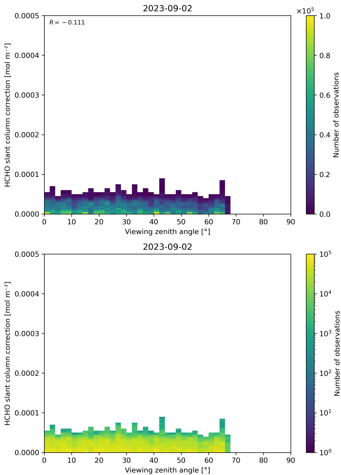
Figure 187: Scatter density plot of “Viewing zenith angle” against “HCHO slant column correction” for 2023-09-01 to 2023-09-03.
