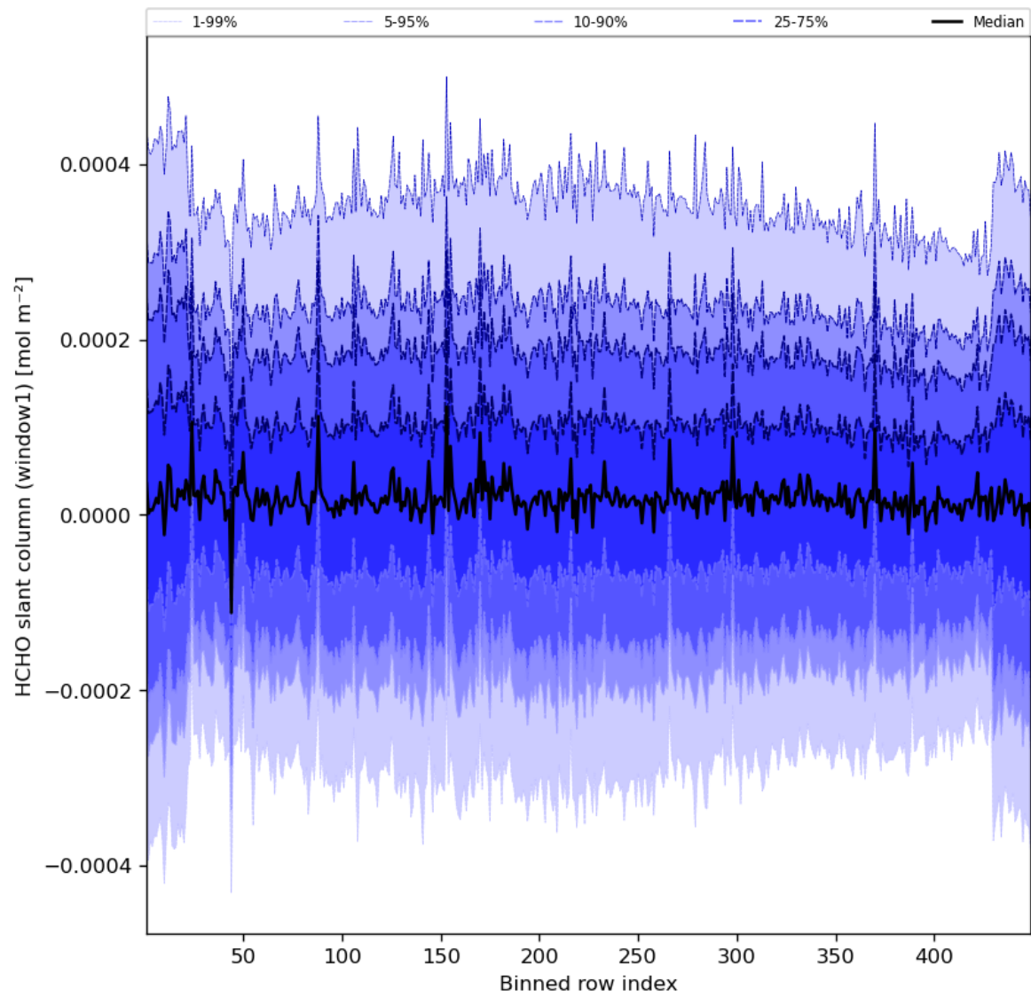
Figure 52: Along track statistics of "HCHO slant column (window1)" for 2023-09-01 to 2023-09-03
