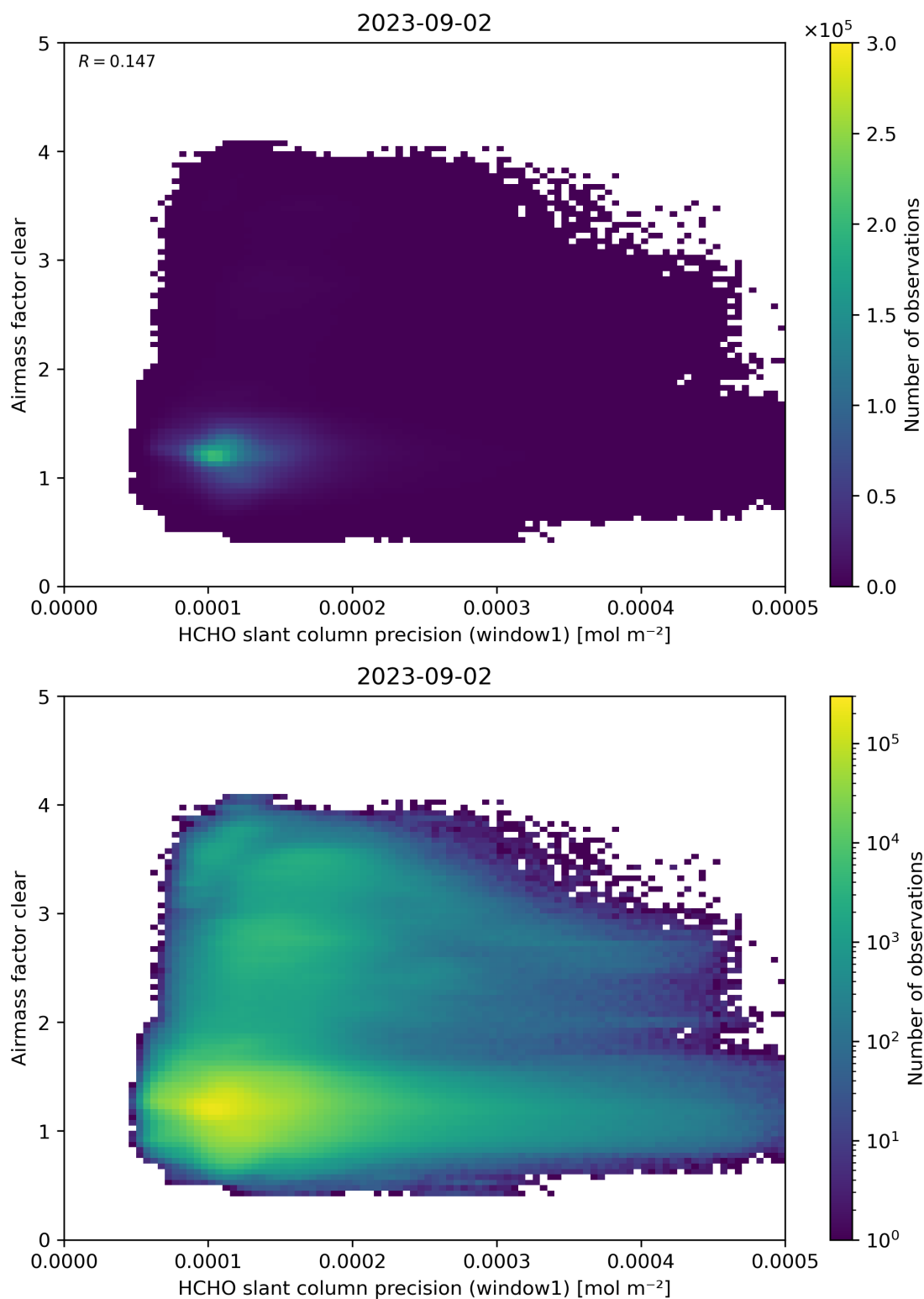
Figure 91: Scatter density plot of “HCHO slant column precision (window1)” against “Airmass factor clear” for 2023-09-01 to 2023-09-03.
