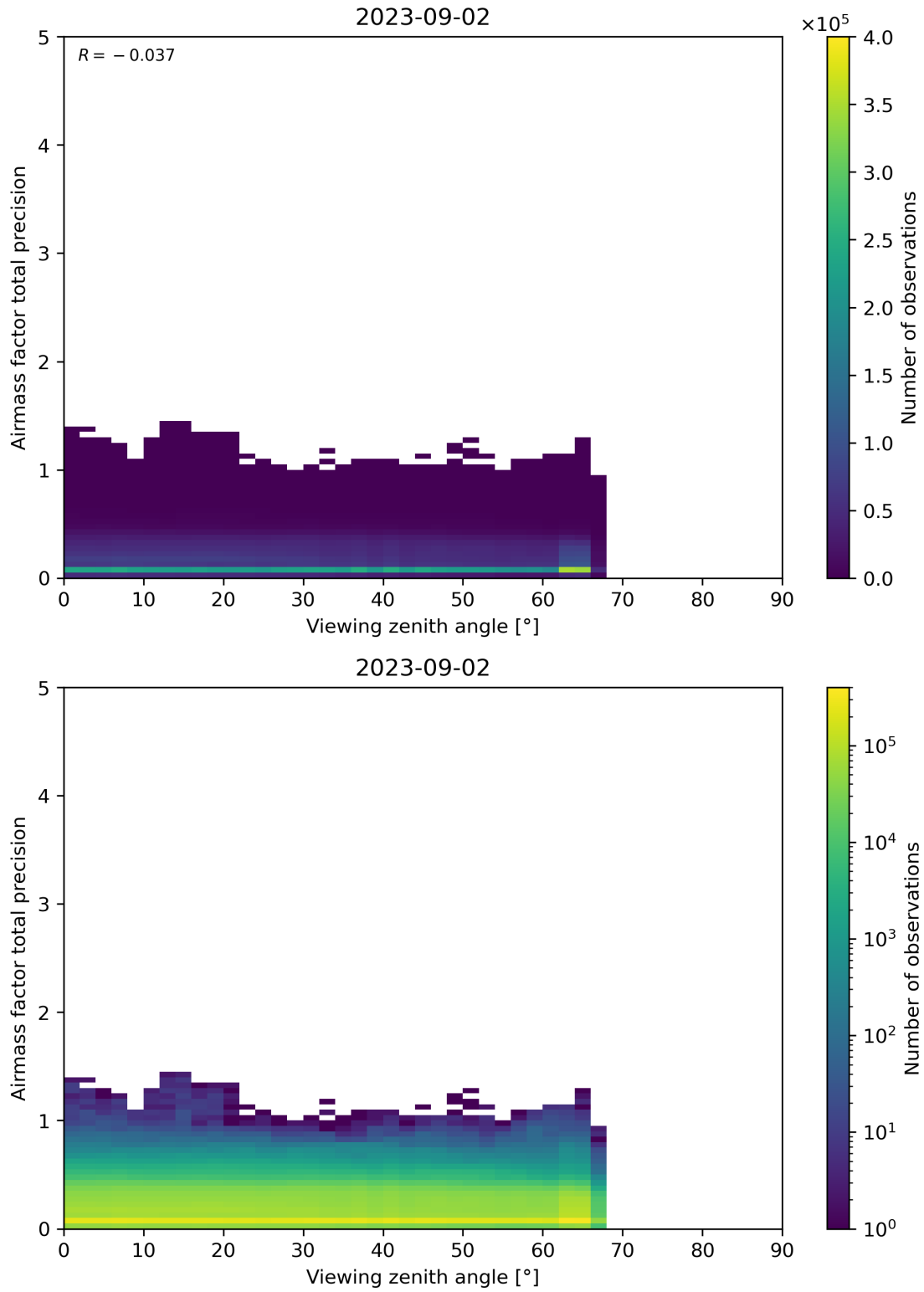
Figure 191: Scatter density plot of “Viewing zenith angle” against “Airmass factor total precision” for 2023-09-01 to 2023-09-03.
