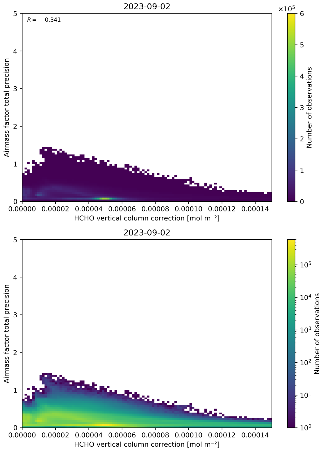
Figure 121: Scatter density plot of “HCHO vertical column correction” against “Airmass factor total precision” for 2023-09-01 to 2023-09-03.
