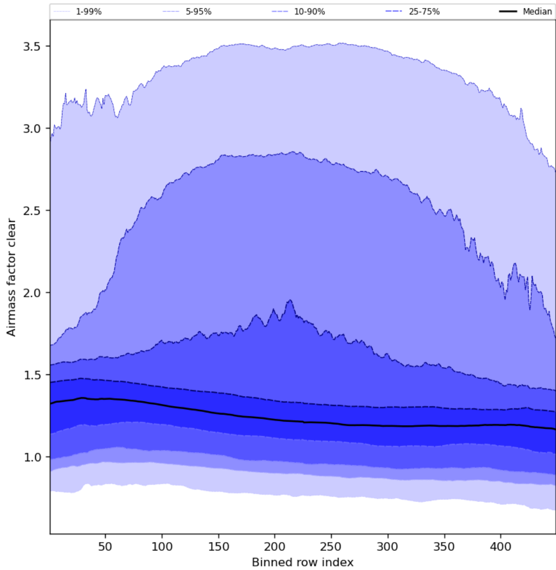
Figure 56: Along track statistics of “Airmass factor clear” for 2023-09-01 to 2023-09-03
