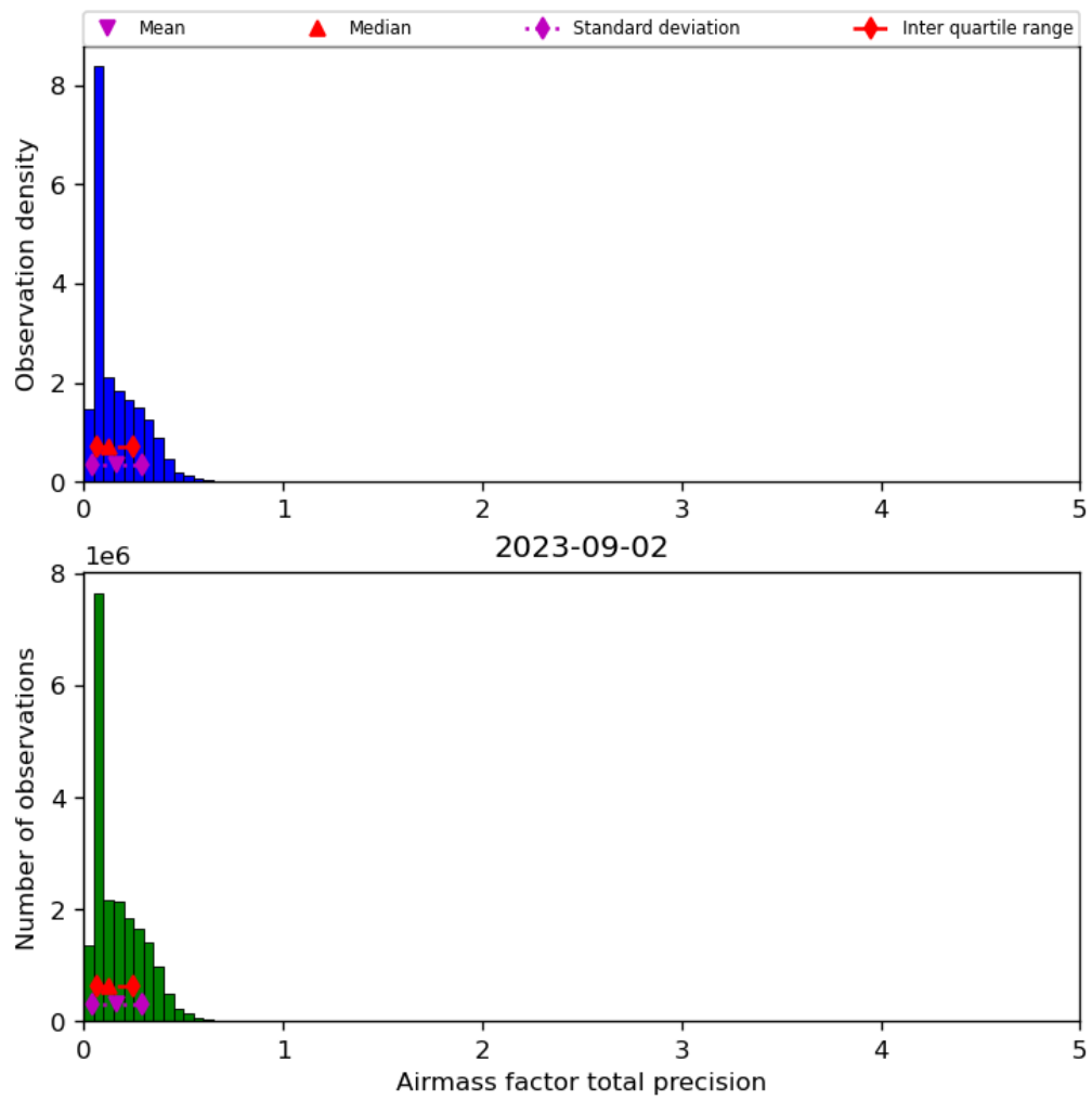
Figure 41: Histogram of “Airmass factor total precision” for 2023-09-01 to 2023-09-03
