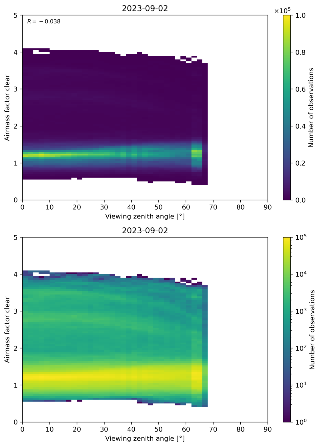
Figure 185: Scatter density plot of “Viewing zenith angle” against “Airmass factor clear” for 2023-09-01 to 2023-09-03.
