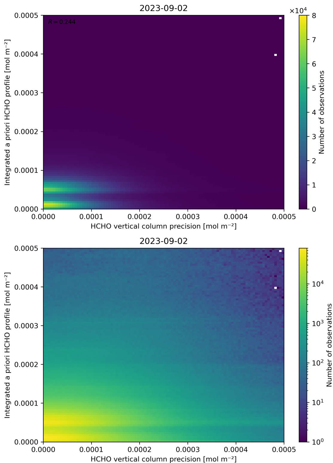
Figure 147: Scatter density plot of “HCHO vertical column precision” against “Integrated a priori HCHO profile” for 2023-09-01 to 2023-09-03.
