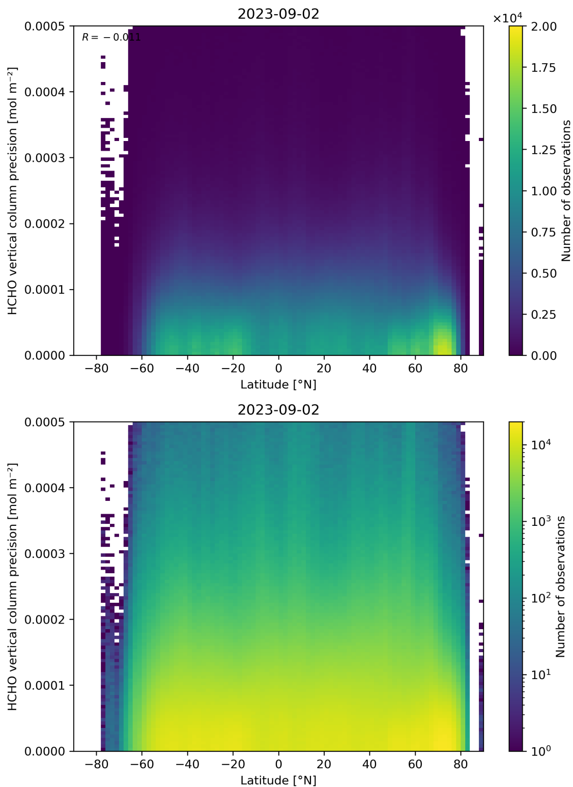
Figure 165: Scatter density plot of “Latitude” against “HCHO vertical column precision” for 2023-09-01 to 2023-09-03.
