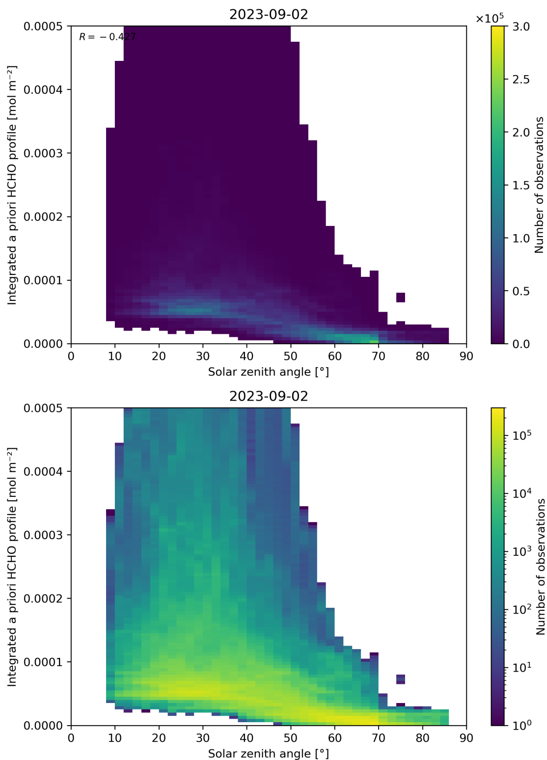
Figure 180: Scatter density plot of “Solar zenith angle” against “Integrated a priori HCHO profile” for 2023-09-01 to 2023-09-03.
