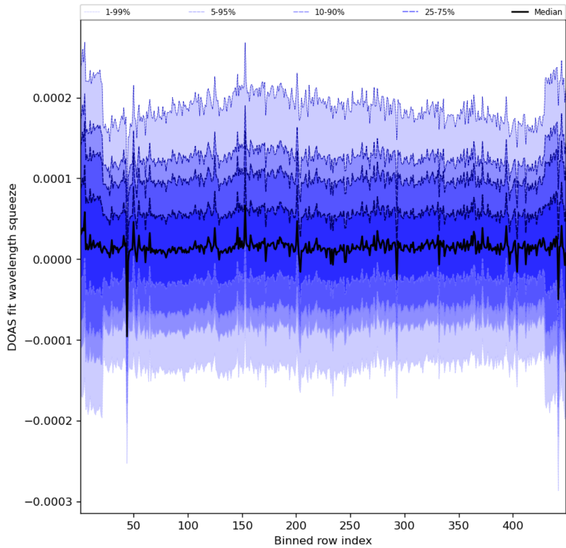
Figure 59: Along track statistics of “DOAS fit wavelength squeeze” for 2023-09-01 to 2023-09-03
