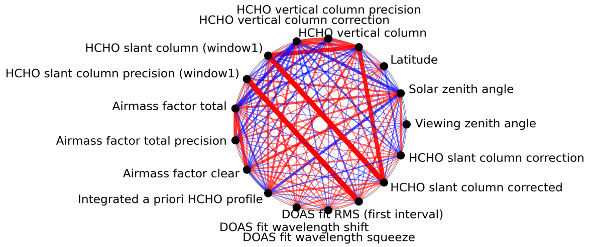
Figure 1: Map of correlation graph for 2023-09-01 to 2023-09-03.
