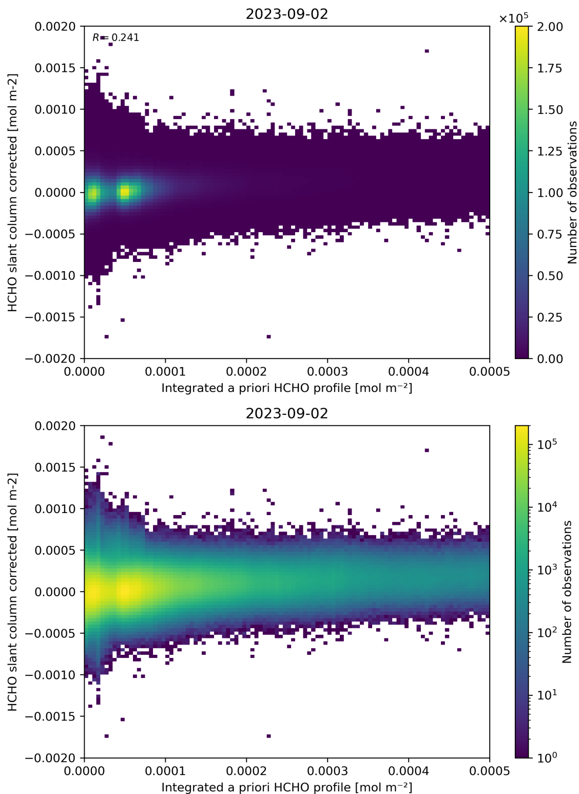
Figure 151: Scatter density plot of “Integrated a priori HCHO profile” against “HCHO slant column corrected” for 2023-09-01 to 2023-09-03.
