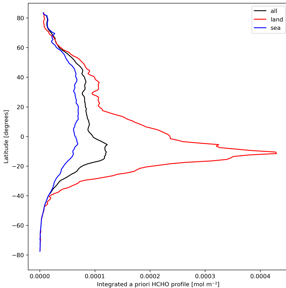
Figure 29: Zonal average of “Integrated a priori HCHO profile” for 2023-09-01 to 2023-09-03.
