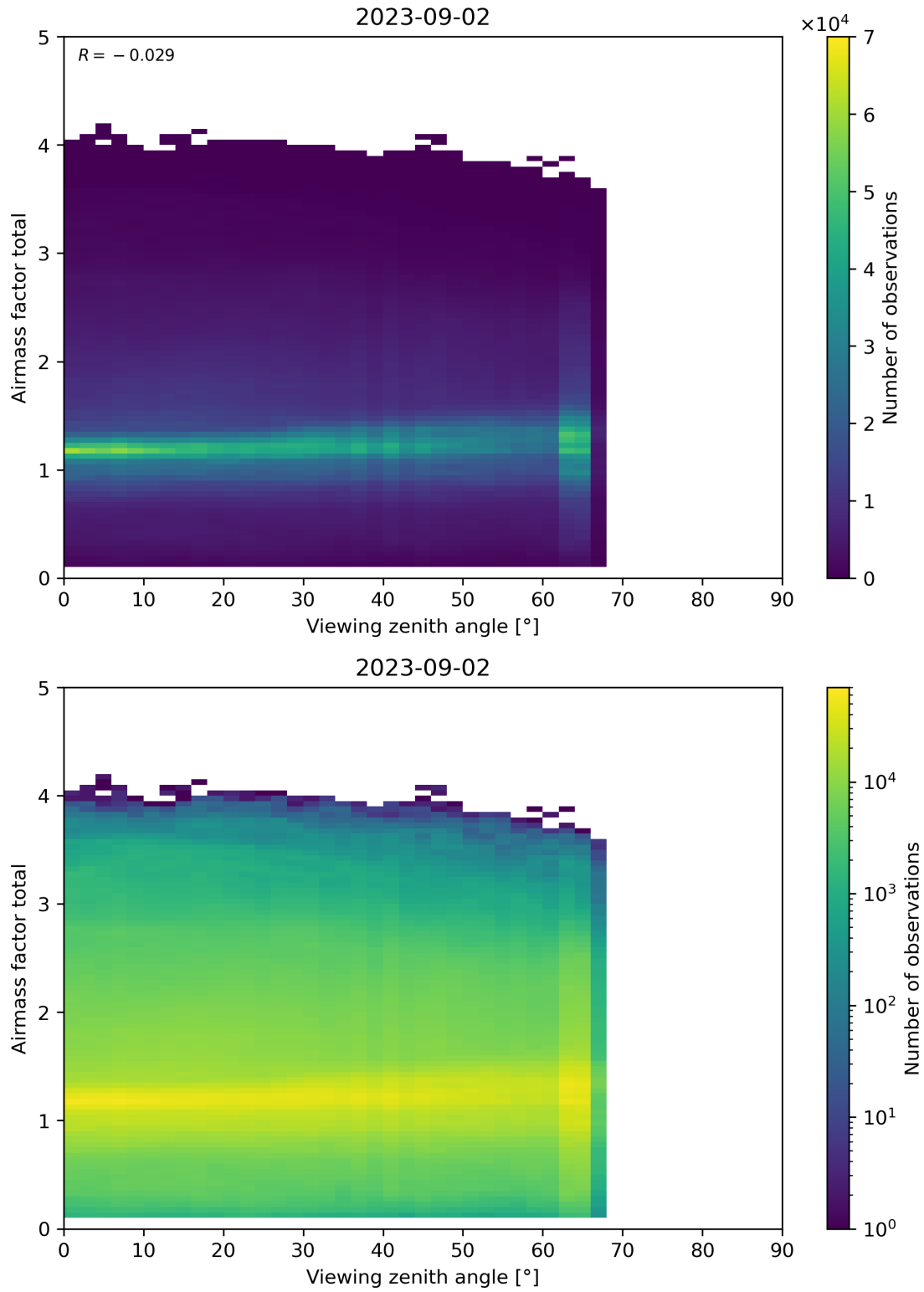
Figure 190: Scatter density plot of “Viewing zenith angle” against “Airmass factor total” for 2023-09-01 to 2023-09-03.
