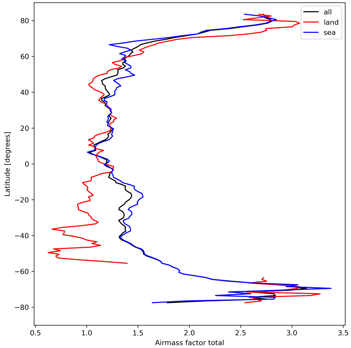
Figure 26: Zonal average of “Airmass factor total” for 2023-09-01 to 2023-09-03.
