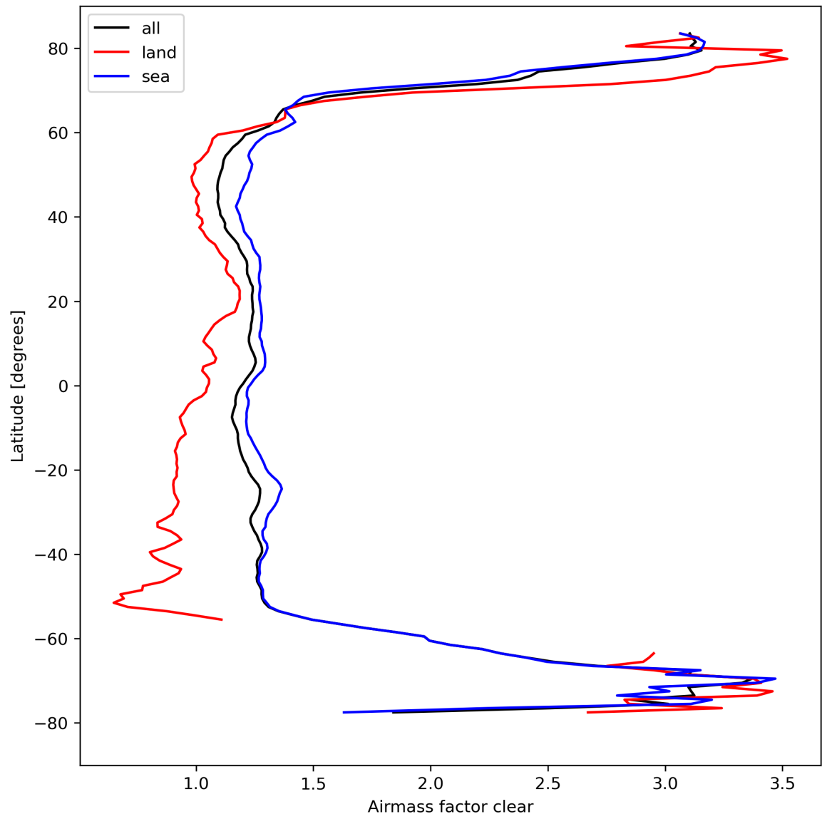
Figure 28: Zonal average of “Airmass factor clear” for 2023-09-01 to 2023-09-03.
