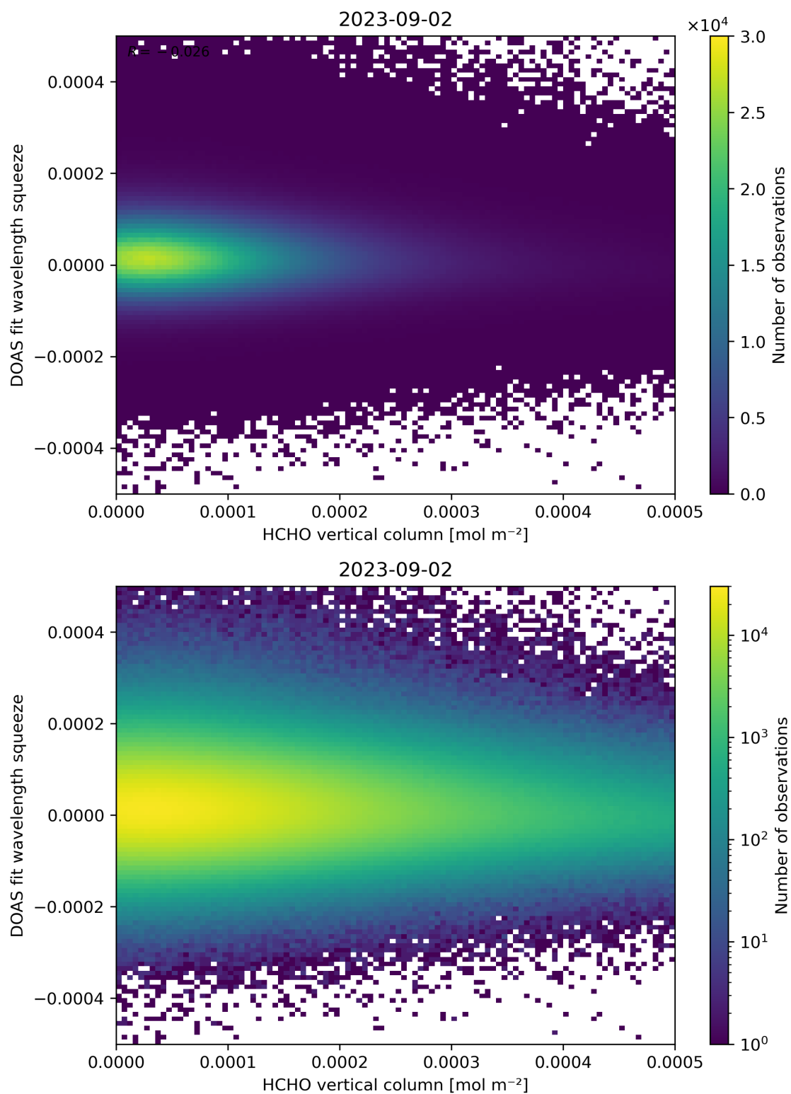
Figure 125: Scatter density plot of “HCHO vertical column” against “DOAS fit wavelength squeeze” for 2023-09-01 to 2023-09-03.
