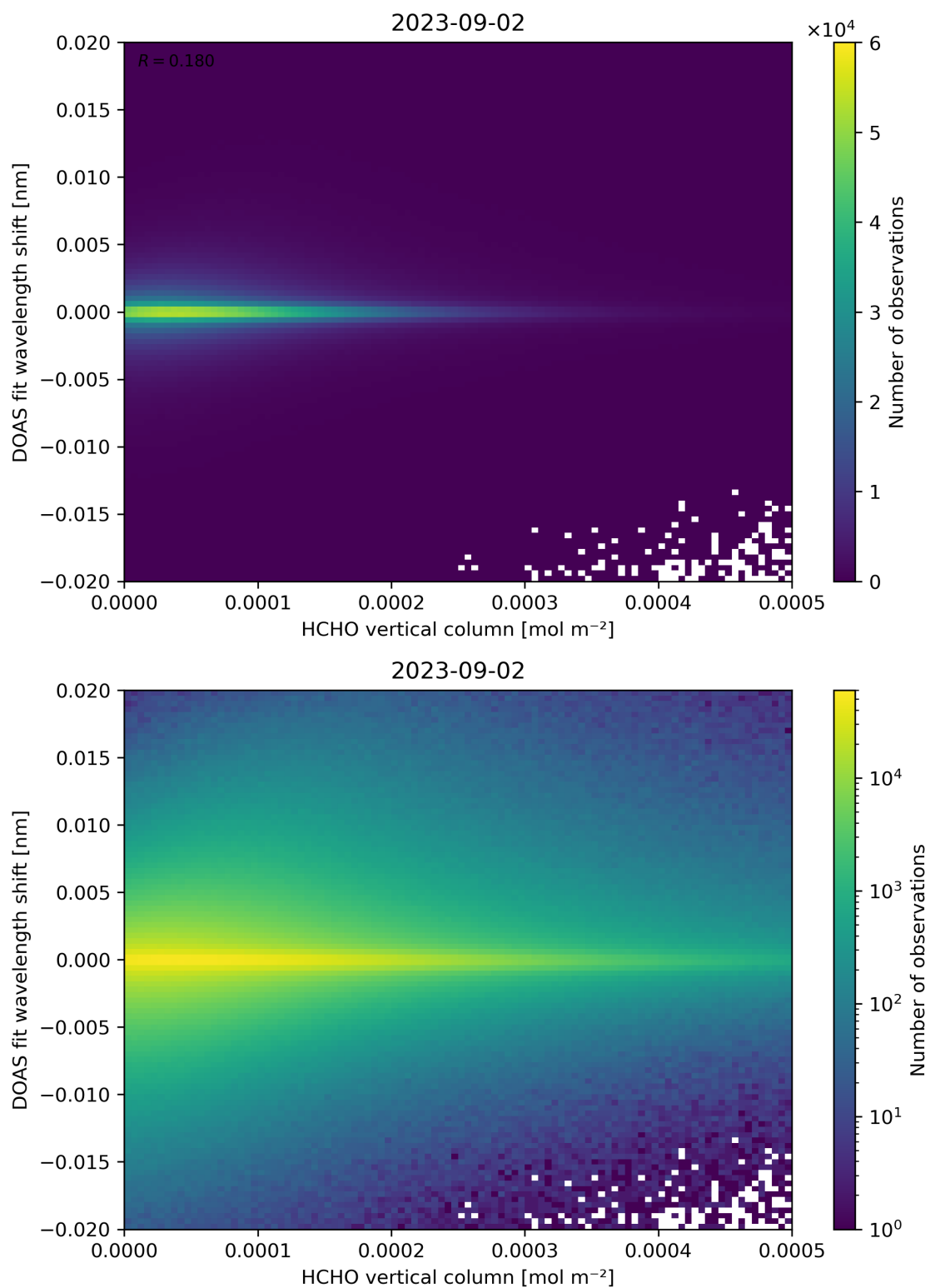
Figure 124: Scatter density plot of “HCHO vertical column” against “DOAS fit wavelength shift” for 2023-09-01 to 2023-09-03.
