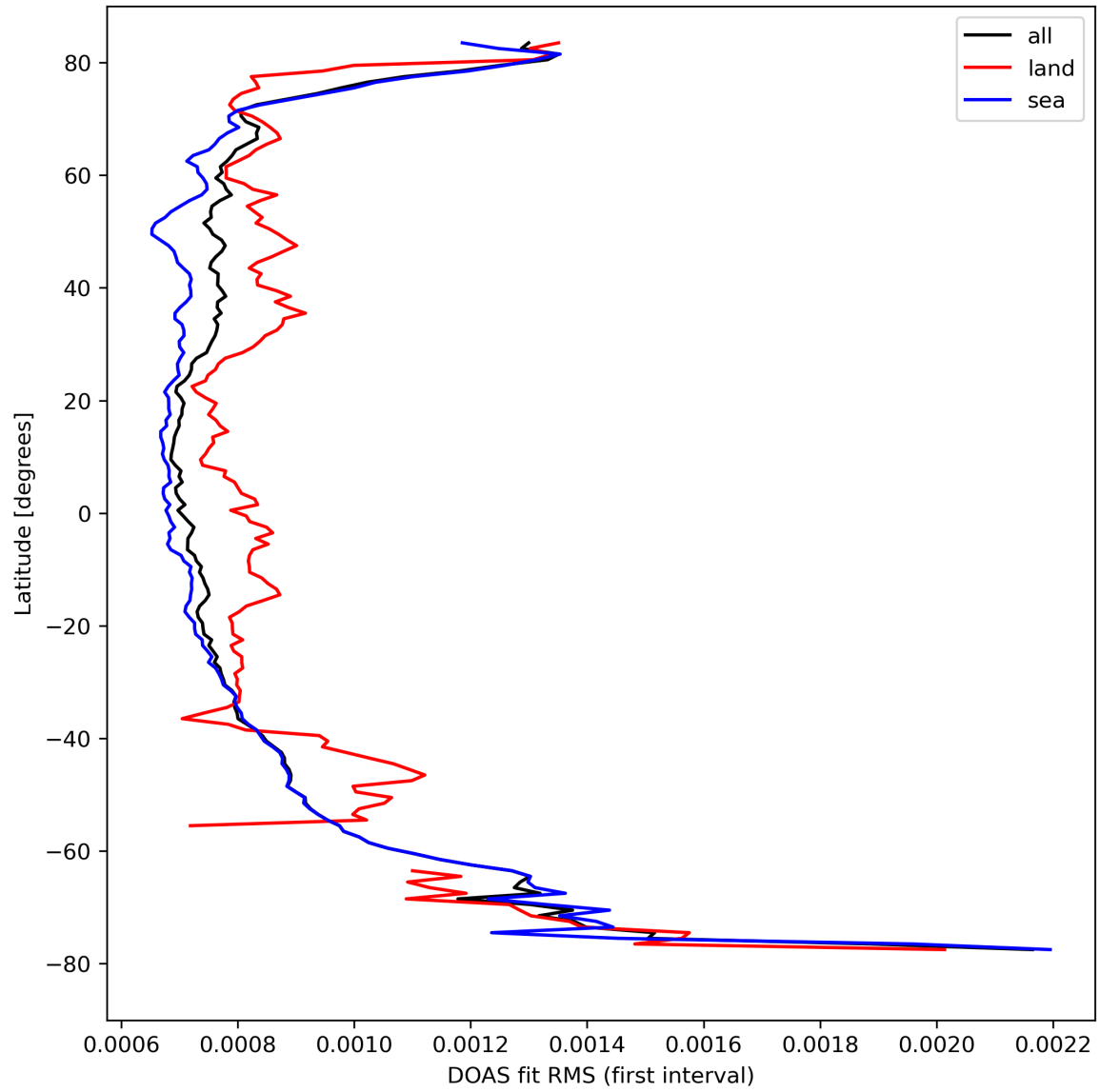
Figure 32: Zonal average of “DOAS fit RMS (first interval)” for 2023-09-01 to 2023-09-03.
