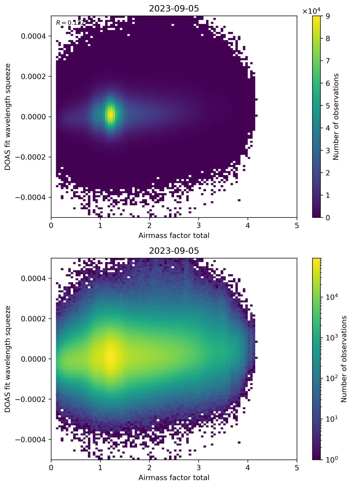
Figure 99: Scatter density plot of “Airmass factor total” against “DOAS fit wavelength squeeze” for 2023-09-05 to 2023-09-06.
