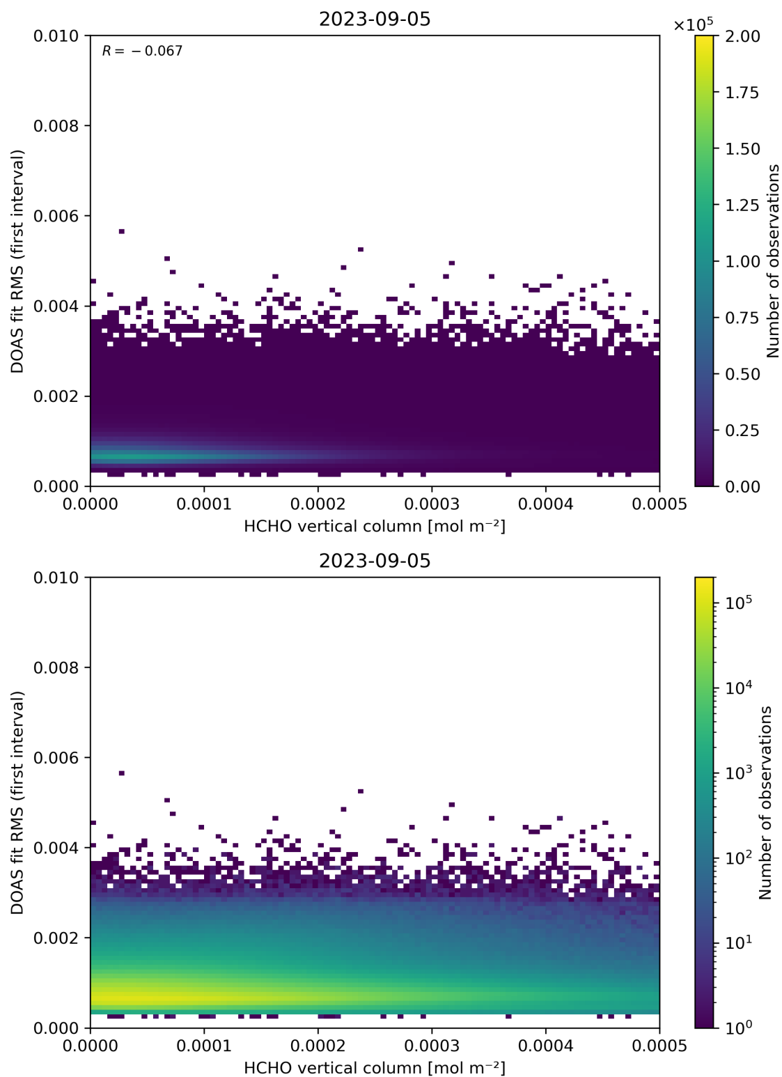
Figure 123: Scatter density plot of “HCHO vertical column” against “DOAS fit RMS (first interval)” for 2023-09-05 to 2023-09-06.
