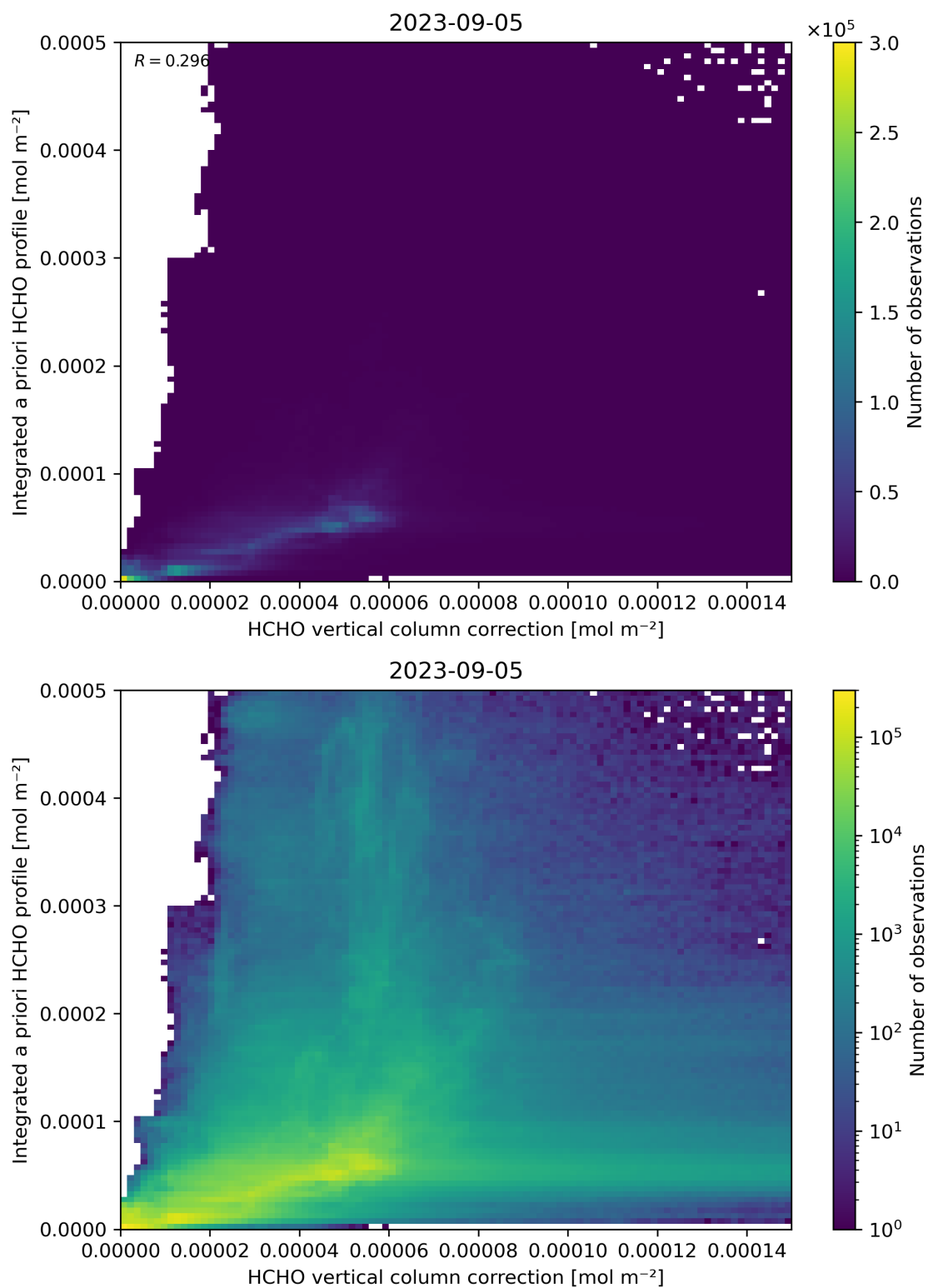
Figure 122: Scatter density plot of “HCHO vertical column correction” against “Integrated a priori HCHO profile” for 2023-09-05 to 2023-09-06.
