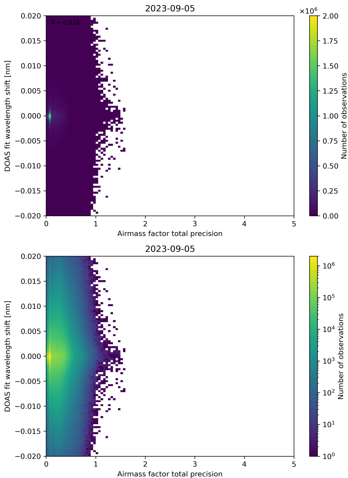
Figure 106: Scatter density plot of “Airmass factor total precision” against “DOAS fit wavelength shift” for 2023-09-05 to 2023-09-06.
