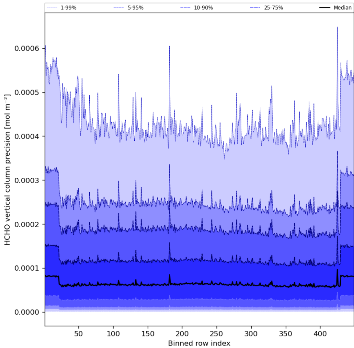
Figure 50: Along track statistics of “HCHO vertical column precision” for 2023-09-05 to 2023-09-06
