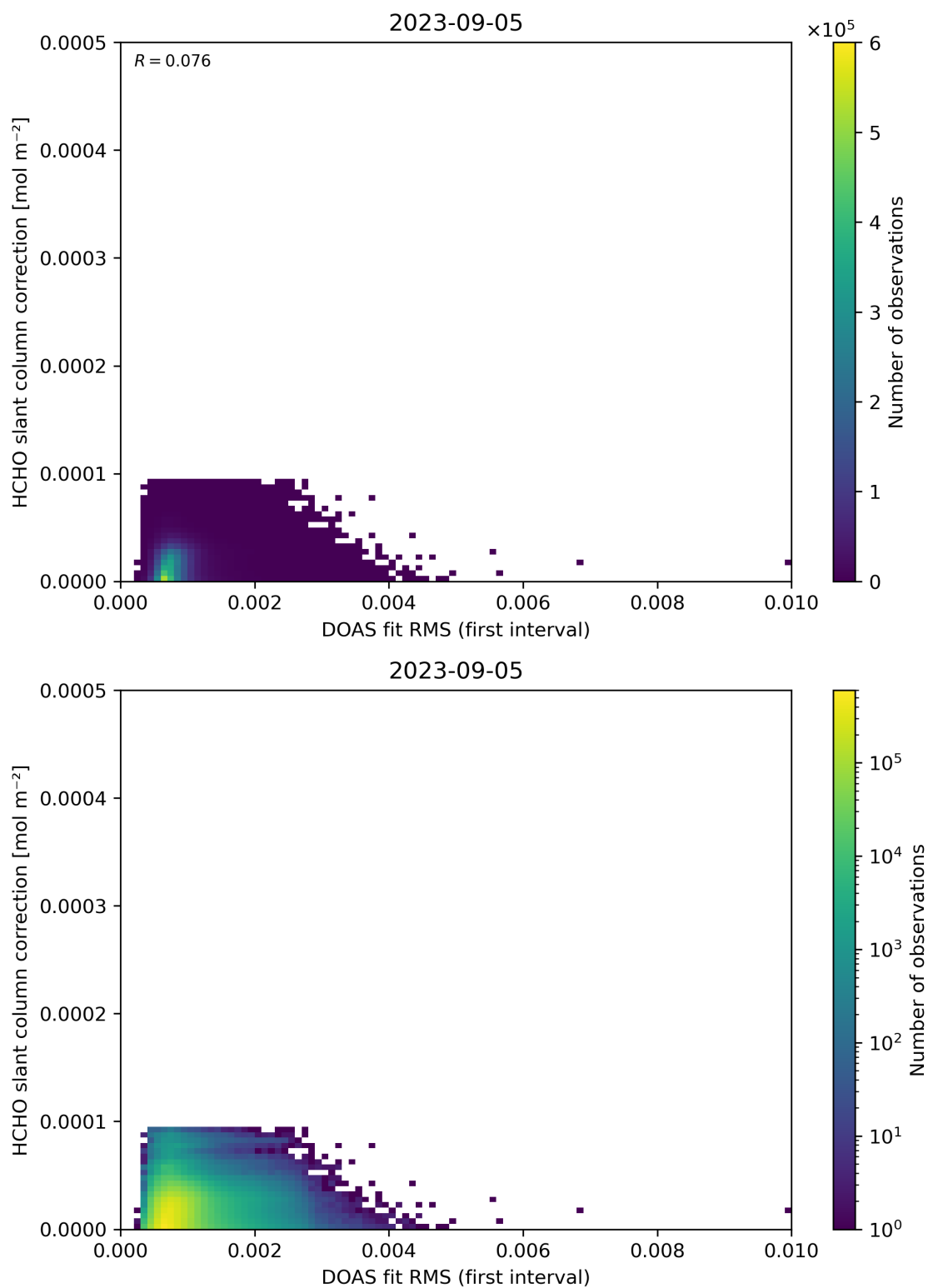
Figure 63: Scatter density plot of “DOAS fit RMS (first interval)” against “HCHO slant column correction” for 2023-09-05 to 2023-09-06.
