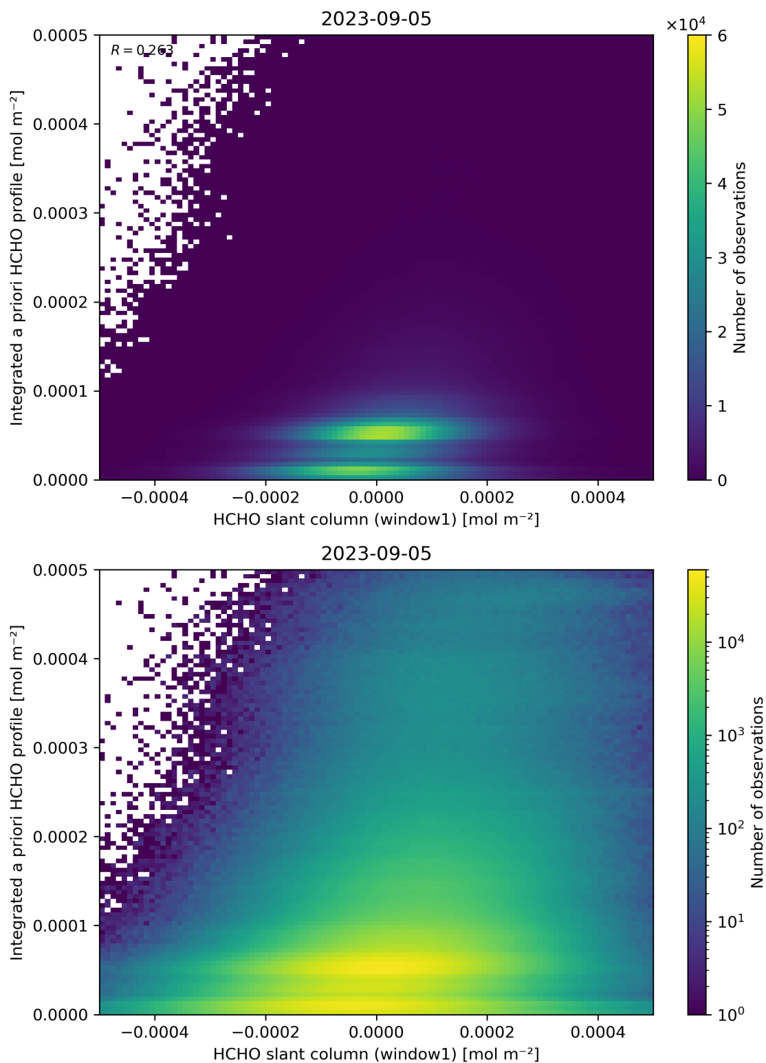
Figure 87: Scatter density plot of “HCHO slant column (window1)” against “Integrated a priori HCHO profile” for 2023-09-05 to 2023-09-06.
