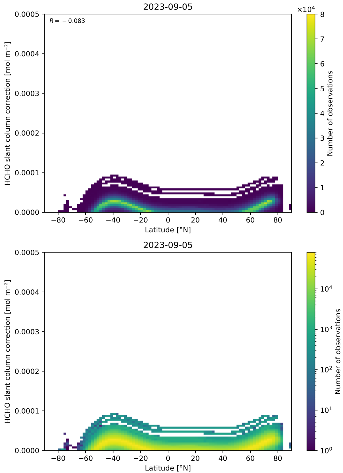
Figure 158: Scatter density plot of “Latitude” against “HCHO slant column correction” for 2023-09-05 to 2023-09-06.
