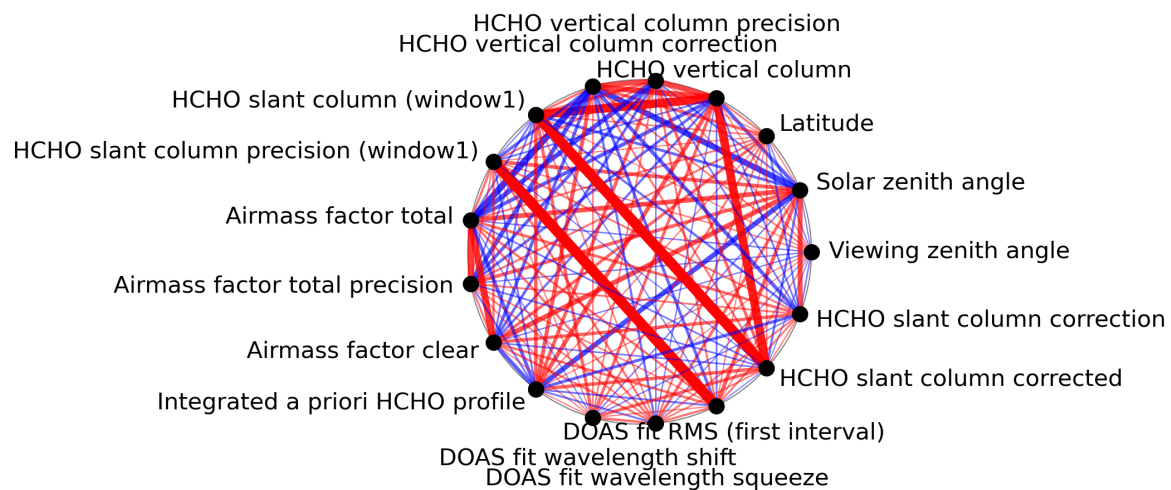
Figure 1: Map of correlation graph for 2023-09-05 to 2023-09-06.
