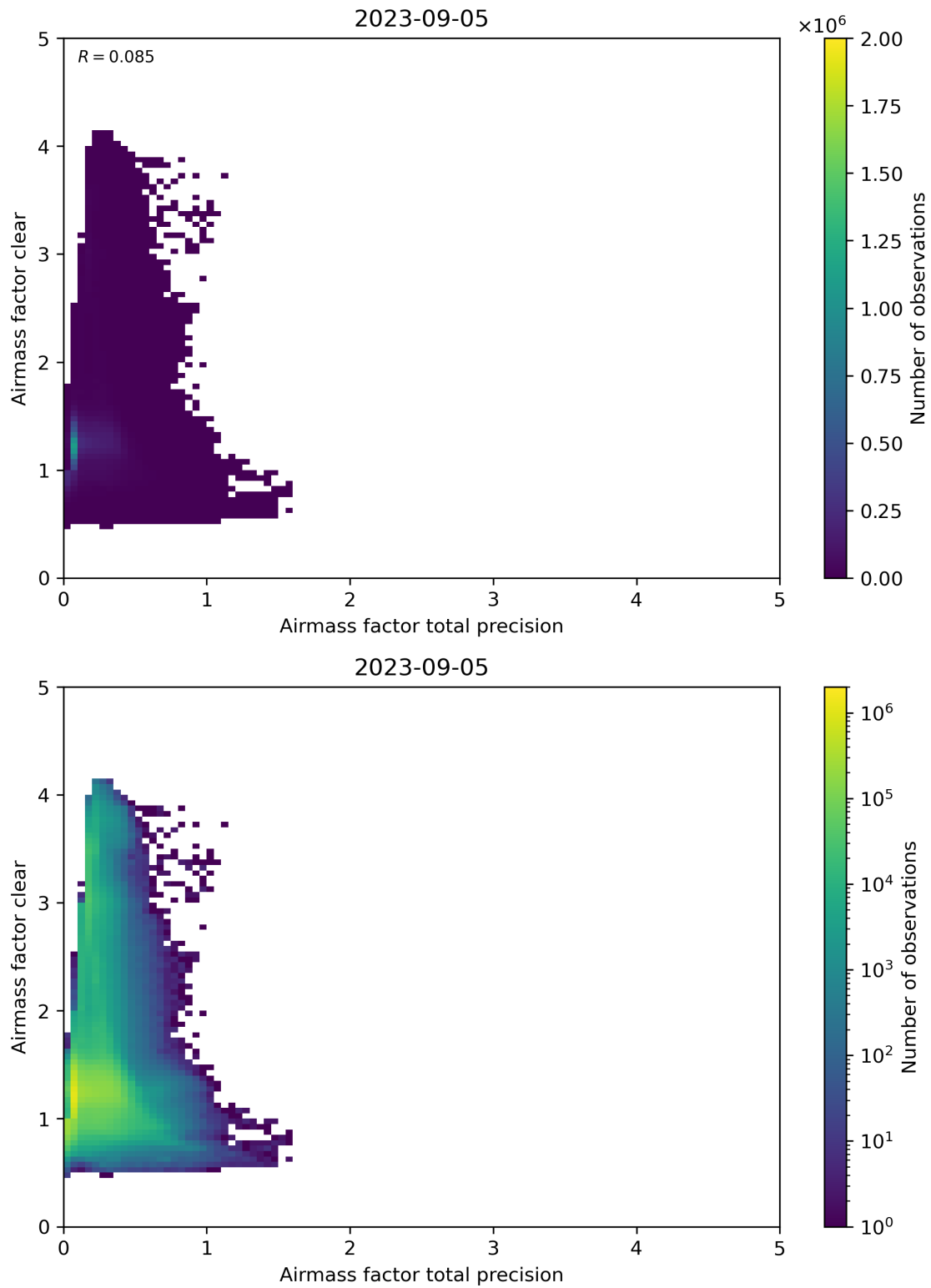
Figure 108: Scatter density plot of “Airmass factor total precision” against “Airmass factor clear” for 2023-09-05 to 2023-09-06.
