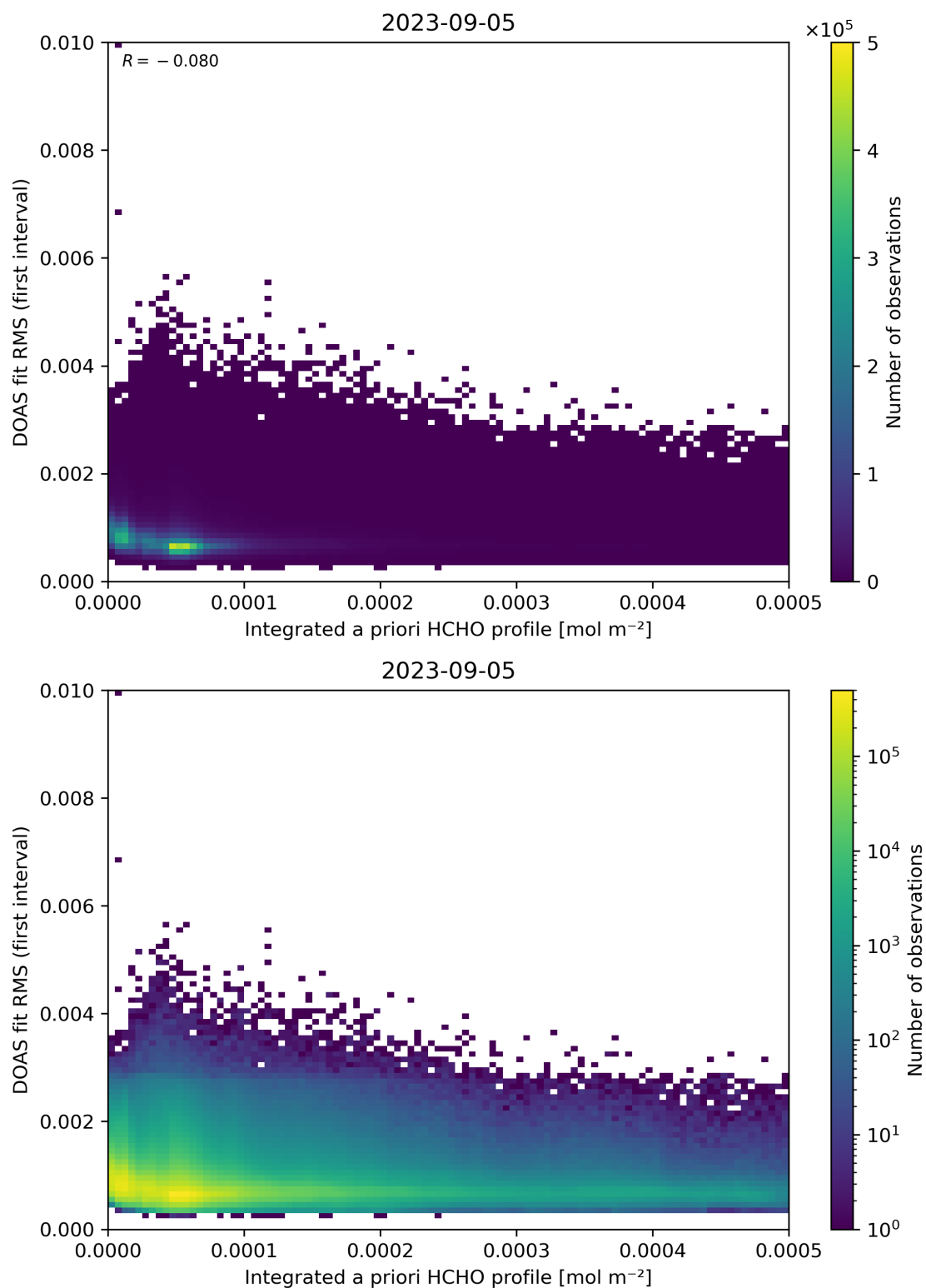
Figure 148: Scatter density plot of “Integrated a priori HCHO profile” against “DOAS fit RMS (first interval)” for 2023-09-05 to 2023-09-06.
