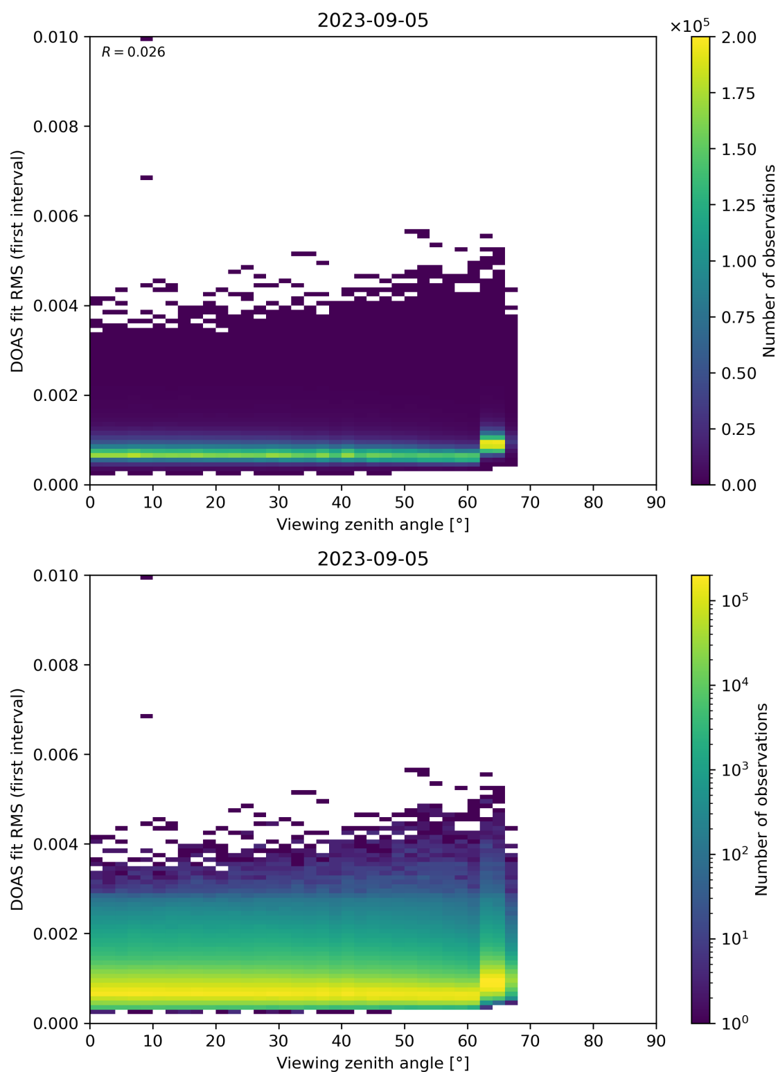
Figure 182: Scatter density plot of “Viewing zenith angle” against “DOAS fit RMS (first interval)” for 2023-09-05 to 2023-09-06.
