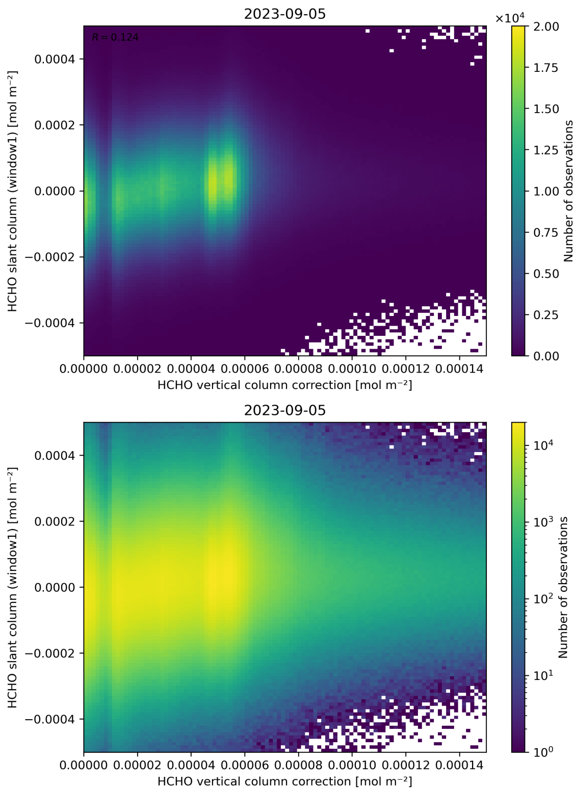
Figure 118: Scatter density plot of “HCHO vertical column correction” against “HCHO slant column (window1)” for 2023-09-05 to 2023-09-06.
