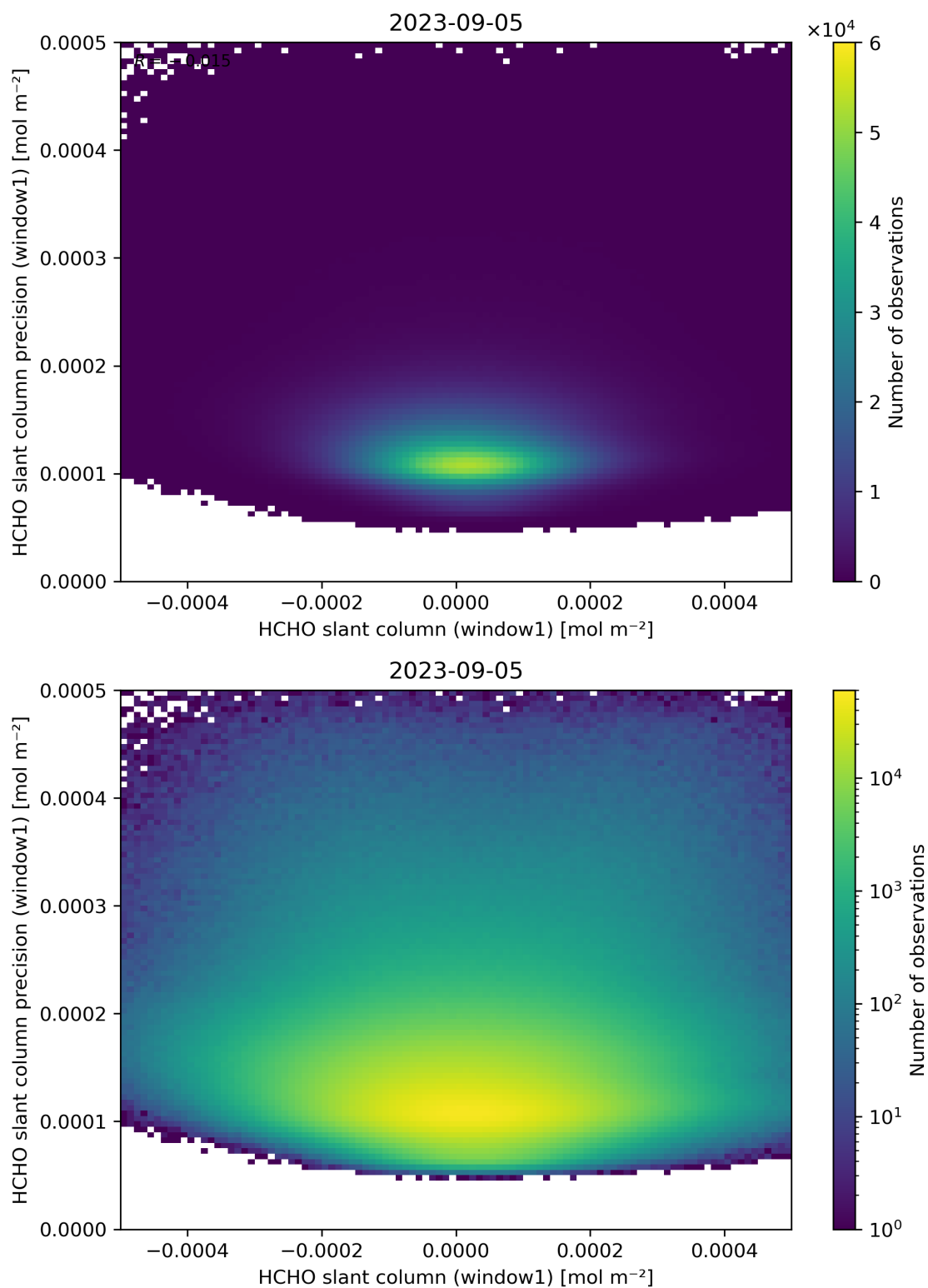
Figure 84: Scatter density plot of “HCHO slant column (window1)” against “HCHO slant column precision (window1)” for 2023-09-05 to 2023-09-06.
