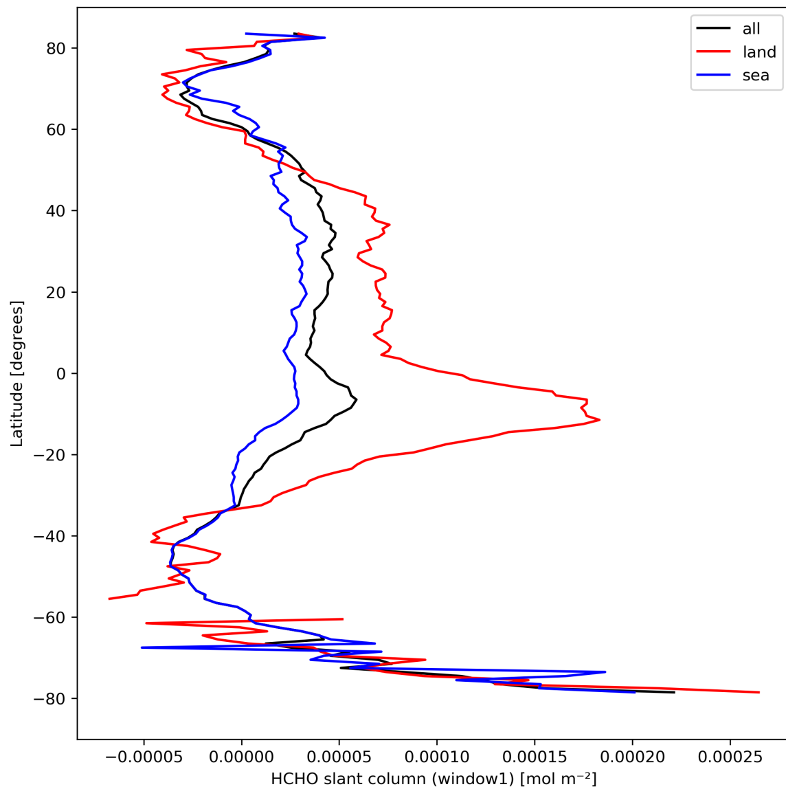
Figure 24: Zonal average of “HCHO slant column (window1)” for 2023-09-05 to 2023-09-06.
