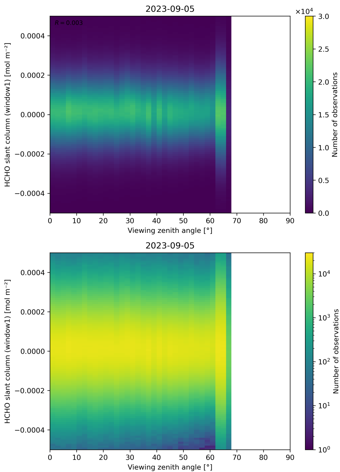
Figure 188: Scatter density plot of “Viewing zenith angle” against “HCHO slant column (window1)” for 2023-09-05 to 2023-09-06.
