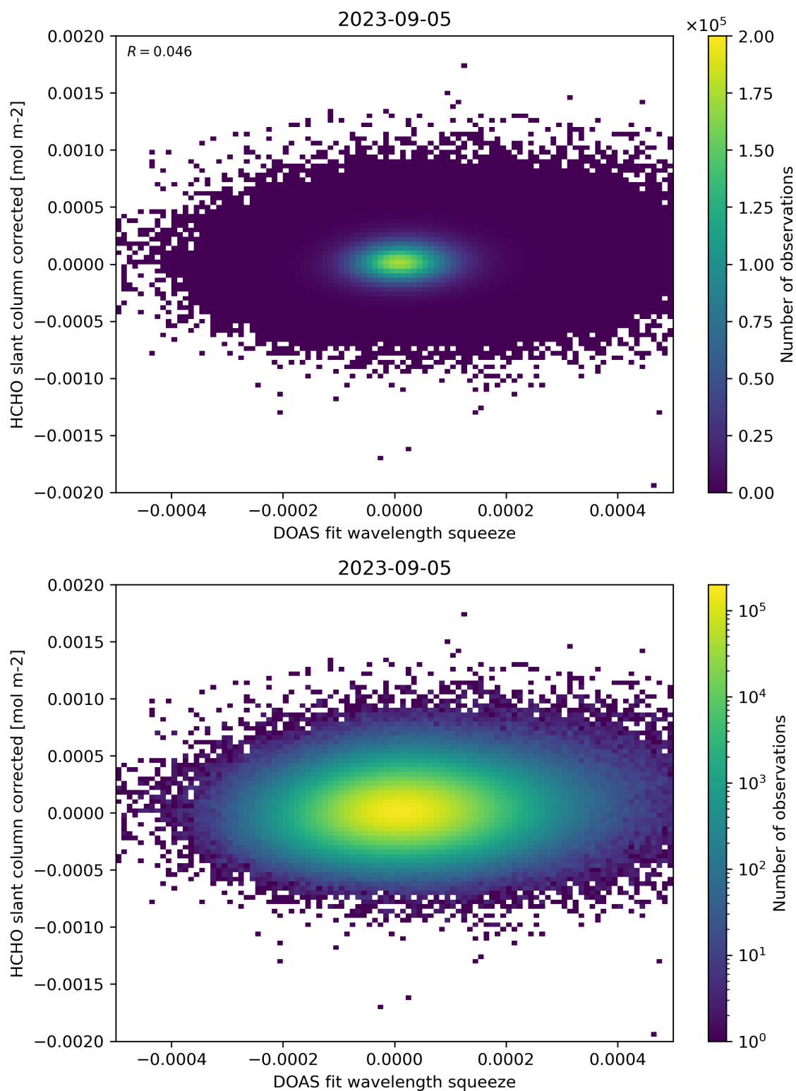
Figure 69: Scatter density plot of “DOAS fit wavelength squeeze” against “HCHO slant column corrected” for 2023-09-05 to 2023-09-06.
