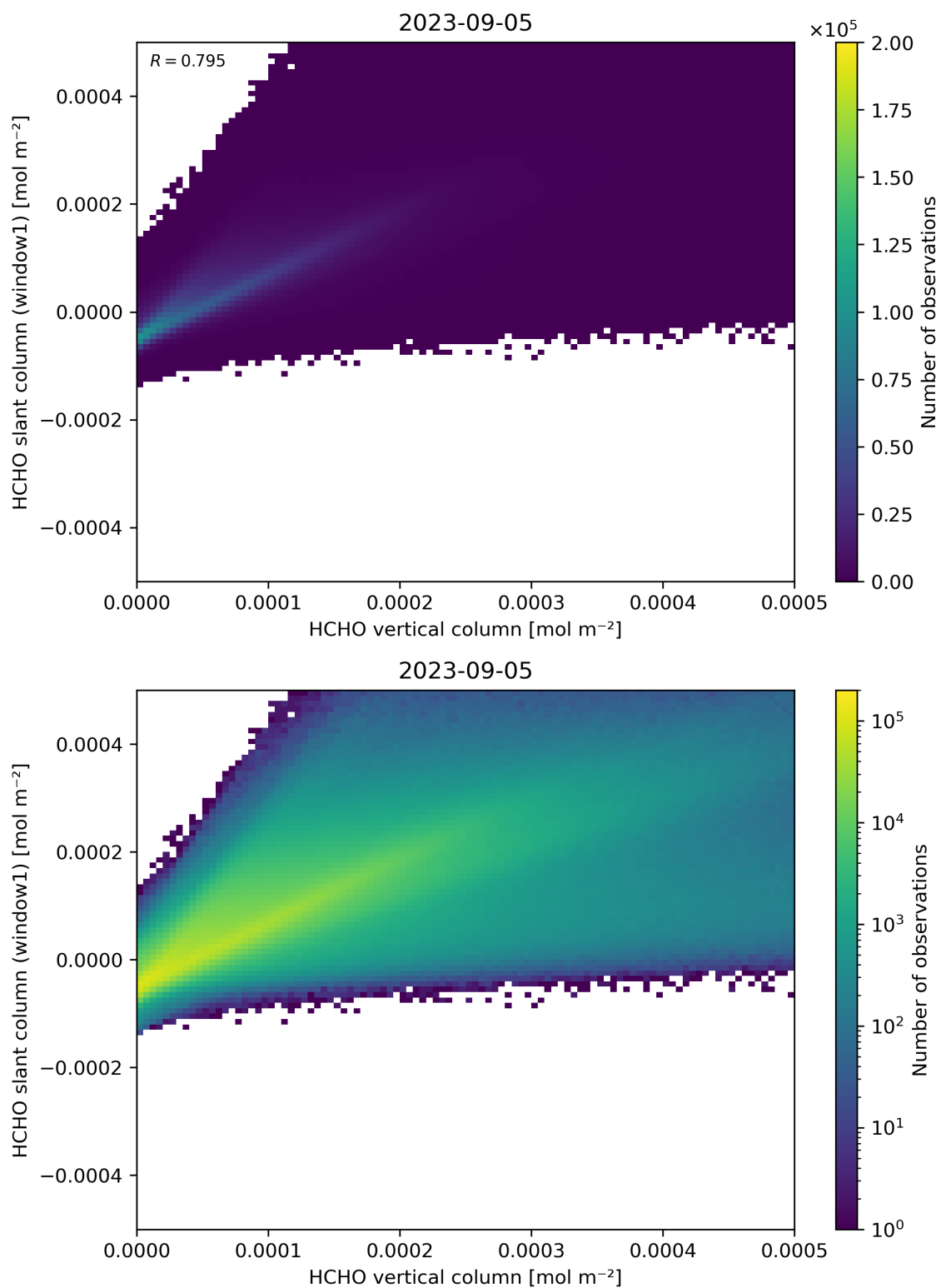
Figure 129: Scatter density plot of “HCHO vertical column” against “HCHO slant column (window1)” for 2023-09-05 to 2023-09-06.
