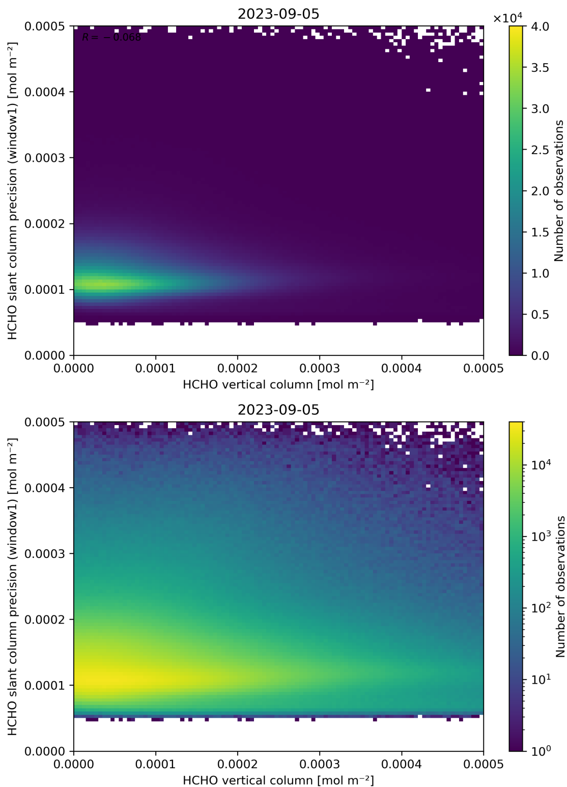
Figure 130: Scatter density plot of “HCHO vertical column” against “HCHO slant column precision (window1)” for 2023-09-05 to 2023-09-06.
