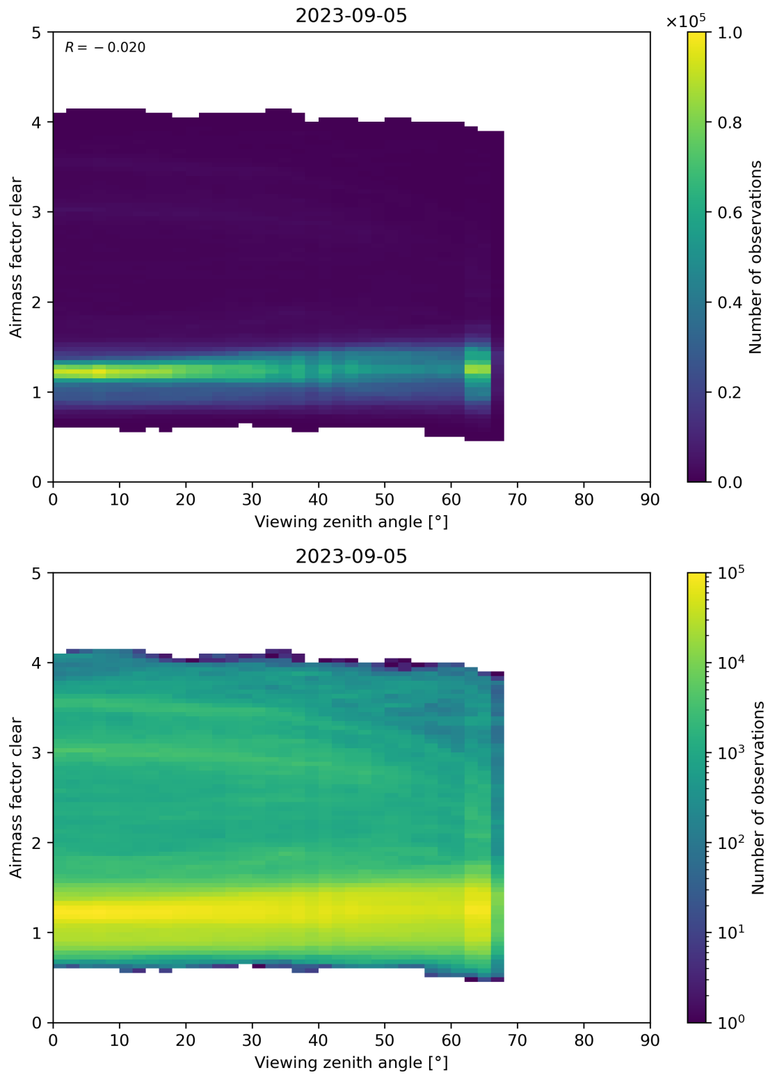
Figure 185: Scatter density plot of “Viewing zenith angle” against “Airmass factor clear” for 2023-09-05 to 2023-09-06.
