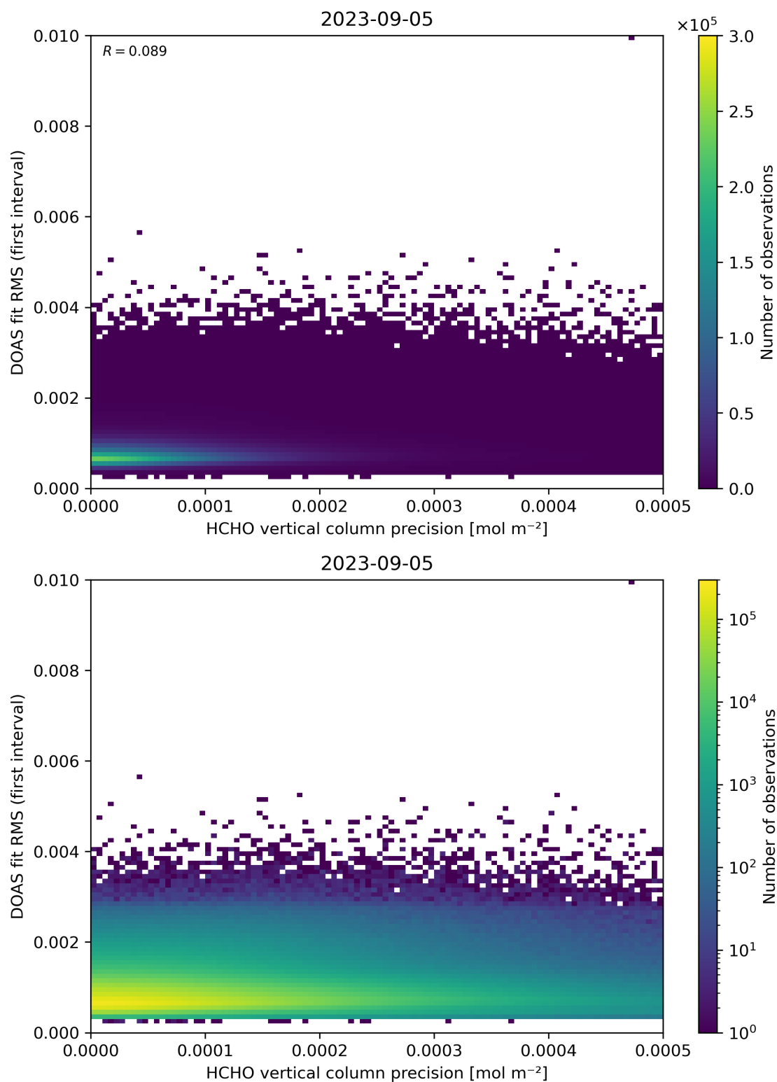
Figure 136: Scatter density plot of “HCHO vertical column precision” against “DOAS fit RMS (first interval)” for 2023-09-05 to 2023-09-06.
