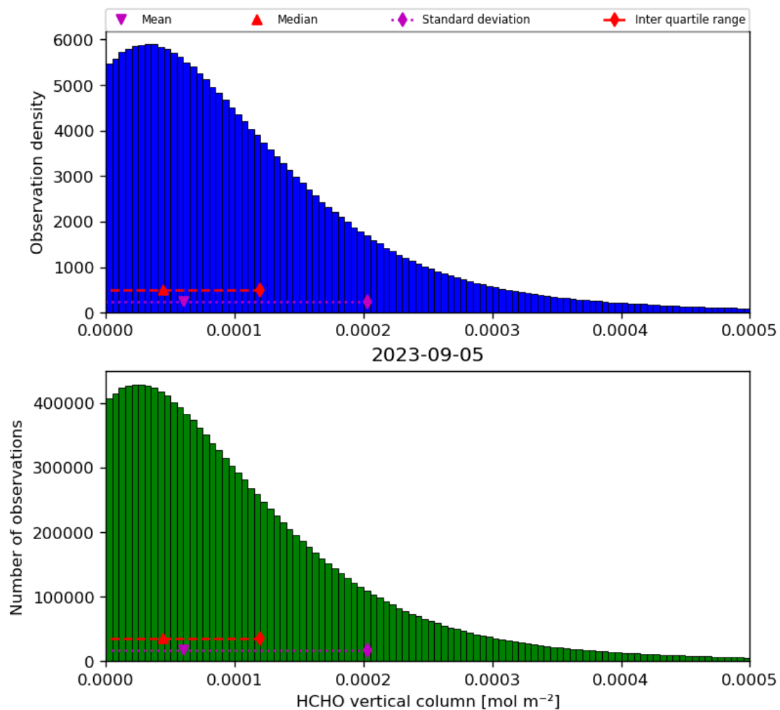
Figure 35: Histogram of “HCHO vertical column” for 2023-09-05 to 2023-09-06
