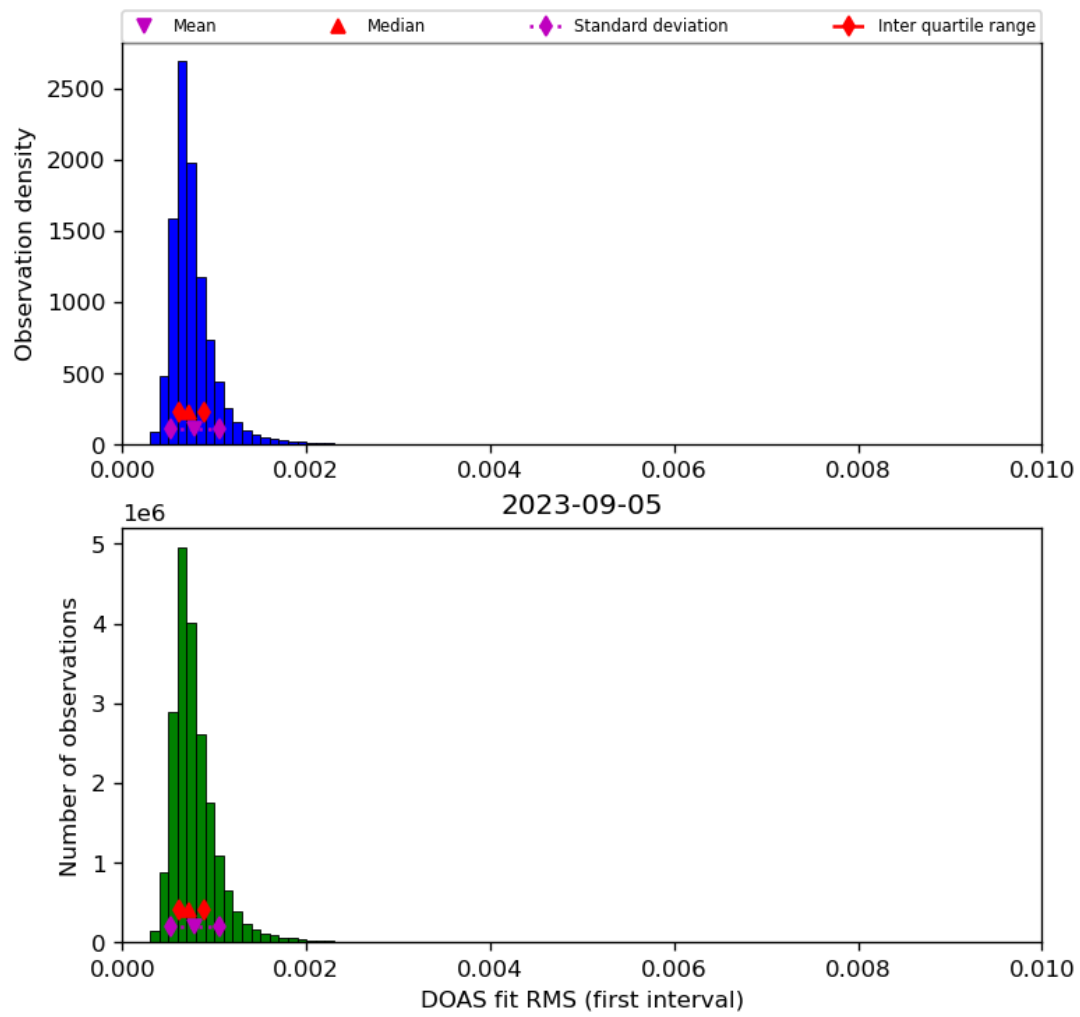
Figure 46: Histogram of “DOAS fit RMS (first interval)” for 2023-09-05 to 2023-09-06
