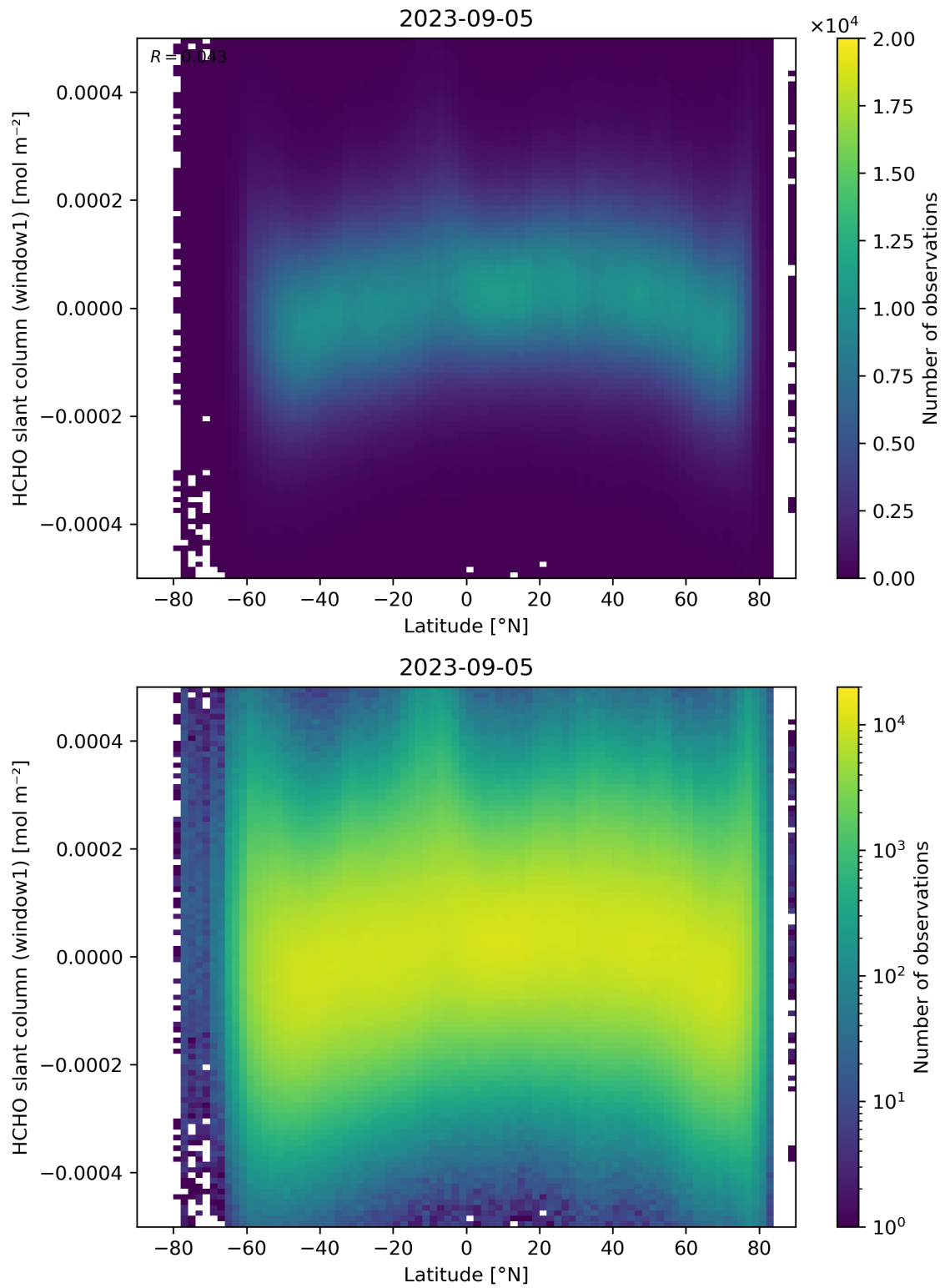
Figure 159: Scatter density plot of “Latitude” against “HCHO slant column (window1)” for 2023-09-05 to 2023-09-06.
