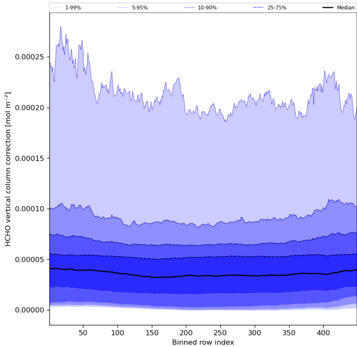
Figure 51: Along track statistics of “HCHO vertical column correction” for 2023-09-05 to 2023-09-06
