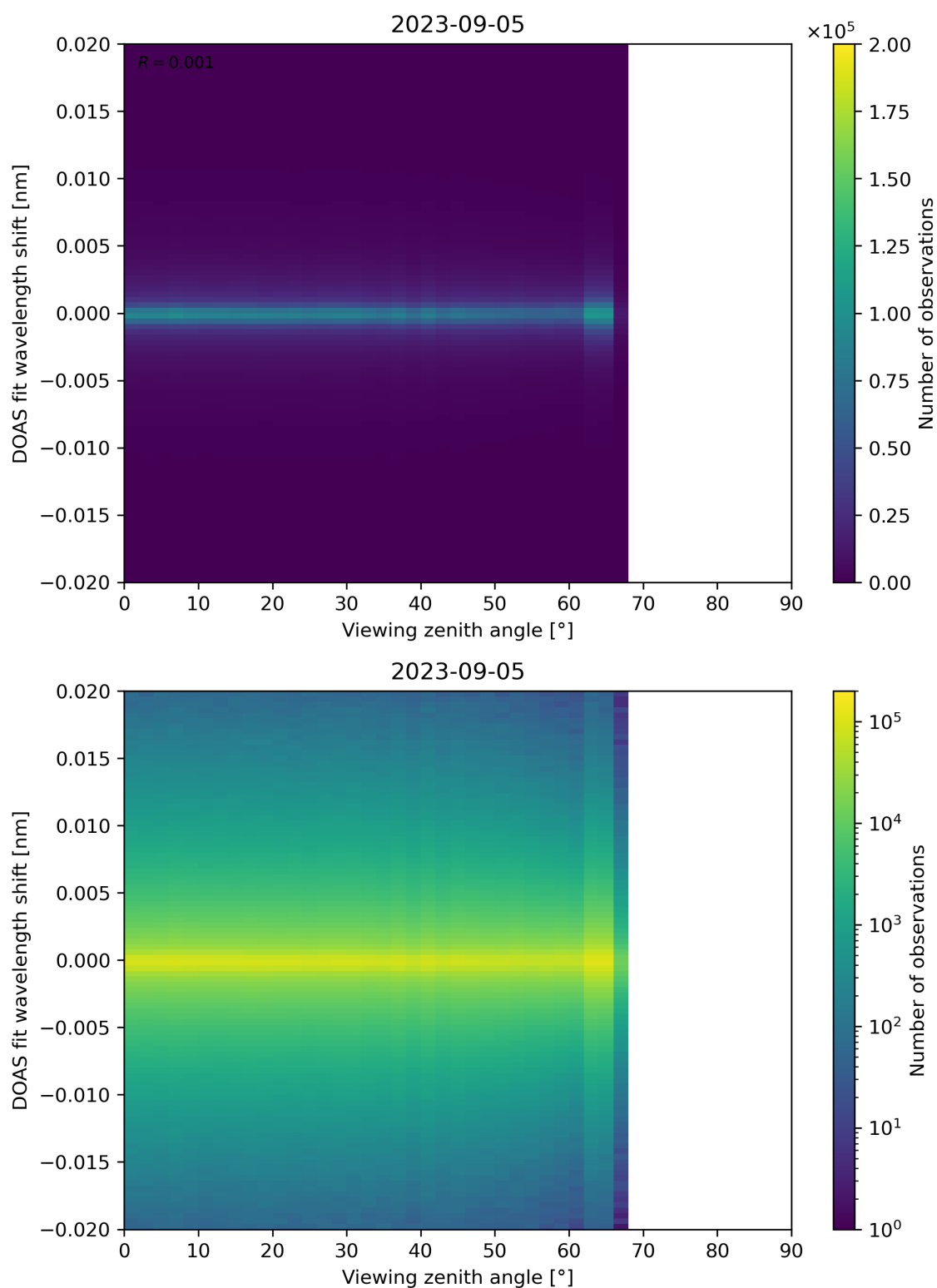
Figure 183: Scatter density plot of “Viewing zenith angle” against “DOAS fit wavelength shift” for 2023-09-05 to 2023-09-06.
