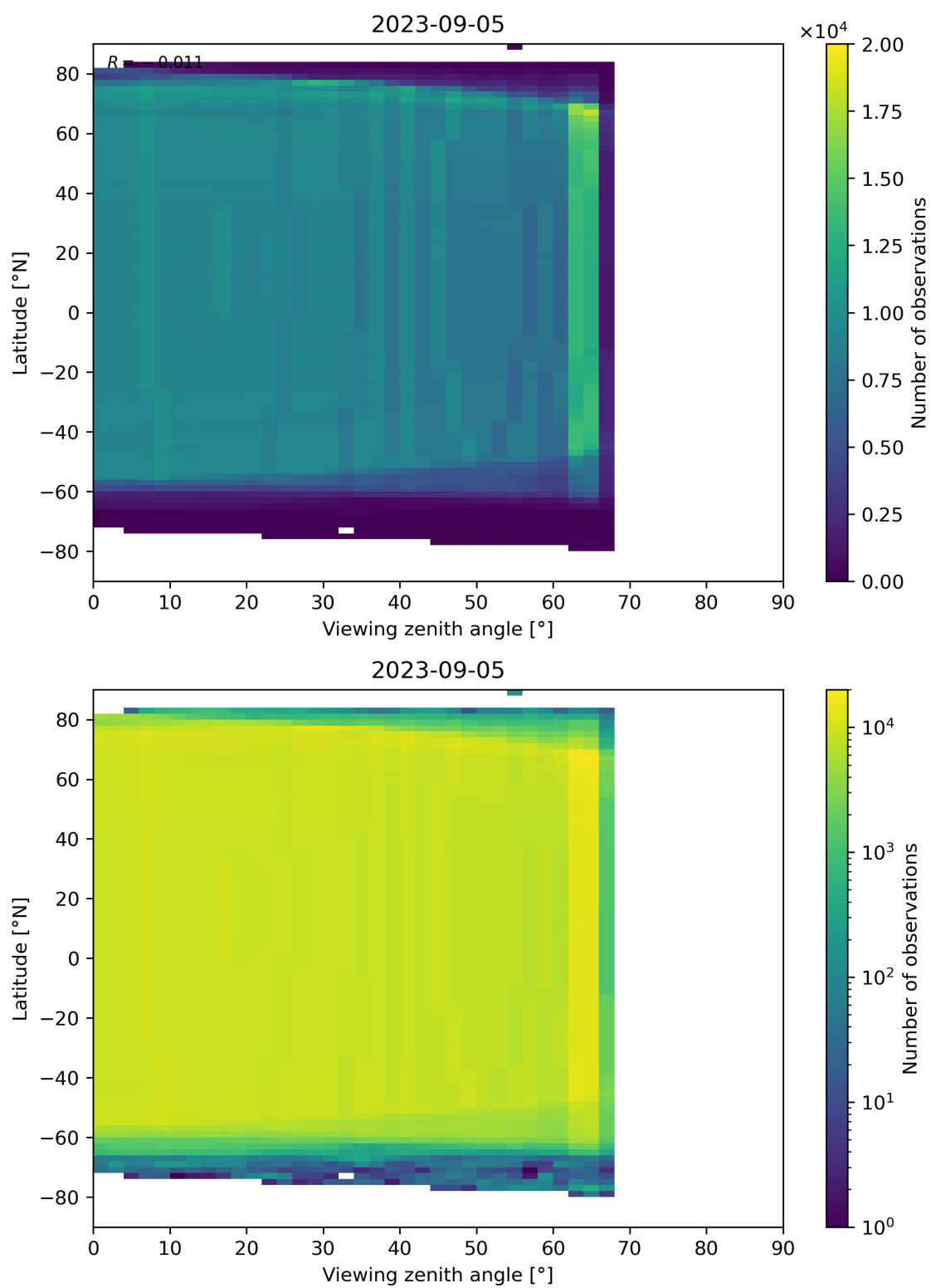
Figure 196: Scatter density plot of “Viewing zenith angle” against “Latitude” for 2023-09-05 to 2023-09-06.
