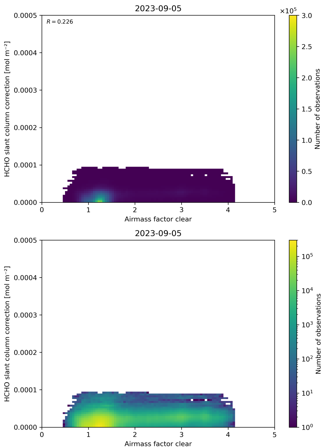
Figure 75: Scatter density plot of “Airmass factor clear” against “HCHO slant column correction” for 2023-09-05 to 2023-09-06.
