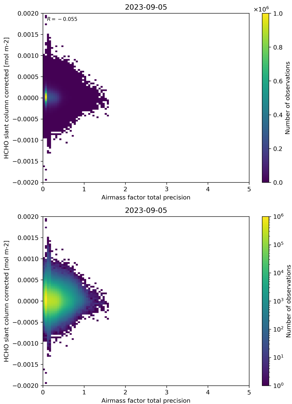
Figure 109: Scatter density plot of “Airmass factor total precision” against “HCHO slant column corrected” for 2023-09-05 to 2023-09-06.
