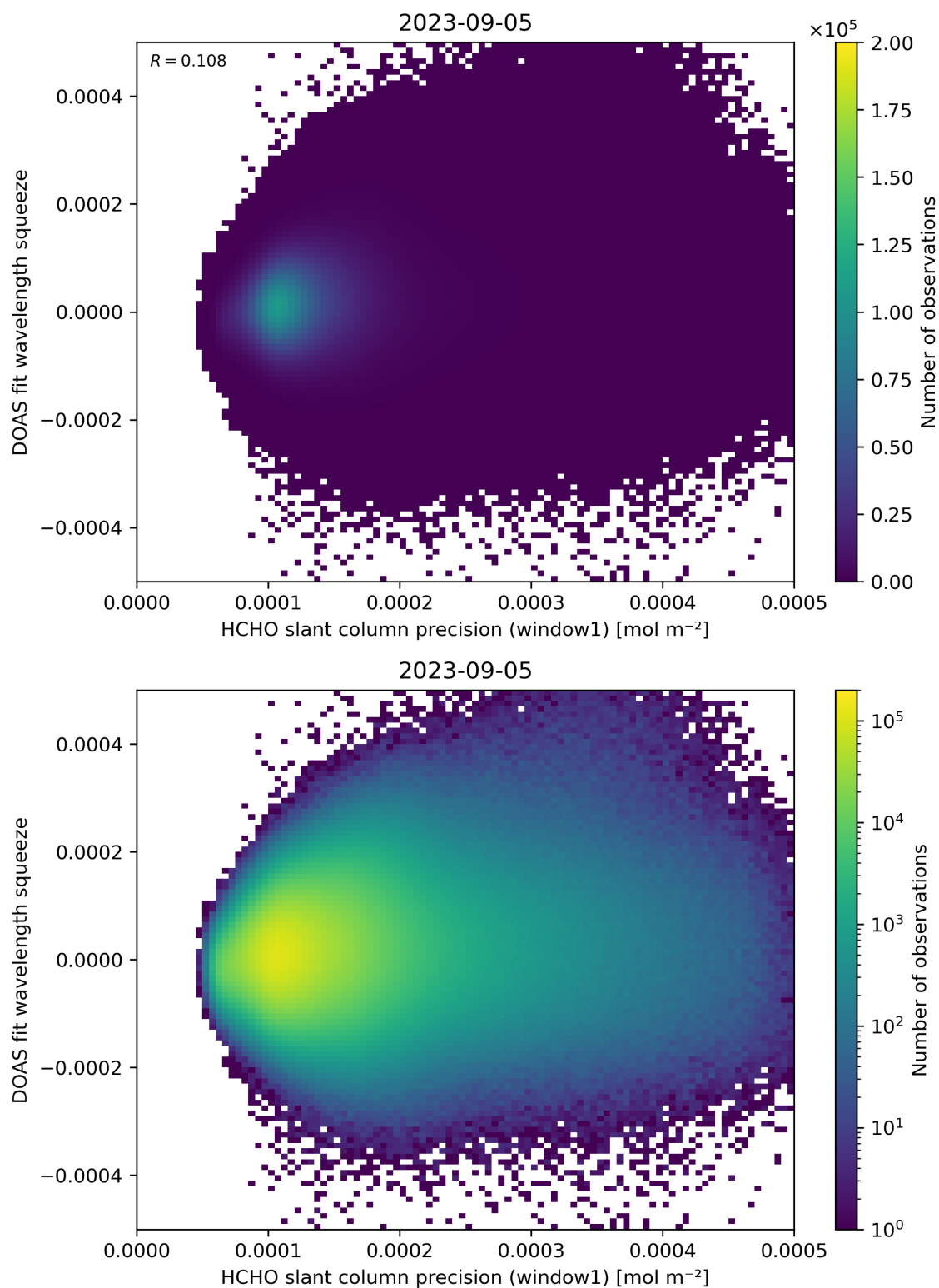
Figure 90: Scatter density plot of “HCHO slant column precision (window1)” against “DOAS fit wavelength squeeze” for 2023-09-05 to 2023-09-06.
