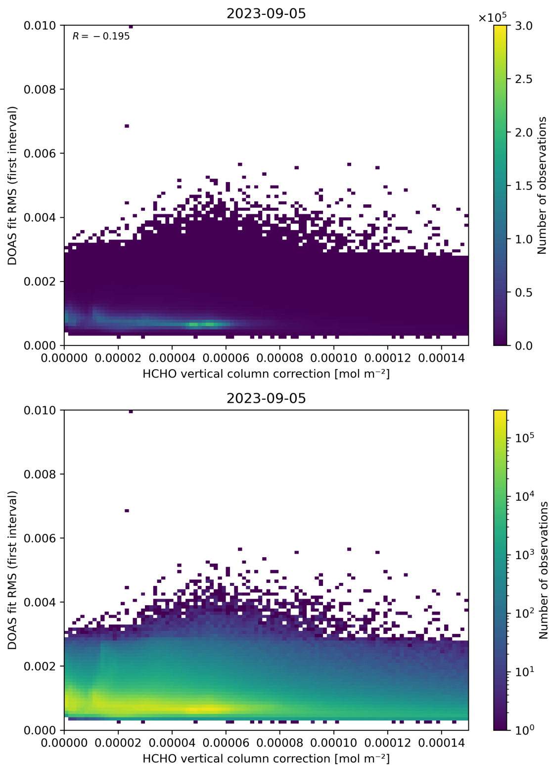
Figure 112: Scatter density plot of “HCHO vertical column correction” against “DOAS fit RMS (first interval)” for 2023-09-05 to 2023-09-06.
