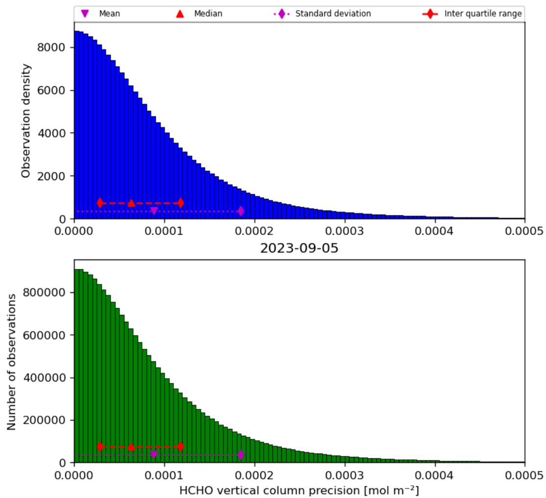
Figure 36: Histogram of “HCHO vertical column precision” for 2023-09-05 to 2023-09-06
