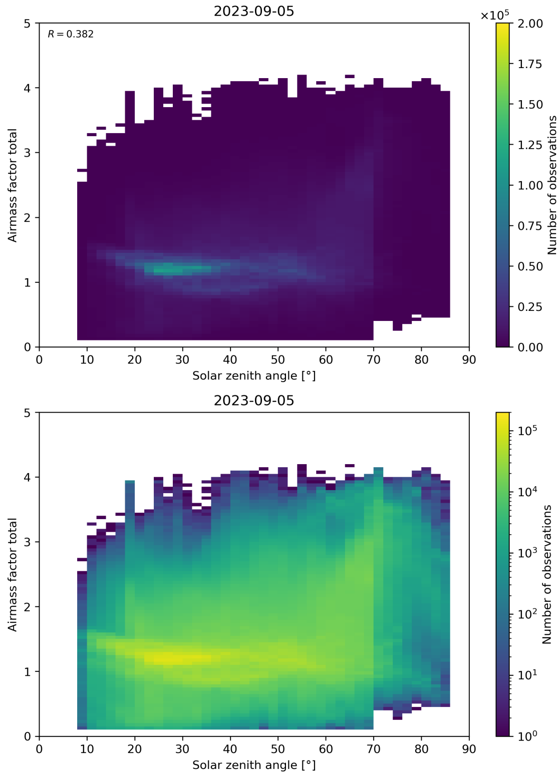
Figure 175: Scatter density plot of “Solar zenith angle” against “Airmass factor total” for 2023-09-05 to 2023-09-06.
