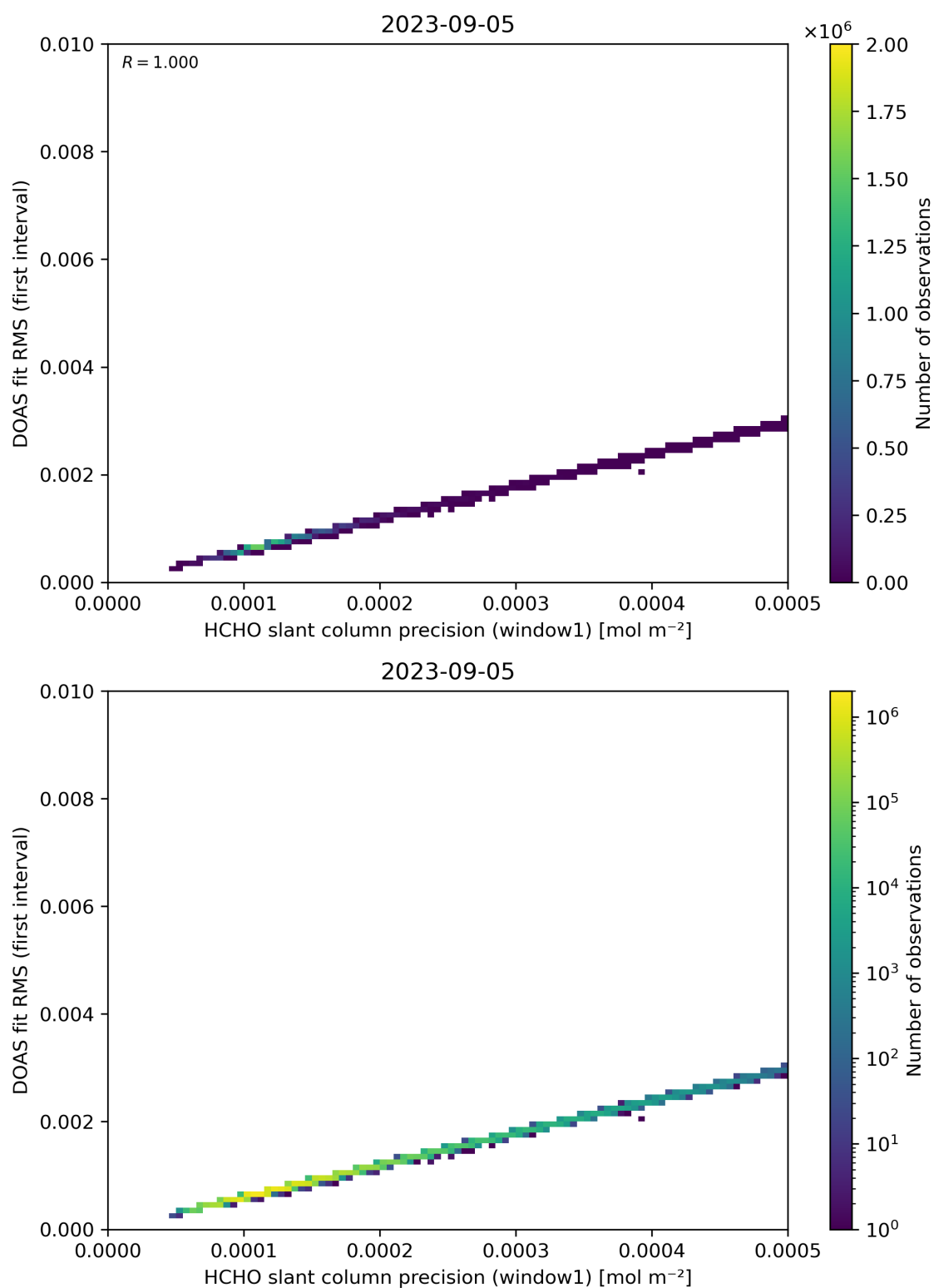
Figure 88: Scatter density plot of “HCHO slant column precision (window1)” against “DOAS fit RMS (first interval)” for 2023-09-05 to 2023-09-06.
