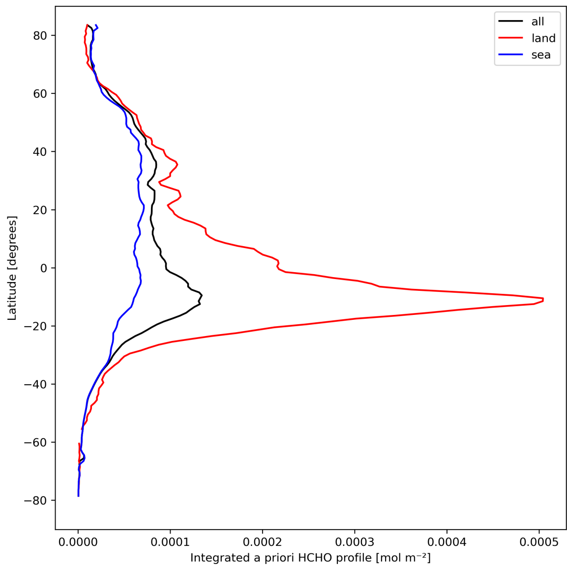
Figure 29: Zonal average of “Integrated a priori HCHO profile” for 2023-09-05 to 2023-09-06.
