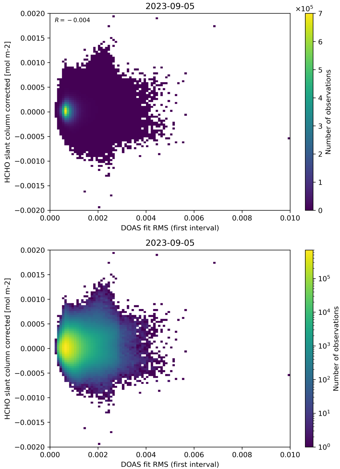
Figure 62: Scatter density plot of “DOAS fit RMS (first interval)” against “HCHO slant column corrected” for 2023-09-05 to 2023-09-06.
