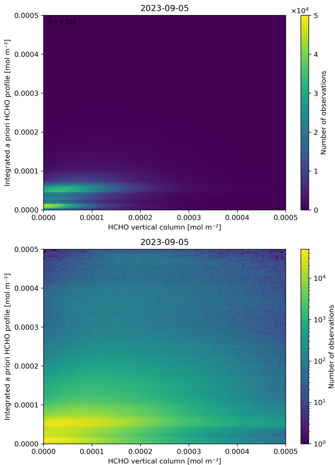
Figure 135: Scatter density plot of “HCHO vertical column” against “Integrated a priori HCHO profile” for 2023-09-05 to 2023-09-06.
