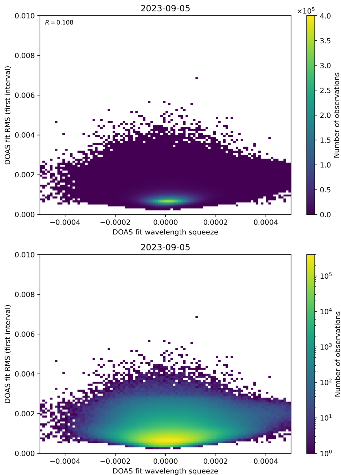
Figure 68: Scatter density plot of “DOAS fit wavelength squeeze” against “DOAS fit RMS (first interval)” for 2023-09-05 to 2023-09-06.
