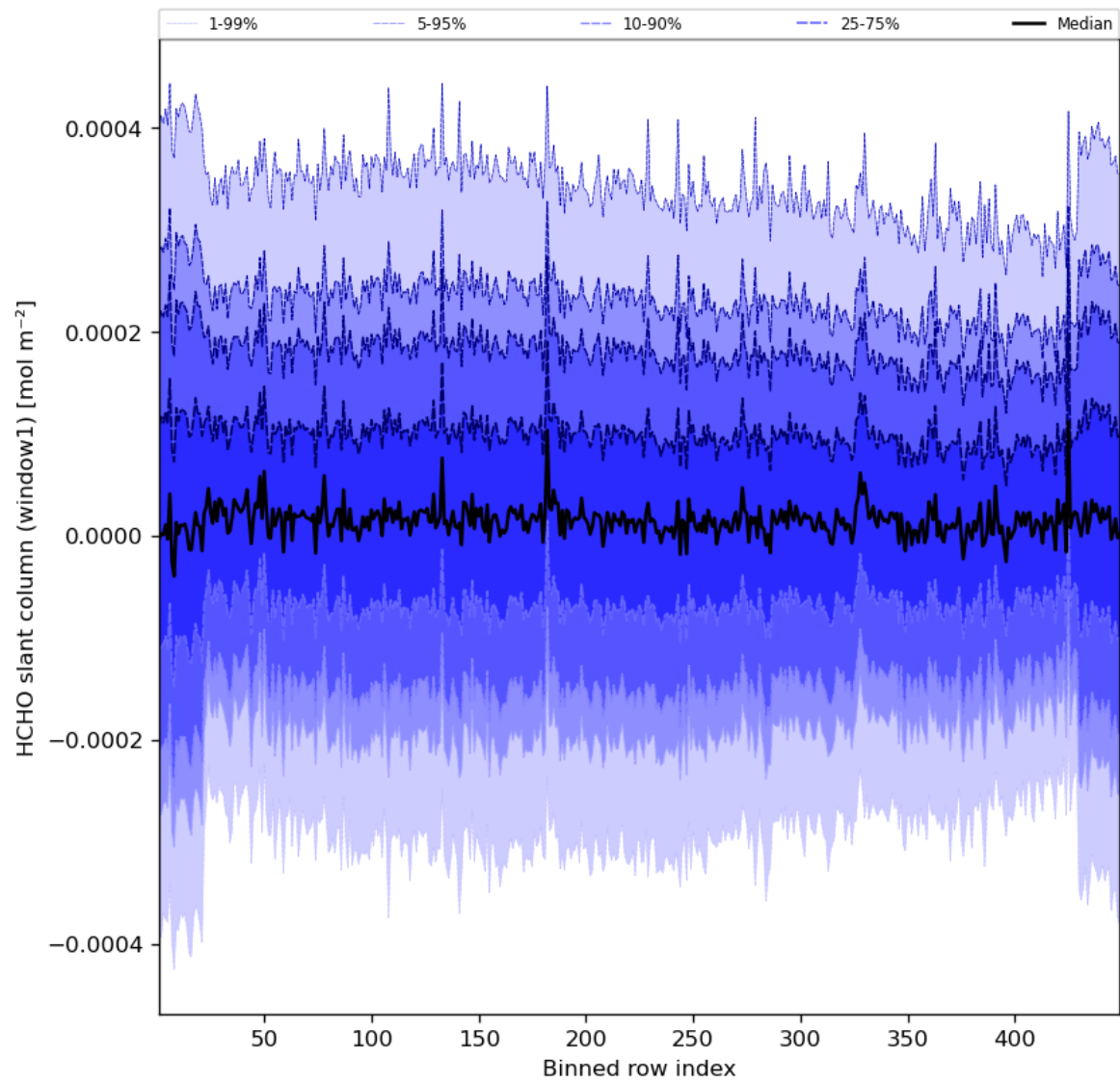
Figure 52: Along track statistics of “HCHO slant column (window1)” for 2023-09-05 to 2023-09-06
