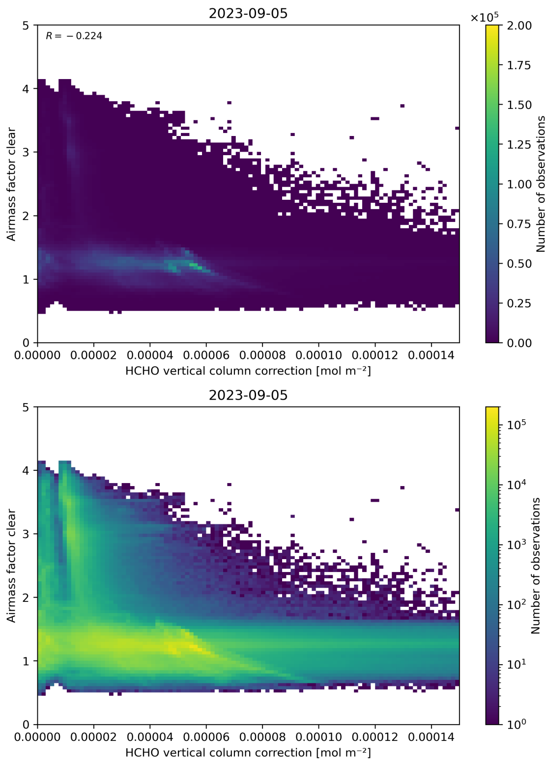
Figure 115: Scatter density plot of “HCHO vertical column correction” against “Airmass factor clear” for 2023-09-05 to 2023-09-06.
