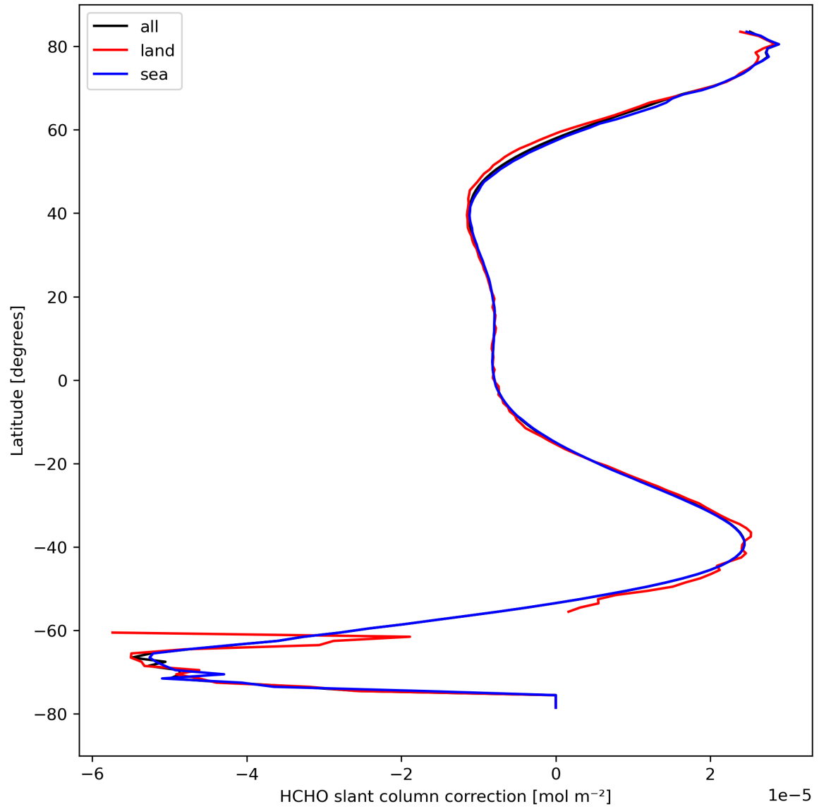
Figure 33: Zonal average of “HCHO slant column correction” for 2023-09-05 to 2023-09-06.
