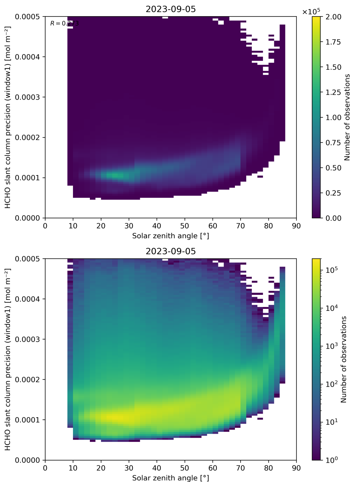
Figure 174: Scatter density plot of “Solar zenith angle” against “HCHO slant column precision (window1)” for 2023-09-05 to 2023-09-06.
