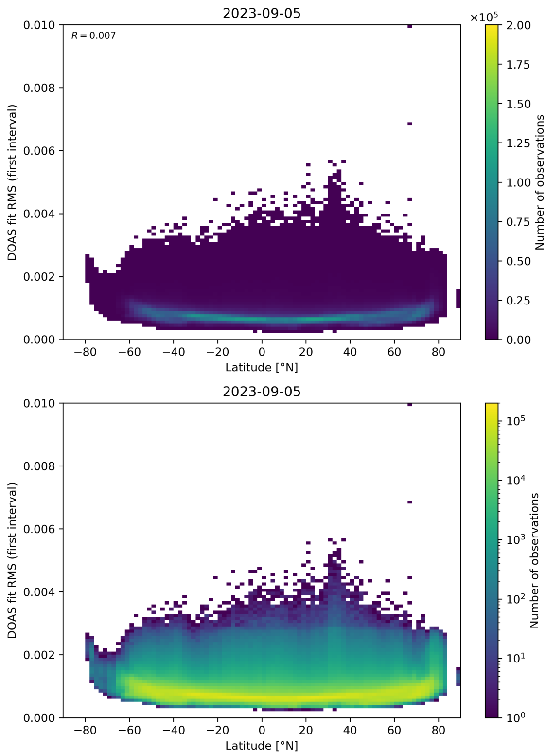
Figure 153: Scatter density plot of “Latitude” against “DOAS fit RMS (first interval)” for 2023-09-05 to 2023-09-06.
