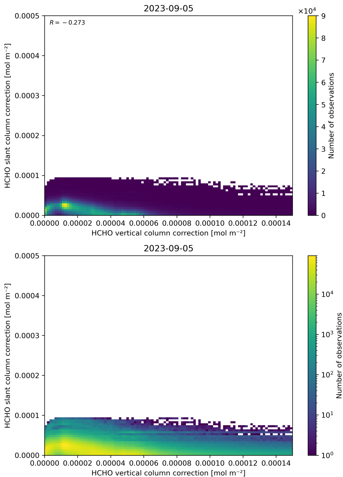
Figure 117: Scatter density plot of “HCHO vertical column correction” against “HCHO slant column correction” for 2023-09-05 to 2023-09-06.
