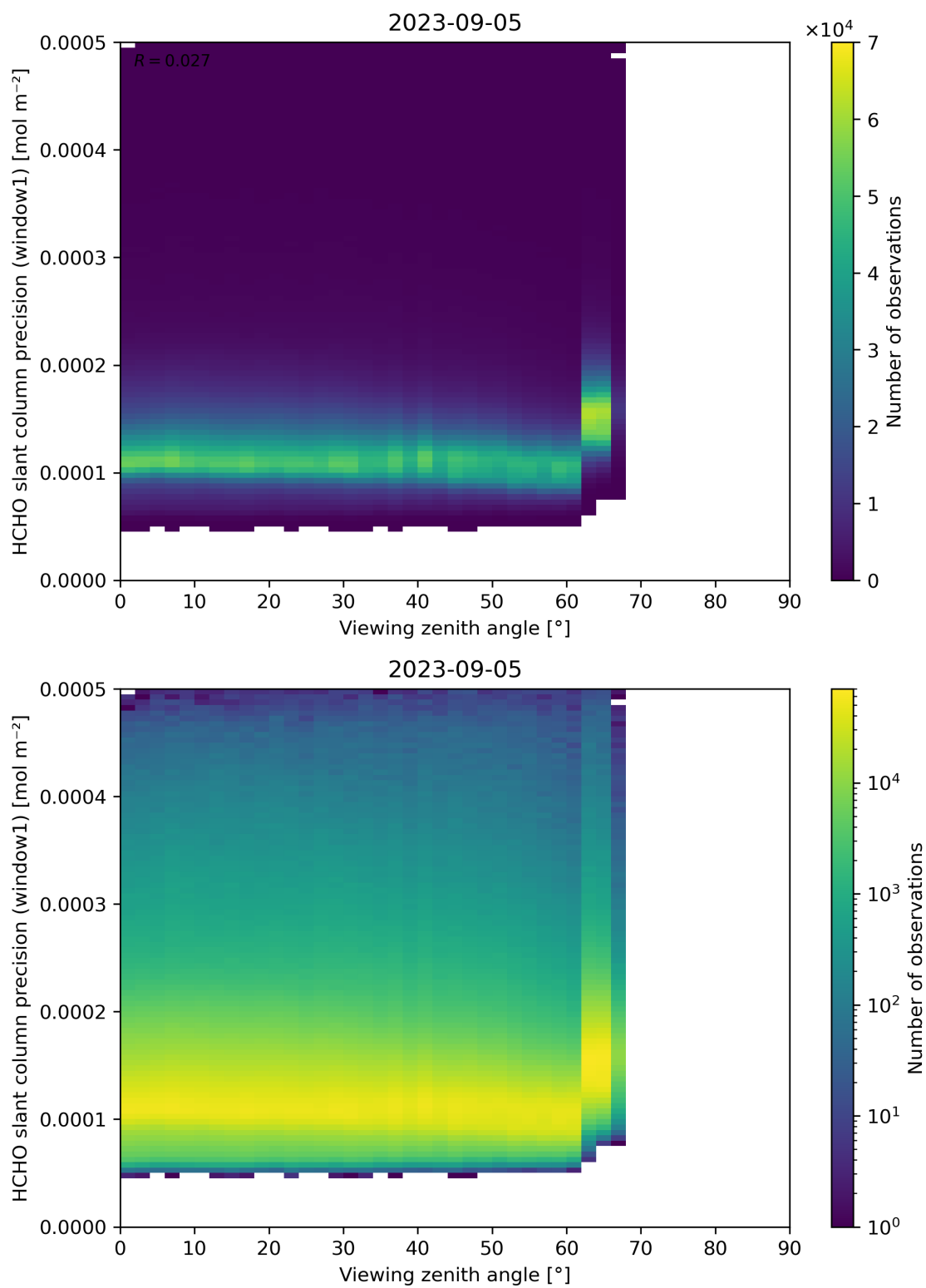
Figure 189: Scatter density plot of “Viewing zenith angle” against “HCHO slant column precision (window1)” for 2023-09-05 to 2023-09-06.
