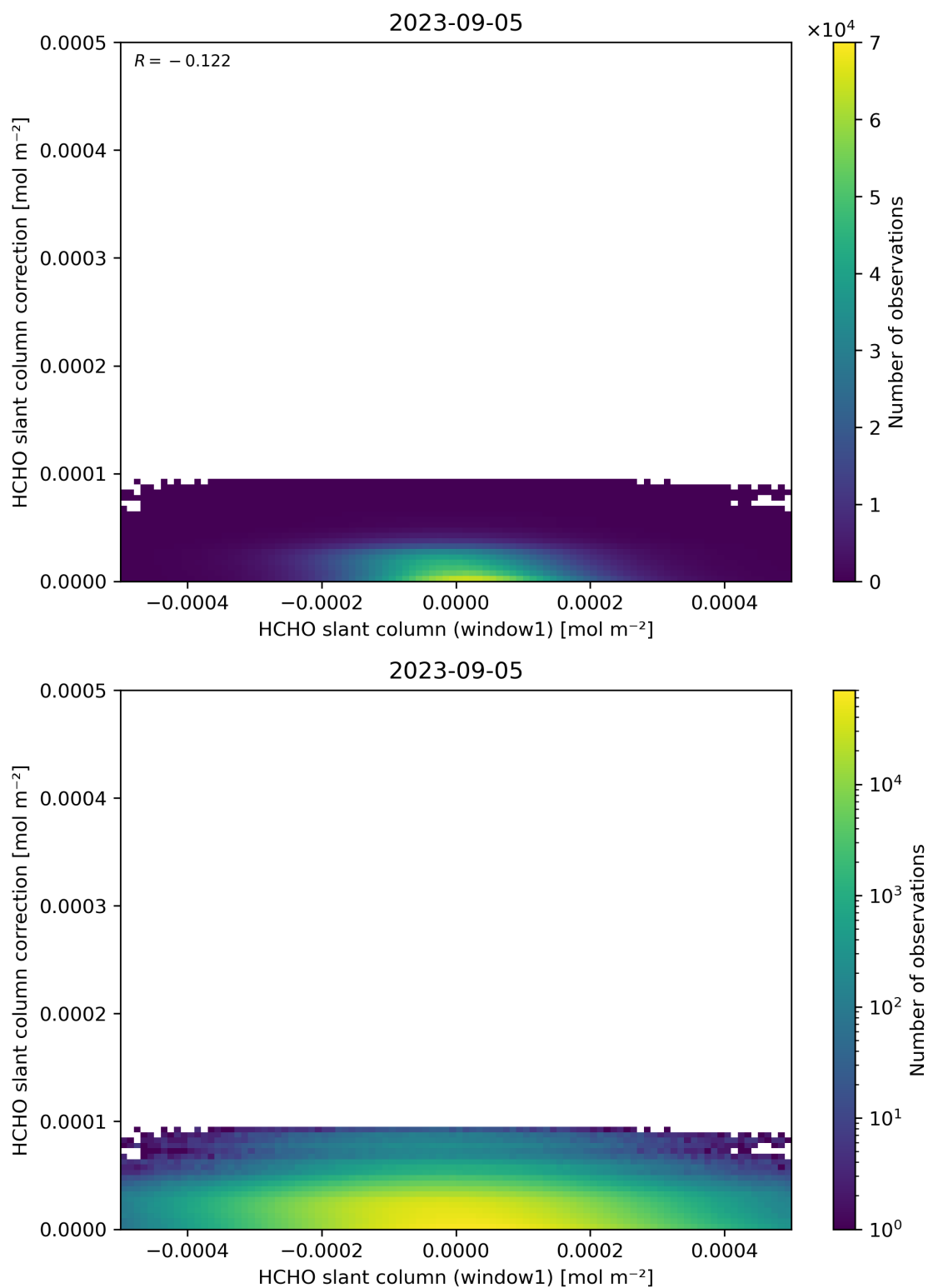
Figure 83: Scatter density plot of “HCHO slant column (window1)” against “HCHO slant column correction” for 2023-09-05 to 2023-09-06.
