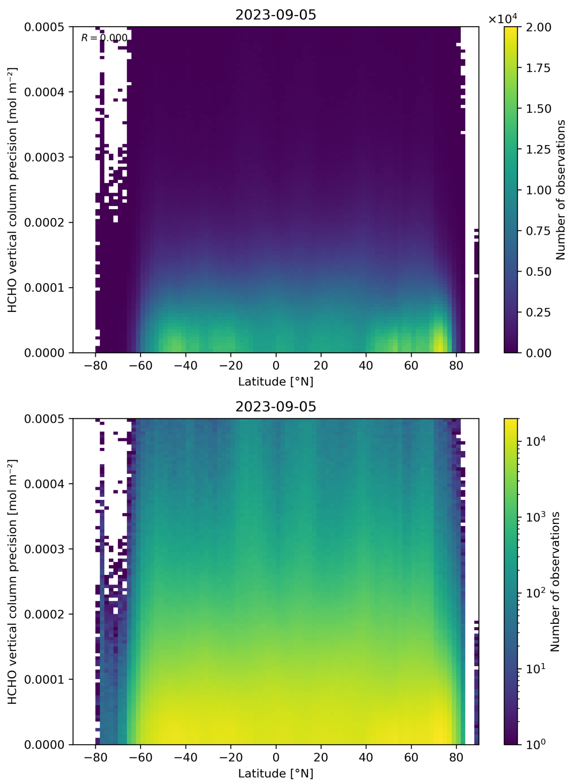
Figure 165: Scatter density plot of “Latitude” against “HCHO vertical column precision” for 2023-09-05 to 2023-09-06.
