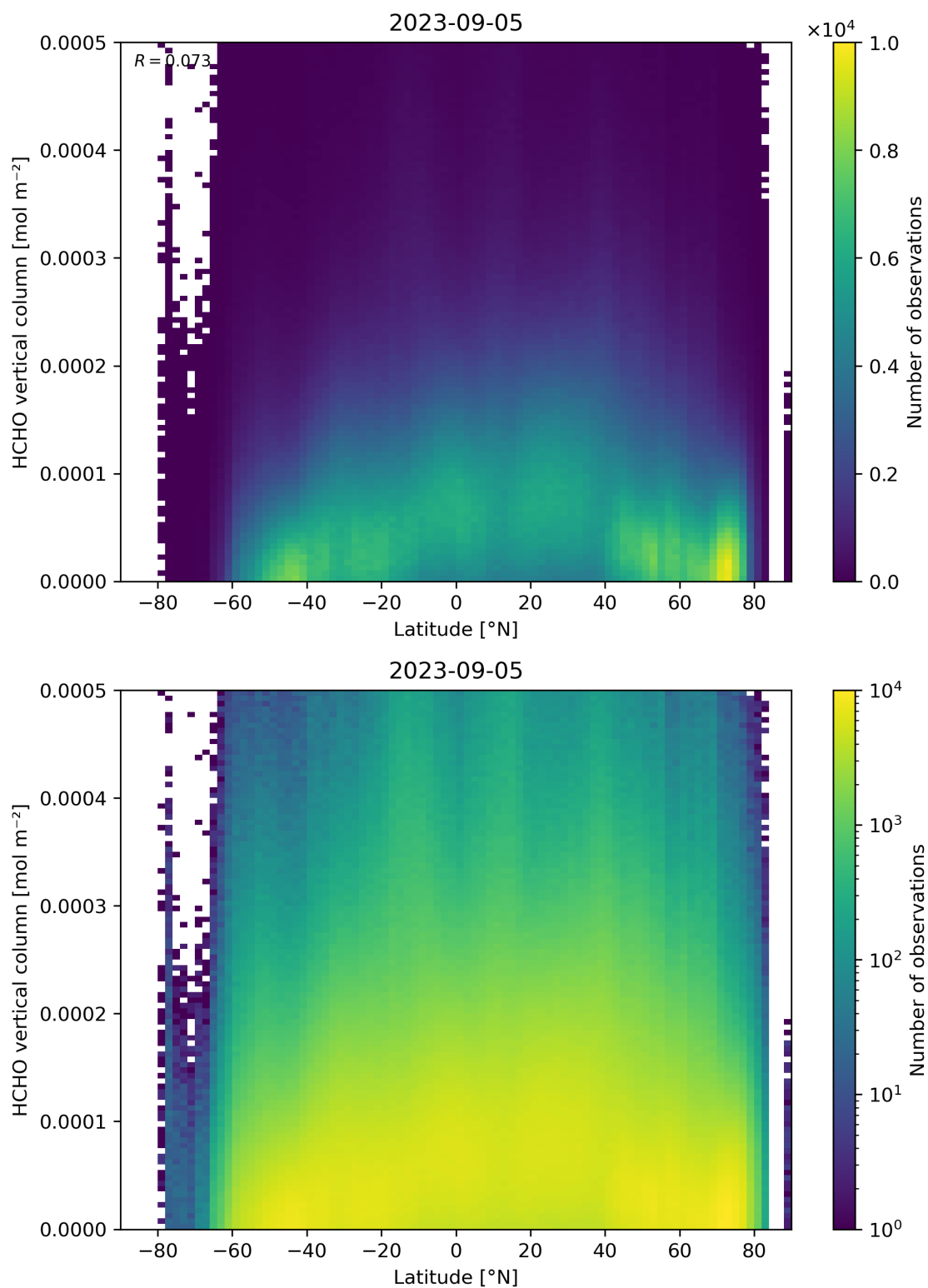
Figure 163: Scatter density plot of “Latitude” against “HCHO vertical column” for 2023-09-05 to 2023-09-06.
