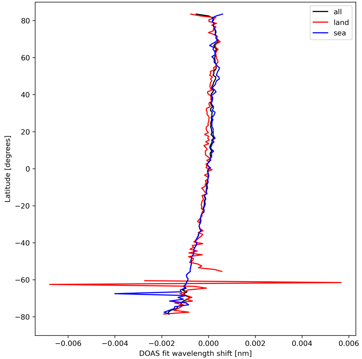
Figure 30: Zonal average of “DOAS fit wavelength shift” for 2023-09-05 to 2023-09-06.
