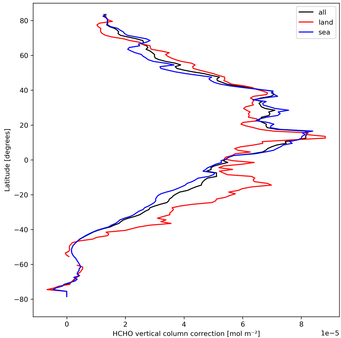
Figure 23: Zonal average of “HCHO vertical column correction” for 2023-09-05 to 2023-09-06.
