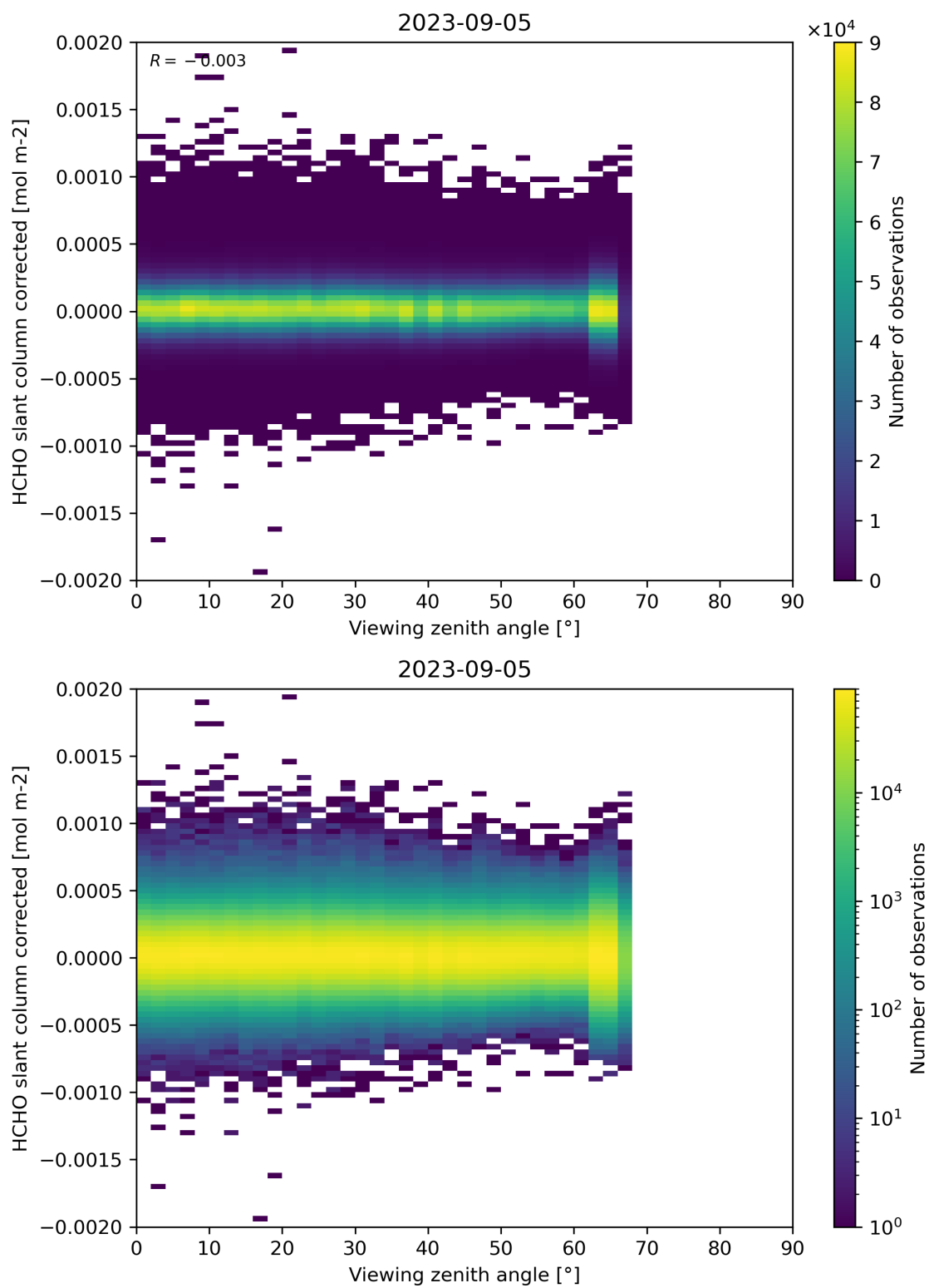
Figure 186: Scatter density plot of “Viewing zenith angle” against “HCHO slant column corrected” for 2023-09-05 to 2023-09-06.
