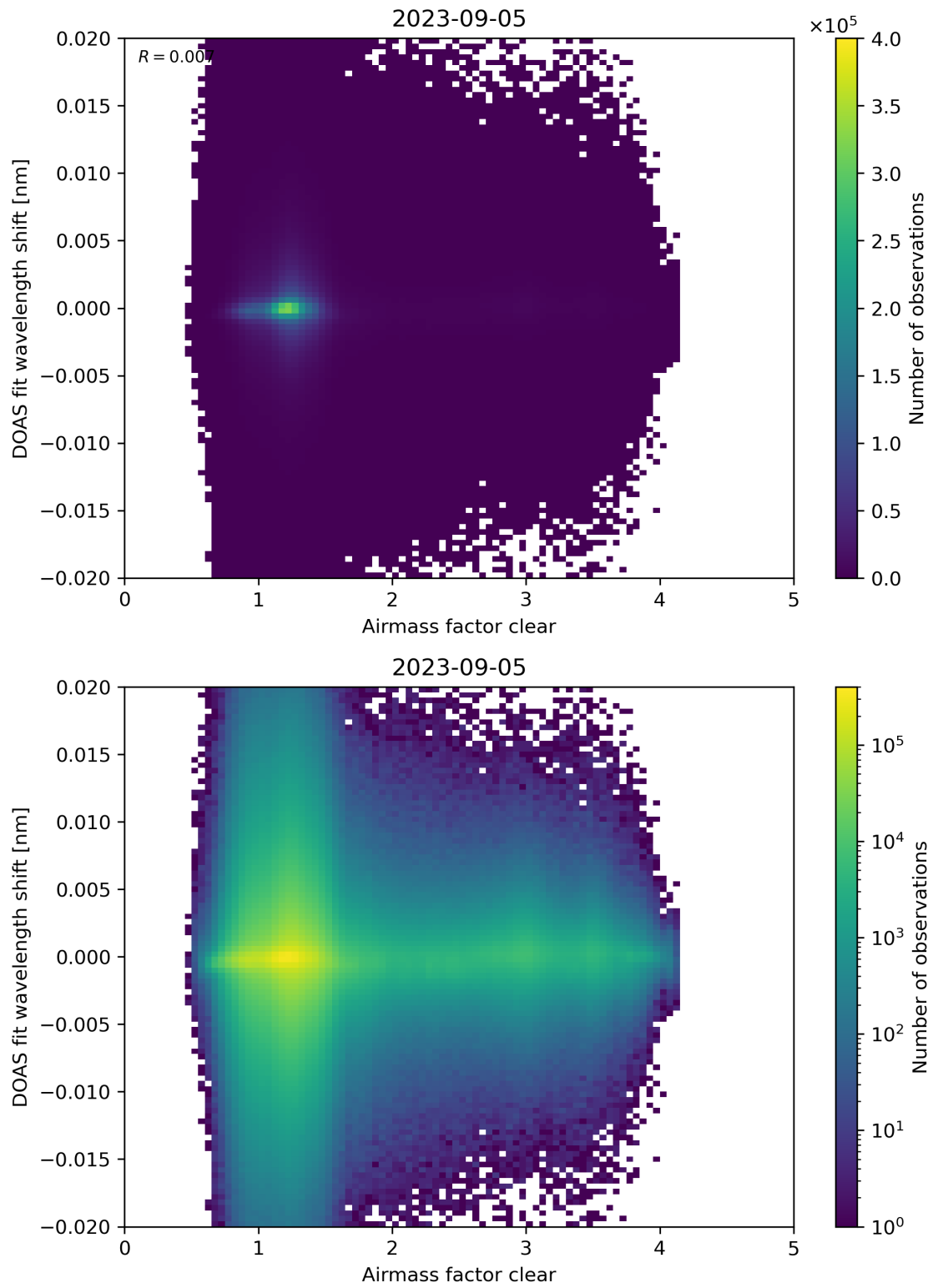
Figure 72: Scatter density plot of “Airmass factor clear” against “DOAS fit wavelength shift” for 2023-09-05 to 2023-09-06.
