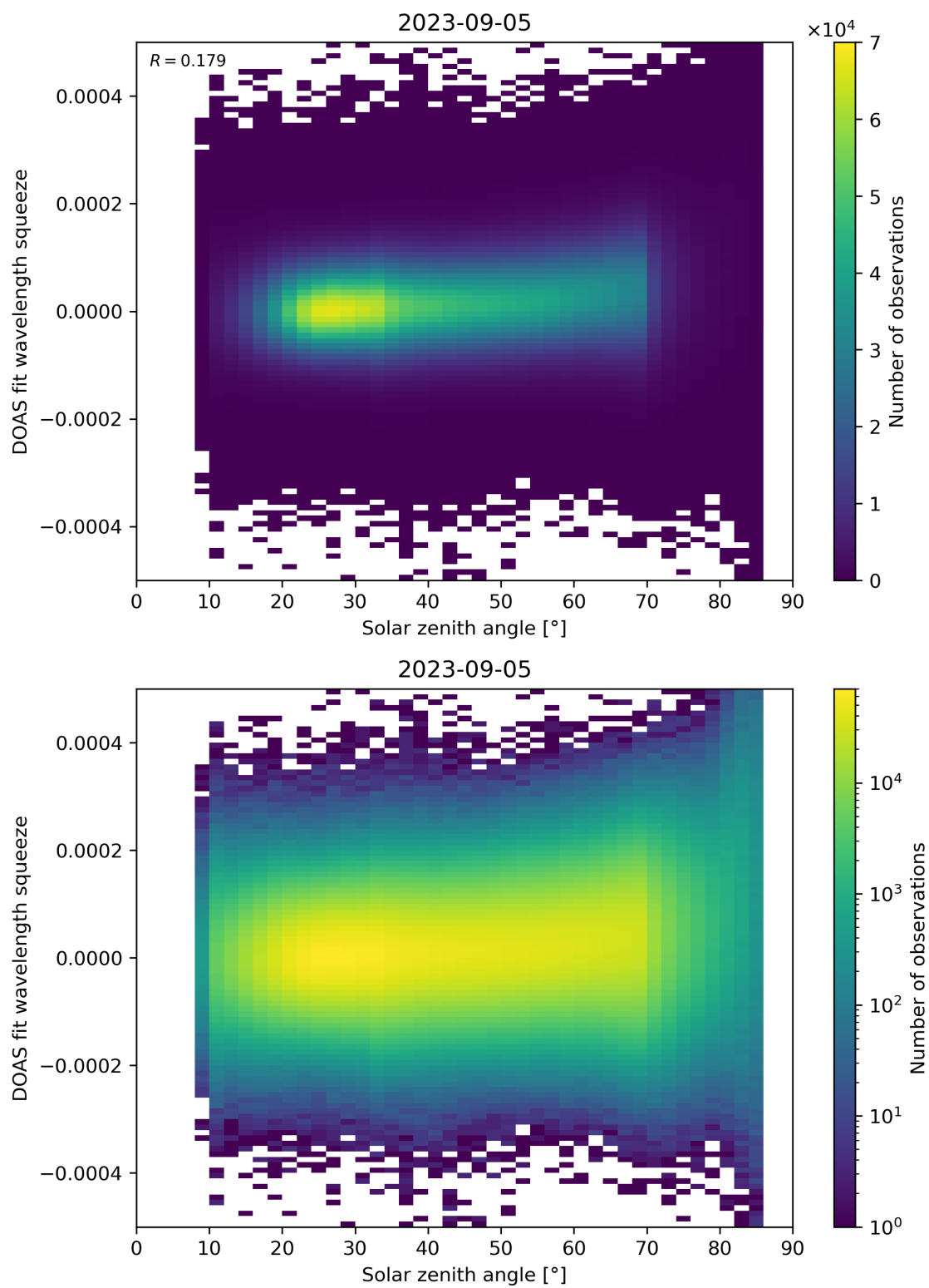
Figure 169: Scatter density plot of “Solar zenith angle” against “DOAS fit wavelength squeeze” for 2023-09-05 to 2023-09-06.
