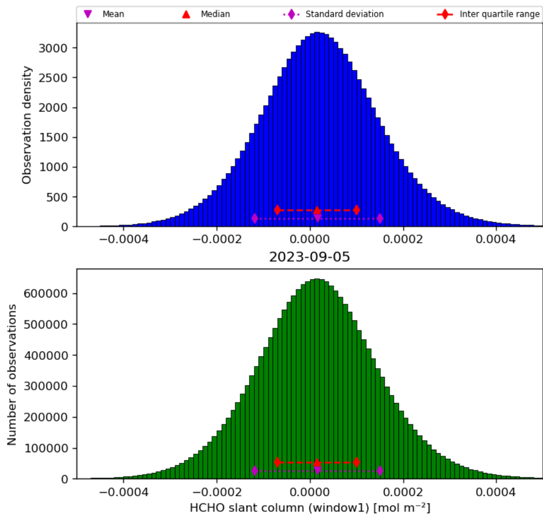
Figure 38: Histogram of “HCHO slant column (window1)” for 2023-09-05 to 2023-09-06
