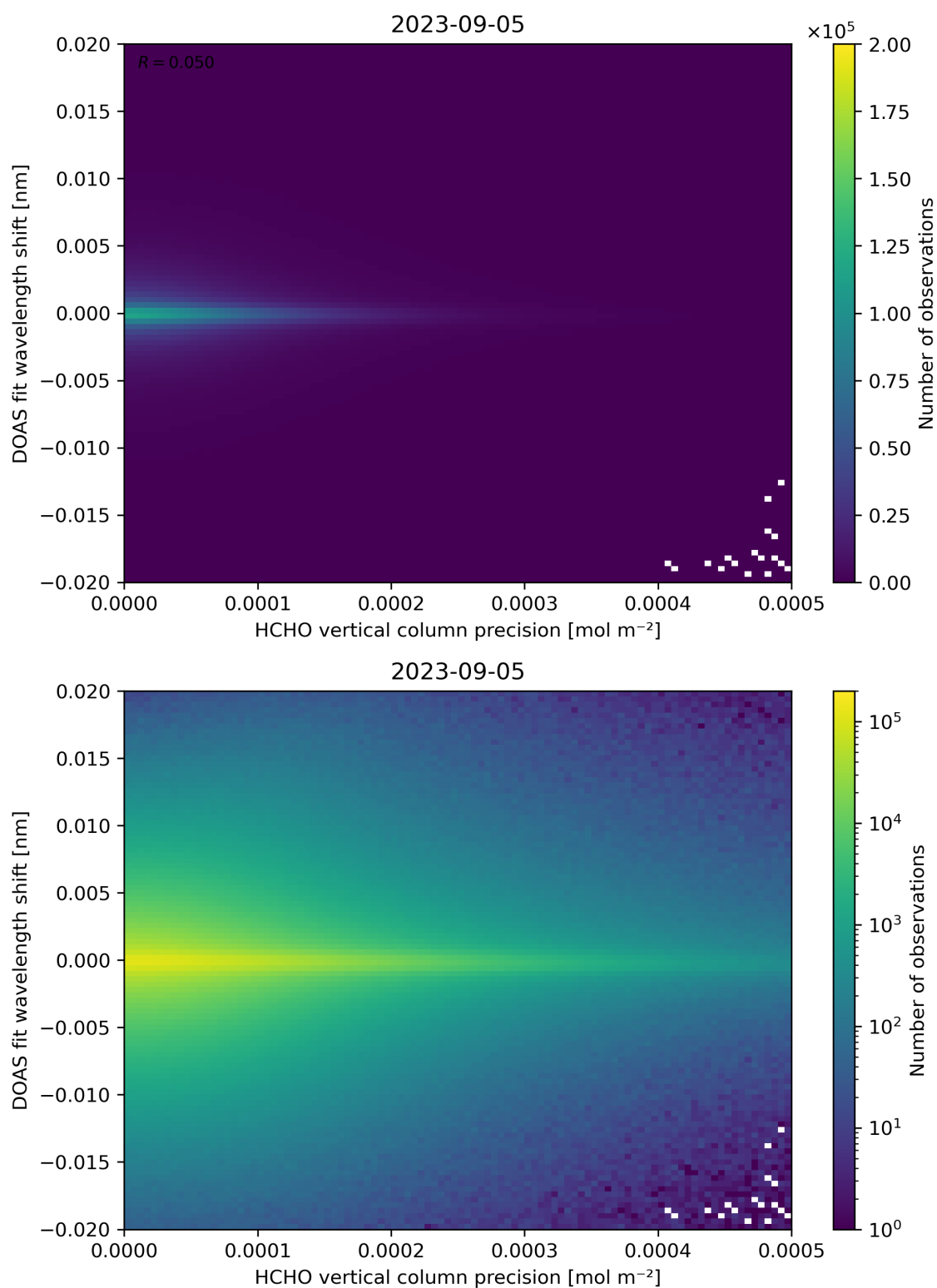
Figure 137: Scatter density plot of “HCHO vertical column precision” against “DOAS fit wavelength shift” for 2023-09-05 to 2023-09-06.
