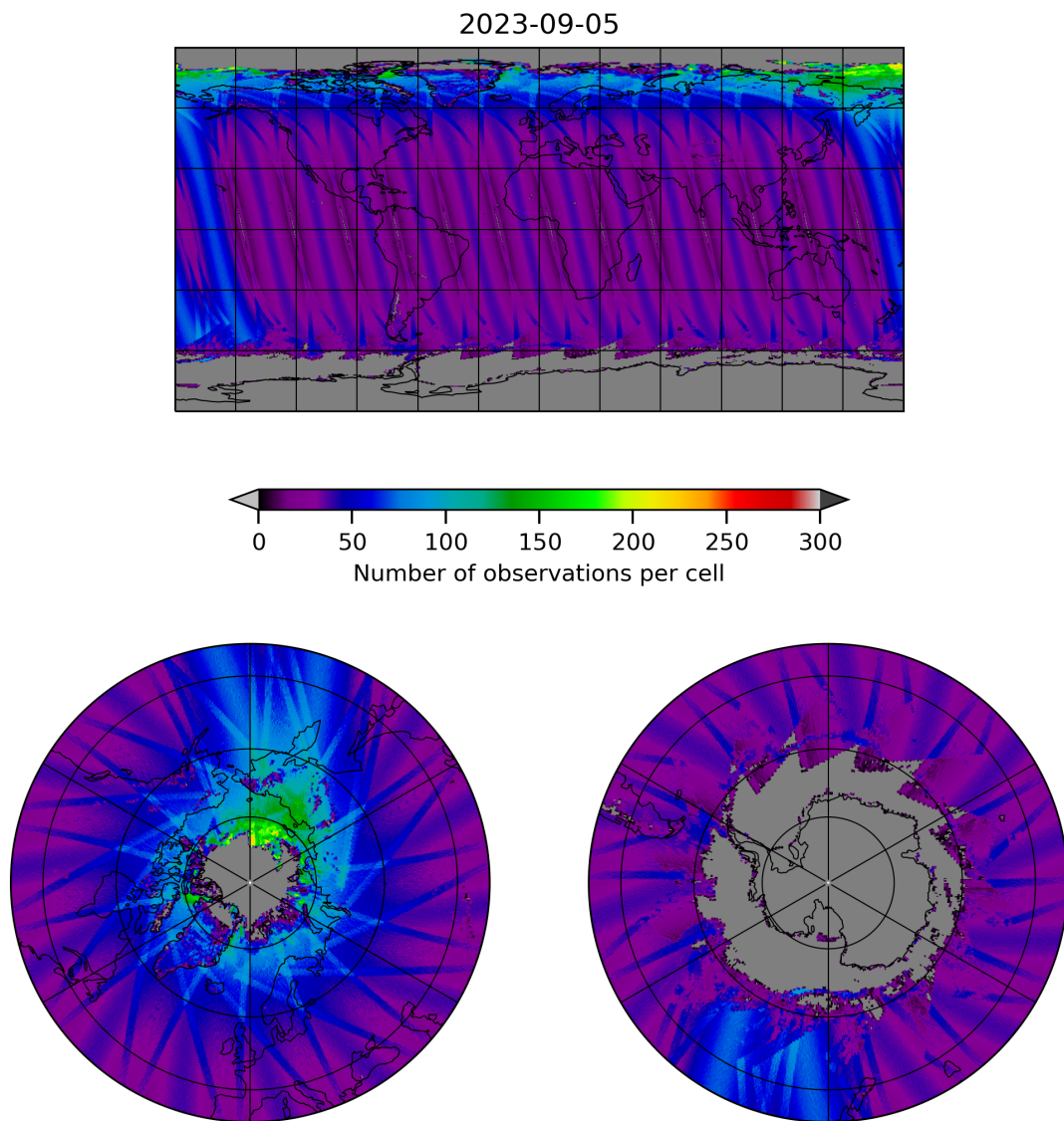
Figure 19: Map of the number of observations for 2023-09-05 to 2023-09-06
