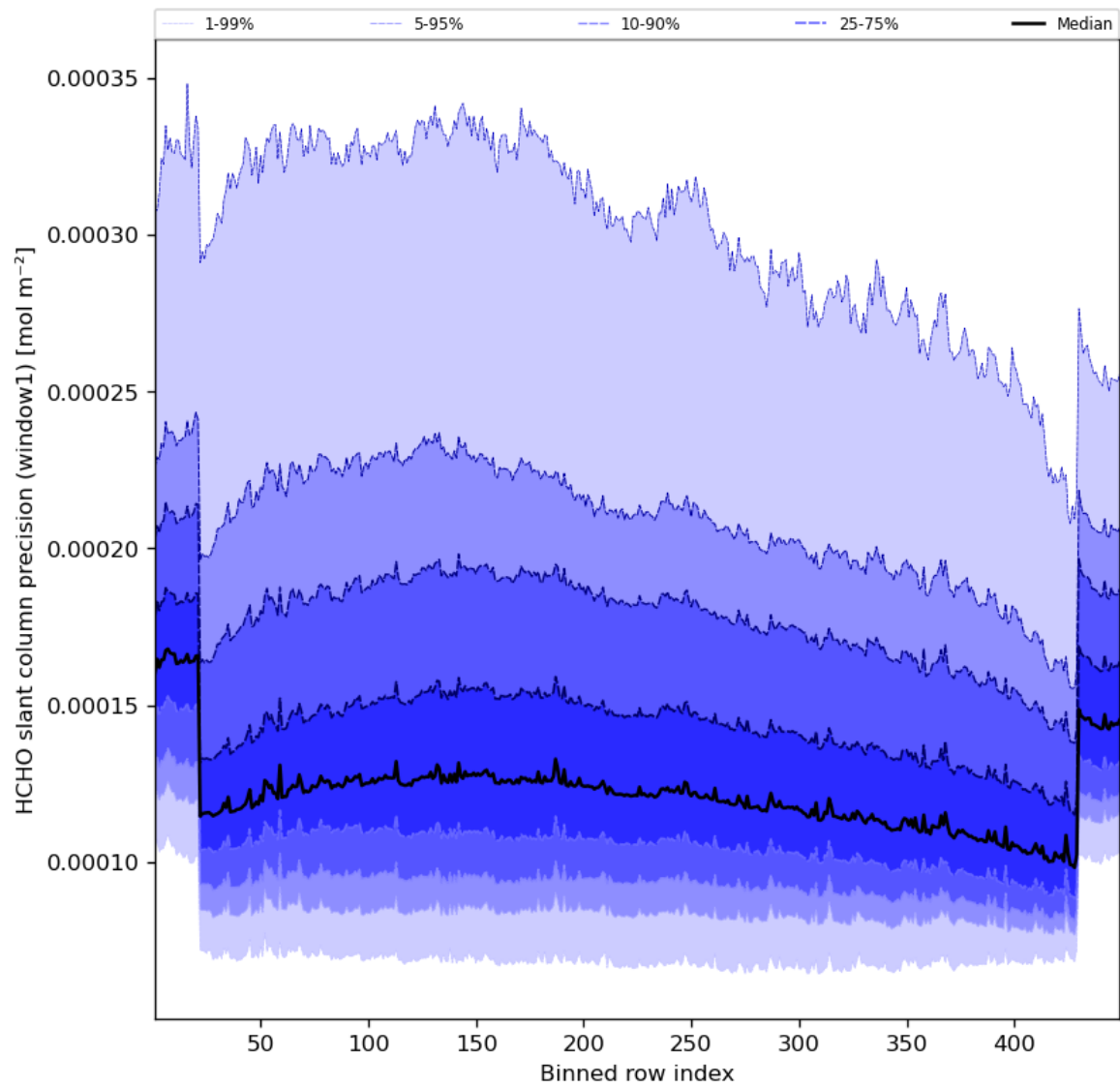
Figure 53: Along track statistics of “HCHO slant column precision (window1)” for 2023-09-05 to 2023-09-06
