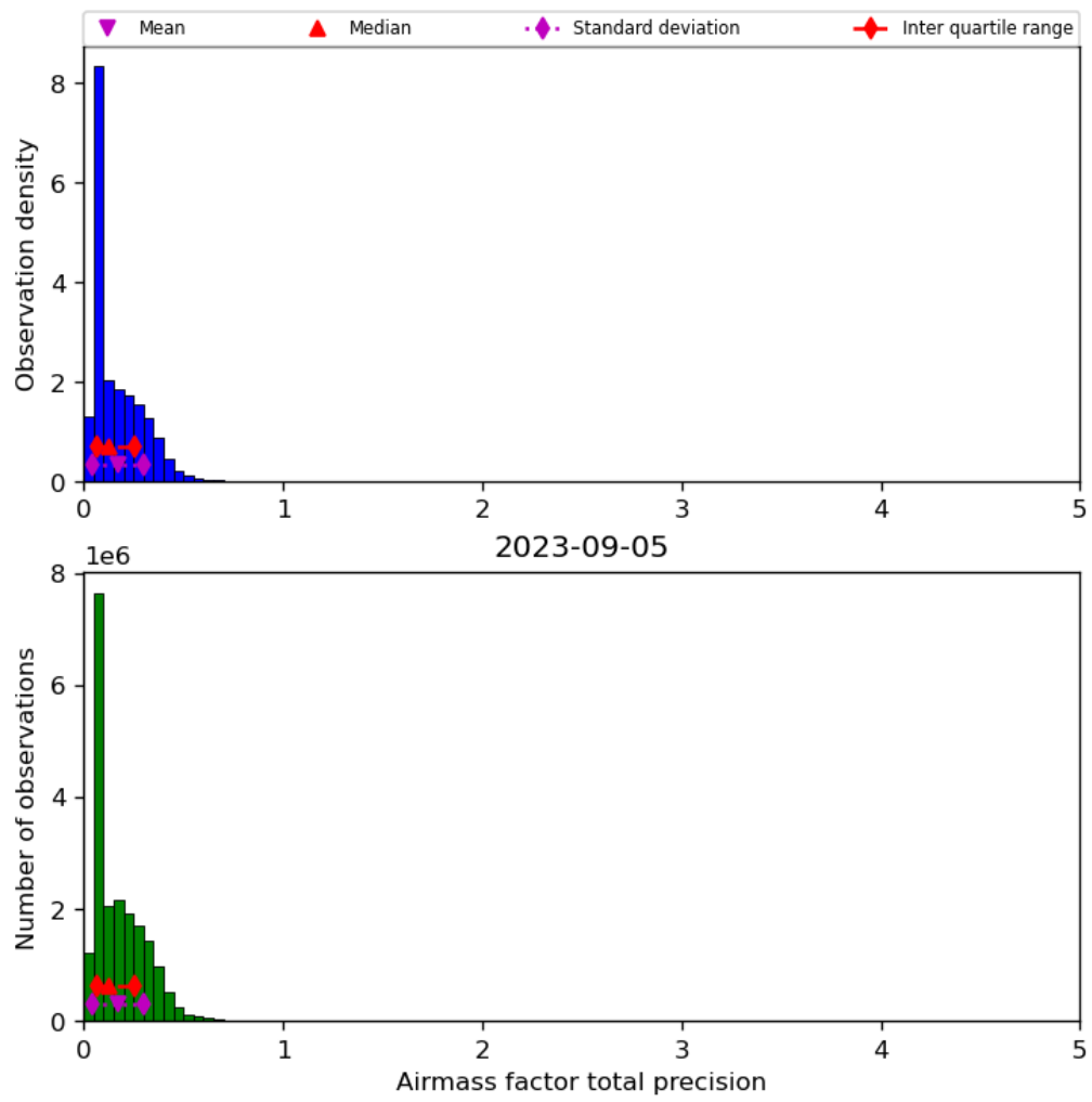
Figure 41: Histogram of “Airmass factor total precision” for 2023-09-05 to 2023-09-06
