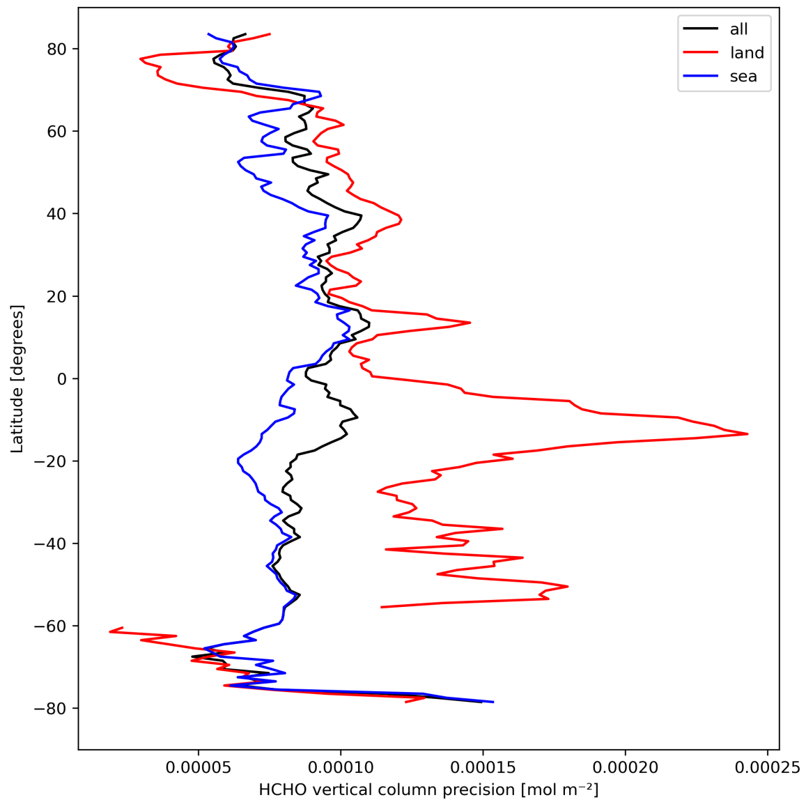
Figure 22: Zonal average of “HCHO vertical column precision” for 2023-09-05 to 2023-09-06.
