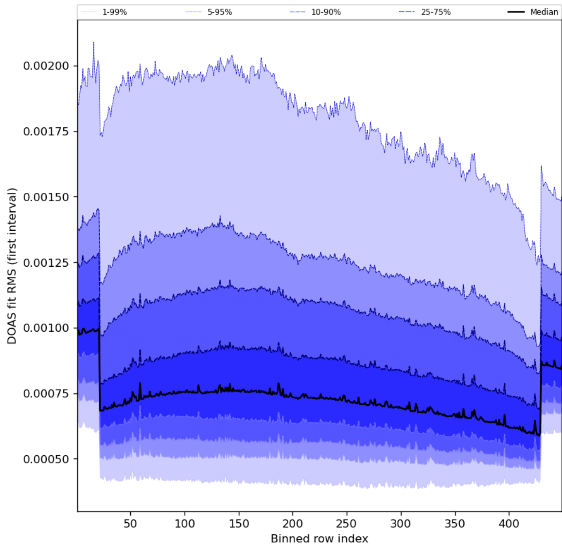
Figure 60: Along track statistics of “DOAS fit RMS (first interval)” for 2023-09-05 to 2023-09-06
