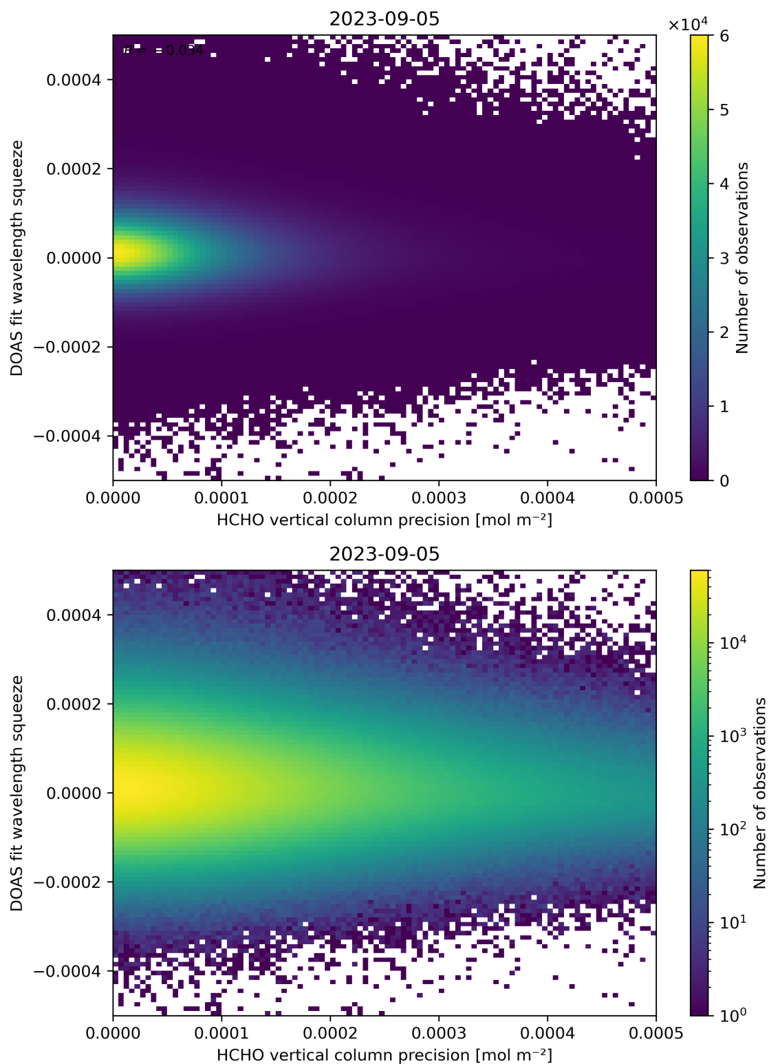
Figure 138: Scatter density plot of “HCHO vertical column precision” against “DOAS fit wavelength squeeze” for 2023-09-05 to 2023-09-06.
