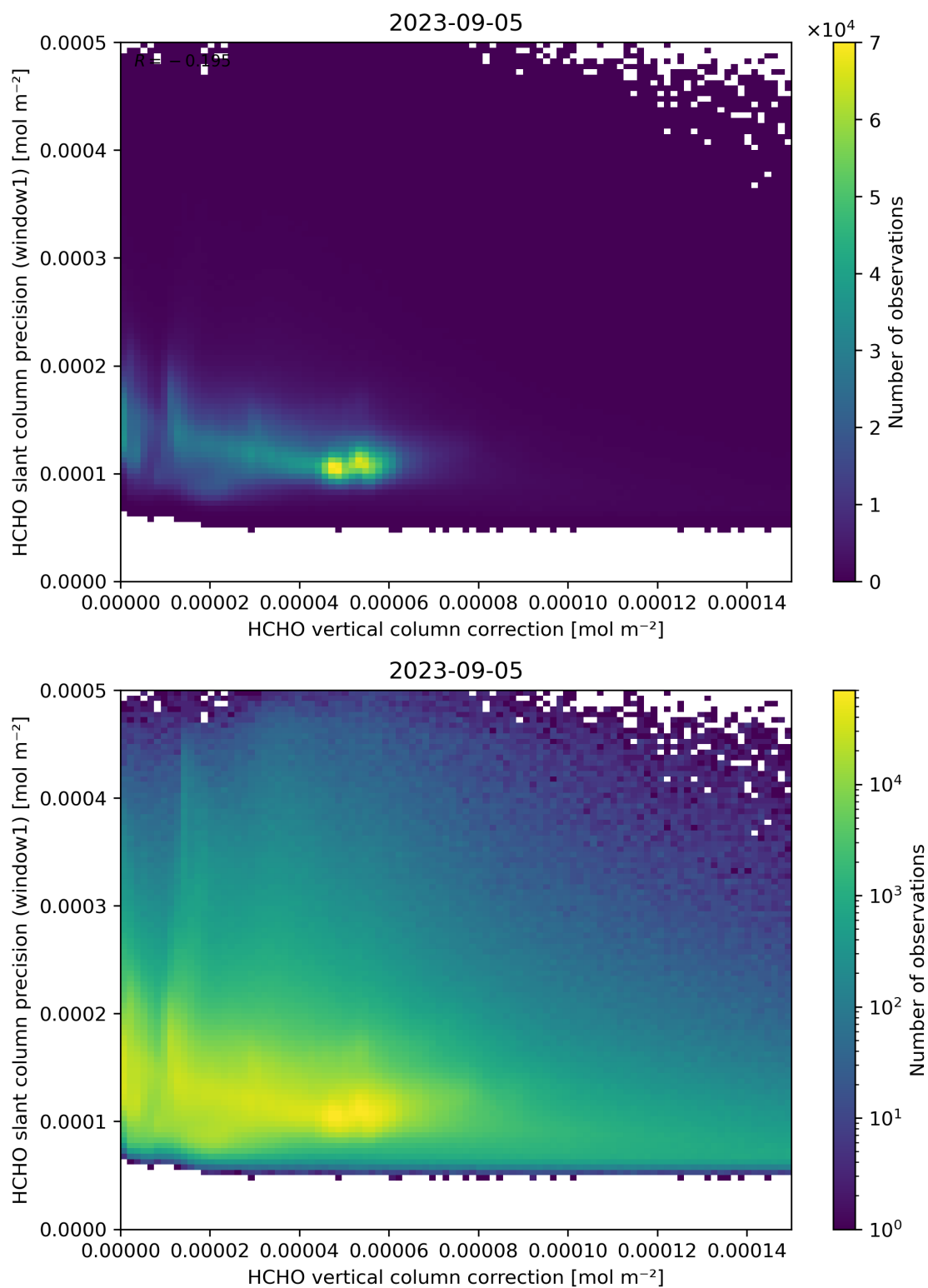
Figure 119: Scatter density plot of “HCHO vertical column correction” against “HCHO slant column precision (window1)” for 2023-09-05 to 2023-09-06.
