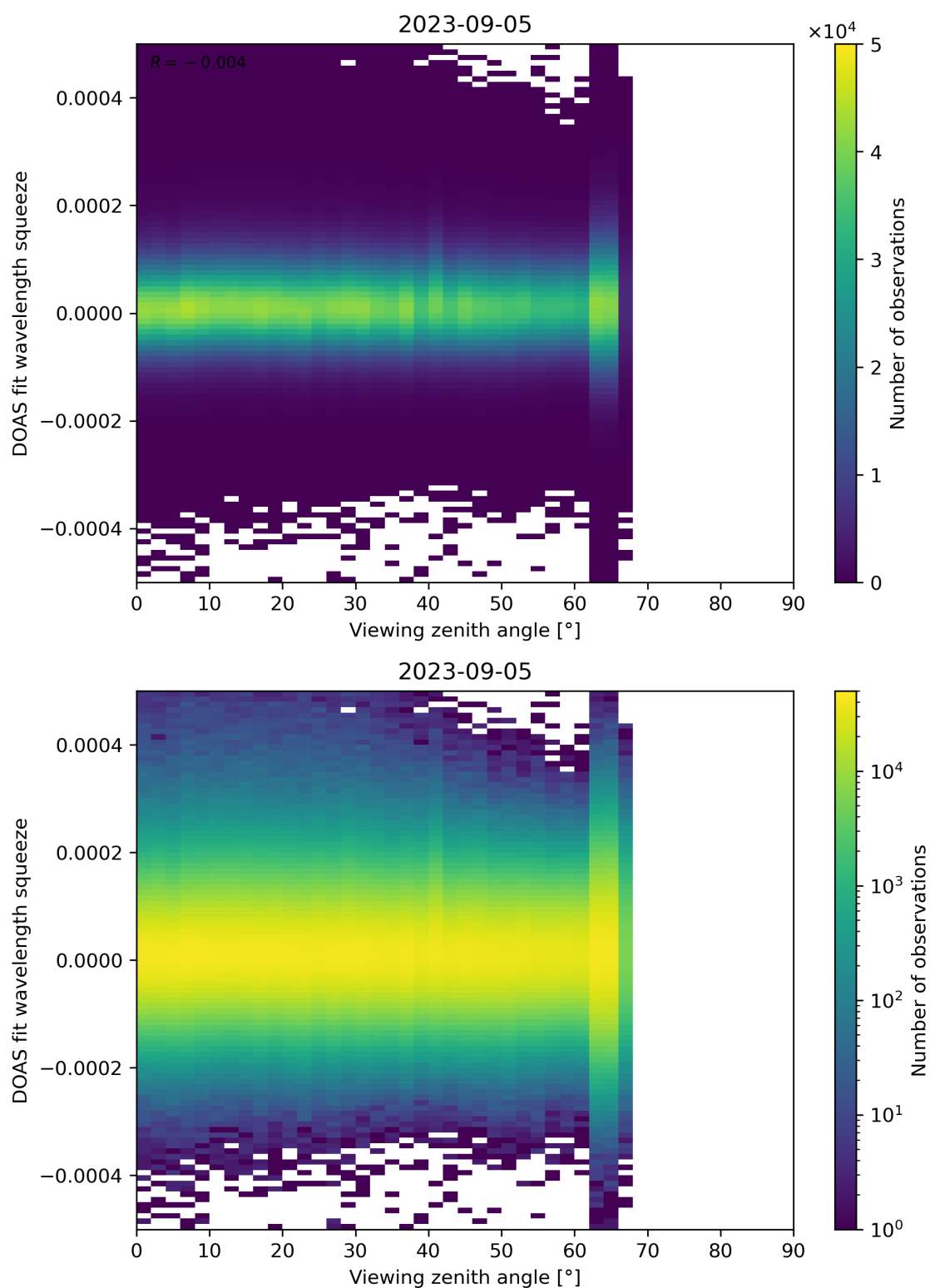
Figure 184: Scatter density plot of “Viewing zenith angle” against “DOAS fit wavelength squeeze” for 2023-09-05 to 2023-09-06.
