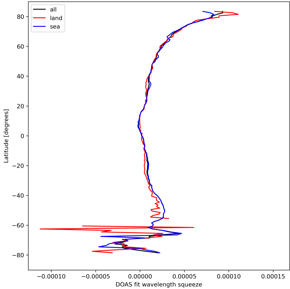
Figure 31: Zonal average of “DOAS fit wavelength squeeze” for 2023-09-05 to 2023-09-06.
