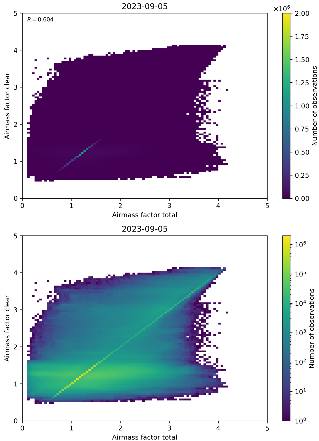
Figure 100: Scatter density plot of “Airmass factor total” against “Airmass factor clear” for 2023-09-05 to 2023-09-06.
