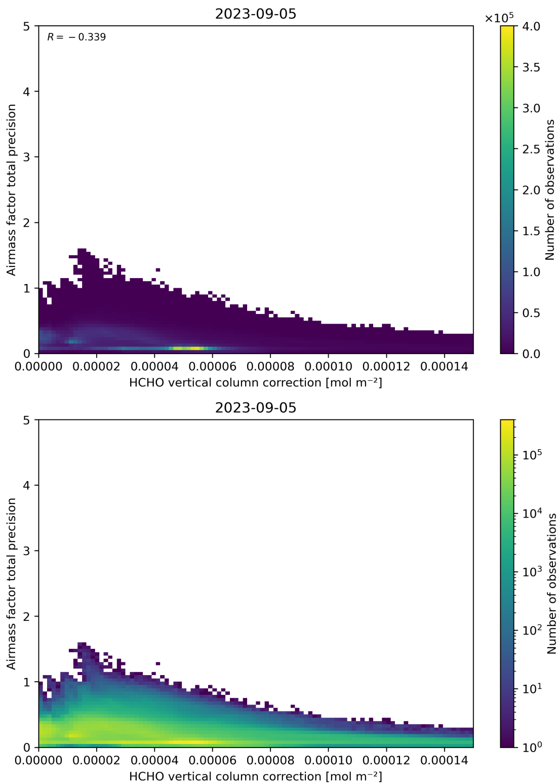
Figure 121: Scatter density plot of “HCHO vertical column correction” against “Airmass factor total precision” for 2023-09-05 to 2023-09-06.
