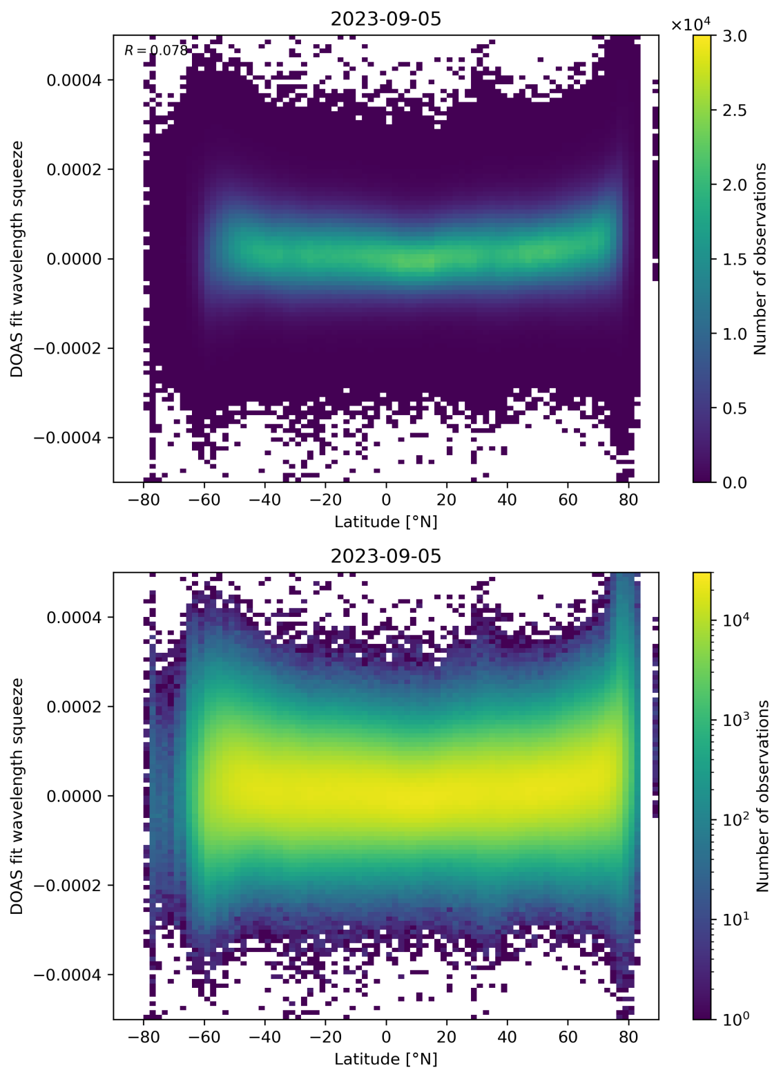
Figure 155: Scatter density plot of “Latitude” against “DOAS fit wavelength squeeze” for 2023-09-05 to 2023-09-06.
