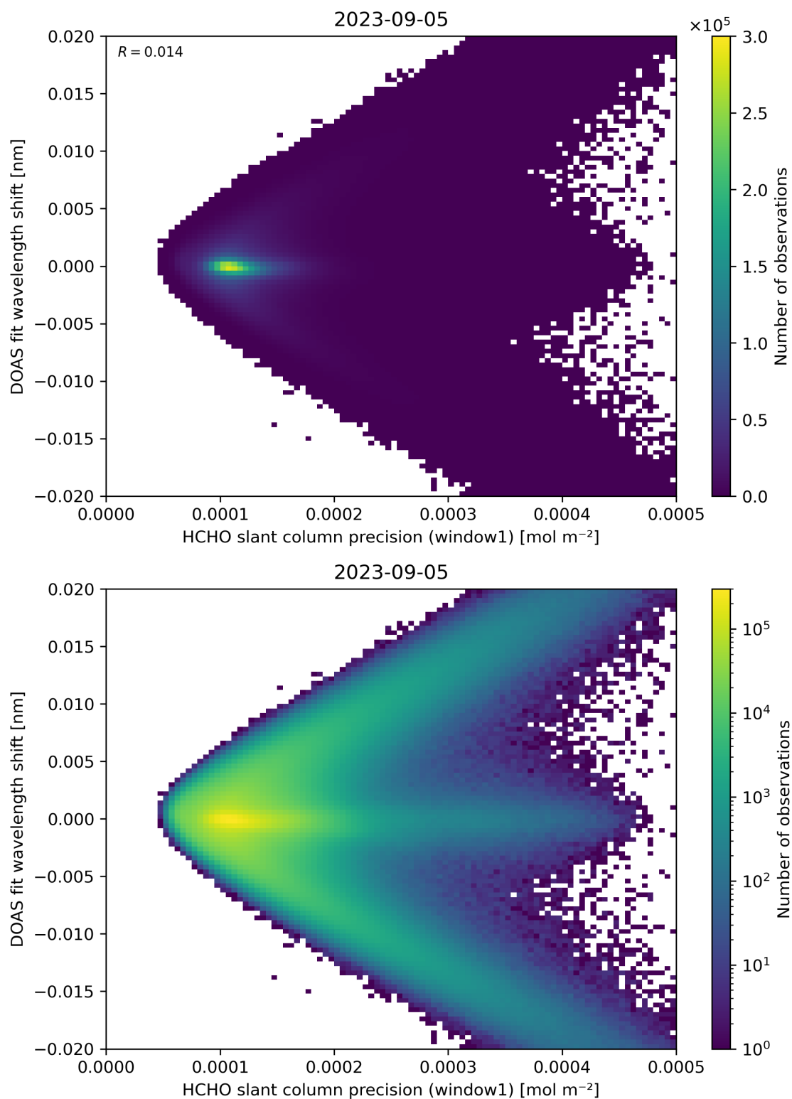
Figure 89: Scatter density plot of “HCHO slant column precision (window1)” against “DOAS fit wavelength shift” for 2023-09-05 to 2023-09-06.
