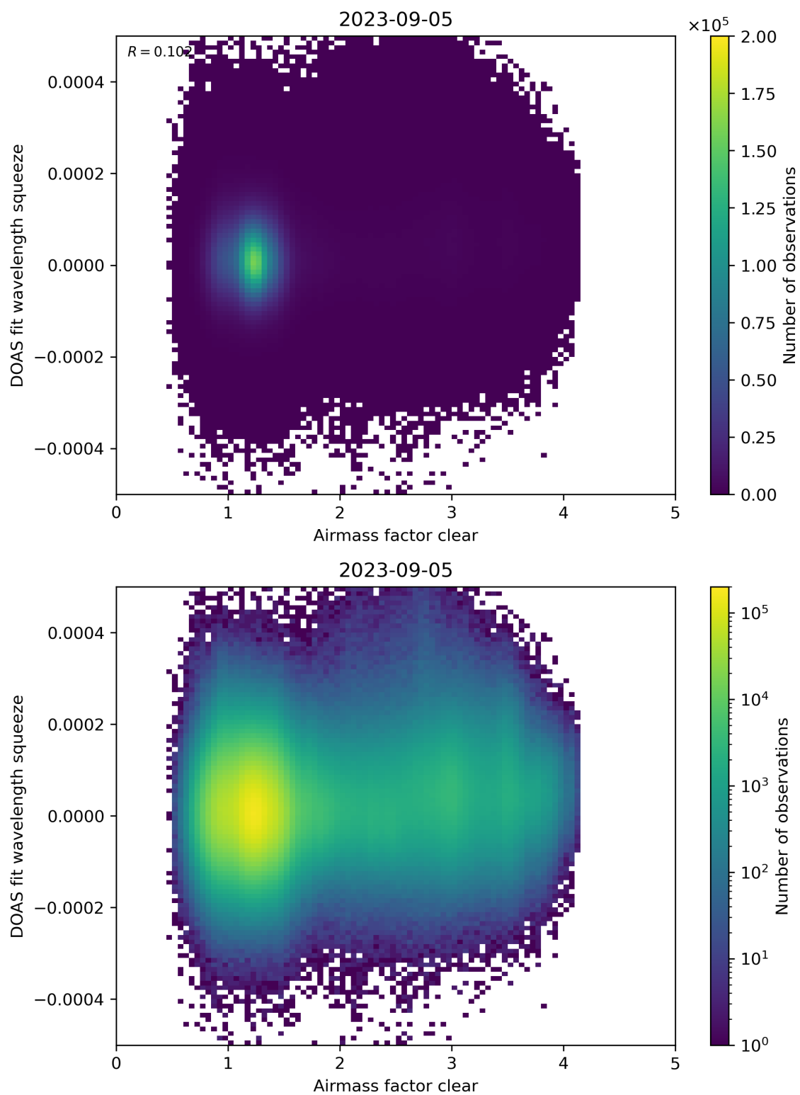
Figure 73: Scatter density plot of “Airmass factor clear” against “DOAS fit wavelength squeeze” for 2023-09-05 to 2023-09-06.
