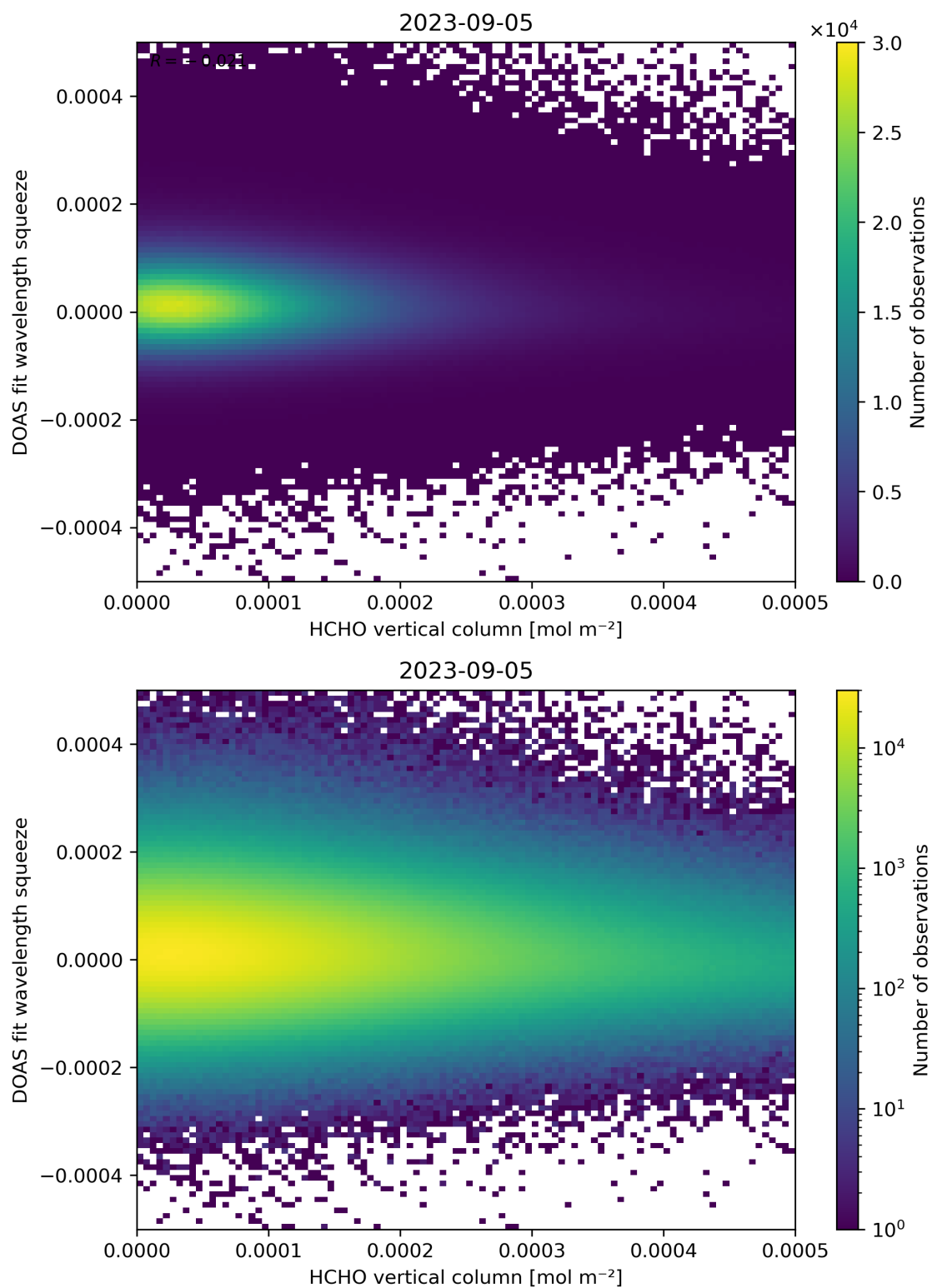
Figure 125: Scatter density plot of “HCHO vertical column” against “DOAS fit wavelength squeeze” for 2023-09-05 to 2023-09-06.
