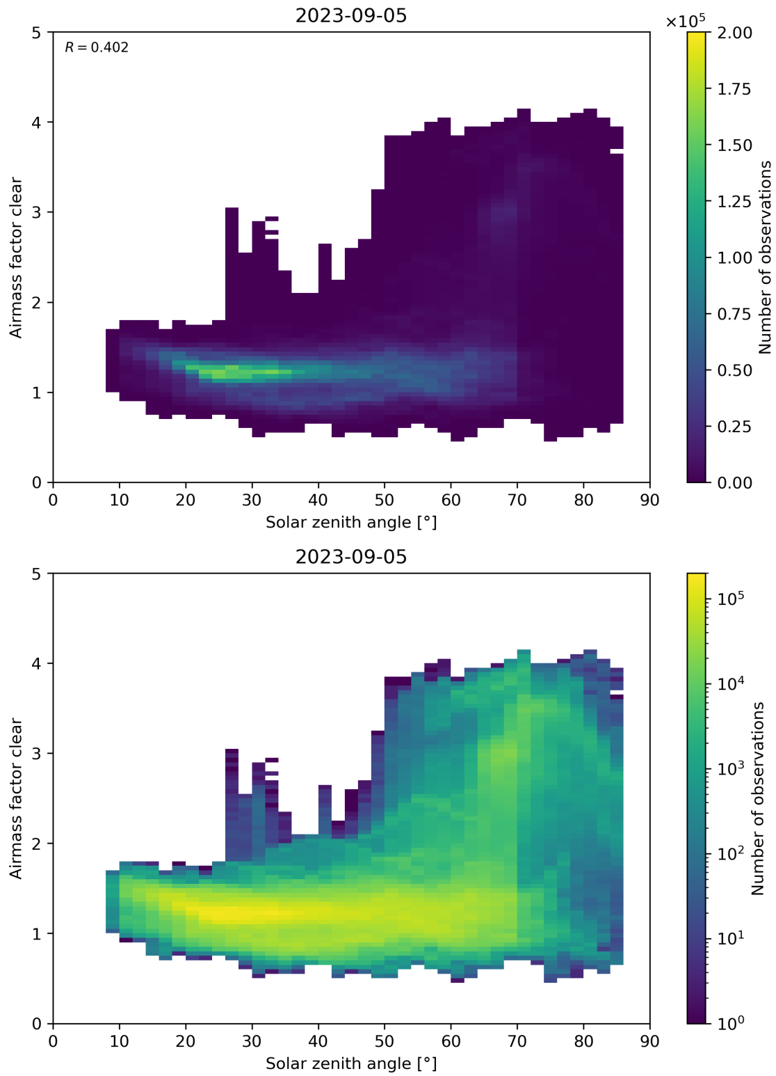
Figure 170: Scatter density plot of “Solar zenith angle” against “Airmass factor clear” for 2023-09-05 to 2023-09-06.
