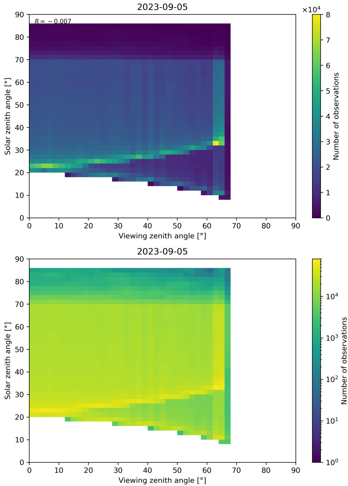
Figure 197: Scatter density plot of “Viewing zenith angle” against “Solar zenith angle” for 2023-09-05 to 2023-09-06.
