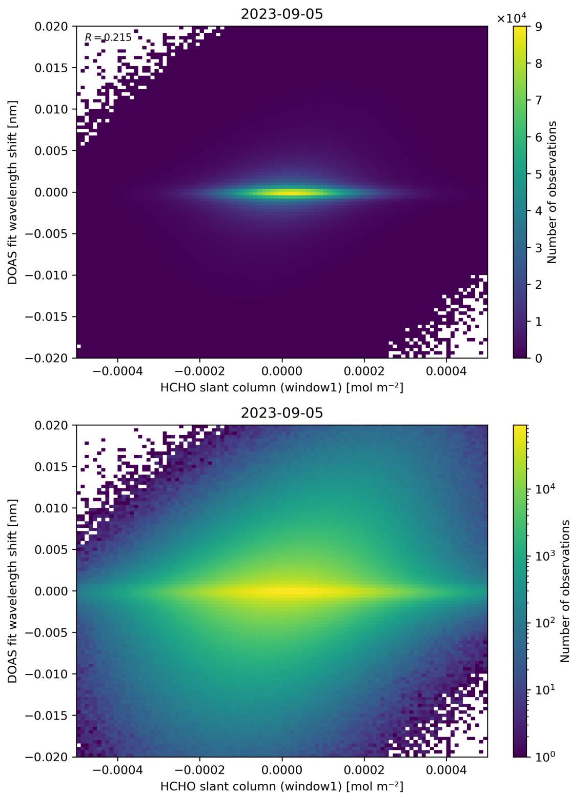
Figure 79: Scatter density plot of “HCHO slant column (window1)” against “DOAS fit wavelength shift” for 2023-09-05 to 2023-09-06.
