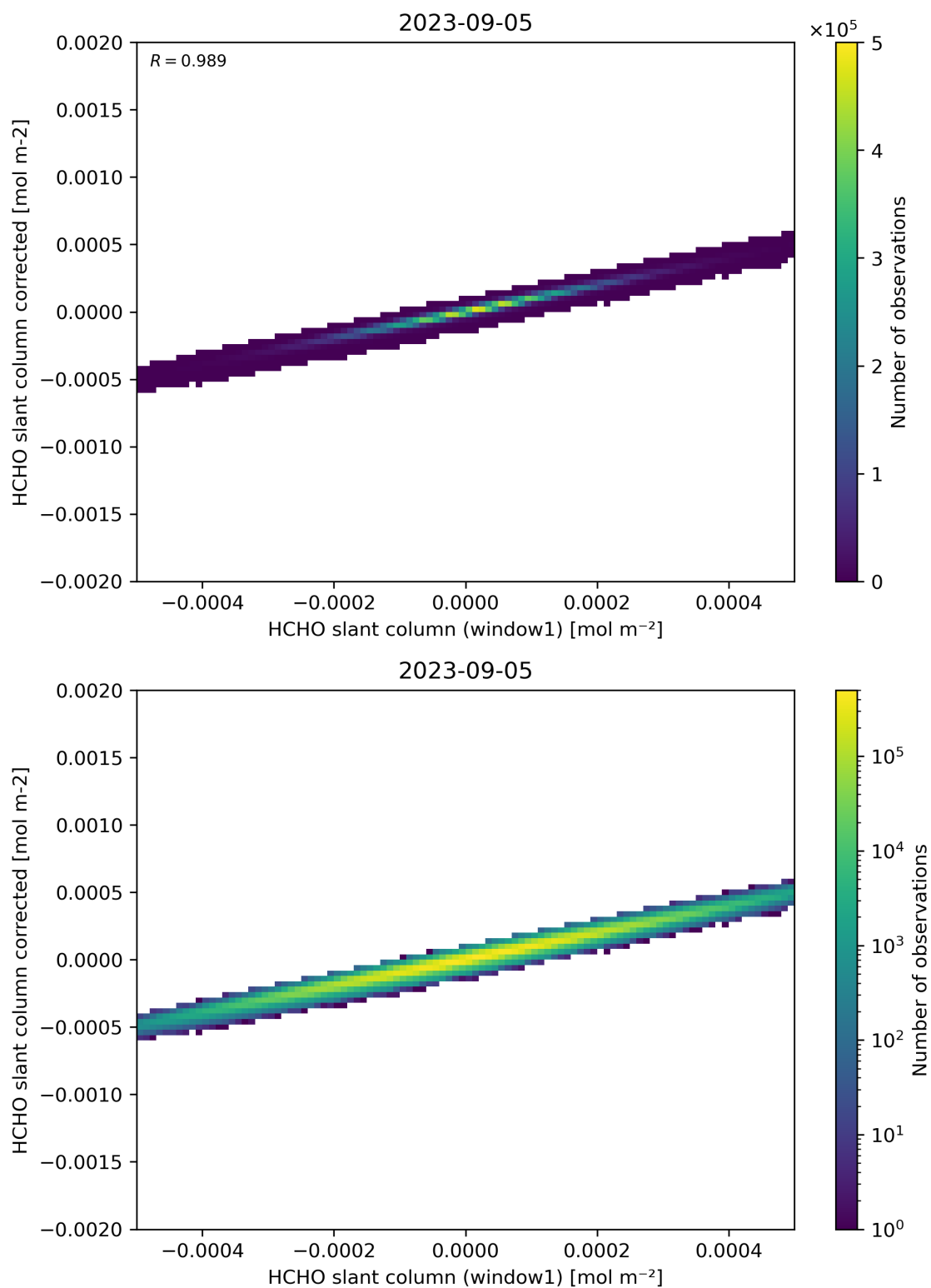
Figure 82: Scatter density plot of “HCHO slant column (window1)” against “HCHO slant column corrected” for 2023-09-05 to 2023-09-06.
