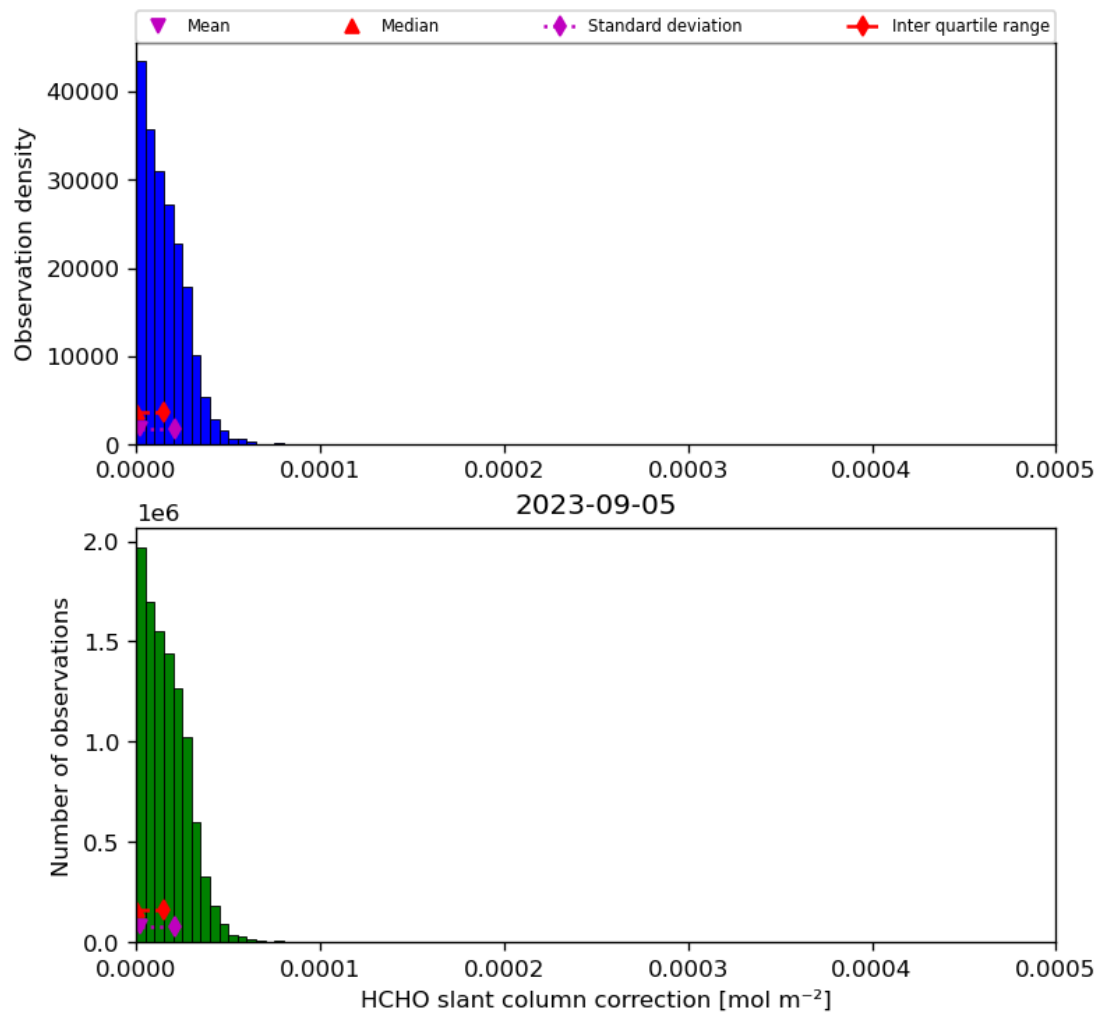
Figure 47: Histogram of “HCHO slant column correction” for 2023-09-05 to 2023-09-06
