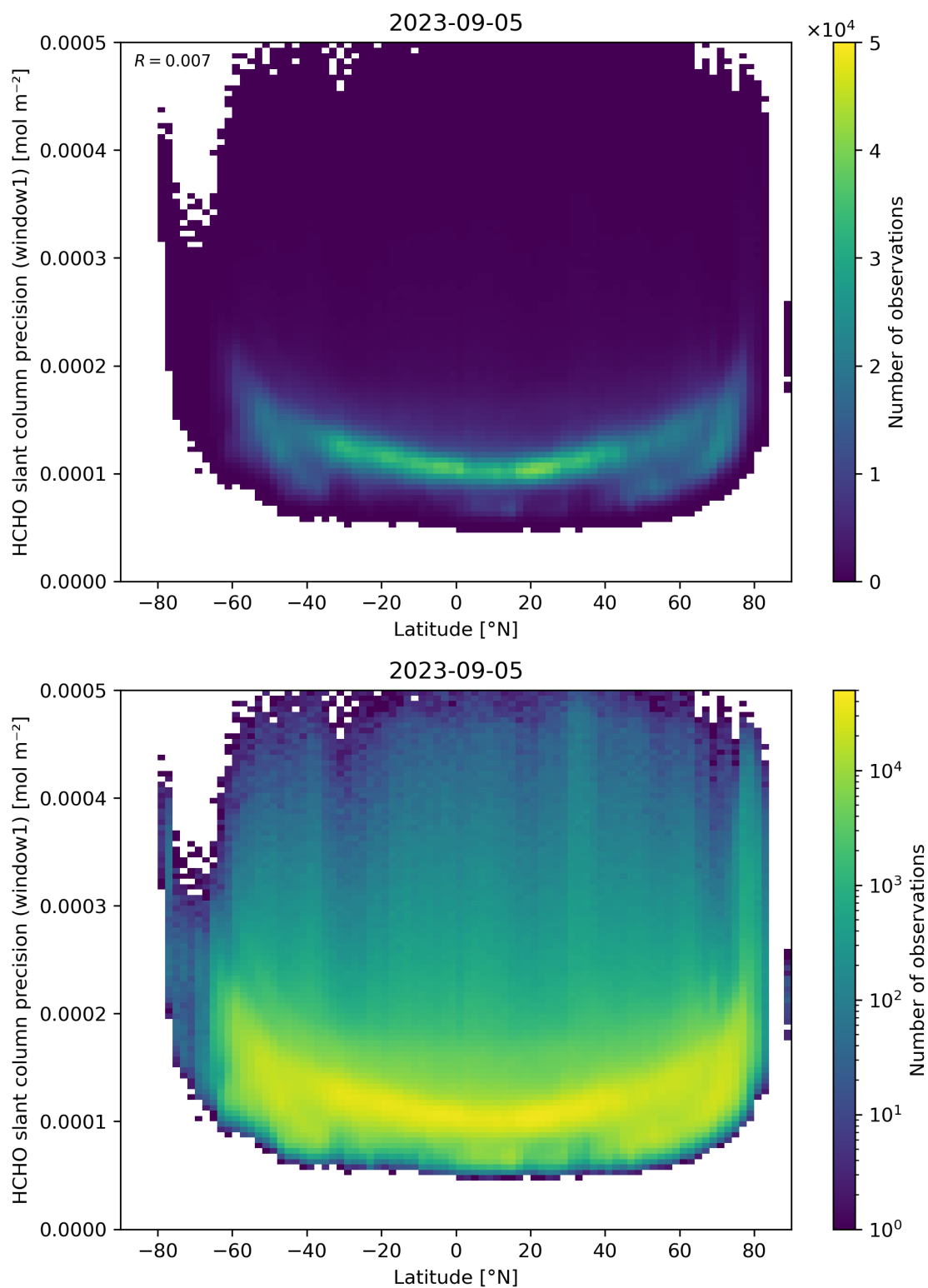
Figure 160: Scatter density plot of “Latitude” against “HCHO slant column precision (window1)” for 2023-09-05 to 2023-09-06.
