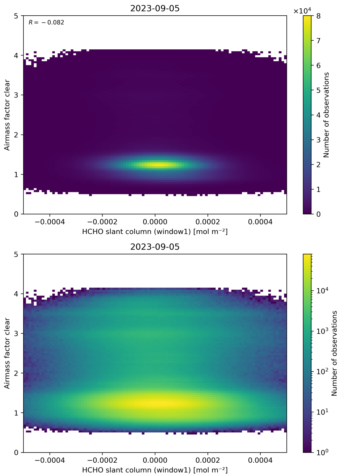
Figure 81: Scatter density plot of “HCHO slant column (window1)” against “Airmass factor clear” for 2023-09-05 to 2023-09-06.
