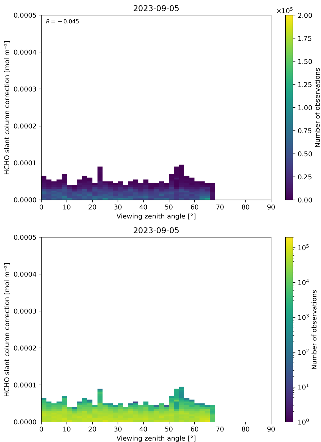
Figure 187: Scatter density plot of “Viewing zenith angle” against “HCHO slant column correction” for 2023-09-05 to 2023-09-06.
