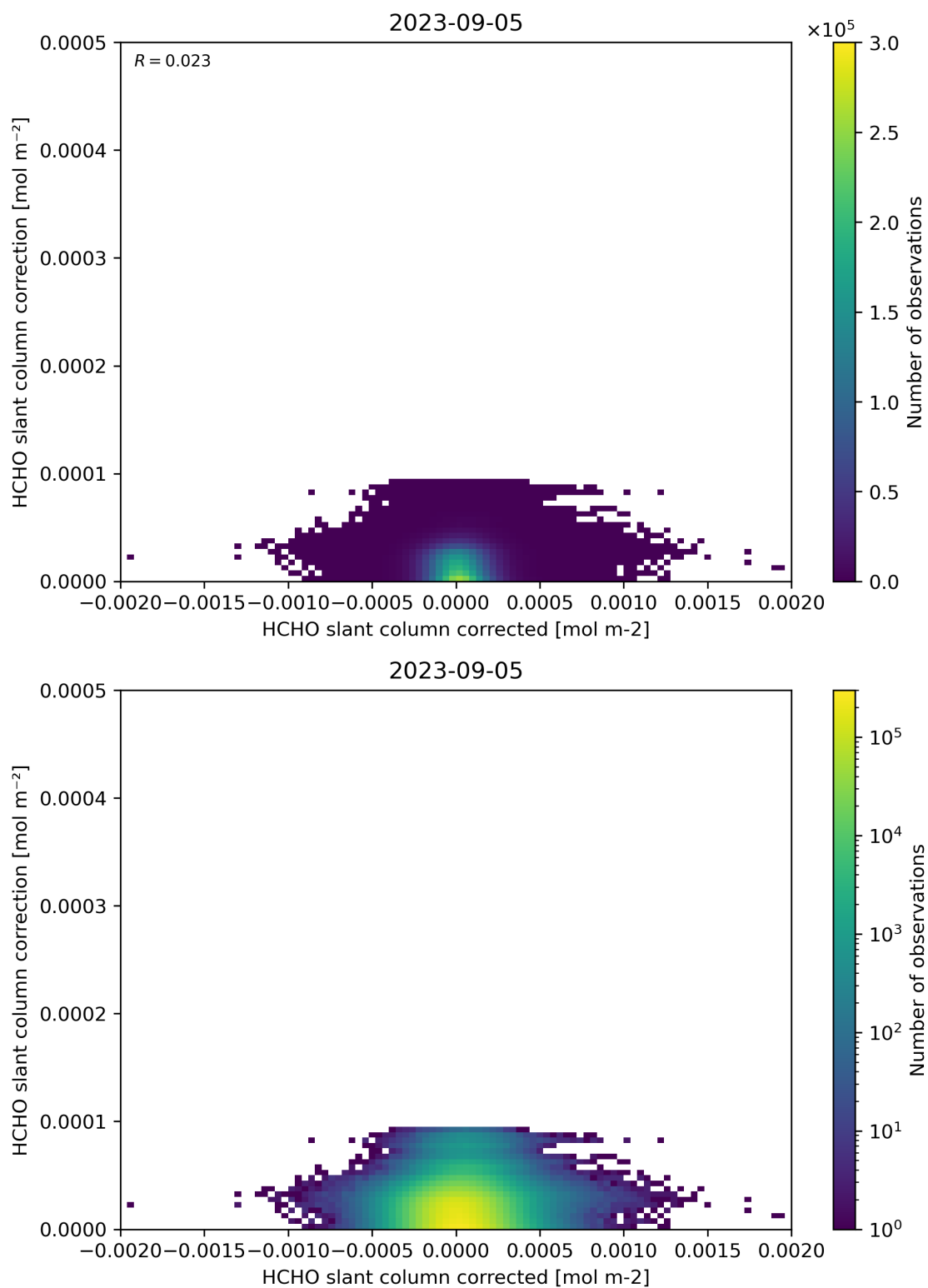
Figure 77: Scatter density plot of “HCHO slant column corrected” against “HCHO slant column correction” for 2023-09-05 to 2023-09-06.
