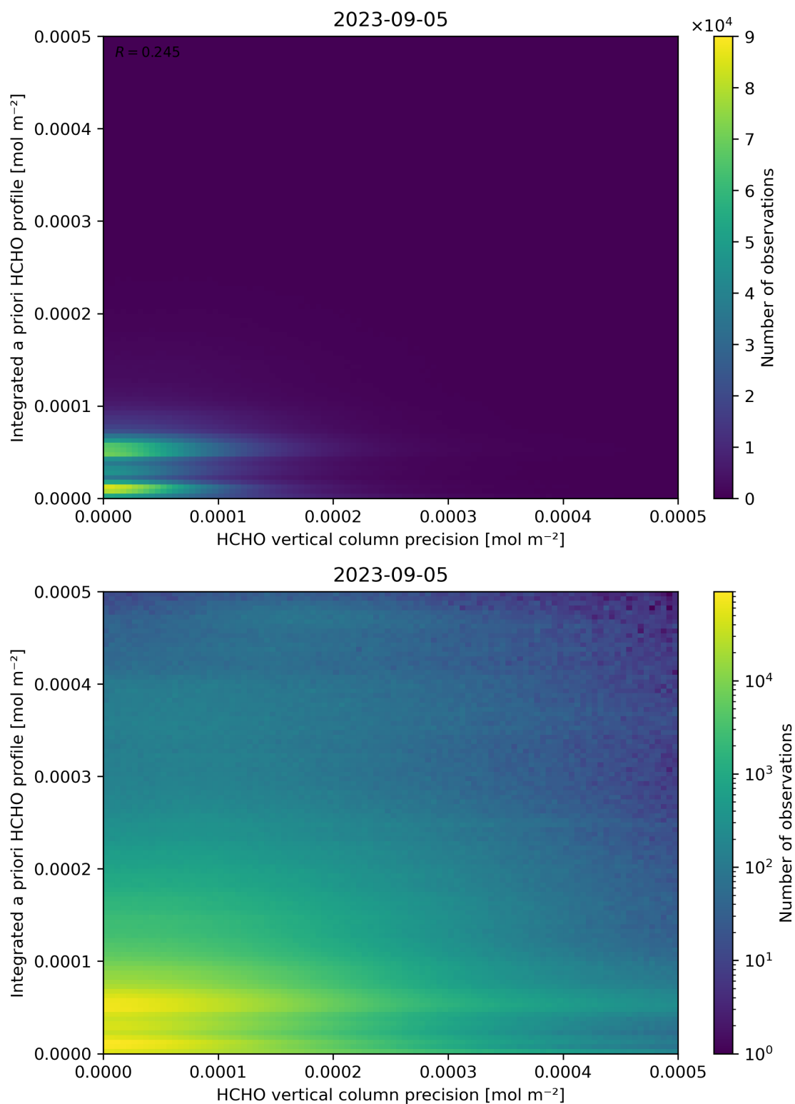
Figure 147: Scatter density plot of “HCHO vertical column precision” against “Integrated a priori HCHO profile” for 2023-09-05 to 2023-09-06.
