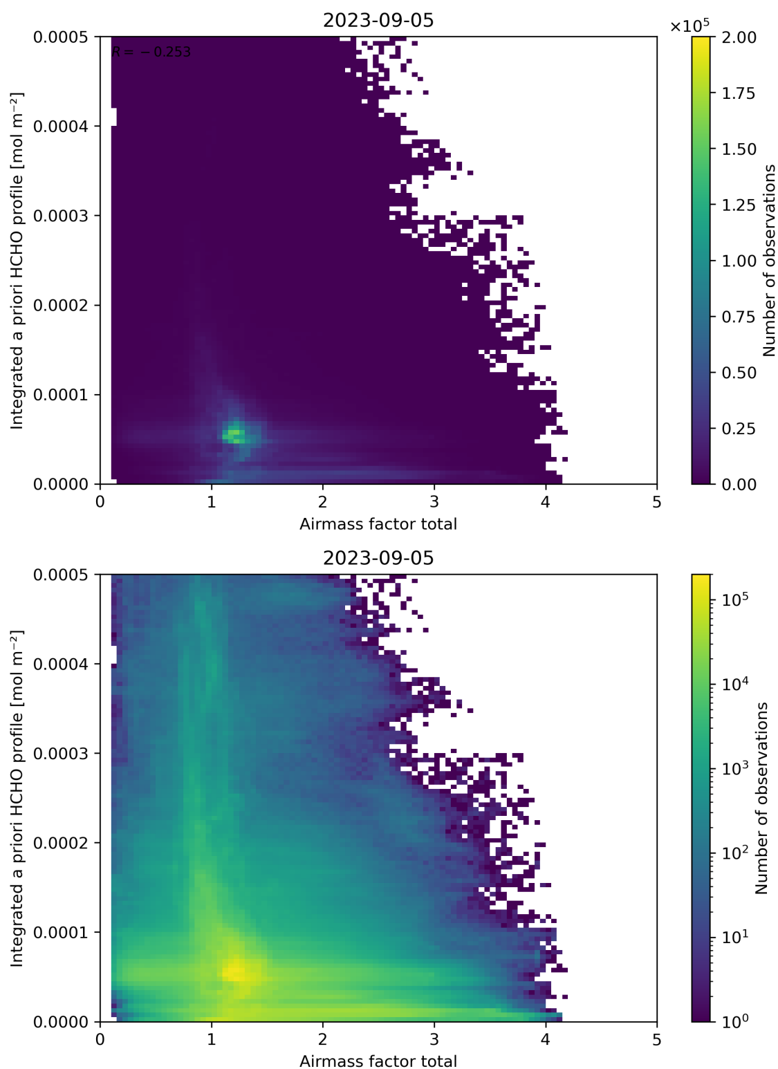
Figure 104: Scatter density plot of “Airmass factor total” against “Integrated a priori HCHO profile” for 2023-09-05 to 2023-09-06.
