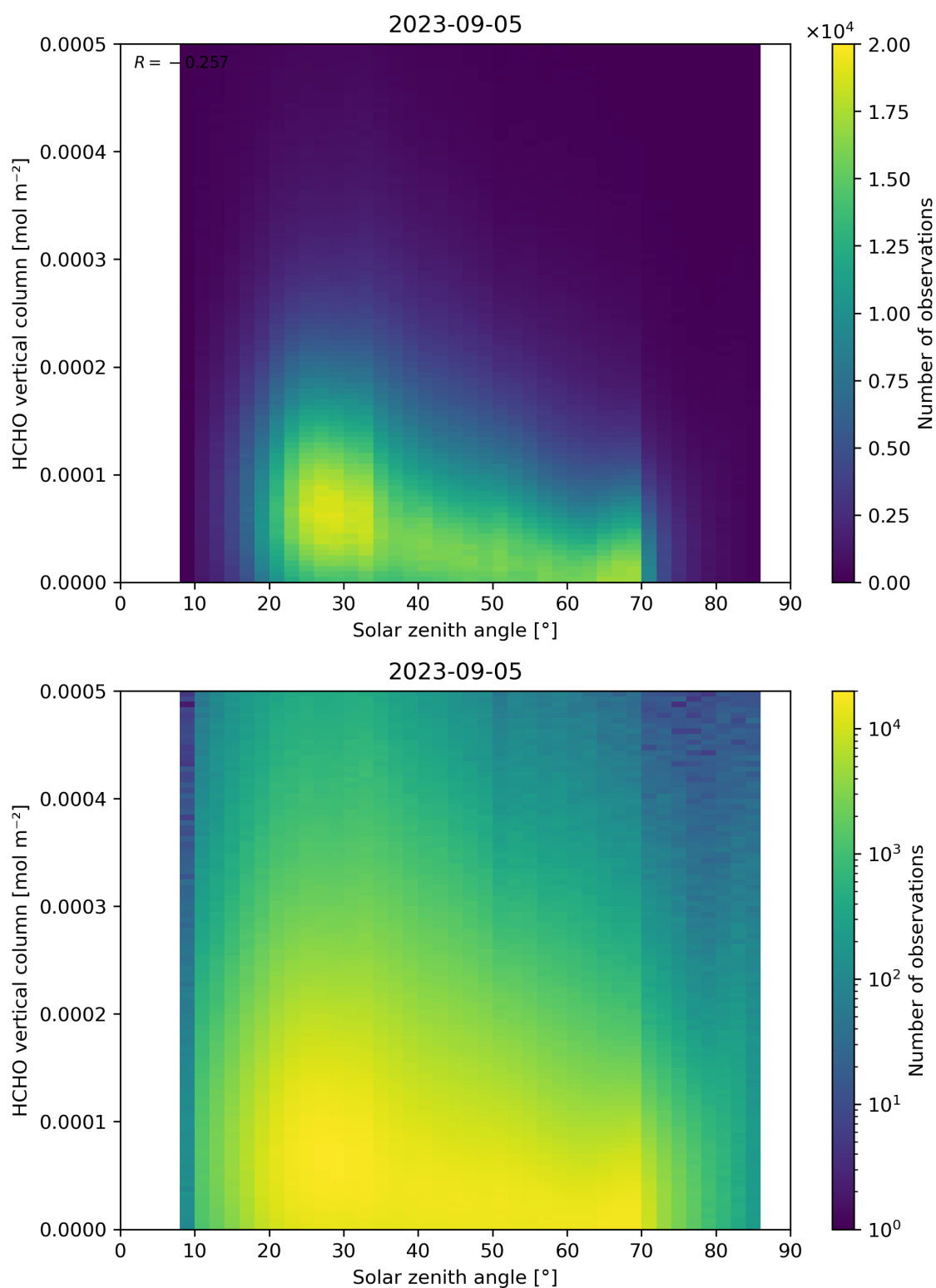
Figure 177: Scatter density plot of “Solar zenith angle” against “HCHO vertical column” for 2023-09-05 to 2023-09-06.
