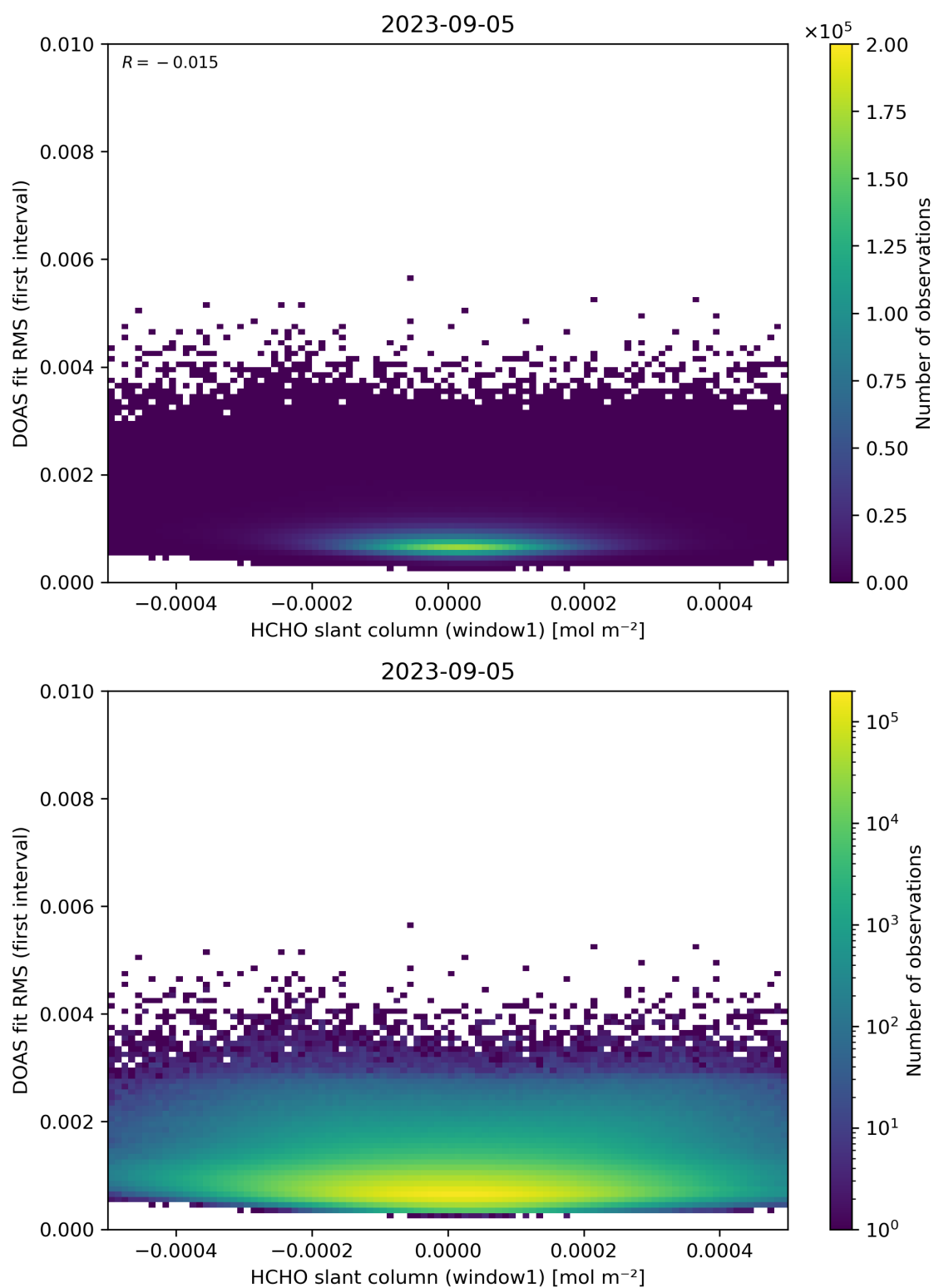
Figure 78: Scatter density plot of “HCHO slant column (window1)” against “DOAS fit RMS (first interval)” for 2023-09-05 to 2023-09-06.
