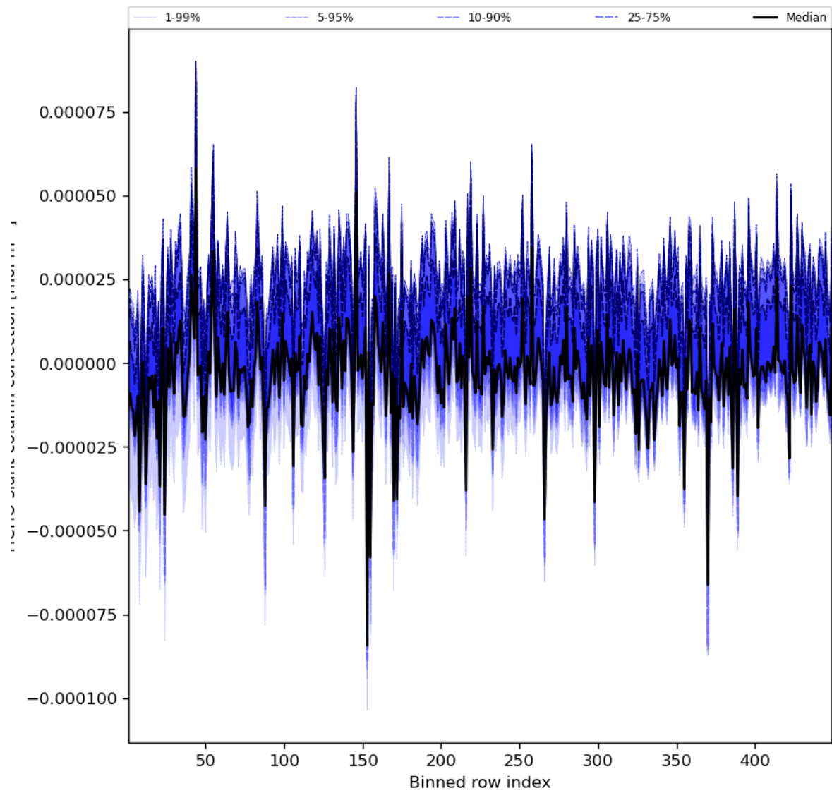
Figure 61: Along track statistics of “HCHO slant column correction” for 2023-09-05 to 2023-09-06
