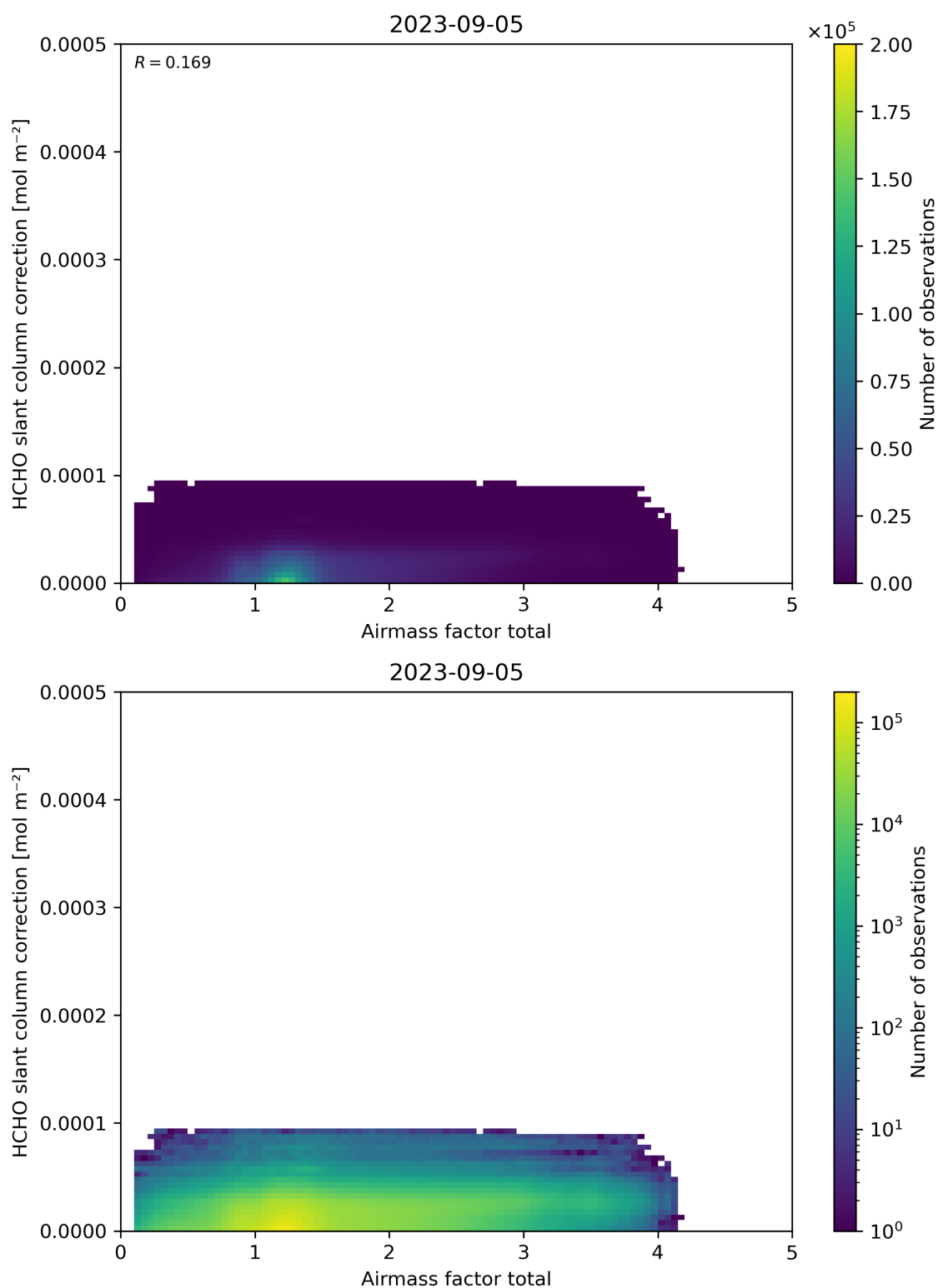
Figure 102: Scatter density plot of “Airmass factor total” against “HCHO slant column correction” for 2023-09-05 to 2023-09-06.
