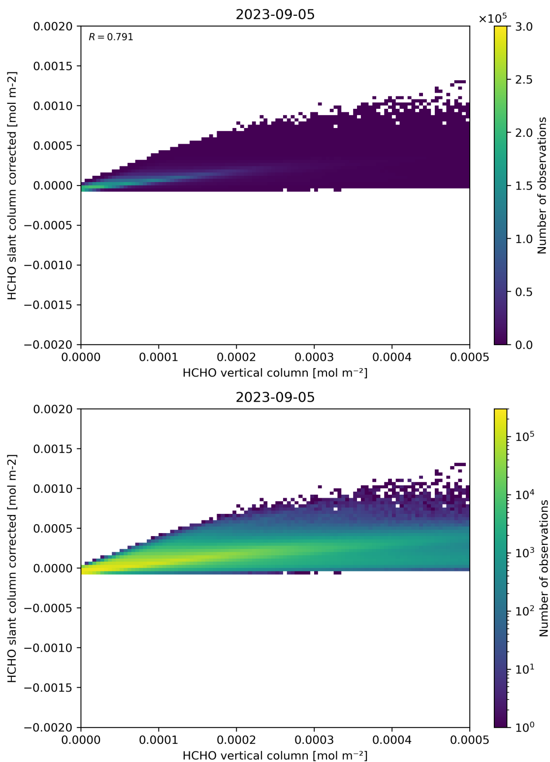
Figure 127: Scatter density plot of “HCHO vertical column” against “HCHO slant column corrected” for 2023-09-05 to 2023-09-06.
