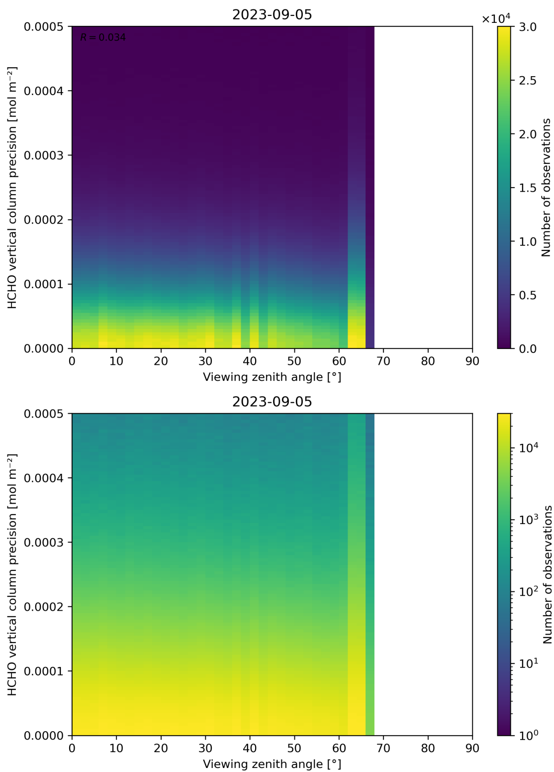
Figure 194: Scatter density plot of “Viewing zenith angle” against “HCHO vertical column precision” for 2023-09-05 to 2023-09-06.
