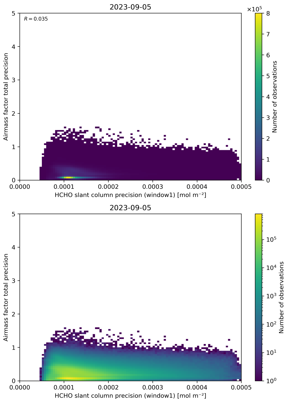
Figure 95: Scatter density plot of “HCHO slant column precision (window1)” against “Airmass factor total precision” for 2023-09-05 to 2023-09-06.
