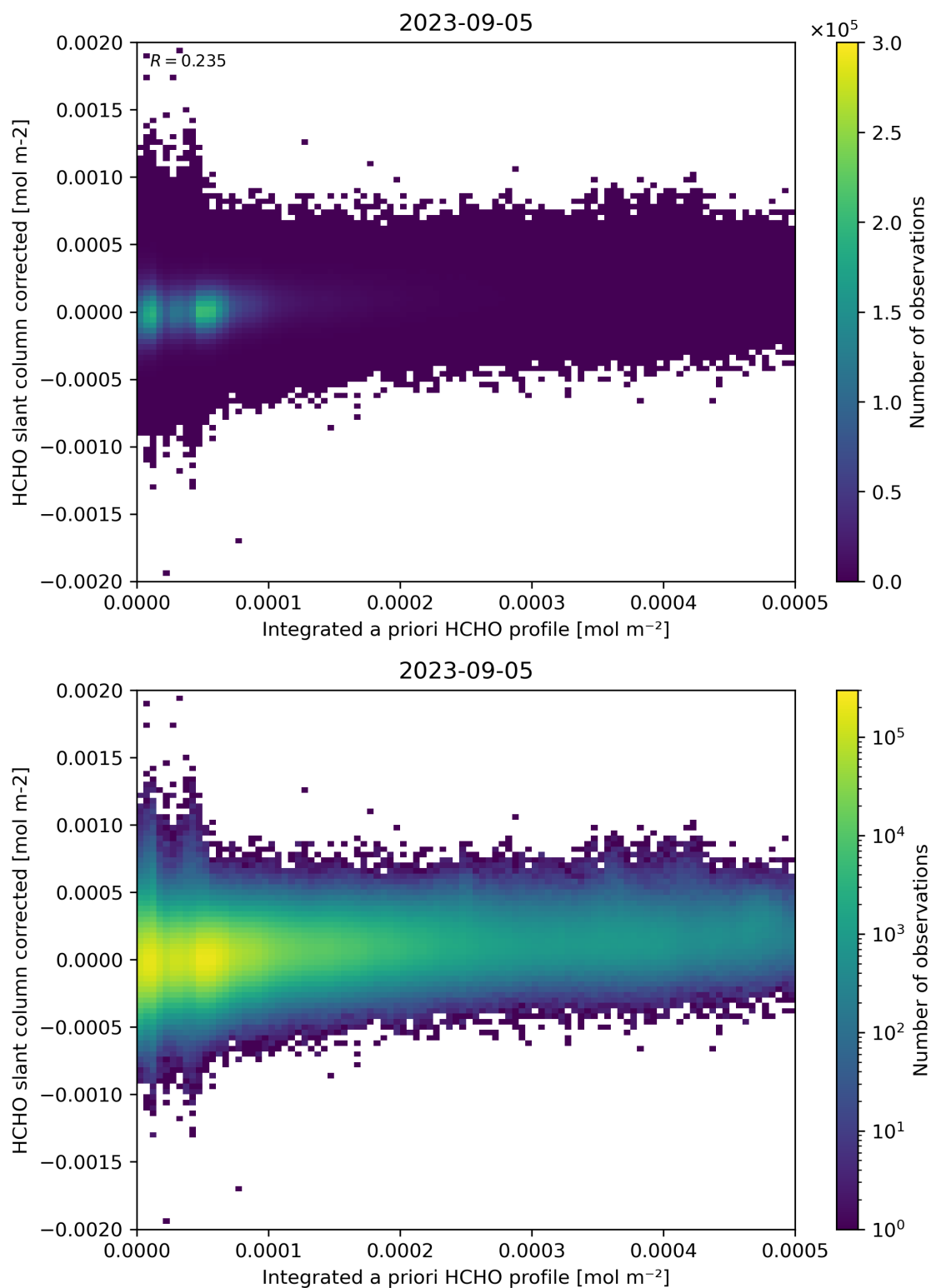
Figure 151: Scatter density plot of “Integrated a priori HCHO profile” against “HCHO slant column corrected” for 2023-09-05 to 2023-09-06.
