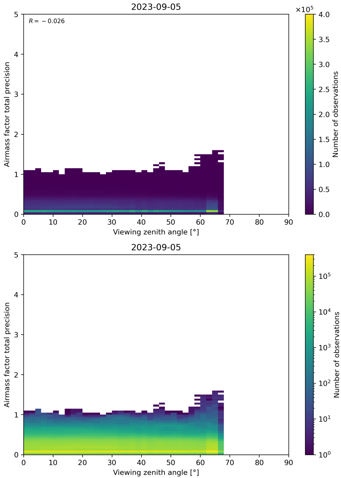
Figure 191: Scatter density plot of “Viewing zenith angle” against “Airmass factor total precision” for 2023-09-05 to 2023-09-06.
