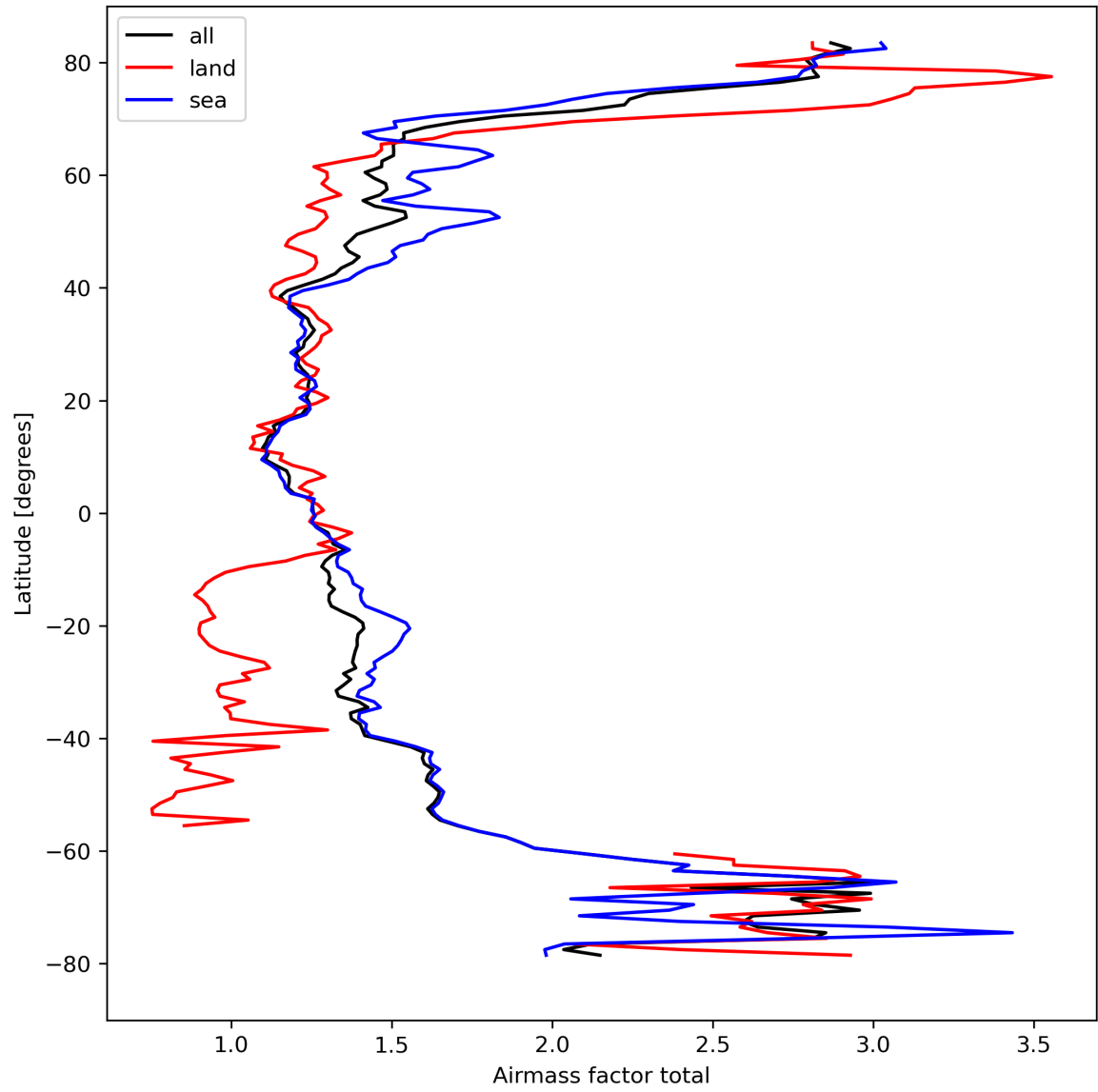
Figure 26: Zonal average of “Airmass factor total” for 2023-09-05 to 2023-09-06.
