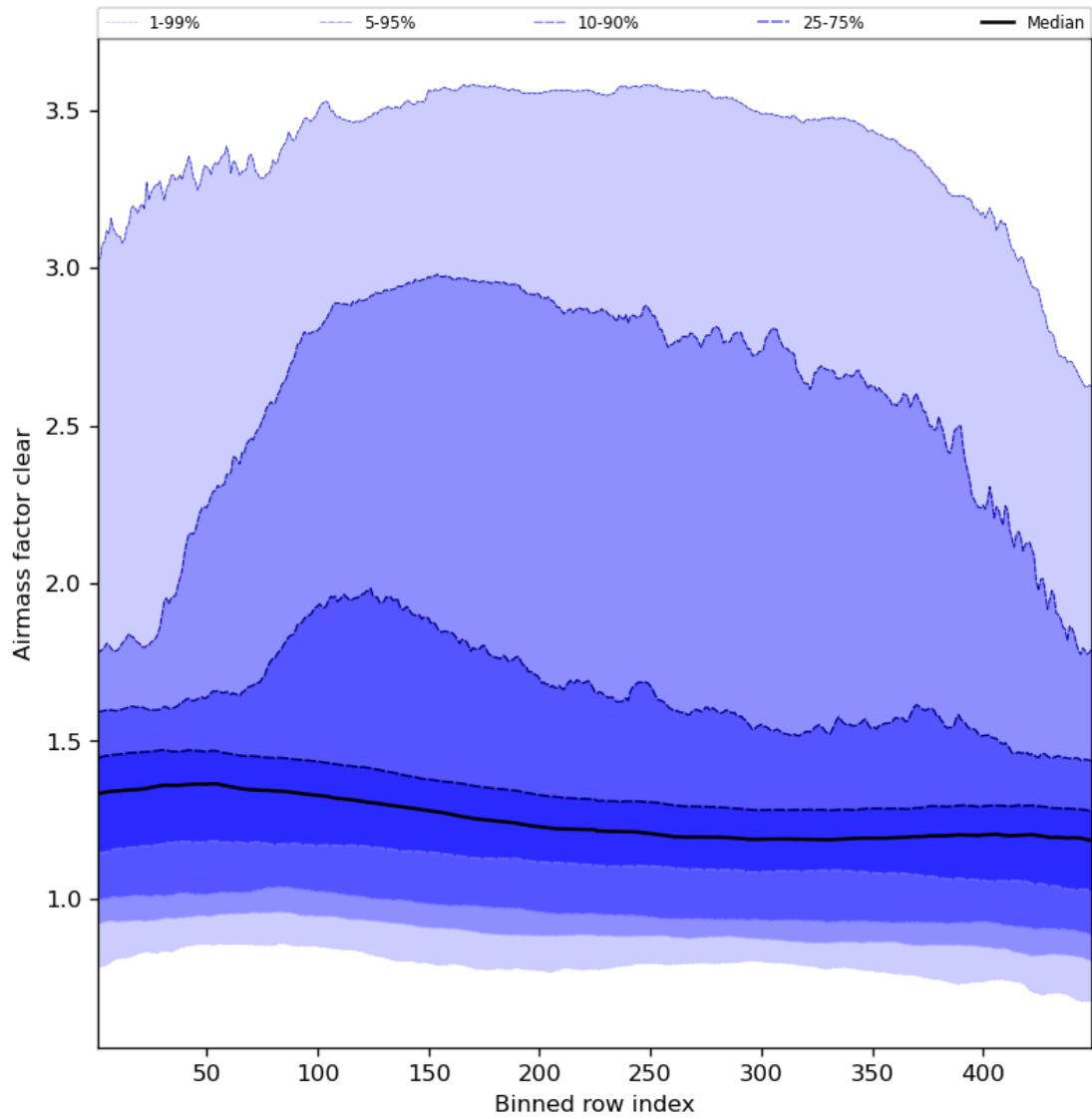
Figure 56: Along track statistics of “Airmass factor clear” for 2023-09-05 to 2023-09-06
