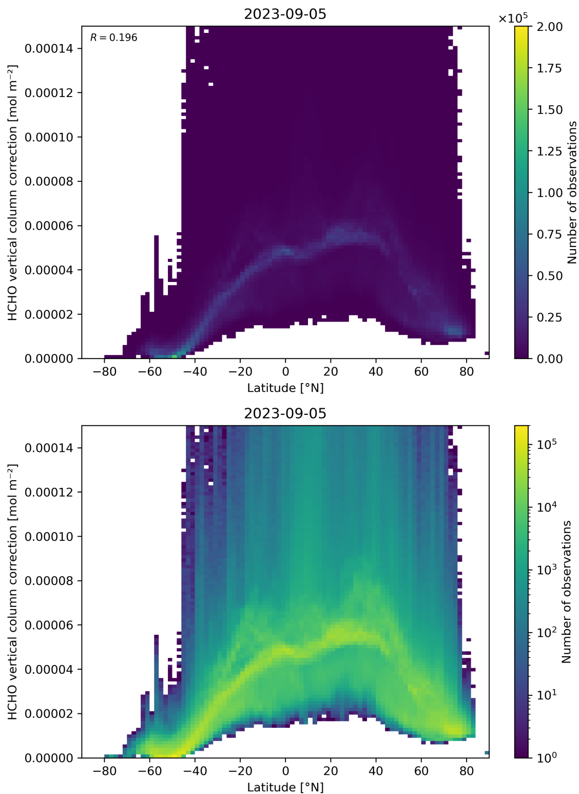
Figure 164: Scatter density plot of “Latitude” against “HCHO vertical column correction” for 2023-09-05 to 2023-09-06.
