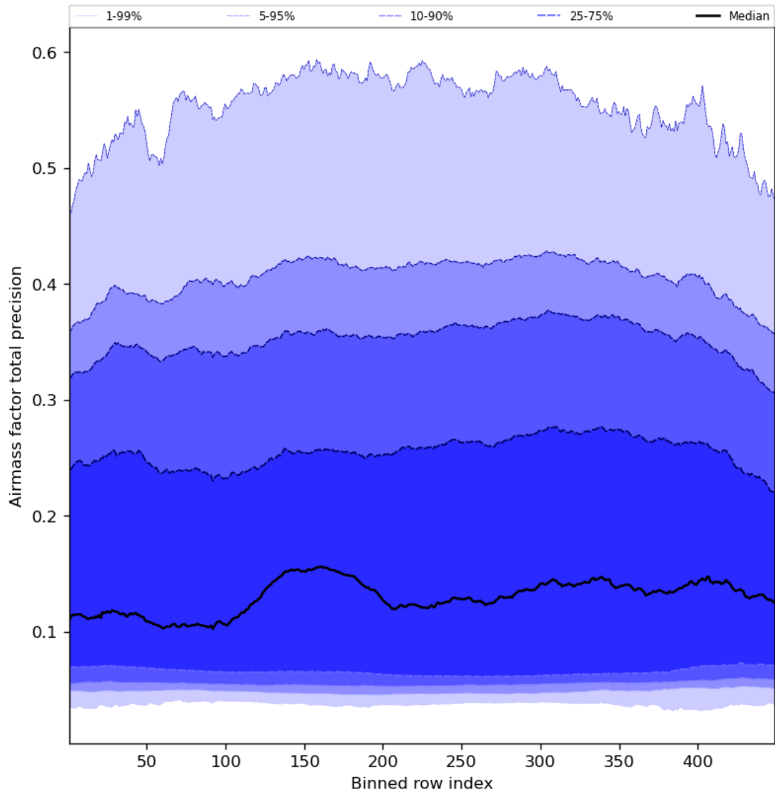
Figure 55: Along track statistics of “Airmass factor total precision” for 2023-09-05 to 2023-09-06
