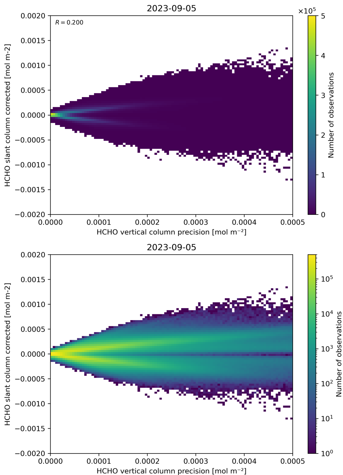
Figure 140: Scatter density plot of “HCHO vertical column precision” against “HCHO slant column corrected” for 2023-09-05 to 2023-09-06.
