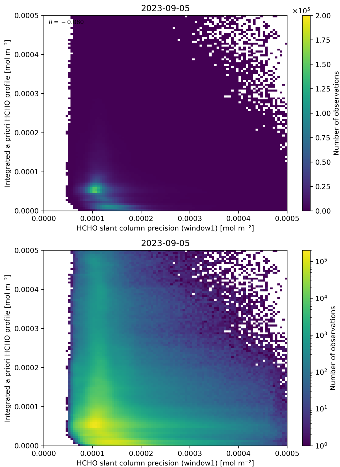
Figure 96: Scatter density plot of “HCHO slant column precision (window1)” against “Integrated a priori HCHO profile” for 2023-09-05 to 2023-09-06.
