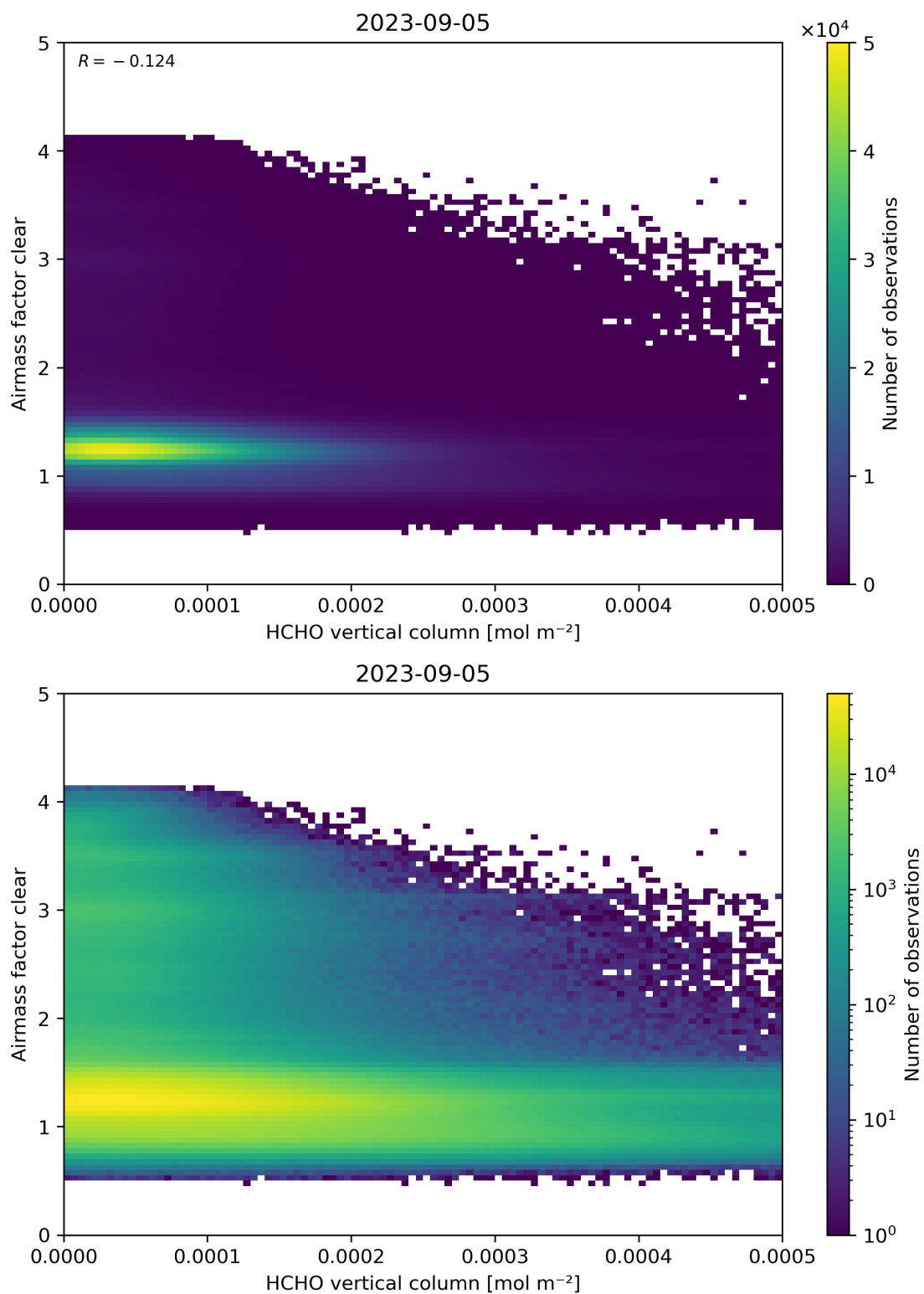
Figure 126: Scatter density plot of “HCHO vertical column” against “Airmass factor clear” for 2023-09-05 to 2023-09-06.
