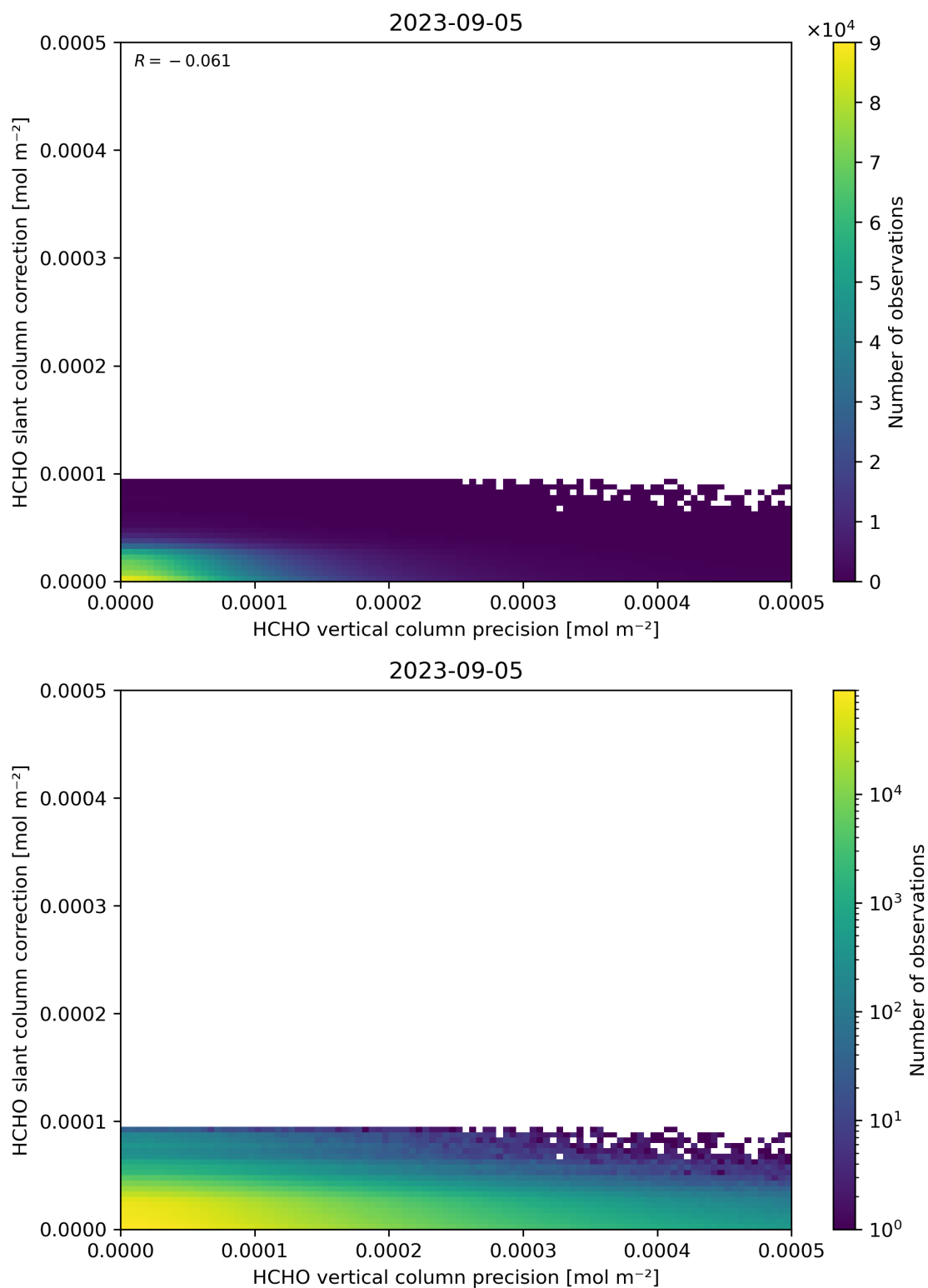
Figure 141: Scatter density plot of “HCHO vertical column precision” against “HCHO slant column correction” for 2023-09-05 to 2023-09-06.
