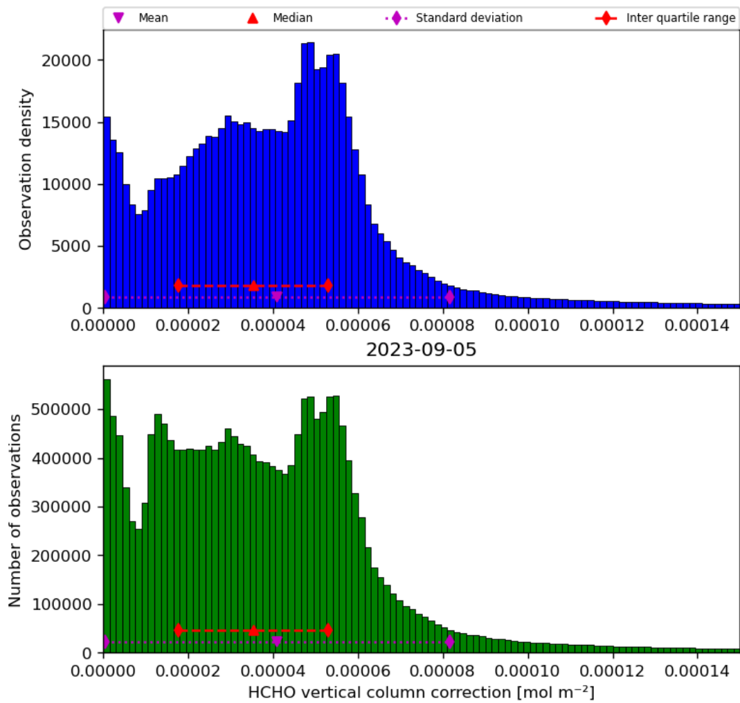
Figure 37: Histogram of “HCHO vertical column correction” for 2023-09-05 to 2023-09-06
