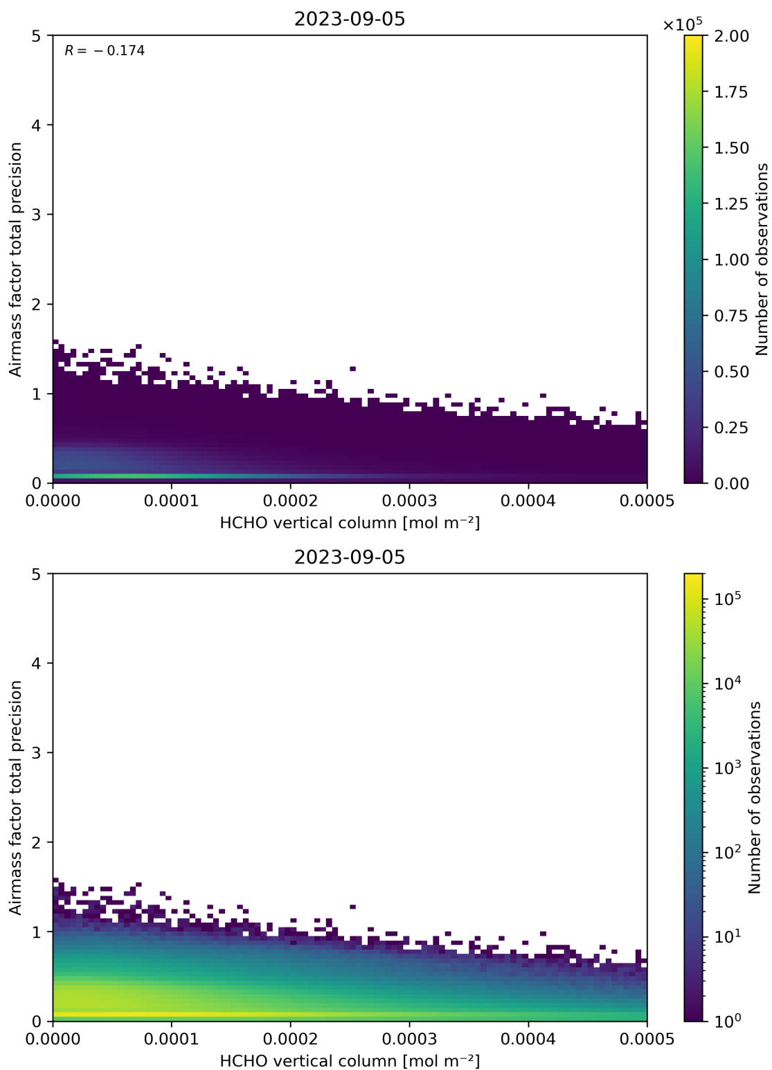
Figure 132: Scatter density plot of “HCHO vertical column” against “Airmass factor total precision” for 2023-09-05 to 2023-09-06.
