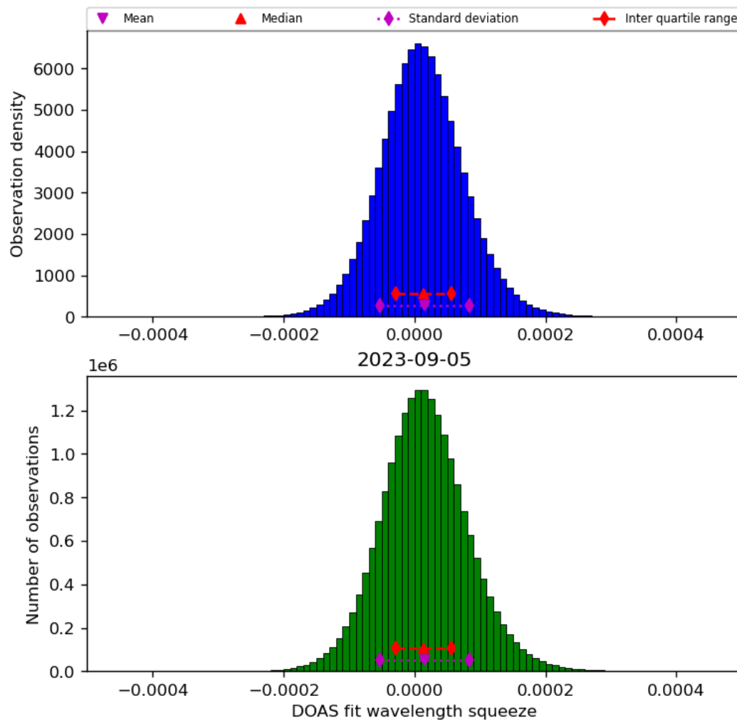
Figure 45: Histogram of “DOAS fit wavelength squeeze” for 2023-09-05 to 2023-09-06
