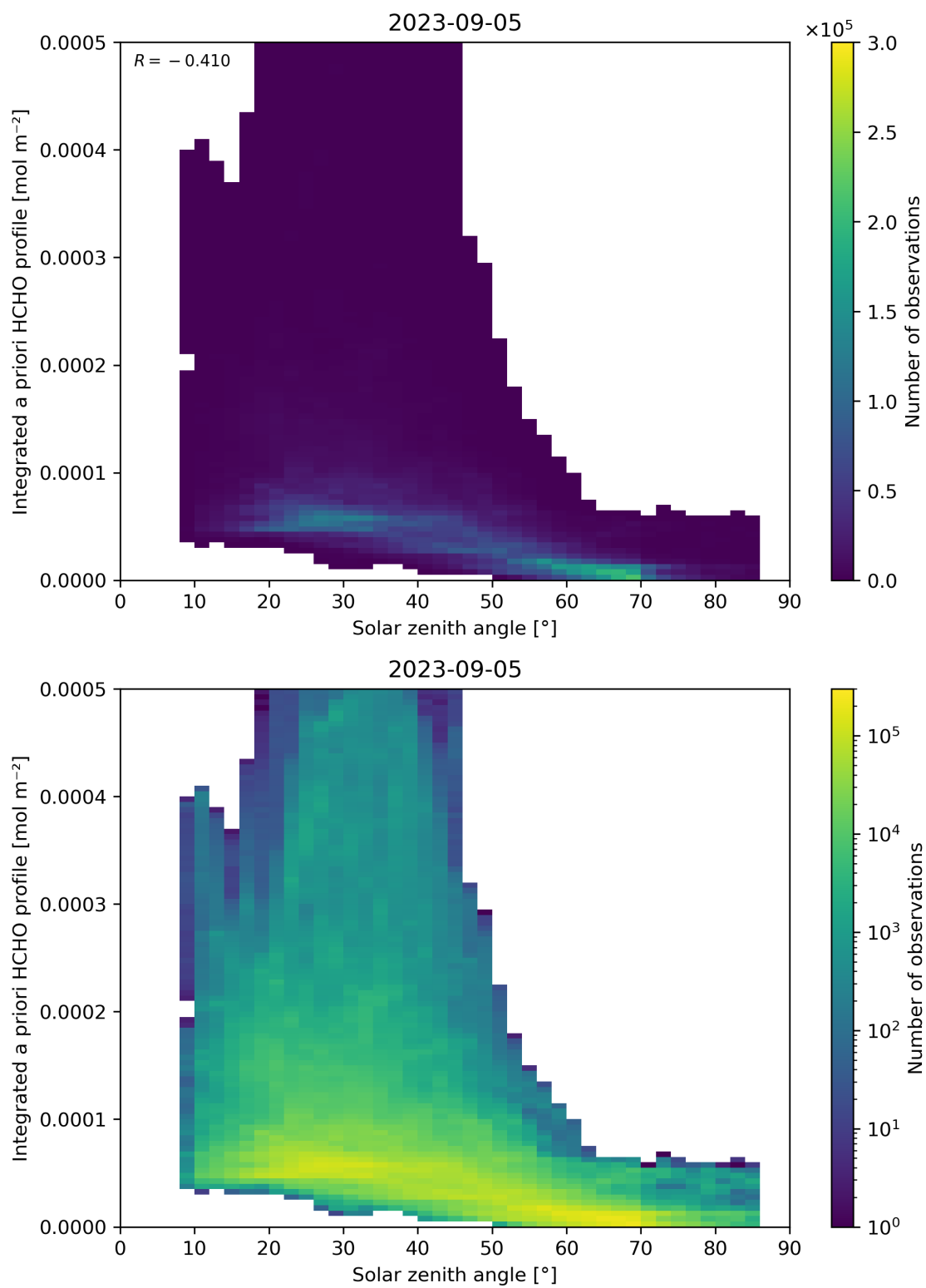
Figure 180: Scatter density plot of “Solar zenith angle” against “Integrated a priori HCHO profile” for 2023-09-05 to 2023-09-06.
