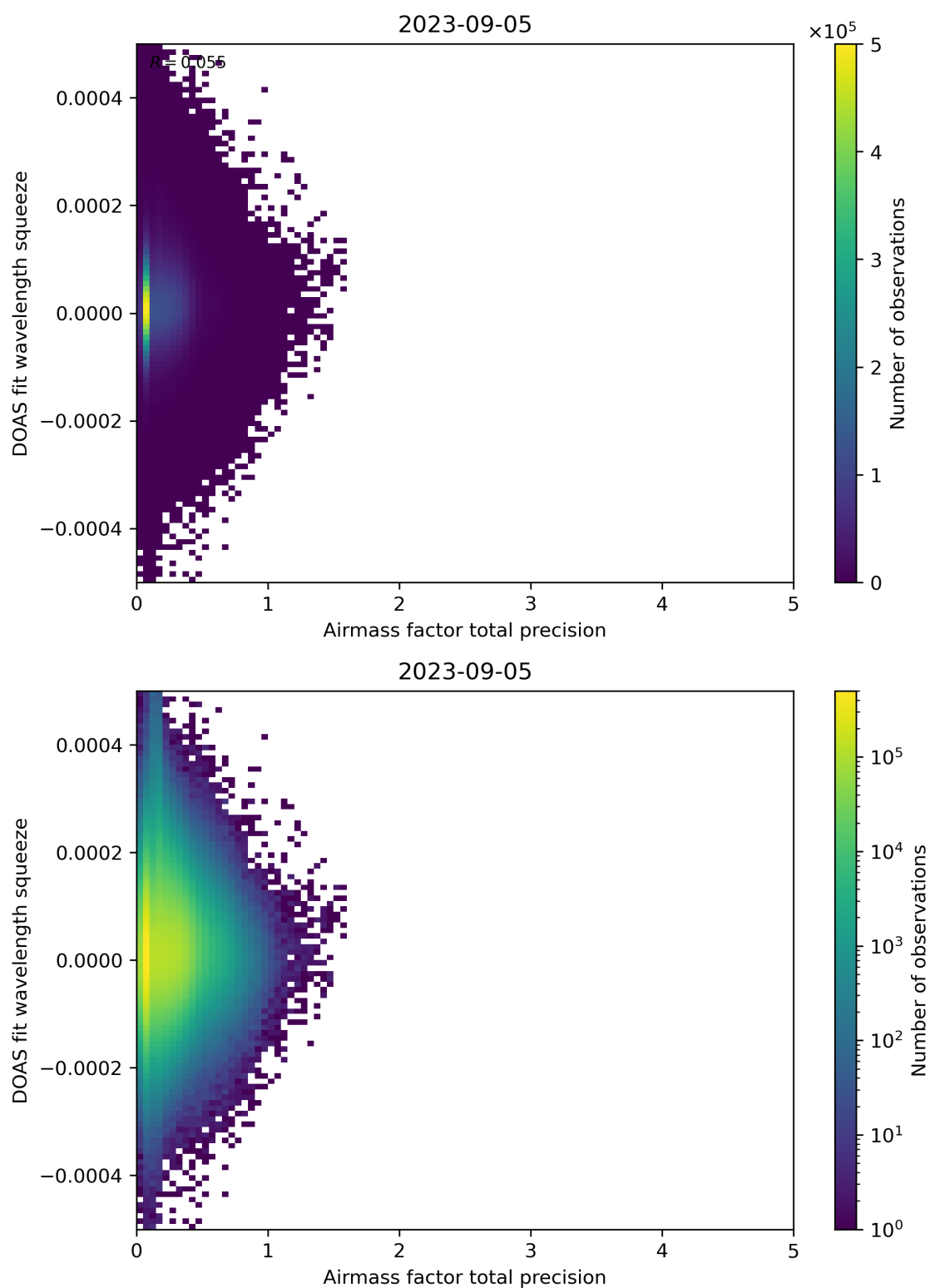
Figure 107: Scatter density plot of “Airmass factor total precision” against “DOAS fit wavelength squeeze” for 2023-09-05 to 2023-09-06.
