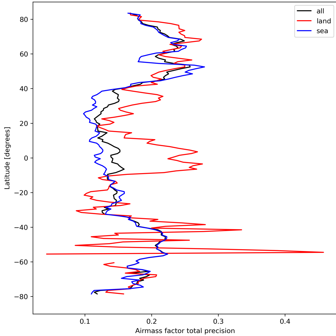
Figure 27: Zonal average of “Airmass factor total precision” for 2023-09-05 to 2023-09-06.
