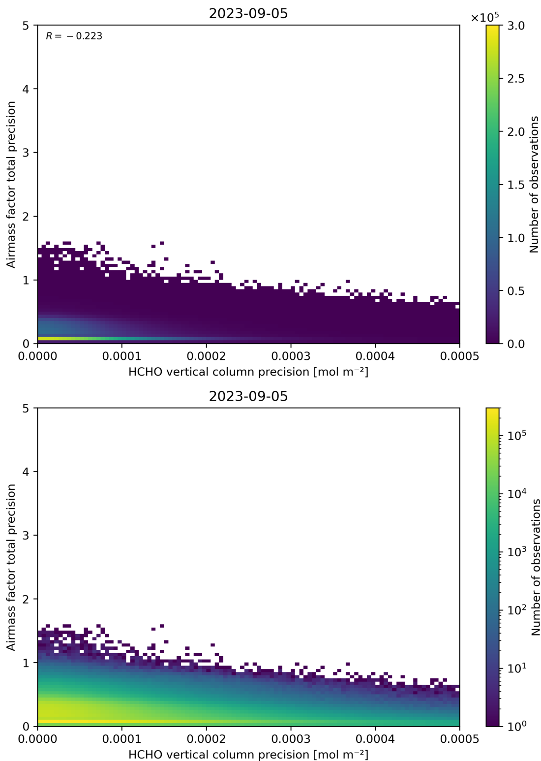
Figure 145: Scatter density plot of “HCHO vertical column precision” against “Airmass factor total precision” for 2023-09-05 to 2023-09-06.
