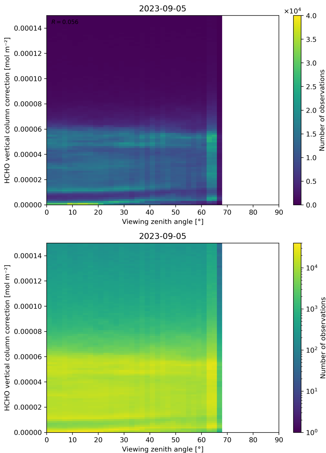
Figure 193: Scatter density plot of “Viewing zenith angle” against “HCHO vertical column correction” for 2023-09-05 to 2023-09-06.
