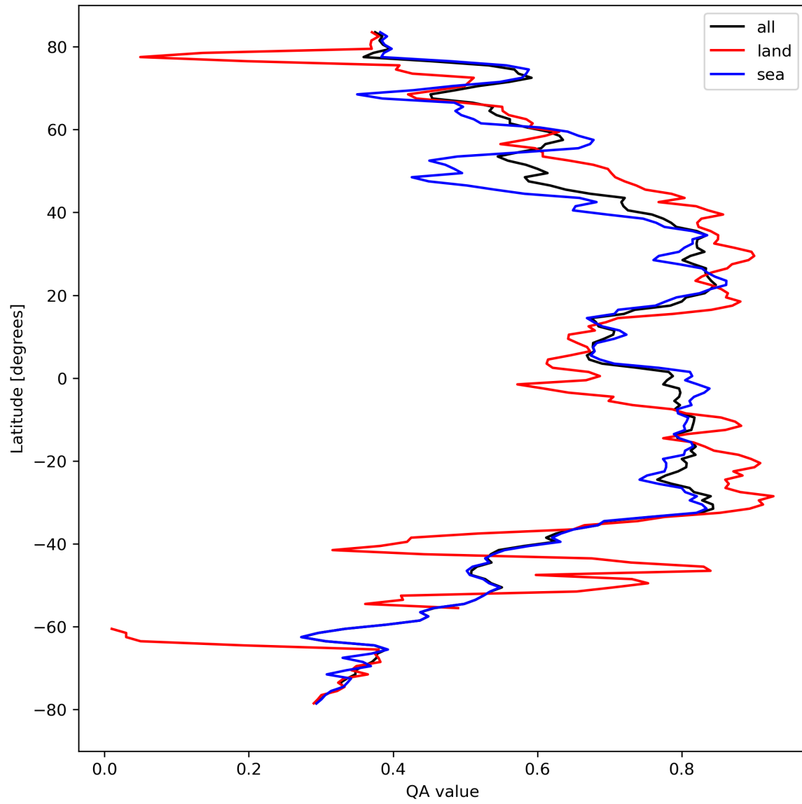
Figure 20: Zonal average of “QA value” for 2023-09-05 to 2023-09-06.
