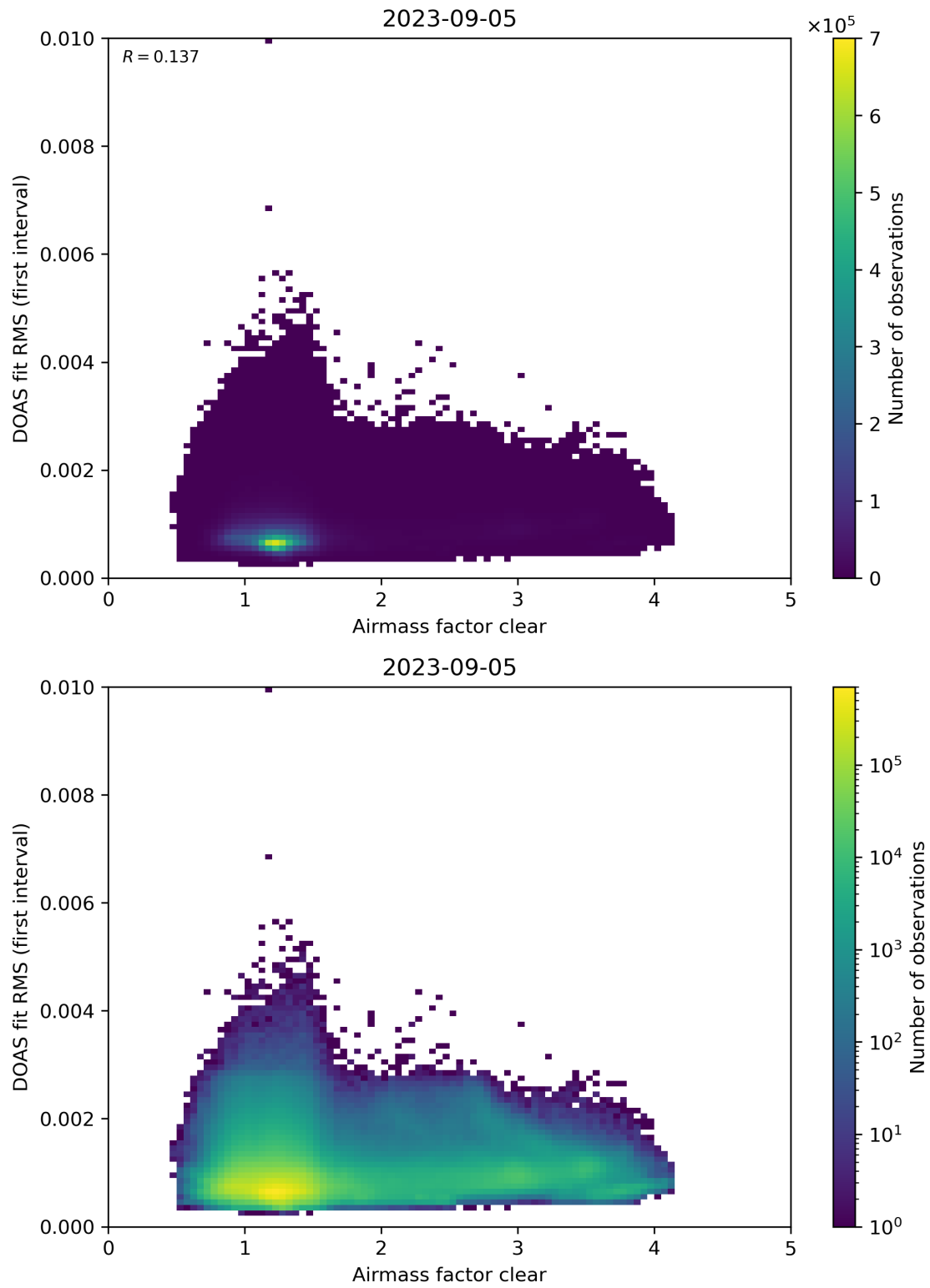
Figure 71: Scatter density plot of “Airmass factor clear” against “DOAS fit RMS (first interval)” for 2023-09-05 to 2023-09-06.
