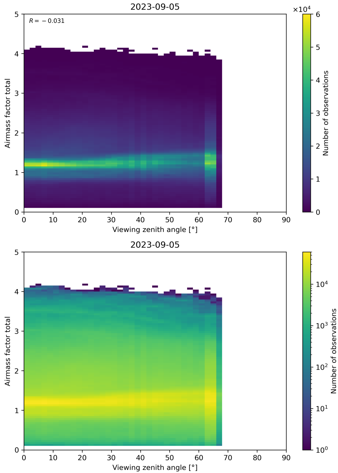
Figure 190: Scatter density plot of “Viewing zenith angle” against “Airmass factor total” for 2023-09-05 to 2023-09-06.
