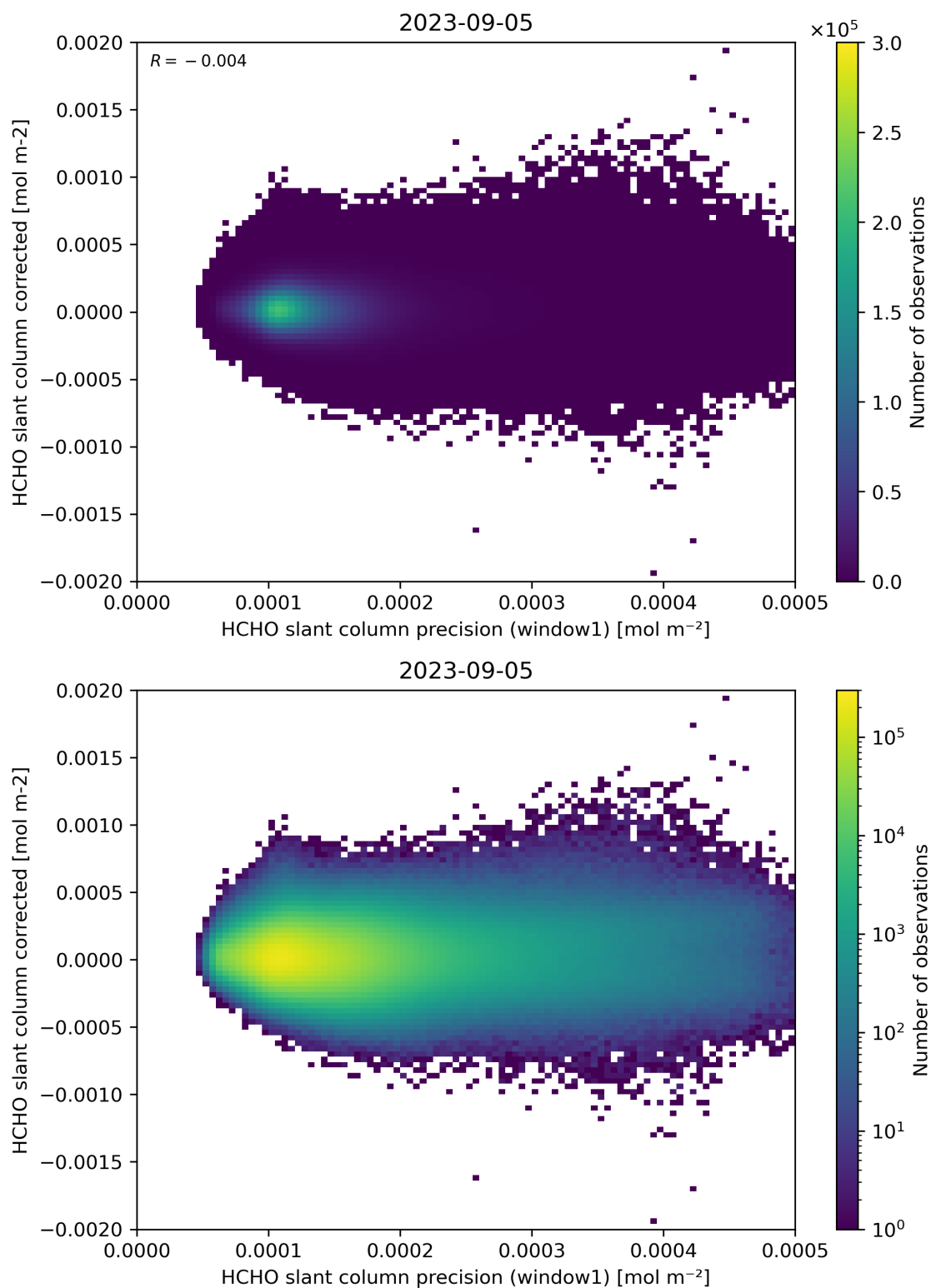
Figure 92: Scatter density plot of “HCHO slant column precision (window1)” against “HCHO slant column corrected” for 2023-09-05 to 2023-09-06.
