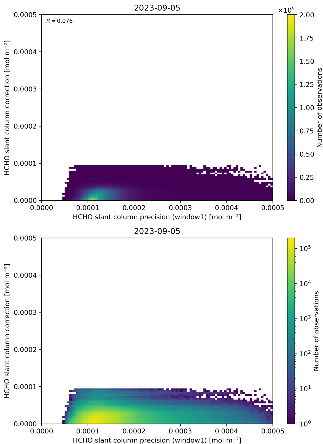
Figure 93: Scatter density plot of “HCHO slant column precision (window1)” against “HCHO slant column correction” for 2023-09-05 to 2023-09-06.
