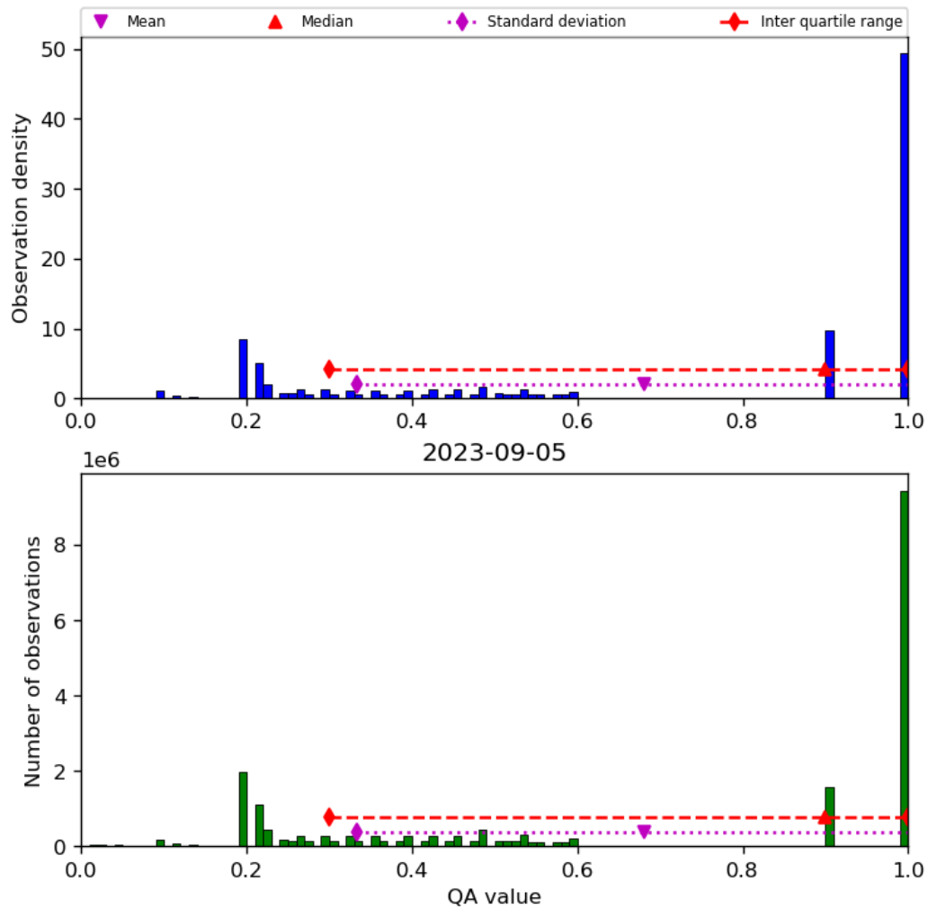
Figure 34: Histogram of “QA value” for 2023-09-05 to 2023-09-06
