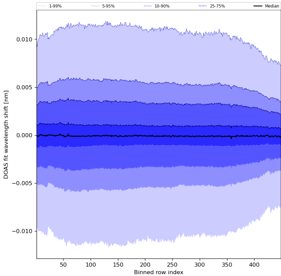
Figure 58: Along track statistics of “DOAS fit wavelength shift” for 2023-09-05 to 2023-09-06
