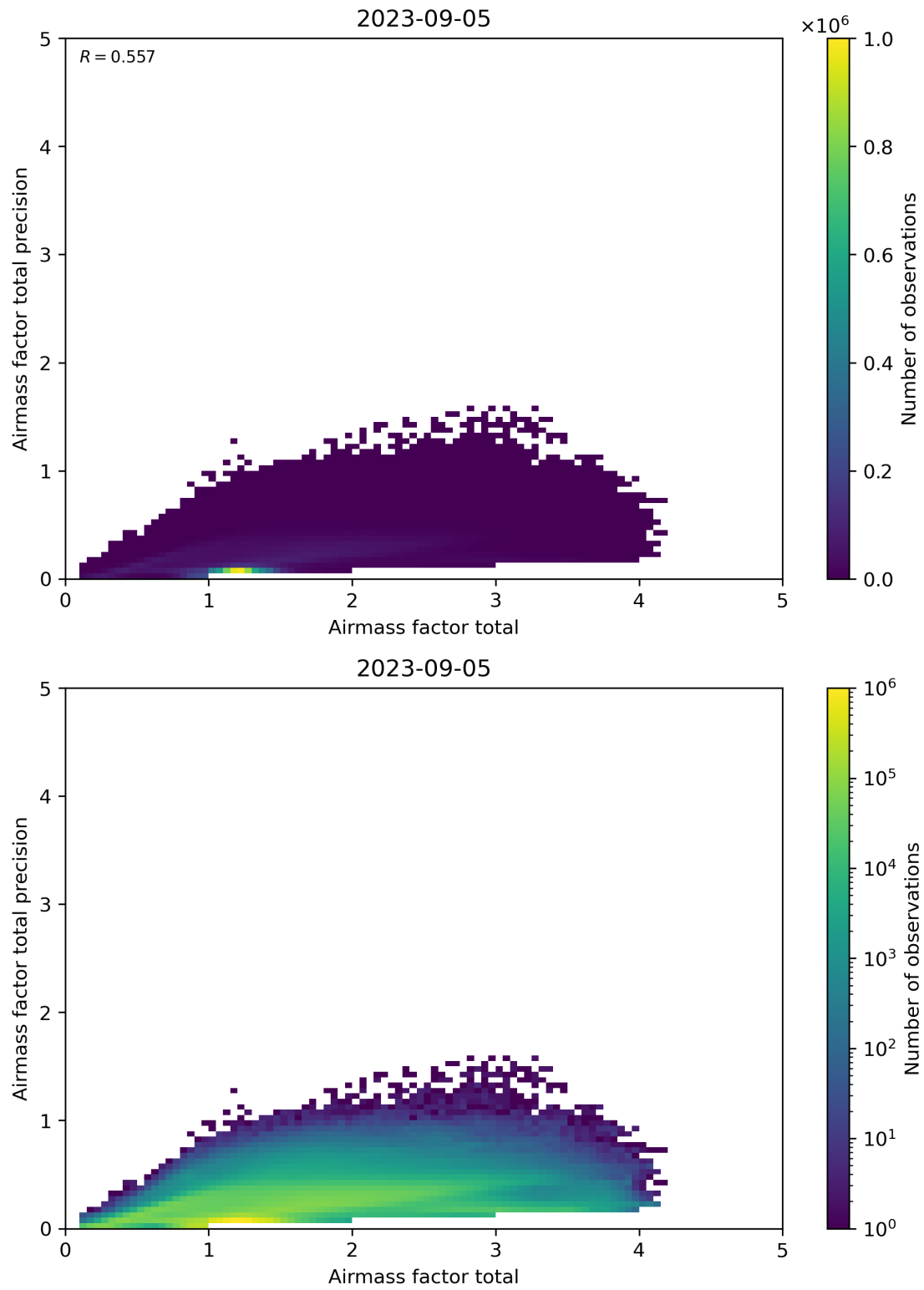
Figure 103: Scatter density plot of “Airmass factor total” against “Airmass factor total precision” for 2023-09-05 to 2023-09-06.
