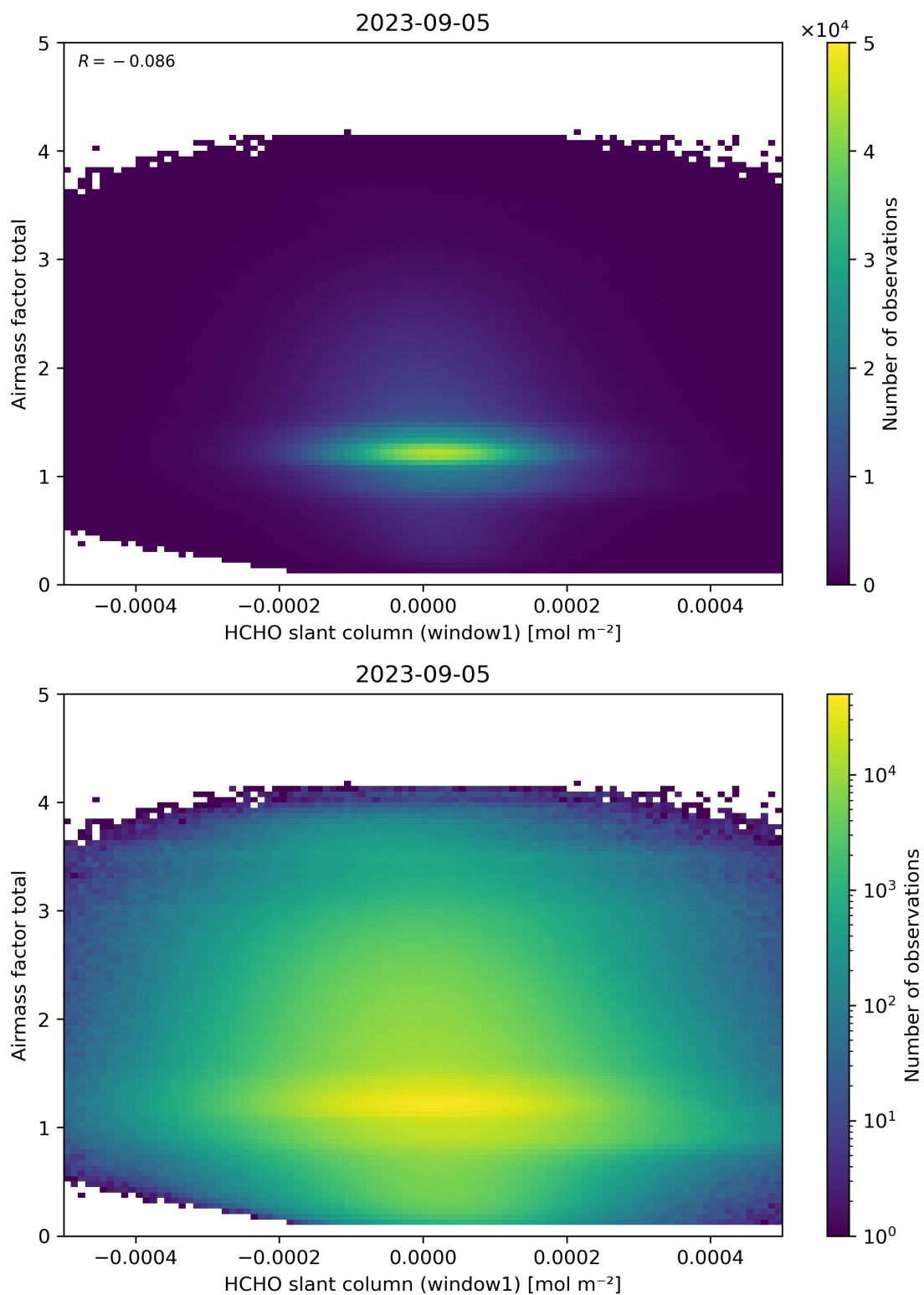
Figure 85: Scatter density plot of “HCHO slant column (window1)” against “Airmass factor total” for 2023-09-05 to 2023-09-06.
