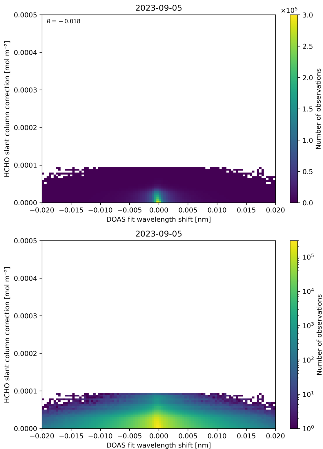
Figure 67: Scatter density plot of “DOAS fit wavelength shift” against “HCHO slant column correction” for 2023-09-05 to 2023-09-06.
