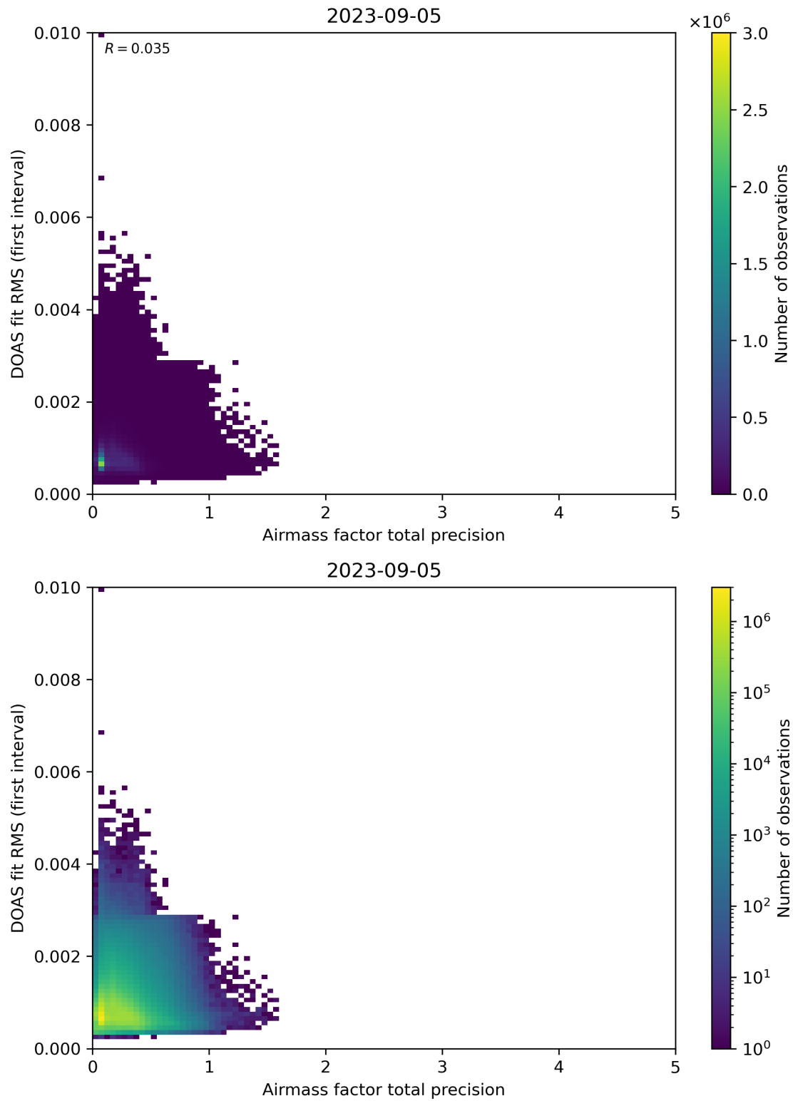
Figure 105: Scatter density plot of “Airmass factor total precision” against “DOAS fit RMS (first interval)” for 2023-09-05 to 2023-09-06.
