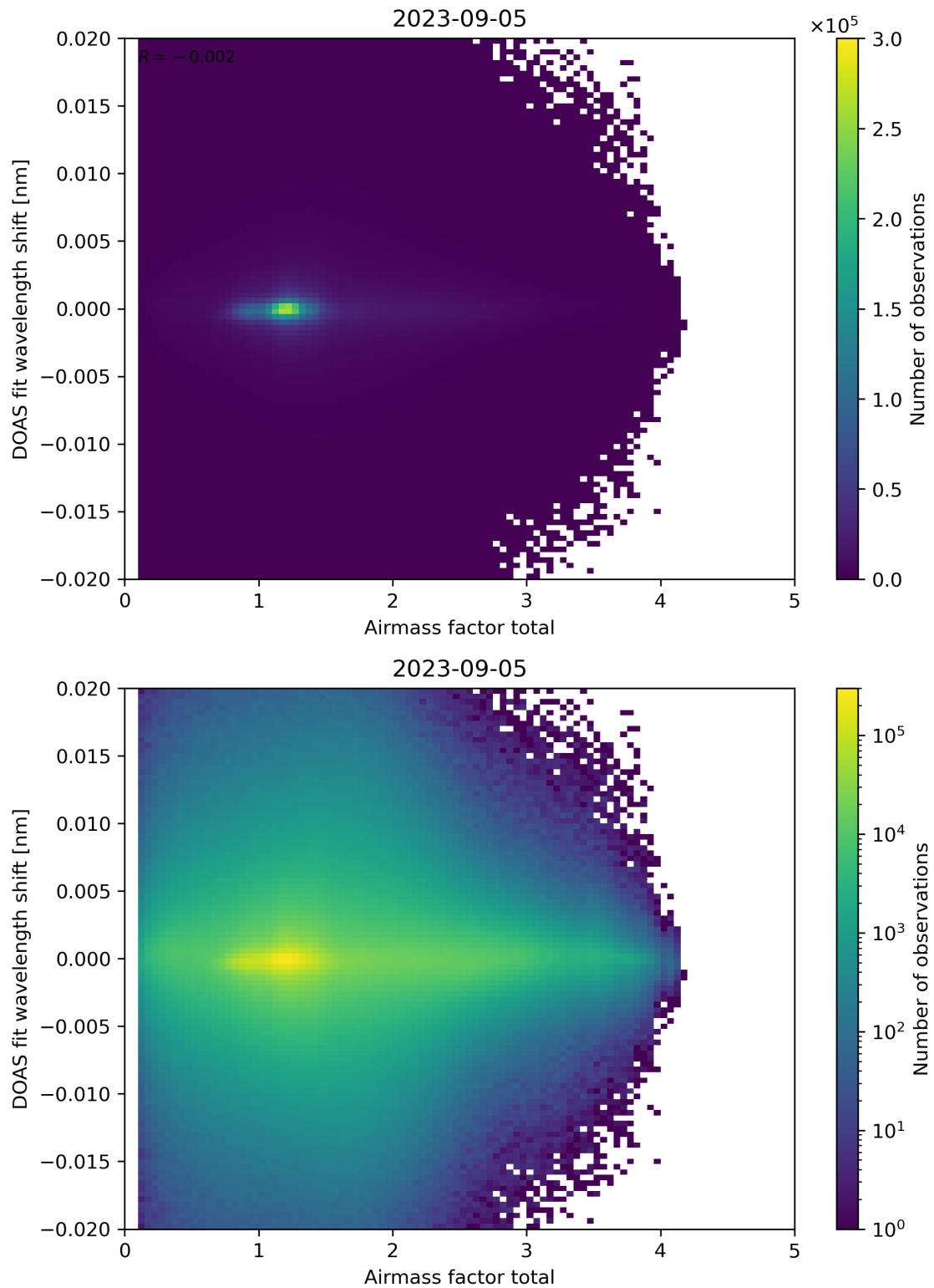
Figure 98: Scatter density plot of “Airmass factor total” against “DOAS fit wavelength shift” for 2023-09-05 to 2023-09-06.
