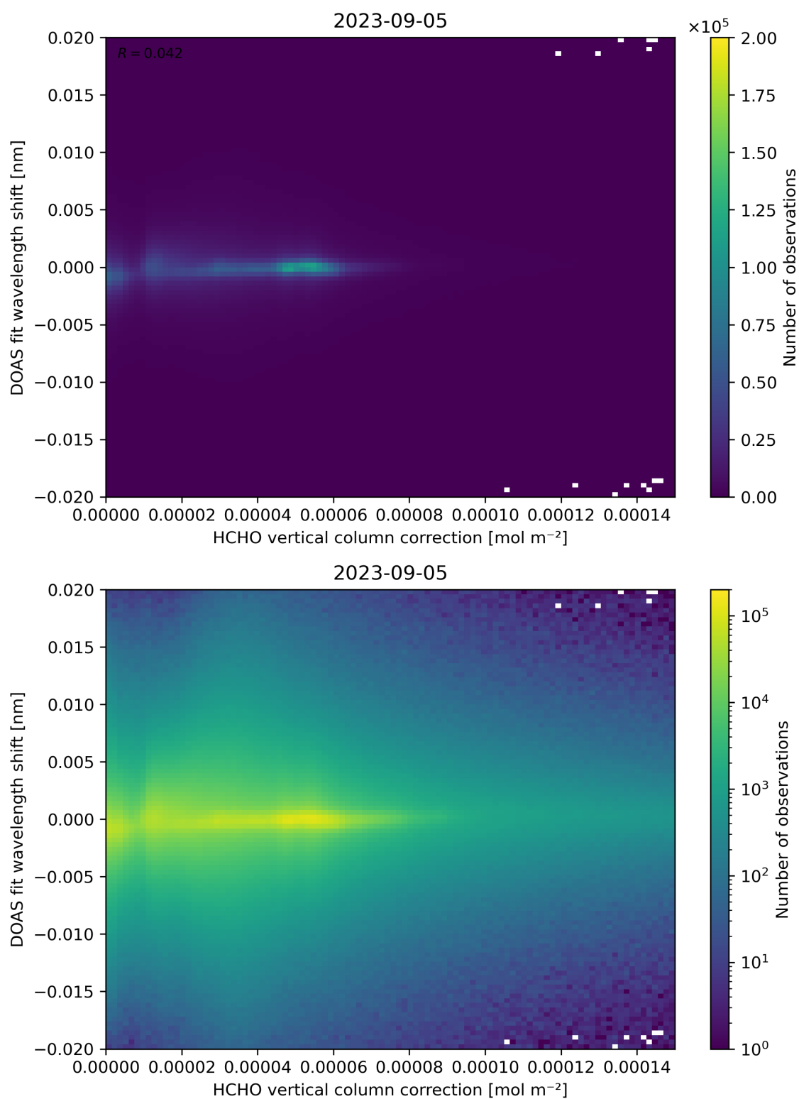
Figure 113: Scatter density plot of “HCHO vertical column correction” against “DOAS fit wavelength shift” for 2023-09-05 to 2023-09-06.
