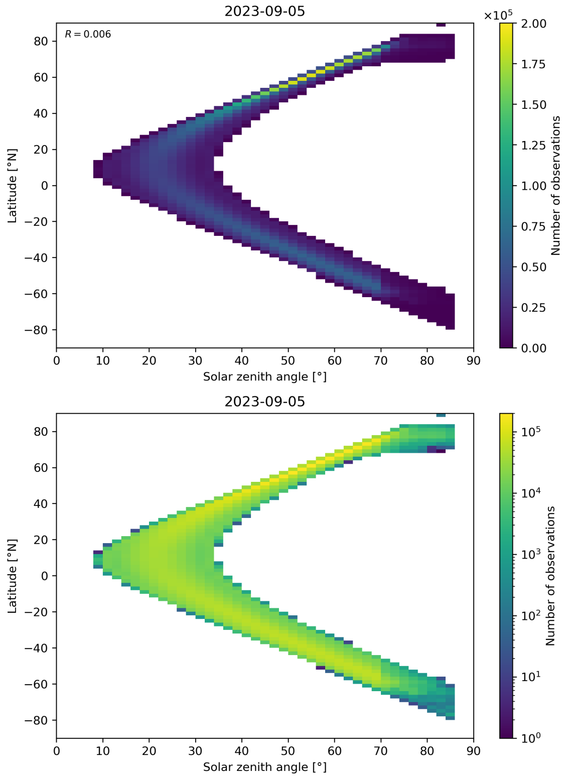
Figure 181: Scatter density plot of “Solar zenith angle” against “Latitude” for 2023-09-05 to 2023-09-06.
