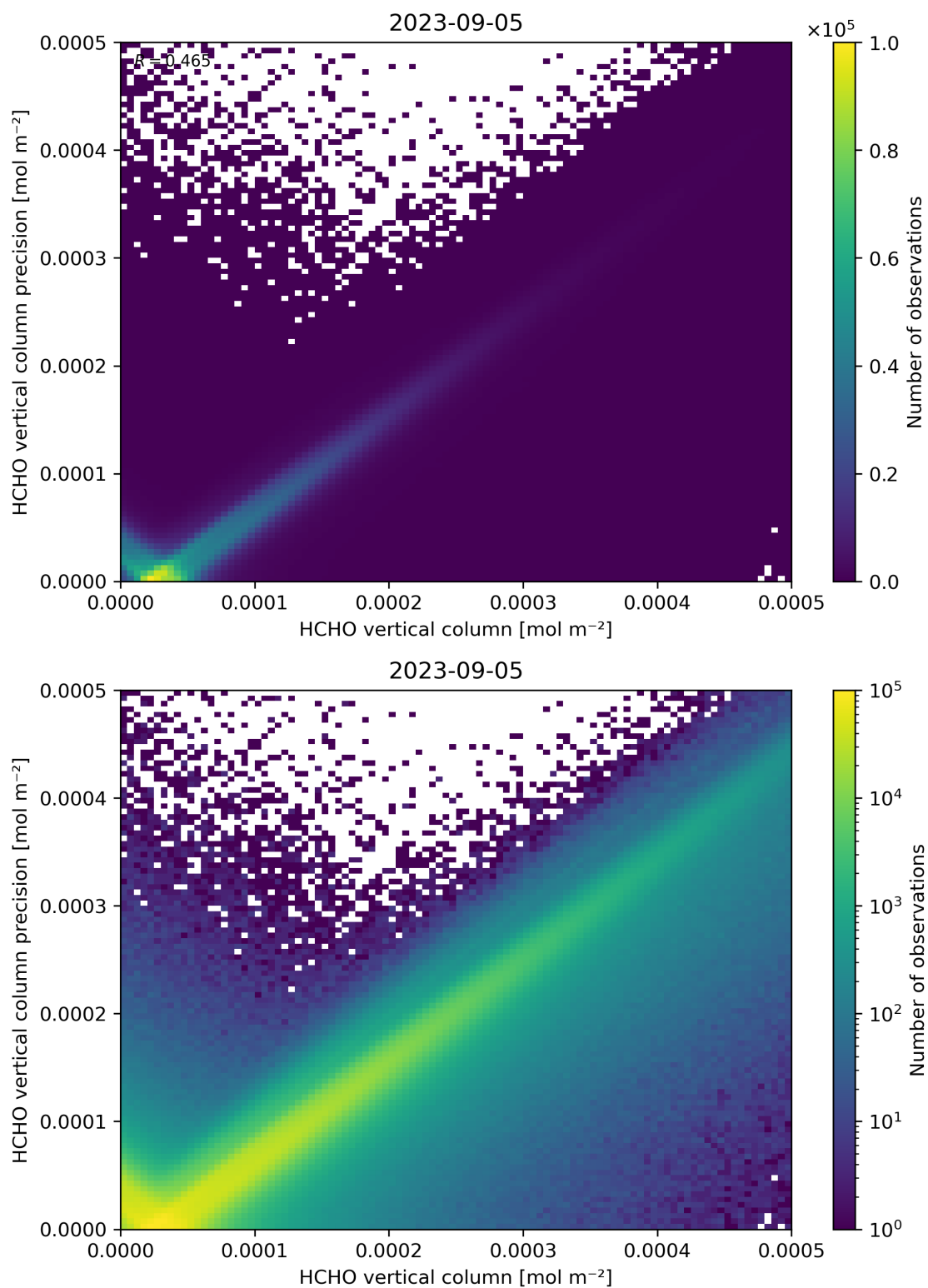
Figure 134: Scatter density plot of “HCHO vertical column” against “HCHO vertical column precision” for 2023-09-05 to 2023-09-06.
