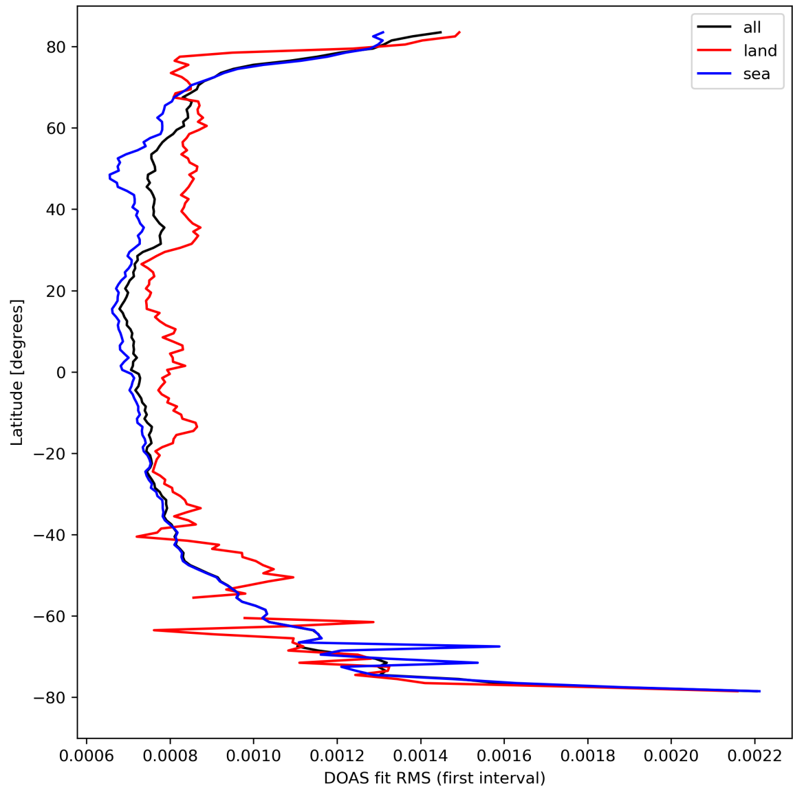
Figure 32: Zonal average of “DOAS fit RMS (first interval)” for 2023-09-05 to 2023-09-06.
