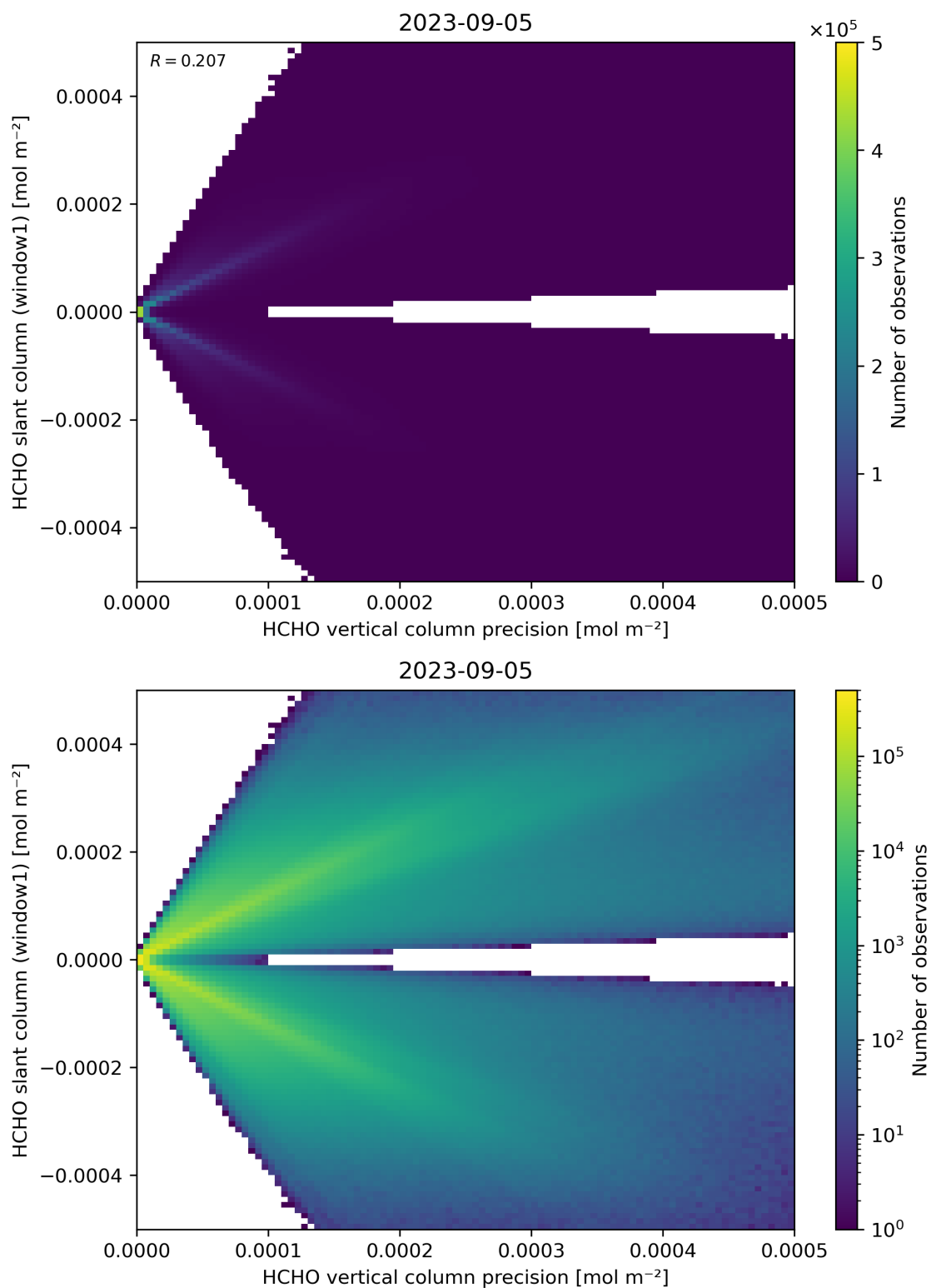
Figure 142: Scatter density plot of “HCHO vertical column precision” against “HCHO slant column (window1)” for 2023-09-05 to 2023-09-06.
