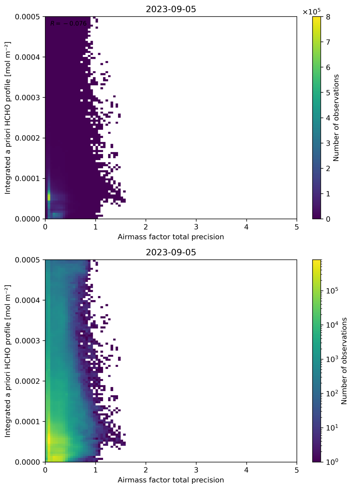
Figure 111: Scatter density plot of “Airmass factor total precision” against “Integrated a priori HCHO profile” for 2023-09-05 to 2023-09-06.
