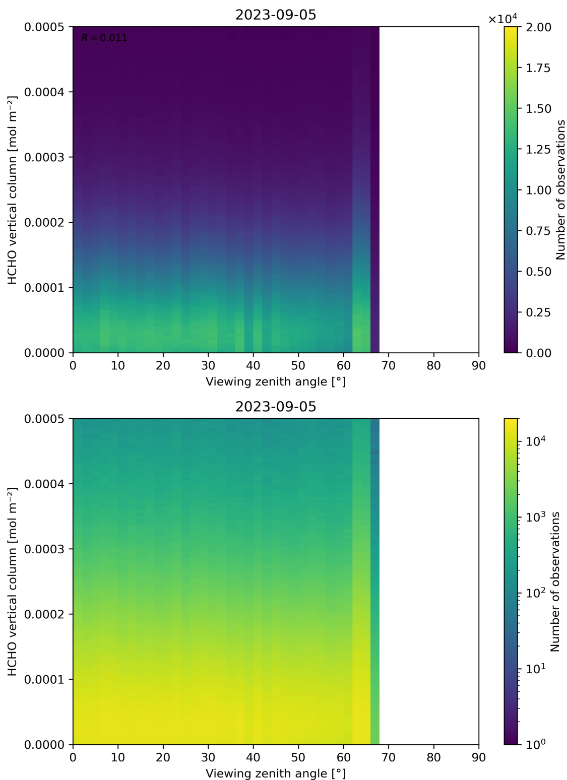
Figure 192: Scatter density plot of “Viewing zenith angle” against “HCHO vertical column” for 2023-09-05 to 2023-09-06.
