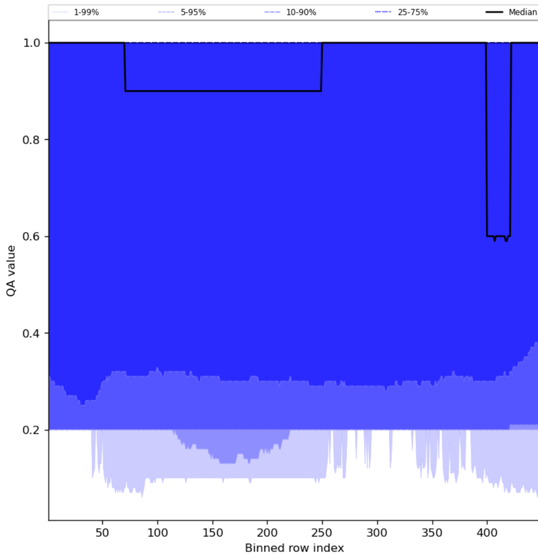
Figure 48: Along track statistics of “QA value” for 2023-09-05 to 2023-09-06
