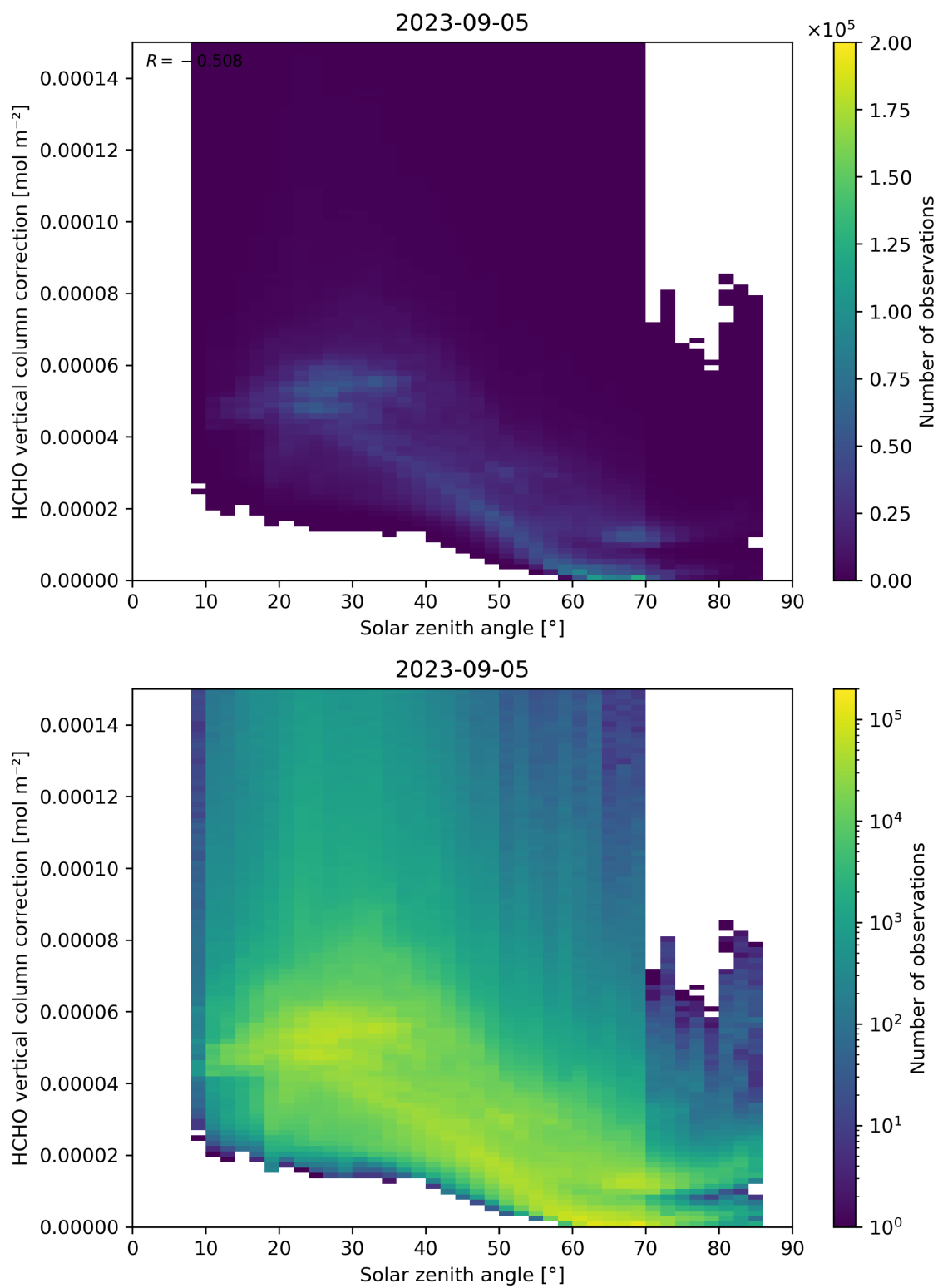
Figure 178: Scatter density plot of “Solar zenith angle” against “HCHO vertical column correction” for 2023-09-05 to 2023-09-06.
