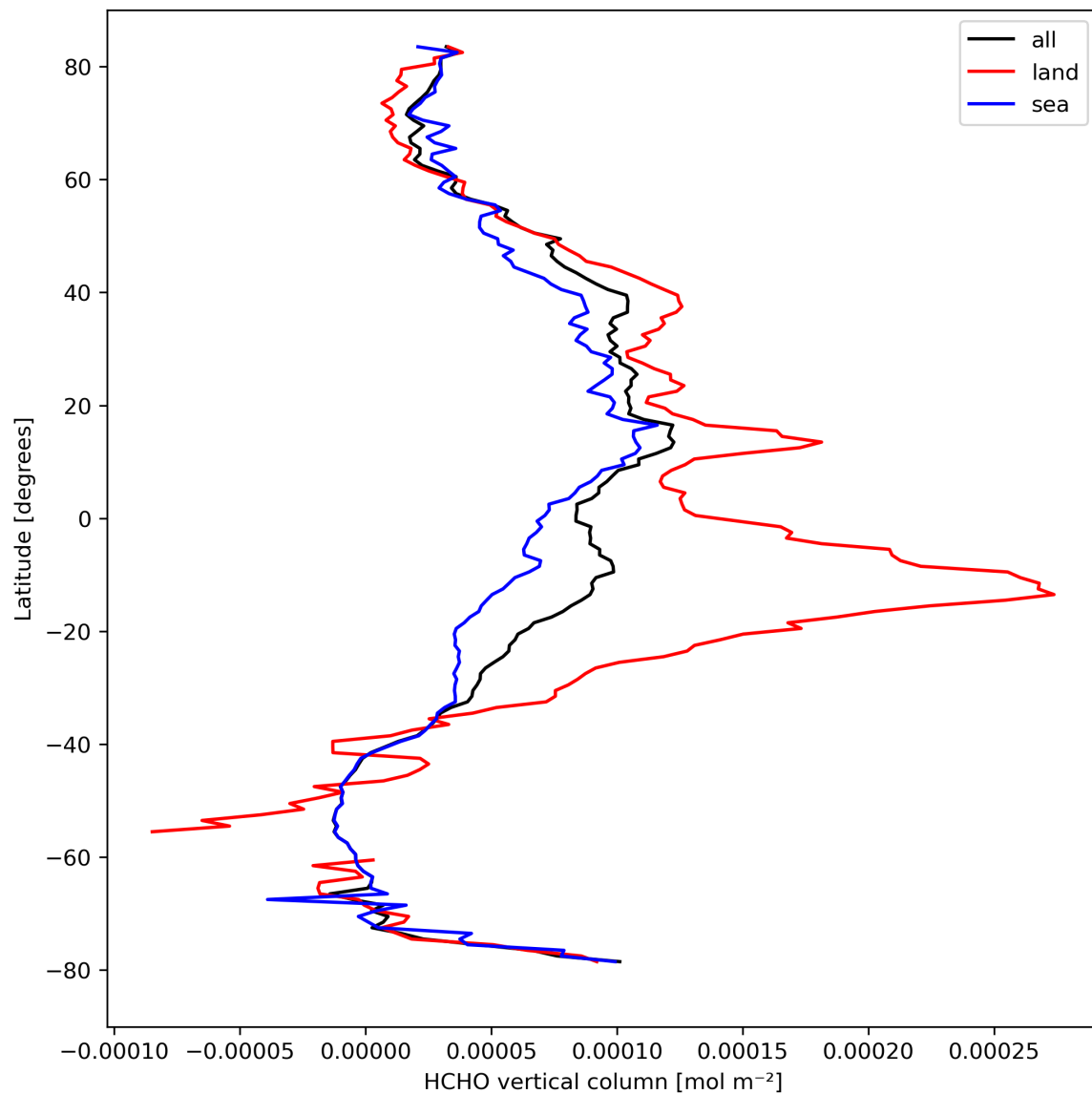
Figure 21: Zonal average of “HCHO vertical column” for 2023-09-05 to 2023-09-06.
