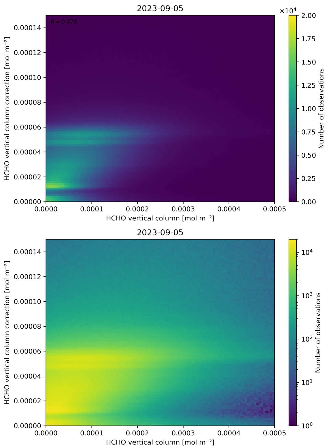
Figure 133: Scatter density plot of “HCHO vertical column” against “HCHO vertical column correction” for 2023-09-05 to 2023-09-06.
