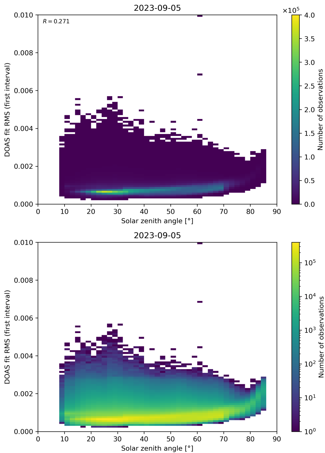
Figure 167: Scatter density plot of “Solar zenith angle” against “DOAS fit RMS (first interval)” for 2023-09-05 to 2023-09-06.
