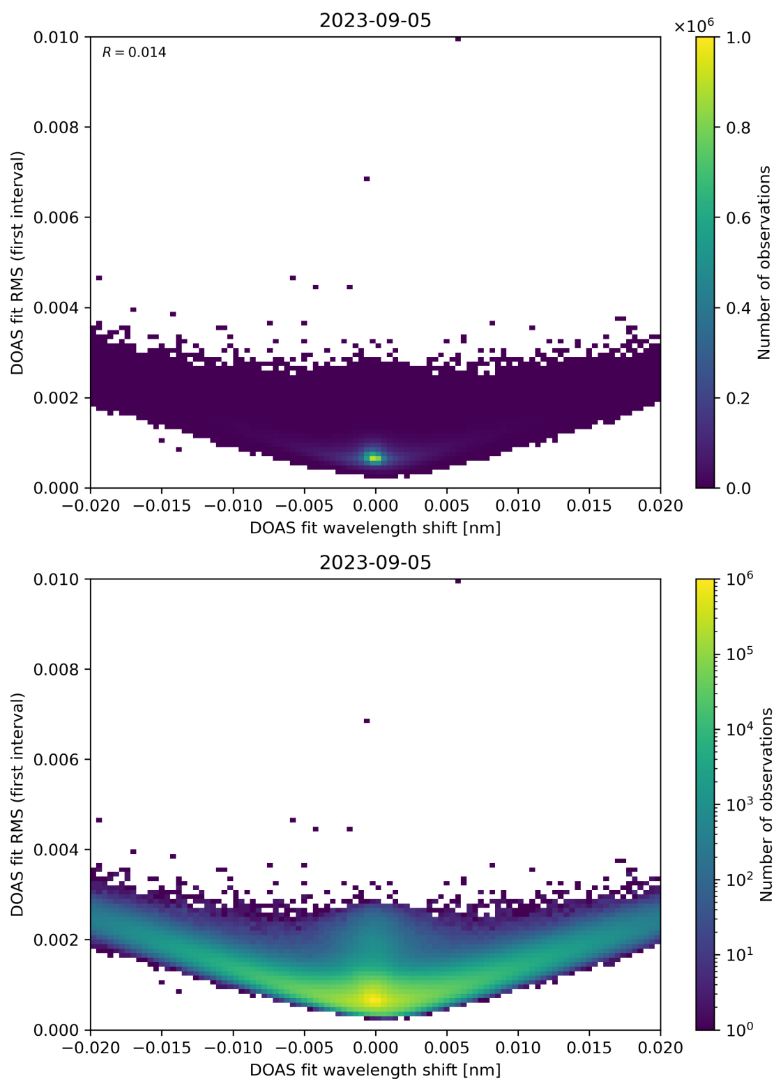
Figure 64: Scatter density plot of “DOAS fit wavelength shift” against “DOAS fit RMS (first interval)” for 2023-09-05 to 2023-09-06.
