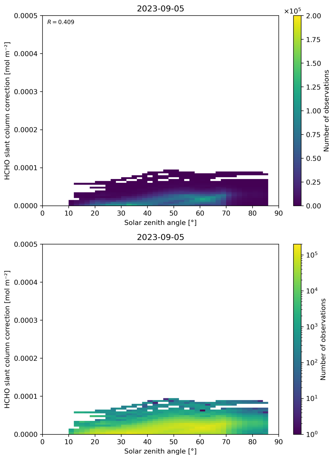
Figure 172: Scatter density plot of “Solar zenith angle” against “HCHO slant column correction” for 2023-09-05 to 2023-09-06.
