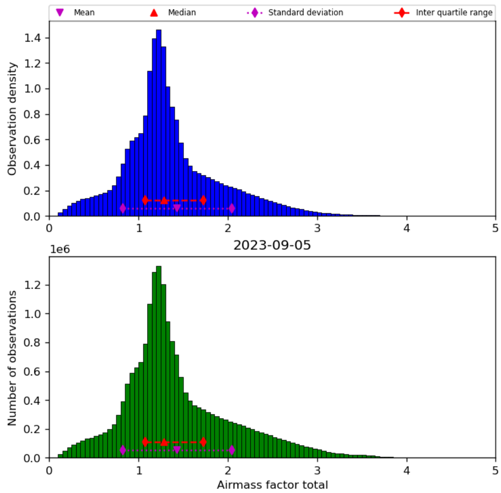
Figure 40: Histogram of “Airmass factor total” for 2023-09-05 to 2023-09-06
