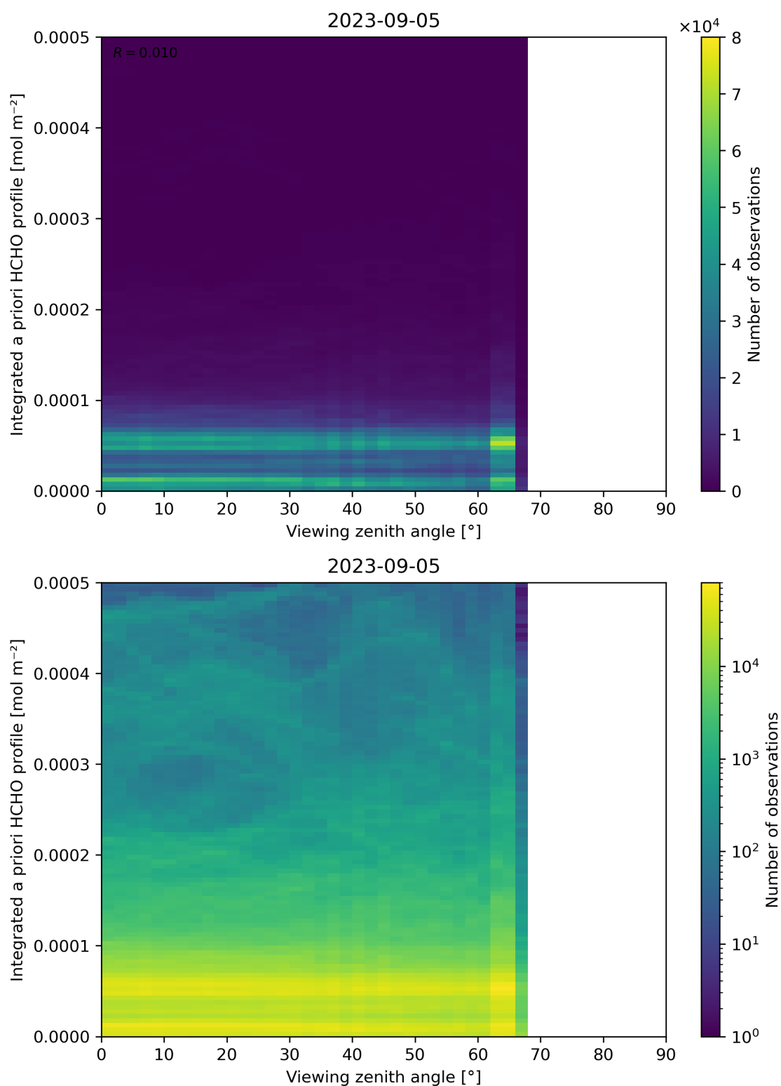
Figure 195: Scatter density plot of “Viewing zenith angle” against “Integrated a priori HCHO profile” for 2023-09-05 to 2023-09-06.
