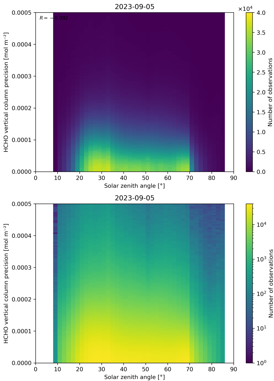
Figure 179: Scatter density plot of “Solar zenith angle” against “HCHO vertical column precision” for 2023-09-05 to 2023-09-06.
