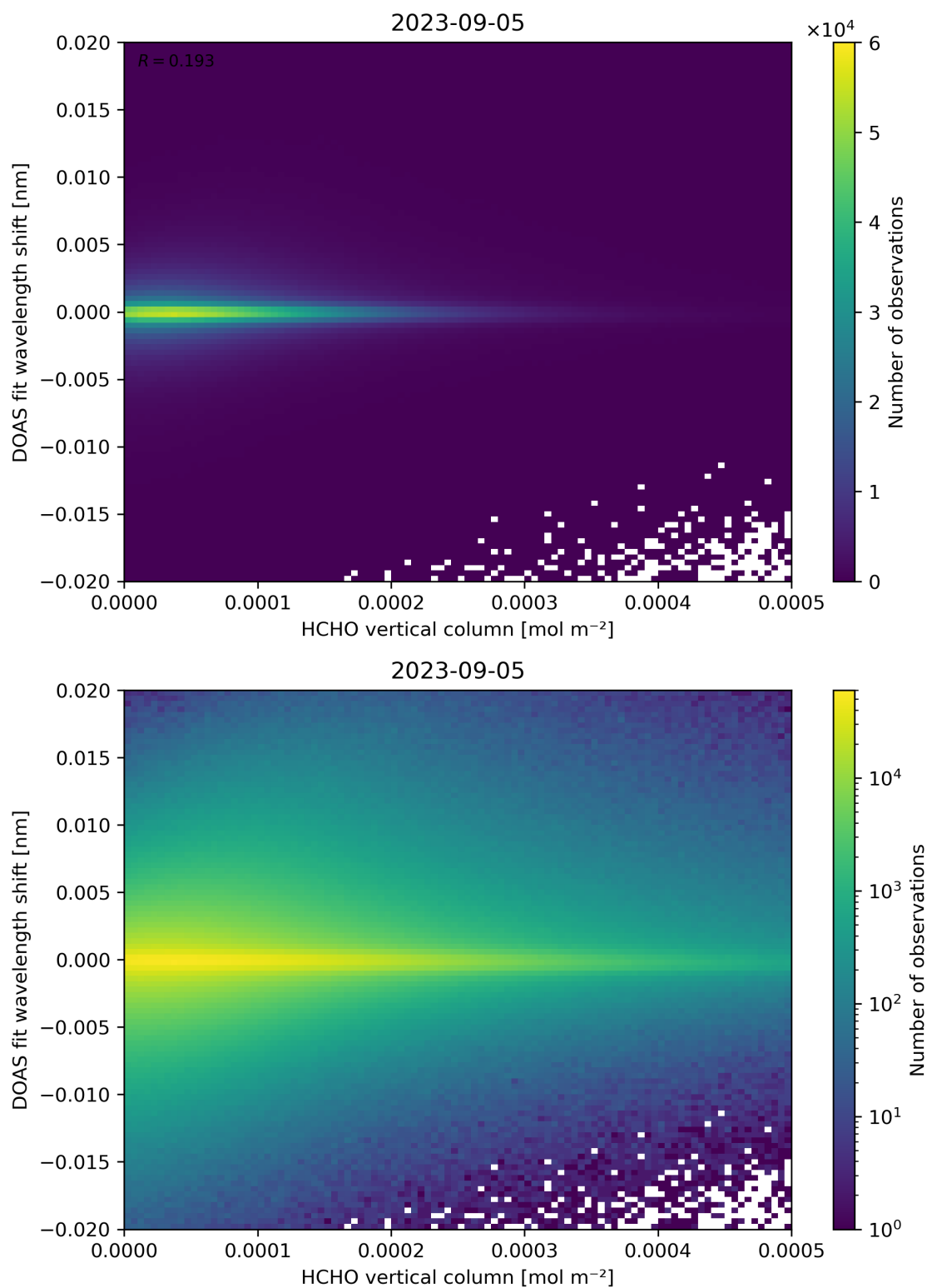
Figure 124: Scatter density plot of “HCHO vertical column” against “DOAS fit wavelength shift” for 2023-09-05 to 2023-09-06.
