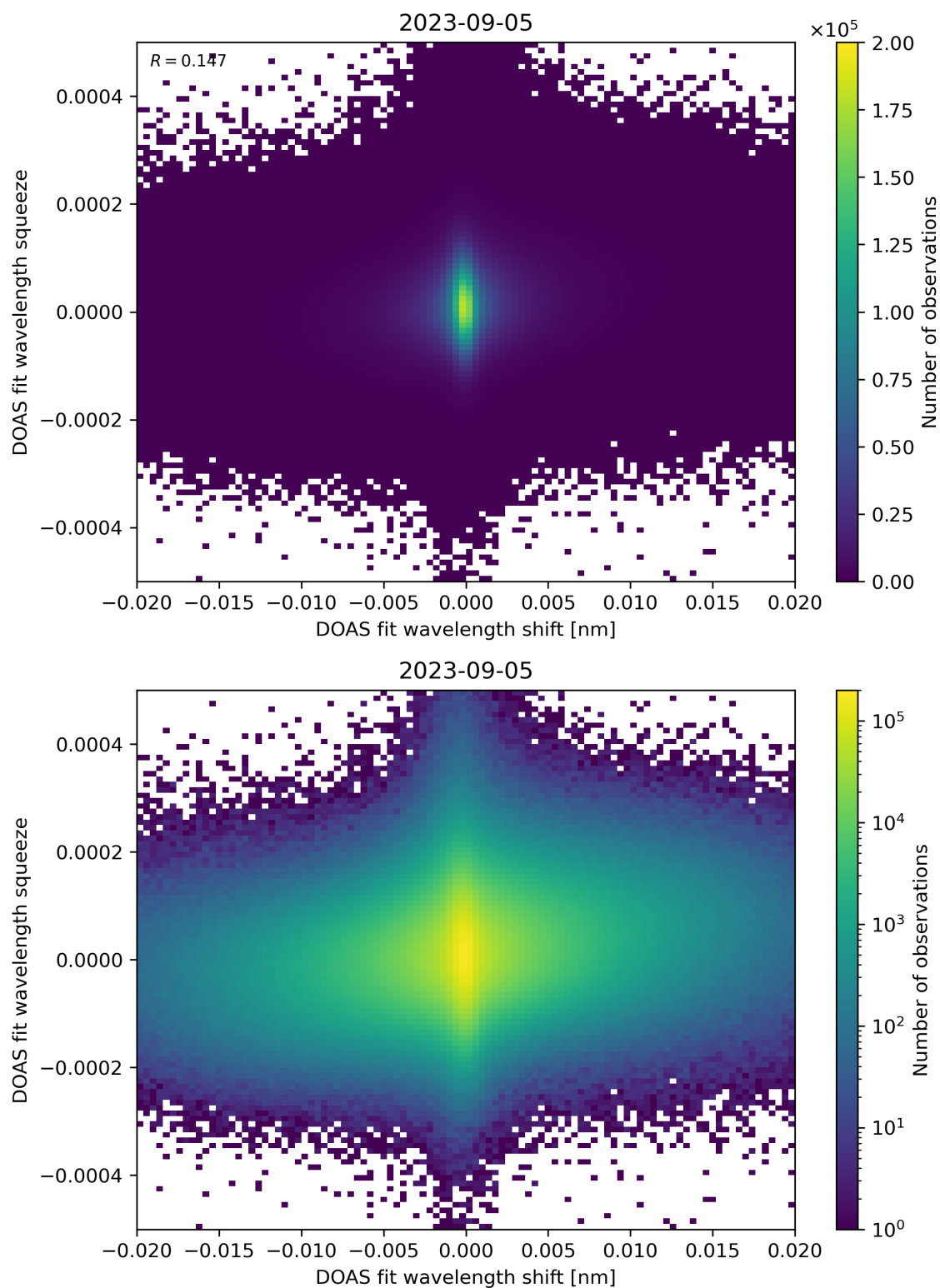
Figure 65: Scatter density plot of “DOAS fit wavelength shift” against “DOAS fit wavelength squeeze” for 2023-09-05 to 2023-09-06.
