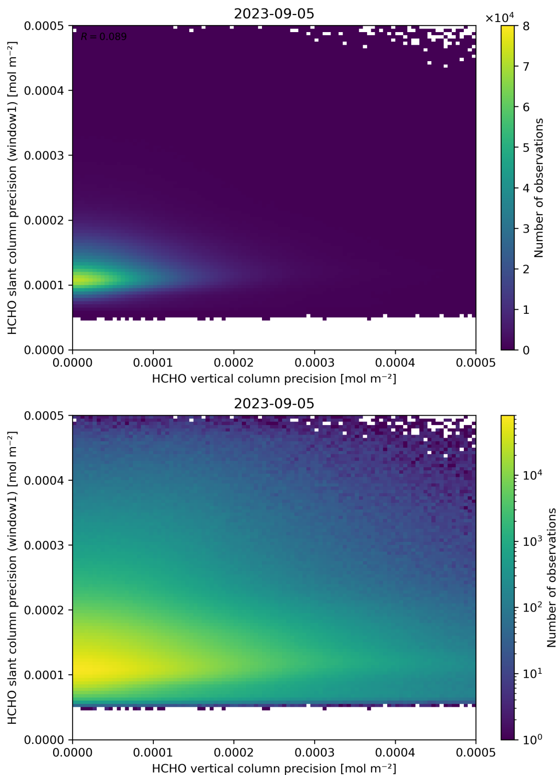
Figure 143: Scatter density plot of “HCHO vertical column precision” against “HCHO slant column precision (window1)” for 2023-09-05 to 2023-09-06.
