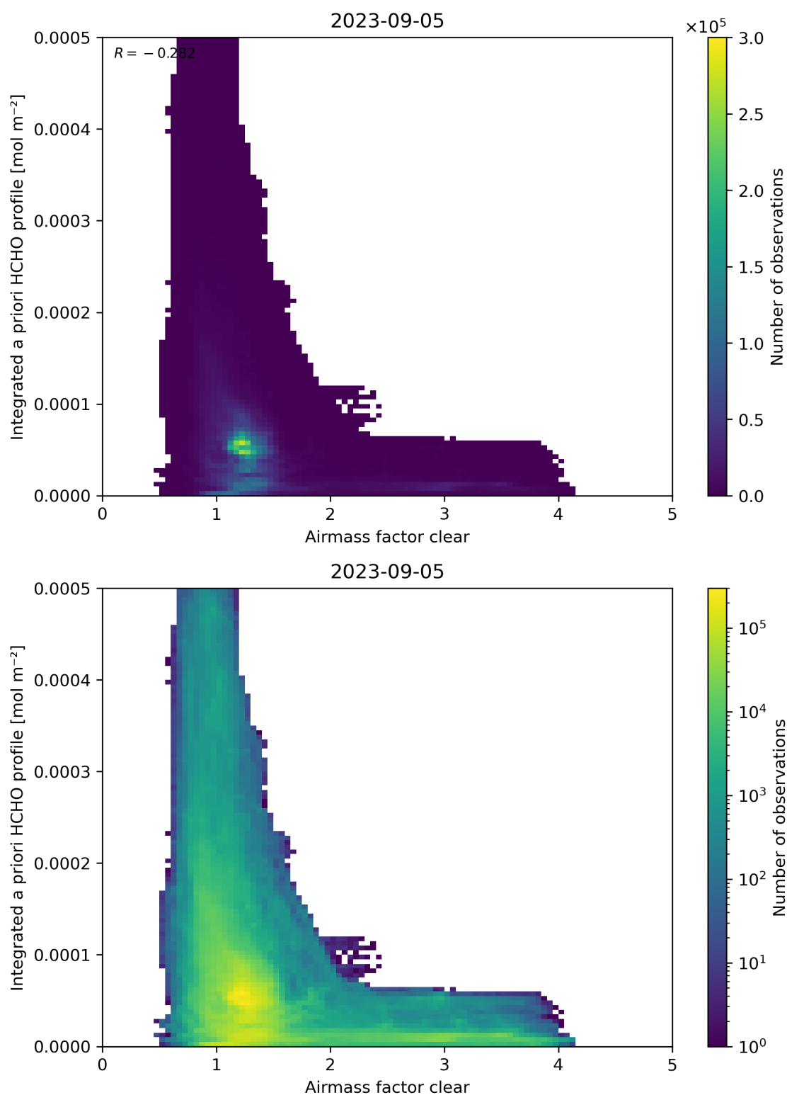
Figure 76: Scatter density plot of “Airmass factor clear” against “Integrated a priori HCHO profile” for 2023-09-05 to 2023-09-06.
