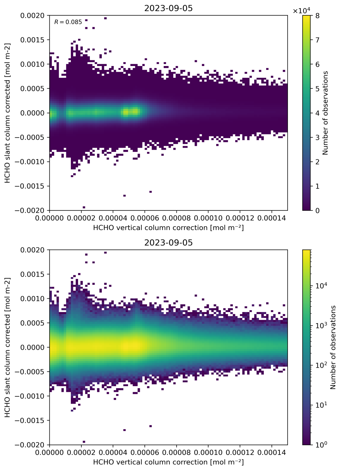
Figure 116: Scatter density plot of “HCHO vertical column correction” against “HCHO slant column corrected” for 2023-09-05 to 2023-09-06.
