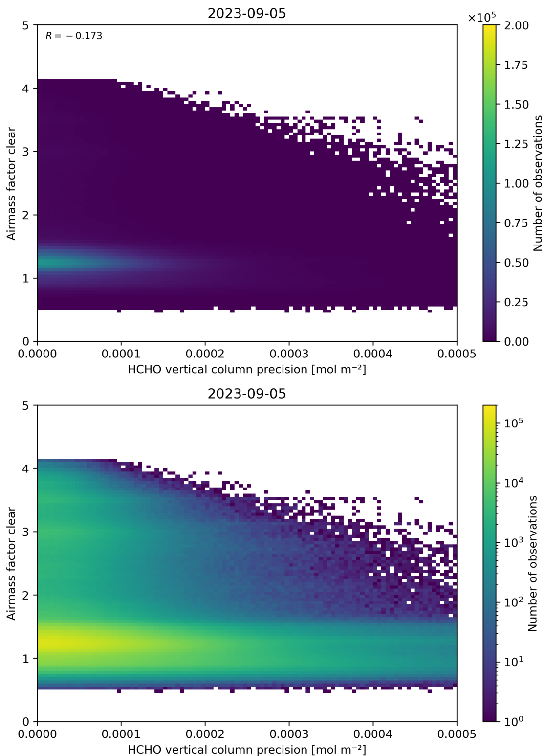
Figure 139: Scatter density plot of “HCHO vertical column precision” against “Airmass factor clear” for 2023-09-05 to 2023-09-06.
