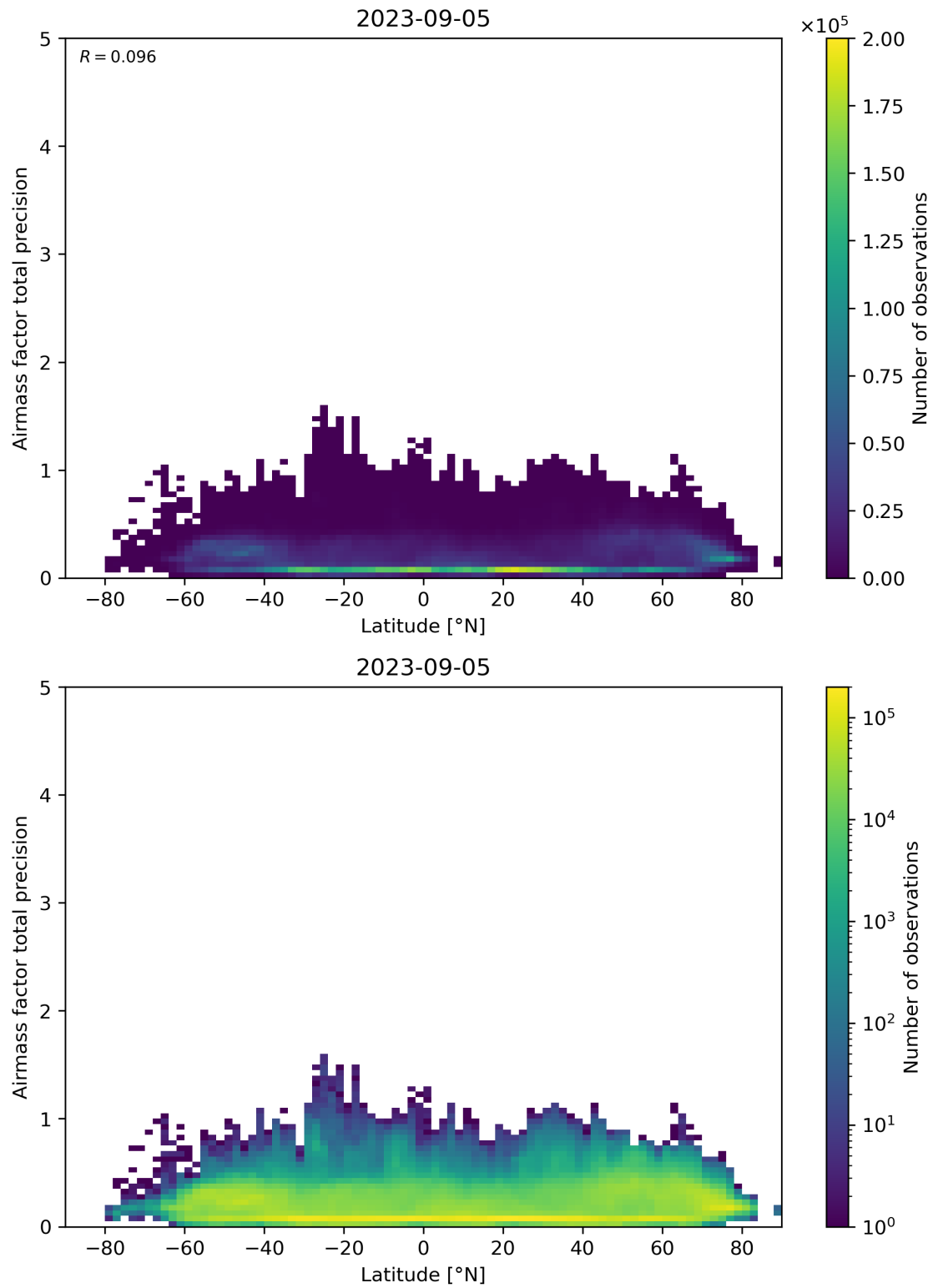
Figure 162: Scatter density plot of “Latitude” against “Airmass factor total precision” for 2023-09-05 to 2023-09-06.
