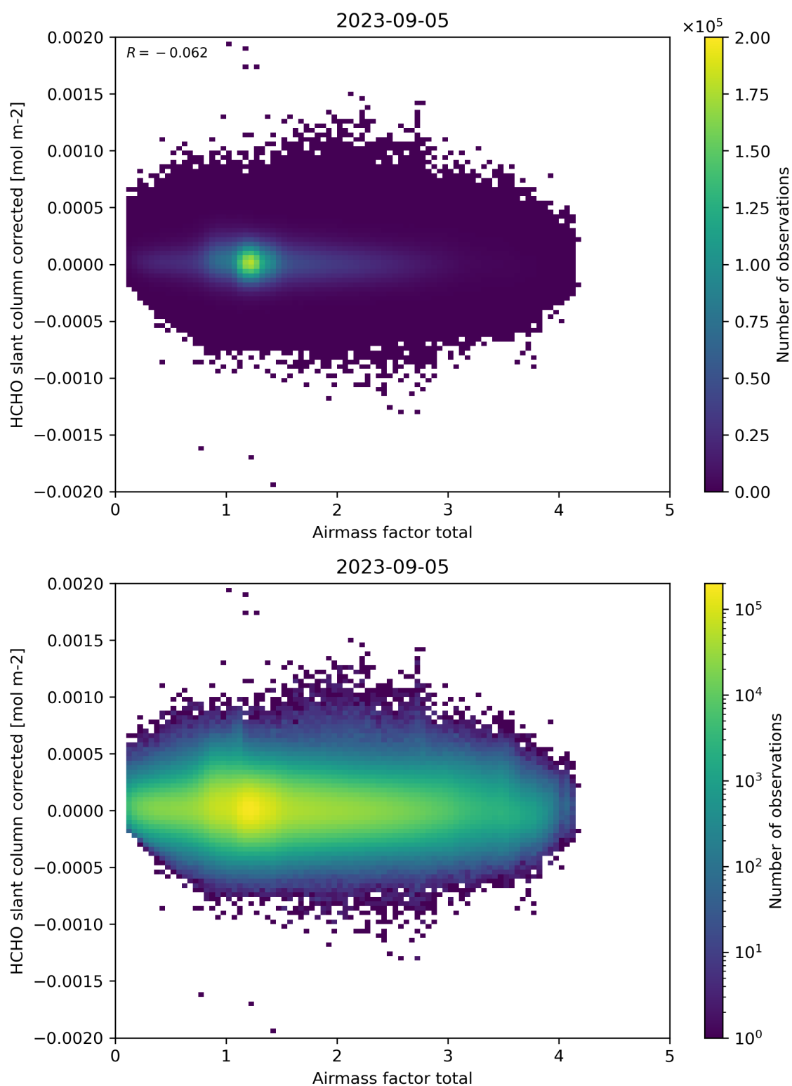
Figure 101: Scatter density plot of “Airmass factor total” against “HCHO slant column corrected” for 2023-09-05 to 2023-09-06.
