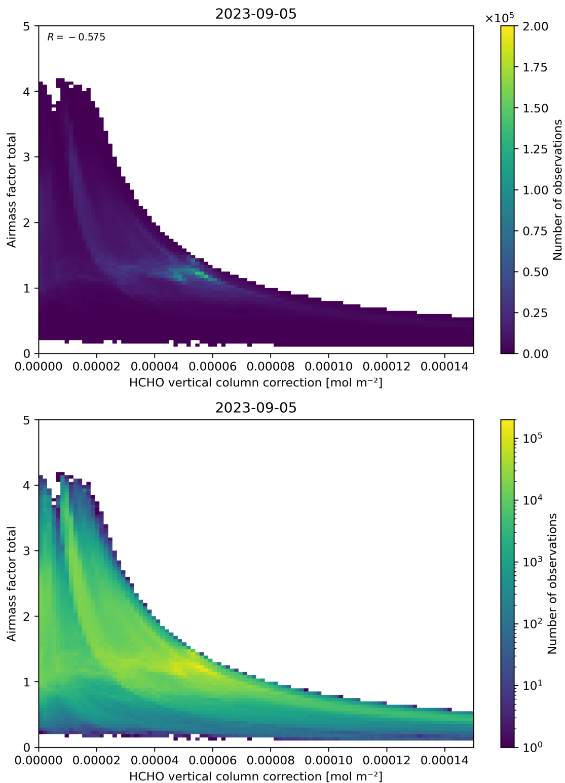
Figure 120: Scatter density plot of “HCHO vertical column correction” against “Airmass factor total” for 2023-09-05 to 2023-09-06.
