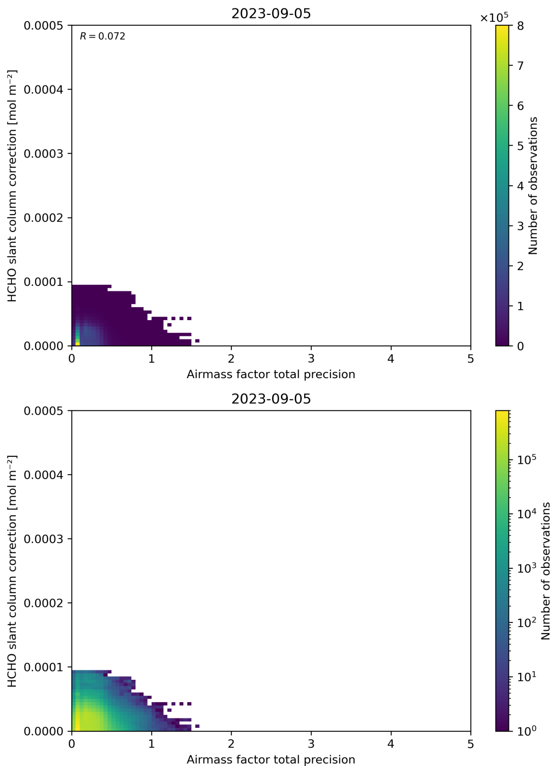
Figure 110: Scatter density plot of “Airmass factor total precision” against “HCHO slant column correction” for 2023-09-05 to 2023-09-06.
