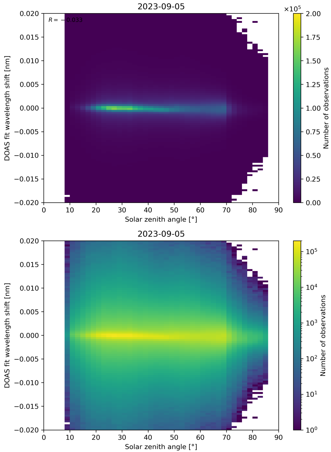
Figure 168: Scatter density plot of “Solar zenith angle” against “DOAS fit wavelength shift” for 2023-09-05 to 2023-09-06.
