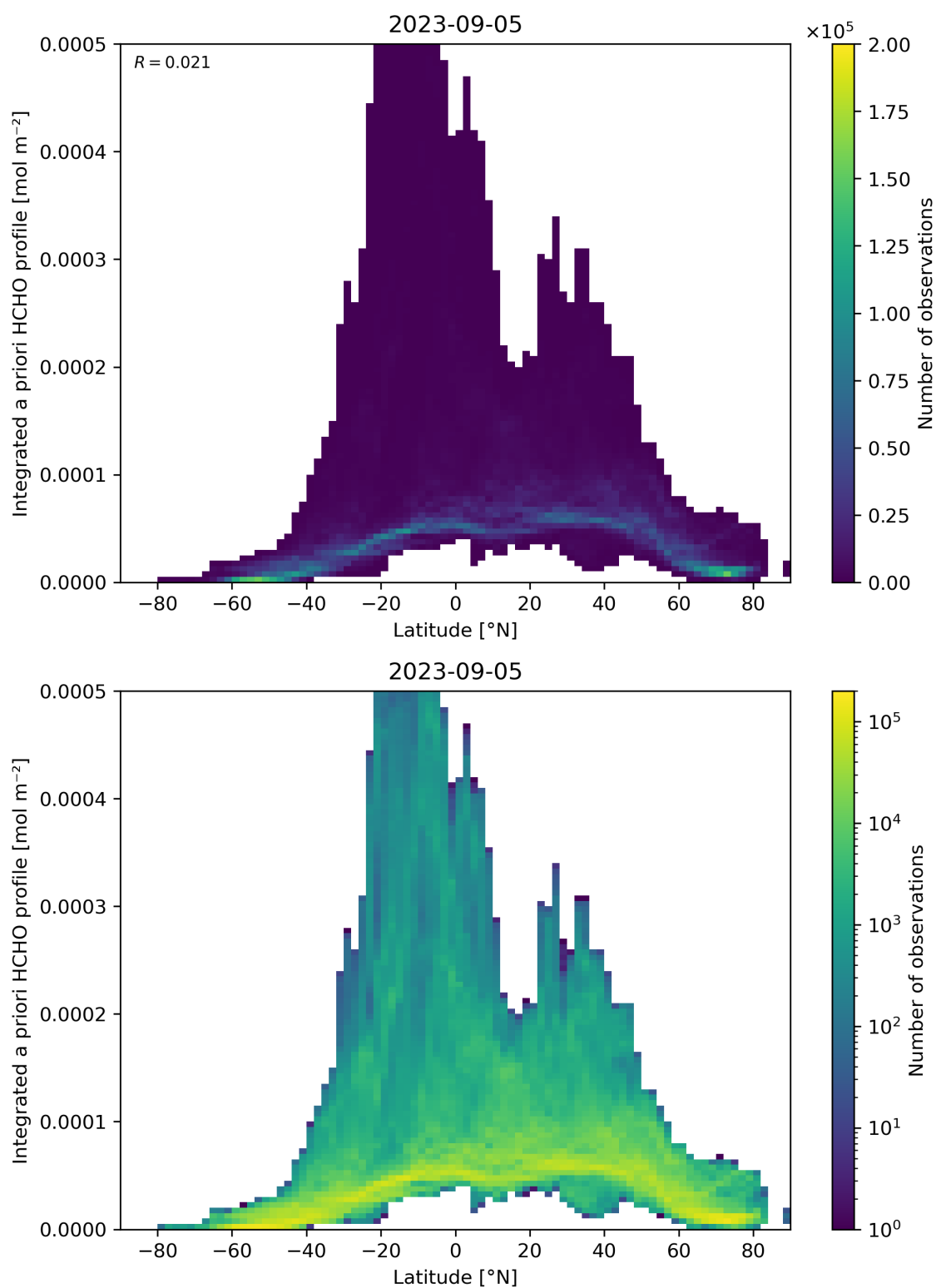
Figure 166: Scatter density plot of “Latitude” against “Integrated a priori HCHO profile” for 2023-09-05 to 2023-09-06.
