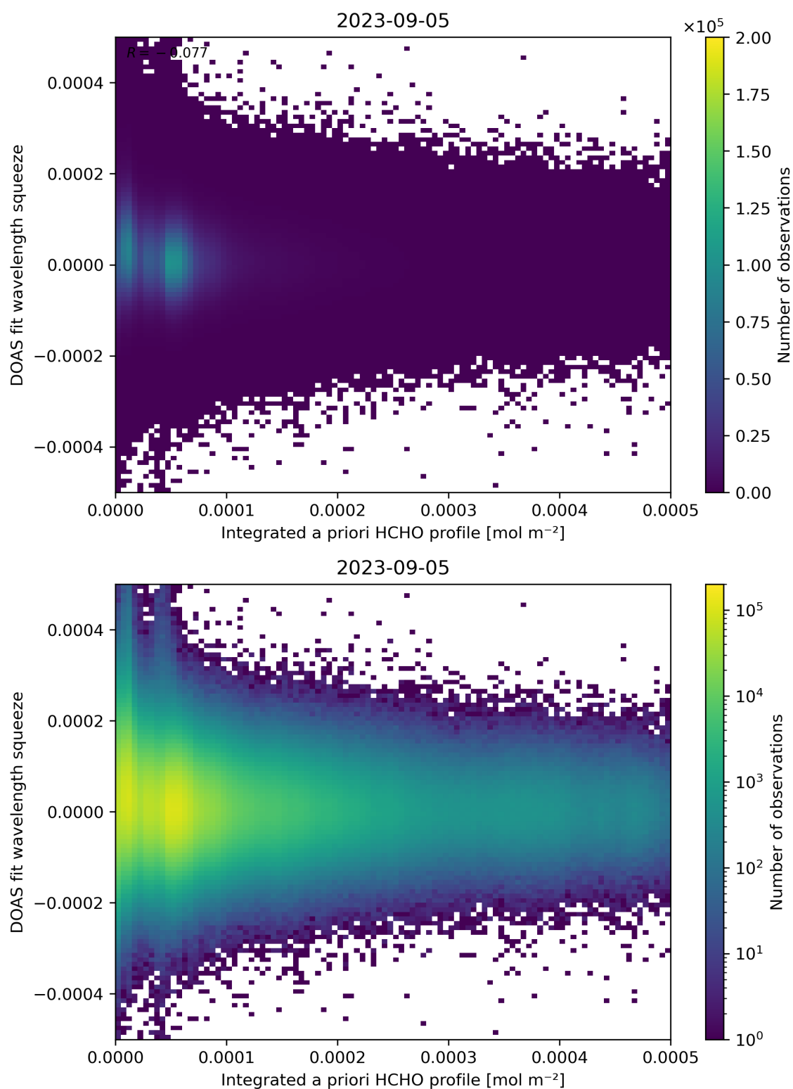
Figure 150: Scatter density plot of “Integrated a priori HCHO profile” against “DOAS fit wavelength squeeze” for 2023-09-05 to 2023-09-06.
