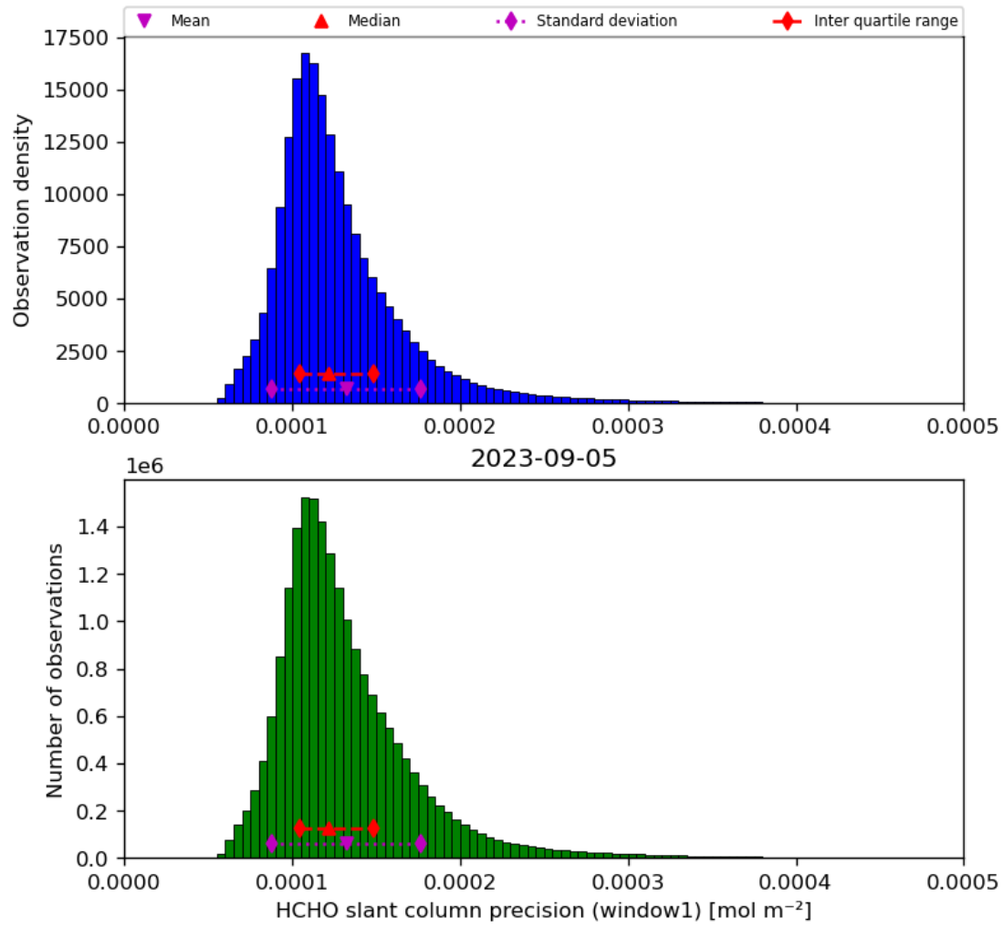
Figure 39: Histogram of “HCHO slant column precision (window1)” for 2023-09-05 to 2023-09-06
