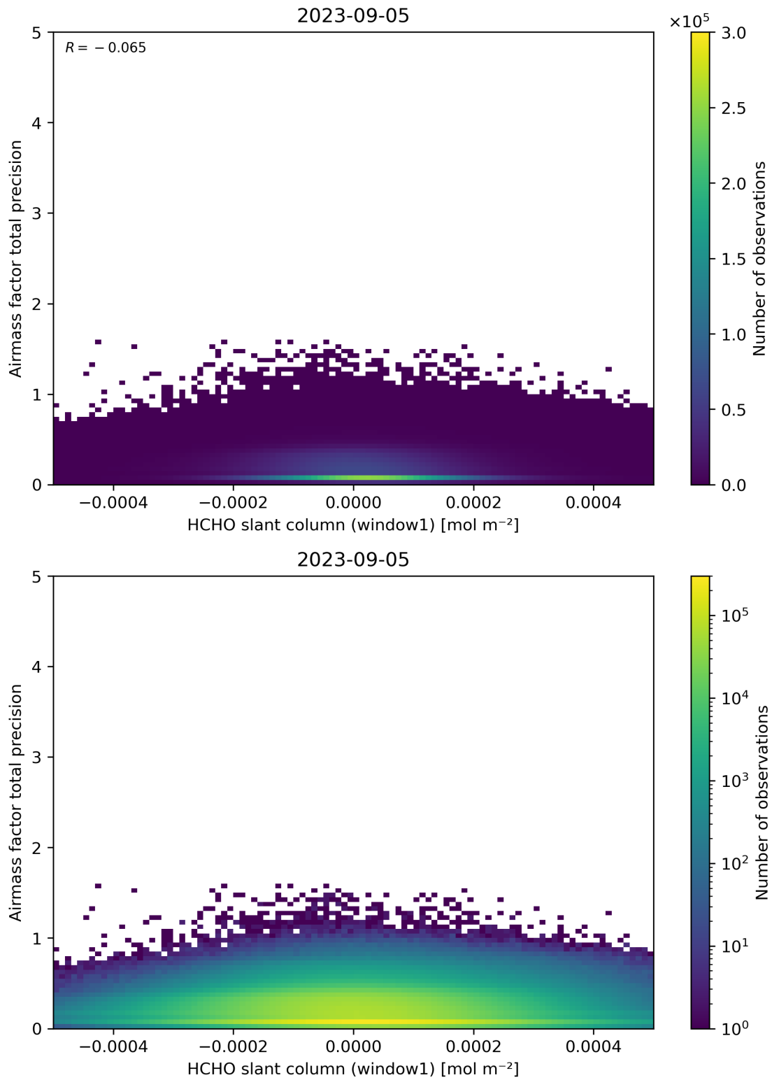
Figure 86: Scatter density plot of “HCHO slant column (window1)” against “Airmass factor total precision” for 2023-09-05 to 2023-09-06.
