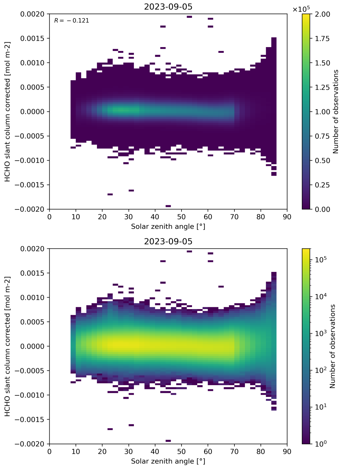
Figure 171: Scatter density plot of “Solar zenith angle” against “HCHO slant column corrected” for 2023-09-05 to 2023-09-06.
