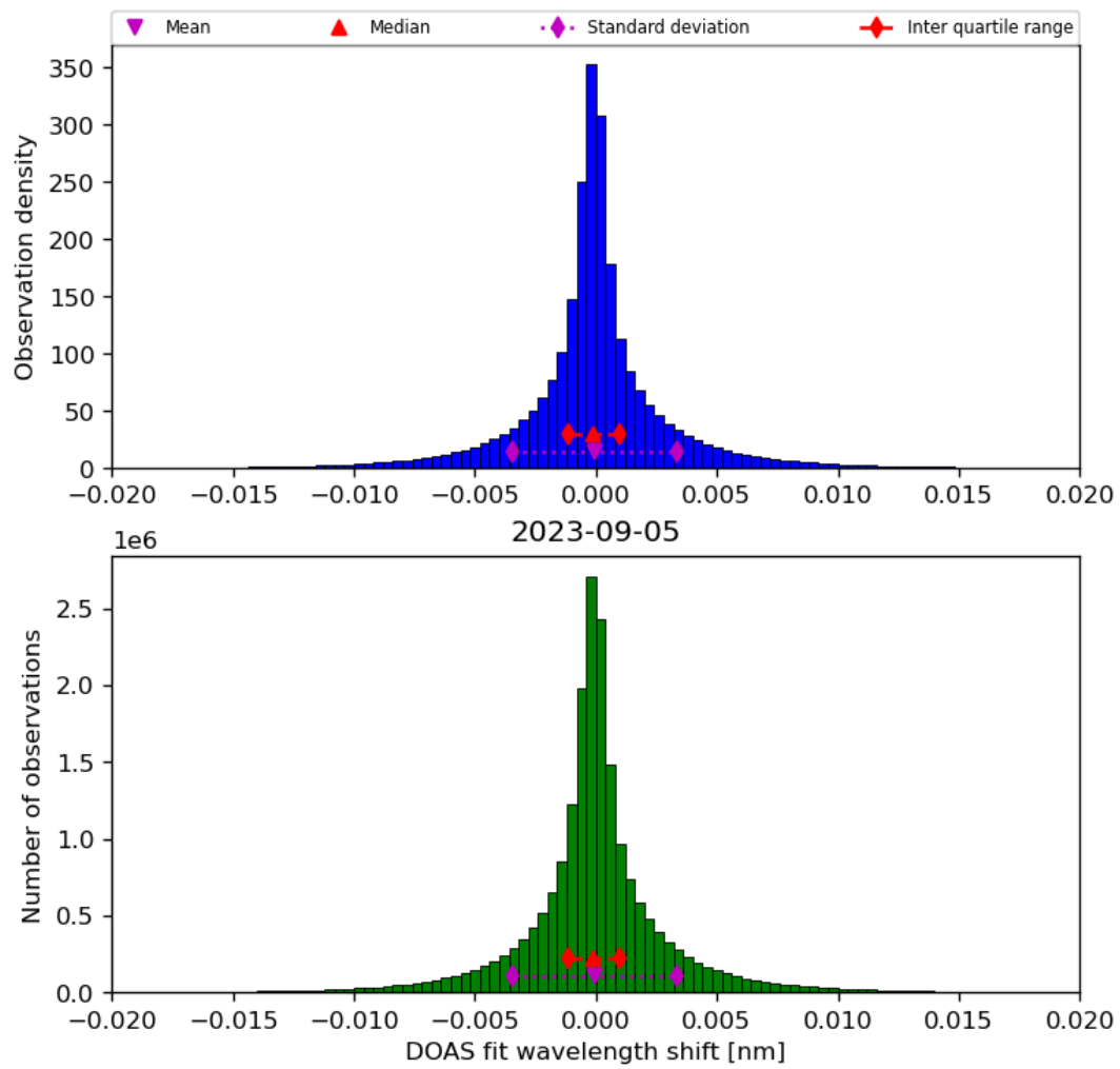
Figure 44: Histogram of “DOAS fit wavelength shift” for 2023-09-05 to 2023-09-06
