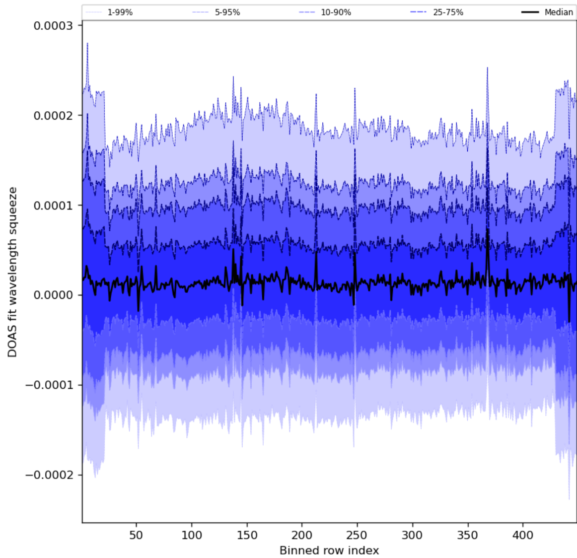
Figure 59: Along track statistics of “DOAS fit wavelength squeeze” for 2023-09-05 to 2023-09-06
