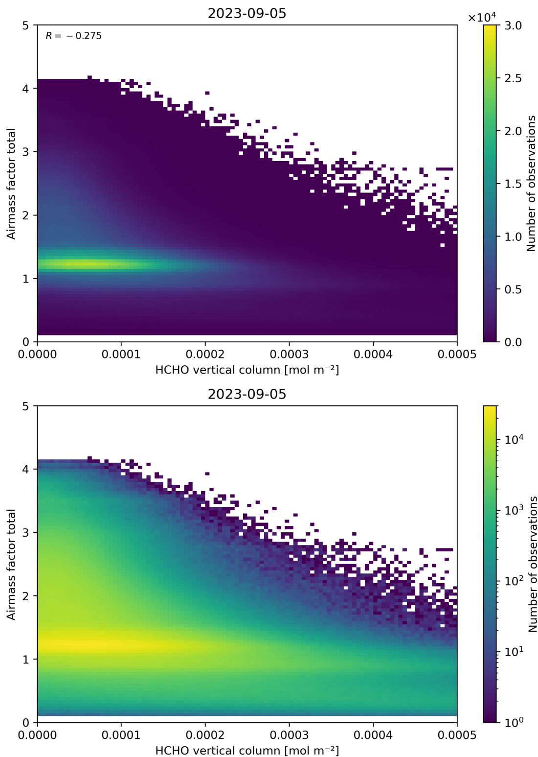
Figure 131: Scatter density plot of “HCHO vertical column” against “Airmass factor total” for 2023-09-05 to 2023-09-06.
