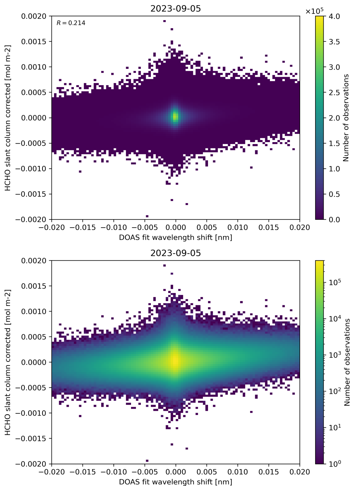
Figure 66: Scatter density plot of “DOAS fit wavelength shift” against “HCHO slant column corrected” for 2023-09-05 to 2023-09-06.
