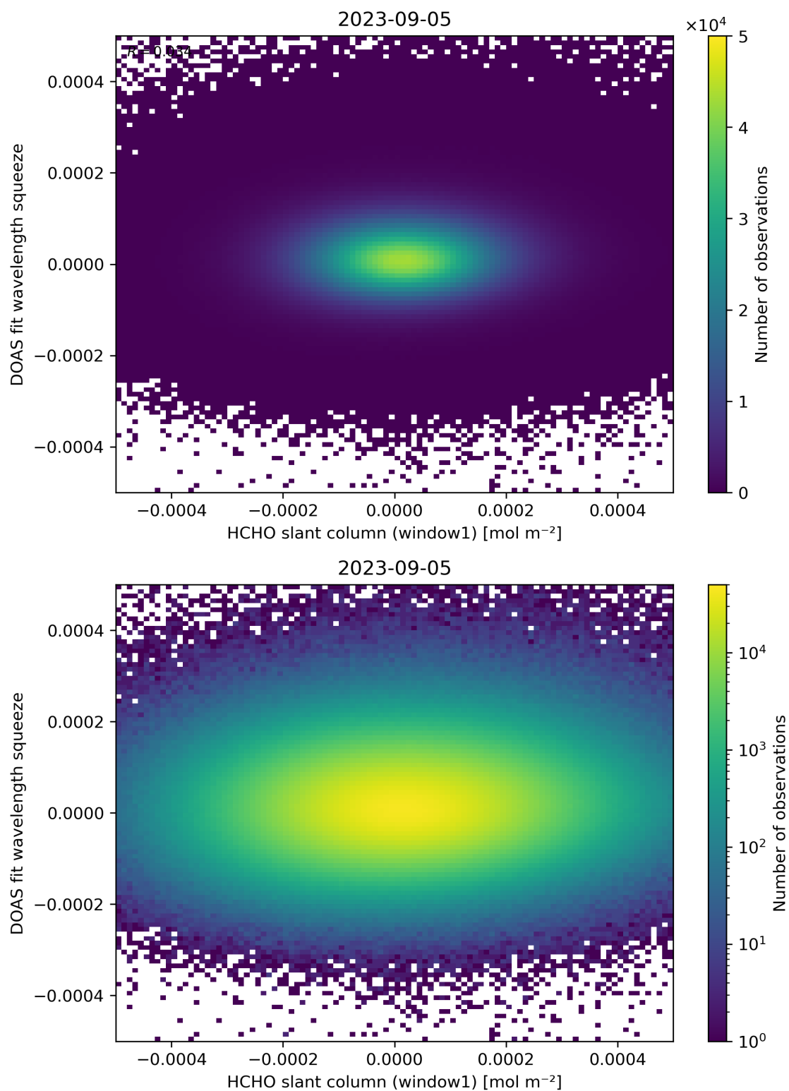
Figure 80: Scatter density plot of “HCHO slant column (window1)” against “DOAS fit wavelength squeeze” for 2023-09-05 to 2023-09-06.
