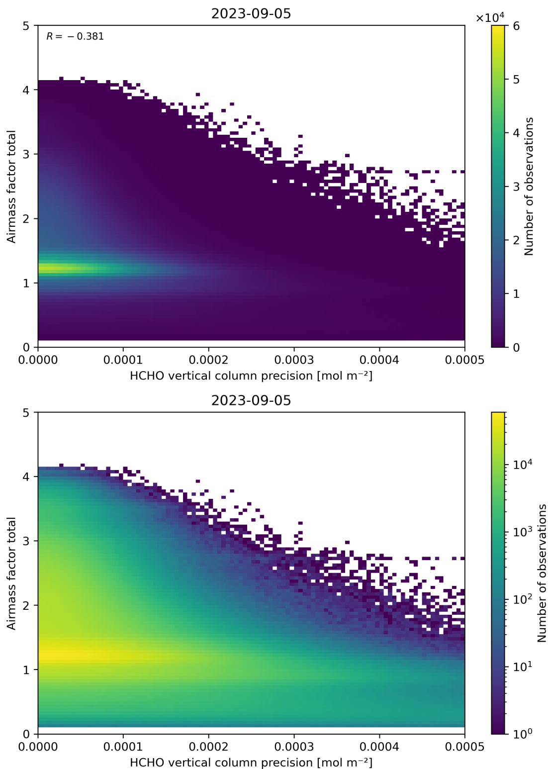
Figure 144: Scatter density plot of “HCHO vertical column precision” against “Airmass factor total” for 2023-09-05 to 2023-09-06.
