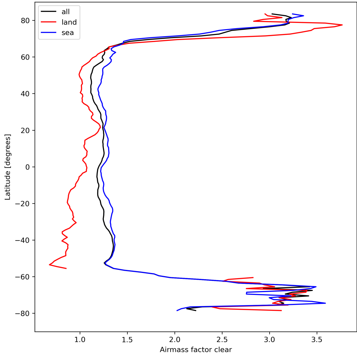
Figure 28: Zonal average of “Airmass factor clear” for 2023-09-05 to 2023-09-06.
