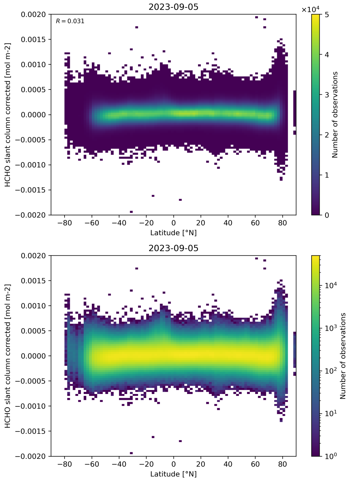
Figure 157: Scatter density plot of “Latitude” against “HCHO slant column corrected” for 2023-09-05 to 2023-09-06.
