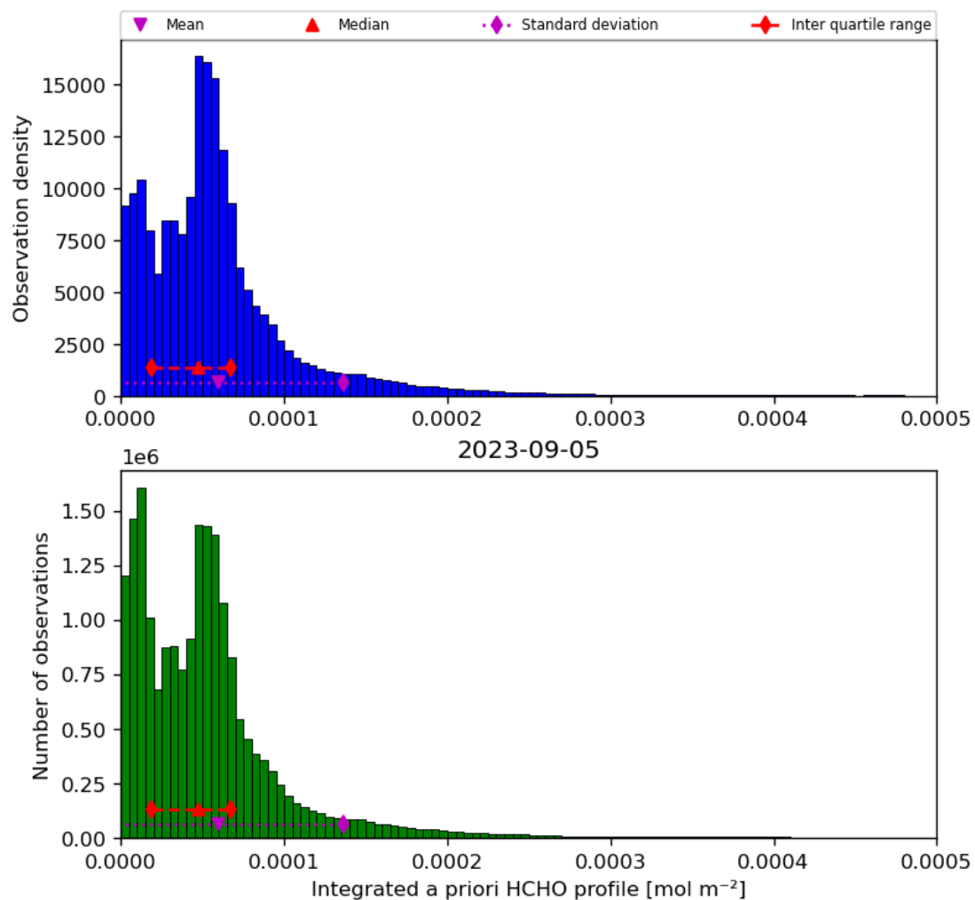
Figure 43: Histogram of “Integrated a priori HCHO profile” for 2023-09-05 to 2023-09-06
