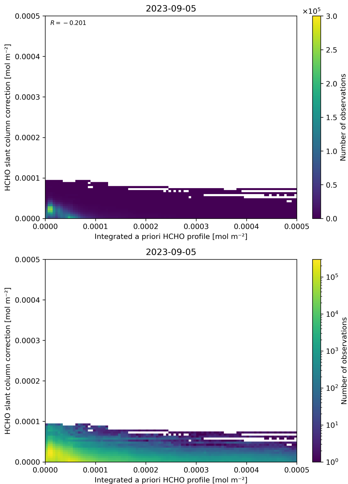
Figure 152: Scatter density plot of “Integrated a priori HCHO profile” against “HCHO slant column correction” for 2023-09-05 to 2023-09-06.
