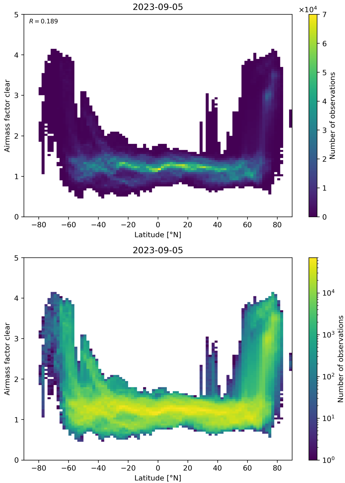
Figure 156: Scatter density plot of “Latitude” against “Airmass factor clear” for 2023-09-05 to 2023-09-06.
