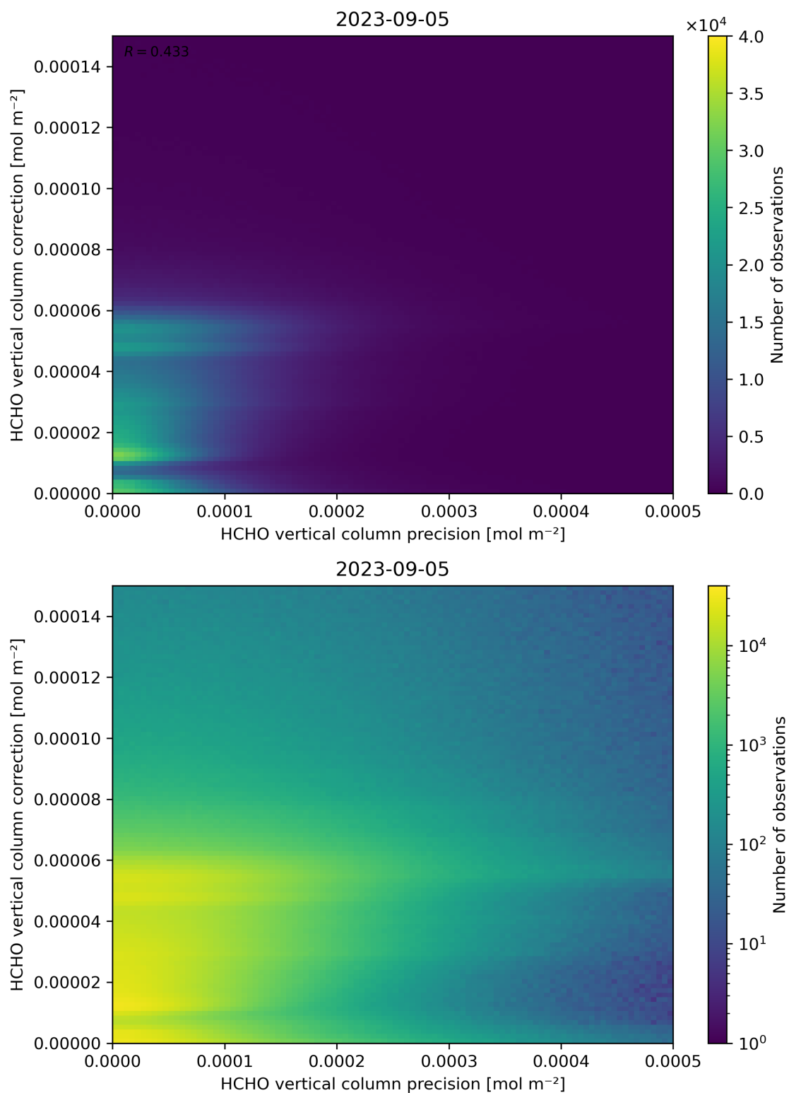
Figure 146: Scatter density plot of “HCHO vertical column precision” against “HCHO vertical column correction” for 2023-09-05 to 2023-09-06.
