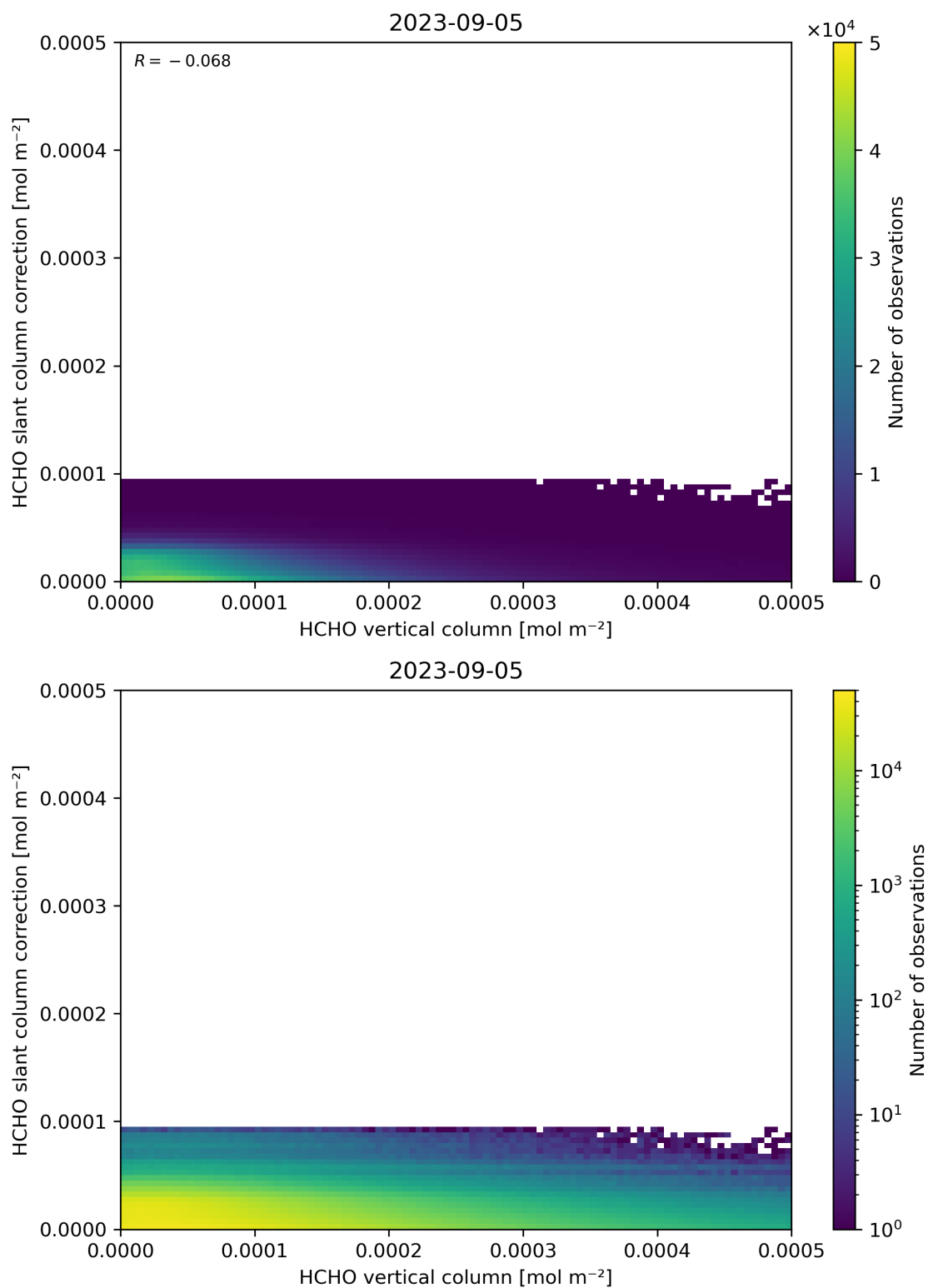
Figure 128: Scatter density plot of “HCHO vertical column” against “HCHO slant column correction” for 2023-09-05 to 2023-09-06.
