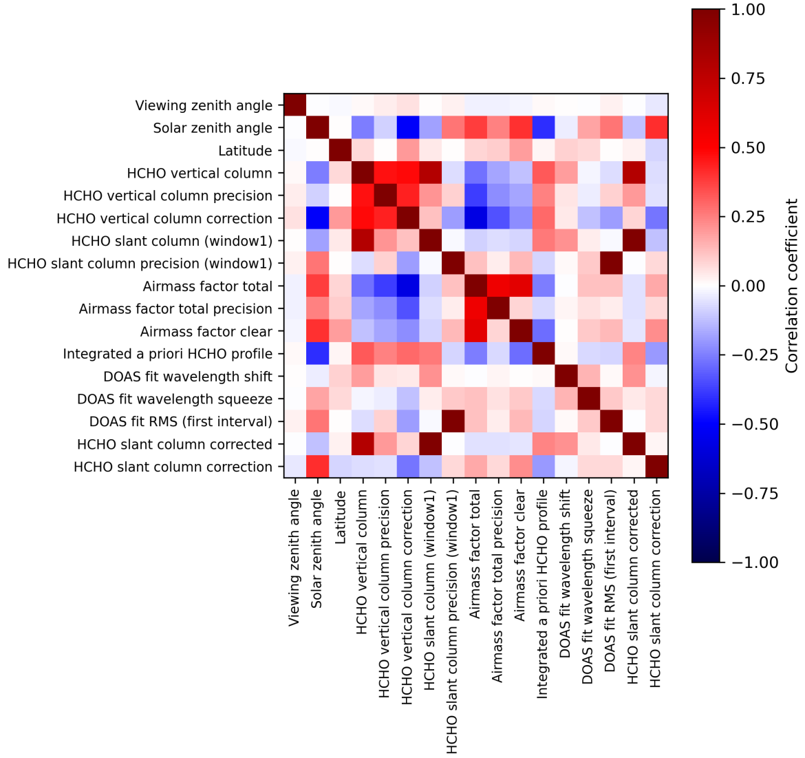
Figure 2: Map of correlation matrix for 2023-09-05 to 2023-09-06.
