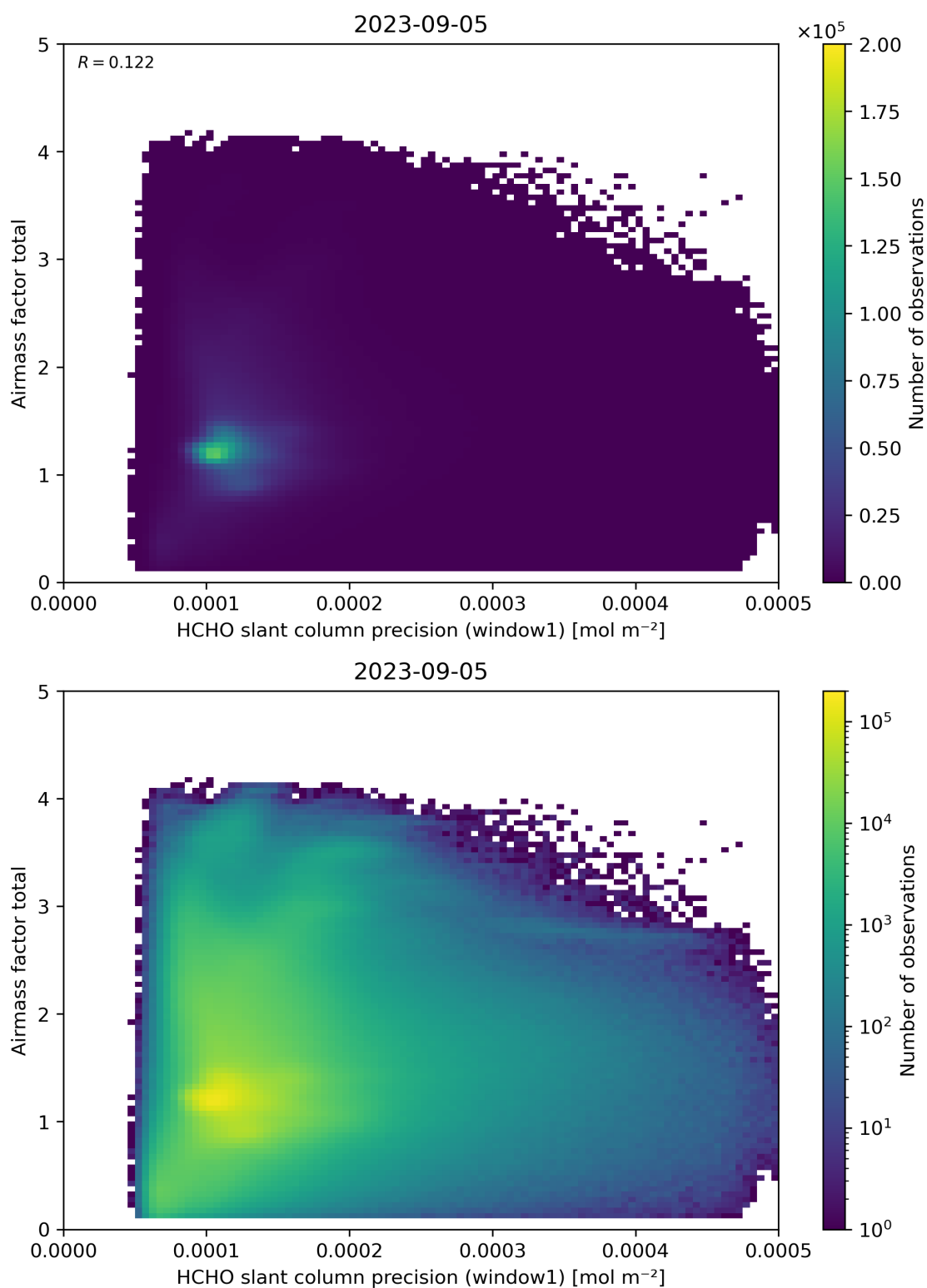
Figure 94: Scatter density plot of “HCHO slant column precision (window1)” against “Airmass factor total” for 2023-09-05 to 2023-09-06.
