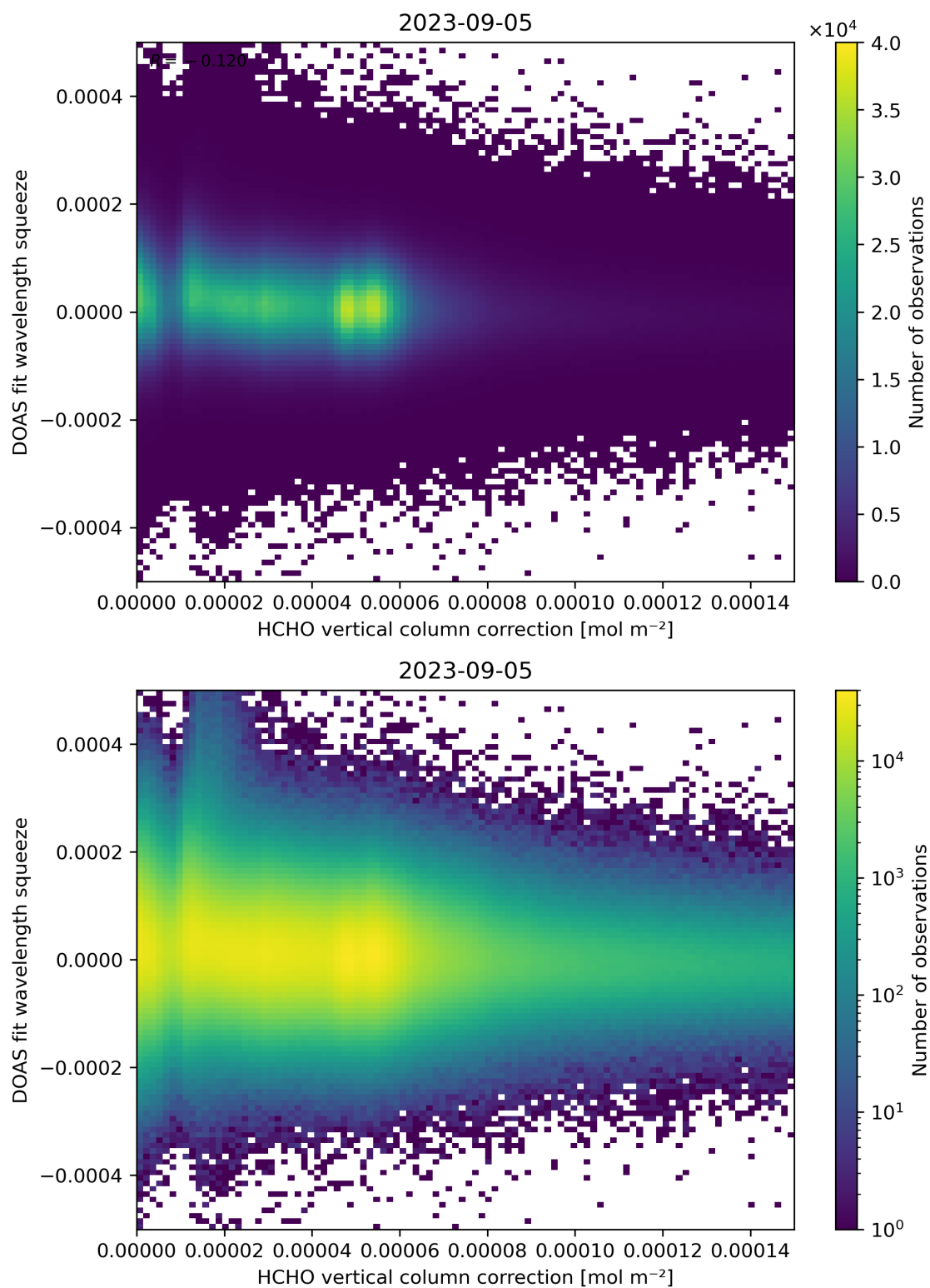
Figure 114: Scatter density plot of “HCHO vertical column correction” against “DOAS fit wavelength squeeze” for 2023-09-05 to 2023-09-06.
