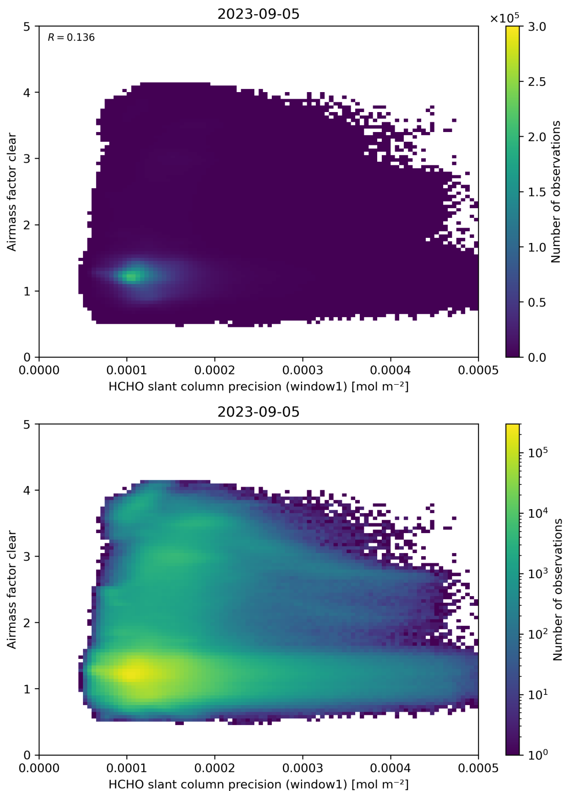
Figure 91: Scatter density plot of “HCHO slant column precision (window1)” against “Airmass factor clear” for 2023-09-05 to 2023-09-06.
