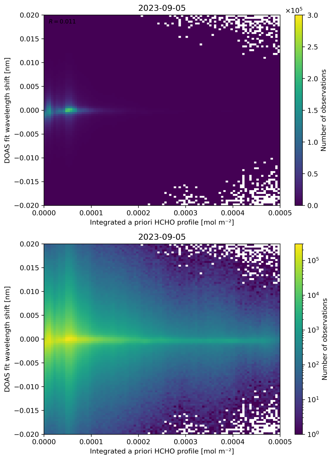
Figure 149: Scatter density plot of “Integrated a priori HCHO profile” against “DOAS fit wavelength shift” for 2023-09-05 to 2023-09-06.
