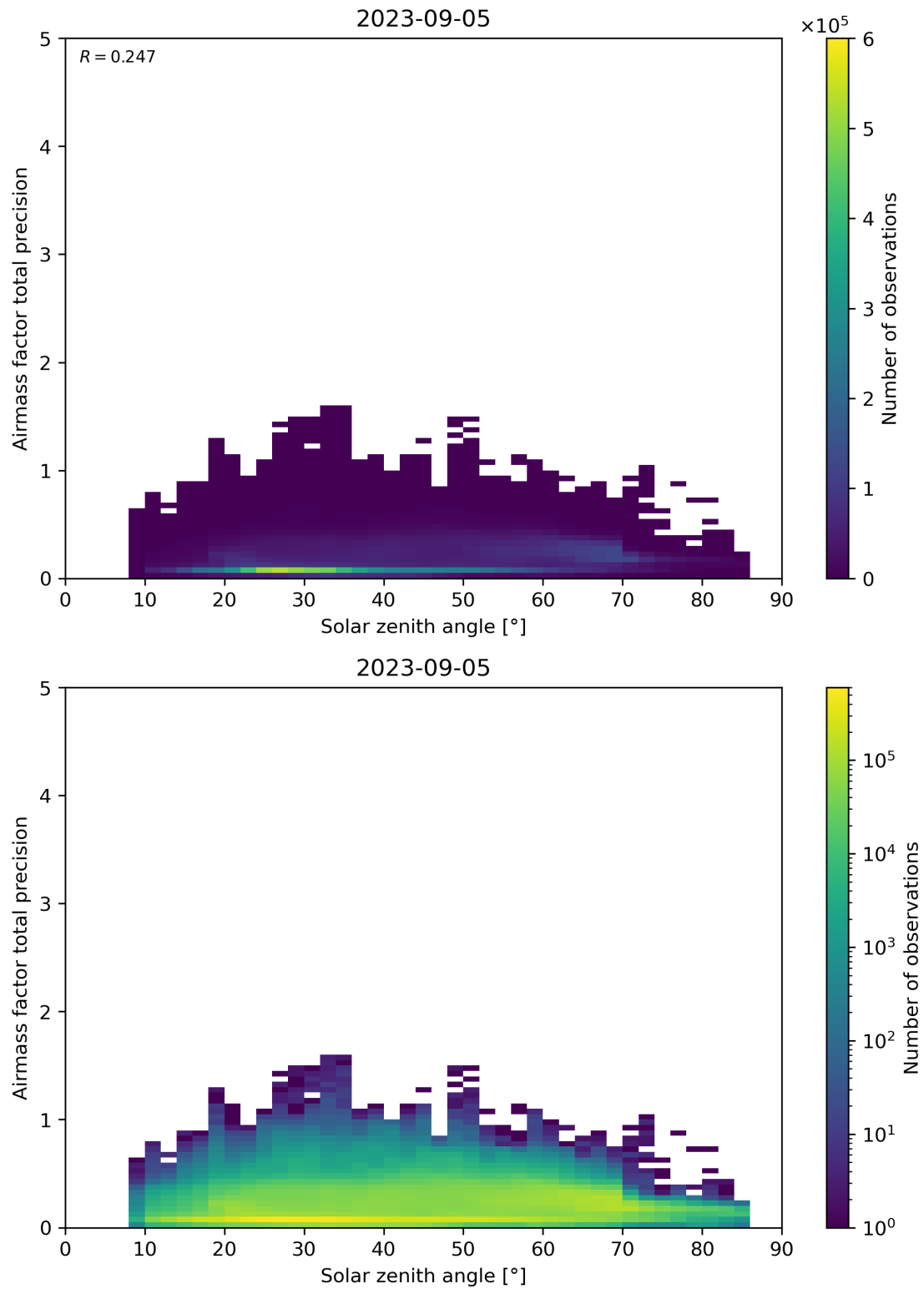
Figure 176: Scatter density plot of “Solar zenith angle” against “Airmass factor total precision” for 2023-09-05 to 2023-09-06.
