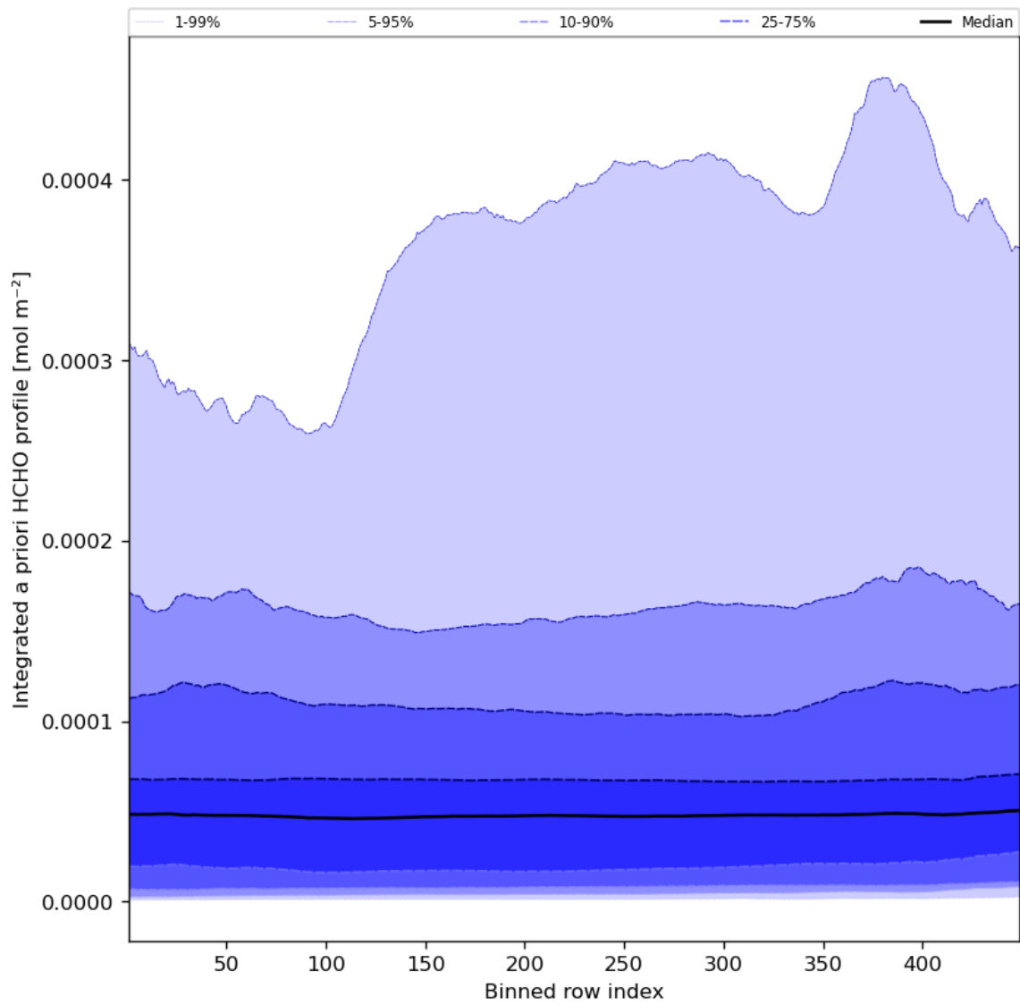
Figure 57: Along track statistics of “Integrated a priori HCHO profile” for 2023-09-05 to 2023-09-06
