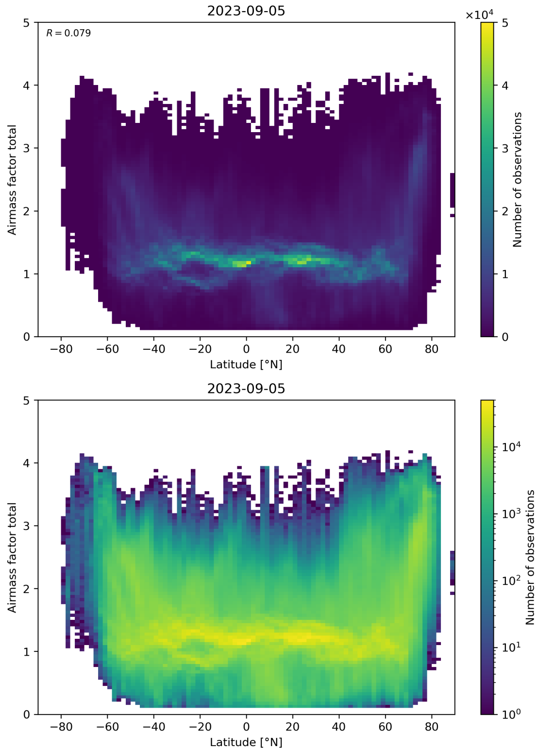
Figure 161: Scatter density plot of “Latitude” against “Airmass factor total” for 2023-09-05 to 2023-09-06.
