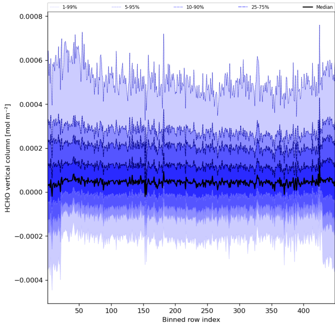
Figure 49: Along track statistics of “HCHO vertical column” for 2023-09-05 to 2023-09-06
