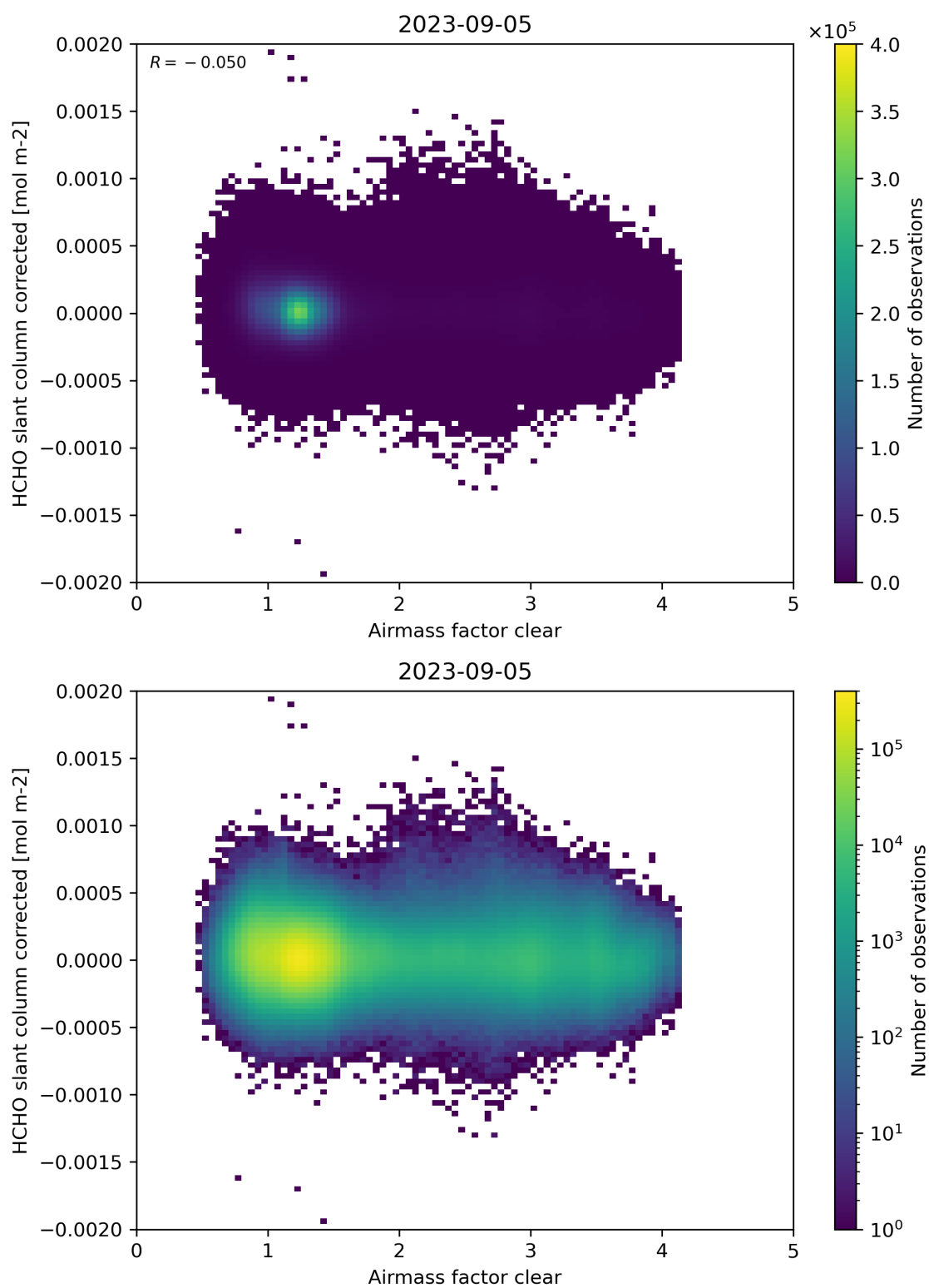
Figure 74: Scatter density plot of “Airmass factor clear” against “HCHO slant column corrected” for 2023-09-05 to 2023-09-06.
