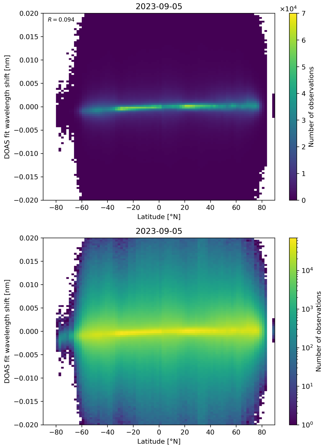
Figure 154: Scatter density plot of “Latitude” against “DOAS fit wavelength shift” for 2023-09-05 to 2023-09-06.
