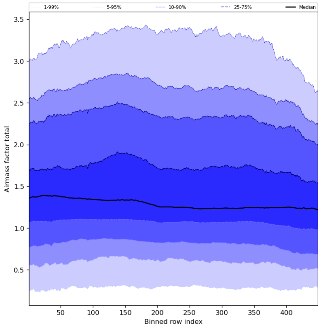
Figure 54: Along track statistics of “Airmass factor total” for 2023-09-05 to 2023-09-06
