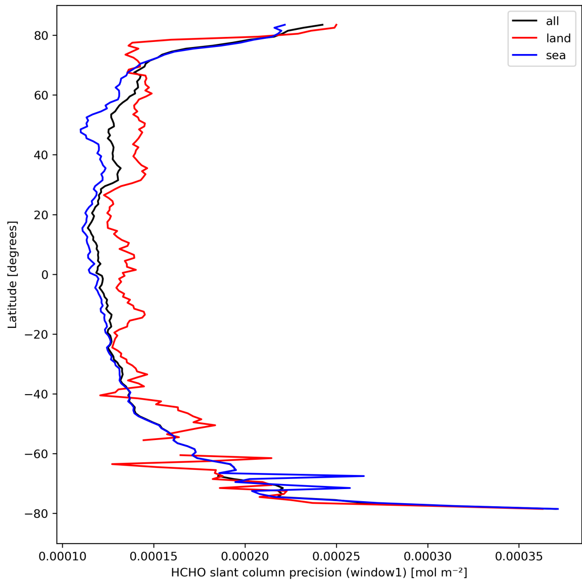
Figure 25: Zonal average of “HCHO slant column precision (window1)” for 2023-09-05 to 2023-09-06.
