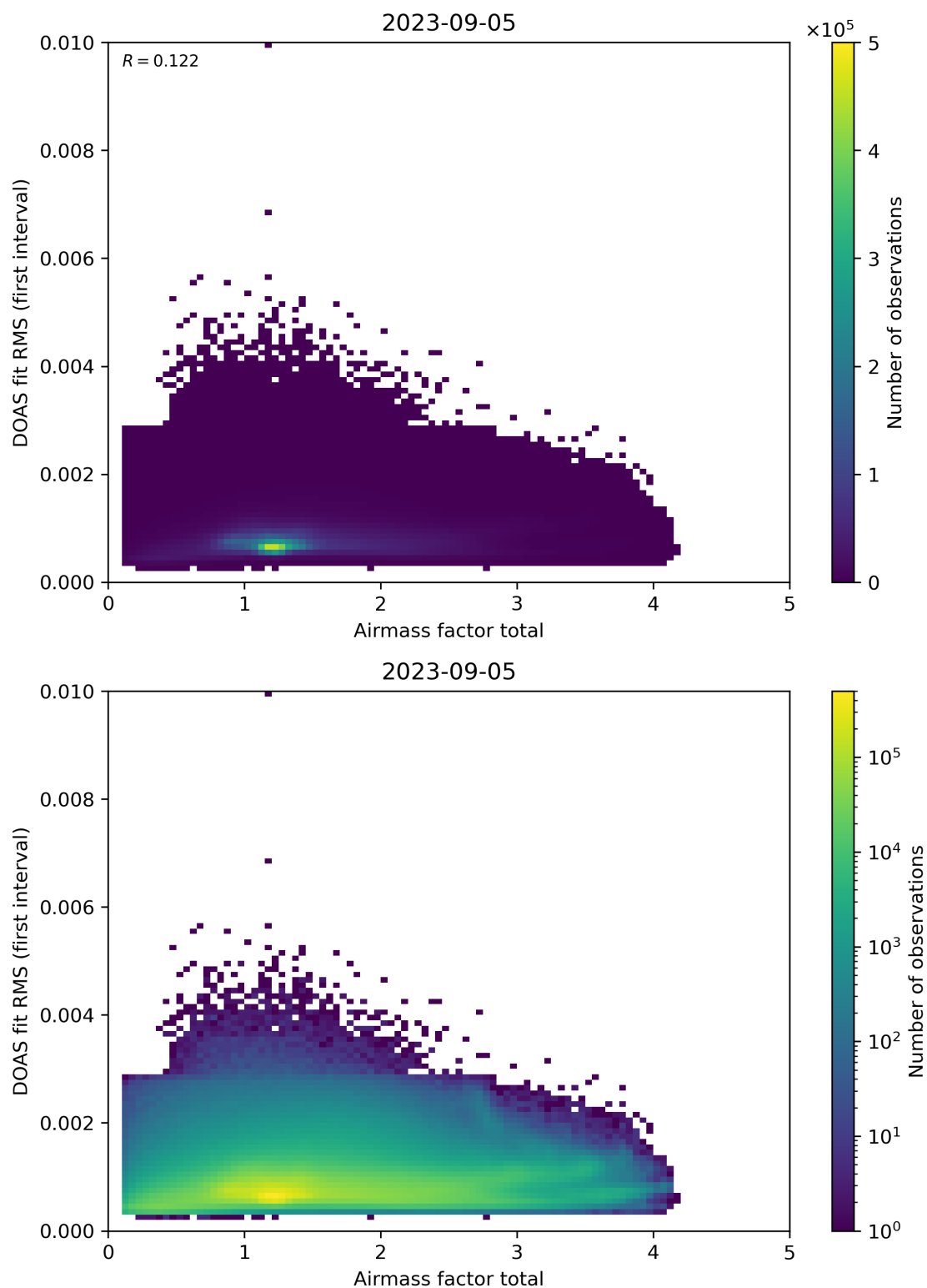
Figure 97: Scatter density plot of “Airmass factor total” against “DOAS fit RMS (first interval)” for 2023-09-05 to 2023-09-06.
