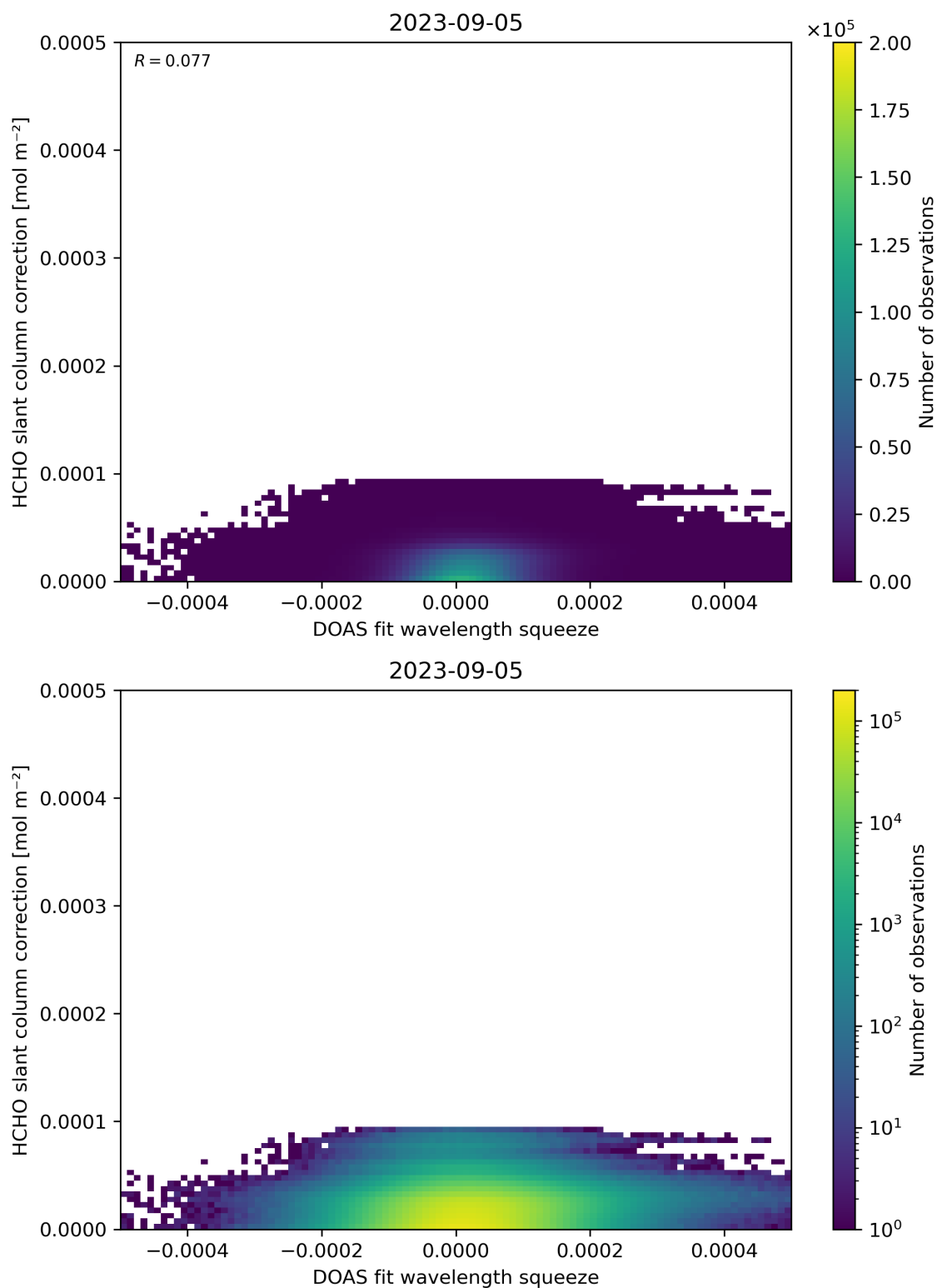
Figure 70: Scatter density plot of “DOAS fit wavelength squeeze” against “HCHO slant column correction” for 2023-09-05 to 2023-09-06.
