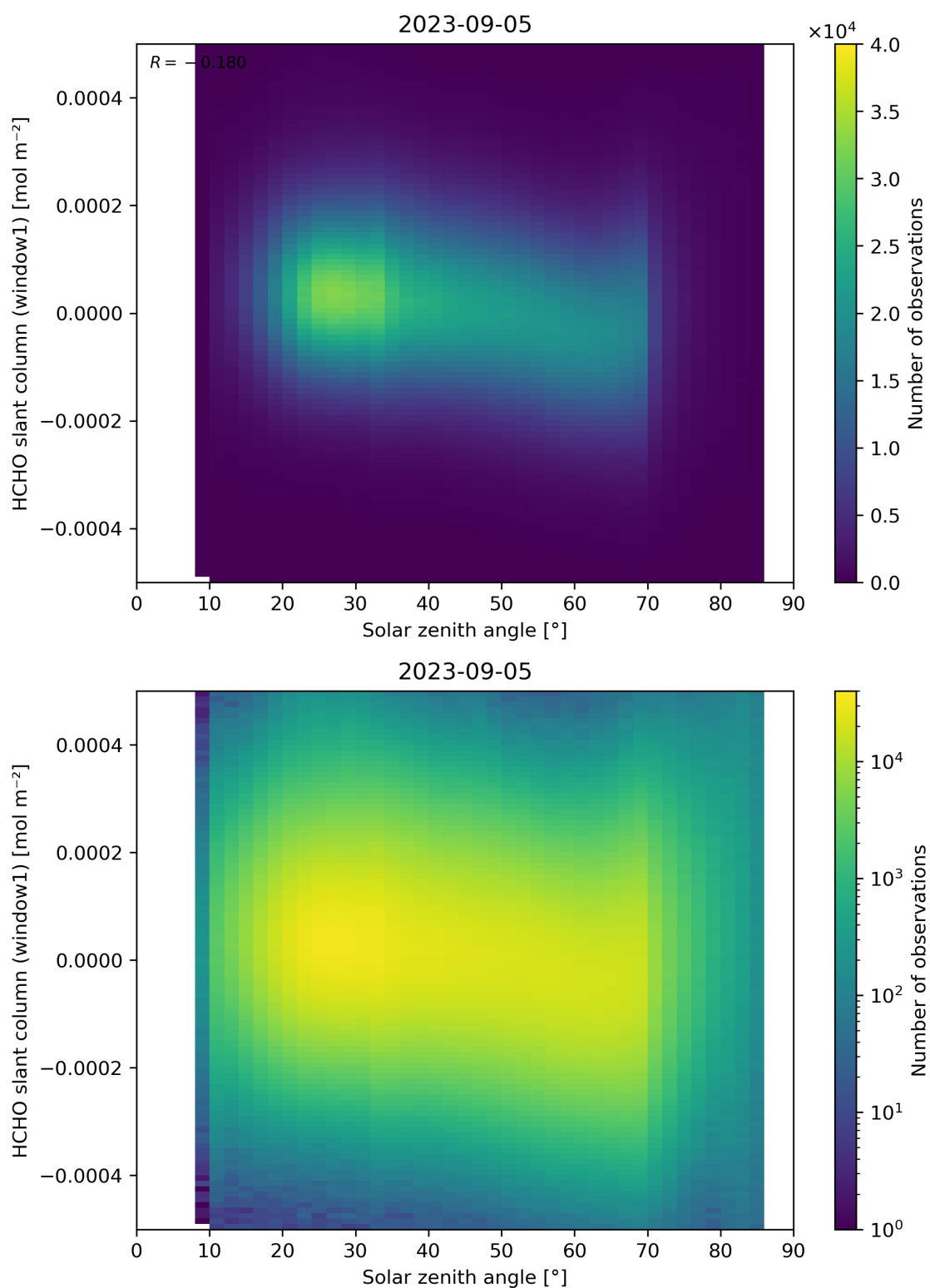
Figure 173: Scatter density plot of “Solar zenith angle” against “HCHO slant column (window1)” for 2023-09-05 to 2023-09-06.
