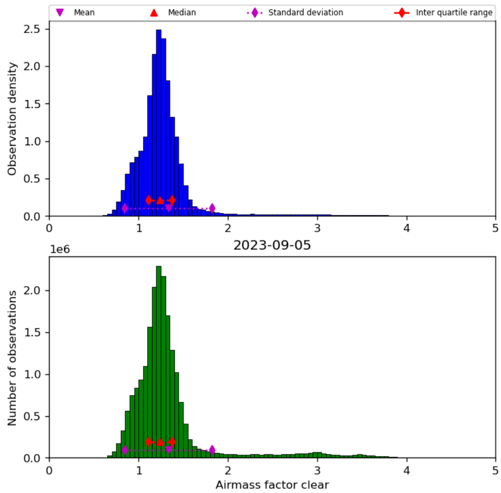
Figure 42: Histogram of “Airmass factor clear” for 2023-09-05 to 2023-09-06
