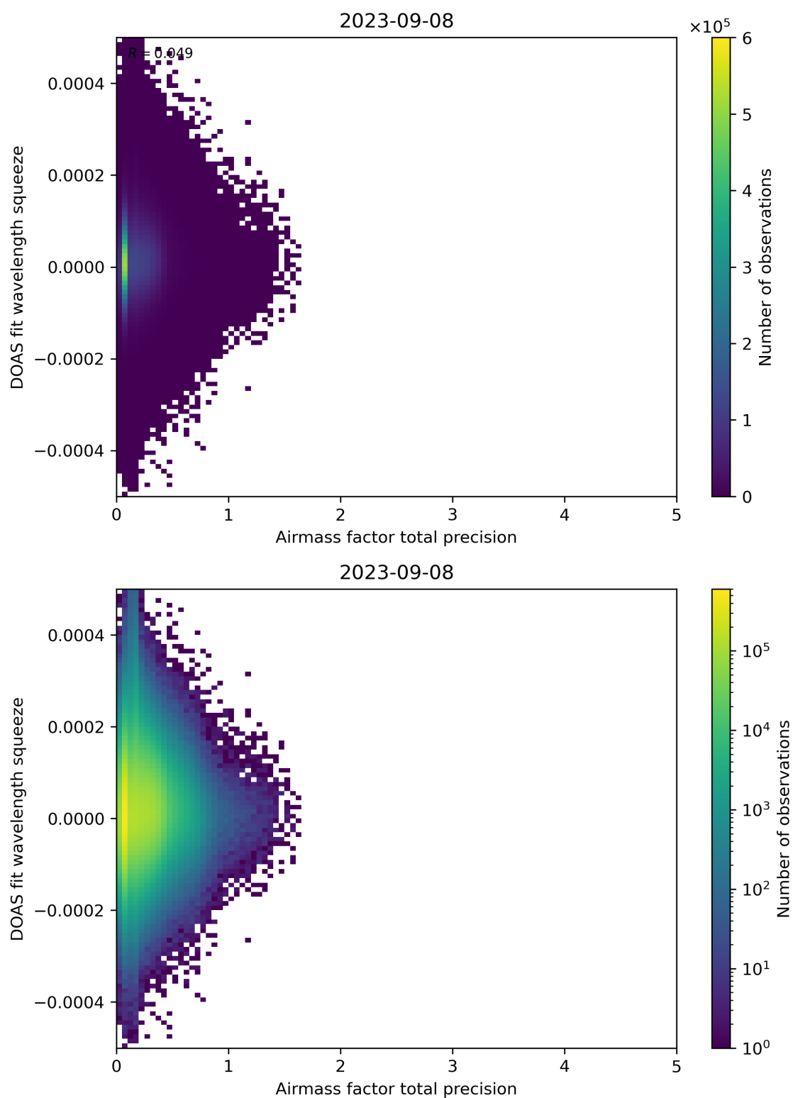
Figure 107: Scatter density plot of “Airmass factor total precision” against “DOAS fit wavelength squeeze” for 2023-09-07 to 2023-09-09.
