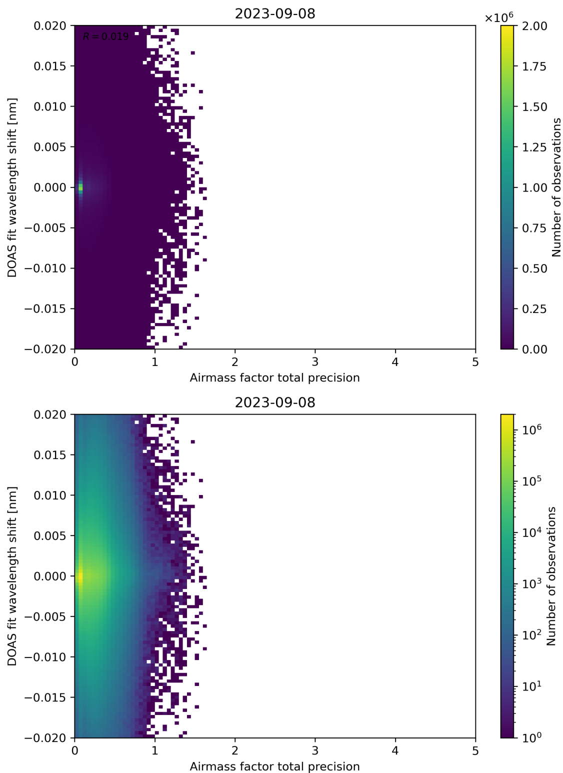
Figure 106: Scatter density plot of “Airmass factor total precision” against “DOAS fit wavelength shift” for 2023-09-07 to 2023-09-09.
