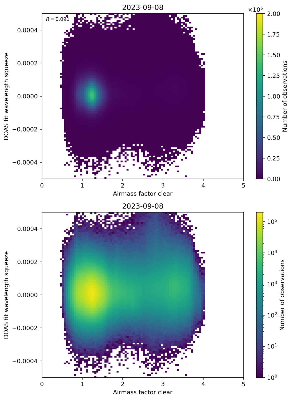
Figure 73: Scatter density plot of “Airmass factor clear” against “DOAS fit wavelength squeeze” for 2023-09-07 to 2023-09-09.
