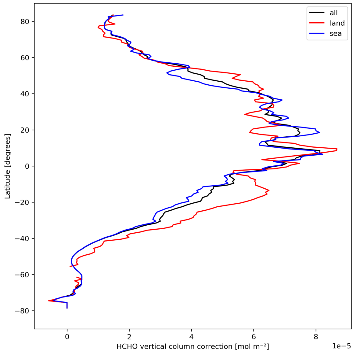
Figure 23: Zonal average of “HCHO vertical column correction” for 2023-09-07 to 2023-09-09.
