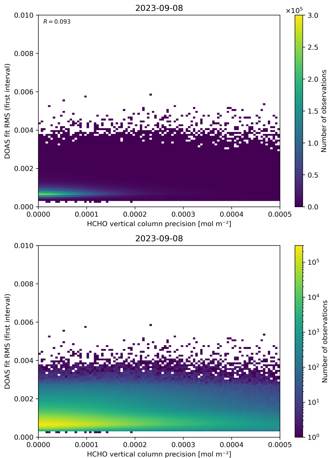
Figure 136: Scatter density plot of “HCHO vertical column precision” against “DOAS fit RMS (first interval)” for 2023-09-07 to 2023-09-09.
