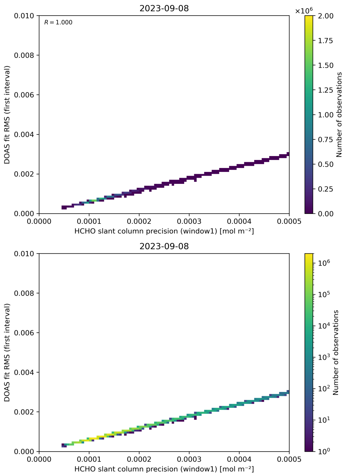
Figure 88: Scatter density plot of “HCHO slant column precision (window1)” against “DOAS fit RMS (first interval)” for 2023-09-07 to 2023-09-09.
