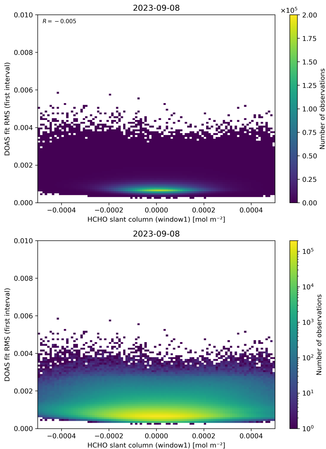
Figure 78: Scatter density plot of “HCHO slant column (window1)” against “DOAS fit RMS (first interval)” for 2023-09-07 to 2023-09-09.
