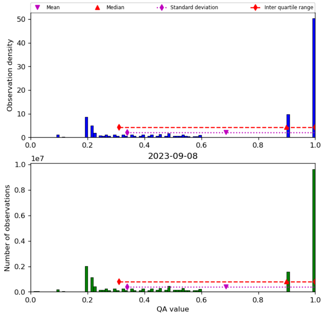
Figure 34: Histogram of “QA value” for 2023-09-07 to 2023-09-09
