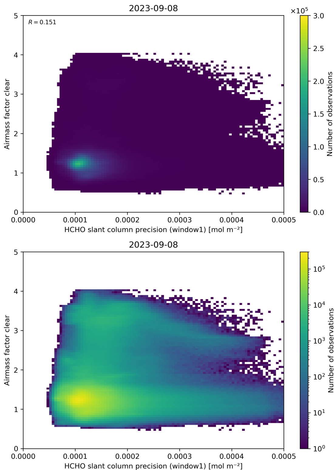
Figure 91: Scatter density plot of “HCHO slant column precision (window1)” against “Airmass factor clear” for 2023-09-07 to 2023-09-09.
