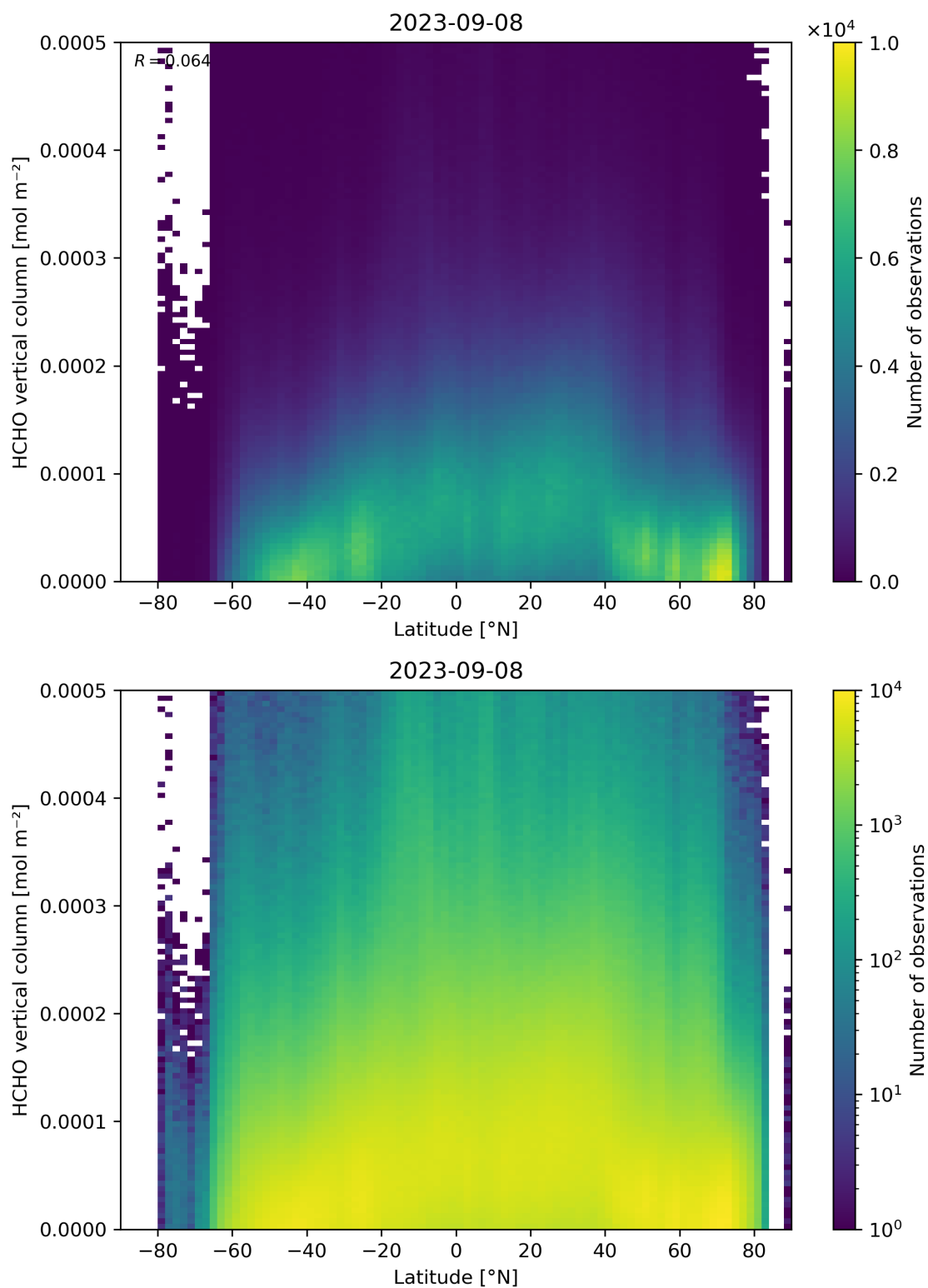
Figure 163: Scatter density plot of “Latitude” against “HCHO vertical column” for 2023-09-07 to 2023-09-09.
