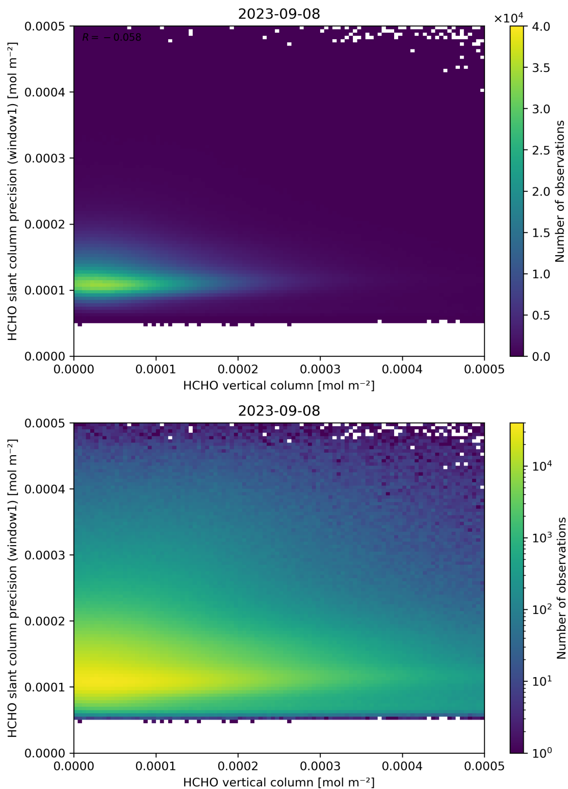
Figure 130: Scatter density plot of “HCHO vertical column” against “HCHO slant column precision (window1)” for 2023-09-07 to 2023-09-09.
