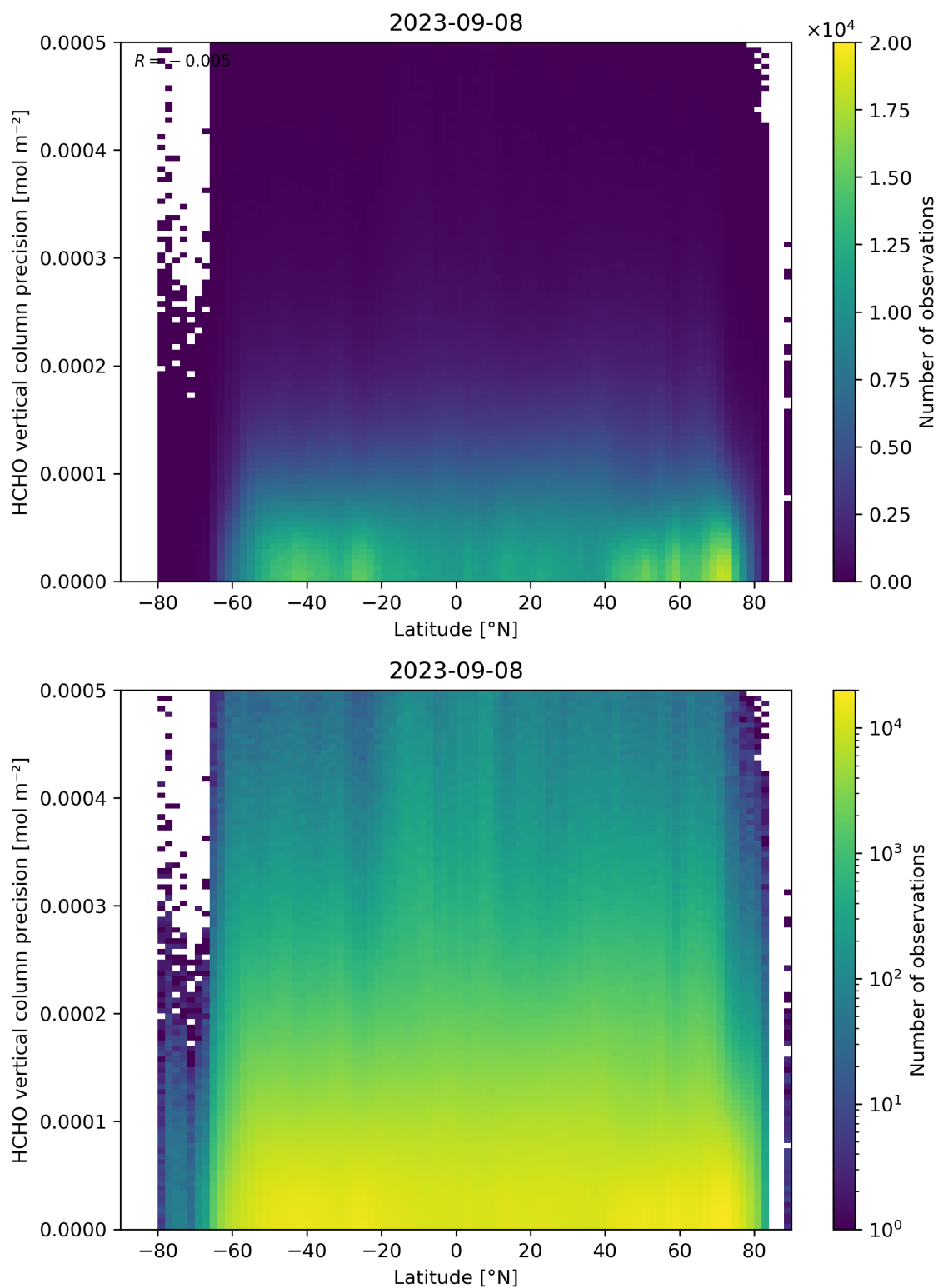
Figure 165: Scatter density plot of “Latitude” against “HCHO vertical column precision” for 2023-09-07 to 2023-09-09.
