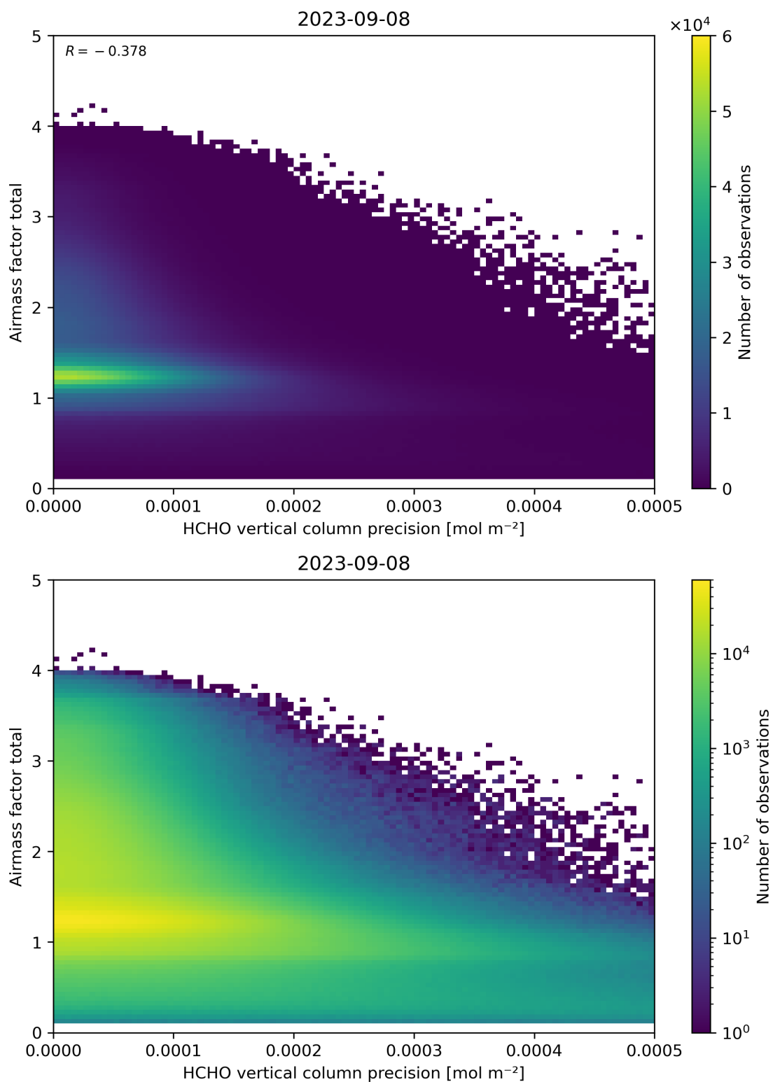
Figure 144: Scatter density plot of “HCHO vertical column precision” against “Airmass factor total” for 2023-09-07 to 2023-09-09.
