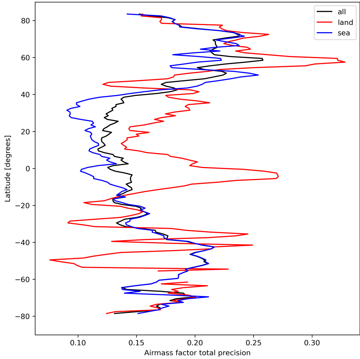
Figure 27: Zonal average of “Airmass factor total precision” for 2023-09-07 to 2023-09-09.
