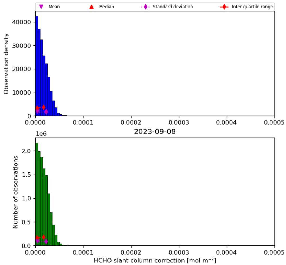
Figure 47: Histogram of “HCHO slant column correction” for 2023-09-07 to 2023-09-09
