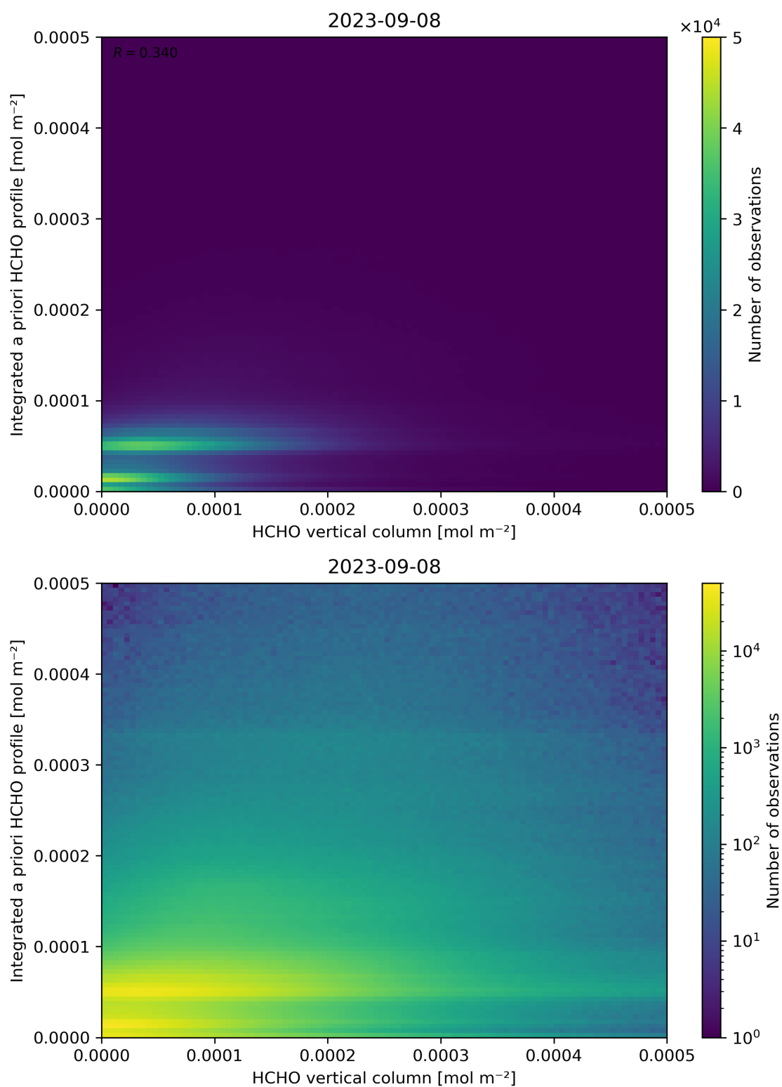
Figure 135: Scatter density plot of “HCHO vertical column” against “Integrated a priori HCHO profile” for 2023-09-07 to 2023-09-09.
