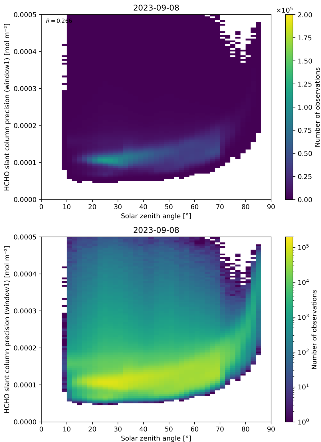
Figure 174: Scatter density plot of “Solar zenith angle” against “HCHO slant column precision (window1)” for 2023-09-07 to 2023-09-09.
