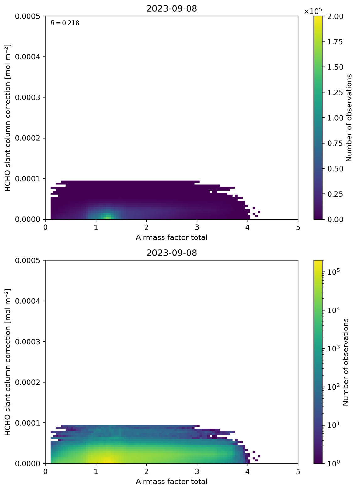
Figure 102: Scatter density plot of “Airmass factor total” against “HCHO slant column correction” for 2023-09-07 to 2023-09-09.
