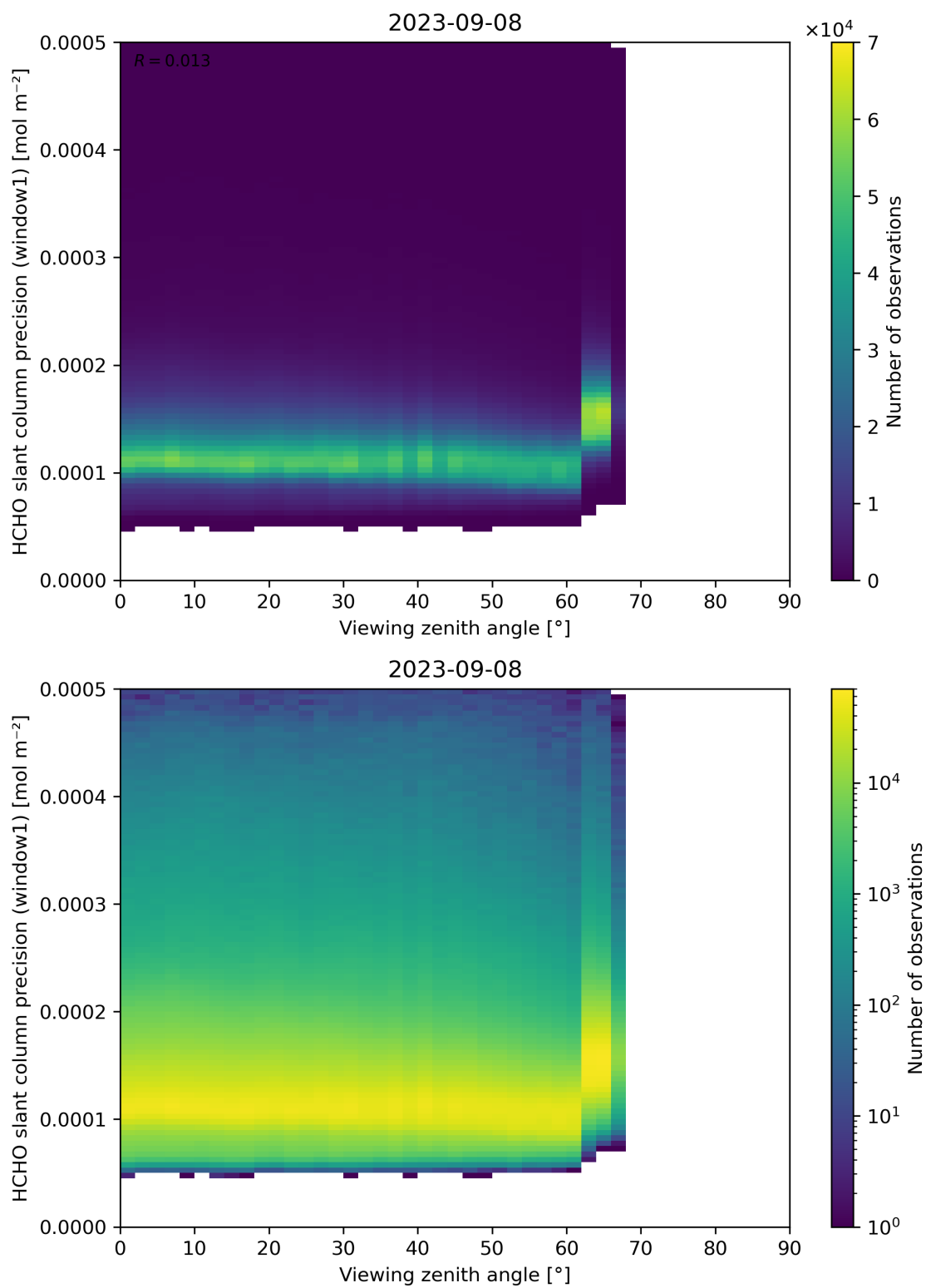
Figure 189: Scatter density plot of “Viewing zenith angle” against “HCHO slant column precision (window1)” for 2023-09-07 to 2023-09-09.
