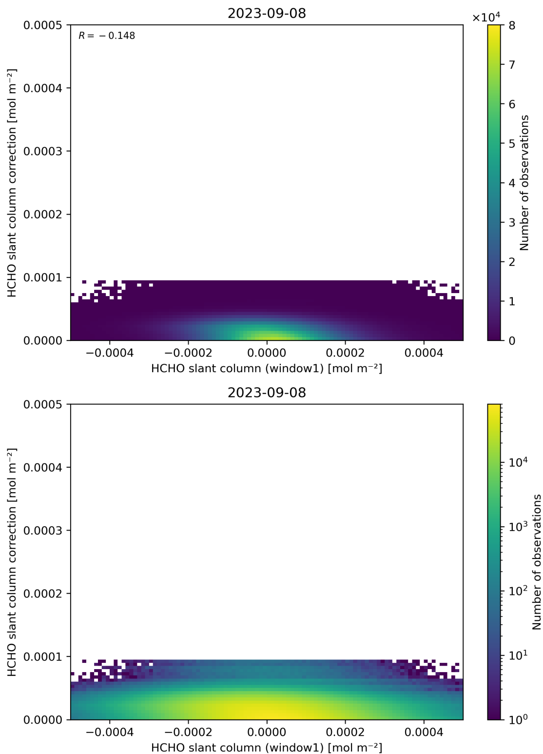
Figure 83: Scatter density plot of “HCHO slant column (window1)” against “HCHO slant column correction” for 2023-09-07 to 2023-09-09.
