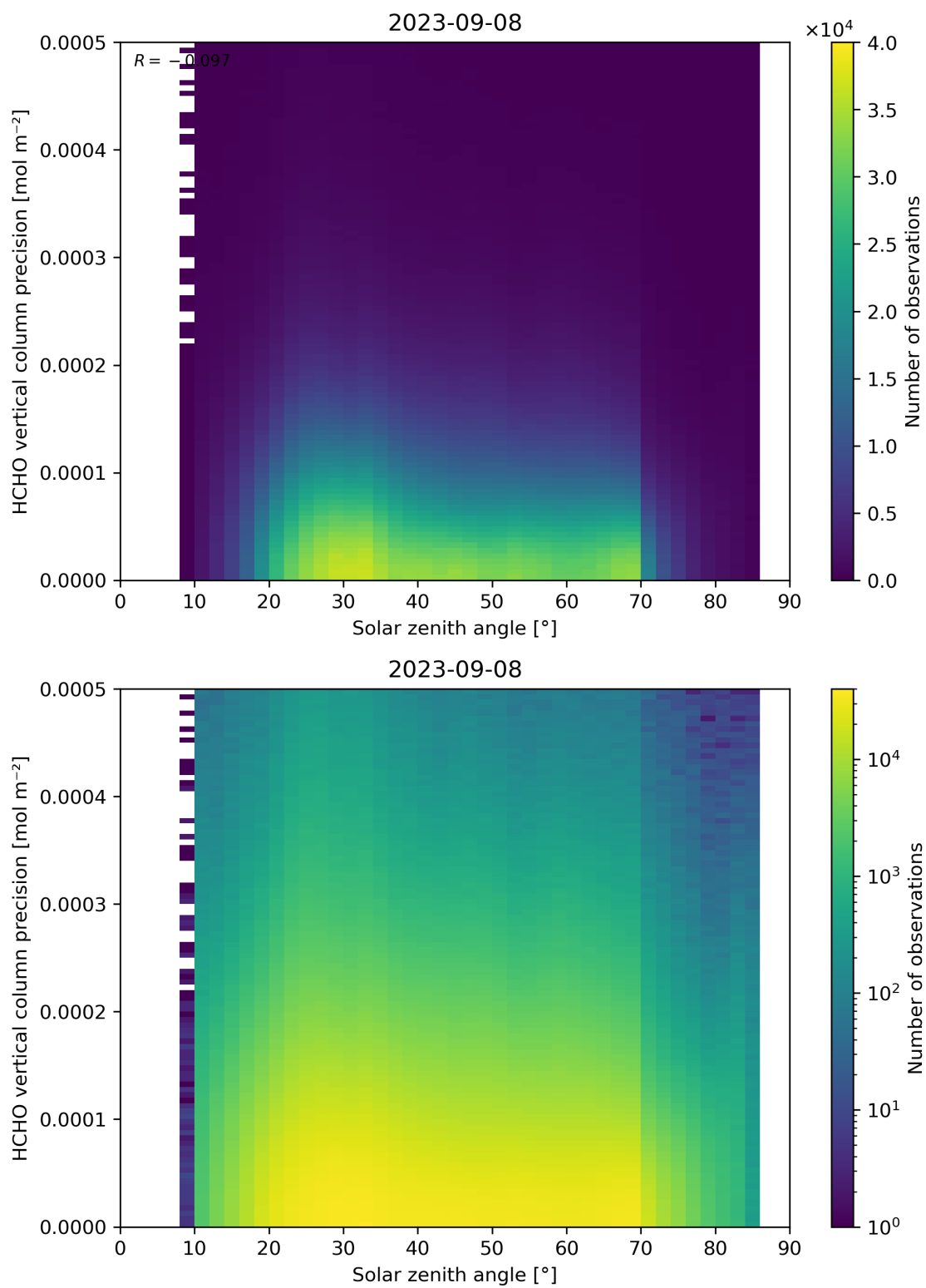
Figure 179: Scatter density plot of “Solar zenith angle” against “HCHO vertical column precision” for 2023-09-07 to 2023-09-09.
