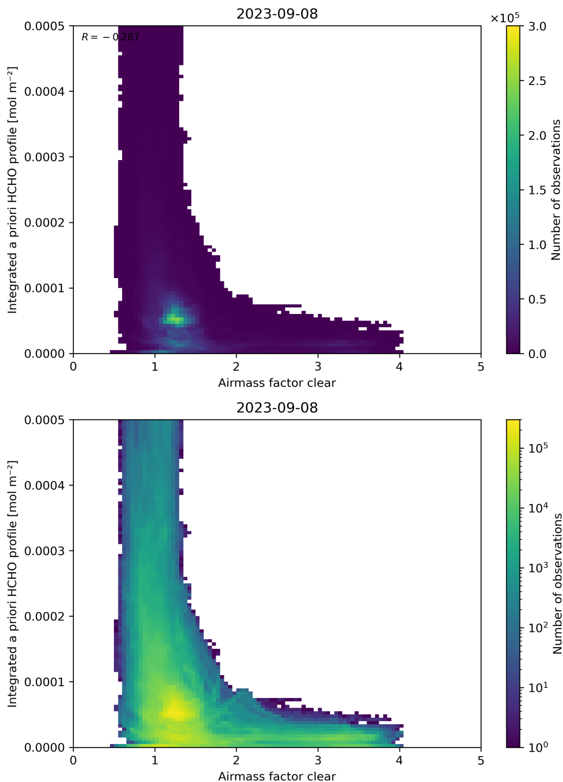
Figure 76: Scatter density plot of “Airmass factor clear” against “Integrated a priori HCHO profile” for 2023-09-07 to 2023-09-09.
