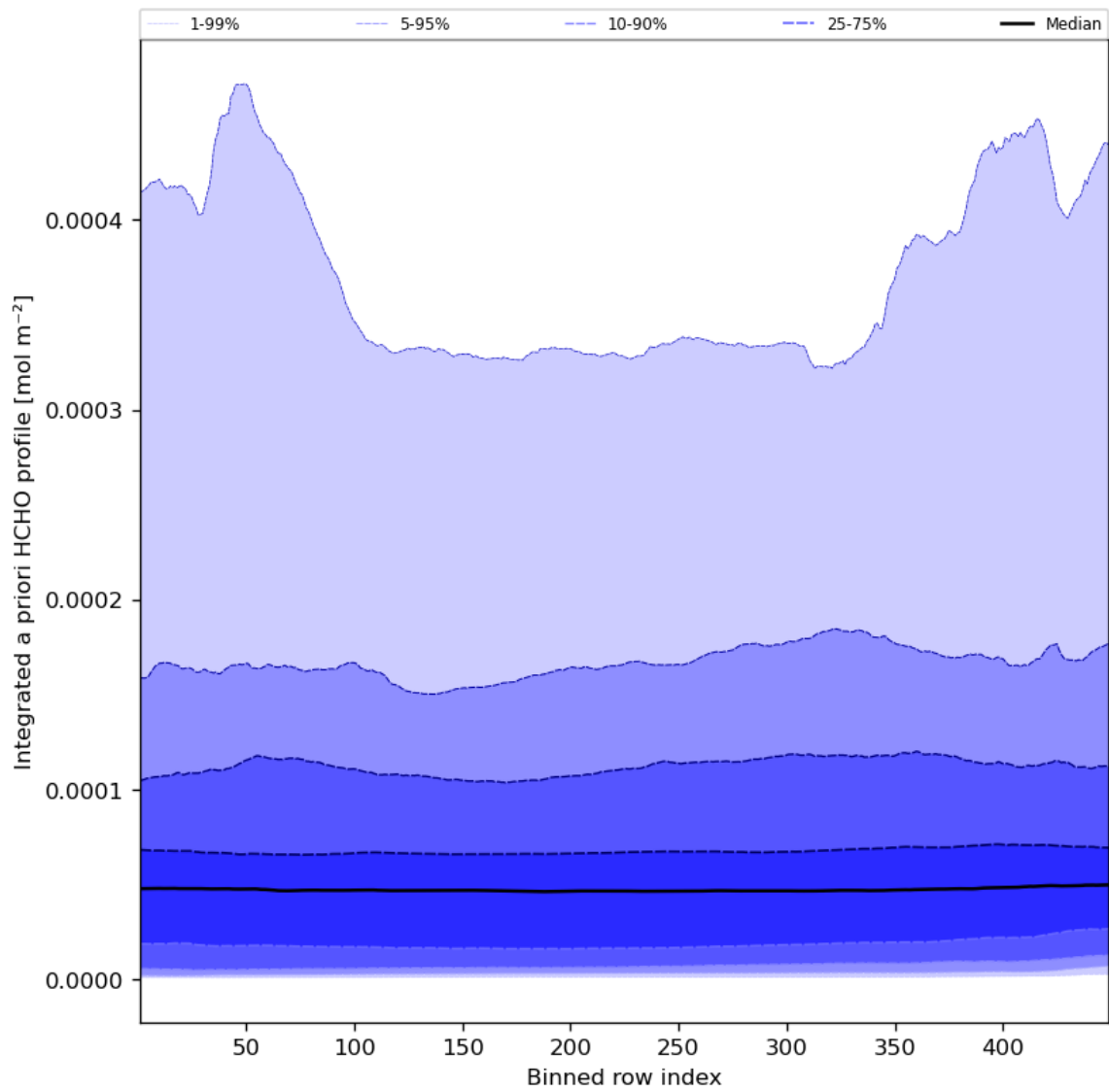
Figure 57: Along track statistics of “Integrated a priori HCHO profile” for 2023-09-07 to 2023-09-09
