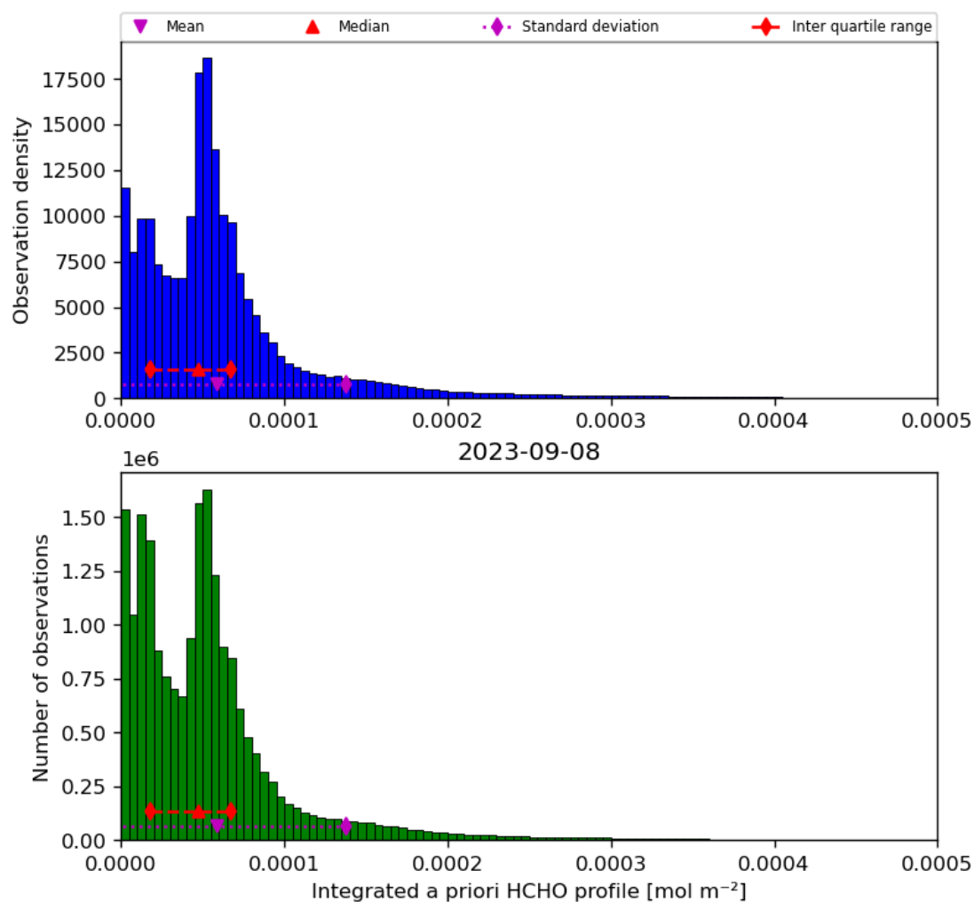
Figure 43: Histogram of “Integrated a priori HCHO profile” for 2023-09-07 to 2023-09-09
