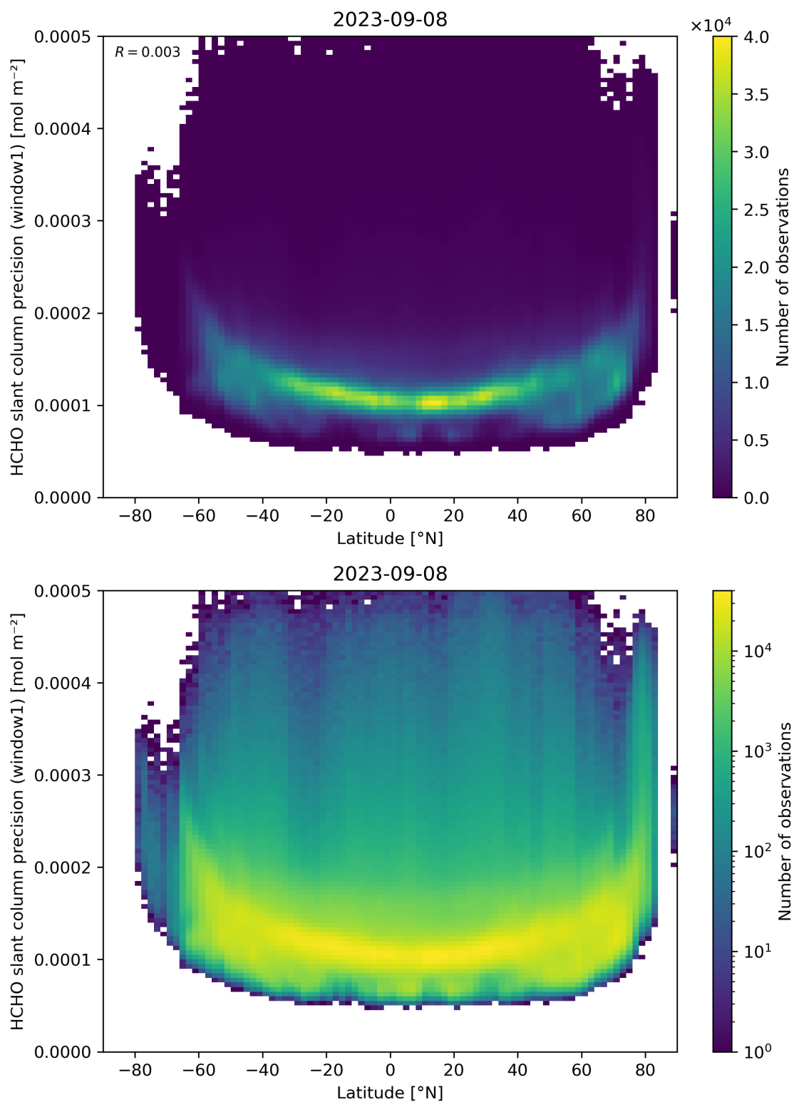
Figure 160: Scatter density plot of “Latitude” against “HCHO slant column precision (window1)” for 2023-09-07 to 2023-09-09.
