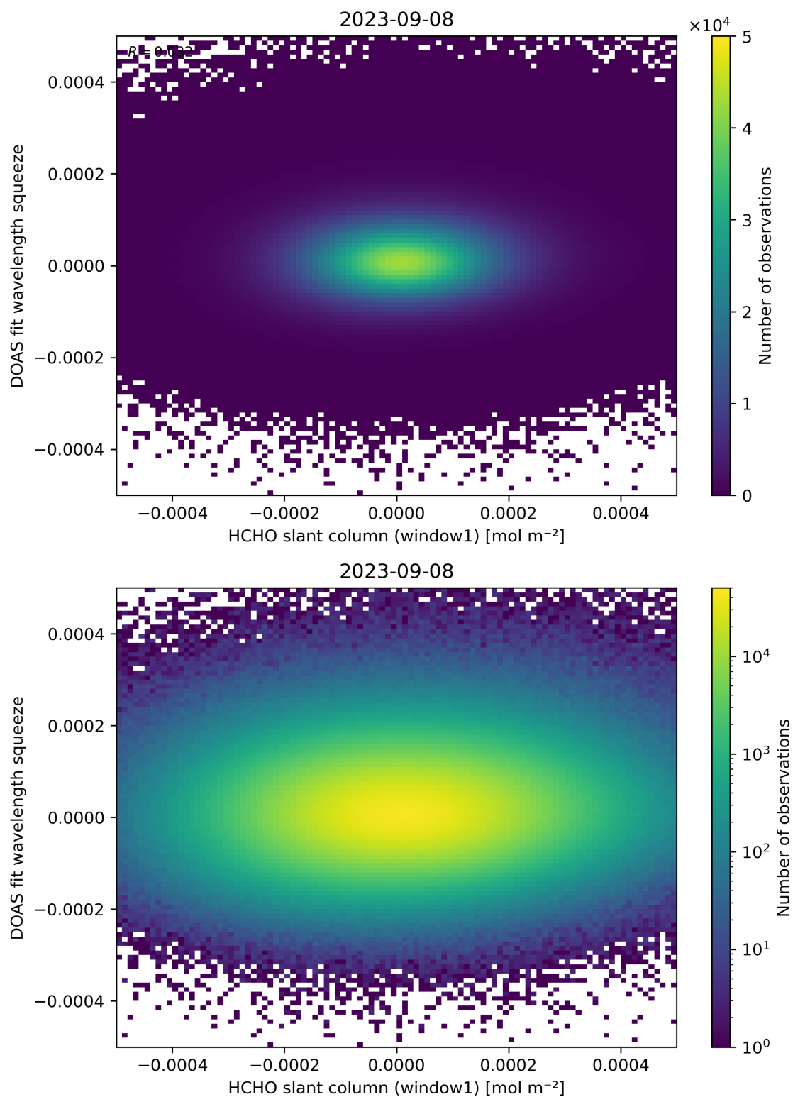
Figure 80: Scatter density plot of “HCHO slant column (window1)” against “DOAS fit wavelength squeeze” for 2023-09-07 to 2023-09-09.
