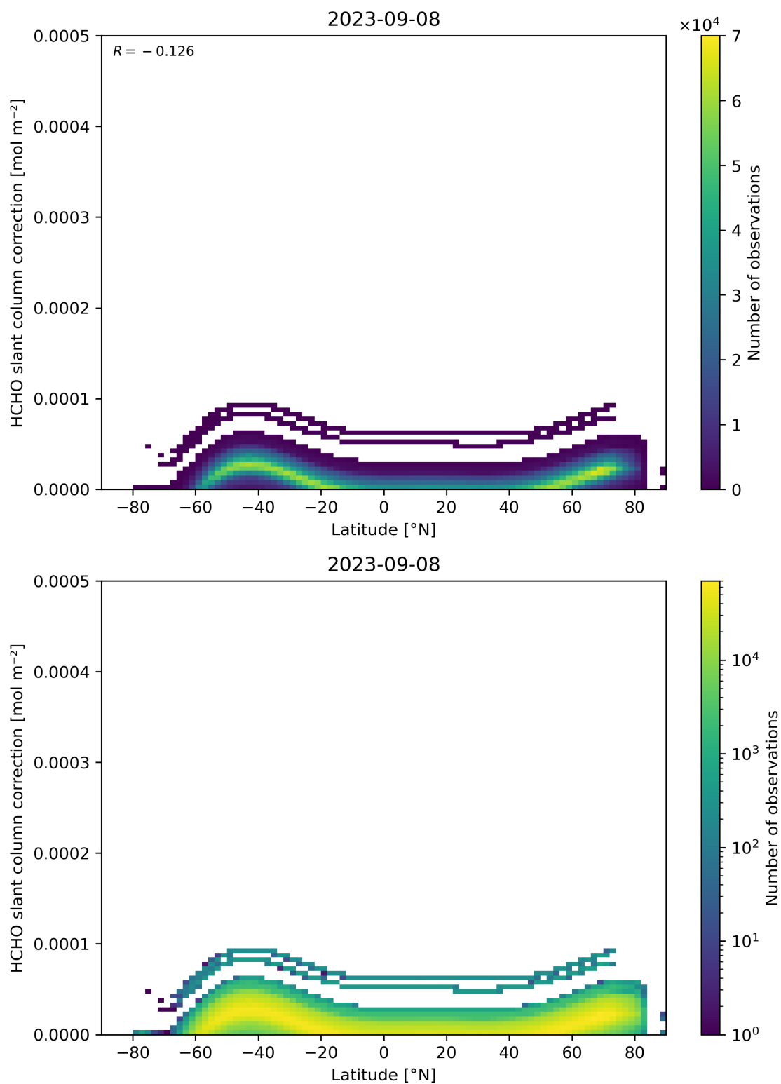
Figure 158: Scatter density plot of “Latitude” against “HCHO slant column correction” for 2023-09-07 to 2023-09-09.
