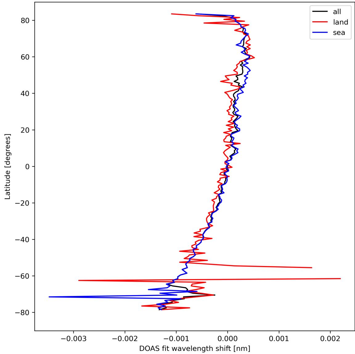
Figure 30: Zonal average of “DOAS fit wavelength shift” for 2023-09-07 to 2023-09-09.
