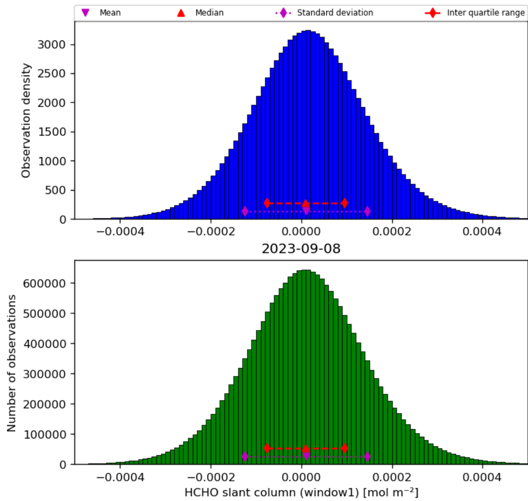
Figure 38: Histogram of “HCHO slant column (window1)” for 2023-09-07 to 2023-09-09
