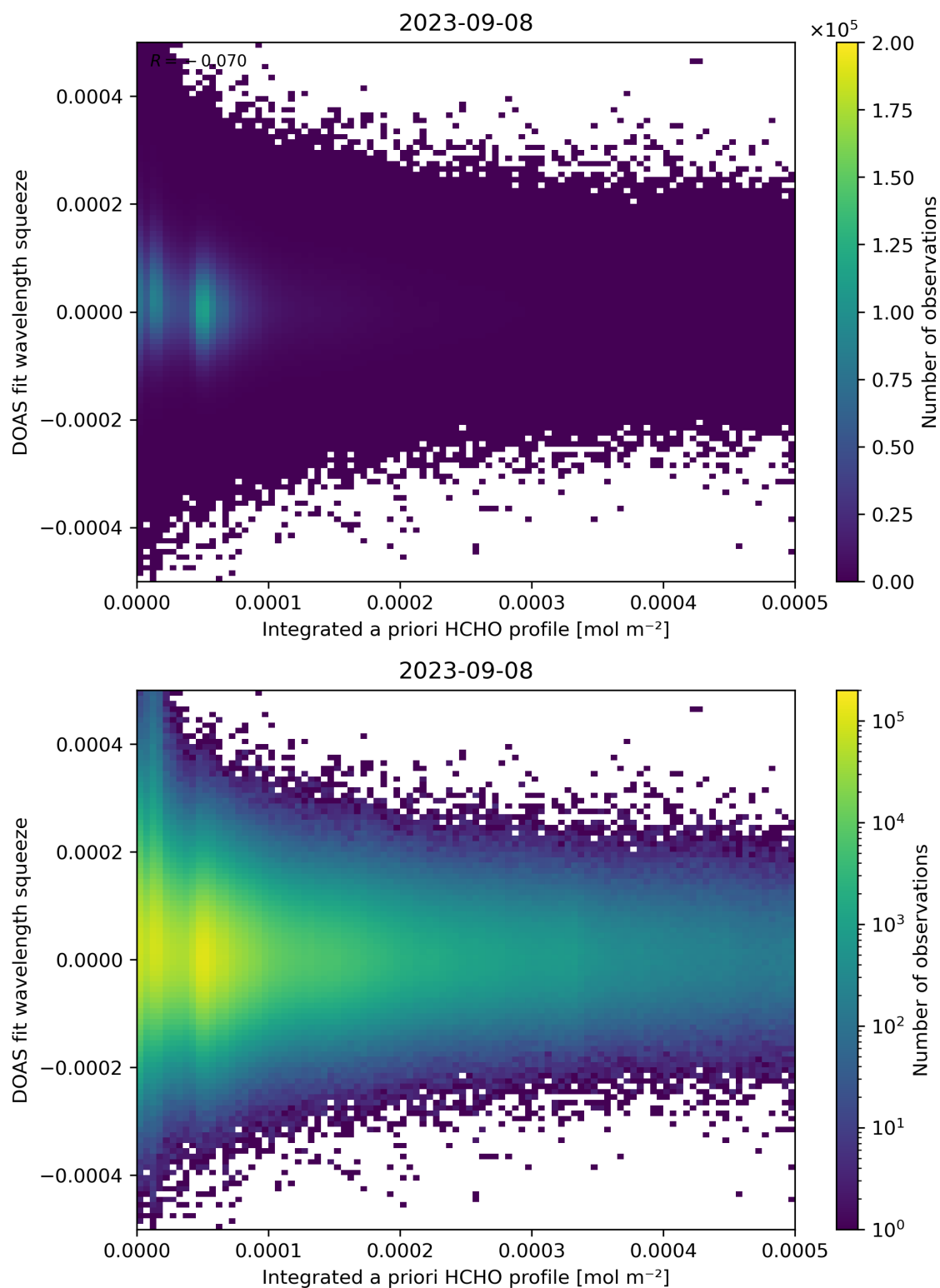
Figure 150: Scatter density plot of “Integrated a priori HCHO profile” against “DOAS fit wavelength squeeze” for 2023-09-07 to 2023-09-09.
