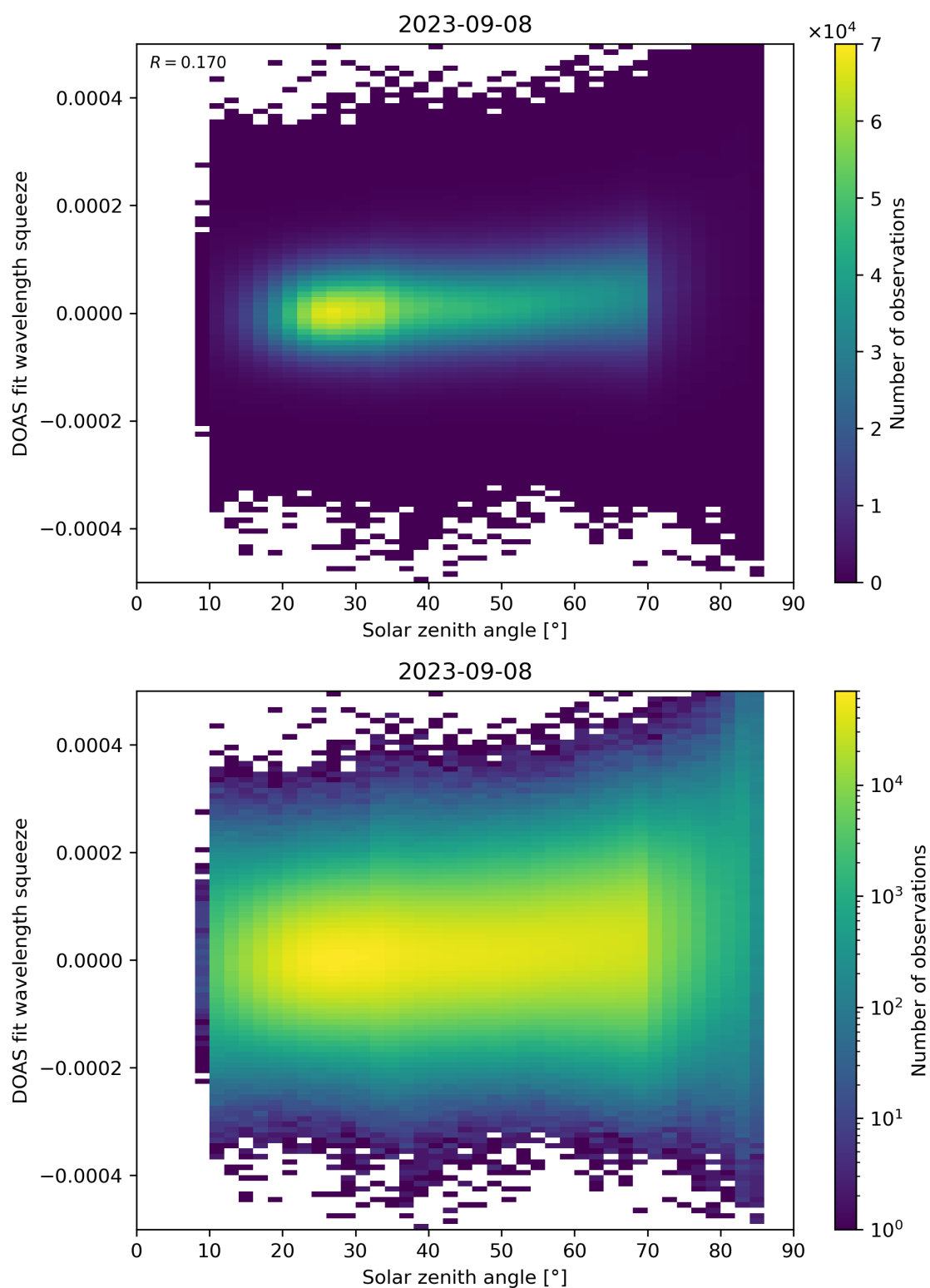
Figure 169: Scatter density plot of “Solar zenith angle” against “DOAS fit wavelength squeeze” for 2023-09-07 to 2023-09-09.
