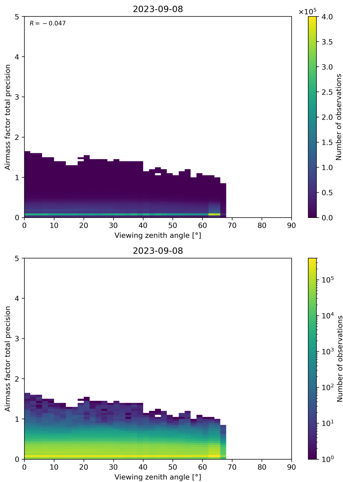
Figure 191: Scatter density plot of “Viewing zenith angle” against “Airmass factor total precision” for 2023-09-07 to 2023-09-09.
