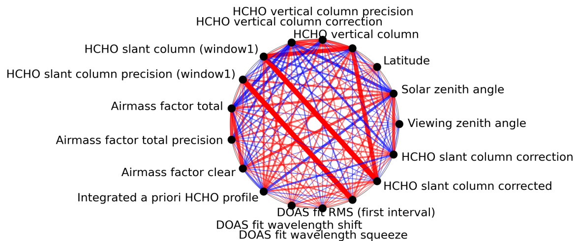
Figure 1: Map of correlation graph for 2023-09-07 to 2023-09-09.
