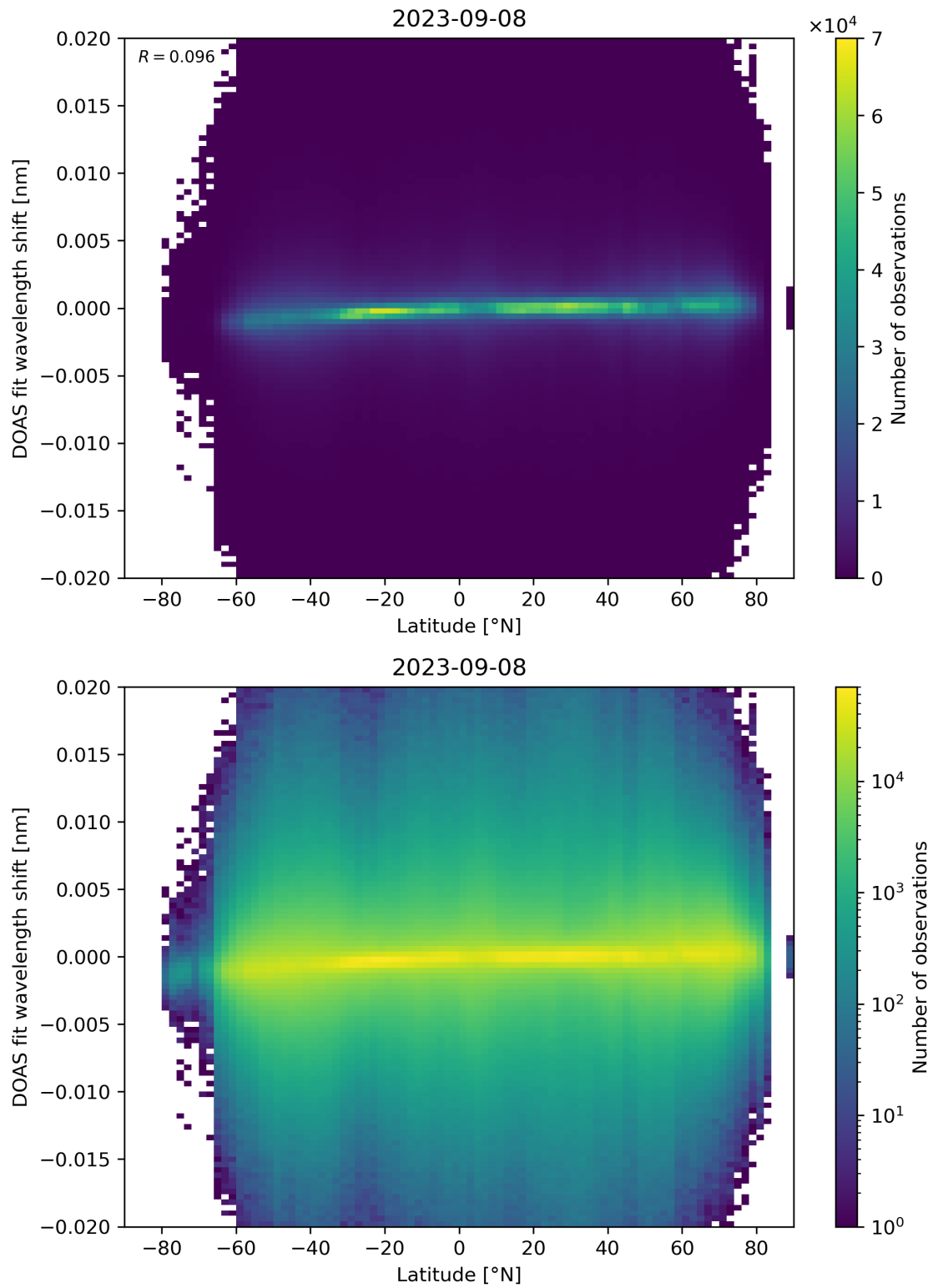
Figure 154: Scatter density plot of “Latitude” against “DOAS fit wavelength shift” for 2023-09-07 to 2023-09-09.
