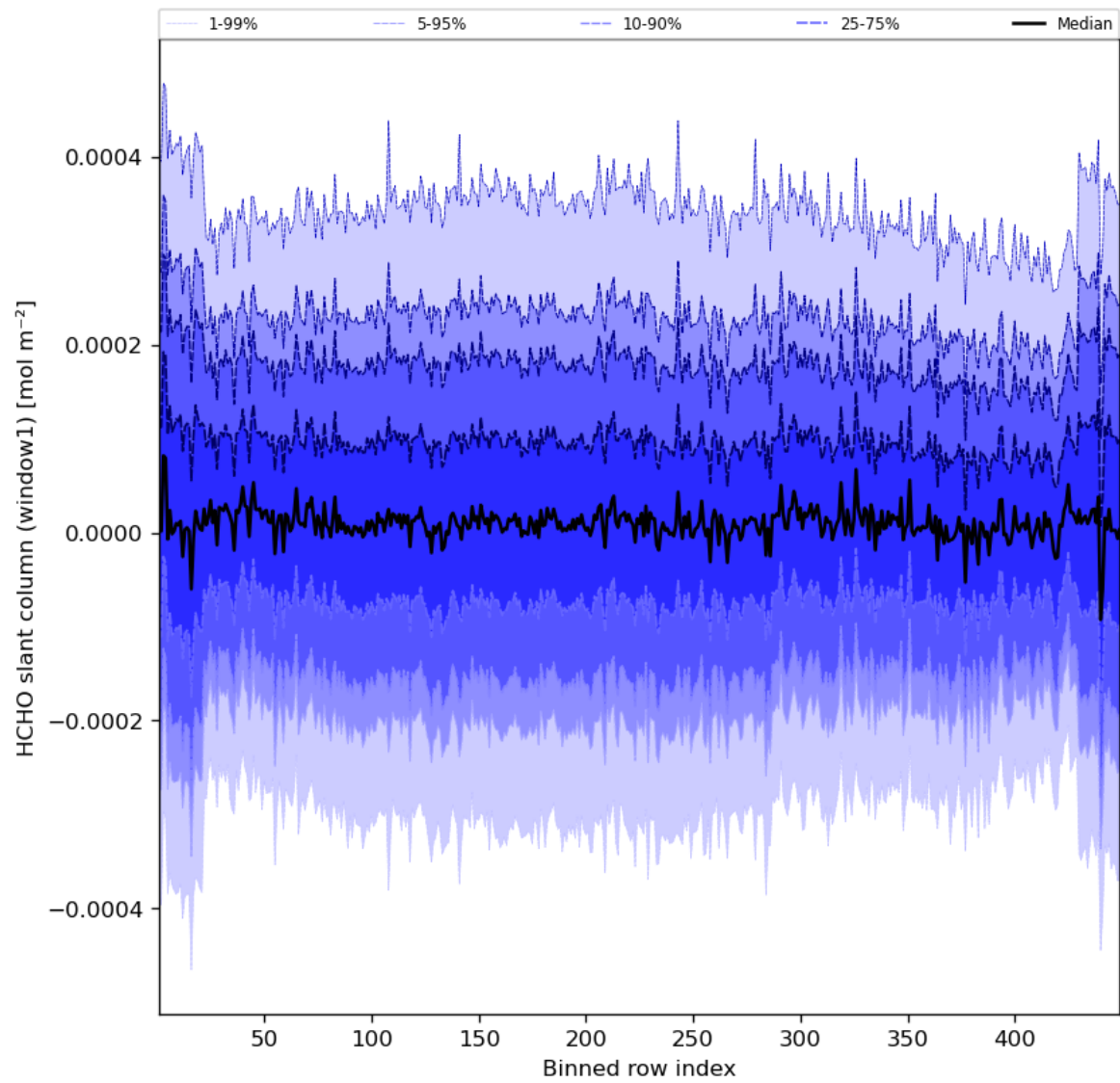
Figure 52: Along track statistics of “HCHO slant column (window1)” for 2023-09-07 to 2023-09-09
