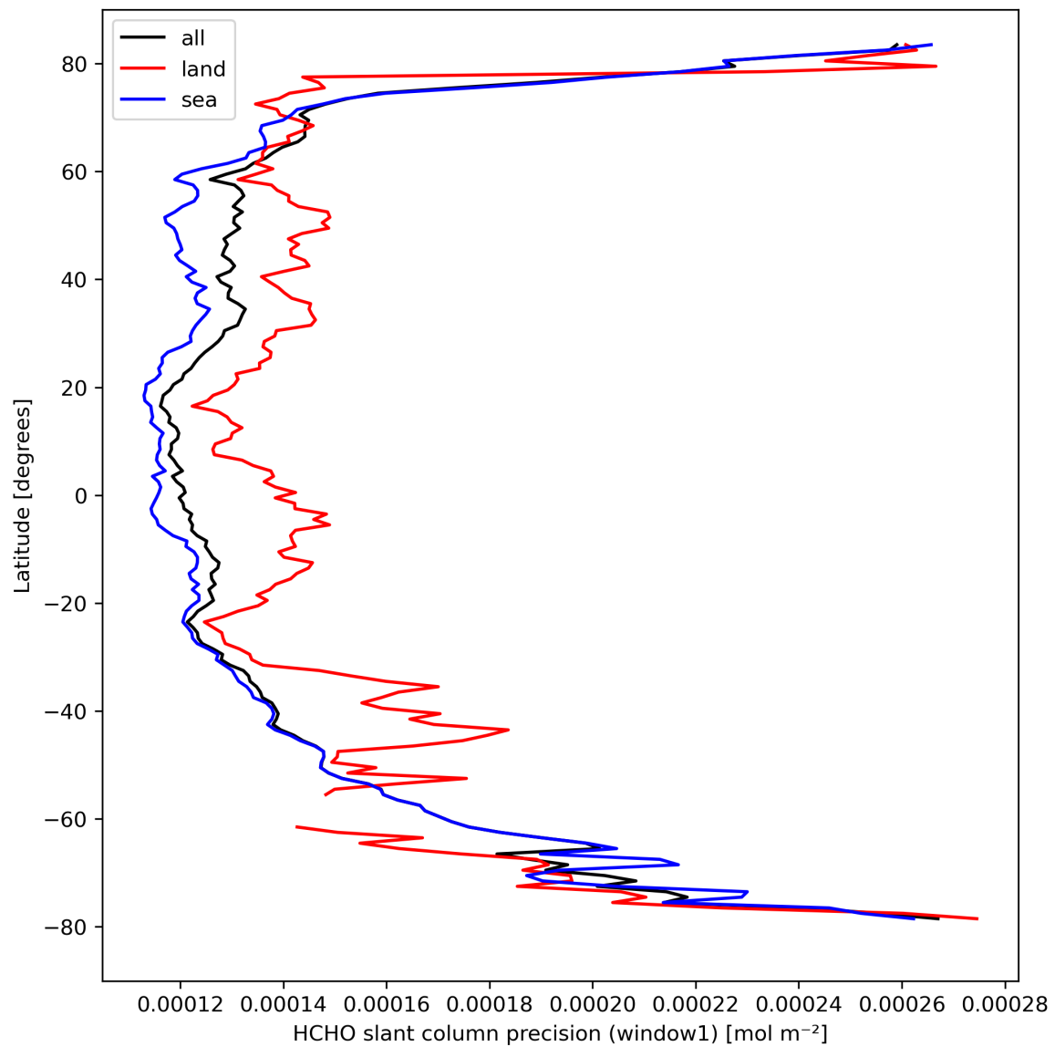
Figure 25: Zonal average of “HCHO slant column precision (window1)” for 2023-09-07 to 2023-09-09.
