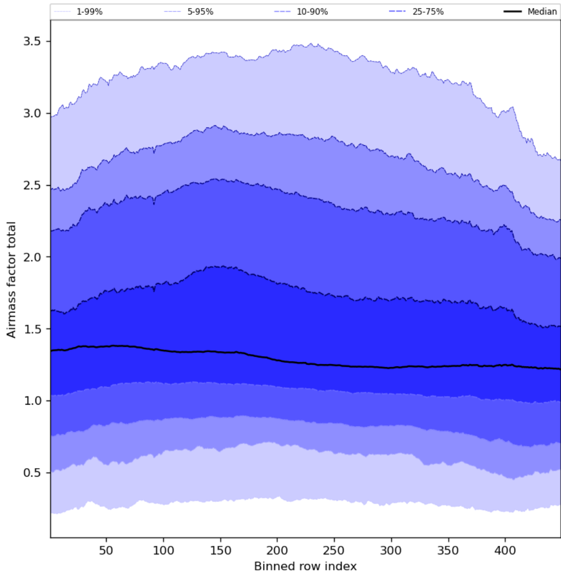
Figure 54: Along track statistics of “Airmass factor total” for 2023-09-07 to 2023-09-09
