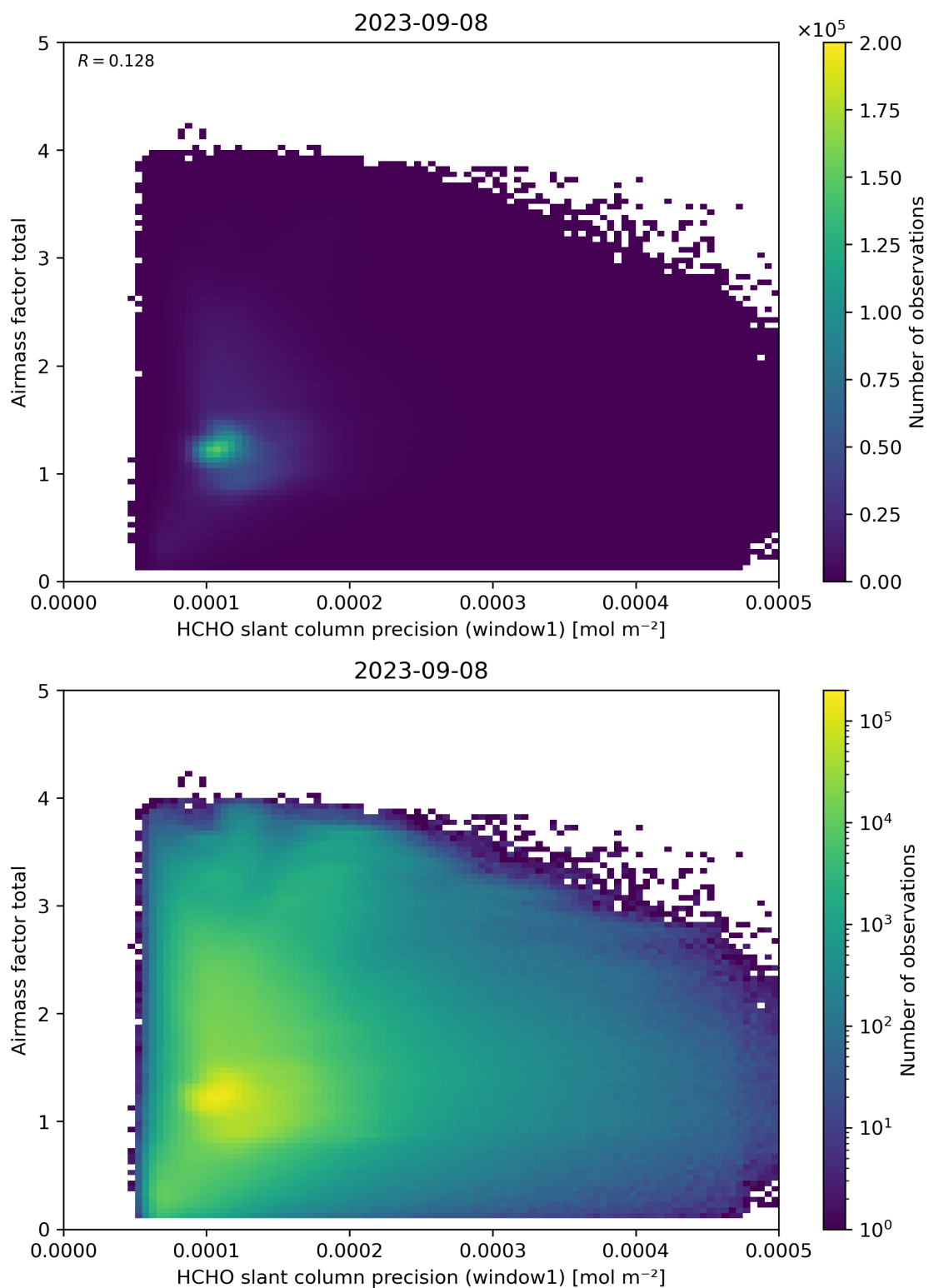
Figure 94: Scatter density plot of “HCHO slant column precision (window1)” against “Airmass factor total” for 2023-09-07 to 2023-09-09.
