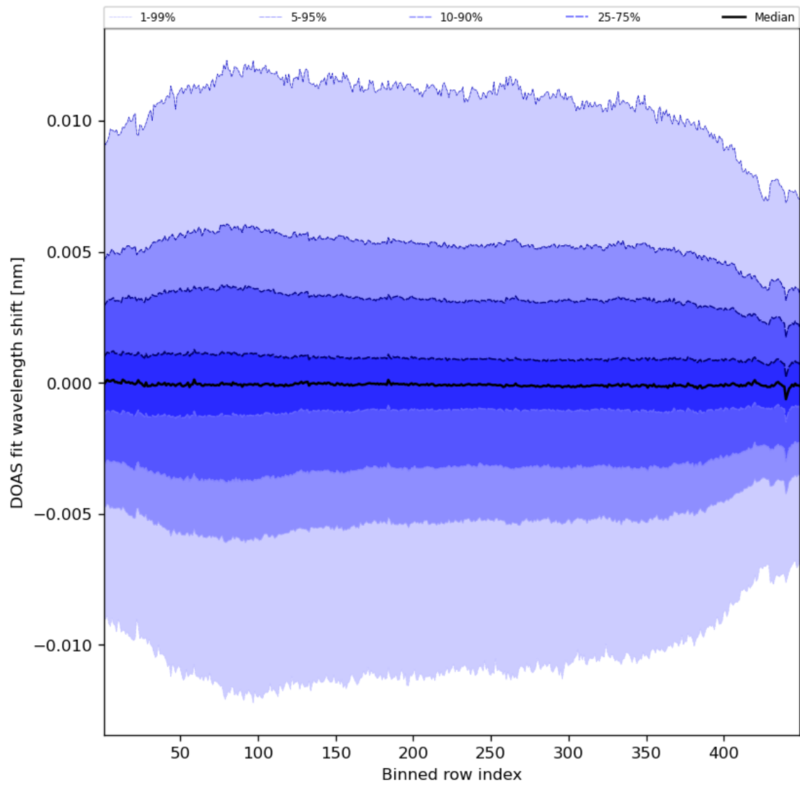
Figure 58: Along track statistics of “DOAS fit wavelength shift” for 2023-09-07 to 2023-09-09
