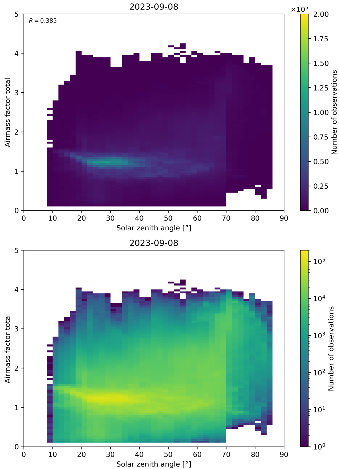
Figure 175: Scatter density plot of “Solar zenith angle” against “Airmass factor total” for 2023-09-07 to 2023-09-09.
