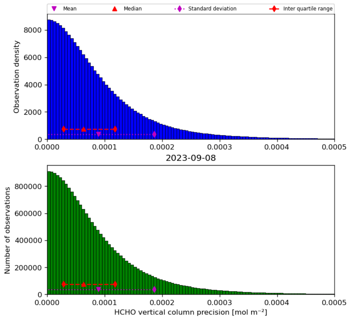
Figure 36: Histogram of “HCHO vertical column precision” for 2023-09-07 to 2023-09-09
