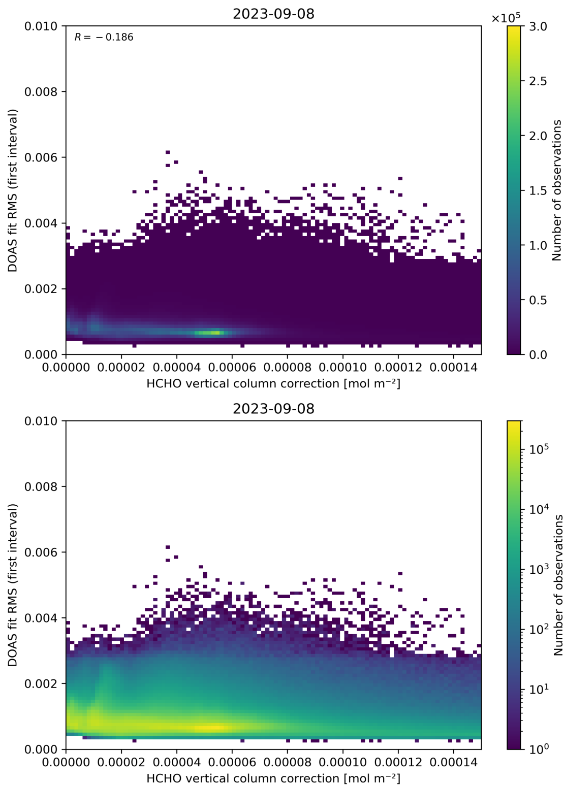
Figure 112: Scatter density plot of “HCHO vertical column correction” against “DOAS fit RMS (first interval)” for 2023-09-07 to 2023-09-09.
