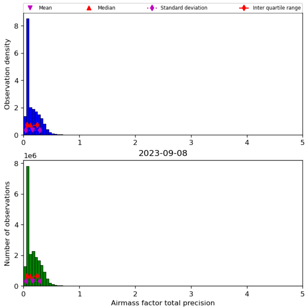
Figure 41: Histogram of "Airmass factor total precision" for 2023-09-07 to 2023-09-09
