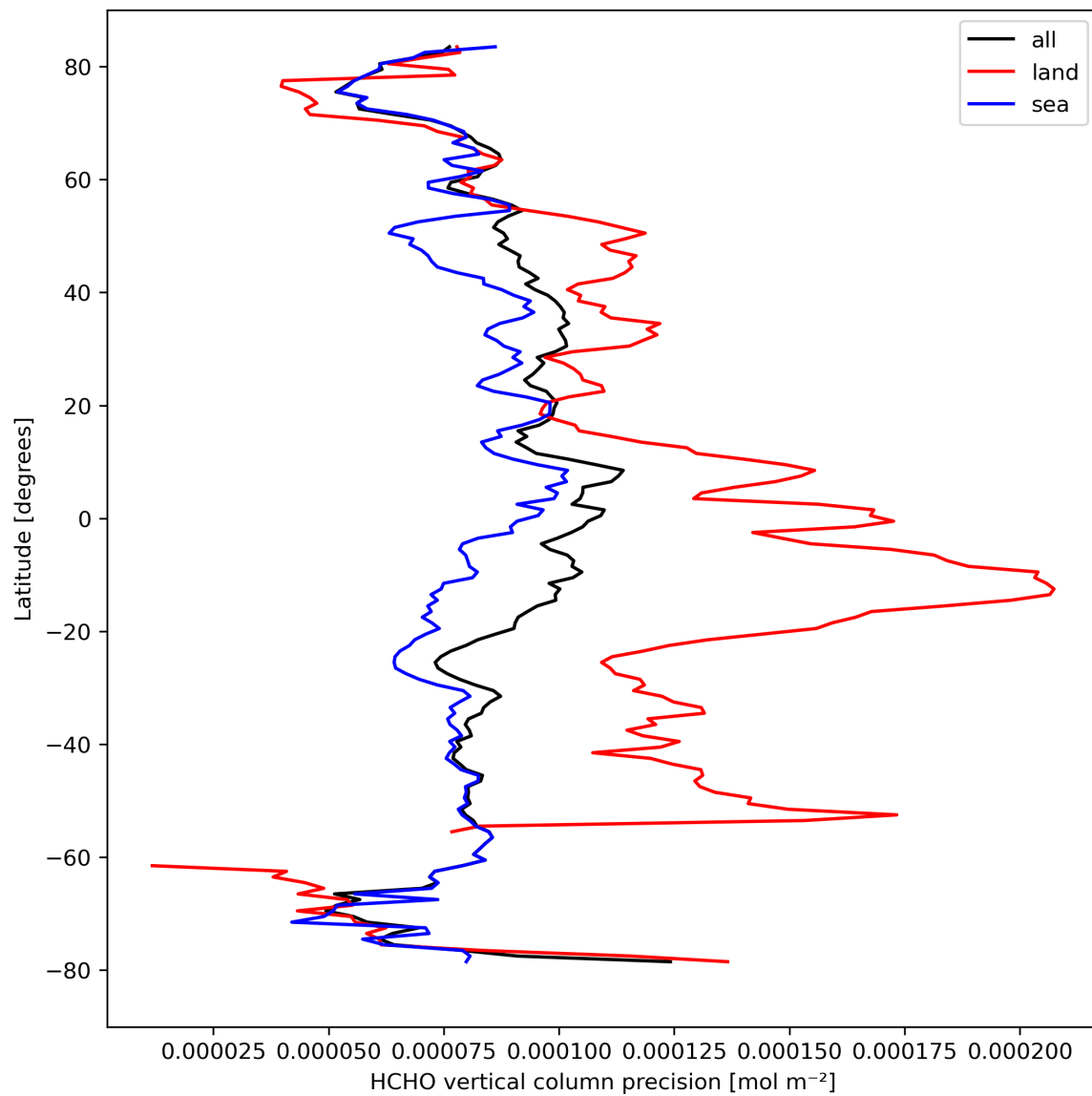
Figure 22: Zonal average of “HCHO vertical column precision” for 2023-09-07 to 2023-09-09.
