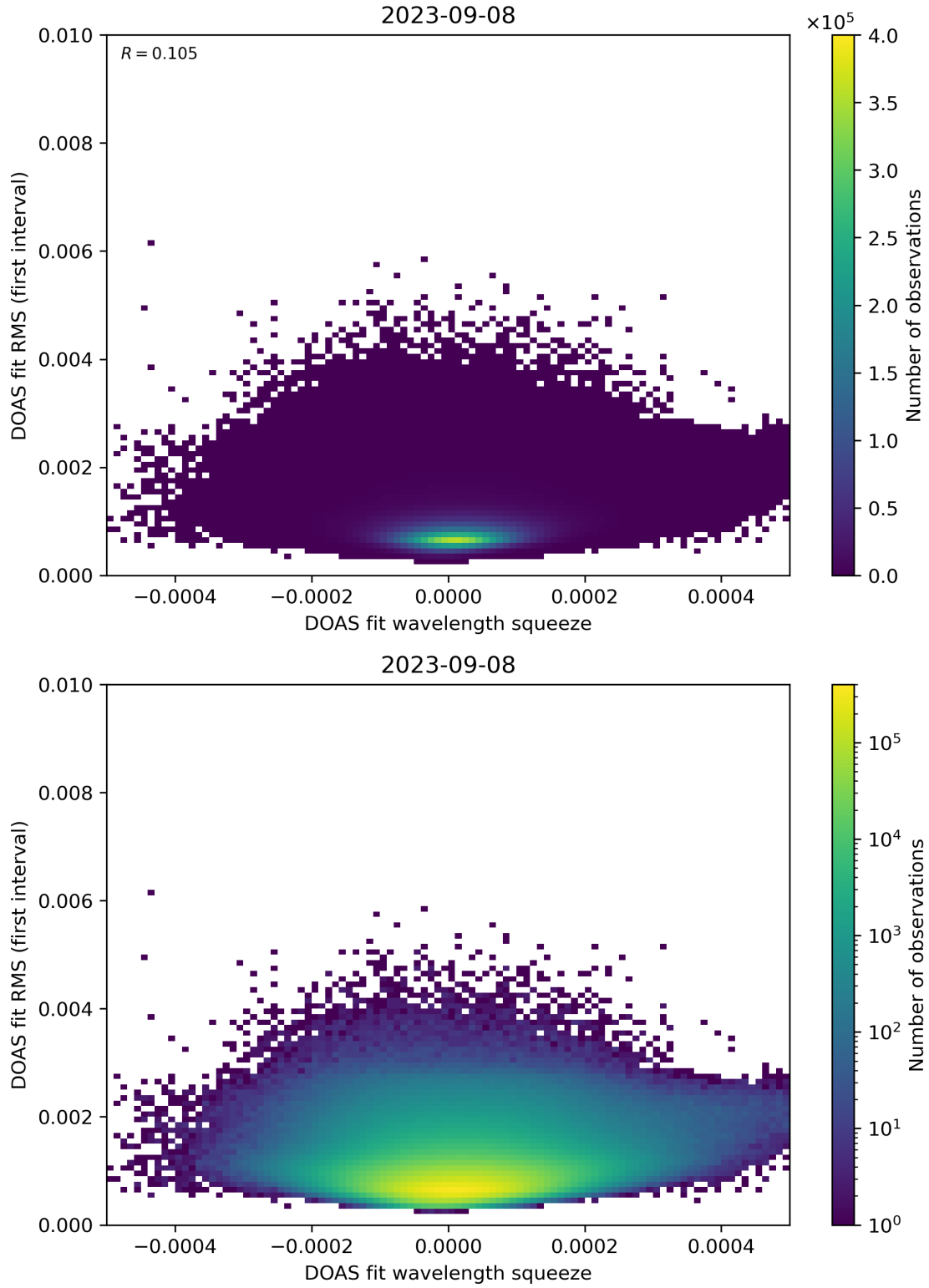
Figure 68: Scatter density plot of “DOAS fit wavelength squeeze” against “DOAS fit RMS (first interval)” for 2023-09-07 to 2023-09-09.
