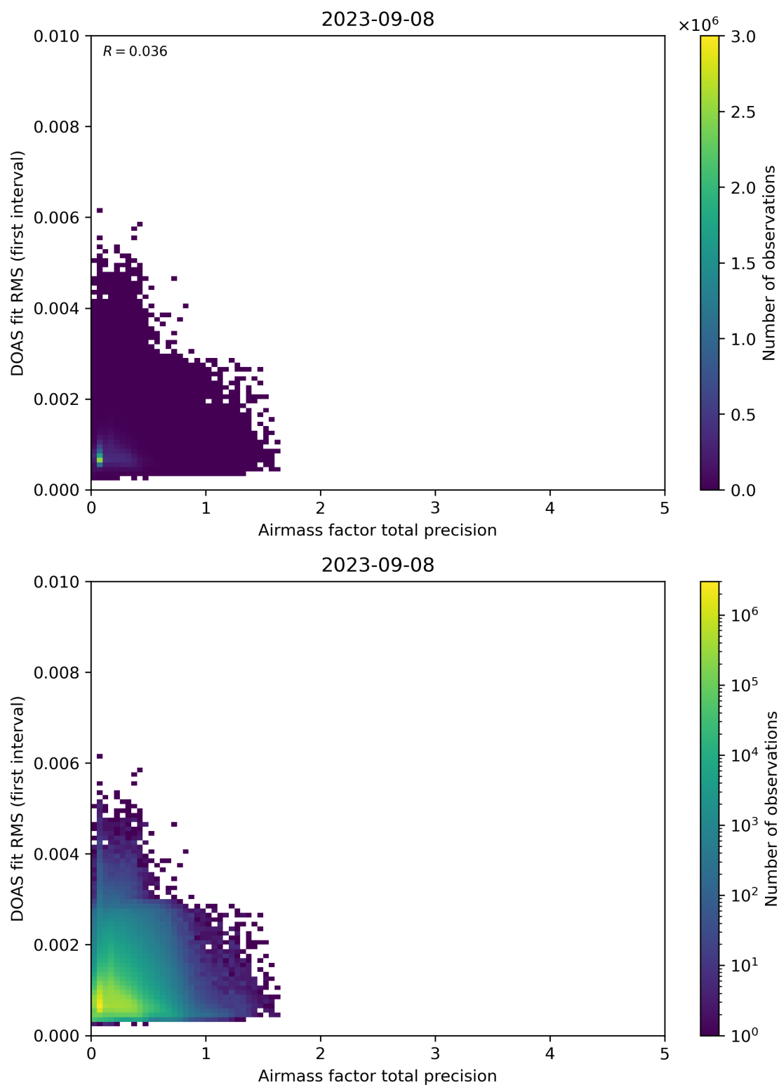
Figure 105: Scatter density plot of “Airmass factor total precision” against “DOAS fit RMS (first interval)” for 2023-09-07 to 2023-09-09.
