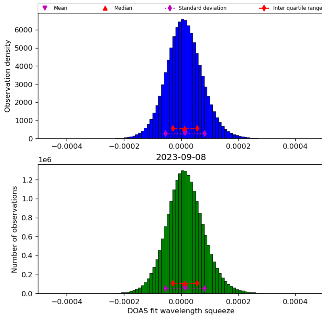
Figure 45: Histogram of “DOAS fit wavelength squeeze” for 2023-09-07 to 2023-09-09
