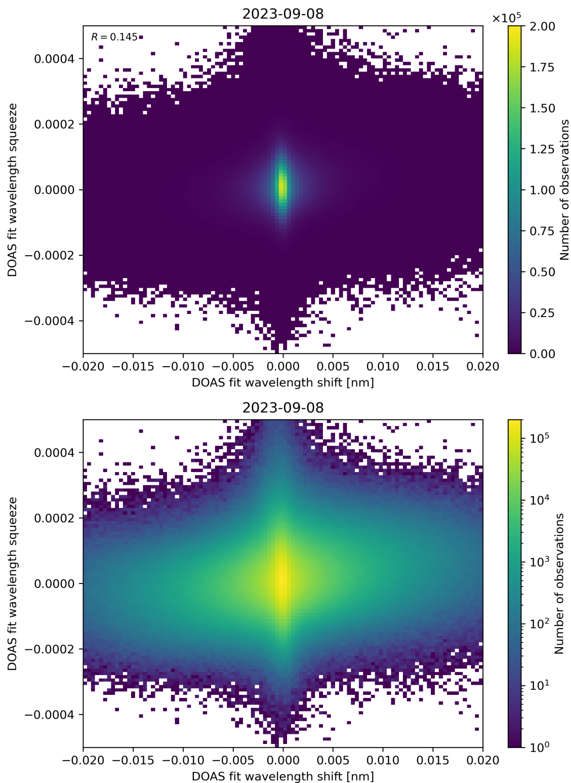
Figure 65: Scatter density plot of “DOAS fit wavelength shift” against “DOAS fit wavelength squeeze” for 2023-09-07 to 2023-09-09.
