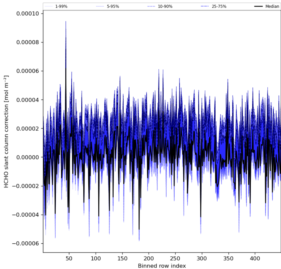
Figure 61: Along track statistics of “HCHO slant column correction” for 2023-09-07 to 2023-09-09
