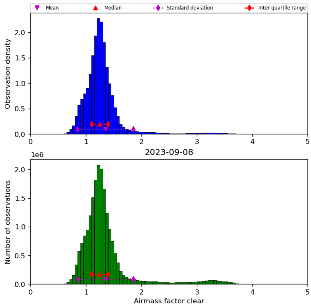
Figure 42: Histogram of "Airmass factor clear" for 2023-09-07 to 2023-09-09
