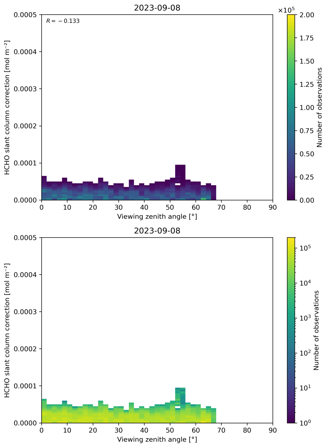
Figure 187: Scatter density plot of “Viewing zenith angle” against “HCHO slant column correction” for 2023-09-07 to 2023-09-09.
