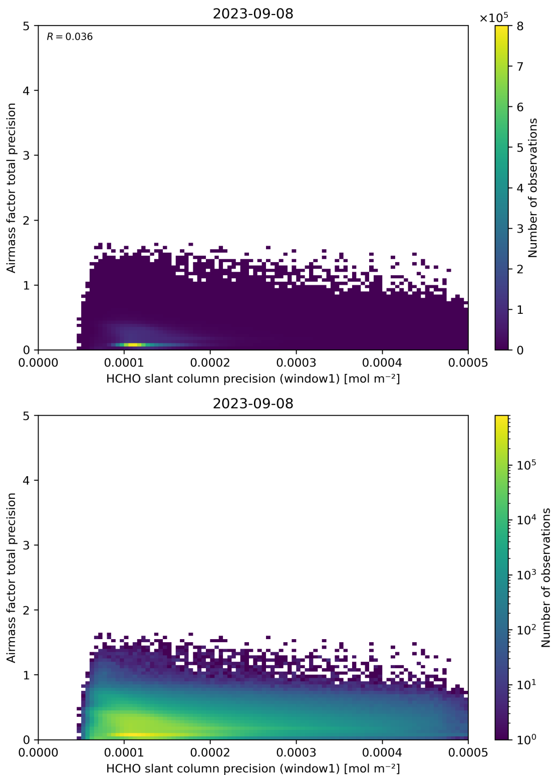
Figure 95: Scatter density plot of “HCHO slant column precision (window1)” against “Airmass factor total precision” for 2023-09-07 to 2023-09-09.
