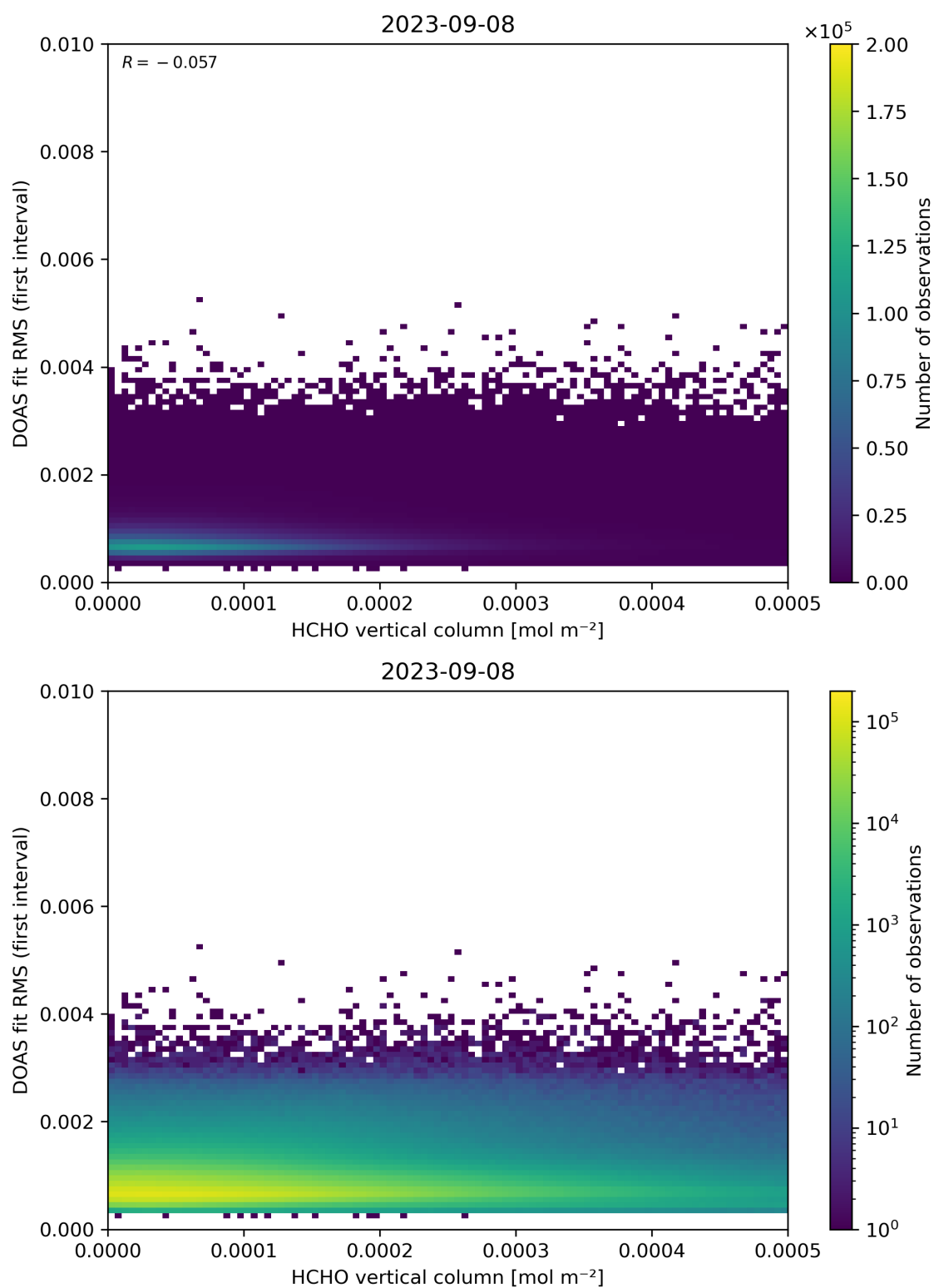
Figure 123: Scatter density plot of “HCHO vertical column” against “DOAS fit RMS (first interval)” for 2023-09-07 to 2023-09-09.
