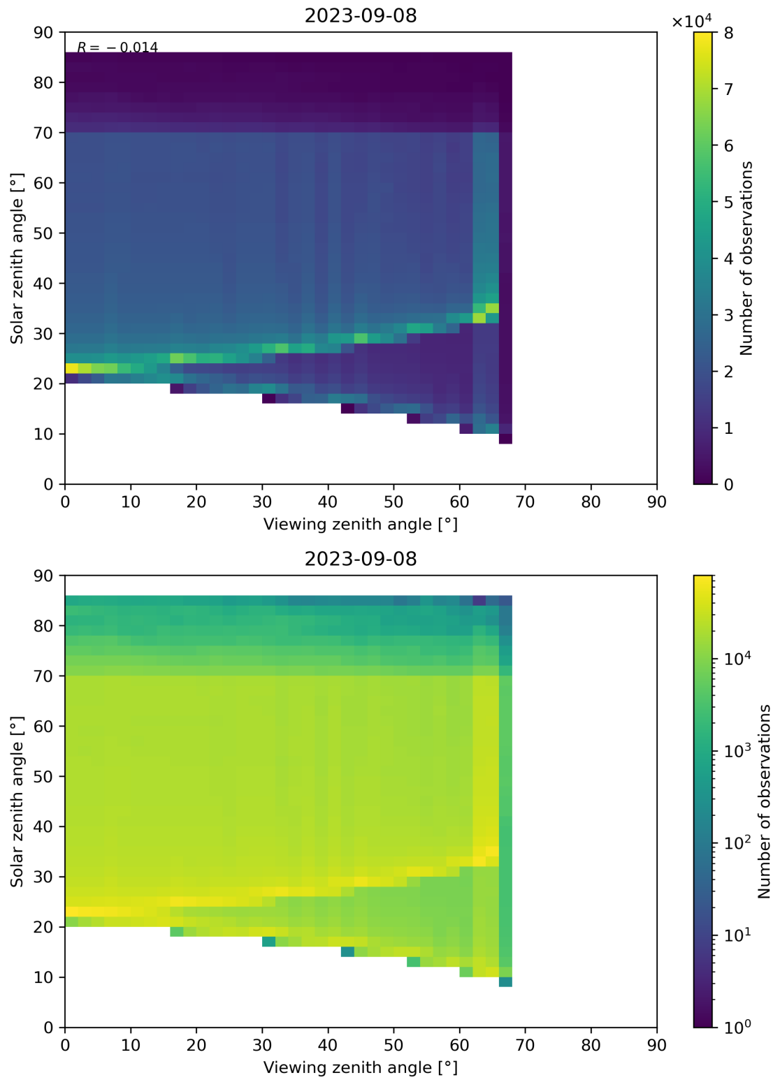
Figure 197: Scatter density plot of “Viewing zenith angle” against “Solar zenith angle” for 2023-09-07 to 2023-09-09.
