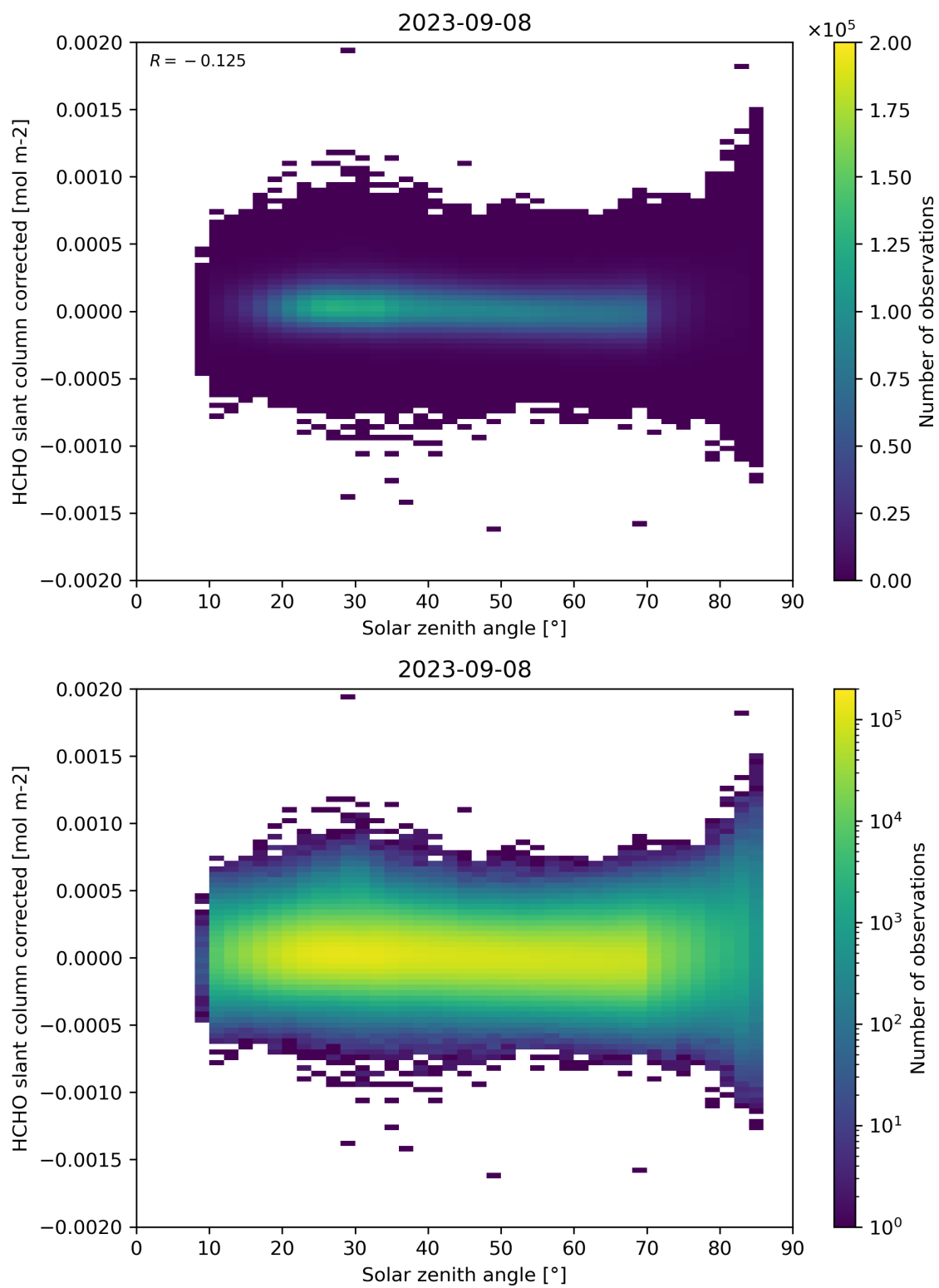
Figure 171: Scatter density plot of “Solar zenith angle” against “HCHO slant column corrected” for 2023-09-07 to 2023-09-09.
