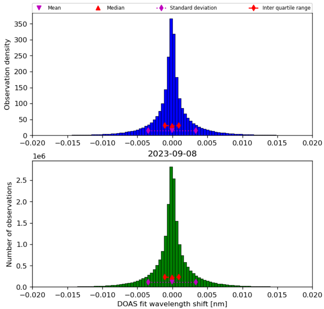
Figure 44: Histogram of “DOAS fit wavelength shift” for 2023-09-07 to 2023-09-09
