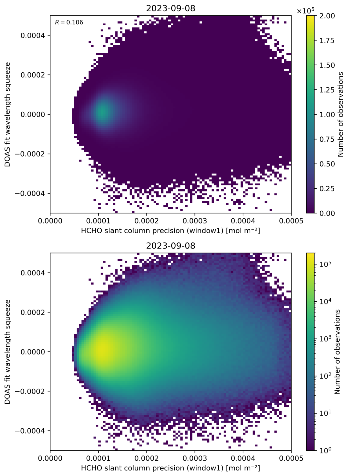
Figure 90: Scatter density plot of “HCHO slant column precision (window1)” against “DOAS fit wavelength squeeze” for 2023-09-07 to 2023-09-09.
