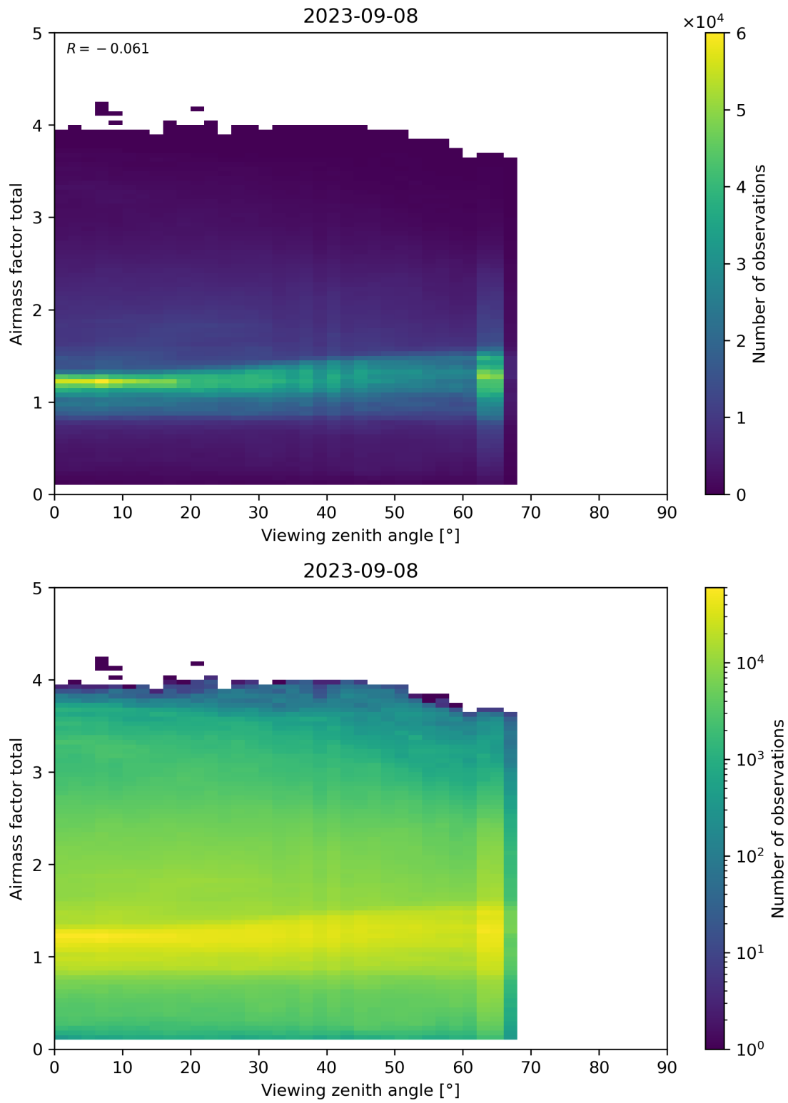
Figure 190: Scatter density plot of “Viewing zenith angle” against “Airmass factor total” for 2023-09-07 to 2023-09-09.
