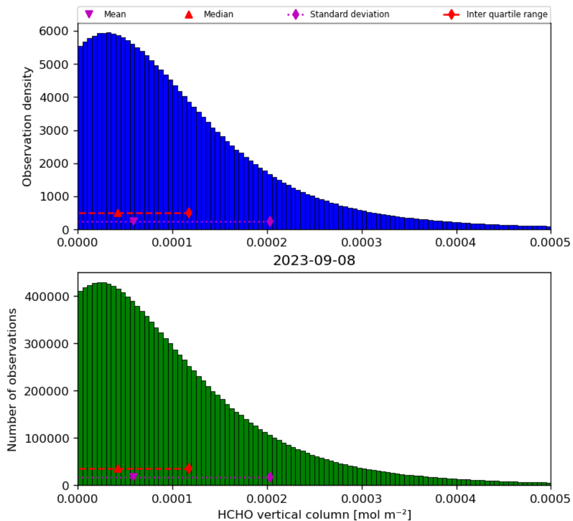
Figure 35: Histogram of “HCHO vertical column” for 2023-09-07 to 2023-09-09
