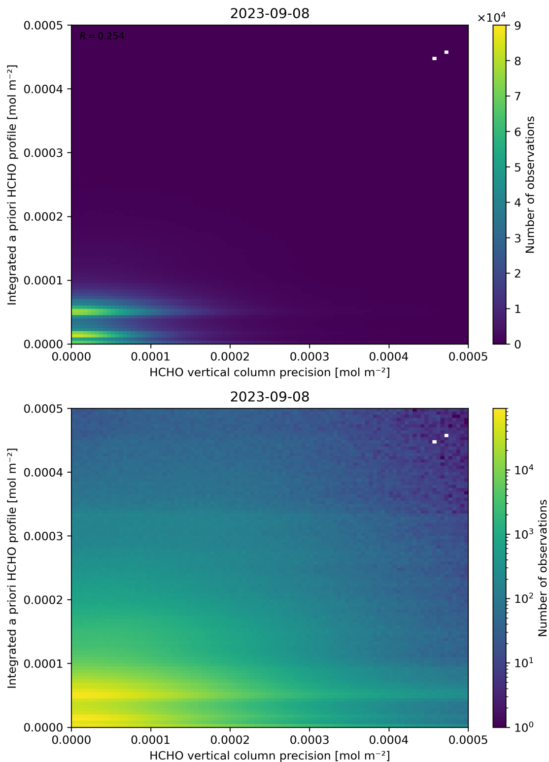
Figure 147: Scatter density plot of “HCHO vertical column precision” against “Integrated a priori HCHO profile” for 2023-09-07 to 2023-09-09.
