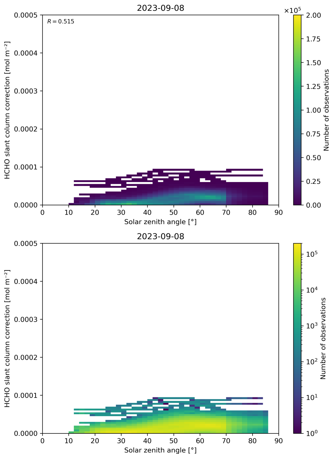
Figure 172: Scatter density plot of “Solar zenith angle” against “HCHO slant column correction” for 2023-09-07 to 2023-09-09.
