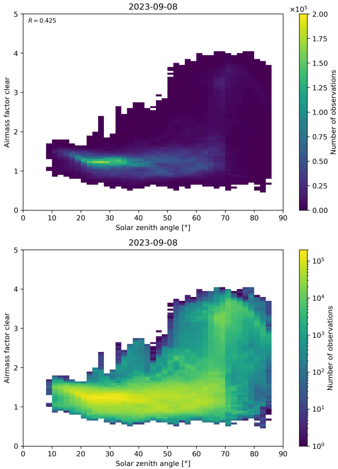
Figure 170: Scatter density plot of “Solar zenith angle” against “Airmass factor clear” for 2023-09-07 to 2023-09-09.
