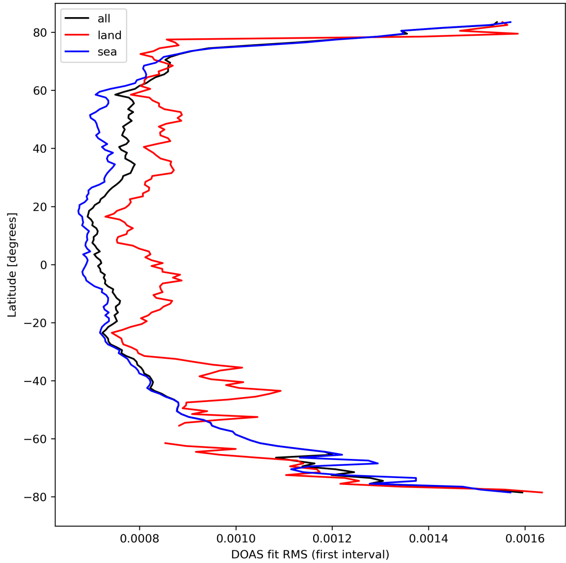
Figure 32: Zonal average of "DOAS fit RMS (first interval)" for 2023-09-07 to 2023-09-09.
