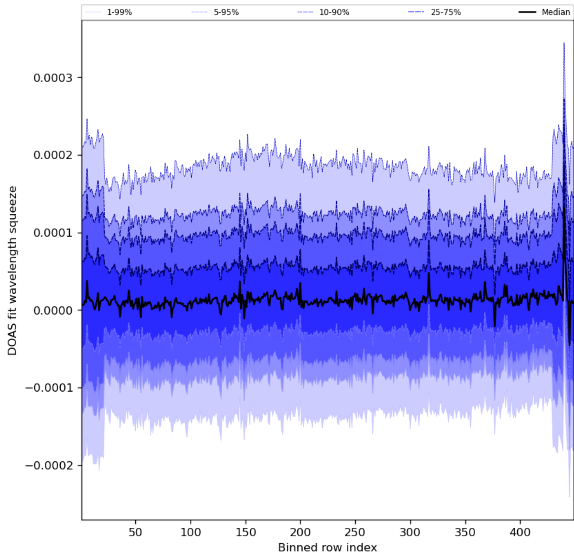
Figure 59: Along track statistics of “DOAS fit wavelength squeeze” for 2023-09-07 to 2023-09-09
