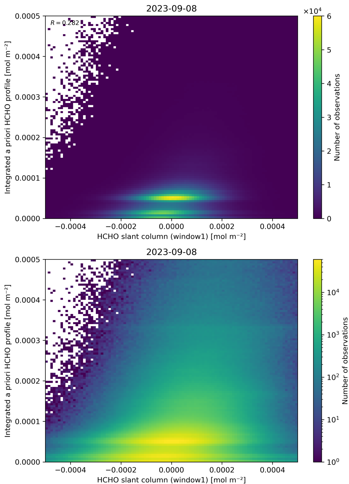
Figure 87: Scatter density plot of “HCHO slant column (window1)” against “Integrated a priori HCHO profile” for 2023-09-07 to 2023-09-09.
