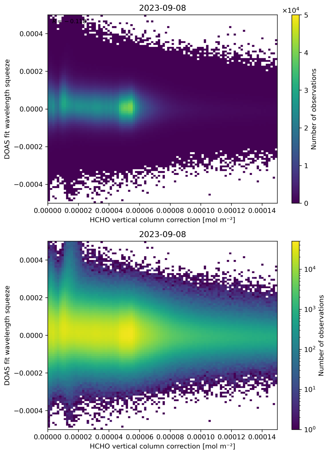
Figure 114: Scatter density plot of “HCHO vertical column correction” against “DOAS fit wavelength squeeze” for 2023-09-07 to 2023-09-09.
