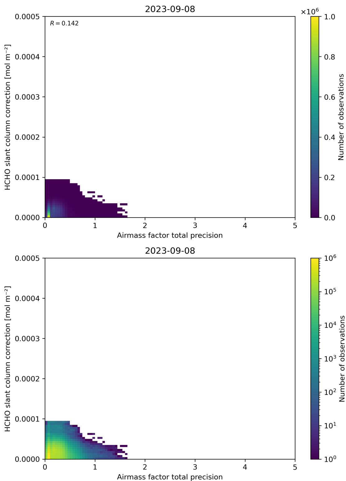
Figure 110: Scatter density plot of “Airmass factor total precision” against “HCHO slant column correction” for 2023-09-07 to 2023-09-09.
