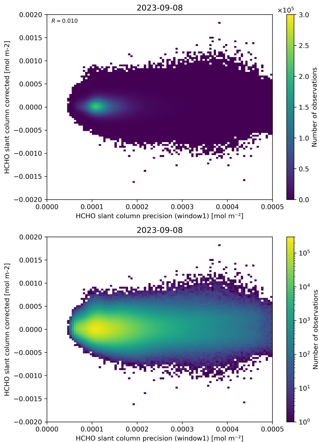
Figure 92: Scatter density plot of “HCHO slant column precision (window1)” against “HCHO slant column corrected” for 2023-09-07 to 2023-09-09.
