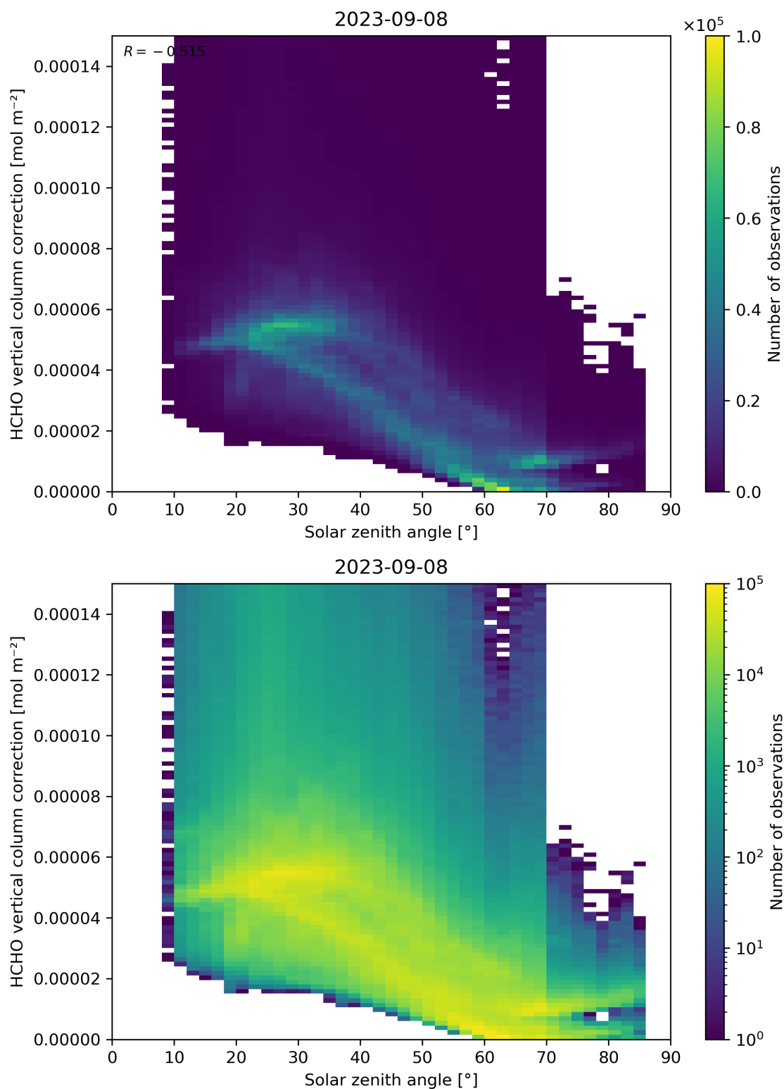
Figure 178: Scatter density plot of “Solar zenith angle” against “HCHO vertical column correction” for 2023-09-07 to 2023-09-09.
