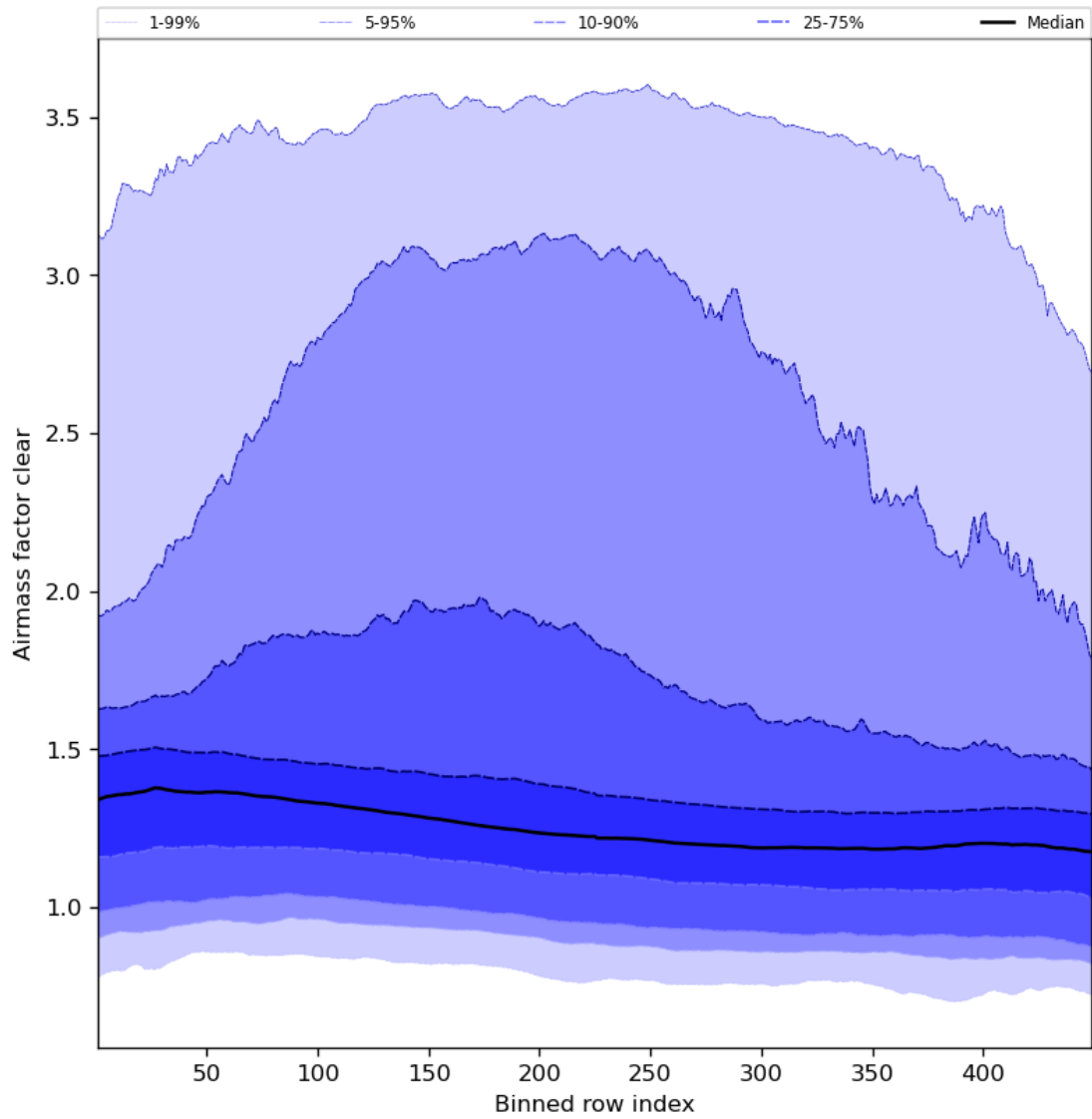
Figure 56: Along track statistics of “Airmass factor clear” for 2023-09-07 to 2023-09-09
