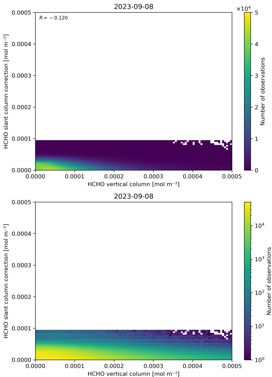
Figure 128: Scatter density plot of “HCHO vertical column” against “HCHO slant column correction” for 2023-09-07 to 2023-09-09.
