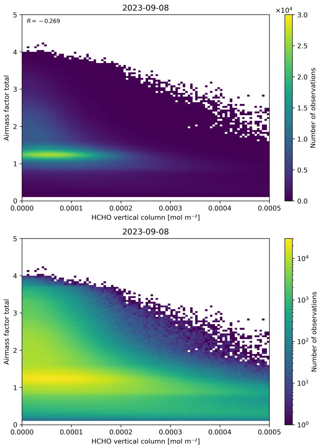
Figure 131: Scatter density plot of “HCHO vertical column” against “Airmass factor total” for 2023-09-07 to 2023-09-09.
