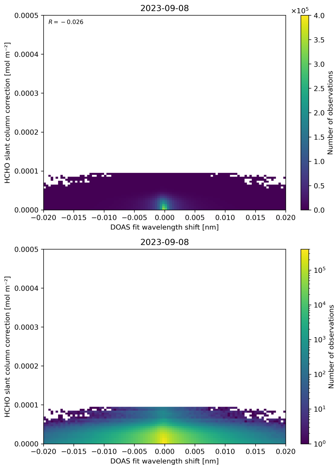
Figure 67: Scatter density plot of “DOAS fit wavelength shift” against “HCHO slant column correction” for 2023-09-07 to 2023-09-09.
