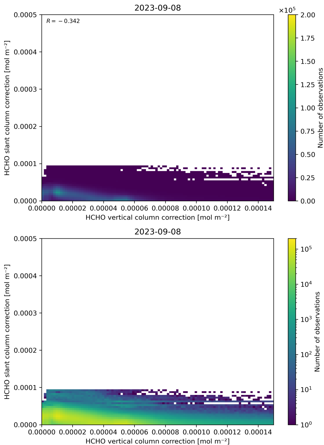
Figure 117: Scatter density plot of “HCHO vertical column correction” against “HCHO slant column correction” for 2023-09-07 to 2023-09-09.
