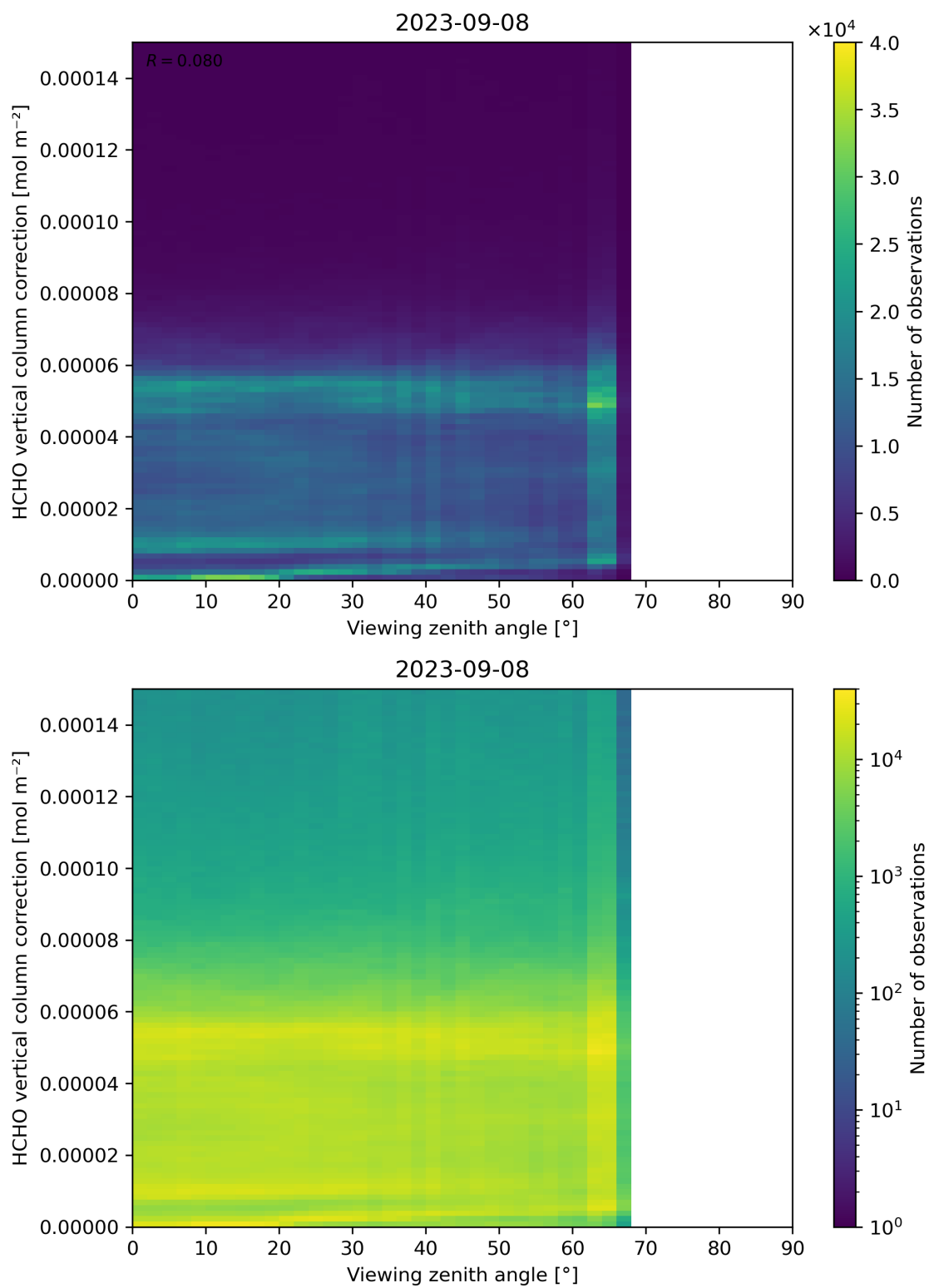
Figure 193: Scatter density plot of “Viewing zenith angle” against “HCHO vertical column correction” for 2023-09-07 to 2023-09-09.
