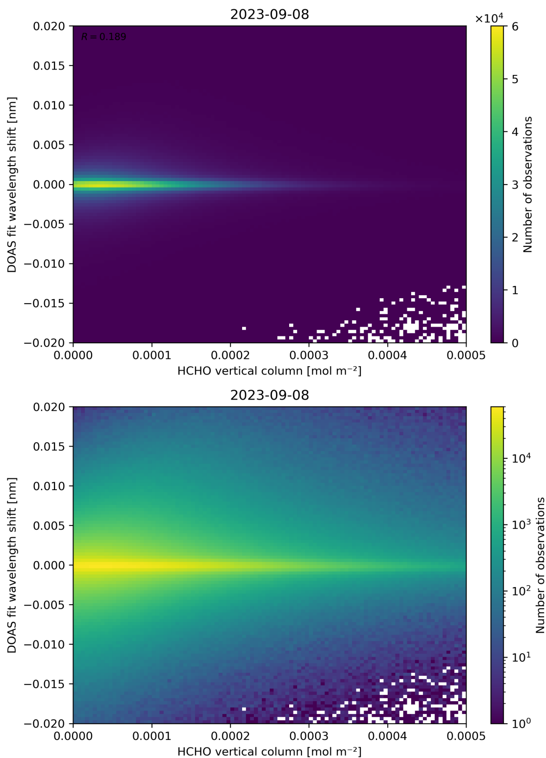
Figure 124: Scatter density plot of “HCHO vertical column” against “DOAS fit wavelength shift” for 2023-09-07 to 2023-09-09.
