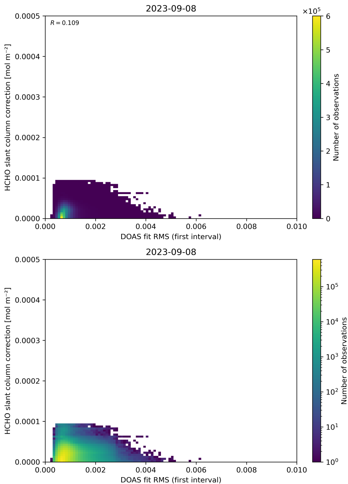
Figure 63: Scatter density plot of “DOAS fit RMS (first interval)” against “HCHO slant column correction” for 2023-09-07 to 2023-09-09.
