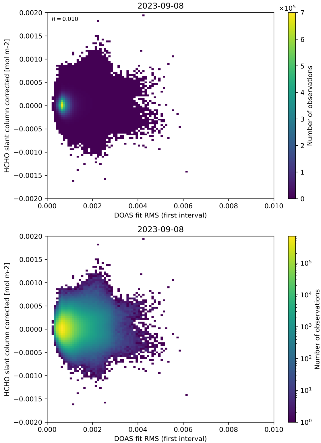
Figure 62: Scatter density plot of “DOAS fit RMS (first interval)” against “HCHO slant column corrected” for 2023-09-07 to 2023-09-09.
