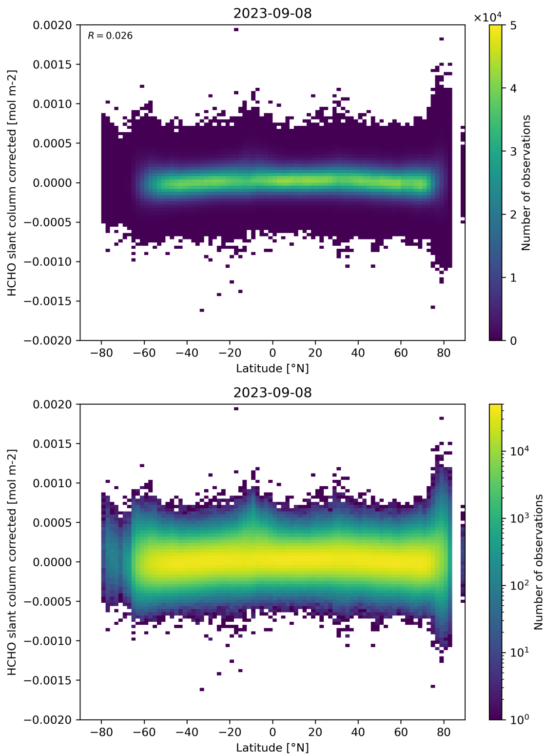
Figure 157: Scatter density plot of “Latitude” against “HCHO slant column corrected” for 2023-09-07 to 2023-09-09.
