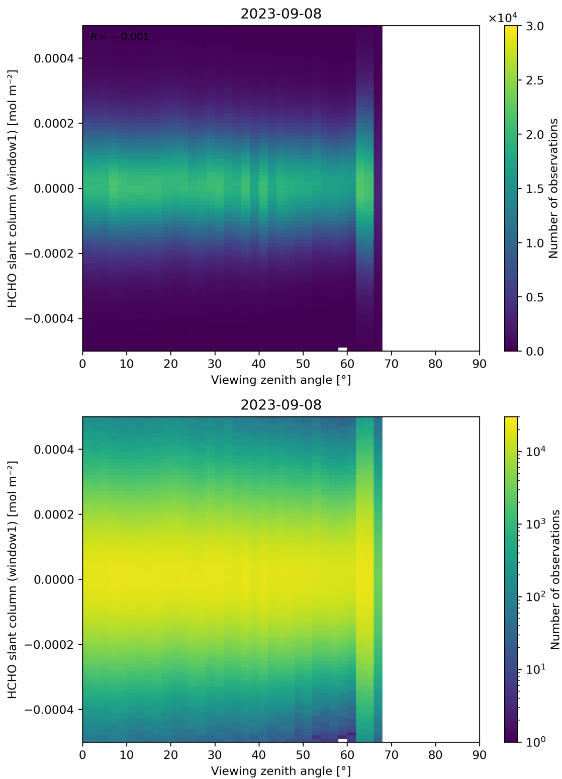
Figure 188: Scatter density plot of “Viewing zenith angle” against “HCHO slant column (window1)” for 2023-09-07 to 2023-09-09.
