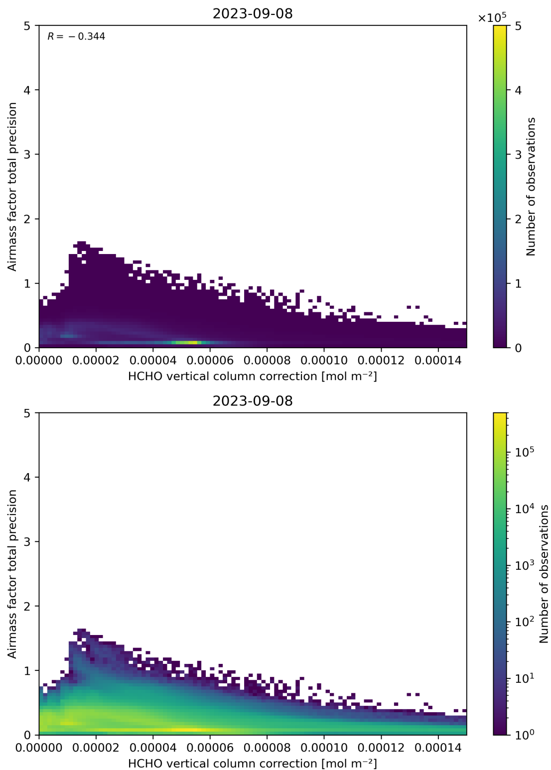
Figure 121: Scatter density plot of “HCHO vertical column correction” against “Airmass factor total precision” for 2023-09-07 to 2023-09-09.
