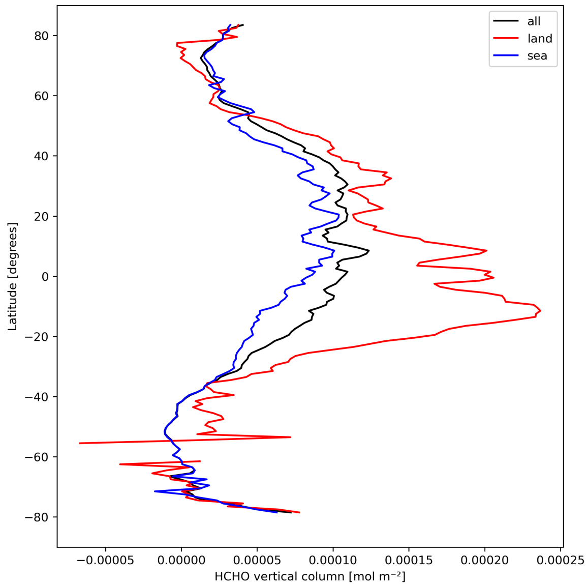
Figure 21: Zonal average of “HCHO vertical column” for 2023-09-07 to 2023-09-09.
