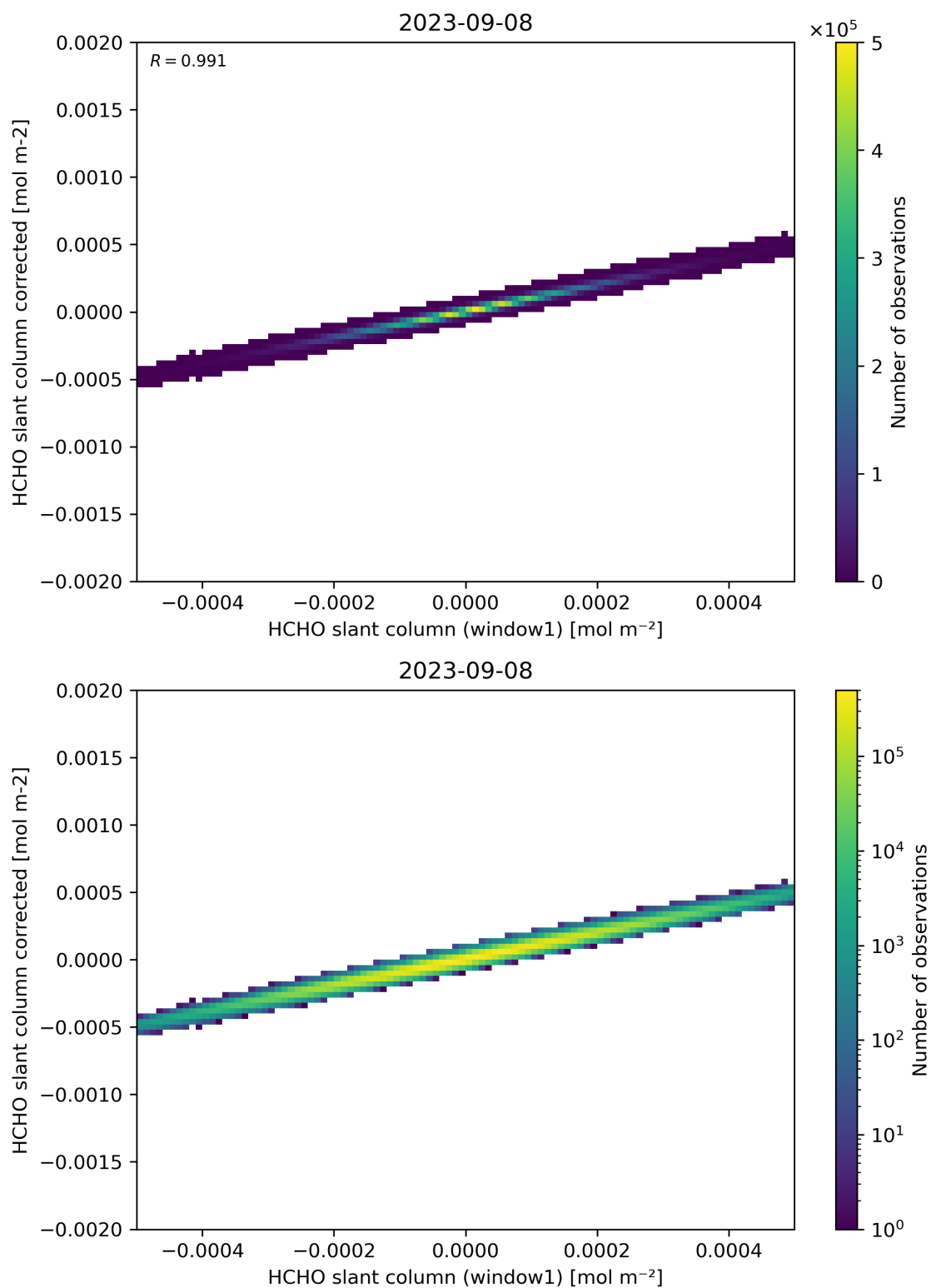
Figure 82: Scatter density plot of “HCHO slant column (window1)” against “HCHO slant column corrected” for 2023-09-07 to 2023-09-09.
