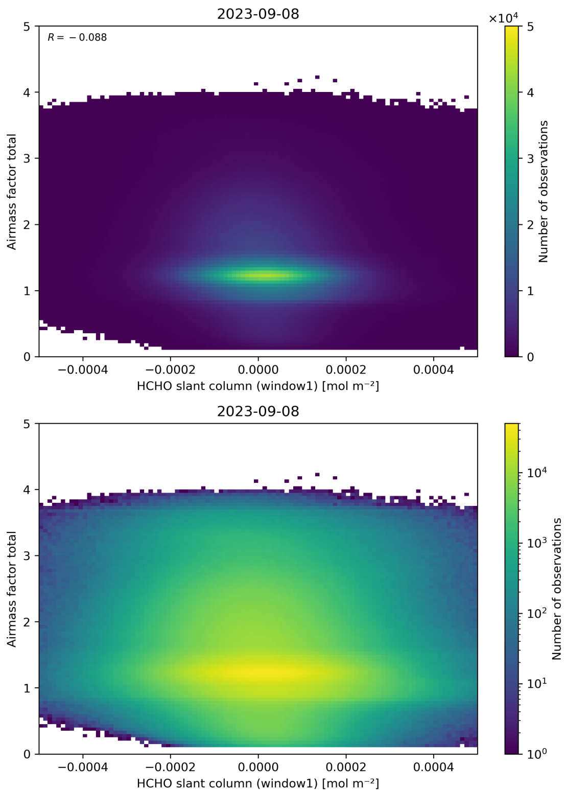
Figure 85: Scatter density plot of “HCHO slant column (window1)” against “Airmass factor total” for 2023-09-07 to 2023-09-09.
