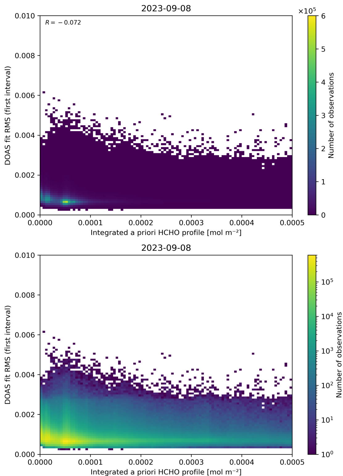
Figure 148: Scatter density plot of “Integrated a priori HCHO profile” against “DOAS fit RMS (first interval)” for 2023-09-07 to 2023-09-09.
