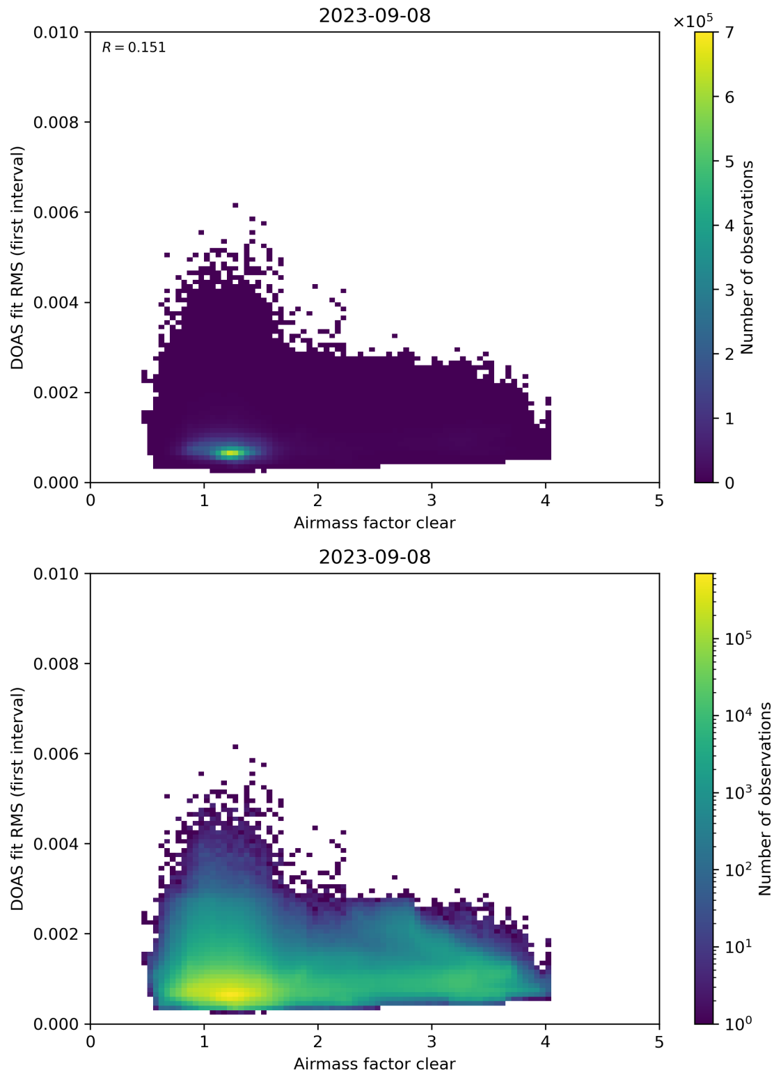
Figure 71: Scatter density plot of “Airmass factor clear” against “DOAS fit RMS (first interval)” for 2023-09-07 to 2023-09-09.
