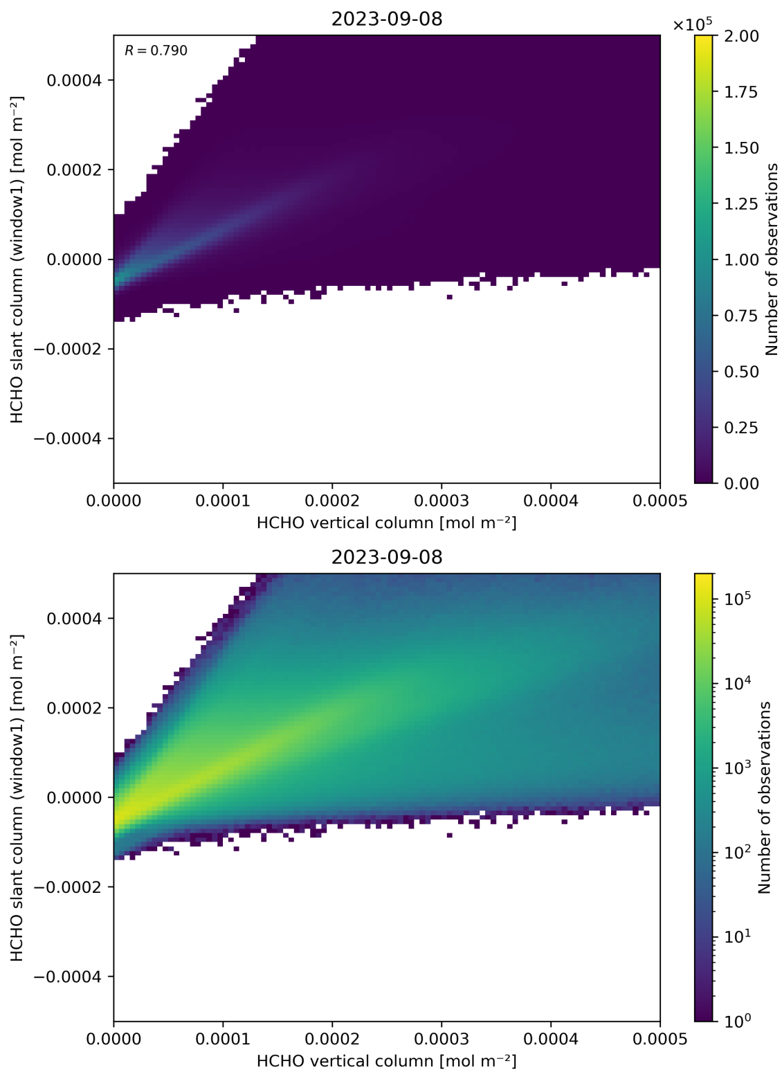
Figure 129: Scatter density plot of “HCHO vertical column” against “HCHO slant column (window1)” for 2023-09-07 to 2023-09-09.
