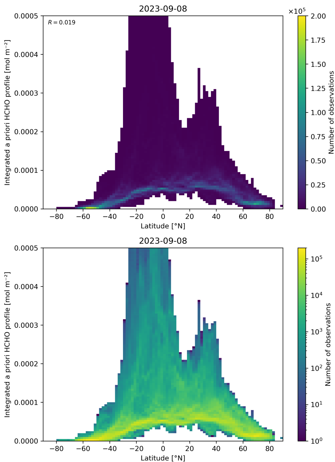
Figure 166: Scatter density plot of “Latitude” against “Integrated a priori HCHO profile” for 2023-09-07 to 2023-09-09.
