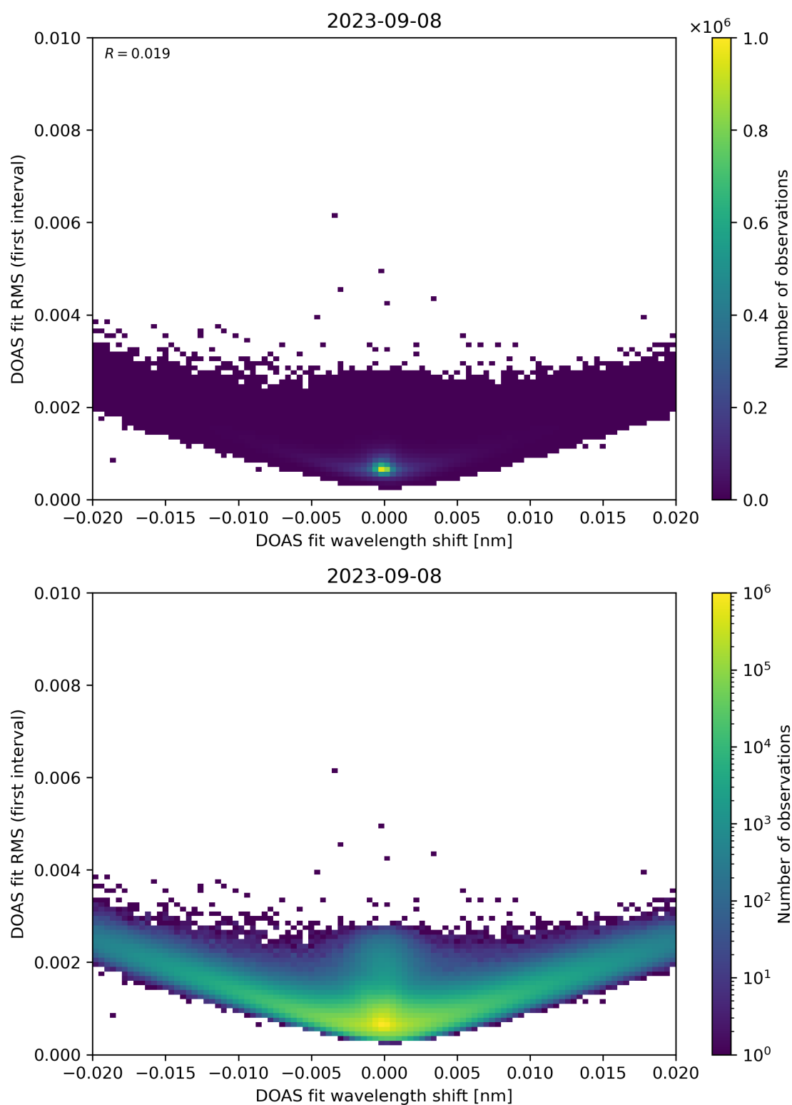
Figure 64: Scatter density plot of “DOAS fit wavelength shift” against “DOAS fit RMS (first interval)” for 2023-09-07 to 2023-09-09.
