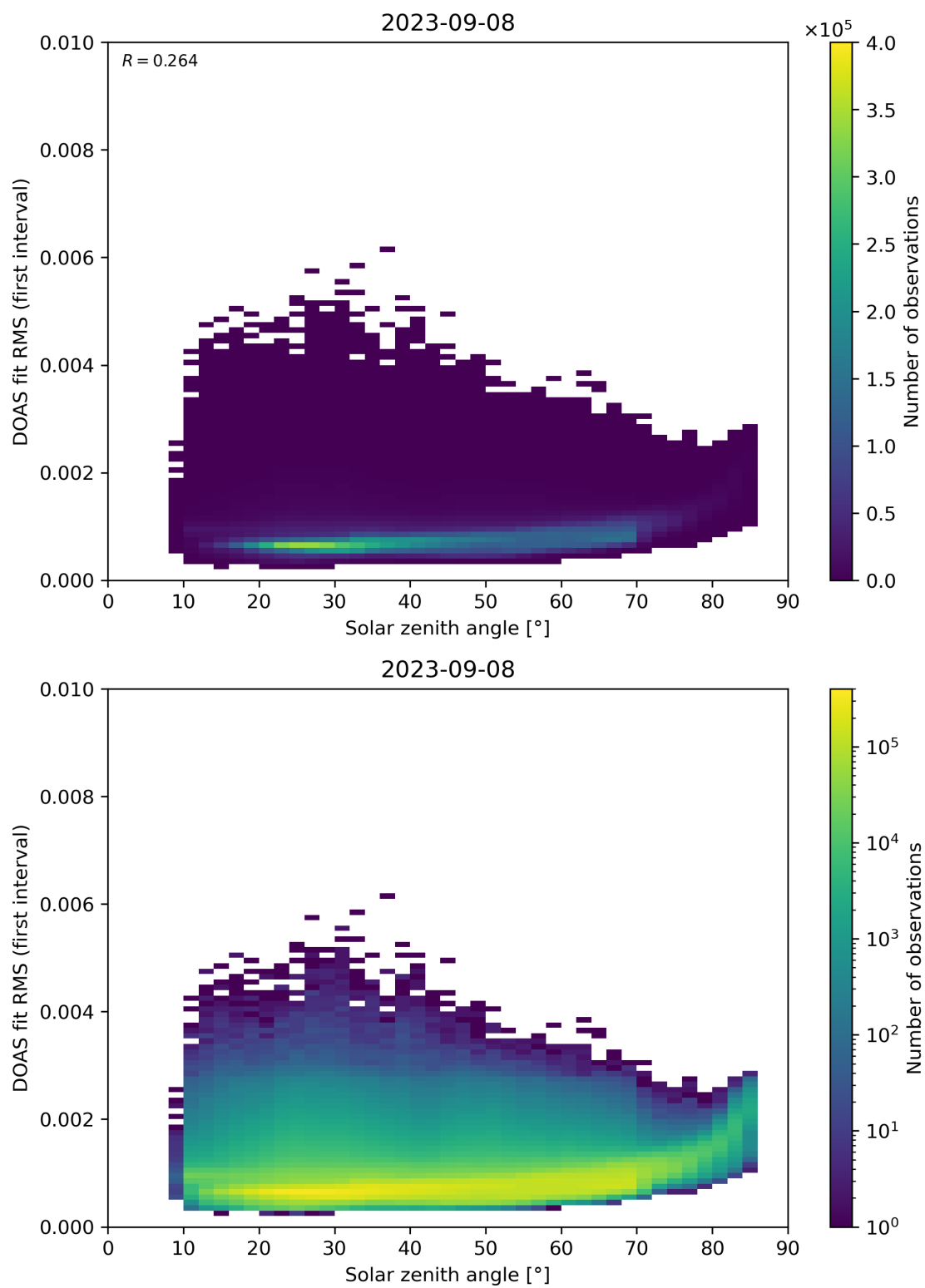
Figure 167: Scatter density plot of “Solar zenith angle” against “DOAS fit RMS (first interval)” for 2023-09-07 to 2023-09-09.
