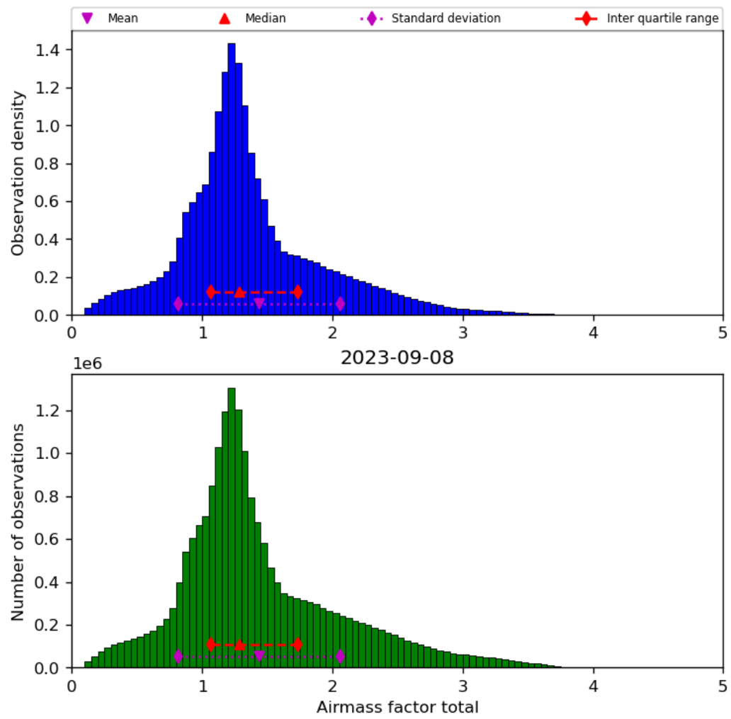
Figure 40: Histogram of “Airmass factor total” for 2023-09-07 to 2023-09-09
