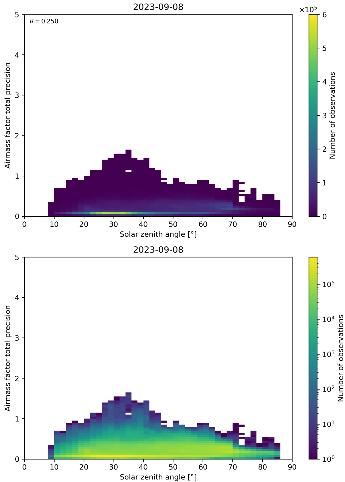
Figure 176: Scatter density plot of “Solar zenith angle” against “Airmass factor total precision” for 2023-09-07 to 2023-09-09.
