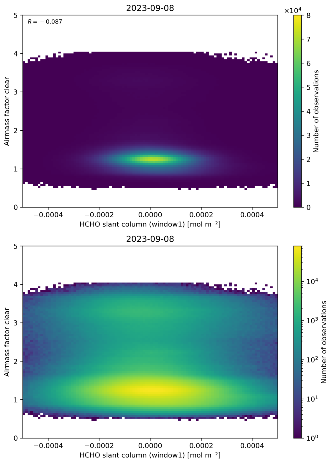
Figure 81: Scatter density plot of “HCHO slant column (window1)” against “Airmass factor clear” for 2023-09-07 to 2023-09-09.
