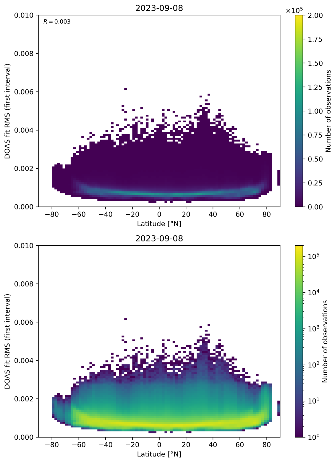
Figure 153: Scatter density plot of “Latitude” against “DOAS fit RMS (first interval)” for 2023-09-07 to 2023-09-09.
