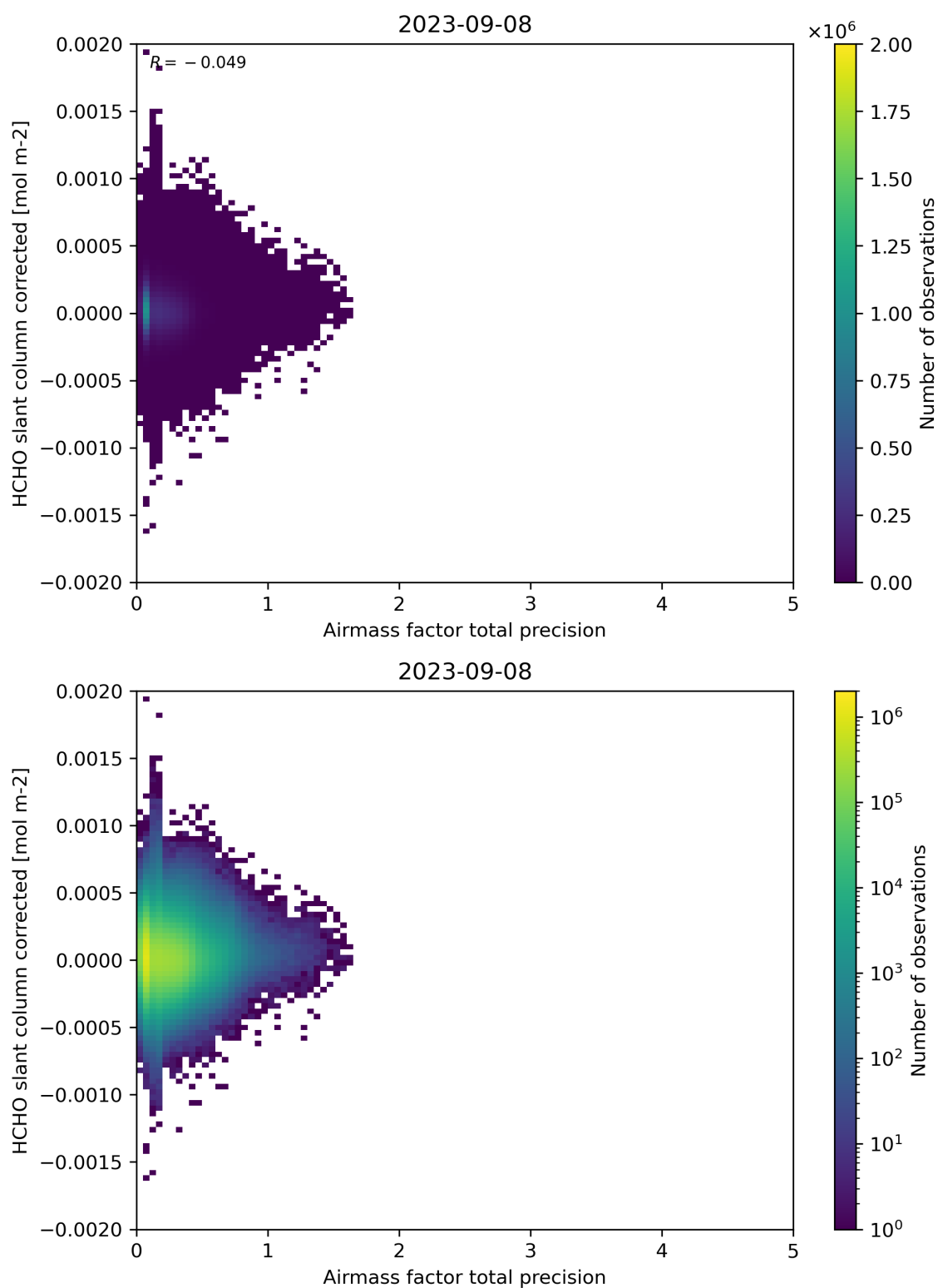
Figure 109: Scatter density plot of “Airmass factor total precision” against “HCHO slant column corrected” for 2023-09-07 to 2023-09-09.
