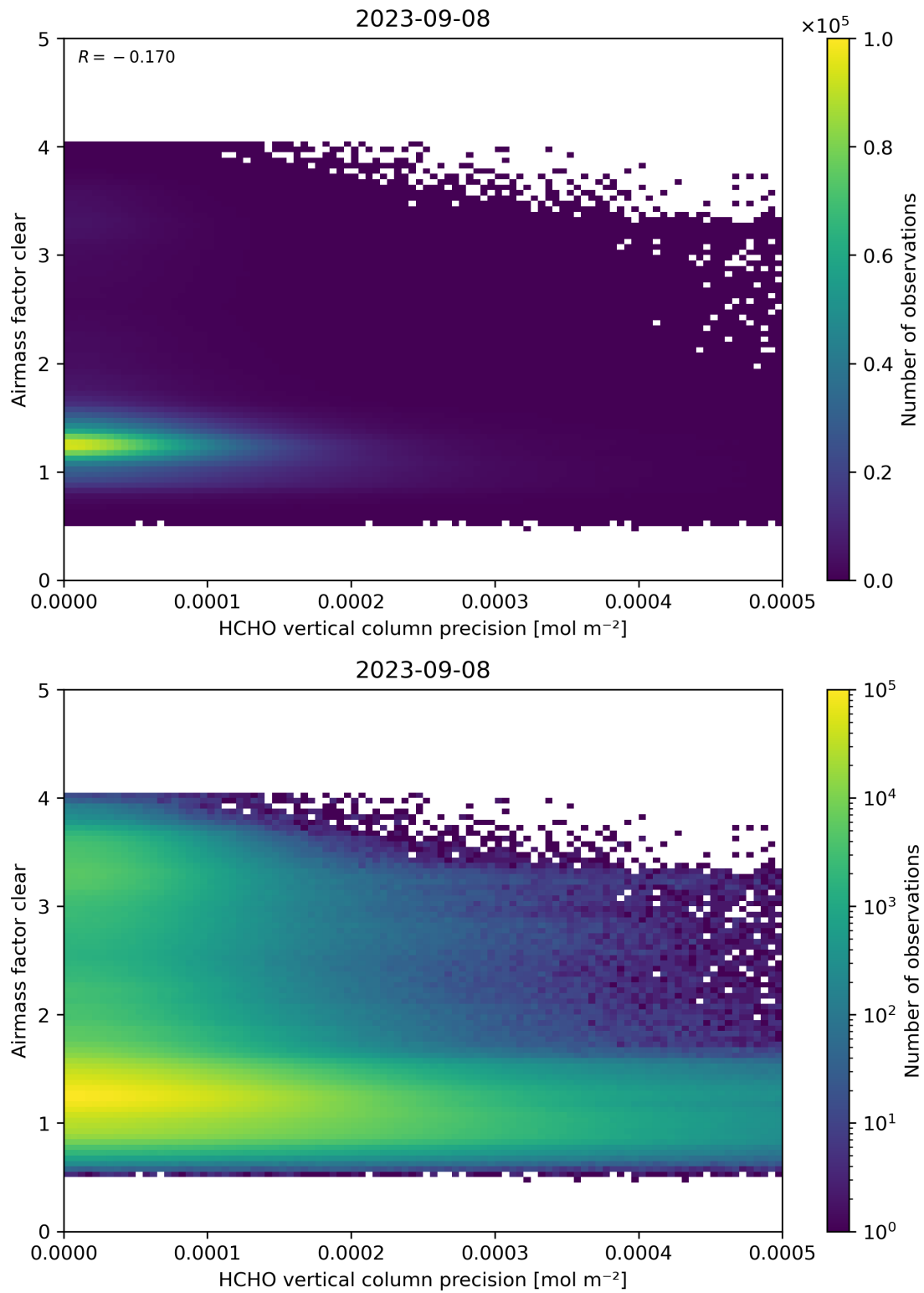
Figure 139: Scatter density plot of “HCHO vertical column precision” against “Airmass factor clear” for 2023-09-07 to 2023-09-09.
