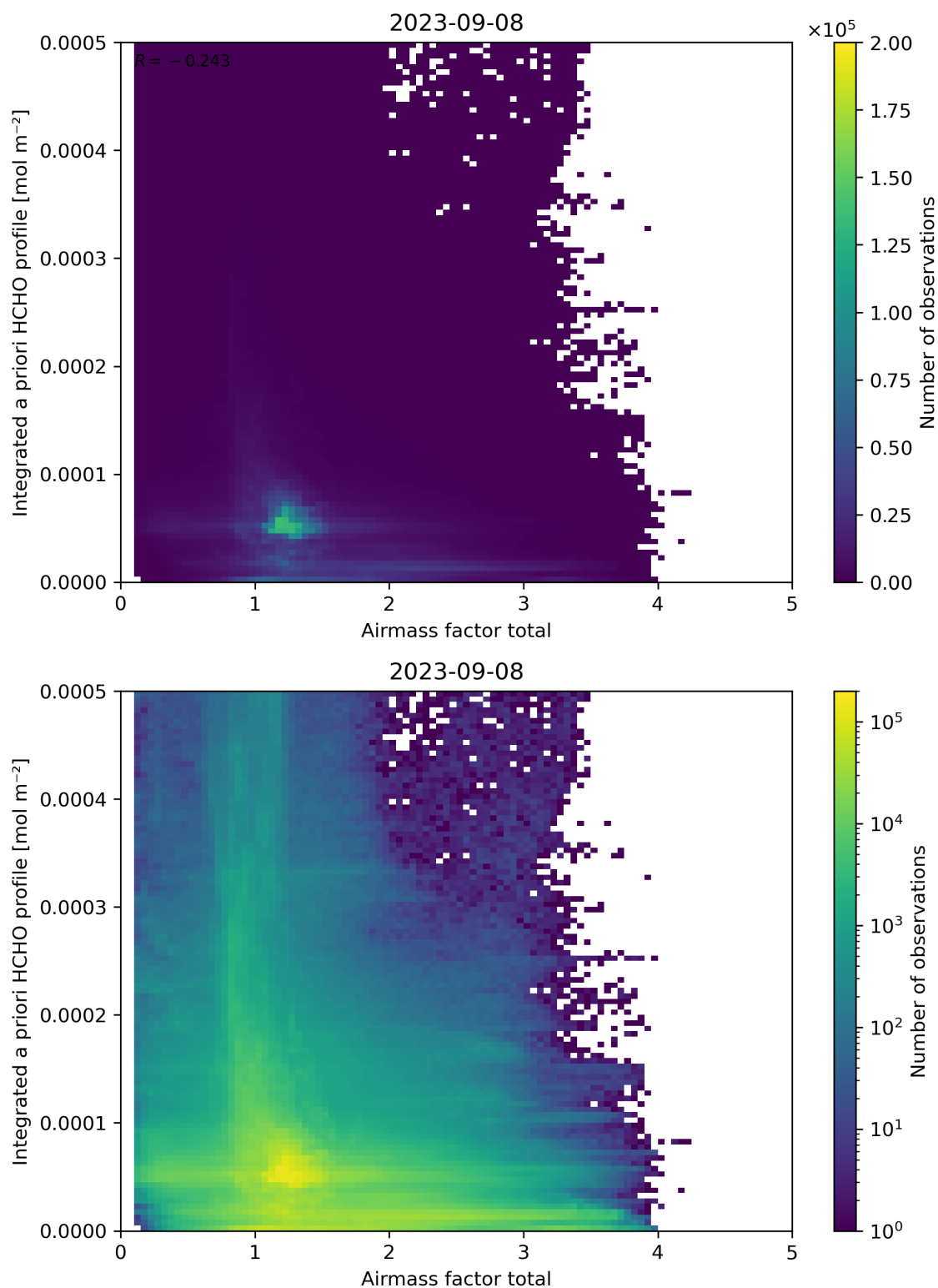
Figure 104: Scatter density plot of “Airmass factor total” against “Integrated a priori HCHO profile” for 2023-09-07 to 2023-09-09.
