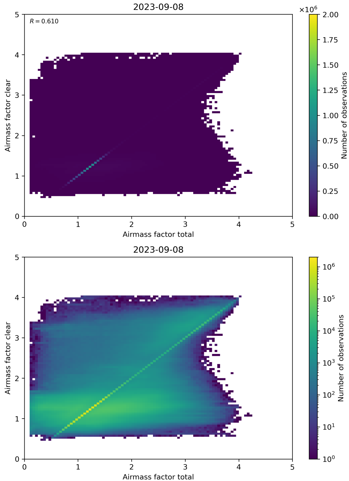
Figure 100: Scatter density plot of “Airmass factor total” against “Airmass factor clear” for 2023-09-07 to 2023-09-09.
