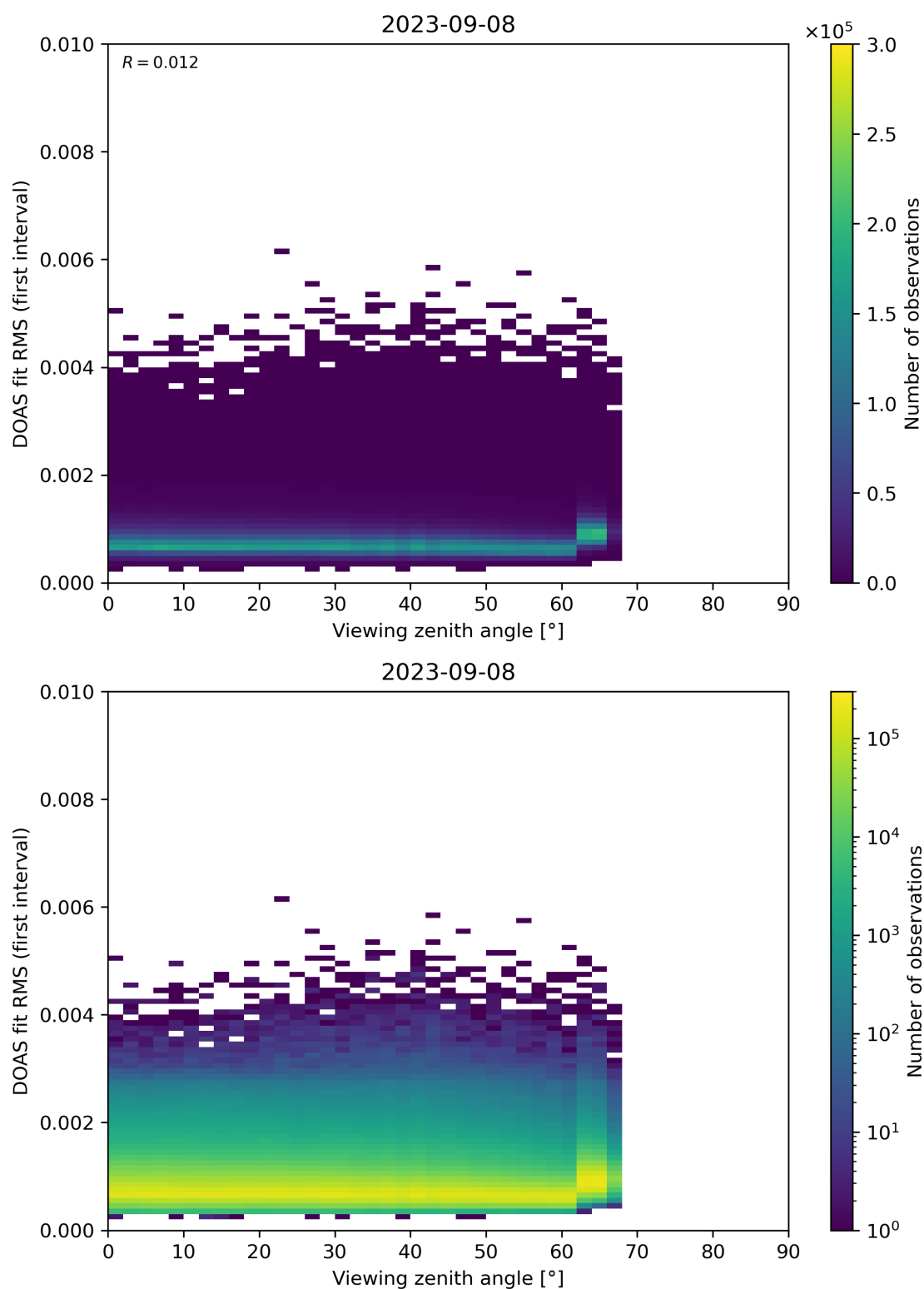
Figure 182: Scatter density plot of “Viewing zenith angle” against “DOAS fit RMS (first interval)” for 2023-09-07 to 2023-09-09.
