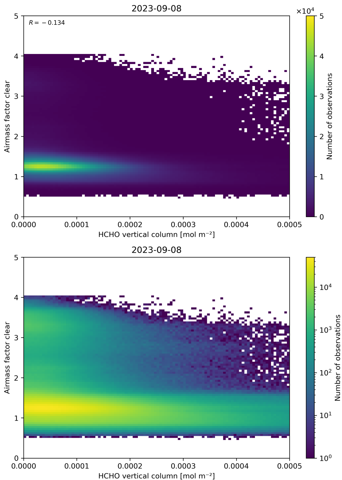
Figure 126: Scatter density plot of “HCHO vertical column” against “Airmass factor clear” for 2023-09-07 to 2023-09-09.
