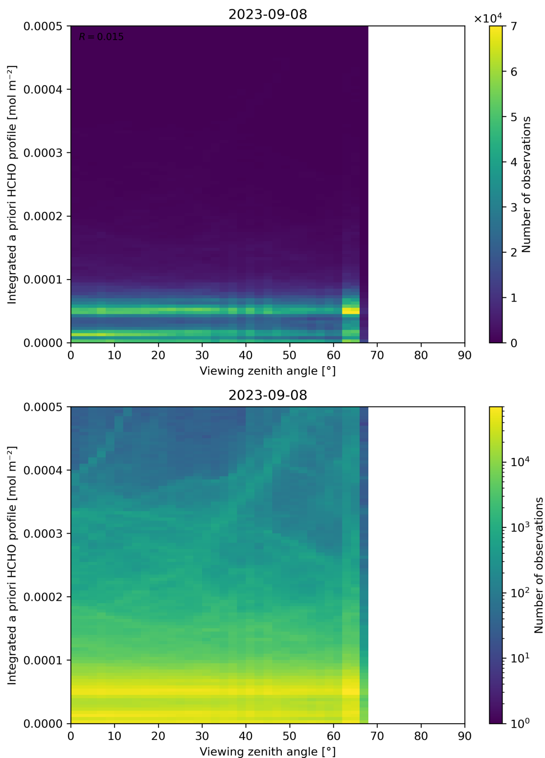
Figure 195: Scatter density plot of “Viewing zenith angle” against “Integrated a priori HCHO profile” for 2023-09-07 to 2023-09-09.
