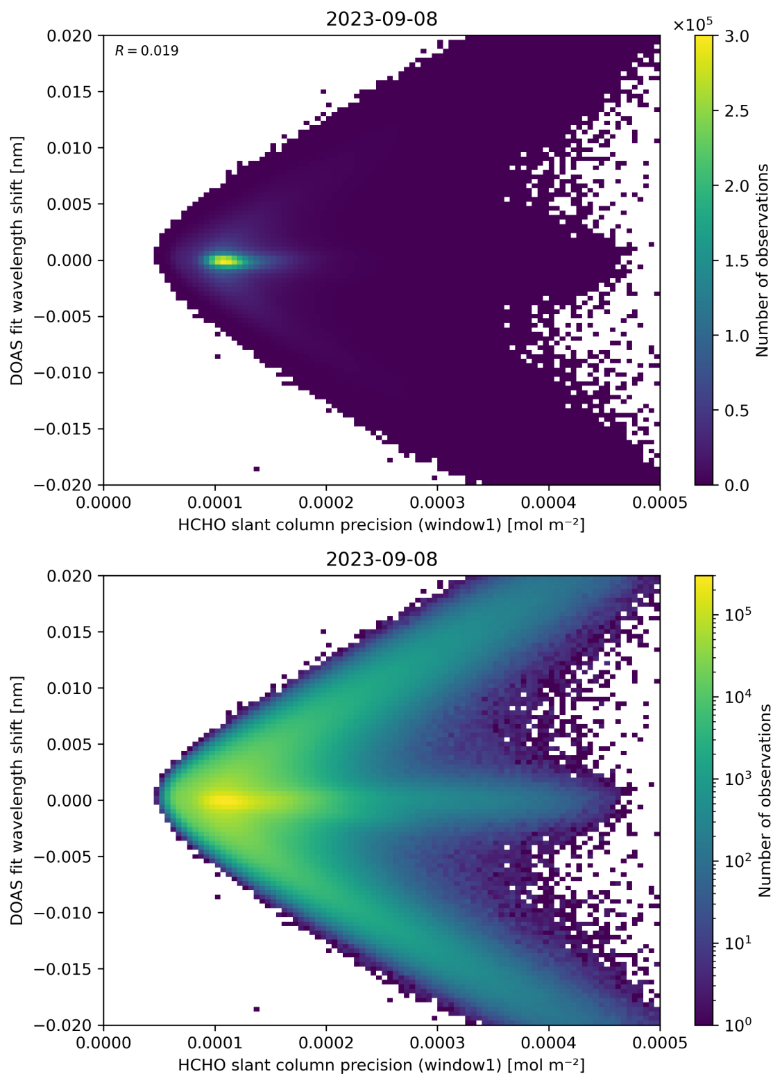
Figure 89: Scatter density plot of “HCHO slant column precision (window1)” against “DOAS fit wavelength shift” for 2023-09-07 to 2023-09-09.
