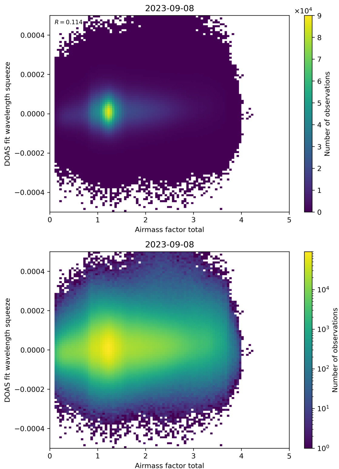
Figure 99: Scatter density plot of “Airmass factor total” against “DOAS fit wavelength squeeze” for 2023-09-07 to 2023-09-09.
