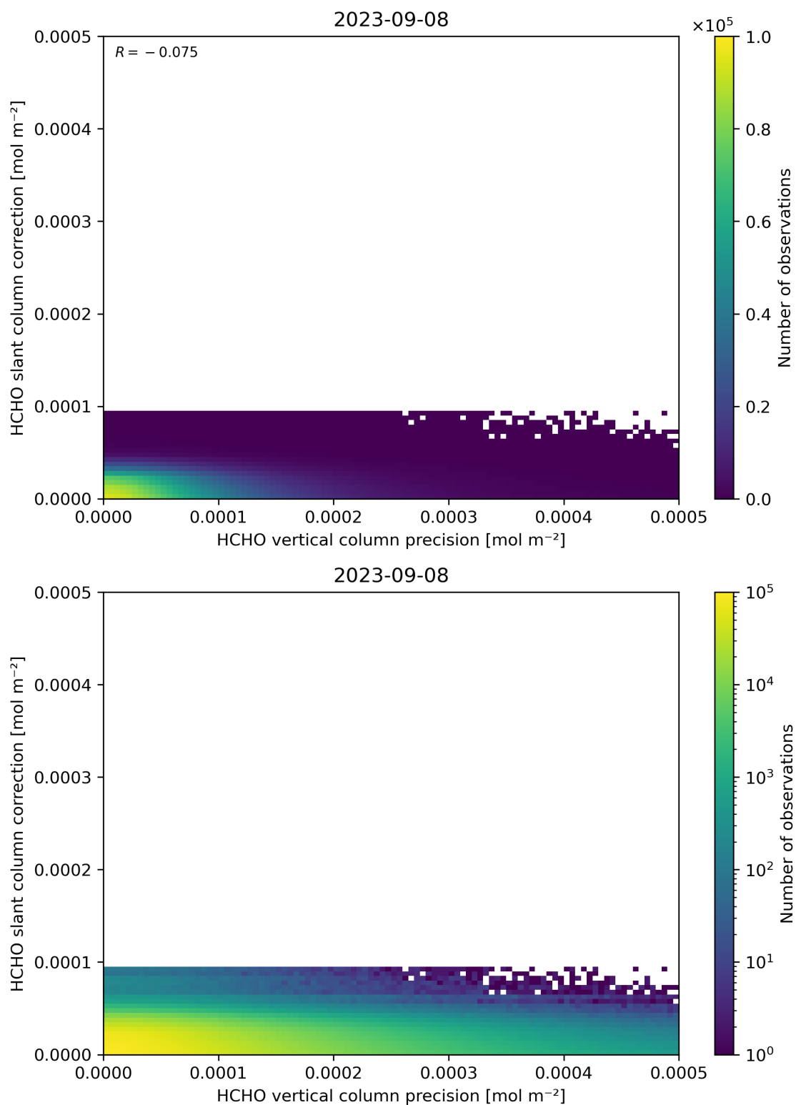
Figure 141: Scatter density plot of “HCHO vertical column precision” against “HCHO slant column correction” for 2023-09-07 to 2023-09-09.
