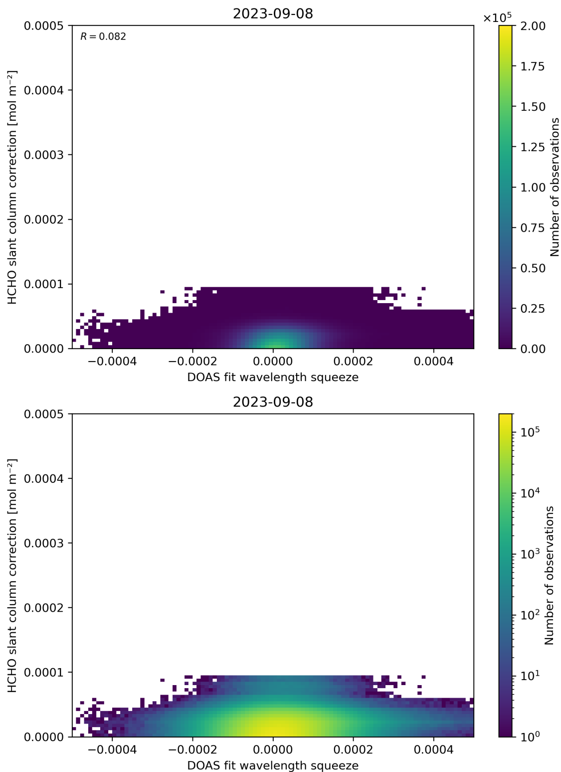
Figure 70: Scatter density plot of “DOAS fit wavelength squeeze” against “HCHO slant column correction” for 2023-09-07 to 2023-09-09.
