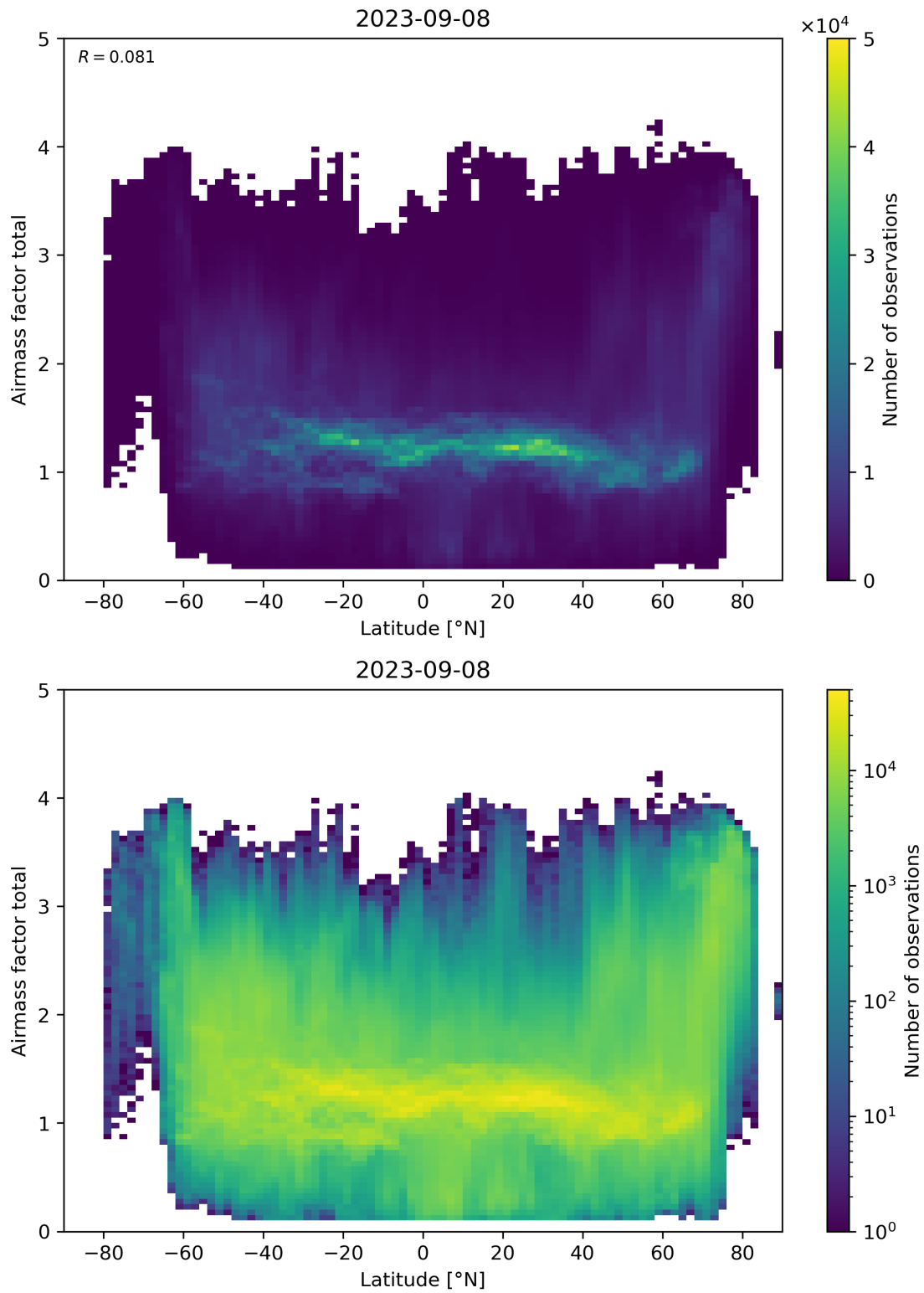
Figure 161: Scatter density plot of “Latitude” against “Airmass factor total” for 2023-09-07 to 2023-09-09.
