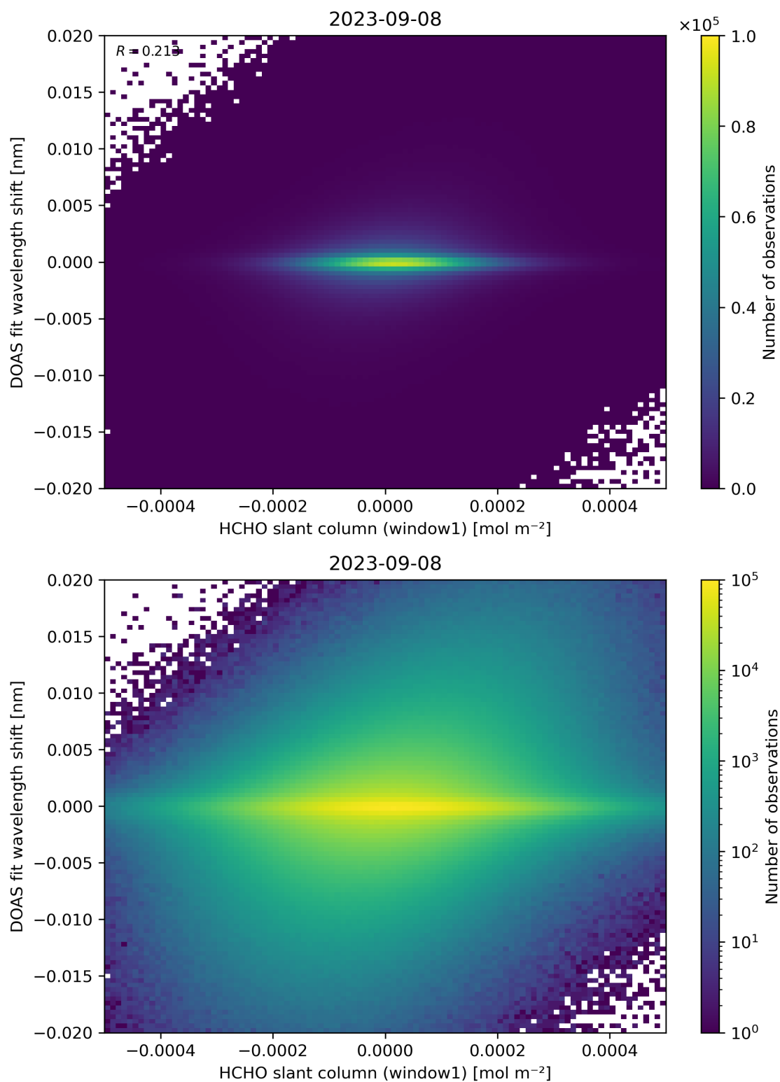
Figure 79: Scatter density plot of “HCHO slant column (window1)” against “DOAS fit wavelength shift” for 2023-09-07 to 2023-09-09.
