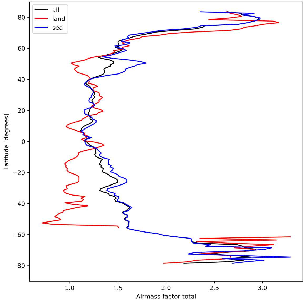
Figure 26: Zonal average of “Airmass factor total” for 2023-09-07 to 2023-09-09.
