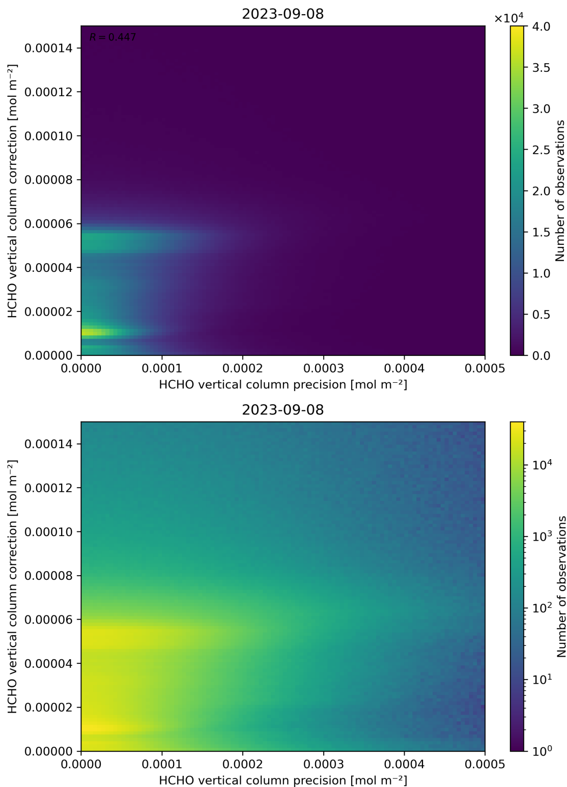
Figure 146: Scatter density plot of “HCHO vertical column precision” against “HCHO vertical column correction” for 2023-09-07 to 2023-09-09.
