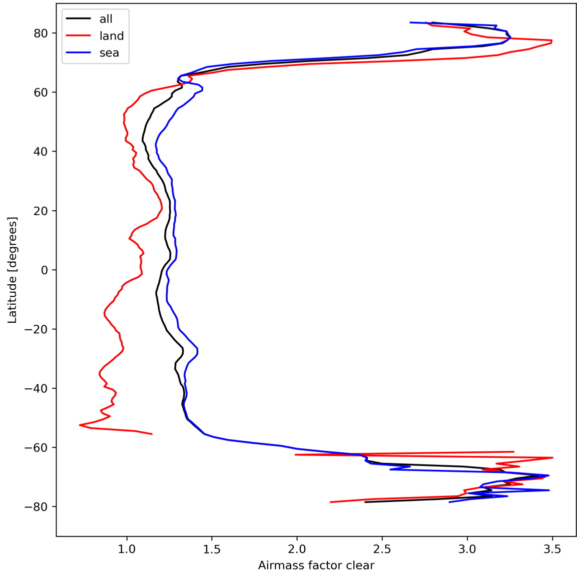
Figure 28: Zonal average of “Airmass factor clear” for 2023-09-07 to 2023-09-09.
