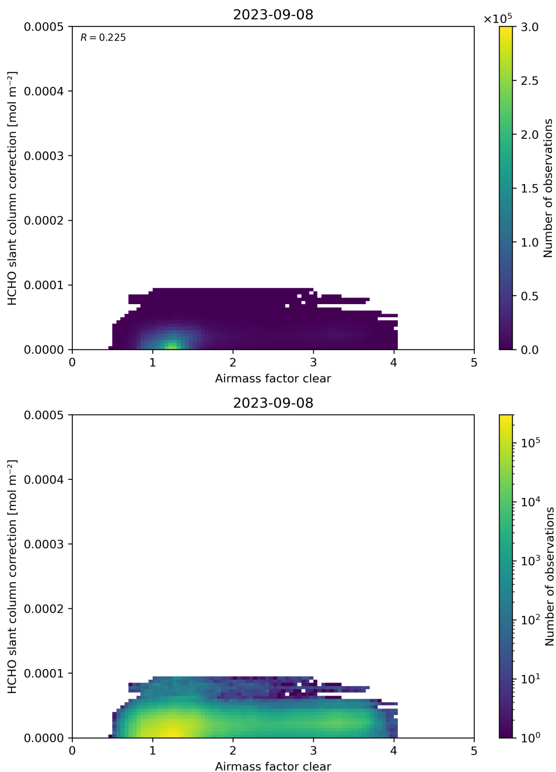
Figure 75: Scatter density plot of “Airmass factor clear” against “HCHO slant column correction” for 2023-09-07 to 2023-09-09.
