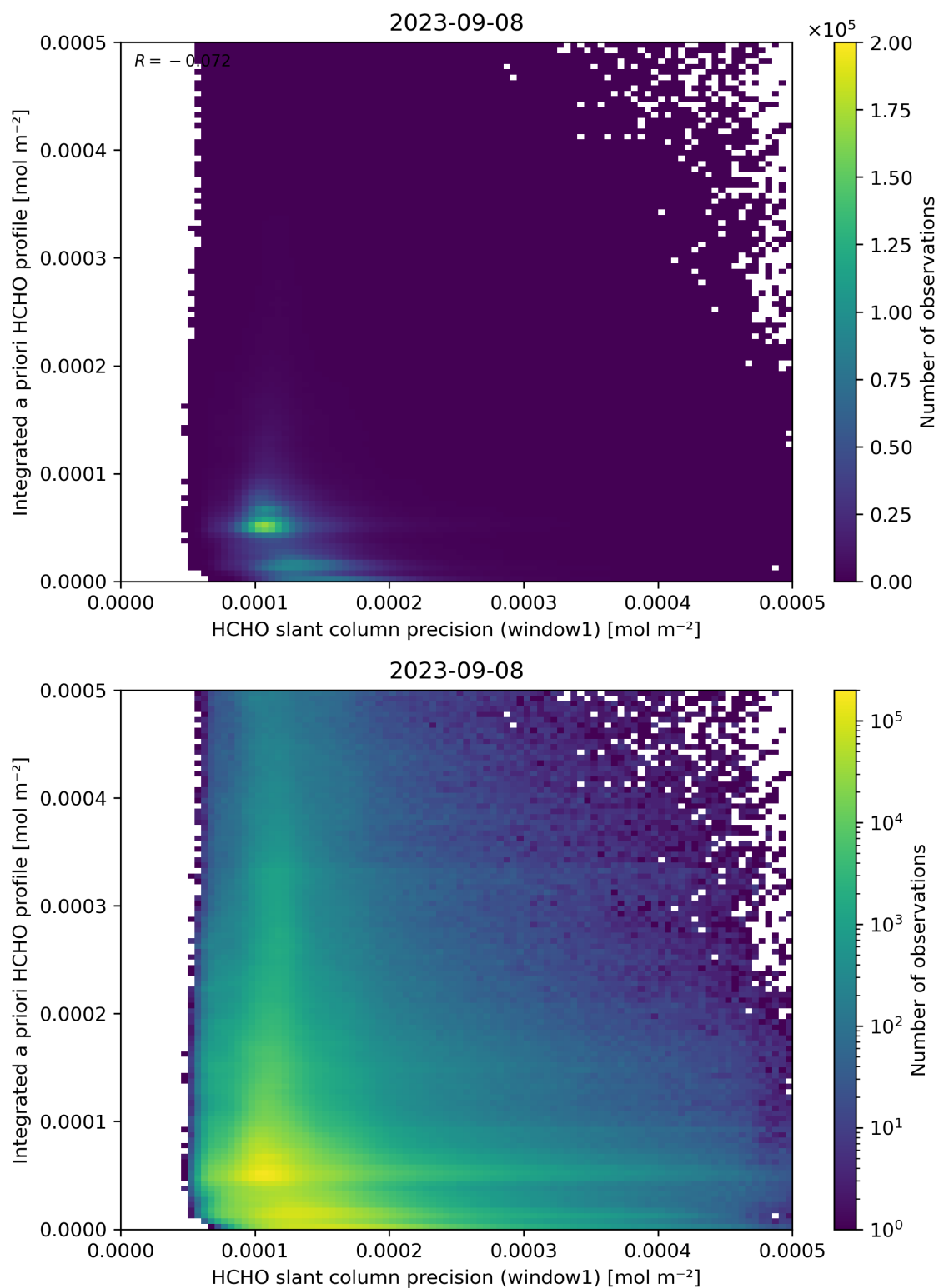
Figure 96: Scatter density plot of “HCHO slant column precision (window1)” against “Integrated a priori HCHO profile” for 2023-09-07 to 2023-09-09.
