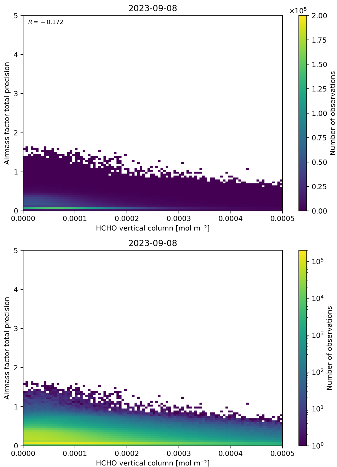
Figure 132: Scatter density plot of “HCHO vertical column” against “Airmass factor total precision” for 2023-09-07 to 2023-09-09.
