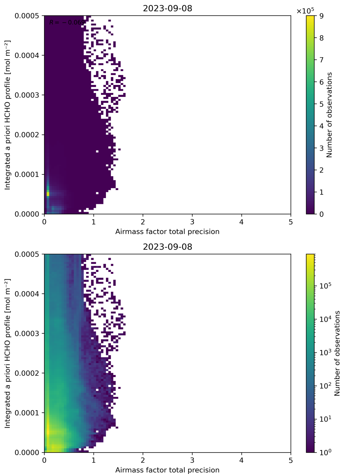
Figure 111: Scatter density plot of “Airmass factor total precision” against “Integrated a priori HCHO profile” for 2023-09-07 to 2023-09-09.
