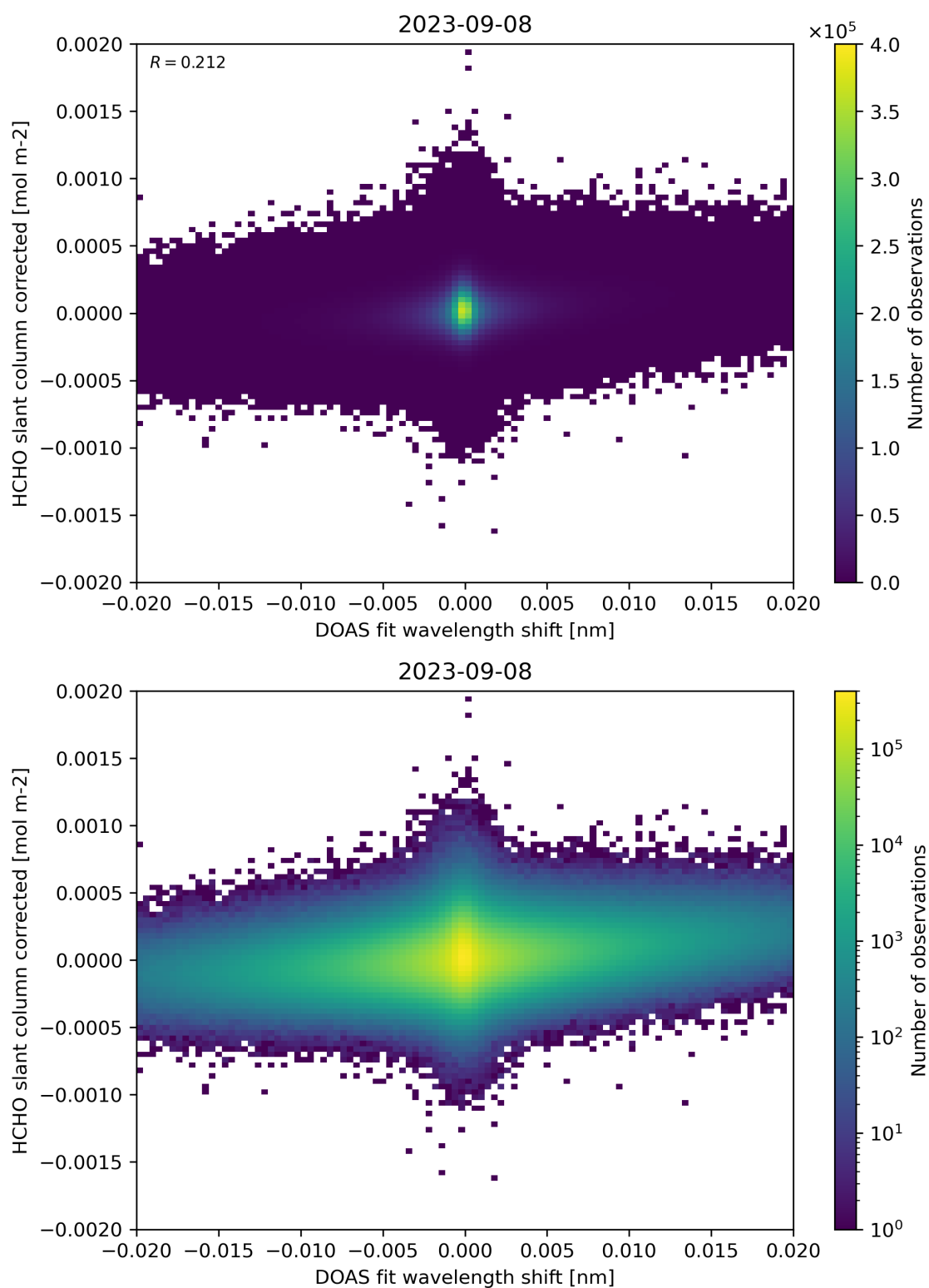
Figure 66: Scatter density plot of “DOAS fit wavelength shift” against “HCHO slant column corrected” for 2023-09-07 to 2023-09-09.
