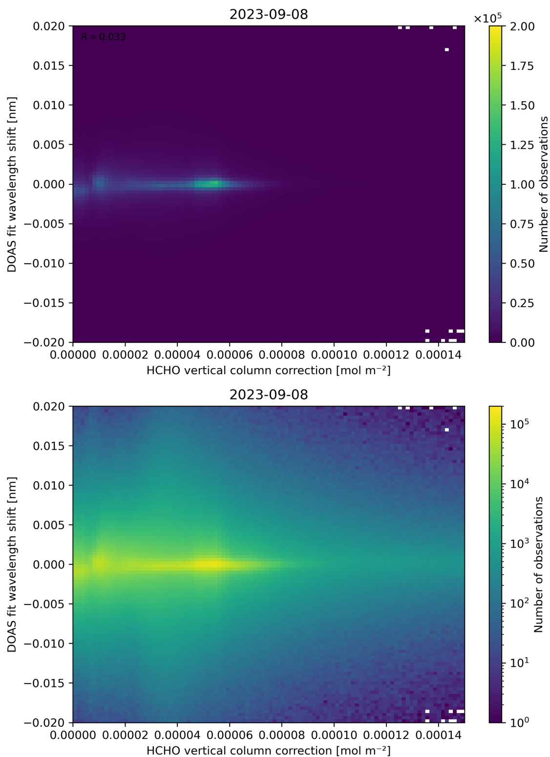
Figure 113: Scatter density plot of “HCHO vertical column correction” against “DOAS fit wavelength shift” for 2023-09-07 to 2023-09-09.
