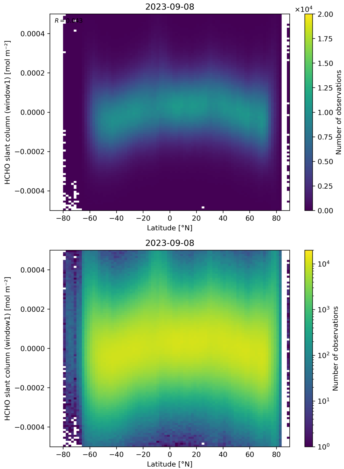
Figure 159: Scatter density plot of “Latitude” against “HCHO slant column (window1)” for 2023-09-07 to 2023-09-09.
