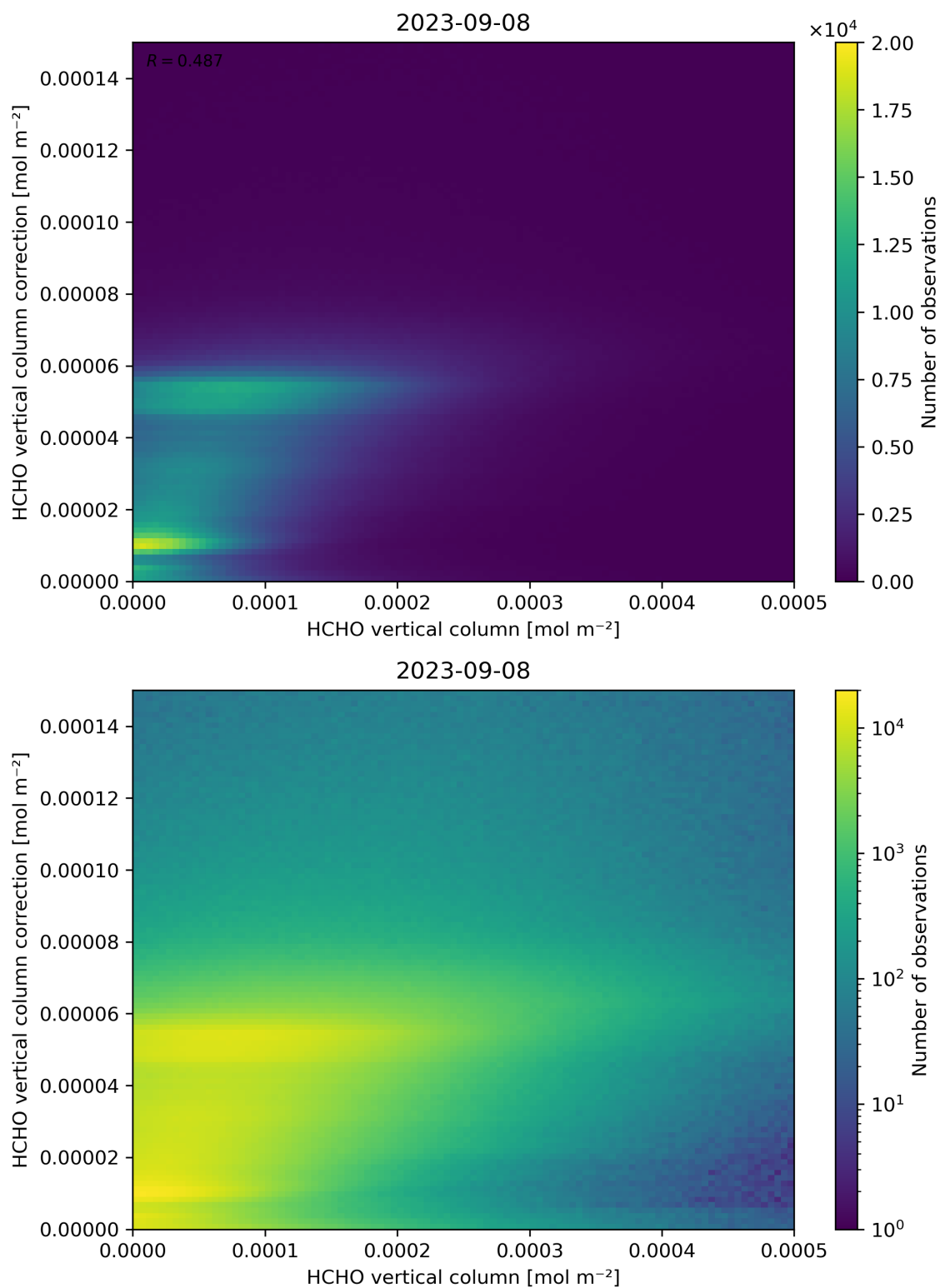
Figure 133: Scatter density plot of “HCHO vertical column” against “HCHO vertical column correction” for 2023-09-07 to 2023-09-09.
