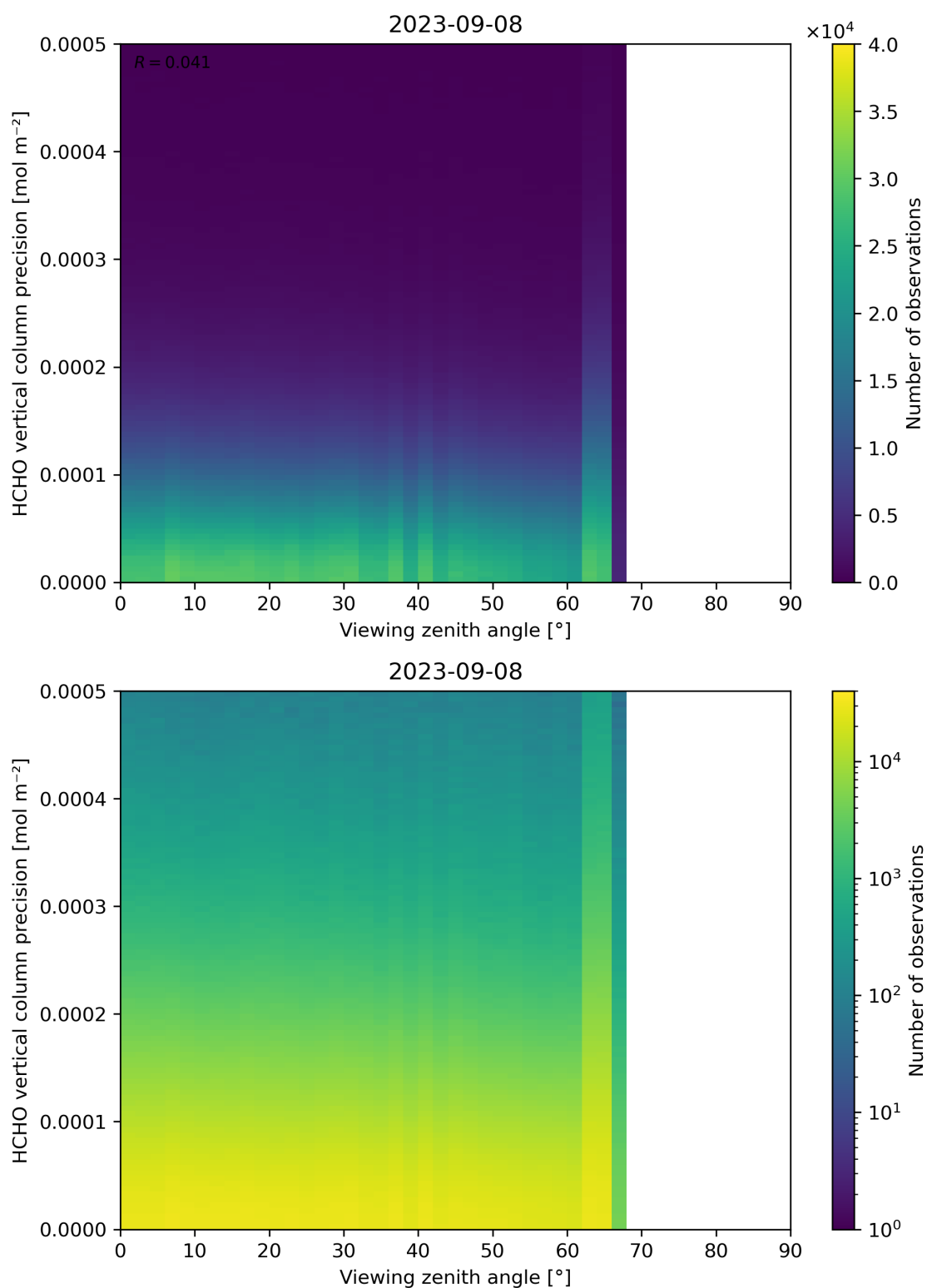
Figure 194: Scatter density plot of “Viewing zenith angle” against “HCHO vertical column precision” for 2023-09-07 to 2023-09-09.
