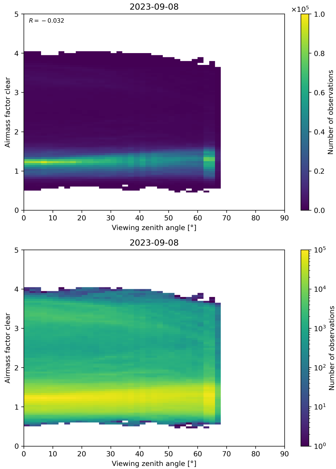
Figure 185: Scatter density plot of “Viewing zenith angle” against “Airmass factor clear” for 2023-09-07 to 2023-09-09.
