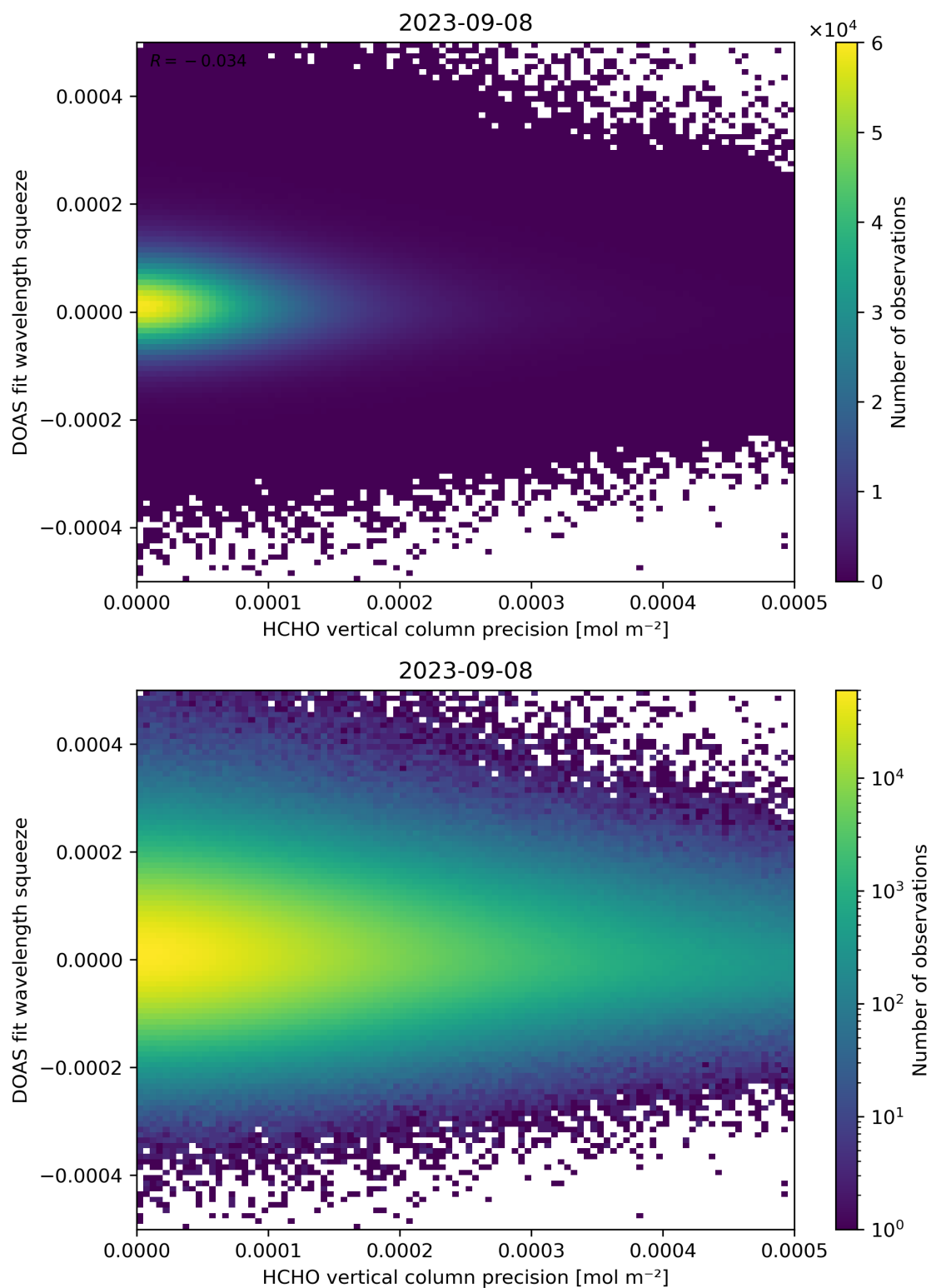
Figure 138: Scatter density plot of “HCHO vertical column precision” against “DOAS fit wavelength squeeze” for 2023-09-07 to 2023-09-09.
