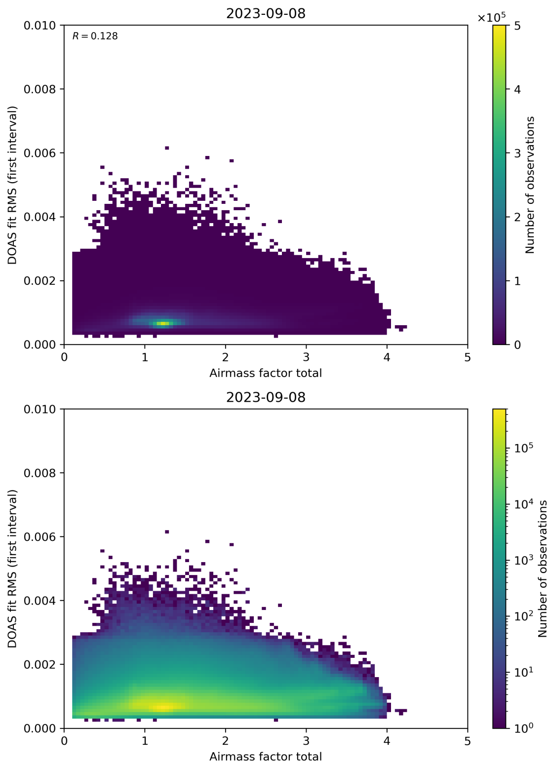
Figure 97: Scatter density plot of “Airmass factor total” against “DOAS fit RMS (first interval)” for 2023-09-07 to 2023-09-09.
