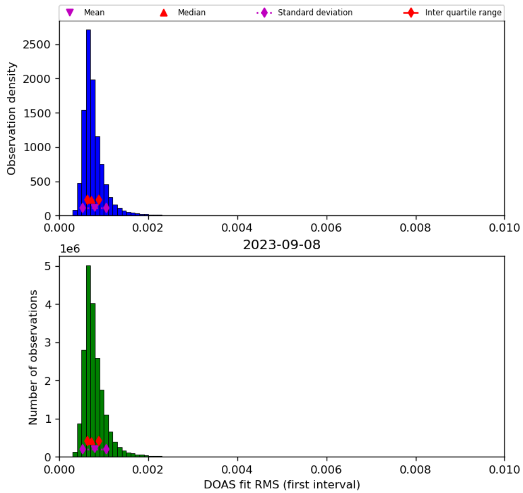
Figure 46: Histogram of “DOAS fit RMS (first interval)” for 2023-09-07 to 2023-09-09
