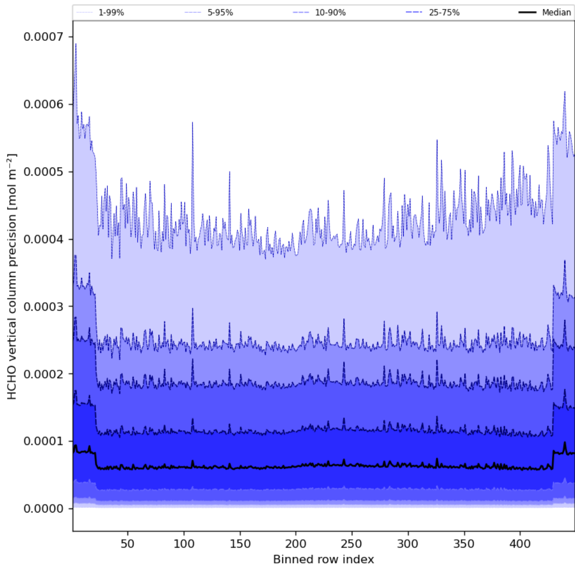
Figure 50: Along track statistics of “HCHO vertical column precision” for 2023-09-07 to 2023-09-09
