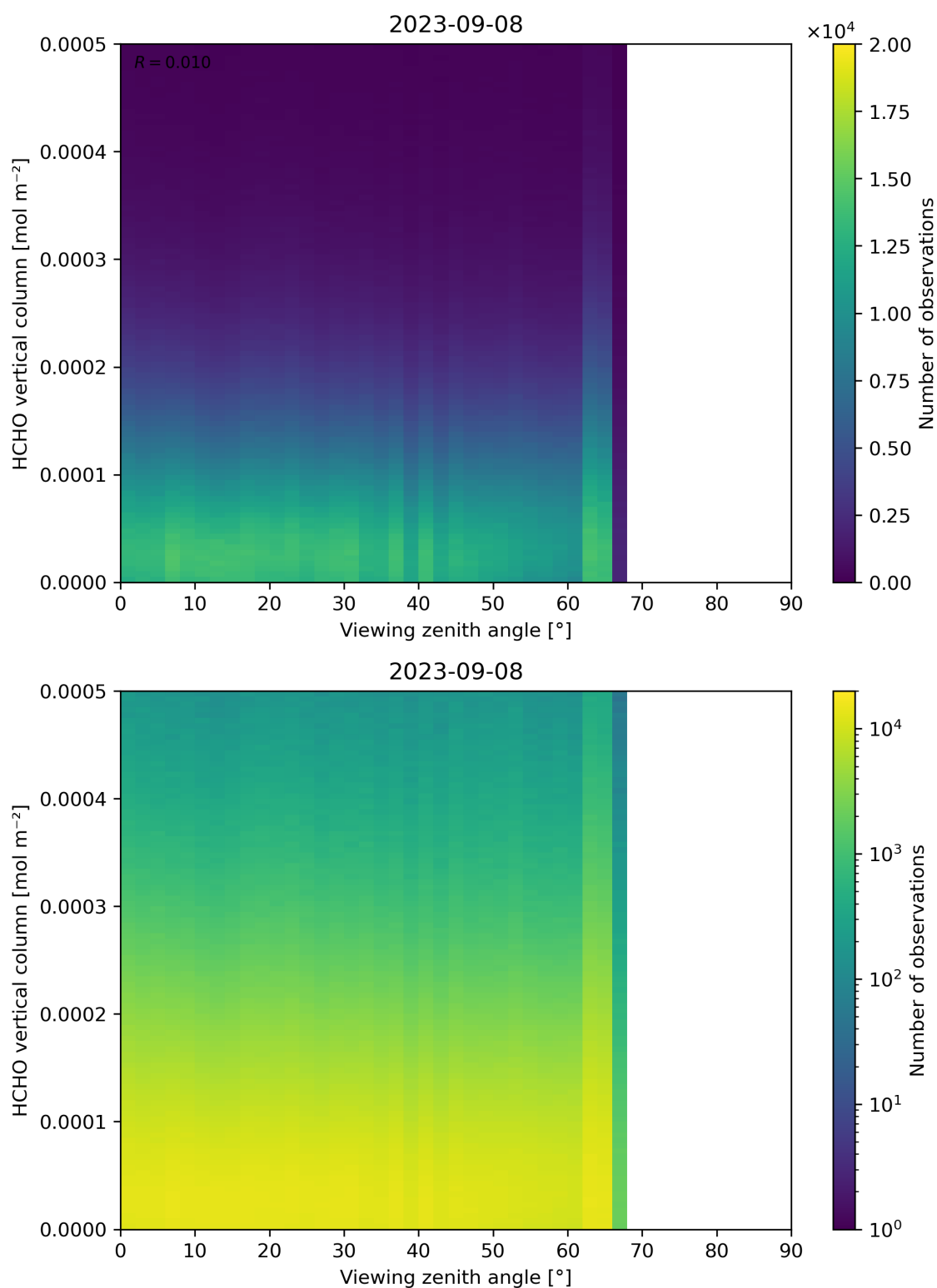
Figure 192: Scatter density plot of “Viewing zenith angle” against “HCHO vertical column” for 2023-09-07 to 2023-09-09.
