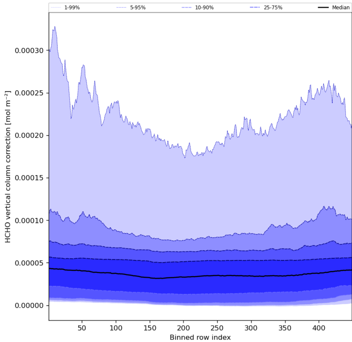
Figure 51: Along track statistics of “HCHO vertical column correction” for 2023-09-07 to 2023-09-09
