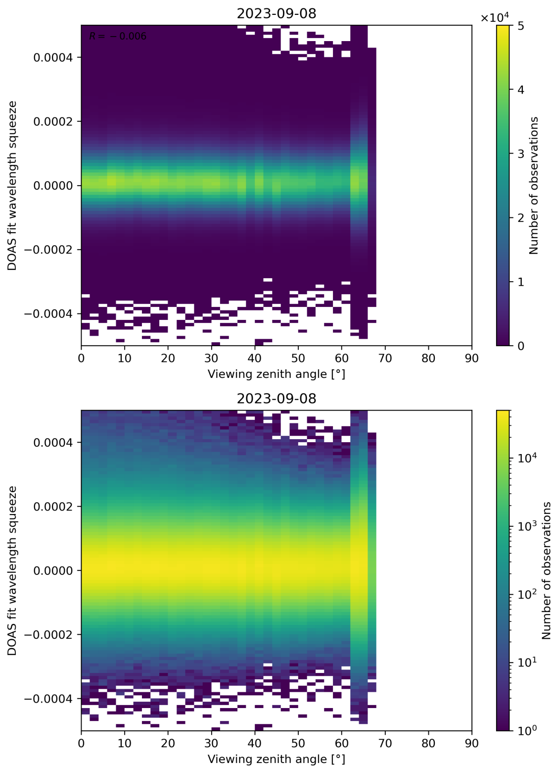
Figure 184: Scatter density plot of “Viewing zenith angle” against “DOAS fit wavelength squeeze” for 2023-09-07 to 2023-09-09.
