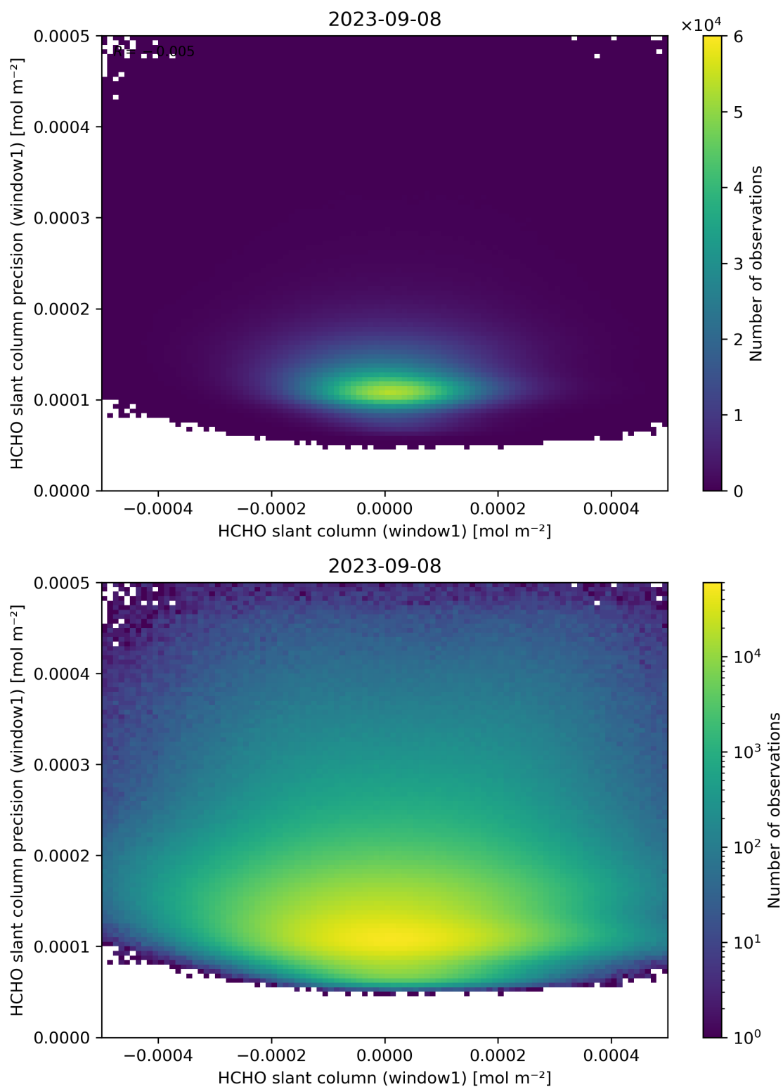
Figure 84: Scatter density plot of “HCHO slant column (window1)” against “HCHO slant column precision (window1)” for 2023-09-07 to 2023-09-09.
