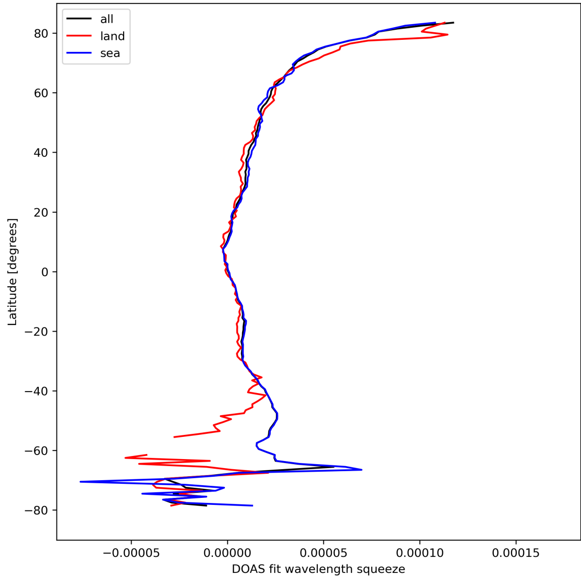
Figure 31: Zonal average of “DOAS fit wavelength squeeze” for 2023-09-07 to 2023-09-09.
