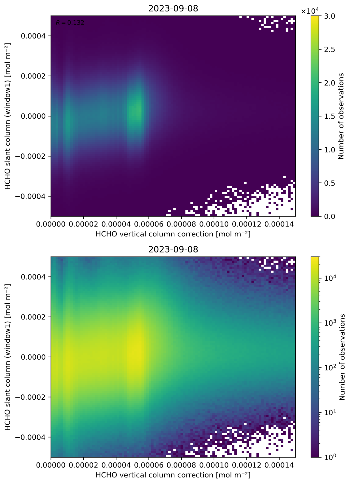
Figure 118: Scatter density plot of “HCHO vertical column correction” against “HCHO slant column (window1)” for 2023-09-07 to 2023-09-09.
