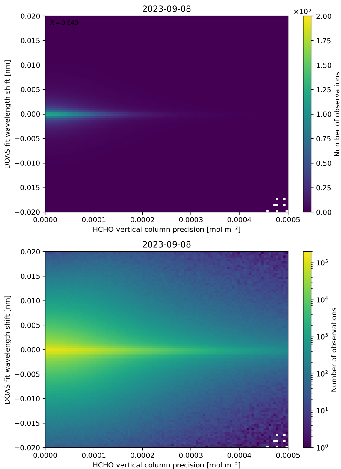
Figure 137: Scatter density plot of “HCHO vertical column precision” against “DOAS fit wavelength shift” for 2023-09-07 to 2023-09-09.
