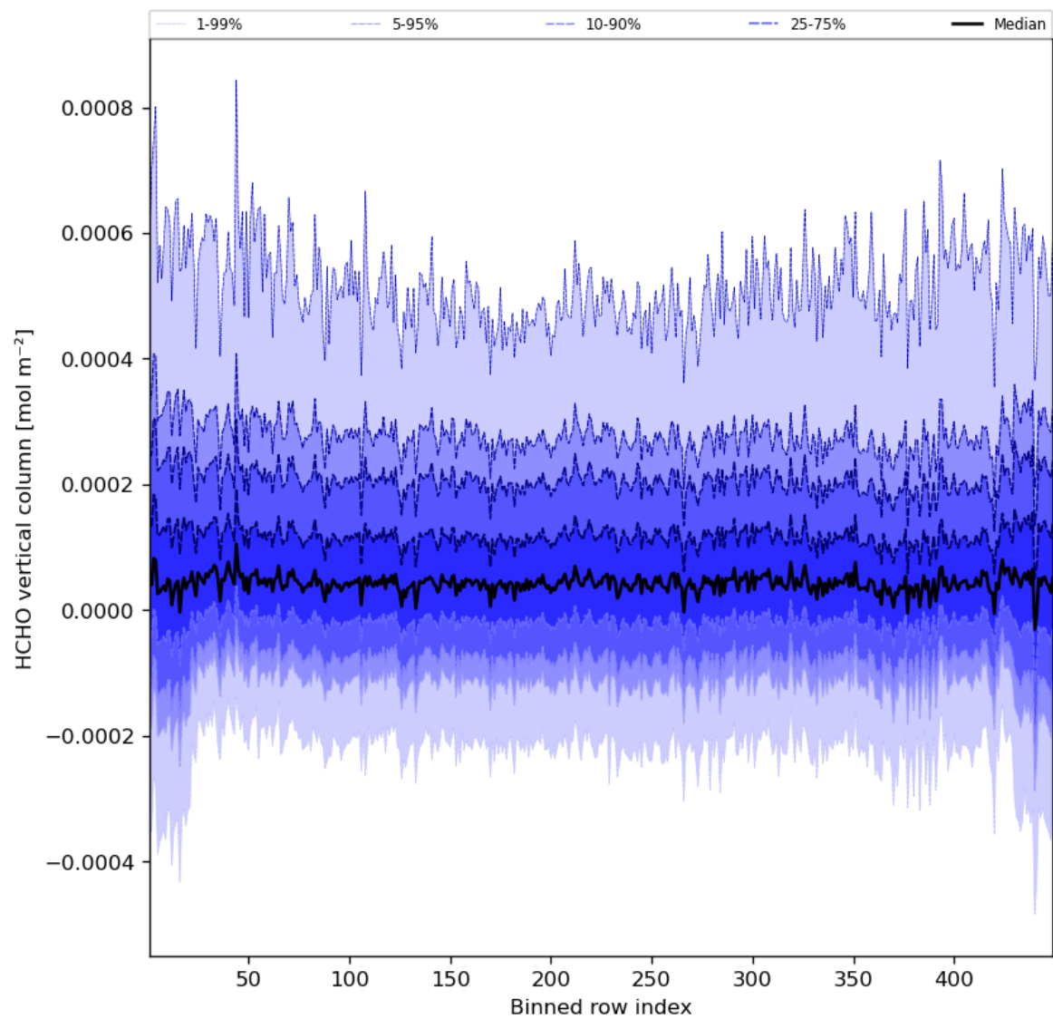
Figure 49: Along track statistics of “HCHO vertical column” for 2023-09-07 to 2023-09-09
