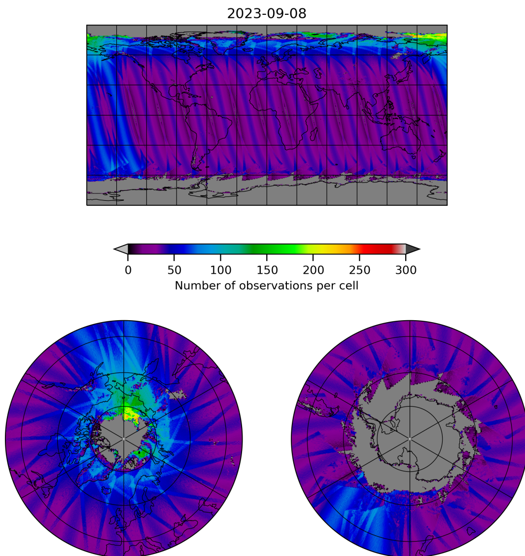
Figure 19: Map of the number of observations for 2023-09-07 to 2023-09-09
