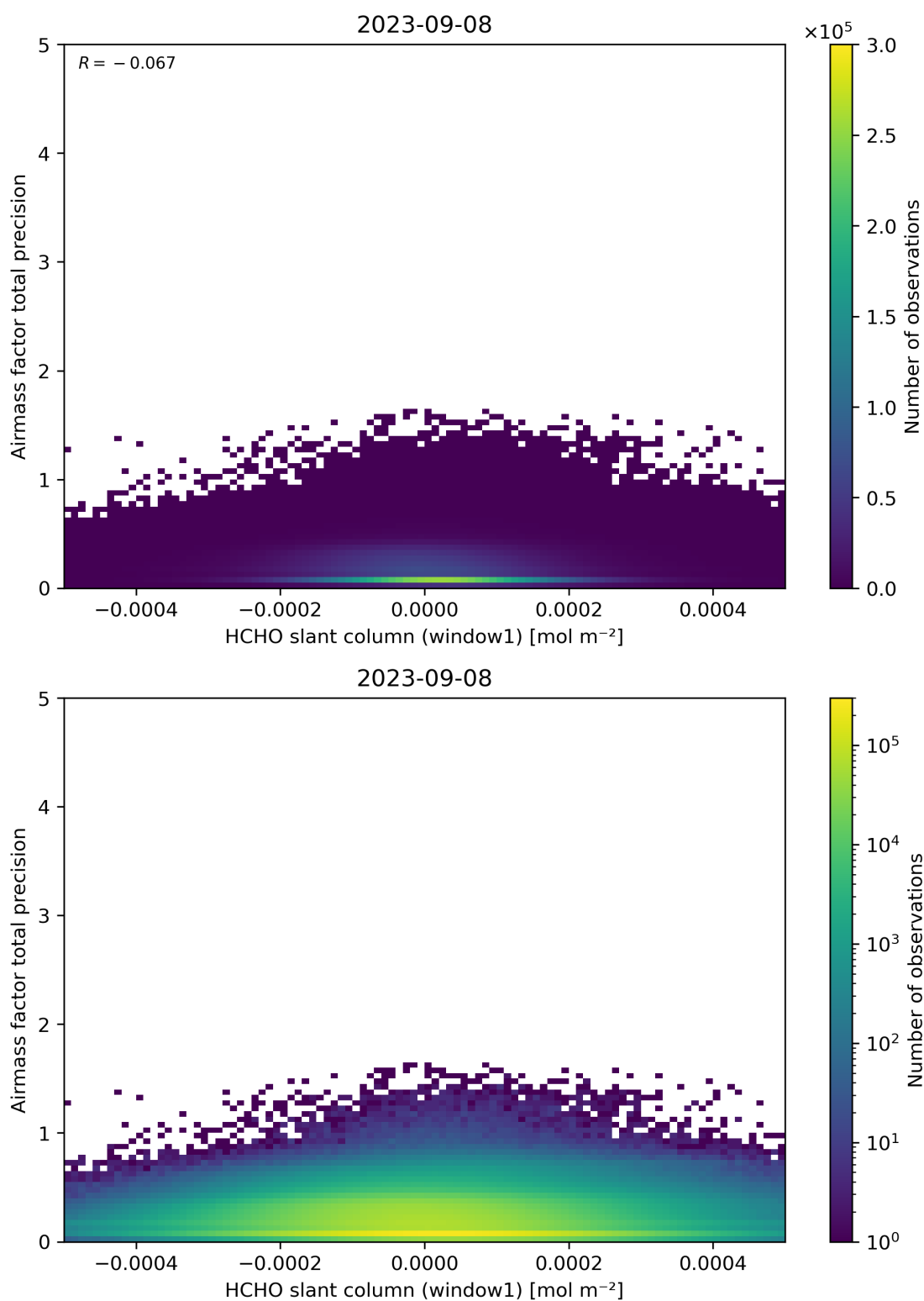
Figure 86: Scatter density plot of “HCHO slant column (window1)” against “Airmass factor total precision” for 2023-09-07 to 2023-09-09.
