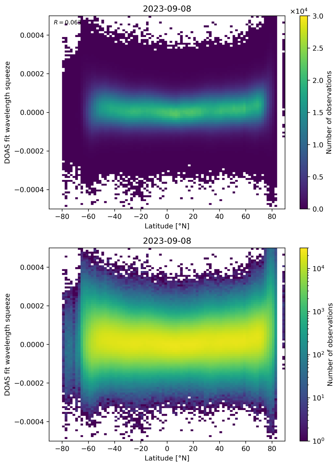
Figure 155: Scatter density plot of “Latitude” against “DOAS fit wavelength squeeze” for 2023-09-07 to 2023-09-09.
