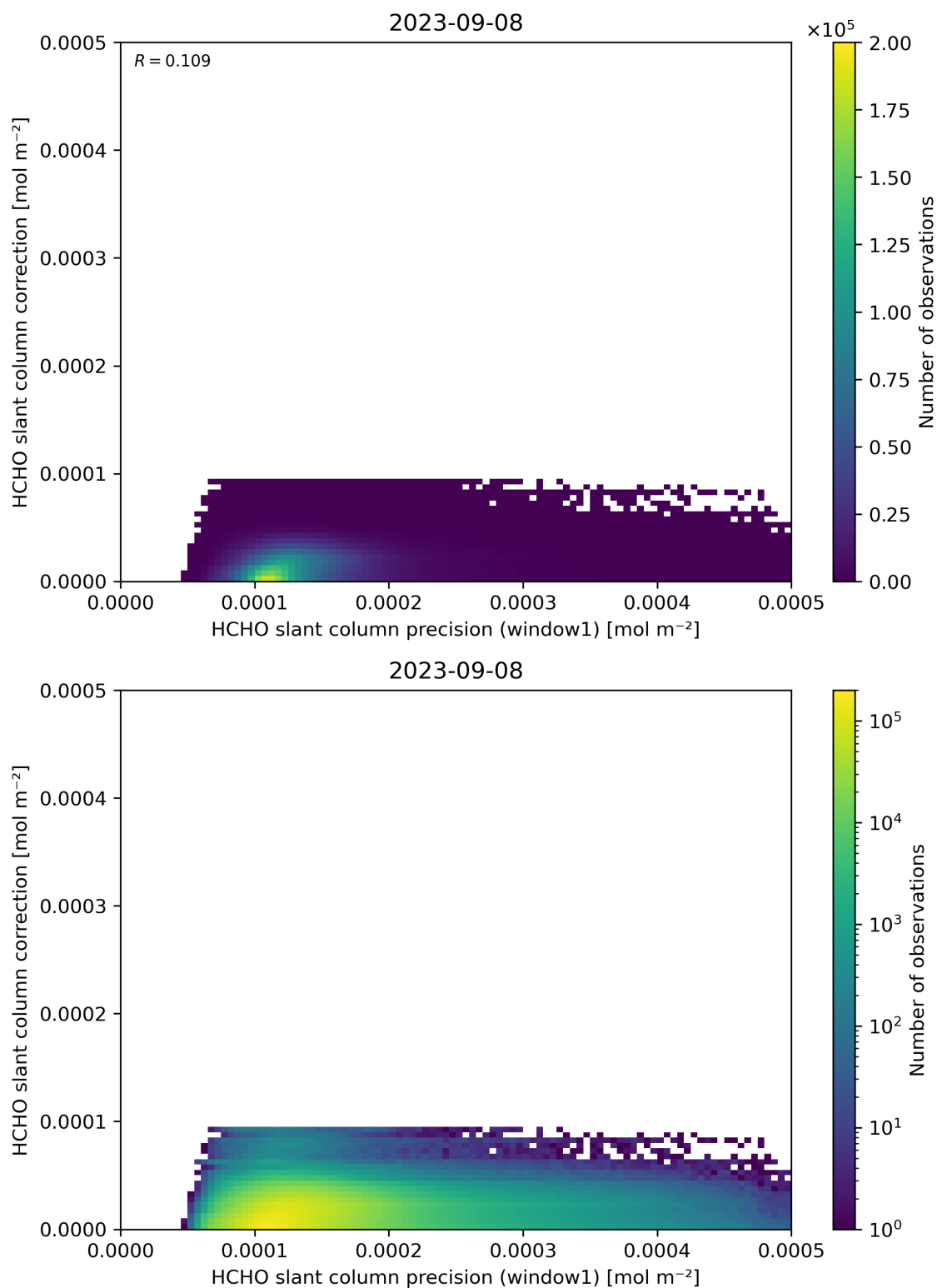
Figure 93: Scatter density plot of “HCHO slant column precision (window1)” against “HCHO slant column correction” for 2023-09-07 to 2023-09-09.
