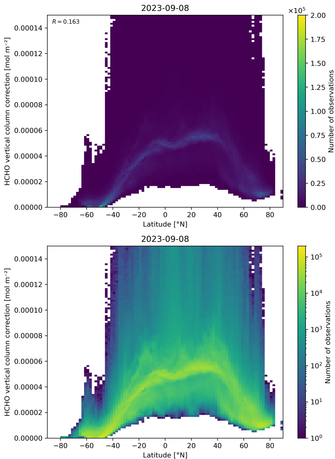
Figure 164: Scatter density plot of “Latitude” against “HCHO vertical column correction” for 2023-09-07 to 2023-09-09.
