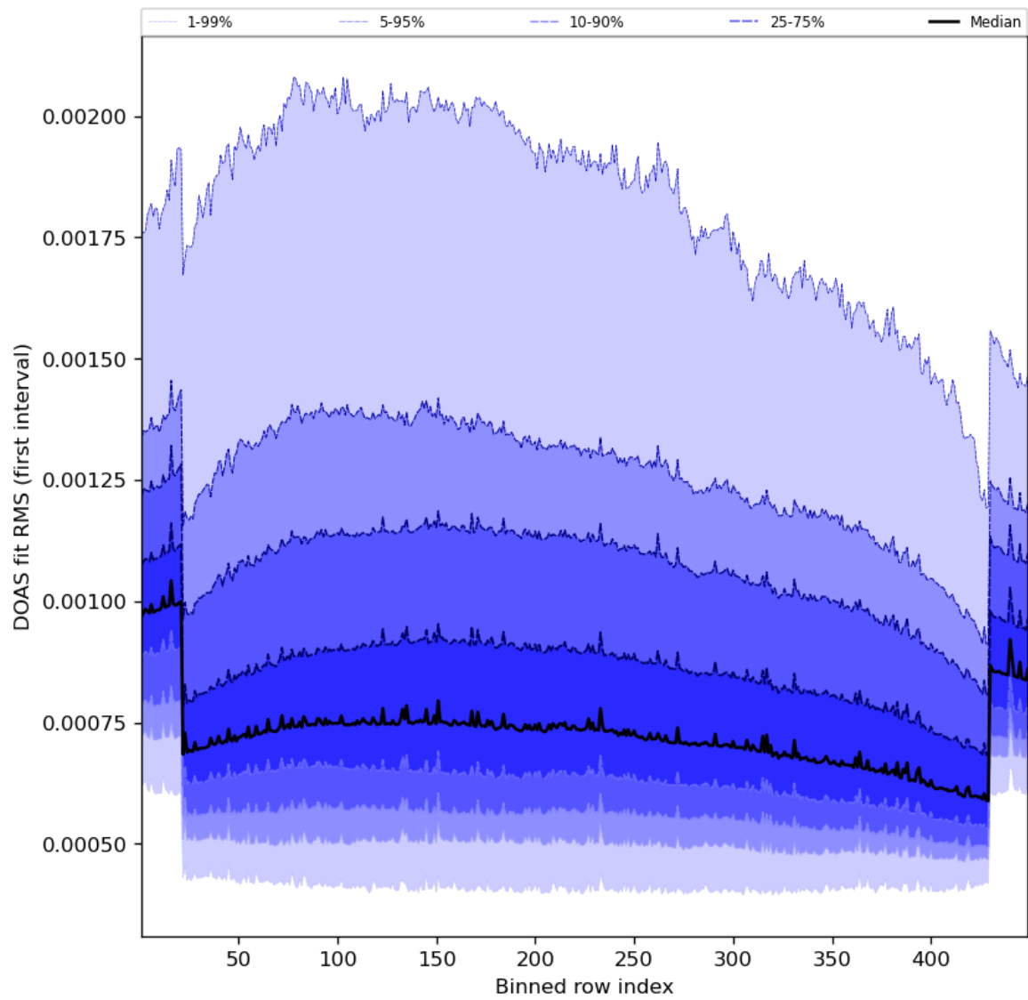
Figure 60: Along track statistics of “DOAS fit RMS (first interval)” for 2023-09-07 to 2023-09-09
