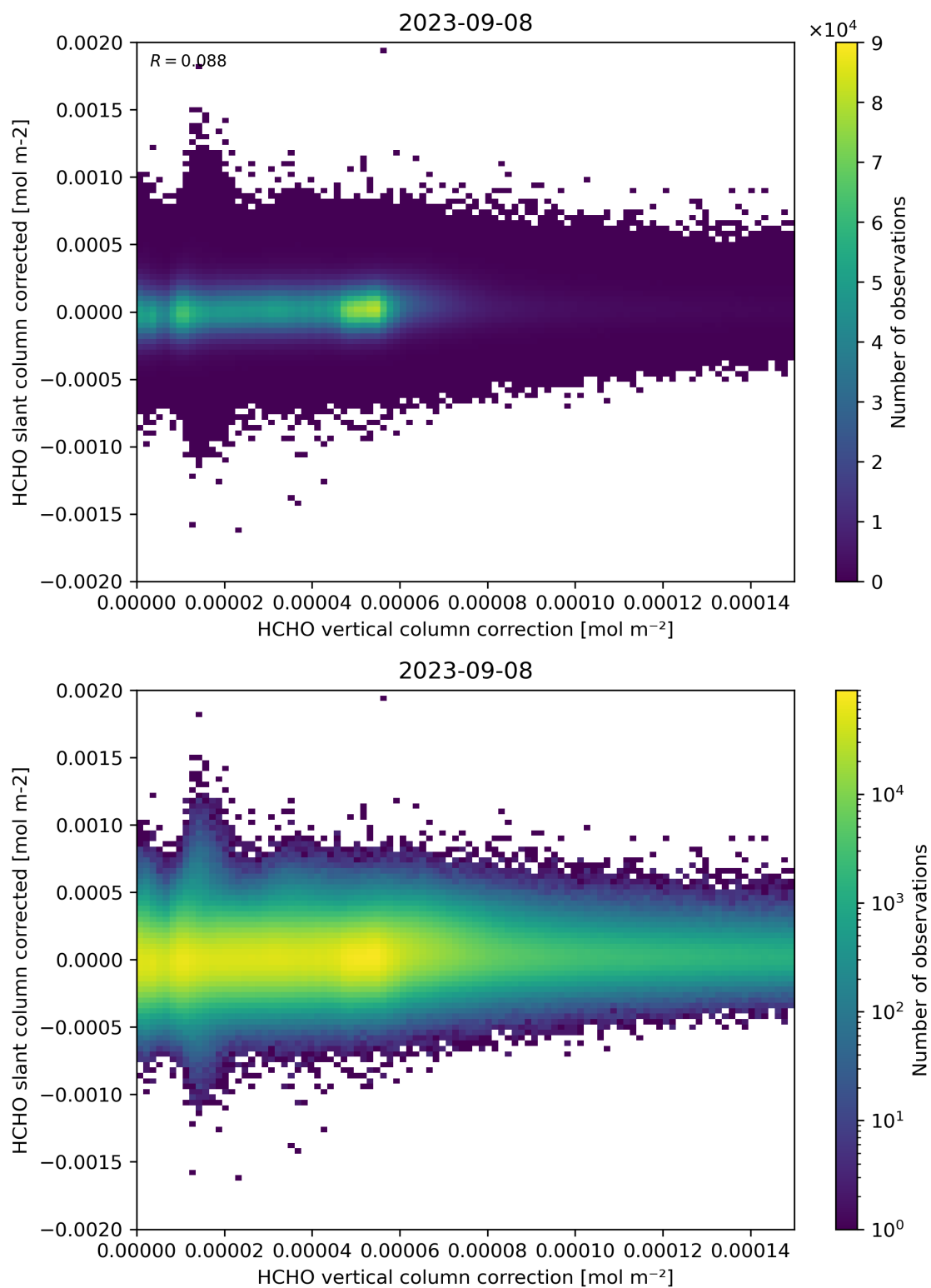
Figure 116: Scatter density plot of “HCHO vertical column correction” against “HCHO slant column corrected” for 2023-09-07 to 2023-09-09.
