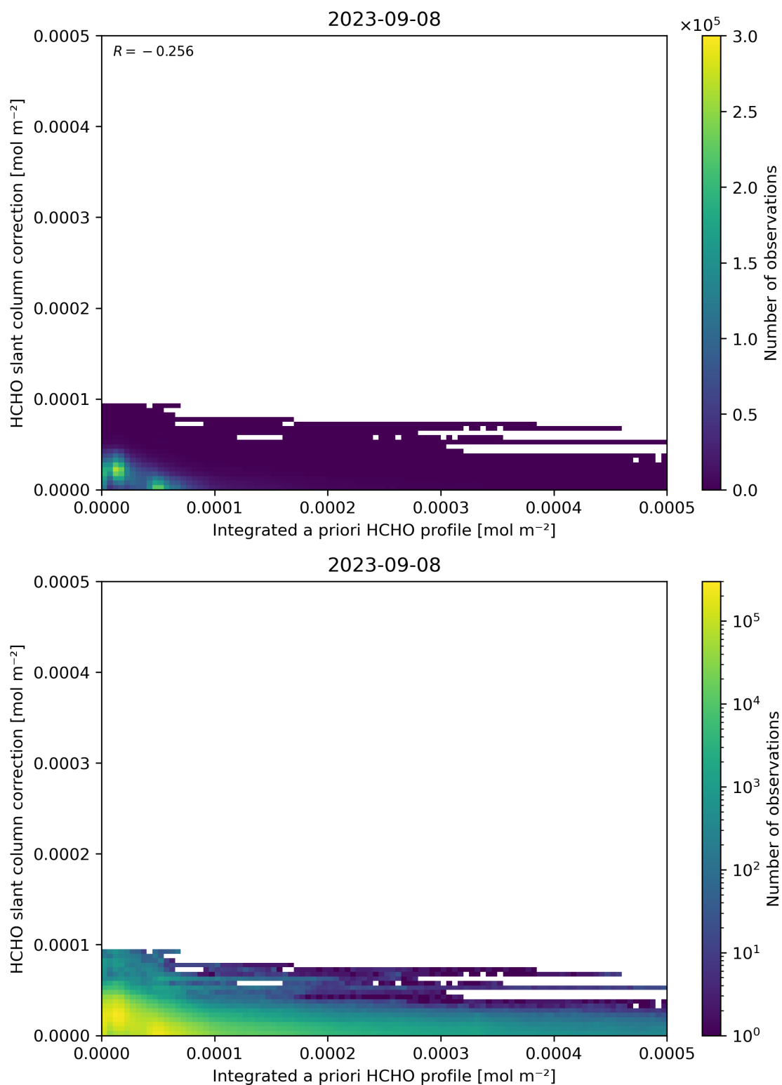
Figure 152: Scatter density plot of “Integrated a priori HCHO profile” against “HCHO slant column correction” for 2023-09-07 to 2023-09-09.
