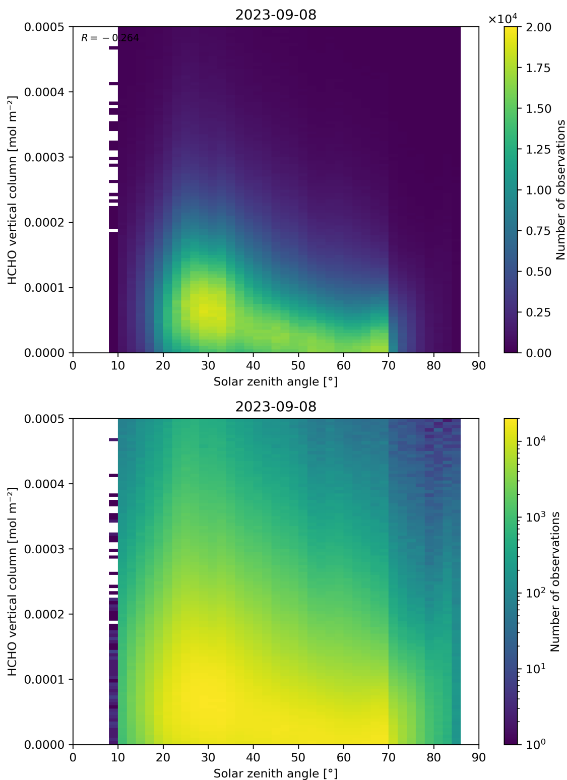
Figure 177: Scatter density plot of “Solar zenith angle” against “HCHO vertical column” for 2023-09-07 to 2023-09-09.
