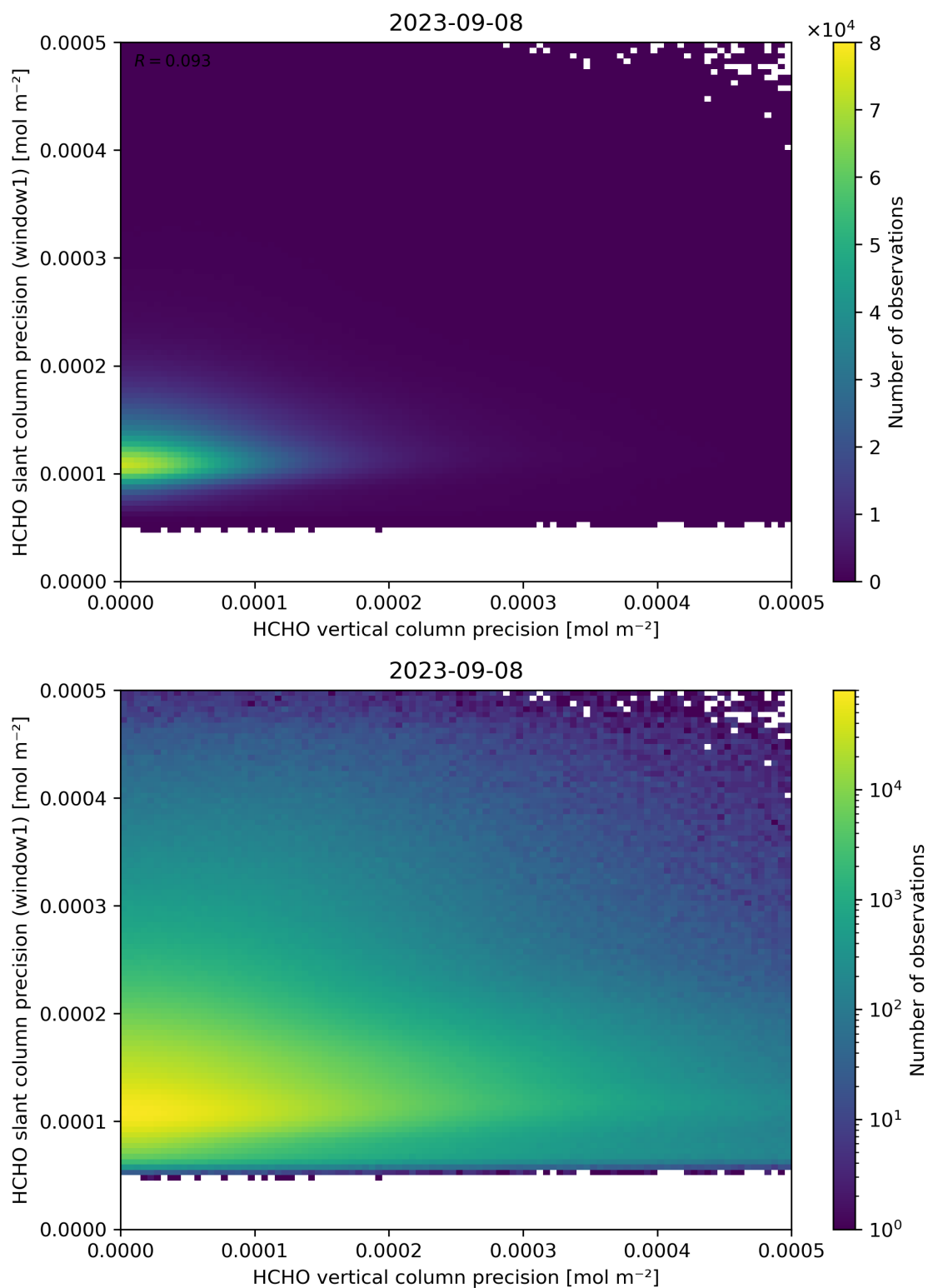
Figure 143: Scatter density plot of “HCHO vertical column precision” against “HCHO slant column precision (window1)” for 2023-09-07 to 2023-09-09.
