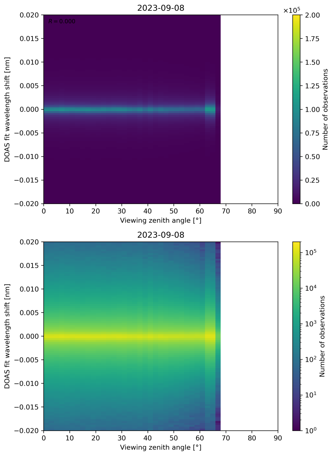
Figure 183: Scatter density plot of “Viewing zenith angle” against “DOAS fit wavelength shift” for 2023-09-07 to 2023-09-09.
