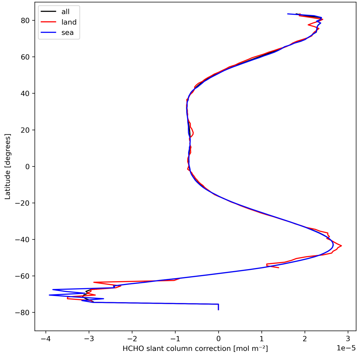
Figure 33: Zonal average of “HCHO slant column correction” for 2023-09-07 to 2023-09-09.
