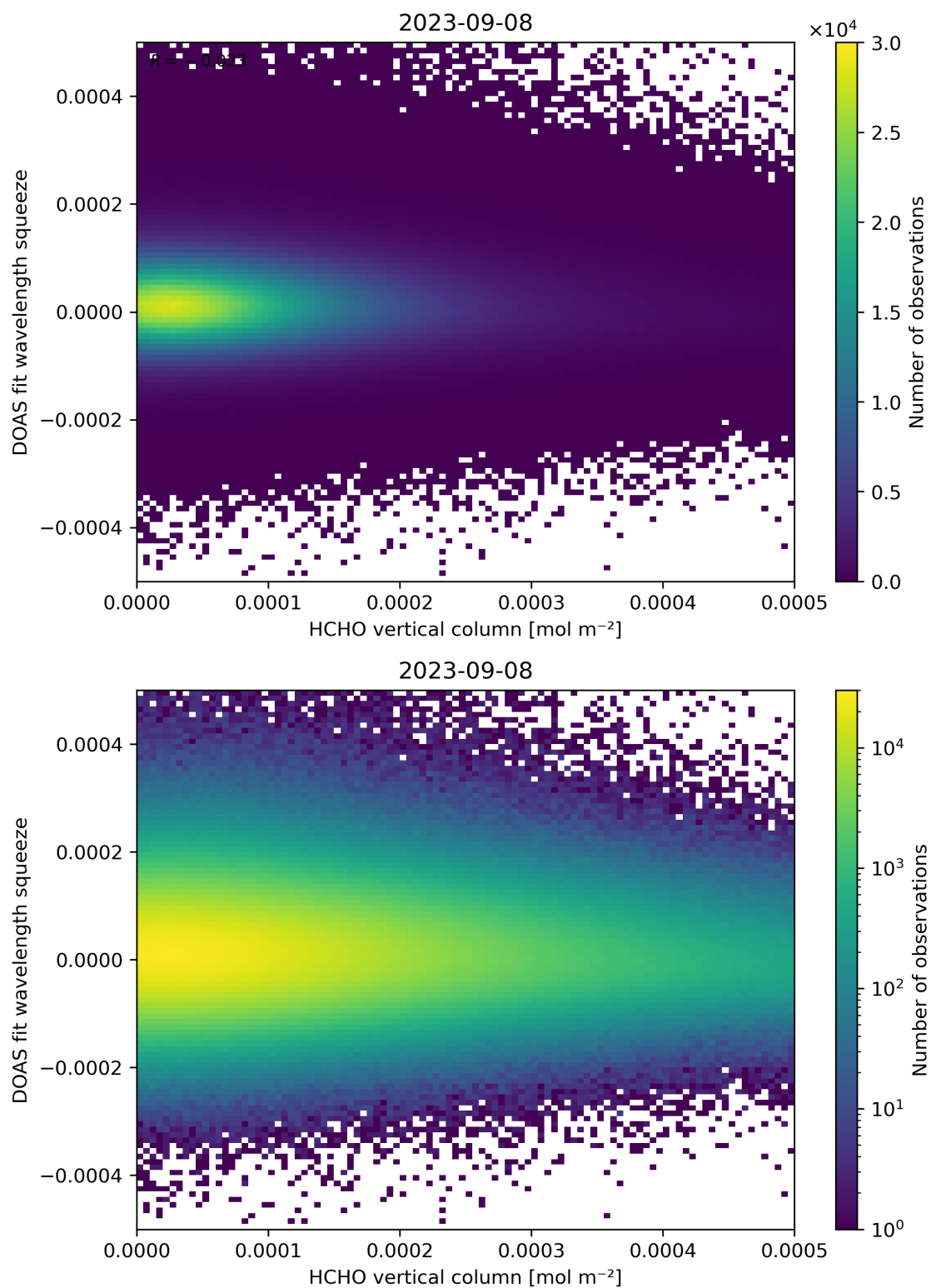
Figure 125: Scatter density plot of “HCHO vertical column” against “DOAS fit wavelength squeeze” for 2023-09-07 to 2023-09-09.
