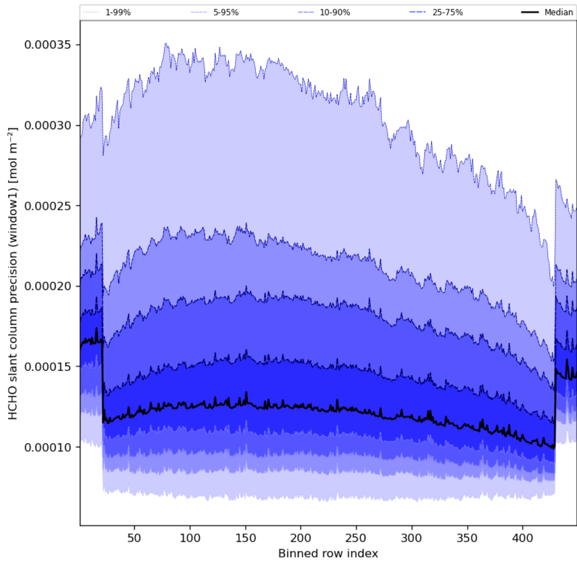
Figure 53: Along track statistics of “HCHO slant column precision (window1)” for 2023-09-07 to 2023-09-09
