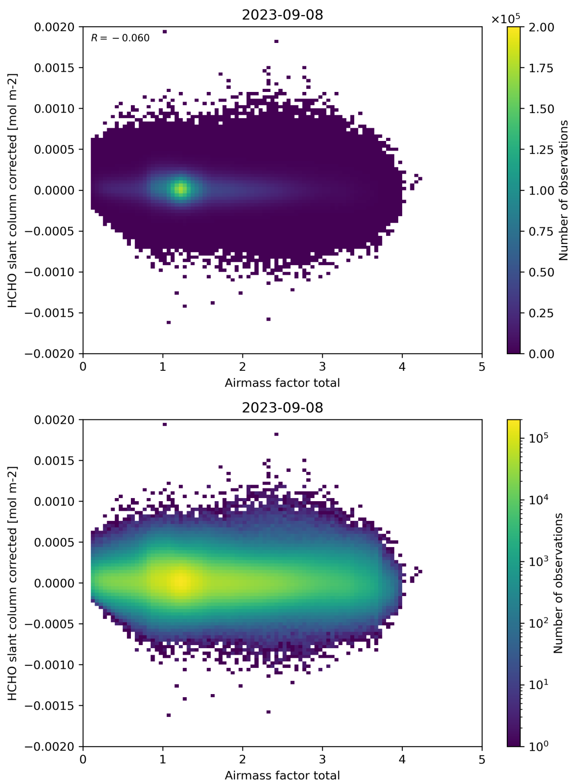
Figure 101: Scatter density plot of “Airmass factor total” against “HCHO slant column corrected” for 2023-09-07 to 2023-09-09.
