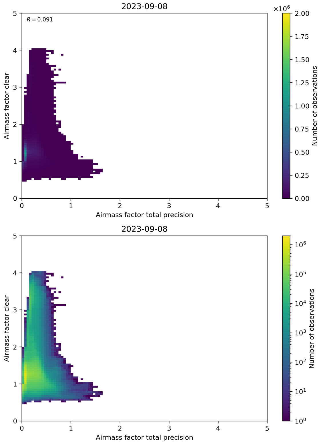
Figure 108: Scatter density plot of “Airmass factor total precision” against “Airmass factor clear” for 2023-09-07 to 2023-09-09.
