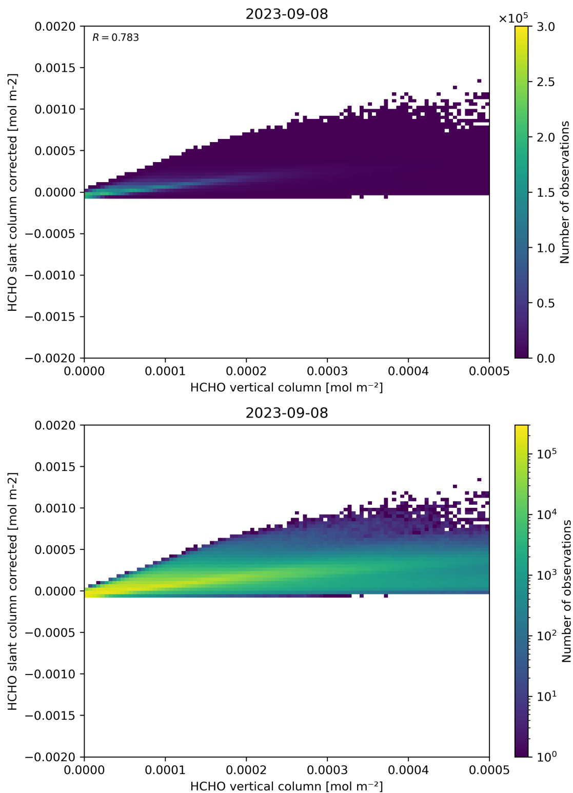
Figure 127: Scatter density plot of “HCHO vertical column” against “HCHO slant column corrected” for 2023-09-07 to 2023-09-09.
