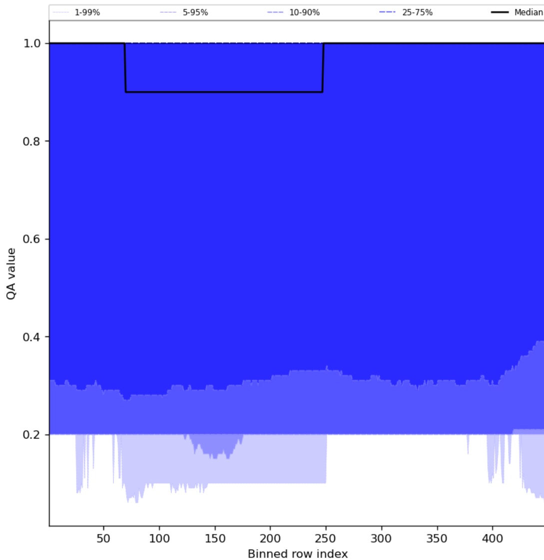
Figure 48: Along track statistics of “QA value” for 2023-09-07 to 2023-09-09
