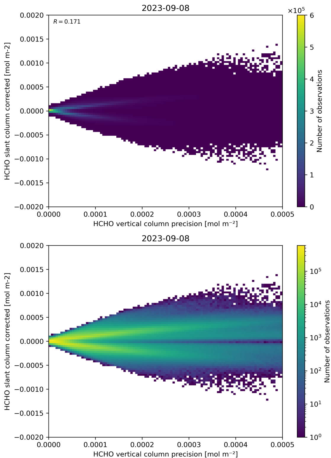
Figure 140: Scatter density plot of “HCHO vertical column precision” against “HCHO slant column corrected” for 2023-09-07 to 2023-09-09.
