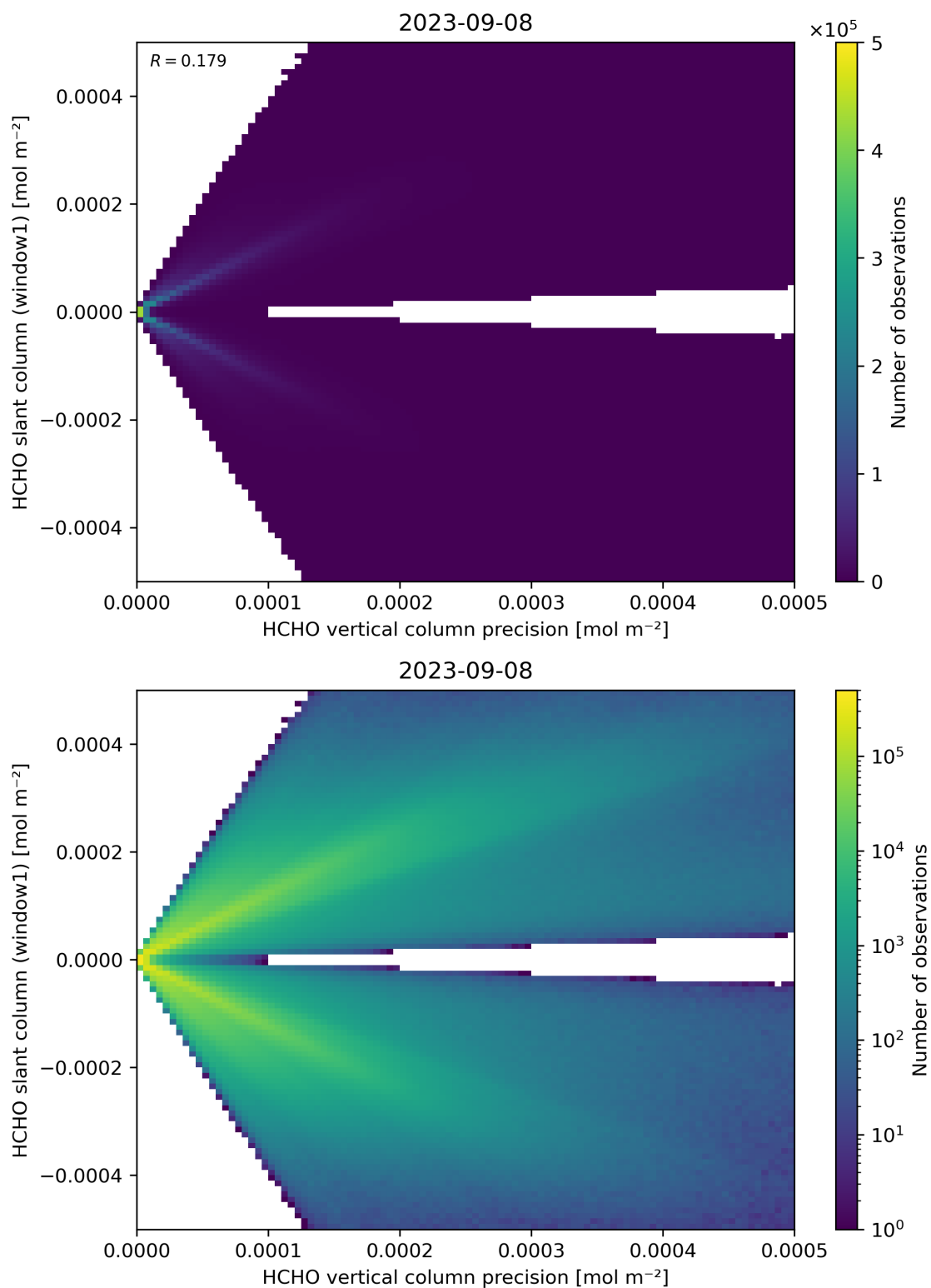
Figure 142: Scatter density plot of “HCHO vertical column precision” against “HCHO slant column (window1)” for 2023-09-07 to 2023-09-09.
