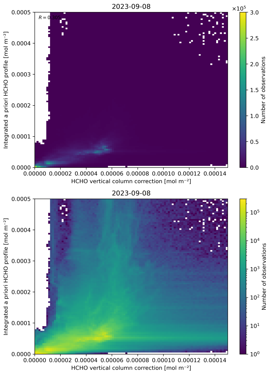
Figure 122: Scatter density plot of “HCHO vertical column correction” against “Integrated a priori HCHO profile” for 2023-09-07 to 2023-09-09.
