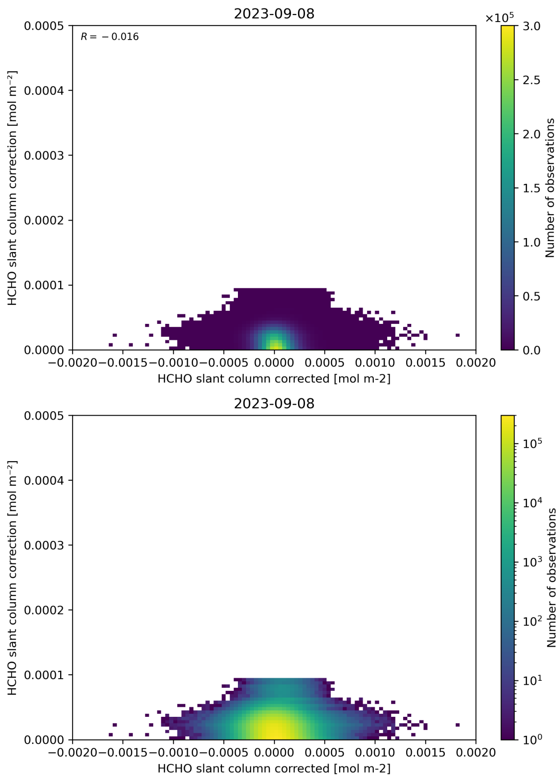
Figure 77: Scatter density plot of “HCHO slant column corrected” against “HCHO slant column correction” for 2023-09-07 to 2023-09-09.
