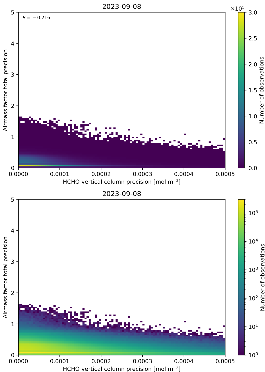
Figure 145: Scatter density plot of “HCHO vertical column precision” against “Airmass factor total precision” for 2023-09-07 to 2023-09-09.
