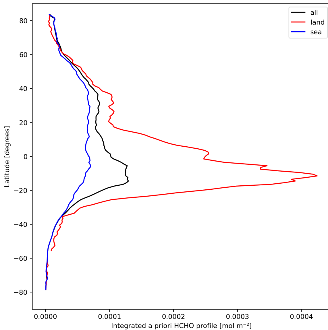
Figure 29: Zonal average of “Integrated a priori HCHO profile” for 2023-09-07 to 2023-09-09.
