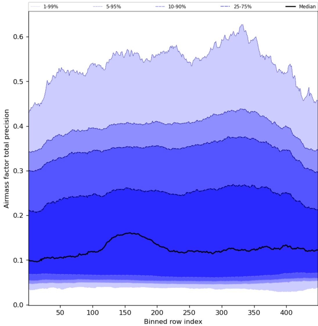
Figure 55: Along track statistics of “Airmass factor total precision” for 2023-09-07 to 2023-09-09
