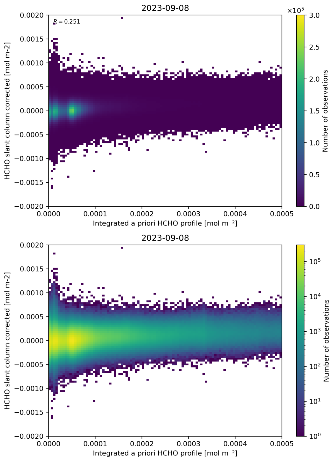
Figure 151: Scatter density plot of “Integrated a priori HCHO profile” against “HCHO slant column corrected” for 2023-09-07 to 2023-09-09.
