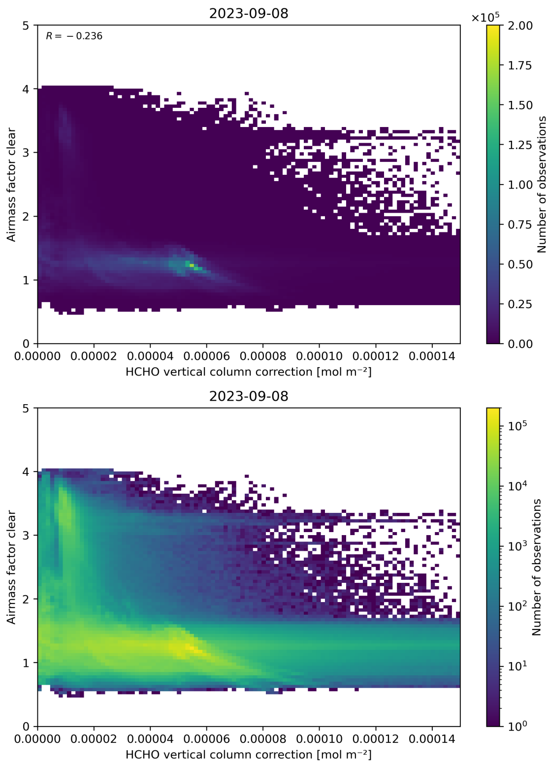
Figure 115: Scatter density plot of “HCHO vertical column correction” against “Airmass factor clear” for 2023-09-07 to 2023-09-09.
