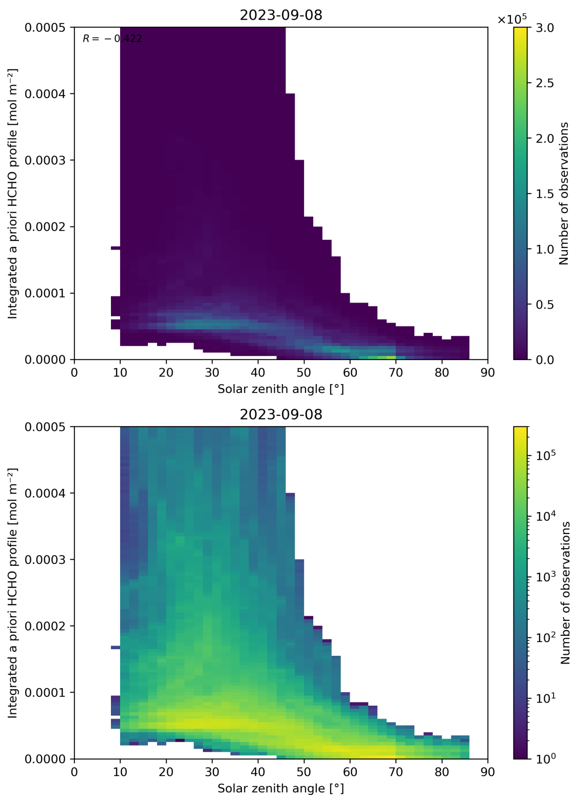
Figure 180: Scatter density plot of “Solar zenith angle” against “Integrated a priori HCHO profile” for 2023-09-07 to 2023-09-09.
