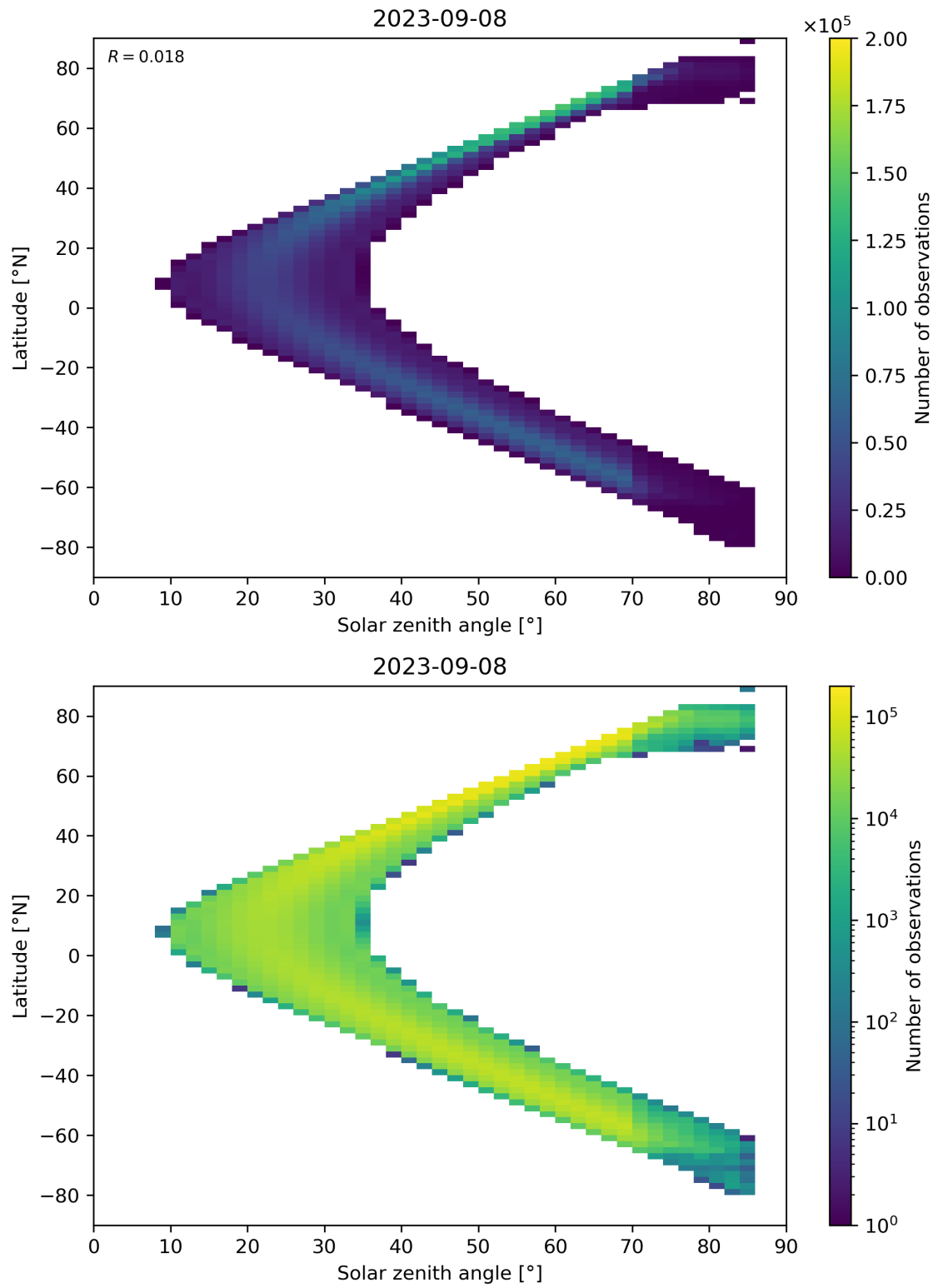
Figure 181: Scatter density plot of “Solar zenith angle” against “Latitude” for 2023-09-07 to 2023-09-09.
