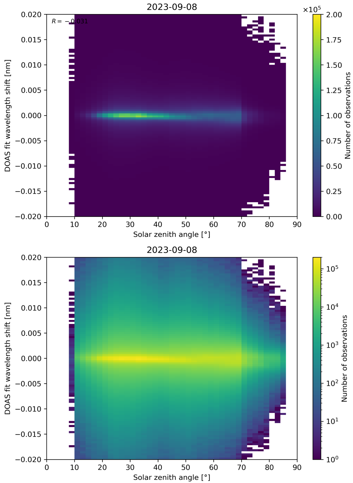
Figure 168: Scatter density plot of “Solar zenith angle” against “DOAS fit wavelength shift” for 2023-09-07 to 2023-09-09.
