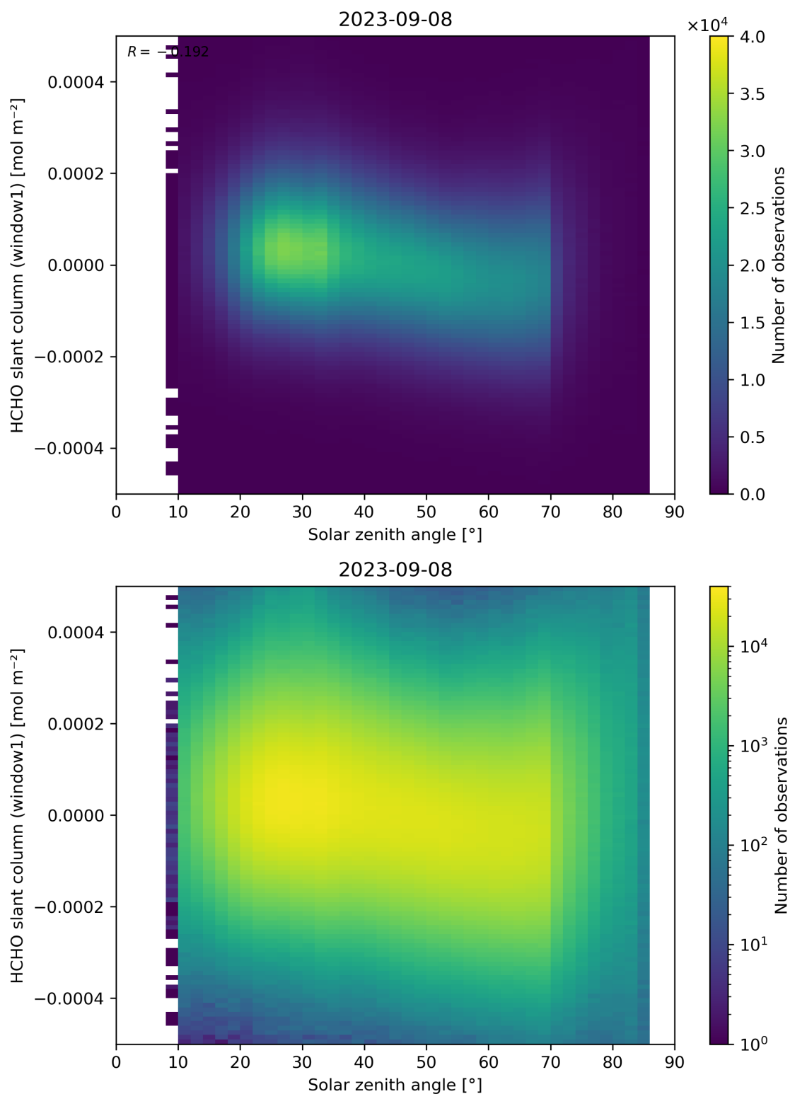
Figure 173: Scatter density plot of “Solar zenith angle” against “HCHO slant column (window1)” for 2023-09-07 to 2023-09-09.
