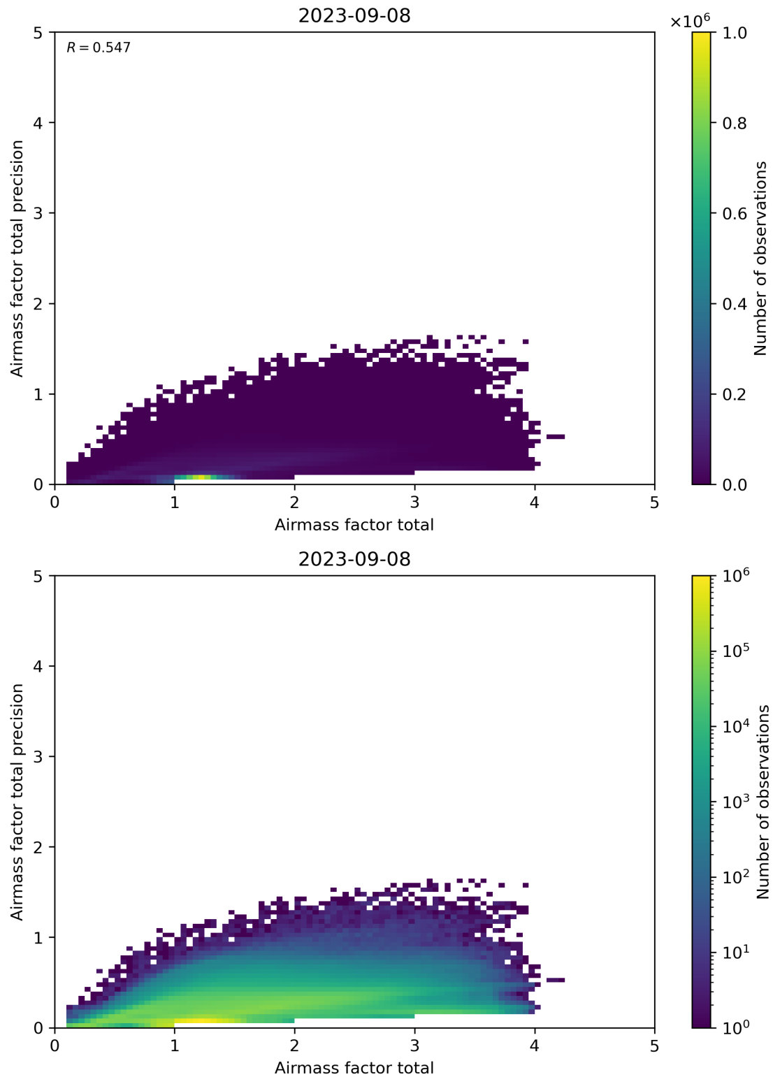
Figure 103: Scatter density plot of “Airmass factor total” against “Airmass factor total precision” for 2023-09-07 to 2023-09-09.
