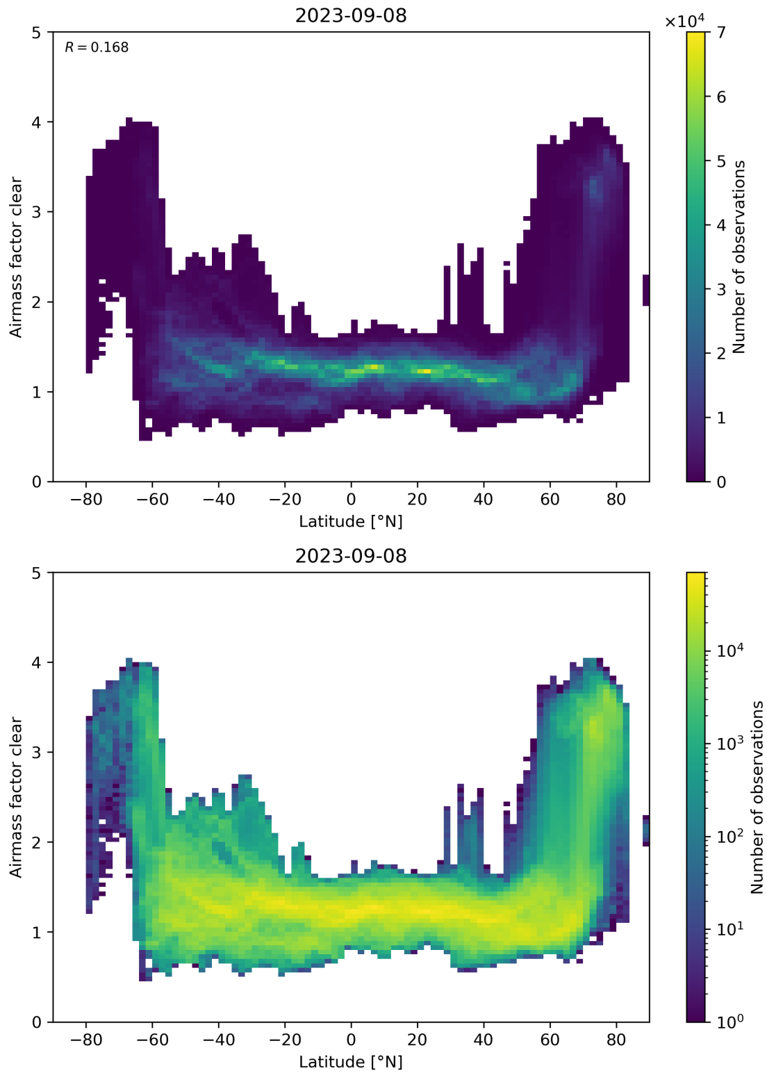
Figure 156: Scatter density plot of “Latitude” against “Airmass factor clear” for 2023-09-07 to 2023-09-09.
