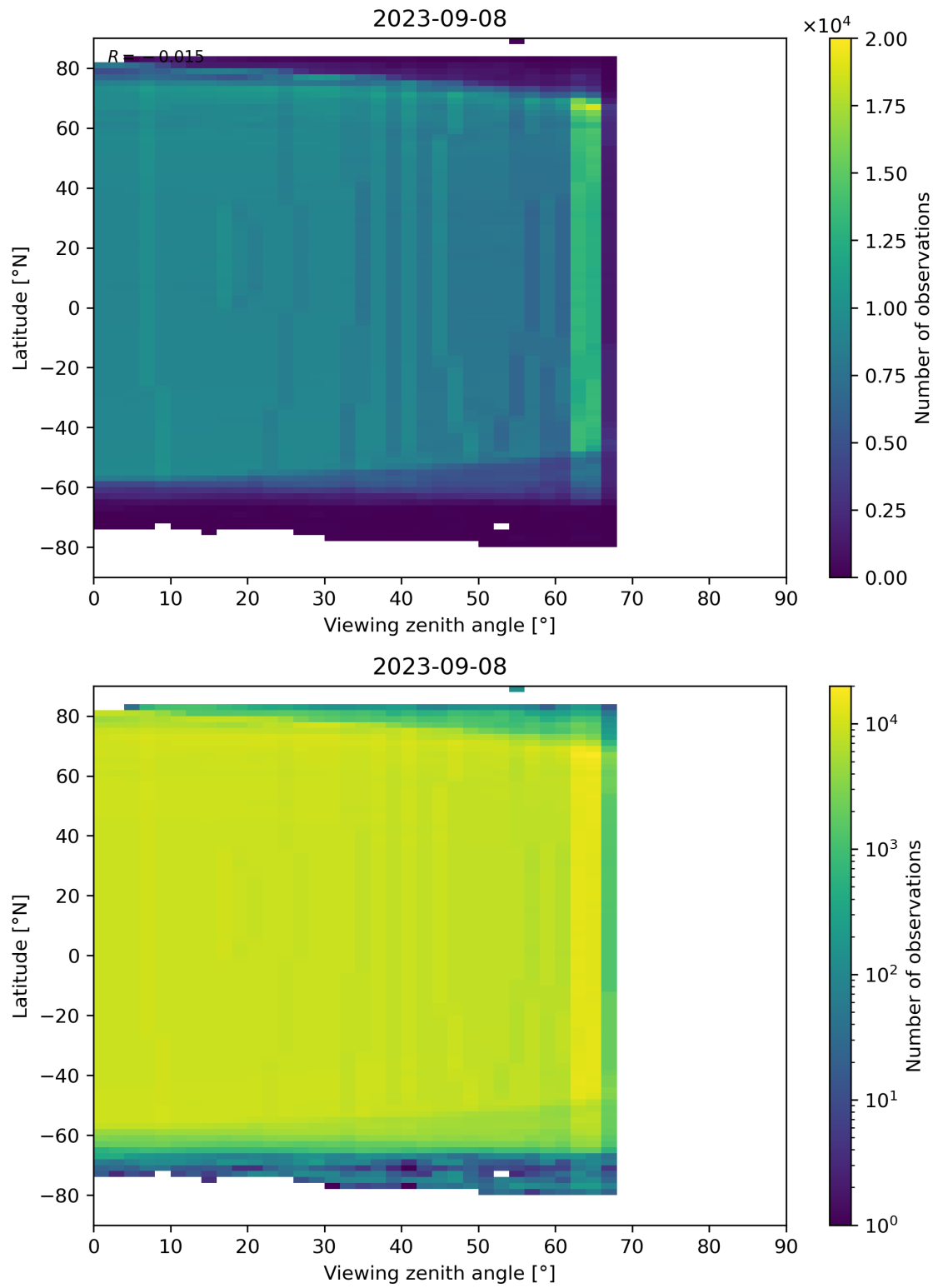
Figure 196: Scatter density plot of “Viewing zenith angle” against “Latitude” for 2023-09-07 to 2023-09-09.
