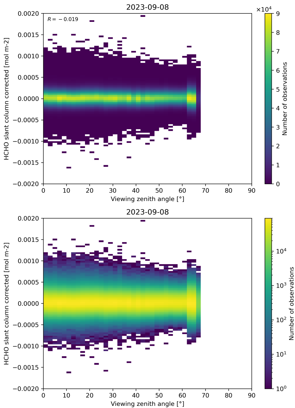
Figure 186: Scatter density plot of “Viewing zenith angle” against “HCHO slant column corrected” for 2023-09-07 to 2023-09-09.
