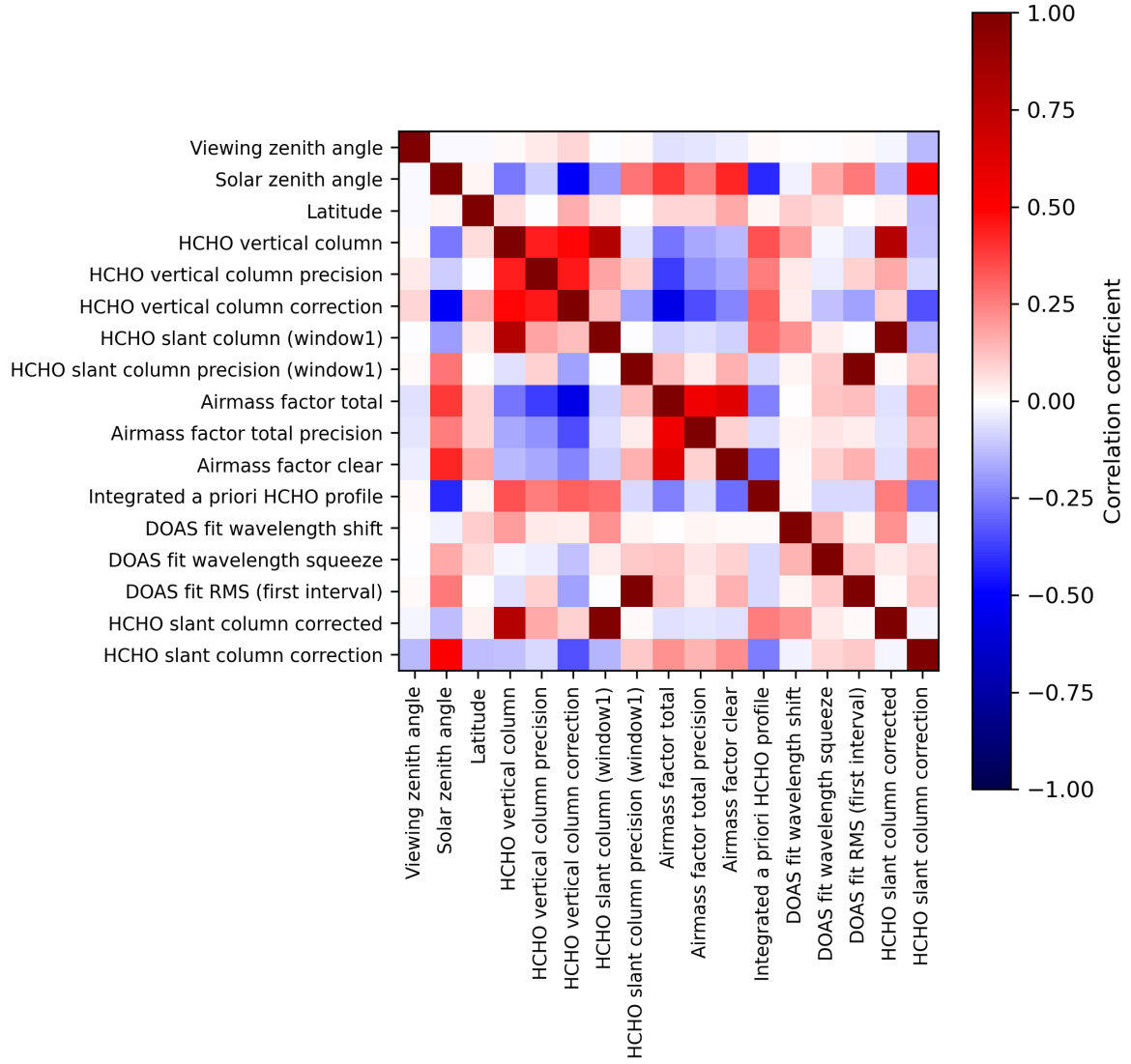
Figure 2: Map of correlation matrix for 2023-09-07 to 2023-09-09.
