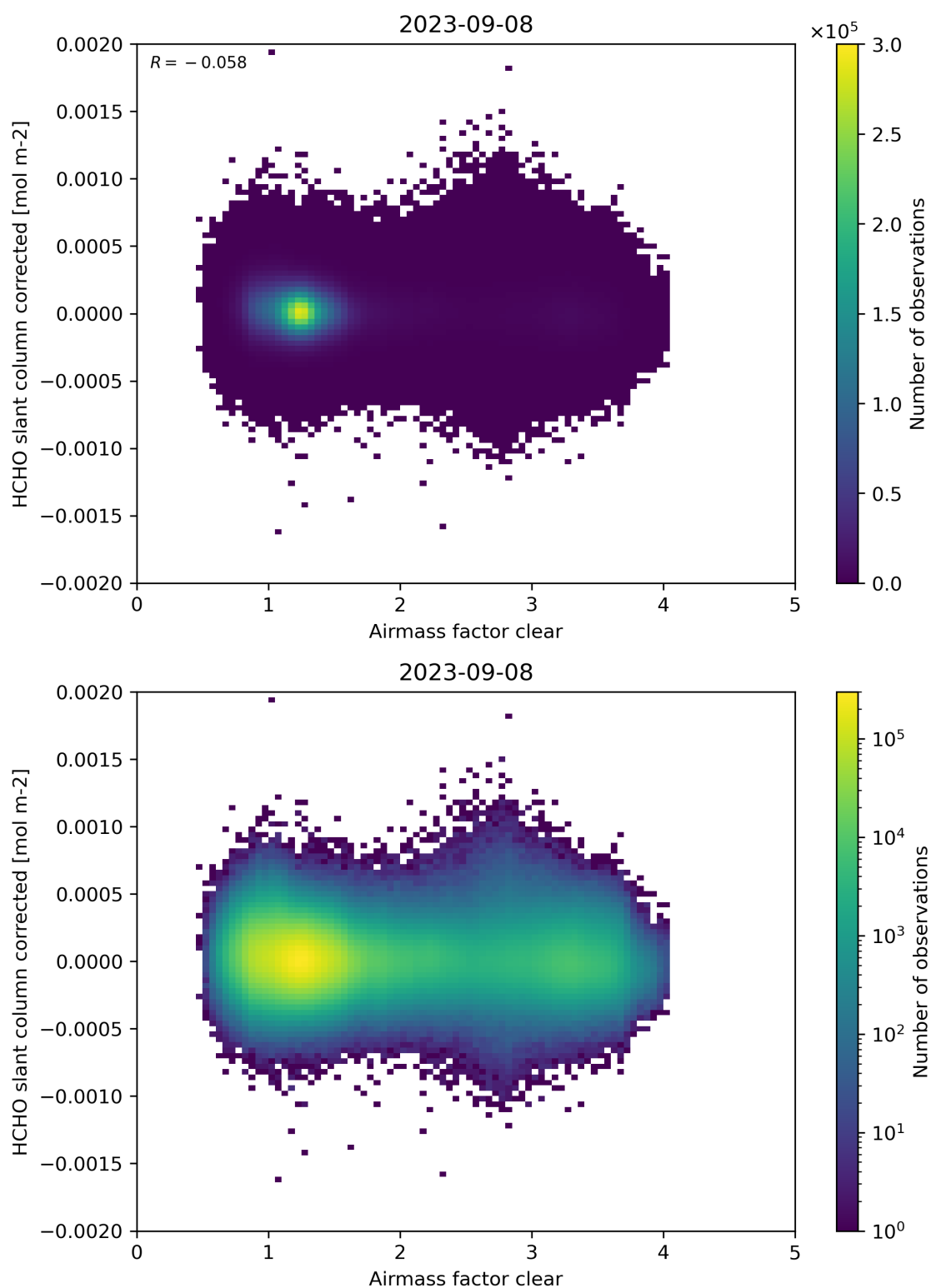
Figure 74: Scatter density plot of “Airmass factor clear” against “HCHO slant column corrected” for 2023-09-07 to 2023-09-09.
