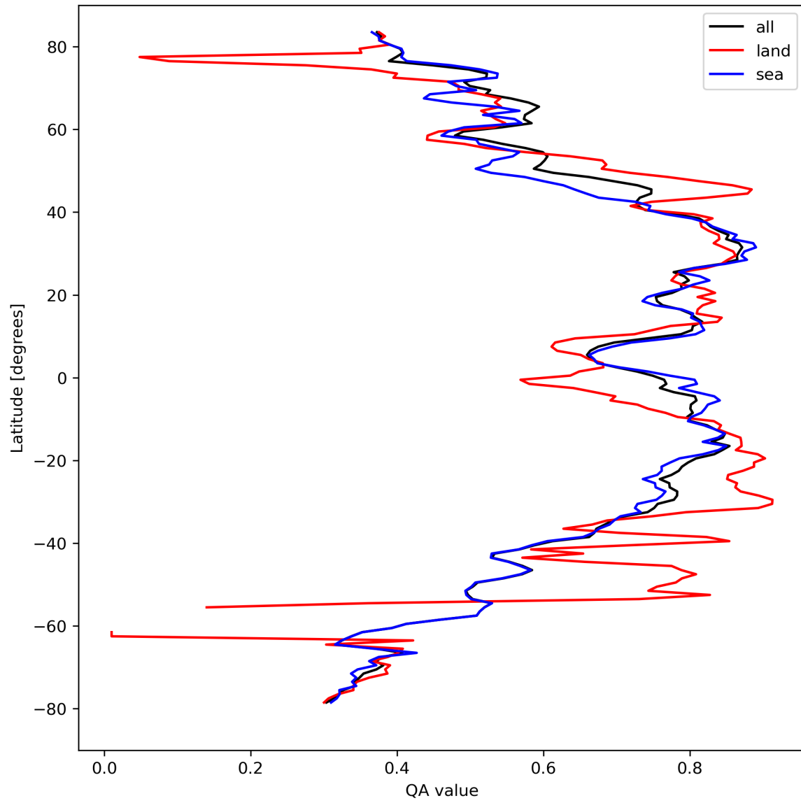
Figure 20: Zonal average of “QA value” for 2023-09-07 to 2023-09-09.
