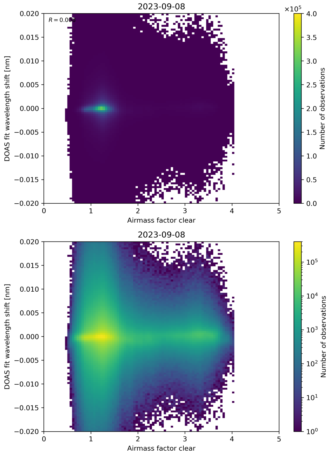
Figure 72: Scatter density plot of “Airmass factor clear” against “DOAS fit wavelength shift” for 2023-09-07 to 2023-09-09.
