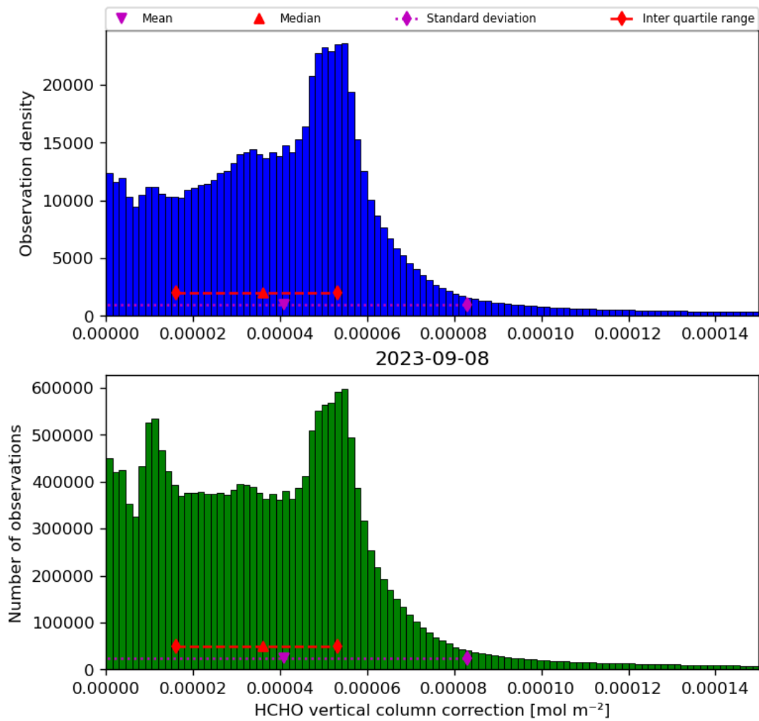
Figure 37: Histogram of “HCHO vertical column correction” for 2023-09-07 to 2023-09-09
