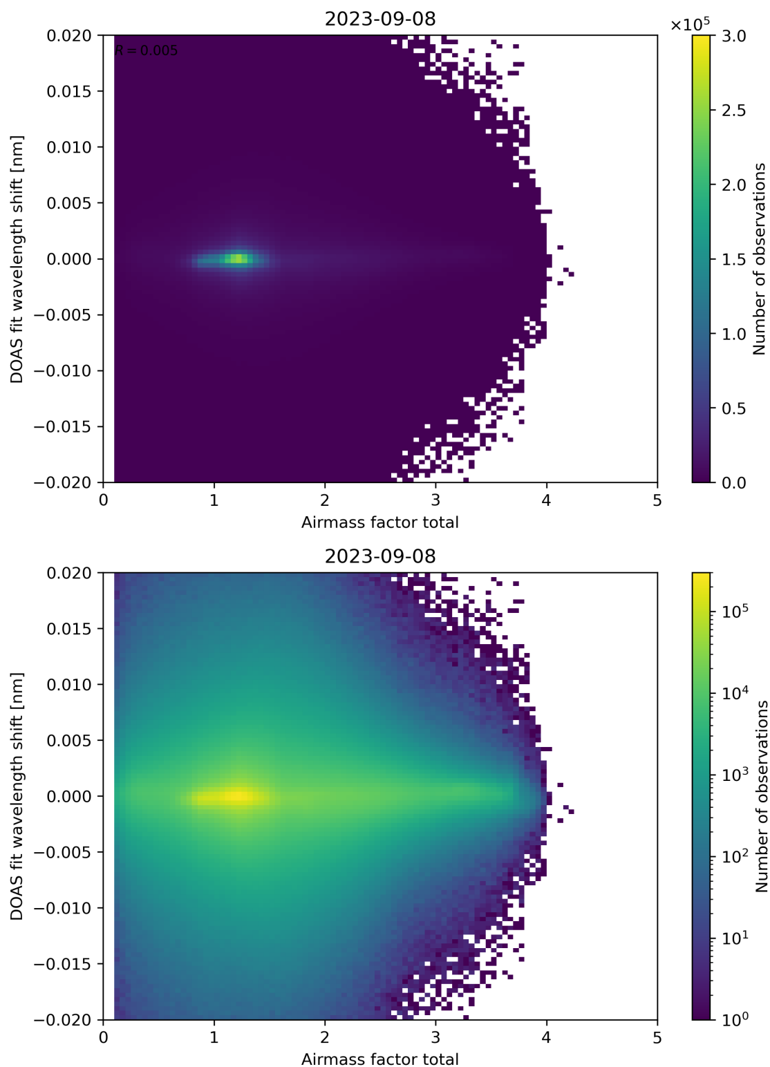
Figure 98: Scatter density plot of “Airmass factor total” against “DOAS fit wavelength shift” for 2023-09-07 to 2023-09-09.
