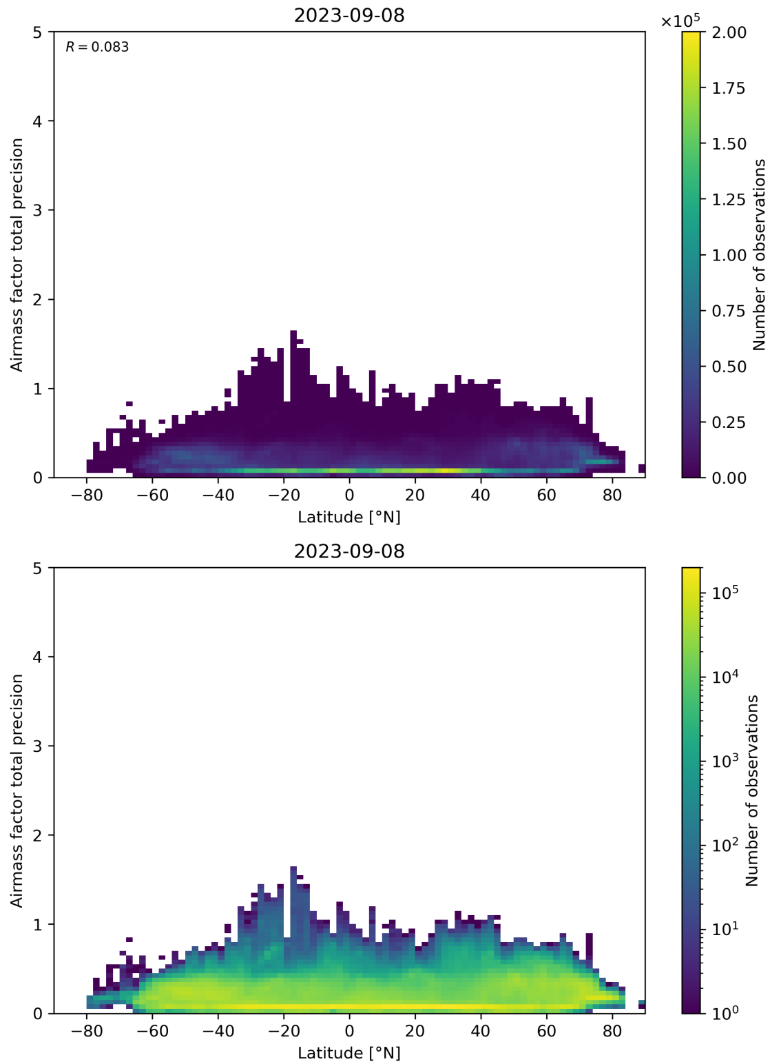
Figure 162: Scatter density plot of “Latitude” against “Airmass factor total precision” for 2023-09-07 to 2023-09-09.
