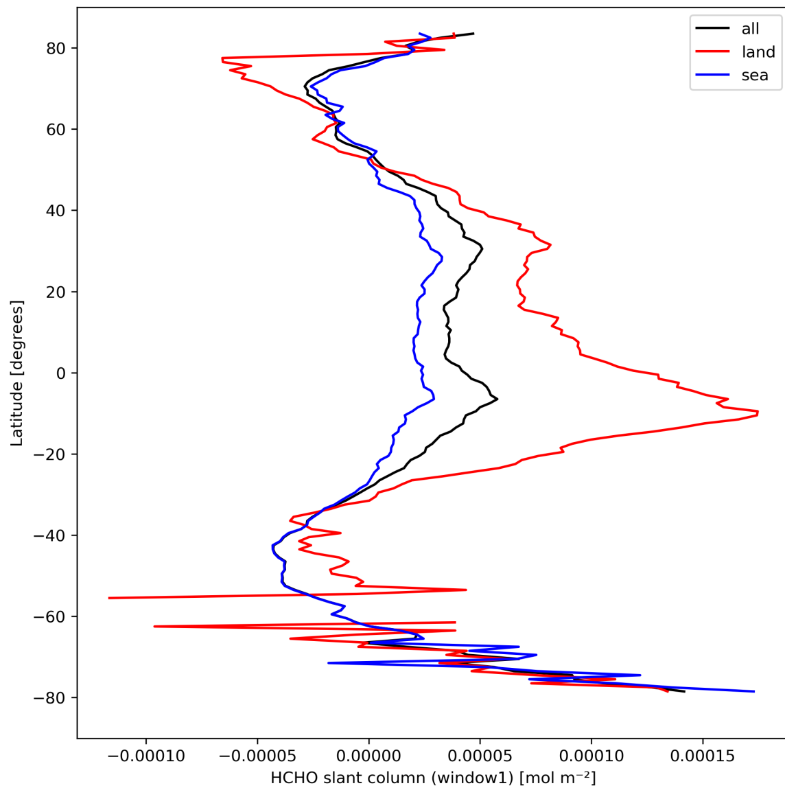
Figure 24: Zonal average of “HCHO slant column (window1)” for 2023-09-07 to 2023-09-09.
