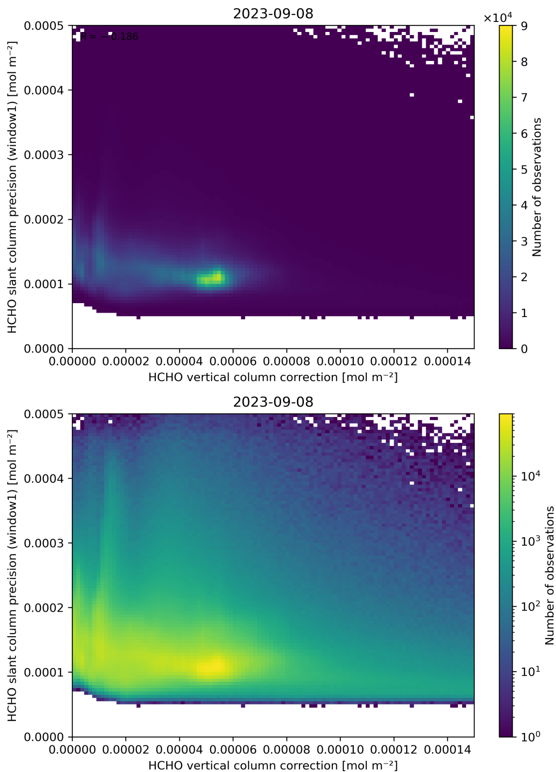
Figure 119: Scatter density plot of “HCHO vertical column correction” against “HCHO slant column precision (window1)” for 2023-09-07 to 2023-09-09.
