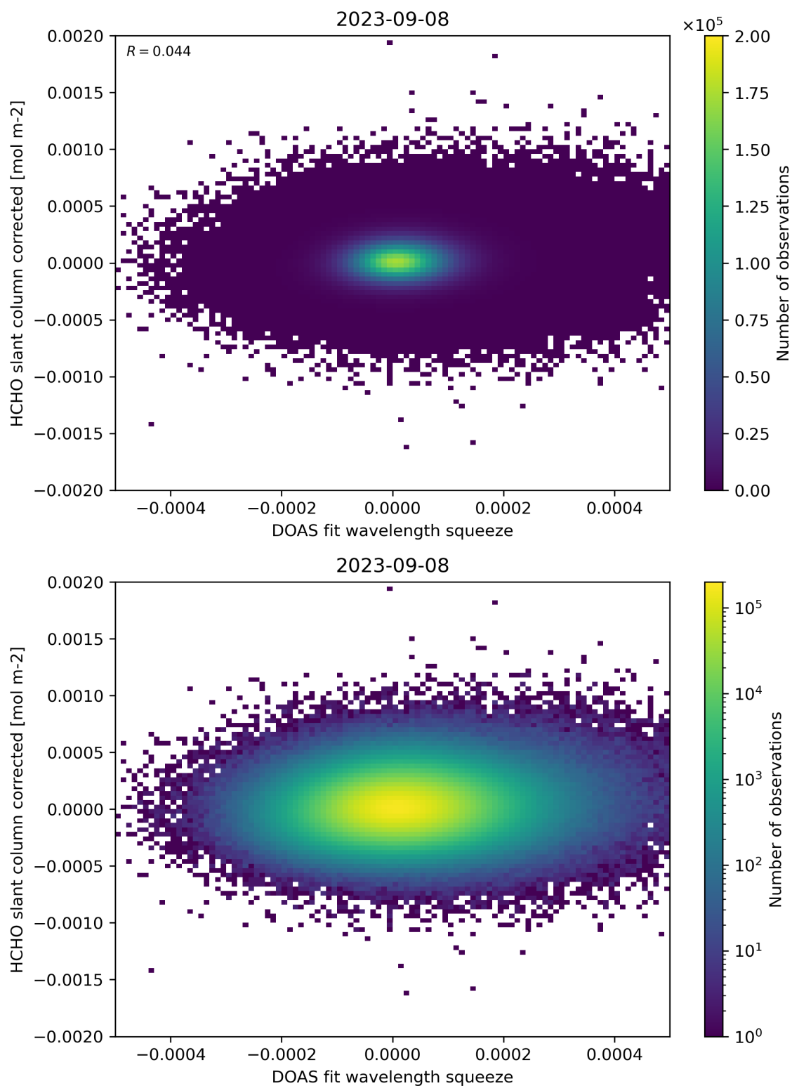
Figure 69: Scatter density plot of “DOAS fit wavelength squeeze” against “HCHO slant column corrected” for 2023-09-07 to 2023-09-09.
