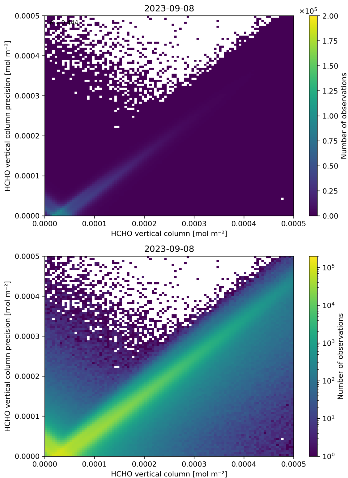
Figure 134: Scatter density plot of “HCHO vertical column” against “HCHO vertical column precision” for 2023-09-07 to 2023-09-09.
