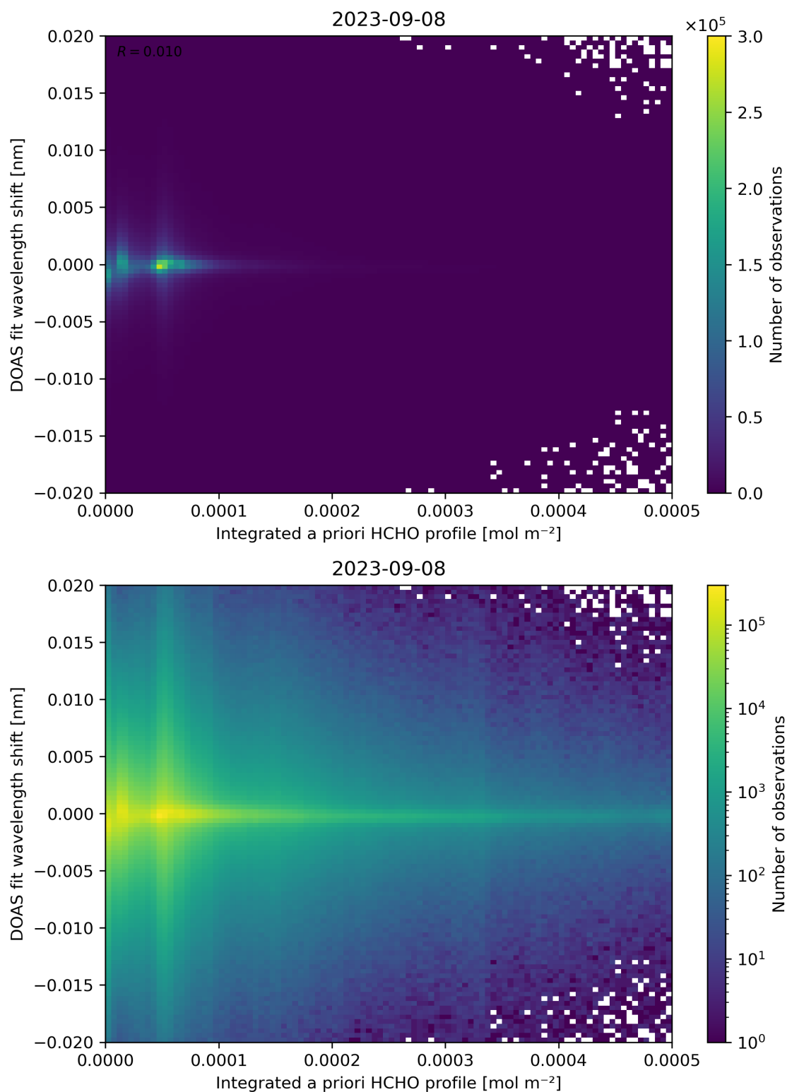
Figure 149: Scatter density plot of “Integrated a priori HCHO profile” against “DOAS fit wavelength shift” for 2023-09-07 to 2023-09-09.
