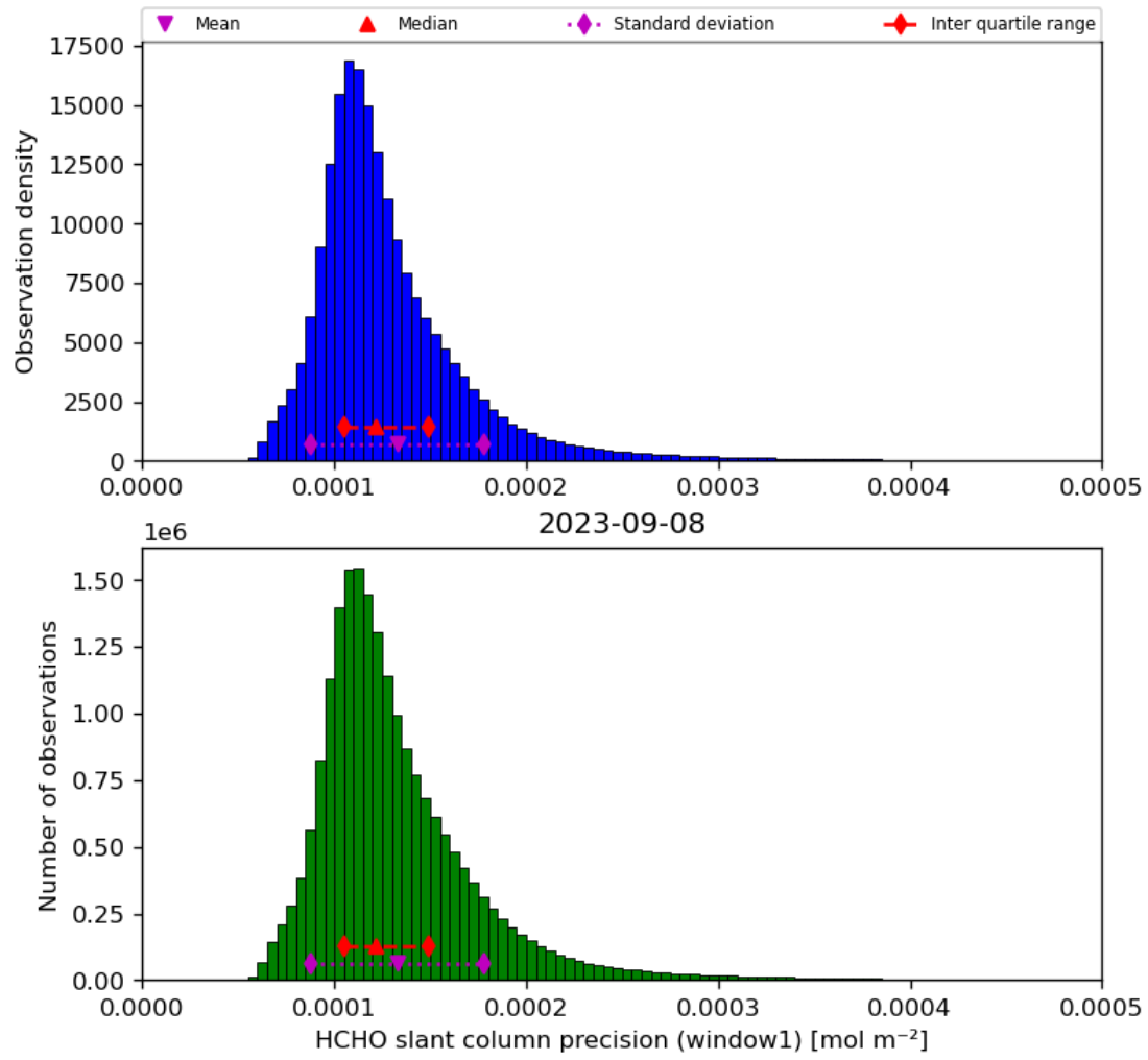
Figure 39: Histogram of “HCHO slant column precision (window1)” for 2023-09-07 to 2023-09-09
