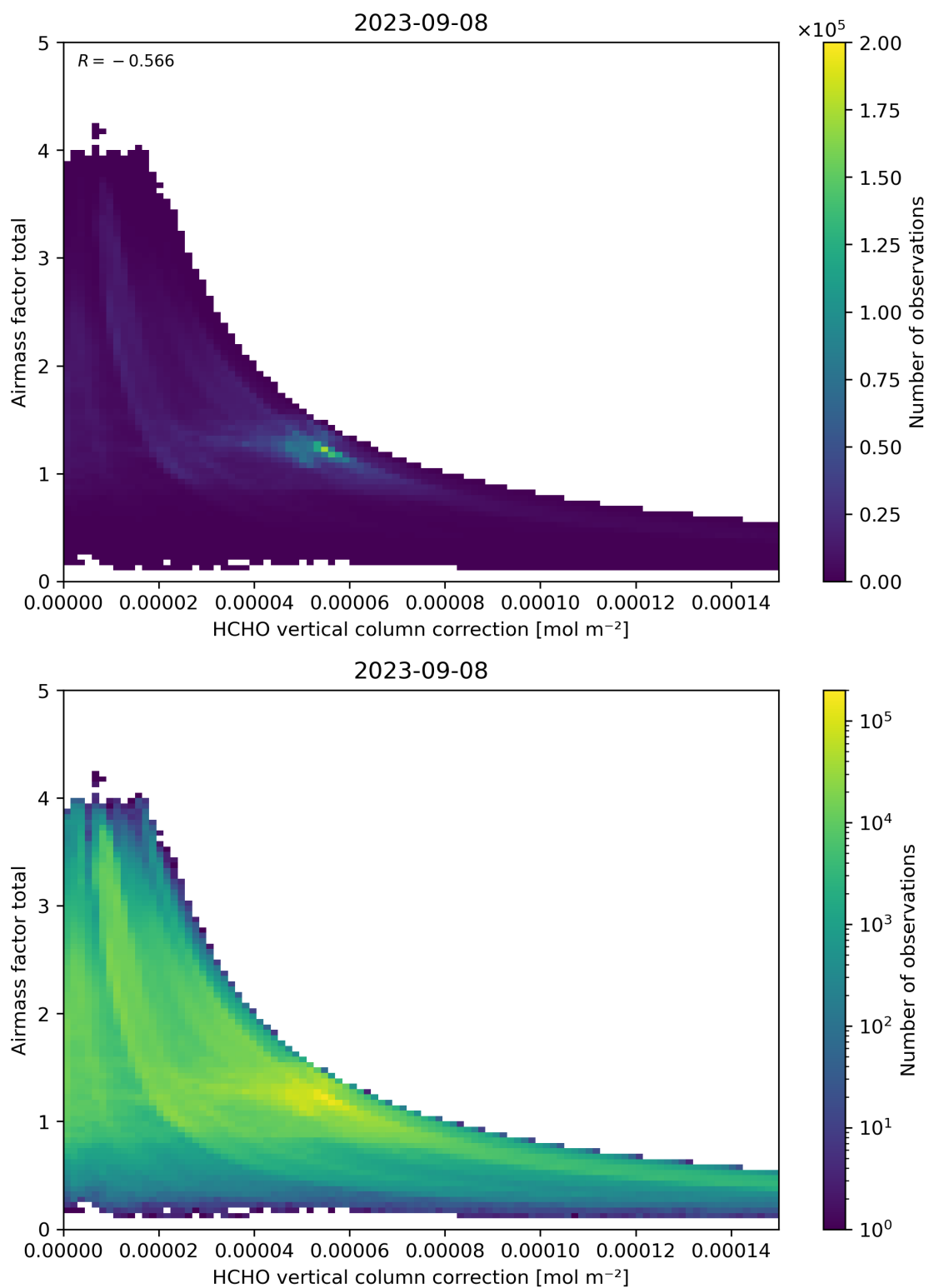
Figure 120: Scatter density plot of “HCHO vertical column correction” against “Airmass factor total” for 2023-09-07 to 2023-09-09.
