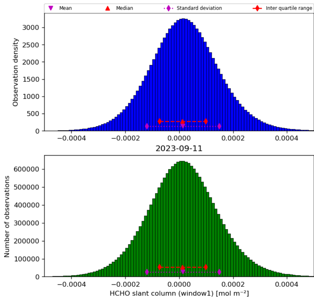
Figure 38: Histogram of “HCHO slant column (window1)” for 2023-09-10 to 2023-09-12
