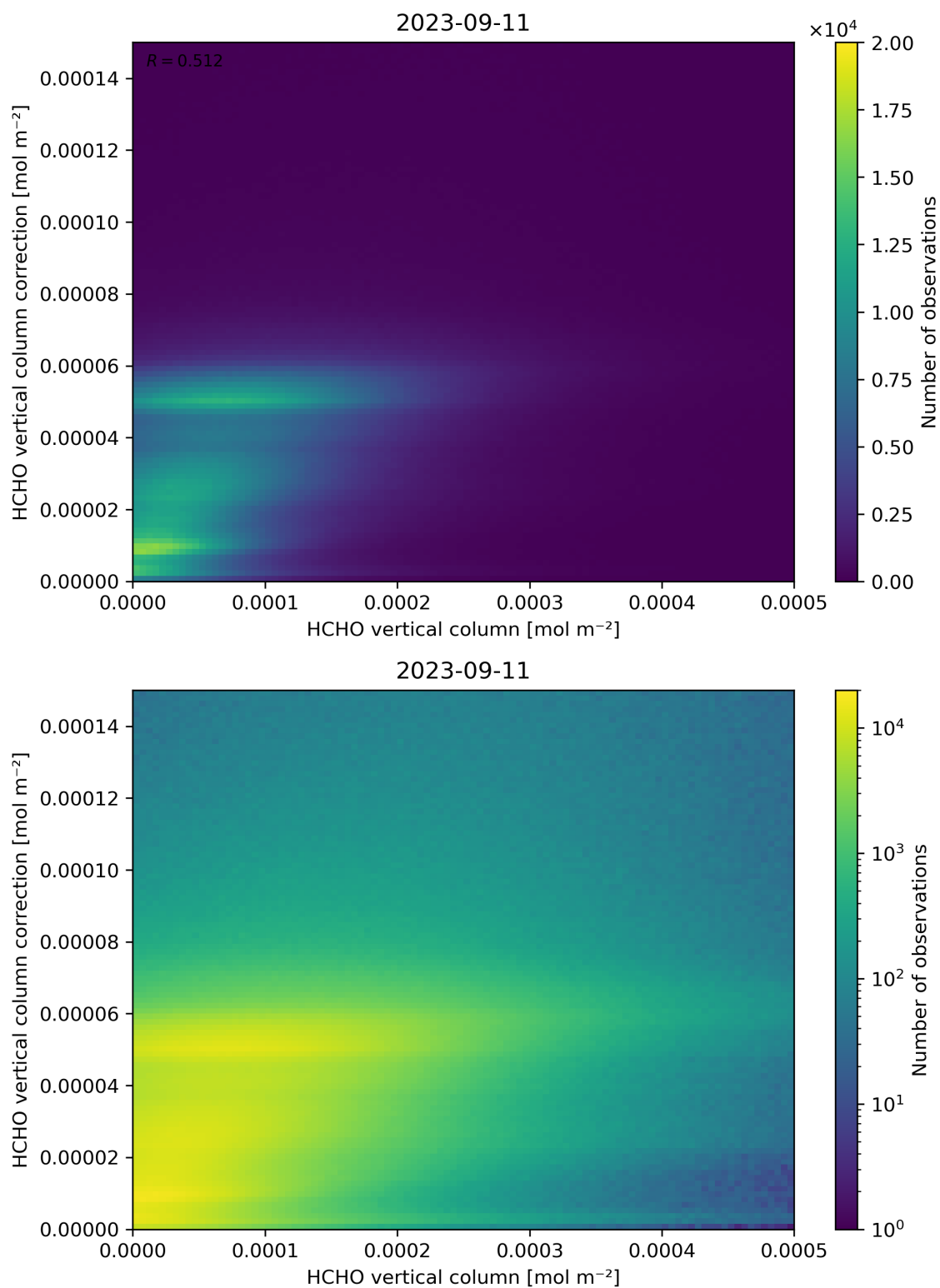
Figure 133: Scatter density plot of “HCHO vertical column” against “HCHO vertical column correction” for 2023-09-10 to 2023-09-12.
