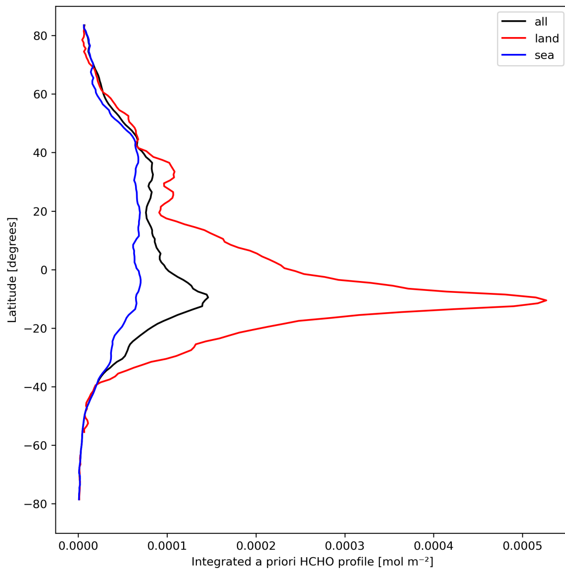
Figure 29: Zonal average of “Integrated a priori HCHO profile” for 2023-09-10 to 2023-09-12.
