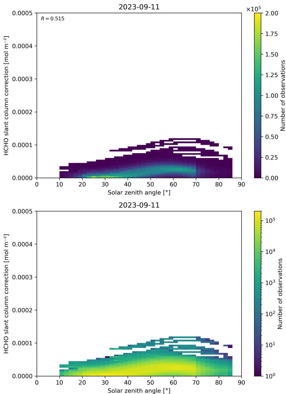
Figure 172: Scatter density plot of “Solar zenith angle” against “HCHO slant column correction” for 2023-09-10 to 2023-09-12.
