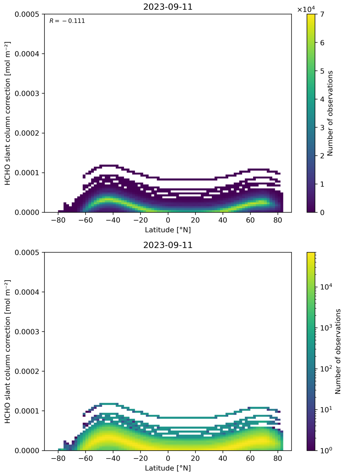
Figure 158: Scatter density plot of “Latitude” against “HCHO slant column correction” for 2023-09-10 to 2023-09-12.
