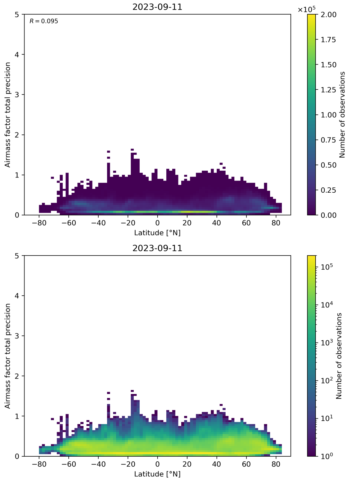
Figure 162: Scatter density plot of “Latitude” against “Airmass factor total precision” for 2023-09-10 to 2023-09-12.
