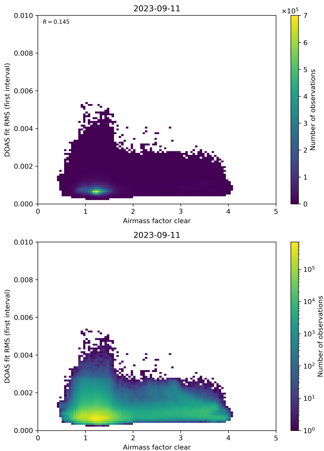
Figure 71: Scatter density plot of “Airmass factor clear” against “DOAS fit RMS (first interval)” for 2023-09-10 to 2023-09-12.
