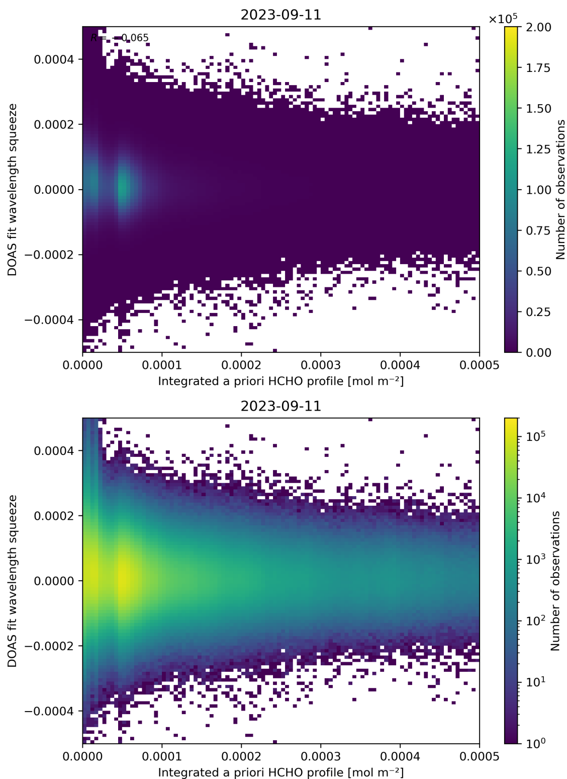
Figure 150: Scatter density plot of “Integrated a priori HCHO profile” against “DOAS fit wavelength squeeze” for 2023-09-10 to 2023-09-12.
