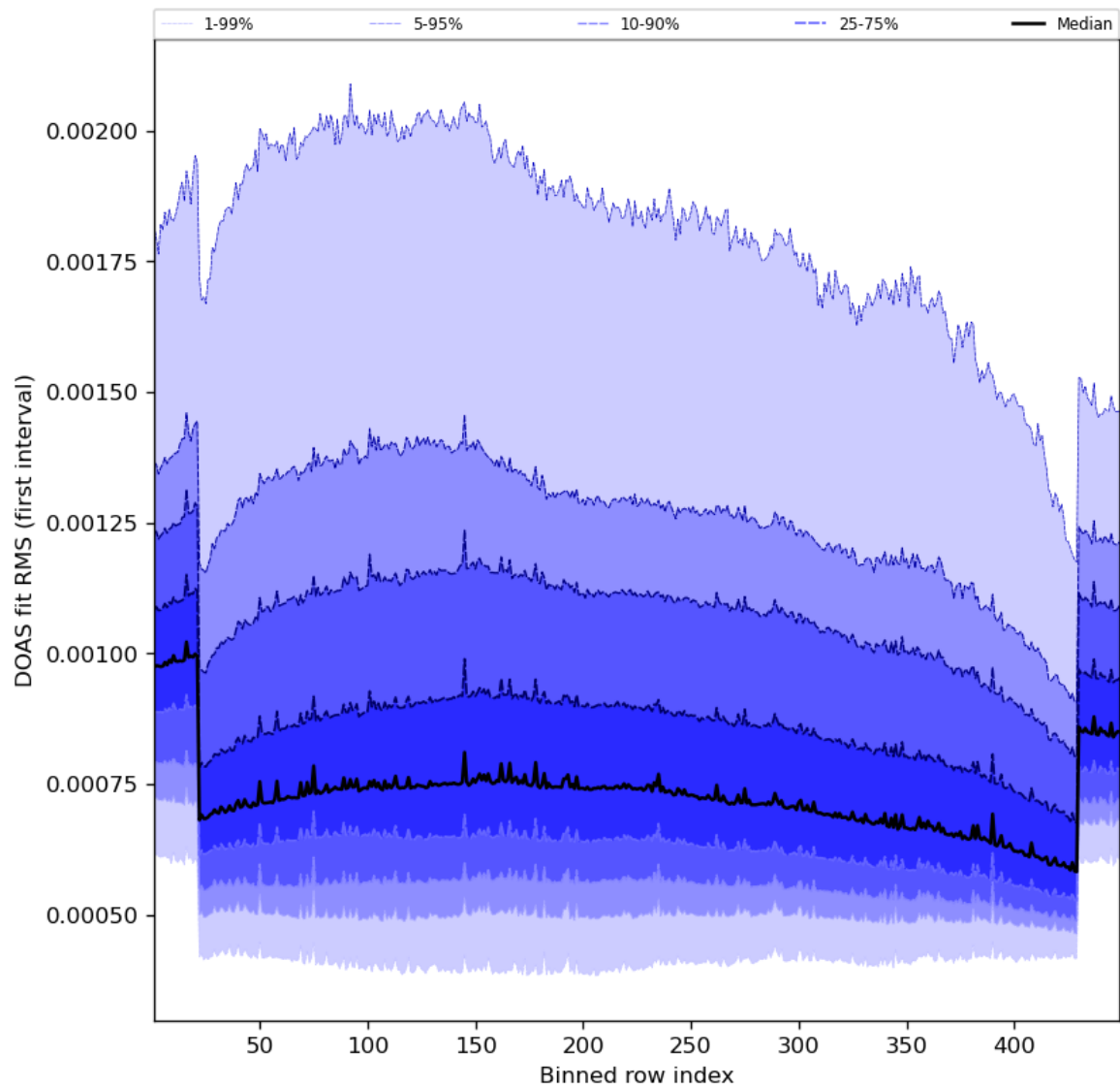
Figure 60: Along track statistics of “DOAS fit RMS (first interval)” for 2023-09-10 to 2023-09-12
