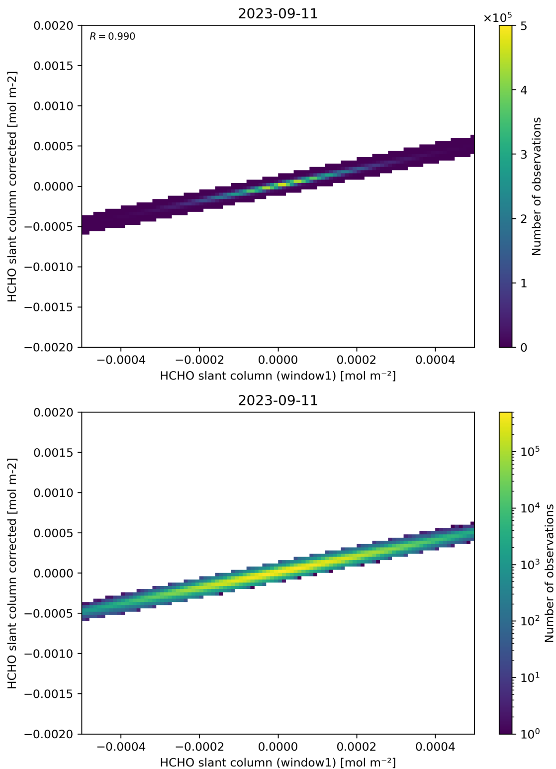
Figure 82: Scatter density plot of “HCHO slant column (window1)” against “HCHO slant column corrected” for 2023-09-10 to 2023-09-12.
