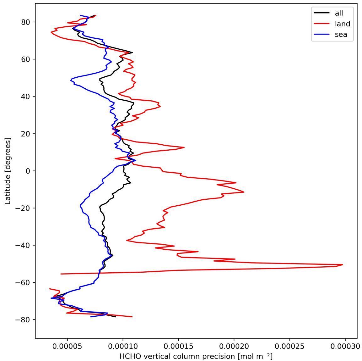
Figure 22: Zonal average of “HCHO vertical column precision” for 2023-09-10 to 2023-09-12.
