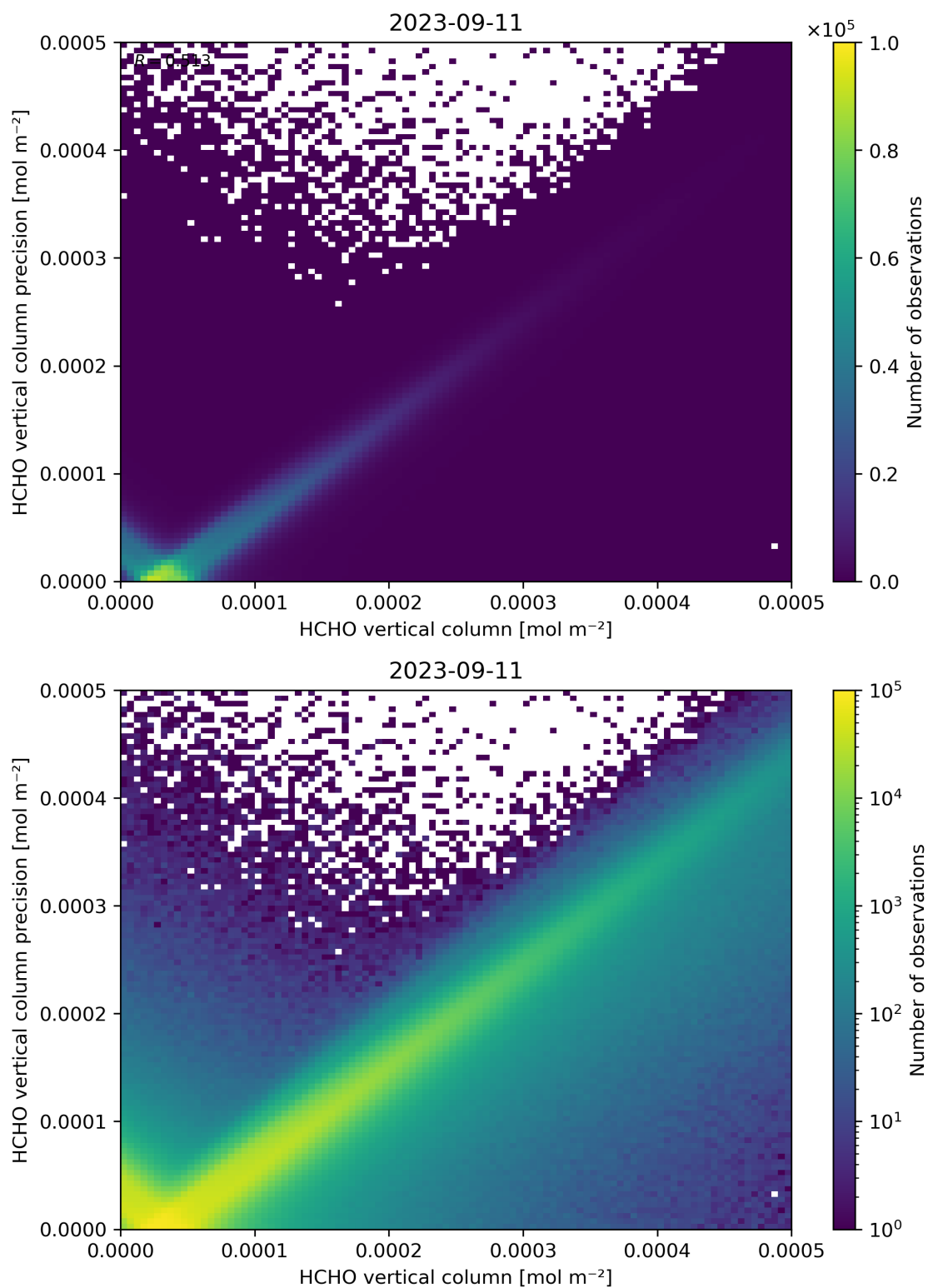
Figure 134: Scatter density plot of “HCHO vertical column” against “HCHO vertical column precision” for 2023-09-10 to 2023-09-12.
