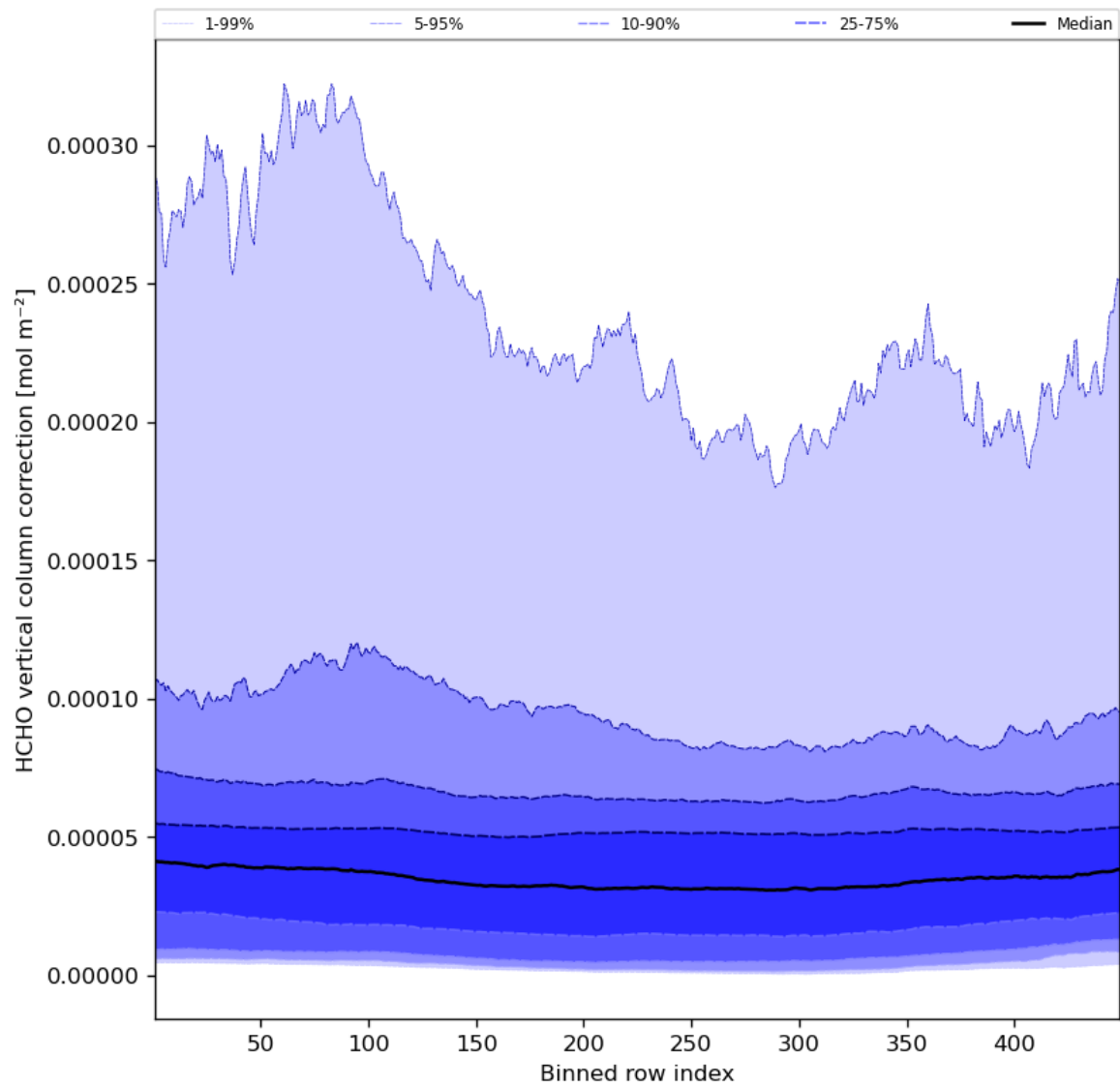
Figure 51: Along track statistics of “HCHO vertical column correction” for 2023-09-10 to 2023-09-12
