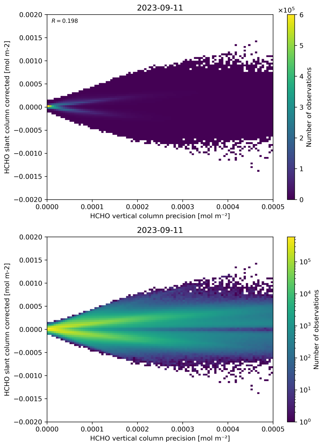
Figure 140: Scatter density plot of “HCHO vertical column precision” against “HCHO slant column corrected” for 2023-09-10 to 2023-09-12.
