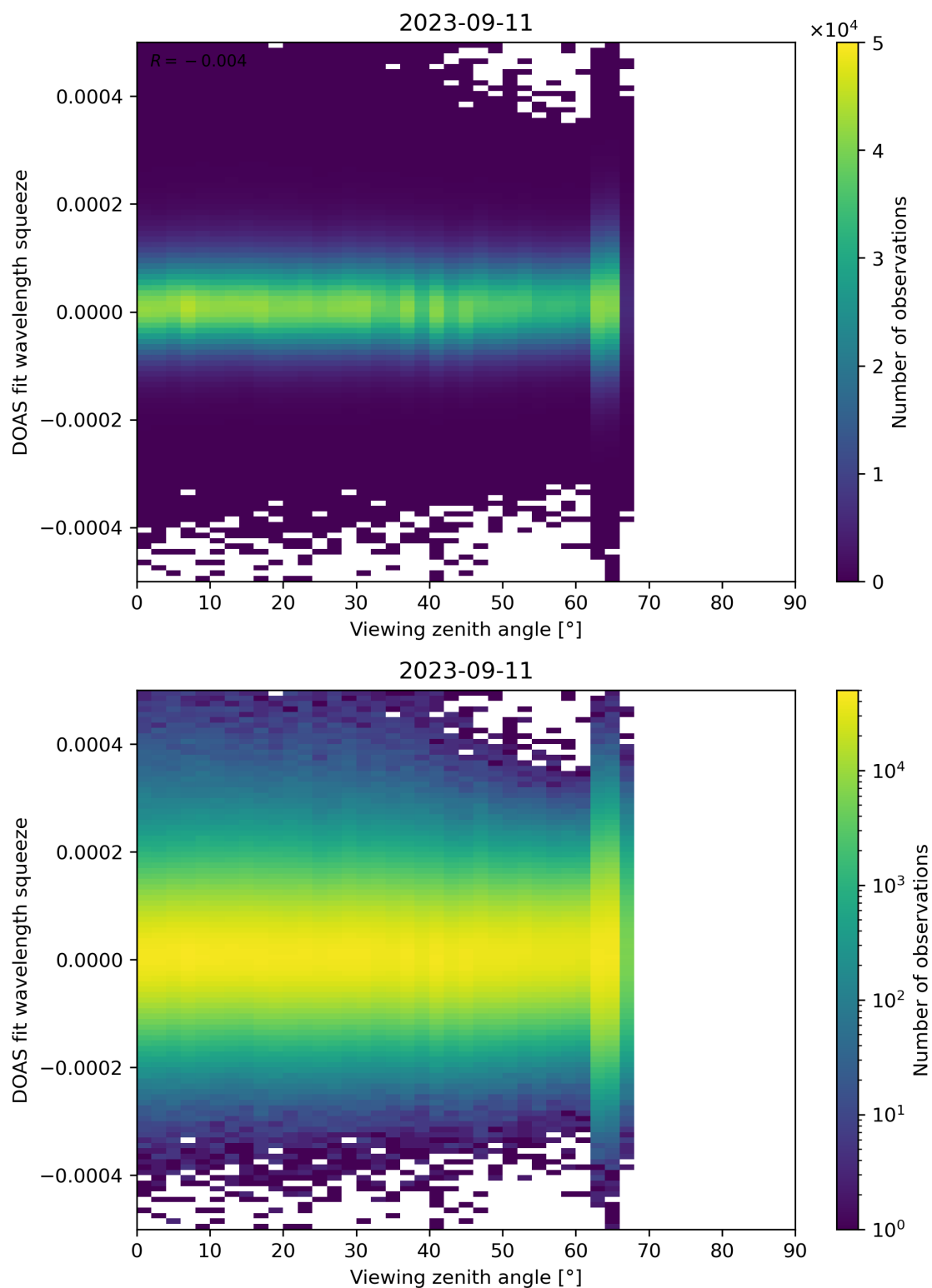
Figure 184: Scatter density plot of “Viewing zenith angle” against “DOAS fit wavelength squeeze” for 2023-09-10 to 2023-09-12.
