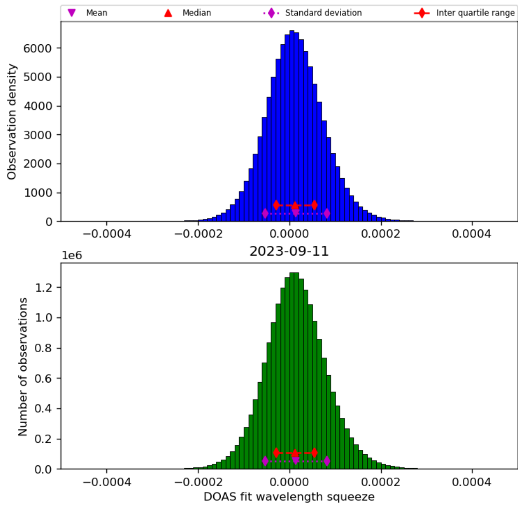
Figure 45: Histogram of “DOAS fit wavelength squeeze” for 2023-09-10 to 2023-09-12
