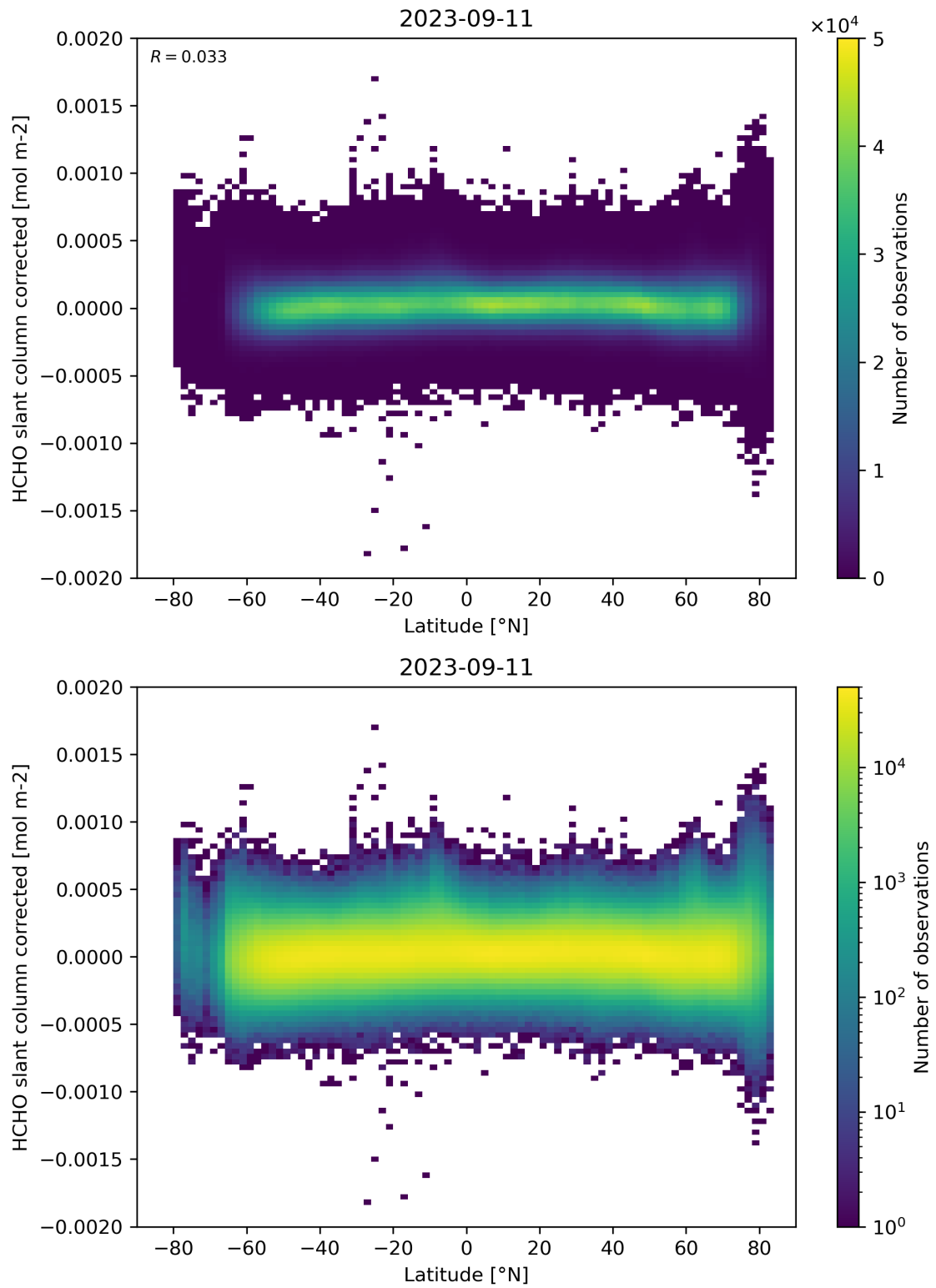
Figure 157: Scatter density plot of “Latitude” against “HCHO slant column corrected” for 2023-09-10 to 2023-09-12.
