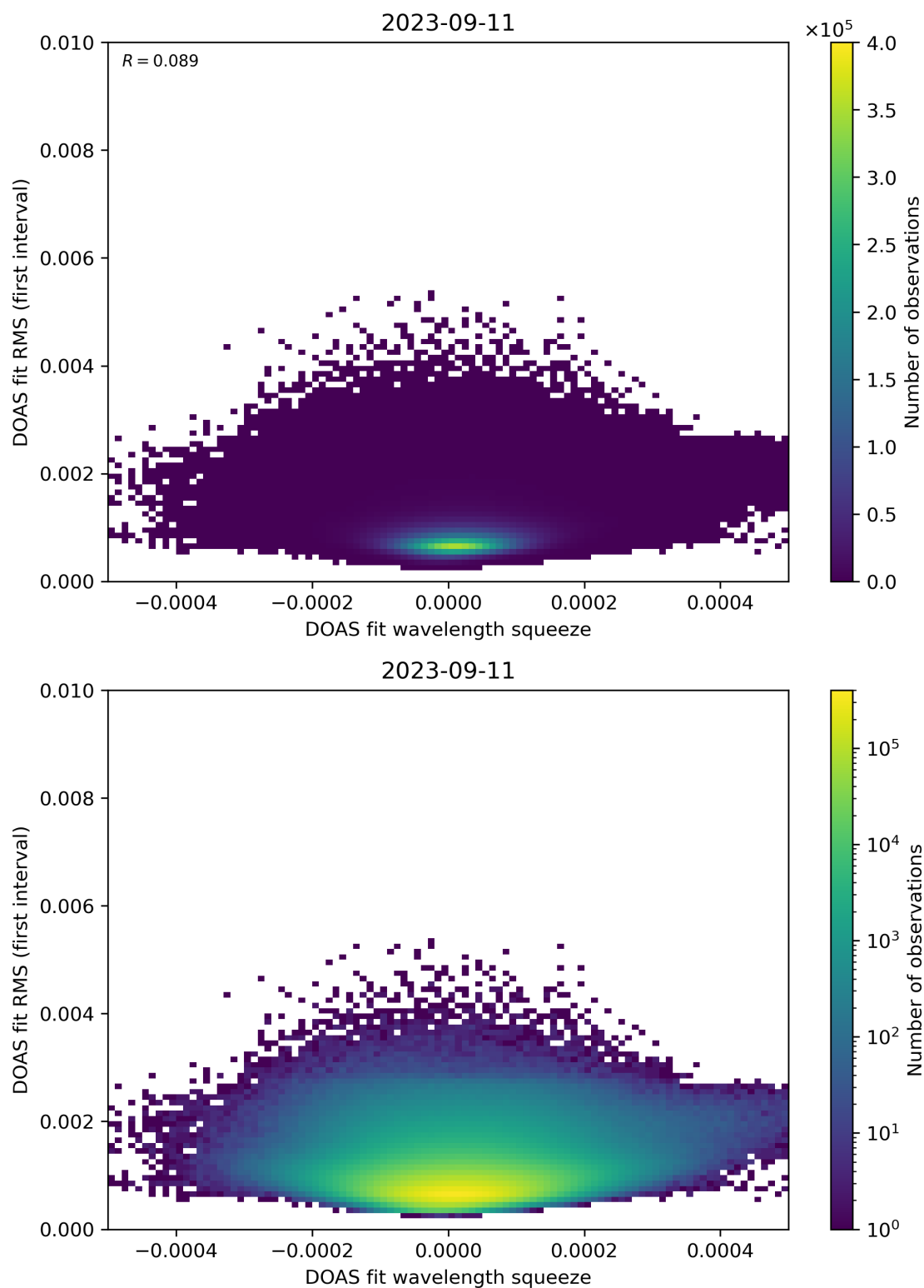
Figure 68: Scatter density plot of “DOAS fit wavelength squeeze” against “DOAS fit RMS (first interval)” for 2023-09-10 to 2023-09-12.
