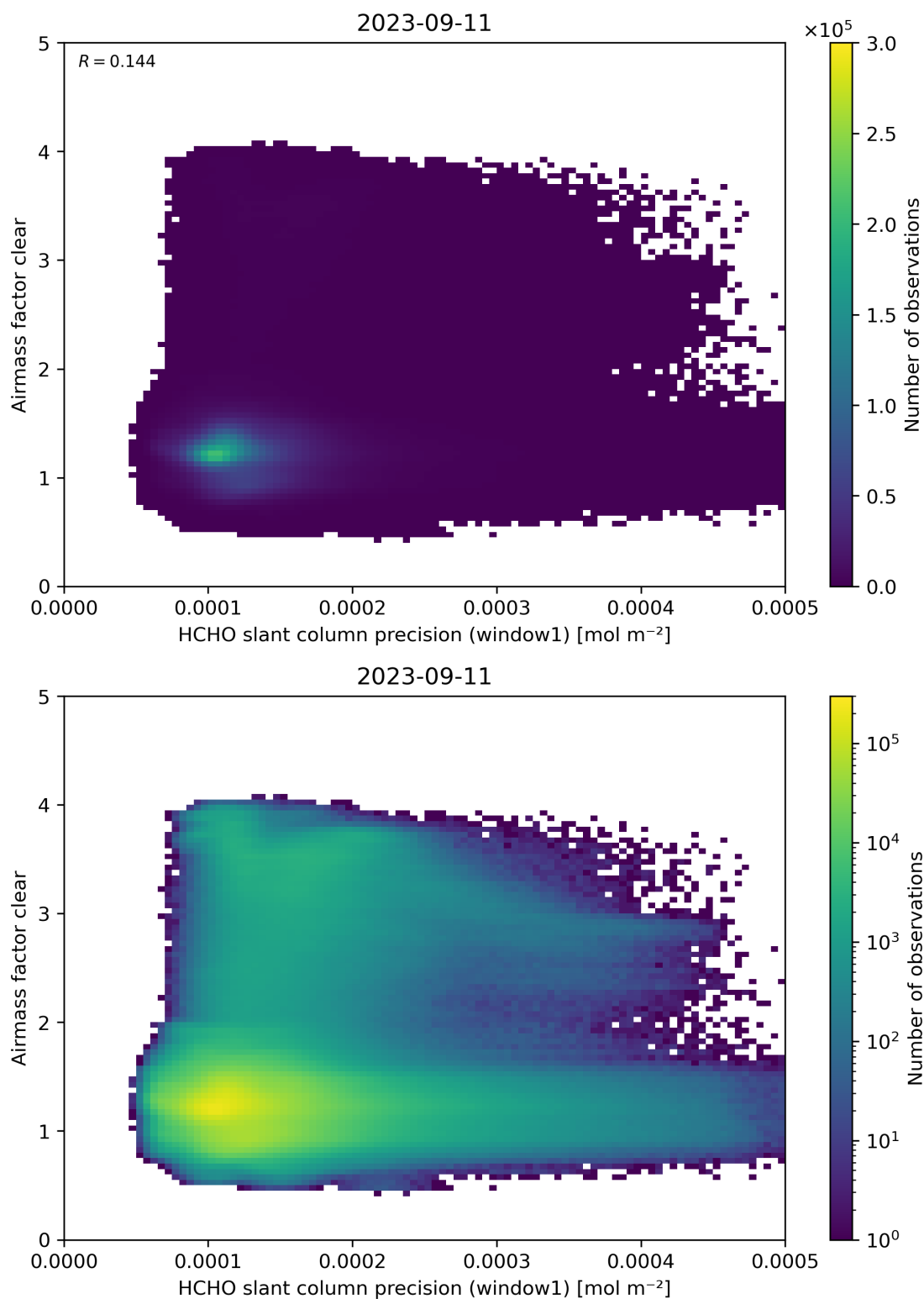
Figure 91: Scatter density plot of “HCHO slant column precision (window1)” against “Airmass factor clear” for 2023-09-10 to 2023-09-12.
