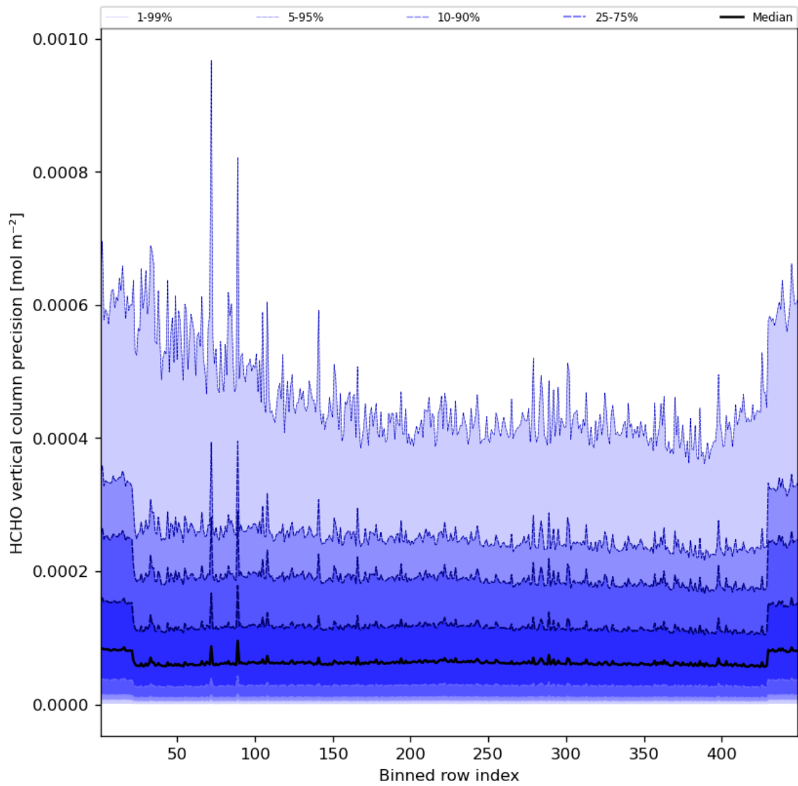
Figure 50: Along track statistics of “HCHO vertical column precision” for 2023-09-10 to 2023-09-12
