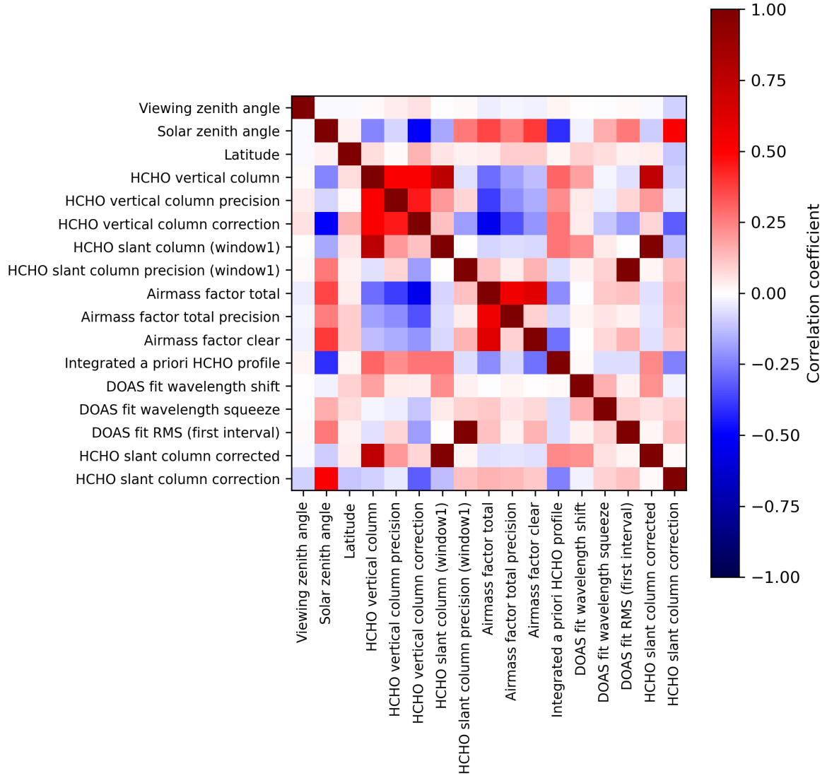
Figure 2: Map of correlation matrix for 2023-09-10 to 2023-09-12.
