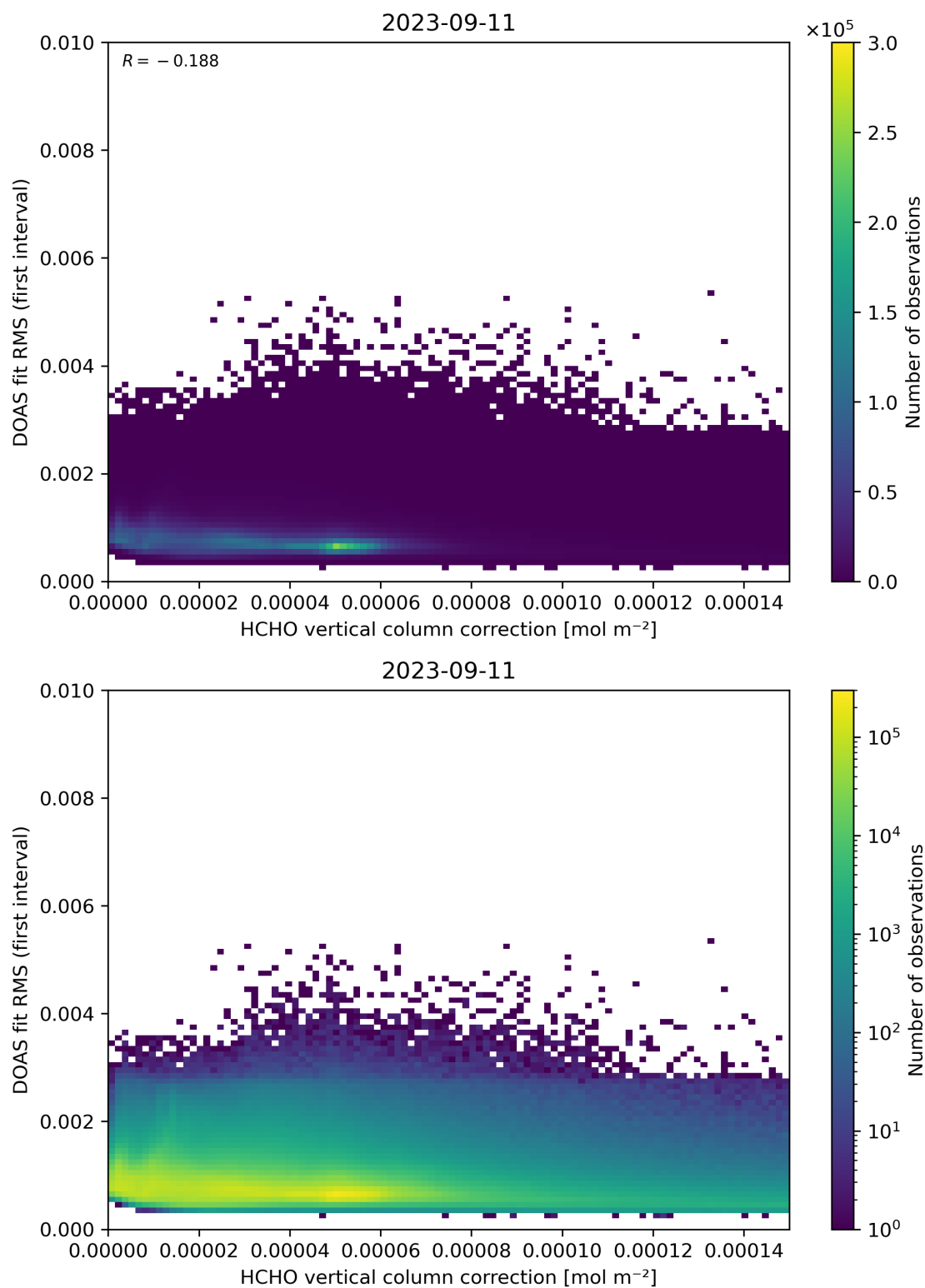
Figure 112: Scatter density plot of “HCHO vertical column correction” against “DOAS fit RMS (first interval)” for 2023-09-10 to 2023-09-12.
