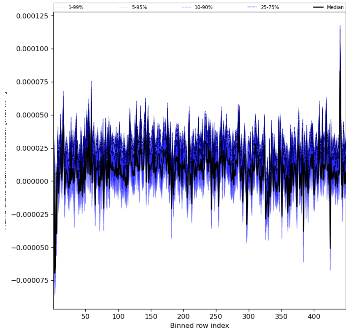
Figure 61: Along track statistics of “HCHO slant column correction” for 2023-09-10 to 2023-09-12
