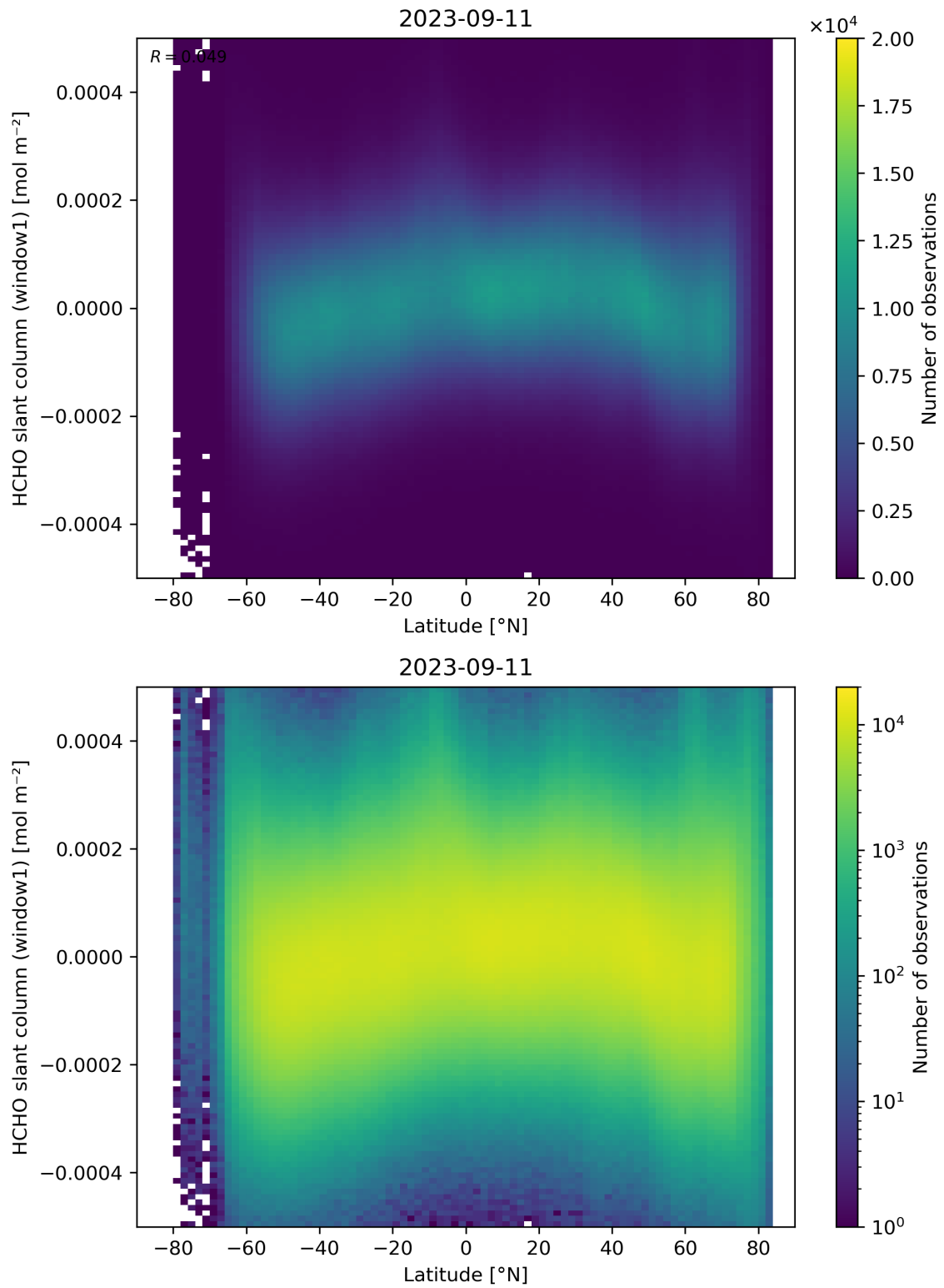
Figure 159: Scatter density plot of “Latitude” against “HCHO slant column (window1)” for 2023-09-10 to 2023-09-12.
