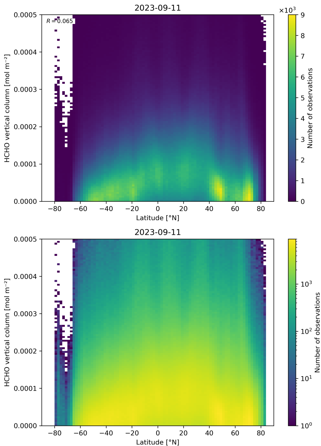
Figure 163: Scatter density plot of “Latitude” against “HCHO vertical column” for 2023-09-10 to 2023-09-12.
