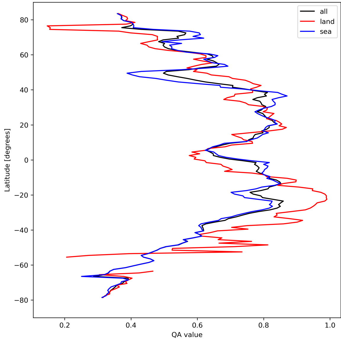
Figure 20: Zonal average of “QA value” for 2023-09-10 to 2023-09-12.
