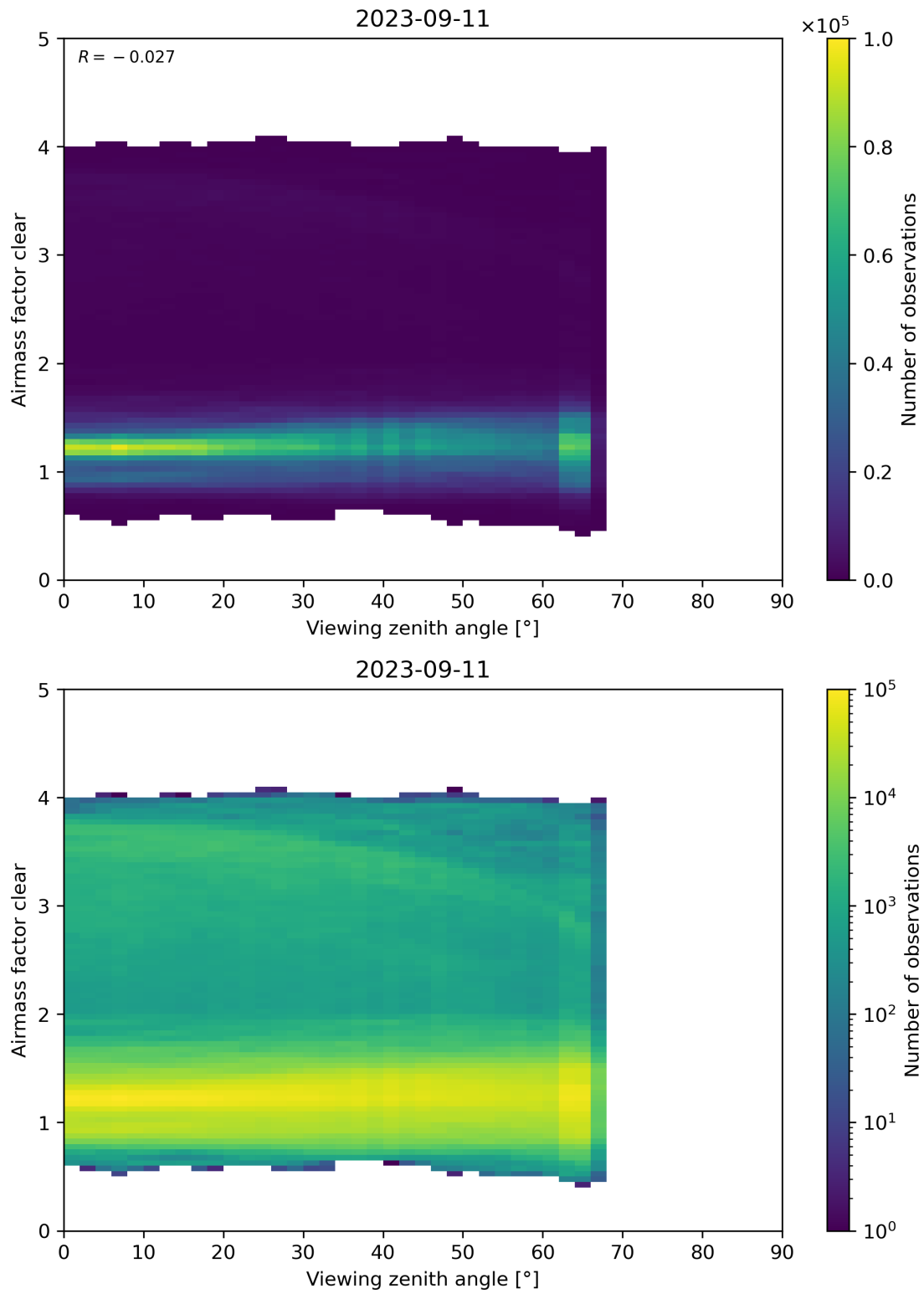
Figure 185: Scatter density plot of “Viewing zenith angle” against “Airmass factor clear” for 2023-09-10 to 2023-09-12.
