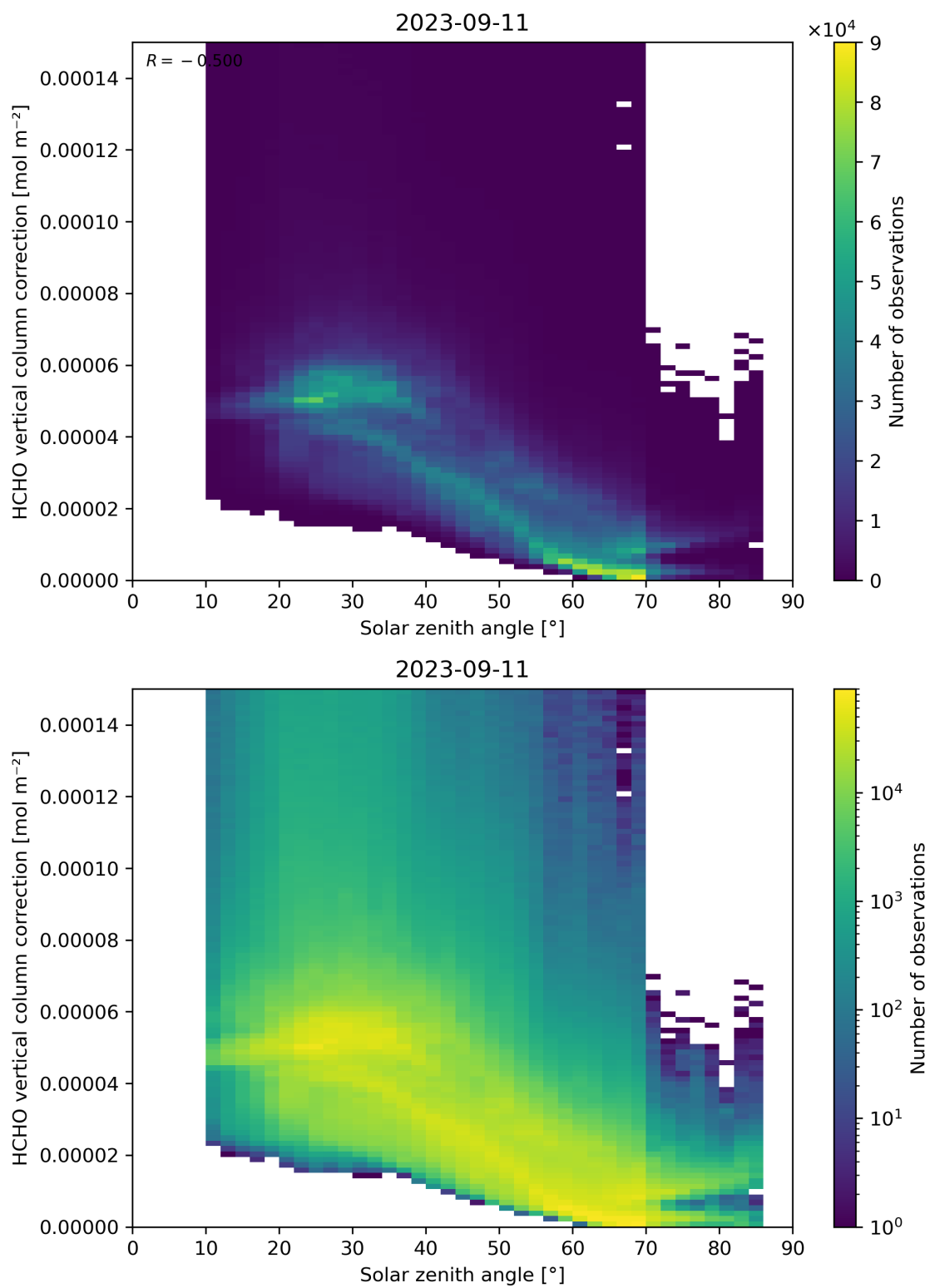
Figure 178: Scatter density plot of “Solar zenith angle” against “HCHO vertical column correction” for 2023-09-10 to 2023-09-12.
