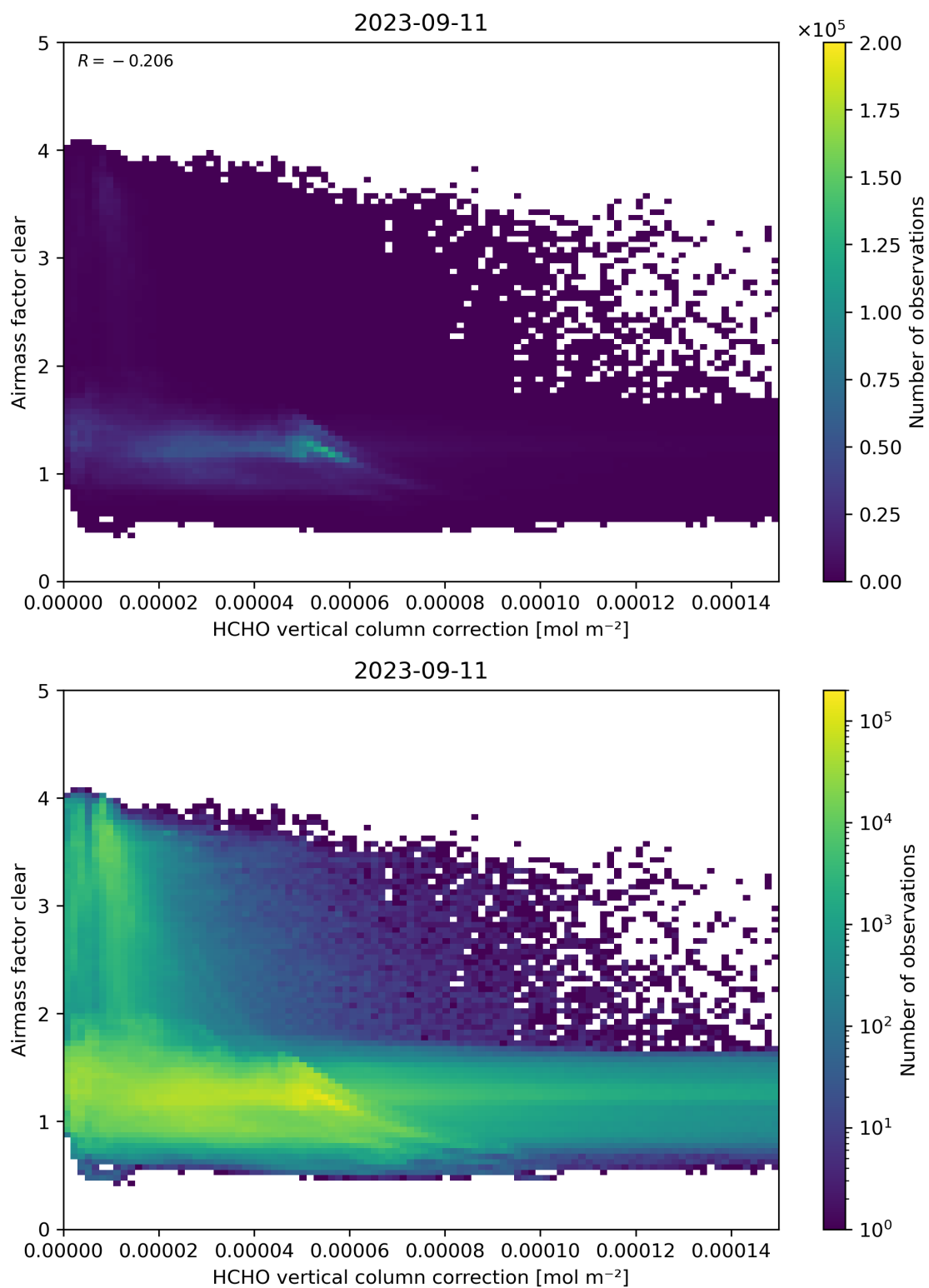
Figure 115: Scatter density plot of “HCHO vertical column correction” against “Airmass factor clear” for 2023-09-10 to 2023-09-12.
