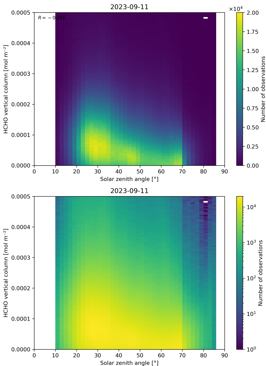
Figure 177: Scatter density plot of “Solar zenith angle” against “HCHO vertical column” for 2023-09-10 to 2023-09-12.
