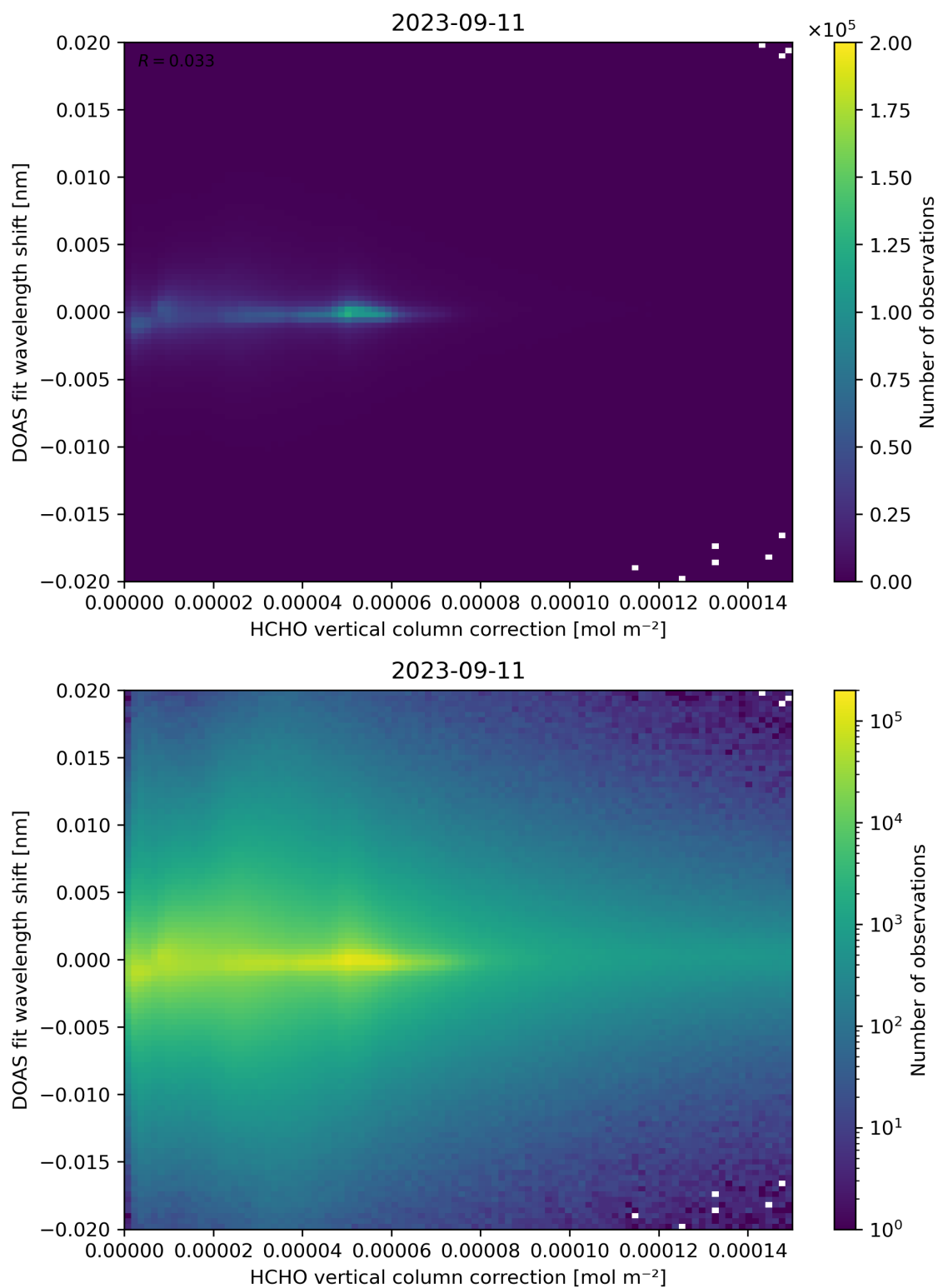
Figure 113: Scatter density plot of “HCHO vertical column correction” against “DOAS fit wavelength shift” for 2023-09-10 to 2023-09-12.
