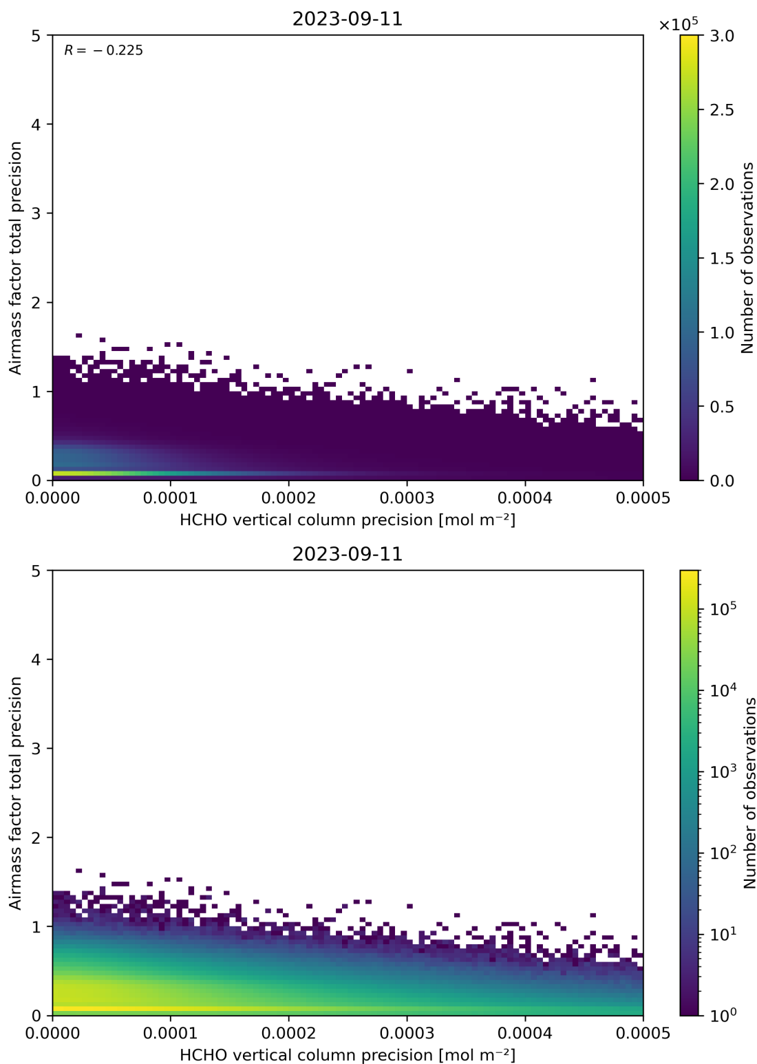
Figure 145: Scatter density plot of “HCHO vertical column precision” against “Airmass factor total precision” for 2023-09-10 to 2023-09-12.
