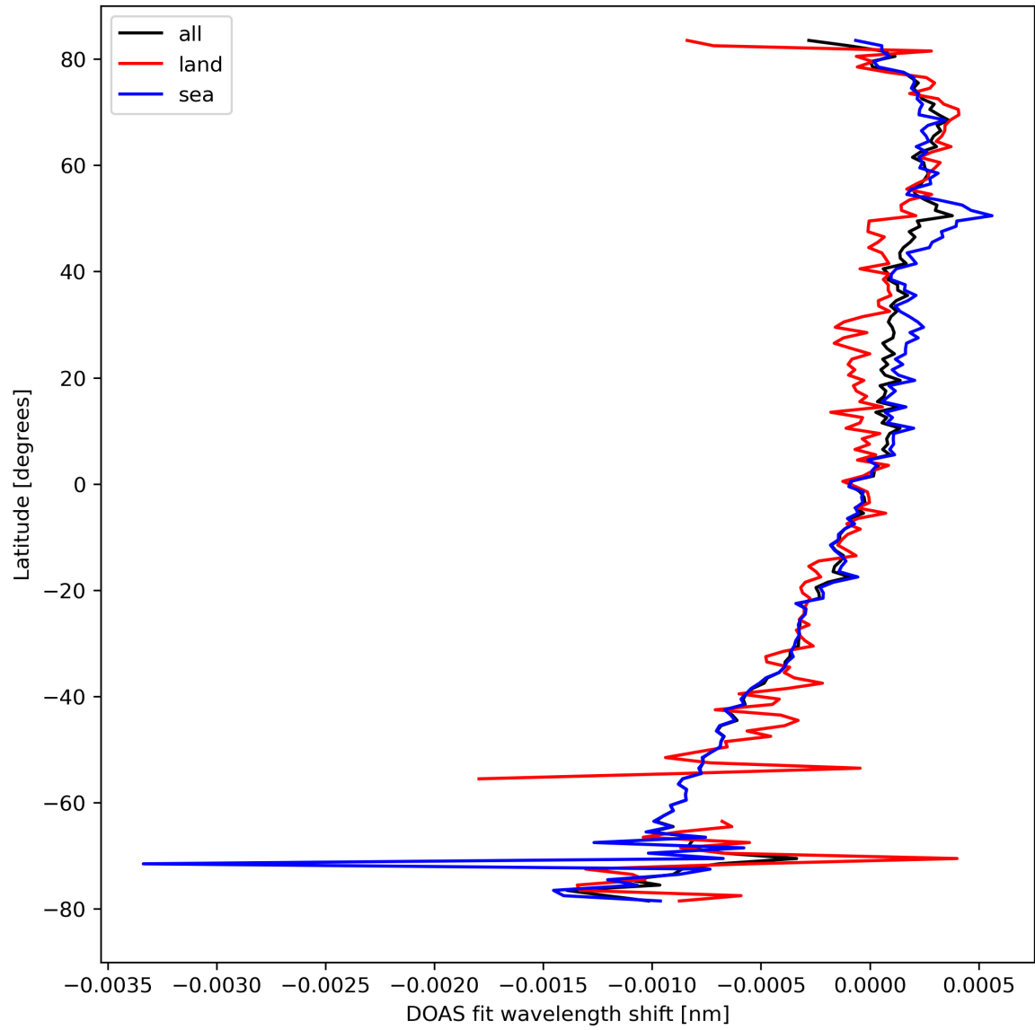
Figure 30: Zonal average of “DOAS fit wavelength shift” for 2023-09-10 to 2023-09-12.
