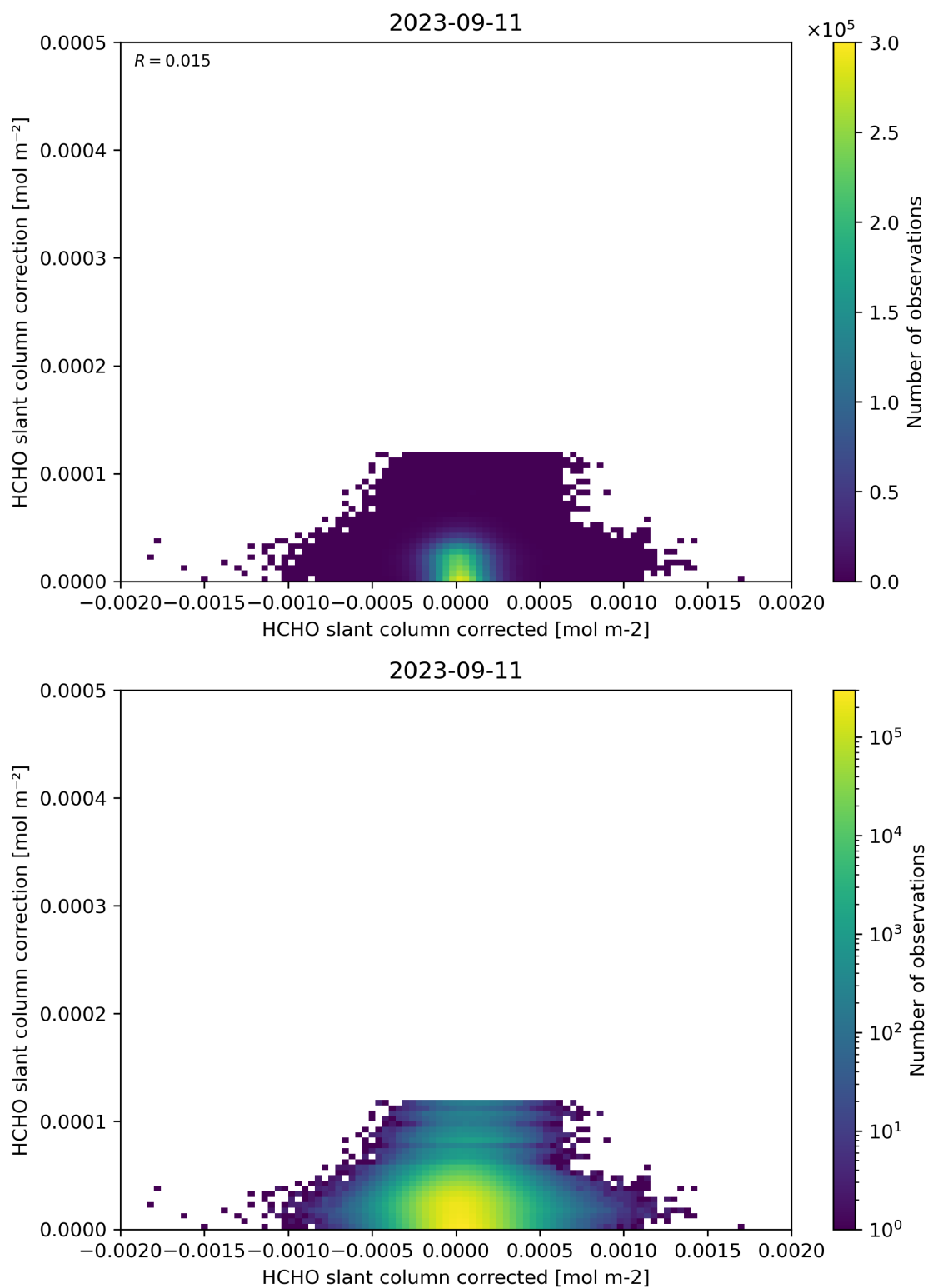
Figure 77: Scatter density plot of “HCHO slant column corrected” against “HCHO slant column correction” for 2023-09-10 to 2023-09-12.
