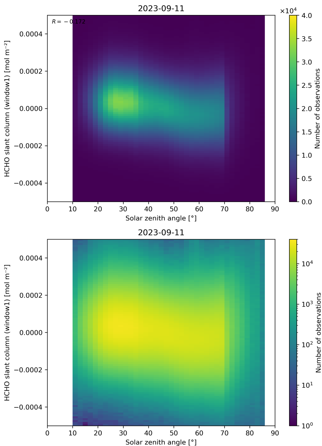
Figure 173: Scatter density plot of “Solar zenith angle” against “HCHO slant column (window1)” for 2023-09-10 to 2023-09-12.
