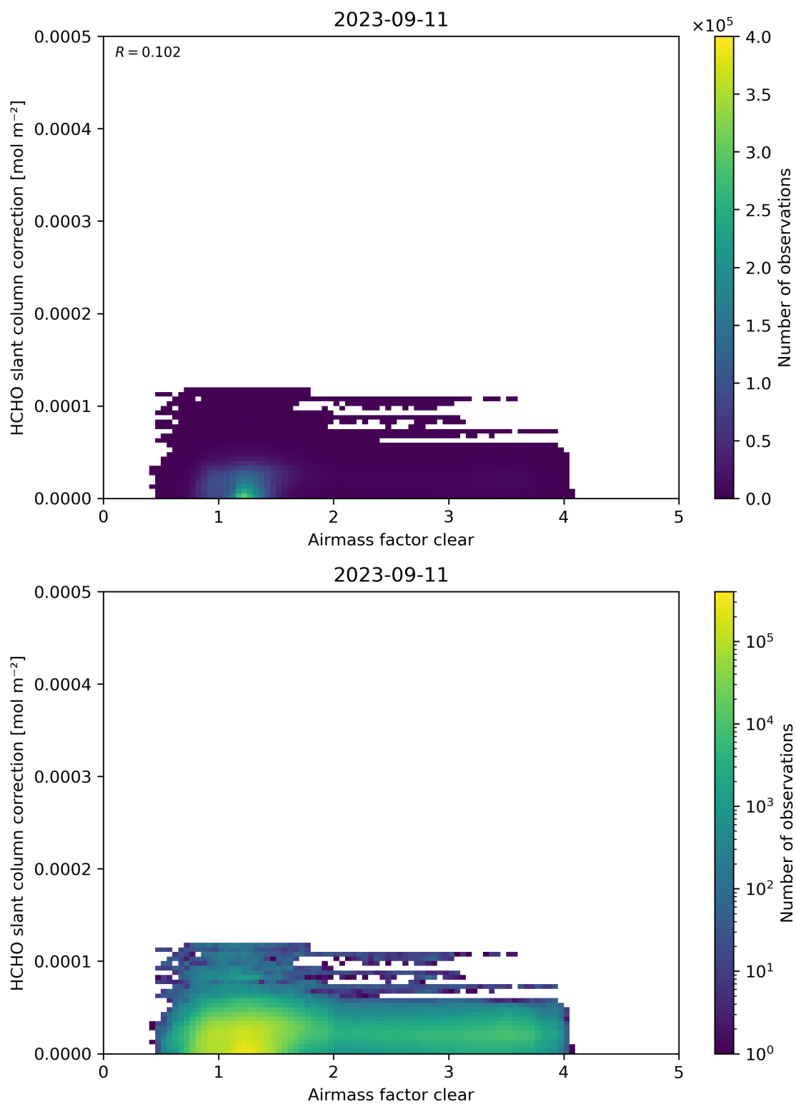
Figure 75: Scatter density plot of “Airmass factor clear” against “HCHO slant column correction” for 2023-09-10 to 2023-09-12.
