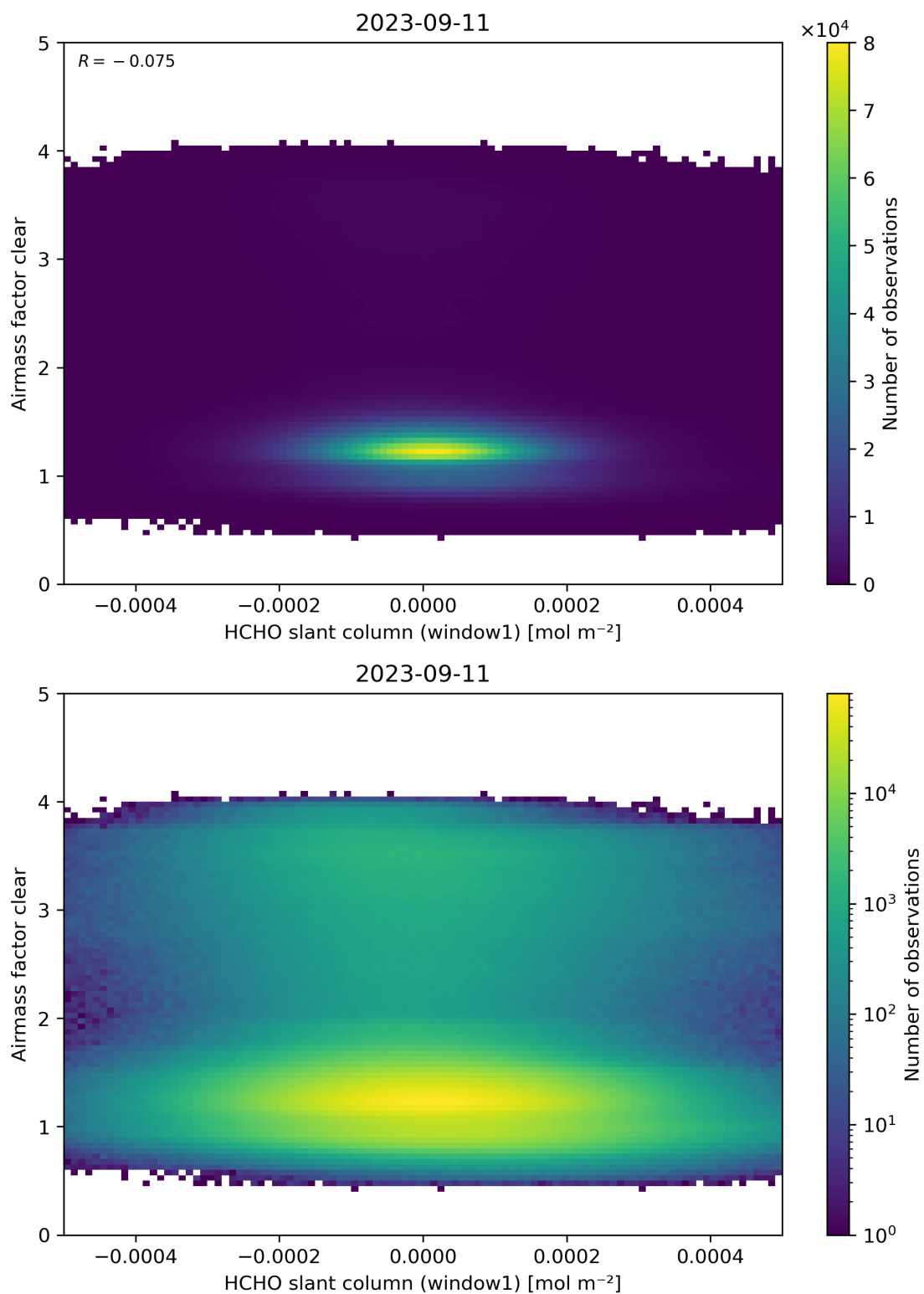
Figure 81: Scatter density plot of “HCHO slant column (window1)” against “Airmass factor clear” for 2023-09-10 to 2023-09-12.
