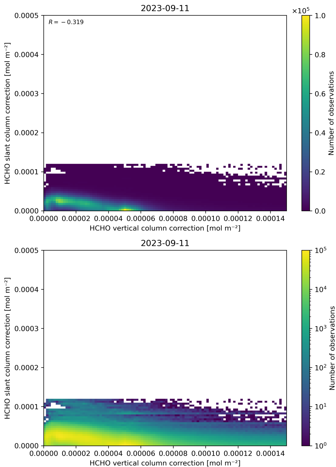
Figure 117: Scatter density plot of “HCHO vertical column correction” against “HCHO slant column correction” for 2023-09-10 to 2023-09-12.
