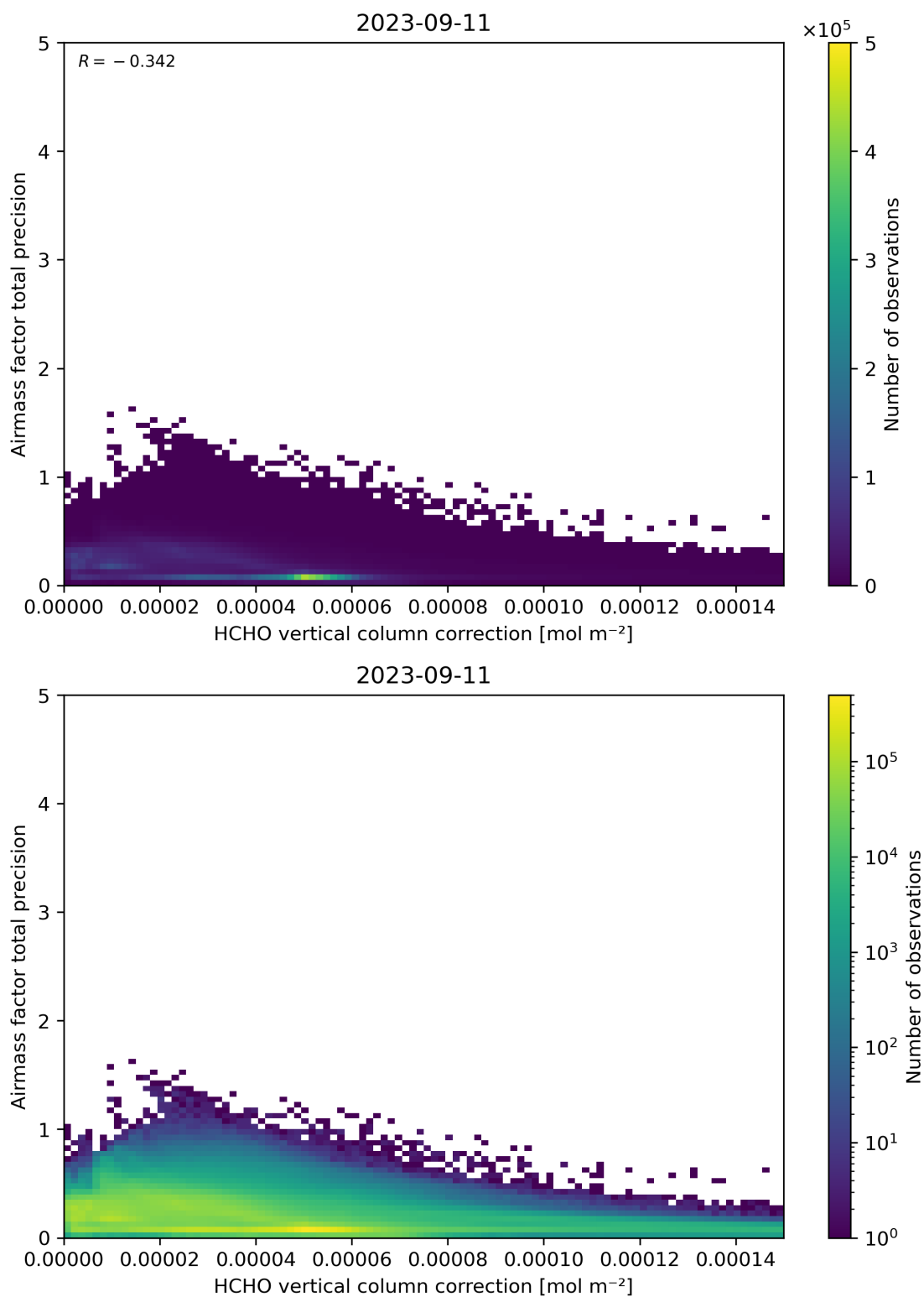
Figure 121: Scatter density plot of “HCHO vertical column correction” against “Airmass factor total precision” for 2023-09-10 to 2023-09-12.
