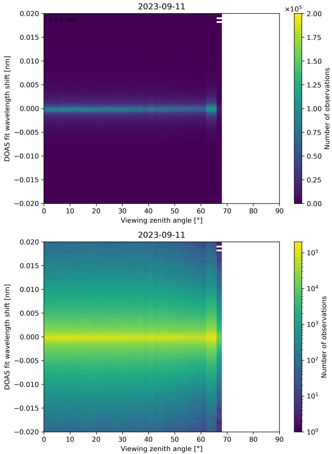
Figure 183: Scatter density plot of “Viewing zenith angle” against “DOAS fit wavelength shift” for 2023-09-10 to 2023-09-12.
