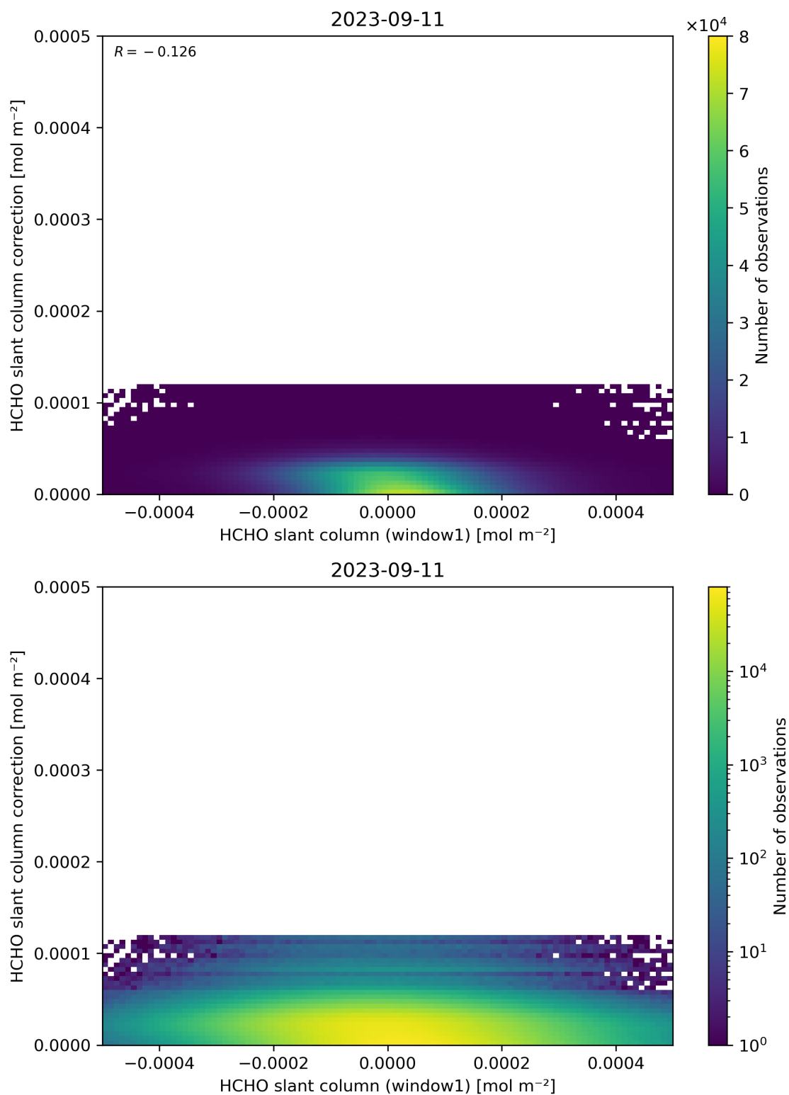
Figure 83: Scatter density plot of “HCHO slant column (window1)” against “HCHO slant column correction” for 2023-09-10 to 2023-09-12.
