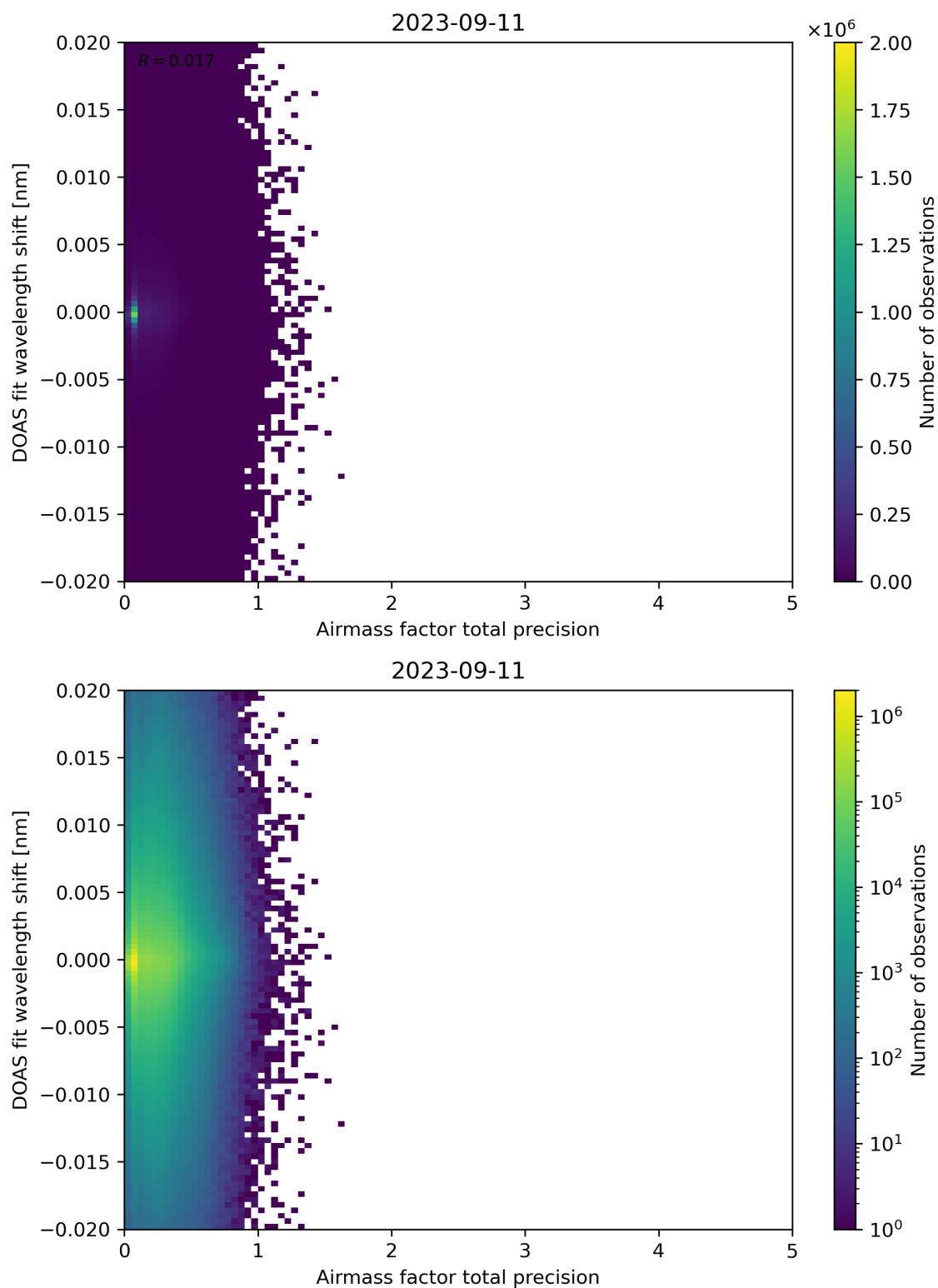
Figure 106: Scatter density plot of “Airmass factor total precision” against “DOAS fit wavelength shift” for 2023-09-10 to 2023-09-12.
