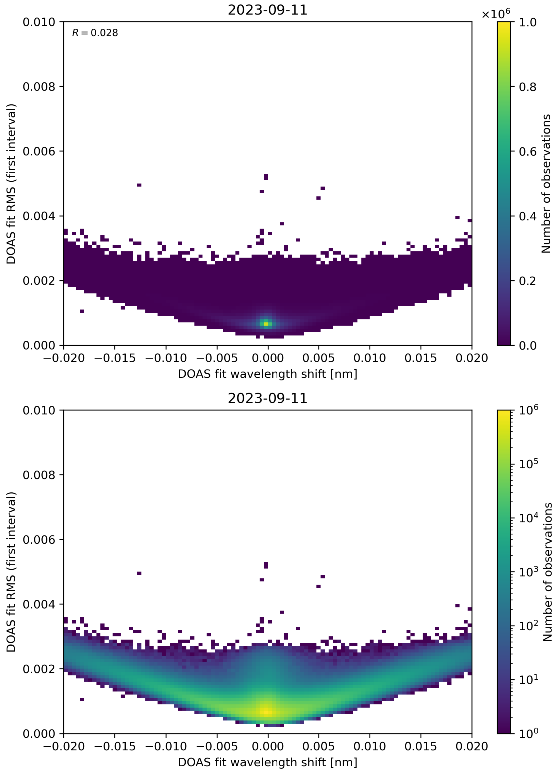
Figure 64: Scatter density plot of “DOAS fit wavelength shift” against “DOAS fit RMS (first interval)” for 2023-09-10 to 2023-09-12.
