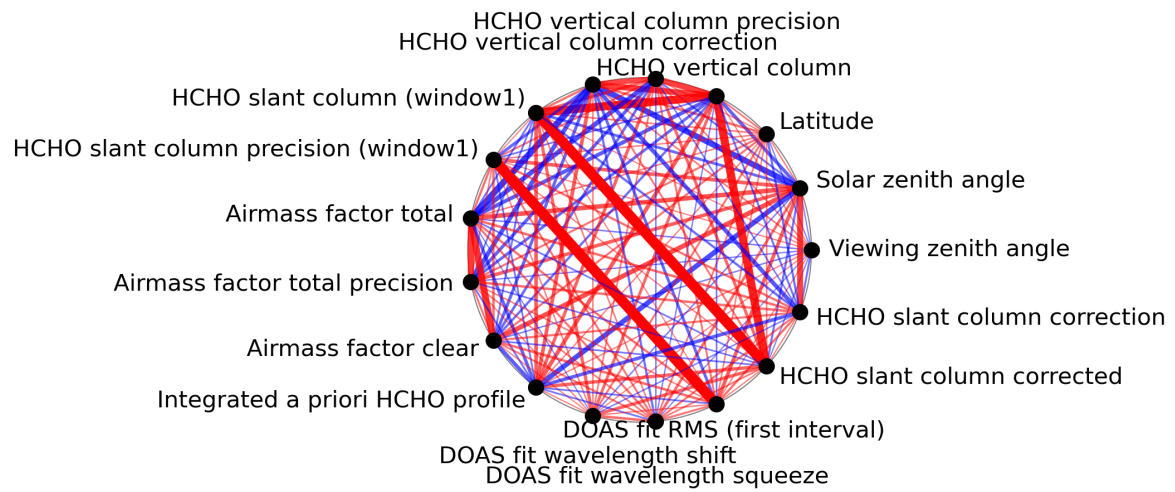
Figure 1: Map of correlation graph for 2023-09-10 to 2023-09-12.
