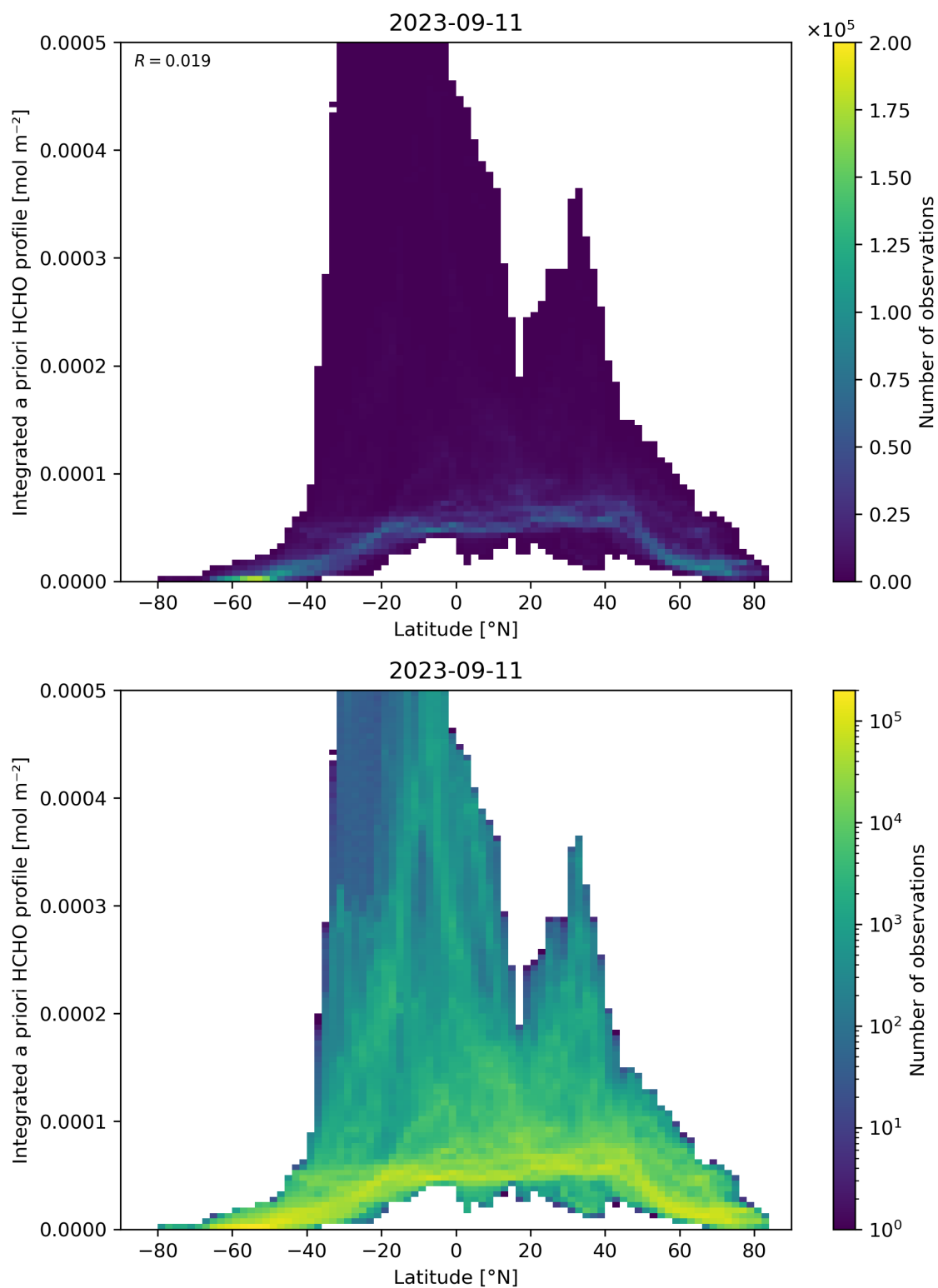
Figure 166: Scatter density plot of “Latitude” against “Integrated a priori HCHO profile” for 2023-09-10 to 2023-09-12.
