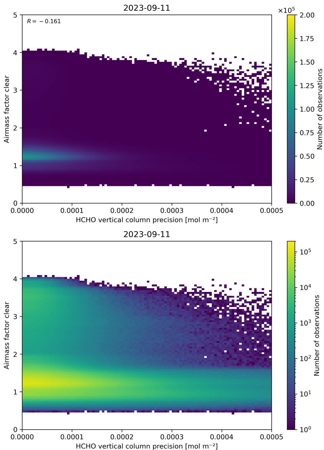
Figure 139: Scatter density plot of “HCHO vertical column precision” against “Airmass factor clear” for 2023-09-10 to 2023-09-12.
