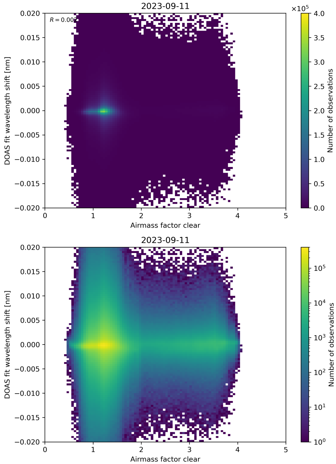
Figure 72: Scatter density plot of “Airmass factor clear” against “DOAS fit wavelength shift” for 2023-09-10 to 2023-09-12.
