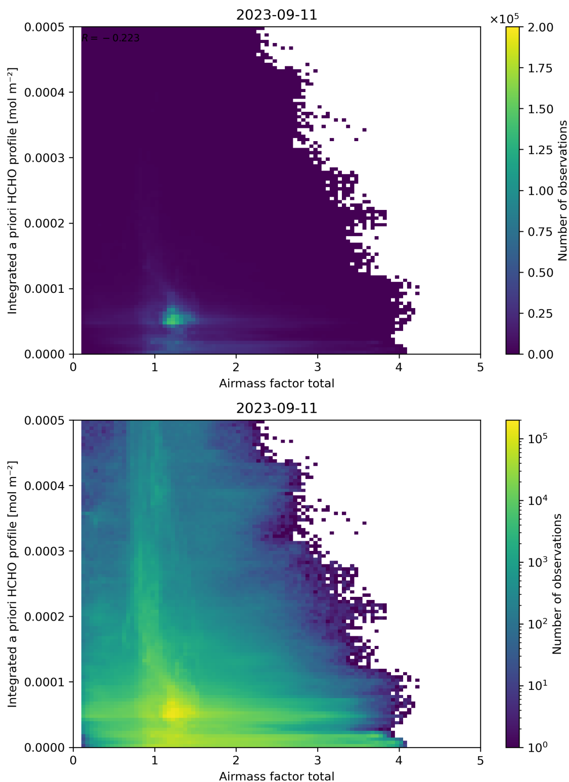
Figure 104: Scatter density plot of “Air mass factor total” against “Integrated a priori HCHO profile” for 2023-09-10 to 2023-09-12.
