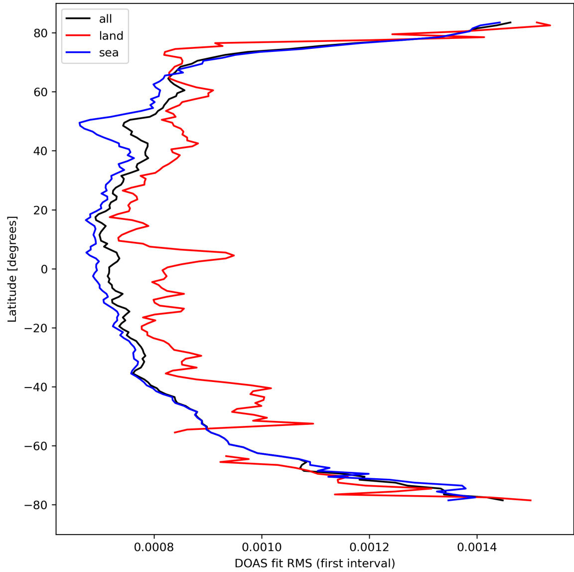
Figure 32: Zonal average of “DOAS fit RMS (first interval)” for 2023-09-10 to 2023-09-12.
