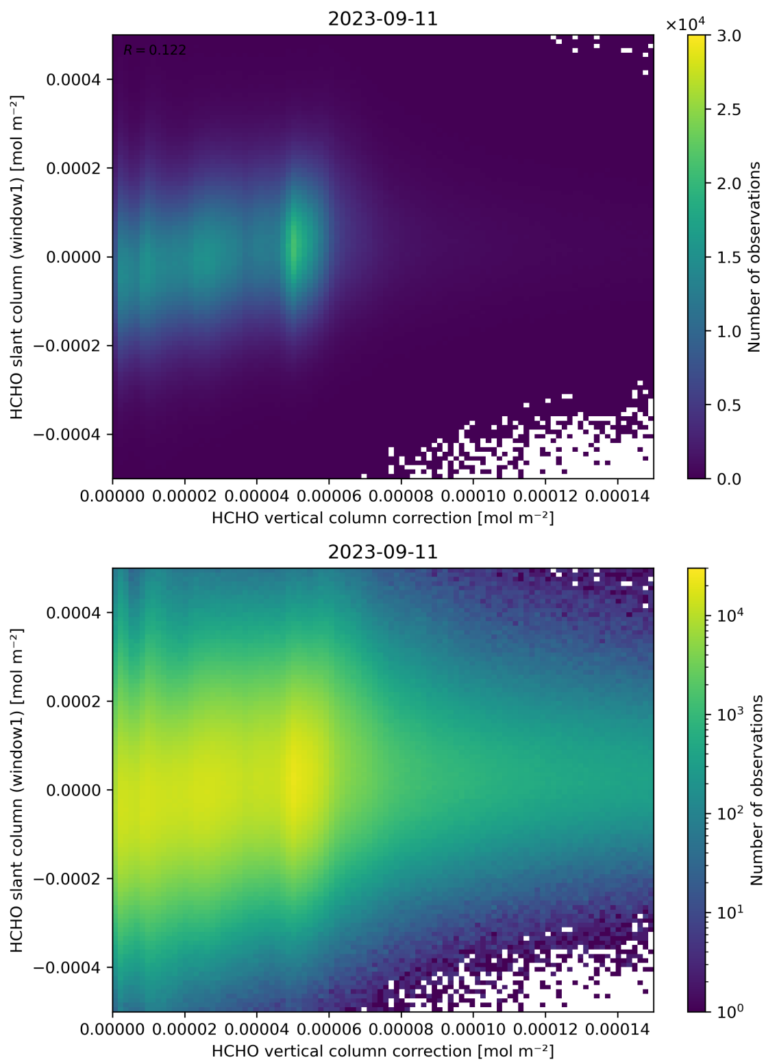
Figure 118: Scatter density plot of “HCHO vertical column correction” against “HCHO slant column (window1)” for 2023-09-10 to 2023-09-12.
