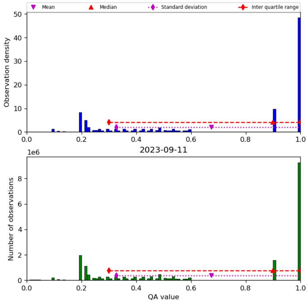
Figure 34: Histogram of “QA value” for 2023-09-10 to 2023-09-12
