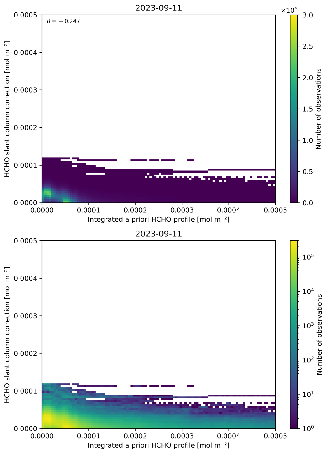
Figure 152: Scatter density plot of “Integrated a priori HCHO profile” against “HCHO slant column correction” for 2023-09-10 to 2023-09-12.
