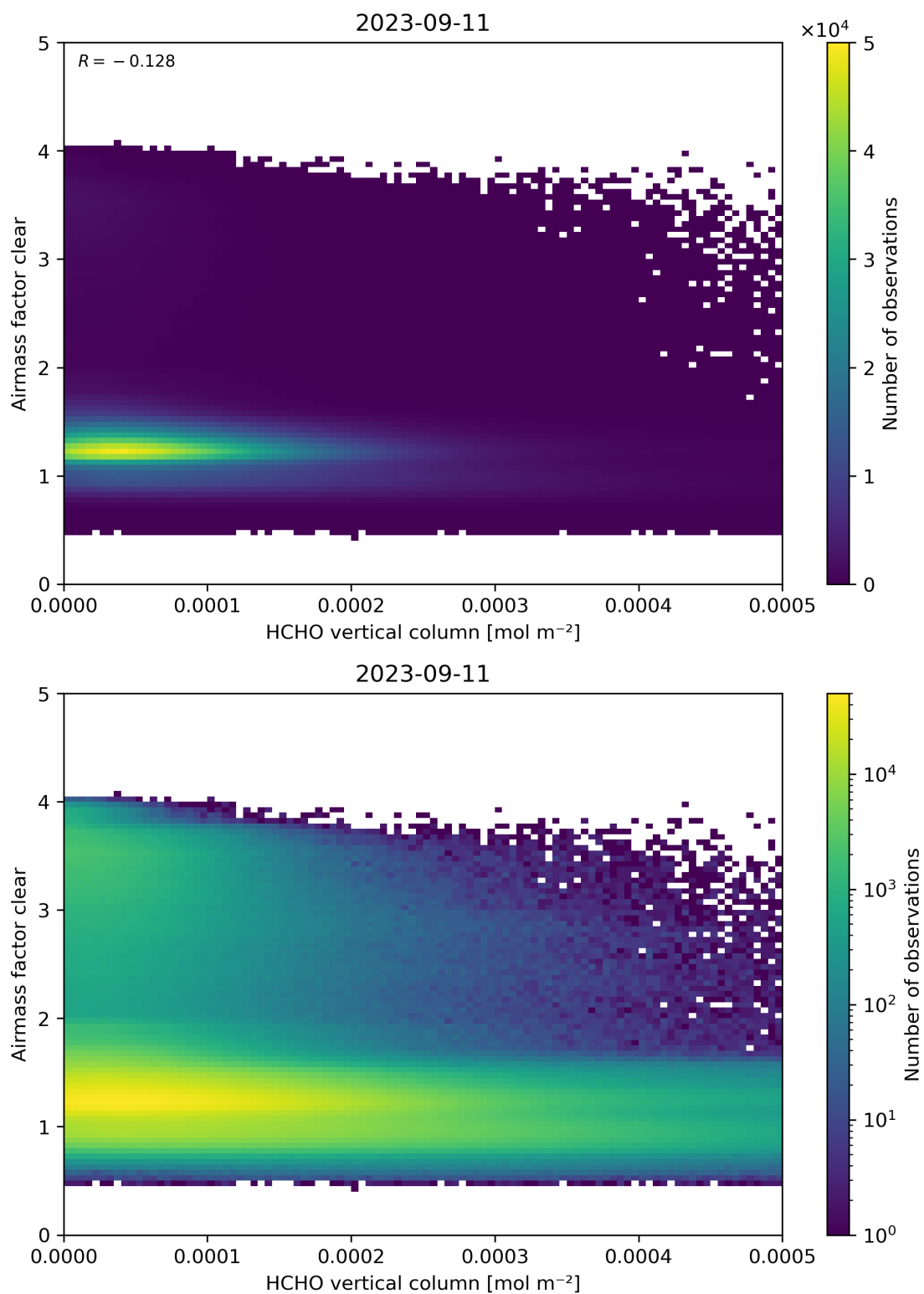
Figure 126: Scatter density plot of “HCHO vertical column” against “Airmass factor clear” for 2023-09-10 to 2023-09-12.
