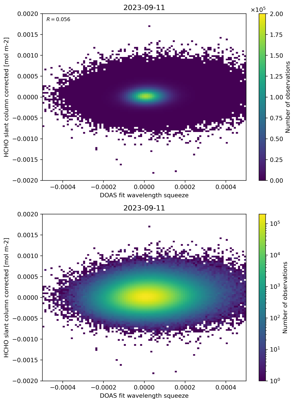
Figure 69: Scatter density plot of “DOAS fit wavelength squeeze” against “HCHO slant column corrected” for 2023-09-10 to 2023-09-12.
