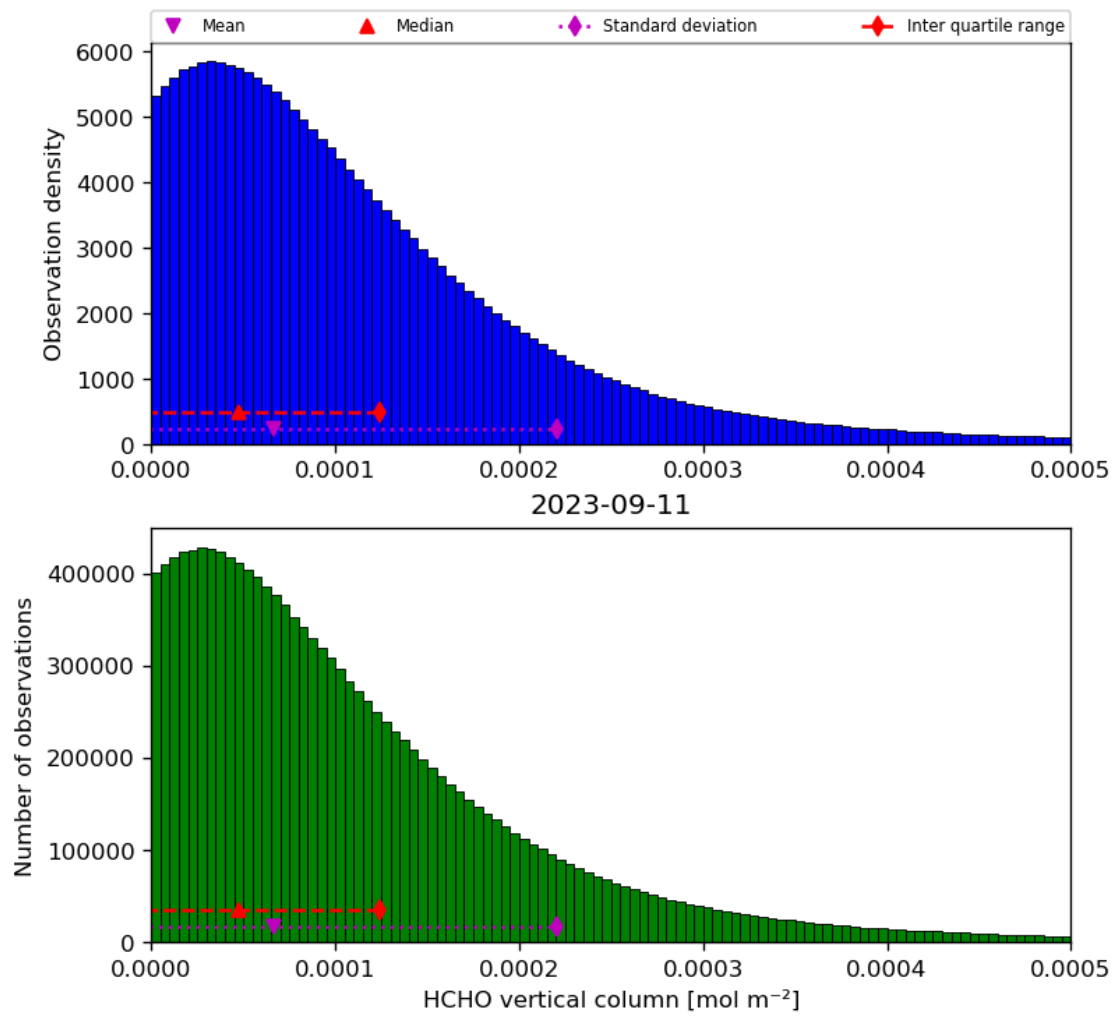
Figure 35: Histogram of “HCHO vertical column” for 2023-09-10 to 2023-09-12
