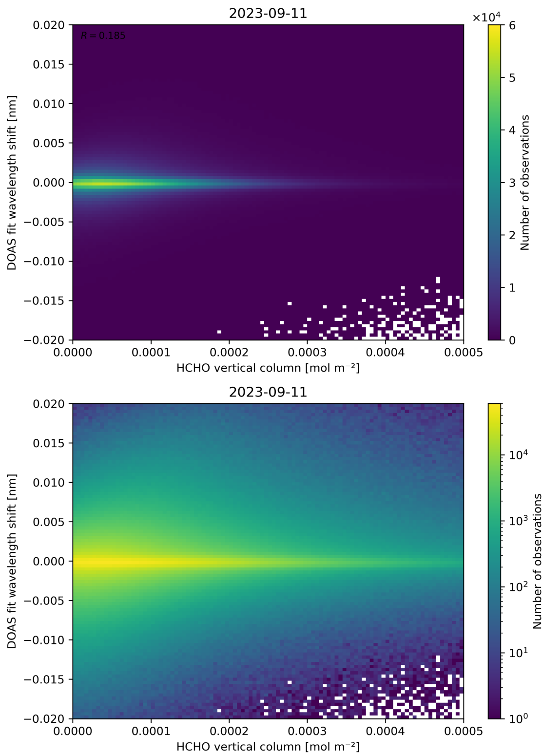
Figure 124: Scatter density plot of “HCHO vertical column” against “DOAS fit wavelength shift” for 2023-09-10 to 2023-09-12.
