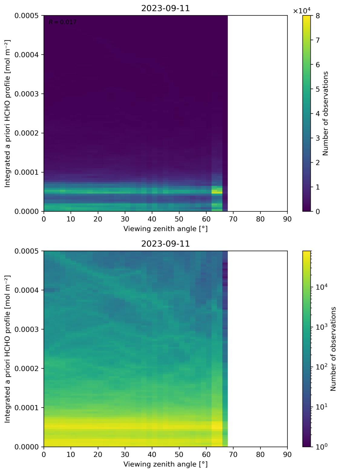
Figure 195: Scatter density plot of “Viewing zenith angle” against “Integrated a priori HCHO profile” for 2023-09-10 to 2023-09-12.
