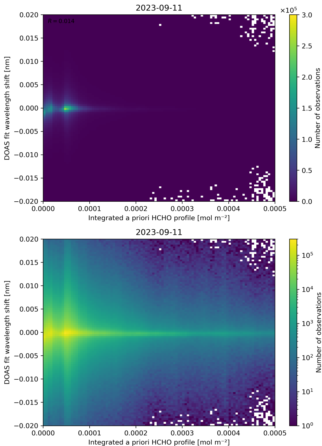
Figure 149: Scatter density plot of “Integrated a priori HCHO profile” against “DOAS fit wavelength shift” for 2023-09-10 to 2023-09-12.
