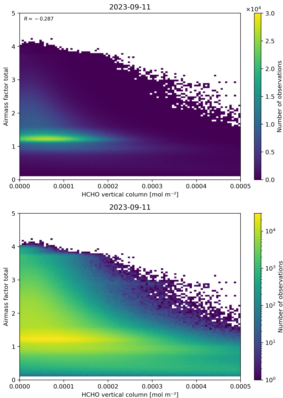
Figure 131: Scatter density plot of “HCHO vertical column” against “Airmass factor total” for 2023-09-10 to 2023-09-12.
