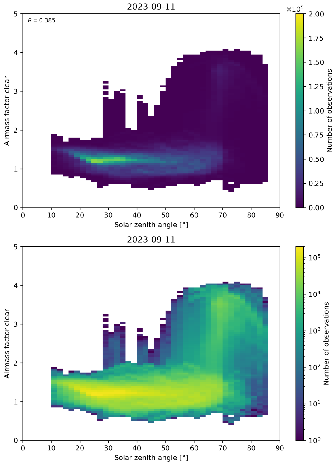
Figure 170: Scatter density plot of “Solar zenith angle” against “Airmass factor clear” for 2023-09-10 to 2023-09-12.
