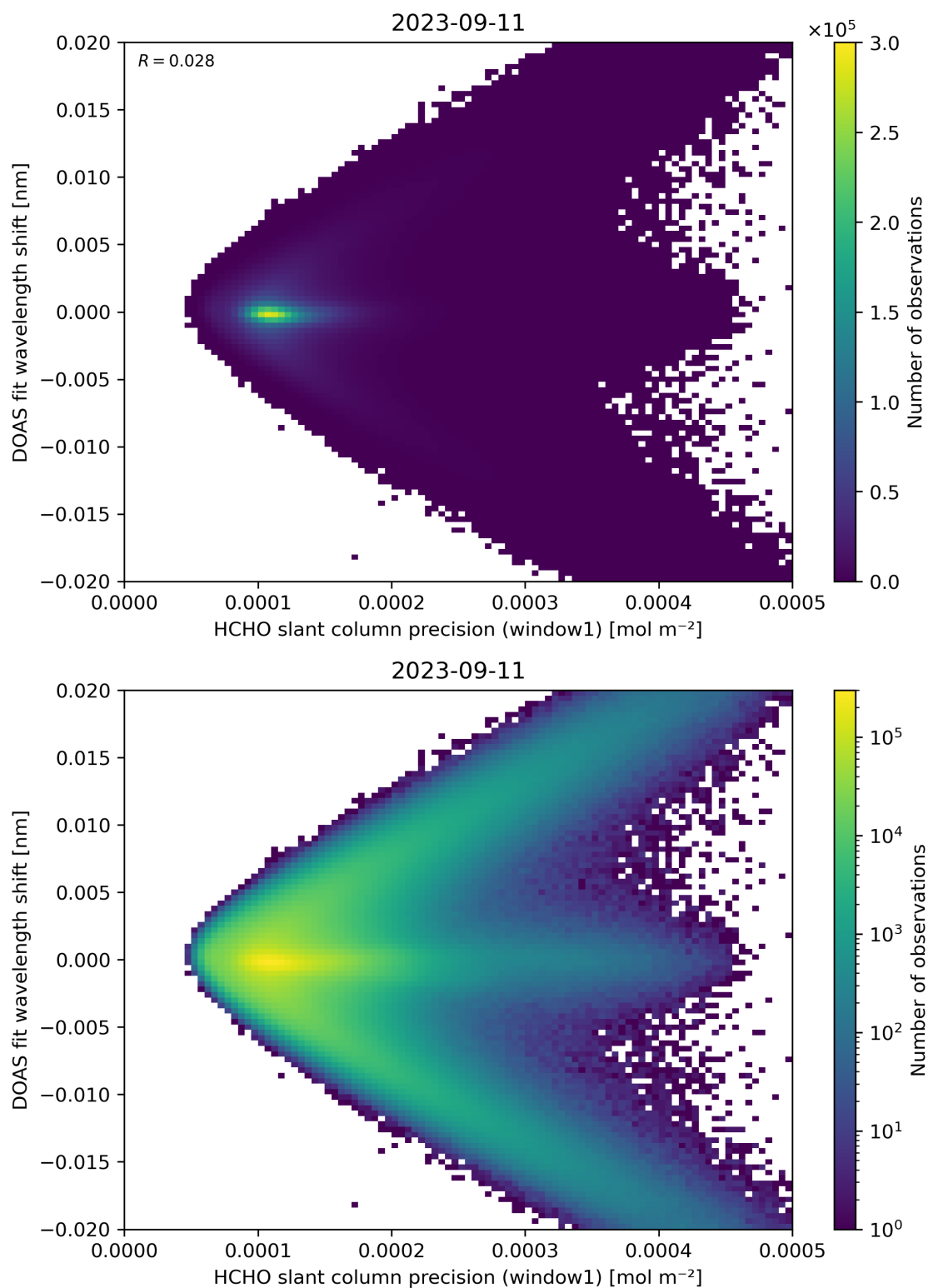
Figure 89: Scatter density plot of “HCHO slant column precision (window1)” against “DOAS fit wavelength shift” for 2023-09-10 to 2023-09-12.
