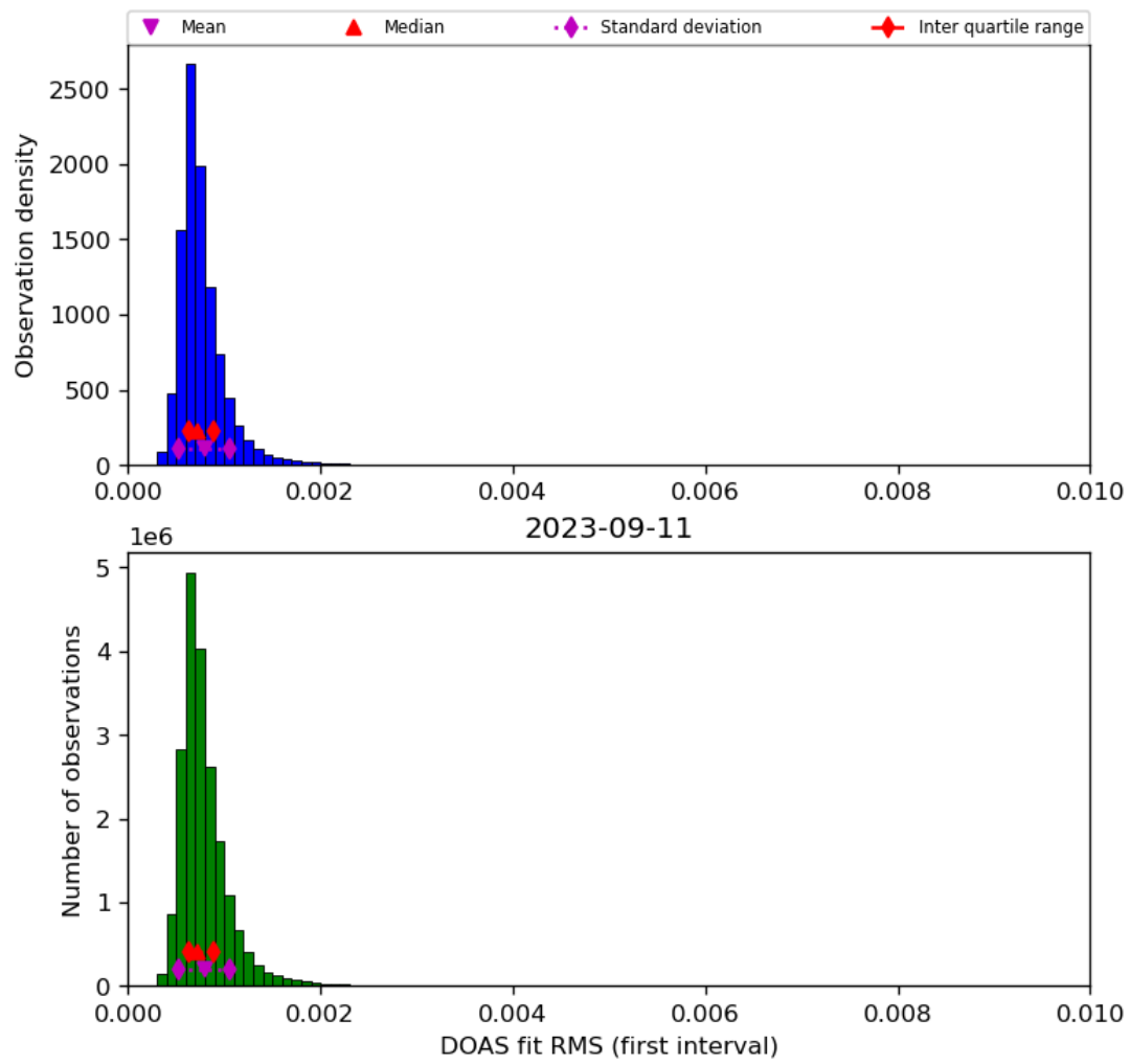
Figure 46: Histogram of “DOAS fit RMS (first interval)” for 2023-09-10 to 2023-09-12
