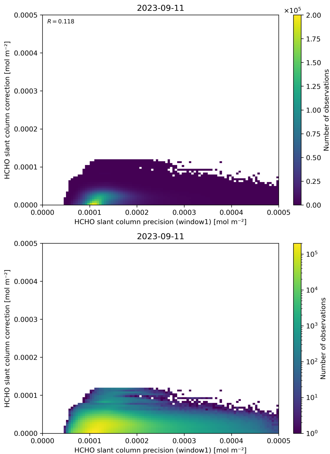
Figure 93: Scatter density plot of “HCHO slant column precision (window1)” against “HCHO slant column correction” for 2023-09-10 to 2023-09-12.
