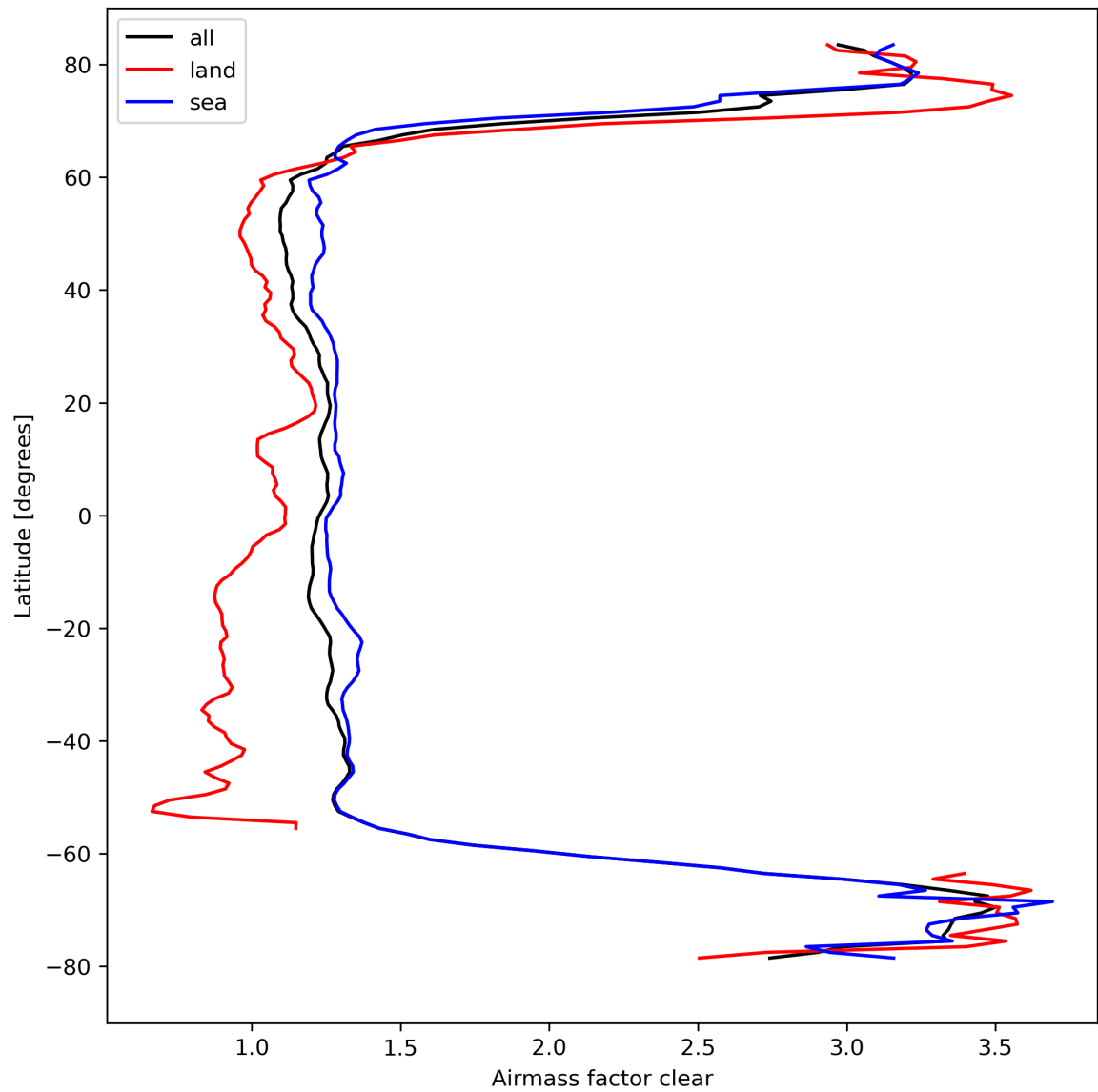
Figure 28: Zonal average of “Airmass factor clear” for 2023-09-10 to 2023-09-12.
