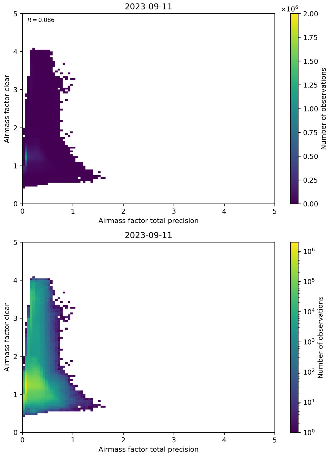
Figure 108: Scatter density plot of “Airmass factor total precision” against “Airmass factor clear” for 2023-09-10 to 2023-09-12.
