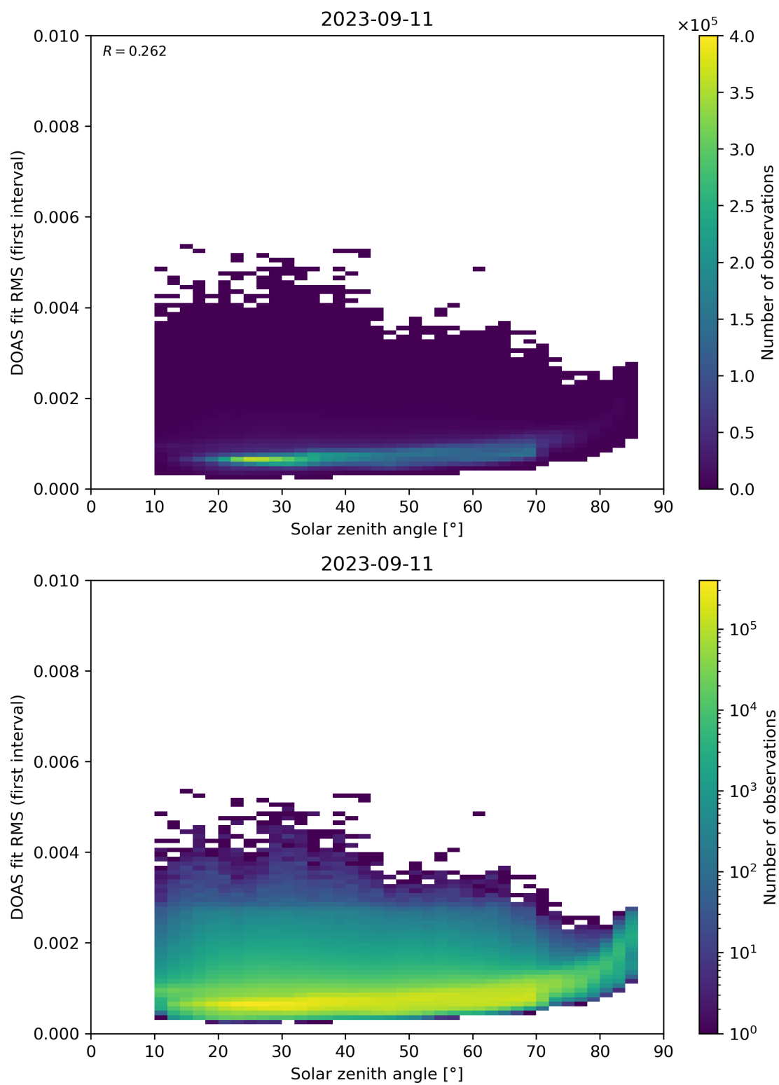
Figure 167: Scatter density plot of “Solar zenith angle” against “DOAS fit RMS (first interval)” for 2023-09-10 to 2023-09-12.
