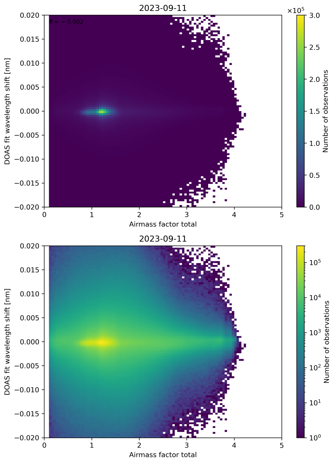
Figure 98: Scatter density plot of “Airmass factor total” against “DOAS fit wavelength shift” for 2023-09-10 to 2023-09-12.
