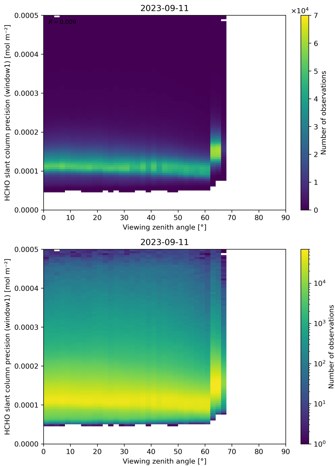
Figure 189: Scatter density plot of “Viewing zenith angle” against “HCHO slant column precision (window1)” for 2023-09-10 to 2023-09-12.
