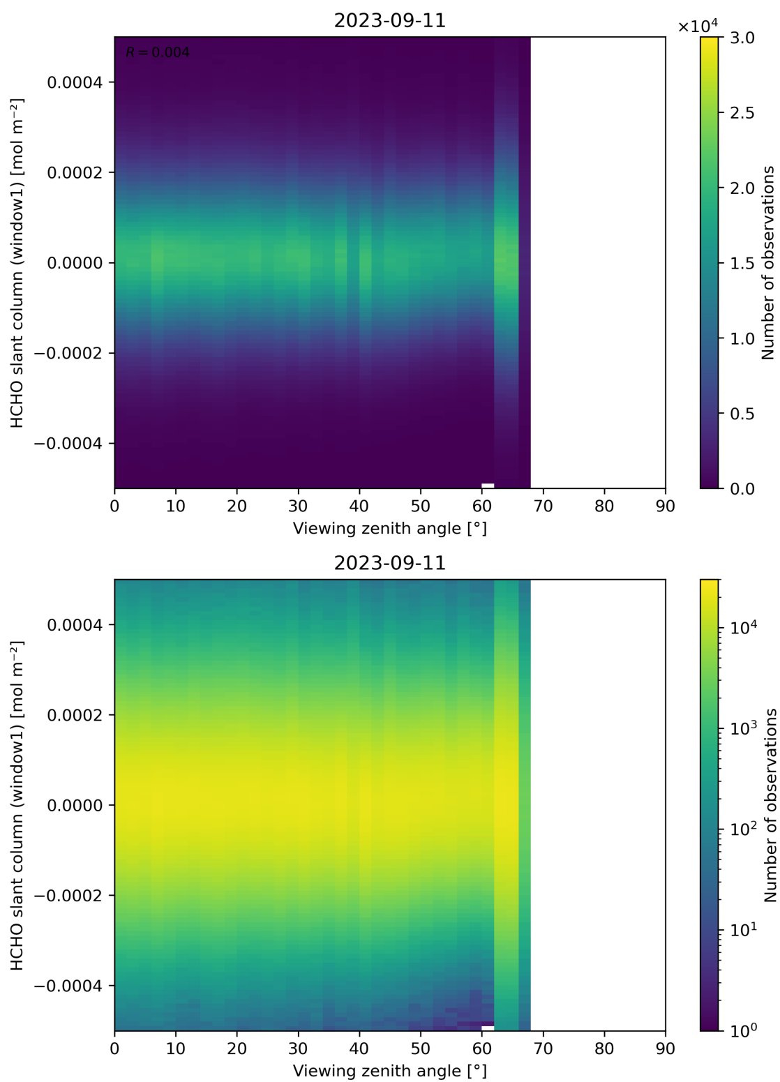
Figure 188: Scatter density plot of “Viewing zenith angle” against “HCHO slant column (window1)” for 2023-09-10 to 2023-09-12.
