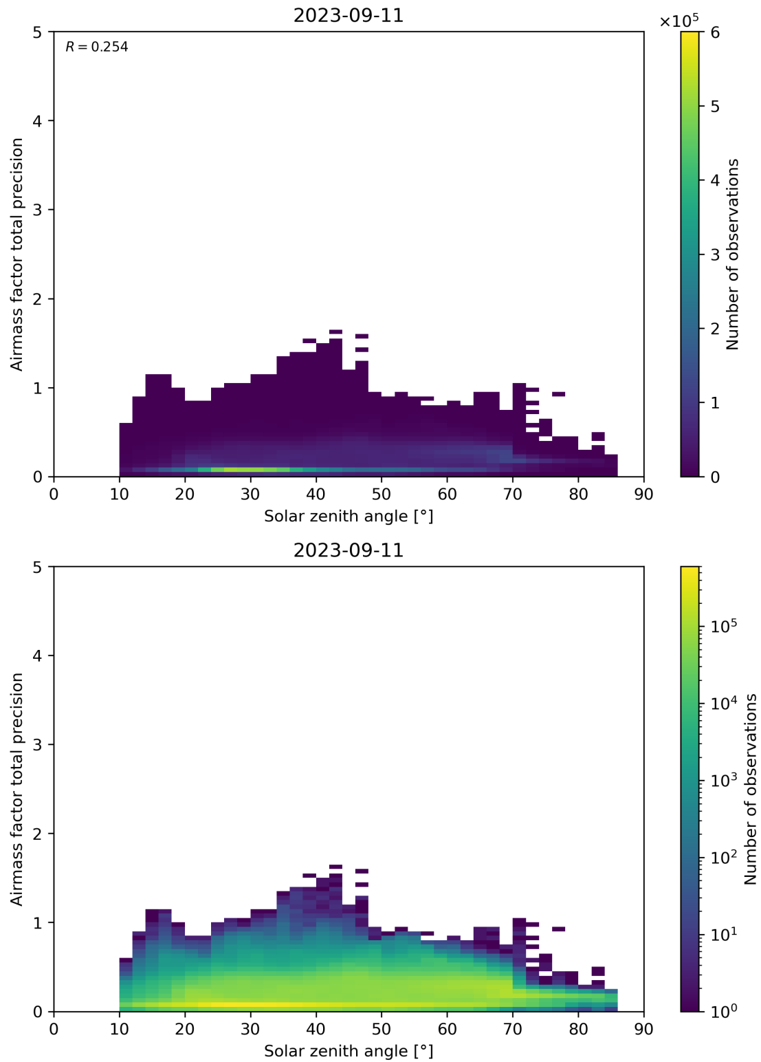
Figure 176: Scatter density plot of “Solar zenith angle” against “Airmass factor total precision” for 2023-09-10 to 2023-09-12.
