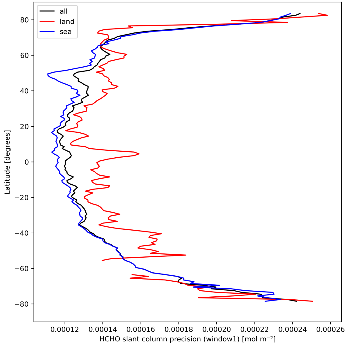
Figure 25: Zonal average of “HCHO slant column precision (window1)” for 2023-09-10 to 2023-09-12.
