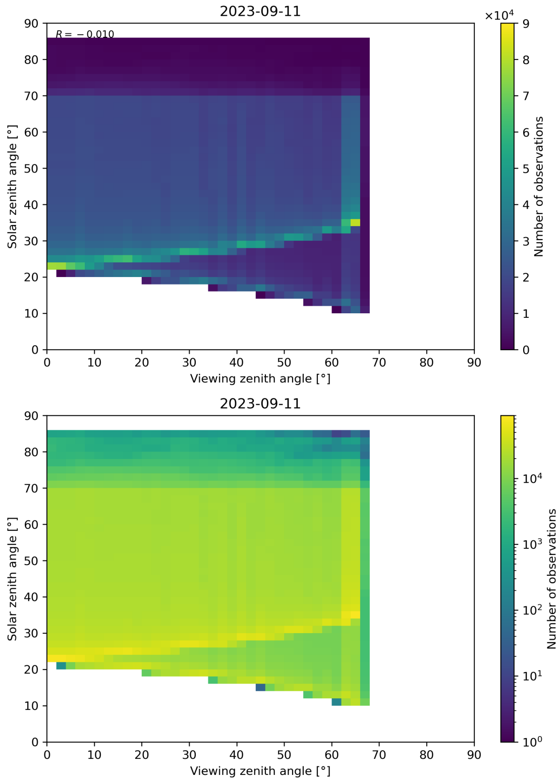
Figure 197: Scatter density plot of “Viewing zenith angle” against “Solar zenith angle” for 2023-09-10 to 2023-09-12.
