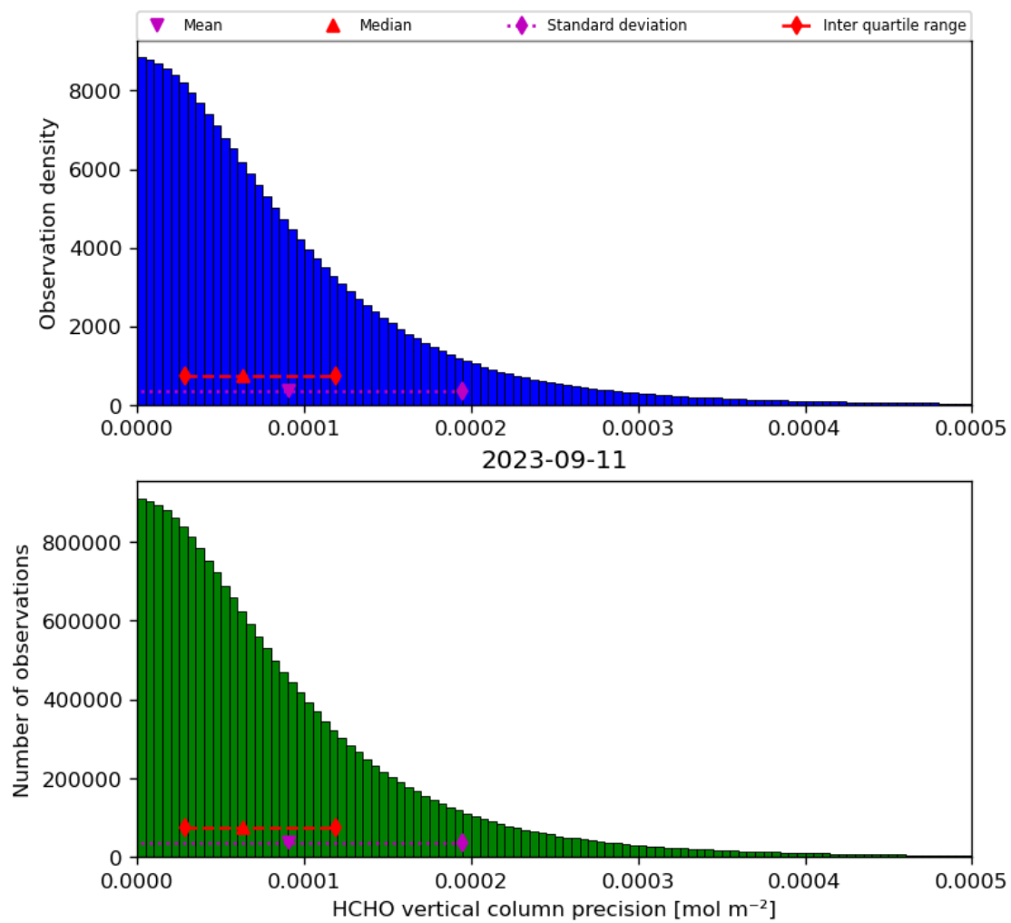
Figure 36: Histogram of “HCHO vertical column precision” for 2023-09-10 to 2023-09-12
