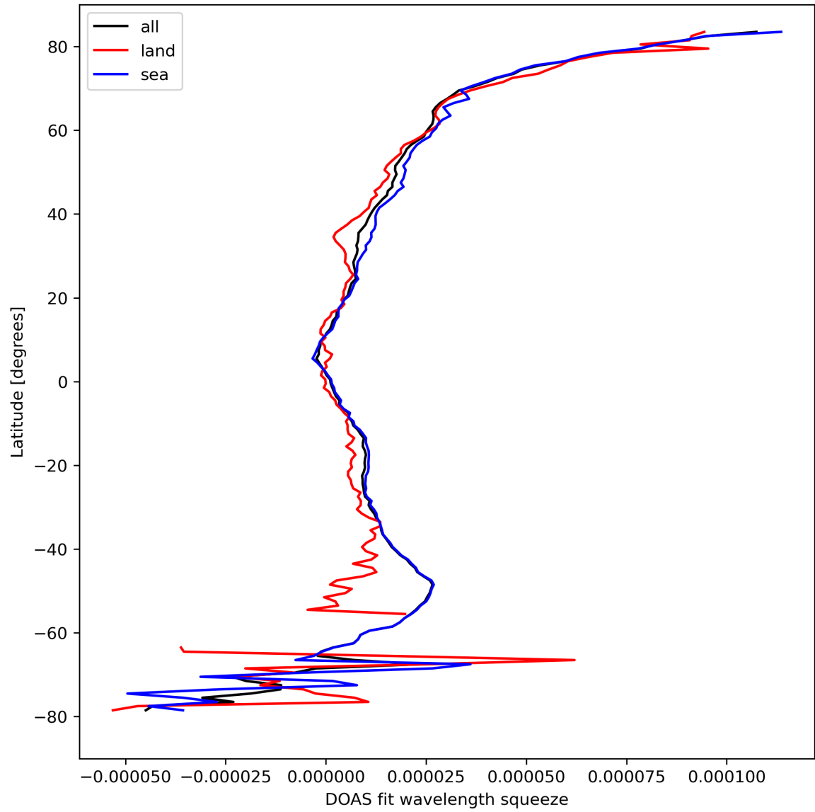
Figure 31: Zonal average of “DOAS fit wavelength squeeze” for 2023-09-10 to 2023-09-12.
