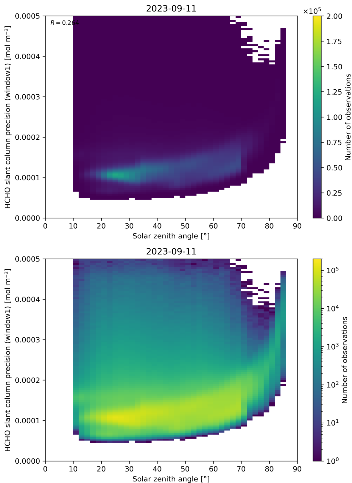
Figure 174: Scatter density plot of “Solar zenith angle” against “HCHO slant column precision (window1)” for 2023-09-10 to 2023-09-12.
