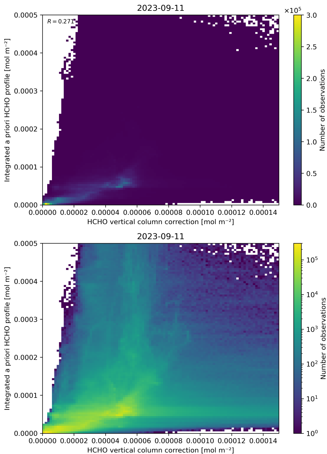
Figure 122: Scatter density plot of “HCHO vertical column correction” against “Integrated a priori HCHO profile” for 2023-09-10 to 2023-09-12.
