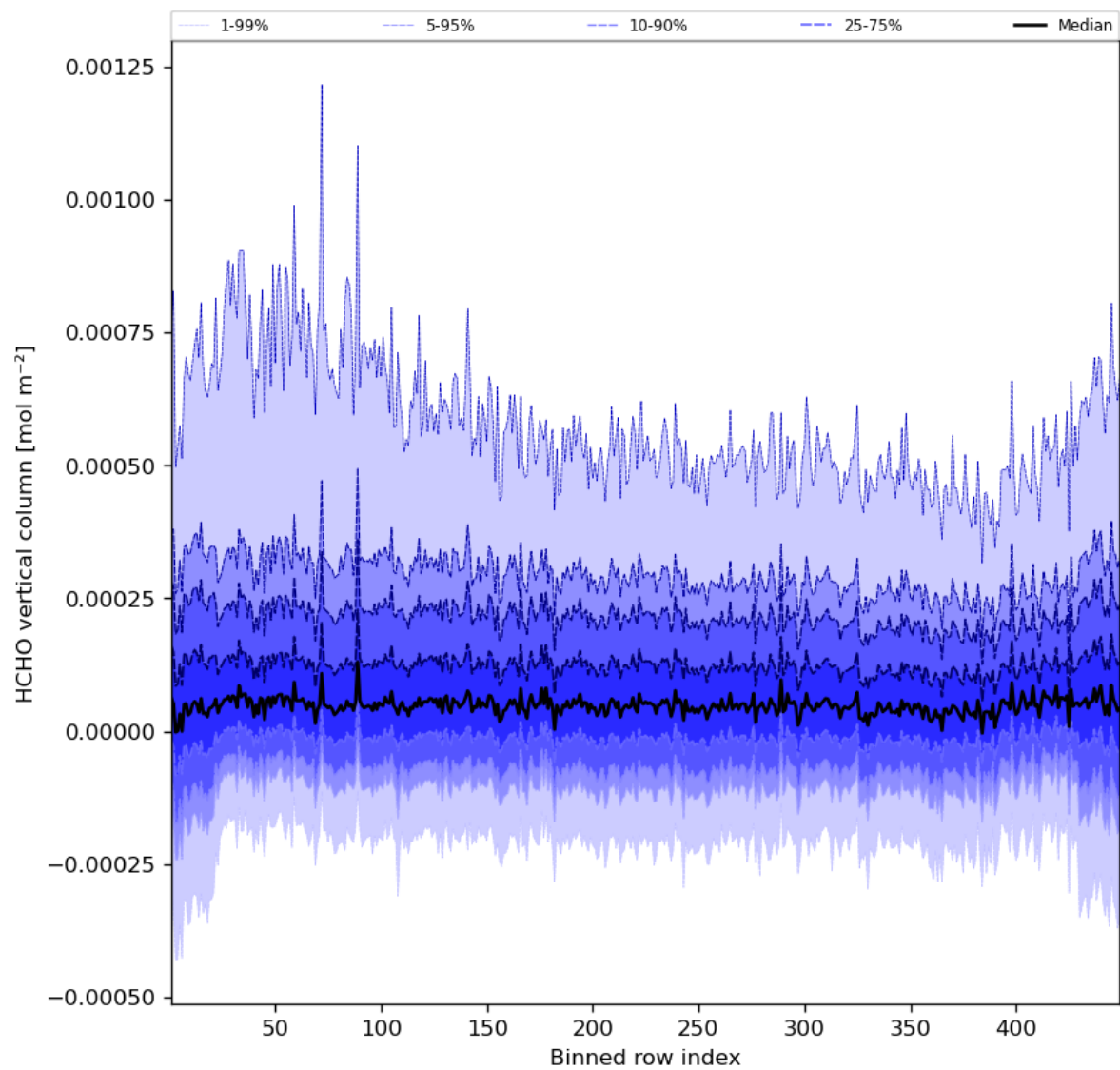
Figure 49: Along track statistics of “HCHO vertical column” for 2023-09-10 to 2023-09-12
