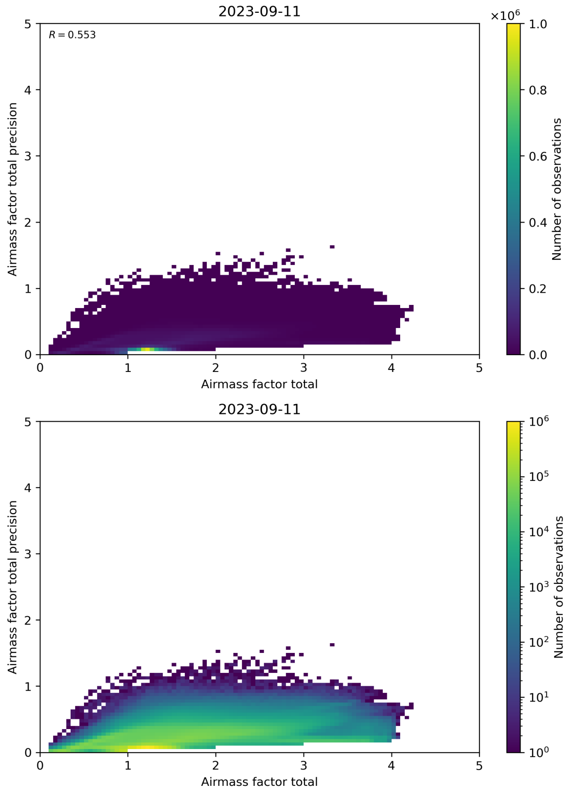
Figure 103: Scatter density plot of “Airmass factor total” against “Airmass factor total precision” for 2023-09-10 to 2023-09-12.
