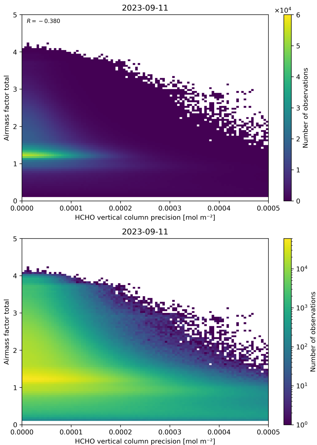
Figure 144: Scatter density plot of “HCHO vertical column precision” against “Airmass factor total” for 2023-09-10 to 2023-09-12.
