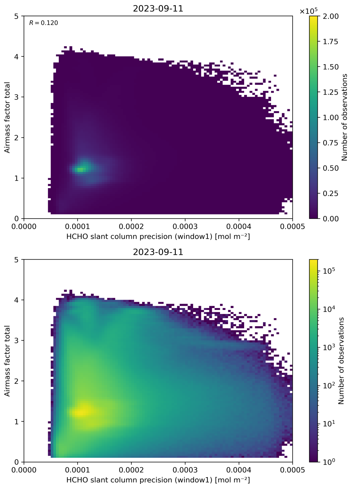
Figure 94: Scatter density plot of “HCHO slant column precision (window1)” against “Airmass factor total” for 2023-09-10 to 2023-09-12.
