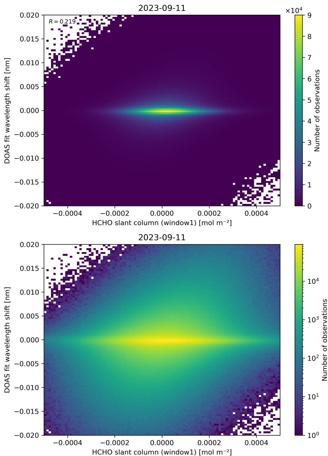
Figure 79: Scatter density plot of “HCHO slant column (window1)” against “DOAS fit wavelength shift” for 2023-09-10 to 2023-09-12.
