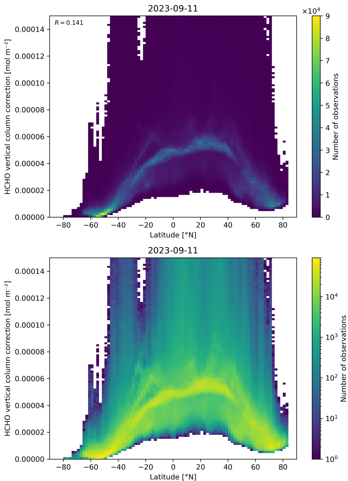
Figure 164: Scatter density plot of “Latitude” against “HCHO vertical column correction” for 2023-09-10 to 2023-09-12.
