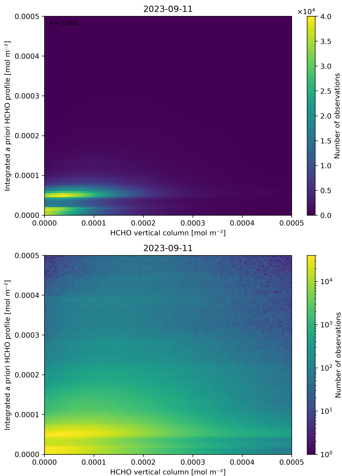
Figure 135: Scatter density plot of “HCHO vertical column” against “Integrated a priori HCHO profile” for 2023-09-10 to 2023-09-12.
