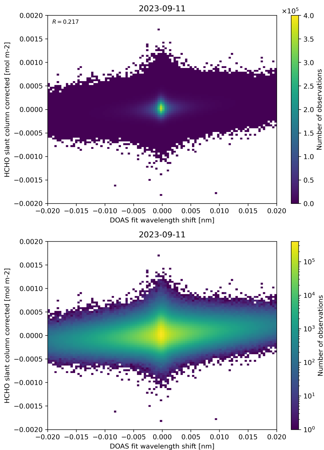
Figure 66: Scatter density plot of “DOAS fit wavelength shift” against “HCHO slant column corrected” for 2023-09-10 to 2023-09-12.
