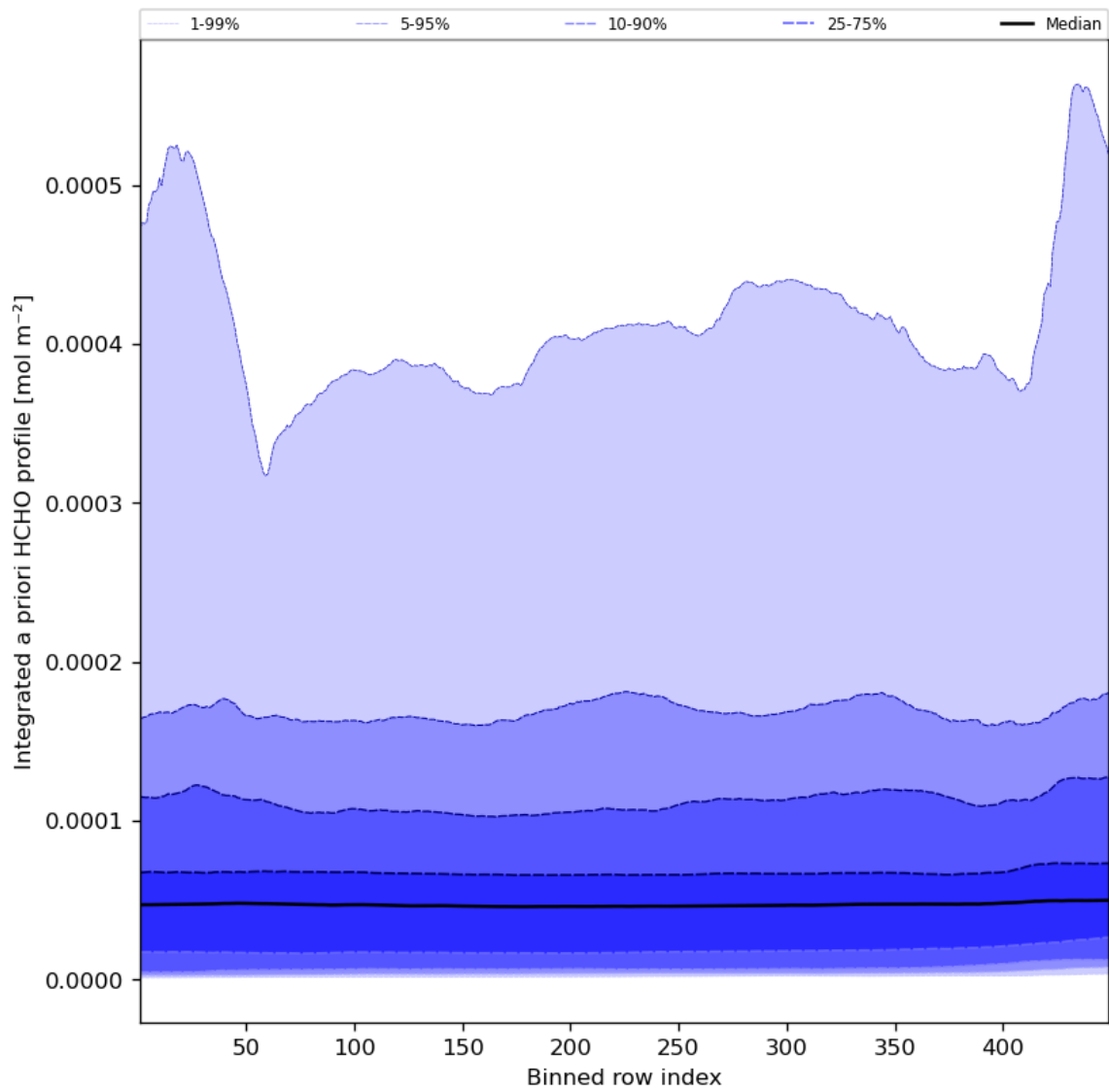
Figure 57: Along track statistics of “Integrated a priori HCHO profile” for 2023-09-10 to 2023-09-12
