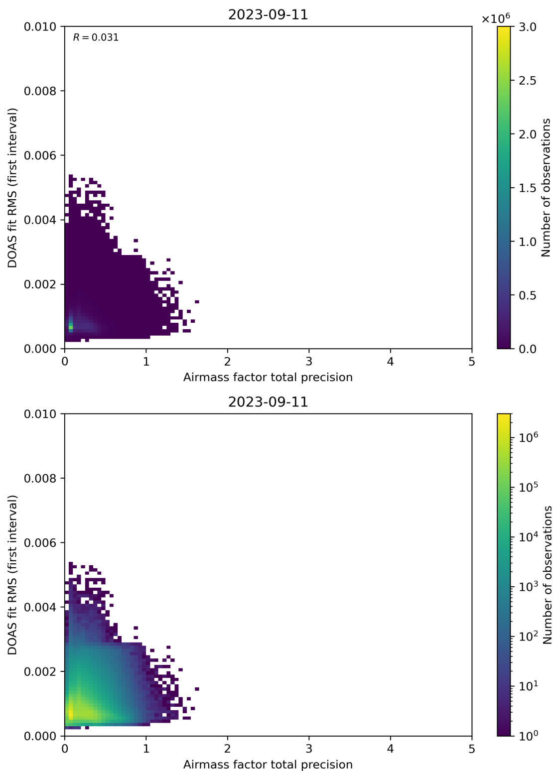
Figure 105: Scatter density plot of “Airmass factor total precision” against “DOAS fit RMS (first interval)” for 2023-09-10 to 2023-09-12.
