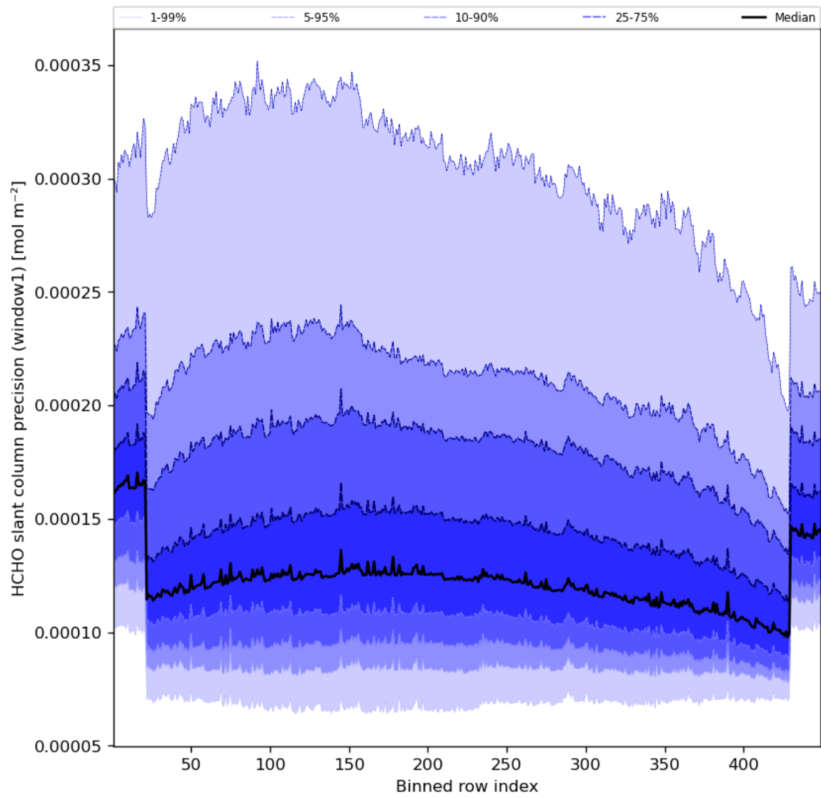
Figure 53: Along track statistics of “HCHO slant column precision (window1)” for 2023-09-10 to 2023-09-12
