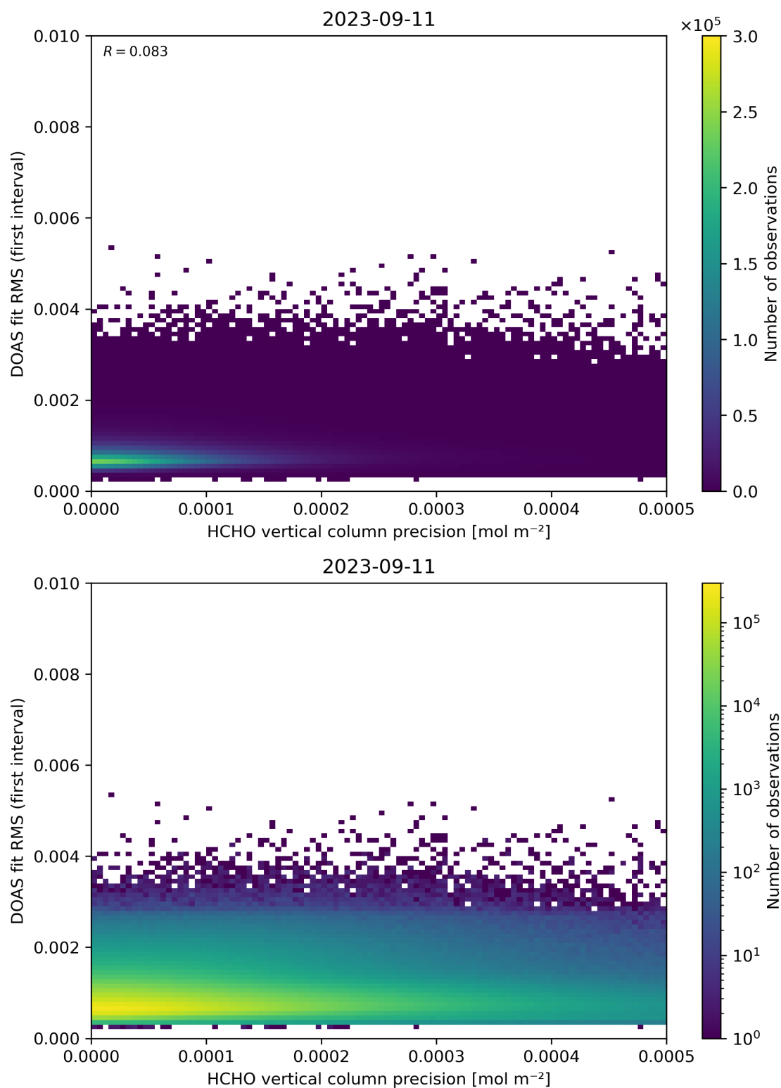
Figure 136: Scatter density plot of “HCHO vertical column precision” against “DOAS fit RMS (first interval)” for 2023-09-10 to 2023-09-12.
