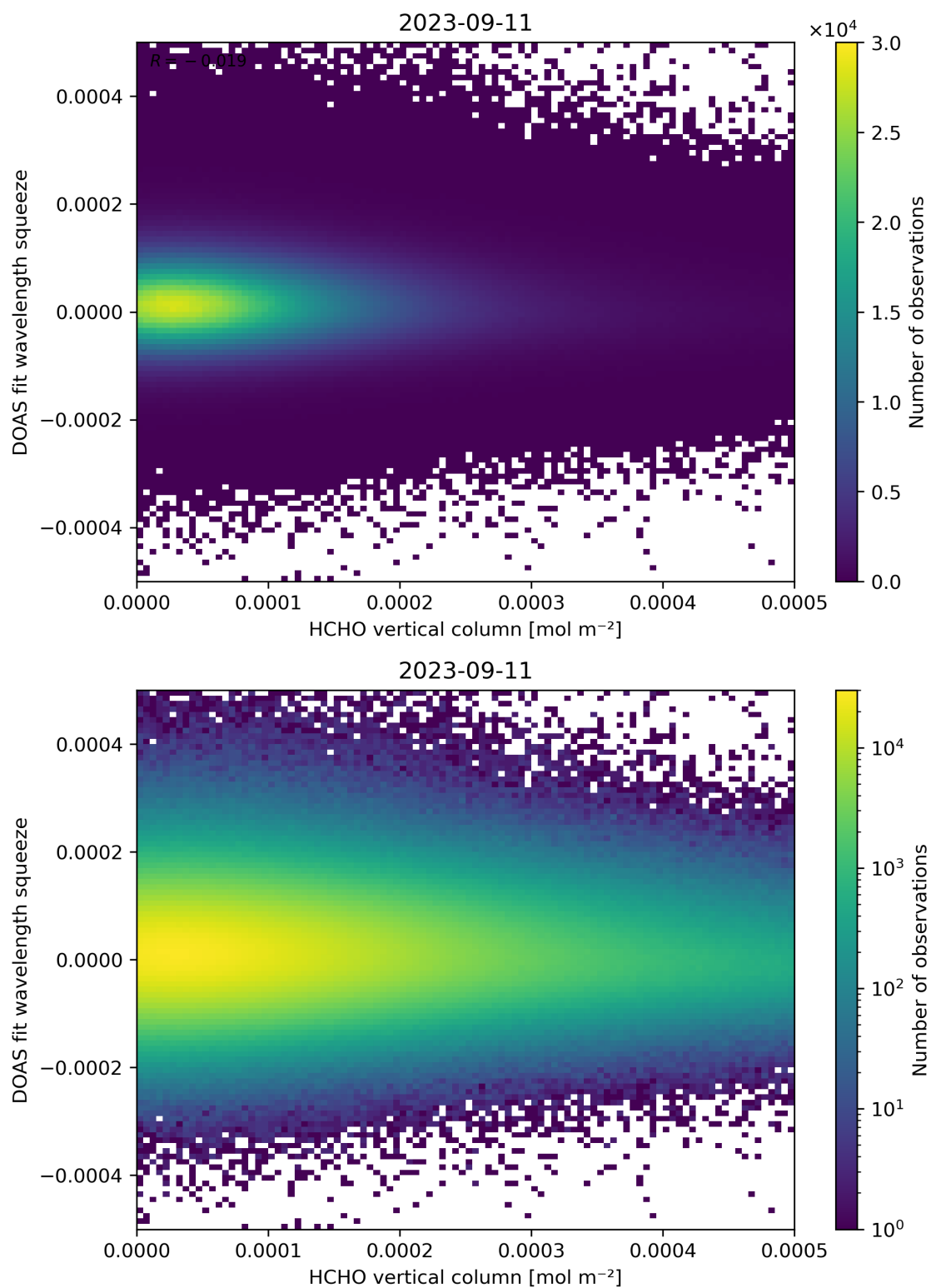
Figure 125: Scatter density plot of “HCHO vertical column” against “DOAS fit wavelength squeeze” for 2023-09-10 to 2023-09-12.
