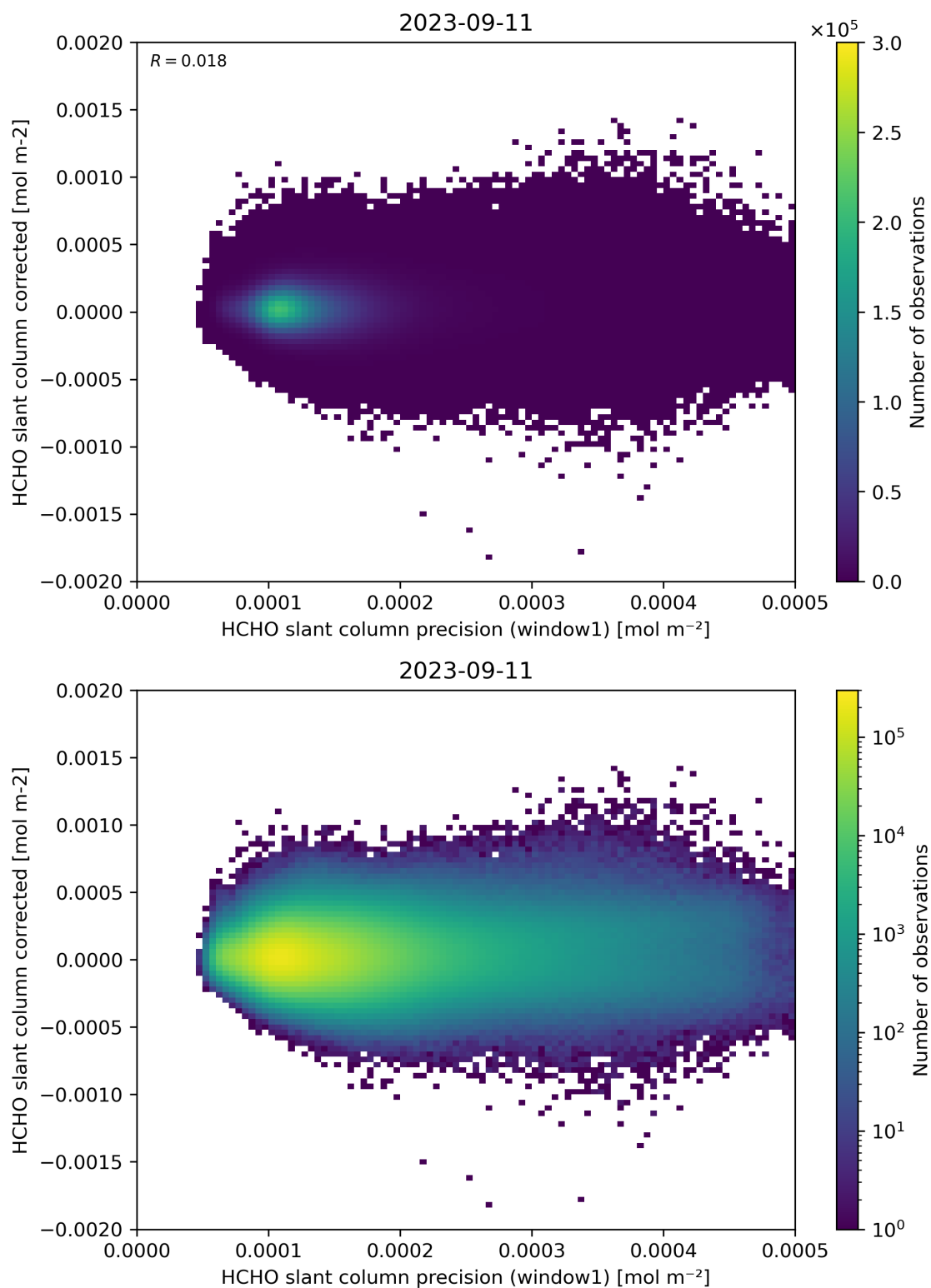
Figure 92: Scatter density plot of “HCHO slant column precision (window1)” against “HCHO slant column corrected” for 2023-09-10 to 2023-09-12.
