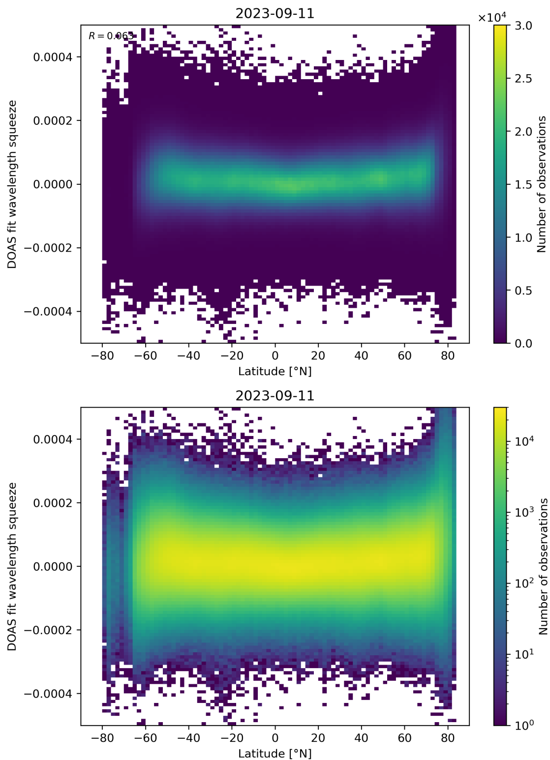
Figure 155: Scatter density plot of “Latitude” against “DOAS fit wavelength squeeze” for 2023-09-10 to 2023-09-12.
