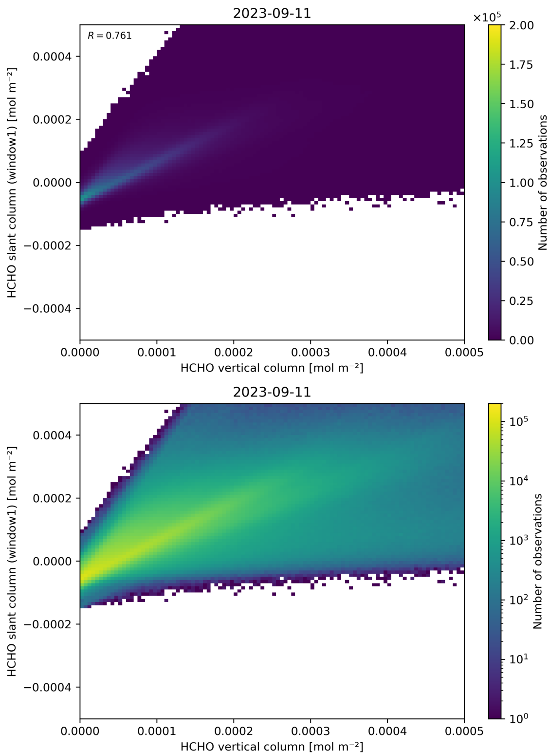
Figure 129: Scatter density plot of “HCHO vertical column” against “HCHO slant column (window1)” for 2023-09-10 to 2023-09-12.
