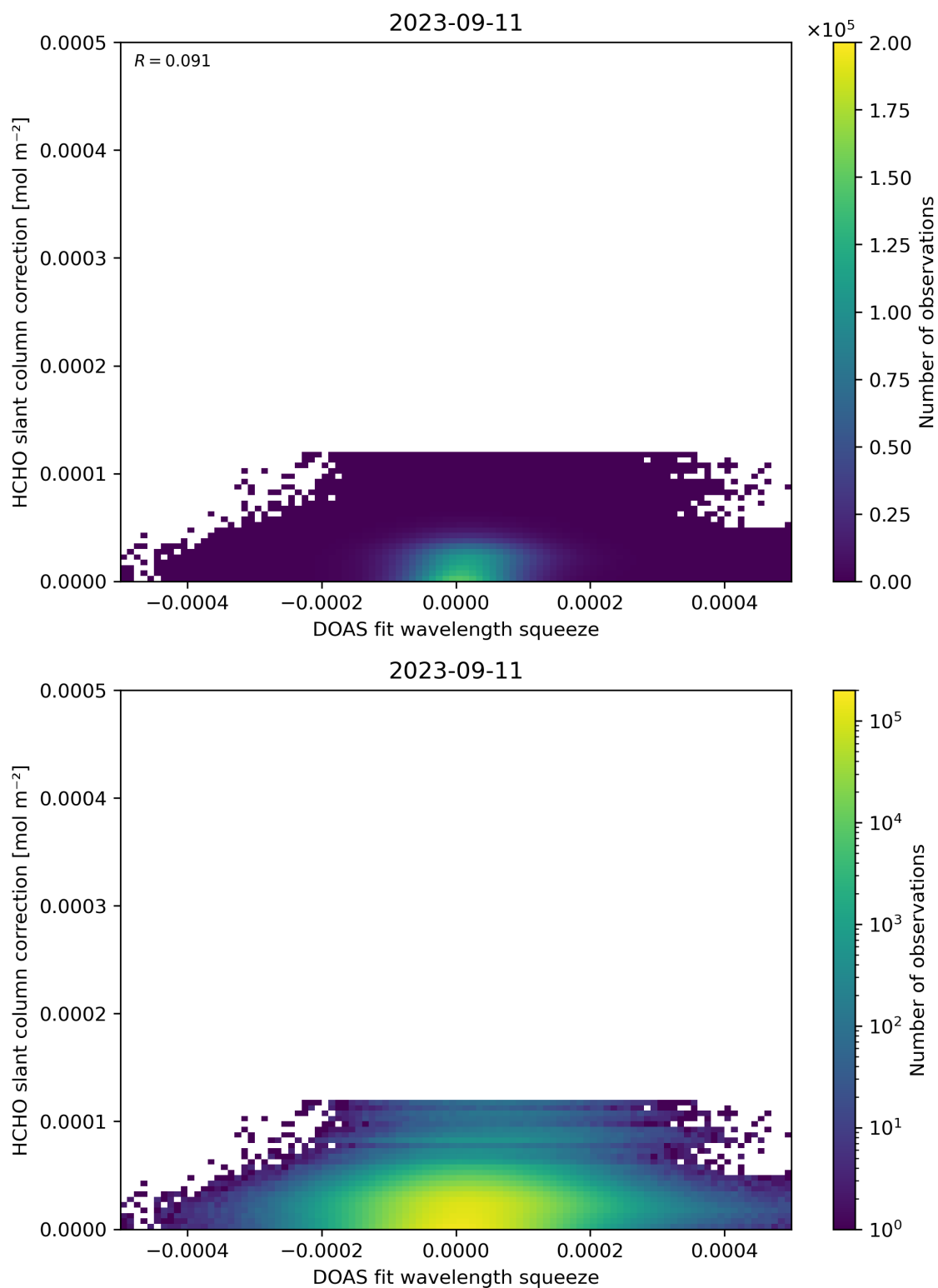
Figure 70: Scatter density plot of “DOAS fit wavelength squeeze” against “HCHO slant column correction” for 2023-09-10 to 2023-09-12.
