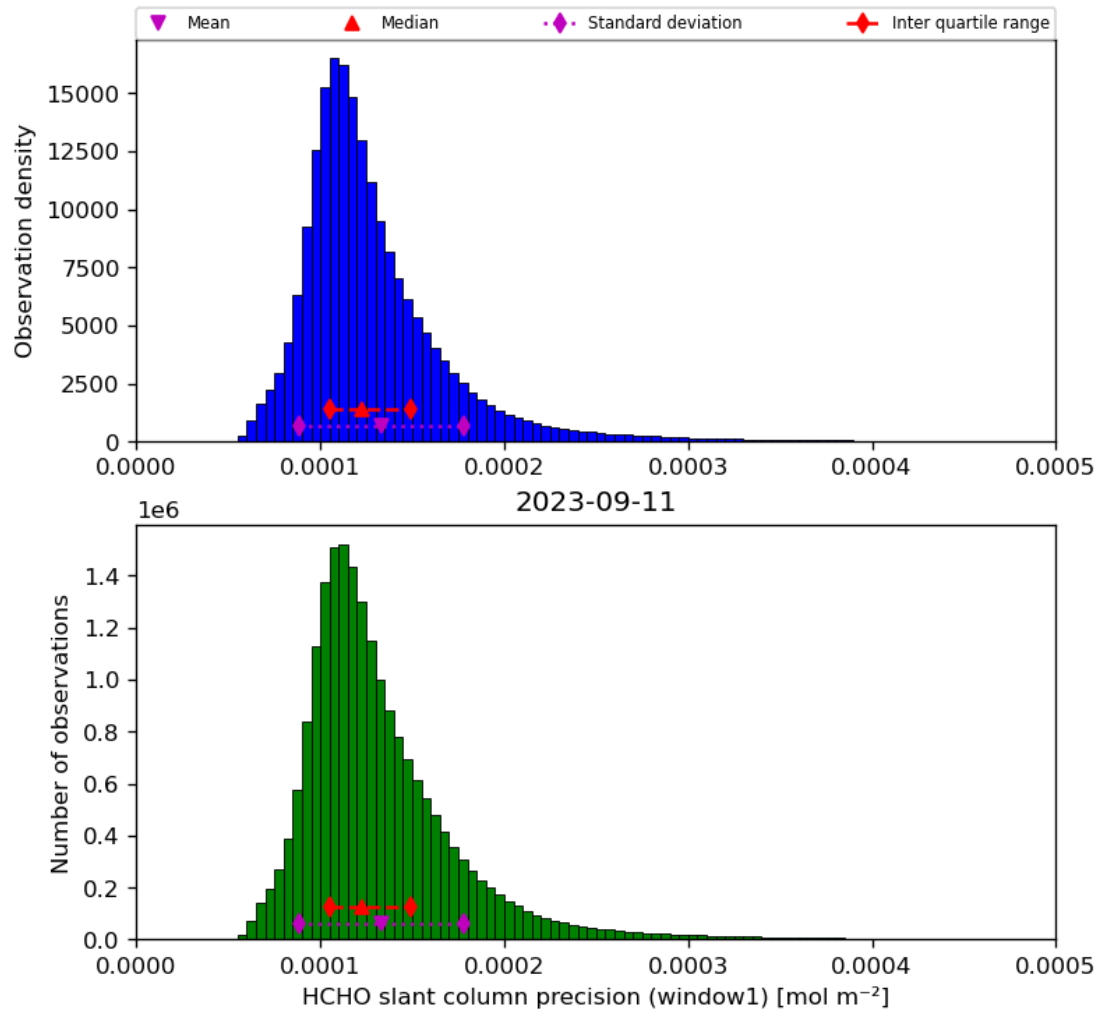
Figure 39: Histogram of “HCHO slant column precision (window1)” for 2023-09-10 to 2023-09-12
