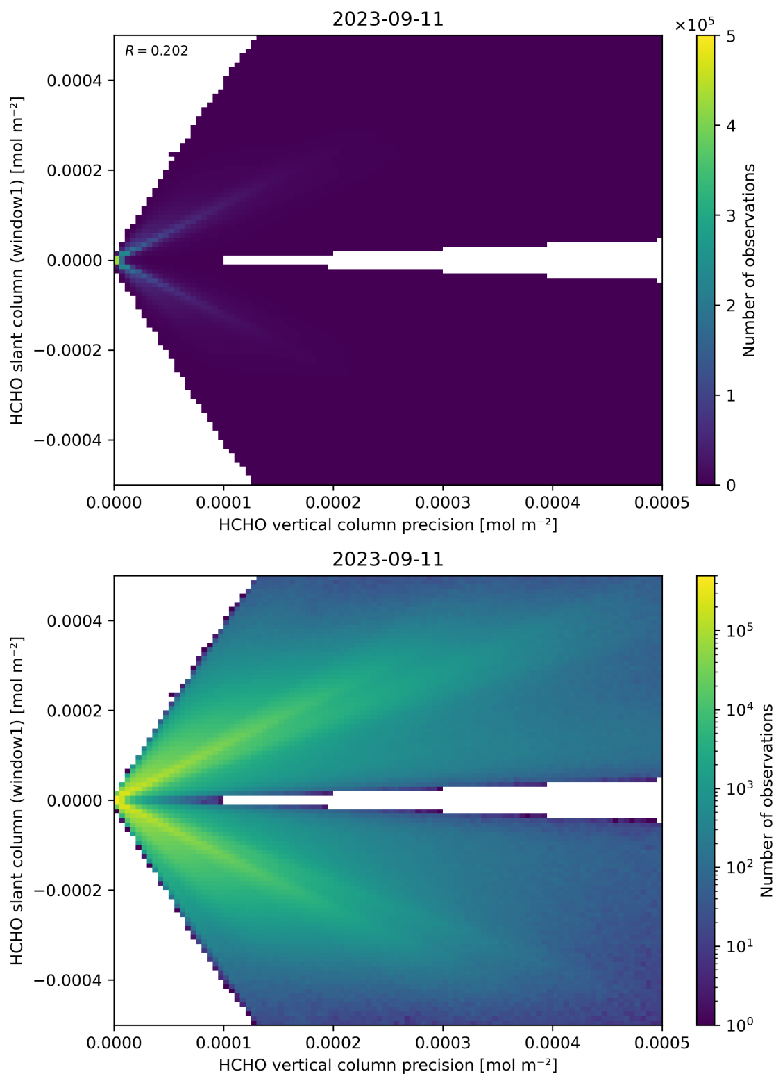
Figure 142: Scatter density plot of “HCHO vertical column precision” against “HCHO slant column (window1)” for 2023-09-10 to 2023-09-12.
