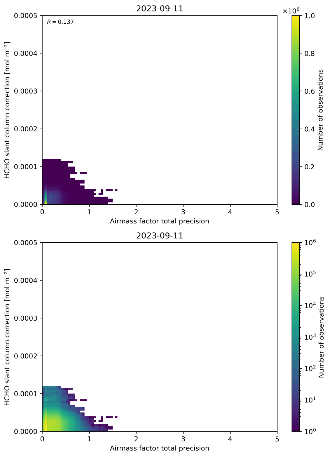
Figure 110: Scatter density plot of “Airmass factor total precision” against “HCHO slant column correction” for 2023-09-10 to 2023-09-12.
