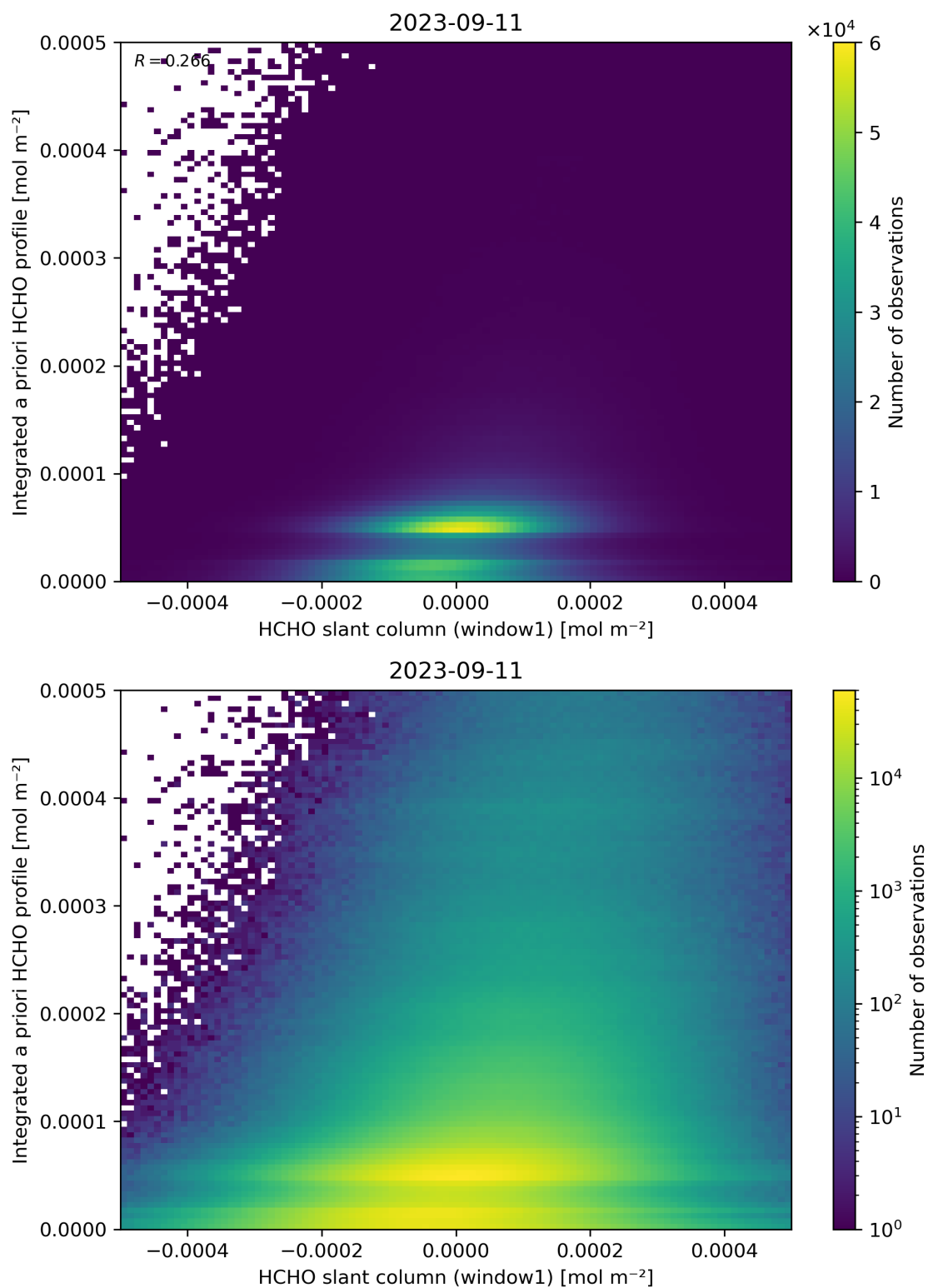
Figure 87: Scatter density plot of “HCHO slant column (window1)” against “Integrated a priori HCHO profile” for 2023-09-10 to 2023-09-12.
