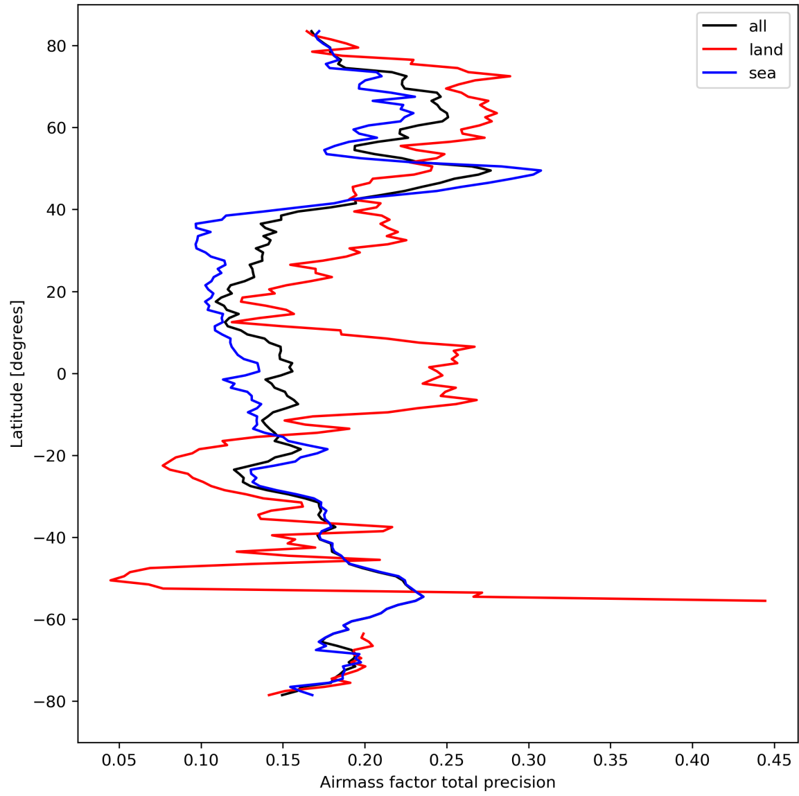
Figure 27: Zonal average of “Airmass factor total precision” for 2023-09-10 to 2023-09-12.
