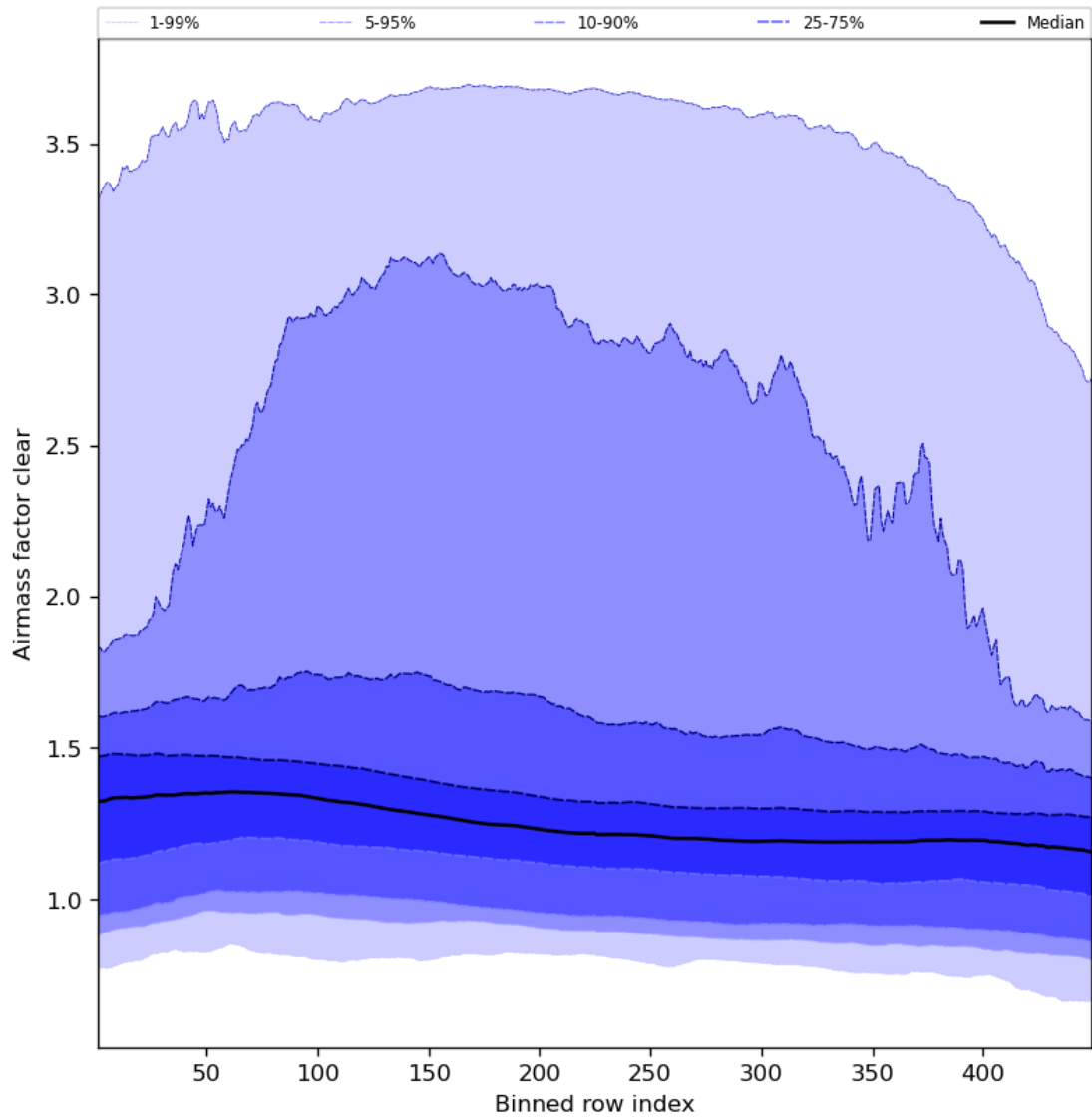
Figure 56: Along track statistics of “Airmass factor clear” for 2023-09-10 to 2023-09-12
