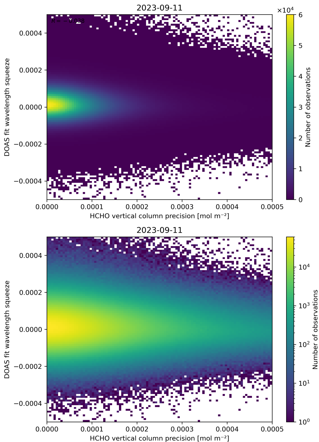
Figure 138: Scatter density plot of “HCHO vertical column precision” against “DOAS fit wavelength squeeze” for 2023-09-10 to 2023-09-12.
