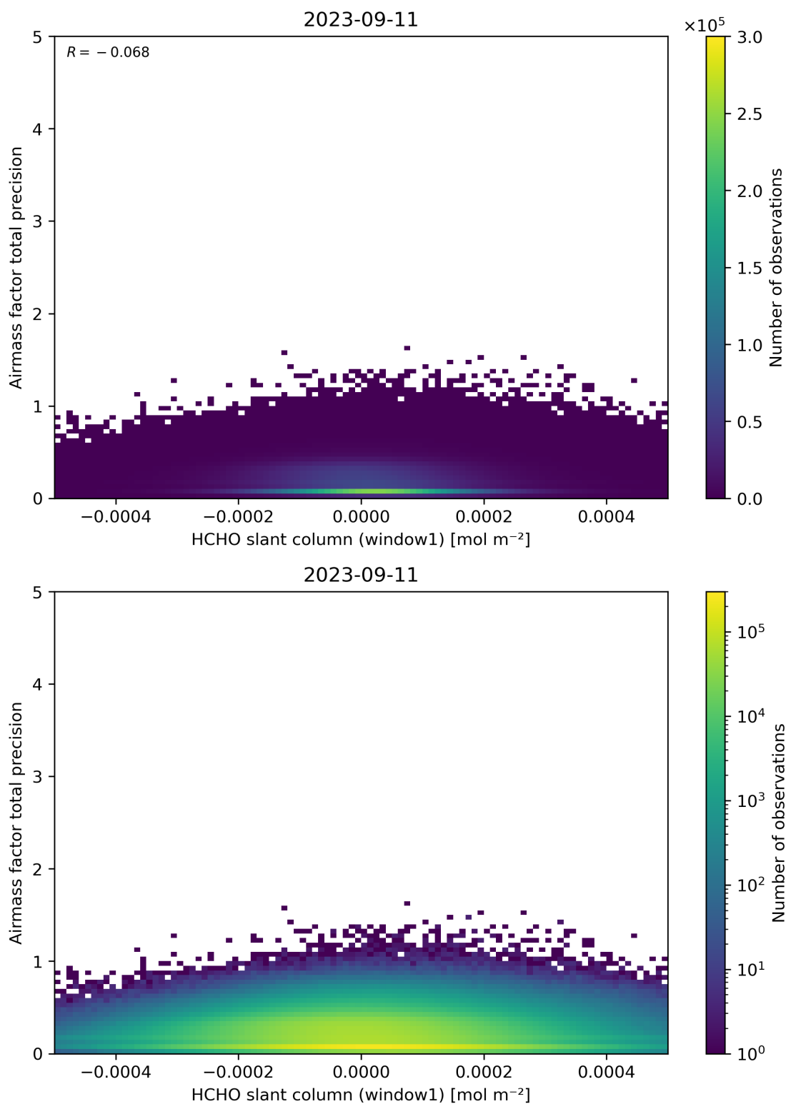
Figure 86: Scatter density plot of “HCHO slant column (window1)” against “Airmass factor total precision” for 2023-09-10 to 2023-09-12.
