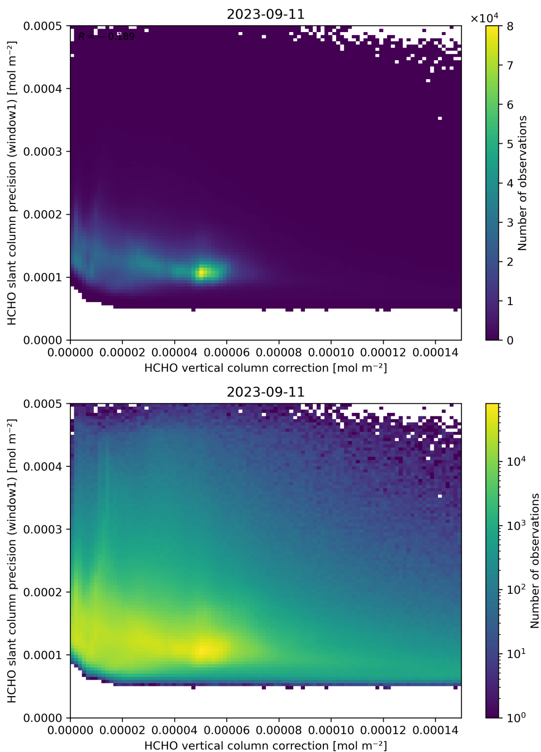
Figure 119: Scatter density plot of “HCHO vertical column correction” against “HCHO slant column precision (window1)” for 2023-09-10 to 2023-09-12.
