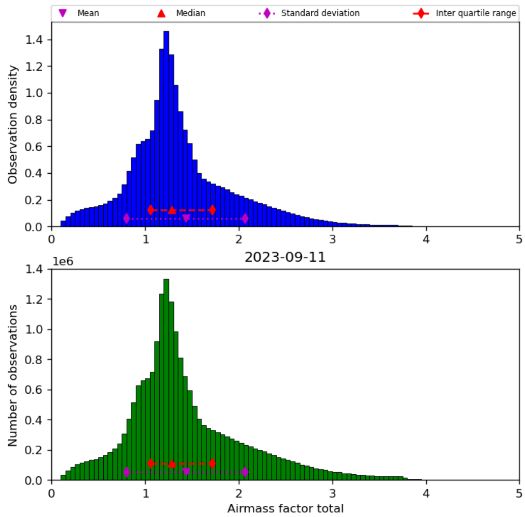
Figure 40: Histogram of “Airmass factor total” for 2023-09-10 to 2023-09-12
