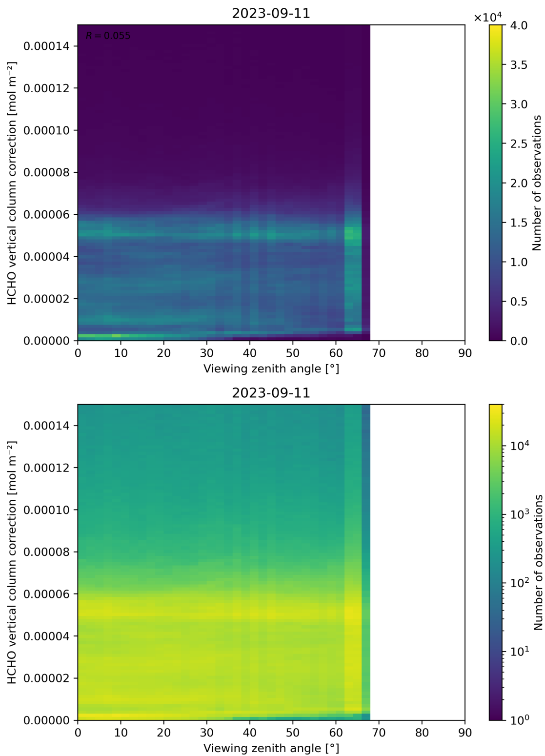
Figure 193: Scatter density plot of “Viewing zenith angle” against “HCHO vertical column correction” for 2023-09-10 to 2023-09-12.
