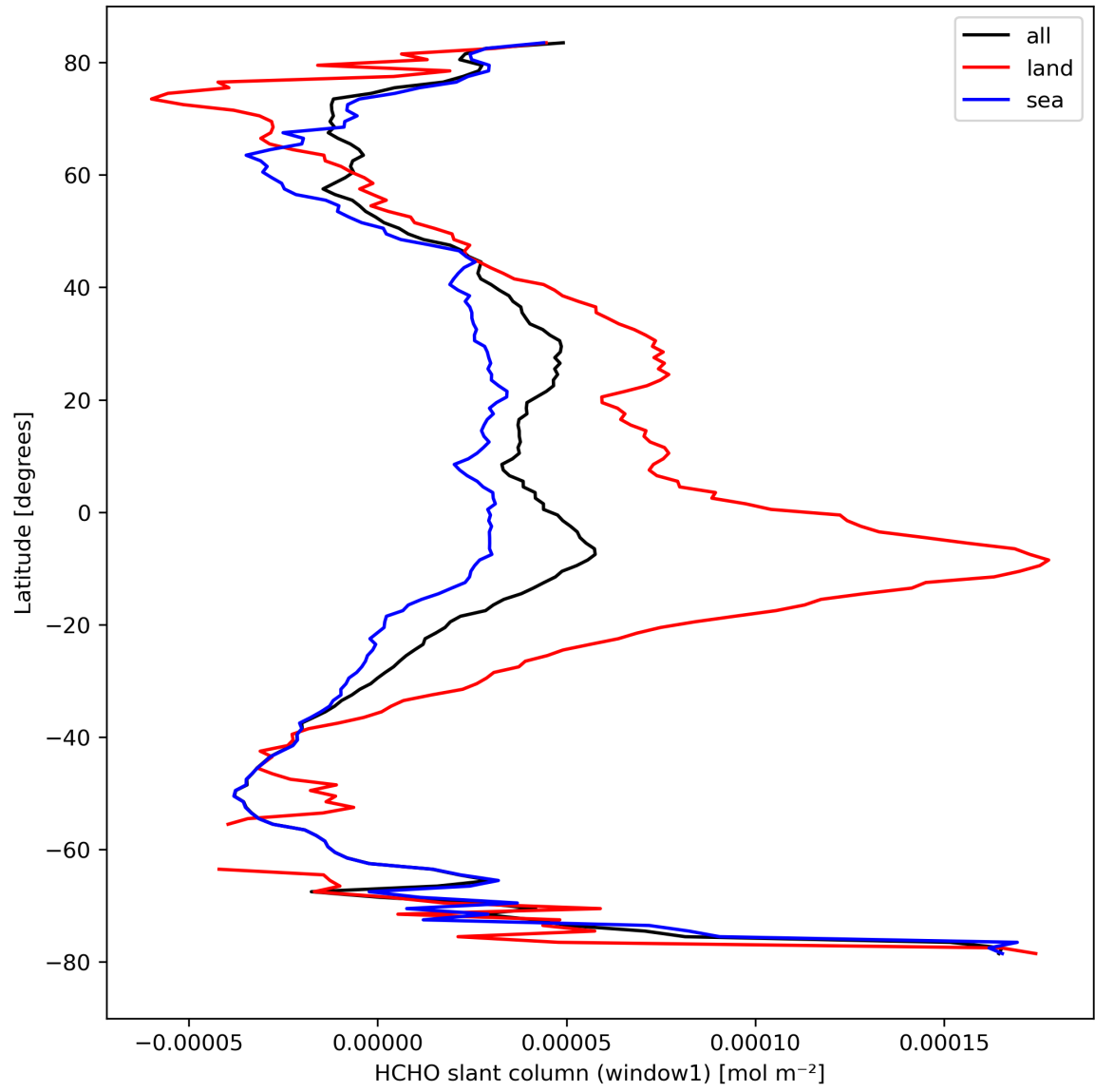
Figure 24: Zonal average of “HCHO slant column (window1)” for 2023-09-10 to 2023-09-12.
