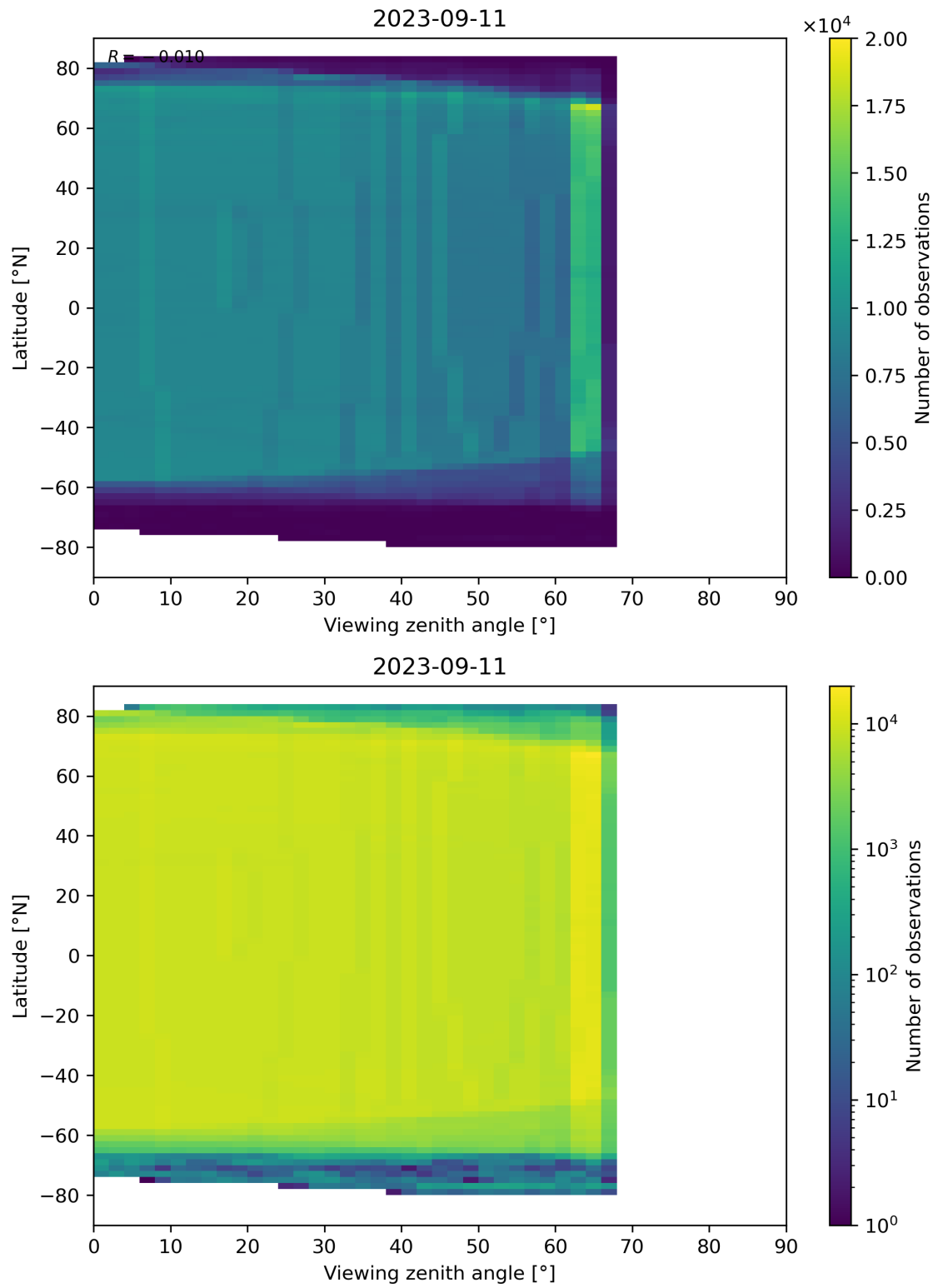
Figure 196: Scatter density plot of “Viewing zenith angle” against “Latitude” for 2023-09-10 to 2023-09-12.
