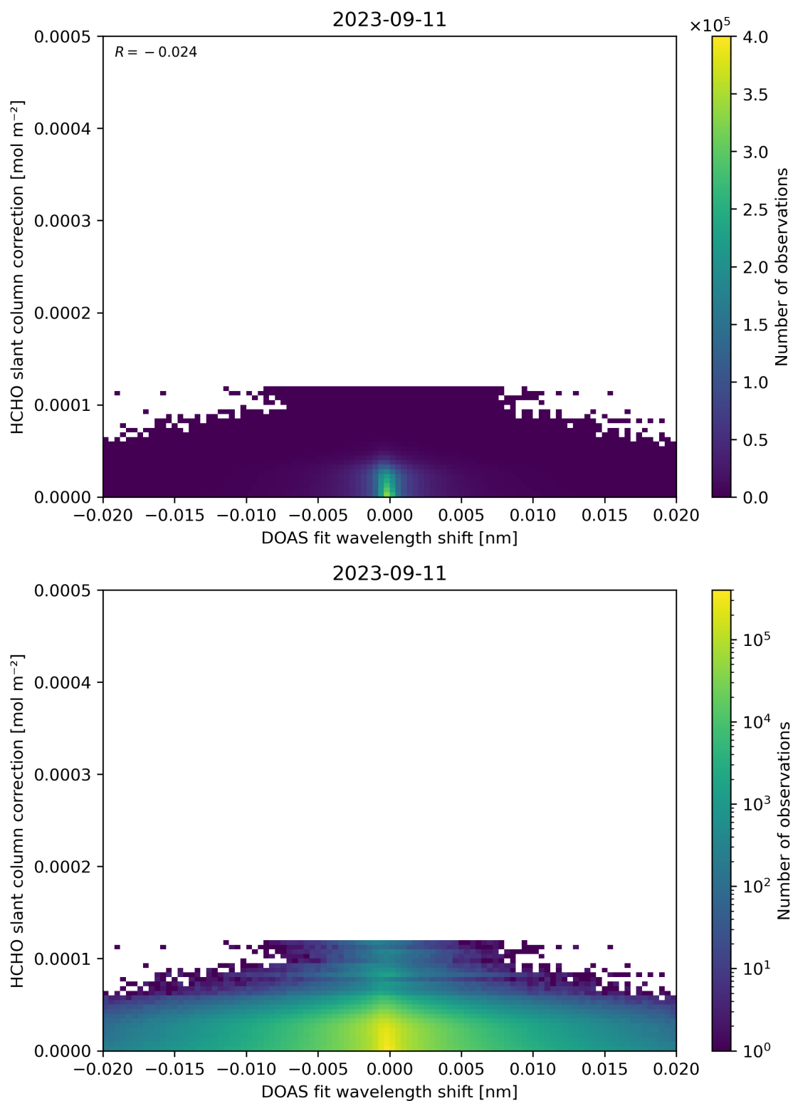
Figure 67: Scatter density plot of “DOAS fit wavelength shift” against “HCHO slant column correction” for 2023-09-10 to 2023-09-12.
