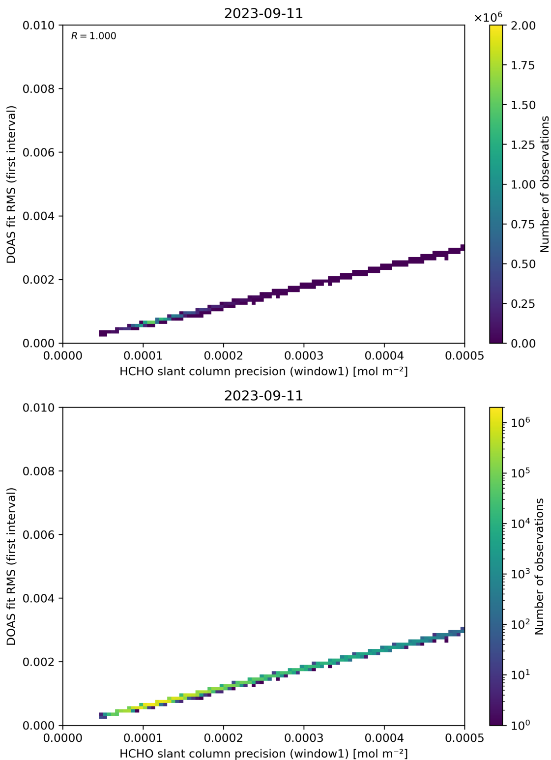
Figure 88: Scatter density plot of “HCHO slant column precision (window1)” against “DOAS fit RMS (first interval)” for 2023-09-10 to 2023-09-12.
