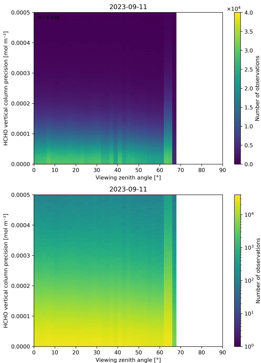
Figure 194: Scatter density plot of “Viewing zenith angle” against “HCHO vertical column precision” for 2023-09-10 to 2023-09-12.
