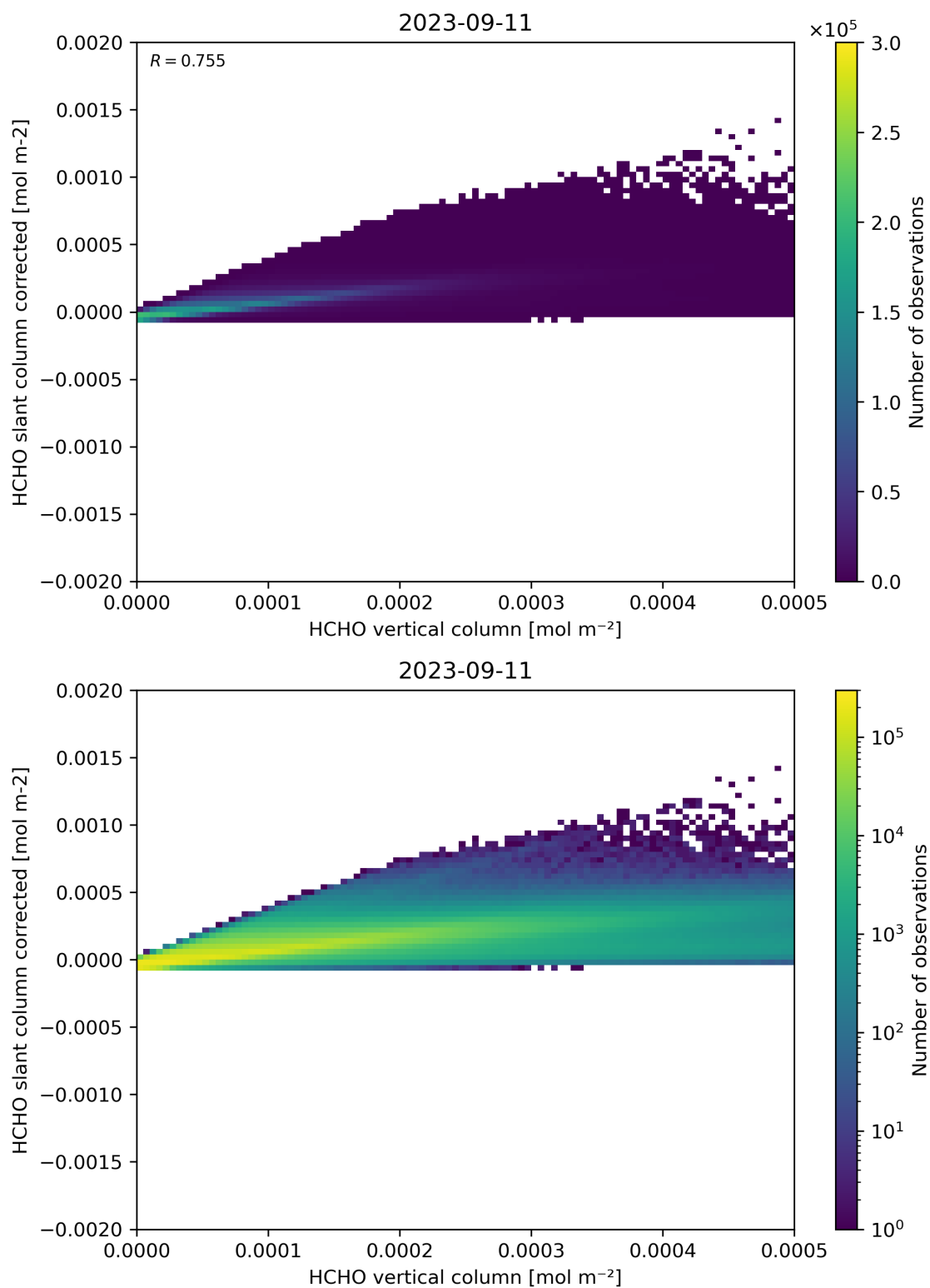
Figure 127: Scatter density plot of “HCHO vertical column” against “HCHO slant column corrected” for 2023-09-10 to 2023-09-12.
