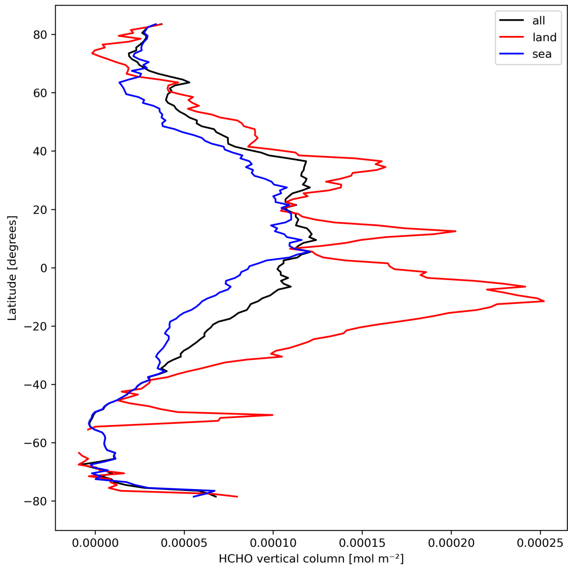
Figure 21: Zonal average of “HCHO vertical column” for 2023-09-10 to 2023-09-12.
