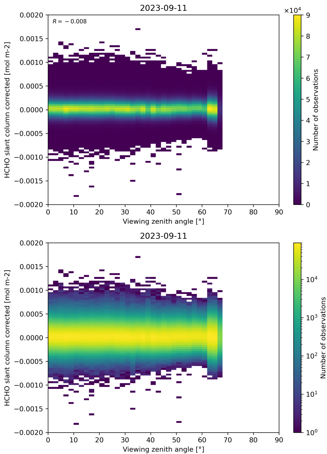
Figure 186: Scatter density plot of “Viewing zenith angle” against “HCHO slant column corrected” for 2023-09-10 to 2023-09-12.
