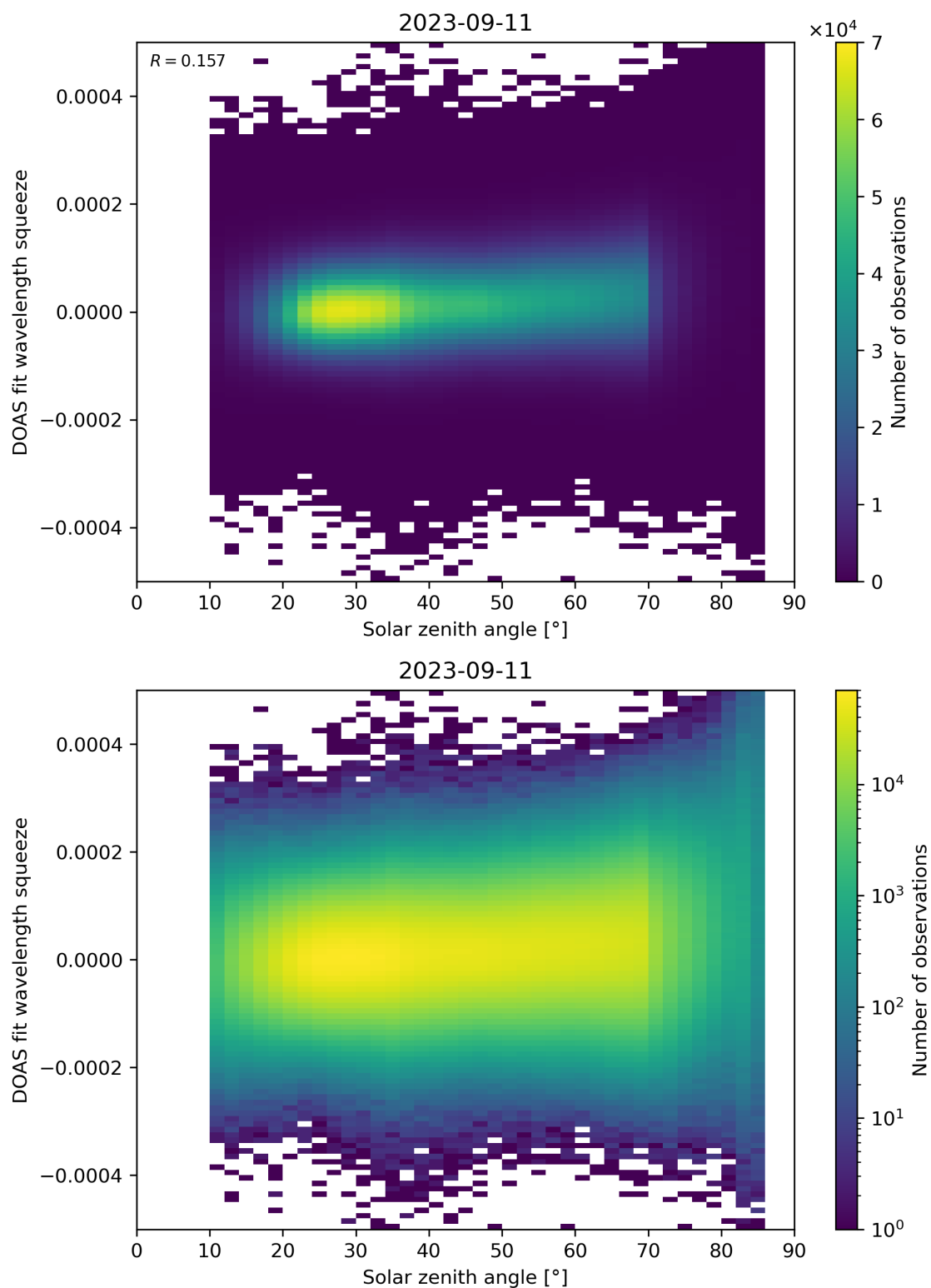
Figure 169: Scatter density plot of “Solar zenith angle” against “DOAS fit wavelength squeeze” for 2023-09-10 to 2023-09-12.
