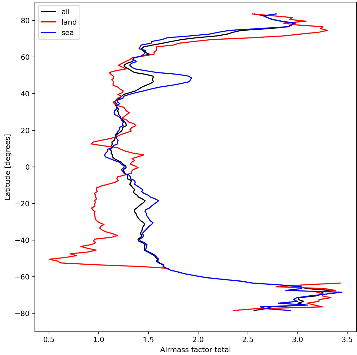
Figure 26: Zonal average of “Airmass factor total” for 2023-09-10 to 2023-09-12.
