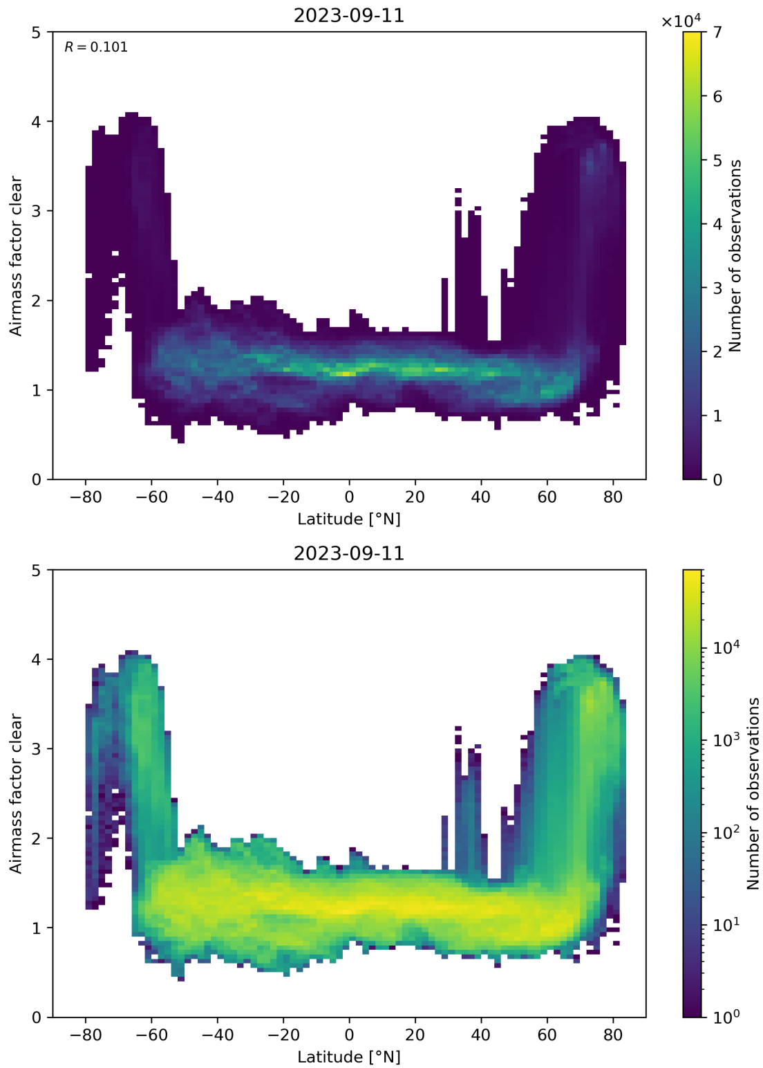
Figure 156: Scatter density plot of “Latitude” against “Airmass factor clear” for 2023-09-10 to 2023-09-12.
