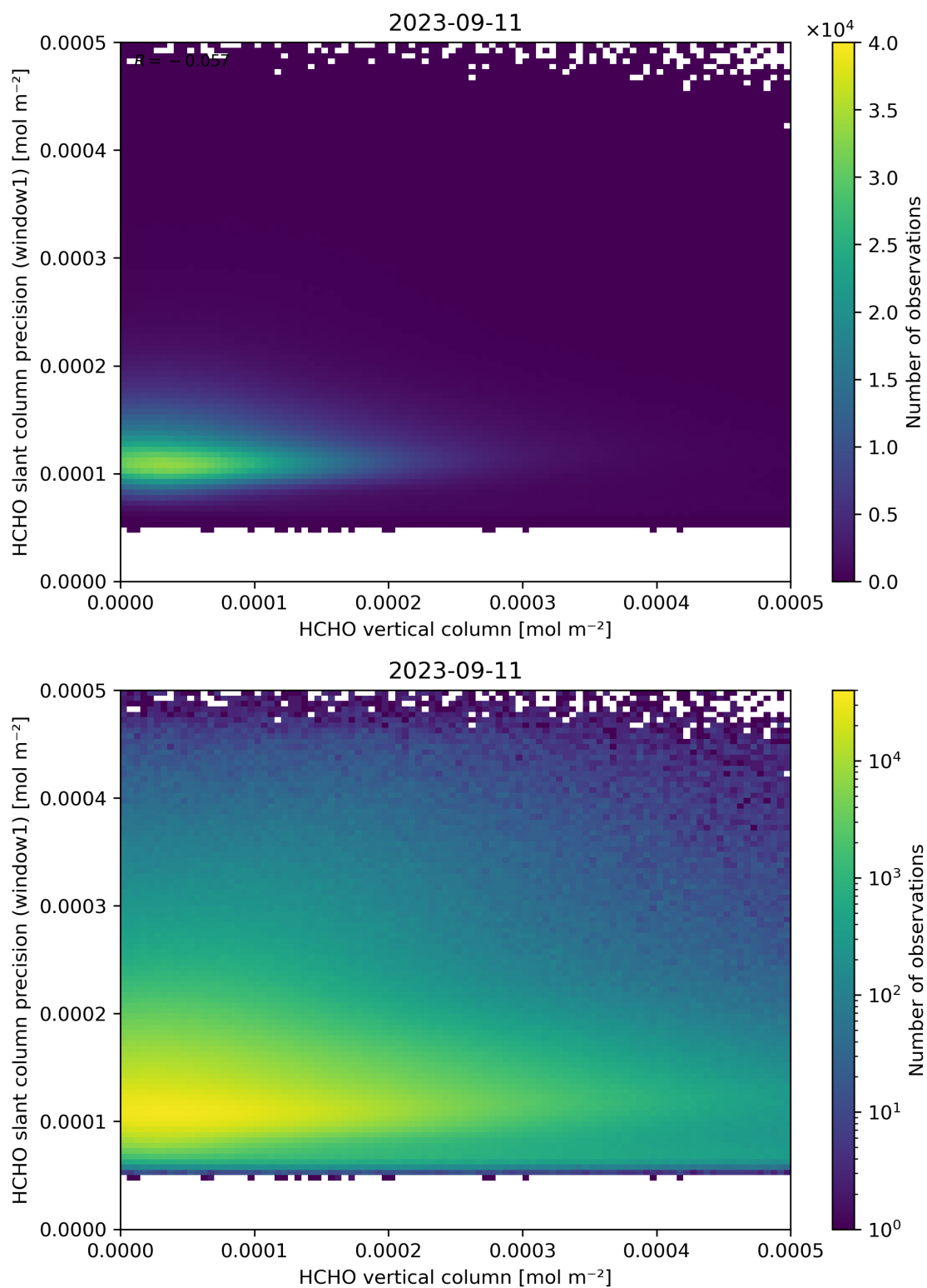
Figure 130: Scatter density plot of “HCHO vertical column” against “HCHO slant column precision (window1)” for 2023-09-10 to 2023-09-12.
