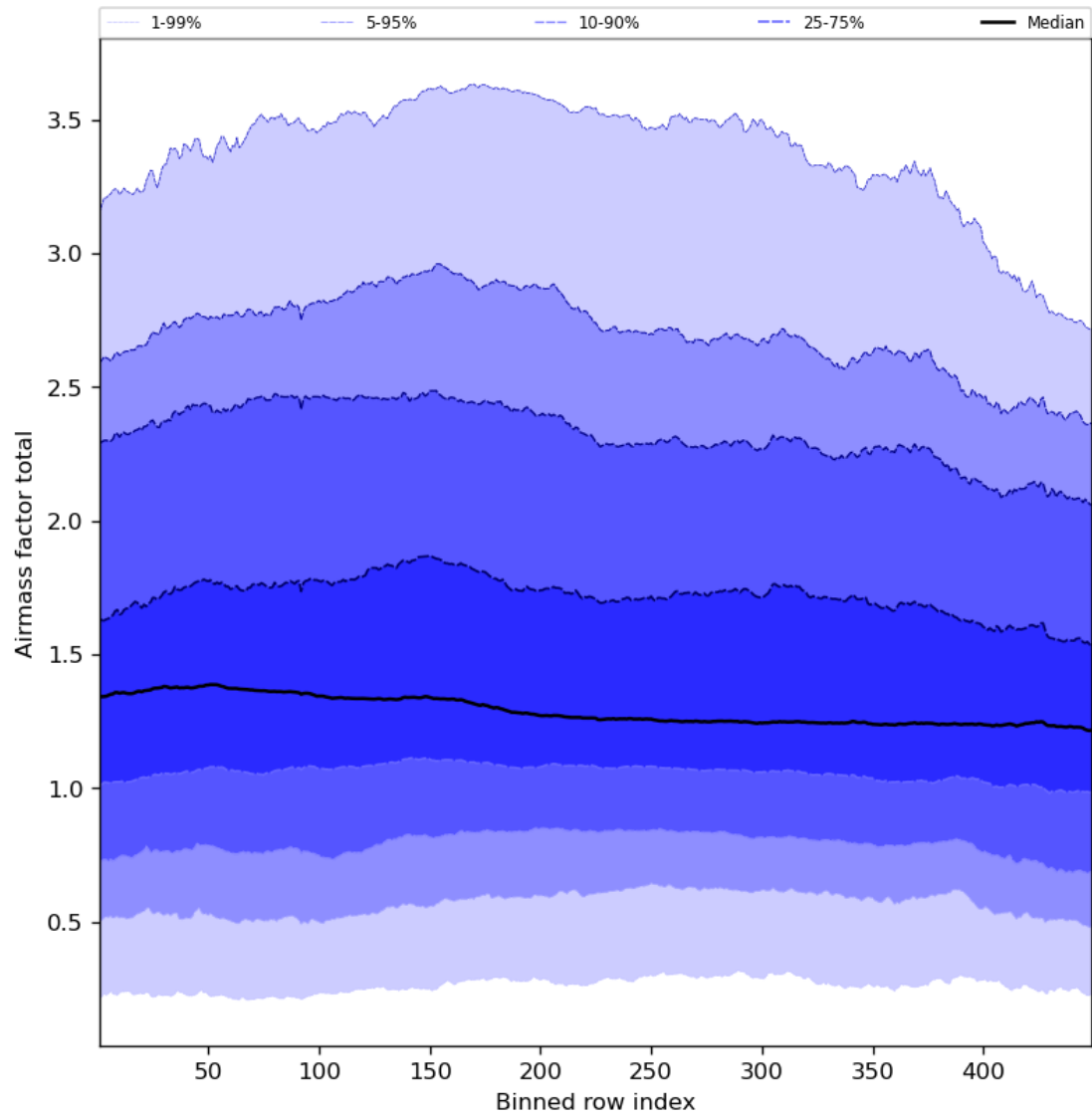
Figure 54: Along track statistics of “Airmass factor total” for 2023-09-10 to 2023-09-12
