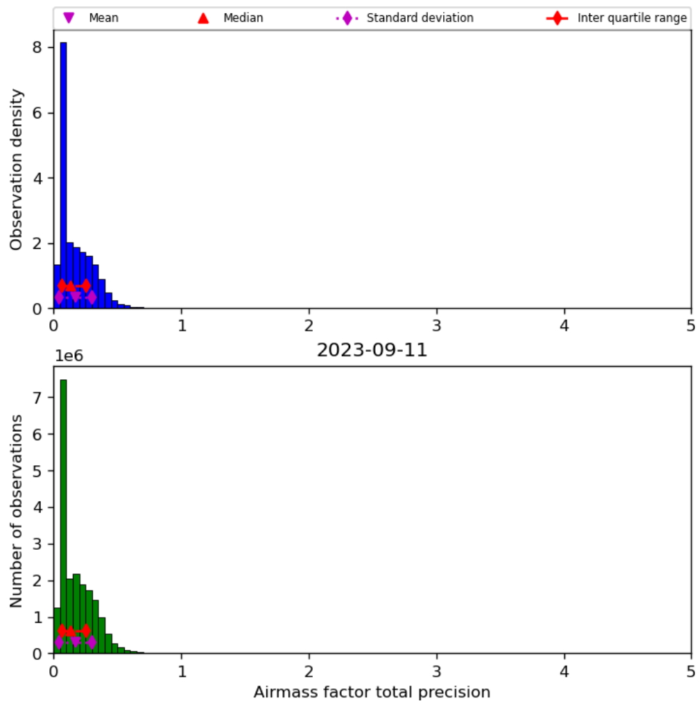
Figure 41: Histogram of “Airmass factor total precision” for 2023-09-10 to 2023-09-12
