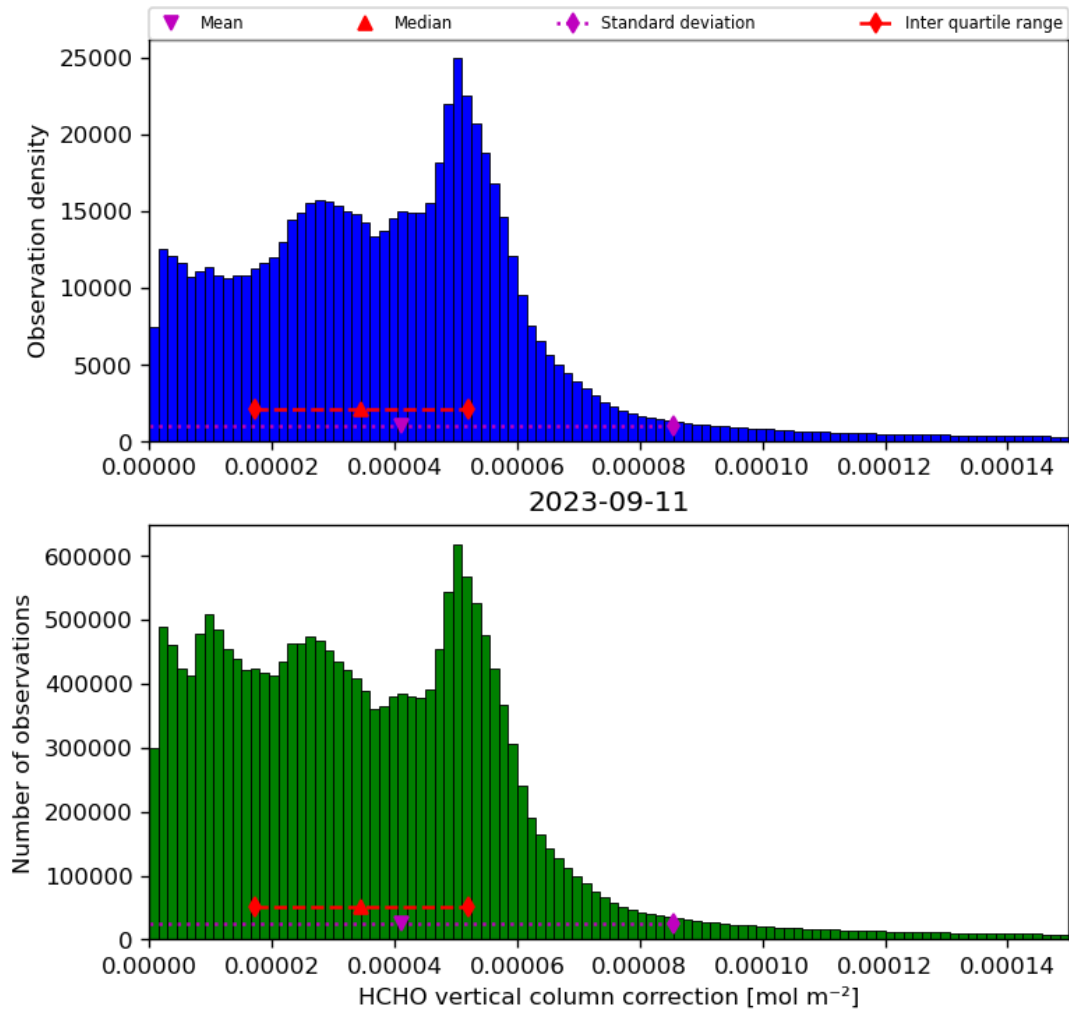
Figure 37: Histogram of “HCHO vertical column correction” for 2023-09-10 to 2023-09-12
