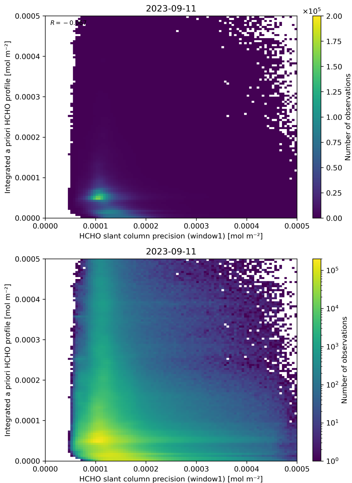
Figure 96: Scatter density plot of “HCHO slant column precision (window1)” against “Integrated a priori HCHO profile” for 2023-09-10 to 2023-09-12.
