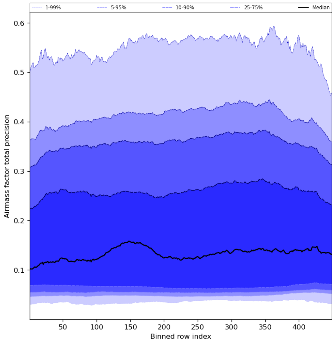
Figure 55: Along track statistics of “Airmass factor total precision” for 2023-09-10 to 2023-09-12
