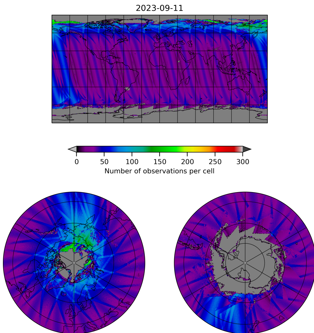
Figure 19: Map of the number of observations for 2023-09-10 to 2023-09-12
