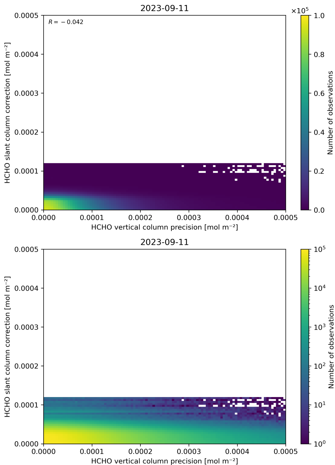
Figure 141: Scatter density plot of “HCHO vertical column precision” against “HCHO slant column correction” for 2023-09-10 to 2023-09-12.
