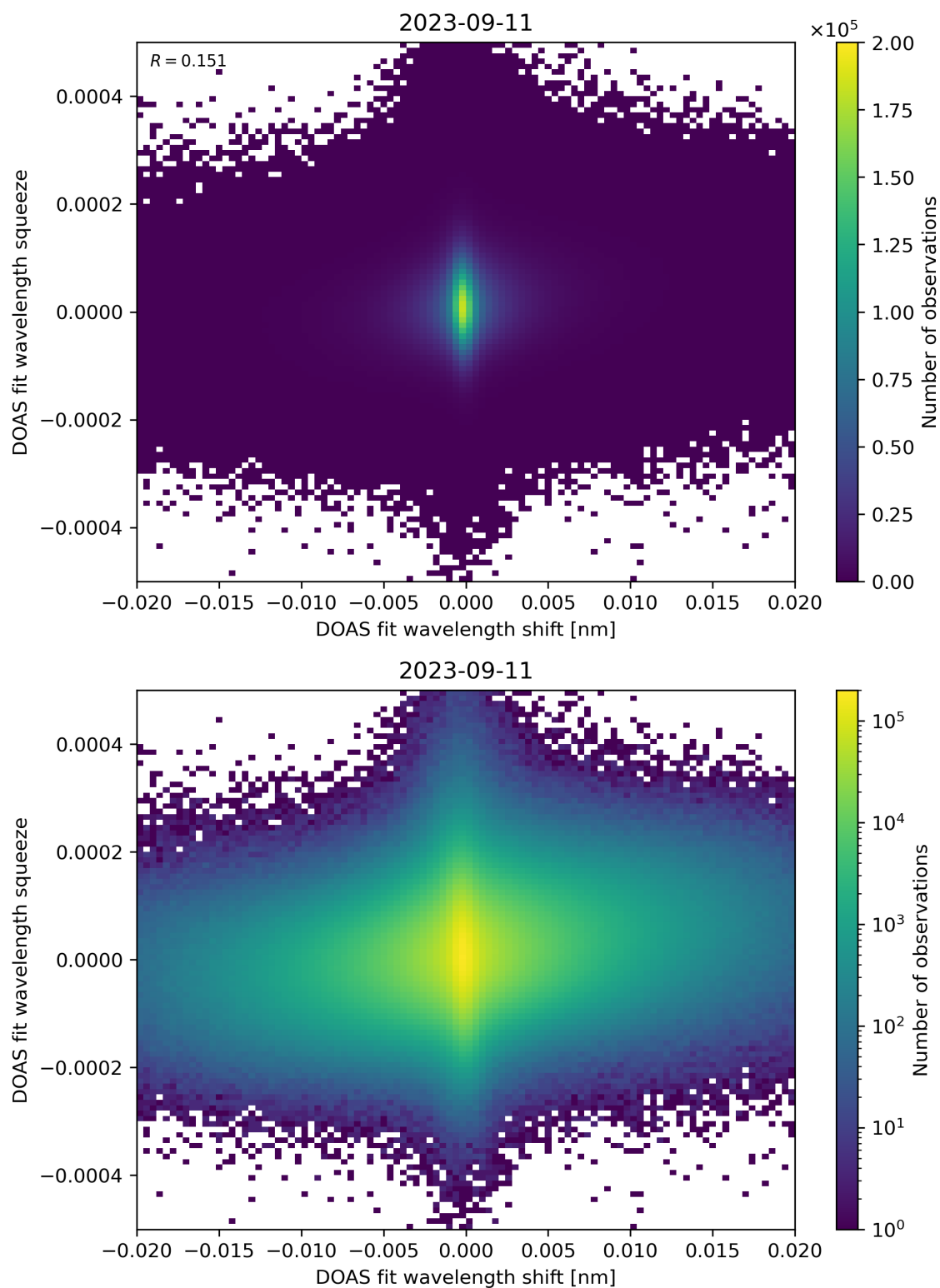
Figure 65: Scatter density plot of “DOAS fit wavelength shift” against “DOAS fit wavelength squeeze” for 2023-09-10 to 2023-09-12.
