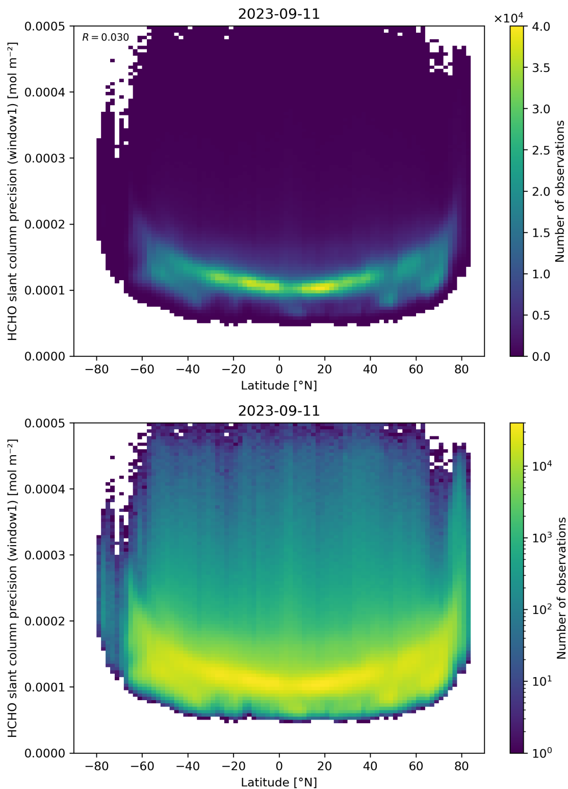
Figure 160: Scatter density plot of “Latitude” against “HCHO slant column precision (window1)” for 2023-09-10 to 2023-09-12.
