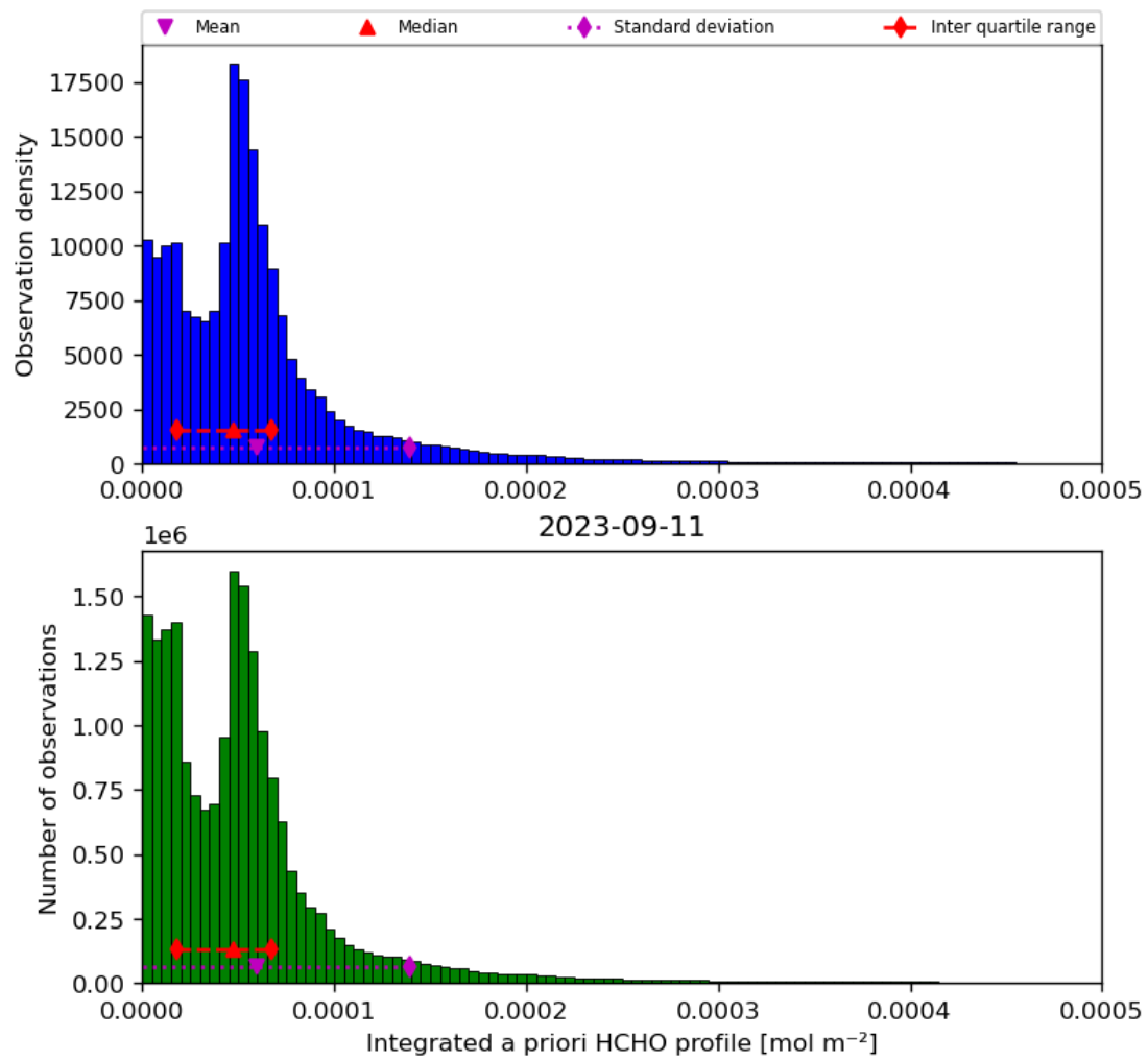
Figure 43: Histogram of “Integrated a priori HCHO profile” for 2023-09-10 to 2023-09-12
