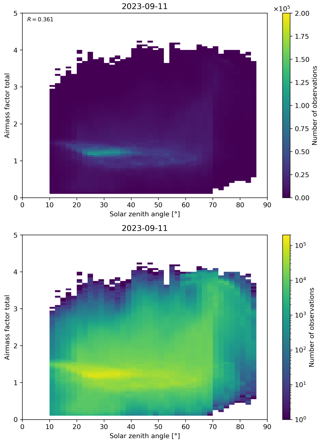
Figure 175: Scatter density plot of “Solar zenith angle” against “Airmass factor total” for 2023-09-10 to 2023-09-12.
