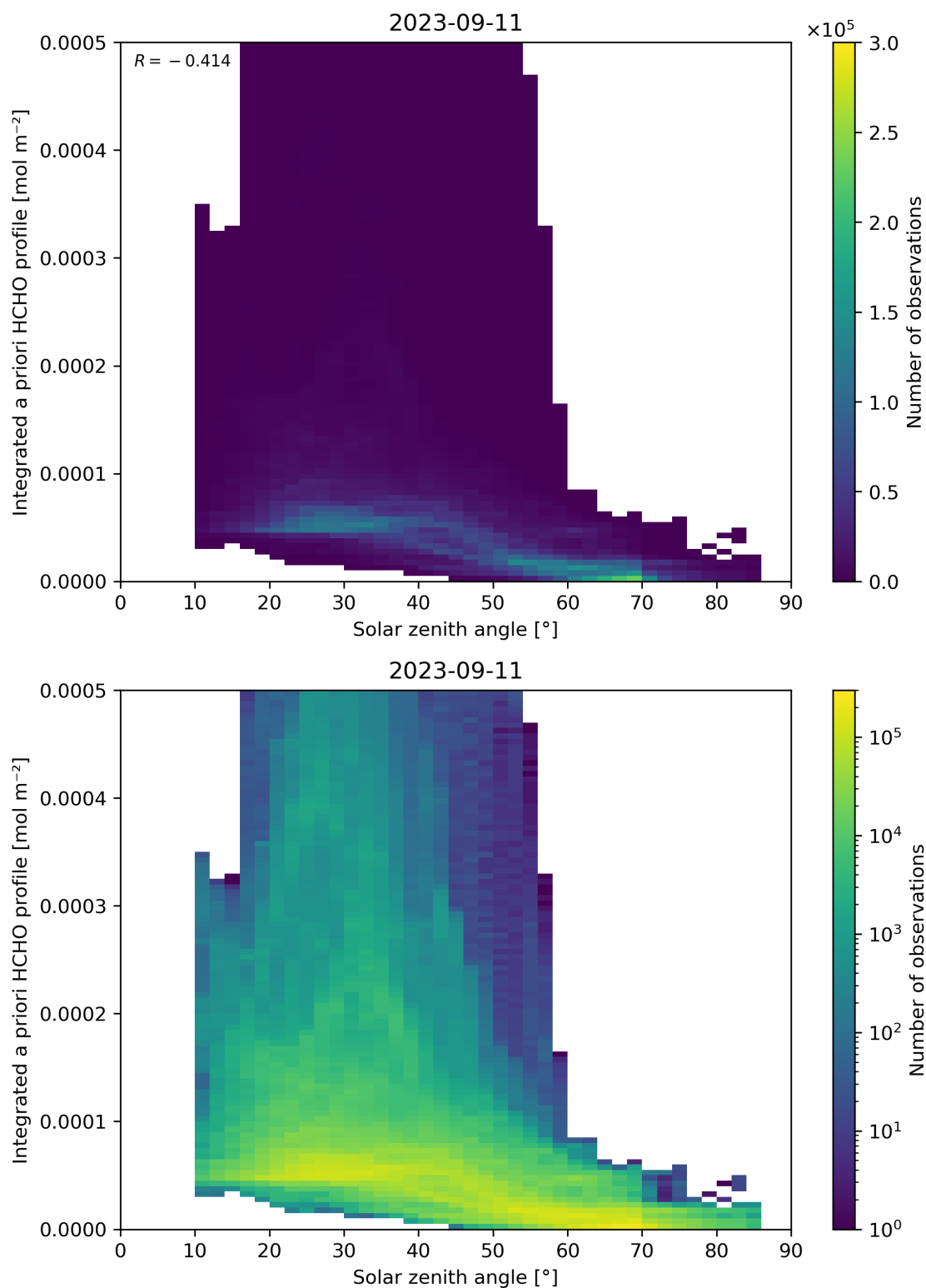
Figure 180: Scatter density plot of “Solar zenith angle” against “Integrated a priori HCHO profile” for 2023-09-10 to 2023-09-12.
