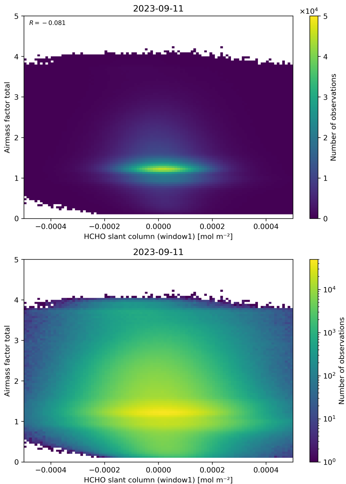
Figure 85: Scatter density plot of “HCHO slant column (window1)” against “Airmass factor total” for 2023-09-10 to 2023-09-12.
