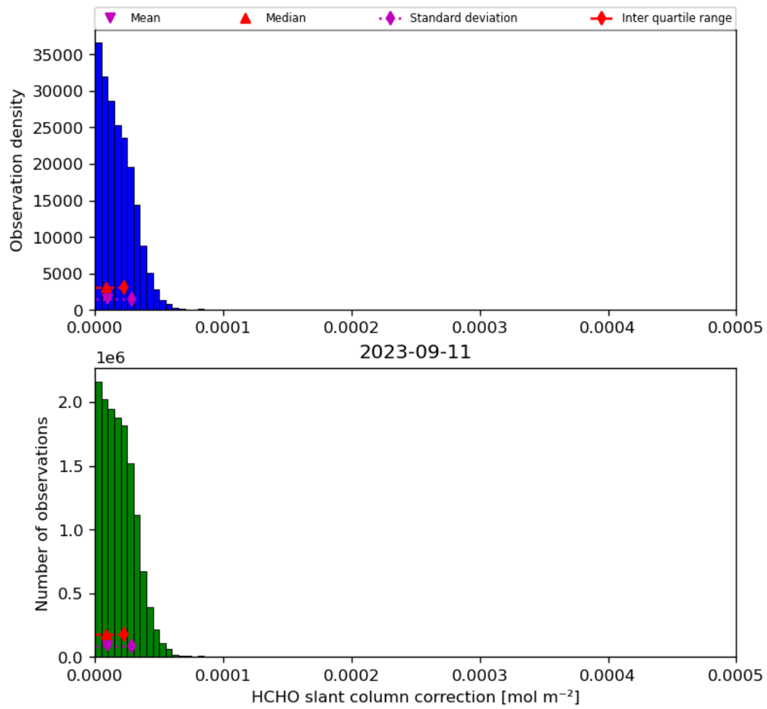
Figure 47: Histogram of “HCHO slant column correction” for 2023-09-10 to 2023-09-12
