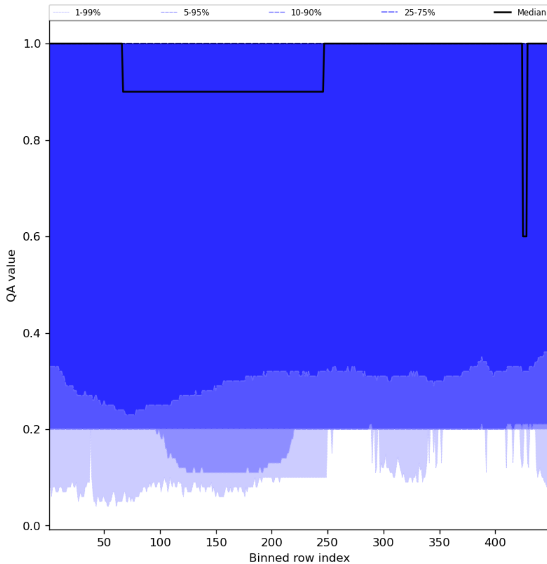
Figure 48: Along track statistics of “QA value” for 2023-09-10 to 2023-09-12
