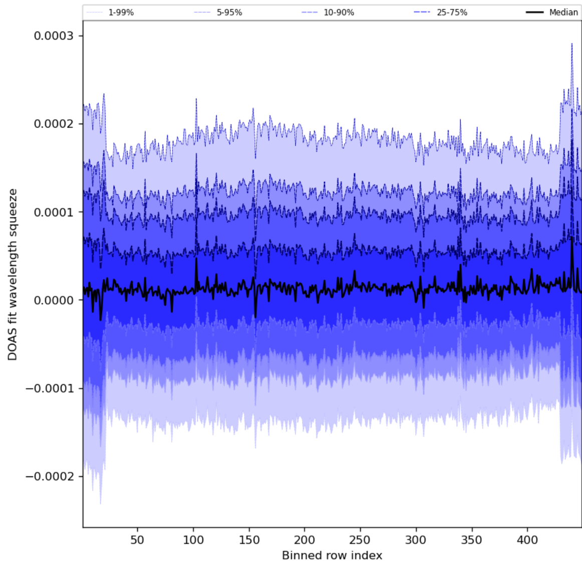
Figure 59: Along track statistics of “DOAS fit wavelength squeeze” for 2023-09-10 to 2023-09-12
