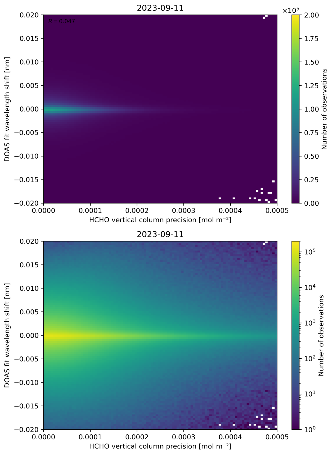
Figure 137: Scatter density plot of “HCHO vertical column precision” against “DOAS fit wavelength shift” for 2023-09-10 to 2023-09-12.
