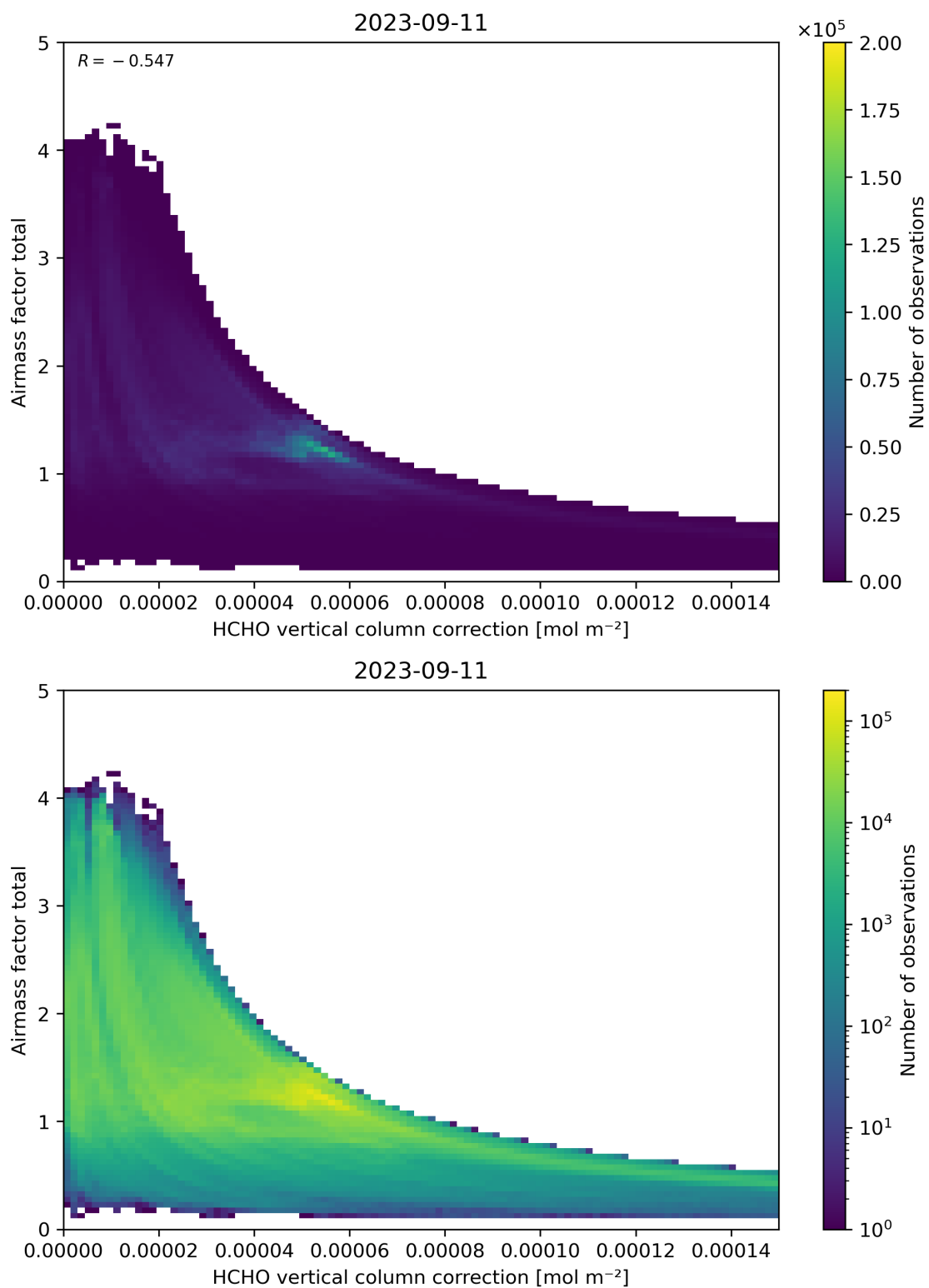
Figure 120: Scatter density plot of “HCHO vertical column correction” against “Airmass factor total” for 2023-09-10 to 2023-09-12.
