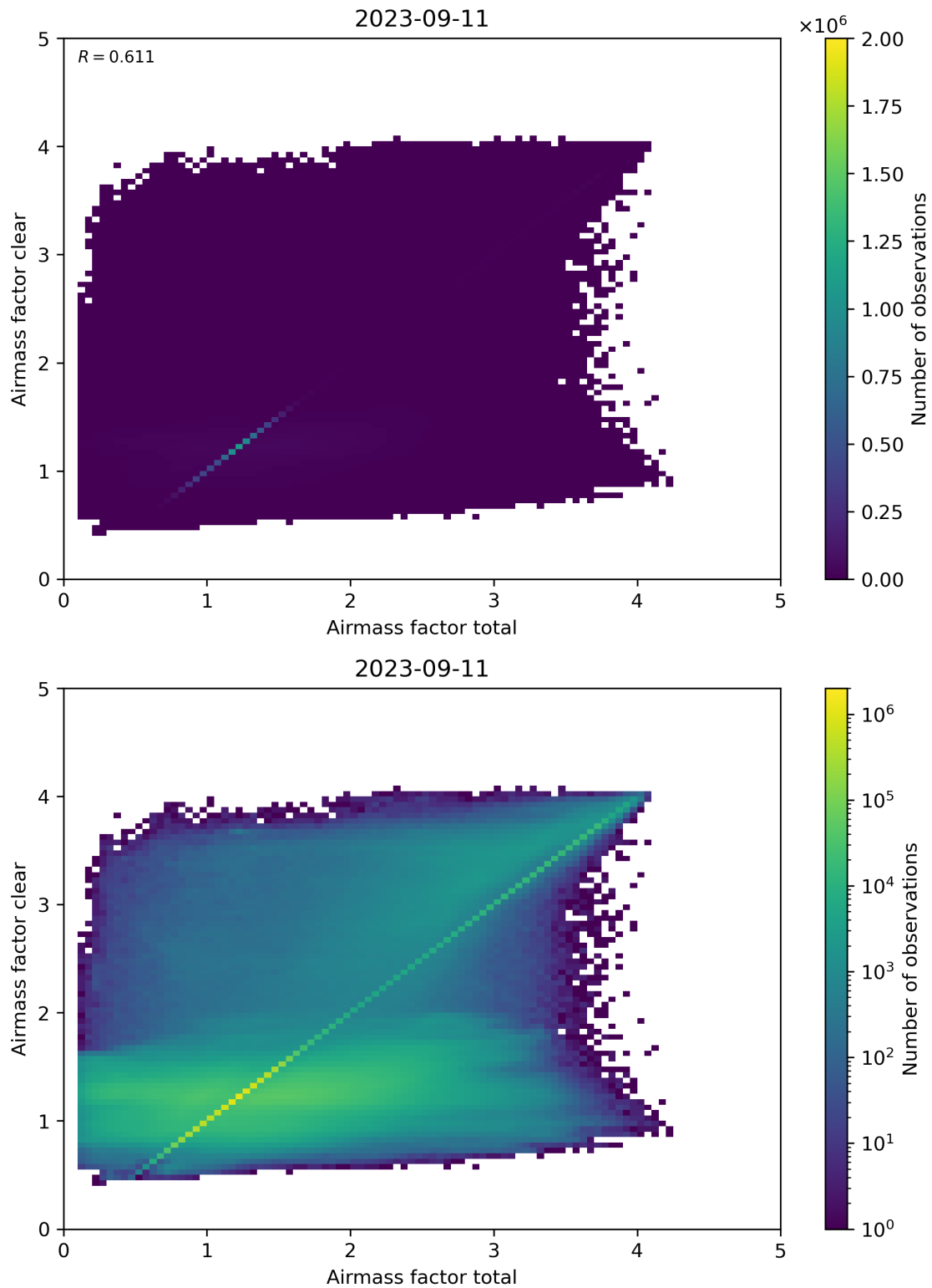
Figure 100: Scatter density plot of “Airmass factor total” against “Airmass factor clear” for 2023-09-10 to 2023-09-12.
