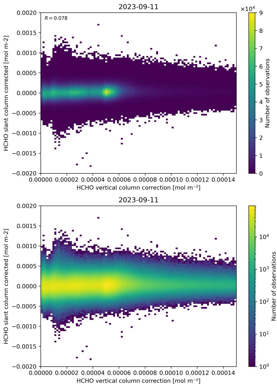
Figure 116: Scatter density plot of “HCHO vertical column correction” against “HCHO slant column corrected” for 2023-09-10 to 2023-09-12.
