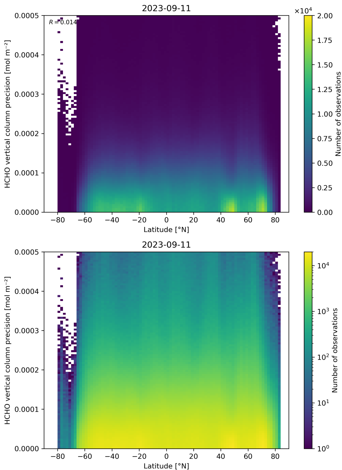
Figure 165: Scatter density plot of “Latitude” against “HCHO vertical column precision” for 2023-09-10 to 2023-09-12.
