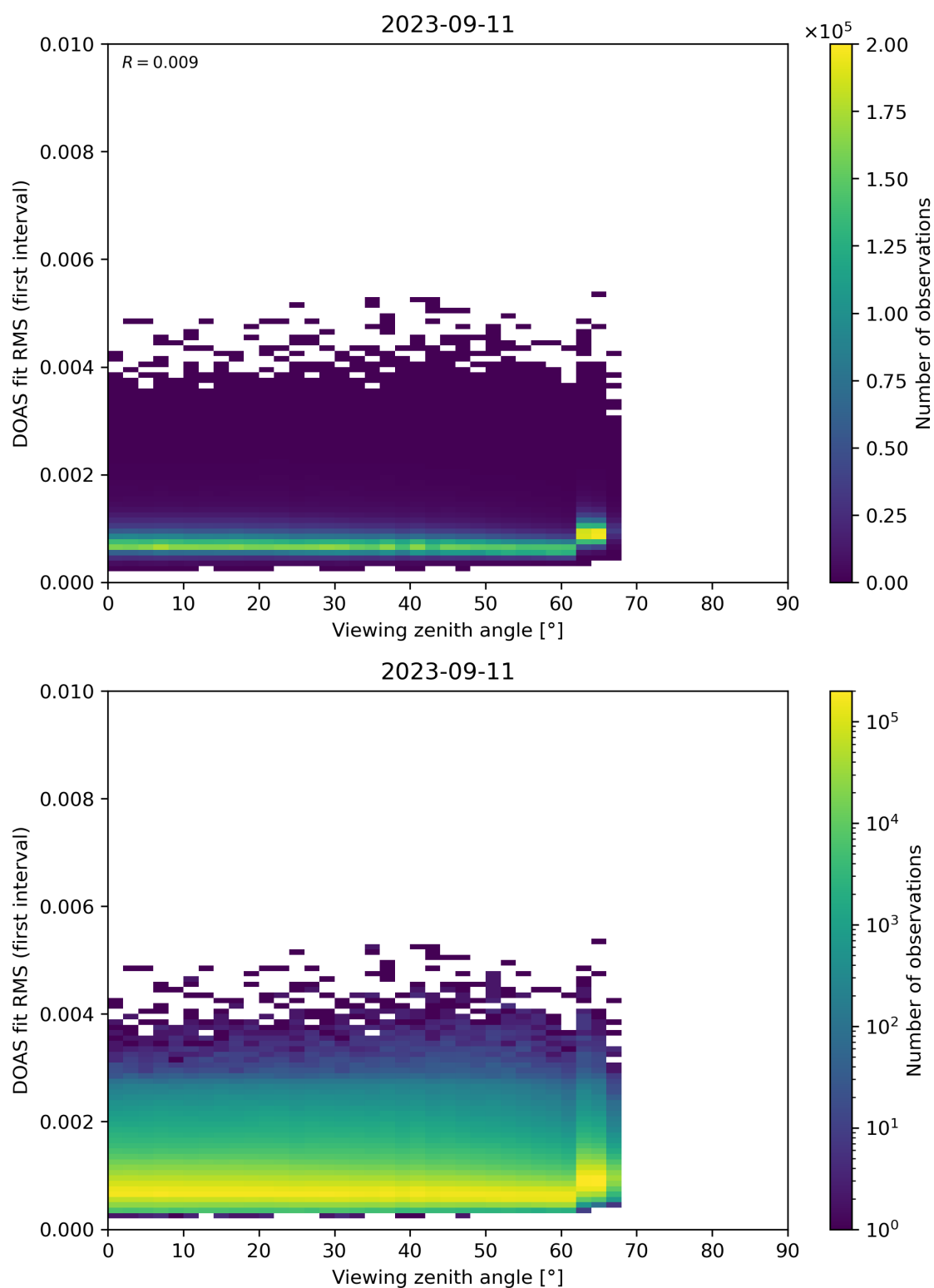
Figure 182: Scatter density plot of “Viewing zenith angle” against “DOAS fit RMS (first interval)” for 2023-09-10 to 2023-09-12.
