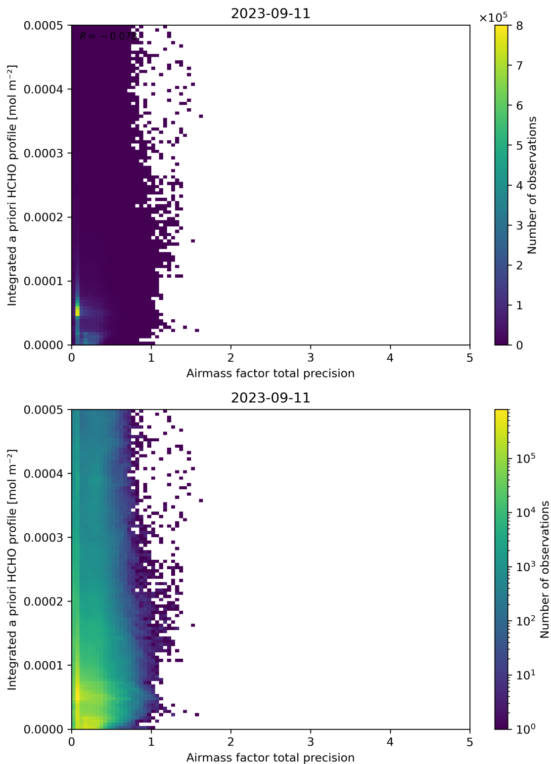
Figure 111: Scatter density plot of “Airmass factor total precision” against “Integrated a priori HCHO profile” for 2023-09-10 to 2023-09-12.
