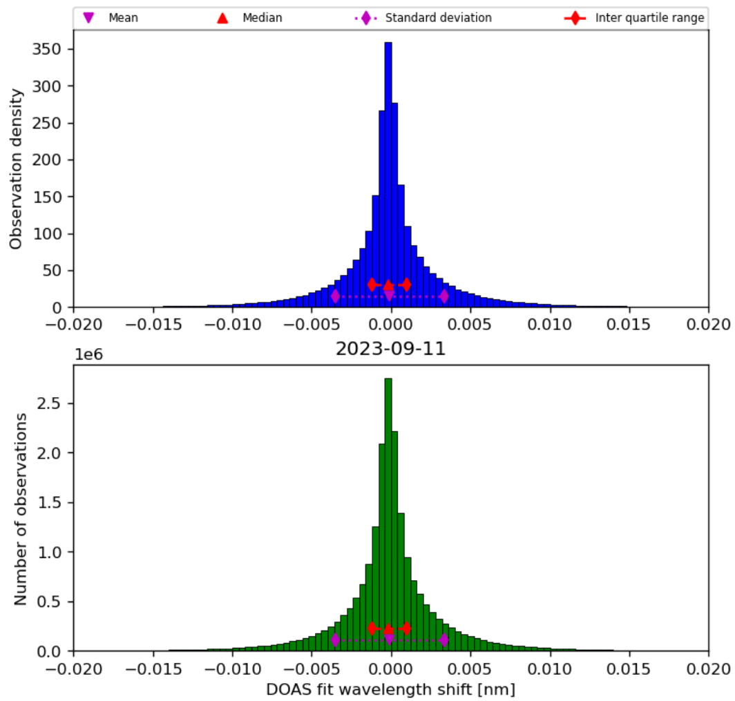
Figure 44: Histogram of “DOAS fit wavelength shift” for 2023-09-10 to 2023-09-12
