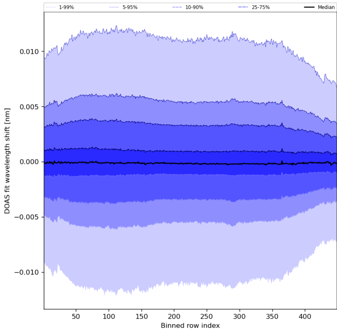
Figure 58: Along track statistics of “DOAS fit wavelength shift” for 2023-09-10 to 2023-09-12
