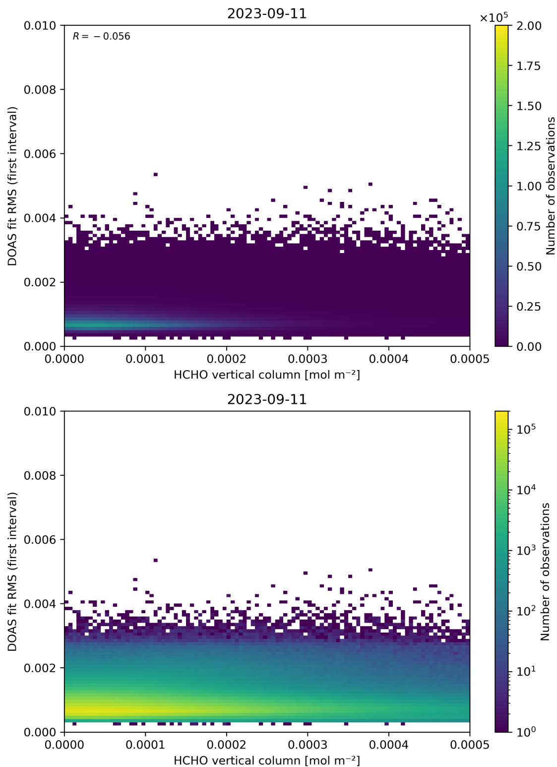
Figure 123: Scatter density plot of “HCHO vertical column” against “DOAS fit RMS (first interval)” for 2023-09-10 to 2023-09-12.
