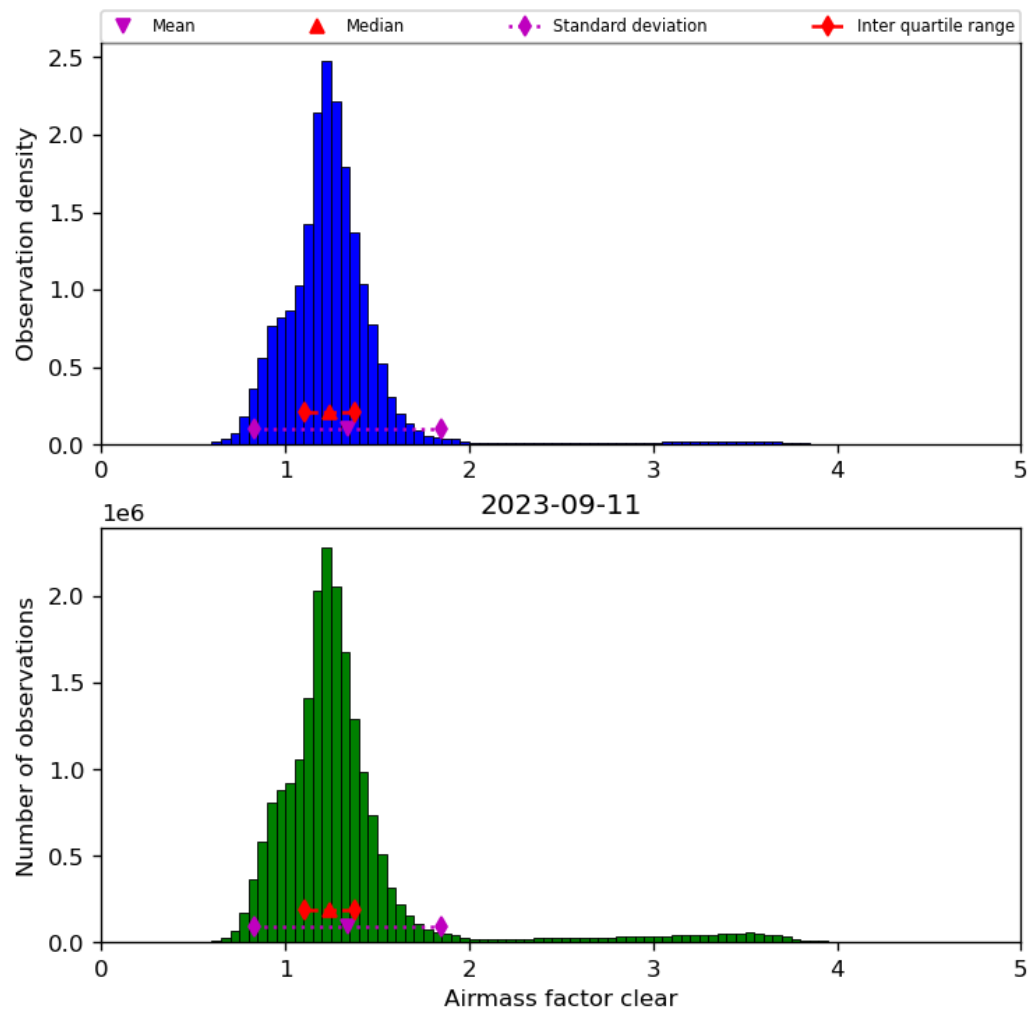
Figure 42: Histogram of “Airmass factor clear” for 2023-09-10 to 2023-09-12
