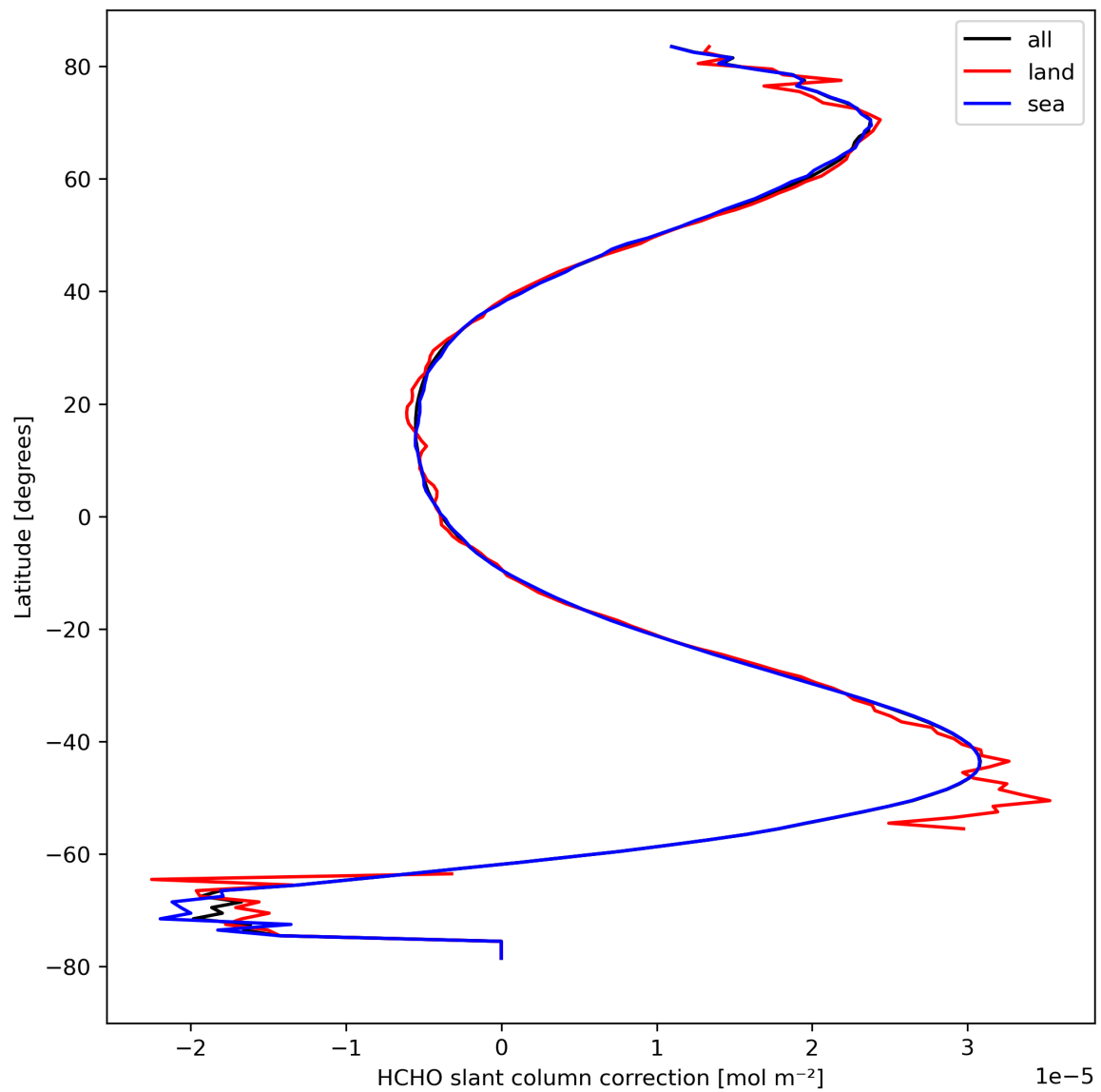
Figure 33: Zonal average of “HCHO slant column correction” for 2023-09-10 to 2023-09-12.
