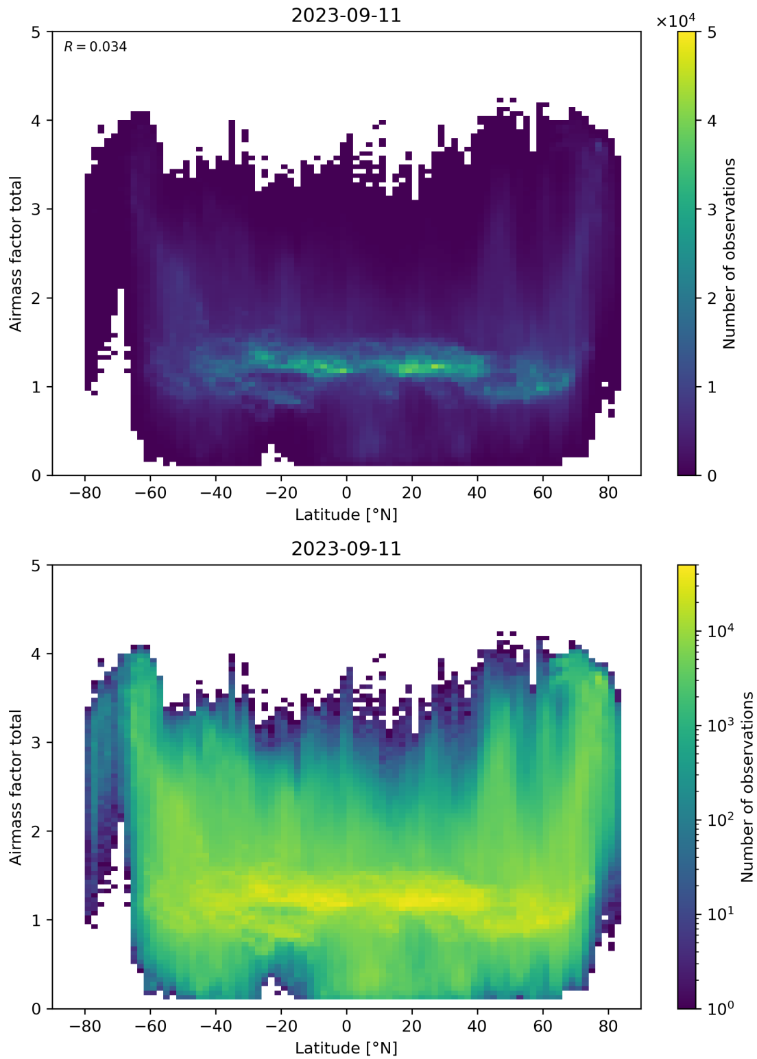
Figure 161: Scatter density plot of “Latitude” against “Airmass factor total” for 2023-09-10 to 2023-09-12.
