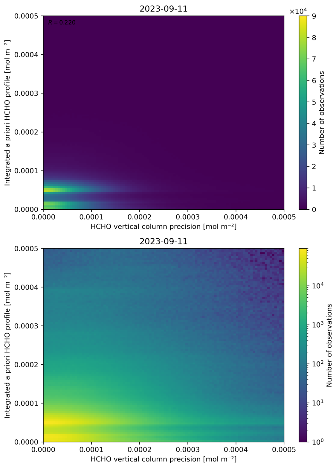
Figure 147: Scatter density plot of “HCHO vertical column precision” against “Integrated a priori HCHO profile” for 2023-09-10 to 2023-09-12.
