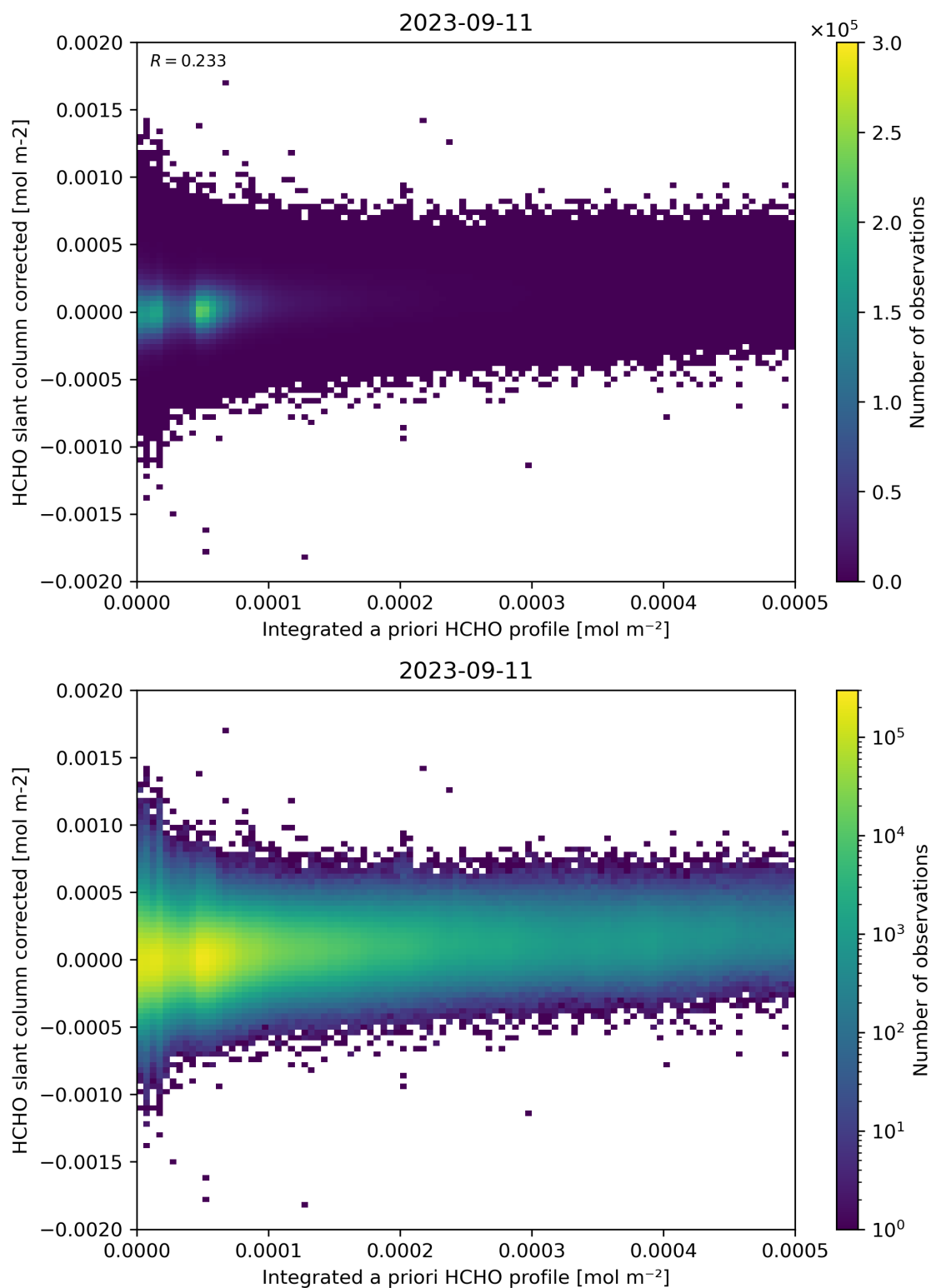
Figure 151: Scatter density plot of “Integrated a priori HCHO profile” against “HCHO slant column corrected” for 2023-09-10 to 2023-09-12.
