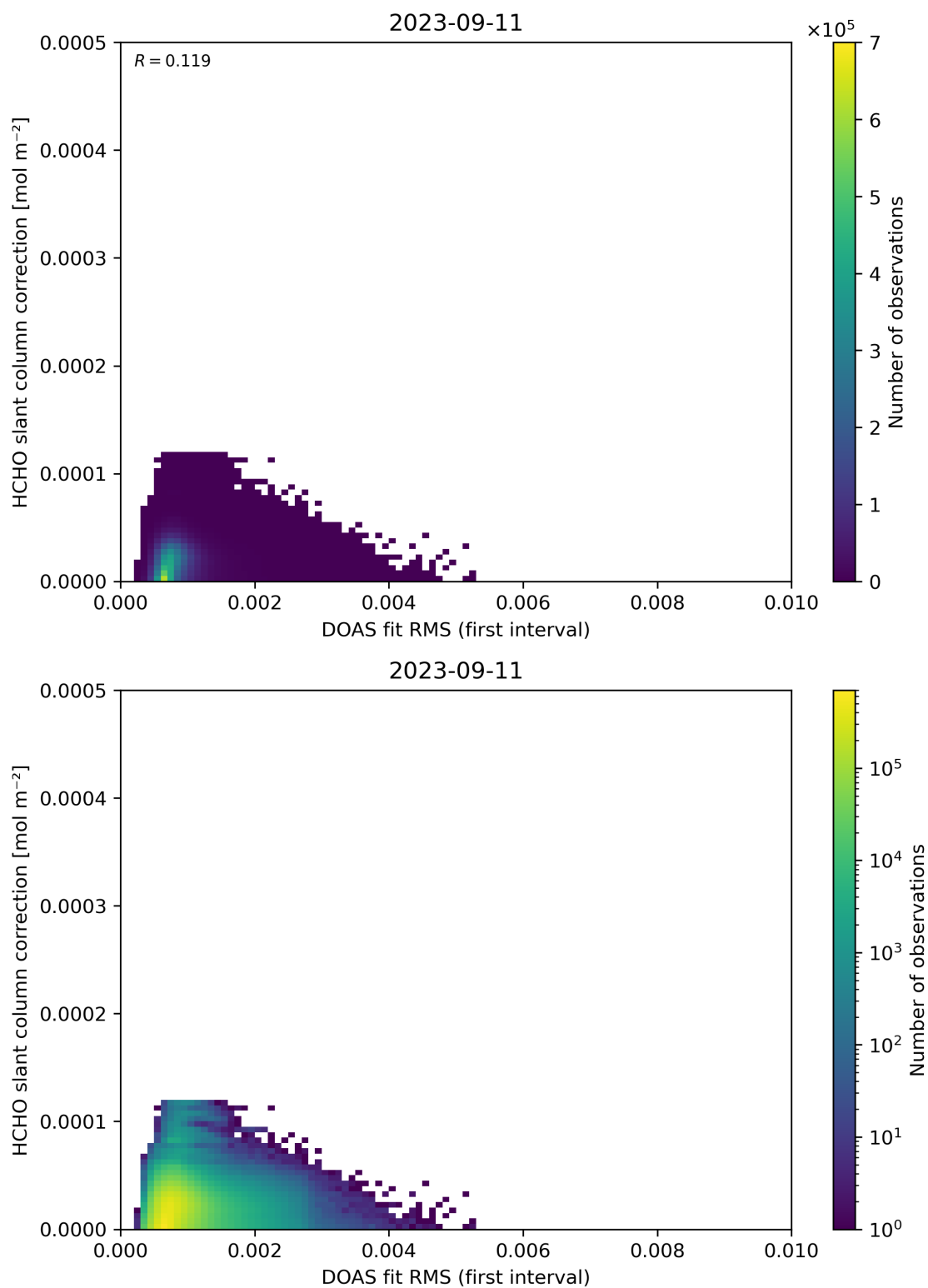
Figure 63: Scatter density plot of “DOAS fit RMS (first interval)” against “HCHO slant column correction” for 2023-09-10 to 2023-09-12.
