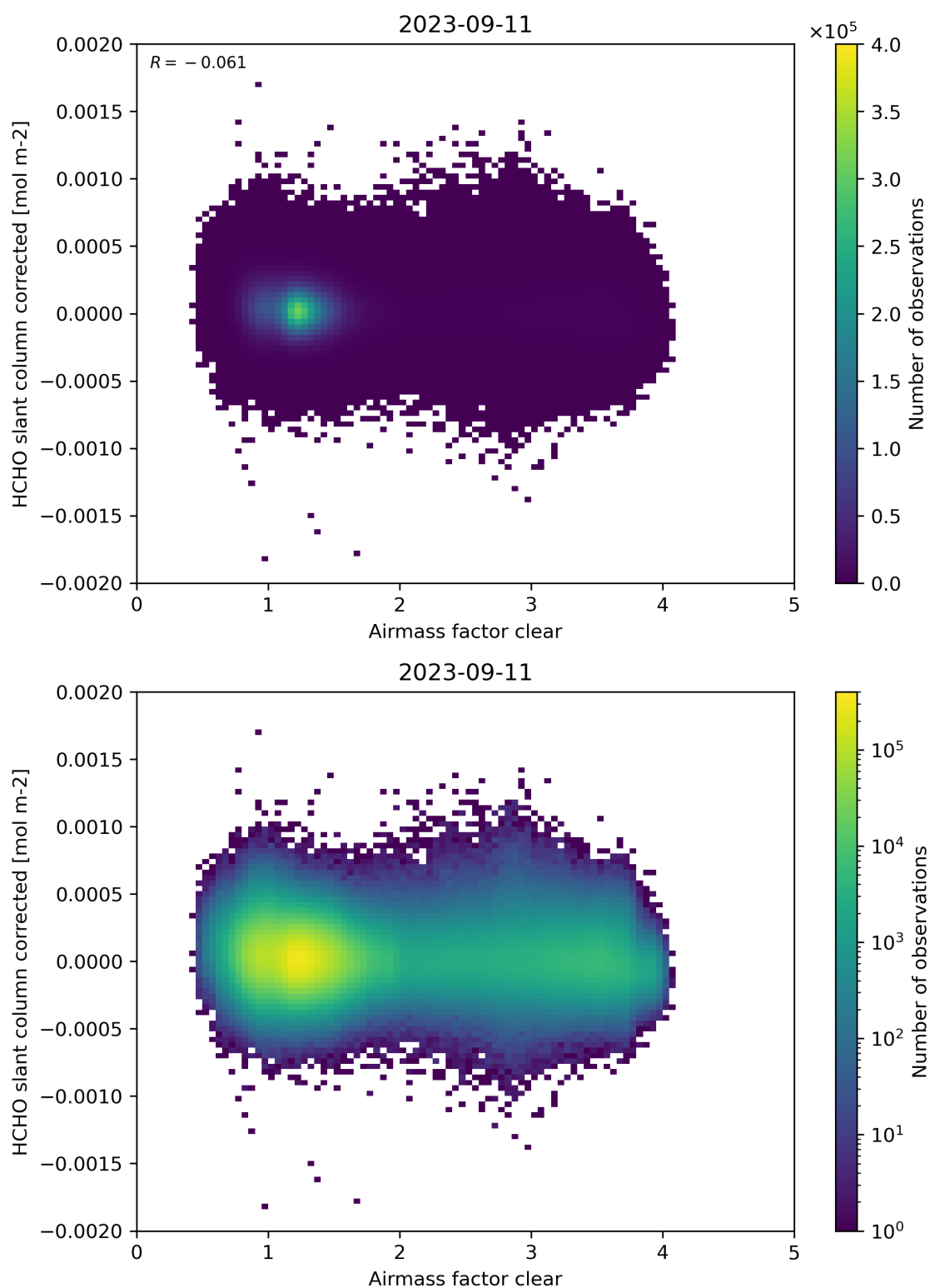
Figure 74: Scatter density plot of “Airmass factor clear” against “HCHO slant column corrected” for 2023-09-10 to 2023-09-12.
