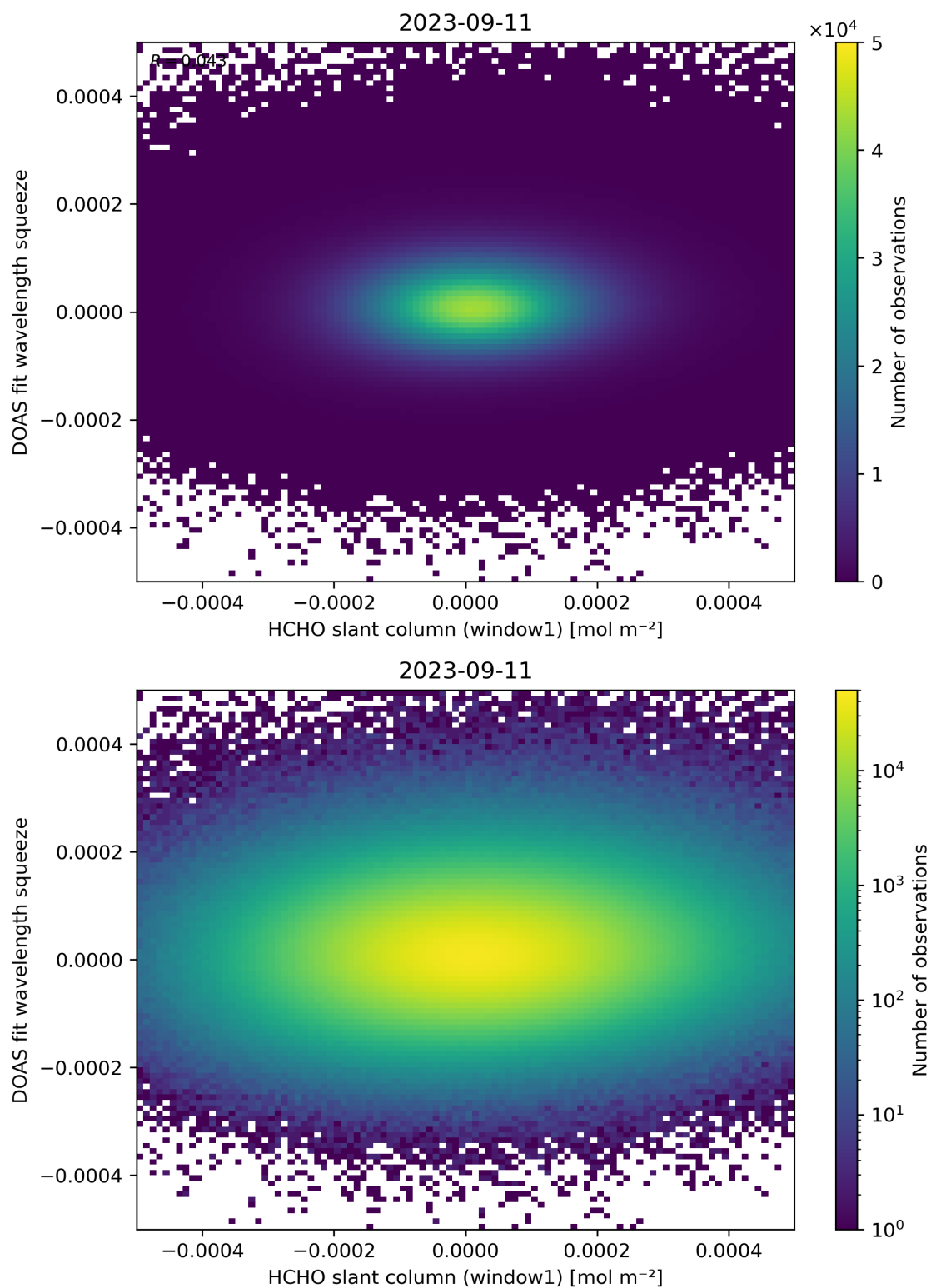
Figure 80: Scatter density plot of “HCHO slant column (window1)” against “DOAS fit wavelength squeeze” for 2023-09-10 to 2023-09-12.
