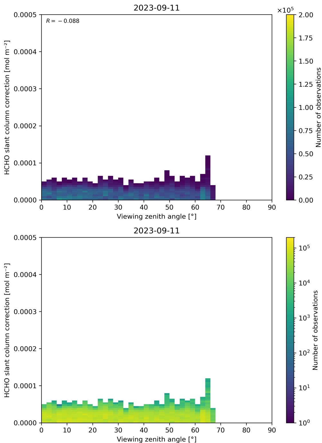
Figure 187: Scatter density plot of “Viewing zenith angle” against “HCHO slant column correction” for 2023-09-10 to 2023-09-12.
