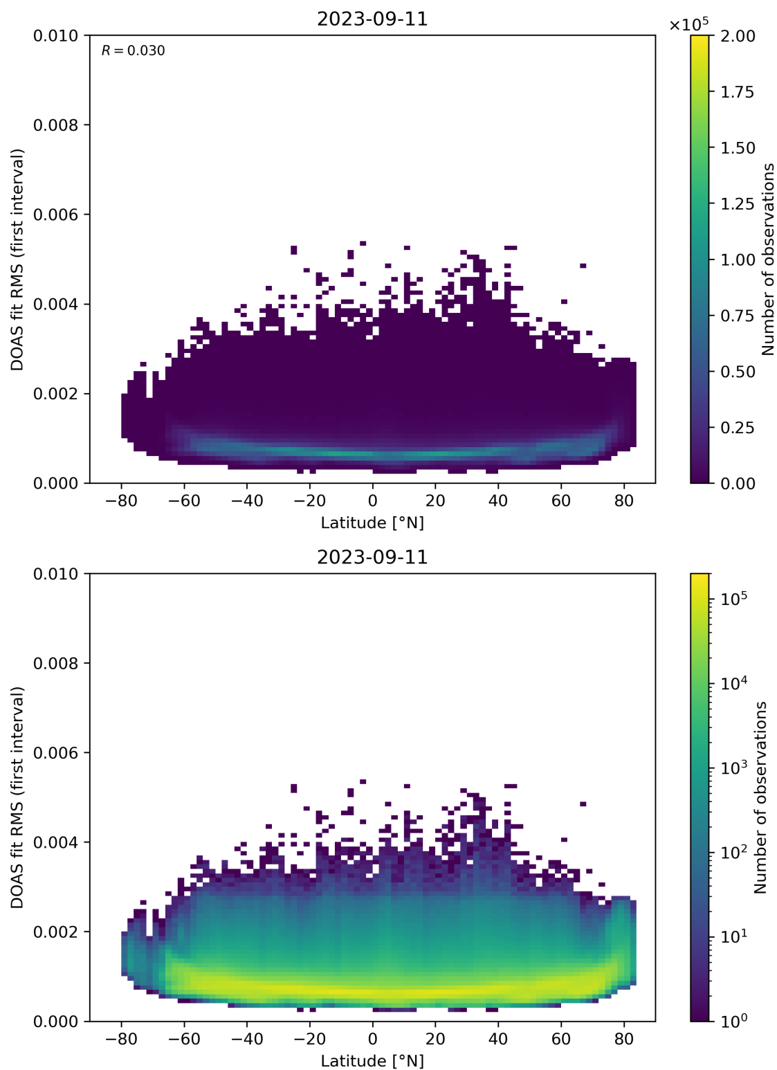
Figure 153: Scatter density plot of “Latitude” against “DOAS fit RMS (first interval)” for 2023-09-10 to 2023-09-12.
