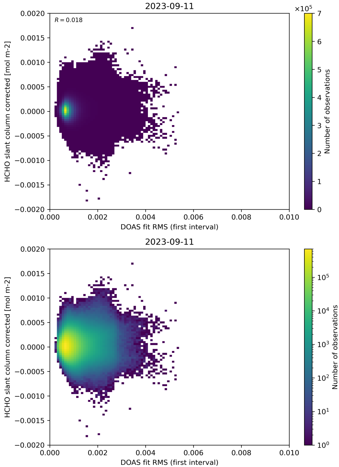
Figure 62: Scatter density plot of “DOAS fit RMS (first interval)” against “HCHO slant column corrected” for 2023-09-10 to 2023-09-12.
