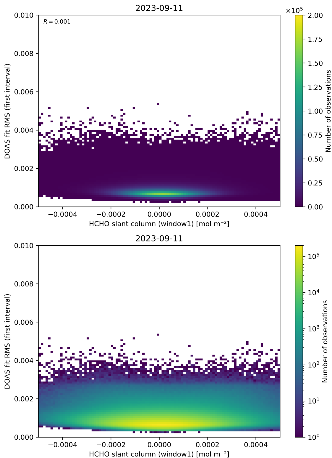
Figure 78: Scatter density plot of “HCHO slant column (window1)” against “DOAS fit RMS (first interval)” for 2023-09-10 to 2023-09-12.
