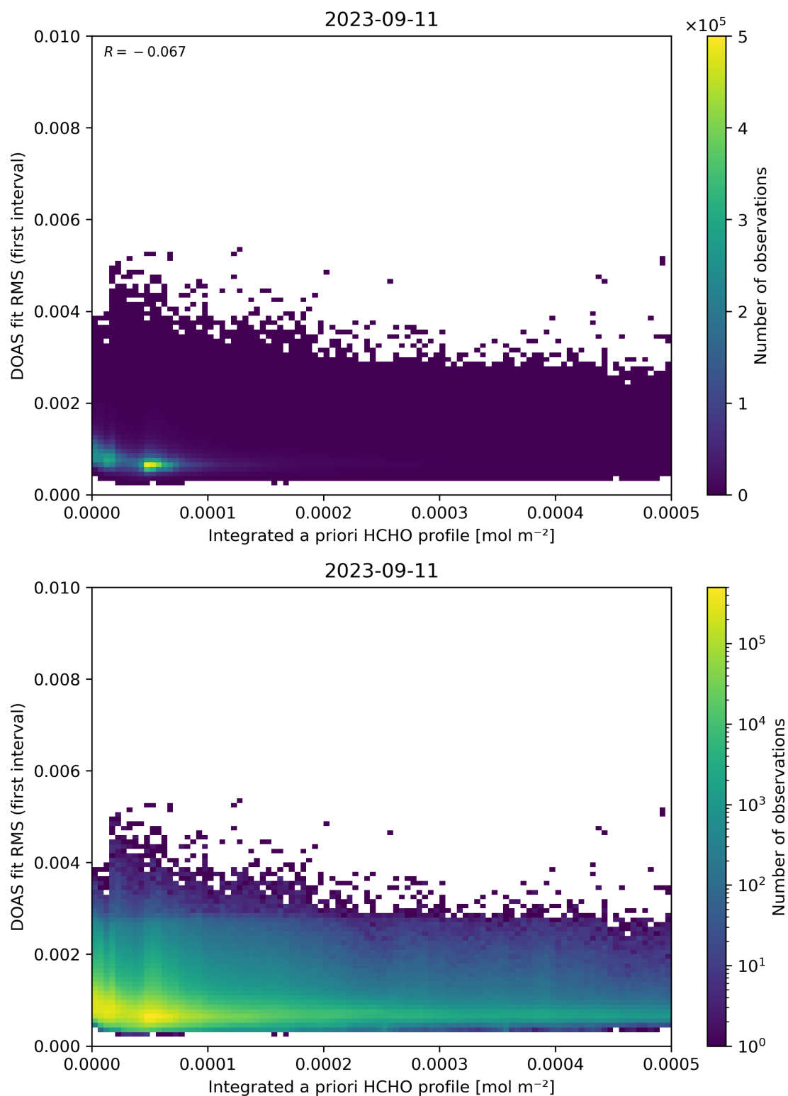
Figure 148: Scatter density plot of “Integrated a priori HCHO profile” against “DOAS fit RMS (first interval)” for 2023-09-10 to 2023-09-12.
