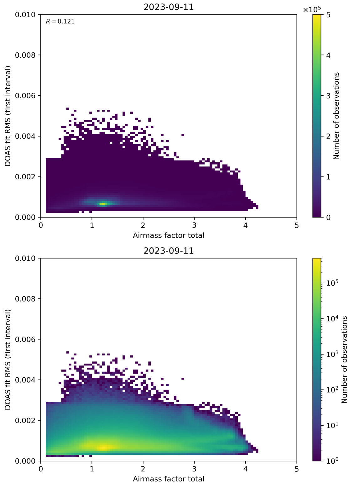
Figure 97: Scatter density plot of “Airmass factor total” against “DOAS fit RMS (first interval)” for 2023-09-10 to 2023-09-12.
