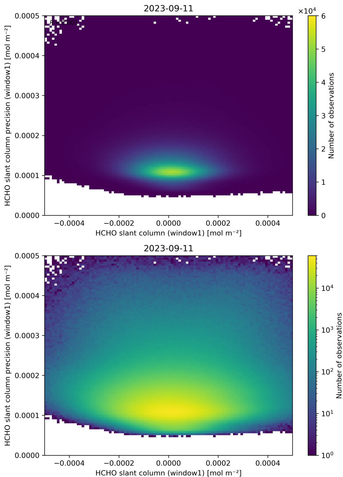
Figure 84: Scatter density plot of “HCHO slant column (window1)” against “HCHO slant column precision (window1)” for 2023-09-10 to 2023-09-12.
