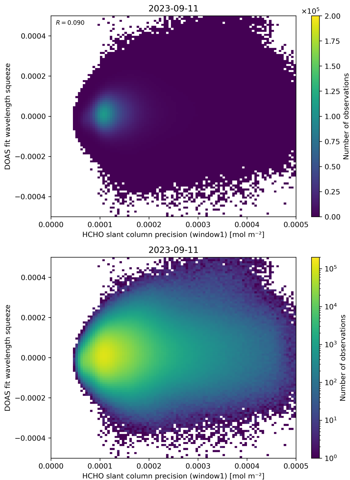
Figure 90: Scatter density plot of “HCHO slant column precision (window1)” against “DOAS fit wavelength squeeze” for 2023-09-10 to 2023-09-12.
