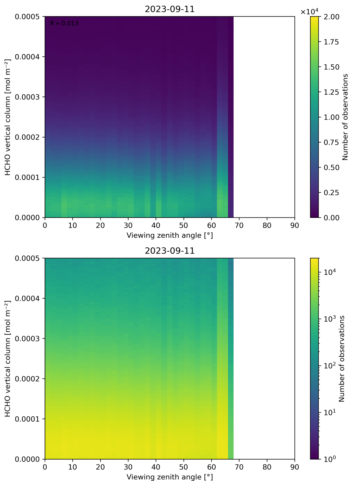
Figure 192: Scatter density plot of “Viewing zenith angle” against “HCHO vertical column” for 2023-09-10 to 2023-09-12.
