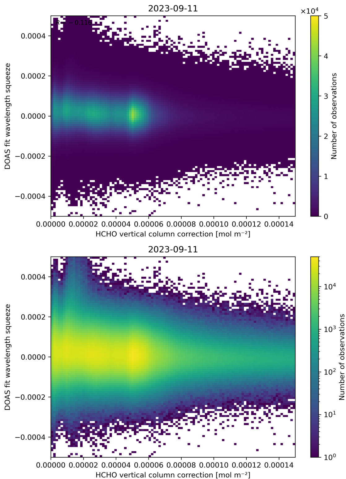
Figure 114: Scatter density plot of “HCHO vertical column correction” against “DOAS fit wavelength squeeze” for 2023-09-10 to 2023-09-12.
