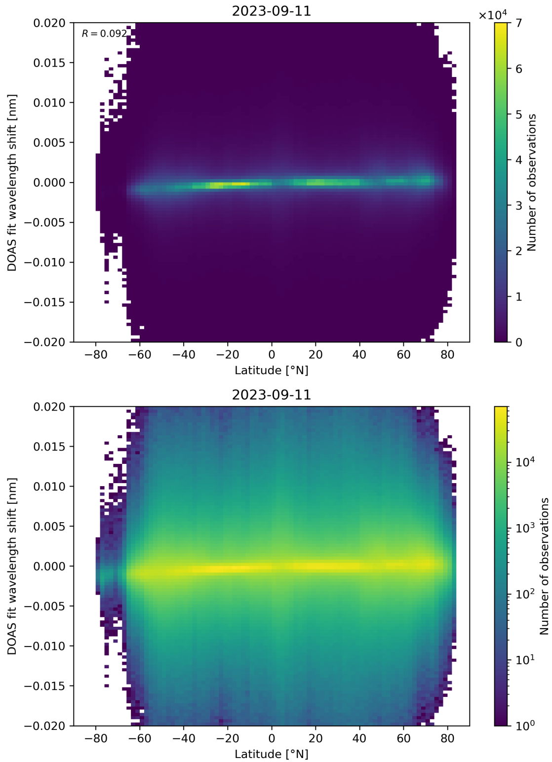
Figure 154: Scatter density plot of “Latitude” against “DOAS fit wavelength shift” for 2023-09-10 to 2023-09-12.
