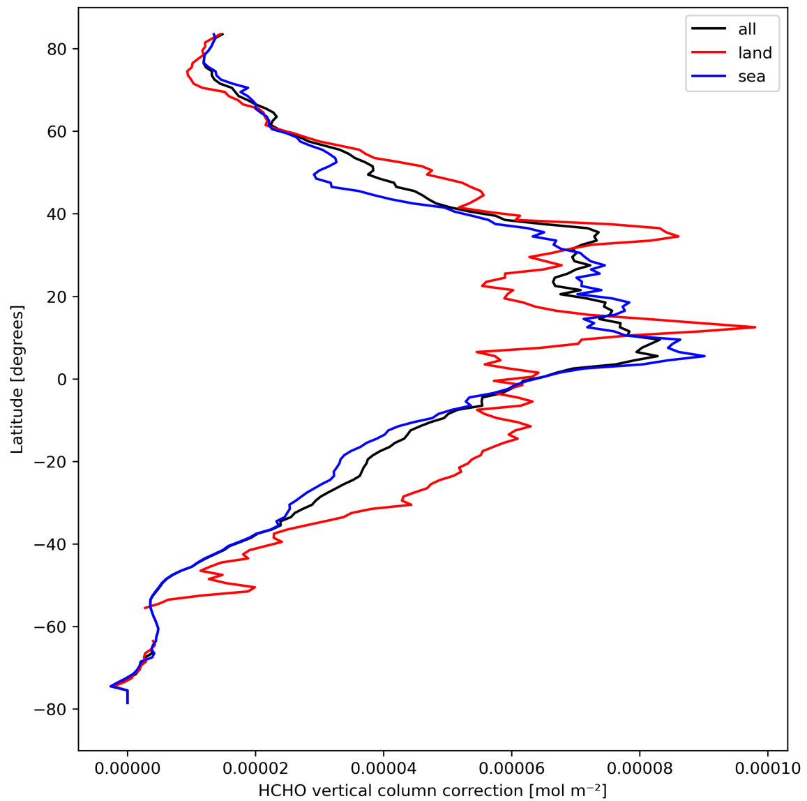
Figure 23: Zonal average of “HCHO vertical column correction” for 2023-09-10 to 2023-09-12.
