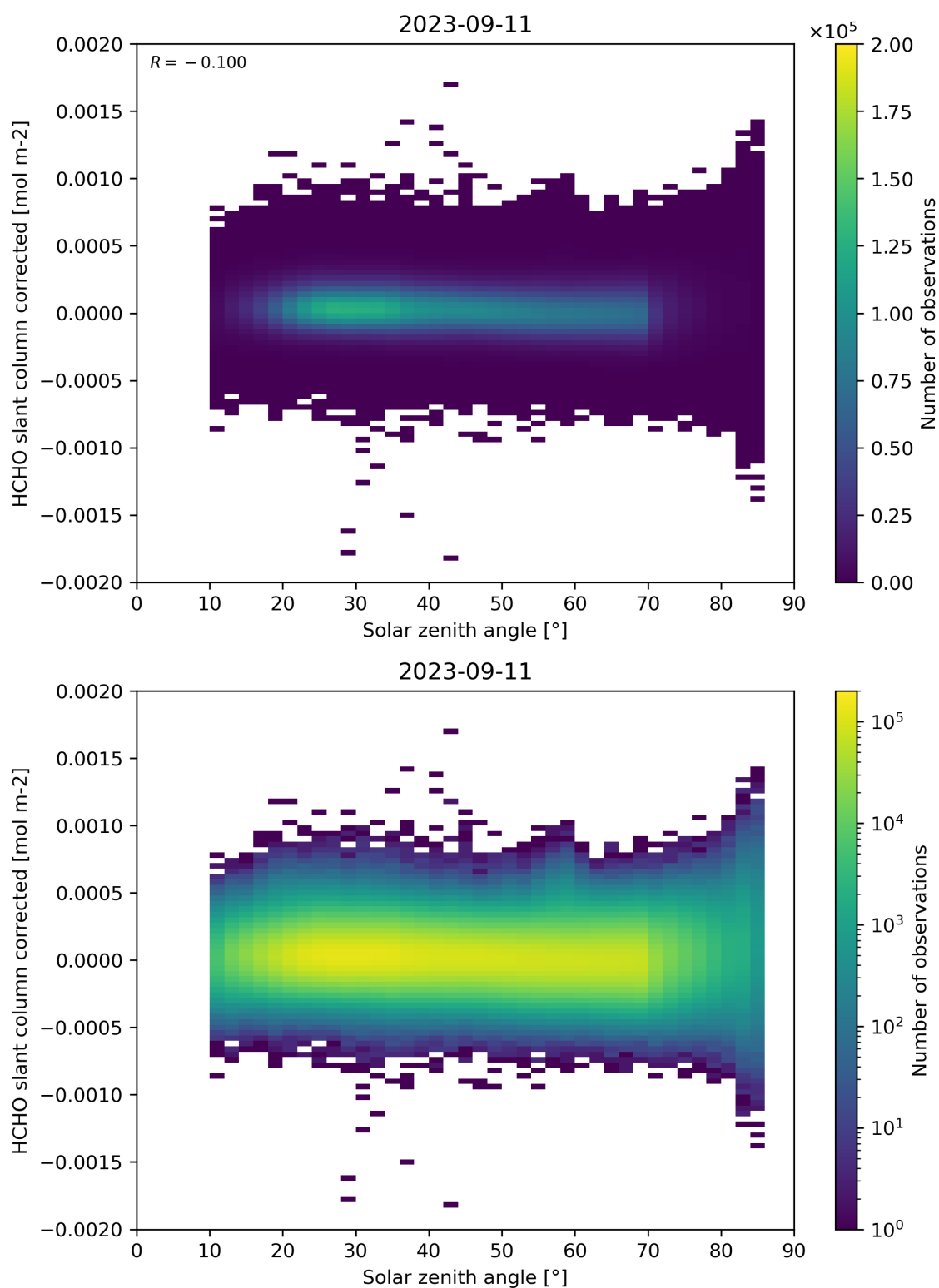
Figure 171: Scatter density plot of “Solar zenith angle” against “HCHO slant column corrected” for 2023-09-10 to 2023-09-12.
