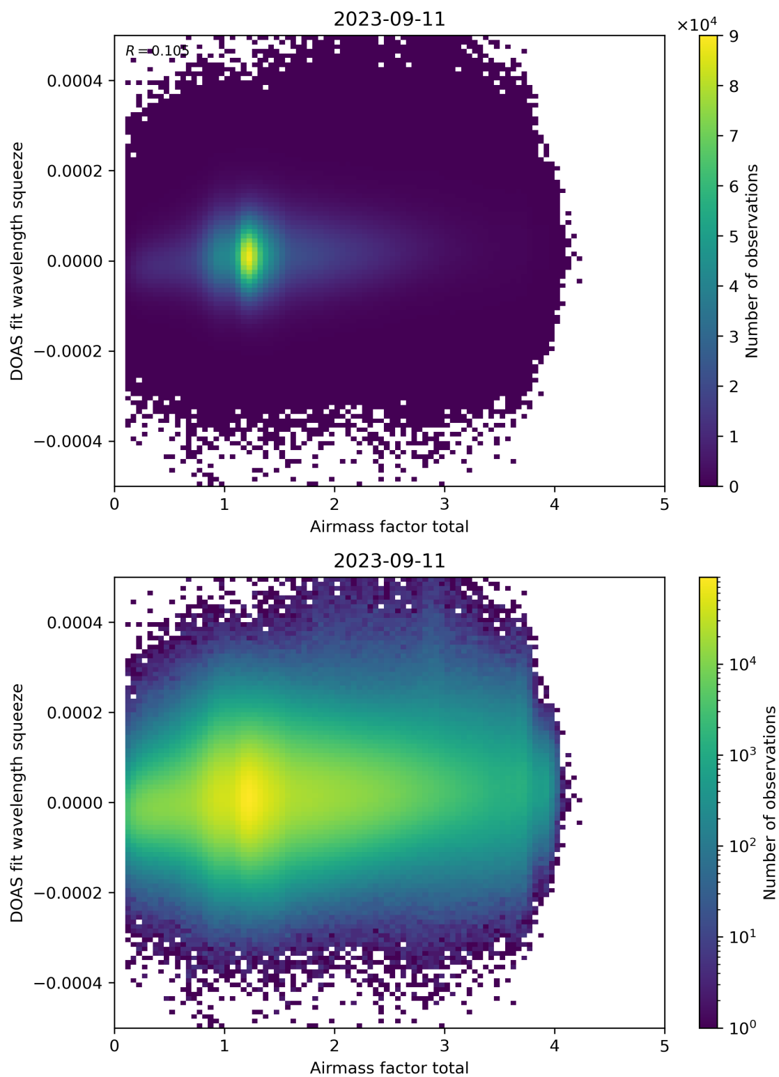
Figure 99: Scatter density plot of “Airmass factor total” against “DOAS fit wavelength squeeze” for 2023-09-10 to 2023-09-12.
