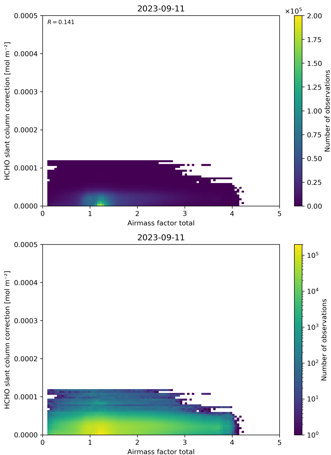
Figure 102: Scatter density plot of “Airmass factor total” against “HCHO slant column correction” for 2023-09-10 to 2023-09-12.
