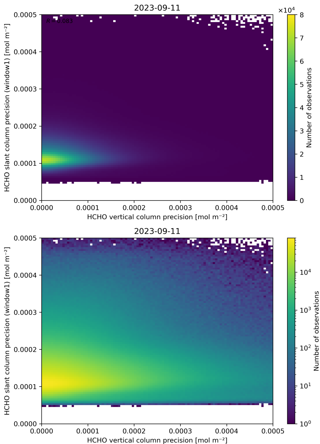
Figure 143: Scatter density plot of “HCHO vertical column precision” against “HCHO slant column precision (window1)” for 2023-09-10 to 2023-09-12.
