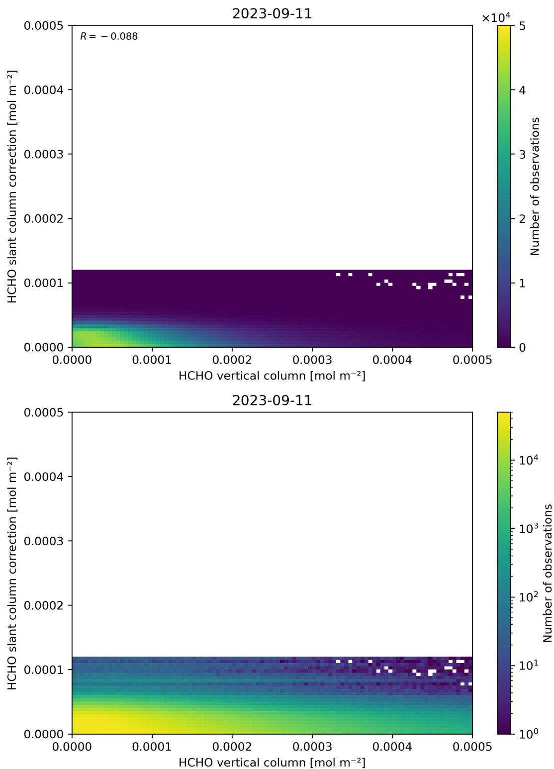
Figure 128: Scatter density plot of “HCHO vertical column” against “HCHO slant column correction” for 2023-09-10 to 2023-09-12.
