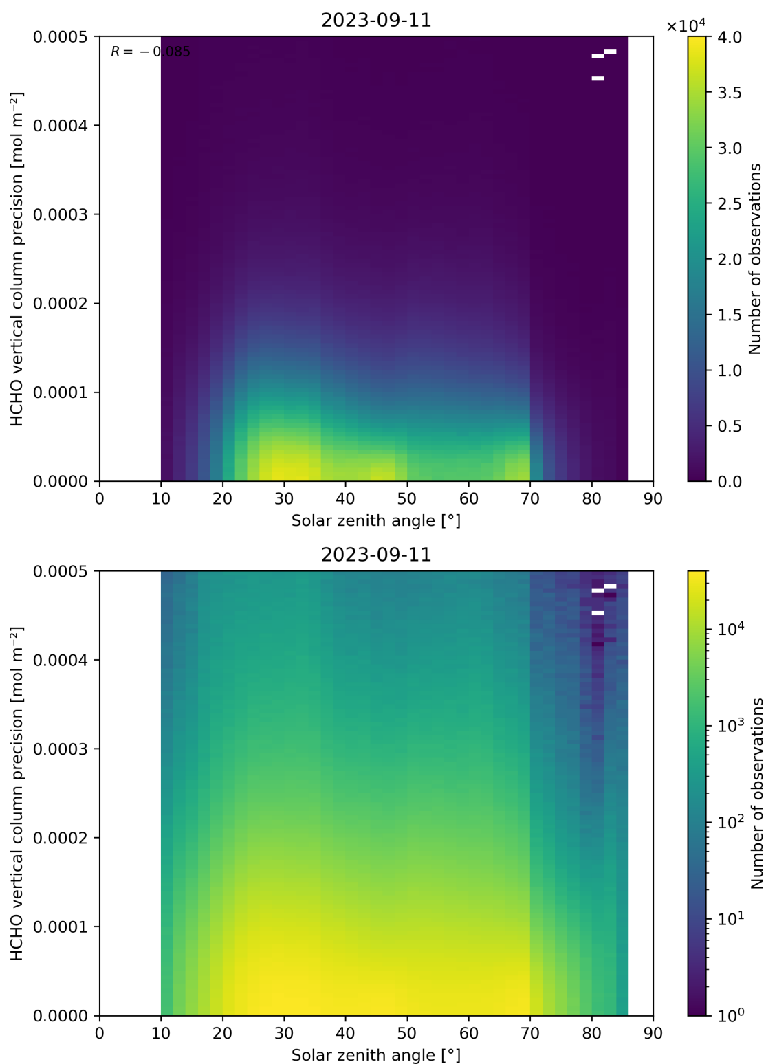
Figure 179: Scatter density plot of “Solar zenith angle” against “HCHO vertical column precision” for 2023-09-10 to 2023-09-12.
