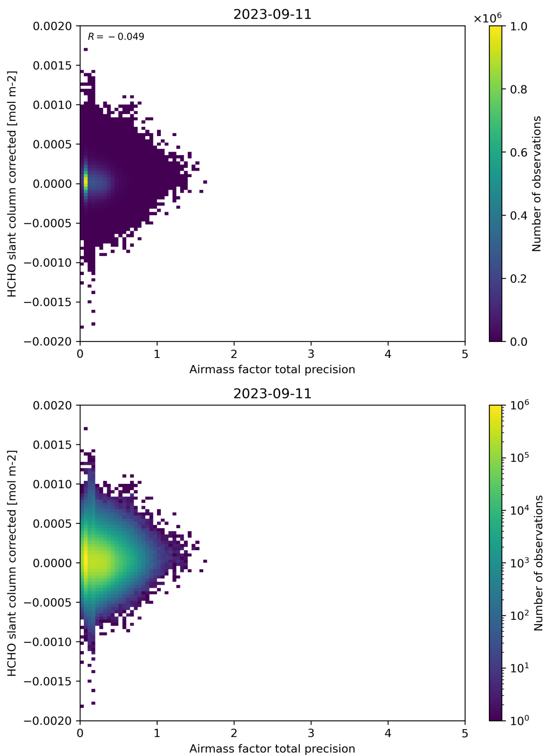
Figure 109: Scatter density plot of “Airmass factor total precision” against “HCHO slant column corrected” for 2023-09-10 to 2023-09-12.
