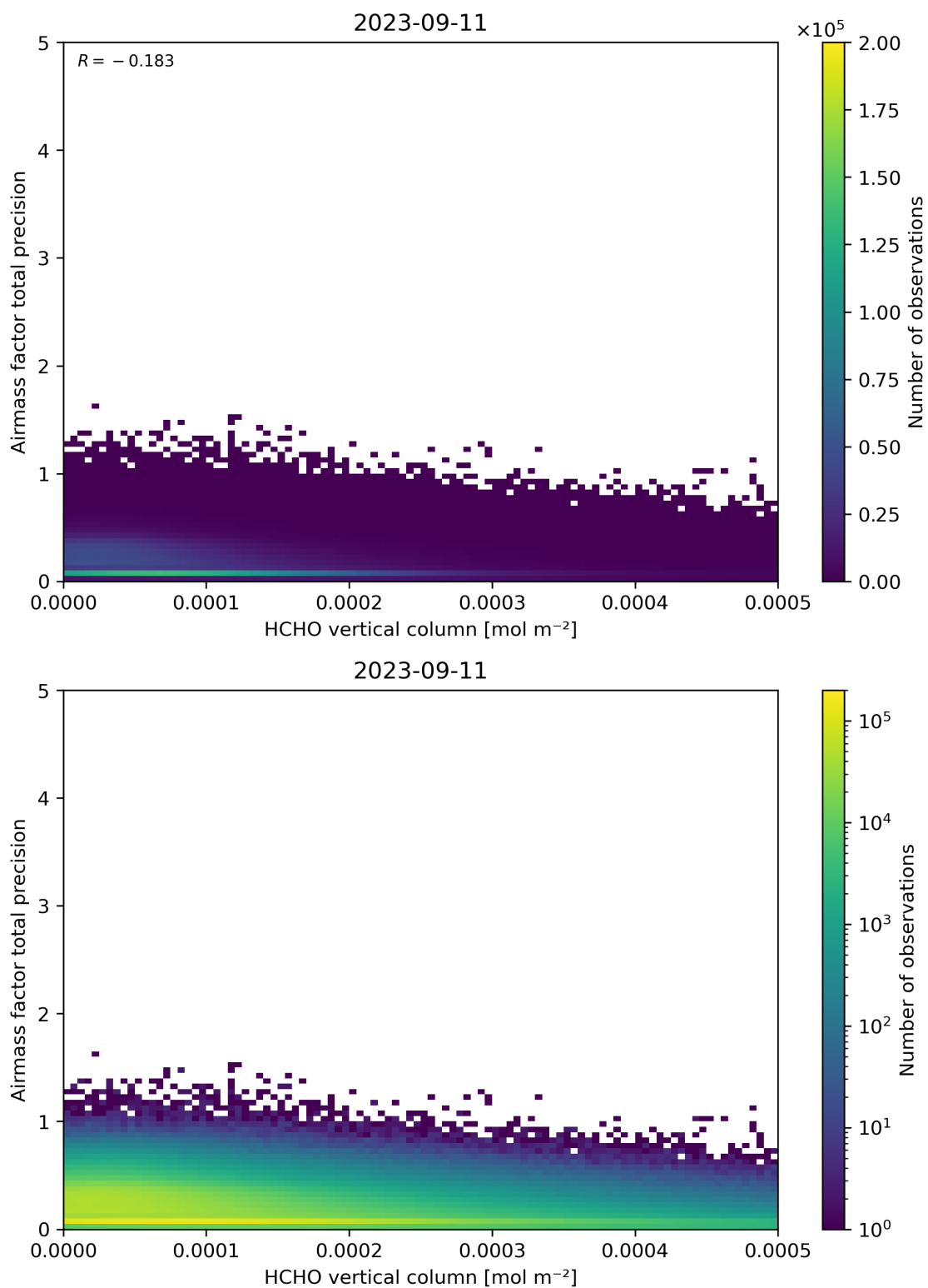
Figure 132: Scatter density plot of “HCHO vertical column” against “Airmass factor total precision” for 2023-09-10 to 2023-09-12.
