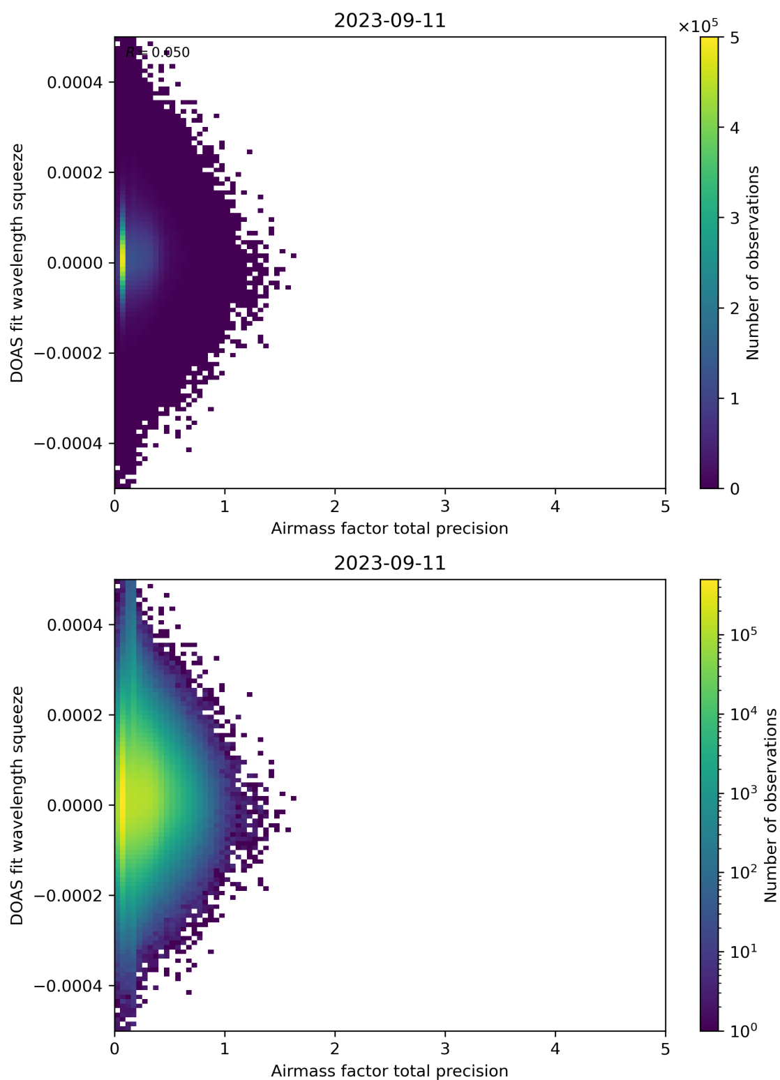
Figure 107: Scatter density plot of “Airmass factor total precision” against “DOAS fit wavelength squeeze” for 2023-09-10 to 2023-09-12.
