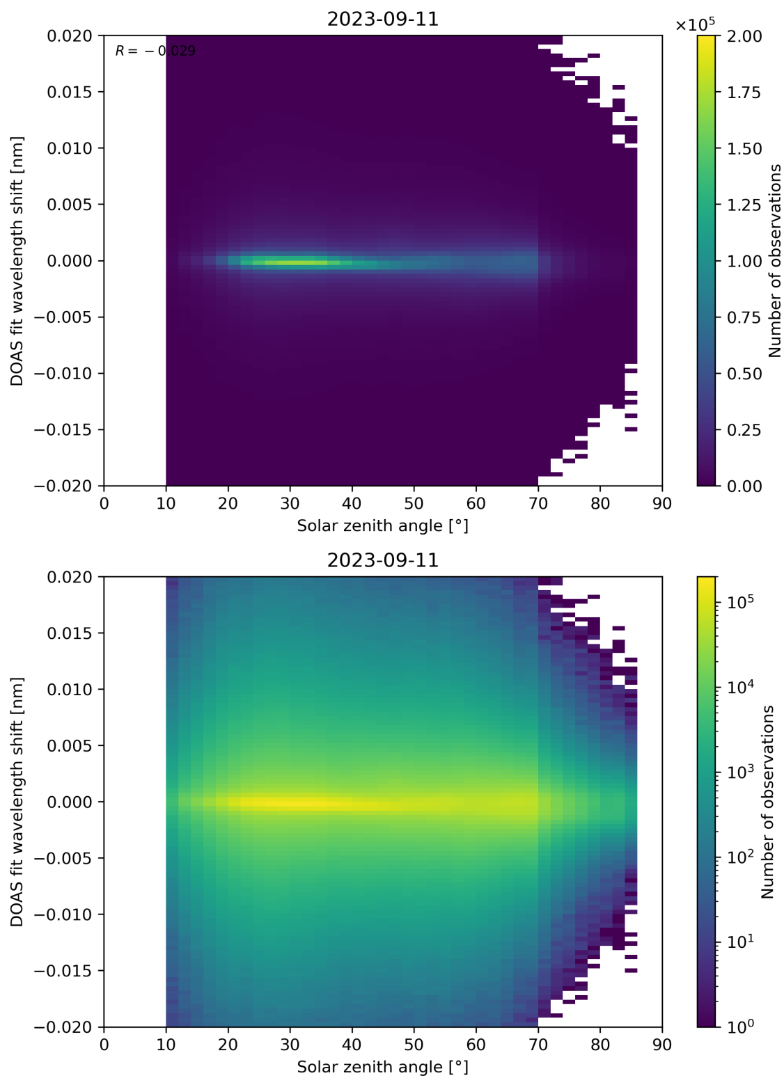
Figure 168: Scatter density plot of “Solar zenith angle” against “DOAS fit wavelength shift” for 2023-09-10 to 2023-09-12.
