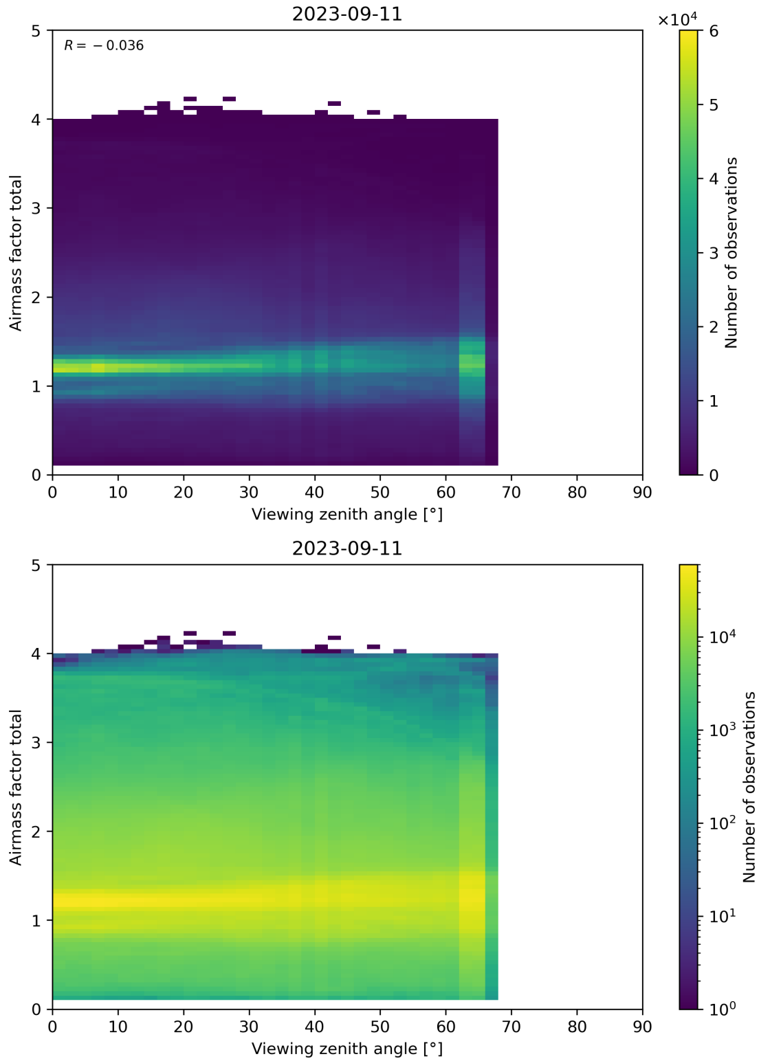
Figure 190: Scatter density plot of “Viewing zenith angle” against “Airmass factor total” for 2023-09-10 to 2023-09-12.
