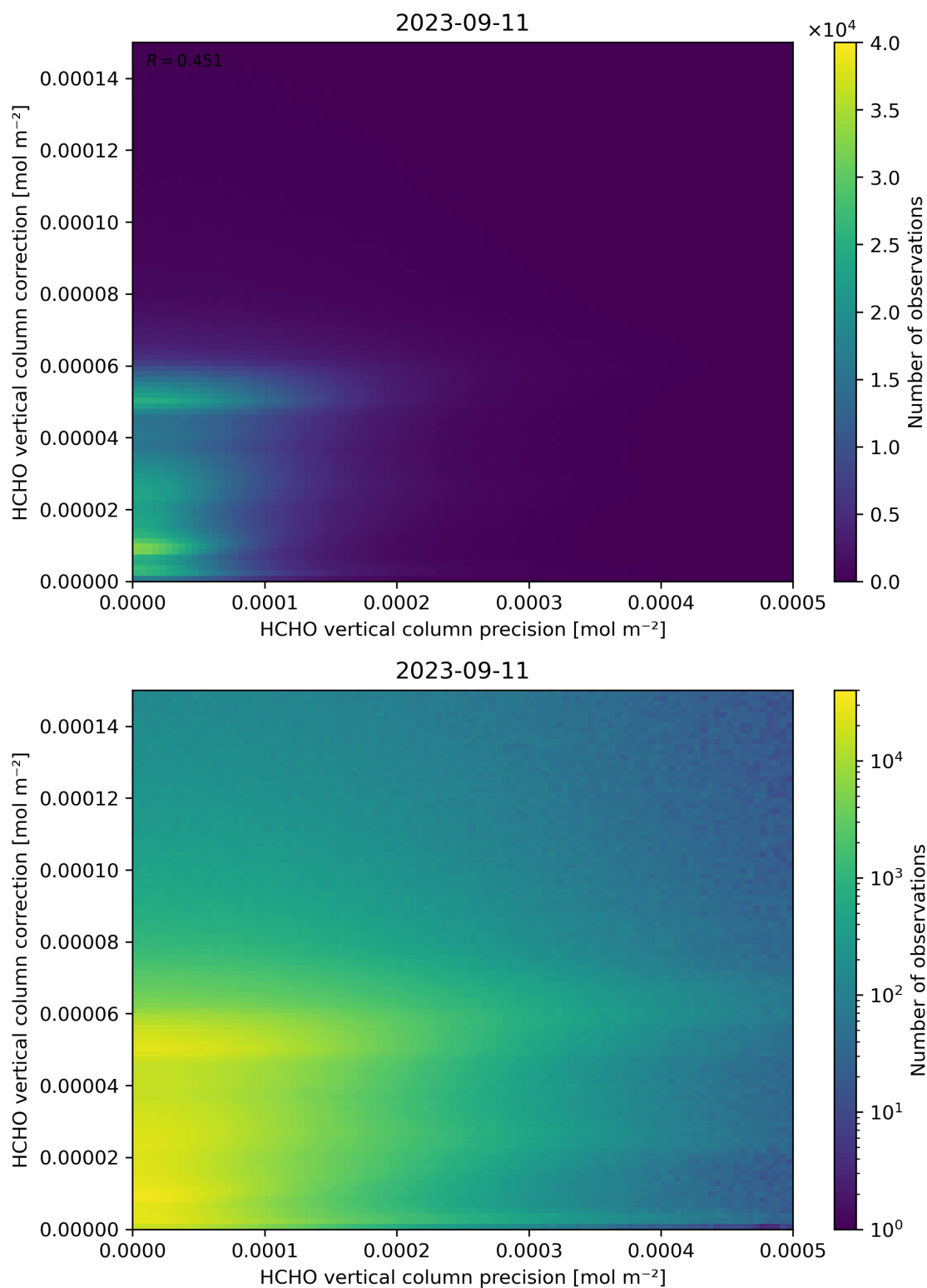
Figure 146: Scatter density plot of “HCHO vertical column precision” against “HCHO vertical column correction” for 2023-09-10 to 2023-09-12.
