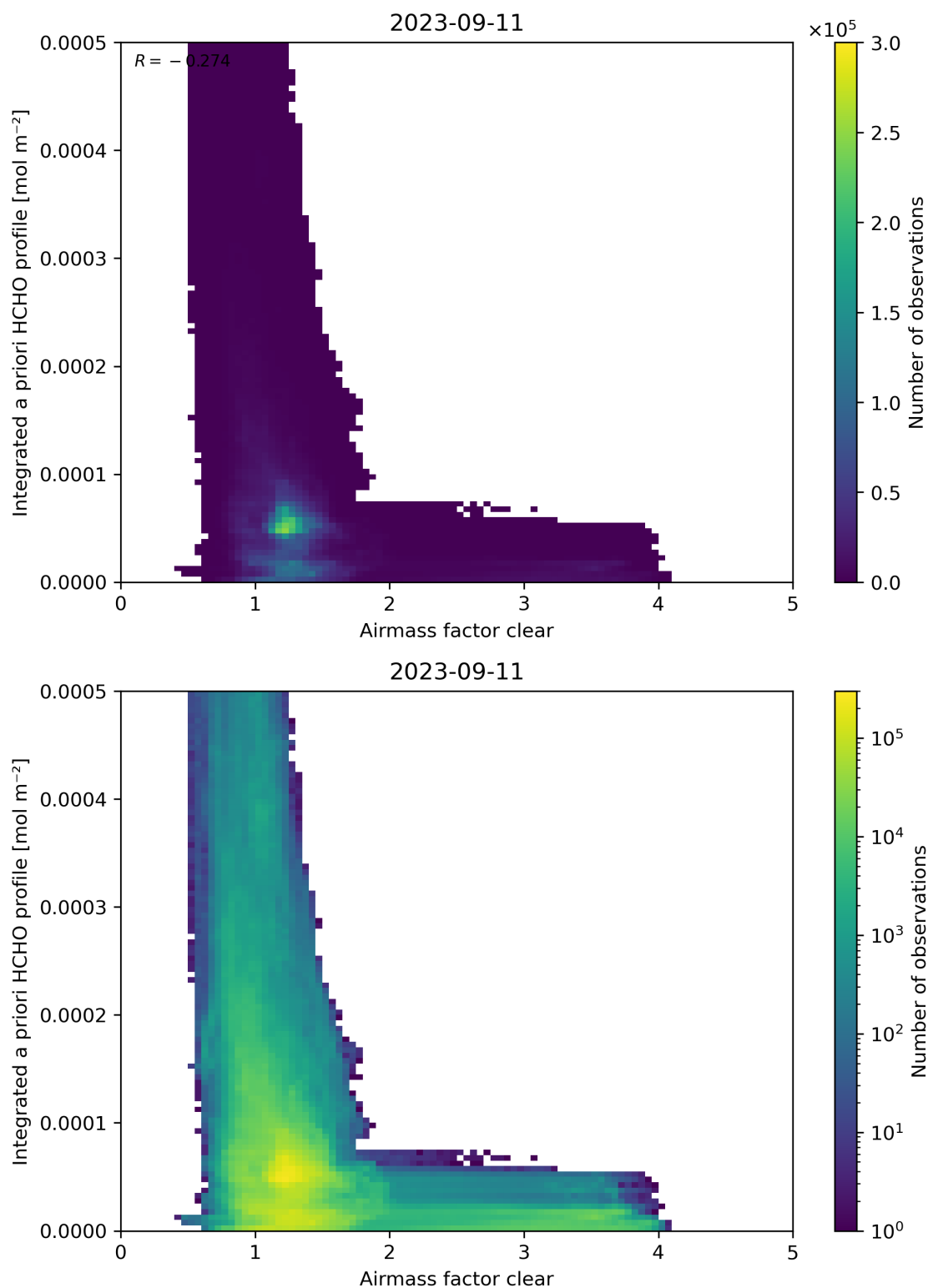
Figure 76: Scatter density plot of “Airmass factor clear” against “Integrated a priori HCHO profile” for 2023-09-10 to 2023-09-12.
