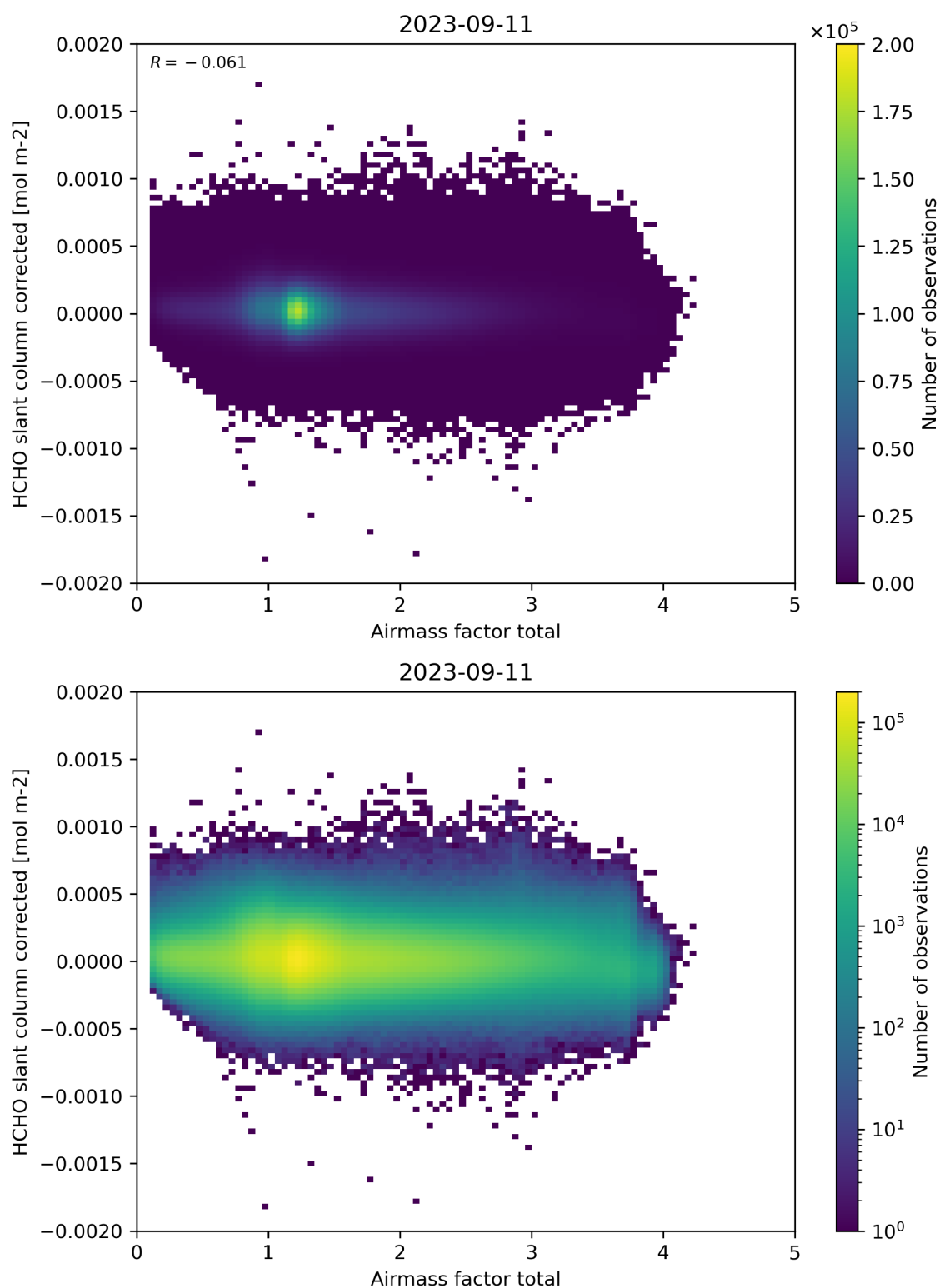
Figure 101: Scatter density plot of “Airmass factor total” against “HCHO slant column corrected” for 2023-09-10 to 2023-09-12.
