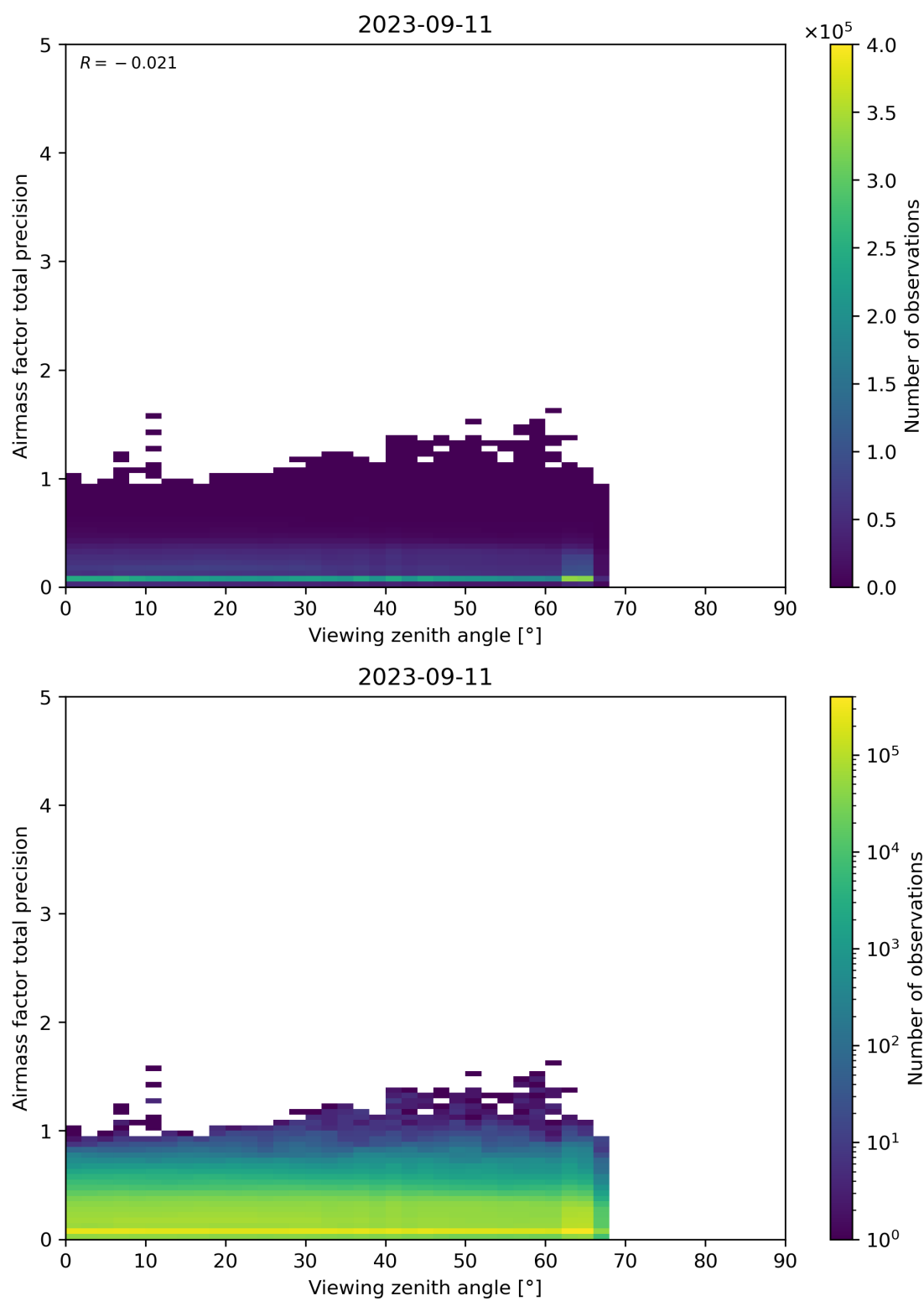
Figure 191: Scatter density plot of “Viewing zenith angle” against “Airmass factor total precision” for 2023-09-10 to 2023-09-12.
