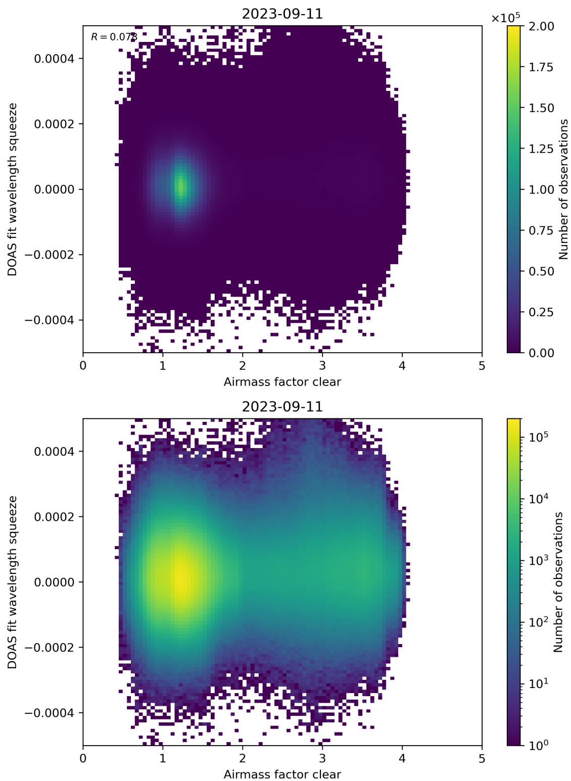
Figure 73: Scatter density plot of “Airmass factor clear” against “DOAS fit wavelength squeeze” for 2023-09-10 to 2023-09-12.
