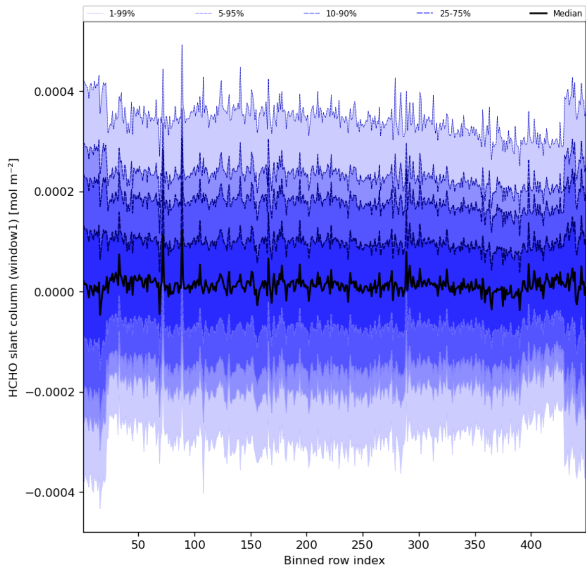
Figure 52: Along track statistics of “HCHO slant column (window1)” for 2023-09-10 to 2023-09-12
