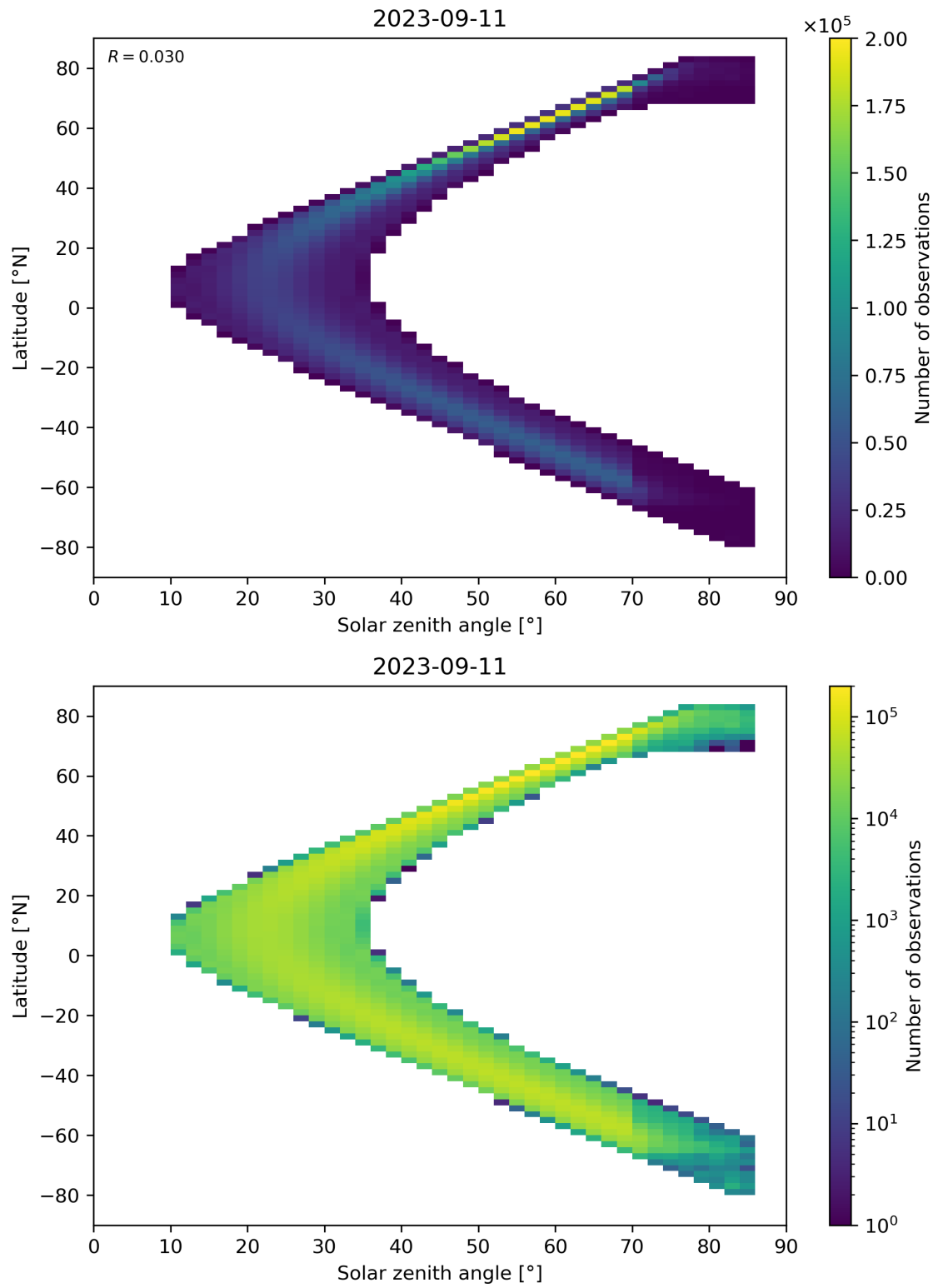
Figure 181: Scatter density plot of “Solar zenith angle” against “Latitude” for 2023-09-10 to 2023-09-12.
