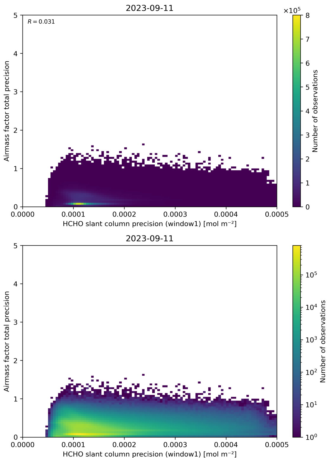
Figure 95: Scatter density plot of “HCHO slant column precision (window1)” against “Airmass factor total precision” for 2023-09-10 to 2023-09-12.
