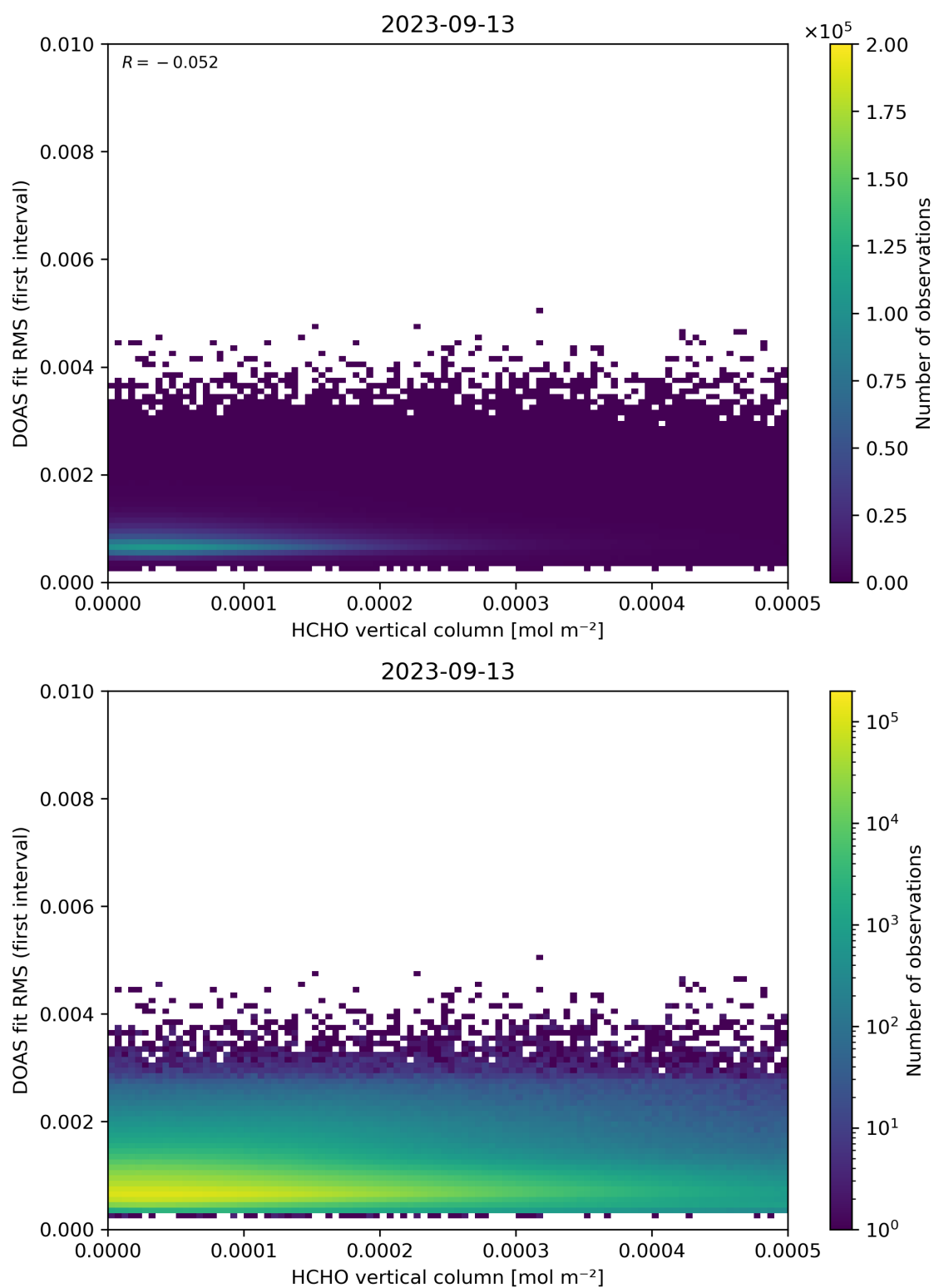
Figure 123: Scatter density plot of “HCHO vertical column” against “DOAS fit RMS (first interval)” for 2023-09-12 to 2023-09-14.
