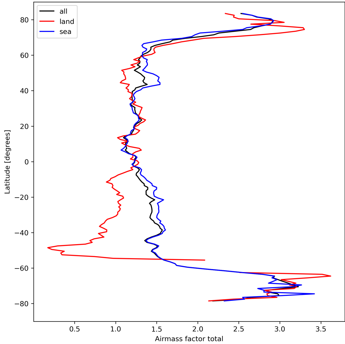
Figure 26: Zonal average of “Airmass factor total” for 2023-09-12 to 2023-09-14.
