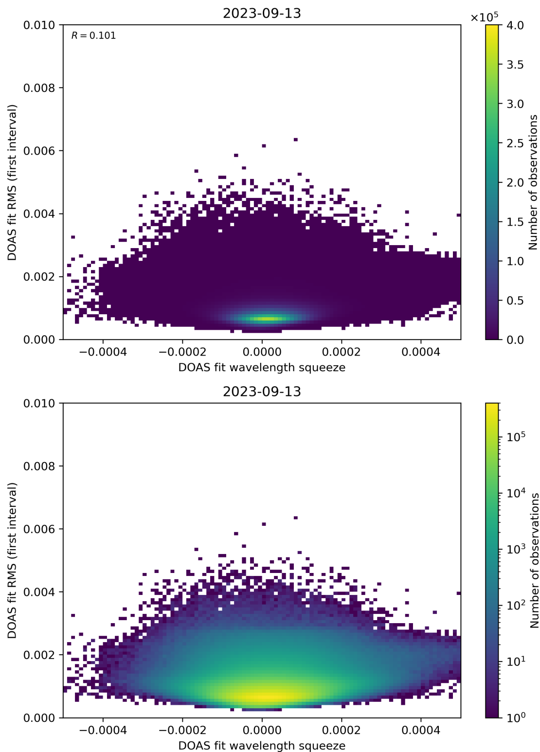
Figure 68: Scatter density plot of “DOAS fit wavelength squeeze” against “DOAS fit RMS (first interval)” for 2023-09-12 to 2023-09-14.
