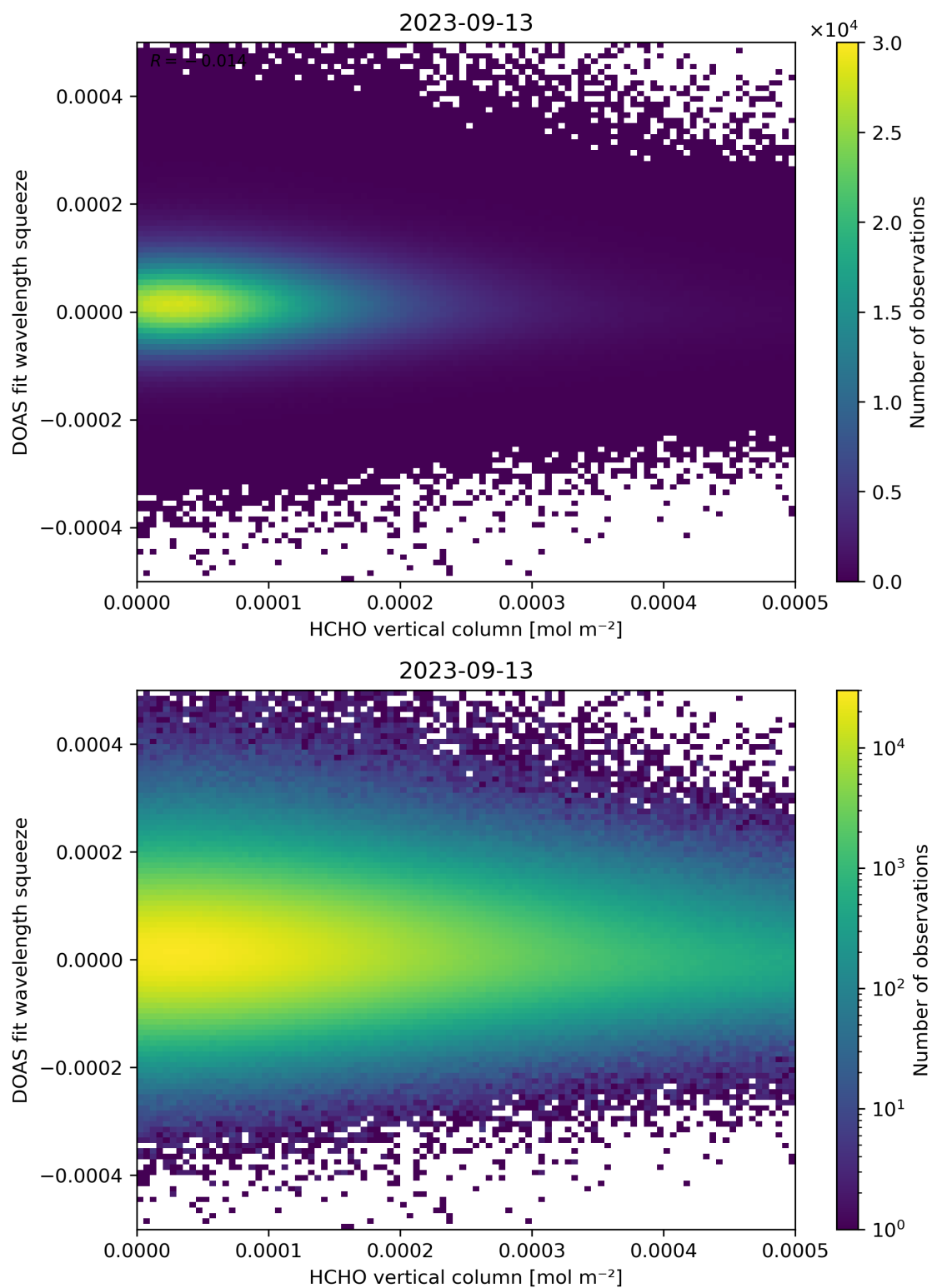
Figure 125: Scatter density plot of “HCHO vertical column” against “DOAS fit wavelength squeeze” for 2023-09-12 to 2023-09-14.
