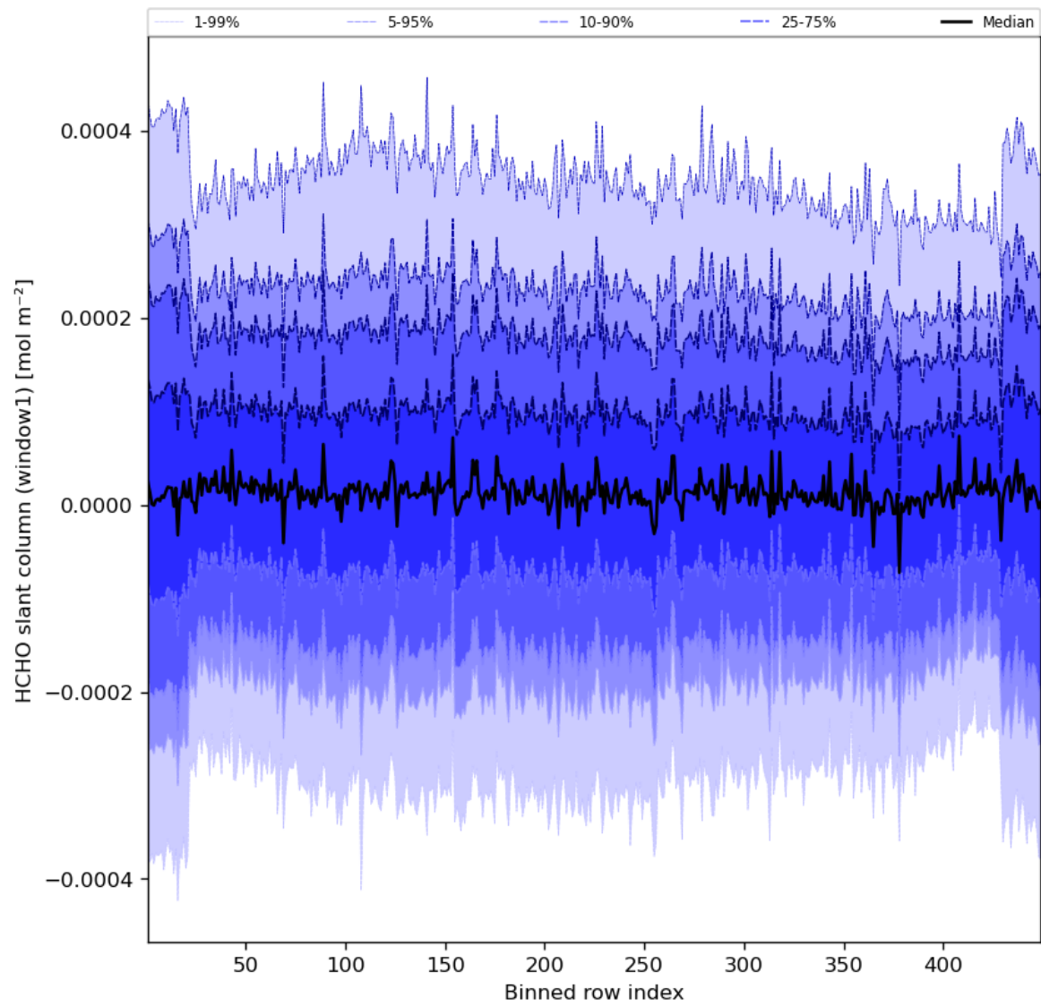
Figure 52: Along track statistics of “HCHO slant column (window1)” for 2023-09-12 to 2023-09-14
