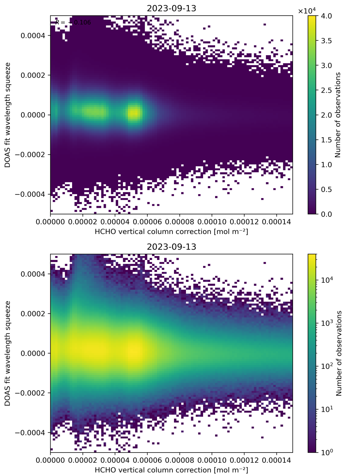
Figure 114: Scatter density plot of “HCHO vertical column correction” against “DOAS fit wavelength squeeze” for 2023-09-12 to 2023-09-14.
