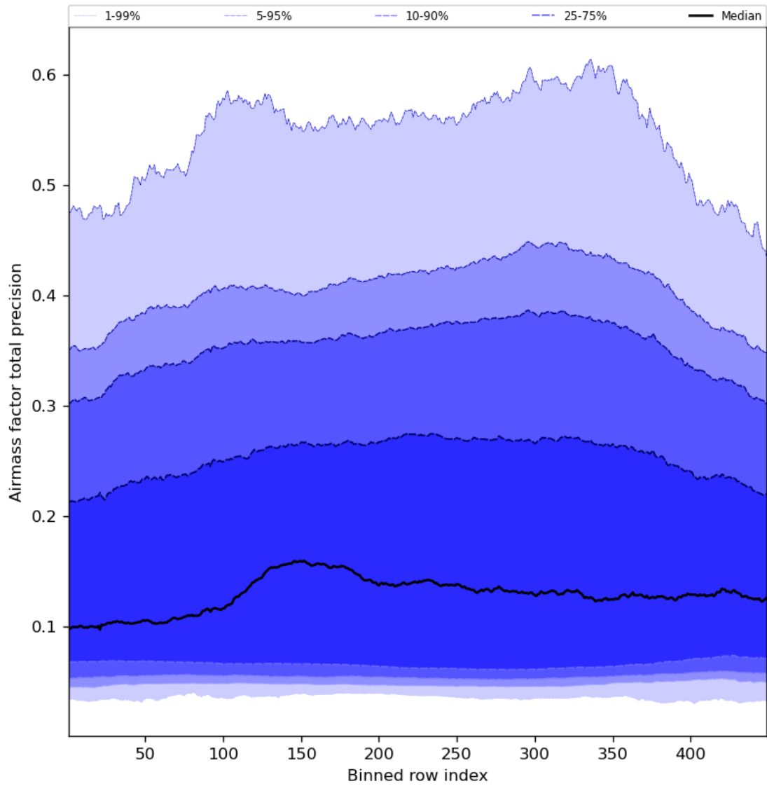
Figure 55: Along track statistics of “Airmass factor total precision” for 2023-09-12 to 2023-09-14
