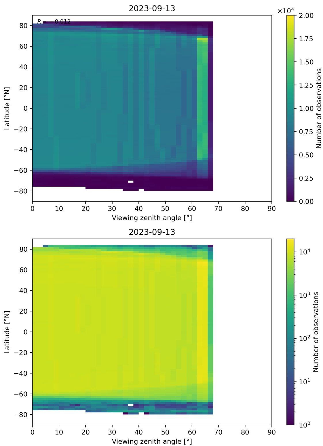
Figure 196: Scatter density plot of “Viewing zenith angle” against “Latitude” for 2023-09-12 to 2023-09-14.
