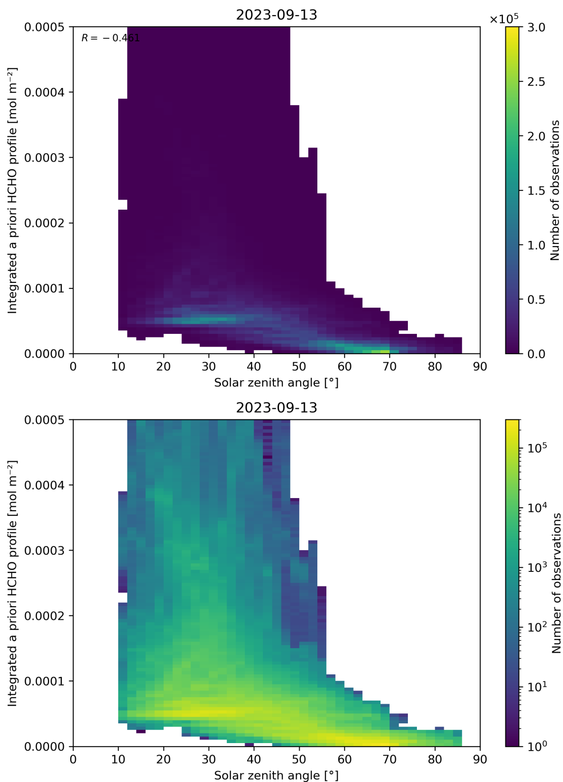
Figure 180: Scatter density plot of “Solar zenith angle” against “Integrated a priori HCHO profile” for 2023-09-12 to 2023-09-14.
