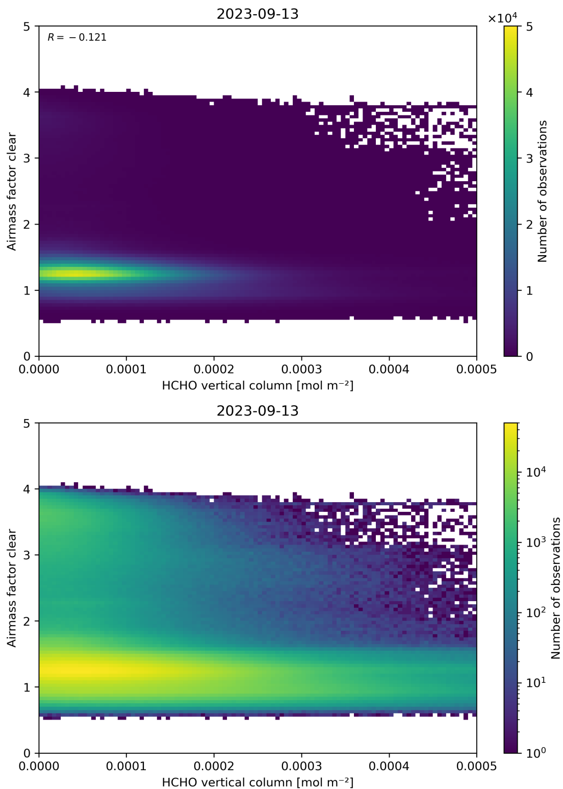
Figure 126: Scatter density plot of “HCHO vertical column” against “Airmass factor clear” for 2023-09-12 to 2023-09-14.
