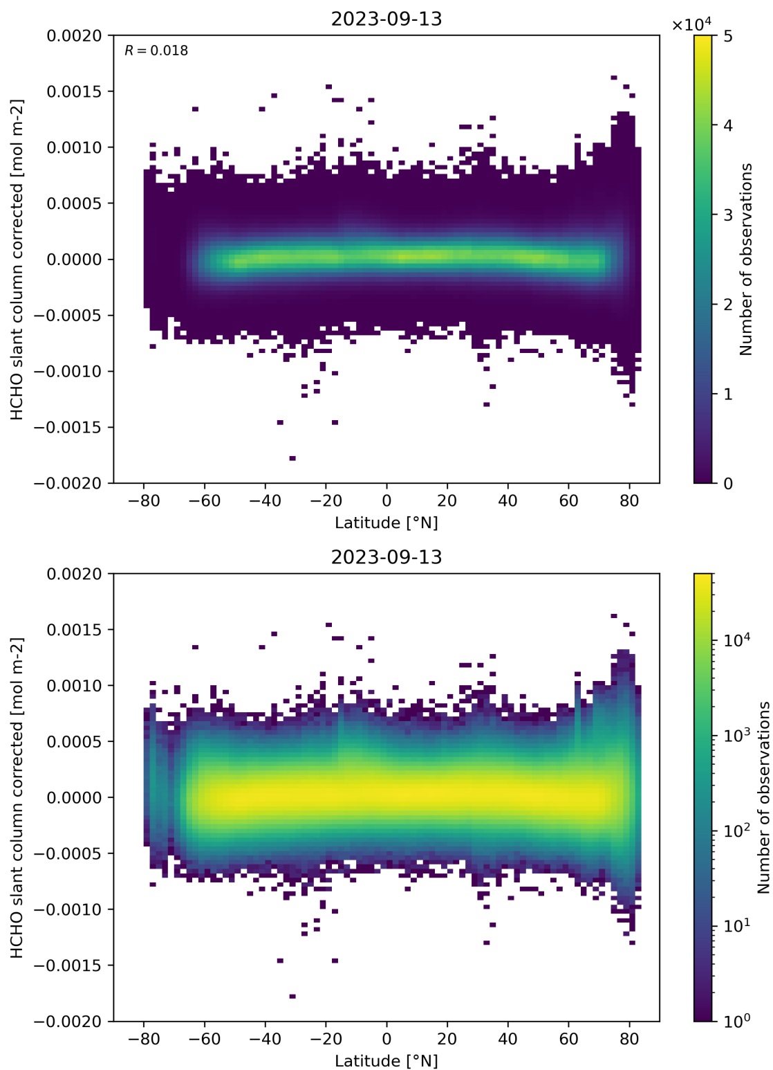
Figure 157: Scatter density plot of “Latitude” against “HCHO slant column corrected” for 2023-09-12 to 2023-09-14.
