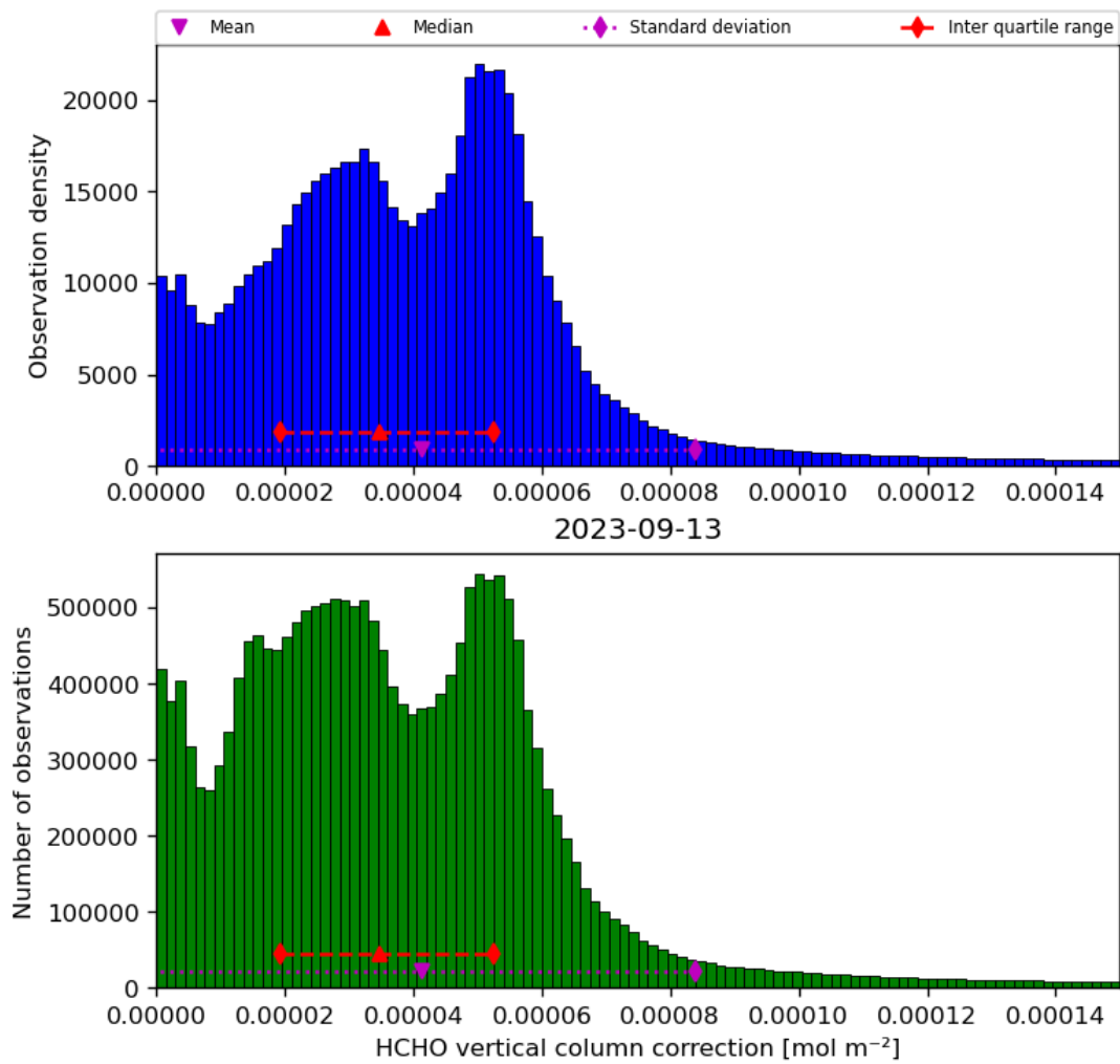
Figure 37: Histogram of “HCHO vertical column correction” for 2023-09-12 to 2023-09-14
