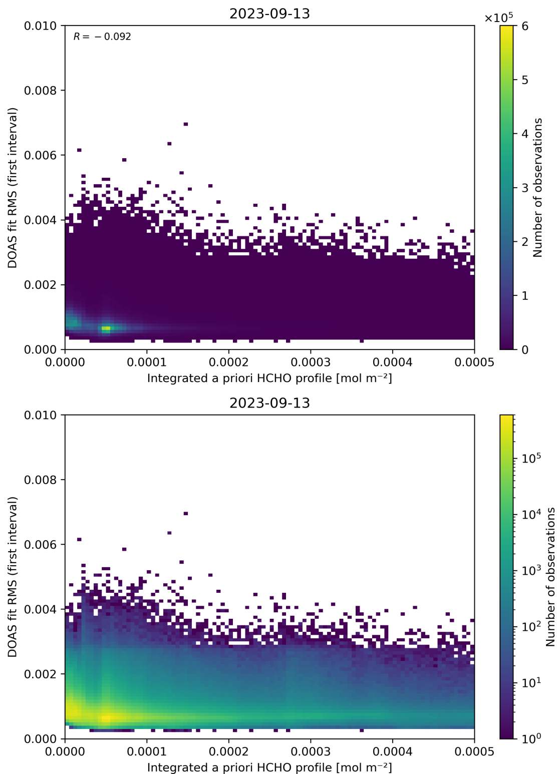
Figure 148: Scatter density plot of “Integrated a priori HCHO profile” against “DOAS fit RMS (first interval)” for 2023-09-12 to 2023-09-14.
