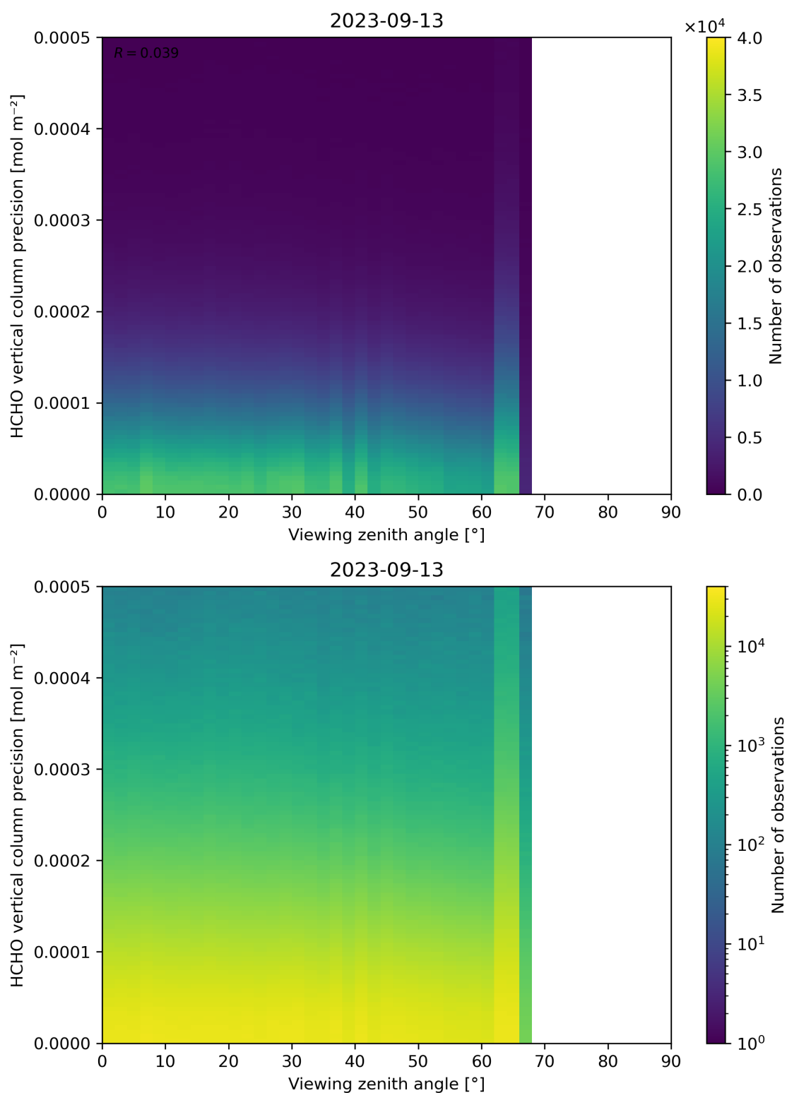
Figure 194: Scatter density plot of “Viewing zenith angle” against “HCHO vertical column precision” for 2023-09-12 to 2023-09-14.
