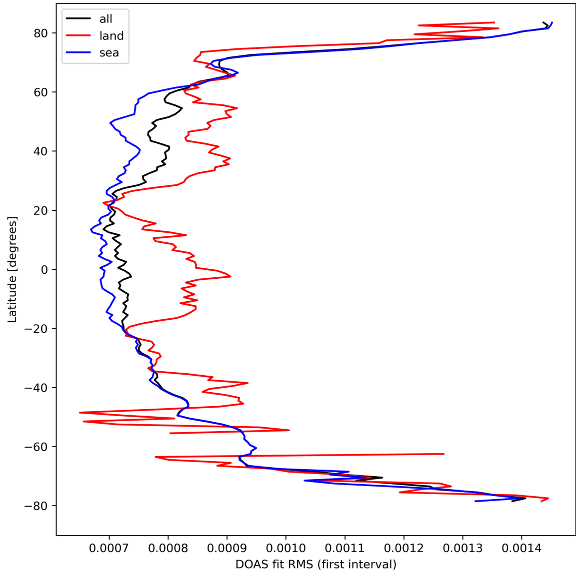
Figure 32: Zonal average of "DOAS fit RMS (first interval)" for 2023-09-12 to 2023-09-14.
