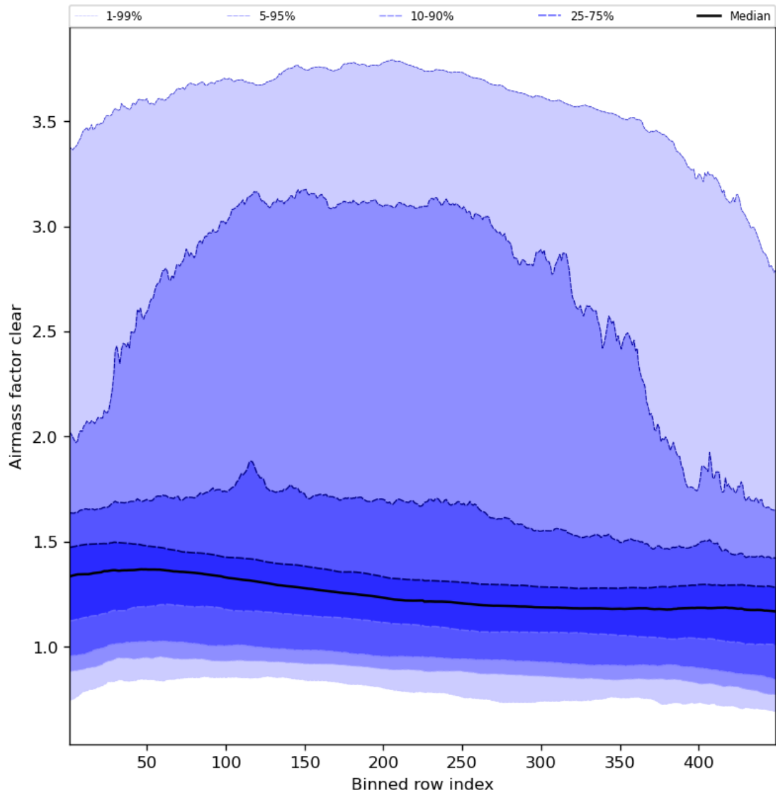
Figure 56: Along track statistics of “Airmass factor clear” for 2023-09-12 to 2023-09-14
