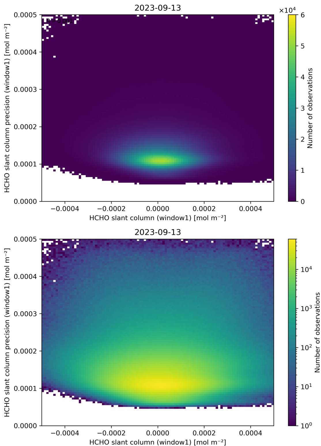
Figure 84: Scatter density plot of “HCHO slant column (window1)” against “HCHO slant column precision (window1)” for 2023-09-12 to 2023-09-14.
