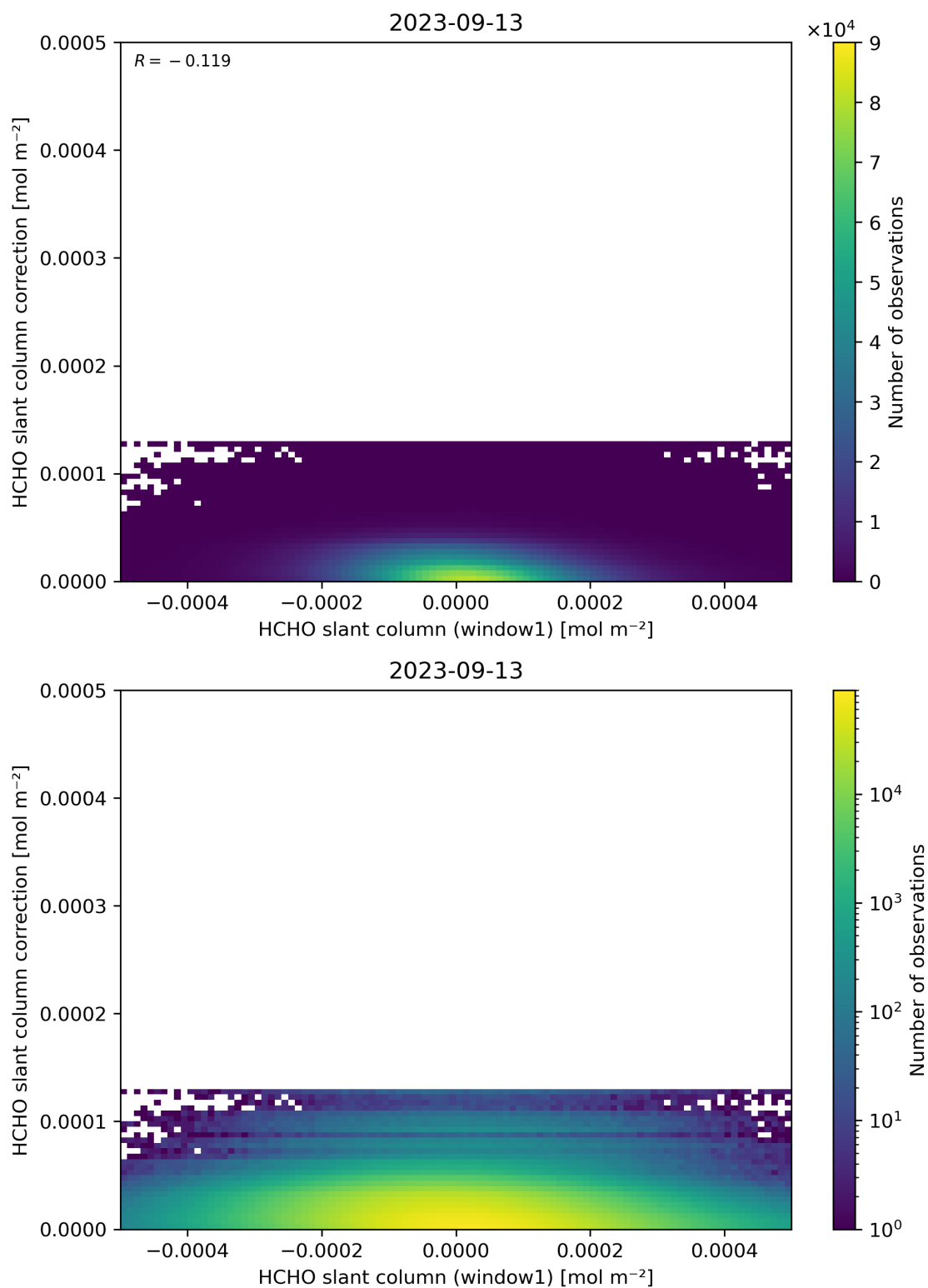
Figure 83: Scatter density plot of “HCHO slant column (window1)” against “HCHO slant column correction” for 2023-09-12 to 2023-09-14.
