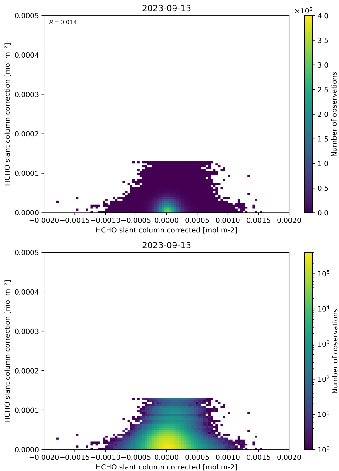
Figure 77: Scatter density plot of “HCHO slant column corrected” against “HCHO slant column correction” for 2023-09-12 to 2023-09-14.
