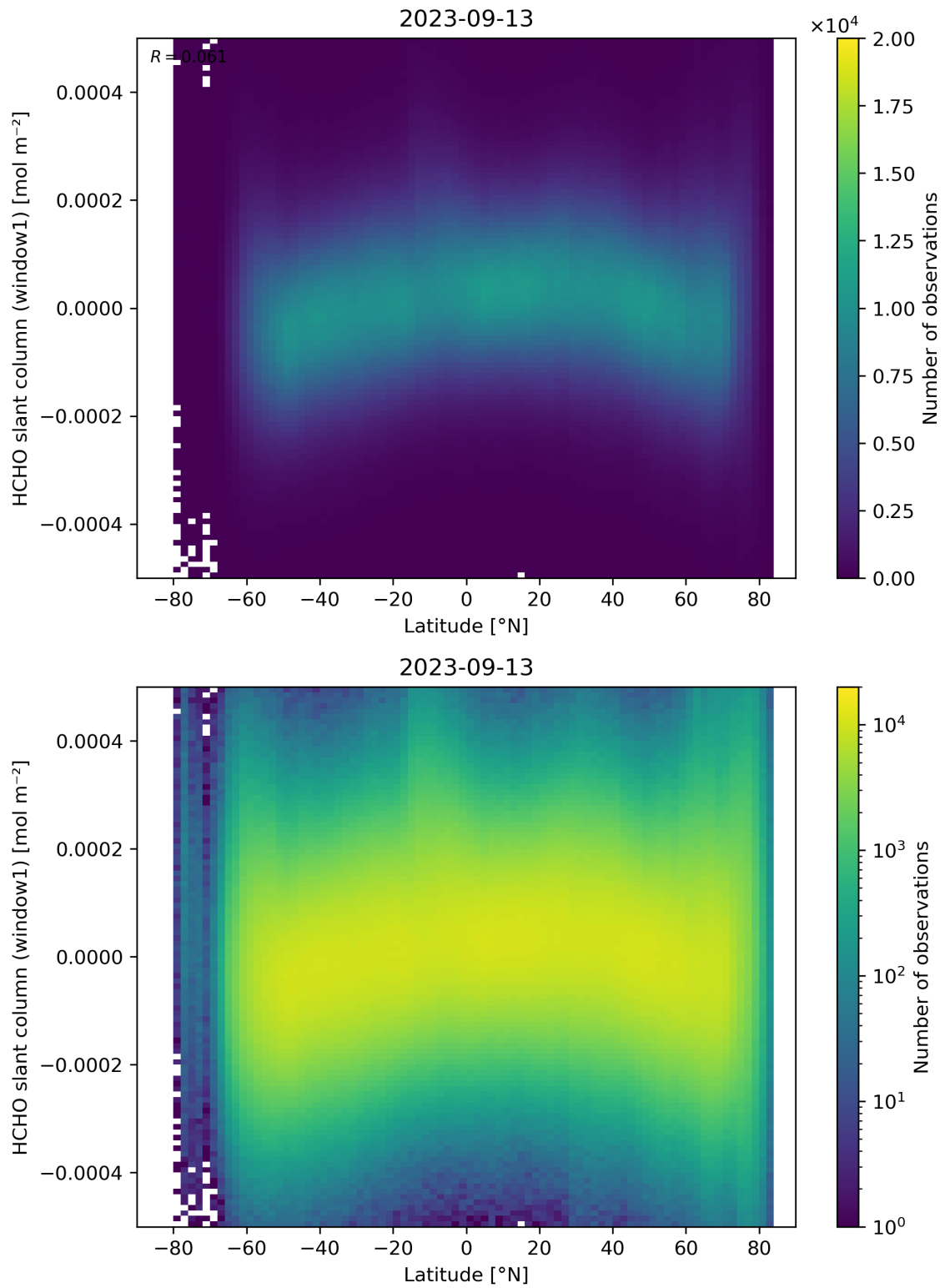
Figure 159: Scatter density plot of “Latitude” against “HCHO slant column (window1)” for 2023-09-12 to 2023-09-14.
