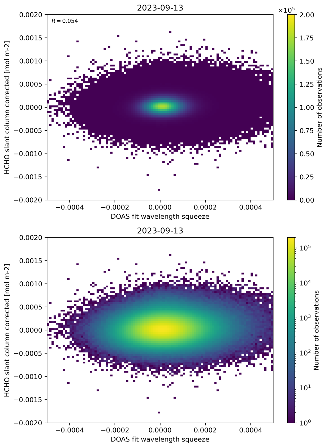
Figure 69: Scatter density plot of “DOAS fit wavelength squeeze” against “HCHO slant column corrected” for 2023-09-12 to 2023-09-14.
