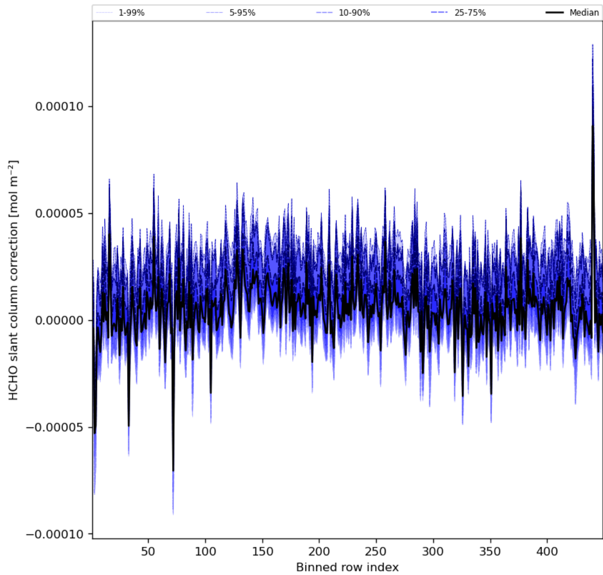
Figure 61: Along track statistics of “HCHO slant column correction” for 2023-09-12 to 2023-09-14
