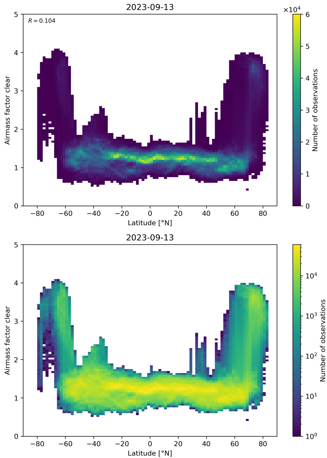
Figure 156: Scatter density plot of “Latitude” against “Airmass factor clear” for 2023-09-12 to 2023-09-14.
