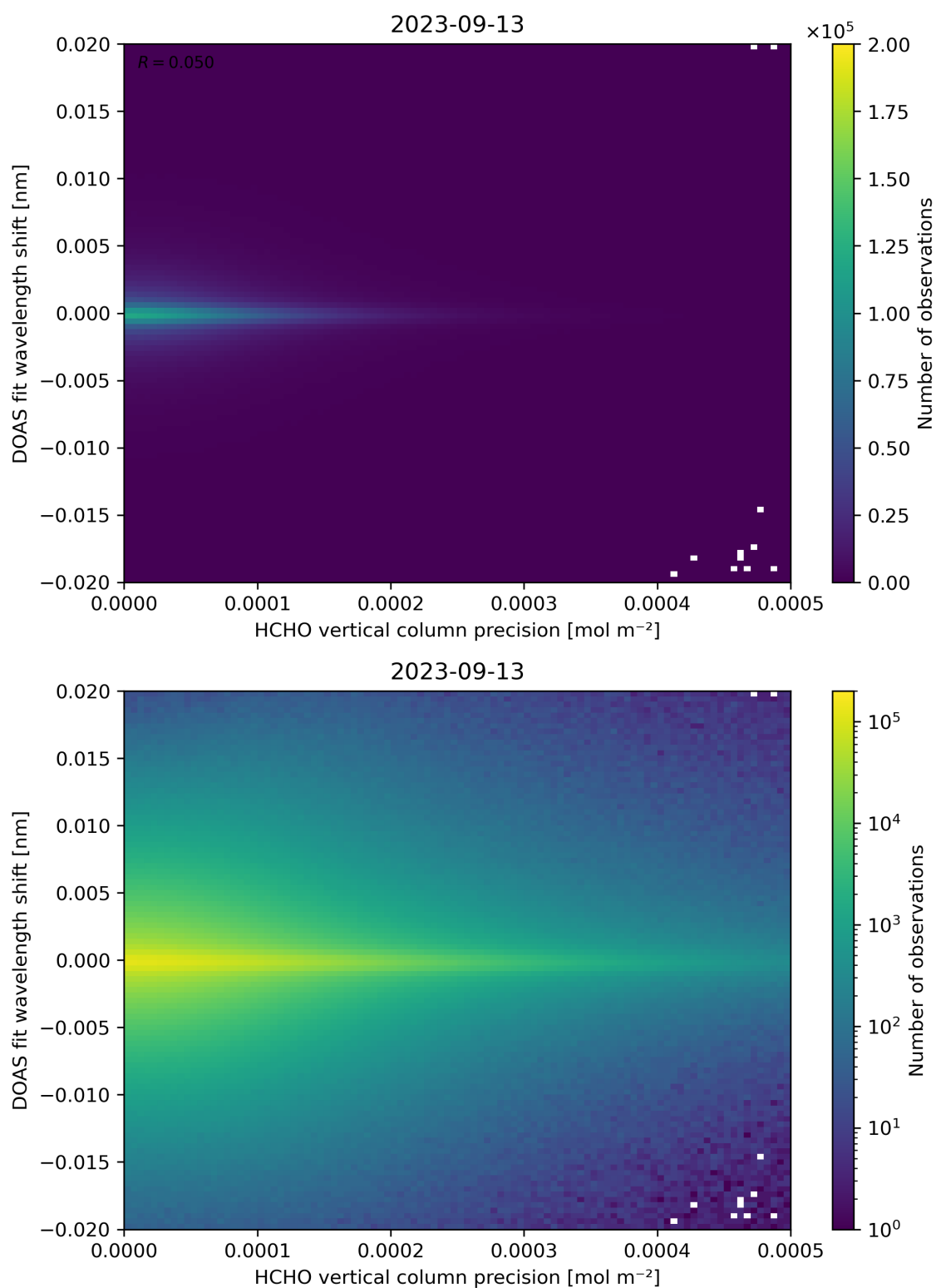
Figure 137: Scatter density plot of “HCHO vertical column precision” against “DOAS fit wavelength shift” for 2023-09-12 to 2023-09-14.
