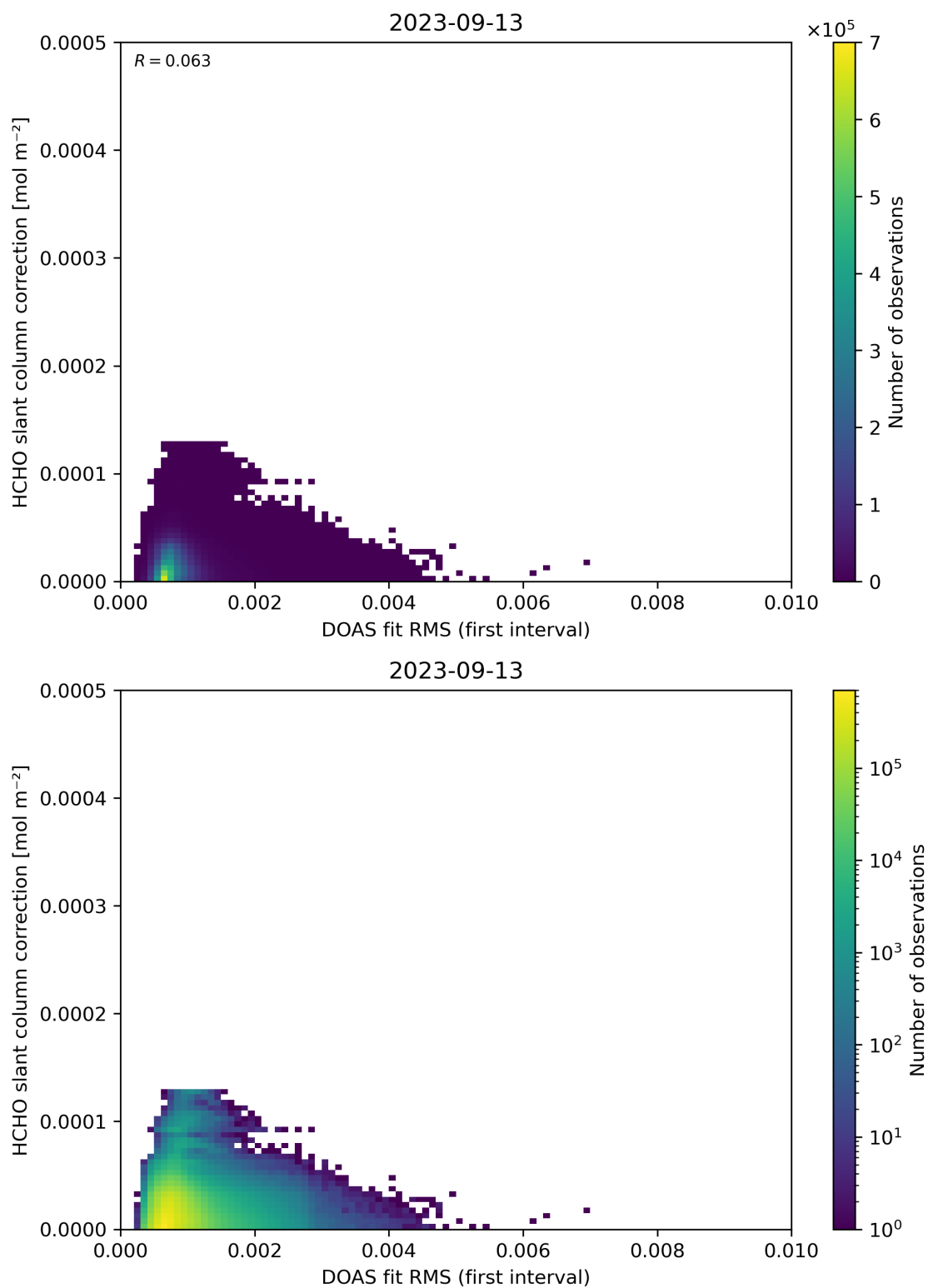
Figure 63: Scatter density plot of “DOAS fit RMS (first interval)” against “HCHO slant column correction” for 2023-09-12 to 2023-09-14.
