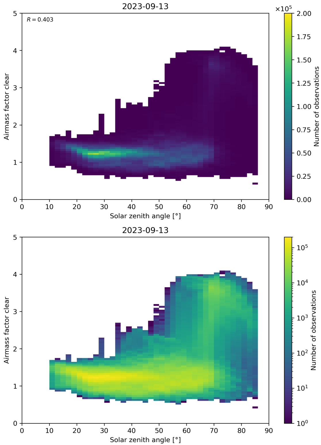
Figure 170: Scatter density plot of “Solar zenith angle” against “Airmass factor clear” for 2023-09-12 to 2023-09-14.
