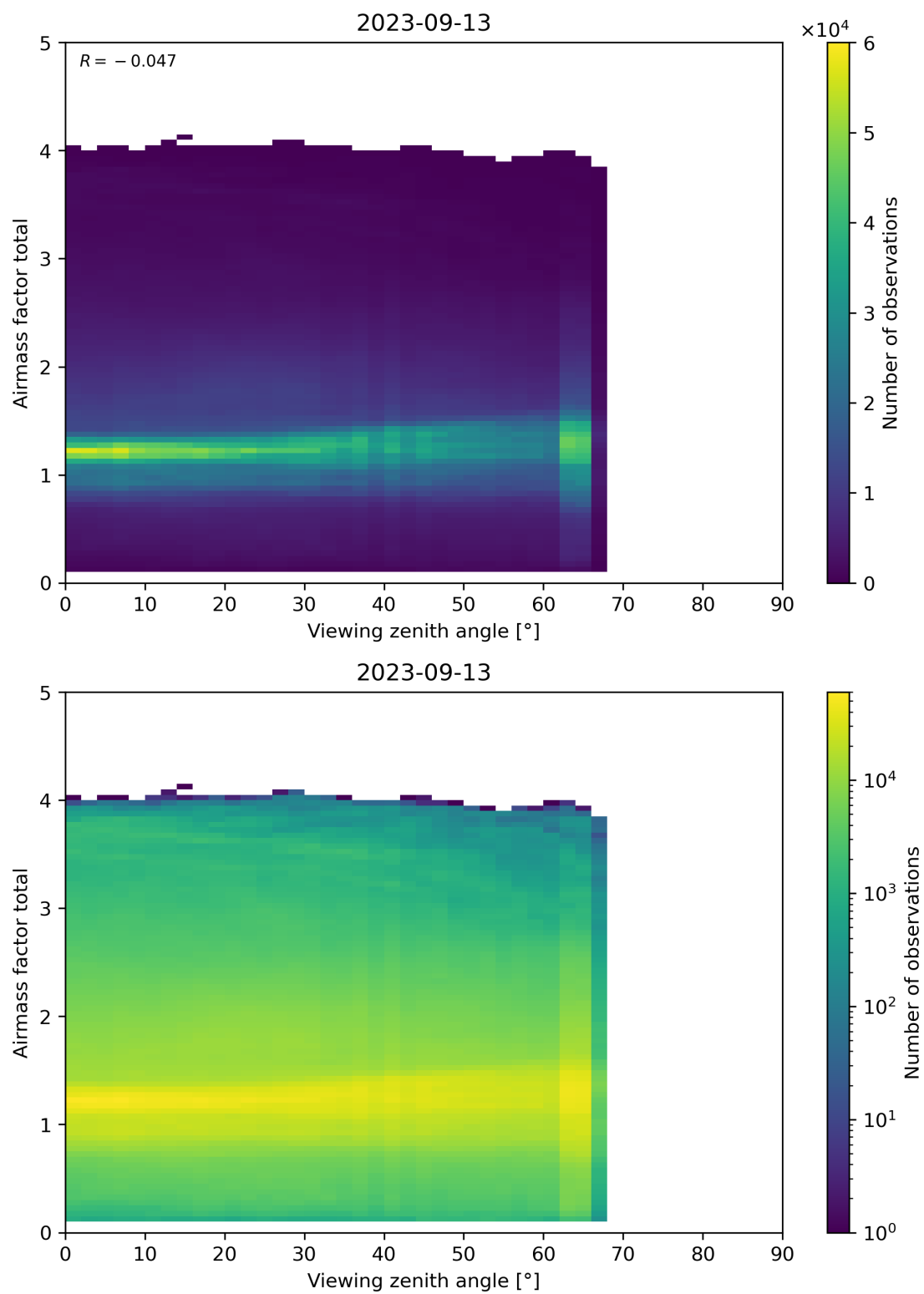
Figure 190: Scatter density plot of “Viewing zenith angle” against “Airmass factor total” for 2023-09-12 to 2023-09-14.
