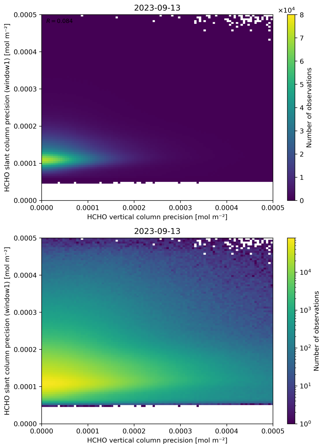
Figure 143: Scatter density plot of “HCHO vertical column precision” against “HCHO slant column precision (window1)” for 2023-09-12 to 2023-09-14.
