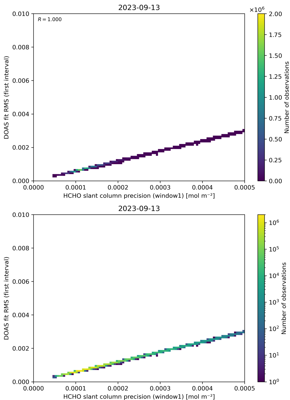
Figure 88: Scatter density plot of “HCHO slant column precision (window1)” against “DOAS fit RMS (first interval)” for 2023-09-12 to 2023-09-14.
