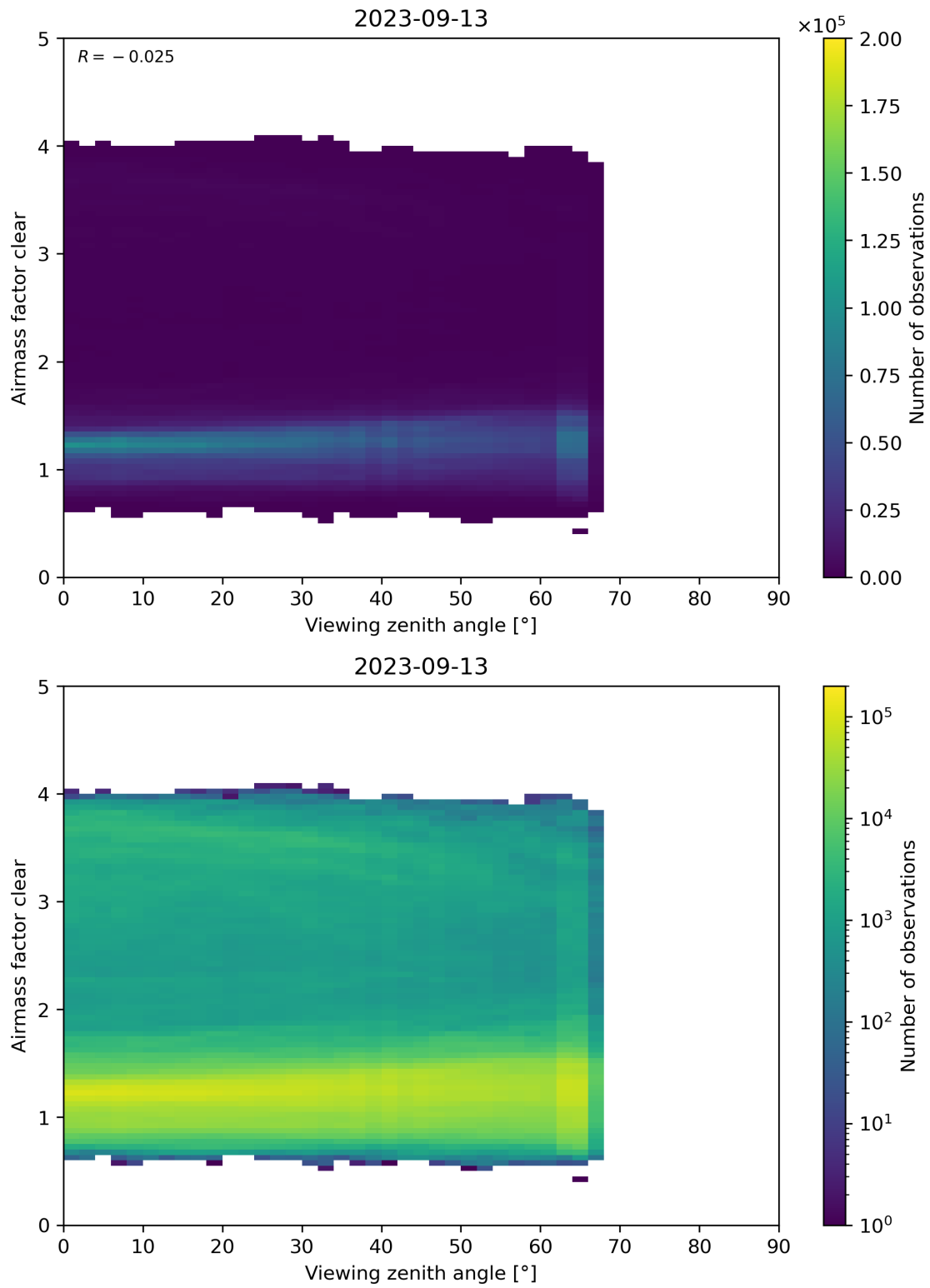
Figure 185: Scatter density plot of “Viewing zenith angle” against “Airmass factor clear” for 2023-09-12 to 2023-09-14.
