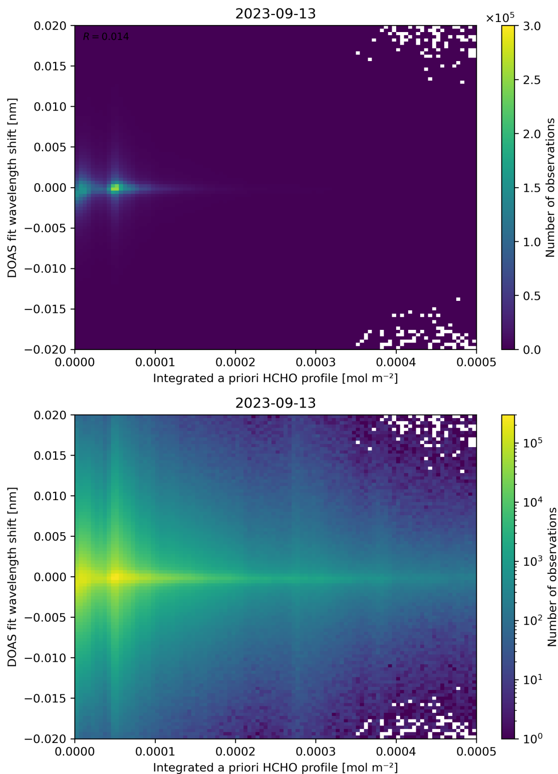
Figure 149: Scatter density plot of “Integrated a priori HCHO profile” against “DOAS fit wavelength shift” for 2023-09-12 to 2023-09-14.
