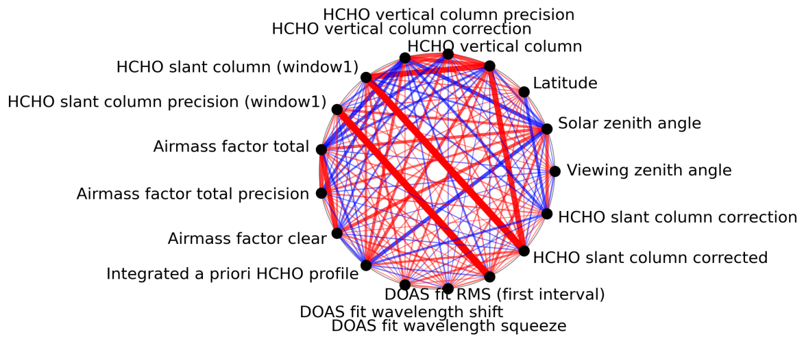
Figure 1: Map of correlation graph for 2023-09-12 to 2023-09-14.
