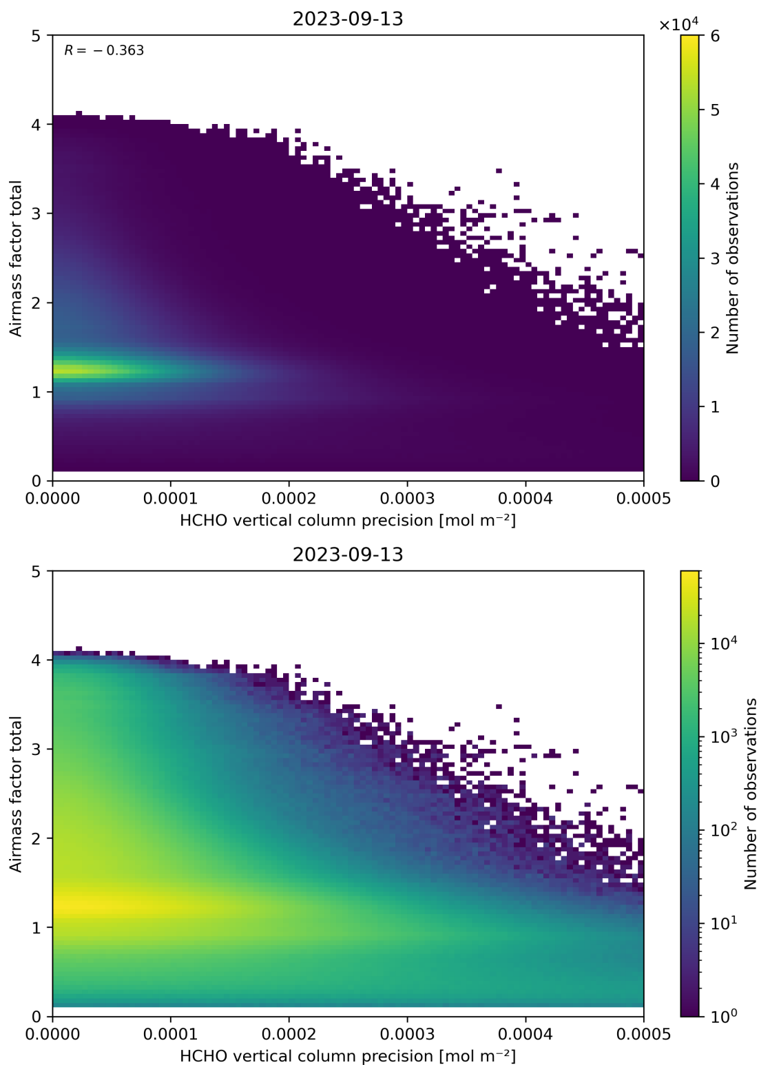
Figure 144: Scatter density plot of “HCHO vertical column precision” against “Airmass factor total” for 2023-09-12 to 2023-09-14.
