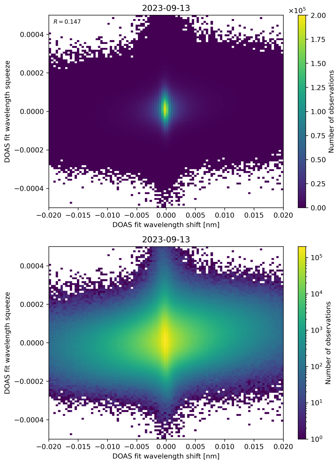
Figure 65: Scatter density plot of “DOAS fit wavelength shift” against “DOAS fit wavelength squeeze” for 2023-09-12 to 2023-09-14.
