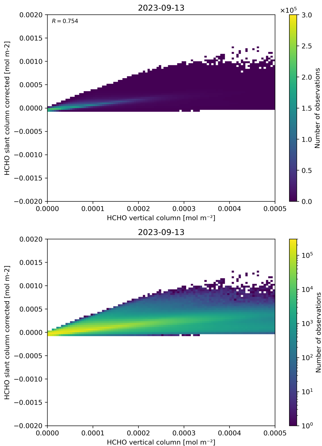
Figure 127: Scatter density plot of “HCHO vertical column” against “HCHO slant column corrected” for 2023-09-12 to 2023-09-14.
