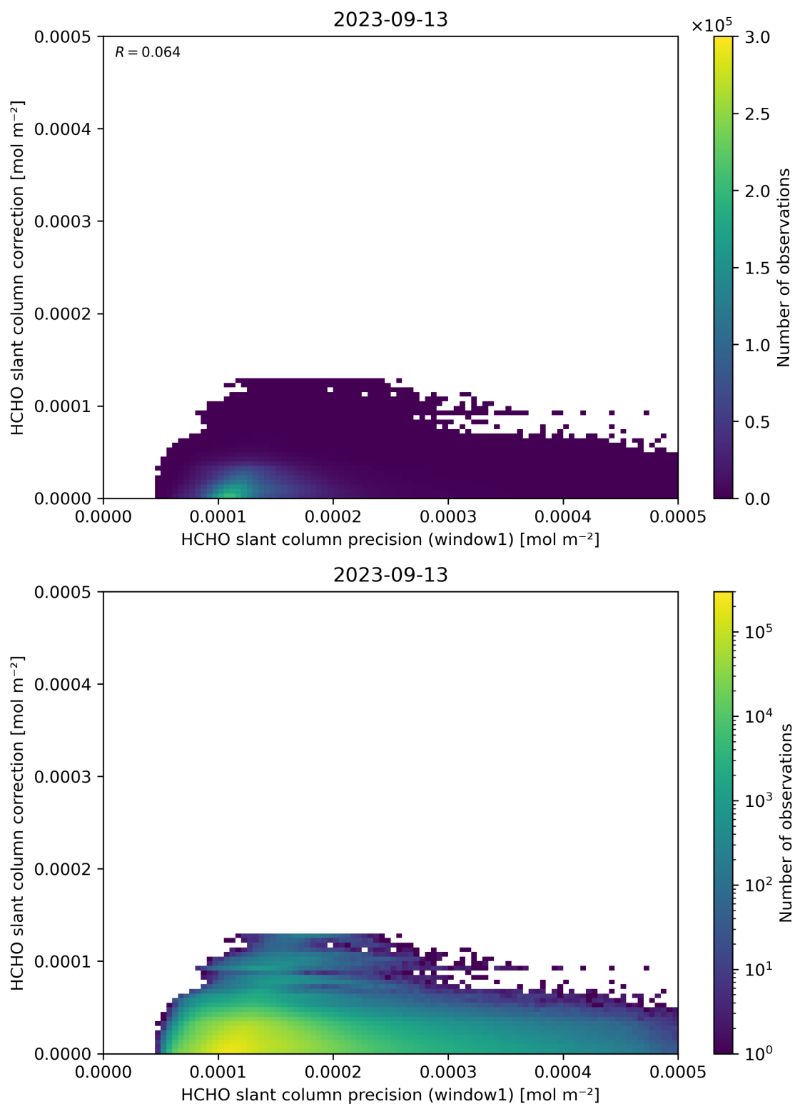
Figure 93: Scatter density plot of “HCHO slant column precision (window1)” against “HCHO slant column correction” for 2023-09-12 to 2023-09-14.
