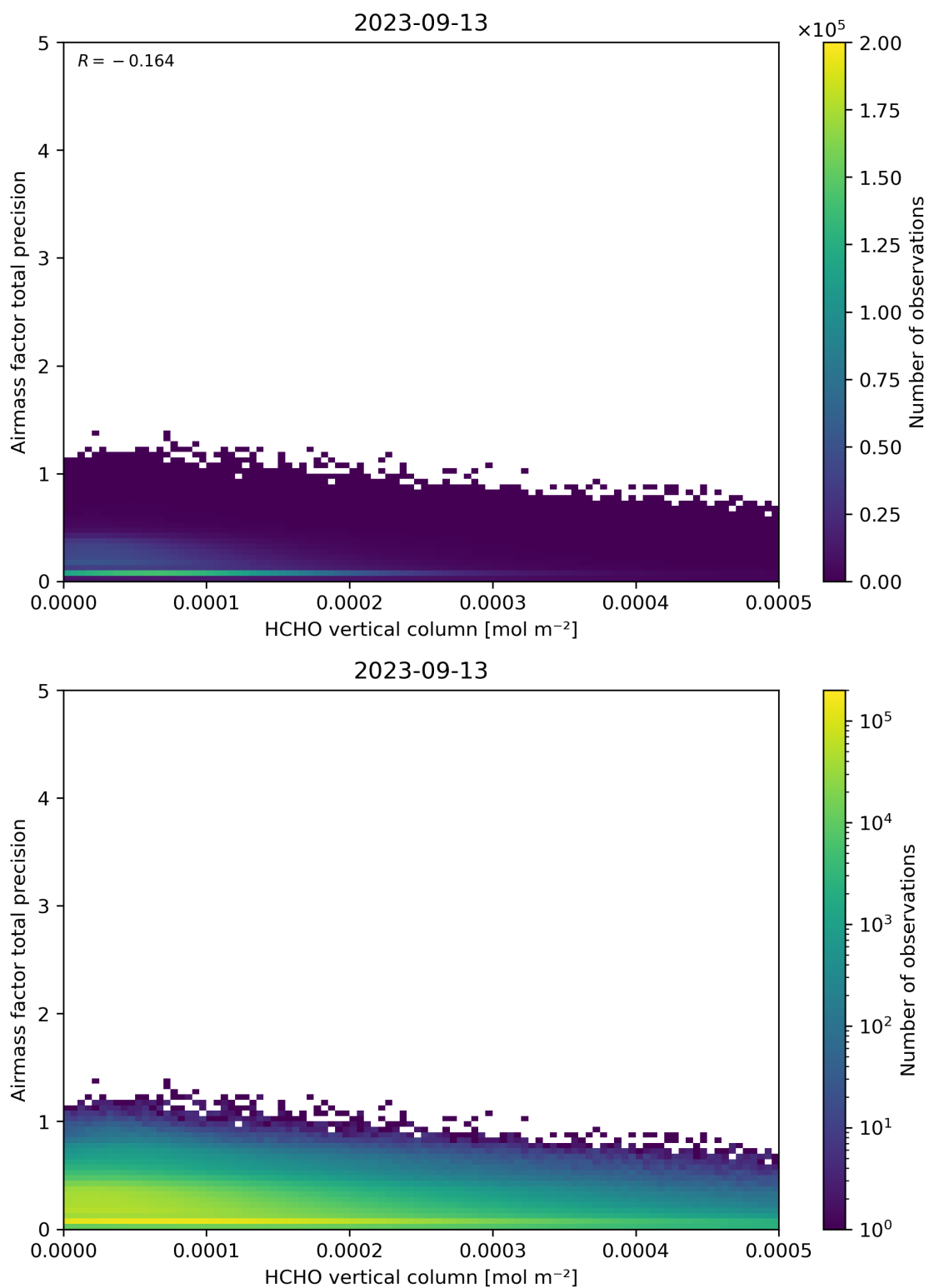
Figure 132: Scatter density plot of “HCHO vertical column” against “Airmass factor total precision” for 2023-09-12 to 2023-09-14.
