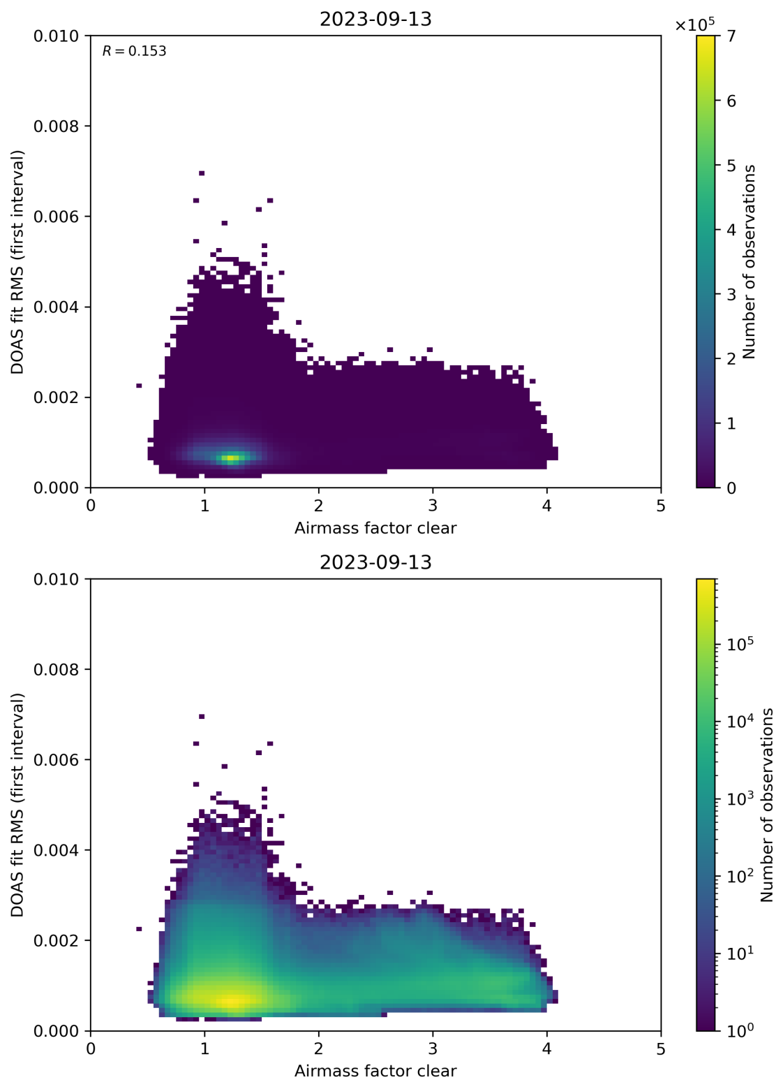
Figure 71: Scatter density plot of “Airmass factor clear” against “DOAS fit RMS (first interval)” for 2023-09-12 to 2023-09-14.
