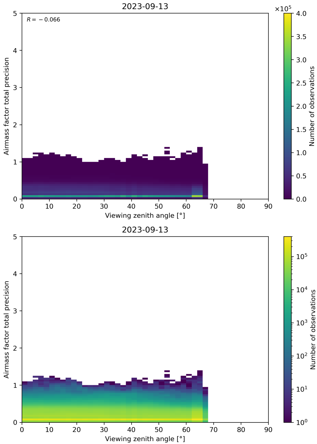
Figure 191: Scatter density plot of “Viewing zenith angle” against “Airmass factor total precision” for 2023-09-12 to 2023-09-14.
