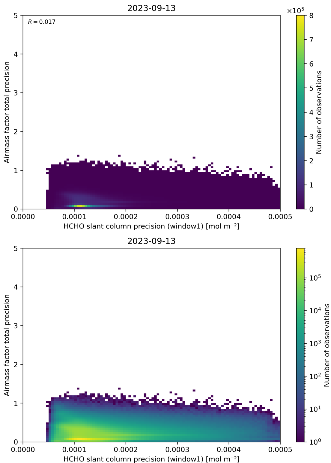
Figure 95: Scatter density plot of “HCHO slant column precision (window1)” against “Airmass factor total precision” for 2023-09-12 to 2023-09-14.
