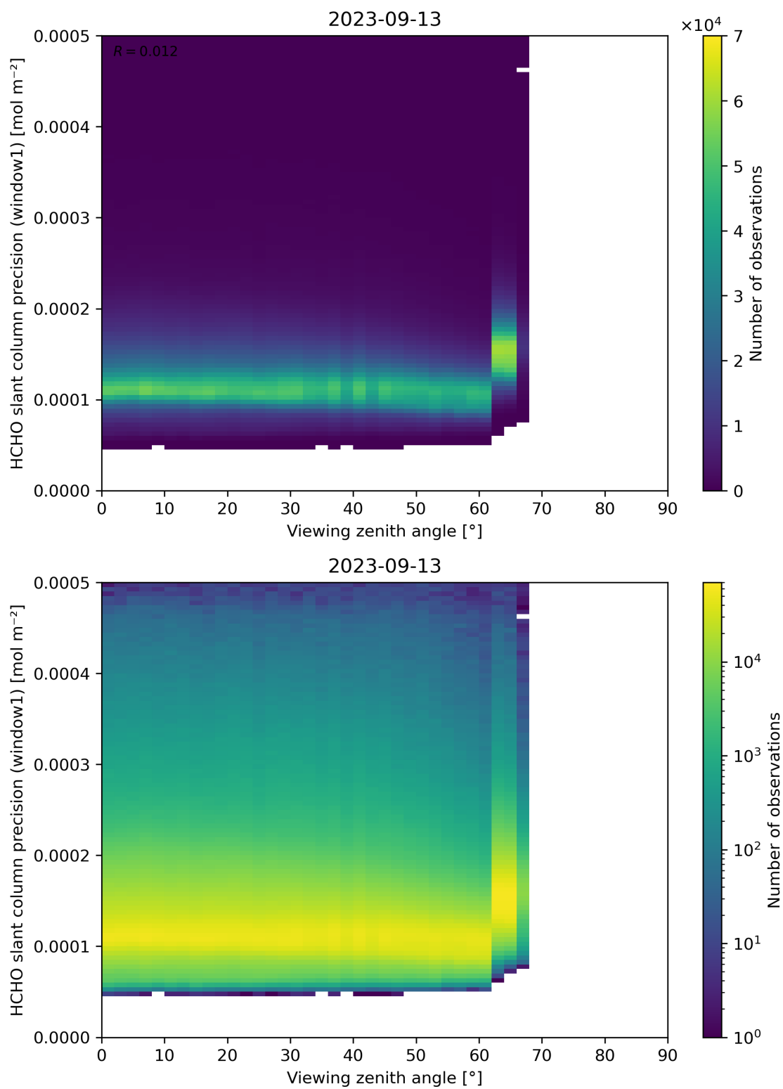
Figure 189: Scatter density plot of “Viewing zenith angle” against “HCHO slant column precision (window1)” for 2023-09-12 to 2023-09-14.
