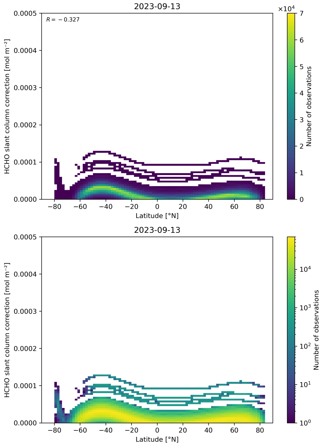
Figure 158: Scatter density plot of “Latitude” against “HCHO slant column correction” for 2023-09-12 to 2023-09-14.
