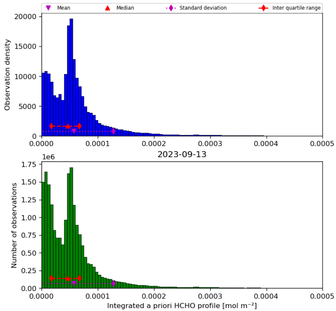
Figure 43: Histogram of “Integrated a priori HCHO profile” for 2023-09-12 to 2023-09-14
