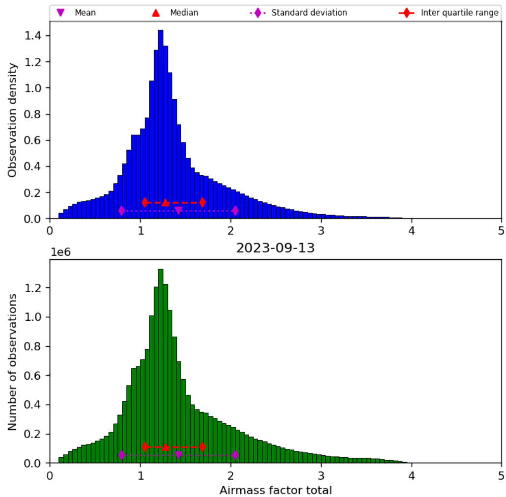
Figure 40: Histogram of “Airmass factor total” for 2023-09-12 to 2023-09-14
