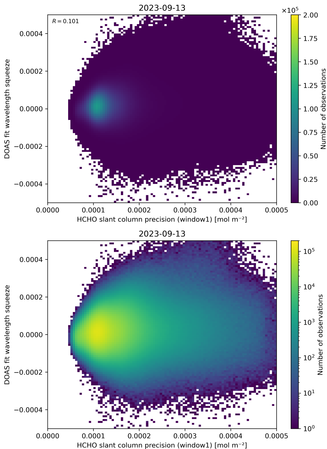
Figure 90: Scatter density plot of “HCHO slant column precision (window1)” against “DOAS fit wavelength squeeze” for 2023-09-12 to 2023-09-14.
