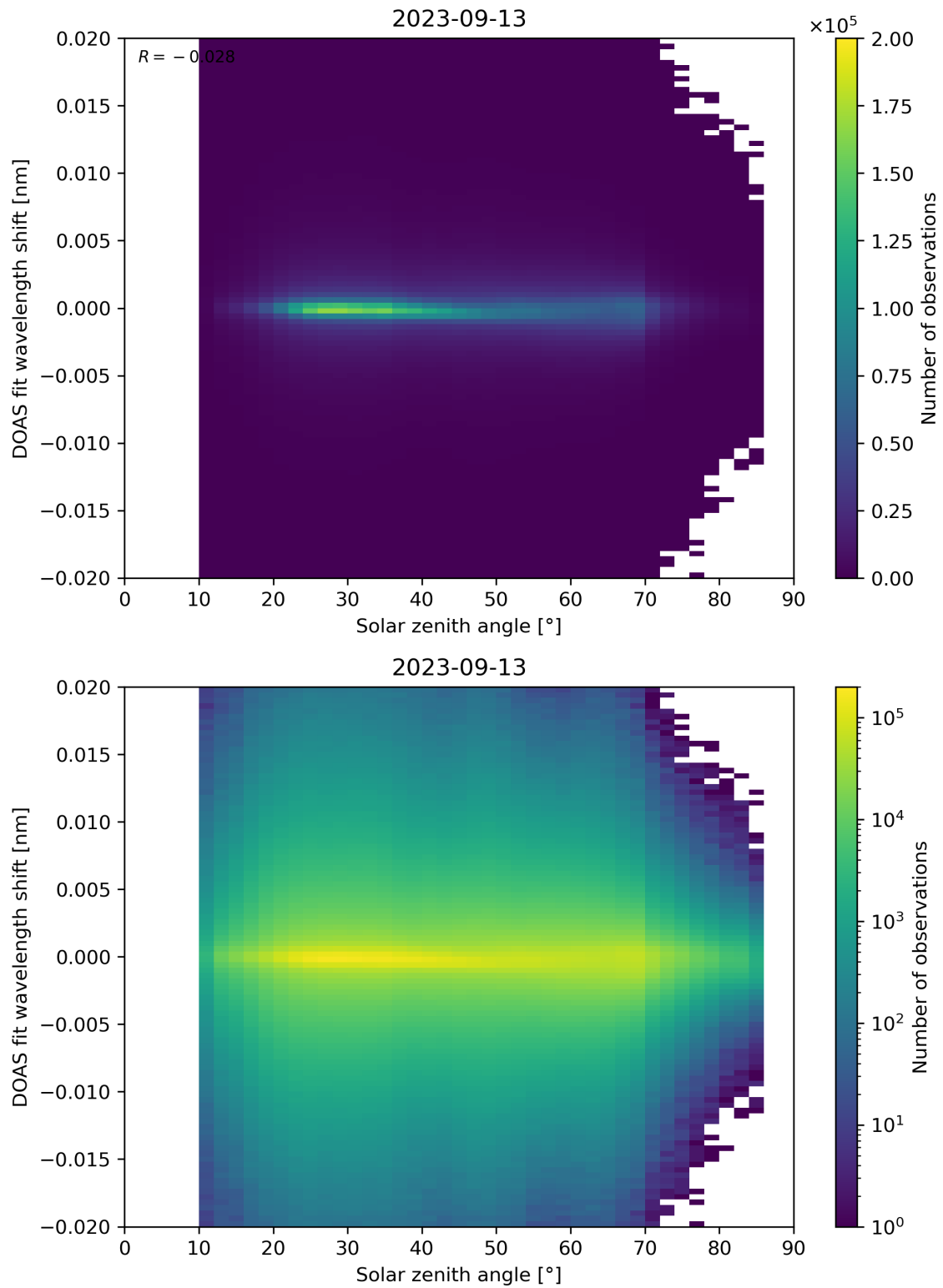
Figure 168: Scatter density plot of “Solar zenith angle” against “DOAS fit wavelength shift” for 2023-09-12 to 2023-09-14.
