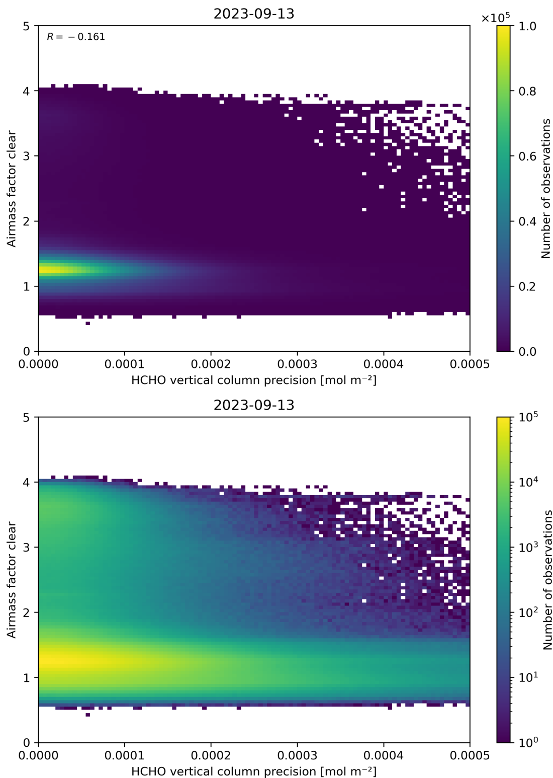
Figure 139: Scatter density plot of “HCHO vertical column precision” against “Airmass factor clear” for 2023-09-12 to 2023-09-14.
