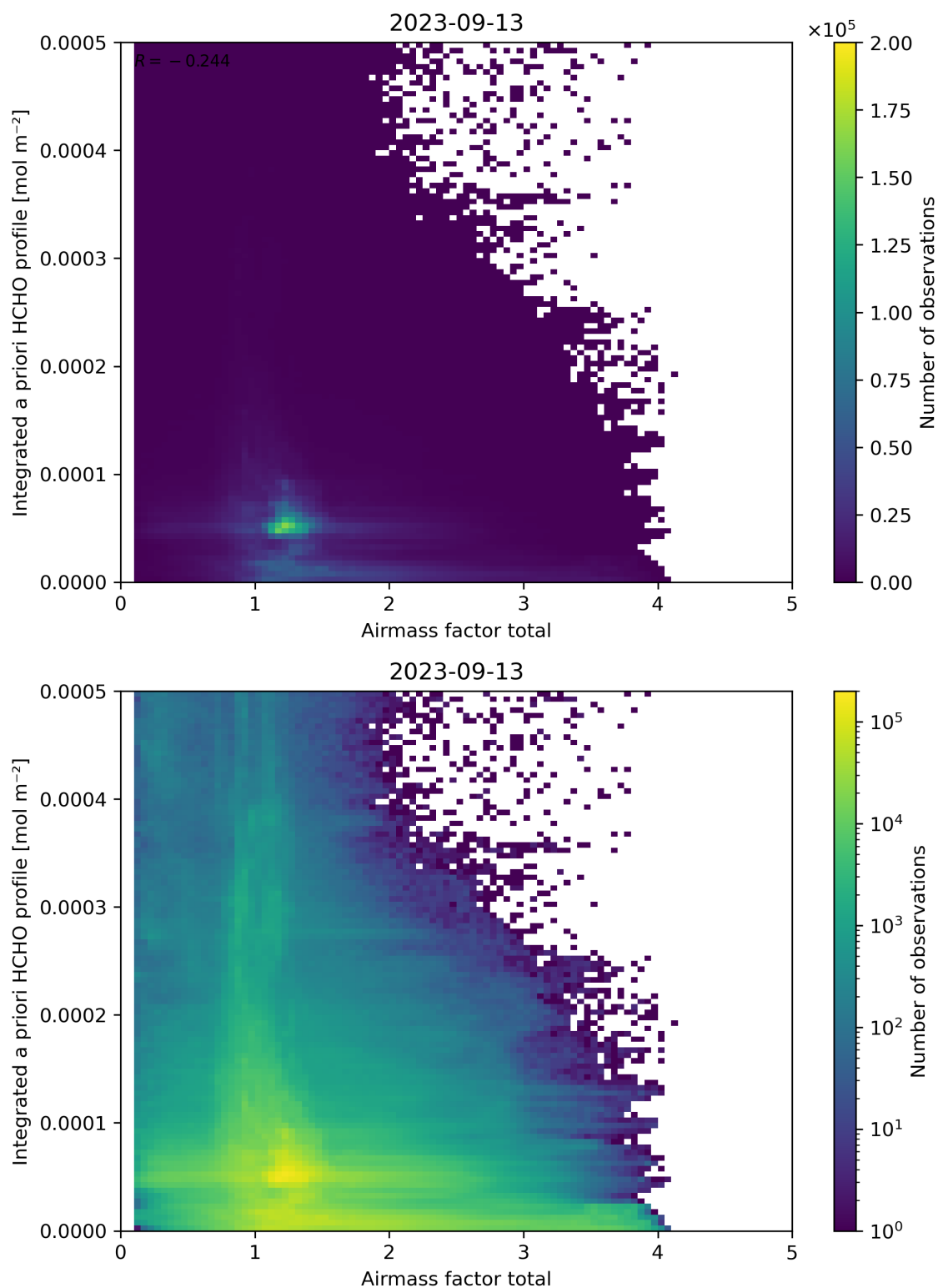
Figure 104: Scatter density plot of “Airmass factor total” against “Integrated a priori HCHO profile” for 2023-09-12 to 2023-09-14.
