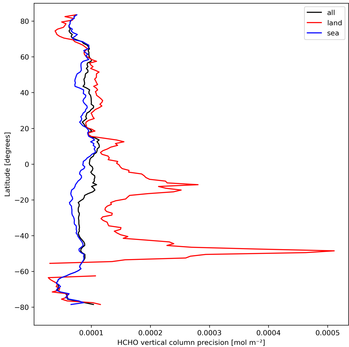
Figure 22: Zonal average of “HCHO vertical column precision” for 2023-09-12 to 2023-09-14.
