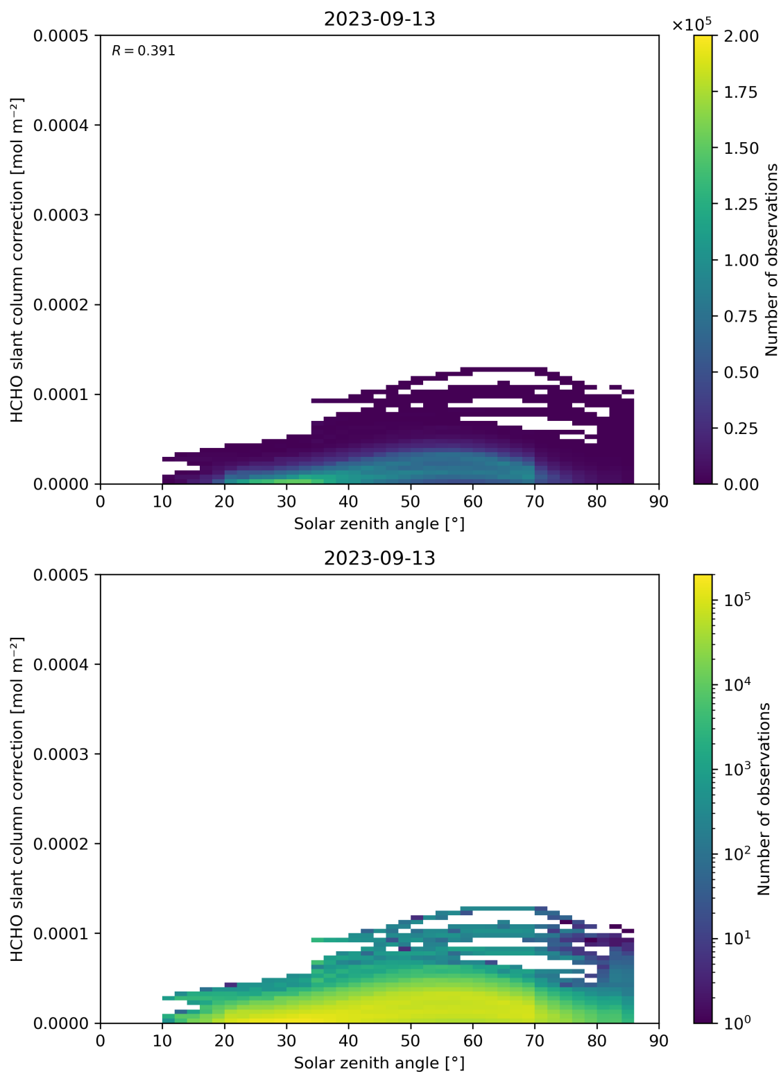
Figure 172: Scatter density plot of “Solar zenith angle” against “HCHO slant column correction” for 2023-09-12 to 2023-09-14.
