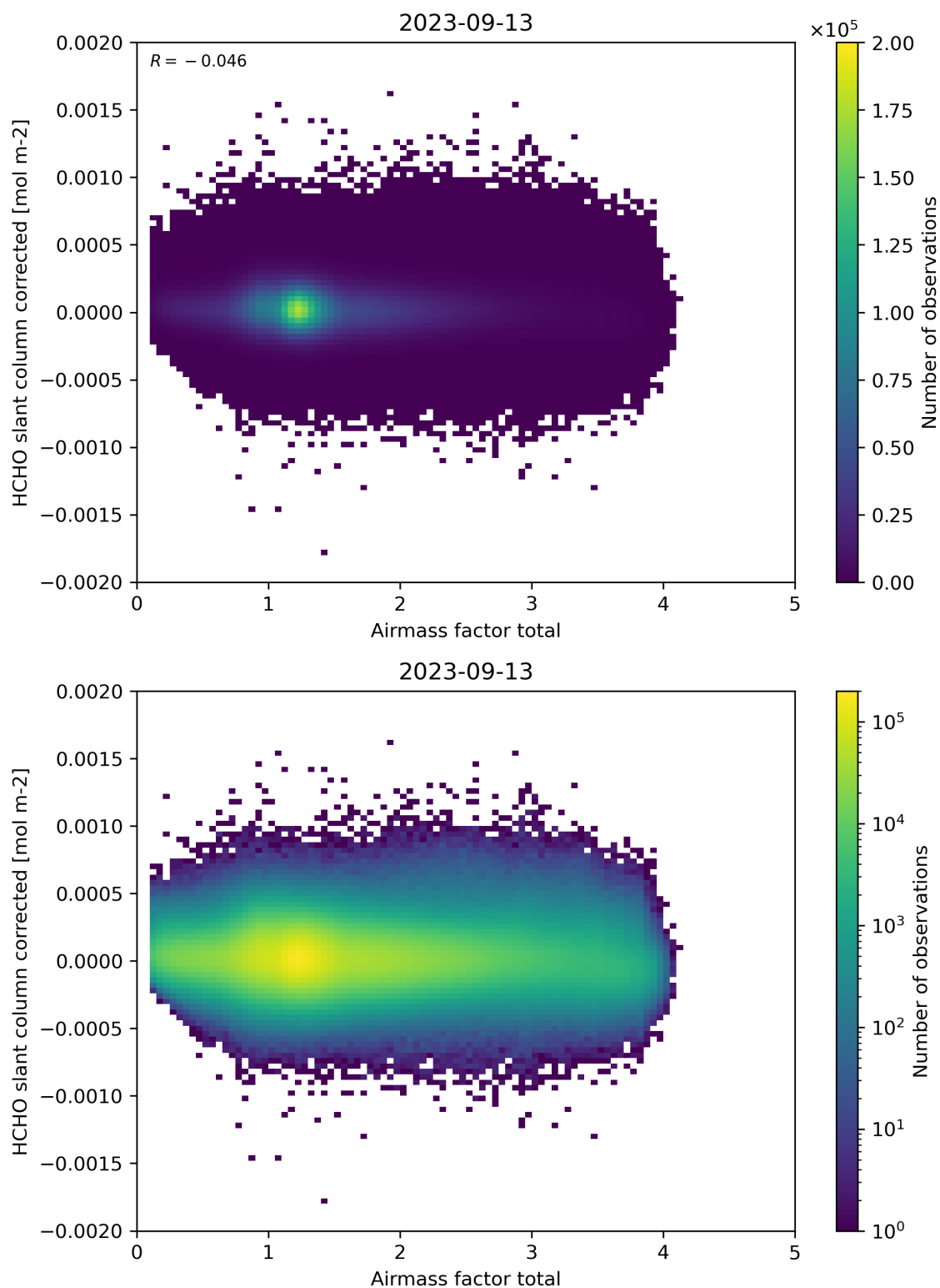
Figure 101: Scatter density plot of “Airmass factor total” against “HCHO slant column corrected” for 2023-09-12 to 2023-09-14.
