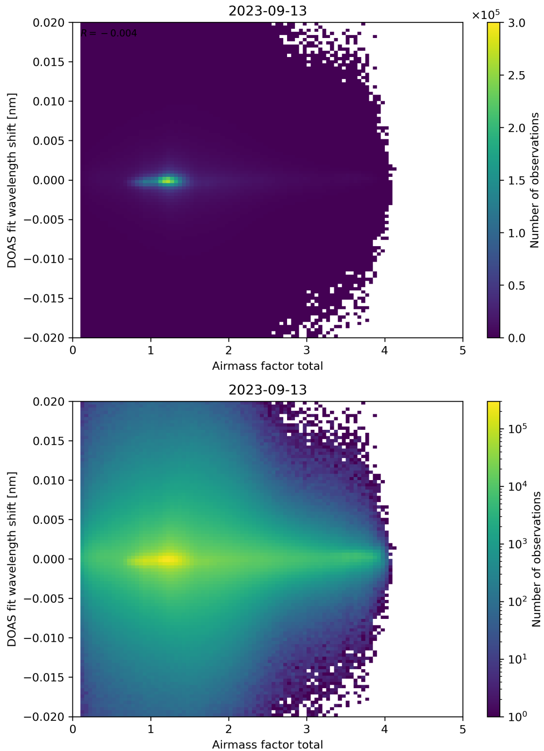
Figure 98: Scatter density plot of “Airmass factor total” against “DOAS fit wavelength shift” for 2023-09-12 to 2023-09-14.
