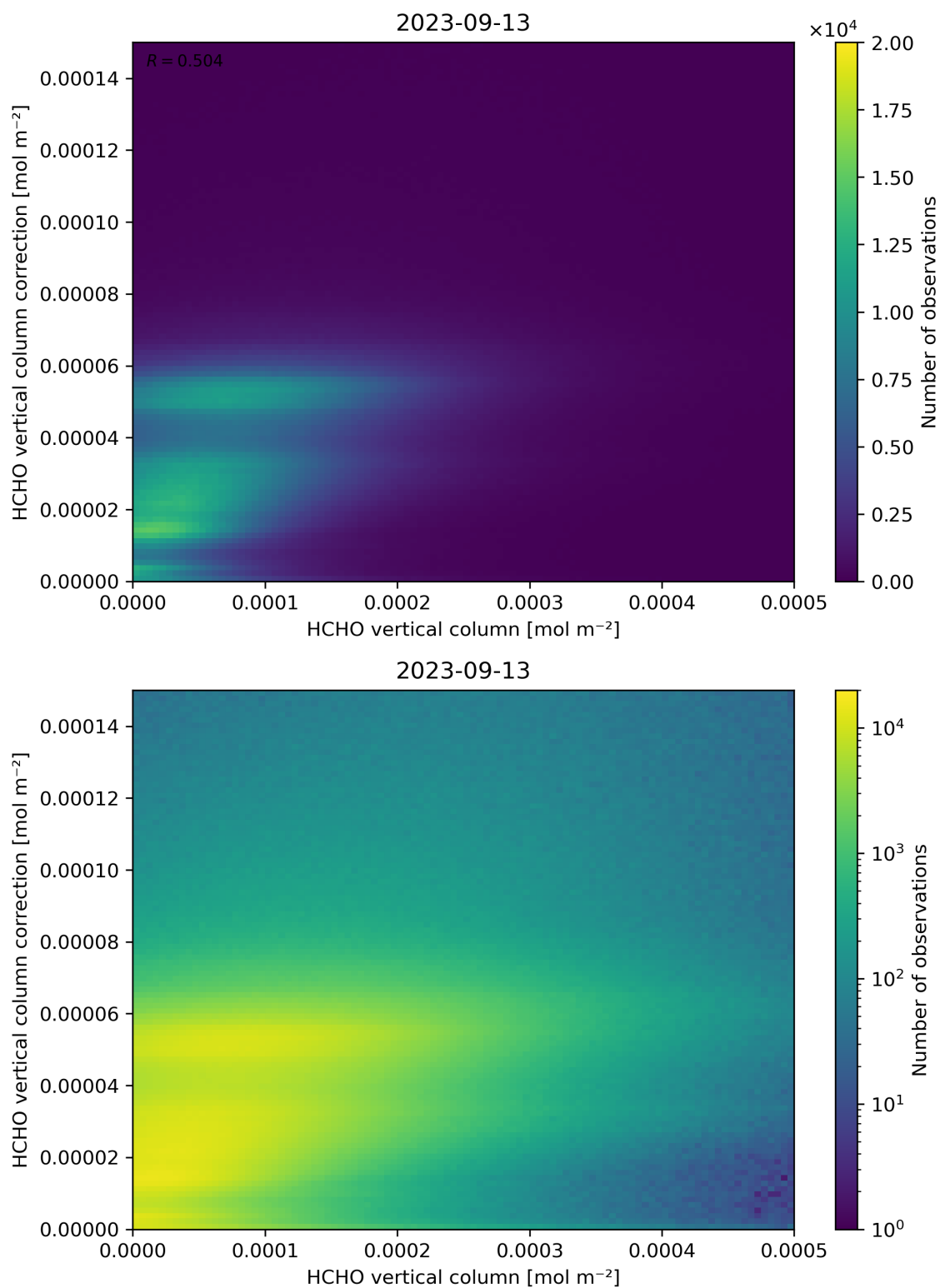
Figure 133: Scatter density plot of “HCHO vertical column” against “HCHO vertical column correction” for 2023-09-12 to 2023-09-14.
