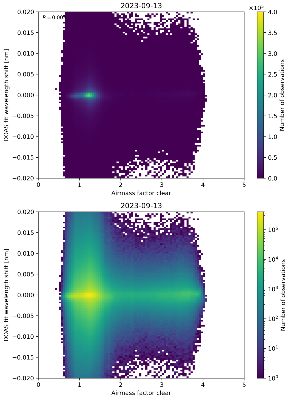
Figure 72: Scatter density plot of “Airmass factor clear” against “DOAS fit wavelength shift” for 2023-09-12 to 2023-09-14.
