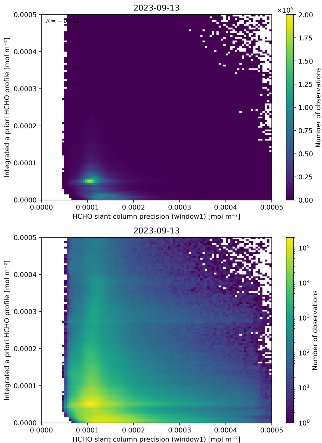
Figure 96: Scatter density plot of “HCHO slant column precision (window1)” against “Integrated a priori HCHO profile” for 2023-09-12 to 2023-09-14.
