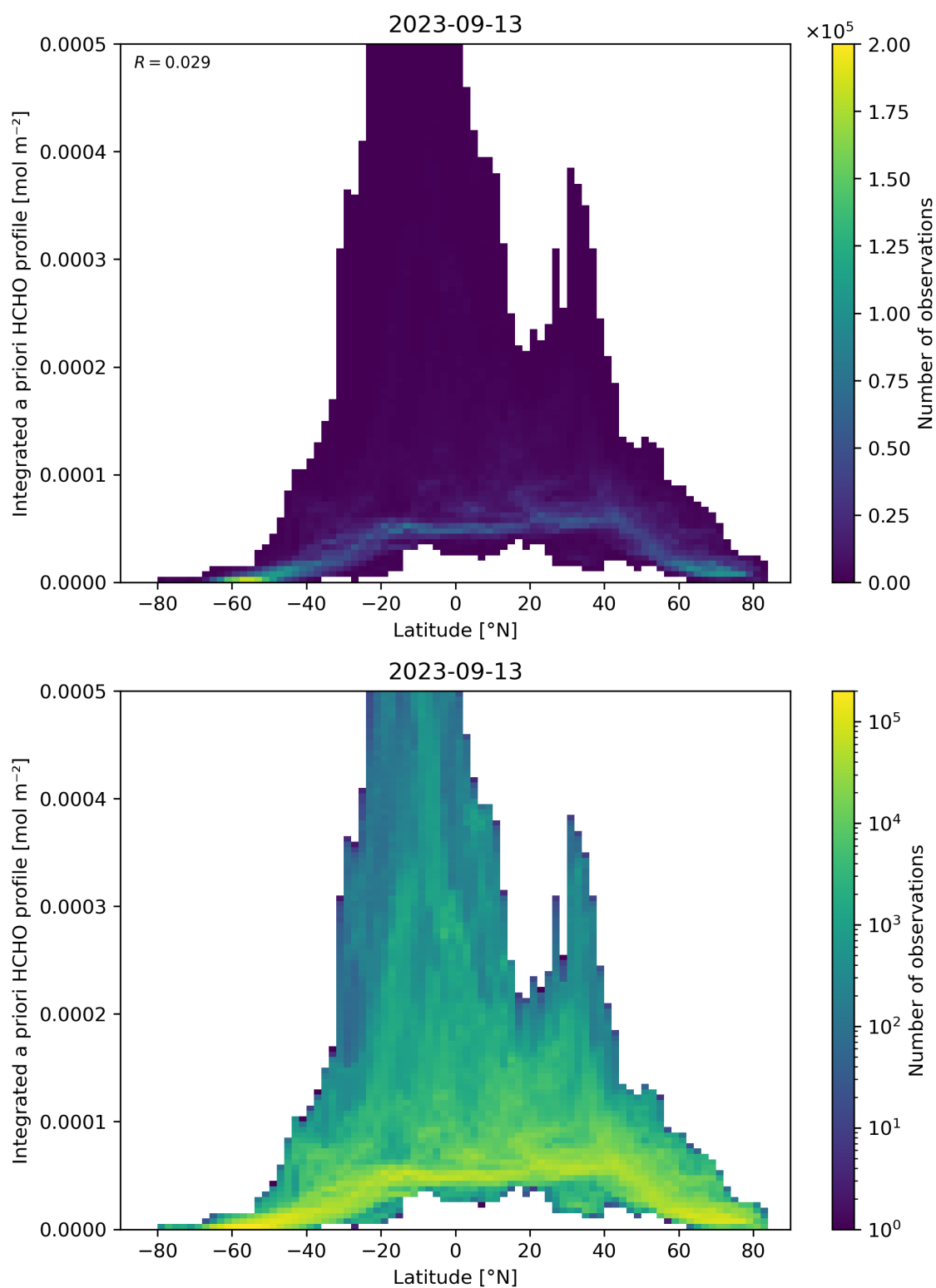
Figure 166: Scatter density plot of “Latitude” against “Integrated a priori HCHO profile” for 2023-09-12 to 2023-09-14.
