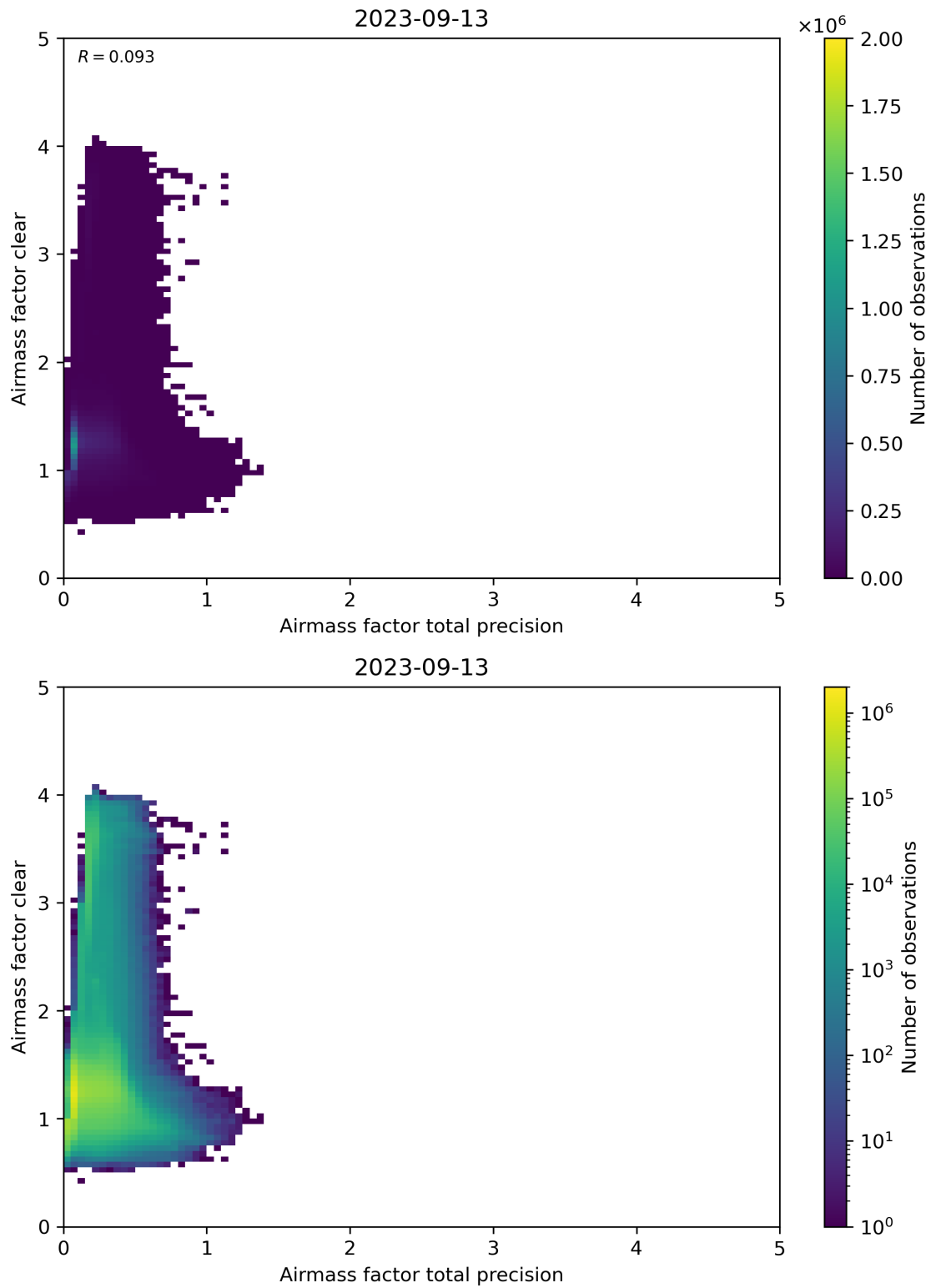
Figure 108: Scatter density plot of “Airmass factor total precision” against “Airmass factor clear” for 2023-09-12 to 2023-09-14.
