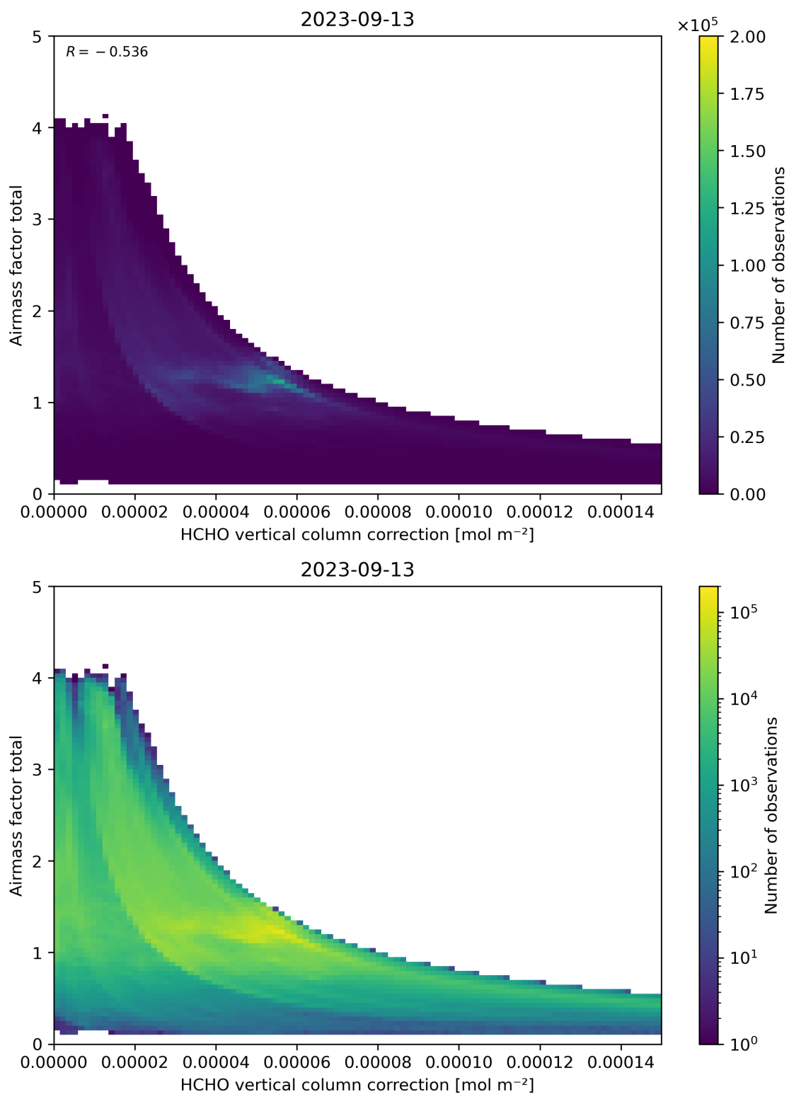
Figure 120: Scatter density plot of “HCHO vertical column correction” against “Airmass factor total” for 2023-09-12 to 2023-09-14.
