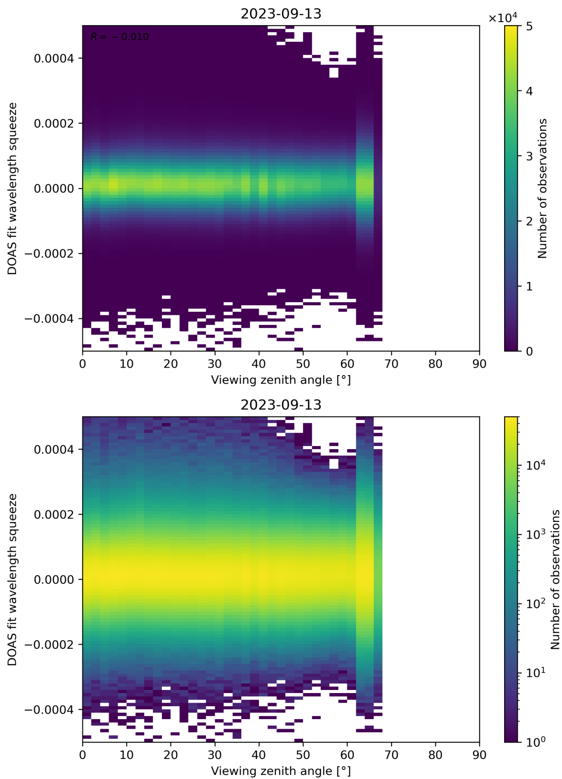
Figure 184: Scatter density plot of “Viewing zenith angle” against “DOAS fit wavelength squeeze” for 2023-09-12 to 2023-09-14.
