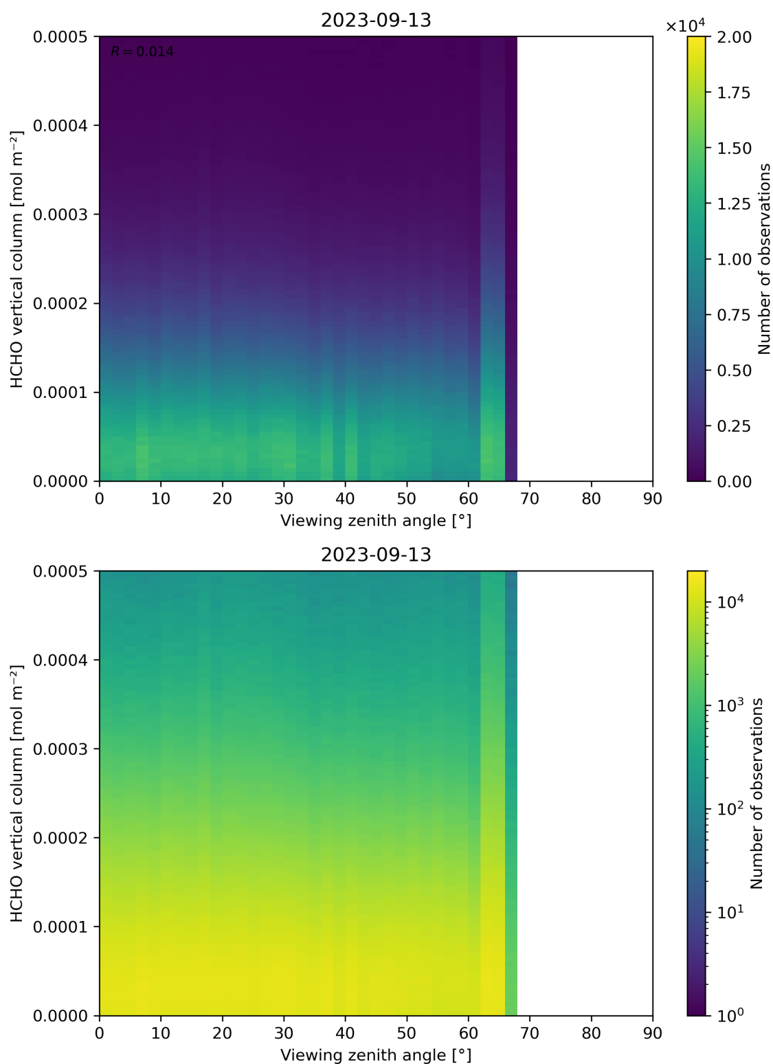
Figure 192: Scatter density plot of “Viewing zenith angle” against “HCHO vertical column” for 2023-09-12 to 2023-09-14.
