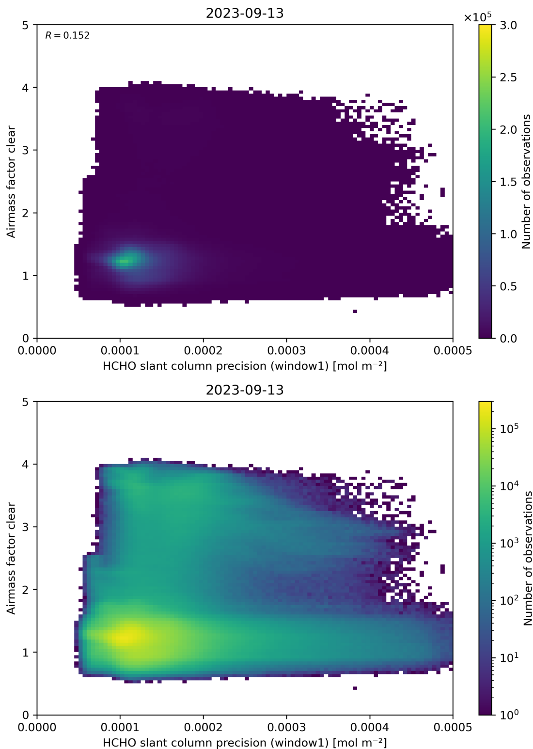
Figure 91: Scatter density plot of “HCHO slant column precision (window1)” against “Airmass factor clear” for 2023-09-12 to 2023-09-14.
