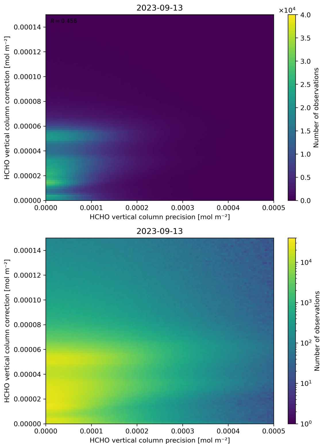
Figure 146: Scatter density plot of “HCHO vertical column precision” against “HCHO vertical column correction” for 2023-09-12 to 2023-09-14.
