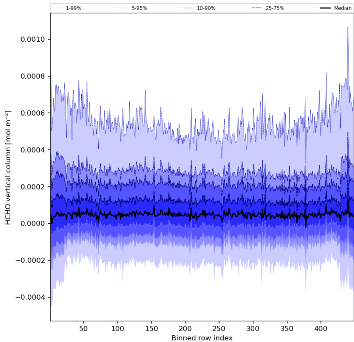
Figure 49: Along track statistics of “HCHO vertical column” for 2023-09-12 to 2023-09-14
