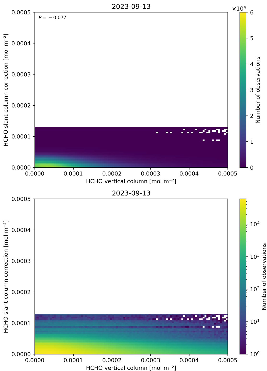
Figure 128: Scatter density plot of “HCHO vertical column” against “HCHO slant column correction” for 2023-09-12 to 2023-09-14.
