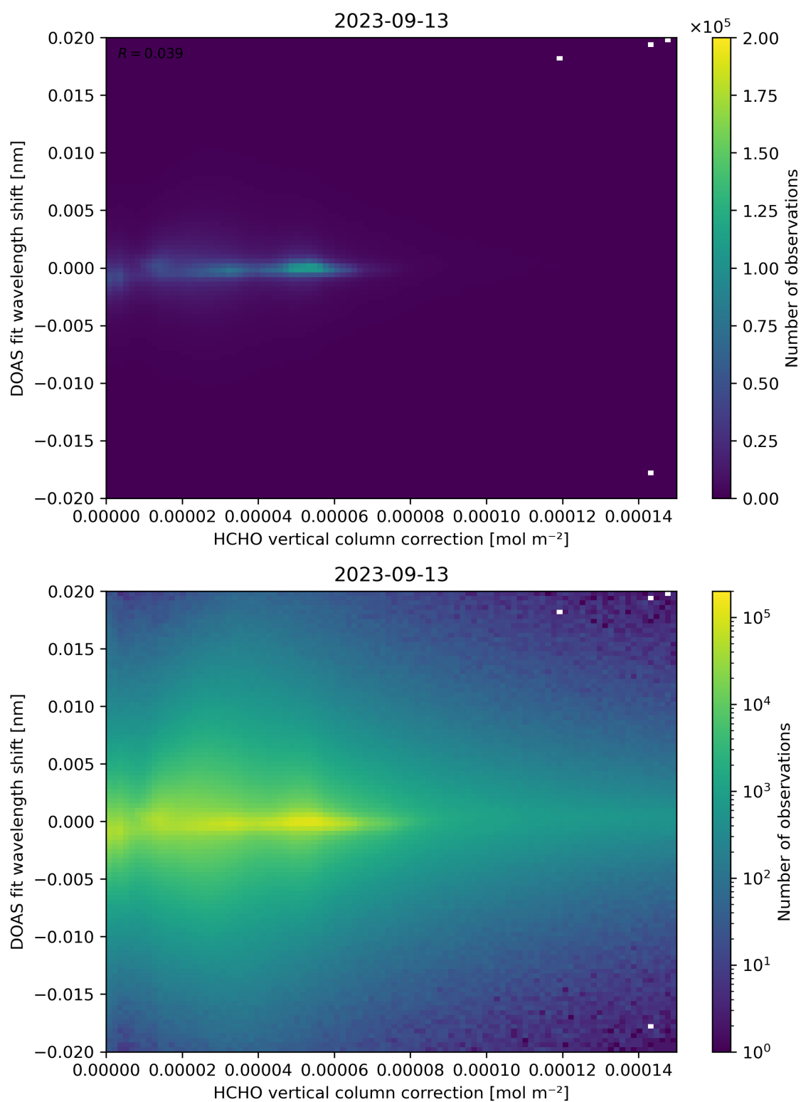
Figure 113: Scatter density plot of “HCHO vertical column correction” against “DOAS fit wavelength shift” for 2023-09-12 to 2023-09-14.
