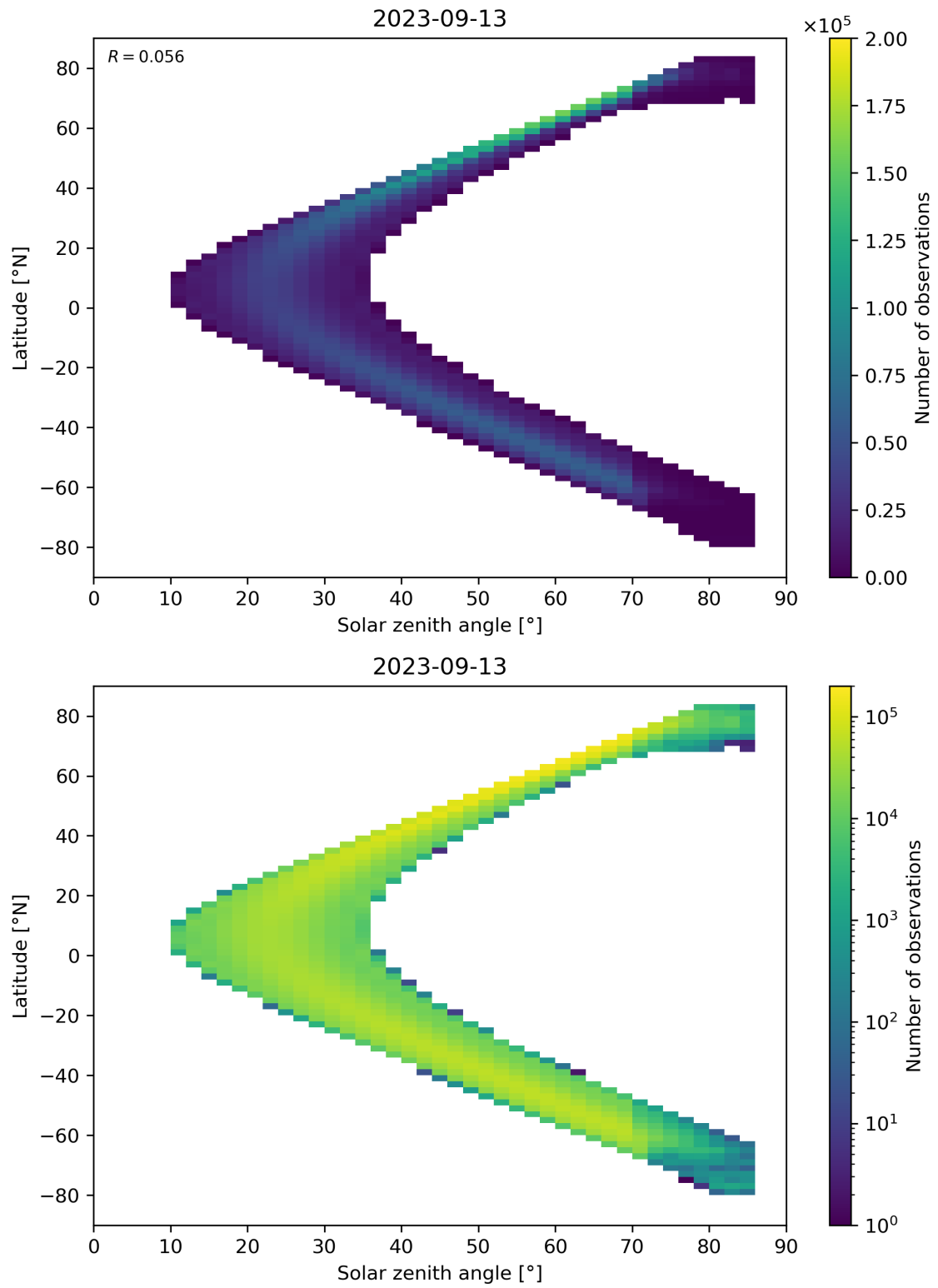
Figure 181: Scatter density plot of “Solar zenith angle” against “Latitude” for 2023-09-12 to 2023-09-14.
