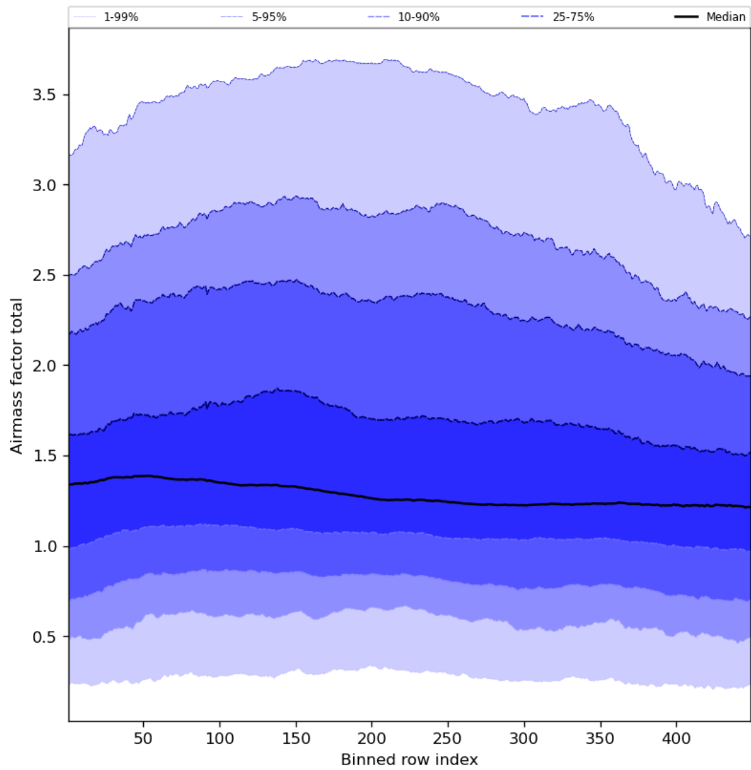
Figure 54: Along track statistics of “Airmass factor total” for 2023-09-12 to 2023-09-14
