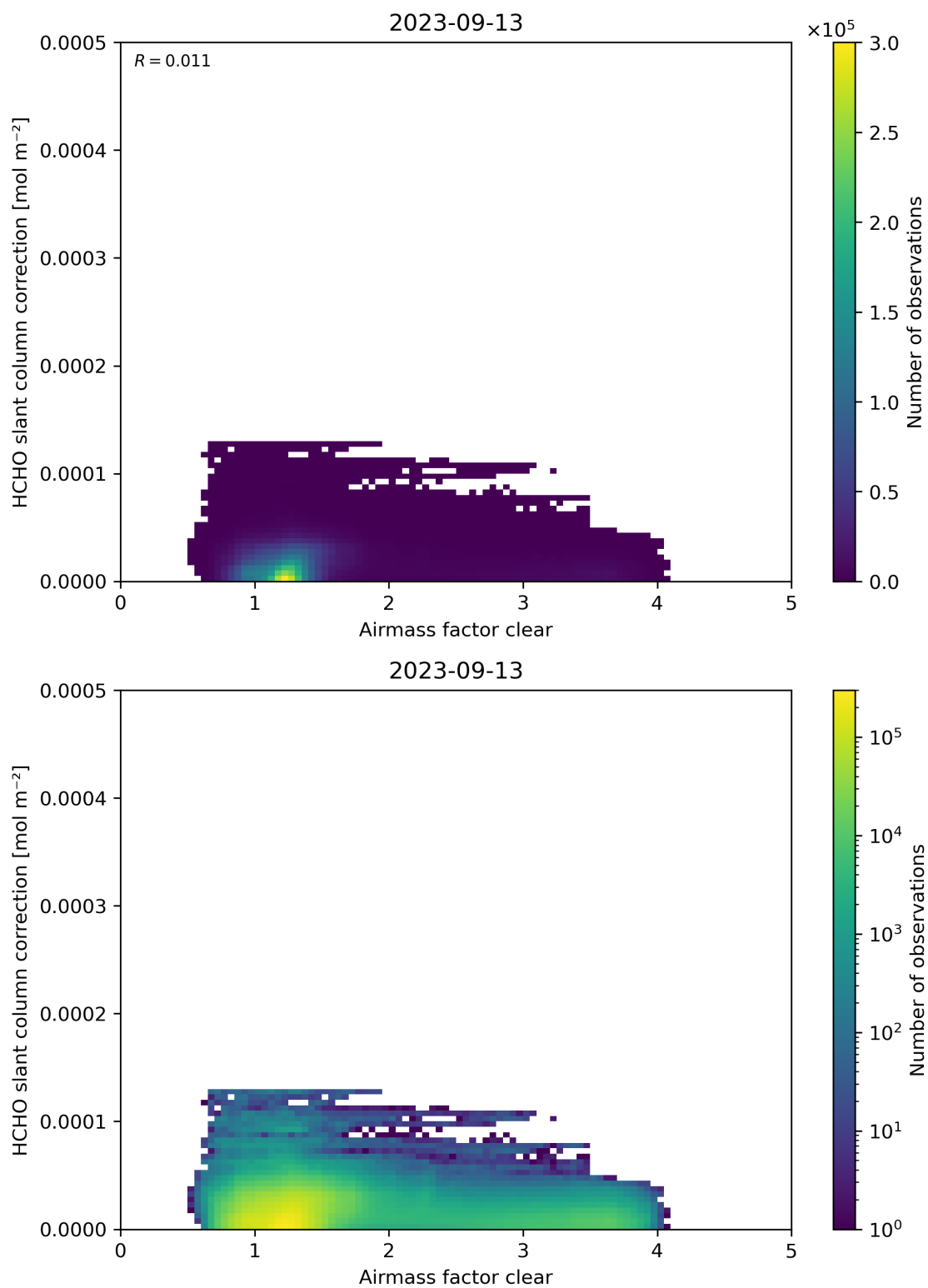
Figure 75: Scatter density plot of “Air mass factor clear” against “HCHO slant column correction” for 2023-09-12 to 2023-09-14.
