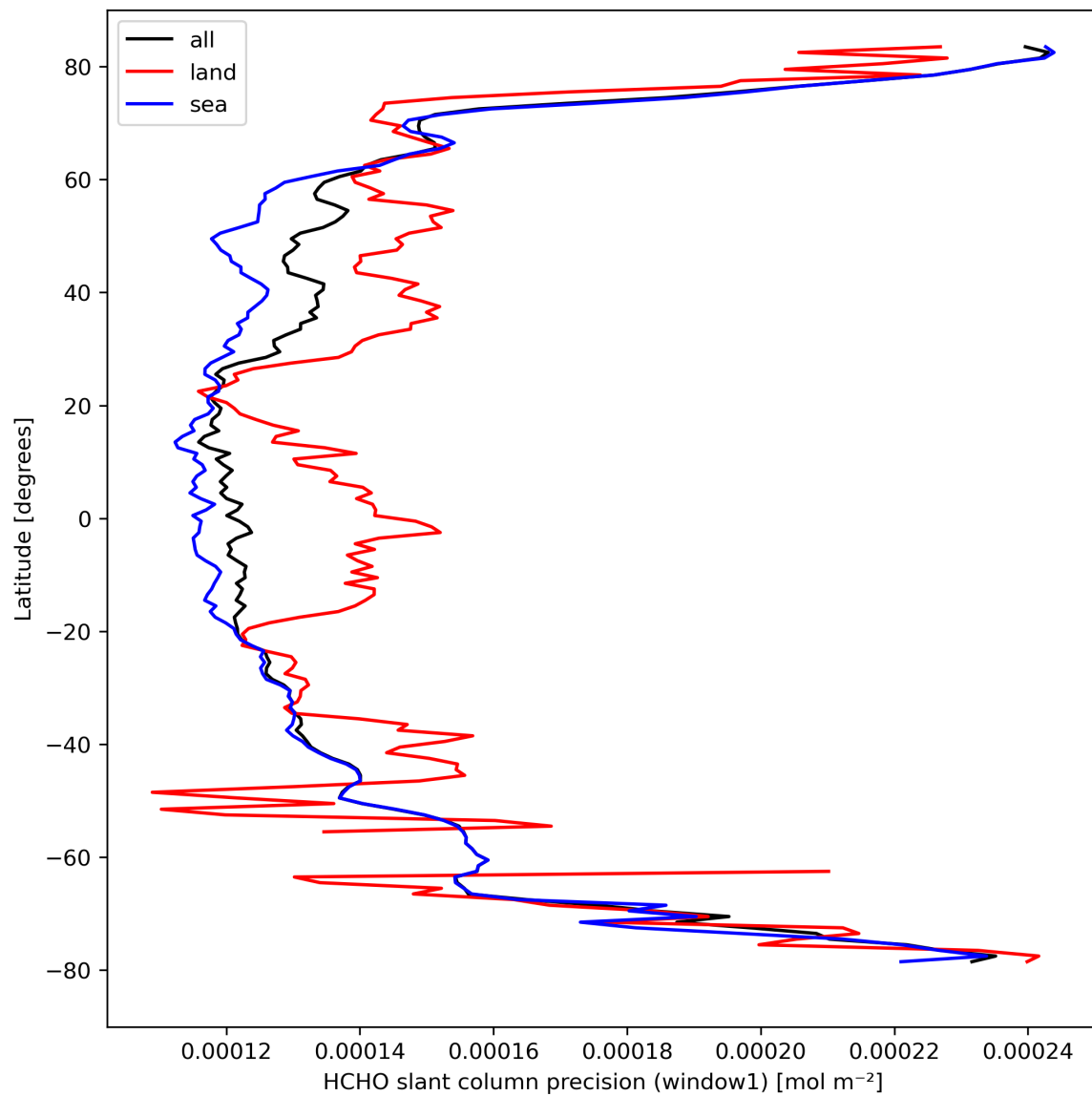
Figure 25: Zonal average of “HCHO slant column precision (window1)” for 2023-09-12 to 2023-09-14.
