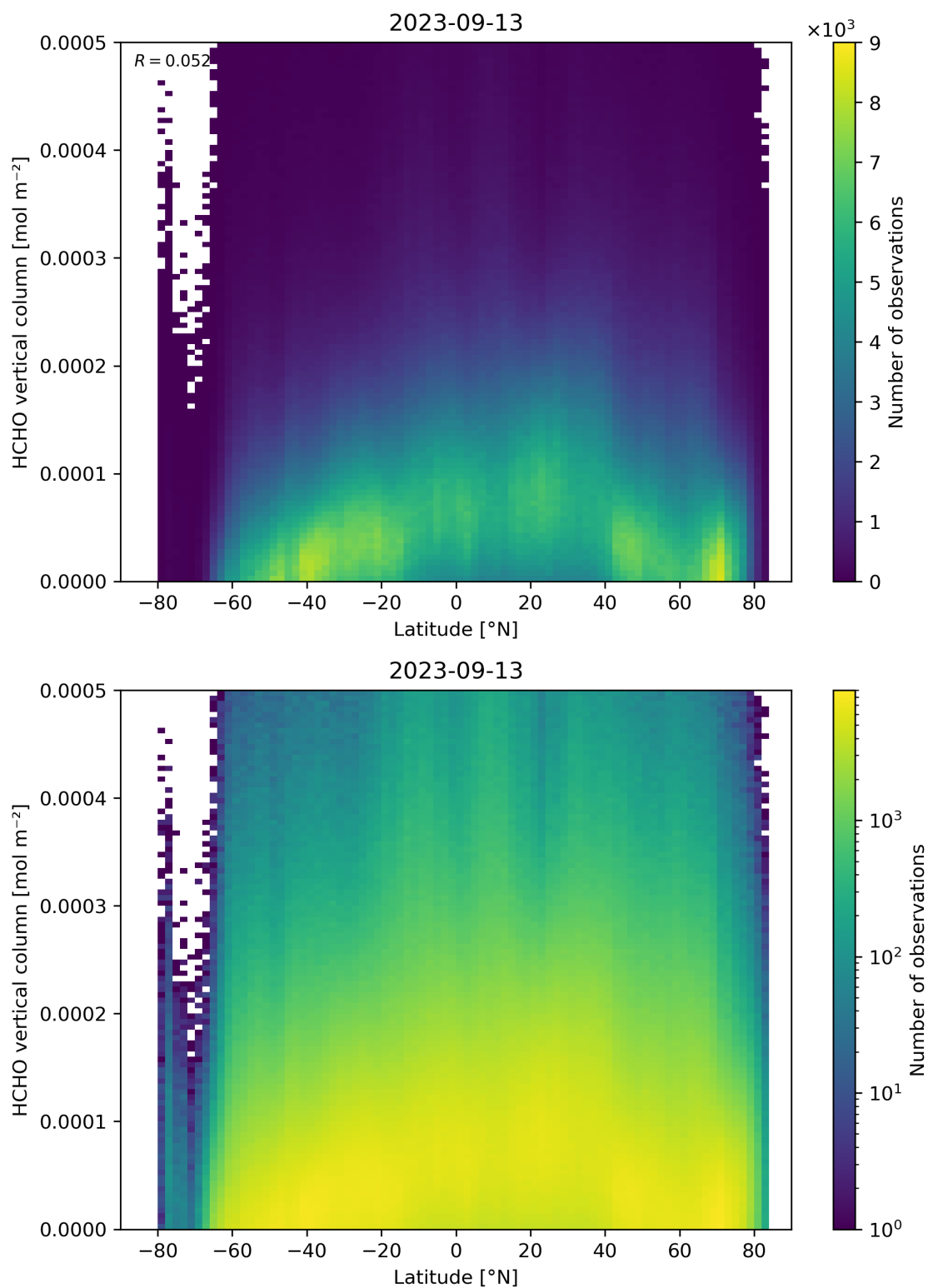
Figure 163: Scatter density plot of “Latitude” against “HCHO vertical column” for 2023-09-12 to 2023-09-14.
