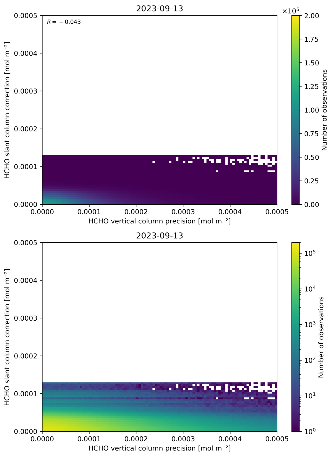
Figure 141: Scatter density plot of “HCHO vertical column precision” against “HCHO slant column correction” for 2023-09-12 to 2023-09-14.
