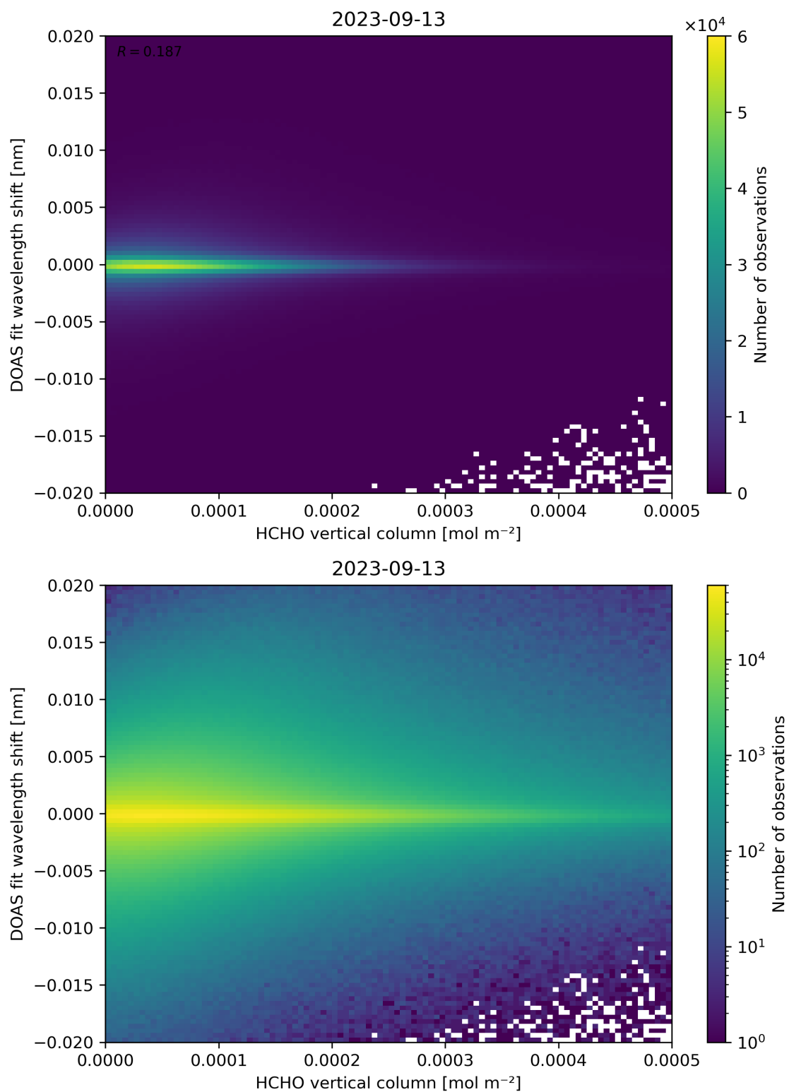
Figure 124: Scatter density plot of “HCHO vertical column” against “DOAS fit wavelength shift” for 2023-09-12 to 2023-09-14.
