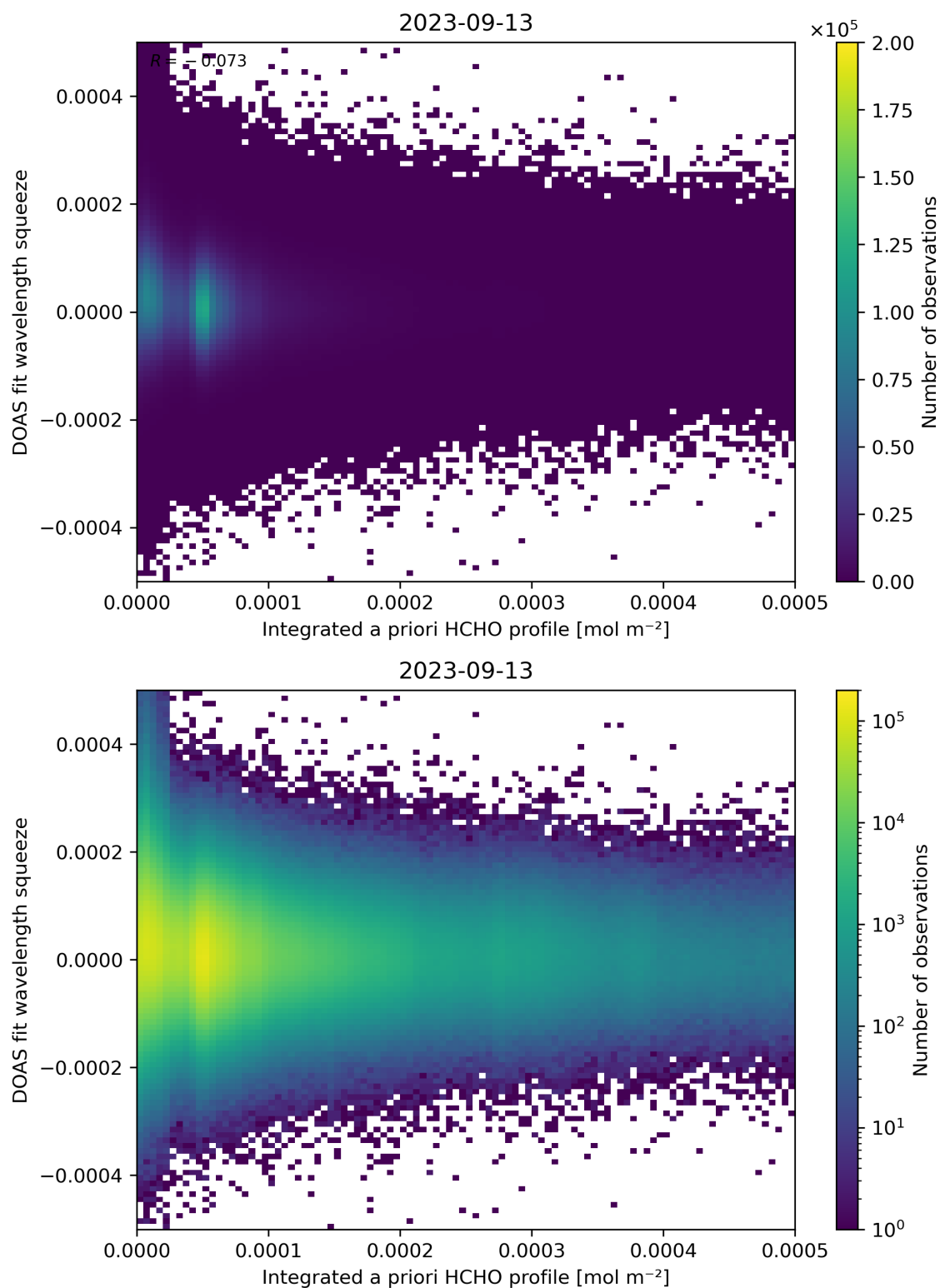
Figure 150: Scatter density plot of “Integrated a priori HCHO profile” against “DOAS fit wavelength squeeze” for 2023-09-12 to 2023-09-14.
