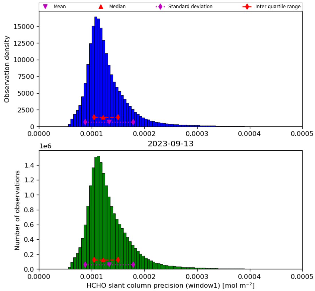
Figure 39: Histogram of “HCHO slant column precision (window1)” for 2023-09-12 to 2023-09-14
