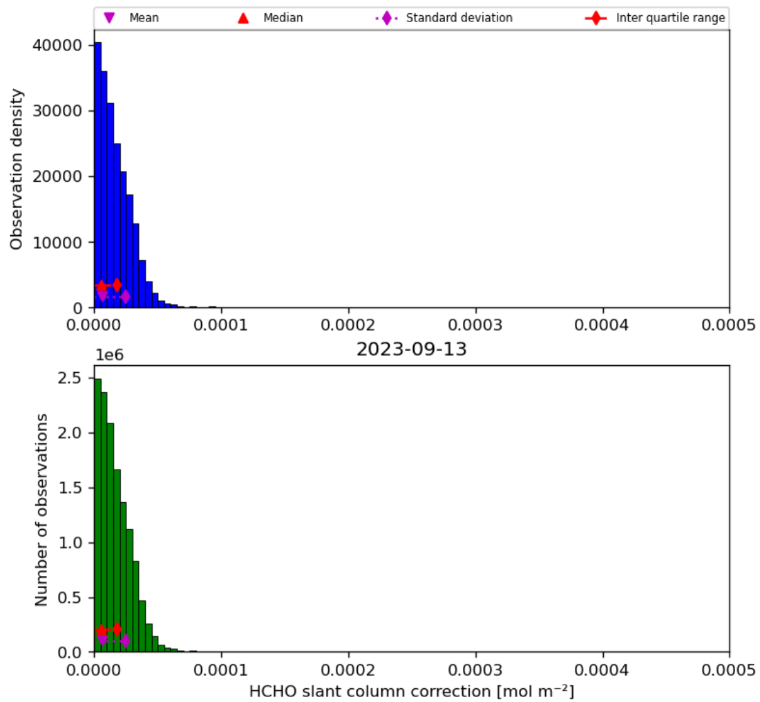
Figure 47: Histogram of “HCHO slant column correction” for 2023-09-12 to 2023-09-14
