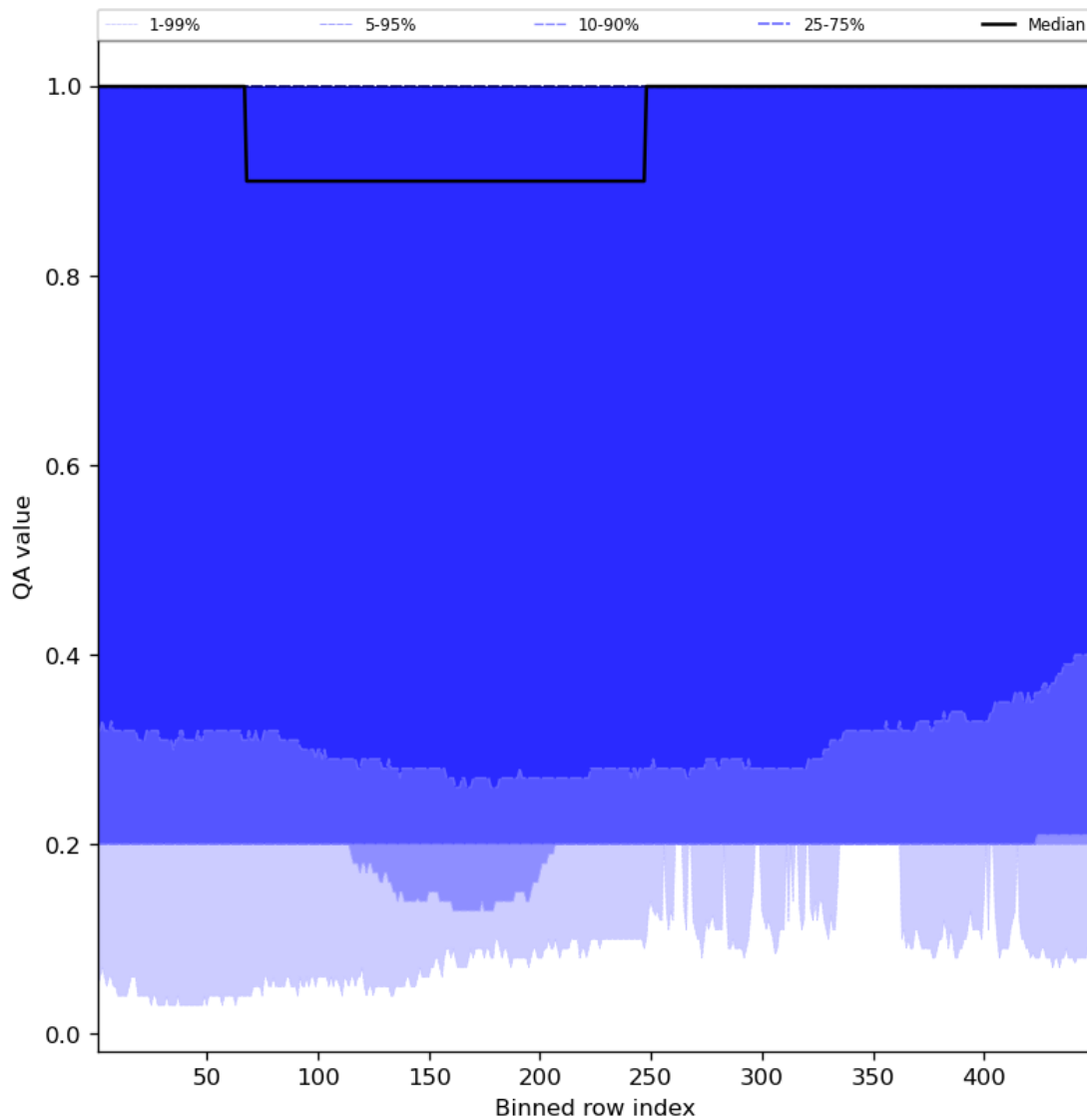
Figure 48: Along track statistics of “QA value” for 2023-09-12 to 2023-09-14
