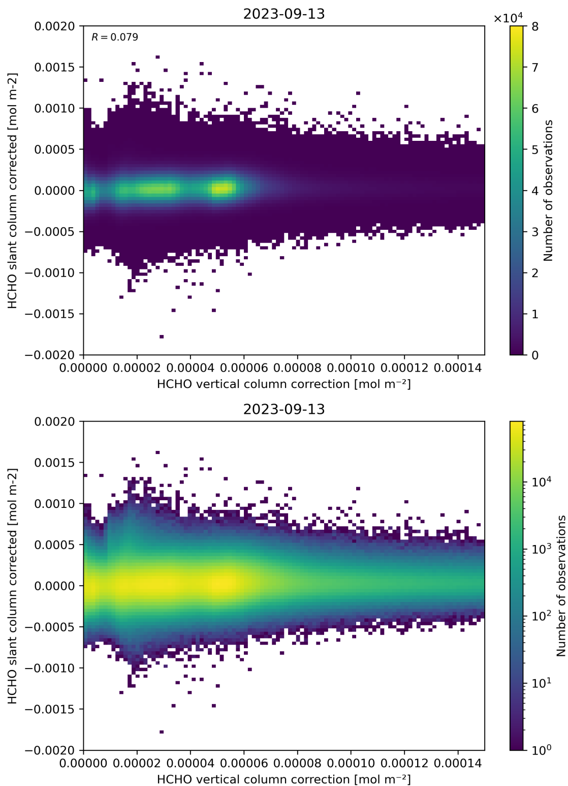
Figure 116: Scatter density plot of “HCHO vertical column correction” against “HCHO slant column corrected” for 2023-09-12 to 2023-09-14.
