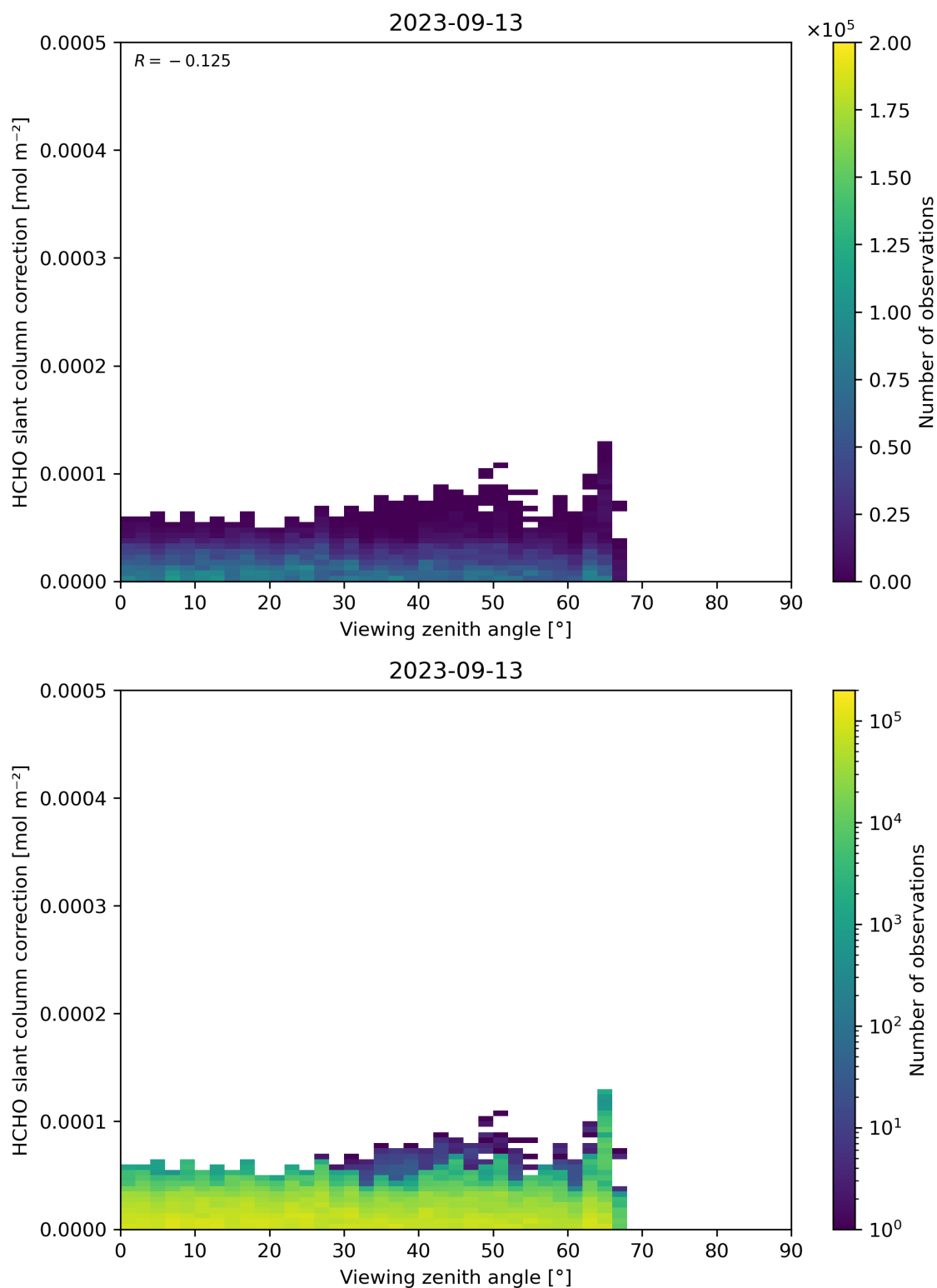
Figure 187: Scatter density plot of “Viewing zenith angle” against “HCHO slant column correction” for 2023-09-12 to 2023-09-14.
