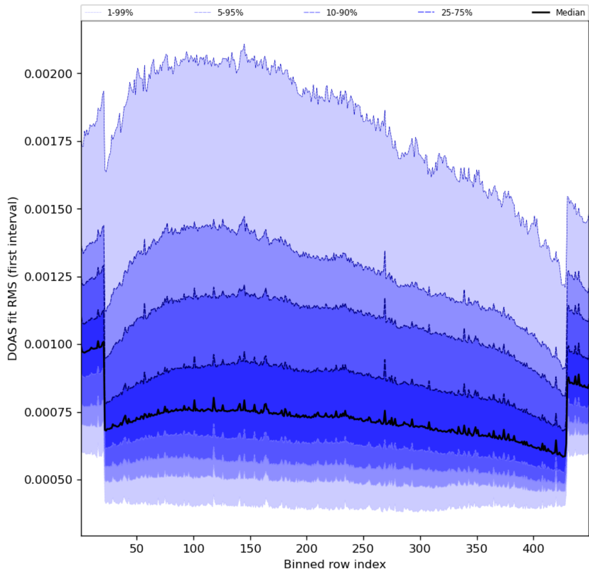
Figure 60: Along track statistics of “DOAS fit RMS (first interval)” for 2023-09-12 to 2023-09-14
