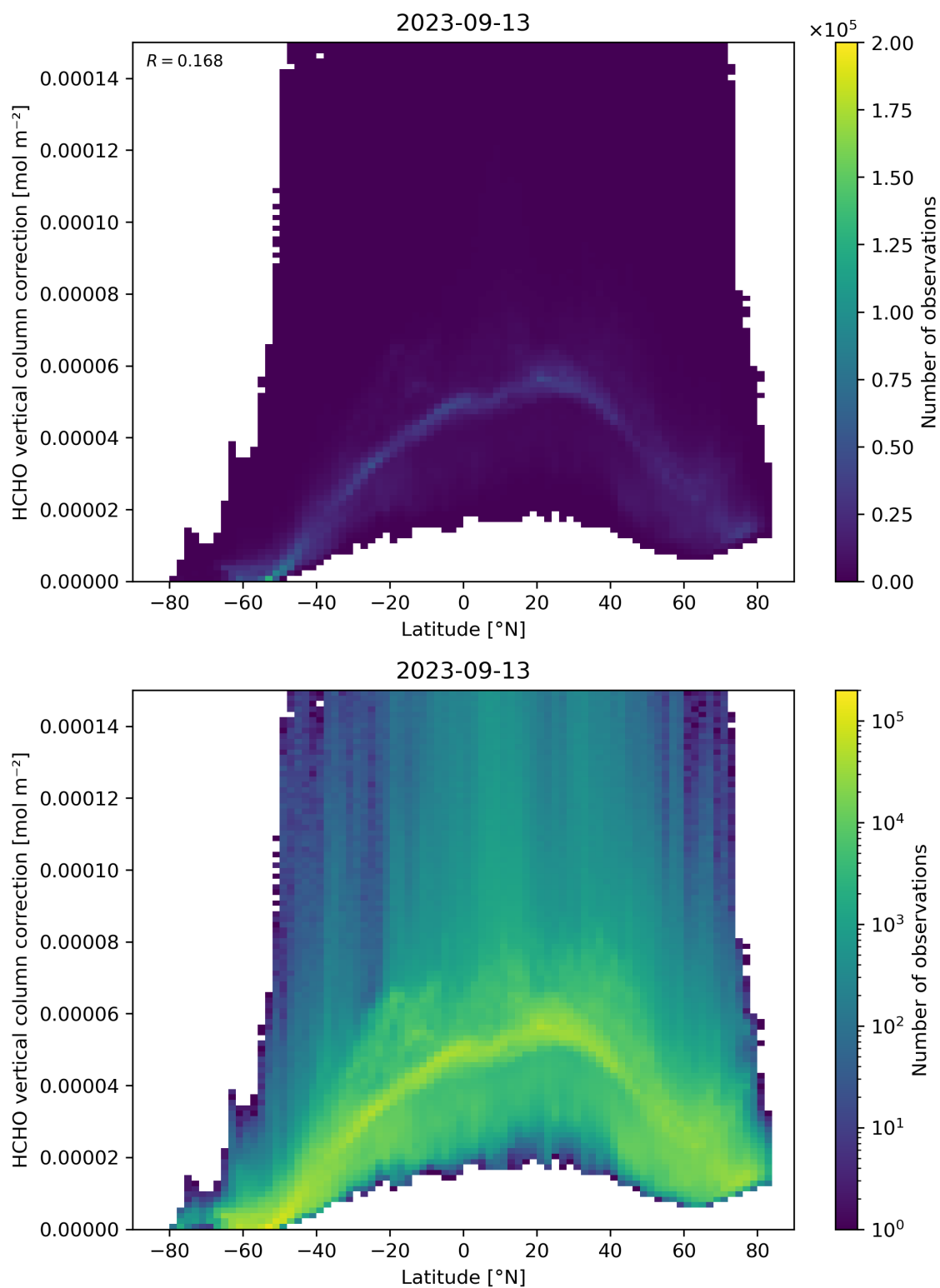
Figure 164: Scatter density plot of “Latitude” against “HCHO vertical column correction” for 2023-09-12 to 2023-09-14.
