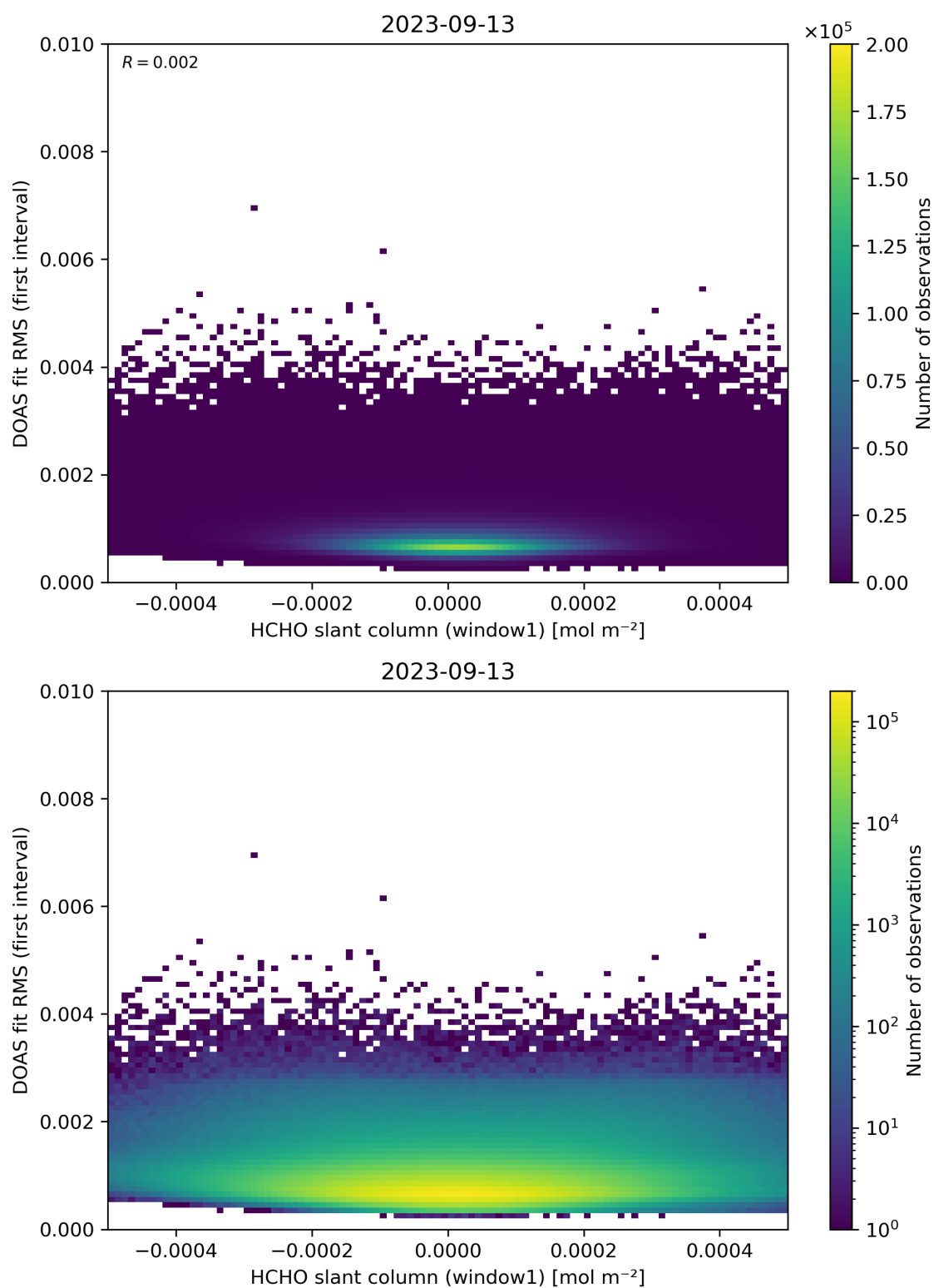
Figure 78: Scatter density plot of “HCHO slant column (window1)” against “DOAS fit RMS (first interval)” for 2023-09-12 to 2023-09-14.
