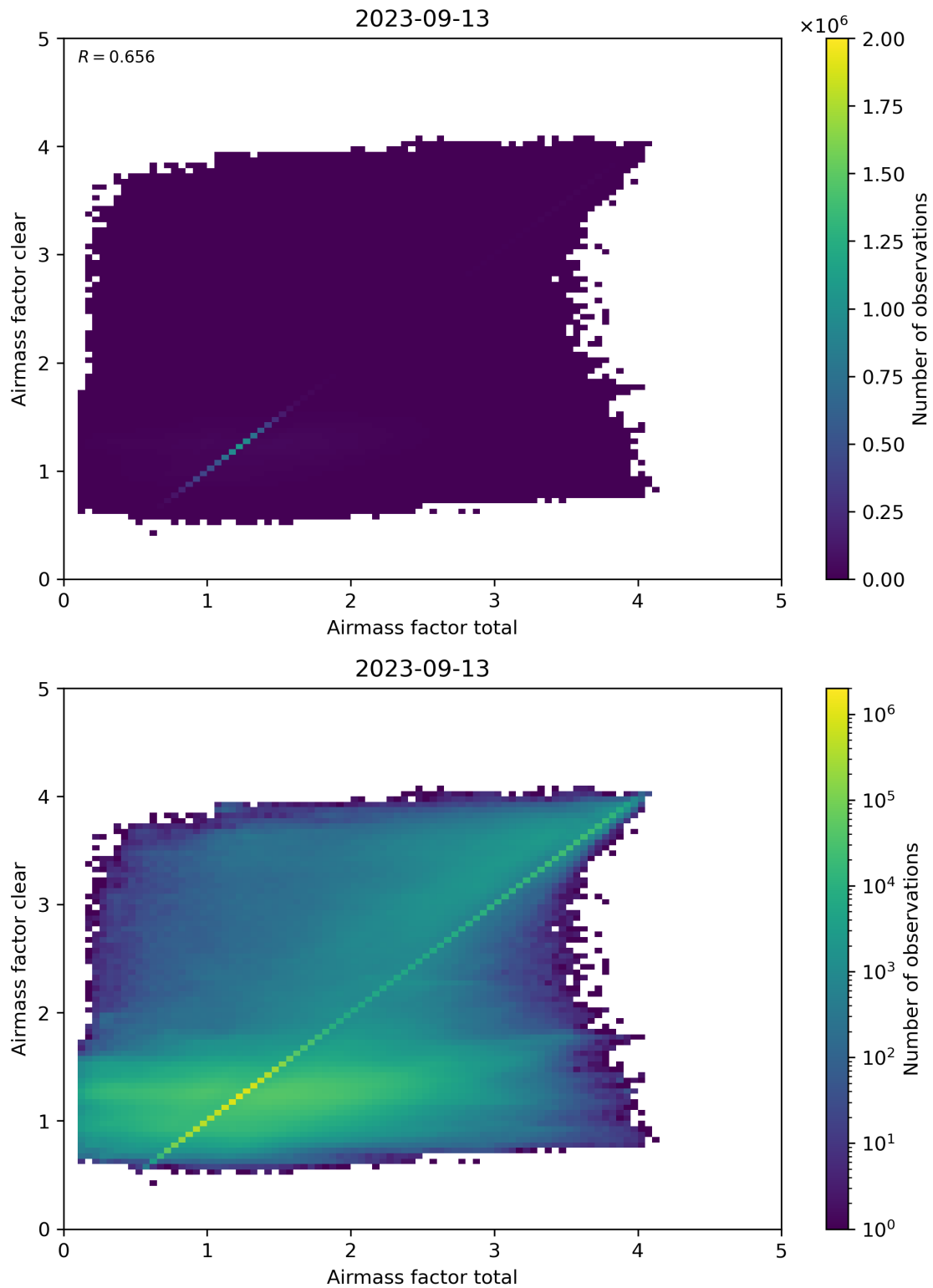
Figure 100: Scatter density plot of “Airmass factor total” against “Airmass factor clear” for 2023-09-12 to 2023-09-14.
