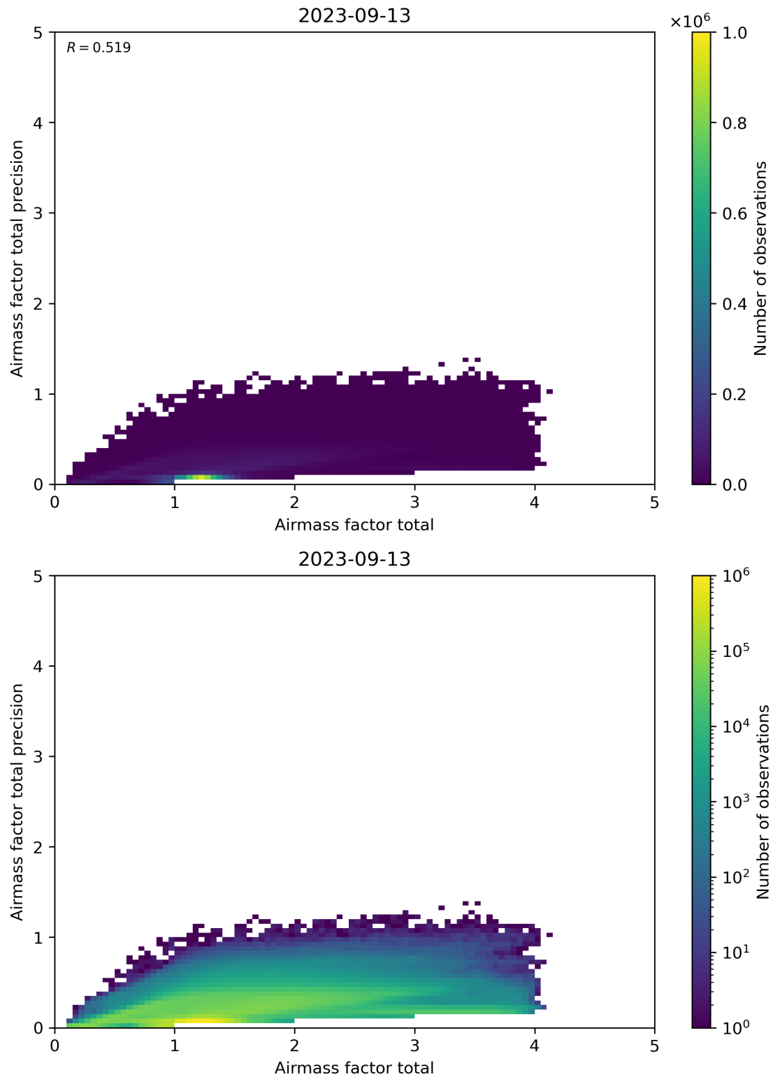
Figure 103: Scatter density plot of “Airmass factor total” against “Airmass factor total precision” for 2023-09-12 to 2023-09-14.
