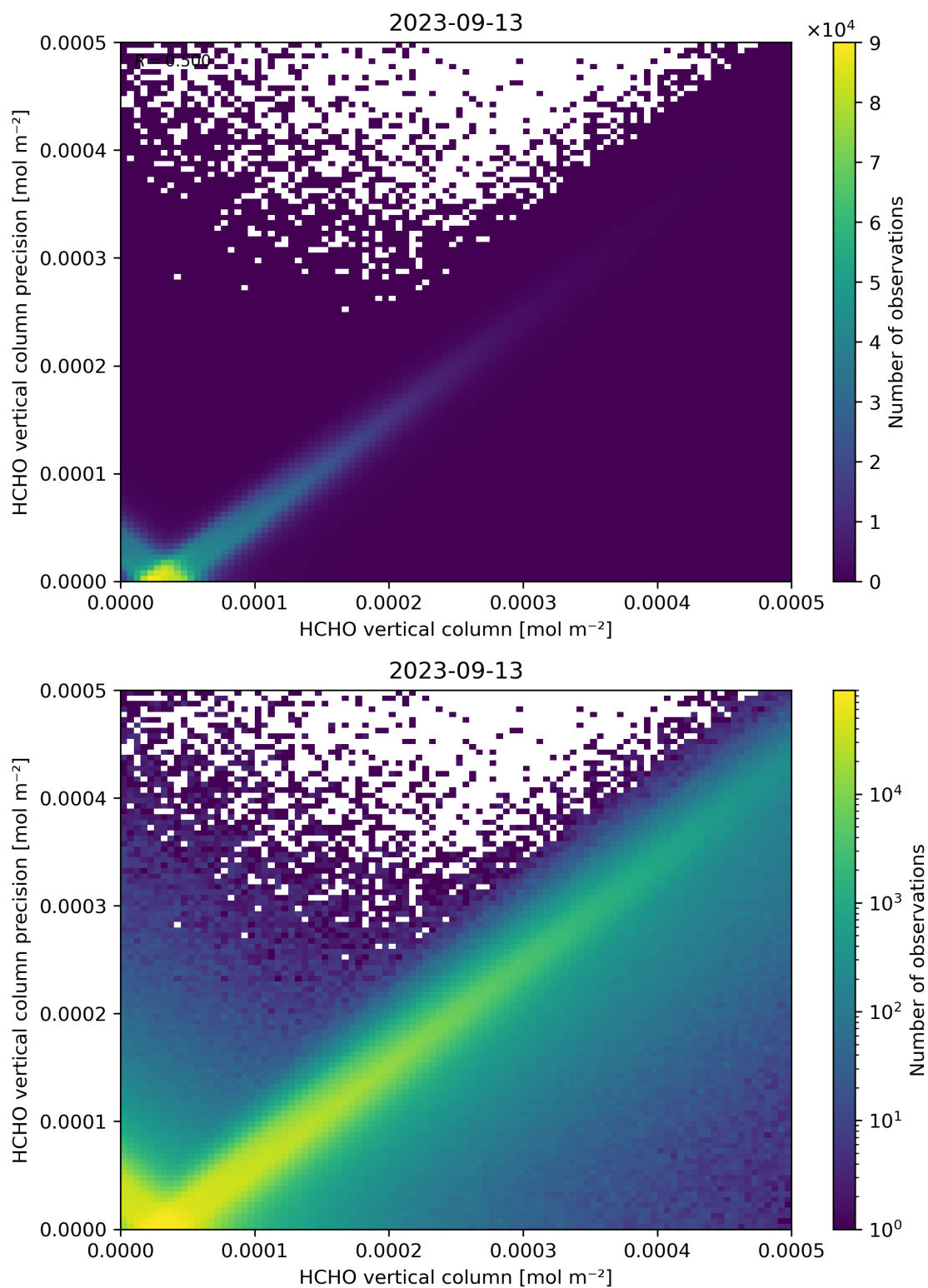
Figure 134: Scatter density plot of “HCHO vertical column” against “HCHO vertical column precision” for 2023-09-12 to 2023-09-14.
