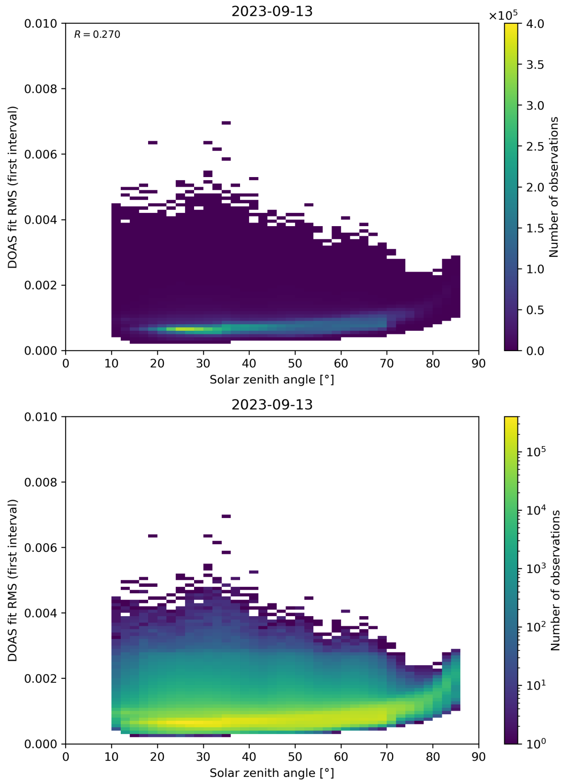
Figure 167: Scatter density plot of “Solar zenith angle” against “DOAS fit RMS (first interval)” for 2023-09-12 to 2023-09-14.
