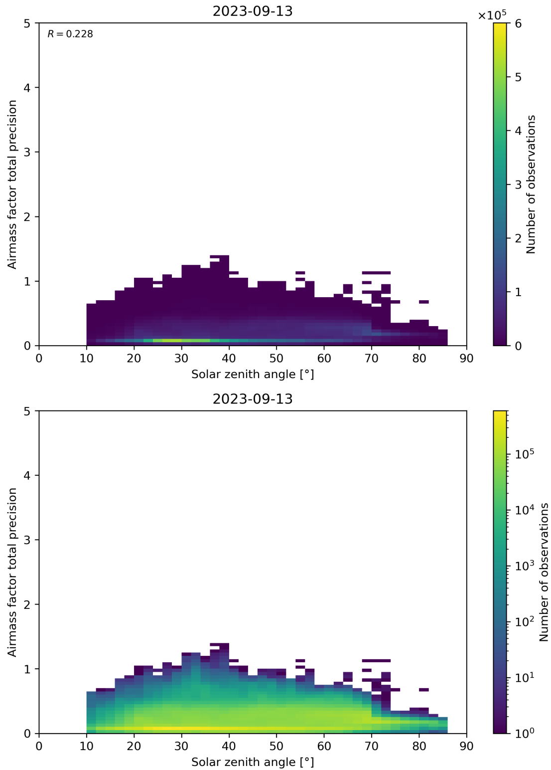
Figure 176: Scatter density plot of “Solar zenith angle” against “Airmass factor total precision” for 2023-09-12 to 2023-09-14.
