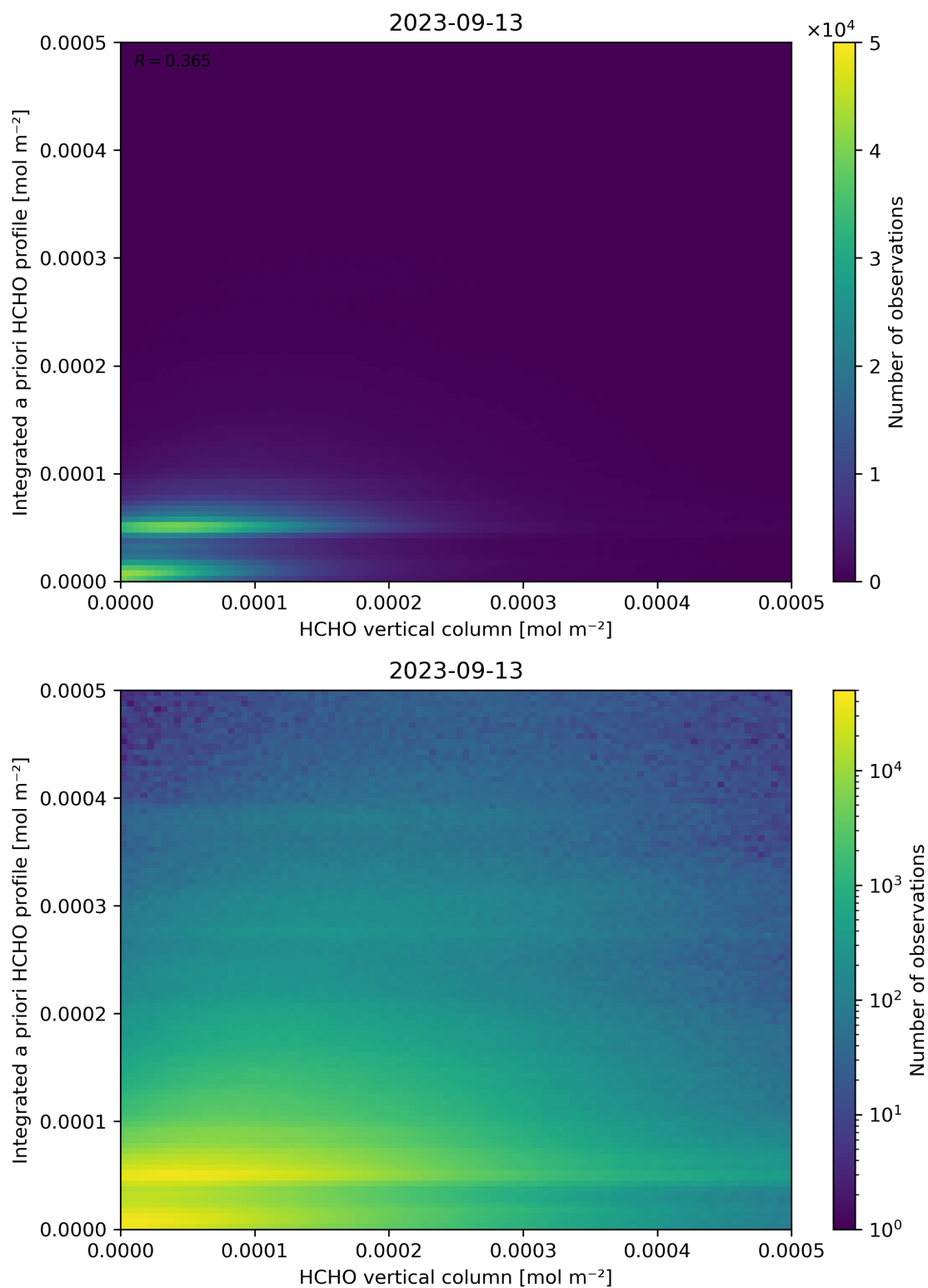
Figure 135: Scatter density plot of “HCHO vertical column” against “Integrated a priori HCHO profile” for 2023-09-12 to 2023-09-14.
