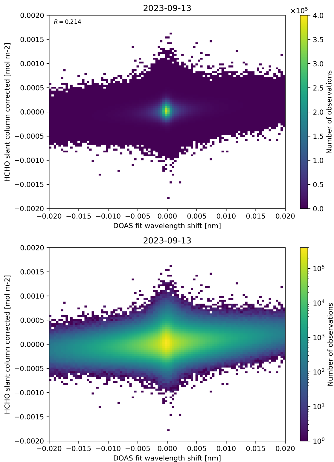
Figure 66: Scatter density plot of “DOAS fit wavelength shift” against “HCHO slant column corrected” for 2023-09-12 to 2023-09-14.
