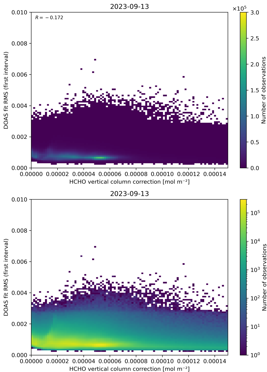
Figure 112: Scatter density plot of “HCHO vertical column correction” against “DOAS fit RMS (first interval)” for 2023-09-12 to 2023-09-14.
