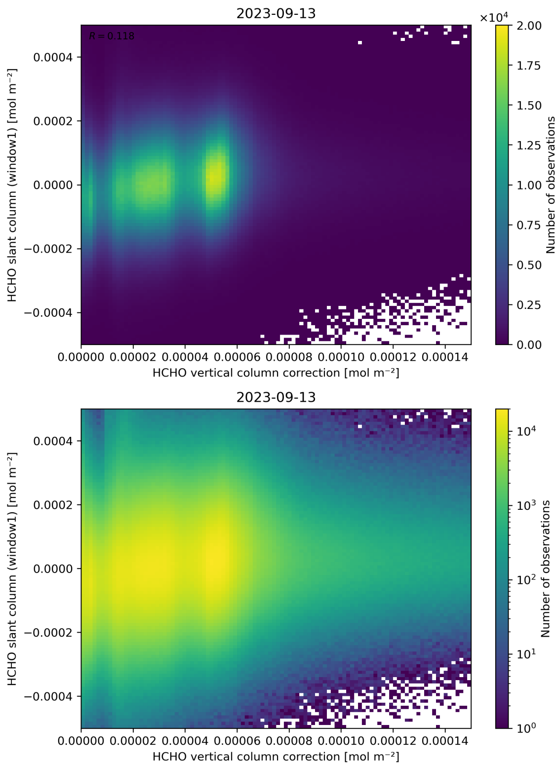
Figure 118: Scatter density plot of “HCHO vertical column correction” against “HCHO slant column (window1)” for 2023-09-12 to 2023-09-14.
