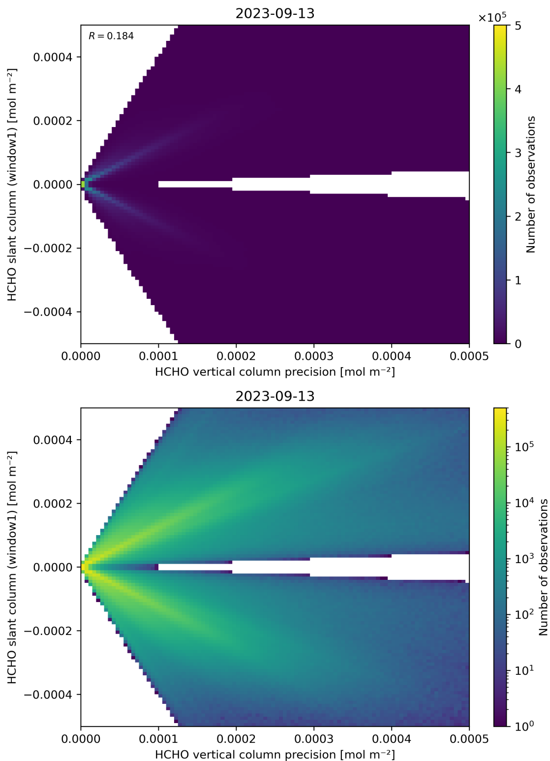
Figure 142: Scatter density plot of “HCHO vertical column precision” against “HCHO slant column (window1)” for 2023-09-12 to 2023-09-14.
