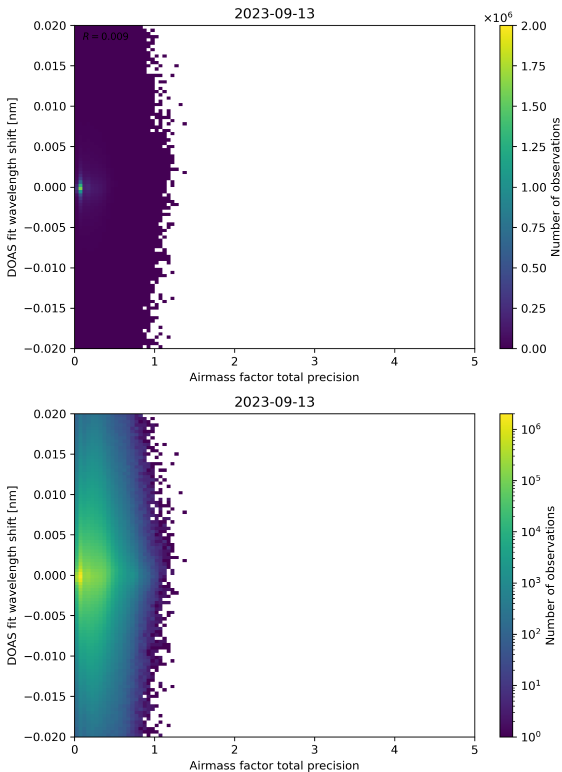
Figure 106: Scatter density plot of “Airmass factor total precision” against “DOAS fit wavelength shift” for 2023-09-12 to 2023-09-14.
