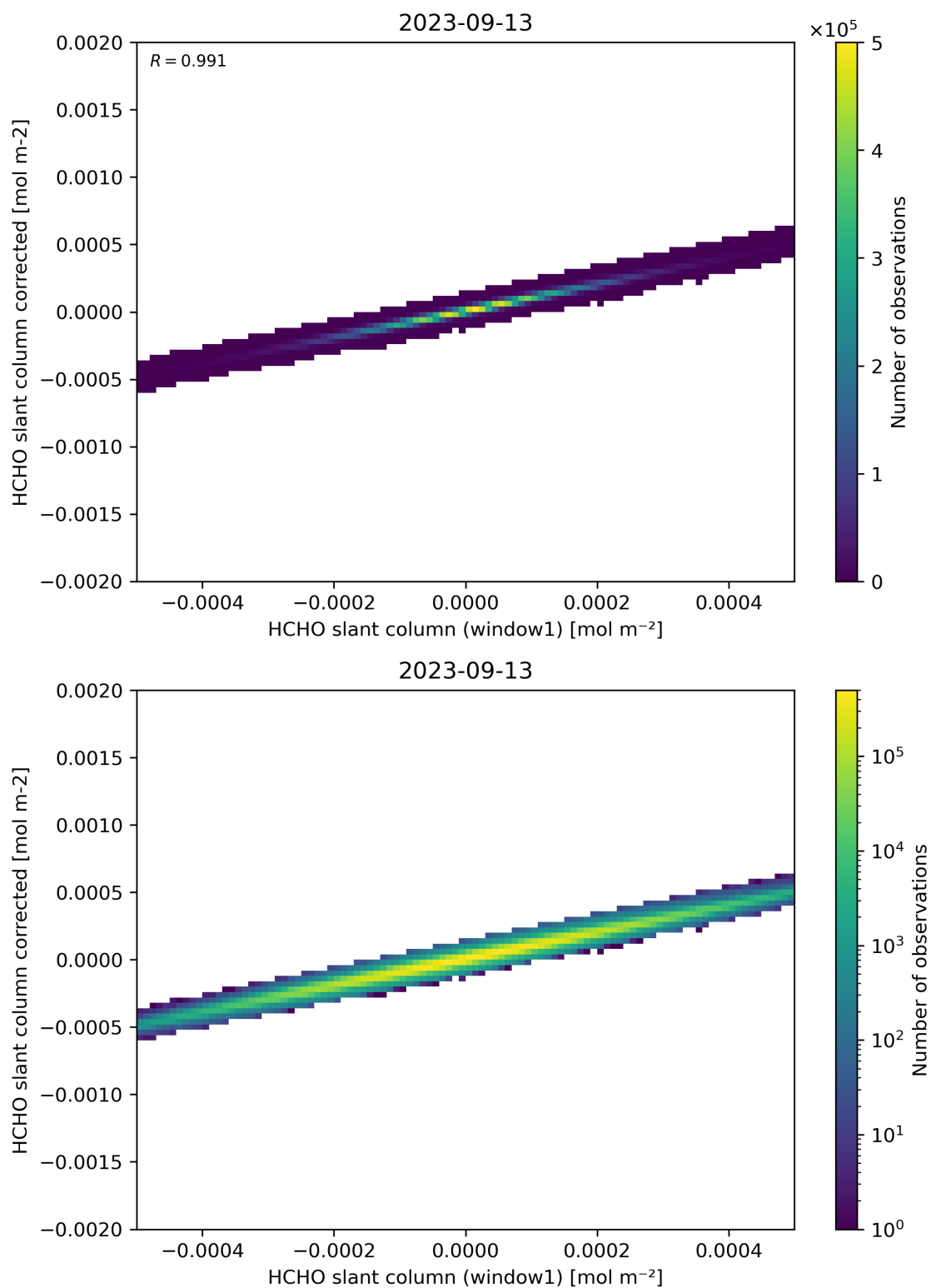
Figure 82: Scatter density plot of “HCHO slant column (window1)” against “HCHO slant column corrected” for 2023-09-12 to 2023-09-14.
