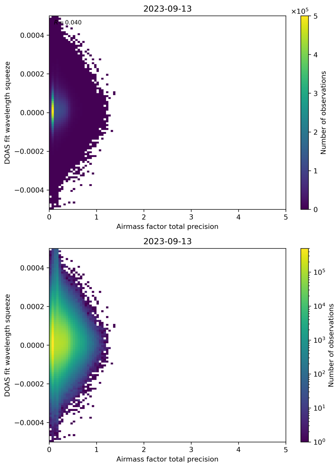
Figure 107: Scatter density plot of “Airmass factor total precision” against “DOAS fit wavelength squeeze” for 2023-09-12 to 2023-09-14.
