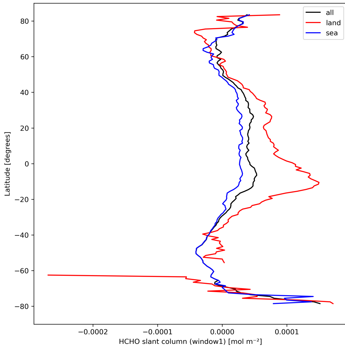
Figure 24: Zonal average of “HCHO slant column (window1)” for 2023-09-12 to 2023-09-14.
