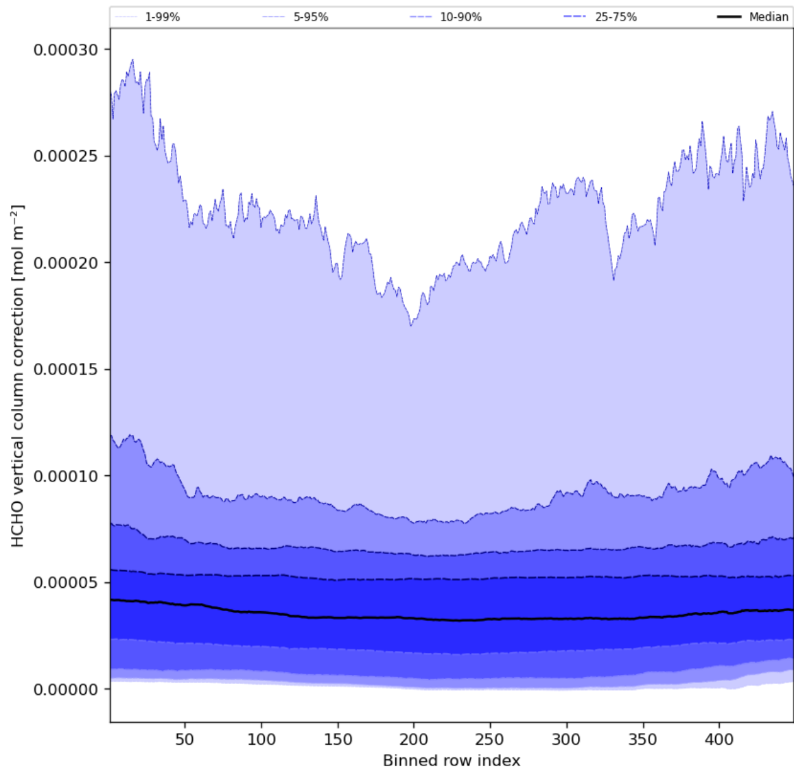
Figure 51: Along track statistics of “HCHO vertical column correction” for 2023-09-12 to 2023-09-14
