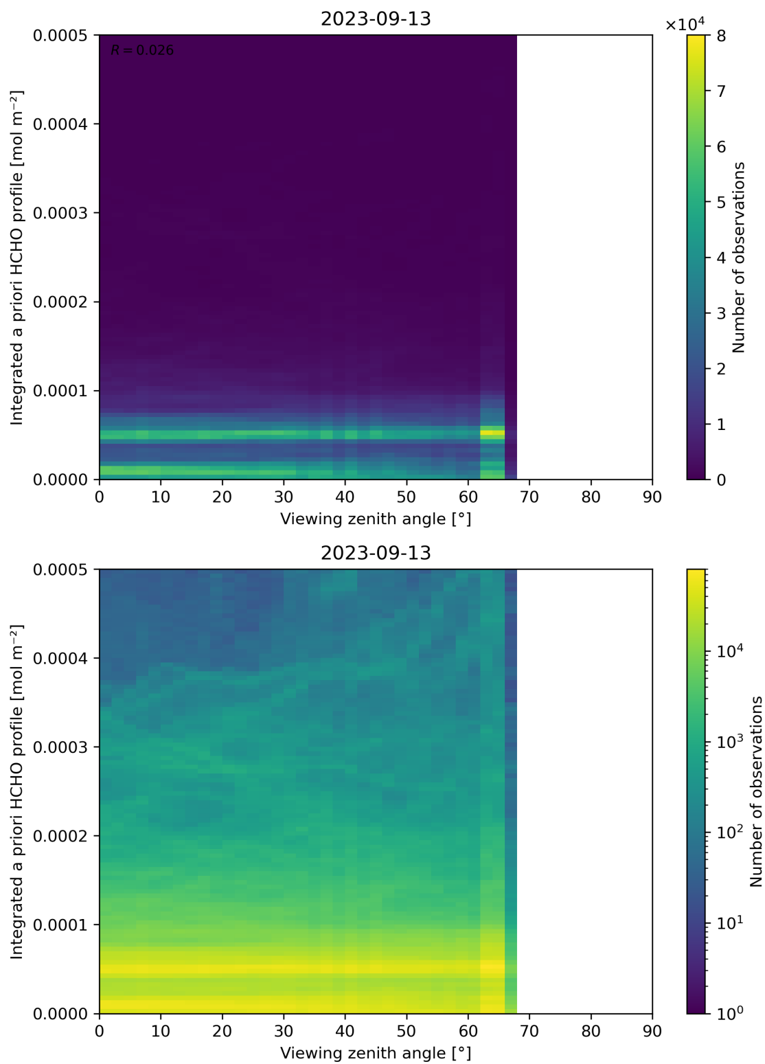
Figure 195: Scatter density plot of “Viewing zenith angle” against “Integrated a priori HCHO profile” for 2023-09-12 to 2023-09-14.
