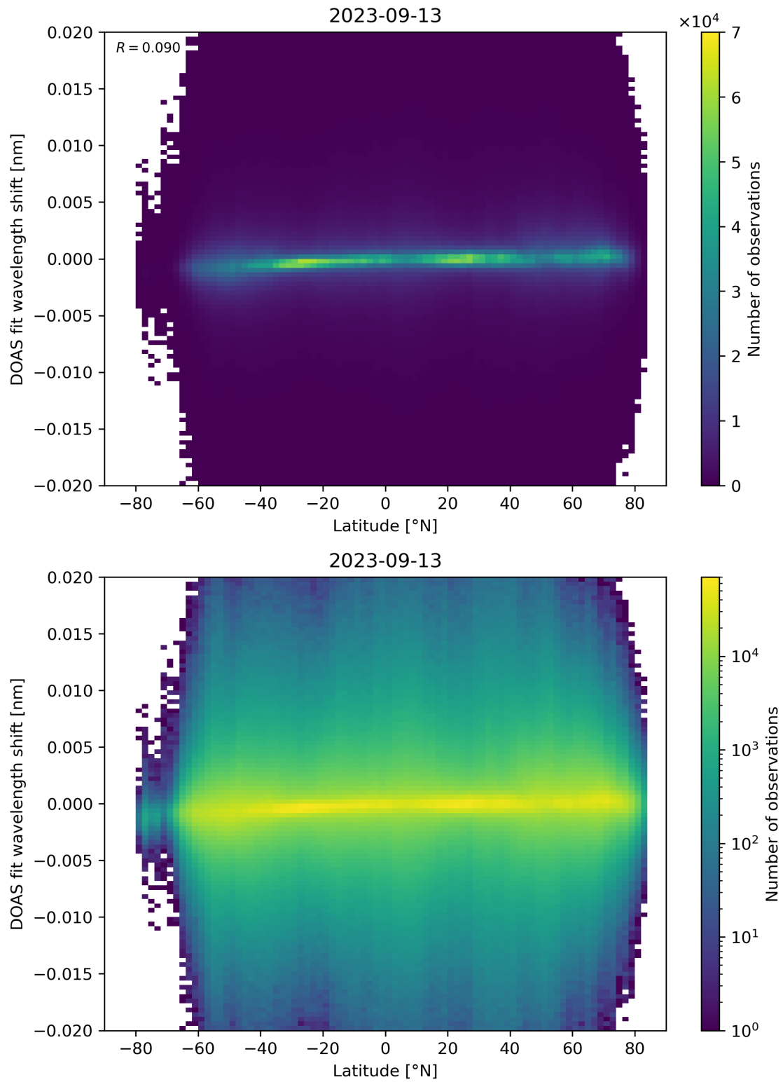
Figure 154: Scatter density plot of “Latitude” against “DOAS fit wavelength shift” for 2023-09-12 to 2023-09-14.
