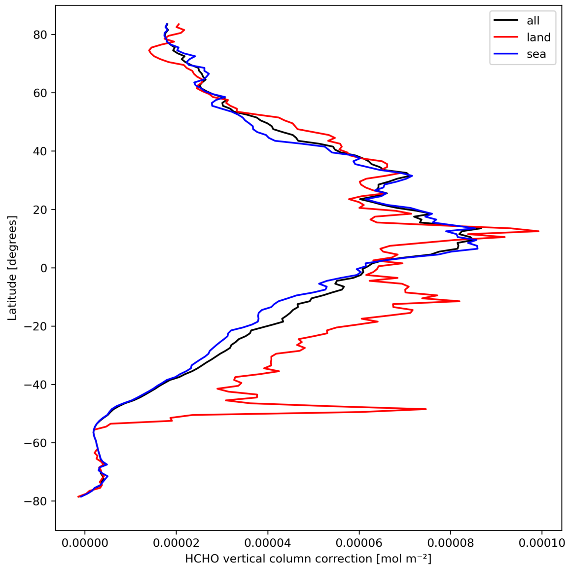
Figure 23: Zonal average of “HCHO vertical column correction” for 2023-09-12 to 2023-09-14.
