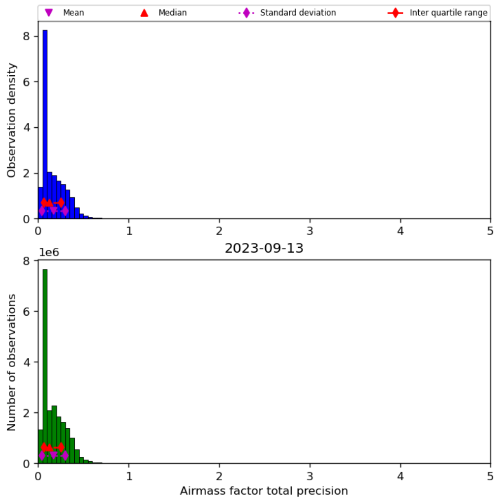
Figure 41: Histogram of “Airmass factor total precision” for 2023-09-12 to 2023-09-14
