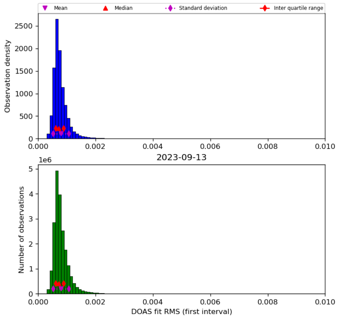
Figure 46: Histogram of “DOAS fit RMS (first interval)” for 2023-09-12 to 2023-09-14
