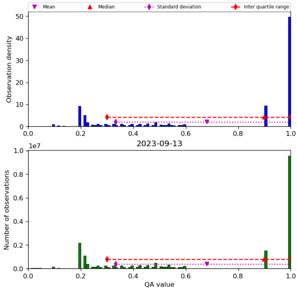
Figure 34: Histogram of “QA value” for 2023-09-12 to 2023-09-14
