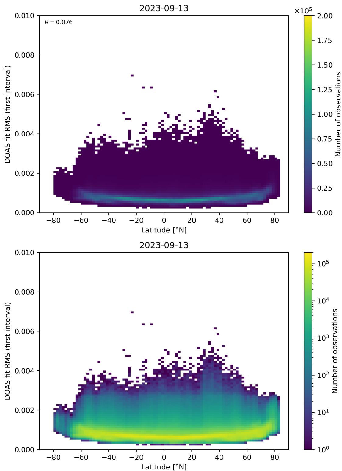
Figure 153: Scatter density plot of “Latitude” against “DOAS fit RMS (first interval)” for 2023-09-12 to 2023-09-14.
