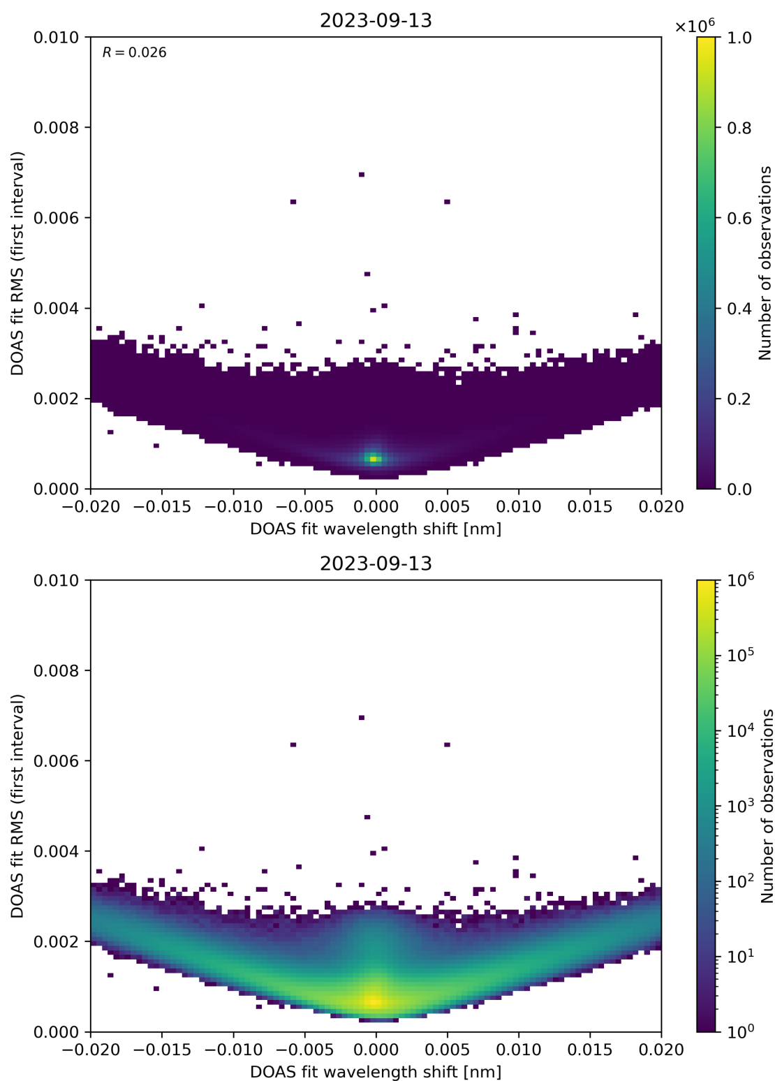
Figure 64: Scatter density plot of “DOAS fit wavelength shift” against “DOAS fit RMS (first interval)” for 2023-09-12 to 2023-09-14.
