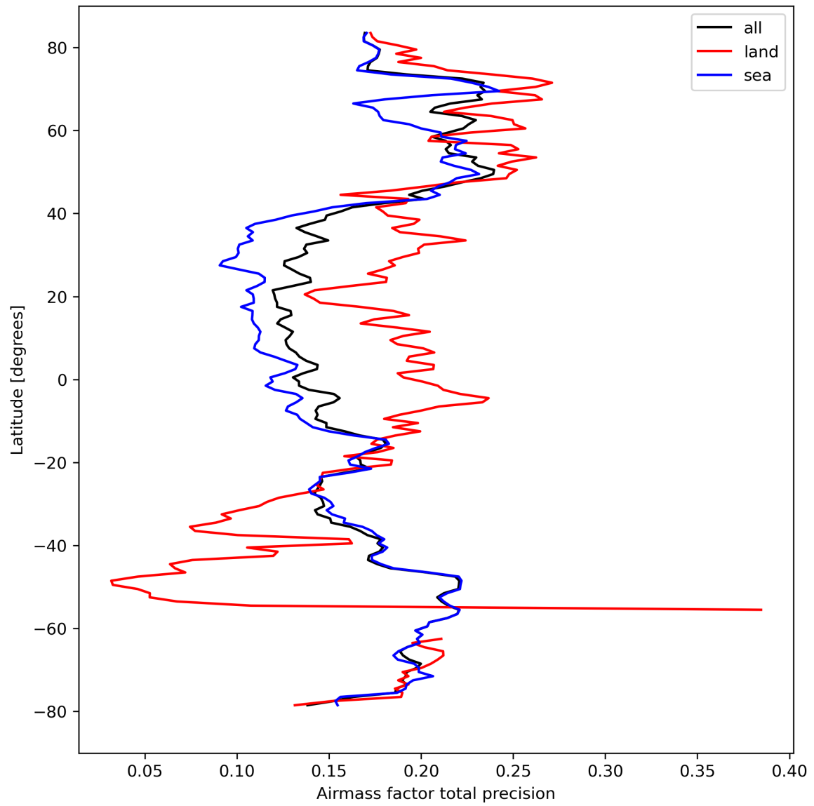
Figure 27: Zonal average of “Airmass factor total precision” for 2023-09-12 to 2023-09-14.
