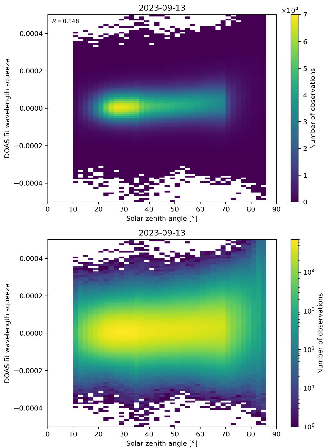
Figure 169: Scatter density plot of “Solar zenith angle” against “DOAS fit wavelength squeeze” for 2023-09-12 to 2023-09-14.
