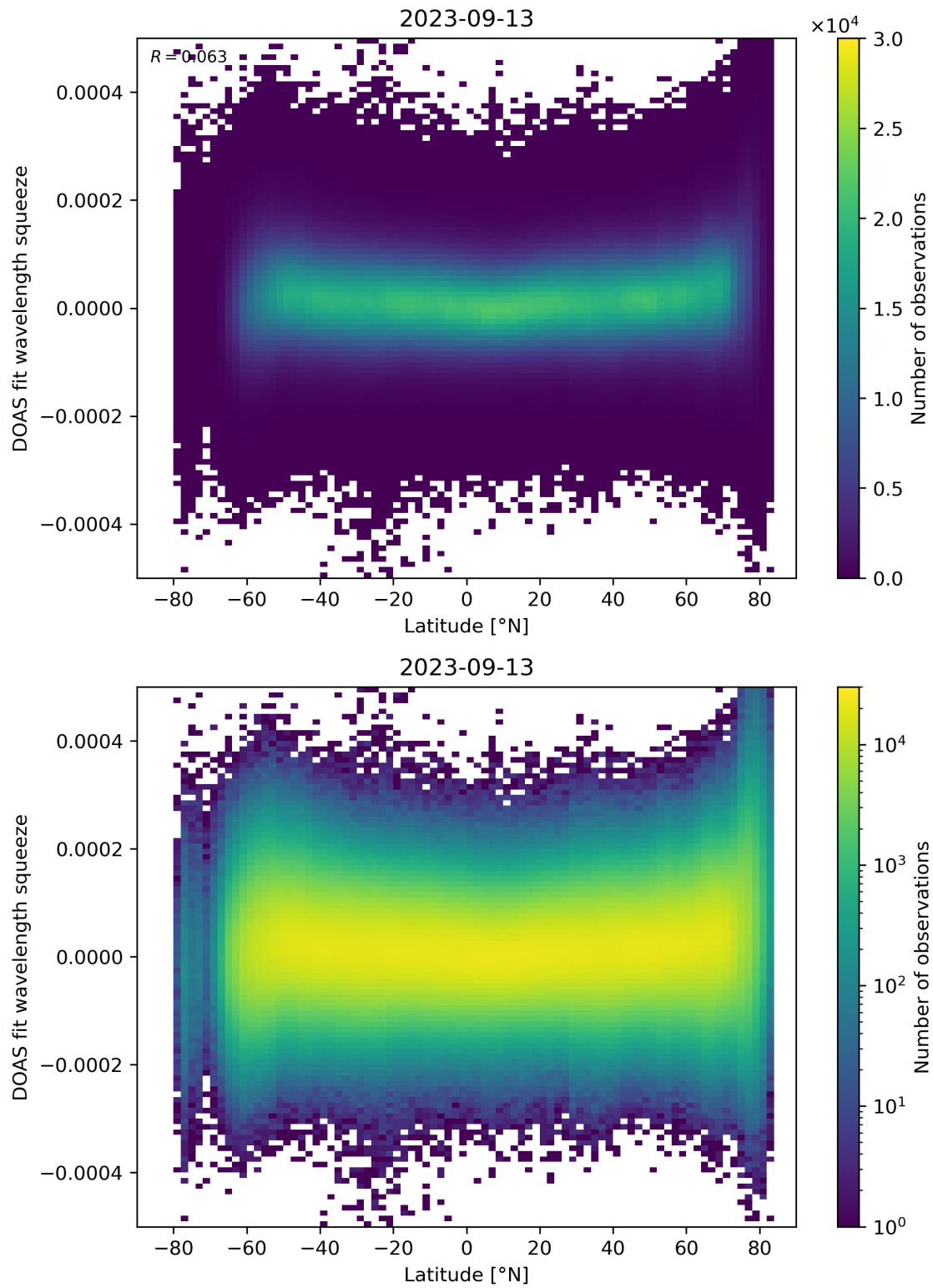
Figure 155: Scatter density plot of “Latitude” against “DOAS fit wavelength squeeze” for 2023-09-12 to 2023-09-14.
