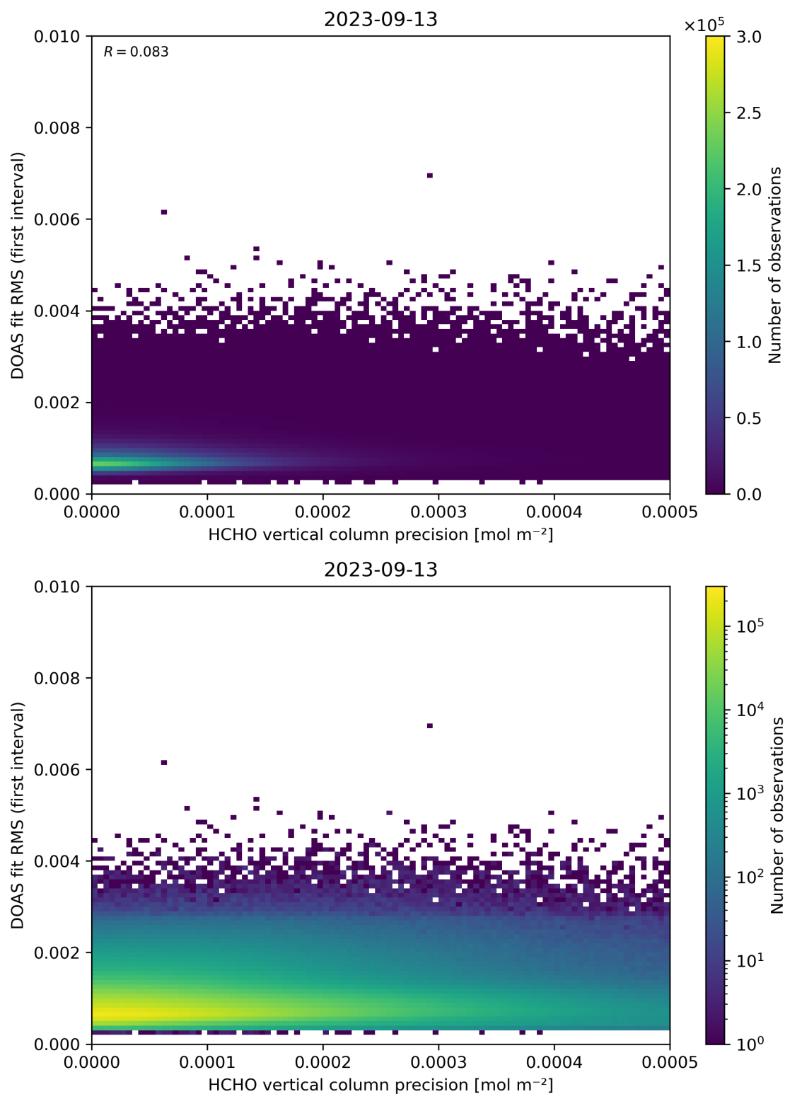
Figure 136: Scatter density plot of “HCHO vertical column precision” against “DOAS fit RMS (first interval)” for 2023-09-12 to 2023-09-14.
