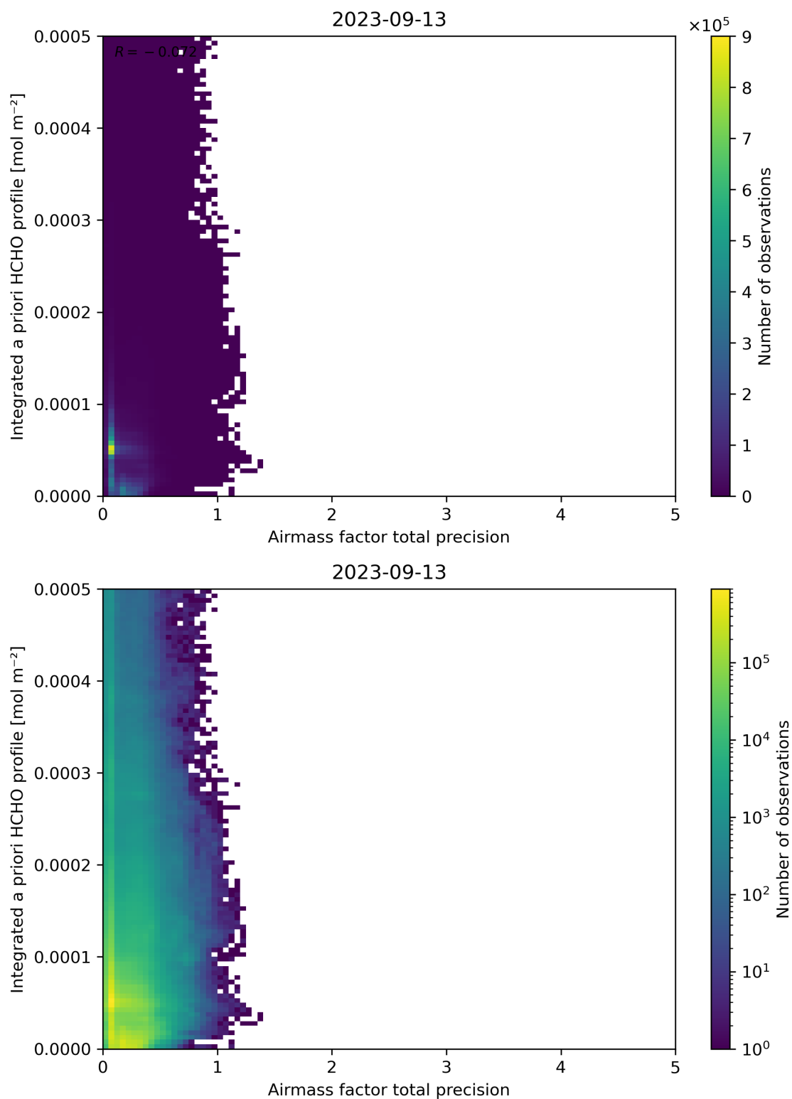
Figure 111: Scatter density plot of “Airmass factor total precision” against “Integrated a priori HCHO profile” for 2023-09-12 to 2023-09-14.
