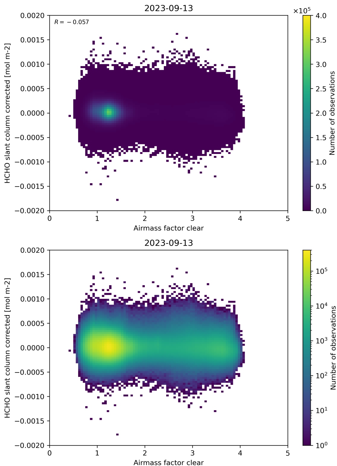
Figure 74: Scatter density plot of “Airmass factor clear” against “HCHO slant column corrected” for 2023-09-12 to 2023-09-14.
