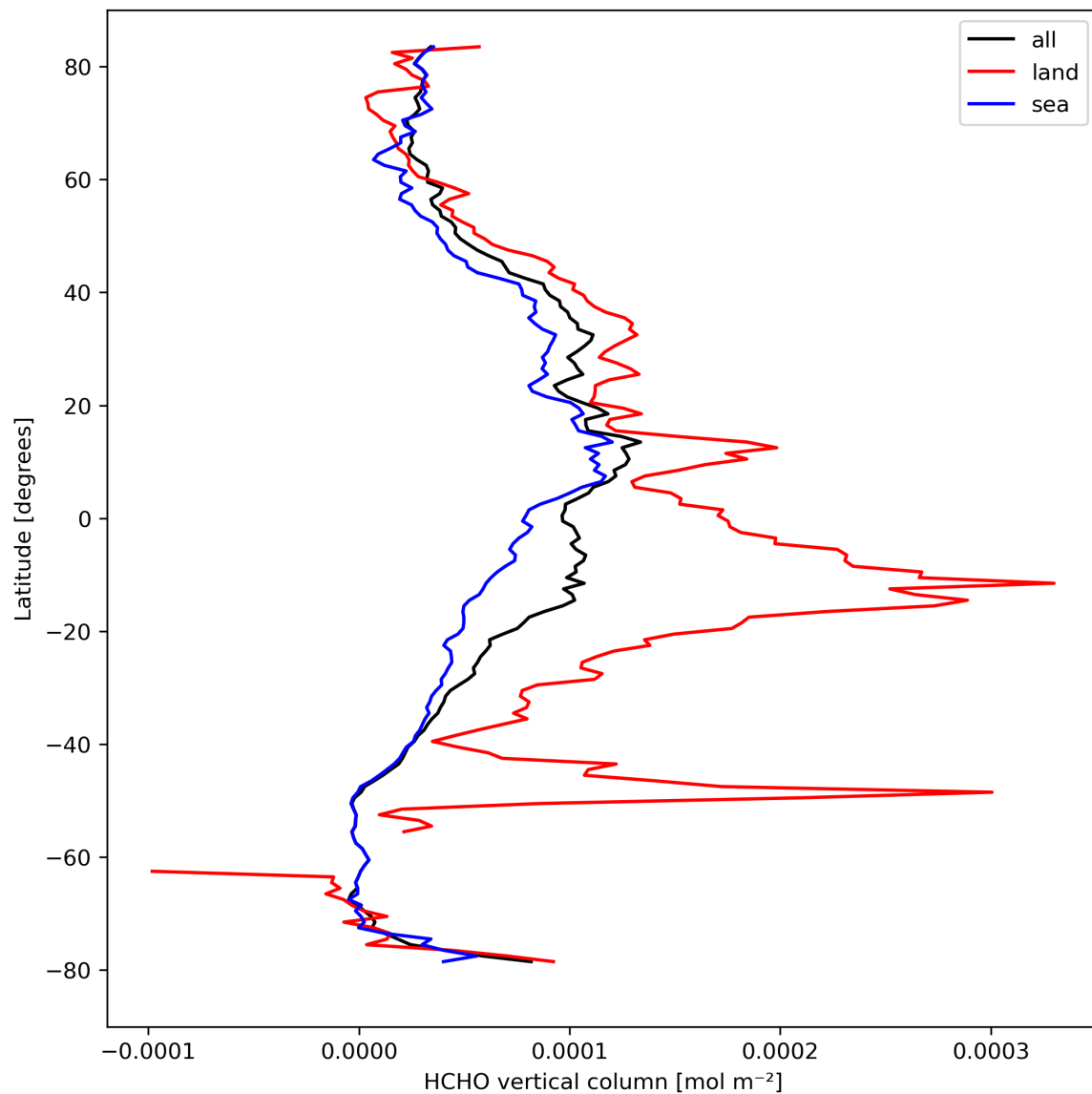
Figure 21: Zonal average of “HCHO vertical column” for 2023-09-12 to 2023-09-14.
