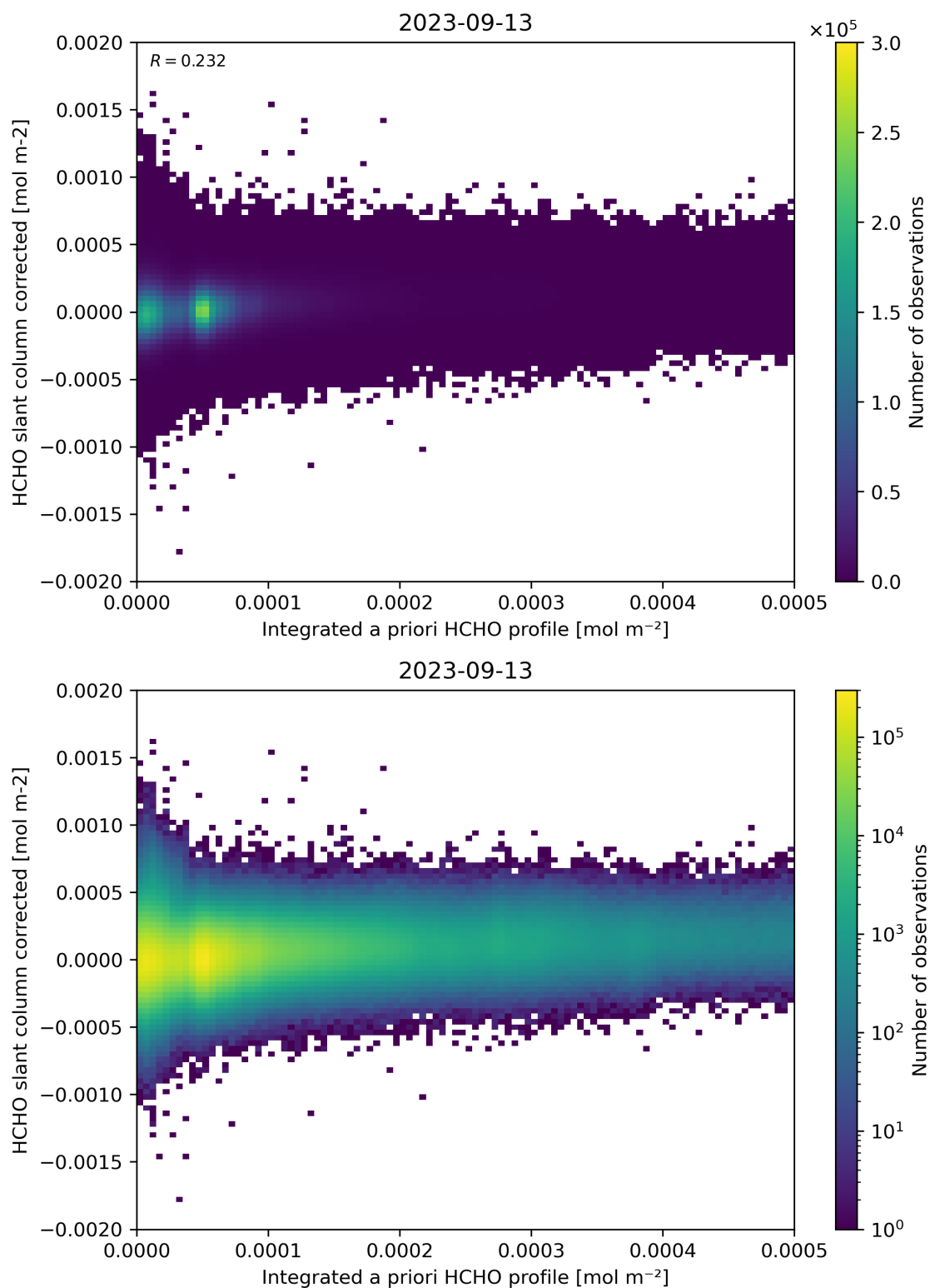
Figure 151: Scatter density plot of “Integrated a priori HCHO profile” against “HCHO slant column corrected” for 2023-09-12 to 2023-09-14.
