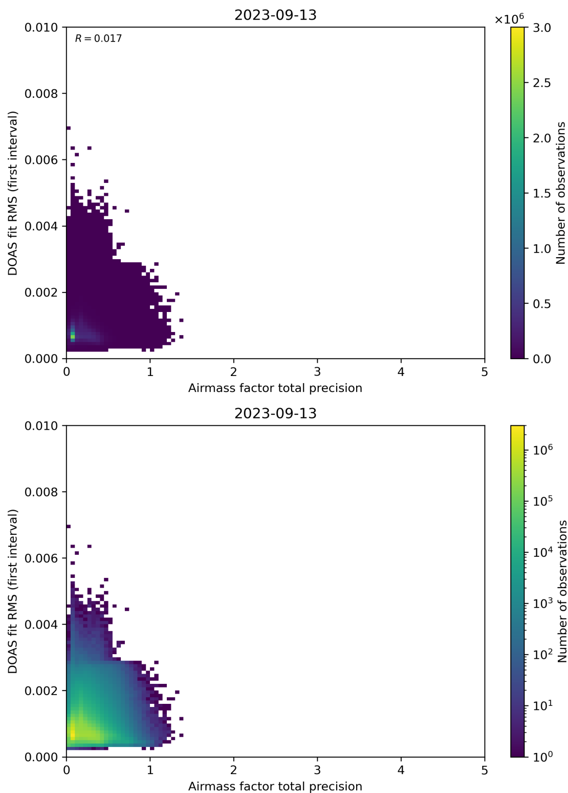
Figure 105: Scatter density plot of “Airmass factor total precision” against “DOAS fit RMS (first interval)” for 2023-09-12 to 2023-09-14.
