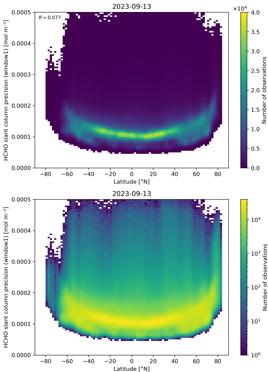
Figure 160: Scatter density plot of “Latitude” against “HCHO slant column precision (window1)” for 2023-09-12 to 2023-09-14.
