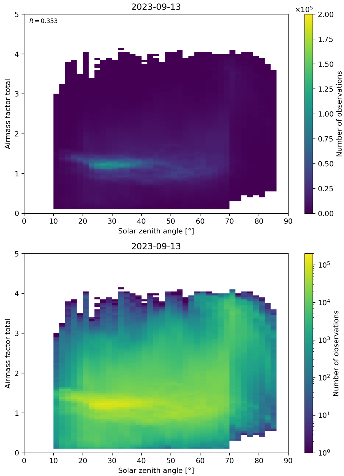
Figure 175: Scatter density plot of “Solar zenith angle” against “Airmass factor total” for 2023-09-12 to 2023-09-14.
