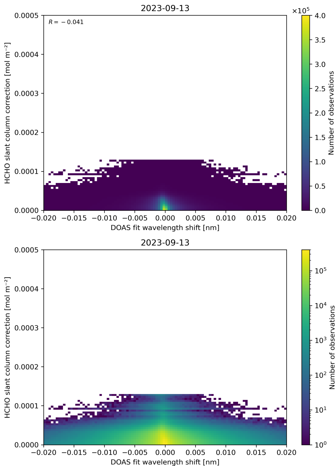
Figure 67: Scatter density plot of “DOAS fit wavelength shift” against “HCHO slant column correction” for 2023-09-12 to 2023-09-14.
