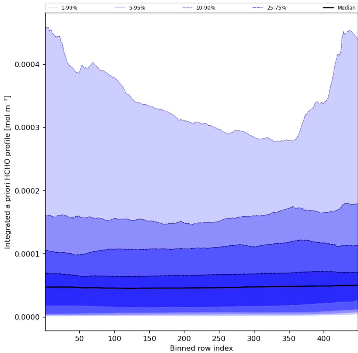
Figure 57: Along track statistics of “Integrated a priori HCHO profile” for 2023-09-12 to 2023-09-14
