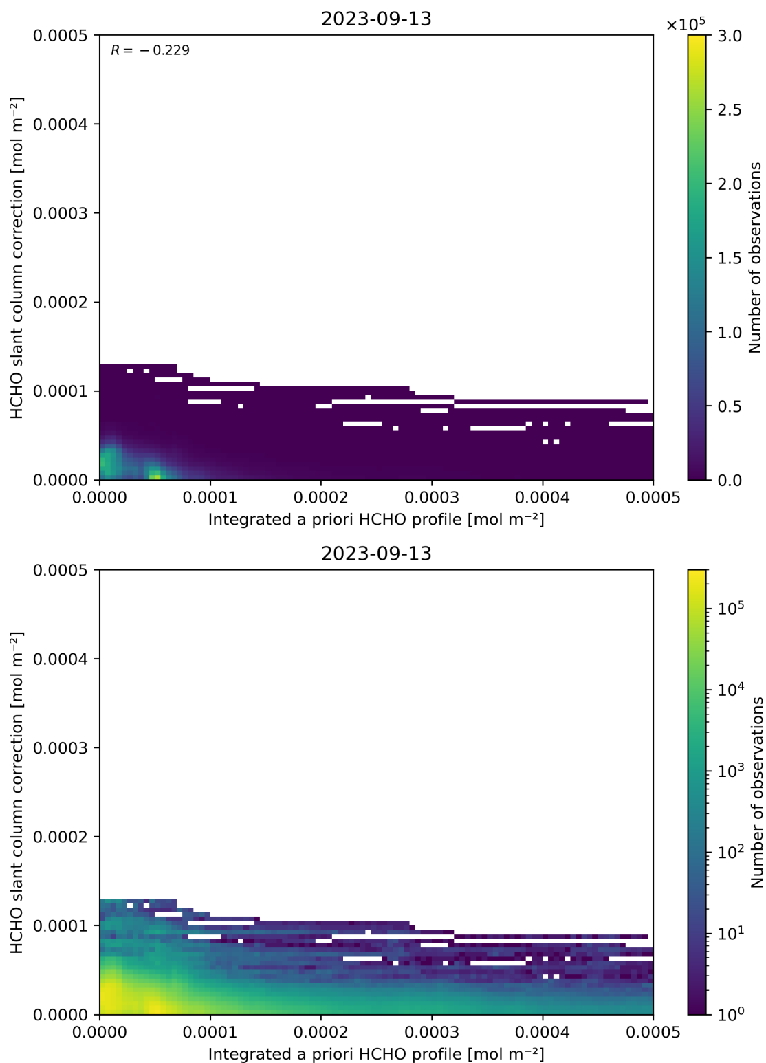
Figure 152: Scatter density plot of “Integrated a priori HCHO profile” against “HCHO slant column correction” for 2023-09-12 to 2023-09-14.
