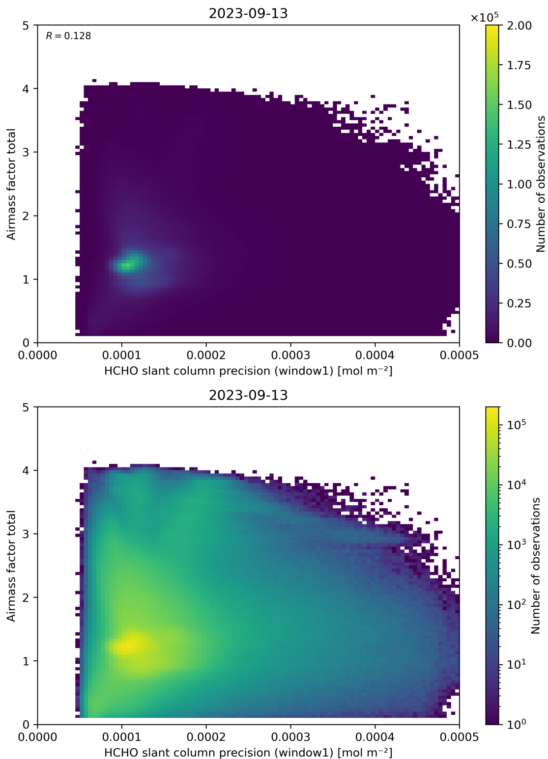
Figure 94: Scatter density plot of “HCHO slant column precision (window1)” against “Airmass factor total” for 2023-09-12 to 2023-09-14.
