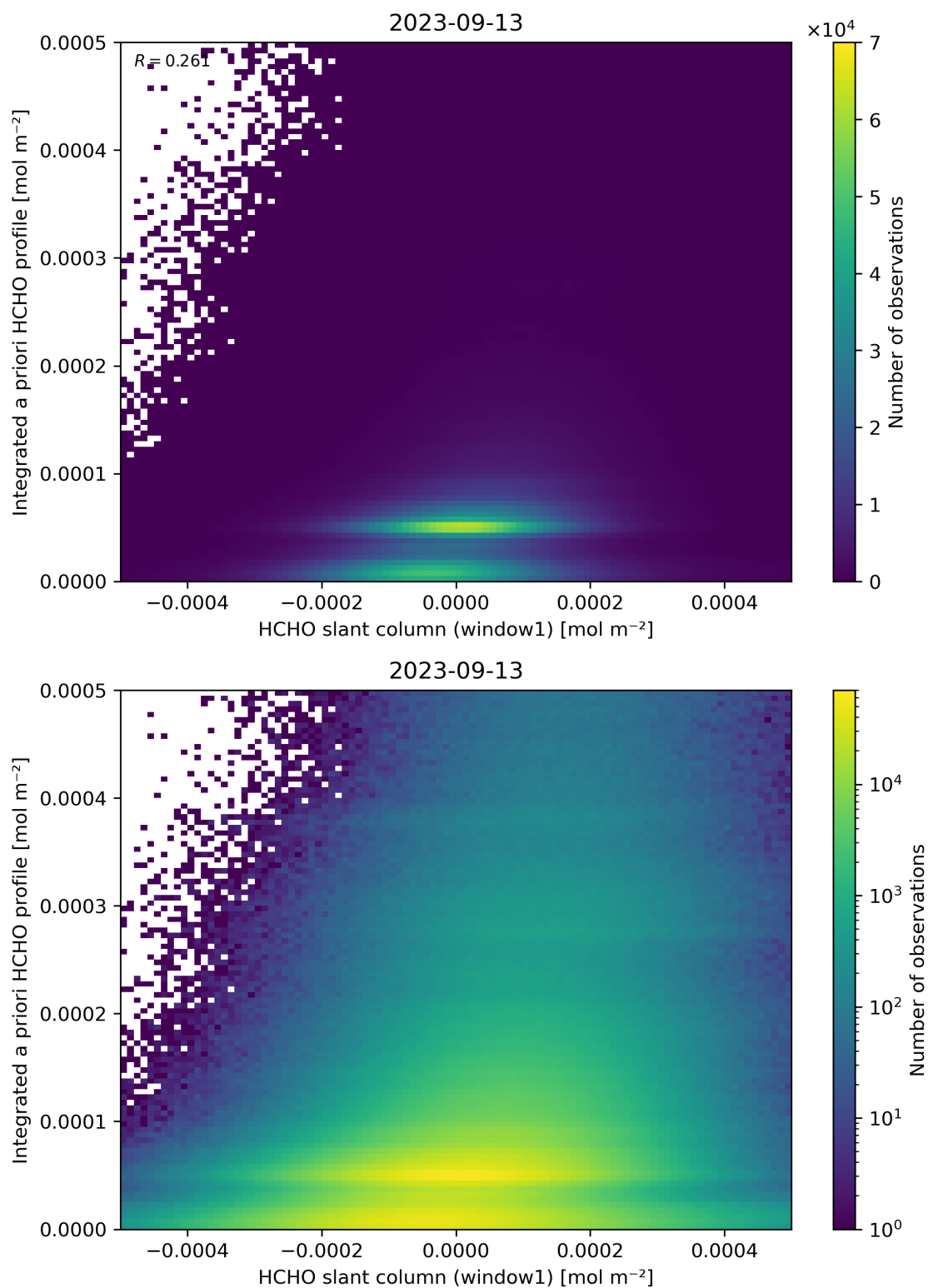
Figure 87: Scatter density plot of “HCHO slant column (window1)” against “Integrated a priori HCHO profile” for 2023-09-12 to 2023-09-14.
