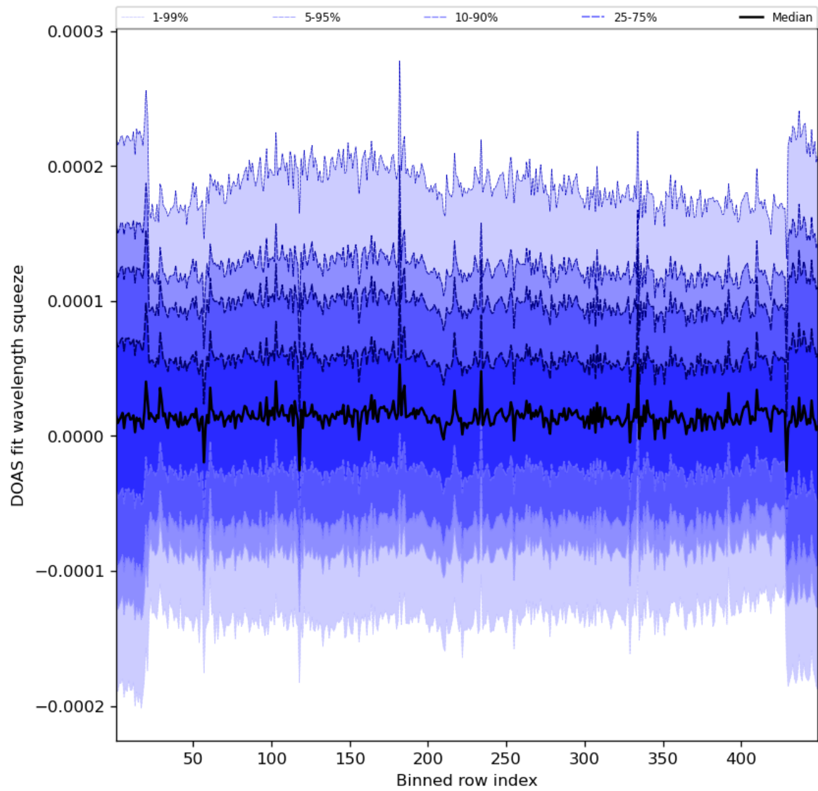
Figure 59: Along track statistics of “DOAS fit wavelength squeeze” for 2023-09-12 to 2023-09-14
