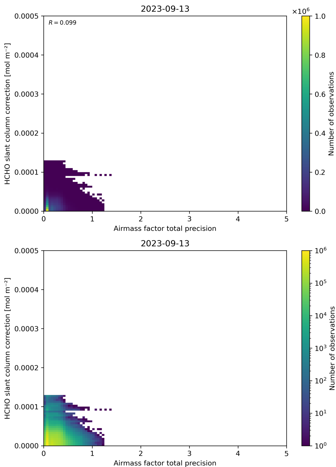
Figure 110: Scatter density plot of “Airmass factor total precision” against “HCHO slant column correction” for 2023-09-12 to 2023-09-14.
