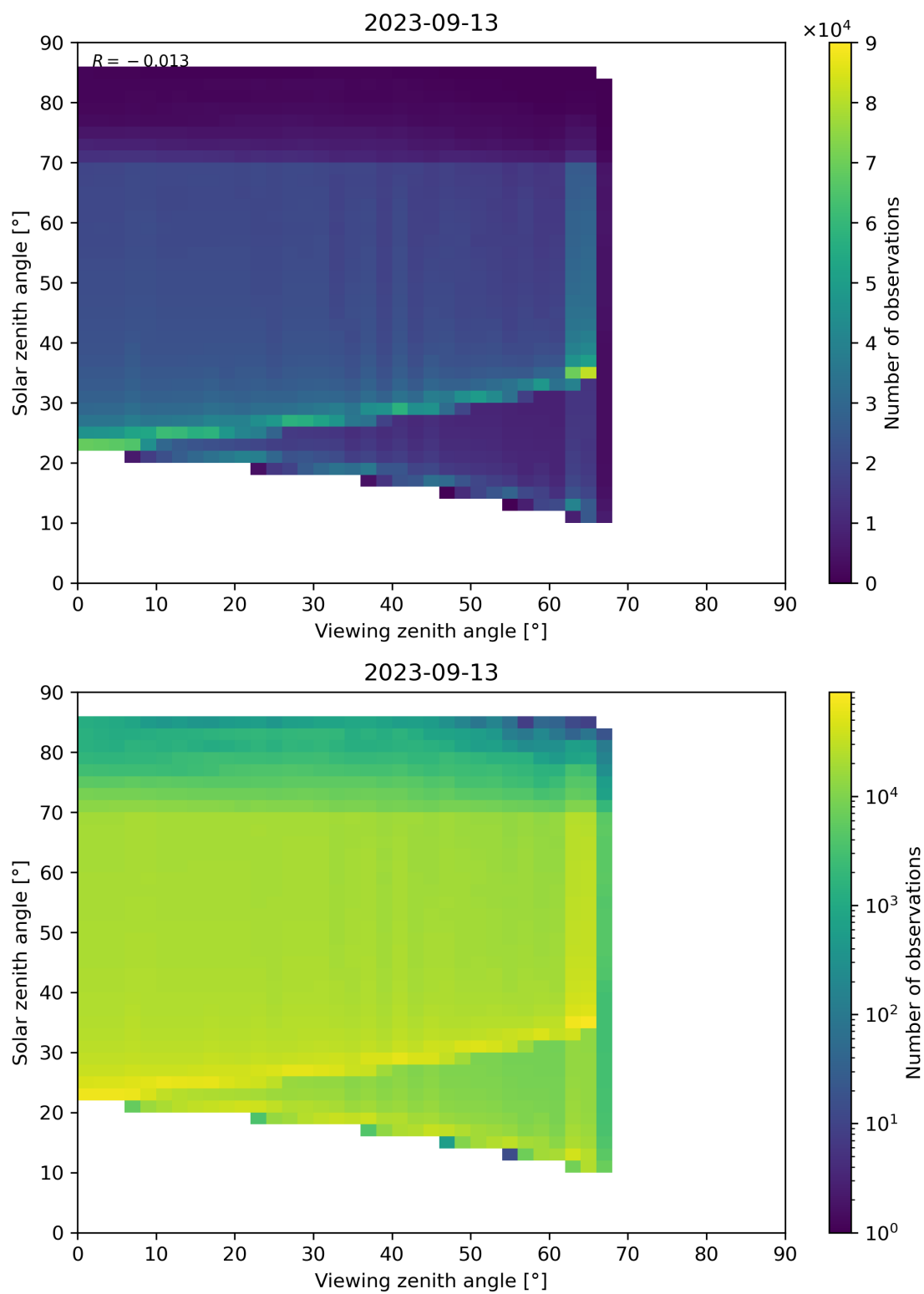
Figure 197: Scatter density plot of “Viewing zenith angle” against “Solar zenith angle” for 2023-09-12 to 2023-09-14.
