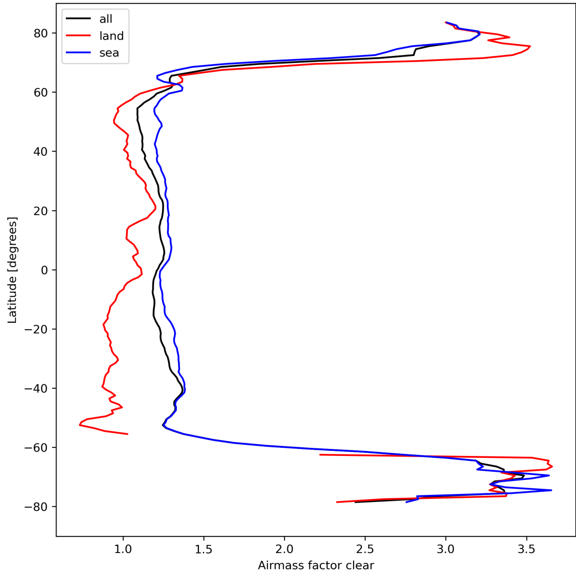
Figure 28: Zonal average of “Airmass factor clear” for 2023-09-12 to 2023-09-14.
