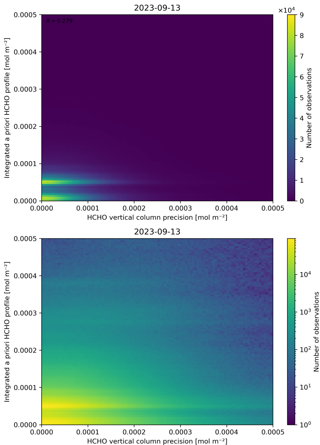
Figure 147: Scatter density plot of “HCHO vertical column precision” against “Integrated a priori HCHO profile” for 2023-09-12 to 2023-09-14.
