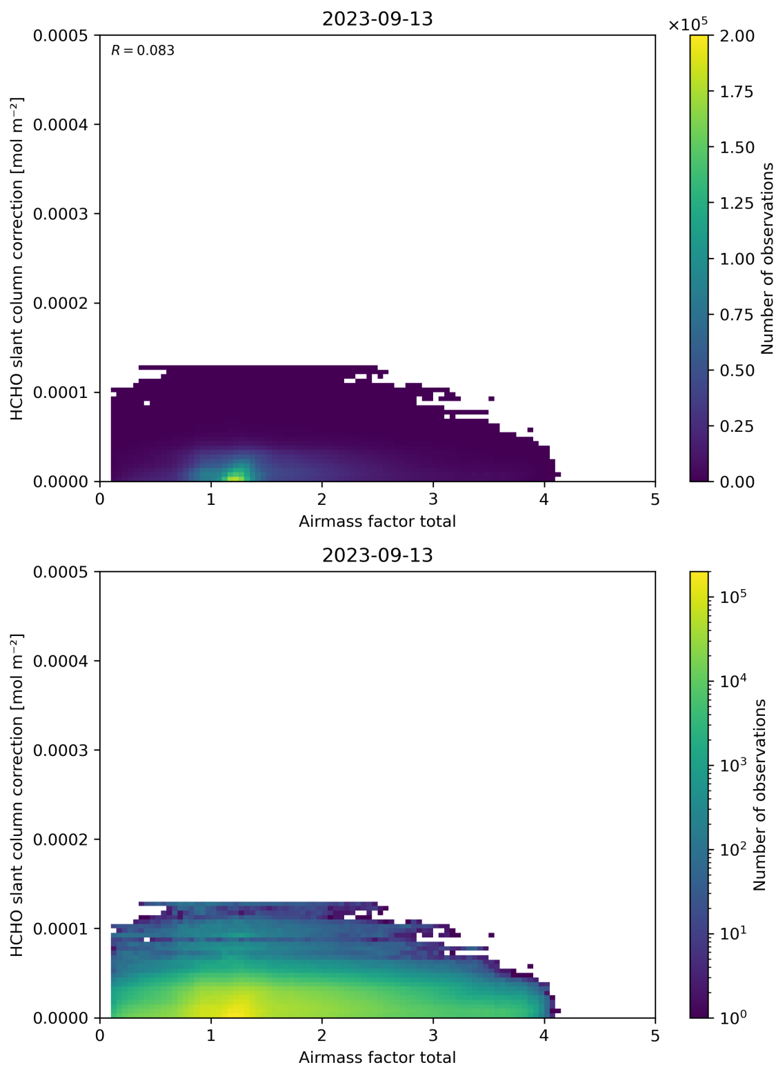
Figure 102: Scatter density plot of “Airmass factor total” against “HCHO slant column correction” for 2023-09-12 to 2023-09-14.
