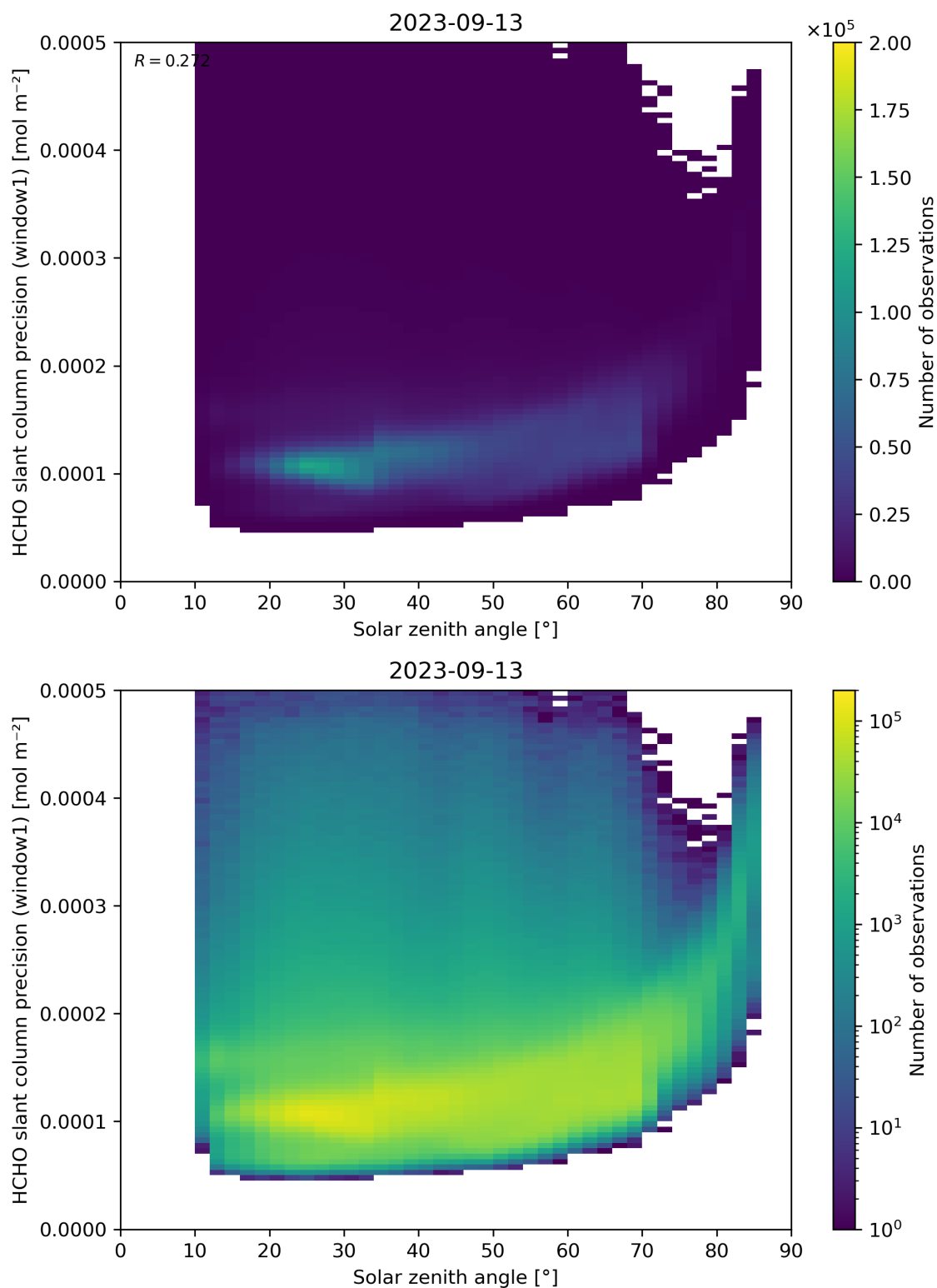
Figure 174: Scatter density plot of “Solar zenith angle” against “HCHO slant column precision (window1)” for 2023-09-12 to 2023-09-14.
