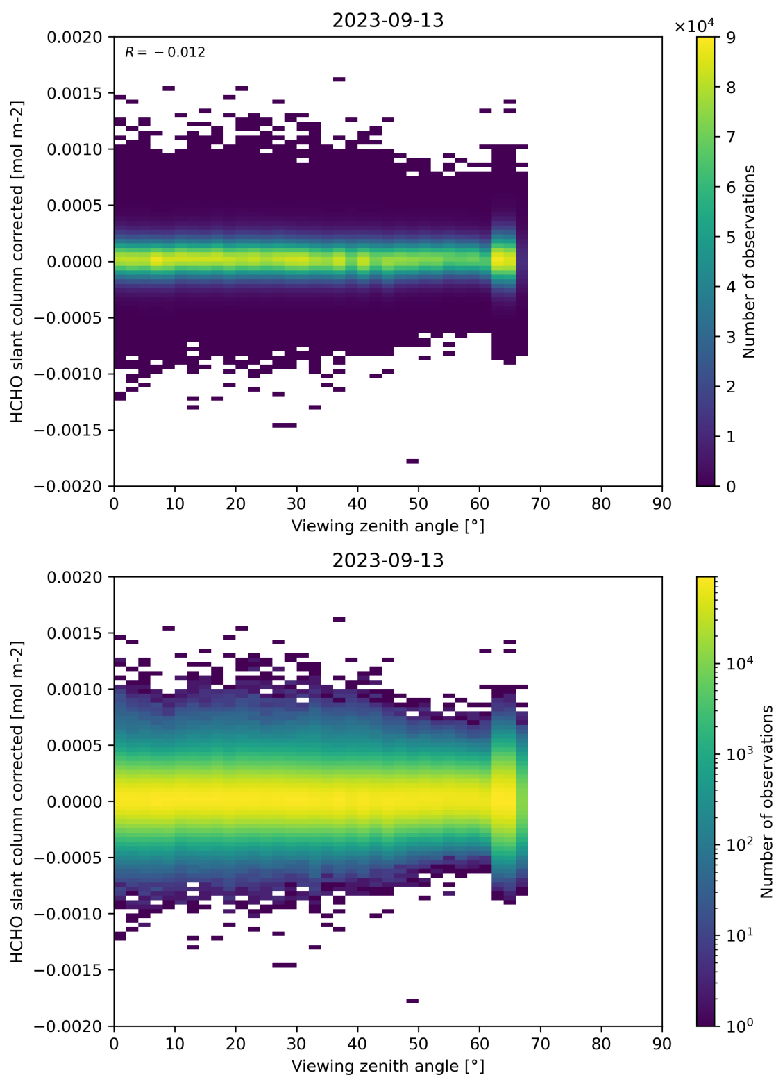
Figure 186: Scatter density plot of “Viewing zenith angle” against “HCHO slant column corrected” for 2023-09-12 to 2023-09-14.
