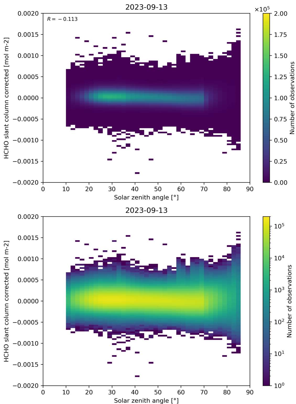
Figure 171: Scatter density plot of “Solar zenith angle” against “HCHO slant column corrected” for 2023-09-12 to 2023-09-14.
