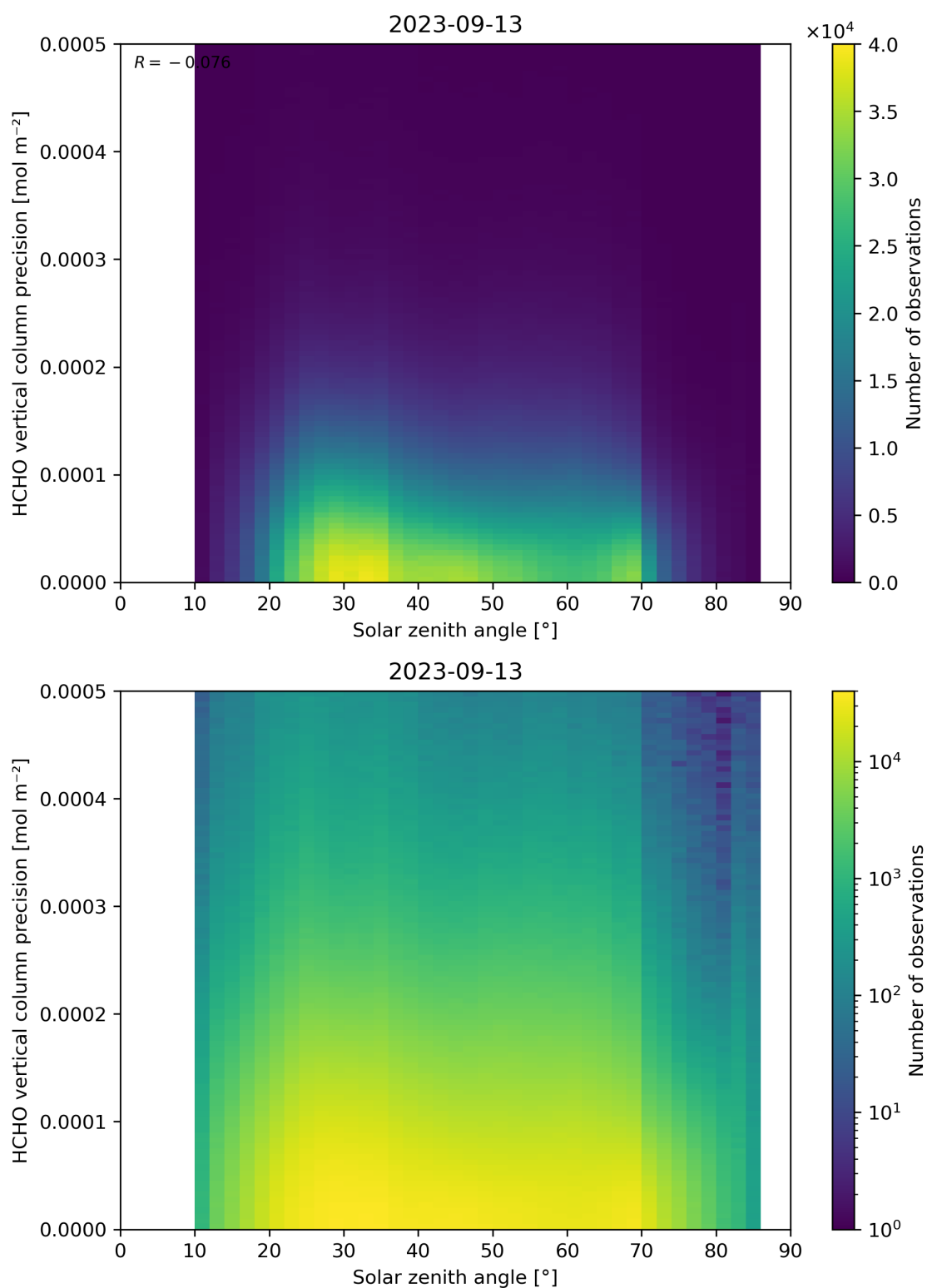
Figure 179: Scatter density plot of “Solar zenith angle” against “HCHO vertical column precision” for 2023-09-12 to 2023-09-14.
