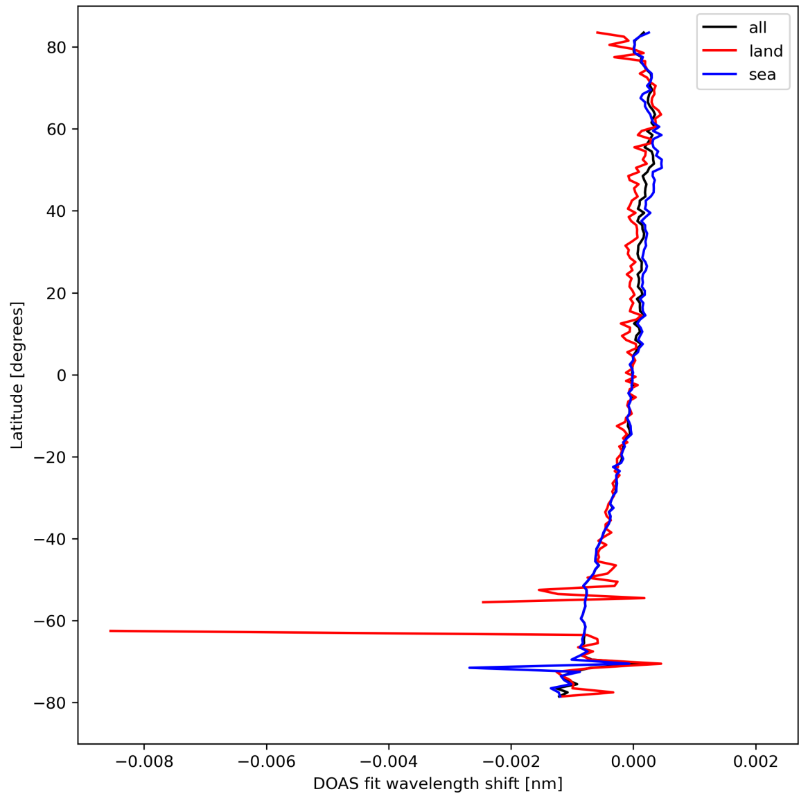
Figure 30: Zonal average of “DOAS fit wavelength shift” for 2023-09-12 to 2023-09-14.
