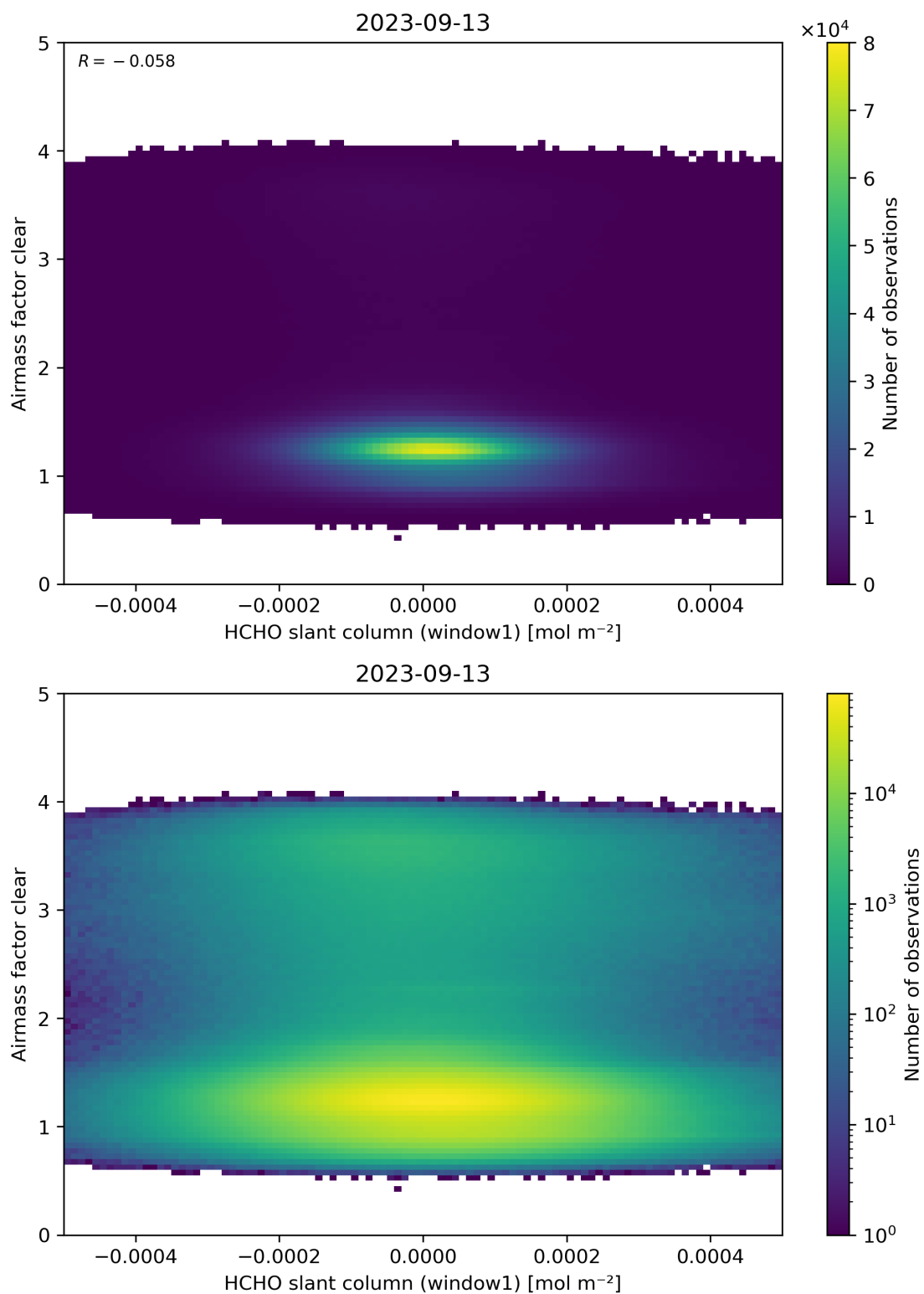
Figure 81: Scatter density plot of “HCHO slant column (window1)” against “Airmass factor clear” for 2023-09-12 to 2023-09-14.
