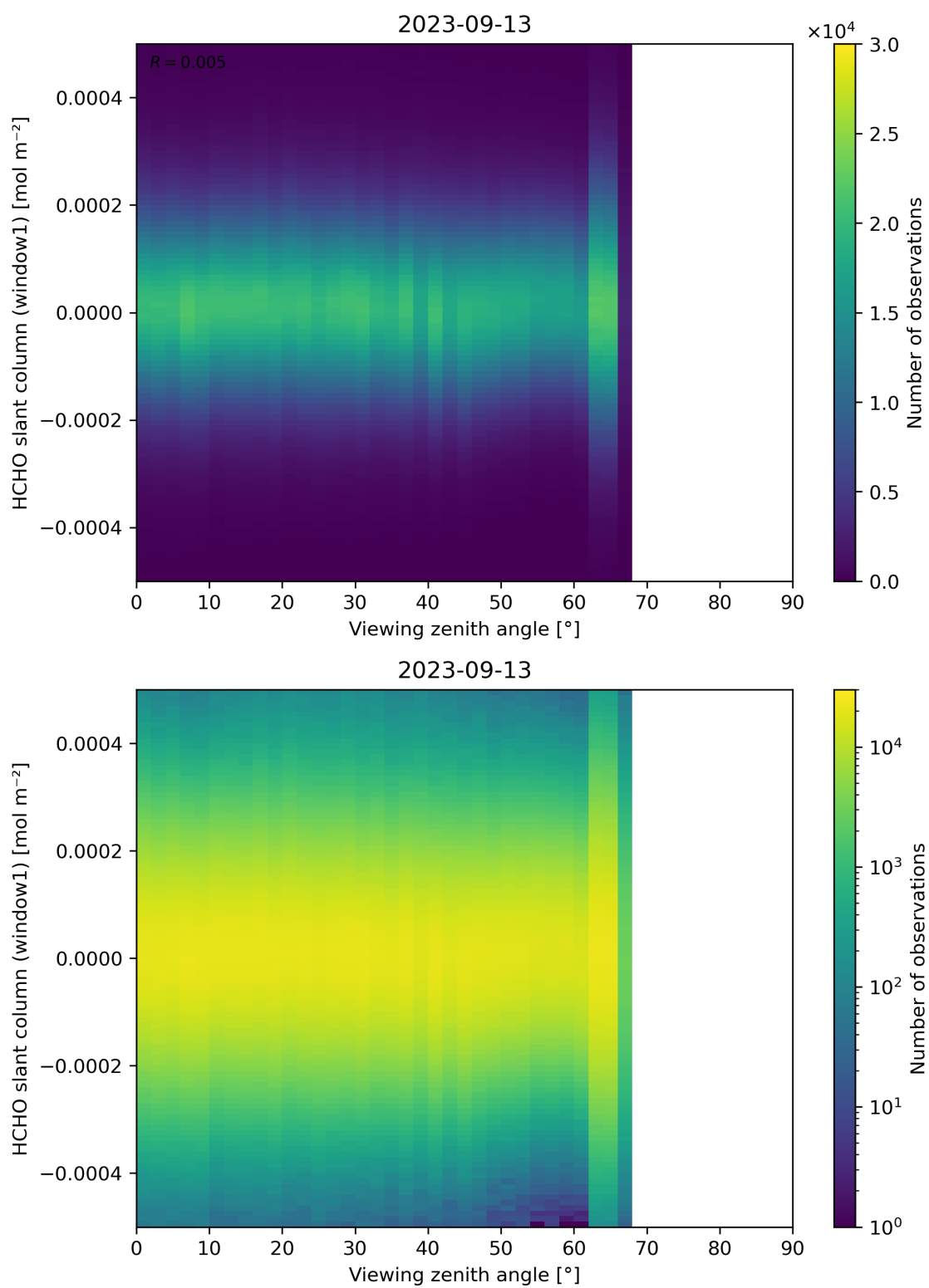
Figure 188: Scatter density plot of “Viewing zenith angle” against “HCHO slant column (window1)” for 2023-09-12 to 2023-09-14.
