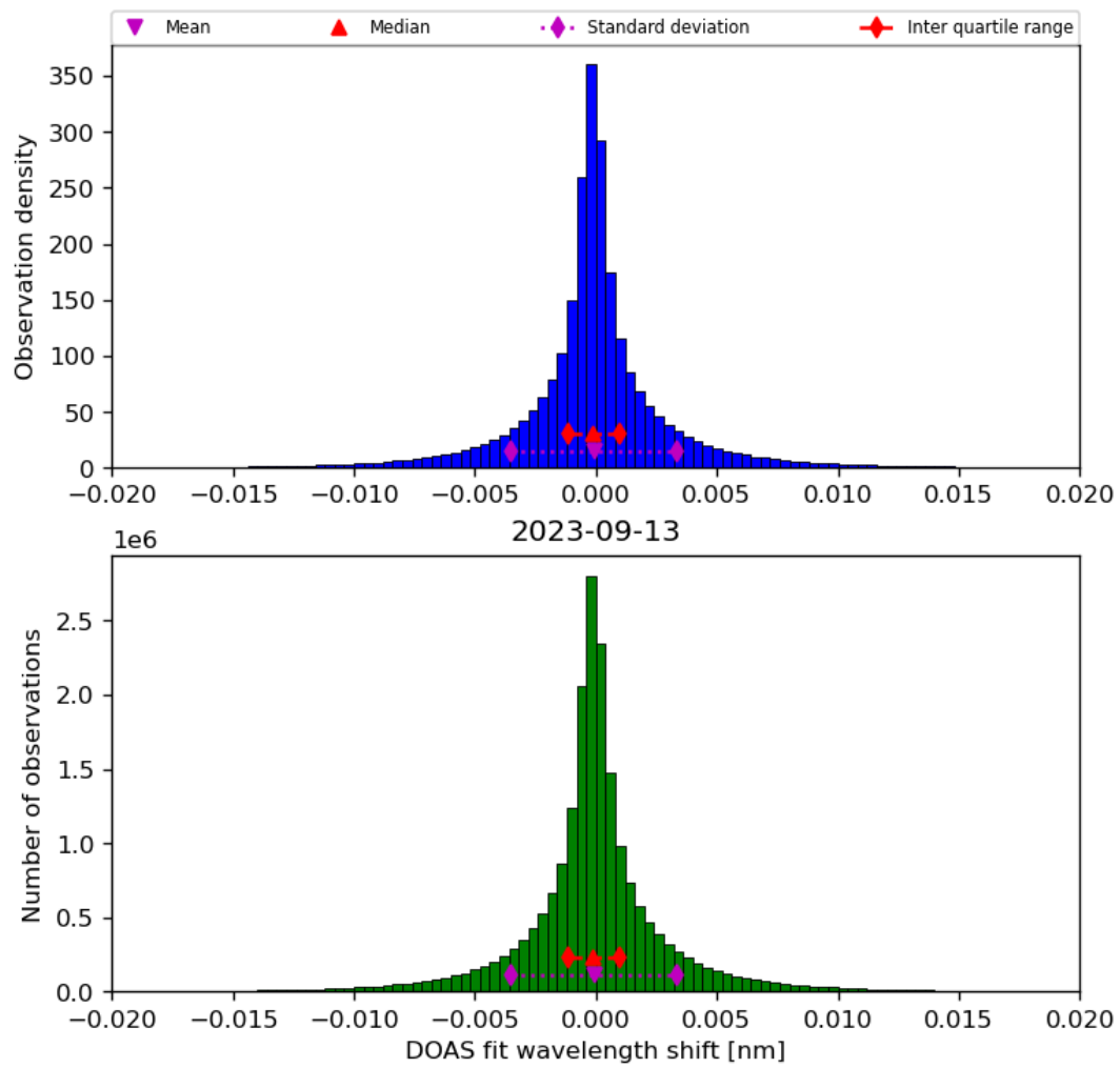
Figure 44: Histogram of “DOAS fit wavelength shift” for 2023-09-12 to 2023-09-14
