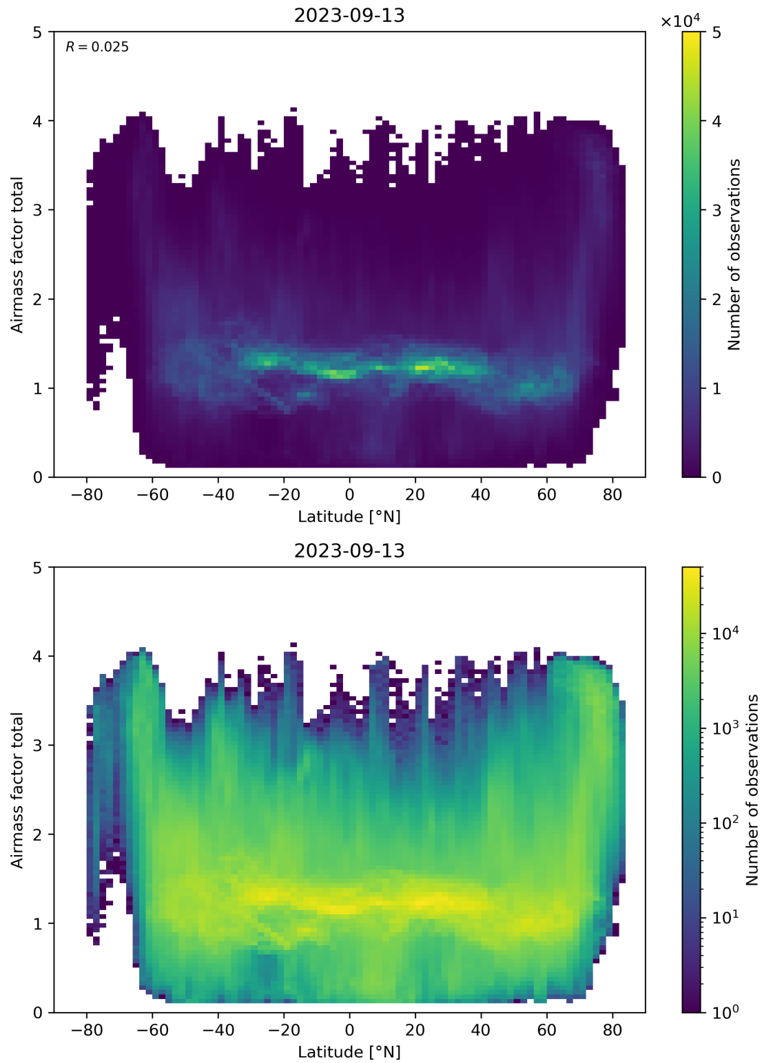
Figure 161: Scatter density plot of “Latitude” against “Airmass factor total” for 2023-09-12 to 2023-09-14.
