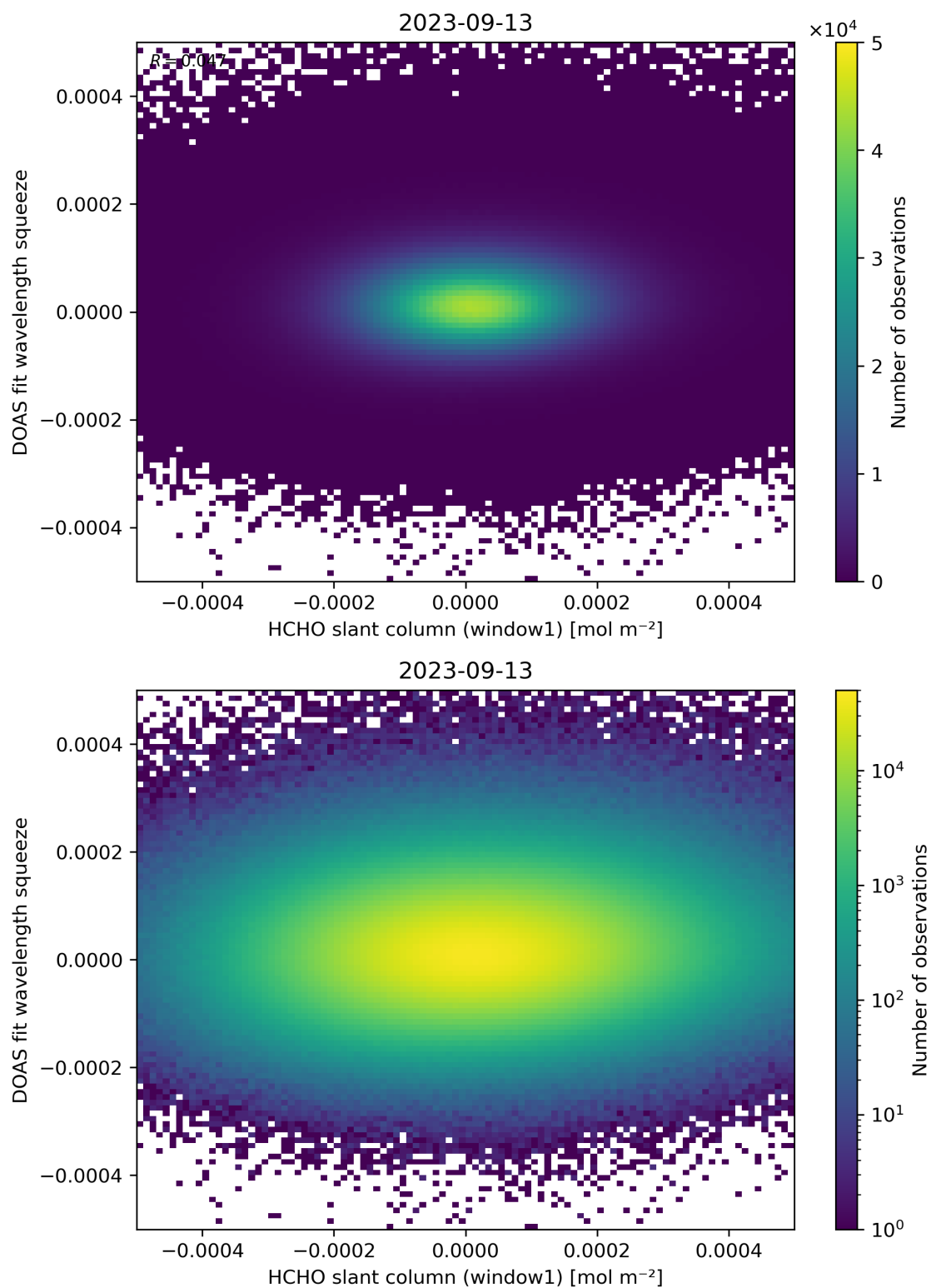
Figure 80: Scatter density plot of “HCHO slant column (window1)” against “DOAS fit wavelength squeeze” for 2023-09-12 to 2023-09-14.
