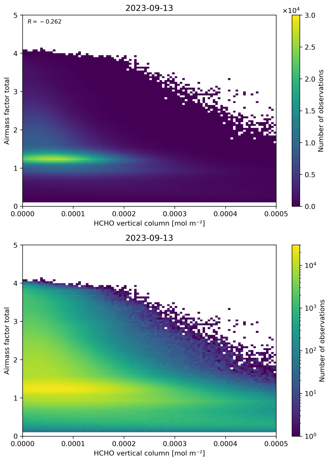
Figure 131: Scatter density plot of “HCHO vertical column” against “Airmass factor total” for 2023-09-12 to 2023-09-14.
