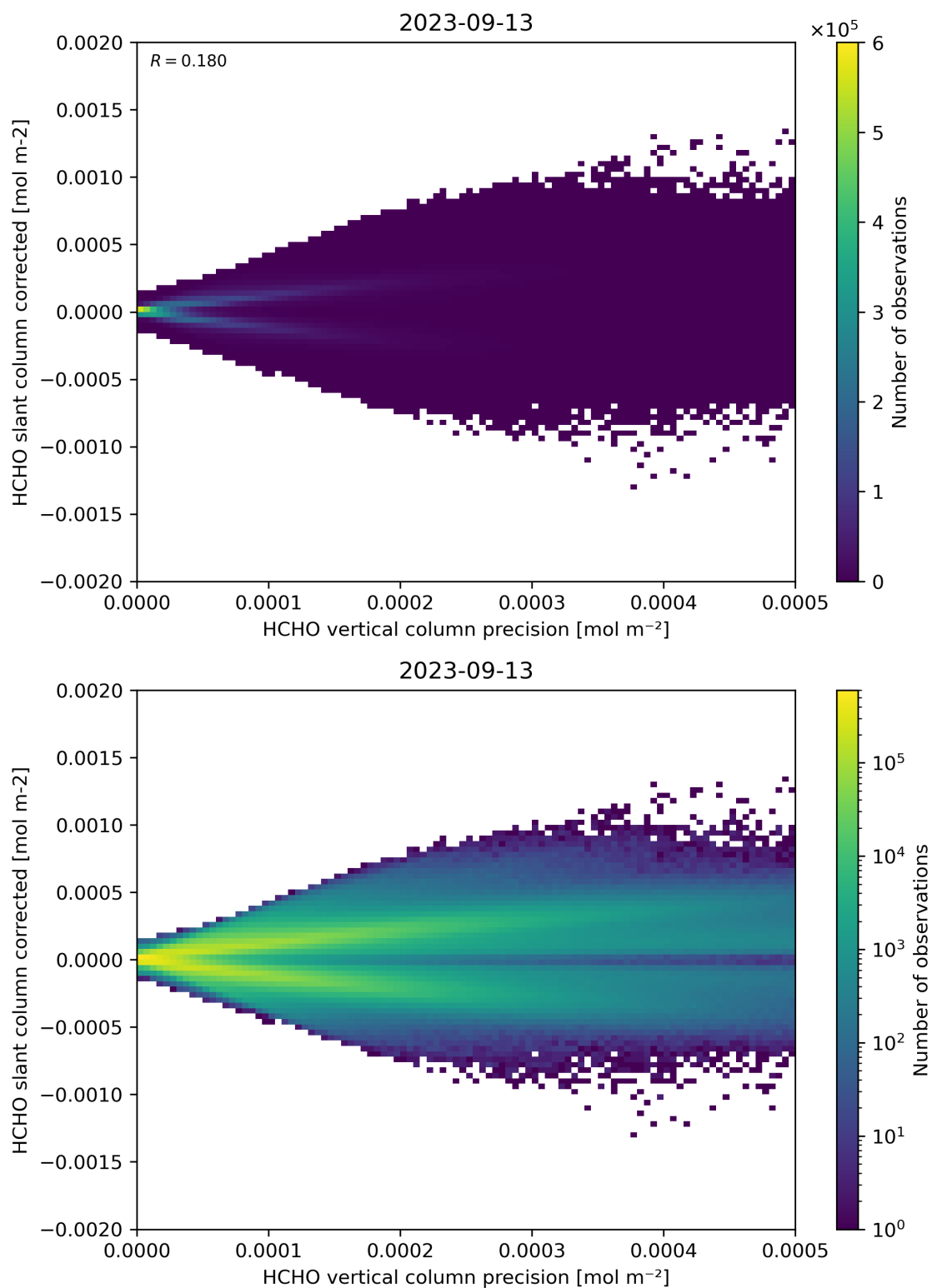
Figure 140: Scatter density plot of “HCHO vertical column precision” against “HCHO slant column corrected” for 2023-09-12 to 2023-09-14.
