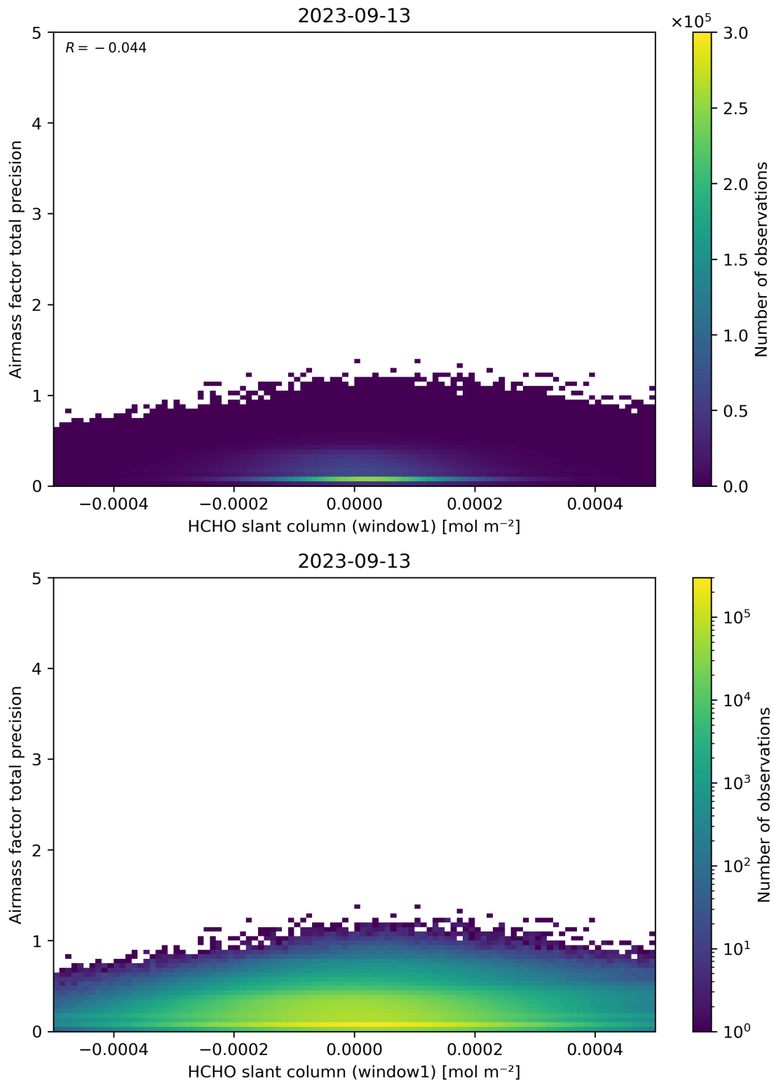
Figure 86: Scatter density plot of “HCHO slant column (window1)” against “Airmass factor total precision” for 2023-09-12 to 2023-09-14.
