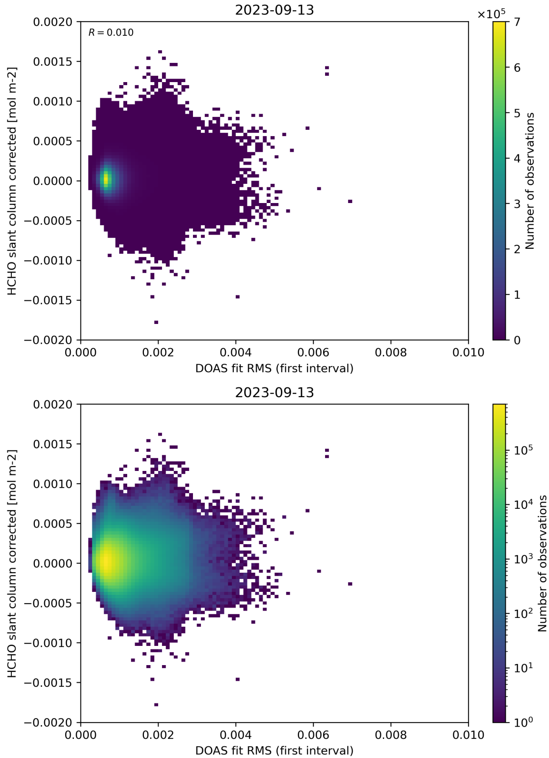
Figure 62: Scatter density plot of “DOAS fit RMS (first interval)” against “HCHO slant column corrected” for 2023-09-12 to 2023-09-14.
