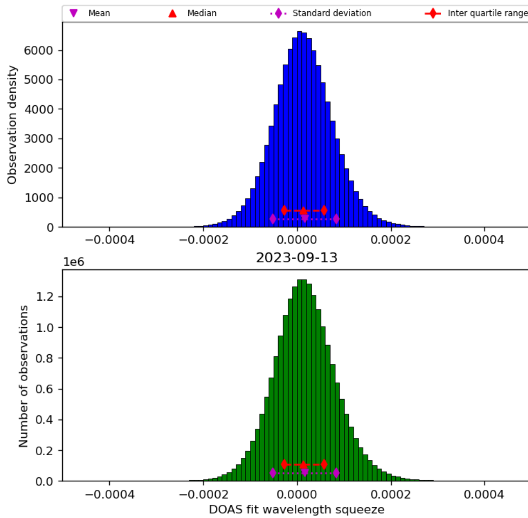
Figure 45: Histogram of “DOAS fit wavelength squeeze” for 2023-09-12 to 2023-09-14
