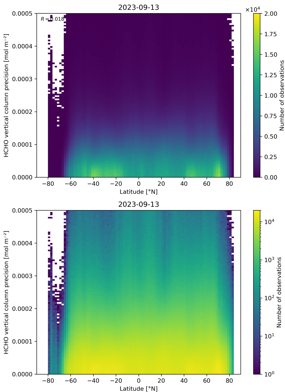
Figure 165: Scatter density plot of “Latitude” against “HCHO vertical column precision” for 2023-09-12 to 2023-09-14.
