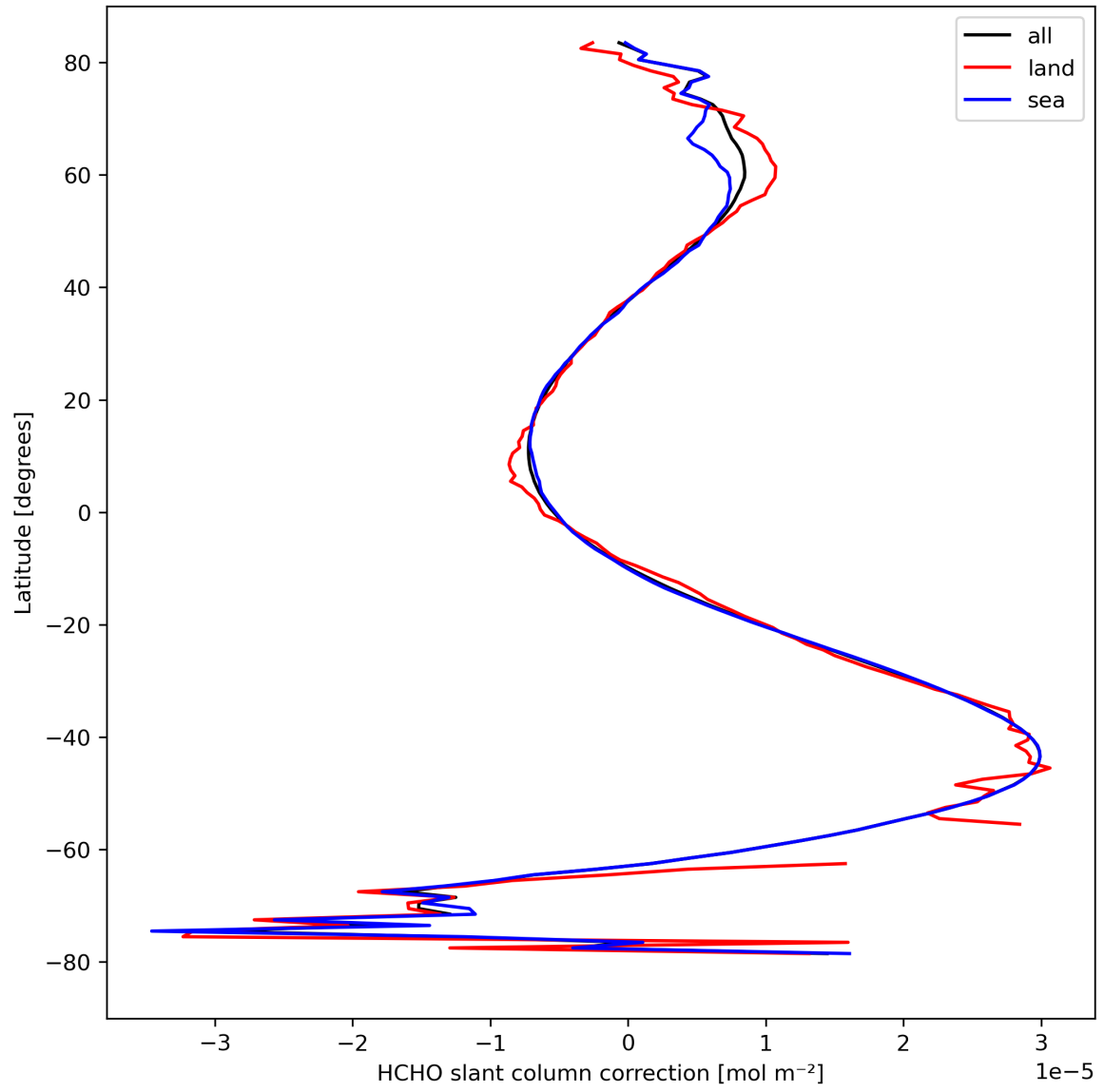
Figure 33: Zonal average of “HCHO slant column correction” for 2023-09-12 to 2023-09-14.
