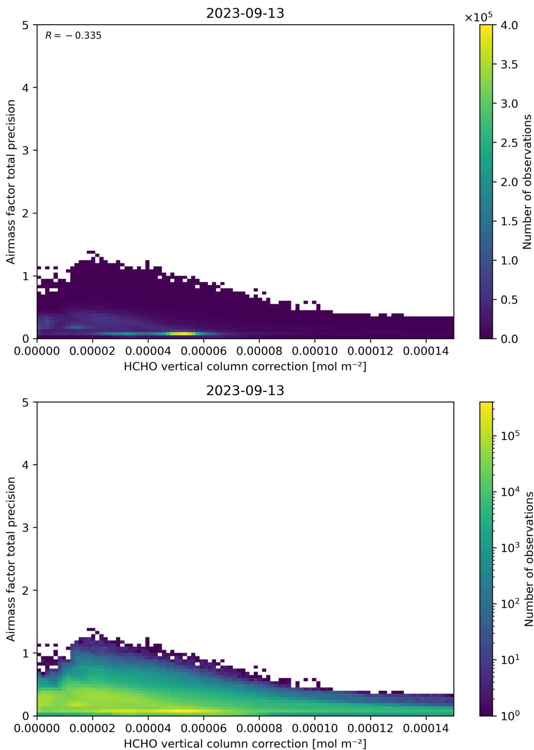
Figure 121: Scatter density plot of “HCHO vertical column correction” against “Airmass factor total precision” for 2023-09-12 to 2023-09-14.
