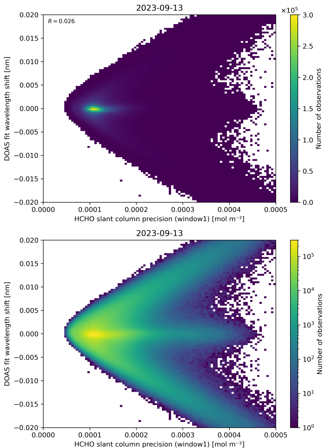
Figure 89: Scatter density plot of “HCHO slant column precision (window1)” against “DOAS fit wavelength shift” for 2023-09-12 to 2023-09-14.
