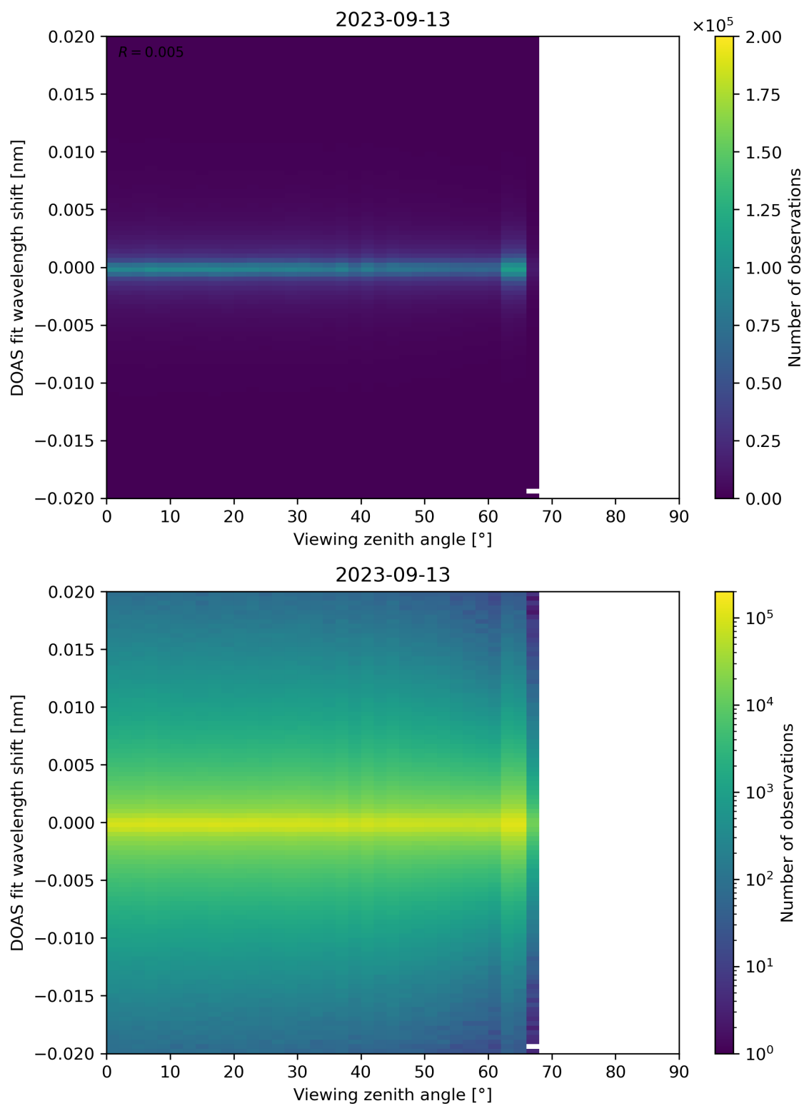
Figure 183: Scatter density plot of “Viewing zenith angle” against “DOAS fit wavelength shift” for 2023-09-12 to 2023-09-14.
