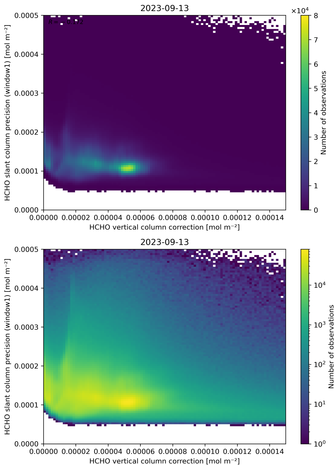
Figure 119: Scatter density plot of “HCHO vertical column correction” against “HCHO slant column precision (window1)” for 2023-09-12 to 2023-09-14.
