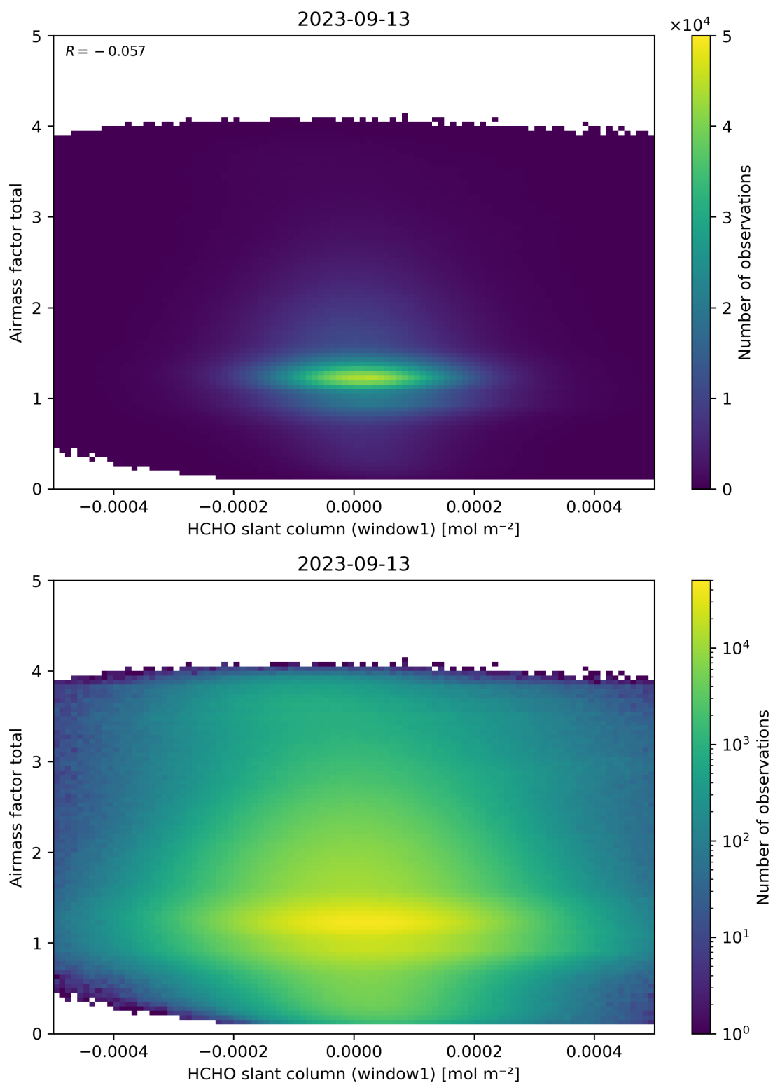
Figure 85: Scatter density plot of “HCHO slant column (window1)” against “Airmass factor total” for 2023-09-12 to 2023-09-14.
