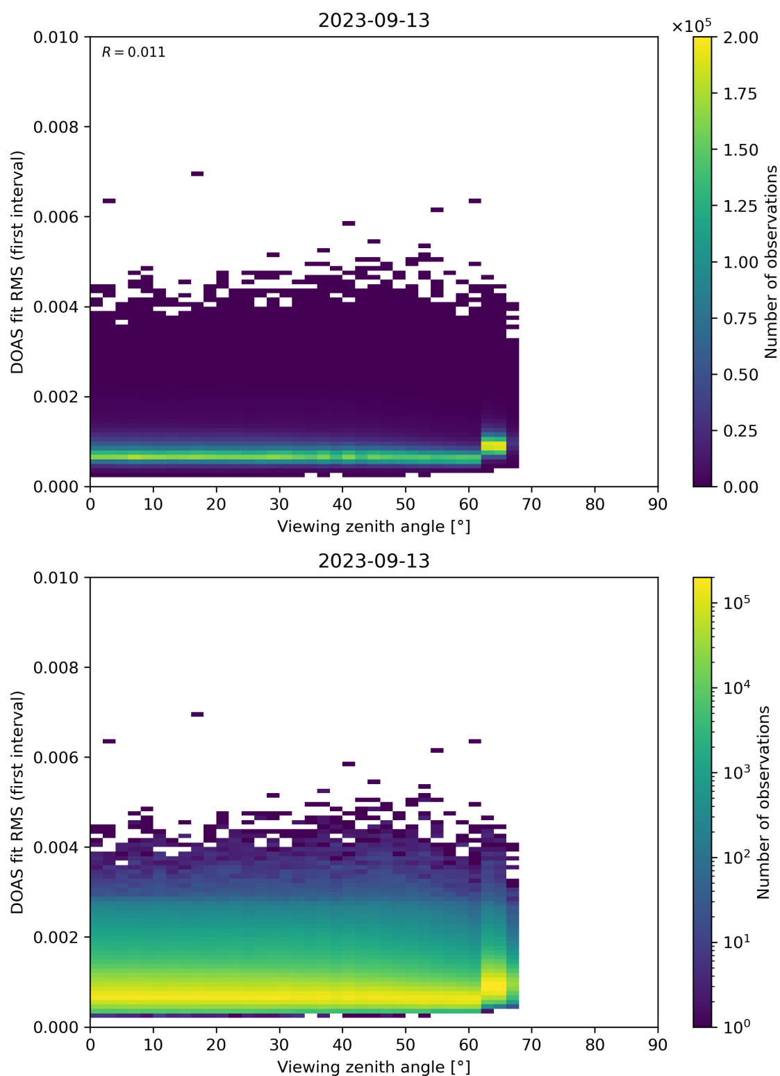
Figure 182: Scatter density plot of “Viewing zenith angle” against “DOAS fit RMS (first interval)” for 2023-09-12 to 2023-09-14.
