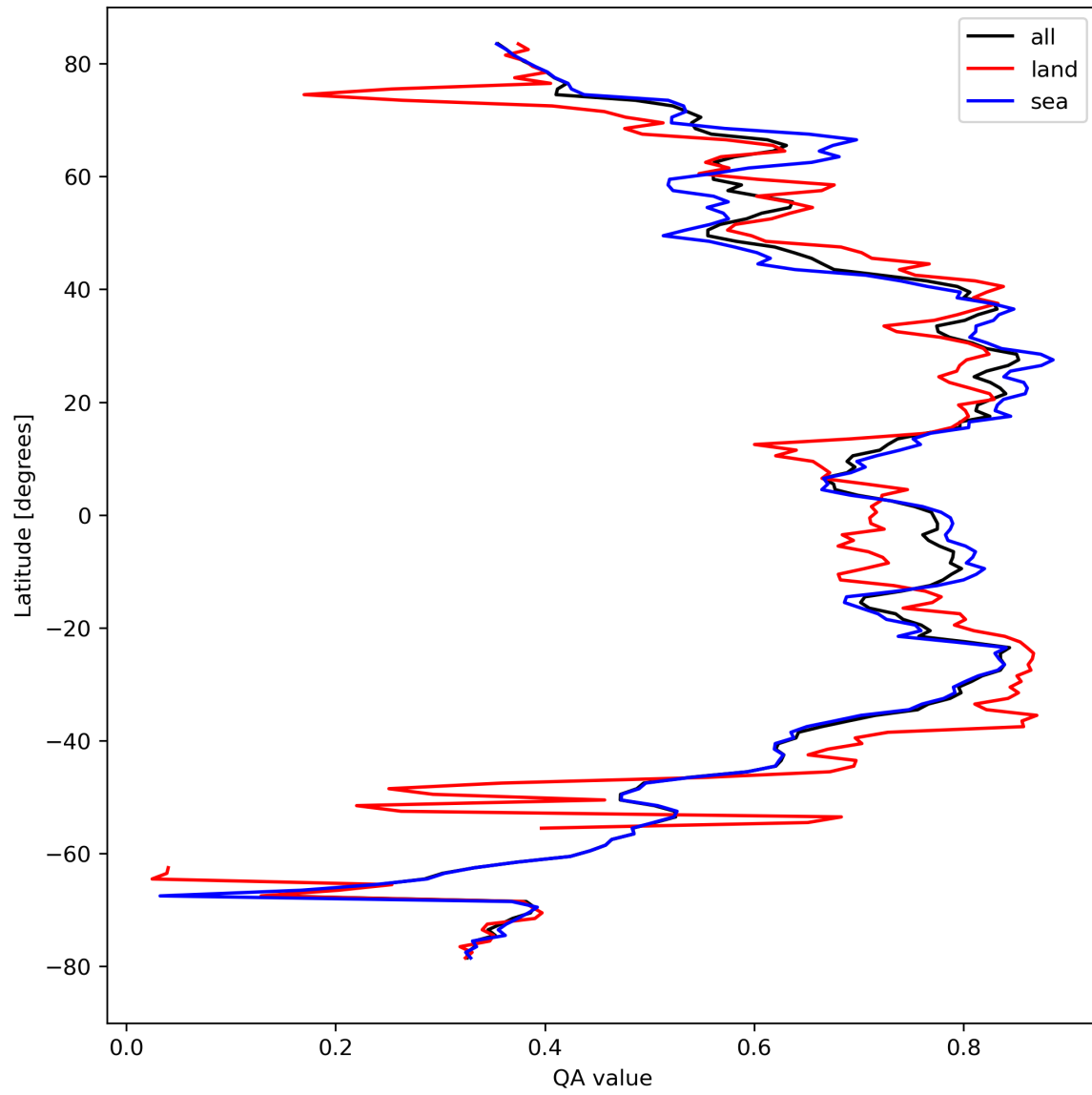
Figure 20: Zonal average of “QA value” for 2023-09-12 to 2023-09-14.
