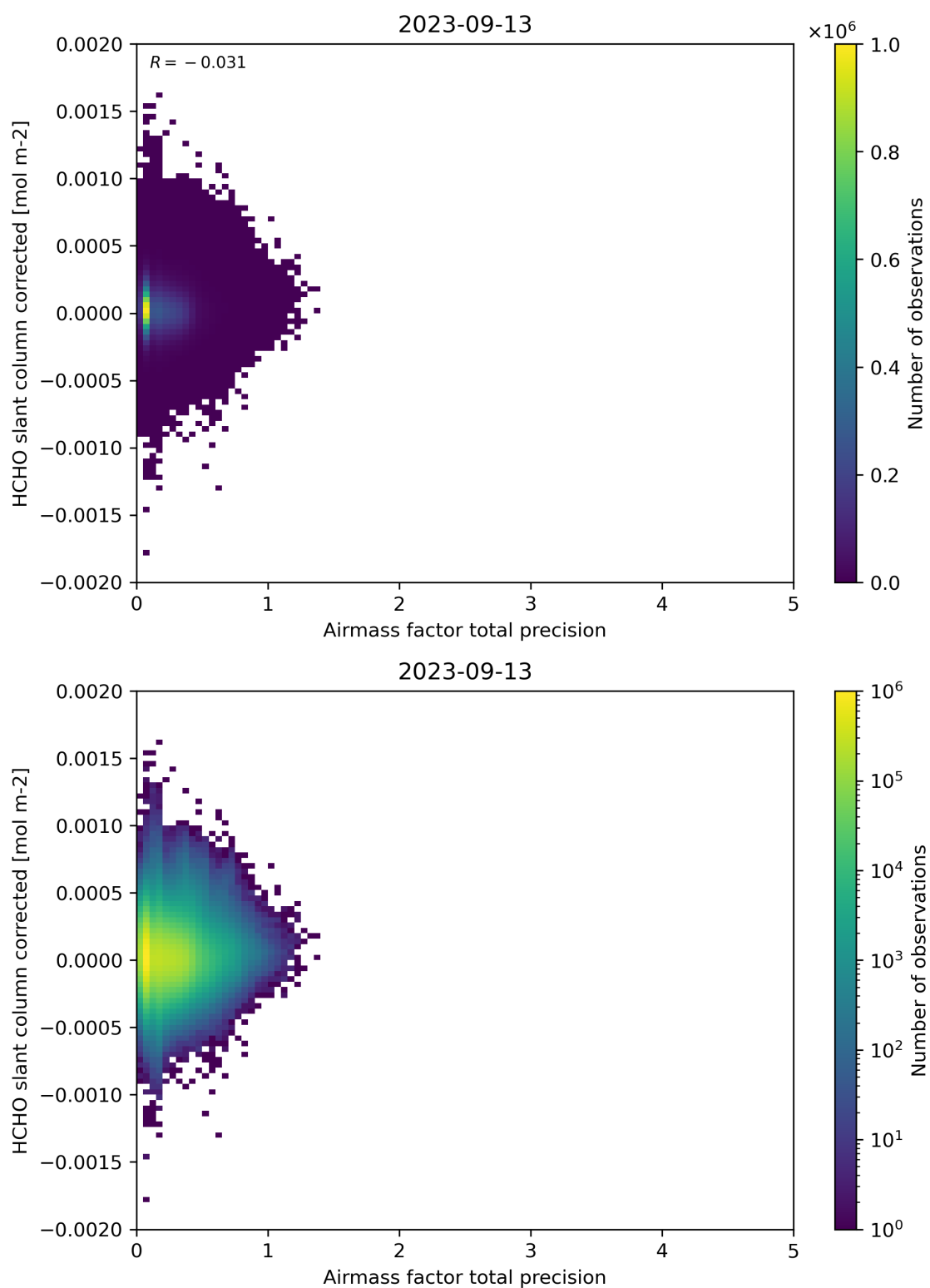
Figure 109: Scatter density plot of “Airmass factor total precision” against “HCHO slant column corrected” for 2023-09-12 to 2023-09-14.
