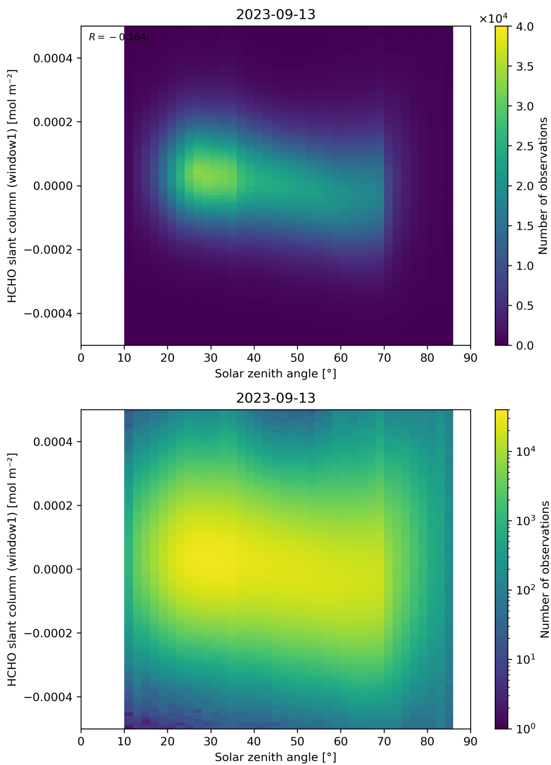
Figure 173: Scatter density plot of “Solar zenith angle” against “HCHO slant column (window1)” for 2023-09-12 to 2023-09-14.
