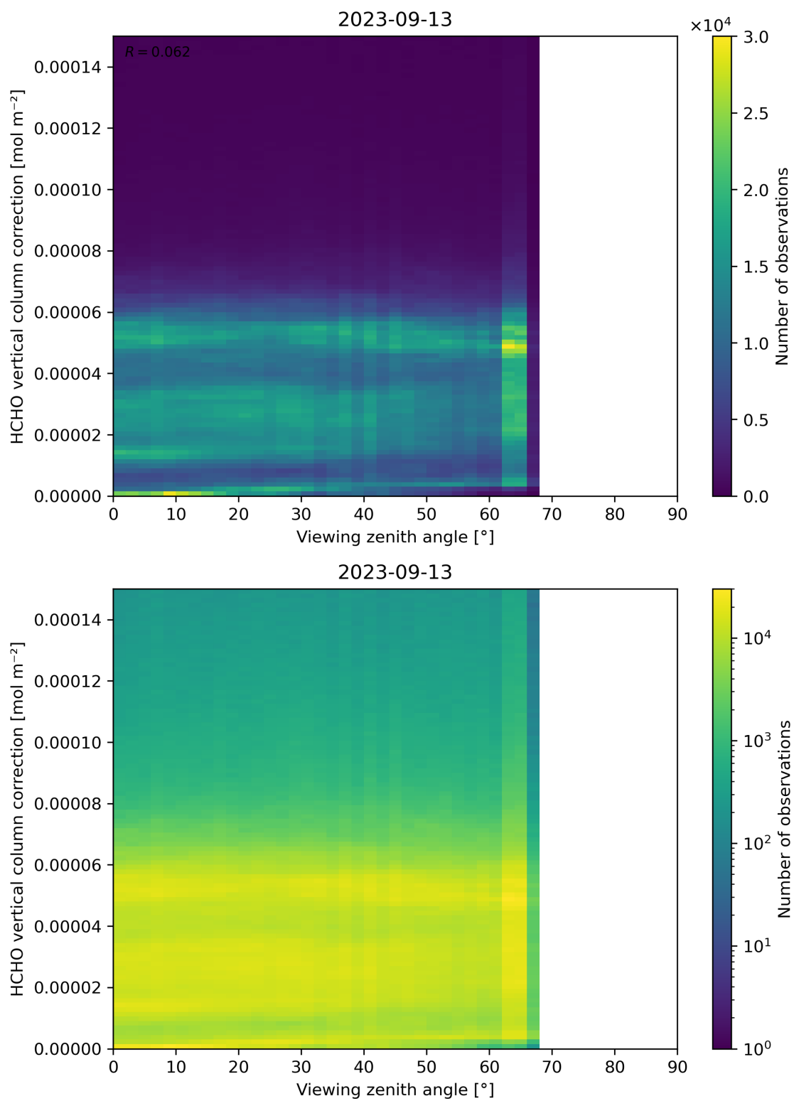
Figure 193: Scatter density plot of “Viewing zenith angle” against “HCHO vertical column correction” for 2023-09-12 to 2023-09-14.
