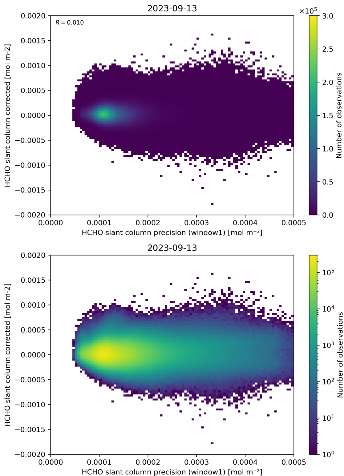
Figure 92: Scatter density plot of “HCHO slant column precision (window1)” against “HCHO slant column corrected” for 2023-09-12 to 2023-09-14.
