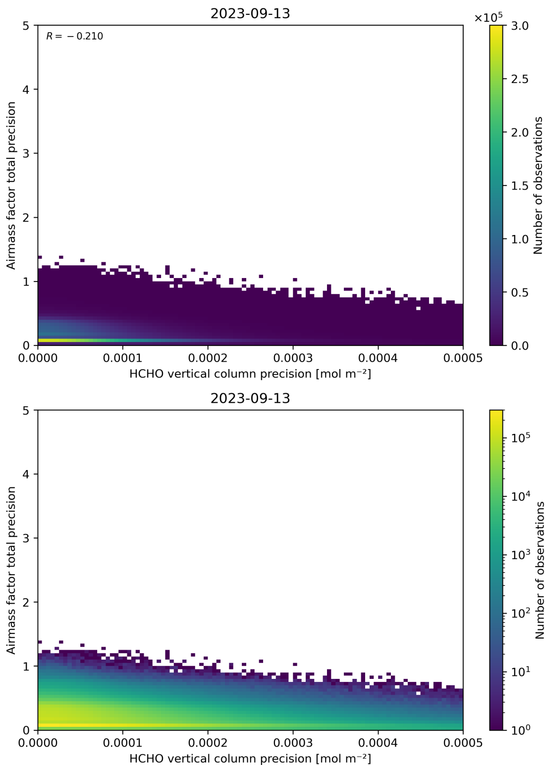
Figure 145: Scatter density plot of “HCHO vertical column precision” against “Airmass factor total precision” for 2023-09-12 to 2023-09-14.
