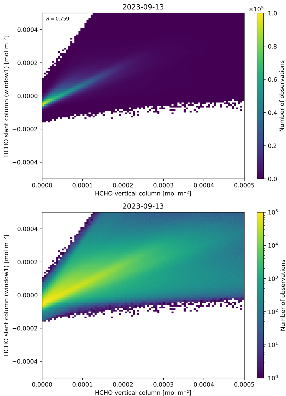
Figure 129: Scatter density plot of “HCHO vertical column” against “HCHO slant column (window1)” for 2023-09-12 to 2023-09-14.
