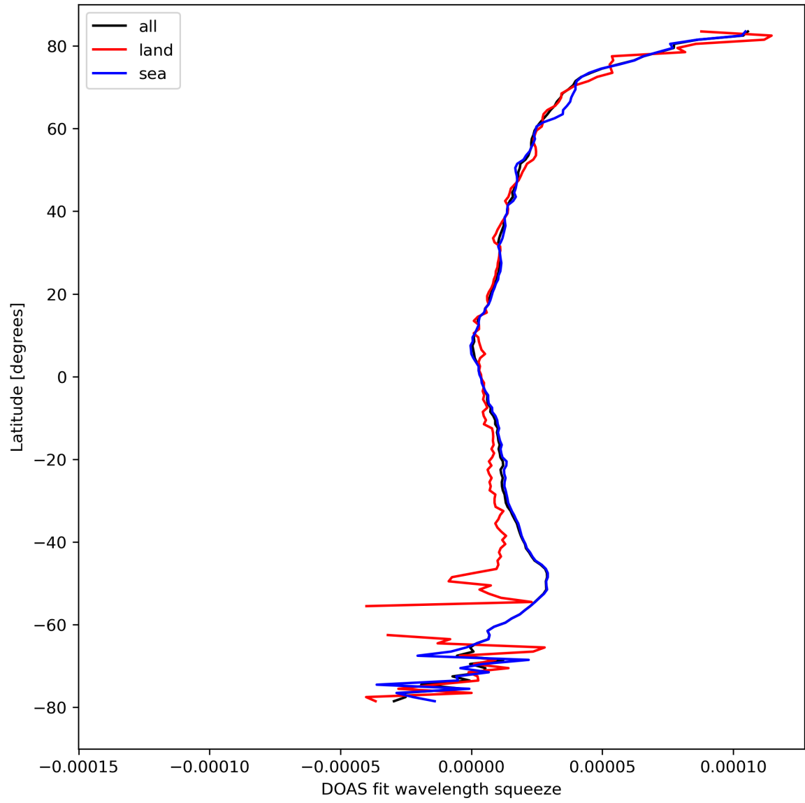
Figure 31: Zonal average of “DOAS fit wavelength squeeze” for 2023-09-12 to 2023-09-14.
