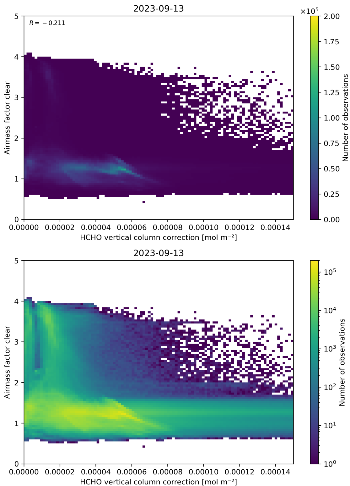
Figure 115: Scatter density plot of “HCHO vertical column correction” against “Airmass factor clear” for 2023-09-12 to 2023-09-14.
