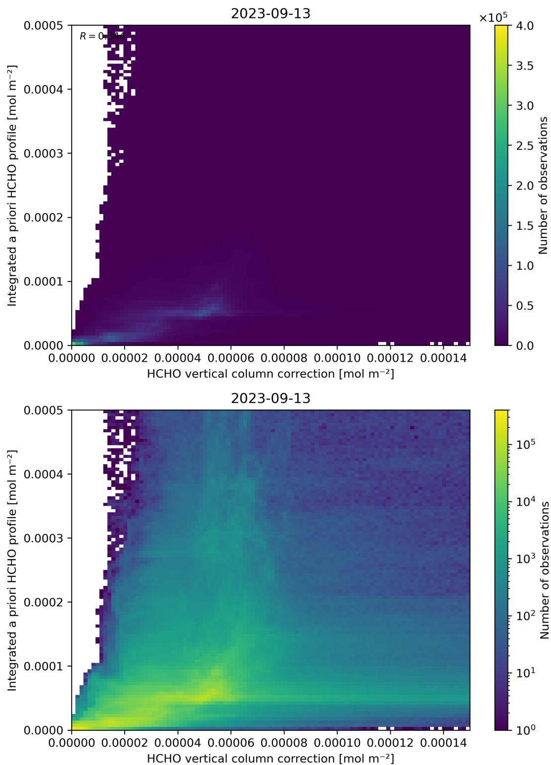
Figure 122: Scatter density plot of “HCHO vertical column correction” against “Integrated a priori HCHO profile” for 2023-09-12 to 2023-09-14.
