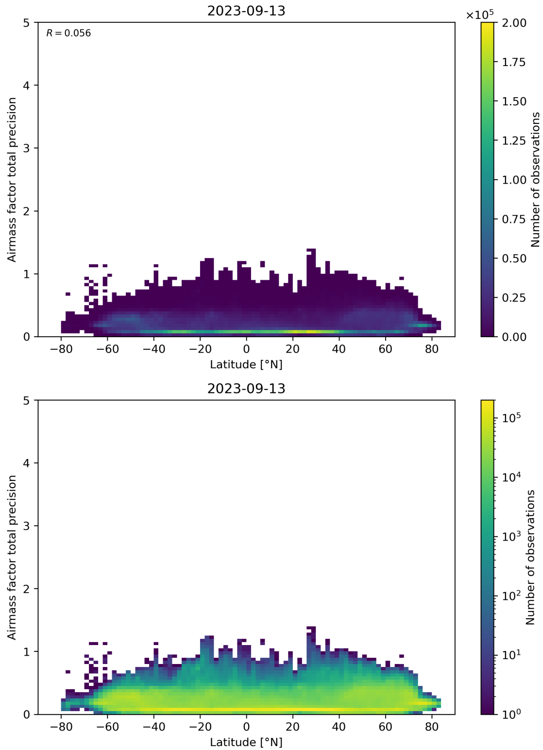
Figure 162: Scatter density plot of “Latitude” against “Airmass factor total precision” for 2023-09-12 to 2023-09-14.
