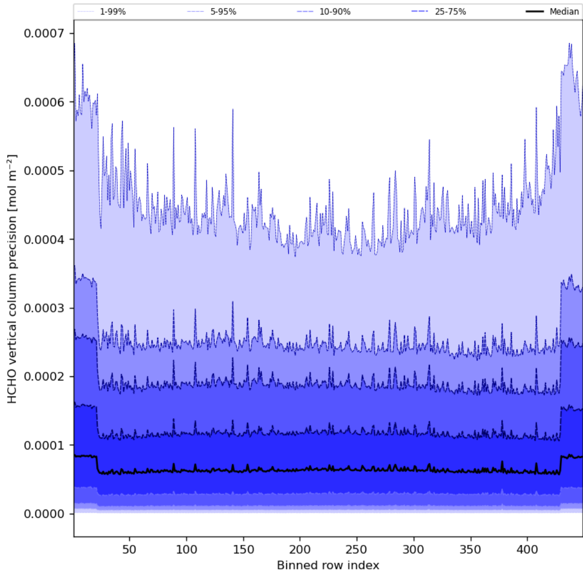
Figure 50: Along track statistics of “HCHO vertical column precision” for 2023-09-12 to 2023-09-14
