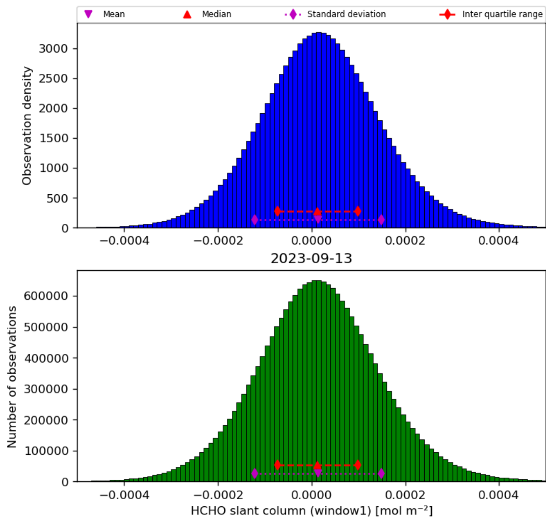
Figure 38: Histogram of “HCHO slant column (window1)” for 2023-09-12 to 2023-09-14
