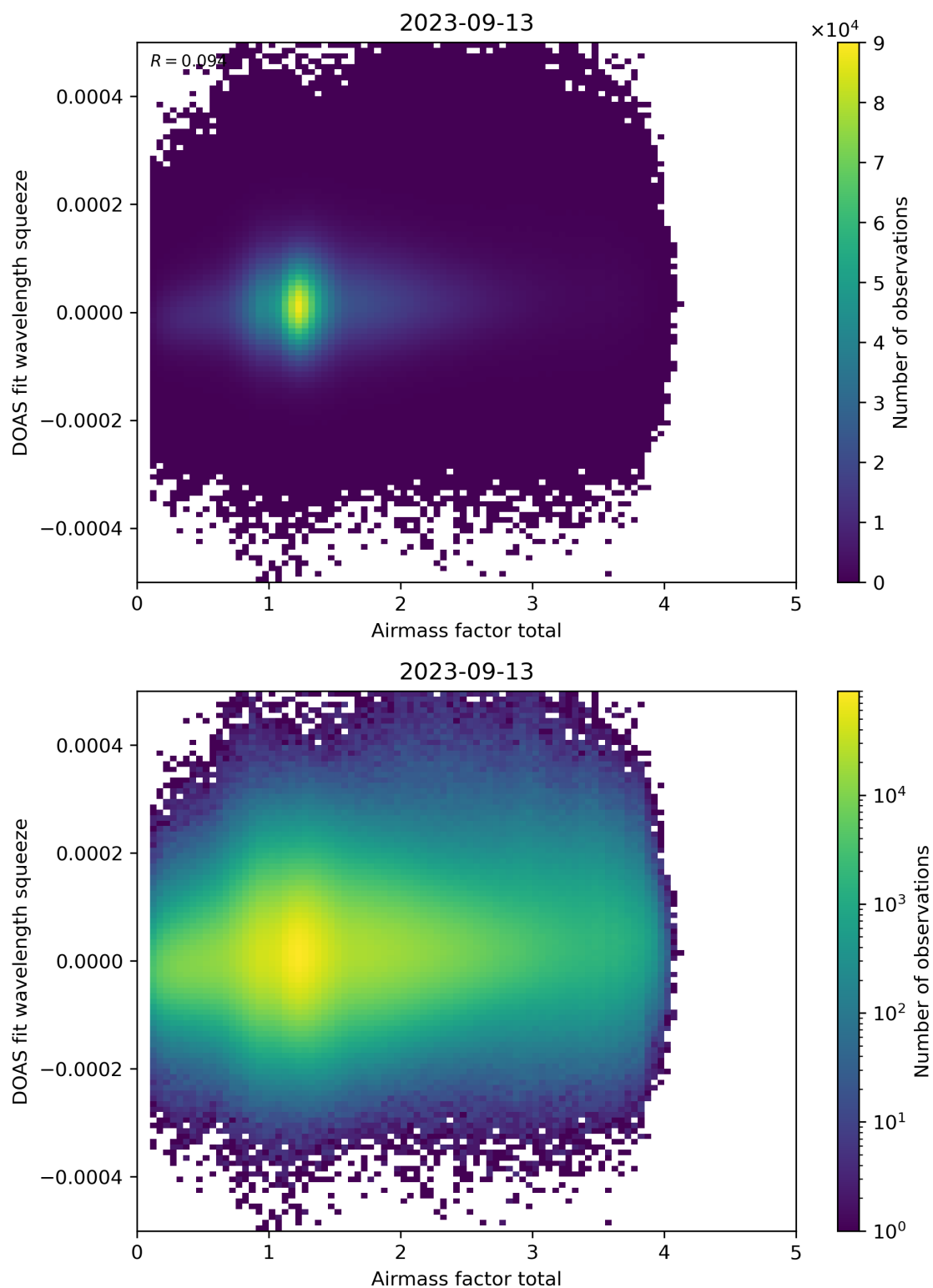
Figure 99: Scatter density plot of “Airmass factor total” against “DOAS fit wavelength squeeze” for 2023-09-12 to 2023-09-14.
