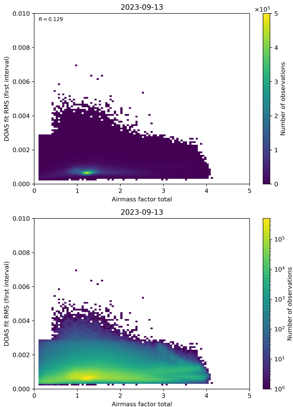
Figure 97: Scatter density plot of “Airmass factor total” against “DOAS fit RMS (first interval)” for 2023-09-12 to 2023-09-14.
