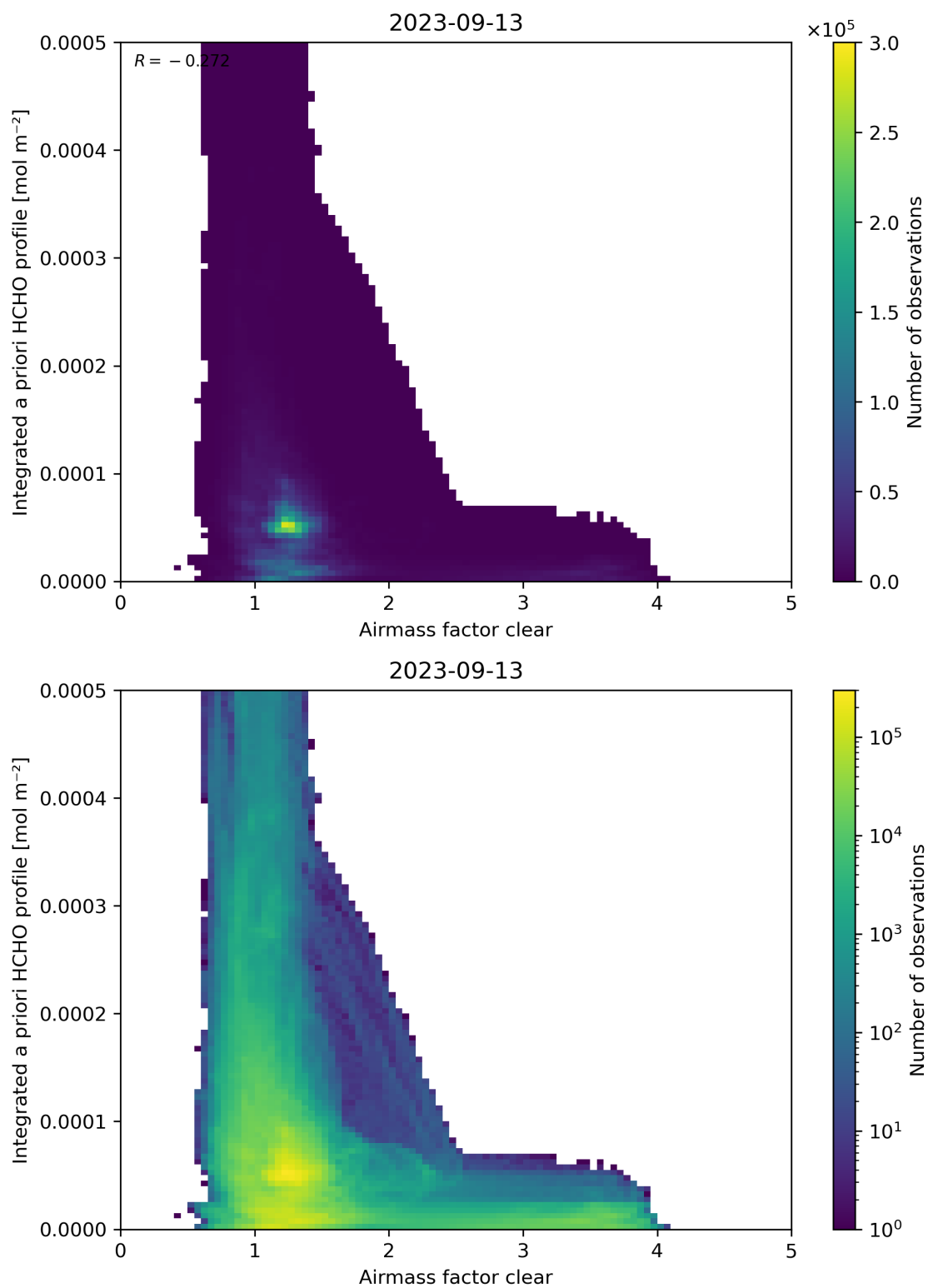
Figure 76: Scatter density plot of “Airmass factor clear” against “Integrated a priori HCHO profile” for 2023-09-12 to 2023-09-14.
