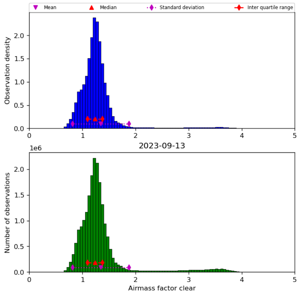
Figure 42: Histogram of “Airmass factor clear” for 2023-09-12 to 2023-09-14
