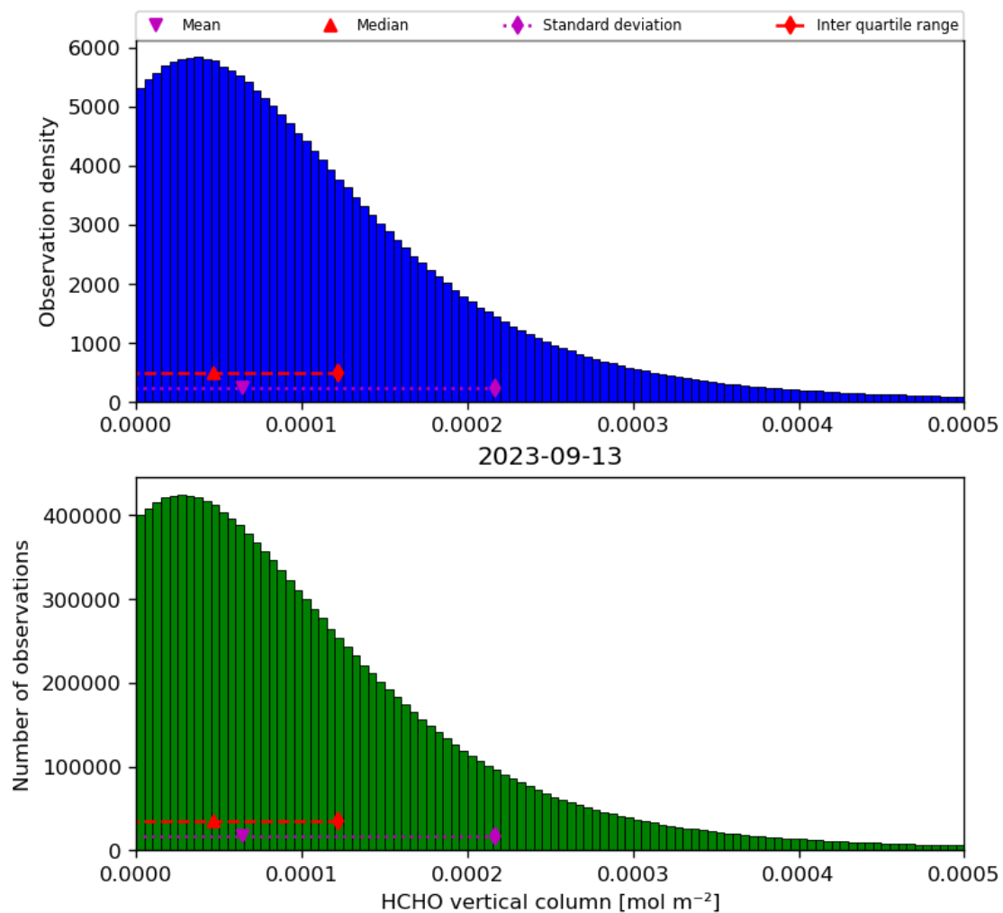
Figure 35: Histogram of “HCHO vertical column” for 2023-09-12 to 2023-09-14
