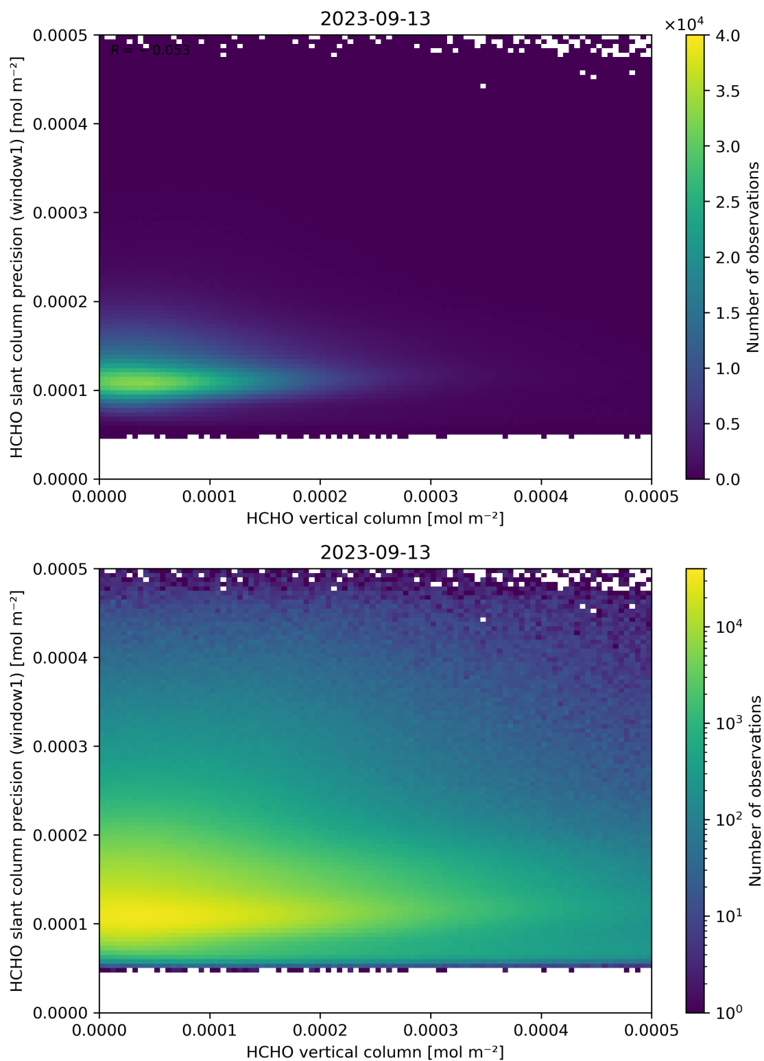
Figure 130: Scatter density plot of “HCHO vertical column” against “HCHO slant column precision (window1)” for 2023-09-12 to 2023-09-14.
