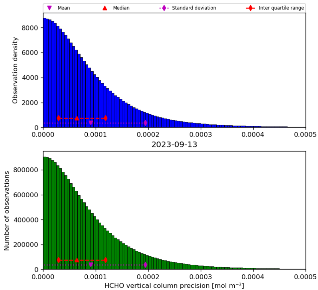
Figure 36: Histogram of “HCHO vertical column precision” for 2023-09-12 to 2023-09-14
