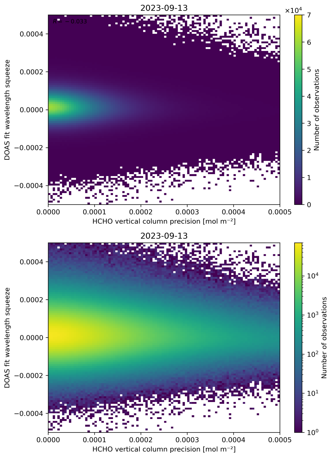
Figure 138: Scatter density plot of “HCHO vertical column precision” against “DOAS fit wavelength squeeze” for 2023-09-12 to 2023-09-14.
