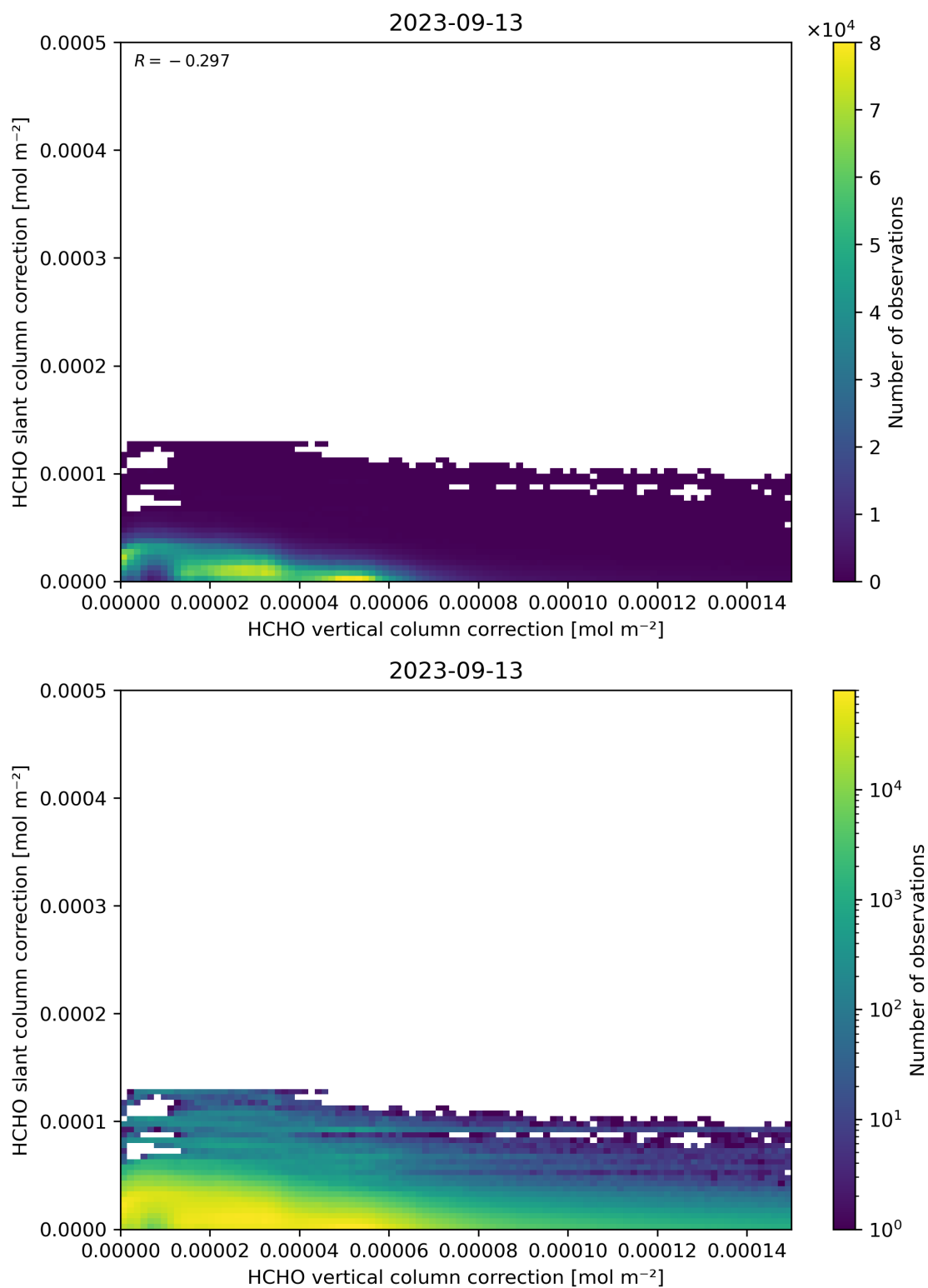
Figure 117: Scatter density plot of “HCHO vertical column correction” against “HCHO slant column correction” for 2023-09-12 to 2023-09-14.
