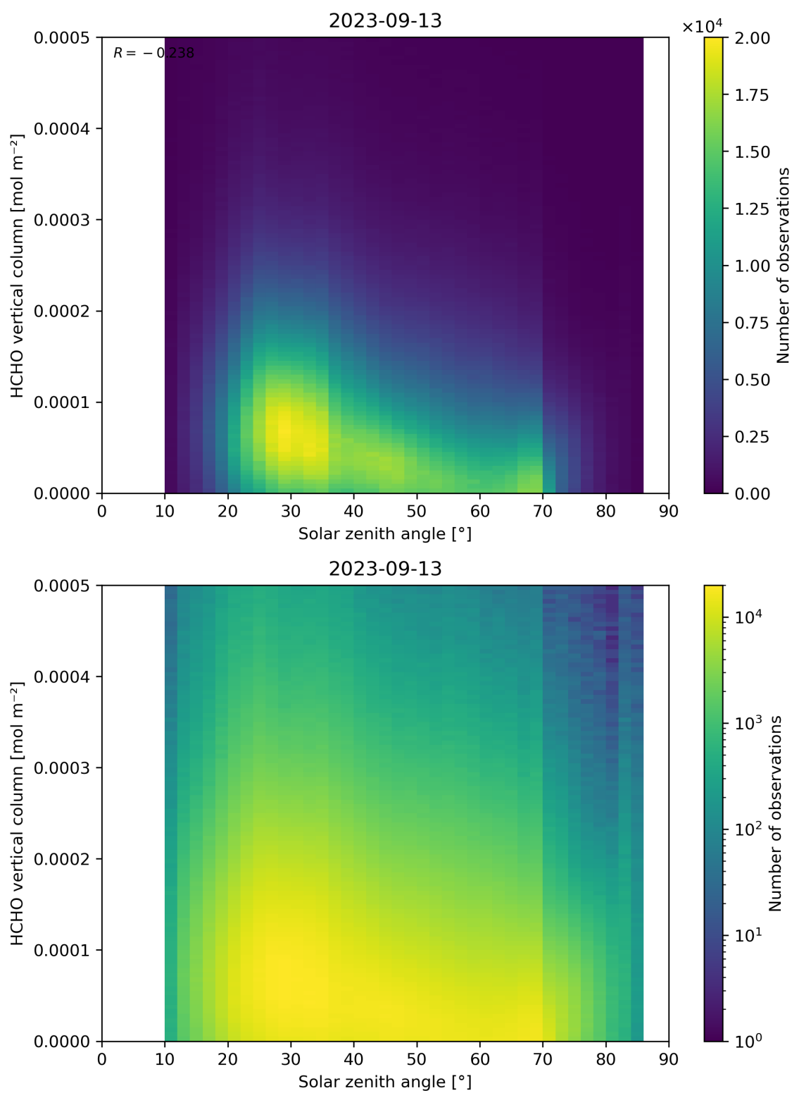
Figure 177: Scatter density plot of “Solar zenith angle” against “HCHO vertical column” for 2023-09-12 to 2023-09-14.
