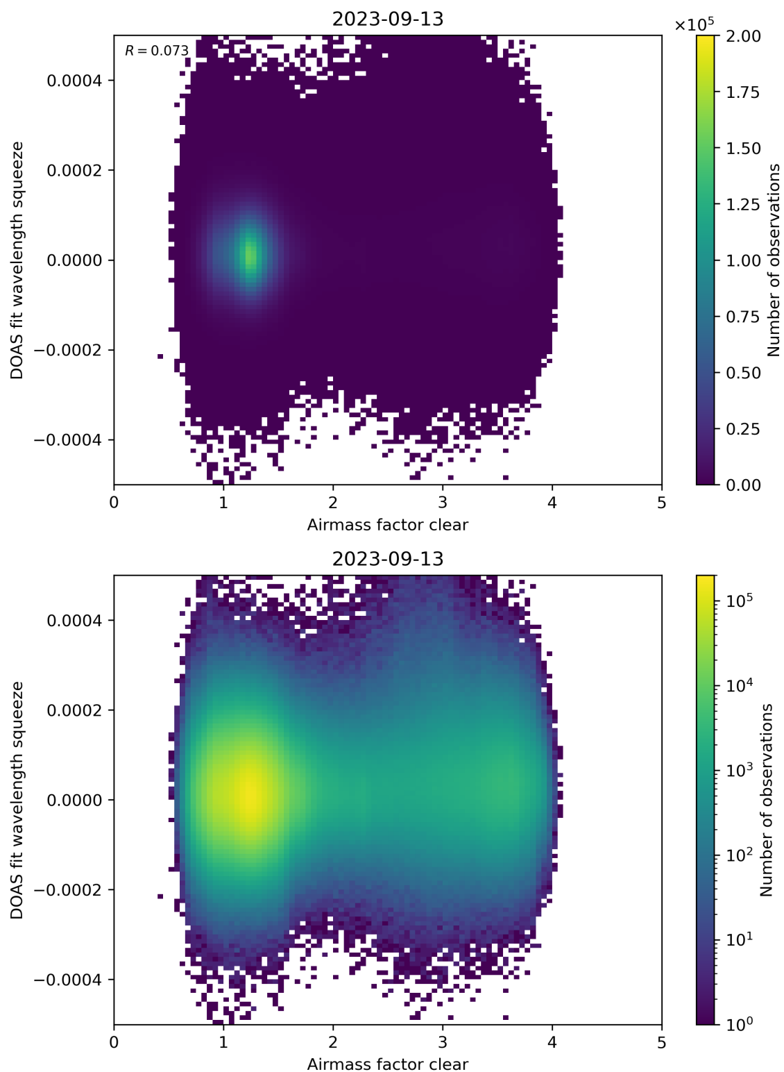
Figure 73: Scatter density plot of “Airmass factor clear” against “DOAS fit wavelength squeeze” for 2023-09-12 to 2023-09-14.
