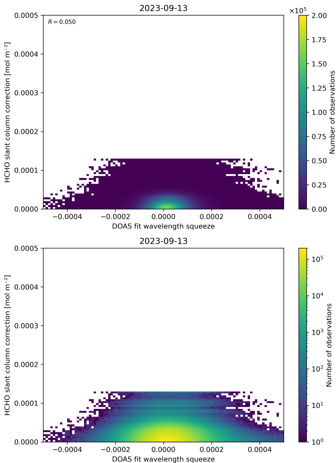
Figure 70: Scatter density plot of “DOAS fit wavelength squeeze” against “HCHO slant column correction” for 2023-09-12 to 2023-09-14.
