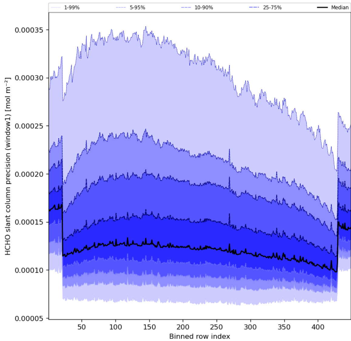
Figure 53: Along track statistics of “HCHO slant column precision (window1)” for 2023-09-12 to 2023-09-14
