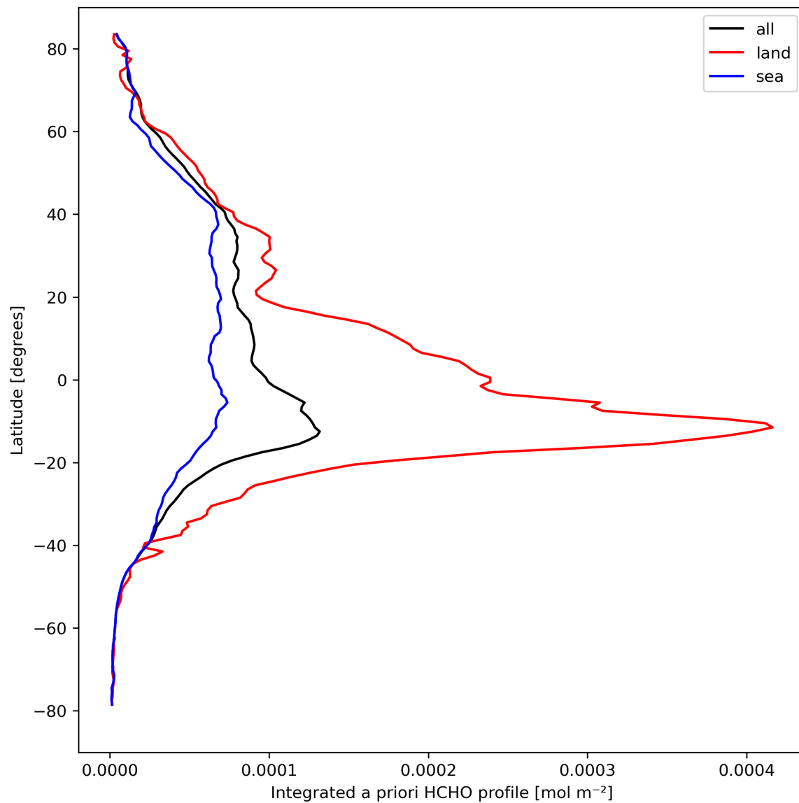
Figure 29: Zonal average of “Integrated a priori HCHO profile” for 2023-09-12 to 2023-09-14.
