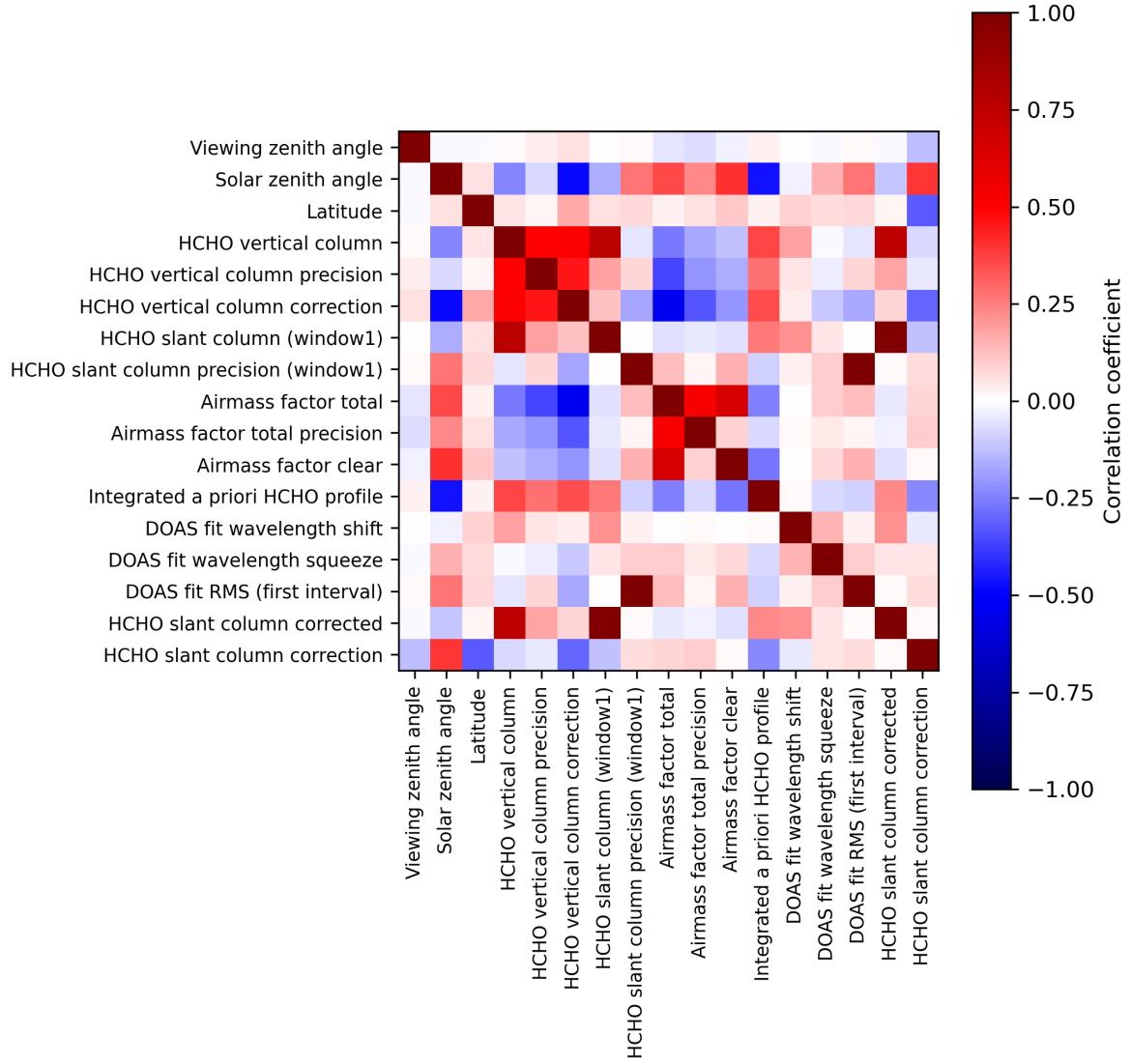
Figure 2: Map of correlation matrix for 2023-09-12 to 2023-09-14.
