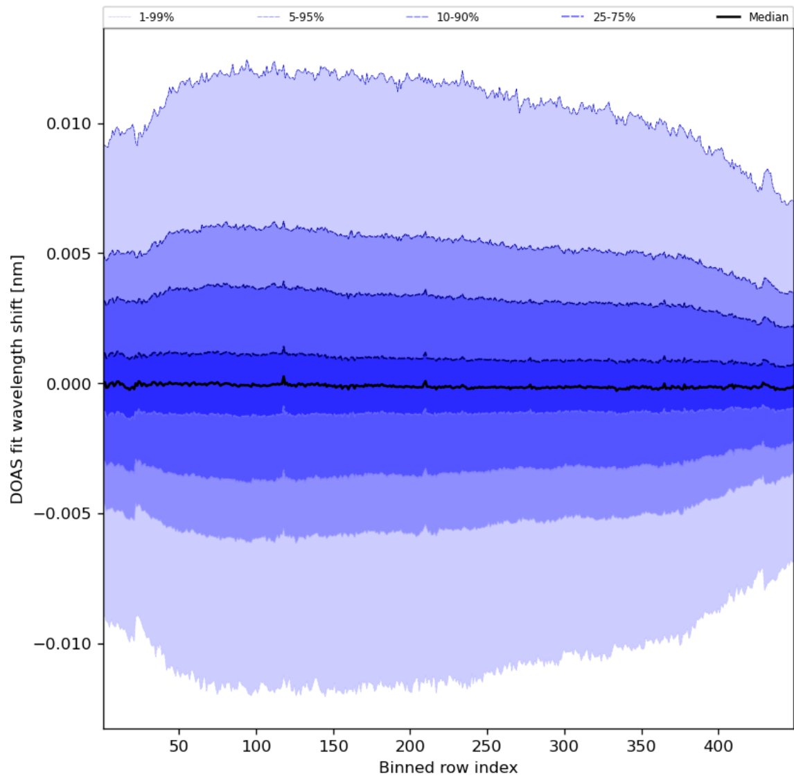
Figure 58: Along track statistics of “DOAS fit wavelength shift” for 2023-09-12 to 2023-09-14
