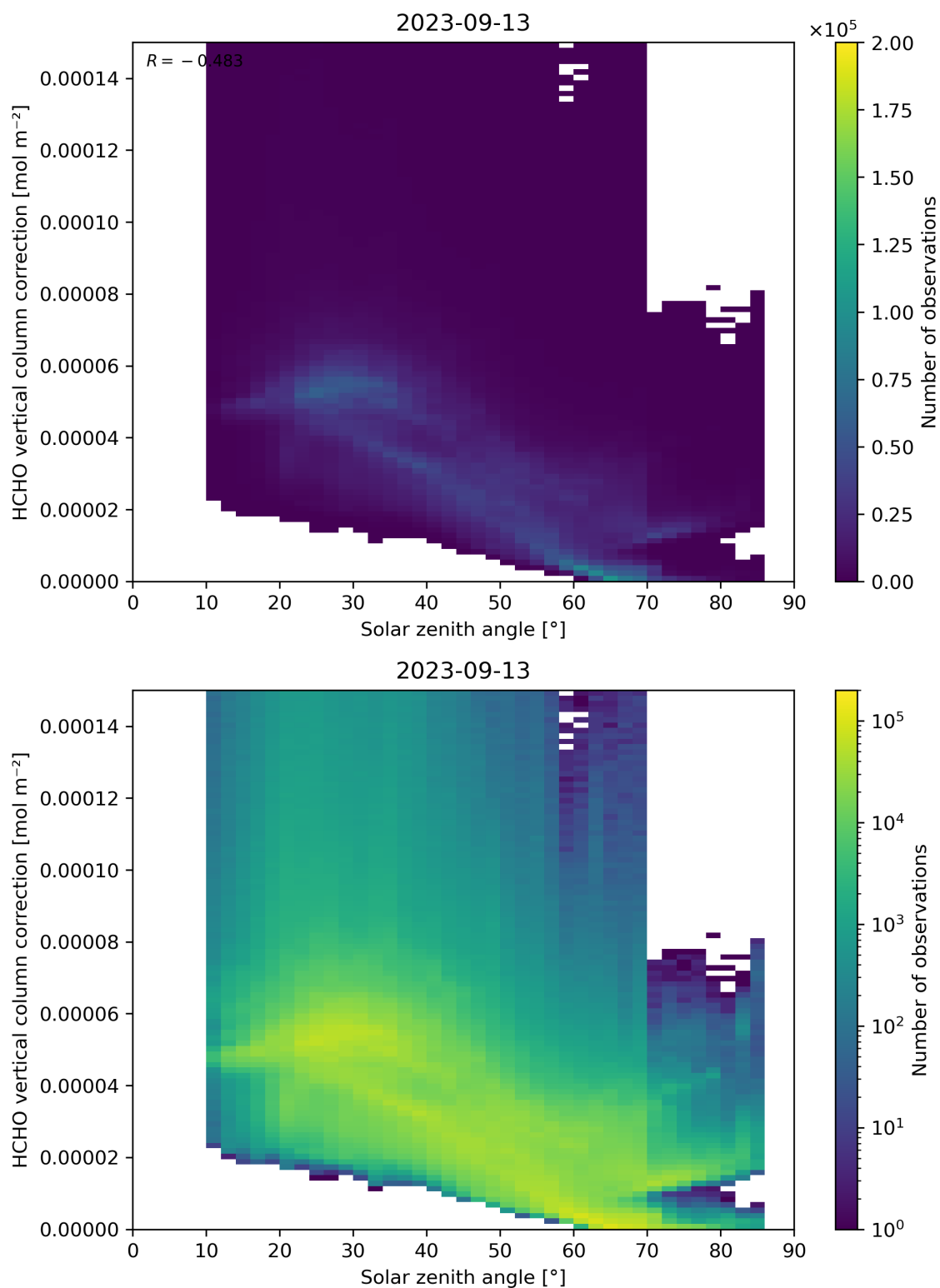
Figure 178: Scatter density plot of “Solar zenith angle” against “HCHO vertical column correction” for 2023-09-12 to 2023-09-14.
