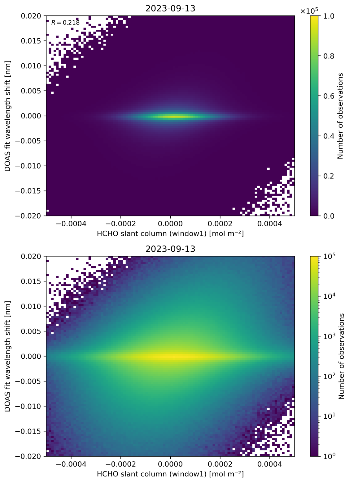
Figure 79: Scatter density plot of “HCHO slant column (window1)” against “DOAS fit wavelength shift” for 2023-09-12 to 2023-09-14.
