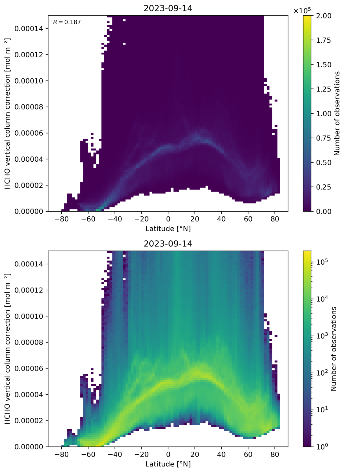
Figure 164: Scatter density plot of “Latitude” against “HCHO vertical column correction” for 2023-09-13 to 2023-09-15.
