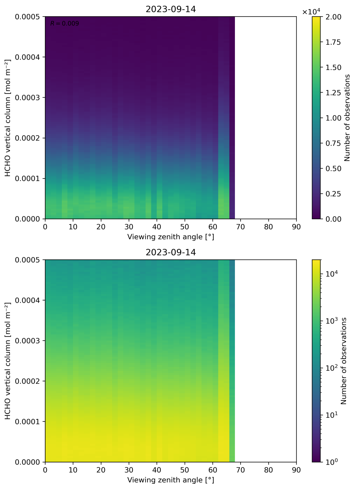
Figure 192: Scatter density plot of “Viewing zenith angle” against “HCHO vertical column” for 2023-09-13 to 2023-09-15.
