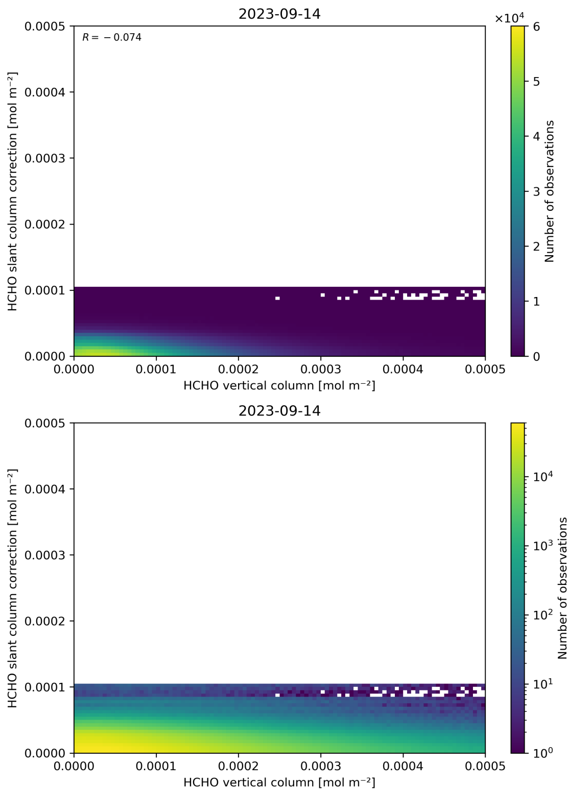
Figure 128: Scatter density plot of “HCHO vertical column” against “HCHO slant column correction” for 2023-09-13 to 2023-09-15.
