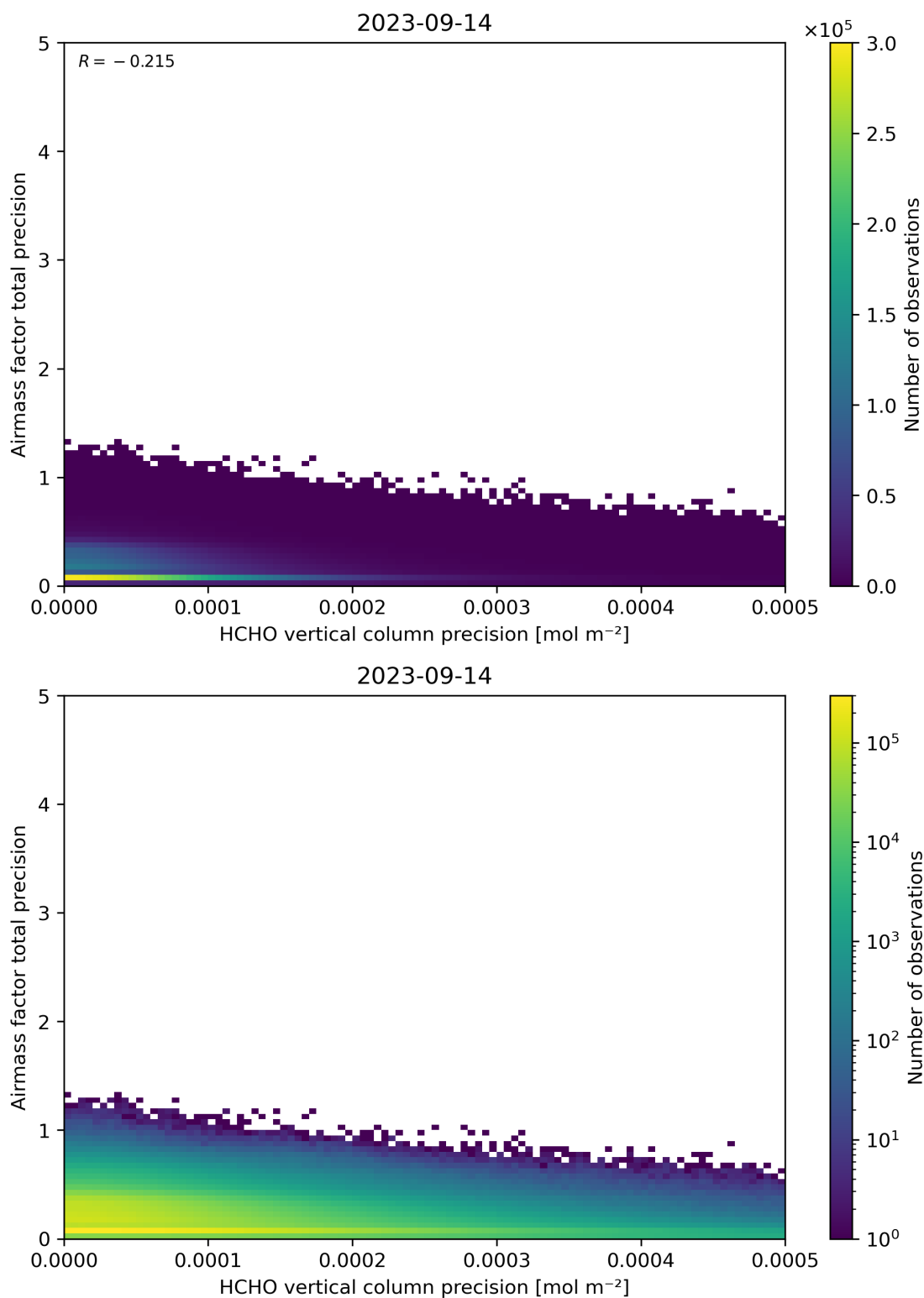
Figure 145: Scatter density plot of “HCHO vertical column precision” against “Airmass factor total precision” for 2023-09-13 to 2023-09-15.
