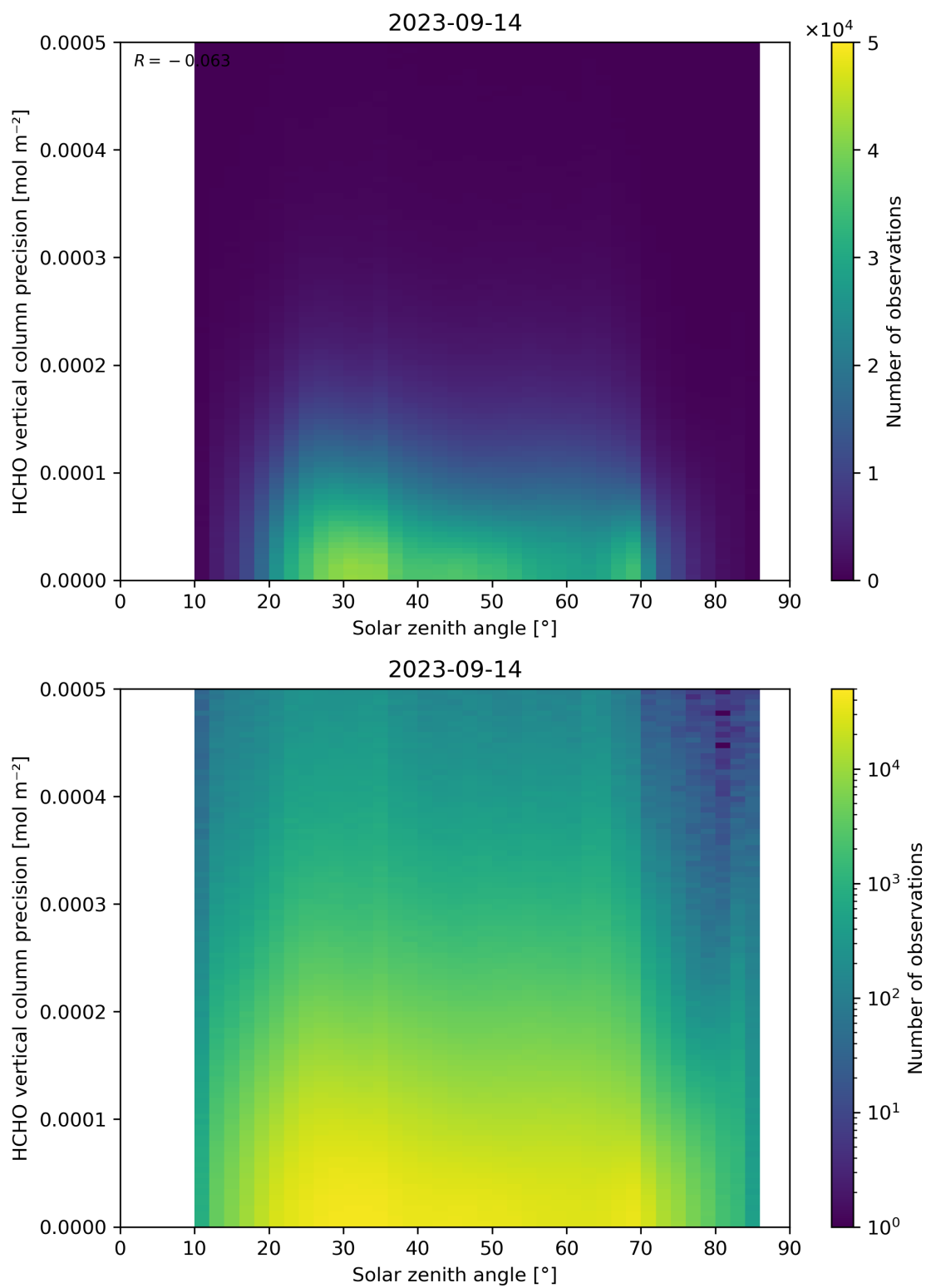
Figure 179: Scatter density plot of “Solar zenith angle” against “HCHO vertical column precision” for 2023-09-13 to 2023-09-15.
