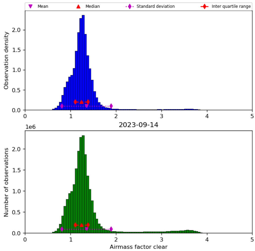
Figure 42: Histogram of “Airmass factor clear” for 2023-09-13 to 2023-09-15
