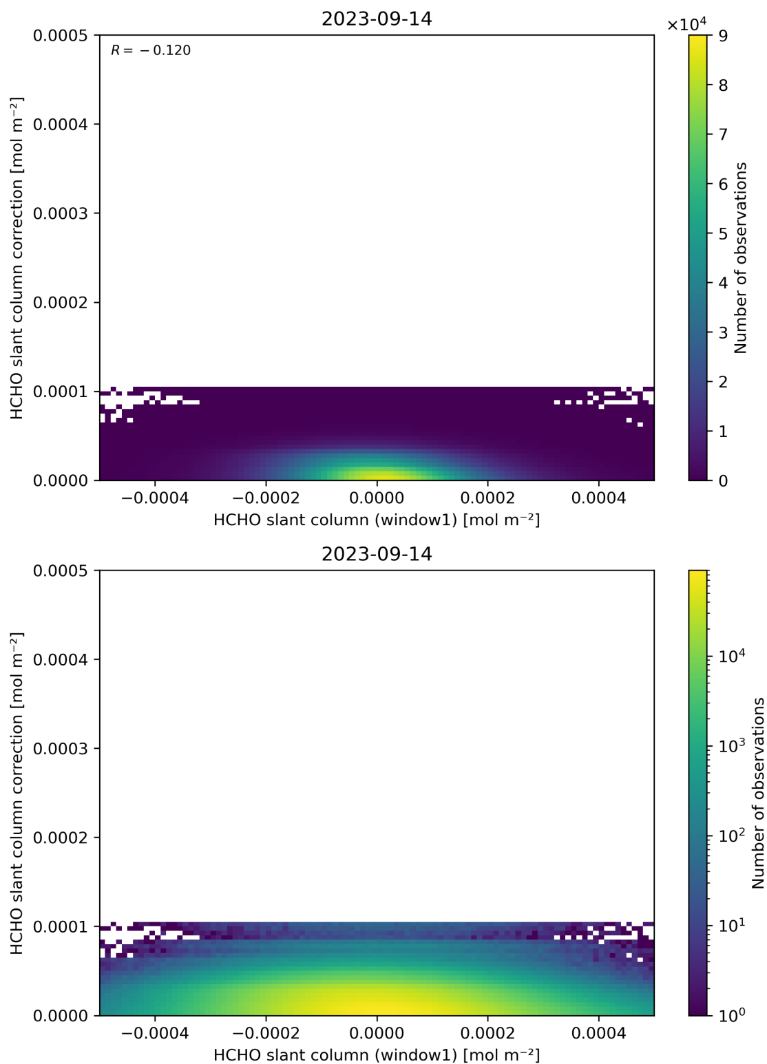
Figure 83: Scatter density plot of “HCHO slant column (window1)” against “HCHO slant column correction” for 2023-09-13 to 2023-09-15.
