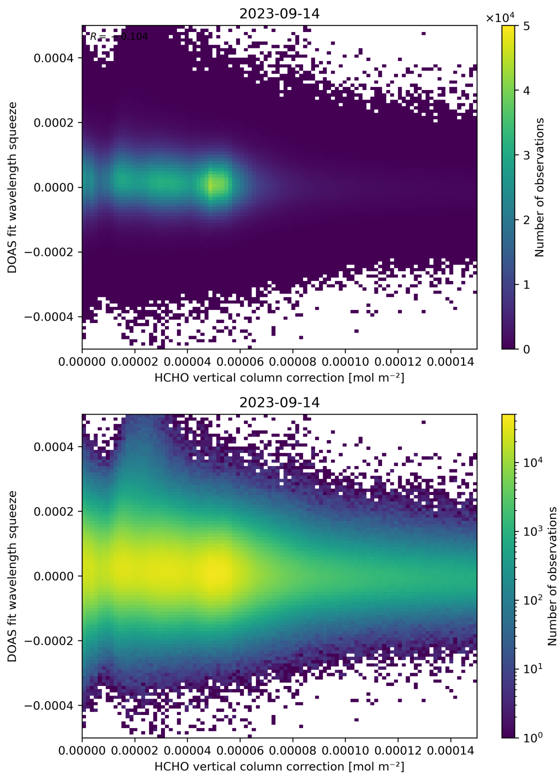
Figure 114: Scatter density plot of “HCHO vertical column correction” against “DOAS fit wavelength squeeze” for 2023-09-13 to 2023-09-15.
