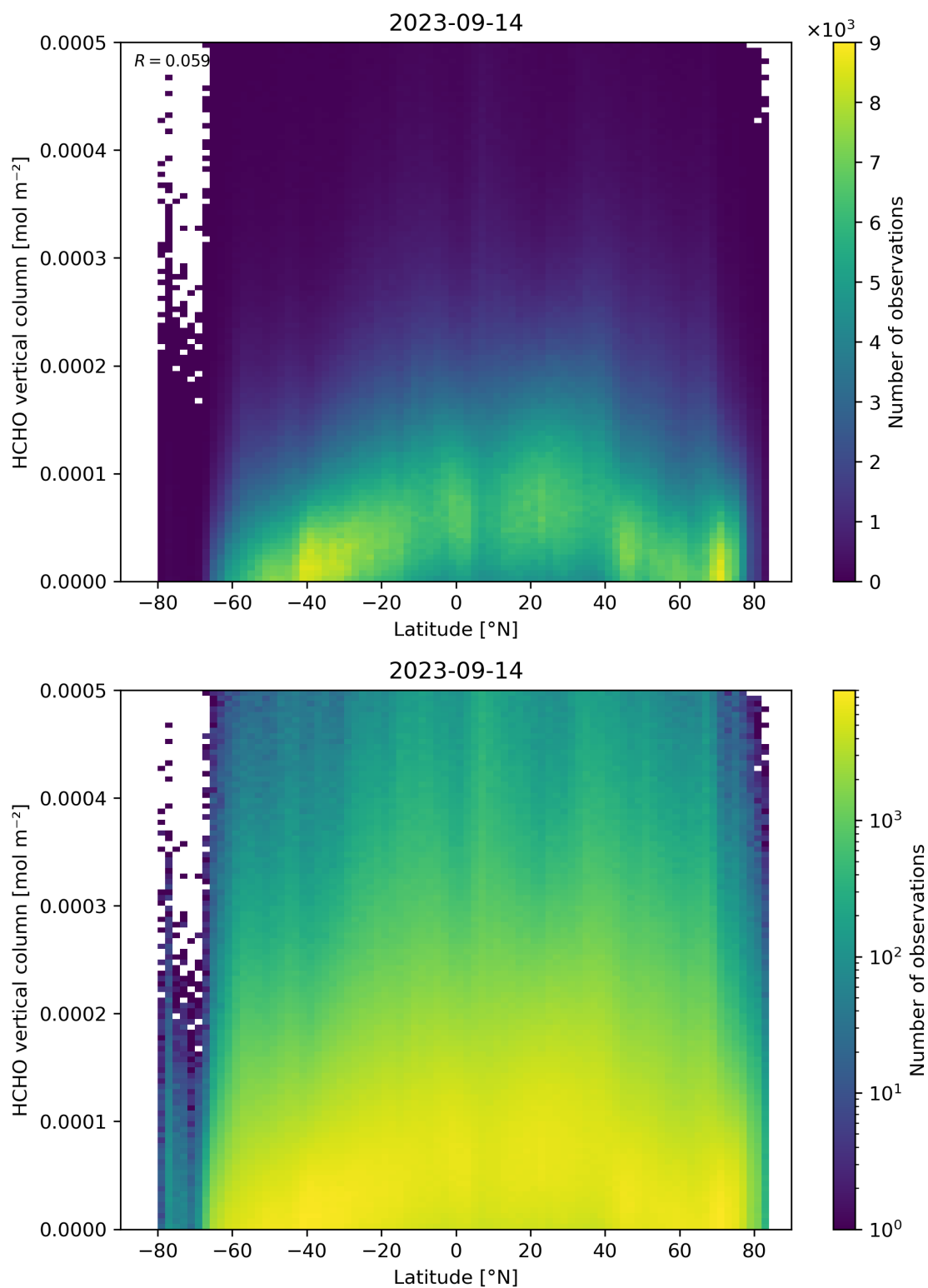
Figure 163: Scatter density plot of “Latitude” against “HCHO vertical column” for 2023-09-13 to 2023-09-15.
