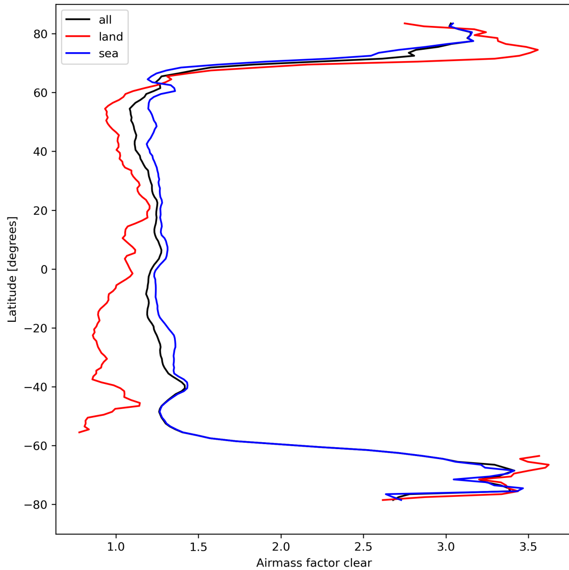
Figure 28: Zonal average of “Airmass factor clear” for 2023-09-13 to 2023-09-15.
