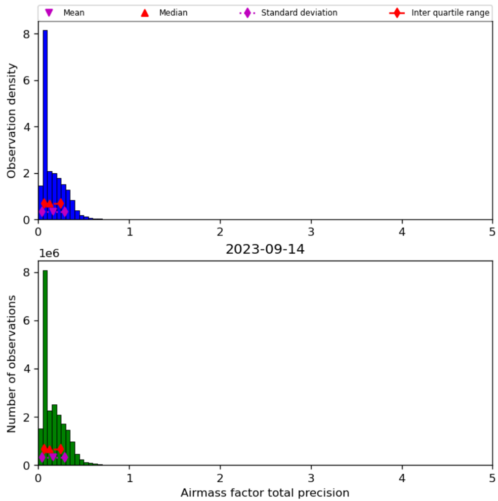
Figure 41: Histogram of “Airmass factor total precision” for 2023-09-13 to 2023-09-15
