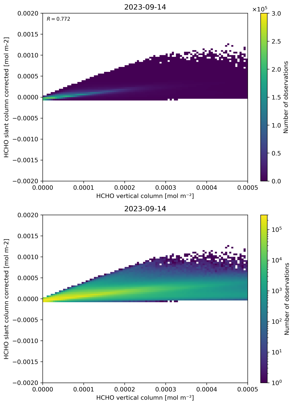
Figure 127: Scatter density plot of “HCHO vertical column” against “HCHO slant column corrected” for 2023-09-13 to 2023-09-15.
