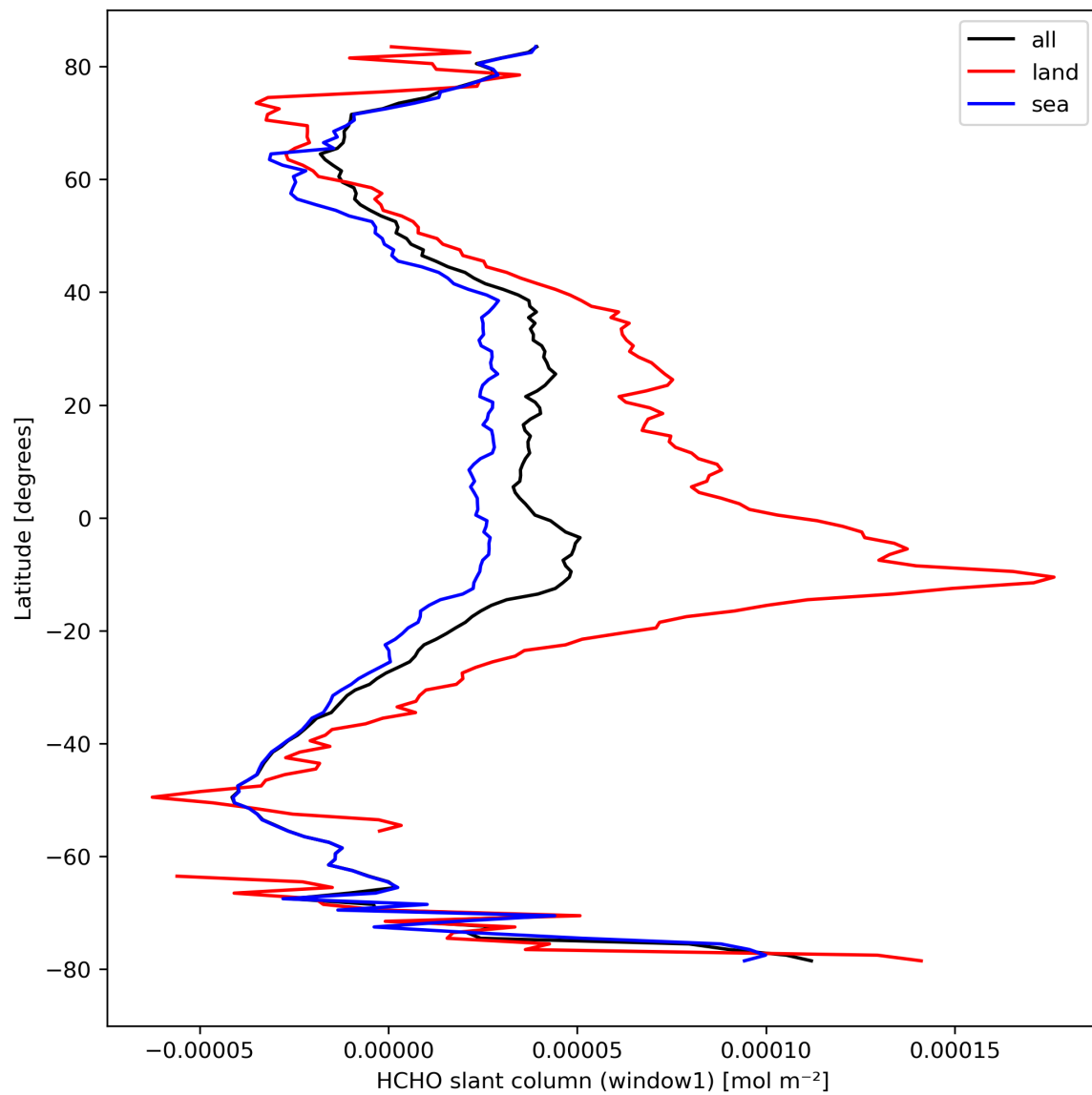
Figure 24: Zonal average of “HCHO slant column (window1)” for 2023-09-13 to 2023-09-15.
