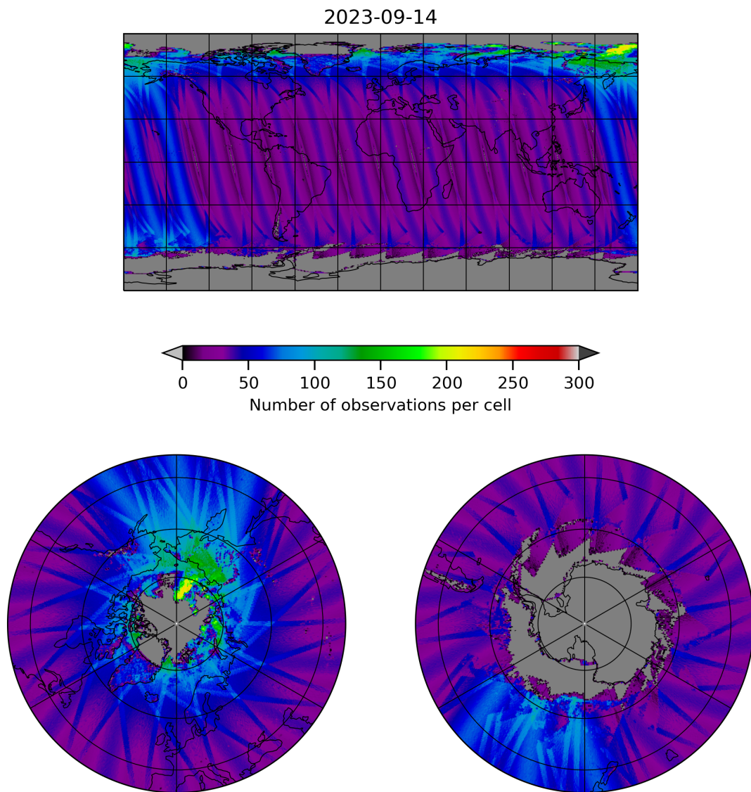
Figure 19: Map of the number of observations for 2023-09-13 to 2023-09-15
