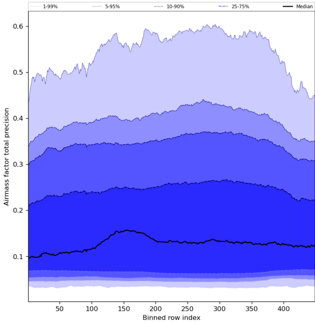
Figure 55: Along track statistics of “Airmass factor total precision” for 2023-09-13 to 2023-09-15
