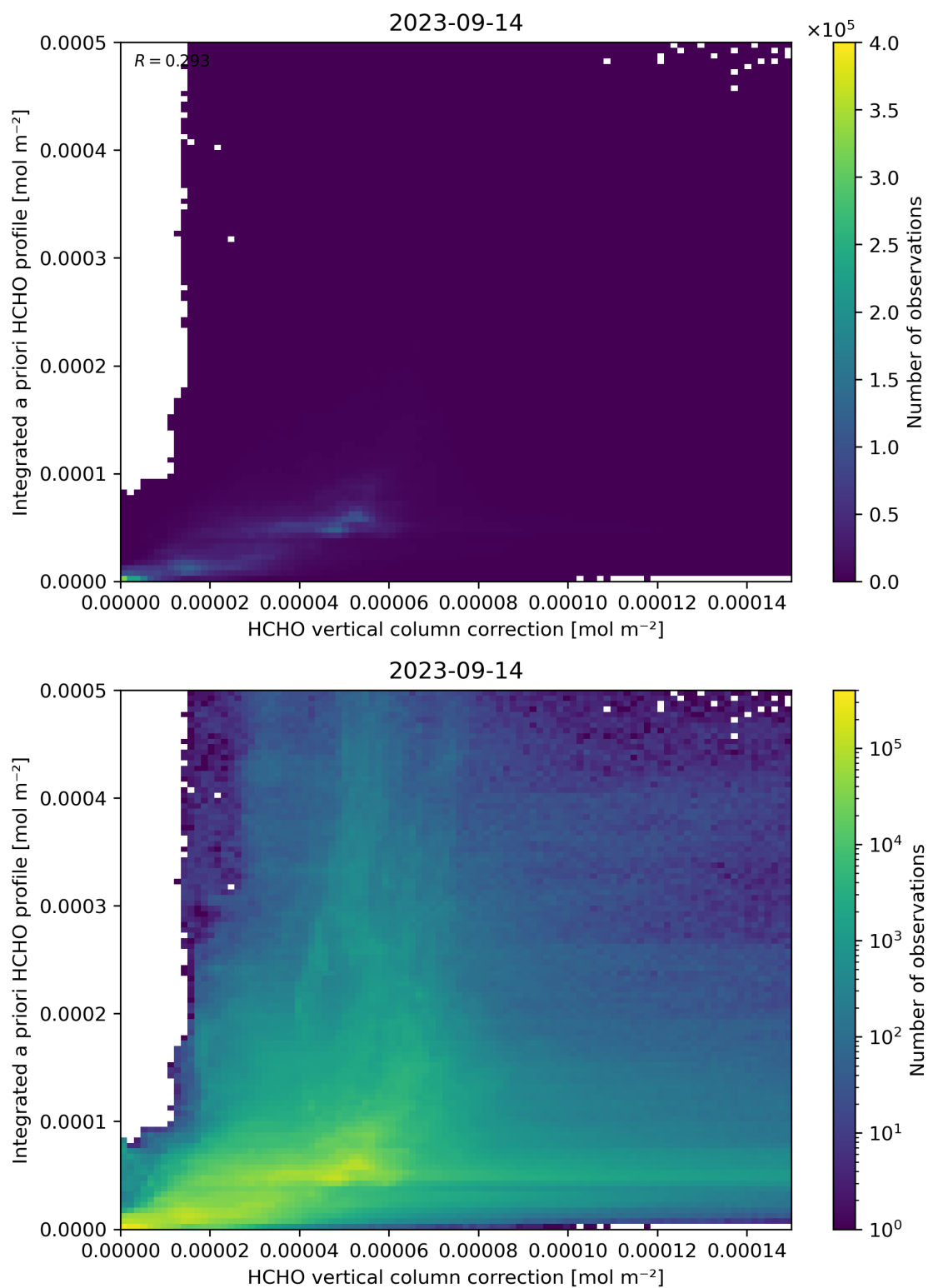
Figure 122: Scatter density plot of “HCHO vertical column correction” against “Integrated a priori HCHO profile” for 2023-09-13 to 2023-09-15.
