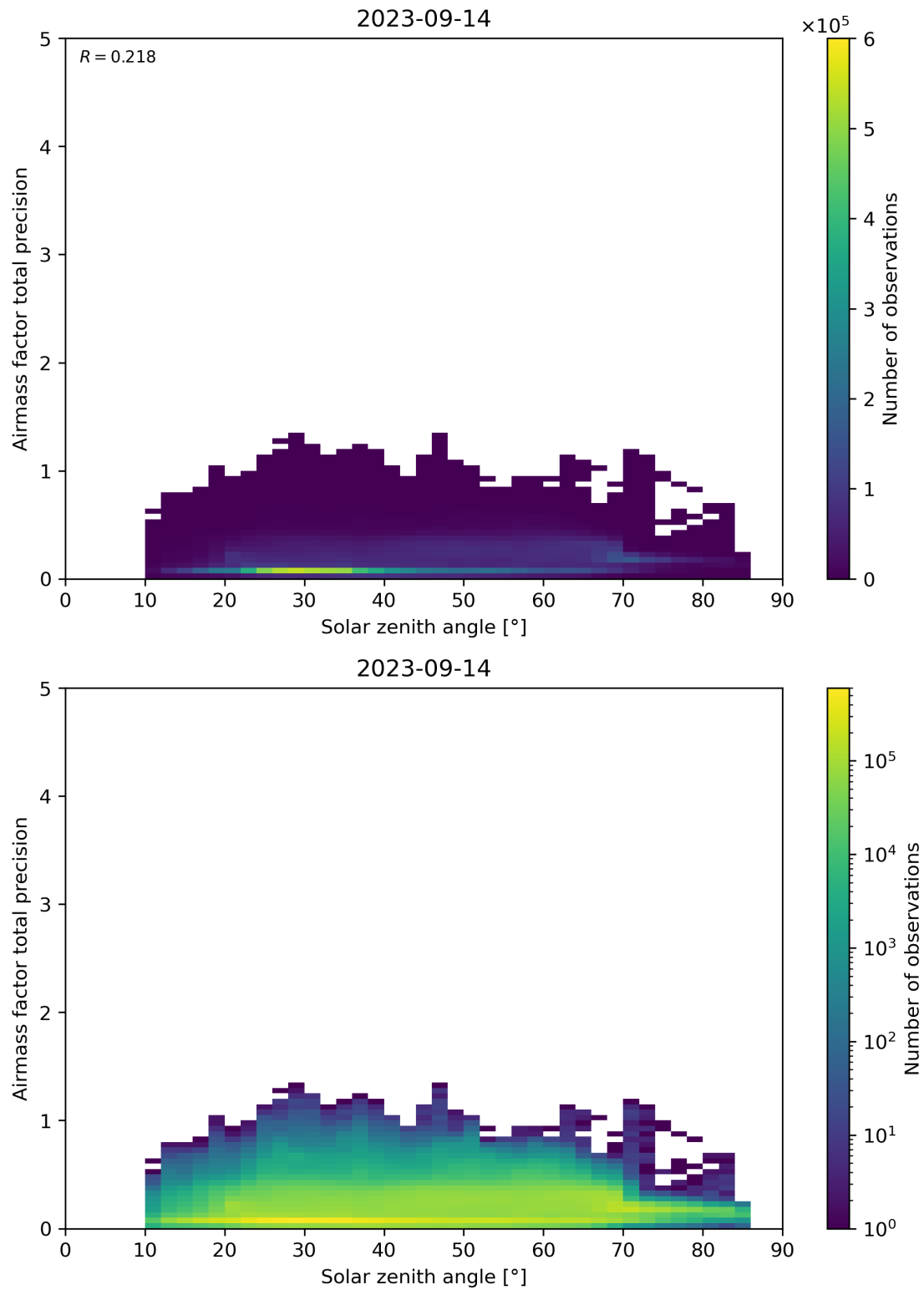
Figure 176: Scatter density plot of “Solar zenith angle” against “Airmass factor total precision” for 2023-09-13 to 2023-09-15.
