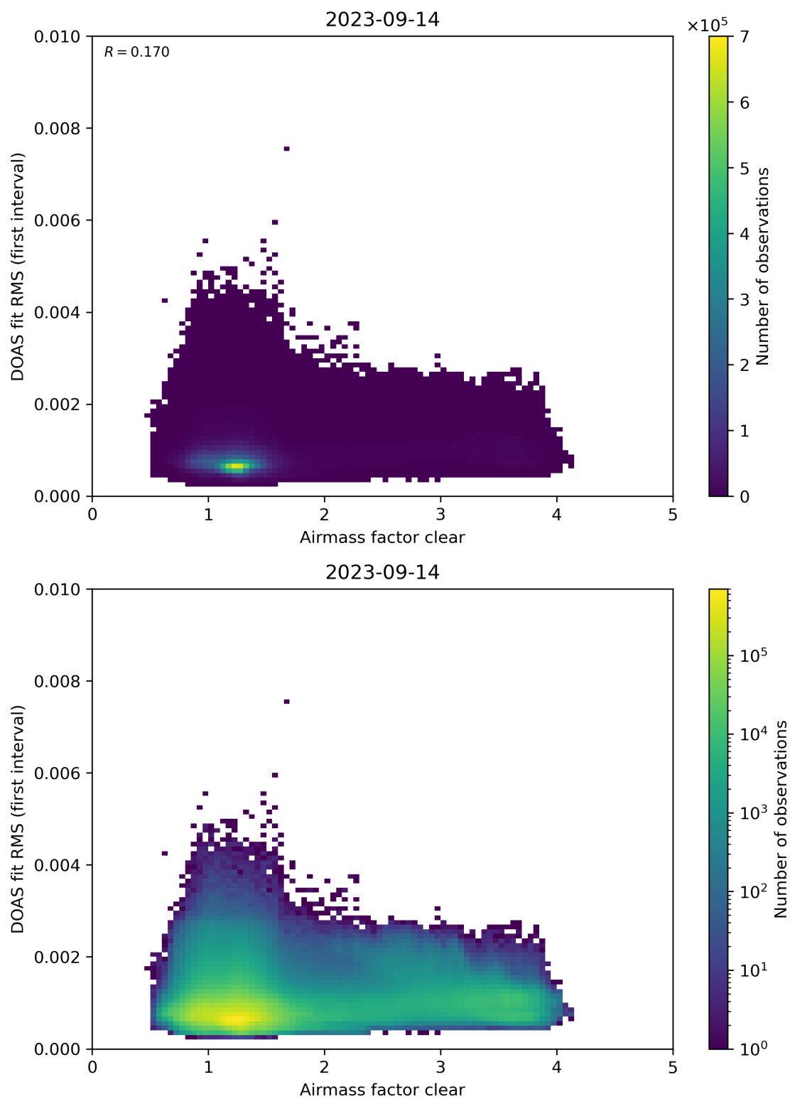
Figure 71: Scatter density plot of “Airmass factor clear” against “DOAS fit RMS (first interval)” for 2023-09-13 to 2023-09-15.
