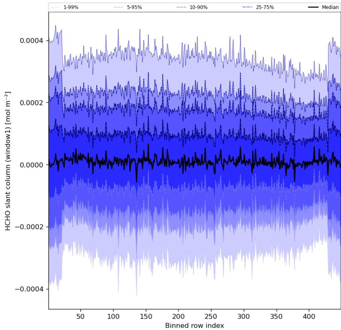
Figure 52: Along track statistics of “HCHO slant column (window1)” for 2023-09-13 to 2023-09-15
