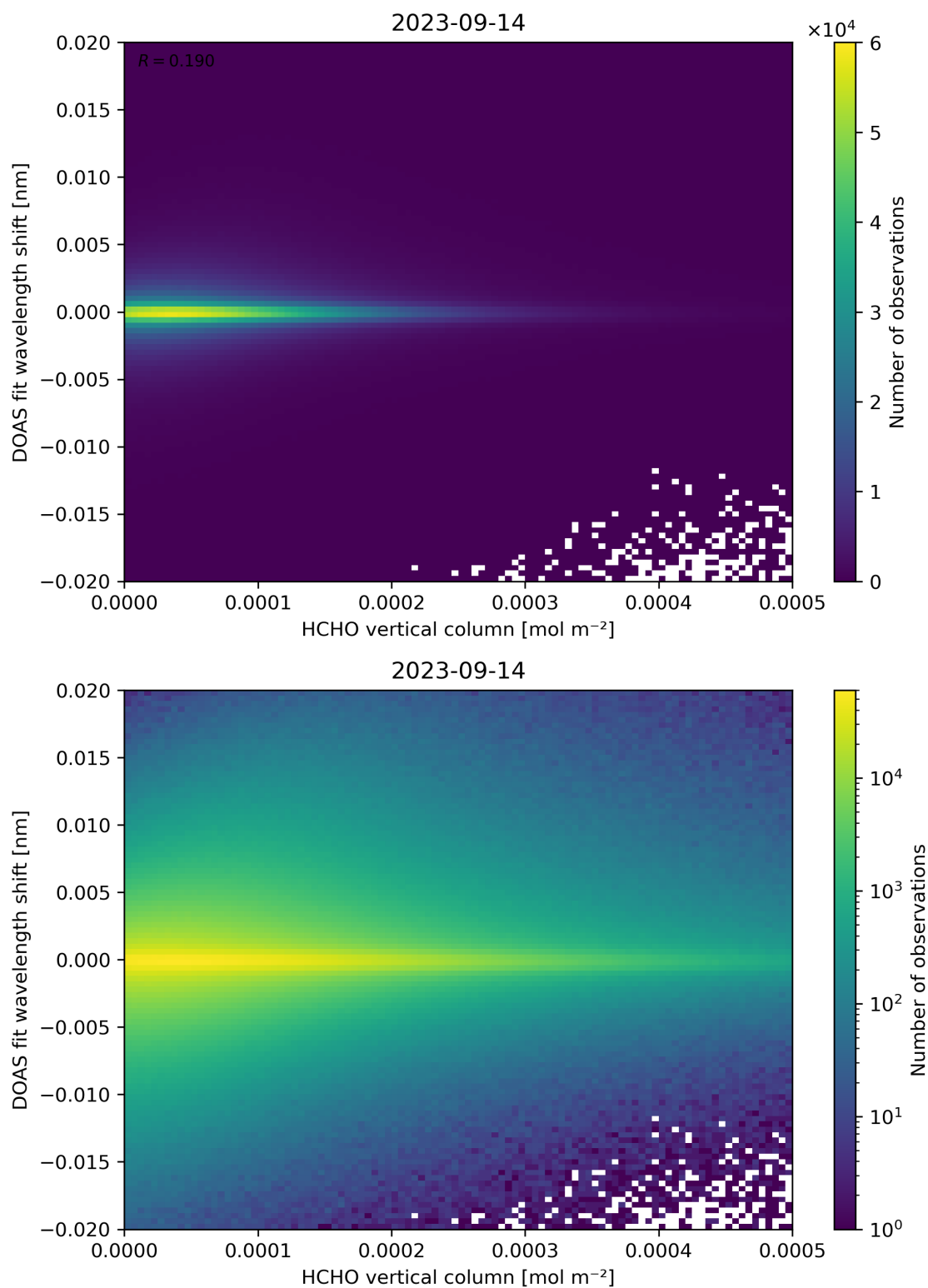
Figure 124: Scatter density plot of “HCHO vertical column” against “DOAS fit wavelength shift” for 2023-09-13 to 2023-09-15.
