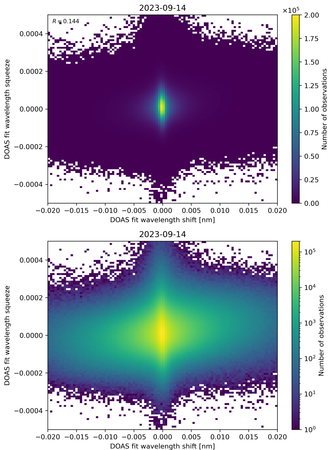
Figure 65: Scatter density plot of “DOAS fit wavelength shift” against “DOAS fit wavelength squeeze” for 2023-09-13 to 2023-09-15.
