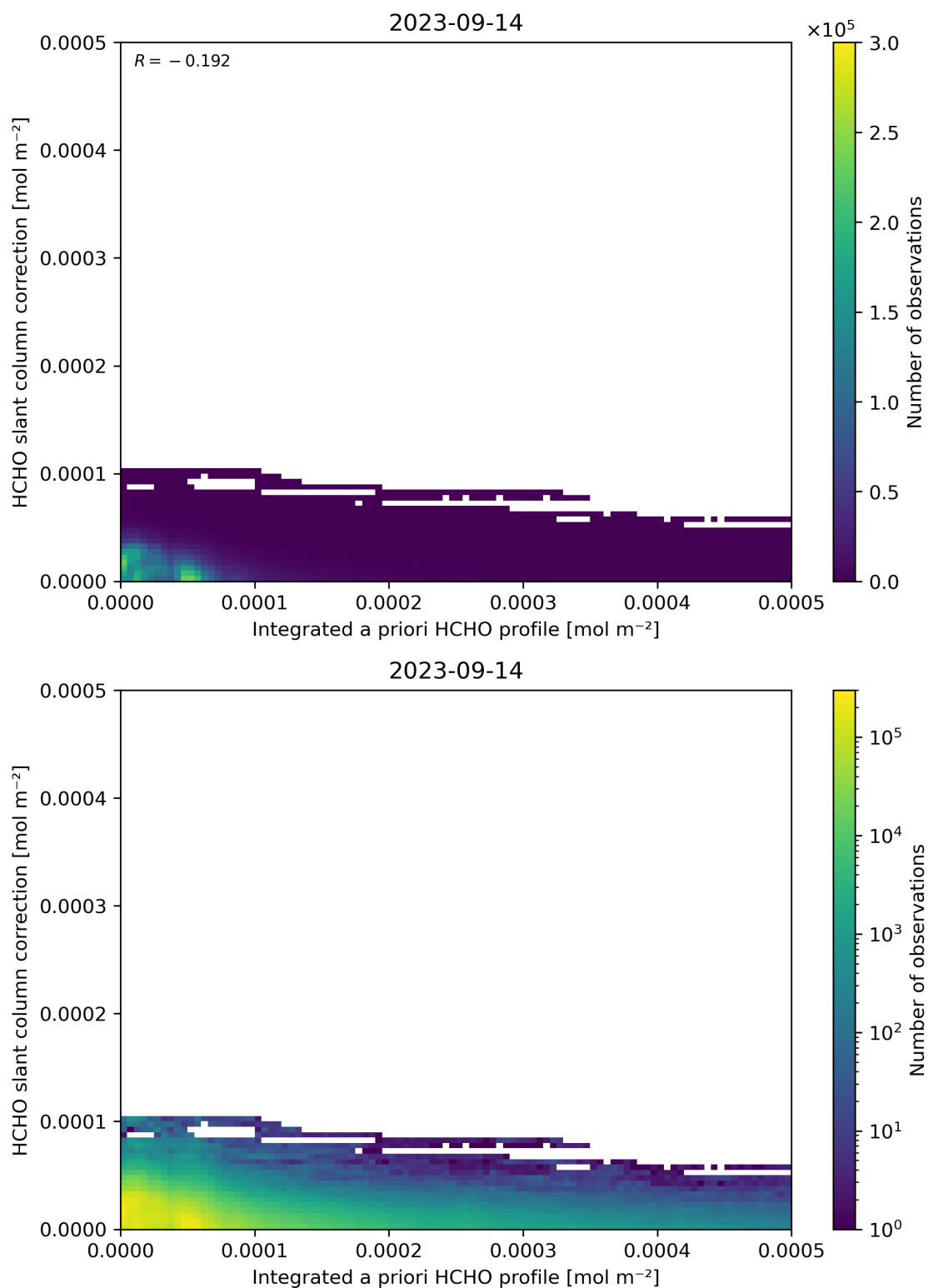
Figure 152: Scatter density plot of “Integrated a priori HCHO profile” against “HCHO slant column correction” for 2023-09-13 to 2023-09-15.
