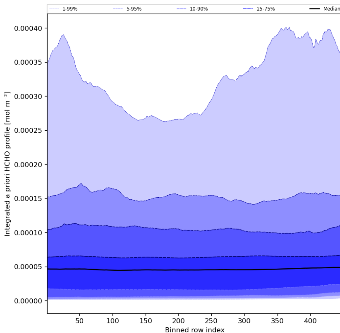
Figure 57: Along track statistics of “Integrated a priori HCHO profile” for 2023-09-13 to 2023-09-15
