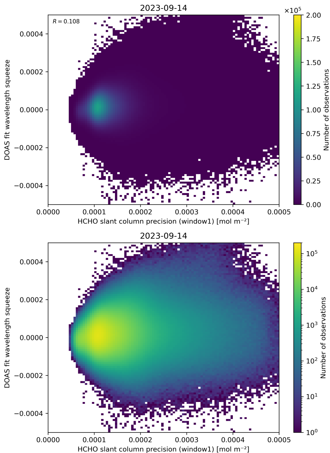
Figure 90: Scatter density plot of “HCHO slant column precision (window1)” against “DOAS fit wavelength squeeze” for 2023-09-13 to 2023-09-15.
