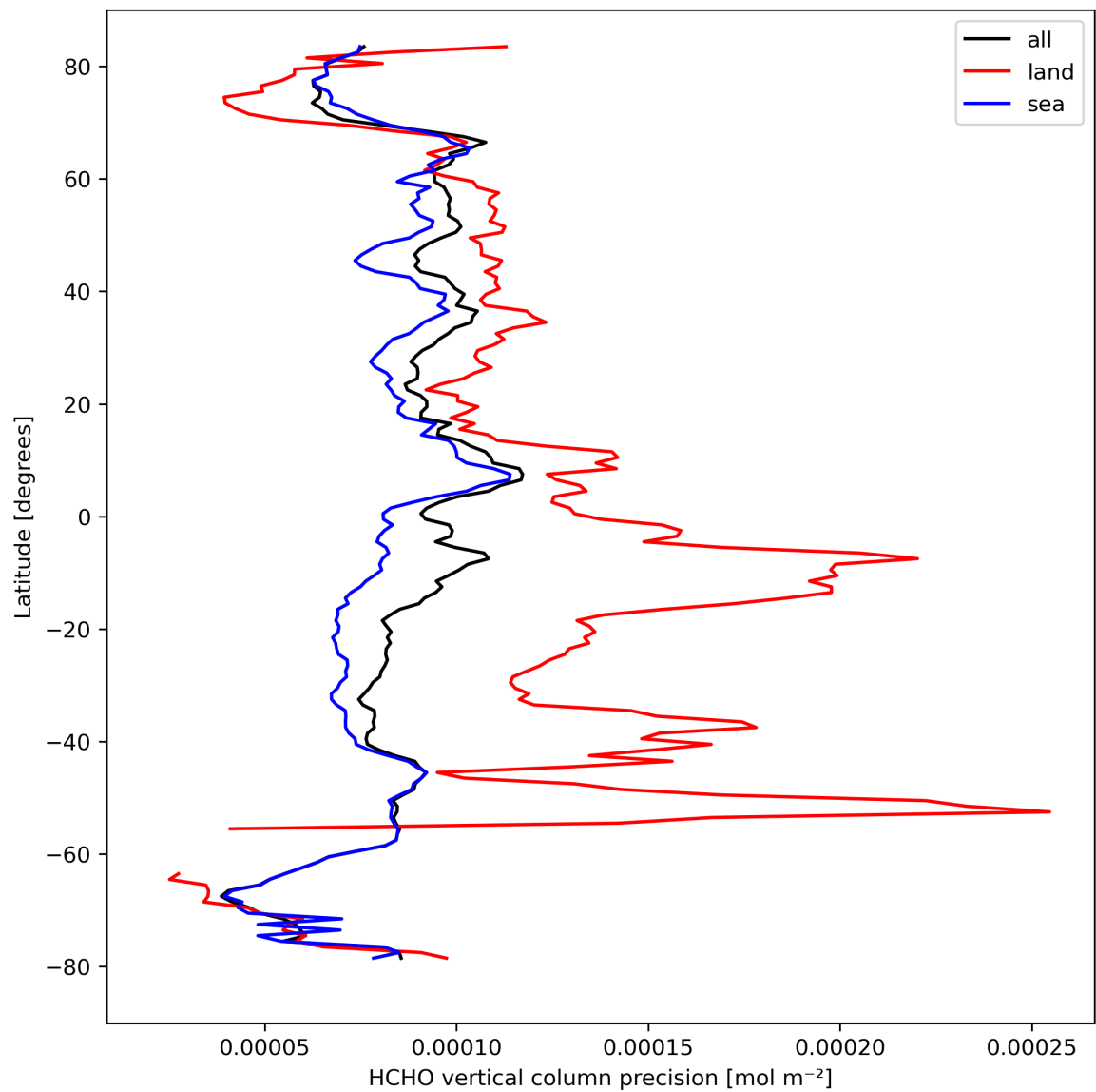
Figure 22: Zonal average of “HCHO vertical column precision” for 2023-09-13 to 2023-09-15.
