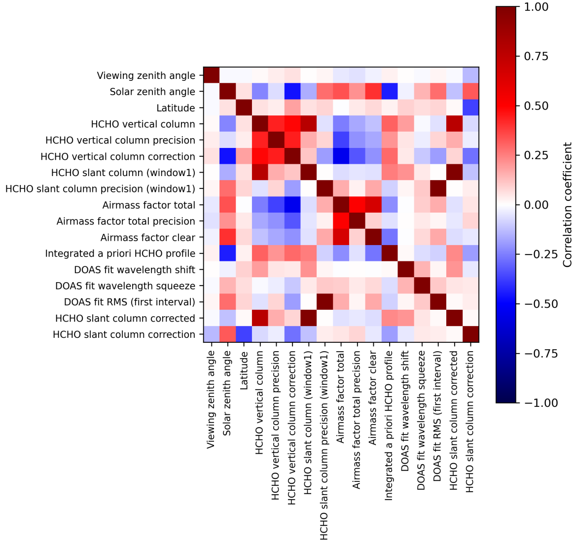
Figure 2: Map of correlation matrix for 2023-09-13 to 2023-09-15.
