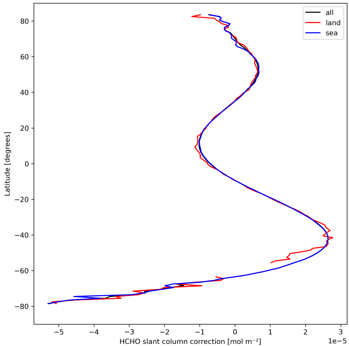
Figure 33: Zonal average of “HCHO slant column correction” for 2023-09-13 to 2023-09-15.
