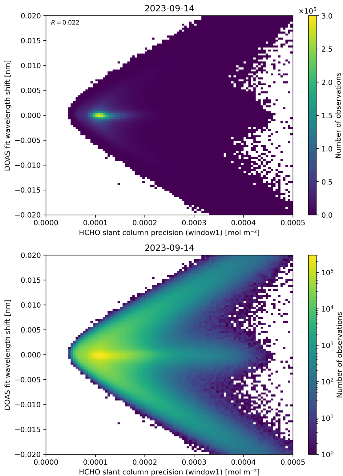
Figure 89: Scatter density plot of “HCHO slant column precision (window1)” against “DOAS fit wavelength shift” for 2023-09-13 to 2023-09-15.
