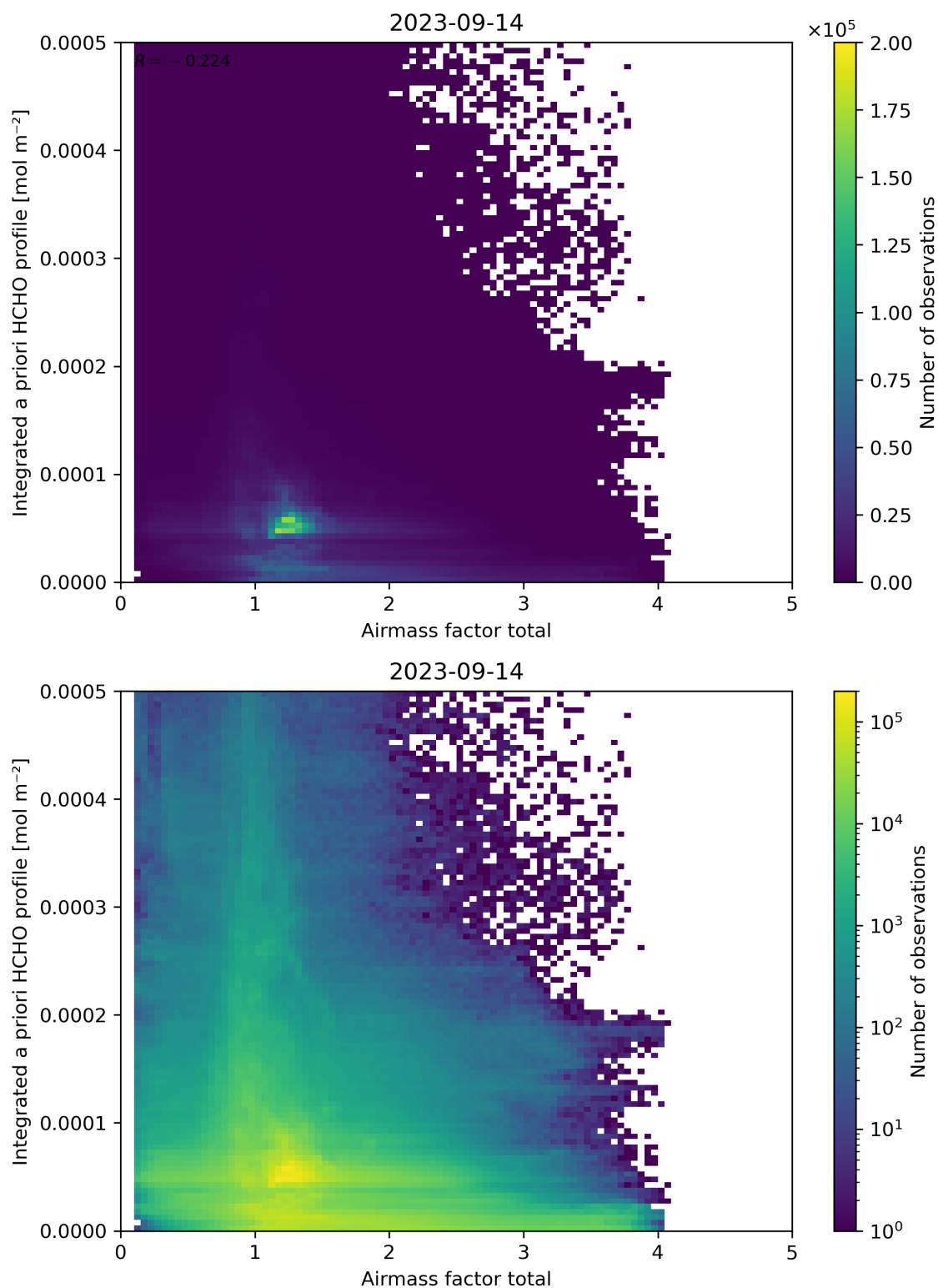
Figure 104: Scatter density plot of “Airmass factor total” against “Integrated a priori HCHO profile” for 2023-09-13 to 2023-09-15.
