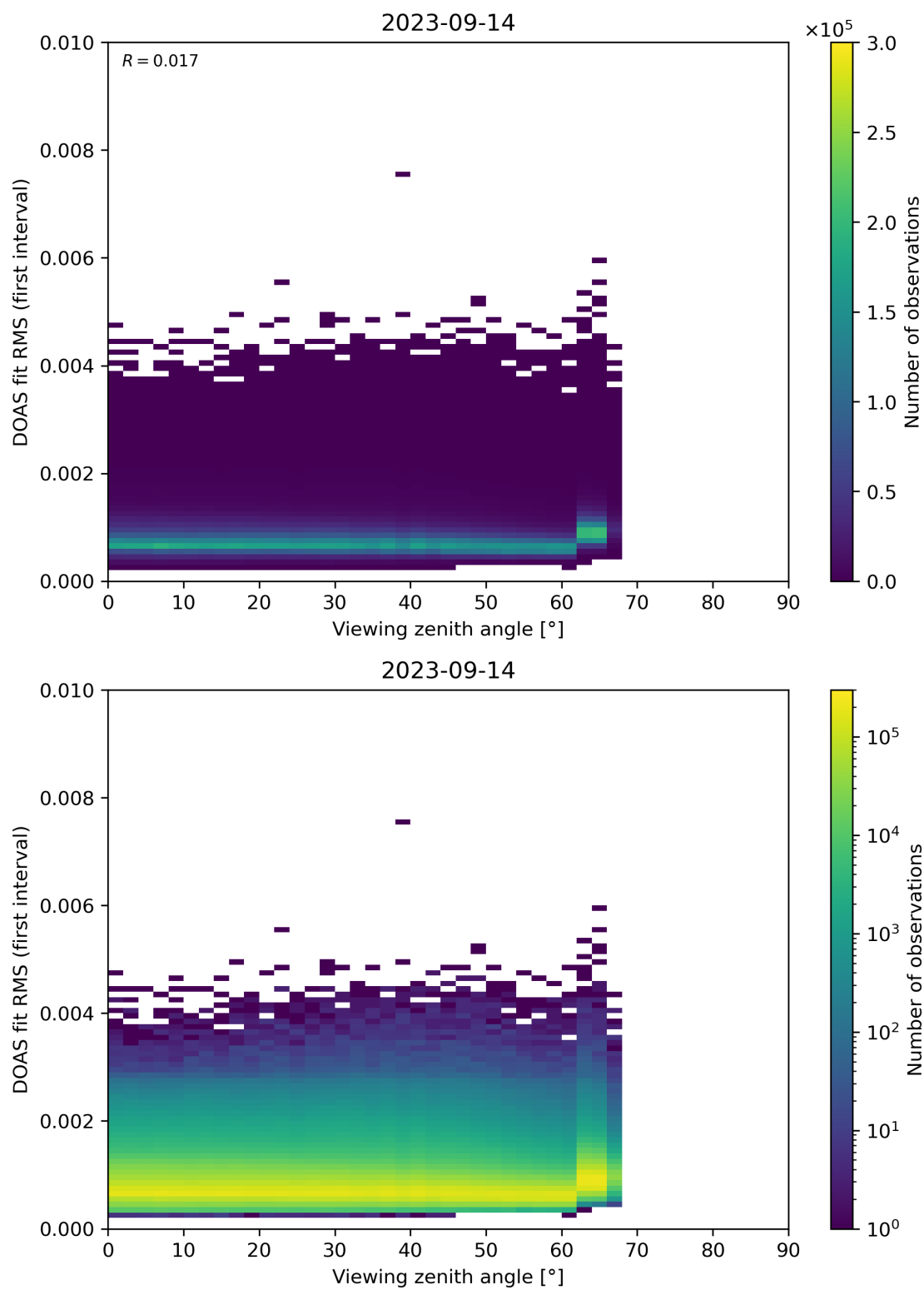
Figure 182: Scatter density plot of “Viewing zenith angle” against “DOAS fit RMS (first interval)” for 2023-09-13 to 2023-09-15.
