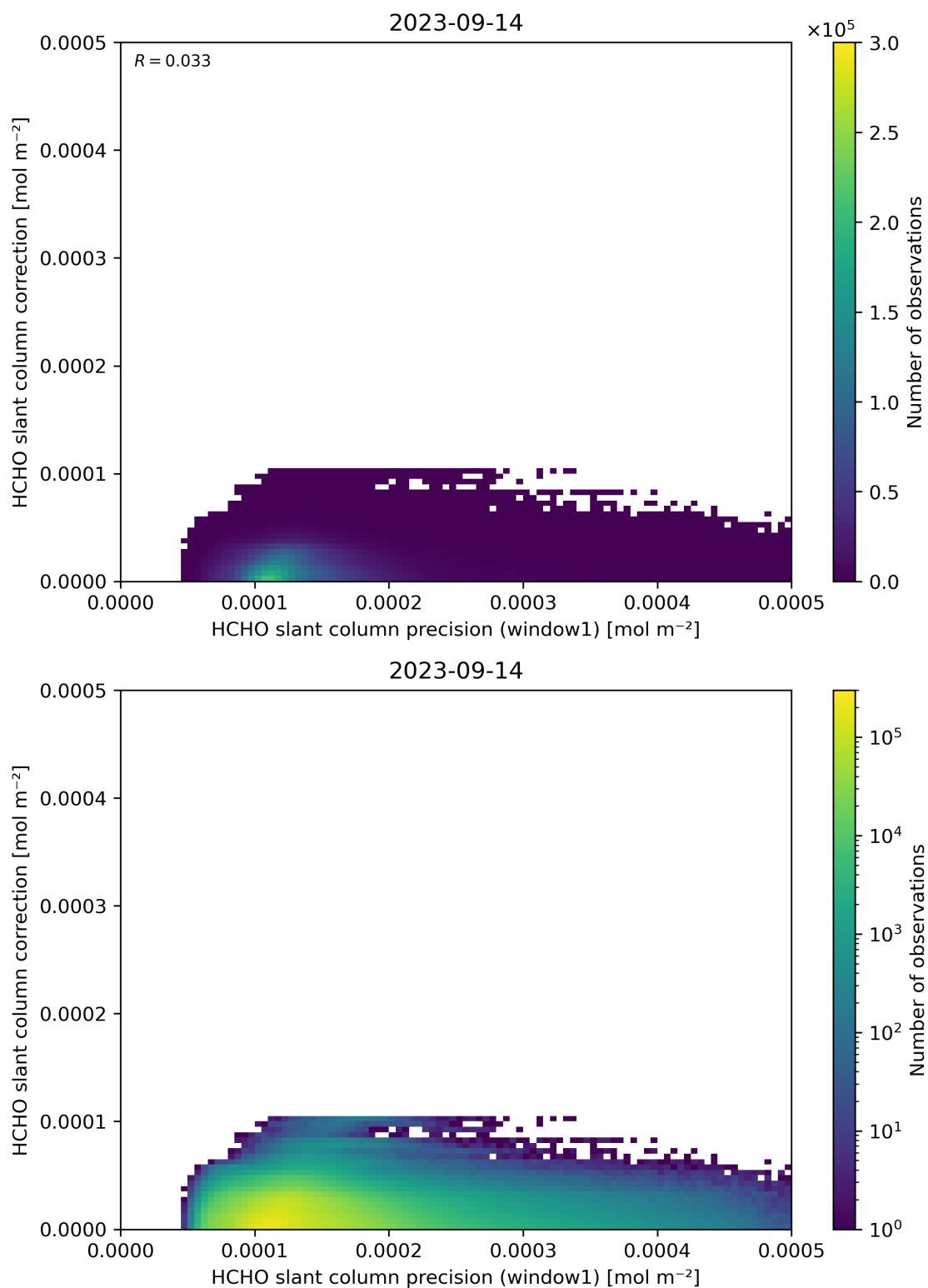
Figure 93: Scatter density plot of “HCHO slant column precision (window1)” against “HCHO slant column correction” for 2023-09-13 to 2023-09-15.
