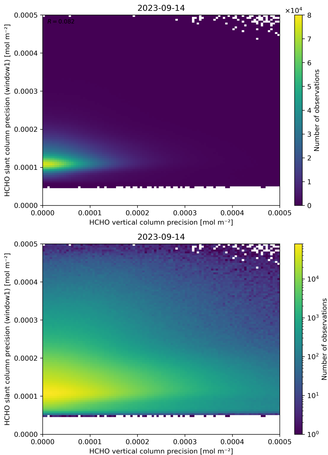
Figure 143: Scatter density plot of “HCHO vertical column precision” against “HCHO slant column precision (window1)” for 2023-09-13 to 2023-09-15.
