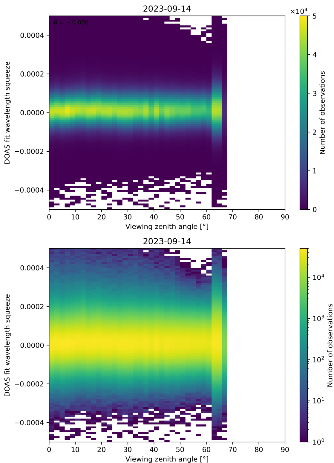
Figure 184: Scatter density plot of “Viewing zenith angle” against “DOAS fit wavelength squeeze” for 2023-09-13 to 2023-09-15.
