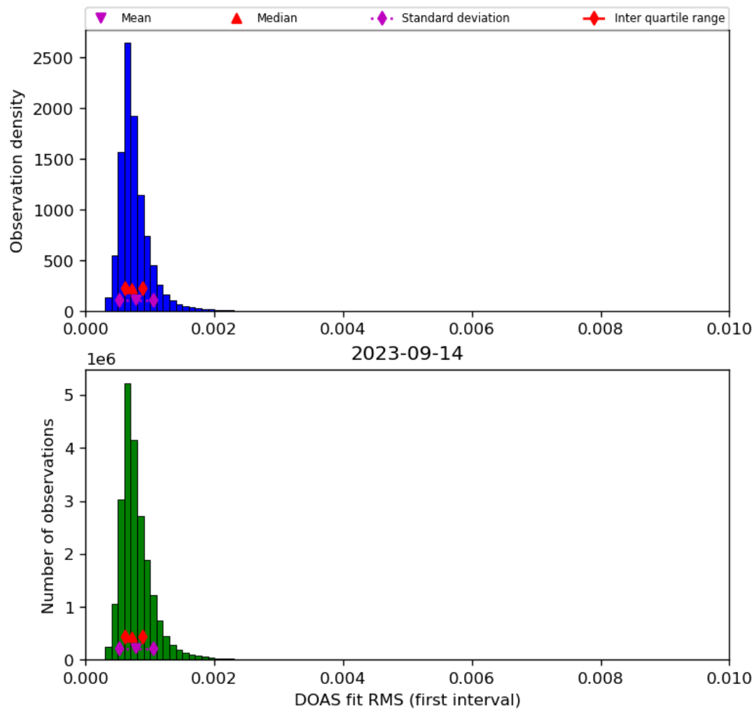
Figure 46: Histogram of “DOAS fit RMS (first interval)” for 2023-09-13 to 2023-09-15
