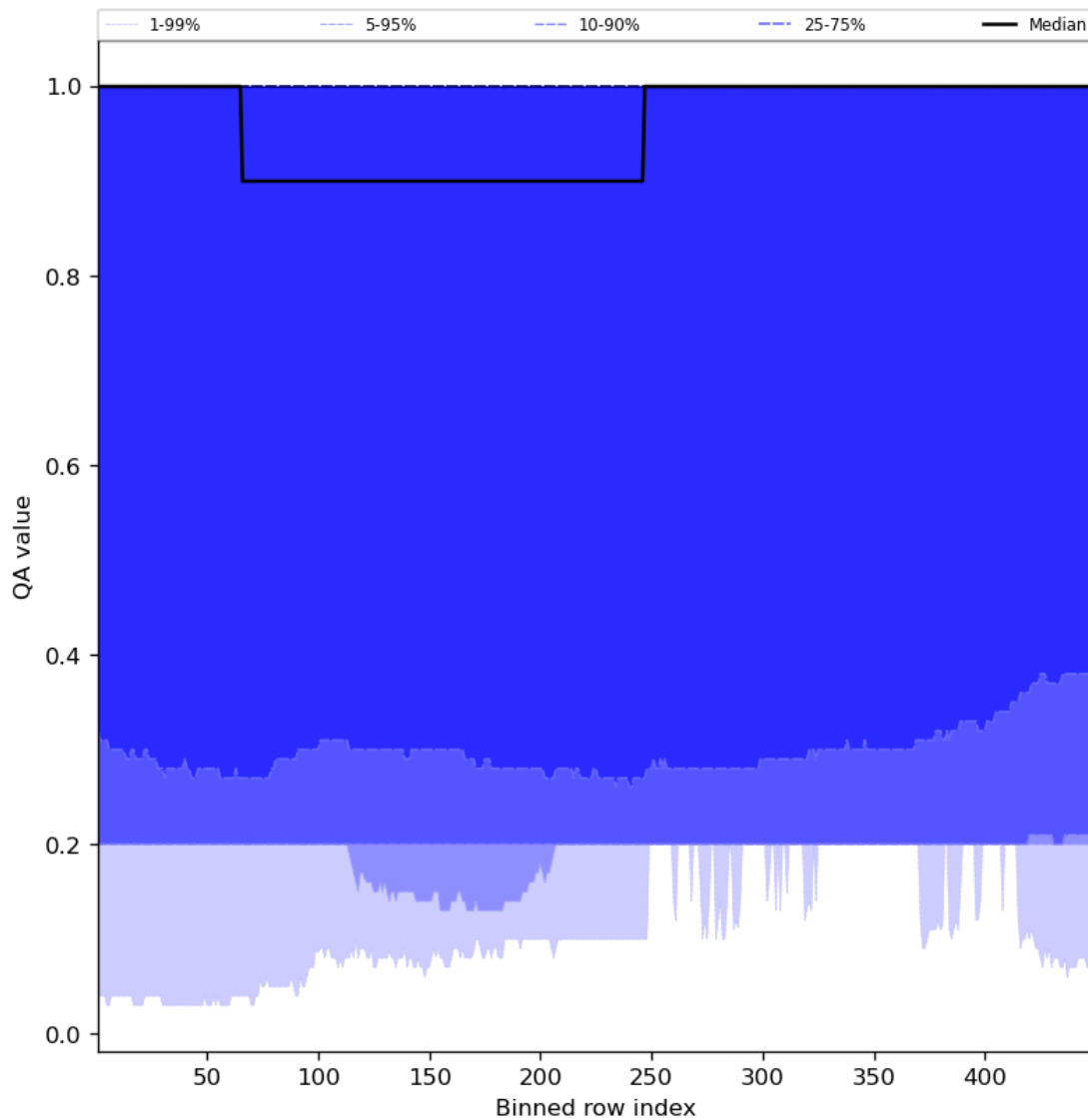
Figure 48: Along track statistics of “QA value” for 2023-09-13 to 2023-09-15
