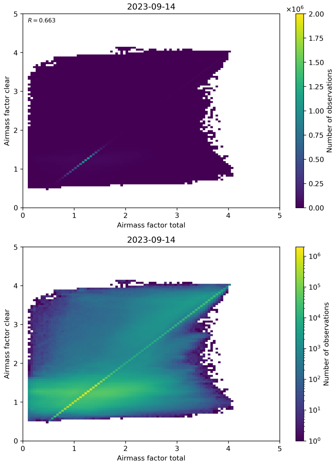
Figure 100: Scatter density plot of “Airmass factor total” against “Airmass factor clear” for 2023-09-13 to 2023-09-15.
