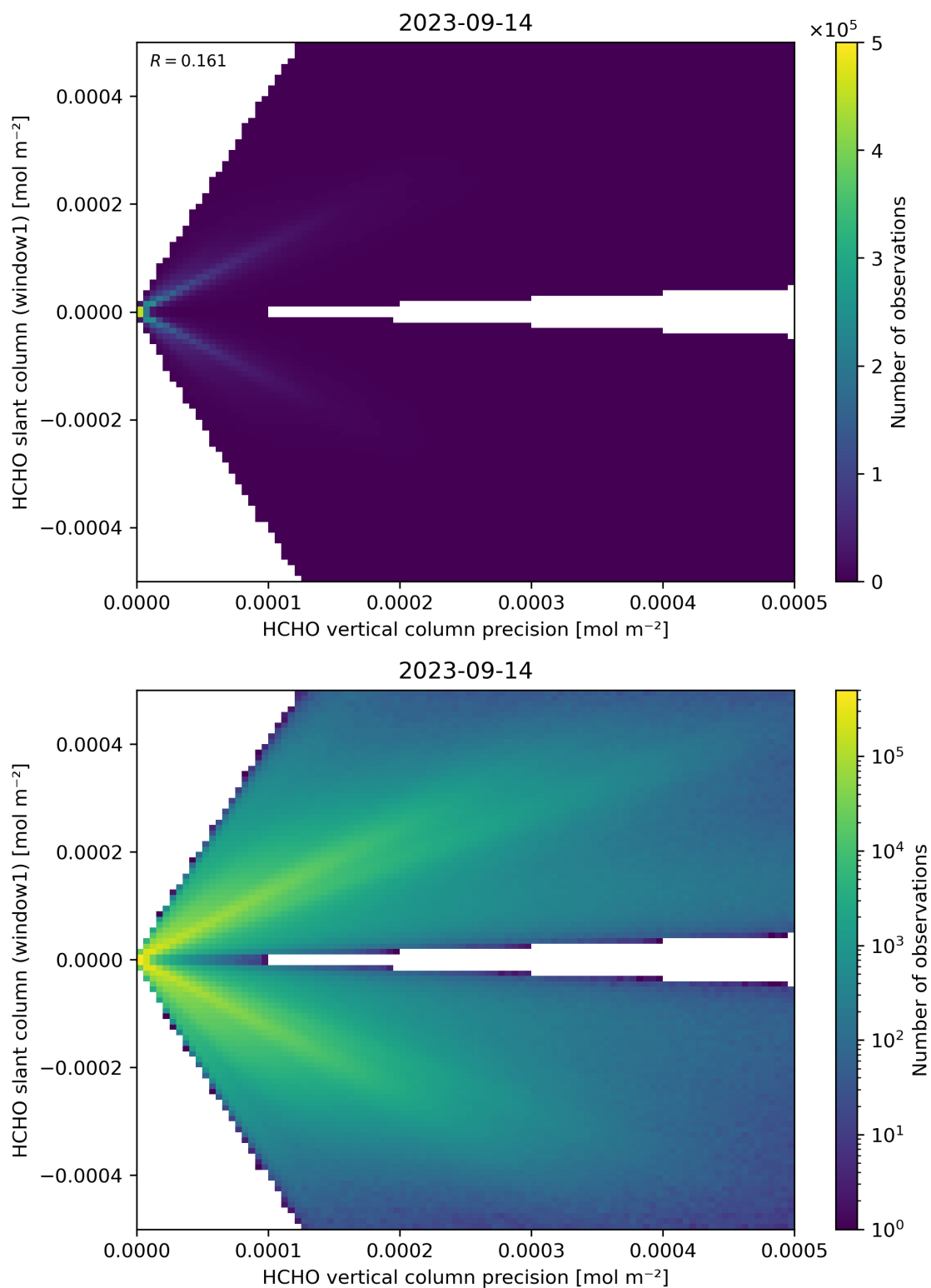
Figure 142: Scatter density plot of “HCHO vertical column precision” against “HCHO slant column (window1)” for 2023-09-13 to 2023-09-15.
