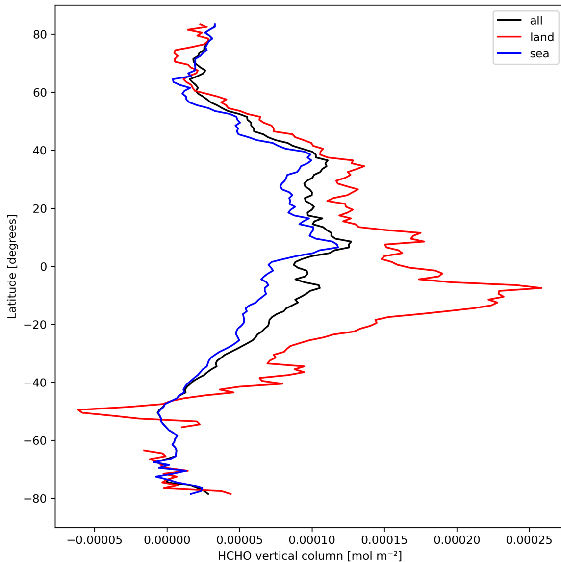
Figure 21: Zonal average of “HCHO vertical column” for 2023-09-13 to 2023-09-15.
