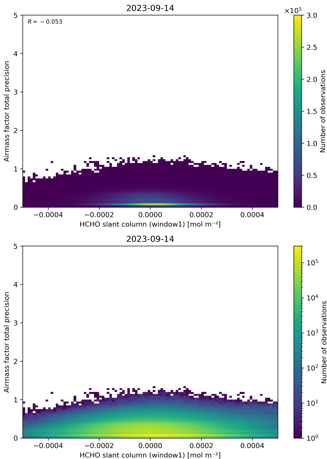
Figure 86: Scatter density plot of “HCHO slant column (window1)” against “Airmass factor total precision” for 2023-09-13 to 2023-09-15.
