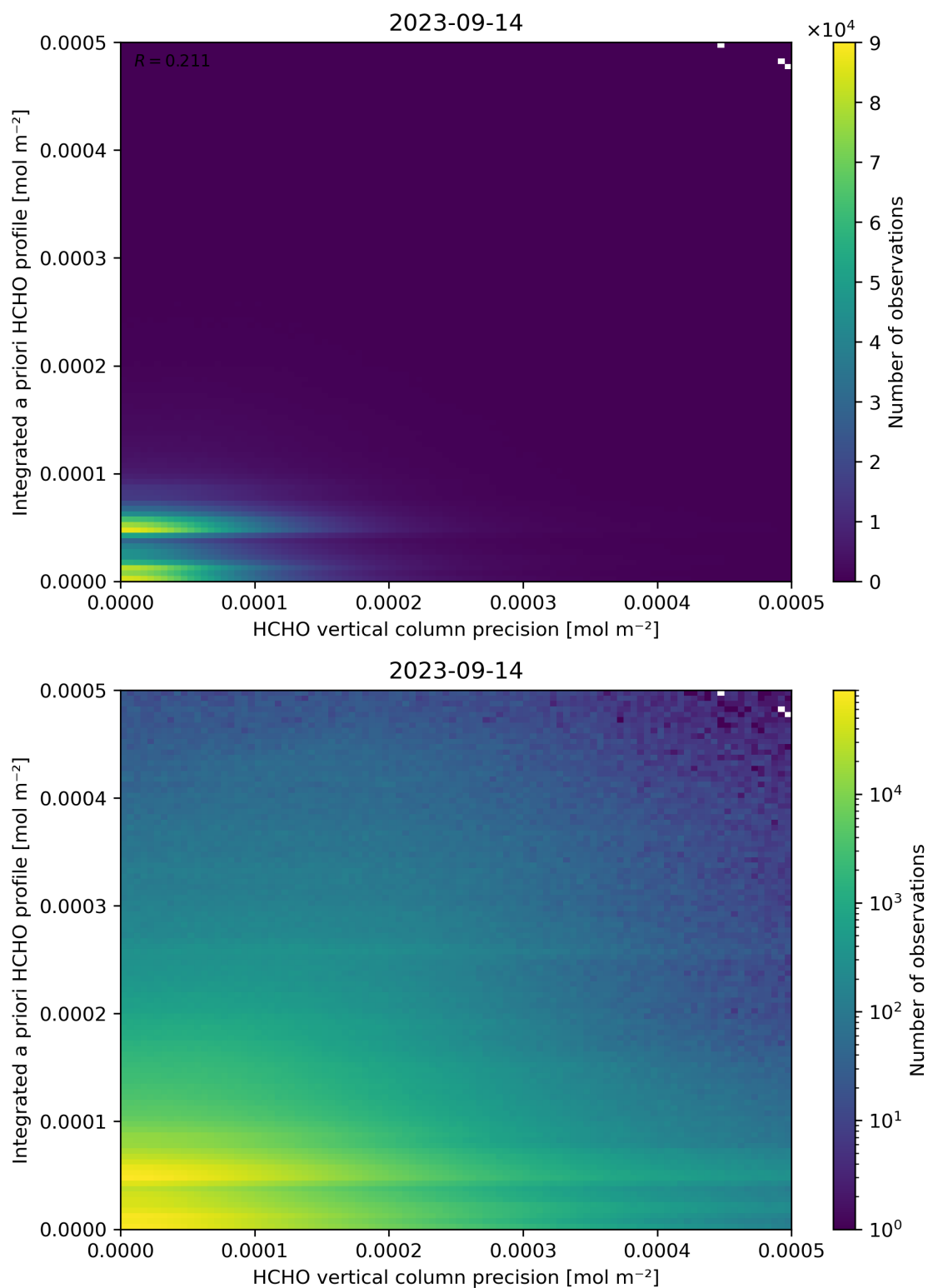
Figure 147: Scatter density plot of “HCHO vertical column precision” against “Integrated a priori HCHO profile” for 2023-09-13 to 2023-09-15.
