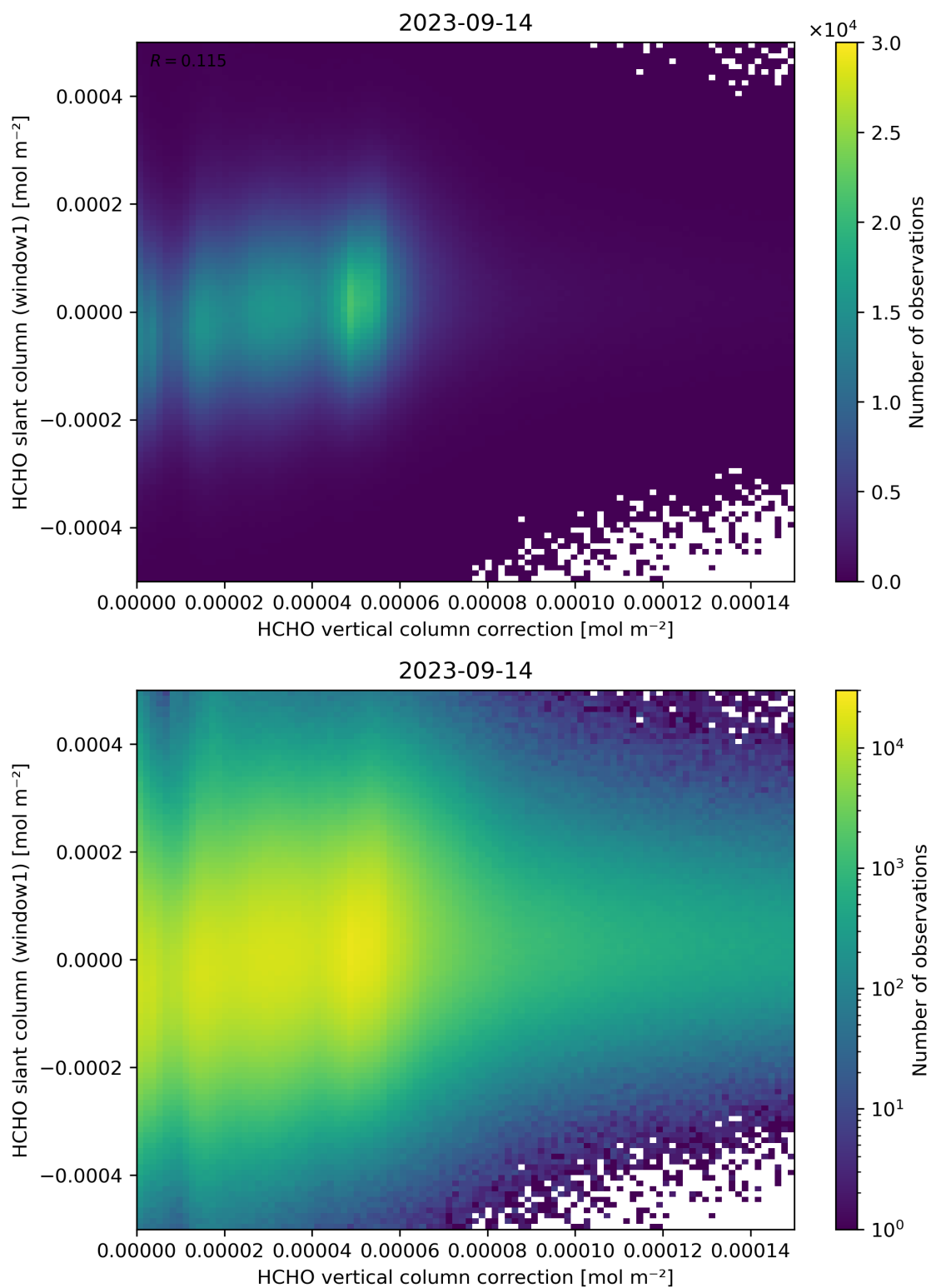
Figure 118: Scatter density plot of “HCHO vertical column correction” against “HCHO slant column (window1)” for 2023-09-13 to 2023-09-15.
