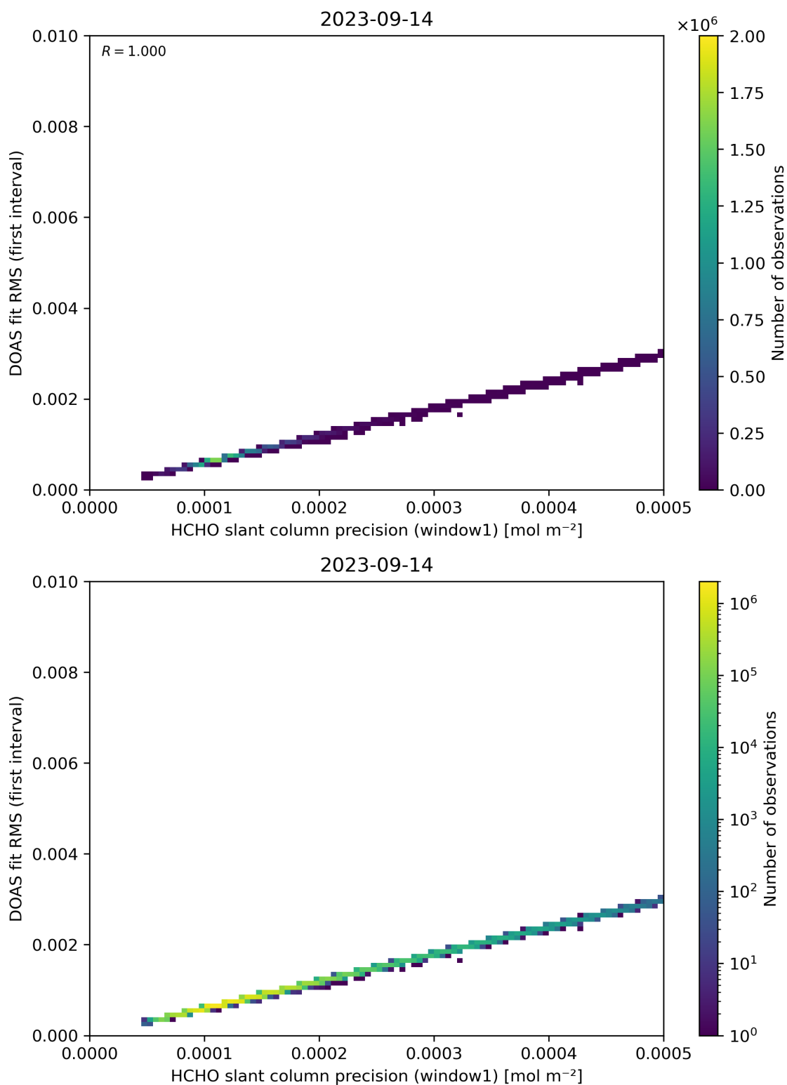
Figure 88: Scatter density plot of “HCHO slant column precision (window1)” against “DOAS fit RMS (first interval)” for 2023-09-13 to 2023-09-15.
