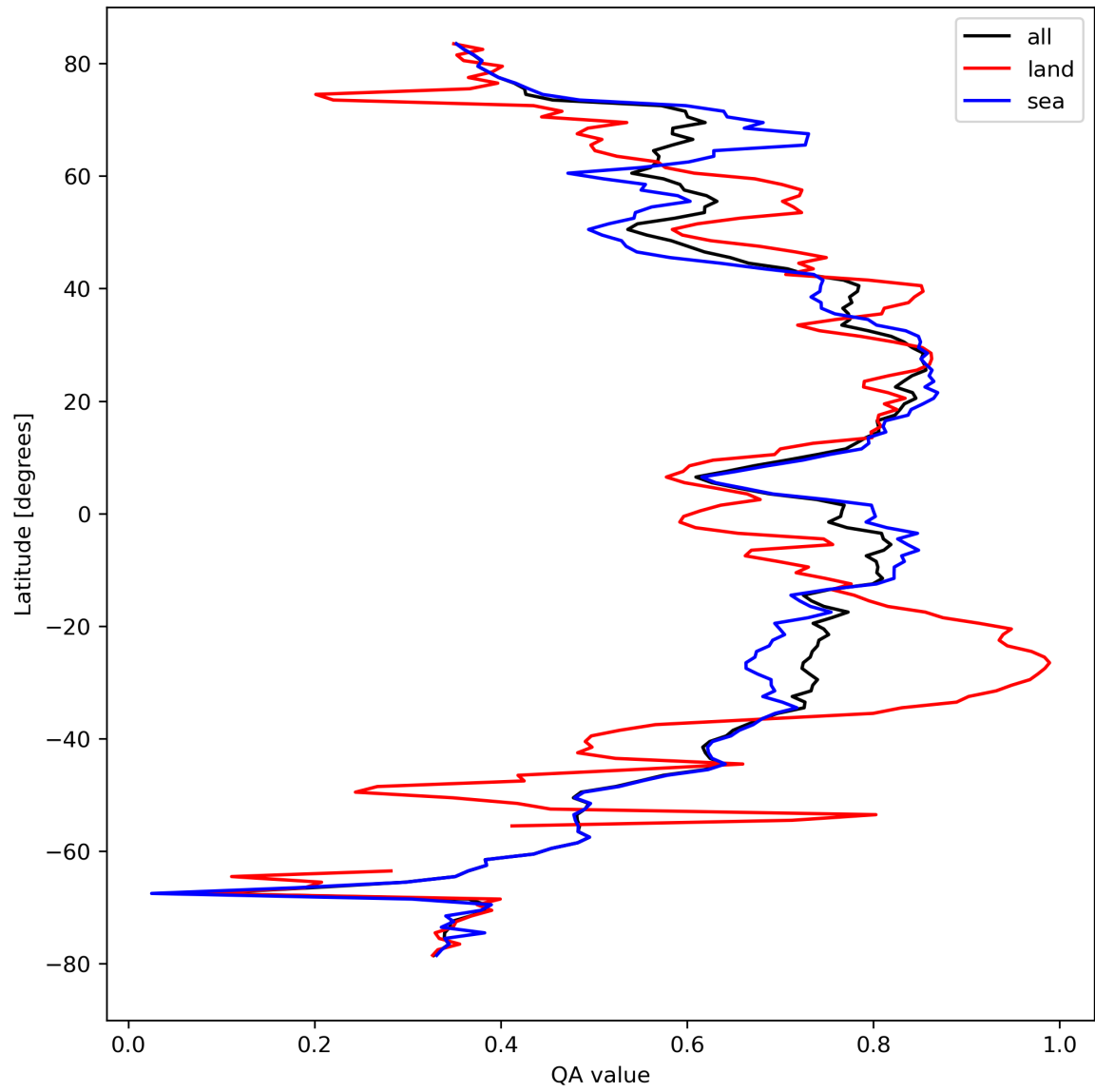
Figure 20: Zonal average of “QA value” for 2023-09-13 to 2023-09-15.
