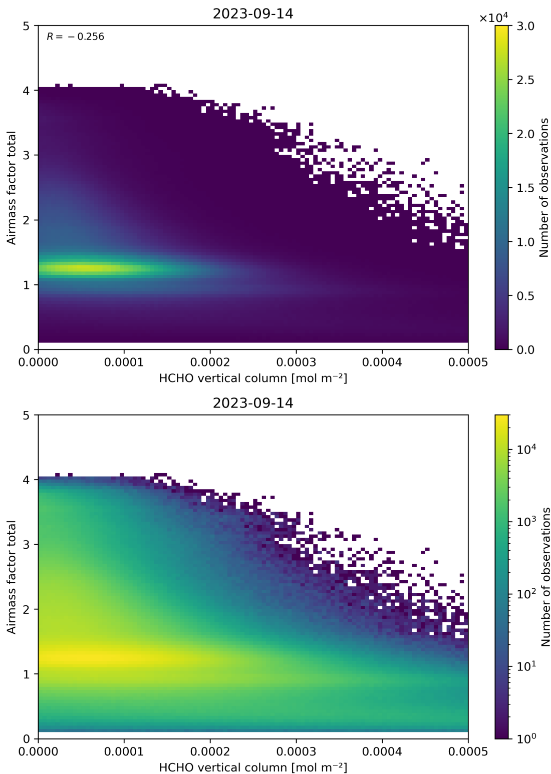
Figure 131: Scatter density plot of “HCHO vertical column” against “Airmass factor total” for 2023-09-13 to 2023-09-15.
