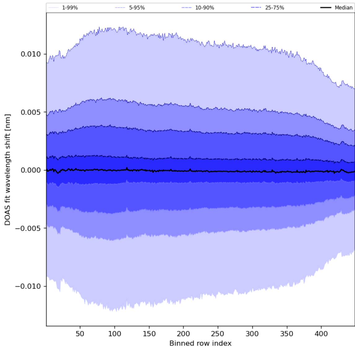
Figure 58: Along track statistics of “DOAS fit wavelength shift” for 2023-09-13 to 2023-09-15
