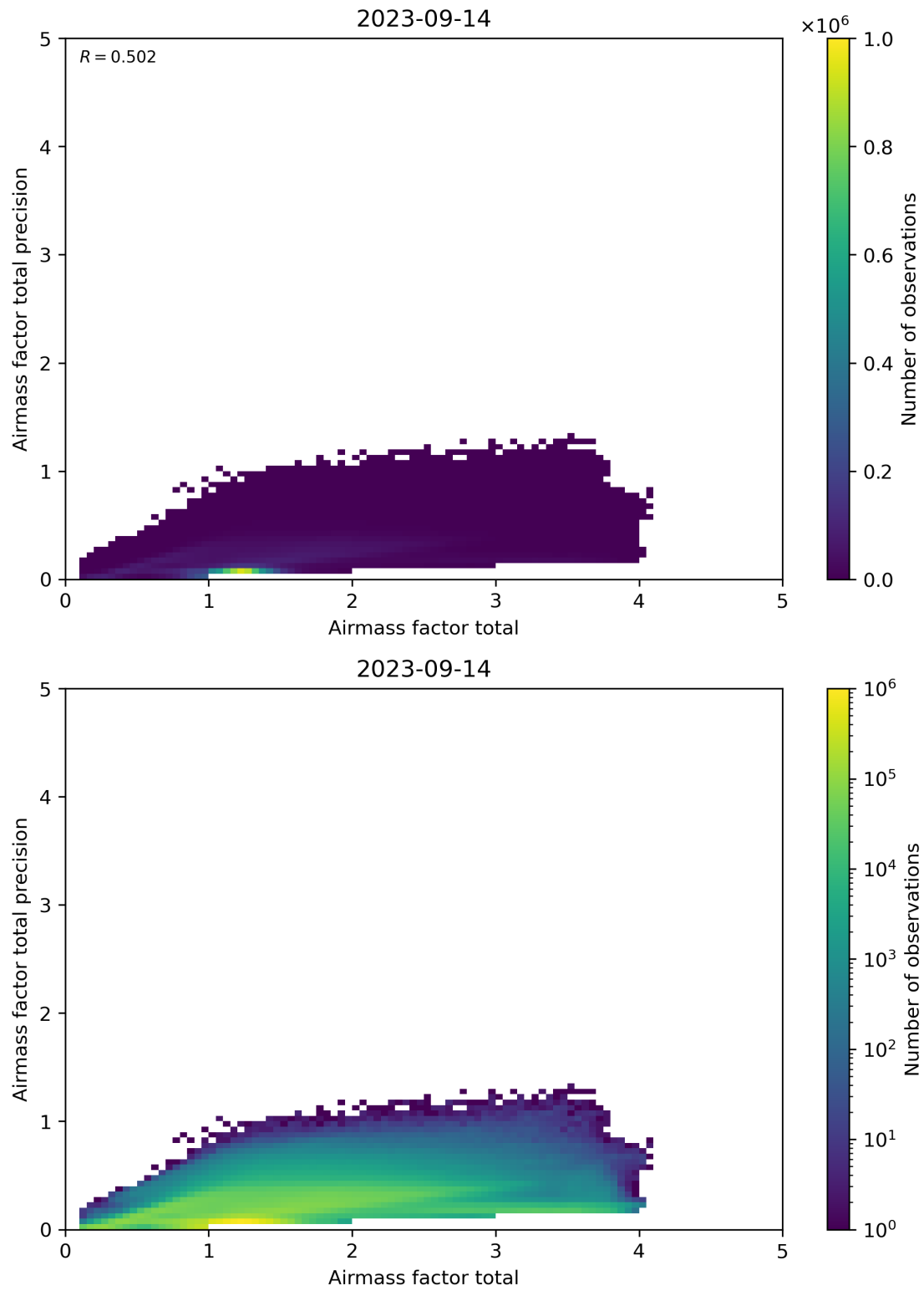
Figure 103: Scatter density plot of “Airmass factor total” against “Airmass factor total precision” for 2023-09-13 to 2023-09-15.
