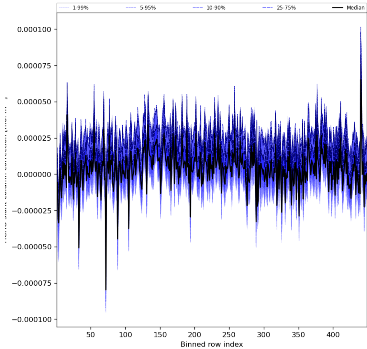
Figure 61: Along track statistics of “HCHO slant column correction” for 2023-09-13 to 2023-09-15
