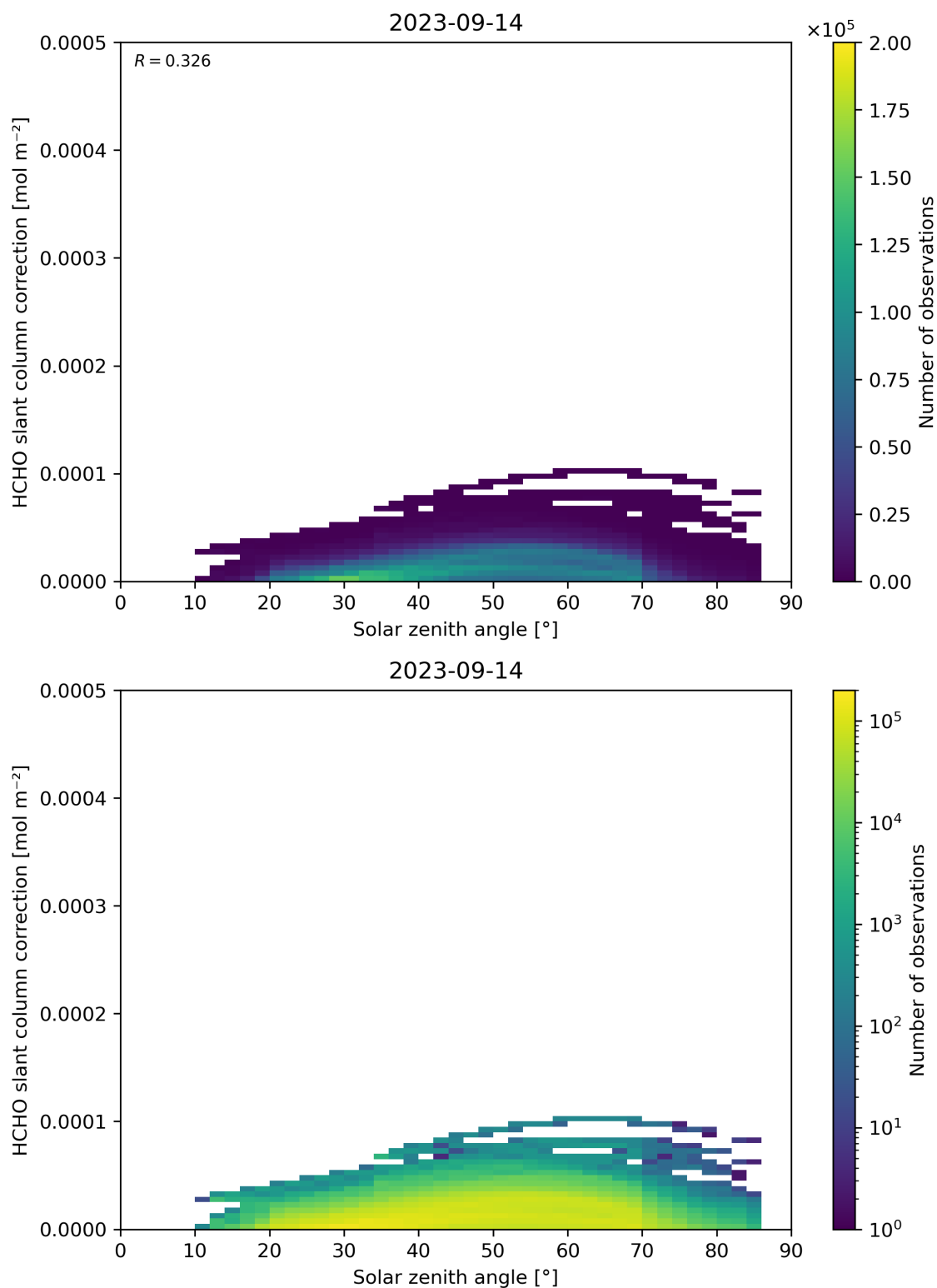
Figure 172: Scatter density plot of “Solar zenith angle” against “HCHO slant column correction” for 2023-09-13 to 2023-09-15.
