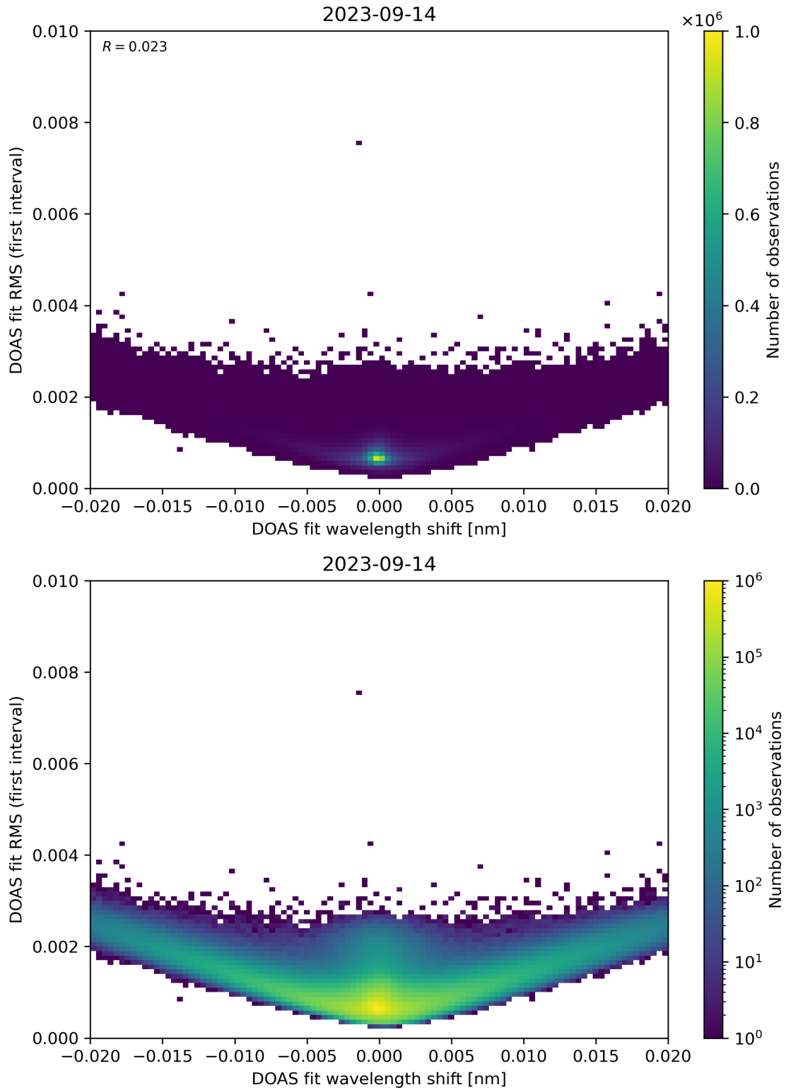
Figure 64: Scatter density plot of “DOAS fit wavelength shift” against “DOAS fit RMS (first interval)” for 2023-09-13 to 2023-09-15.
