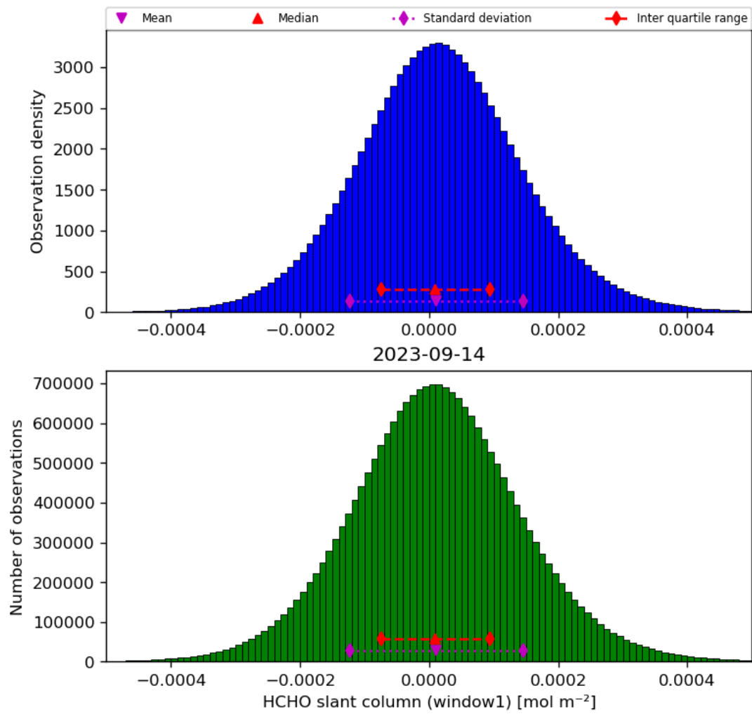
Figure 38: Histogram of “HCHO slant column (window1)” for 2023-09-13 to 2023-09-15
