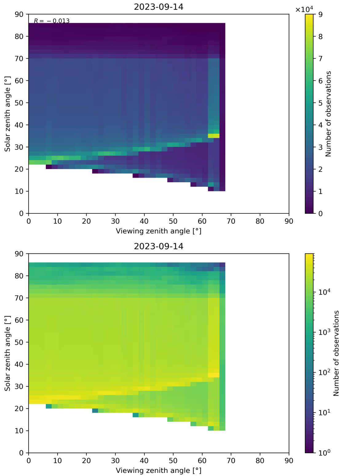
Figure 197: Scatter density plot of “Viewing zenith angle” against “Solar zenith angle” for 2023-09-13 to 2023-09-15.
