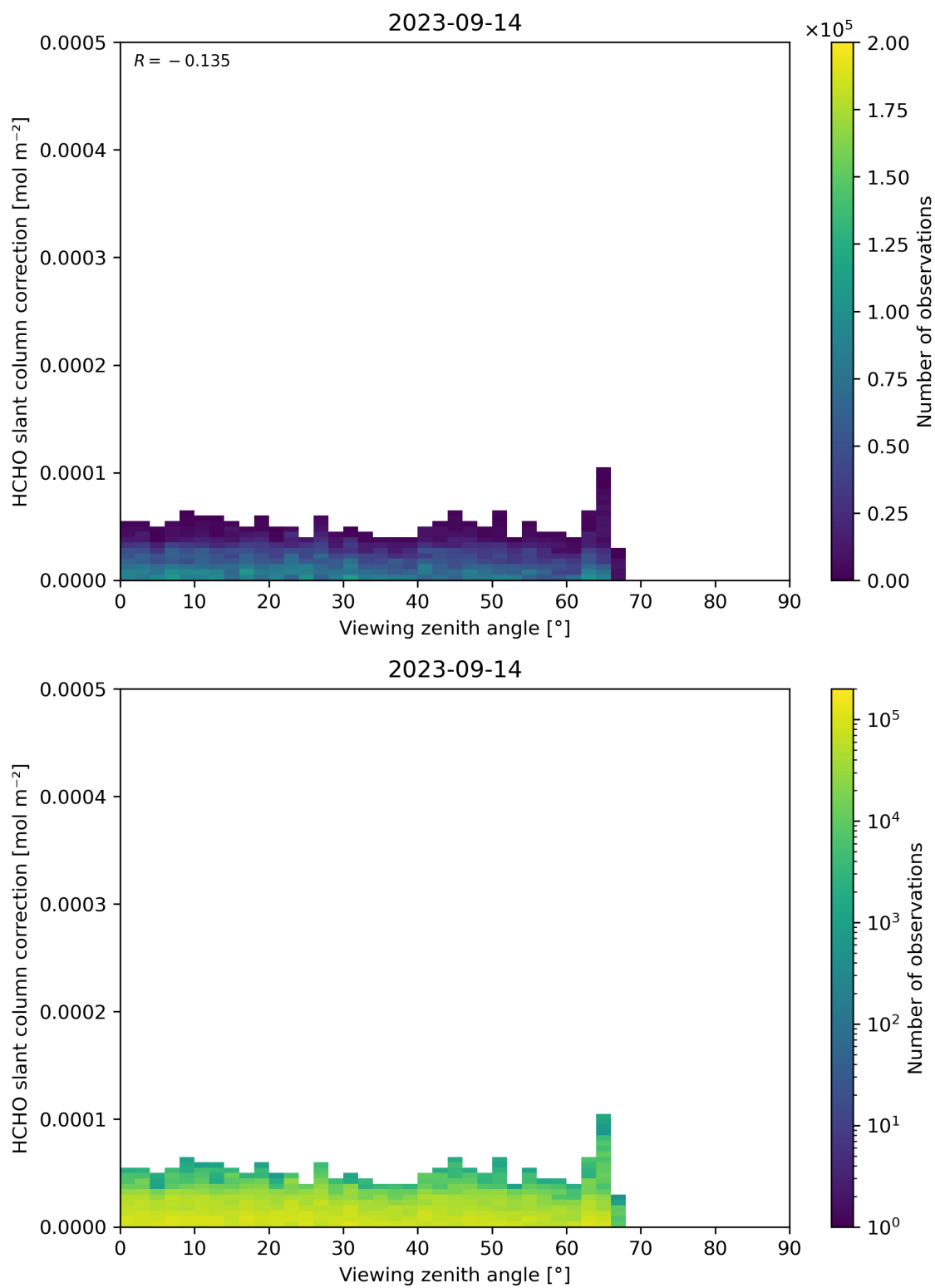
Figure 187: Scatter density plot of “Viewing zenith angle” against “HCHO slant column correction” for 2023-09-13 to 2023-09-15.
