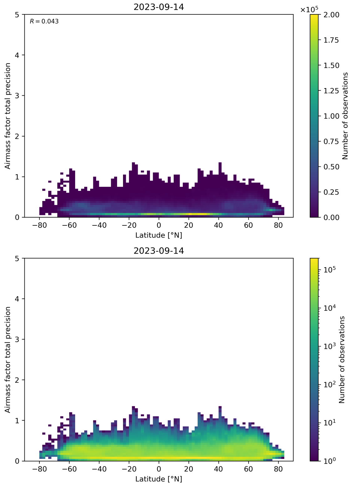
Figure 162: Scatter density plot of “Latitude” against “Airmass factor total precision” for 2023-09-13 to 2023-09-15.
