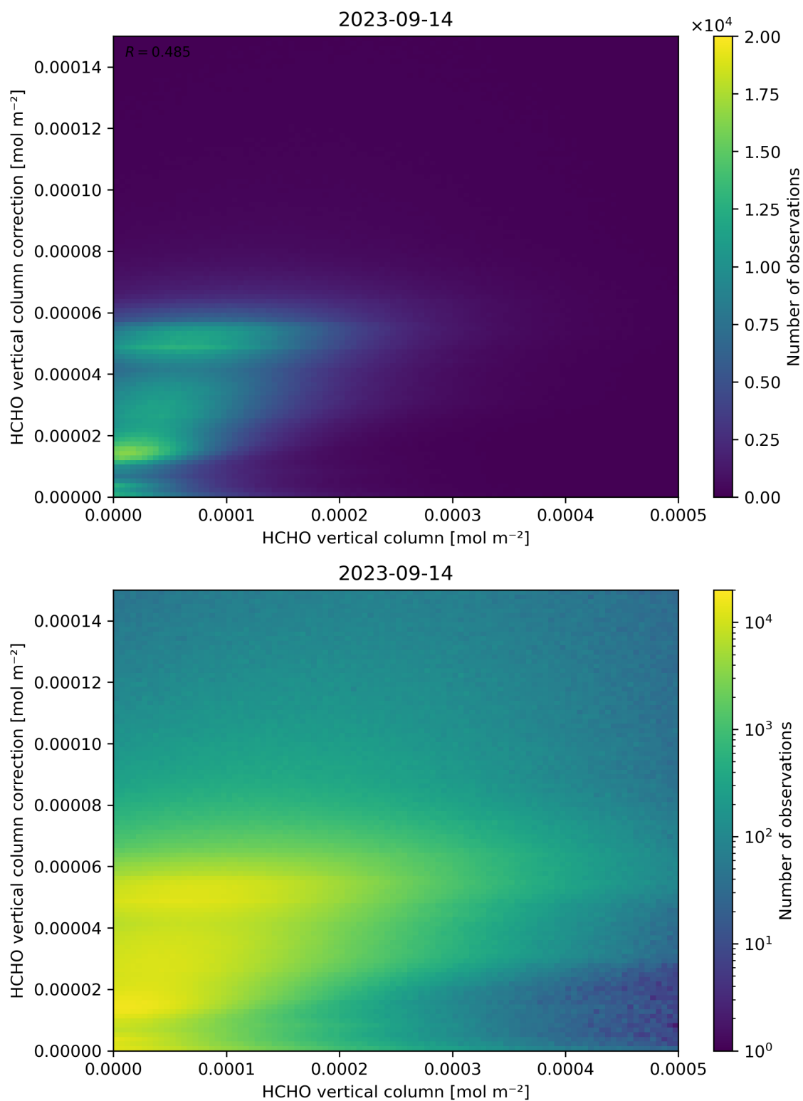
Figure 133: Scatter density plot of “HCHO vertical column” against “HCHO vertical column correction” for 2023-09-13 to 2023-09-15.
