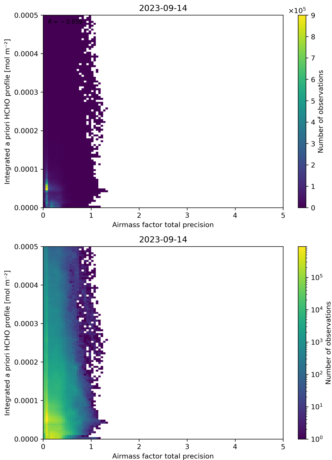
Figure 111: Scatter density plot of “Airmass factor total precision” against “Integrated a priori HCHO profile” for 2023-09-13 to 2023-09-15.
