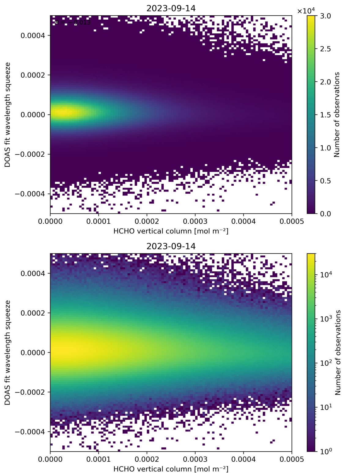
Figure 125: Scatter density plot of “HCHO vertical column” against “DOAS fit wavelength squeeze” for 2023-09-13 to 2023-09-15.
