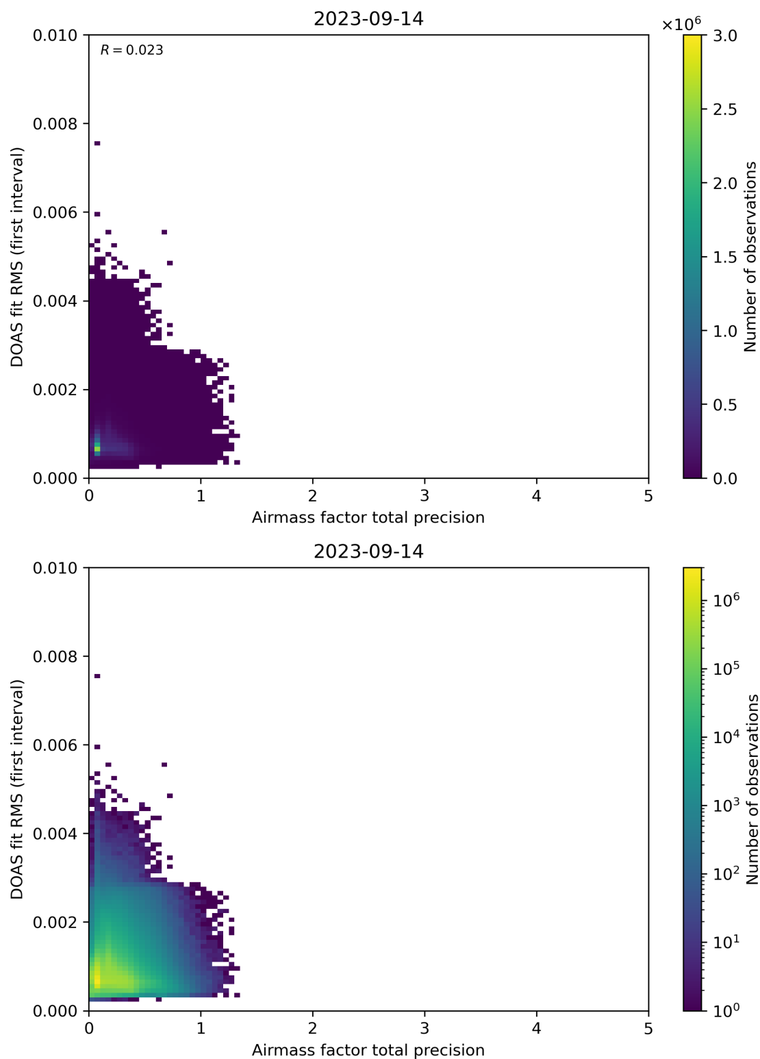
Figure 105: Scatter density plot of “Airmass factor total precision” against “DOAS fit RMS (first interval)” for 2023-09-13 to 2023-09-15.
