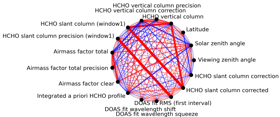
Figure 1: Map of correlation graph for 2023-09-13 to 2023-09-15.
