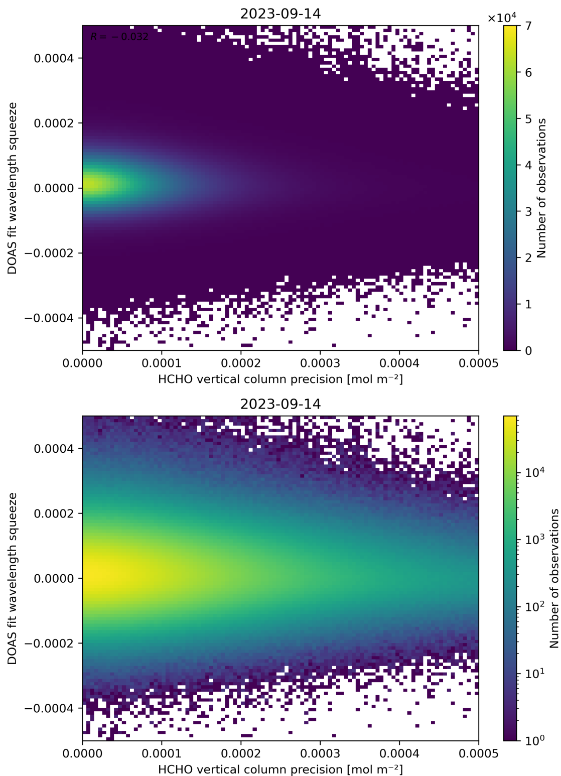
Figure 138: Scatter density plot of “HCHO vertical column precision” against “DOAS fit wavelength squeeze” for 2023-09-13 to 2023-09-15.
