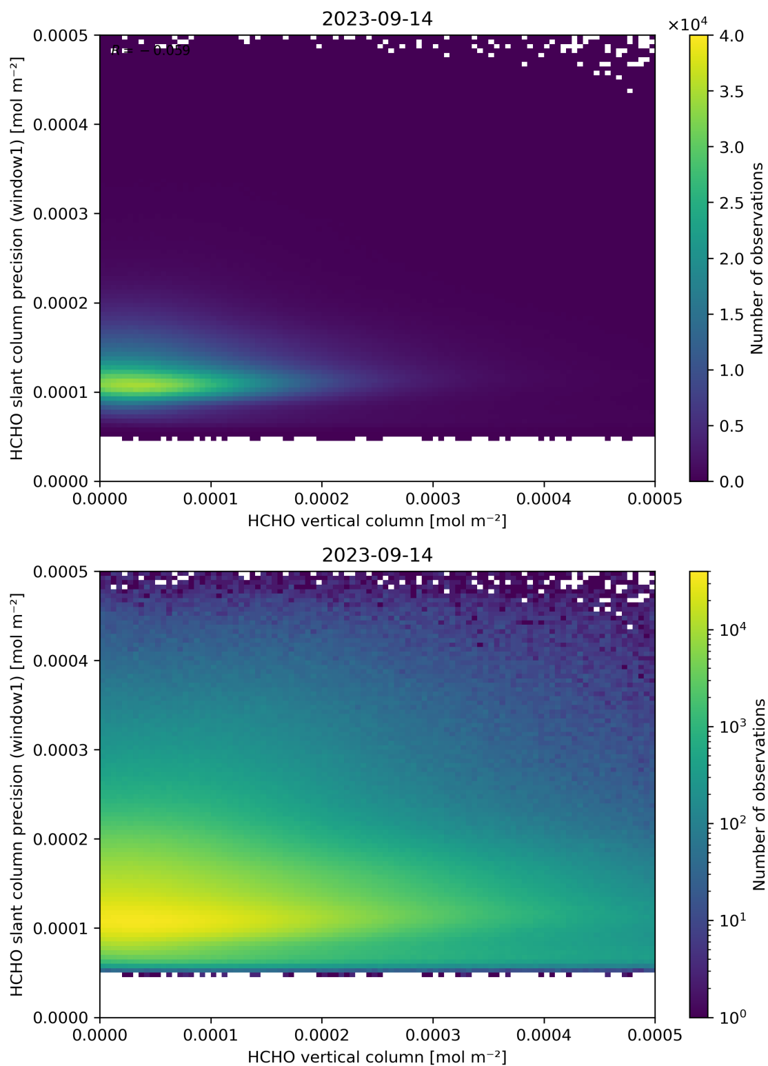
Figure 130: Scatter density plot of “HCHO vertical column” against “HCHO slant column precision (window1)” for 2023-09-13 to 2023-09-15.
