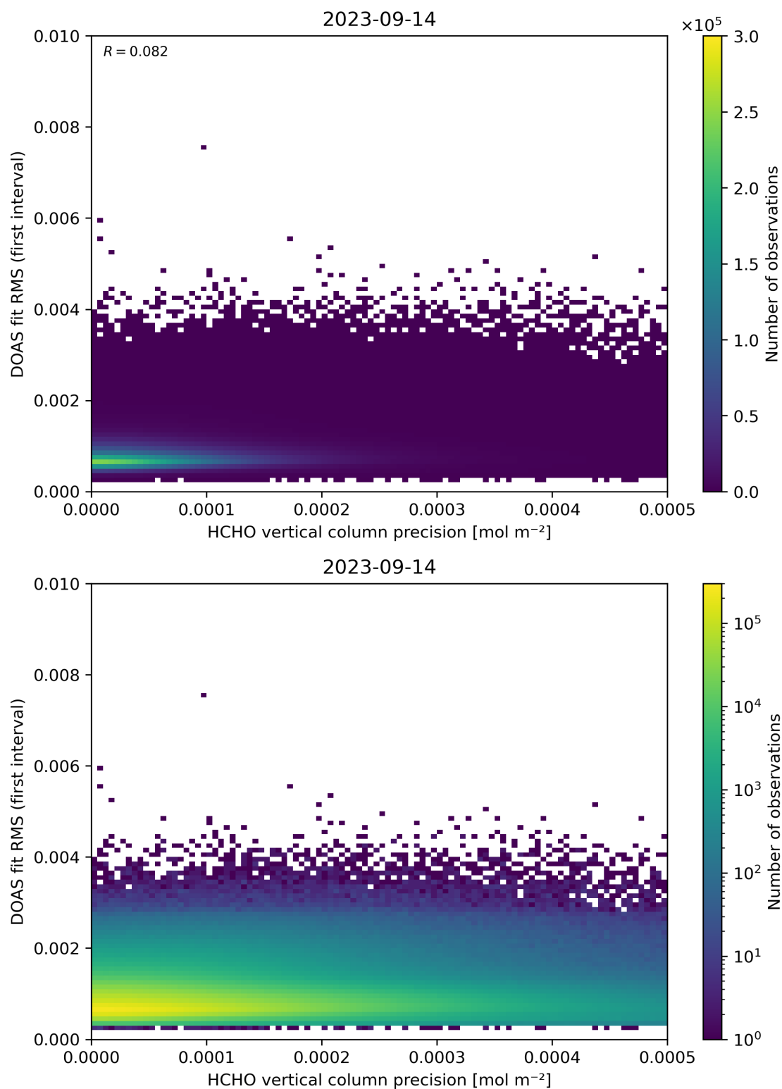
Figure 136: Scatter density plot of “HCHO vertical column precision” against “DOAS fit RMS (first interval)” for 2023-09-13 to 2023-09-15.
