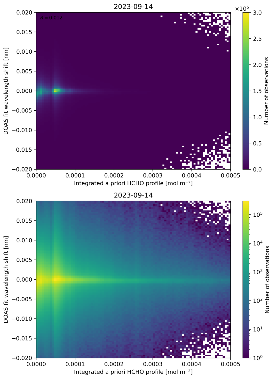
Figure 149: Scatter density plot of “Integrated a priori HCHO profile” against “DOAS fit wavelength shift” for 2023-09-13 to 2023-09-15.
