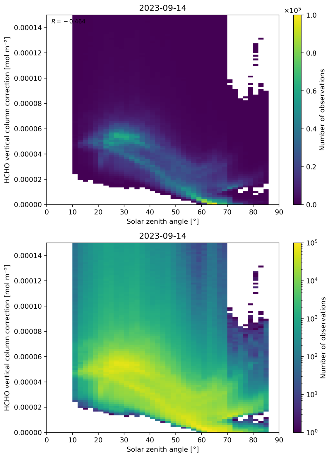
Figure 178: Scatter density plot of “Solar zenith angle” against “HCHO vertical column correction” for 2023-09-13 to 2023-09-15.
