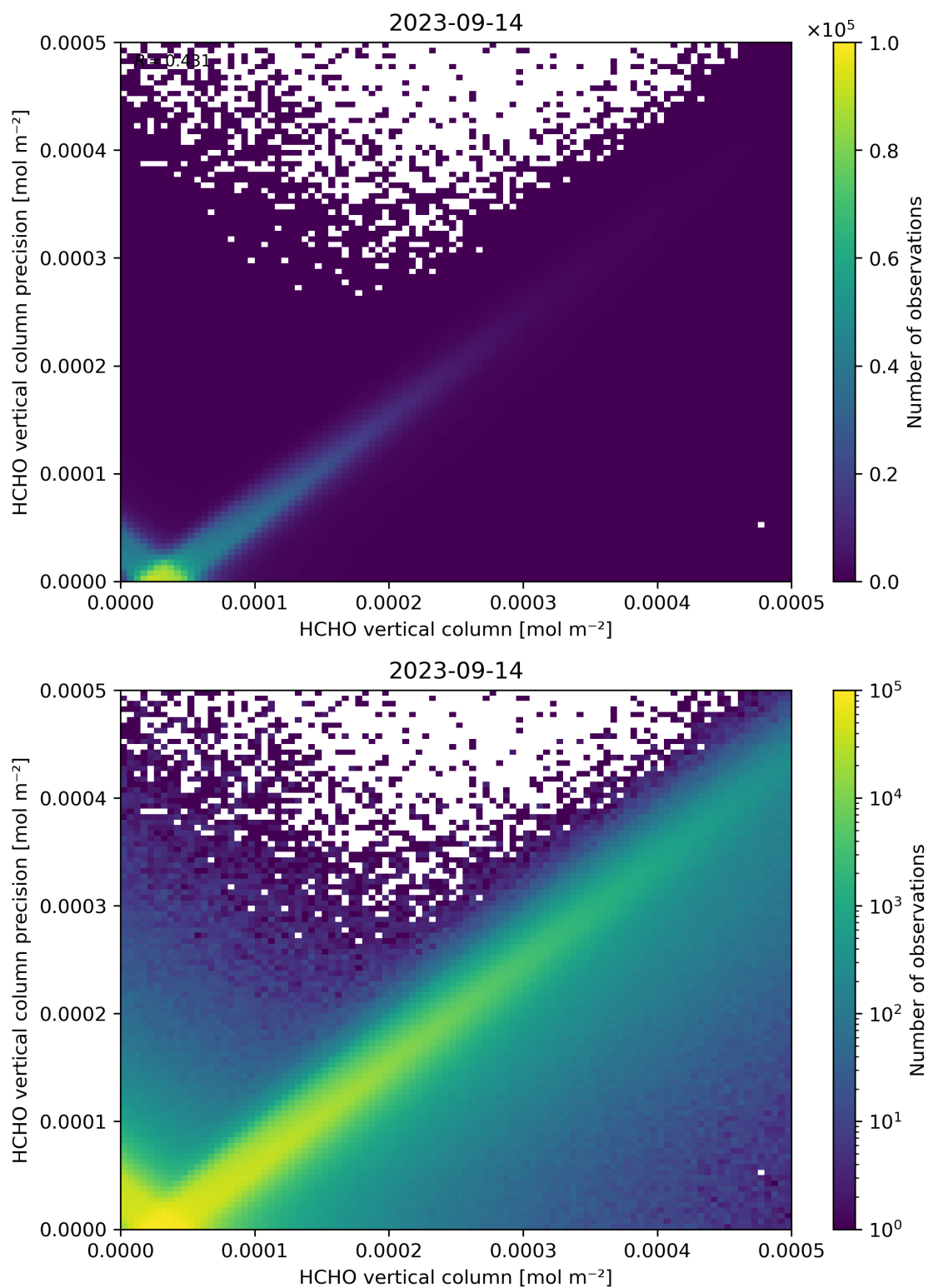
Figure 134: Scatter density plot of “HCHO vertical column” against “HCHO vertical column precision” for 2023-09-13 to 2023-09-15.
