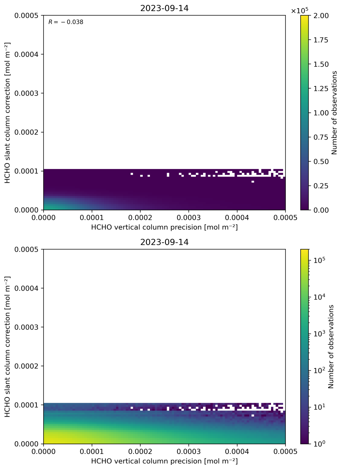
Figure 141: Scatter density plot of “HCHO vertical column precision” against “HCHO slant column correction” for 2023-09-13 to 2023-09-15.
