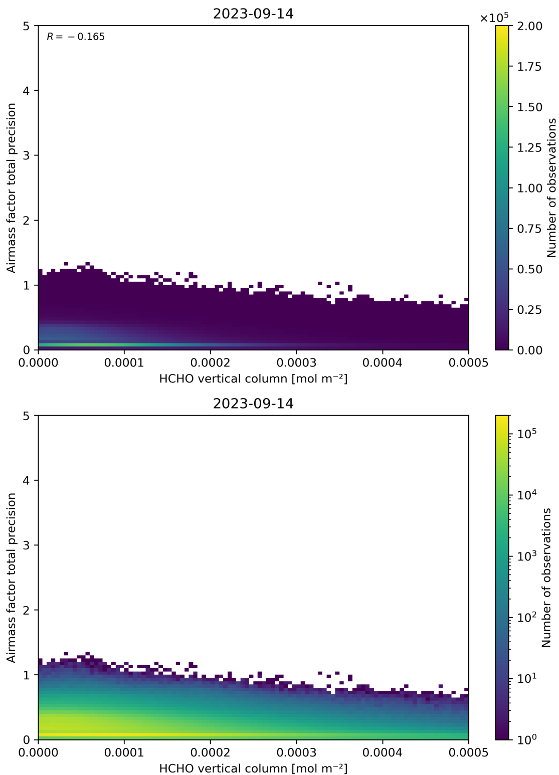
Figure 132: Scatter density plot of “HCHO vertical column” against “Airmass factor total precision” for 2023-09-13 to 2023-09-15.
