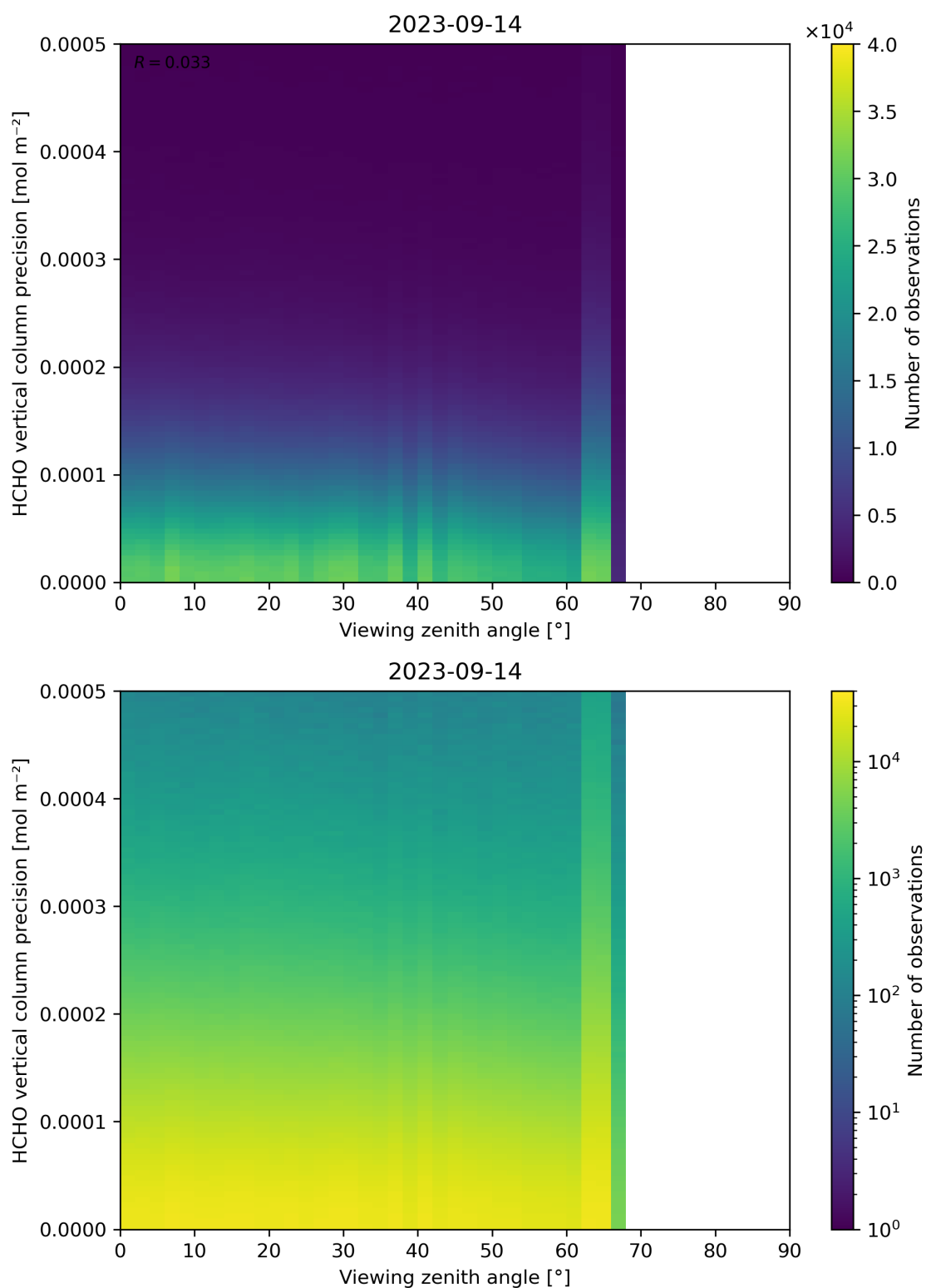
Figure 194: Scatter density plot of “Viewing zenith angle” against “HCHO vertical column precision” for 2023-09-13 to 2023-09-15.
