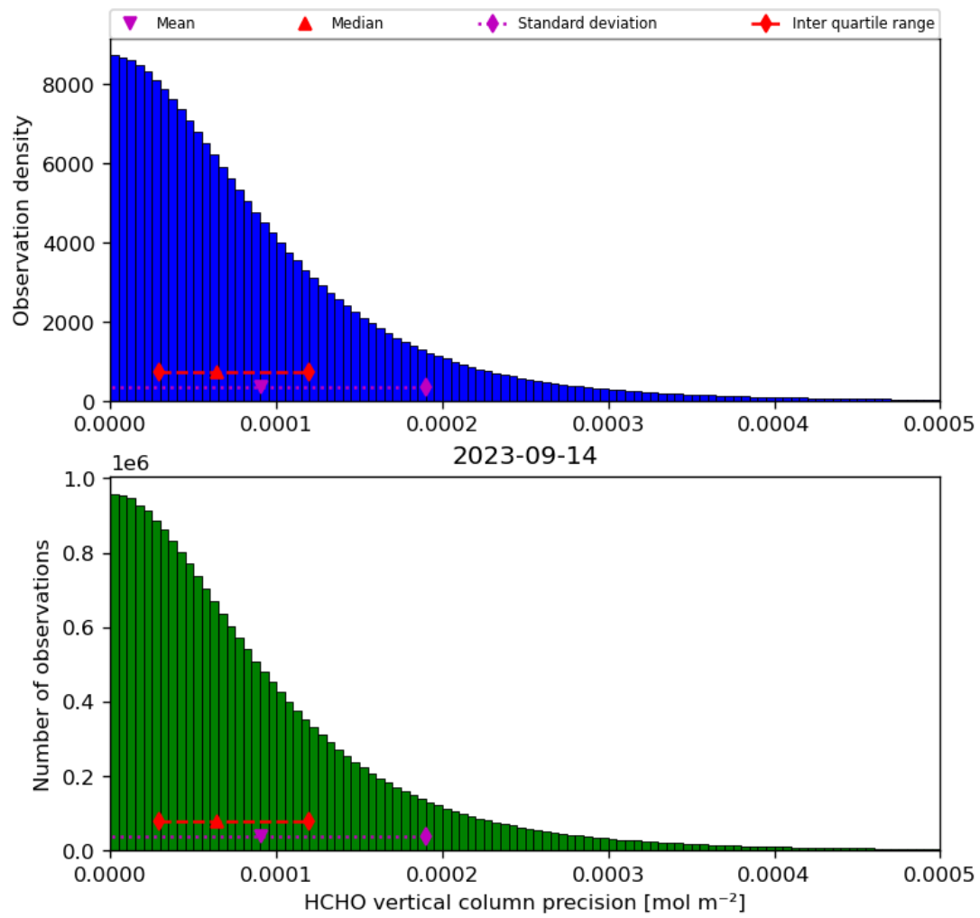
Figure 36: Histogram of “HCHO vertical column precision” for 2023-09-13 to 2023-09-15
