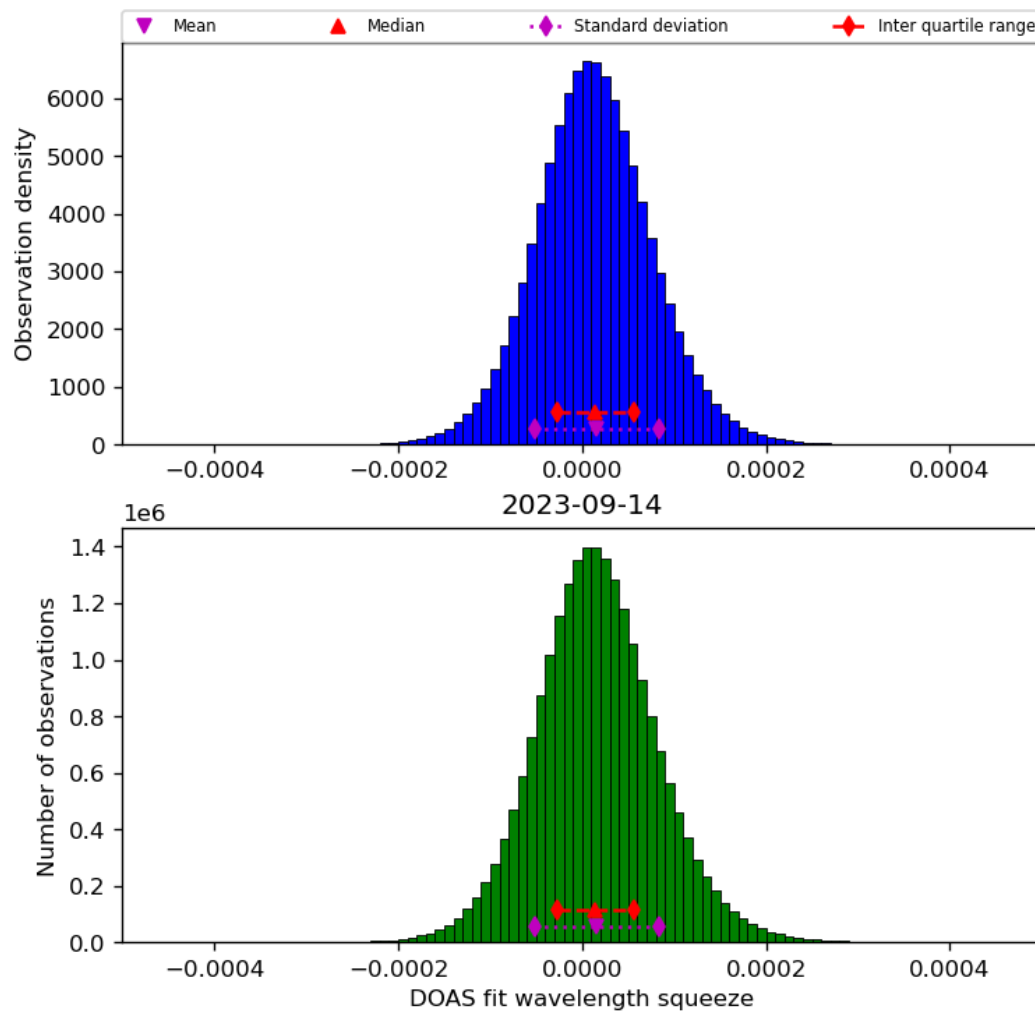
Figure 45: Histogram of “DOAS fit wavelength squeeze” for 2023-09-13 to 2023-09-15
