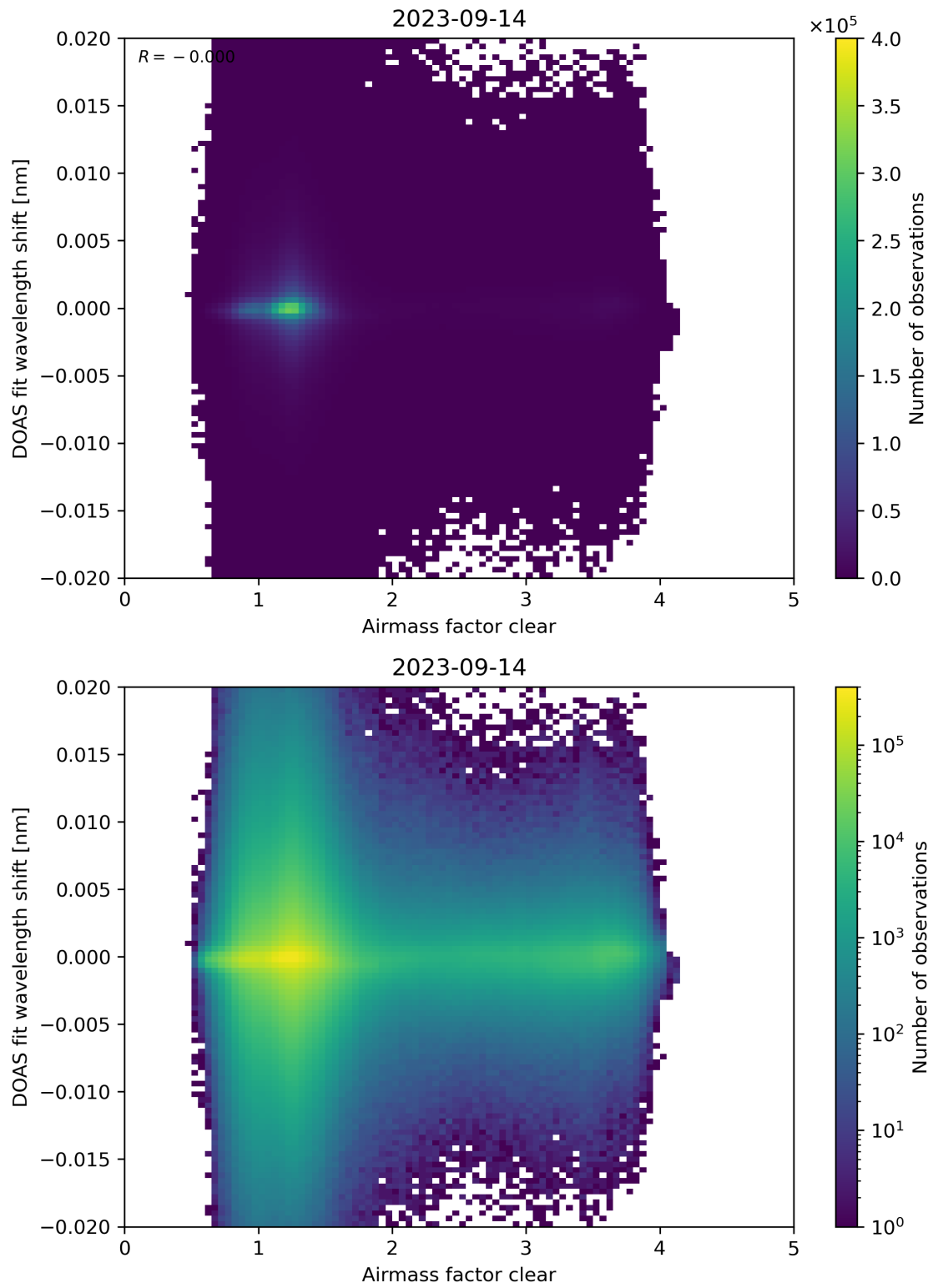
Figure 72: Scatter density plot of “Airmass factor clear” against “DOAS fit wavelength shift” for 2023-09-13 to 2023-09-15.
