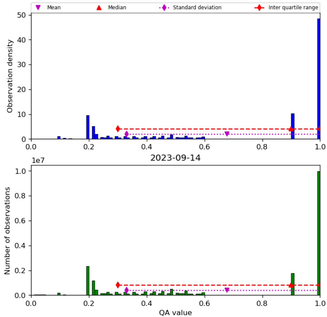
Figure 34: Histogram of “QA value” for 2023-09-13 to 2023-09-15
