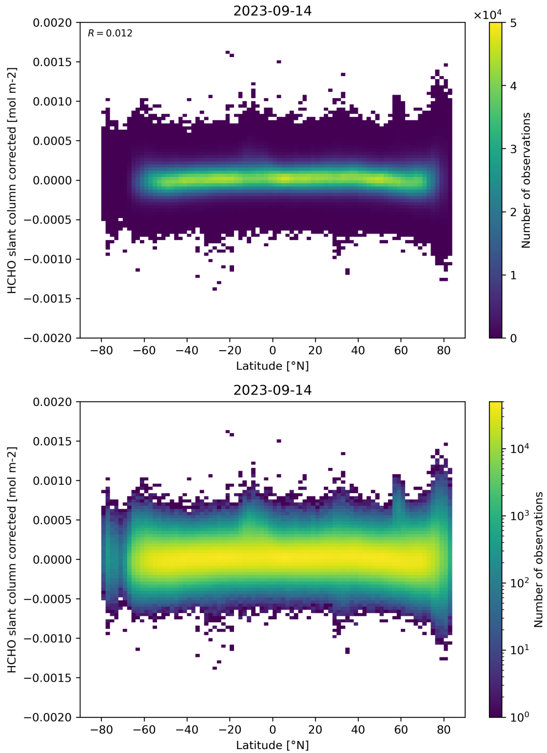
Figure 157: Scatter density plot of “Latitude” against “HCHO slant column corrected” for 2023-09-13 to 2023-09-15.
