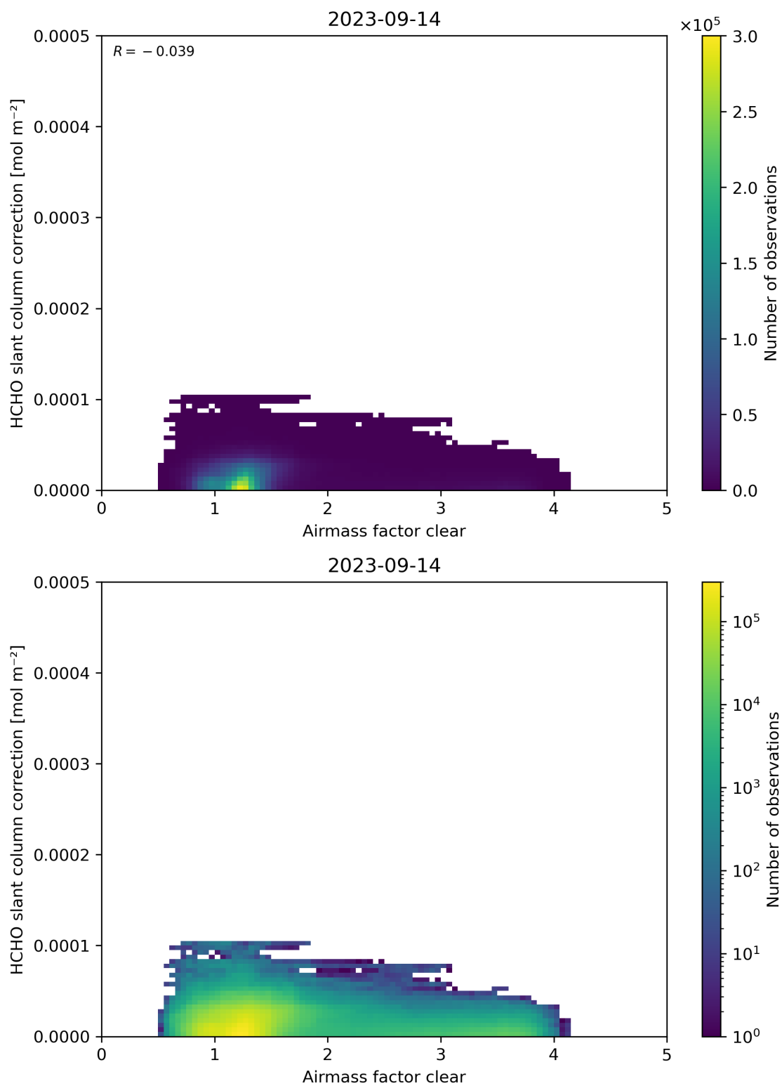
Figure 75: Scatter density plot of “Airmass factor clear” against “HCHO slant column correction” for 2023-09-13 to 2023-09-15.
