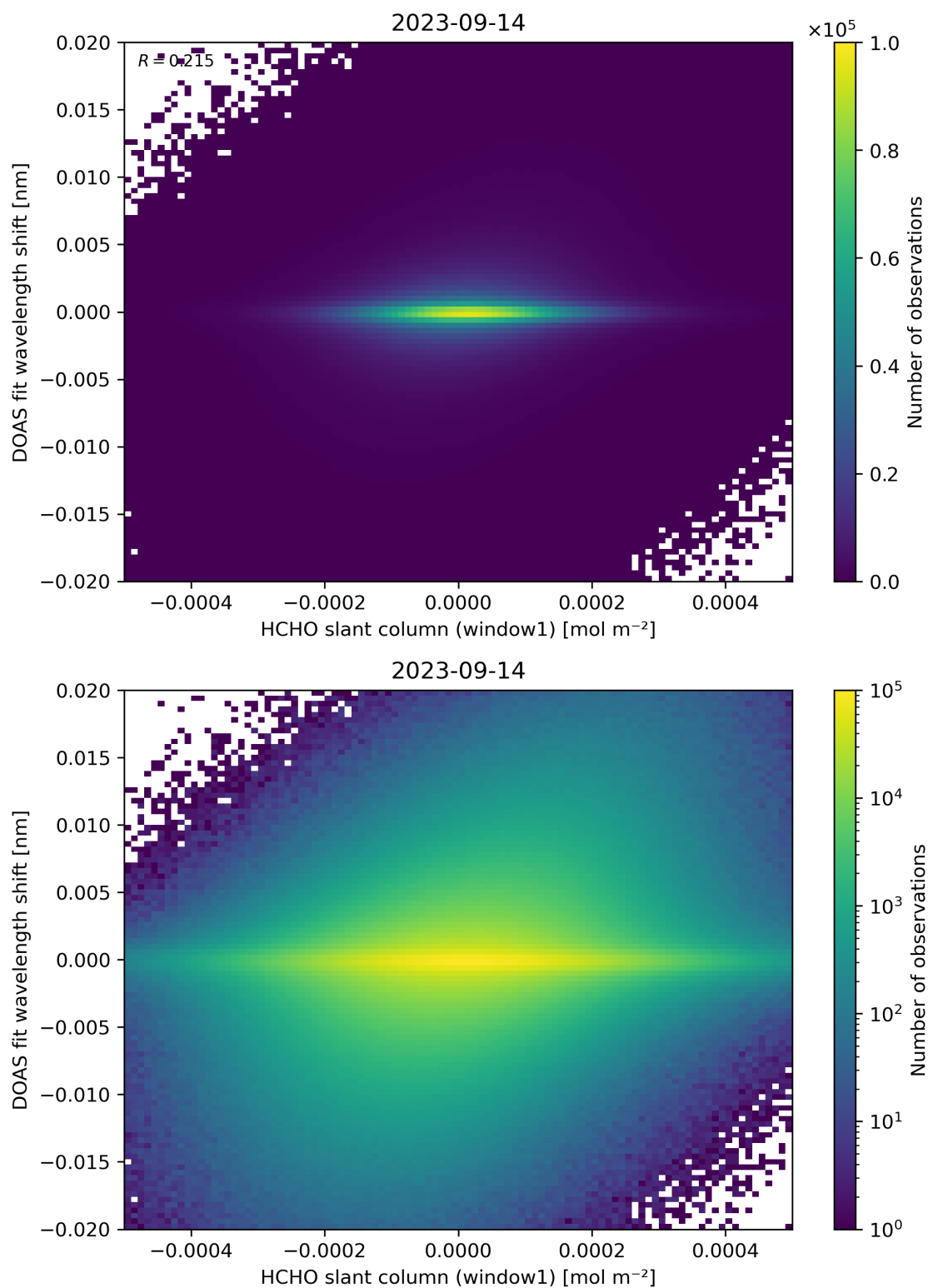
Figure 79: Scatter density plot of “HCHO slant column (window1)” against “DOAS fit wavelength shift” for 2023-09-13 to 2023-09-15.
