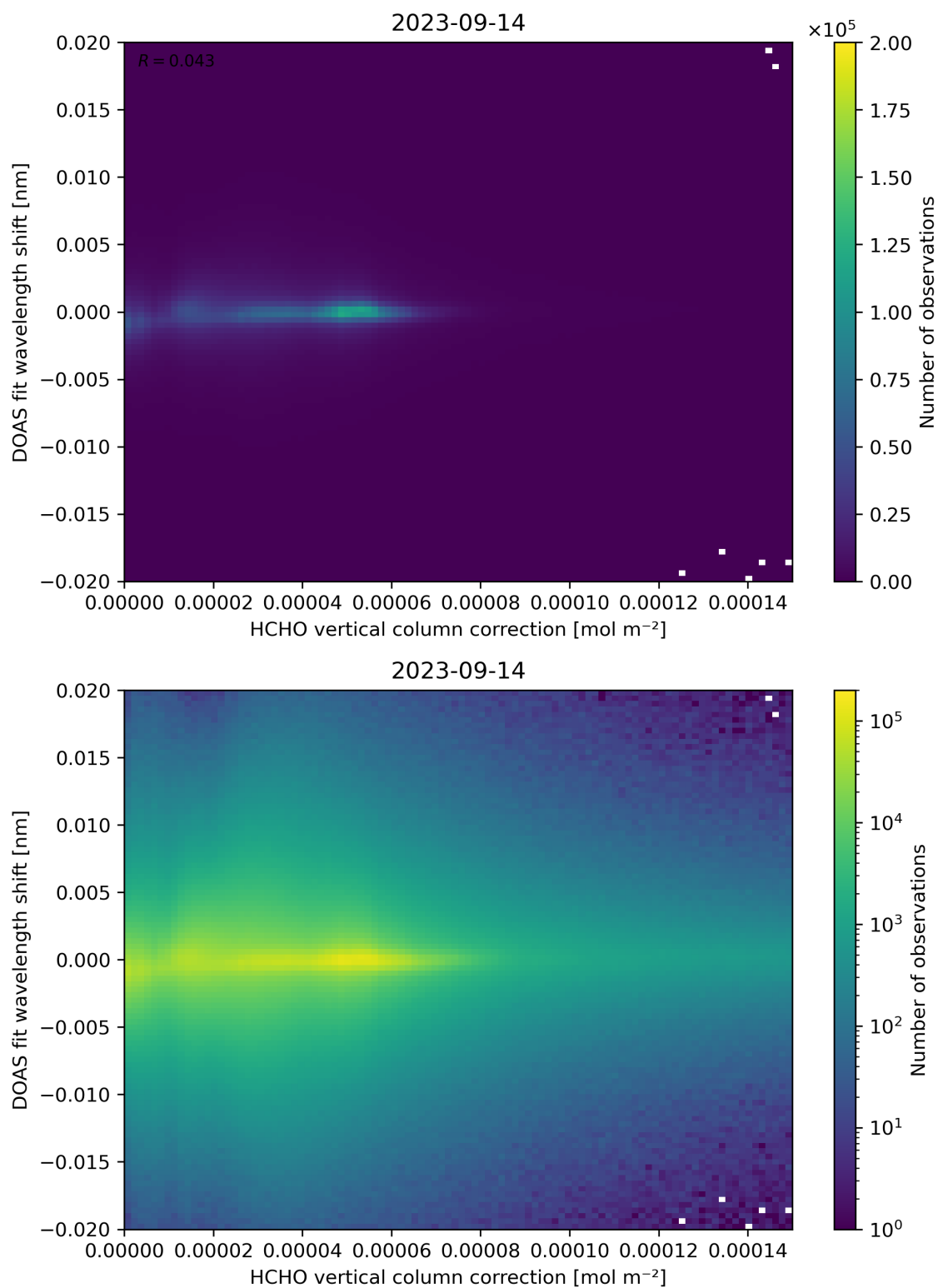
Figure 113: Scatter density plot of “HCHO vertical column correction” against “DOAS fit wavelength shift” for 2023-09-13 to 2023-09-15.
