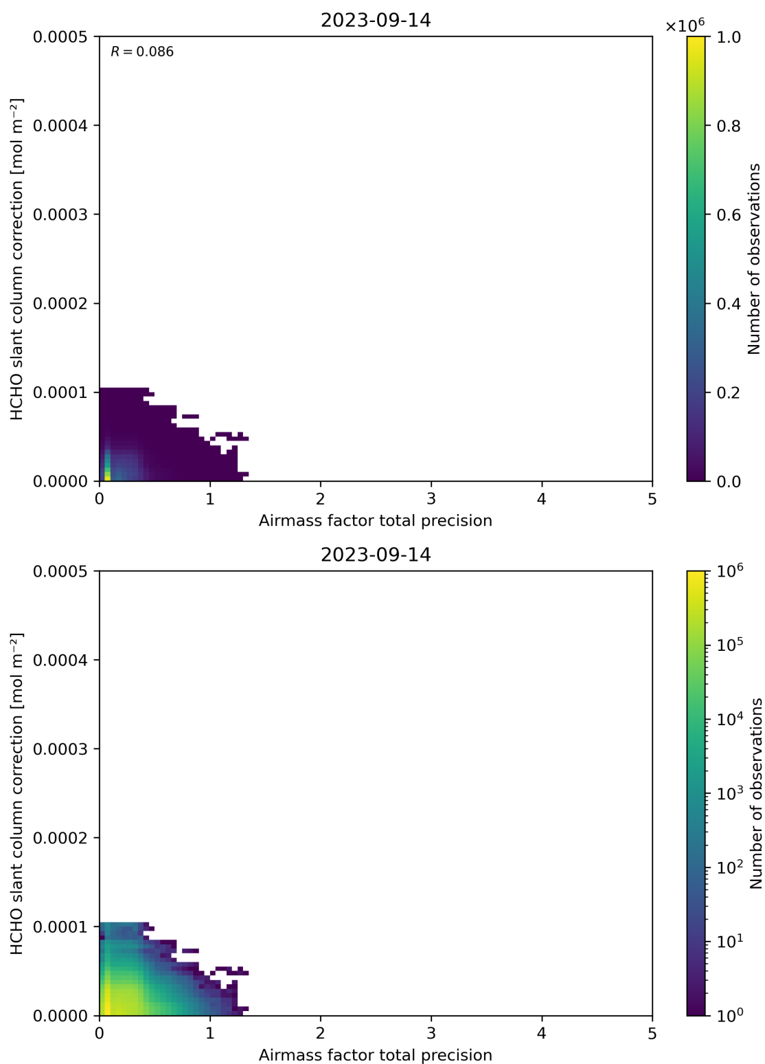
Figure 110: Scatter density plot of “Airmass factor total precision” against “HCHO slant column correction” for 2023-09-13 to 2023-09-15.
