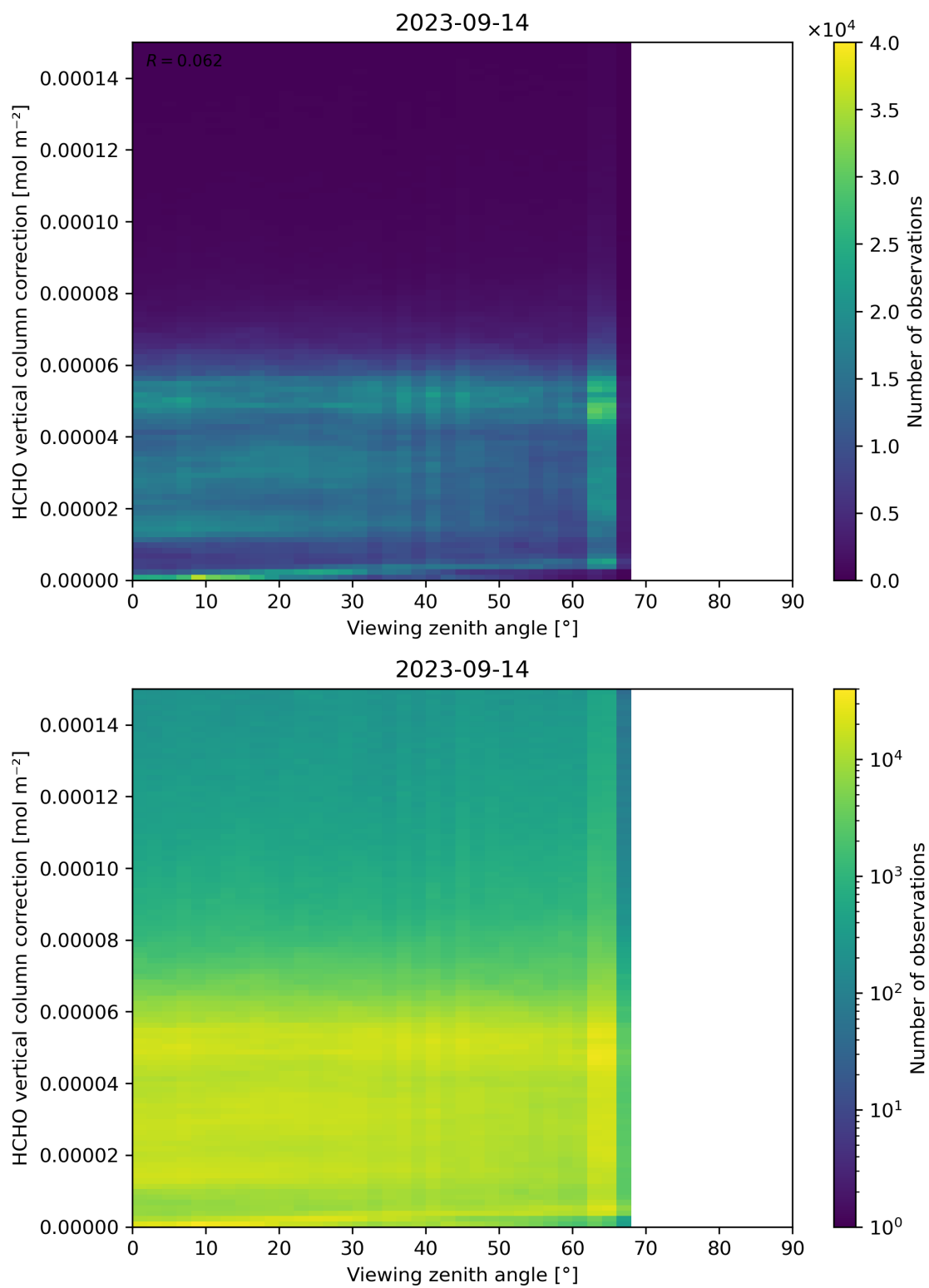
Figure 193: Scatter density plot of “Viewing zenith angle” against “HCHO vertical column correction” for 2023-09-13 to 2023-09-15.
