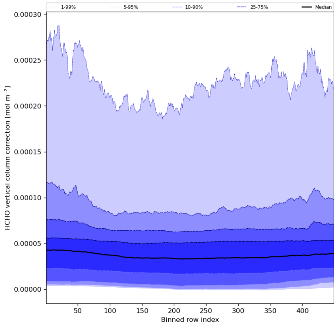
Figure 51: Along track statistics of “HCHO vertical column correction” for 2023-09-13 to 2023-09-15
