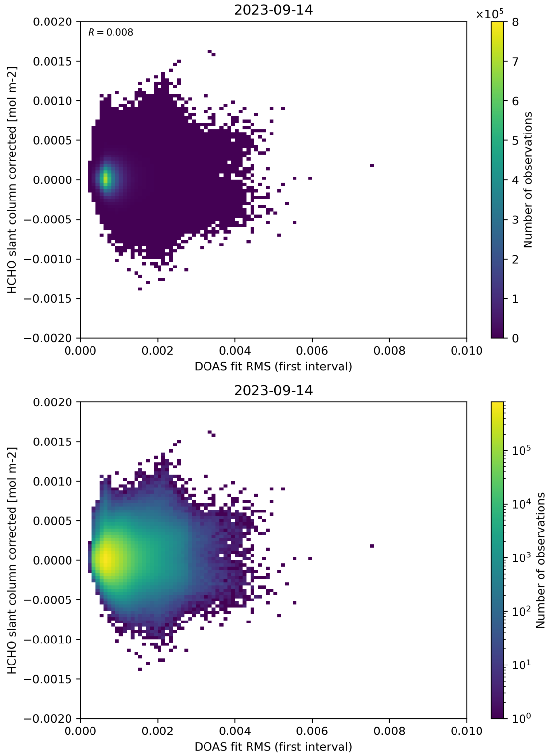
Figure 62: Scatter density plot of “DOAS fit RMS (first interval)” against “HCHO slant column corrected” for 2023-09-13 to 2023-09-15.
