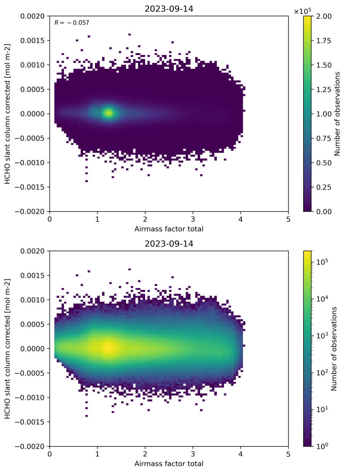
Figure 101: Scatter density plot of “Airmass factor total” against “HCHO slant column corrected” for 2023-09-13 to 2023-09-15.
