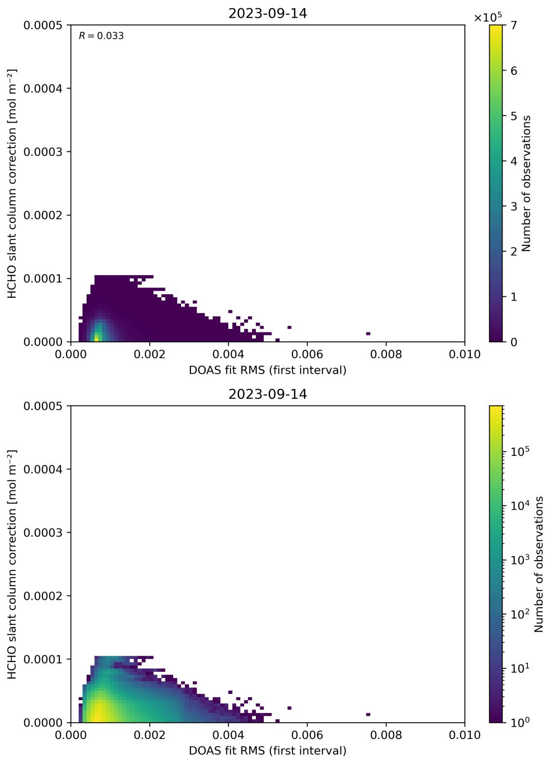
Figure 63: Scatter density plot of “DOAS fit RMS (first interval)” against “HCHO slant column correction” for 2023-09-13 to 2023-09-15.
