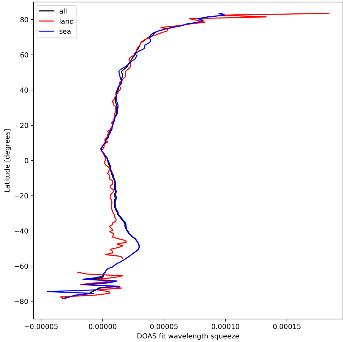
Figure 31: Zonal average of “DOAS fit wavelength squeeze” for 2023-09-13 to 2023-09-15.
