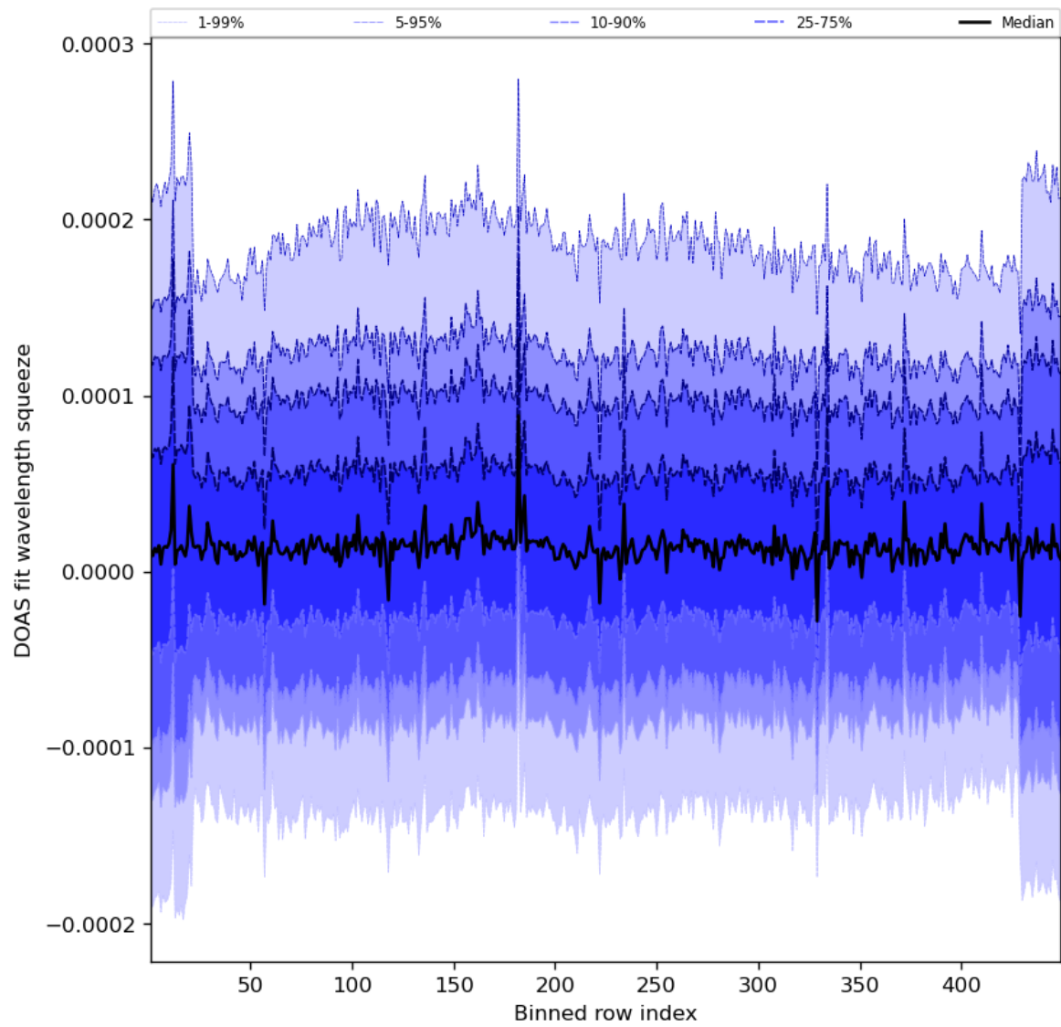
Figure 59: Along track statistics of “DOAS fit wavelength squeeze” for 2023-09-13 to 2023-09-15
