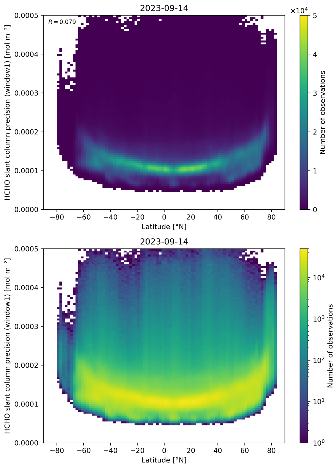
Figure 160: Scatter density plot of “Latitude” against “HCHO slant column precision (window1)” for 2023-09-13 to 2023-09-15.
