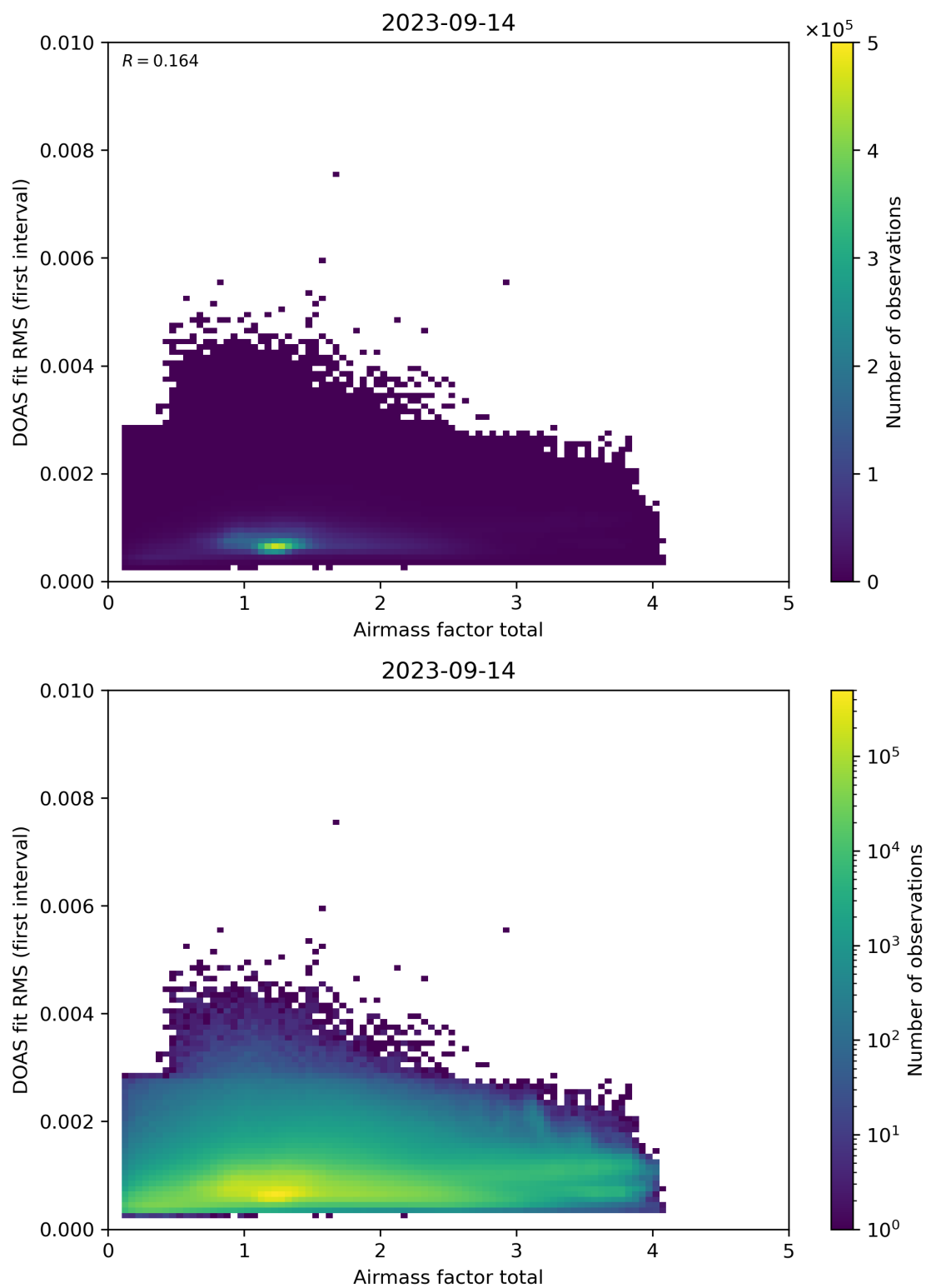
Figure 97: Scatter density plot of “Airmass factor total” against “DOAS fit RMS (first interval)” for 2023-09-13 to 2023-09-15.
