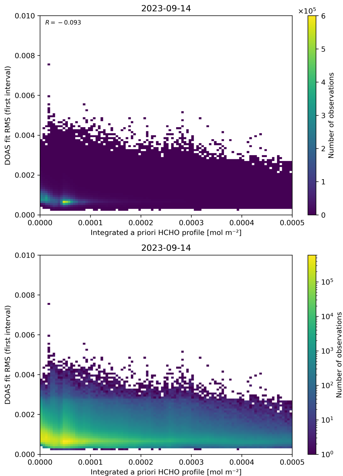
Figure 148: Scatter density plot of “Integrated a priori HCHO profile” against “DOAS fit RMS (first interval)” for 2023-09-13 to 2023-09-15.
