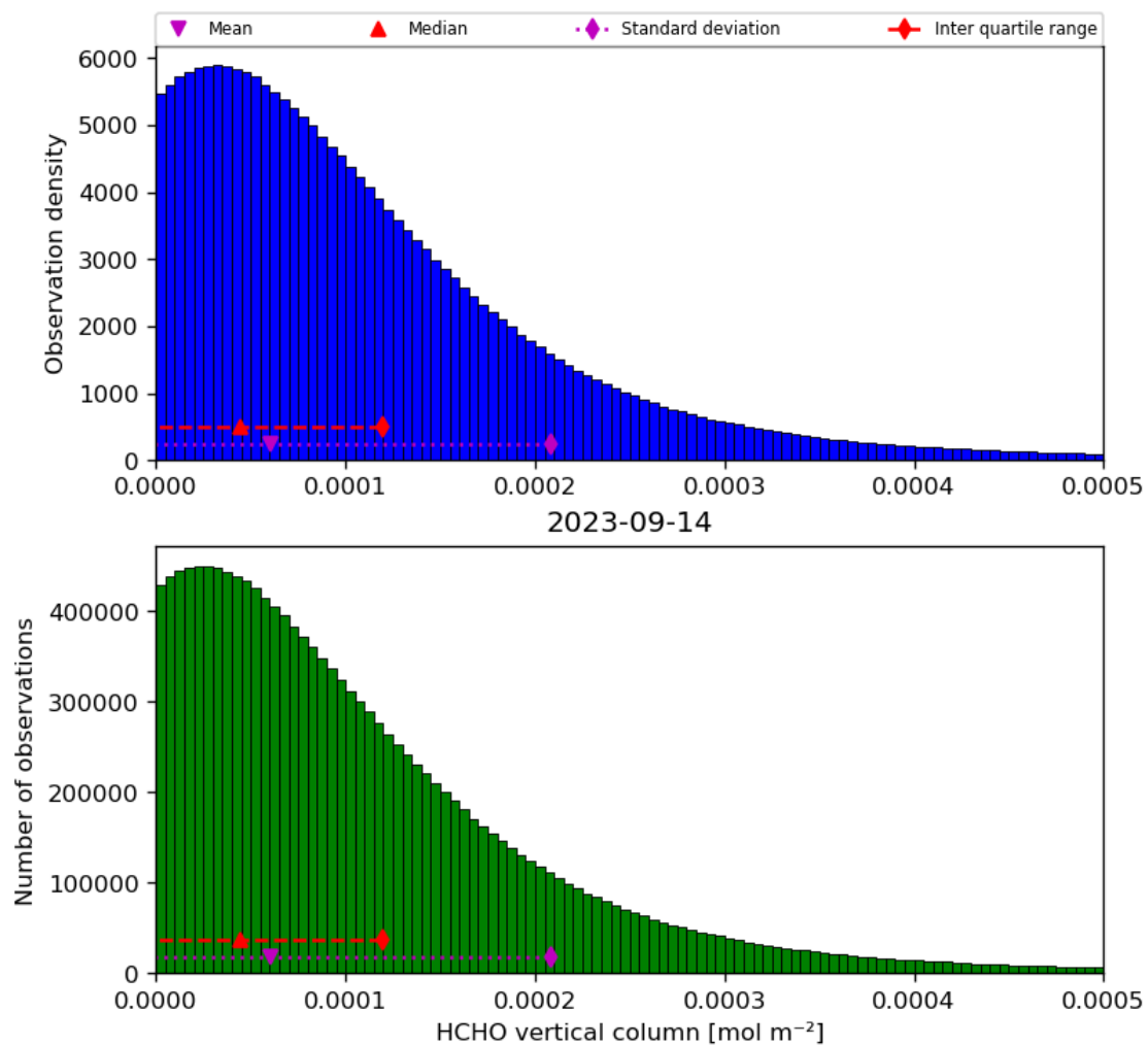
Figure 35: Histogram of “HCHO vertical column” for 2023-09-13 to 2023-09-15
