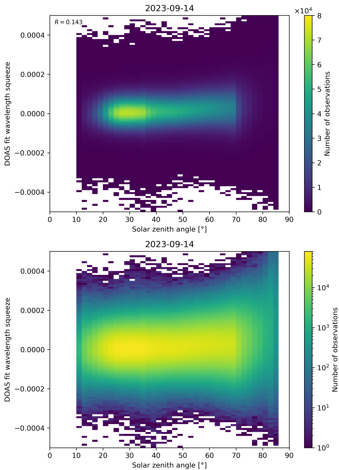
Figure 169: Scatter density plot of “Solar zenith angle” against “DOAS fit wavelength squeeze” for 2023-09-13 to 2023-09-15.
