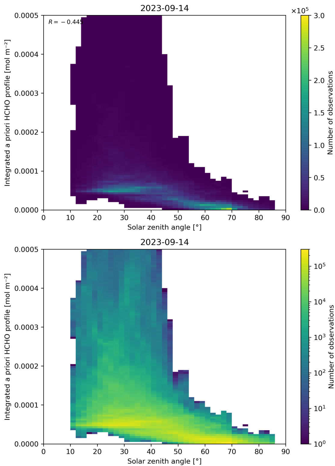
Figure 180: Scatter density plot of “Solar zenith angle” against “Integrated a priori HCHO profile” for 2023-09-13 to 2023-09-15.
