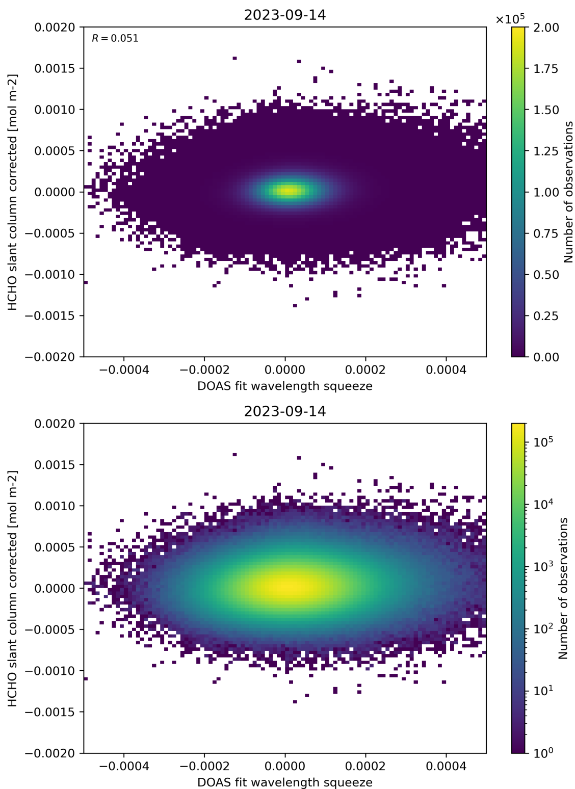
Figure 69: Scatter density plot of “DOAS fit wavelength squeeze” against “HCHO slant column corrected” for 2023-09-13 to 2023-09-15.
