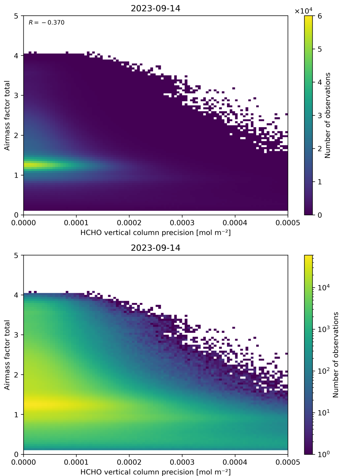
Figure 144: Scatter density plot of “HCHO vertical column precision” against “Airmass factor total” for 2023-09-13 to 2023-09-15.
