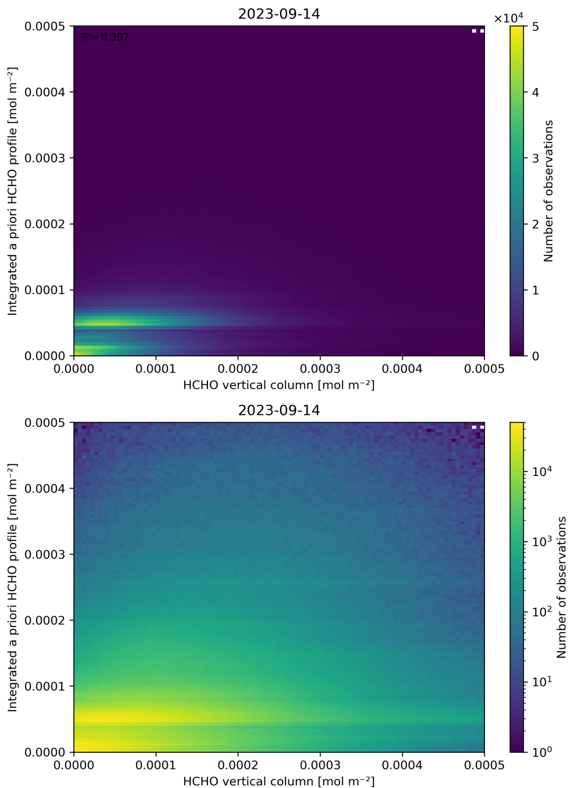
Figure 135: Scatter density plot of “HCHO vertical column” against “Integrated a priori HCHO profile” for 2023-09-13 to 2023-09-15.
