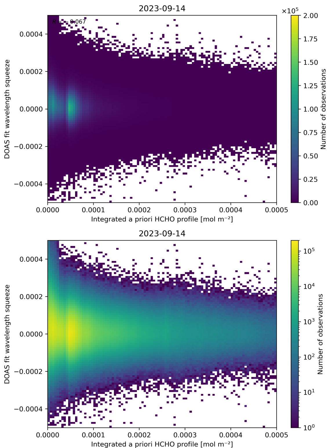
Figure 150: Scatter density plot of “Integrated a priori HCHO profile” against “DOAS fit wavelength squeeze” for 2023-09-13 to 2023-09-15.
