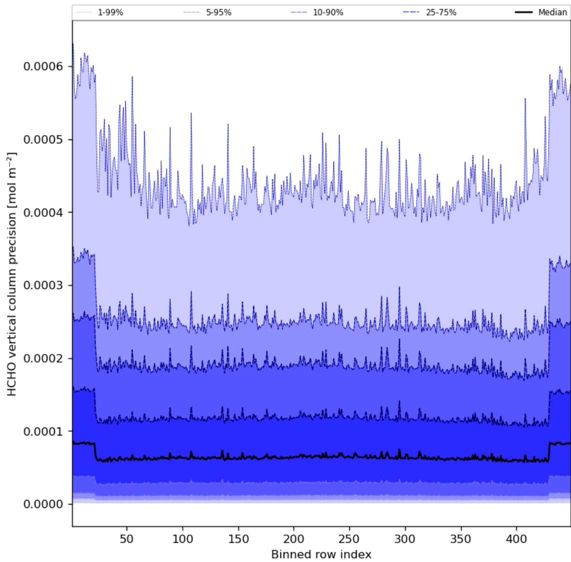
Figure 50: Along track statistics of “HCHO vertical column precision” for 2023-09-13 to 2023-09-15
