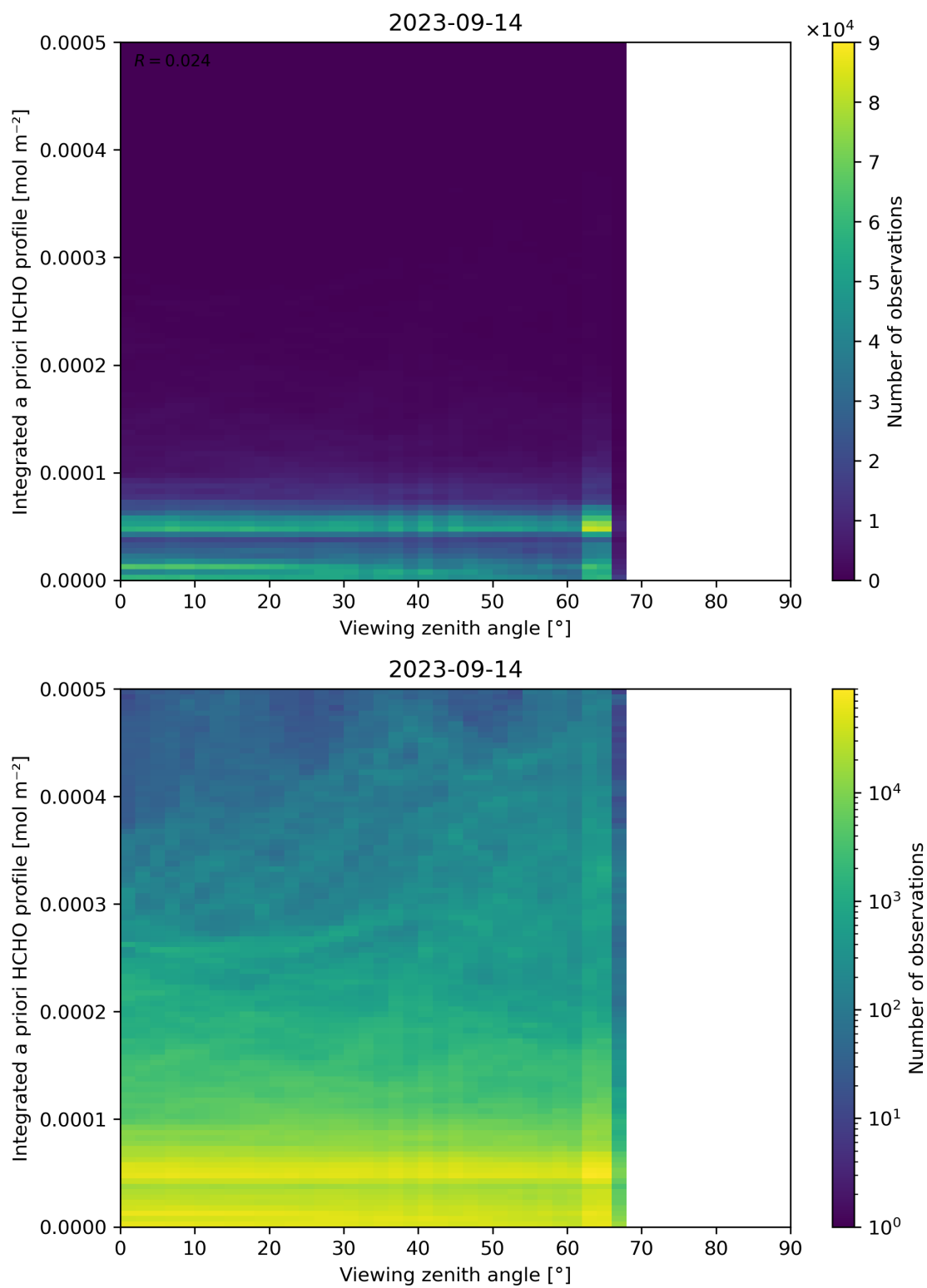
Figure 195: Scatter density plot of “Viewing zenith angle” against “Integrated a priori HCHO profile” for 2023-09-13 to 2023-09-15.
