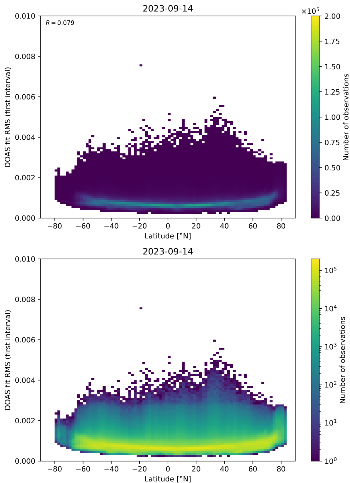
Figure 153: Scatter density plot of “Latitude” against “DOAS fit RMS (first interval)” for 2023-09-13 to 2023-09-15.
