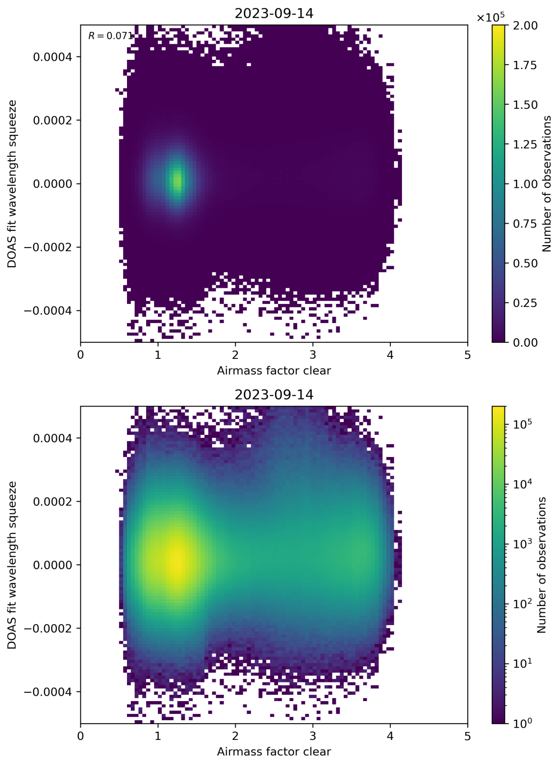
Figure 73: Scatter density plot of “Airmass factor clear” against “DOAS fit wavelength squeeze” for 2023-09-13 to 2023-09-15.
