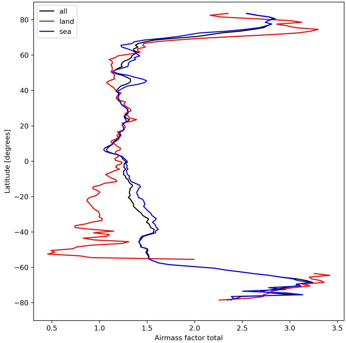
Figure 26: Zonal average of “Airmass factor total” for 2023-09-13 to 2023-09-15.
