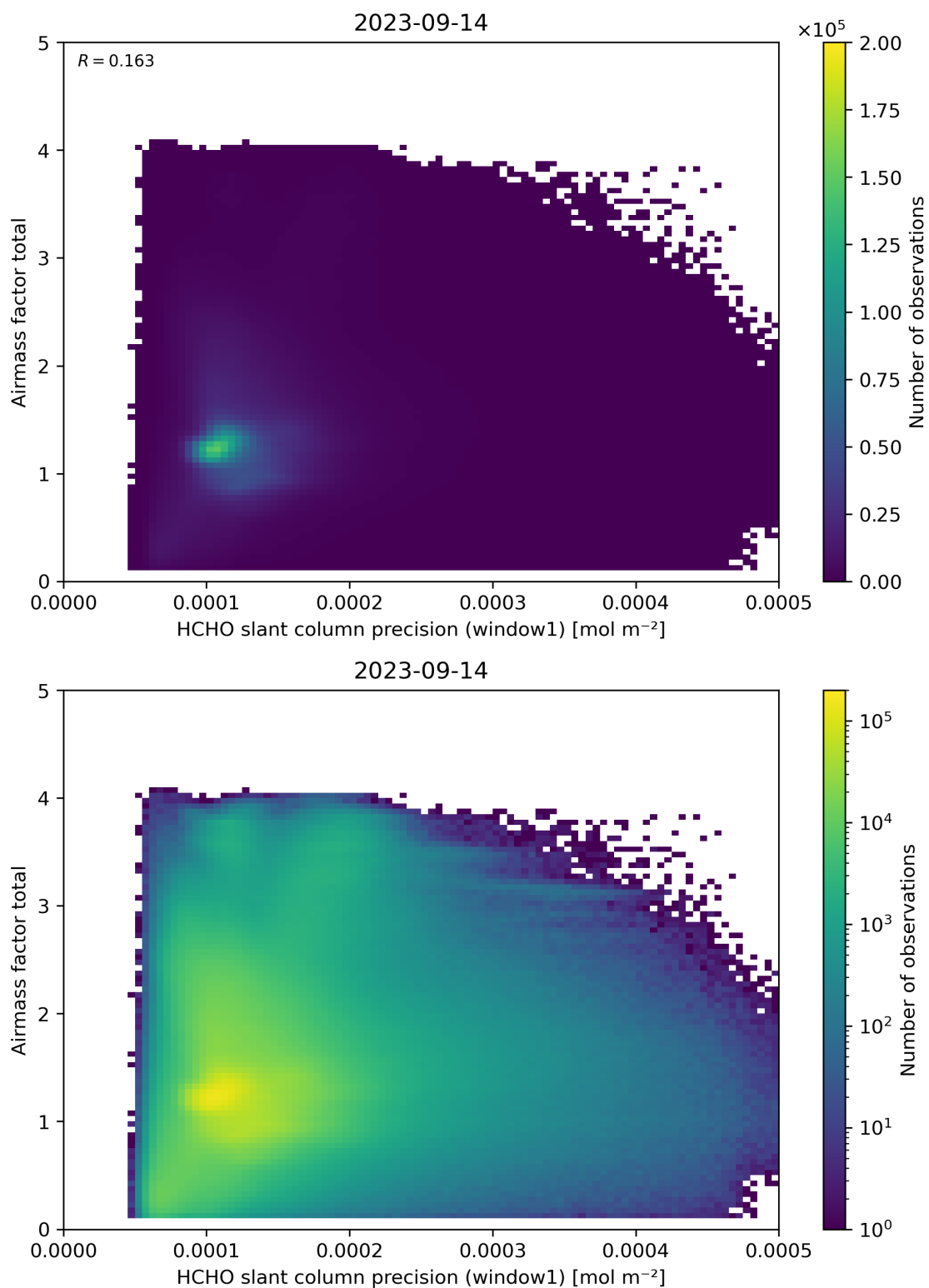
Figure 94: Scatter density plot of “HCHO slant column precision (window1)” against “Airmass factor total” for 2023-09-13 to 2023-09-15.
