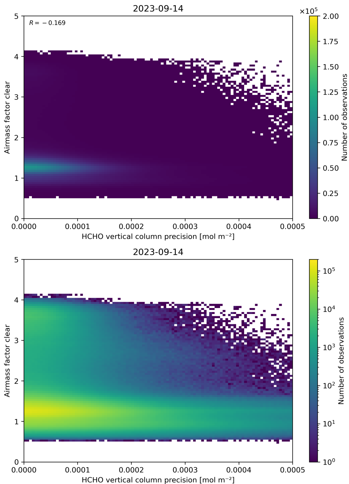
Figure 139: Scatter density plot of “HCHO vertical column precision” against “Airmass factor clear” for 2023-09-13 to 2023-09-15.
