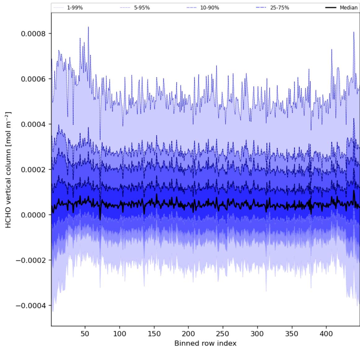
Figure 49: Along track statistics of “HCHO vertical column” for 2023-09-13 to 2023-09-15
