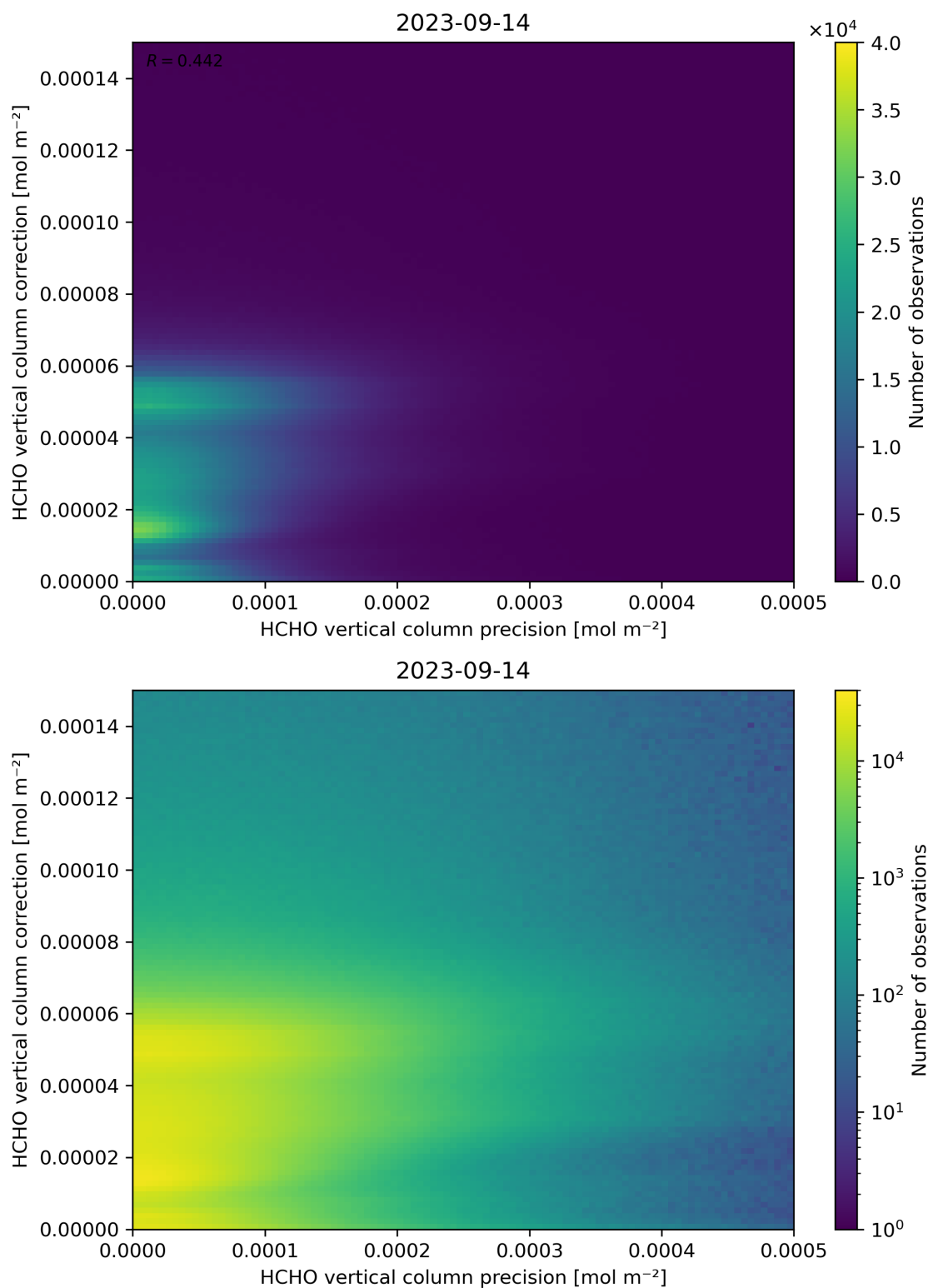
Figure 146: Scatter density plot of “HCHO vertical column precision” against “HCHO vertical column correction” for 2023-09-13 to 2023-09-15.
