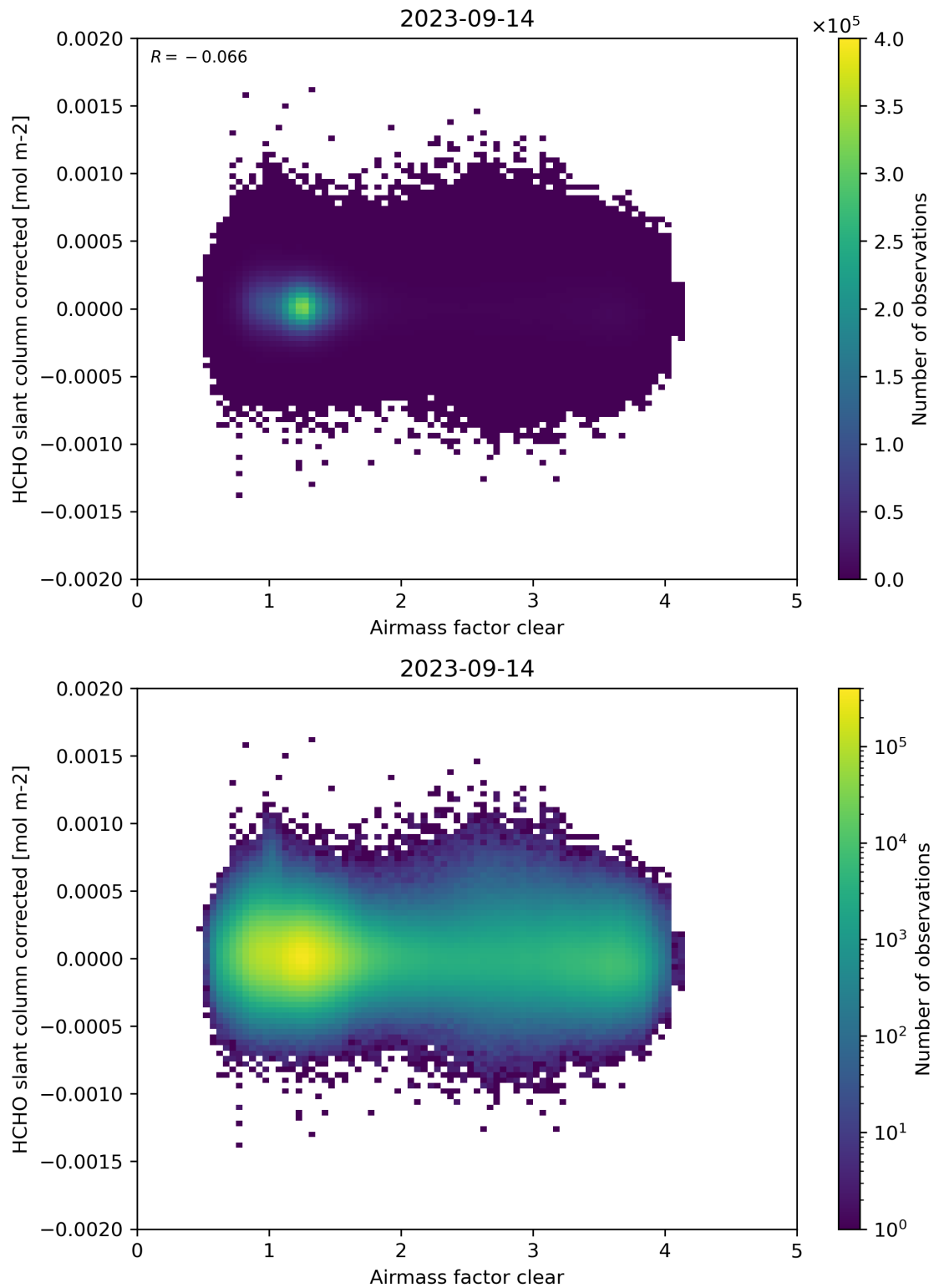
Figure 74: Scatter density plot of “Airmass factor clear” against “HCHO slant column corrected” for 2023-09-13 to 2023-09-15.
