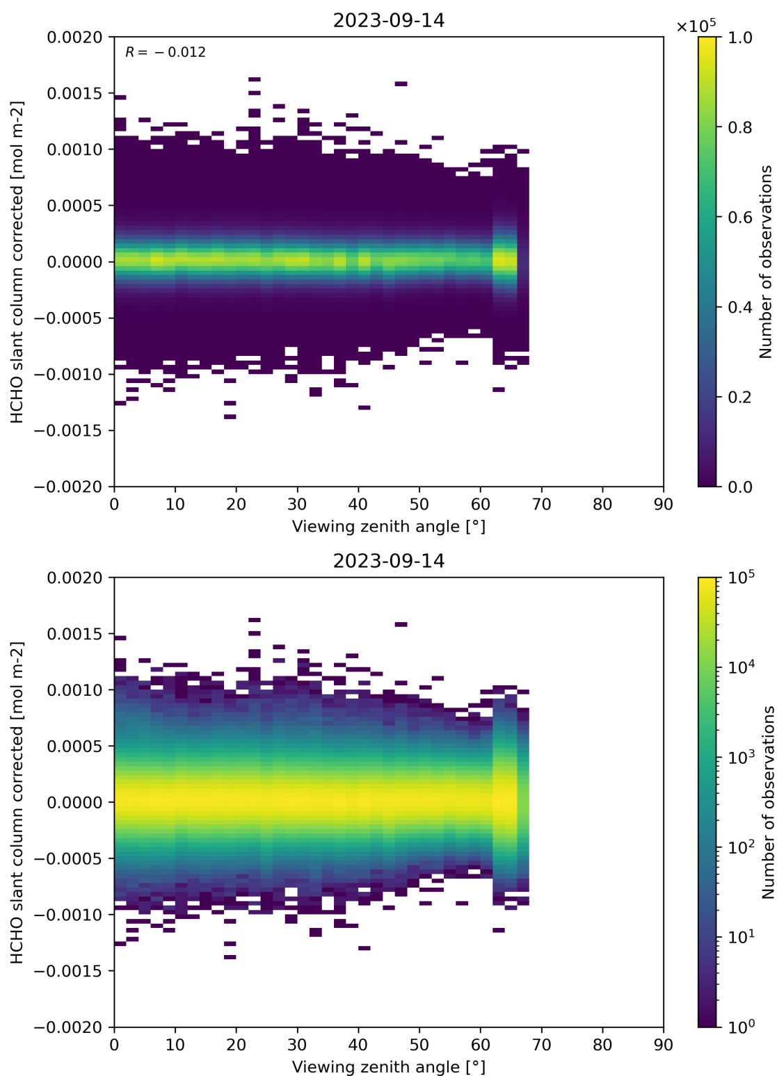
Figure 186: Scatter density plot of “Viewing zenith angle” against “HCHO slant column corrected” for 2023-09-13 to 2023-09-15.
