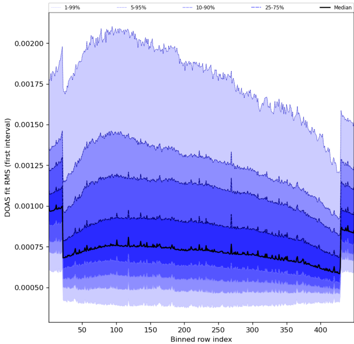
Figure 60: Along track statistics of “DOAS fit RMS (first interval)” for 2023-09-13 to 2023-09-15
