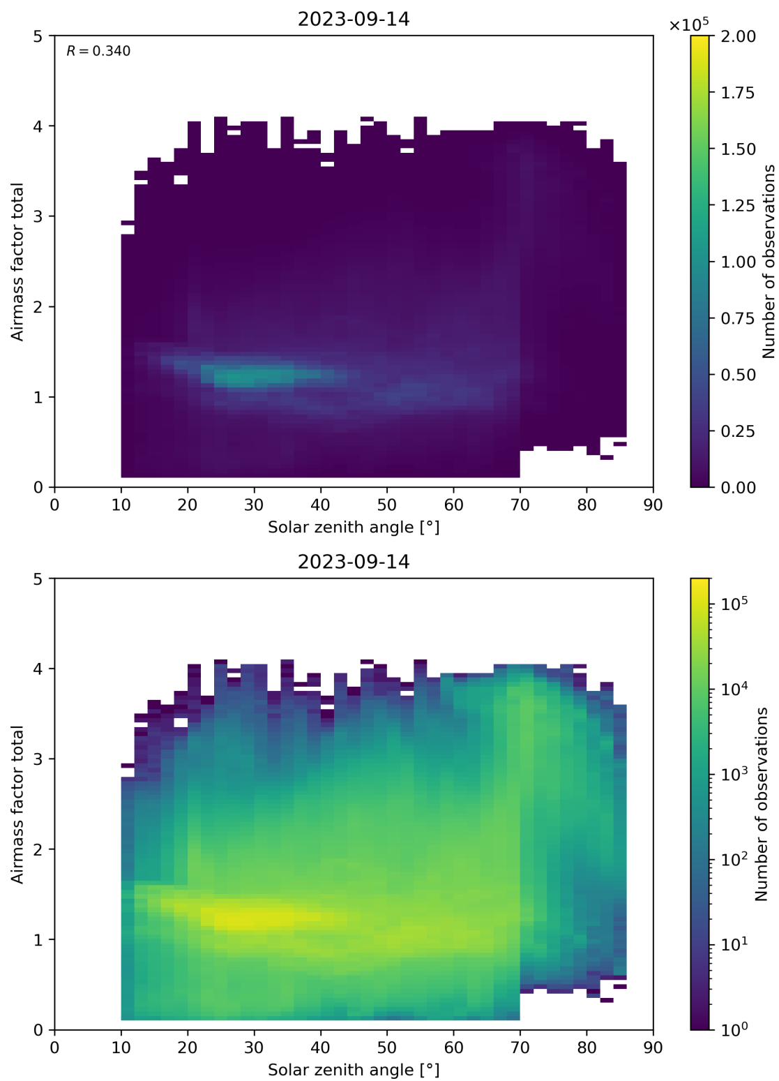
Figure 175: Scatter density plot of “Solar zenith angle” against “Airmass factor total” for 2023-09-13 to 2023-09-15.
