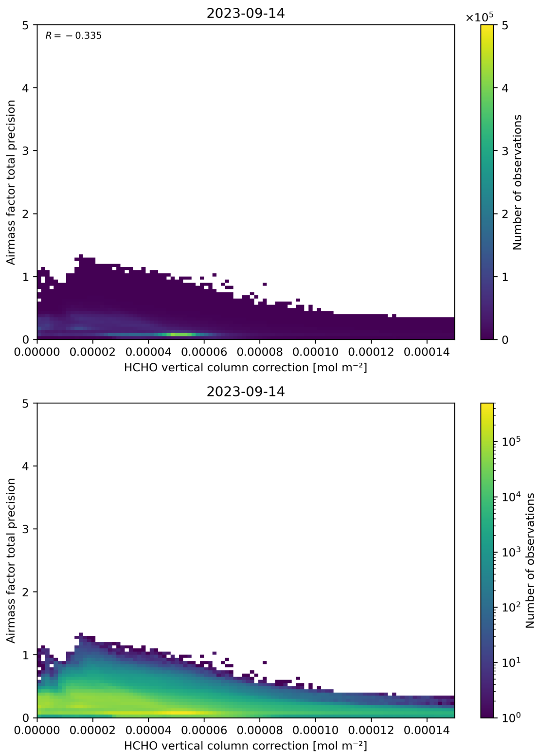
Figure 121: Scatter density plot of “HCHO vertical column correction” against “Airmass factor total precision” for 2023-09-13 to 2023-09-15.
