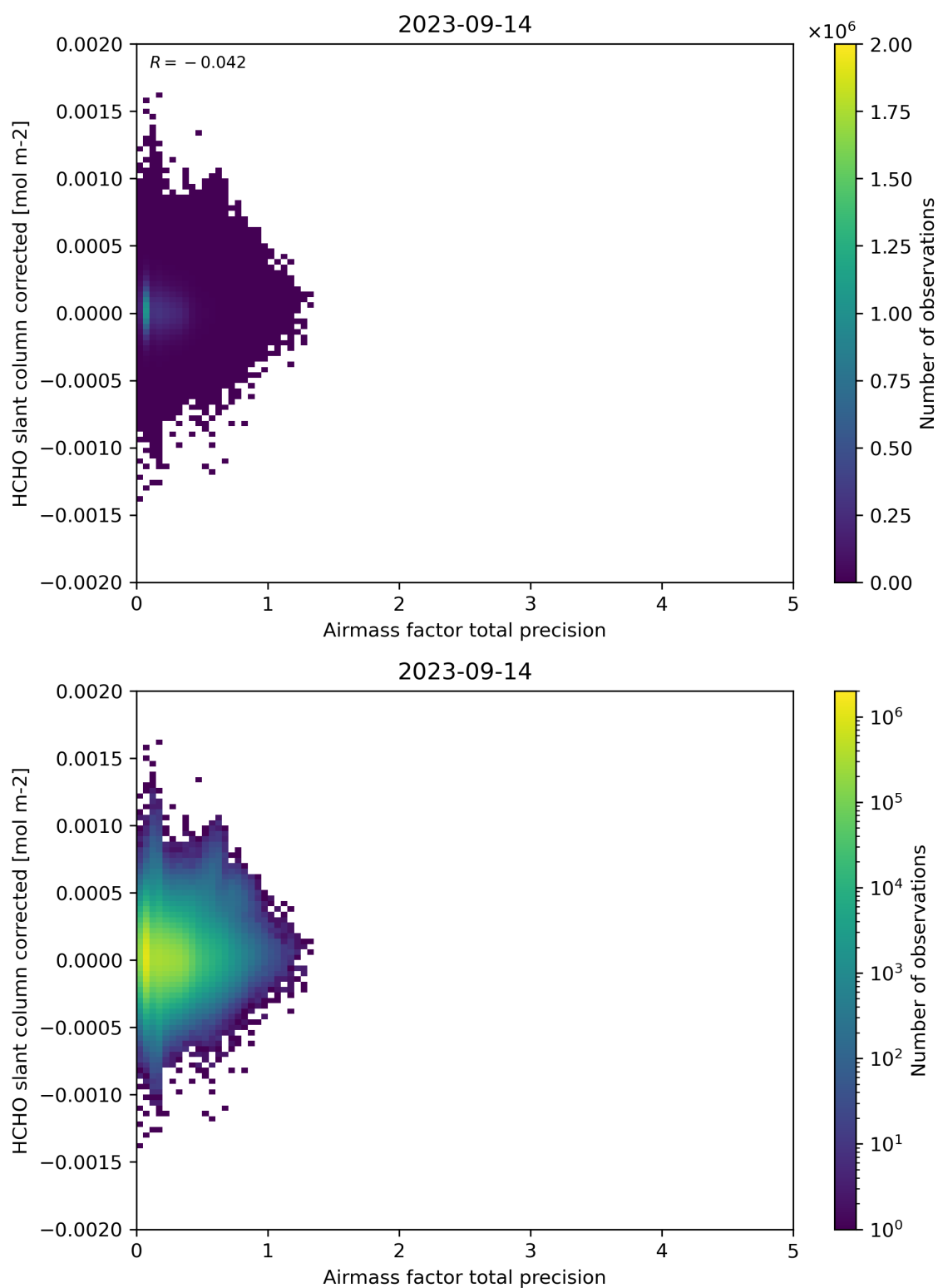
Figure 109: Scatter density plot of “Airmass factor total precision” against “HCHO slant column corrected” for 2023-09-13 to 2023-09-15.
