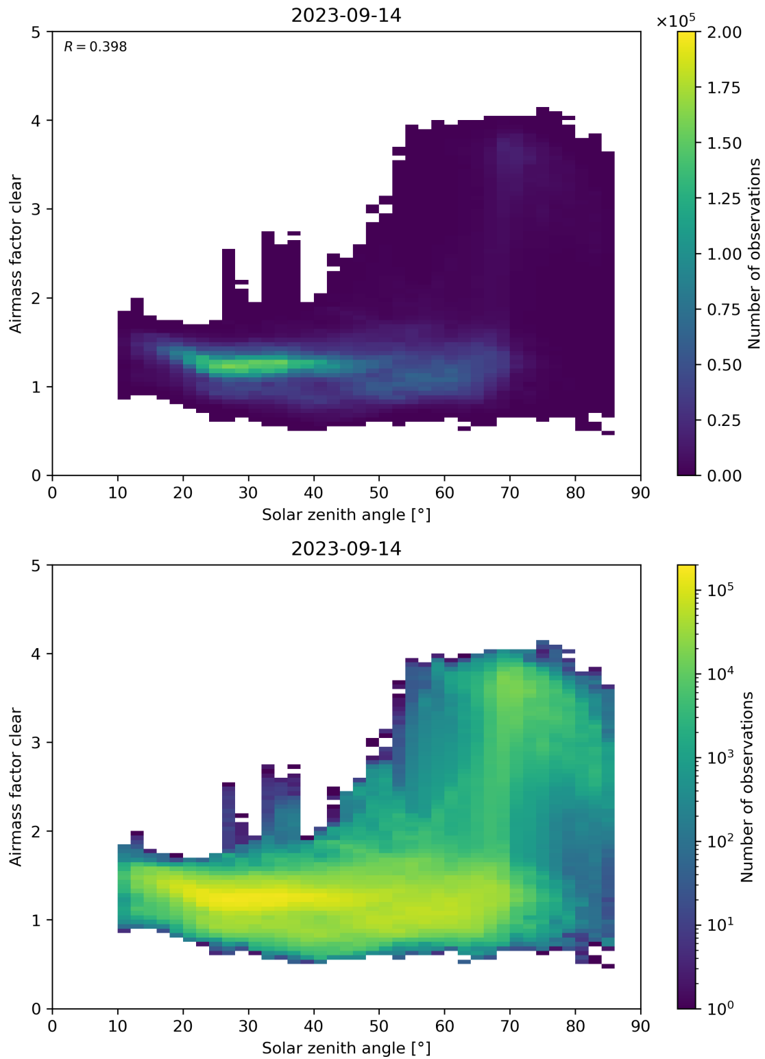
Figure 170: Scatter density plot of “Solar zenith angle” against “Airmass factor clear” for 2023-09-13 to 2023-09-15.
