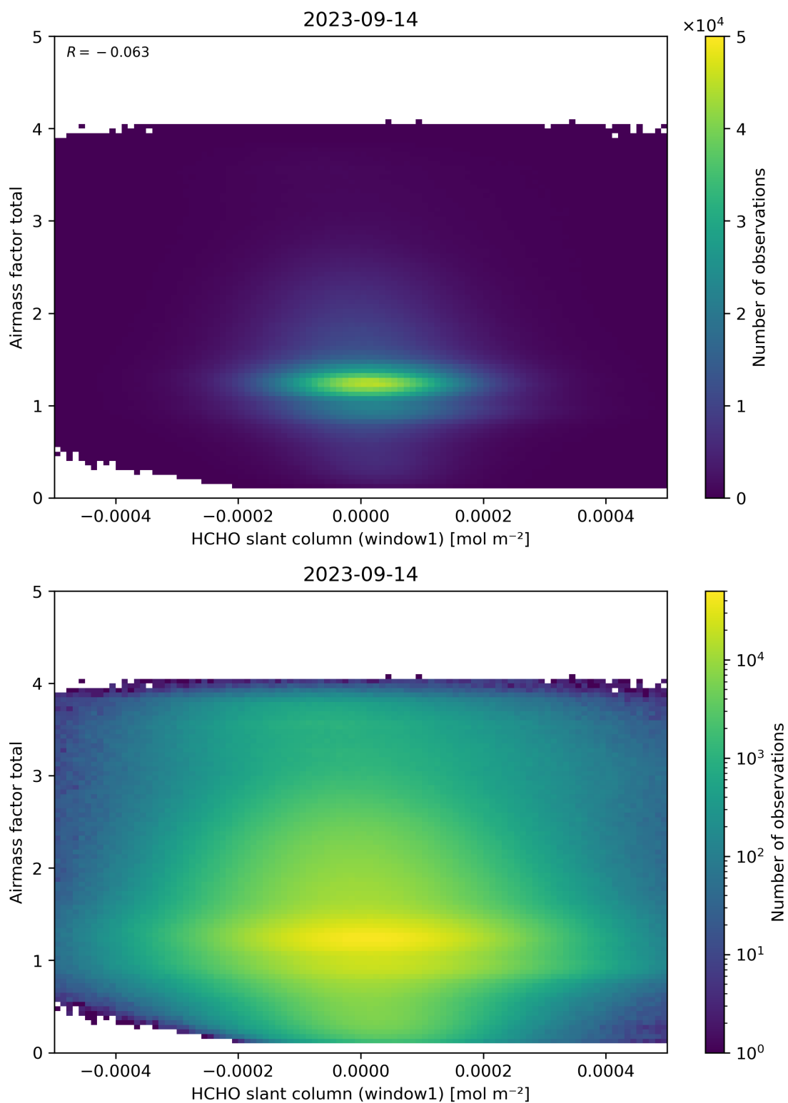
Figure 85: Scatter density plot of “HCHO slant column (window1)” against “Airmass factor total” for 2023-09-13 to 2023-09-15.
