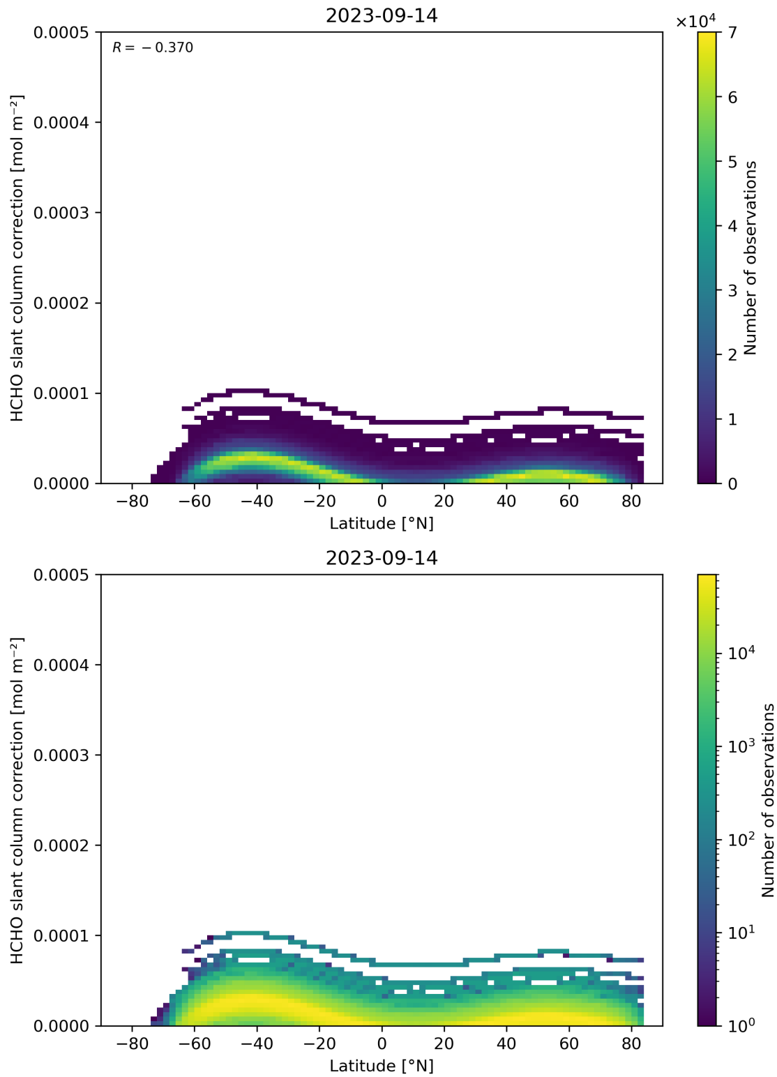
Figure 158: Scatter density plot of “Latitude” against “HCHO slant column correction” for 2023-09-13 to 2023-09-15.
