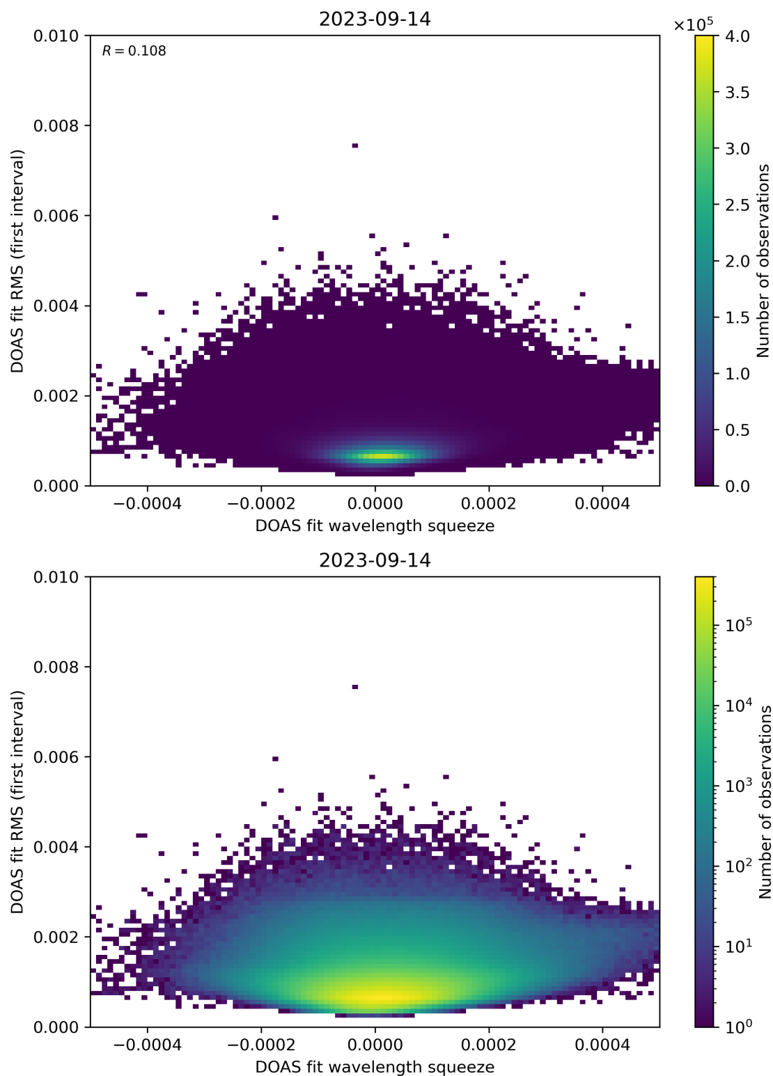
Figure 68: Scatter density plot of “DOAS fit wavelength squeeze” against “DOAS fit RMS (first interval)” for 2023-09-13 to 2023-09-15.
