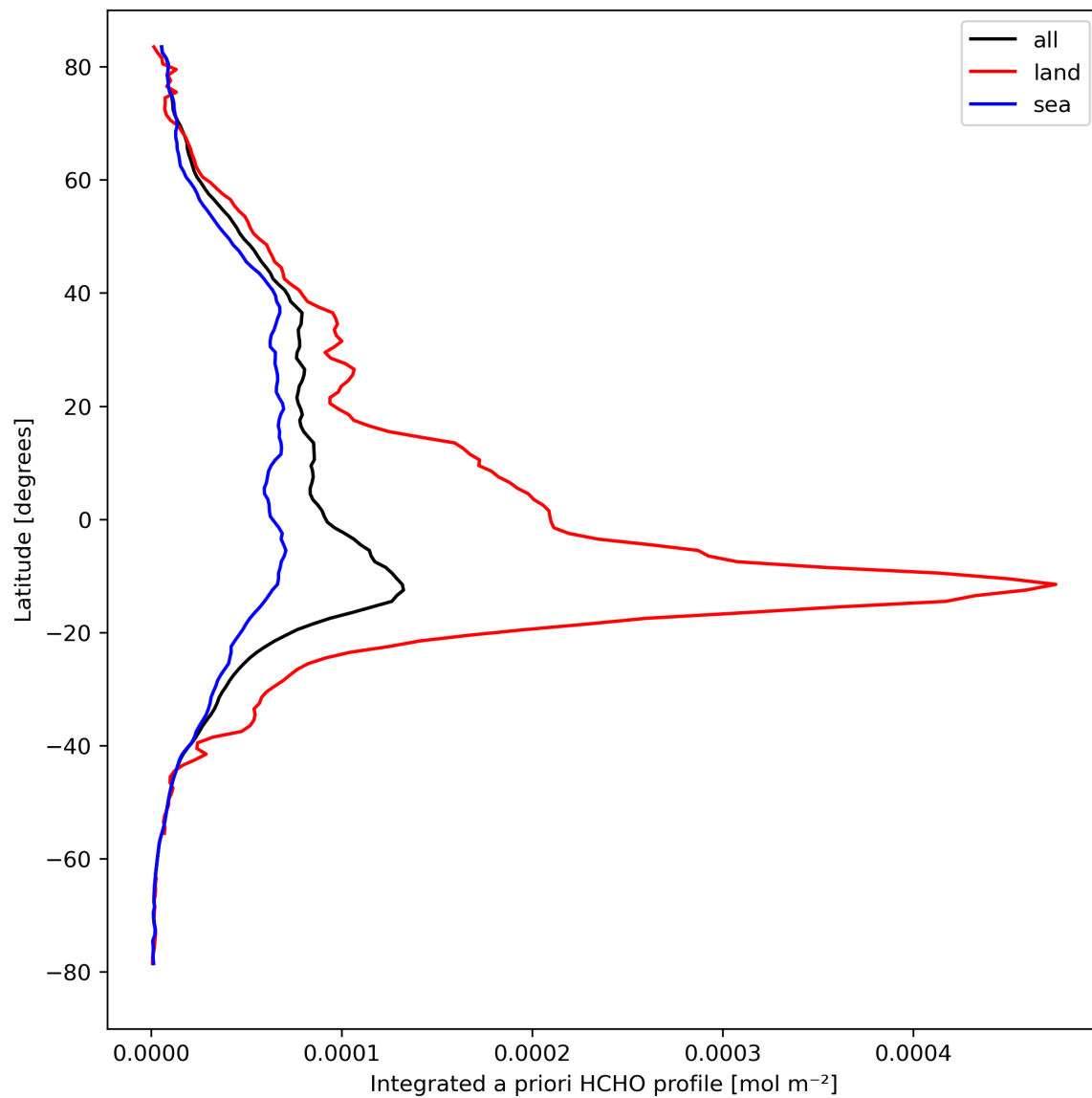
Figure 29: Zonal average of “Integrated a priori HCHO profile” for 2023-09-13 to 2023-09-15.
