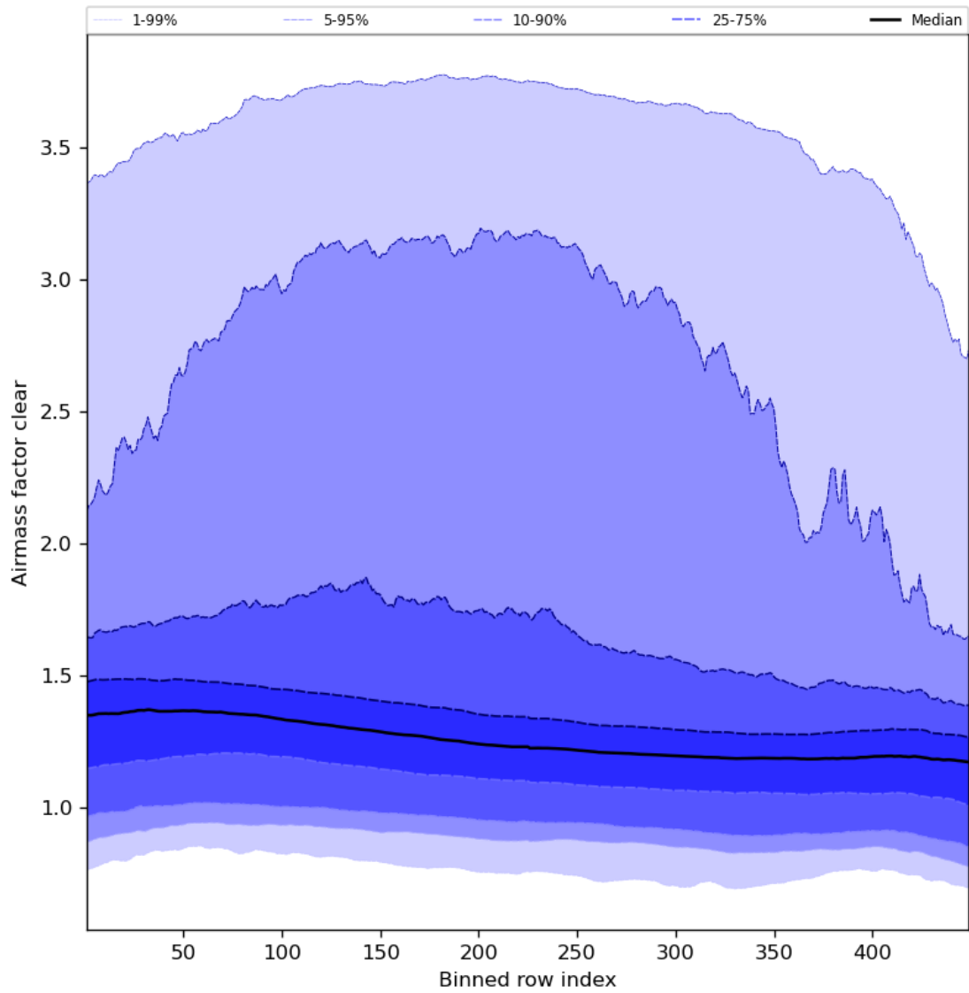
Figure 56: Along track statistics of “Airmass factor clear” for 2023-09-13 to 2023-09-15
