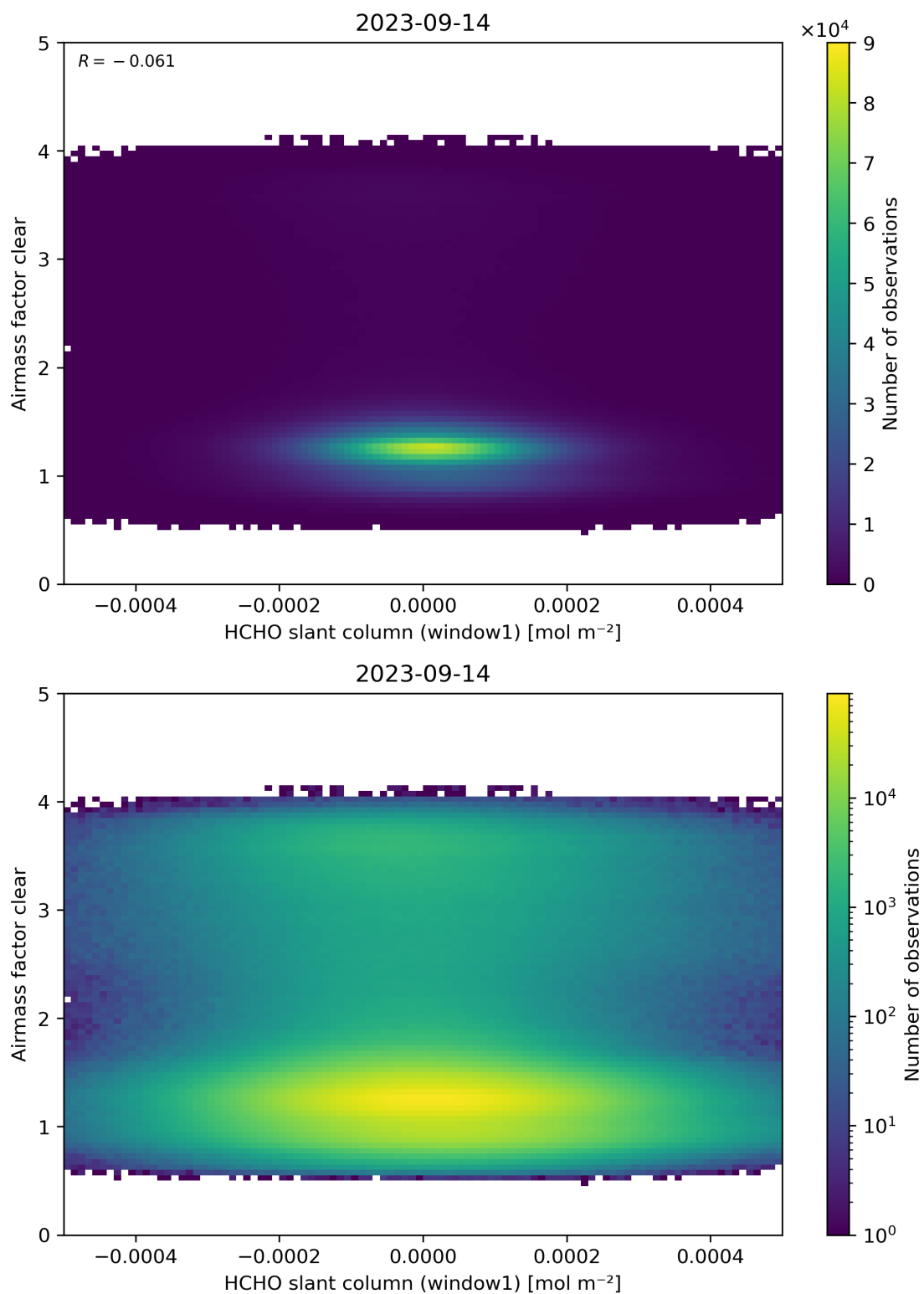
Figure 81: Scatter density plot of “HCHO slant column (window1)” against “Airmass factor clear” for 2023-09-13 to 2023-09-15.
