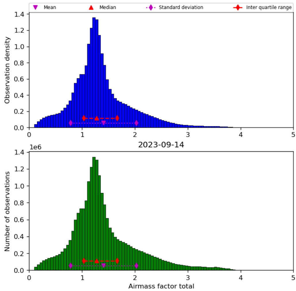
Figure 40: Histogram of “Airmass factor total” for 2023-09-13 to 2023-09-15
