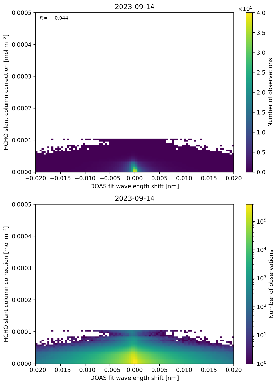
Figure 67: Scatter density plot of “DOAS fit wavelength shift” against “HCHO slant column correction” for 2023-09-13 to 2023-09-15.
