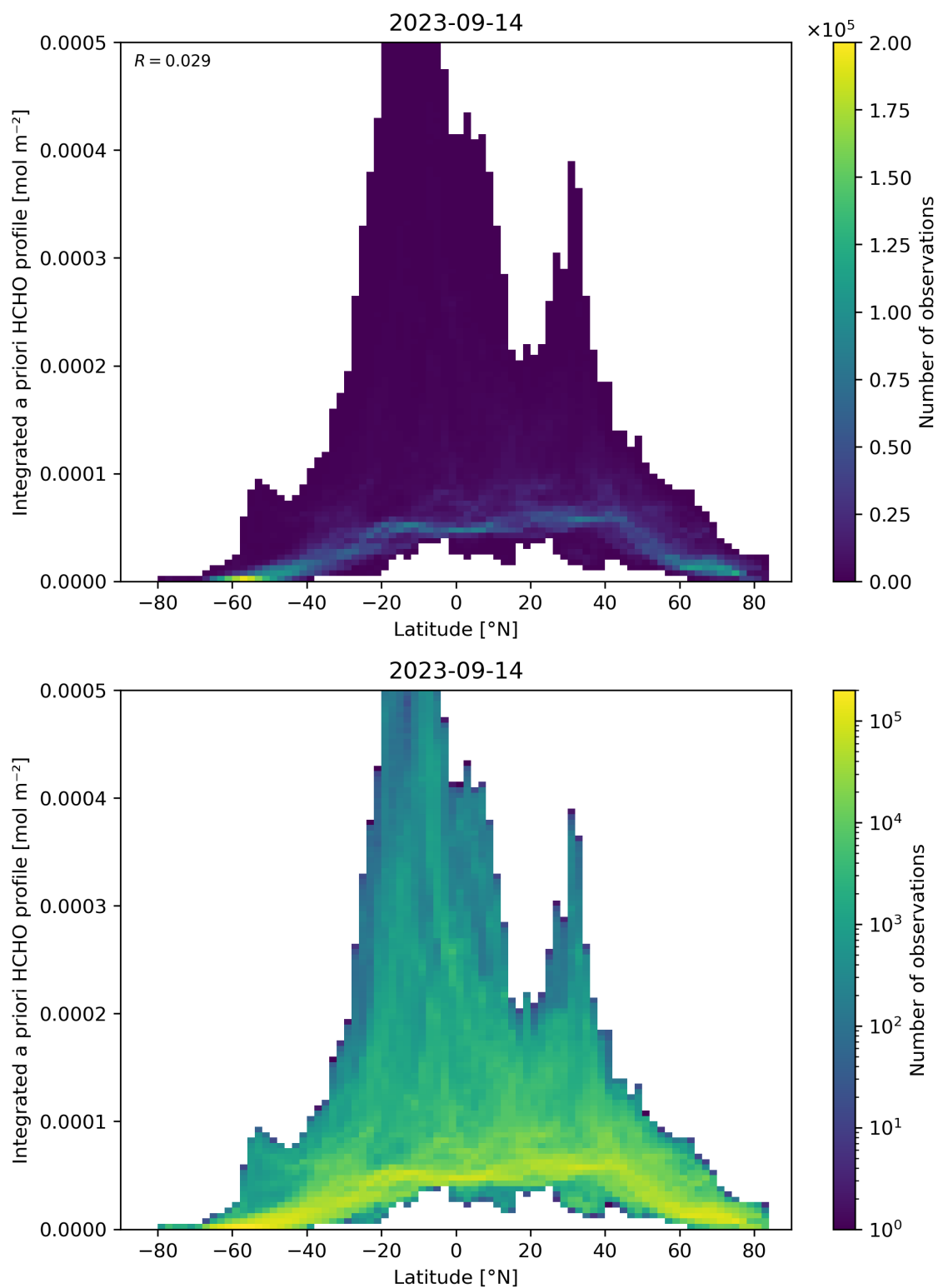
Figure 166: Scatter density plot of “Latitude” against “Integrated a priori HCHO profile” for 2023-09-13 to 2023-09-15.
