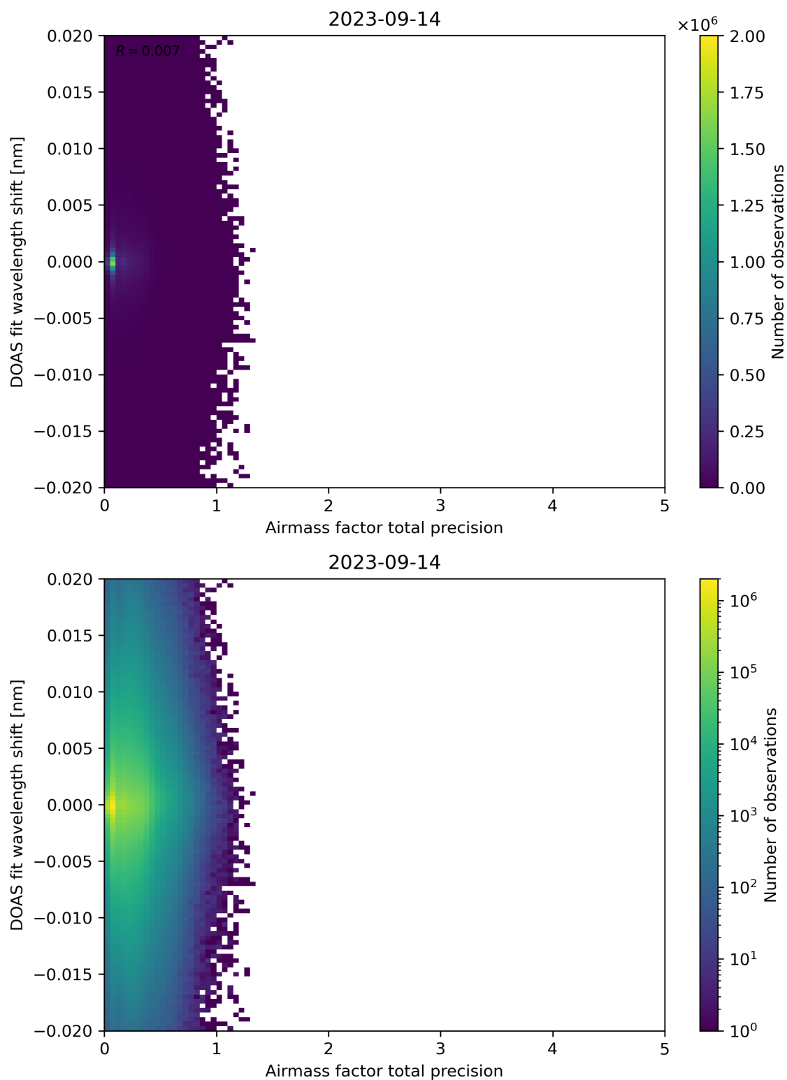
Figure 106: Scatter density plot of “Airmass factor total precision” against “DOAS fit wavelength shift” for 2023-09-13 to 2023-09-15.
