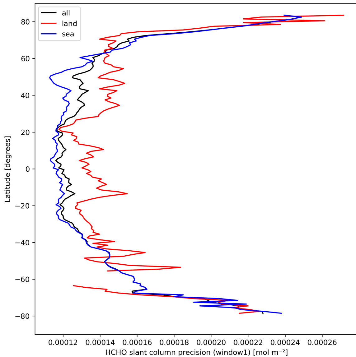
Figure 25: Zonal average of “HCHO slant column precision (window1)” for 2023-09-13 to 2023-09-15.
