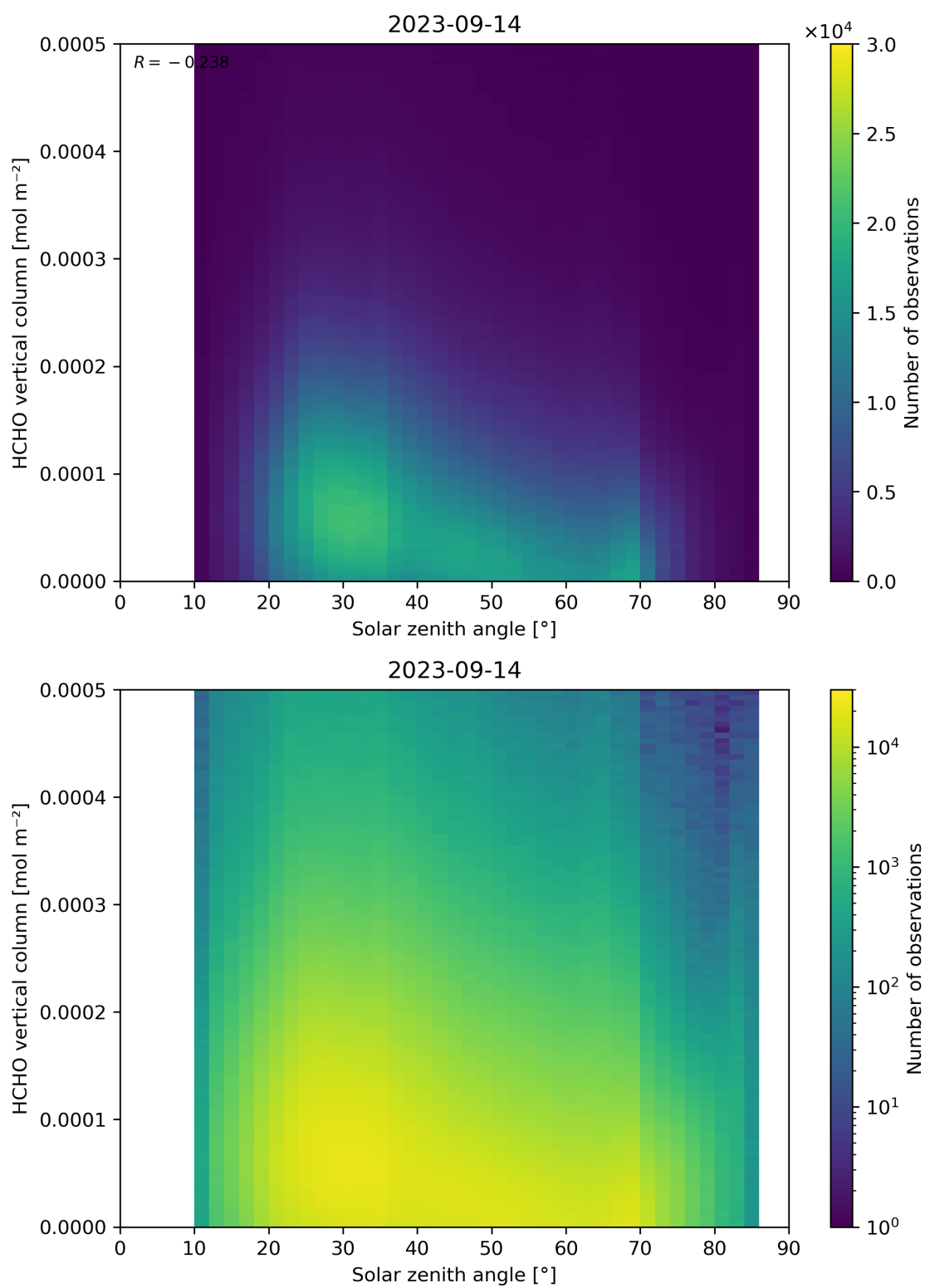
Figure 177: Scatter density plot of “Solar zenith angle” against “HCHO vertical column” for 2023-09-13 to 2023-09-15.
