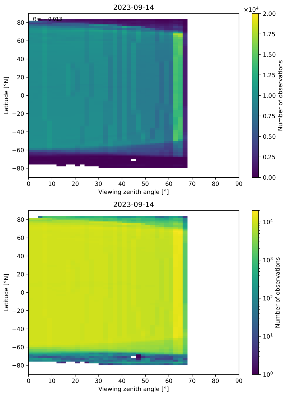
Figure 196: Scatter density plot of “Viewing zenith angle” against “Latitude” for 2023-09-13 to 2023-09-15.
