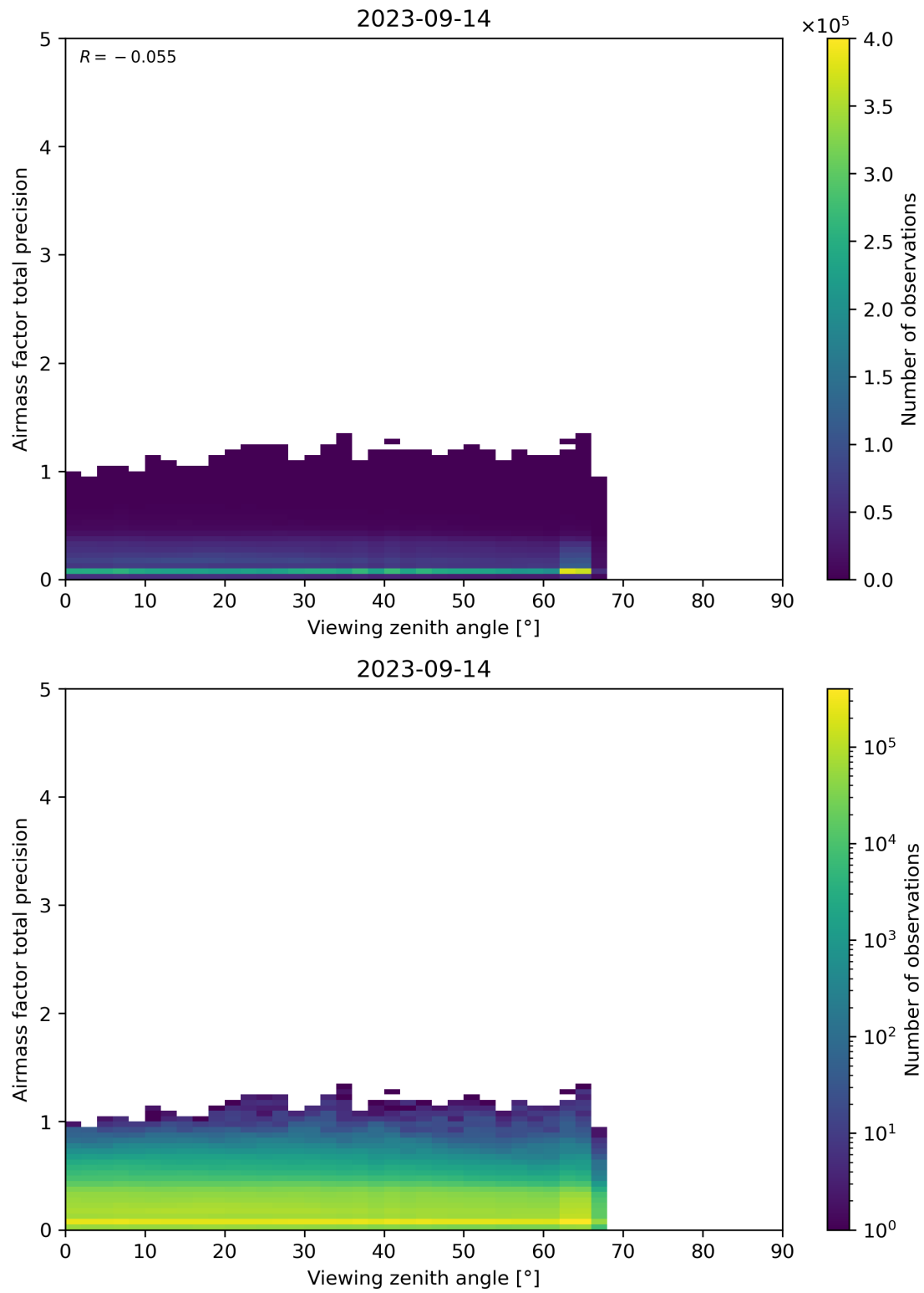
Figure 191: Scatter density plot of “Viewing zenith angle” against “Airmass factor total precision” for 2023-09-13 to 2023-09-15.
