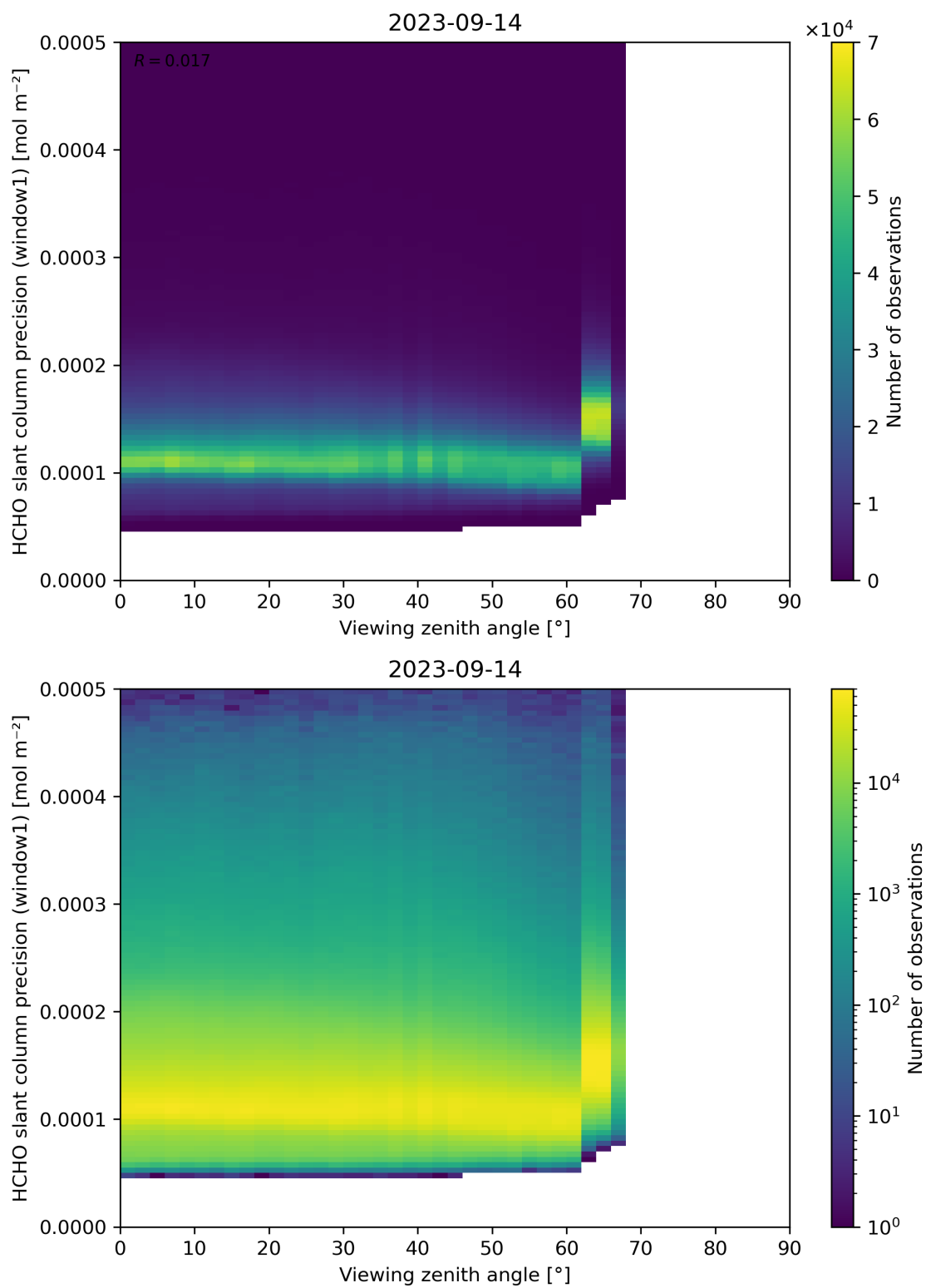
Figure 189: Scatter density plot of “Viewing zenith angle” against “HCHO slant column precision (window1)” for 2023-09-13 to 2023-09-15.
