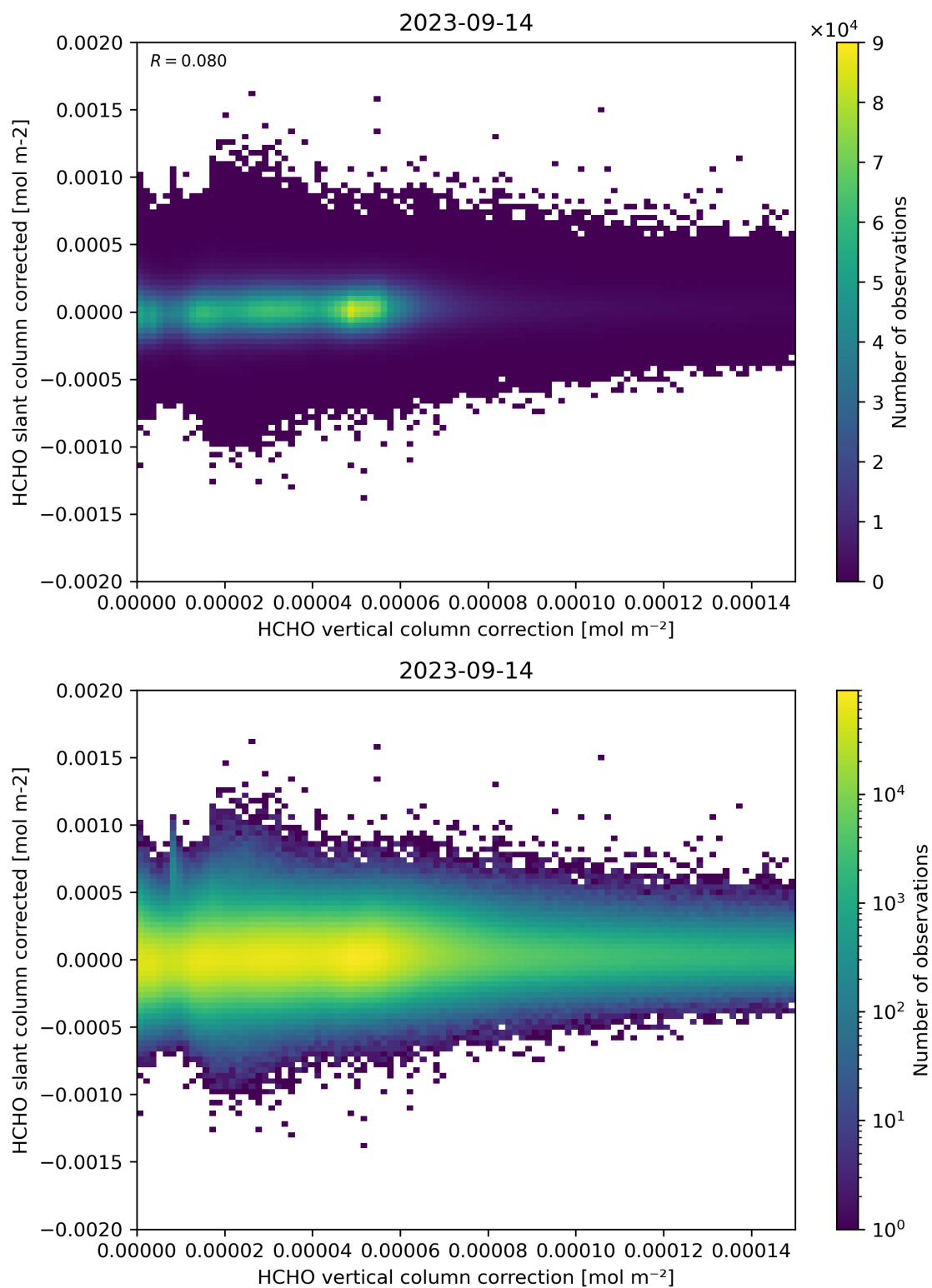
Figure 116: Scatter density plot of “HCHO vertical column correction” against “HCHO slant column corrected” for 2023-09-13 to 2023-09-15.
