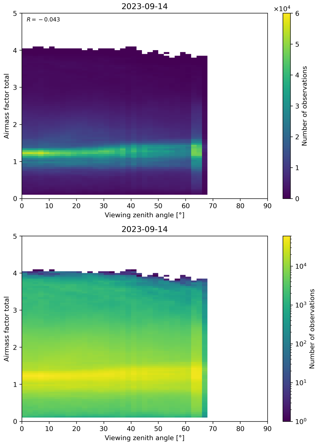
Figure 190: Scatter density plot of “Viewing zenith angle” against “Airmass factor total” for 2023-09-13 to 2023-09-15.
