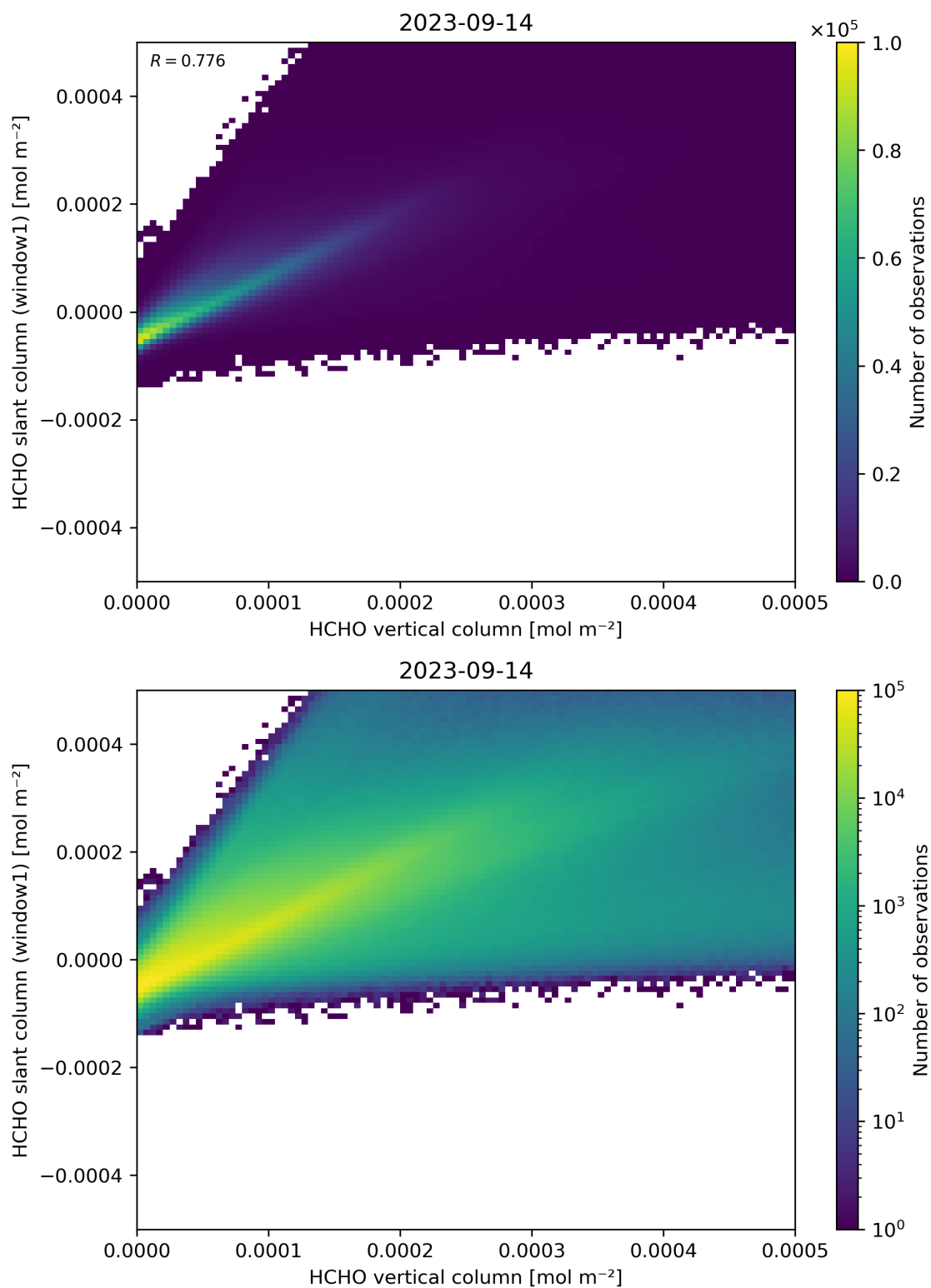
Figure 129: Scatter density plot of “HCHO vertical column” against “HCHO slant column (window1)” for 2023-09-13 to 2023-09-15.
