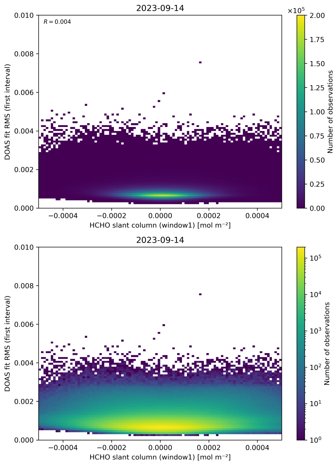
Figure 78: Scatter density plot of “HCHO slant column (window1)” against “DOAS fit RMS (first interval)” for 2023-09-13 to 2023-09-15.
