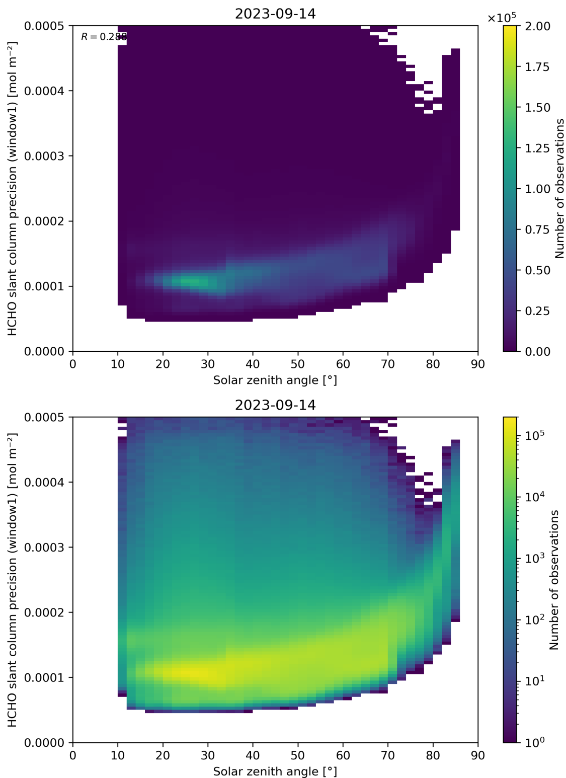
Figure 174: Scatter density plot of “Solar zenith angle” against “HCHO slant column precision (window1)” for 2023-09-13 to 2023-09-15.
