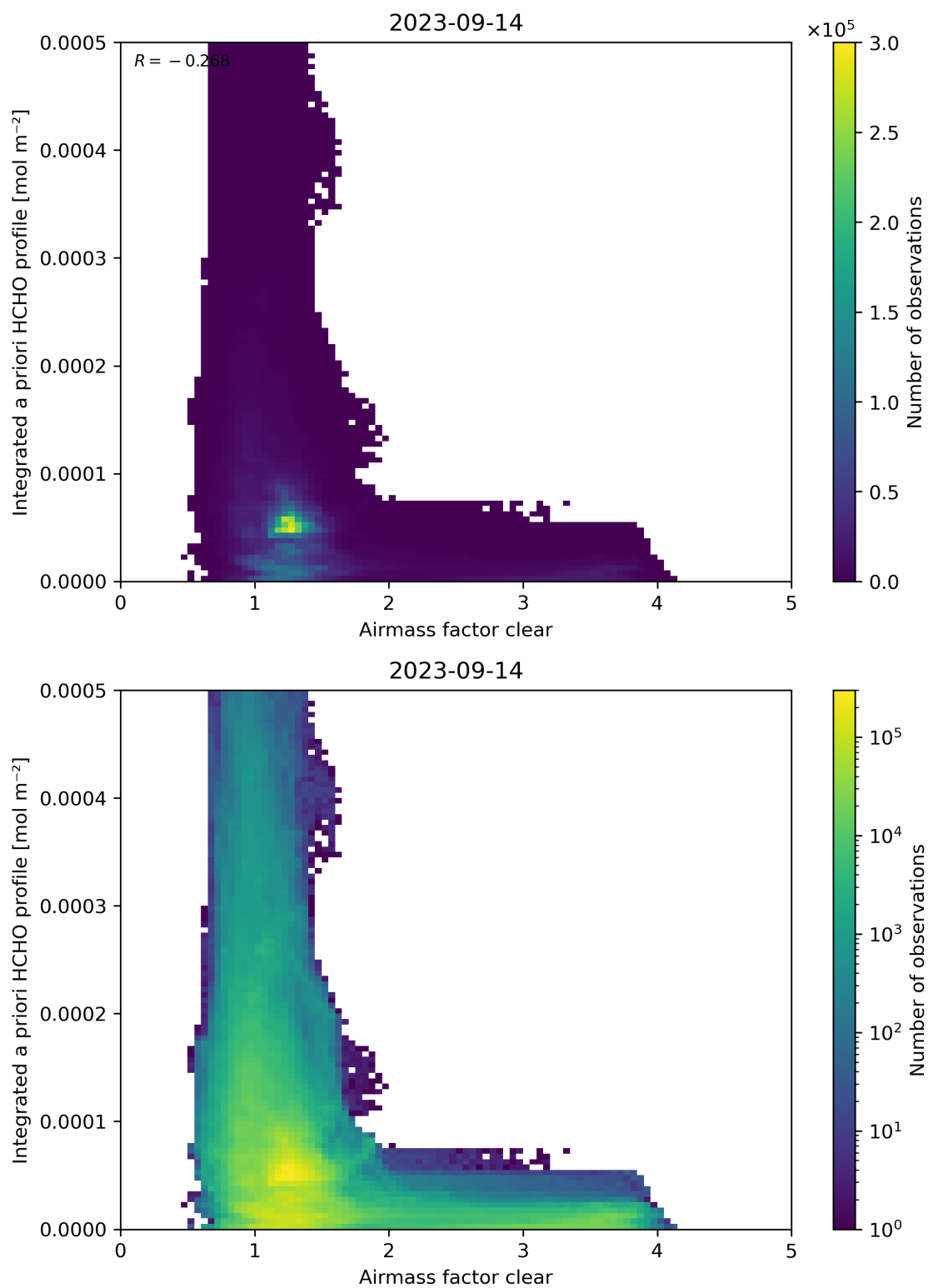
Figure 76: Scatter density plot of “Airmass factor clear” against “Integrated a priori HCHO profile” for 2023-09-13 to 2023-09-15.
