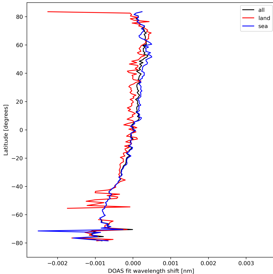
Figure 30: Zonal average of “DOAS fit wavelength shift” for 2023-09-13 to 2023-09-15.
