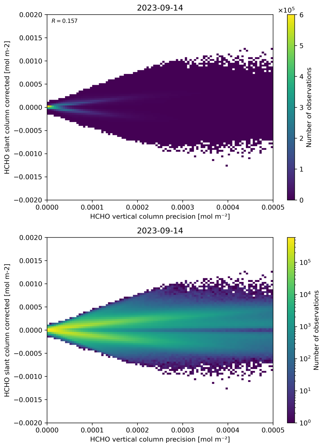
Figure 140: Scatter density plot of “HCHO vertical column precision” against “HCHO slant column corrected” for 2023-09-13 to 2023-09-15.
