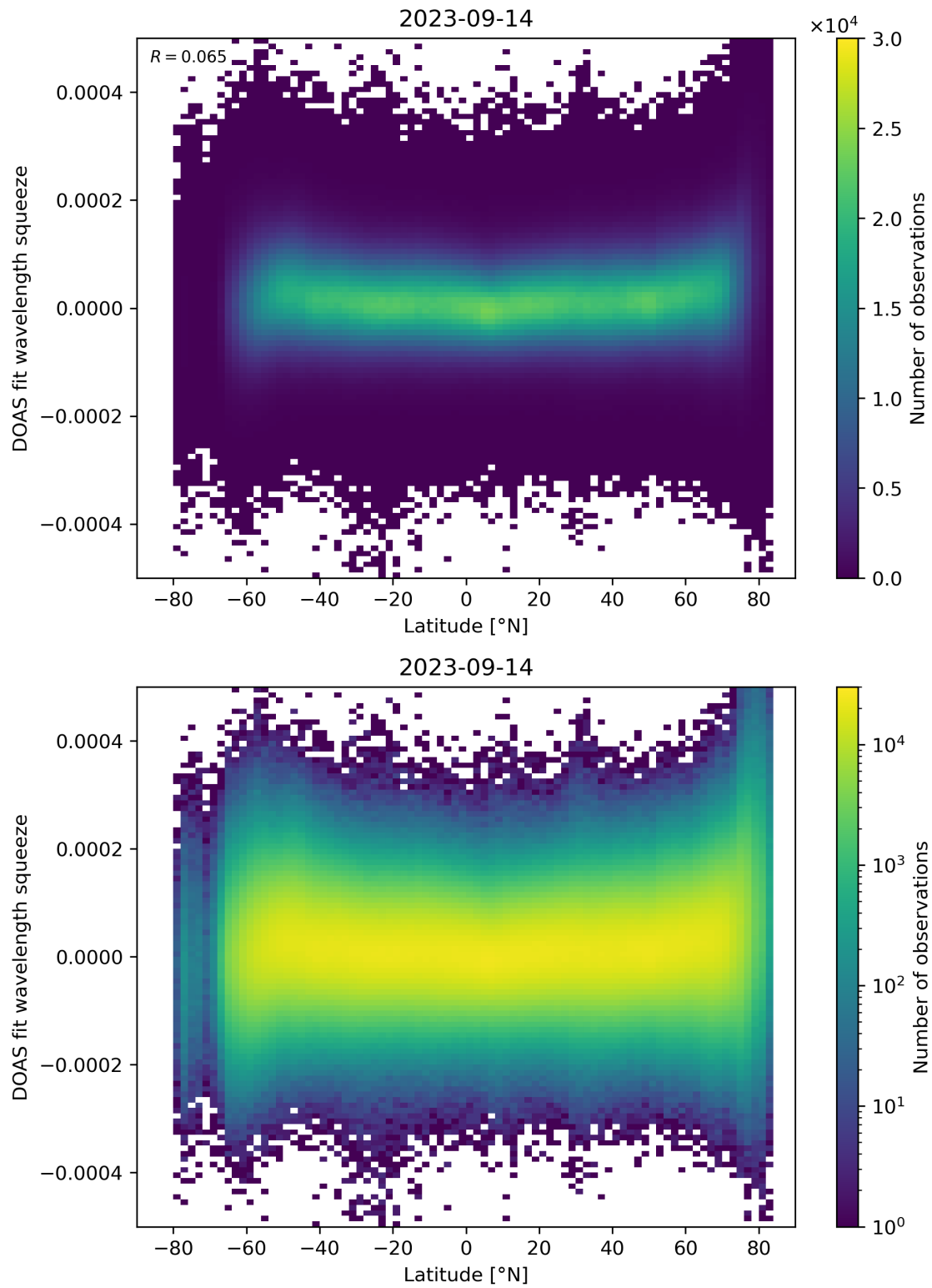
Figure 155: Scatter density plot of “Latitude” against “DOAS fit wavelength squeeze” for 2023-09-13 to 2023-09-15.
