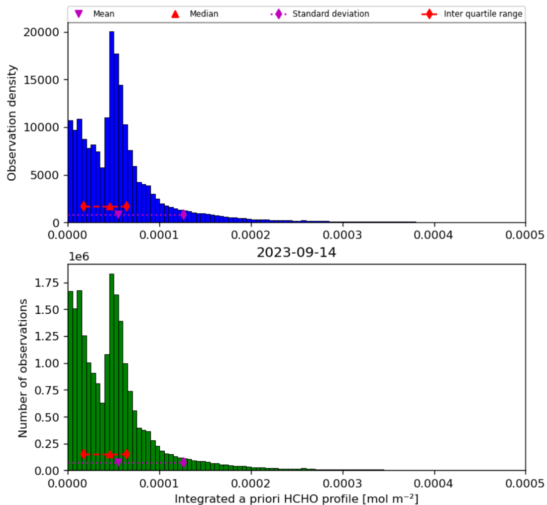
Figure 43: Histogram of “Integrated a priori HCHO profile” for 2023-09-13 to 2023-09-15
