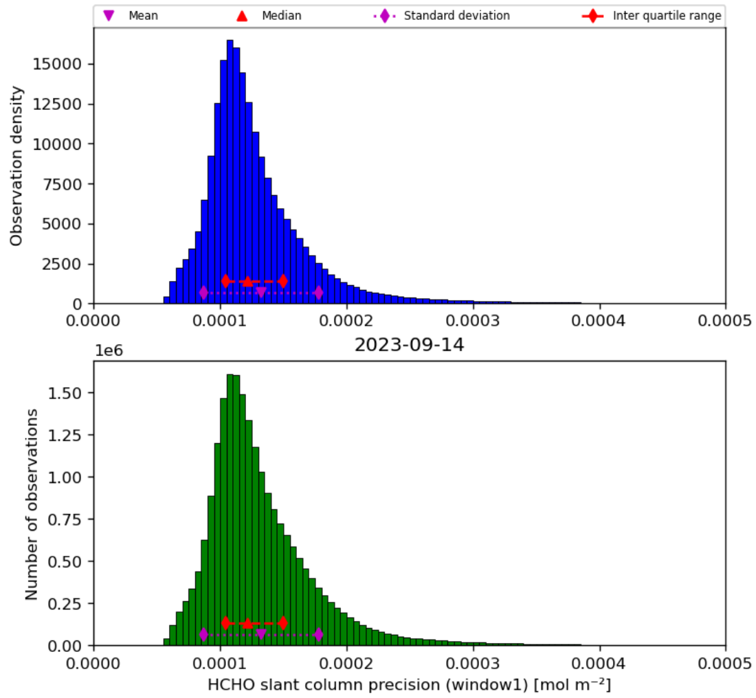
Figure 39: Histogram of “HCHO slant column precision (window1)” for 2023-09-13 to 2023-09-15
