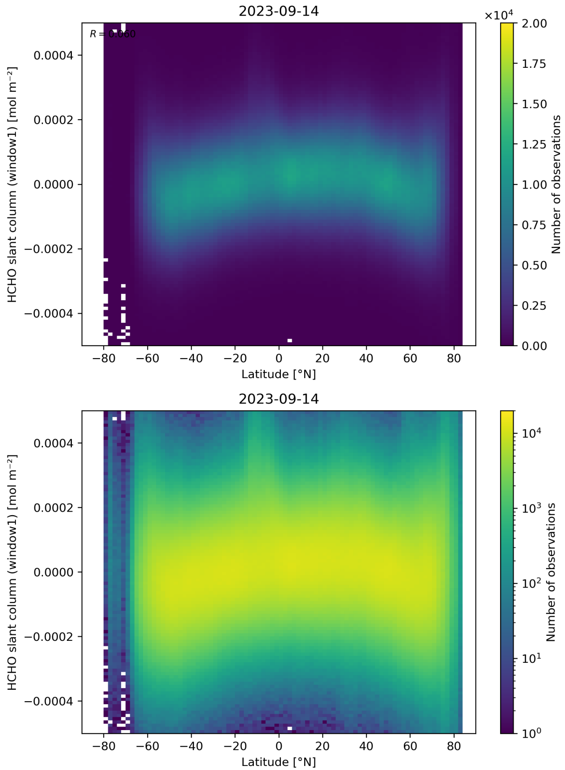
Figure 159: Scatter density plot of “Latitude” against “HCHO slant column (window1)” for 2023-09-13 to 2023-09-15.
