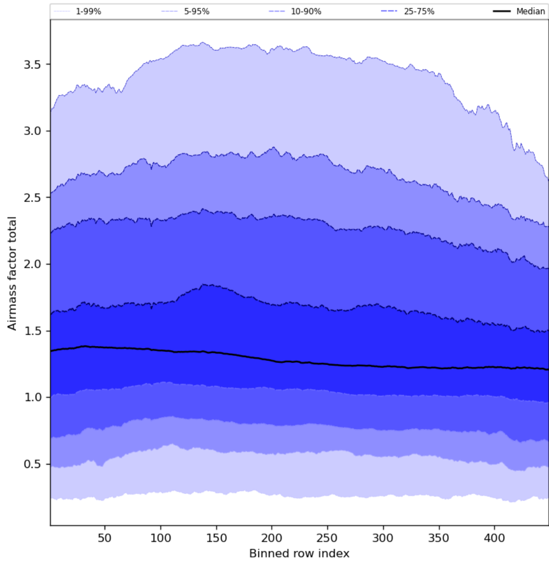
Figure 54: Along track statistics of “Airmass factor total” for 2023-09-13 to 2023-09-15
