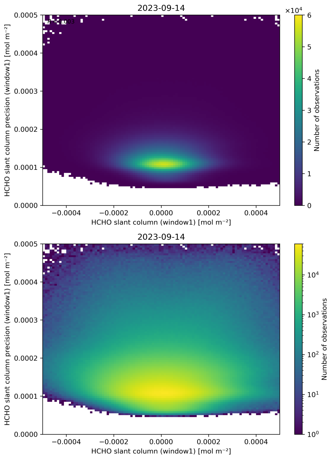
Figure 84: Scatter density plot of “HCHO slant column (window1)” against “HCHO slant column precision (window1)” for 2023-09-13 to 2023-09-15.
