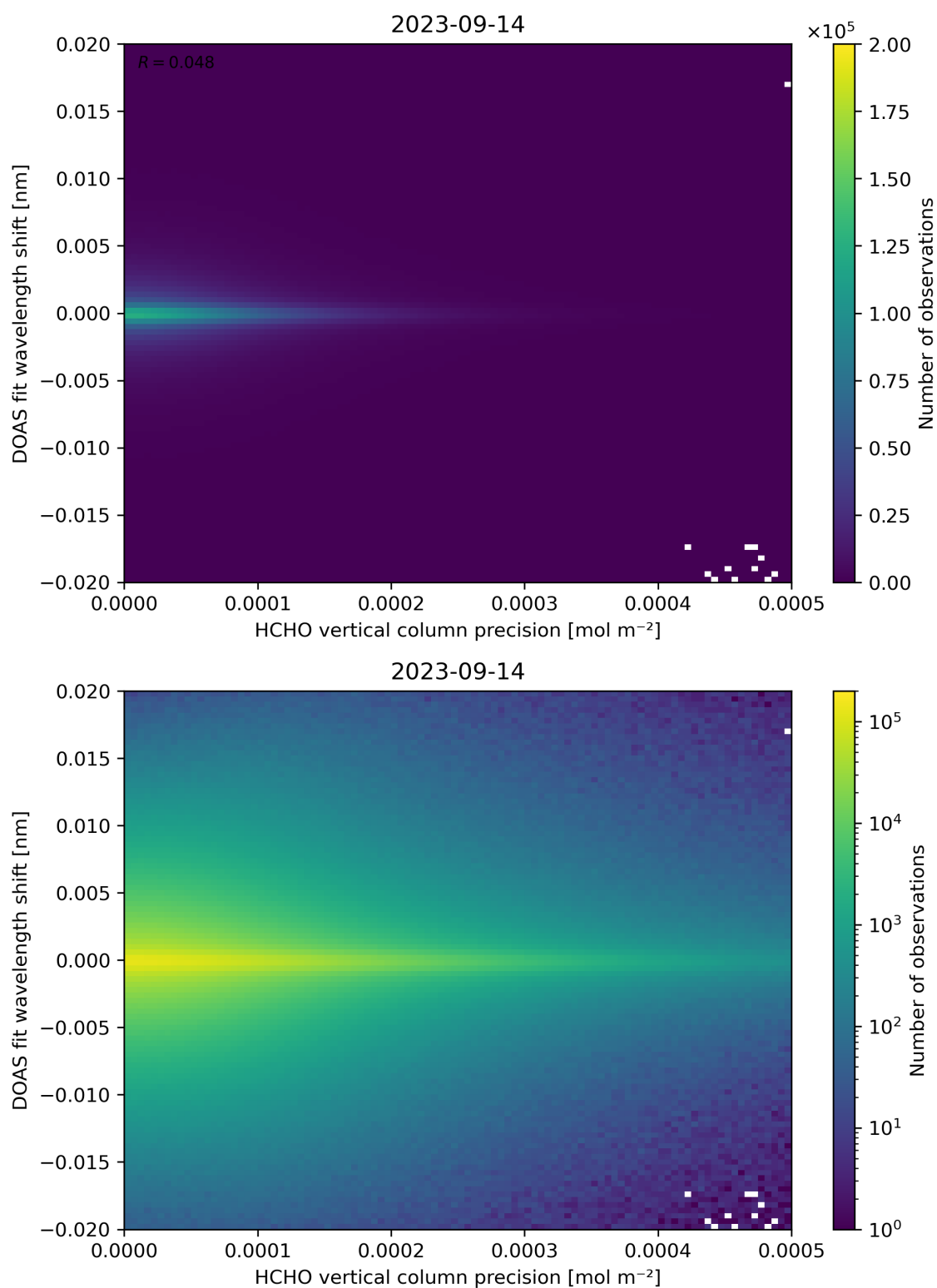
Figure 137: Scatter density plot of “HCHO vertical column precision” against “DOAS fit wavelength shift” for 2023-09-13 to 2023-09-15.
