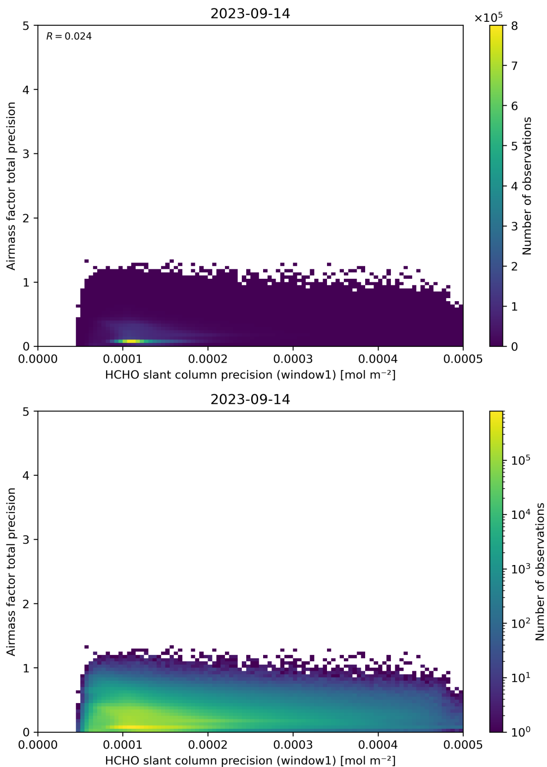
Figure 95: Scatter density plot of “HCHO slant column precision (window1)” against “Airmass factor total precision” for 2023-09-13 to 2023-09-15.
