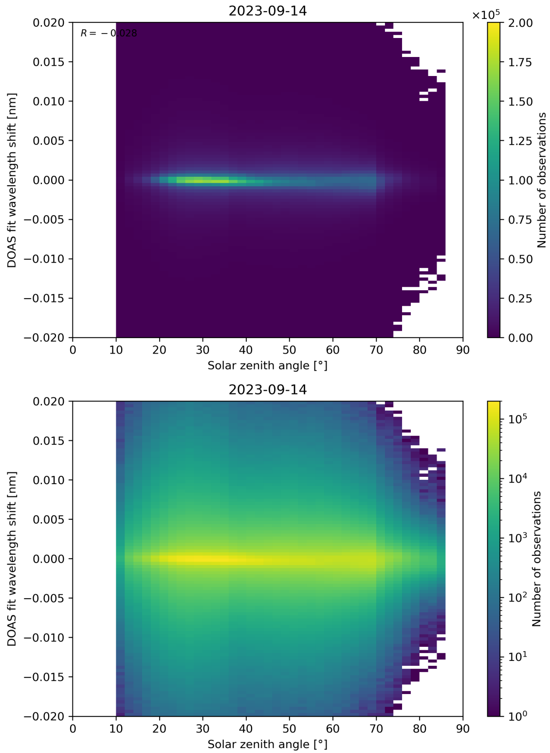
Figure 168: Scatter density plot of “Solar zenith angle” against “DOAS fit wavelength shift” for 2023-09-13 to 2023-09-15.
