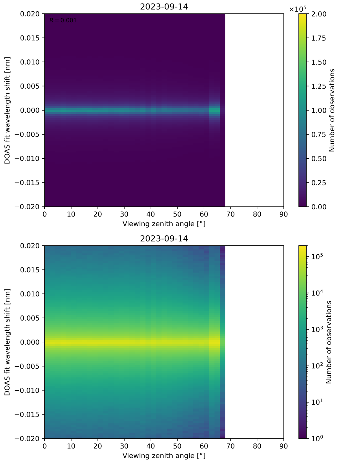
Figure 183: Scatter density plot of “Viewing zenith angle” against “DOAS fit wavelength shift” for 2023-09-13 to 2023-09-15.
