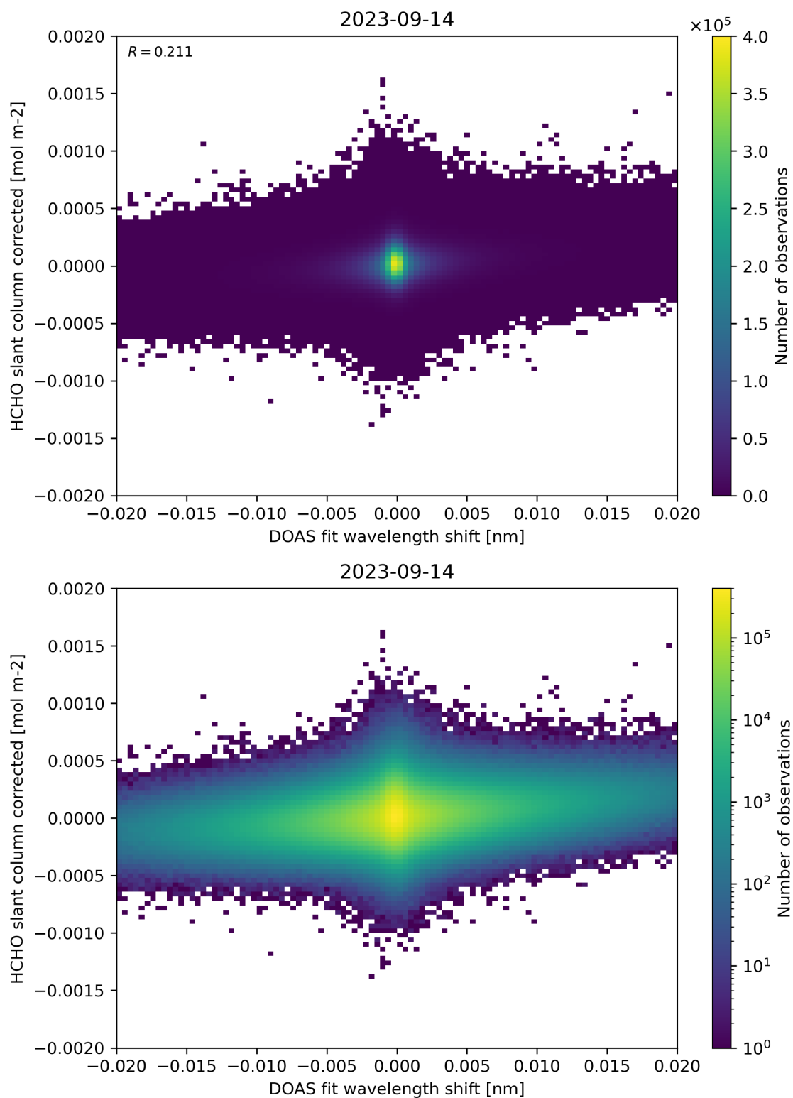
Figure 66: Scatter density plot of “DOAS fit wavelength shift” against “HCHO slant column corrected” for 2023-09-13 to 2023-09-15.
