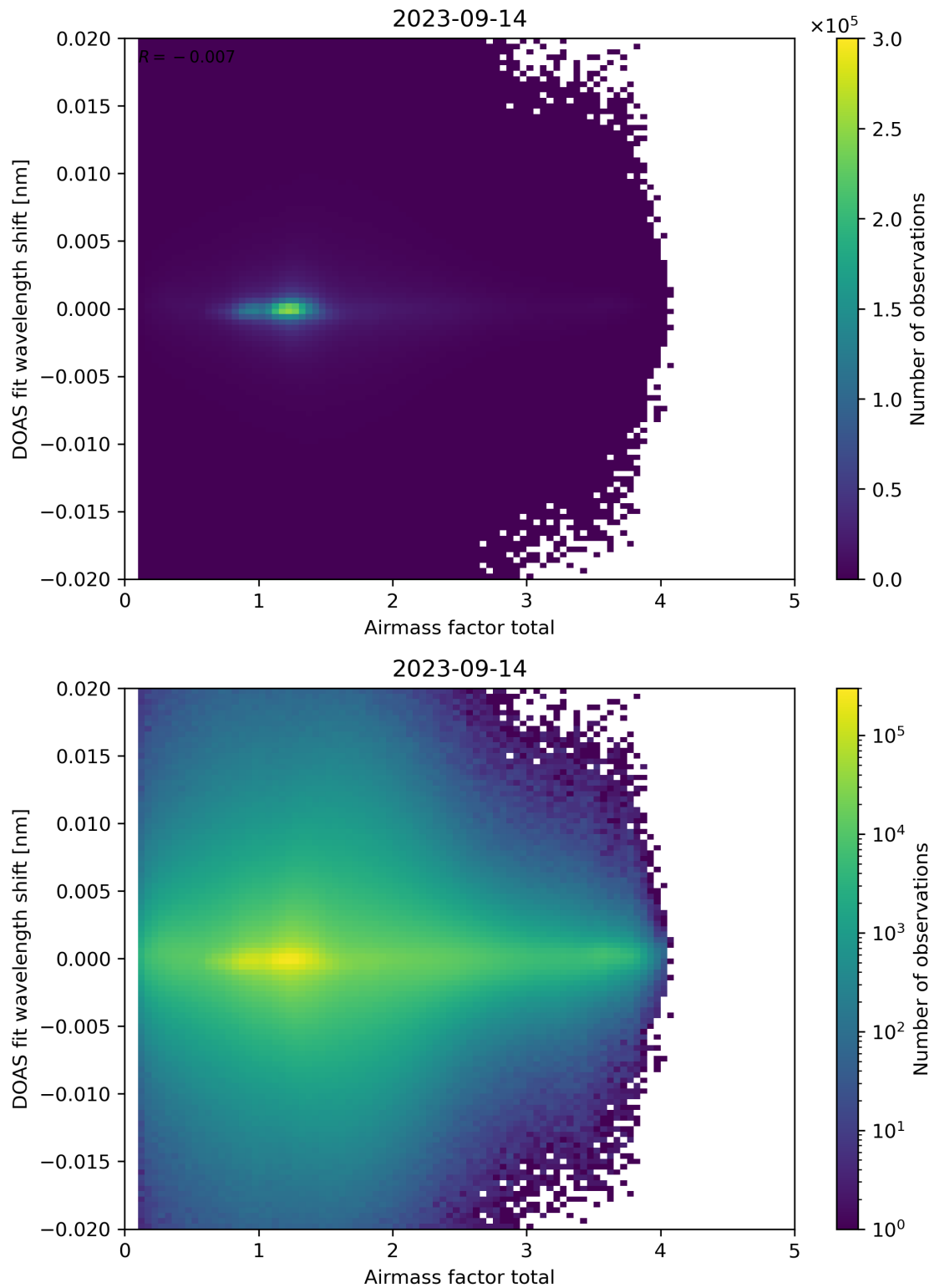
Figure 98: Scatter density plot of “Airmass factor total” against “DOAS fit wavelength shift” for 2023-09-13 to 2023-09-15.
