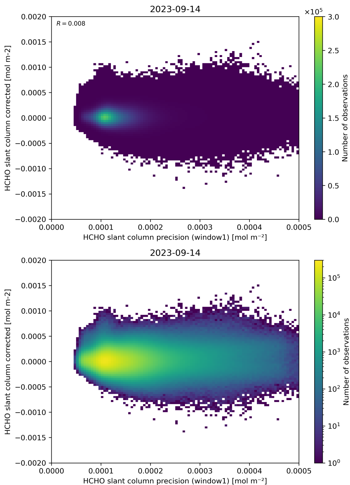
Figure 92: Scatter density plot of “HCHO slant column precision (window1)” against “HCHO slant column corrected” for 2023-09-13 to 2023-09-15.
