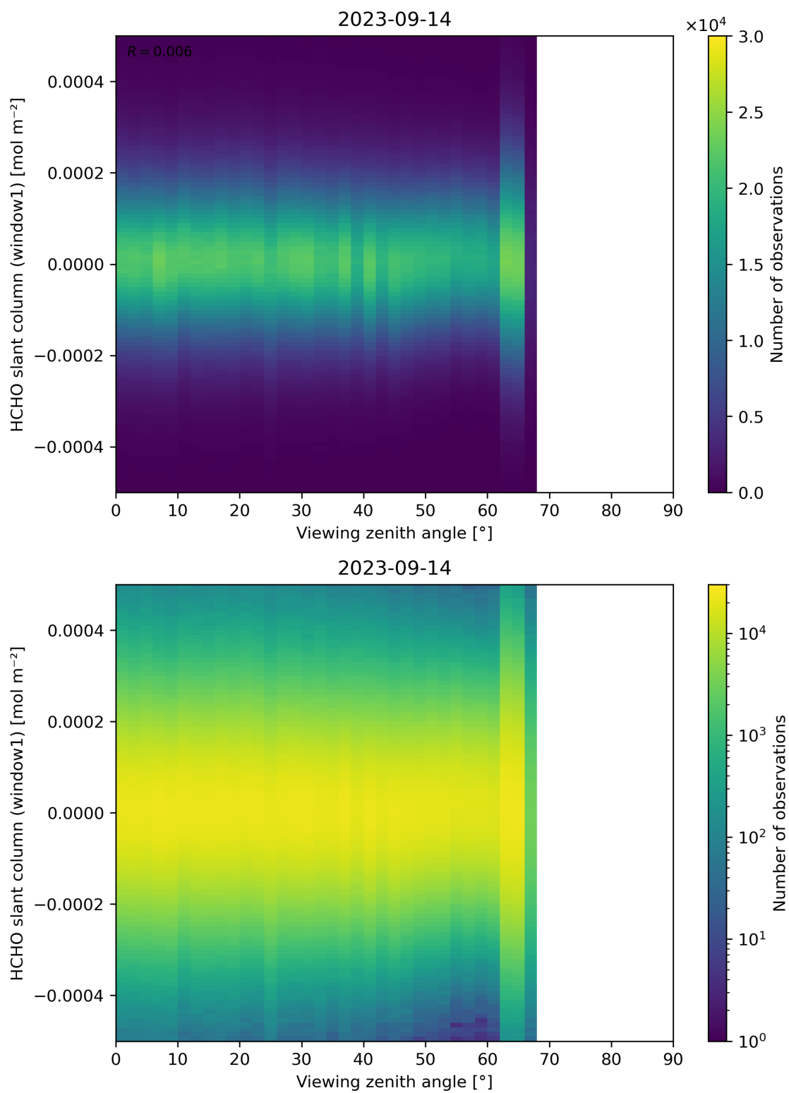
Figure 188: Scatter density plot of “Viewing zenith angle” against “HCHO slant column (window1)” for 2023-09-13 to 2023-09-15.
