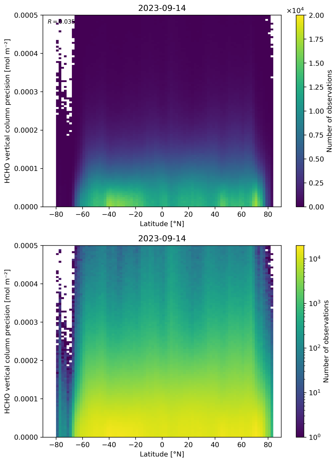
Figure 165: Scatter density plot of “Latitude” against “HCHO vertical column precision” for 2023-09-13 to 2023-09-15.
