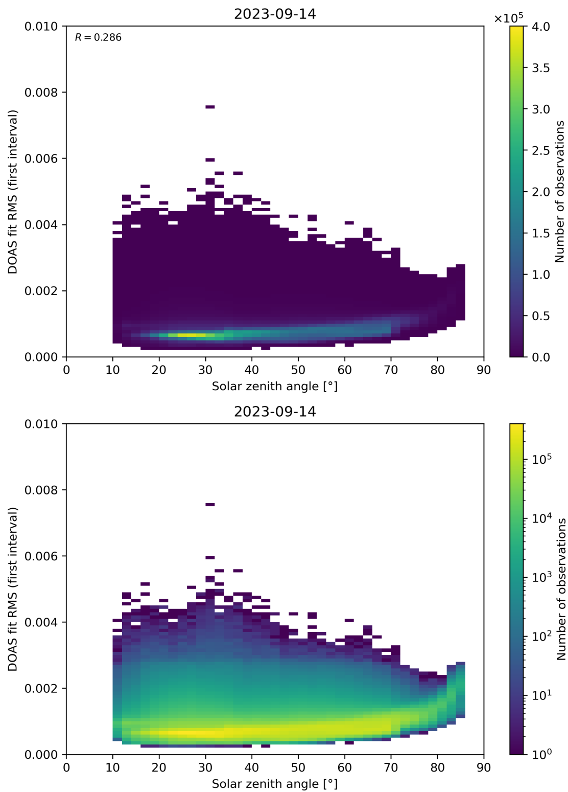
Figure 167: Scatter density plot of “Solar zenith angle” against “DOAS fit RMS (first interval)” for 2023-09-13 to 2023-09-15.
