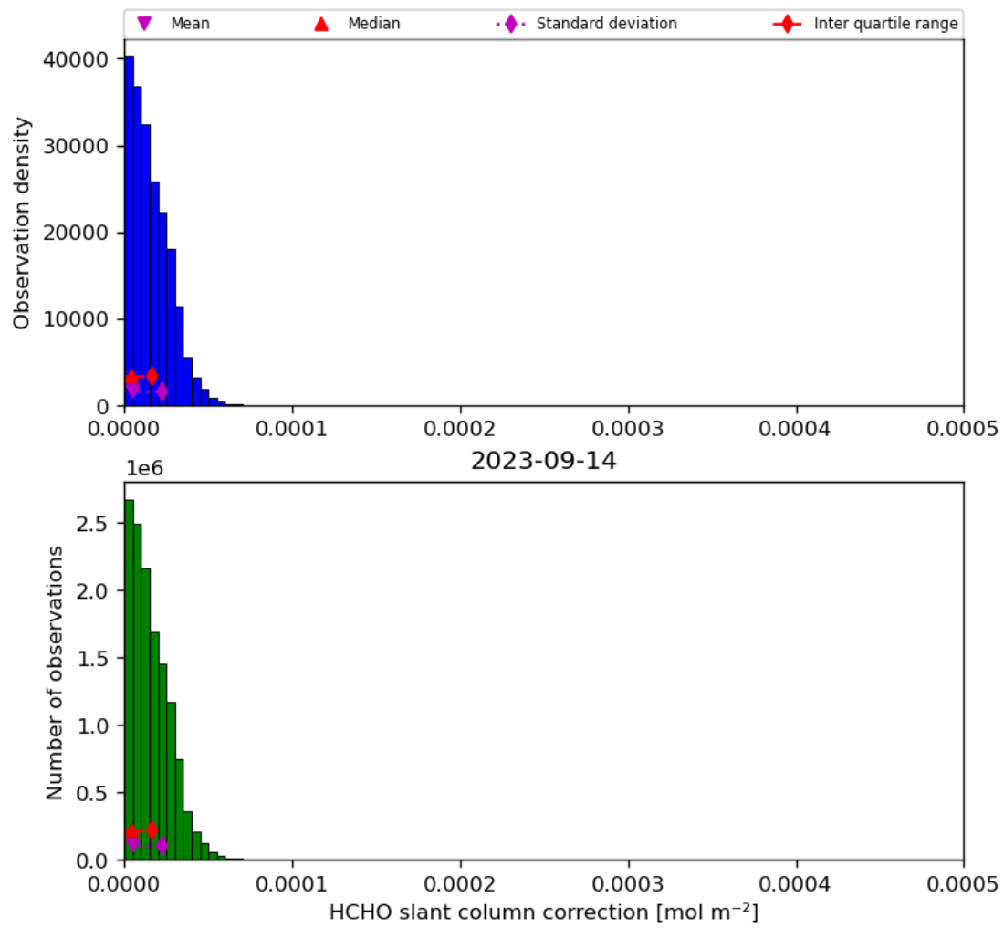
Figure 47: Histogram of “HCHO slant column correction” for 2023-09-13 to 2023-09-15
