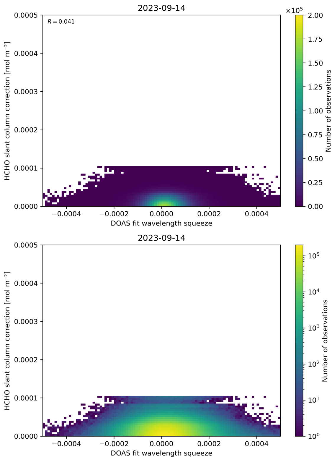
Figure 70: Scatter density plot of “DOAS fit wavelength squeeze” against “HCHO slant column correction” for 2023-09-13 to 2023-09-15.
