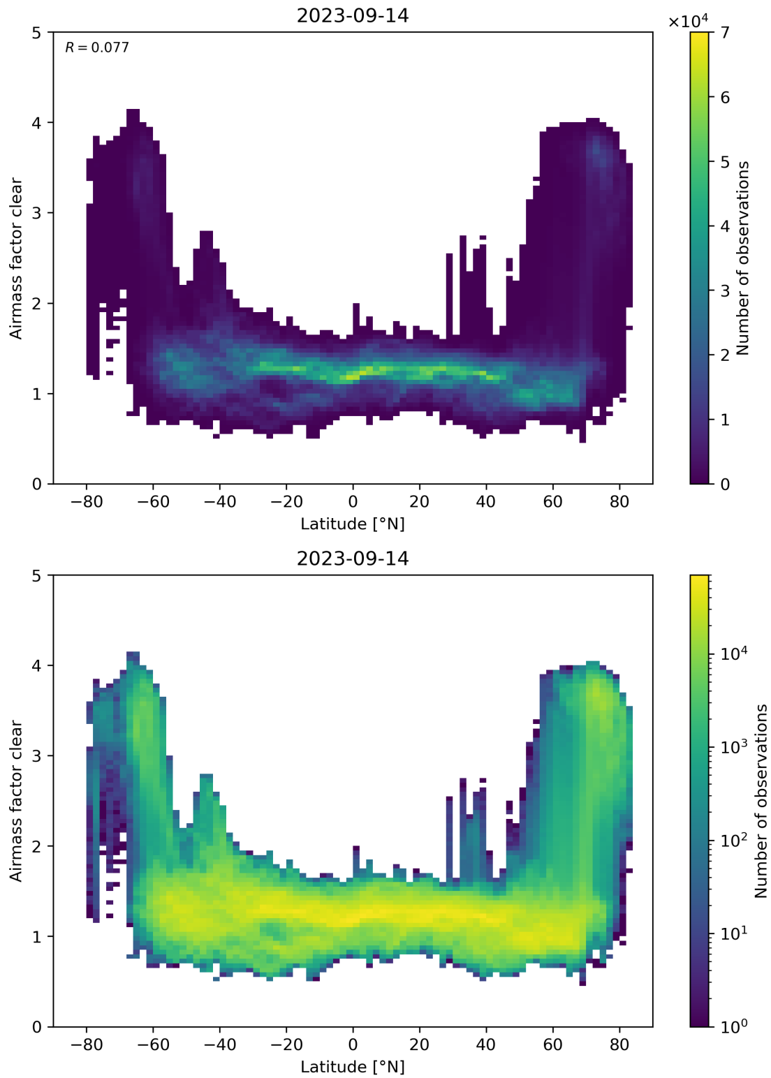
Figure 156: Scatter density plot of “Latitude” against “Airmass factor clear” for 2023-09-13 to 2023-09-15.
