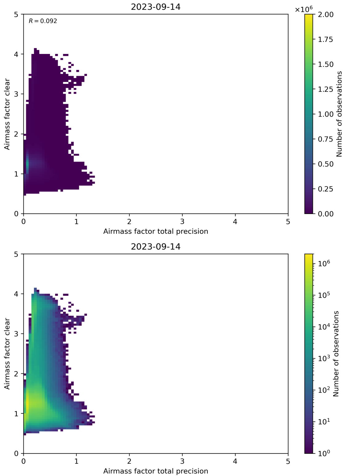
Figure 108: Scatter density plot of “Airmass factor total precision” against “Airmass factor clear” for 2023-09-13 to 2023-09-15.
