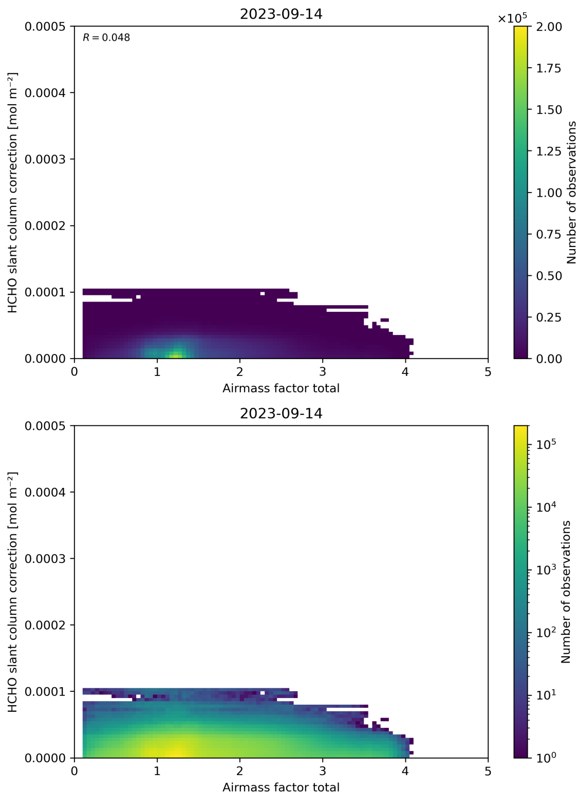
Figure 102: Scatter density plot of “Airmass factor total” against “HCHO slant column correction” for 2023-09-13 to 2023-09-15.
