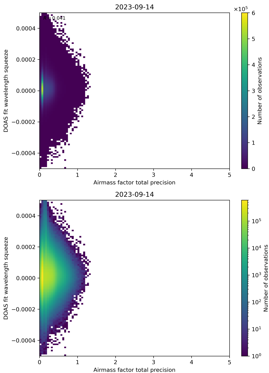
Figure 107: Scatter density plot of “Airmass factor total precision” against “DOAS fit wavelength squeeze” for 2023-09-13 to 2023-09-15.
