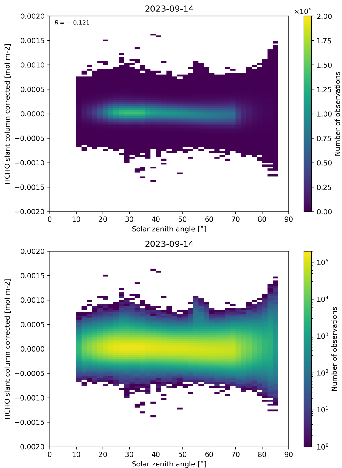
Figure 171: Scatter density plot of “Solar zenith angle” against “HCHO slant column corrected” for 2023-09-13 to 2023-09-15.
