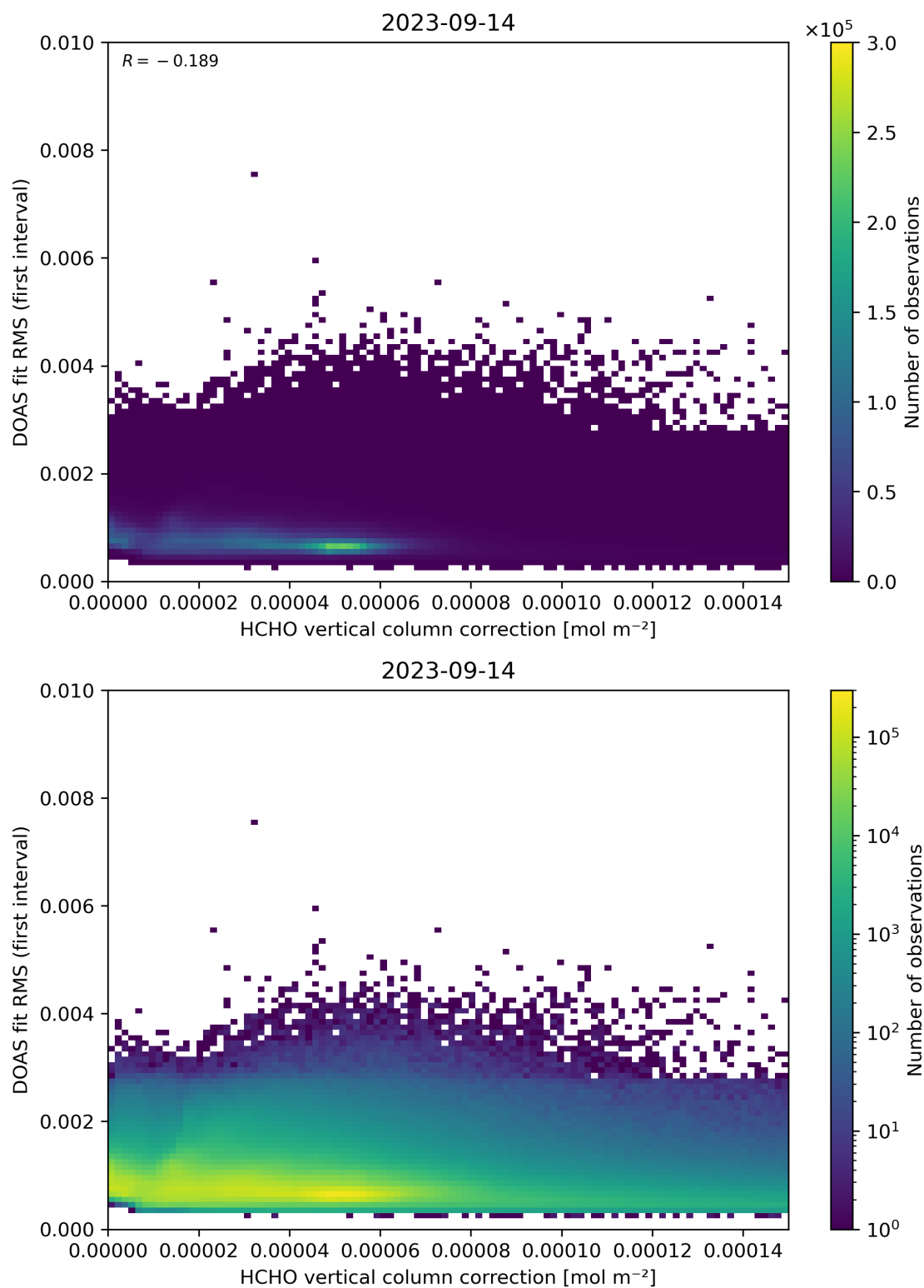
Figure 112: Scatter density plot of “HCHO vertical column correction” against “DOAS fit RMS (first interval)” for 2023-09-13 to 2023-09-15.
