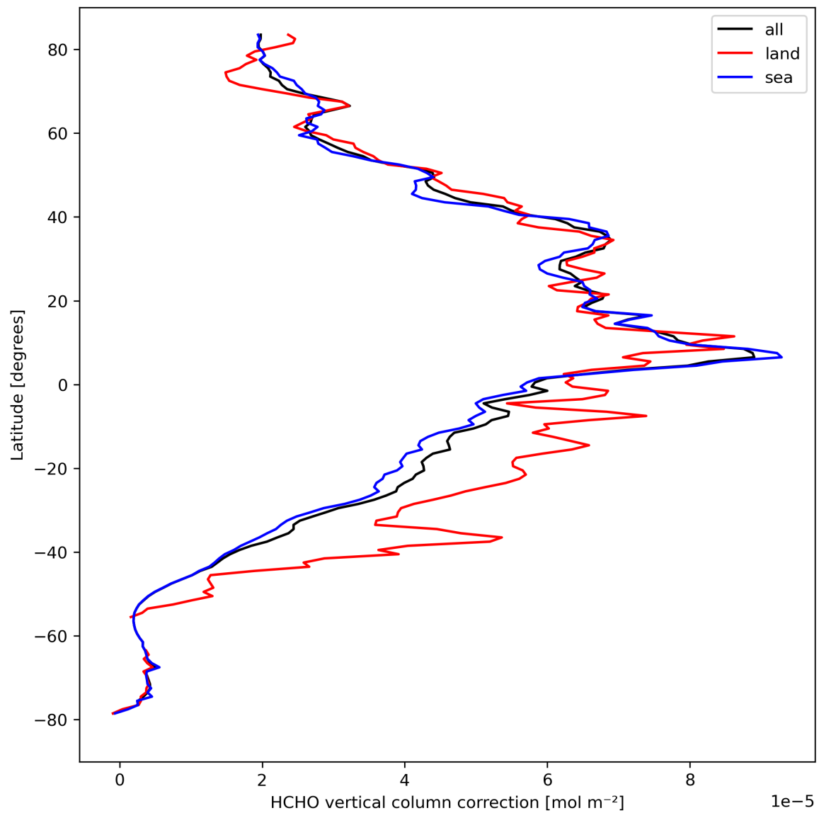
Figure 23: Zonal average of “HCHO vertical column correction” for 2023-09-13 to 2023-09-15.
