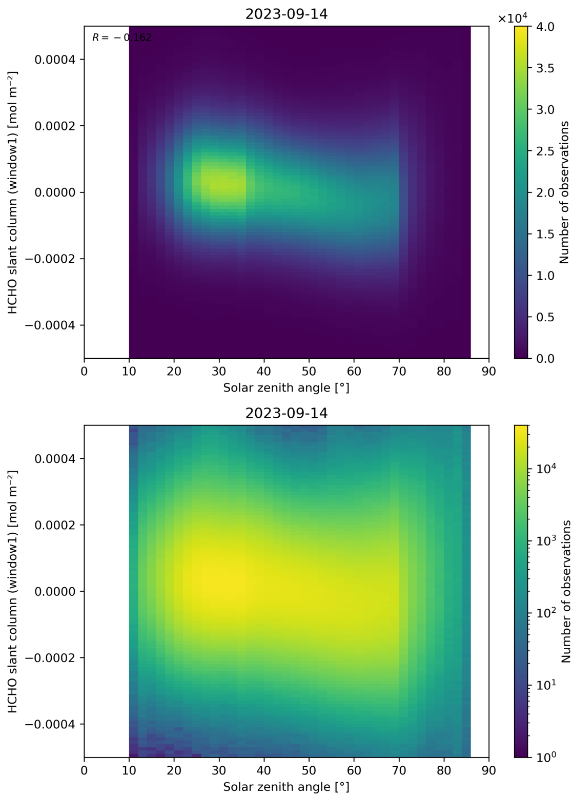
Figure 173: Scatter density plot of “Solar zenith angle” against “HCHO slant column (window1)” for 2023-09-13 to 2023-09-15.
