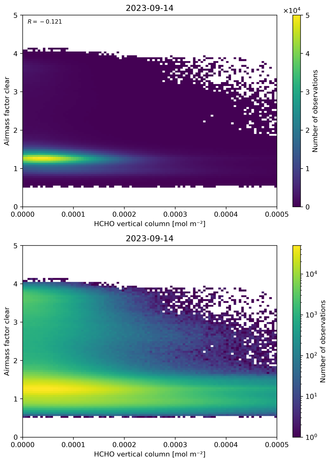
Figure 126: Scatter density plot of “HCHO vertical column” against “Airmass factor clear” for 2023-09-13 to 2023-09-15.
