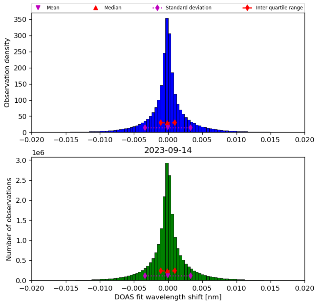
Figure 44: Histogram of “DOAS fit wavelength shift” for 2023-09-13 to 2023-09-15
