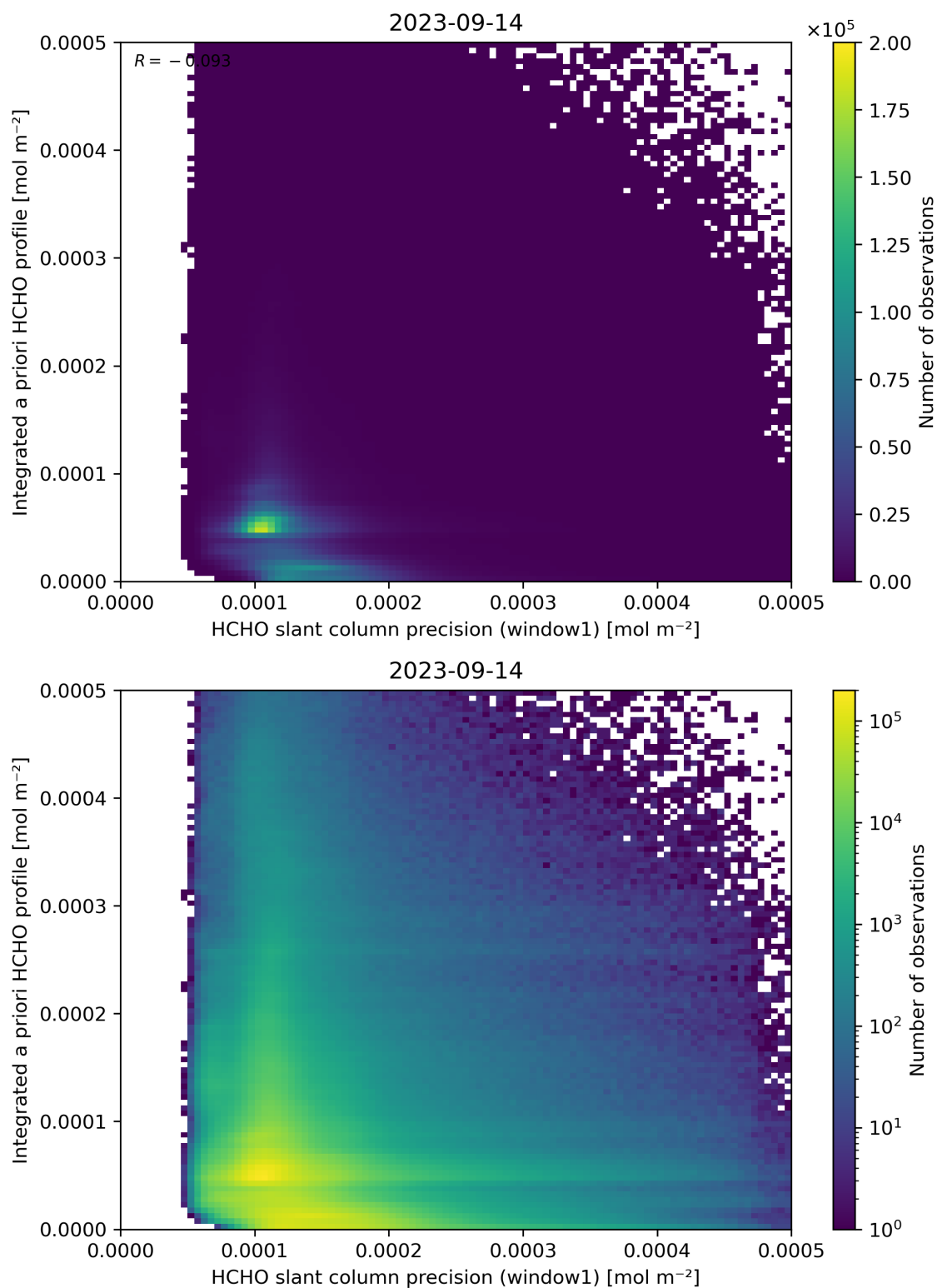
Figure 96: Scatter density plot of “HCHO slant column precision (window1)” against “Integrated a priori HCHO profile” for 2023-09-13 to 2023-09-15.
