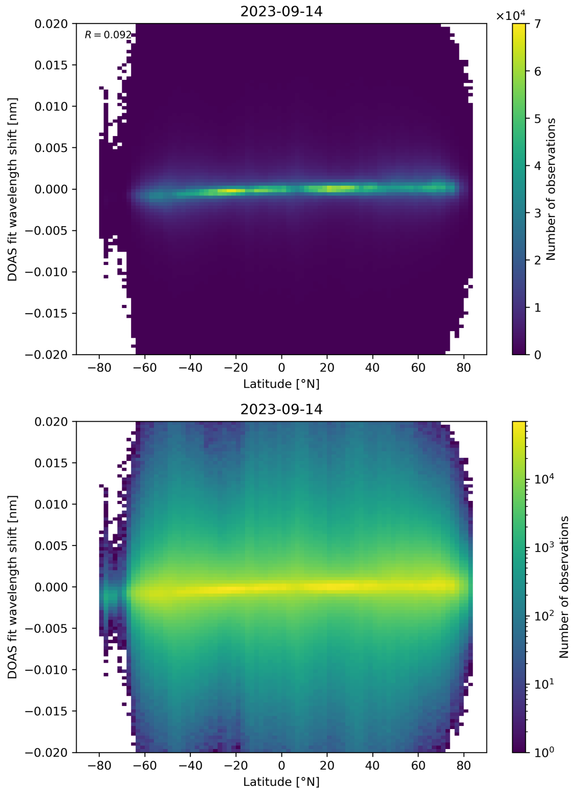
Figure 154: Scatter density plot of “Latitude” against “DOAS fit wavelength shift” for 2023-09-13 to 2023-09-15.
