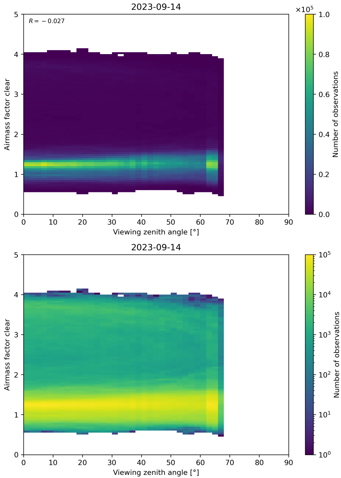
Figure 185: Scatter density plot of “Viewing zenith angle” against “Airmass factor clear” for 2023-09-13 to 2023-09-15.
