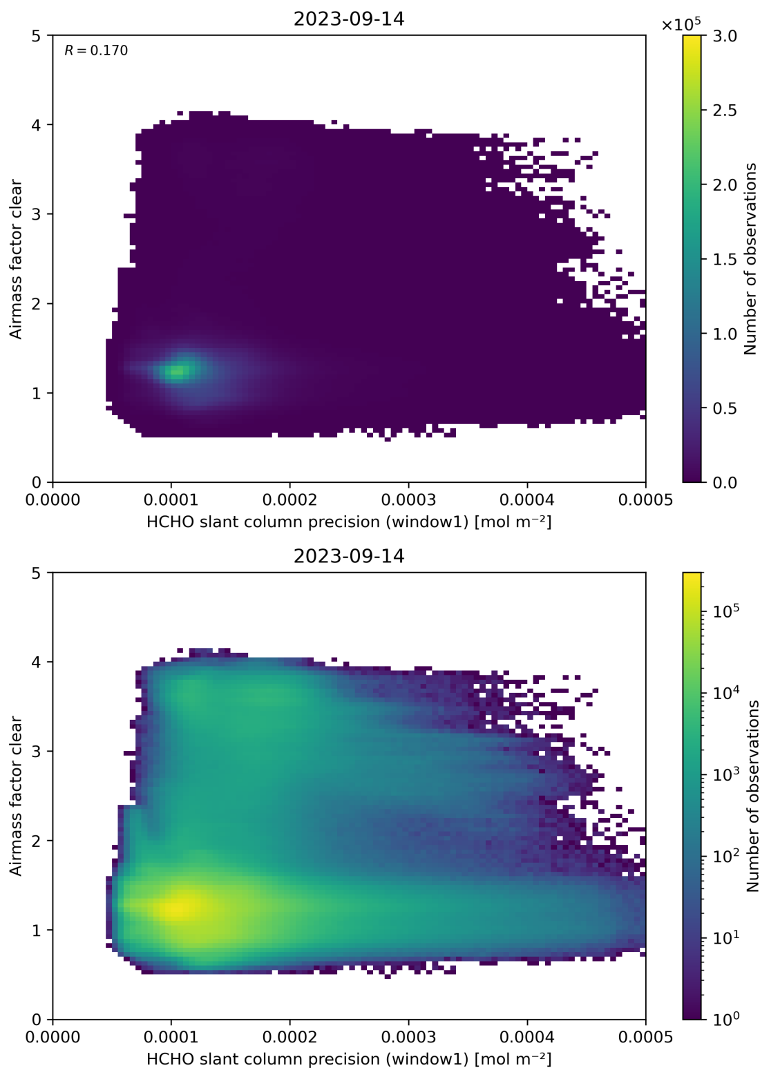
Figure 91: Scatter density plot of “HCHO slant column precision (window1)” against “Airmass factor clear” for 2023-09-13 to 2023-09-15.
