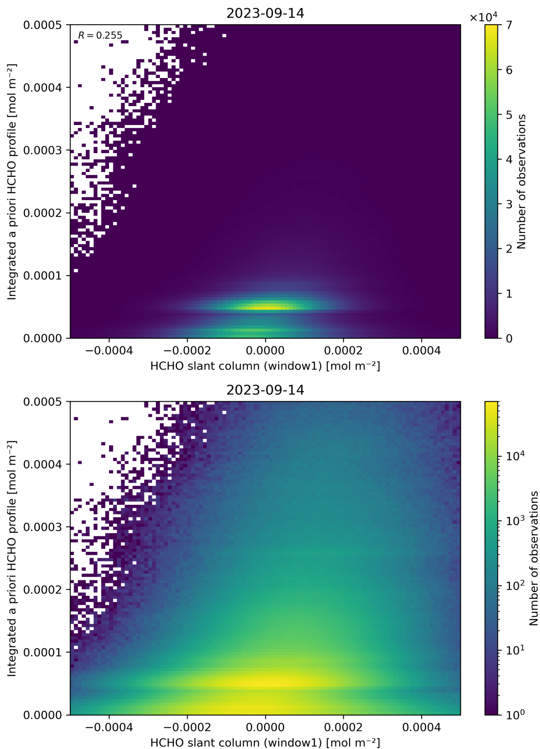
Figure 87: Scatter density plot of “HCHO slant column (window1)” against “Integrated a priori HCHO profile” for 2023-09-13 to 2023-09-15.
