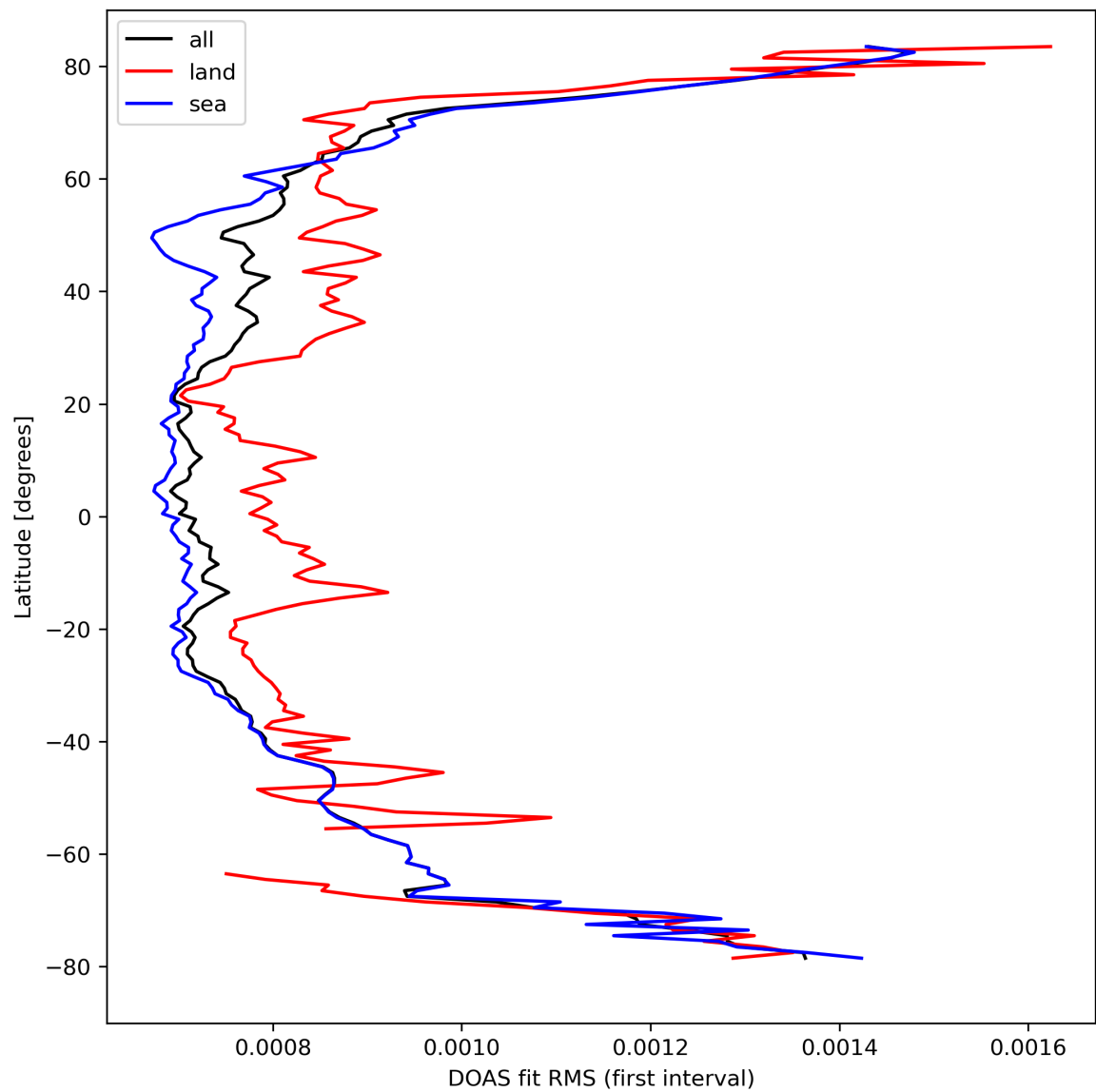
Figure 32: Zonal average of “DOAS fit RMS (first interval)” for 2023-09-13 to 2023-09-15.
