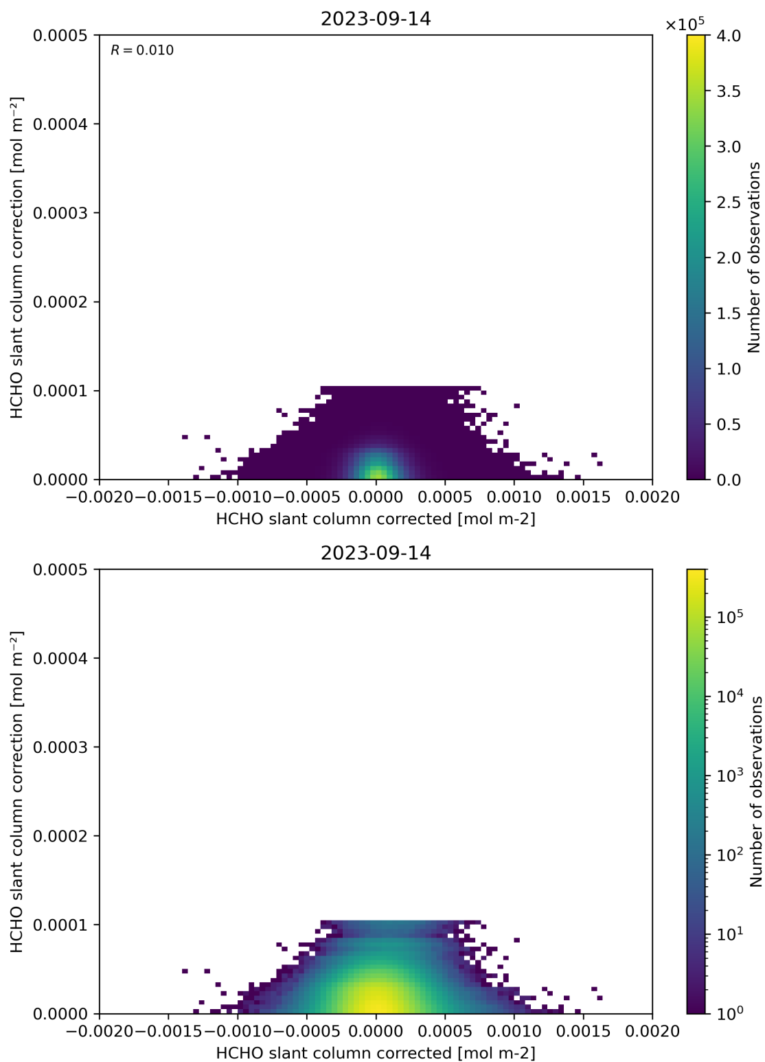
Figure 77: Scatter density plot of “HCHO slant column corrected” against “HCHO slant column correction” for 2023-09-13 to 2023-09-15.
