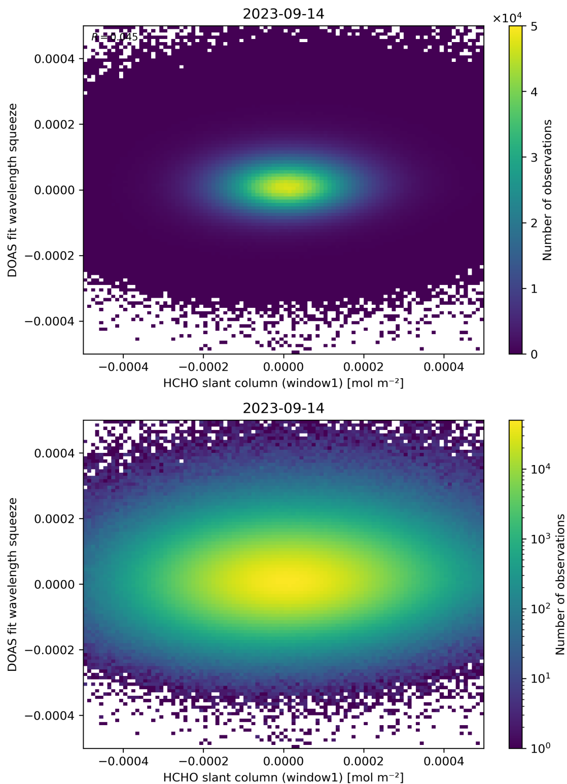
Figure 80: Scatter density plot of “HCHO slant column (window1)” against “DOAS fit wavelength squeeze” for 2023-09-13 to 2023-09-15.
