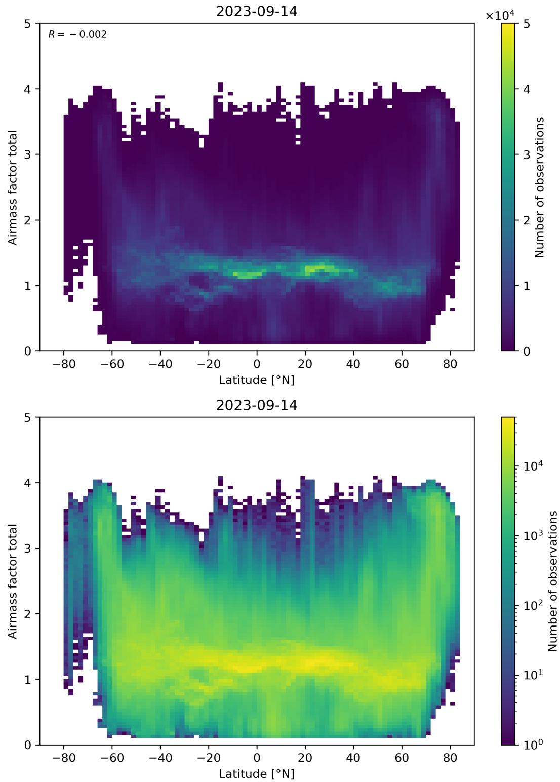
Figure 161: Scatter density plot of “Latitude” against “Airmass factor total” for 2023-09-13 to 2023-09-15.
