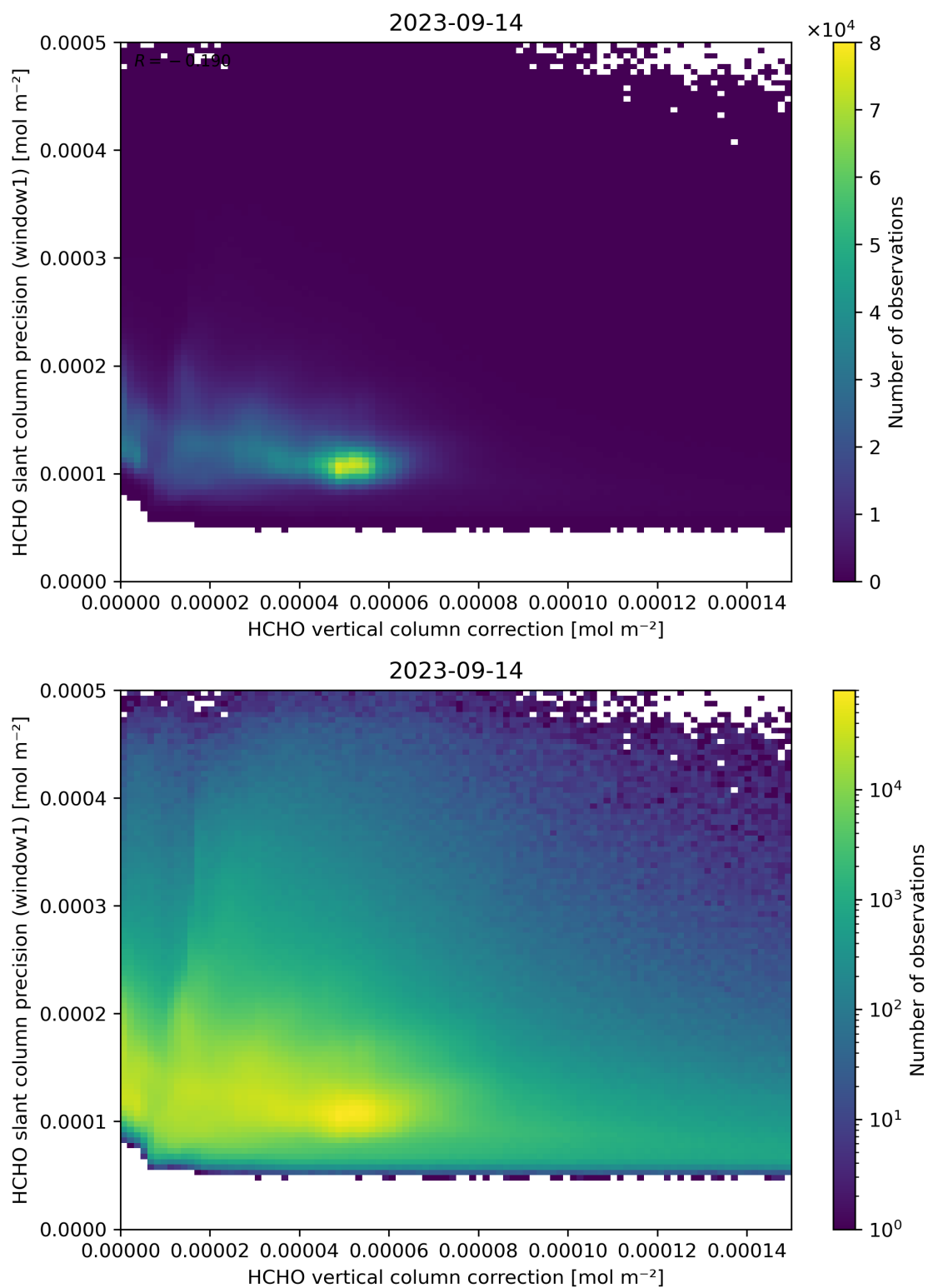
Figure 119: Scatter density plot of “HCHO vertical column correction” against “HCHO slant column precision (window1)” for 2023-09-13 to 2023-09-15.
