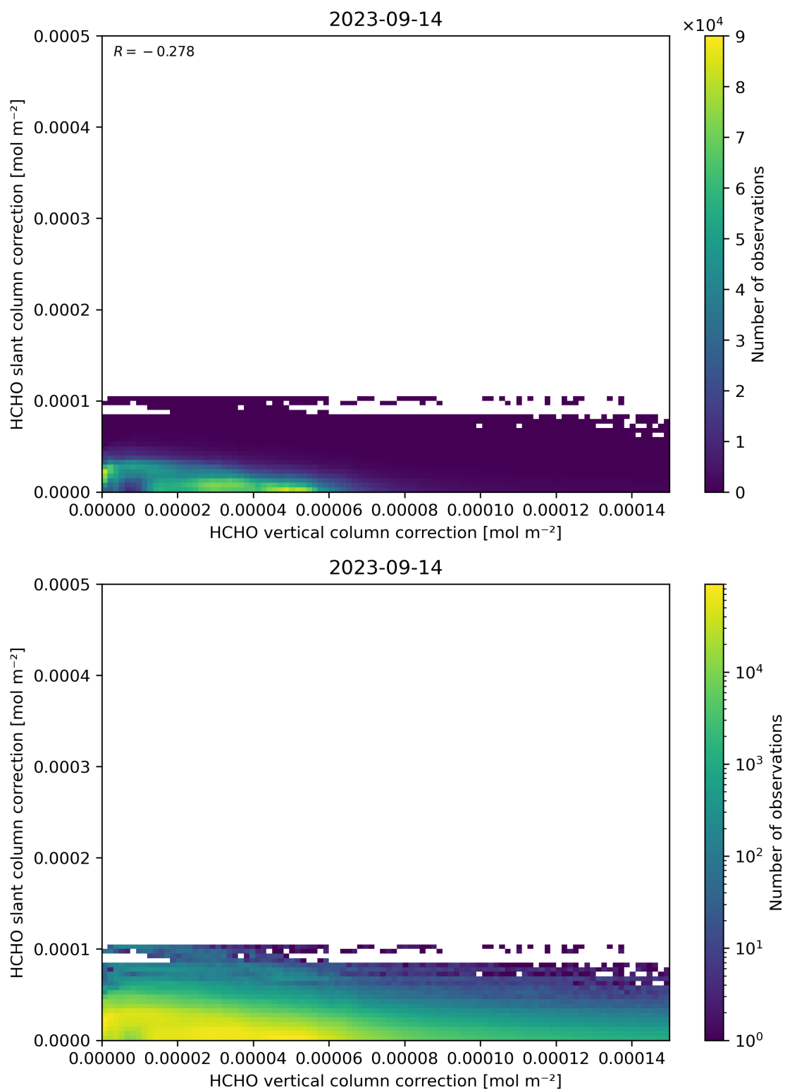
Figure 117: Scatter density plot of “HCHO vertical column correction” against “HCHO slant column correction” for 2023-09-13 to 2023-09-15.
