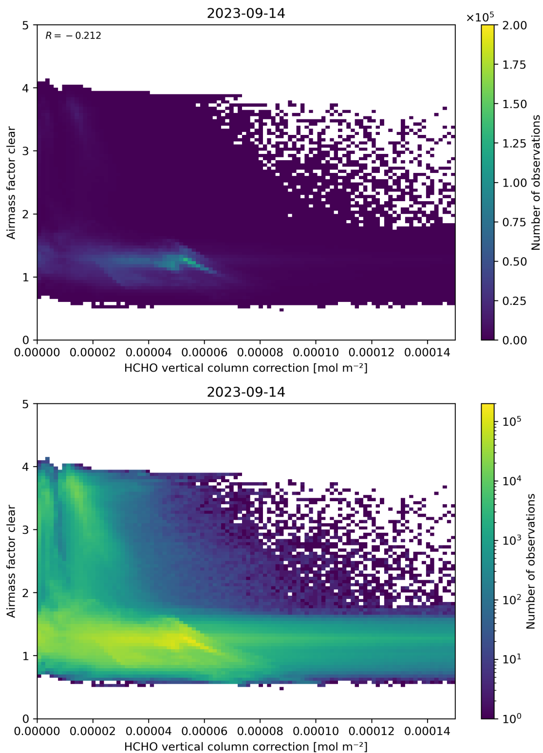
Figure 115: Scatter density plot of “HCHO vertical column correction” against “Airmass factor clear” for 2023-09-13 to 2023-09-15.
