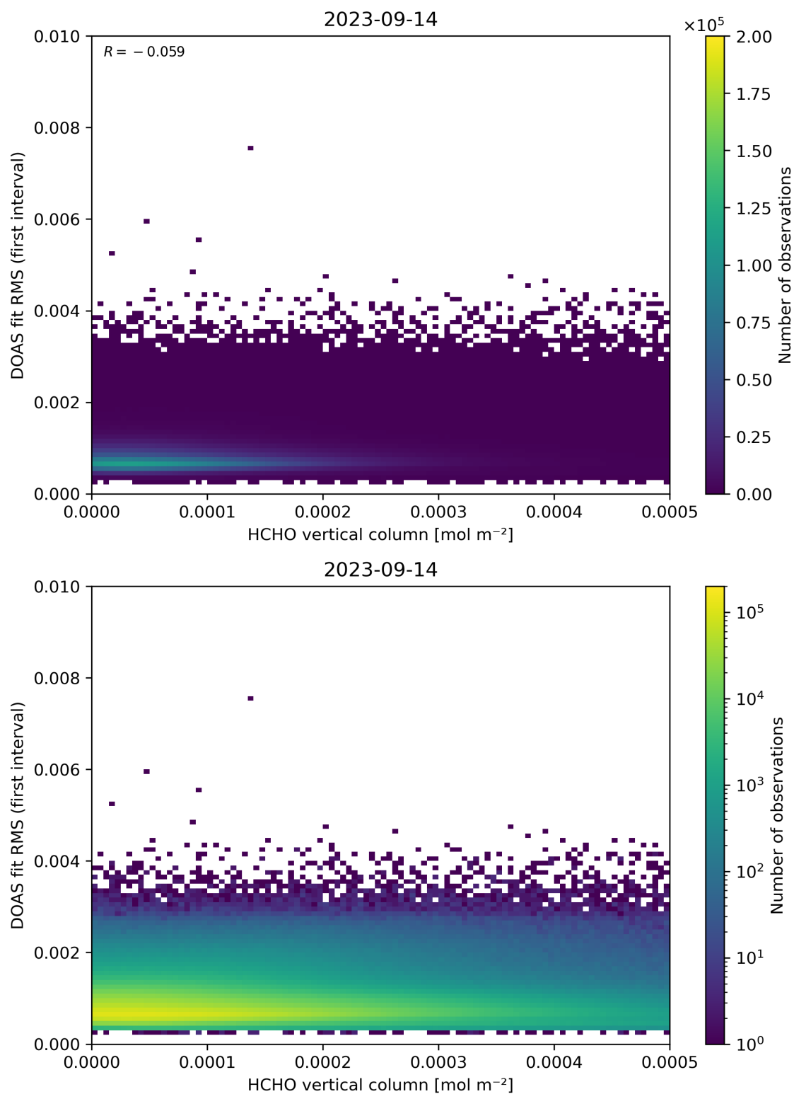
Figure 123: Scatter density plot of “HCHO vertical column” against “DOAS fit RMS (first interval)” for 2023-09-13 to 2023-09-15.
