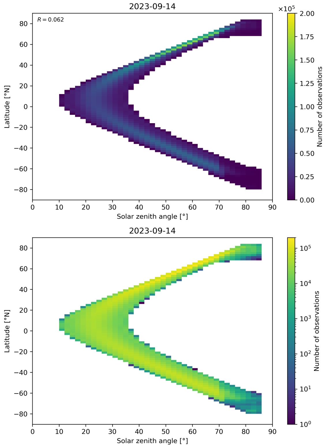
Figure 181: Scatter density plot of “Solar zenith angle” against “Latitude” for 2023-09-13 to 2023-09-15.
