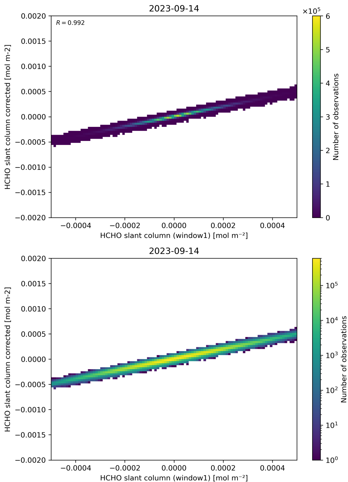
Figure 82: Scatter density plot of “HCHO slant column (window1)” against “HCHO slant column corrected” for 2023-09-13 to 2023-09-15.
