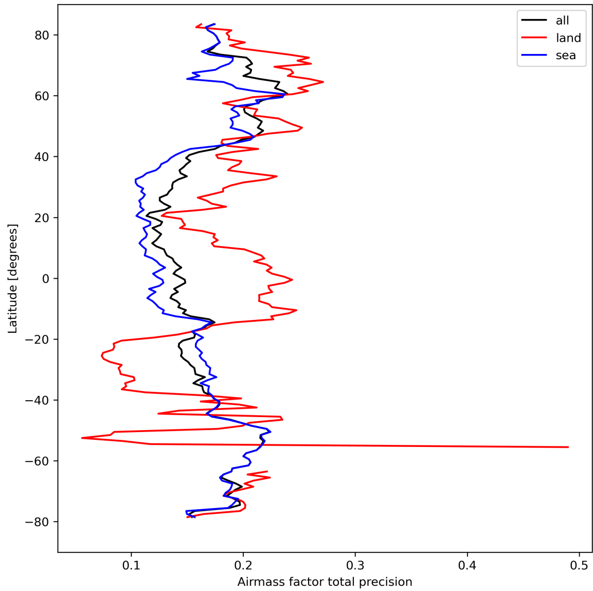
Figure 27: Zonal average of “Airmass factor total precision” for 2023-09-13 to 2023-09-15.
