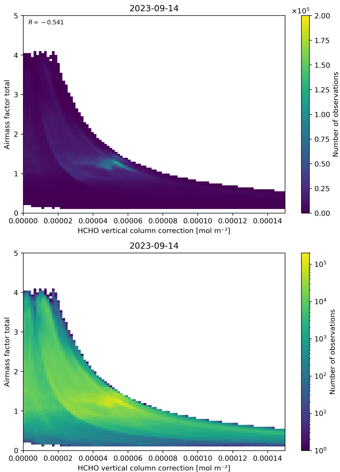
Figure 120: Scatter density plot of “HCHO vertical column correction” against “Airmass factor total” for 2023-09-13 to 2023-09-15.
