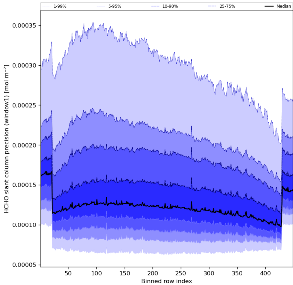
Figure 53: Along track statistics of “HCHO slant column precision (window1)” for 2023-09-13 to 2023-09-15
