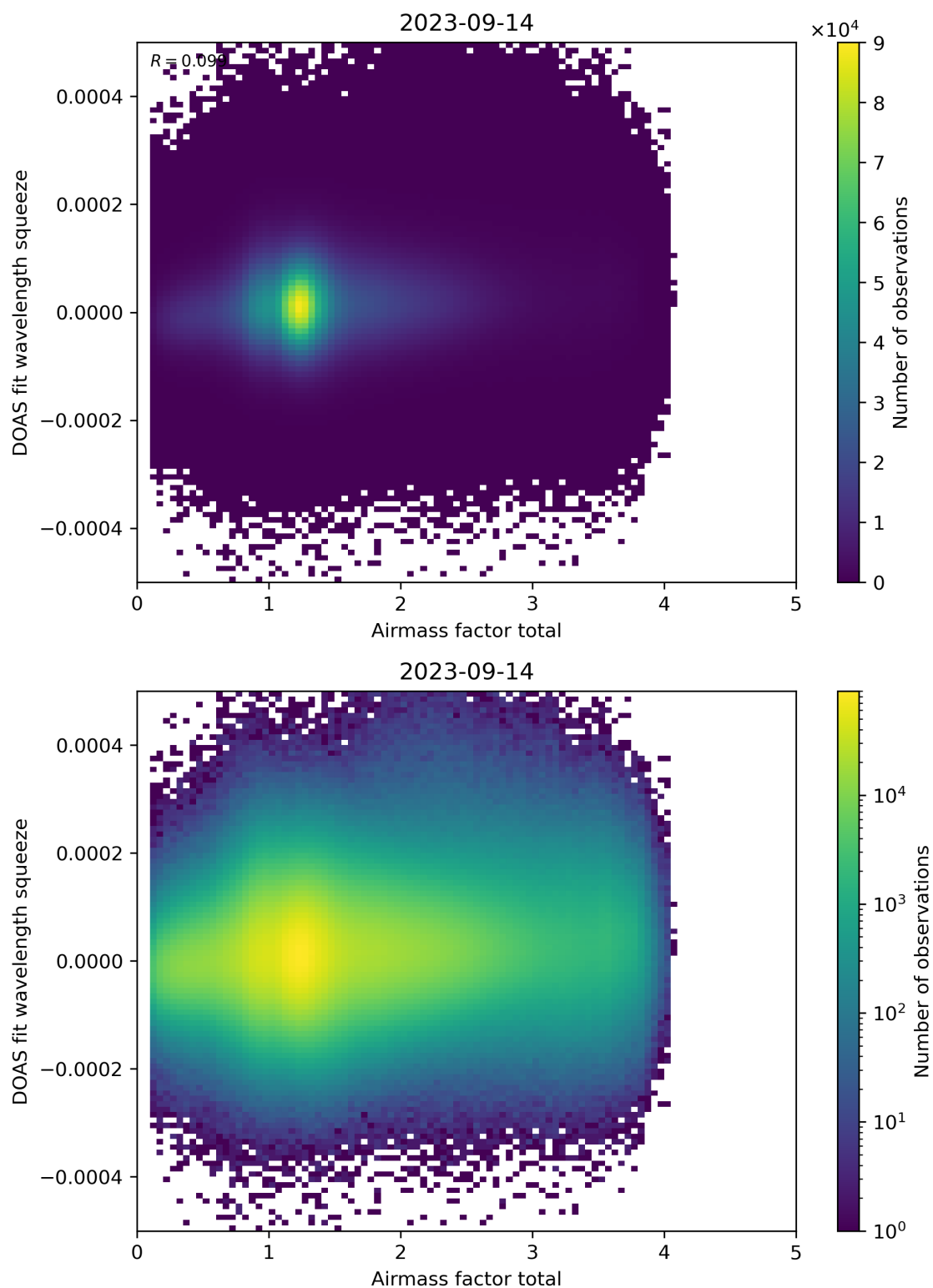
Figure 99: Scatter density plot of “Airmass factor total” against “DOAS fit wavelength squeeze” for 2023-09-13 to 2023-09-15.
