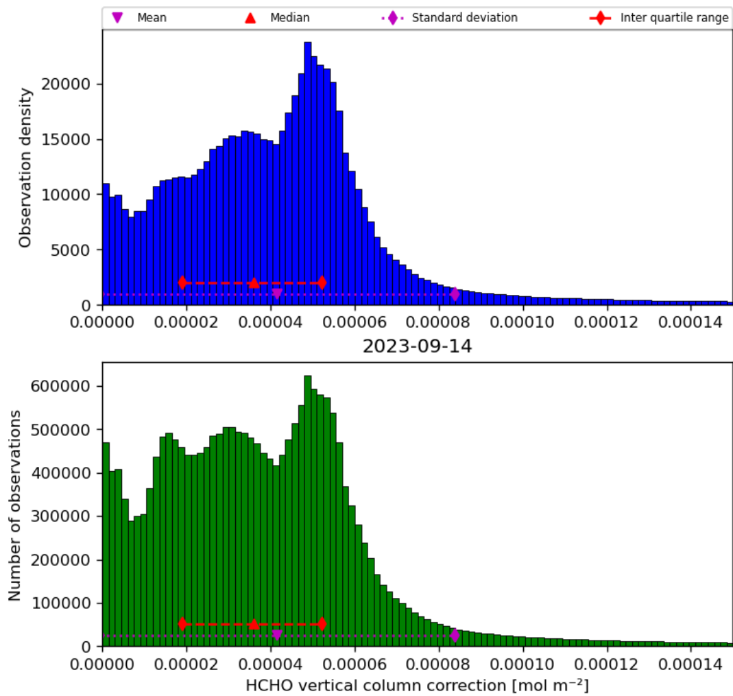
Figure 37: Histogram of “HCHO vertical column correction” for 2023-09-13 to 2023-09-15
