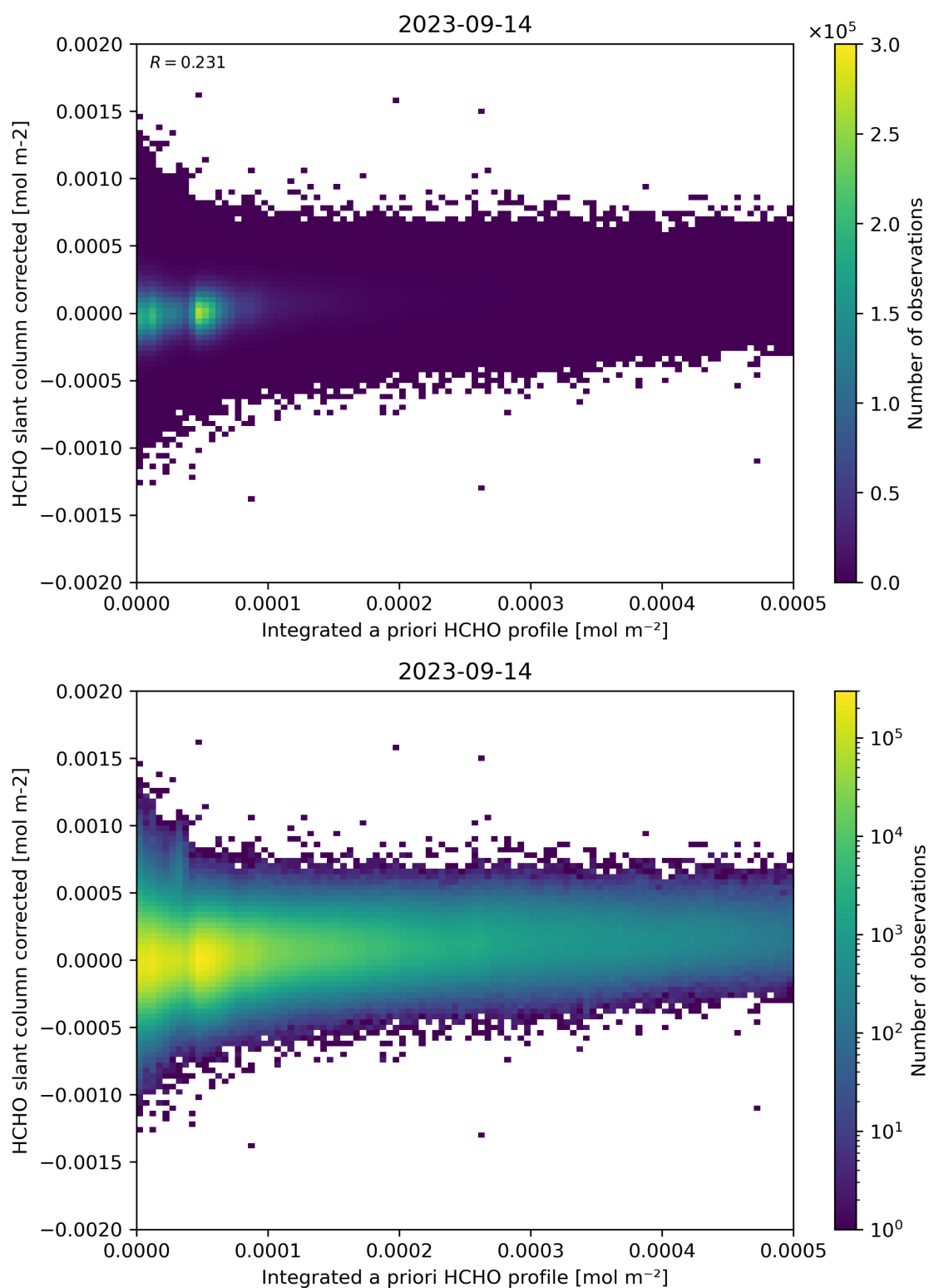
Figure 151: Scatter density plot of “Integrated a priori HCHO profile” against “HCHO slant column corrected” for 2023-09-13 to 2023-09-15.
