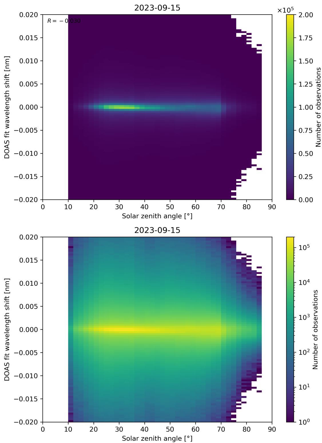
Figure 168: Scatter density plot of “Solar zenith angle” against “DOAS fit wavelength shift” for 2023-09-15 to 2023-09-16.
