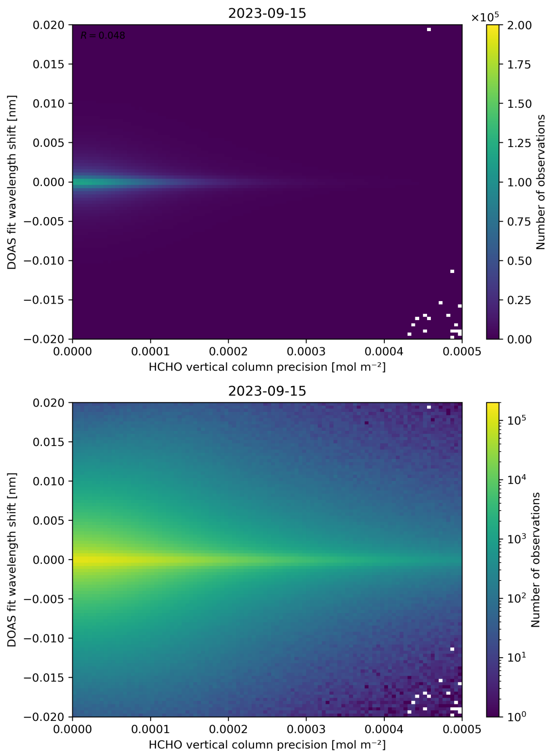
Figure 137: Scatter density plot of “HCHO vertical column precision” against “DOAS fit wavelength shift” for 2023-09-15 to 2023-09-16.
