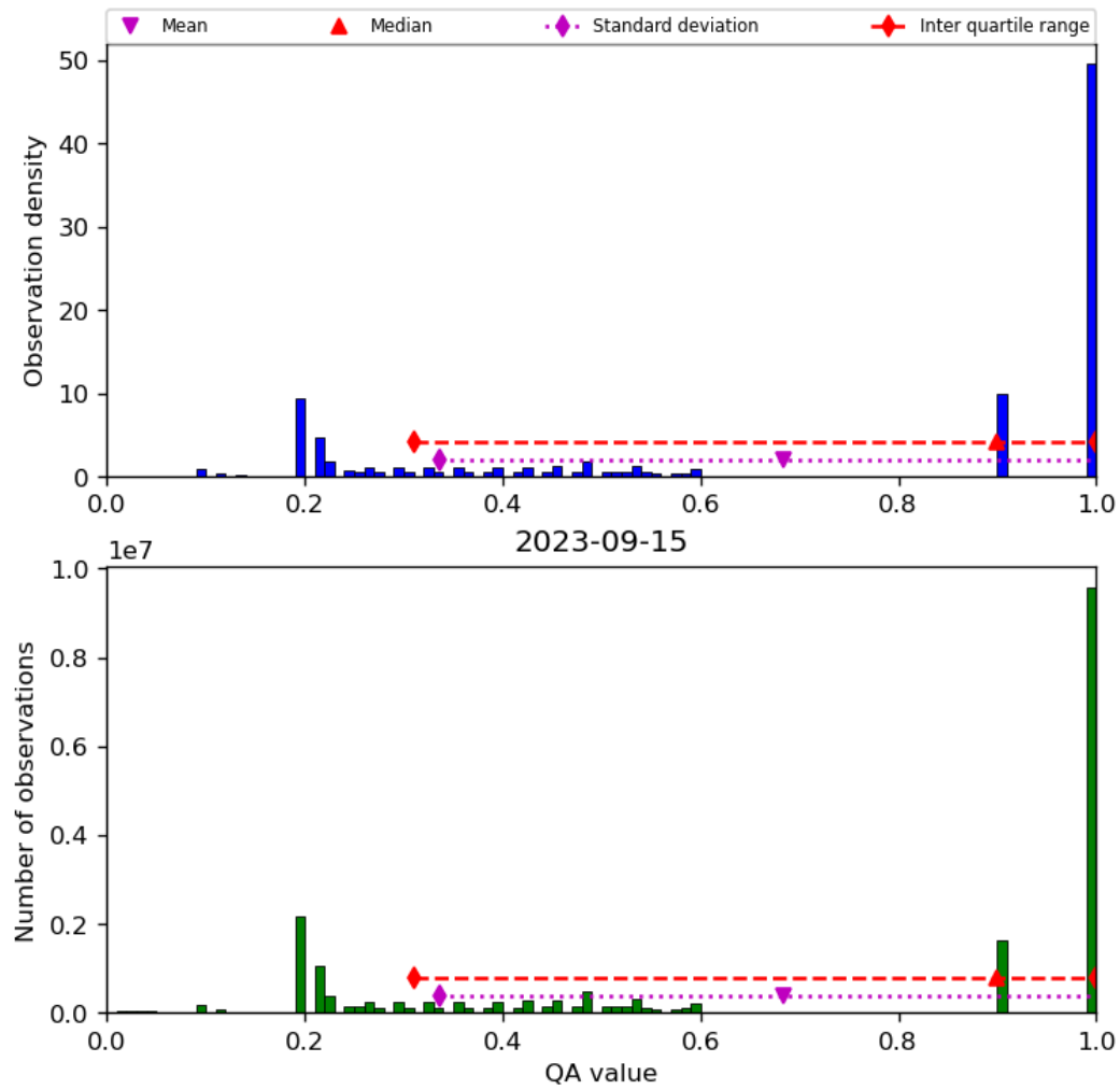
Figure 34: Histogram of “QA value” for 2023-09-15 to 2023-09-16
