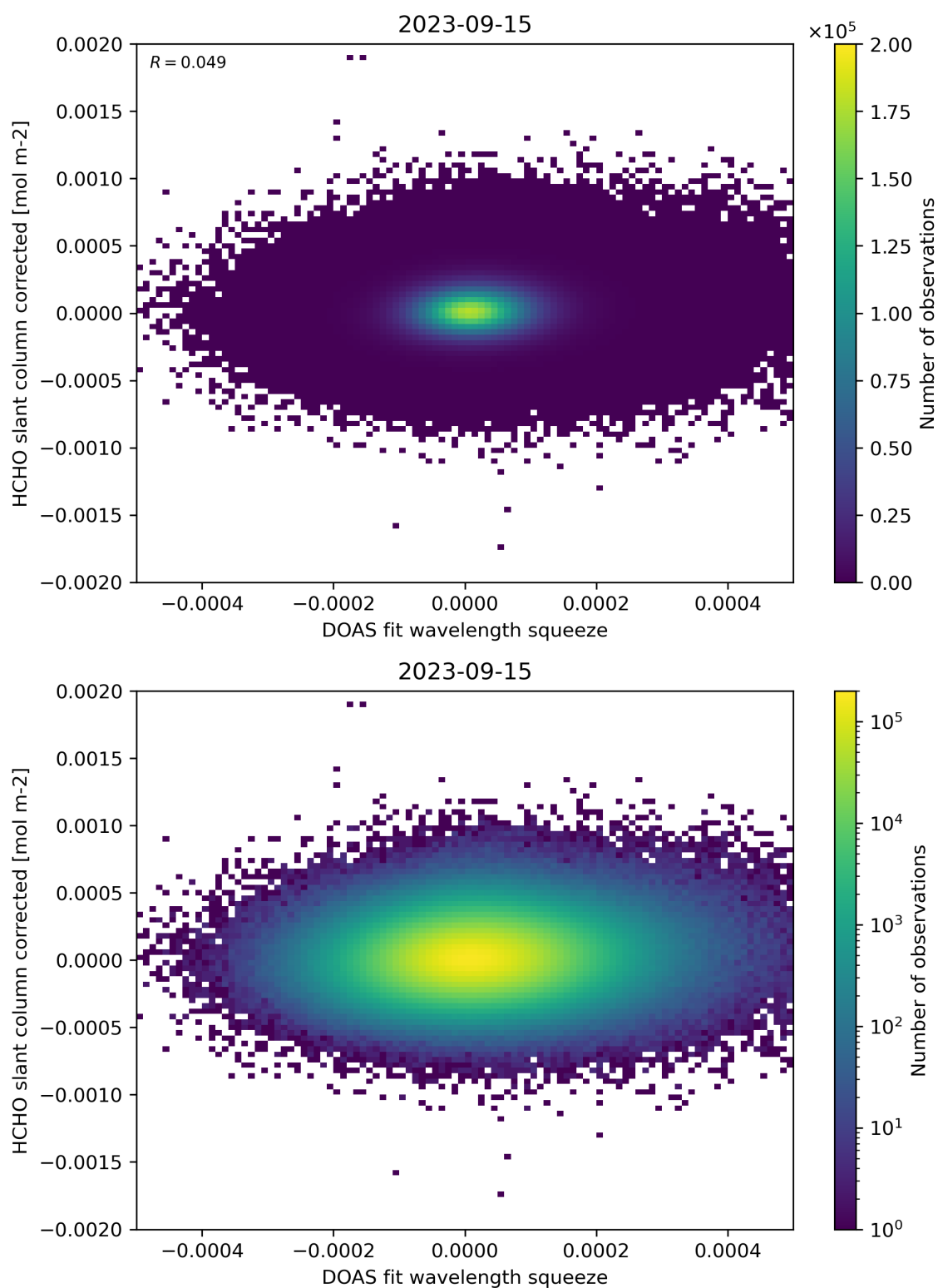
Figure 69: Scatter density plot of “DOAS fit wavelength squeeze” against “HCHO slant column corrected” for 2023-09-15 to 2023-09-16.
