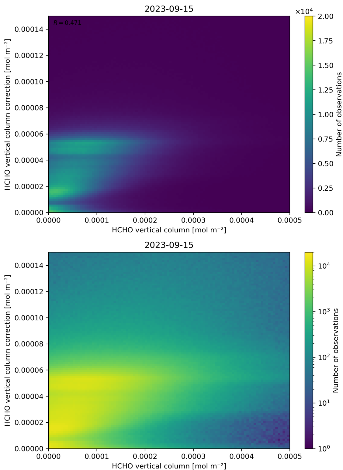
Figure 133: Scatter density plot of “HCHO vertical column” against “HCHO vertical column correction” for 2023-09-15 to 2023-09-16.
