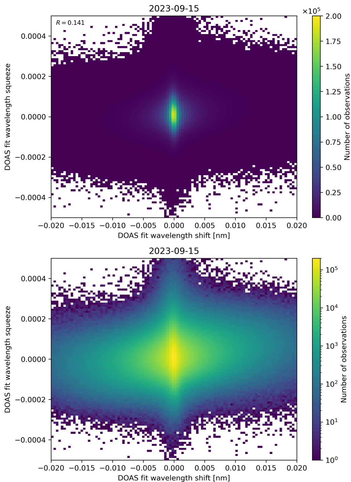
Figure 65: Scatter density plot of “DOAS fit wavelength shift” against “DOAS fit wavelength squeeze” for 2023-09-15 to 2023-09-16.
