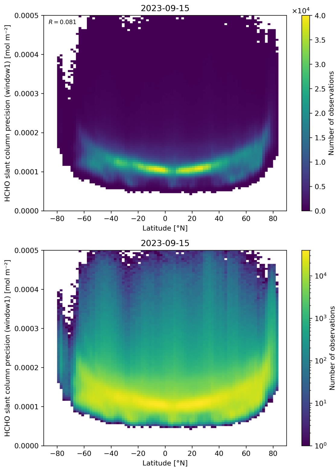
Figure 160: Scatter density plot of “Latitude” against “HCHO slant column precision (window1)” for 2023-09-15 to 2023-09-16.
