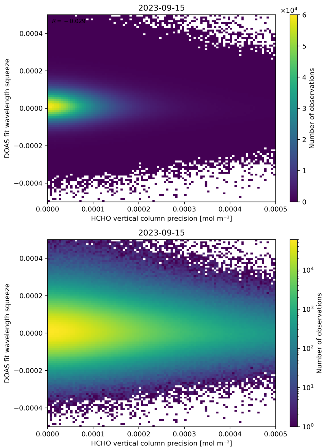
Figure 138: Scatter density plot of “HCHO vertical column precision” against “DOAS fit wavelength squeeze” for 2023-09-15 to 2023-09-16.
