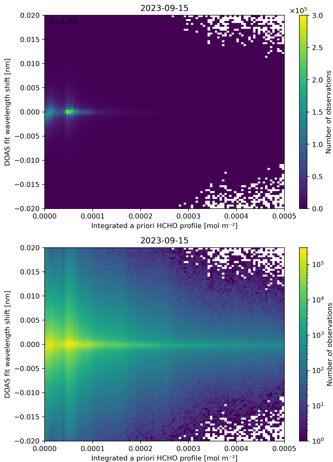
Figure 149: Scatter density plot of “Integrated a priori HCHO profile” against “DOAS fit wavelength shift” for 2023-09-15 to 2023-09-16.
