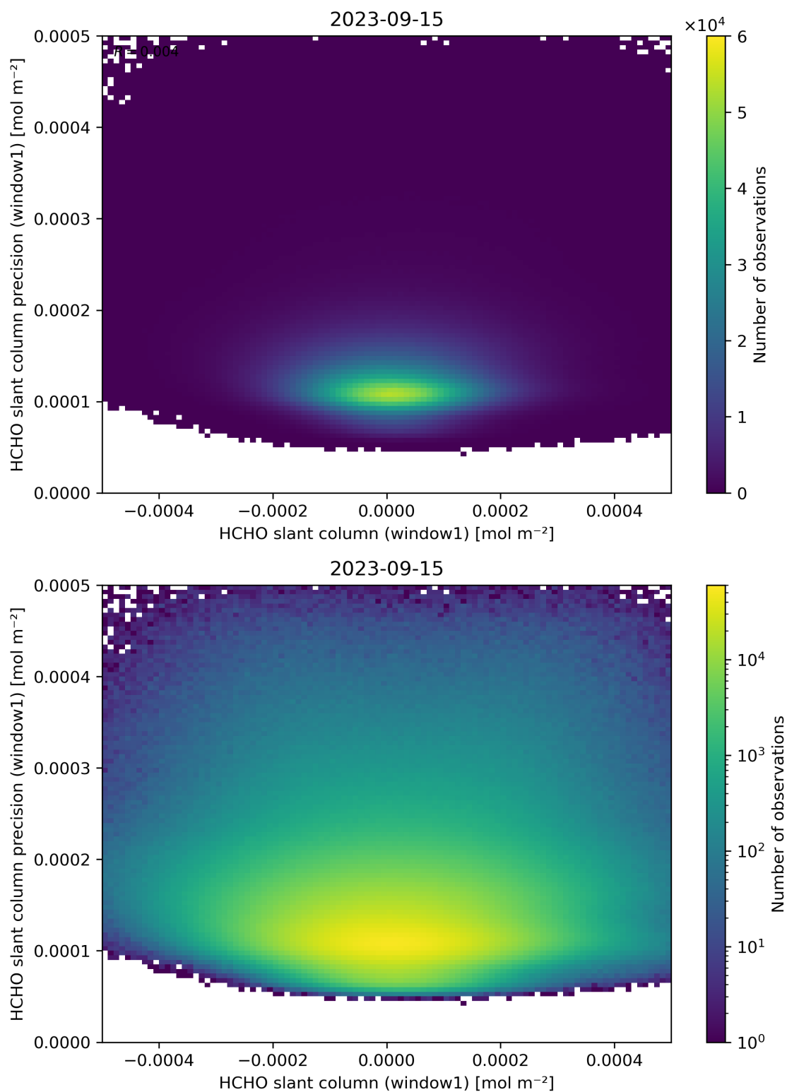
Figure 84: Scatter density plot of “HCHO slant column (window1)” against “HCHO slant column precision (window1)” for 2023-09-15 to 2023-09-16.
