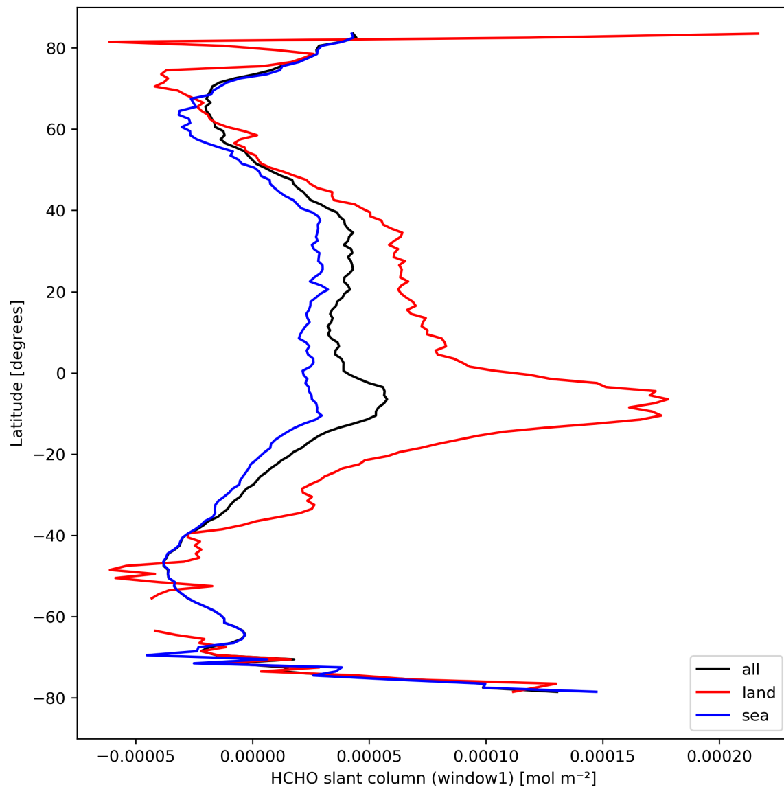
Figure 24: Zonal average of “HCHO slant column (window1)” for 2023-09-15 to 2023-09-16.
