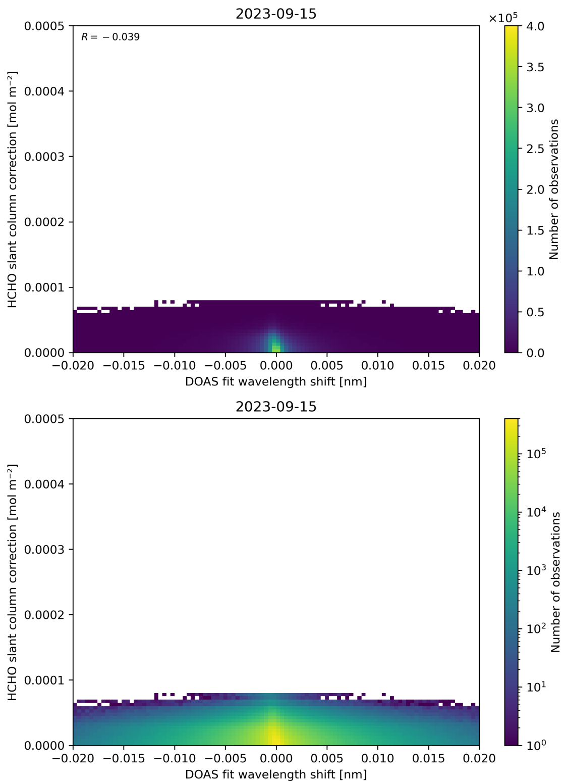
Figure 67: Scatter density plot of “DOAS fit wavelength shift” against “HCHO slant column correction” for 2023-09-15 to 2023-09-16.
