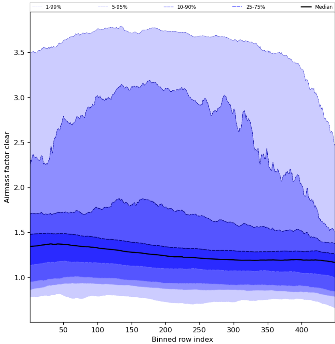
Figure 56: Along track statistics of “Airmass factor clear” for 2023-09-15 to 2023-09-16
