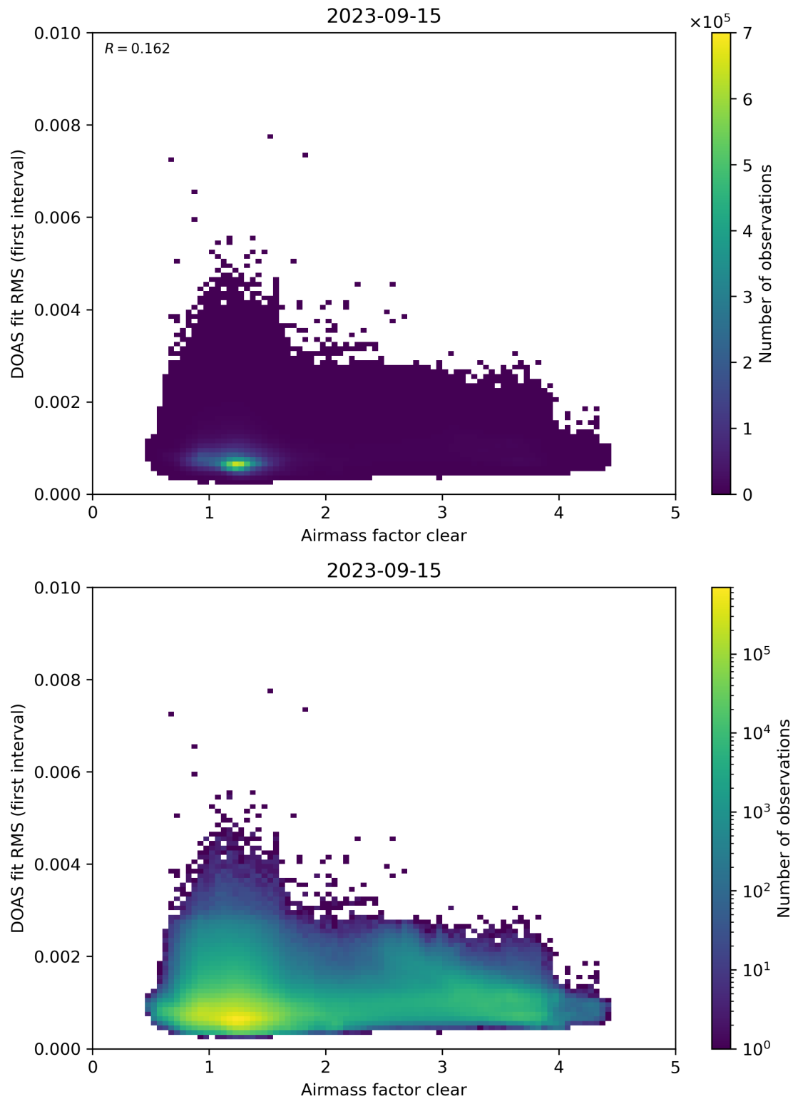
Figure 71: Scatter density plot of “Airmass factor clear” against “DOAS fit RMS (first interval)” for 2023-09-15 to 2023-09-16.
