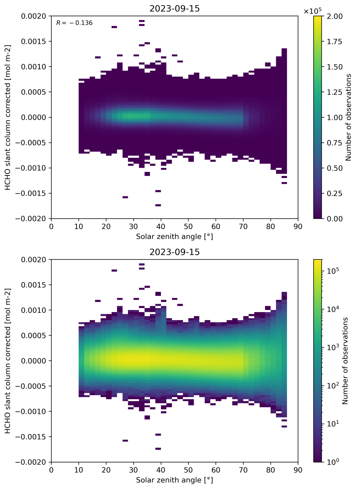
Figure 171: Scatter density plot of “Solar zenith angle” against “HCHO slant column corrected” for 2023-09-15 to 2023-09-16.
