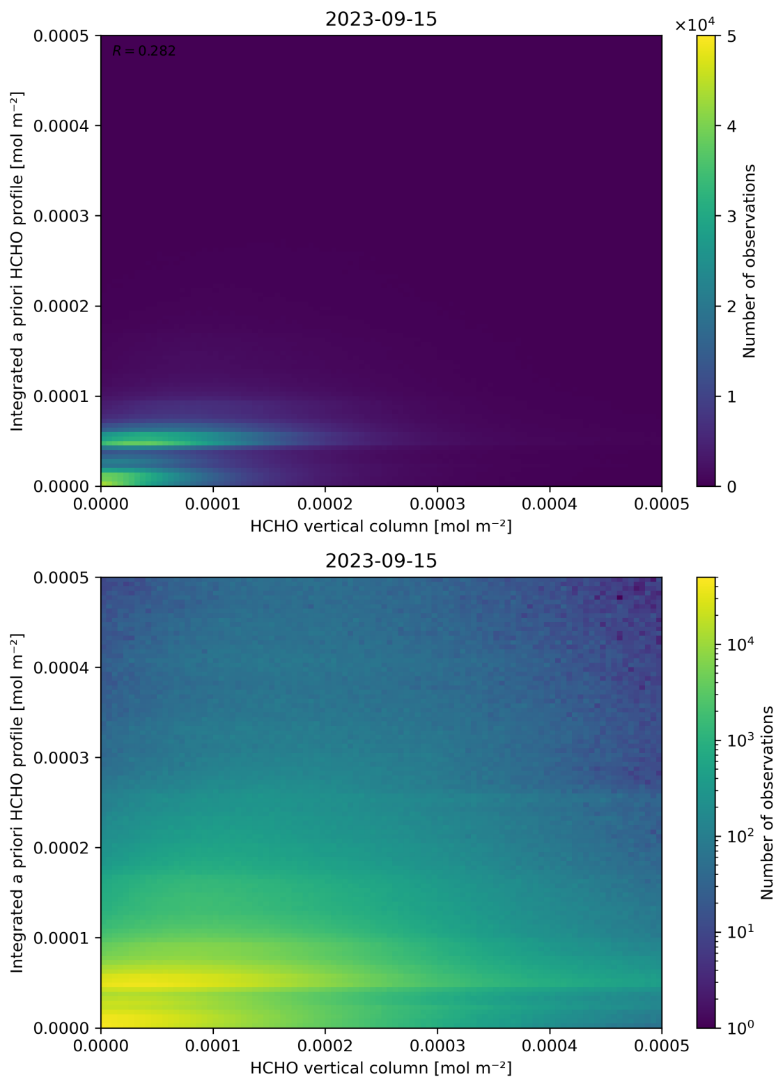
Figure 135: Scatter density plot of “HCHO vertical column” against “Integrated a priori HCHO profile” for 2023-09-15 to 2023-09-16.
