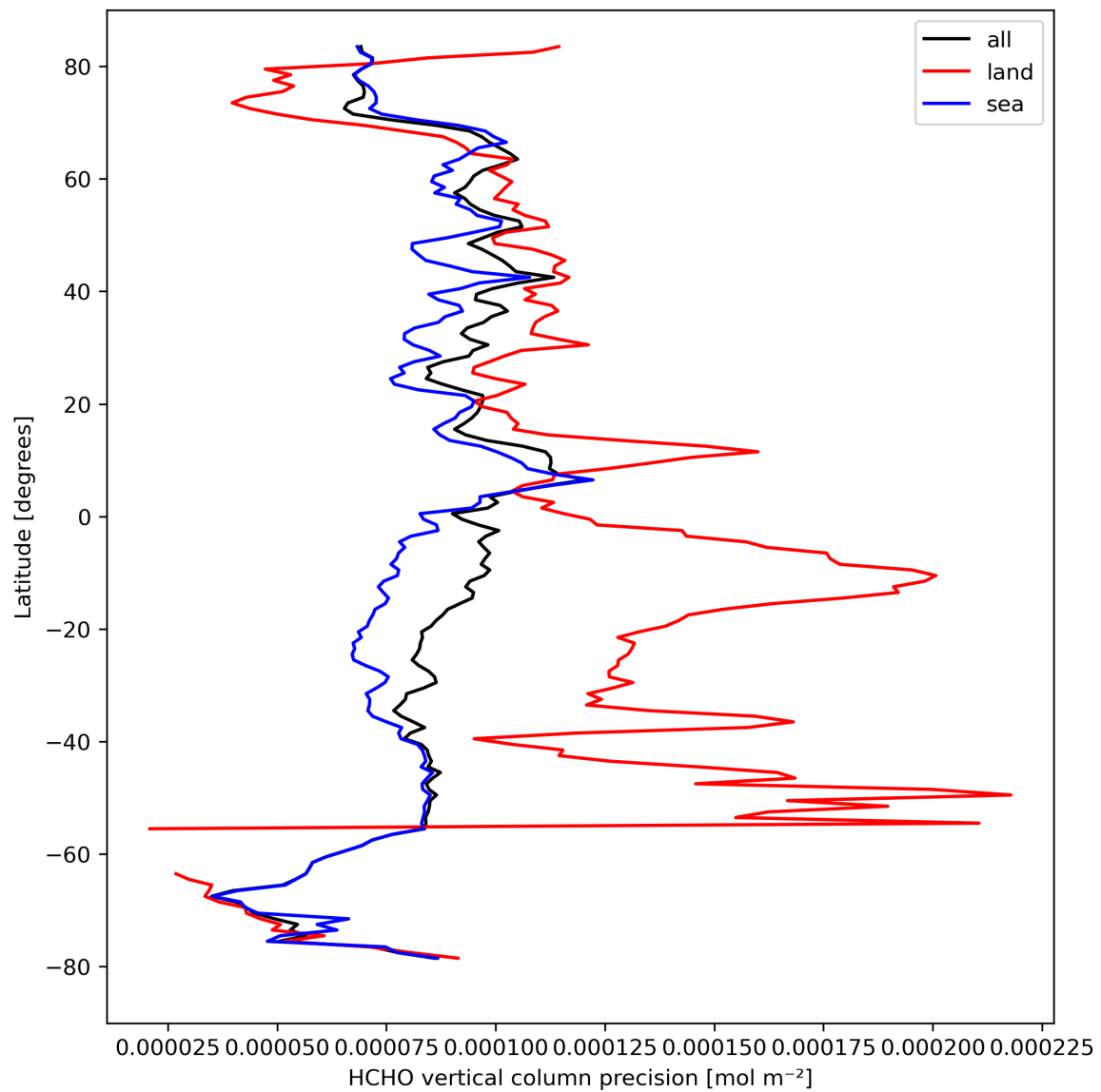
Figure 22: Zonal average of “HCHO vertical column precision” for 2023-09-15 to 2023-09-16.
