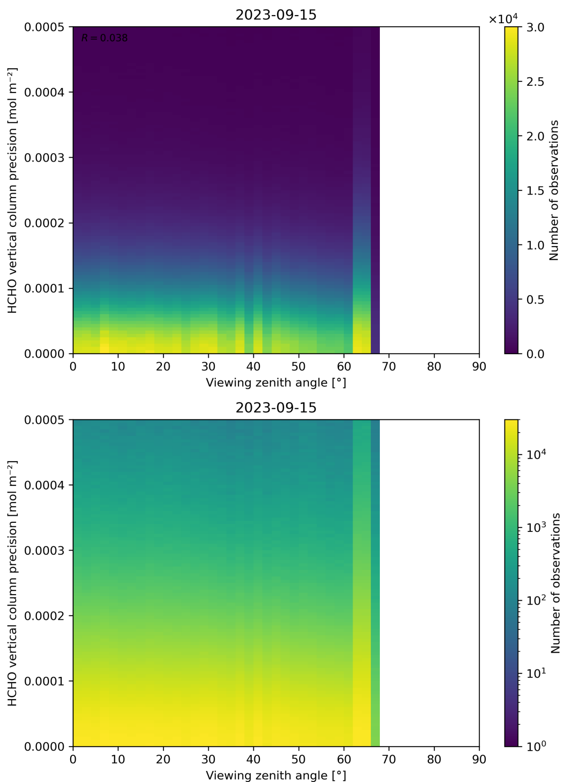
Figure 194: Scatter density plot of “Viewing zenith angle” against “HCHO vertical column precision” for 2023-09-15 to 2023-09-16.
