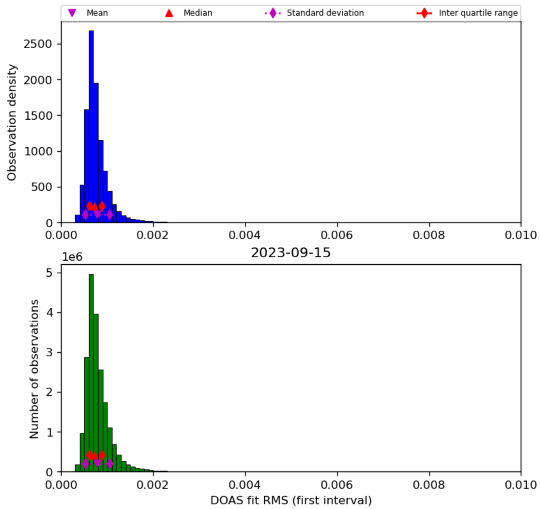
Figure 46: Histogram of “DOAS fit RMS (first interval)” for 2023-09-15 to 2023-09-16
