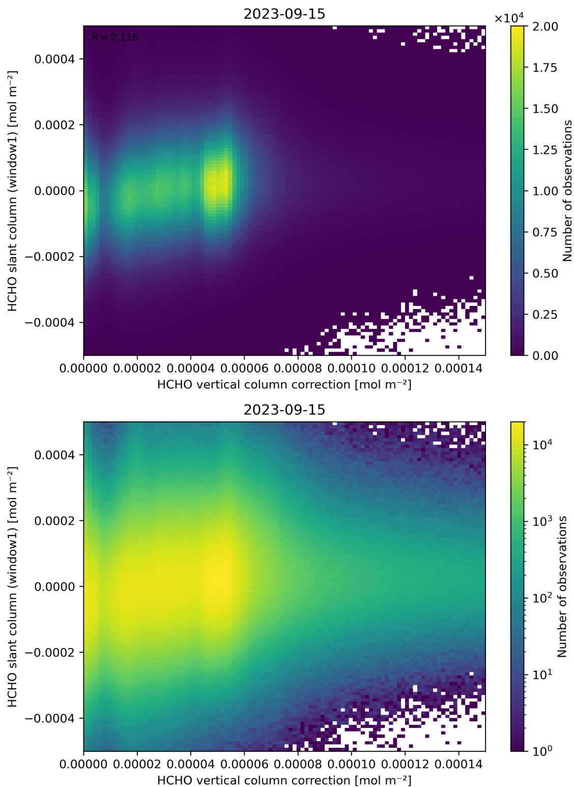
Figure 118: Scatter density plot of “HCHO vertical column correction” against “HCHO slant column (window1)” for 2023-09-15 to 2023-09-16.
