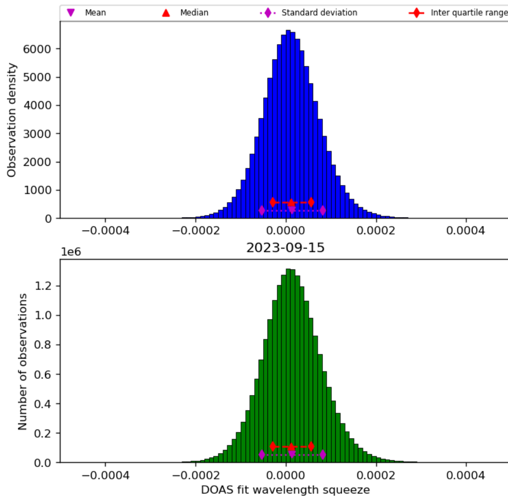
Figure 45: Histogram of “DOAS fit wavelength squeeze” for 2023-09-15 to 2023-09-16
