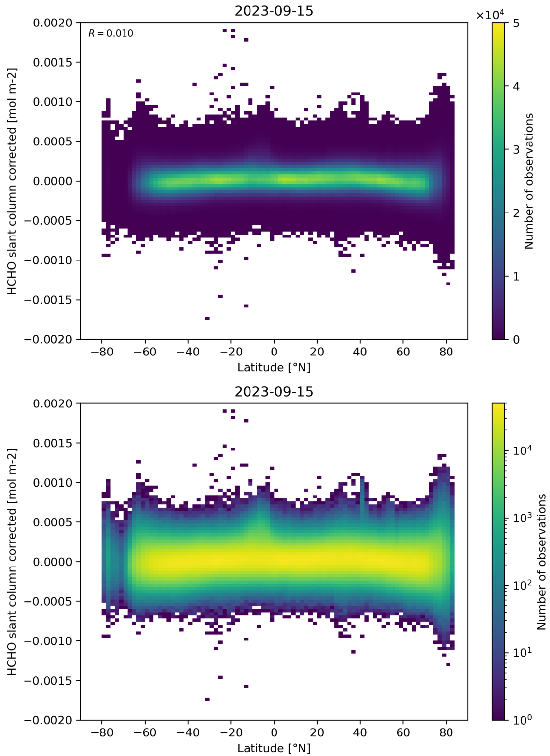
Figure 157: Scatter density plot of “Latitude” against “HCHO slant column corrected” for 2023-09-15 to 2023-09-16.
