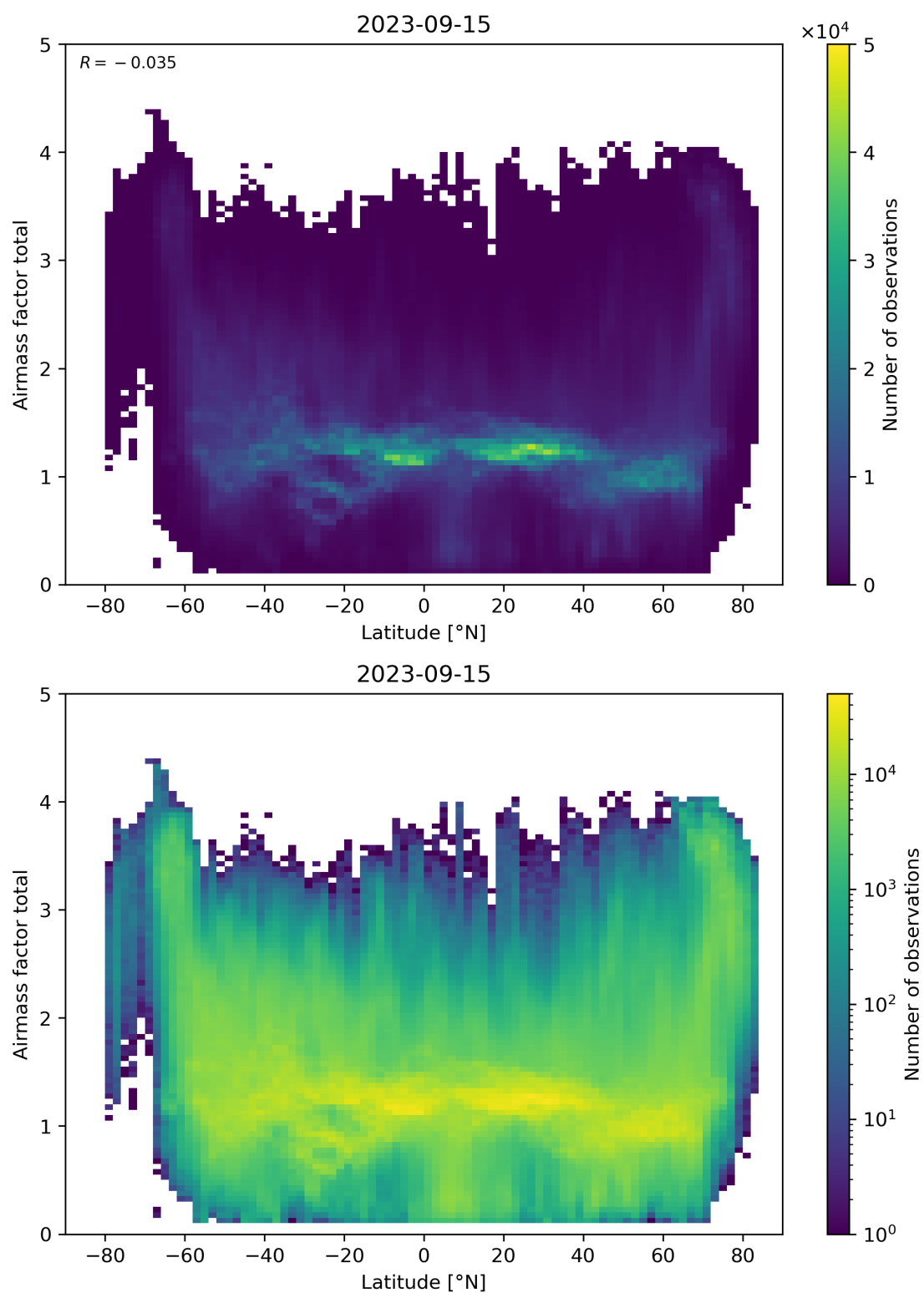
Figure 161: Scatter density plot of “Latitude” against “Airmass factor total” for 2023-09-15 to 2023-09-16.
