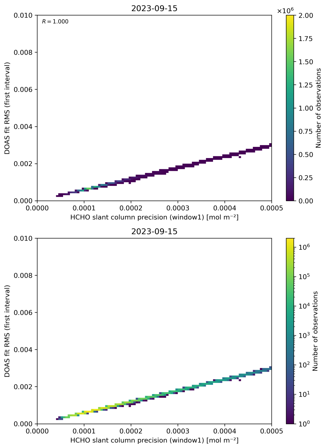
Figure 88: Scatter density plot of “HCHO slant column precision (window1)” against “DOAS fit RMS (first interval)” for 2023-09-15 to 2023-09-16.
