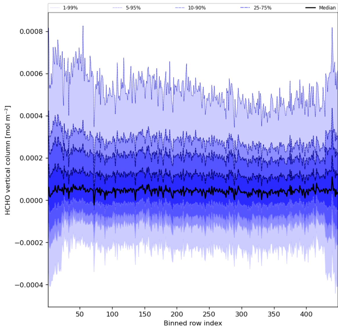
Figure 49: Along track statistics of “HCHO vertical column” for 2023-09-15 to 2023-09-16
