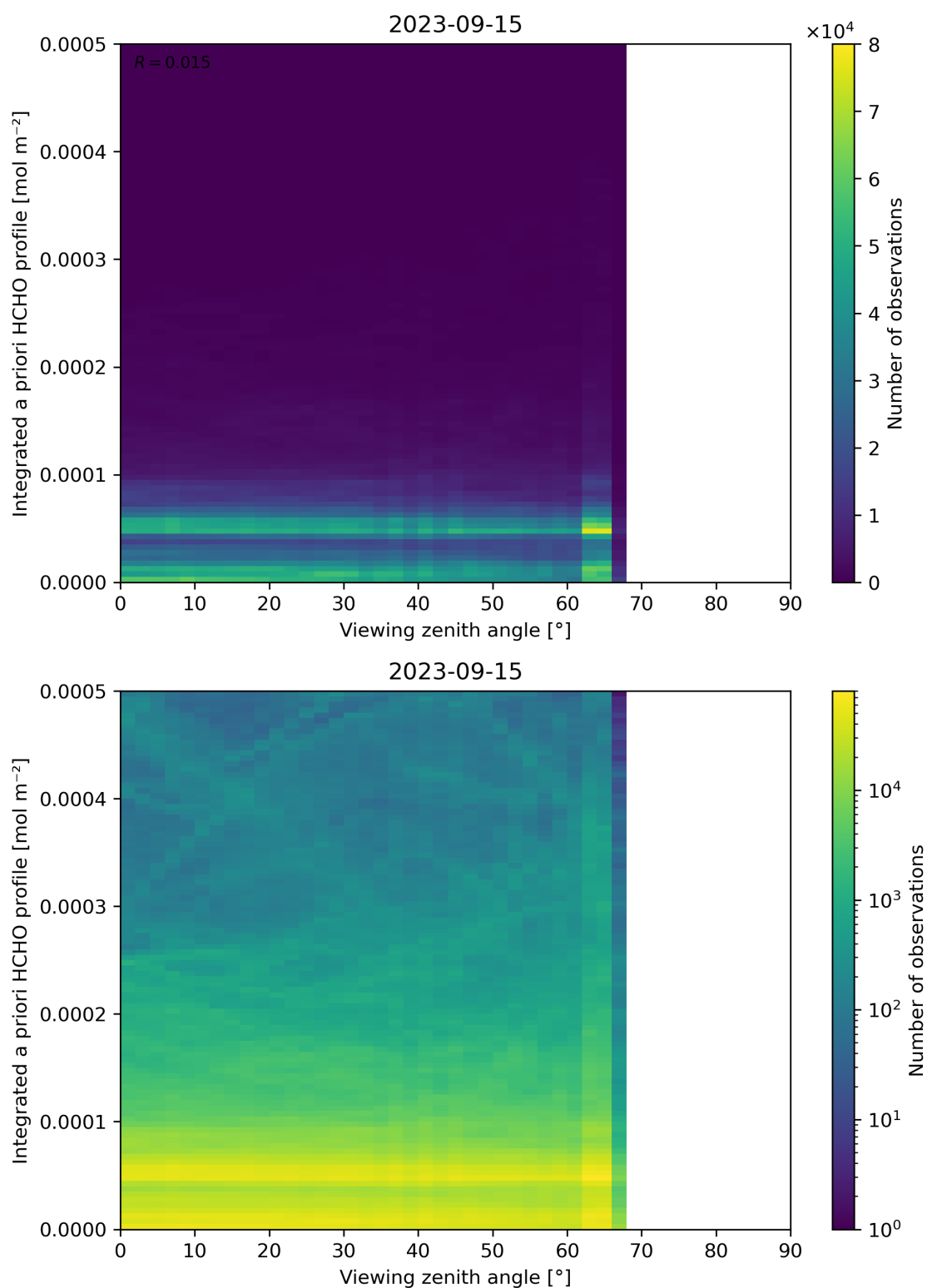
Figure 195: Scatter density plot of “Viewing zenith angle” against “Integrated a priori HCHO profile” for 2023-09-15 to 2023-09-16.
