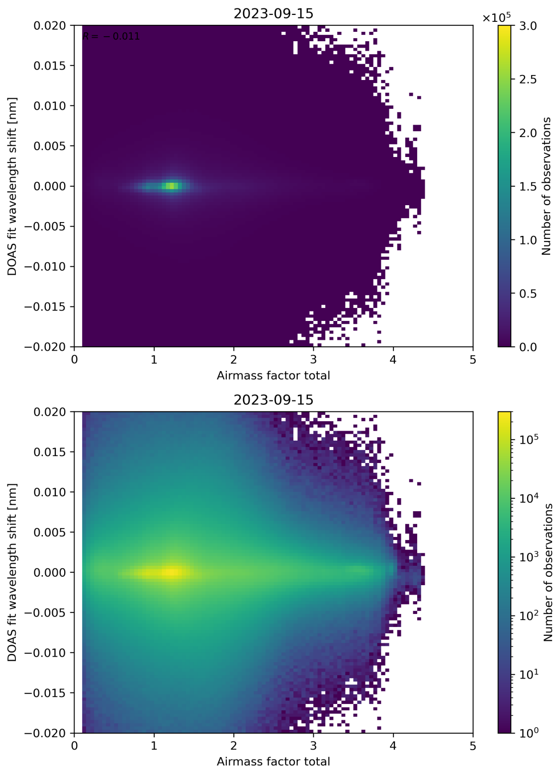
Figure 98: Scatter density plot of “Airmass factor total” against “DOAS fit wavelength shift” for 2023-09-15 to 2023-09-16.
