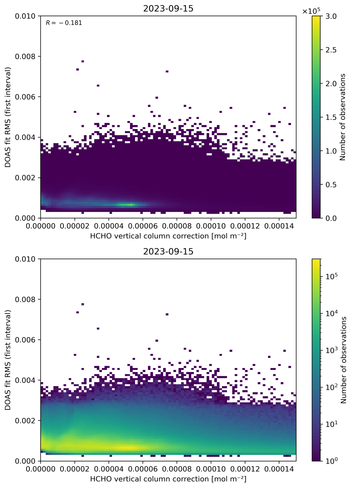
Figure 112: Scatter density plot of “HCHO vertical column correction” against “DOAS fit RMS (first interval)” for 2023-09-15 to 2023-09-16.
