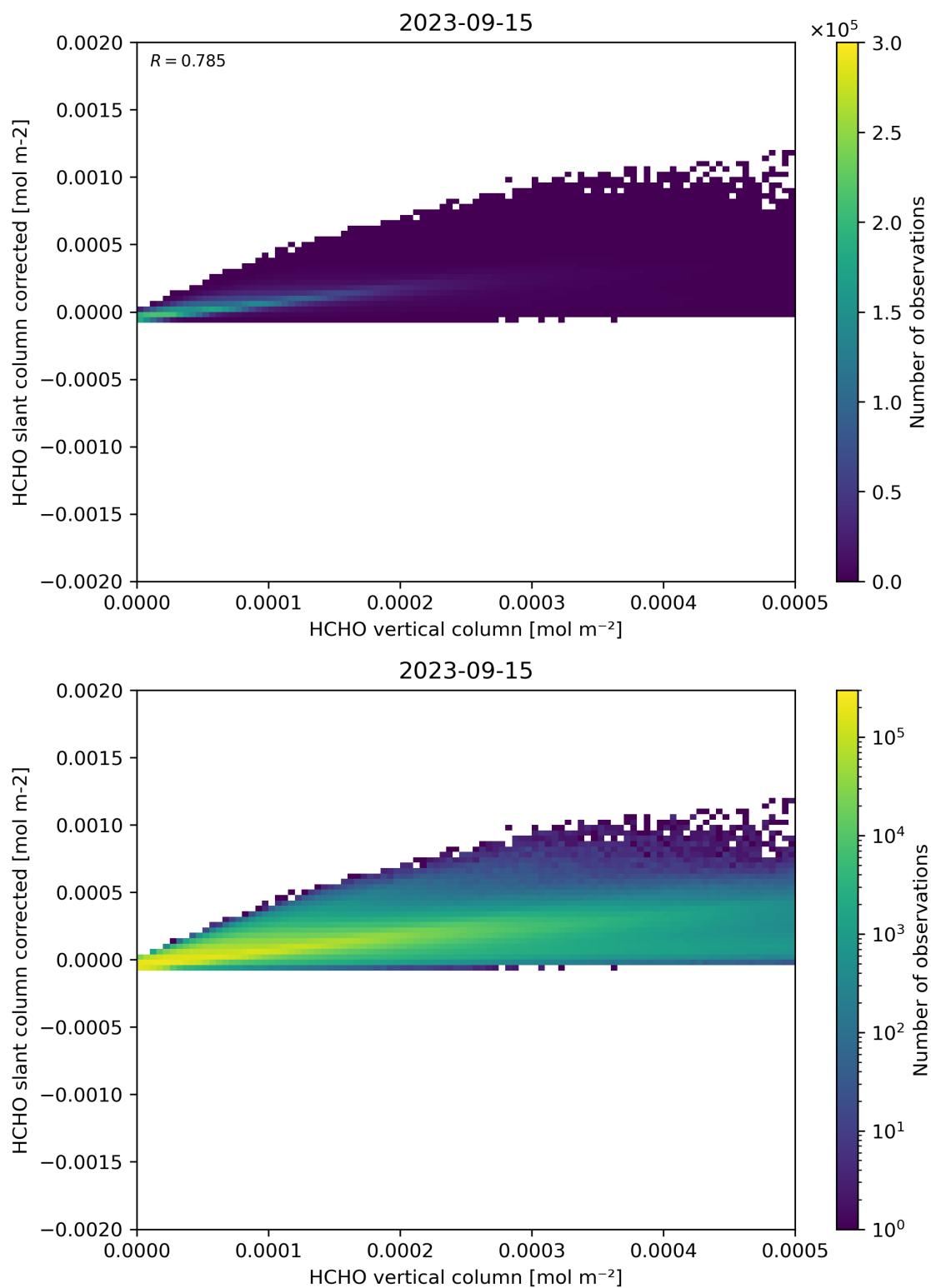
Figure 127: Scatter density plot of “HCHO vertical column” against “HCHO slant column corrected” for 2023-09-15 to 2023-09-16.
