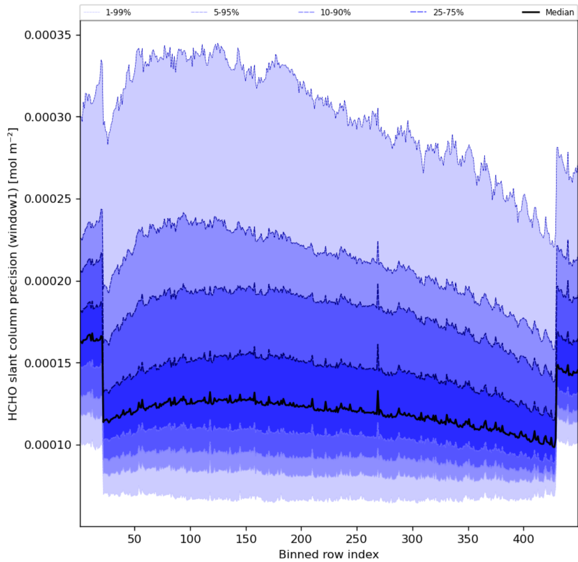
Figure 53: Along track statistics of “HCHO slant column precision (window1)” for 2023-09-15 to 2023-09-16
