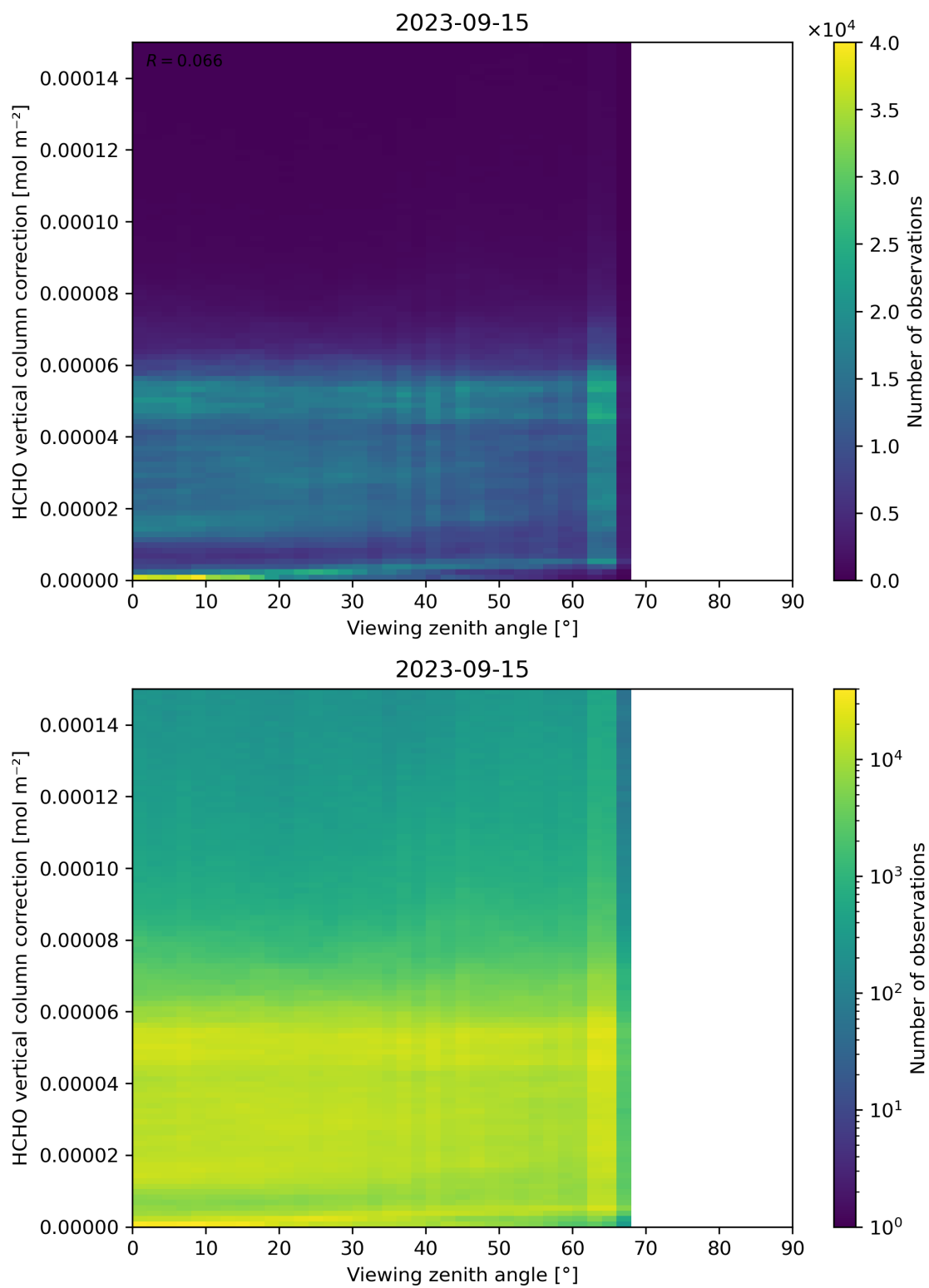
Figure 193: Scatter density plot of “Viewing zenith angle” against “HCHO vertical column correction” for 2023-09-15 to 2023-09-16.
