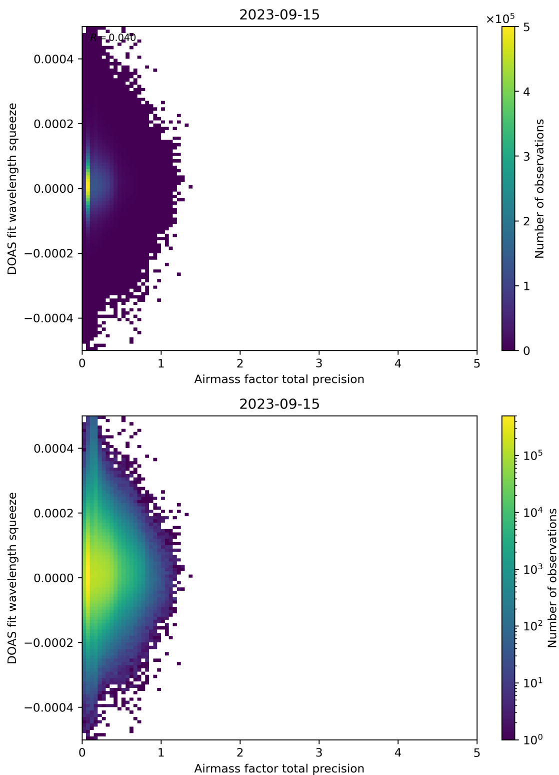
Figure 107: Scatter density plot of “Airmass factor total precision” against “DOAS fit wavelength squeeze” for 2023-09-15 to 2023-09-16.
