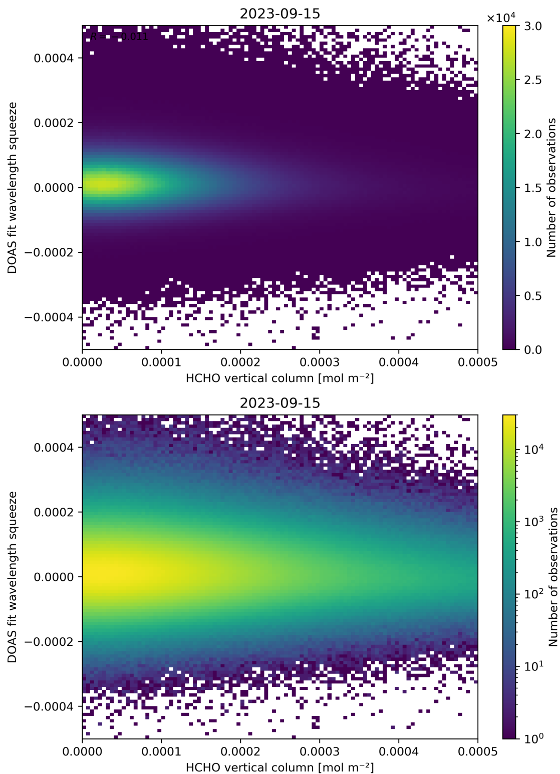
Figure 125: Scatter density plot of “HCHO vertical column” against “DOAS fit wavelength squeeze” for 2023-09-15 to 2023-09-16.
