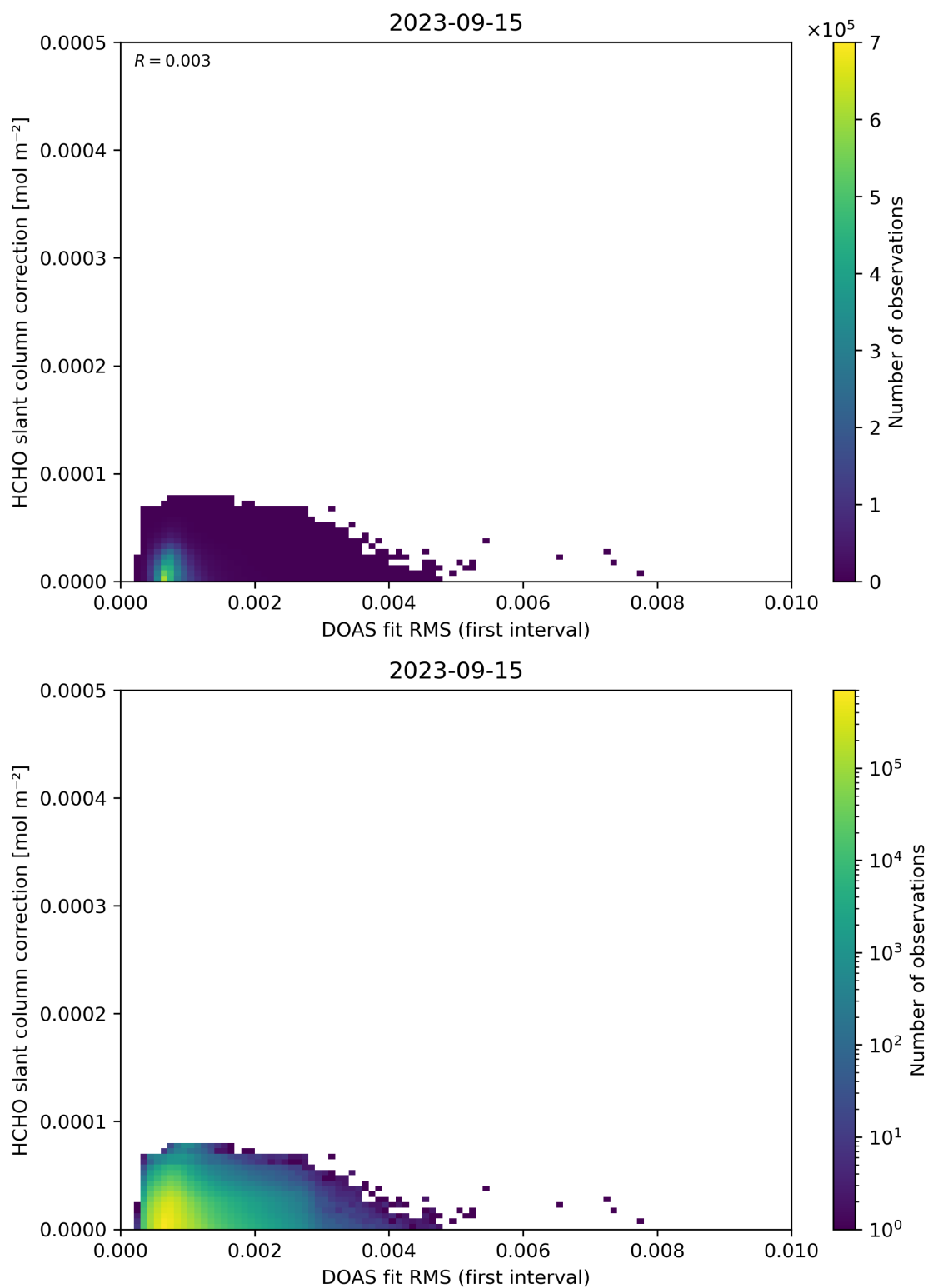
Figure 63: Scatter density plot of “DOAS fit RMS (first interval)” against “HCHO slant column correction” for 2023-09-15 to 2023-09-16.
