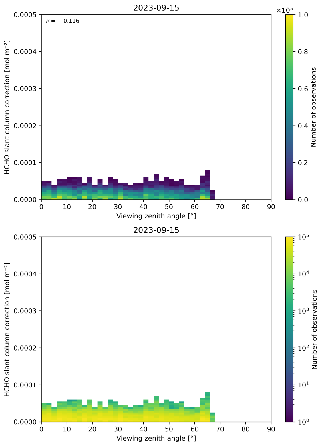
Figure 187: Scatter density plot of “Viewing zenith angle” against “HCHO slant column correction” for 2023-09-15 to 2023-09-16.
