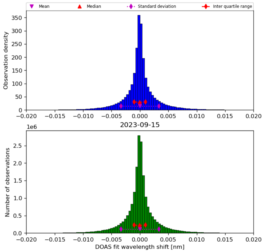
Figure 44: Histogram of “DOAS fit wavelength shift” for 2023-09-15 to 2023-09-16
