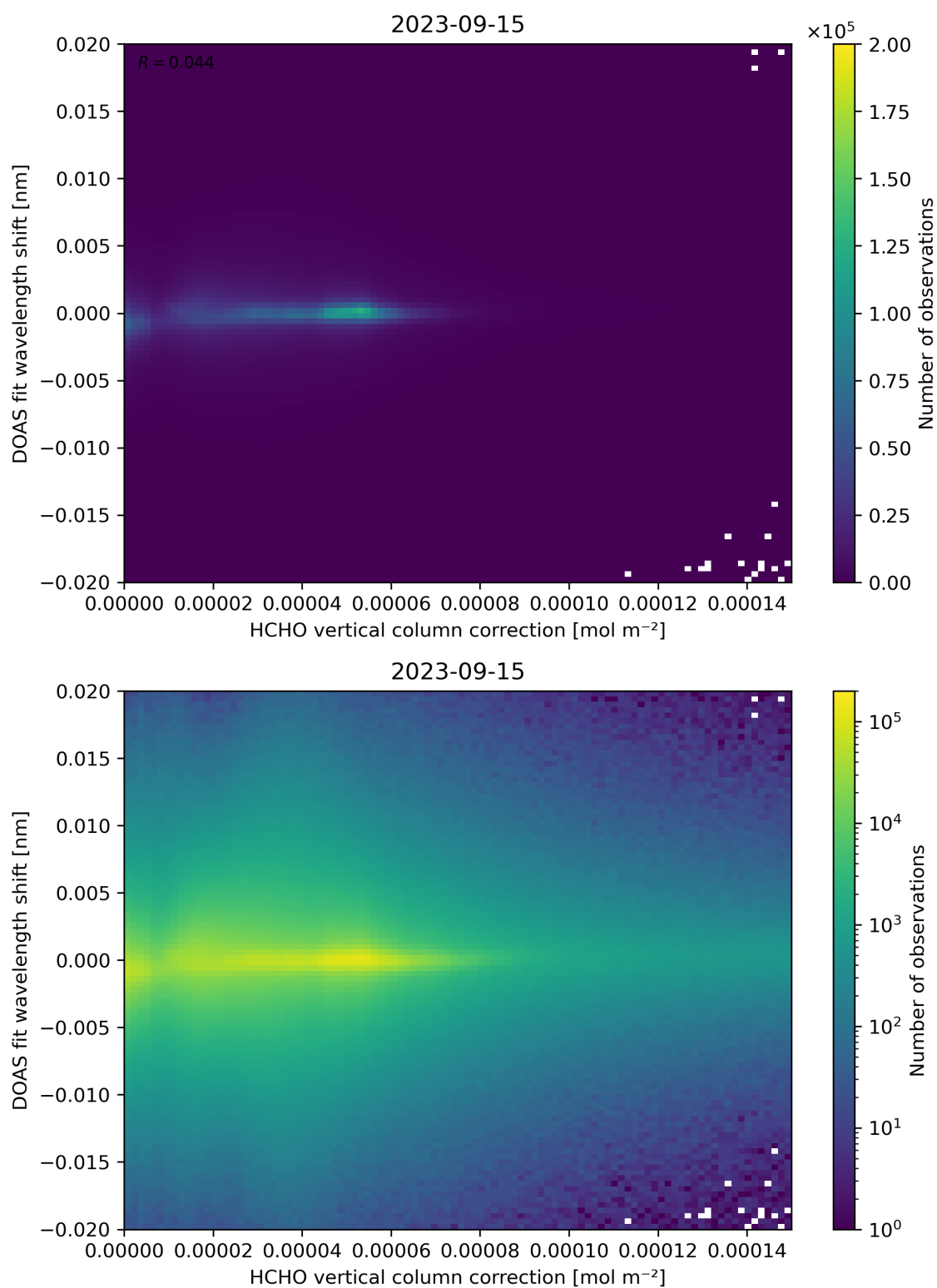
Figure 113: Scatter density plot of “HCHO vertical column correction” against “DOAS fit wavelength shift” for 2023-09-15 to 2023-09-16.
