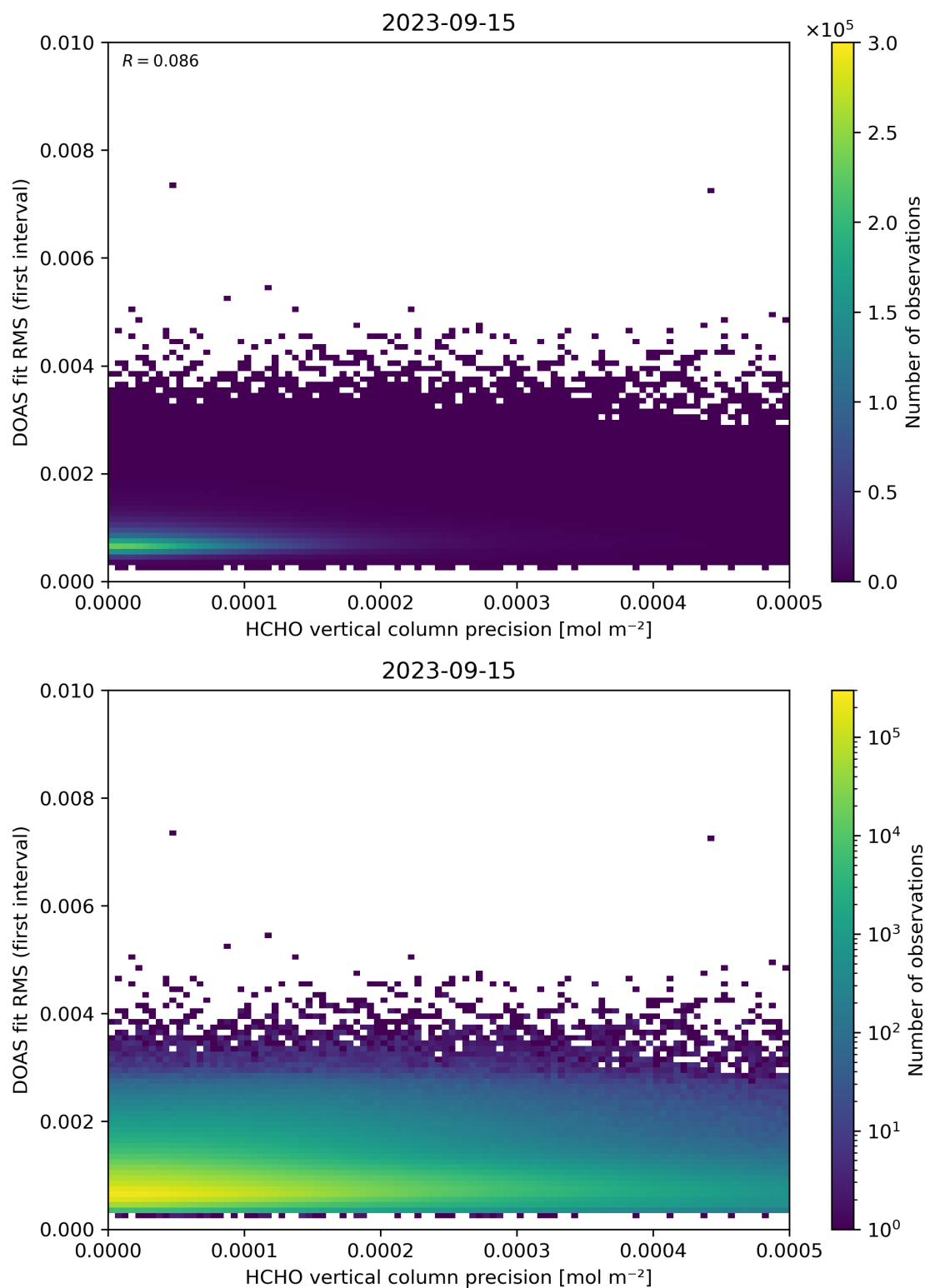
Figure 136: Scatter density plot of “HCHO vertical column precision” against “DOAS fit RMS (first interval)” for 2023-09-15 to 2023-09-16.
