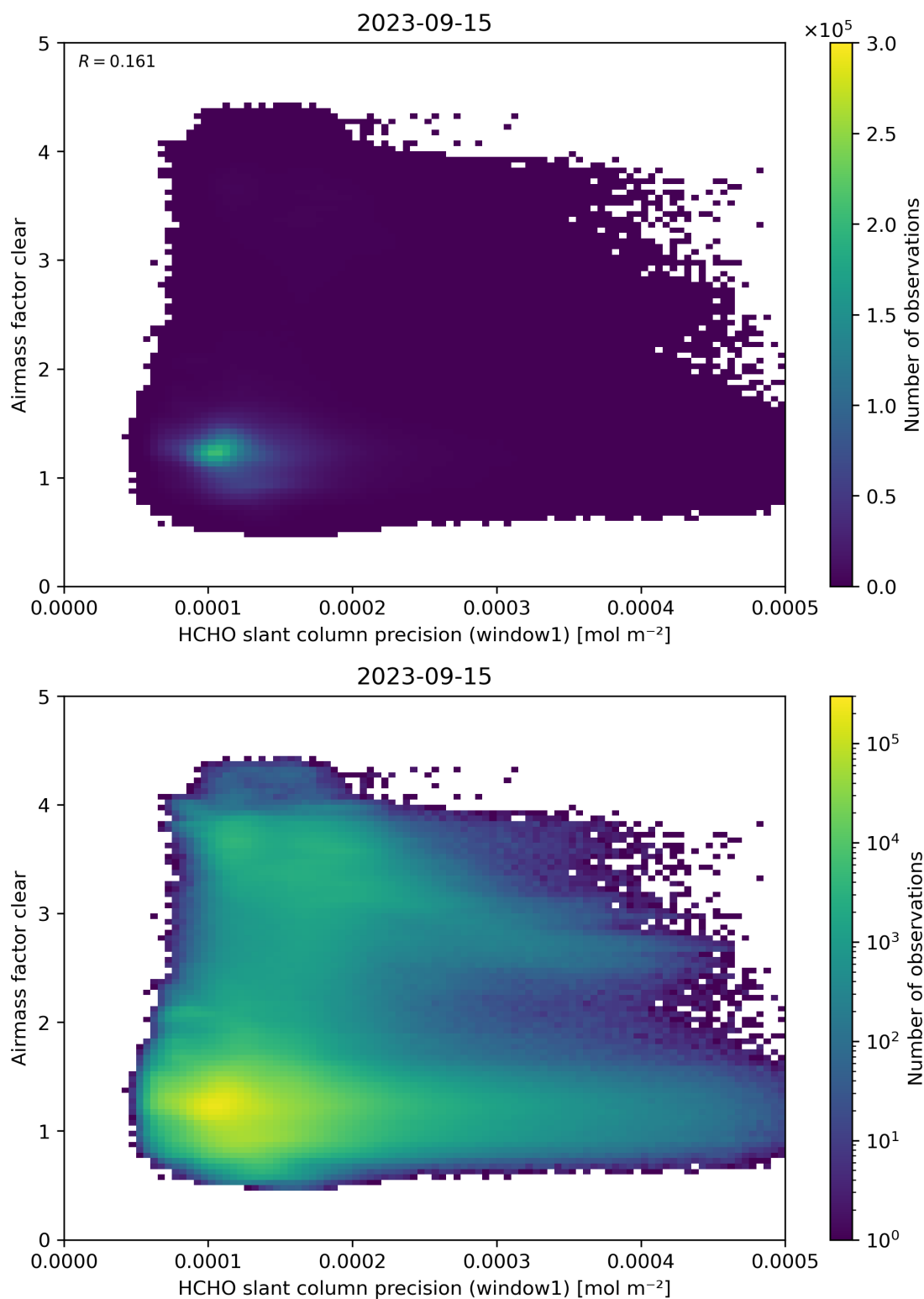
Figure 91: Scatter density plot of “HCHO slant column precision (window1)” against “Airmass factor clear” for 2023-09-15 to 2023-09-16.
