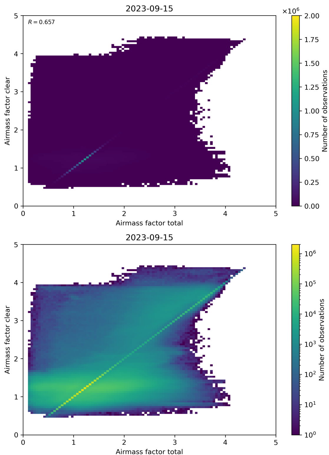
Figure 100: Scatter density plot of “Airmass factor total” against “Airmass factor clear” for 2023-09-15 to 2023-09-16.
