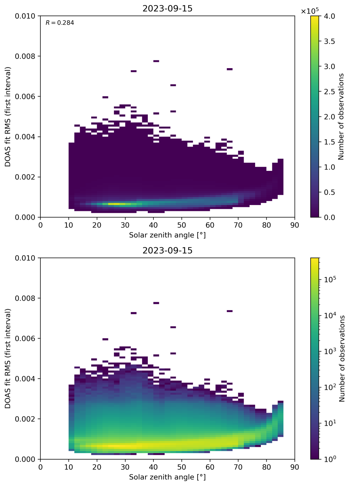
Figure 167: Scatter density plot of “Solar zenith angle” against “DOAS fit RMS (first interval)” for 2023-09-15 to 2023-09-16.
