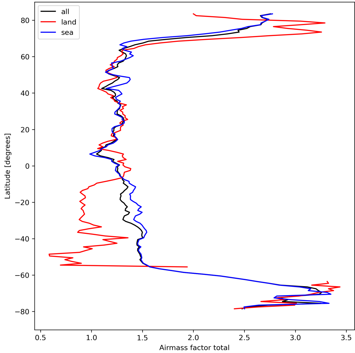
Figure 26: Zonal average of “Airmass factor total” for 2023-09-15 to 2023-09-16.
