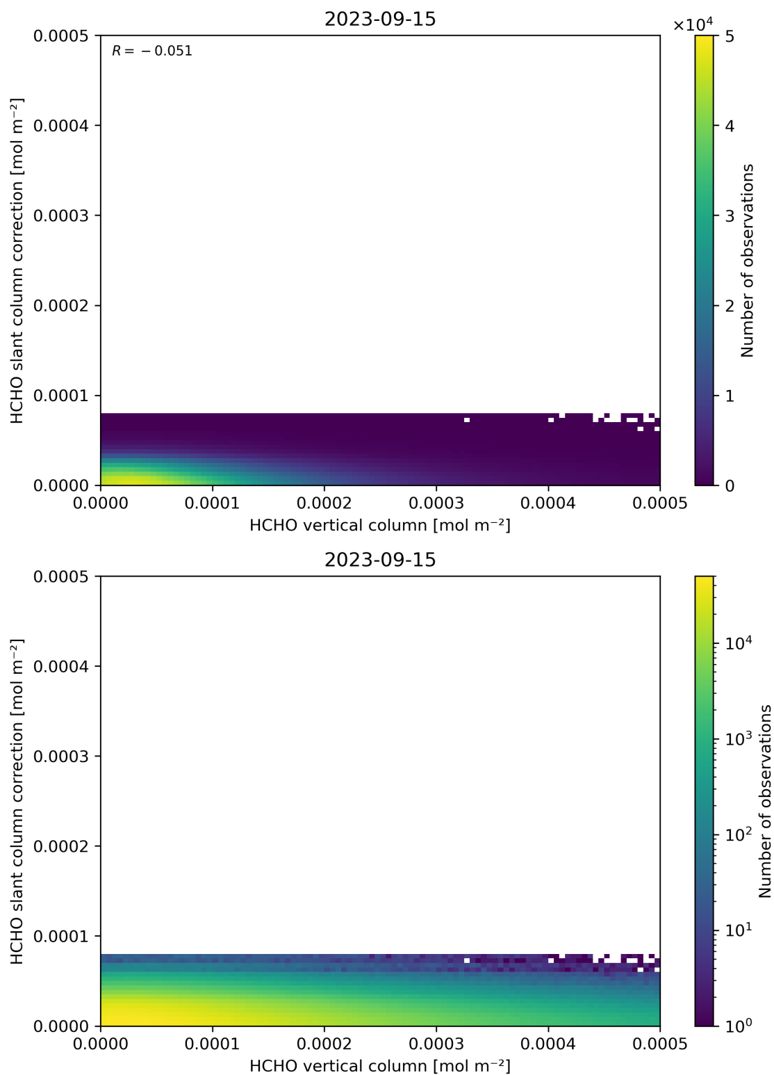
Figure 128: Scatter density plot of “HCHO vertical column” against “HCHO slant column correction” for 2023-09-15 to 2023-09-16.
