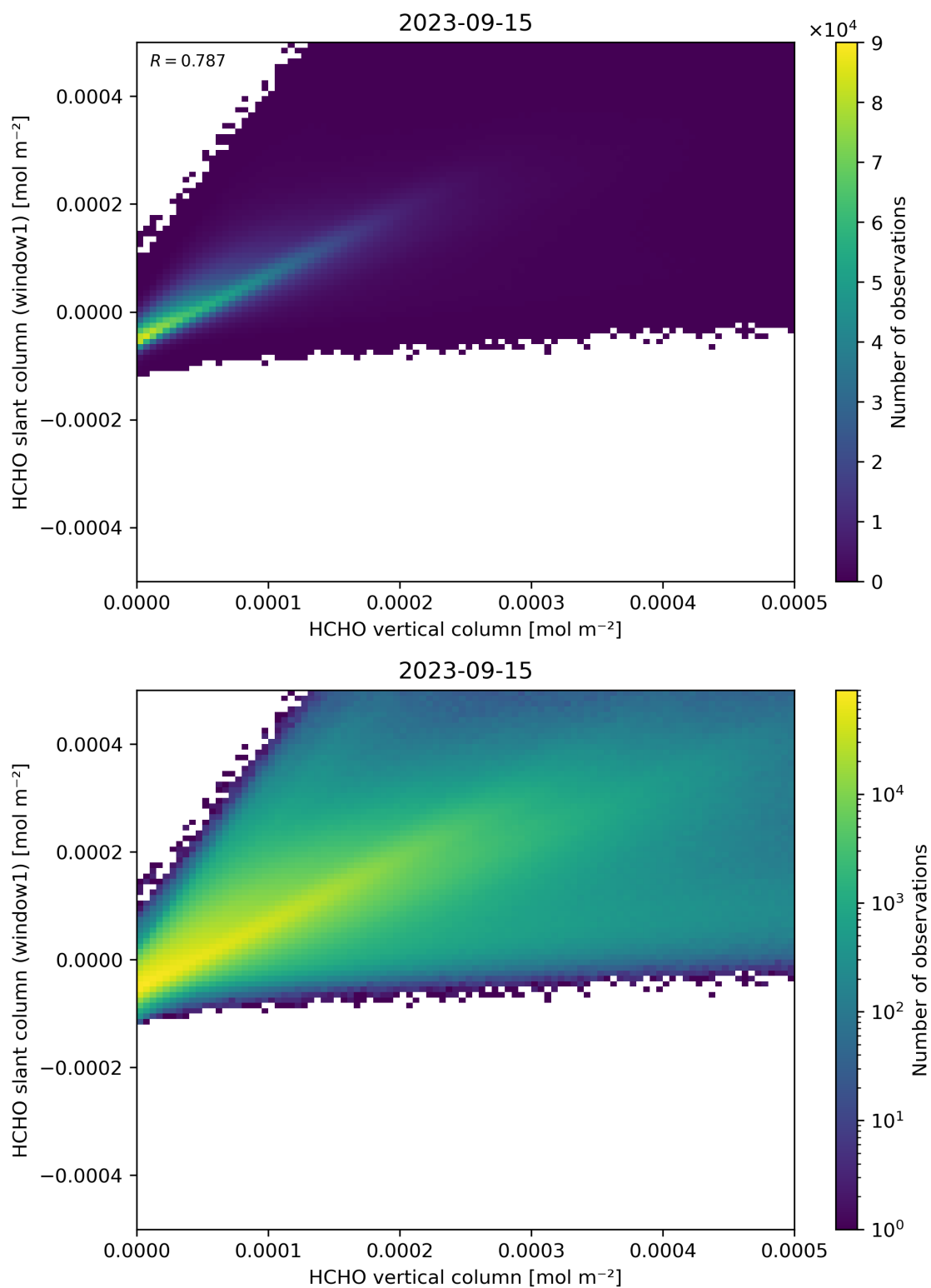
Figure 129: Scatter density plot of “HCHO vertical column” against “HCHO slant column (window1)” for 2023-09-15 to 2023-09-16.
