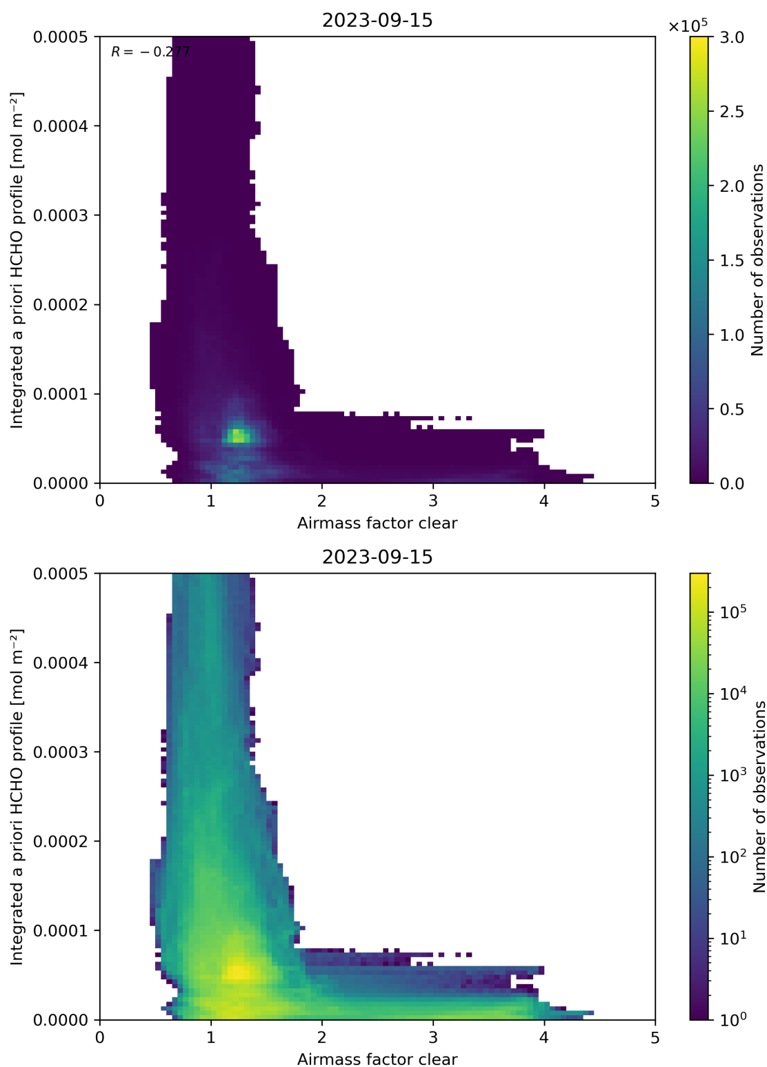
Figure 76: Scatter density plot of “Airmass factor clear” against “Integrated a priori HCHO profile” for 2023-09-15 to 2023-09-16.
