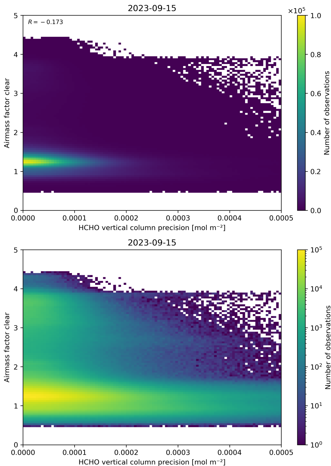
Figure 139: Scatter density plot of “HCHO vertical column precision” against “Airmass factor clear” for 2023-09-15 to 2023-09-16.
