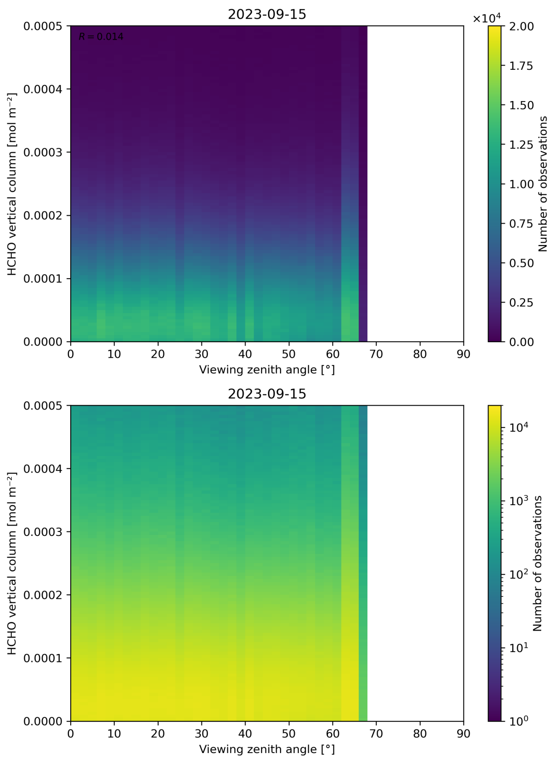
Figure 192: Scatter density plot of “Viewing zenith angle” against “HCHO vertical column” for 2023-09-15 to 2023-09-16.
