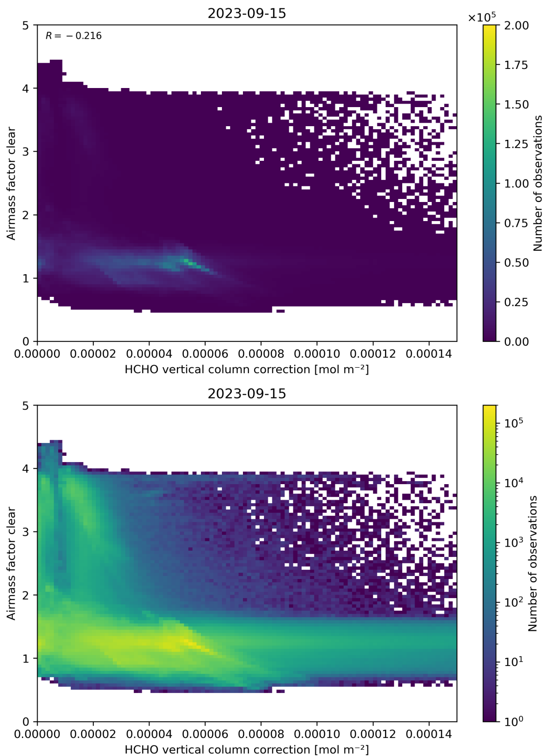
Figure 115: Scatter density plot of “HCHO vertical column correction” against “Airmass factor clear” for 2023-09-15 to 2023-09-16.
