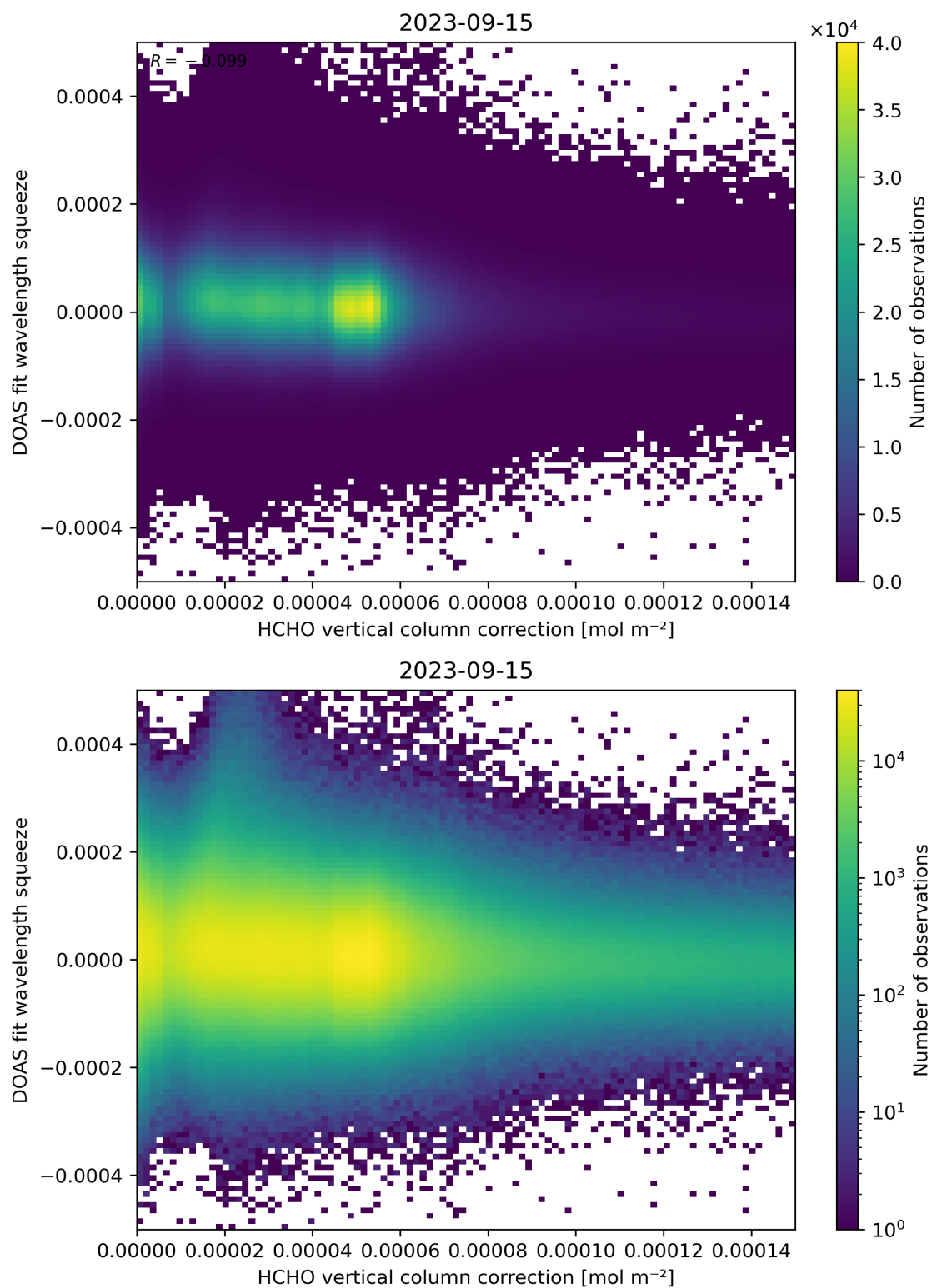
Figure 114: Scatter density plot of “HCHO vertical column correction” against “DOAS fit wavelength squeeze” for 2023-09-15 to 2023-09-16.
