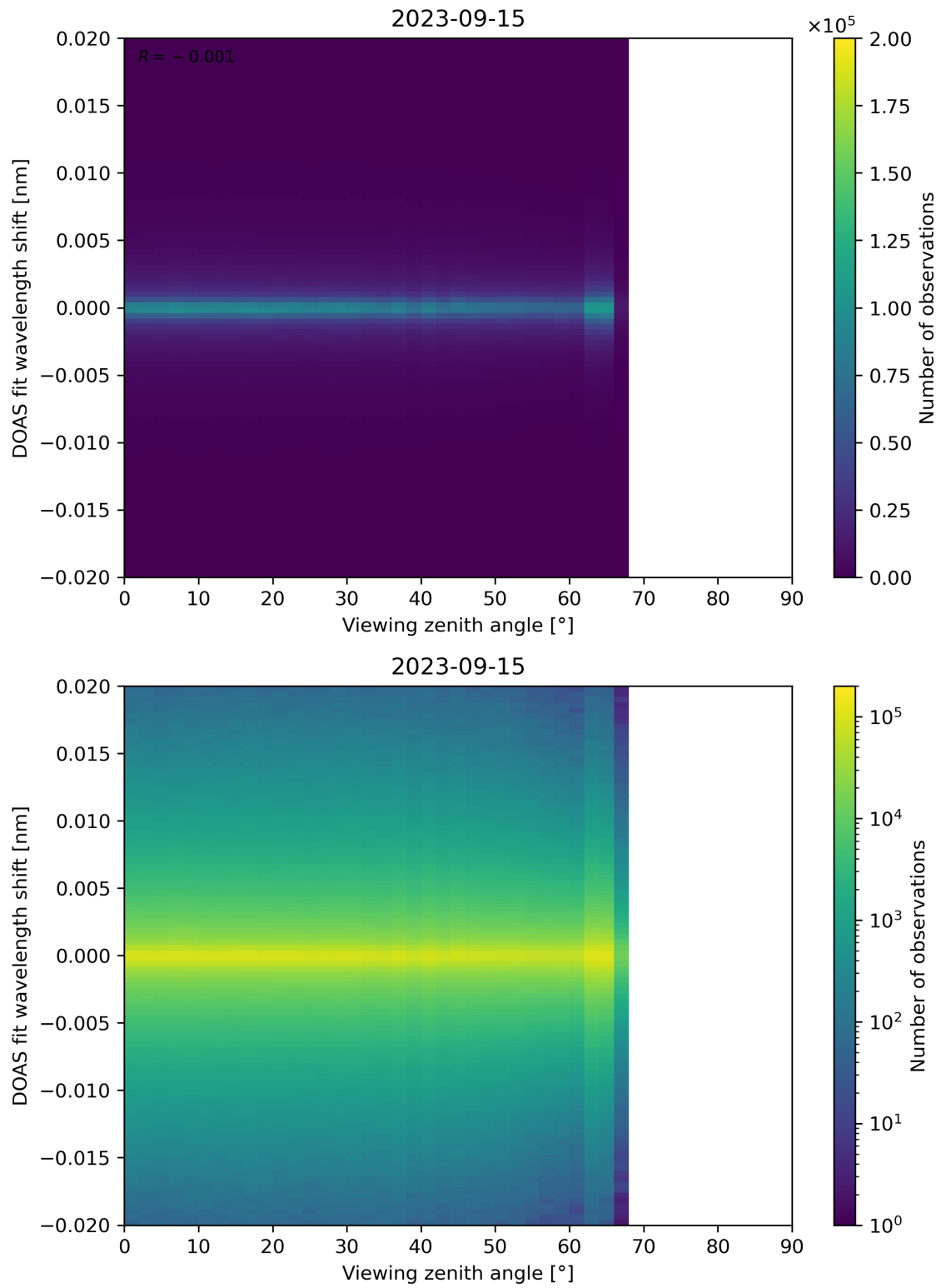
Figure 183: Scatter density plot of “Viewing zenith angle” against “DOAS fit wavelength shift” for 2023-09-15 to 2023-09-16.
