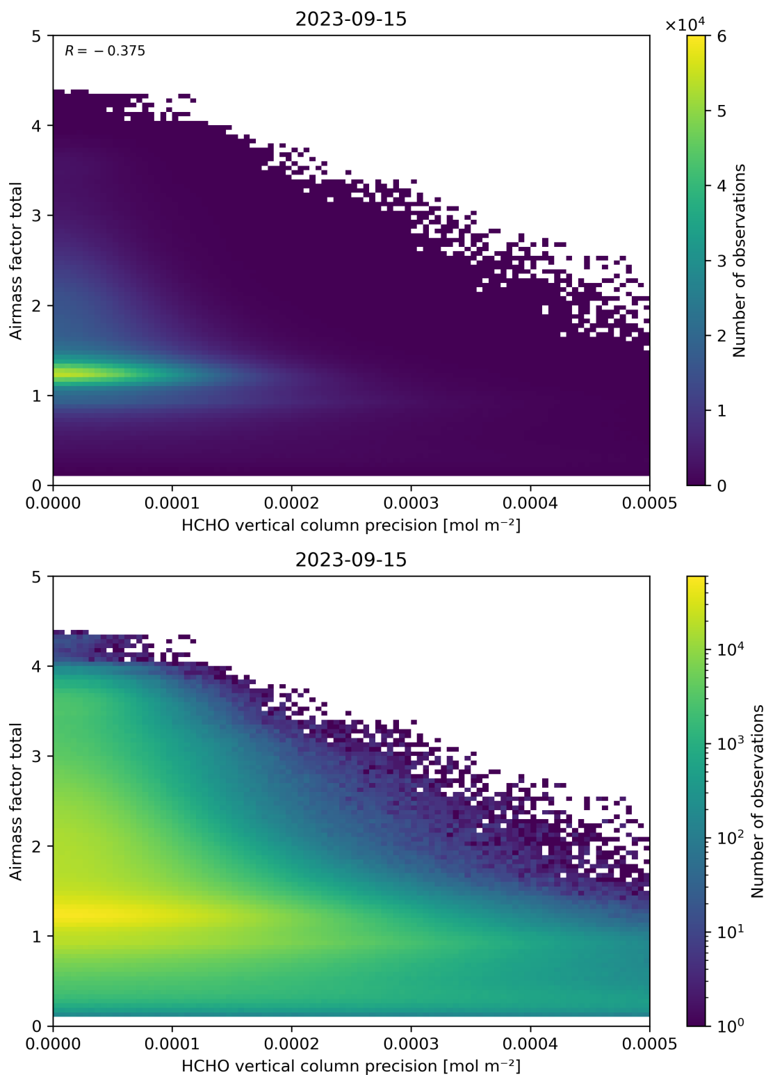
Figure 144: Scatter density plot of “HCHO vertical column precision” against “Airmass factor total” for 2023-09-15 to 2023-09-16.
