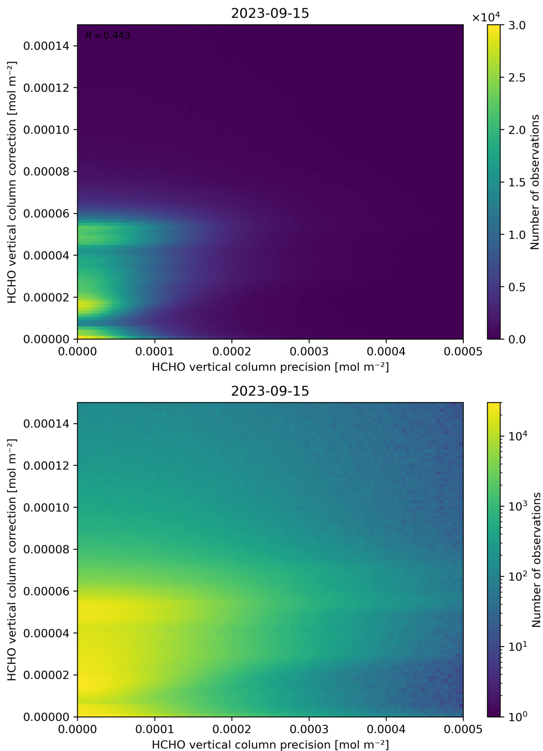
Figure 146: Scatter density plot of “HCHO vertical column precision” against “HCHO vertical column correction” for 2023-09-15 to 2023-09-16.
