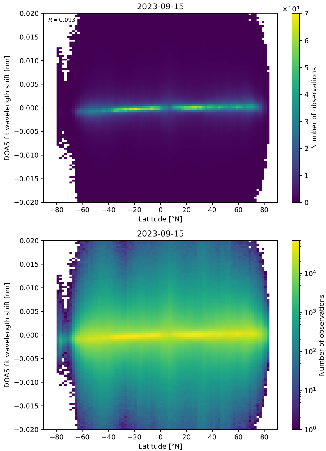
Figure 154: Scatter density plot of “Latitude” against “DOAS fit wavelength shift” for 2023-09-15 to 2023-09-16.
