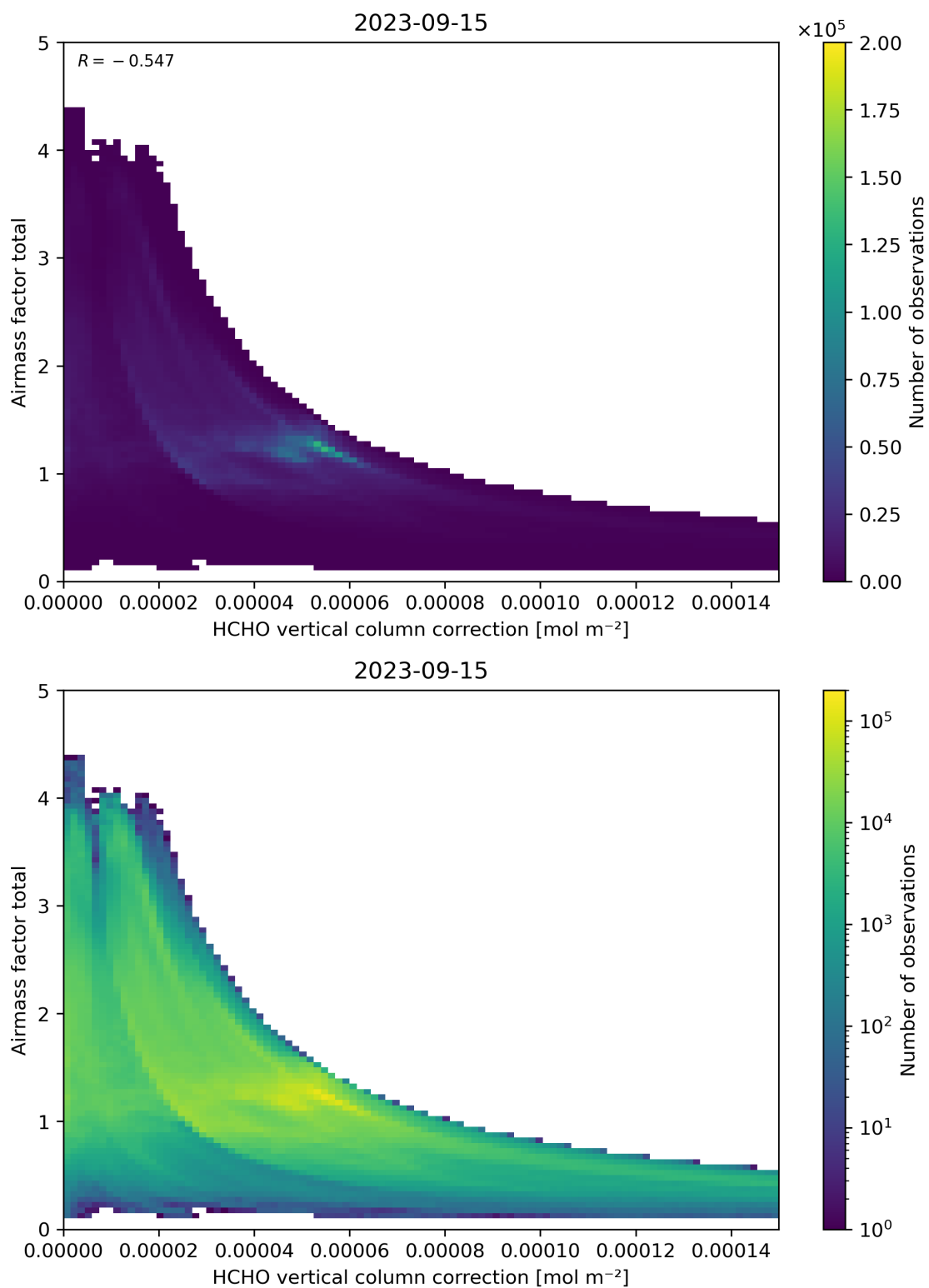
Figure 120: Scatter density plot of “HCHO vertical column correction” against “Airmass factor total” for 2023-09-15 to 2023-09-16.
