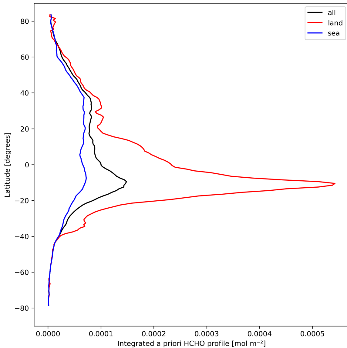
Figure 29: Zonal average of “Integrated a priori HCHO profile” for 2023-09-15 to 2023-09-16.
