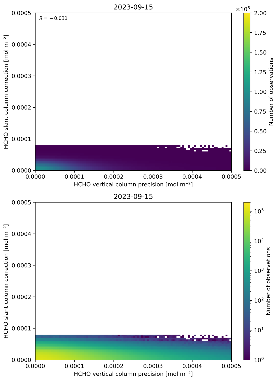
Figure 141: Scatter density plot of “HCHO vertical column precision” against “HCHO slant column correction” for 2023-09-15 to 2023-09-16.
