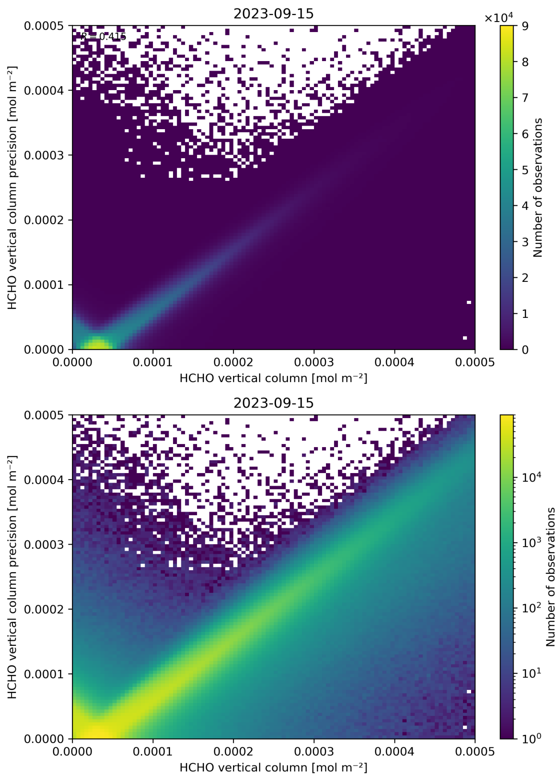
Figure 134: Scatter density plot of “HCHO vertical column” against “HCHO vertical column precision” for 2023-09-15 to 2023-09-16.
