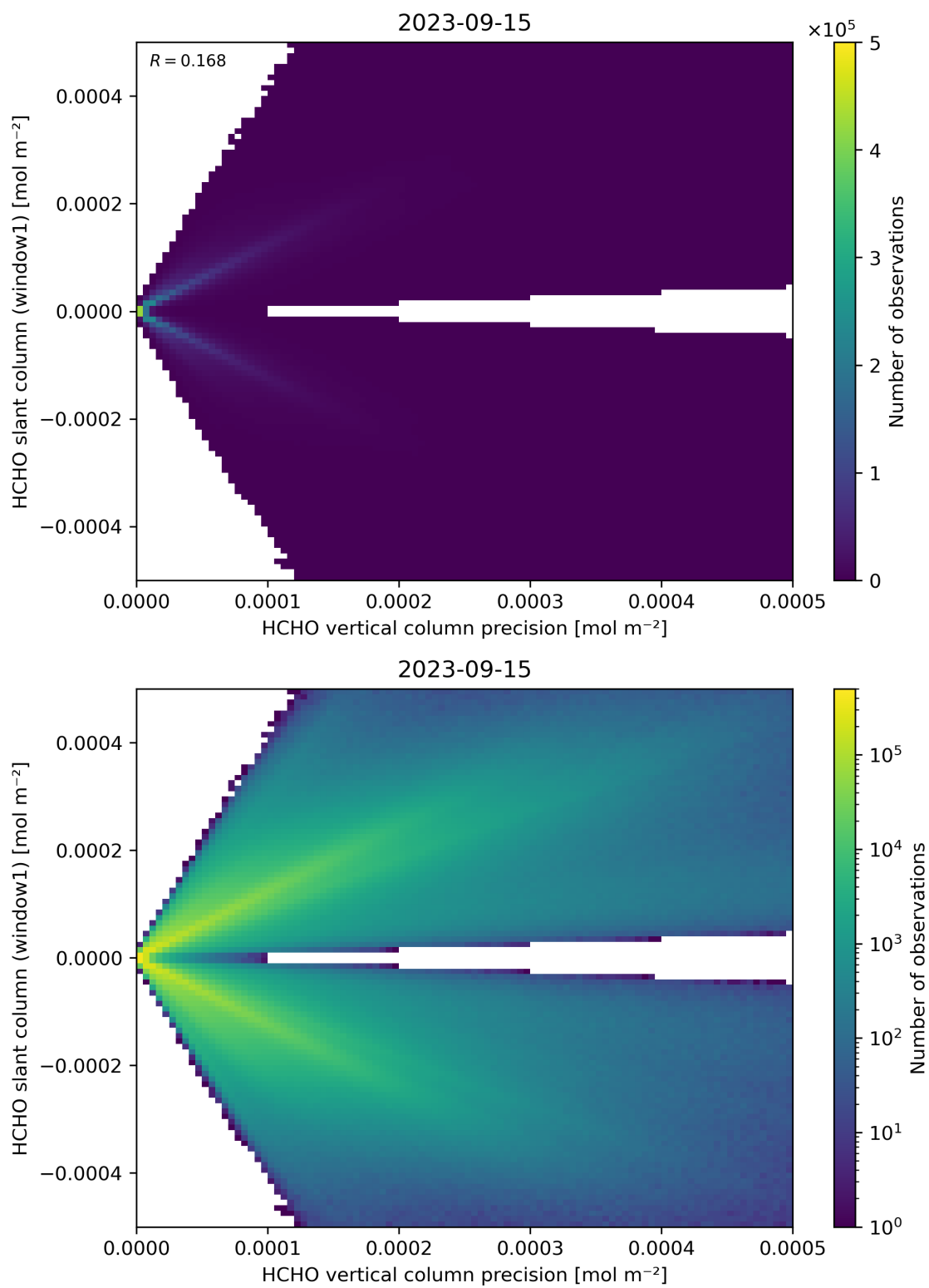
Figure 142: Scatter density plot of “HCHO vertical column precision” against “HCHO slant column (window1)” for 2023-09-15 to 2023-09-16.
