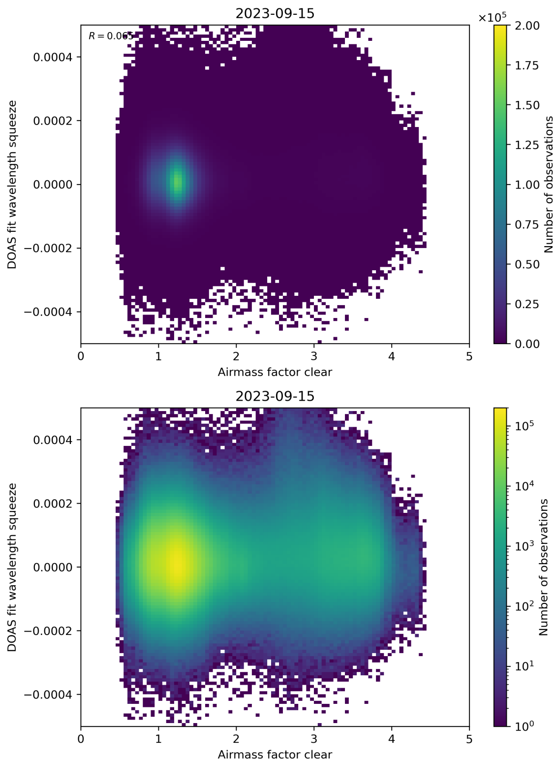
Figure 73: Scatter density plot of “Airmass factor clear” against “DOAS fit wavelength squeeze” for 2023-09-15 to 2023-09-16.
