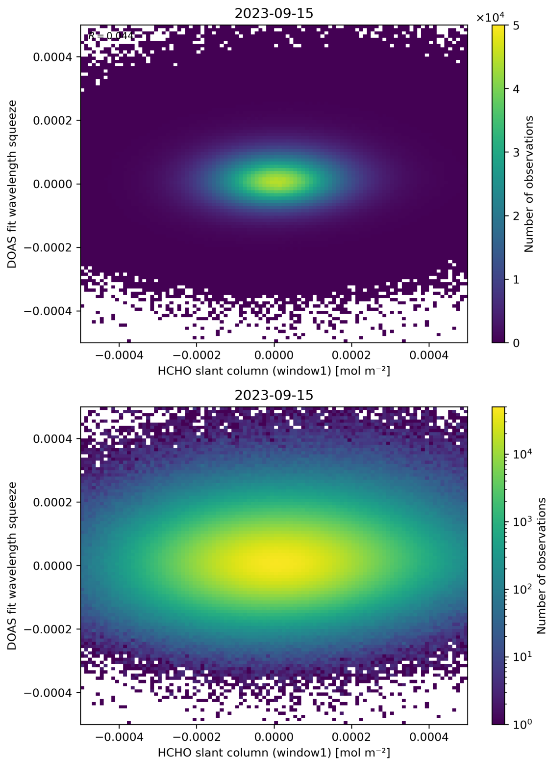
Figure 80: Scatter density plot of “HCHO slant column (window1)” against “DOAS fit wavelength squeeze” for 2023-09-15 to 2023-09-16.
