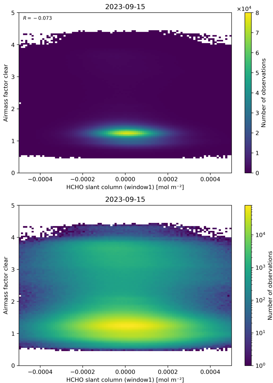
Figure 81: Scatter density plot of “HCHO slant column (window1)” against “Airmass factor clear” for 2023-09-15 to 2023-09-16.
