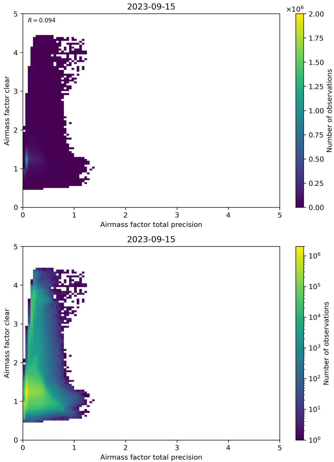
Figure 108: Scatter density plot of “Airmass factor total precision” against “Airmass factor clear” for 2023-09-15 to 2023-09-16.
