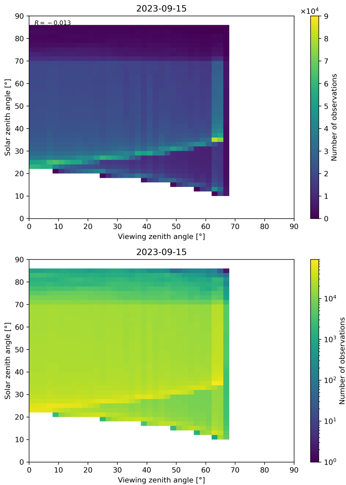
Figure 197: Scatter density plot of “Viewing zenith angle” against “Solar zenith angle” for 2023-09-15 to 2023-09-16.
