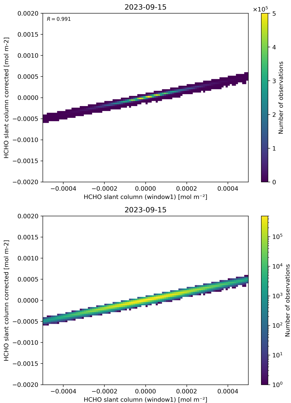
Figure 82: Scatter density plot of “HCHO slant column (window1)” against “HCHO slant column corrected” for 2023-09-15 to 2023-09-16.
