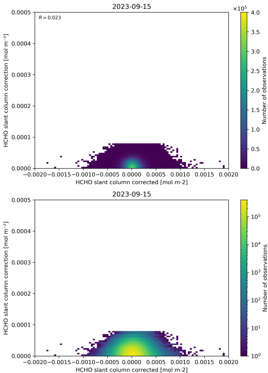
Figure 77: Scatter density plot of “HCHO slant column corrected” against “HCHO slant column correction” for 2023-09-15 to 2023-09-16.
