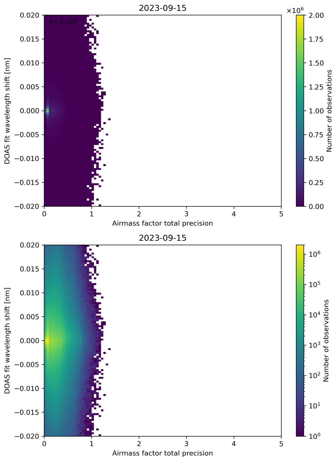
Figure 106: Scatter density plot of “Airmass factor total precision” against “DOAS fit wavelength shift” for 2023-09-15 to 2023-09-16.
