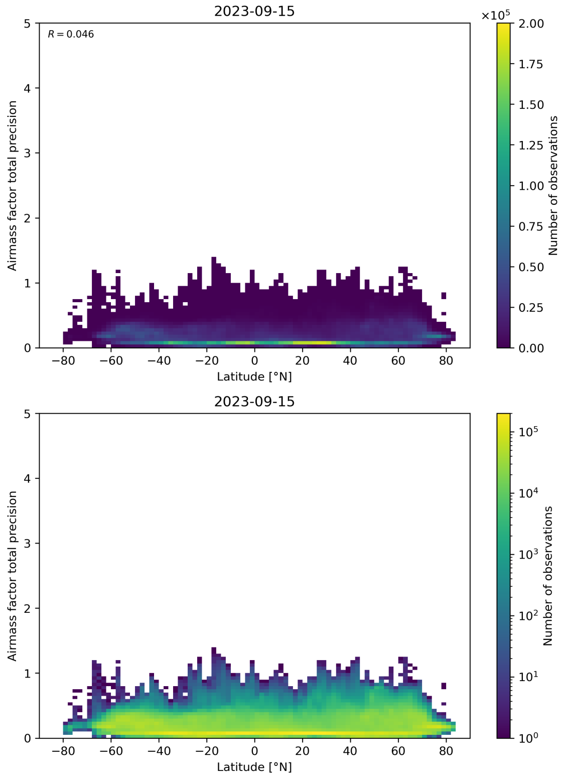
Figure 162: Scatter density plot of “Latitude” against “Airmass factor total precision” for 2023-09-15 to 2023-09-16.
