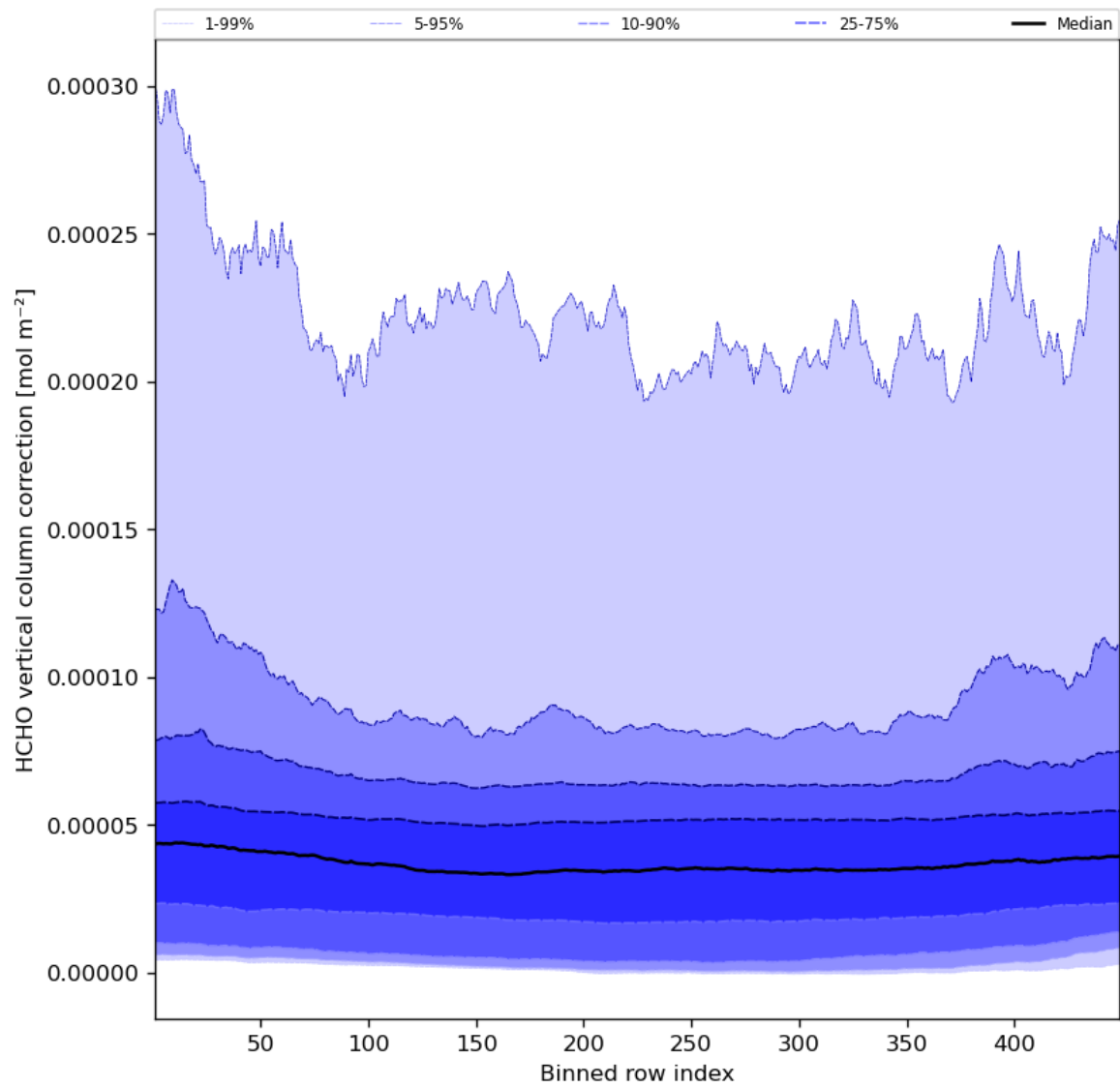
Figure 51: Along track statistics of “HCHO vertical column correction” for 2023-09-15 to 2023-09-16
