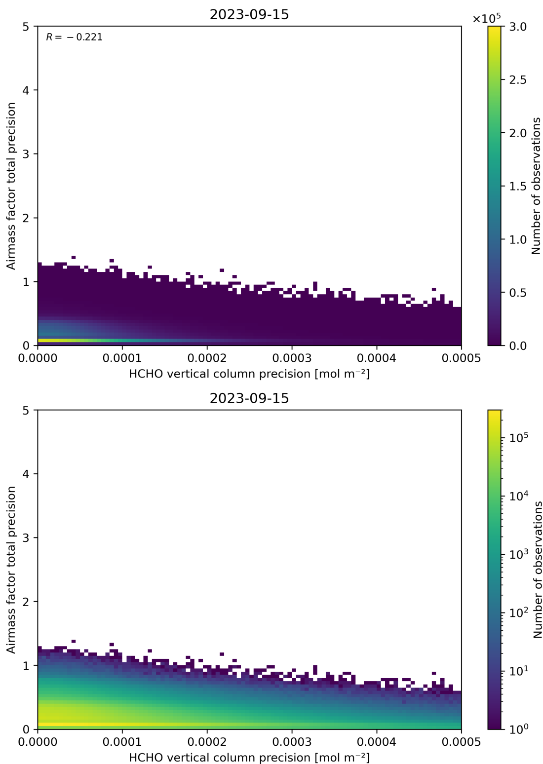
Figure 145: Scatter density plot of “HCHO vertical column precision” against “Airmass factor total precision” for 2023-09-15 to 2023-09-16.
