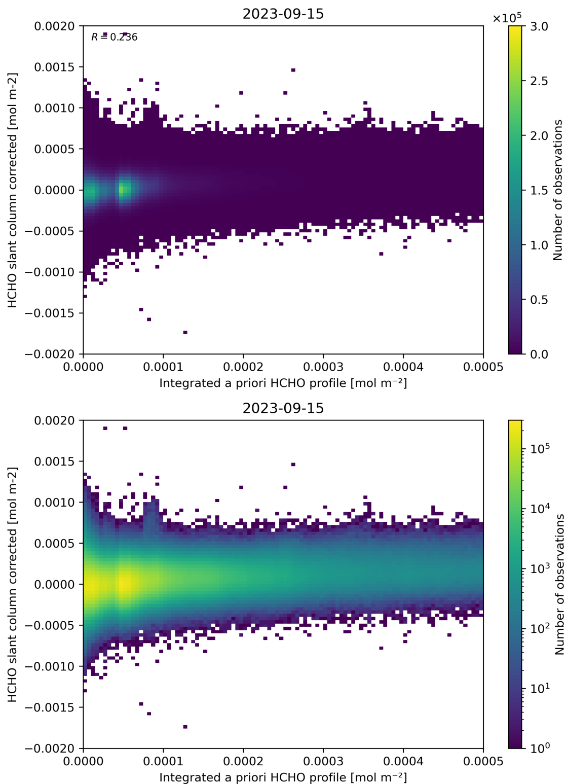
Figure 151: Scatter density plot of “Integrated a priori HCHO profile” against “HCHO slant column corrected” for 2023-09-15 to 2023-09-16.
