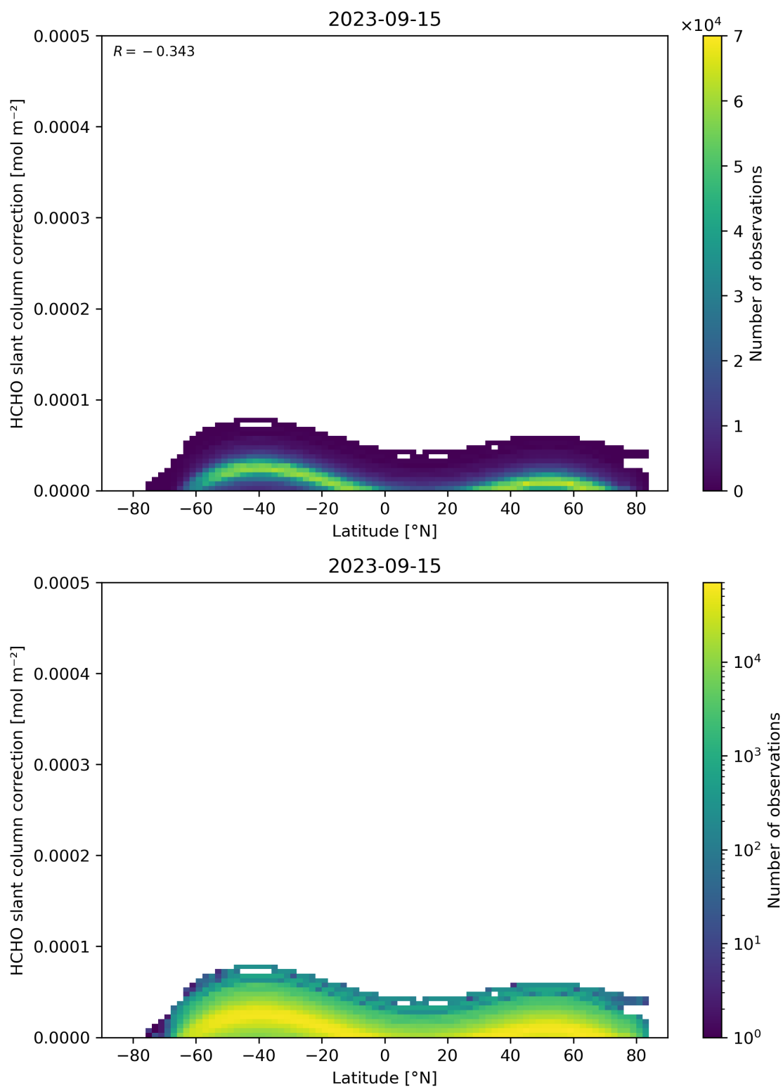
Figure 158: Scatter density plot of “Latitude” against “HCHO slant column correction” for 2023-09-15 to 2023-09-16.
