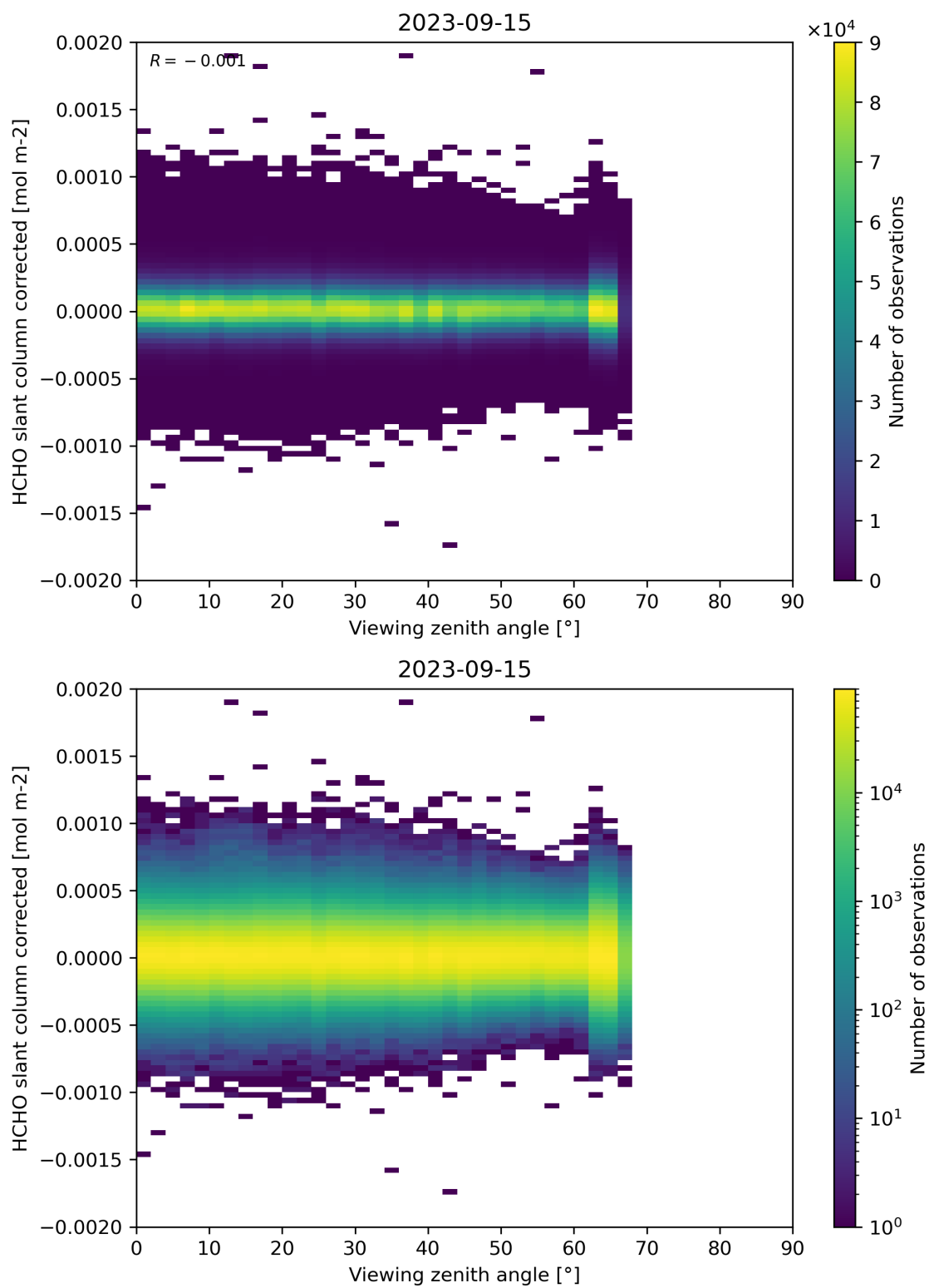
Figure 186: Scatter density plot of “Viewing zenith angle” against “HCHO slant column corrected” for 2023-09-15 to 2023-09-16.
