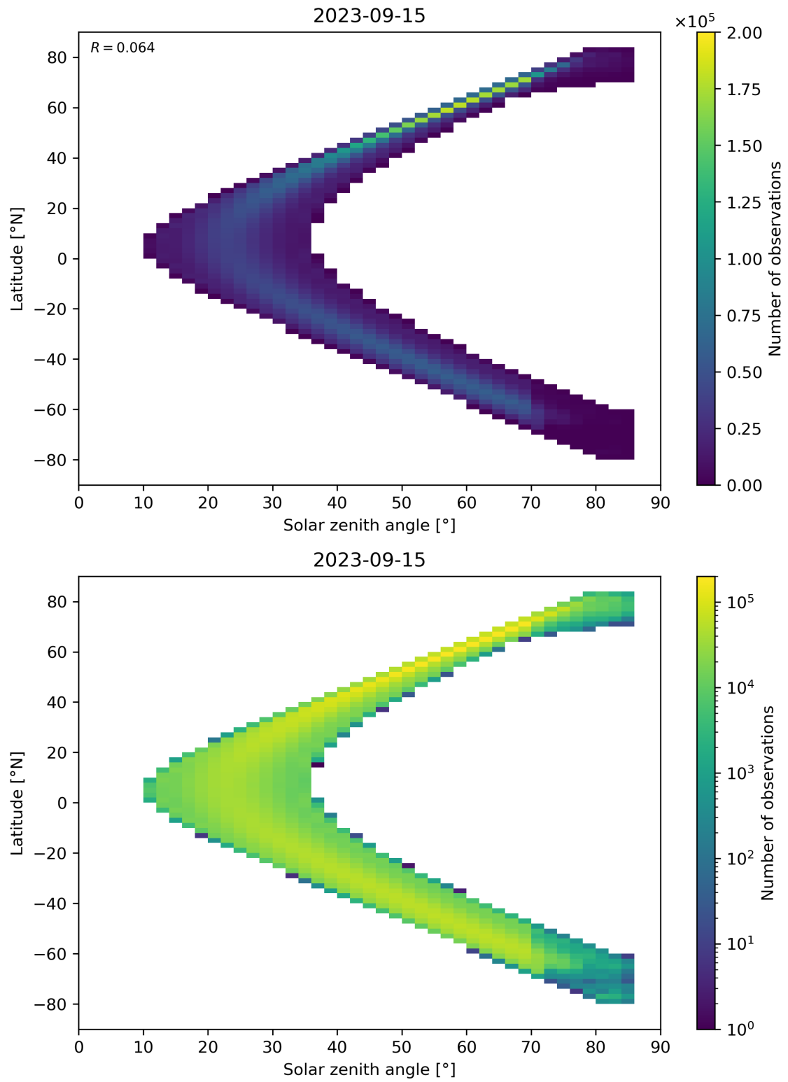
Figure 181: Scatter density plot of “Solar zenith angle” against “Latitude” for 2023-09-15 to 2023-09-16.
