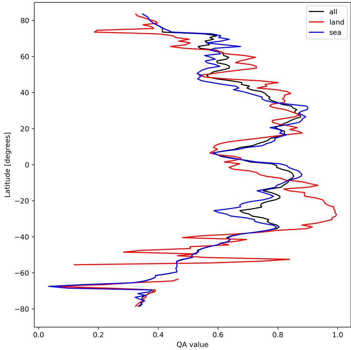
Figure 20: Zonal average of “QA value” for 2023-09-15 to 2023-09-16.
