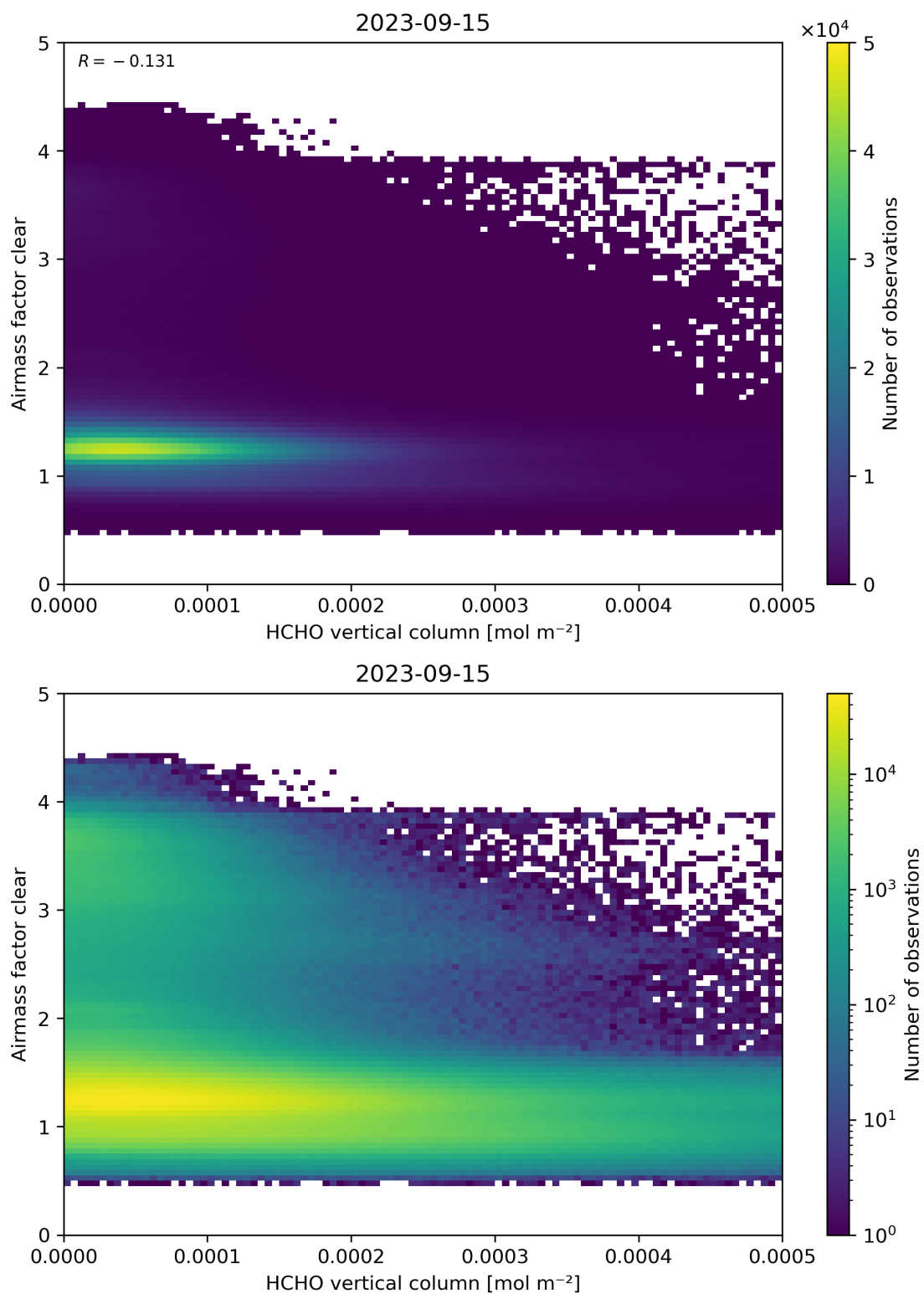
Figure 126: Scatter density plot of “HCHO vertical column” against “Airmass factor clear” for 2023-09-15 to 2023-09-16.
