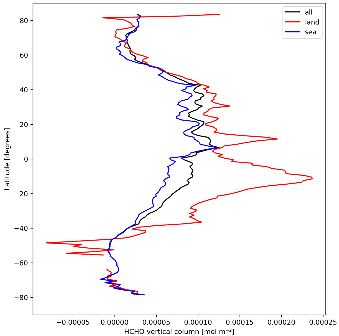
Figure 21: Zonal average of “HCHO vertical column” for 2023-09-15 to 2023-09-16.
