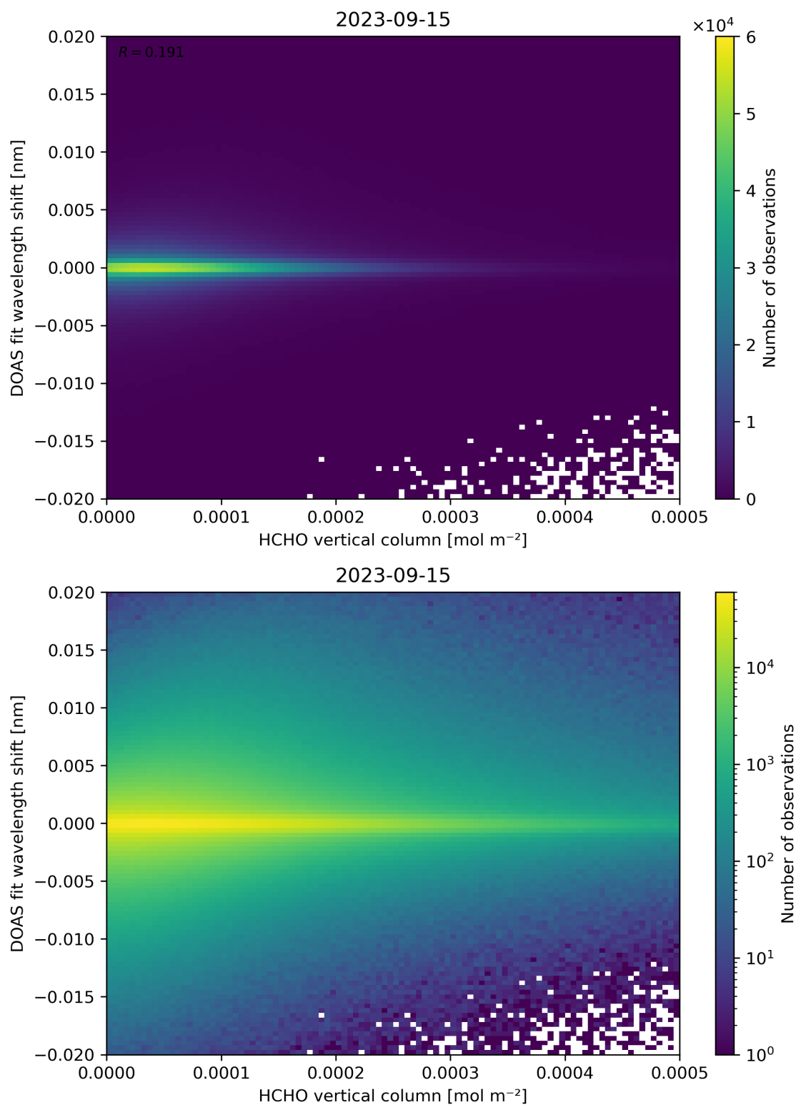
Figure 124: Scatter density plot of “HCHO vertical column” against “DOAS fit wavelength shift” for 2023-09-15 to 2023-09-16.
