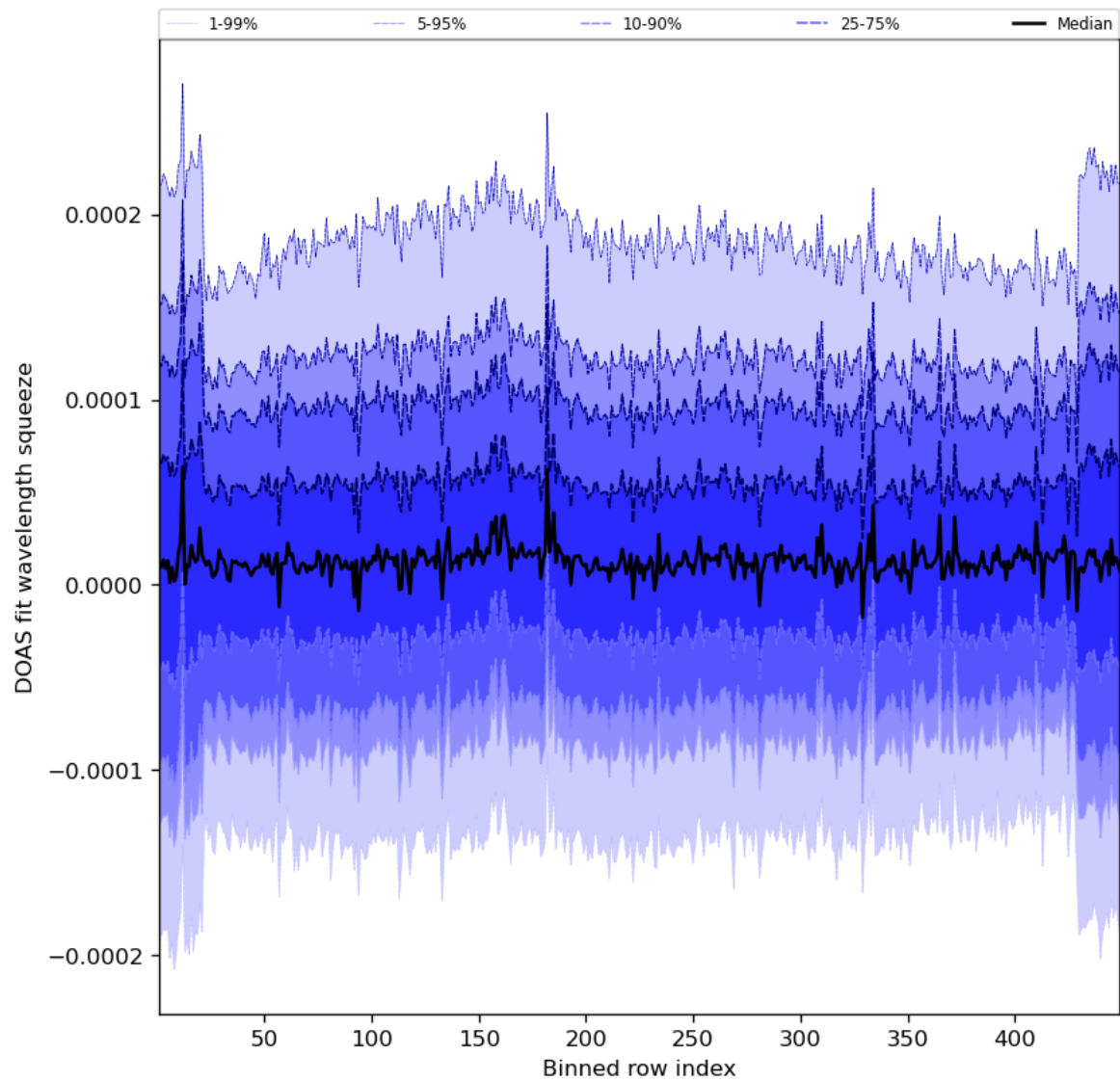
Figure 59: Along track statistics of “DOAS fit wavelength squeeze” for 2023-09-15 to 2023-09-16
