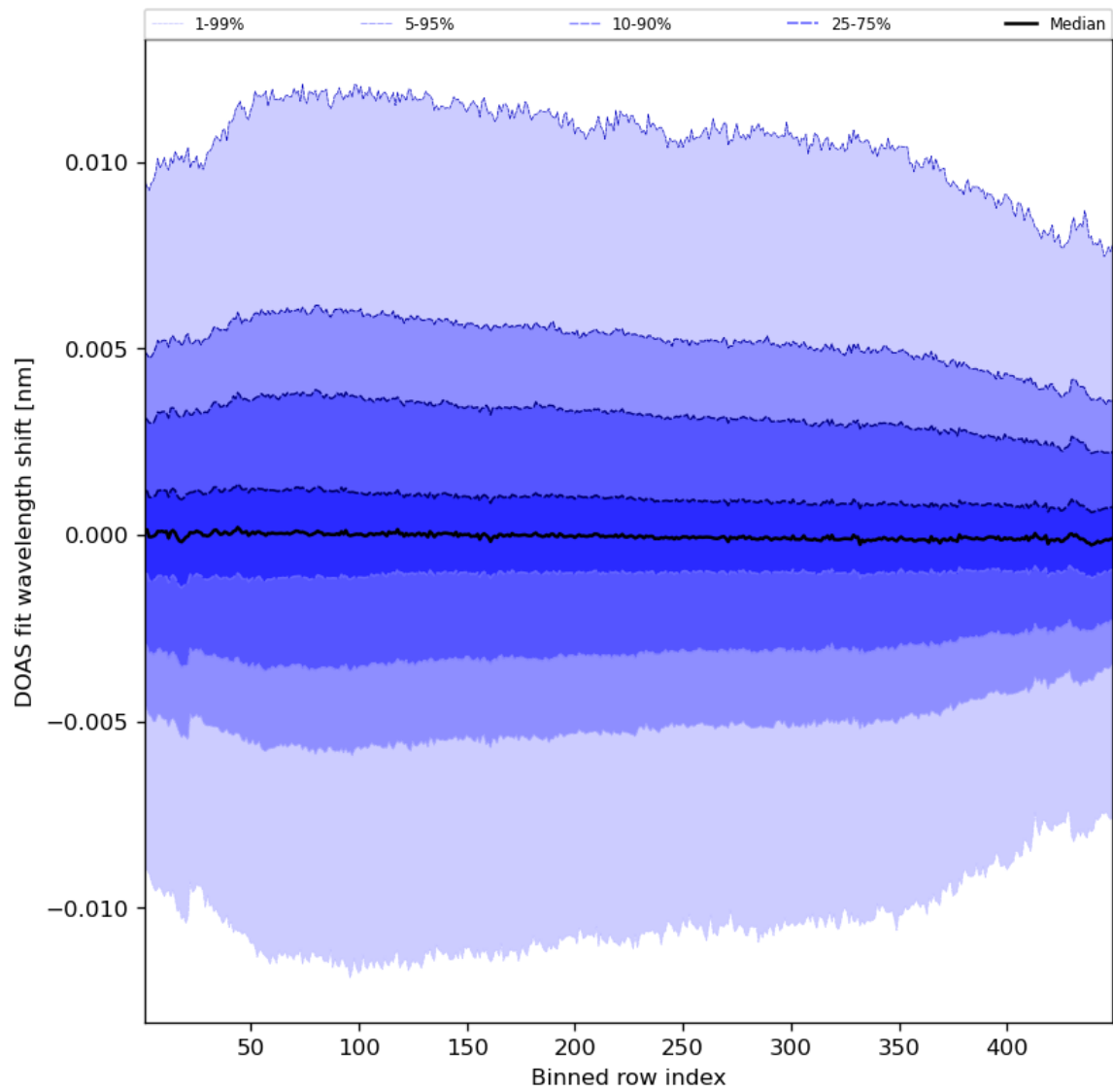
Figure 58: Along track statistics of “DOAS fit wavelength shift” for 2023-09-15 to 2023-09-16
