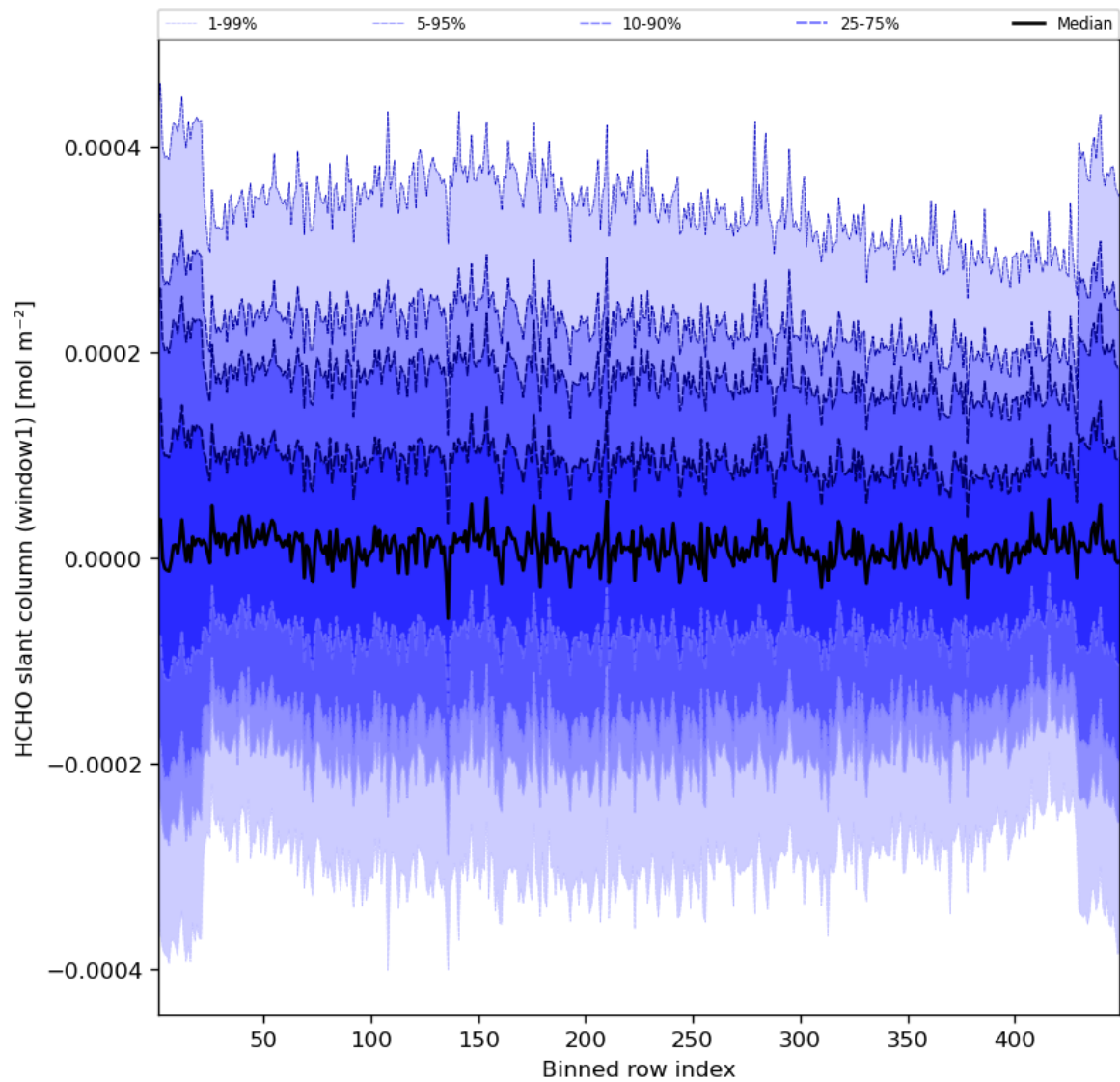
Figure 52: Along track statistics of “HCHO slant column (window1)” for 2023-09-15 to 2023-09-16
