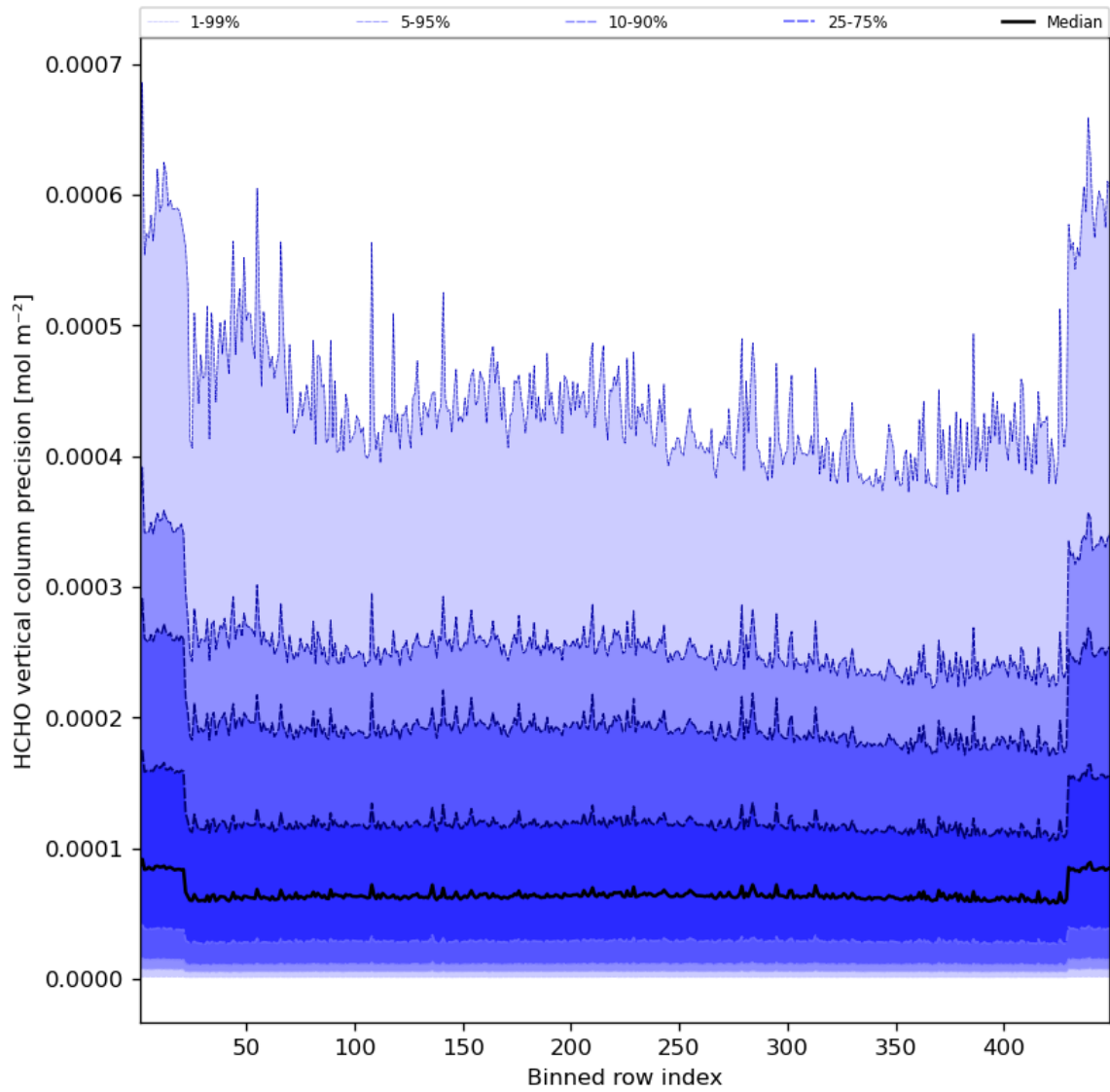
Figure 50: Along track statistics of “HCHO vertical column precision” for 2023-09-15 to 2023-09-16
