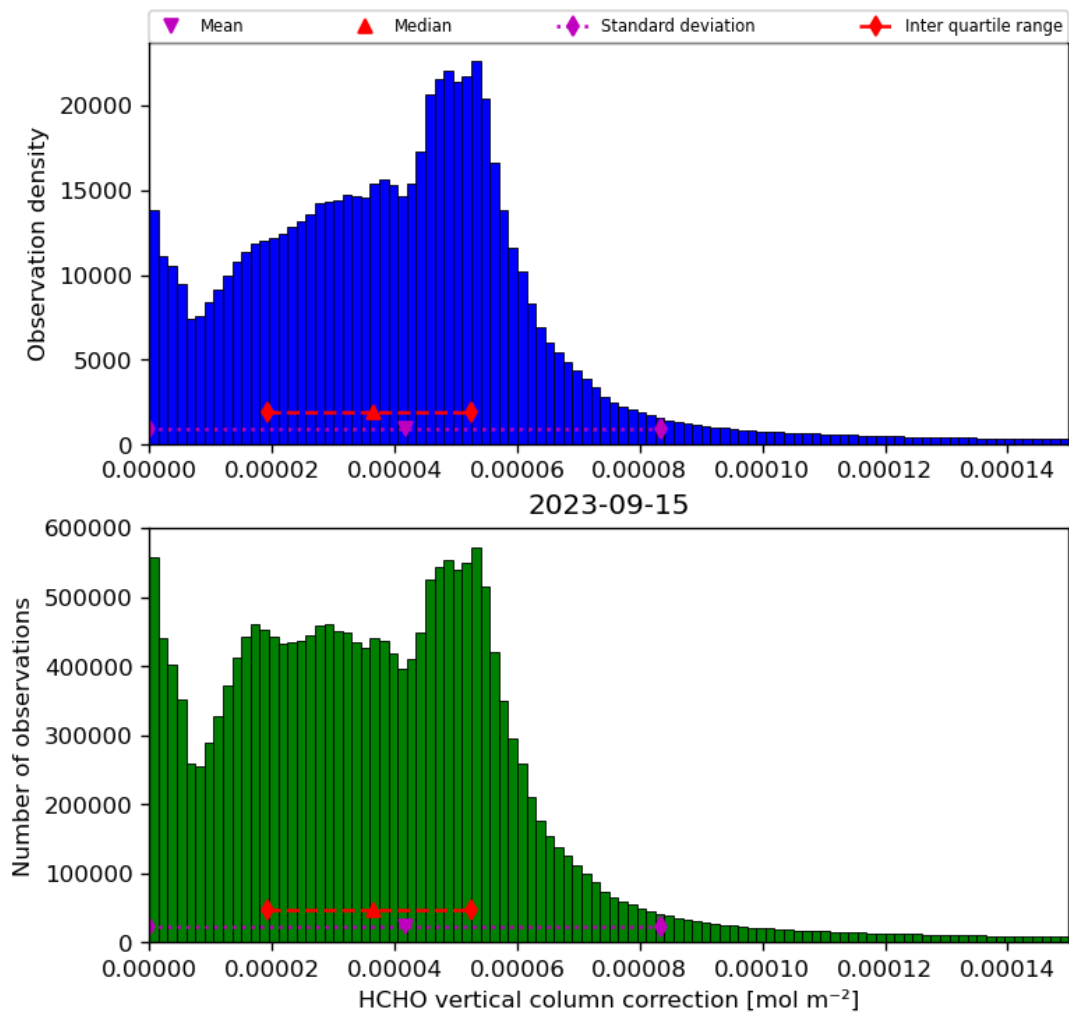
Figure 37: Histogram of “HCHO vertical column correction” for 2023-09-15 to 2023-09-16
