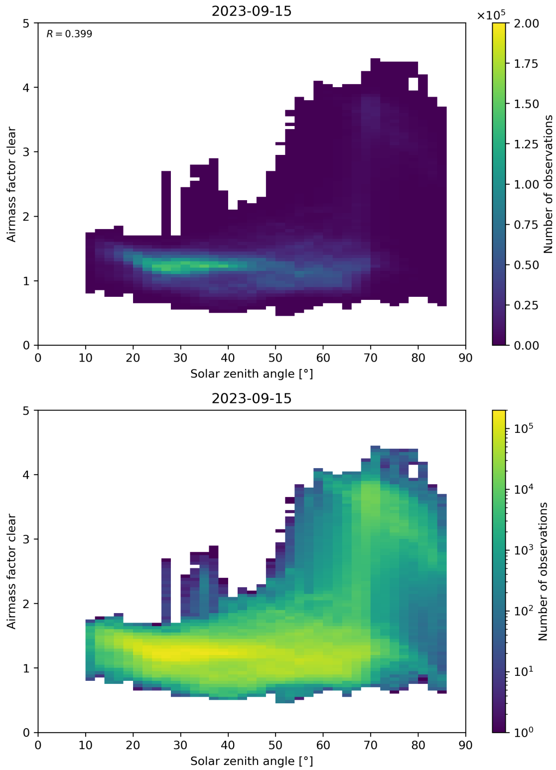
Figure 170: Scatter density plot of “Solar zenith angle” against “Airmass factor clear” for 2023-09-15 to 2023-09-16.
