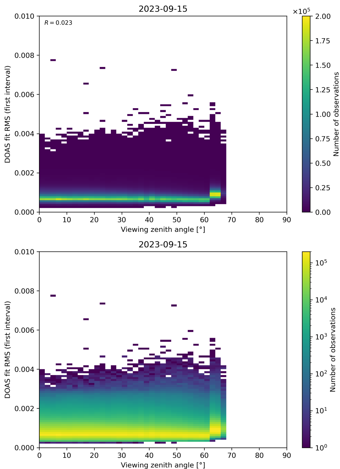
Figure 182: Scatter density plot of “Viewing zenith angle” against “DOAS fit RMS (first interval)” for 2023-09-15 to 2023-09-16.
