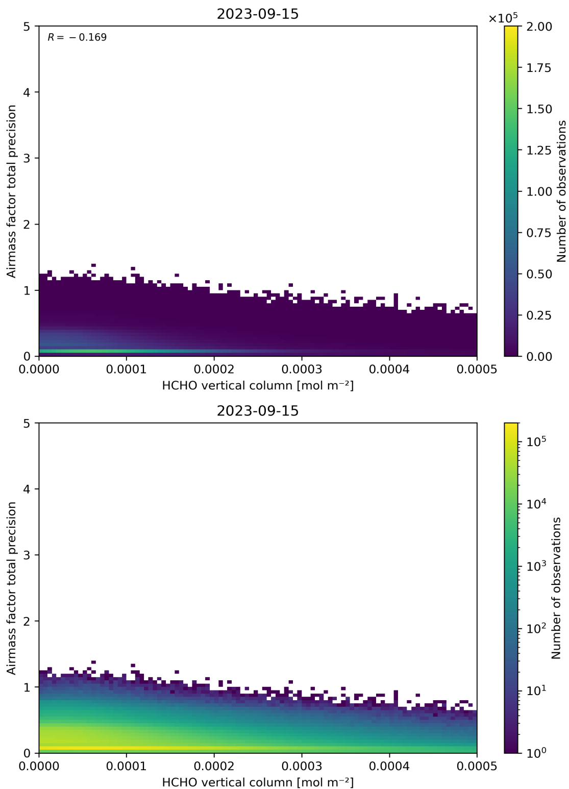
Figure 132: Scatter density plot of “HCHO vertical column” against “Airmass factor total precision” for 2023-09-15 to 2023-09-16.
