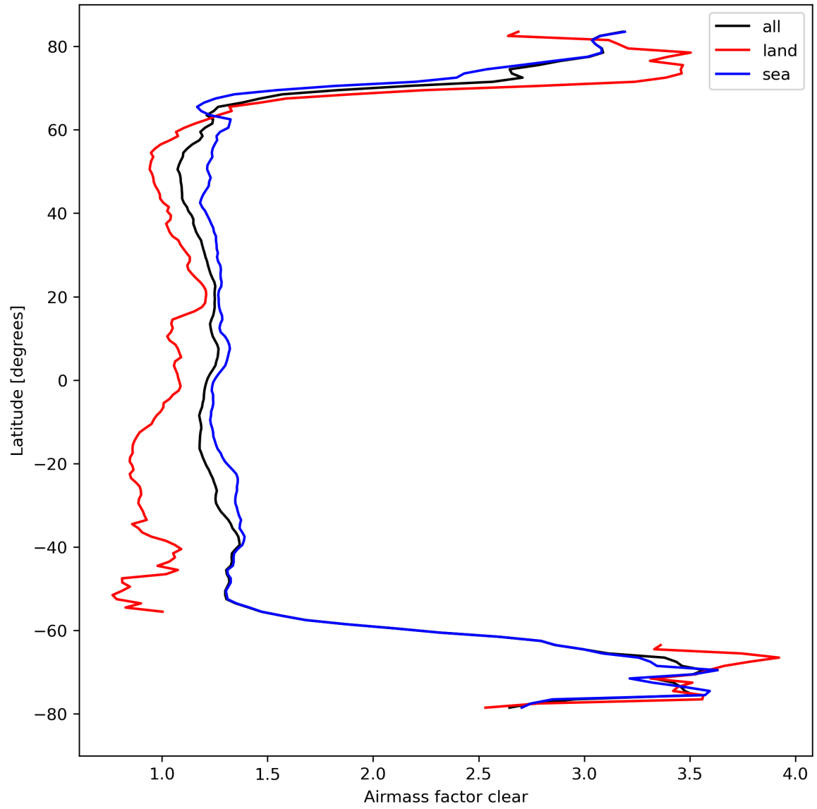
Figure 28: Zonal average of “Airmass factor clear” for 2023-09-15 to 2023-09-16.
