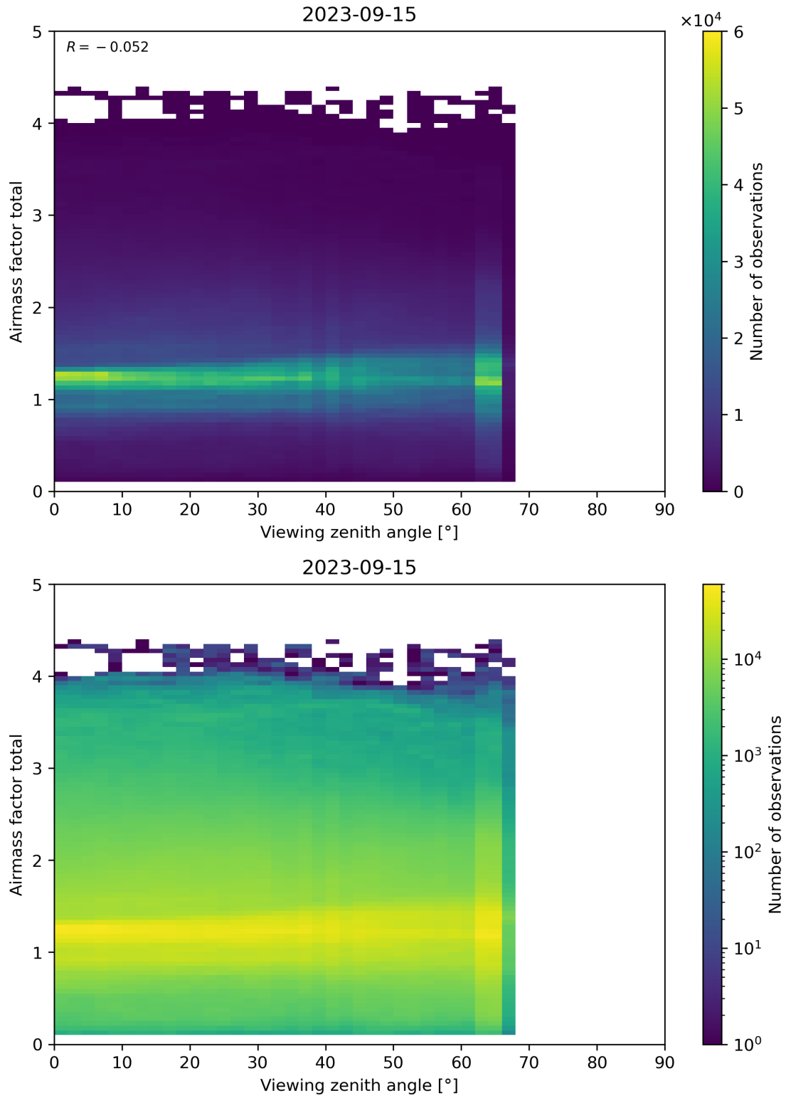
Figure 190: Scatter density plot of “Viewing zenith angle” against “Airmass factor total” for 2023-09-15 to 2023-09-16.
