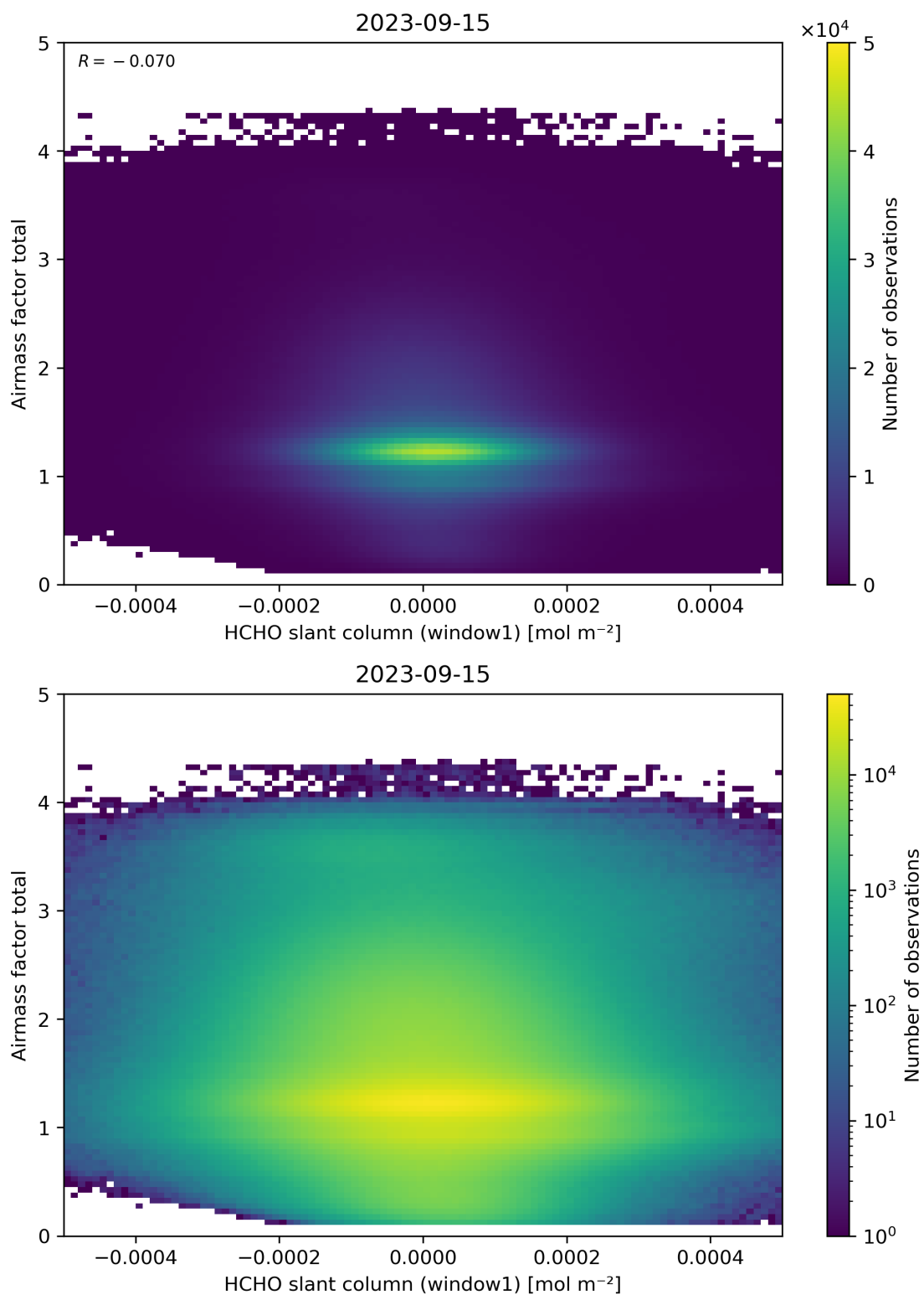
Figure 85: Scatter density plot of “HCHO slant column (window1)” against “Airmass factor total” for 2023-09-15 to 2023-09-16.
