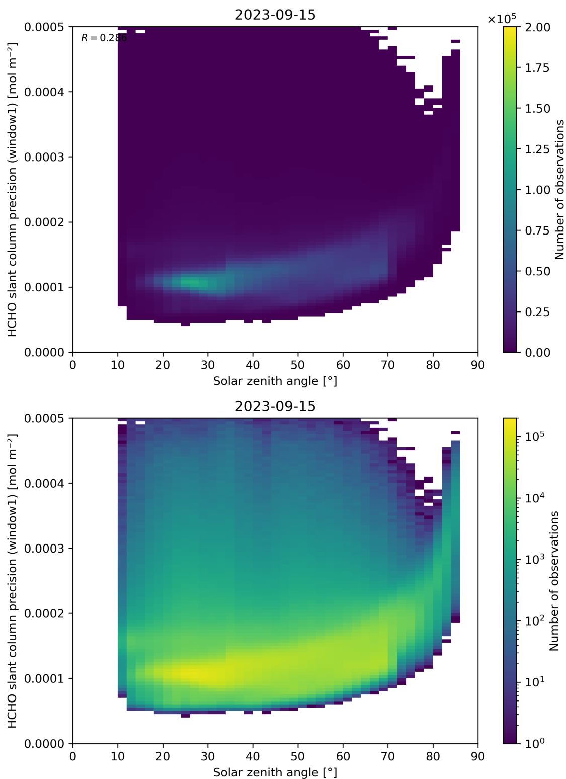
Figure 174: Scatter density plot of “Solar zenith angle” against “HCHO slant column precision (window1)” for 2023-09-15 to 2023-09-16.
