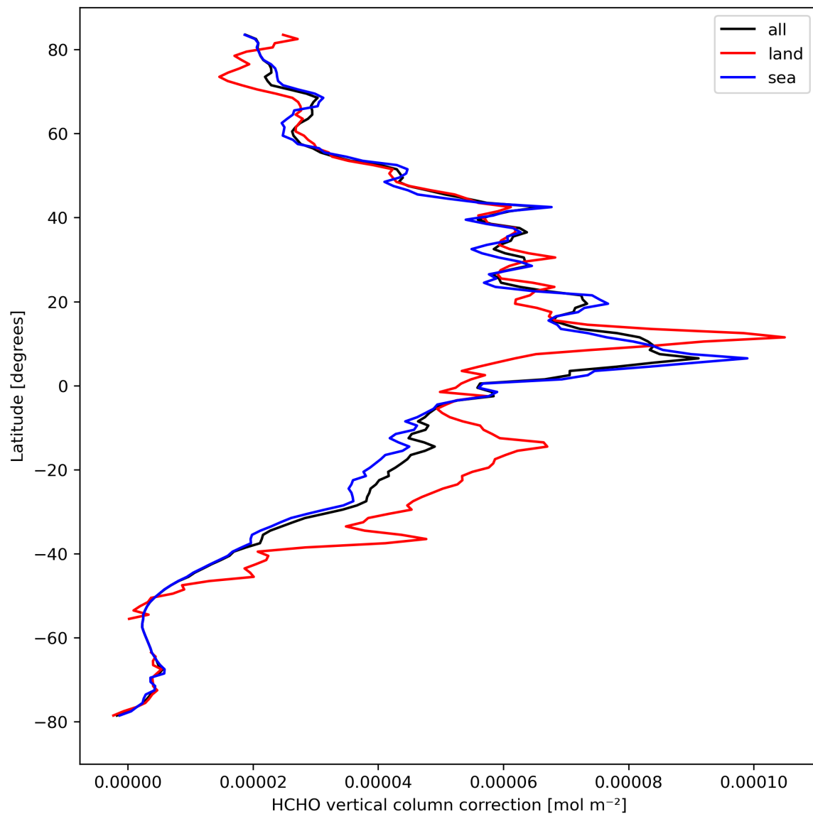
Figure 23: Zonal average of “HCHO vertical column correction” for 2023-09-15 to 2023-09-16.
