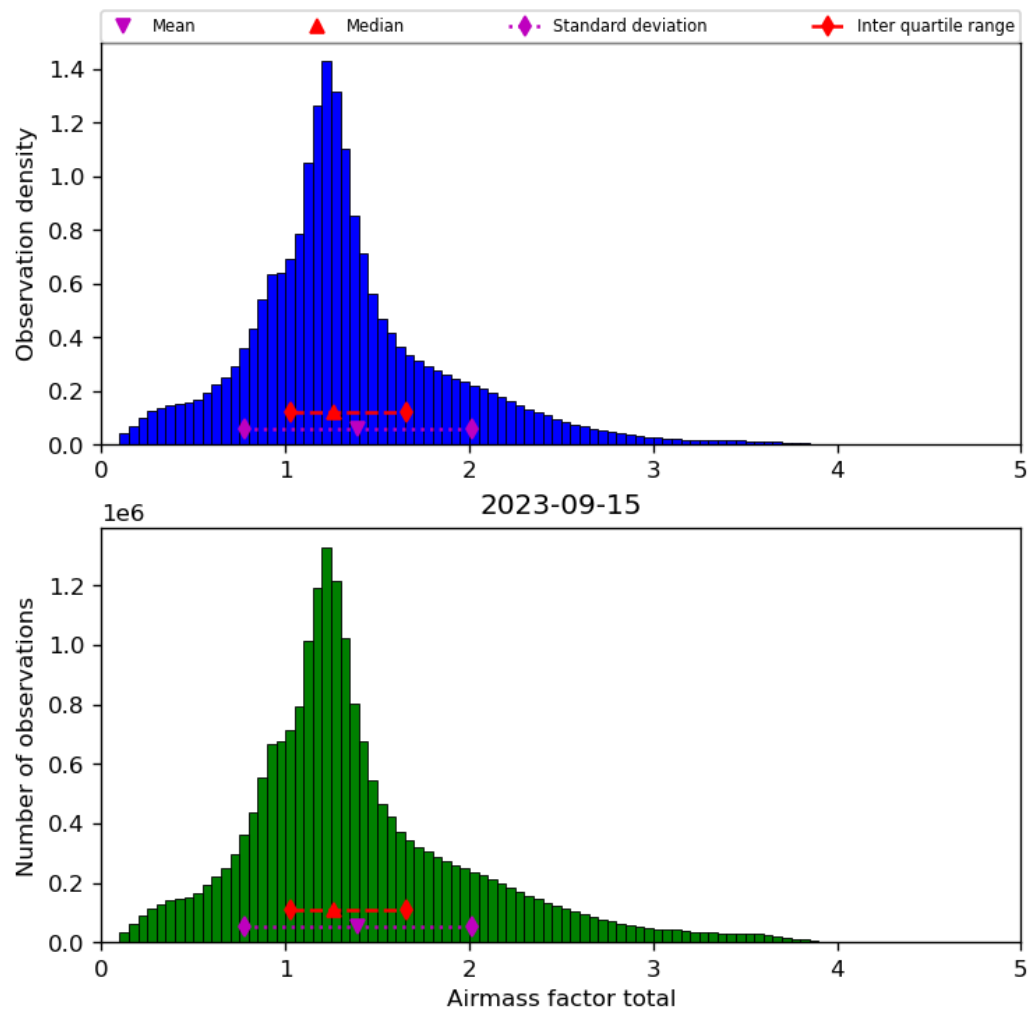
Figure 40: Histogram of “Airmass factor total” for 2023-09-15 to 2023-09-16
