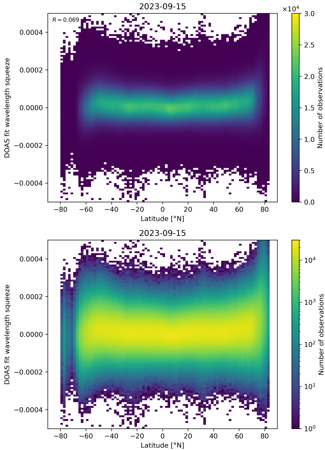
Figure 155: Scatter density plot of “Latitude” against “DOAS fit wavelength squeeze” for 2023-09-15 to 2023-09-16.
