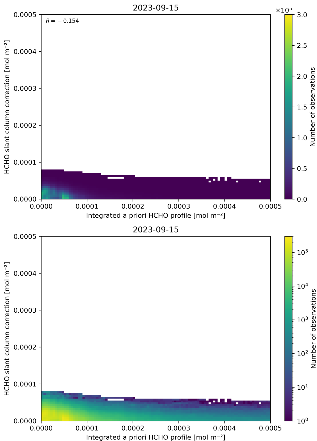
Figure 152: Scatter density plot of “Integrated a priori HCHO profile” against “HCHO slant column correction” for 2023-09-15 to 2023-09-16.
