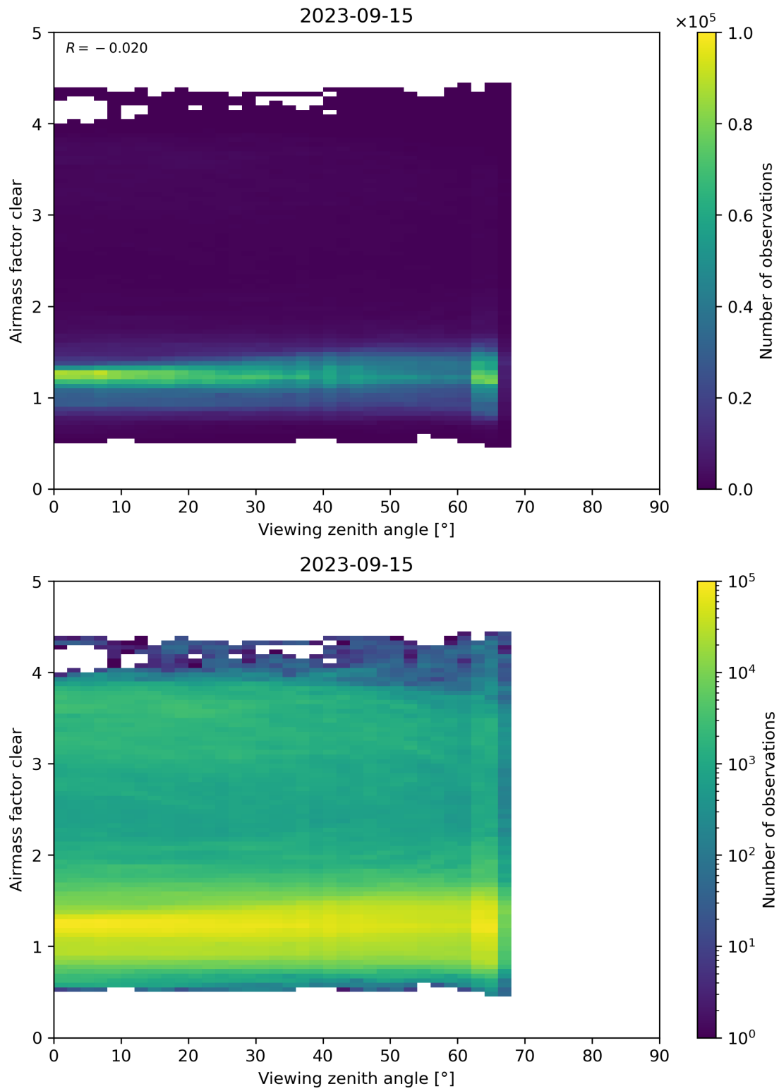
Figure 185: Scatter density plot of “Viewing zenith angle” against “Airmass factor clear” for 2023-09-15 to 2023-09-16.
