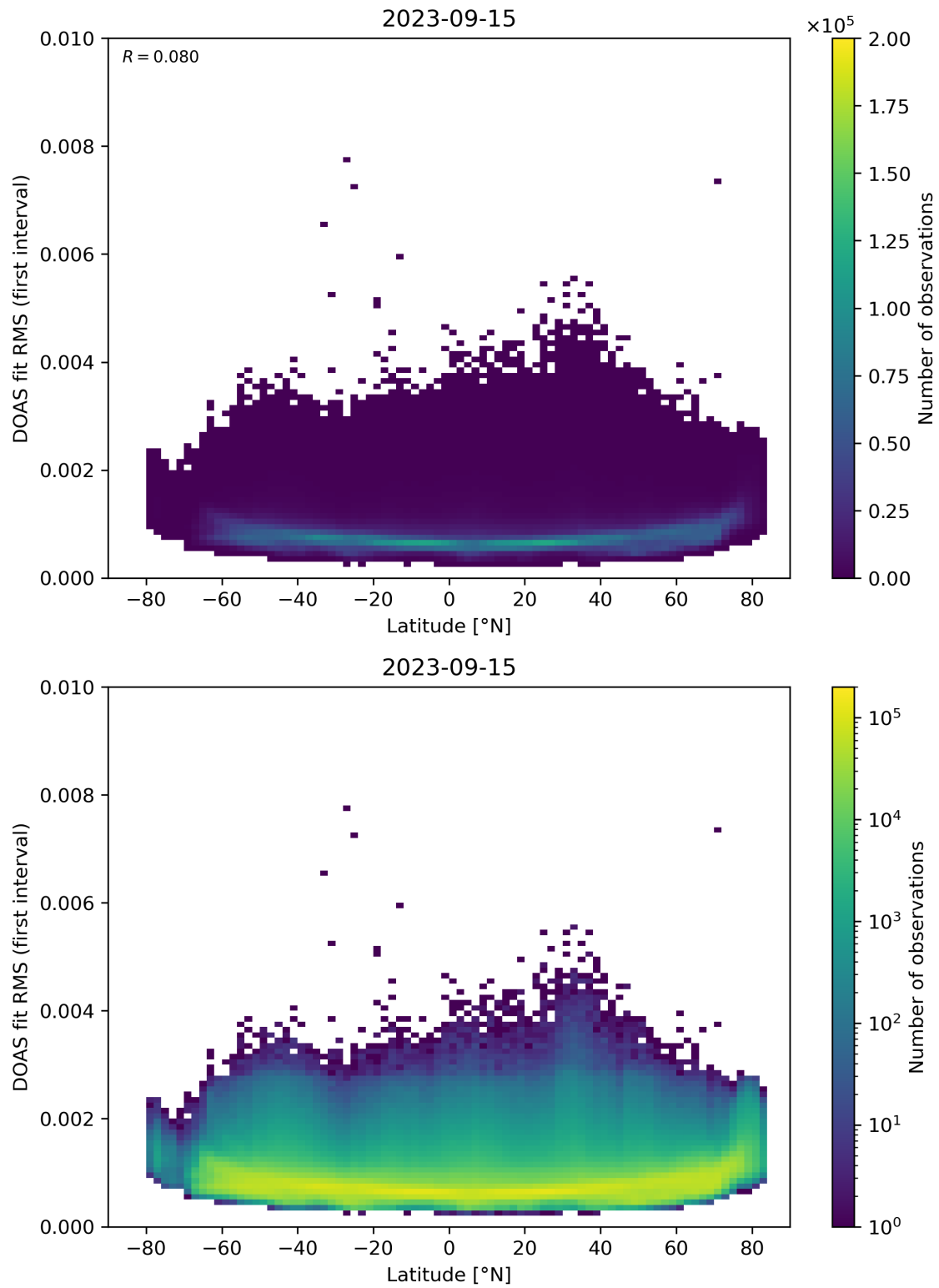
Figure 153: Scatter density plot of “Latitude” against “DOAS fit RMS (first interval)” for 2023-09-15 to 2023-09-16.
