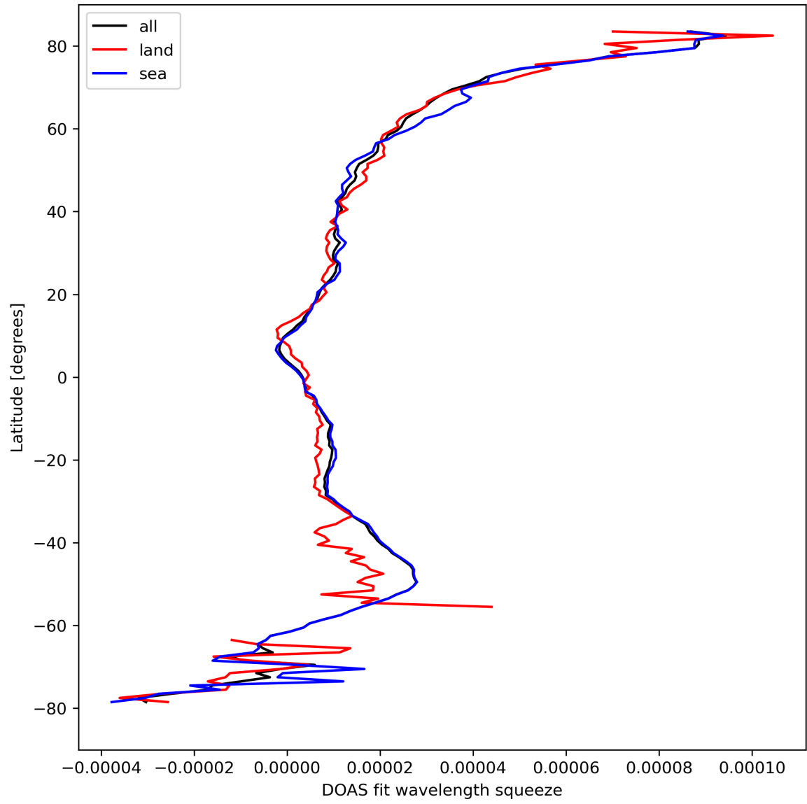
Figure 31: Zonal average of “DOAS fit wavelength squeeze” for 2023-09-15 to 2023-09-16.
