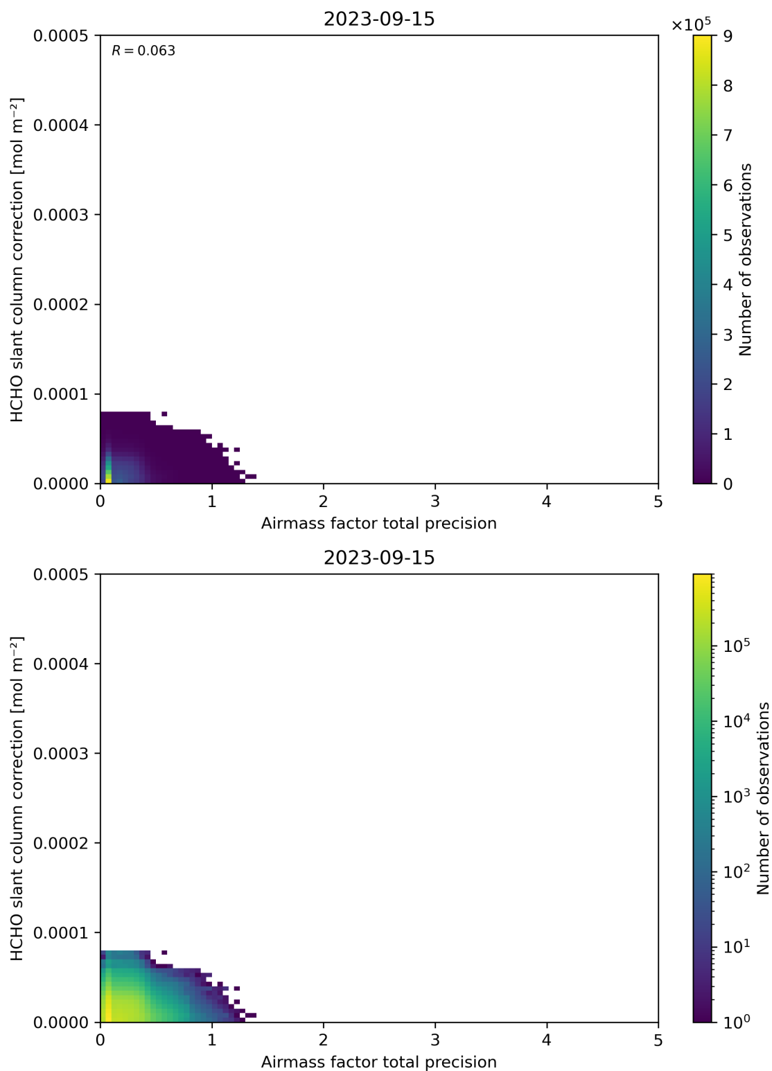
Figure 110: Scatter density plot of “Airmass factor total precision” against “HCHO slant column correction” for 2023-09-15 to 2023-09-16.
