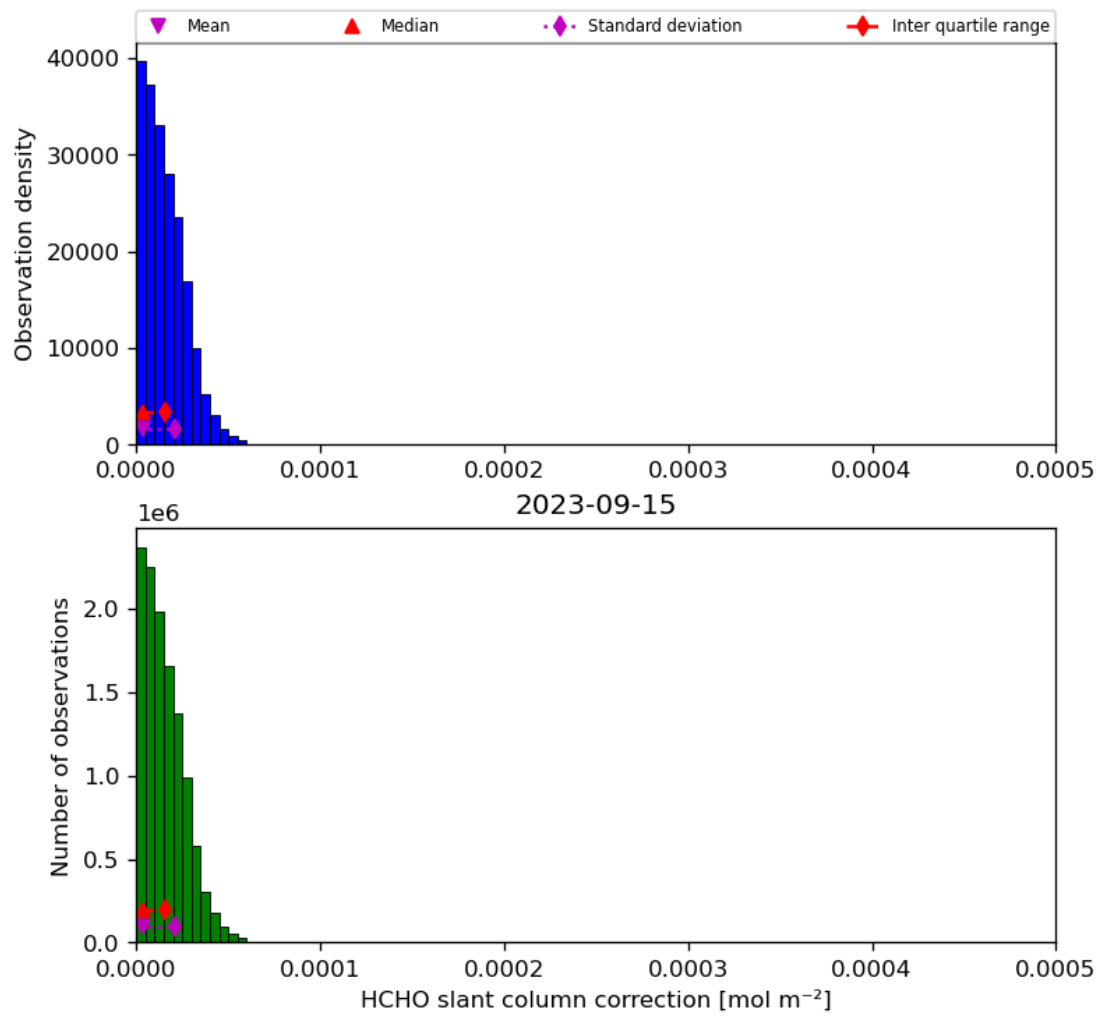
Figure 47: Histogram of “HCHO slant column correction” for 2023-09-15 to 2023-09-16
