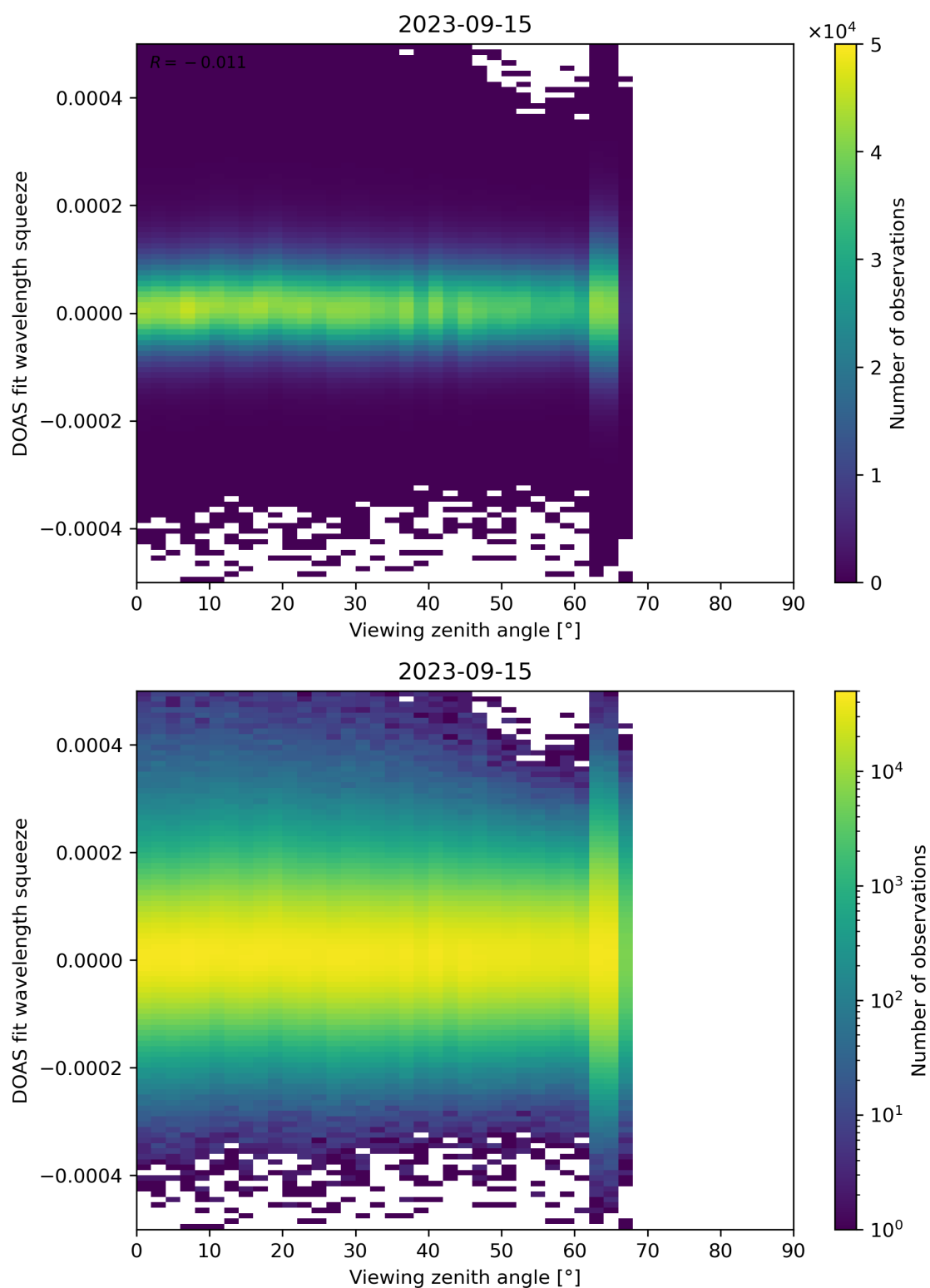
Figure 184: Scatter density plot of “Viewing zenith angle” against “DOAS fit wavelength squeeze” for 2023-09-15 to 2023-09-16.
