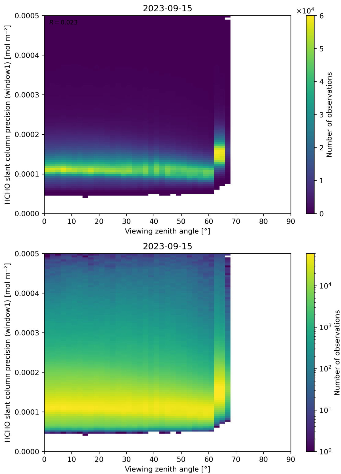
Figure 189: Scatter density plot of “Viewing zenith angle” against “HCHO slant column precision (window1)” for 2023-09-15 to 2023-09-16.
