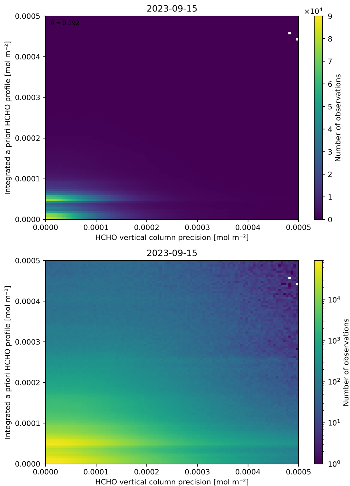
Figure 147: Scatter density plot of “HCHO vertical column precision” against “Integrated a priori HCHO profile” for 2023-09-15 to 2023-09-16.
