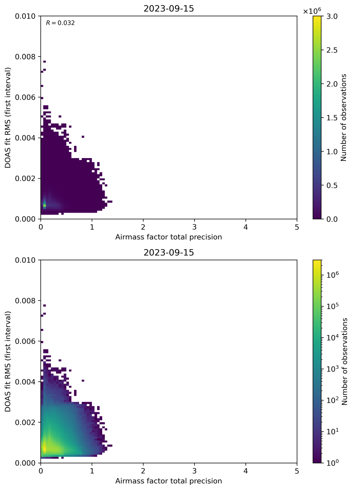
Figure 105: Scatter density plot of “Airmass factor total precision” against “DOAS fit RMS (first interval)” for 2023-09-15 to 2023-09-16.
