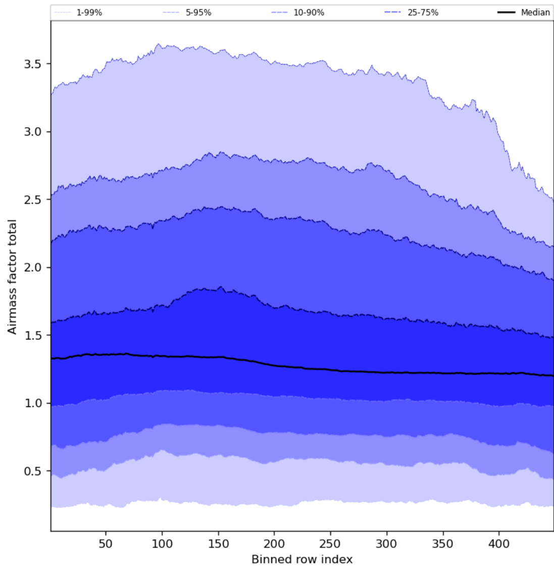
Figure 54: Along track statistics of “Airmass factor total” for 2023-09-15 to 2023-09-16
