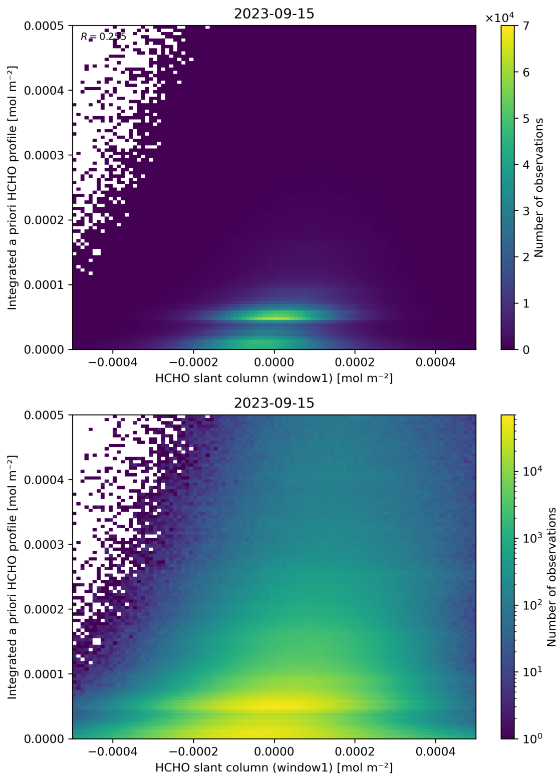
Figure 87: Scatter density plot of “HCHO slant column (window1)” against “Integrated a priori HCHO profile” for 2023-09-15 to 2023-09-16.
