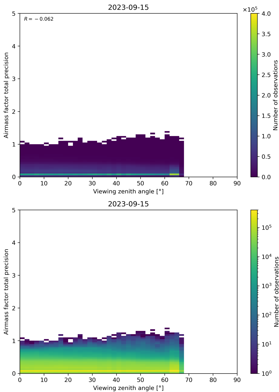
Figure 191: Scatter density plot of “Viewing zenith angle” against “Airmass factor total precision” for 2023-09-15 to 2023-09-16.
