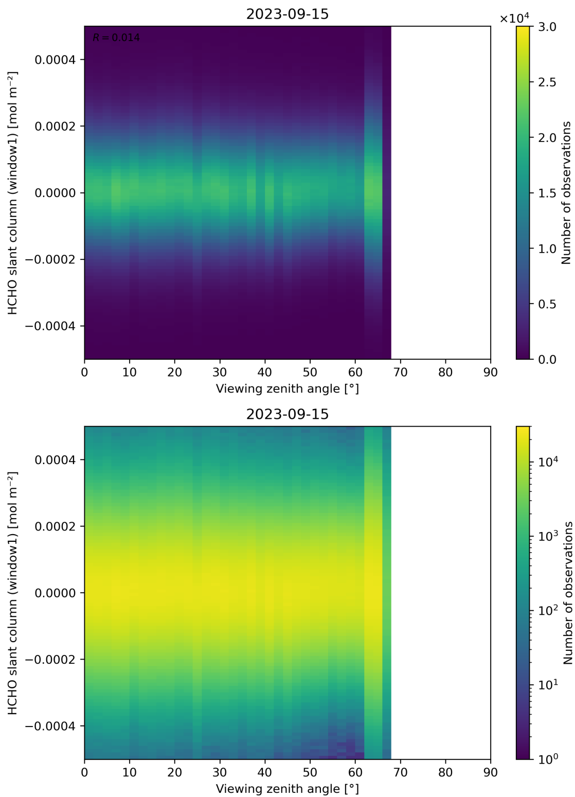
Figure 188: Scatter density plot of “Viewing zenith angle” against “HCHO slant column (window1)” for 2023-09-15 to 2023-09-16.
