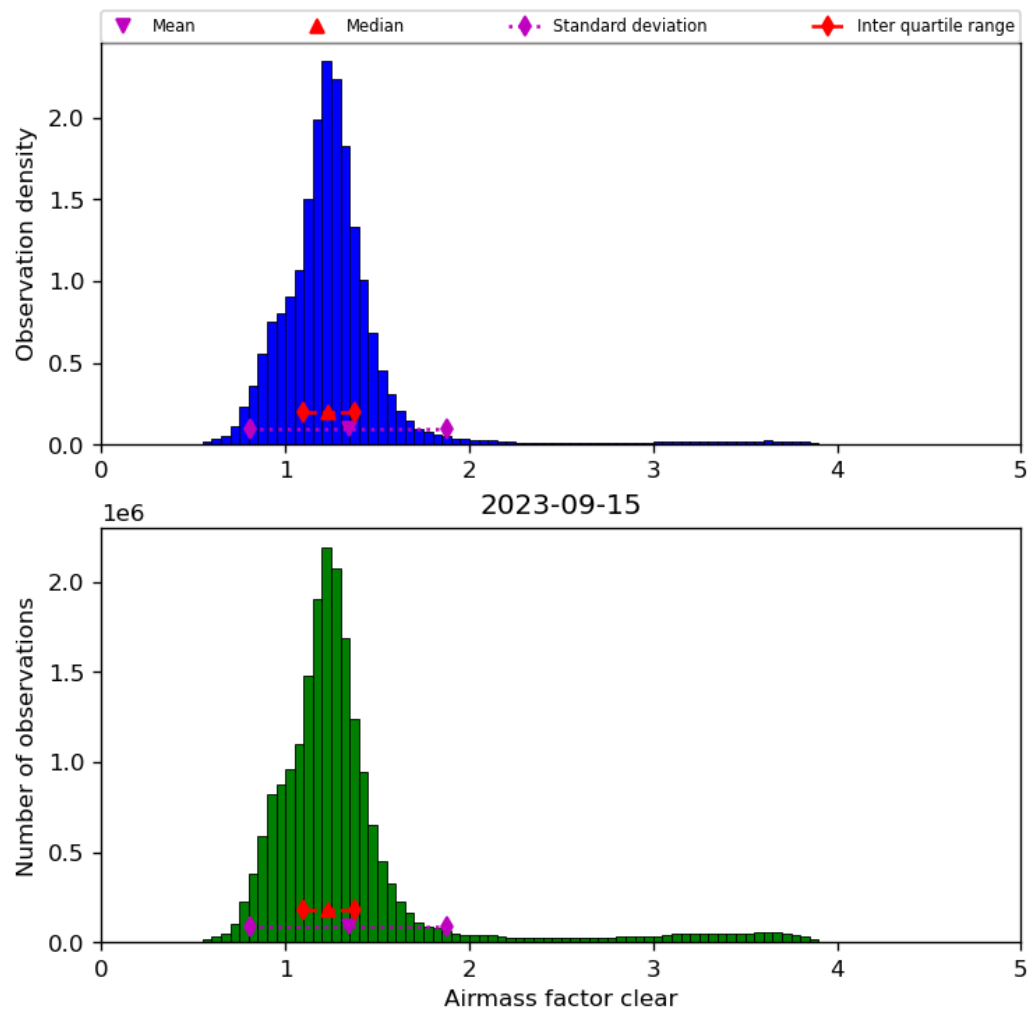
Figure 42: Histogram of “Airmass factor clear” for 2023-09-15 to 2023-09-16
