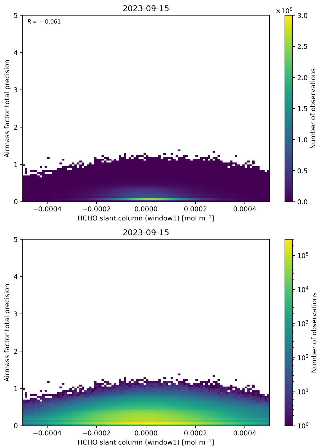
Figure 86: Scatter density plot of “HCHO slant column (window1)” against “Airmass factor total precision” for 2023-09-15 to 2023-09-16.
