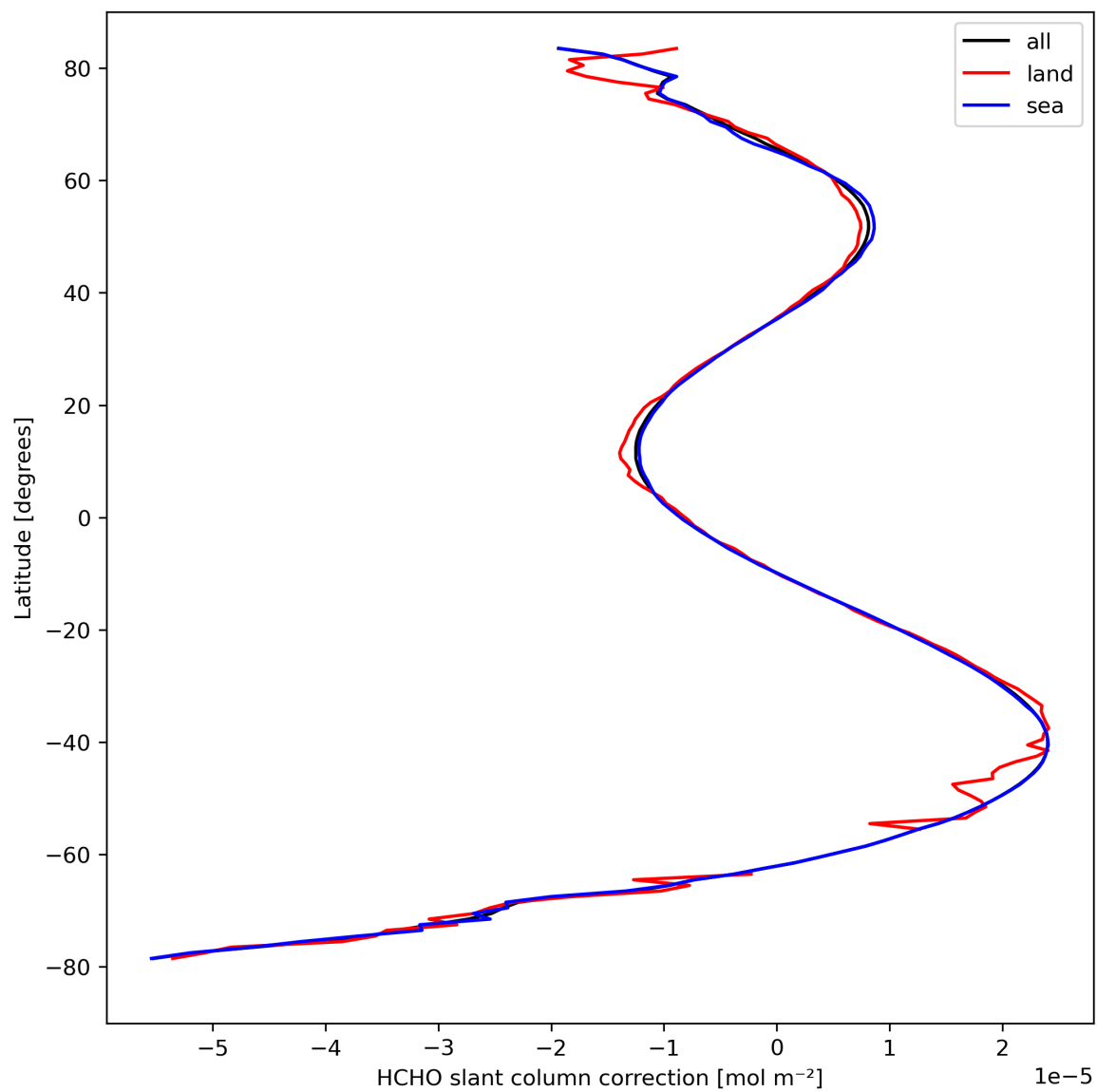
Figure 33: Zonal average of “HCHO slant column correction” for 2023-09-15 to 2023-09-16.
