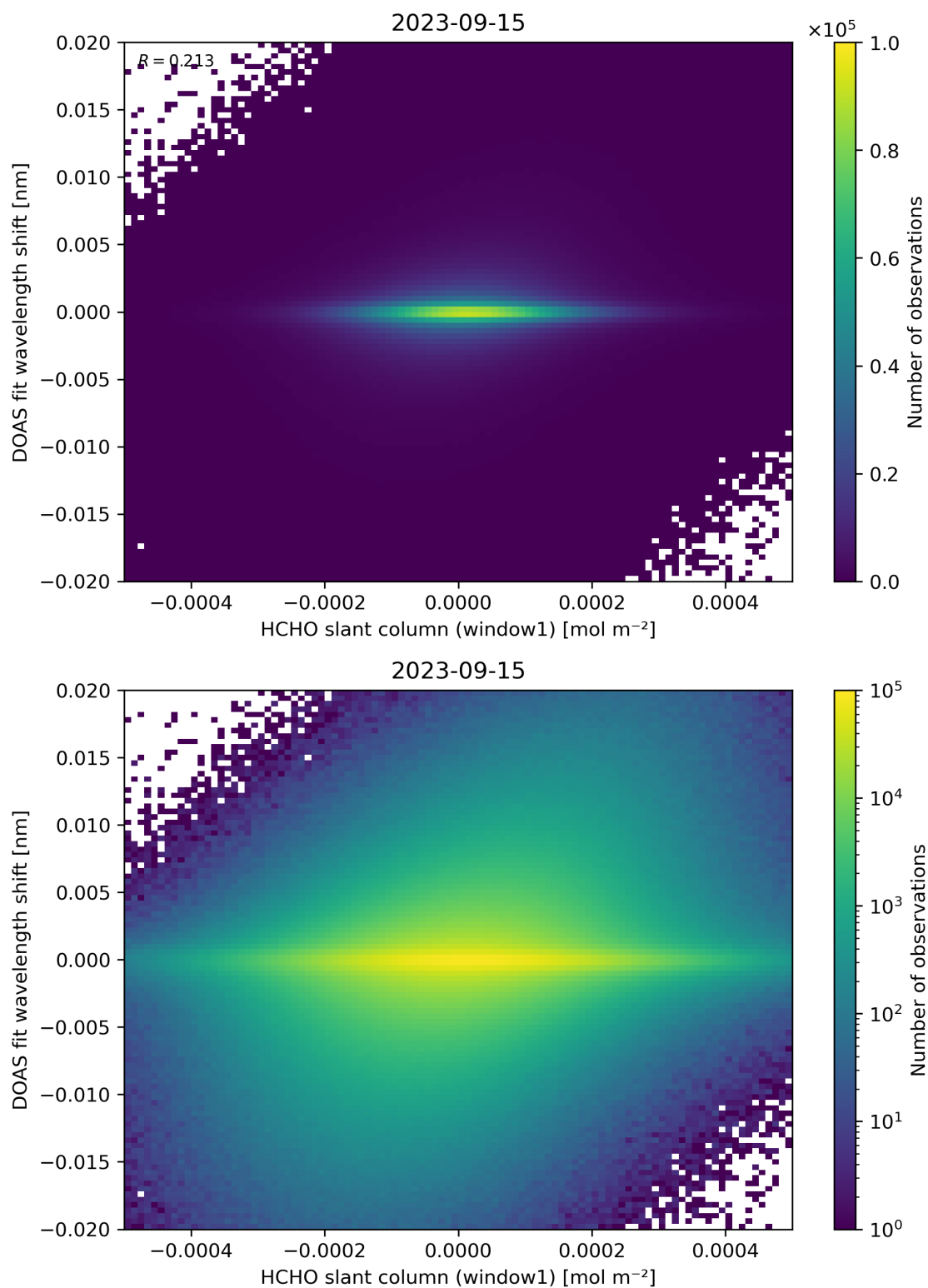
Figure 79: Scatter density plot of “HCHO slant column (window1)” against “DOAS fit wavelength shift” for 2023-09-15 to 2023-09-16.
