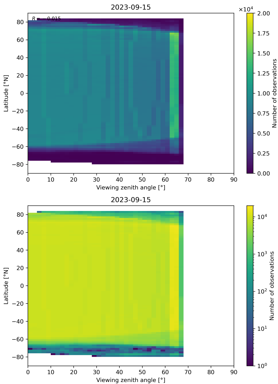
Figure 196: Scatter density plot of “Viewing zenith angle” against “Latitude” for 2023-09-15 to 2023-09-16.
