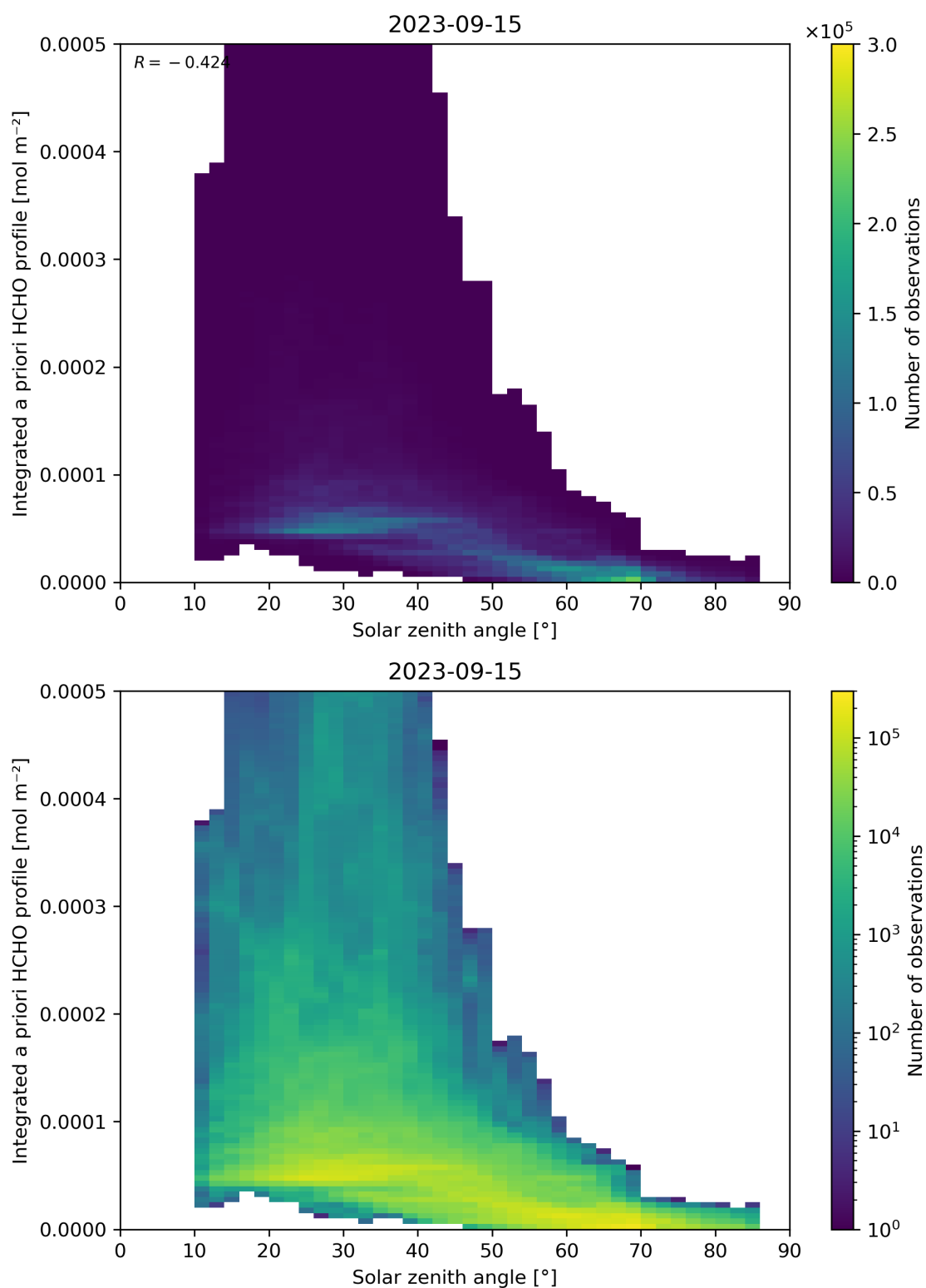
Figure 180: Scatter density plot of “Solar zenith angle” against “Integrated a priori HCHO profile” for 2023-09-15 to 2023-09-16.
