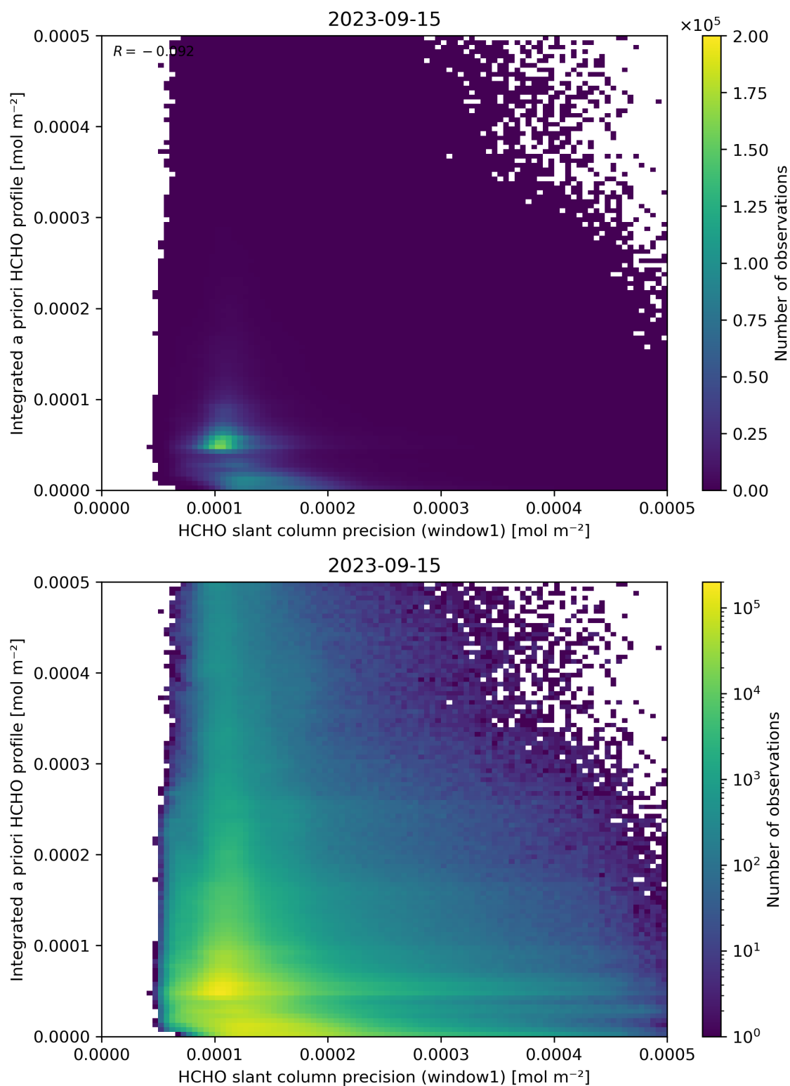
Figure 96: Scatter density plot of “HCHO slant column precision (window1)” against “Integrated a priori HCHO profile” for 2023-09-15 to 2023-09-16.
