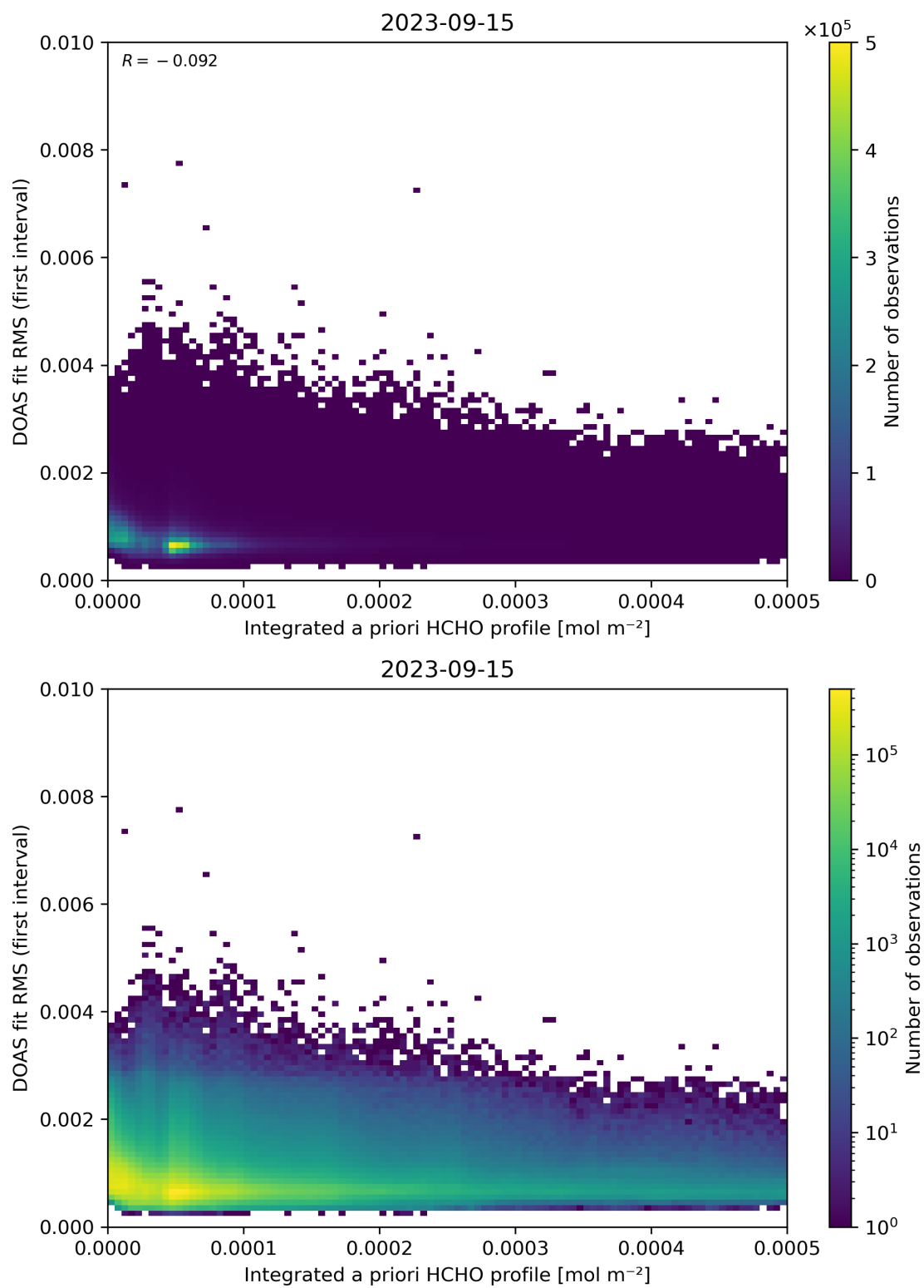
Figure 148: Scatter density plot of “Integrated a priori HCHO profile” against “DOAS fit RMS (first interval)” for 2023-09-15 to 2023-09-16.
