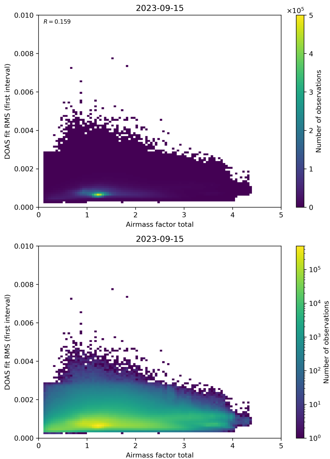
Figure 97: Scatter density plot of “Airmass factor total” against “DOAS fit RMS (first interval)” for 2023-09-15 to 2023-09-16.
