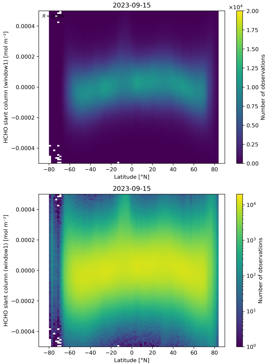
Figure 159: Scatter density plot of “Latitude” against “HCHO slant column (window1)” for 2023-09-15 to 2023-09-16.
