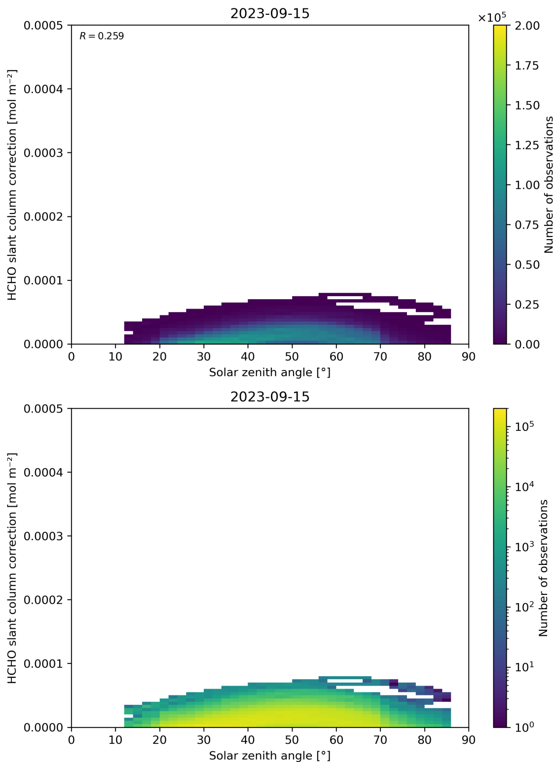
Figure 172: Scatter density plot of “Solar zenith angle” against “HCHO slant column correction” for 2023-09-15 to 2023-09-16.
