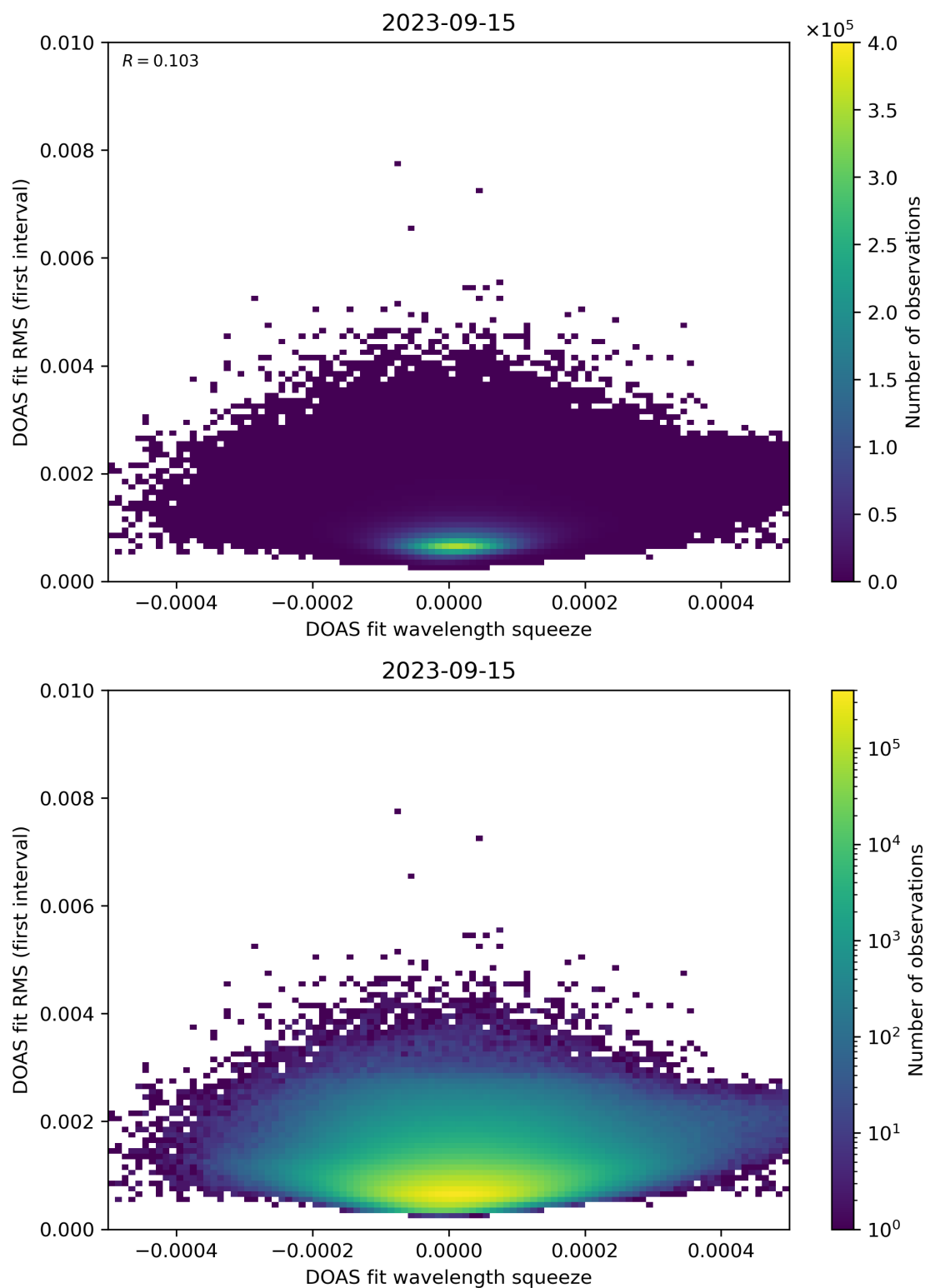
Figure 68: Scatter density plot of “DOAS fit wavelength squeeze” against “DOAS fit RMS (first interval)” for 2023-09-15 to 2023-09-16.
