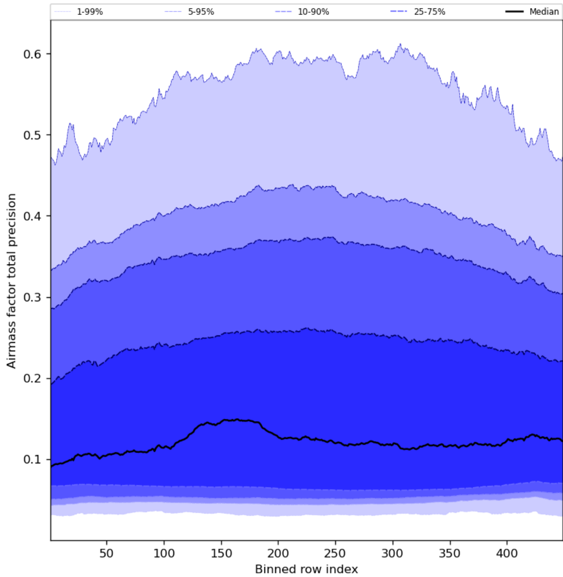
Figure 55: Along track statistics of “Airmass factor total precision” for 2023-09-15 to 2023-09-16
