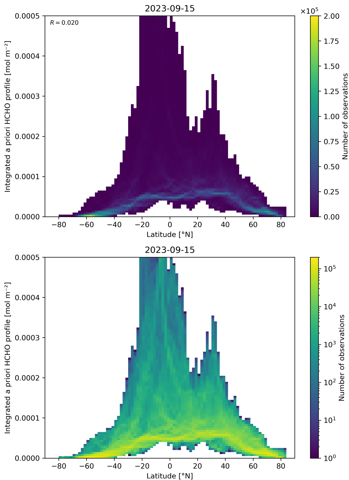
Figure 166: Scatter density plot of “Latitude” against “Integrated a priori HCHO profile” for 2023-09-15 to 2023-09-16.
