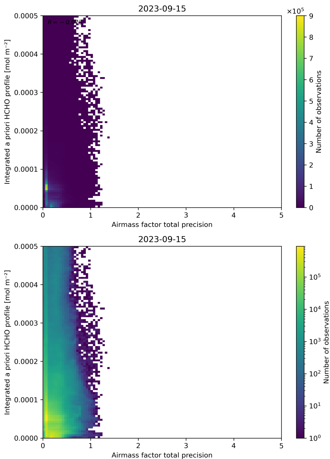
Figure 111: Scatter density plot of “Airmass factor total precision” against “Integrated a priori HCHO profile” for 2023-09-15 to 2023-09-16.
