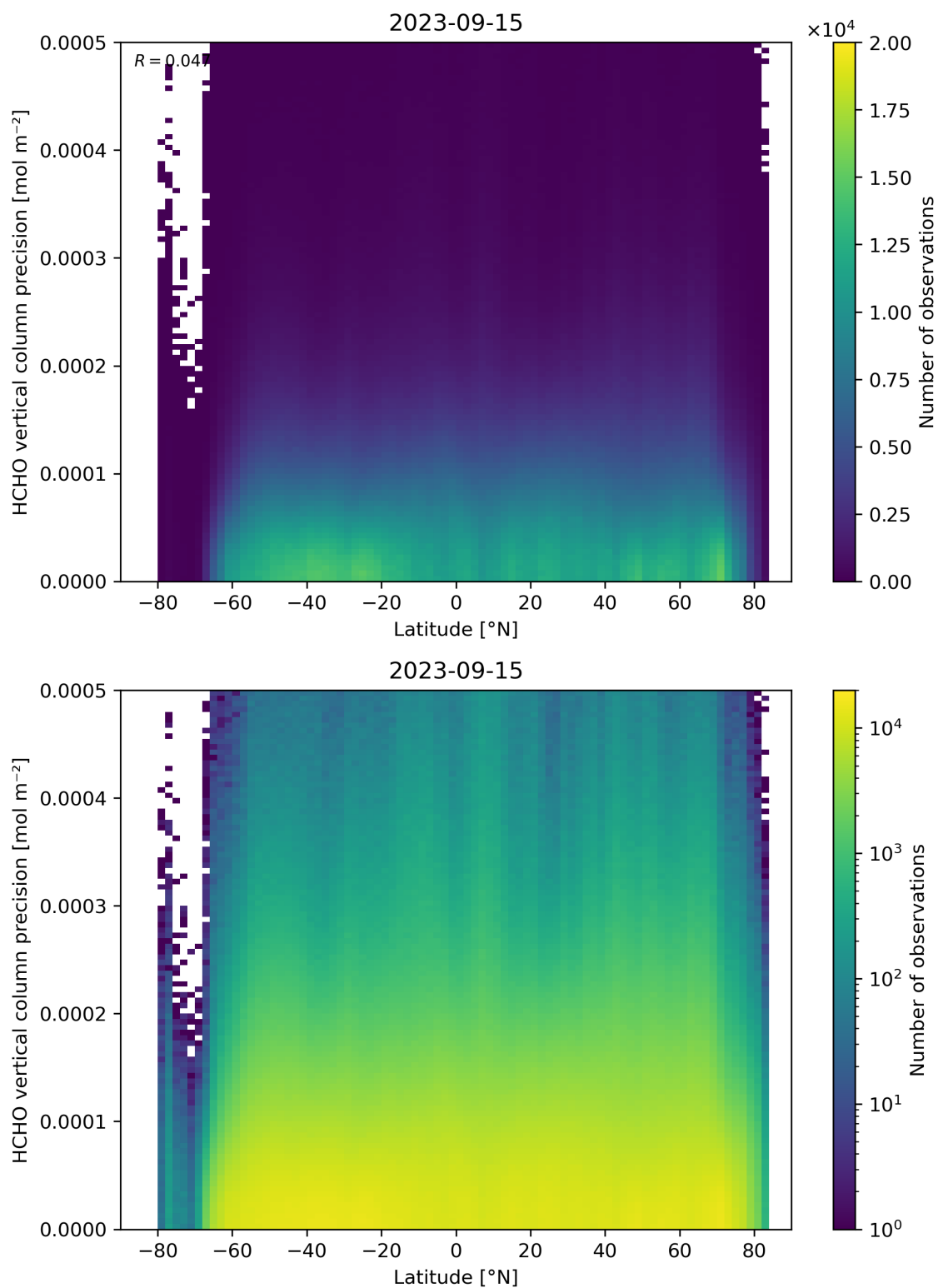
Figure 165: Scatter density plot of “Latitude” against “HCHO vertical column precision” for 2023-09-15 to 2023-09-16.
