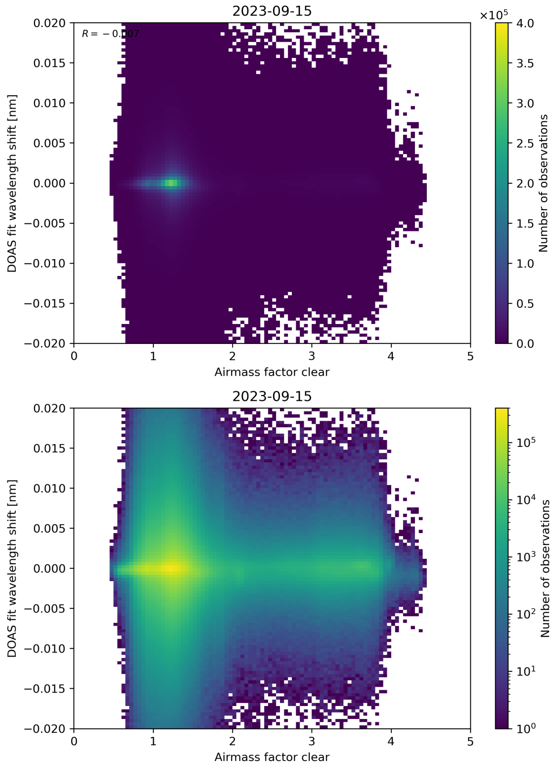
Figure 72: Scatter density plot of “Airmass factor clear” against “DOAS fit wavelength shift” for 2023-09-15 to 2023-09-16.
