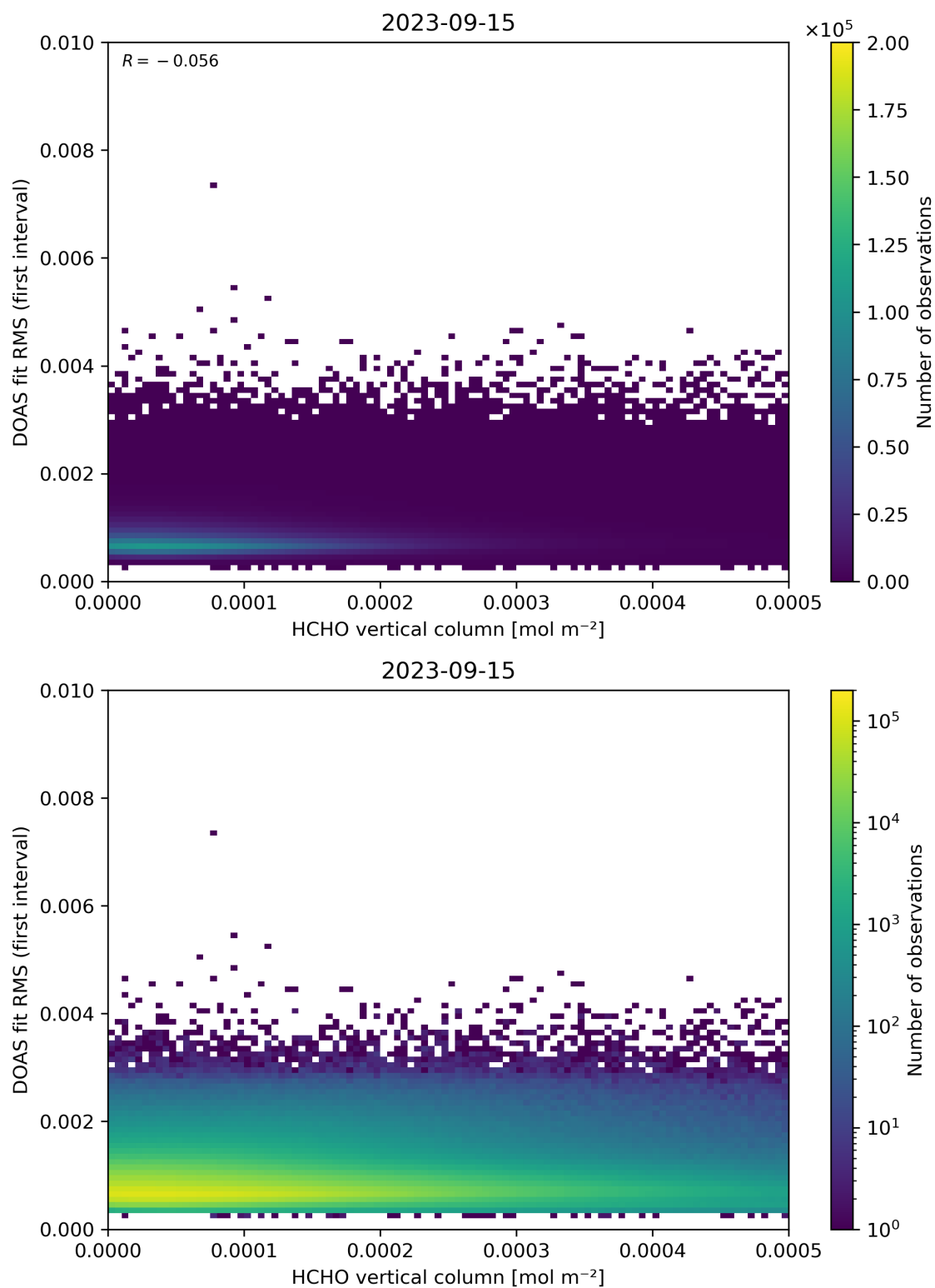
Figure 123: Scatter density plot of “HCHO vertical column” against “DOAS fit RMS (first interval)” for 2023-09-15 to 2023-09-16.
