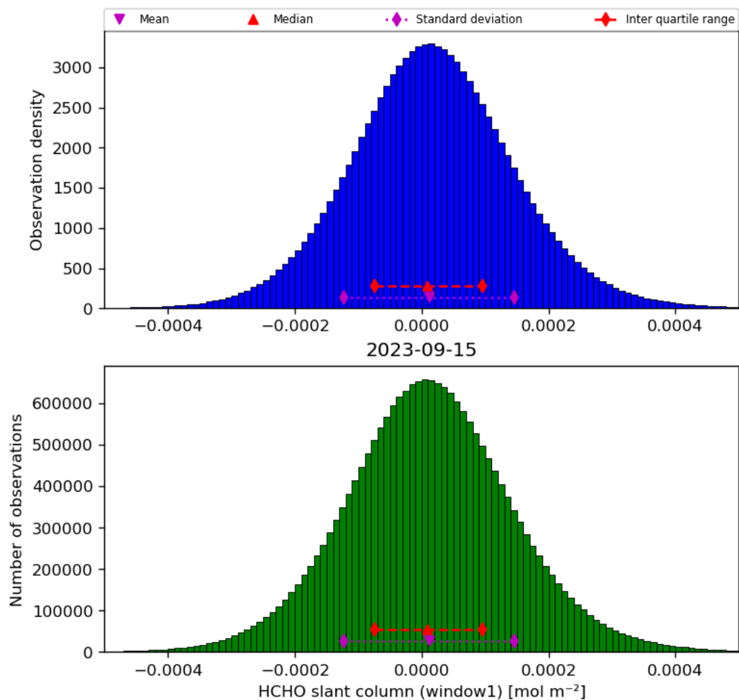
Figure 38: Histogram of “HCHO slant column (window1)” for 2023-09-15 to 2023-09-16
