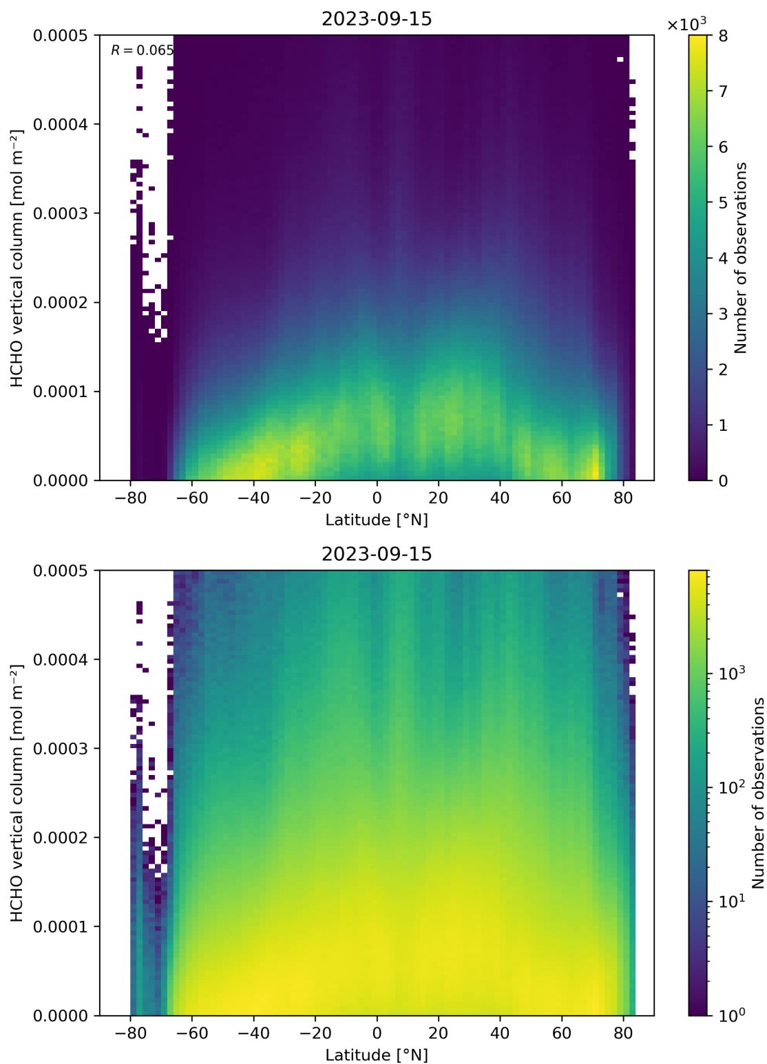
Figure 163: Scatter density plot of “Latitude” against “HCHO vertical column” for 2023-09-15 to 2023-09-16.
