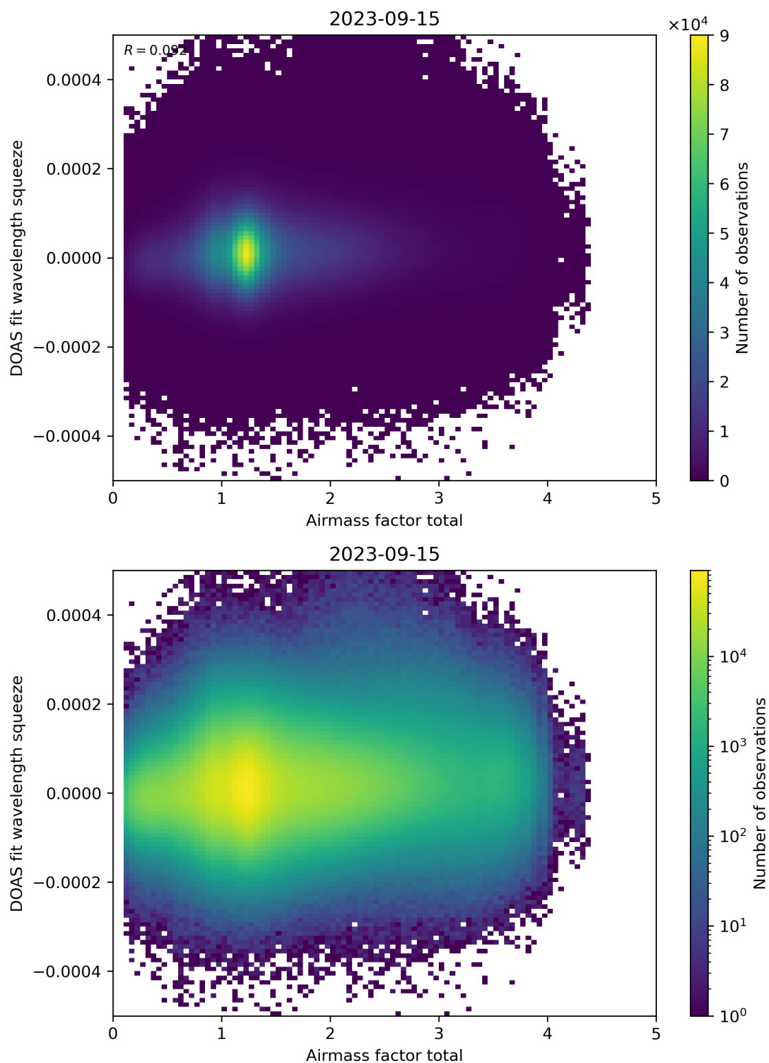
Figure 99: Scatter density plot of “Airmass factor total” against “DOAS fit wavelength squeeze” for 2023-09-15 to 2023-09-16.
