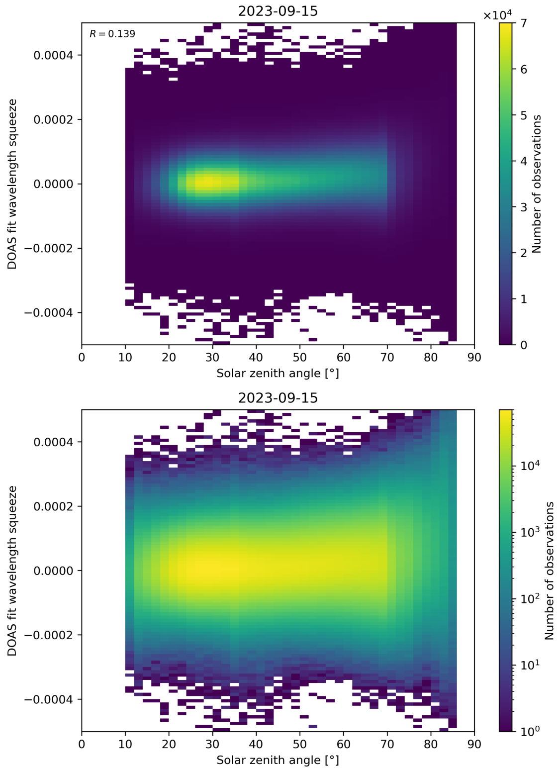
Figure 169: Scatter density plot of “Solar zenith angle” against “DOAS fit wavelength squeeze” for 2023-09-15 to 2023-09-16.
