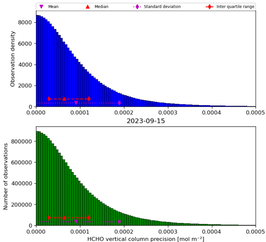
Figure 36: Histogram of “HCHO vertical column precision” for 2023-09-15 to 2023-09-16
