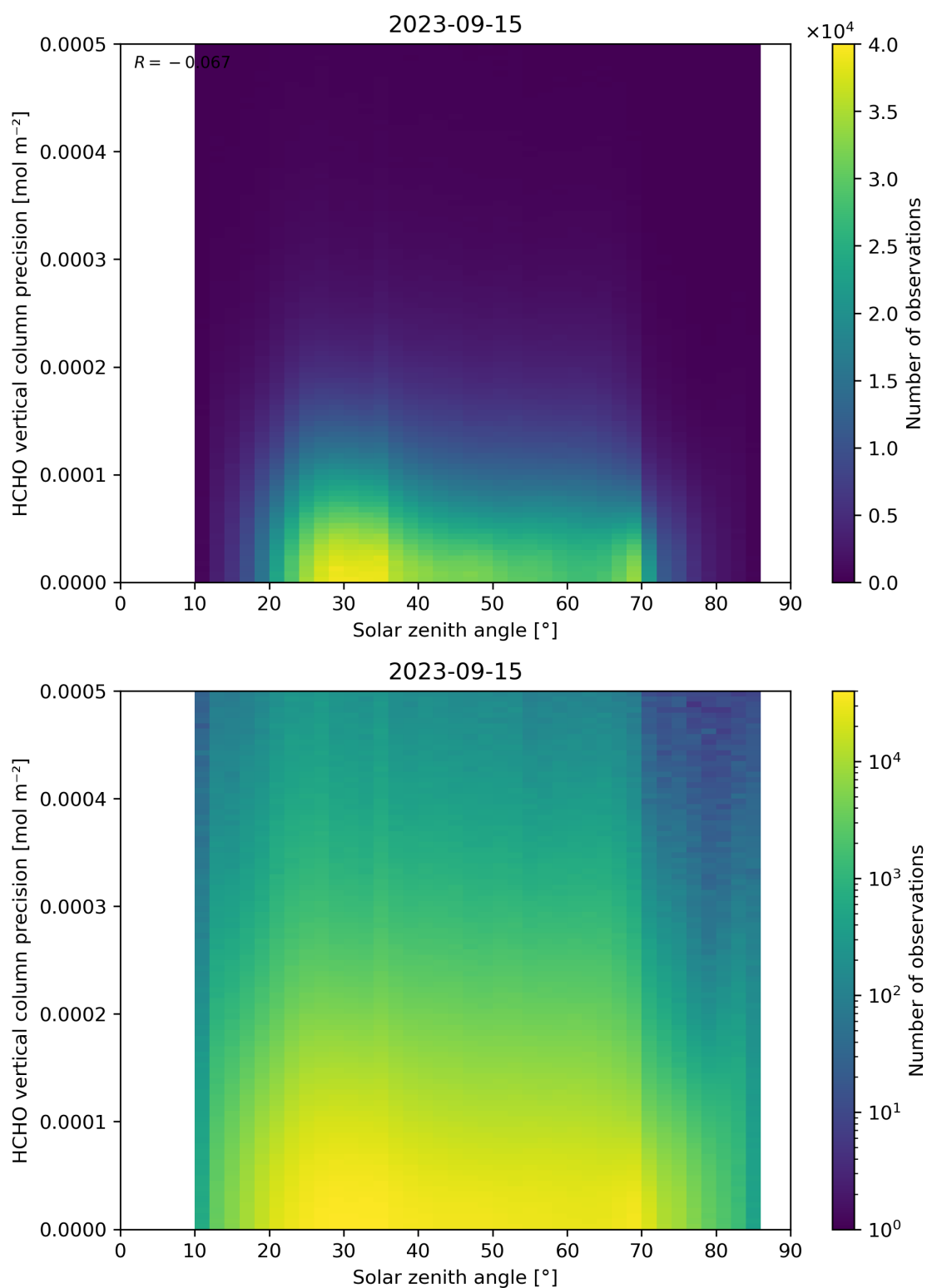
Figure 179: Scatter density plot of “Solar zenith angle” against “HCHO vertical column precision” for 2023-09-15 to 2023-09-16.
