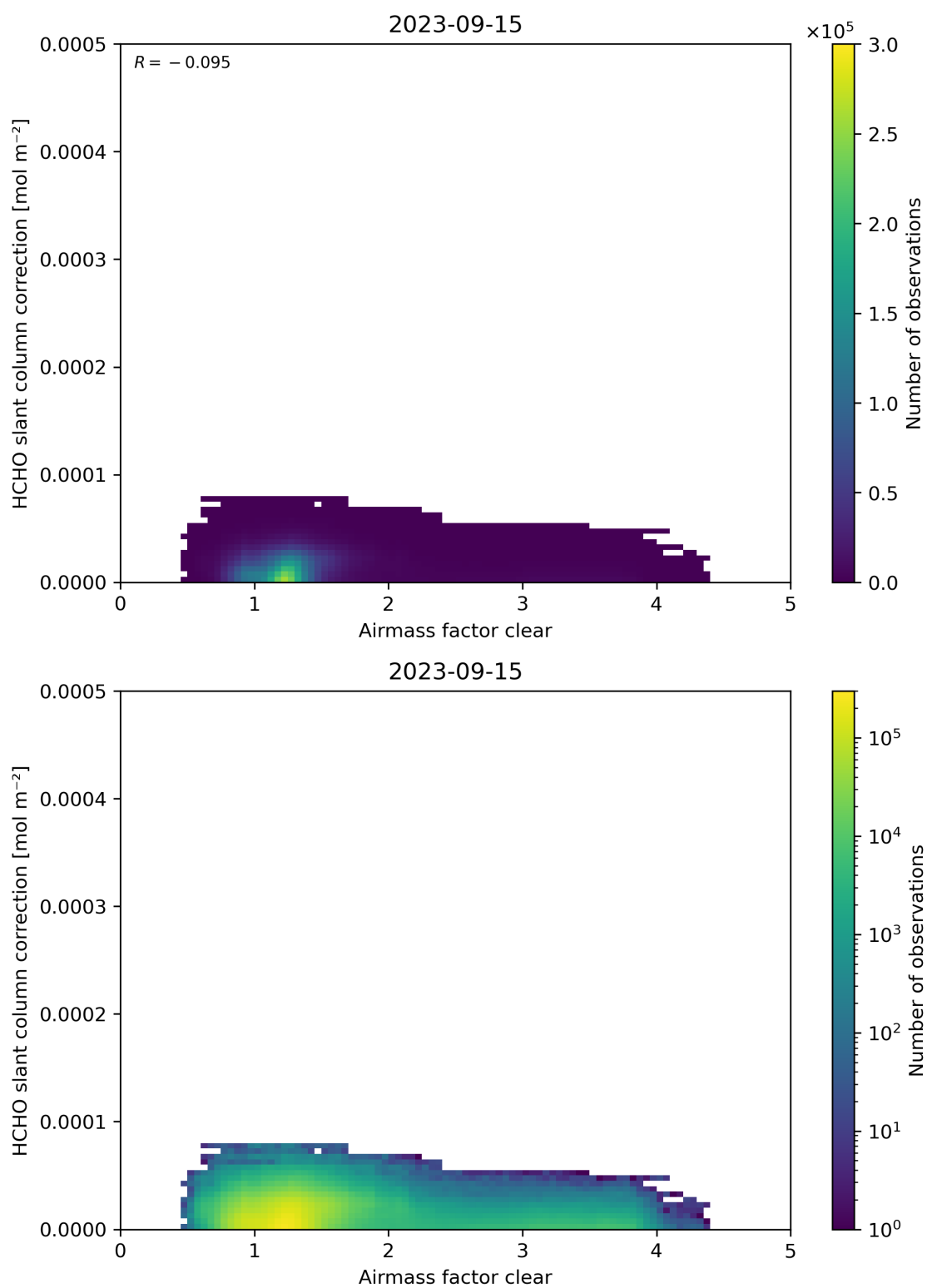
Figure 75: Scatter density plot of “Airmass factor clear” against “HCHO slant column correction” for 2023-09-15 to 2023-09-16.
