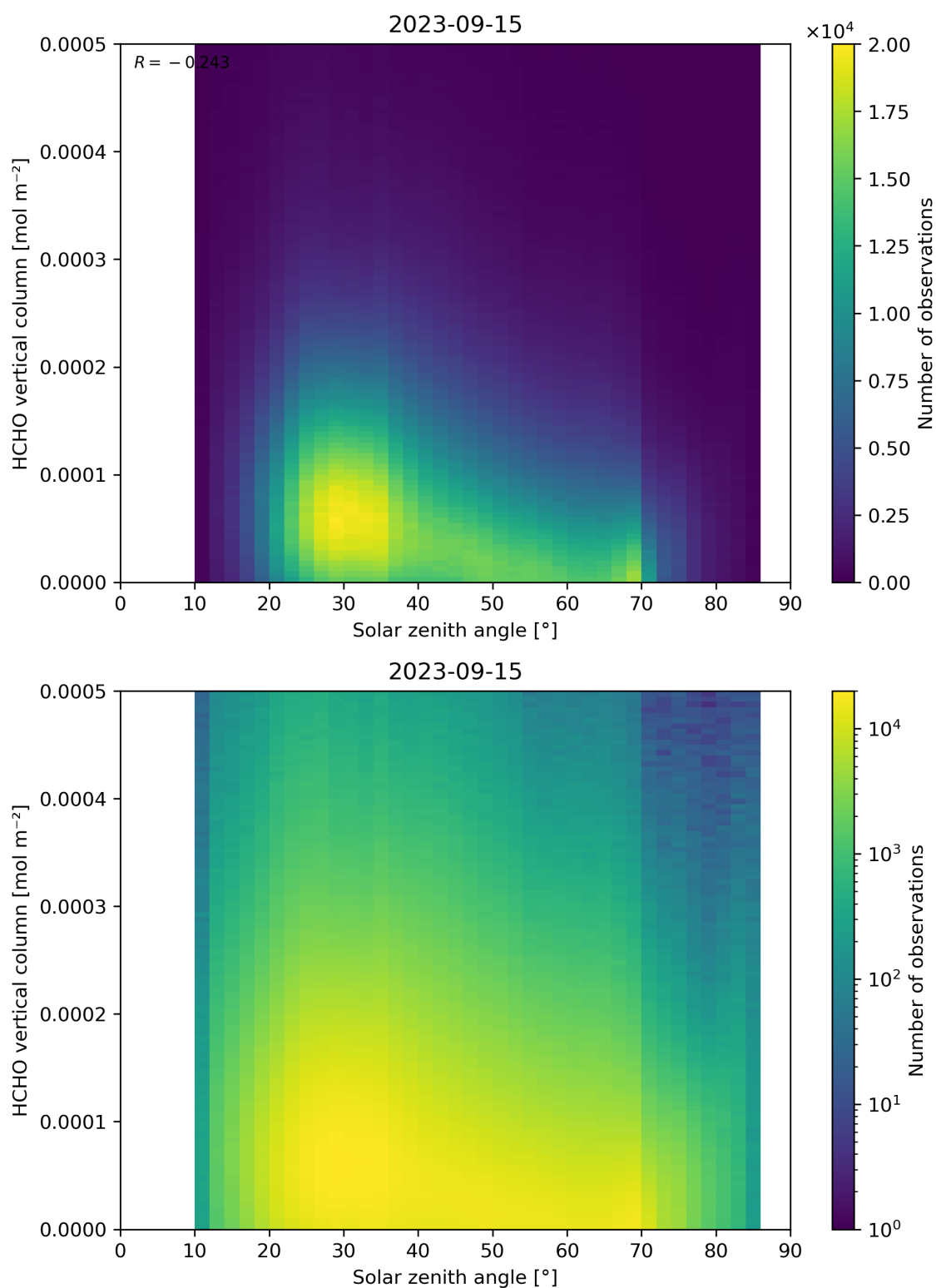
Figure 177: Scatter density plot of “Solar zenith angle” against “HCHO vertical column” for 2023-09-15 to 2023-09-16.
