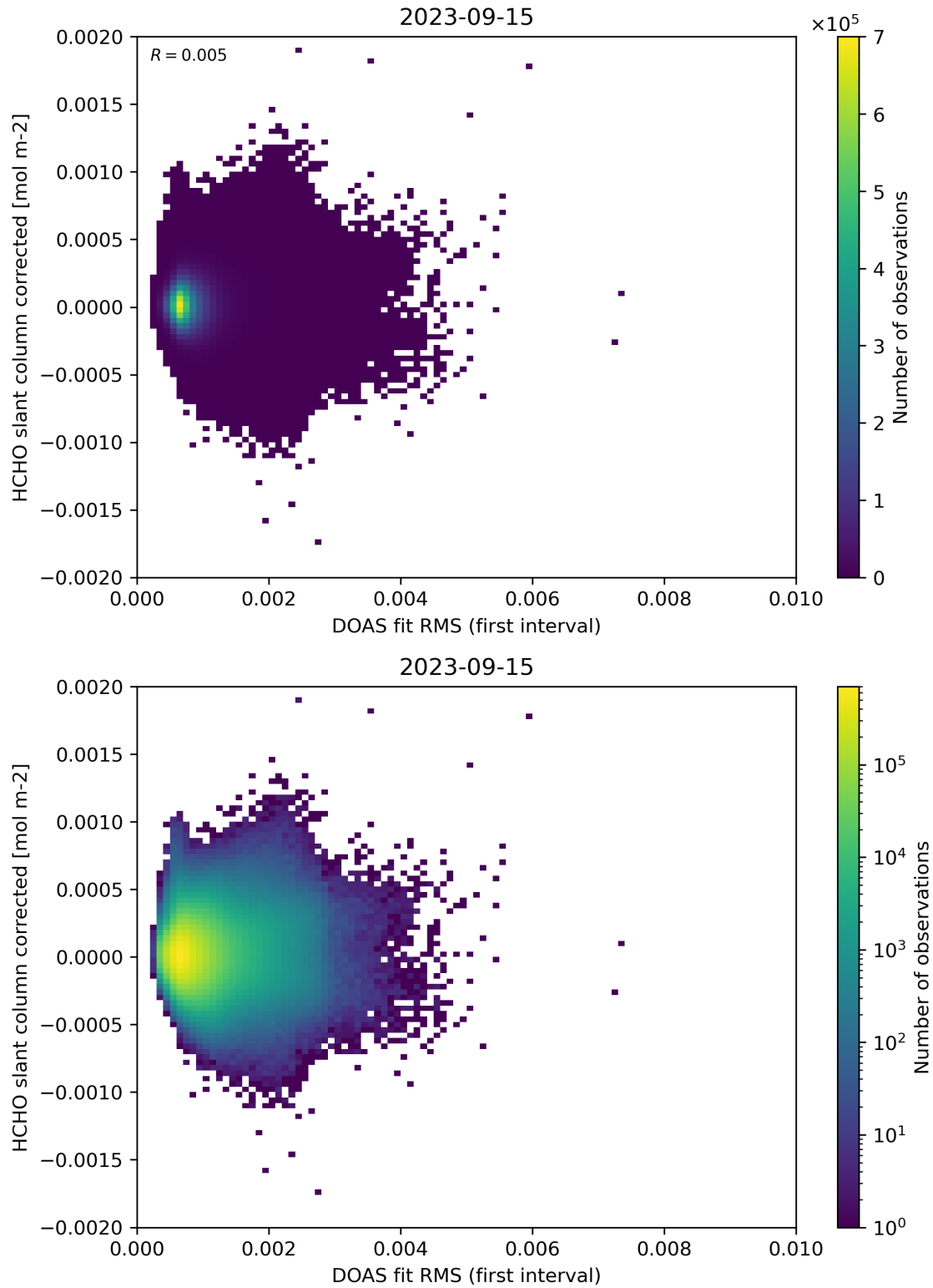
Figure 62: Scatter density plot of “DOAS fit RMS (first interval)” against “HCHO slant column corrected” for 2023-09-15 to 2023-09-16.
