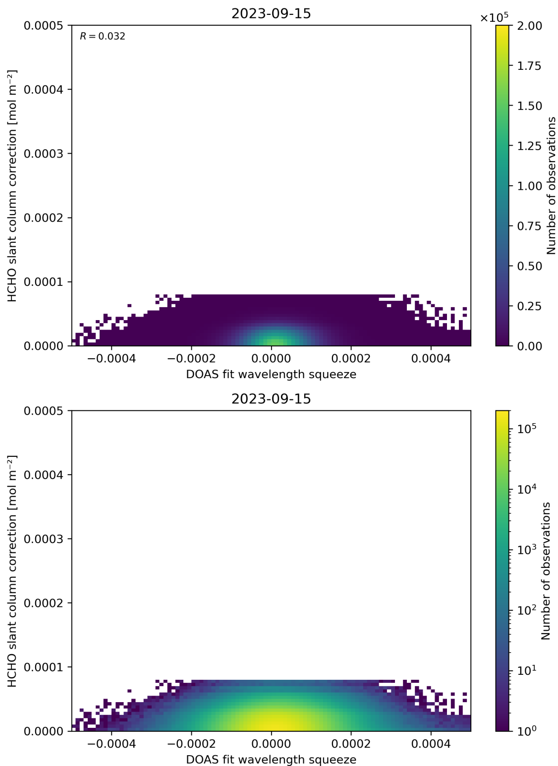
Figure 70: Scatter density plot of “DOAS fit wavelength squeeze” against “HCHO slant column correction” for 2023-09-15 to 2023-09-16.
