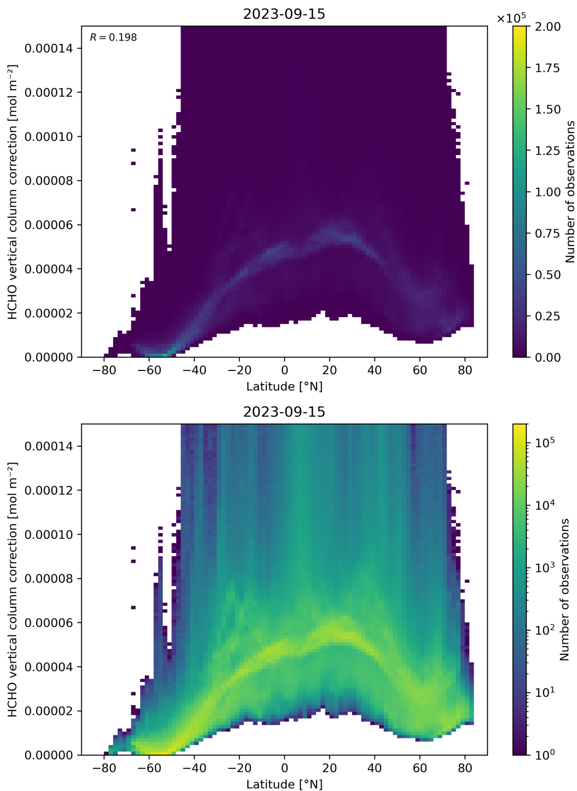
Figure 164: Scatter density plot of “Latitude” against “HCHO vertical column correction” for 2023-09-15 to 2023-09-16.
