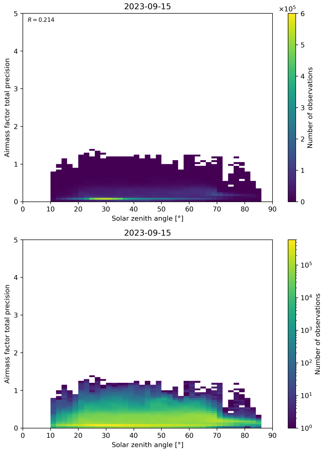
Figure 176: Scatter density plot of “Solar zenith angle” against “Airmass factor total precision” for 2023-09-15 to 2023-09-16.
