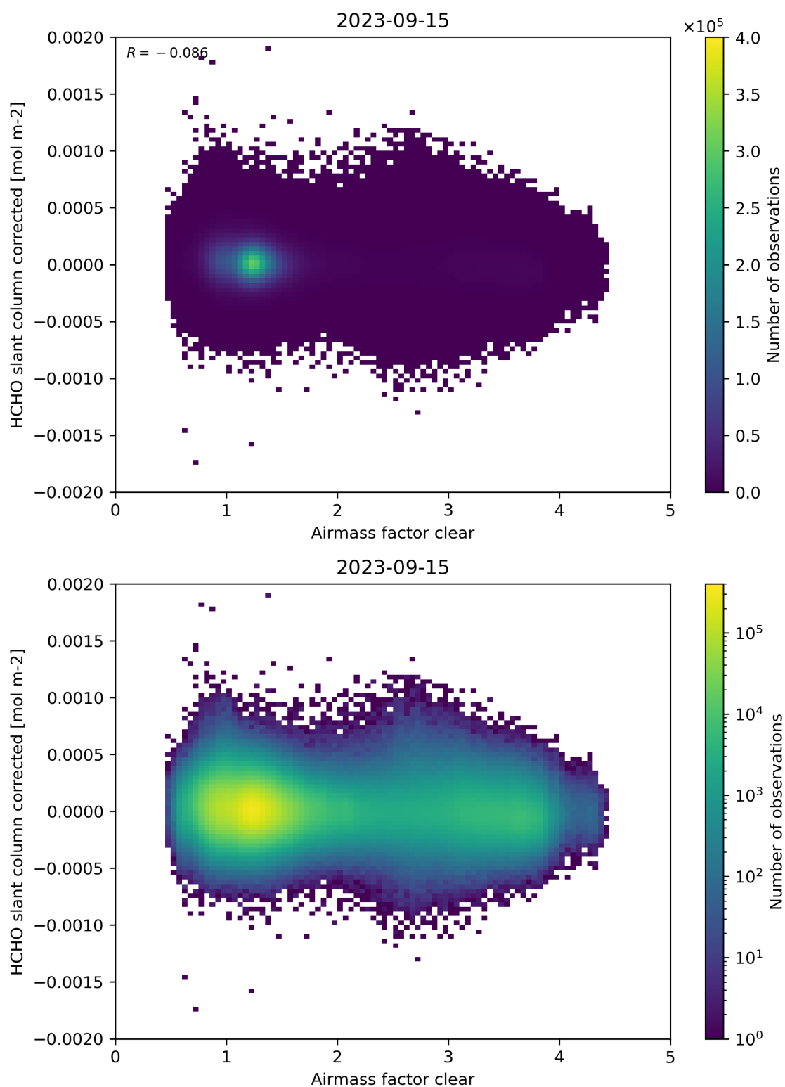
Figure 74: Scatter density plot of “Airmass factor clear” against “HCHO slant column corrected” for 2023-09-15 to 2023-09-16.
