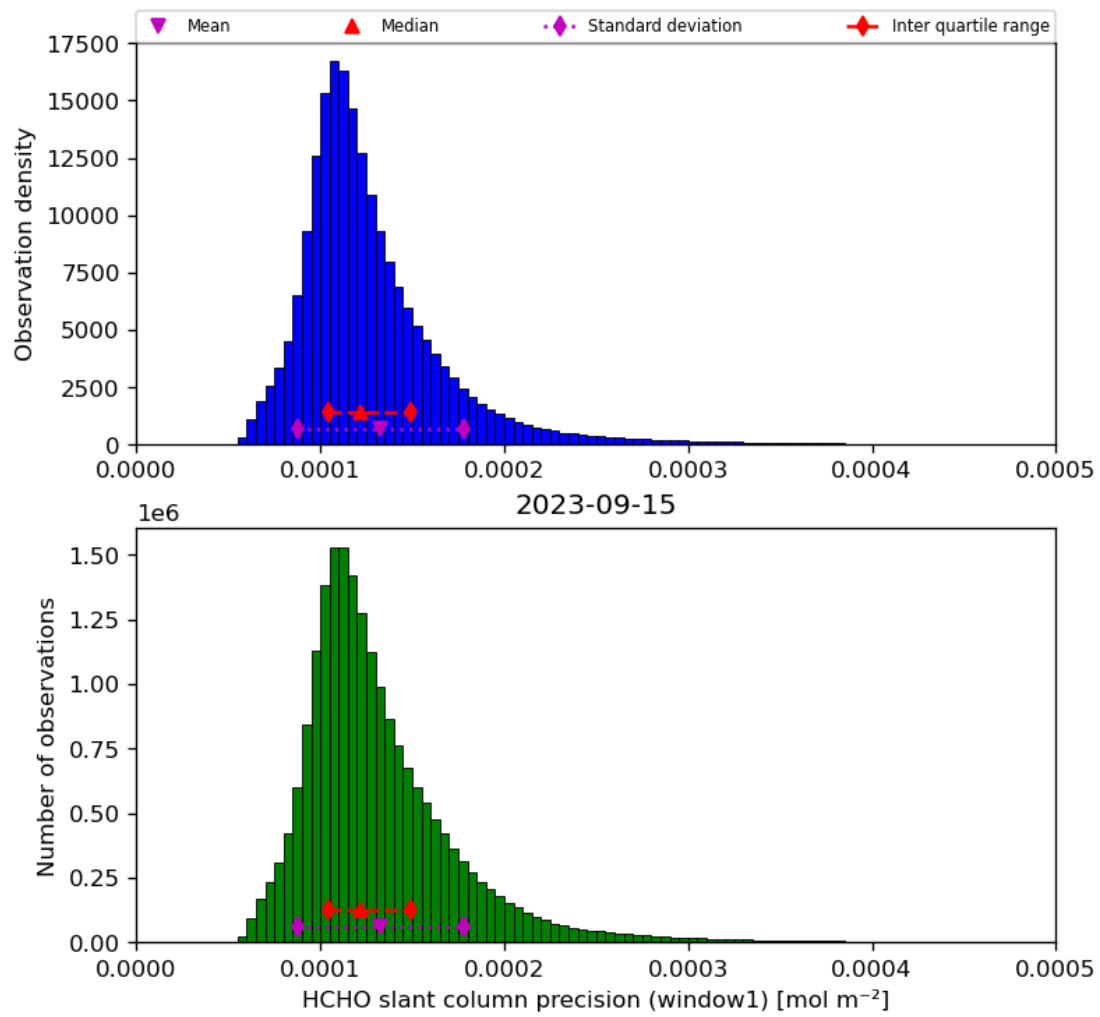
Figure 39: Histogram of “HCHO slant column precision (window1)” for 2023-09-15 to 2023-09-16
