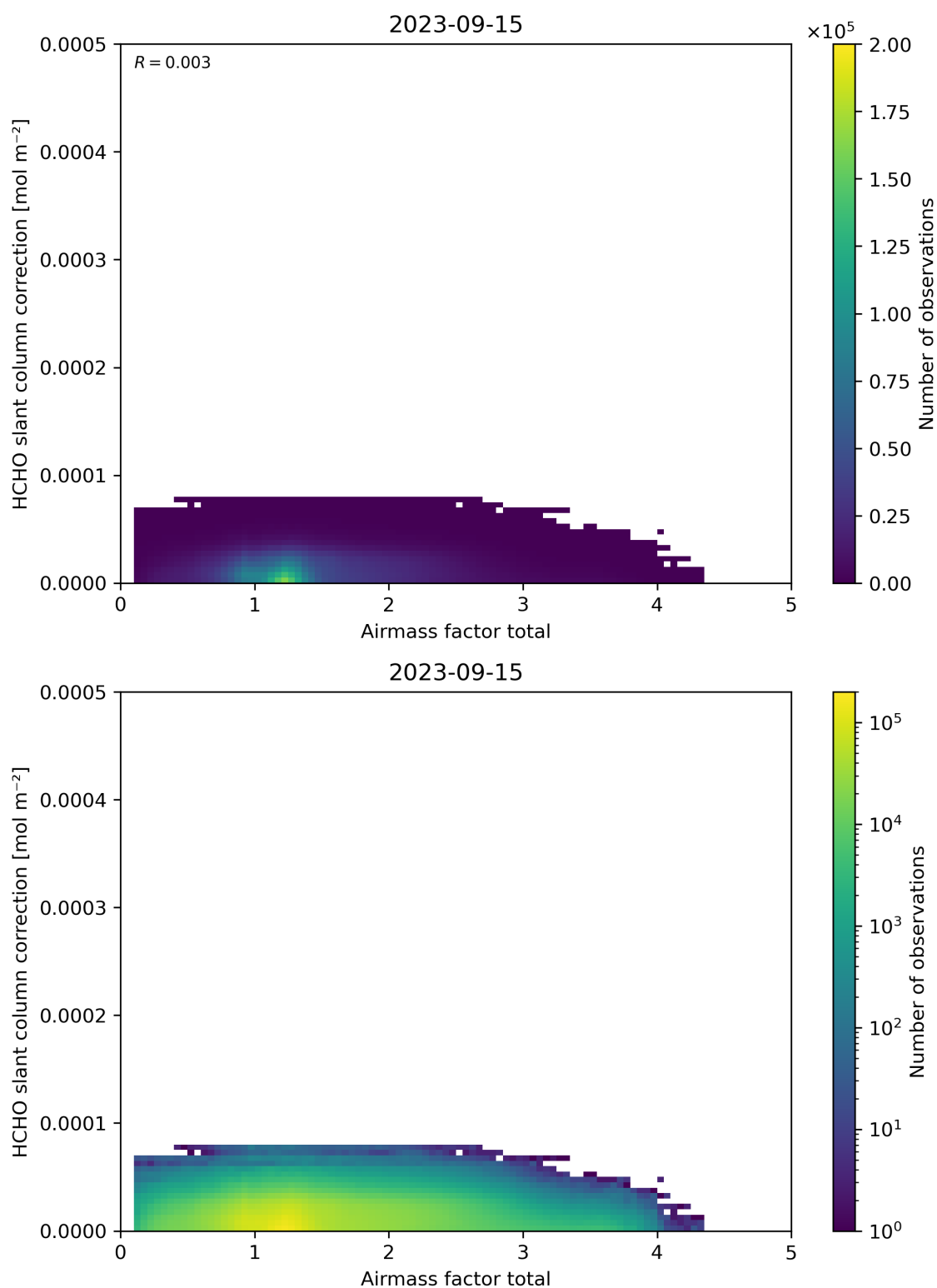
Figure 102: Scatter density plot of “Airmass factor total” against “HCHO slant column correction” for 2023-09-15 to 2023-09-16.
