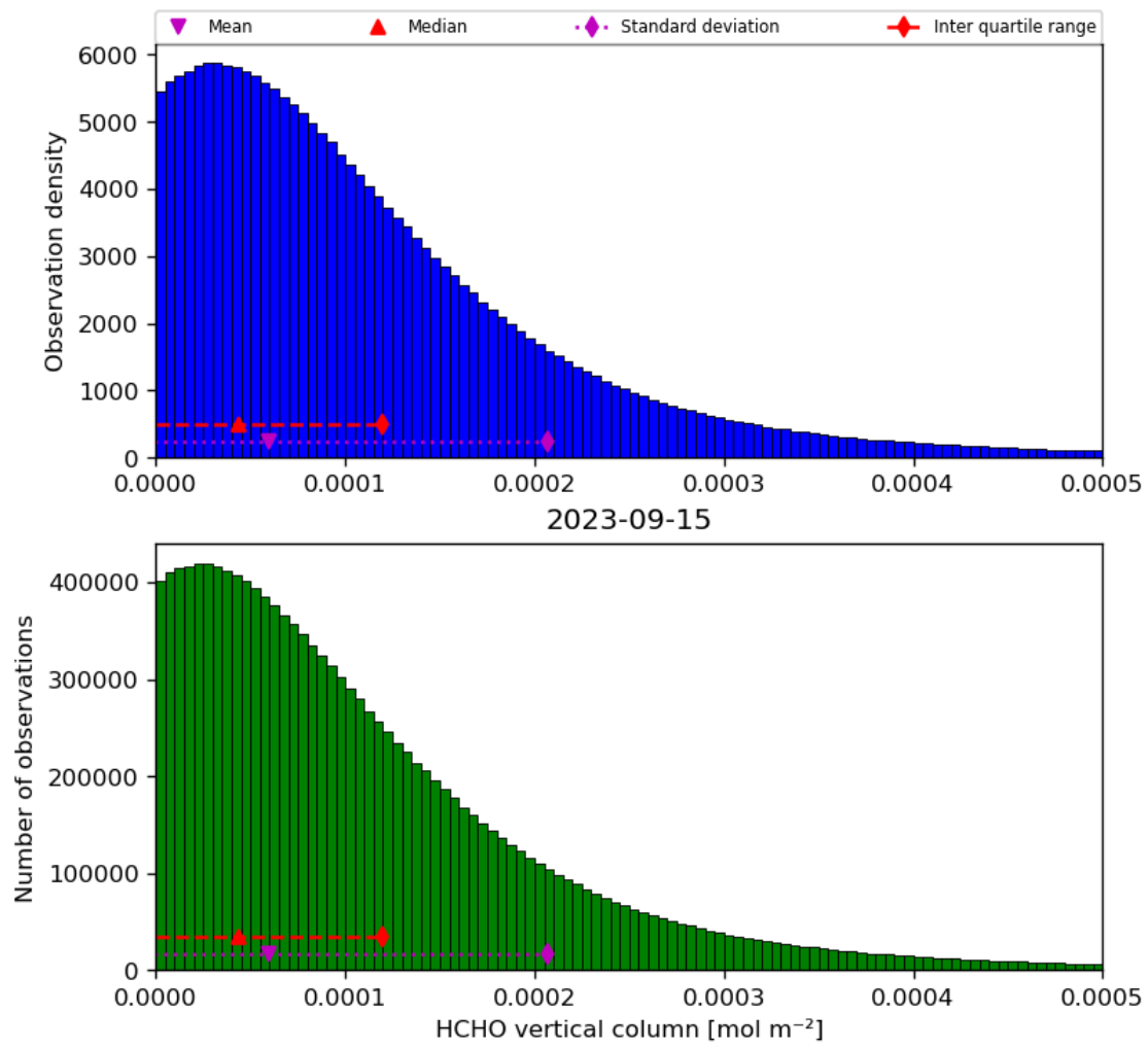
Figure 35: Histogram of “HCHO vertical column” for 2023-09-15 to 2023-09-16
