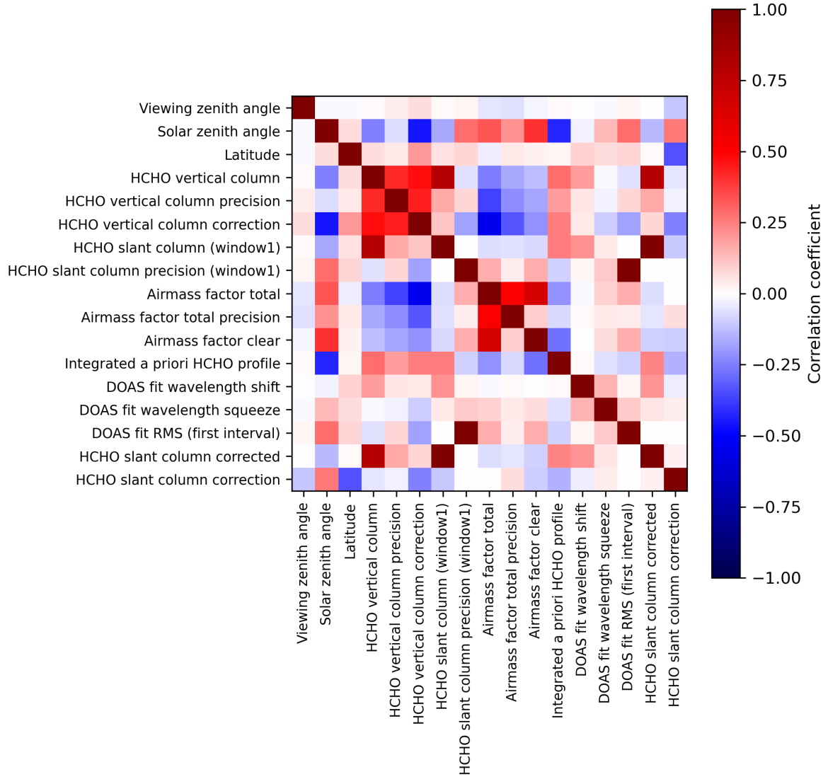
Figure 2: Map of correlation matrix for 2023-09-15 to 2023-09-16.
