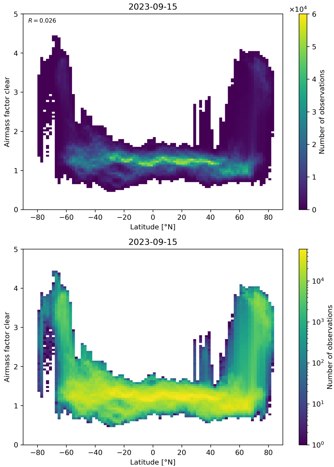
Figure 156: Scatter density plot of “Latitude” against “Airmass factor clear” for 2023-09-15 to 2023-09-16.
