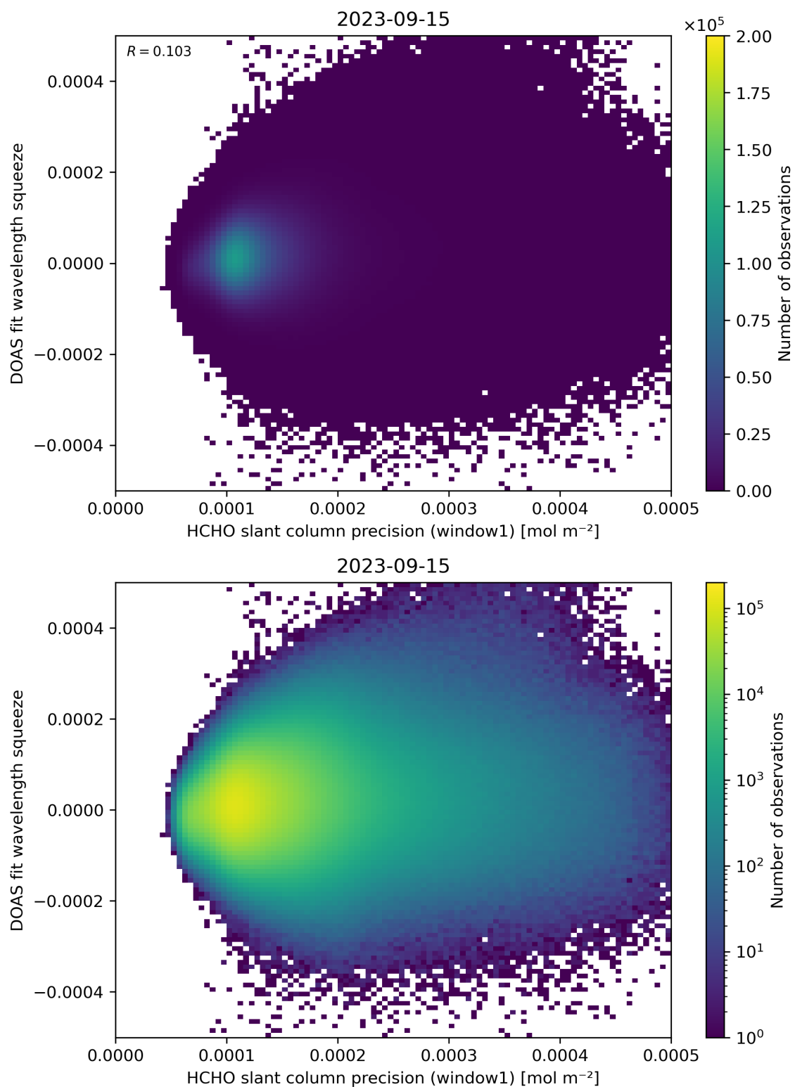
Figure 90: Scatter density plot of “HCHO slant column precision (window1)” against “DOAS fit wavelength squeeze” for 2023-09-15 to 2023-09-16.
