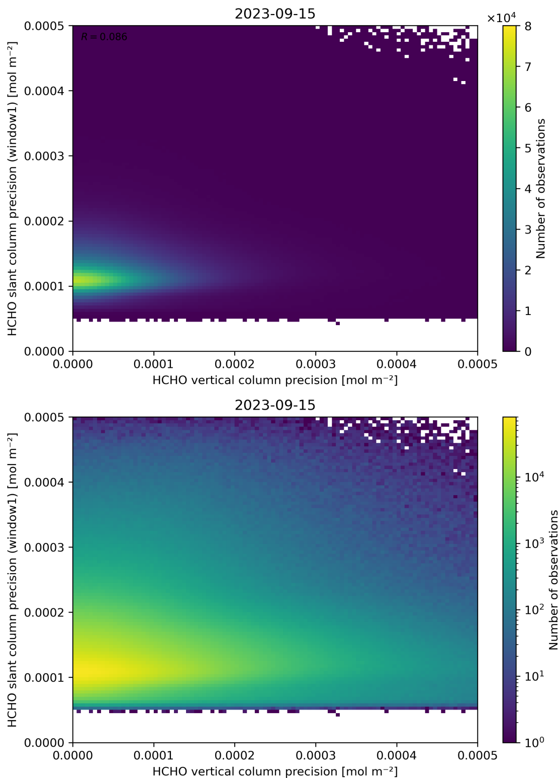
Figure 143: Scatter density plot of “HCHO vertical column precision” against “HCHO slant column precision (window1)” for 2023-09-15 to 2023-09-16.
