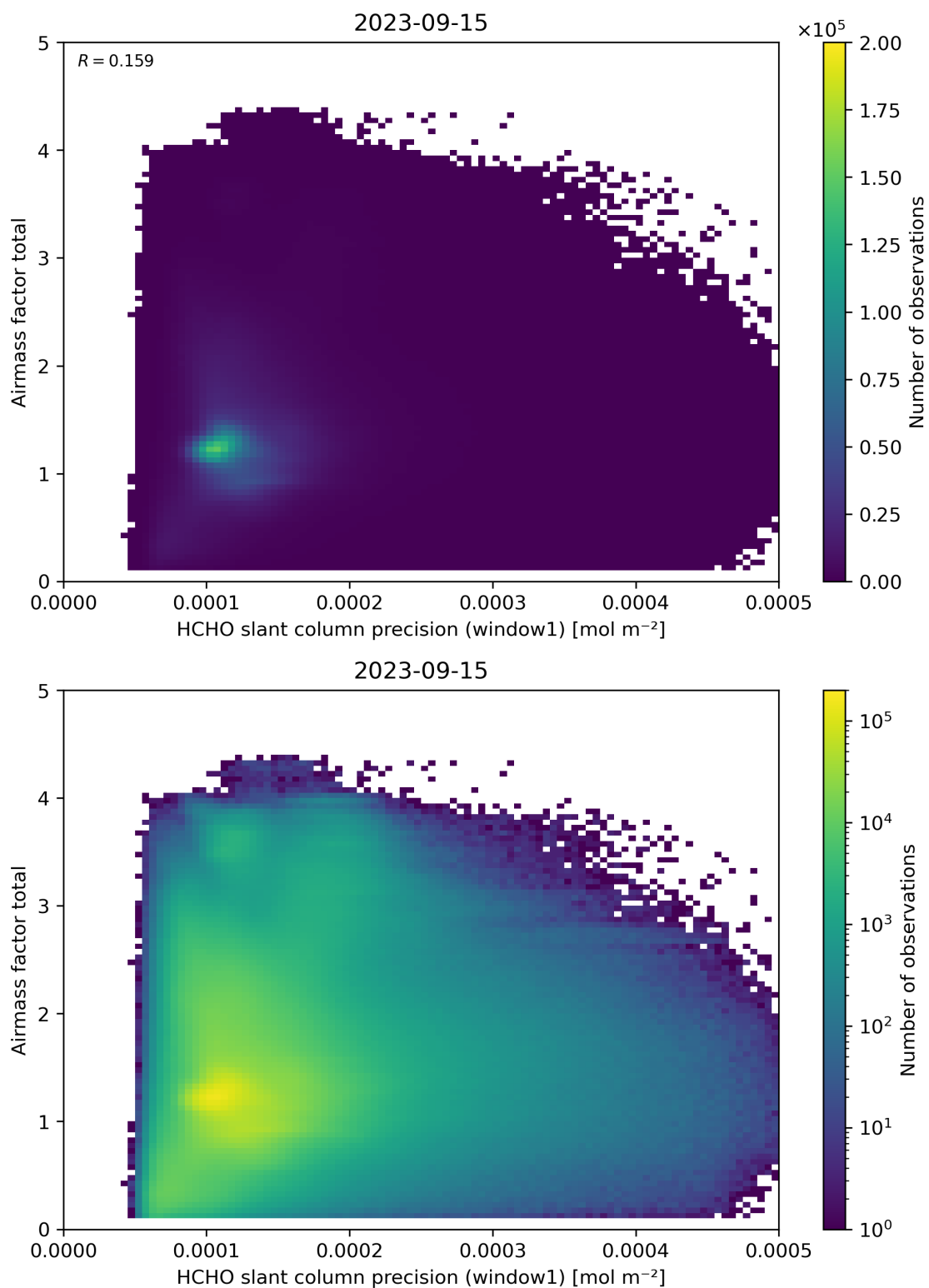
Figure 94: Scatter density plot of “HCHO slant column precision (window1)” against “Airmass factor total” for 2023-09-15 to 2023-09-16.
