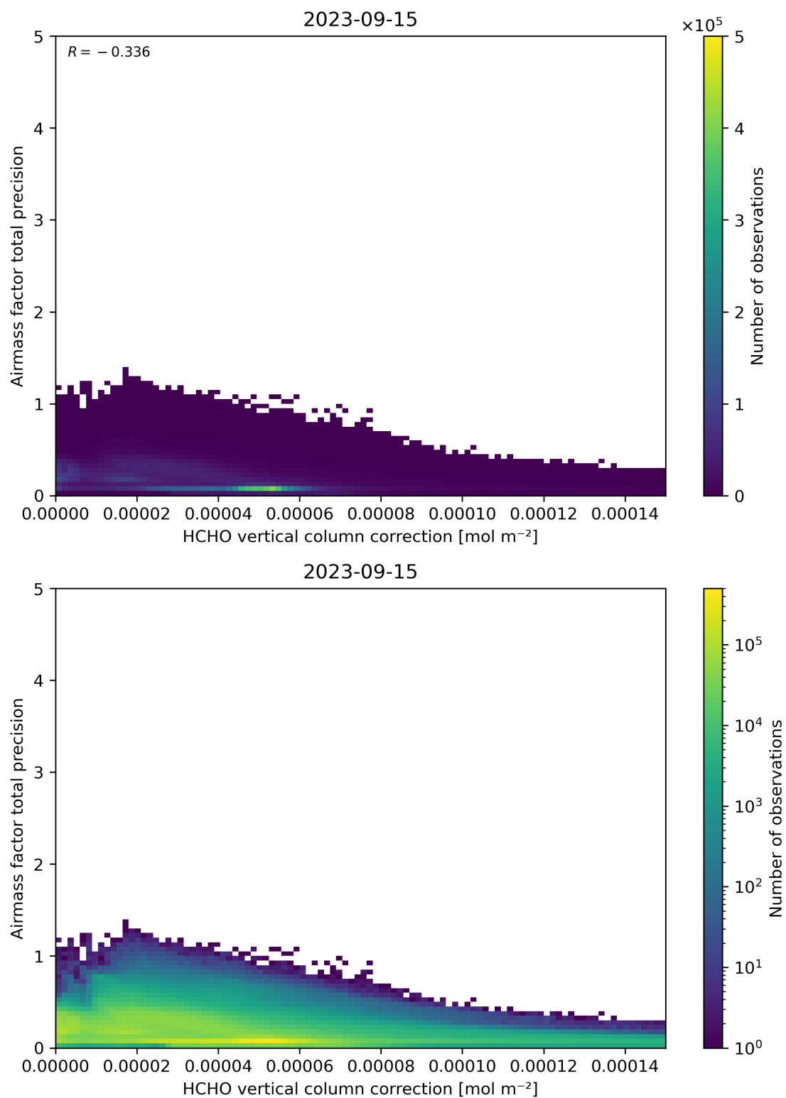
Figure 121: Scatter density plot of “HCHO vertical column correction” against “Airmass factor total precision” for 2023-09-15 to 2023-09-16.
