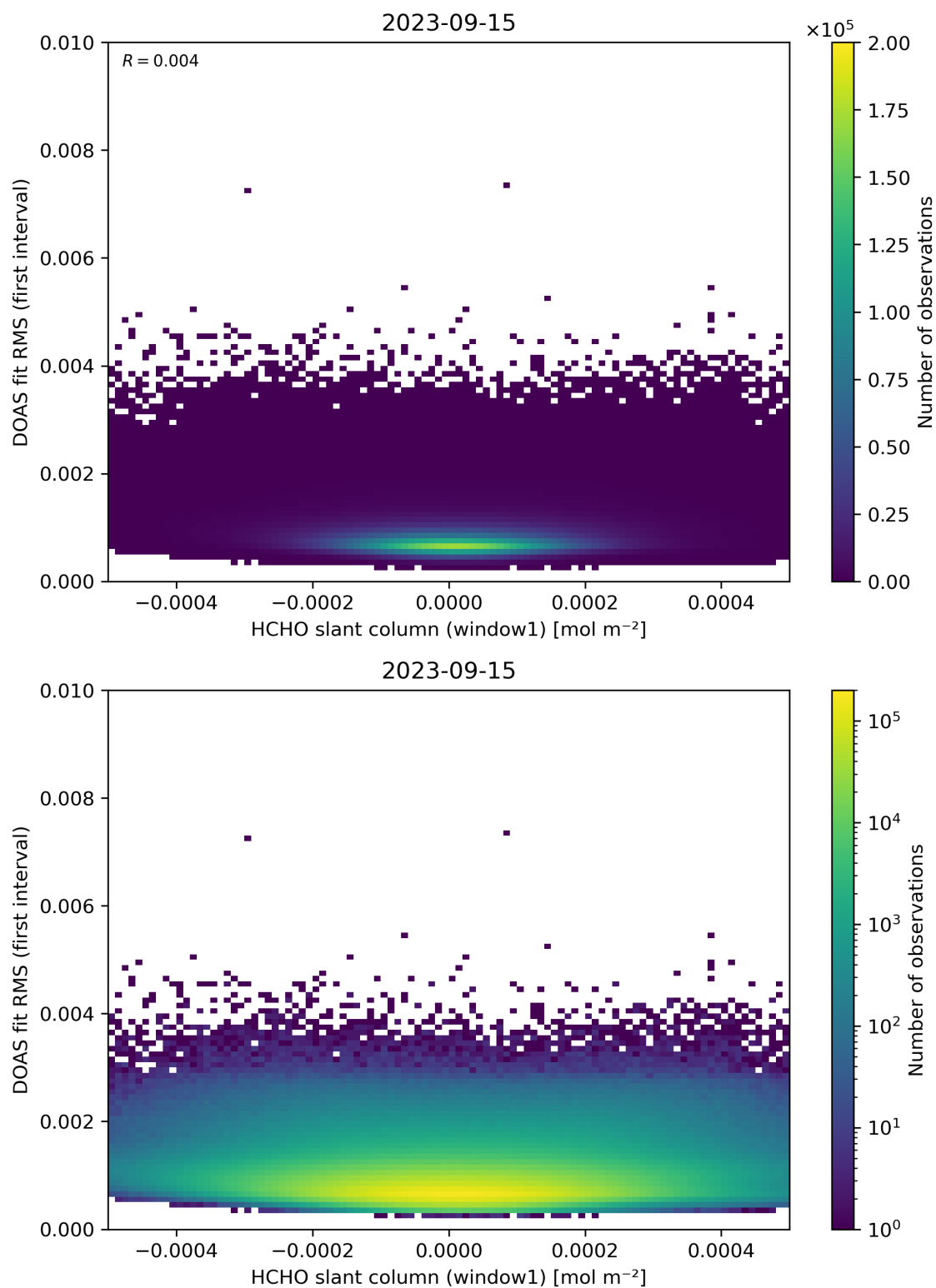
Figure 78: Scatter density plot of “HCHO slant column (window1)” against “DOAS fit RMS (first interval)” for 2023-09-15 to 2023-09-16.
