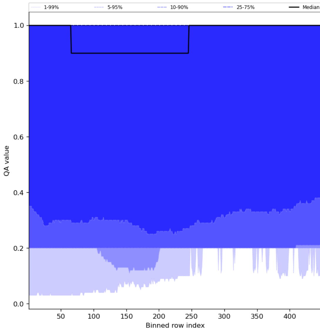
Figure 48: Along track statistics of “QA value” for 2023-09-15 to 2023-09-16
