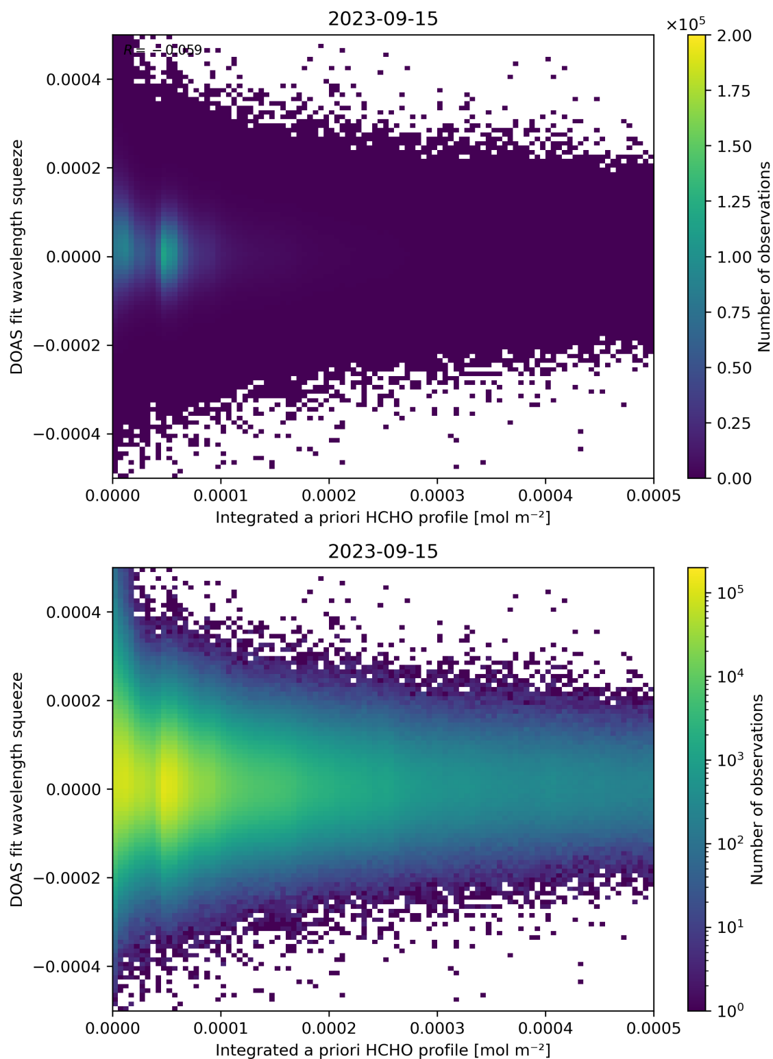
Figure 150: Scatter density plot of “Integrated a priori HCHO profile” against “DOAS fit wavelength squeeze” for 2023-09-15 to 2023-09-16.
