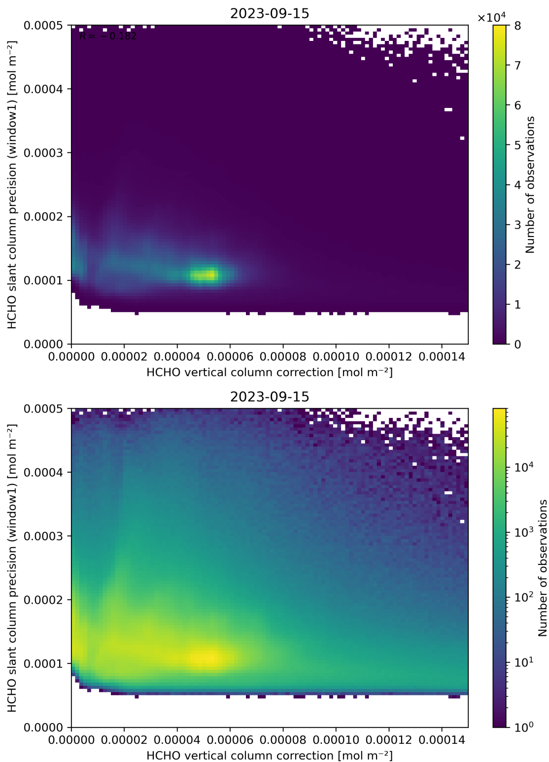
Figure 119: Scatter density plot of “HCHO vertical column correction” against “HCHO slant column precision (window1)” for 2023-09-15 to 2023-09-16.
