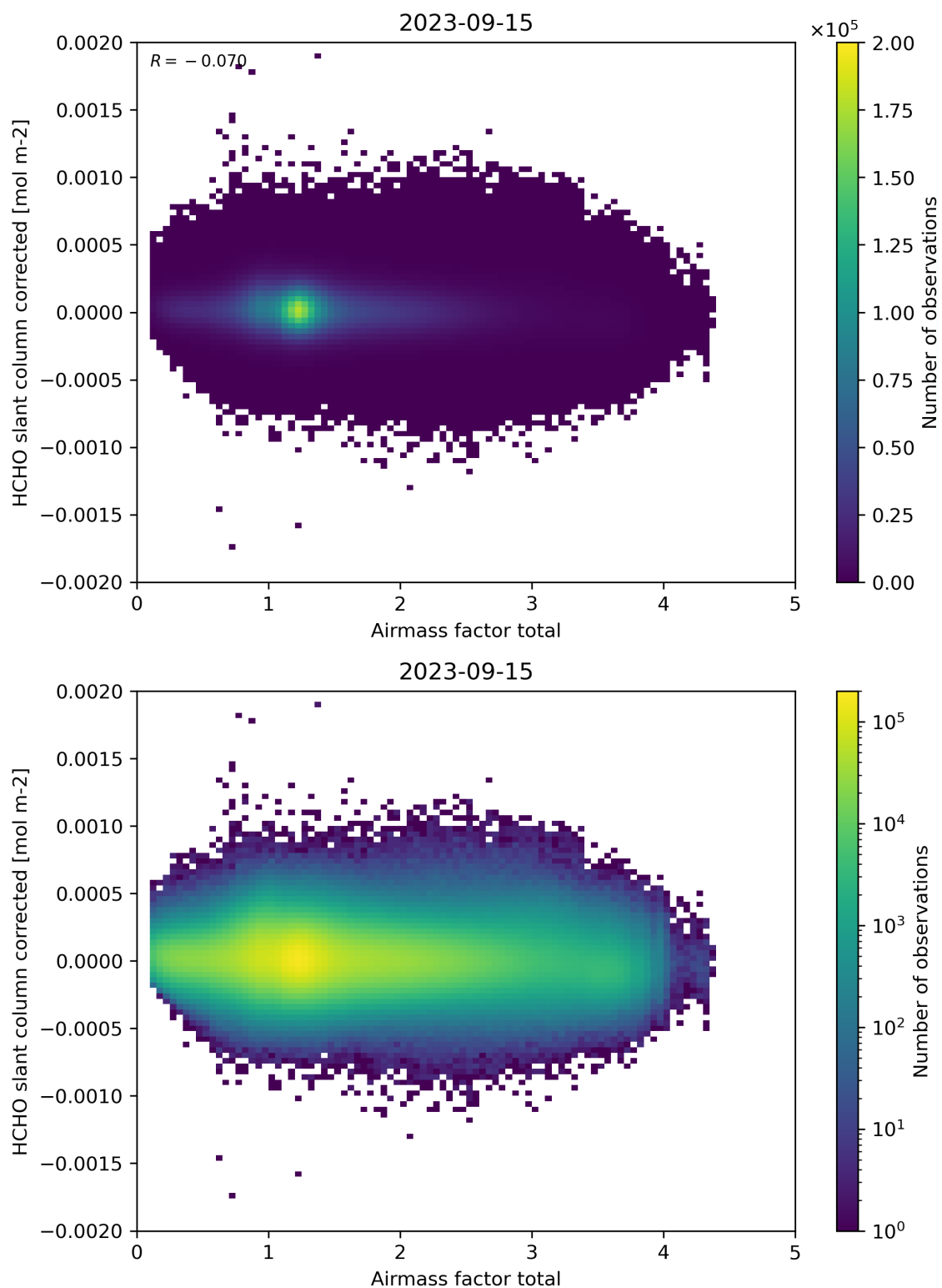
Figure 101: Scatter density plot of “Airmass factor total” against “HCHO slant column corrected” for 2023-09-15 to 2023-09-16.
