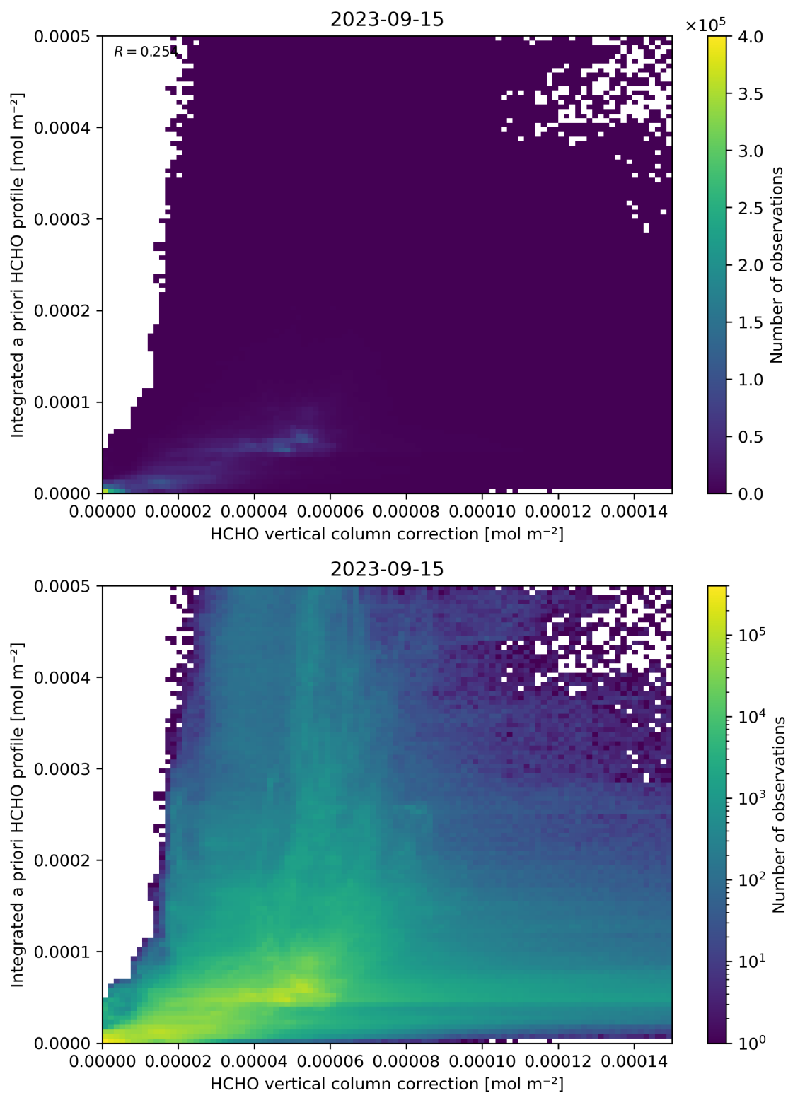
Figure 122: Scatter density plot of “HCHO vertical column correction” against “Integrated a priori HCHO profile” for 2023-09-15 to 2023-09-16.
