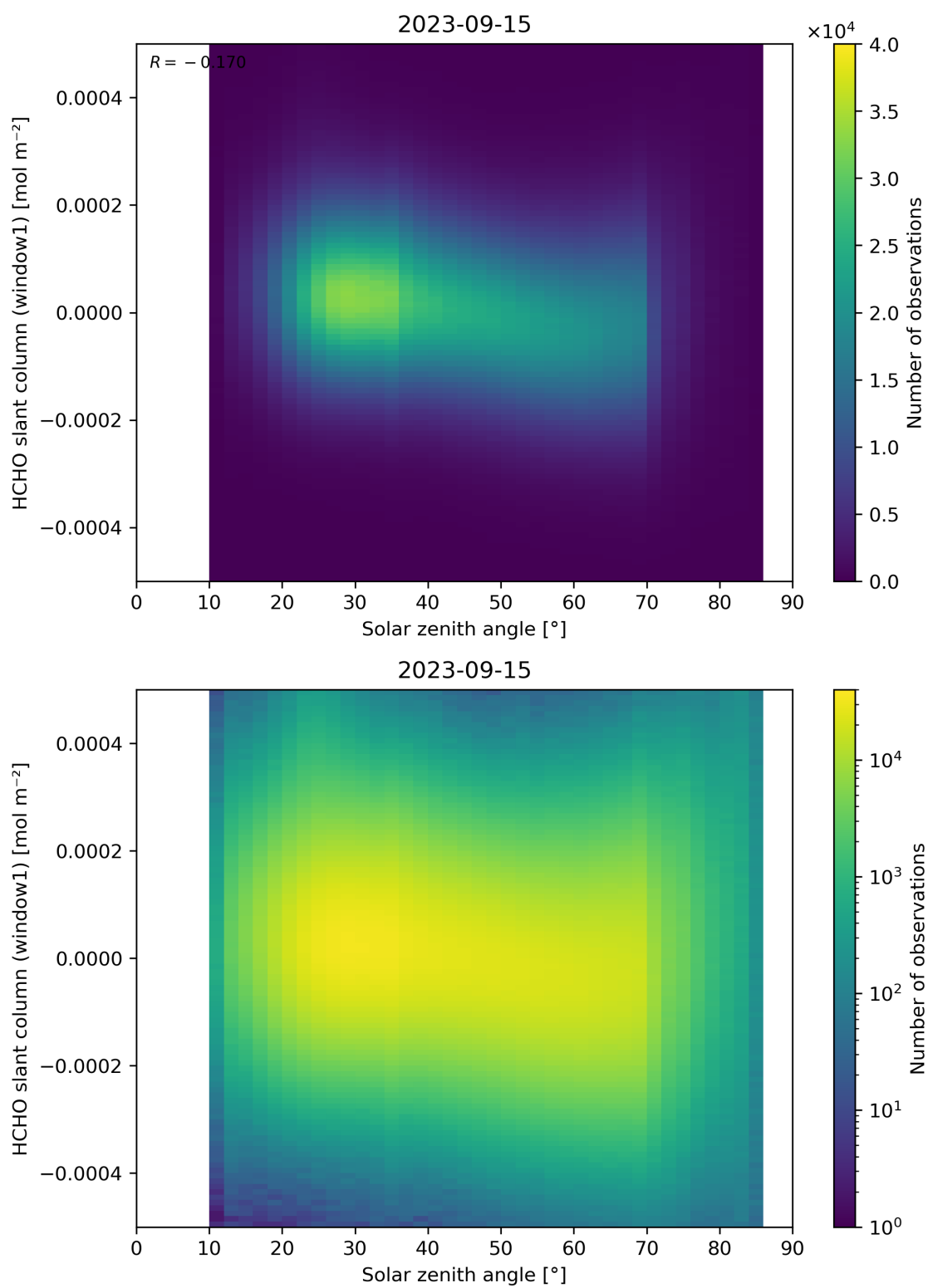
Figure 173: Scatter density plot of “Solar zenith angle” against “HCHO slant column (window1)” for 2023-09-15 to 2023-09-16.
