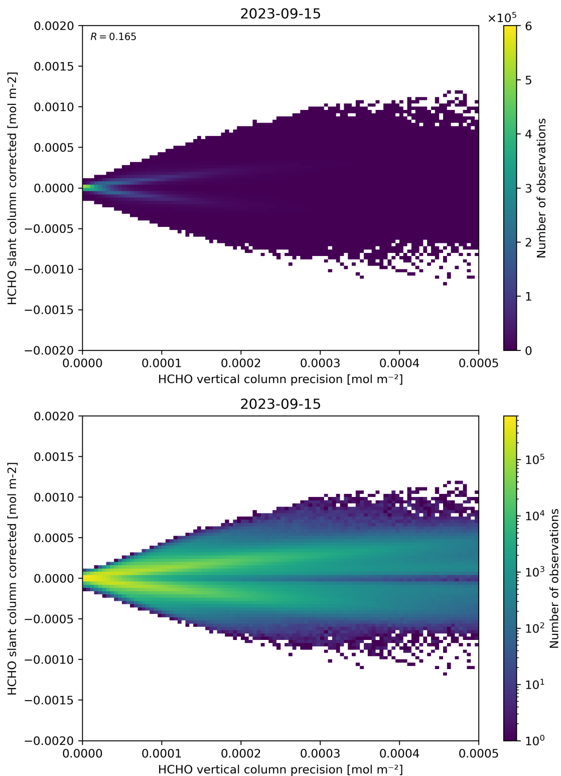
Figure 140: Scatter density plot of “HCHO vertical column precision” against “HCHO slant column corrected” for 2023-09-15 to 2023-09-16.
