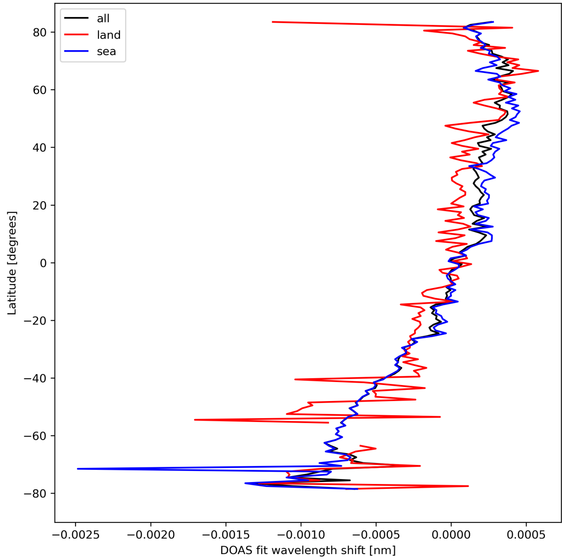
Figure 30: Zonal average of “DOAS fit wavelength shift” for 2023-09-15 to 2023-09-16.
