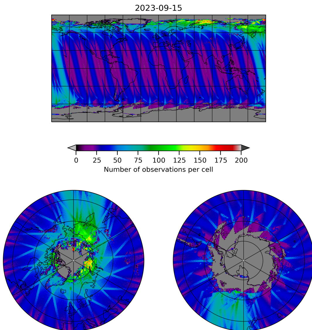
Figure 19: Map of the number of observations for 2023-09-15 to 2023-09-16
