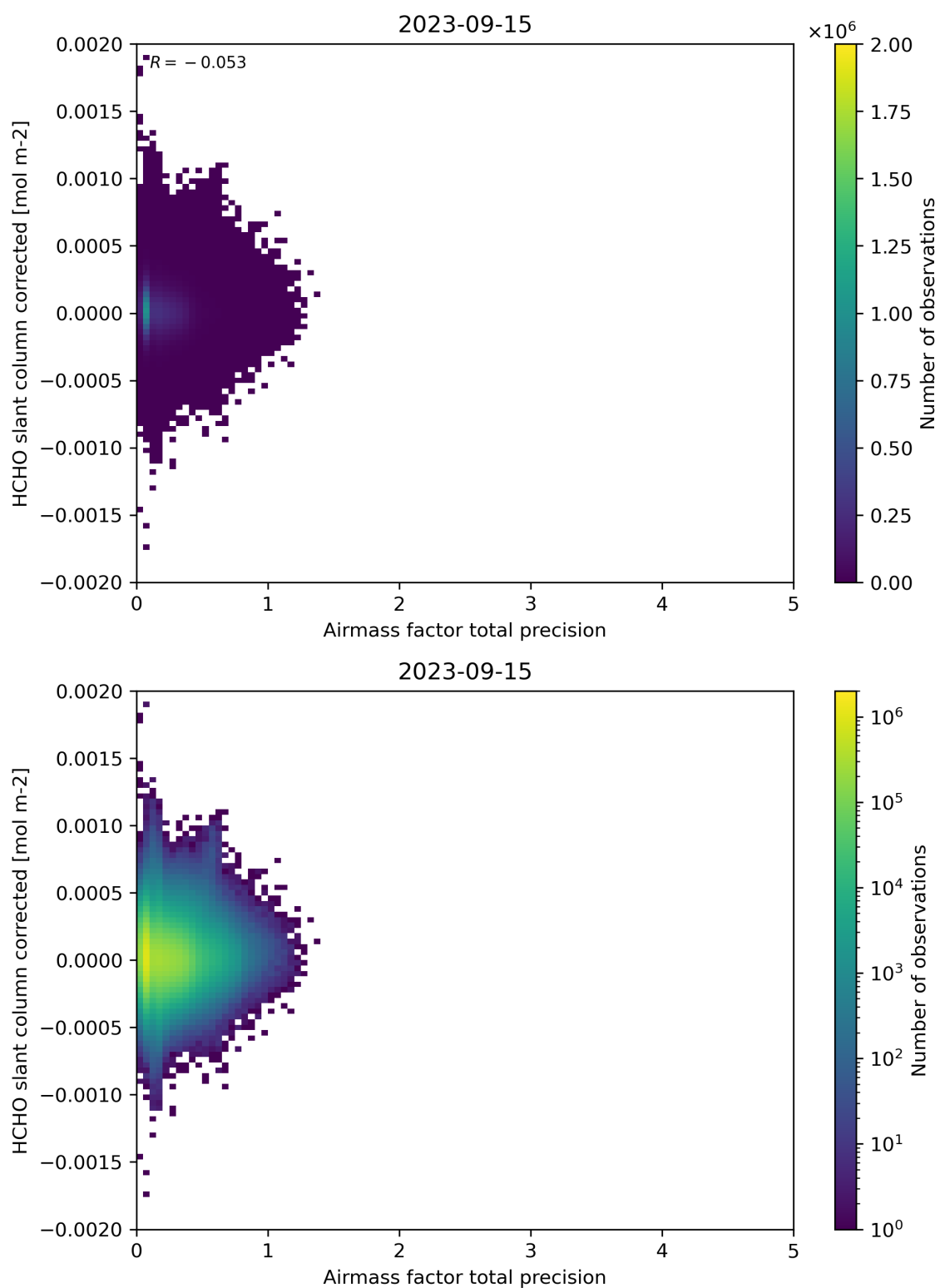
Figure 109: Scatter density plot of “Airmass factor total precision” against “HCHO slant column corrected” for 2023-09-15 to 2023-09-16.
