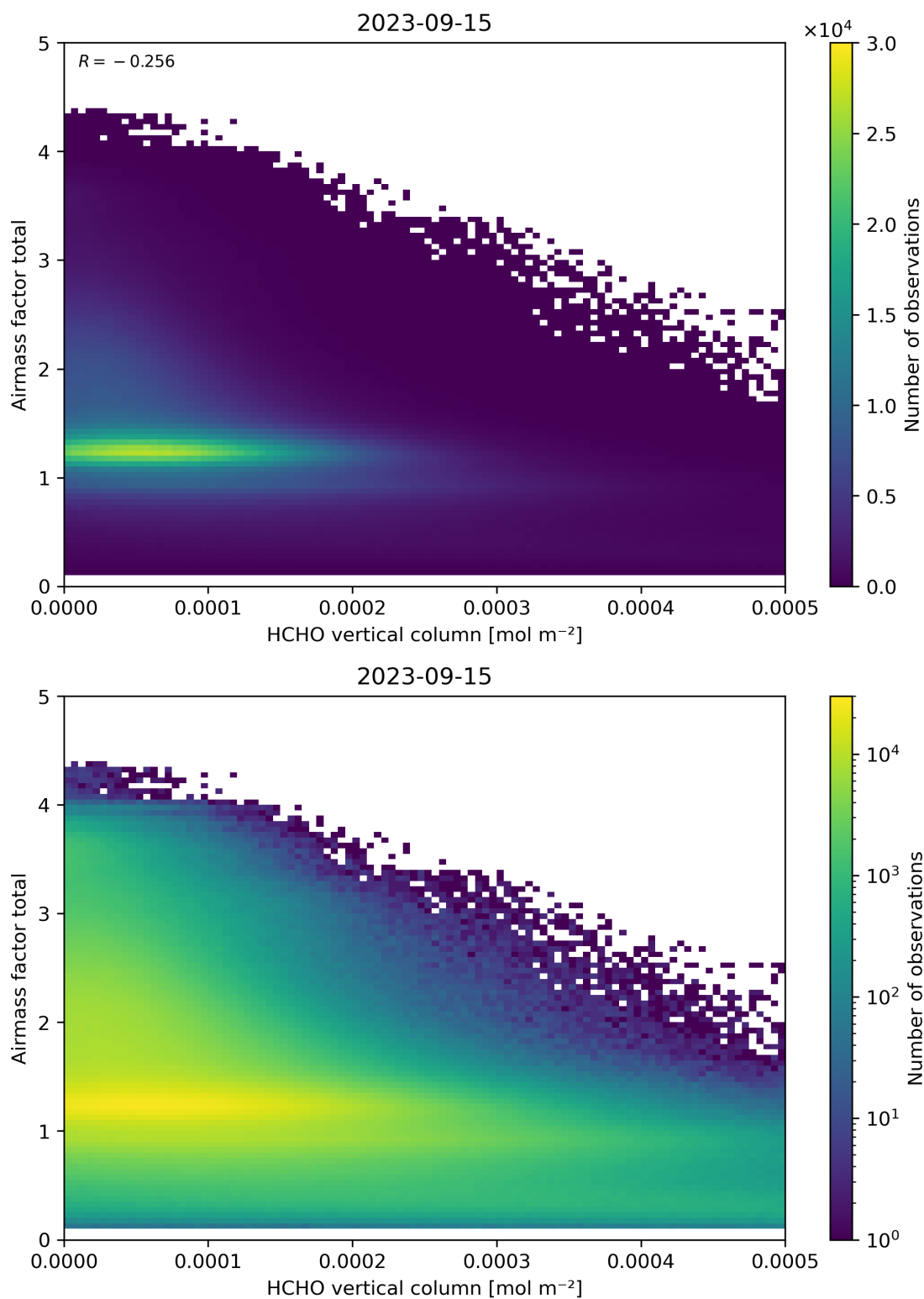
Figure 131: Scatter density plot of “HCHO vertical column” against “Airmass factor total” for 2023-09-15 to 2023-09-16.
