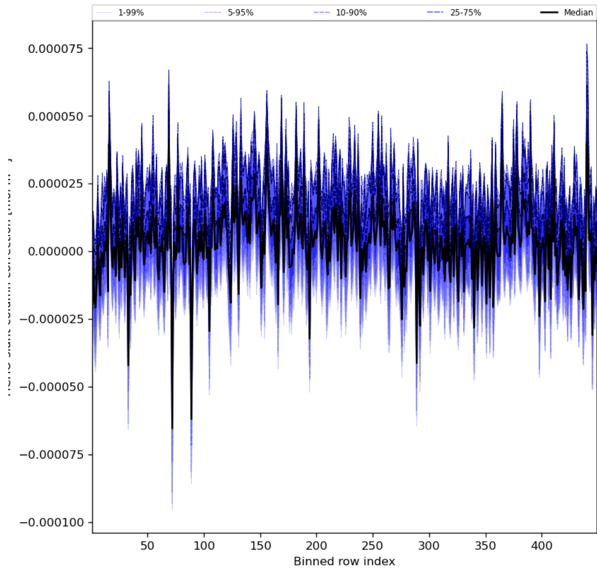
Figure 61: Along track statistics of “HCHO slant column correction” for 2023-09-15 to 2023-09-16
