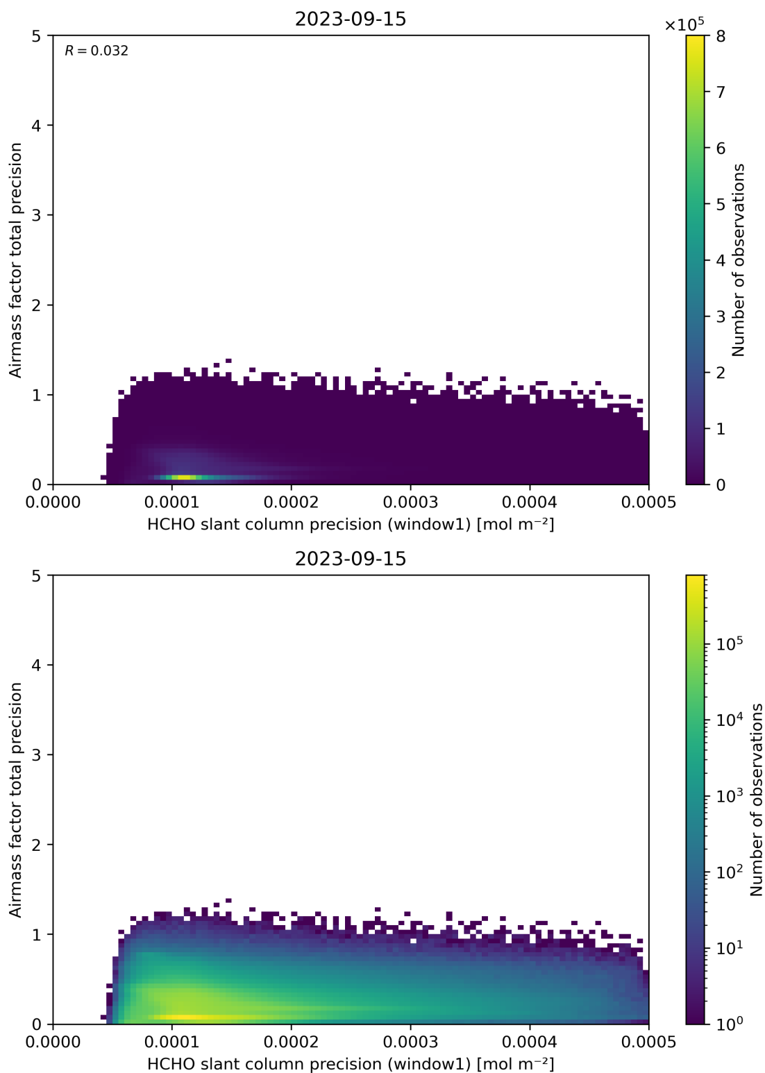
Figure 95: Scatter density plot of “HCHO slant column precision (window1)” against “Airmass factor total precision” for 2023-09-15 to 2023-09-16.
