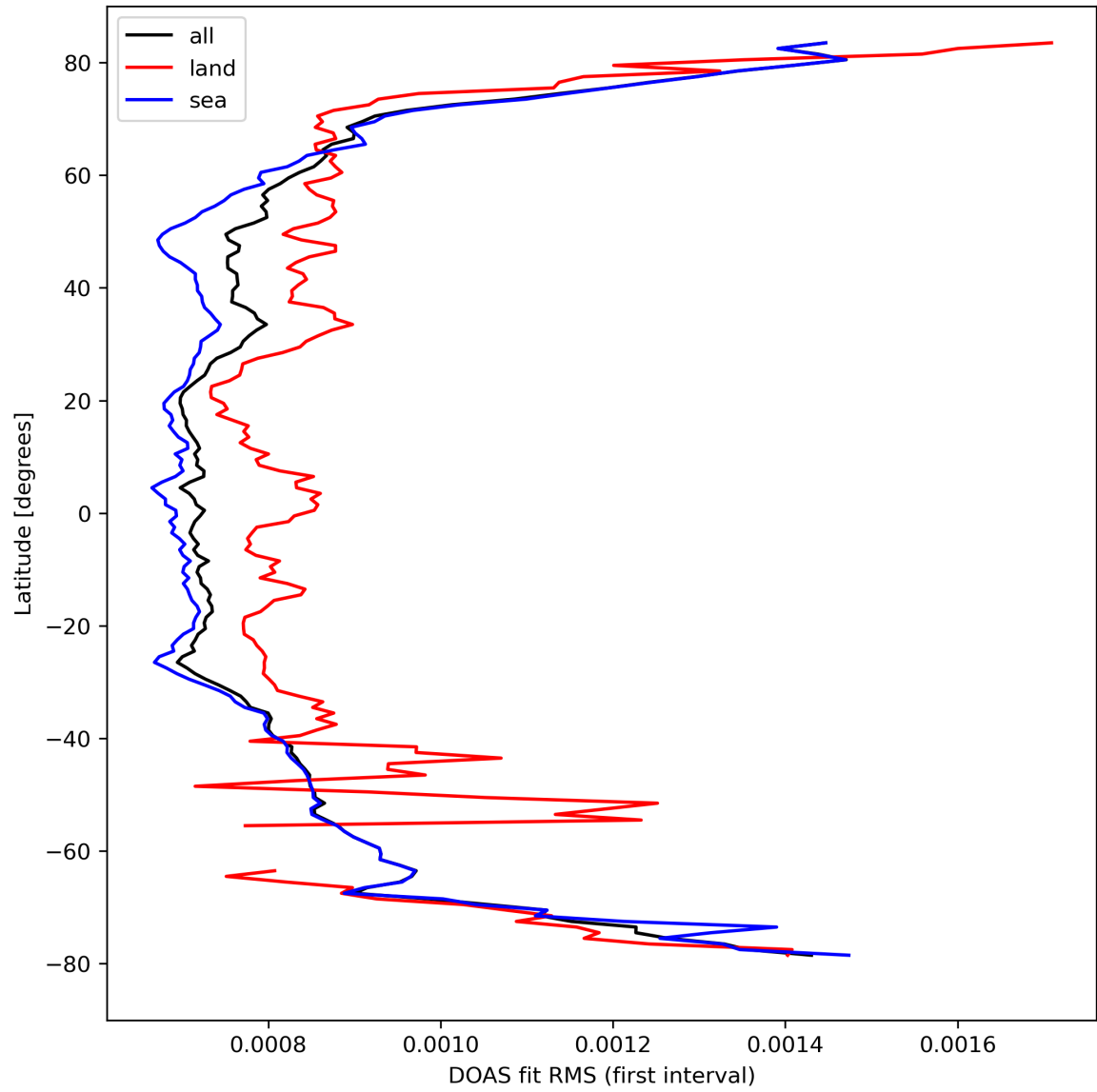
Figure 32: Zonal average of “DOAS fit RMS (first interval)” for 2023-09-15 to 2023-09-16.
