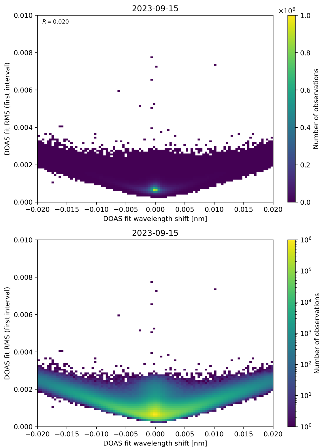
Figure 64: Scatter density plot of “DOAS fit wavelength shift” against “DOAS fit RMS (first interval)” for 2023-09-15 to 2023-09-16.
