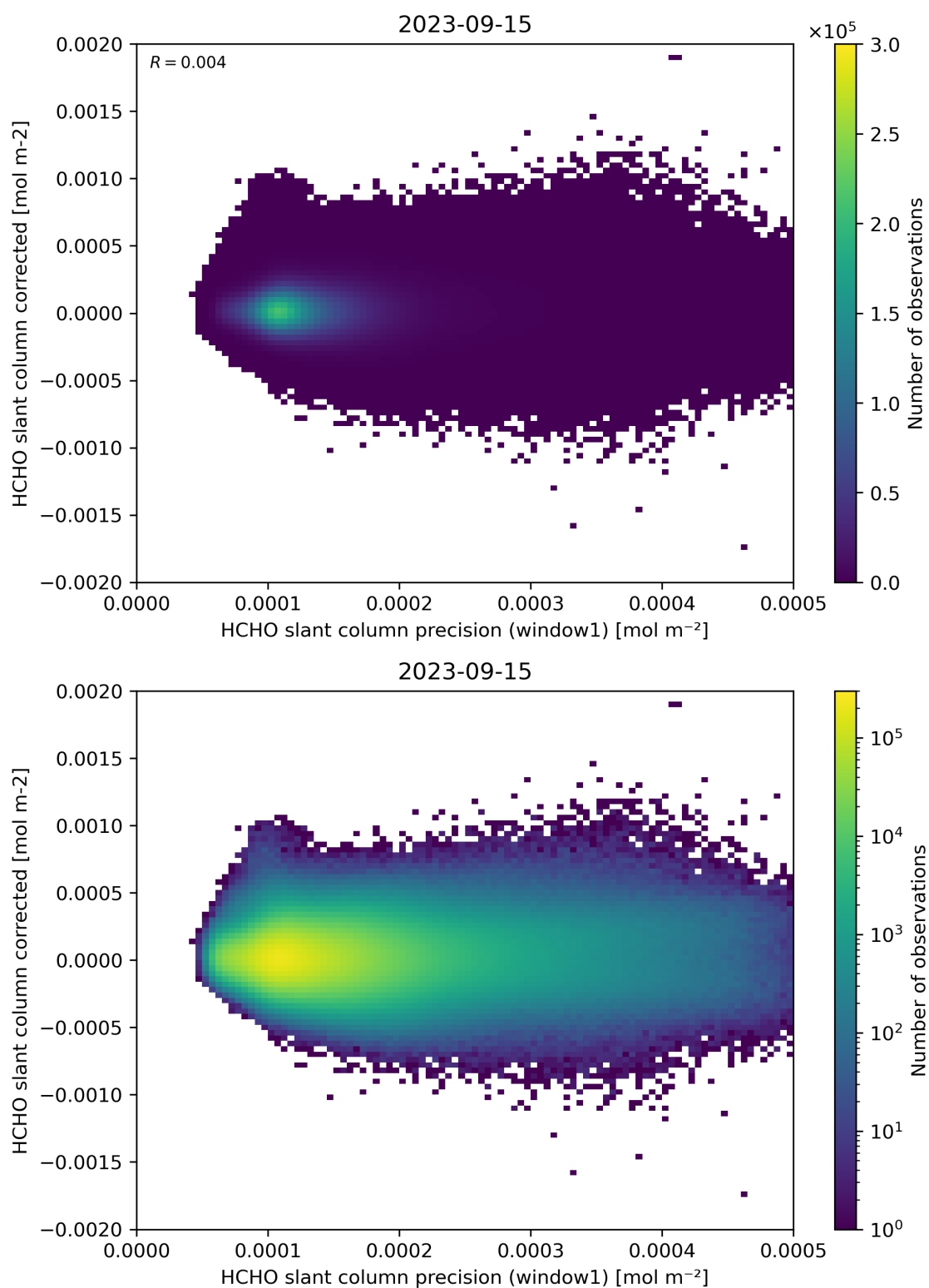
Figure 92: Scatter density plot of “HCHO slant column precision (window1)” against “HCHO slant column corrected” for 2023-09-15 to 2023-09-16.
