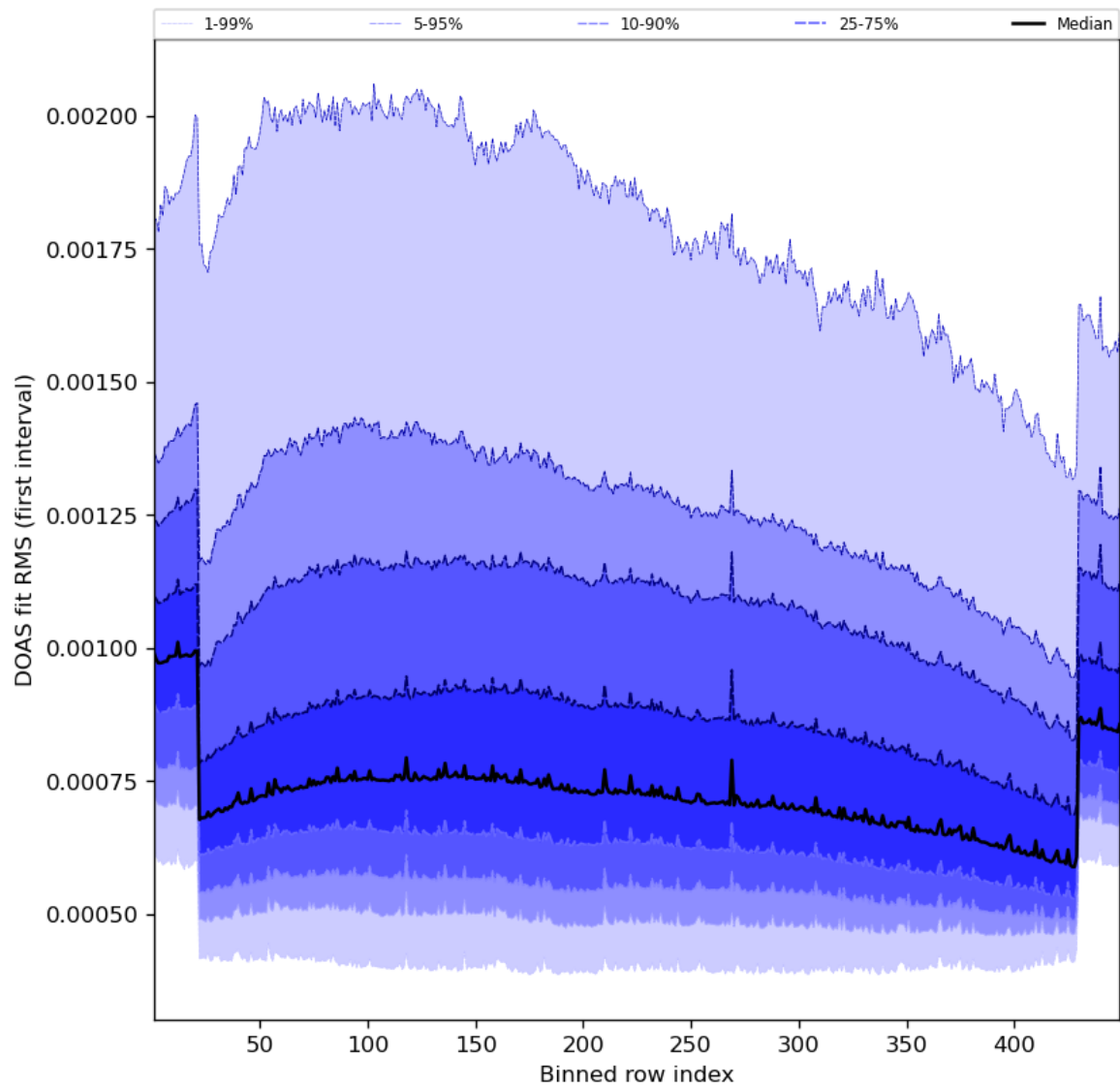
Figure 60: Along track statistics of “DOAS fit RMS (first interval)” for 2023-09-15 to 2023-09-16
