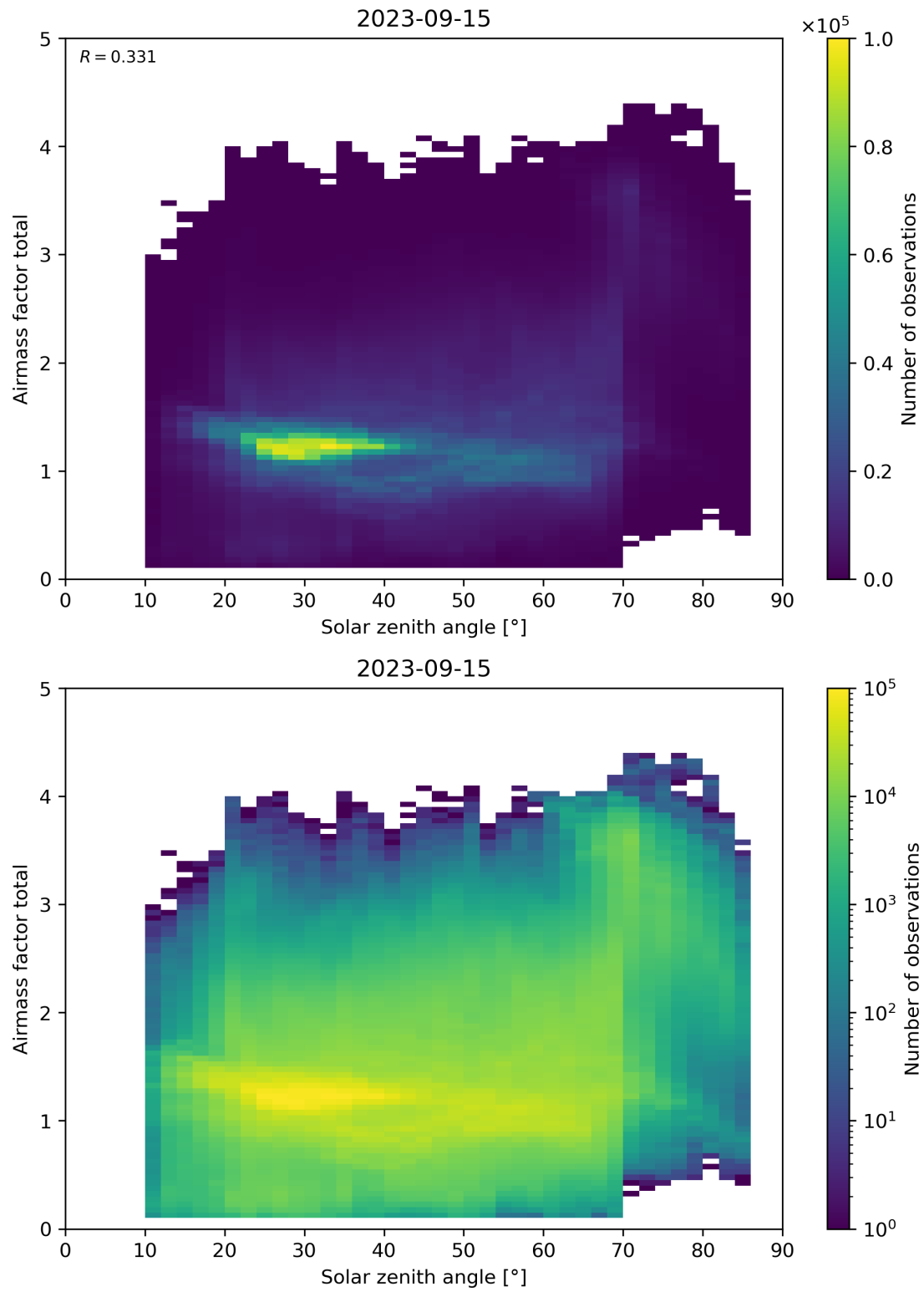
Figure 175: Scatter density plot of “Solar zenith angle” against “Airmass factor total” for 2023-09-15 to 2023-09-16.
