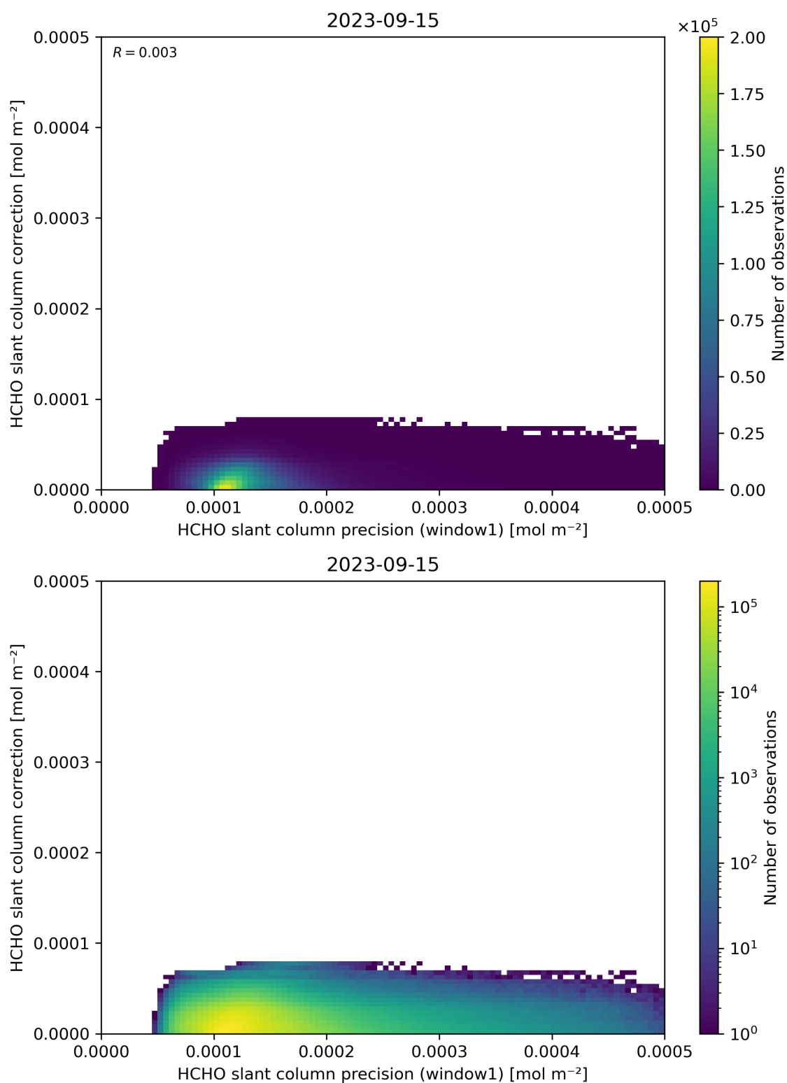
Figure 93: Scatter density plot of “HCHO slant column precision (window1)” against “HCHO slant column correction” for 2023-09-15 to 2023-09-16.
