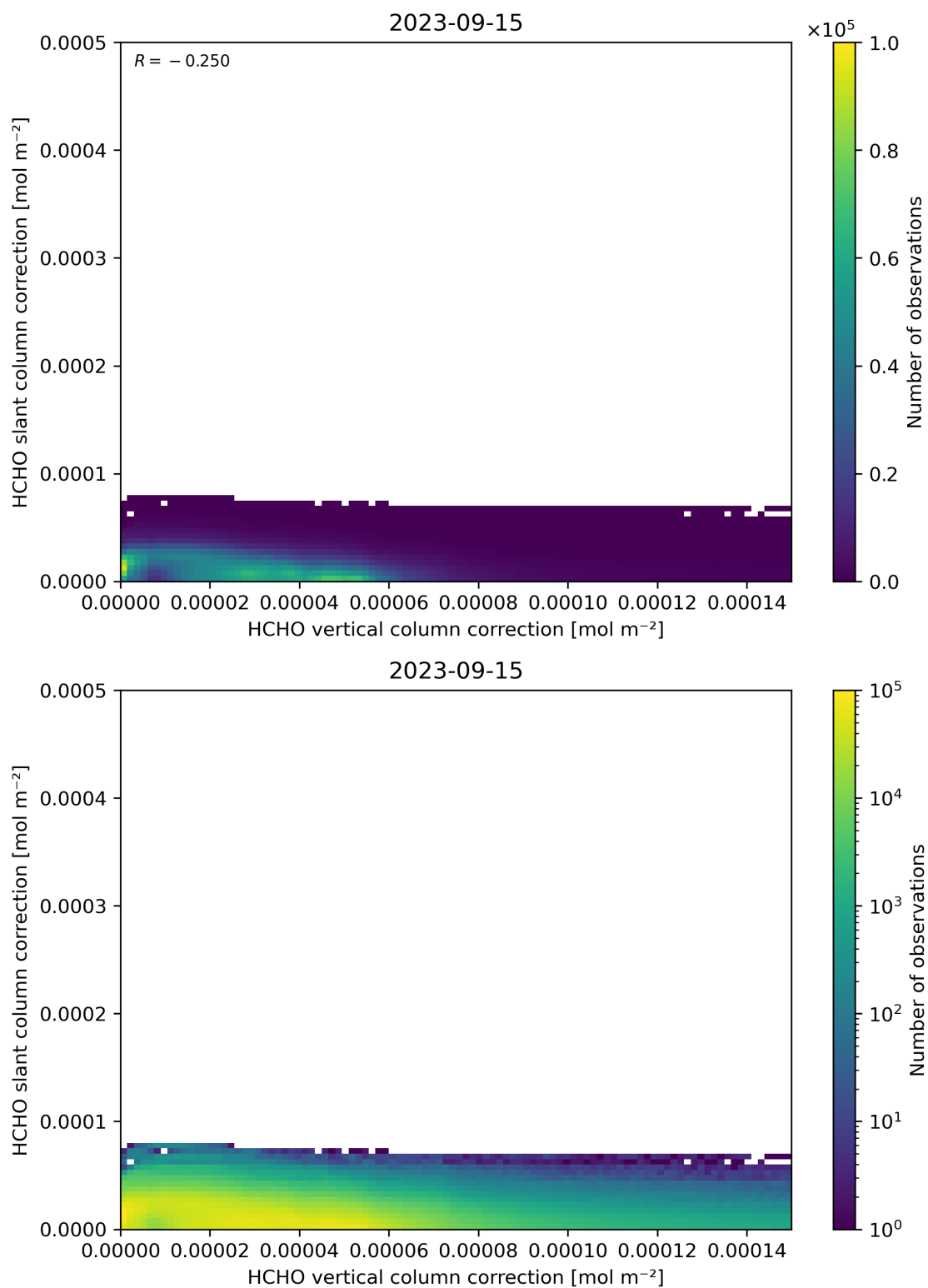
Figure 117: Scatter density plot of “HCHO vertical column correction” against “HCHO slant column correction” for 2023-09-15 to 2023-09-16.
