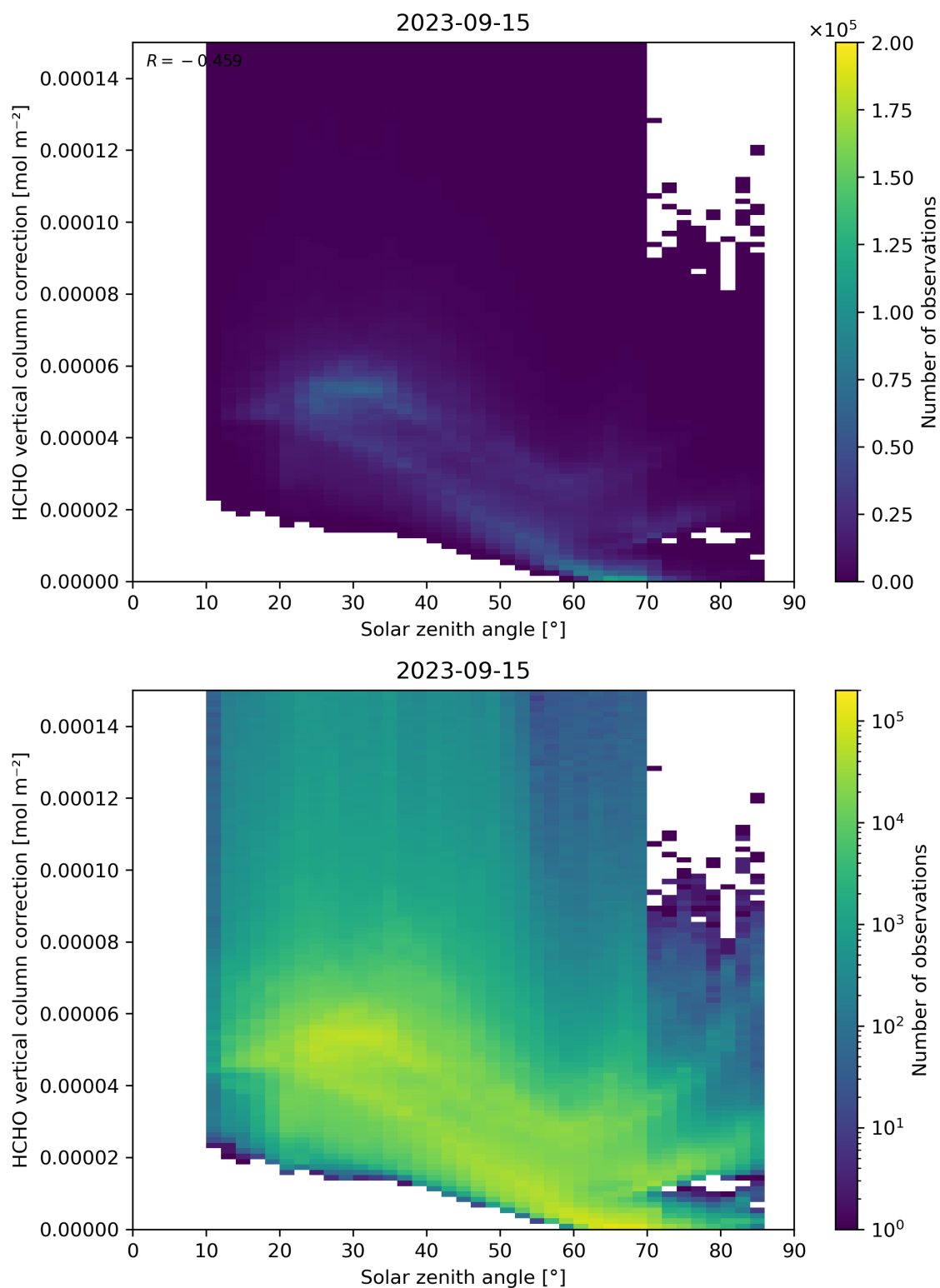
Figure 178: Scatter density plot of “Solar zenith angle” against “HCHO vertical column correction” for 2023-09-15 to 2023-09-16.
