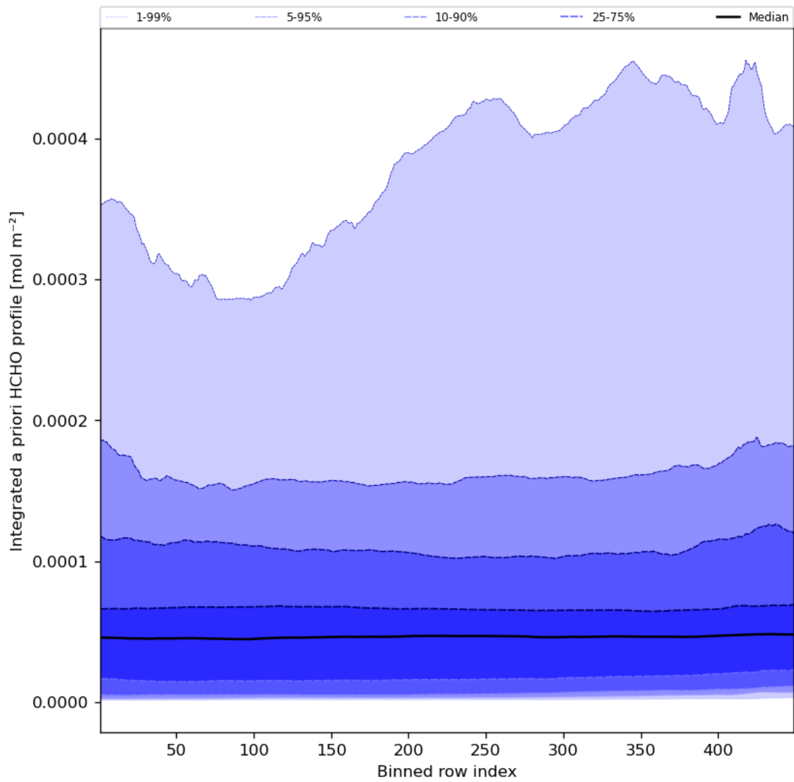
Figure 57: Along track statistics of “Integrated a priori HCHO profile” for 2023-09-15 to 2023-09-16
