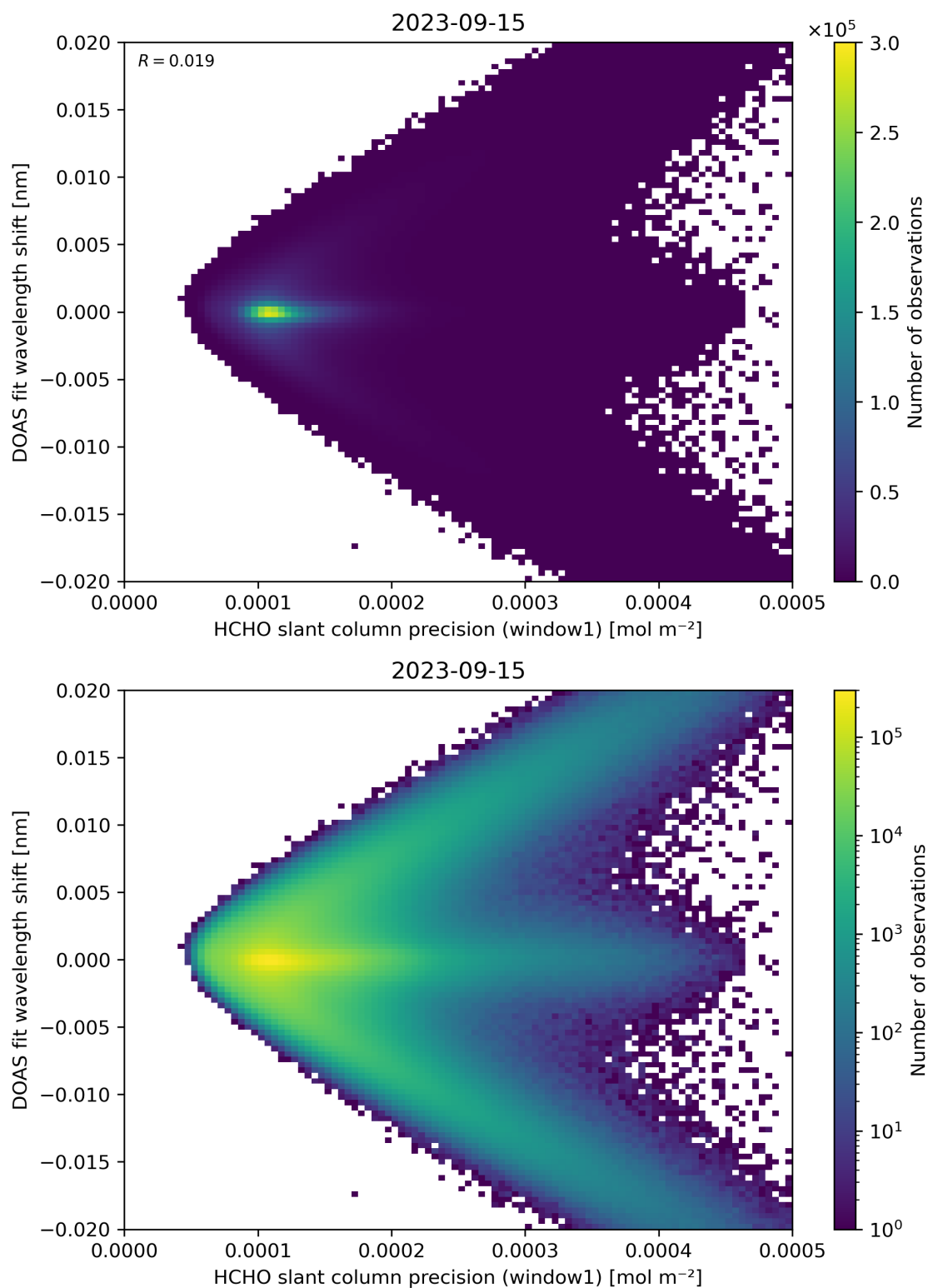
Figure 89: Scatter density plot of “HCHO slant column precision (window1)” against “DOAS fit wavelength shift” for 2023-09-15 to 2023-09-16.
