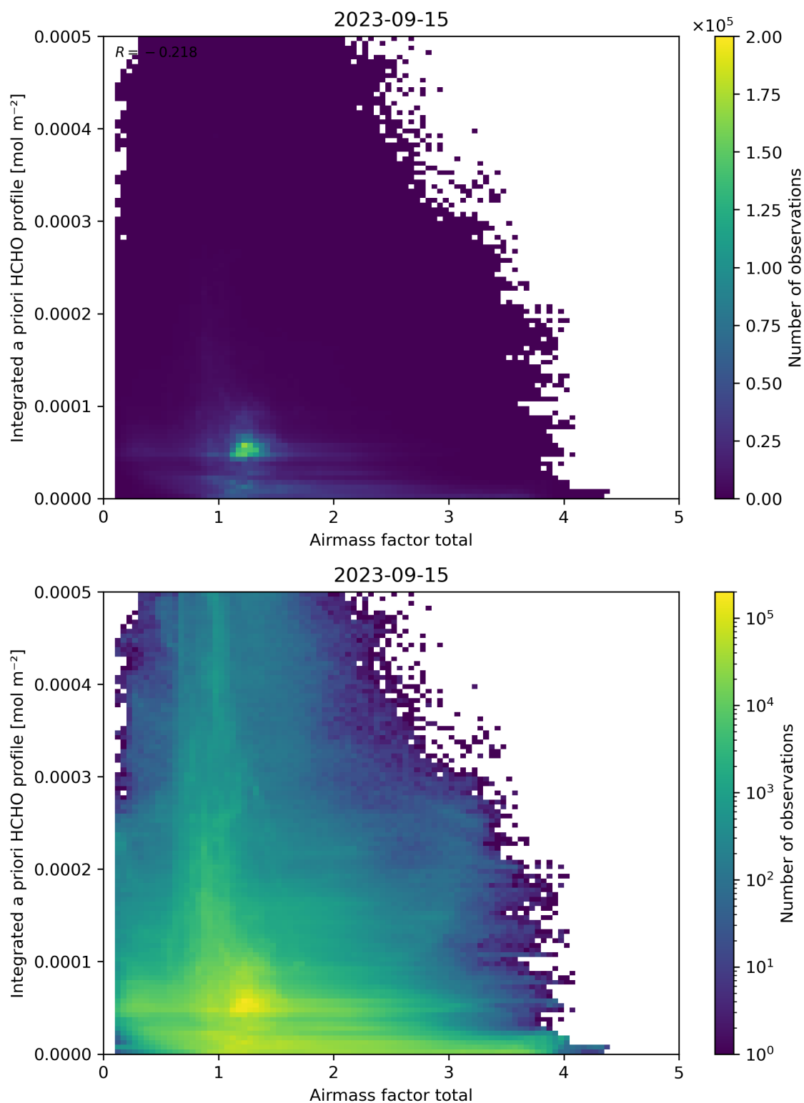
Figure 104: Scatter density plot of “Airmass factor total” against “Integrated a priori HCHO profile” for 2023-09-15 to 2023-09-16.
