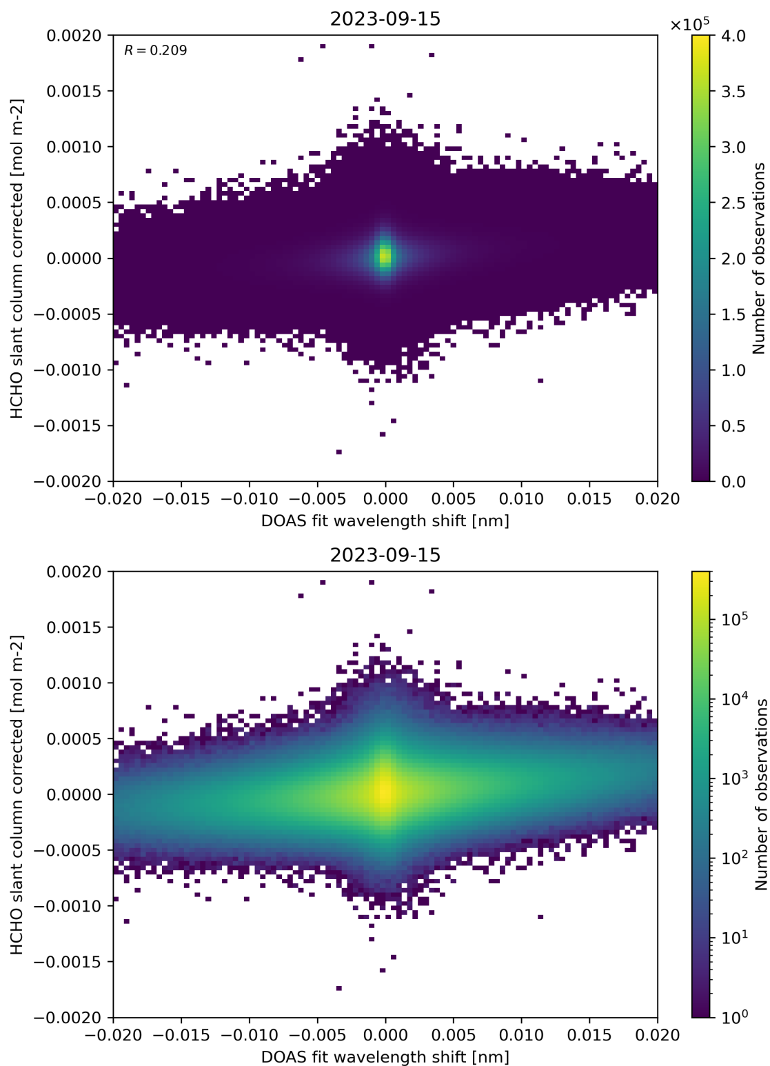
Figure 66: Scatter density plot of “DOAS fit wavelength shift” against “HCHO slant column corrected” for 2023-09-15 to 2023-09-16.
