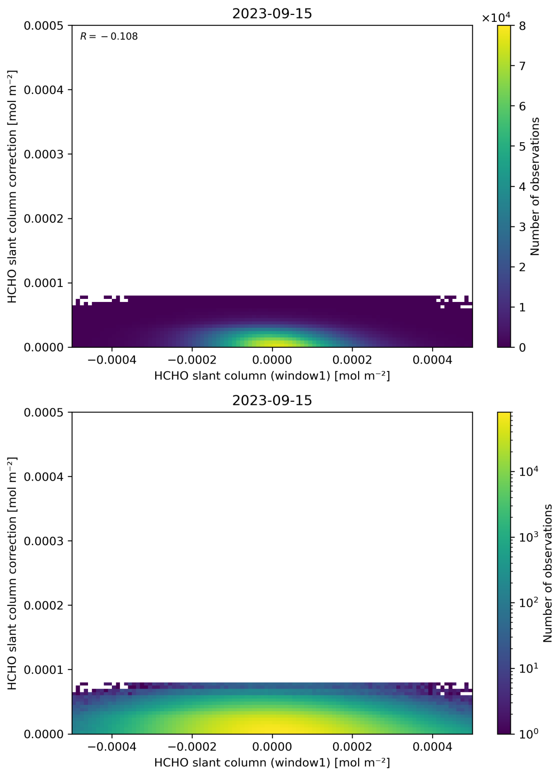
Figure 83: Scatter density plot of “HCHO slant column (window1)” against “HCHO slant column correction” for 2023-09-15 to 2023-09-16.
