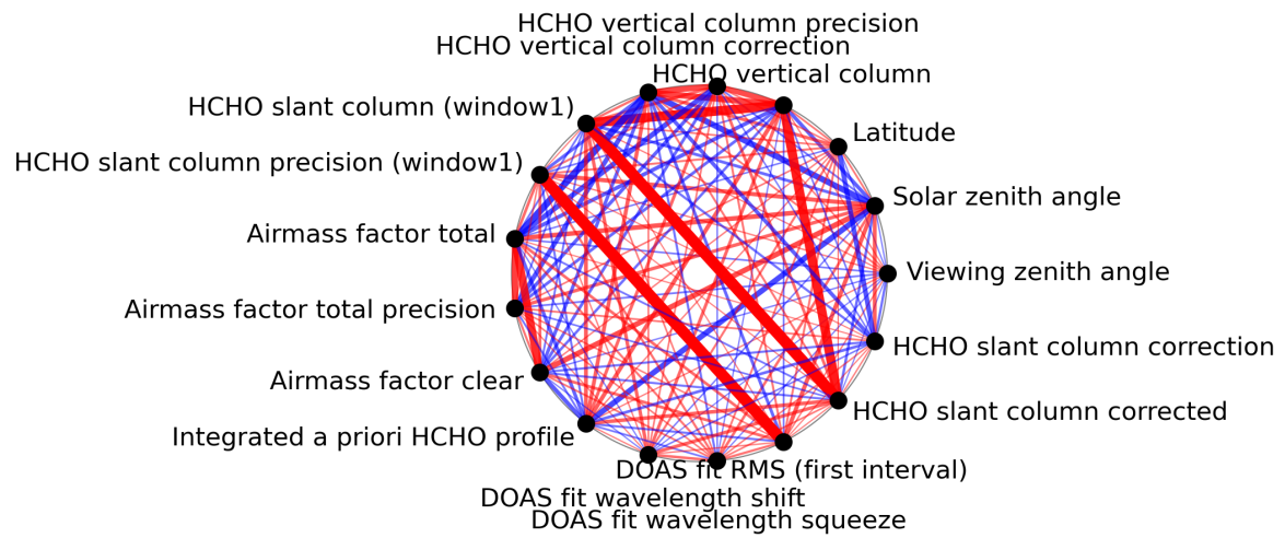
Figure 1: Map of correlation graph for 2023-09-15 to 2023-09-16.
