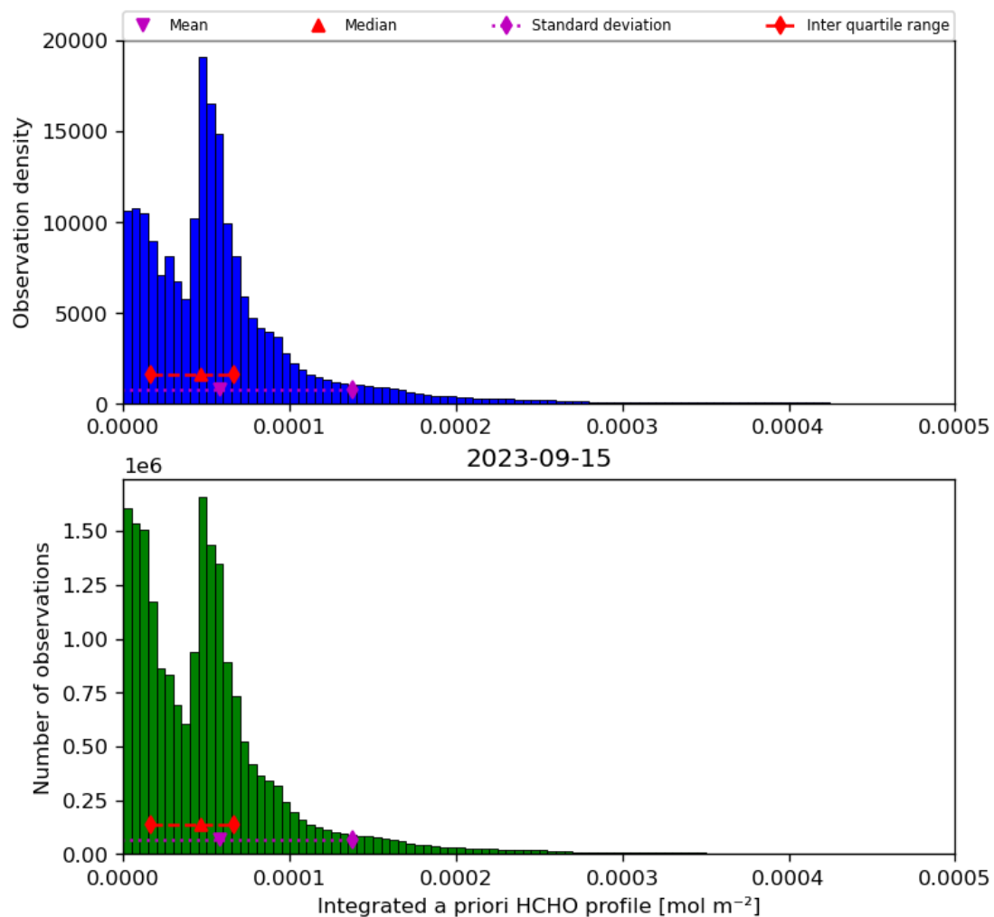
Figure 43: Histogram of “Integrated a priori HCHO profile” for 2023-09-15 to 2023-09-16
