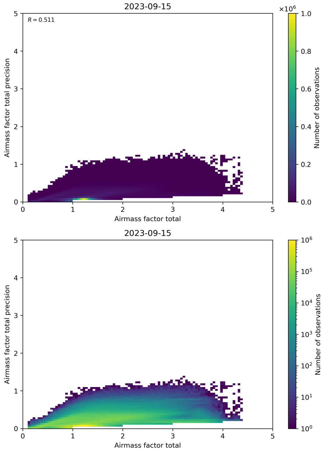
Figure 103: Scatter density plot of “Airmass factor total” against “Airmass factor total precision” for 2023-09-15 to 2023-09-16.
