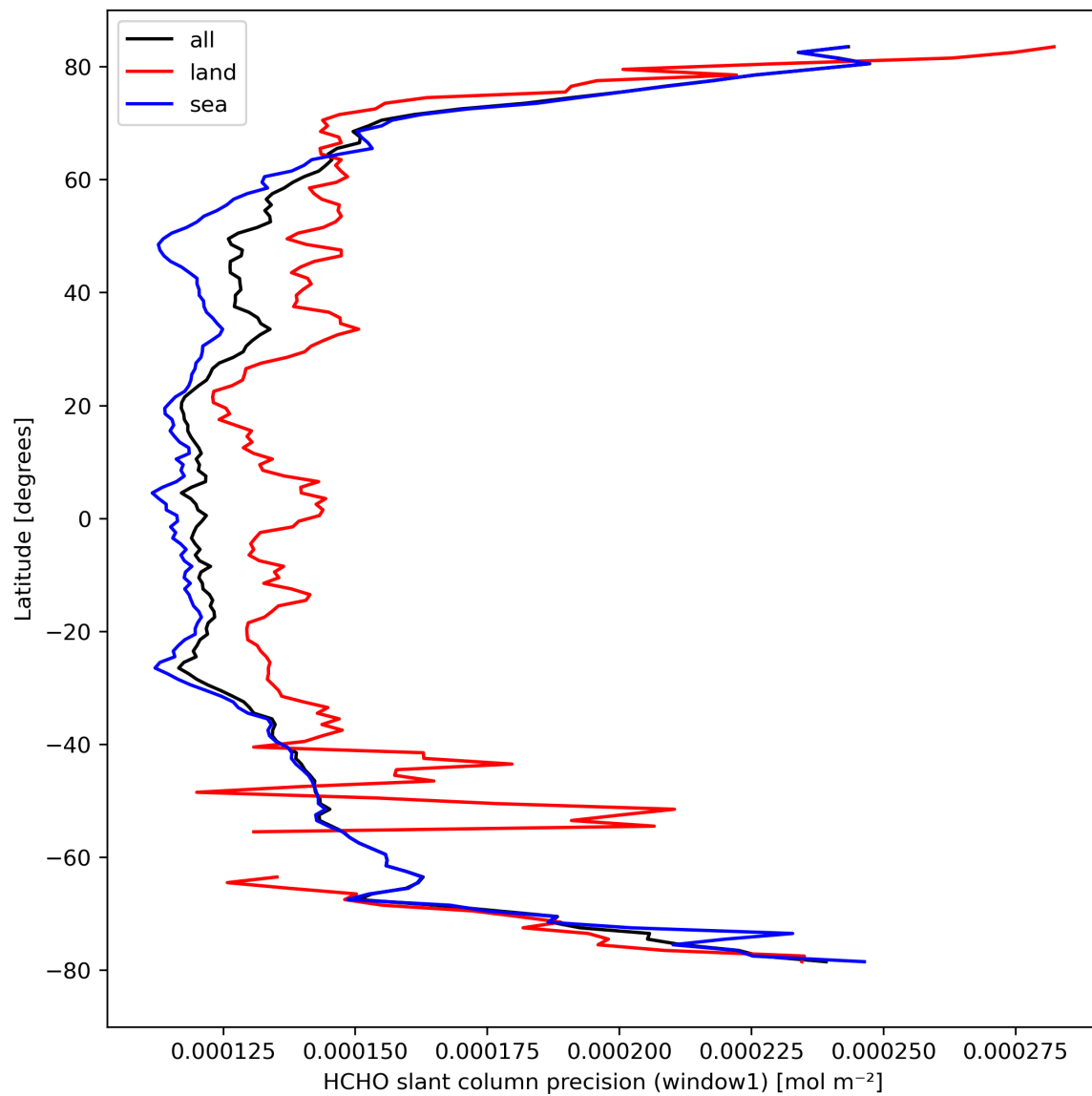
Figure 25: Zonal average of "HCHO slant column precision (window1)" for 2023-09-15 to 2023-09-16.
