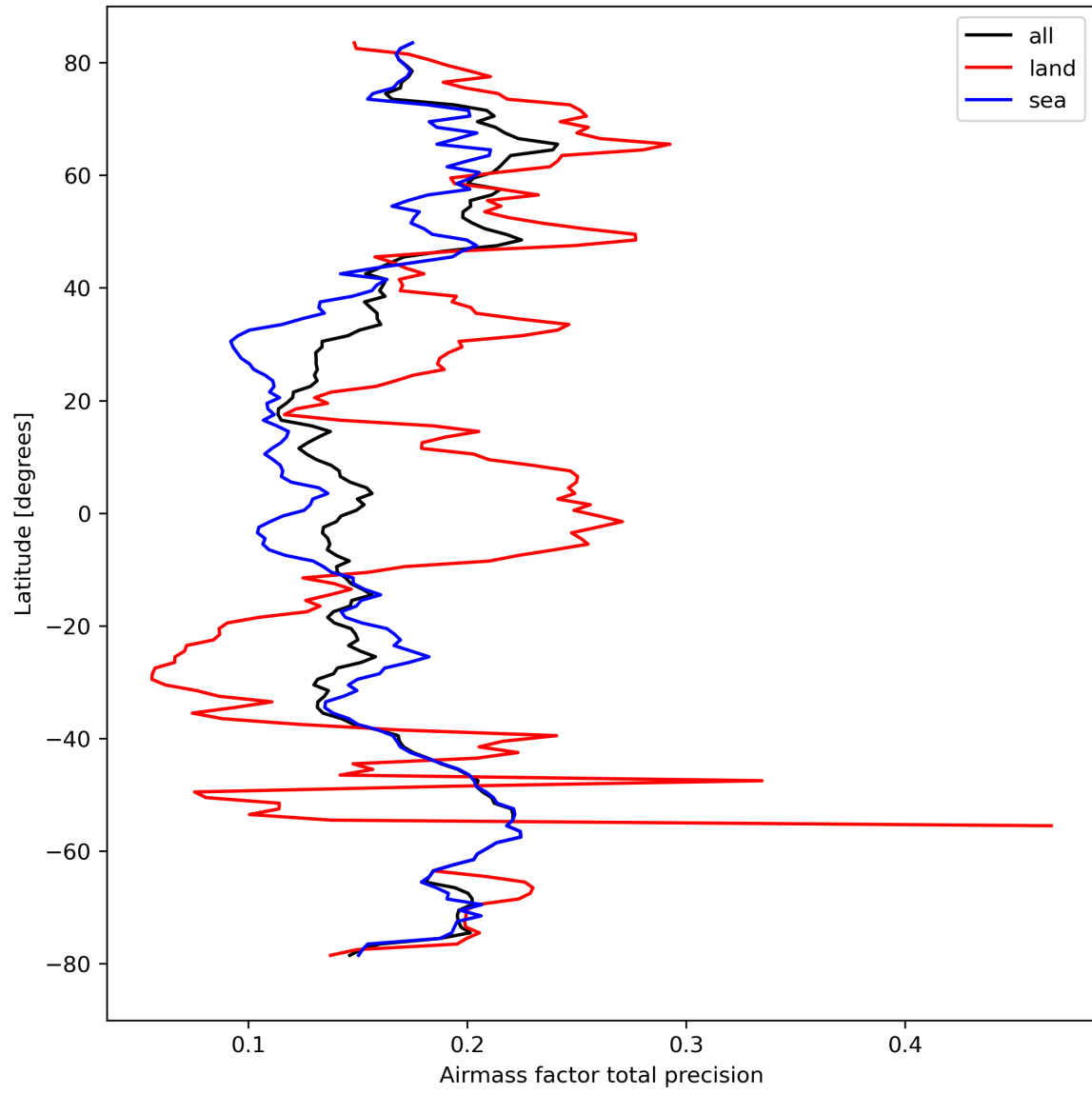
Figure 27: Zonal average of “Airmass factor total precision” for 2023-09-15 to 2023-09-16.
