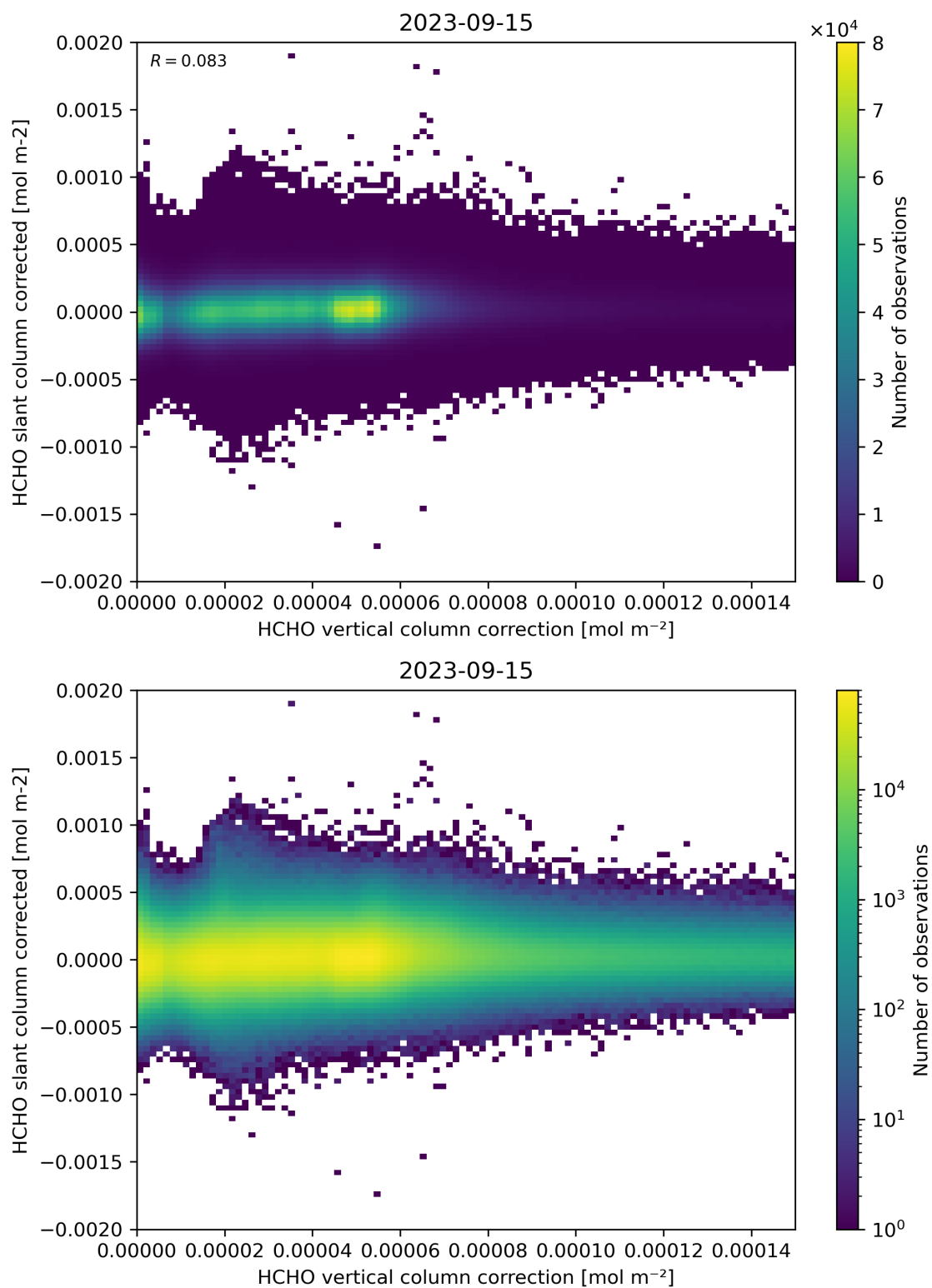
Figure 116: Scatter density plot of “HCHO vertical column correction” against “HCHO slant column corrected” for 2023-09-15 to 2023-09-16.
