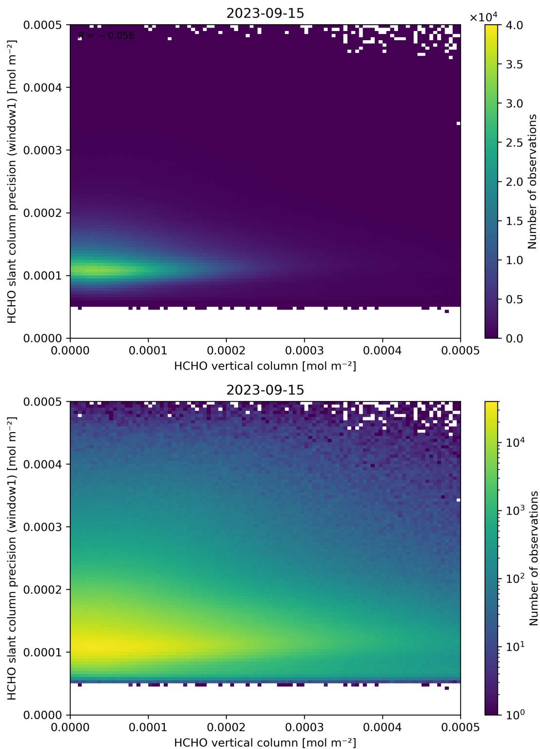
Figure 130: Scatter density plot of “HCHO vertical column” against “HCHO slant column precision (window1)” for 2023-09-15 to 2023-09-16.
