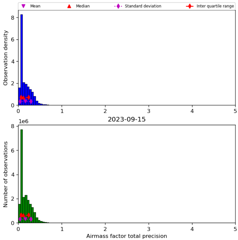
Figure 41: Histogram of “Airmass factor total precision” for 2023-09-15 to 2023-09-16
