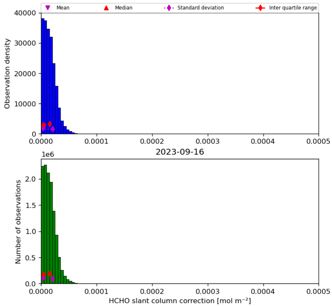
Figure 47: Histogram of “HCHO slant column correction” for 2023-09-15 to 2023-09-17
