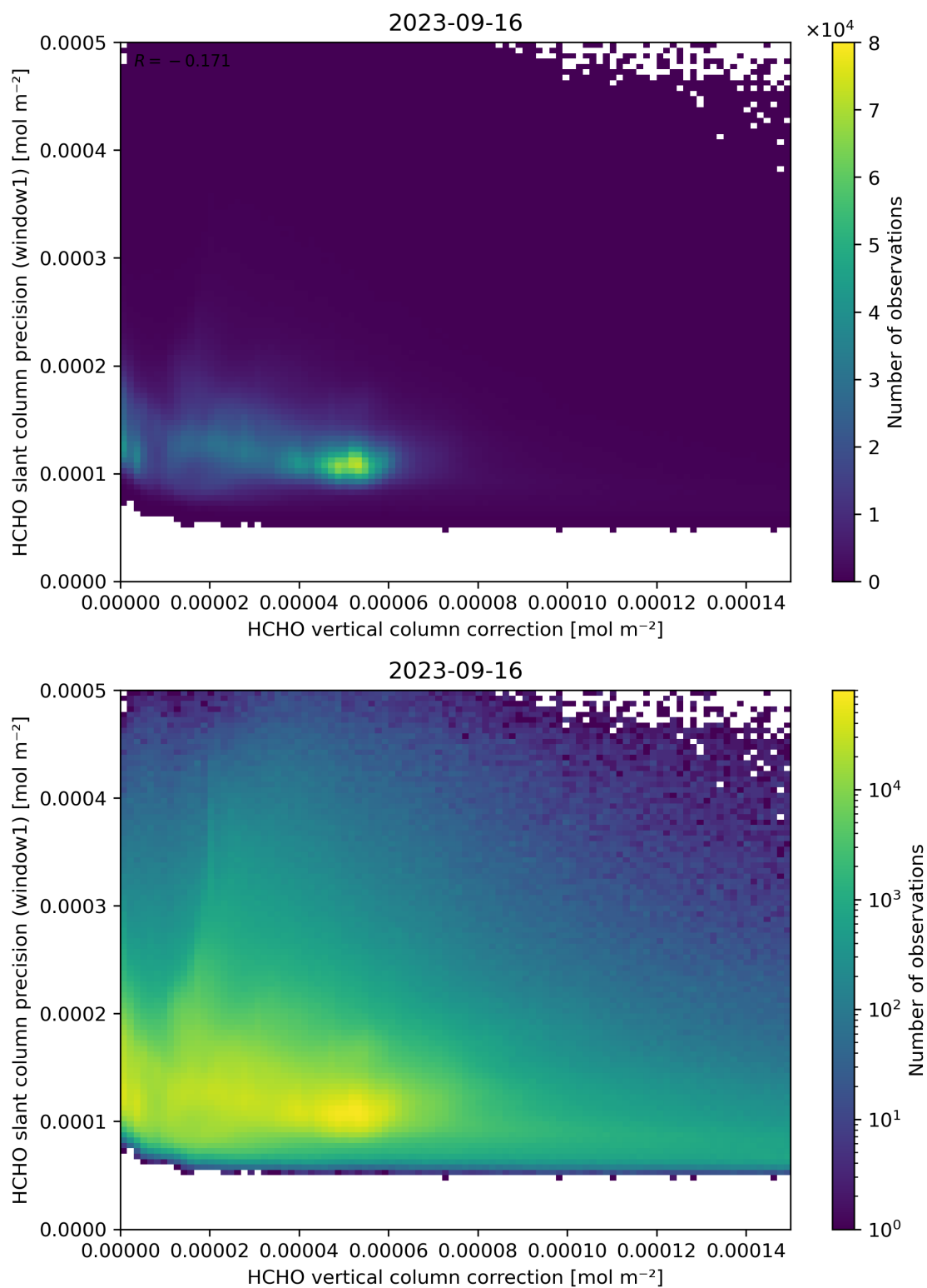
Figure 119: Scatter density plot of “HCHO vertical column correction” against “HCHO slant column precision (window1)” for 2023-09-15 to 2023-09-17.
