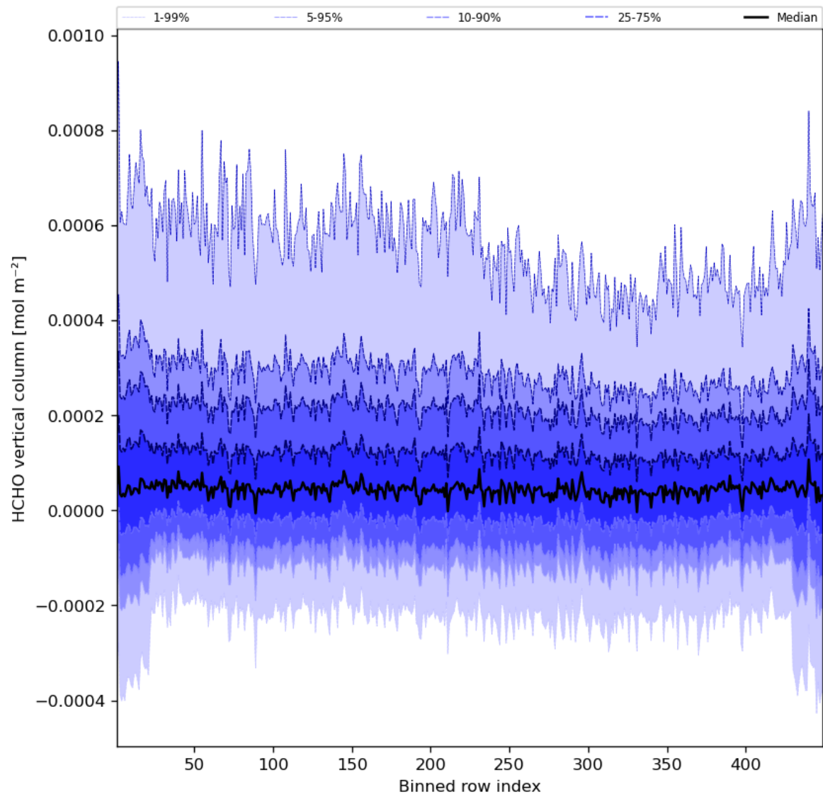
Figure 49: Along track statistics of “HCHO vertical column” for 2023-09-15 to 2023-09-17
