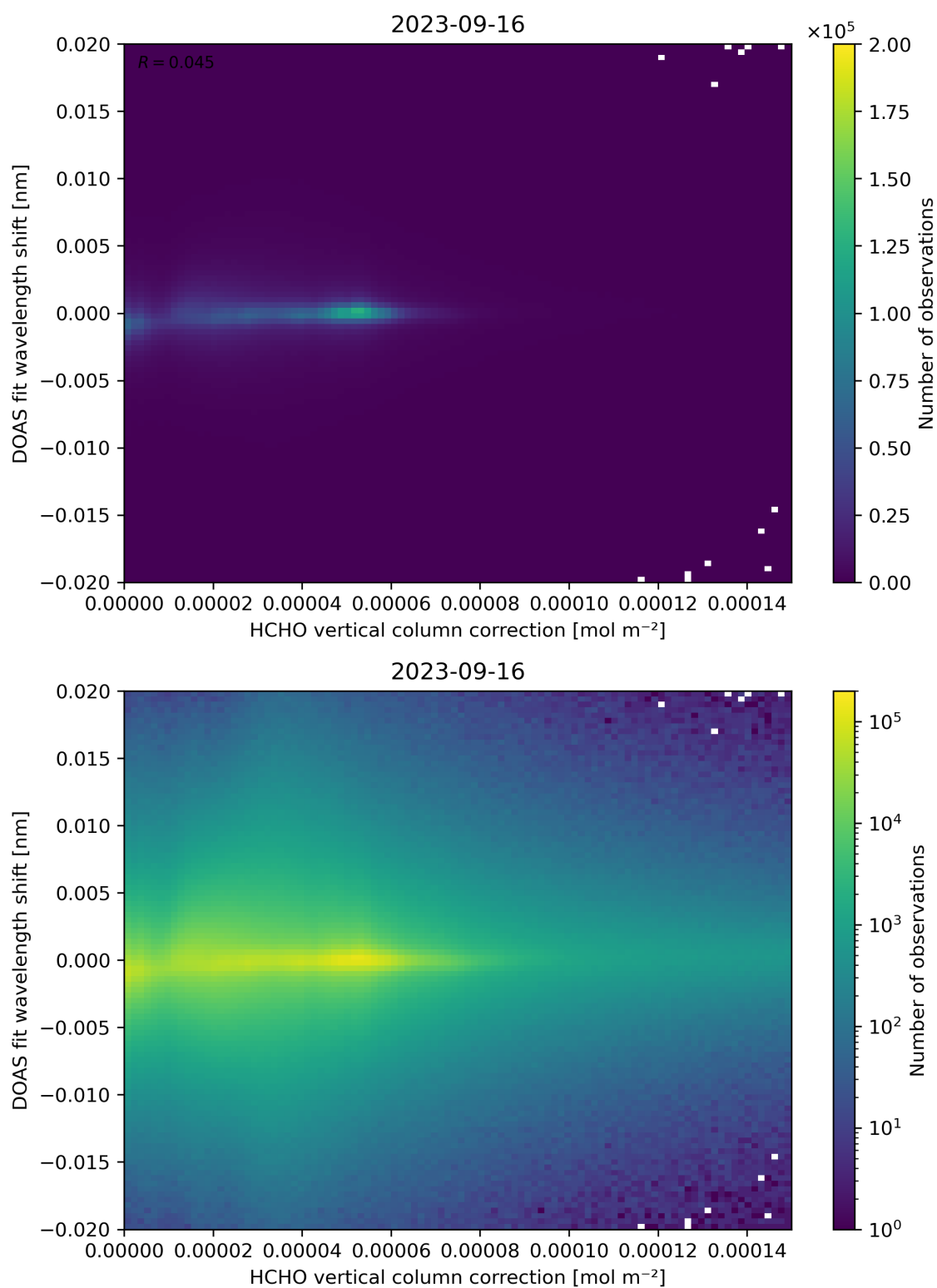
Figure 113: Scatter density plot of “HCHO vertical column correction” against “DOAS fit wavelength shift” for 2023-09-15 to 2023-09-17.
