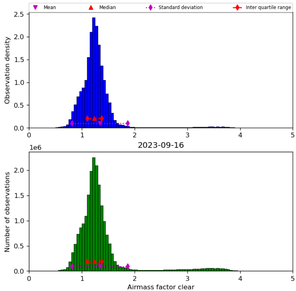
Figure 42: Histogram of “Airmass factor clear” for 2023-09-15 to 2023-09-17
