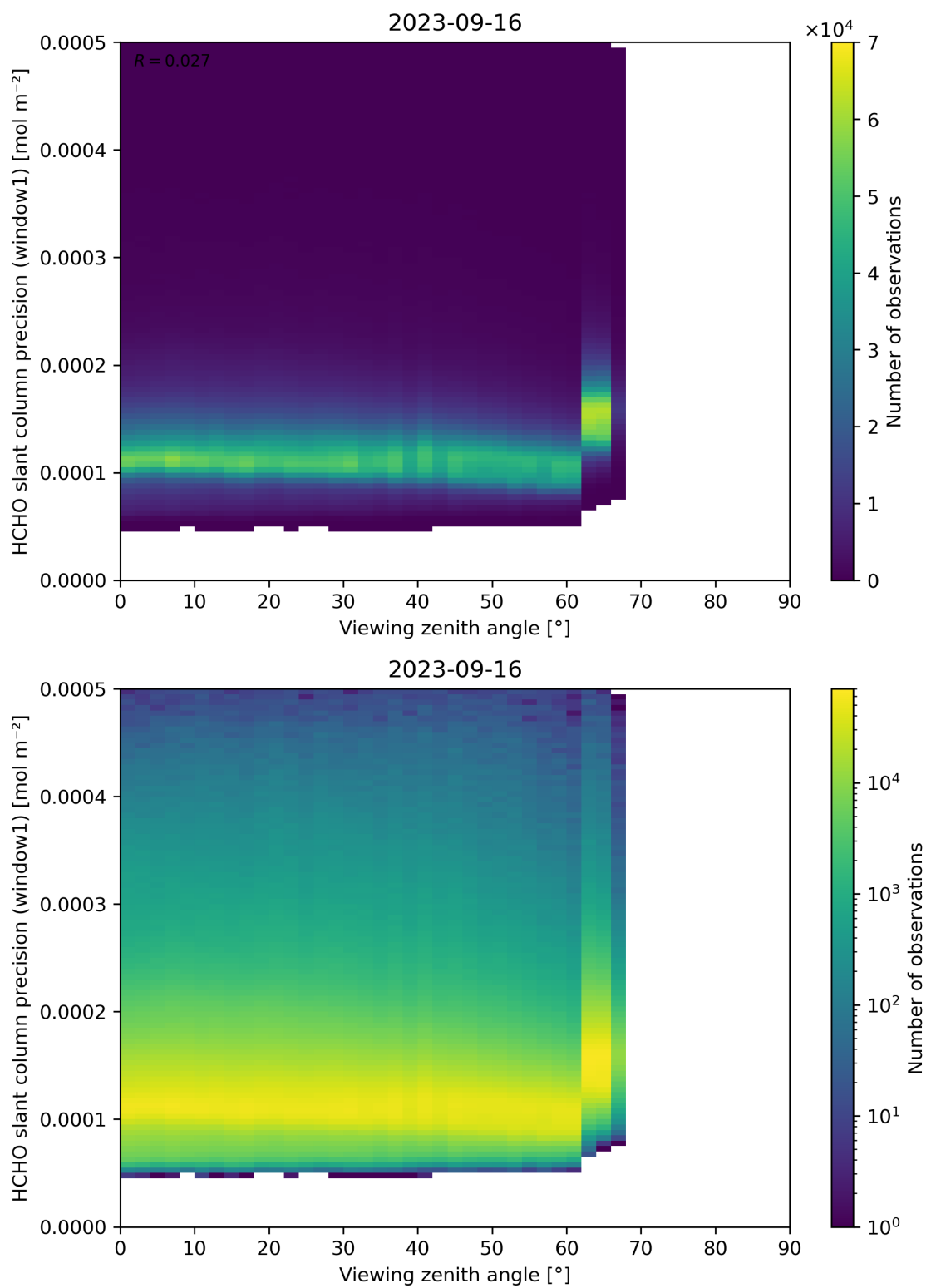
Figure 189: Scatter density plot of “Viewing zenith angle” against “HCHO slant column precision (window1)” for 2023-09-15 to 2023-09-17.
