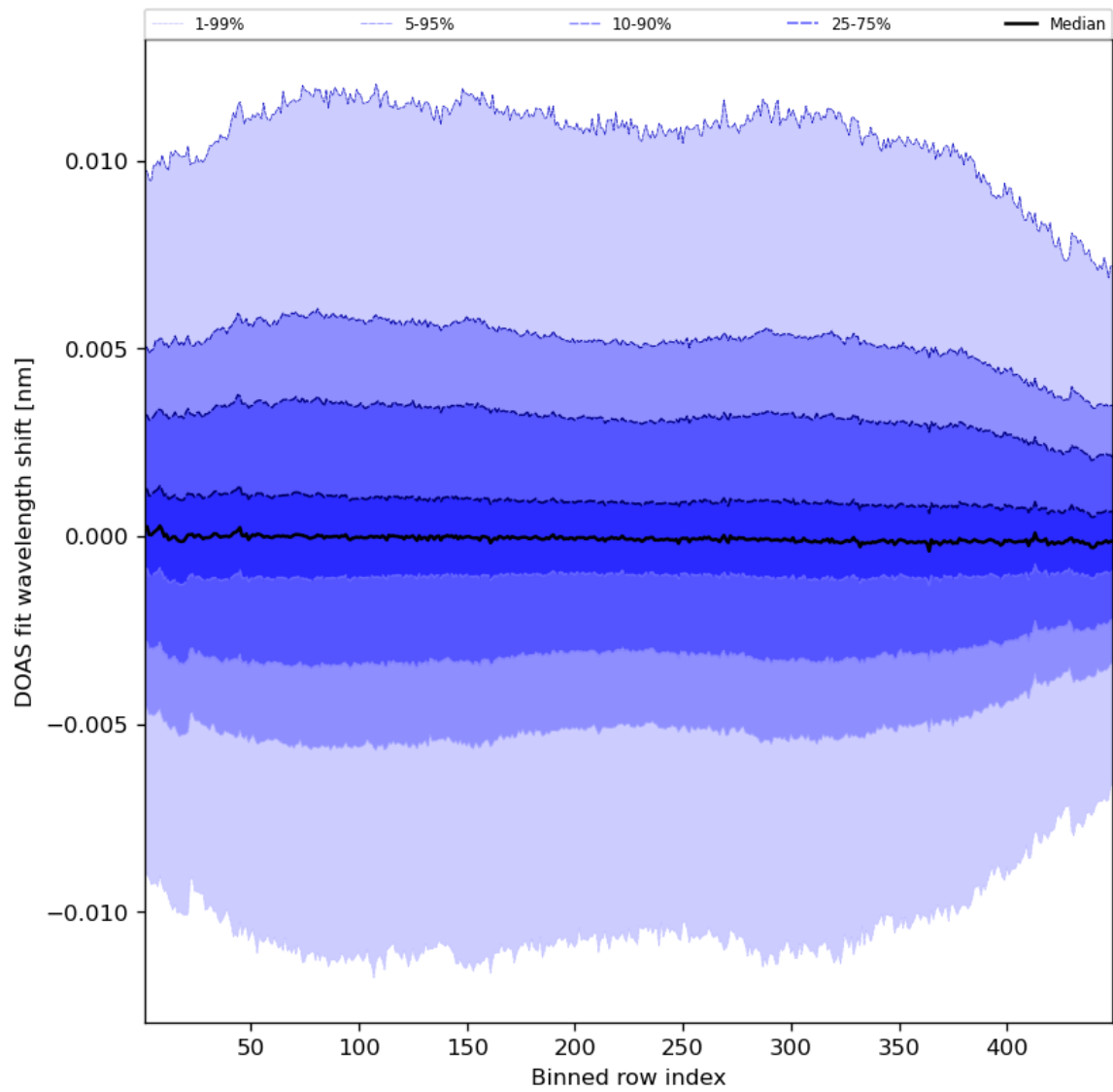
Figure 58: Along track statistics of “DOAS fit wavelength shift” for 2023-09-15 to 2023-09-17
