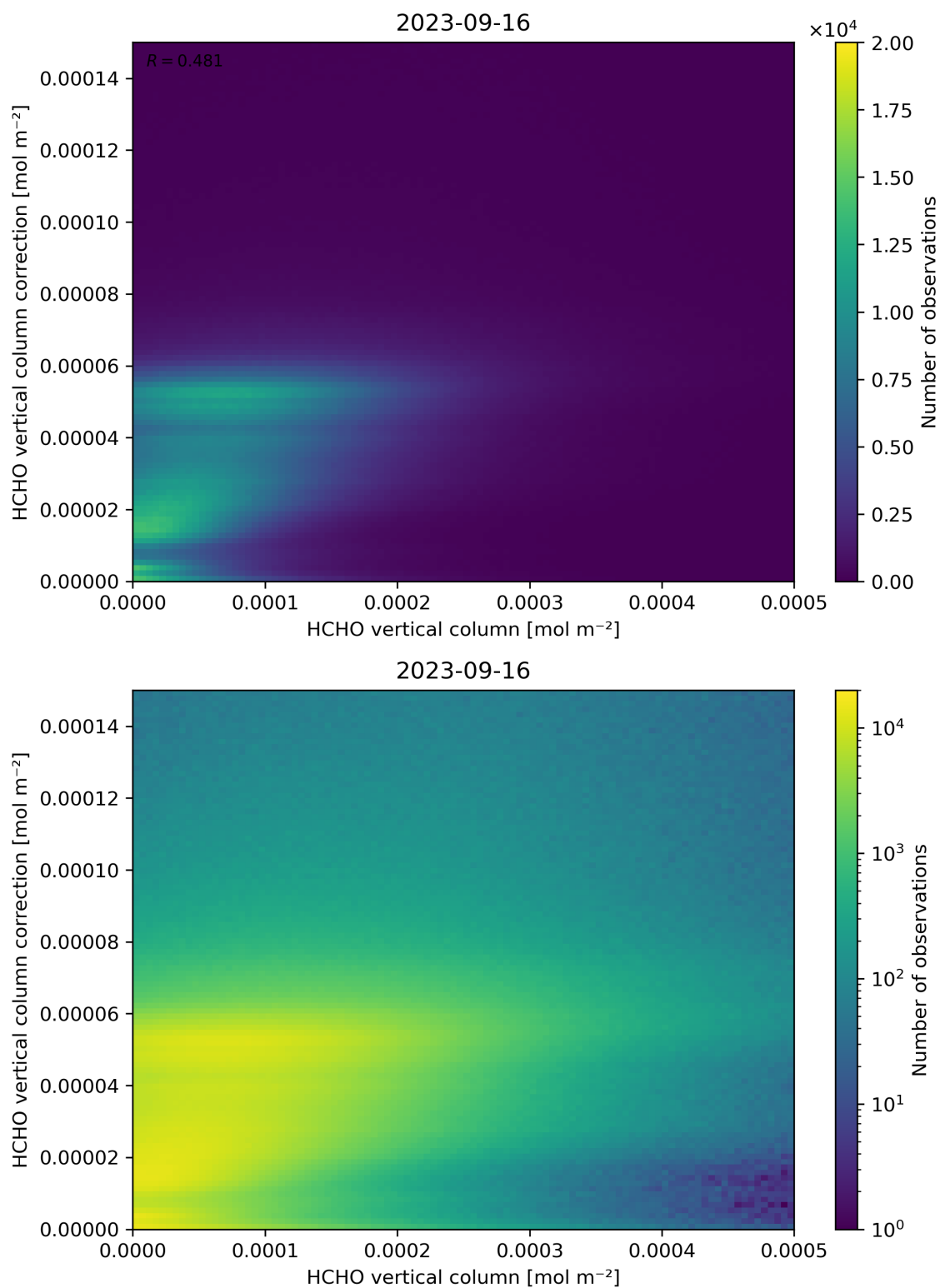
Figure 133: Scatter density plot of “HCHO vertical column” against “HCHO vertical column correction” for 2023-09-15 to 2023-09-17.
