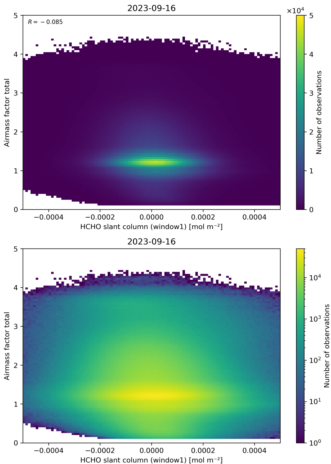
Figure 85: Scatter density plot of “HCHO slant column (window1)” against “Airmass factor total” for 2023-09-15 to 2023-09-17.
