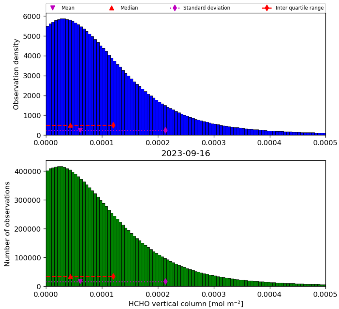
Figure 35: Histogram of “HCHO vertical column” for 2023-09-15 to 2023-09-17
