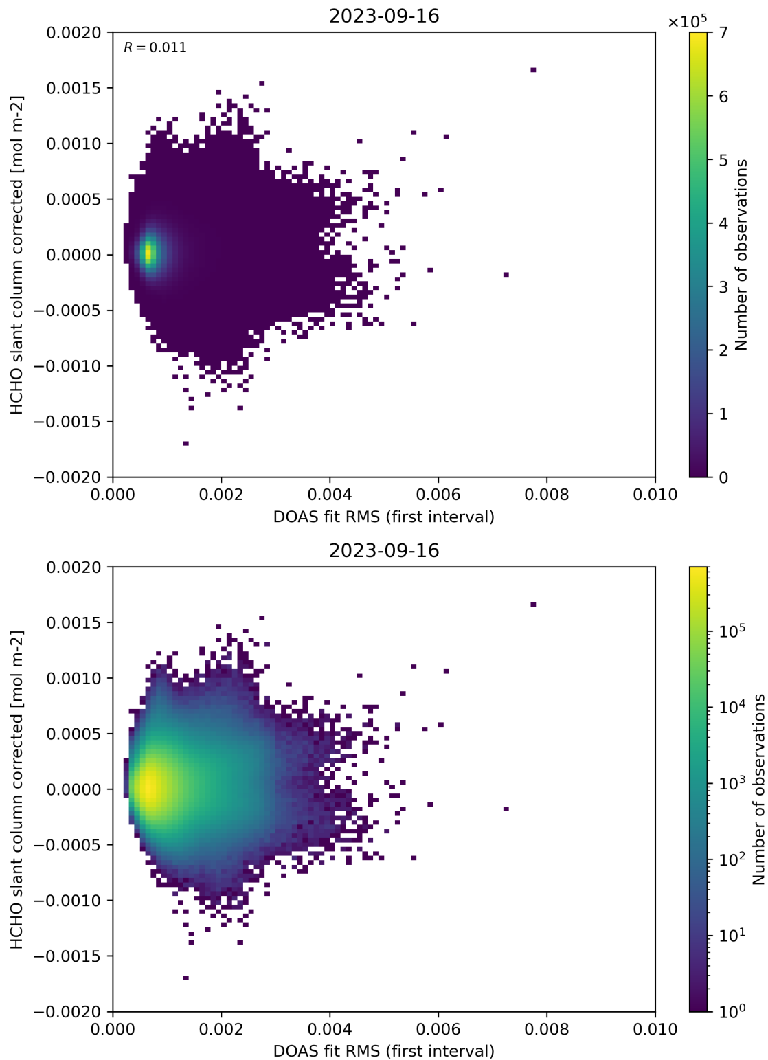
Figure 62: Scatter density plot of “DOAS fit RMS (first interval)” against “HCHO slant column corrected” for 2023-09-15 to 2023-09-17.
