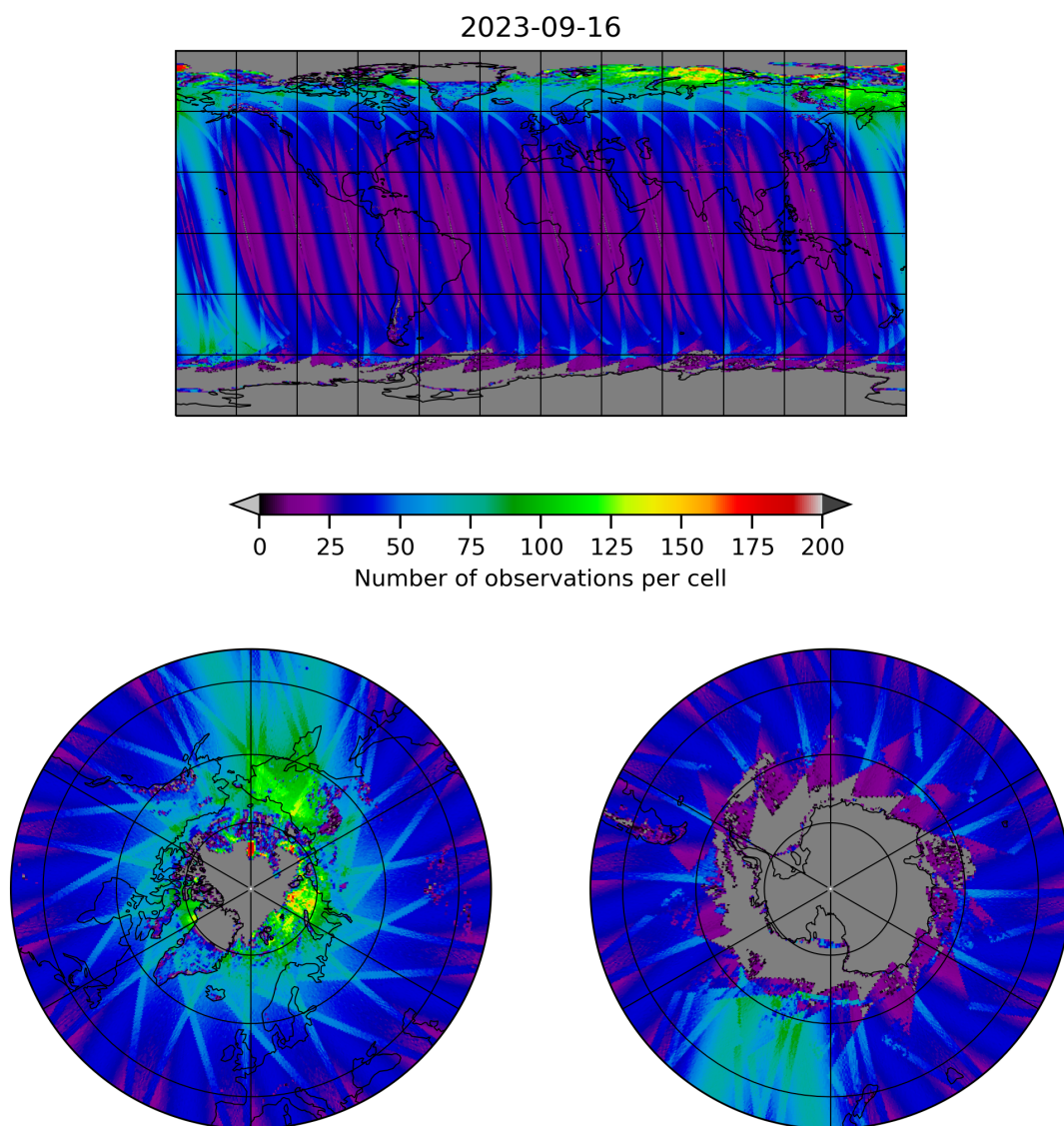
Figure 19: Map of the number of observations for 2023-09-15 to 2023-09-17
