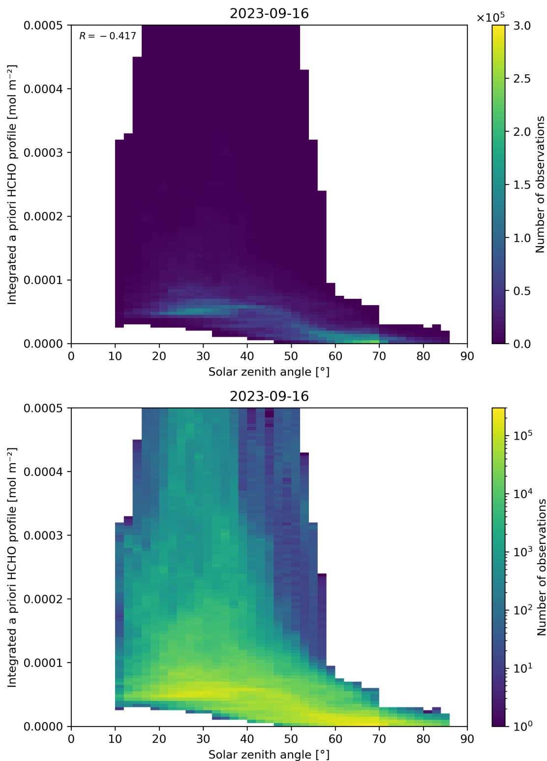
Figure 180: Scatter density plot of “Solar zenith angle” against “Integrated a priori HCHO profile” for 2023-09-15 to 2023-09-17.
