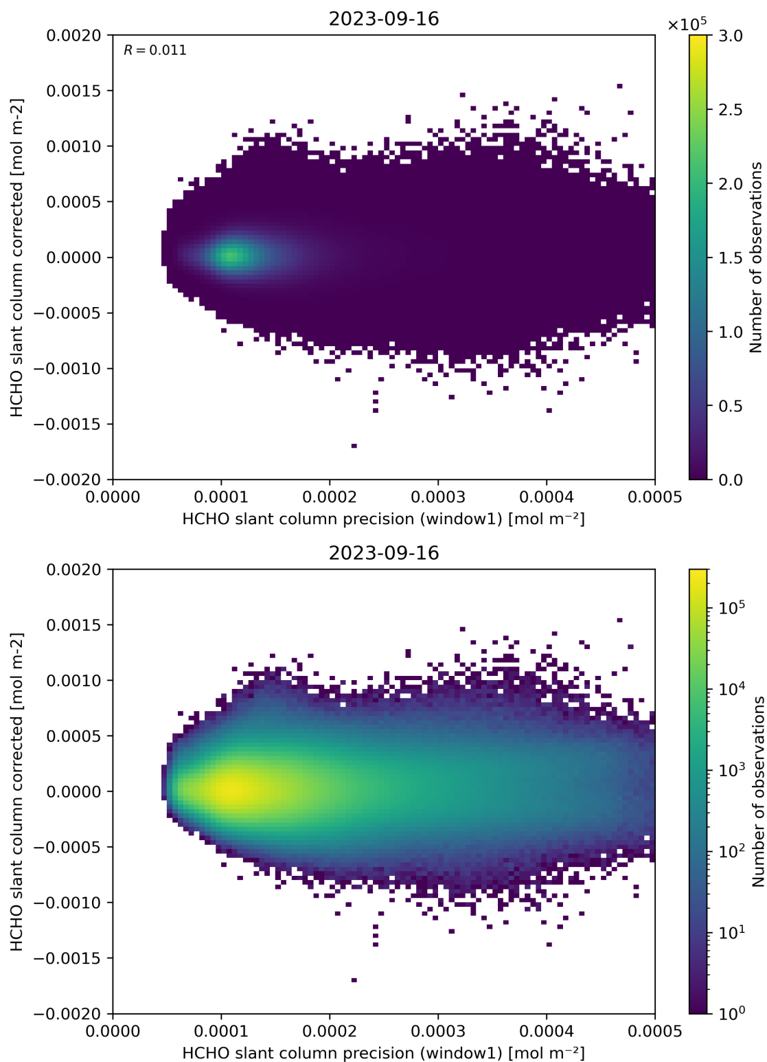
Figure 92: Scatter density plot of “HCHO slant column precision (window1)” against “HCHO slant column corrected” for 2023-09-15 to 2023-09-17.
