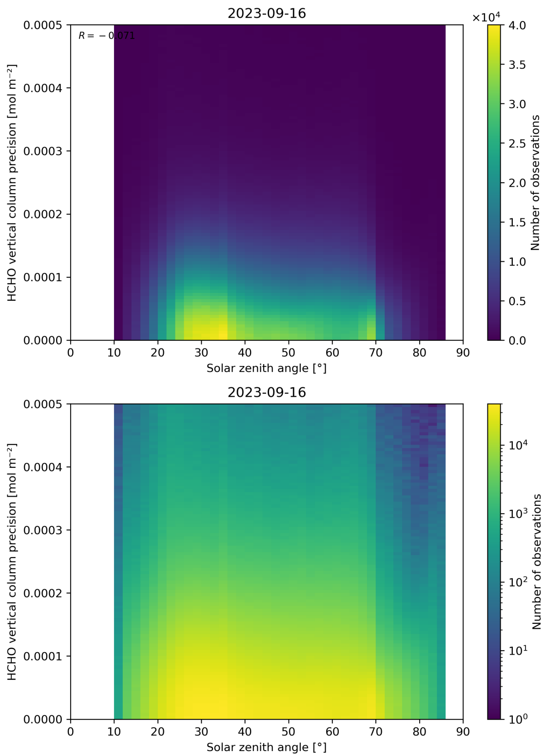
Figure 179: Scatter density plot of “Solar zenith angle” against “HCHO vertical column precision” for 2023-09-15 to 2023-09-17.
