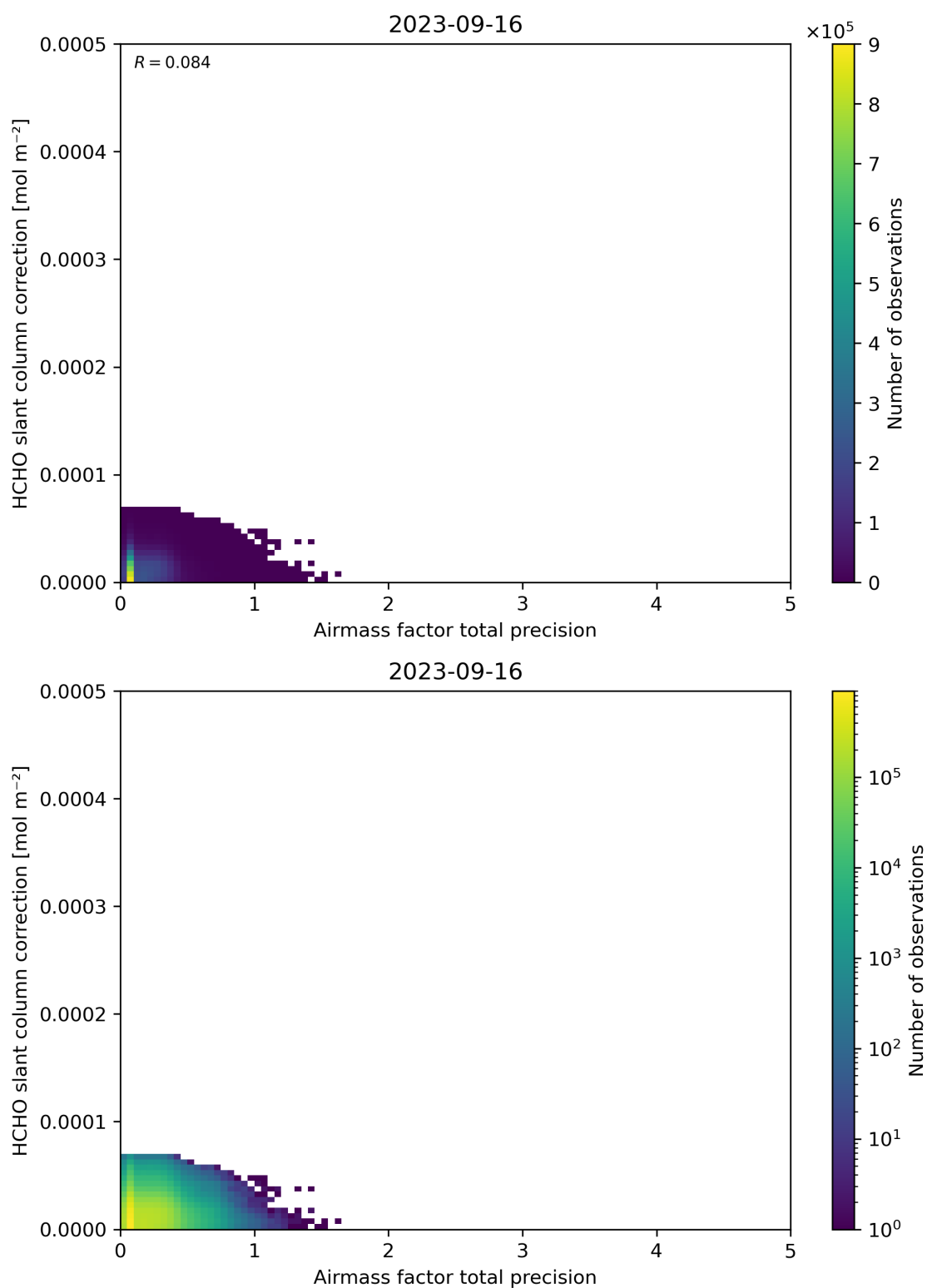
Figure 110: Scatter density plot of “Airmass factor total precision” against “HCHO slant column correction” for 2023-09-15 to 2023-09-17.
