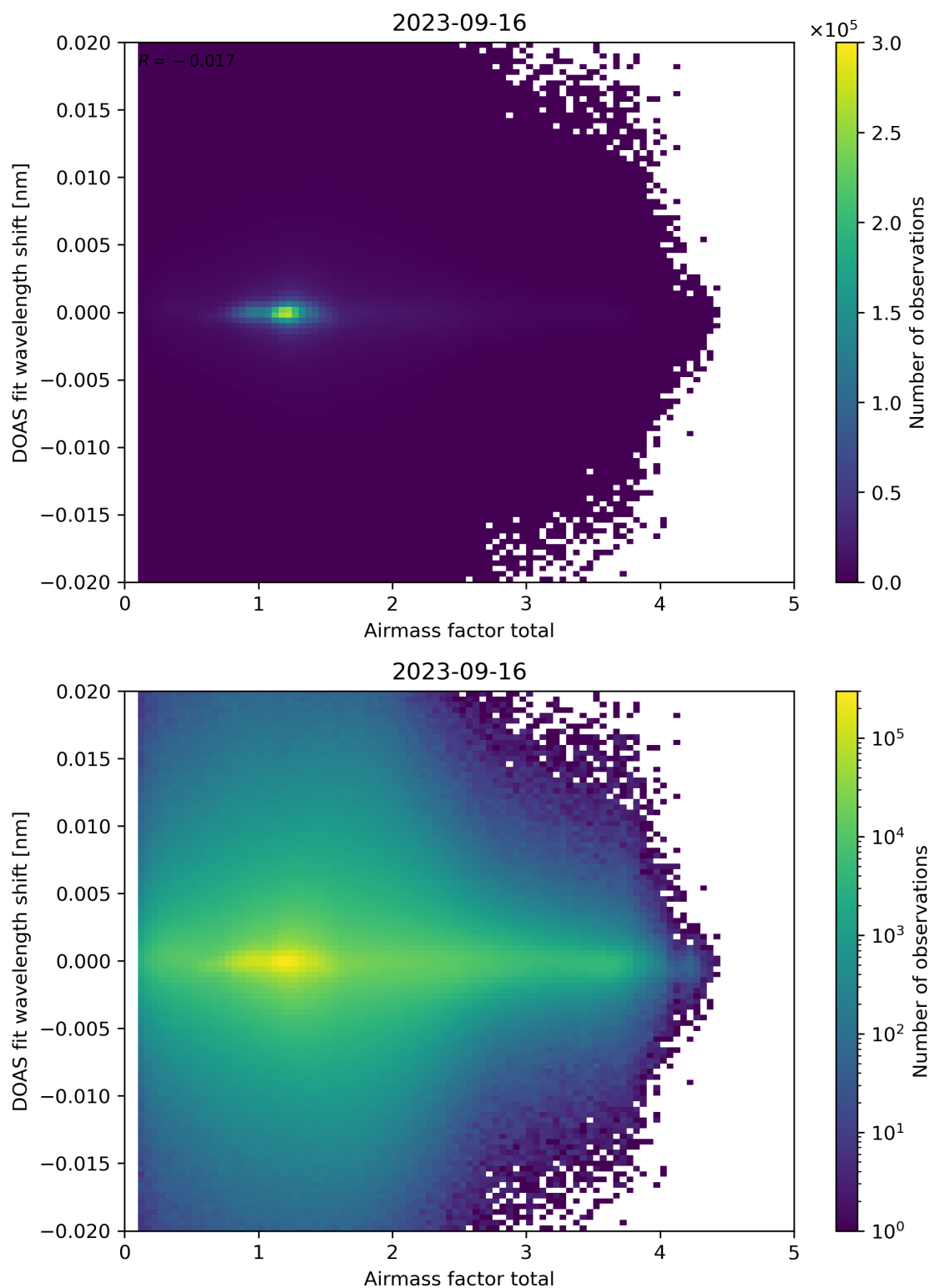
Figure 98: Scatter density plot of “Airmass factor total” against “DOAS fit wavelength shift” for 2023-09-15 to 2023-09-17.
