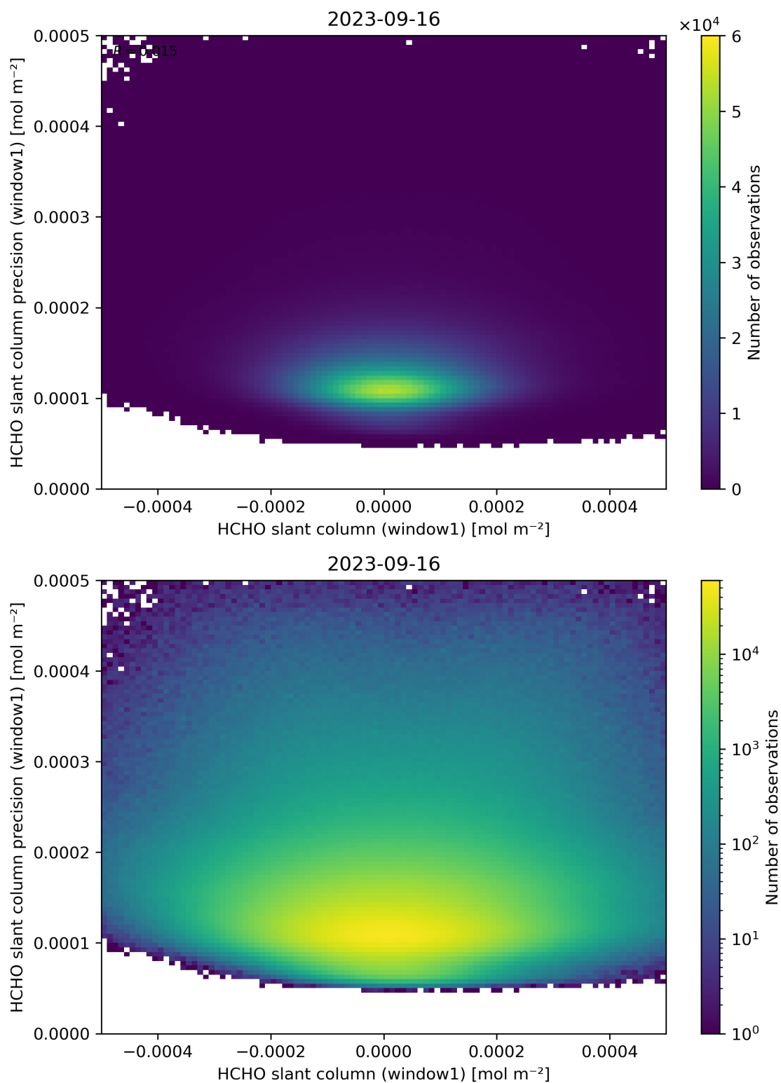
Figure 84: Scatter density plot of “HCHO slant column (window1)” against “HCHO slant column precision (window1)” for 2023-09-15 to 2023-09-17.
