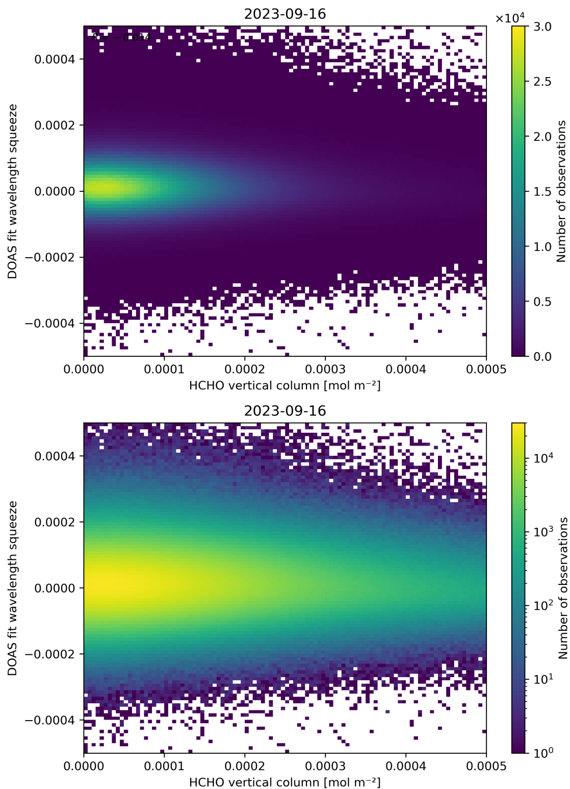
Figure 125: Scatter density plot of “HCHO vertical column” against “DOAS fit wavelength squeeze” for 2023-09-15 to 2023-09-17.
