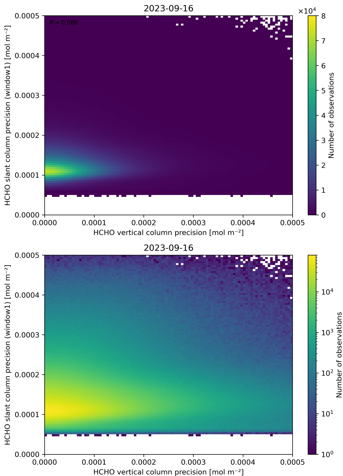
Figure 143: Scatter density plot of “HCHO vertical column precision” against “HCHO slant column precision (window1)” for 2023-09-15 to 2023-09-17.
