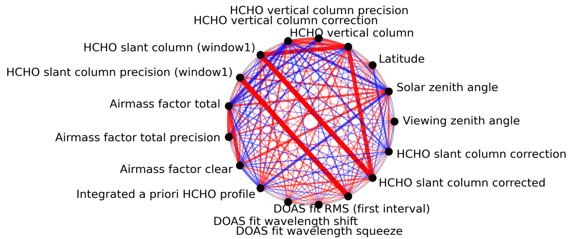
Figure 1: Map of correlation graph for 2023-09-15 to 2023-09-17.
