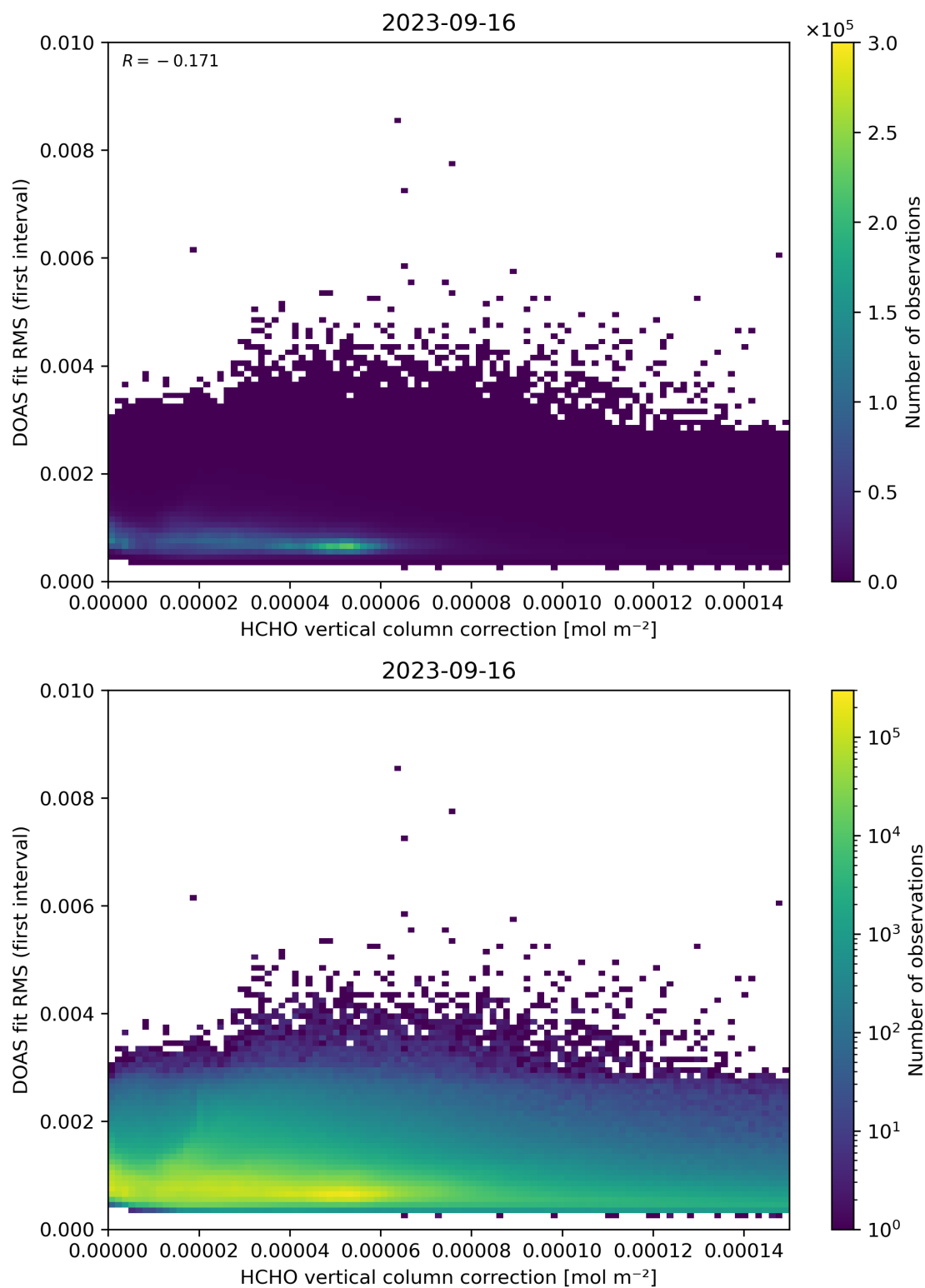
Figure 112: Scatter density plot of “HCHO vertical column correction” against “DOAS fit RMS (first interval)” for 2023-09-15 to 2023-09-17.
