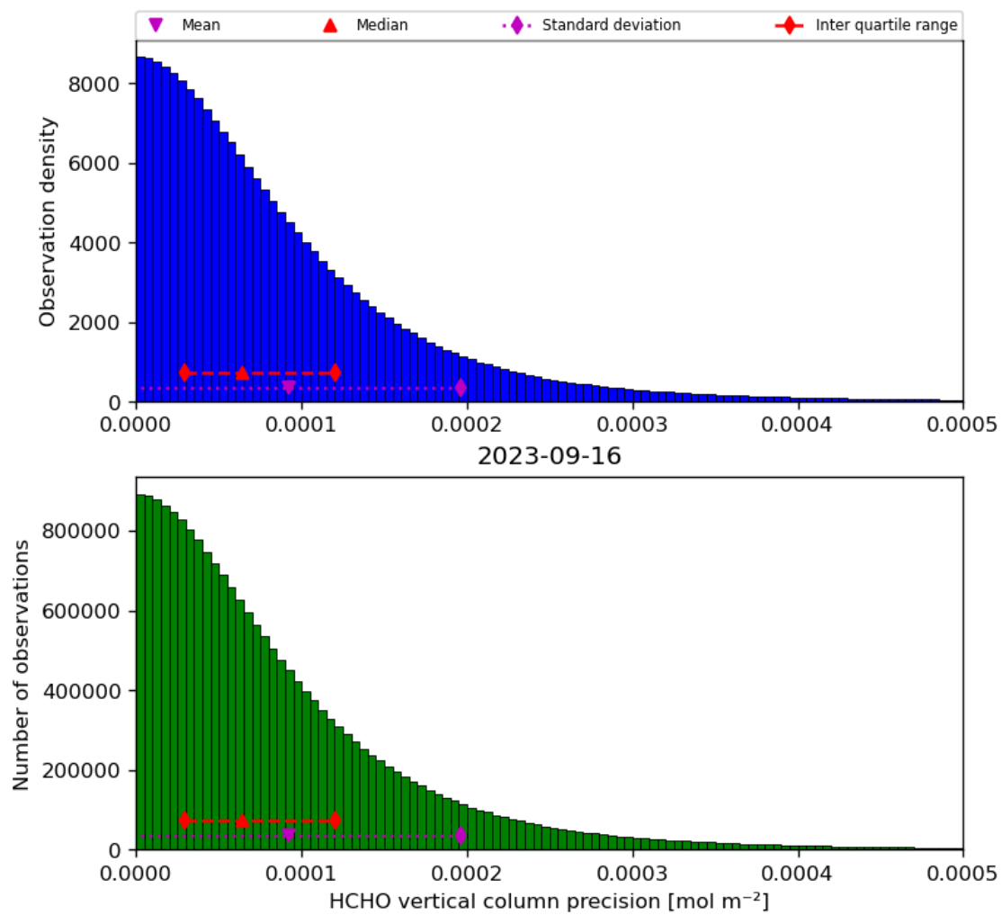
Figure 36: Histogram of “HCHO vertical column precision” for 2023-09-15 to 2023-09-17
