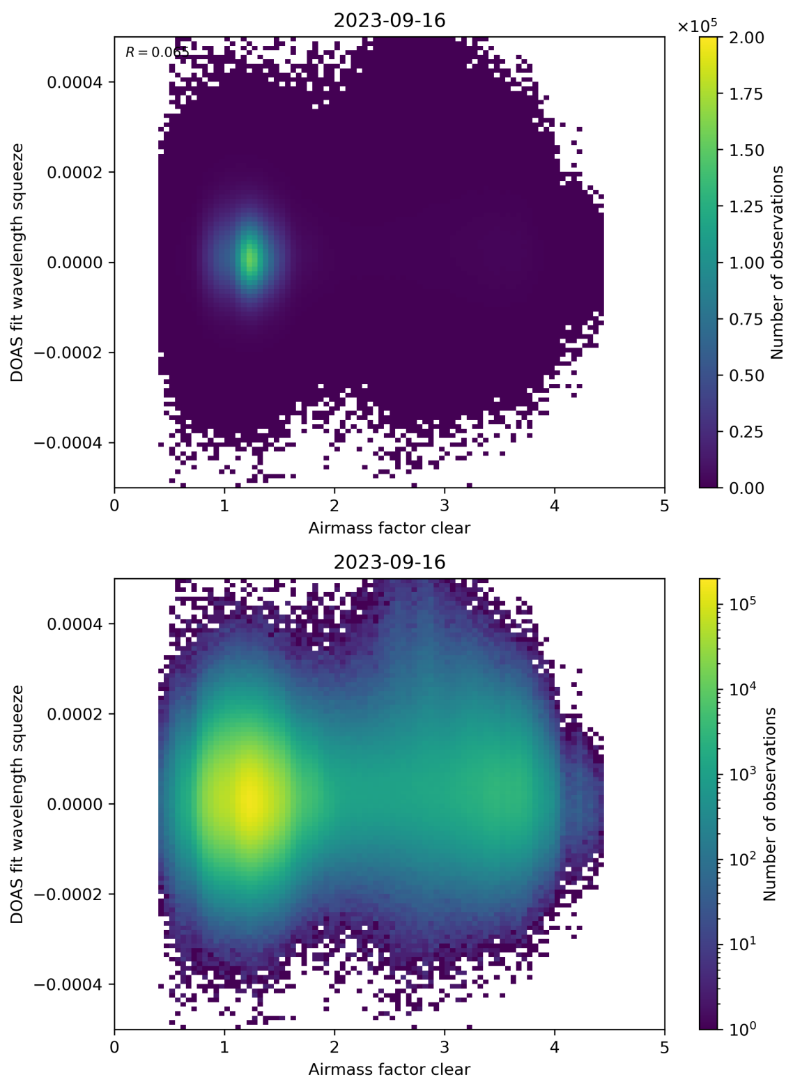
Figure 73: Scatter density plot of “Airmass factor clear” against “DOAS fit wavelength squeeze” for 2023-09-15 to 2023-09-17.
