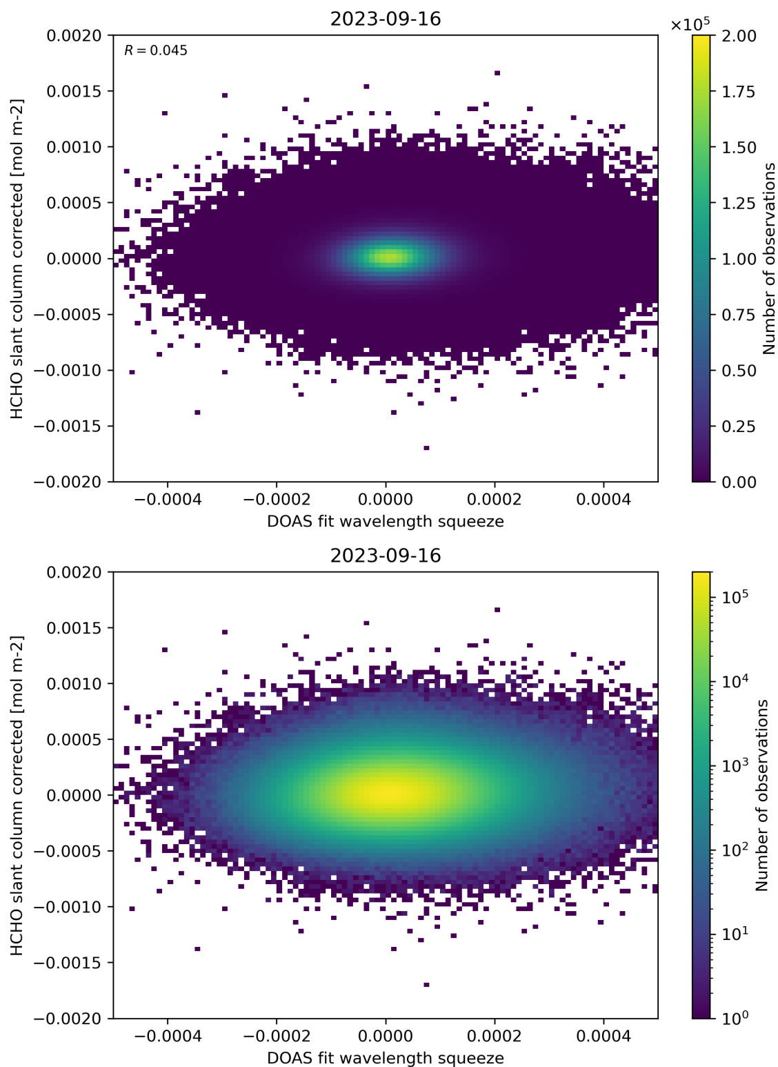
Figure 69: Scatter density plot of “DOAS fit wavelength squeeze” against “HCHO slant column corrected” for 2023-09-15 to 2023-09-17.
