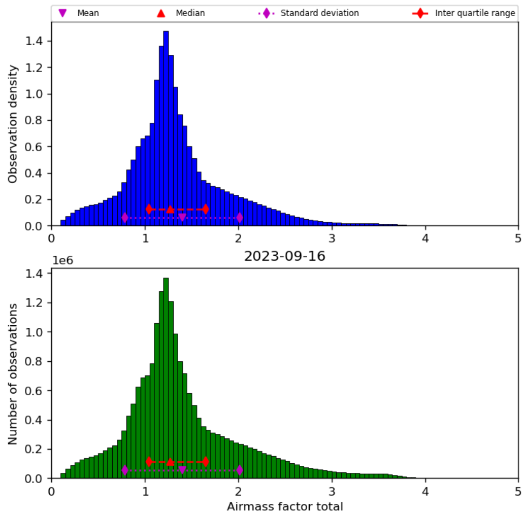
Figure 40: Histogram of “Airmass factor total” for 2023-09-15 to 2023-09-17
