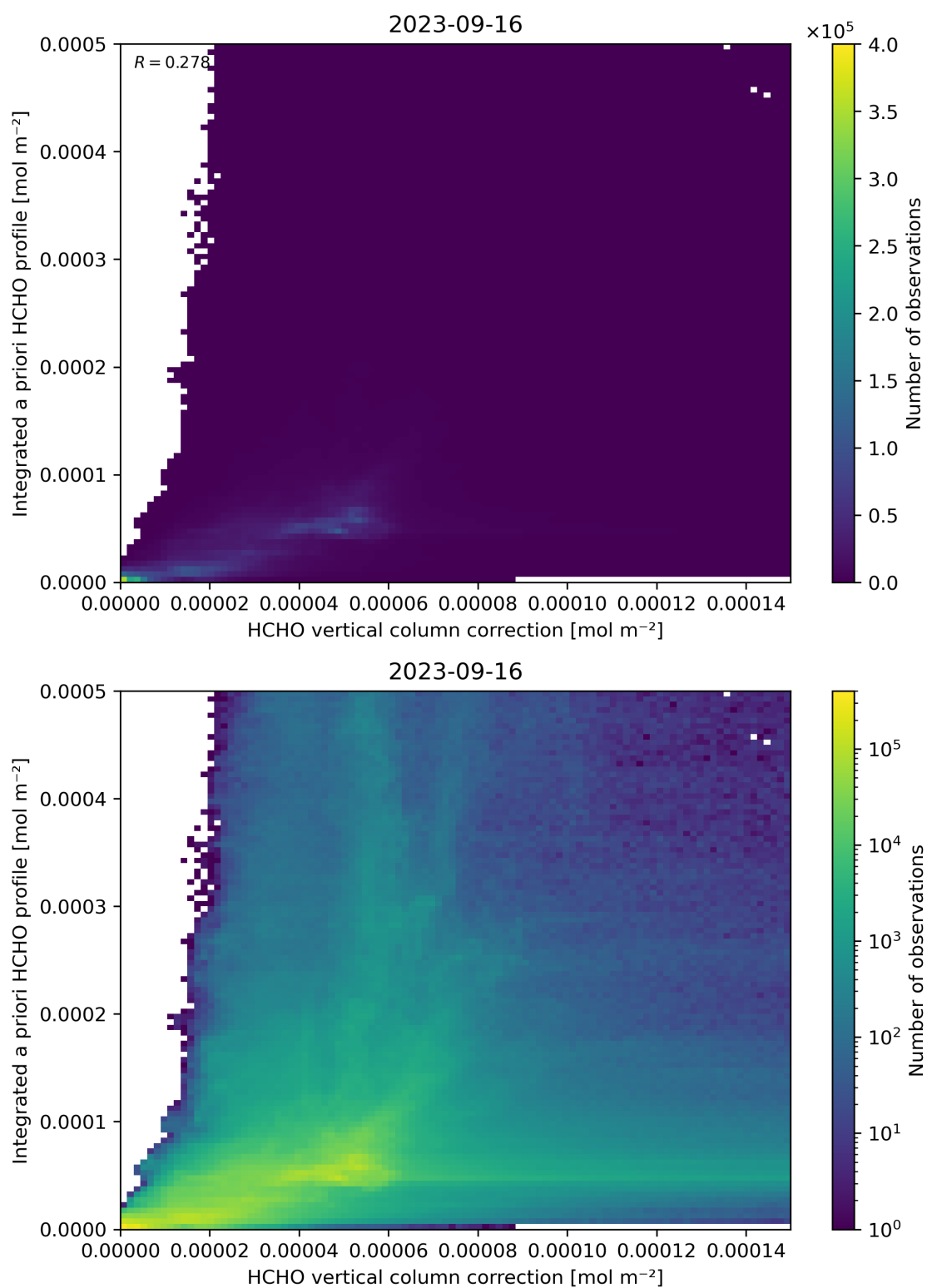
Figure 122: Scatter density plot of “HCHO vertical column correction” against “Integrated a priori HCHO profile” for 2023-09-15 to 2023-09-17.
