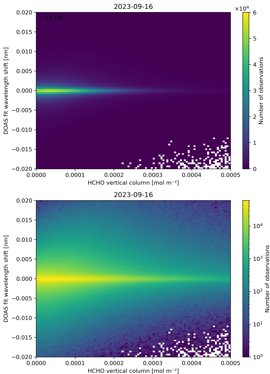
Figure 124: Scatter density plot of “HCHO vertical column” against “DOAS fit wavelength shift” for 2023-09-15 to 2023-09-17.
