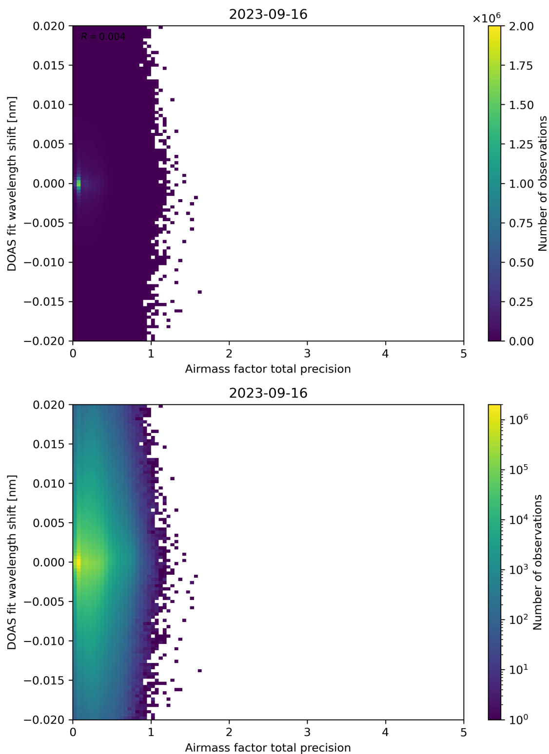
Figure 106: Scatter density plot of “Airmass factor total precision” against “DOAS fit wavelength shift” for 2023-09-15 to 2023-09-17.
