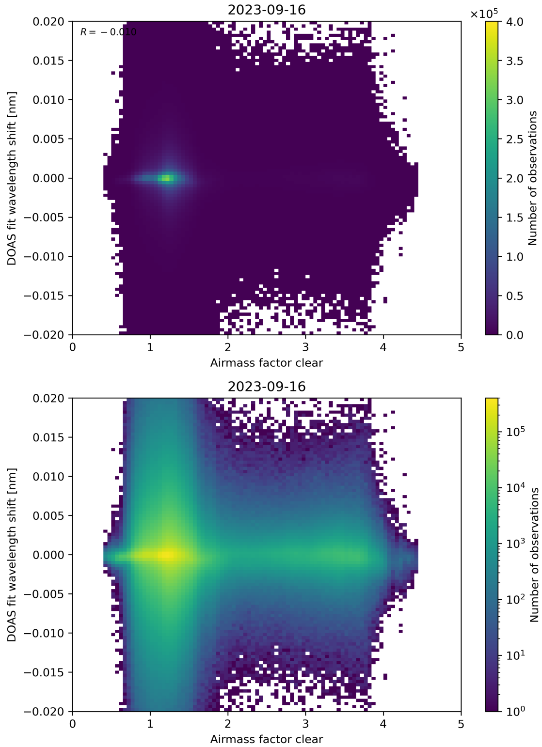
Figure 72: Scatter density plot of “Airmass factor clear” against “DOAS fit wavelength shift” for 2023-09-15 to 2023-09-17.
