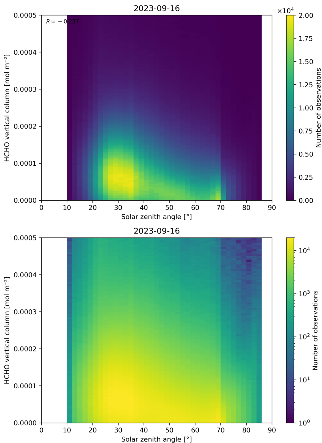
Figure 177: Scatter density plot of “Solar zenith angle” against “HCHO vertical column” for 2023-09-15 to 2023-09-17.
