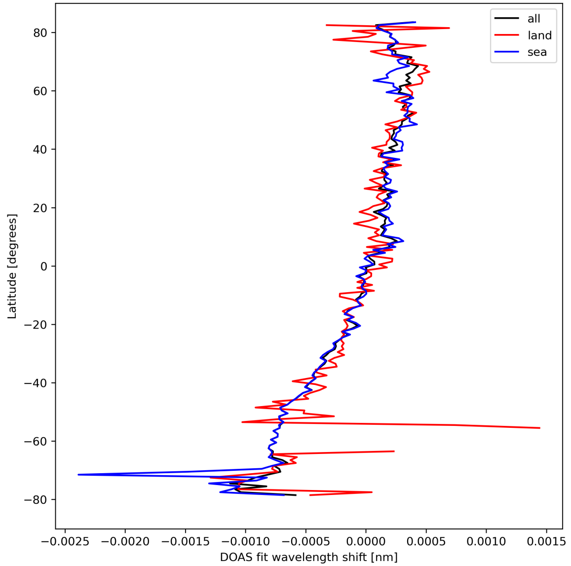
Figure 30: Zonal average of “DOAS fit wavelength shift” for 2023-09-15 to 2023-09-17.
