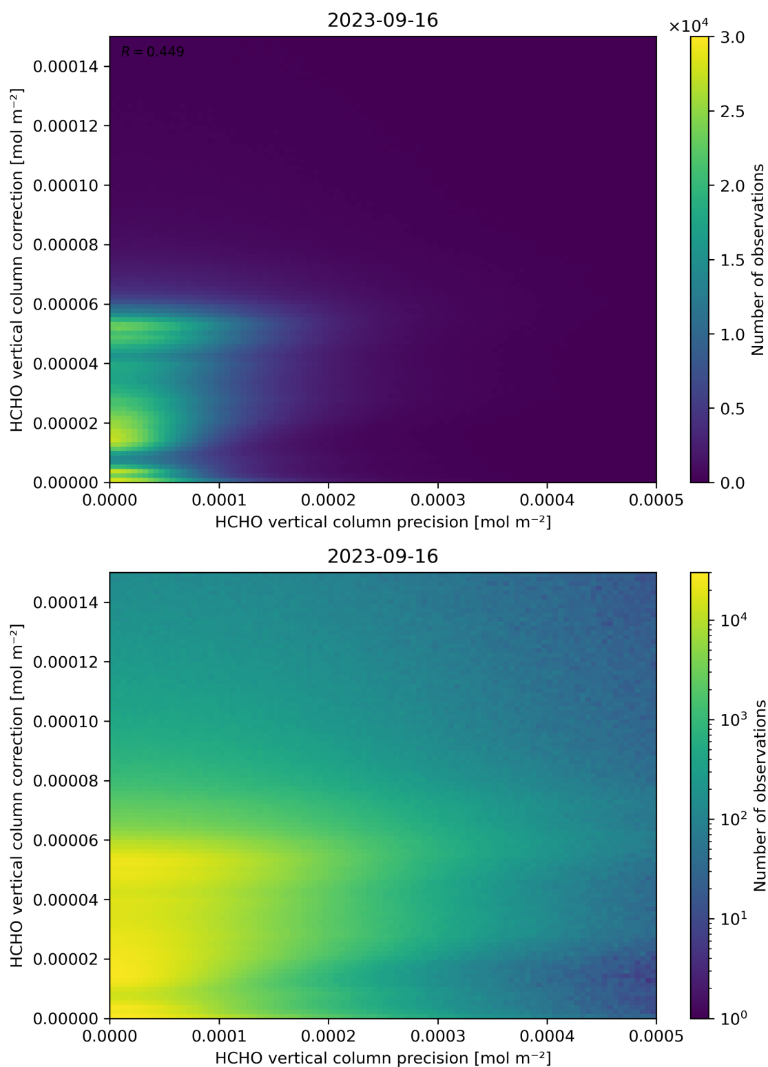
Figure 146: Scatter density plot of “HCHO vertical column precision” against “HCHO vertical column correction” for 2023-09-15 to 2023-09-17.
