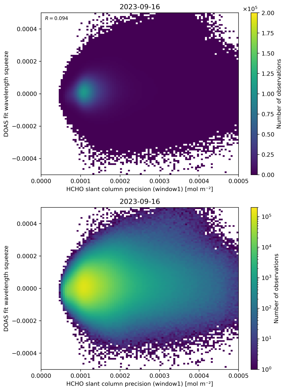
Figure 90: Scatter density plot of “HCHO slant column precision (window1)” against “DOAS fit wavelength squeeze” for 2023-09-15 to 2023-09-17.
