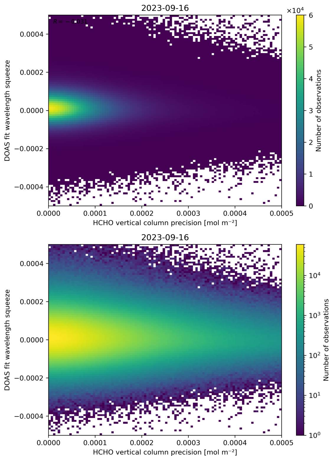
Figure 138: Scatter density plot of “HCHO vertical column precision” against “DOAS fit wavelength squeeze” for 2023-09-15 to 2023-09-17.
