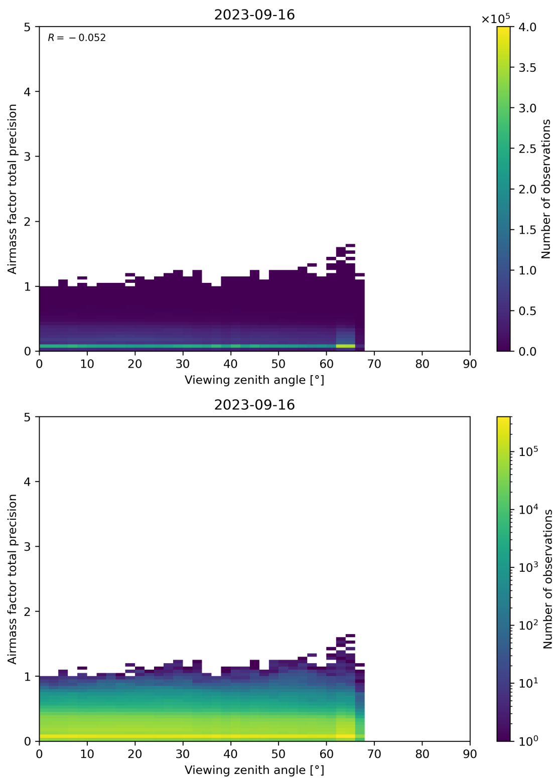
Figure 191: Scatter density plot of “Viewing zenith angle” against “Airmass factor total precision” for 2023-09-15 to 2023-09-17.
