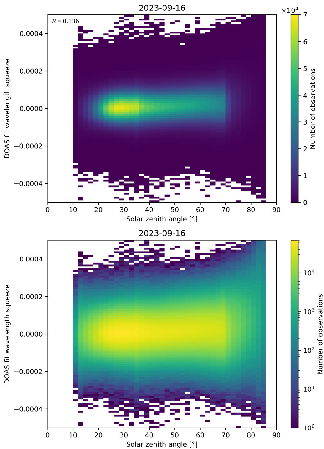
Figure 169: Scatter density plot of “Solar zenith angle” against “DOAS fit wavelength squeeze” for 2023-09-15 to 2023-09-17.
