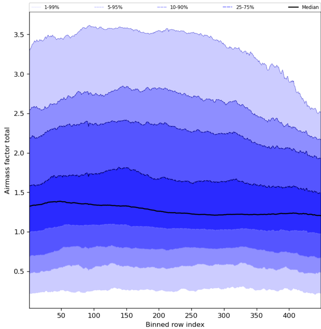
Figure 54: Along track statistics of “Airmass factor total” for 2023-09-15 to 2023-09-17
