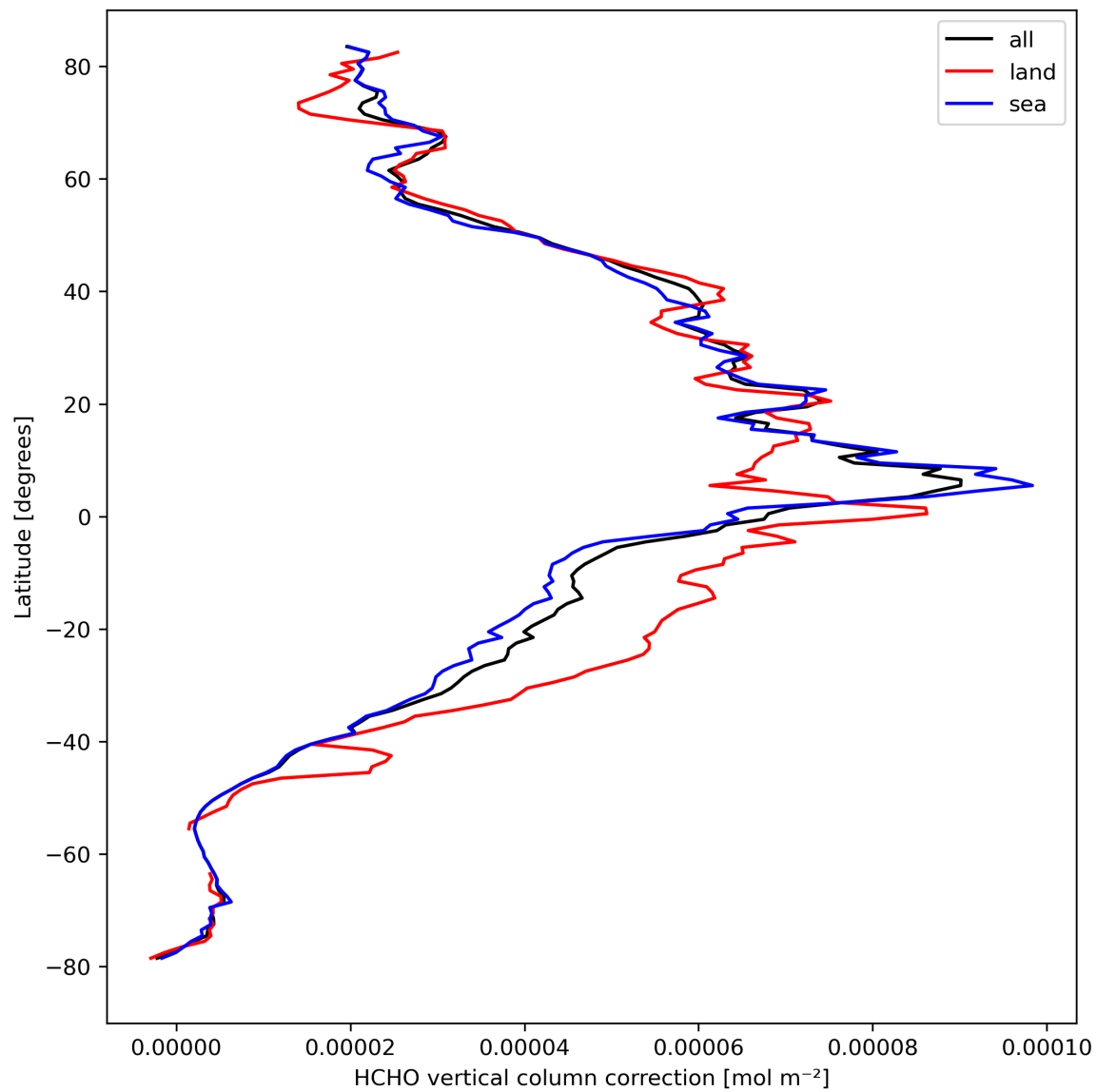
Figure 23: Zonal average of “HCHO vertical column correction” for 2023-09-15 to 2023-09-17.
