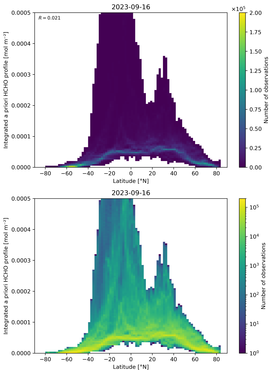
Figure 166: Scatter density plot of “Latitude” against “Integrated a priori HCHO profile” for 2023-09-15 to 2023-09-17.
