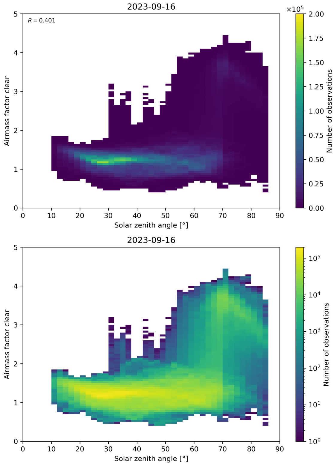
Figure 170: Scatter density plot of “Solar zenith angle” against “Airmass factor clear” for 2023-09-15 to 2023-09-17.
