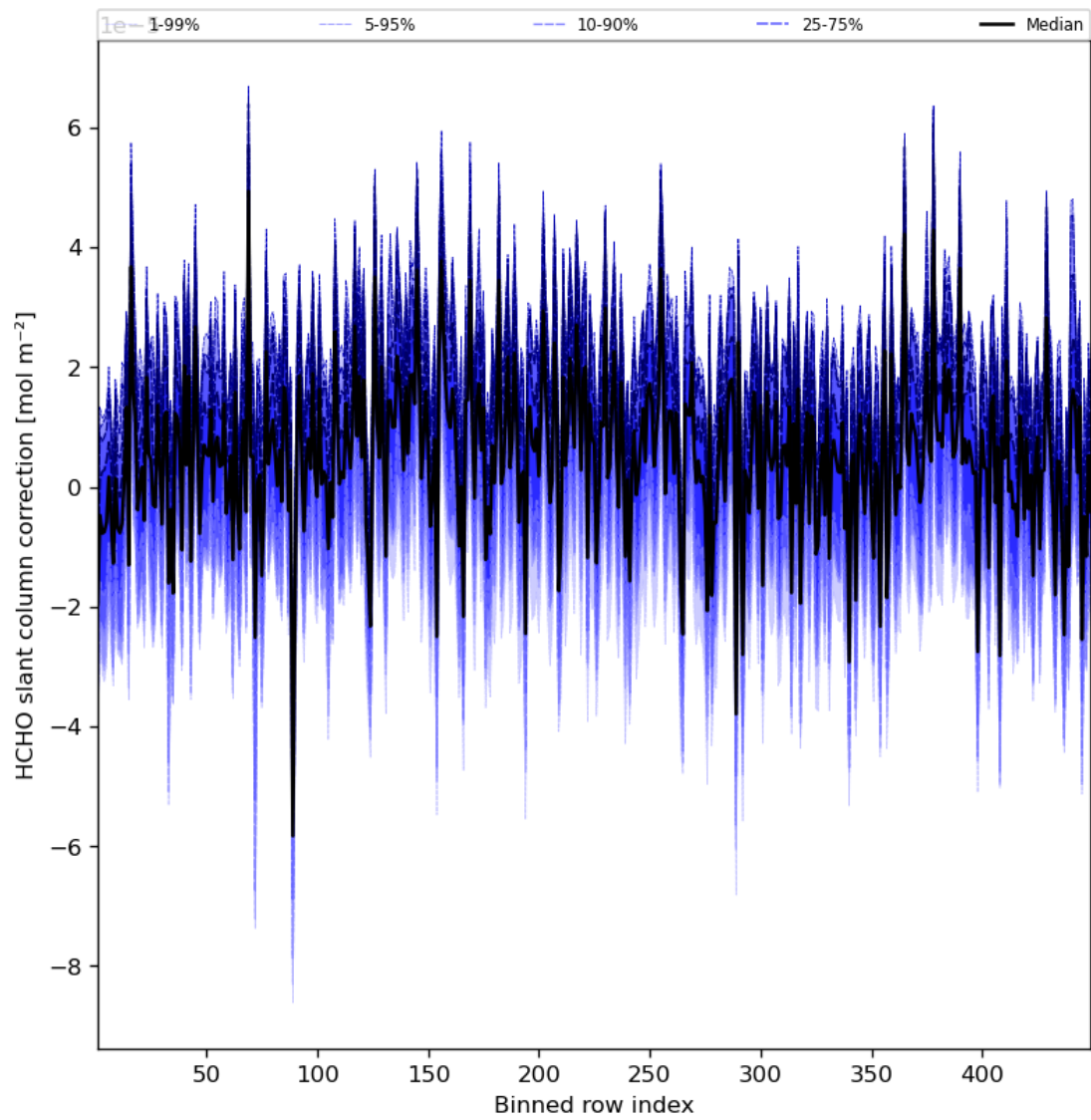
Figure 61: Along track statistics of “HCHO slant column correction” for 2023-09-15 to 2023-09-17
