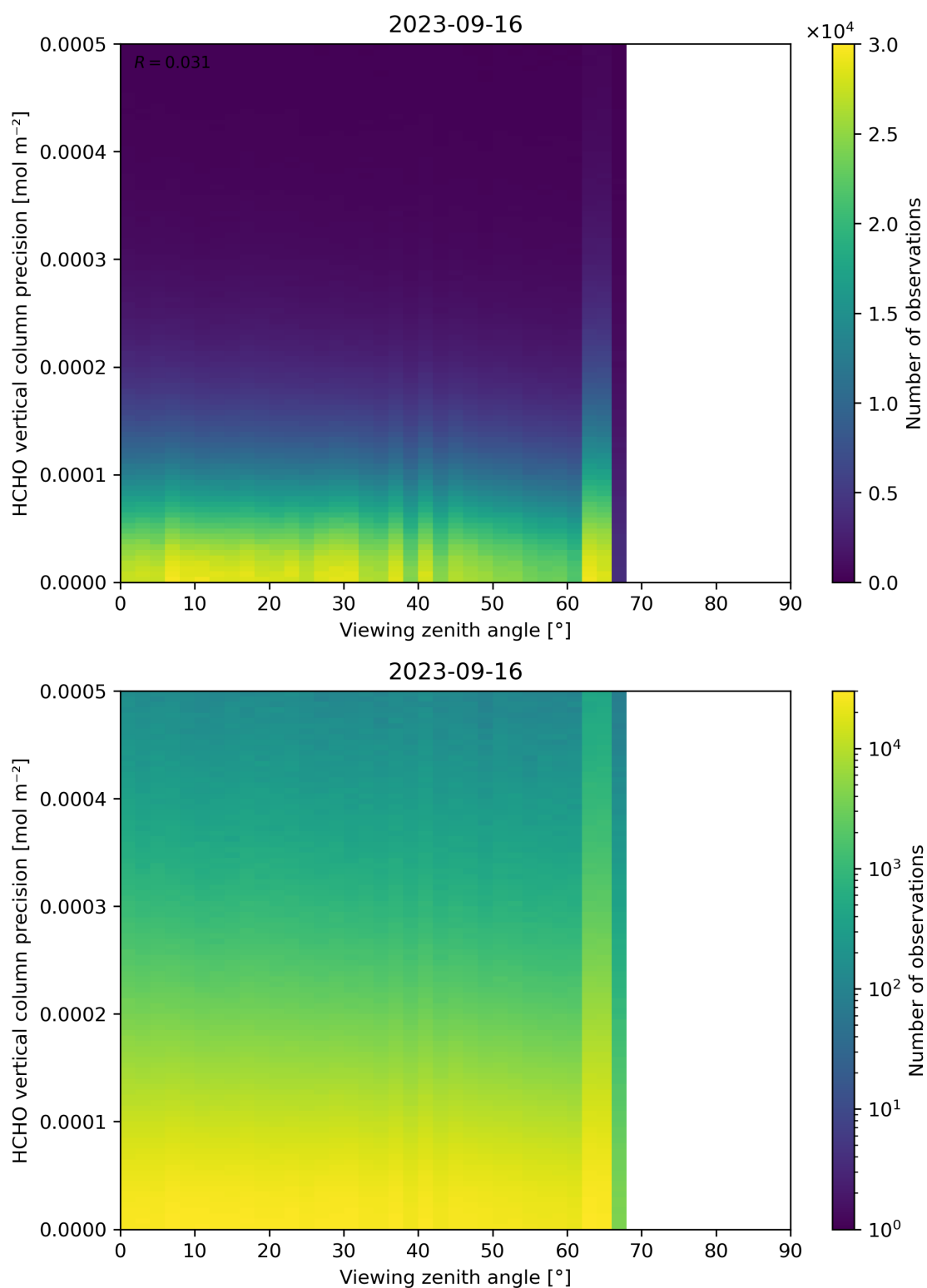
Figure 194: Scatter density plot of “Viewing zenith angle” against “HCHO vertical column precision” for 2023-09-15 to 2023-09-17.
