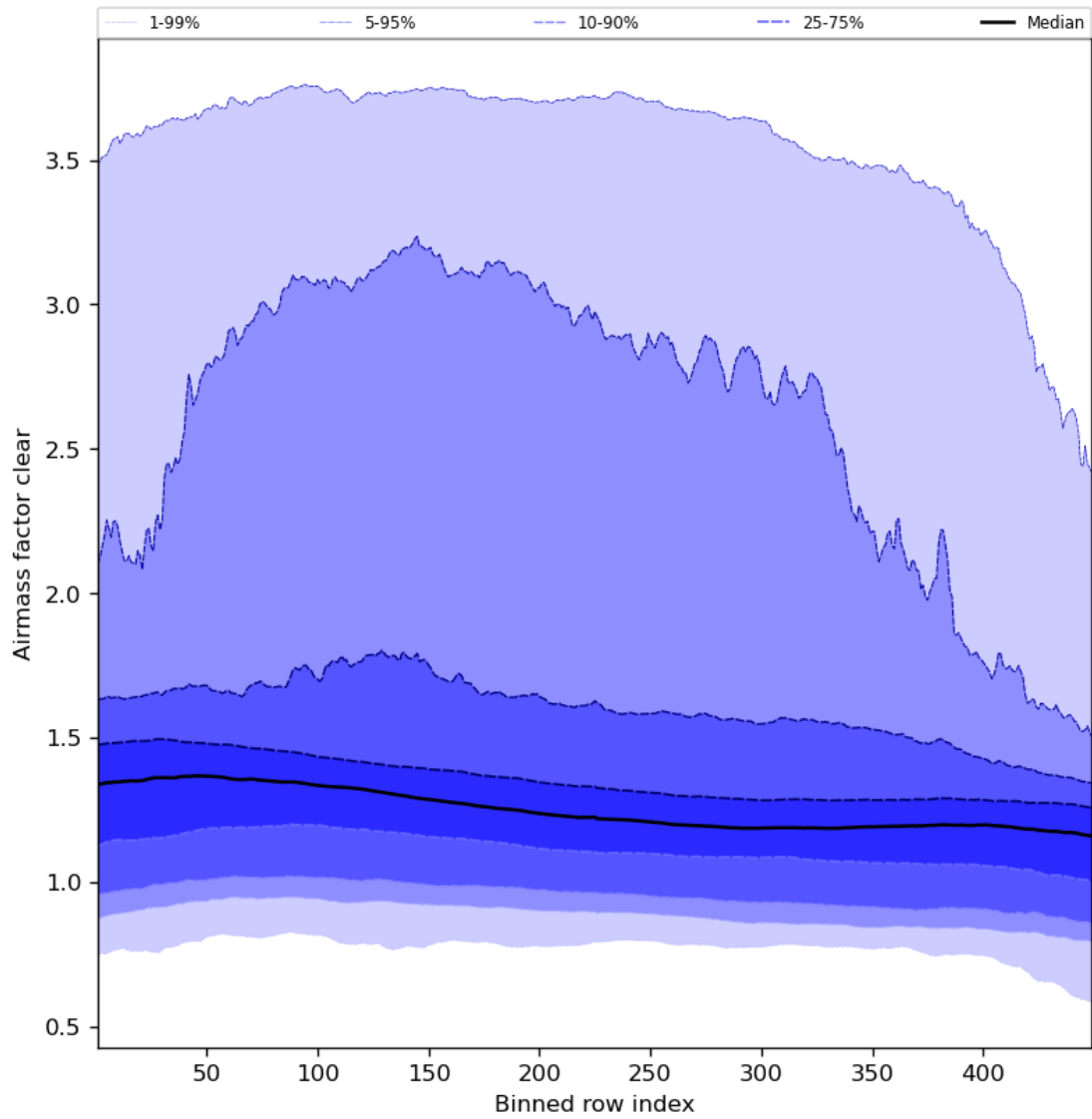
Figure 56: Along track statistics of “Airmass factor clear” for 2023-09-15 to 2023-09-17
