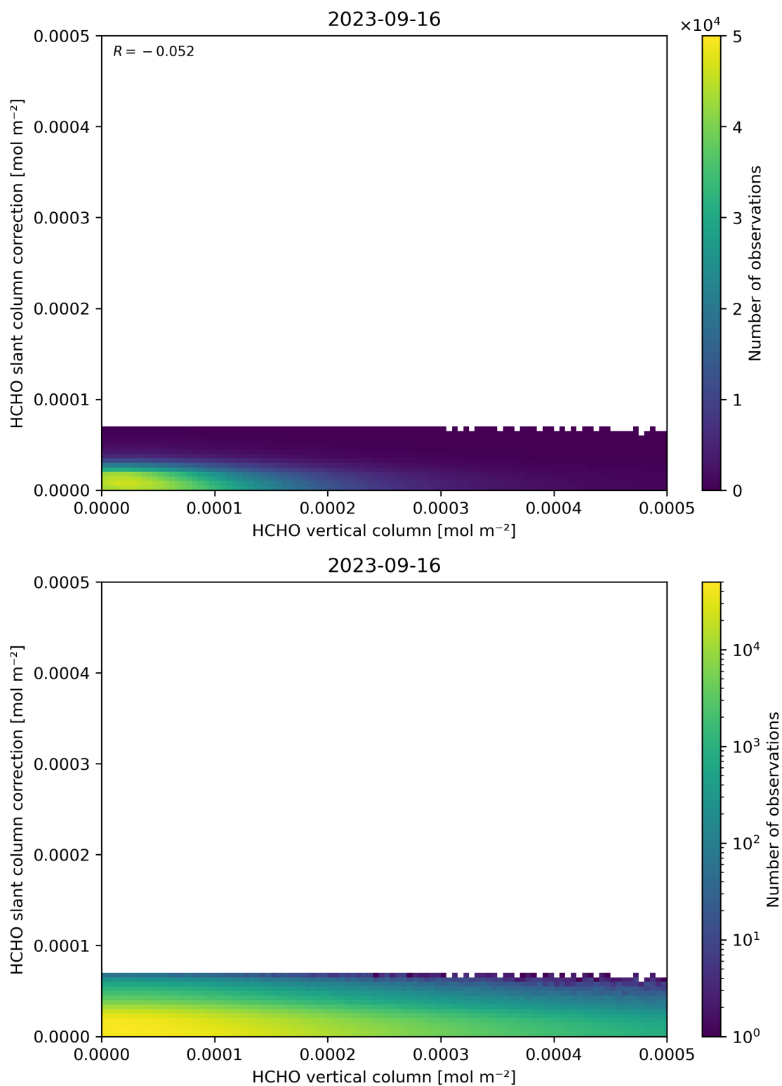
Figure 128: Scatter density plot of “HCHO vertical column” against “HCHO slant column correction” for 2023-09-15 to 2023-09-17.
