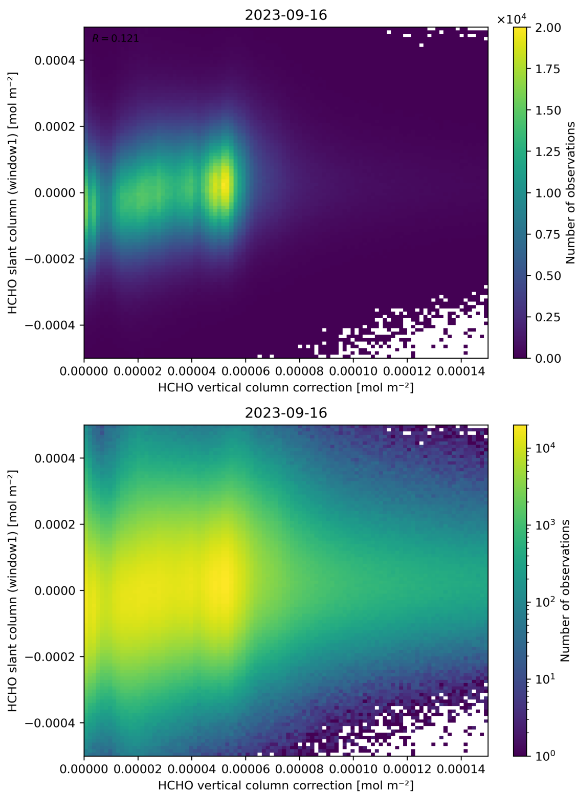
Figure 118: Scatter density plot of “HCHO vertical column correction” against “HCHO slant column (window1)” for 2023-09-15 to 2023-09-17.
