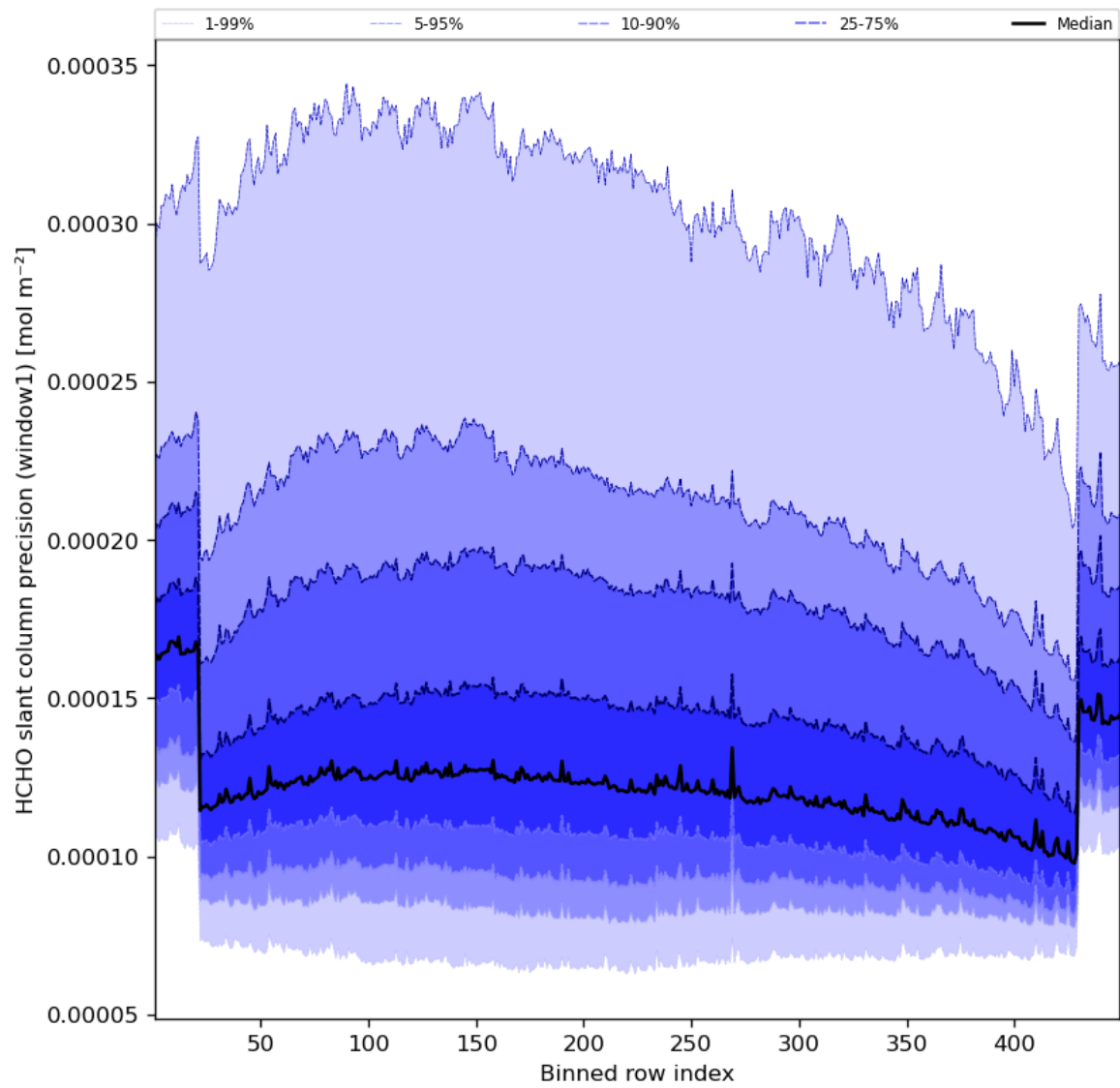
Figure 53: Along track statistics of "HCHO slant column precision (window1)" for 2023-09-15 to 2023-09-17
