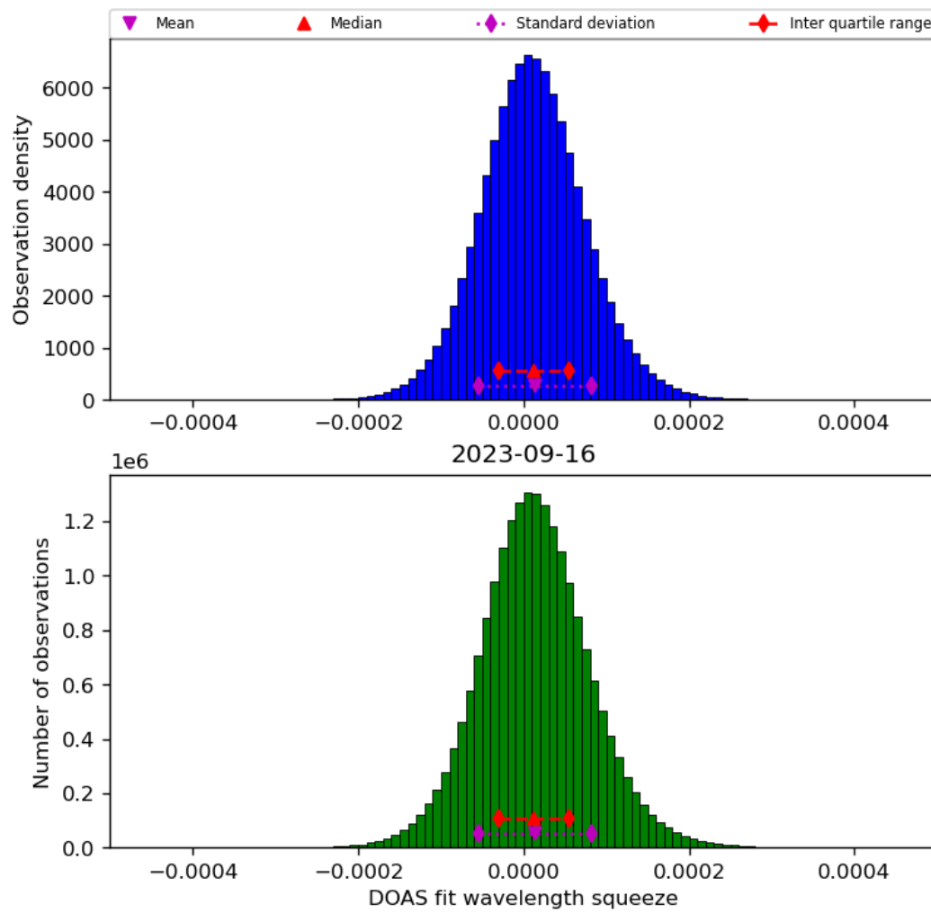
Figure 45: Histogram of “DOAS fit wavelength squeeze” for 2023-09-15 to 2023-09-17
