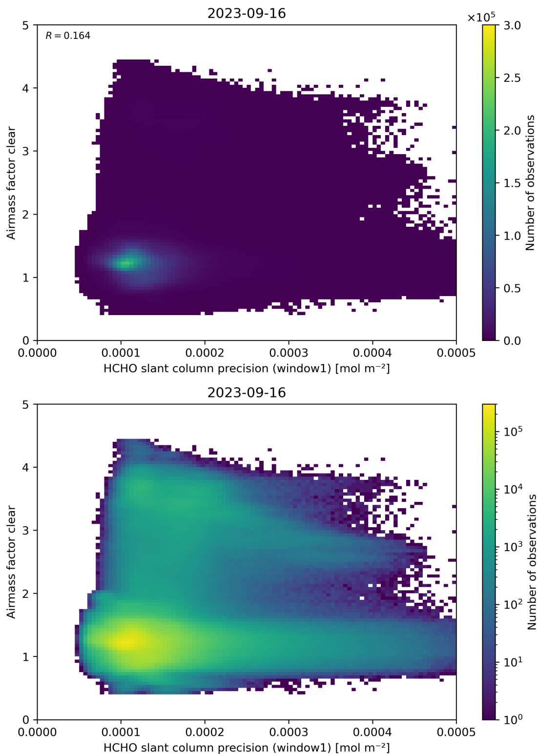
Figure 91: Scatter density plot of “HCHO slant column precision (window1)” against “Airmass factor clear” for 2023-09-15 to 2023-09-17.
