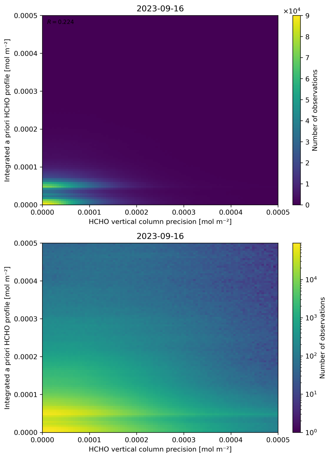
Figure 147: Scatter density plot of “HCHO vertical column precision” against “Integrated a priori HCHO profile” for 2023-09-15 to 2023-09-17.
