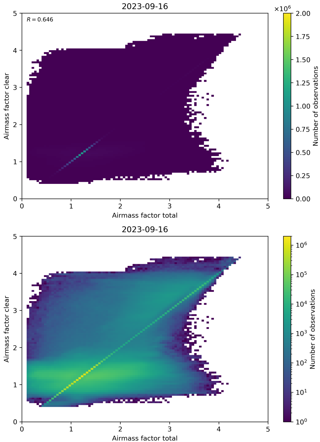
Figure 100: Scatter density plot of “Airmass factor total” against “Airmass factor clear” for 2023-09-15 to 2023-09-17.
