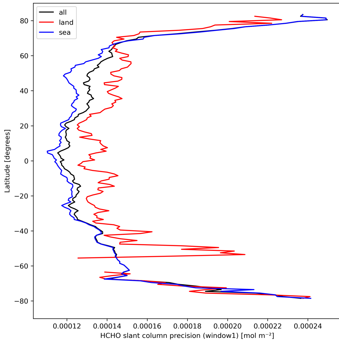
Figure 25: Zonal average of “HCHO slant column precision (window1)” for 2023-09-15 to 2023-09-17.
