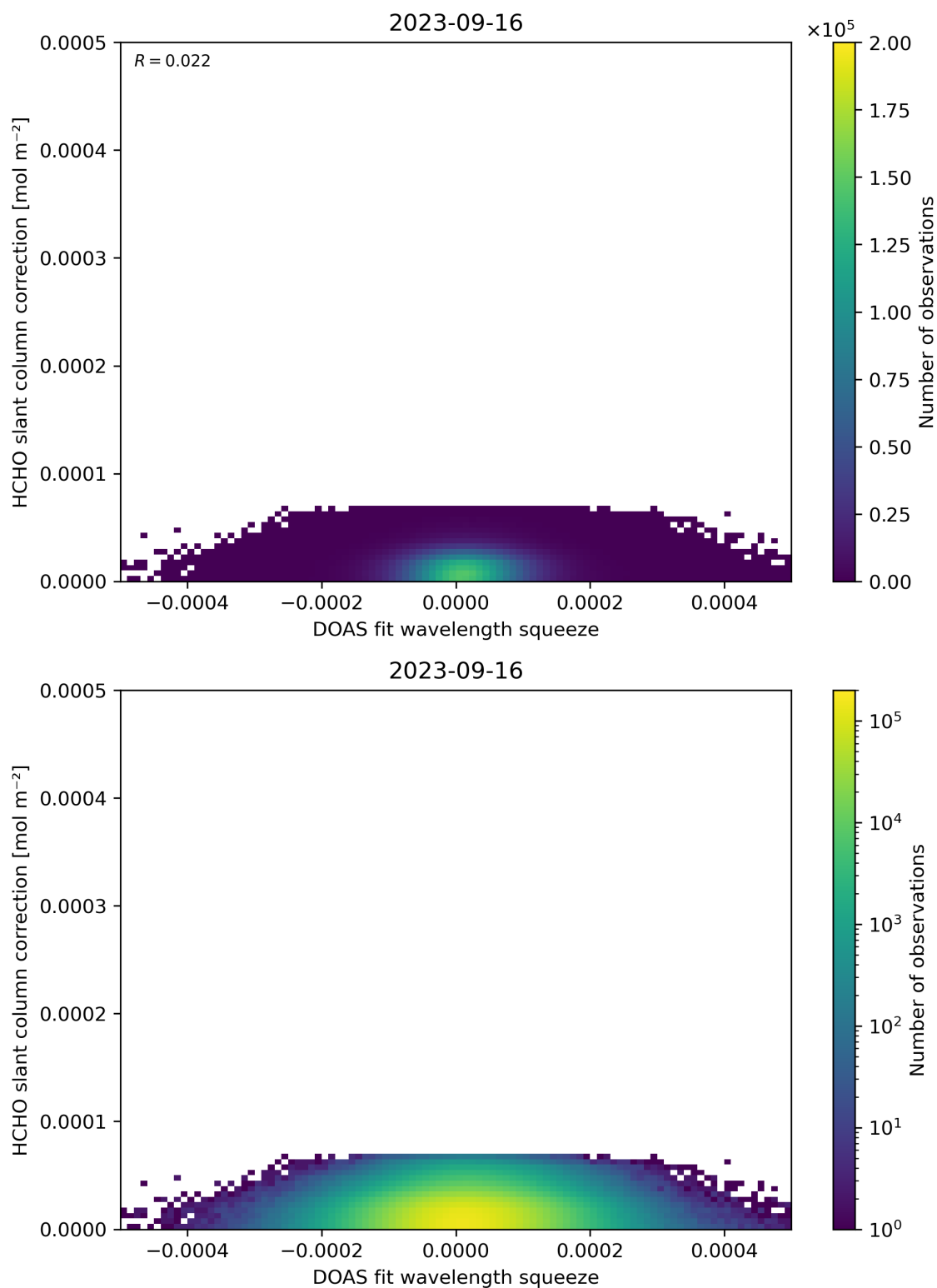
Figure 70: Scatter density plot of “DOAS fit wavelength squeeze” against “HCHO slant column correction” for 2023-09-15 to 2023-09-17.
