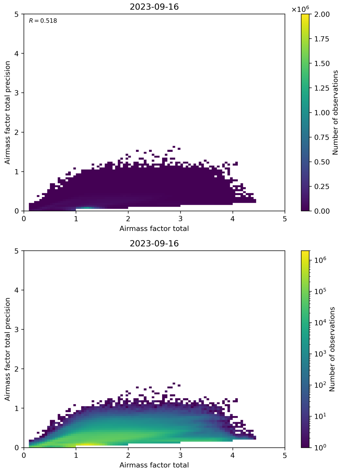
Figure 103: Scatter density plot of “Airmass factor total” against “Airmass factor total precision” for 2023-09-15 to 2023-09-17.
