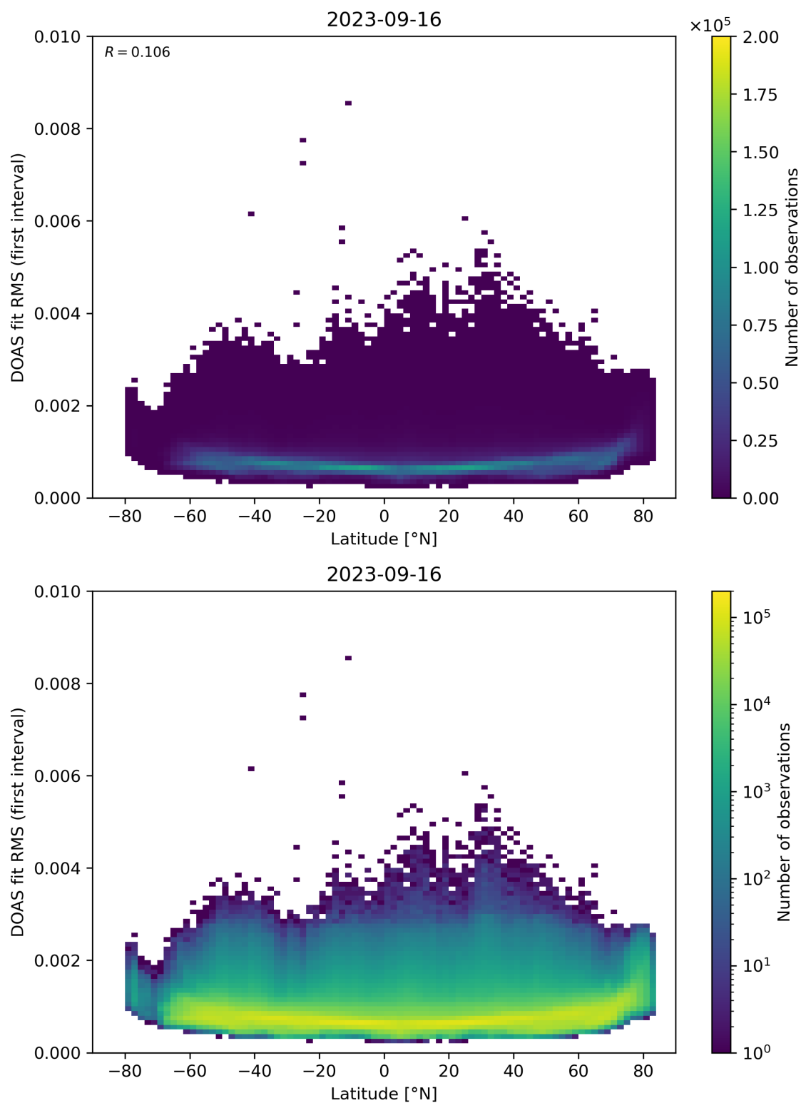
Figure 153: Scatter density plot of “Latitude” against “DOAS fit RMS (first interval)” for 2023-09-15 to 2023-09-17.
