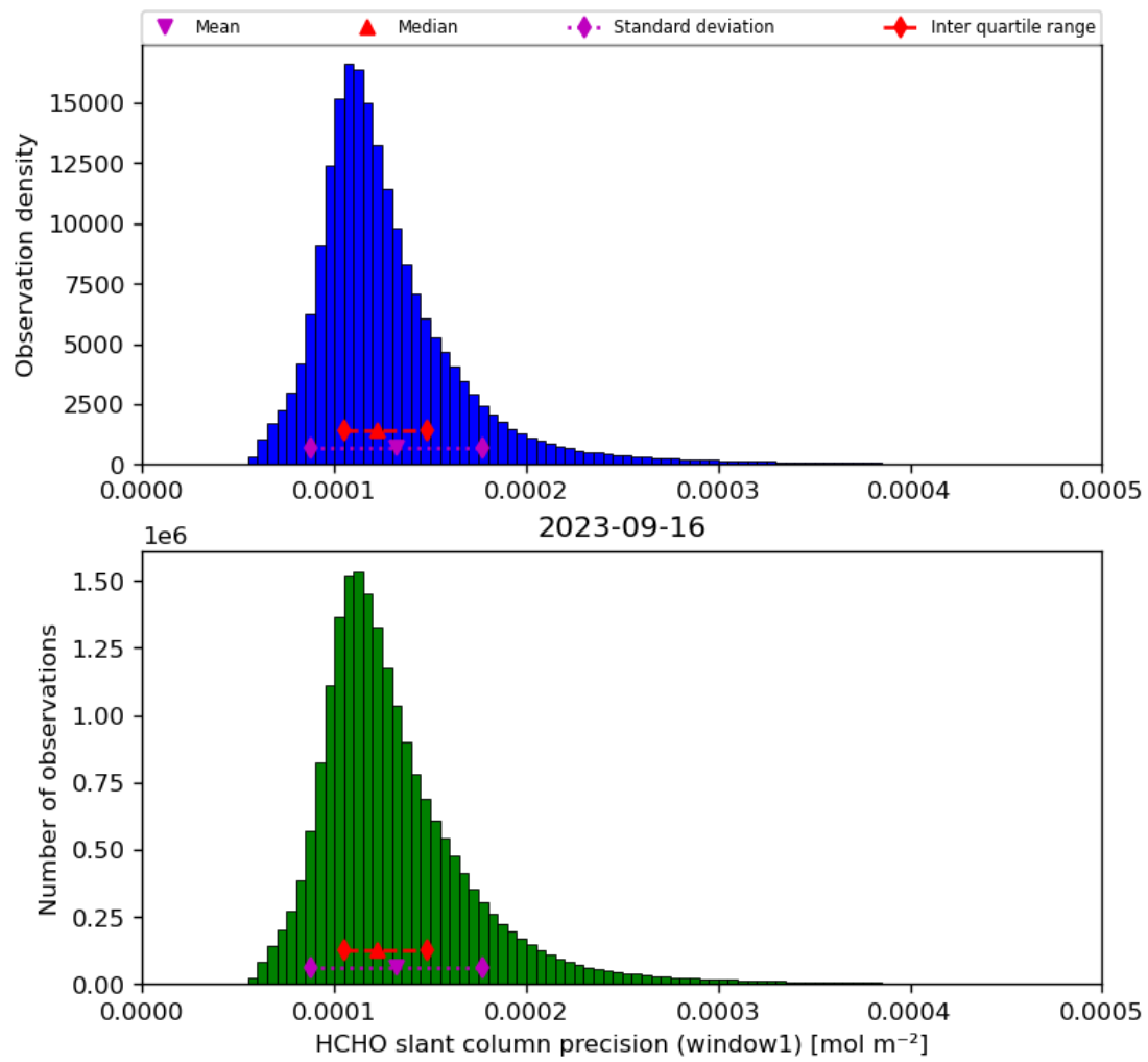
Figure 39: Histogram of “HCHO slant column precision (window1)” for 2023-09-15 to 2023-09-17
