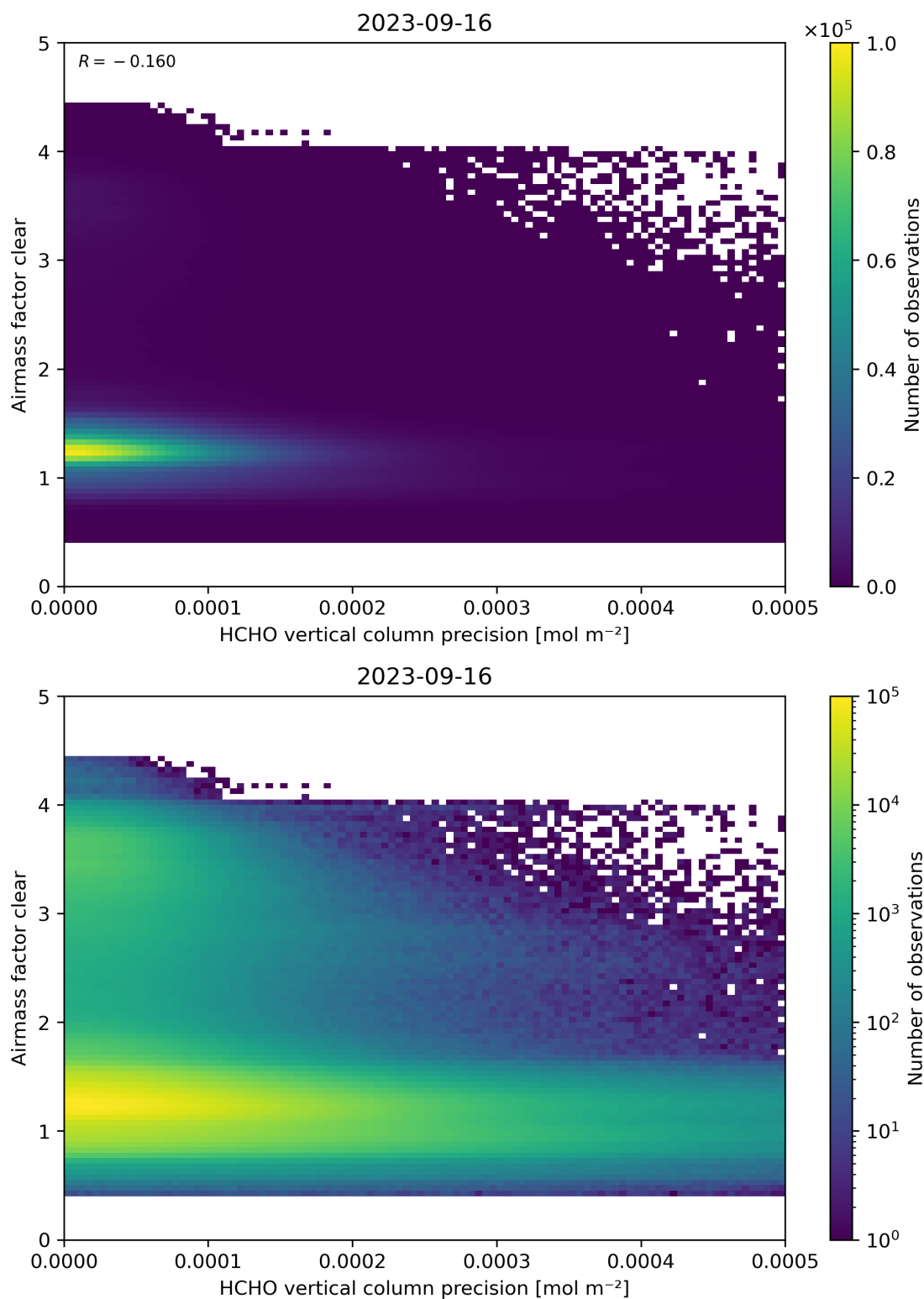
Figure 139: Scatter density plot of “HCHO vertical column precision” against “Airmass factor clear” for 2023-09-15 to 2023-09-17.
