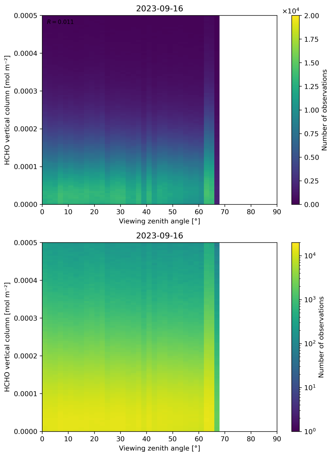
Figure 192: Scatter density plot of “Viewing zenith angle” against “HCHO vertical column” for 2023-09-15 to 2023-09-17.
