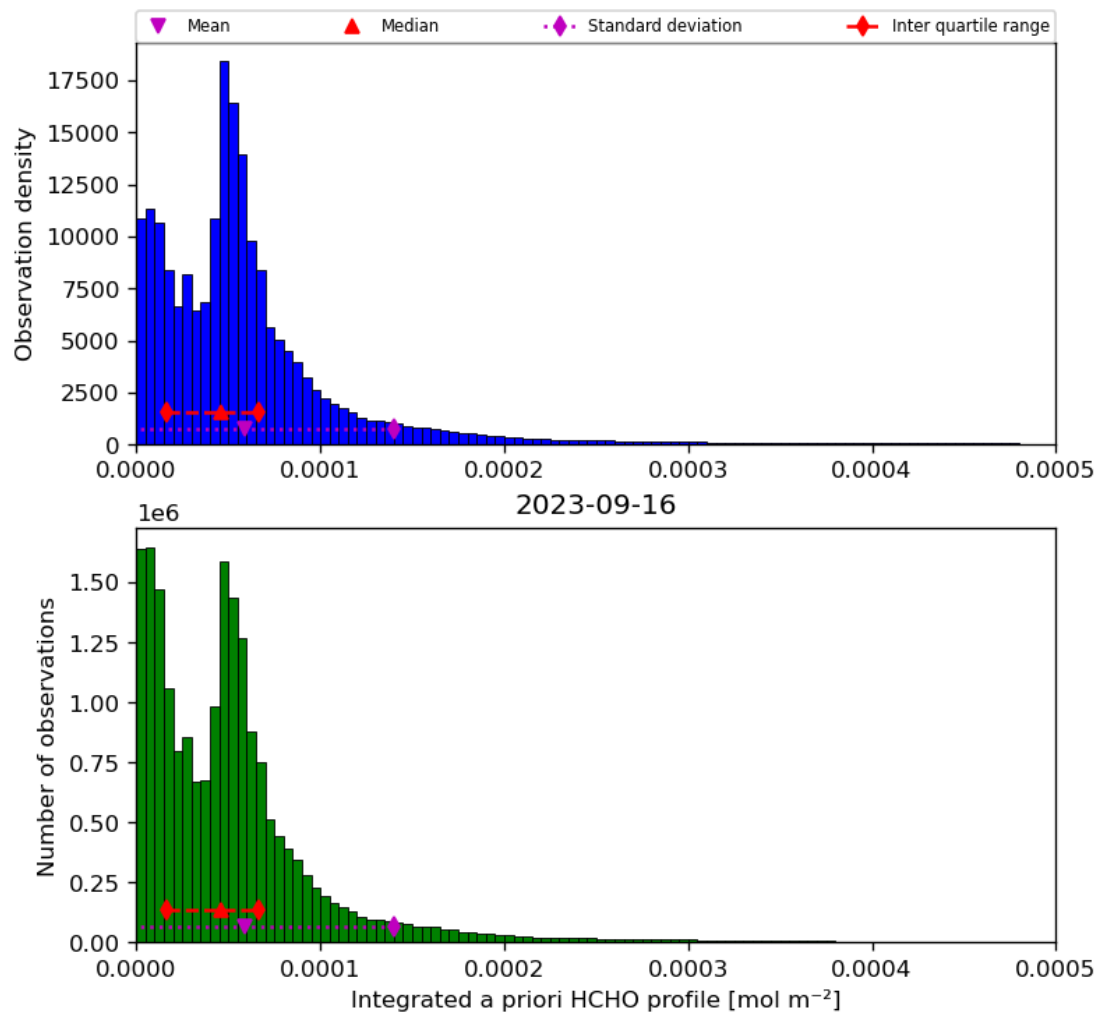
Figure 43: Histogram of “Integrated a priori HCHO profile” for 2023-09-15 to 2023-09-17
