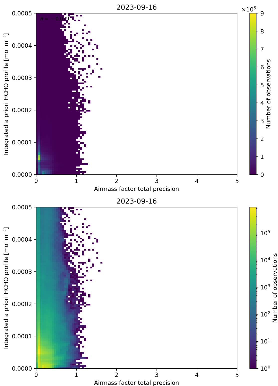
Figure 111: Scatter density plot of “Airmass factor total precision” against “Integrated a priori HCHO profile” for 2023-09-15 to 2023-09-17.
