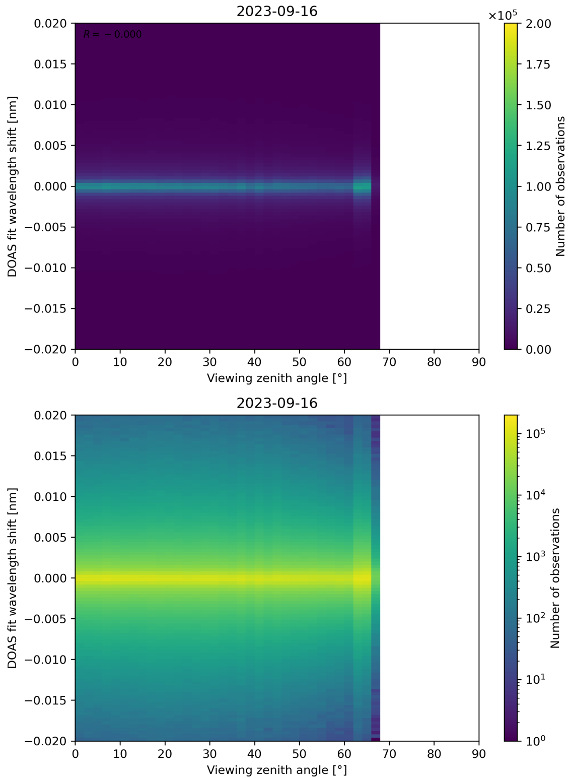
Figure 183: Scatter density plot of “Viewing zenith angle” against “DOAS fit wavelength shift” for 2023-09-15 to 2023-09-17.
