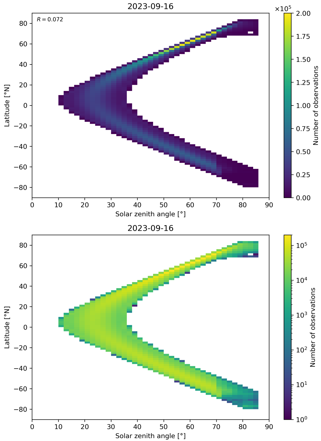
Figure 181: Scatter density plot of “Solar zenith angle” against “Latitude” for 2023-09-15 to 2023-09-17.
