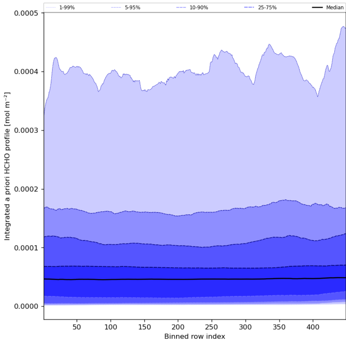
Figure 57: Along track statistics of “Integrated a priori HCHO profile” for 2023-09-15 to 2023-09-17
