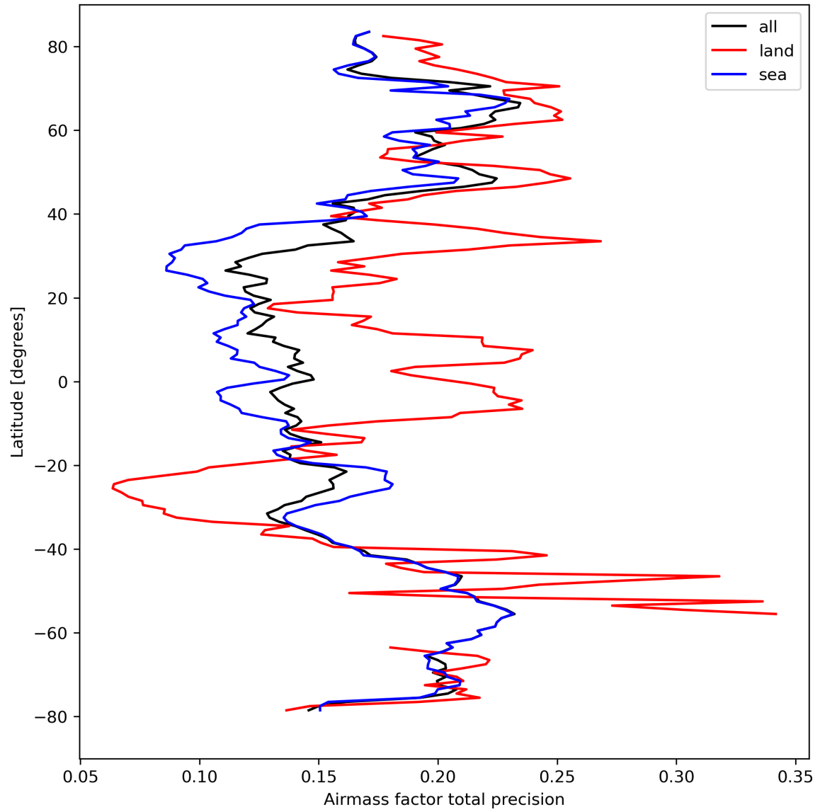
Figure 27: Zonal average of “Airmass factor total precision” for 2023-09-15 to 2023-09-17.
