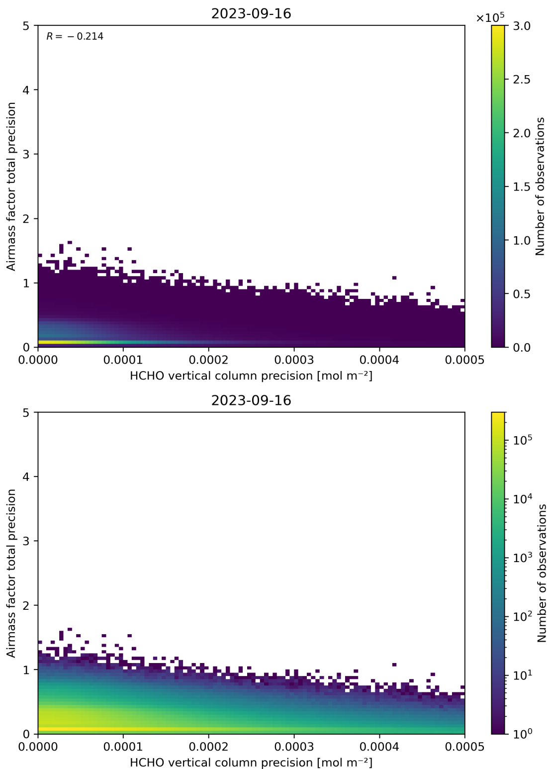
Figure 145: Scatter density plot of “HCHO vertical column precision” against “Airmass factor total precision” for 2023-09-15 to 2023-09-17.
