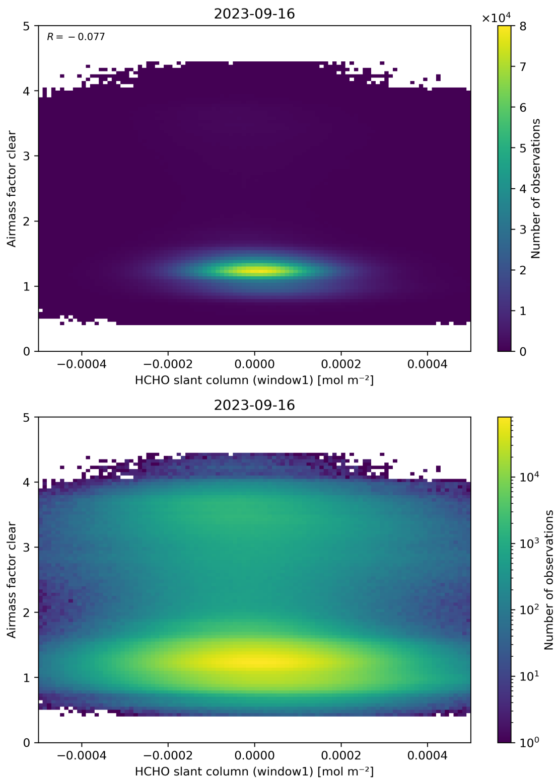
Figure 81: Scatter density plot of “HCHO slant column (window1)” against “Airmass factor clear” for 2023-09-15 to 2023-09-17.
