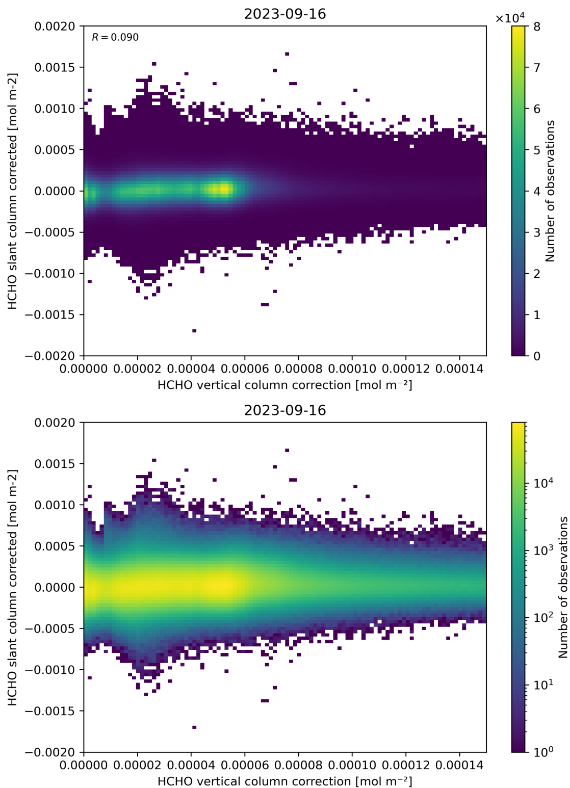
Figure 116: Scatter density plot of “HCHO vertical column correction” against “HCHO slant column corrected” for 2023-09-15 to 2023-09-17.
