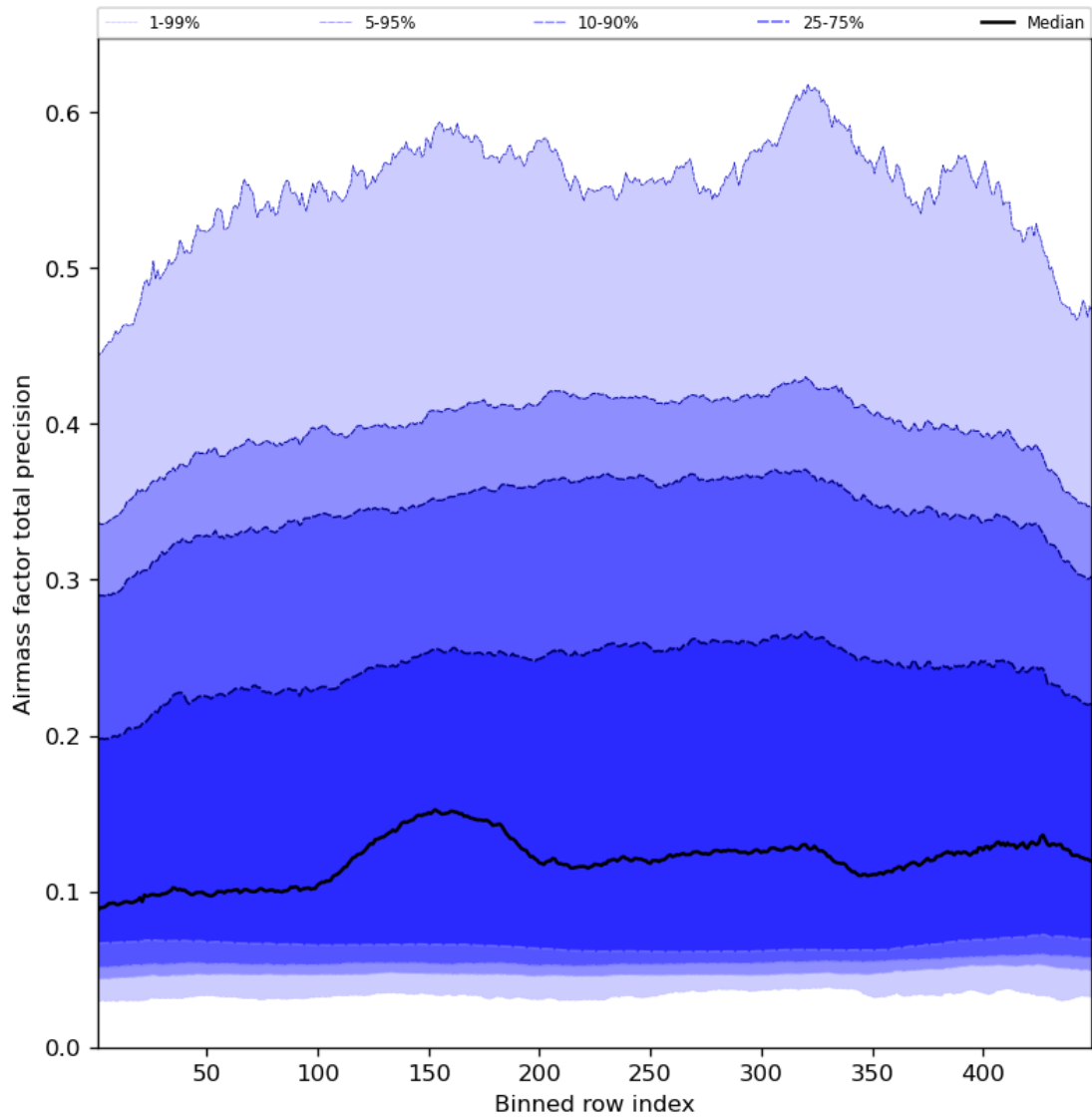
Figure 55: Along track statistics of “Airmass factor total precision” for 2023-09-15 to 2023-09-17
