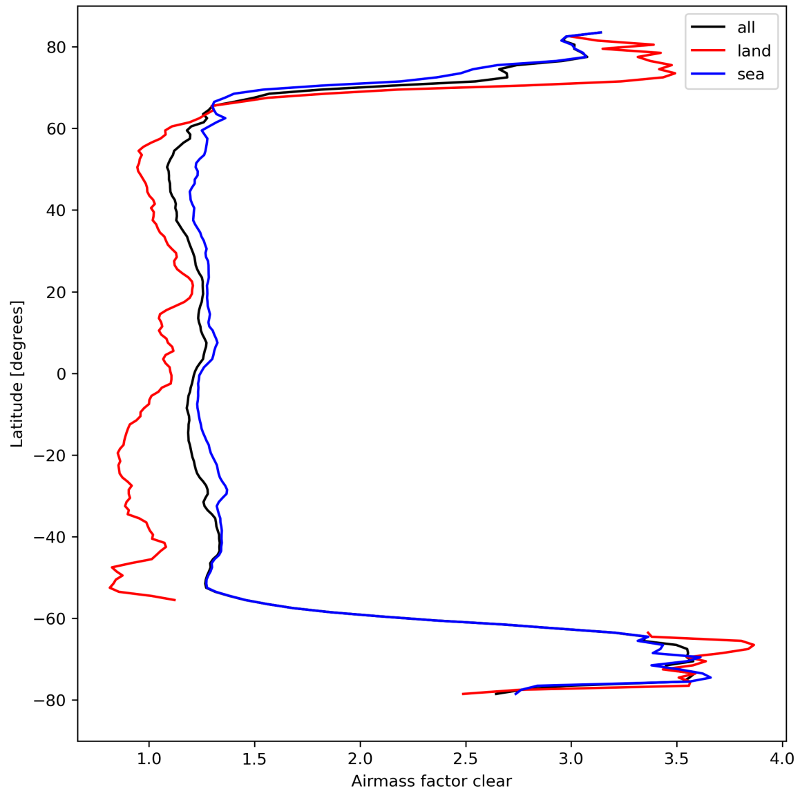
Figure 28: Zonal average of “Airmass factor clear” for 2023-09-15 to 2023-09-17.
