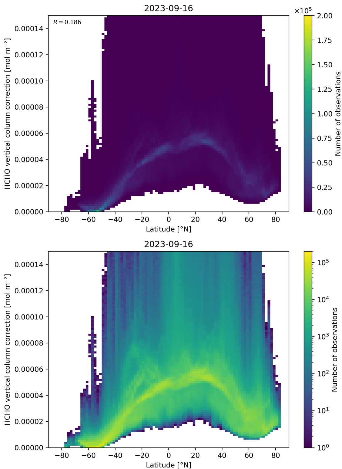
Figure 164: Scatter density plot of “Latitude” against “HCHO vertical column correction” for 2023-09-15 to 2023-09-17.
