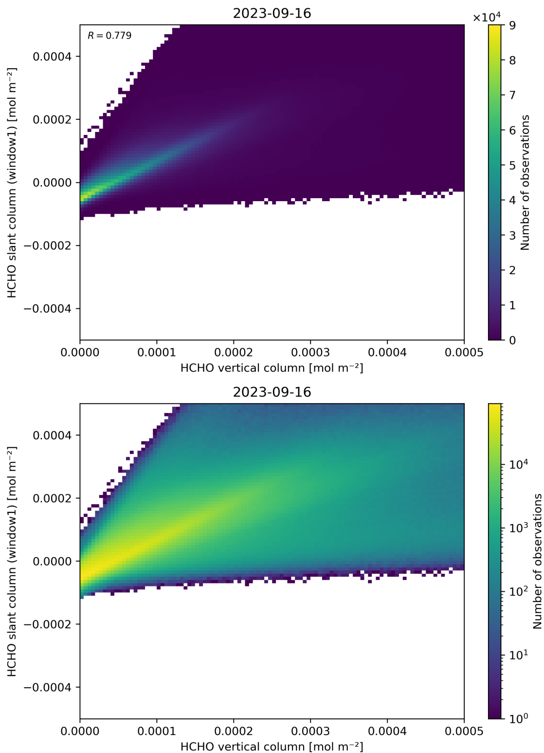
Figure 129: Scatter density plot of “HCHO vertical column” against “HCHO slant column (window1)” for 2023-09-15 to 2023-09-17.
