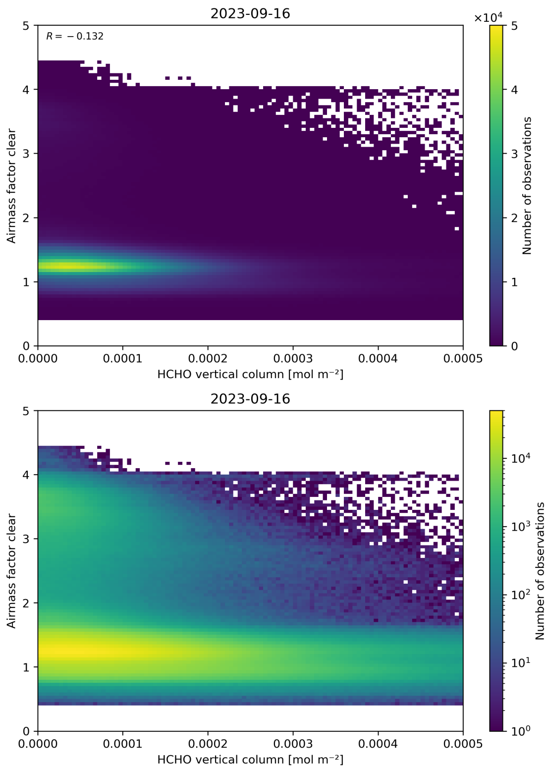
Figure 126: Scatter density plot of “HCHO vertical column” against “Airmass factor clear” for 2023-09-15 to 2023-09-17.
