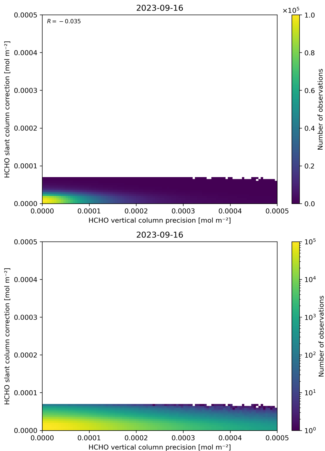
Figure 141: Scatter density plot of “HCHO vertical column precision” against “HCHO slant column correction” for 2023-09-15 to 2023-09-17.
