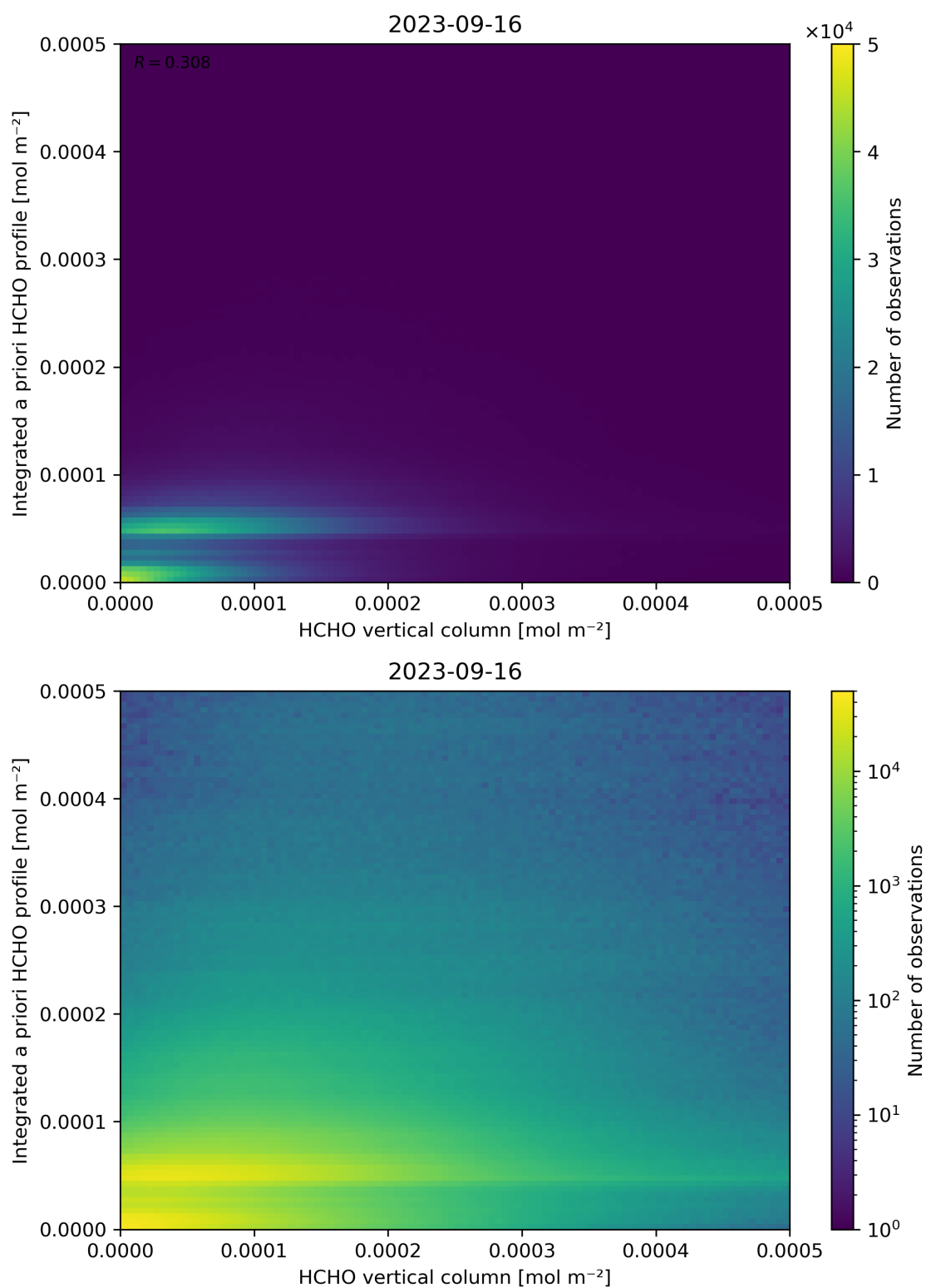
Figure 135: Scatter density plot of “HCHO vertical column” against “Integrated a priori HCHO profile” for 2023-09-15 to 2023-09-17.
