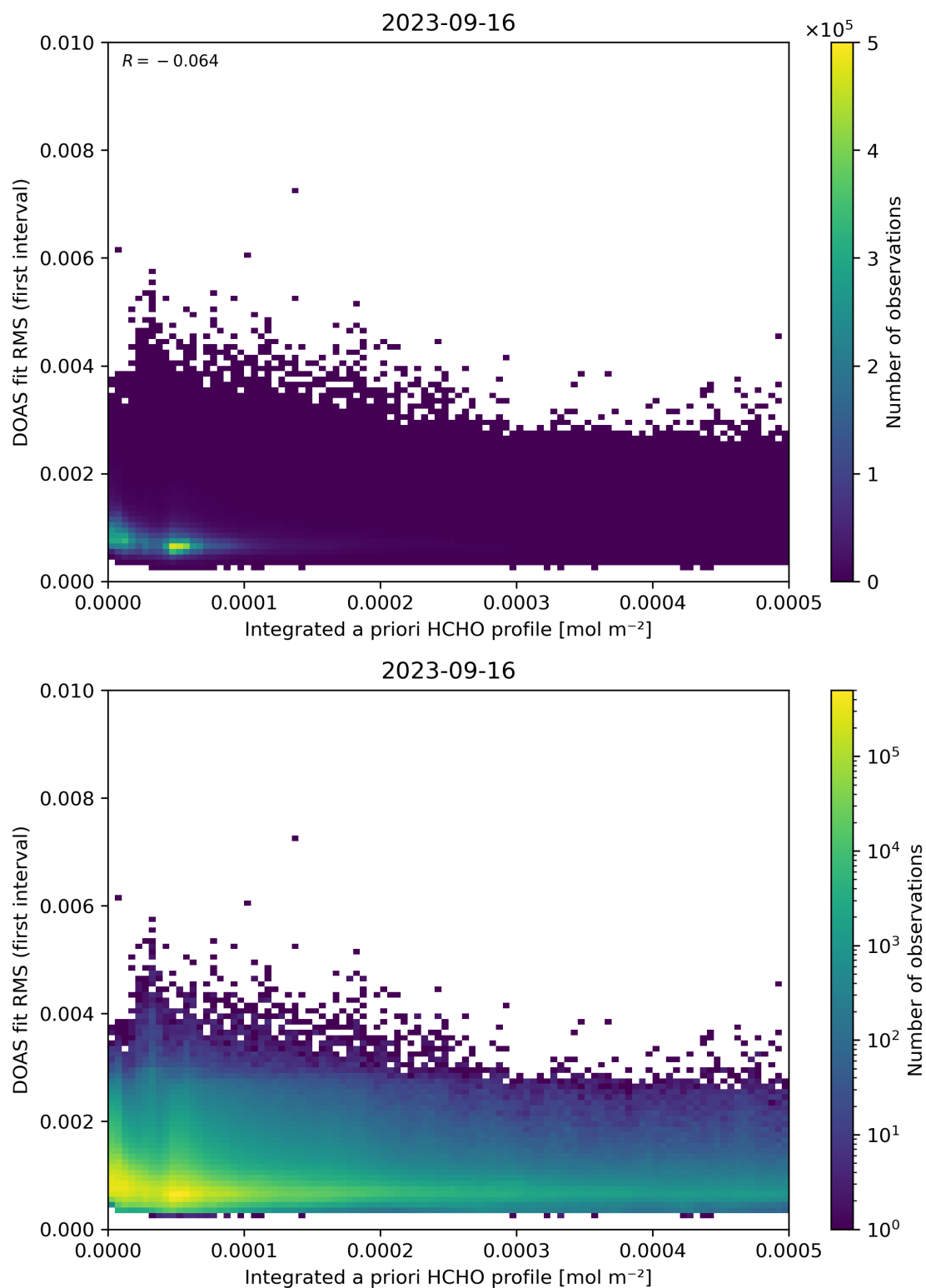
Figure 148: Scatter density plot of “Integrated a priori HCHO profile” against “DOAS fit RMS (first interval)” for 2023-09-15 to 2023-09-17.
