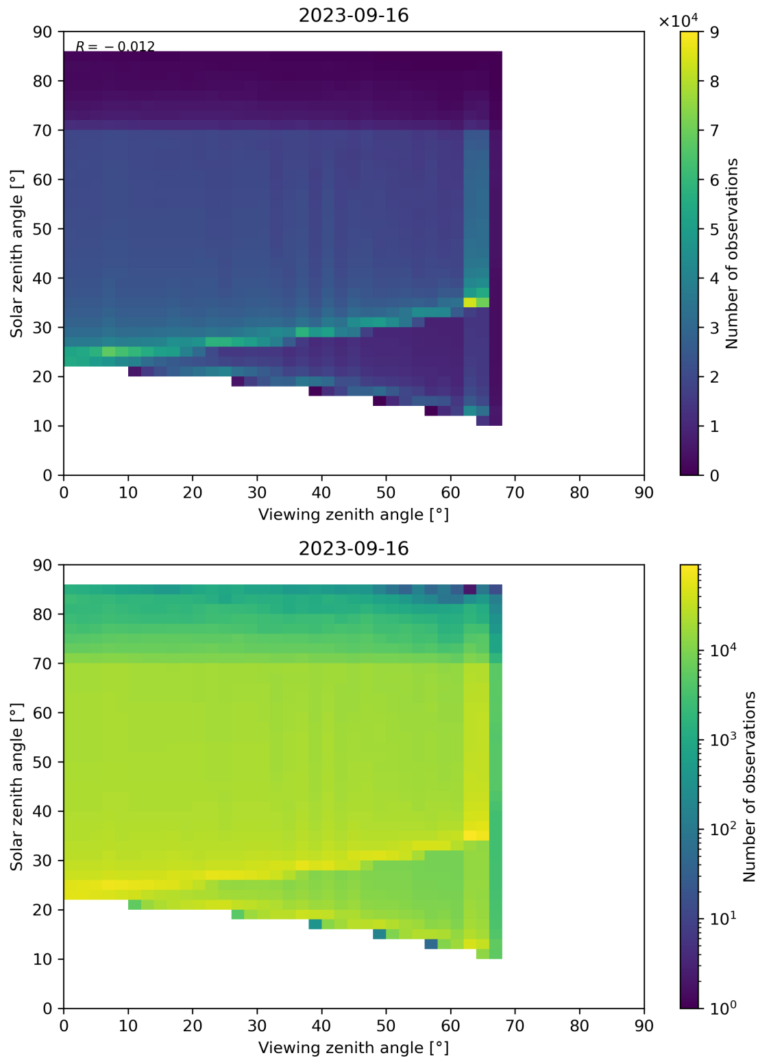
Figure 197: Scatter density plot of “Viewing zenith angle” against “Solar zenith angle” for 2023-09-15 to 2023-09-17.
