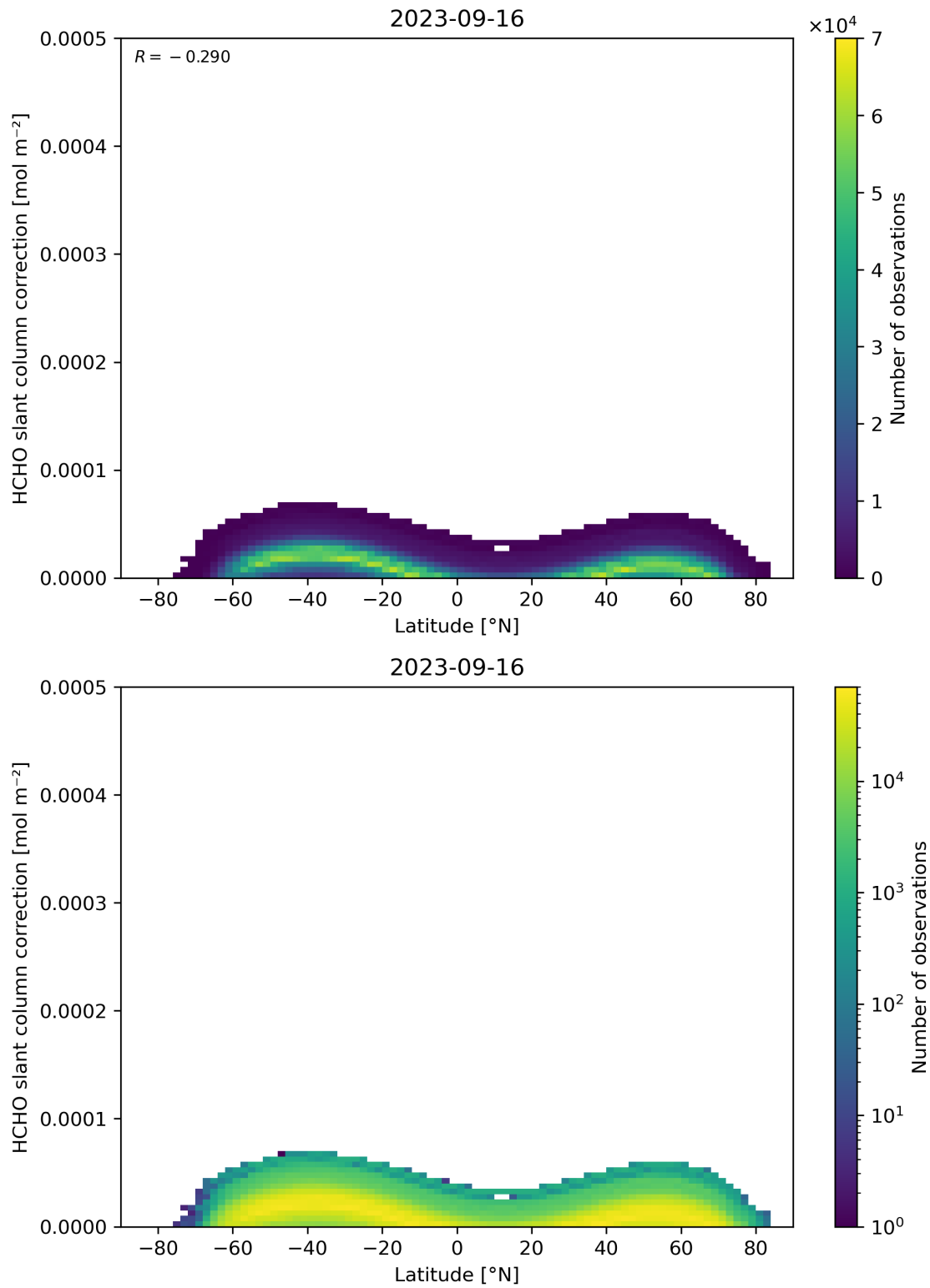
Figure 158: Scatter density plot of “Latitude” against “HCHO slant column correction” for 2023-09-15 to 2023-09-17.
