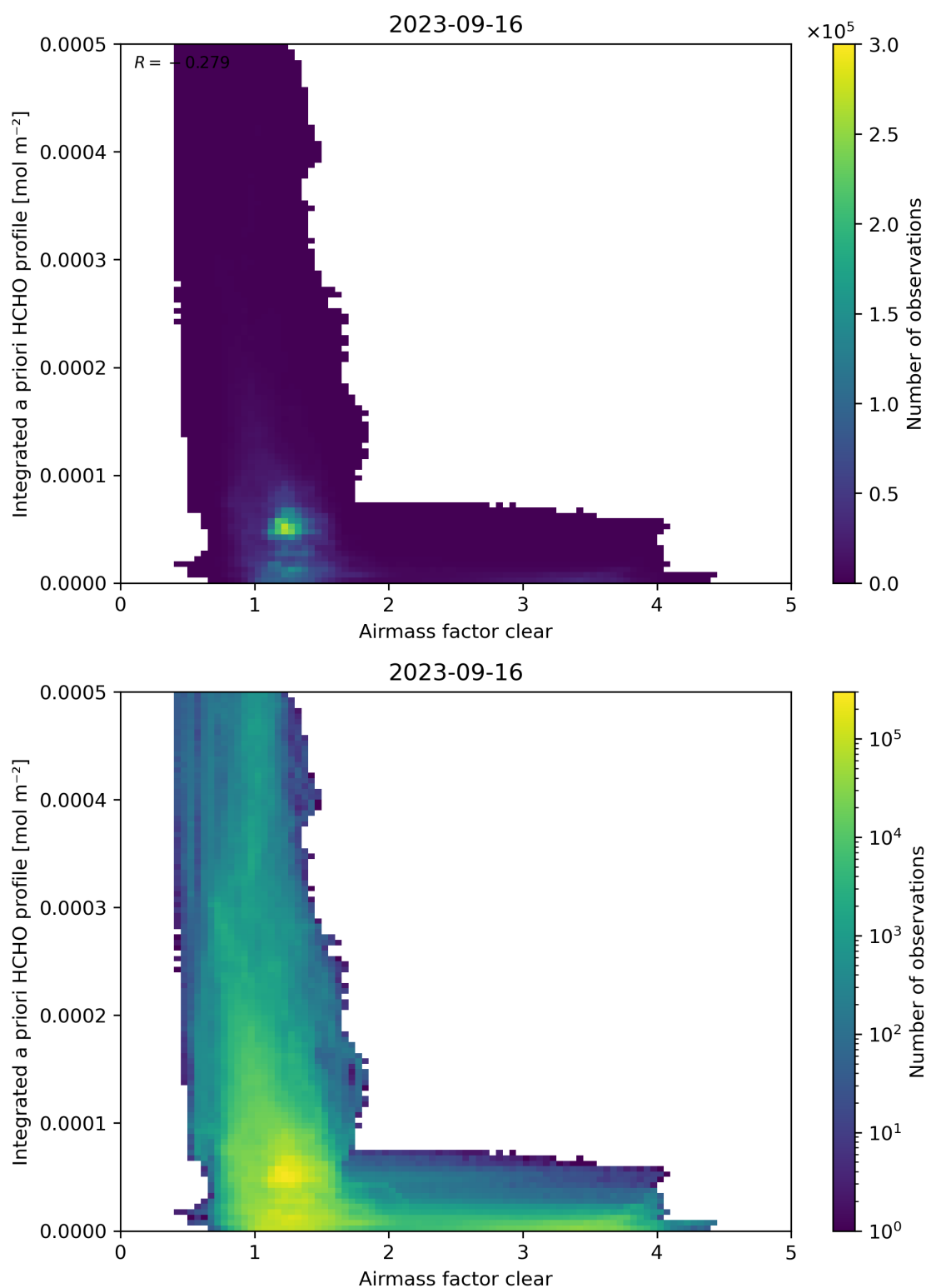
Figure 76: Scatter density plot of “Airmass factor clear” against “Integrated a priori HCHO profile” for 2023-09-15 to 2023-09-17.
