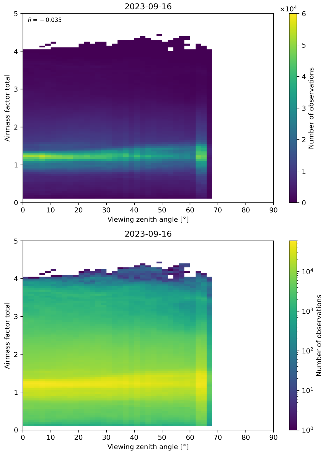
Figure 190: Scatter density plot of “Viewing zenith angle” against “Airmass factor total” for 2023-09-15 to 2023-09-17.
