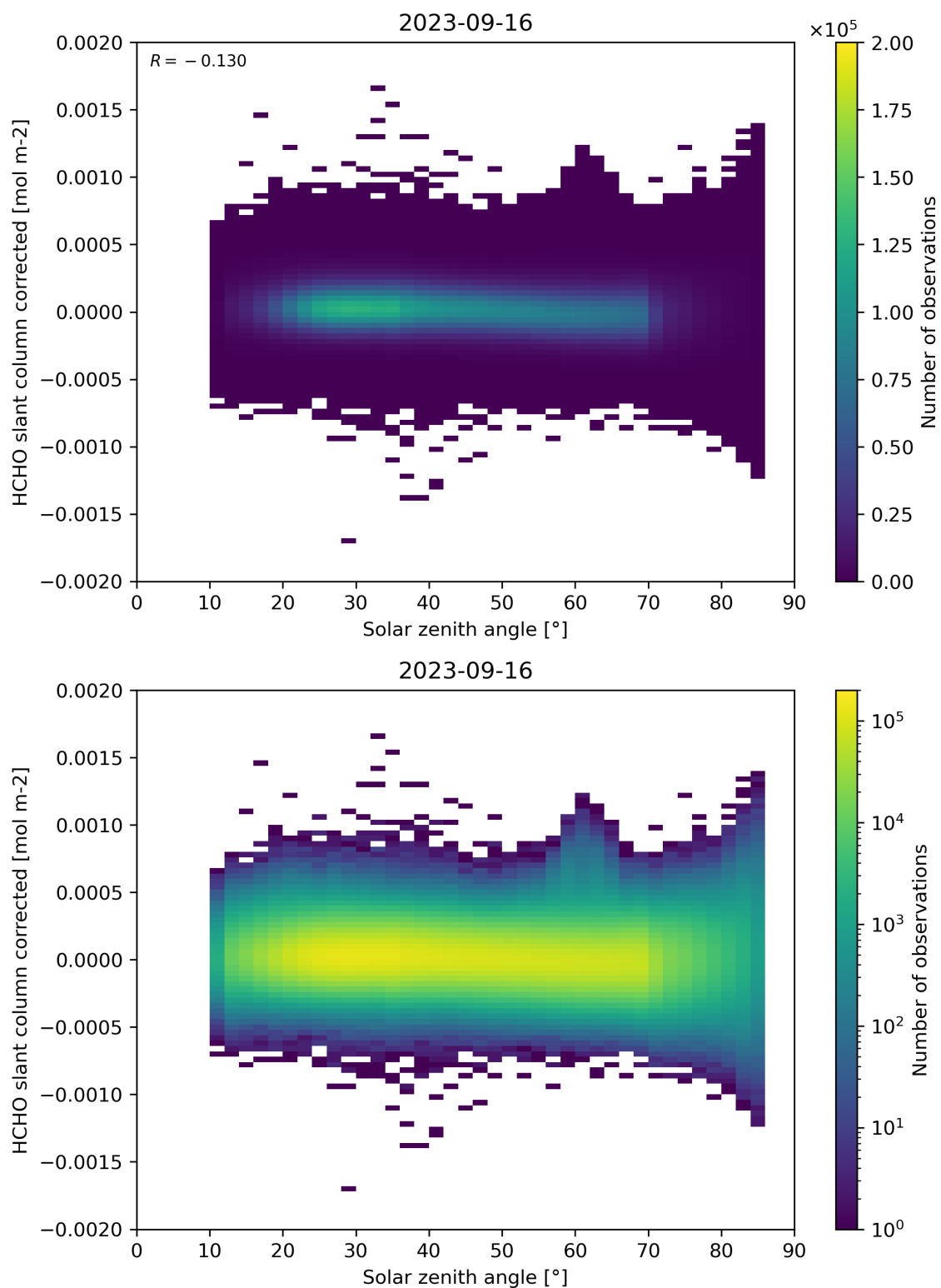
Figure 171: Scatter density plot of “Solar zenith angle” against “HCHO slant column corrected” for 2023-09-15 to 2023-09-17.
