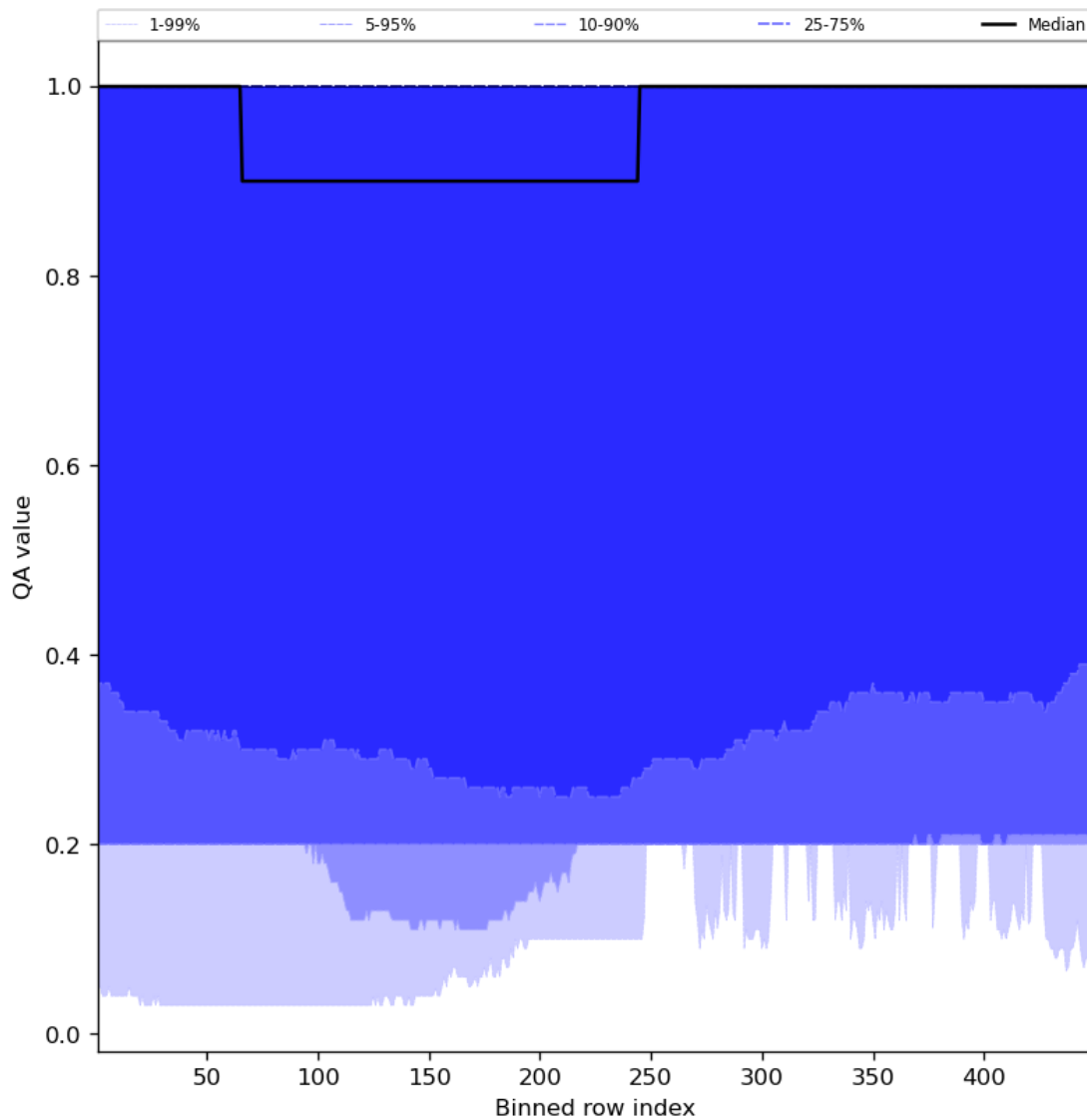
Figure 48: Along track statistics of “QA value” for 2023-09-15 to 2023-09-17
