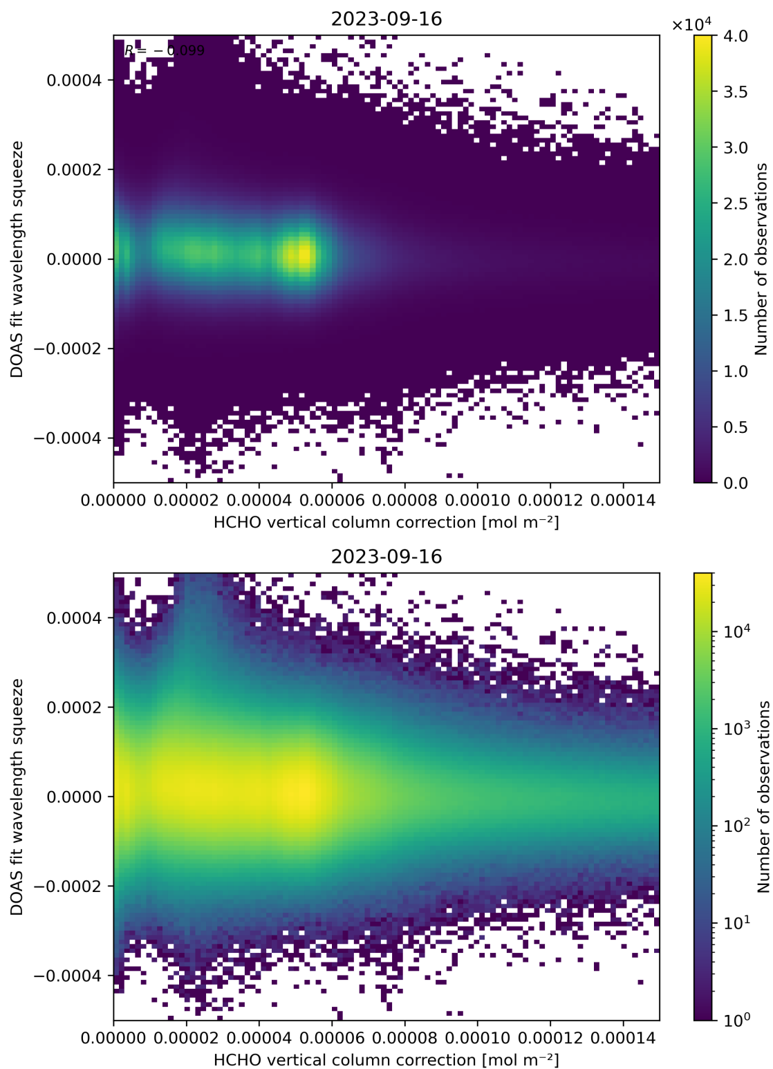
Figure 114: Scatter density plot of “HCHO vertical column correction” against “DOAS fit wavelength squeeze” for 2023-09-15 to 2023-09-17.
