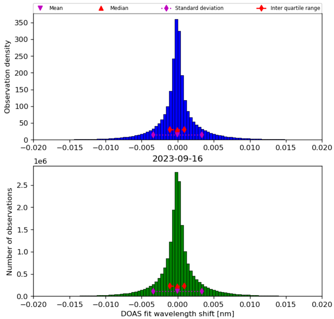
Figure 44: Histogram of “DOAS fit wavelength shift” for 2023-09-15 to 2023-09-17
