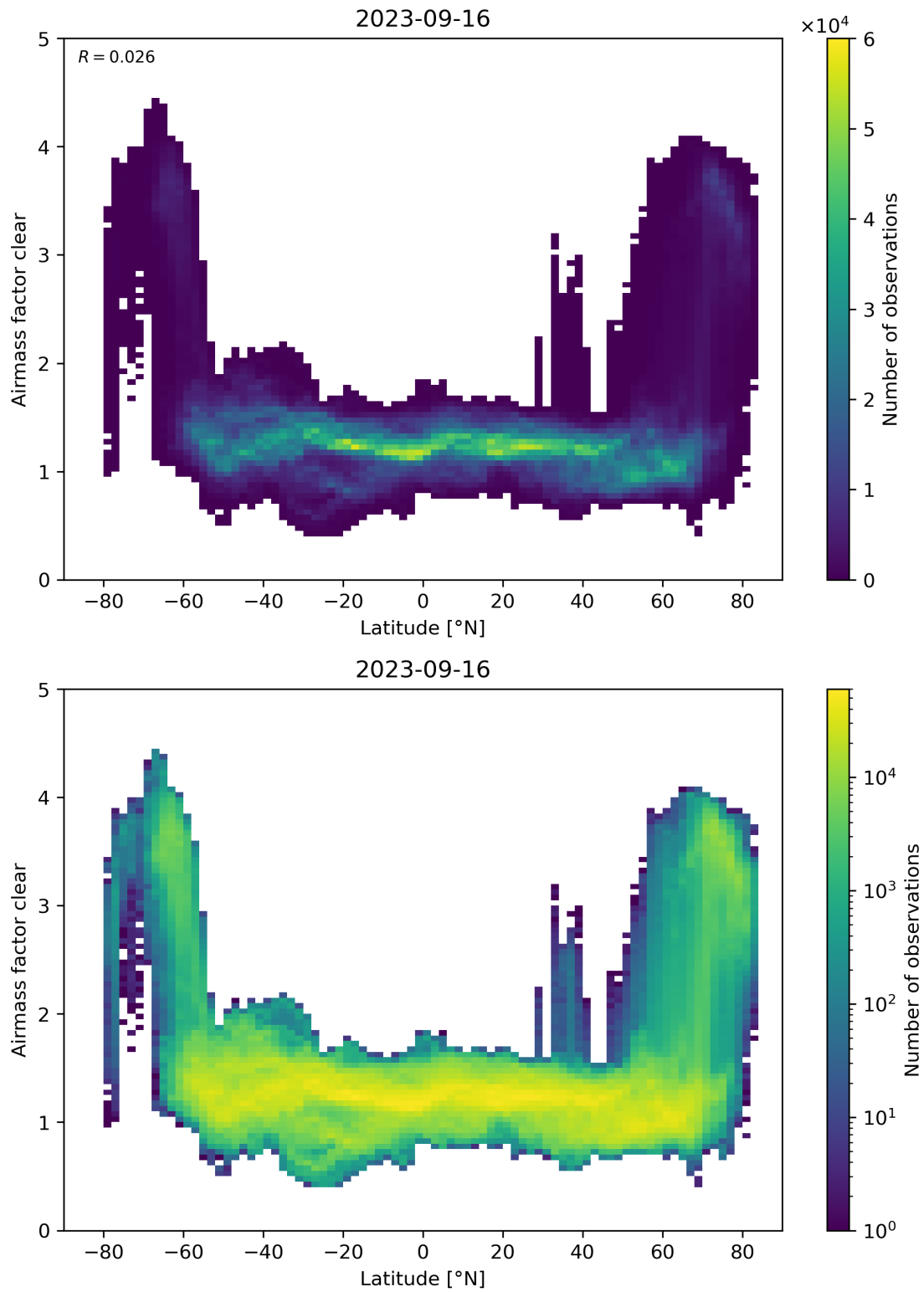
Figure 156: Scatter density plot of “Latitude” against “Airmass factor clear” for 2023-09-15 to 2023-09-17.
