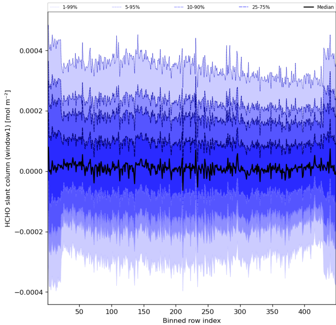
Figure 52: Along track statistics of “HCHO slant column (window1)” for 2023-09-15 to 2023-09-17
