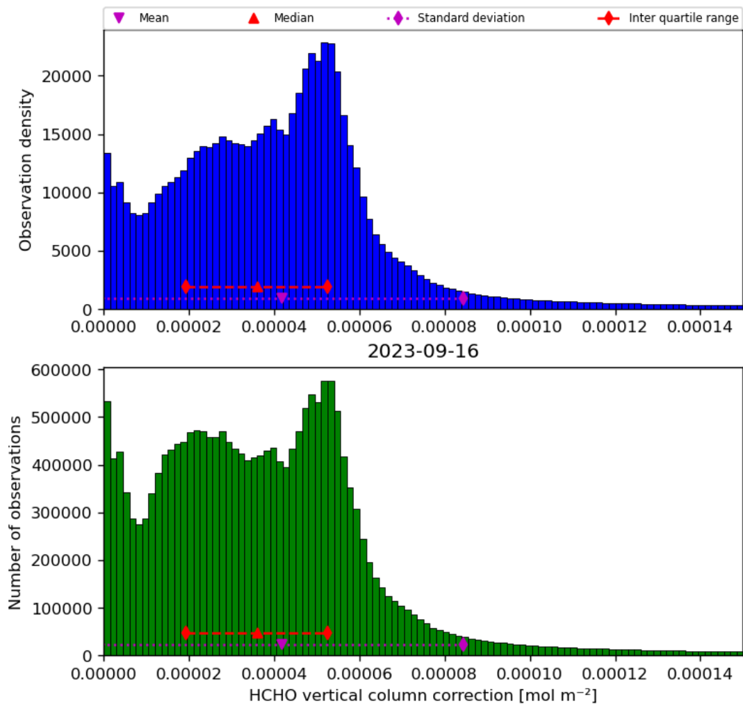
Figure 37: Histogram of “HCHO vertical column correction” for 2023-09-15 to 2023-09-17
