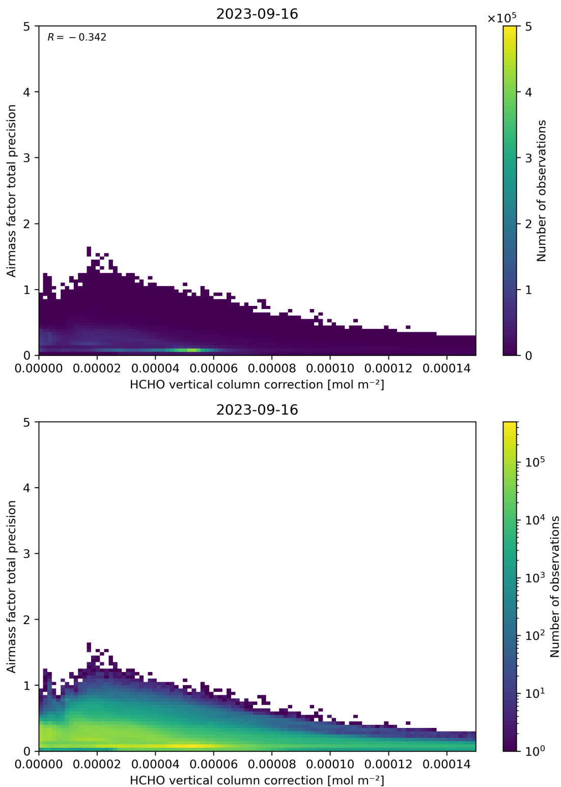
Figure 121: Scatter density plot of “HCHO vertical column correction” against “Airmass factor total precision” for 2023-09-15 to 2023-09-17.
