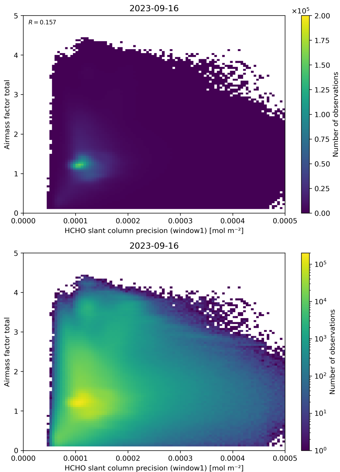
Figure 94: Scatter density plot of “HCHO slant column precision (window1)” against “Airmass factor total” for 2023-09-15 to 2023-09-17.
