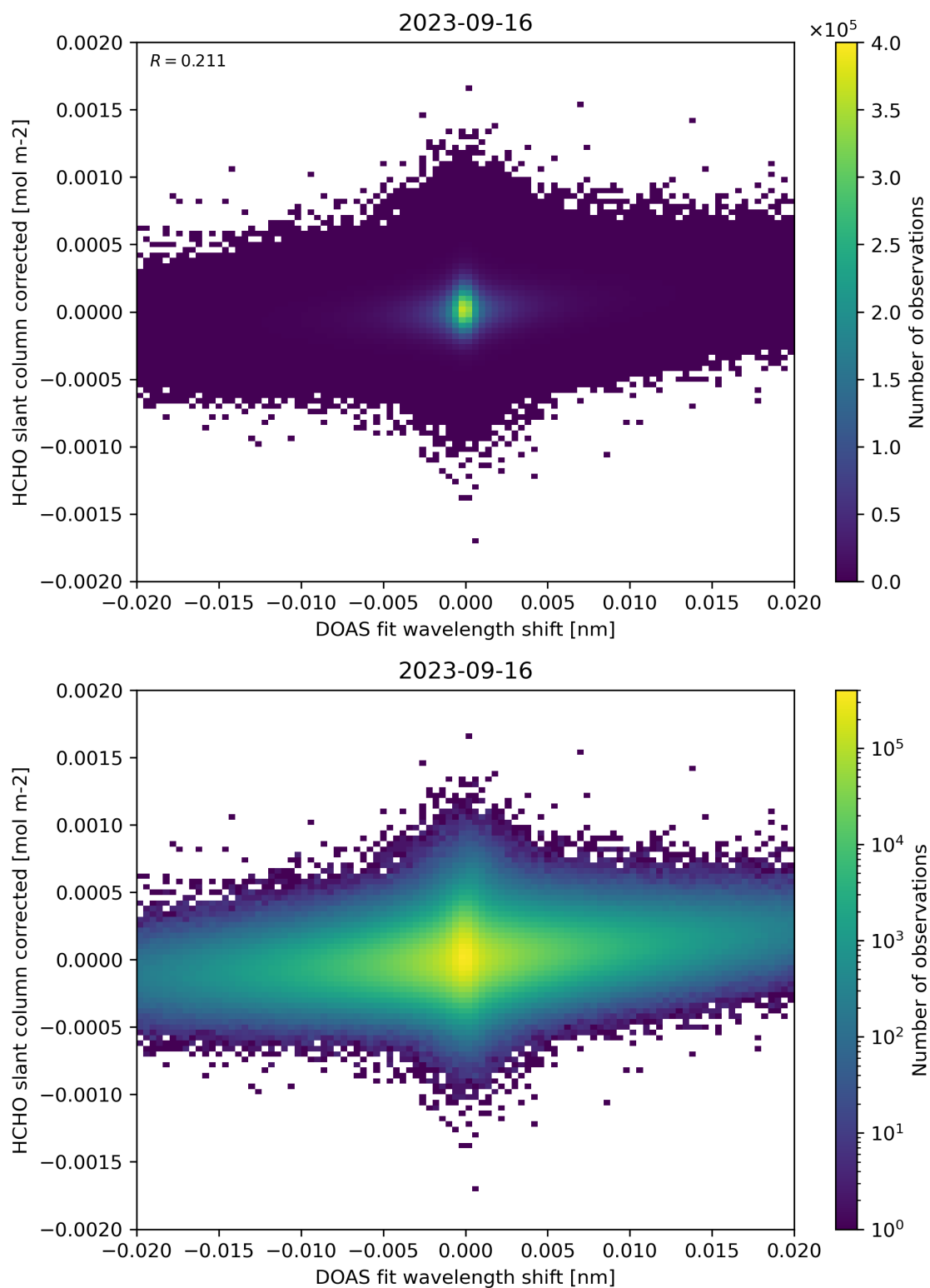
Figure 66: Scatter density plot of “DOAS fit wavelength shift” against “HCHO slant column corrected” for 2023-09-15 to 2023-09-17.
