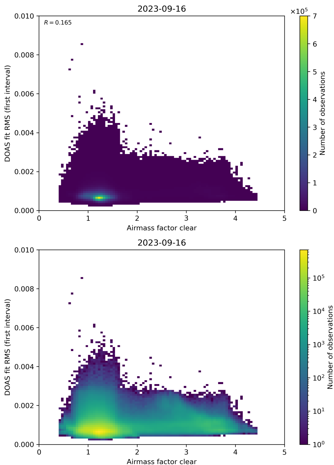
Figure 71: Scatter density plot of “Airmass factor clear” against “DOAS fit RMS (first interval)” for 2023-09-15 to 2023-09-17.
