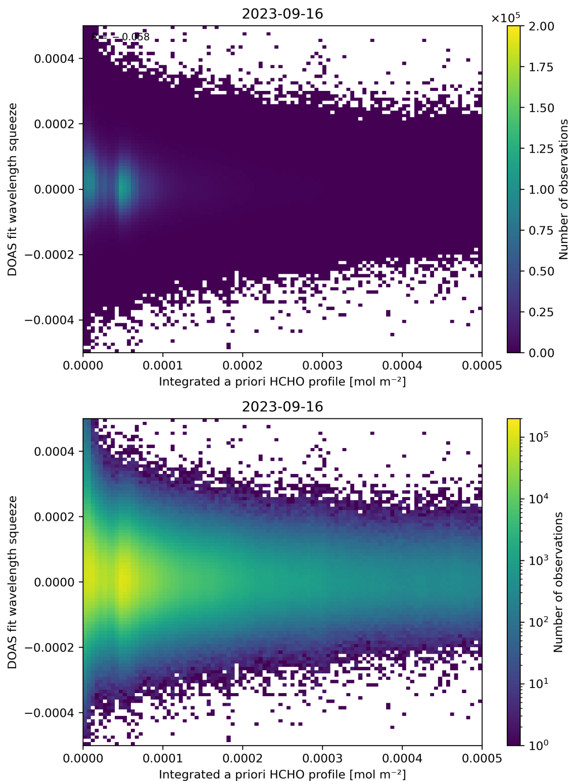
Figure 150: Scatter density plot of “Integrated a priori HCHO profile” against “DOAS fit wavelength squeeze” for 2023-09-15 to 2023-09-17.
