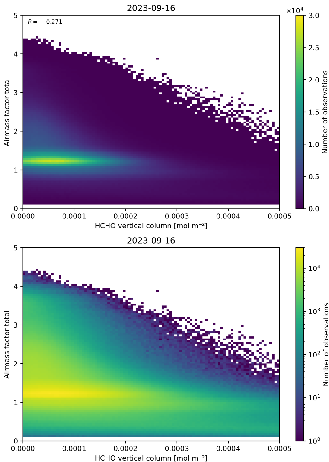
Figure 131: Scatter density plot of “HCHO vertical column” against “Airmass factor total” for 2023-09-15 to 2023-09-17.
