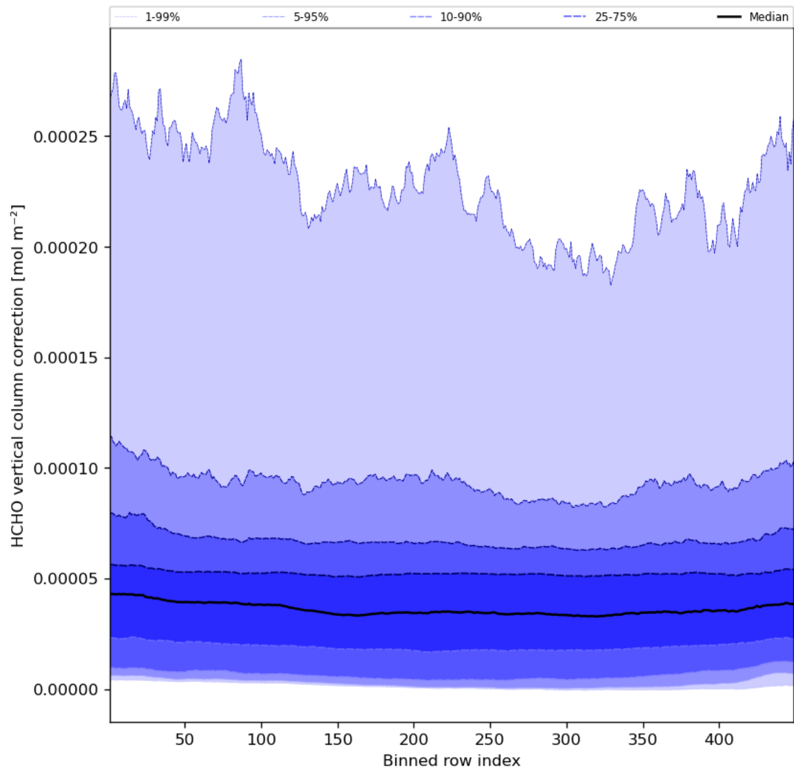
Figure 51: Along track statistics of “HCHO vertical column correction” for 2023-09-15 to 2023-09-17
