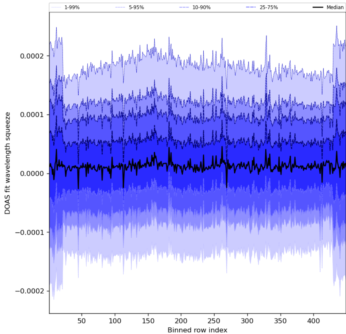
Figure 59: Along track statistics of “DOAS fit wavelength squeeze” for 2023-09-15 to 2023-09-17
