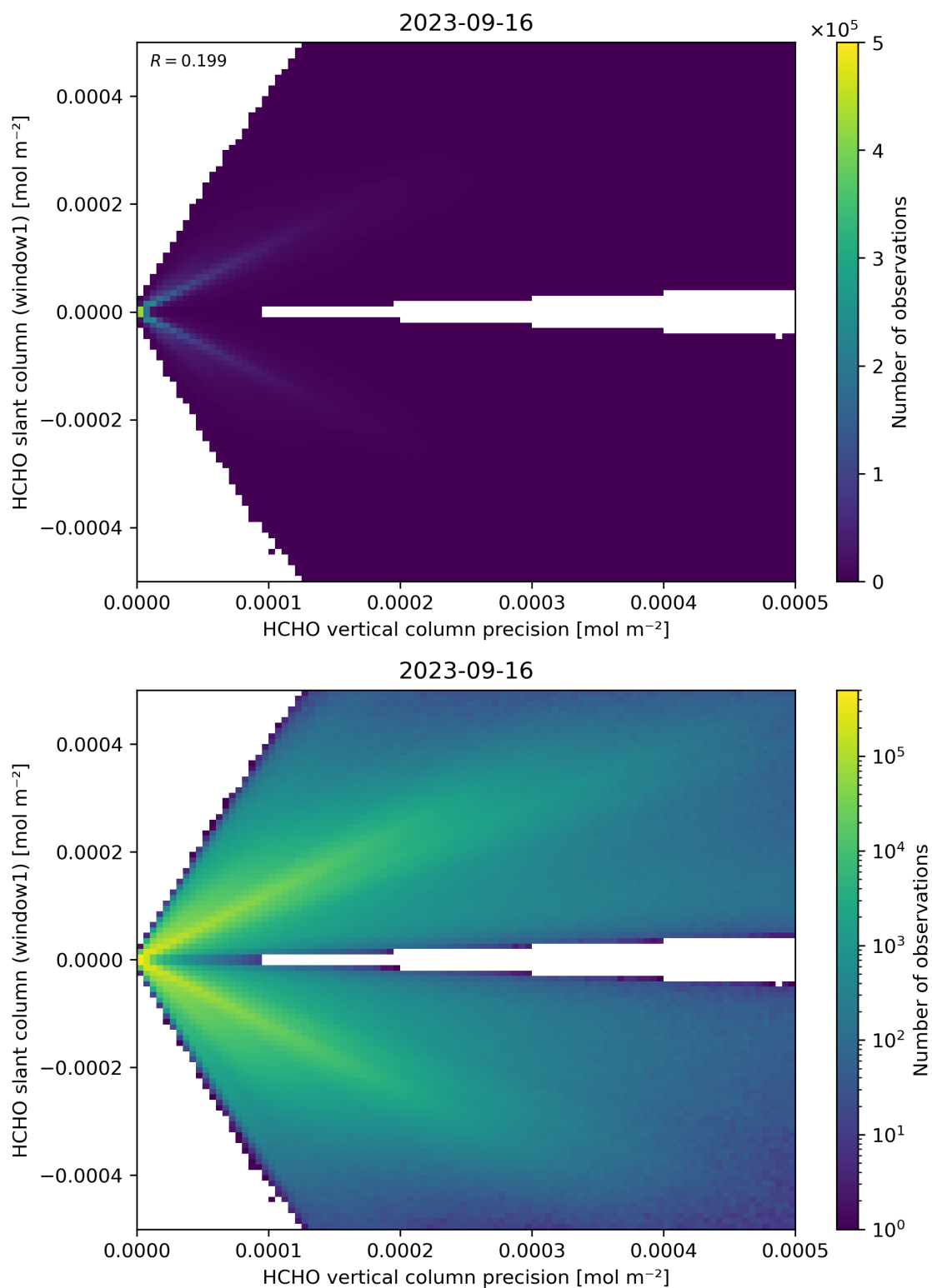
Figure 142: Scatter density plot of “HCHO vertical column precision” against “HCHO slant column (window1)” for 2023-09-15 to 2023-09-17.
