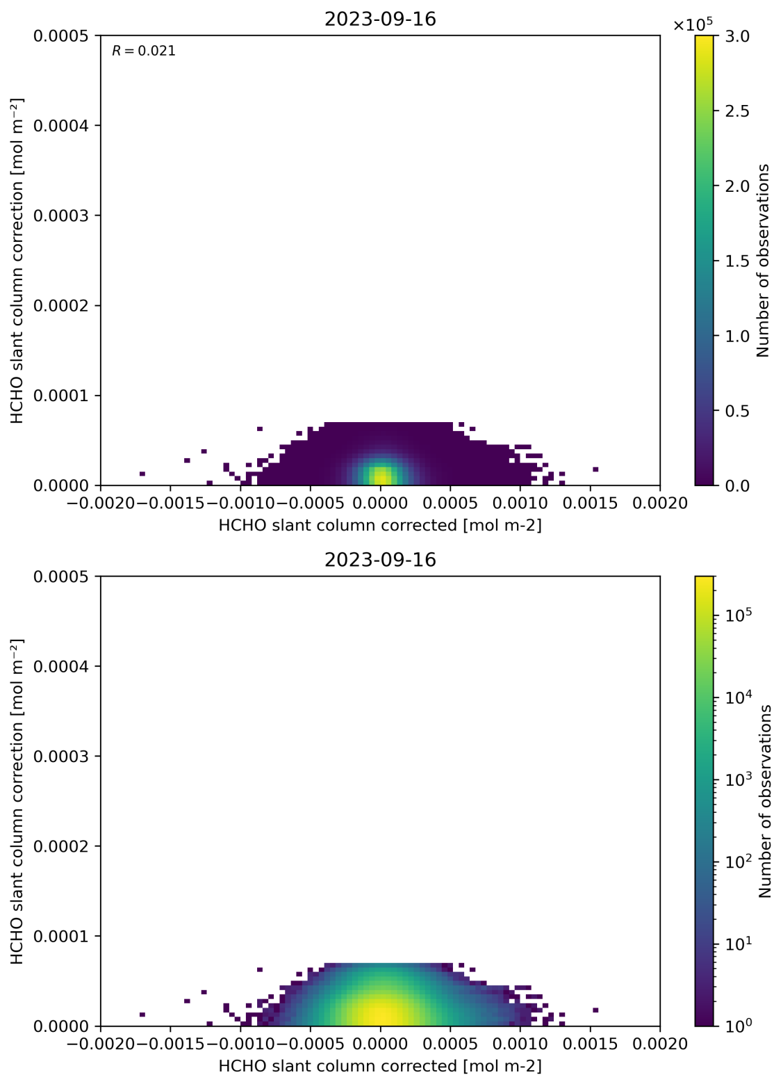
Figure 77: Scatter density plot of “HCHO slant column corrected” against “HCHO slant column correction” for 2023-09-15 to 2023-09-17.
