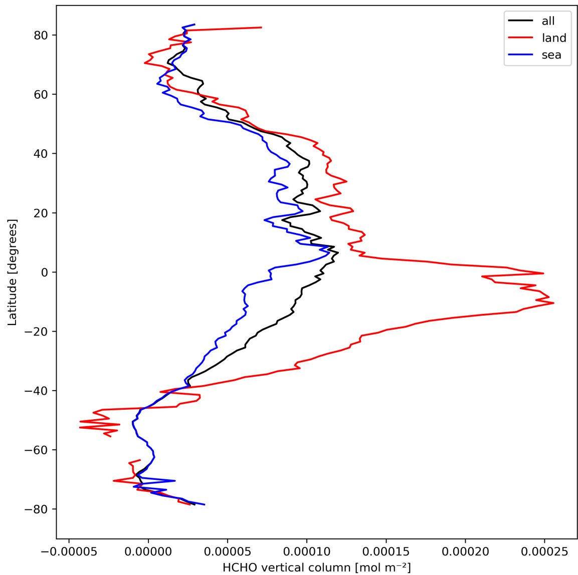
Figure 21: Zonal average of “HCHO vertical column” for 2023-09-15 to 2023-09-17.
