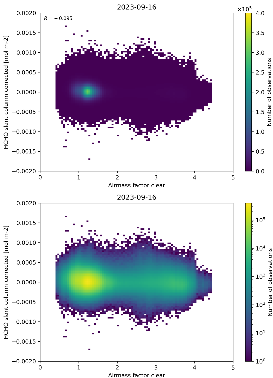
Figure 74: Scatter density plot of “Airmass factor clear” against “HCHO slant column corrected” for 2023-09-15 to 2023-09-17.
