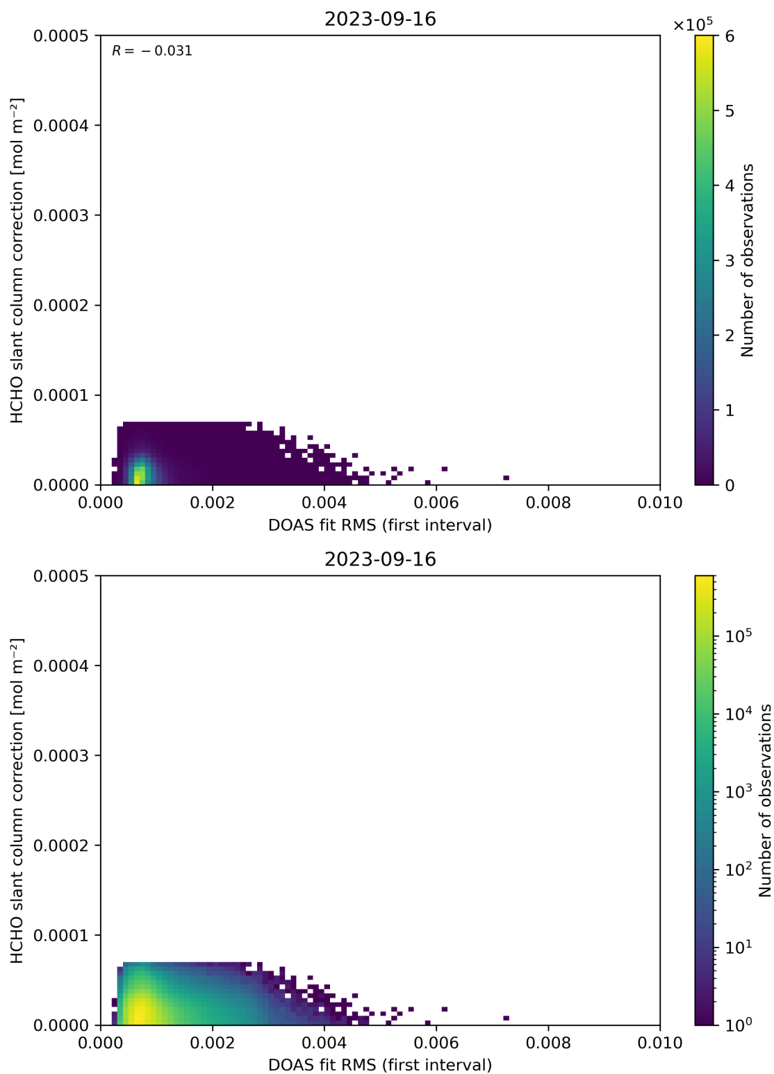
Figure 63: Scatter density plot of “DOAS fit RMS (first interval)” against “HCHO slant column correction” for 2023-09-15 to 2023-09-17.
