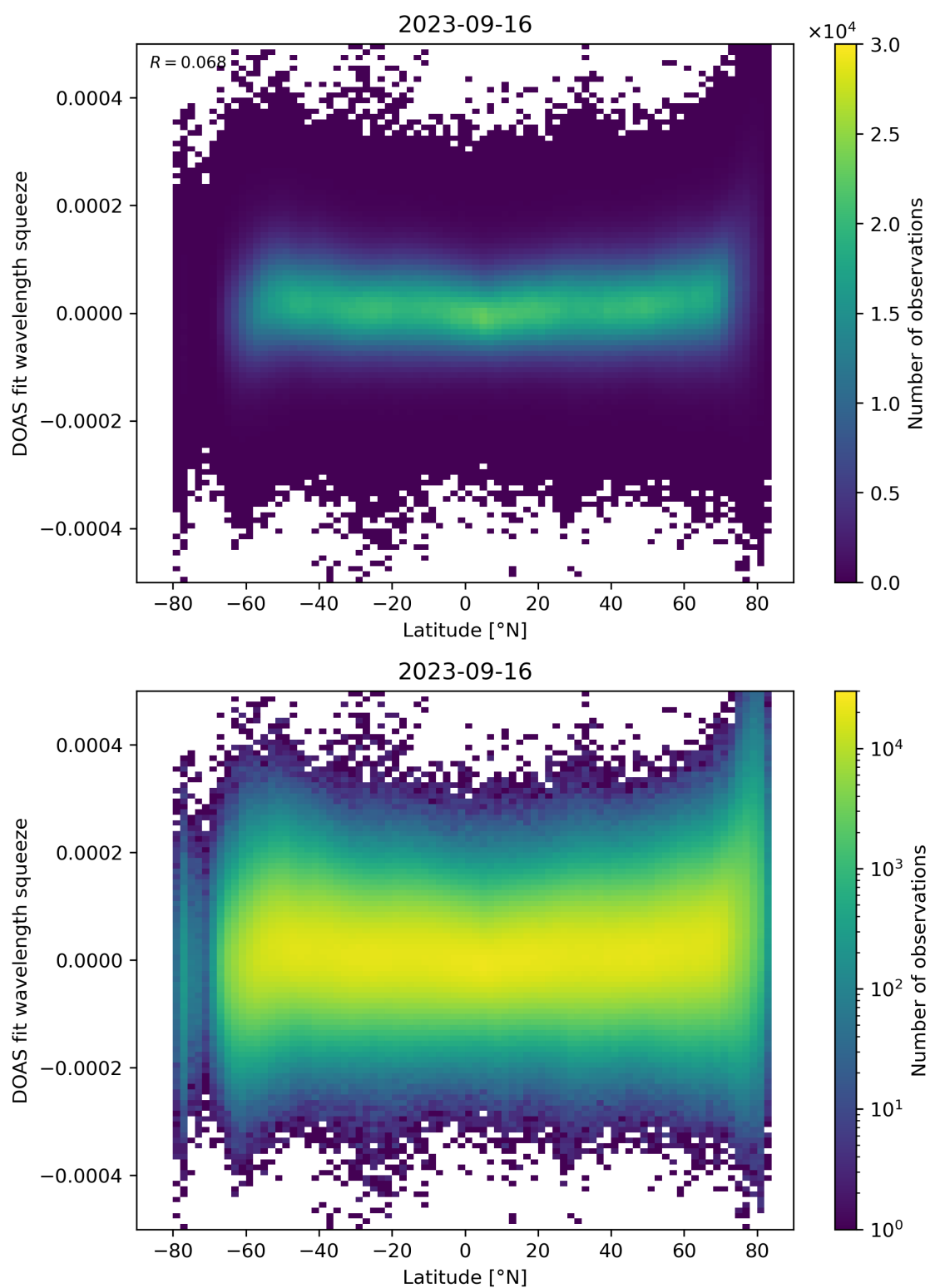
Figure 155: Scatter density plot of “Latitude” against “DOAS fit wavelength squeeze” for 2023-09-15 to 2023-09-17.
