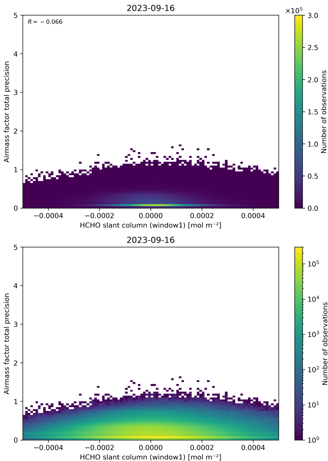
Figure 86: Scatter density plot of “HCHO slant column (window1)” against “Airmass factor total precision” for 2023-09-15 to 2023-09-17.
