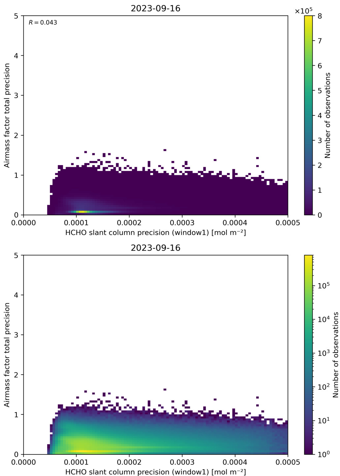
Figure 95: Scatter density plot of “HCHO slant column precision (window1)” against “Airmass factor total precision” for 2023-09-15 to 2023-09-17.
