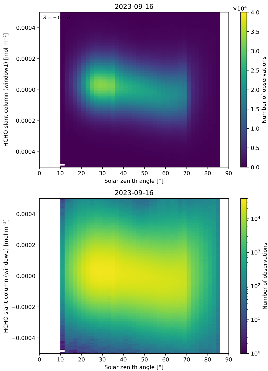
Figure 173: Scatter density plot of “Solar zenith angle” against “HCHO slant column (window1)” for 2023-09-15 to 2023-09-17.
