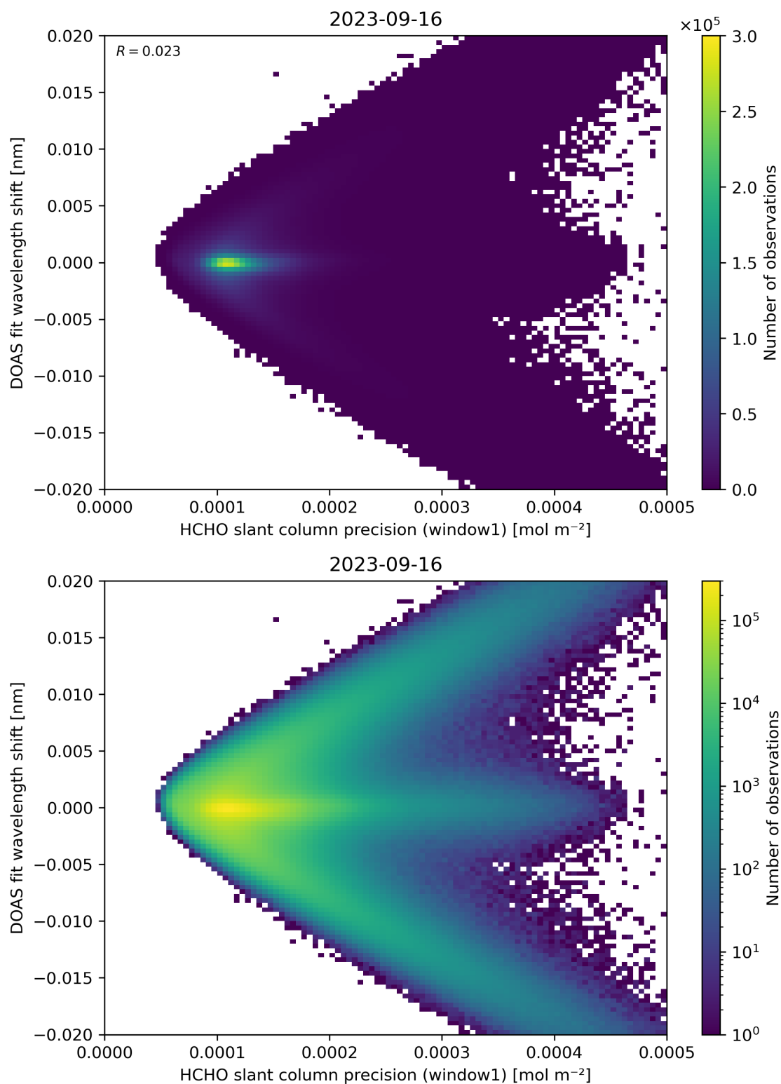
Figure 89: Scatter density plot of “HCHO slant column precision (window1)” against “DOAS fit wavelength shift” for 2023-09-15 to 2023-09-17.
