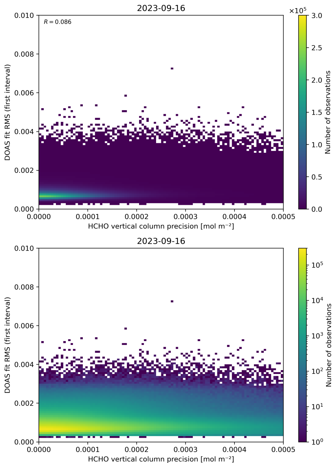
Figure 136: Scatter density plot of “HCHO vertical column precision” against “DOAS fit RMS (first interval)” for 2023-09-15 to 2023-09-17.
