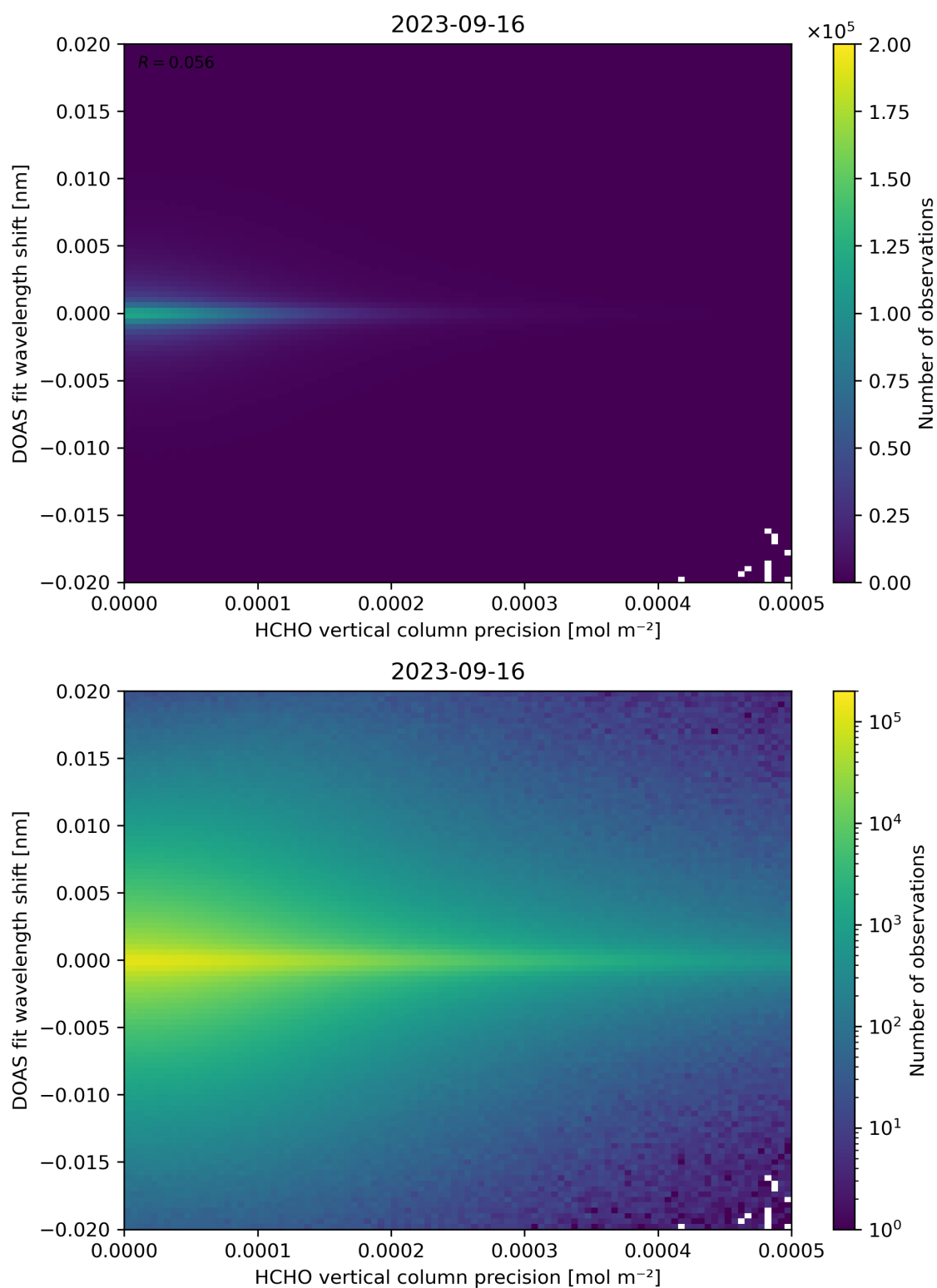
Figure 137: Scatter density plot of “HCHO vertical column precision” against “DOAS fit wavelength shift” for 2023-09-15 to 2023-09-17.
