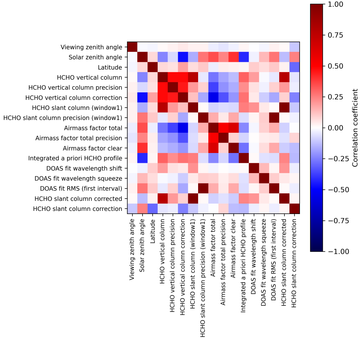
Figure 2: Map of correlation matrix for 2023-09-15 to 2023-09-17.
