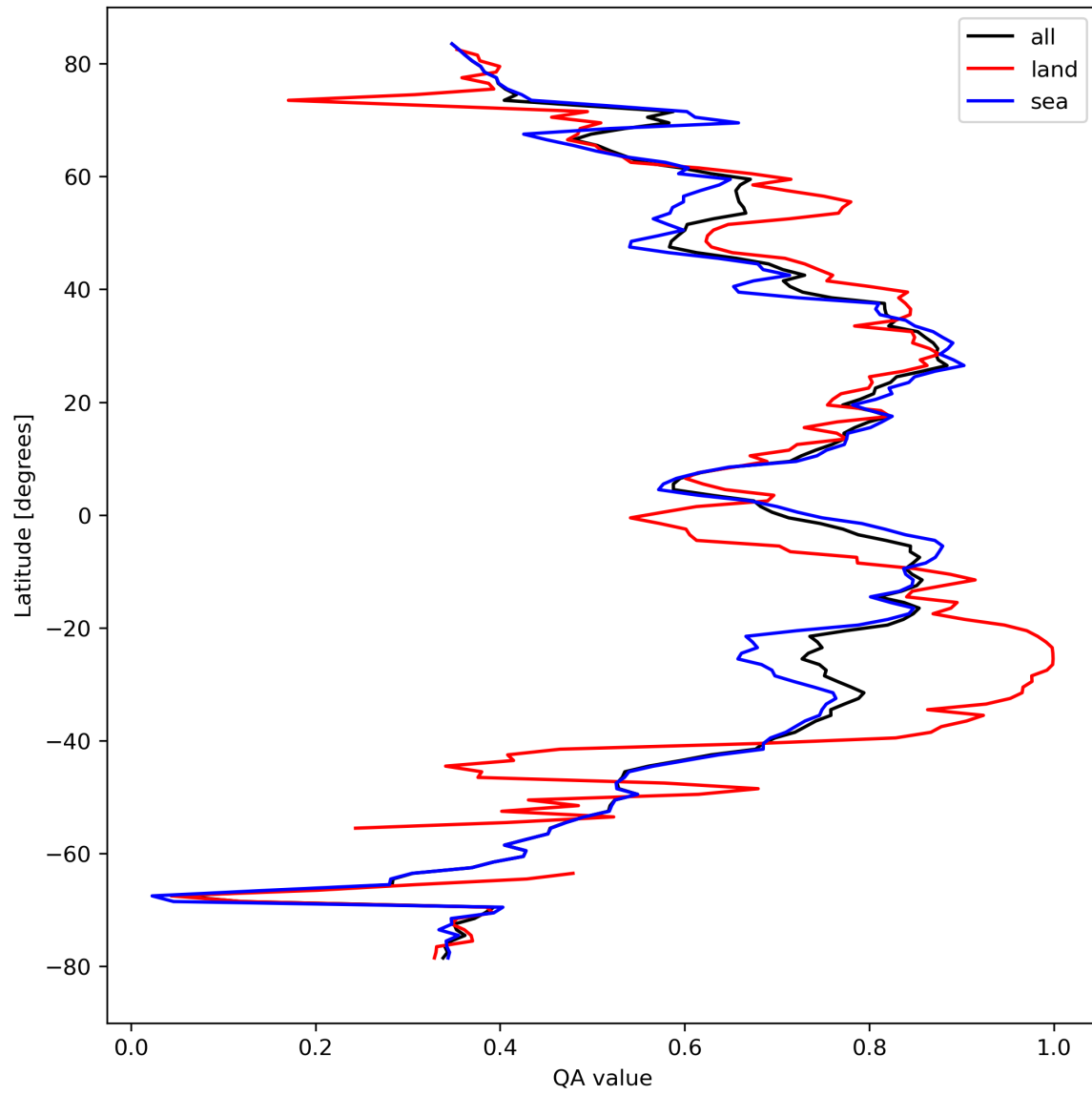
Figure 20: Zonal average of “QA value” for 2023-09-15 to 2023-09-17.
