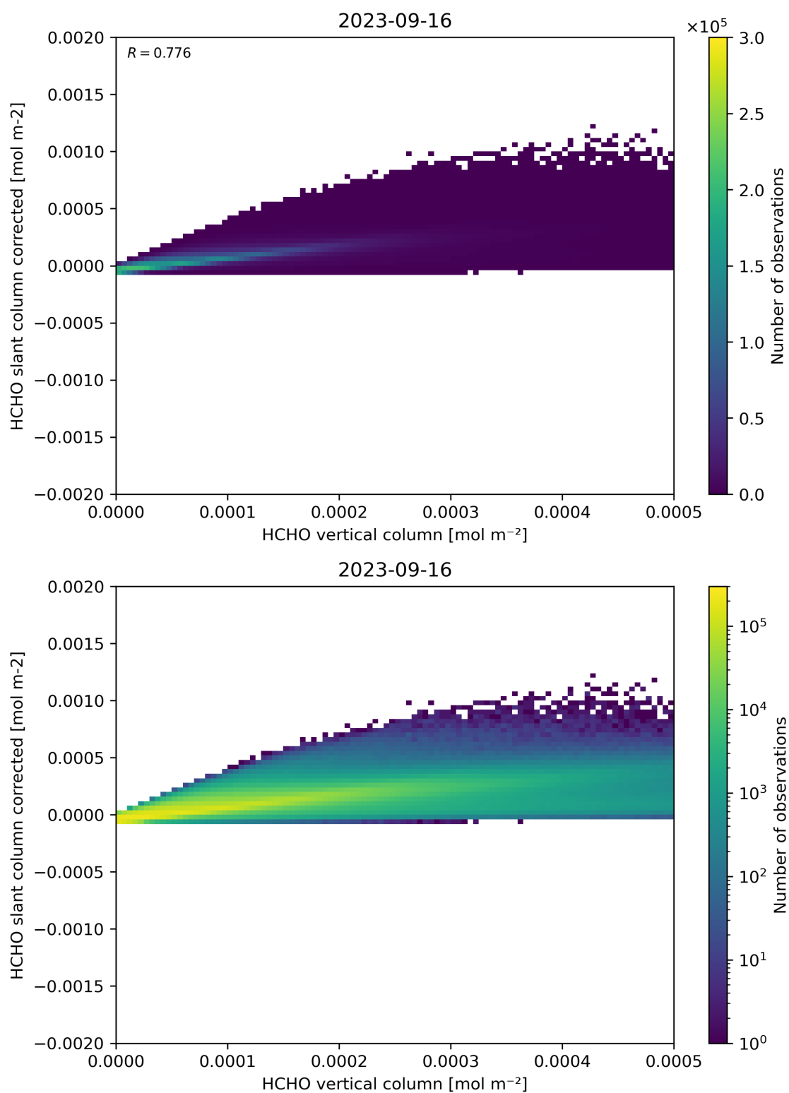
Figure 127: Scatter density plot of “HCHO vertical column” against “HCHO slant column corrected” for 2023-09-15 to 2023-09-17.
