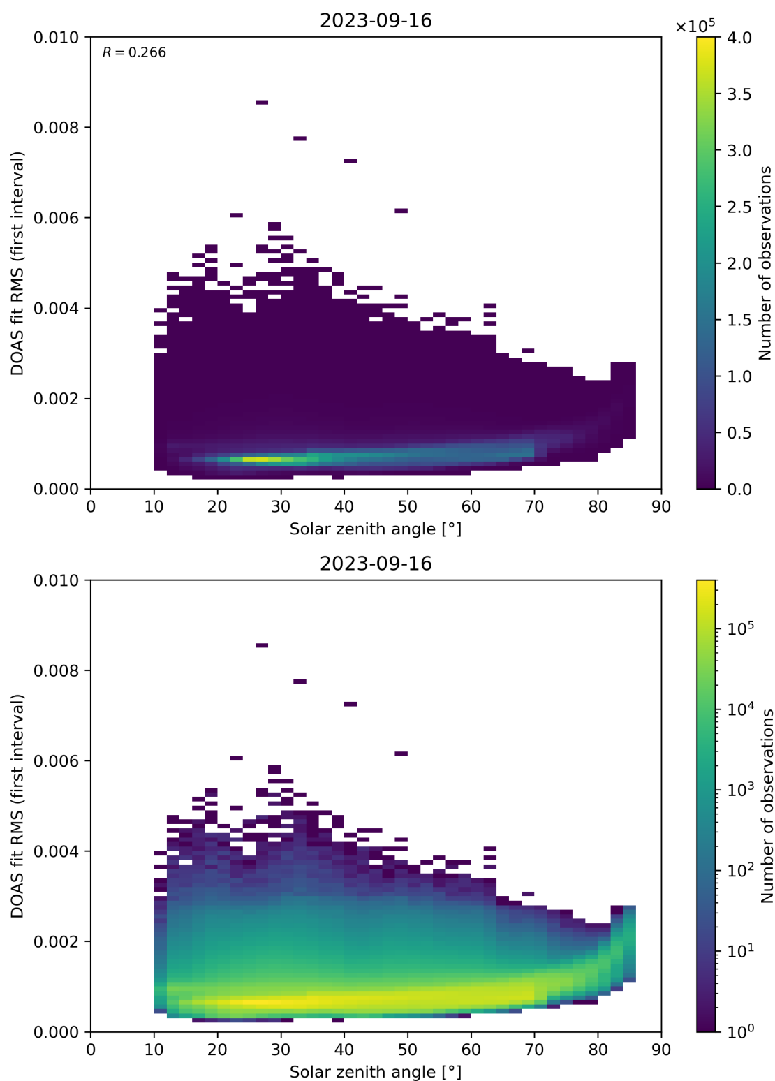
Figure 167: Scatter density plot of “Solar zenith angle” against “DOAS fit RMS (first interval)” for 2023-09-15 to 2023-09-17.
