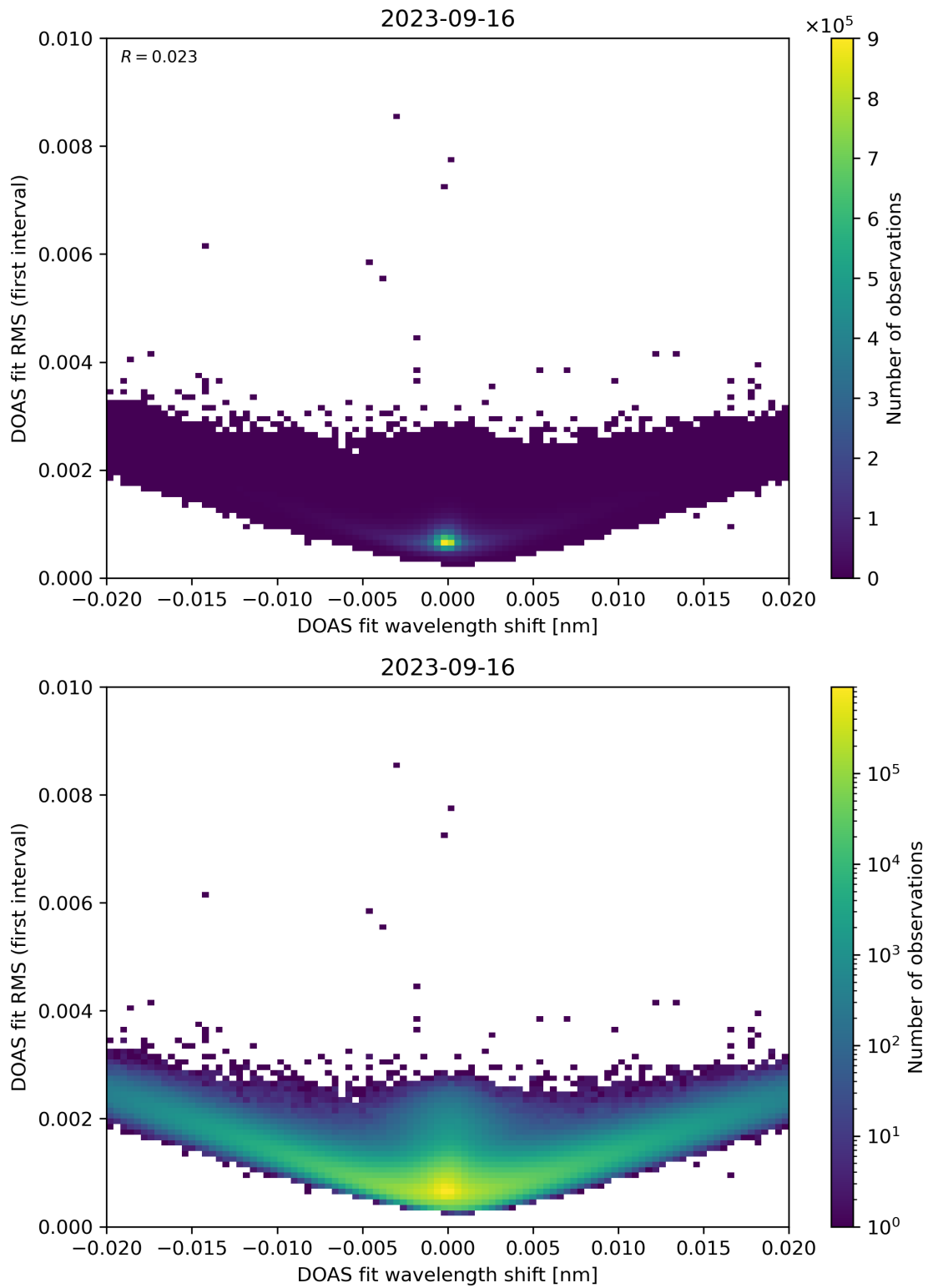
Figure 64: Scatter density plot of “DOAS fit wavelength shift” against “DOAS fit RMS (first interval)” for 2023-09-15 to 2023-09-17.
