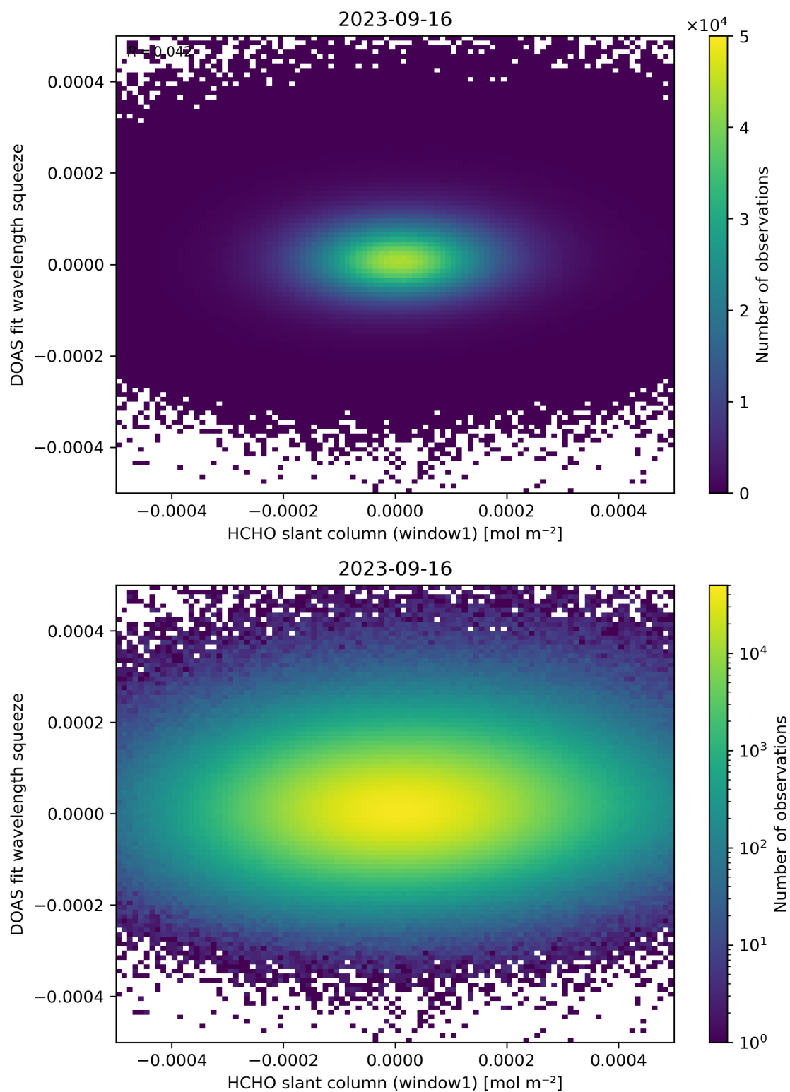
Figure 80: Scatter density plot of “HCHO slant column (window1)” against “DOAS fit wavelength squeeze” for 2023-09-15 to 2023-09-17.
