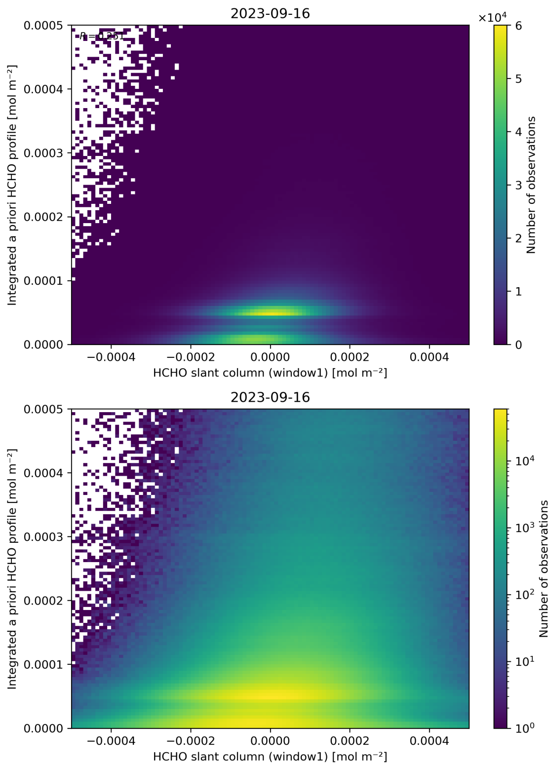
Figure 87: Scatter density plot of “HCHO slant column (window1)” against “Integrated a priori HCHO profile” for 2023-09-15 to 2023-09-17.
