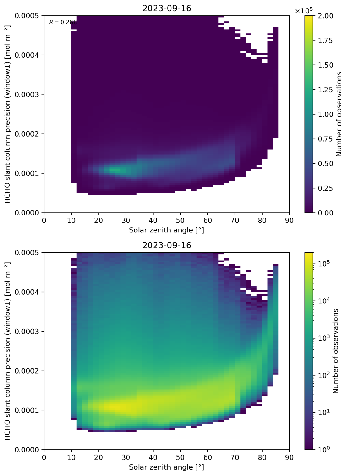
Figure 174: Scatter density plot of “Solar zenith angle” against “HCHO slant column precision (window1)” for 2023-09-15 to 2023-09-17.
