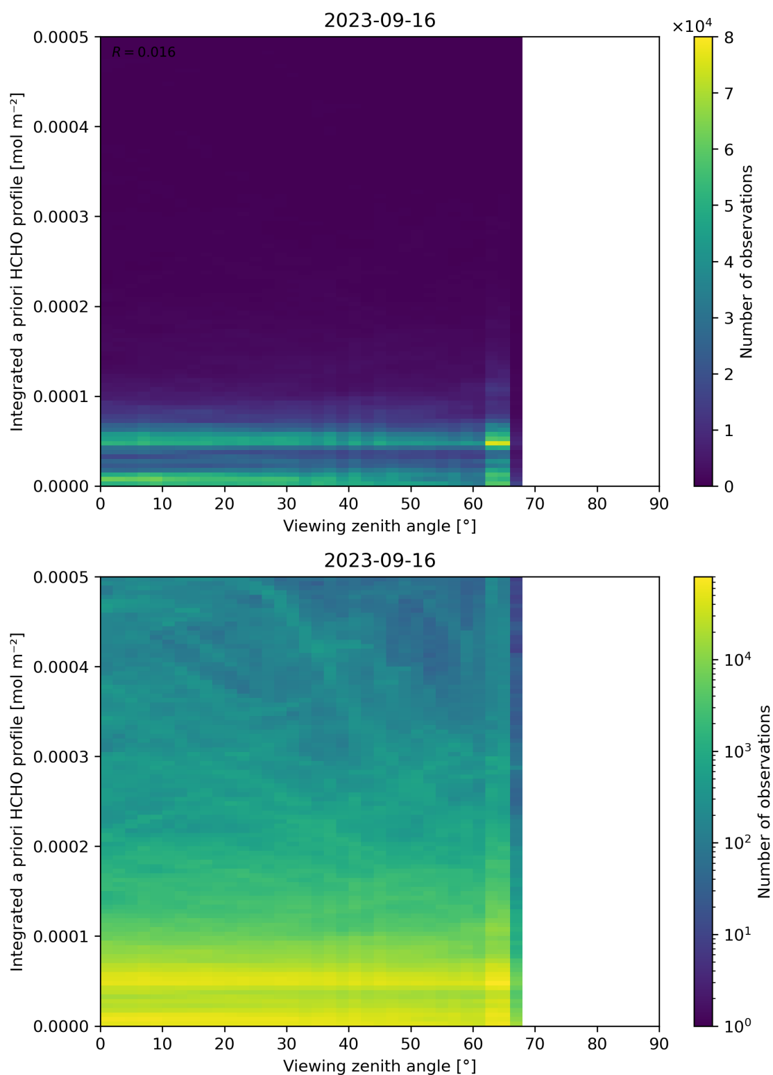
Figure 195: Scatter density plot of “Viewing zenith angle” against “Integrated a priori HCHO profile” for 2023-09-15 to 2023-09-17.
