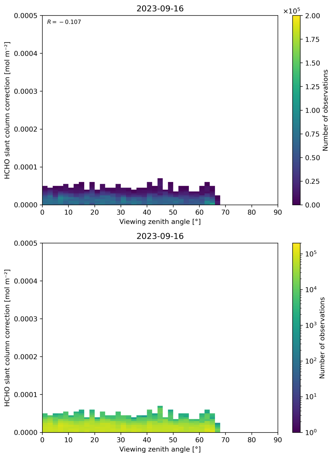
Figure 187: Scatter density plot of “Viewing zenith angle” against “HCHO slant column correction” for 2023-09-15 to 2023-09-17.
