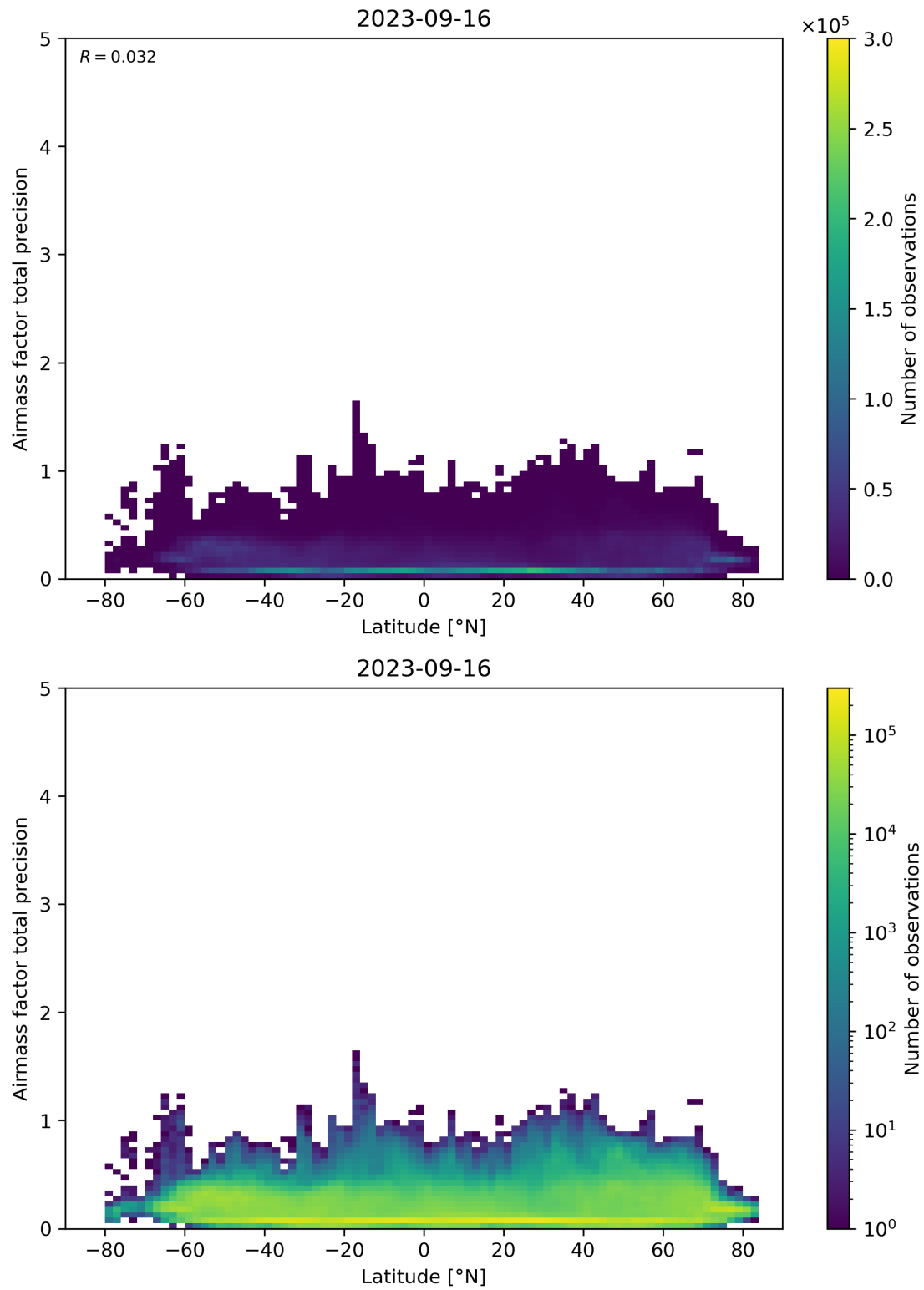
Figure 162: Scatter density plot of “Latitude” against “Airmass factor total precision” for 2023-09-15 to 2023-09-17.
