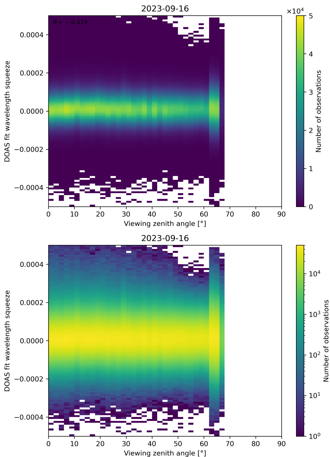
Figure 184: Scatter density plot of “Viewing zenith angle” against “DOAS fit wavelength squeeze” for 2023-09-15 to 2023-09-17.
