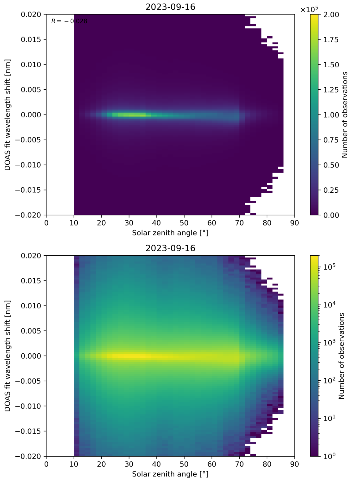
Figure 168: Scatter density plot of “Solar zenith angle” against “DOAS fit wavelength shift” for 2023-09-15 to 2023-09-17.
