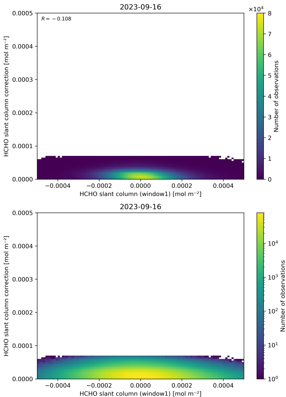
Figure 83: Scatter density plot of “HCHO slant column (window1)” against “HCHO slant column correction” for 2023-09-15 to 2023-09-17.
