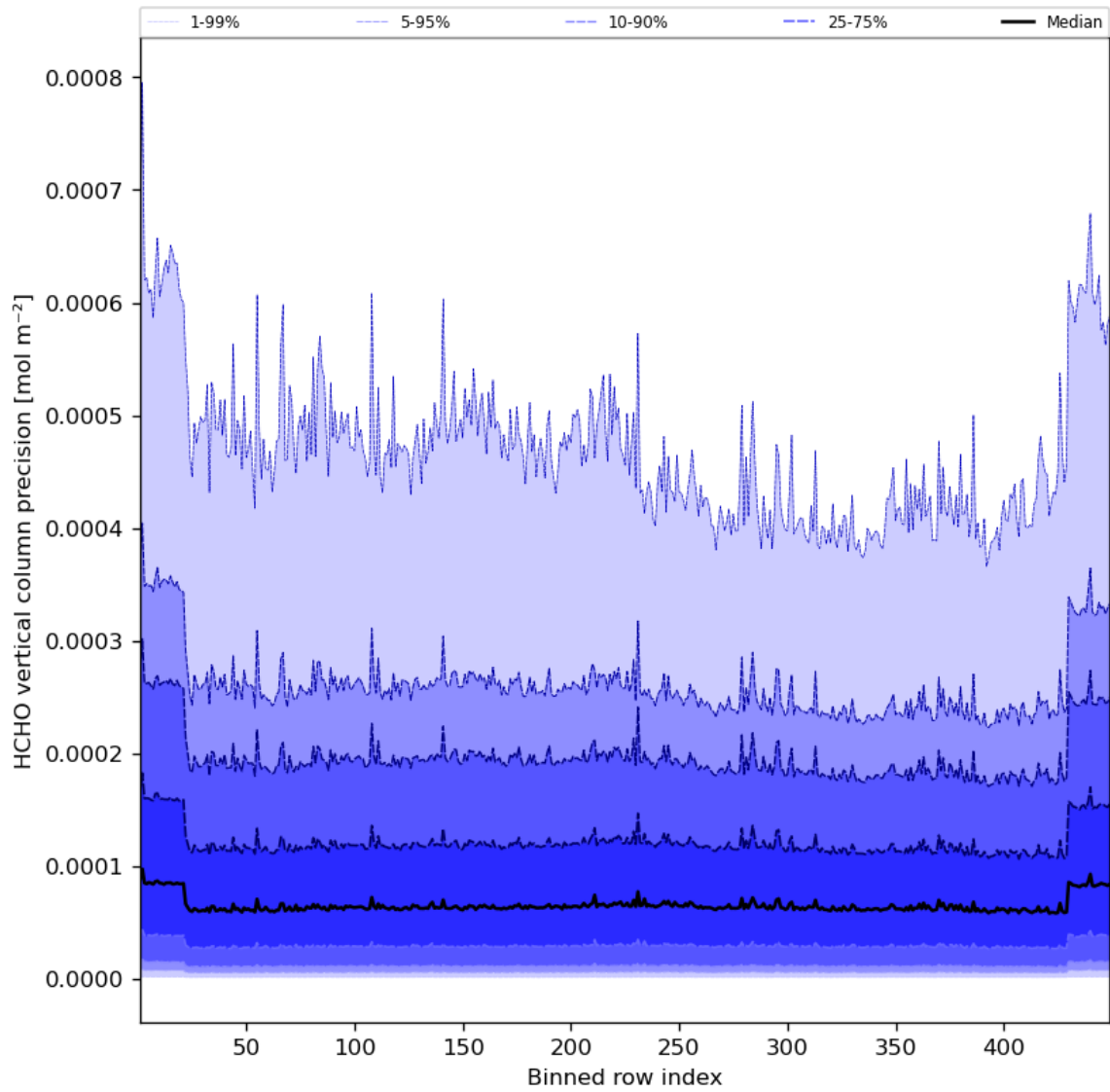
Figure 50: Along track statistics of “HCHO vertical column precision” for 2023-09-15 to 2023-09-17
