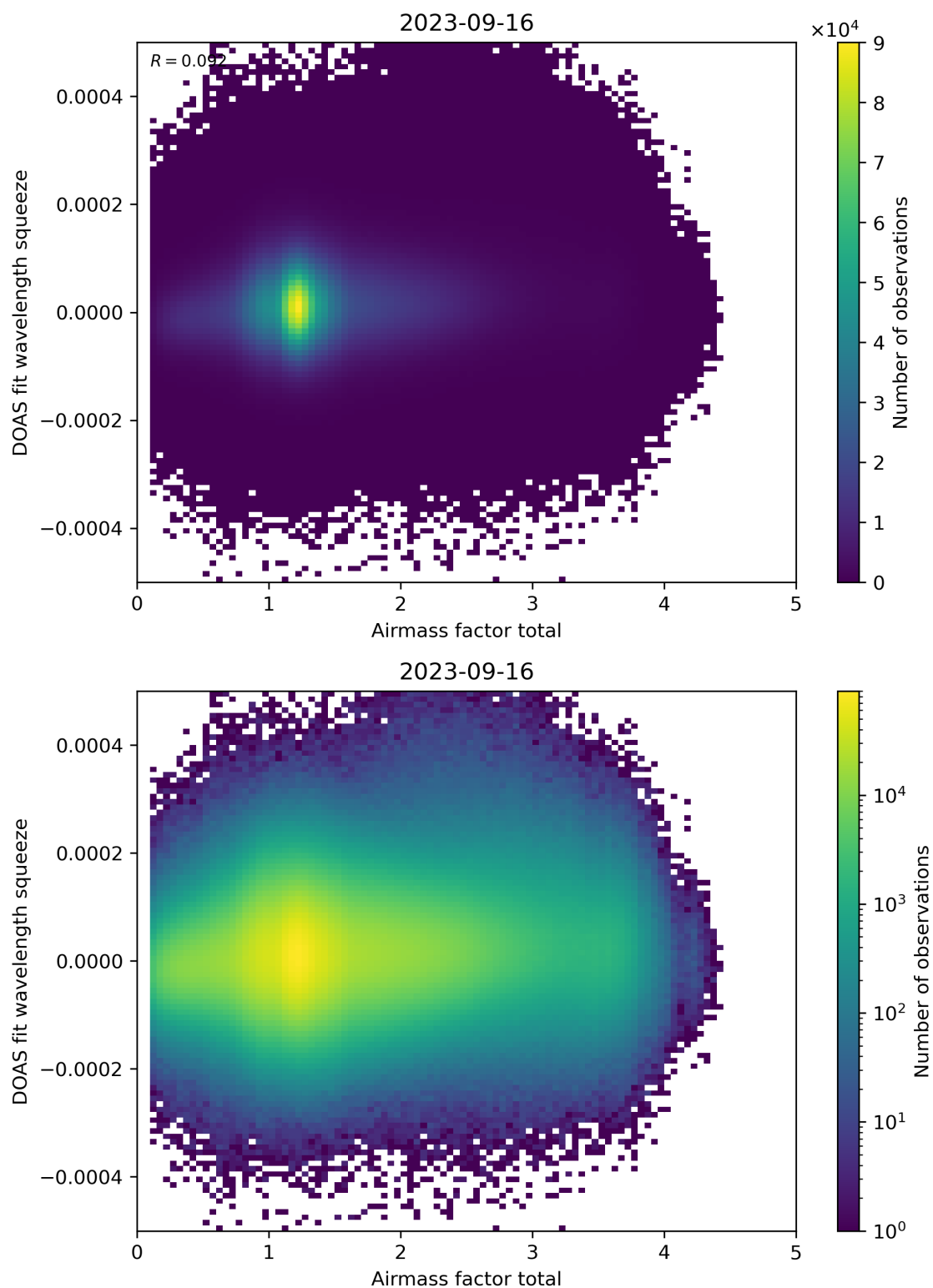
Figure 99: Scatter density plot of “Airmass factor total” against “DOAS fit wavelength squeeze” for 2023-09-15 to 2023-09-17.
