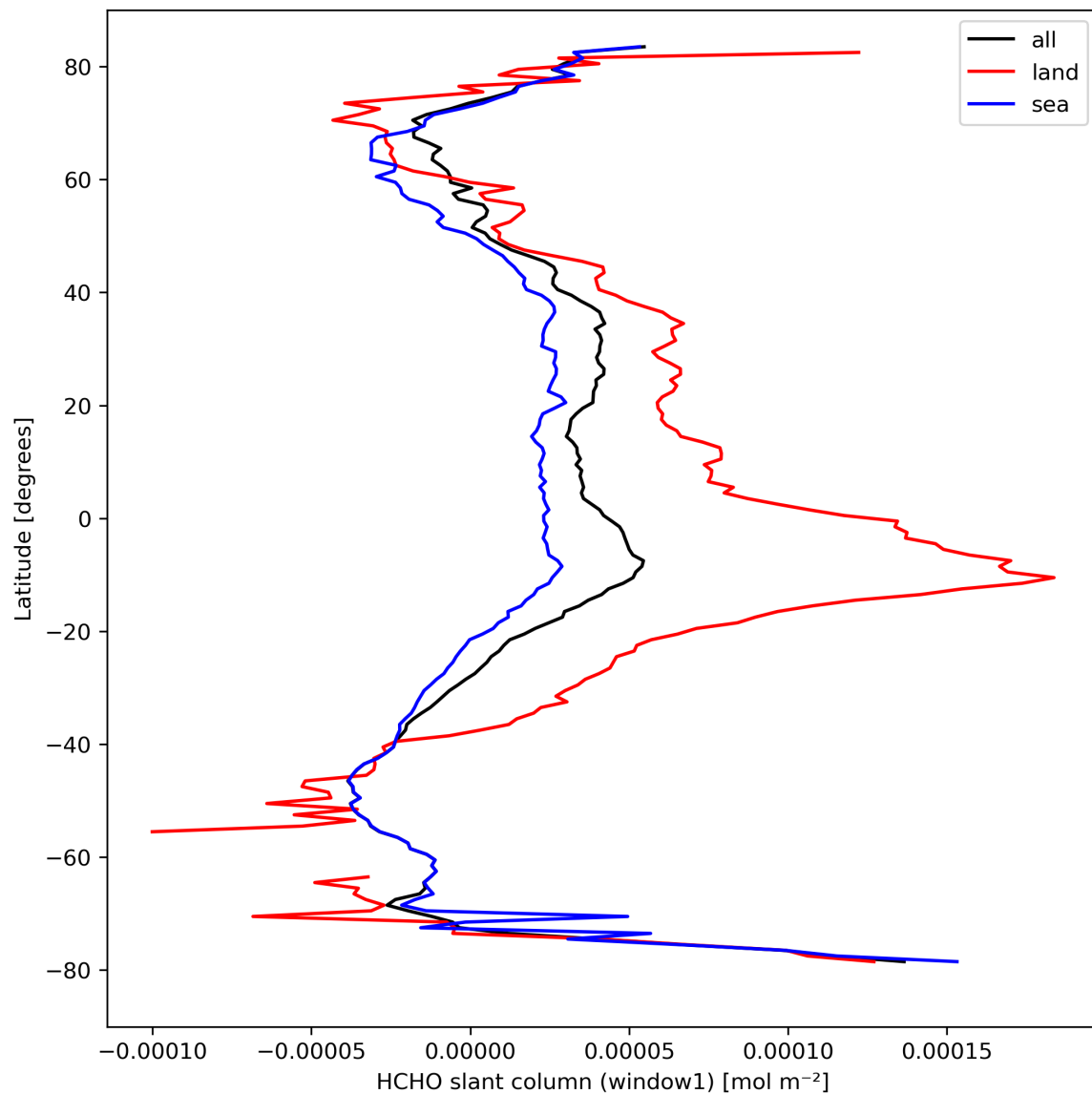
Figure 24: Zonal average of “HCHO slant column (window1)” for 2023-09-15 to 2023-09-17.
