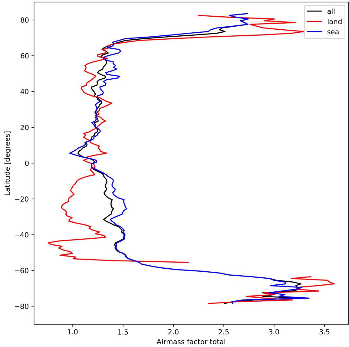
Figure 26: Zonal average of “Airmass factor total” for 2023-09-15 to 2023-09-17.
