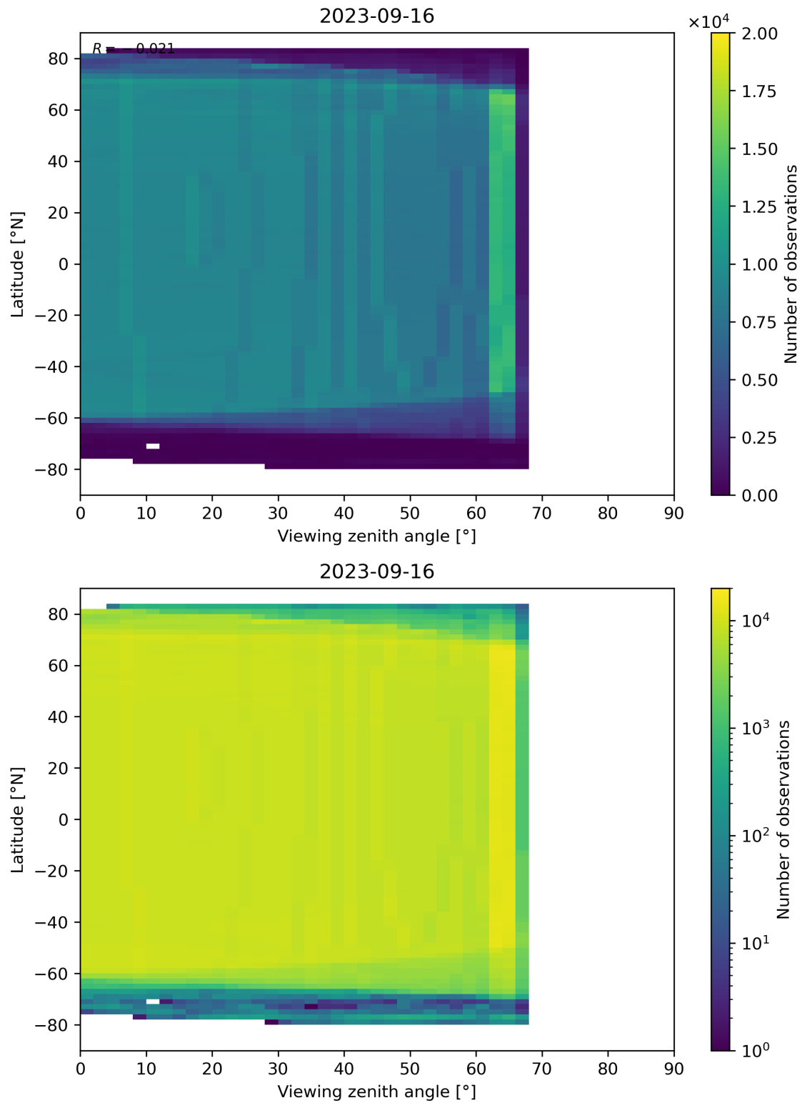
Figure 196: Scatter density plot of “Viewing zenith angle” against “Latitude” for 2023-09-15 to 2023-09-17.
