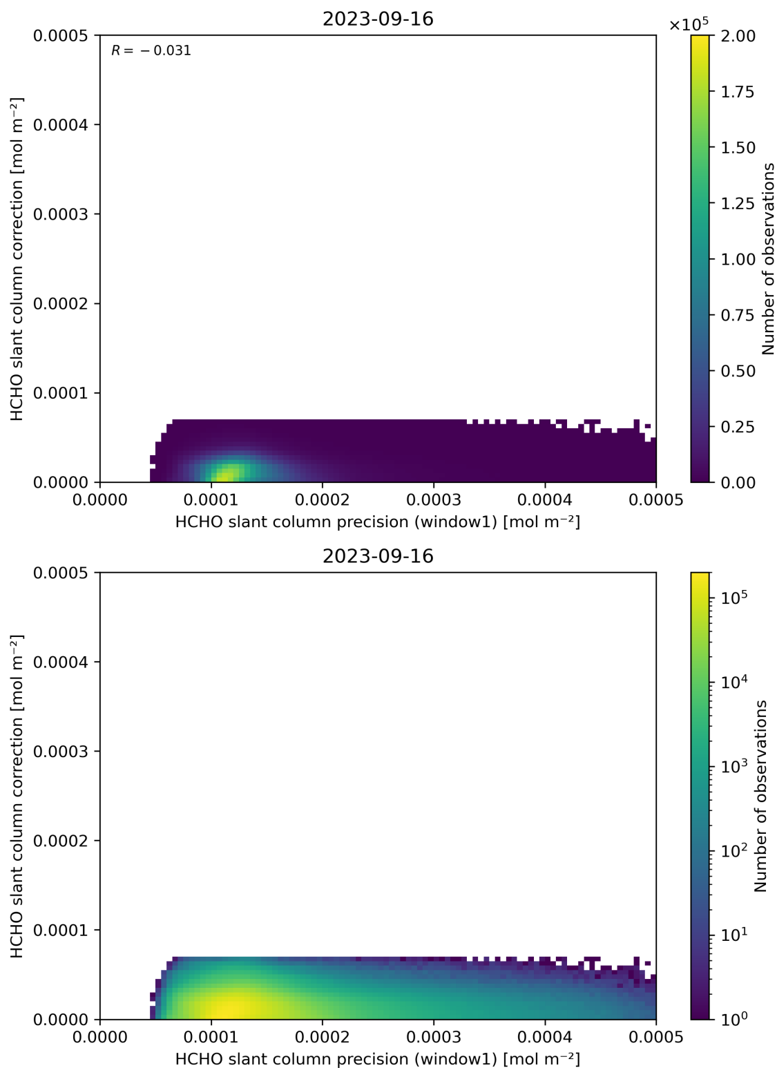
Figure 93: Scatter density plot of “HCHO slant column precision (window1)” against “HCHO slant column correction” for 2023-09-15 to 2023-09-17.
