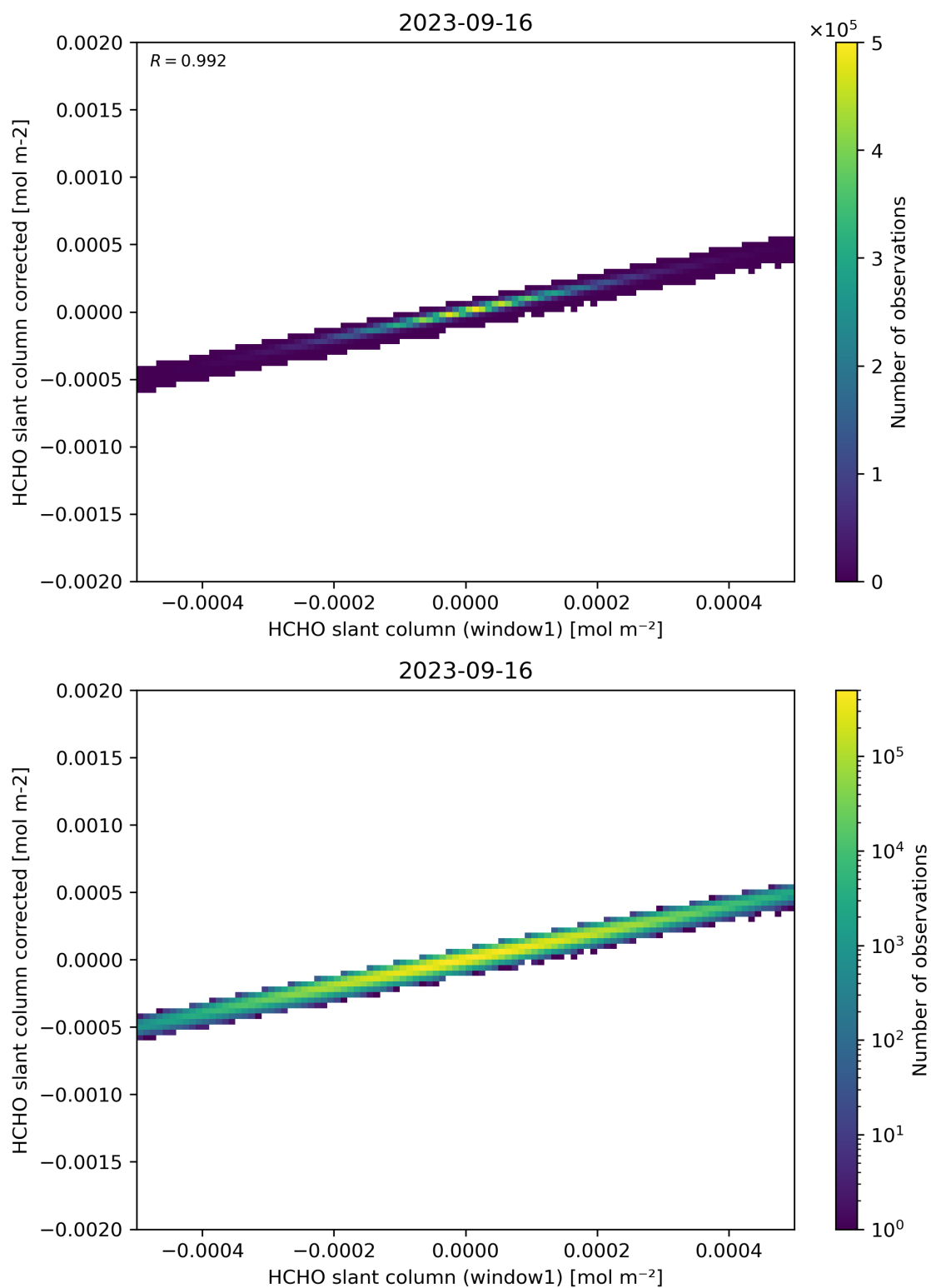
Figure 82: Scatter density plot of “HCHO slant column (window1)” against “HCHO slant column corrected” for 2023-09-15 to 2023-09-17.
