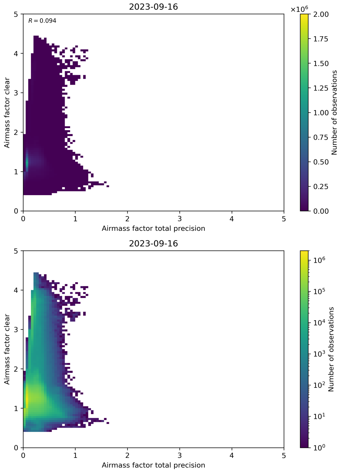
Figure 108: Scatter density plot of “Airmass factor total precision” against “Airmass factor clear” for 2023-09-15 to 2023-09-17.
