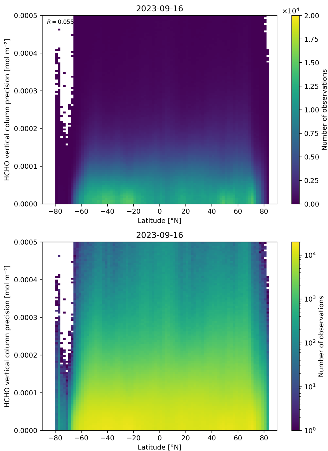
Figure 165: Scatter density plot of “Latitude” against “HCHO vertical column precision” for 2023-09-15 to 2023-09-17.
