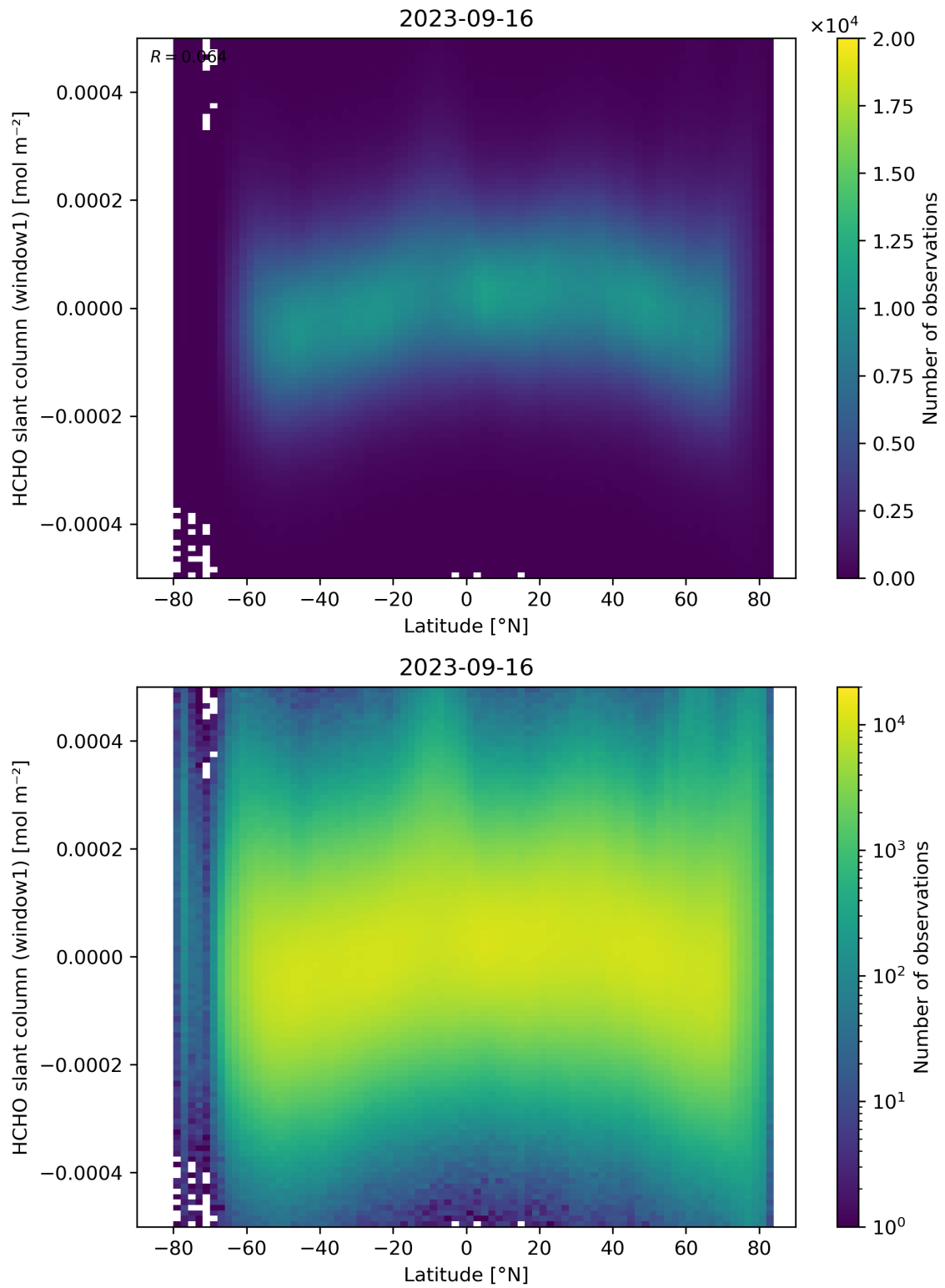
Figure 159: Scatter density plot of “Latitude” against “HCHO slant column (window1)” for 2023-09-15 to 2023-09-17.
