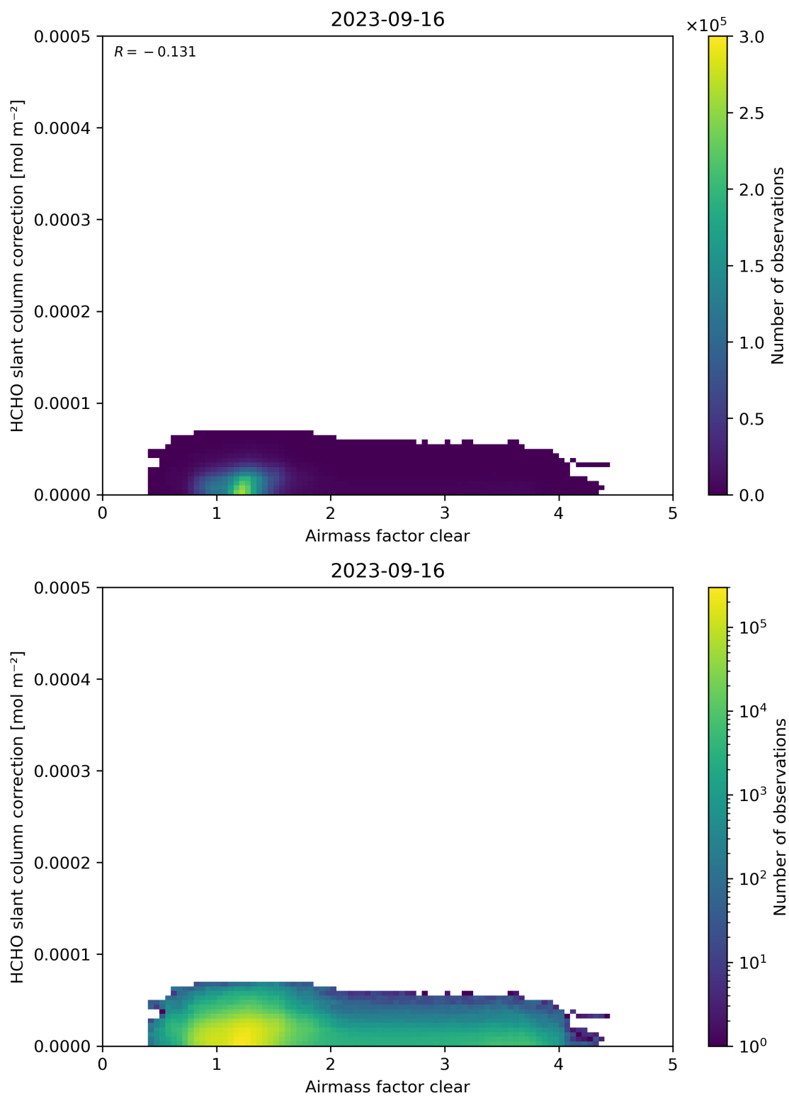
Figure 75: Scatter density plot of “Airmass factor clear” against “HCHO slant column correction” for 2023-09-15 to 2023-09-17.
