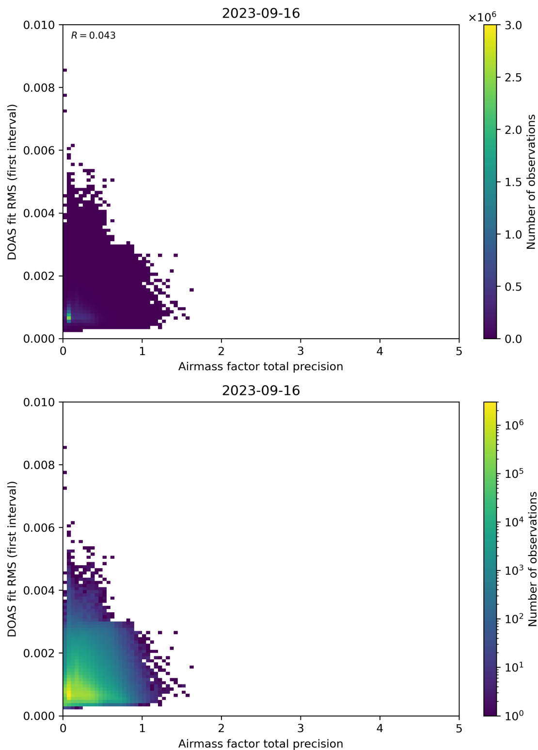
Figure 105: Scatter density plot of “Airmass factor total precision” against “DOAS fit RMS (first interval)” for 2023-09-15 to 2023-09-17.
