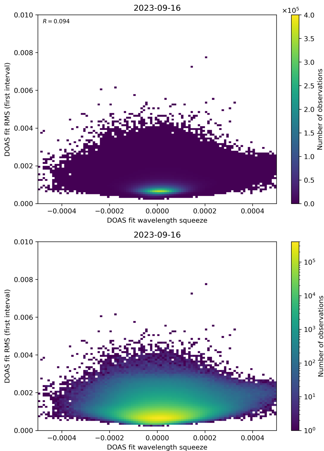
Figure 68: Scatter density plot of “DOAS fit wavelength squeeze” against “DOAS fit RMS (first interval)” for 2023-09-15 to 2023-09-17.
