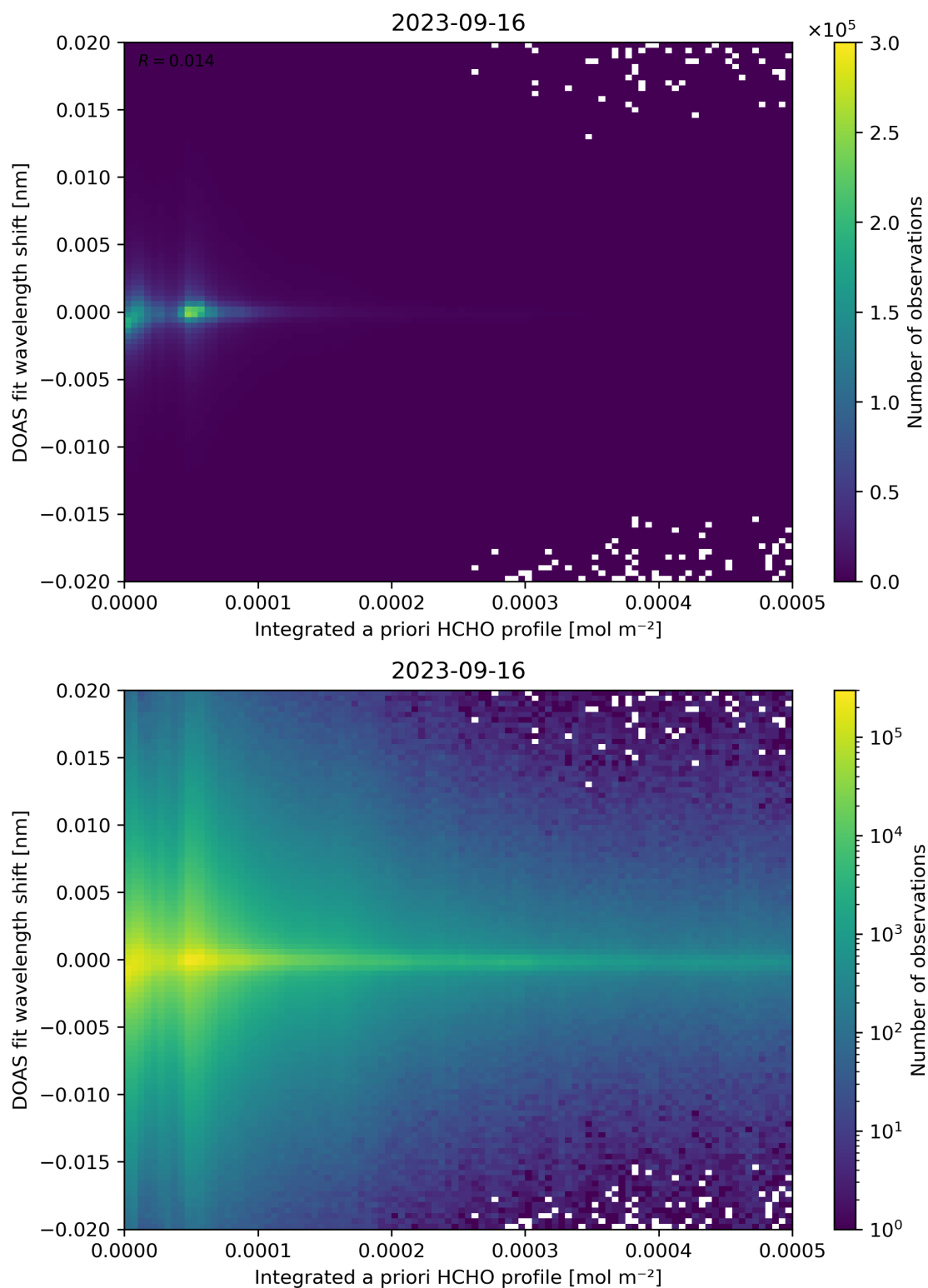
Figure 149: Scatter density plot of “Integrated a priori HCHO profile” against “DOAS fit wavelength shift” for 2023-09-15 to 2023-09-17.
