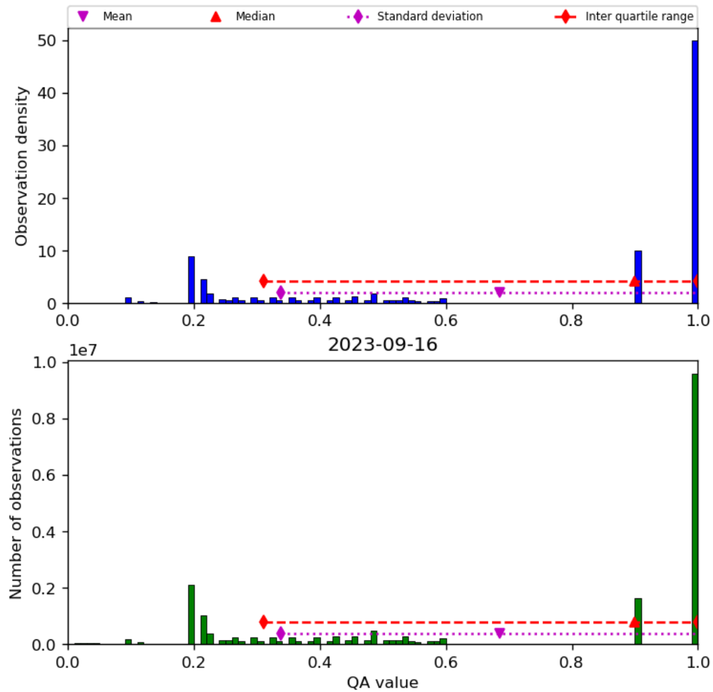
Figure 34: Histogram of “QA value” for 2023-09-15 to 2023-09-17
