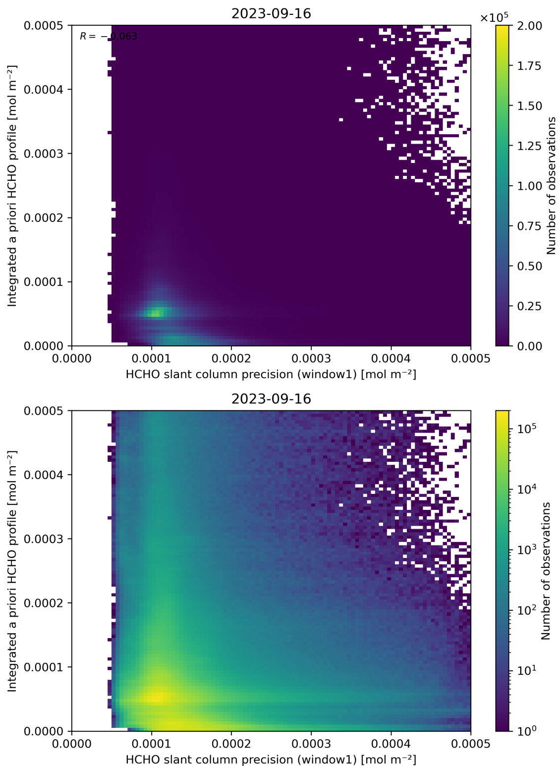
Figure 96: Scatter density plot of “HCHO slant column precision (window1)” against “Integrated a priori HCHO profile” for 2023-09-15 to 2023-09-17.
