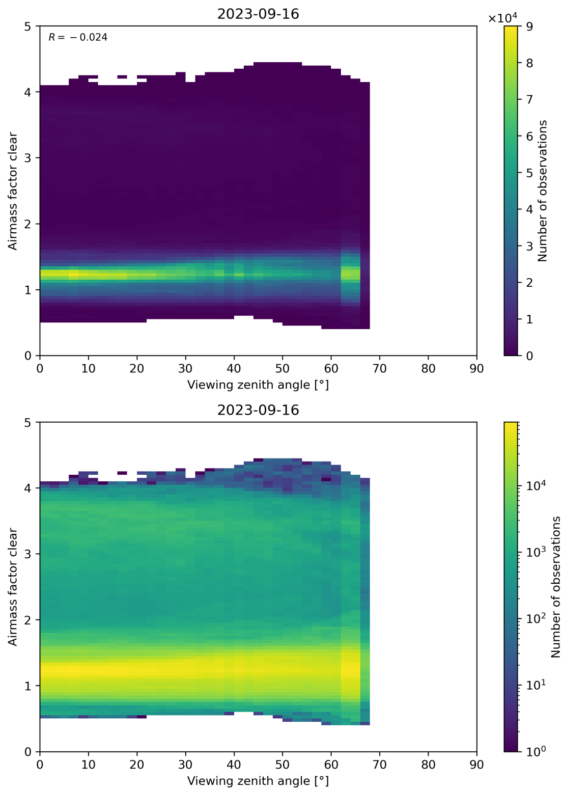
Figure 185: Scatter density plot of “Viewing zenith angle” against “Airmass factor clear” for 2023-09-15 to 2023-09-17.
