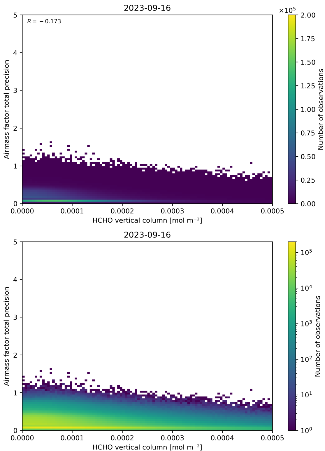
Figure 132: Scatter density plot of “HCHO vertical column” against “Airmass factor total precision” for 2023-09-15 to 2023-09-17.
