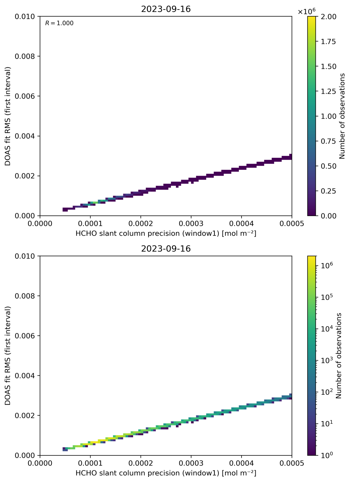
Figure 88: Scatter density plot of “HCHO slant column precision (window1)” against “DOAS fit RMS (first interval)” for 2023-09-15 to 2023-09-17.
