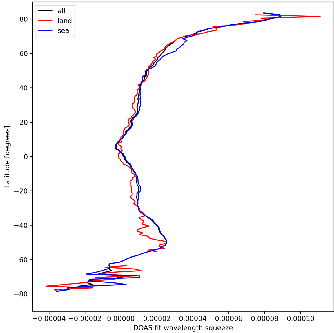
Figure 31: Zonal average of “DOAS fit wavelength squeeze” for 2023-09-15 to 2023-09-17.
