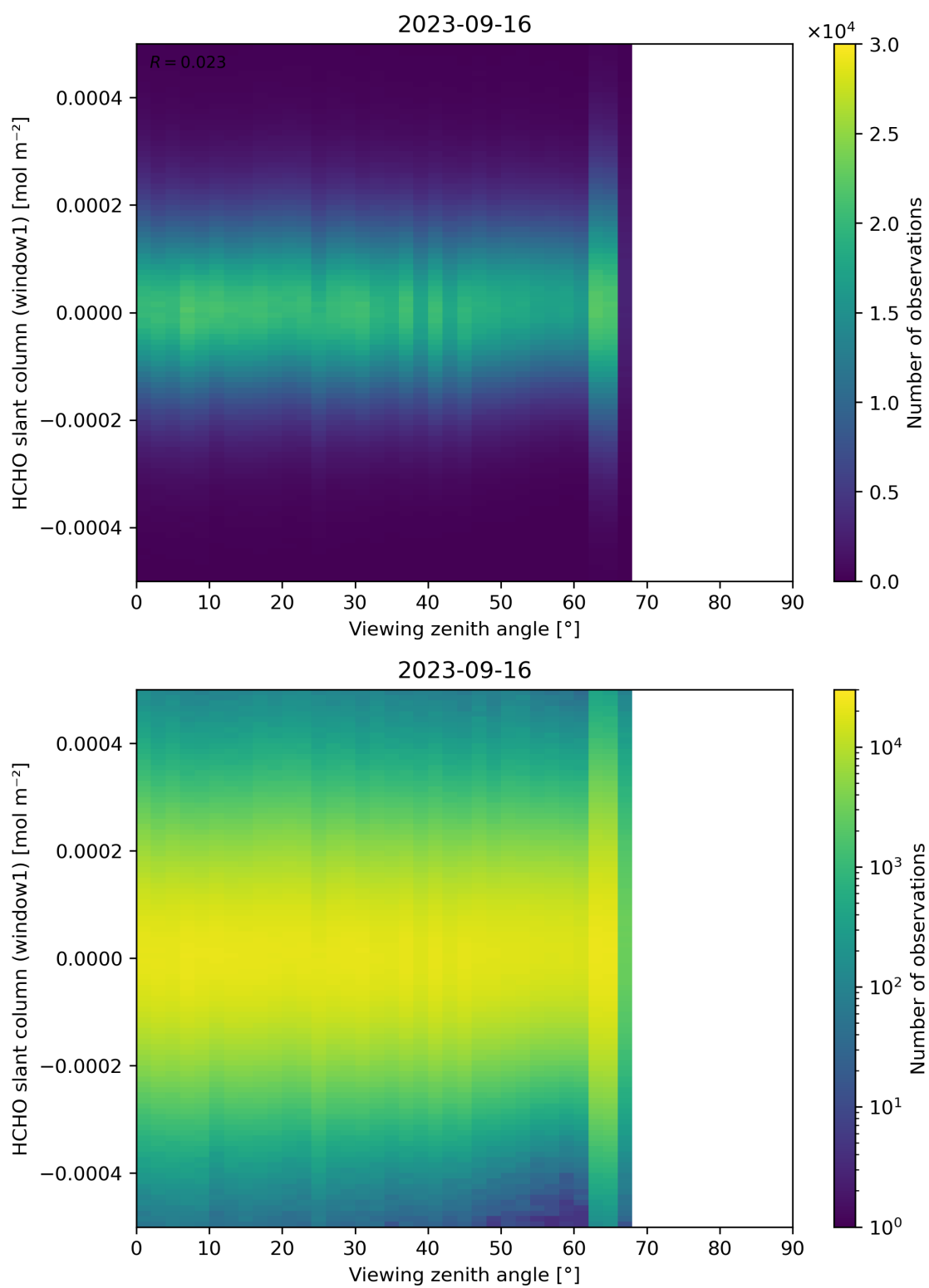
Figure 188: Scatter density plot of “Viewing zenith angle” against “HCHO slant column (window1)” for 2023-09-15 to 2023-09-17.
