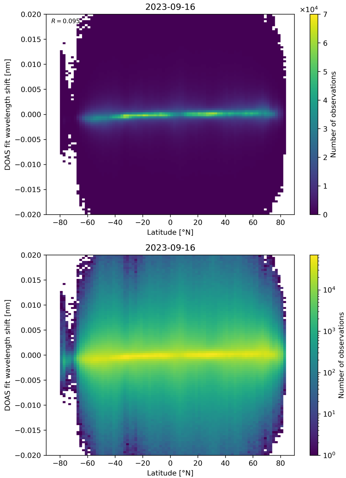
Figure 154: Scatter density plot of “Latitude” against “DOAS fit wavelength shift” for 2023-09-15 to 2023-09-17.
