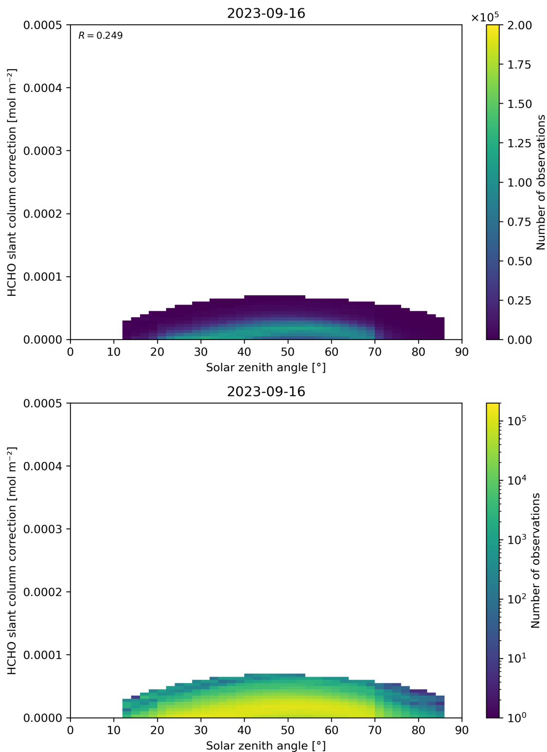
Figure 172: Scatter density plot of “Solar zenith angle” against “HCHO slant column correction” for 2023-09-15 to 2023-09-17.
