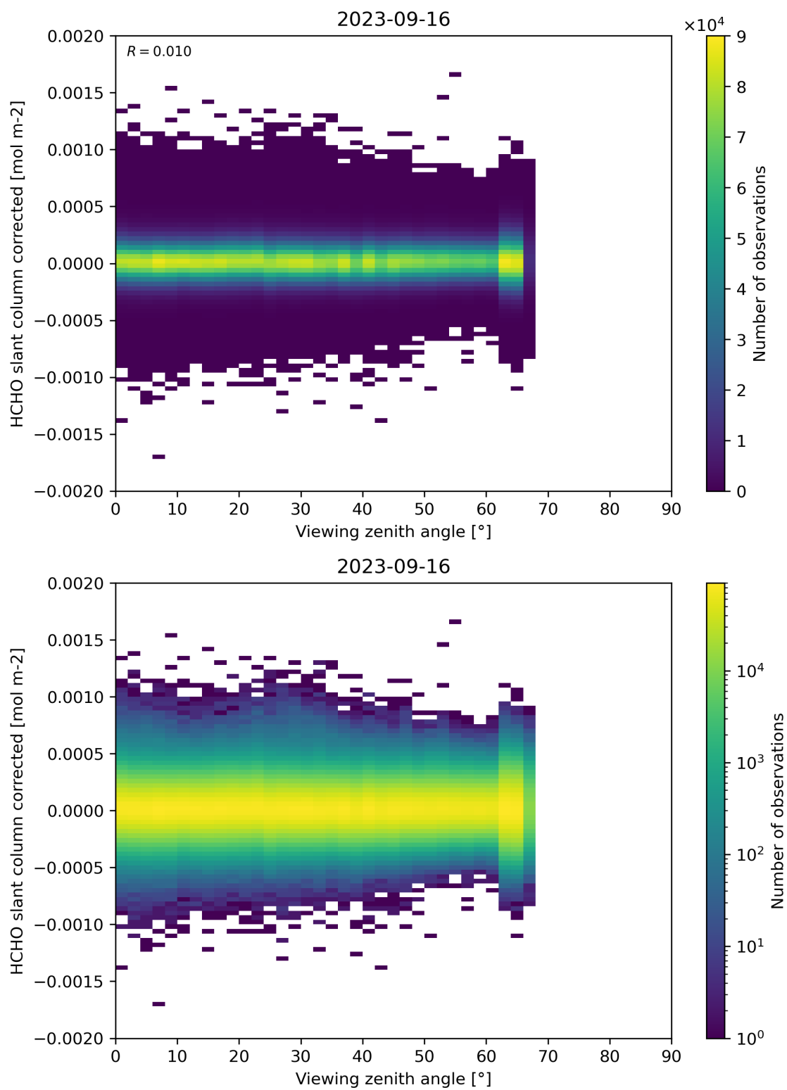
Figure 186: Scatter density plot of “Viewing zenith angle” against “HCHO slant column corrected” for 2023-09-15 to 2023-09-17.
