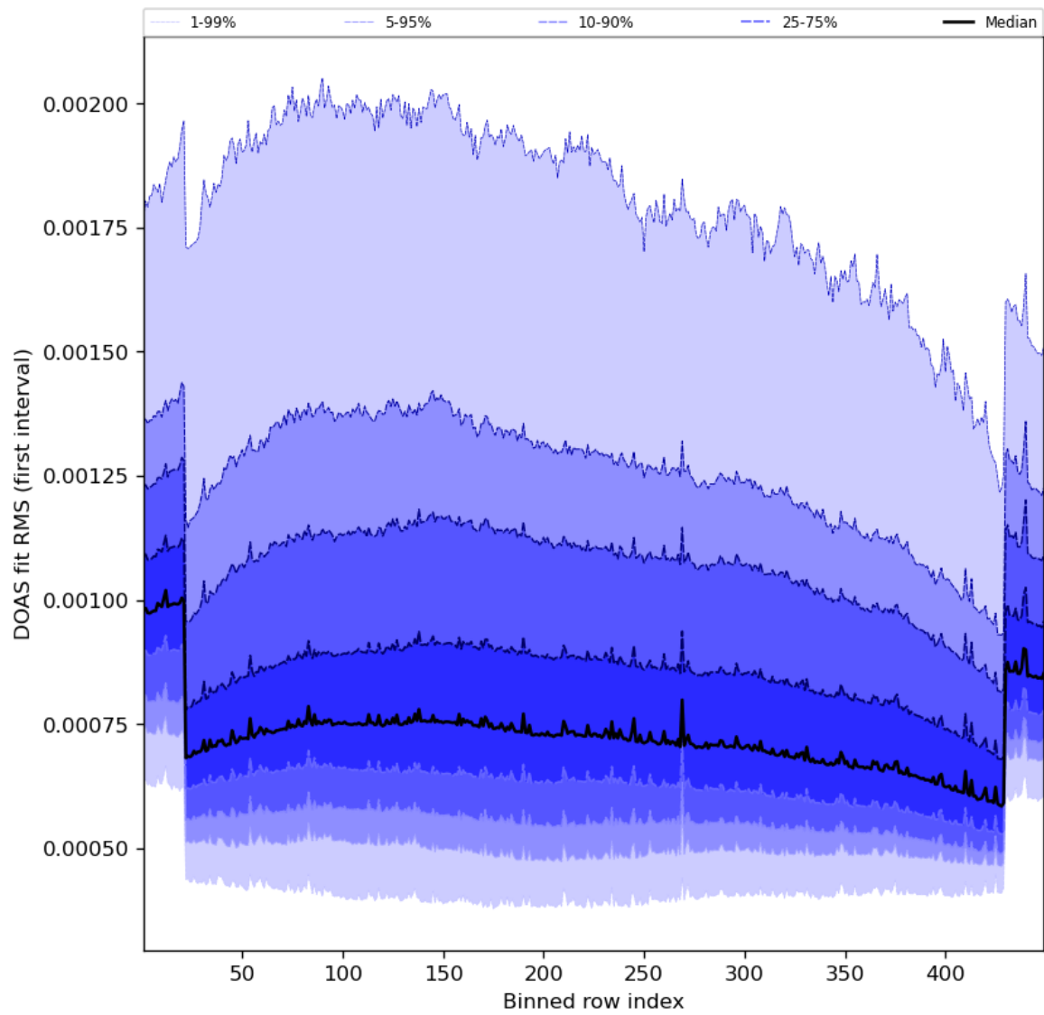
Figure 60: Along track statistics of “DOAS fit RMS (first interval)” for 2023-09-15 to 2023-09-17
