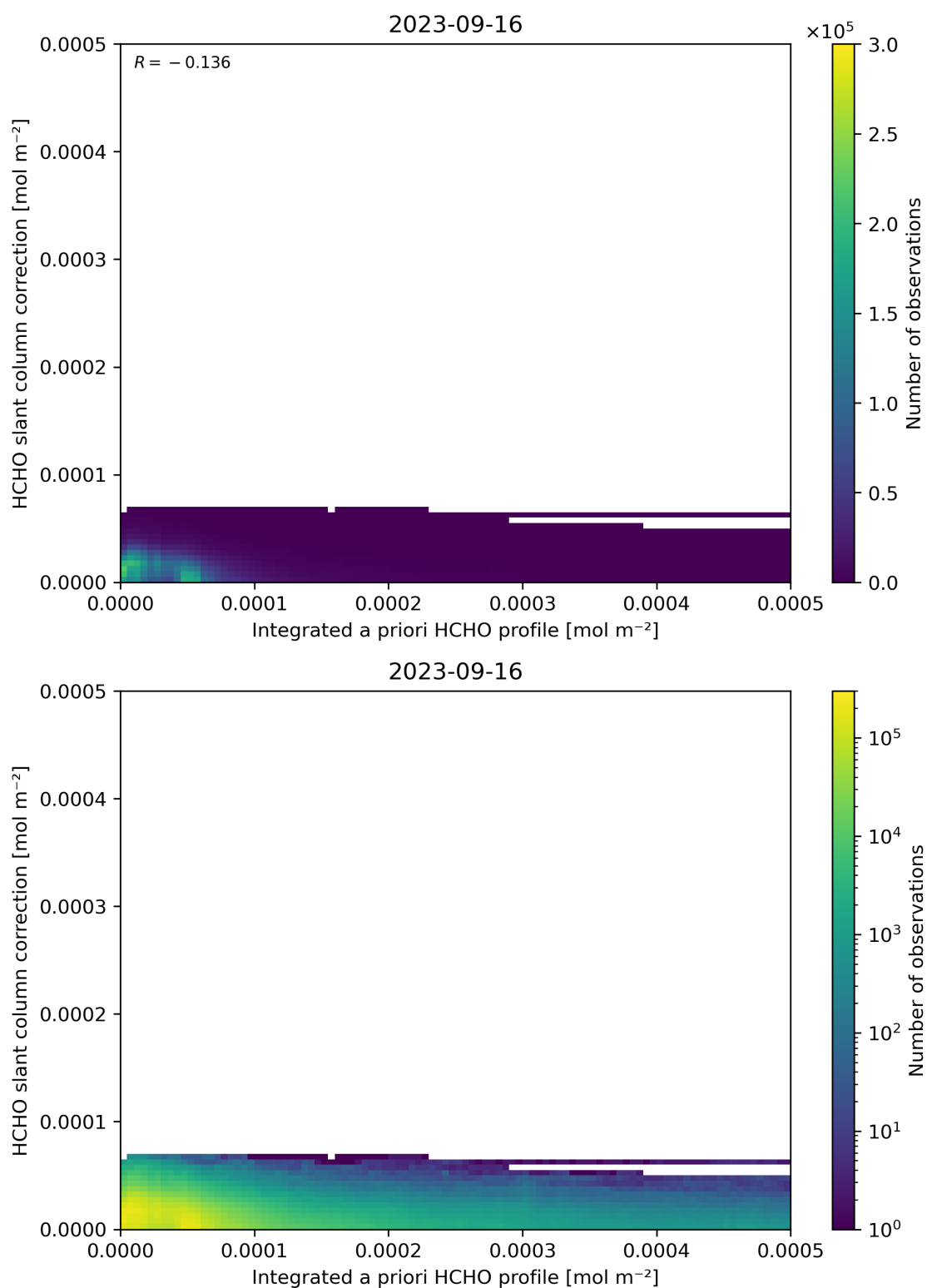
Figure 152: Scatter density plot of “Integrated a priori HCHO profile” against “HCHO slant column correction” for 2023-09-15 to 2023-09-17.
