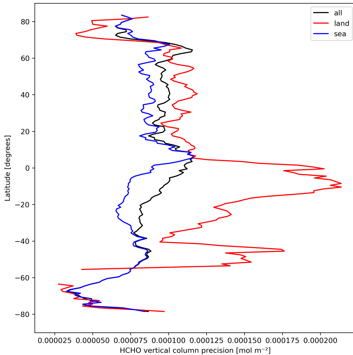
Figure 22: Zonal average of “HCHO vertical column precision” for 2023-09-15 to 2023-09-17.
