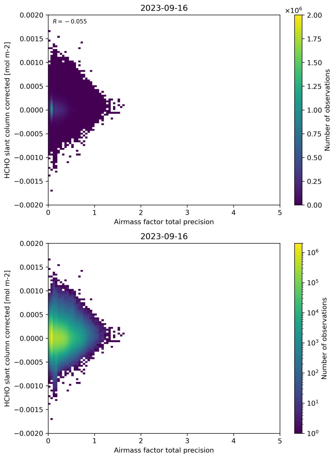
Figure 109: Scatter density plot of “Airmass factor total precision” against “HCHO slant column corrected” for 2023-09-15 to 2023-09-17.
