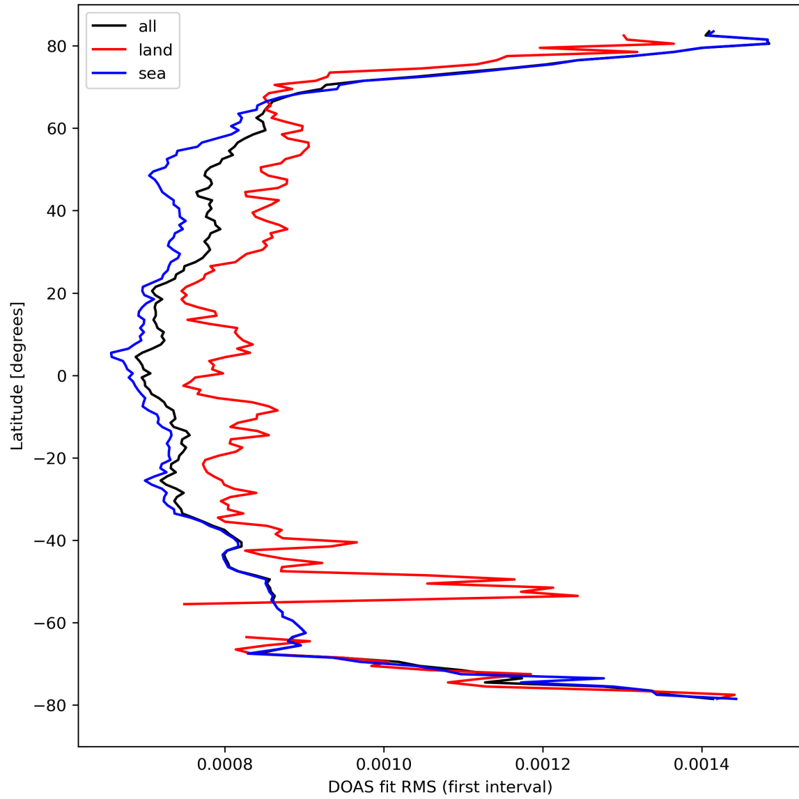
Figure 32: Zonal average of “DOAS fit RMS (first interval)” for 2023-09-15 to 2023-09-17.
