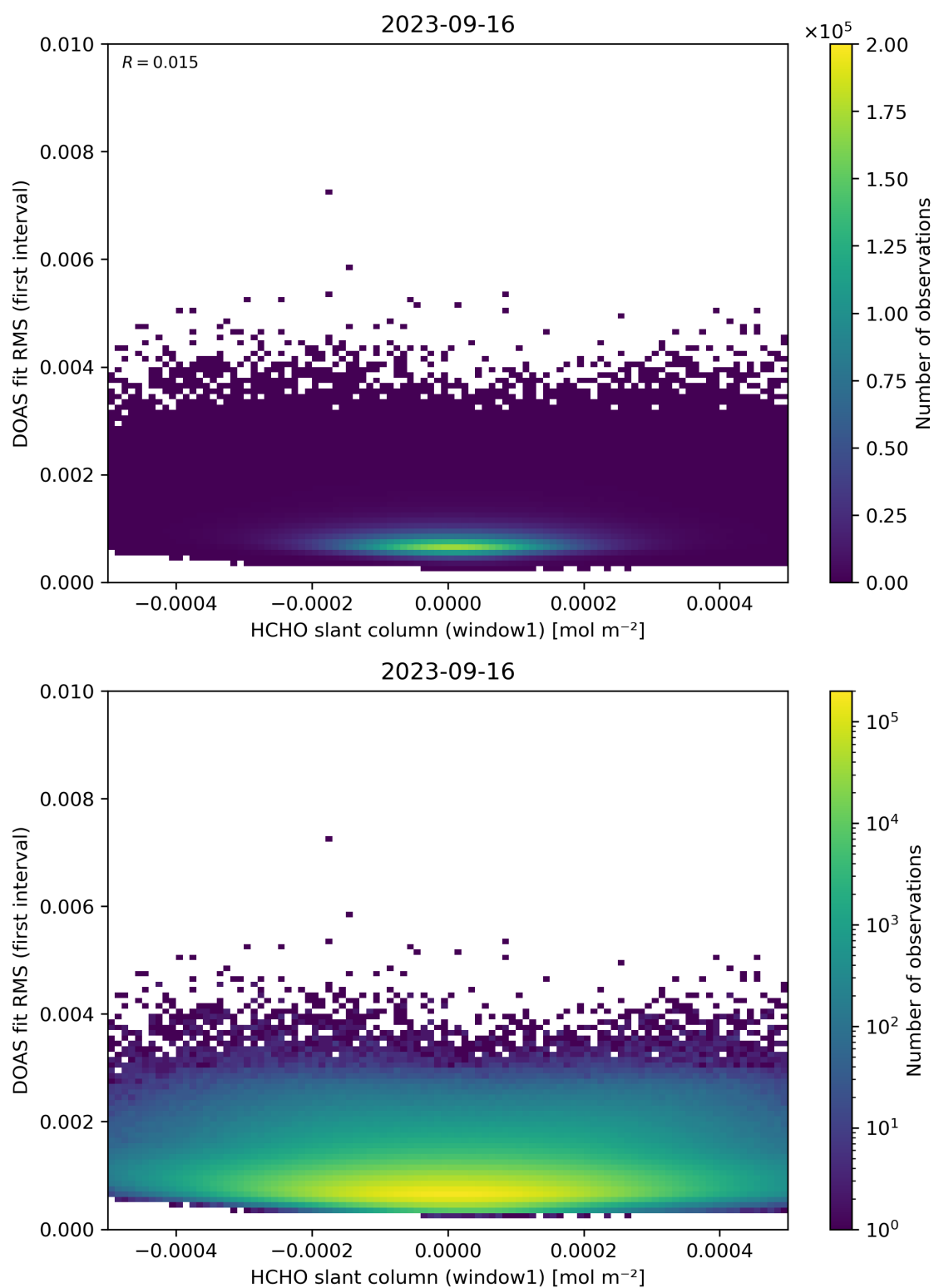
Figure 78: Scatter density plot of “HCHO slant column (window1)” against “DOAS fit RMS (first interval)” for 2023-09-15 to 2023-09-17.
