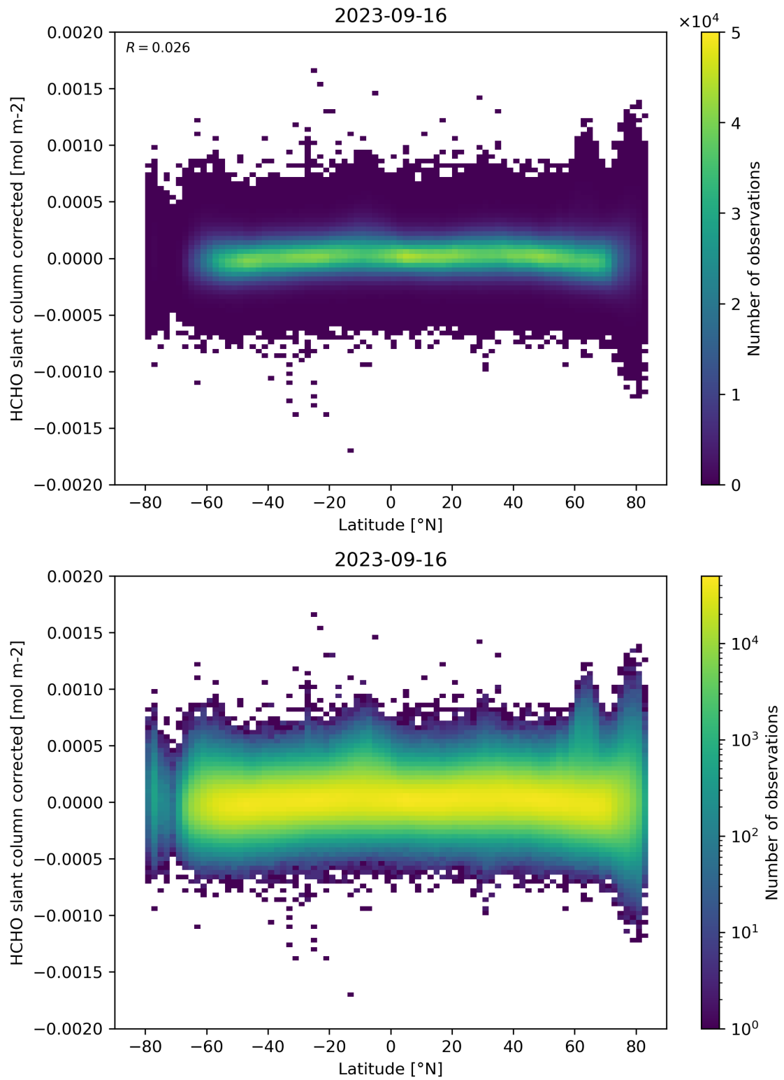
Figure 157: Scatter density plot of “Latitude” against “HCHO slant column corrected” for 2023-09-15 to 2023-09-17.
