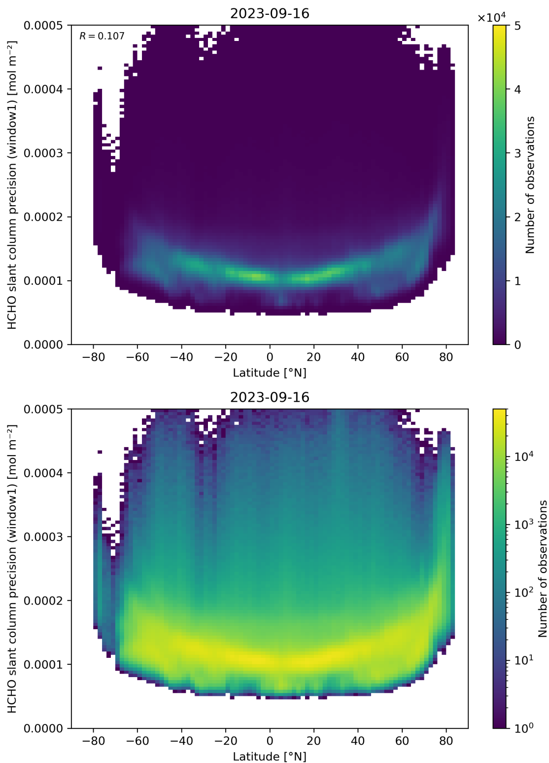
Figure 160: Scatter density plot of “Latitude” against “HCHO slant column precision (window1)” for 2023-09-15 to 2023-09-17.
