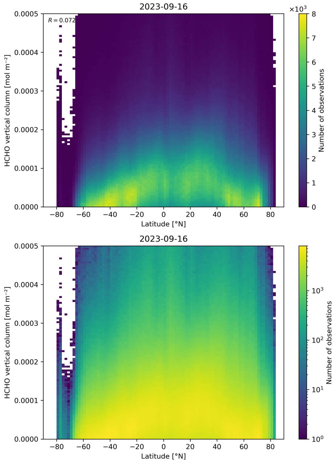
Figure 163: Scatter density plot of “Latitude” against “HCHO vertical column” for 2023-09-15 to 2023-09-17.
