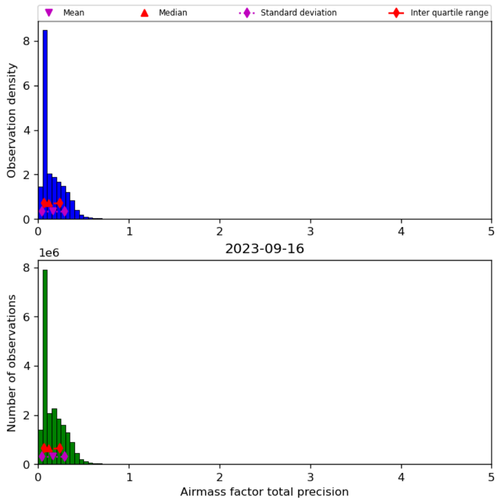
Figure 41: Histogram of “Airmass factor total precision” for 2023-09-15 to 2023-09-17
