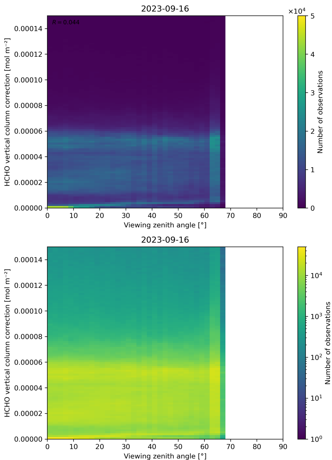
Figure 193: Scatter density plot of “Viewing zenith angle” against “HCHO vertical column correction” for 2023-09-15 to 2023-09-17.
