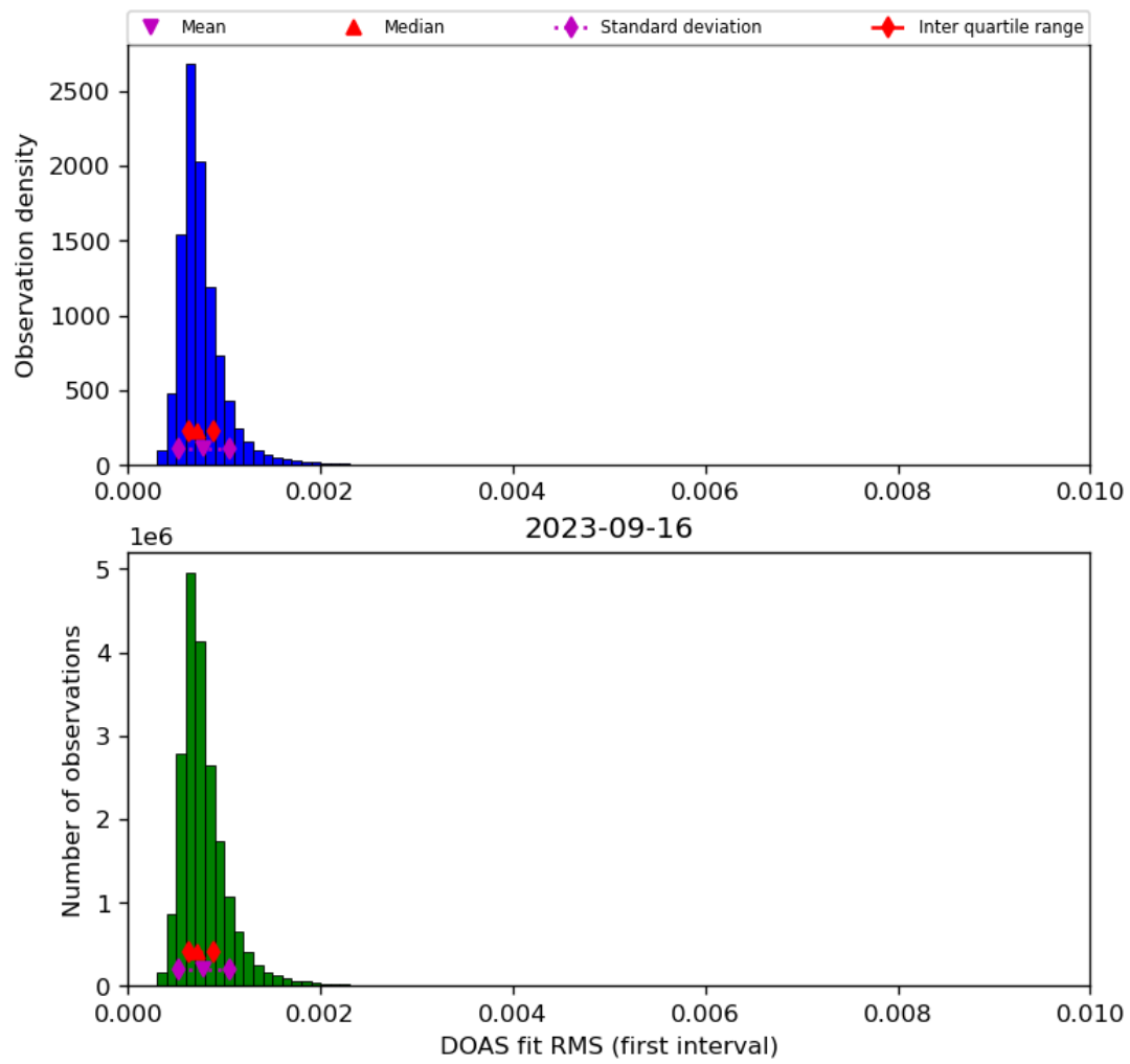
Figure 46: Histogram of “DOAS fit RMS (first interval)” for 2023-09-15 to 2023-09-17
