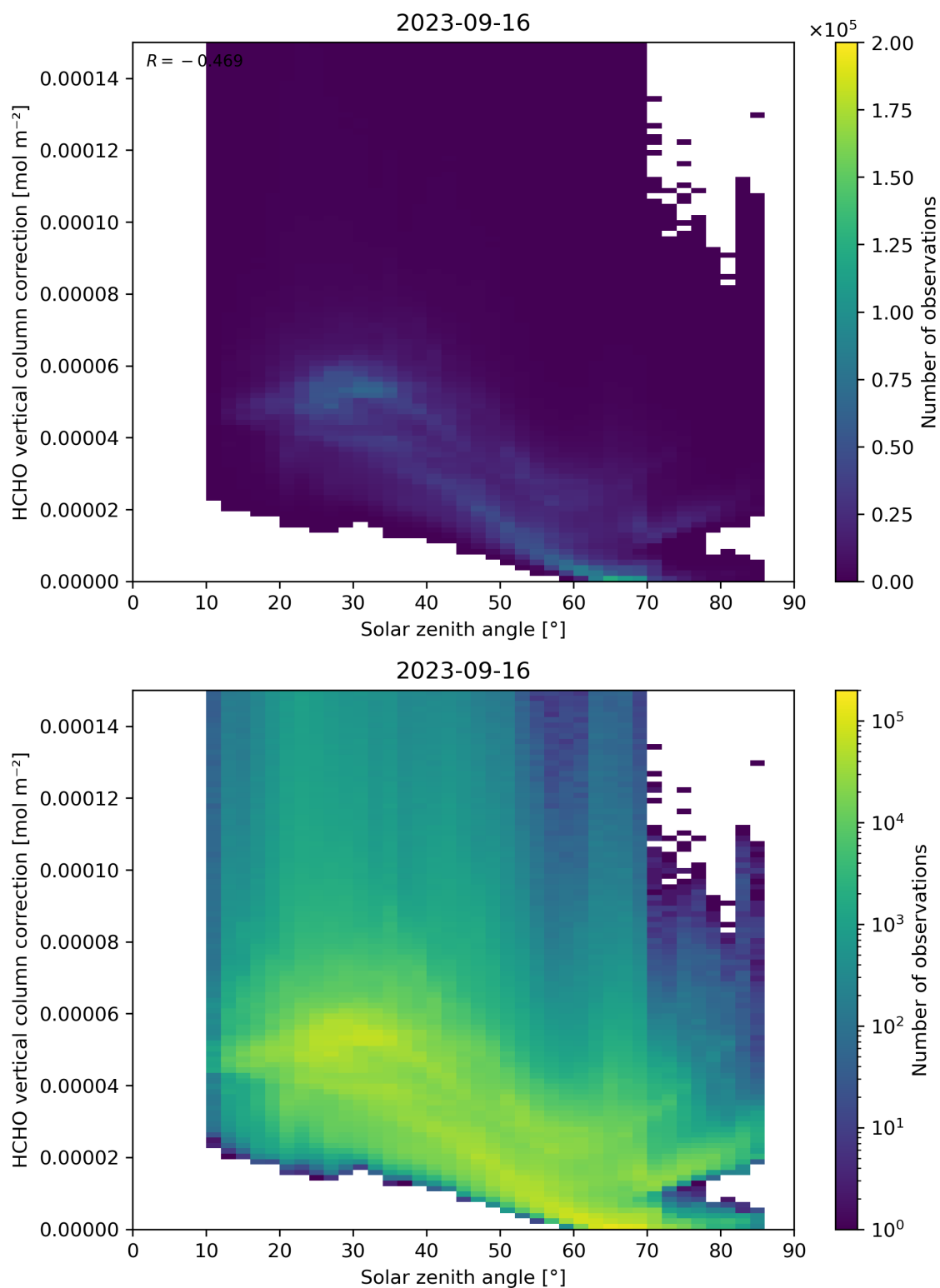
Figure 178: Scatter density plot of “Solar zenith angle” against “HCHO vertical column correction” for 2023-09-15 to 2023-09-17.
