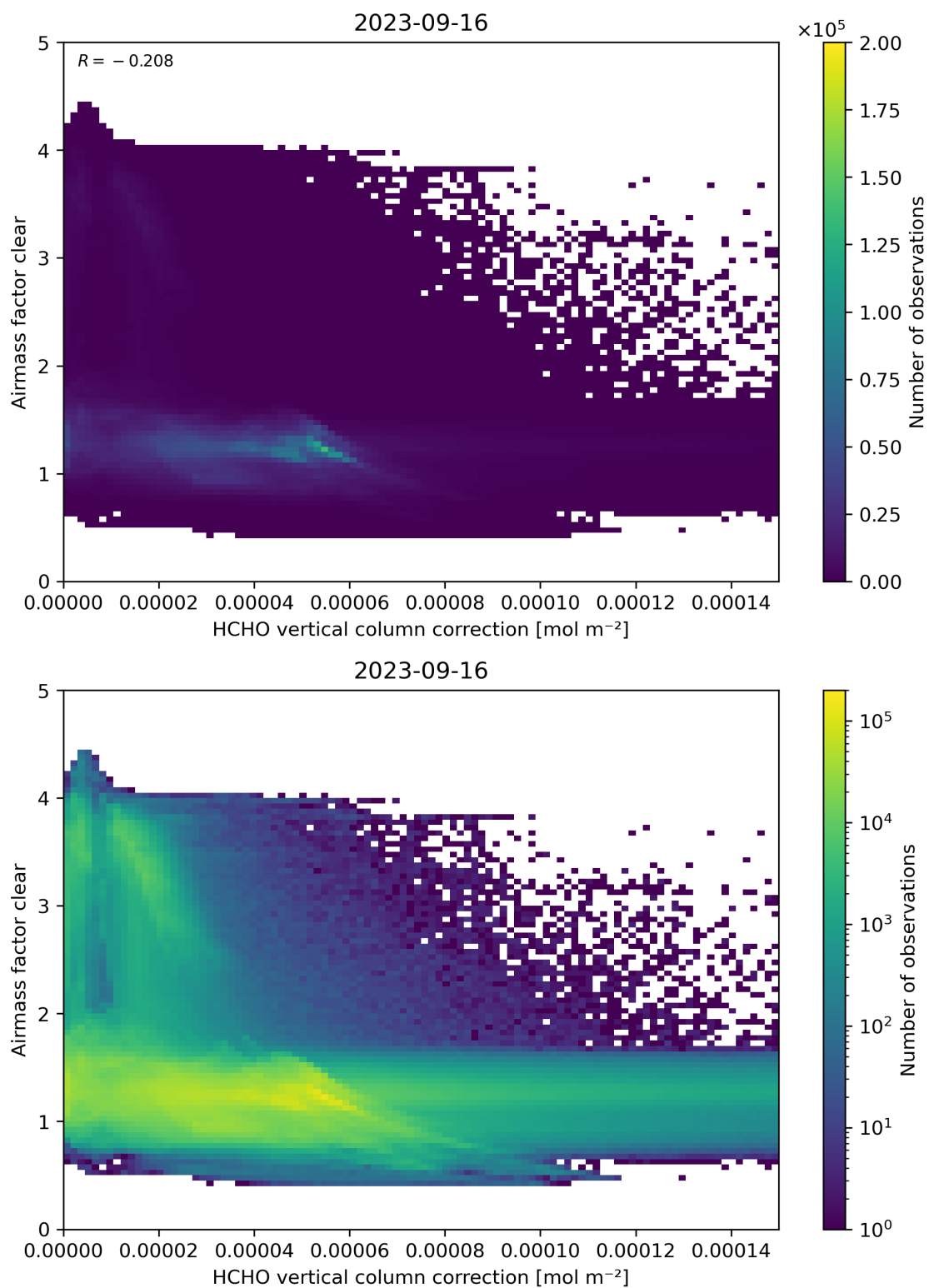
Figure 115: Scatter density plot of “HCHO vertical column correction” against “Airmass factor clear” for 2023-09-15 to 2023-09-17.
