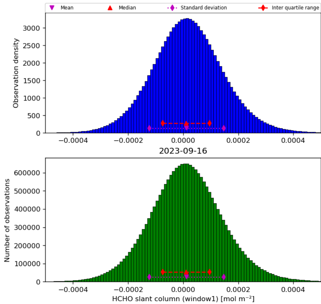
Figure 38: Histogram of “HCHO slant column (window1)” for 2023-09-15 to 2023-09-17
