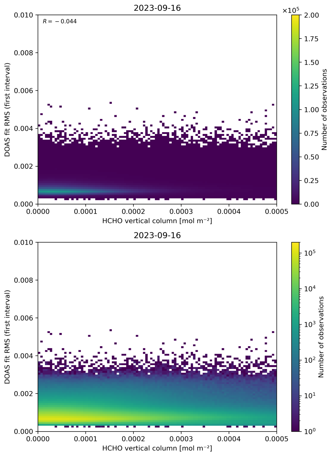
Figure 123: Scatter density plot of “HCHO vertical column” against “DOAS fit RMS (first interval)” for 2023-09-15 to 2023-09-17.
