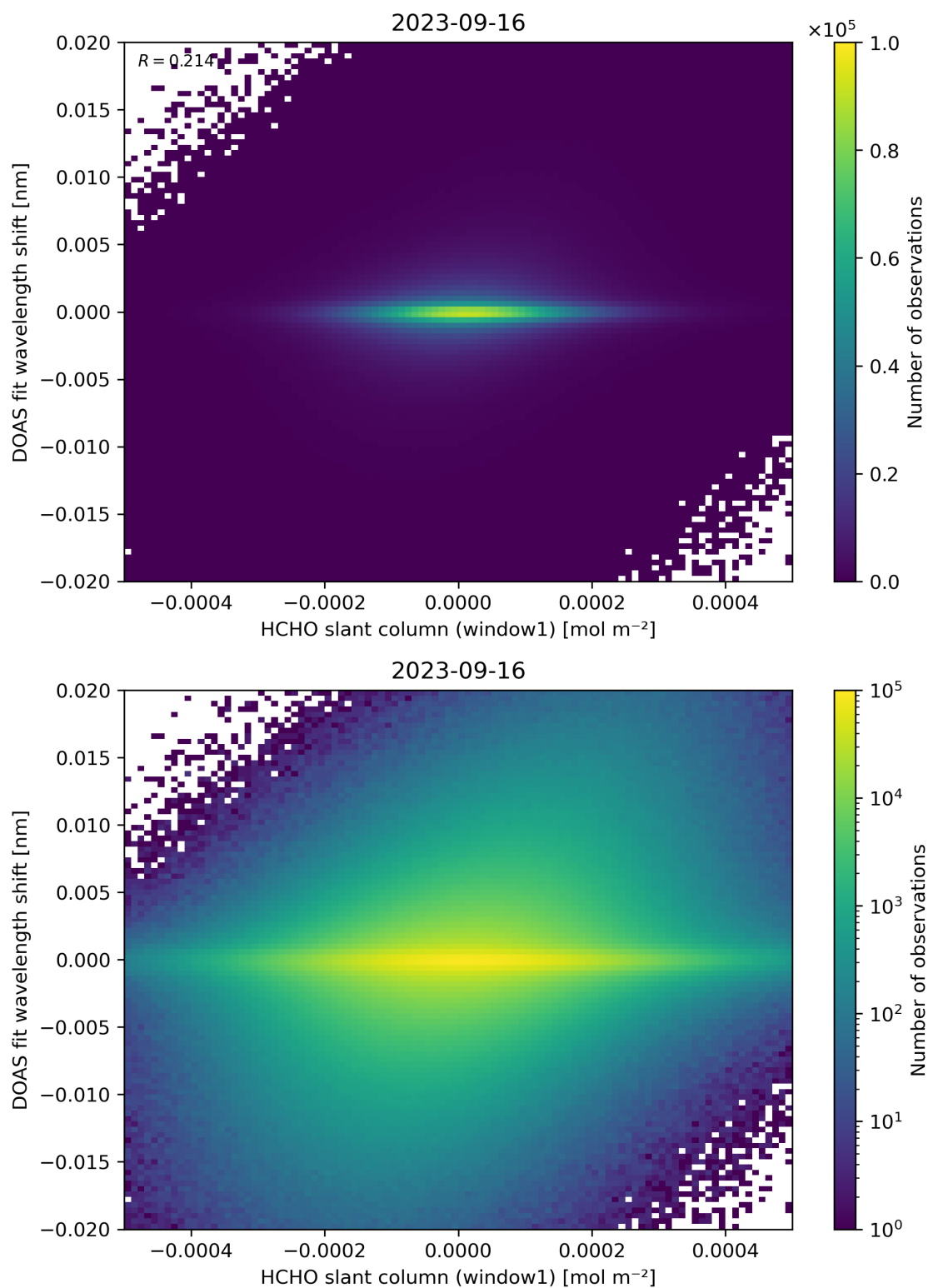
Figure 79: Scatter density plot of “HCHO slant column (window1)” against “DOAS fit wavelength shift” for 2023-09-15 to 2023-09-17.
