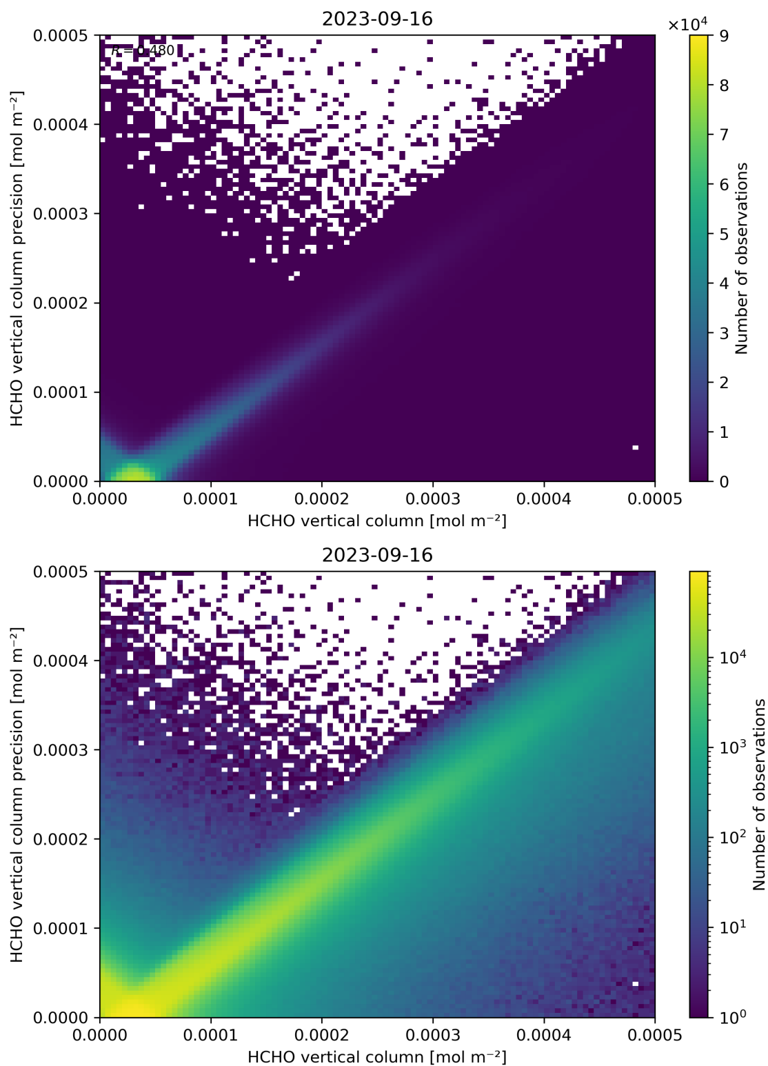
Figure 134: Scatter density plot of “HCHO vertical column” against “HCHO vertical column precision” for 2023-09-15 to 2023-09-17.
