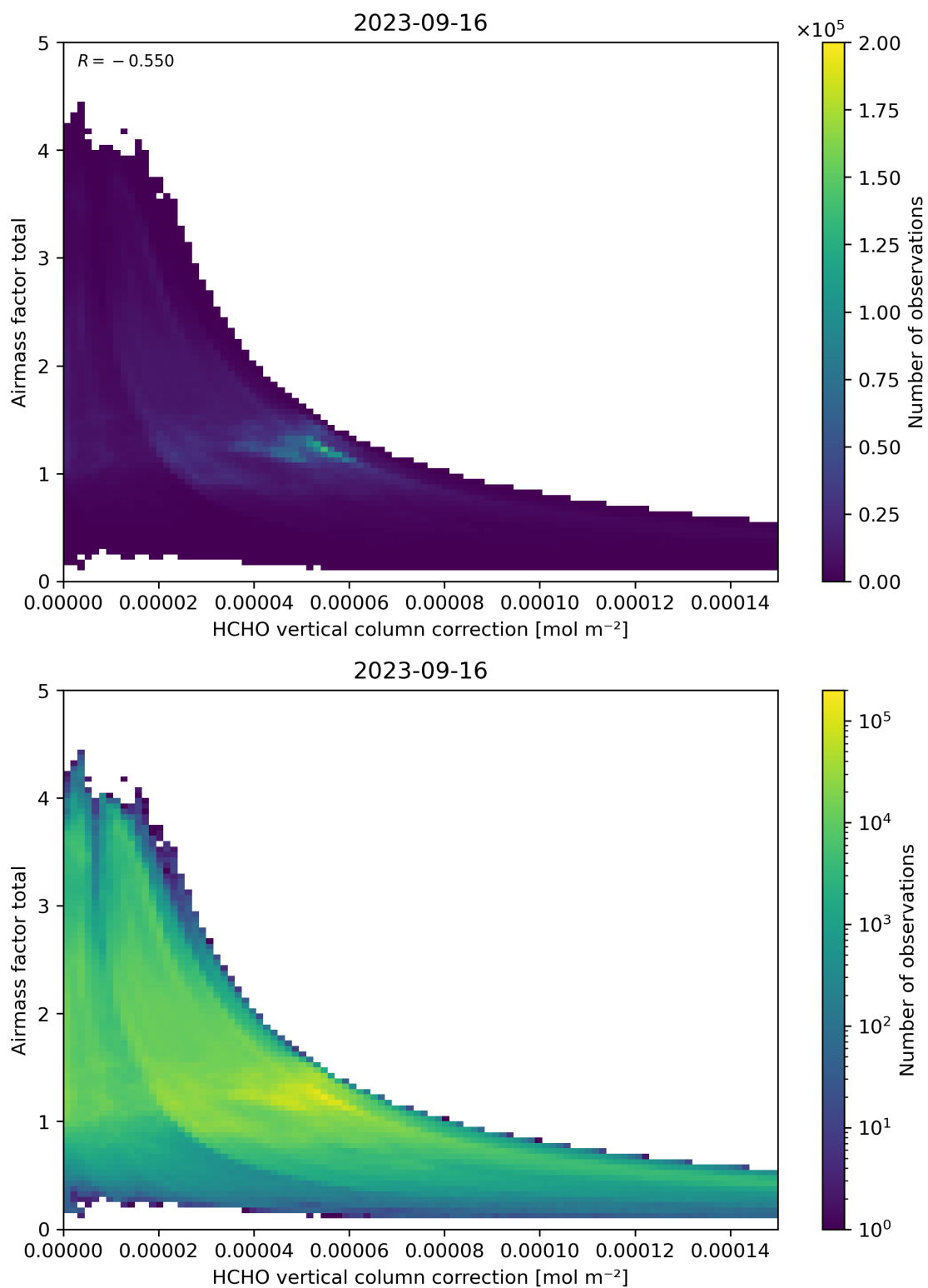
Figure 120: Scatter density plot of “HCHO vertical column correction” against “Airmass factor total” for 2023-09-15 to 2023-09-17.
