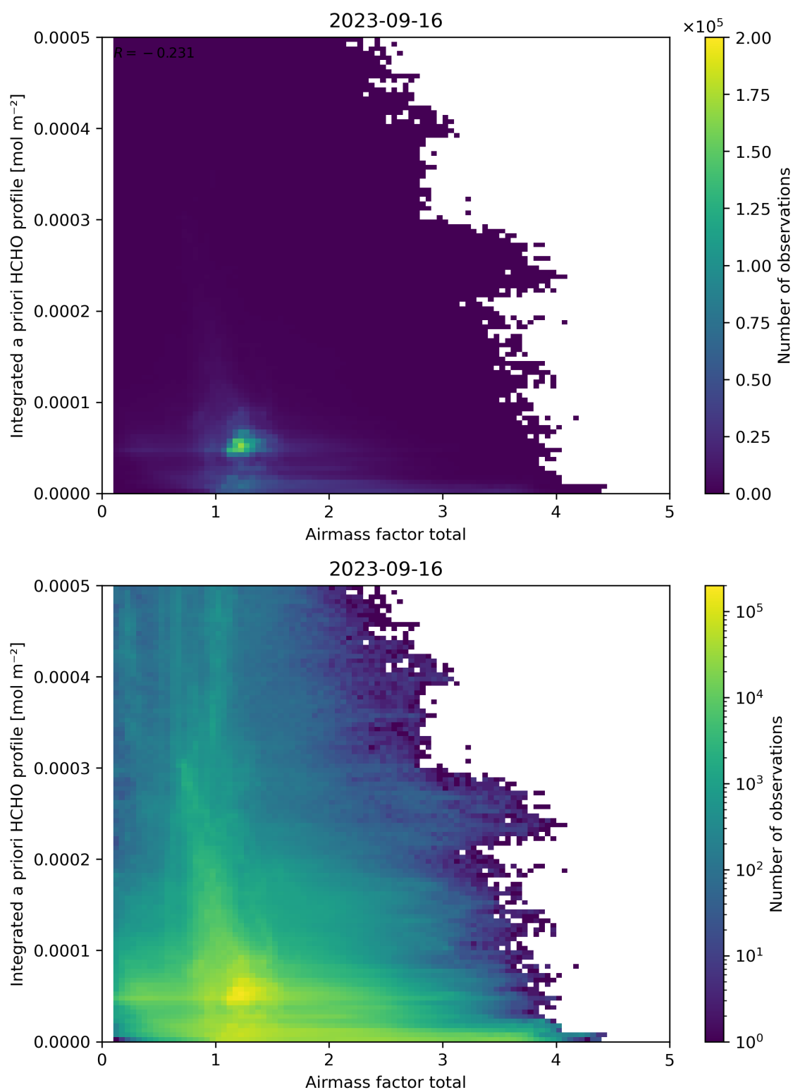
Figure 104: Scatter density plot of “Airmass factor total” against “Integrated a priori HCHO profile” for 2023-09-15 to 2023-09-17.
