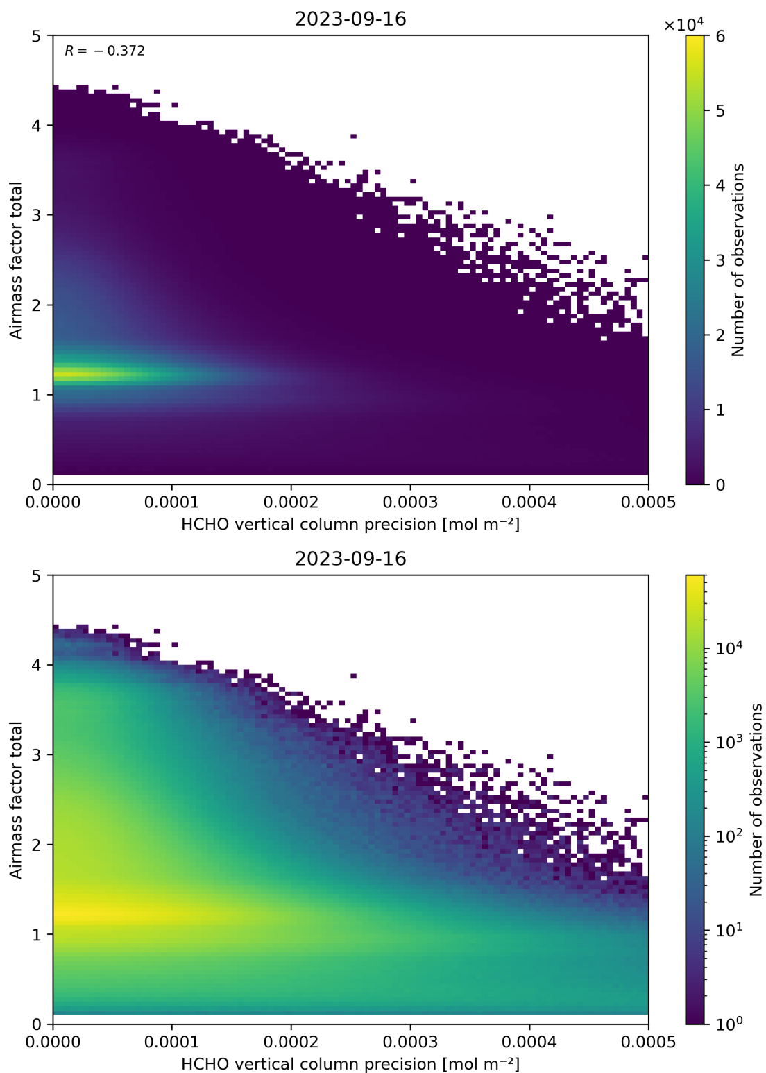
Figure 144: Scatter density plot of “HCHO vertical column precision” against “Airmass factor total” for 2023-09-15 to 2023-09-17.
