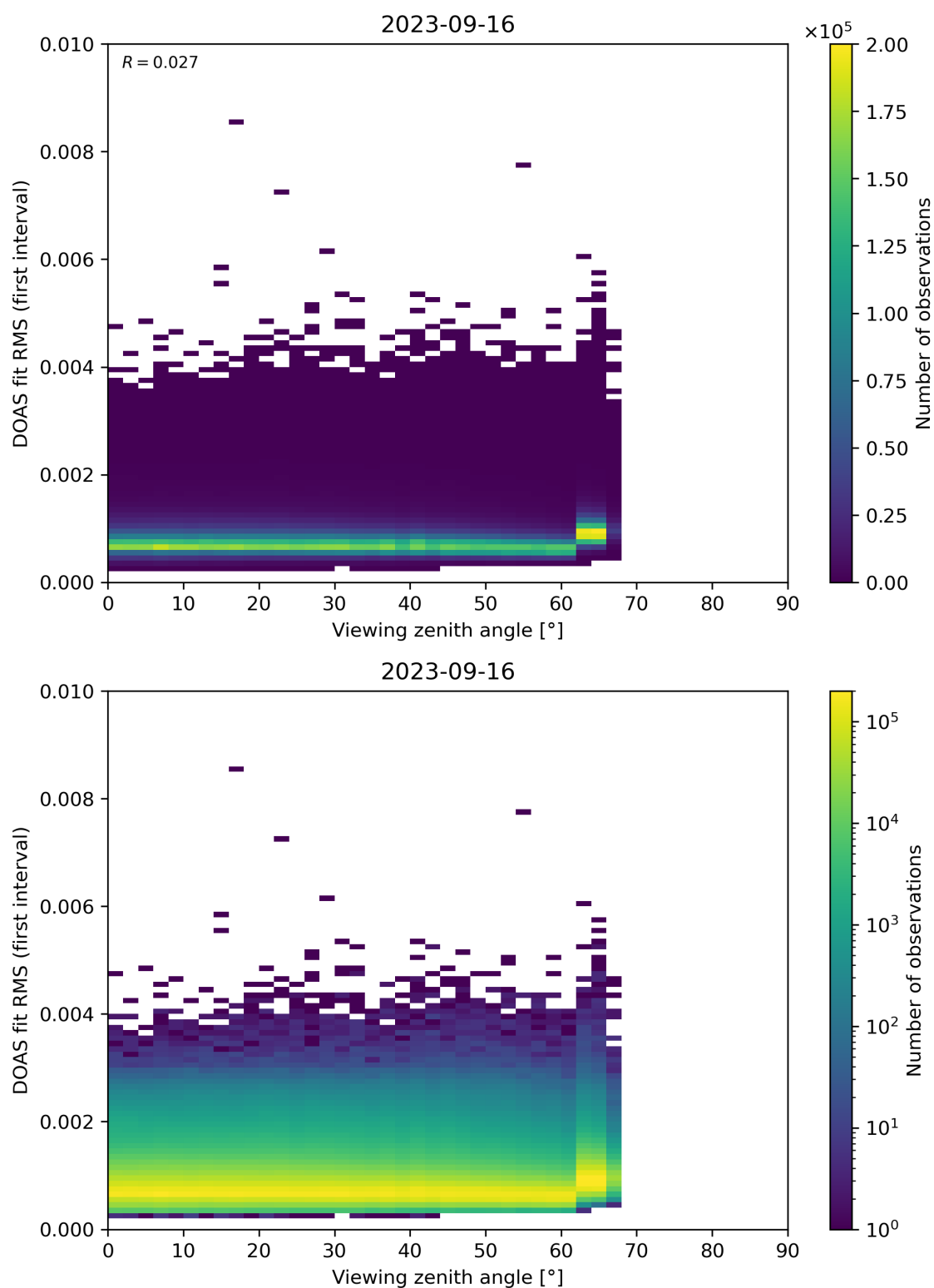
Figure 182: Scatter density plot of “Viewing zenith angle” against “DOAS fit RMS (first interval)” for 2023-09-15 to 2023-09-17.
