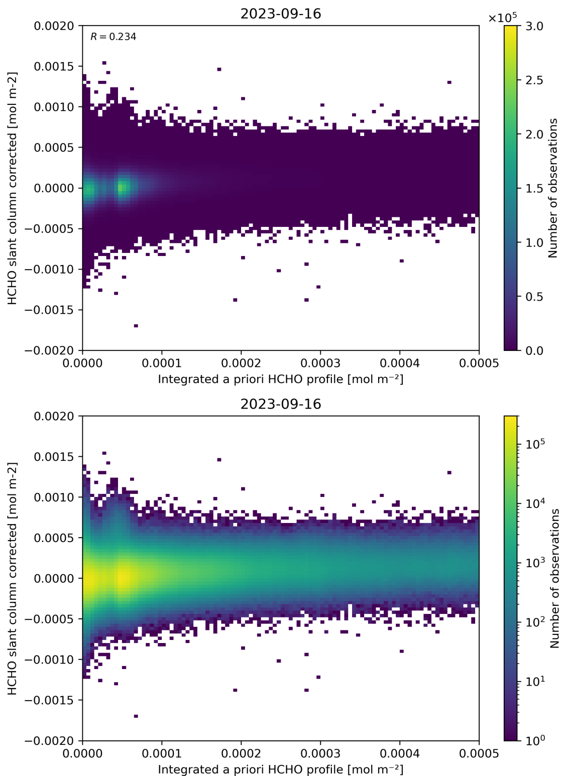
Figure 151: Scatter density plot of “Integrated a priori HCHO profile” against “HCHO slant column corrected” for 2023-09-15 to 2023-09-17.
