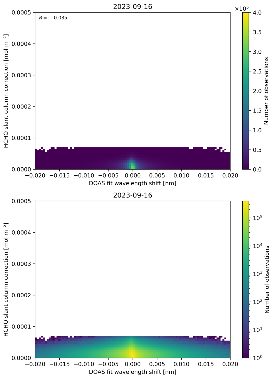
Figure 67: Scatter density plot of “DOAS fit wavelength shift” against “HCHO slant column correction” for 2023-09-15 to 2023-09-17.
