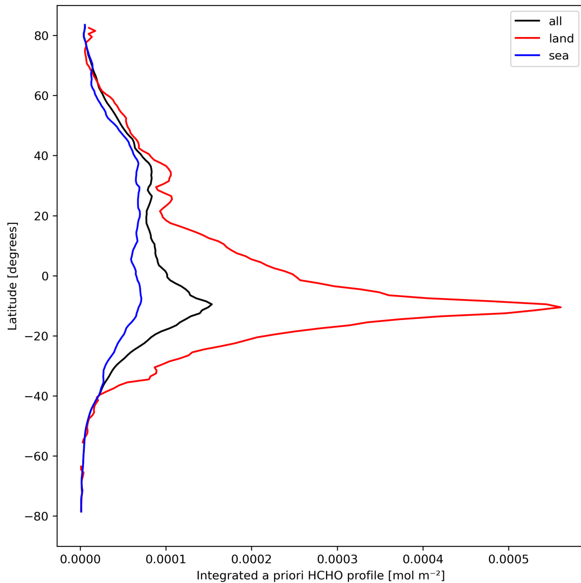
Figure 29: Zonal average of “Integrated a priori HCHO profile” for 2023-09-15 to 2023-09-17.
