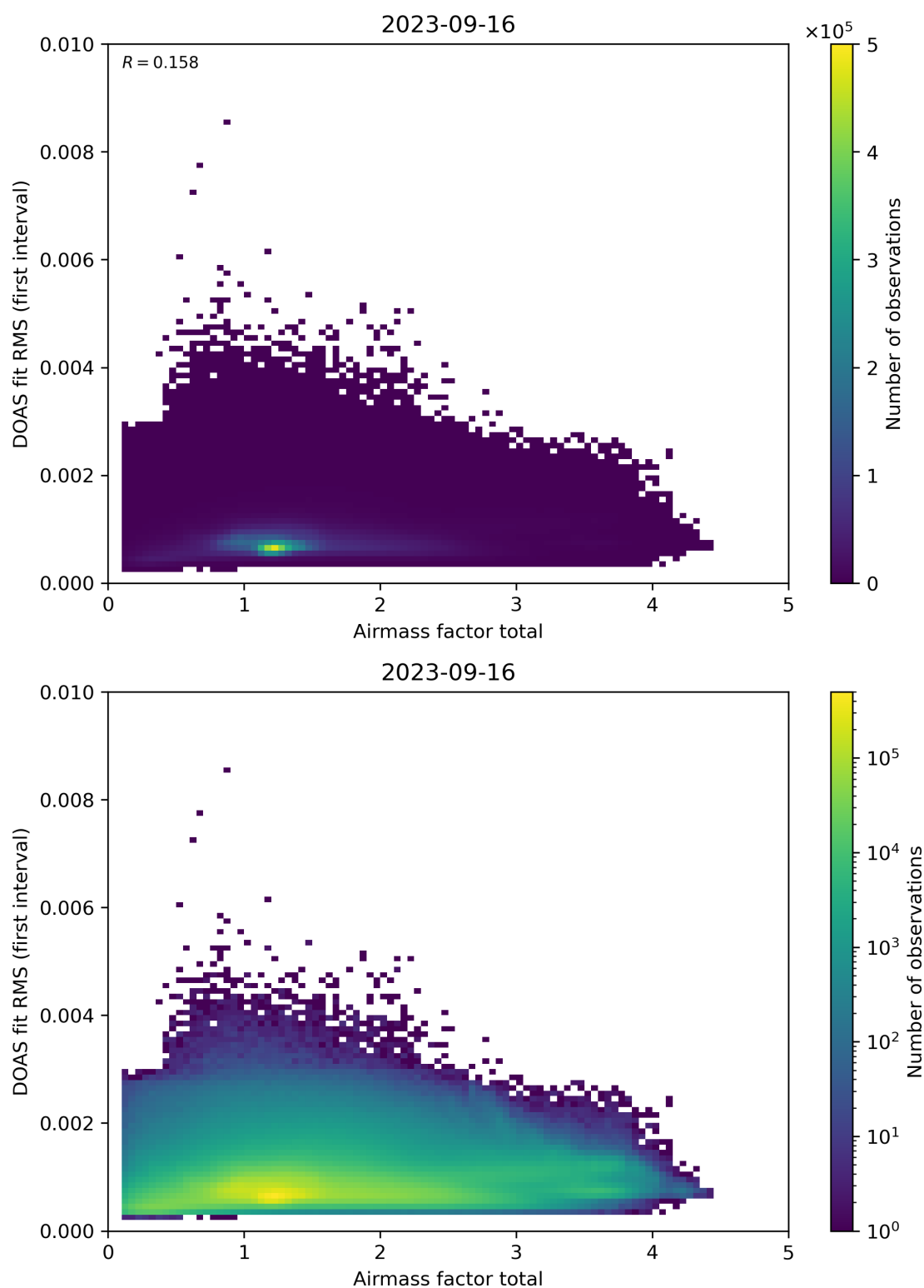
Figure 97: Scatter density plot of “Airmass factor total” against “DOAS fit RMS (first interval)” for 2023-09-15 to 2023-09-17.
