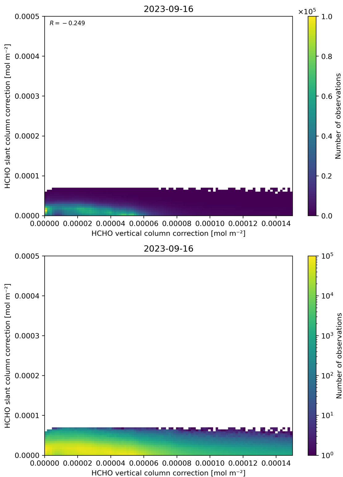
Figure 117: Scatter density plot of “HCHO vertical column correction” against “HCHO slant column correction” for 2023-09-15 to 2023-09-17.
