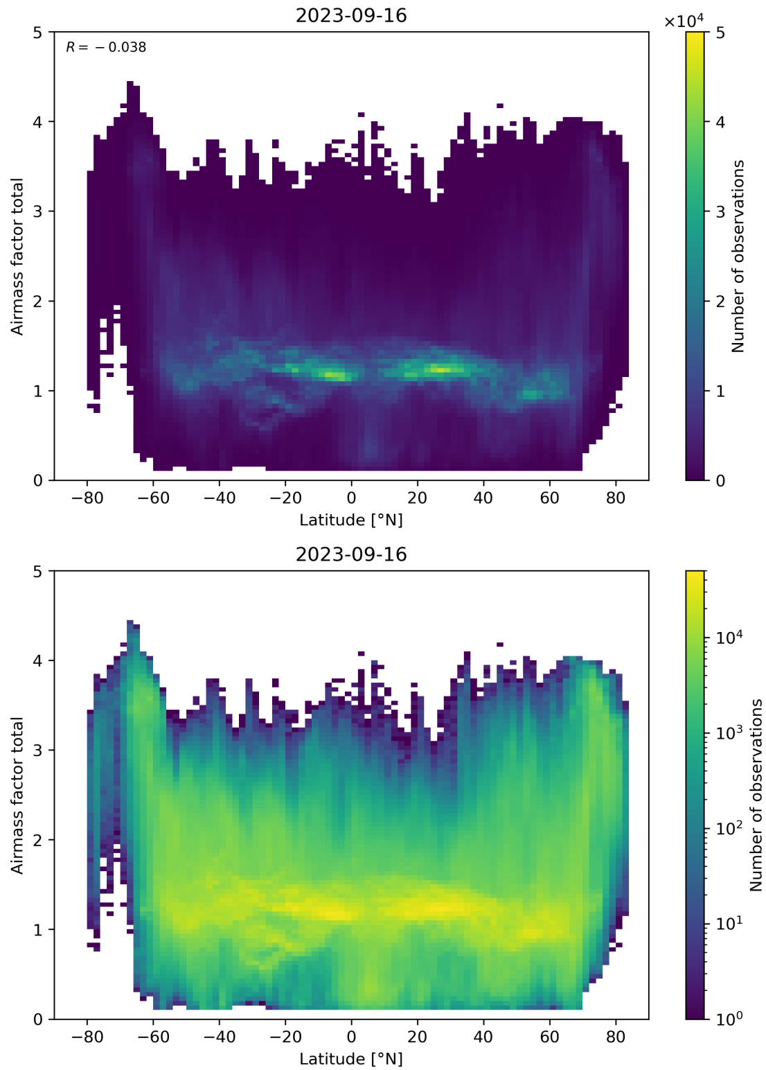
Figure 161: Scatter density plot of “Latitude” against “Airmass factor total” for 2023-09-15 to 2023-09-17.
