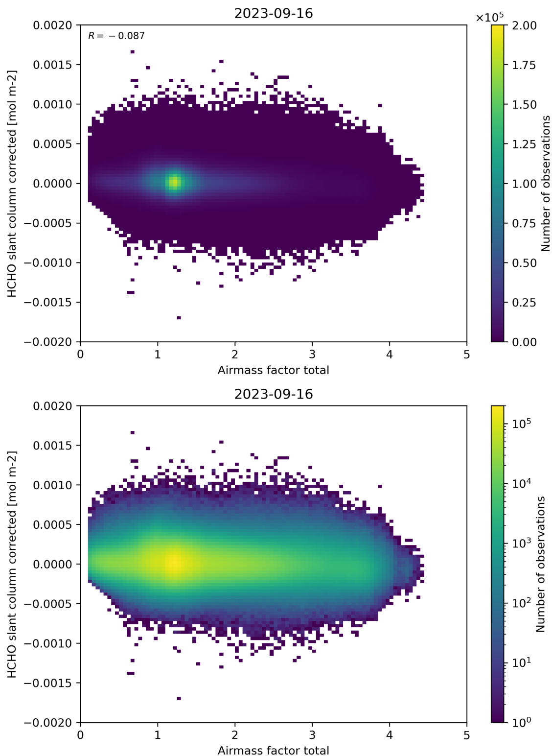
Figure 101: Scatter density plot of “Airmass factor total” against “HCHO slant column corrected” for 2023-09-15 to 2023-09-17.
