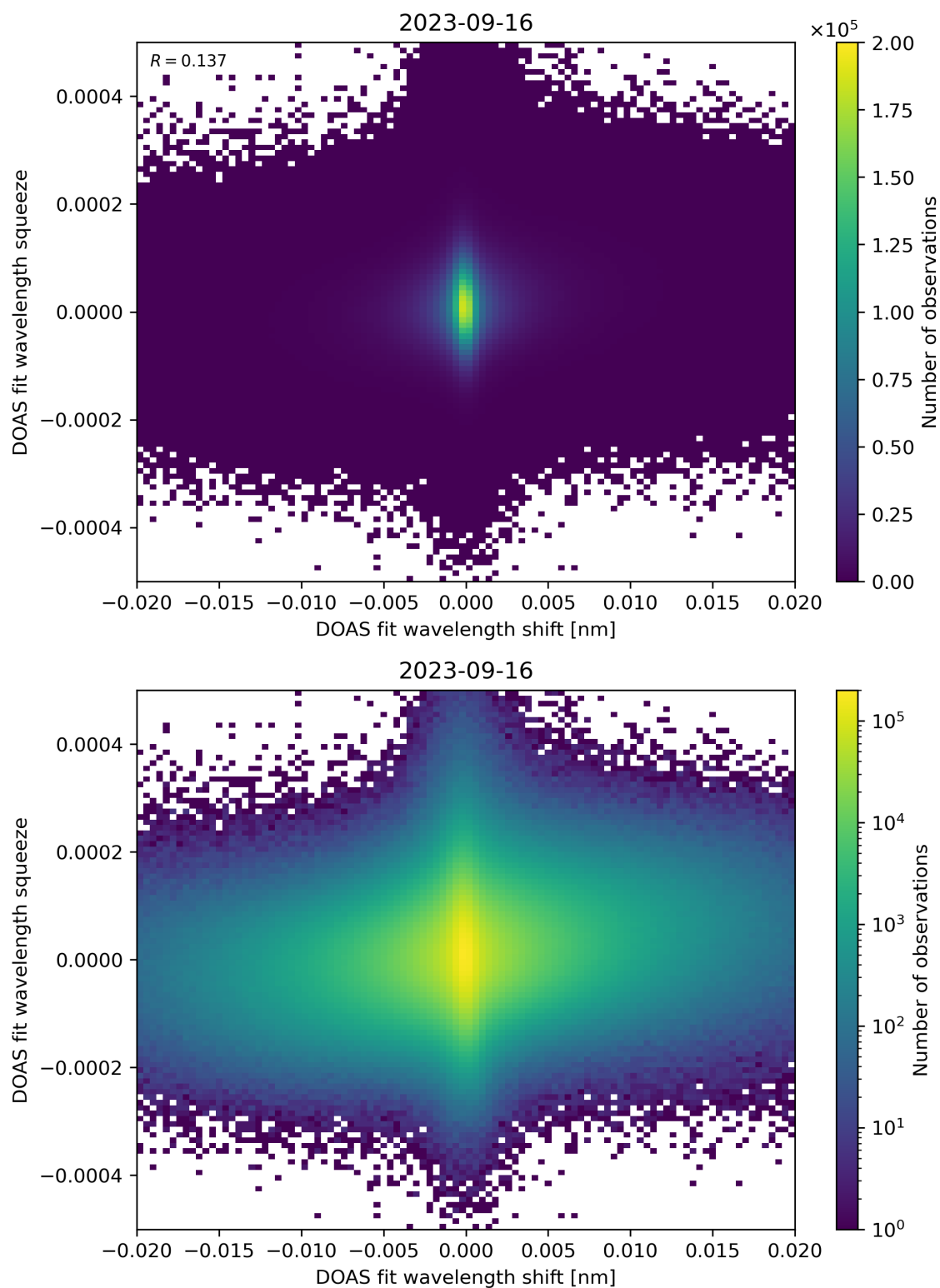
Figure 65: Scatter density plot of “DOAS fit wavelength shift” against “DOAS fit wavelength squeeze” for 2023-09-15 to 2023-09-17.
