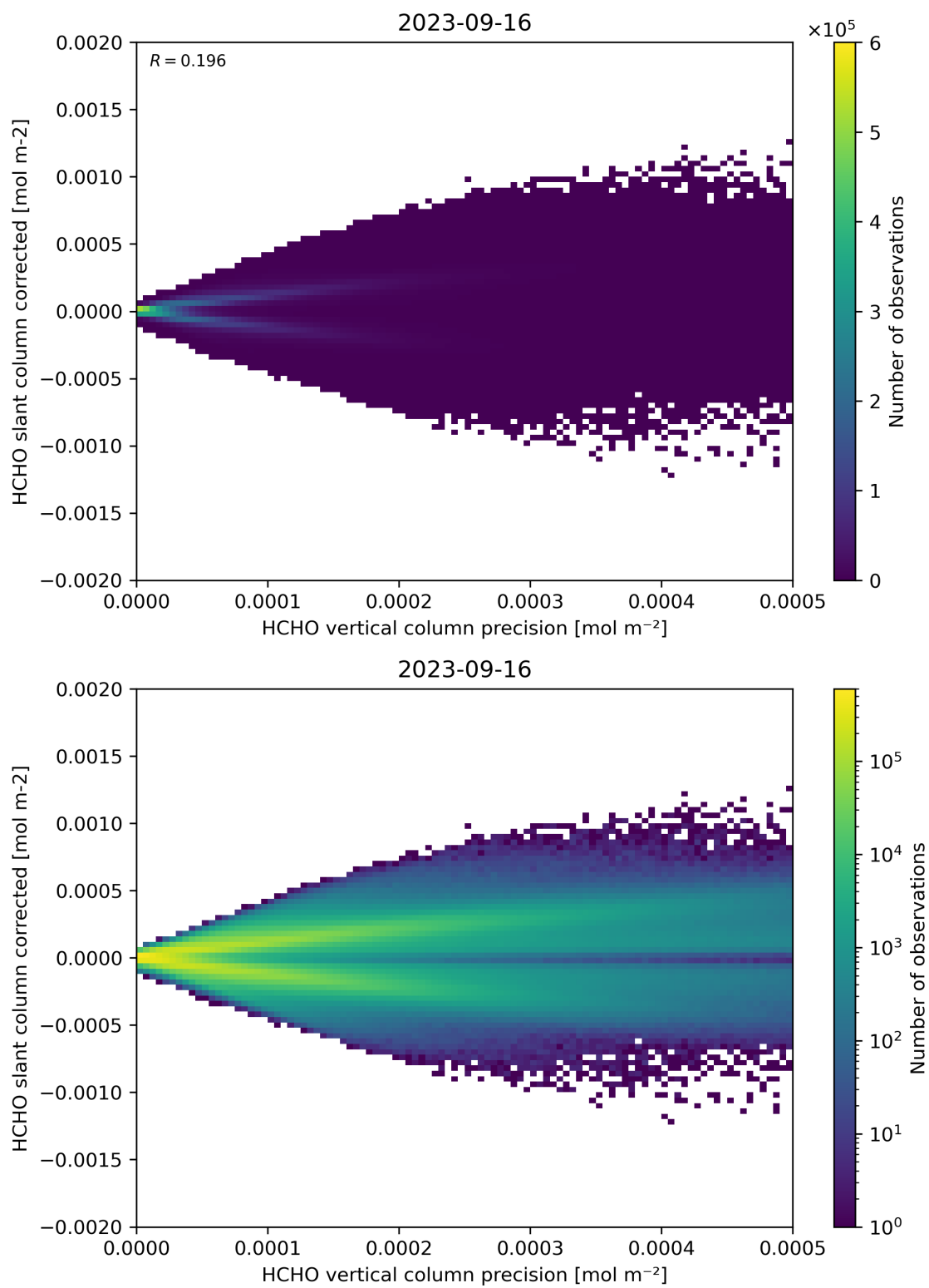
Figure 140: Scatter density plot of “HCHO vertical column precision” against “HCHO slant column corrected” for 2023-09-15 to 2023-09-17.
