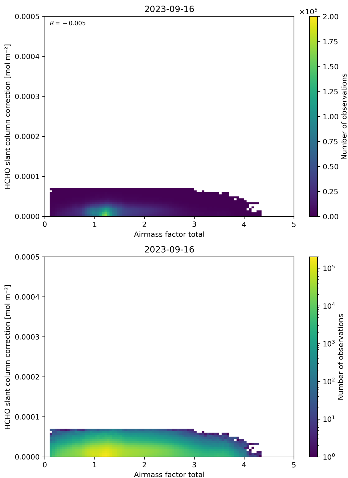
Figure 102: Scatter density plot of “Airmass factor total” against “HCHO slant column correction” for 2023-09-15 to 2023-09-17.
