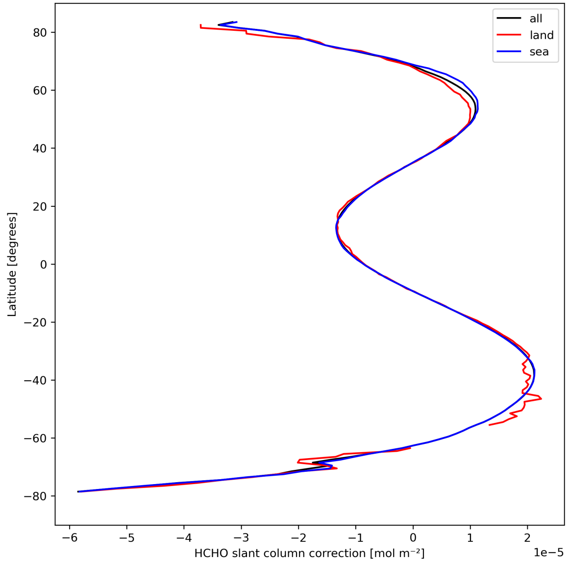
Figure 33: Zonal average of “HCHO slant column correction” for 2023-09-15 to 2023-09-17.
