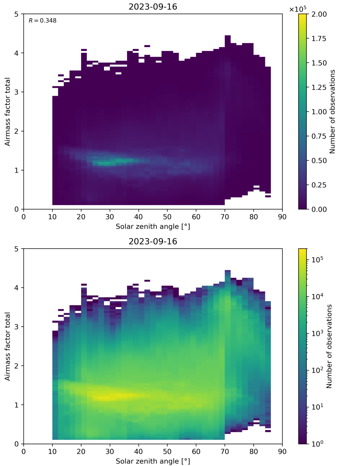
Figure 175: Scatter density plot of “Solar zenith angle” against “Airmass factor total” for 2023-09-15 to 2023-09-17.
