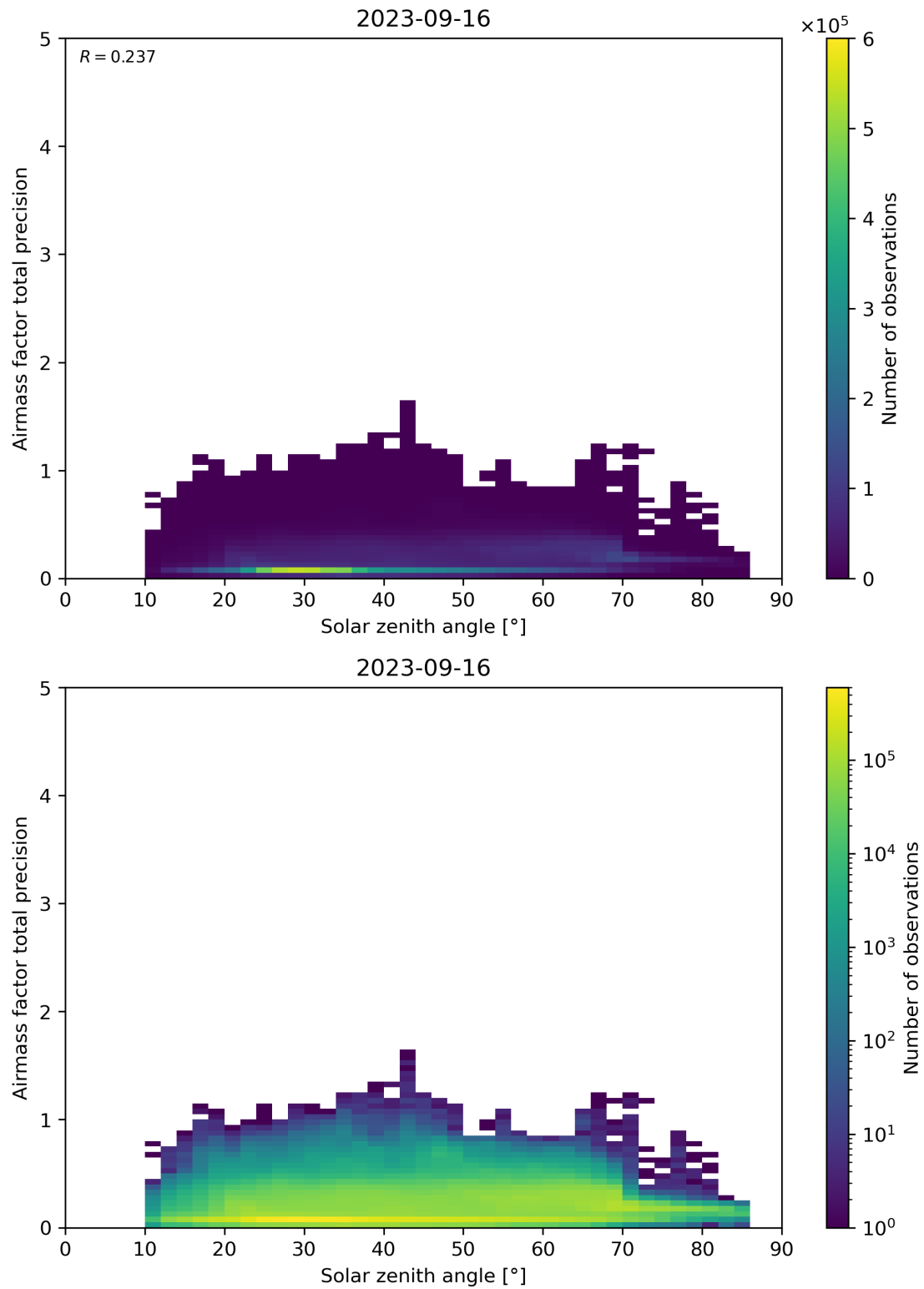
Figure 176: Scatter density plot of “Solar zenith angle” against “Airmass factor total precision” for 2023-09-15 to 2023-09-17.
