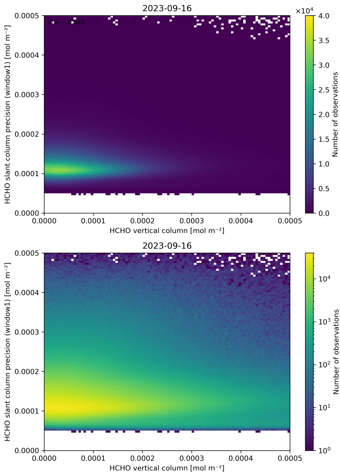
Figure 130: Scatter density plot of “HCHO vertical column” against “HCHO slant column precision (window1)” for 2023-09-15 to 2023-09-17.
