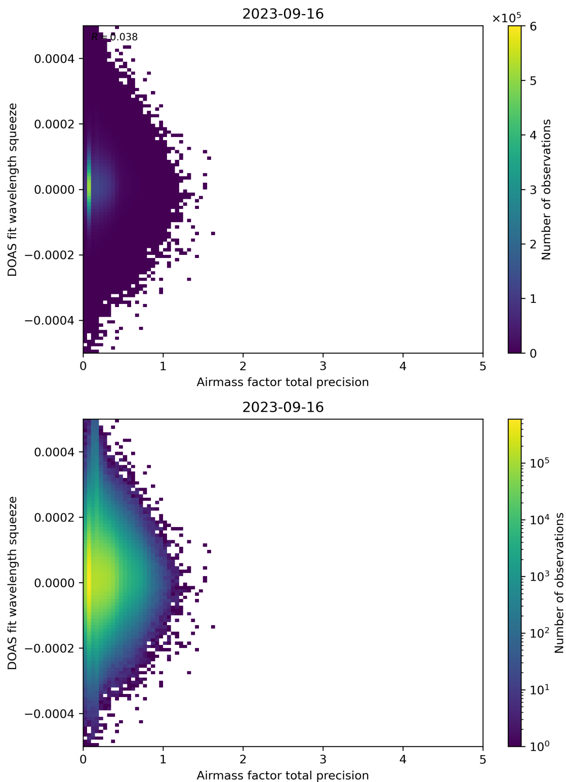
Figure 107: Scatter density plot of “Airmass factor total precision” against “DOAS fit wavelength squeeze” for 2023-09-15 to 2023-09-17.
