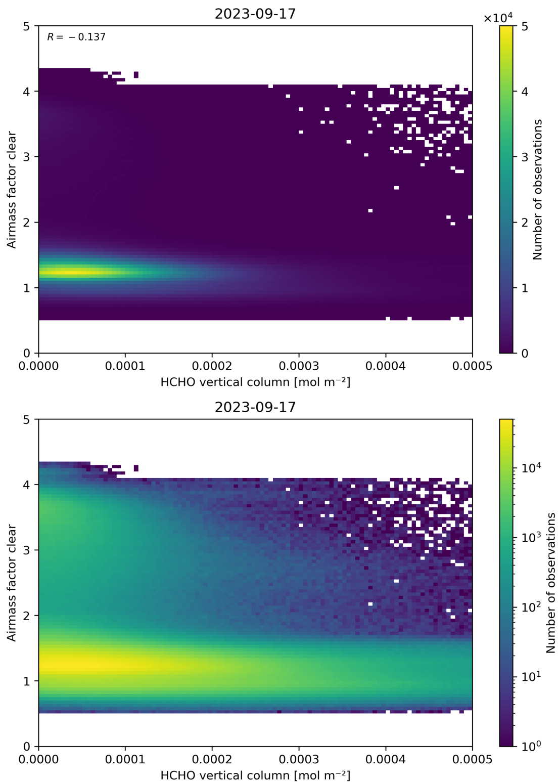
Figure 126: Scatter density plot of “HCHO vertical column” against “Airmass factor clear” for 2023-09-16 to 2023-09-18.
