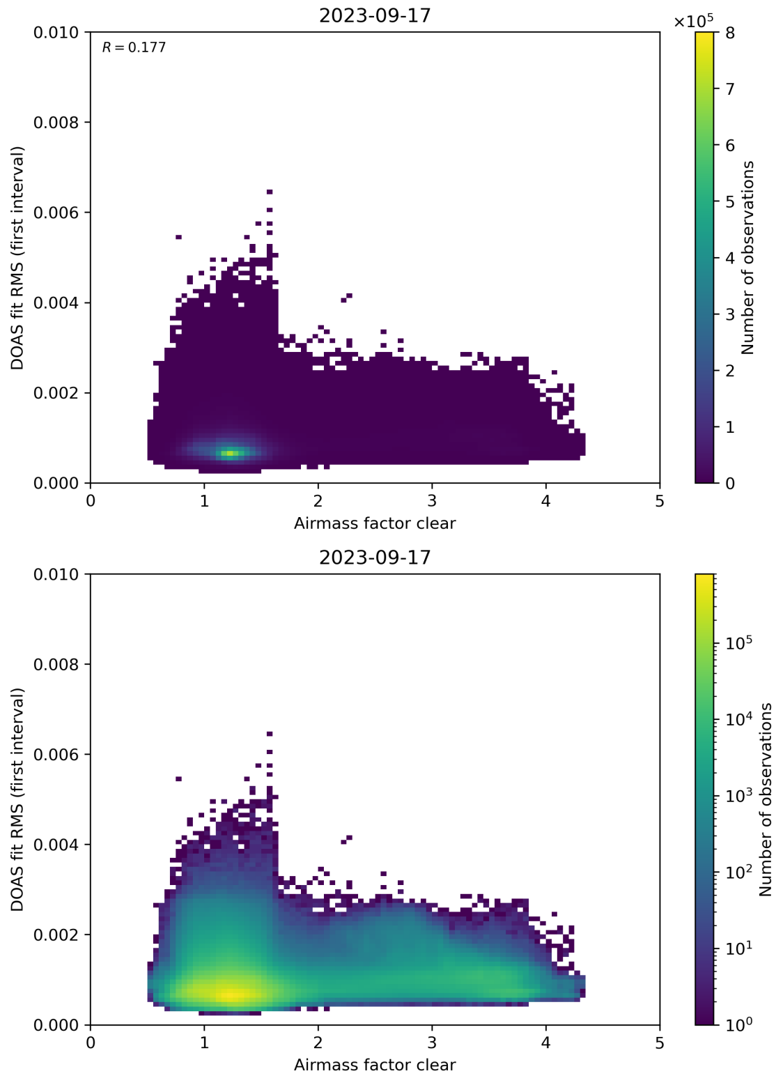
Figure 71: Scatter density plot of “Airmass factor clear” against “DOAS fit RMS (first interval)” for 2023-09-16 to 2023-09-18.
