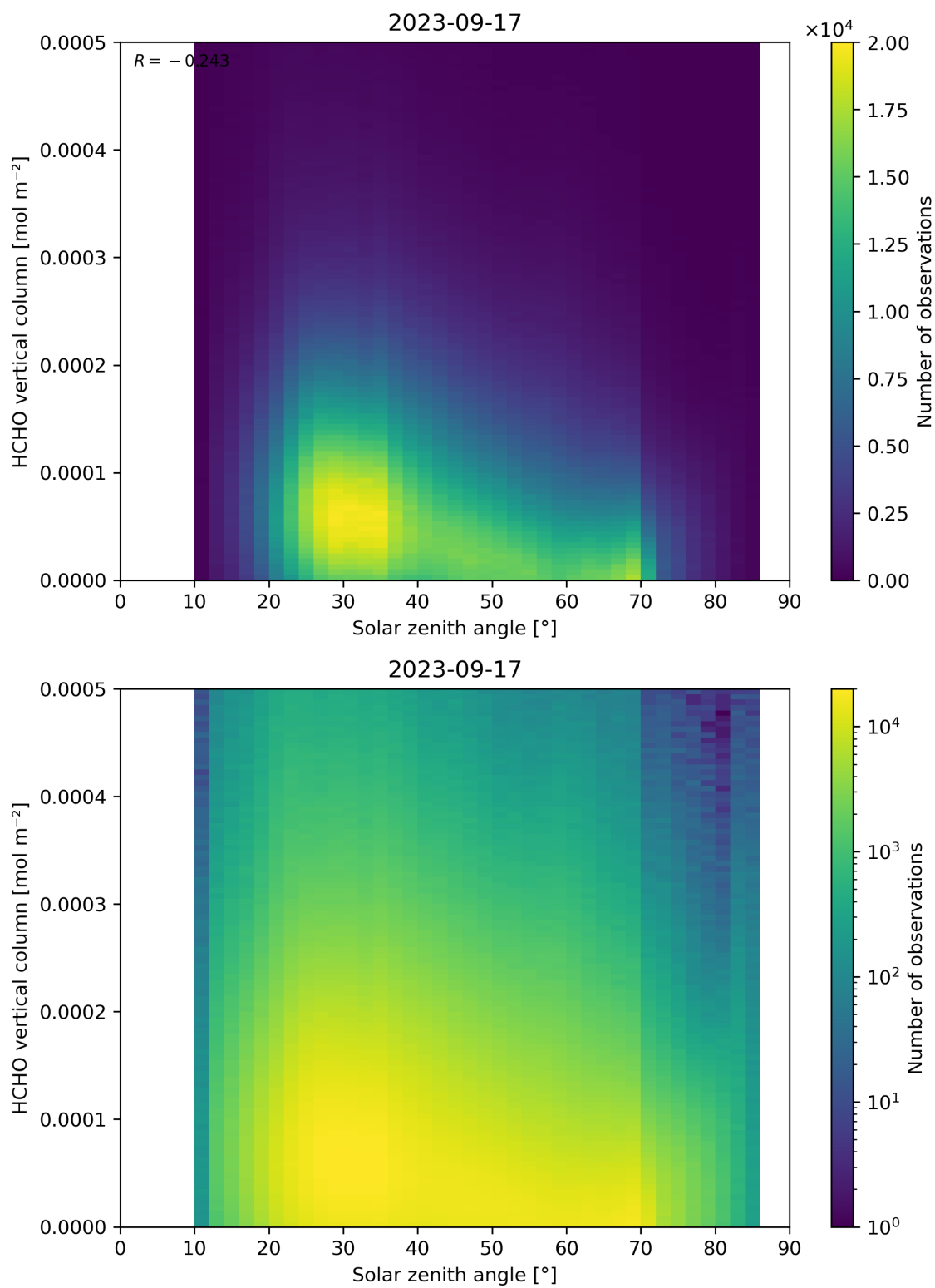
Figure 177: Scatter density plot of “Solar zenith angle” against “HCHO vertical column” for 2023-09-16 to 2023-09-18.
