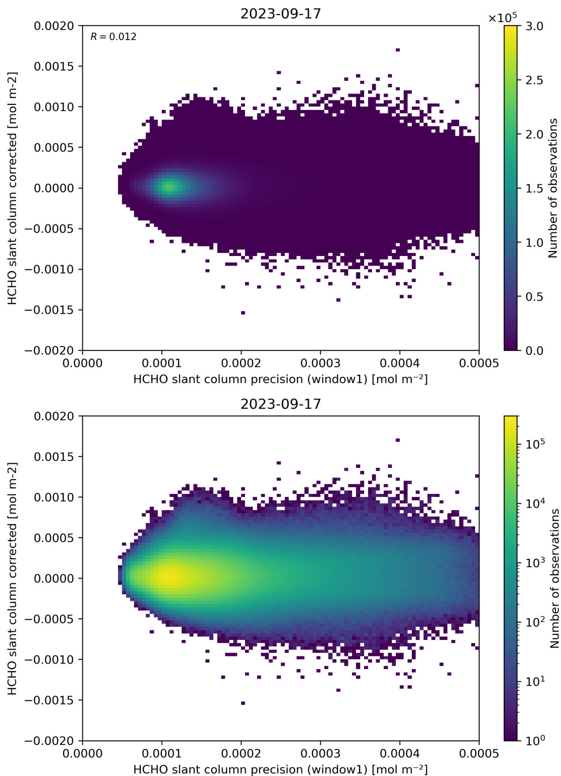
Figure 92: Scatter density plot of “HCHO slant column precision (window1)” against “HCHO slant column corrected” for 2023-09-16 to 2023-09-18.
