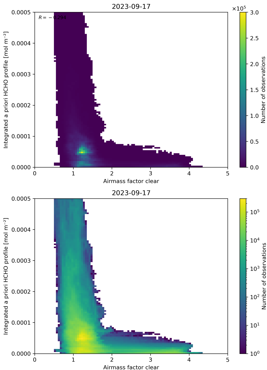
Figure 76: Scatter density plot of “Airmass factor clear” against “Integrated a priori HCHO profile” for 2023-09-16 to 2023-09-18.
