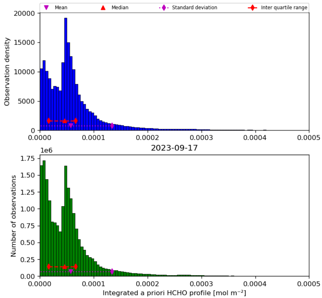
Figure 43: Histogram of “Integrated a priori HCHO profile” for 2023-09-16 to 2023-09-18
