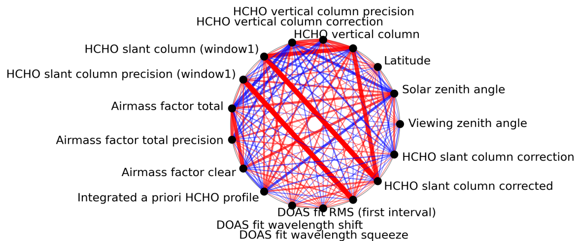
Figure 1: Map of correlation graph for 2023-09-16 to 2023-09-18.
