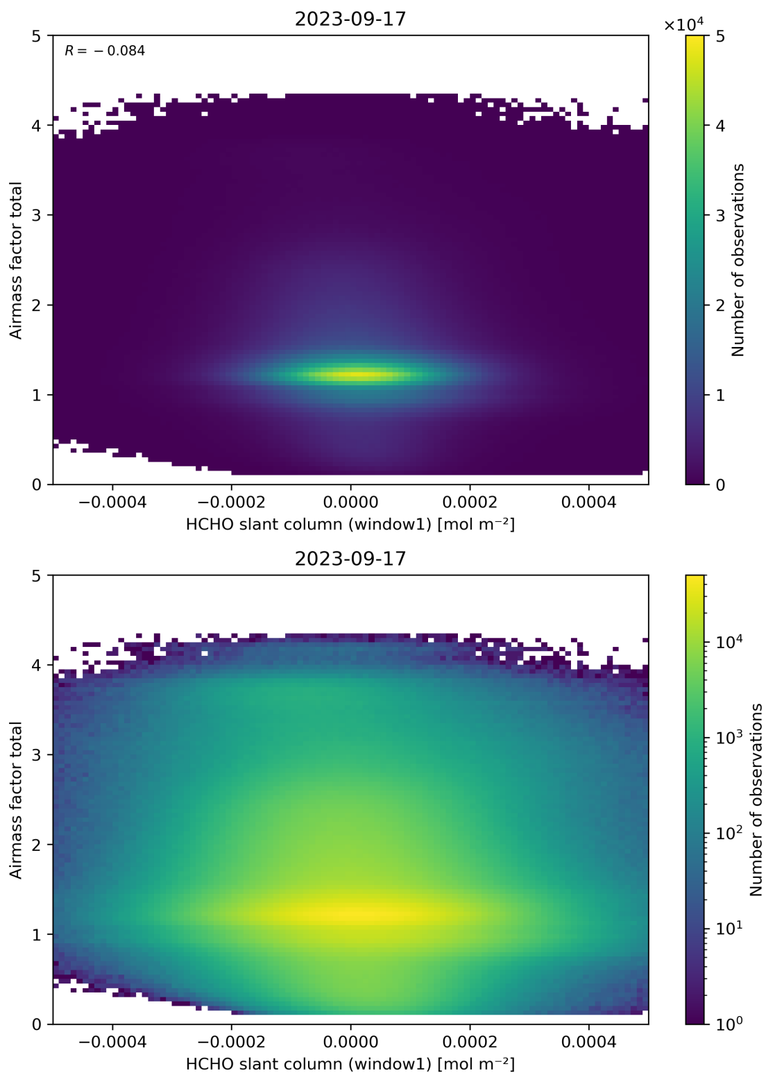
Figure 85: Scatter density plot of “HCHO slant column (window1)” against “Airmass factor total” for 2023-09-16 to 2023-09-18.
