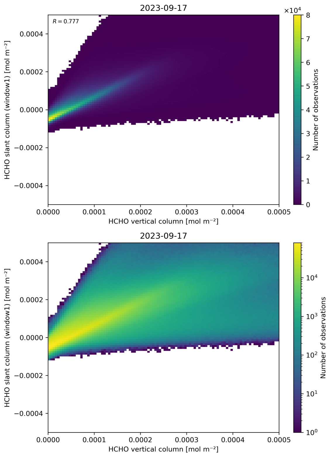
Figure 129: Scatter density plot of “HCHO vertical column” against “HCHO slant column (window1)” for 2023-09-16 to 2023-09-18.
