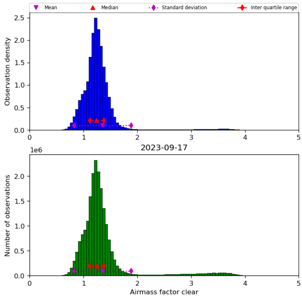
Figure 42: Histogram of “Airmass factor clear” for 2023-09-16 to 2023-09-18
