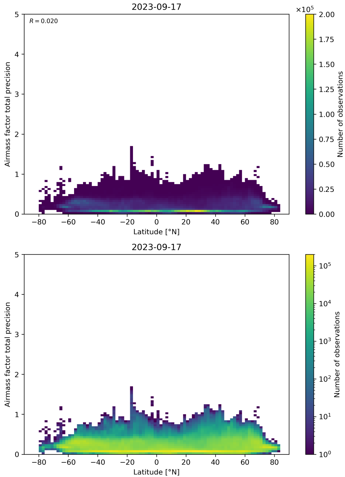
Figure 162: Scatter density plot of “Latitude” against “Airmass factor total precision” for 2023-09-16 to 2023-09-18.
