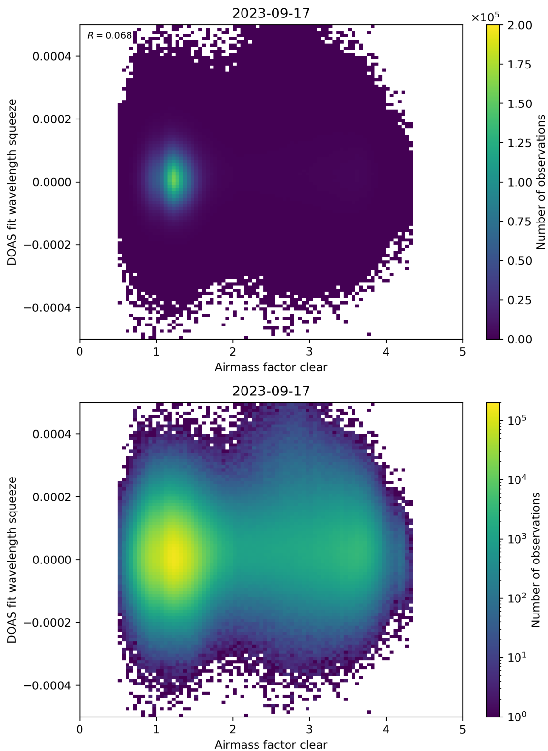
Figure 73: Scatter density plot of “Airmass factor clear” against “DOAS fit wavelength squeeze” for 2023-09-16 to 2023-09-18.
