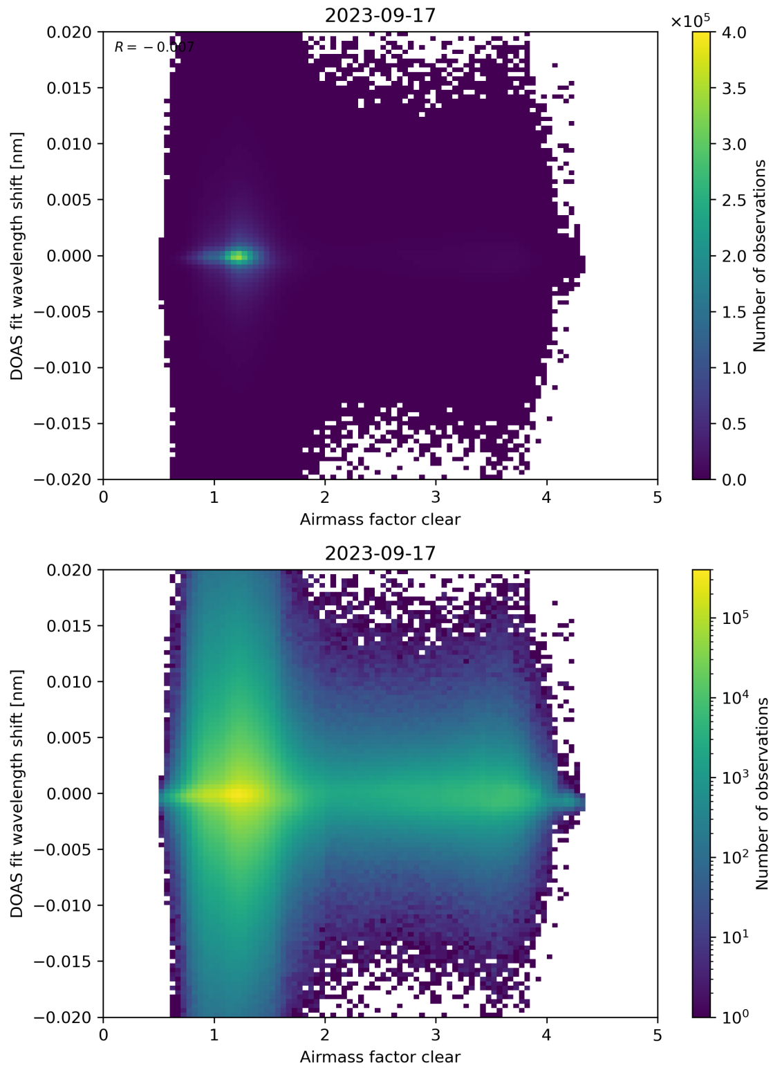
Figure 72: Scatter density plot of “Airmass factor clear” against “DOAS fit wavelength shift” for 2023-09-16 to 2023-09-18.
