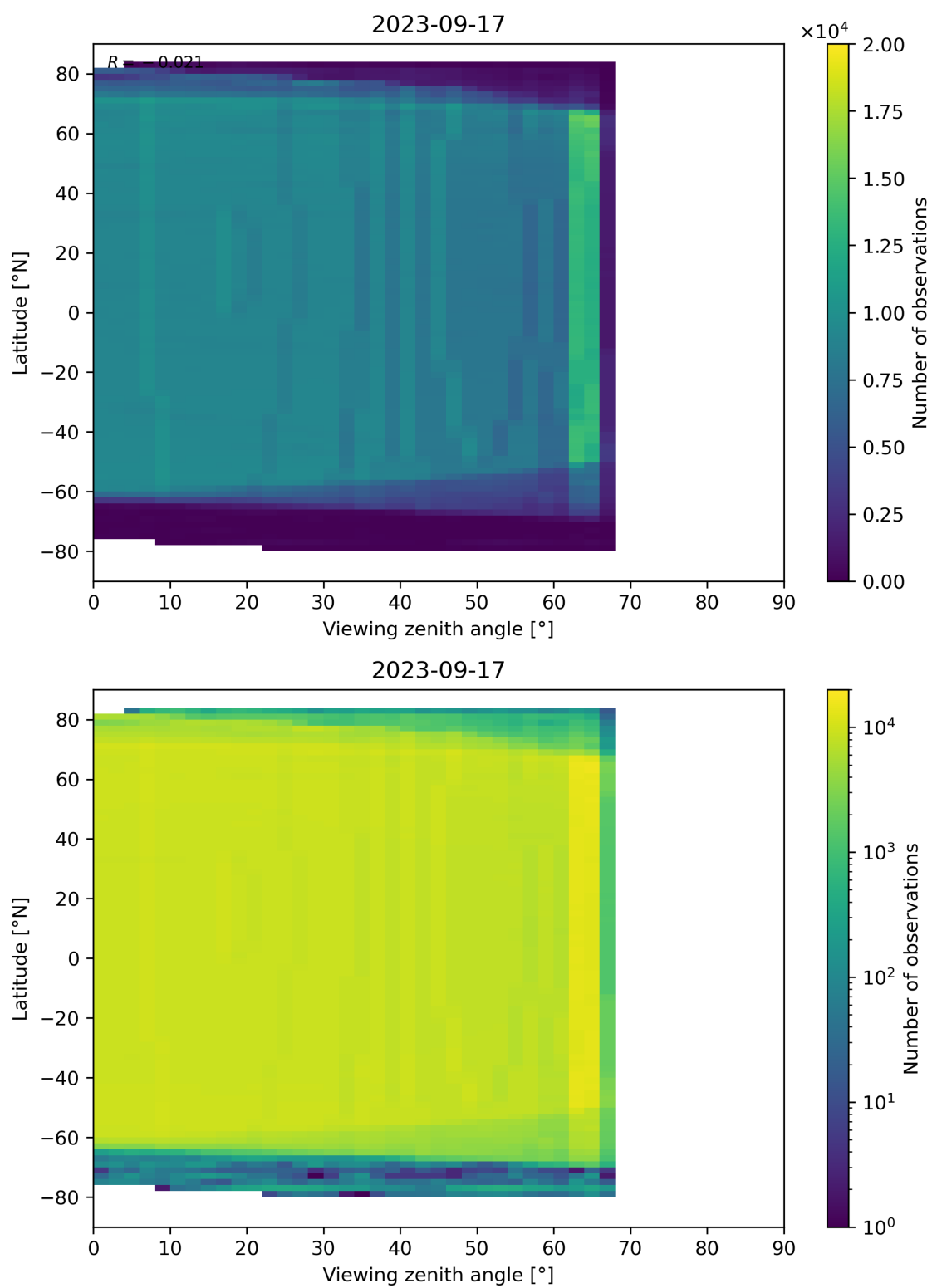
Figure 196: Scatter density plot of “Viewing zenith angle” against “Latitude” for 2023-09-16 to 2023-09-18.
