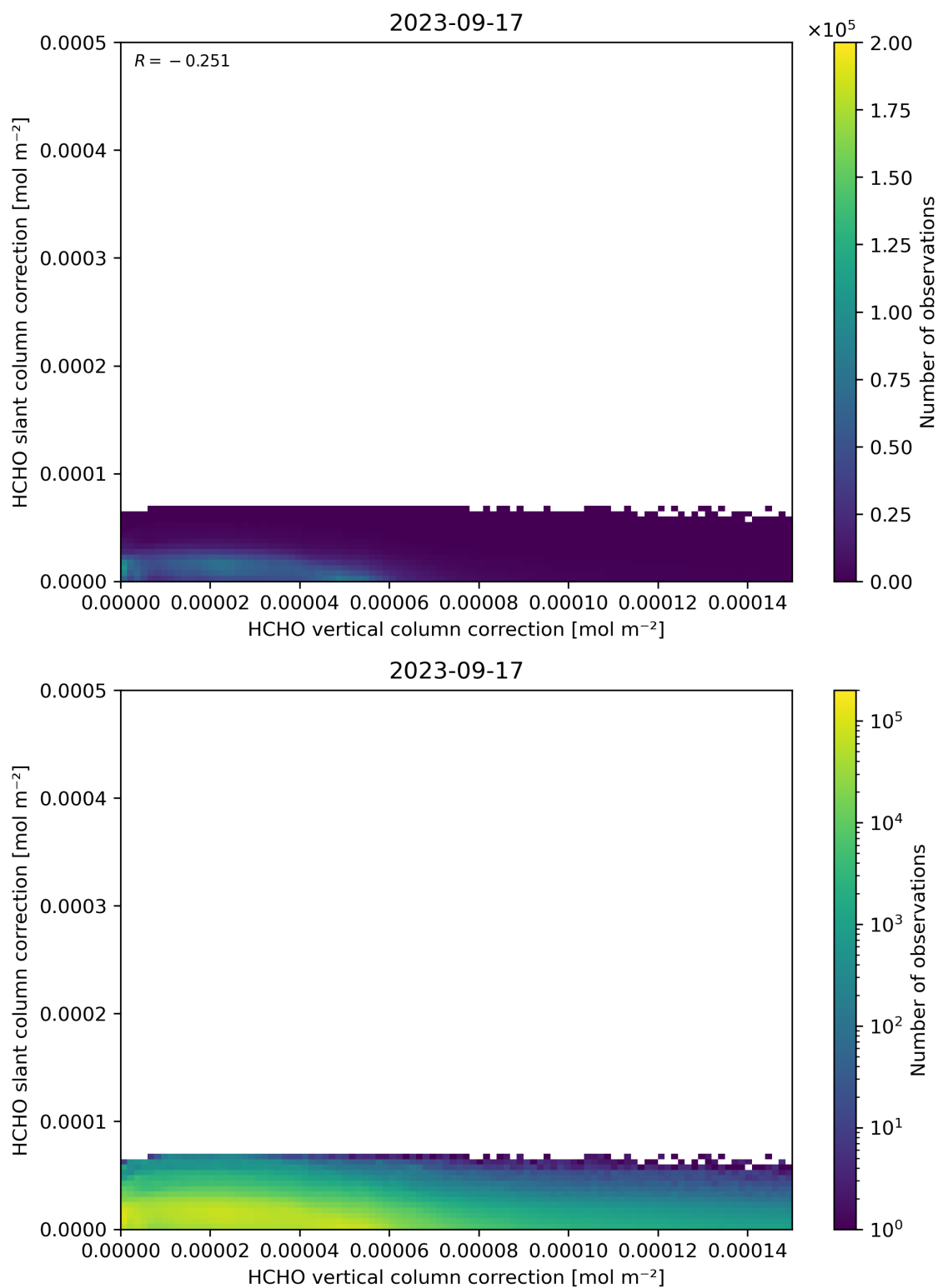
Figure 117: Scatter density plot of “HCHO vertical column correction” against “HCHO slant column correction” for 2023-09-16 to 2023-09-18.
