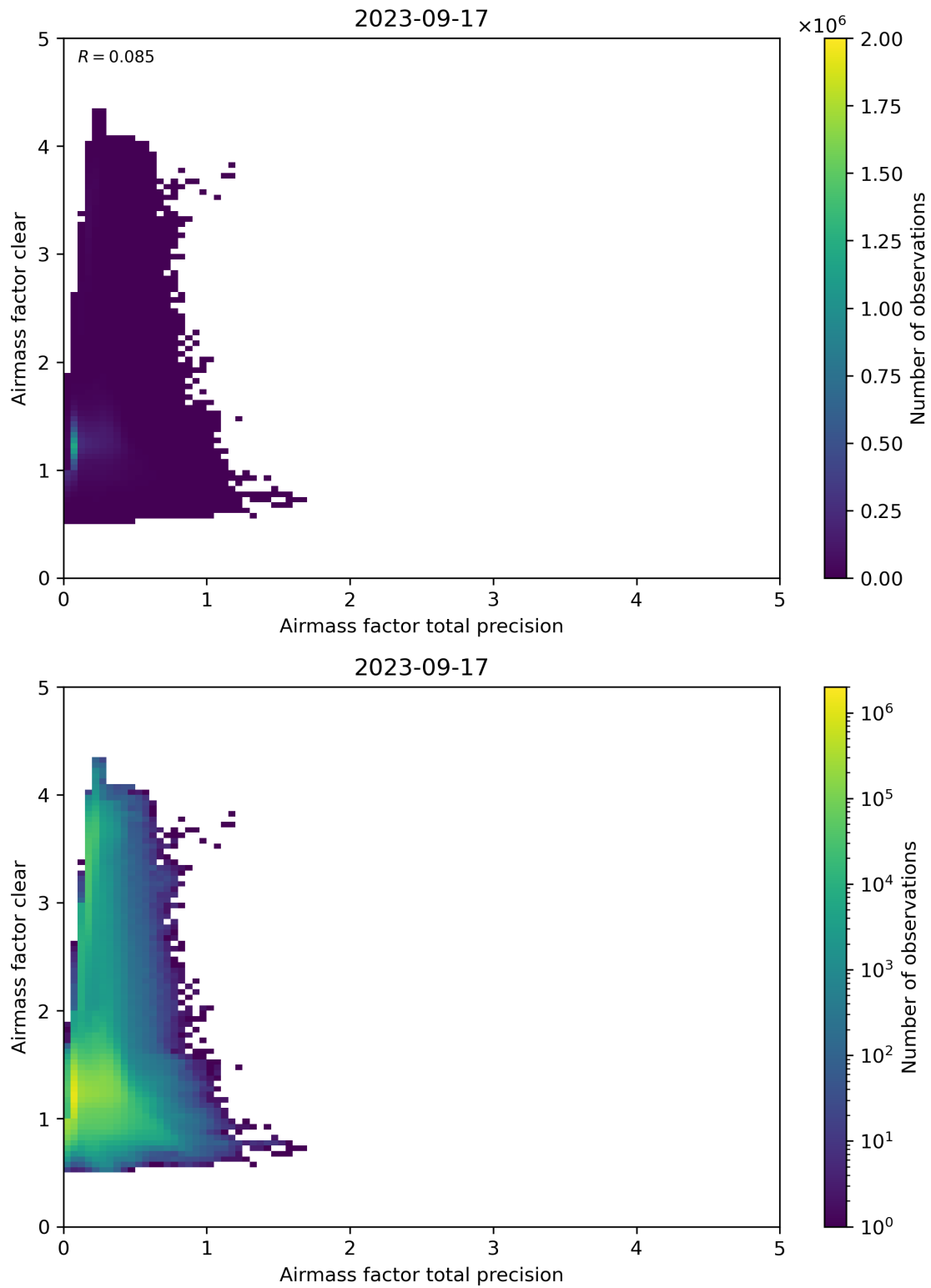
Figure 108: Scatter density plot of “Airmass factor total precision” against “Airmass factor clear” for 2023-09-16 to 2023-09-18.
