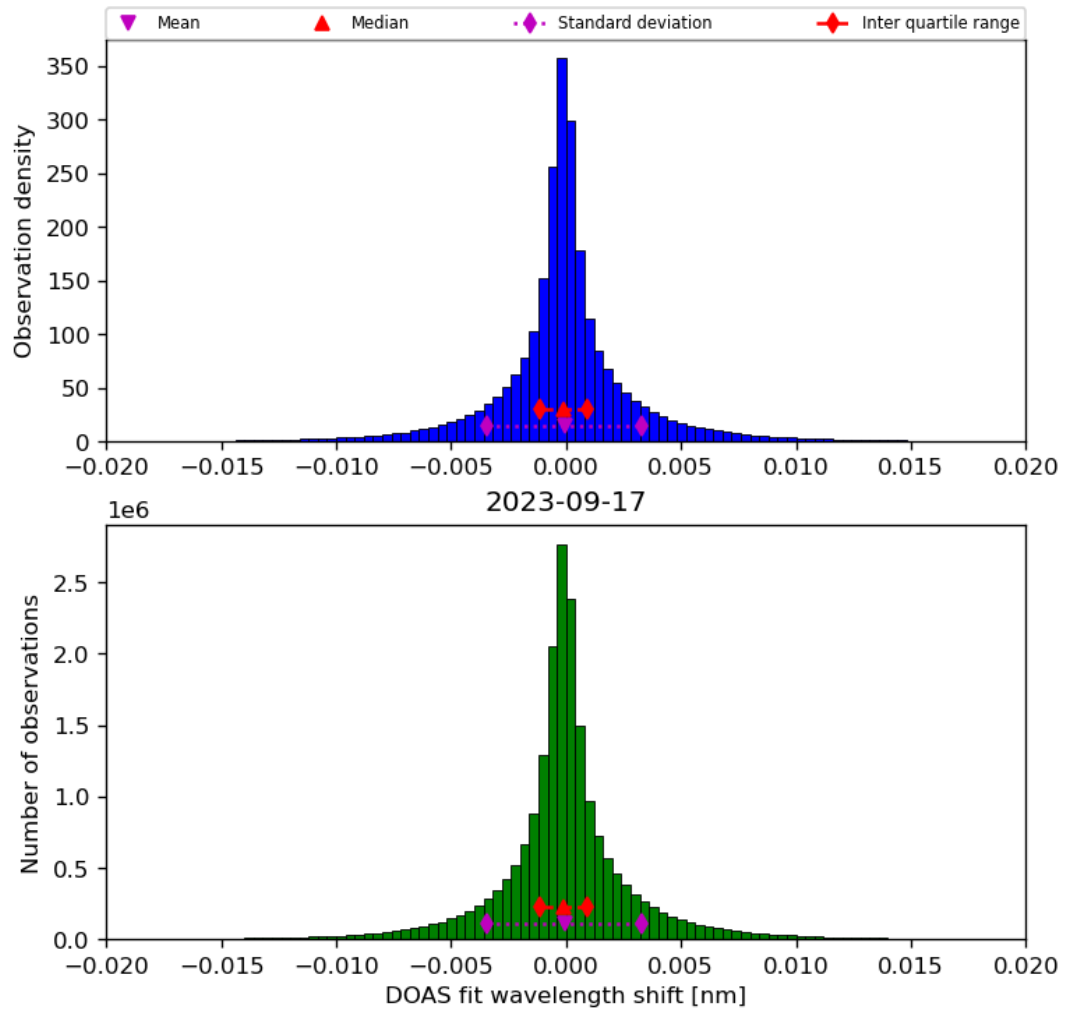
Figure 44: Histogram of “DOAS fit wavelength shift” for 2023-09-16 to 2023-09-18
