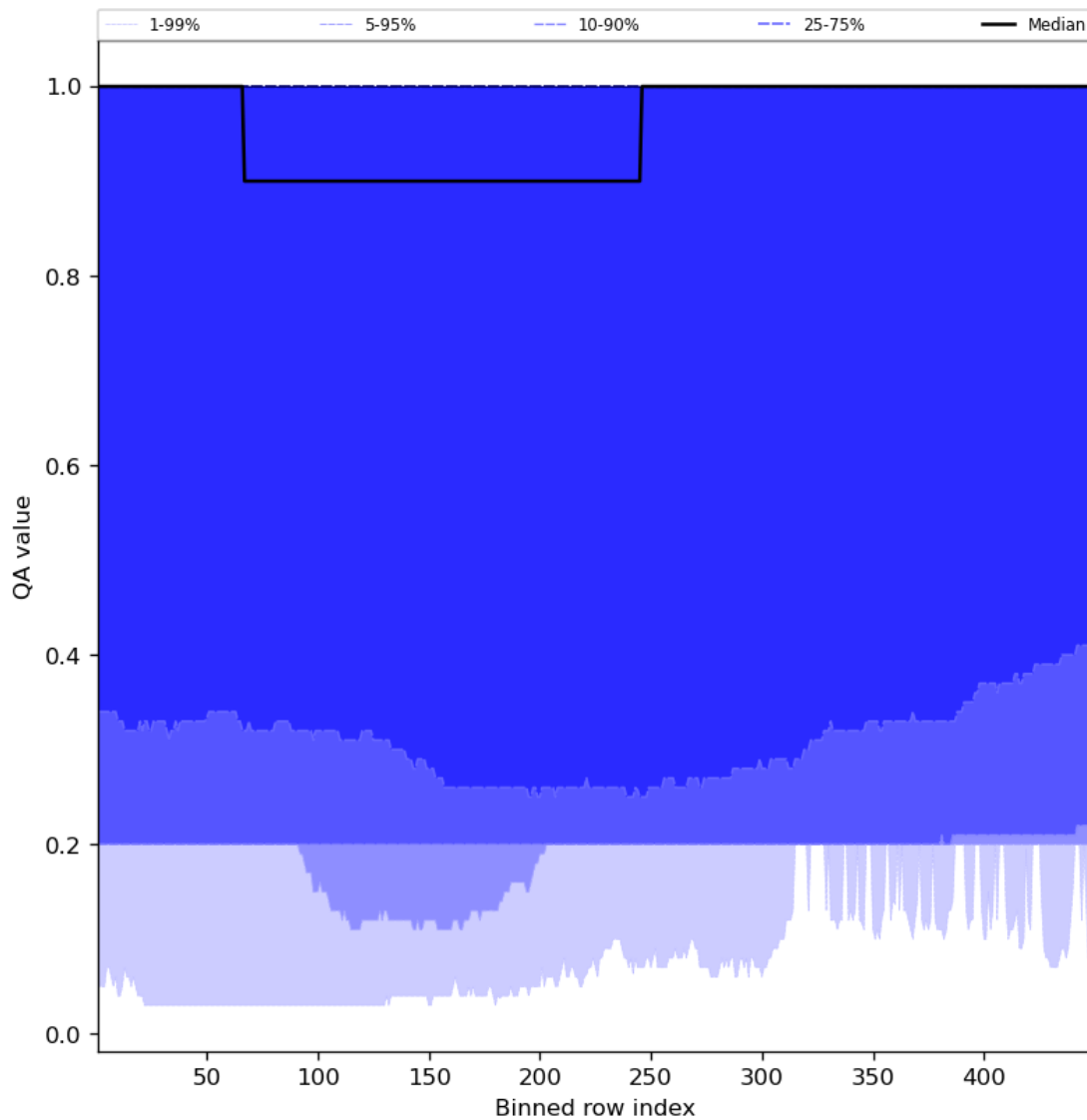
Figure 48: Along track statistics of “QA value” for 2023-09-16 to 2023-09-18
