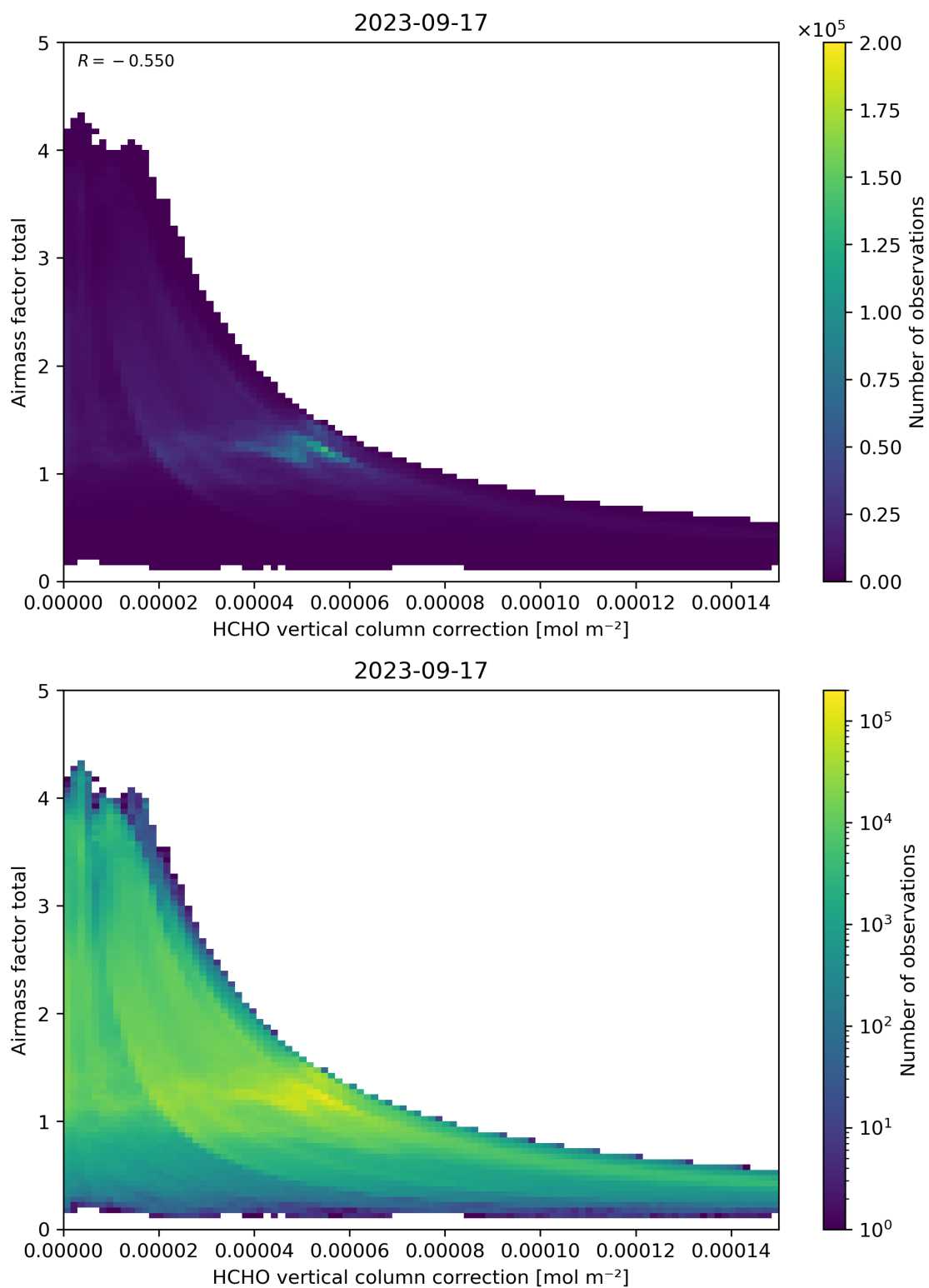
Figure 120: Scatter density plot of “HCHO vertical column correction” against “Airmass factor total” for 2023-09-16 to 2023-09-18.
