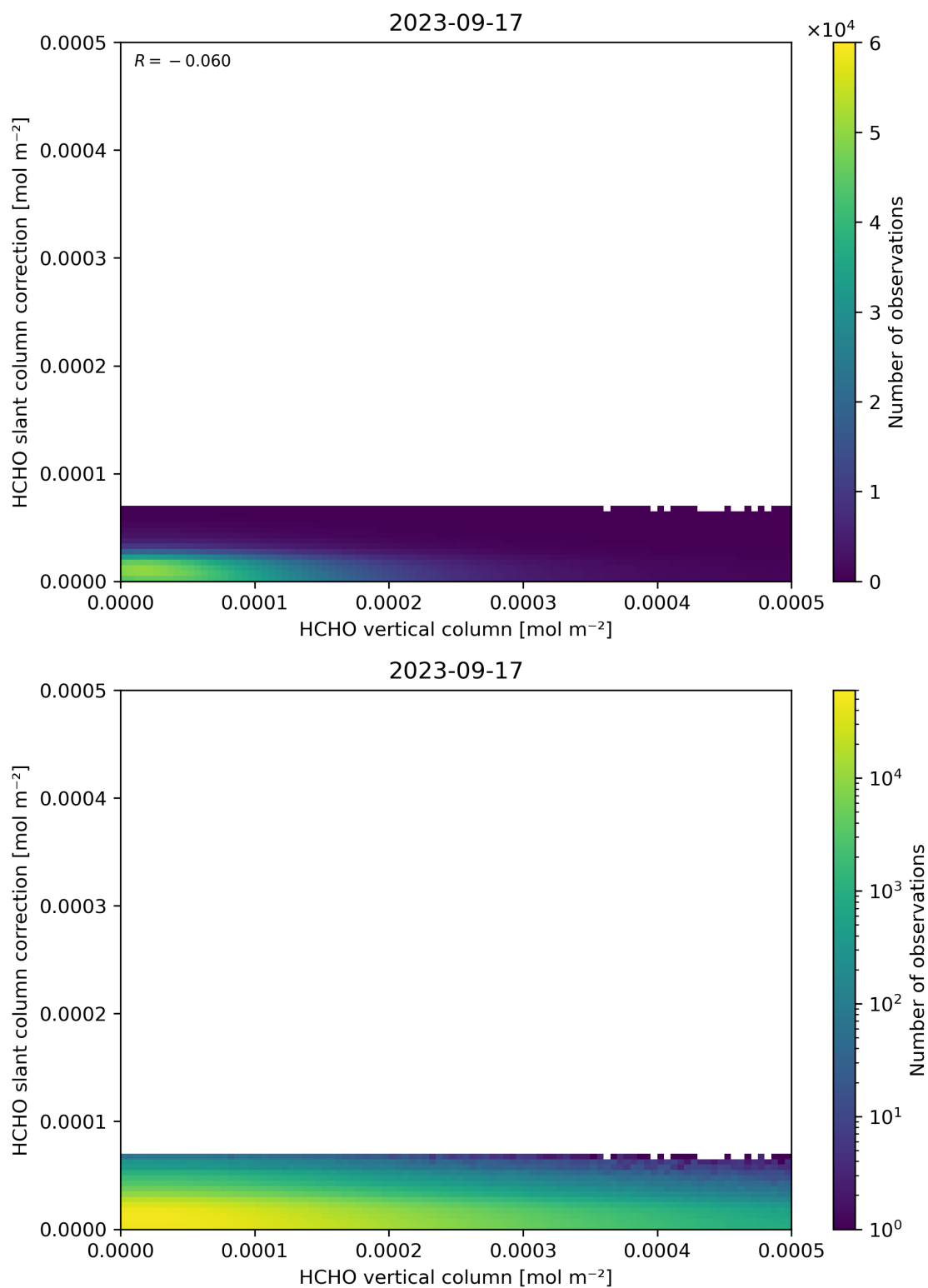
Figure 128: Scatter density plot of “HCHO vertical column” against “HCHO slant column correction” for 2023-09-16 to 2023-09-18.
