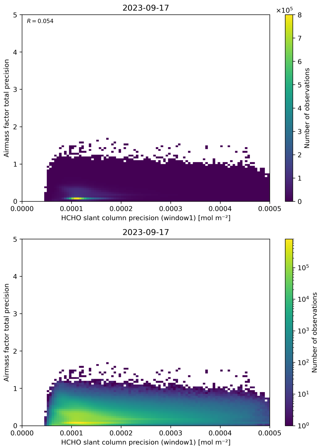
Figure 95: Scatter density plot of “HCHO slant column precision (window1)” against “Airmass factor total precision” for 2023-09-16 to 2023-09-18.
