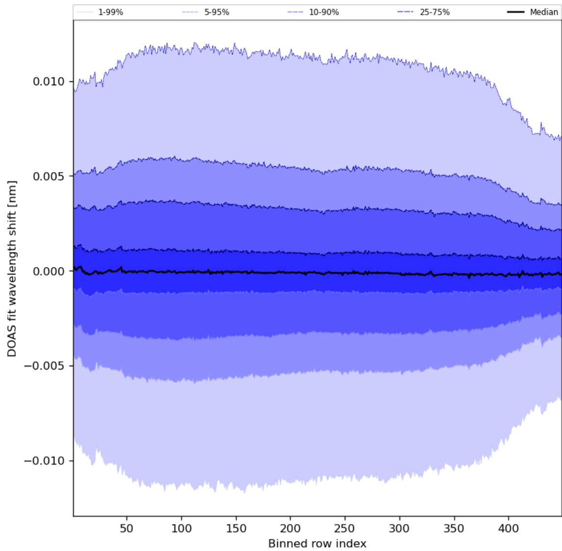
Figure 58: Along track statistics of “DOAS fit wavelength shift” for 2023-09-16 to 2023-09-18
