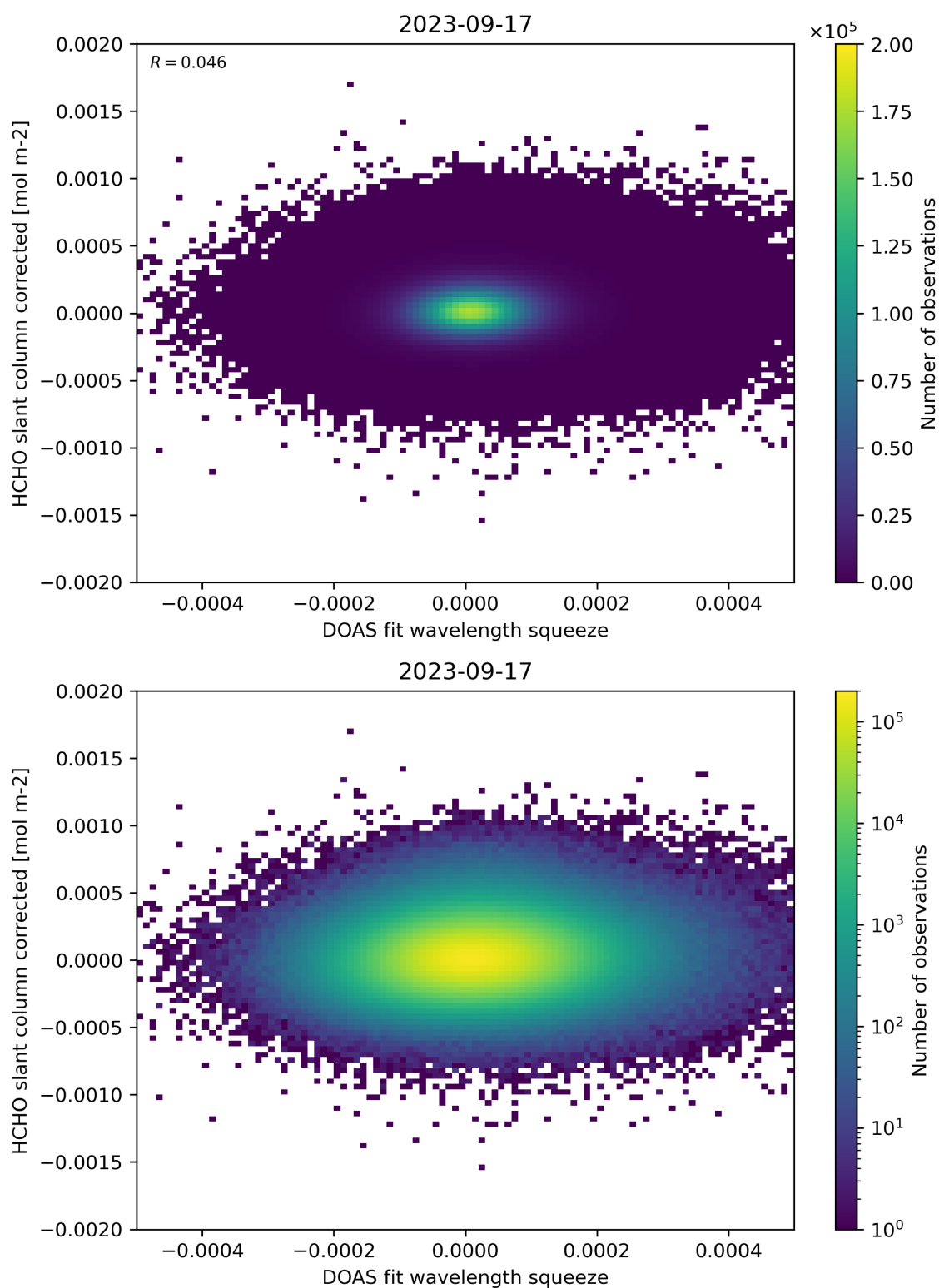
Figure 69: Scatter density plot of “DOAS fit wavelength squeeze” against “HCHO slant column corrected” for 2023-09-16 to 2023-09-18.
