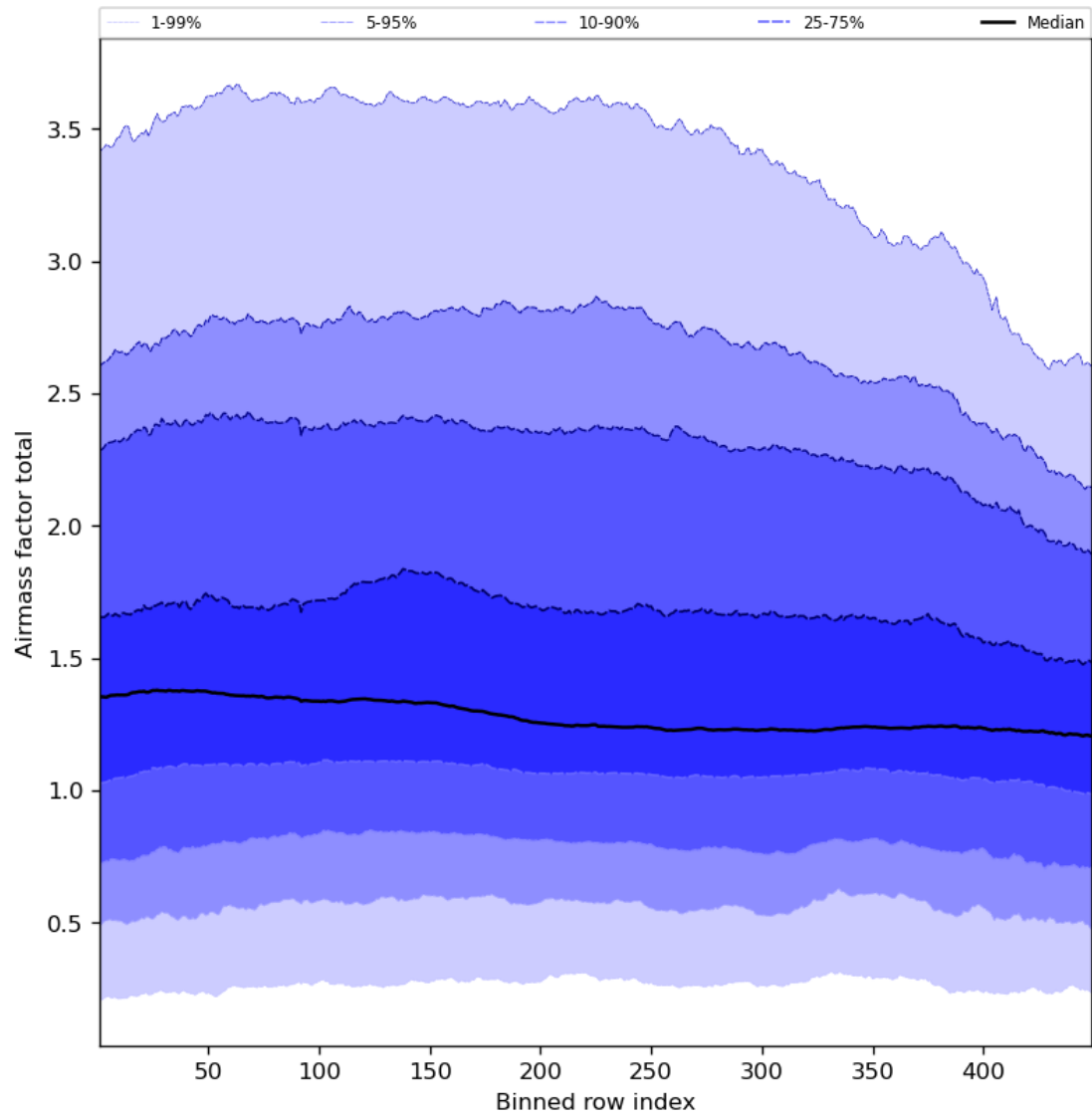
Figure 54: Along track statistics of “Airmass factor total” for 2023-09-16 to 2023-09-18
