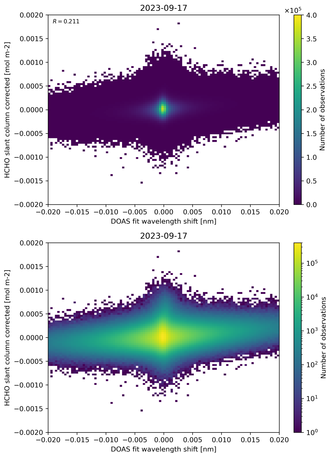
Figure 66: Scatter density plot of “DOAS fit wavelength shift” against “HCHO slant column corrected” for 2023-09-16 to 2023-09-18.
