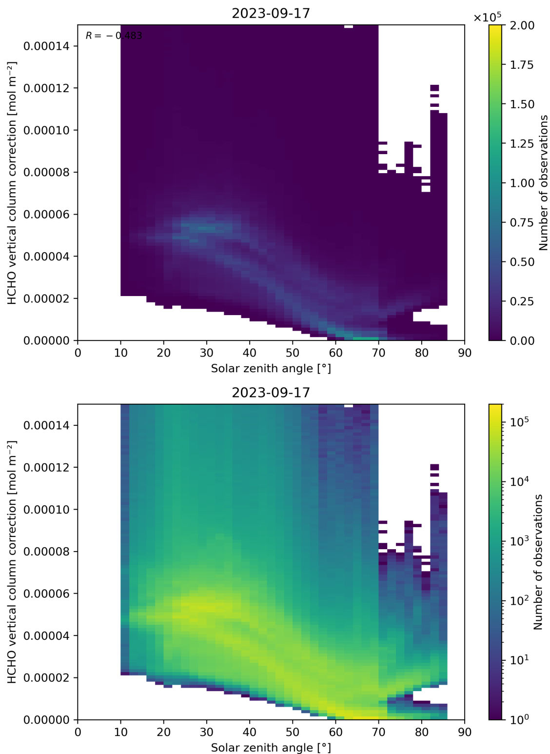
Figure 178: Scatter density plot of “Solar zenith angle” against “HCHO vertical column correction” for 2023-09-16 to 2023-09-18.
