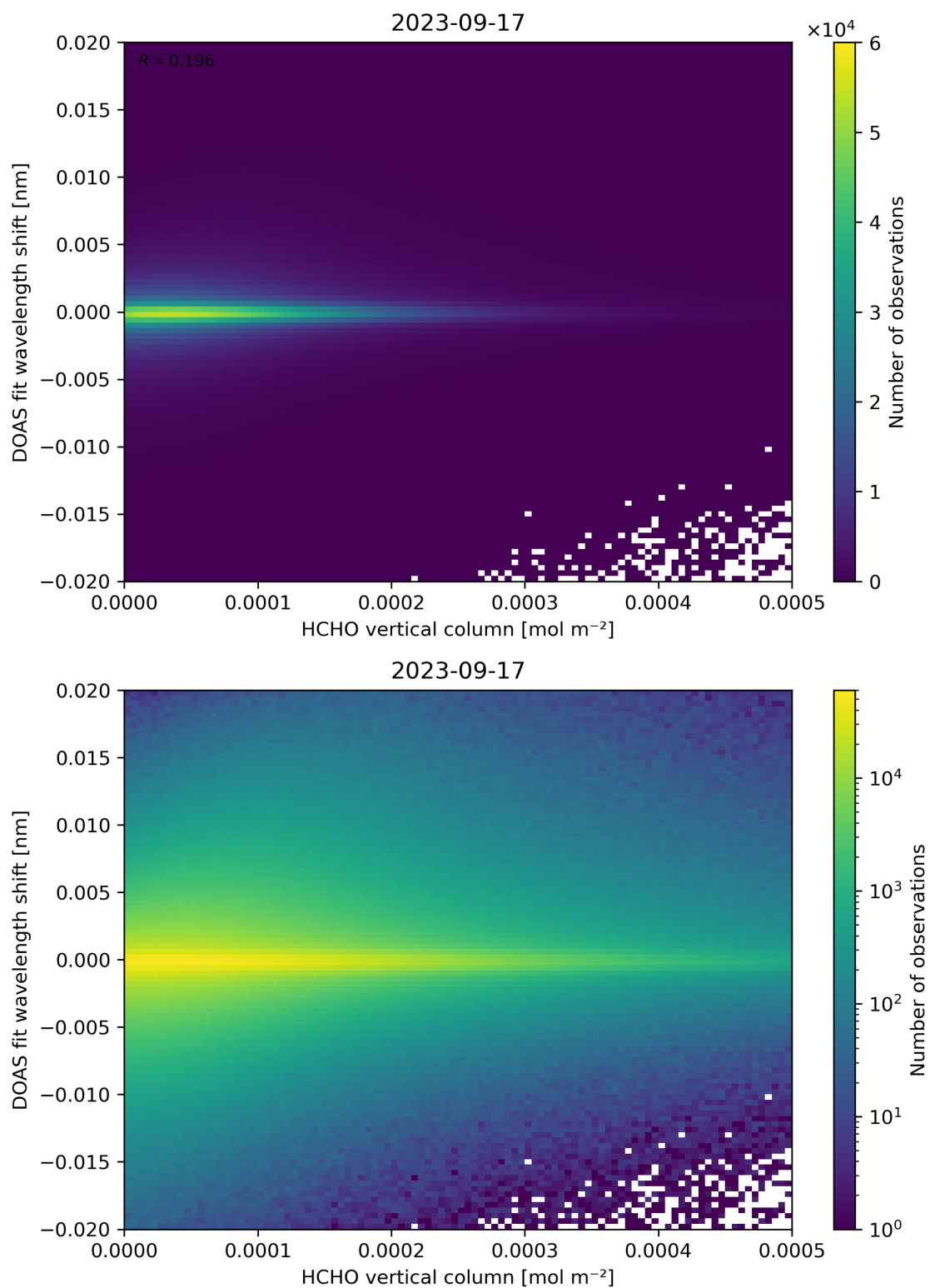
Figure 124: Scatter density plot of “HCHO vertical column” against “DOAS fit wavelength shift” for 2023-09-16 to 2023-09-18.
