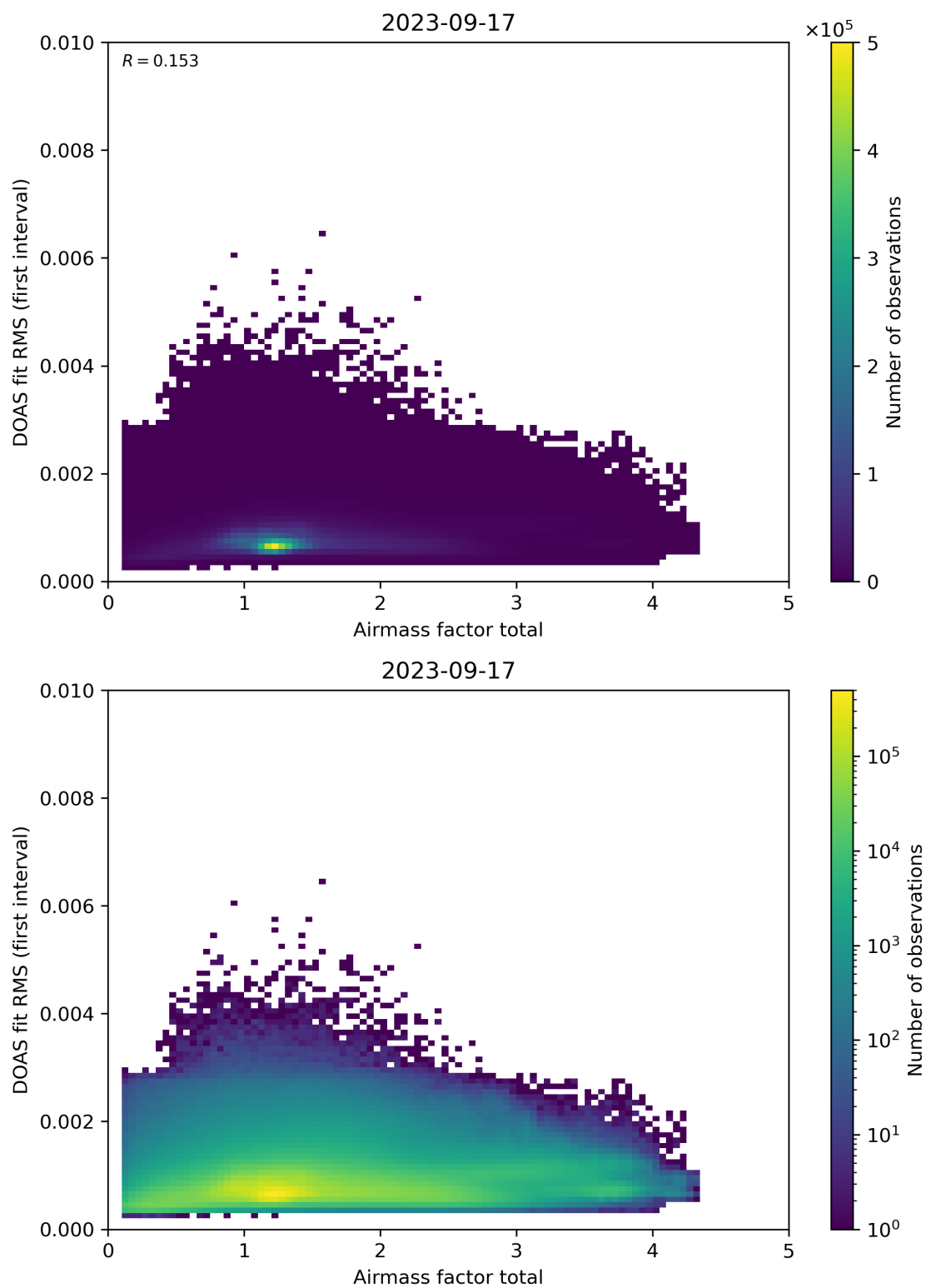
Figure 97: Scatter density plot of “Airmass factor total” against “DOAS fit RMS (first interval)” for 2023-09-16 to 2023-09-18.
