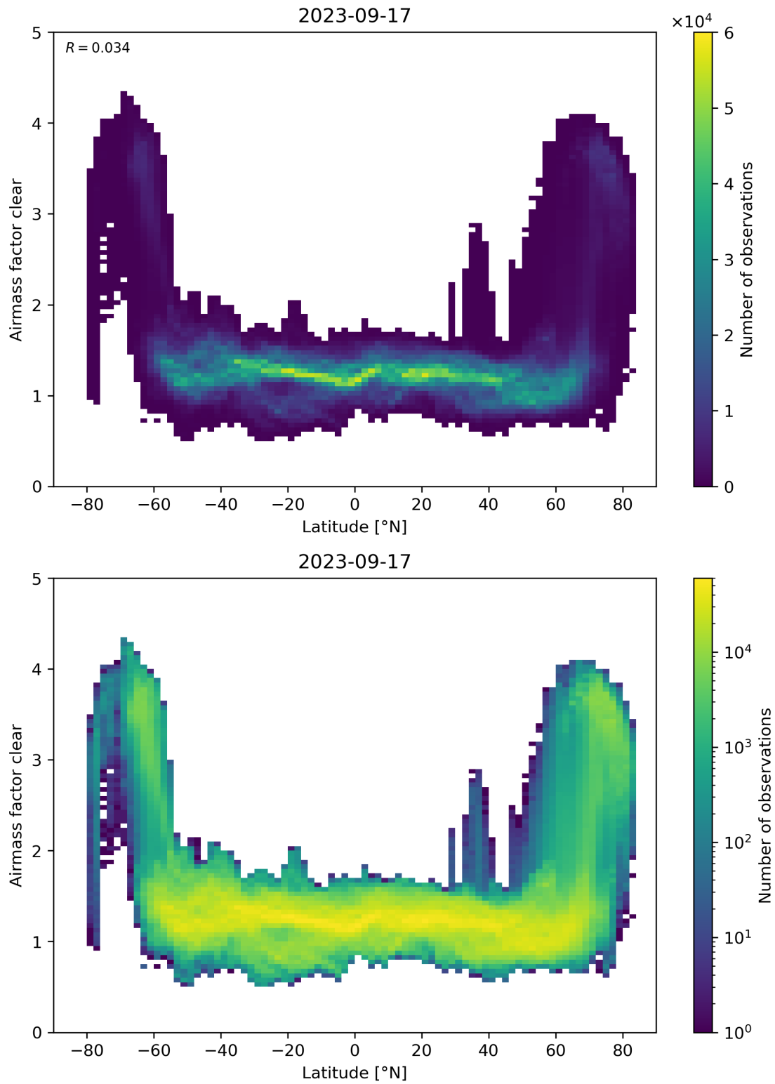
Figure 156: Scatter density plot of “Latitude” against “Airmass factor clear” for 2023-09-16 to 2023-09-18.
