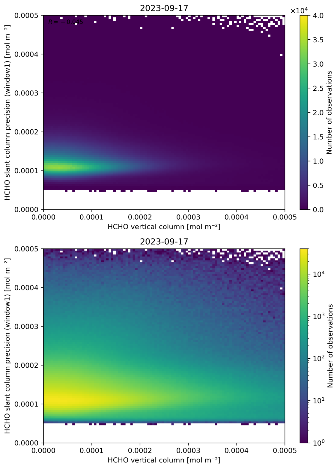
Figure 130: Scatter density plot of “HCHO vertical column” against “HCHO slant column precision (window1)” for 2023-09-16 to 2023-09-18.
