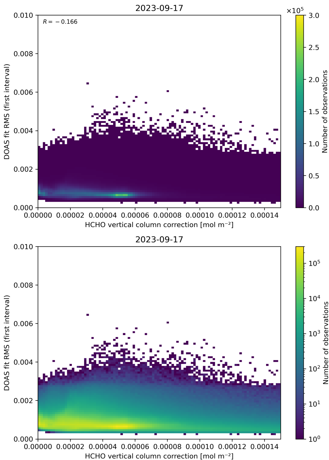
Figure 112: Scatter density plot of “HCHO vertical column correction” against “DOAS fit RMS (first interval)” for 2023-09-16 to 2023-09-18.
