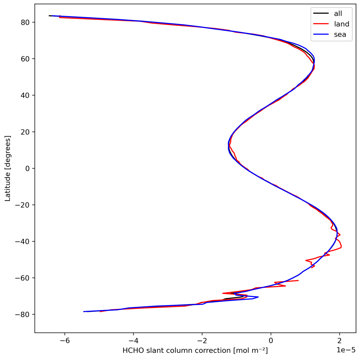
Figure 33: Zonal average of “HCHO slant column correction” for 2023-09-16 to 2023-09-18.
