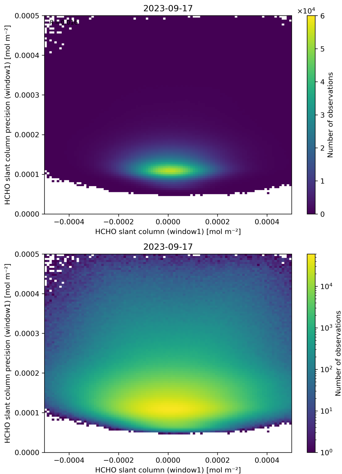
Figure 84: Scatter density plot of “HCHO slant column (window1)” against “HCHO slant column precision (window1)” for 2023-09-16 to 2023-09-18.
