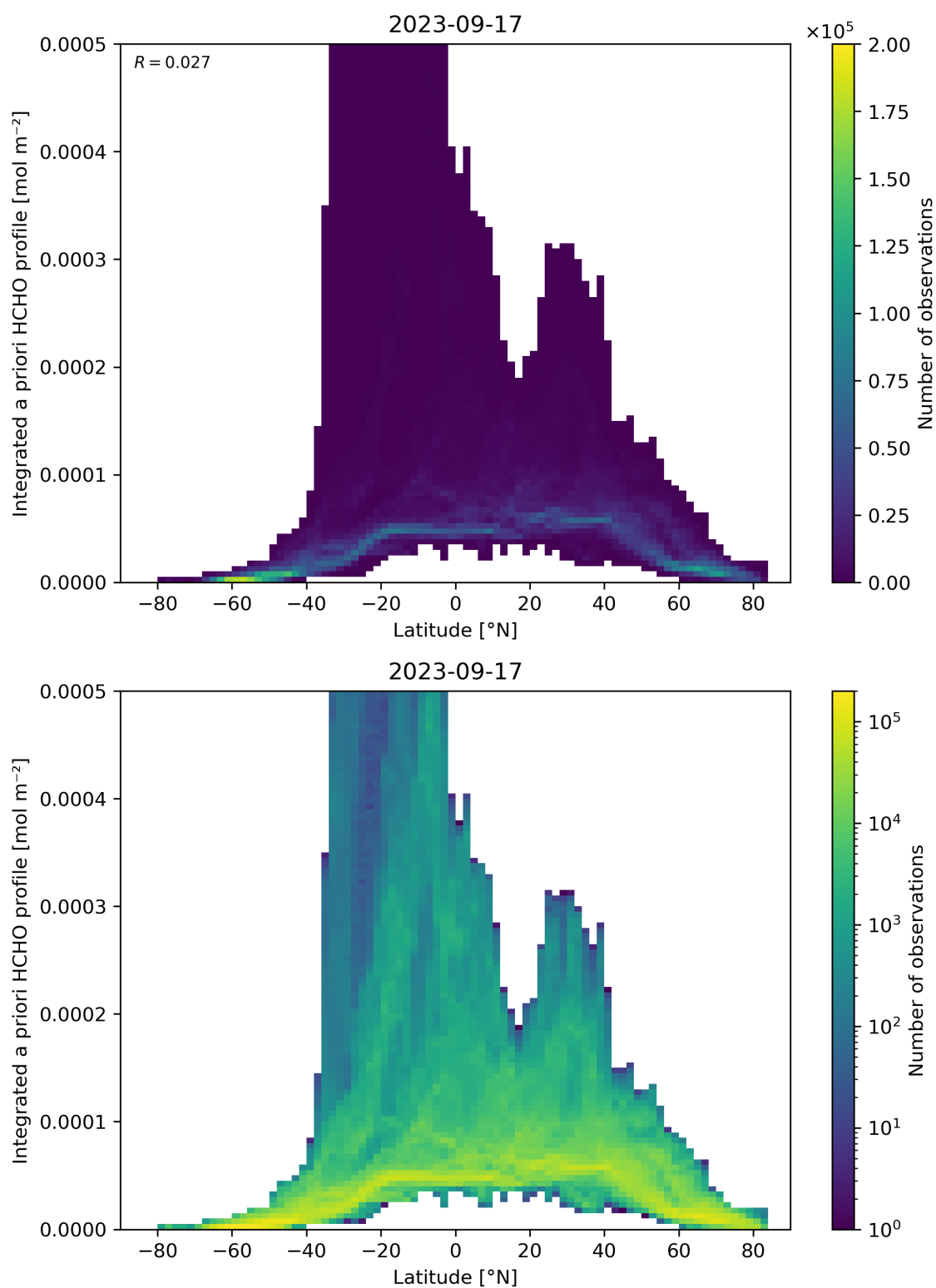
Figure 166: Scatter density plot of “Latitude” against “Integrated a priori HCHO profile” for 2023-09-16 to 2023-09-18.
