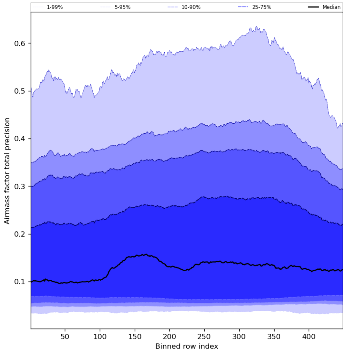
Figure 55: Along track statistics of “Airmass factor total precision” for 2023-09-16 to 2023-09-18
