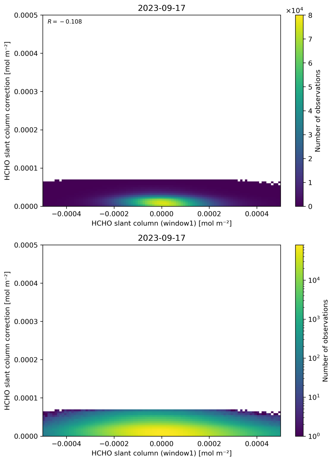
Figure 83: Scatter density plot of “HCHO slant column (window1)” against “HCHO slant column correction” for 2023-09-16 to 2023-09-18.
