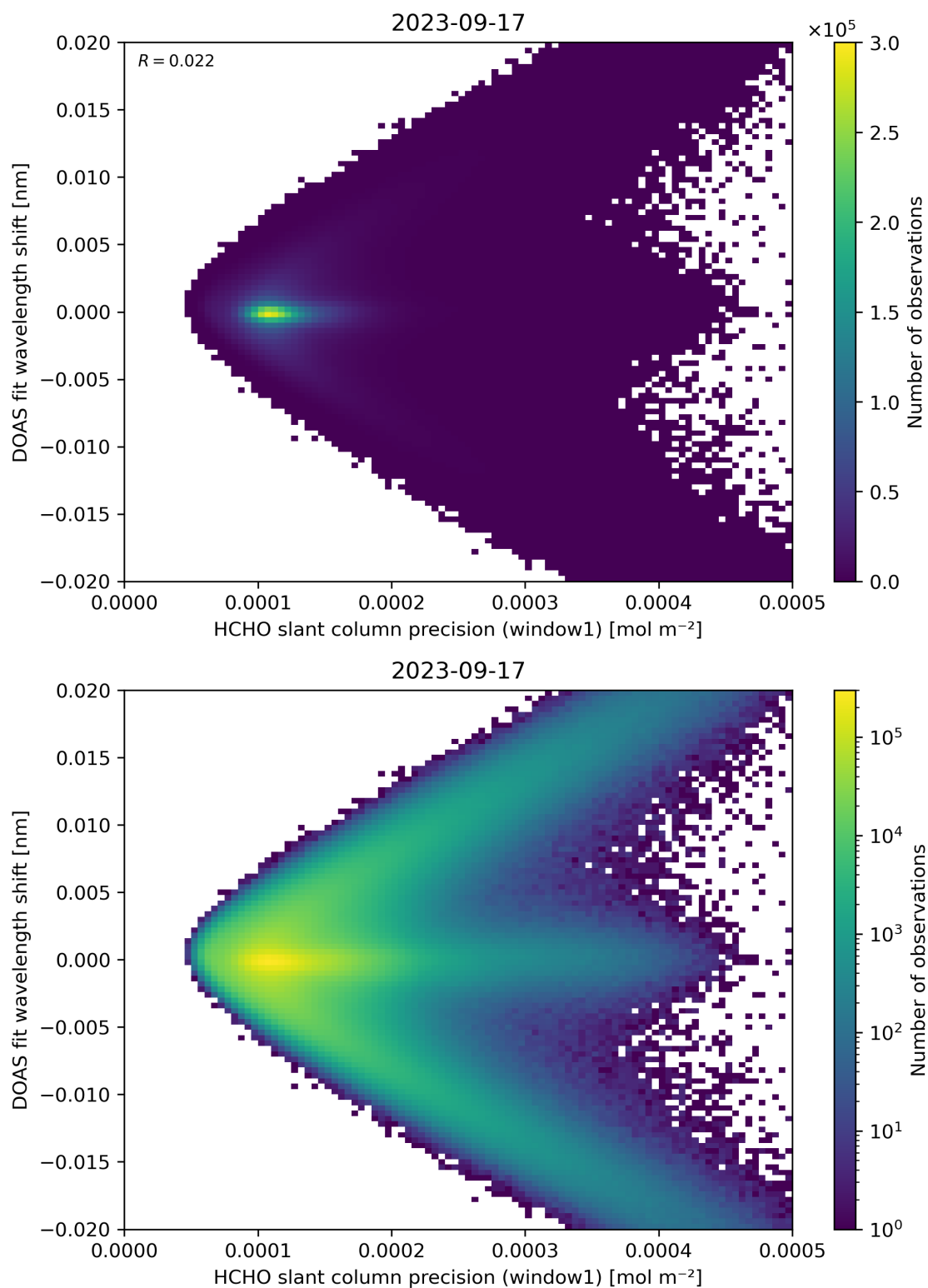
Figure 89: Scatter density plot of “HCHO slant column precision (window1)” against “DOAS fit wavelength shift” for 2023-09-16 to 2023-09-18.
