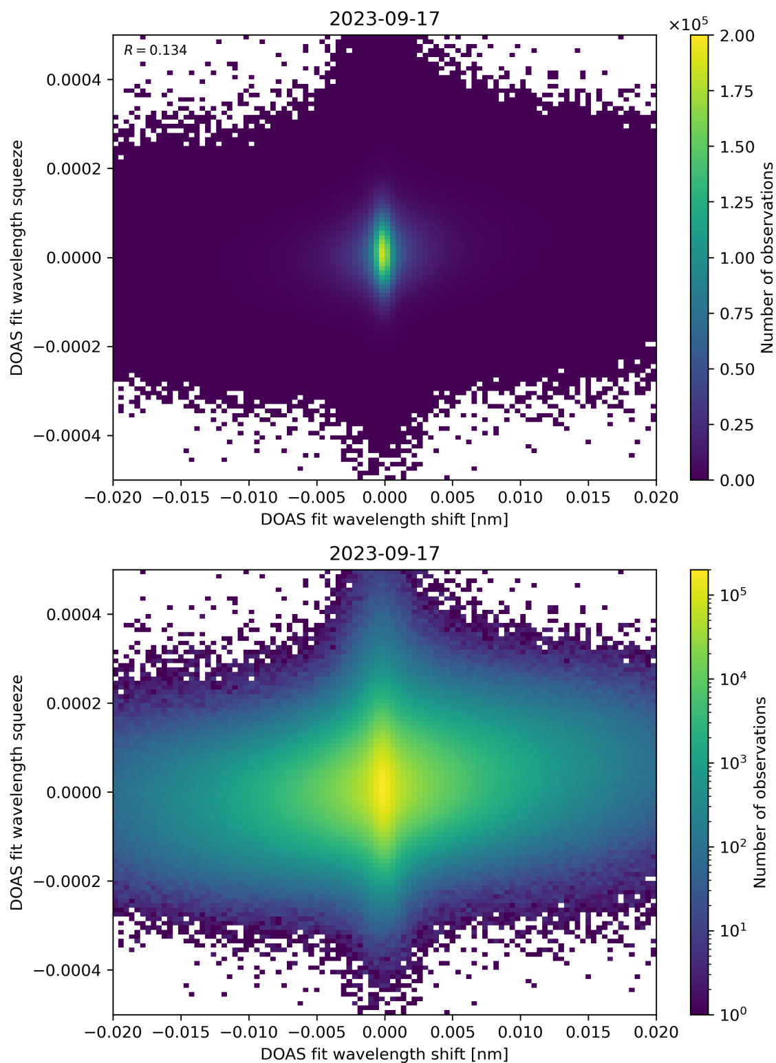
Figure 65: Scatter density plot of “DOAS fit wavelength shift” against “DOAS fit wavelength squeeze” for 2023-09-16 to 2023-09-18.
