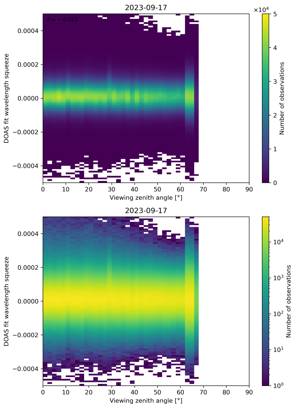
Figure 184: Scatter density plot of “Viewing zenith angle” against “DOAS fit wavelength squeeze” for 2023-09-16 to 2023-09-18.
