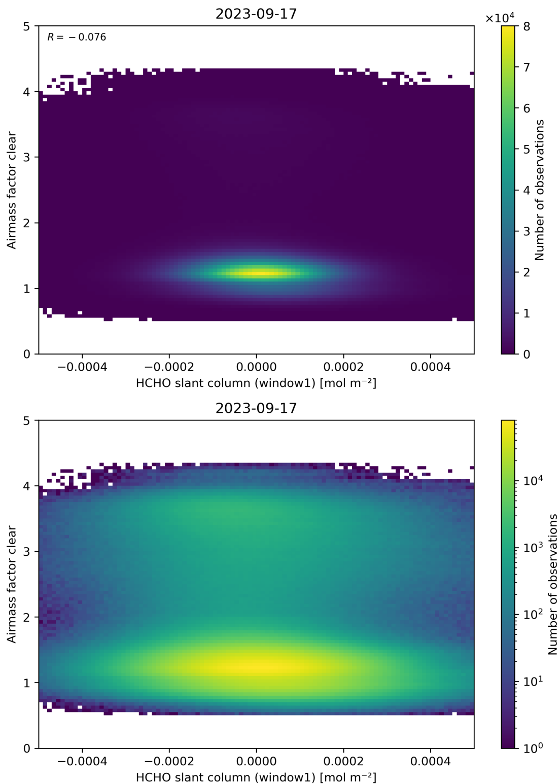
Figure 81: Scatter density plot of “HCHO slant column (window1)” against “Airmass factor clear” for 2023-09-16 to 2023-09-18.
