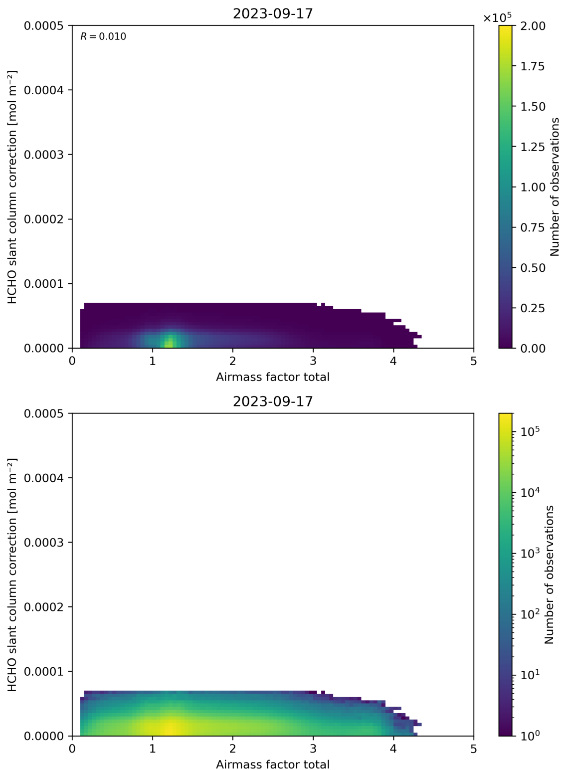
Figure 102: Scatter density plot of “Airmass factor total” against “HCHO slant column correction” for 2023-09-16 to 2023-09-18.
