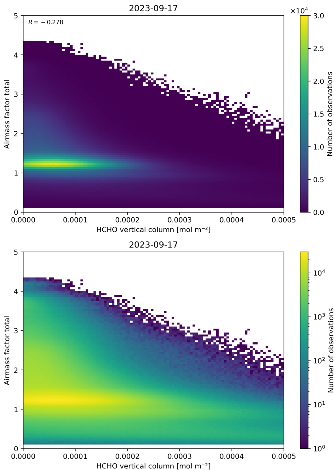
Figure 131: Scatter density plot of “HCHO vertical column” against “Airmass factor total” for 2023-09-16 to 2023-09-18.
