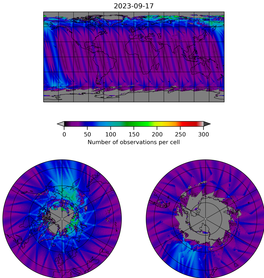
Figure 19: Map of the number of observations for 2023-09-16 to 2023-09-18
