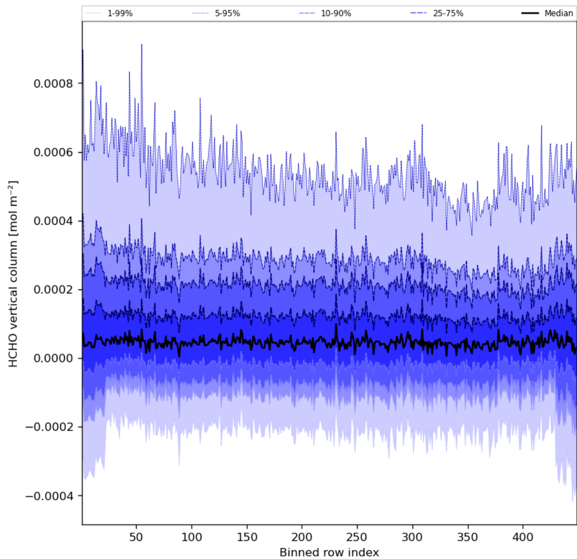
Figure 49: Along track statistics of “HCHO vertical column” for 2023-09-16 to 2023-09-18
