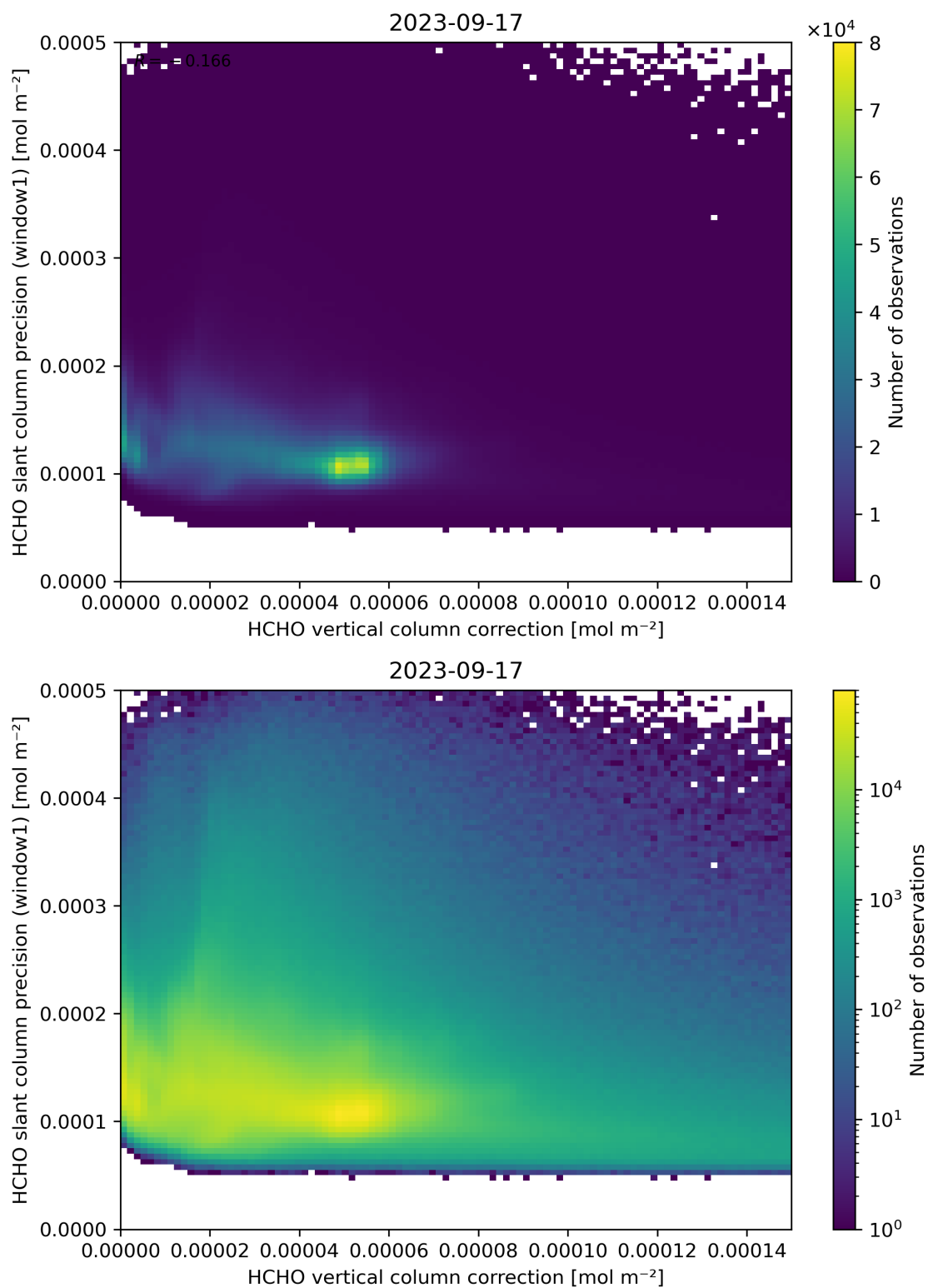
Figure 119: Scatter density plot of “HCHO vertical column correction” against “HCHO slant column precision (window1)” for 2023-09-16 to 2023-09-18.
