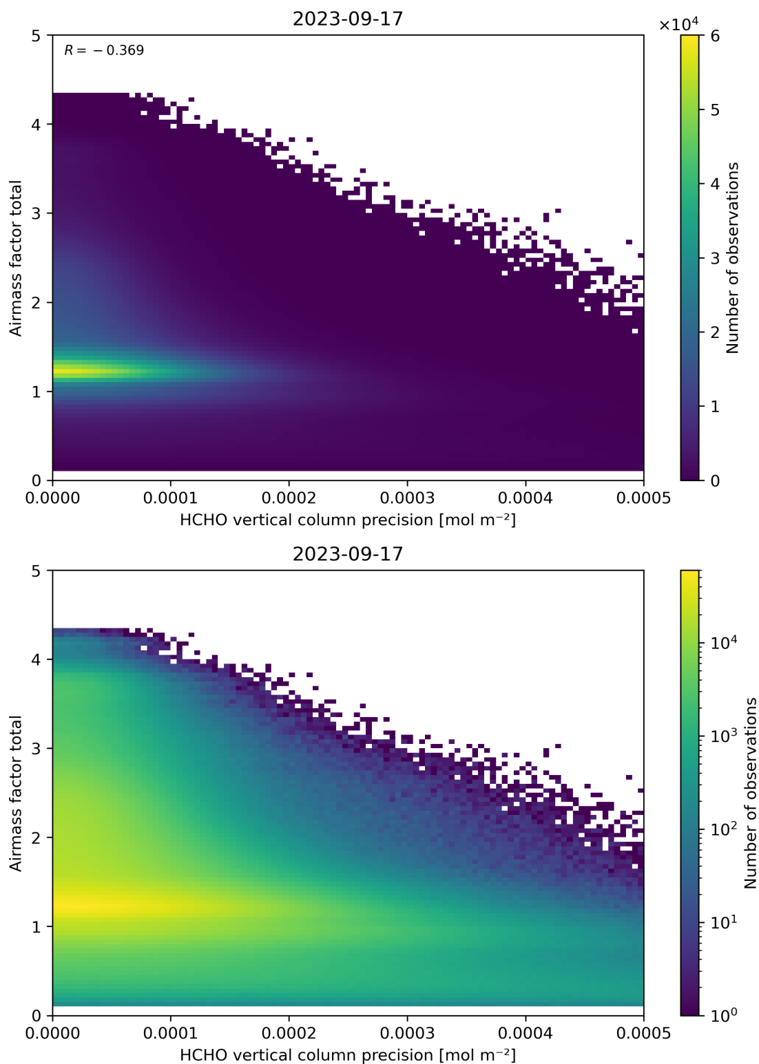
Figure 144: Scatter density plot of “HCHO vertical column precision” against “Airmass factor total” for 2023-09-16 to 2023-09-18.
