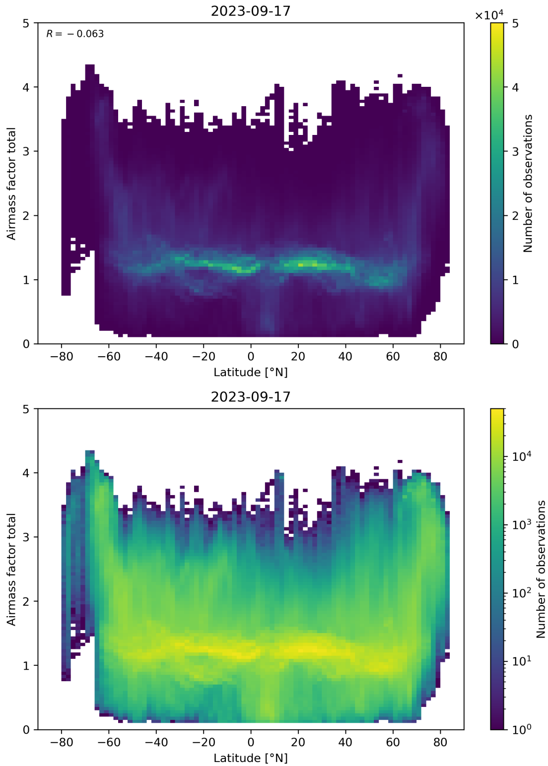
Figure 161: Scatter density plot of “Latitude” against “Airmass factor total” for 2023-09-16 to 2023-09-18.
