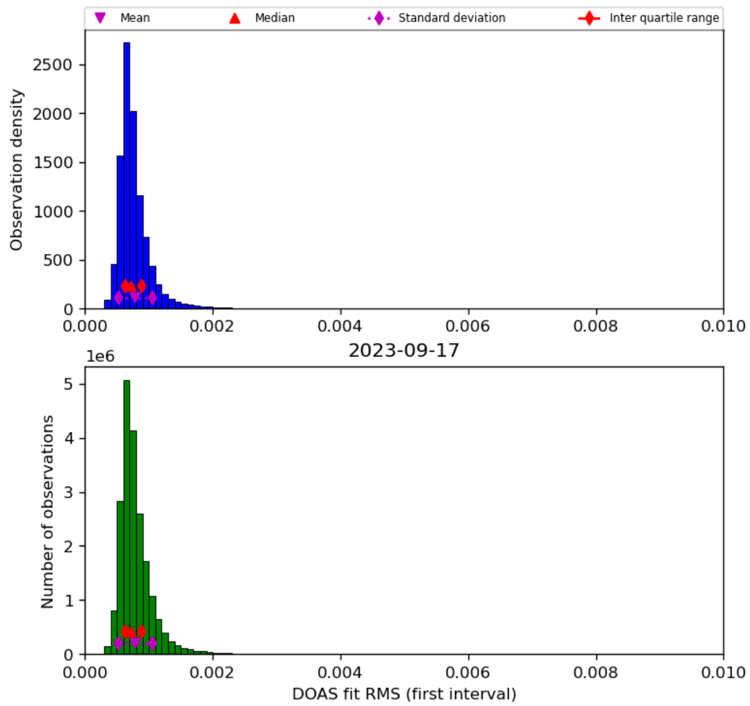
Figure 46: Histogram of “DOAS fit RMS (first interval)” for 2023-09-16 to 2023-09-18
