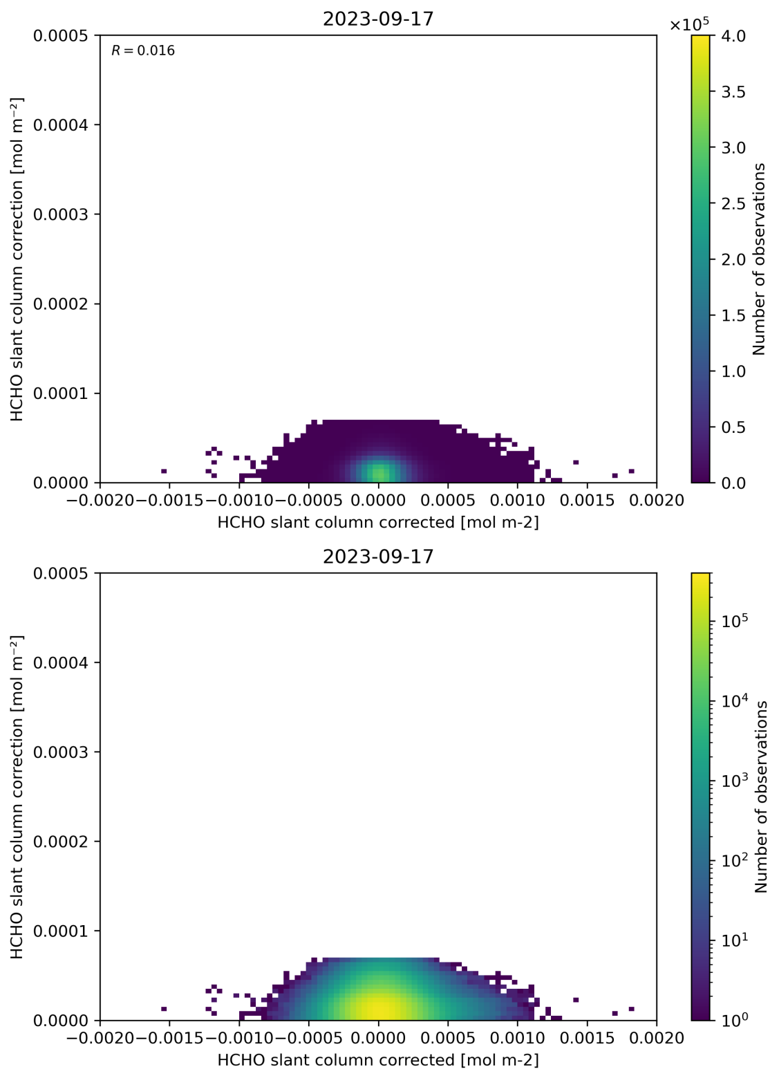
Figure 77: Scatter density plot of “HCHO slant column corrected” against “HCHO slant column correction” for 2023-09-16 to 2023-09-18.
