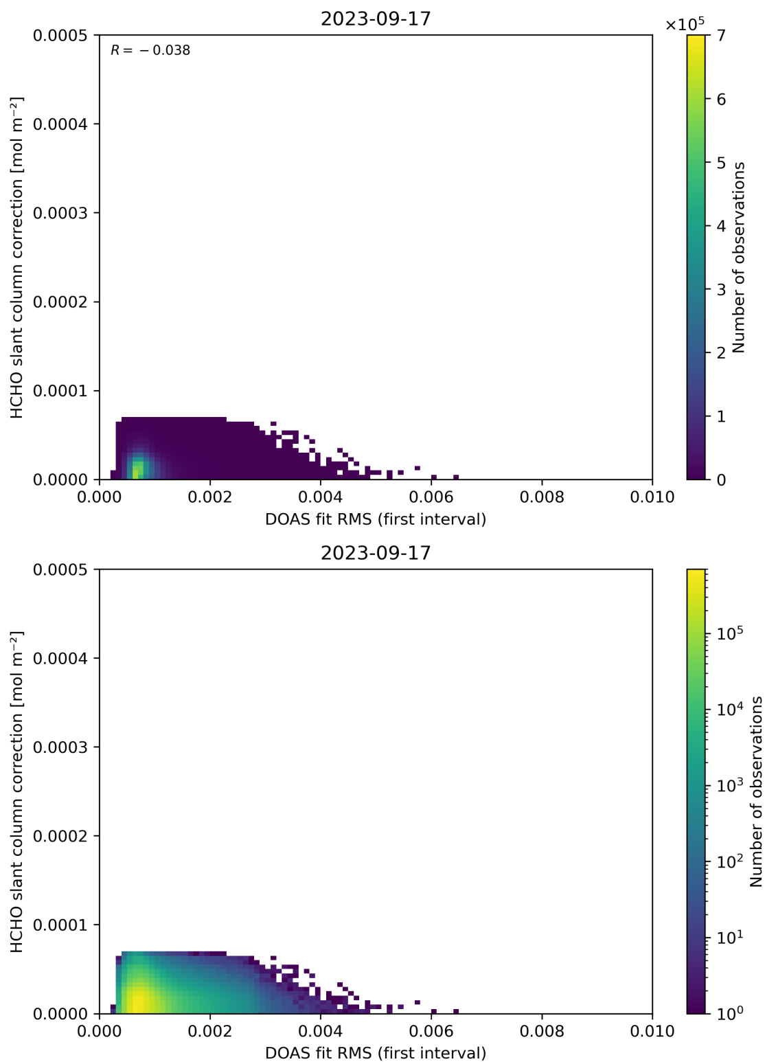
Figure 63: Scatter density plot of “DOAS fit RMS (first interval)” against “HCHO slant column correction” for 2023-09-16 to 2023-09-18.
