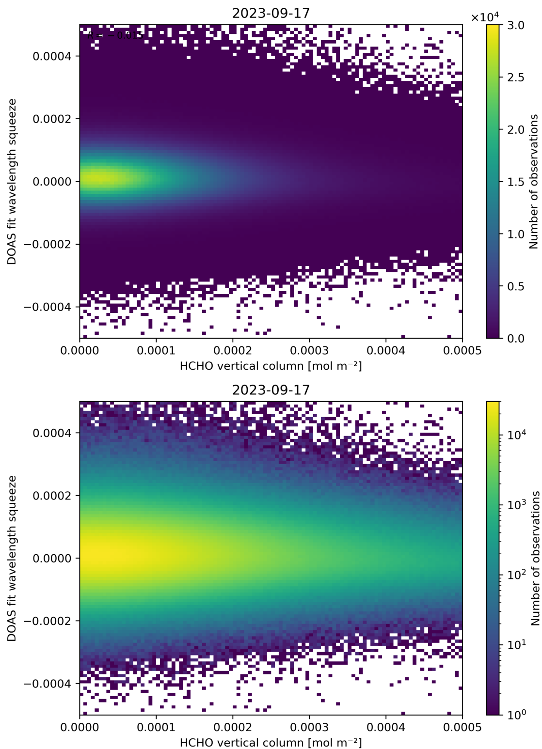
Figure 125: Scatter density plot of “HCHO vertical column” against “DOAS fit wavelength squeeze” for 2023-09-16 to 2023-09-18.
