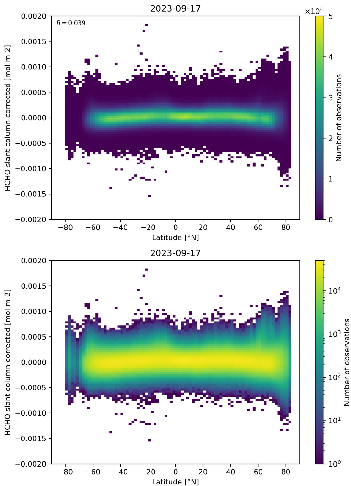
Figure 157: Scatter density plot of “Latitude” against “HCHO slant column corrected” for 2023-09-16 to 2023-09-18.
