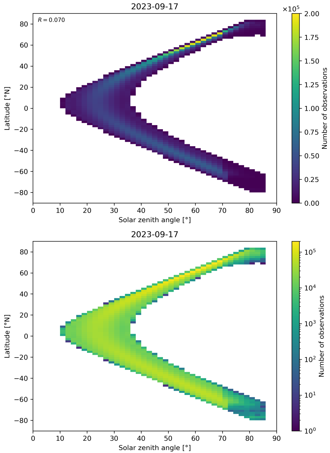
Figure 181: Scatter density plot of “Solar zenith angle” against “Latitude” for 2023-09-16 to 2023-09-18.
