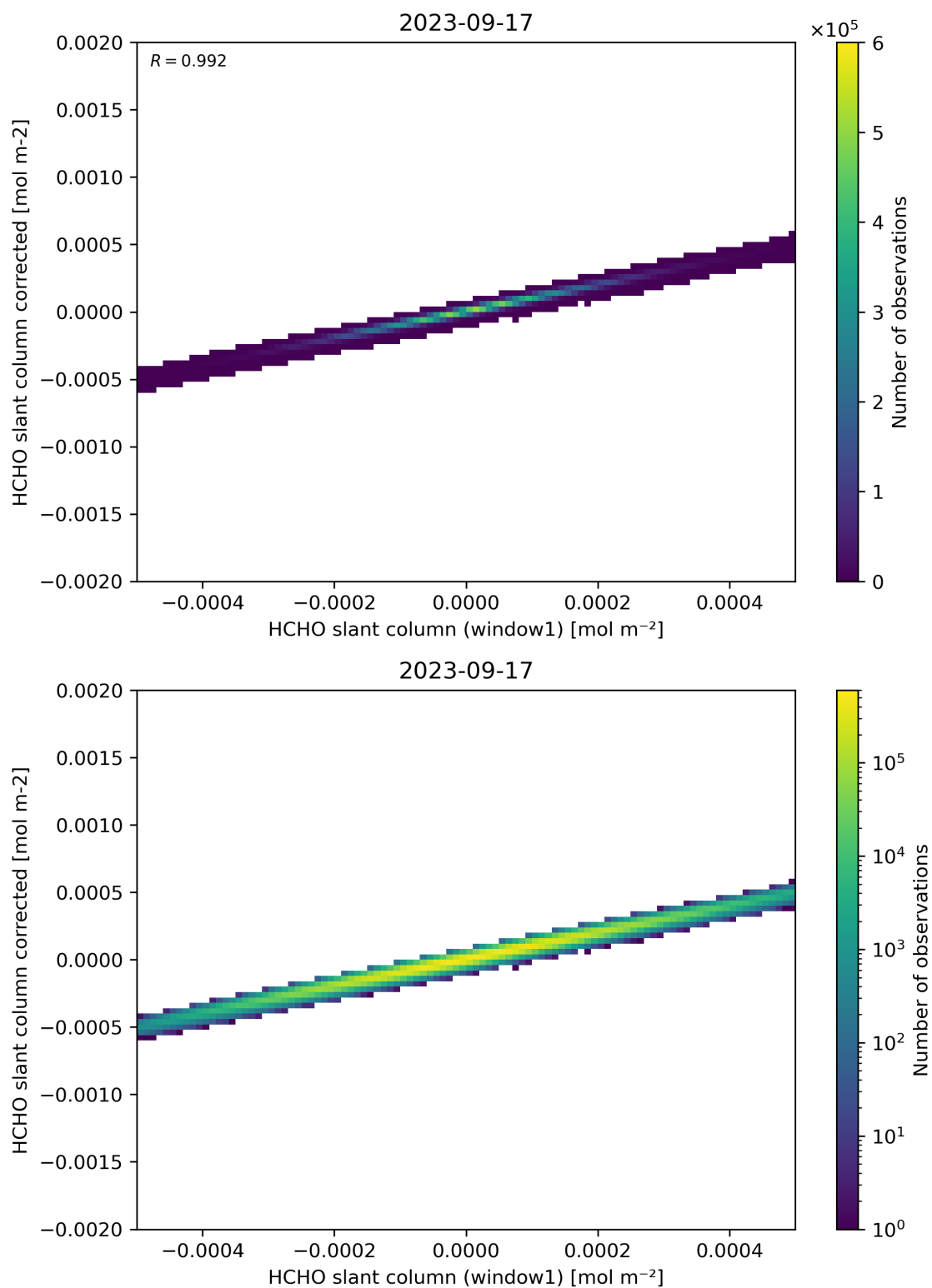
Figure 82: Scatter density plot of “HCHO slant column (window1)” against “HCHO slant column corrected” for 2023-09-16 to 2023-09-18.
