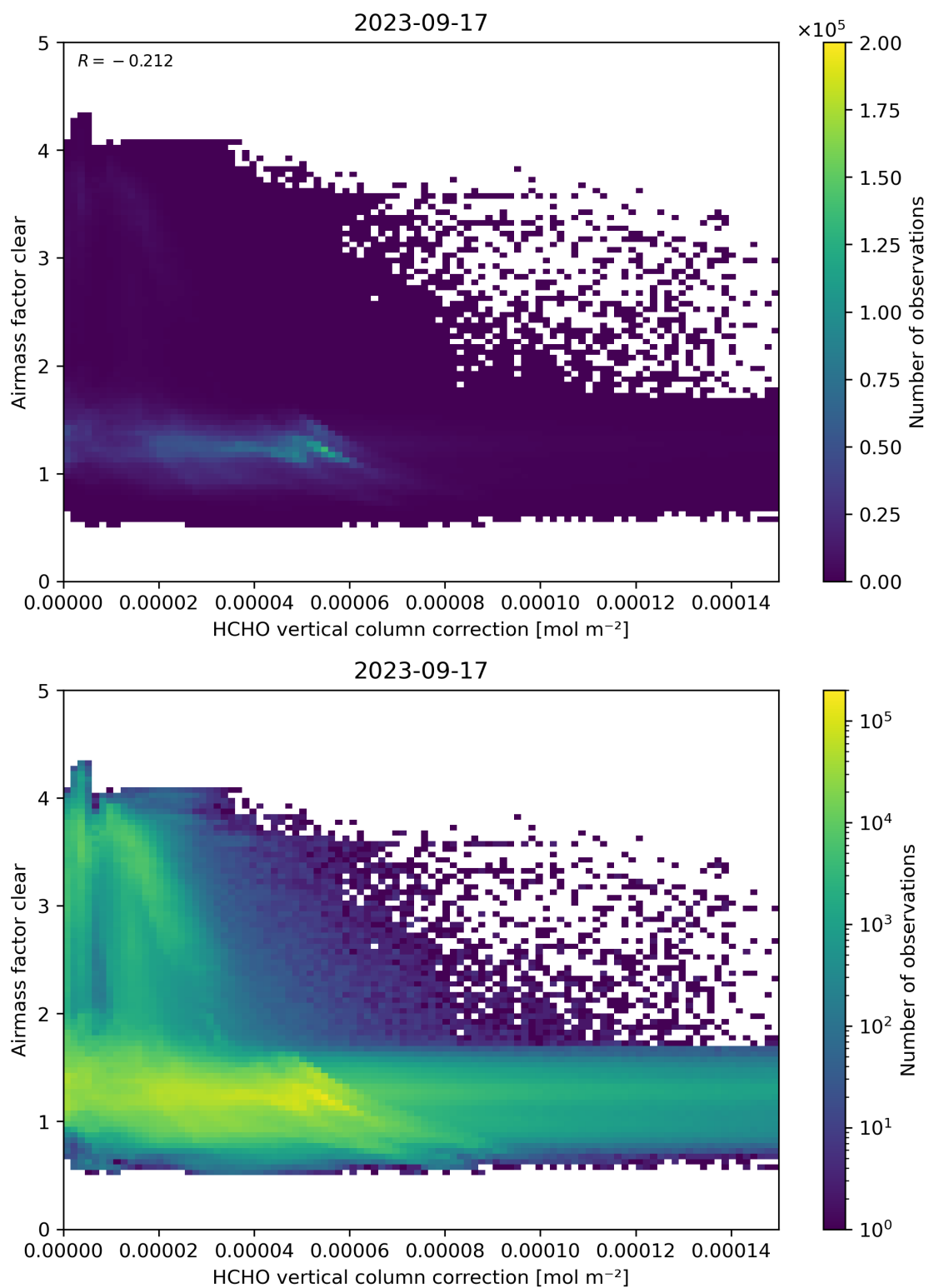
Figure 115: Scatter density plot of “HCHO vertical column correction” against “Airmass factor clear” for 2023-09-16 to 2023-09-18.
