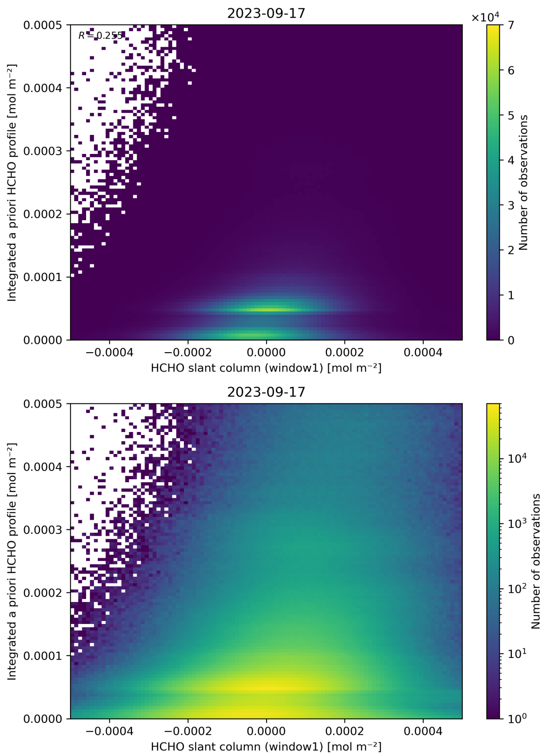
Figure 87: Scatter density plot of “HCHO slant column (window1)” against “Integrated a priori HCHO profile” for 2023-09-16 to 2023-09-18.
