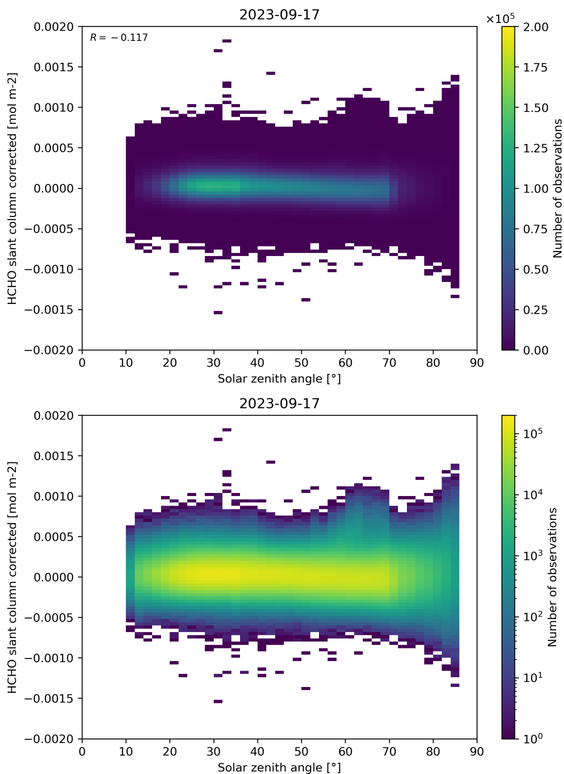
Figure 171: Scatter density plot of “Solar zenith angle” against “HCHO slant column corrected” for 2023-09-16 to 2023-09-18.
