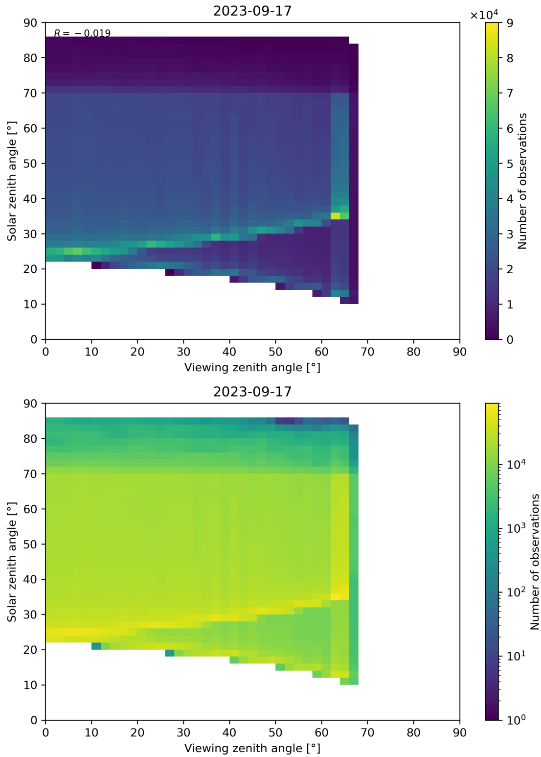
Figure 197: Scatter density plot of “Viewing zenith angle” against “Solar zenith angle” for 2023-09-16 to 2023-09-18.
