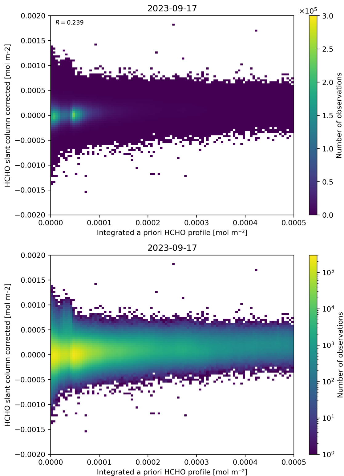
Figure 151: Scatter density plot of “Integrated a priori HCHO profile” against “HCHO slant column corrected” for 2023-09-16 to 2023-09-18.
