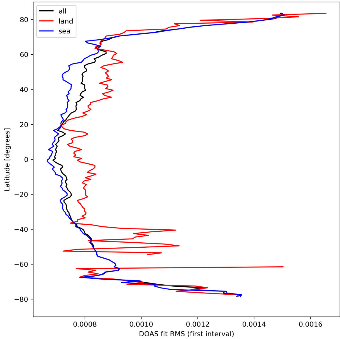
Figure 32: Zonal average of “DOAS fit RMS (first interval)” for 2023-09-16 to 2023-09-18.
