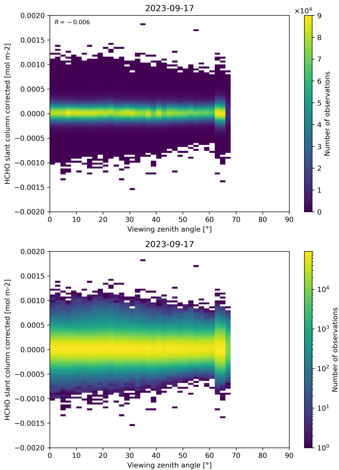
Figure 186: Scatter density plot of “Viewing zenith angle” against “HCHO slant column corrected” for 2023-09-16 to 2023-09-18.
