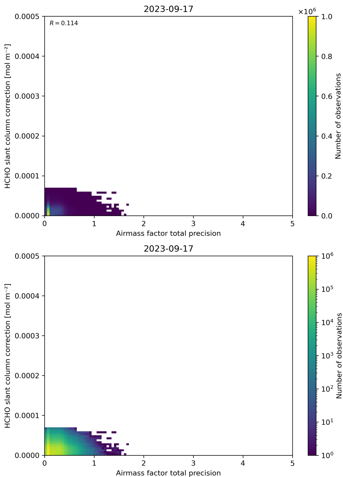
Figure 110: Scatter density plot of “Airmass factor total precision” against “HCHO slant column correction” for 2023-09-16 to 2023-09-18.
