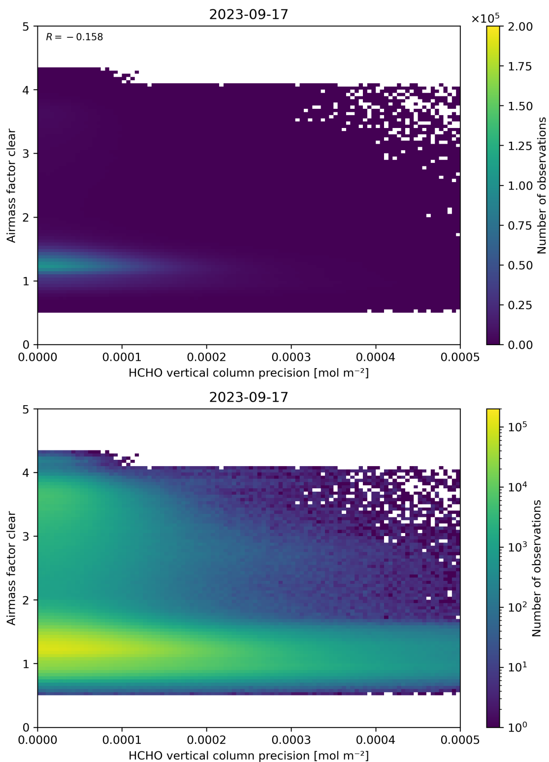
Figure 139: Scatter density plot of “HCHO vertical column precision” against “Airmass factor clear” for 2023-09-16 to 2023-09-18.
