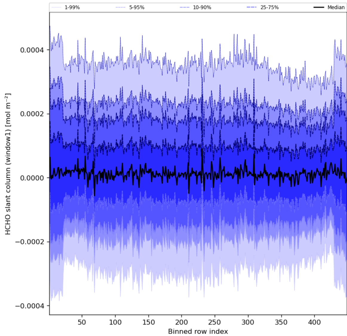
Figure 52: Along track statistics of “HCHO slant column (window1)” for 2023-09-16 to 2023-09-18
