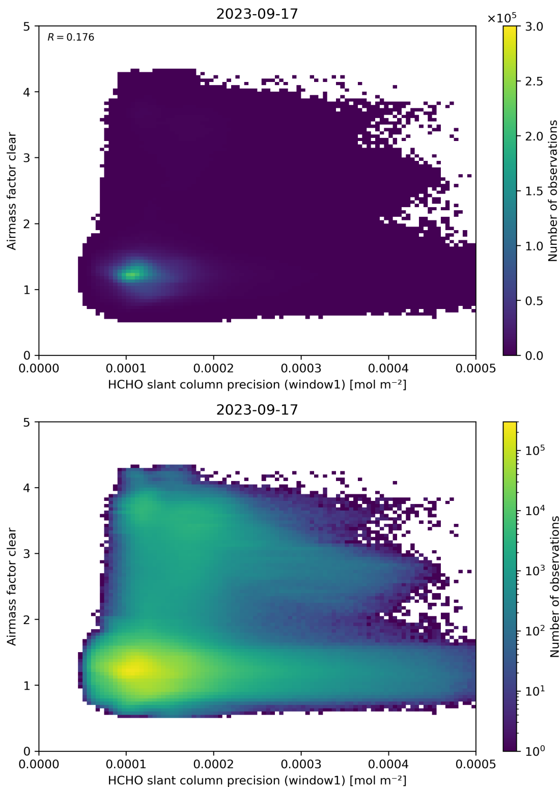
Figure 91: Scatter density plot of “HCHO slant column precision (window1)” against “Airmass factor clear” for 2023-09-16 to 2023-09-18.
