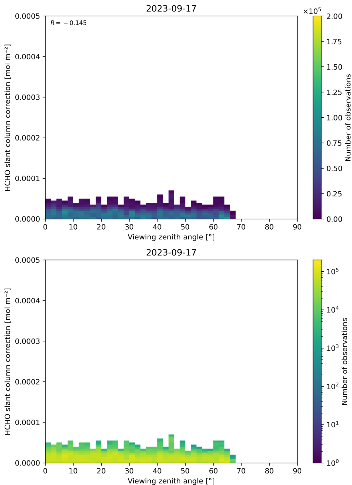
Figure 187: Scatter density plot of “Viewing zenith angle” against “HCHO slant column correction” for 2023-09-16 to 2023-09-18.
