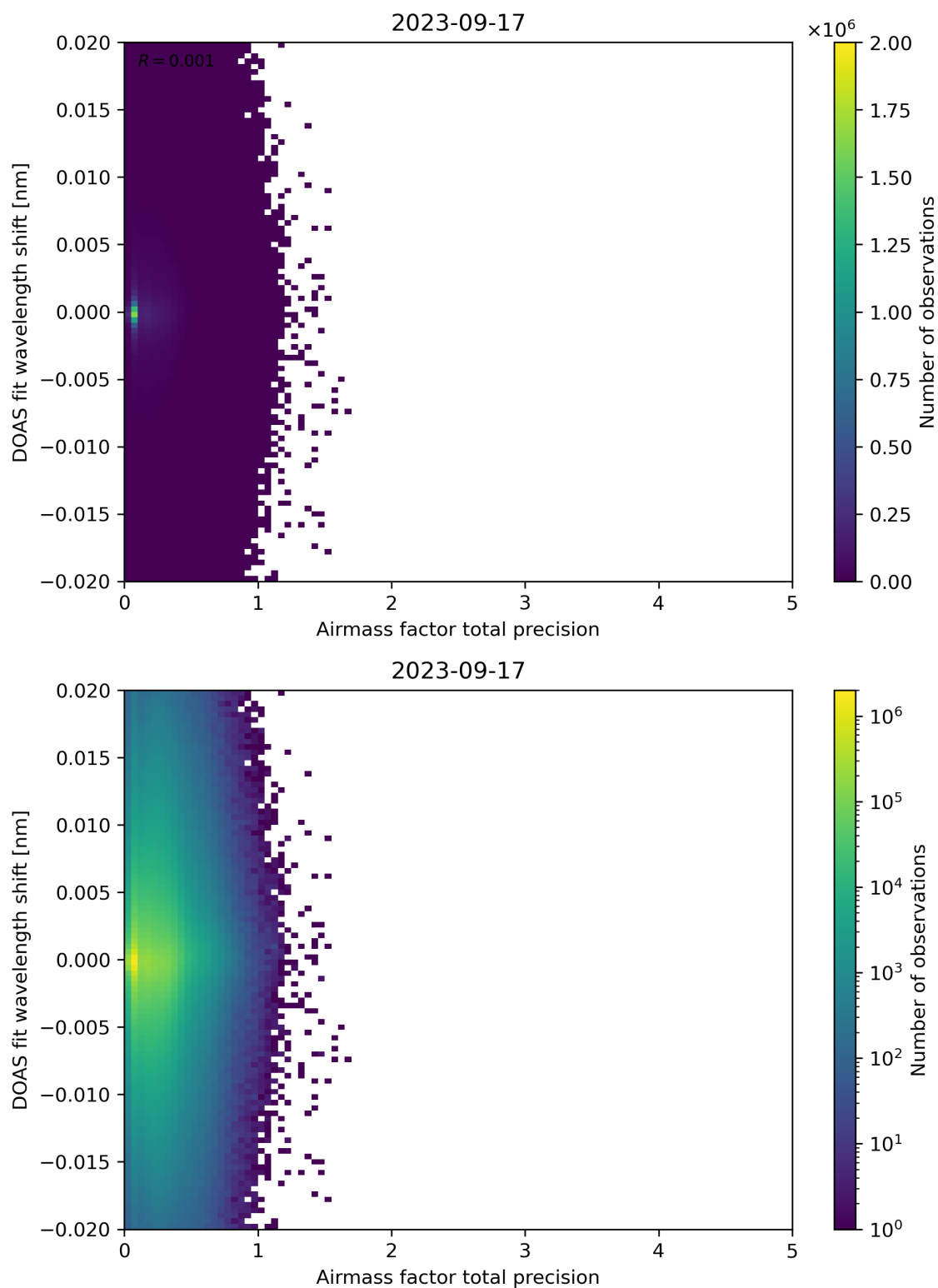
Figure 106: Scatter density plot of “Airmass factor total precision” against “DOAS fit wavelength shift” for 2023-09-16 to 2023-09-18.
