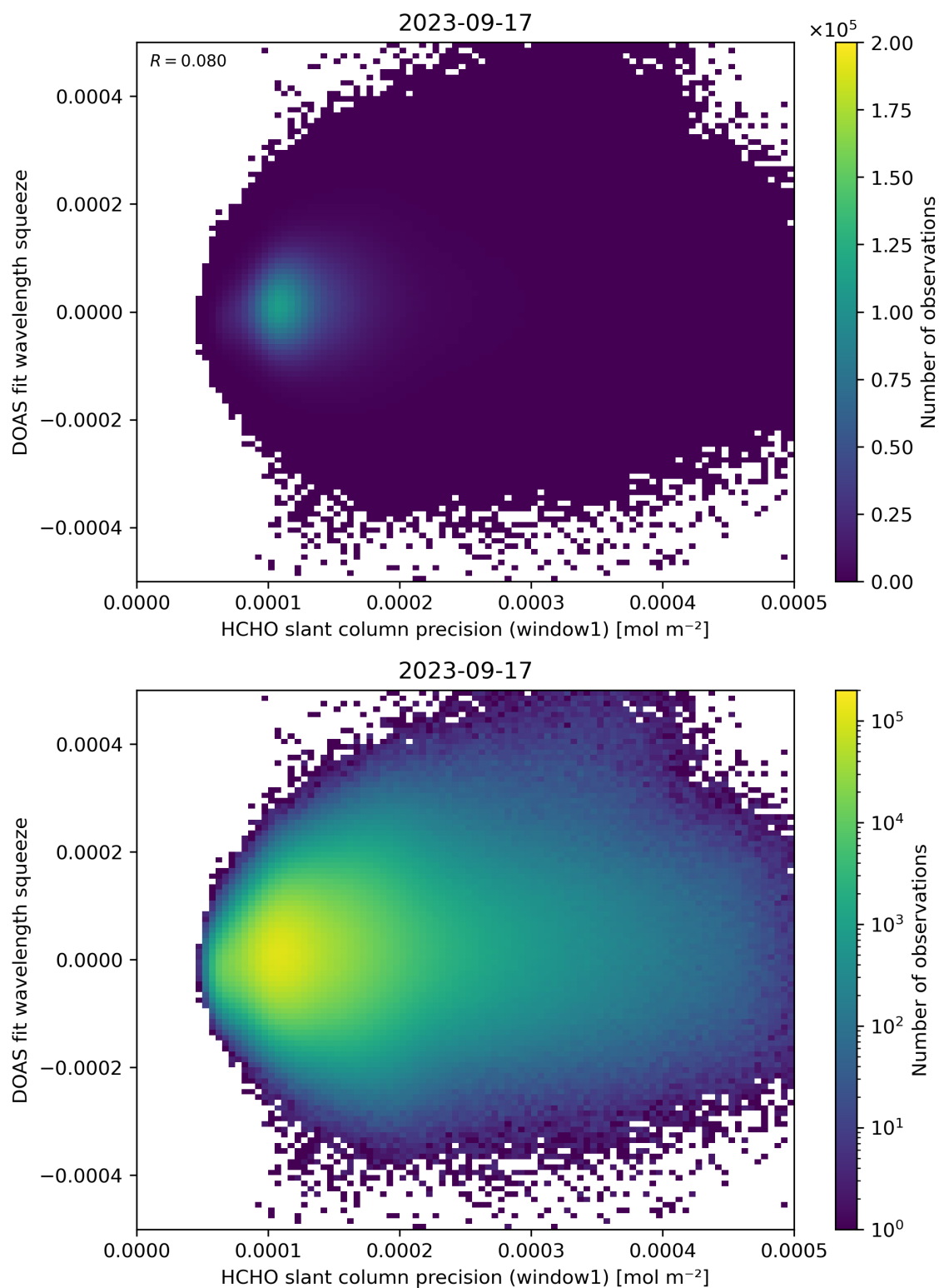
Figure 90: Scatter density plot of “HCHO slant column precision (window1)” against “DOAS fit wavelength squeeze” for 2023-09-16 to 2023-09-18.
