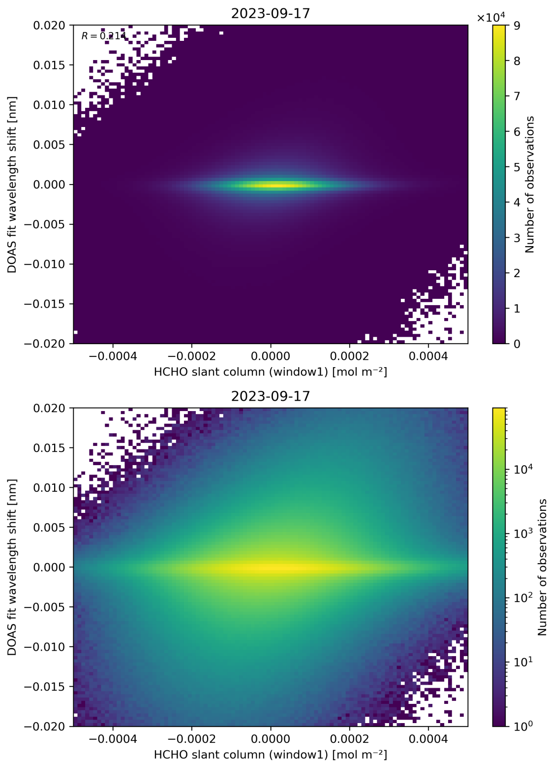
Figure 79: Scatter density plot of “HCHO slant column (window1)” against “DOAS fit wavelength shift” for 2023-09-16 to 2023-09-18.
