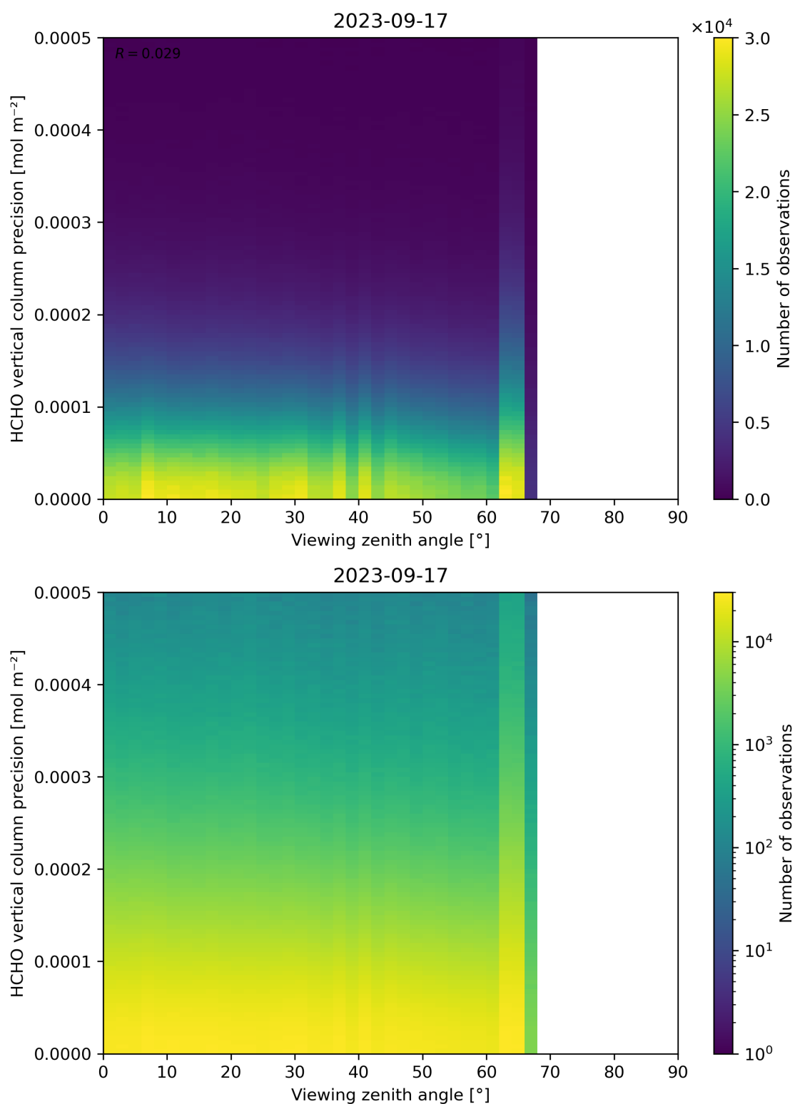
Figure 194: Scatter density plot of “Viewing zenith angle” against “HCHO vertical column precision” for 2023-09-16 to 2023-09-18.
