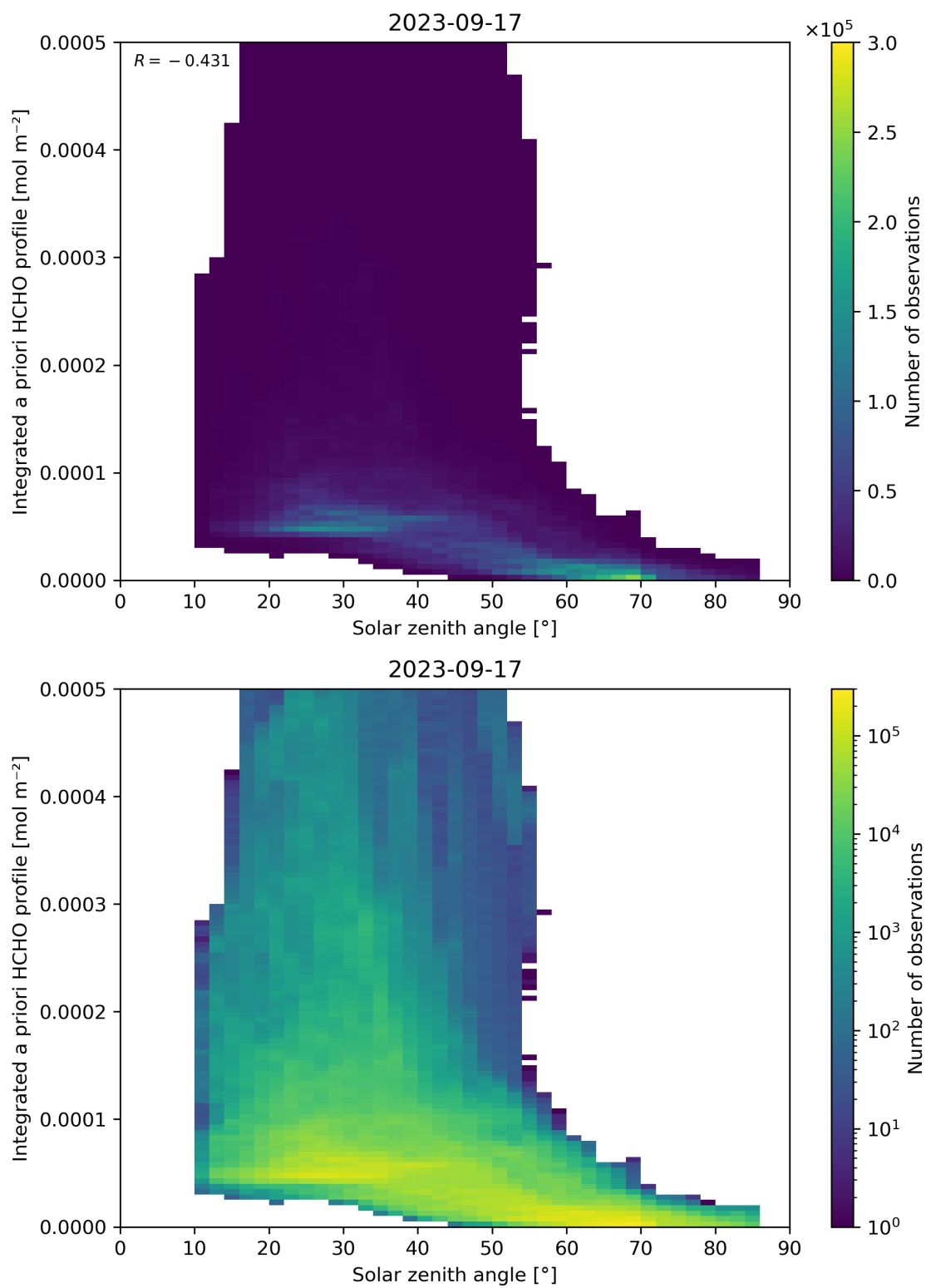
Figure 180: Scatter density plot of “Solar zenith angle” against “Integrated a priori HCHO profile” for 2023-09-16 to 2023-09-18.
