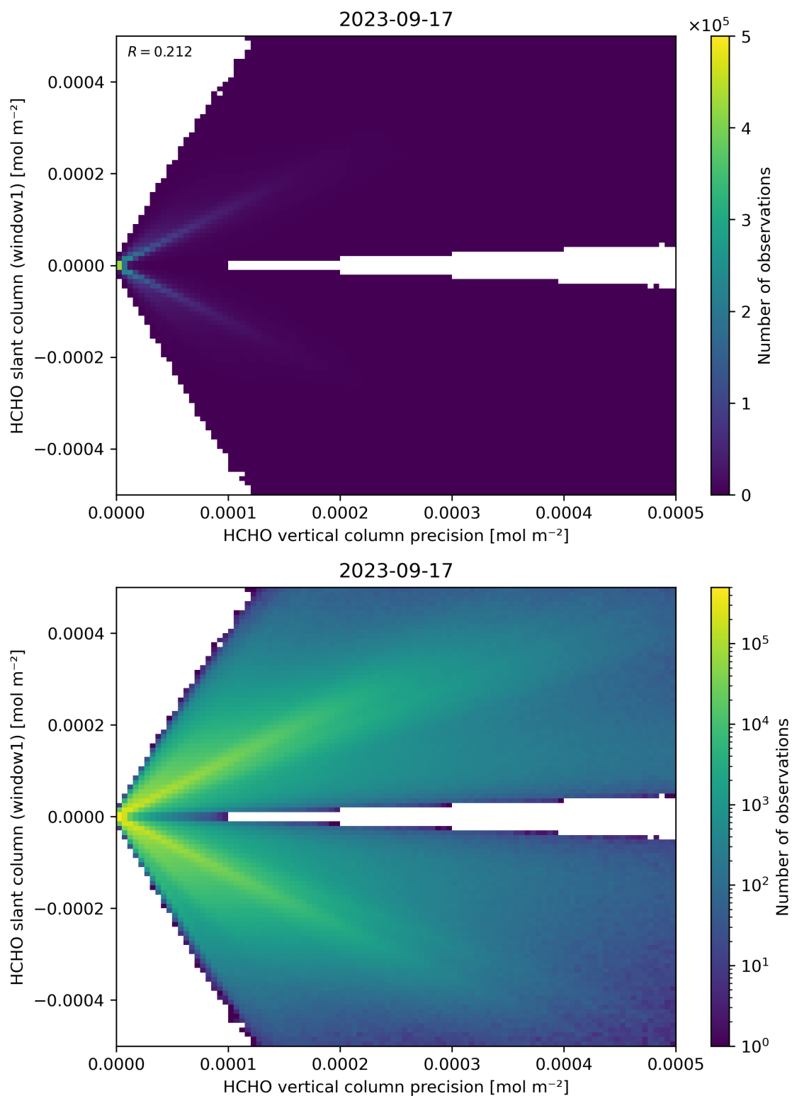
Figure 142: Scatter density plot of “HCHO vertical column precision” against “HCHO slant column (window1)” for 2023-09-16 to 2023-09-18.
