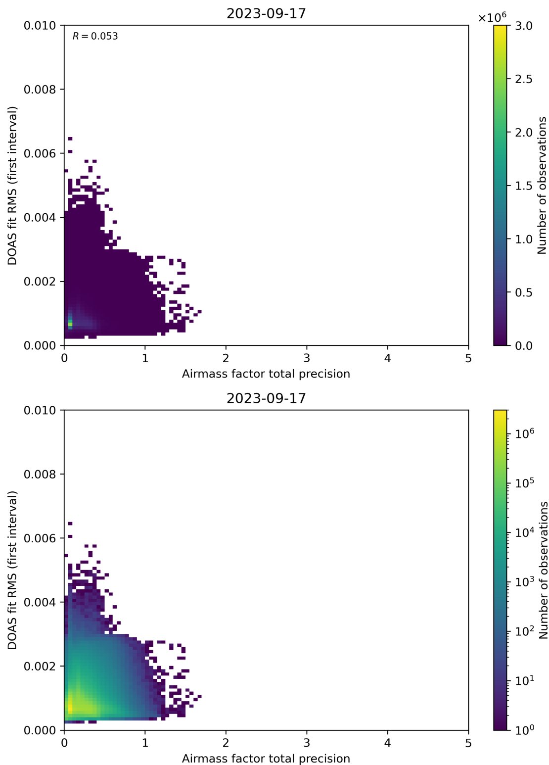
Figure 105: Scatter density plot of “Airmass factor total precision” against “DOAS fit RMS (first interval)” for 2023-09-16 to 2023-09-18.
