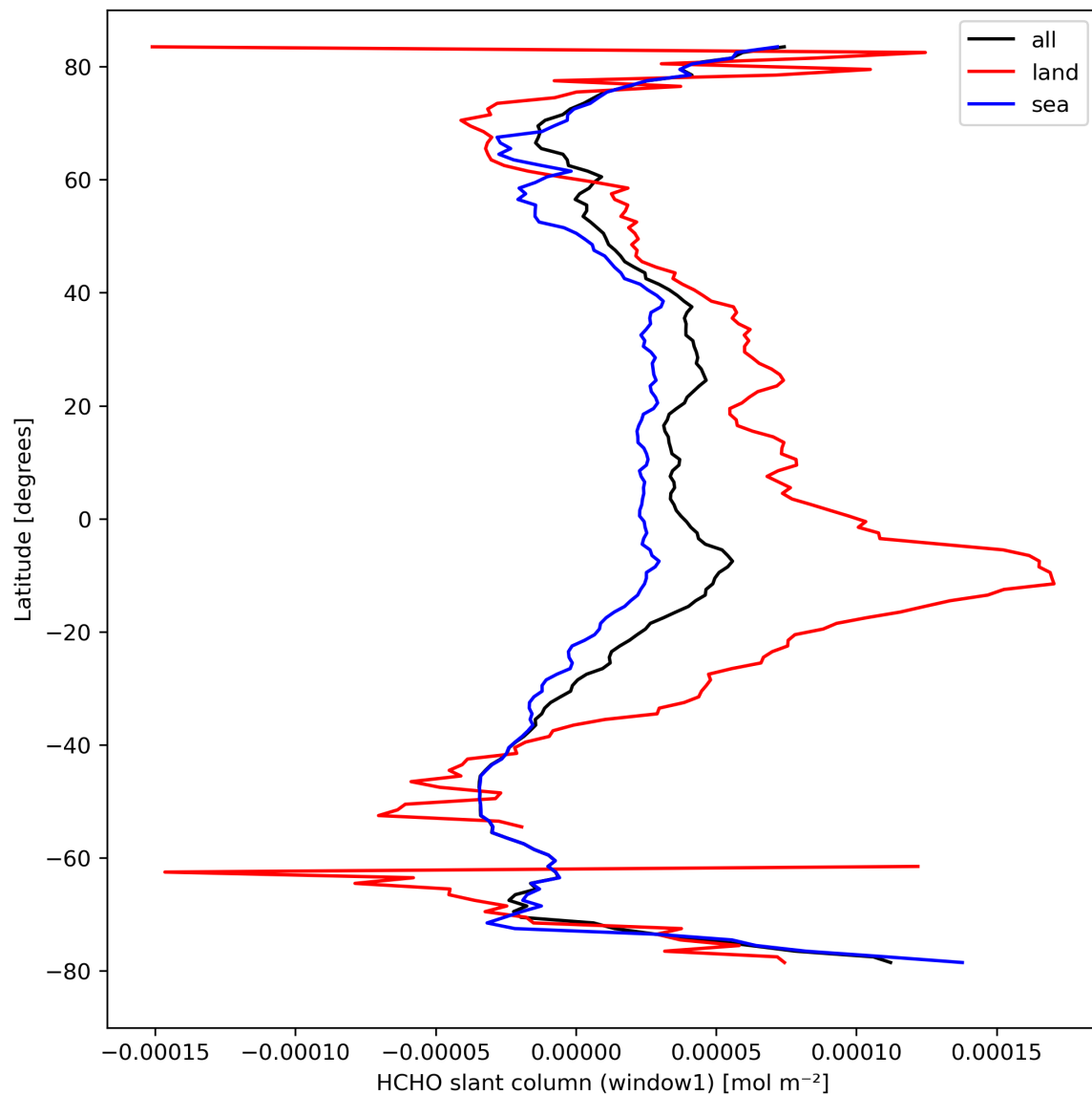
Figure 24: Zonal average of “HCHO slant column (window1)” for 2023-09-16 to 2023-09-18.
