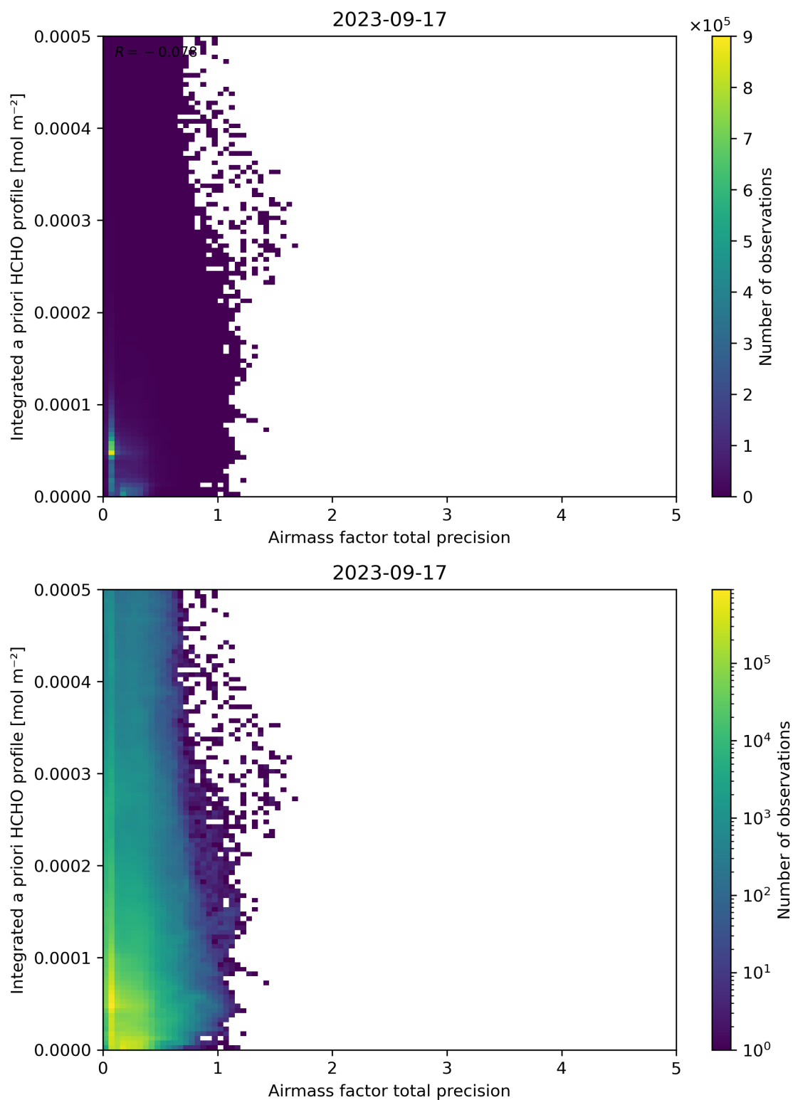
Figure 111: Scatter density plot of “Airmass factor total precision” against “Integrated a priori HCHO profile” for 2023-09-16 to 2023-09-18.
