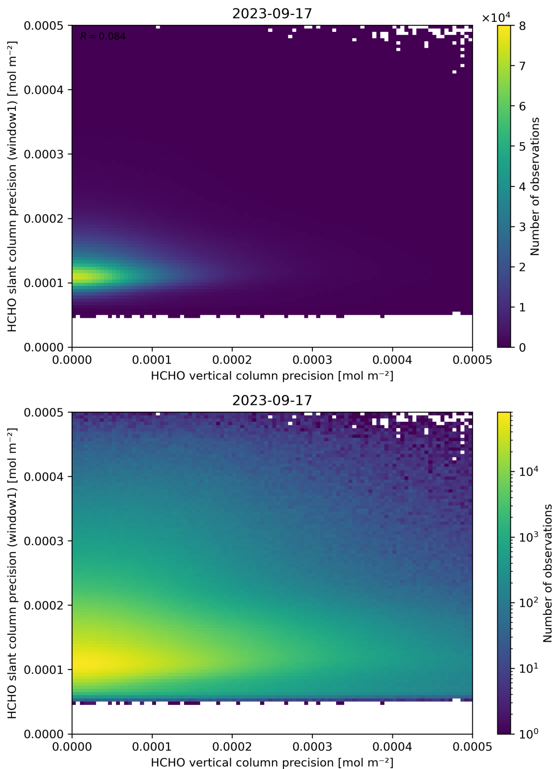
Figure 143: Scatter density plot of “HCHO vertical column precision” against “HCHO slant column precision (window1)” for 2023-09-16 to 2023-09-18.
