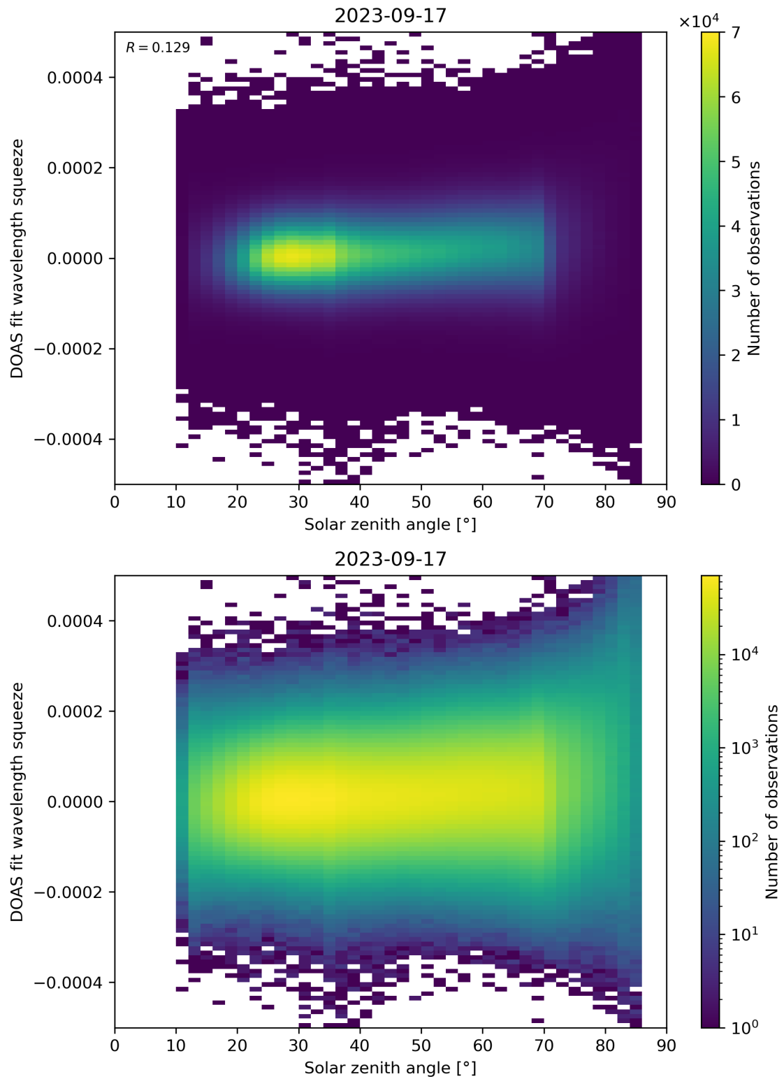
Figure 169: Scatter density plot of “Solar zenith angle” against “DOAS fit wavelength squeeze” for 2023-09-16 to 2023-09-18.
