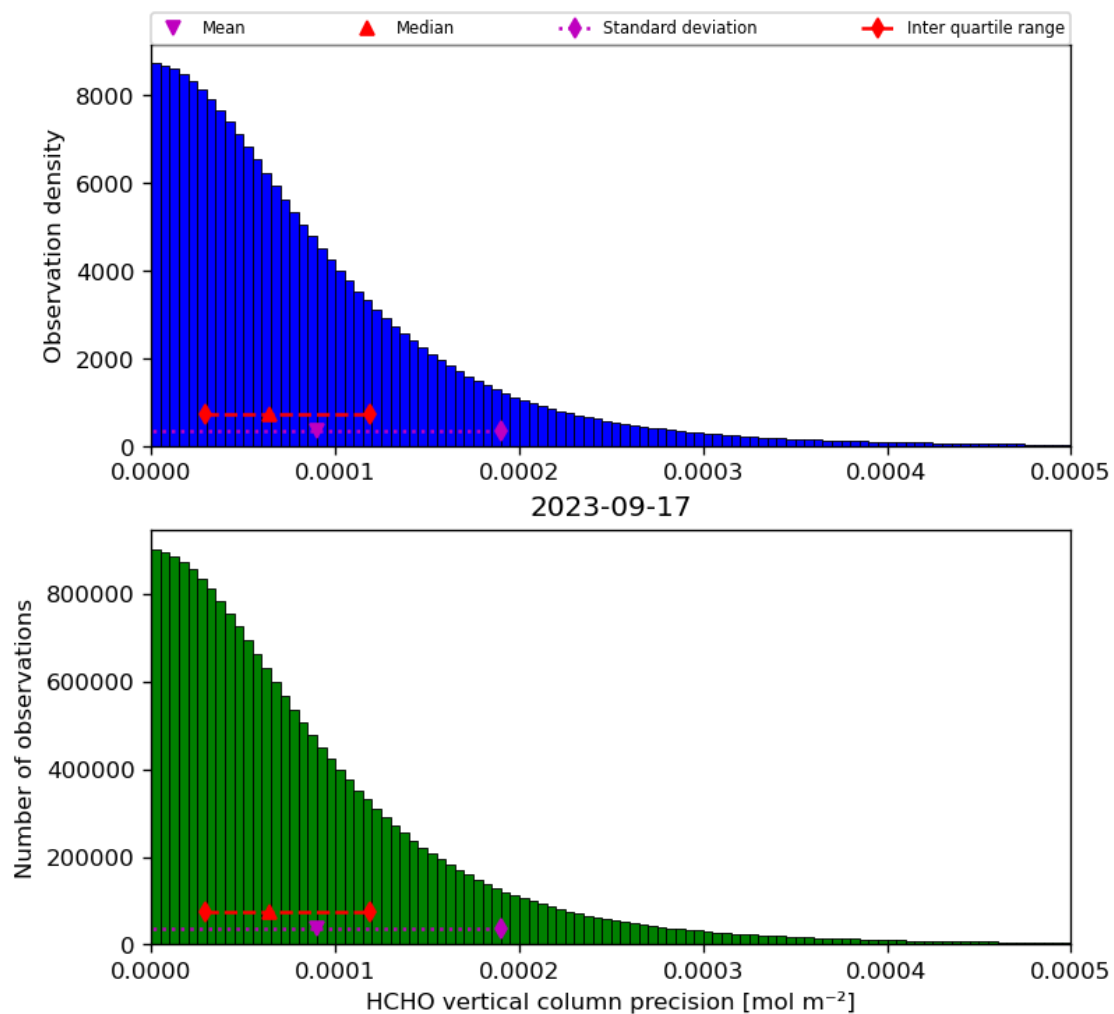
Figure 36: Histogram of “HCHO vertical column precision” for 2023-09-16 to 2023-09-18
