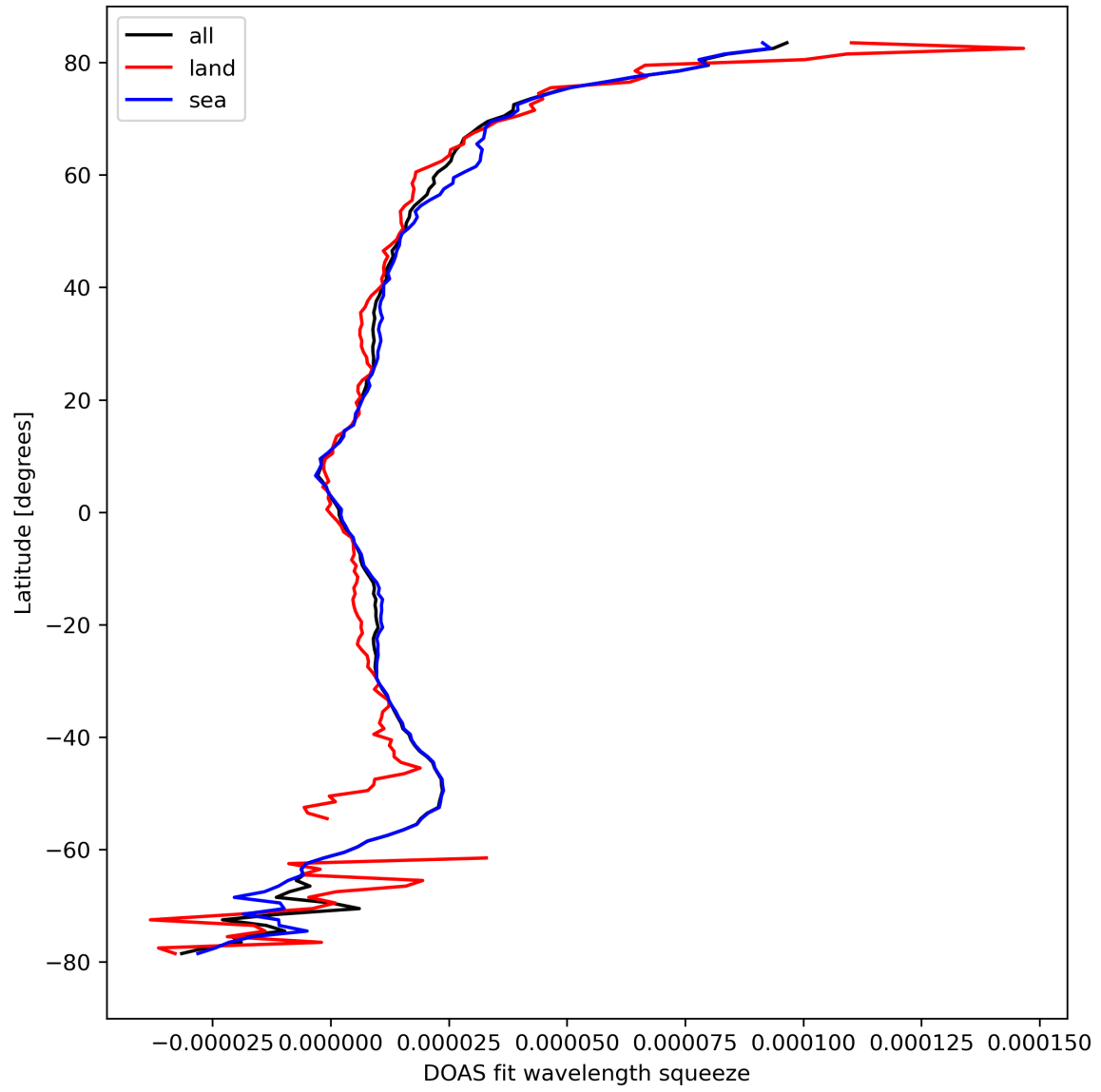
Figure 31: Zonal average of “DOAS fit wavelength squeeze” for 2023-09-16 to 2023-09-18.
