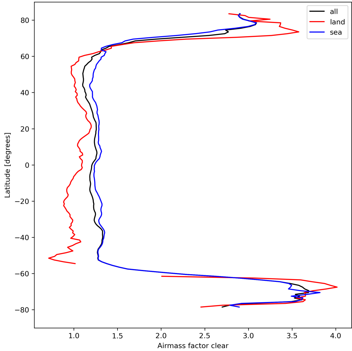
Figure 28: Zonal average of “Airmass factor clear” for 2023-09-16 to 2023-09-18.
