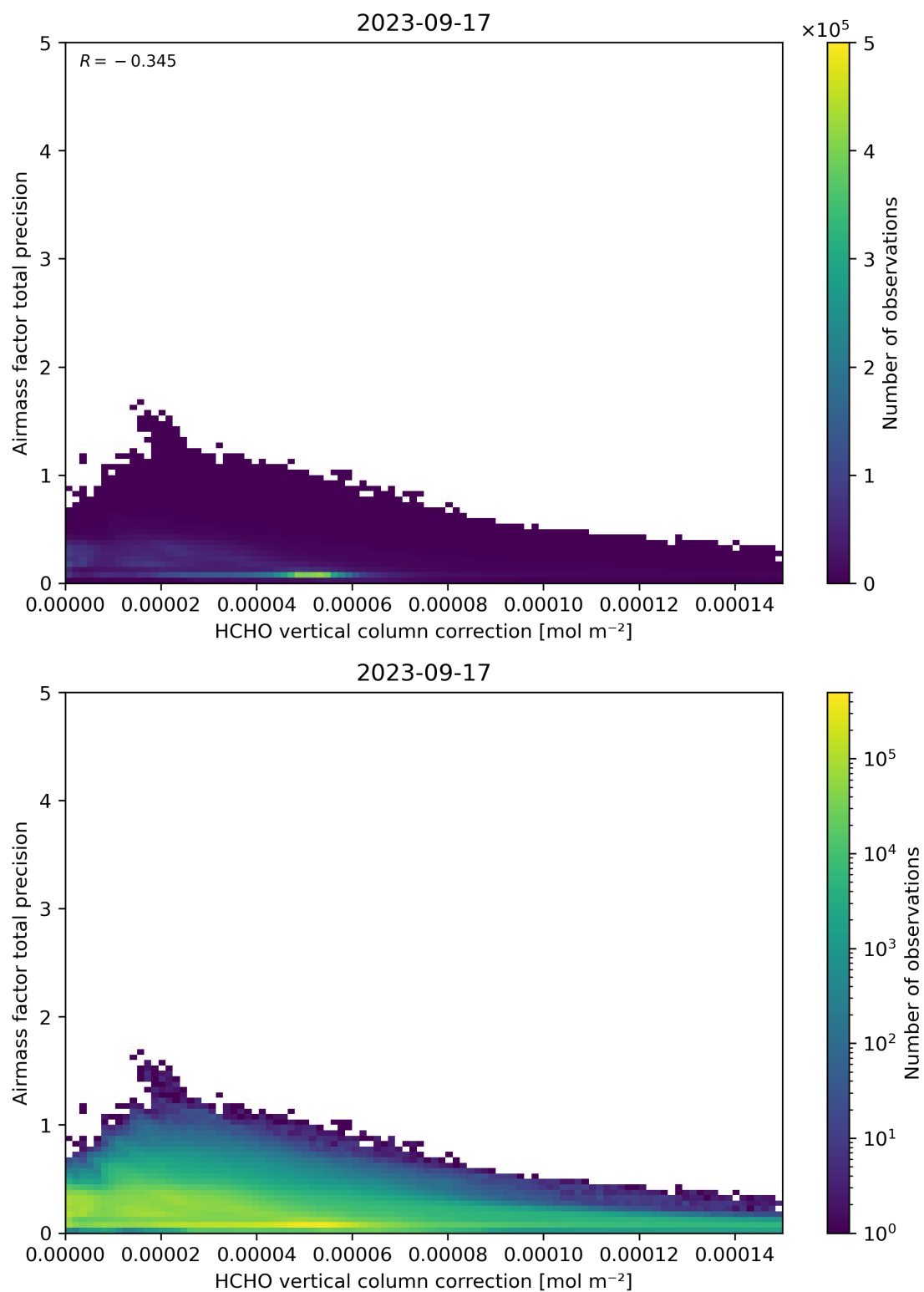
Figure 121: Scatter density plot of “HCHO vertical column correction” against “Airmass factor total precision” for 2023-09-16 to 2023-09-18.
