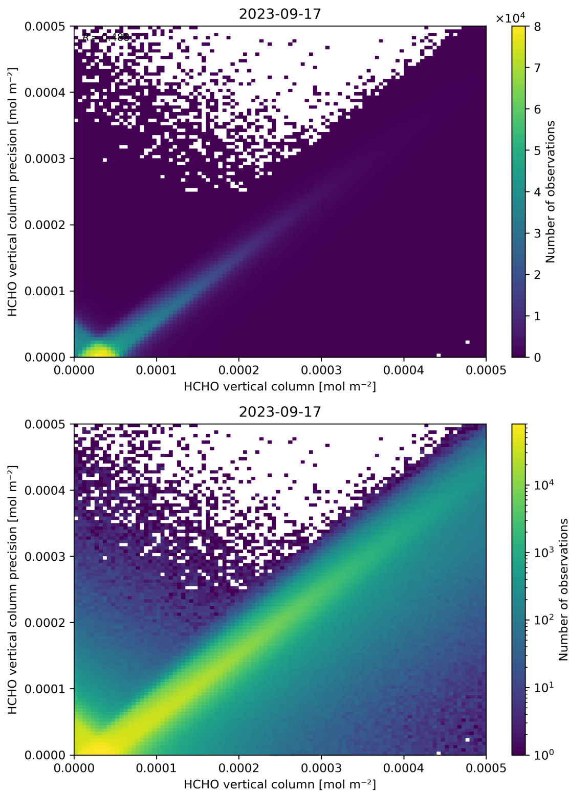
Figure 134: Scatter density plot of “HCHO vertical column” against “HCHO vertical column precision” for 2023-09-16 to 2023-09-18.
