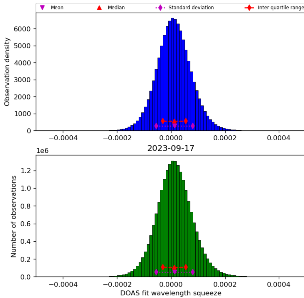
Figure 45: Histogram of “DOAS fit wavelength squeeze” for 2023-09-16 to 2023-09-18
