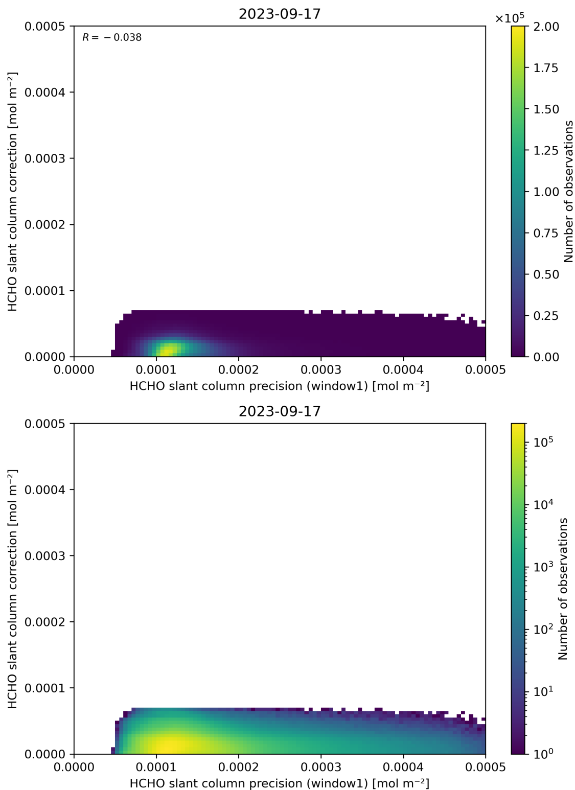
Figure 93: Scatter density plot of “HCHO slant column precision (window1)” against “HCHO slant column correction” for 2023-09-16 to 2023-09-18.
