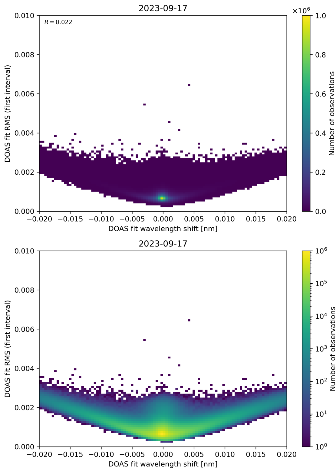
Figure 64: Scatter density plot of “DOAS fit wavelength shift” against “DOAS fit RMS (first interval)” for 2023-09-16 to 2023-09-18.
