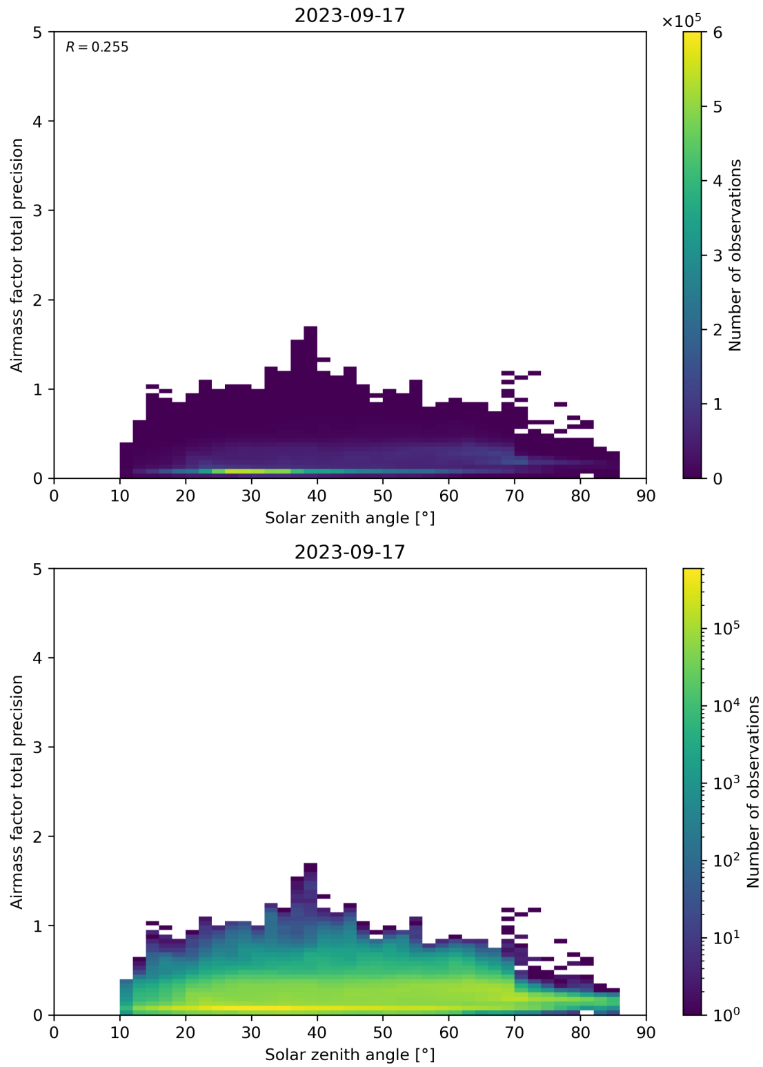
Figure 176: Scatter density plot of “Solar zenith angle” against “Airmass factor total precision” for 2023-09-16 to 2023-09-18.
