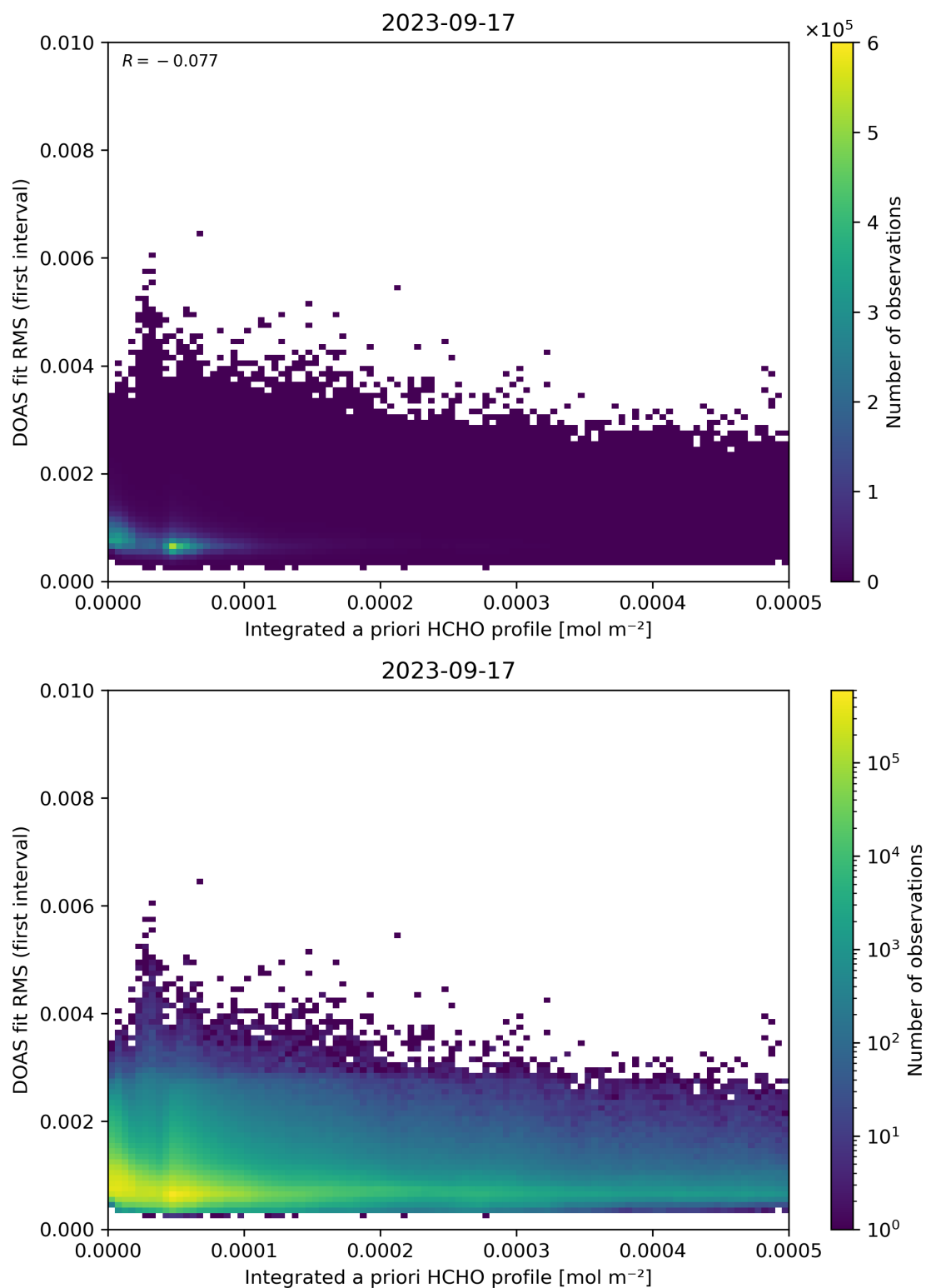
Figure 148: Scatter density plot of “Integrated a priori HCHO profile” against “DOAS fit RMS (first interval)” for 2023-09-16 to 2023-09-18.
