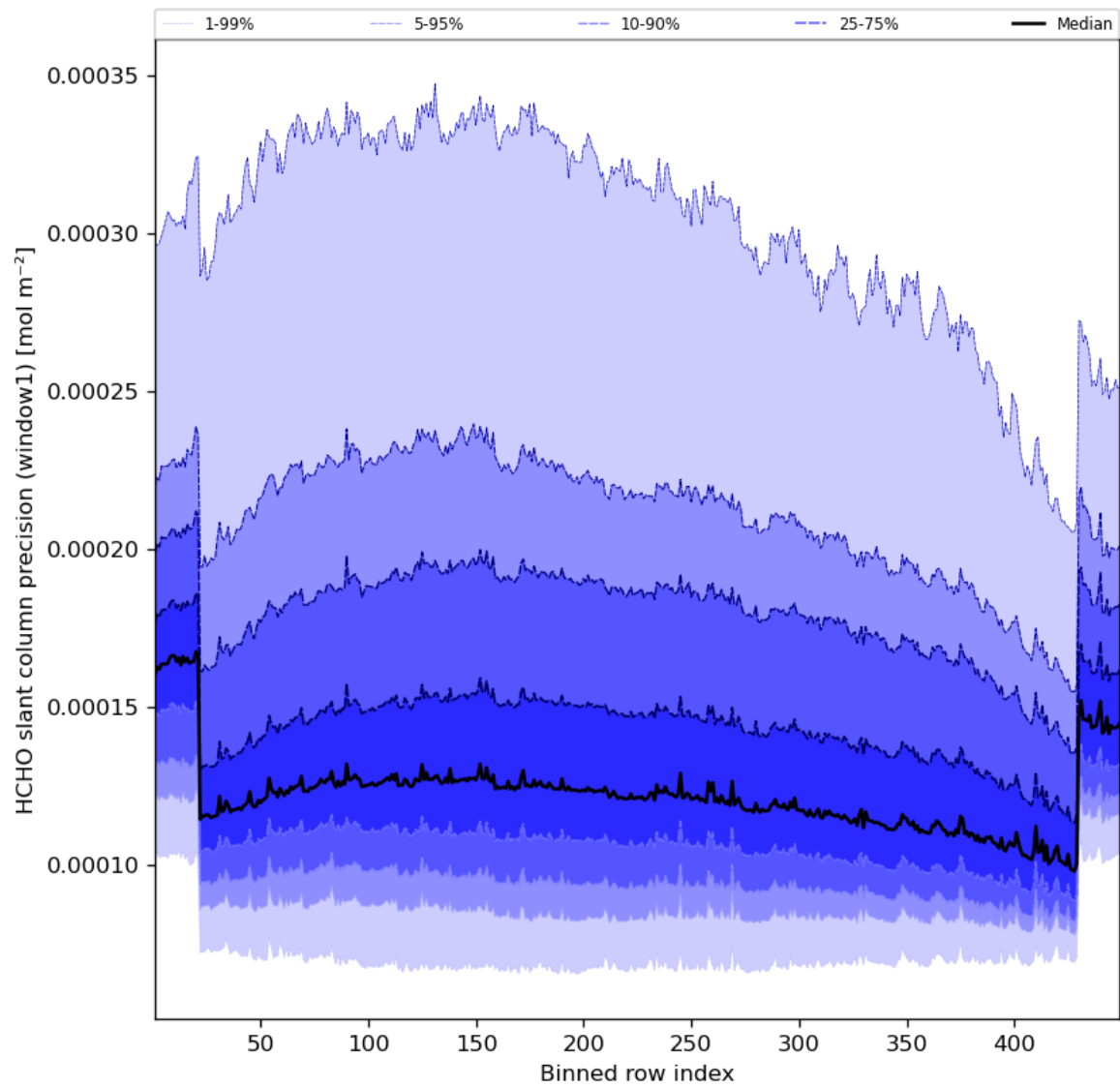
Figure 53: Along track statistics of “HCHO slant column precision (window1)” for 2023-09-16 to 2023-09-18
