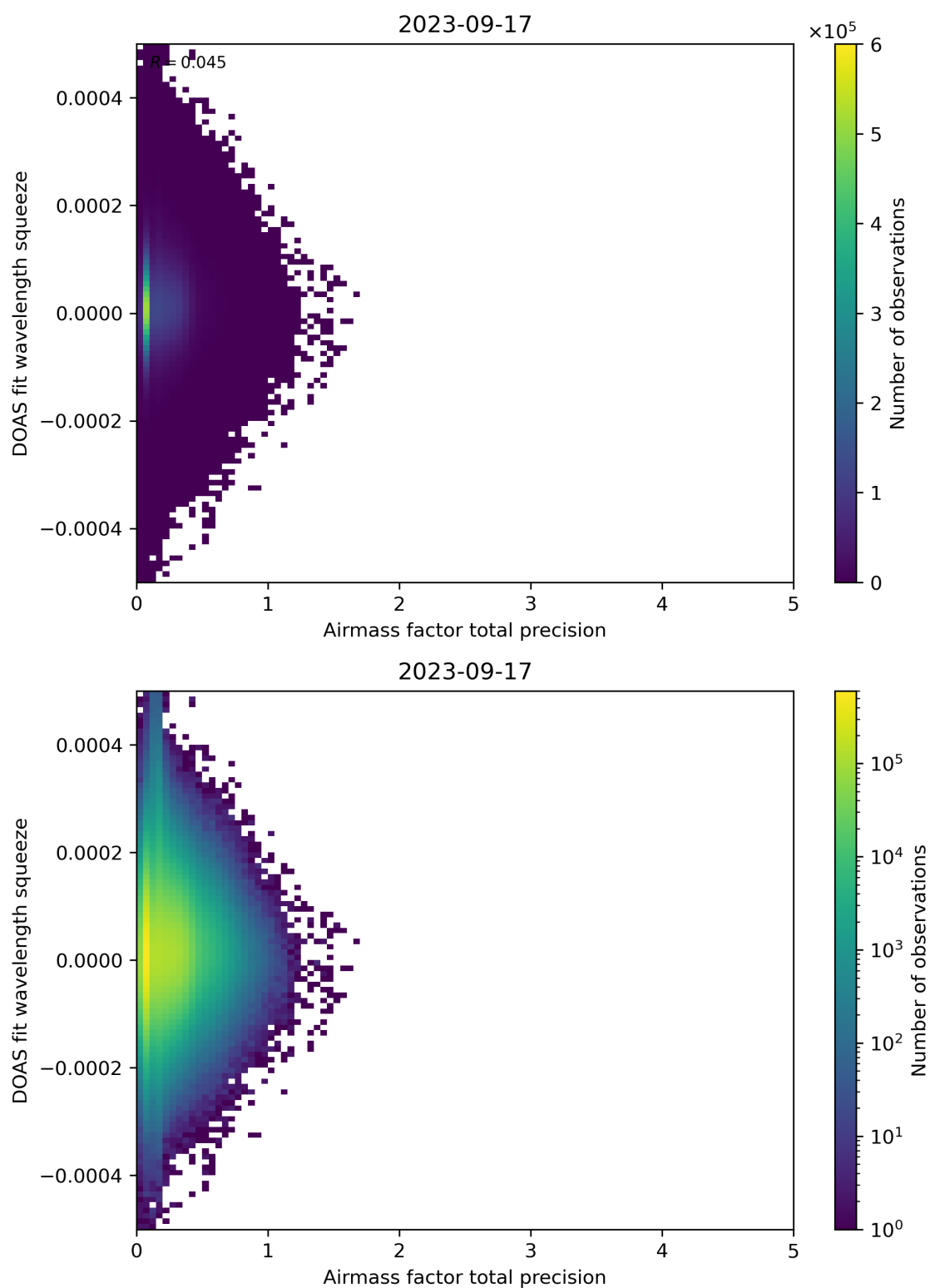
Figure 107: Scatter density plot of “Airmass factor total precision” against “DOAS fit wavelength squeeze” for 2023-09-16 to 2023-09-18.
