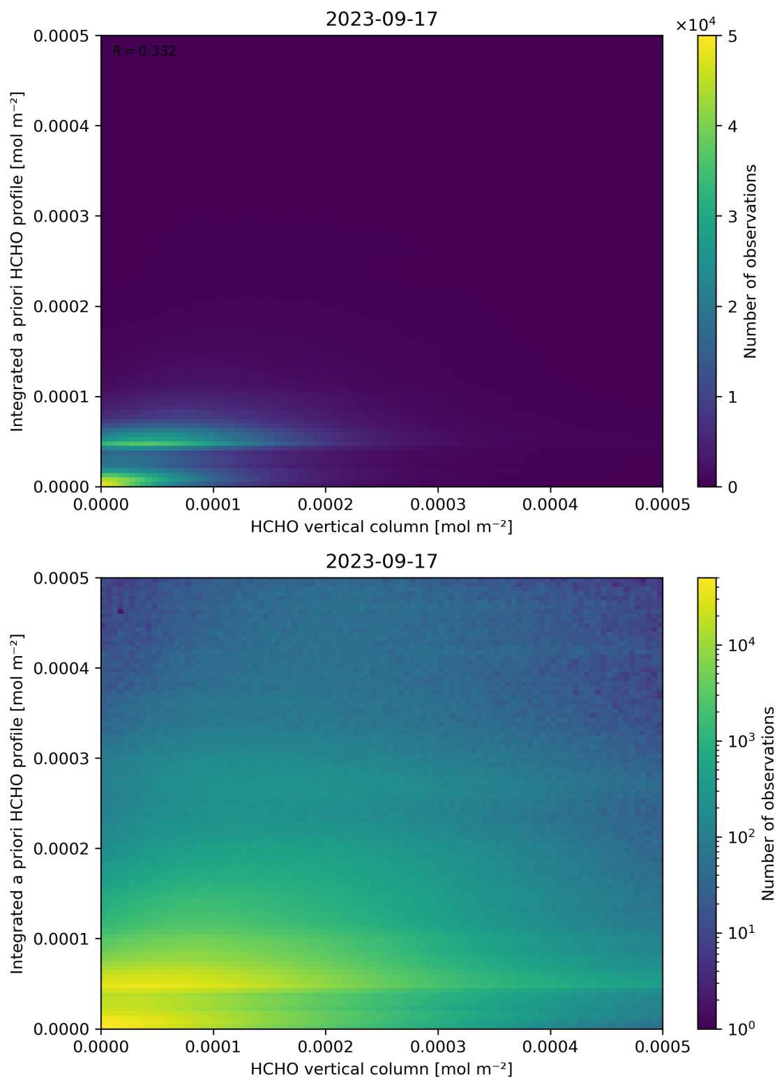
Figure 135: Scatter density plot of “HCHO vertical column” against “Integrated a priori HCHO profile” for 2023-09-16 to 2023-09-18.
