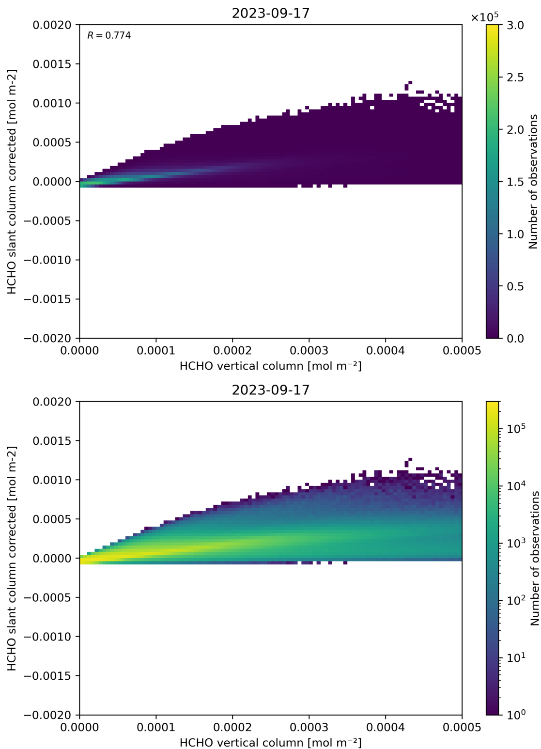
Figure 127: Scatter density plot of “HCHO vertical column” against “HCHO slant column corrected” for 2023-09-16 to 2023-09-18.
