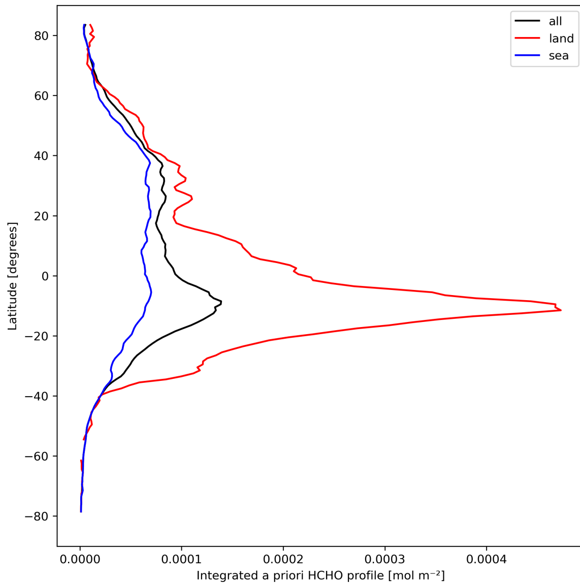
Figure 29: Zonal average of “Integrated a priori HCHO profile” for 2023-09-16 to 2023-09-18.
