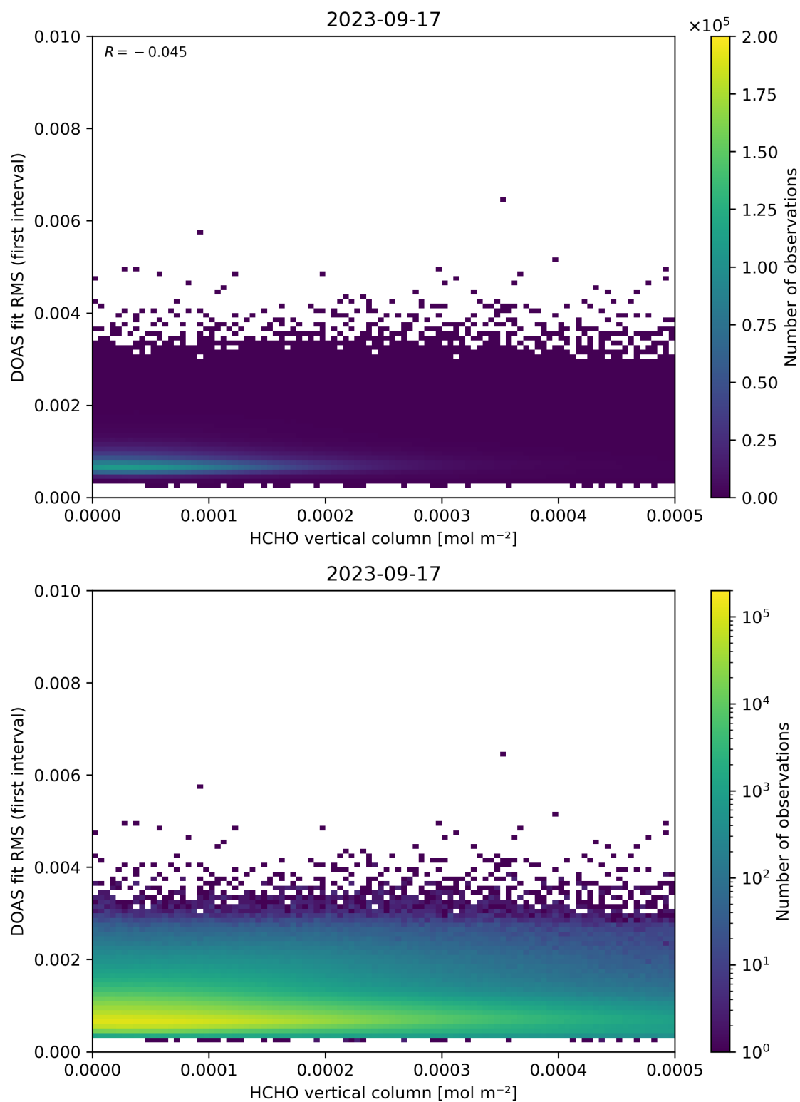
Figure 123: Scatter density plot of “HCHO vertical column” against “DOAS fit RMS (first interval)” for 2023-09-16 to 2023-09-18.
