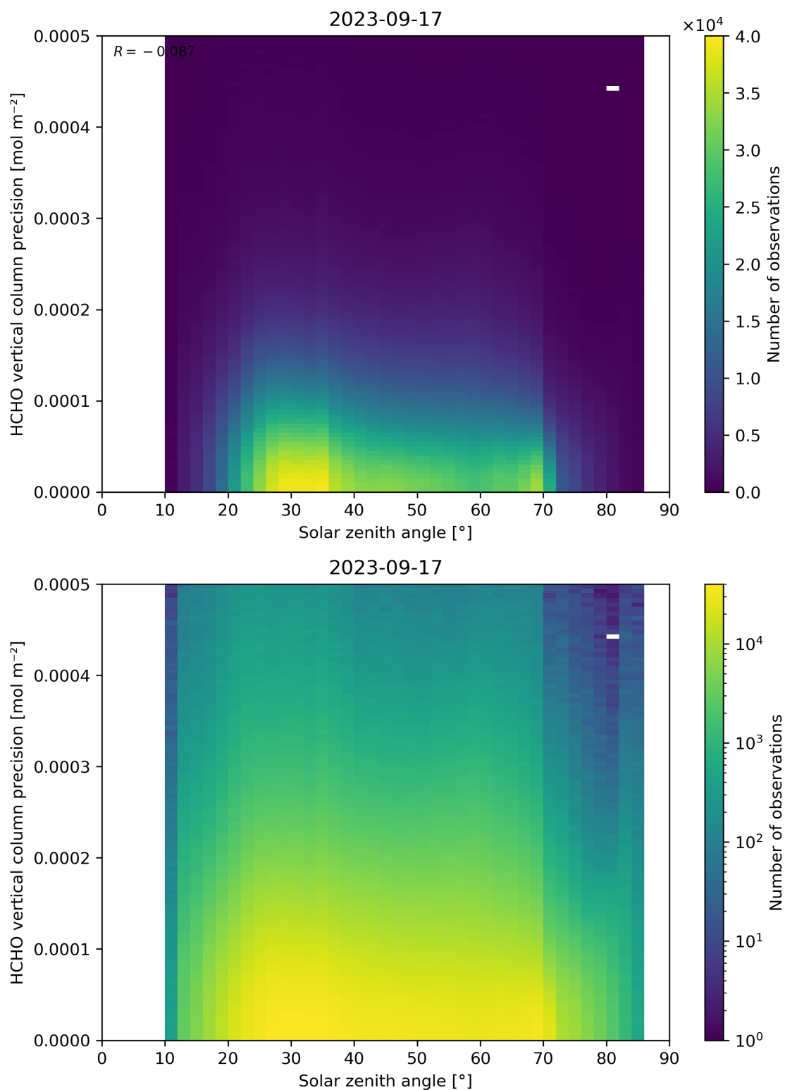
Figure 179: Scatter density plot of “Solar zenith angle” against “HCHO vertical column precision” for 2023-09-16 to 2023-09-18.
