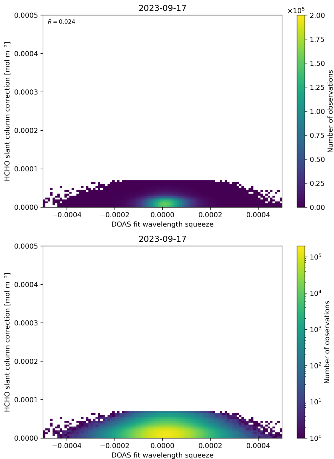
Figure 70: Scatter density plot of “DOAS fit wavelength squeeze” against “HCHO slant column correction” for 2023-09-16 to 2023-09-18.
