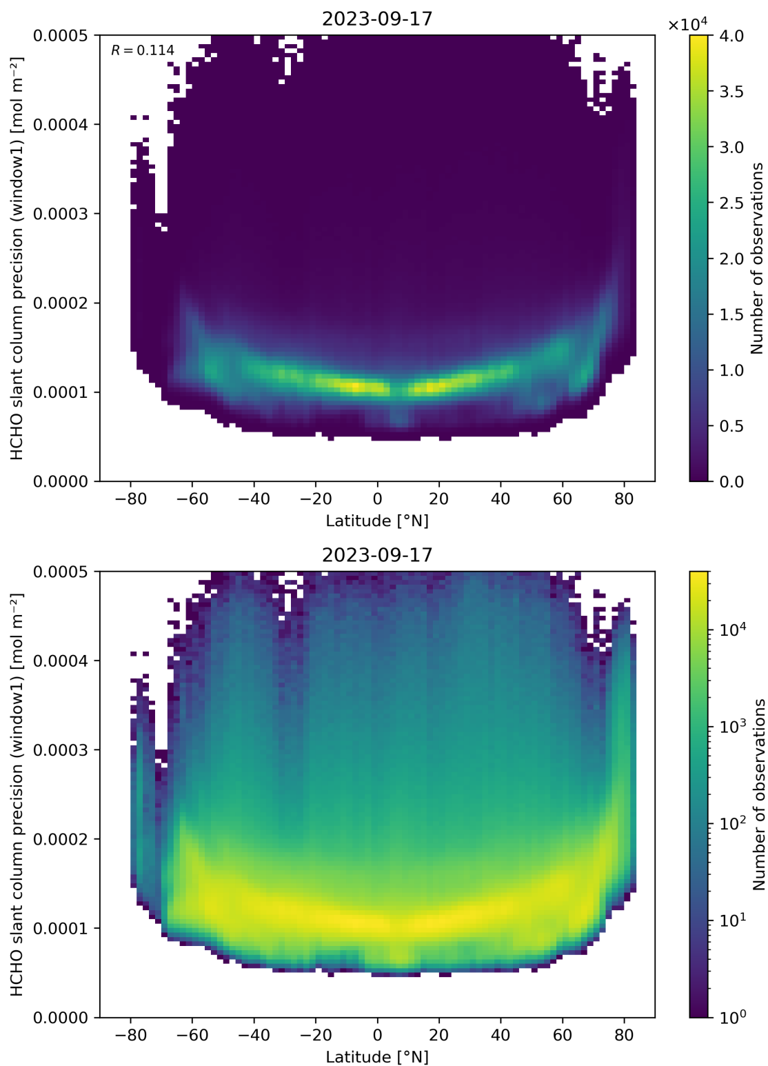
Figure 160: Scatter density plot of “Latitude” against “HCHO slant column precision (window1)” for 2023-09-16 to 2023-09-18.
