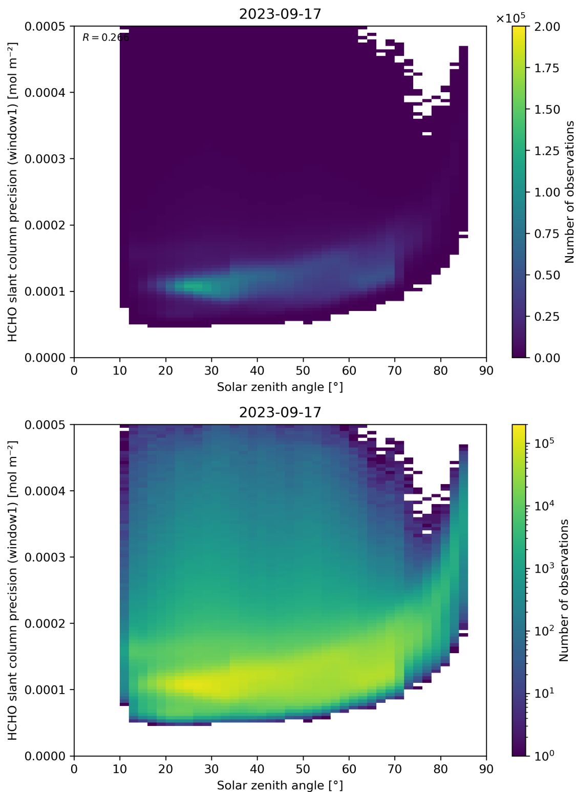
Figure 174: Scatter density plot of “Solar zenith angle” against “HCHO slant column precision (window1)” for 2023-09-16 to 2023-09-18.
