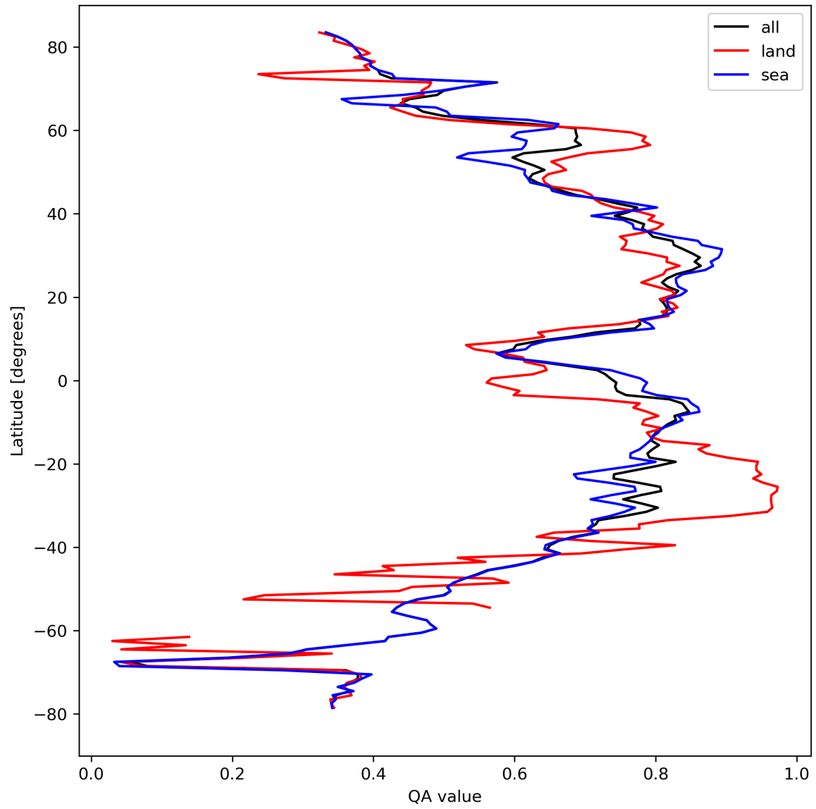
Figure 20: Zonal average of “QA value” for 2023-09-16 to 2023-09-18.
