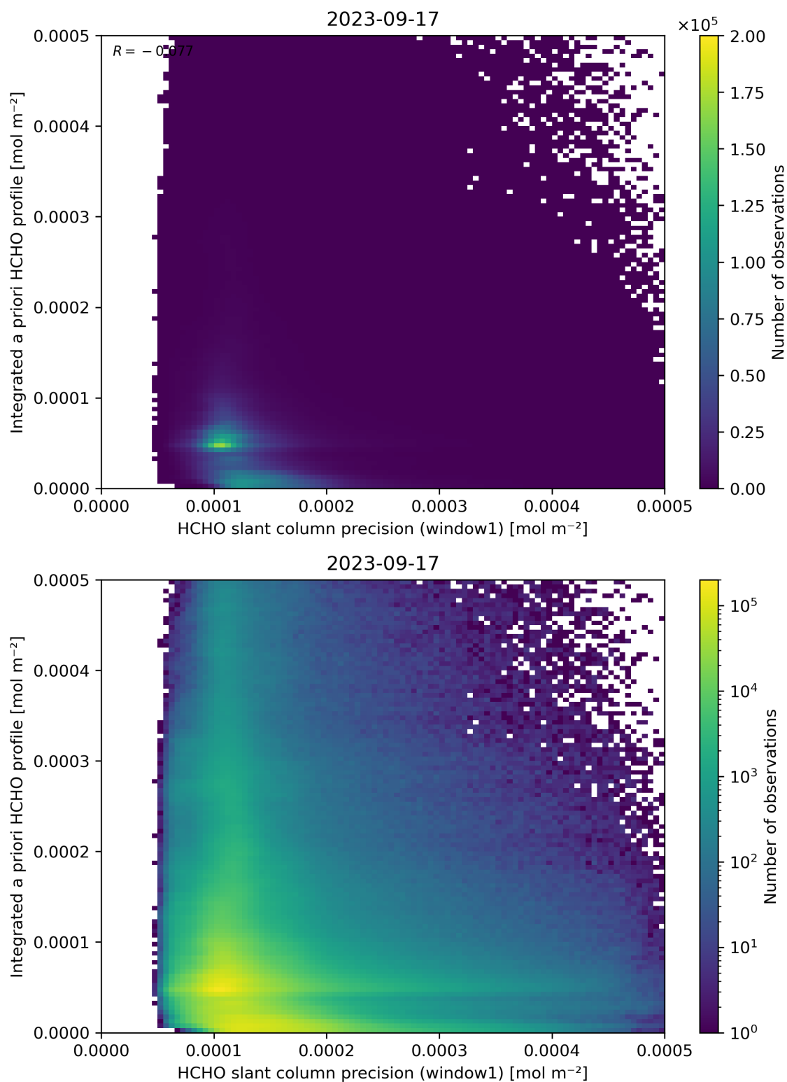
Figure 96: Scatter density plot of “HCHO slant column precision (window1)” against “Integrated a priori HCHO profile” for 2023-09-16 to 2023-09-18.
