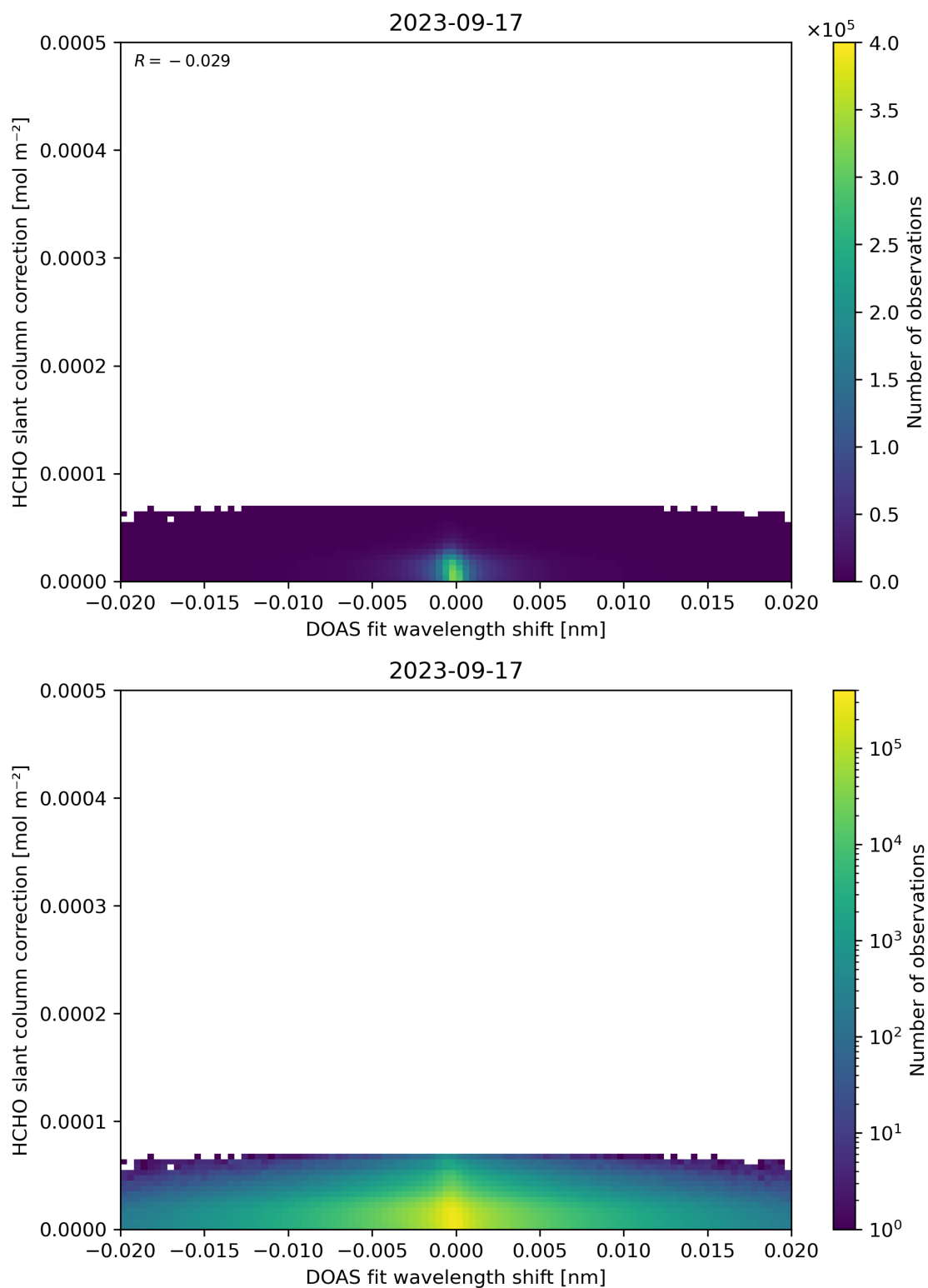
Figure 67: Scatter density plot of “DOAS fit wavelength shift” against “HCHO slant column correction” for 2023-09-16 to 2023-09-18.
