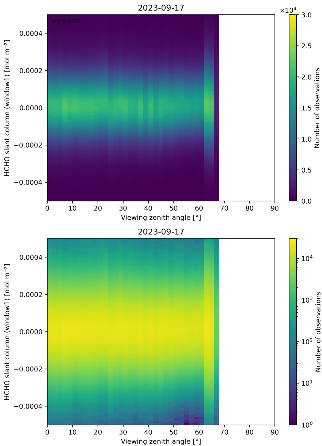
Figure 188: Scatter density plot of “Viewing zenith angle” against “HCHO slant column (window1)” for 2023-09-16 to 2023-09-18.
