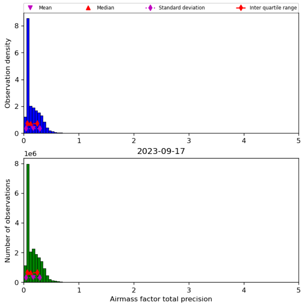
Figure 41: Histogram of “Airmass factor total precision” for 2023-09-16 to 2023-09-18
