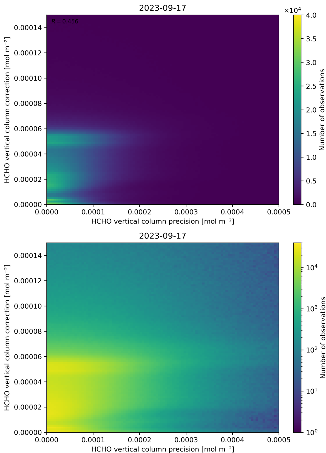
Figure 146: Scatter density plot of “HCHO vertical column precision” against “HCHO vertical column correction” for 2023-09-16 to 2023-09-18.
