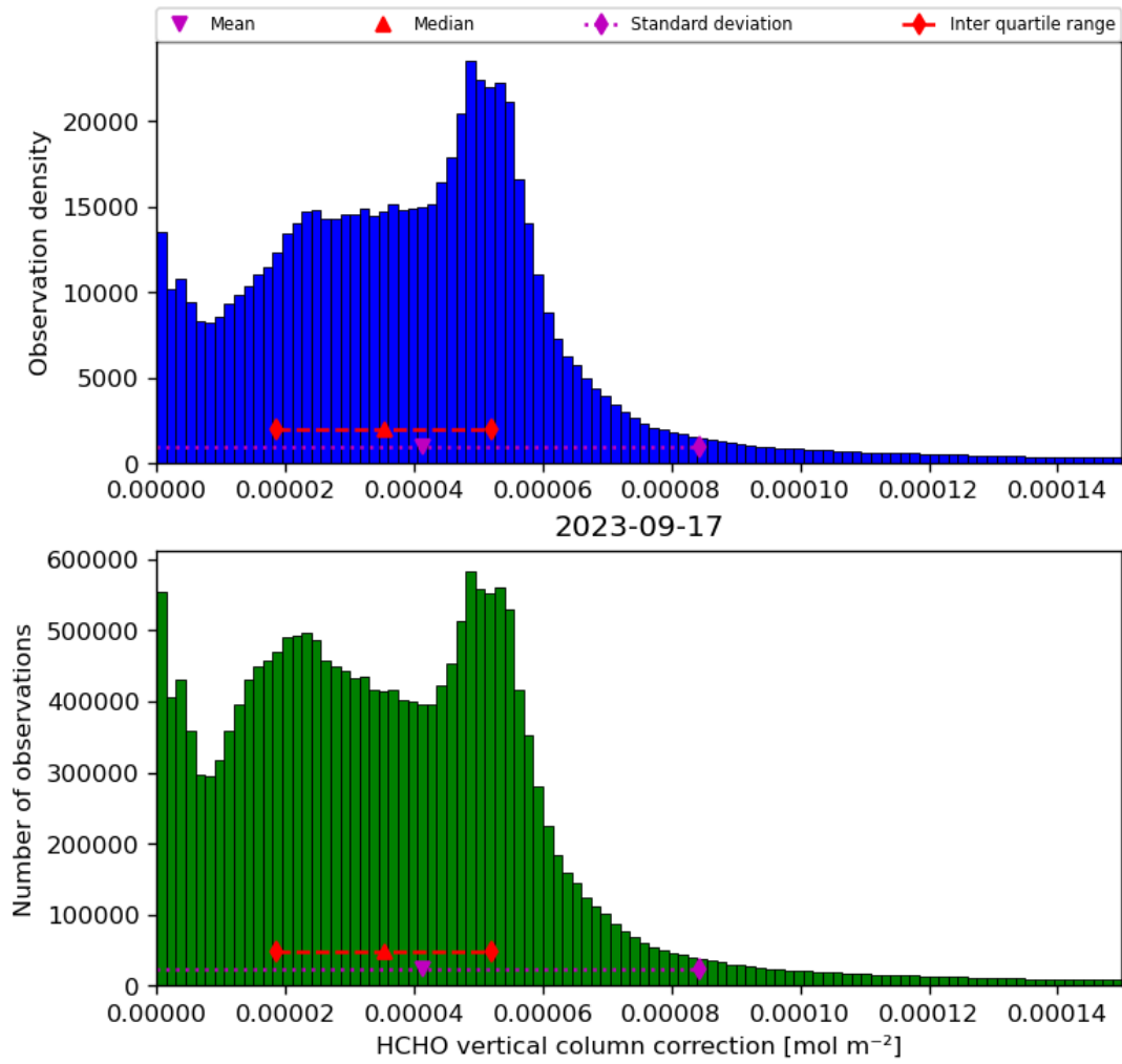
Figure 37: Histogram of “HCHO vertical column correction” for 2023-09-16 to 2023-09-18
