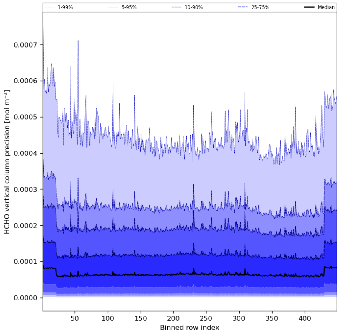
Figure 50: Along track statistics of “HCHO vertical column precision” for 2023-09-16 to 2023-09-18
