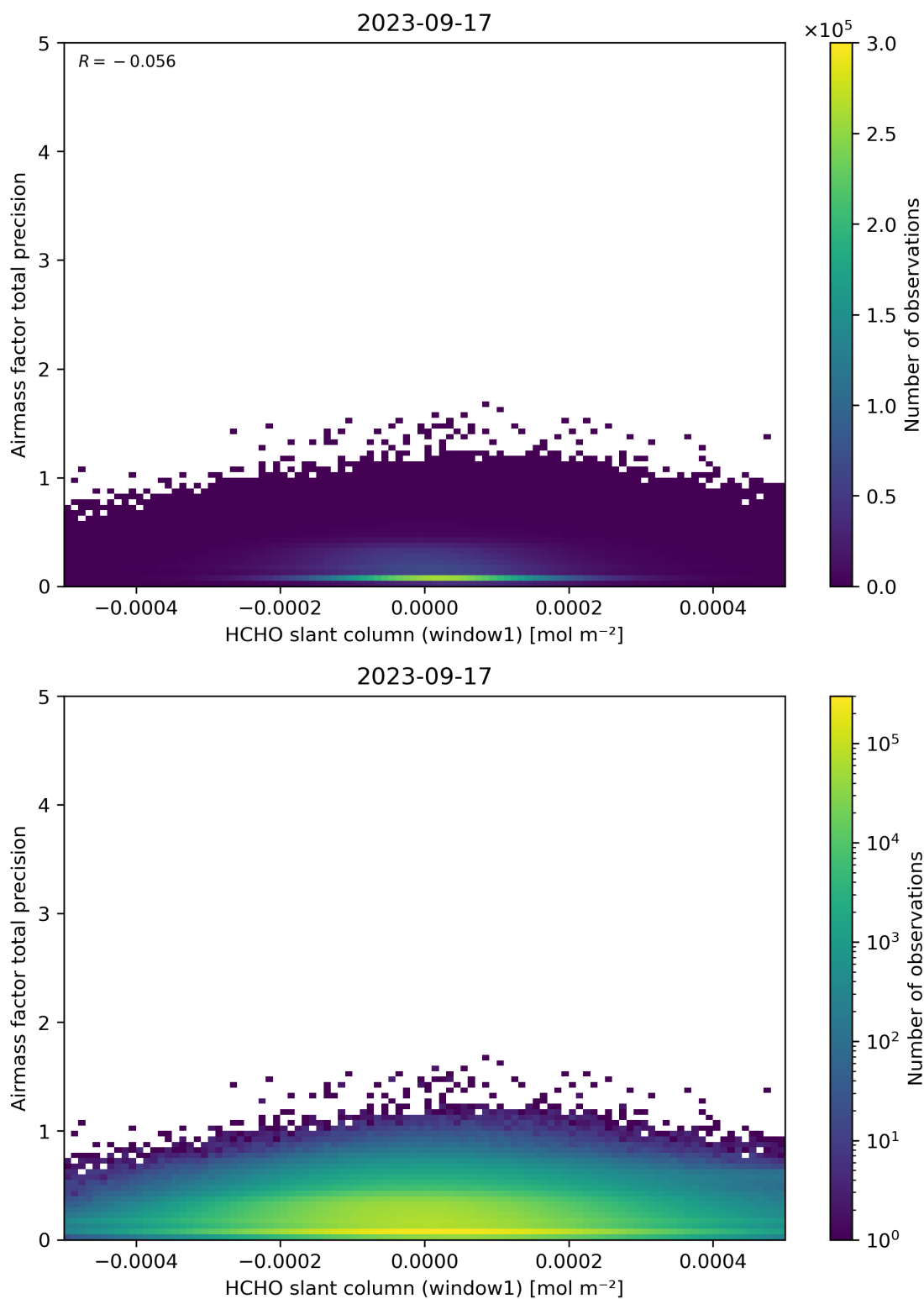
Figure 86: Scatter density plot of “HCHO slant column (window1)” against “Airmass factor total precision” for 2023-09-16 to 2023-09-18.
