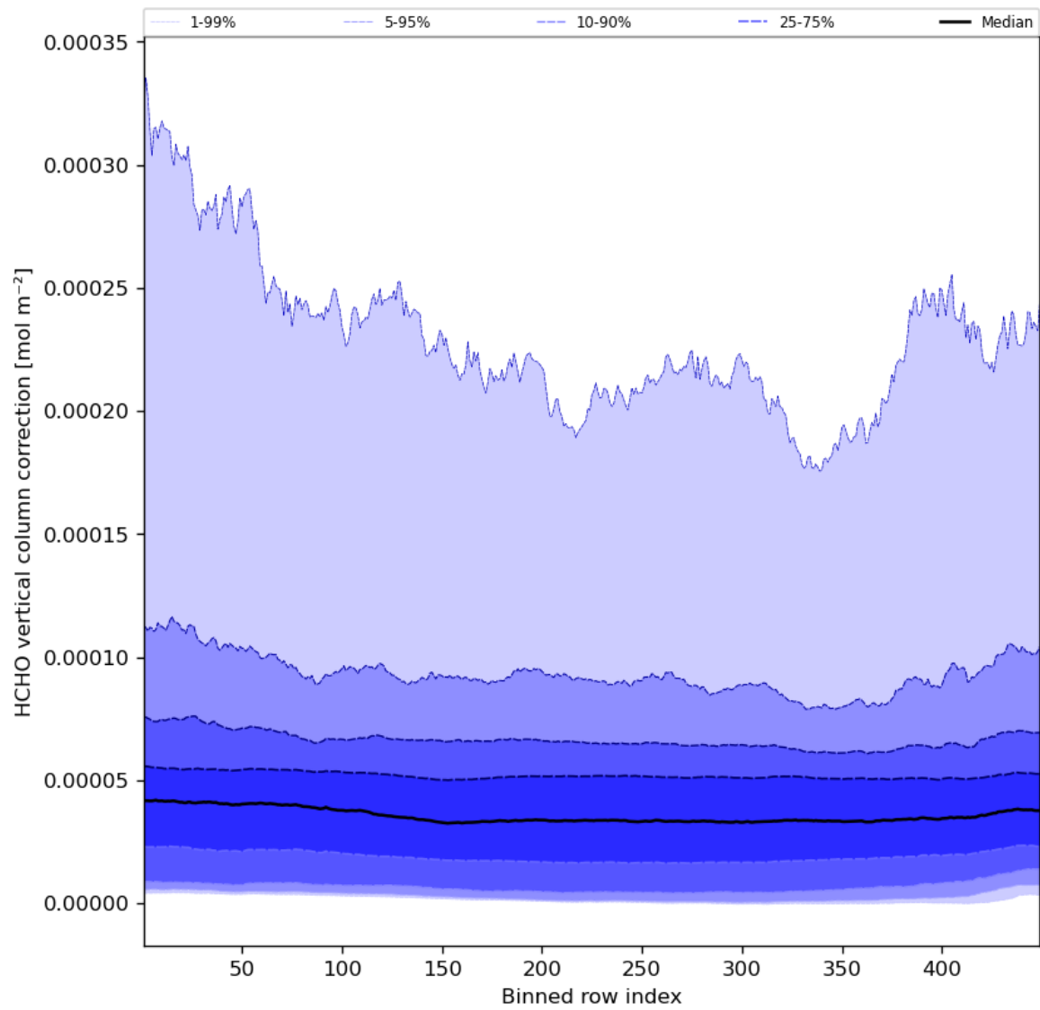
Figure 51: Along track statistics of “HCHO vertical column correction” for 2023-09-16 to 2023-09-18
