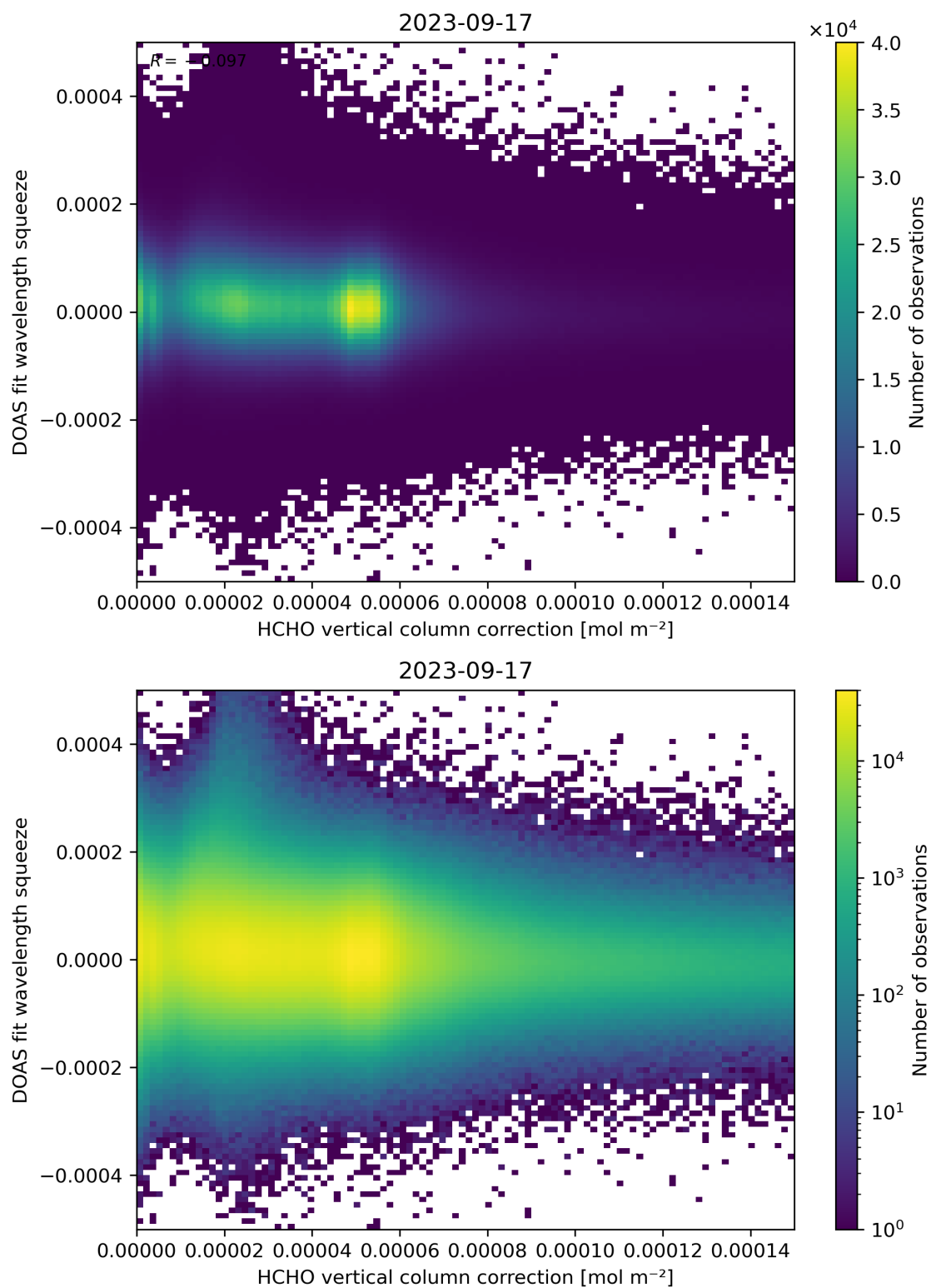
Figure 114: Scatter density plot of “HCHO vertical column correction” against “DOAS fit wavelength squeeze” for 2023-09-16 to 2023-09-18.
