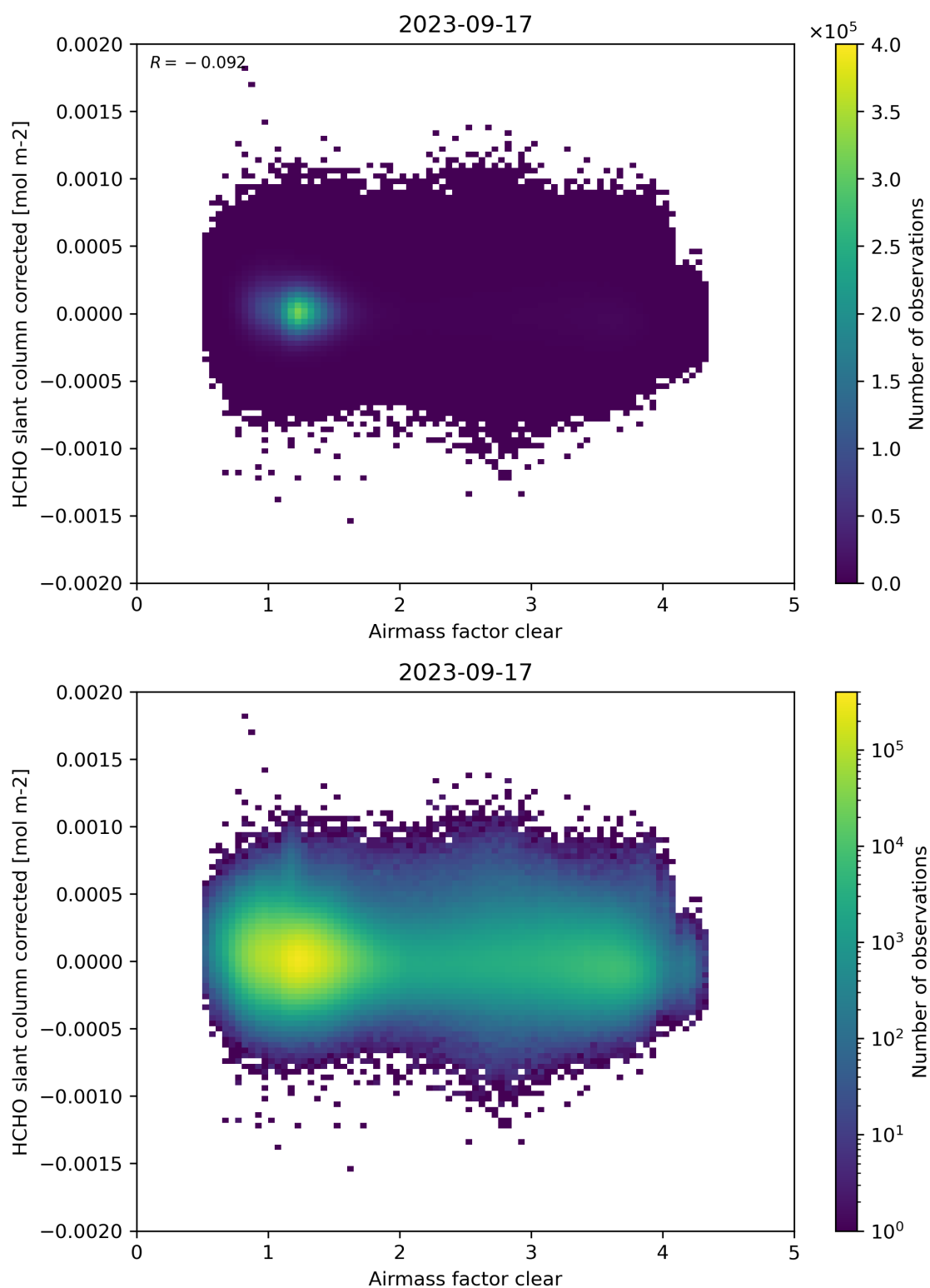
Figure 74: Scatter density plot of “Airmass factor clear” against “HCHO slant column corrected” for 2023-09-16 to 2023-09-18.
