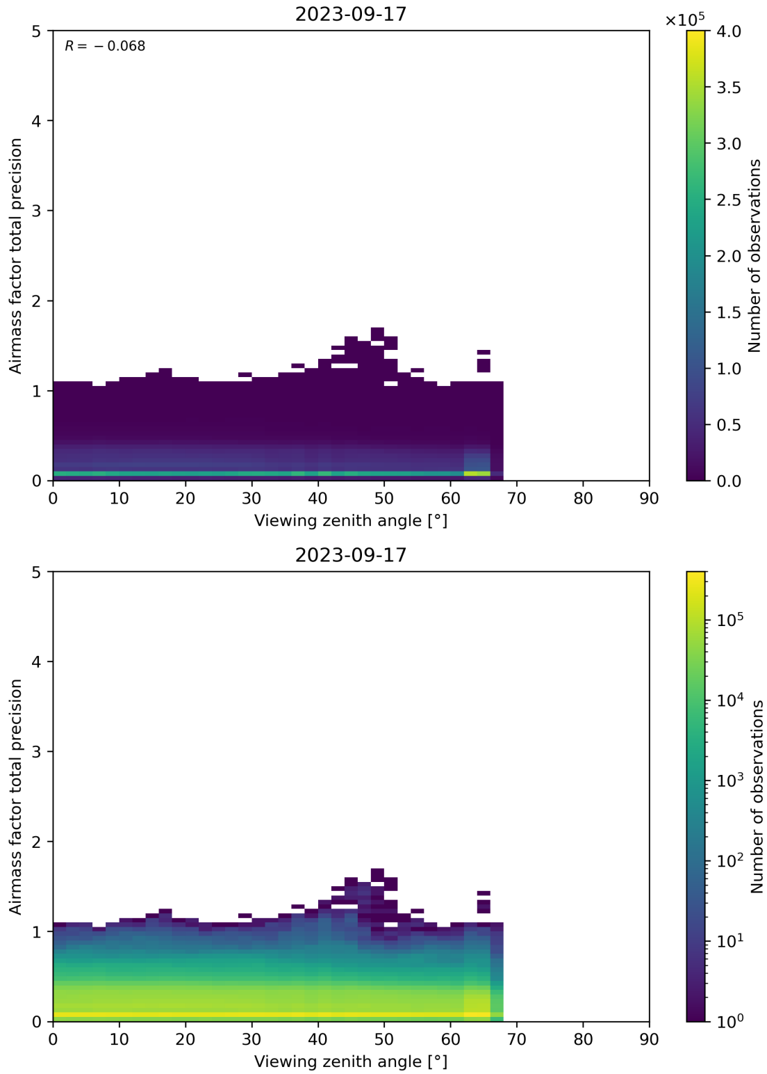
Figure 191: Scatter density plot of “Viewing zenith angle” against “Airmass factor total precision” for 2023-09-16 to 2023-09-18.
