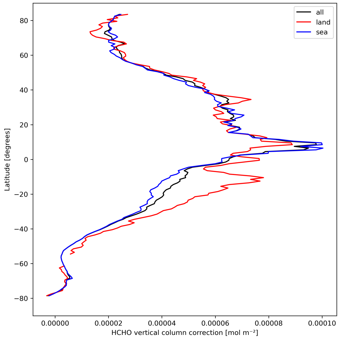
Figure 23: Zonal average of “HCHO vertical column correction” for 2023-09-16 to 2023-09-18.
