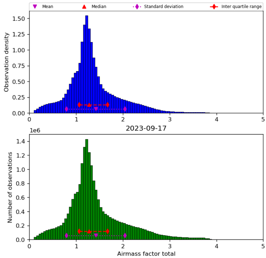
Figure 40: Histogram of “Airmass factor total” for 2023-09-16 to 2023-09-18
