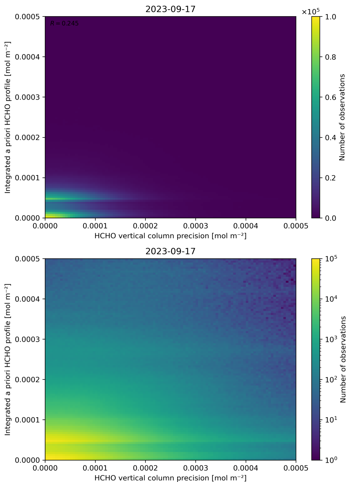
Figure 147: Scatter density plot of “HCHO vertical column precision” against “Integrated a priori HCHO profile” for 2023-09-16 to 2023-09-18.
