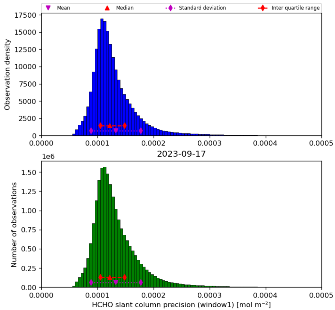
Figure 39: Histogram of “HCHO slant column precision (window1)” for 2023-09-16 to 2023-09-18
