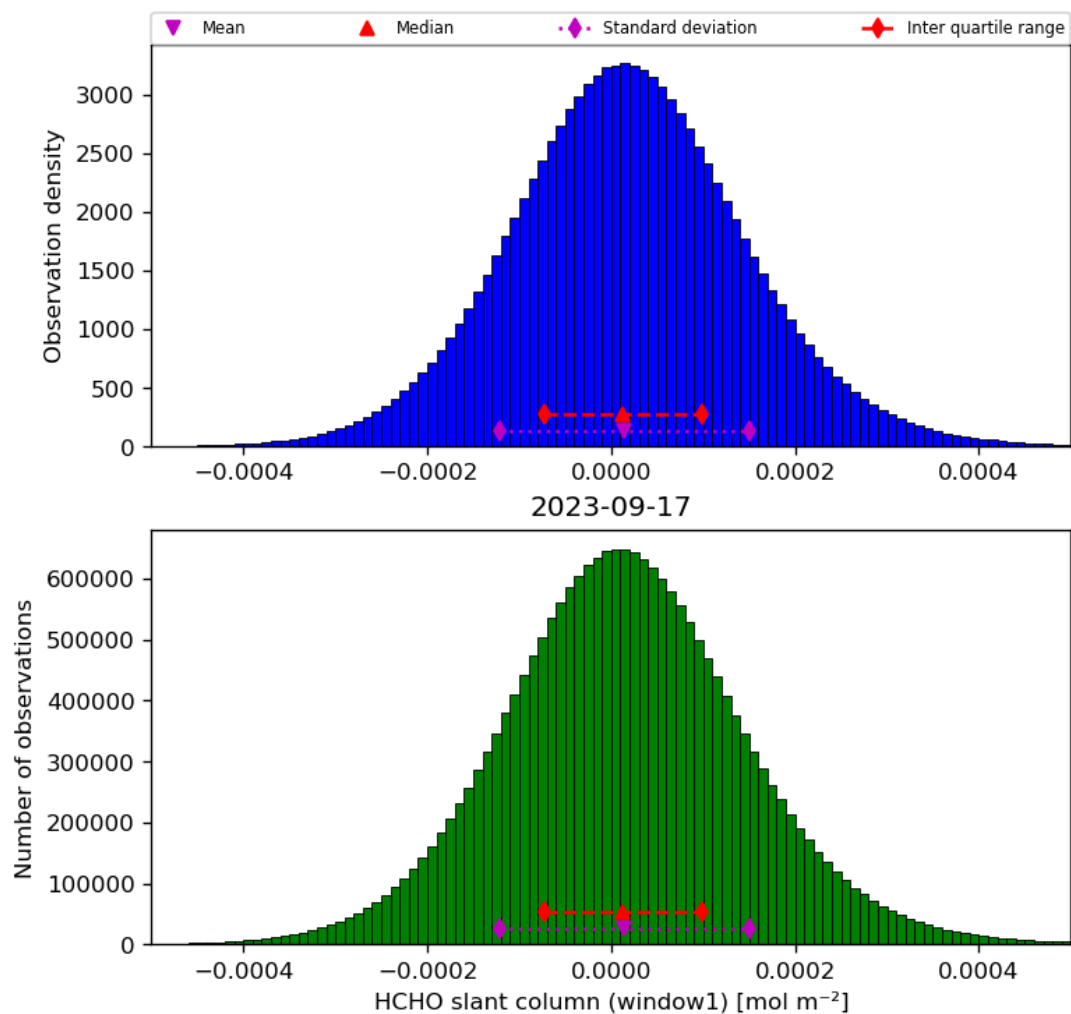
Figure 38: Histogram of “HCHO slant column (window1)” for 2023-09-16 to 2023-09-18
