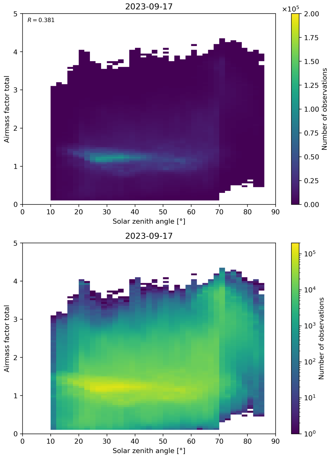
Figure 175: Scatter density plot of “Solar zenith angle” against “Airmass factor total” for 2023-09-16 to 2023-09-18.
