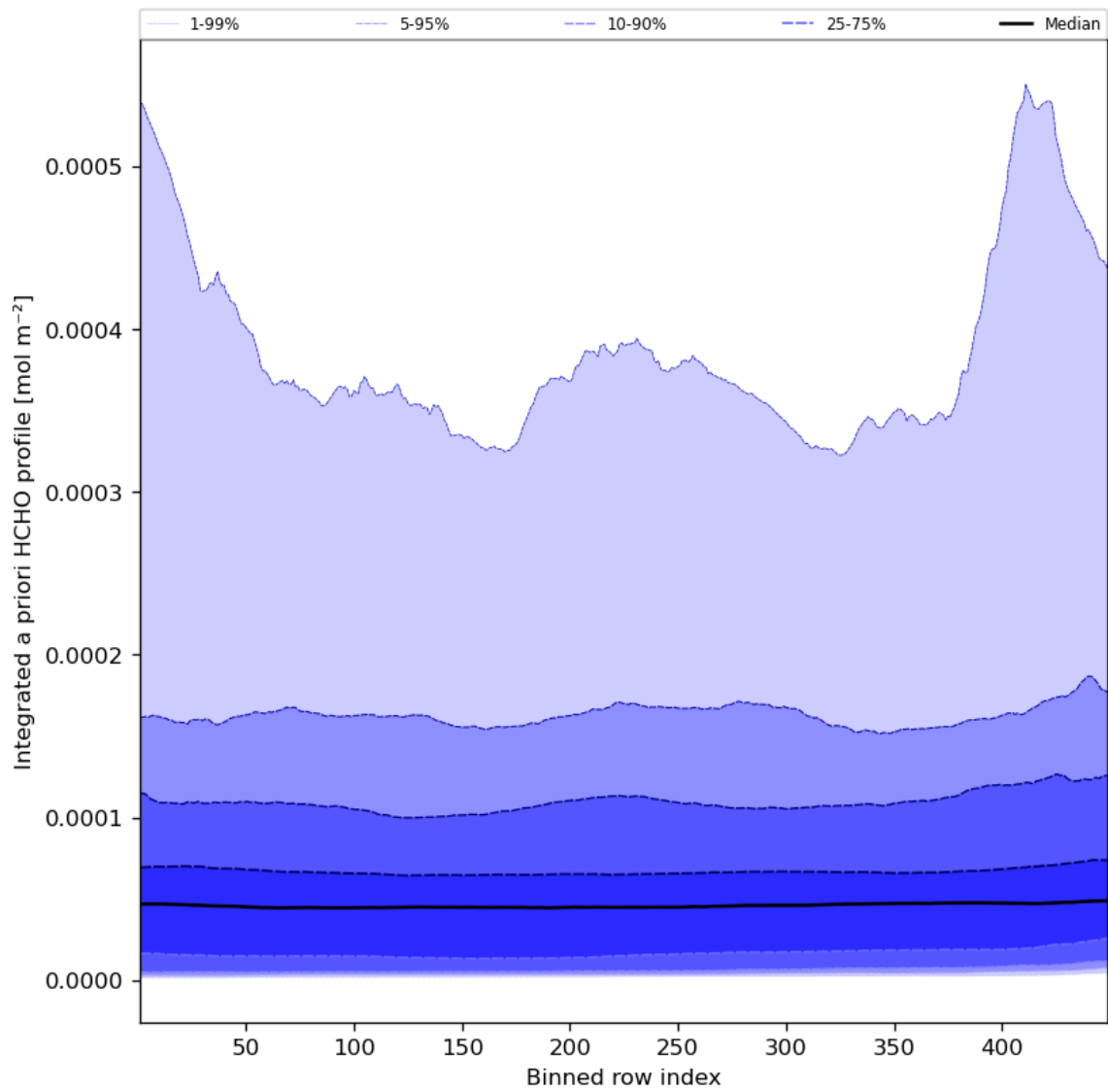
Figure 57: Along track statistics of "Integrated a priori HCHO profile" for 2023-09-16 to 2023-09-18
