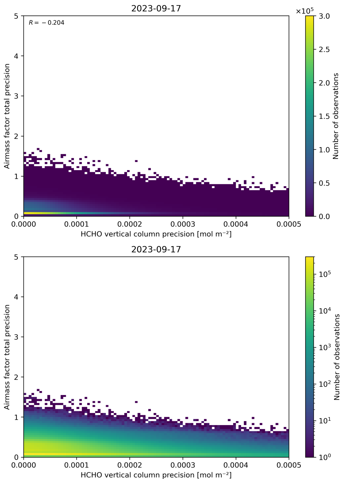
Figure 145: Scatter density plot of “HCHO vertical column precision” against “Airmass factor total precision” for 2023-09-16 to 2023-09-18.
