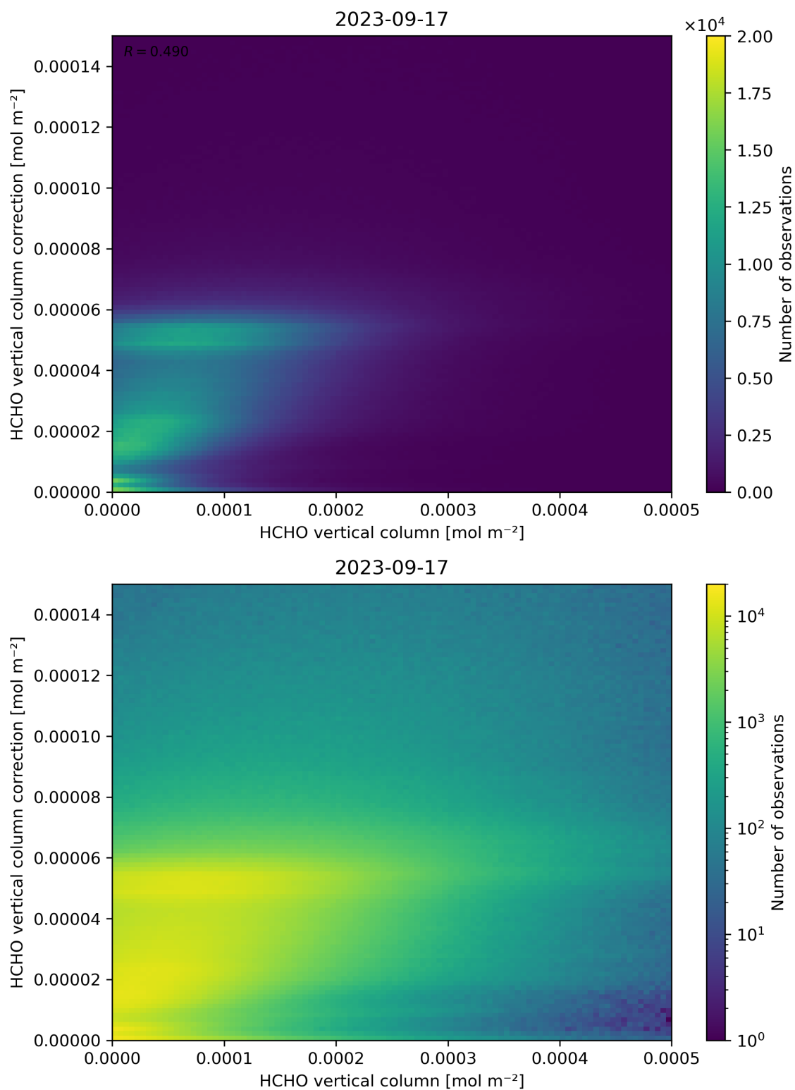
Figure 133: Scatter density plot of “HCHO vertical column” against “HCHO vertical column correction” for 2023-09-16 to 2023-09-18.
