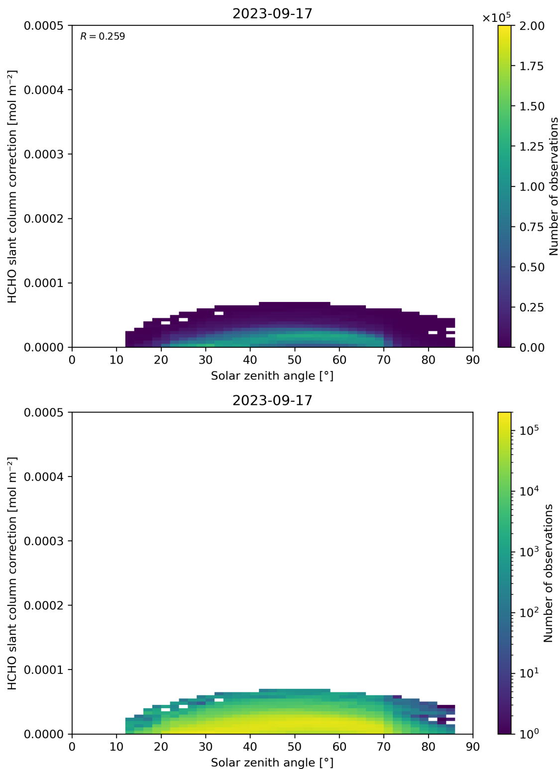
Figure 172: Scatter density plot of “Solar zenith angle” against “HCHO slant column correction” for 2023-09-16 to 2023-09-18.
