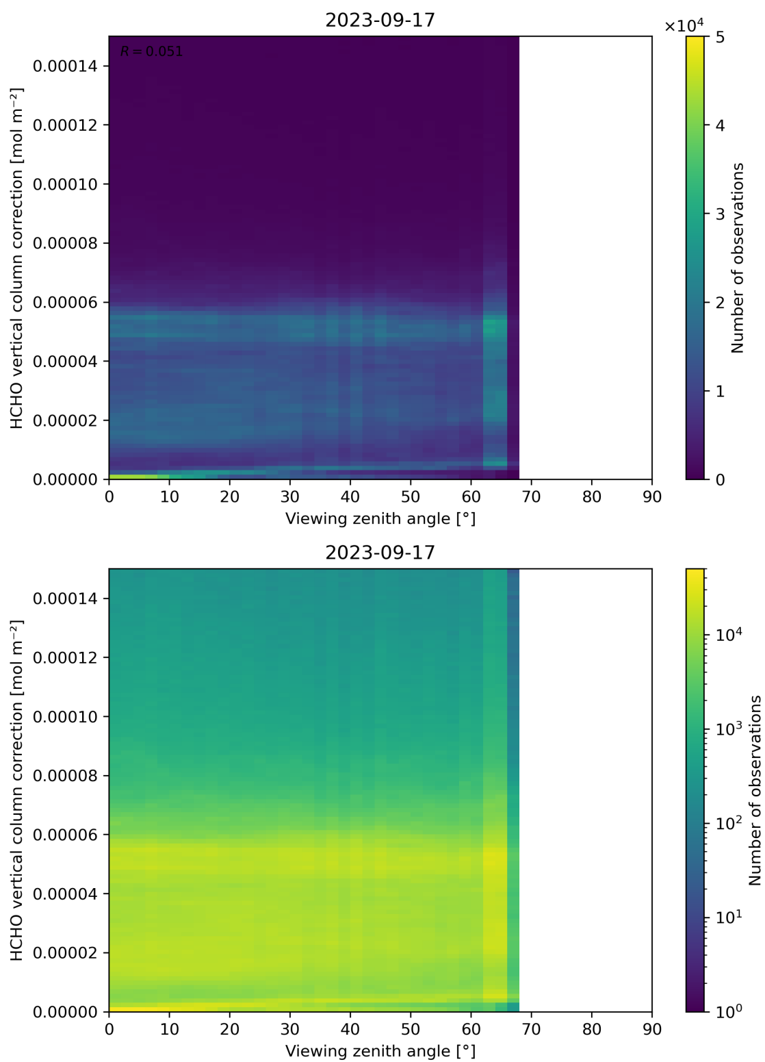
Figure 193: Scatter density plot of “Viewing zenith angle” against “HCHO vertical column correction” for 2023-09-16 to 2023-09-18.
