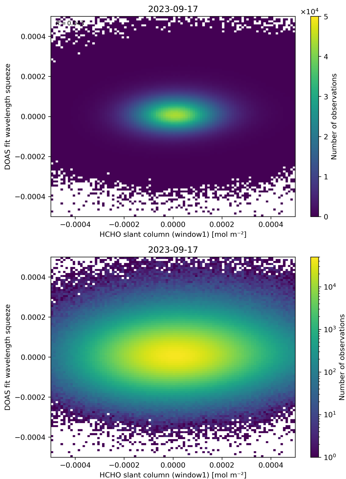
Figure 80: Scatter density plot of “HCHO slant column (window1)” against “DOAS fit wavelength squeeze” for 2023-09-16 to 2023-09-18.
