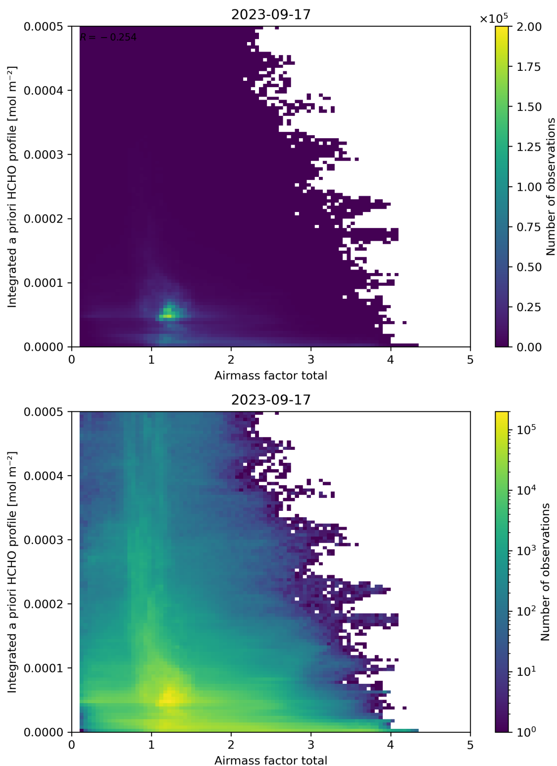
Figure 104: Scatter density plot of “Air mass factor total” against “Integrated a priori HCHO profile” for 2023-09-16 to 2023-09-18.
