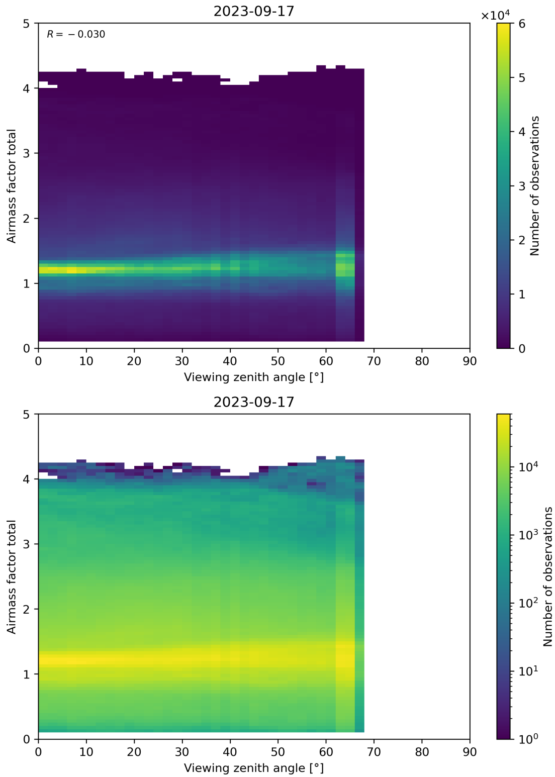
Figure 190: Scatter density plot of “Viewing zenith angle” against “Airmass factor total” for 2023-09-16 to 2023-09-18.
