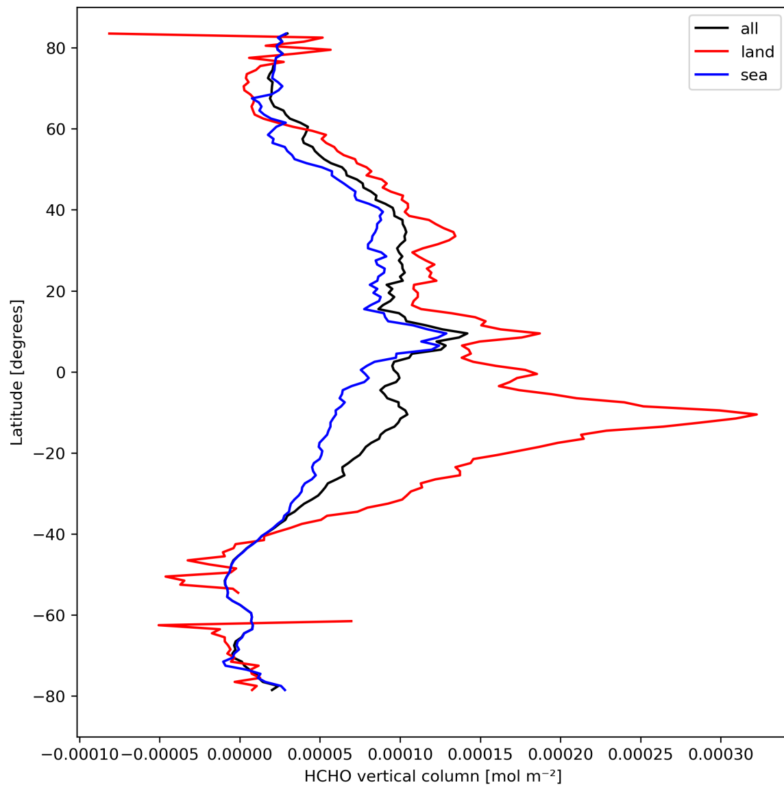
Figure 21: Zonal average of “HCHO vertical column” for 2023-09-16 to 2023-09-18.
