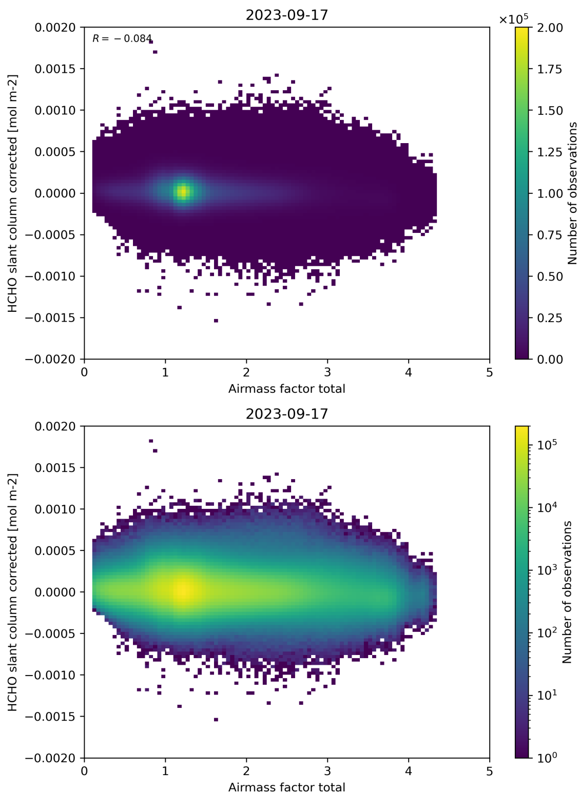
Figure 101: Scatter density plot of “Airmass factor total” against “HCHO slant column corrected” for 2023-09-16 to 2023-09-18.
