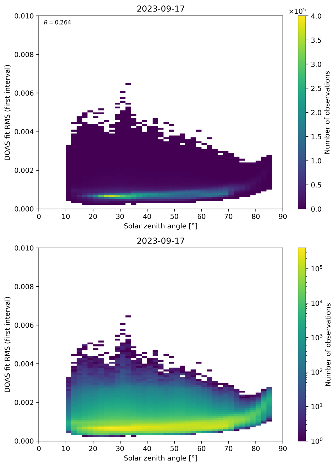
Figure 167: Scatter density plot of “Solar zenith angle” against “DOAS fit RMS (first interval)” for 2023-09-16 to 2023-09-18.
