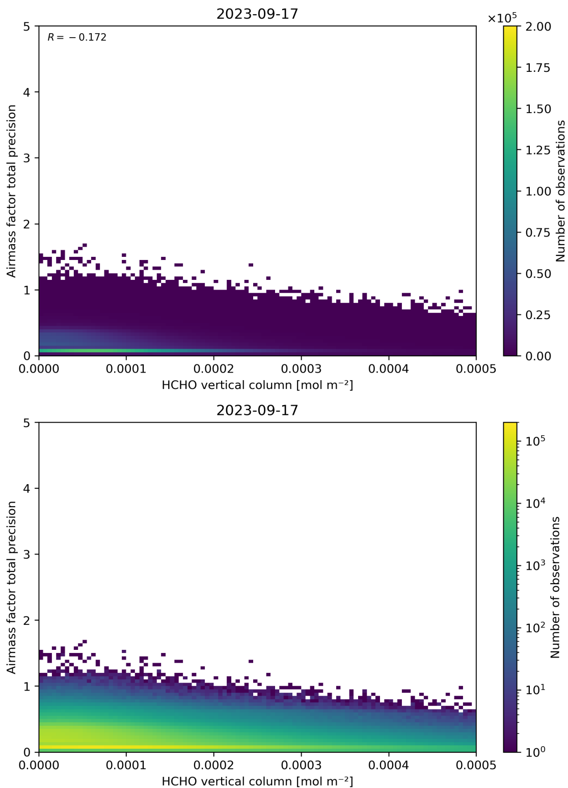
Figure 132: Scatter density plot of “HCHO vertical column” against “Airmass factor total precision” for 2023-09-16 to 2023-09-18.
