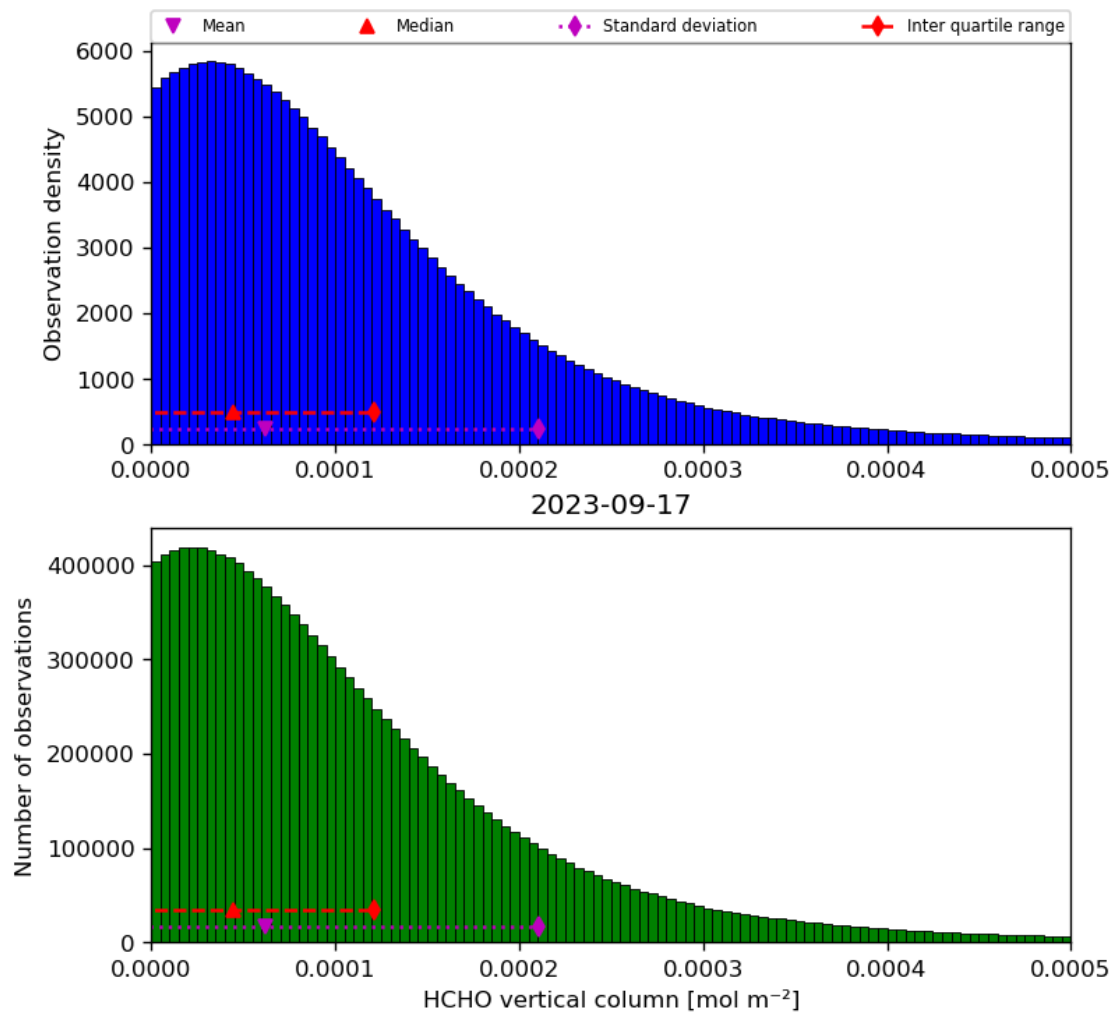
Figure 35: Histogram of “HCHO vertical column” for 2023-09-16 to 2023-09-18
