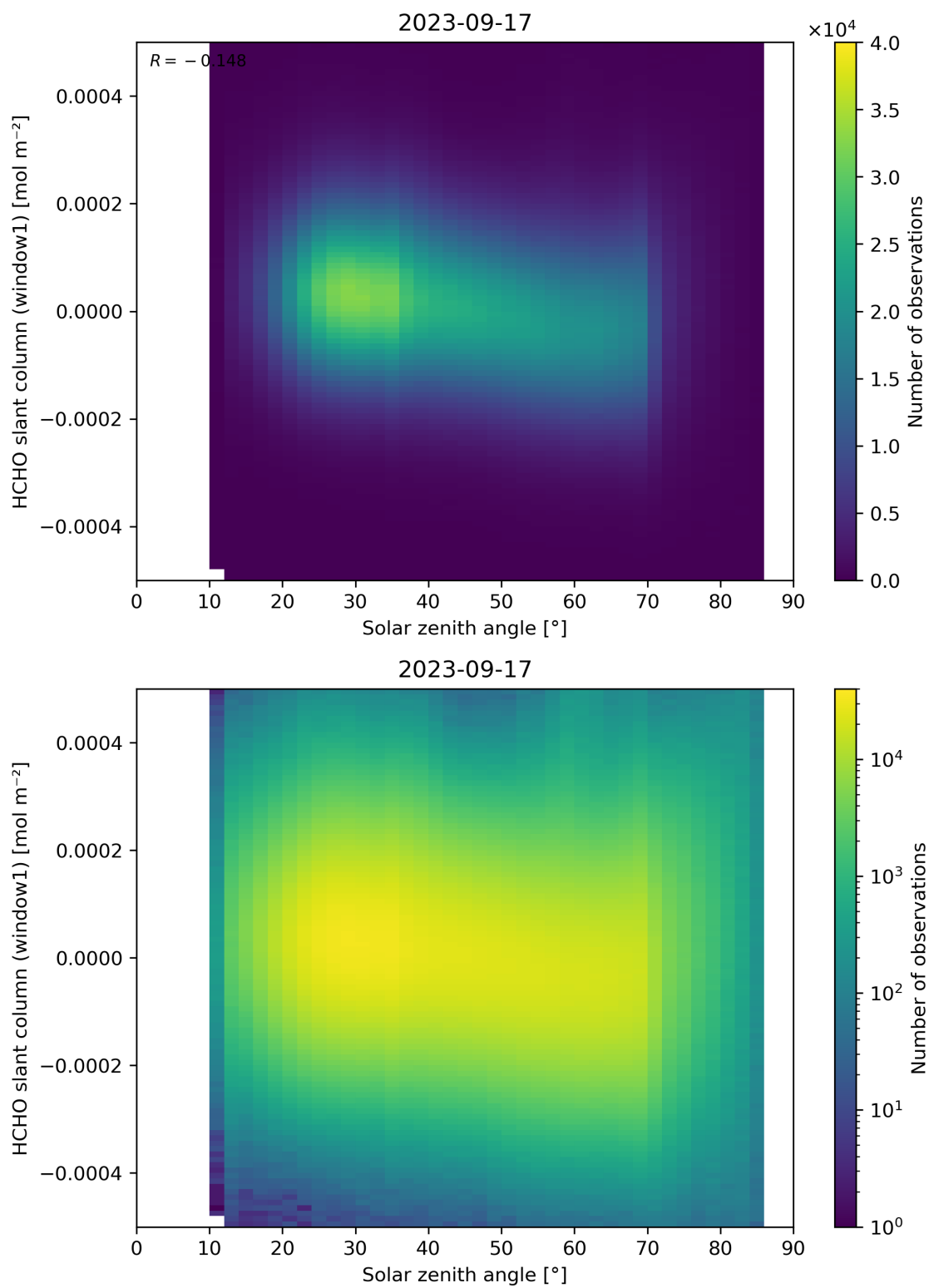
Figure 173: Scatter density plot of “Solar zenith angle” against “HCHO slant column (window1)” for 2023-09-16 to 2023-09-18.
