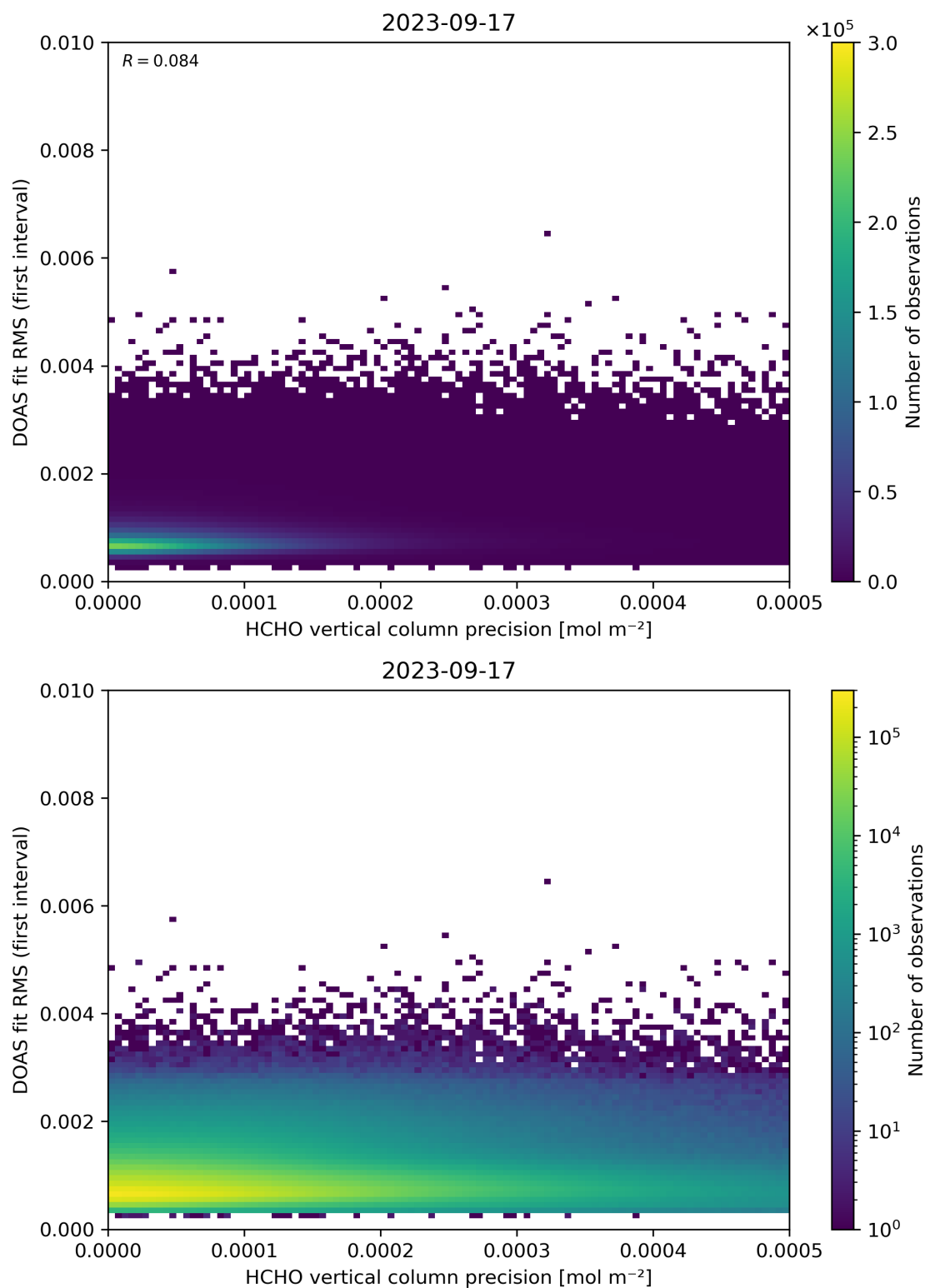
Figure 136: Scatter density plot of “HCHO vertical column precision” against “DOAS fit RMS (first interval)” for 2023-09-16 to 2023-09-18.
