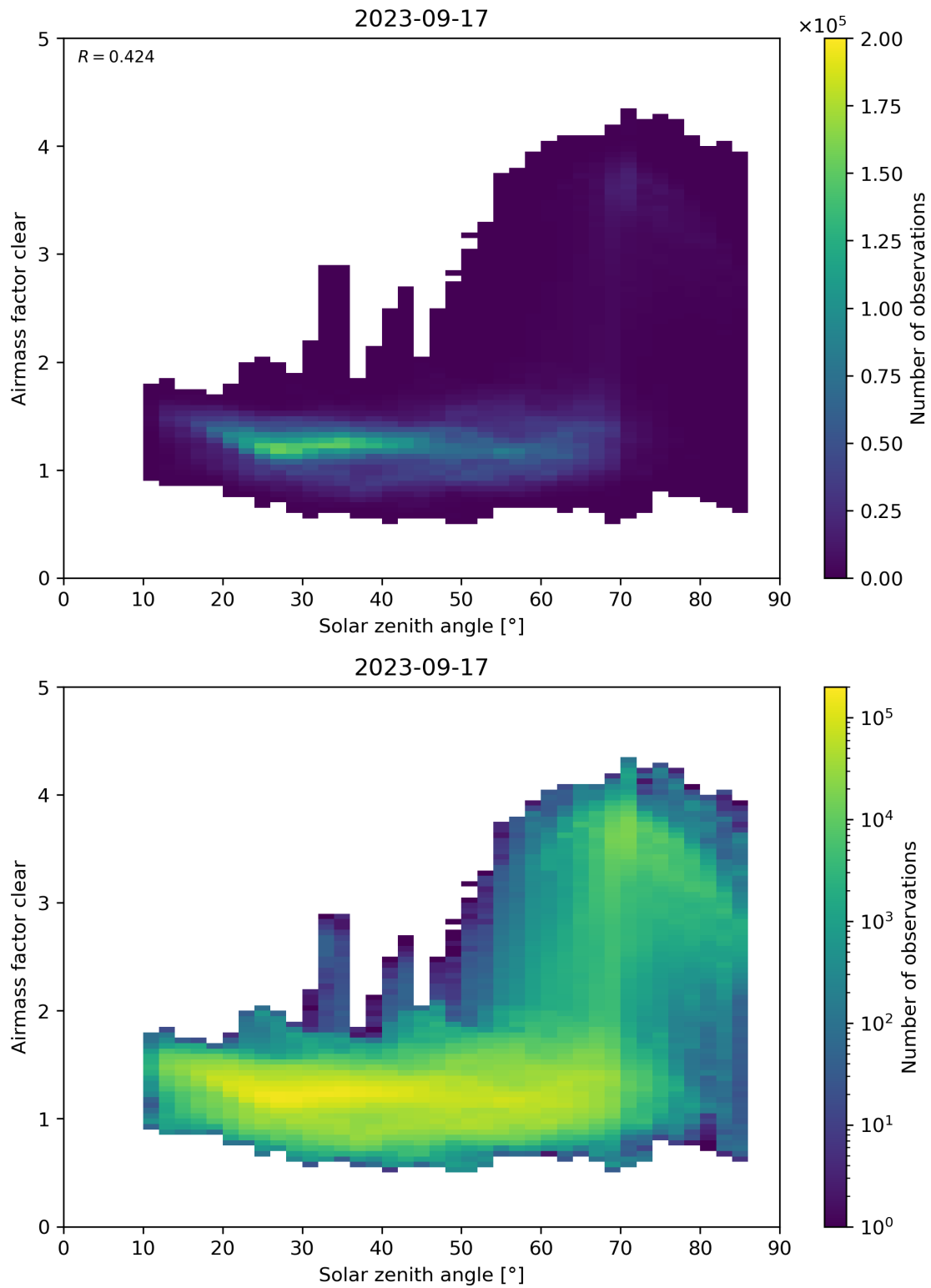
Figure 170: Scatter density plot of “Solar zenith angle” against “Airmass factor clear” for 2023-09-16 to 2023-09-18.
