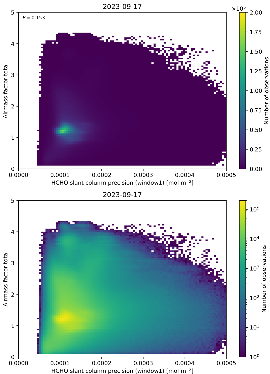
Figure 94: Scatter density plot of “HCHO slant column precision (window1)” against “Airmass factor total” for 2023-09-16 to 2023-09-18.
