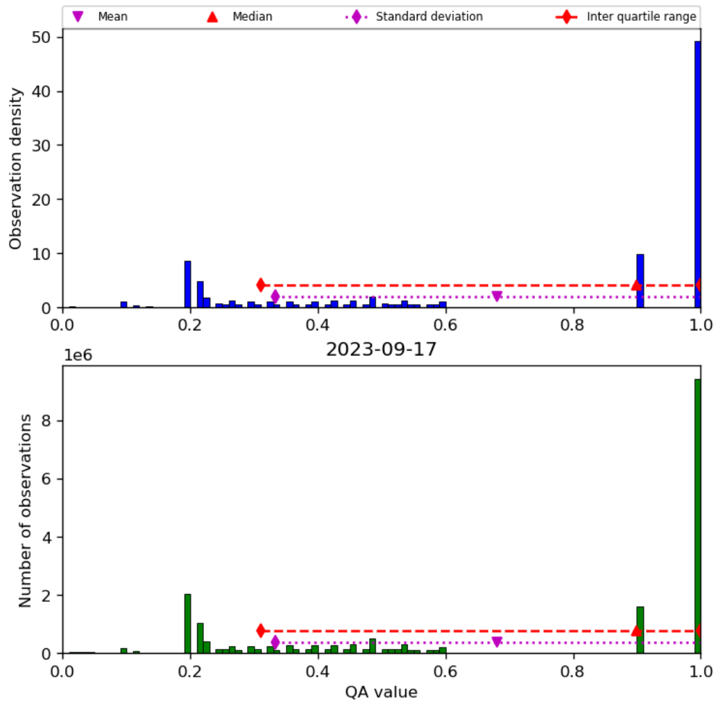
Figure 34: Histogram of “QA value” for 2023-09-16 to 2023-09-18
