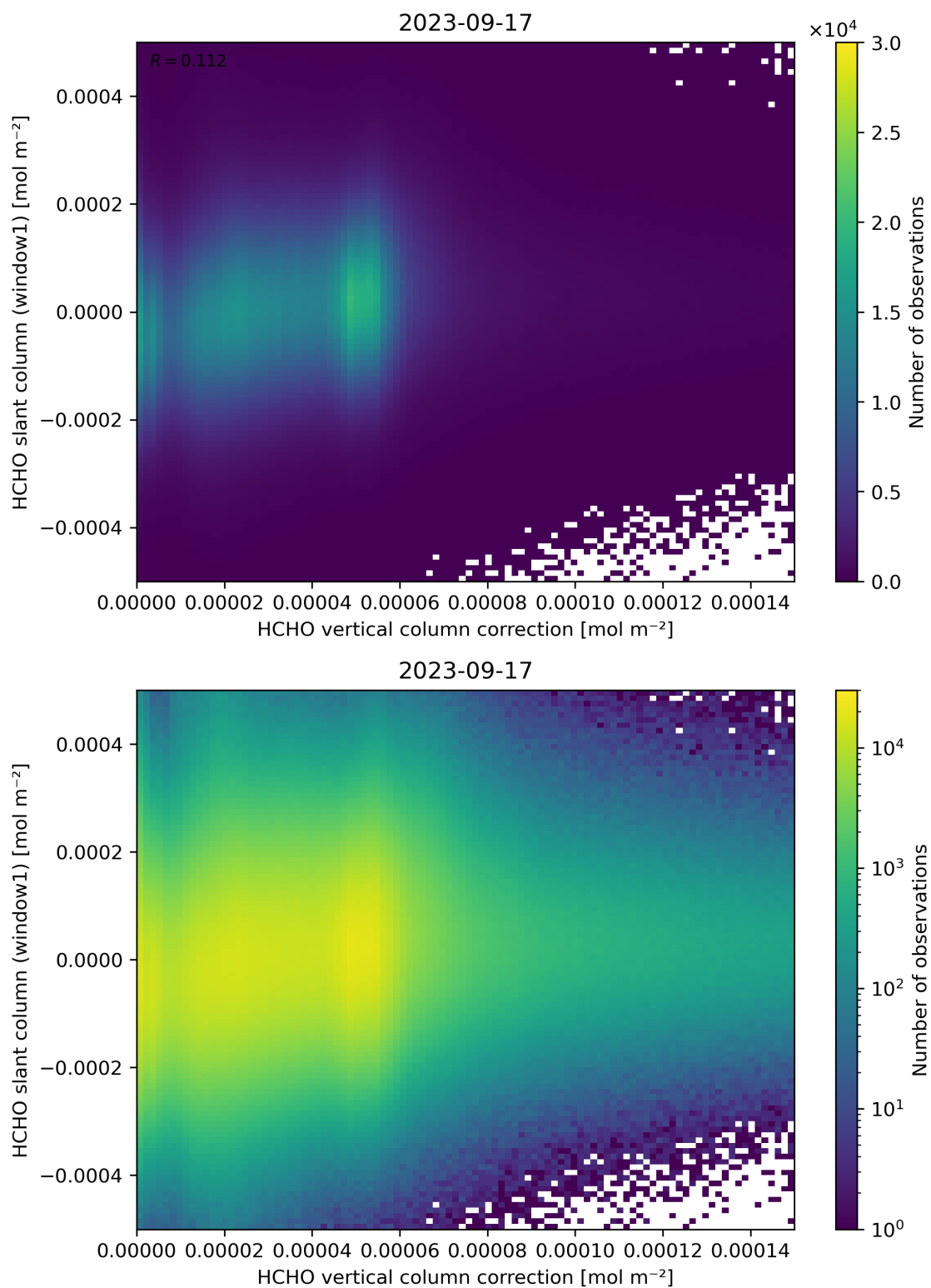
Figure 118: Scatter density plot of “HCHO vertical column correction” against “HCHO slant column (window1)” for 2023-09-16 to 2023-09-18.
