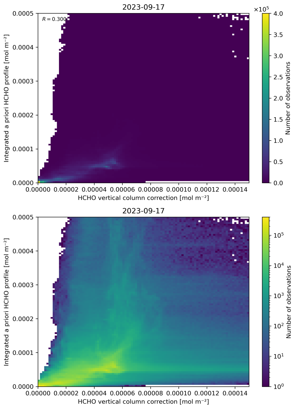
Figure 122: Scatter density plot of “HCHO vertical column correction” against “Integrated a priori HCHO profile” for 2023-09-16 to 2023-09-18.
