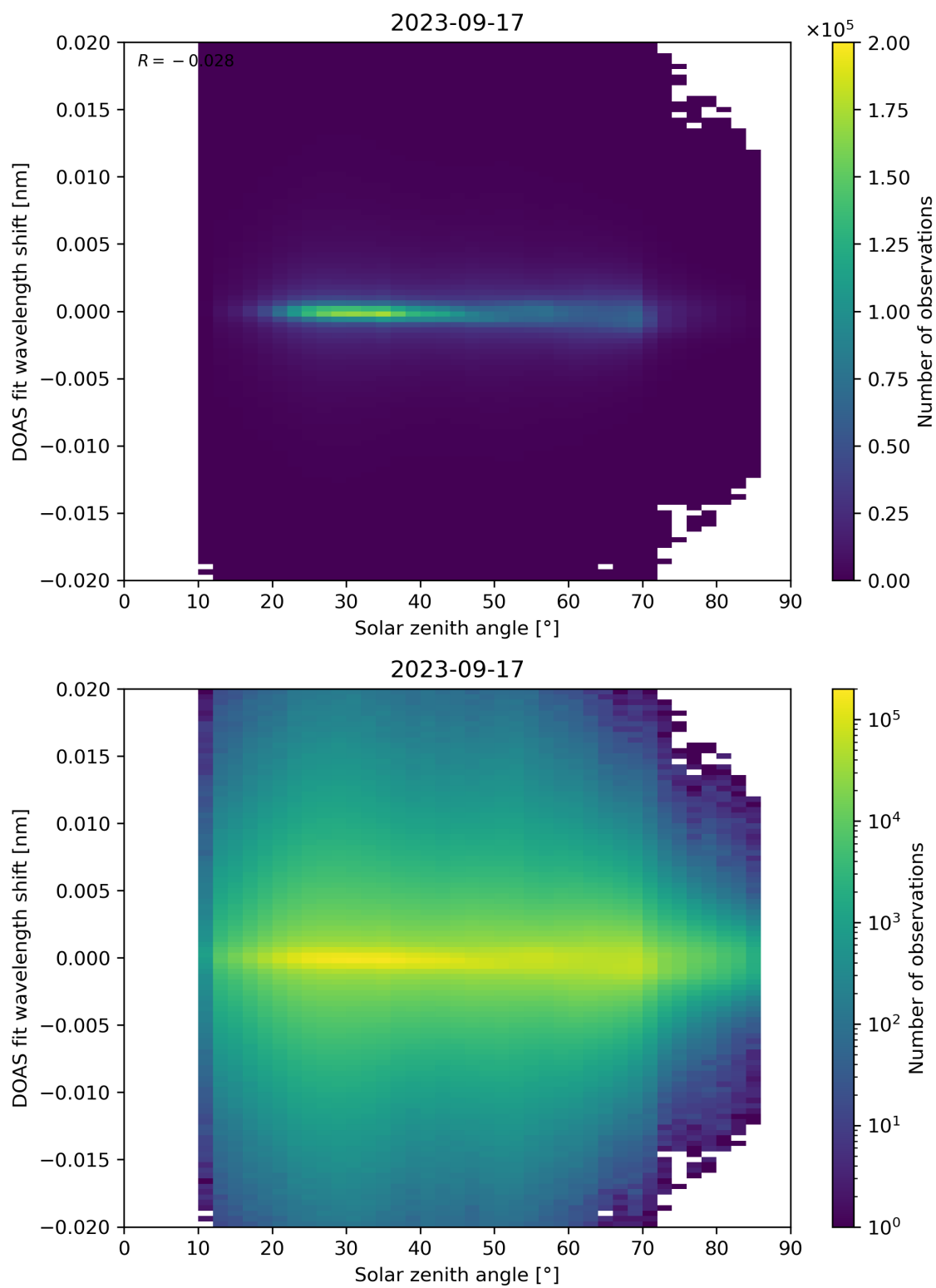
Figure 168: Scatter density plot of “Solar zenith angle” against “DOAS fit wavelength shift” for 2023-09-16 to 2023-09-18.
