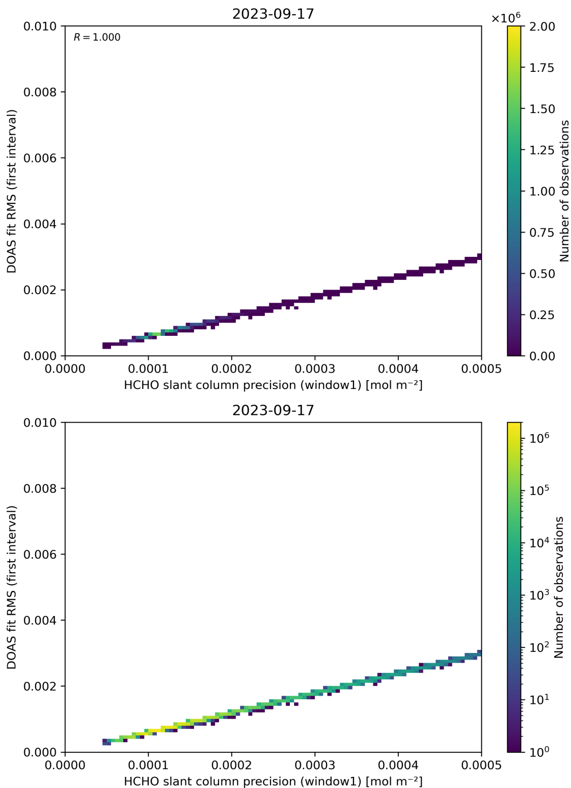
Figure 88: Scatter density plot of “HCHO slant column precision (window1)” against “DOAS fit RMS (first interval)” for 2023-09-16 to 2023-09-18.
