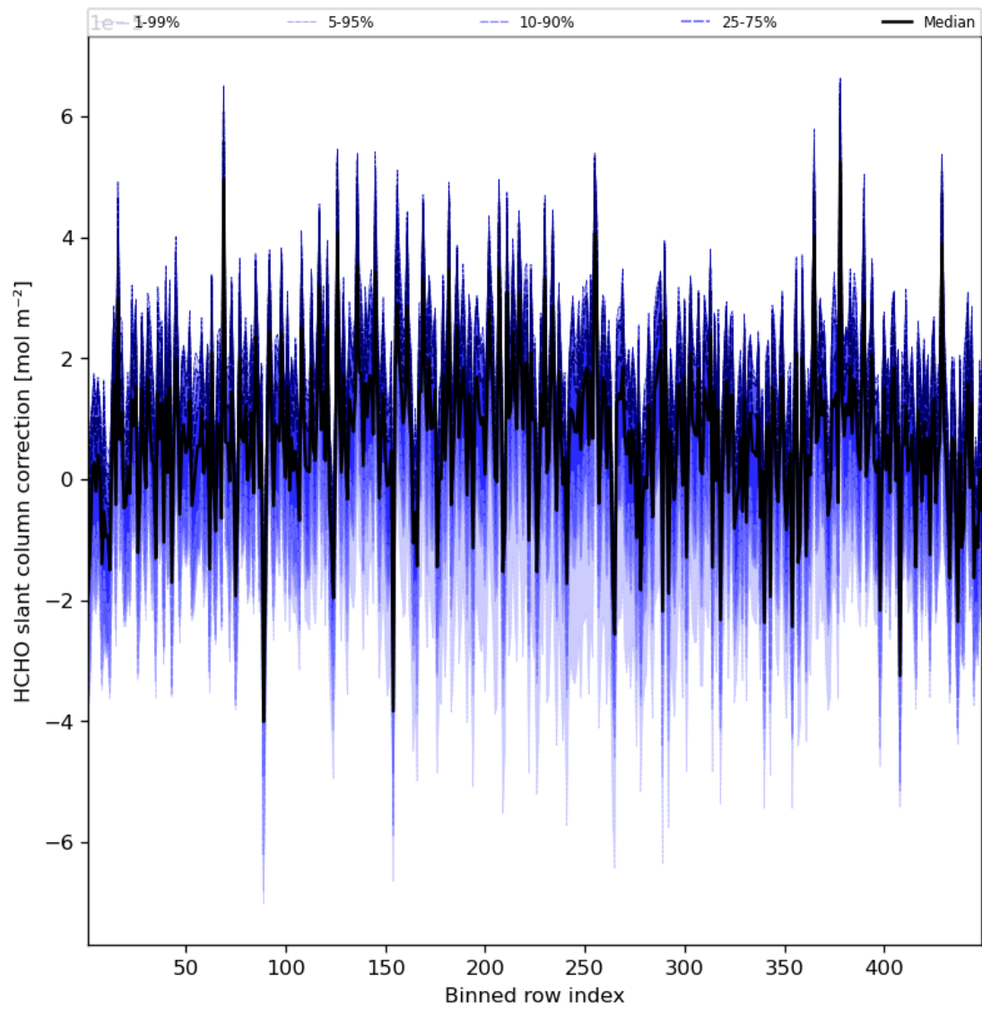
Figure 61: Along track statistics of “HCHO slant column correction” for 2023-09-16 to 2023-09-18
