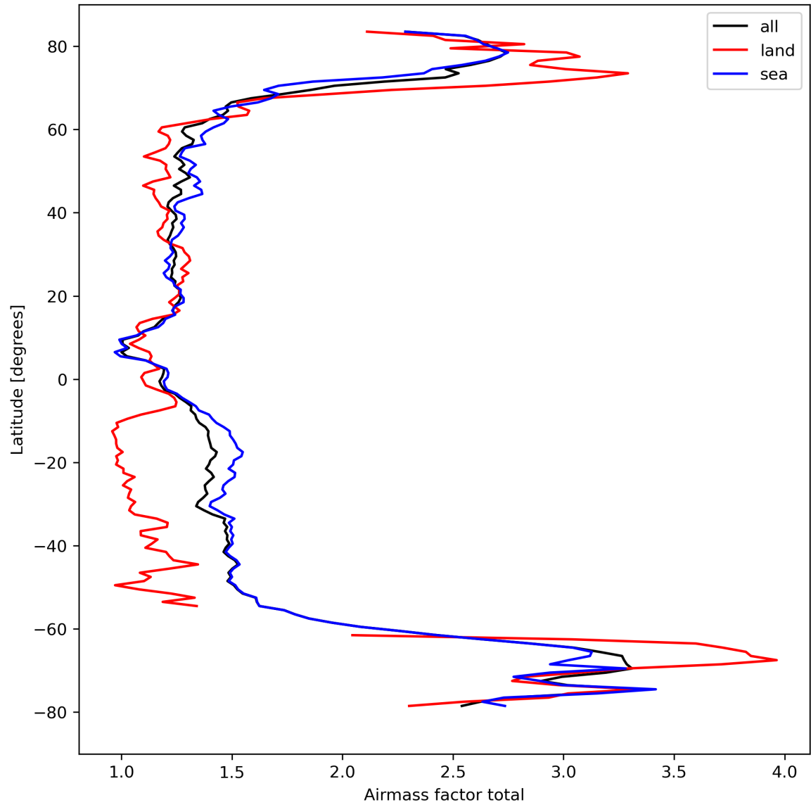
Figure 26: Zonal average of “Airmass factor total” for 2023-09-16 to 2023-09-18.
