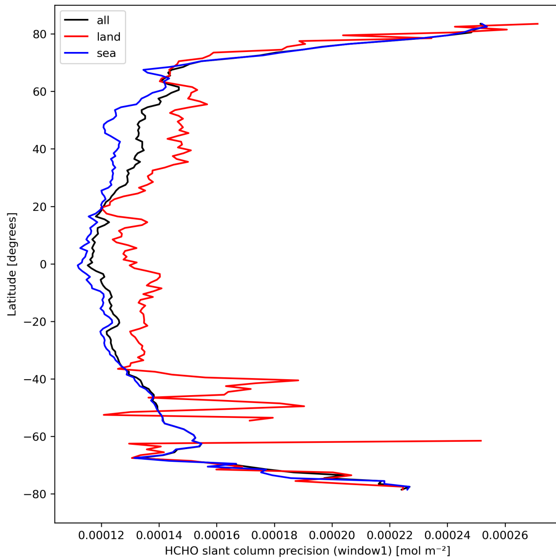
Figure 25: Zonal average of “HCHO slant column precision (window1)” for 2023-09-16 to 2023-09-18.
