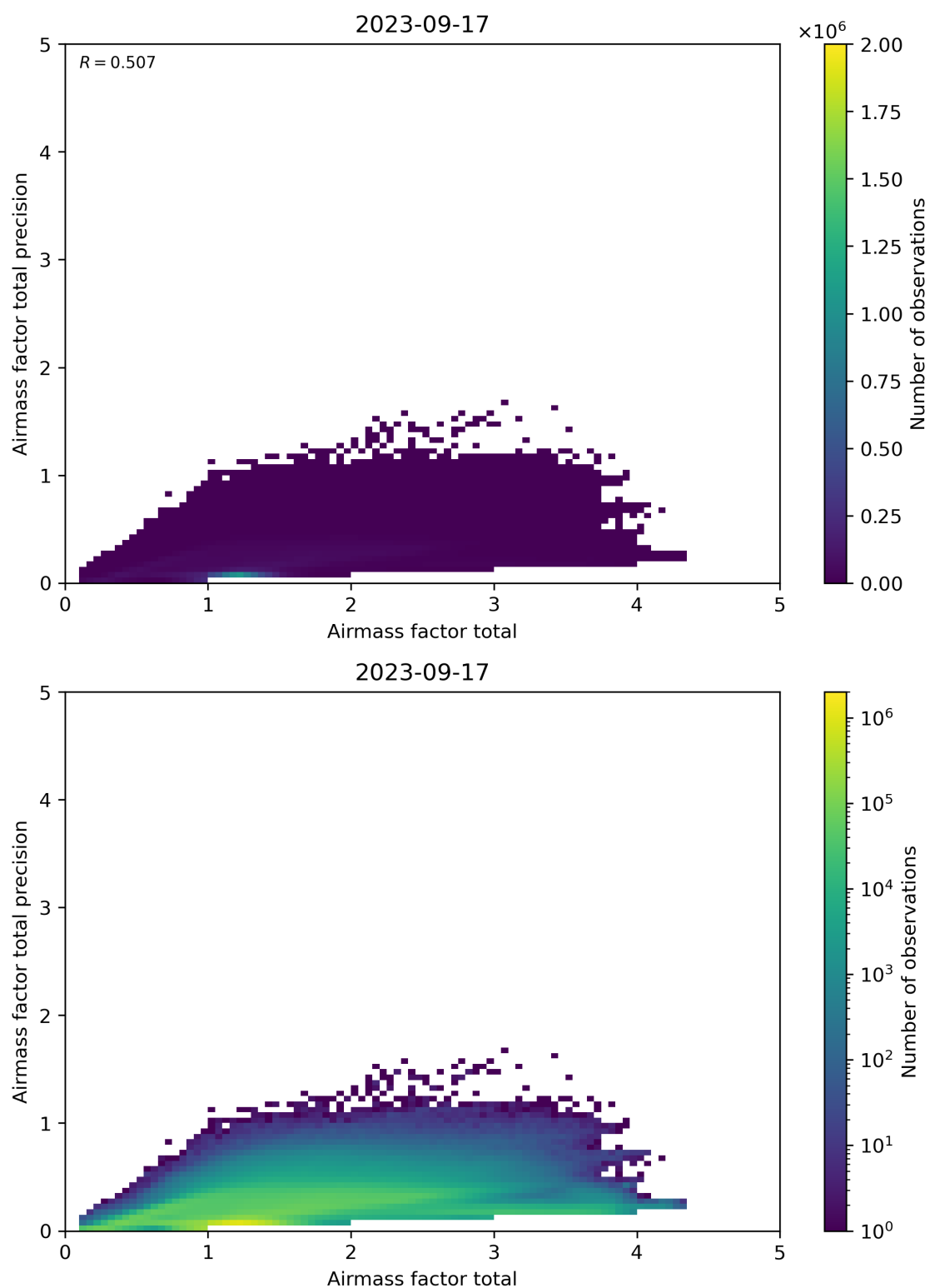
Figure 103: Scatter density plot of “Airmass factor total” against “Airmass factor total precision” for 2023-09-16 to 2023-09-18.
