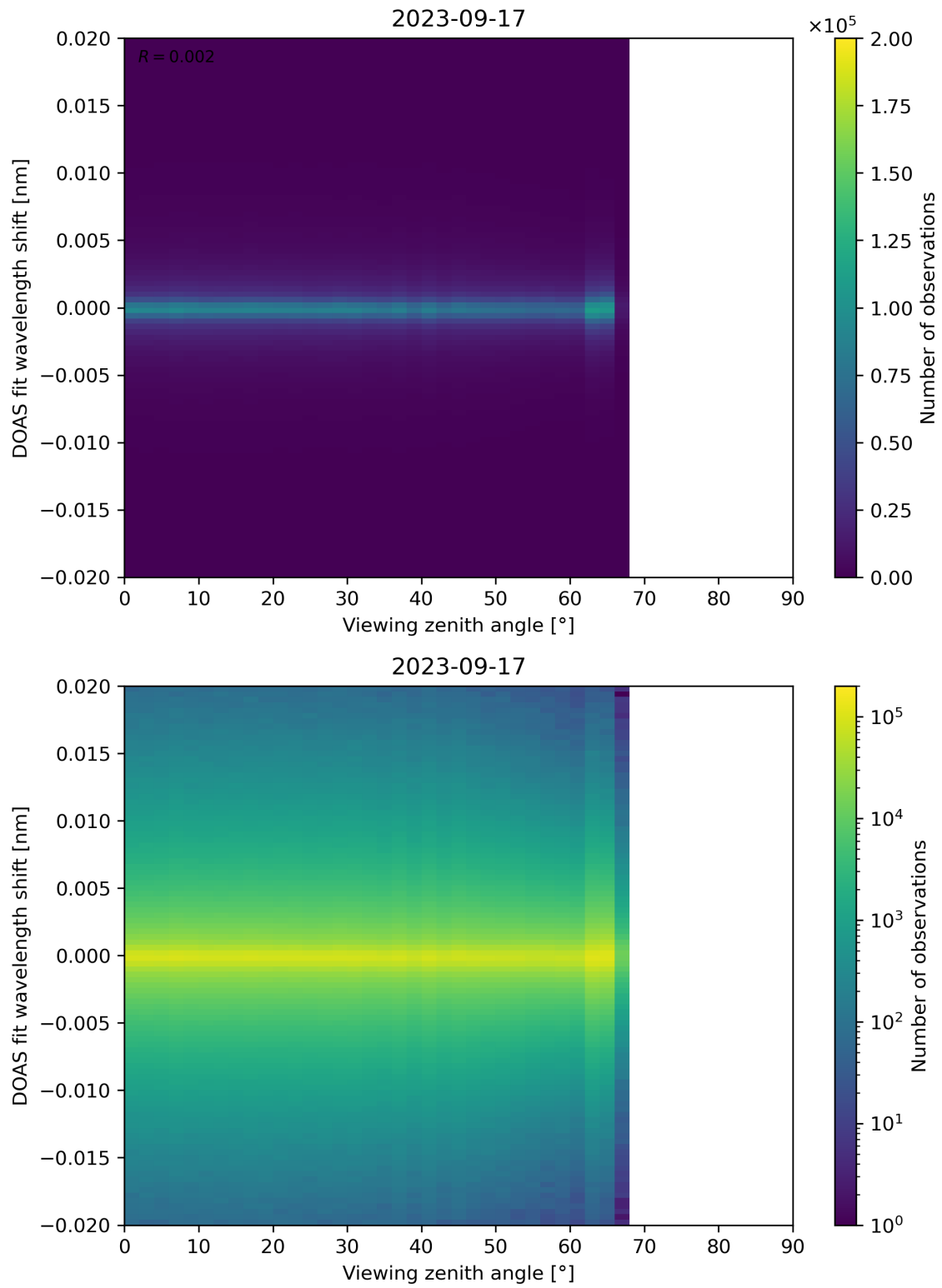
Figure 183: Scatter density plot of “Viewing zenith angle” against “DOAS fit wavelength shift” for 2023-09-16 to 2023-09-18.
