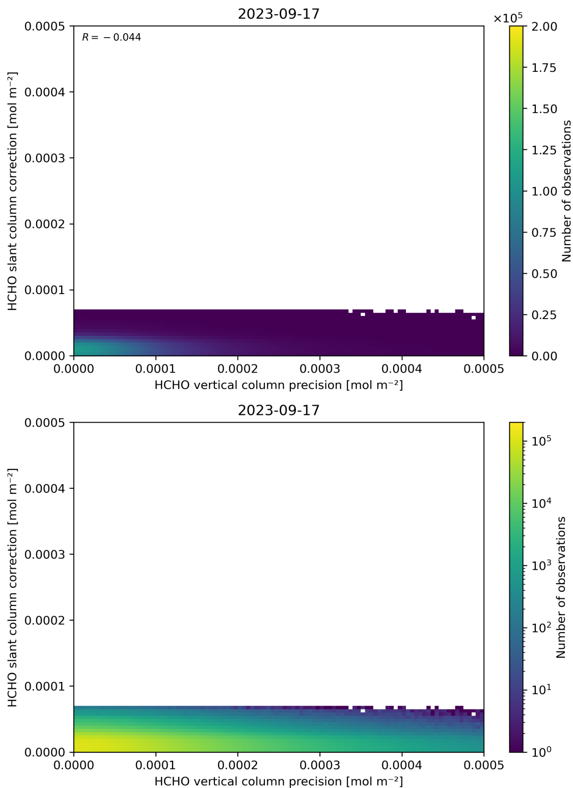
Figure 141: Scatter density plot of “HCHO vertical column precision” against “HCHO slant column correction” for 2023-09-16 to 2023-09-18.
