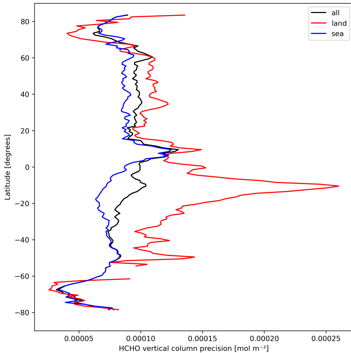
Figure 22: Zonal average of “HCHO vertical column precision” for 2023-09-16 to 2023-09-18.
