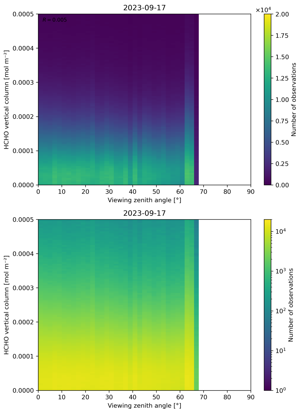
Figure 192: Scatter density plot of “Viewing zenith angle” against “HCHO vertical column” for 2023-09-16 to 2023-09-18.
