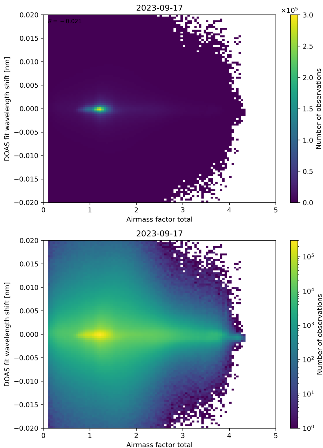
Figure 98: Scatter density plot of “Airmass factor total” against “DOAS fit wavelength shift” for 2023-09-16 to 2023-09-18.
