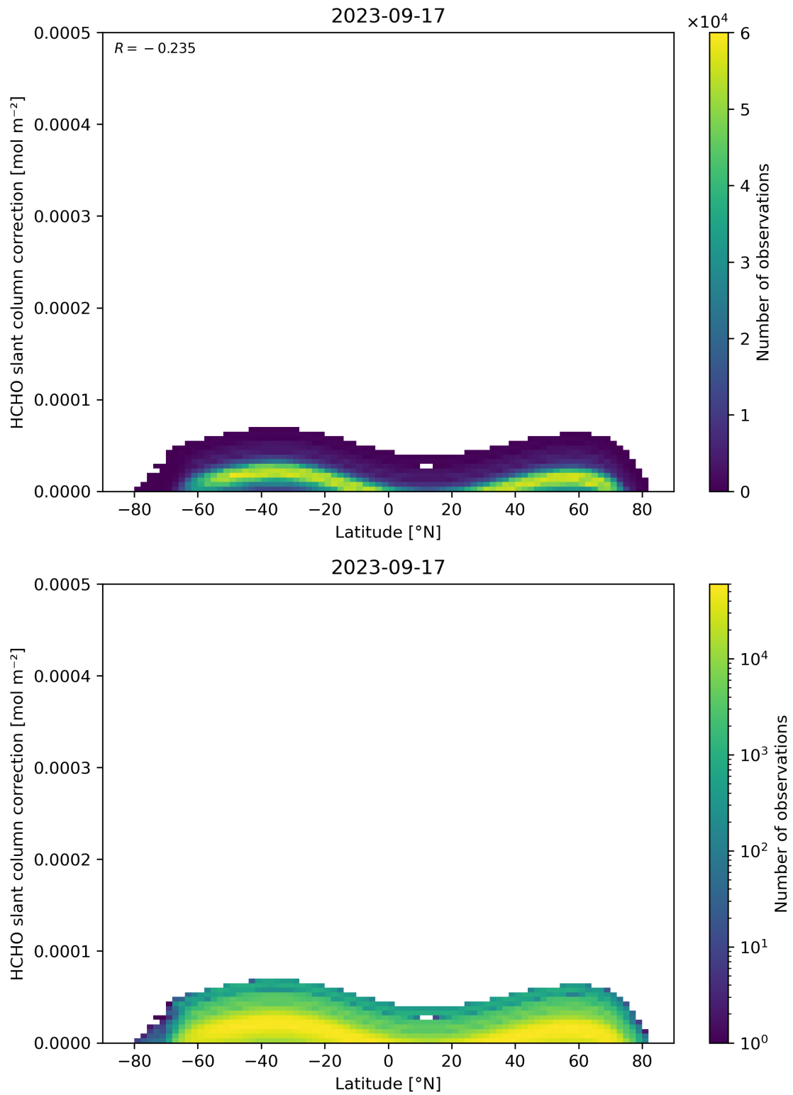
Figure 158: Scatter density plot of “Latitude” against “HCHO slant column correction” for 2023-09-16 to 2023-09-18.
