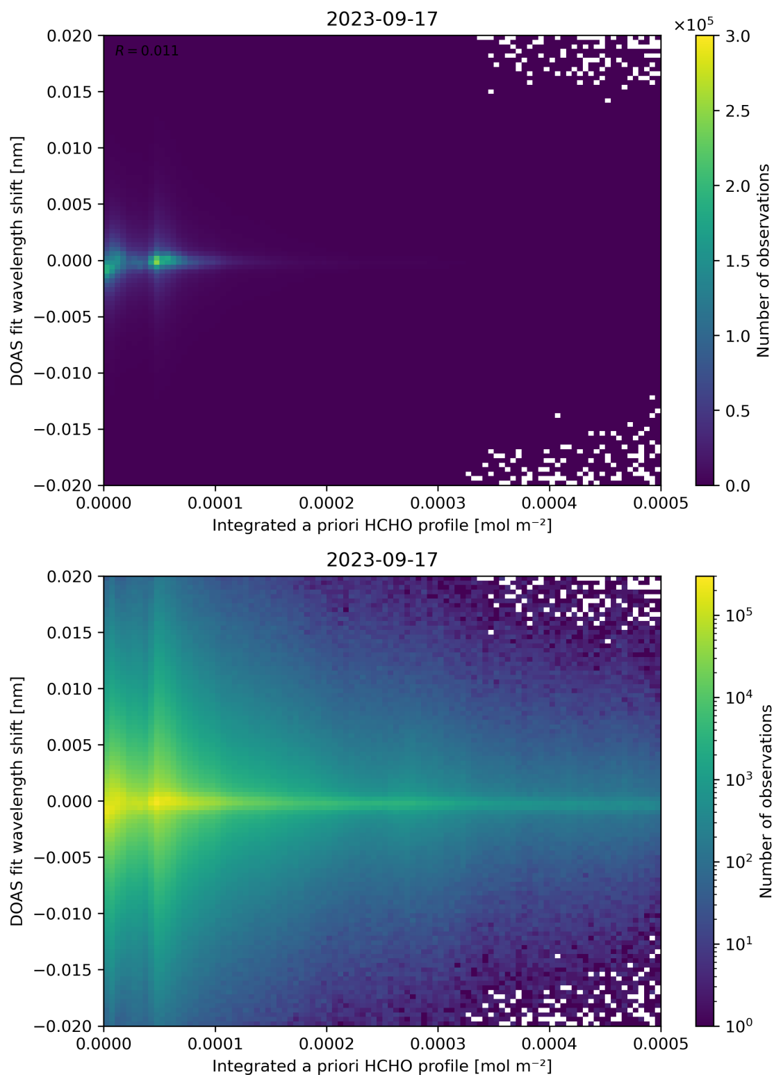
Figure 149: Scatter density plot of “Integrated a priori HCHO profile” against “DOAS fit wavelength shift” for 2023-09-16 to 2023-09-18.
