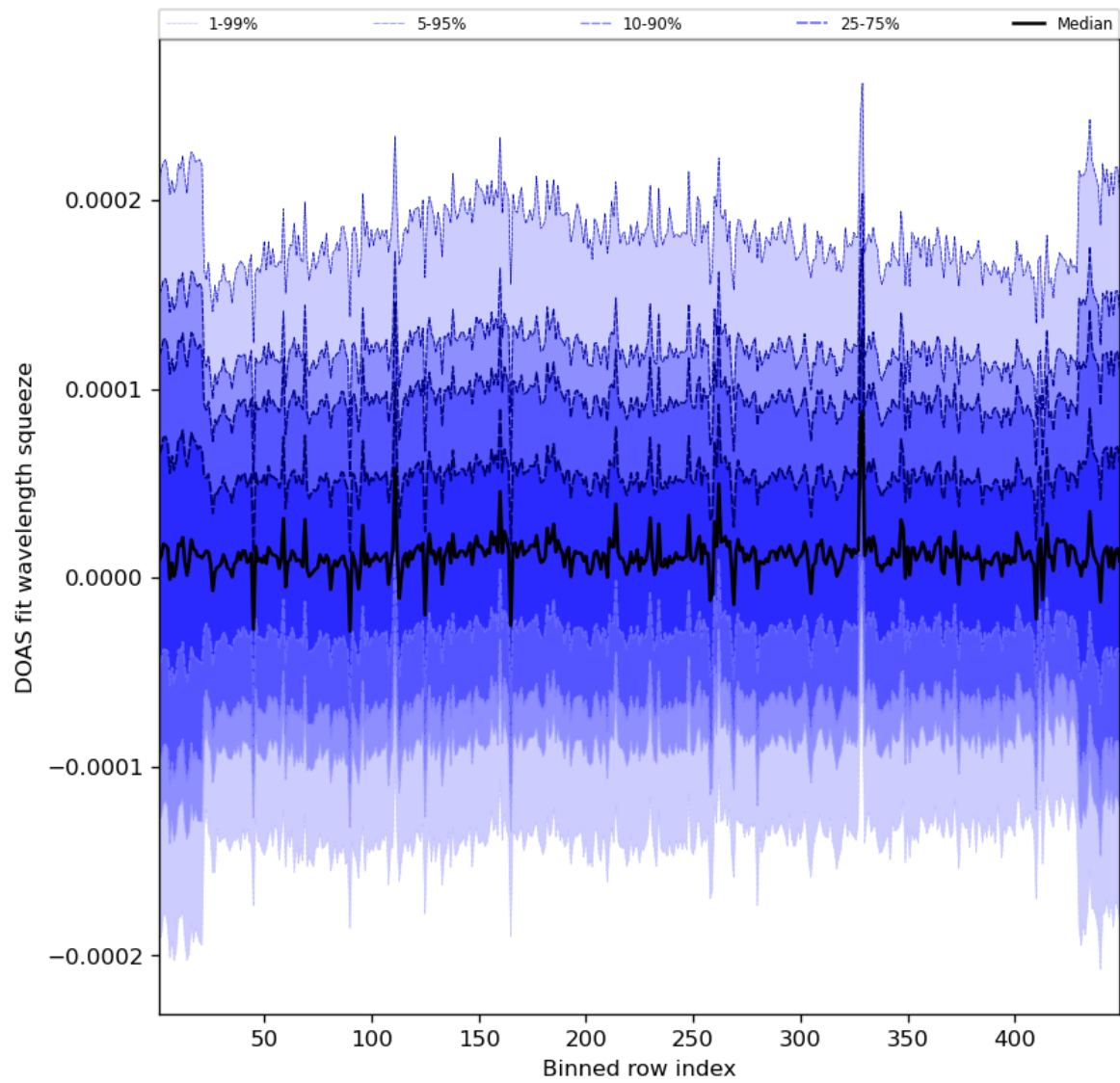
Figure 59: Along track statistics of “DOAS fit wavelength squeeze” for 2023-09-16 to 2023-09-18
