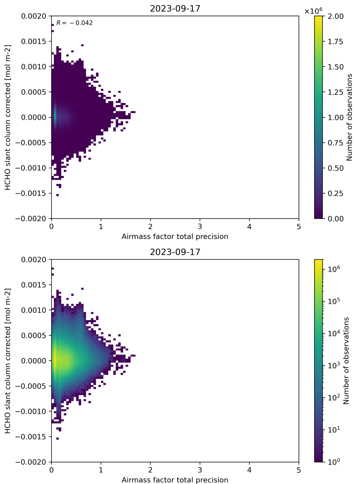
Figure 109: Scatter density plot of “Airmass factor total precision” against “HCHO slant column corrected” for 2023-09-16 to 2023-09-18.
