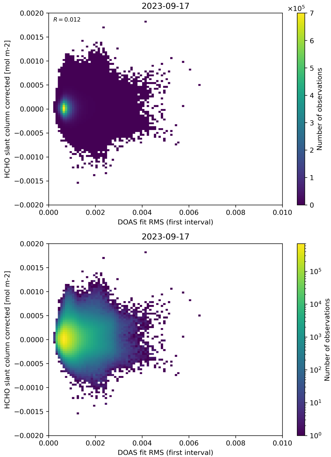
Figure 62: Scatter density plot of “DOAS fit RMS (first interval)” against “HCHO slant column corrected” for 2023-09-16 to 2023-09-18.
