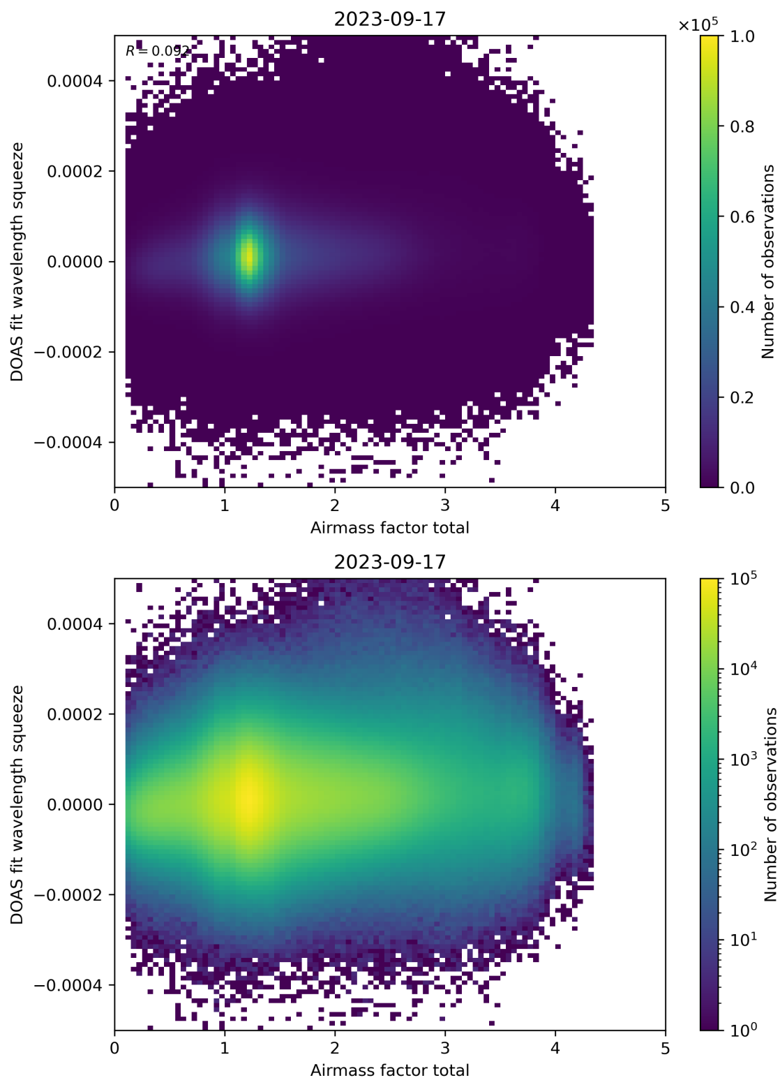
Figure 99: Scatter density plot of “Airmass factor total” against “DOAS fit wavelength squeeze” for 2023-09-16 to 2023-09-18.
