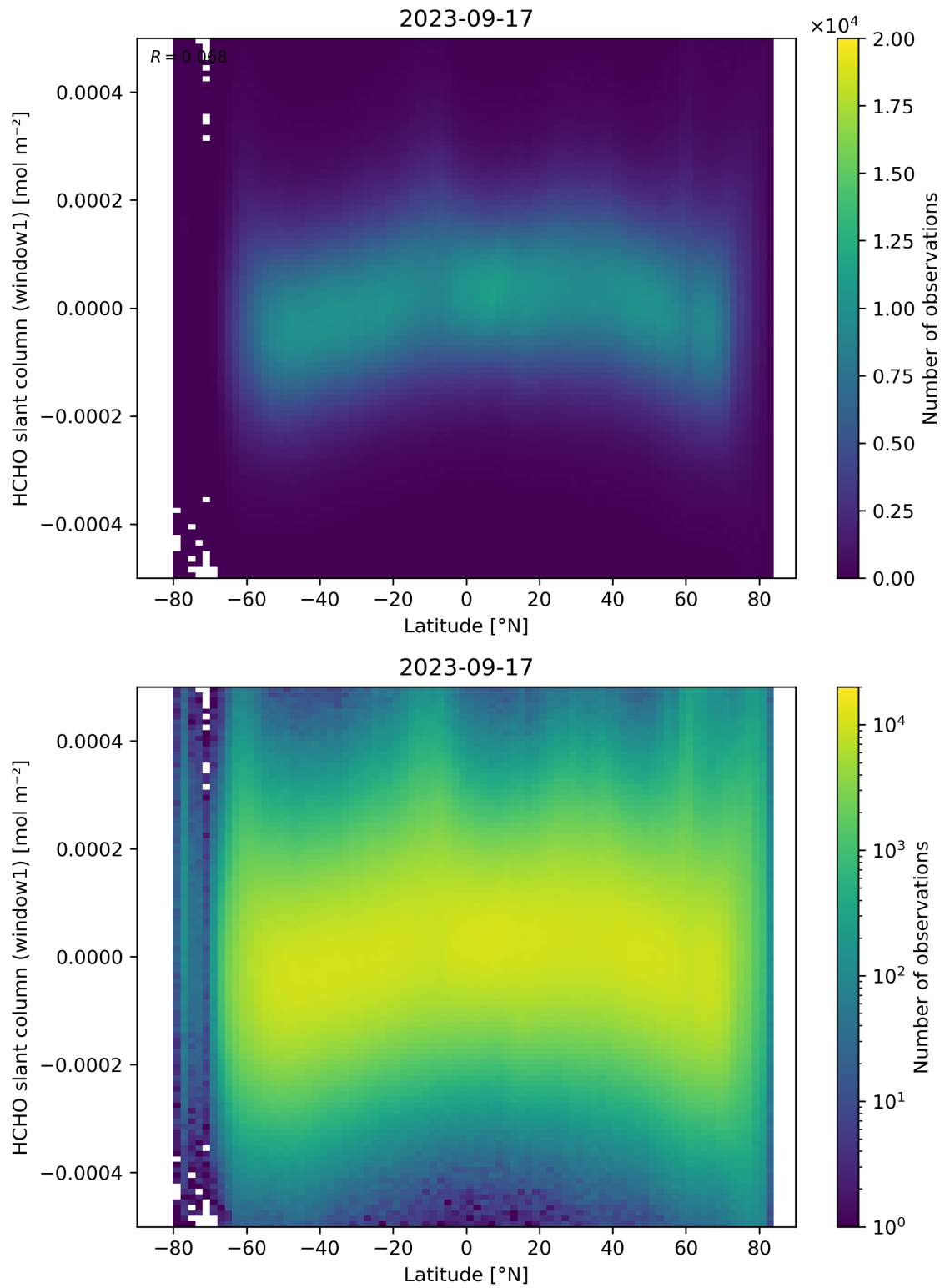
Figure 159: Scatter density plot of “Latitude” against “HCHO slant column (window1)” for 2023-09-16 to 2023-09-18.
