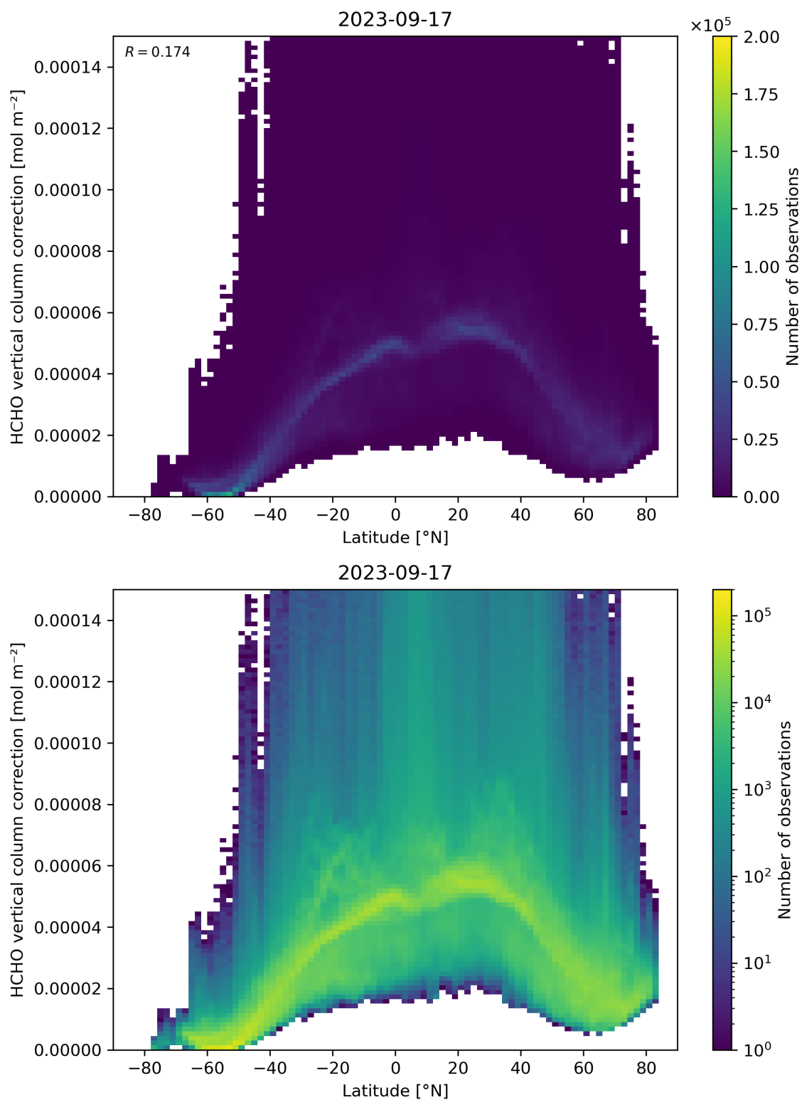
Figure 164: Scatter density plot of “Latitude” against “HCHO vertical column correction” for 2023-09-16 to 2023-09-18.
