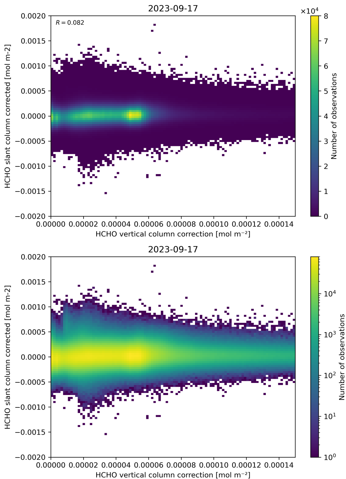
Figure 116: Scatter density plot of “HCHO vertical column correction” against “HCHO slant column corrected” for 2023-09-16 to 2023-09-18.
