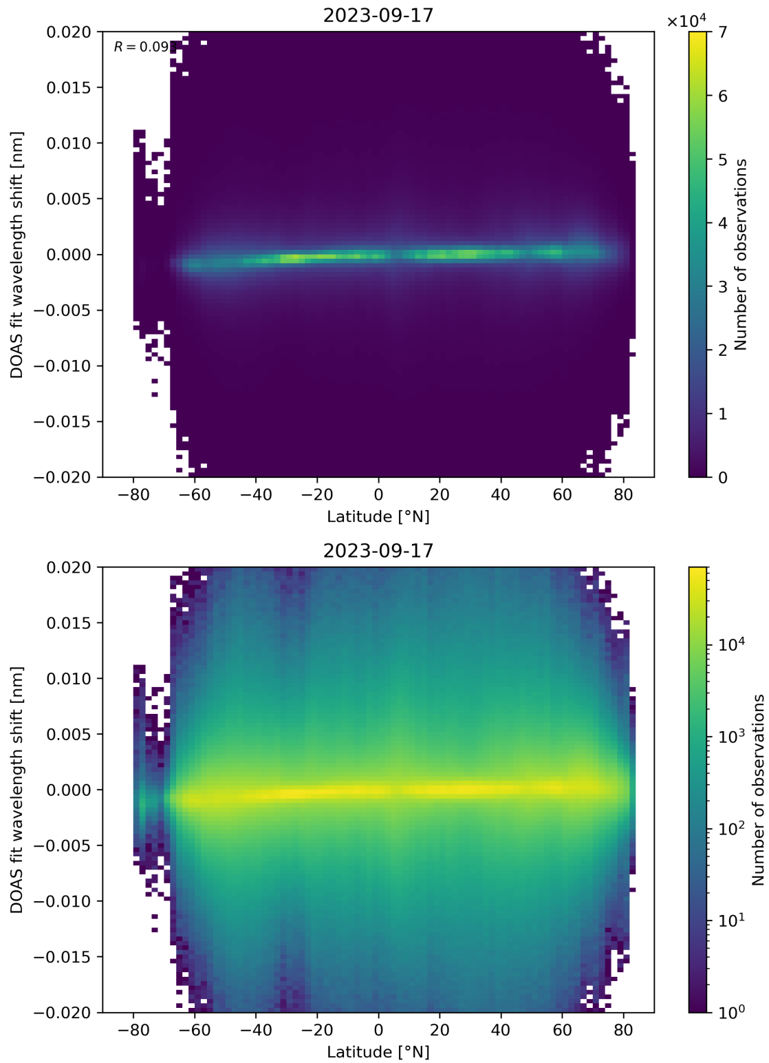
Figure 154: Scatter density plot of “Latitude” against “DOAS fit wavelength shift” for 2023-09-16 to 2023-09-18.
