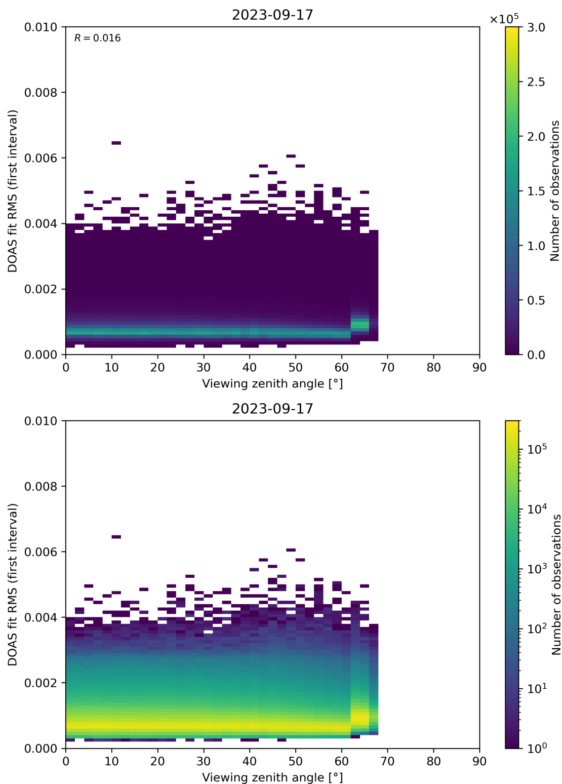
Figure 182: Scatter density plot of “Viewing zenith angle” against “DOAS fit RMS (first interval)” for 2023-09-16 to 2023-09-18.
