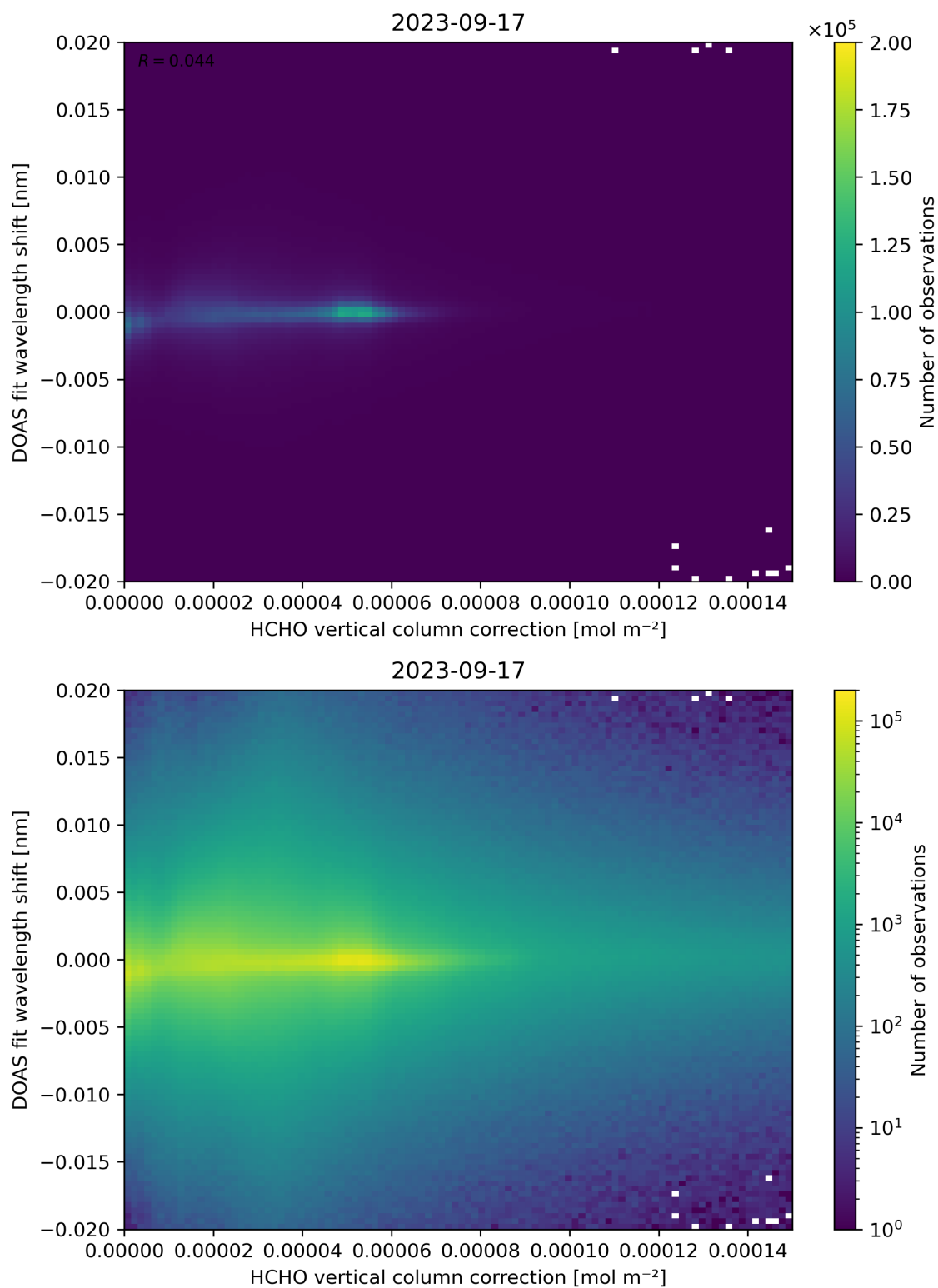
Figure 113: Scatter density plot of “HCHO vertical column correction” against “DOAS fit wavelength shift” for 2023-09-16 to 2023-09-18.
