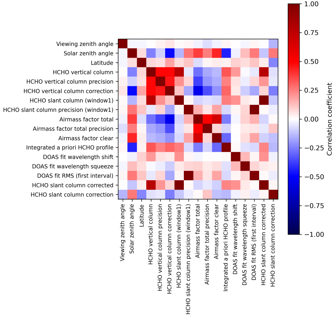
Figure 2: Map of correlation matrix for 2023-09-16 to 2023-09-18.
