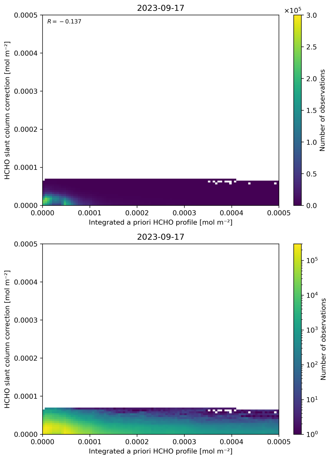
Figure 152: Scatter density plot of “Integrated a priori HCHO profile” against “HCHO slant column correction” for 2023-09-16 to 2023-09-18.
