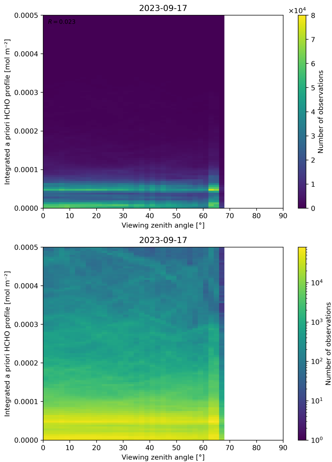
Figure 195: Scatter density plot of “Viewing zenith angle” against “Integrated a priori HCHO profile” for 2023-09-16 to 2023-09-18.
