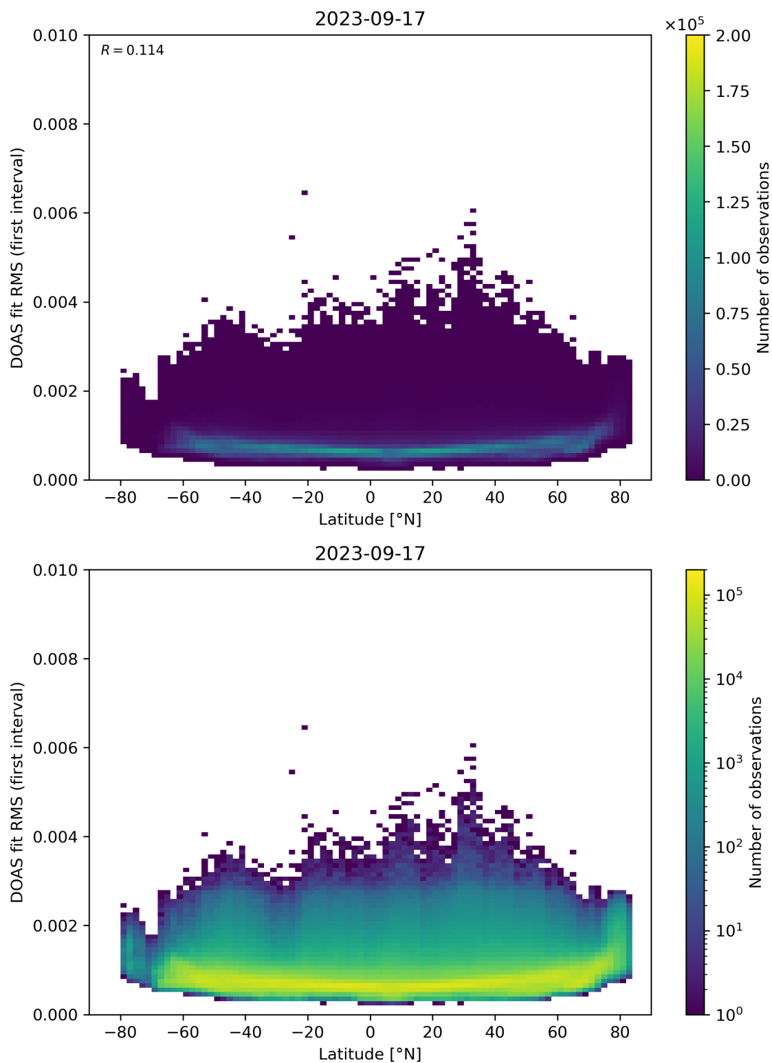
Figure 153: Scatter density plot of “Latitude” against “DOAS fit RMS (first interval)” for 2023-09-16 to 2023-09-18.
