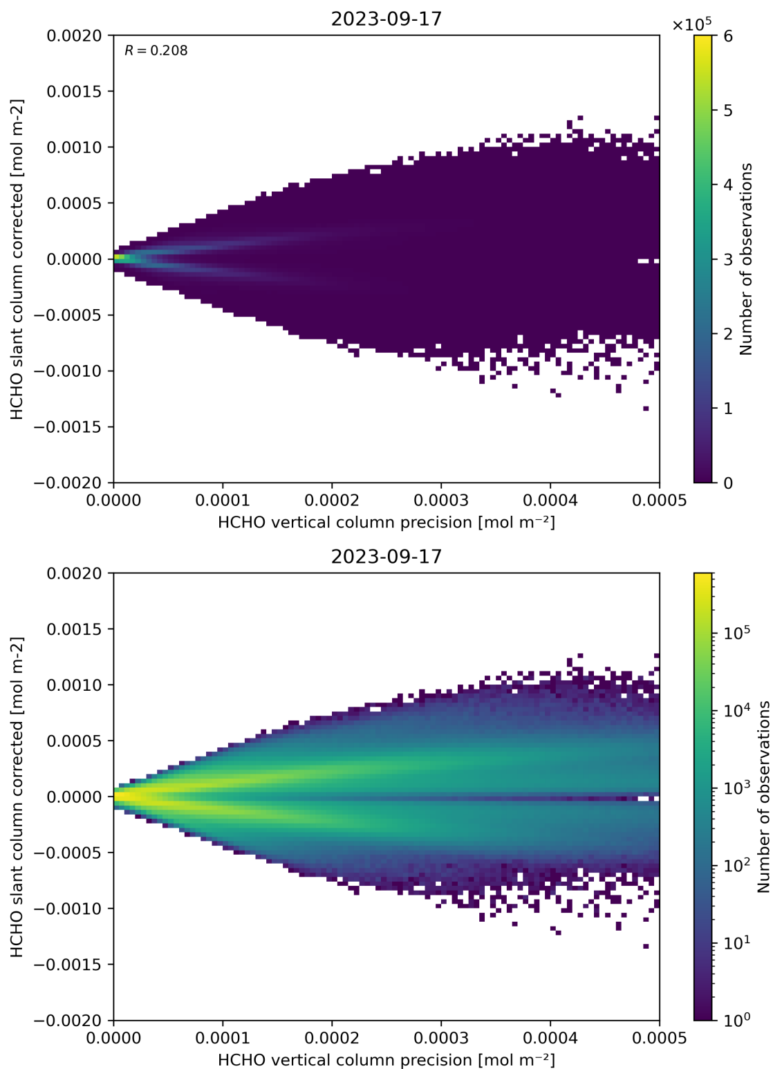
Figure 140: Scatter density plot of “HCHO vertical column precision” against “HCHO slant column corrected” for 2023-09-16 to 2023-09-18.
