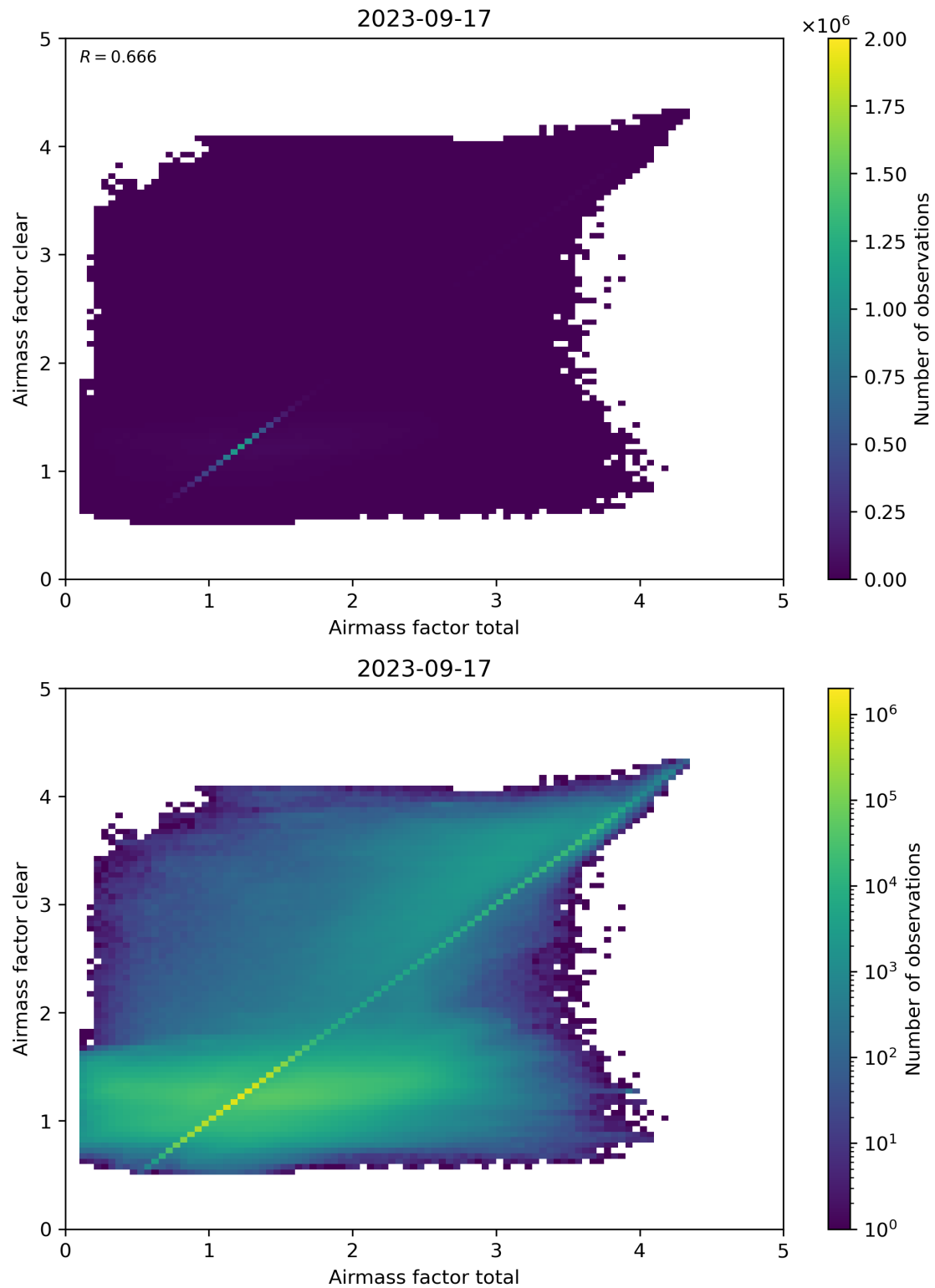
Figure 100: Scatter density plot of “Airmass factor total” against “Airmass factor clear” for 2023-09-16 to 2023-09-18.
