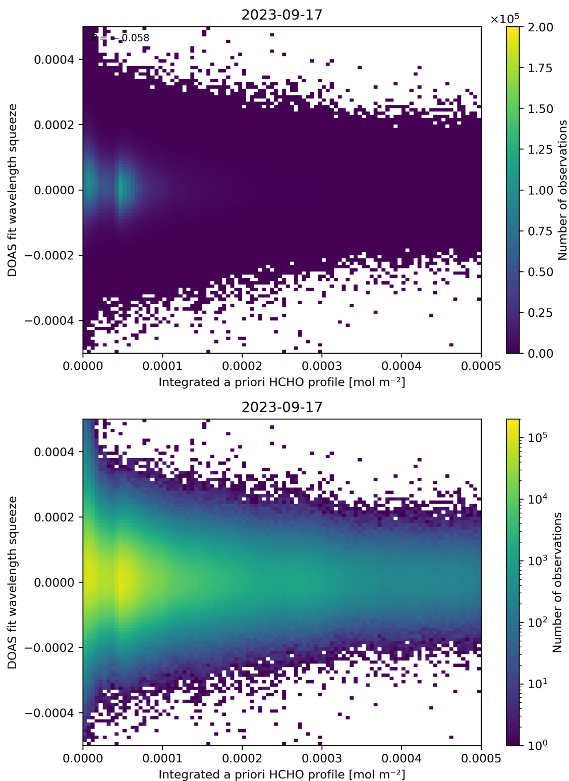
Figure 150: Scatter density plot of “Integrated a priori HCHO profile” against “DOAS fit wavelength squeeze” for 2023-09-16 to 2023-09-18.
