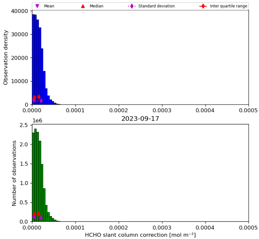
Figure 47: Histogram of “HCHO slant column correction” for 2023-09-16 to 2023-09-18
