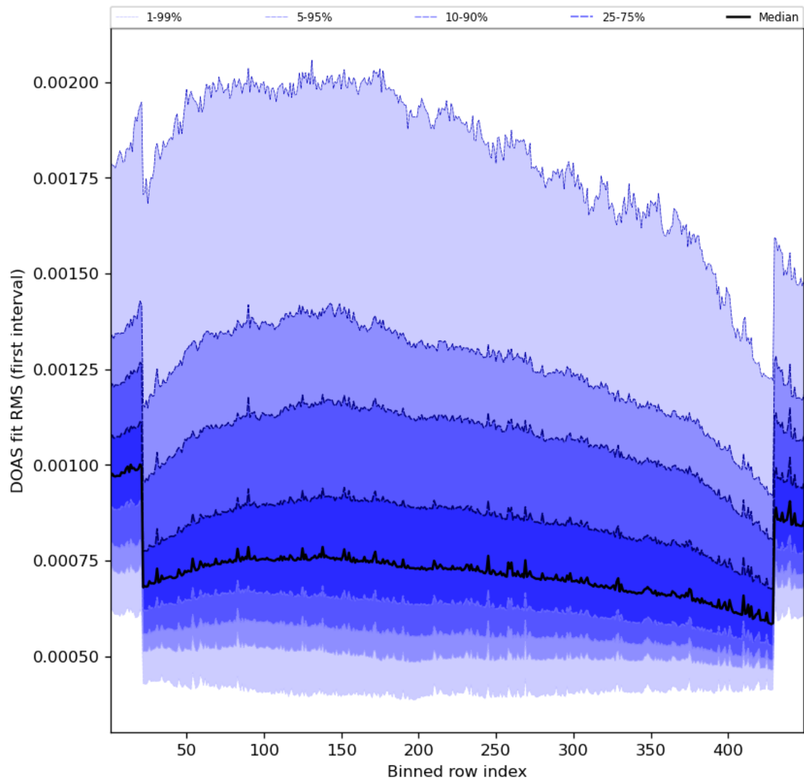
Figure 60: Along track statistics of “DOAS fit RMS (first interval)” for 2023-09-16 to 2023-09-18
