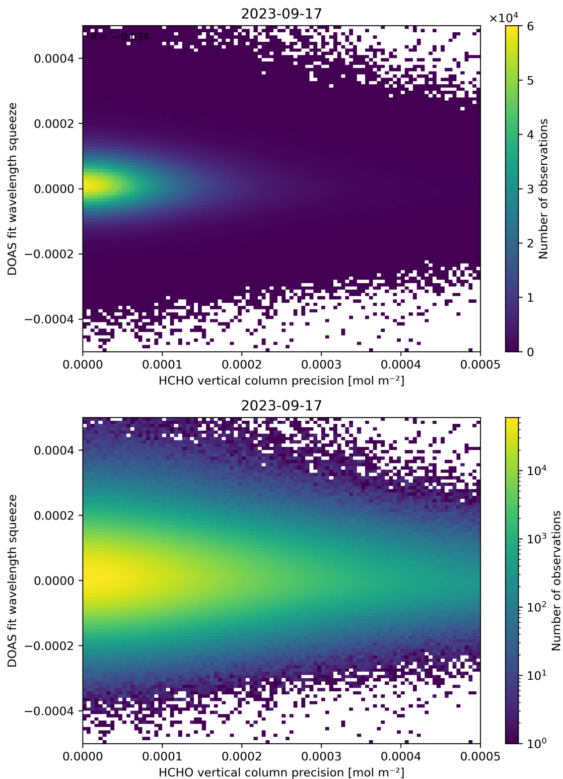
Figure 138: Scatter density plot of “HCHO vertical column precision” against “DOAS fit wavelength squeeze” for 2023-09-16 to 2023-09-18.
