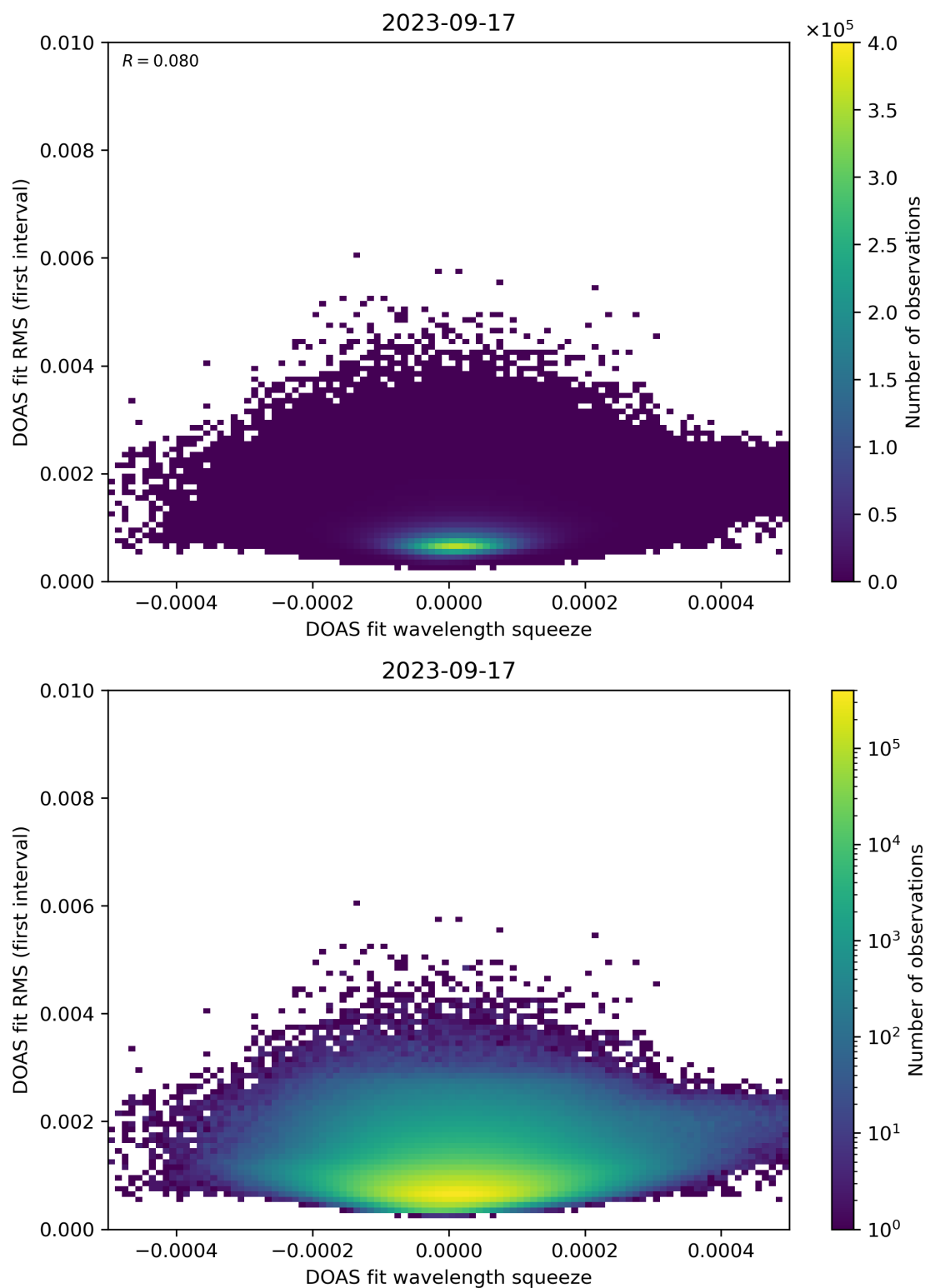
Figure 68: Scatter density plot of “DOAS fit wavelength squeeze” against “DOAS fit RMS (first interval)” for 2023-09-16 to 2023-09-18.
