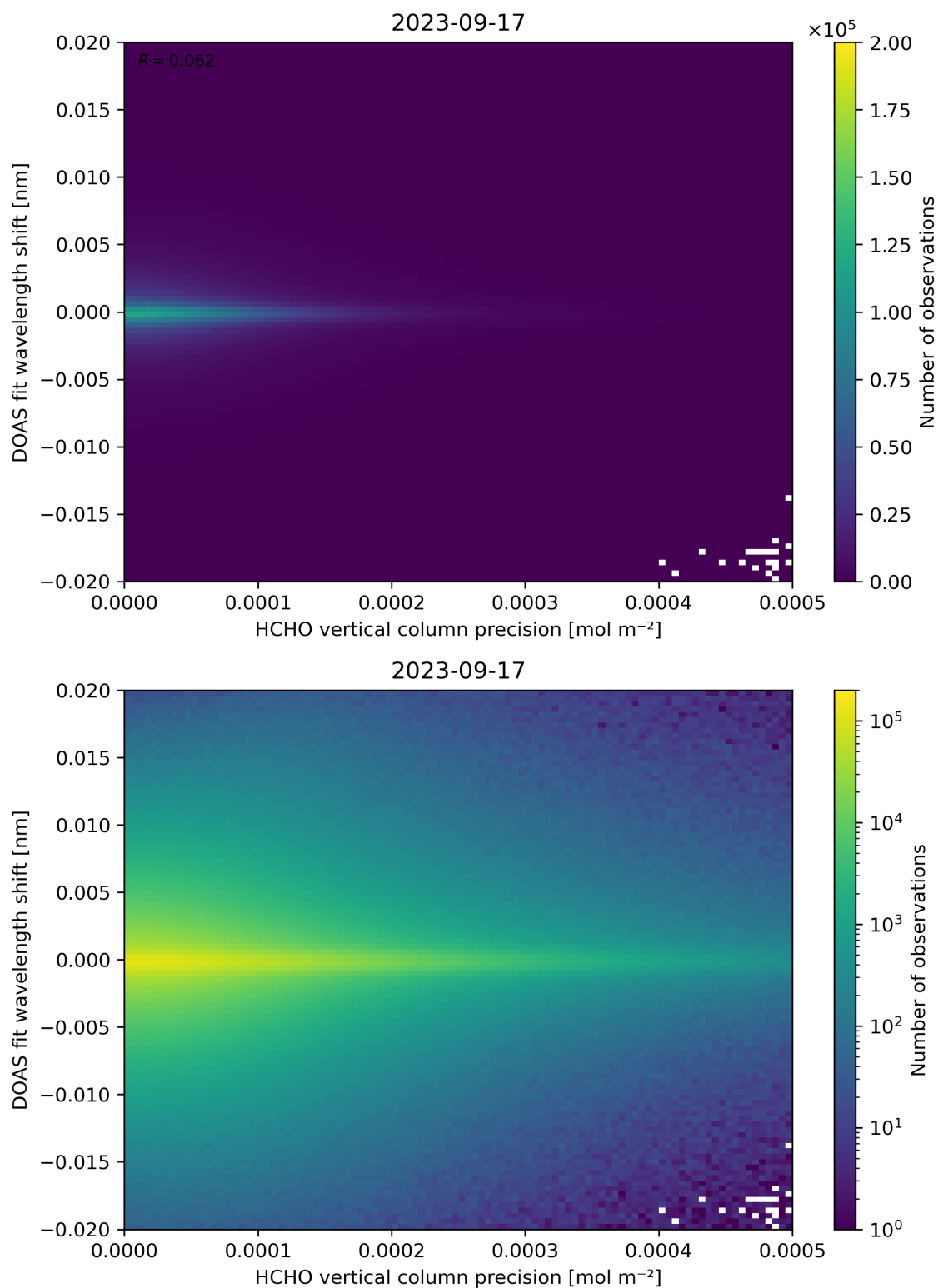
Figure 137: Scatter density plot of “HCHO vertical column precision” against “DOAS fit wavelength shift” for 2023-09-16 to 2023-09-18.
