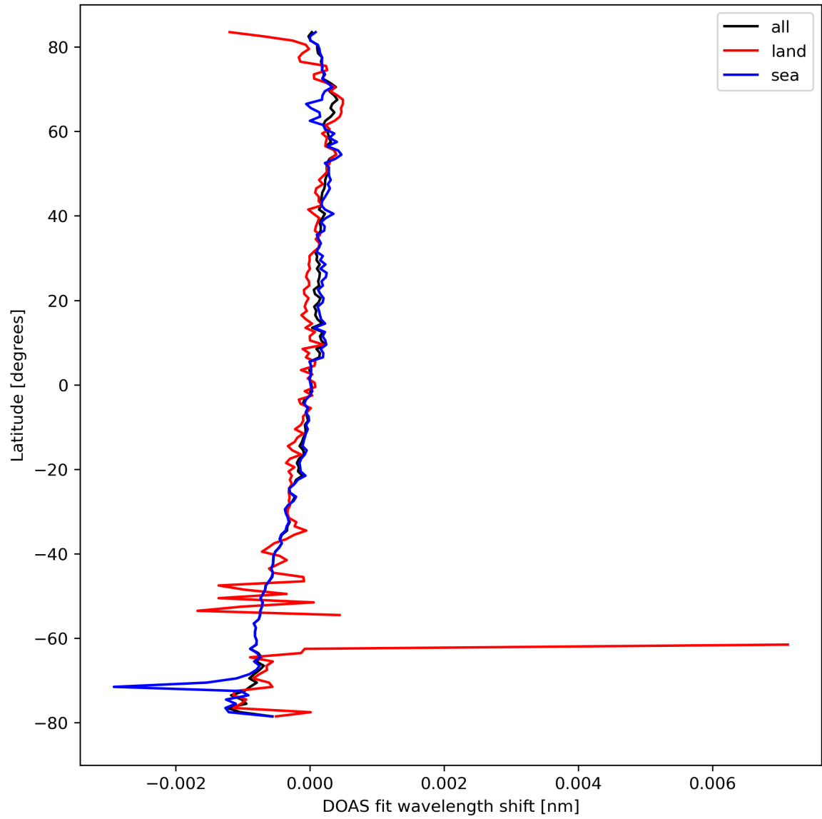
Figure 30: Zonal average of “DOAS fit wavelength shift” for 2023-09-16 to 2023-09-18.
