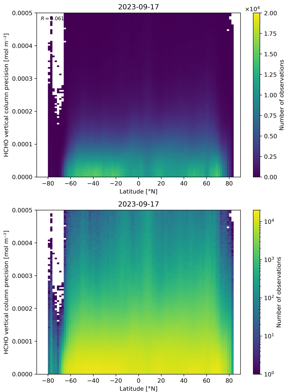
Figure 165: Scatter density plot of “Latitude” against “HCHO vertical column precision” for 2023-09-16 to 2023-09-18.
