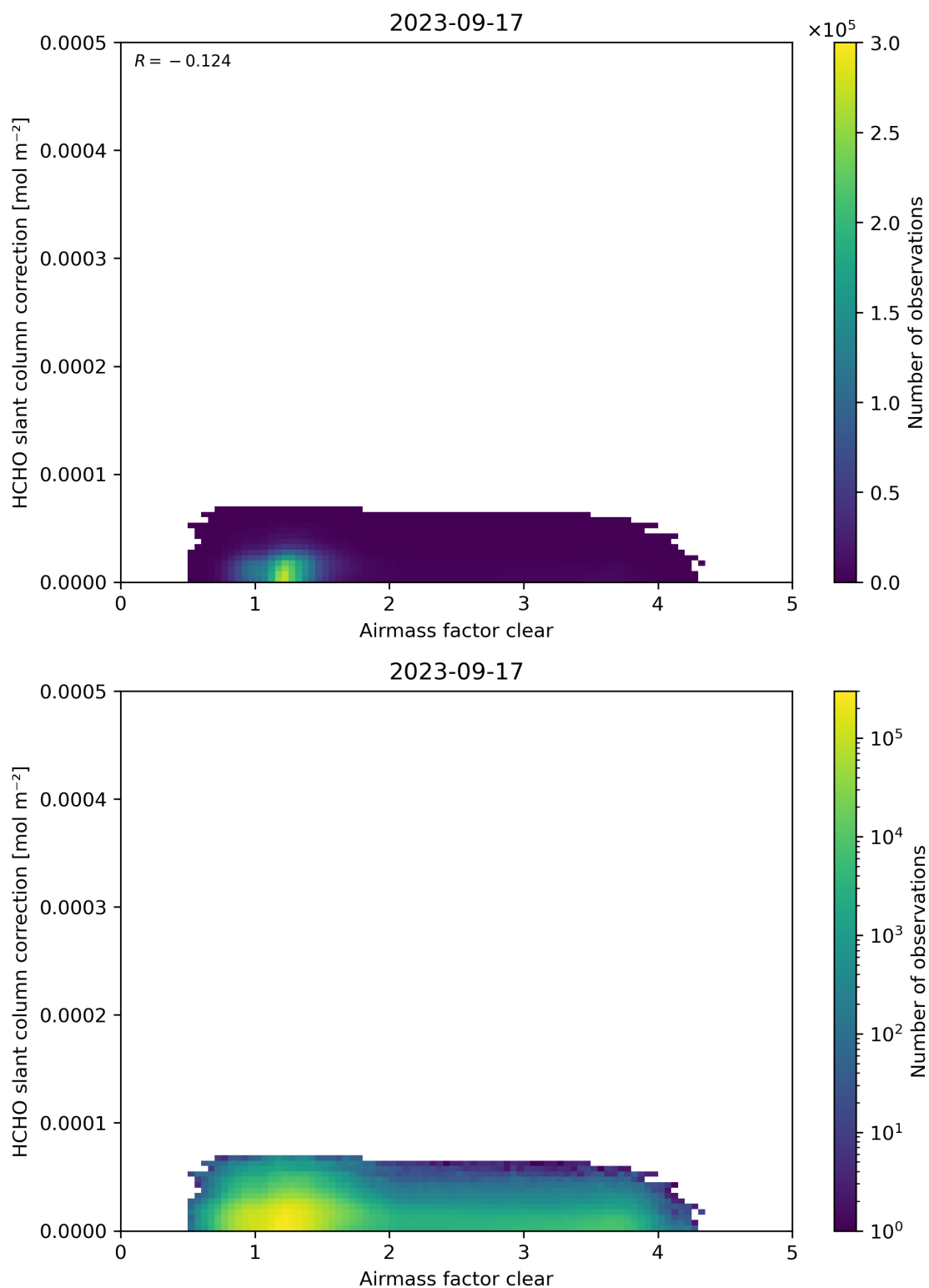
Figure 75: Scatter density plot of “Airmass factor clear” against “HCHO slant column correction” for 2023-09-16 to 2023-09-18.
