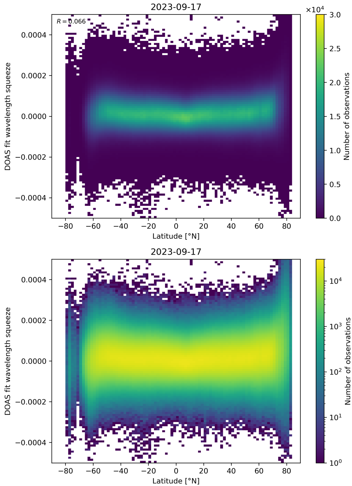
Figure 155: Scatter density plot of “Latitude” against “DOAS fit wavelength squeeze” for 2023-09-16 to 2023-09-18.
