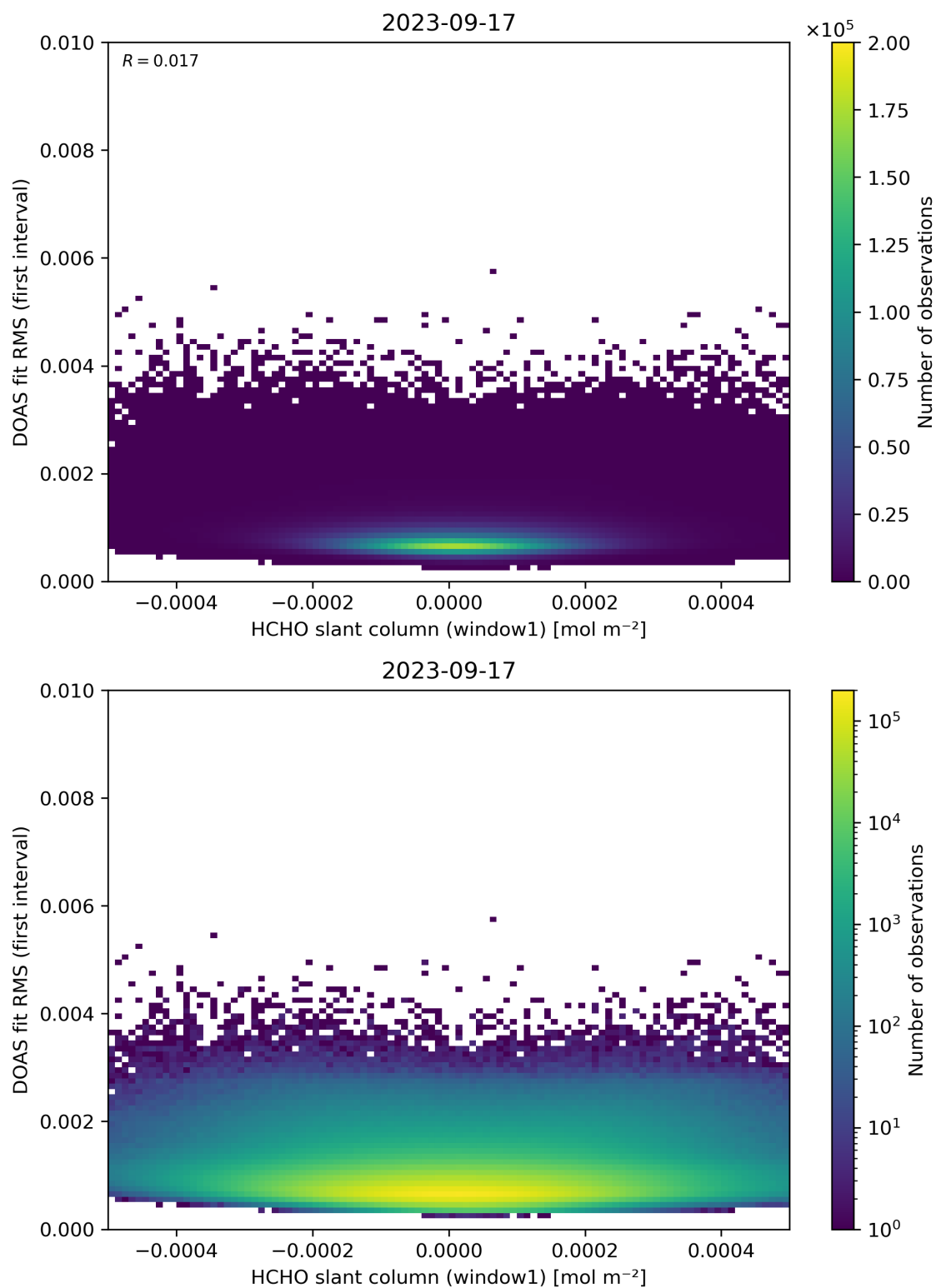
Figure 78: Scatter density plot of “HCHO slant column (window1)” against “DOAS fit RMS (first interval)” for 2023-09-16 to 2023-09-18.
