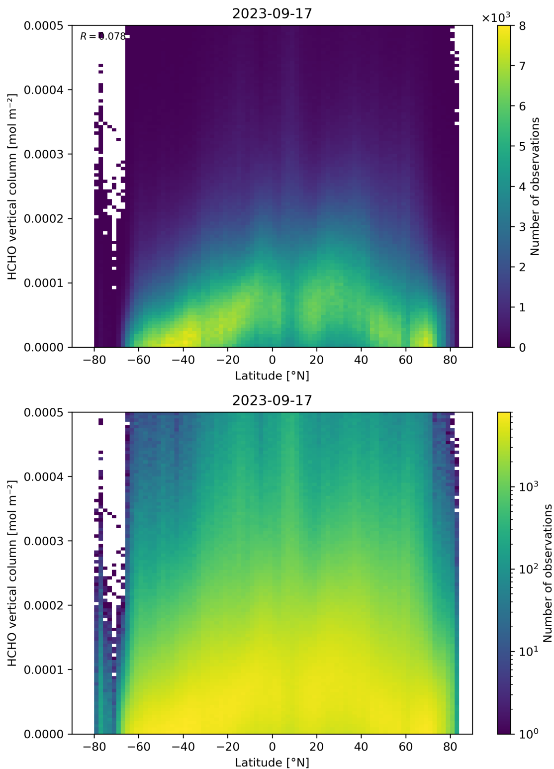
Figure 163: Scatter density plot of “Latitude” against “HCHO vertical column” for 2023-09-16 to 2023-09-18.
