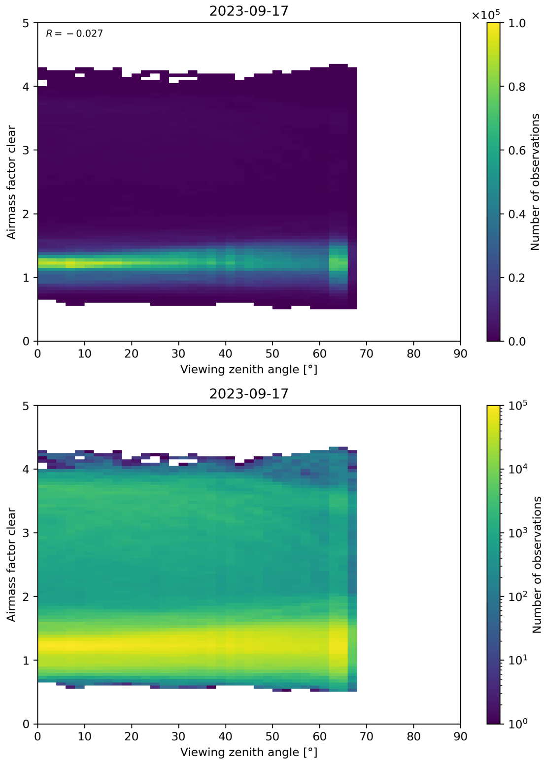
Figure 185: Scatter density plot of “Viewing zenith angle” against “Airmass factor clear” for 2023-09-16 to 2023-09-18.
