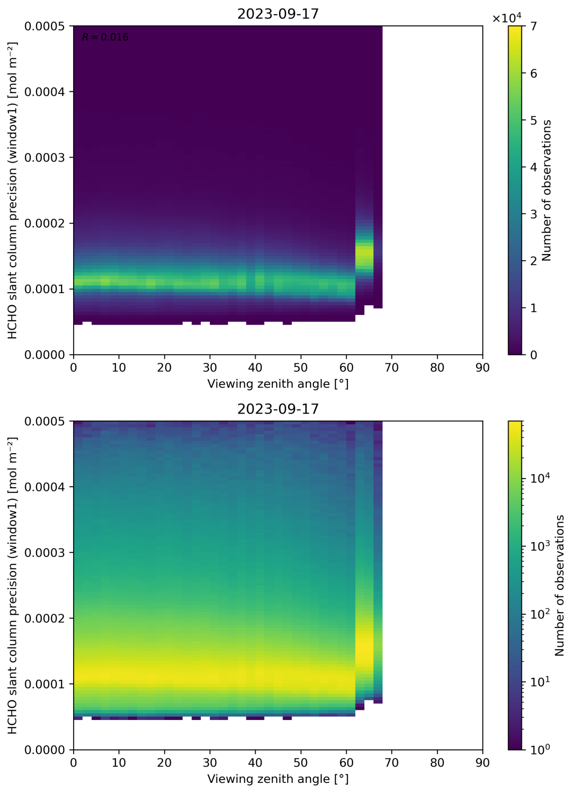
Figure 189: Scatter density plot of “Viewing zenith angle” against “HCHO slant column precision (window1)” for 2023-09-16 to 2023-09-18.
