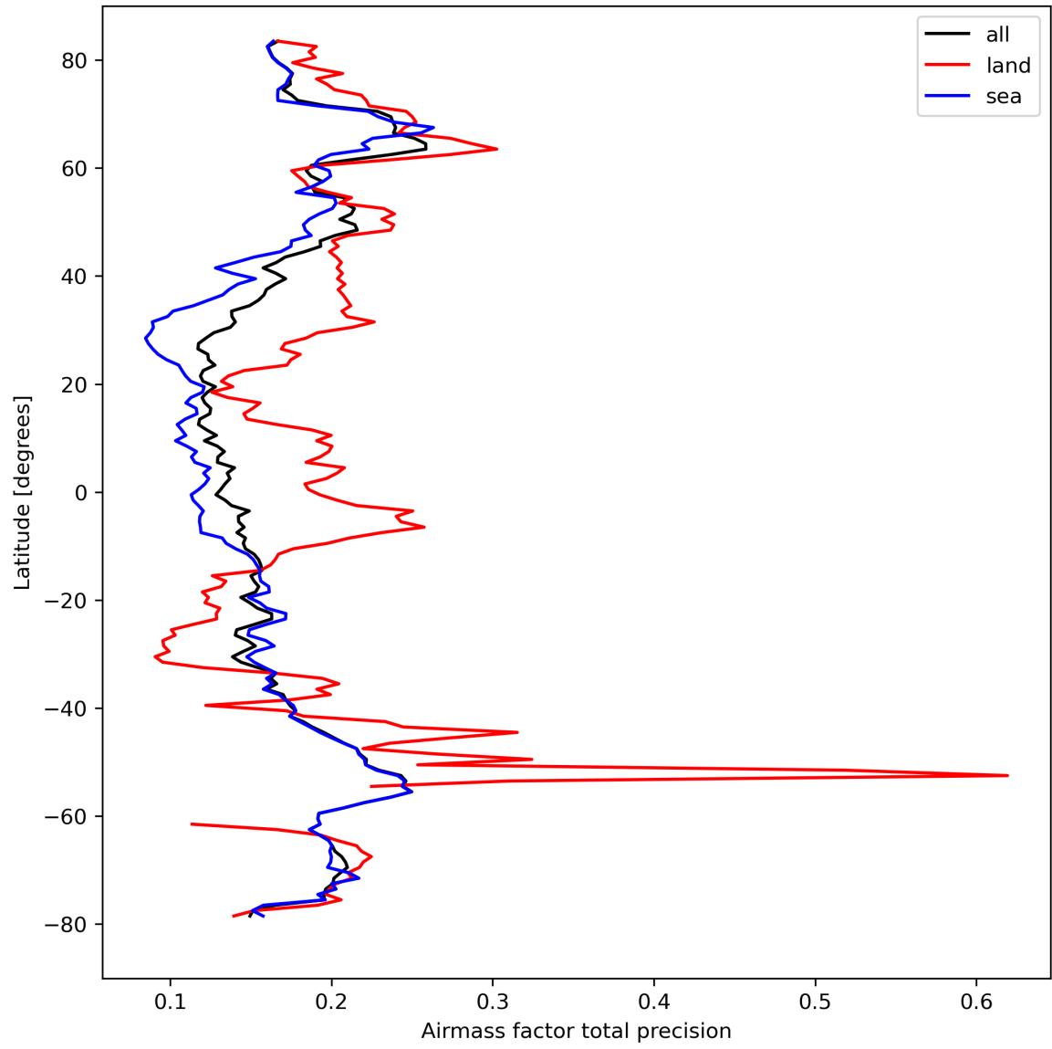
Figure 27: Zonal average of “Airmass factor total precision” for 2023-09-16 to 2023-09-18.
