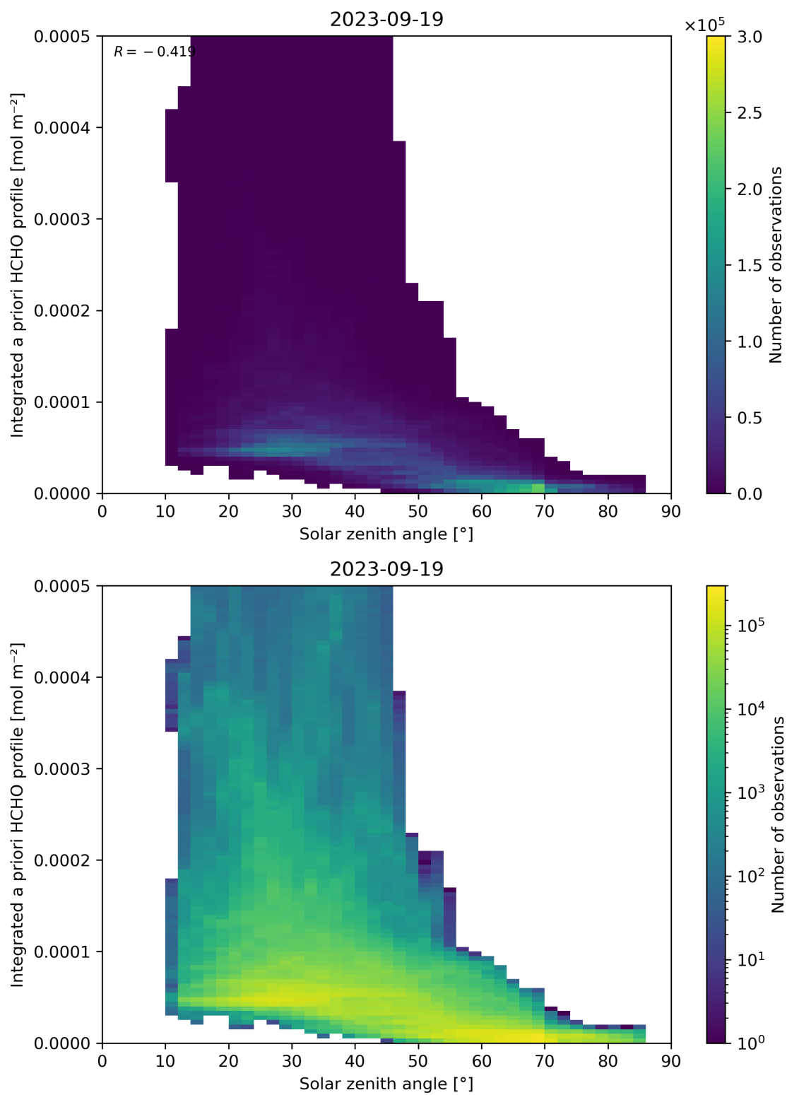
Figure 180: Scatter density plot of “Solar zenith angle” against “Integrated a priori HCHO profile” for 2023-09-18 to 2023-09-20.
