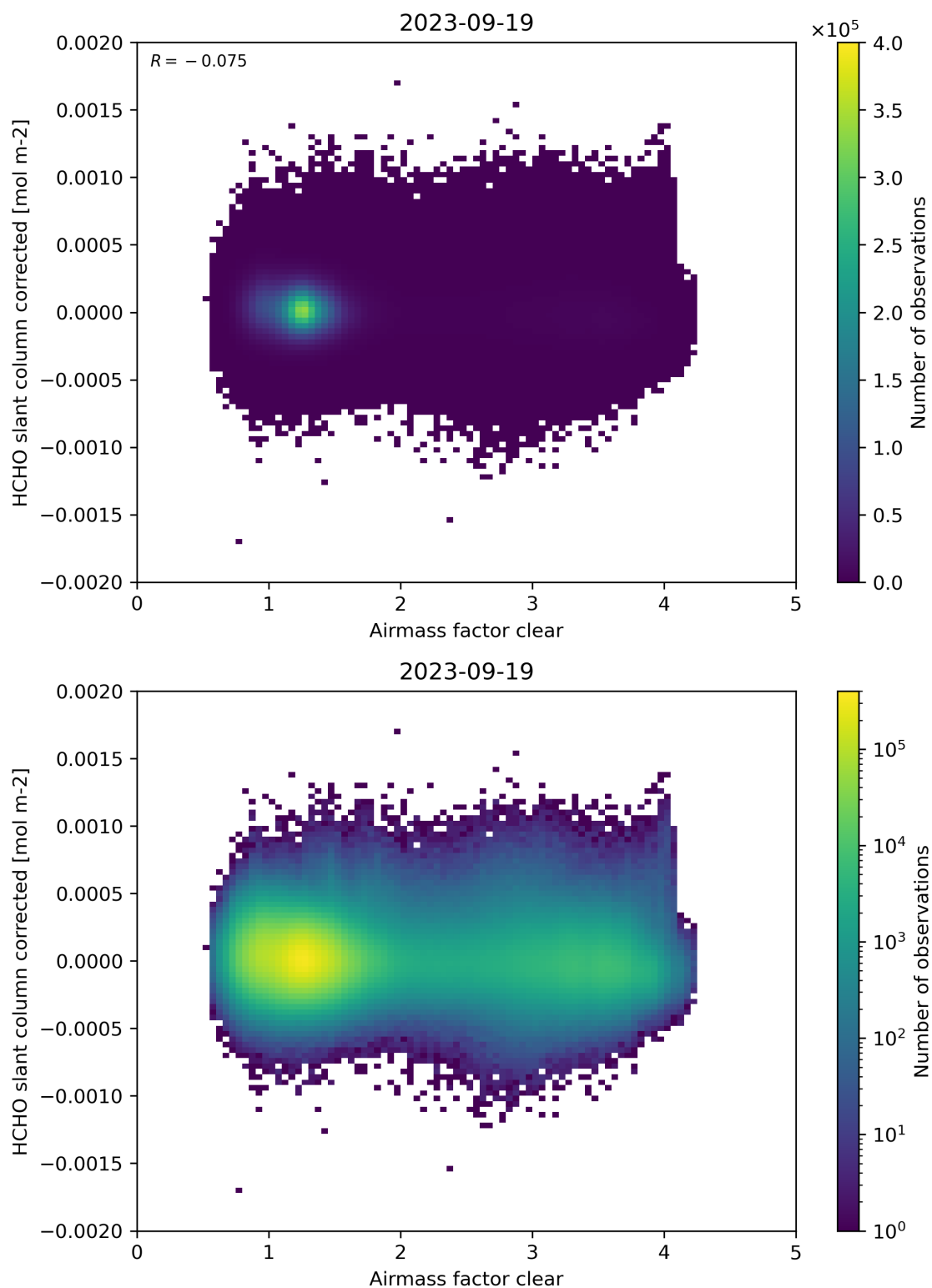
Figure 74: Scatter density plot of “Airmass factor clear” against “HCHO slant column corrected” for 2023-09-18 to 2023-09-20.
