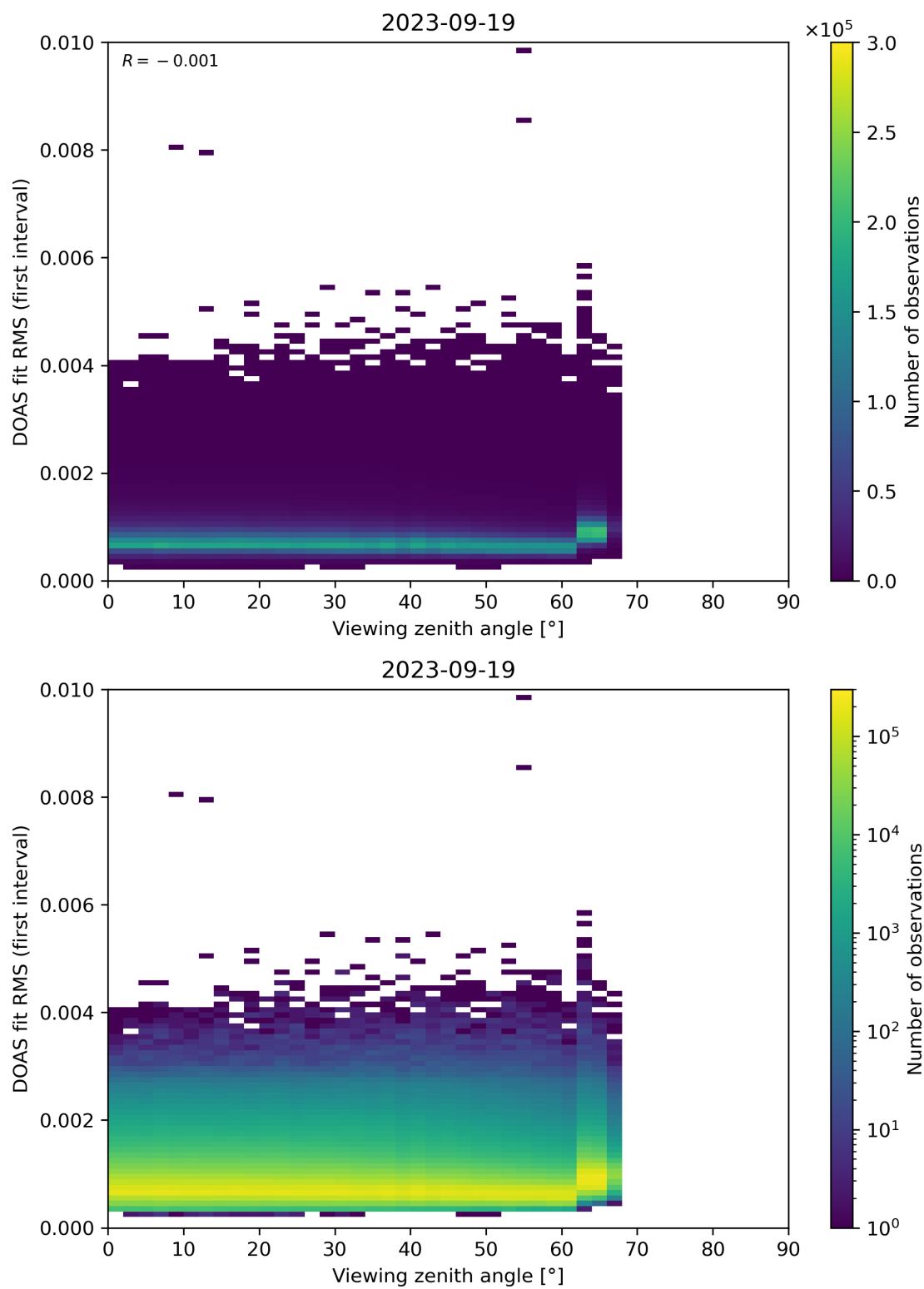
Figure 182: Scatter density plot of “Viewing zenith angle” against “DOAS fit RMS (first interval)” for 2023-09-18 to 2023-09-20.
