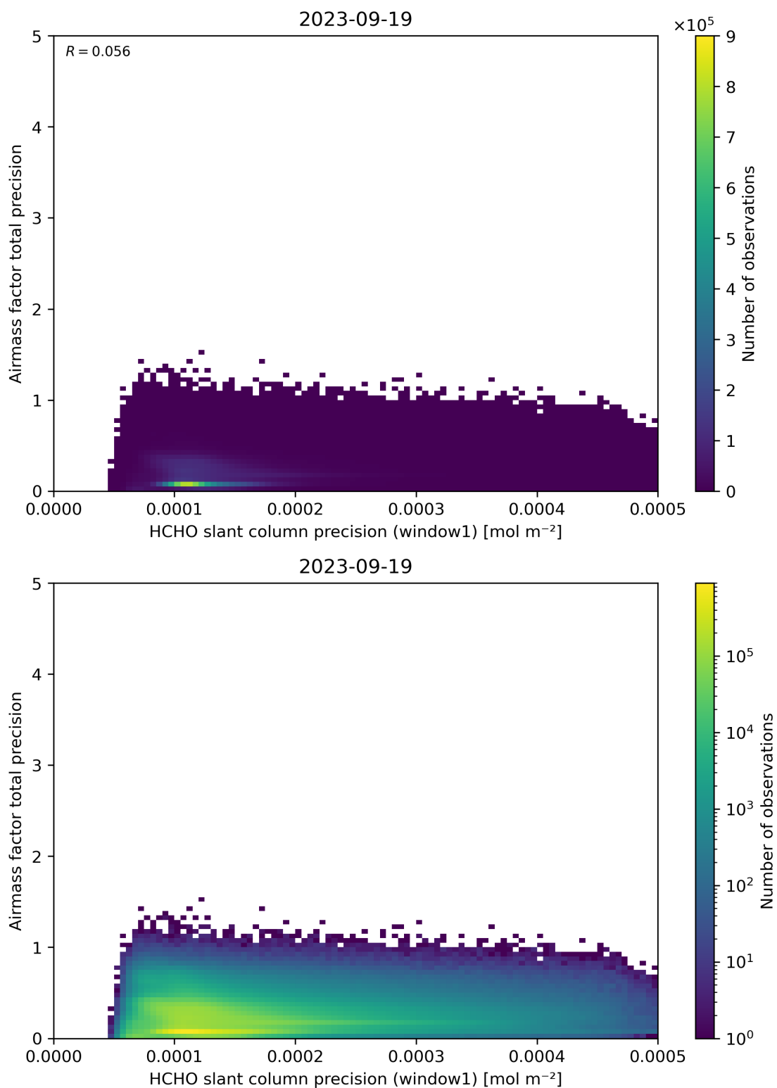
Figure 95: Scatter density plot of “HCHO slant column precision (window1)” against “Airmass factor total precision” for 2023-09-18 to 2023-09-20.
