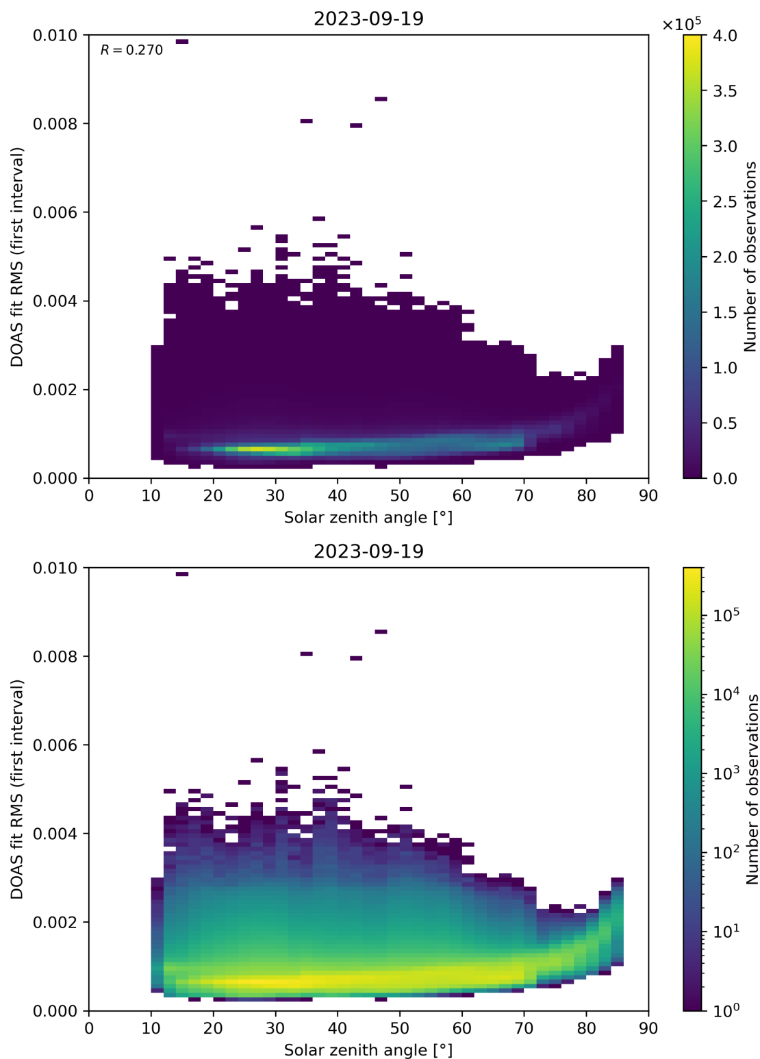
Figure 167: Scatter density plot of “Solar zenith angle” against “DOAS fit RMS (first interval)” for 2023-09-18 to 2023-09-20.
