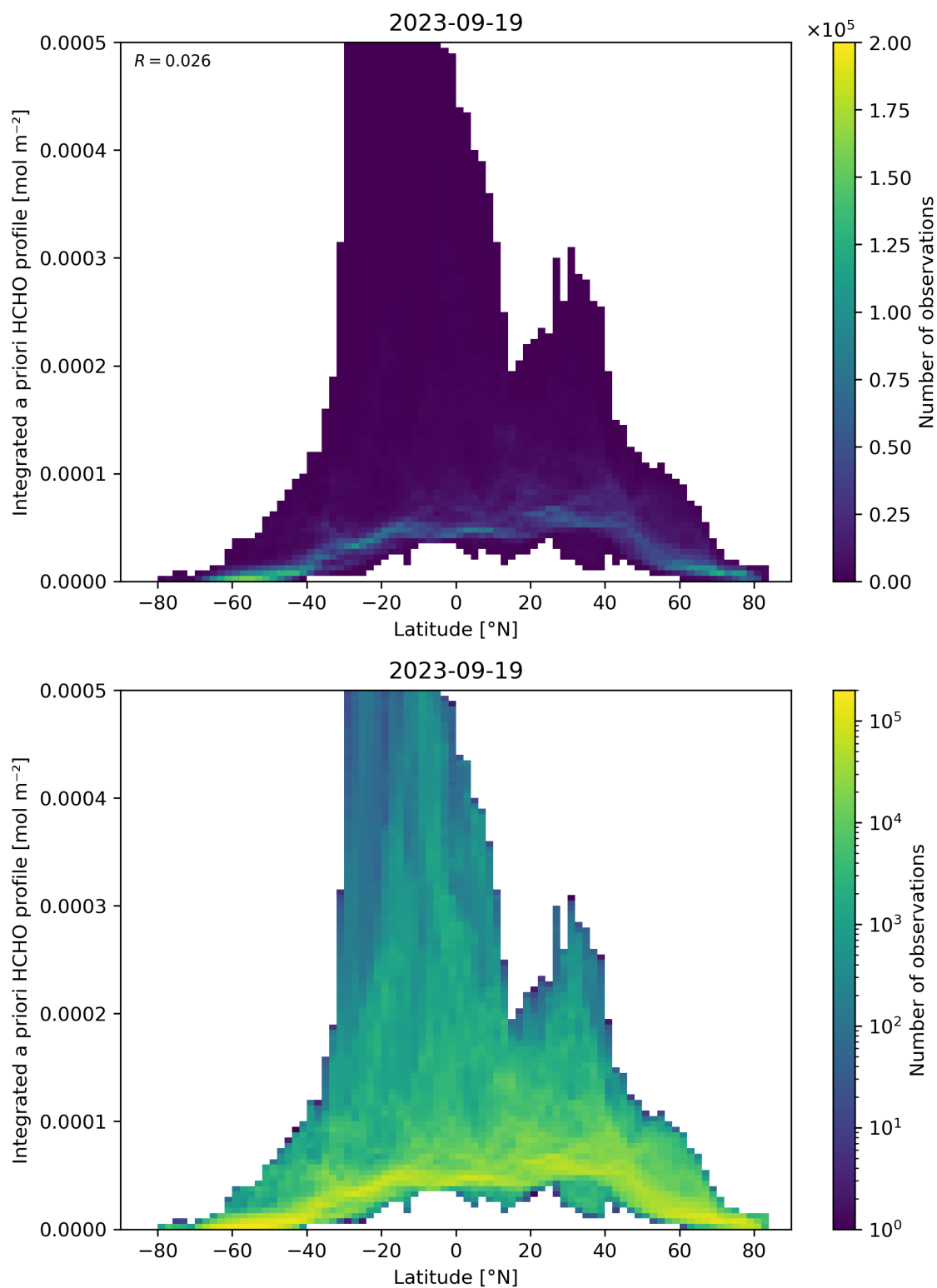
Figure 166: Scatter density plot of “Latitude” against “Integrated a priori HCHO profile” for 2023-09-18 to 2023-09-20.
