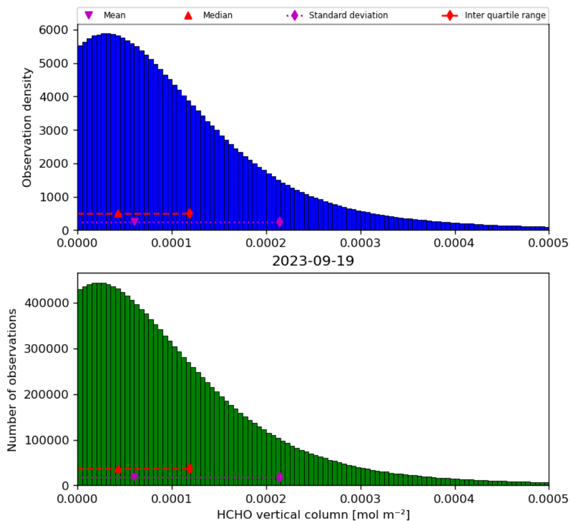
Figure 35: Histogram of “HCHO vertical column” for 2023-09-18 to 2023-09-20
