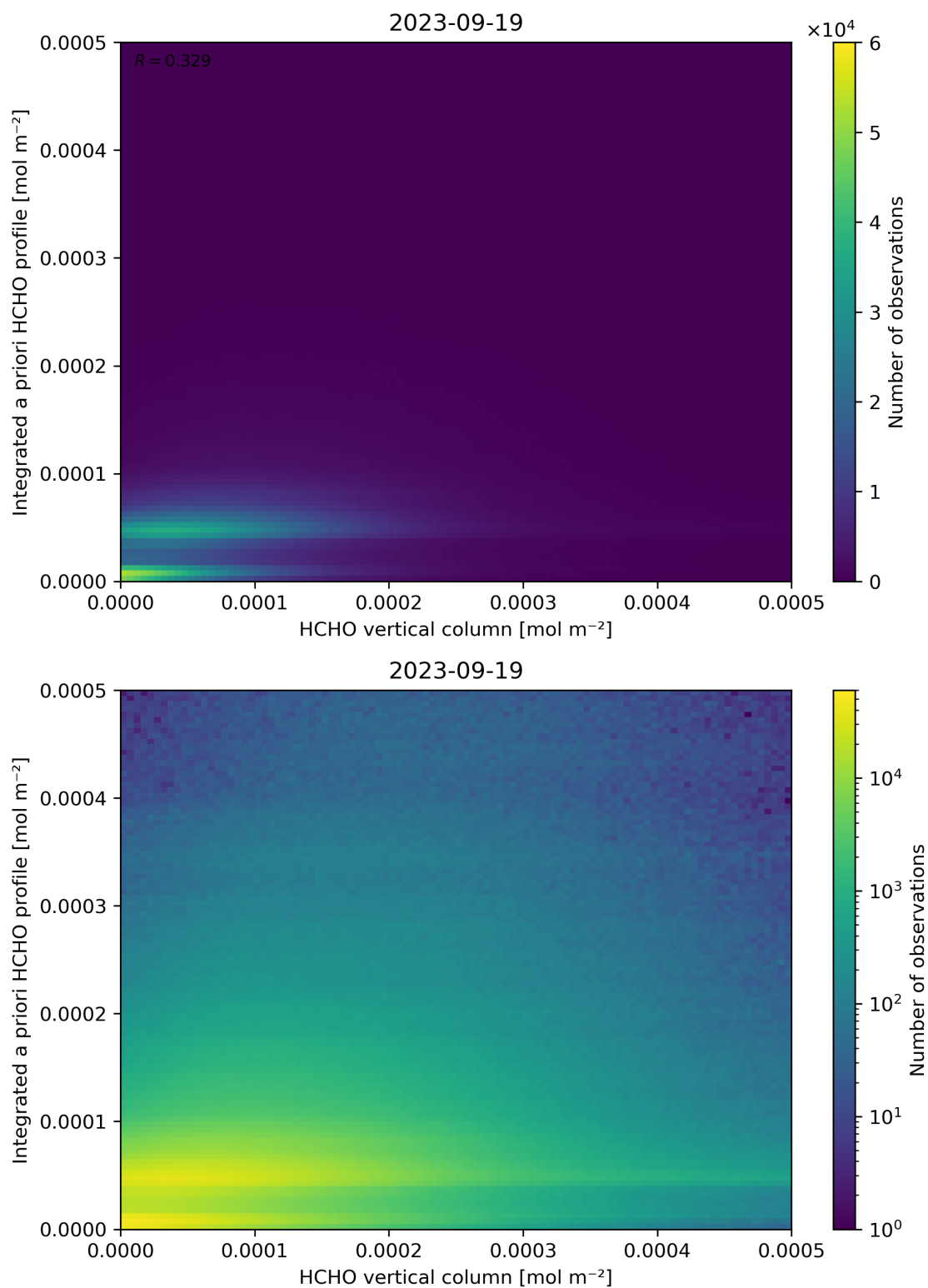
Figure 135: Scatter density plot of “HCHO vertical column” against “Integrated a priori HCHO profile” for 2023-09-18 to 2023-09-20.
