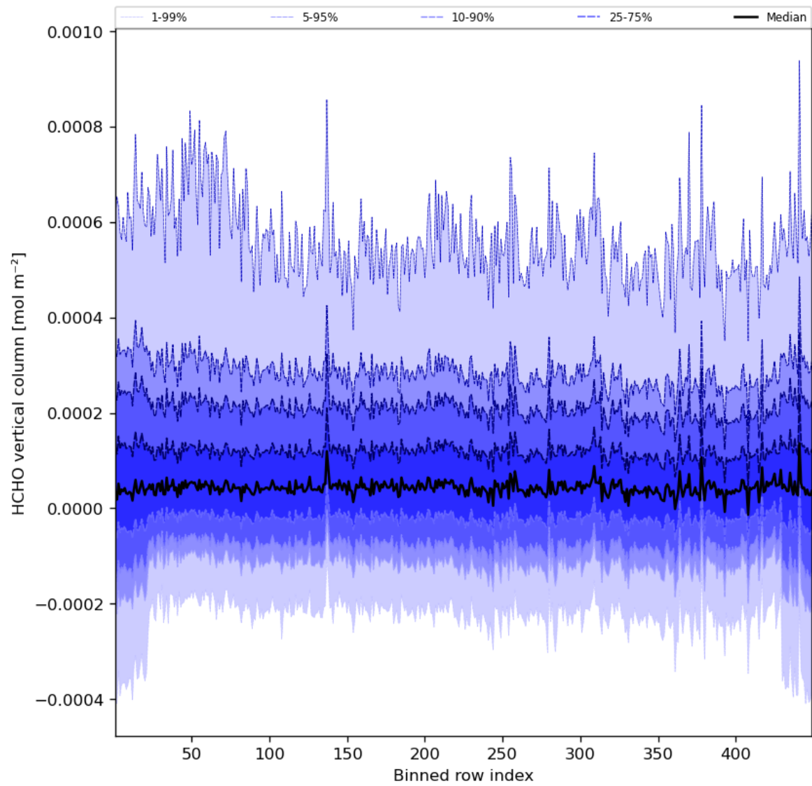
Figure 49: Along track statistics of “HCHO vertical column” for 2023-09-18 to 2023-09-20
