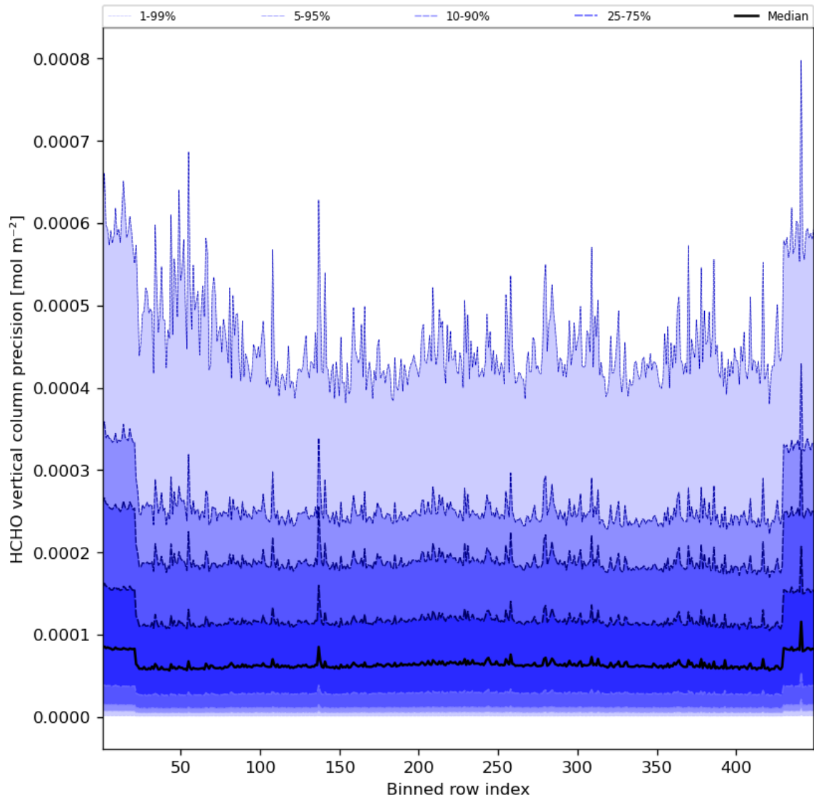
Figure 50: Along track statistics of "HCHO vertical column precision" for 2023-09-18 to 2023-09-20
