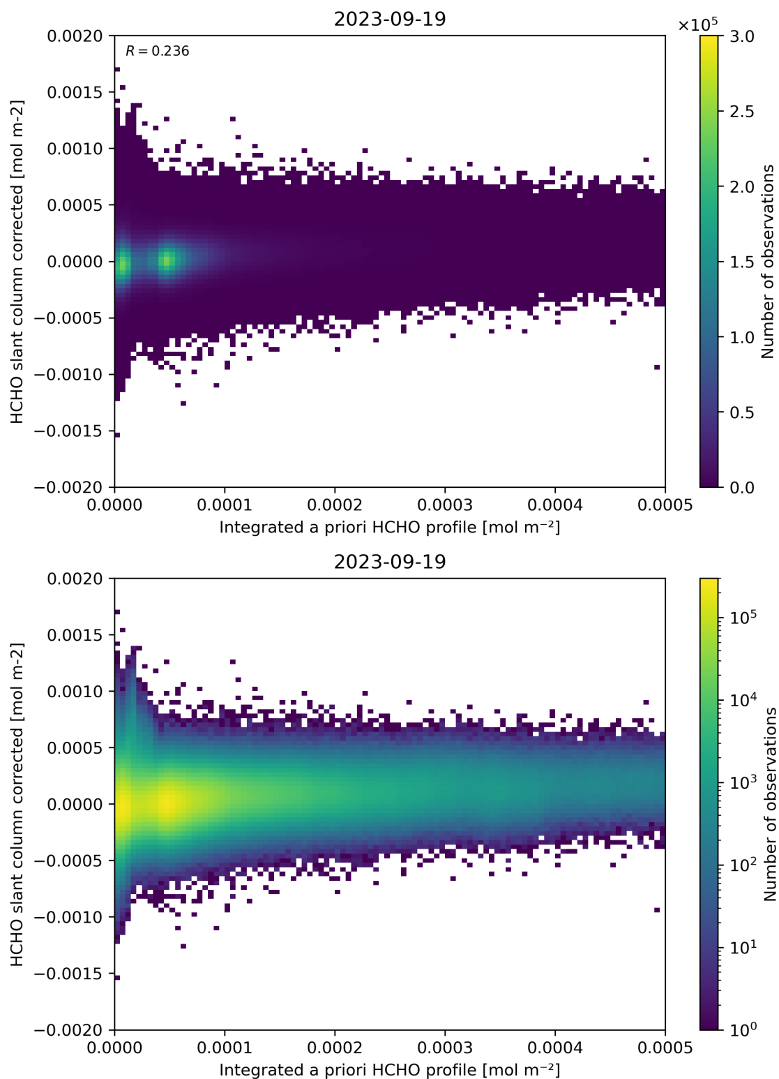
Figure 151: Scatter density plot of “Integrated a priori HCHO profile” against “HCHO slant column corrected” for 2023-09-18 to 2023-09-20.
