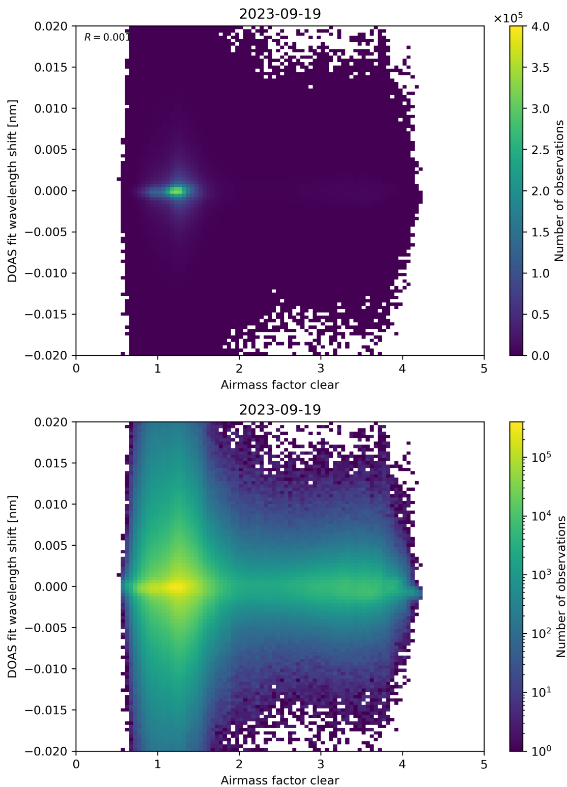
Figure 72: Scatter density plot of “Airmass factor clear” against “DOAS fit wavelength shift” for 2023-09-18 to 2023-09-20.
