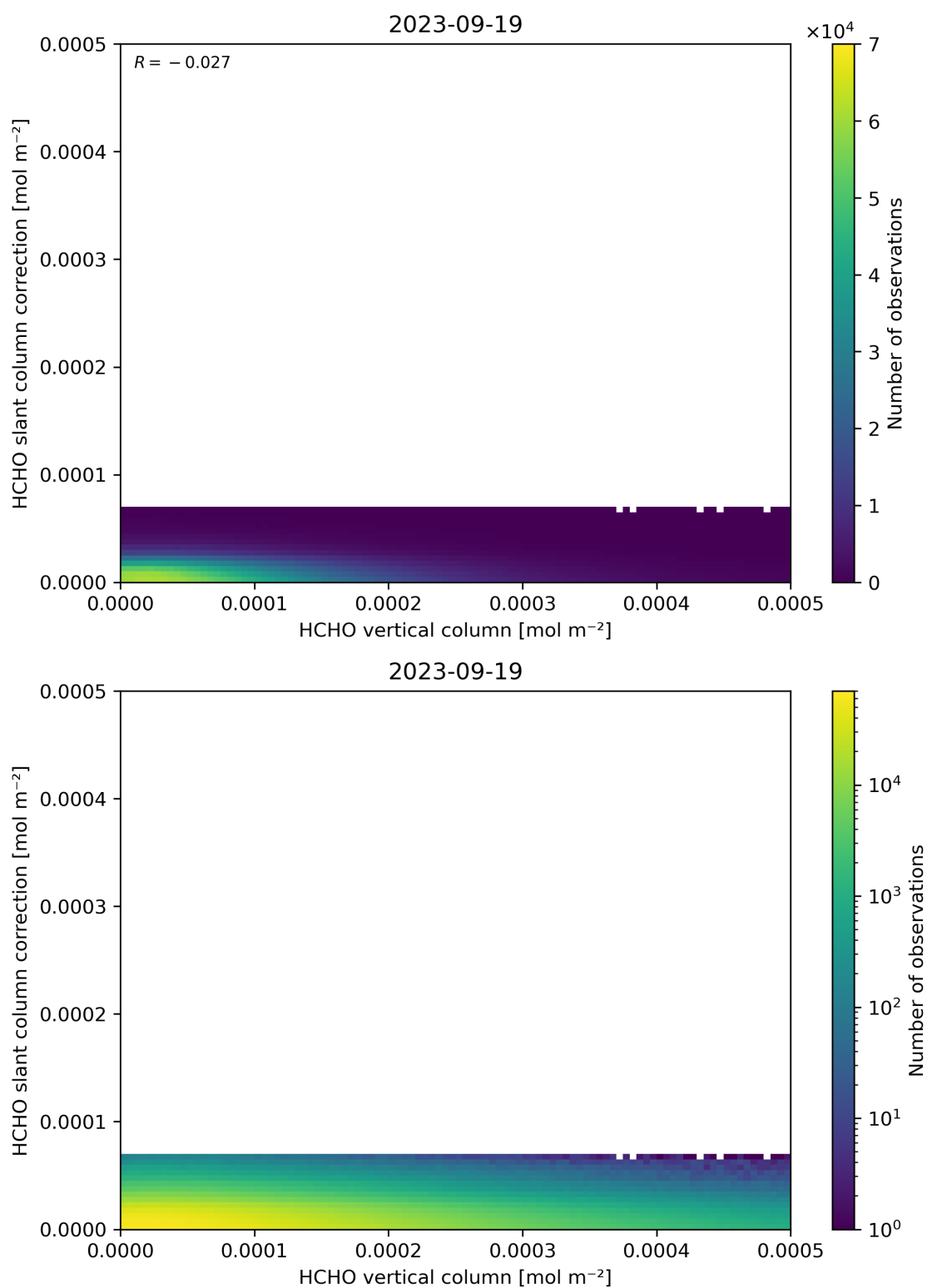
Figure 128: Scatter density plot of “HCHO vertical column” against “HCHO slant column correction” for 2023-09-18 to 2023-09-20.
