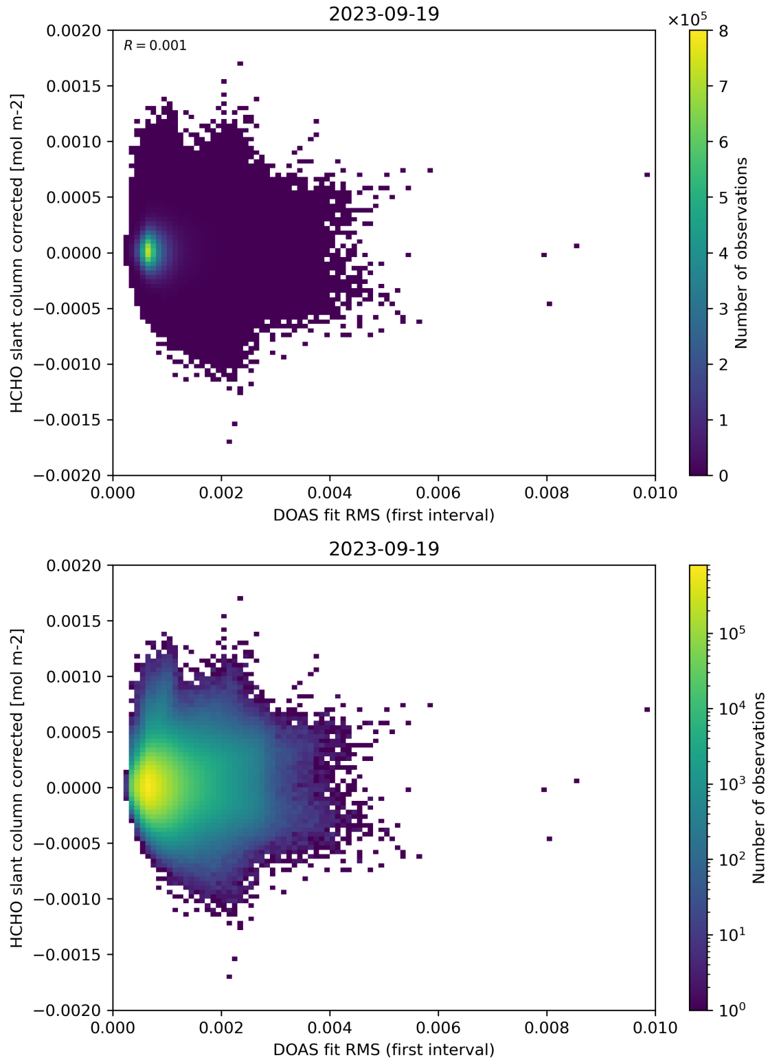
Figure 62: Scatter density plot of “DOAS fit RMS (first interval)” against “HCHO slant column corrected” for 2023-09-18 to 2023-09-20.
