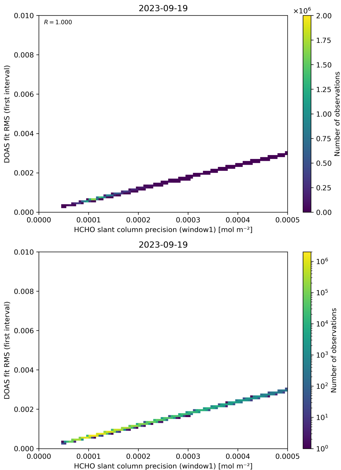
Figure 88: Scatter density plot of “HCHO slant column precision (window1)” against “DOAS fit RMS (first interval)” for 2023-09-18 to 2023-09-20.
