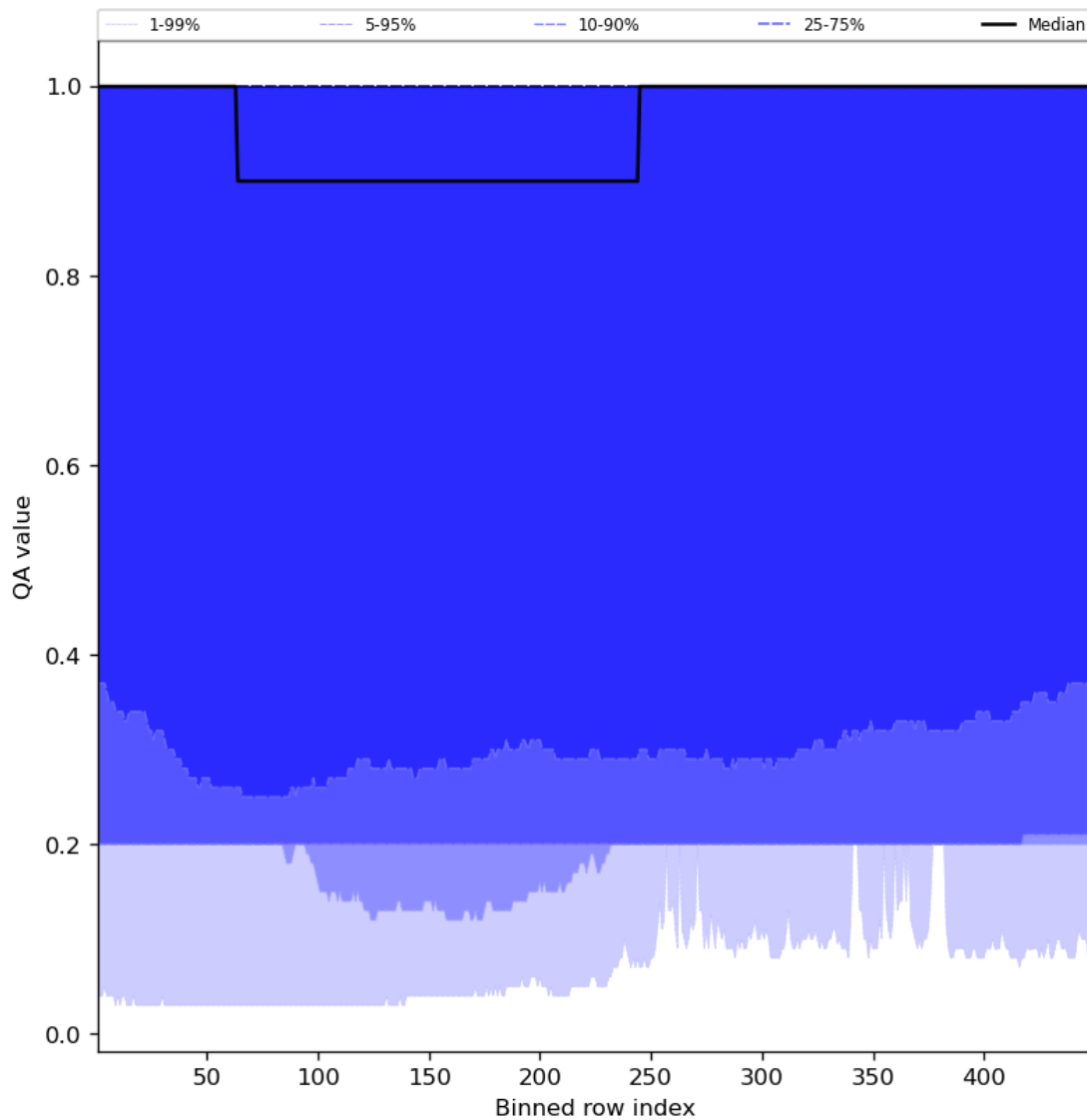
Figure 48: Along track statistics of “QA value” for 2023-09-18 to 2023-09-20
