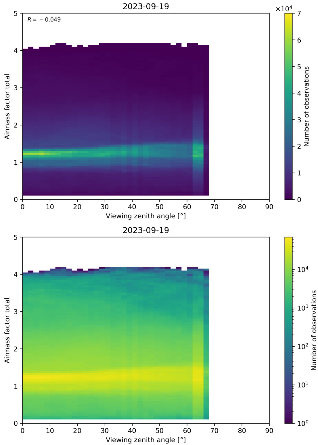
Figure 190: Scatter density plot of “Viewing zenith angle” against “Airmass factor total” for 2023-09-18 to 2023-09-20.
