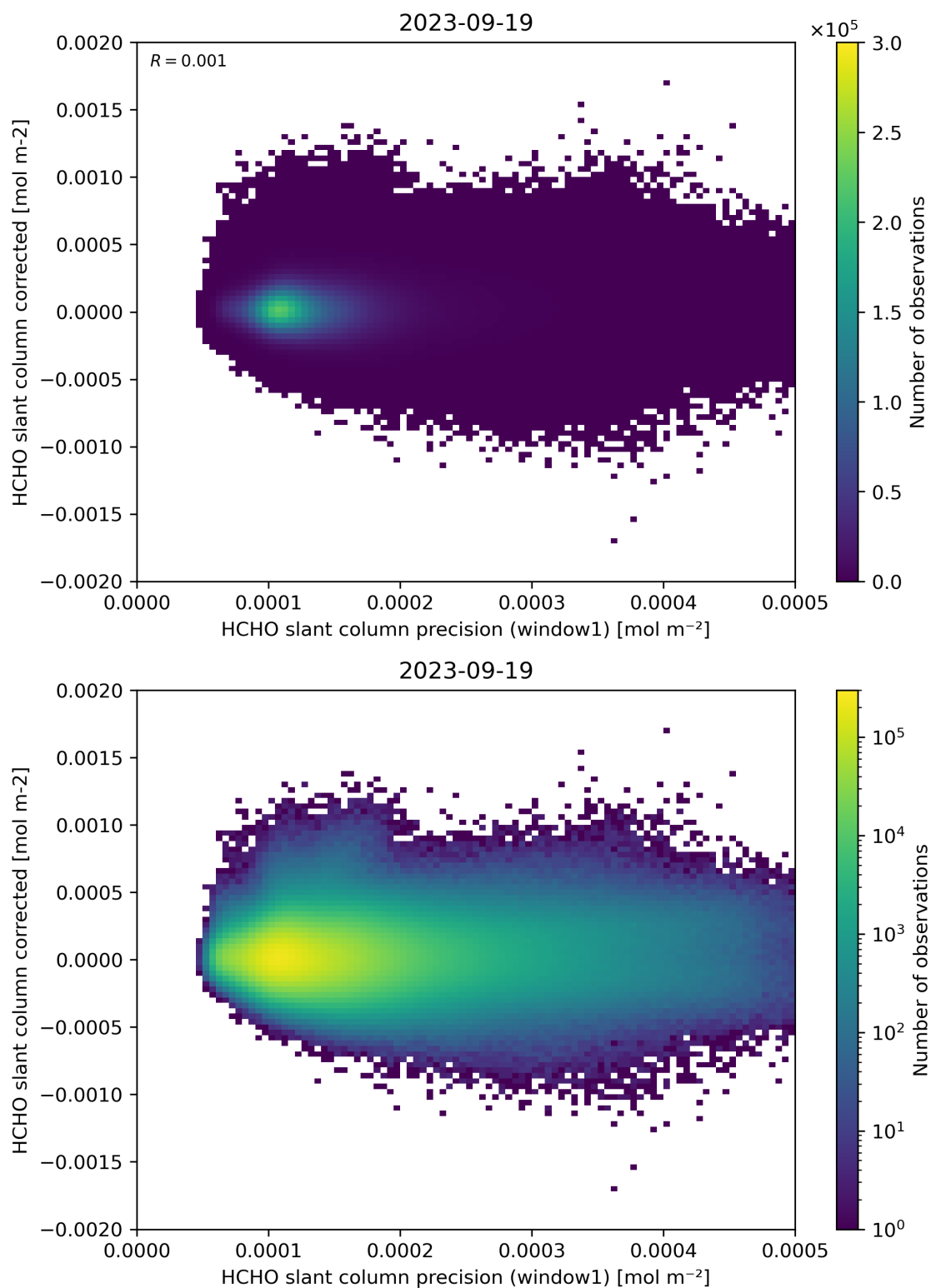
Figure 92: Scatter density plot of “HCHO slant column precision (window1)” against “HCHO slant column corrected” for 2023-09-18 to 2023-09-20.
