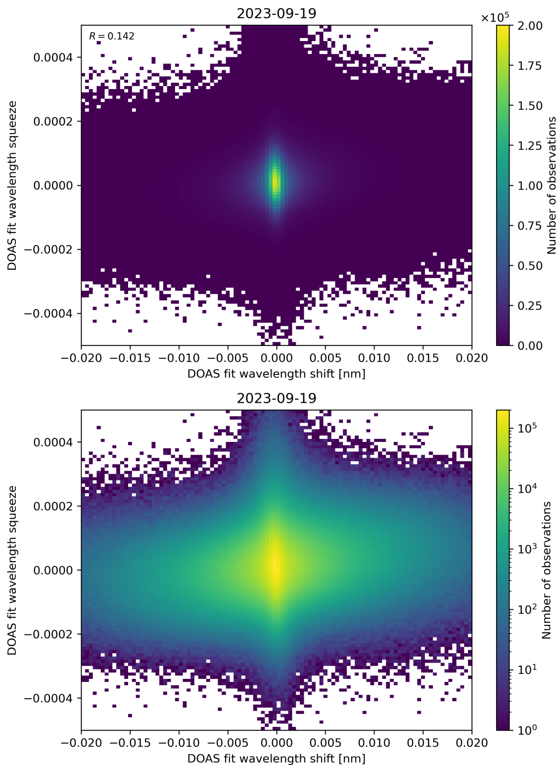
Figure 65: Scatter density plot of “DOAS fit wavelength shift” against “DOAS fit wavelength squeeze” for 2023-09-18 to 2023-09-20.
