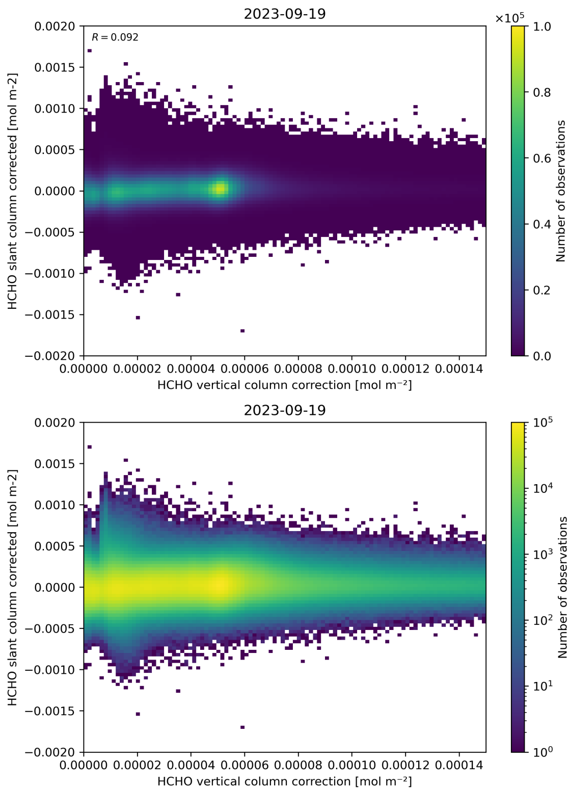
Figure 116: Scatter density plot of “HCHO vertical column correction” against “HCHO slant column corrected” for 2023-09-18 to 2023-09-20.
