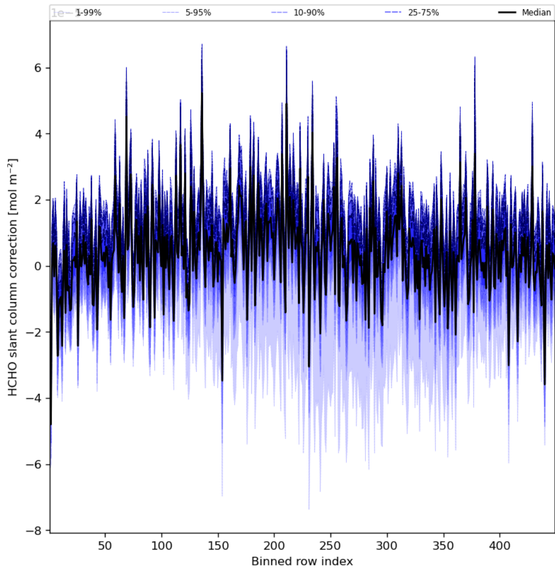
Figure 61: Along track statistics of “HCHO slant column correction” for 2023-09-18 to 2023-09-20
