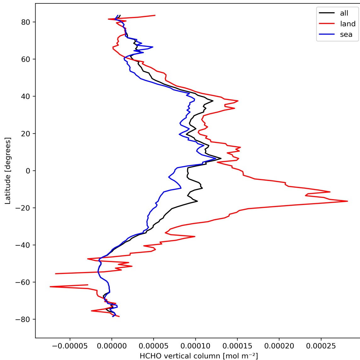
Figure 21: Zonal average of “HCHO vertical column” for 2023-09-18 to 2023-09-20.
