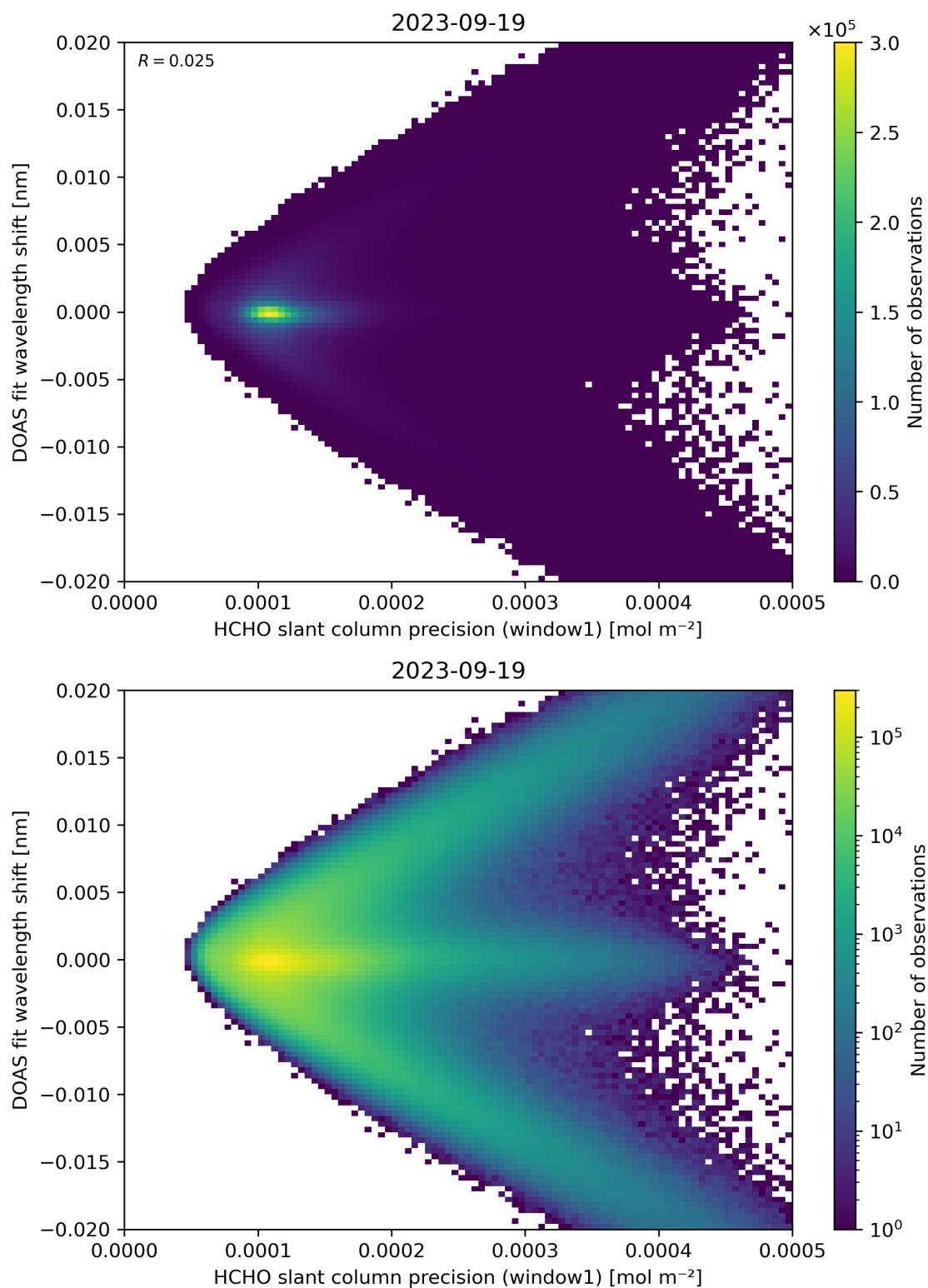
Figure 89: Scatter density plot of “HCHO slant column precision (window1)” against “DOAS fit wavelength shift” for 2023-09-18 to 2023-09-20.
