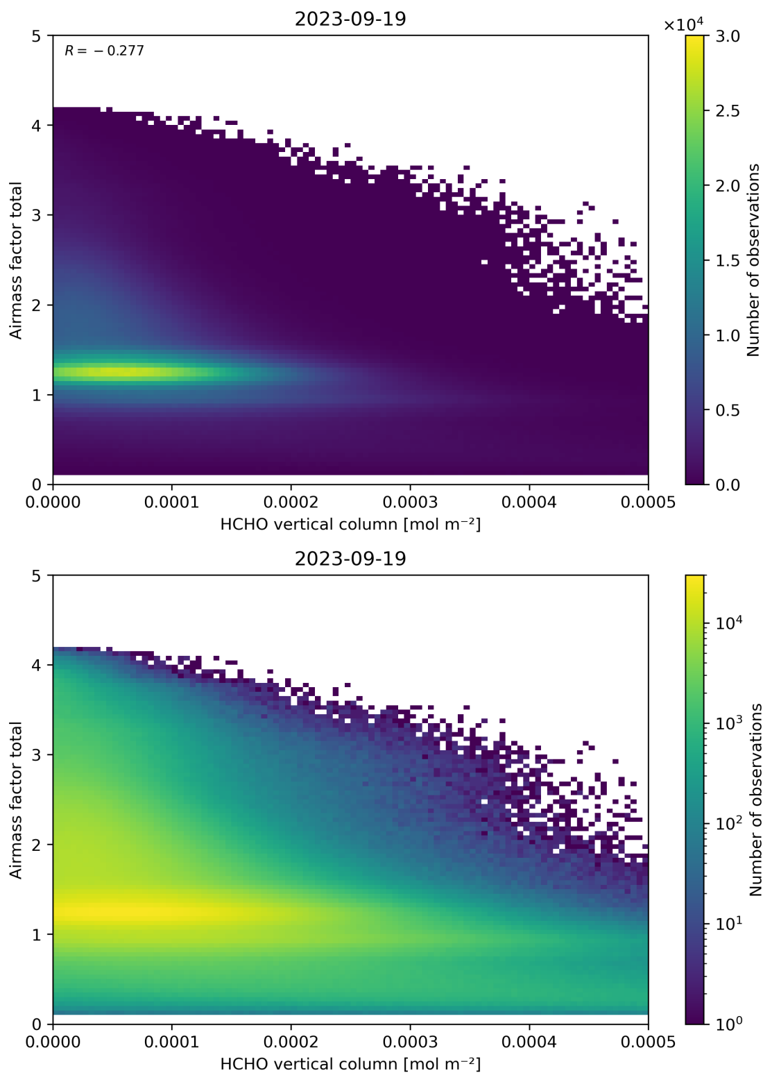
Figure 131: Scatter density plot of “HCHO vertical column” against “Airmass factor total” for 2023-09-18 to 2023-09-20.
