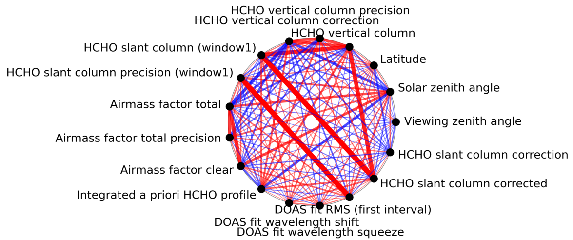
Figure 1: Map of correlation graph for 2023-09-18 to 2023-09-20.
