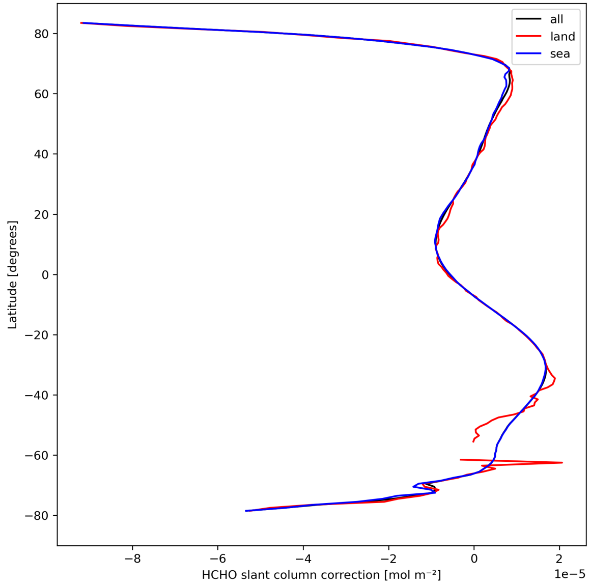
Figure 33: Zonal average of “HCHO slant column correction” for 2023-09-18 to 2023-09-20.
