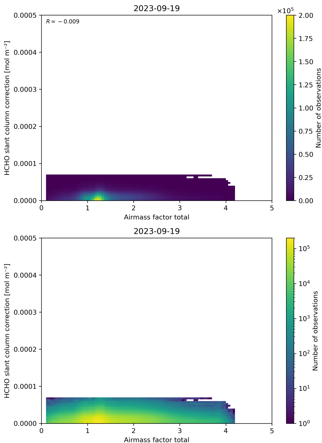
Figure 102: Scatter density plot of “Airmass factor total” against “HCHO slant column correction” for 2023-09-18 to 2023-09-20.
