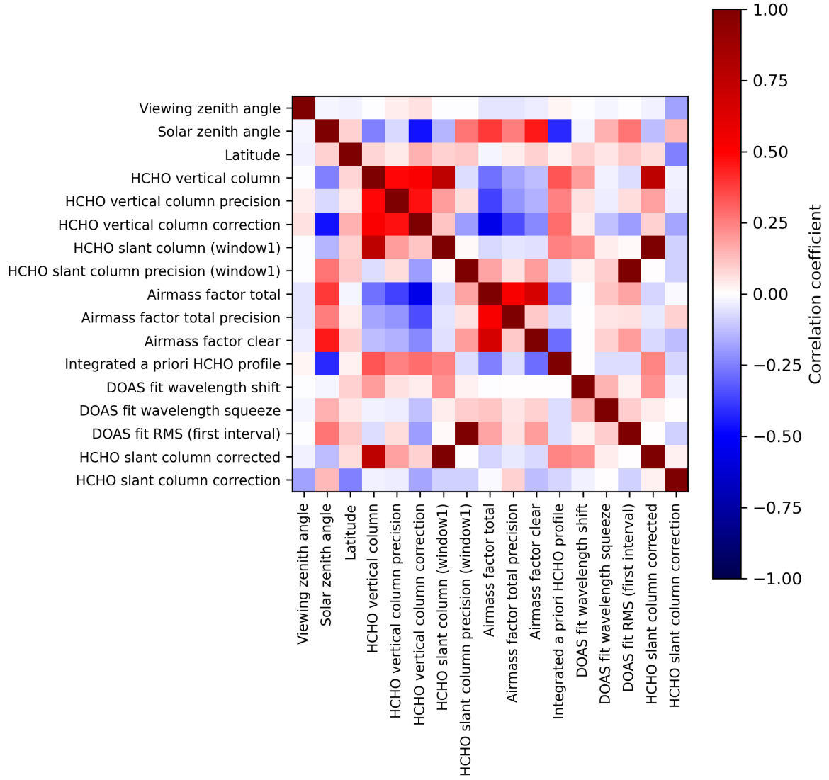
Figure 2: Map of correlation matrix for 2023-09-18 to 2023-09-20.
