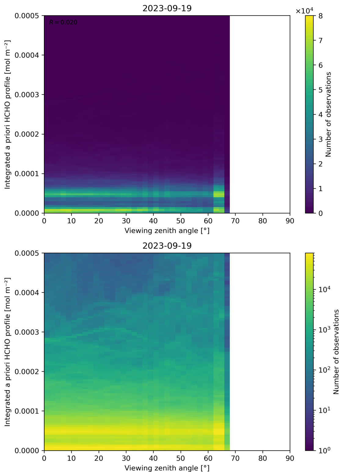
Figure 195: Scatter density plot of “Viewing zenith angle” against “Integrated a priori HCHO profile” for 2023-09-18 to 2023-09-20.
