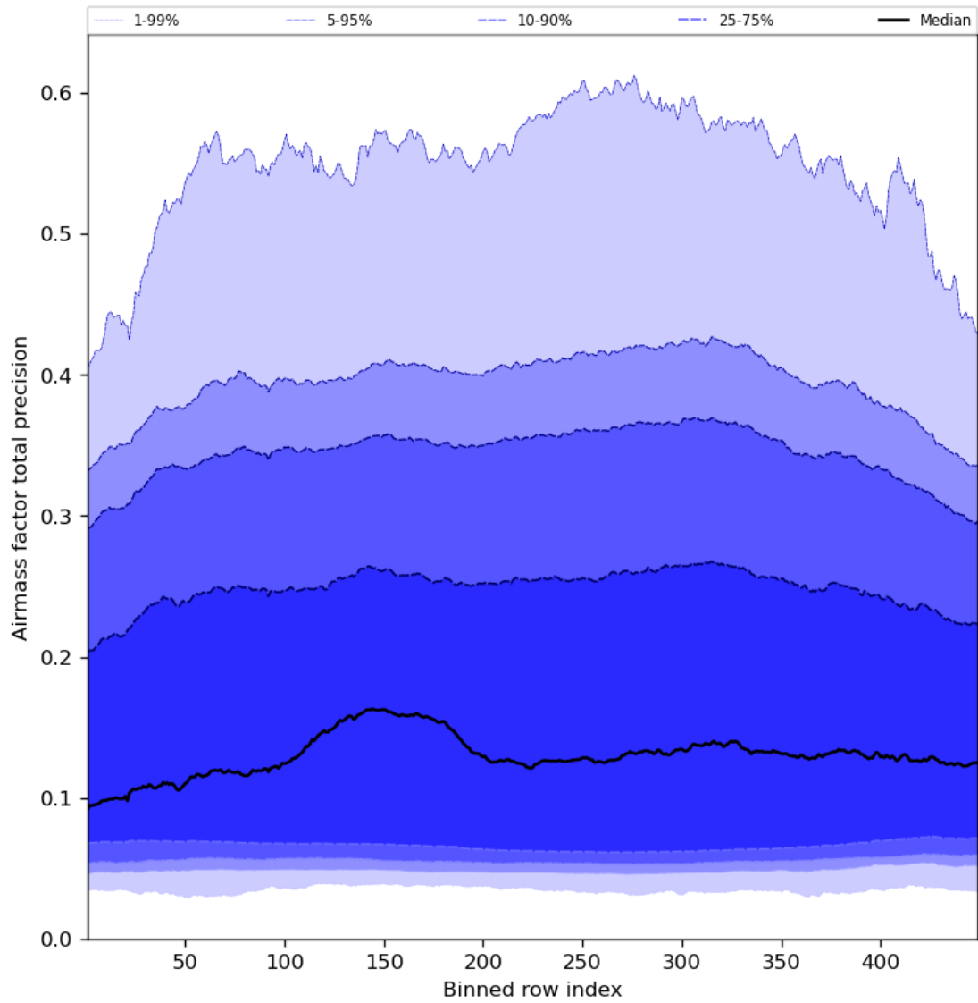
Figure 55: Along track statistics of “Airmass factor total precision” for 2023-09-18 to 2023-09-20
