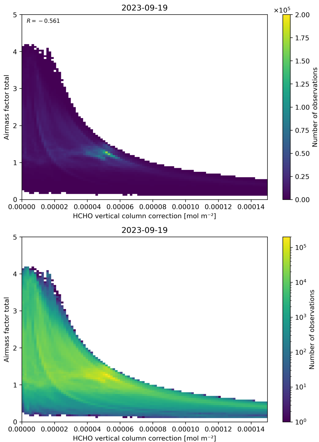
Figure 120: Scatter density plot of “HCHO vertical column correction” against “Airmass factor total” for 2023-09-18 to 2023-09-20.
