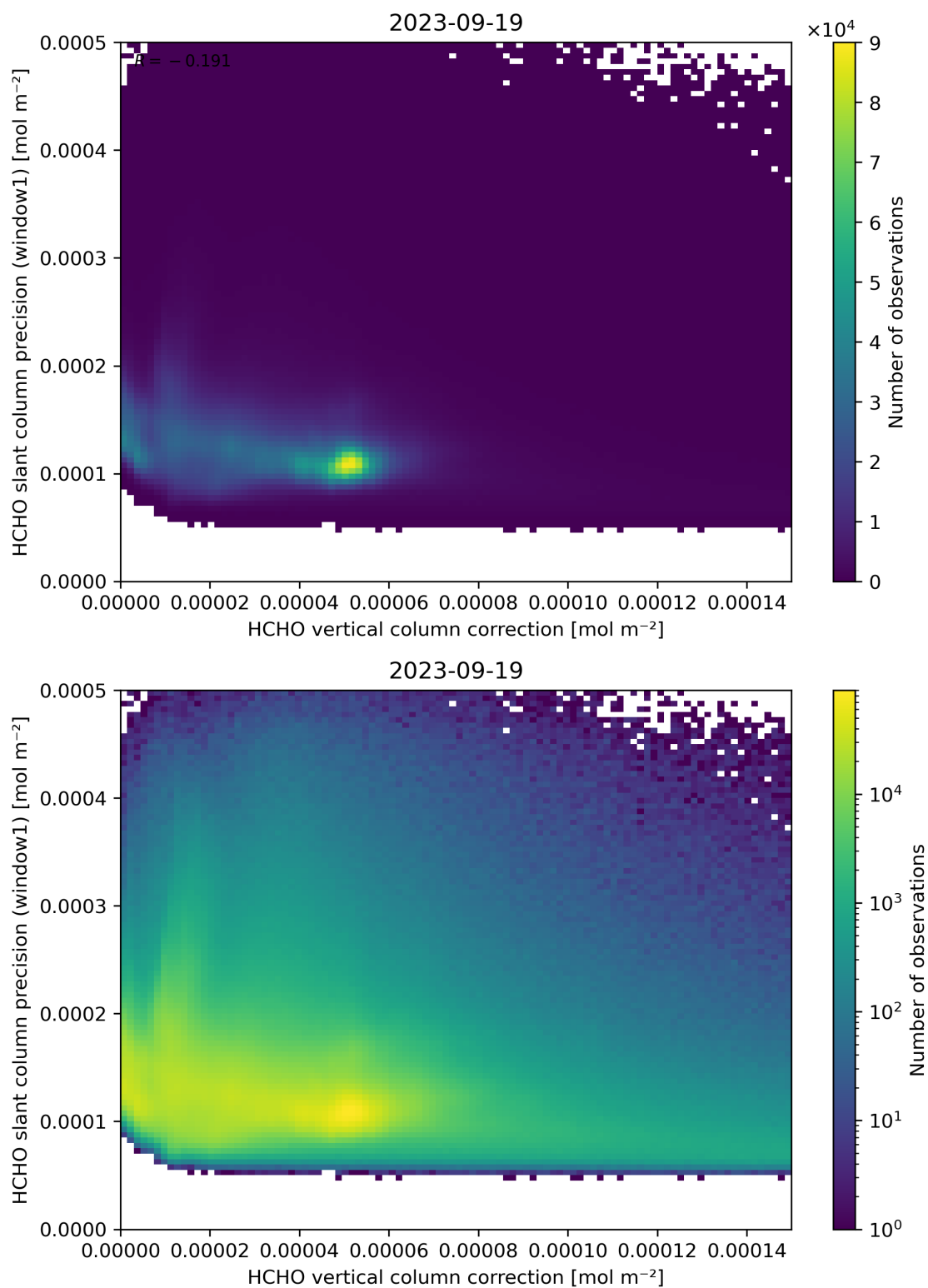
Figure 119: Scatter density plot of “HCHO vertical column correction” against “HCHO slant column precision (window1)” for 2023-09-18 to 2023-09-20.
