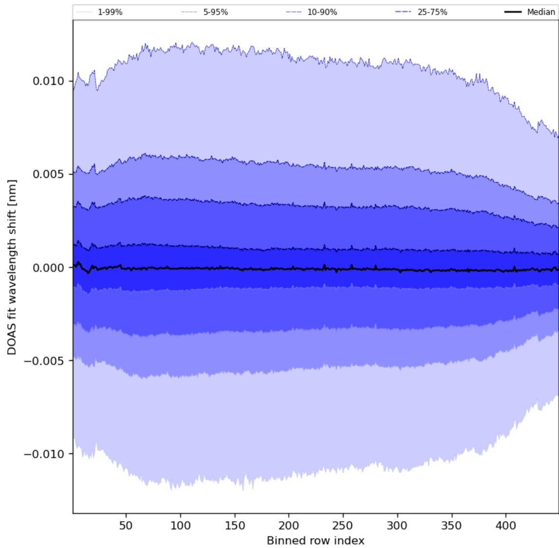
Figure 58: Along track statistics of “DOAS fit wavelength shift” for 2023-09-18 to 2023-09-20
