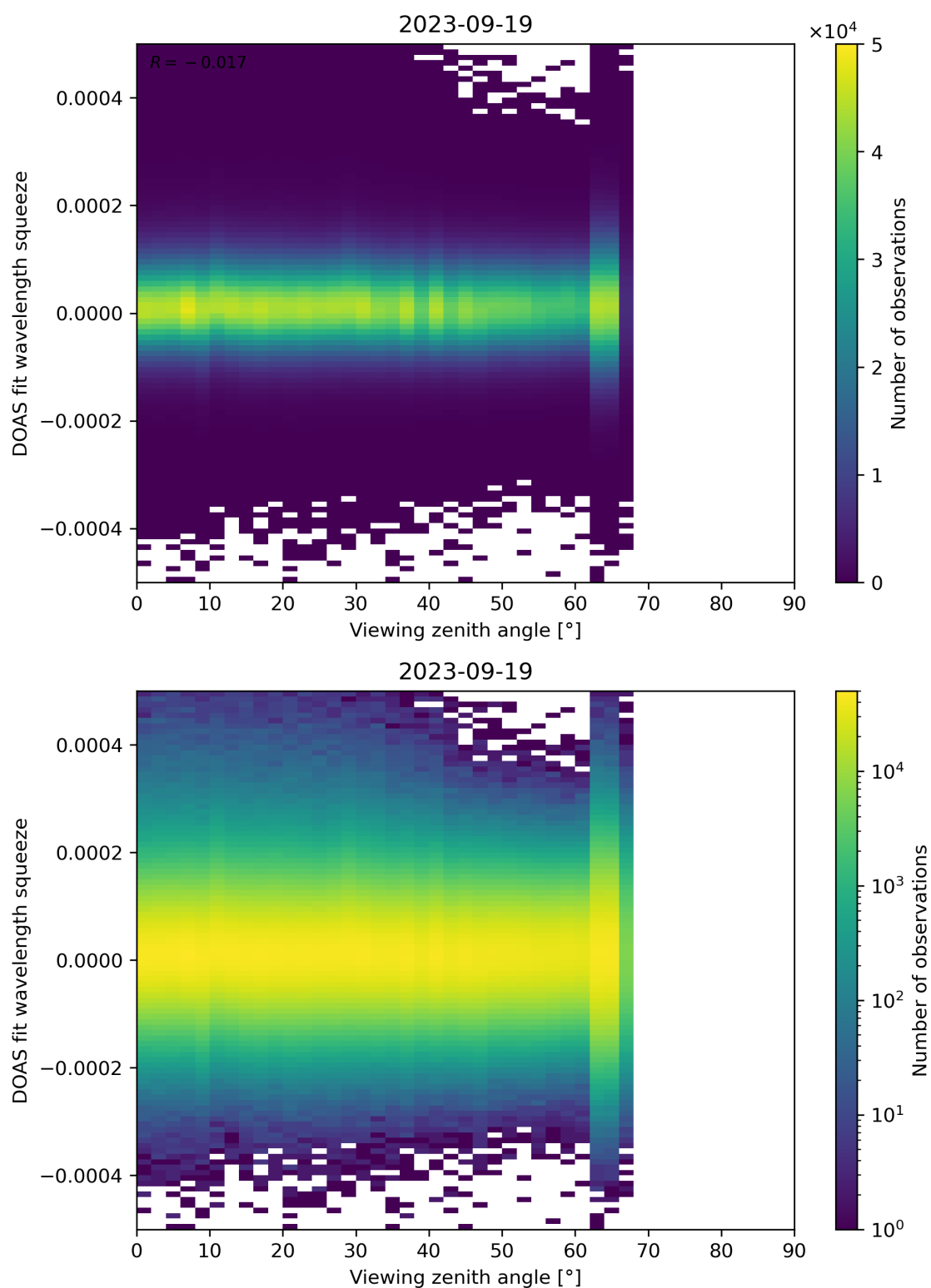
Figure 184: Scatter density plot of “Viewing zenith angle” against “DOAS fit wavelength squeeze” for 2023-09-18 to 2023-09-20.
