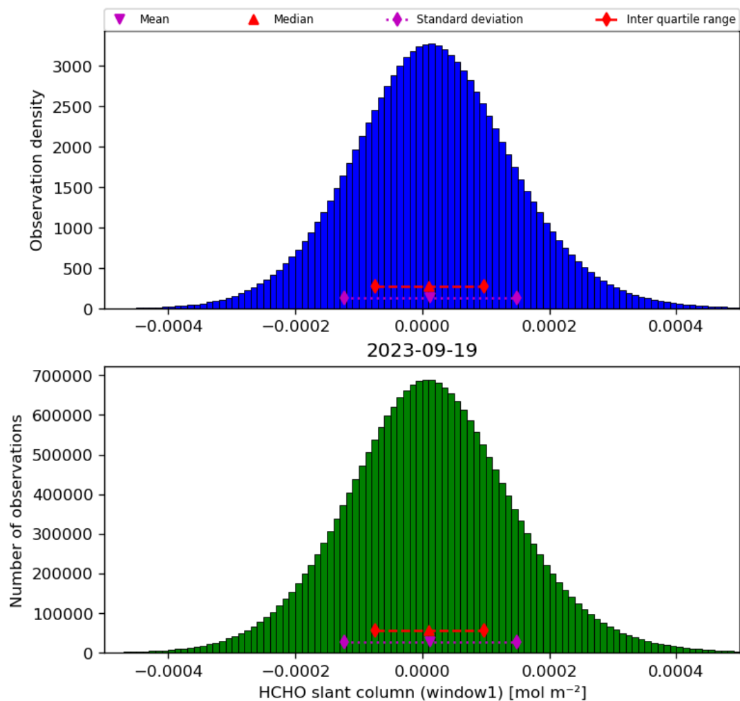
Figure 38: Histogram of “HCHO slant column (window1)” for 2023-09-18 to 2023-09-20
