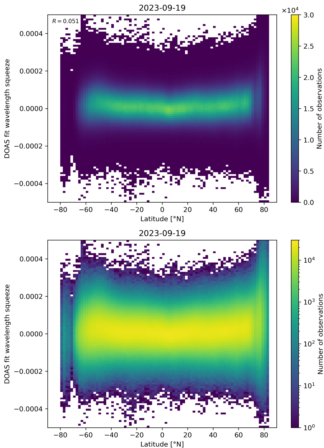
Figure 155: Scatter density plot of “Latitude” against “DOAS fit wavelength squeeze” for 2023-09-18 to 2023-09-20.
