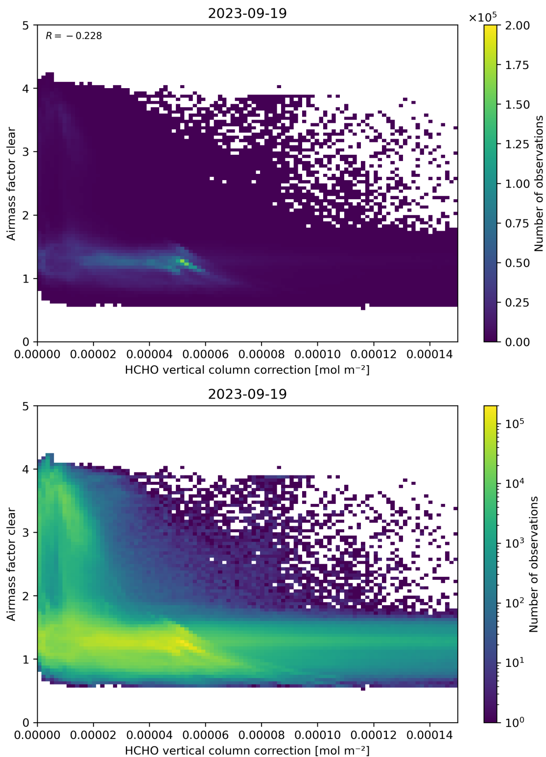
Figure 115: Scatter density plot of “HCHO vertical column correction” against “Airmass factor clear” for 2023-09-18 to 2023-09-20.
