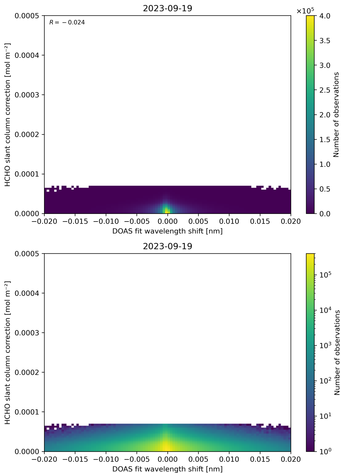
Figure 67: Scatter density plot of “DOAS fit wavelength shift” against “HCHO slant column correction” for 2023-09-18 to 2023-09-20.
