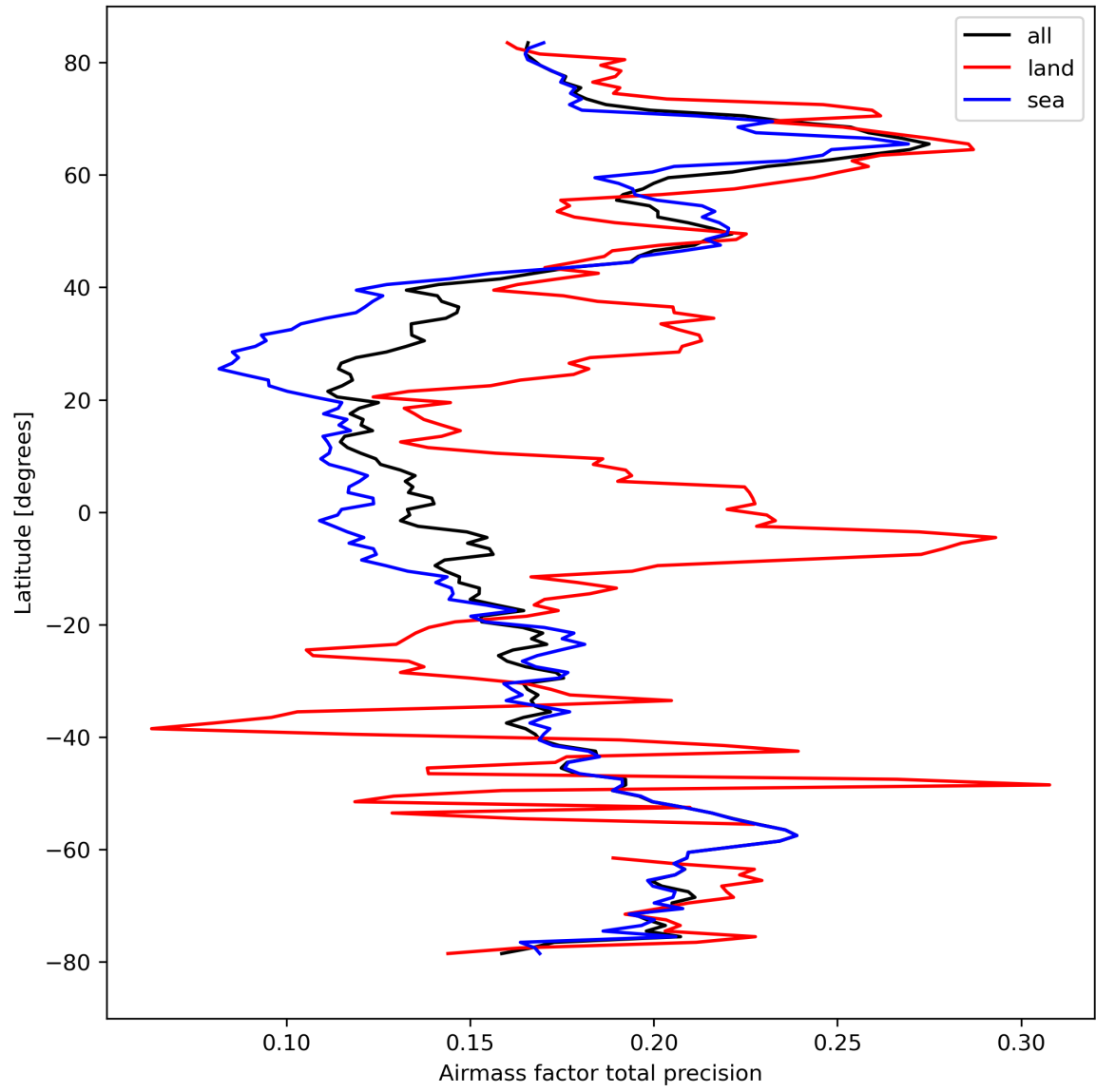
Figure 27: Zonal average of “Airmass factor total precision” for 2023-09-18 to 2023-09-20.
