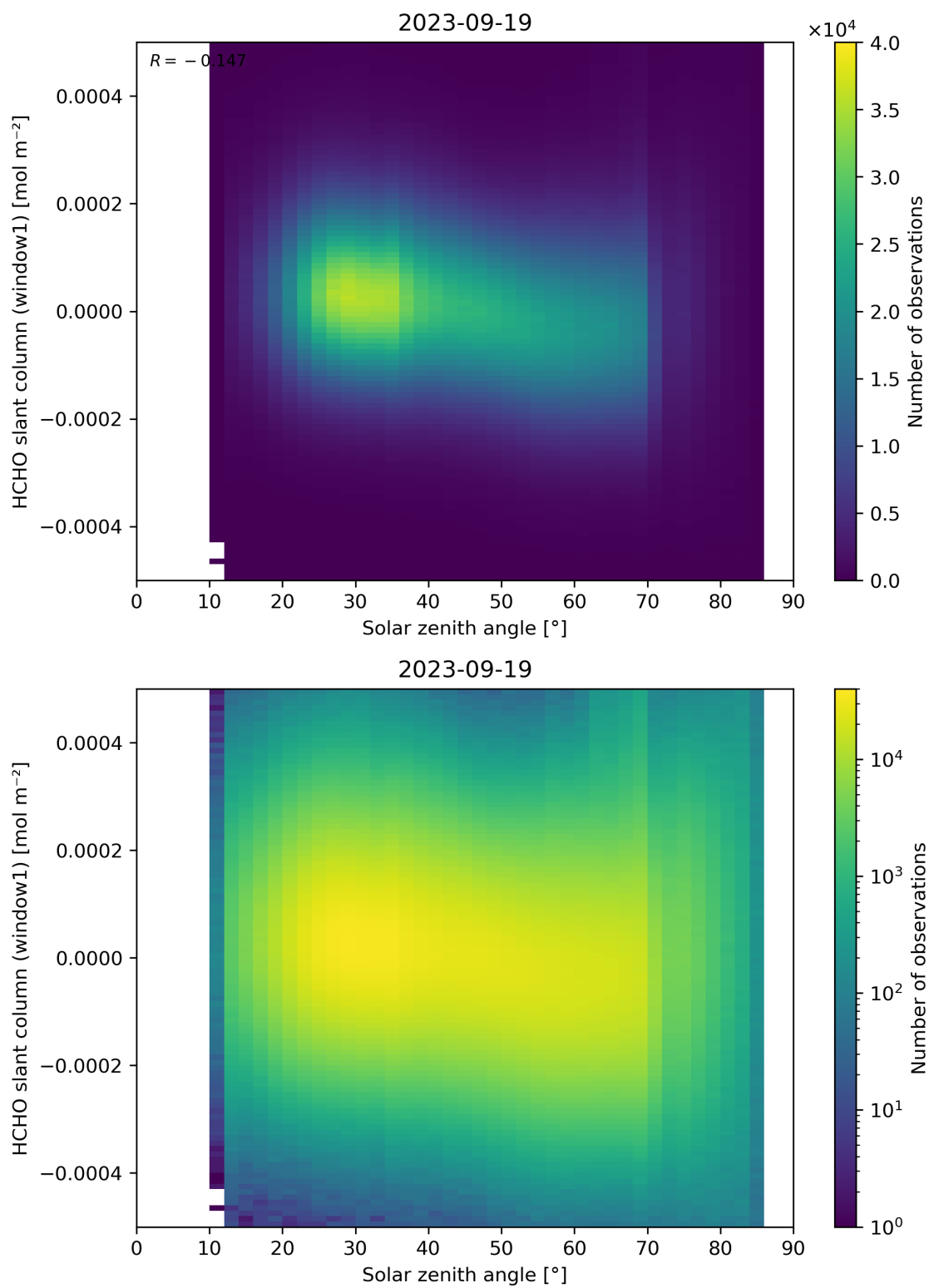
Figure 173: Scatter density plot of “Solar zenith angle” against “HCHO slant column (window1)” for 2023-09-18 to 2023-09-20.
