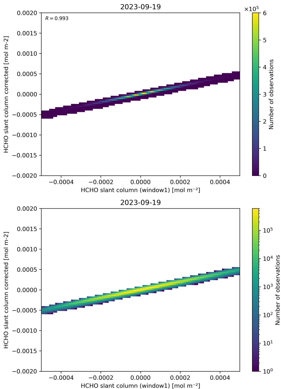
Figure 82: Scatter density plot of “HCHO slant column (window1)” against “HCHO slant column corrected” for 2023-09-18 to 2023-09-20.
