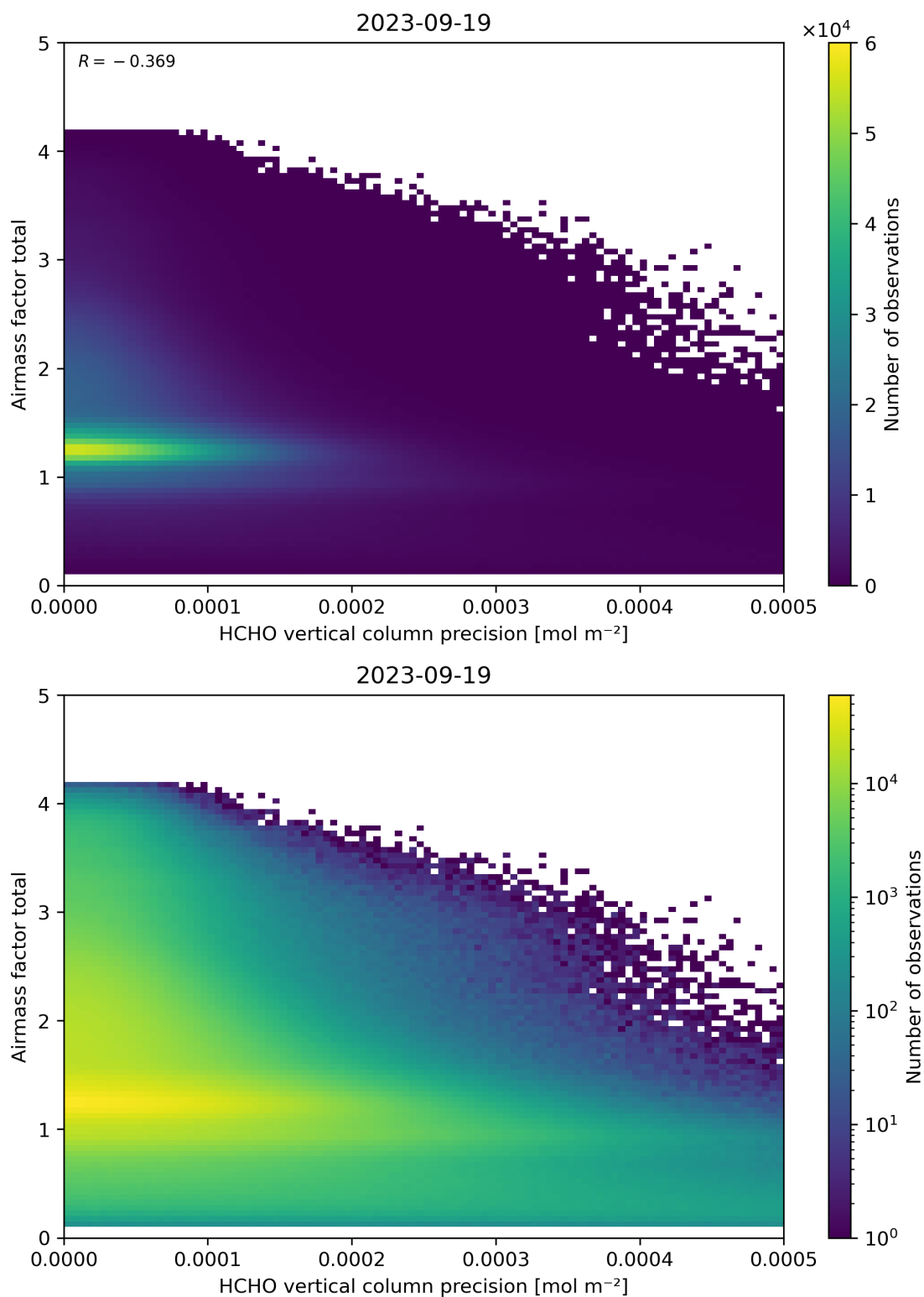
Figure 144: Scatter density plot of “HCHO vertical column precision” against “Airmass factor total” for 2023-09-18 to 2023-09-20.
