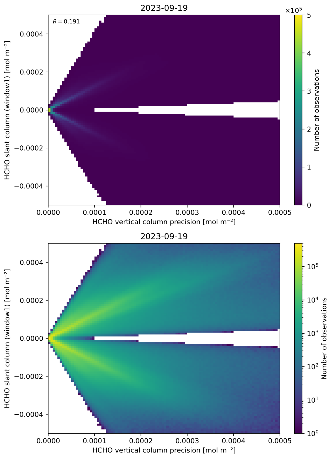
Figure 142: Scatter density plot of “HCHO vertical column precision” against “HCHO slant column (window1)” for 2023-09-18 to 2023-09-20.
