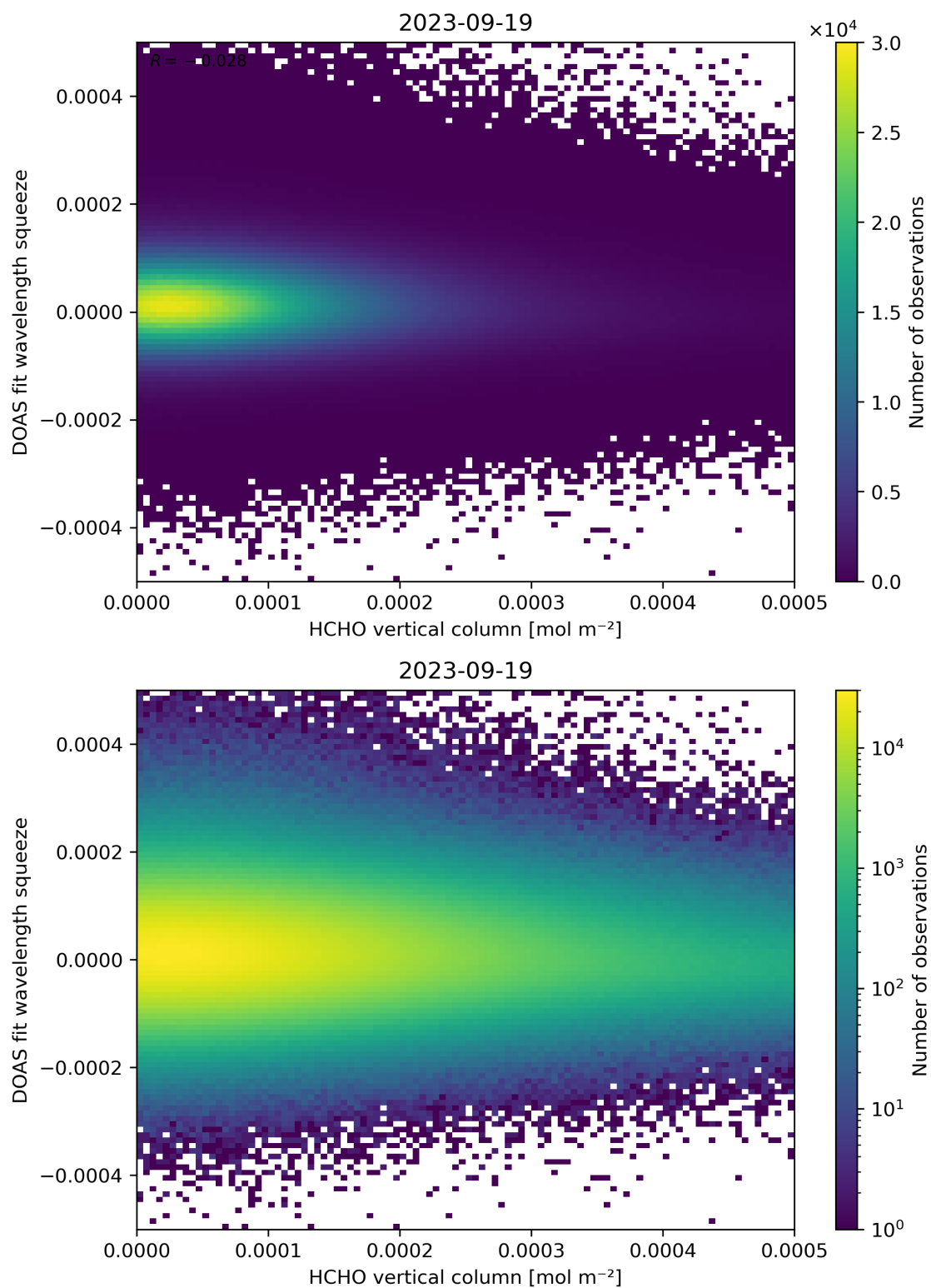
Figure 125: Scatter density plot of “HCHO vertical column” against “DOAS fit wavelength squeeze” for 2023-09-18 to 2023-09-20.
