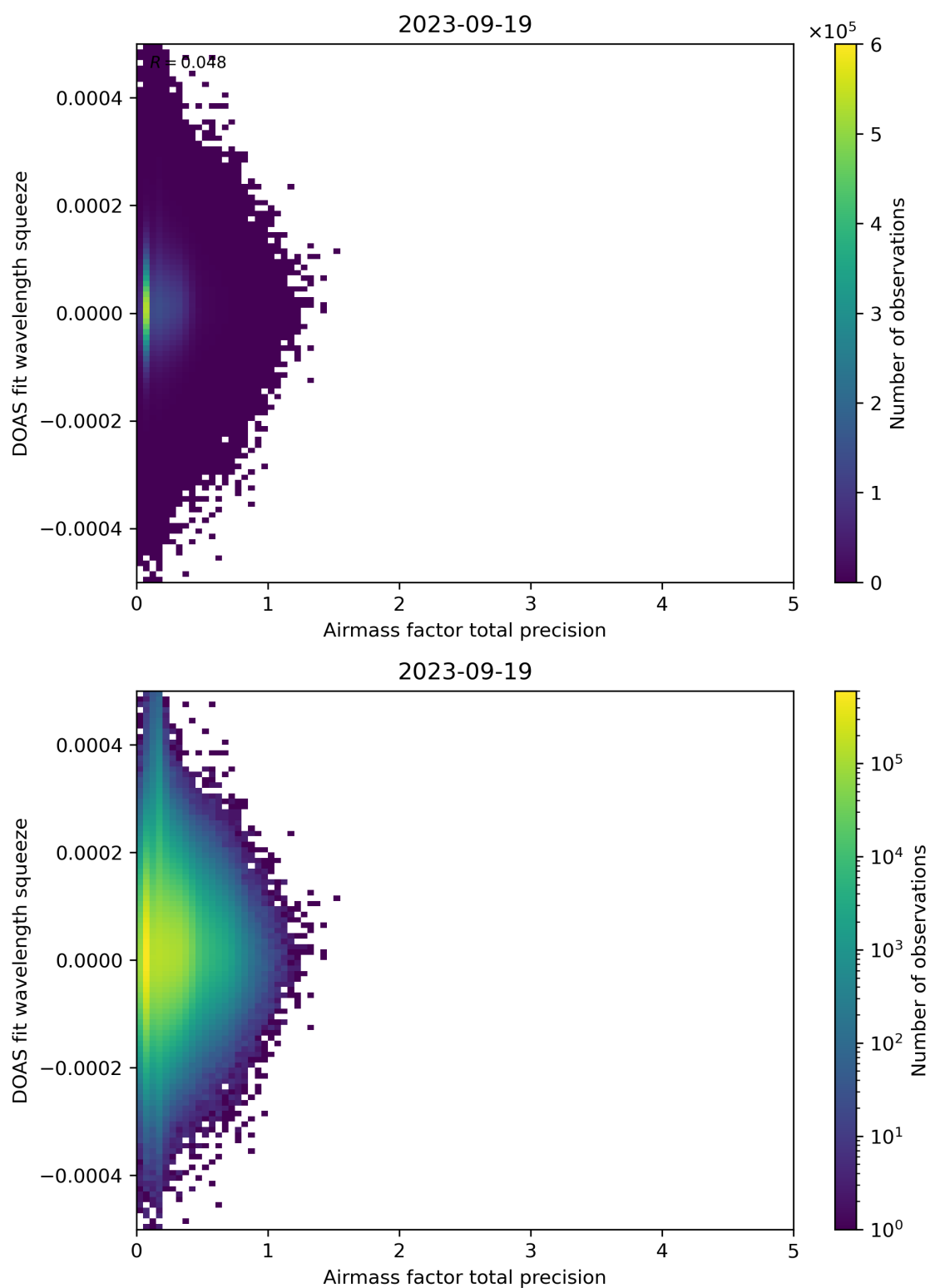
Figure 107: Scatter density plot of “Airmass factor total precision” against “DOAS fit wavelength squeeze” for 2023-09-18 to 2023-09-20.
