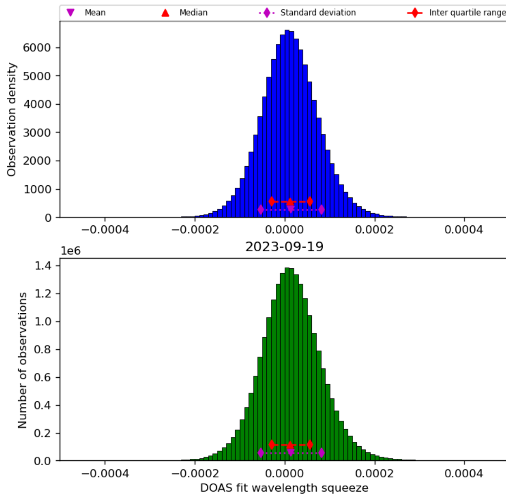
Figure 45: Histogram of “DOAS fit wavelength squeeze” for 2023-09-18 to 2023-09-20
