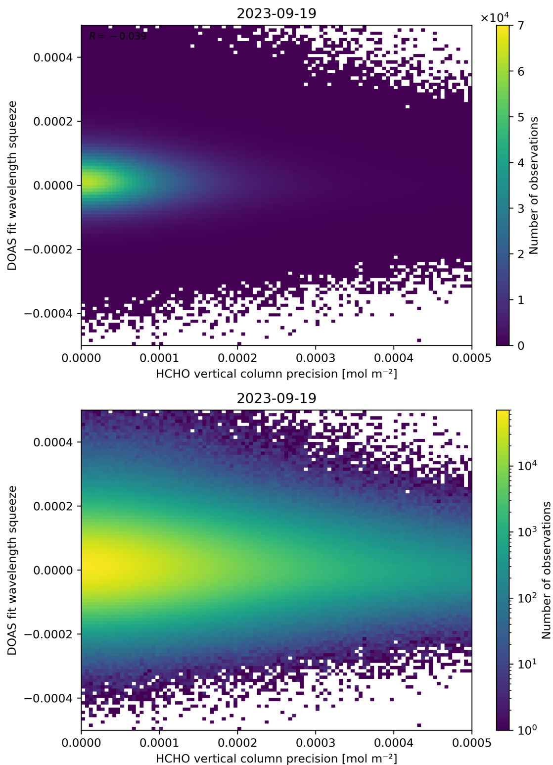
Figure 138: Scatter density plot of “HCHO vertical column precision” against “DOAS fit wavelength squeeze” for 2023-09-18 to 2023-09-20.
