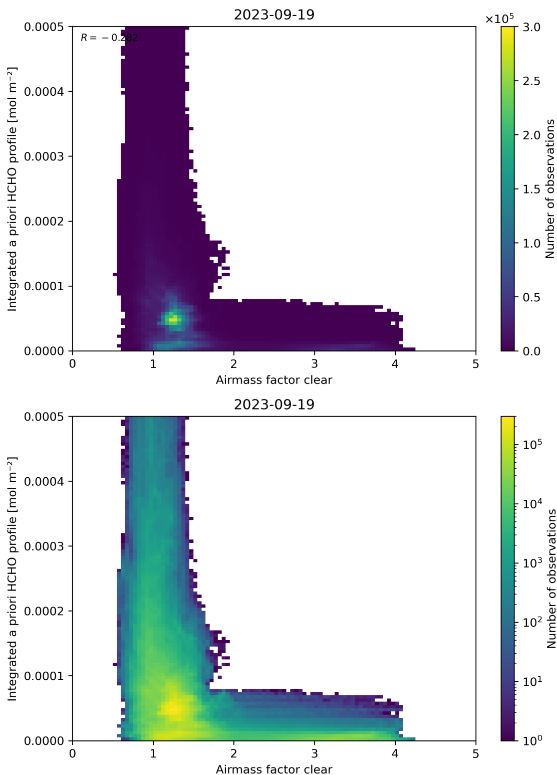
Figure 76: Scatter density plot of “Airmass factor clear” against “Integrated a priori HCHO profile” for 2023-09-18 to 2023-09-20.
