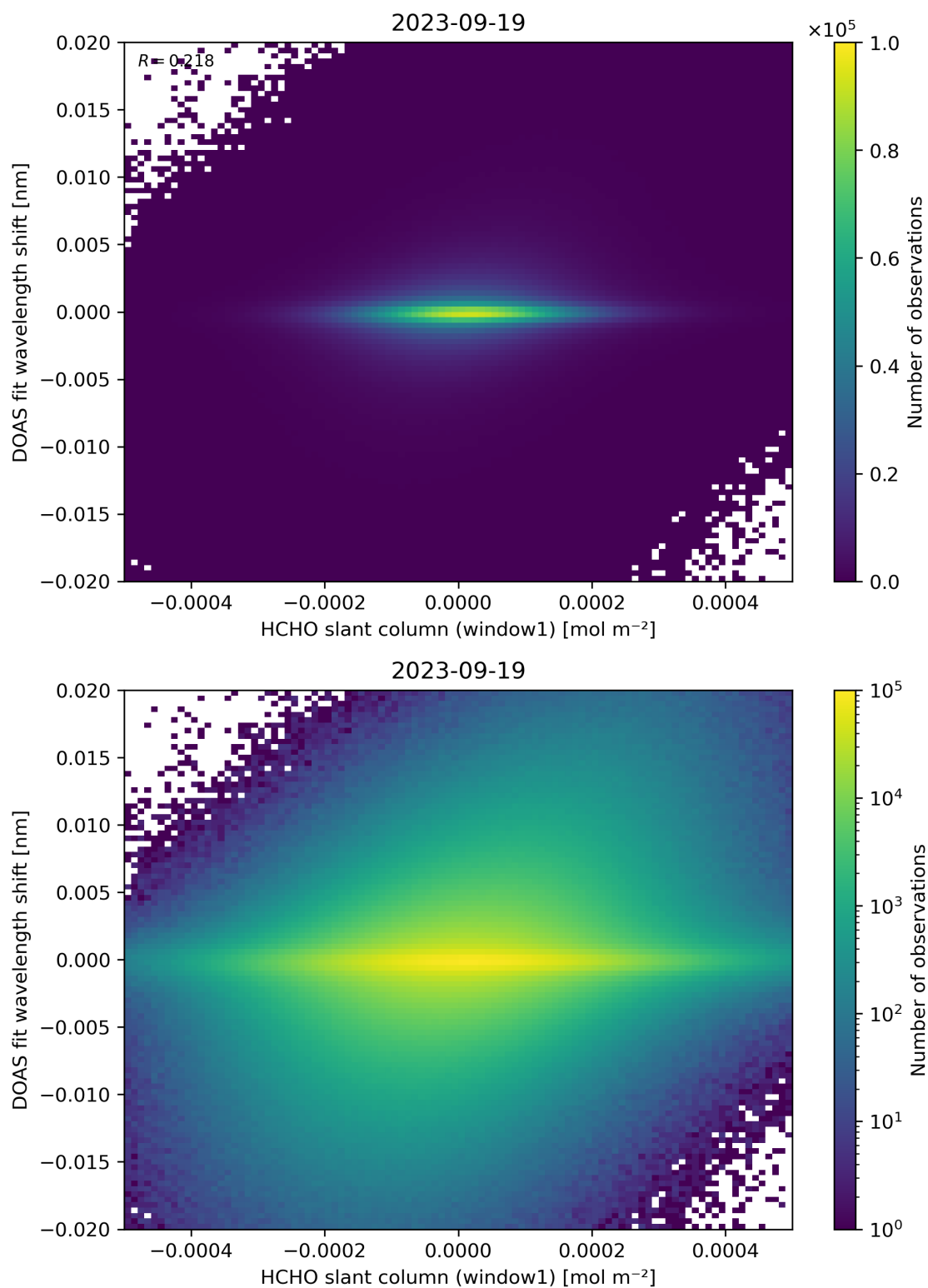
Figure 79: Scatter density plot of “HCHO slant column (window1)” against “DOAS fit wavelength shift” for 2023-09-18 to 2023-09-20.
