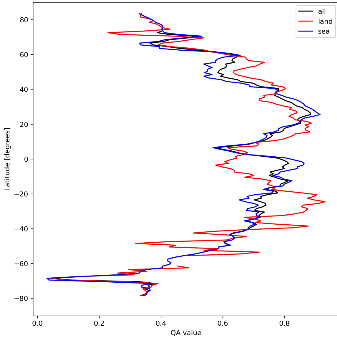
Figure 20: Zonal average of “QA value” for 2023-09-18 to 2023-09-20.
