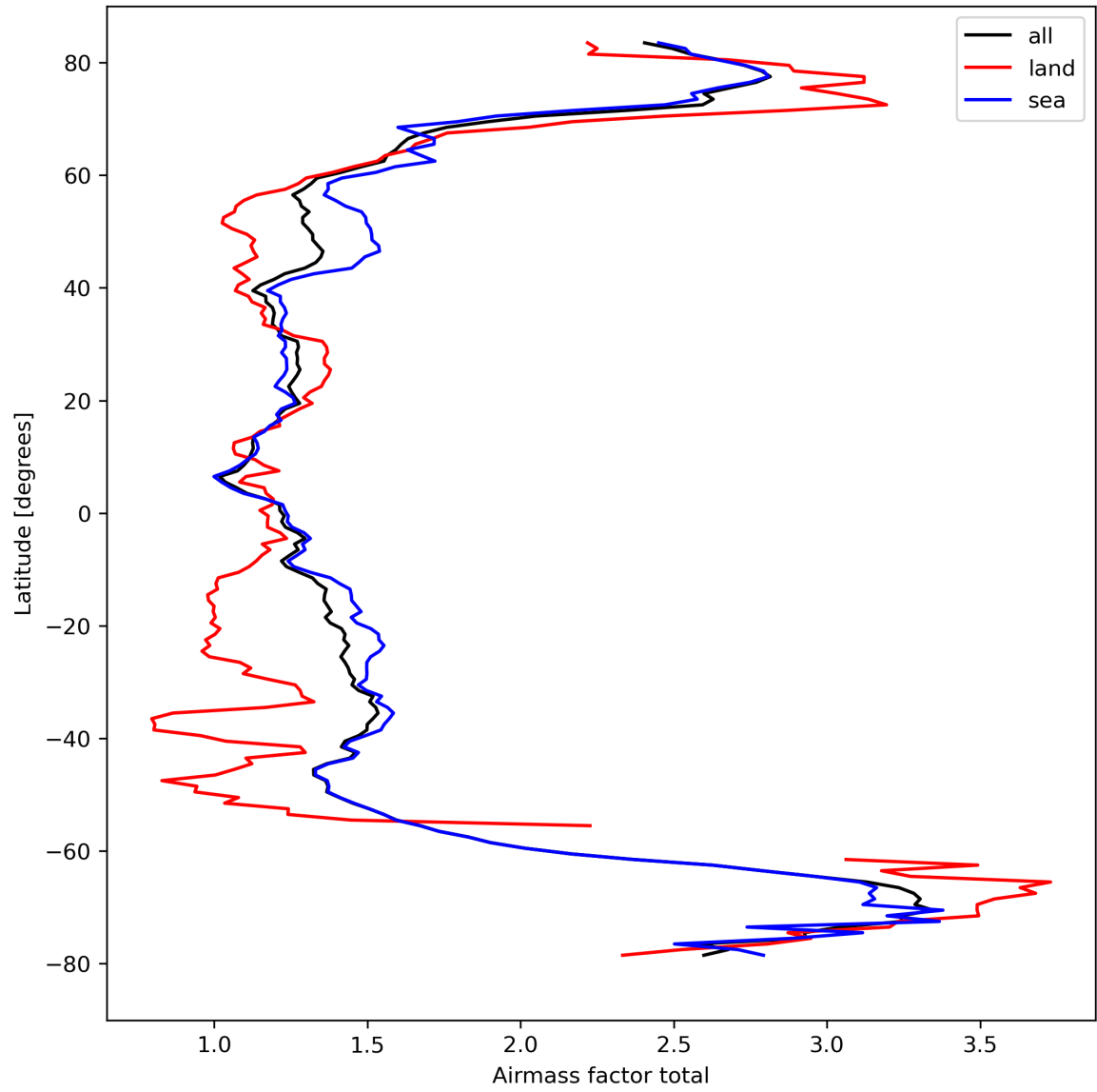
Figure 26: Zonal average of “Airmass factor total” for 2023-09-18 to 2023-09-20.
