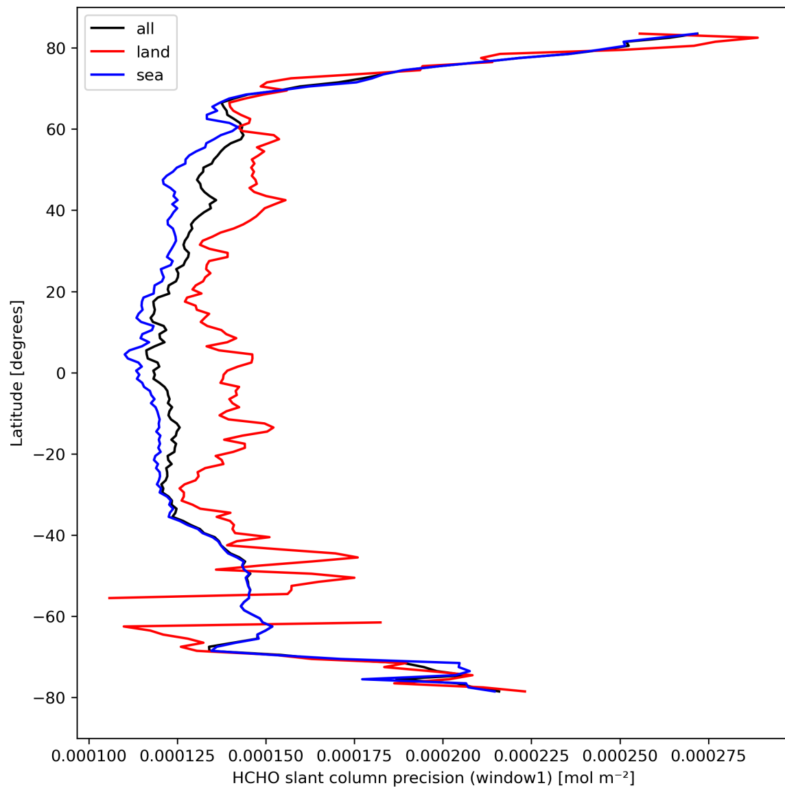
Figure 25: Zonal average of “HCHO slant column precision (window1)” for 2023-09-18 to 2023-09-20.
