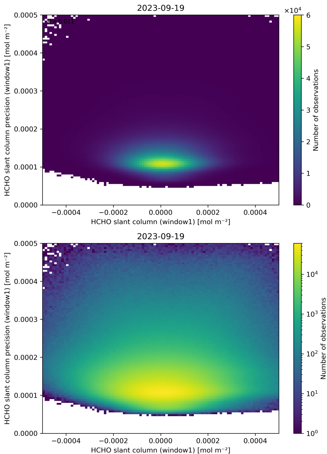
Figure 84: Scatter density plot of “HCHO slant column (window1)” against “HCHO slant column precision (window1)” for 2023-09-18 to 2023-09-20.
