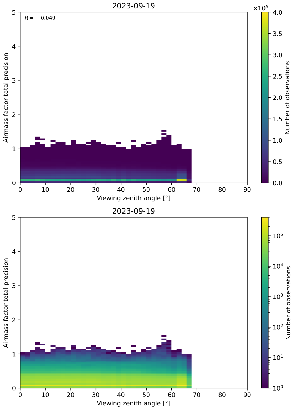
Figure 191: Scatter density plot of “Viewing zenith angle” against “Airmass factor total precision” for 2023-09-18 to 2023-09-20.
