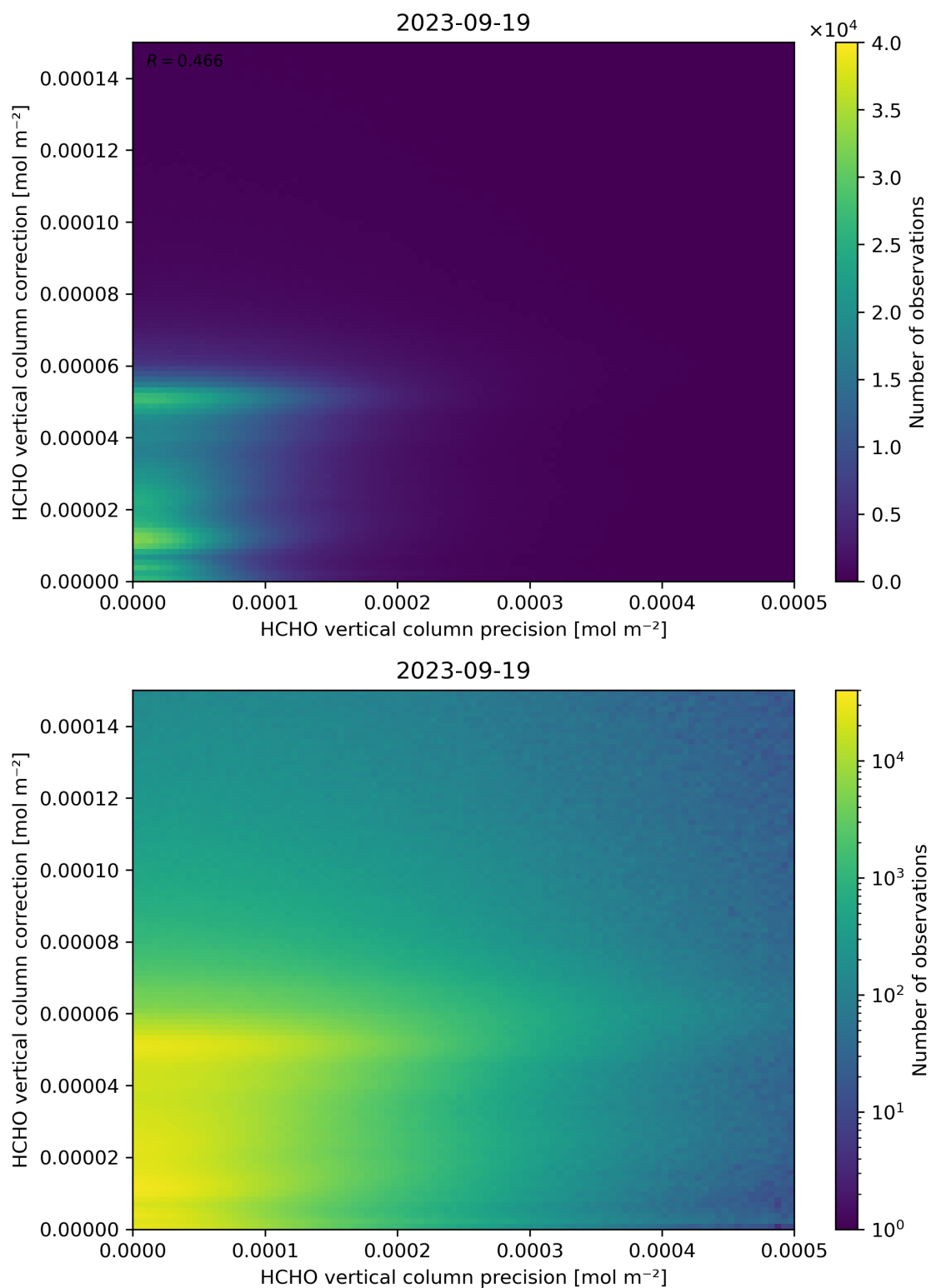
Figure 146: Scatter density plot of “HCHO vertical column precision” against “HCHO vertical column correction” for 2023-09-18 to 2023-09-20.
