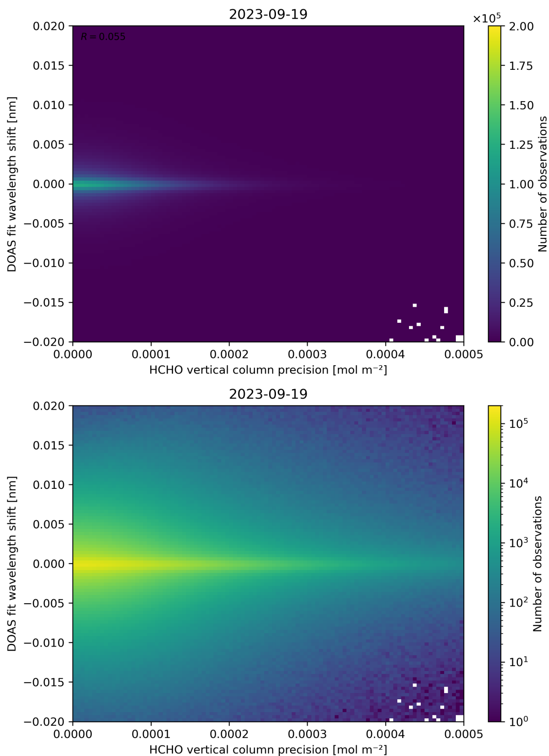
Figure 137: Scatter density plot of “HCHO vertical column precision” against “DOAS fit wavelength shift” for 2023-09-18 to 2023-09-20.
