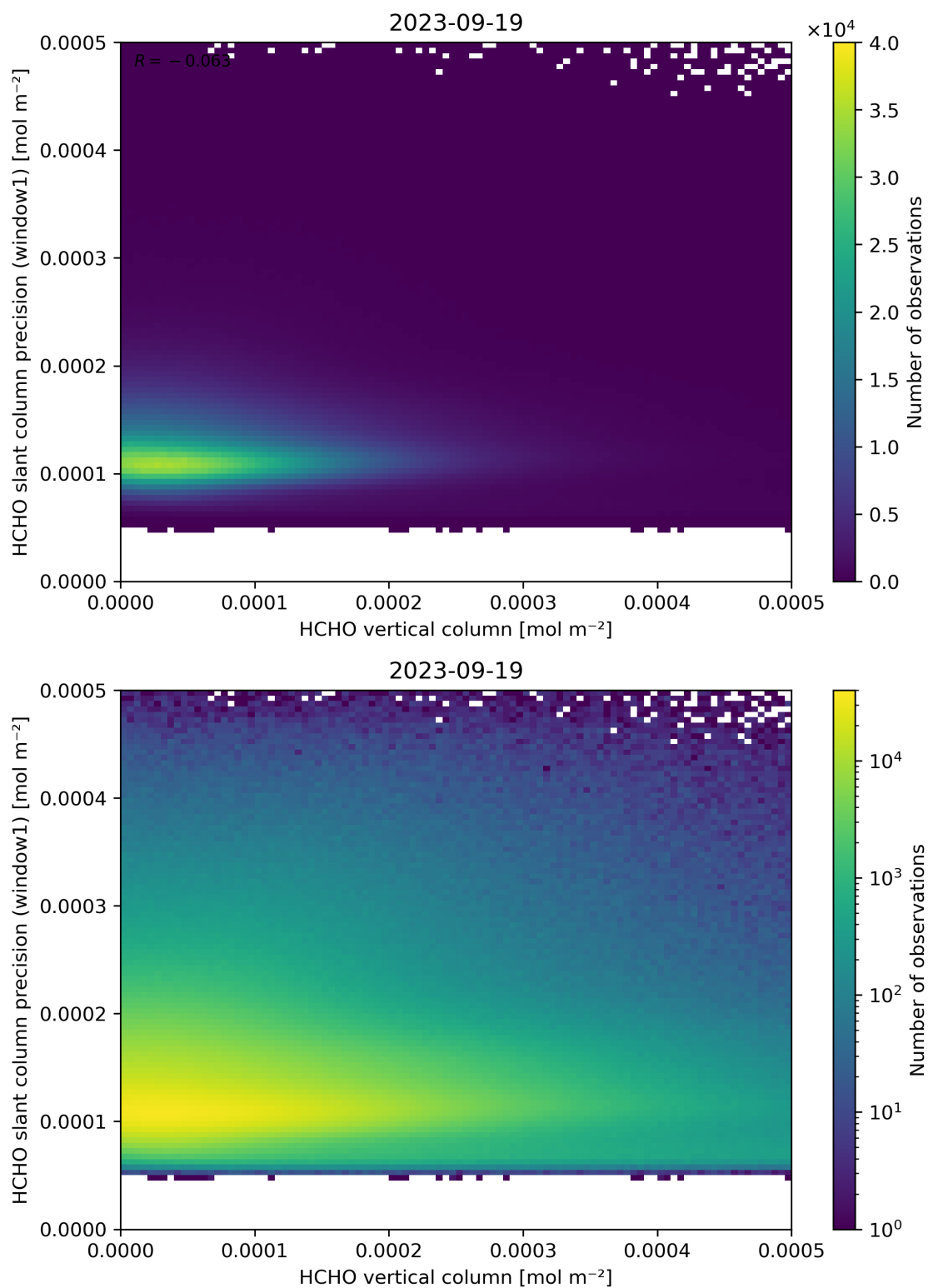
Figure 130: Scatter density plot of “HCHO vertical column” against “HCHO slant column precision (window1)” for 2023-09-18 to 2023-09-20.
