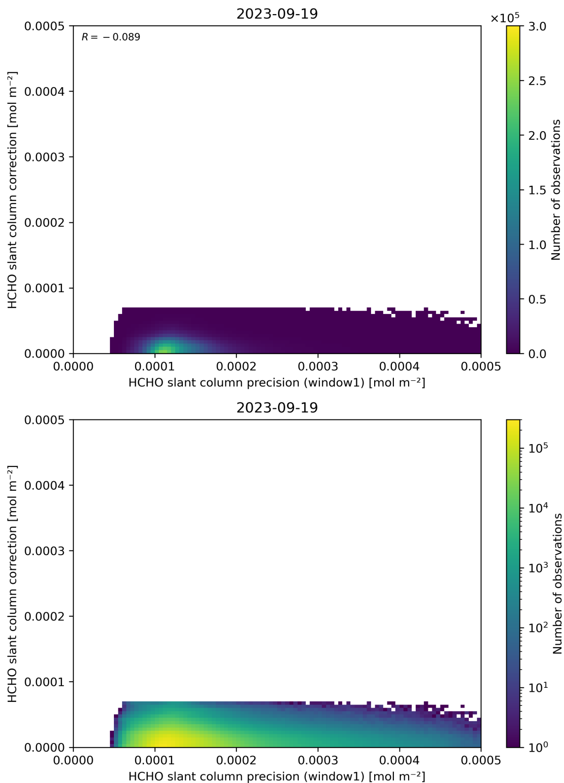
Figure 93: Scatter density plot of “HCHO slant column precision (window1)” against “HCHO slant column correction” for 2023-09-18 to 2023-09-20.
