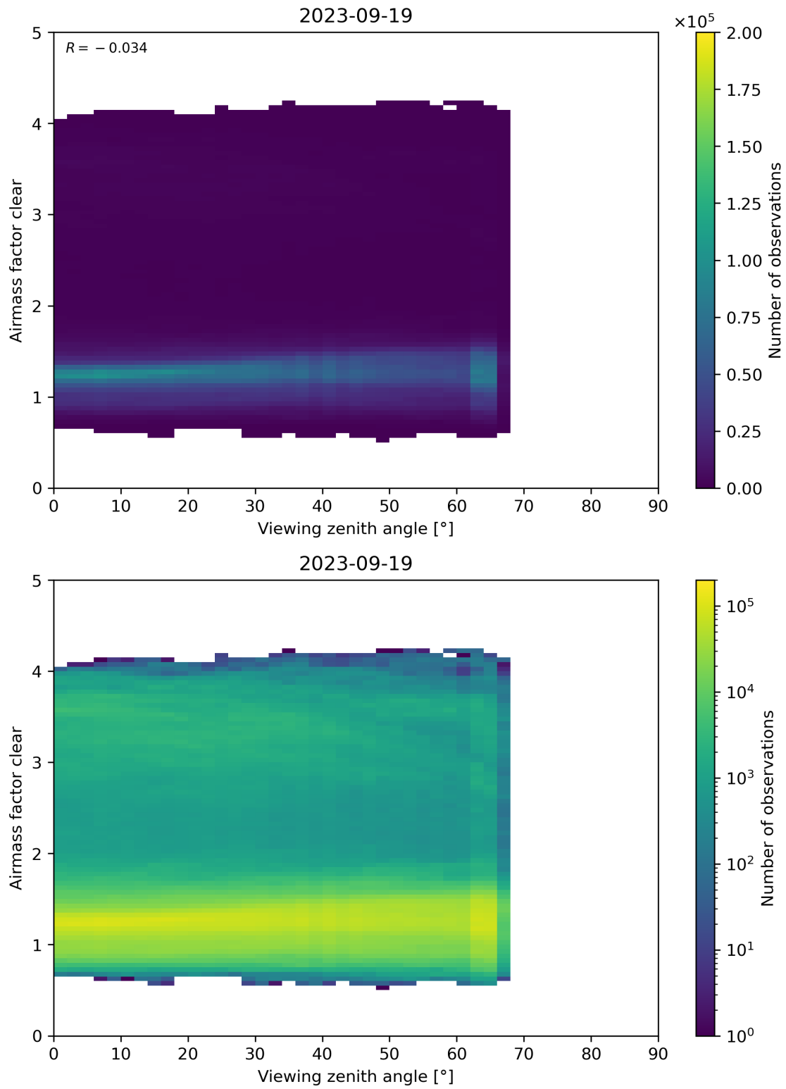
Figure 185: Scatter density plot of “Viewing zenith angle” against “Airmass factor clear” for 2023-09-18 to 2023-09-20.
