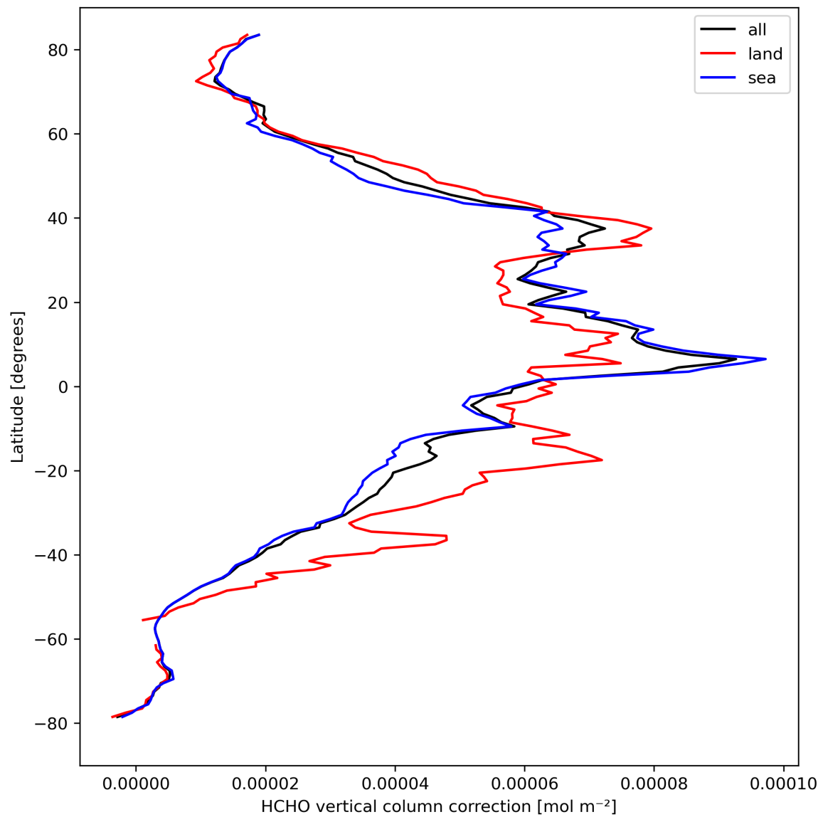
Figure 23: Zonal average of “HCHO vertical column correction” for 2023-09-18 to 2023-09-20.
