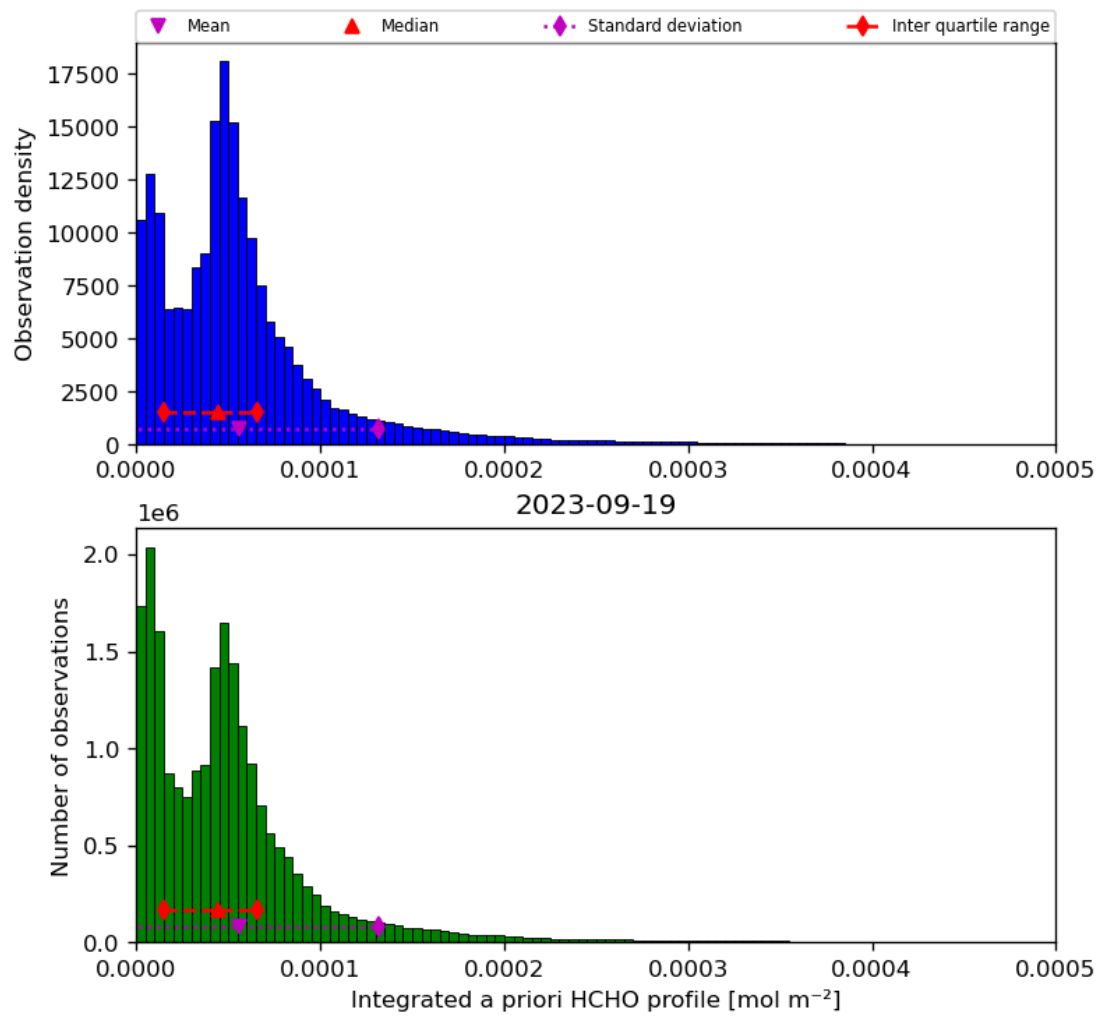
Figure 43: Histogram of “Integrated a priori HCHO profile” for 2023-09-18 to 2023-09-20
