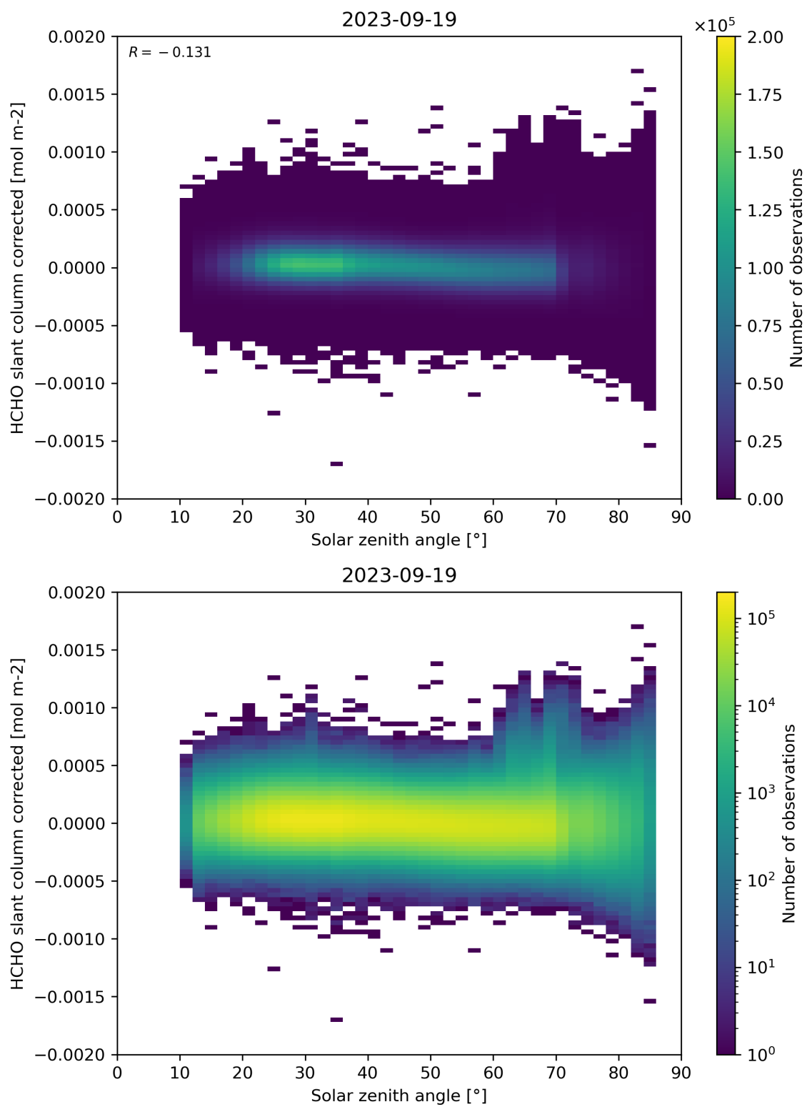
Figure 171: Scatter density plot of “Solar zenith angle” against “HCHO slant column corrected” for 2023-09-18 to 2023-09-20.
