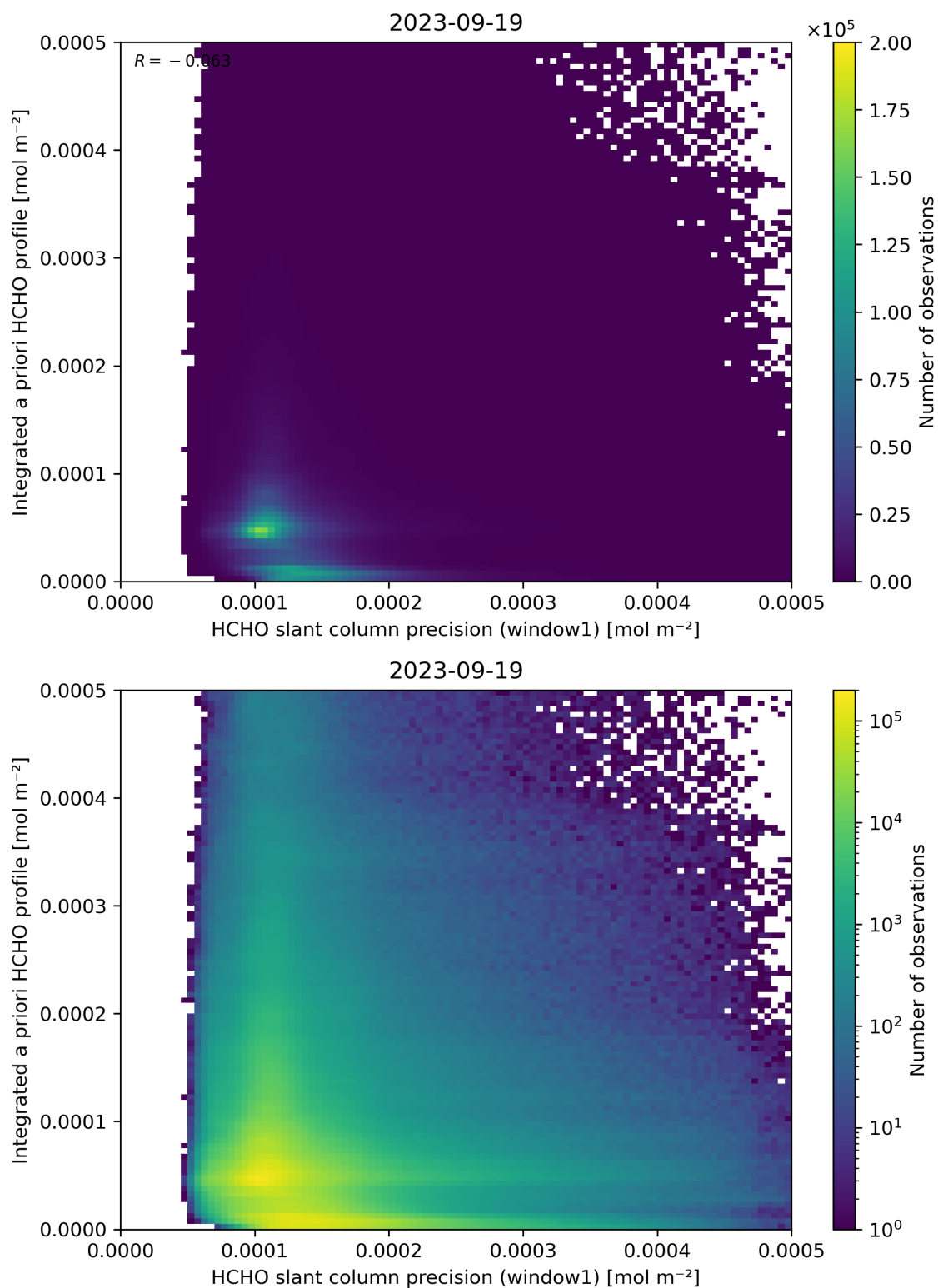
Figure 96: Scatter density plot of “HCHO slant column precision (window1)” against “Integrated a priori HCHO profile” for 2023-09-18 to 2023-09-20.
