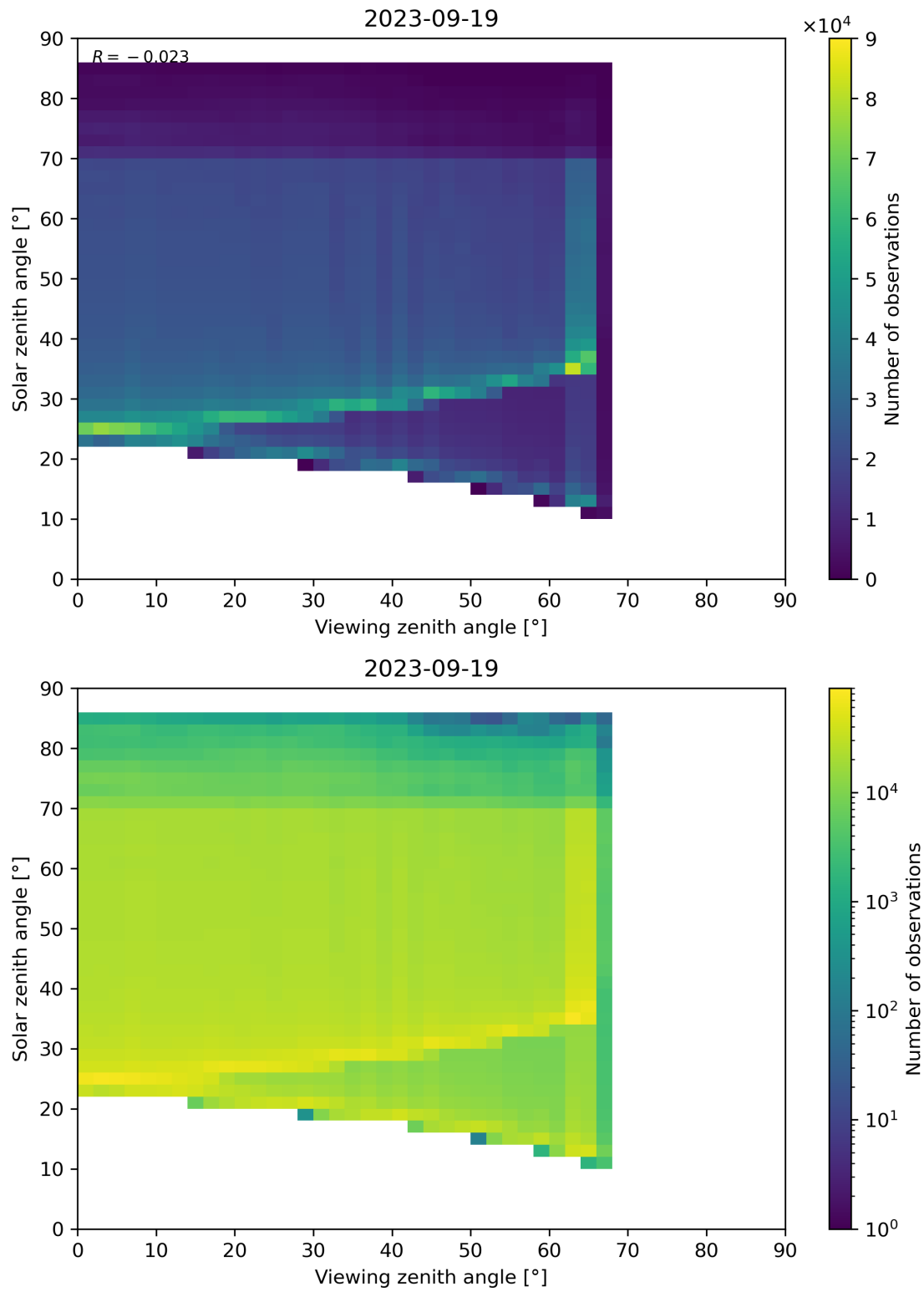
Figure 197: Scatter density plot of “Viewing zenith angle” against “Solar zenith angle” for 2023-09-18 to 2023-09-20.
