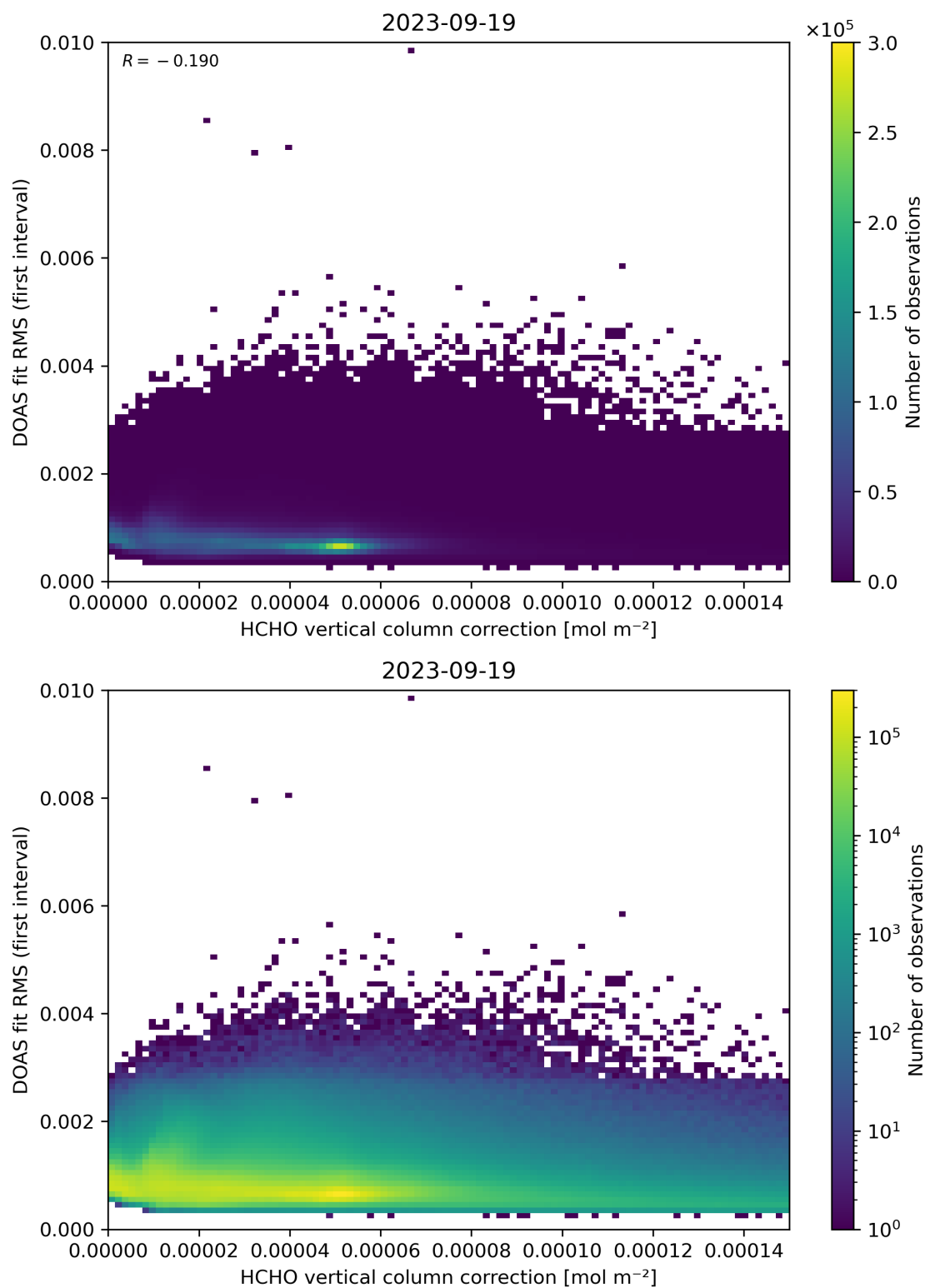
Figure 112: Scatter density plot of “HCHO vertical column correction” against “DOAS fit RMS (first interval)” for 2023-09-18 to 2023-09-20.
