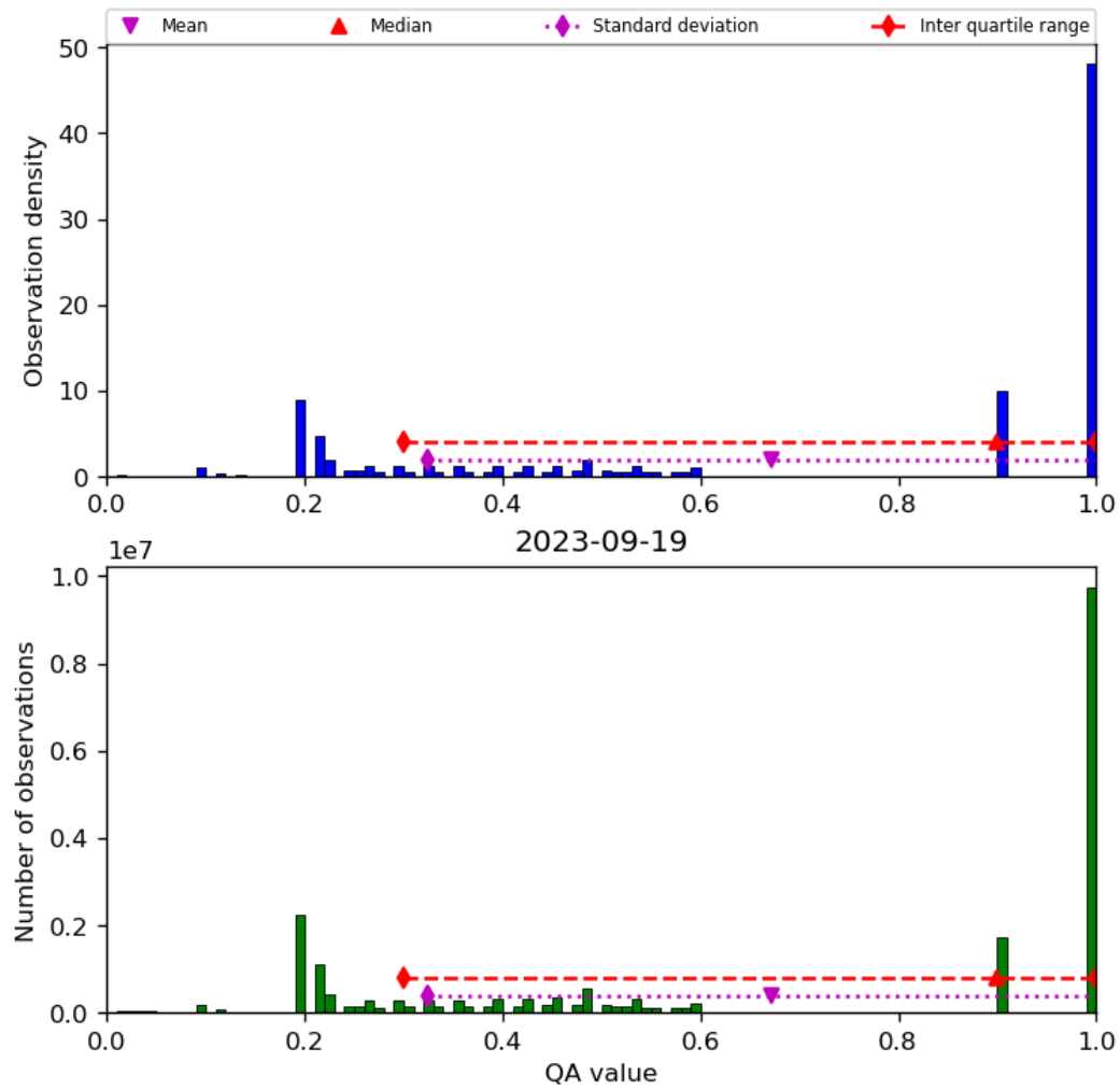
Figure 34: Histogram of “QA value” for 2023-09-18 to 2023-09-20
