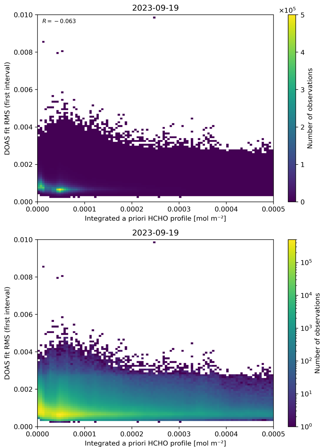
Figure 148: Scatter density plot of “Integrated a priori HCHO profile” against “DOAS fit RMS (first interval)” for 2023-09-18 to 2023-09-20.
