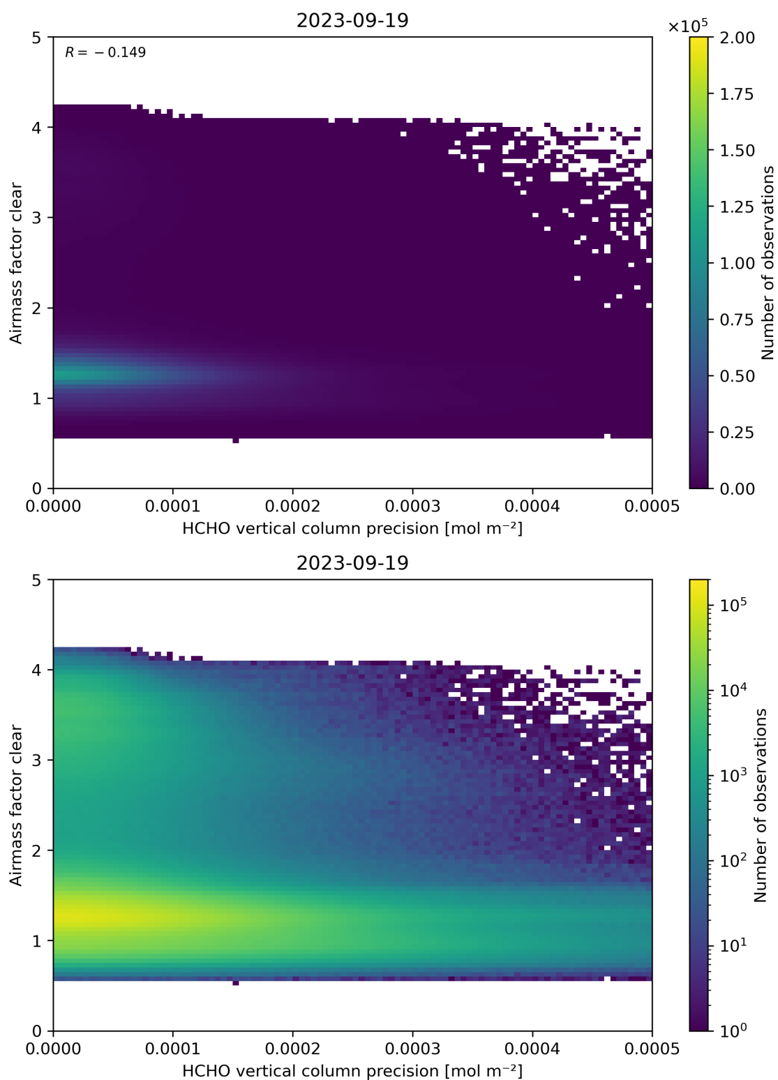
Figure 139: Scatter density plot of “HCHO vertical column precision” against “Airmass factor clear” for 2023-09-18 to 2023-09-20.
