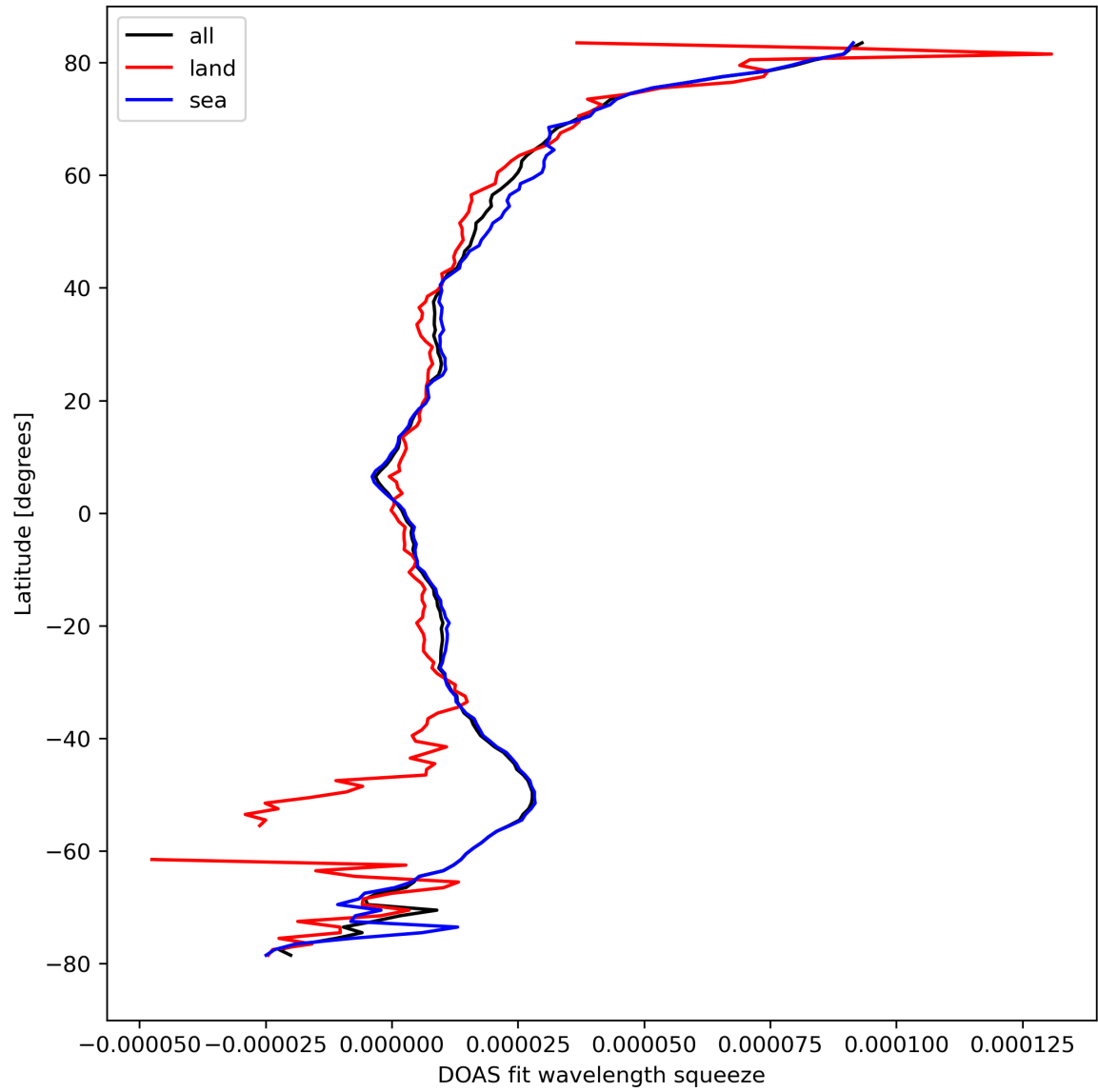
Figure 31: Zonal average of “DOAS fit wavelength squeeze” for 2023-09-18 to 2023-09-20.
