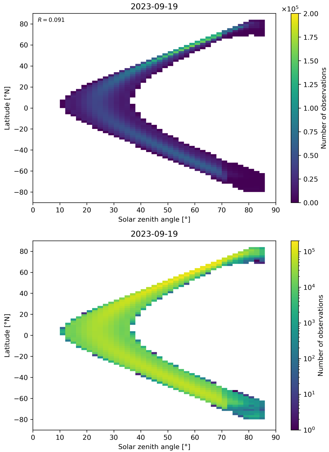
Figure 181: Scatter density plot of “Solar zenith angle” against “Latitude” for 2023-09-18 to 2023-09-20.
