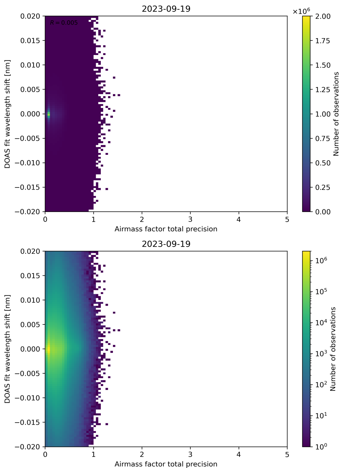
Figure 106: Scatter density plot of “Airmass factor total precision” against “DOAS fit wavelength shift” for 2023-09-18 to 2023-09-20.
