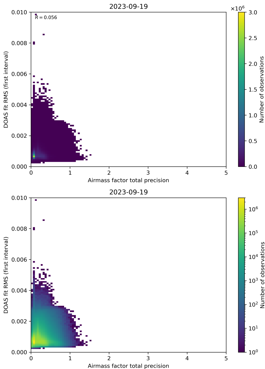
Figure 105: Scatter density plot of “Airmass factor total precision” against “DOAS fit RMS (first interval)” for 2023-09-18 to 2023-09-20.
