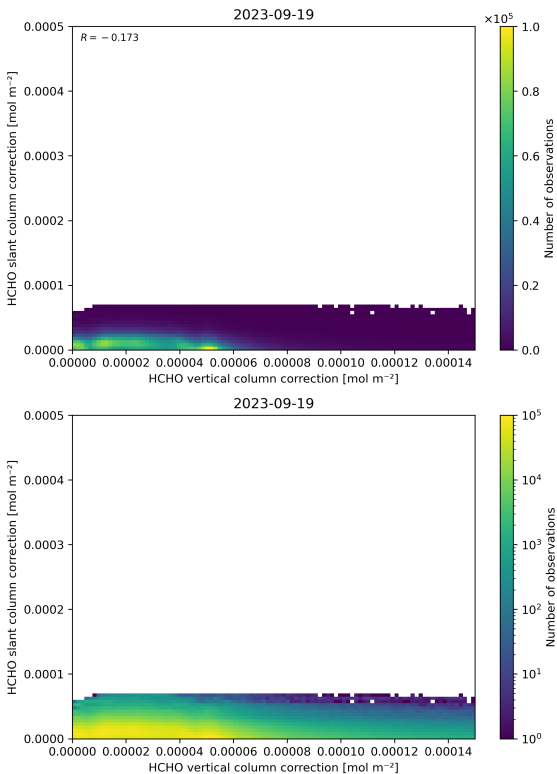
Figure 117: Scatter density plot of “HCHO vertical column correction” against “HCHO slant column correction” for 2023-09-18 to 2023-09-20.
