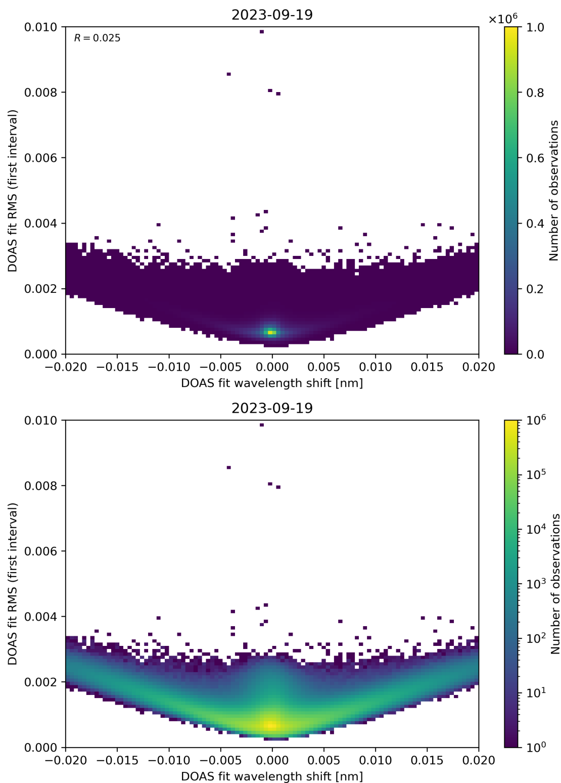
Figure 64: Scatter density plot of “DOAS fit wavelength shift” against “DOAS fit RMS (first interval)” for 2023-09-18 to 2023-09-20.
