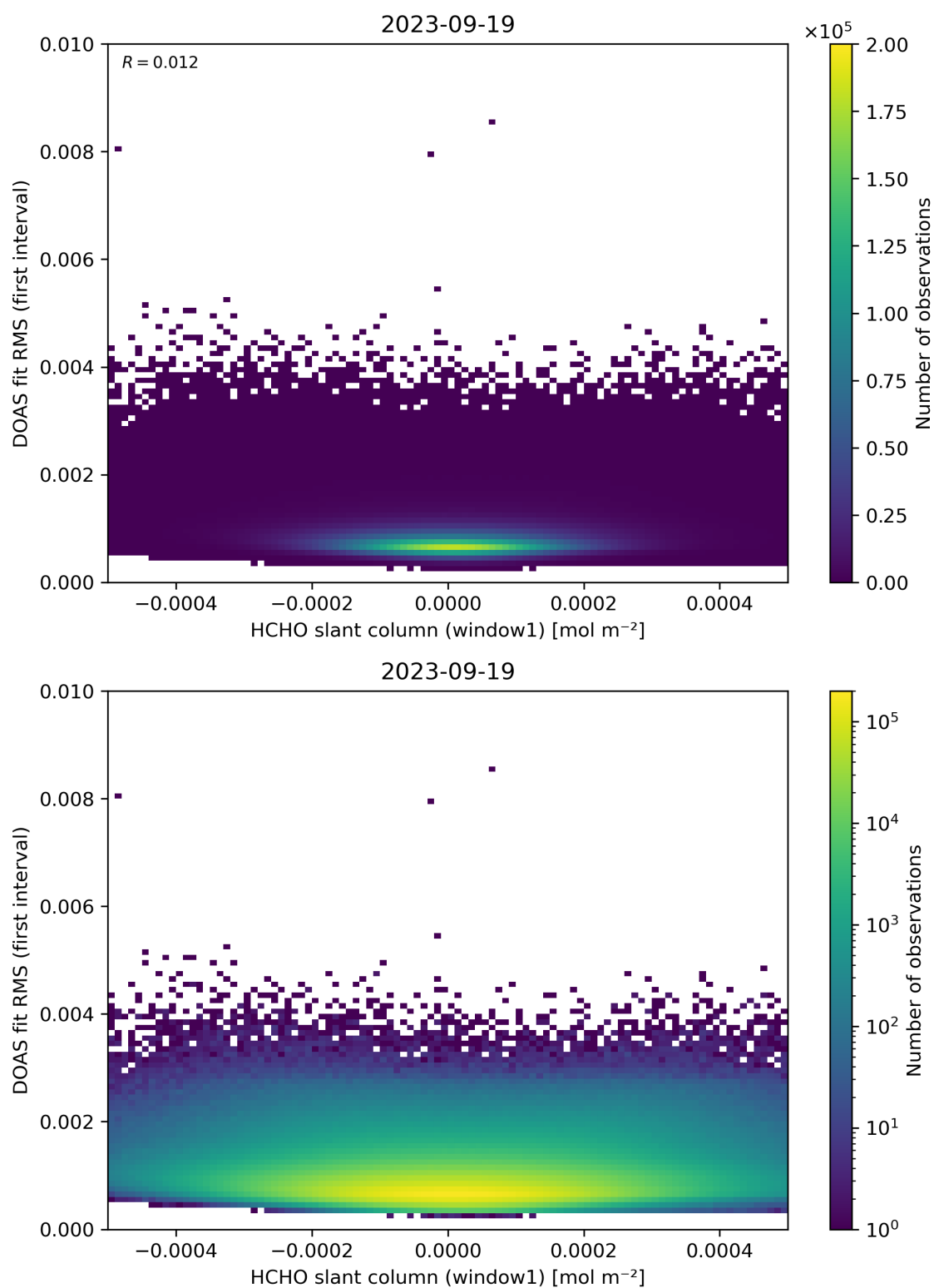
Figure 78: Scatter density plot of “HCHO slant column (window1)” against “DOAS fit RMS (first interval)” for 2023-09-18 to 2023-09-20.
