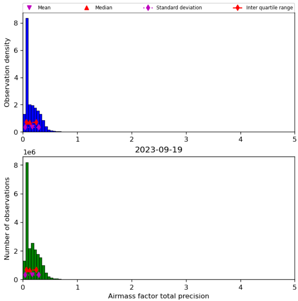
Figure 41: Histogram of “Airmass factor total precision” for 2023-09-18 to 2023-09-20
