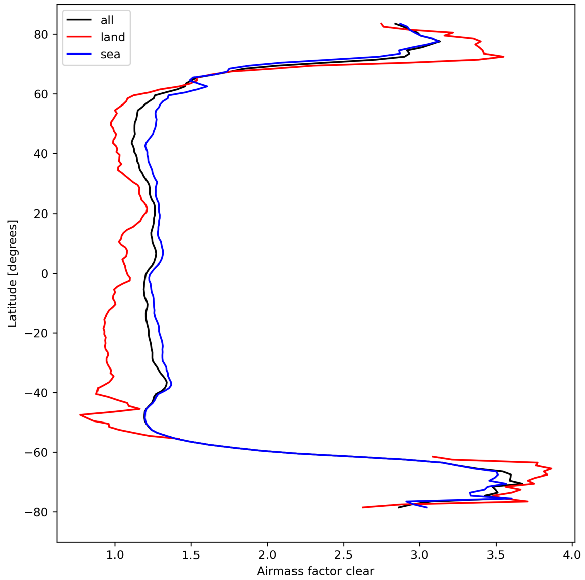
Figure 28: Zonal average of “Airmass factor clear” for 2023-09-18 to 2023-09-20.
