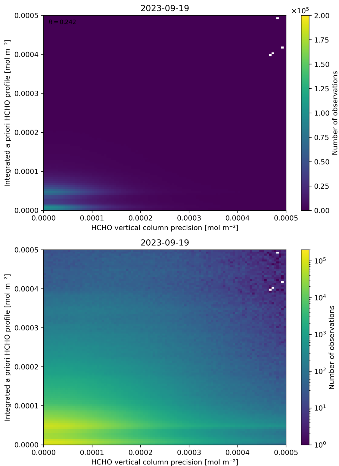
Figure 147: Scatter density plot of “HCHO vertical column precision” against “Integrated a priori HCHO profile” for 2023-09-18 to 2023-09-20.
