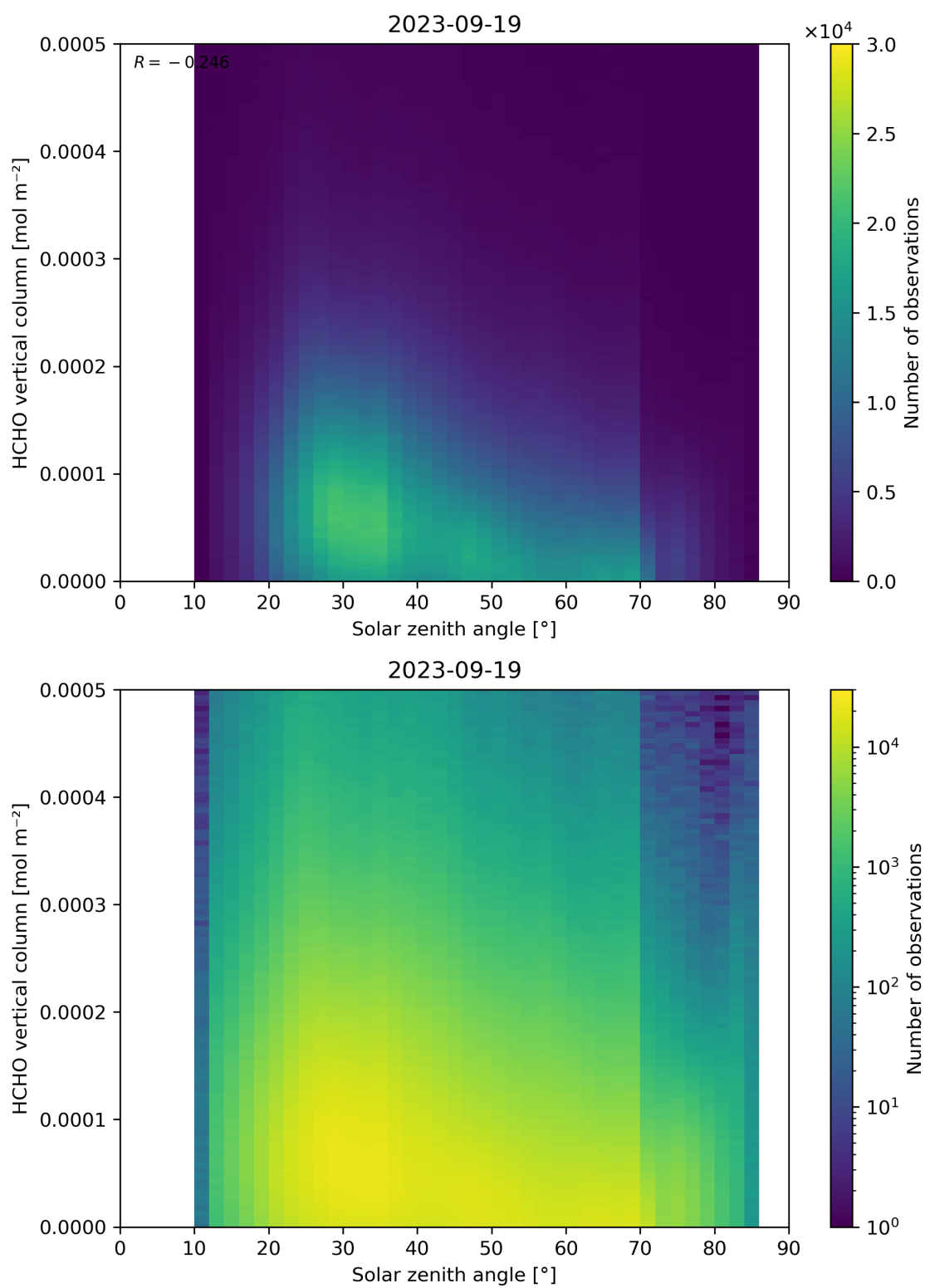
Figure 177: Scatter density plot of “Solar zenith angle” against “HCHO vertical column” for 2023-09-18 to 2023-09-20.
