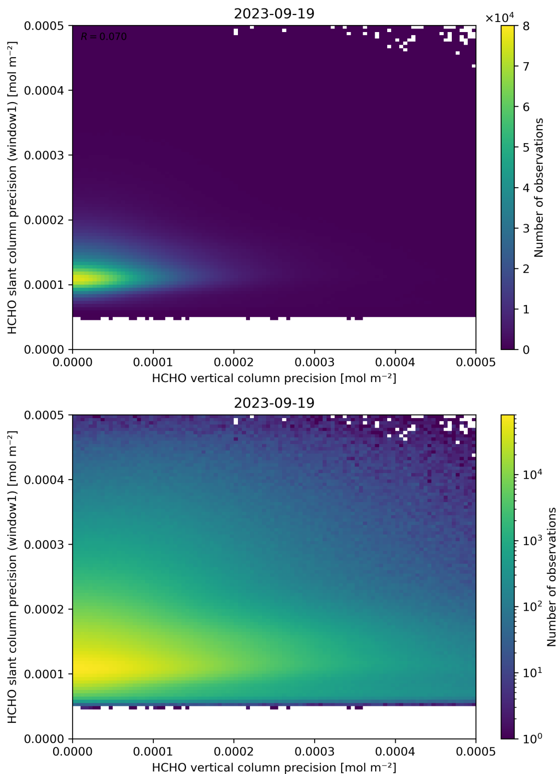
Figure 143: Scatter density plot of “HCHO vertical column precision” against “HCHO slant column precision (window1)” for 2023-09-18 to 2023-09-20.
