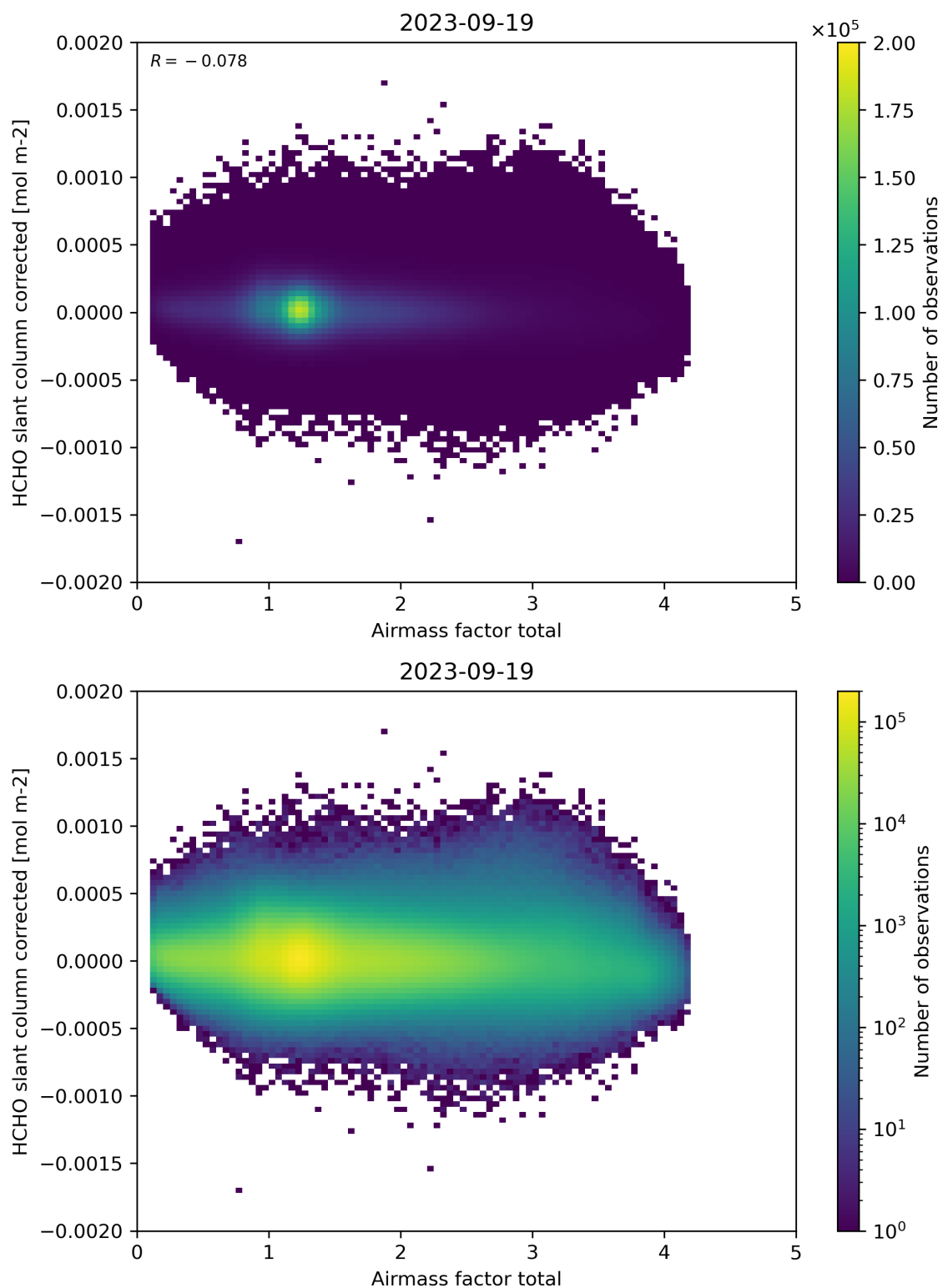
Figure 101: Scatter density plot of “Airmass factor total” against “HCHO slant column corrected” for 2023-09-18 to 2023-09-20.
