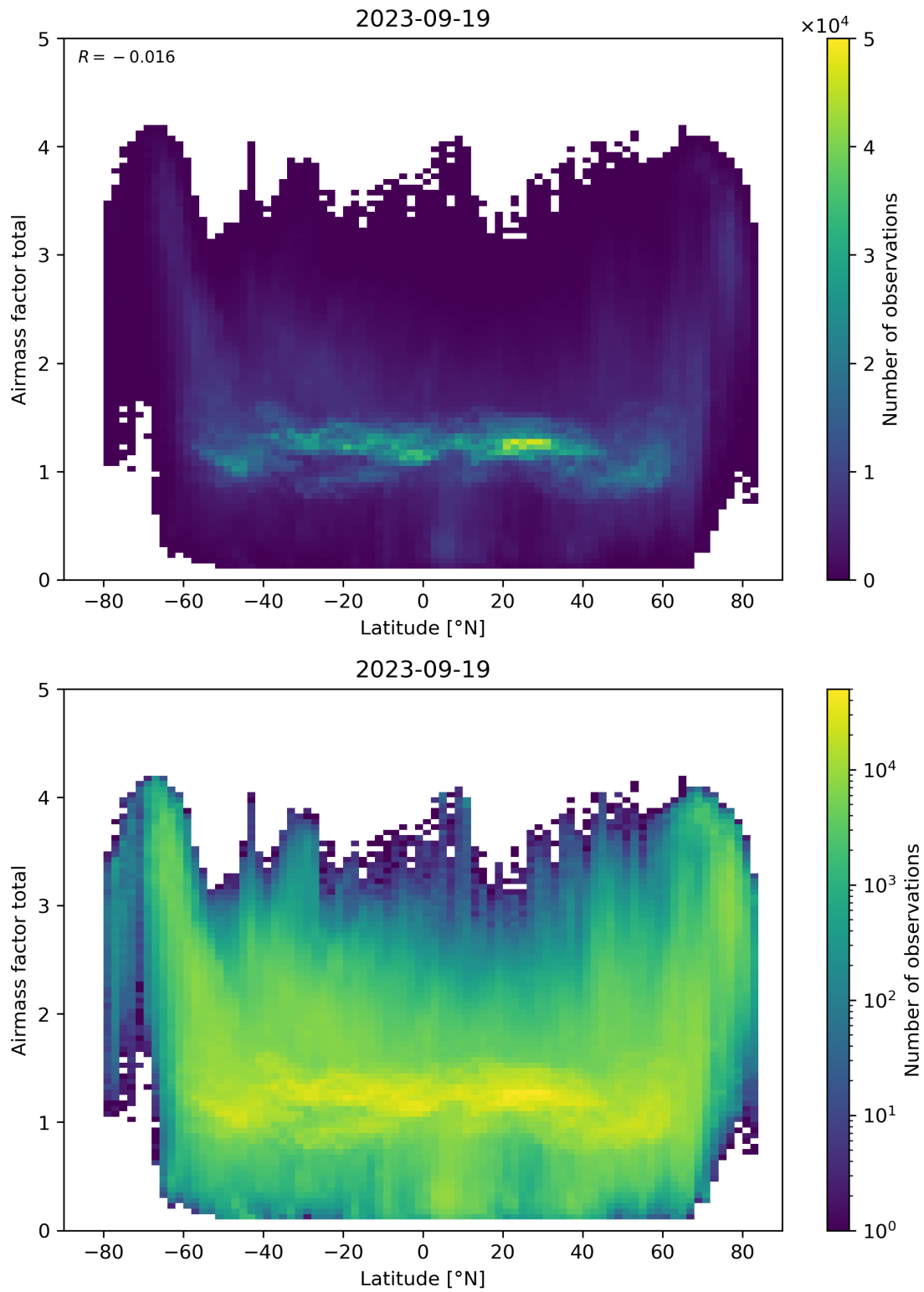
Figure 161: Scatter density plot of “Latitude” against “Airmass factor total” for 2023-09-18 to 2023-09-20.
