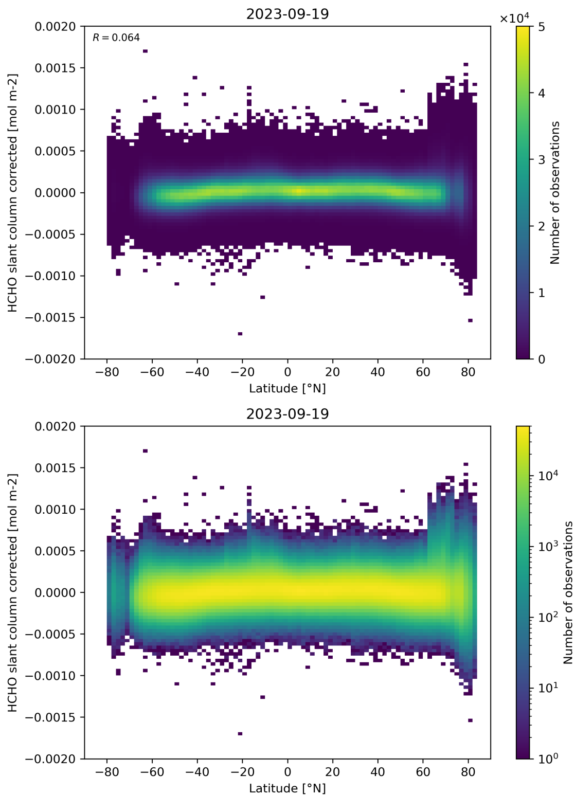
Figure 157: Scatter density plot of “Latitude” against “HCHO slant column corrected” for 2023-09-18 to 2023-09-20.
