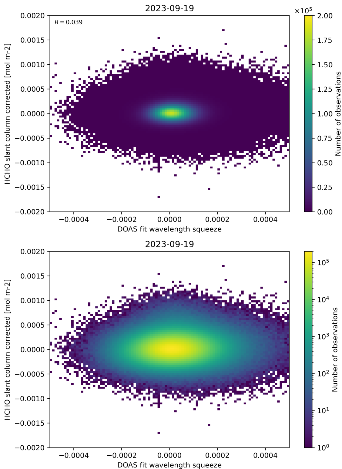
Figure 69: Scatter density plot of “DOAS fit wavelength squeeze” against “HCHO slant column corrected” for 2023-09-18 to 2023-09-20.
