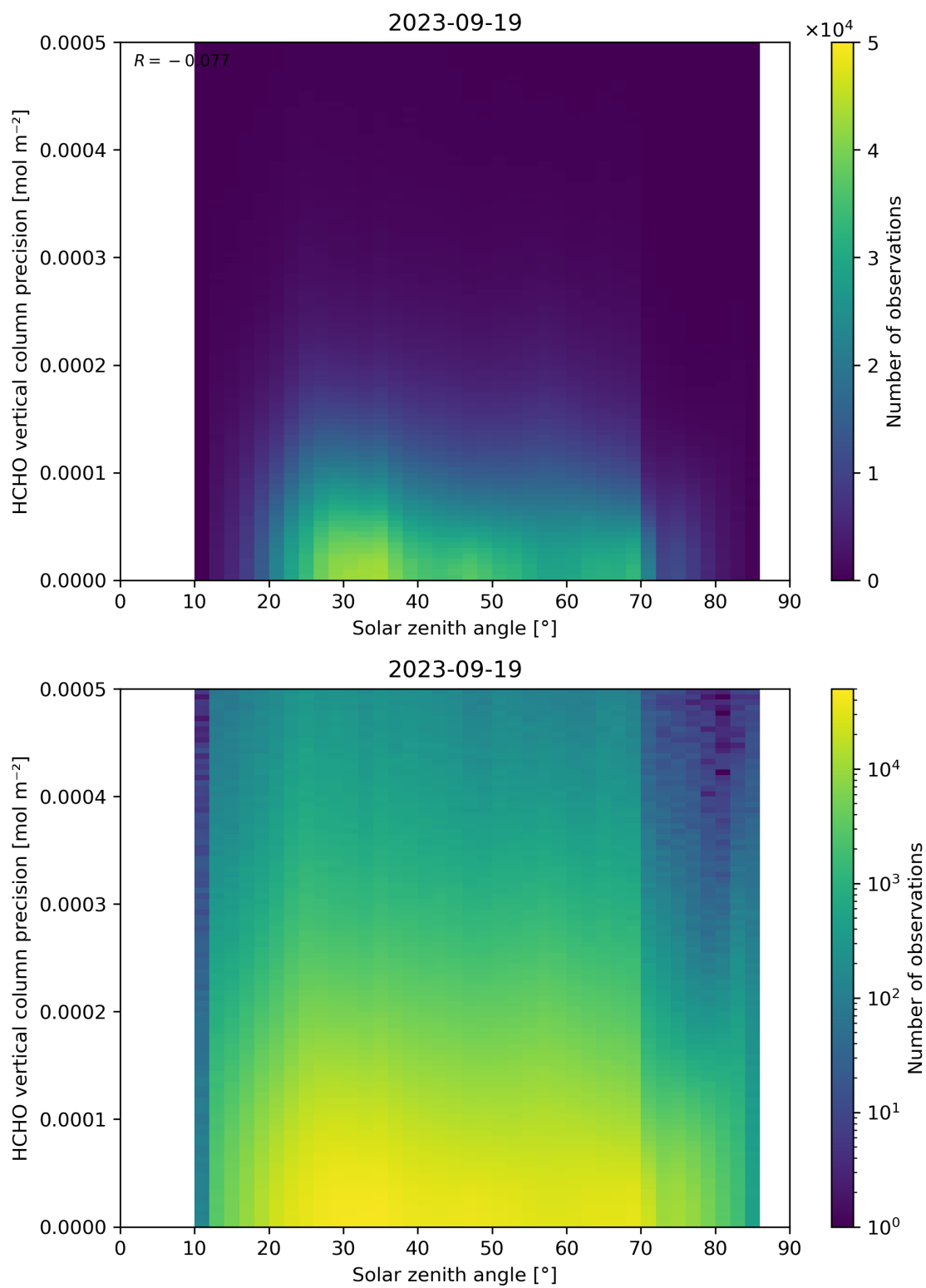
Figure 179: Scatter density plot of “Solar zenith angle” against “HCHO vertical column precision” for 2023-09-18 to 2023-09-20.
