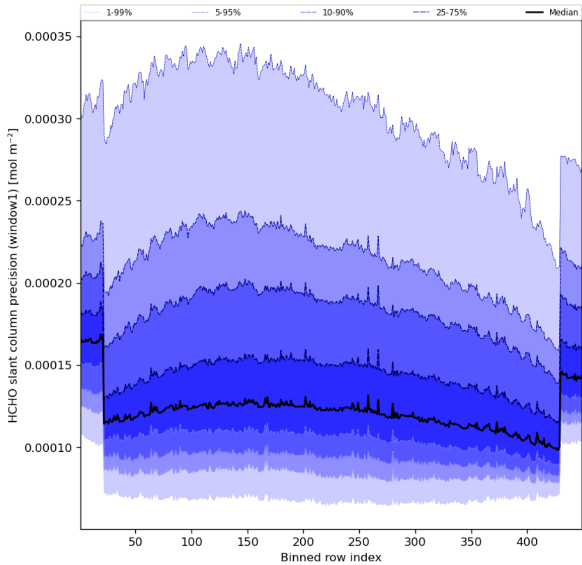
Figure 53: Along track statistics of “HCHO slant column precision (window1)” for 2023-09-18 to 2023-09-20
