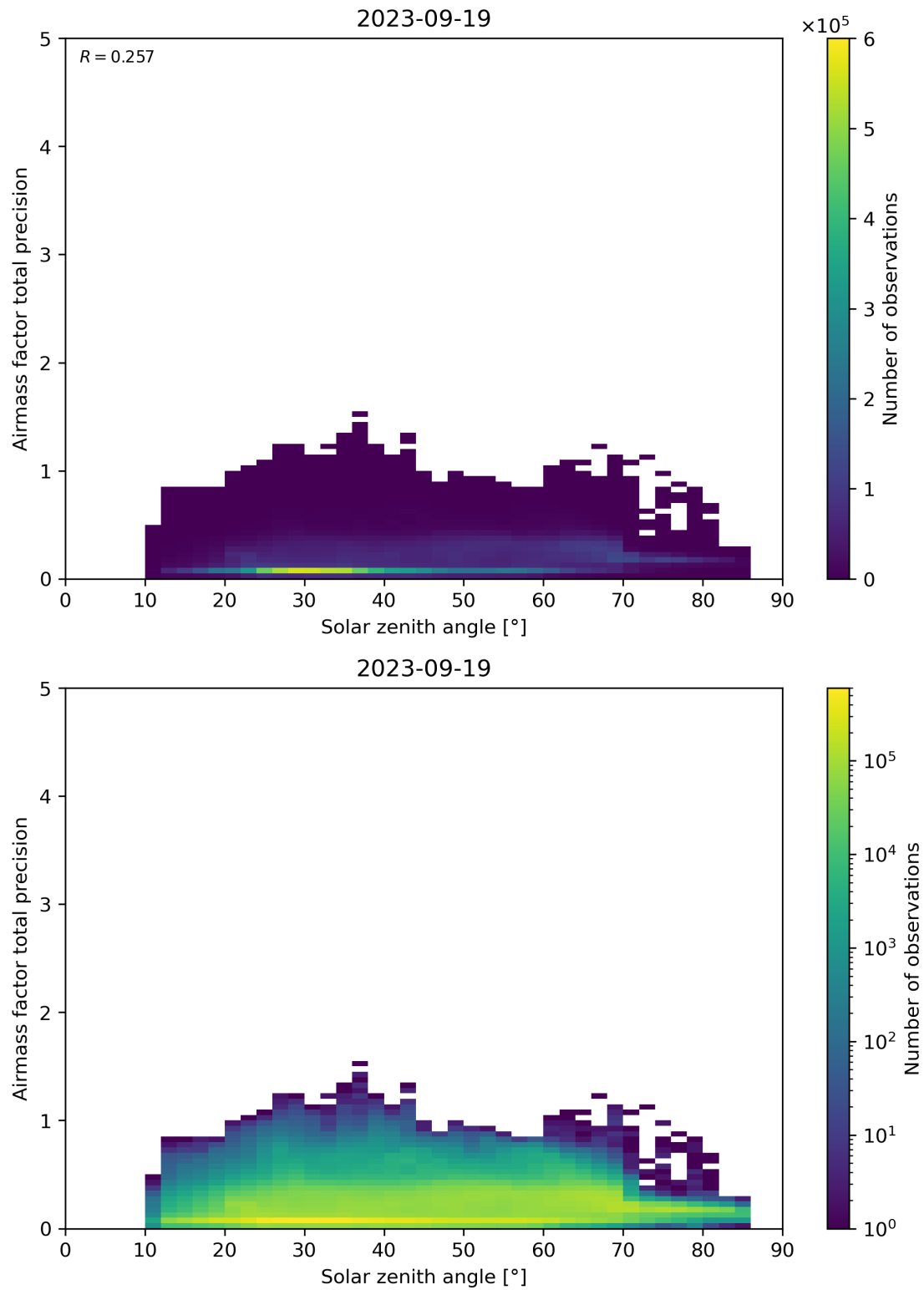
Figure 176: Scatter density plot of “Solar zenith angle” against “Airmass factor total precision” for 2023-09-18 to 2023-09-20.
