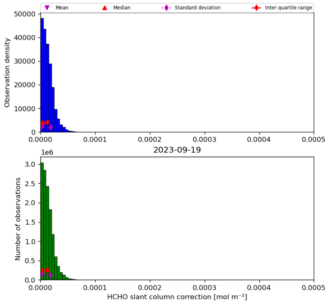
Figure 47: Histogram of “HCHO slant column correction” for 2023-09-18 to 2023-09-20
