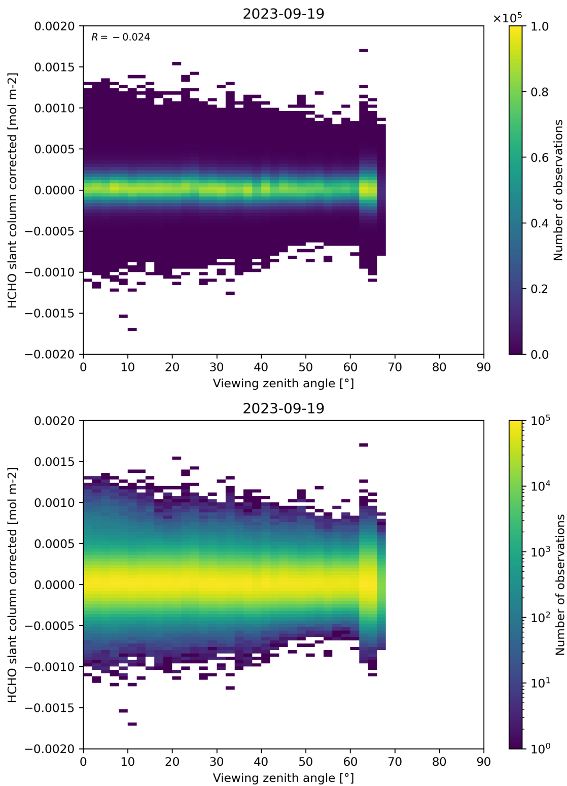
Figure 186: Scatter density plot of “Viewing zenith angle” against “HCHO slant column corrected” for 2023-09-18 to 2023-09-20.
