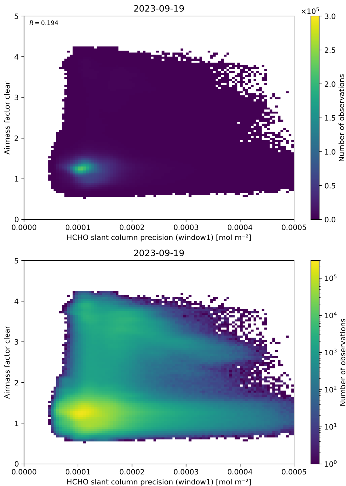
Figure 91: Scatter density plot of “HCHO slant column precision (window1)” against “Airmass factor clear” for 2023-09-18 to 2023-09-20.
