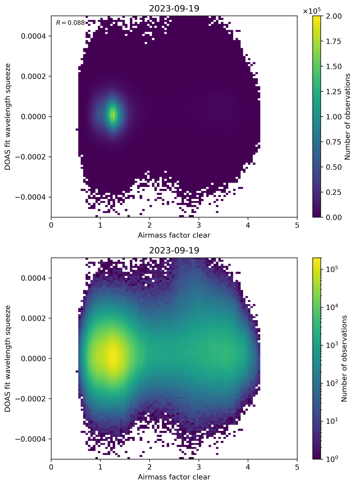
Figure 73: Scatter density plot of “Airmass factor clear” against “DOAS fit wavelength squeeze” for 2023-09-18 to 2023-09-20.
