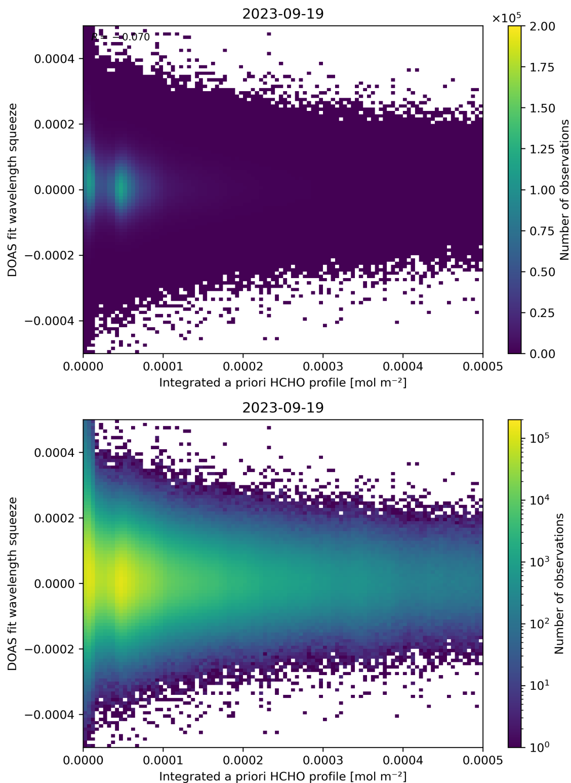
Figure 150: Scatter density plot of “Integrated a priori HCHO profile” against “DOAS fit wavelength squeeze” for 2023-09-18 to 2023-09-20.
