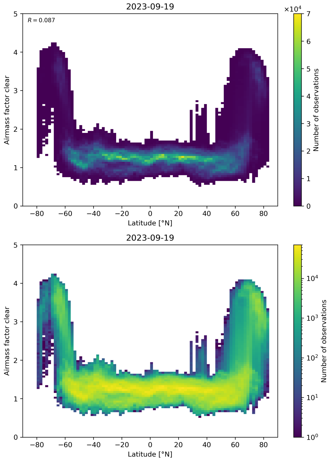
Figure 156: Scatter density plot of “Latitude” against “Airmass factor clear” for 2023-09-18 to 2023-09-20.
