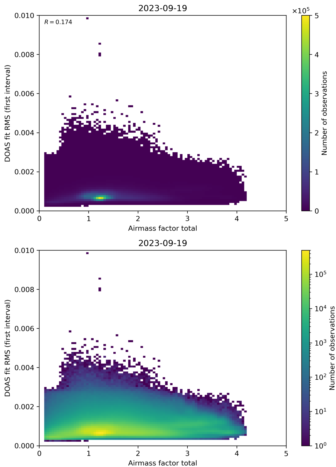
Figure 97: Scatter density plot of “Airmass factor total” against “DOAS fit RMS (first interval)” for 2023-09-18 to 2023-09-20.
