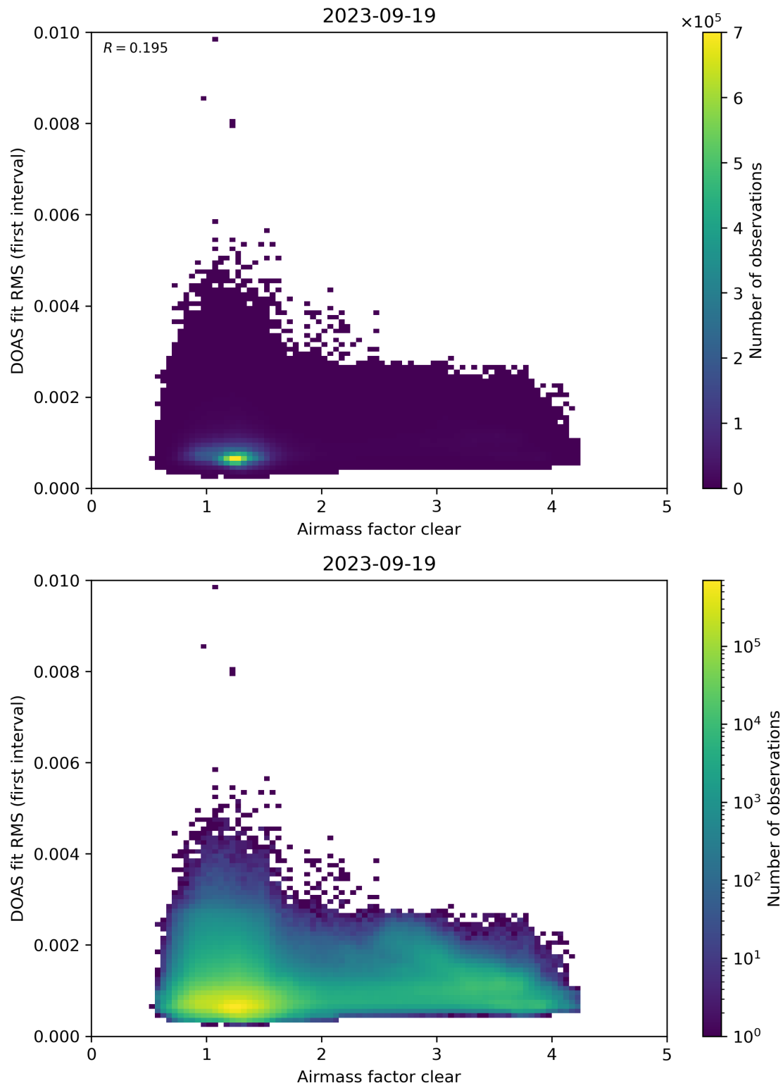
Figure 71: Scatter density plot of “Airmass factor clear” against “DOAS fit RMS (first interval)” for 2023-09-18 to 2023-09-20.
