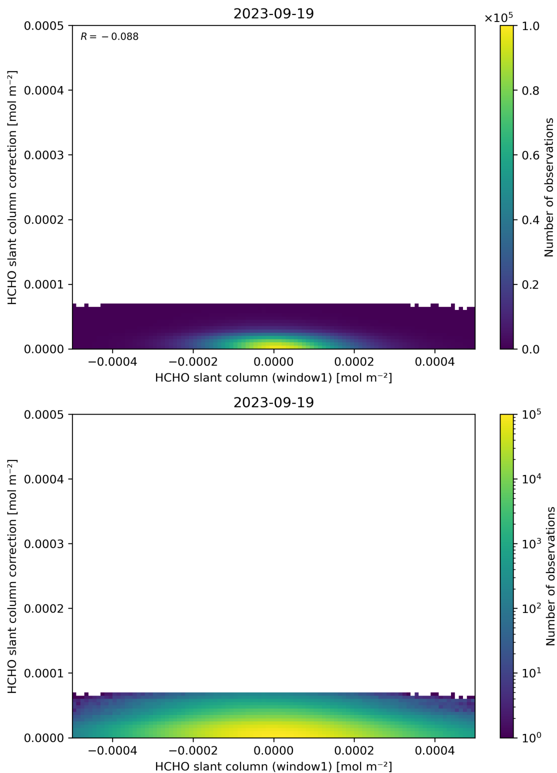
Figure 83: Scatter density plot of “HCHO slant column (window1)” against “HCHO slant column correction” for 2023-09-18 to 2023-09-20.
