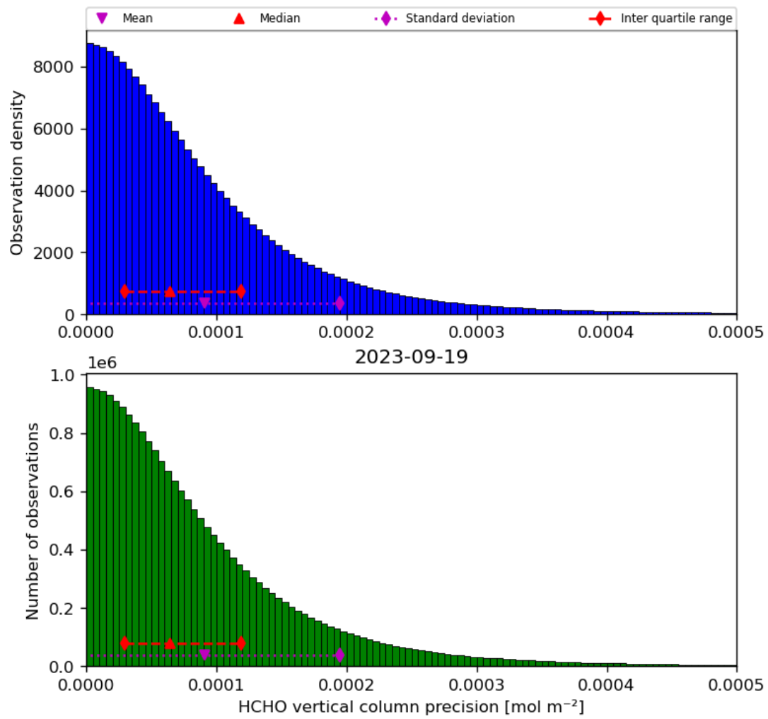
Figure 36: Histogram of “HCHO vertical column precision” for 2023-09-18 to 2023-09-20
