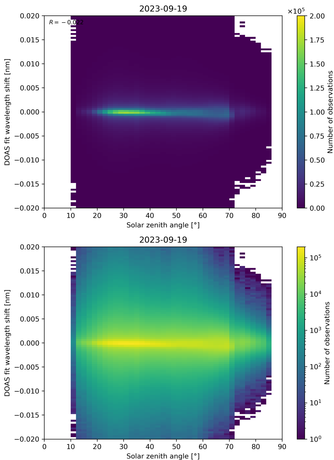
Figure 168: Scatter density plot of “Solar zenith angle” against “DOAS fit wavelength shift” for 2023-09-18 to 2023-09-20.
