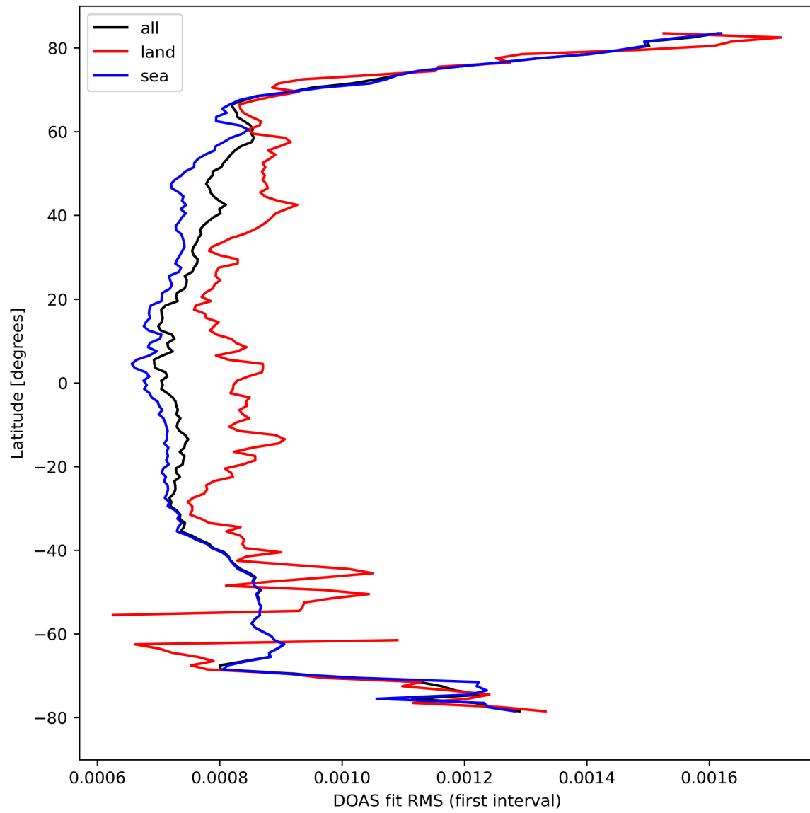
Figure 32: Zonal average of “DOAS fit RMS (first interval)” for 2023-09-18 to 2023-09-20.
