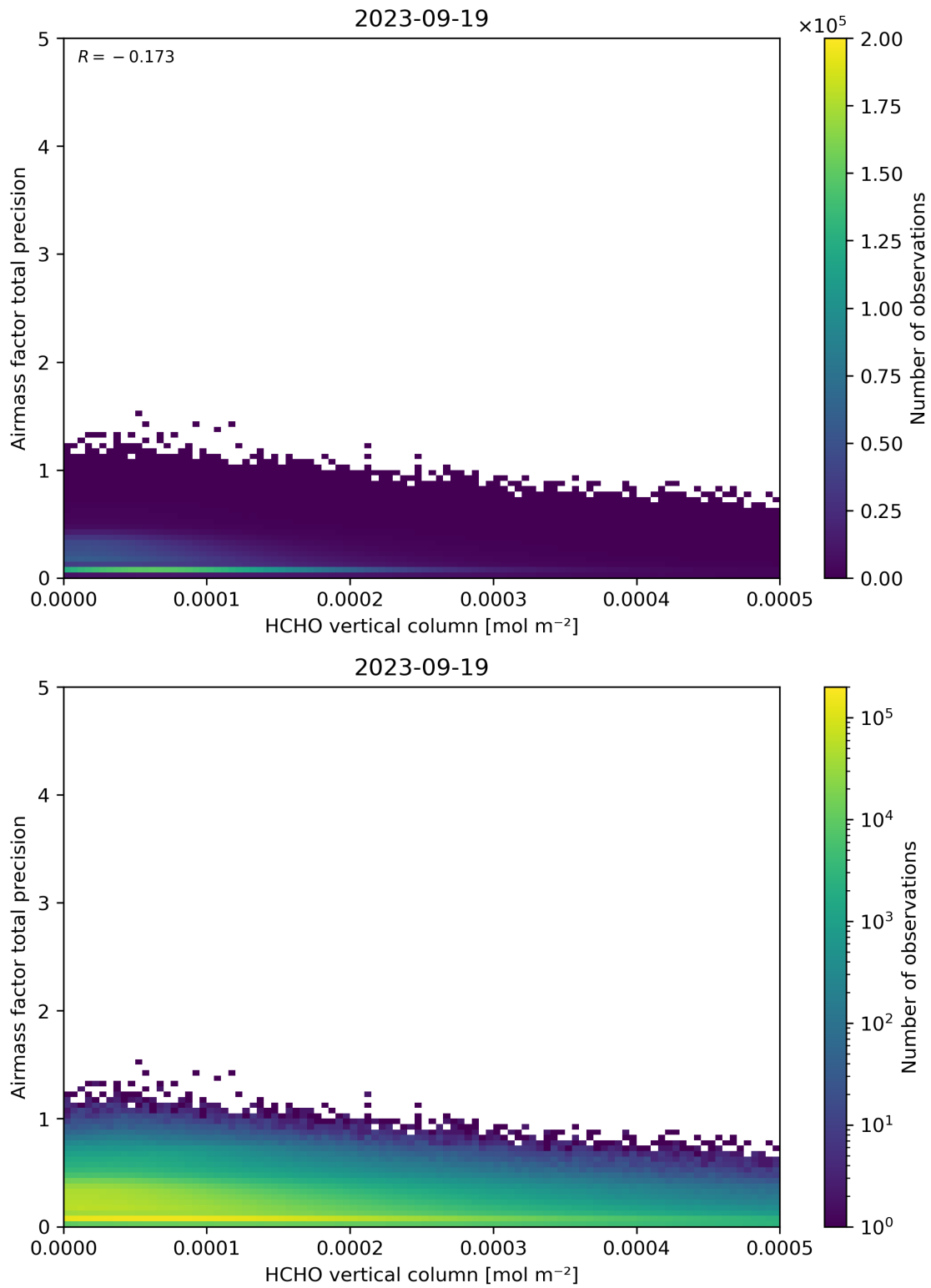
Figure 132: Scatter density plot of “HCHO vertical column” against “Airmass factor total precision” for 2023-09-18 to 2023-09-20.
