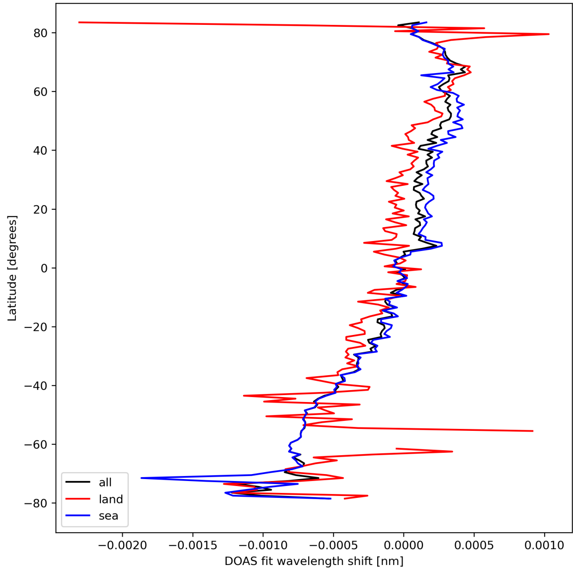
Figure 30: Zonal average of “DOAS fit wavelength shift” for 2023-09-18 to 2023-09-20.
