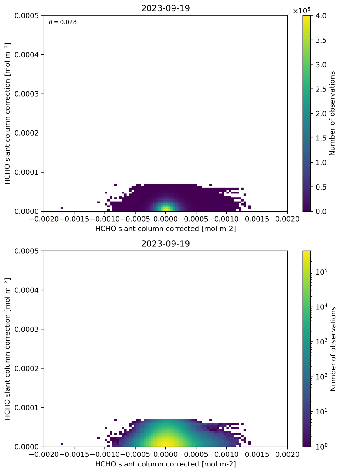
Figure 77: Scatter density plot of “HCHO slant column corrected” against “HCHO slant column correction” for 2023-09-18 to 2023-09-20.
