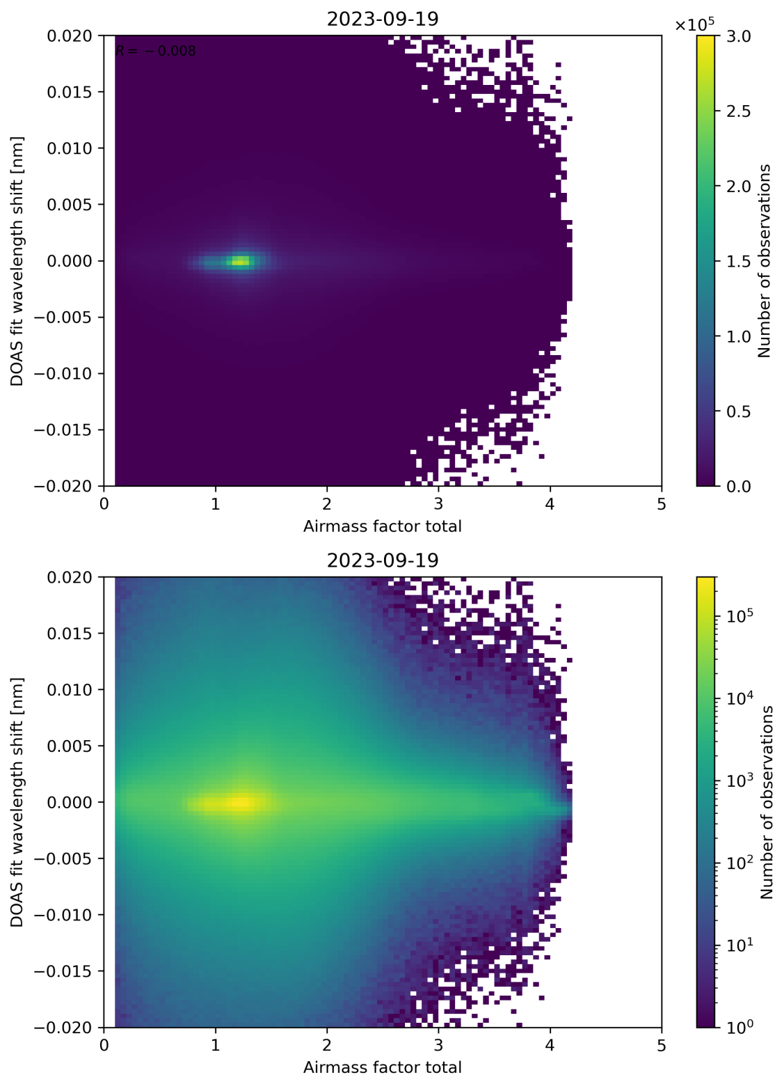
Figure 98: Scatter density plot of “Airmass factor total” against “DOAS fit wavelength shift” for 2023-09-18 to 2023-09-20.
