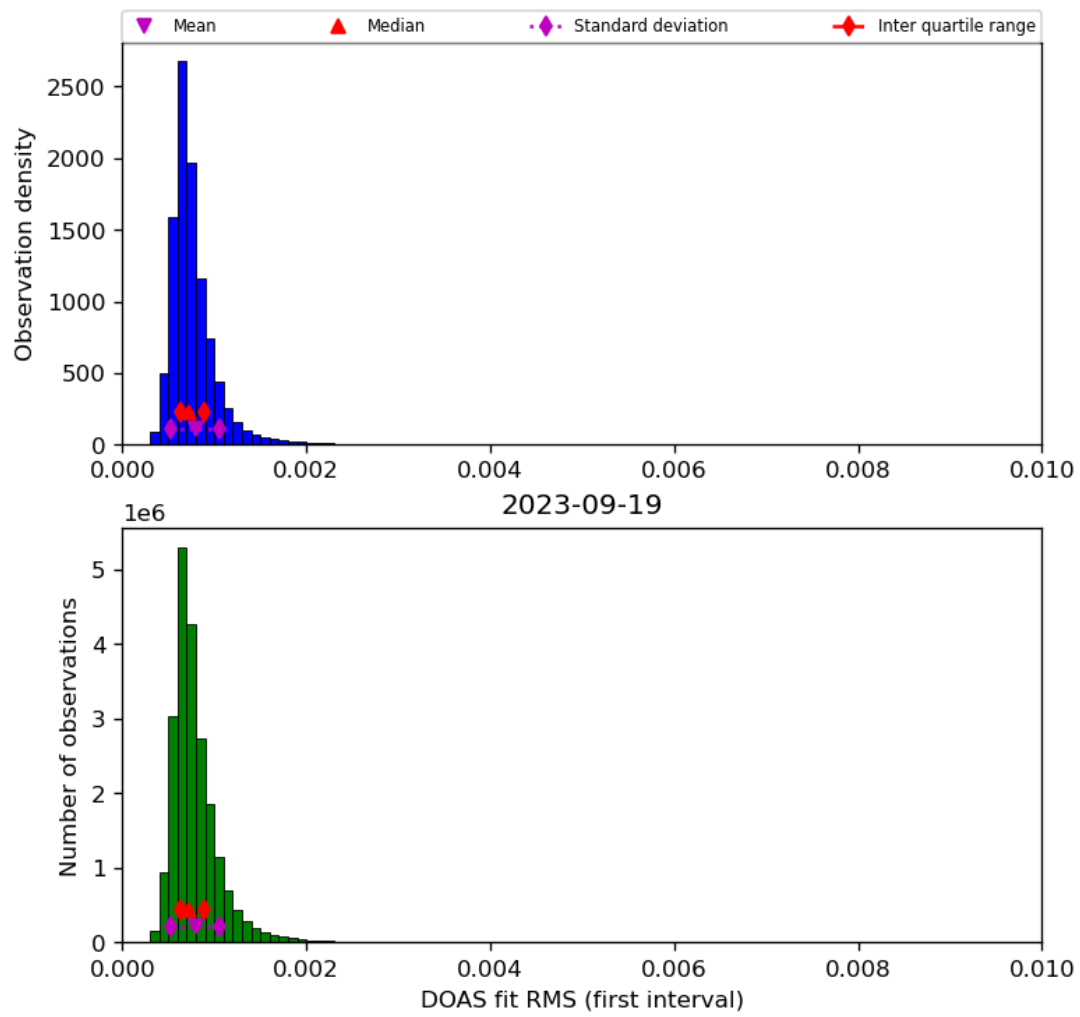
Figure 46: Histogram of “DOAS fit RMS (first interval)” for 2023-09-18 to 2023-09-20
