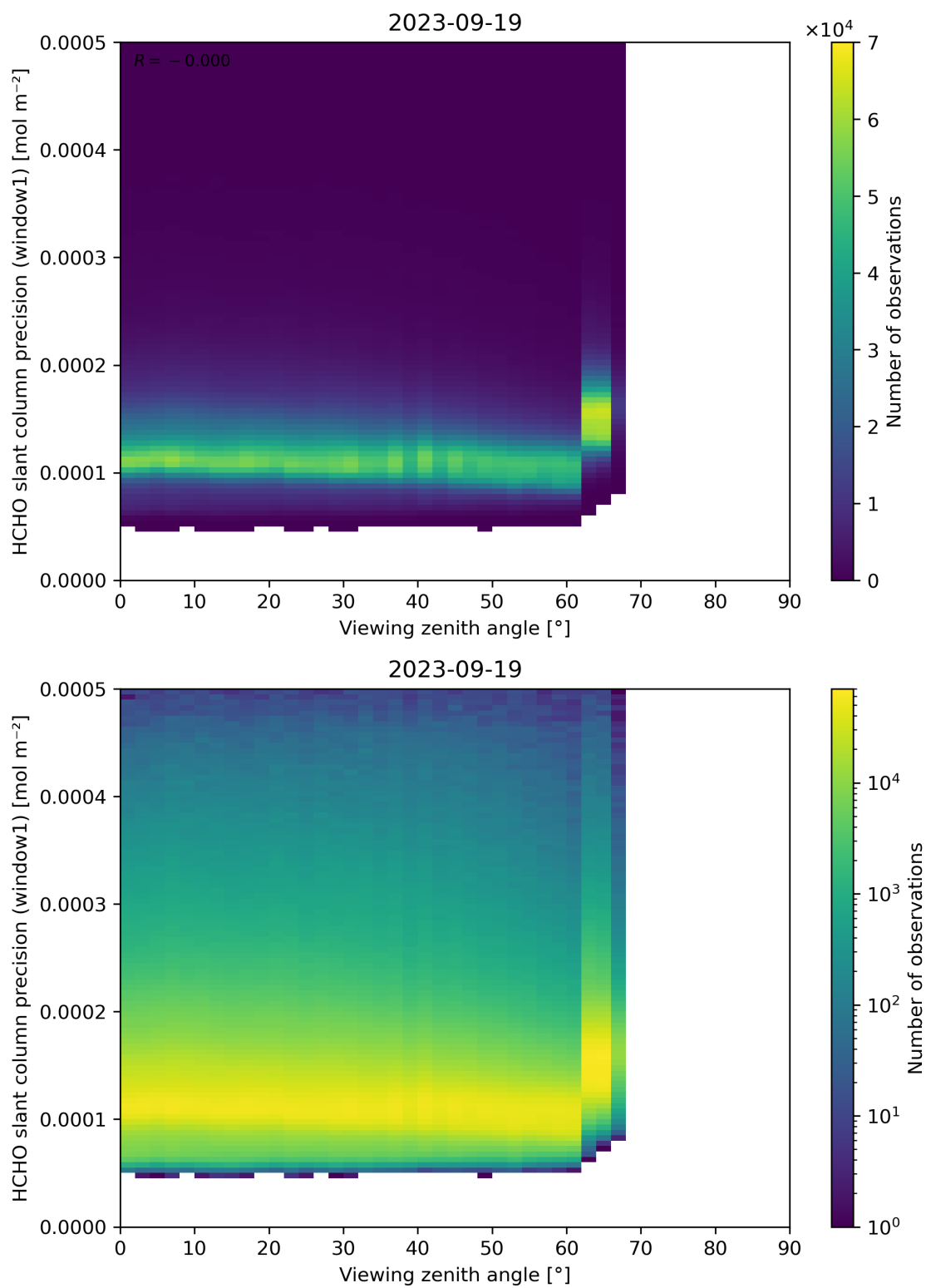
Figure 189: Scatter density plot of “Viewing zenith angle” against “HCHO slant column precision (window1)” for 2023-09-18 to 2023-09-20.
