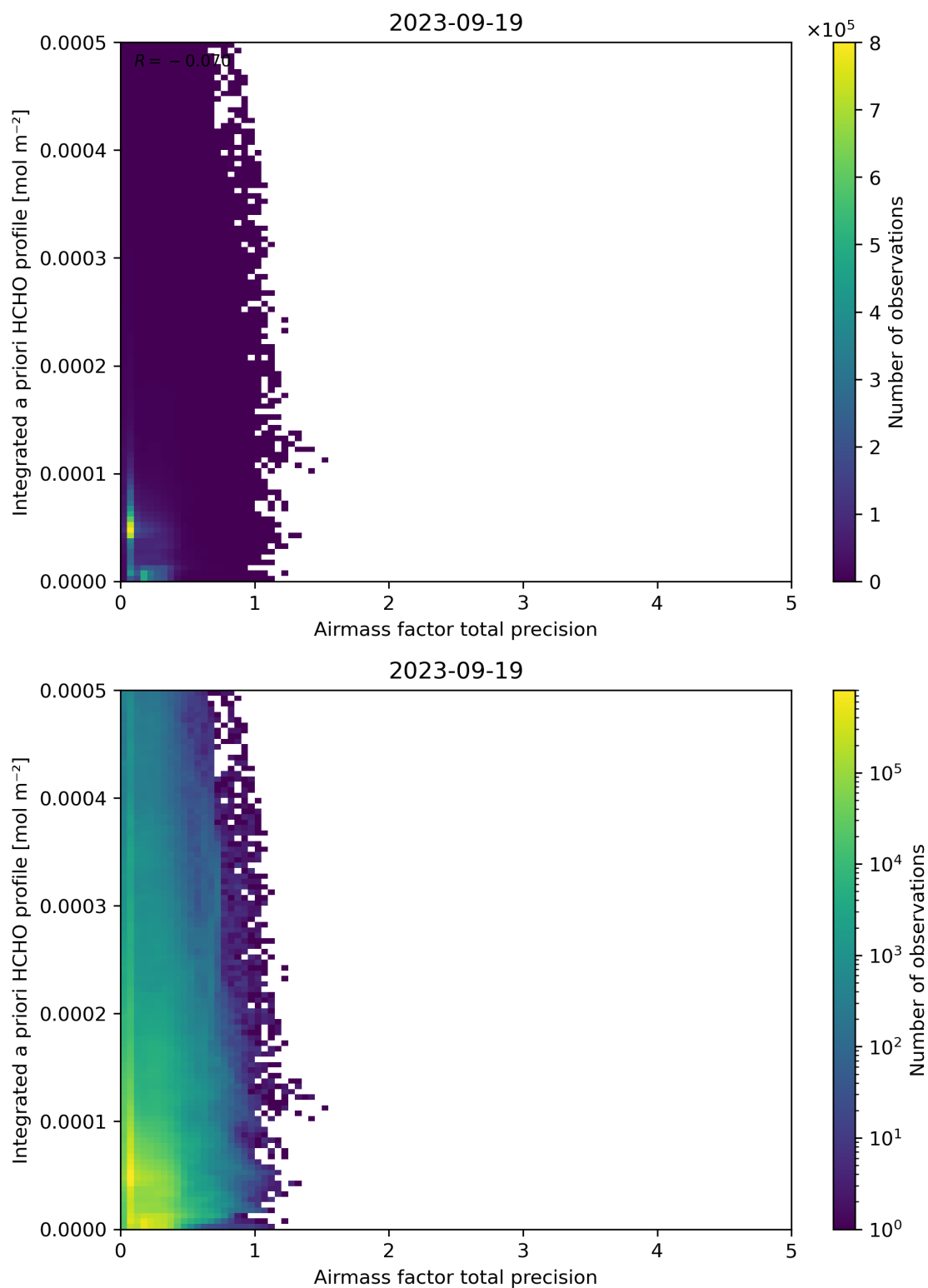
Figure 111: Scatter density plot of “Airmass factor total precision” against “Integrated a priori HCHO profile” for 2023-09-18 to 2023-09-20.
