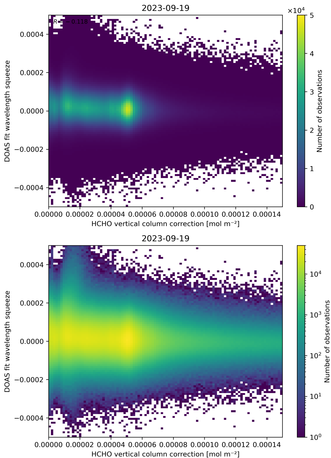
Figure 114: Scatter density plot of “HCHO vertical column correction” against “DOAS fit wavelength squeeze” for 2023-09-18 to 2023-09-20.
