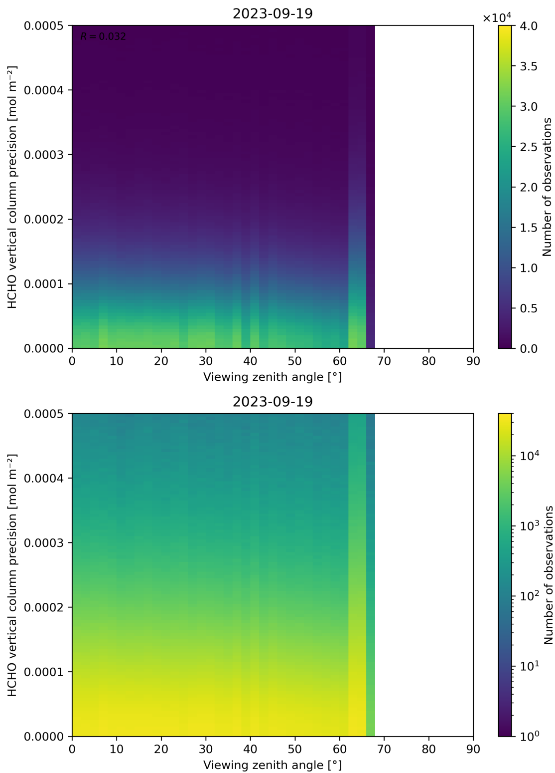
Figure 194: Scatter density plot of “Viewing zenith angle” against “HCHO vertical column precision” for 2023-09-18 to 2023-09-20.
