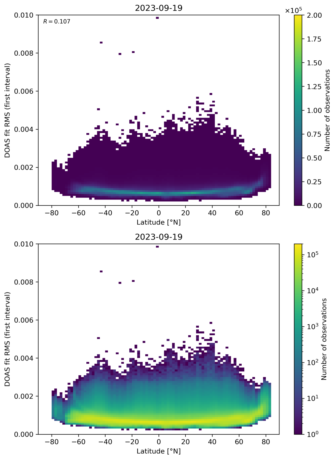
Figure 153: Scatter density plot of “Latitude” against “DOAS fit RMS (first interval)” for 2023-09-18 to 2023-09-20.
