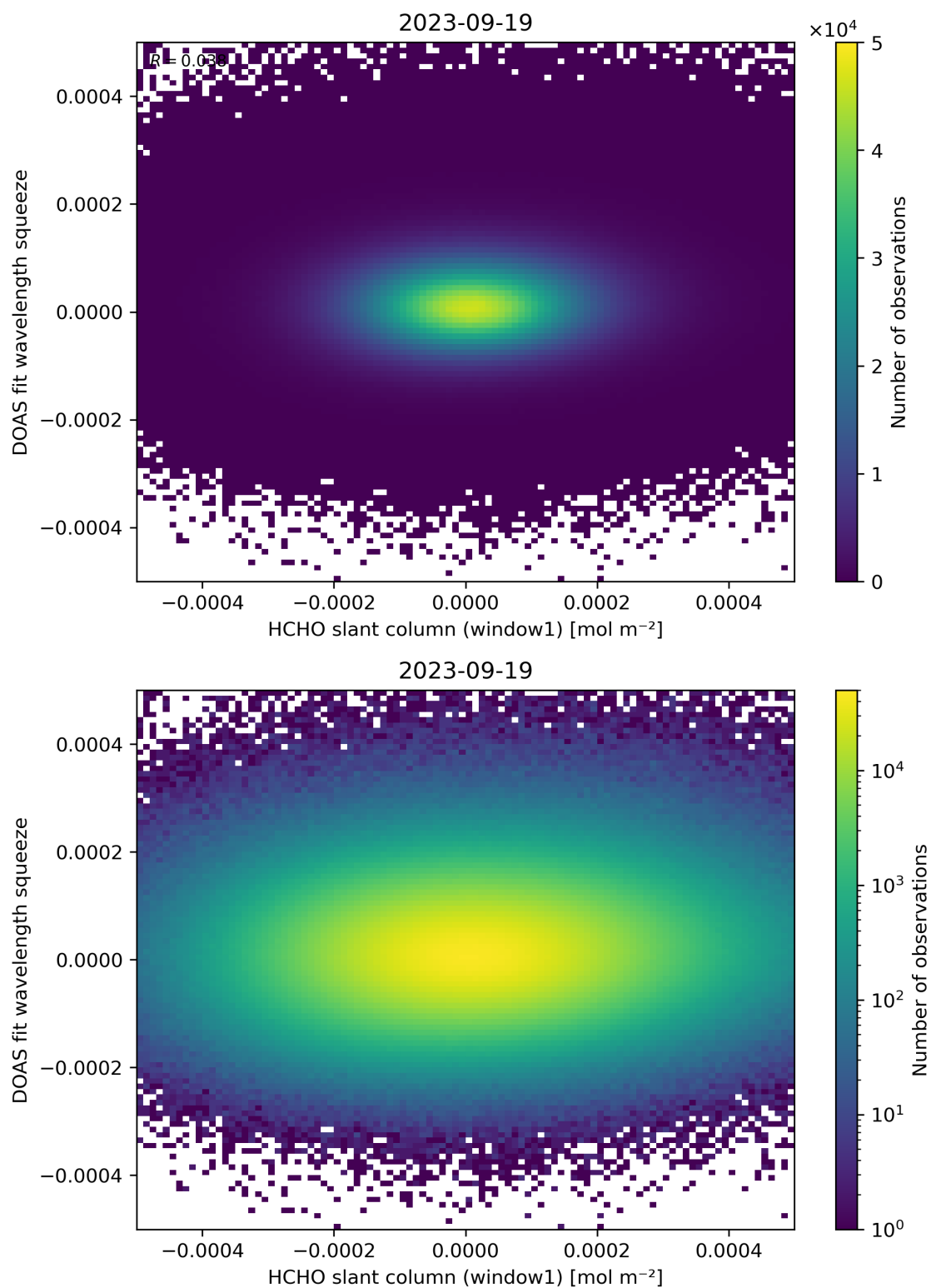
Figure 80: Scatter density plot of “HCHO slant column (window1)” against “DOAS fit wavelength squeeze” for 2023-09-18 to 2023-09-20.
