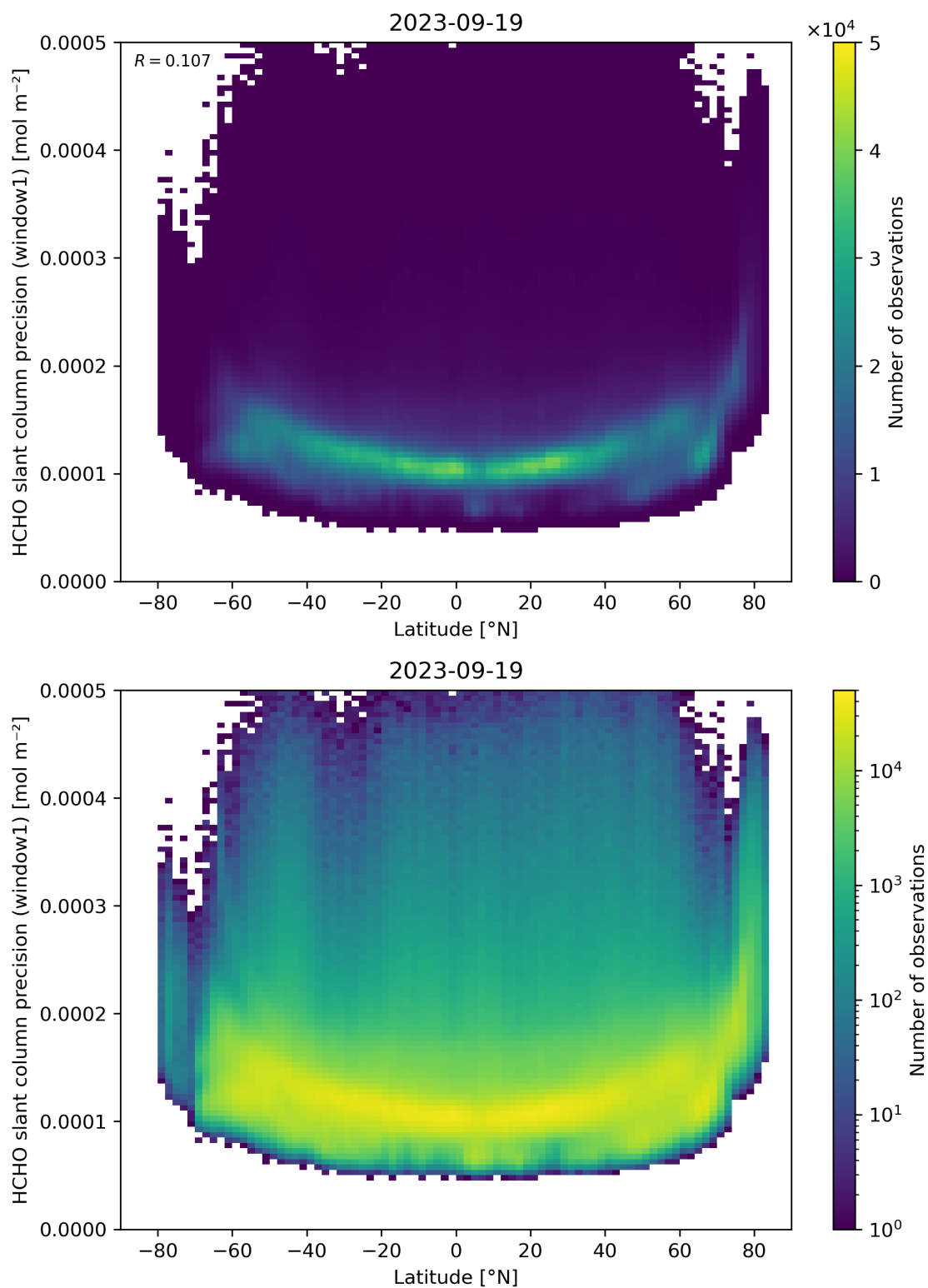
Figure 160: Scatter density plot of “Latitude” against “HCHO slant column precision (window1)” for 2023-09-18 to 2023-09-20.
