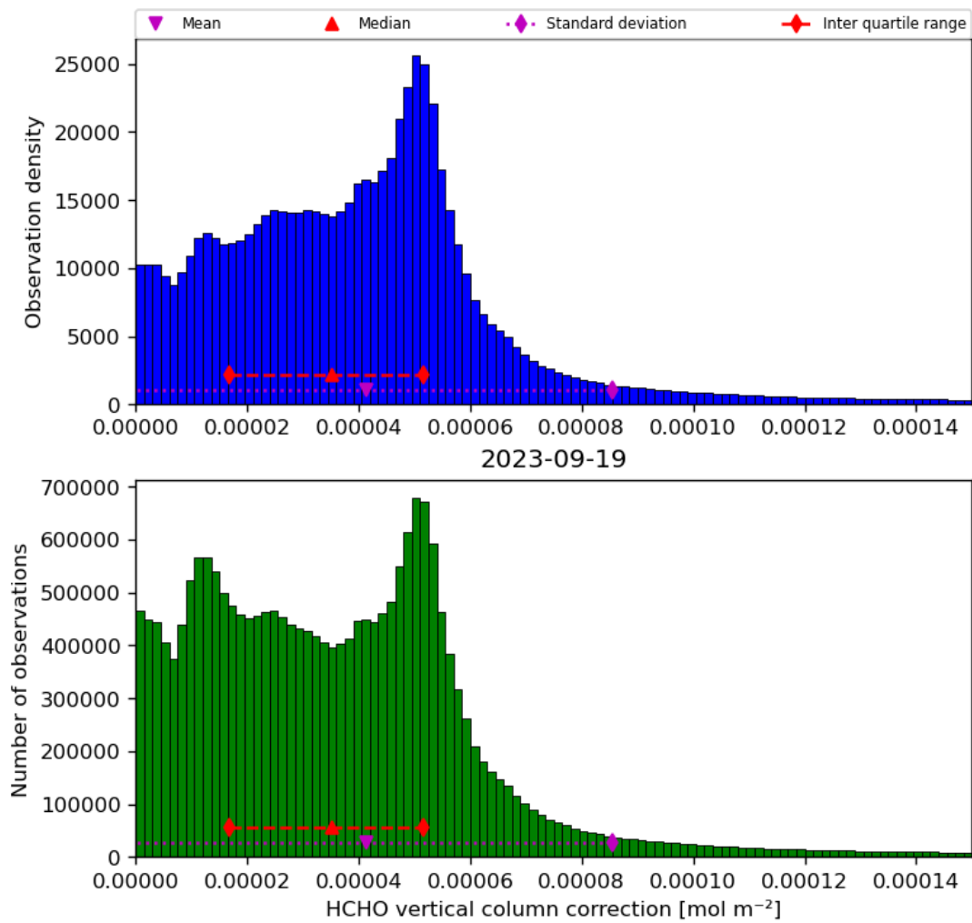
Figure 37: Histogram of “HCHO vertical column correction” for 2023-09-18 to 2023-09-20
