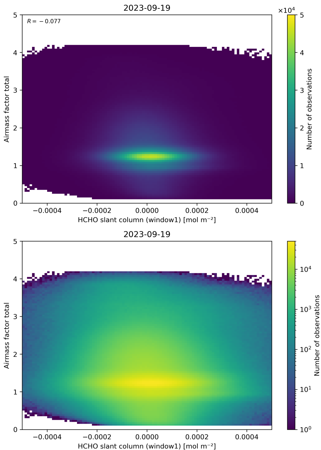
Figure 85: Scatter density plot of “HCHO slant column (window1)” against “Airmass factor total” for 2023-09-18 to 2023-09-20.
