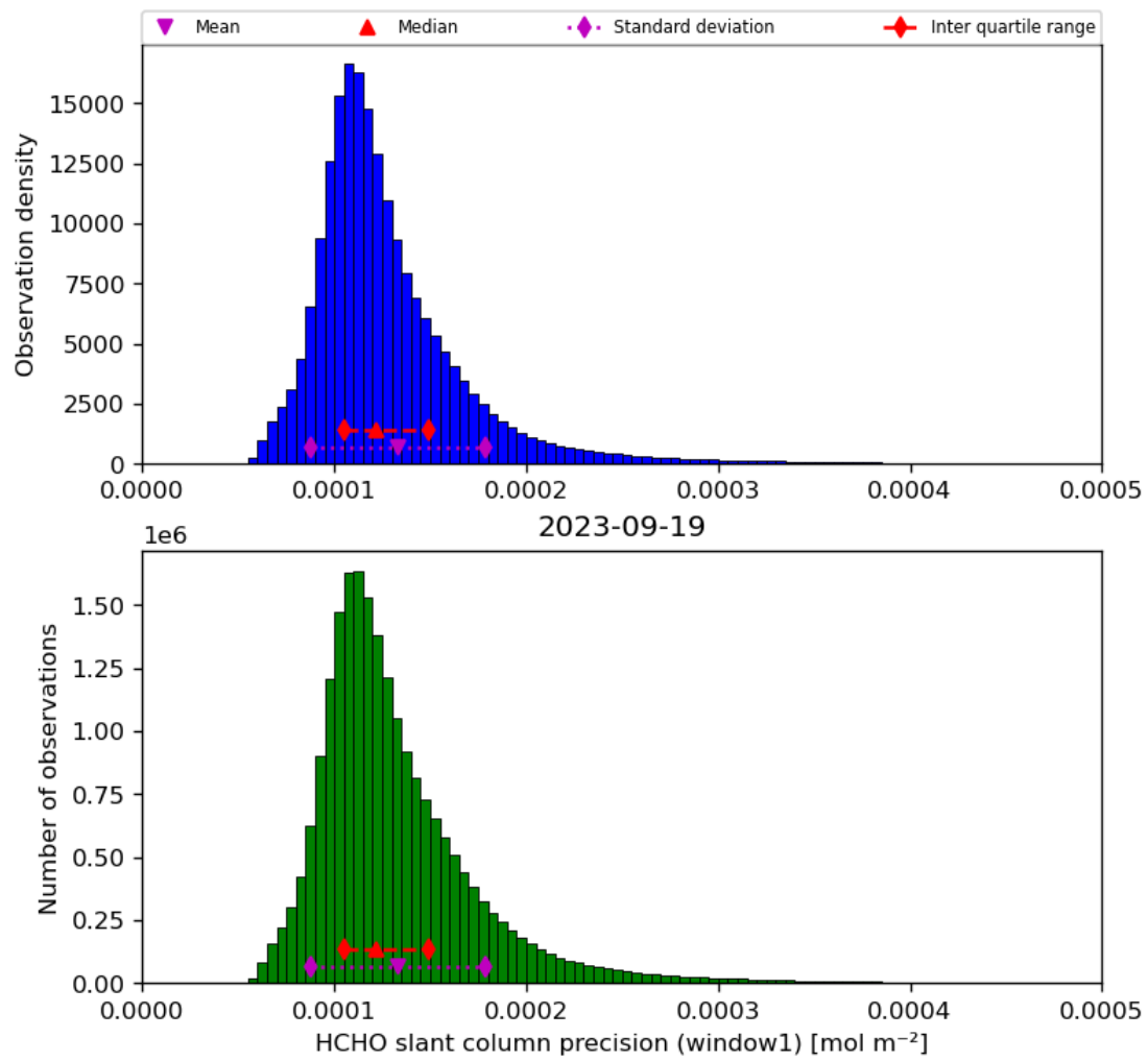
Figure 39: Histogram of “HCHO slant column precision (window1)” for 2023-09-18 to 2023-09-20
