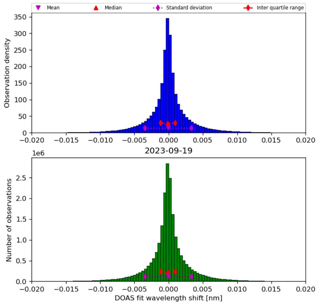
Figure 44: Histogram of “DOAS fit wavelength shift” for 2023-09-18 to 2023-09-20
