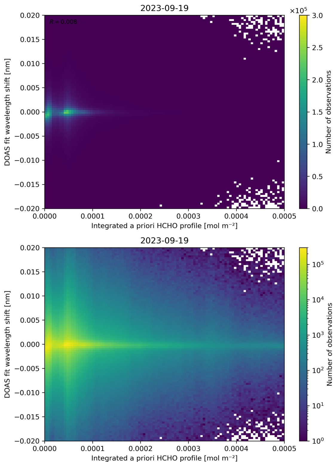
Figure 149: Scatter density plot of “Integrated a priori HCHO profile” against “DOAS fit wavelength shift” for 2023-09-18 to 2023-09-20.
