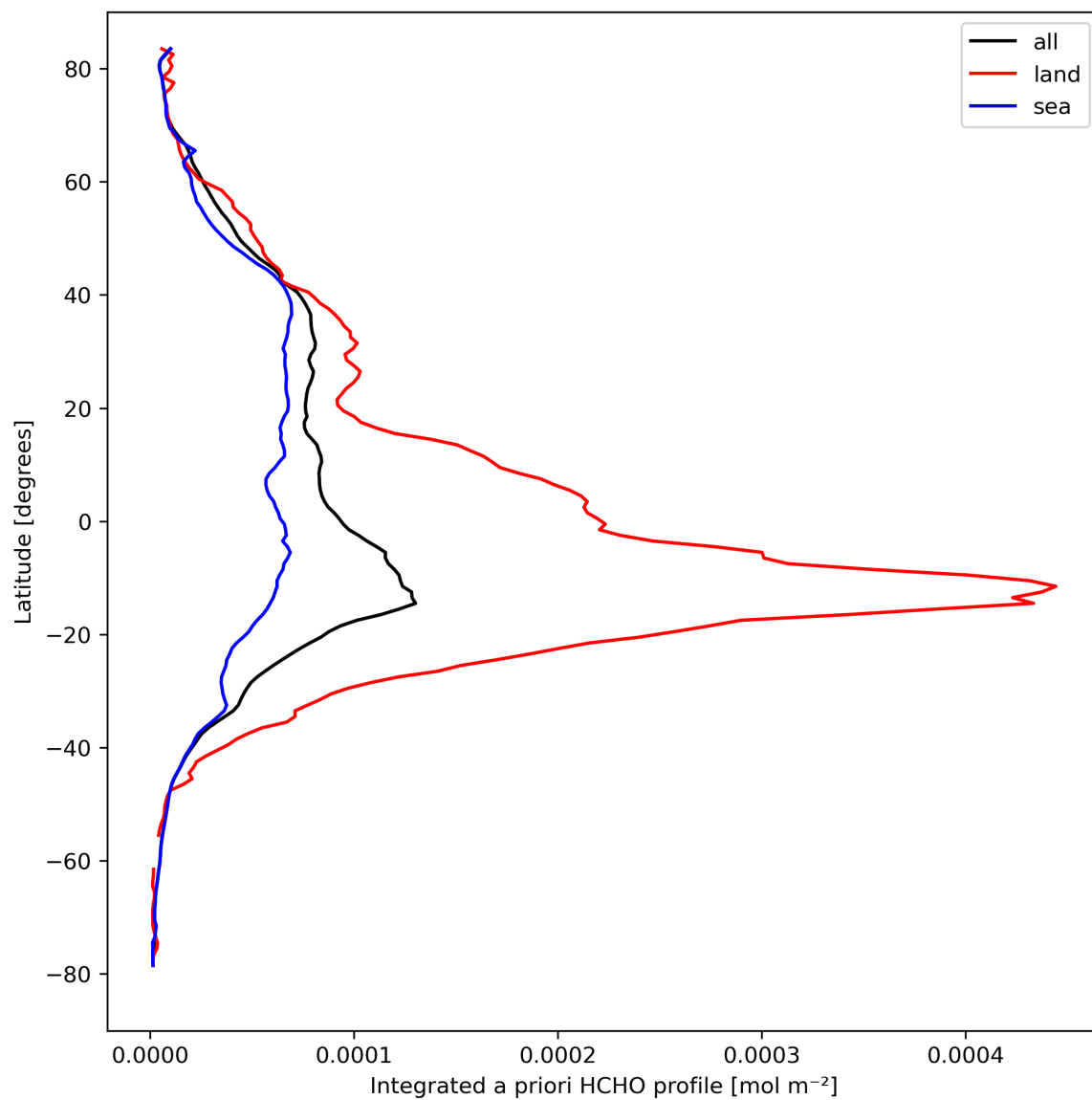
Figure 29: Zonal average of “Integrated a priori HCHO profile” for 2023-09-18 to 2023-09-20.
