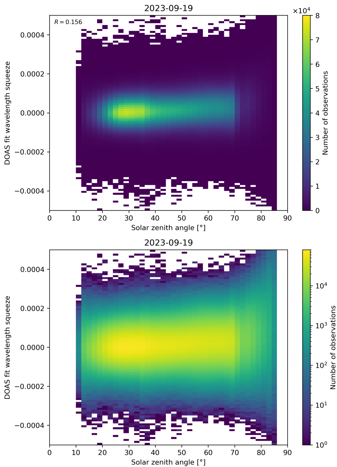
Figure 169: Scatter density plot of “Solar zenith angle” against “DOAS fit wavelength squeeze” for 2023-09-18 to 2023-09-20.
