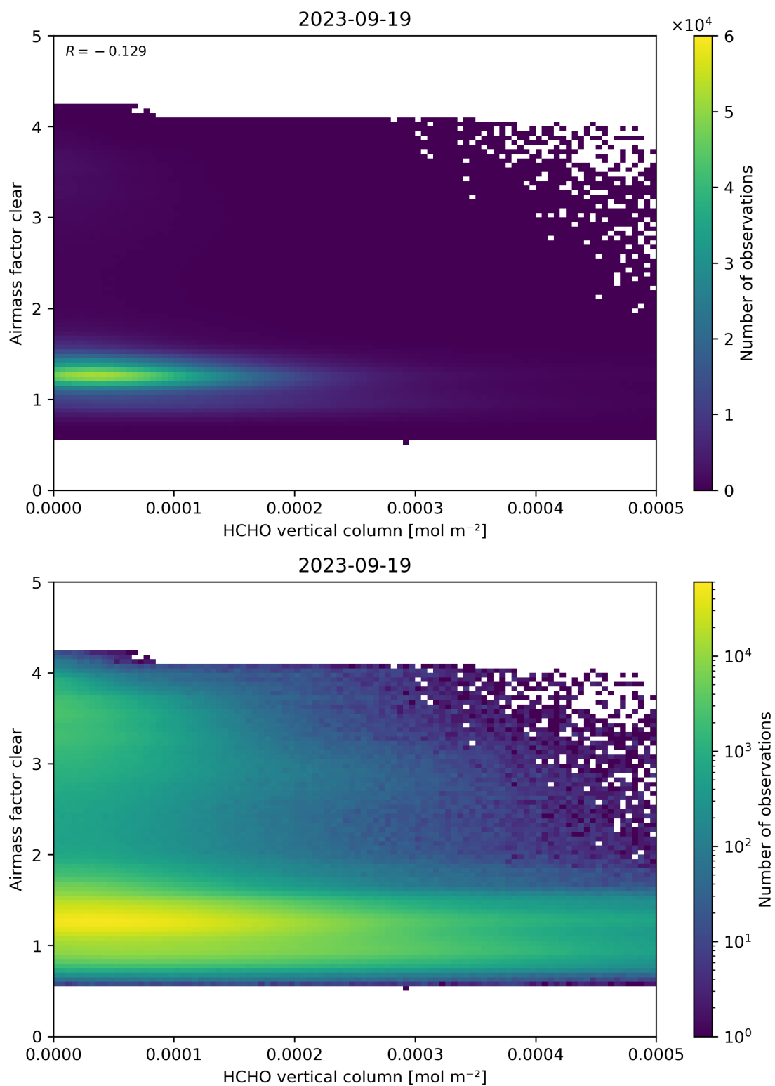
Figure 126: Scatter density plot of “HCHO vertical column” against “Airmass factor clear” for 2023-09-18 to 2023-09-20.
