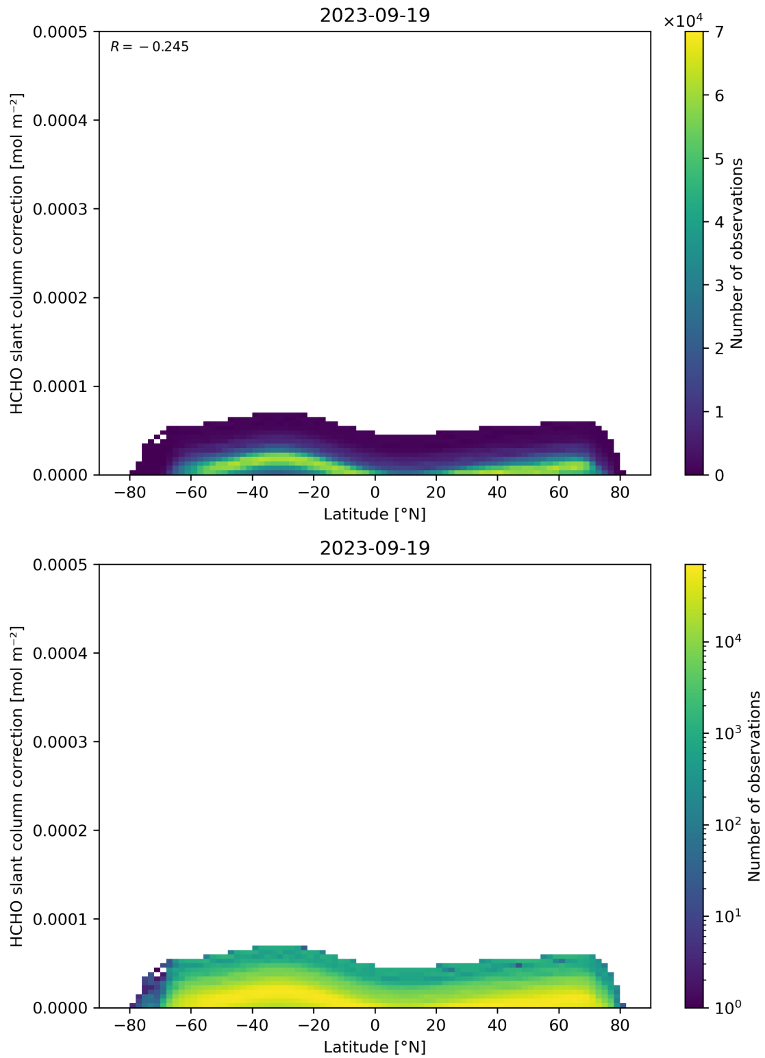
Figure 158: Scatter density plot of “Latitude” against “HCHO slant column correction” for 2023-09-18 to 2023-09-20.
