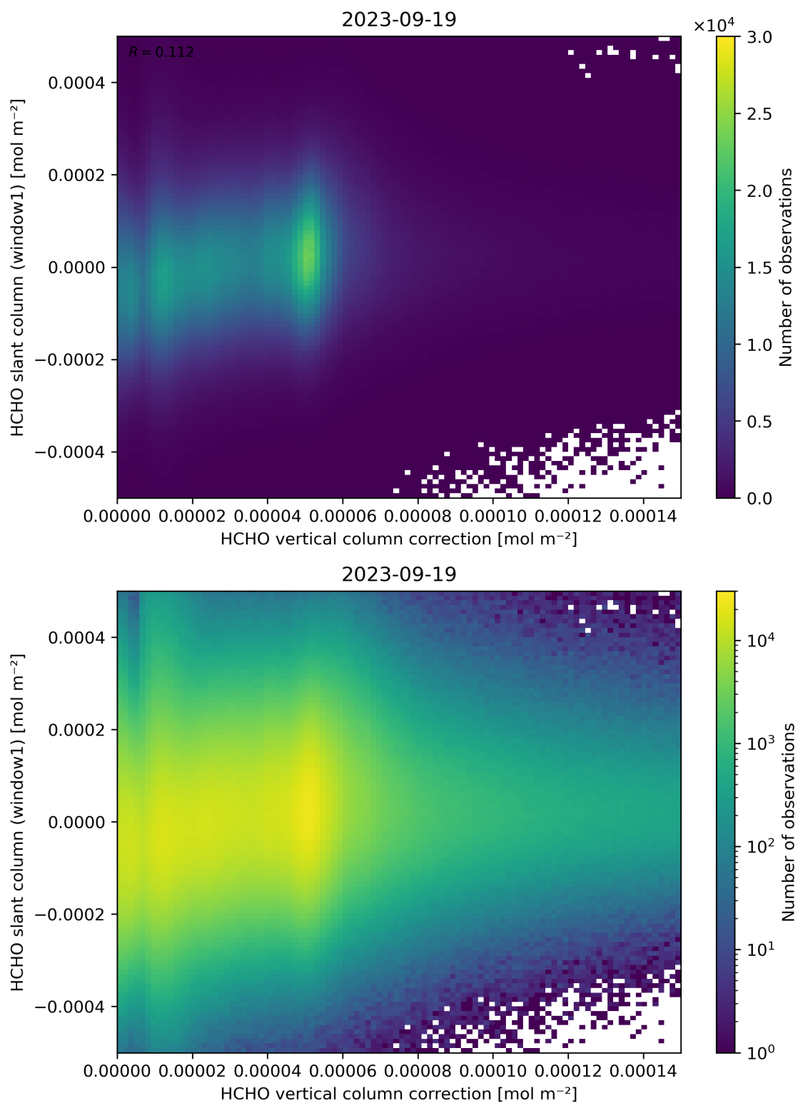
Figure 118: Scatter density plot of “HCHO vertical column correction” against “HCHO slant column (window1)” for 2023-09-18 to 2023-09-20.
