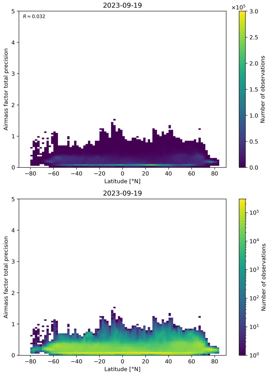
Figure 162: Scatter density plot of “Latitude” against “Airmass factor total precision” for 2023-09-18 to 2023-09-20.
