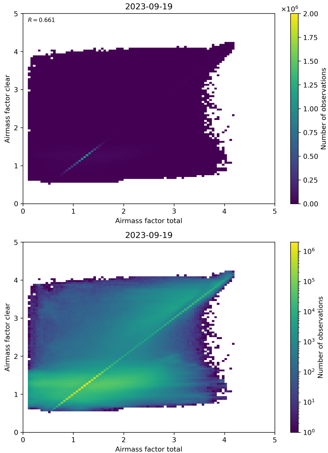
Figure 100: Scatter density plot of “Airmass factor total” against “Airmass factor clear” for 2023-09-18 to 2023-09-20.
