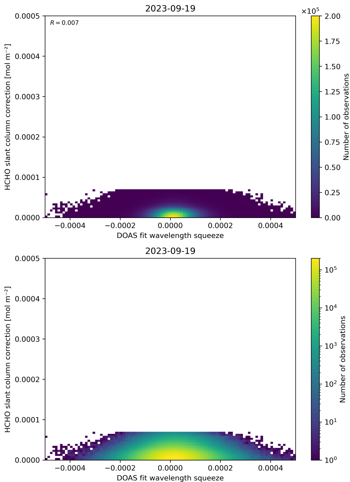
Figure 70: Scatter density plot of “DOAS fit wavelength squeeze” against “HCHO slant column correction” for 2023-09-18 to 2023-09-20.
