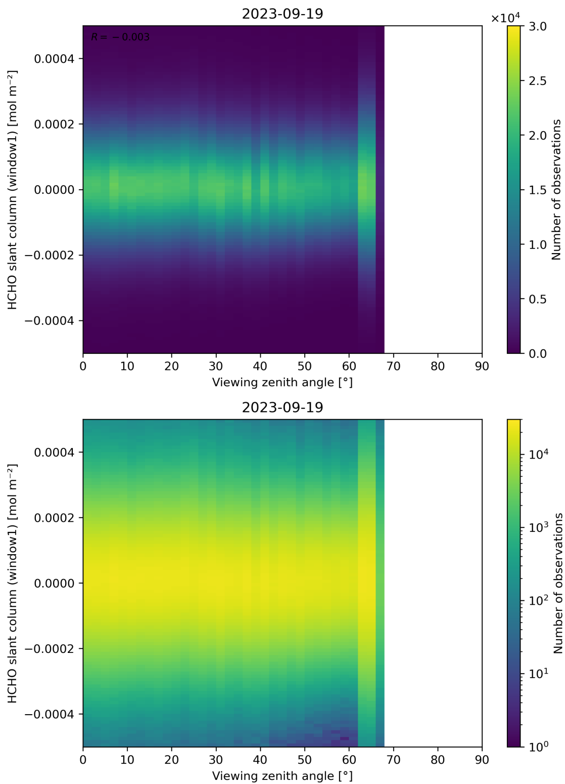
Figure 188: Scatter density plot of “Viewing zenith angle” against “HCHO slant column (window1)” for 2023-09-18 to 2023-09-20.
