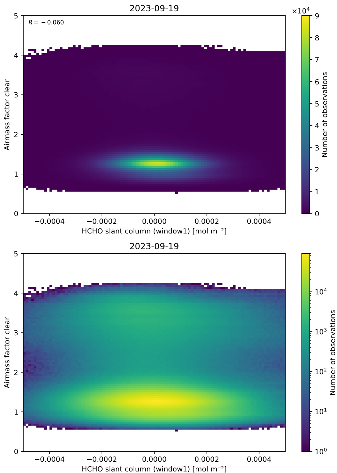
Figure 81: Scatter density plot of “HCHO slant column (window1)” against “Airmass factor clear” for 2023-09-18 to 2023-09-20.
