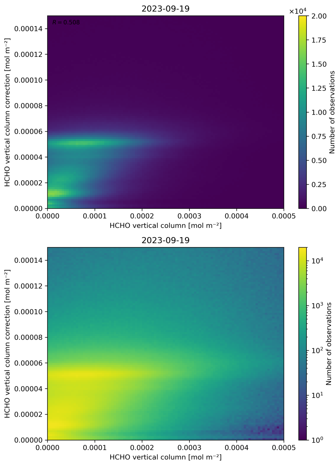
Figure 133: Scatter density plot of “HCHO vertical column” against “HCHO vertical column correction” for 2023-09-18 to 2023-09-20.
