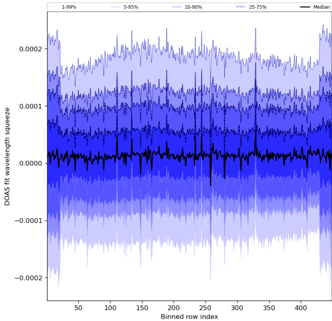
Figure 59: Along track statistics of “DOAS fit wavelength squeeze” for 2023-09-18 to 2023-09-20
