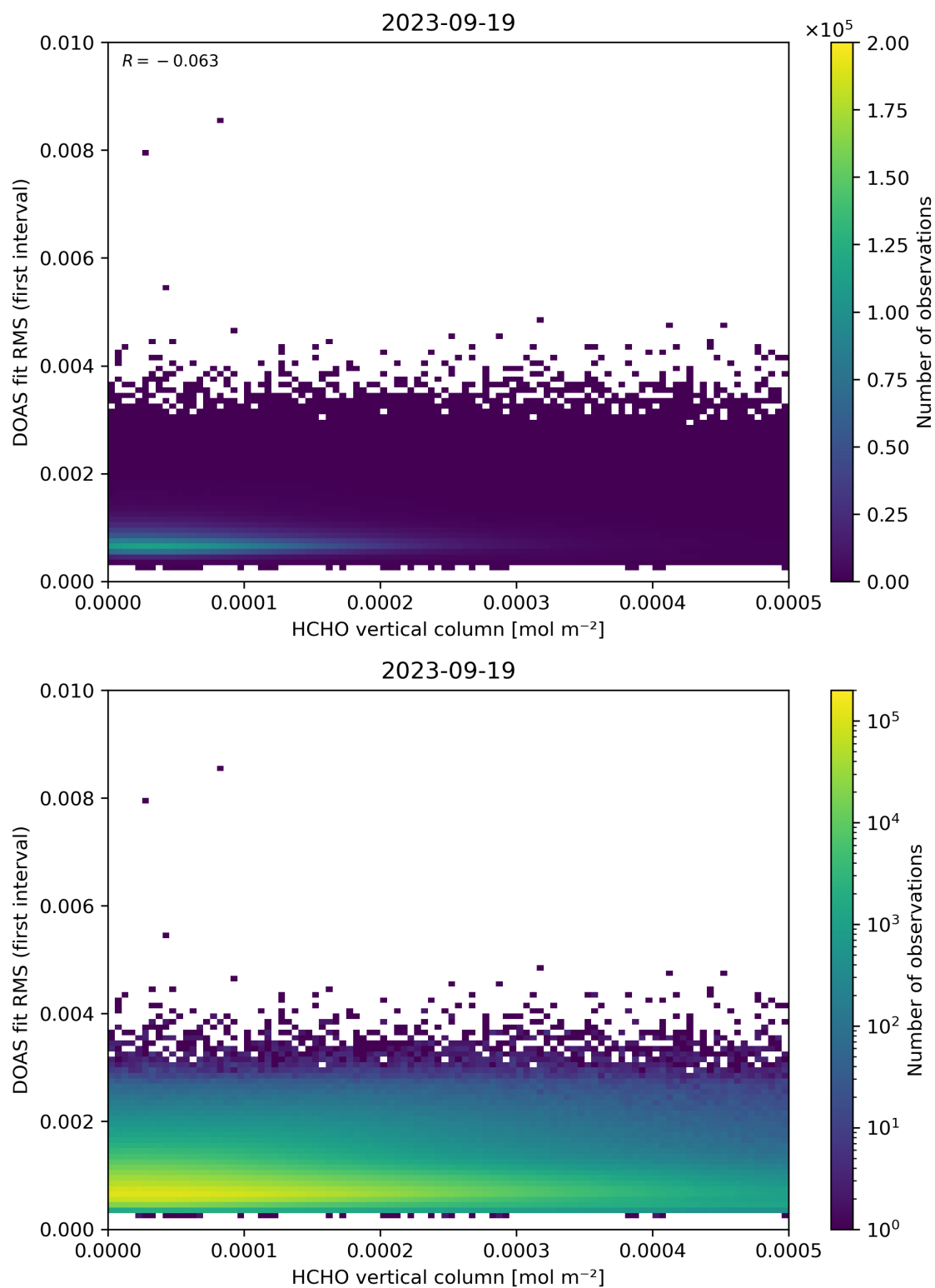
Figure 123: Scatter density plot of “HCHO vertical column” against “DOAS fit RMS (first interval)” for 2023-09-18 to 2023-09-20.
