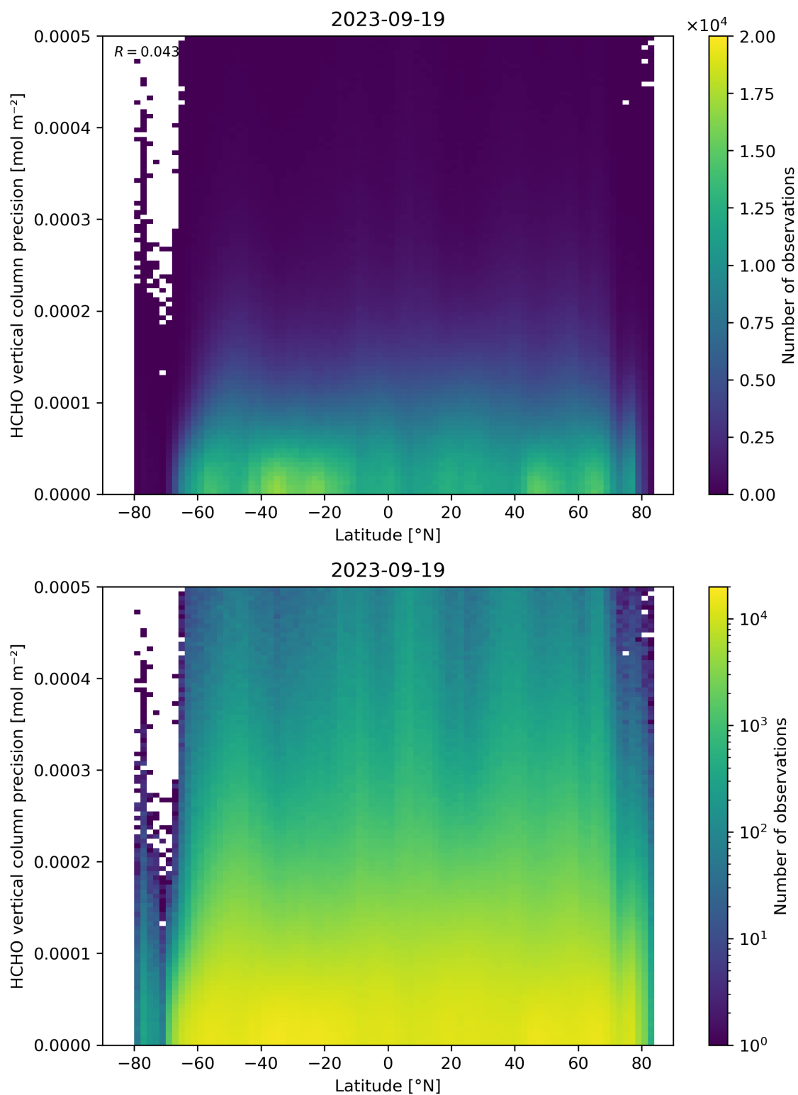
Figure 165: Scatter density plot of “Latitude” against “HCHO vertical column precision” for 2023-09-18 to 2023-09-20.
