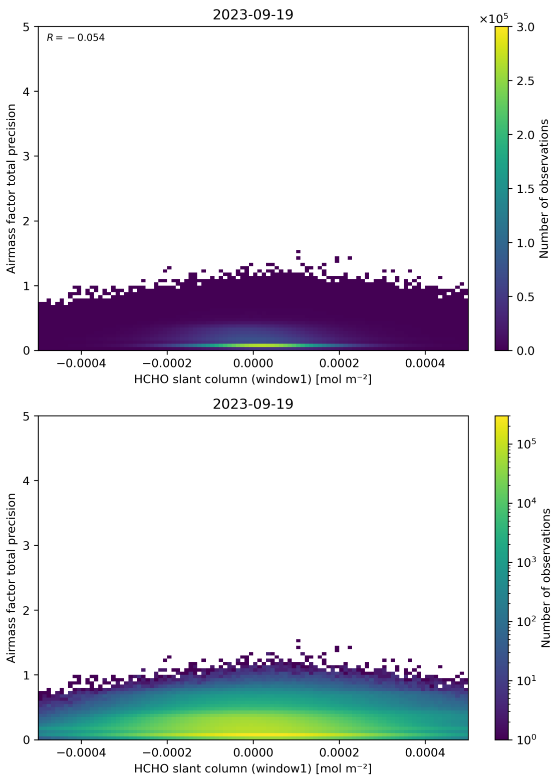
Figure 86: Scatter density plot of “HCHO slant column (window1)” against “Airmass factor total precision” for 2023-09-18 to 2023-09-20.
