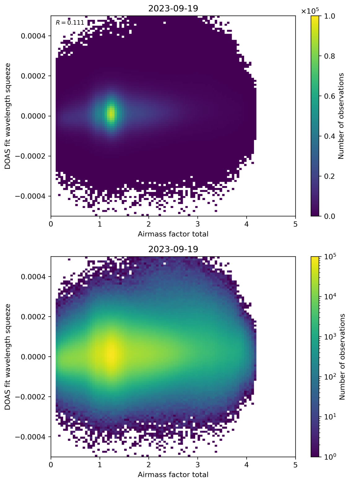
Figure 99: Scatter density plot of “Airmass factor total” against “DOAS fit wavelength squeeze” for 2023-09-18 to 2023-09-20.
