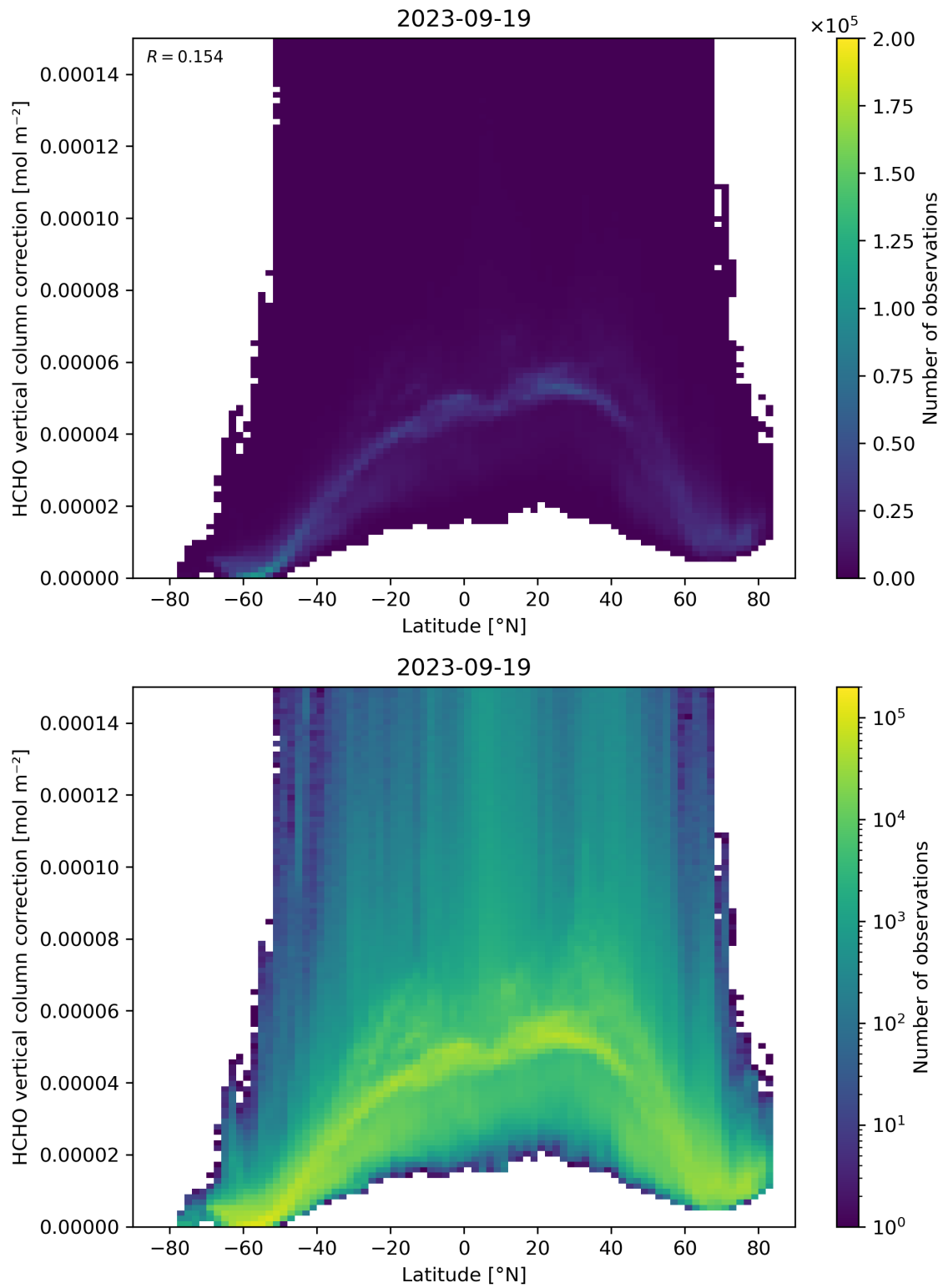
Figure 164: Scatter density plot of “Latitude” against “HCHO vertical column correction” for 2023-09-18 to 2023-09-20.
