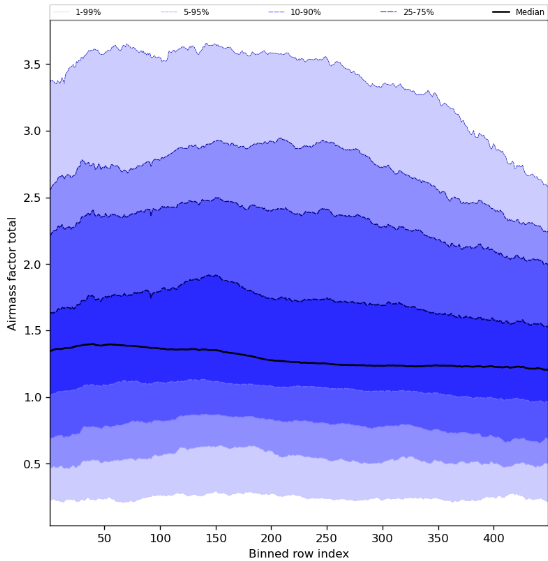
Figure 54: Along track statistics of “Airmass factor total” for 2023-09-18 to 2023-09-20
