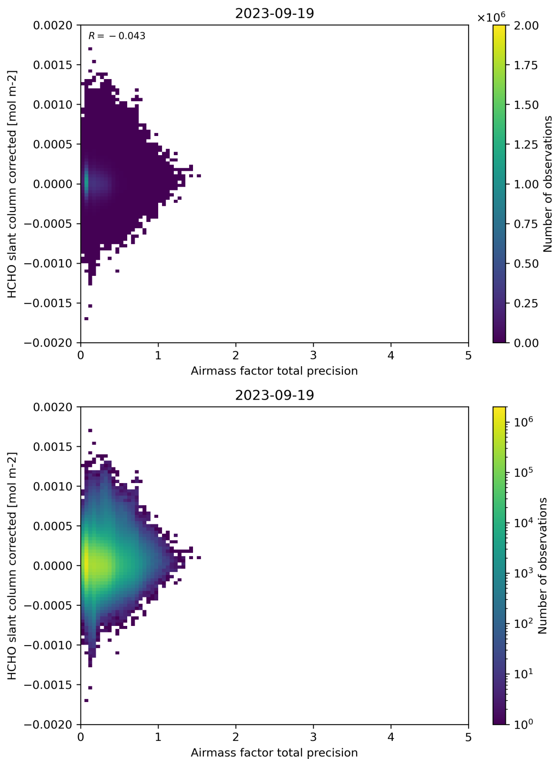
Figure 109: Scatter density plot of “Airmass factor total precision” against “HCHO slant column corrected” for 2023-09-18 to 2023-09-20.
