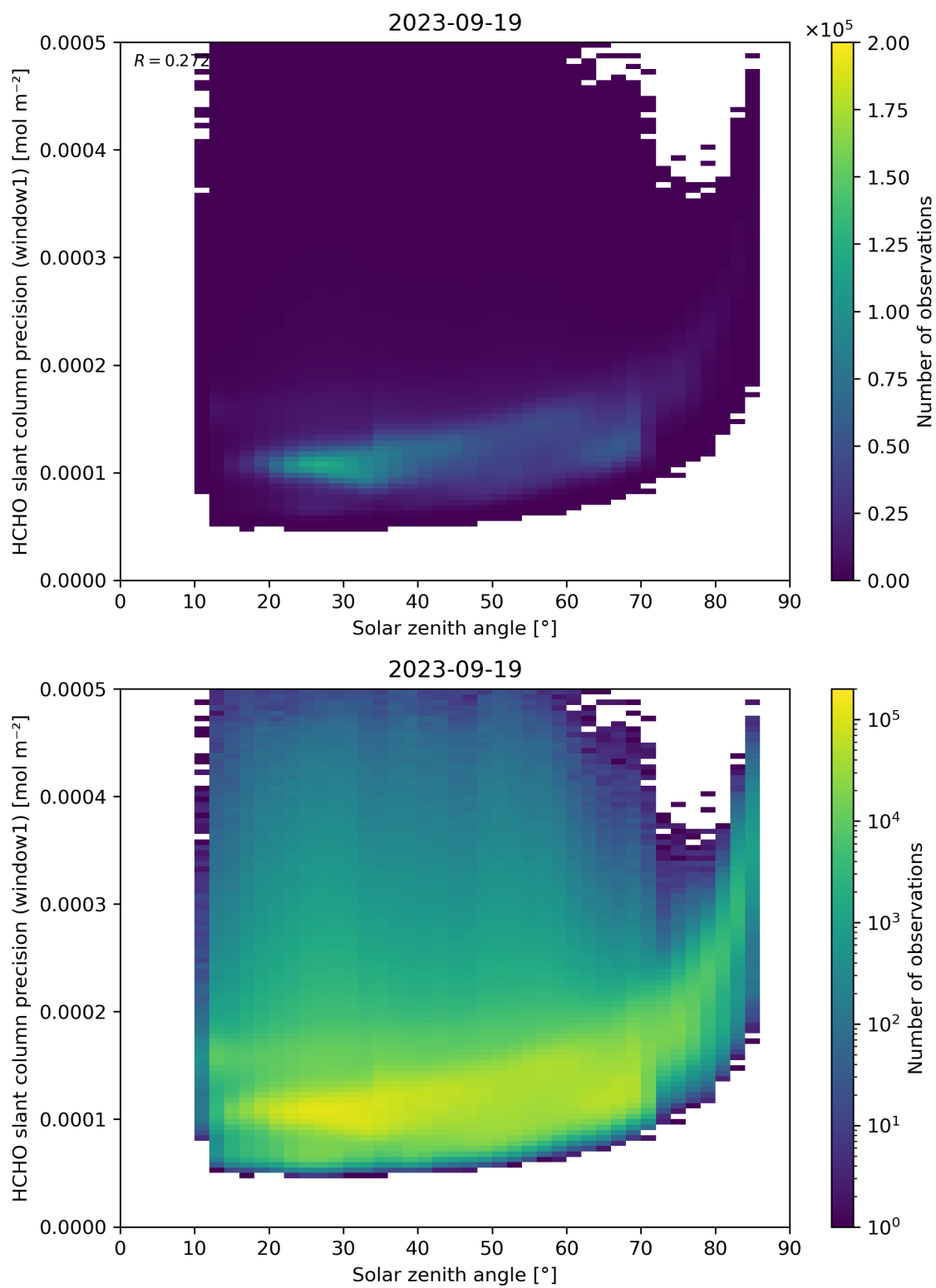
Figure 174: Scatter density plot of “Solar zenith angle” against “HCHO slant column precision (window1)” for 2023-09-18 to 2023-09-20.
