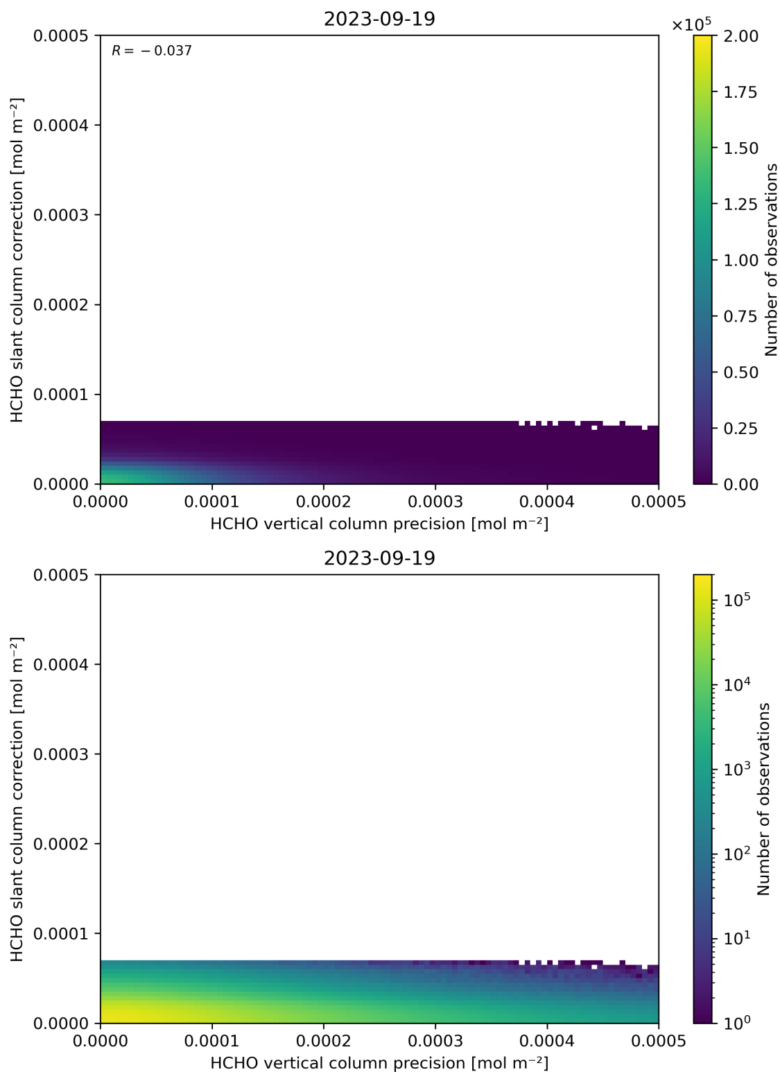
Figure 141: Scatter density plot of “HCHO vertical column precision” against “HCHO slant column correction” for 2023-09-18 to 2023-09-20.
