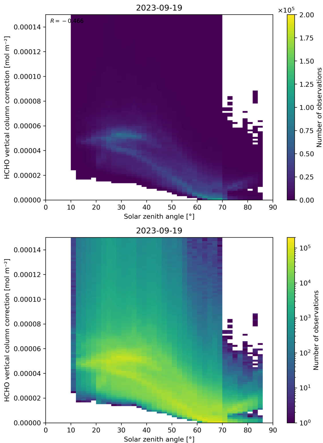
Figure 178: Scatter density plot of “Solar zenith angle” against “HCHO vertical column correction” for 2023-09-18 to 2023-09-20.
