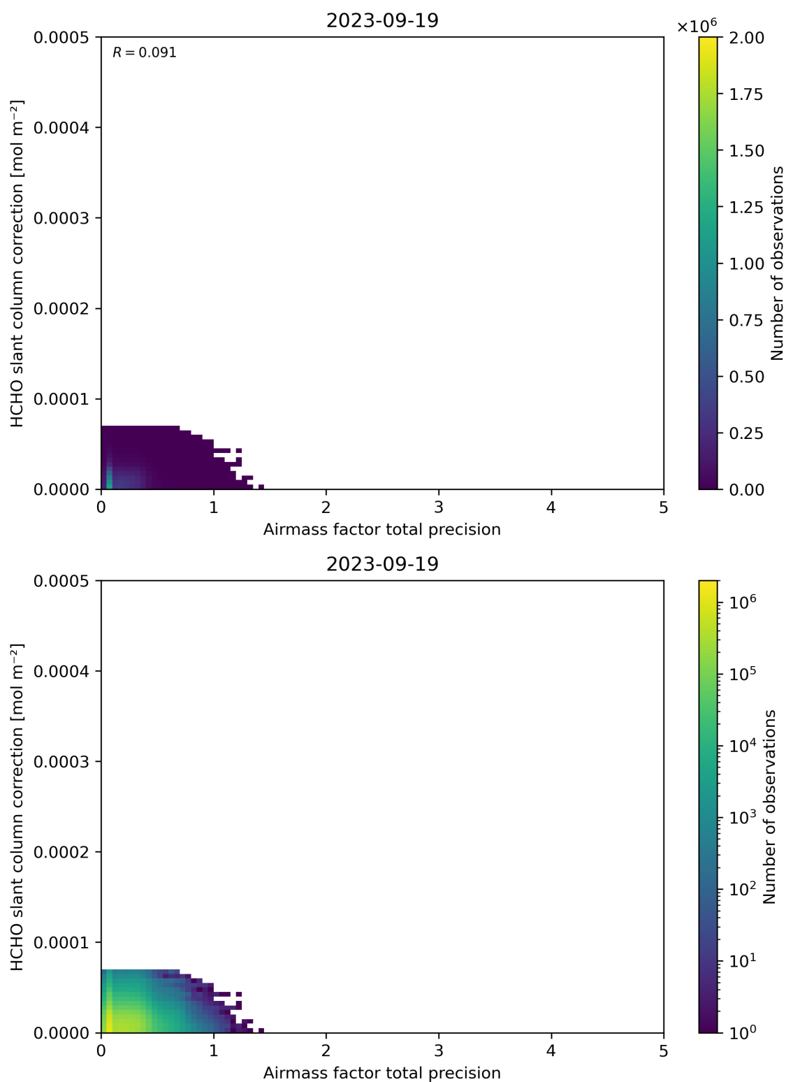
Figure 110: Scatter density plot of “Airmass factor total precision” against “HCHO slant column correction” for 2023-09-18 to 2023-09-20.
