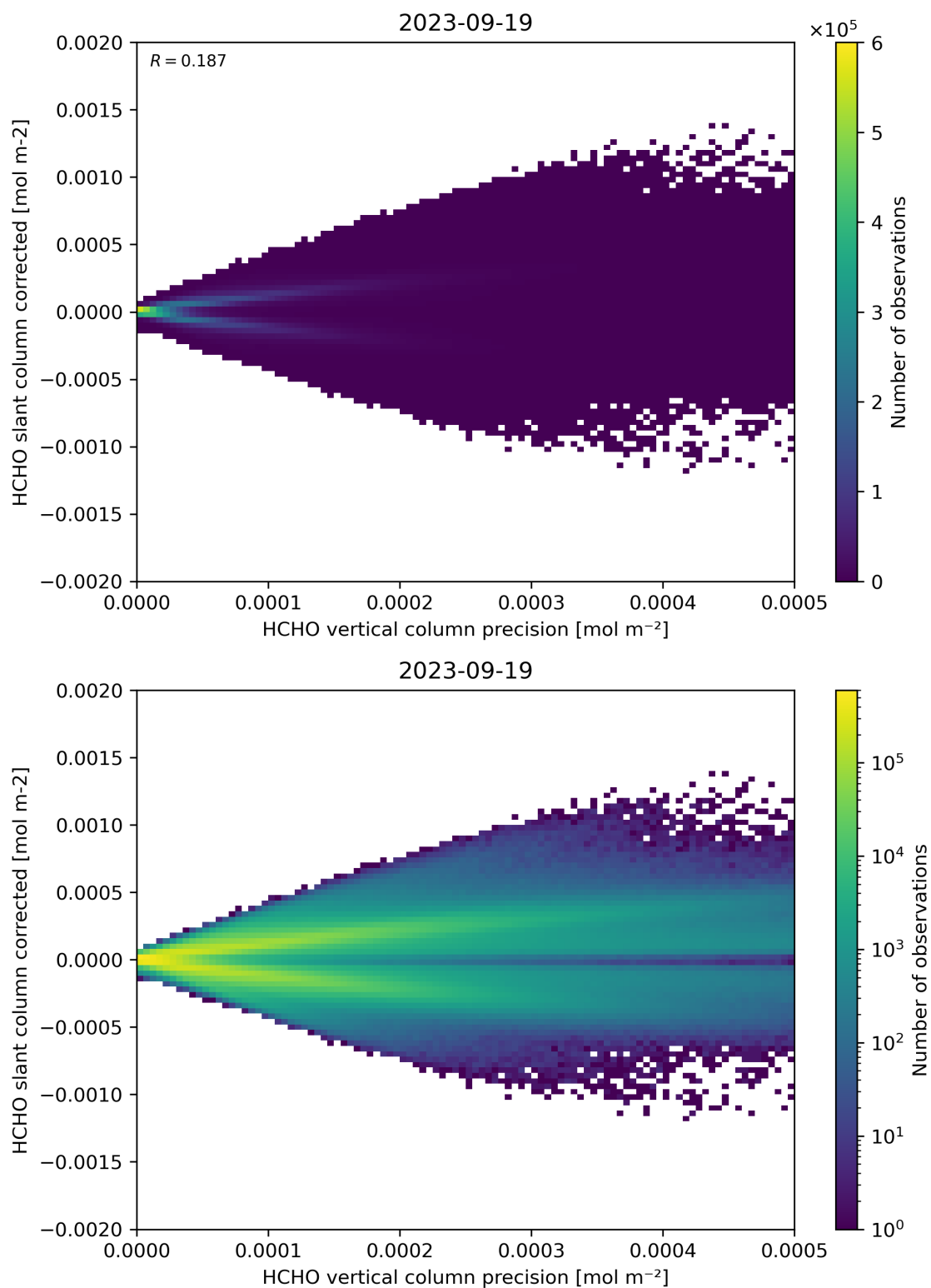
Figure 140: Scatter density plot of “HCHO vertical column precision” against “HCHO slant column corrected” for 2023-09-18 to 2023-09-20.
