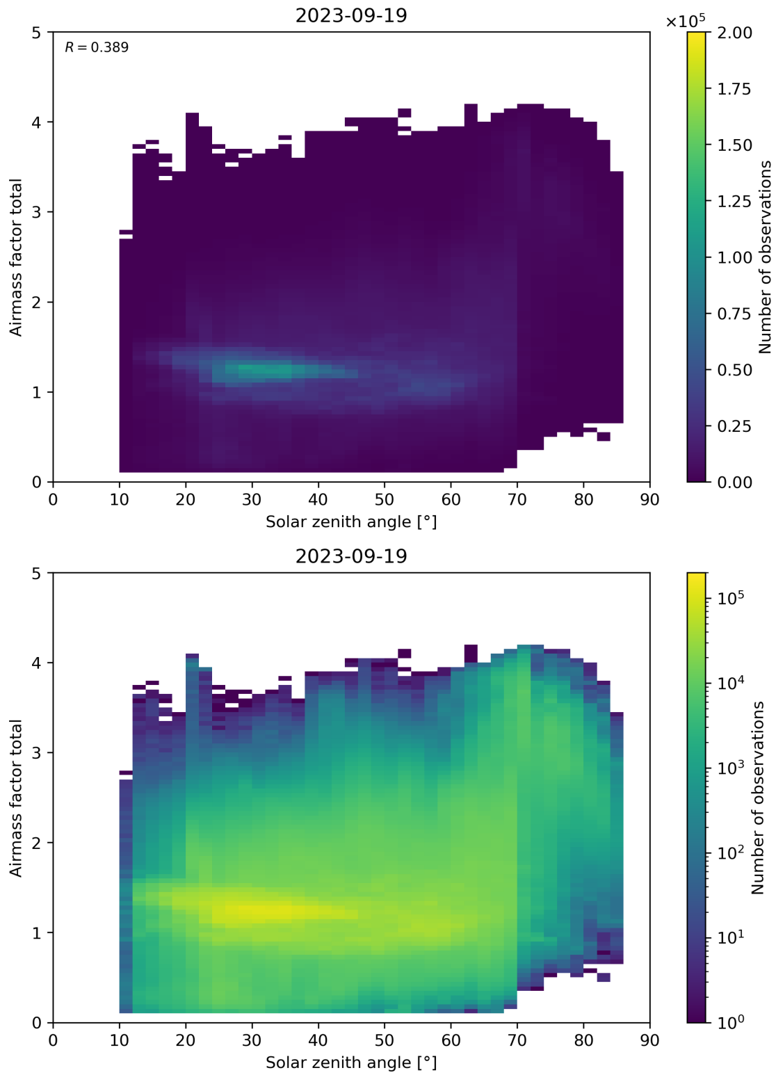
Figure 175: Scatter density plot of “Solar zenith angle” against “Airmass factor total” for 2023-09-18 to 2023-09-20.
