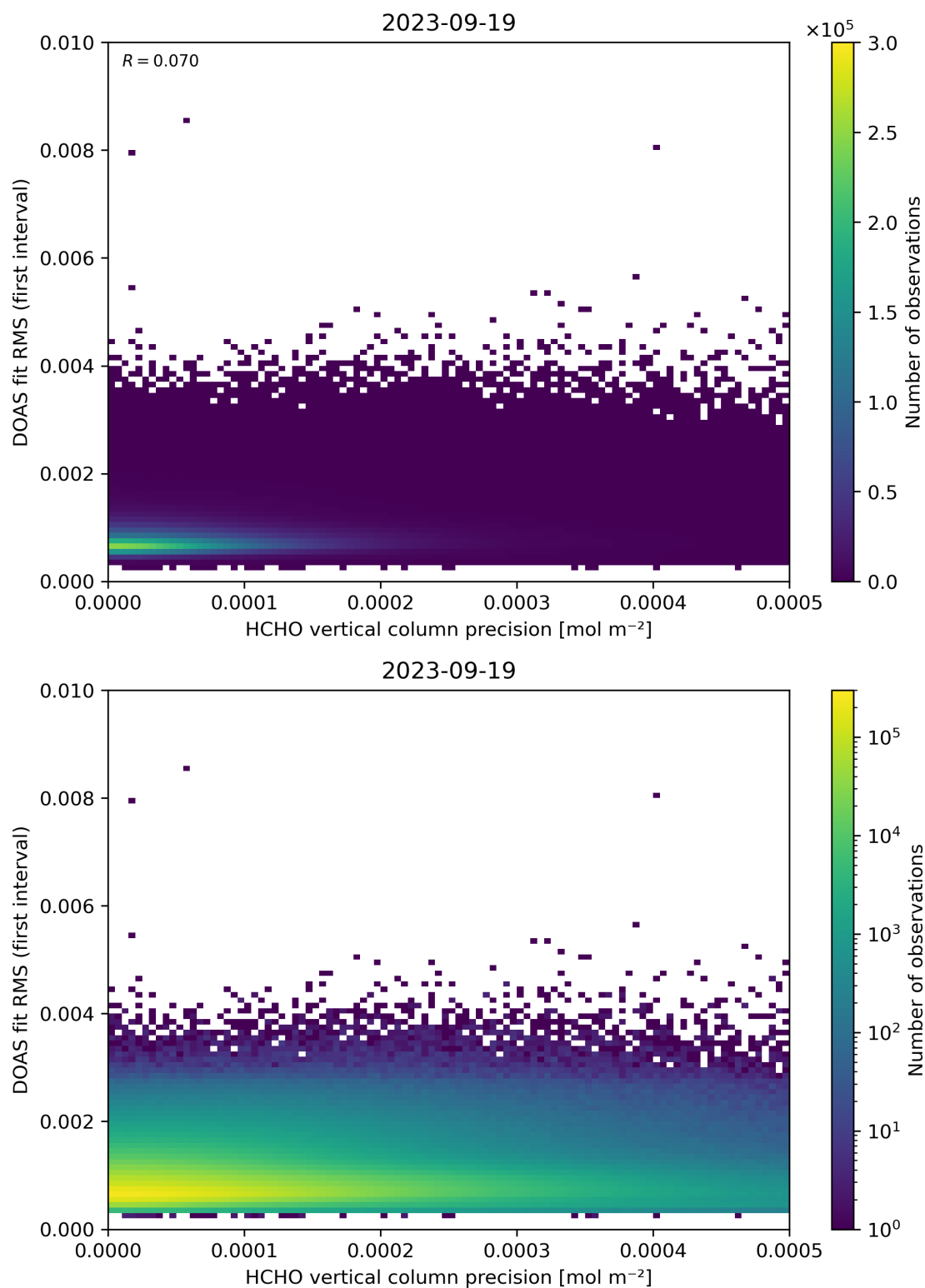
Figure 136: Scatter density plot of “HCHO vertical column precision” against “DOAS fit RMS (first interval)” for 2023-09-18 to 2023-09-20.
