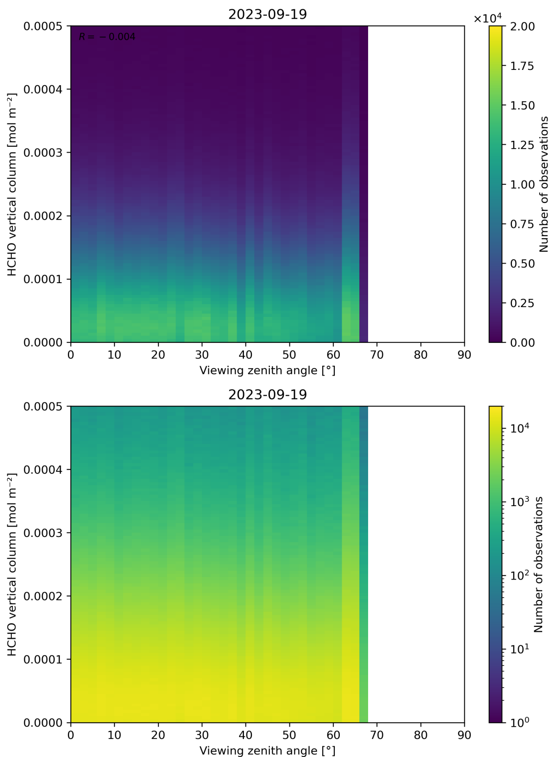
Figure 192: Scatter density plot of “Viewing zenith angle” against “HCHO vertical column” for 2023-09-18 to 2023-09-20.
