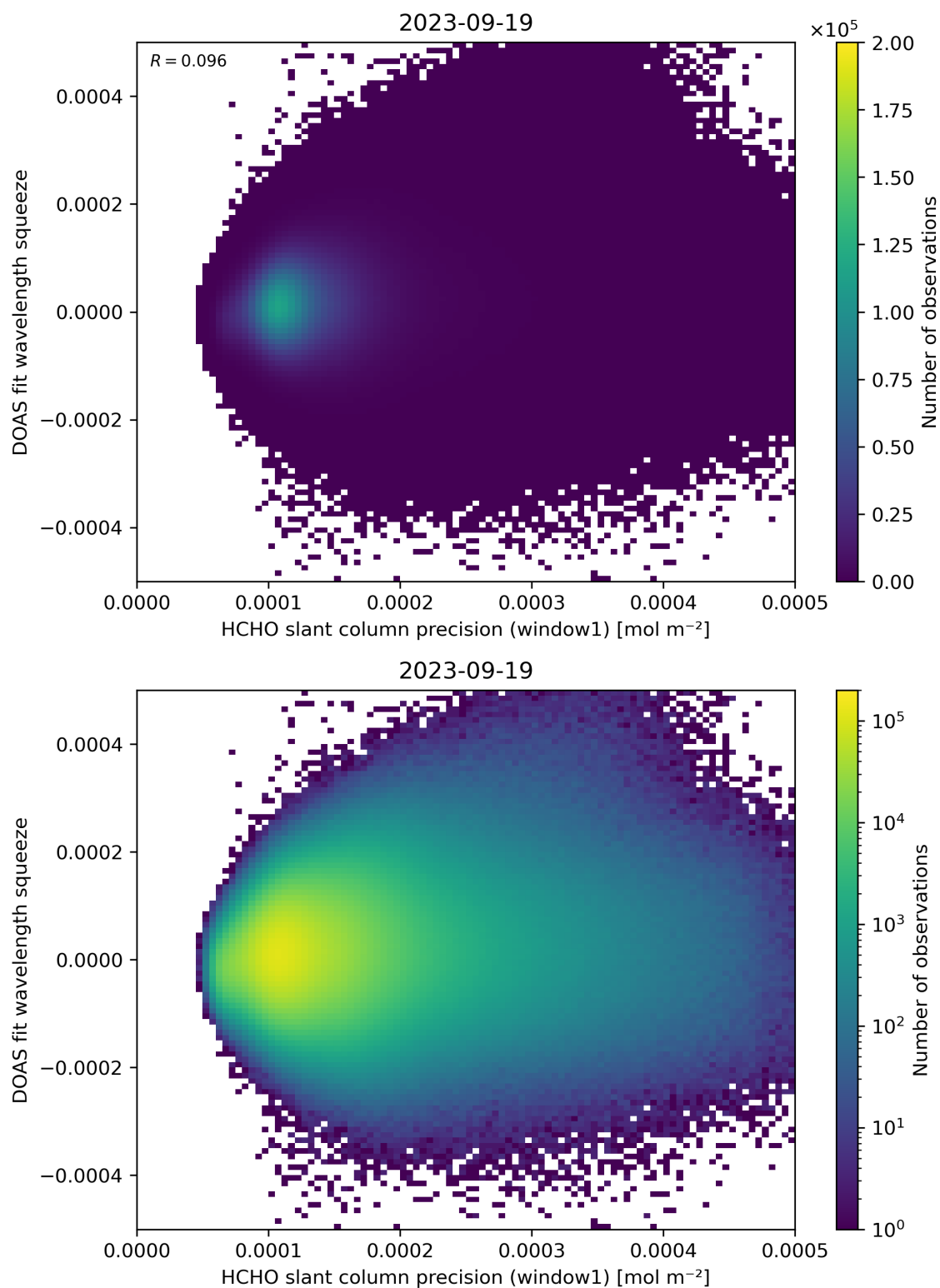
Figure 90: Scatter density plot of “HCHO slant column precision (window1)” against “DOAS fit wavelength squeeze” for 2023-09-18 to 2023-09-20.
