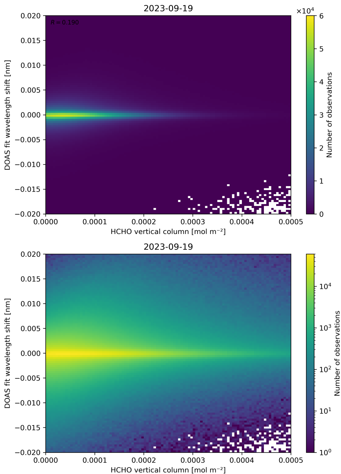
Figure 124: Scatter density plot of “HCHO vertical column” against “DOAS fit wavelength shift” for 2023-09-18 to 2023-09-20.
