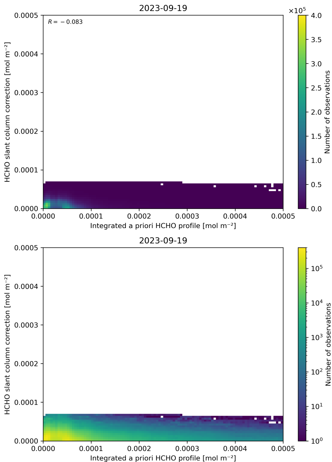
Figure 152: Scatter density plot of “Integrated a priori HCHO profile” against “HCHO slant column correction” for 2023-09-18 to 2023-09-20.
