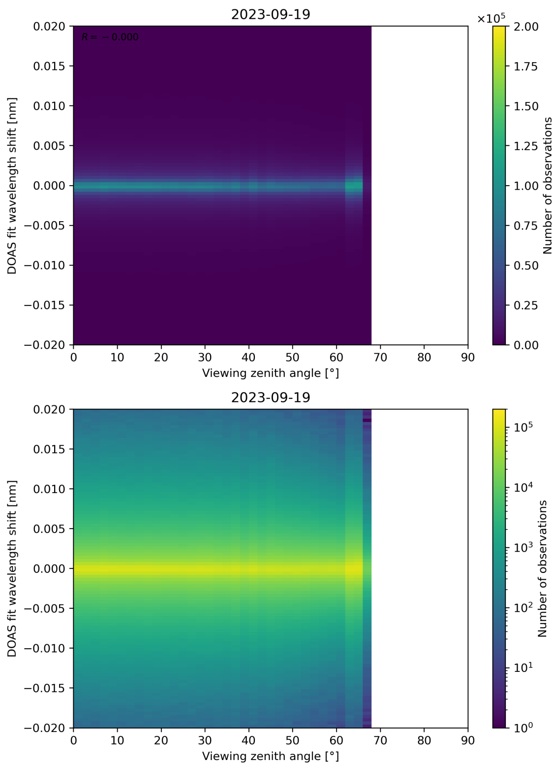
Figure 183: Scatter density plot of “Viewing zenith angle” against “DOAS fit wavelength shift” for 2023-09-18 to 2023-09-20.
