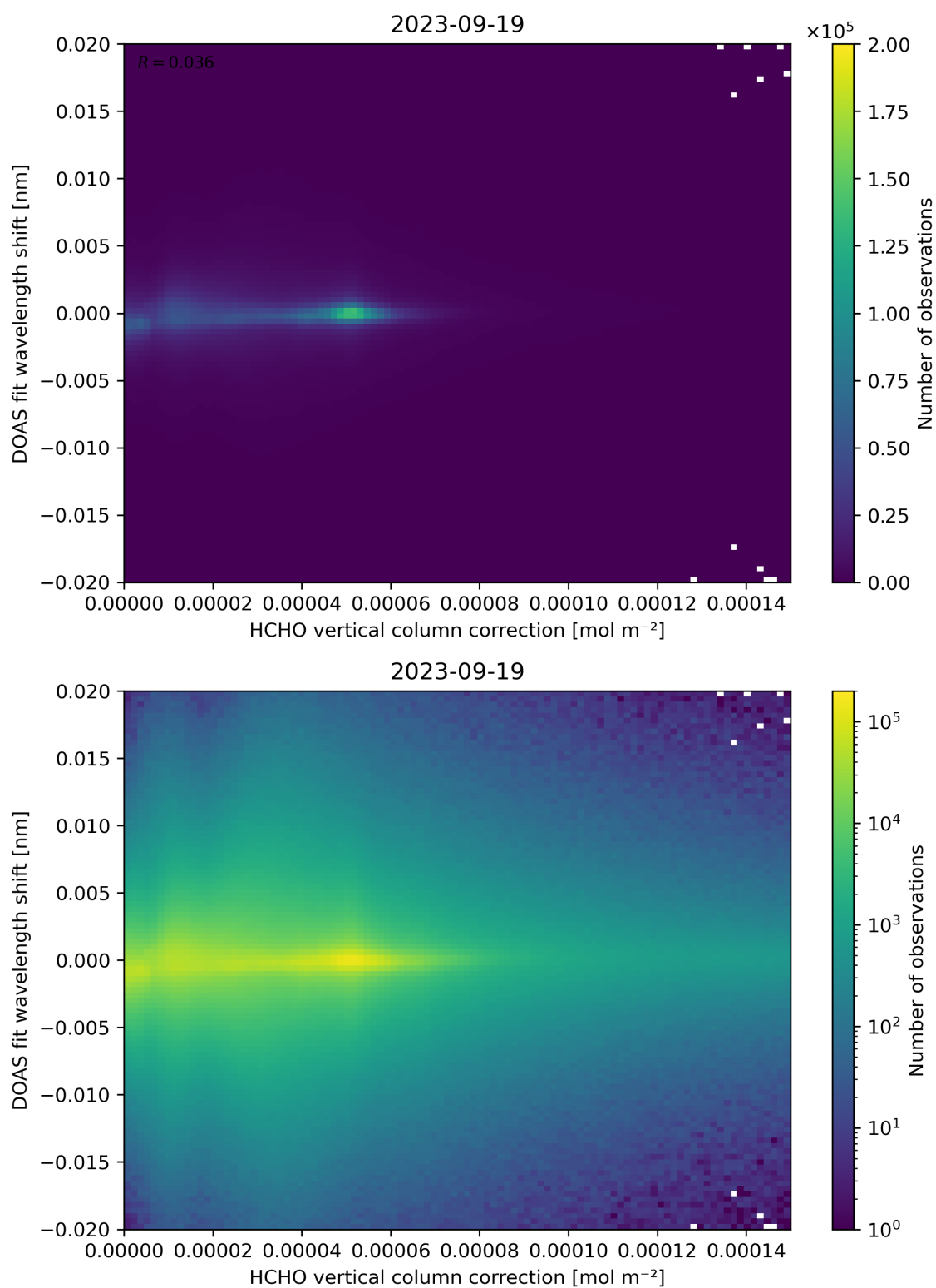
Figure 113: Scatter density plot of “HCHO vertical column correction” against “DOAS fit wavelength shift” for 2023-09-18 to 2023-09-20.
