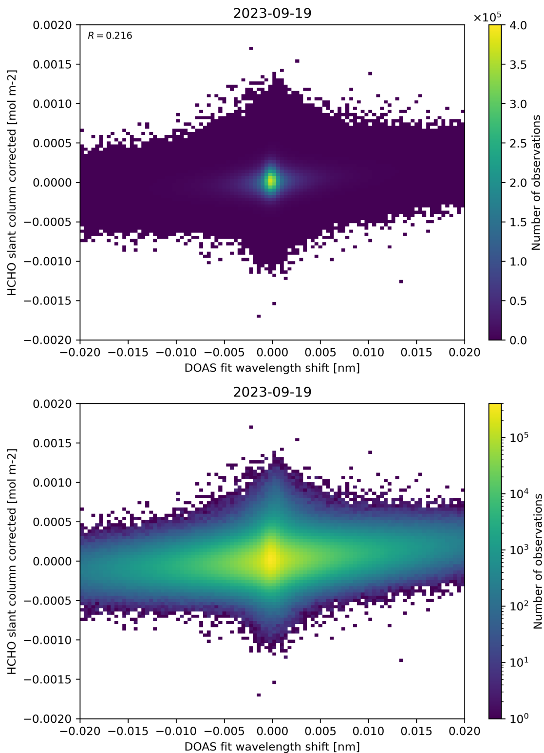
Figure 66: Scatter density plot of “DOAS fit wavelength shift” against “HCHO slant column corrected” for 2023-09-18 to 2023-09-20.
