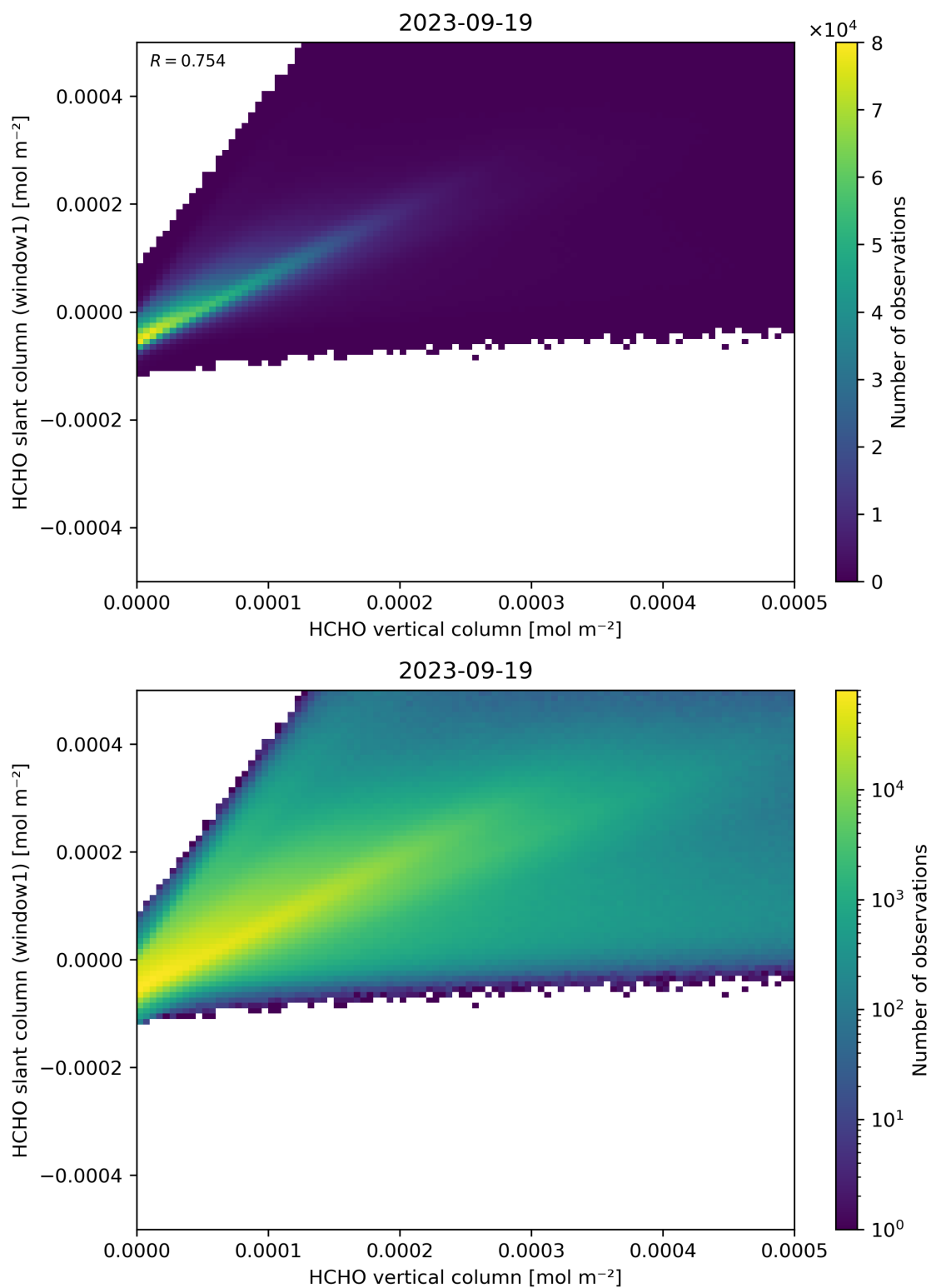
Figure 129: Scatter density plot of “HCHO vertical column” against “HCHO slant column (window1)” for 2023-09-18 to 2023-09-20.
