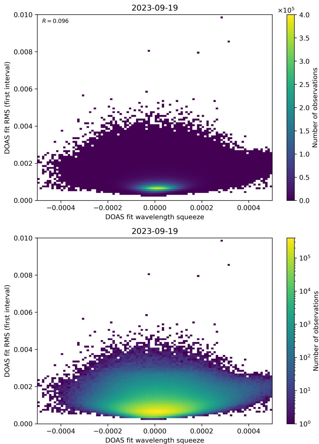
Figure 68: Scatter density plot of “DOAS fit wavelength squeeze” against “DOAS fit RMS (first interval)” for 2023-09-18 to 2023-09-20.
