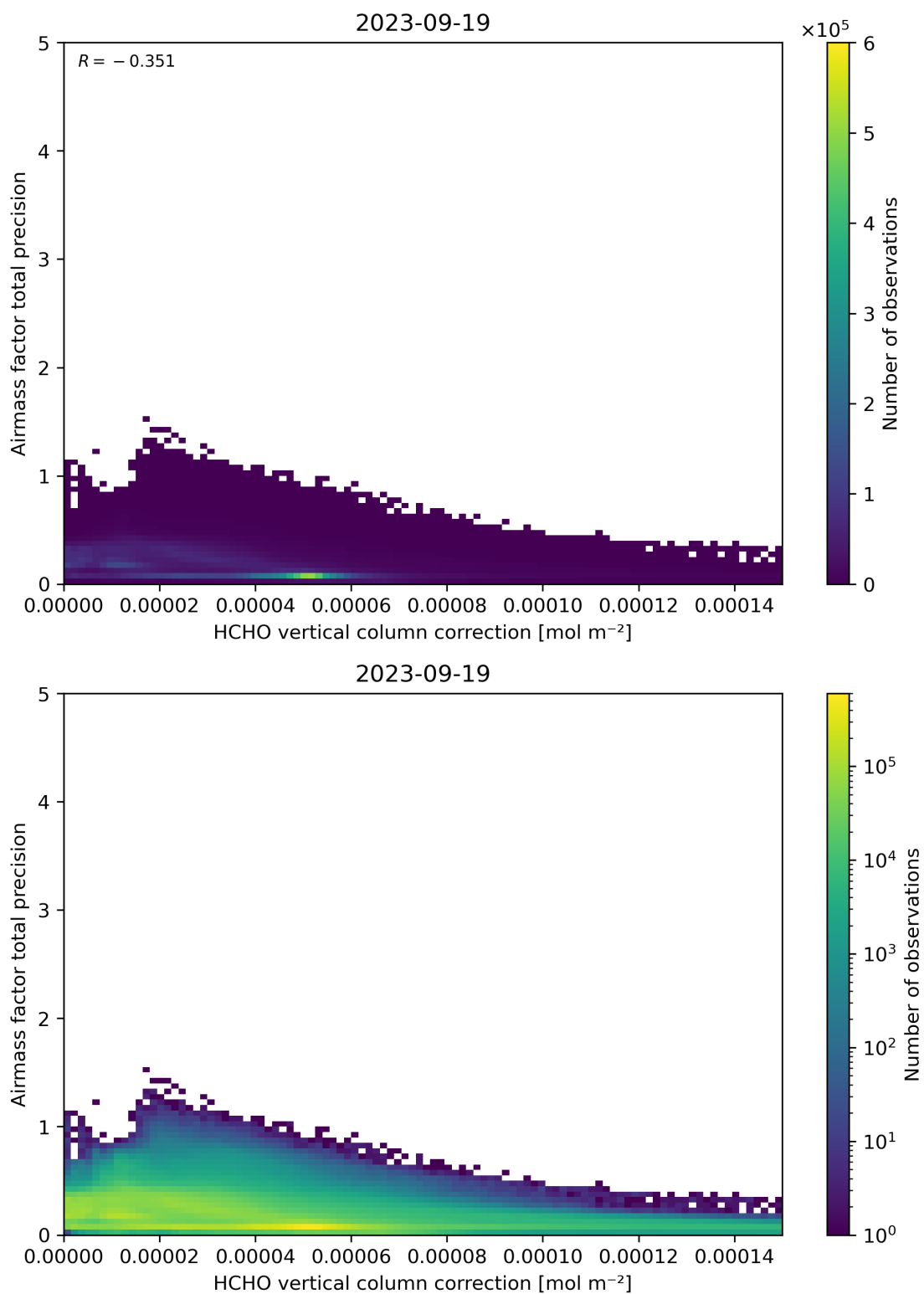
Figure 121: Scatter density plot of “HCHO vertical column correction” against “Airmass factor total precision” for 2023-09-18 to 2023-09-20.
