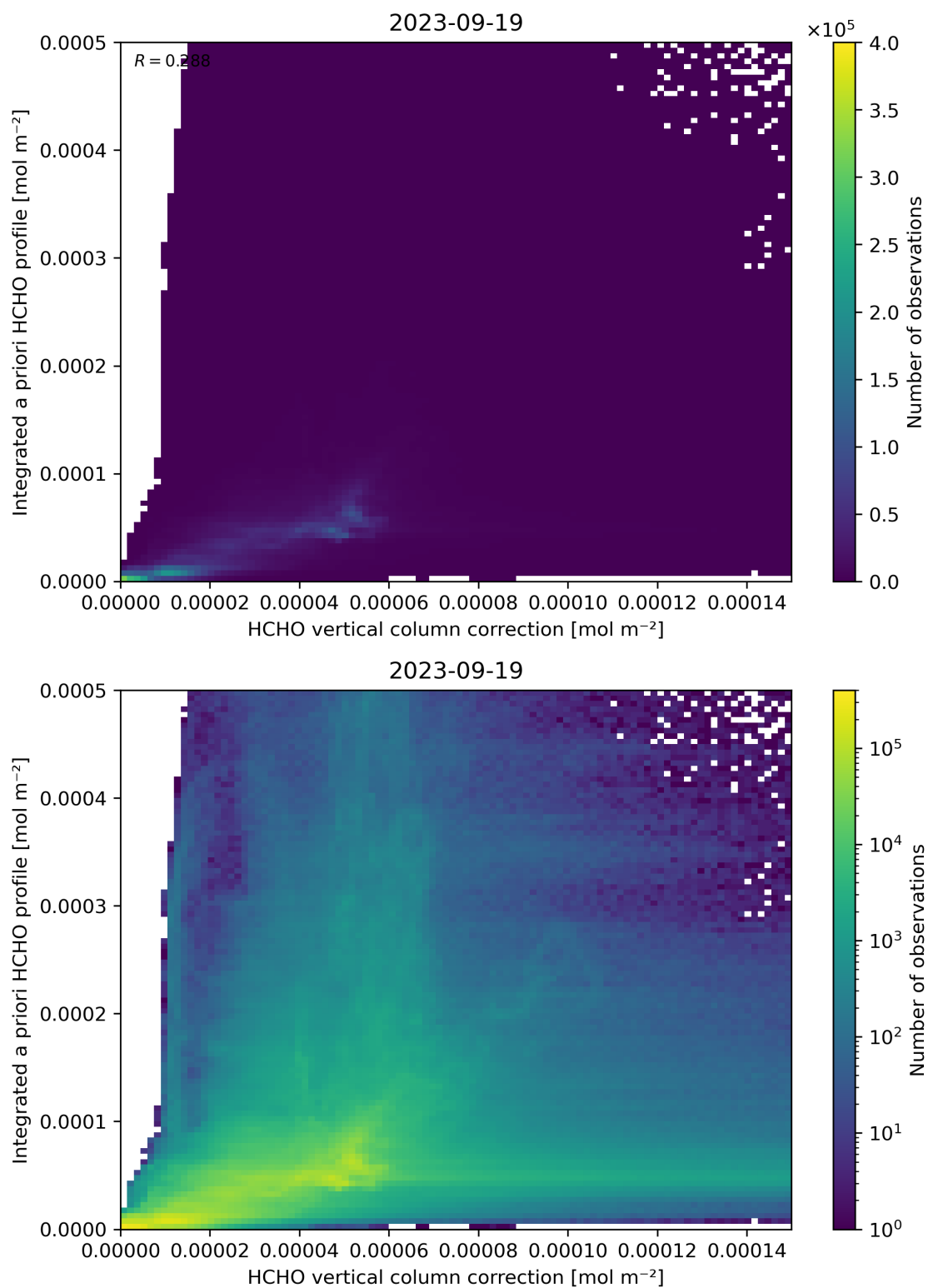
Figure 122: Scatter density plot of “HCHO vertical column correction” against “Integrated a priori HCHO profile” for 2023-09-18 to 2023-09-20.
