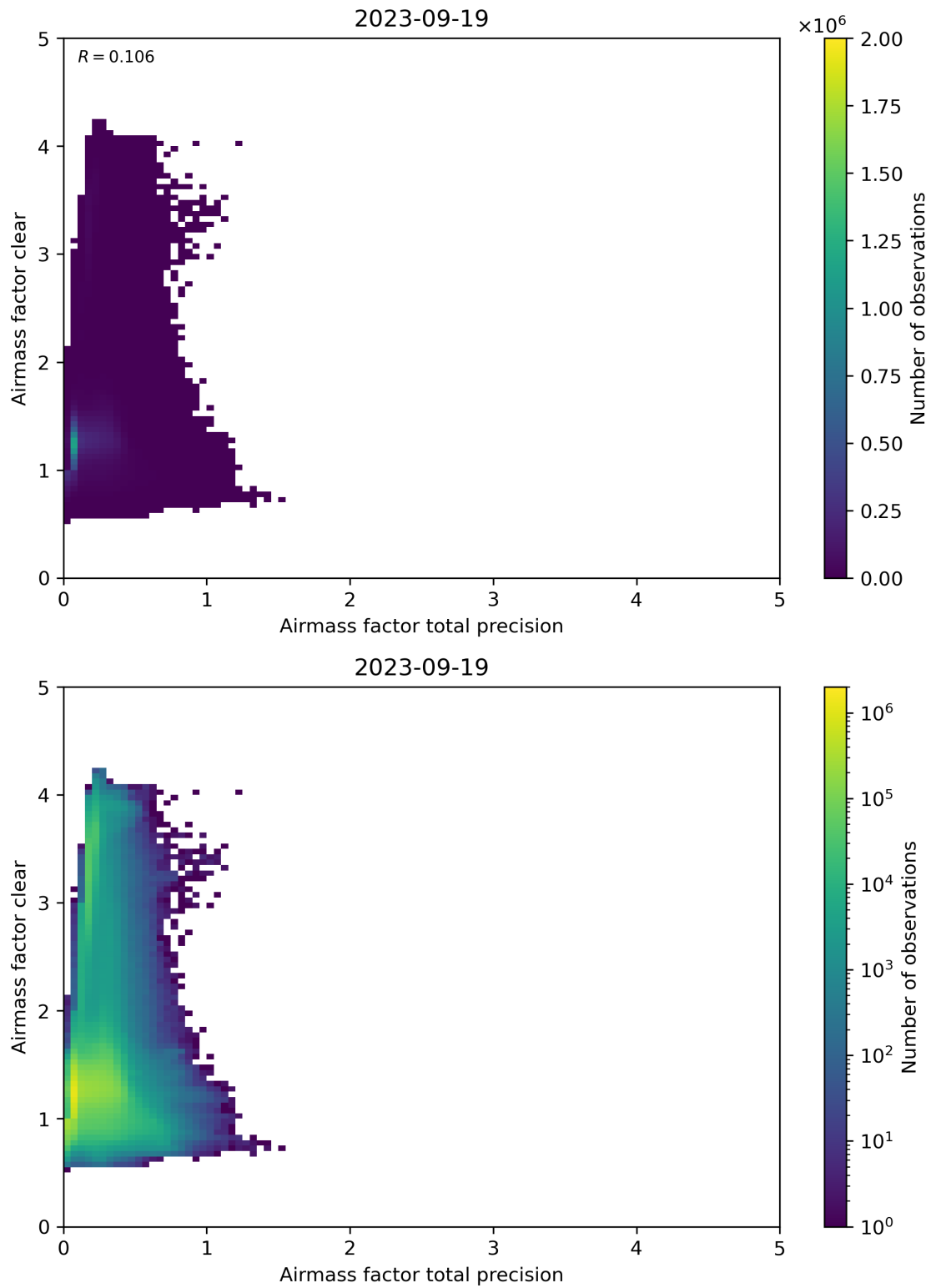
Figure 108: Scatter density plot of “Airmass factor total precision” against “Airmass factor clear” for 2023-09-18 to 2023-09-20.
