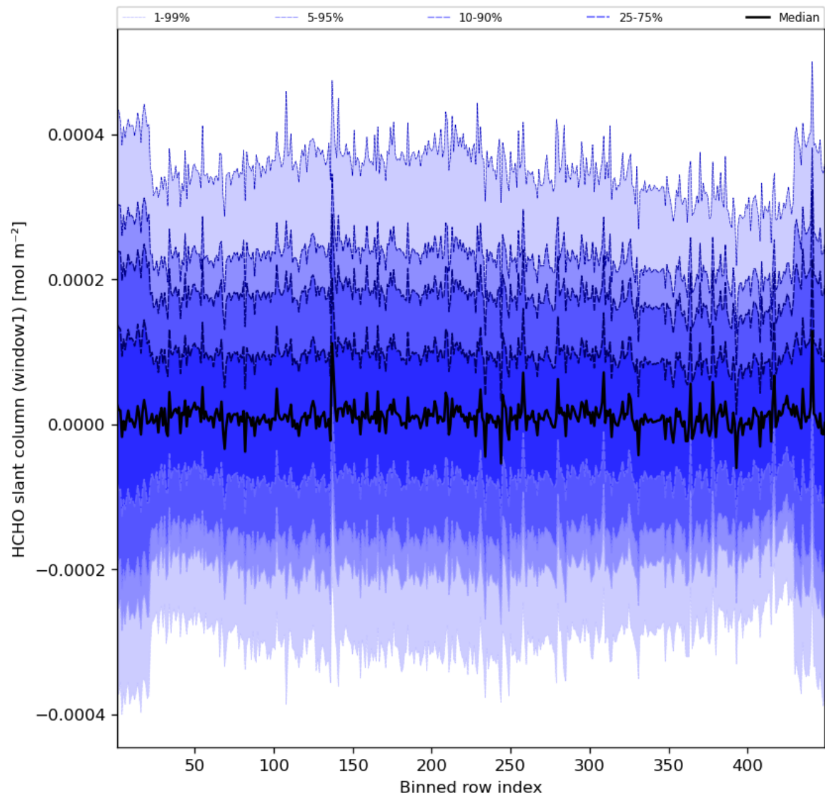
Figure 52: Along track statistics of “HCHO slant column (window1)” for 2023-09-18 to 2023-09-20
