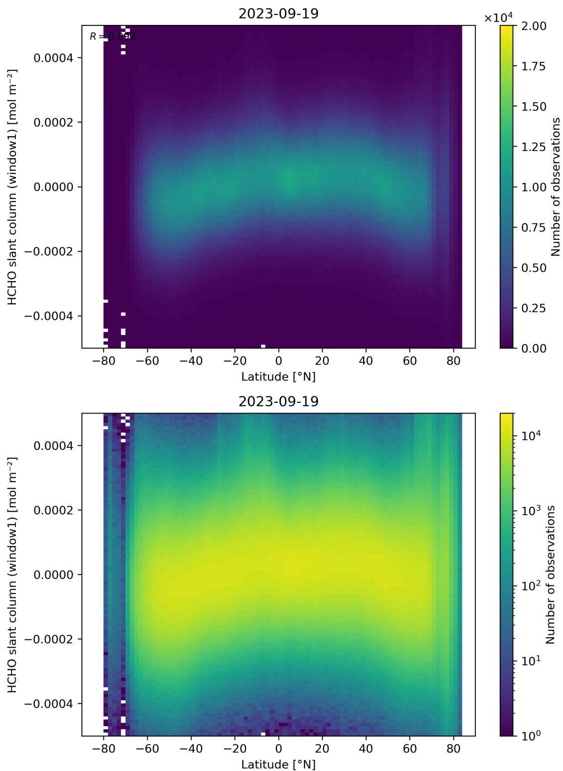
Figure 159: Scatter density plot of “Latitude” against “HCHO slant column (window1)” for 2023-09-18 to 2023-09-20.
