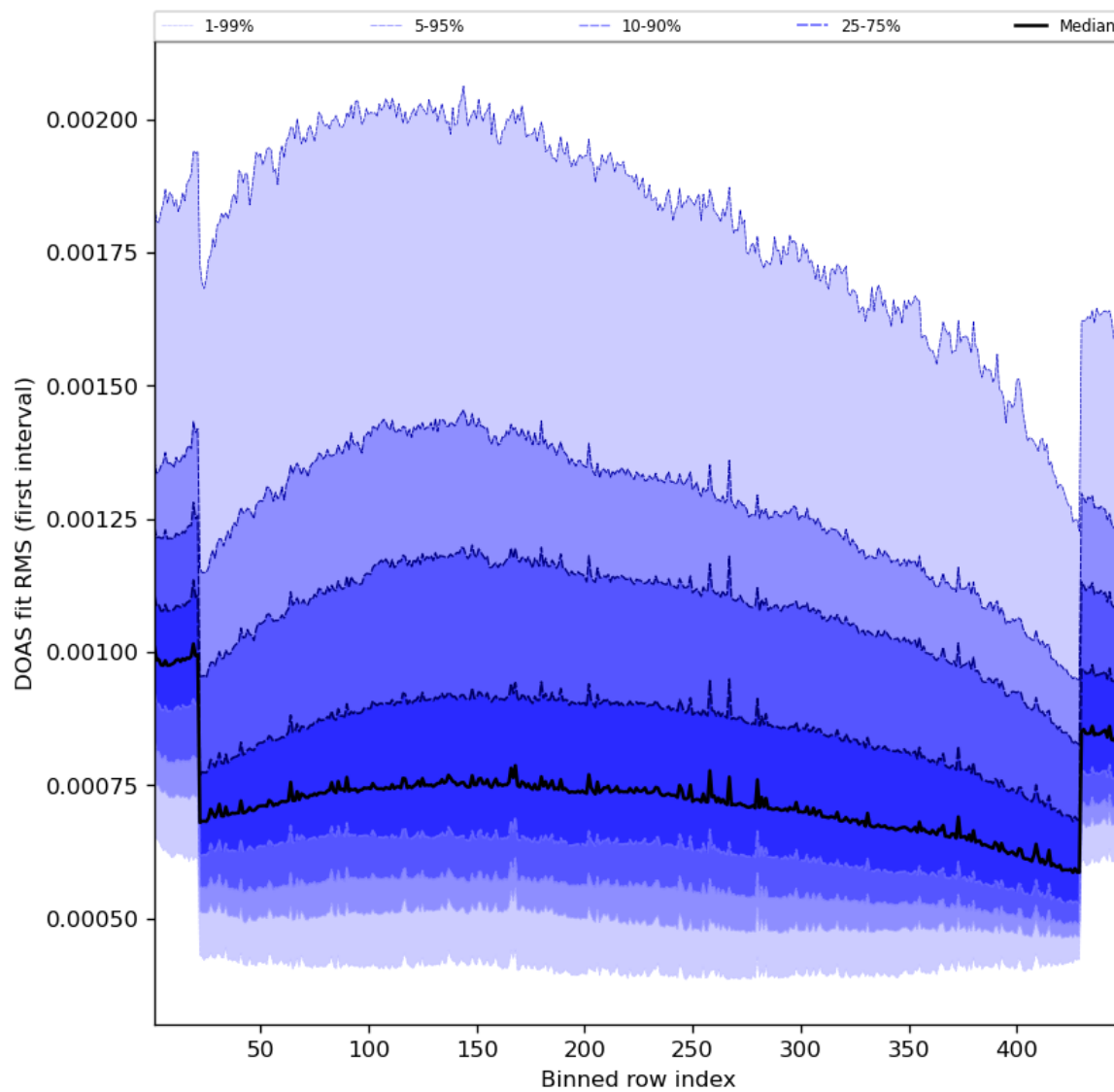
Figure 60: Along track statistics of “DOAS fit RMS (first interval)” for 2023-09-18 to 2023-09-20
