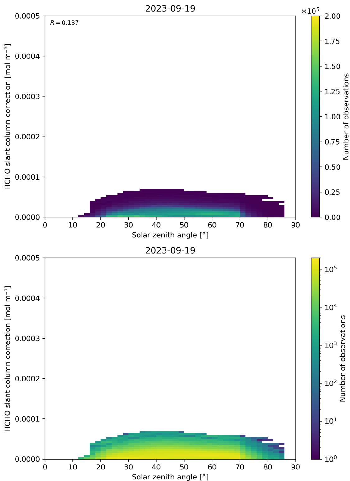
Figure 172: Scatter density plot of “Solar zenith angle” against “HCHO slant column correction” for 2023-09-18 to 2023-09-20.
