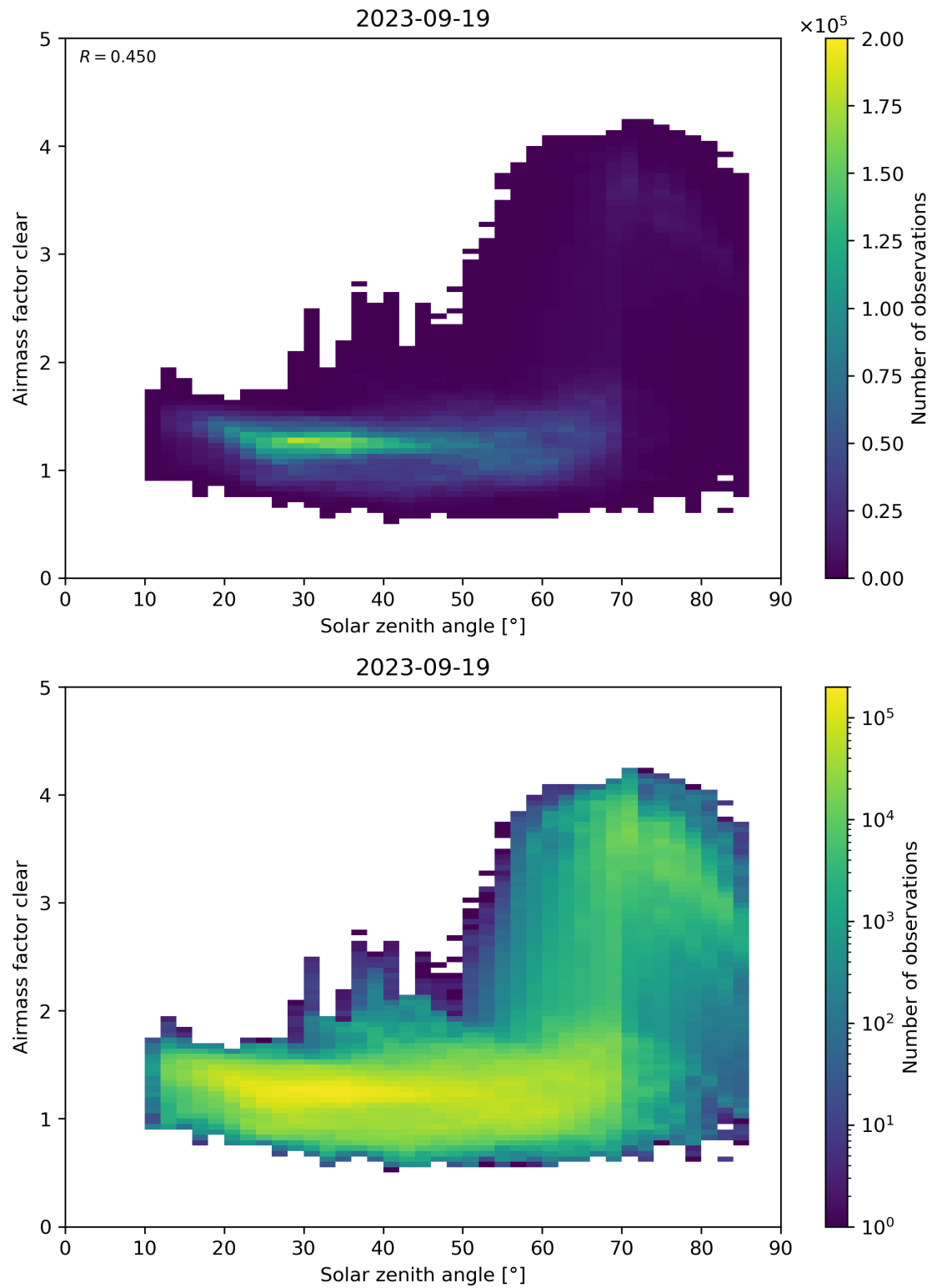
Figure 170: Scatter density plot of “Solar zenith angle” against “Airmass factor clear” for 2023-09-18 to 2023-09-20.
