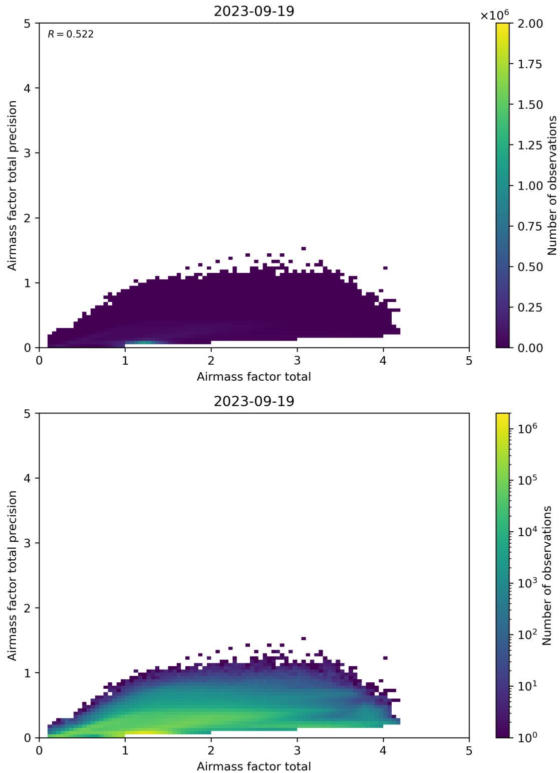
Figure 103: Scatter density plot of “Airmass factor total” against “Airmass factor total precision” for 2023-09-18 to 2023-09-20.
