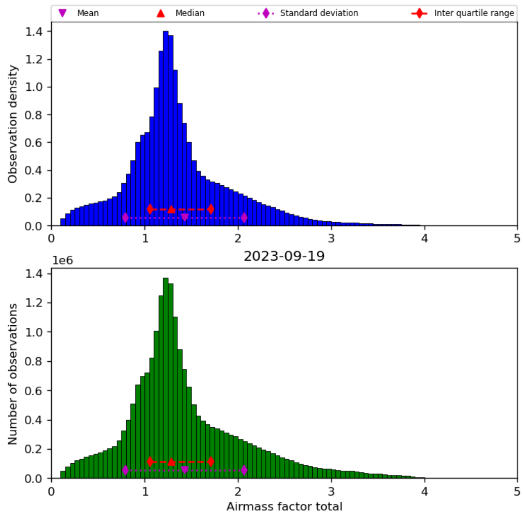
Figure 40: Histogram of “Airmass factor total” for 2023-09-18 to 2023-09-20
