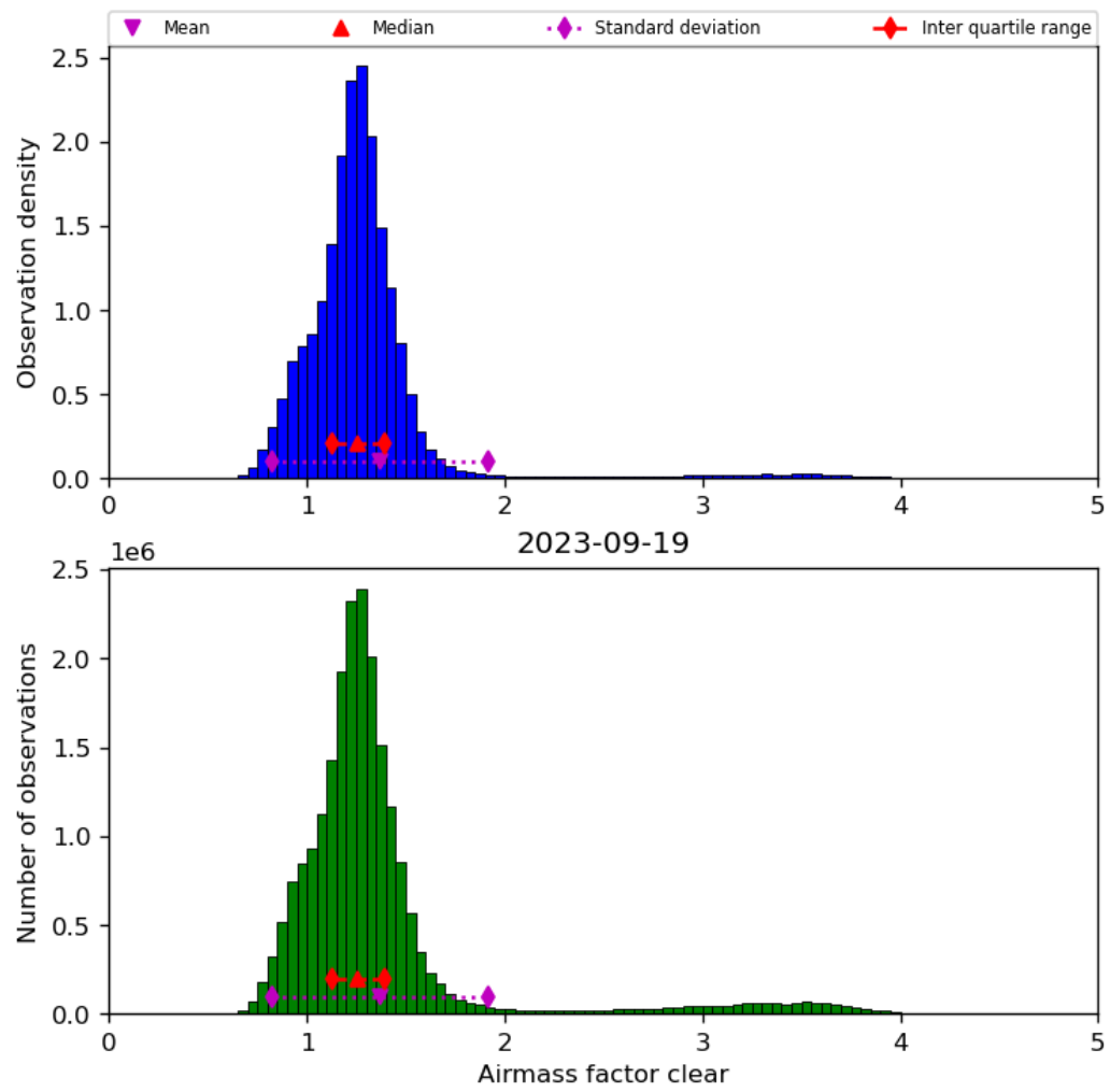
Figure 42: Histogram of “Airmass factor clear” for 2023-09-18 to 2023-09-20
