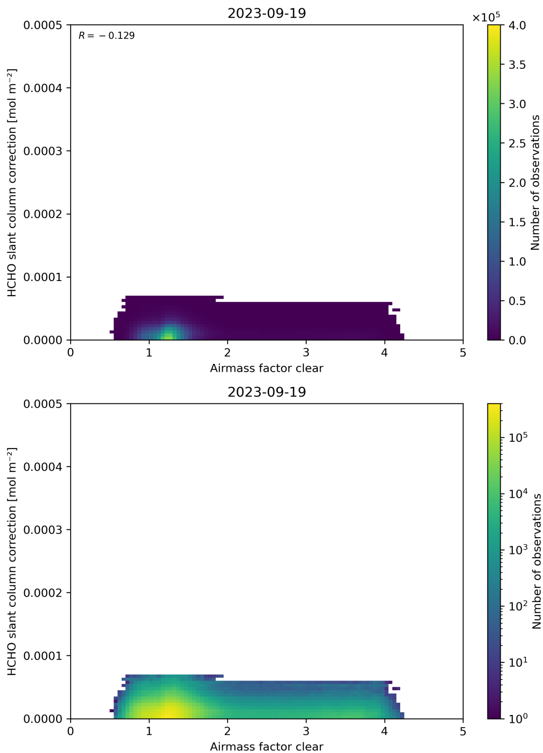
Figure 75: Scatter density plot of “Airmass factor clear” against “HCHO slant column correction” for 2023-09-18 to 2023-09-20.
