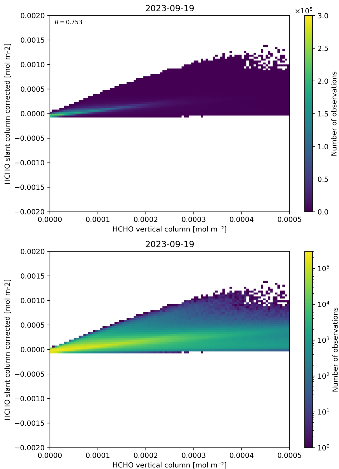
Figure 127: Scatter density plot of “HCHO vertical column” against “HCHO slant column corrected” for 2023-09-18 to 2023-09-20.
