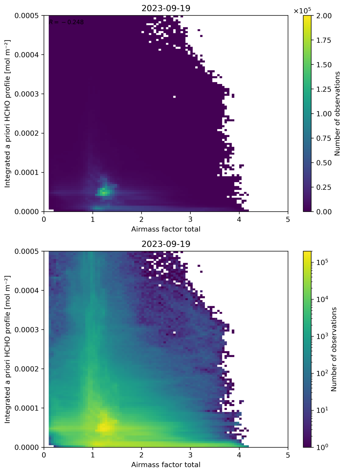
Figure 104: Scatter density plot of “Airmass factor total” against “Integrated a priori HCHO profile” for 2023-09-18 to 2023-09-20.
