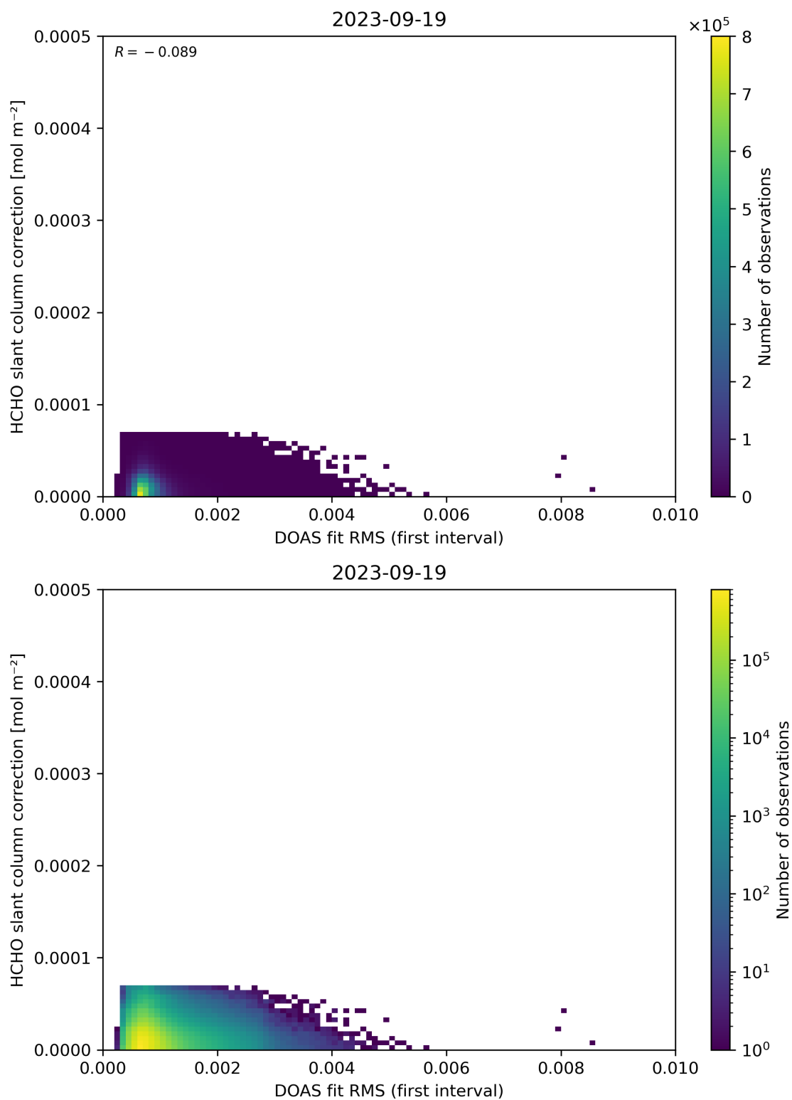
Figure 63: Scatter density plot of “DOAS fit RMS (first interval)” against “HCHO slant column correction” for 2023-09-18 to 2023-09-20.
