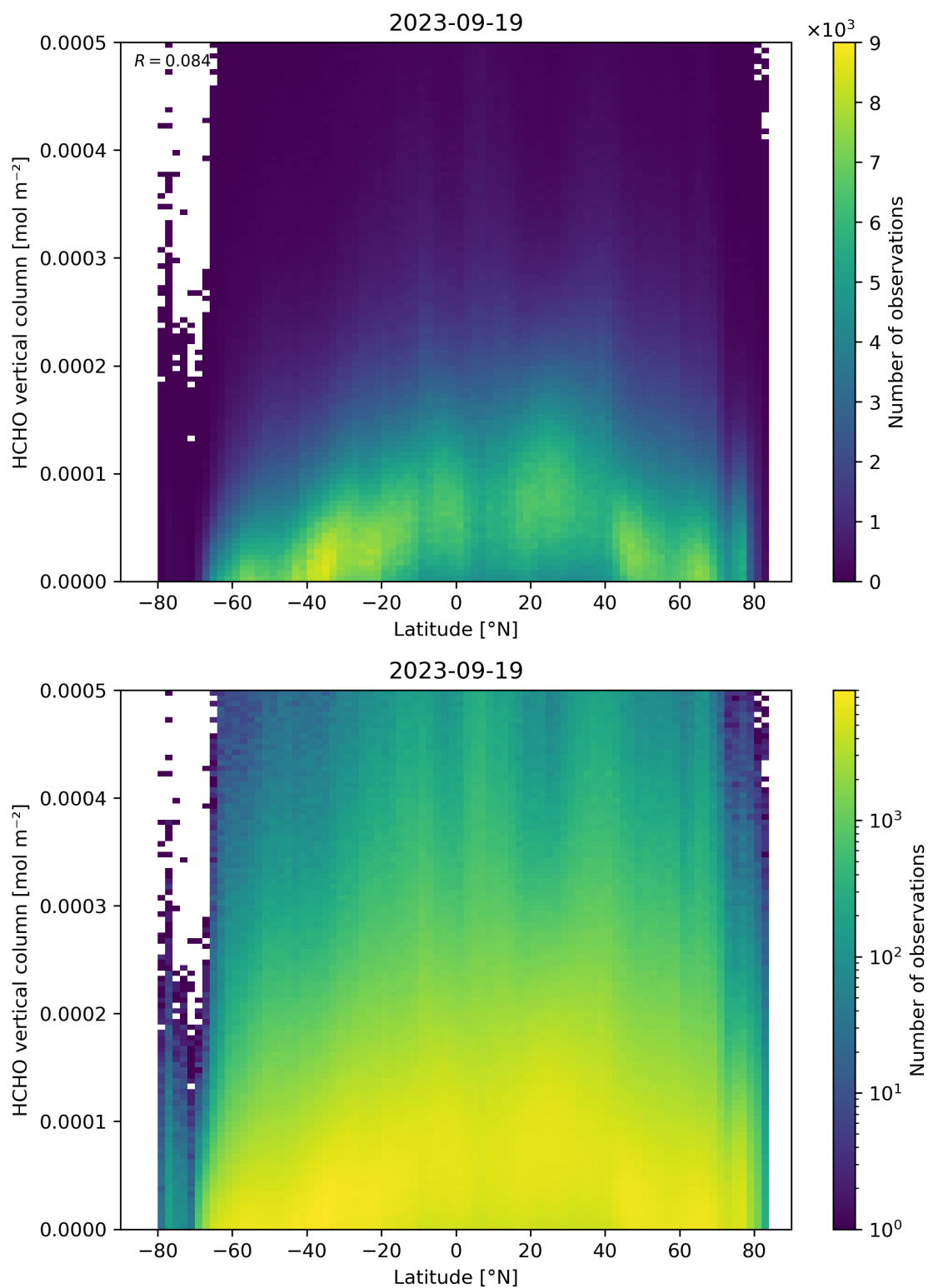
Figure 163: Scatter density plot of “Latitude” against “HCHO vertical column” for 2023-09-18 to 2023-09-20.
