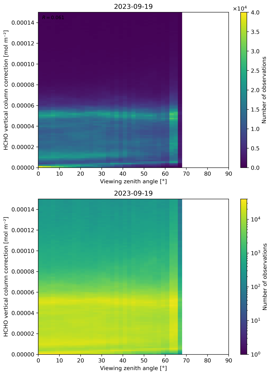
Figure 193: Scatter density plot of “Viewing zenith angle” against “HCHO vertical column correction” for 2023-09-18 to 2023-09-20.
