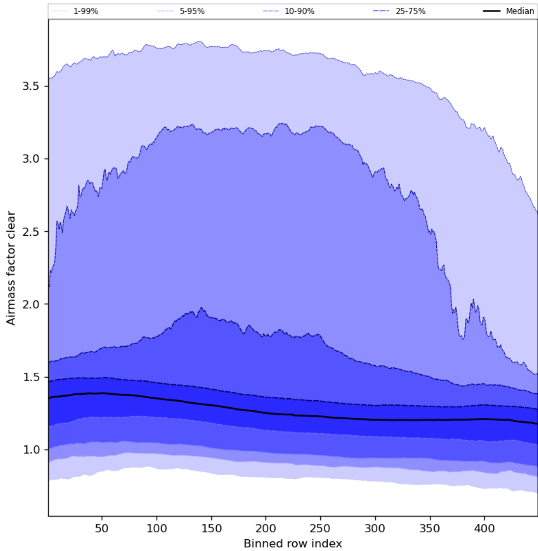
Figure 56: Along track statistics of “Airmass factor clear” for 2023-09-18 to 2023-09-20
