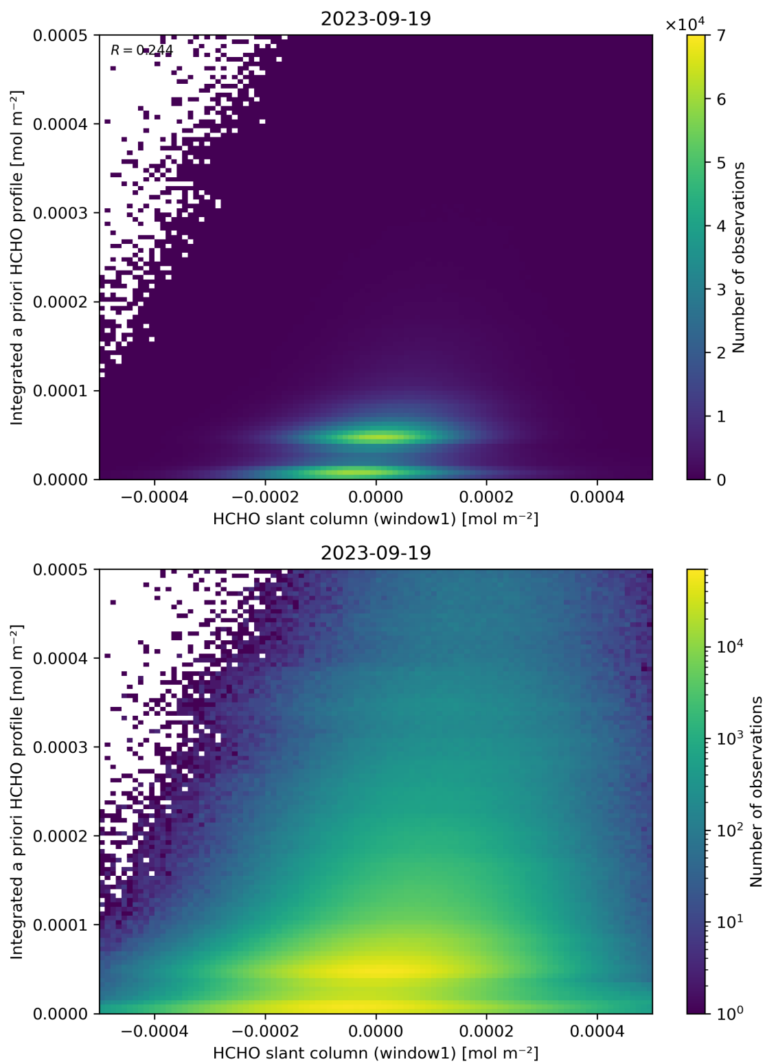
Figure 87: Scatter density plot of “HCHO slant column (window1)” against “Integrated a priori HCHO profile” for 2023-09-18 to 2023-09-20.
