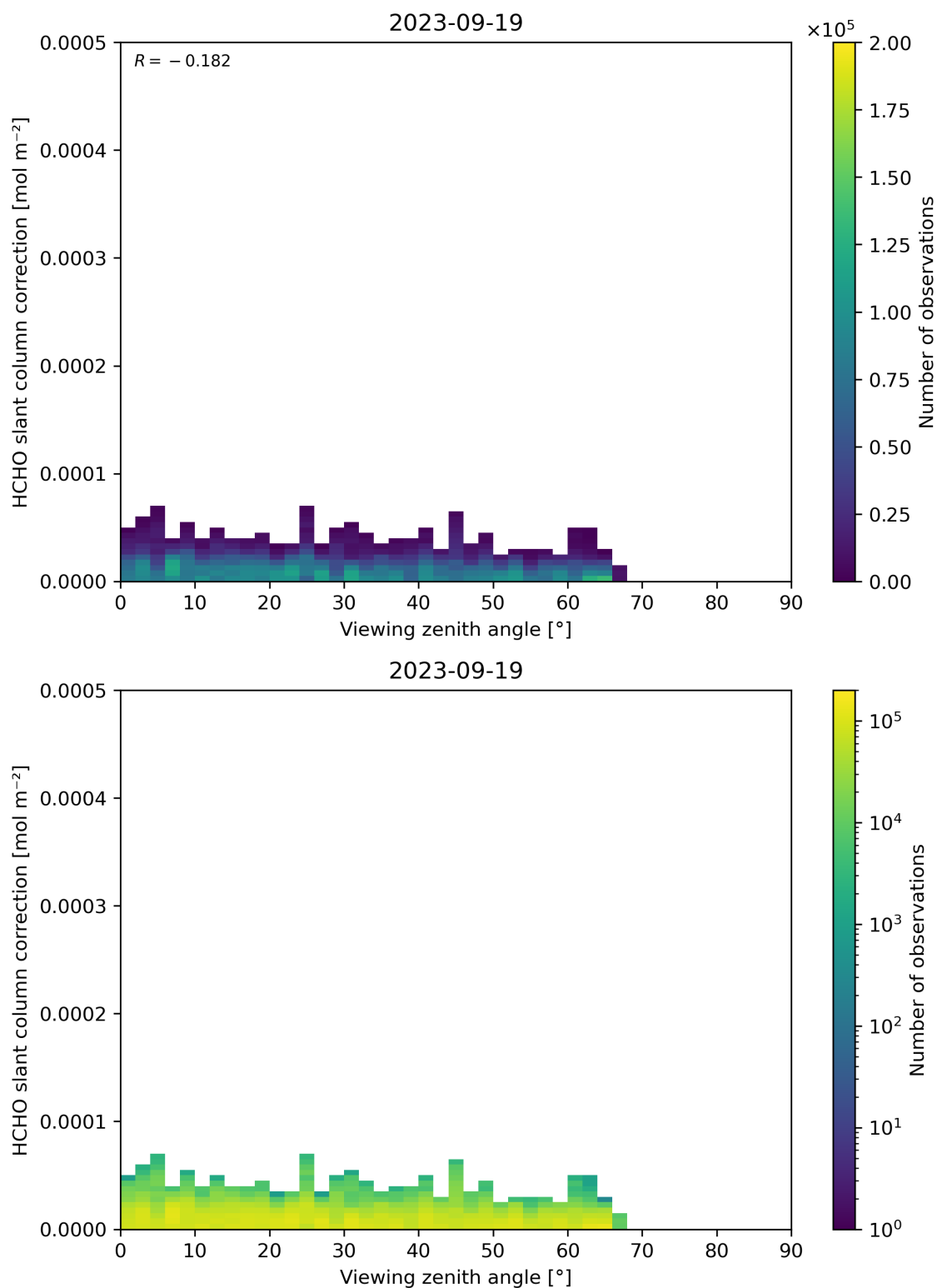
Figure 187: Scatter density plot of “Viewing zenith angle” against “HCHO slant column correction” for 2023-09-18 to 2023-09-20.
