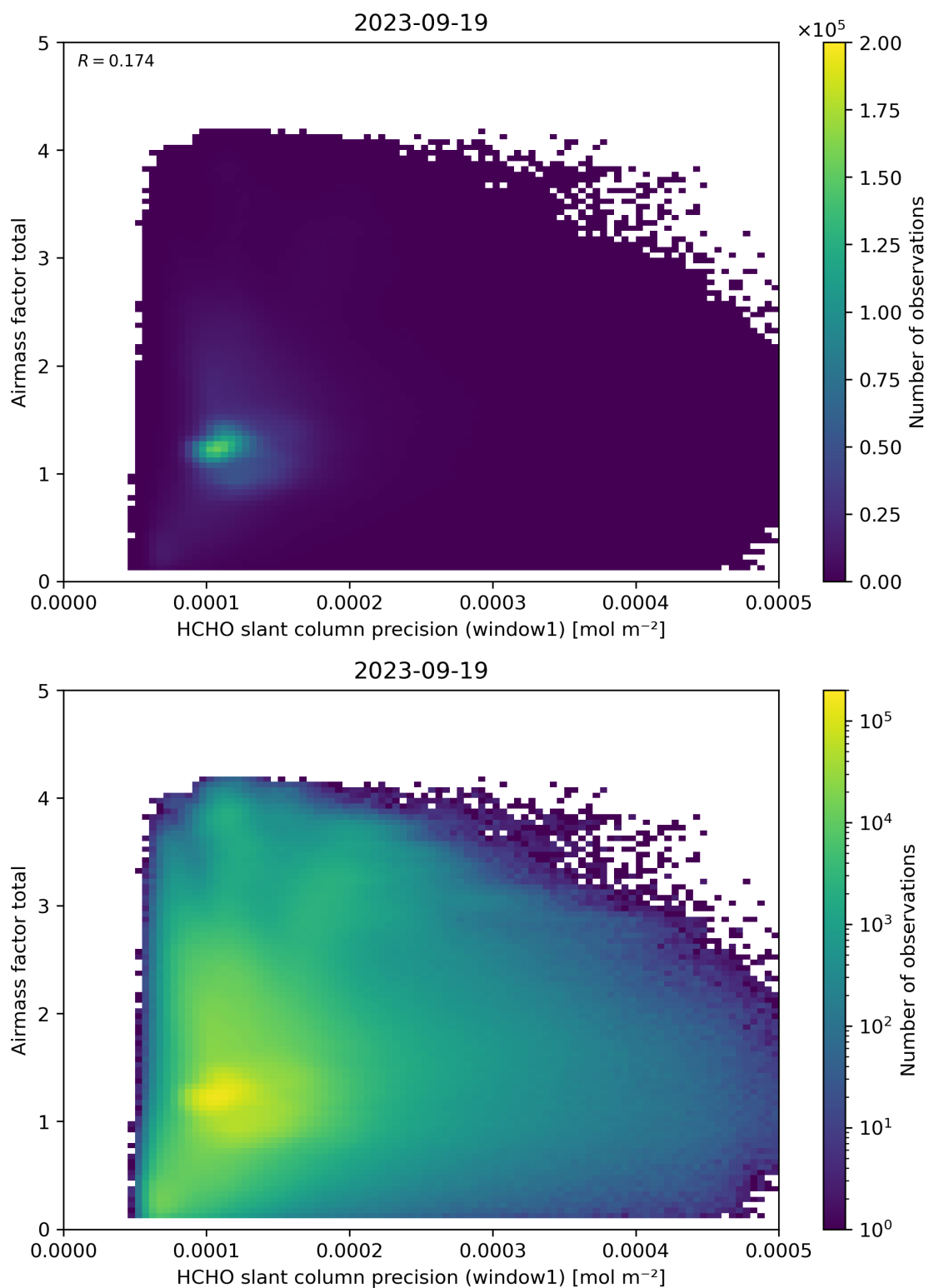
Figure 94: Scatter density plot of “HCHO slant column precision (window1)” against “Airmass factor total” for 2023-09-18 to 2023-09-20.
