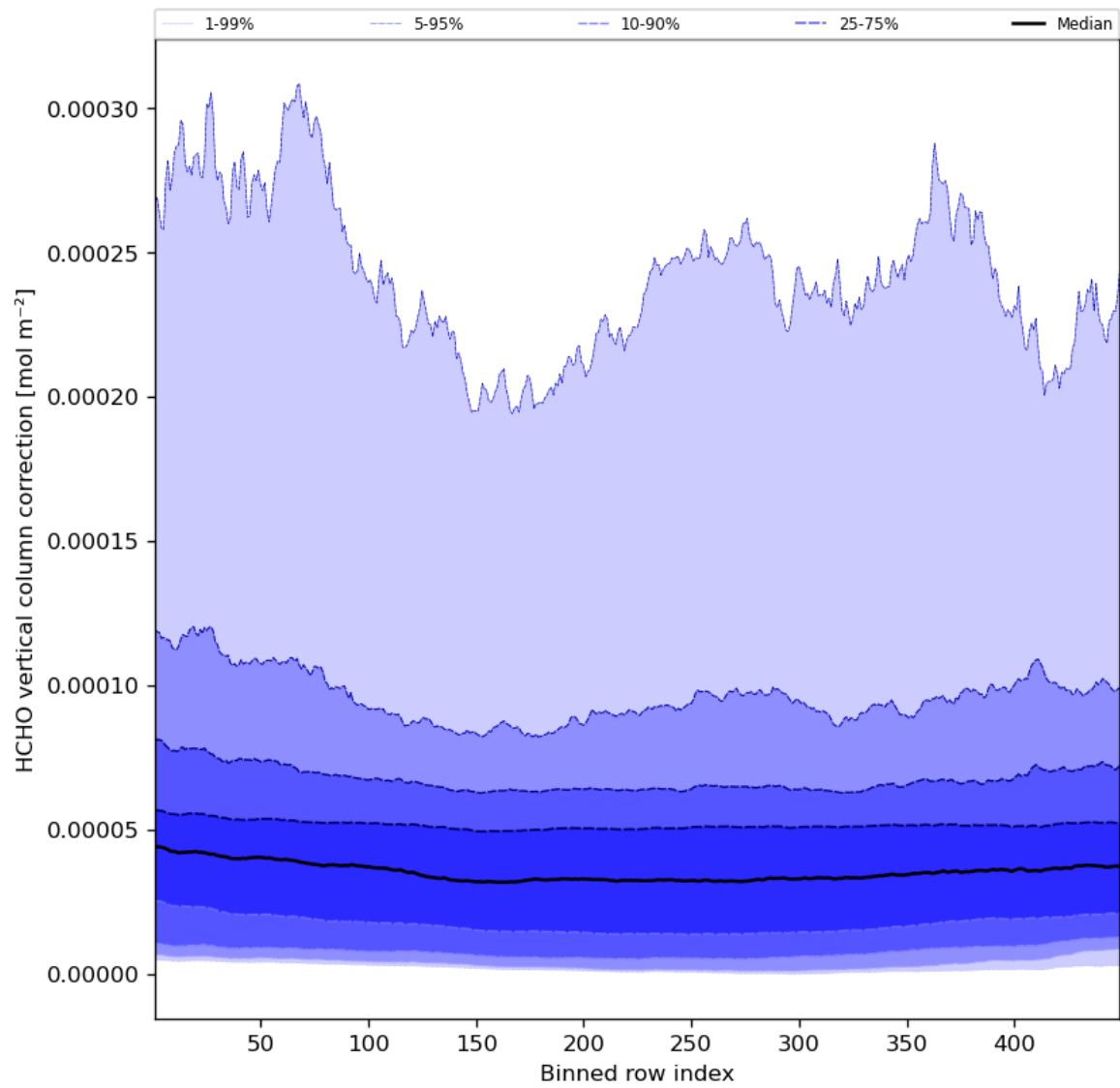
Figure 51: Along track statistics of “HCHO vertical column correction” for 2023-09-18 to 2023-09-20
