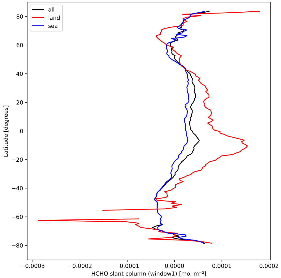
Figure 24: Zonal average of “HCHO slant column (window1)” for 2023-09-18 to 2023-09-20.
