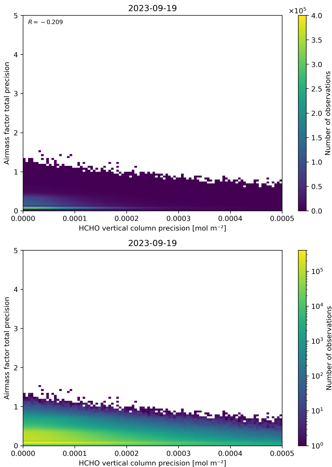
Figure 145: Scatter density plot of “HCHO vertical column precision” against “Airmass factor total precision” for 2023-09-18 to 2023-09-20.
