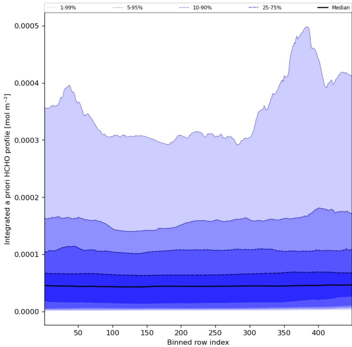
Figure 57: Along track statistics of “Integrated a priori HCHO profile” for 2023-09-18 to 2023-09-20
