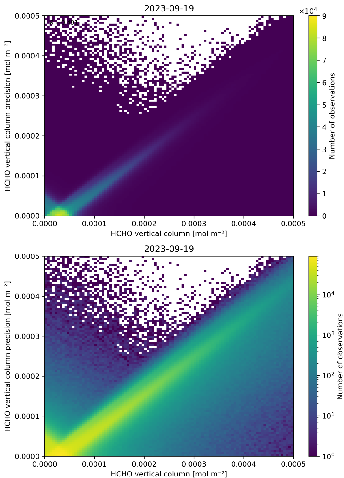
Figure 134: Scatter density plot of “HCHO vertical column” against “HCHO vertical column precision” for 2023-09-18 to 2023-09-20.
