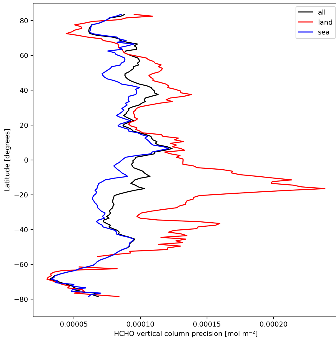
Figure 22: Zonal average of “HCHO vertical column precision” for 2023-09-18 to 2023-09-20.
