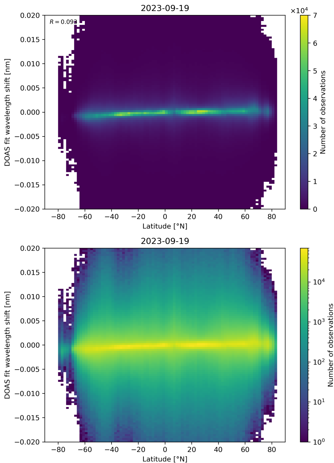
Figure 154: Scatter density plot of “Latitude” against “DOAS fit wavelength shift” for 2023-09-18 to 2023-09-20.
