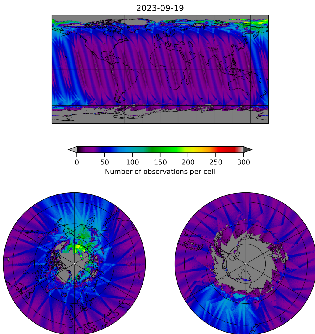
Figure 19: Map of the number of observations for 2023-09-18 to 2023-09-20
