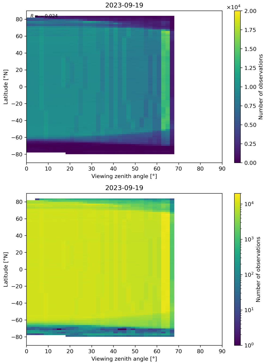
Figure 196: Scatter density plot of “Viewing zenith angle” against “Latitude” for 2023-09-18 to 2023-09-20.
