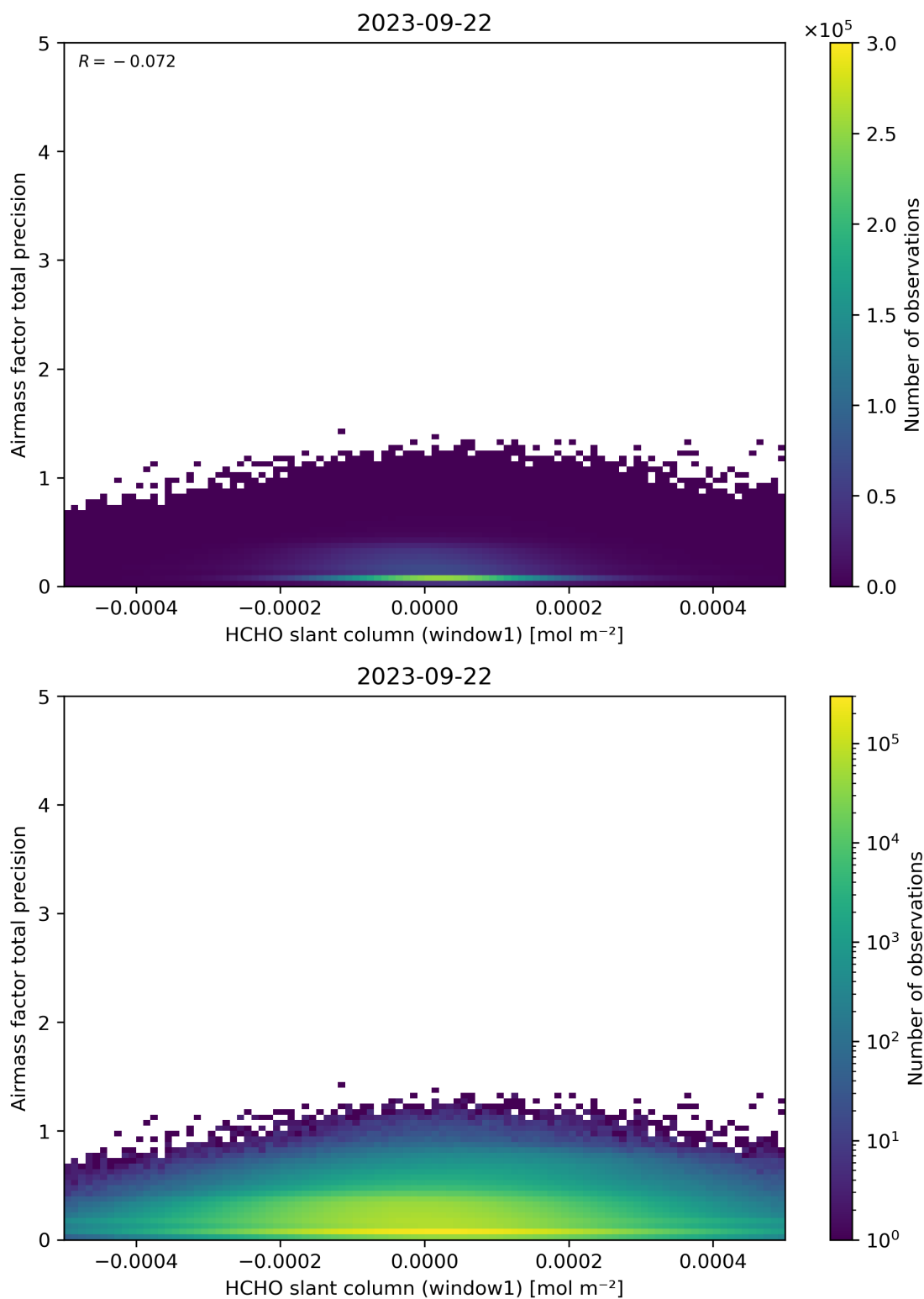
Figure 86: Scatter density plot of “HCHO slant column (window1)” against “Airmass factor total precision” for 2023-09-21 to 2023-09-23.
