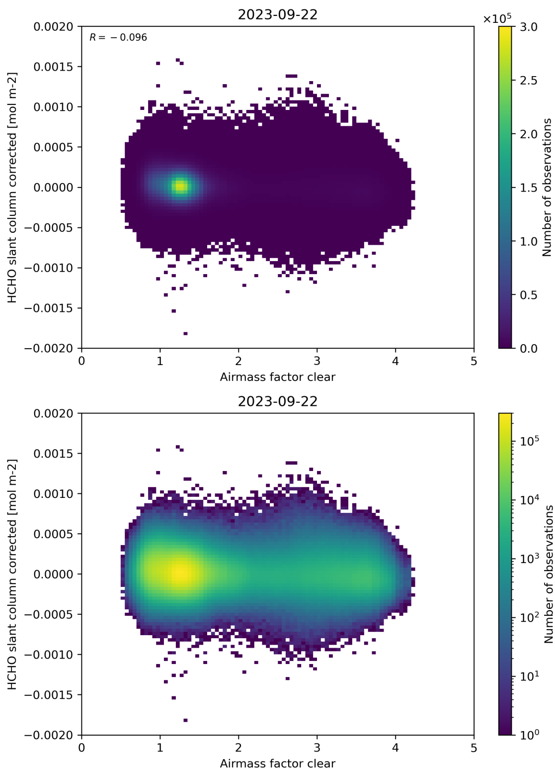
Figure 74: Scatter density plot of “Airmass factor clear” against “HCHO slant column corrected” for 2023-09-21 to 2023-09-23.
