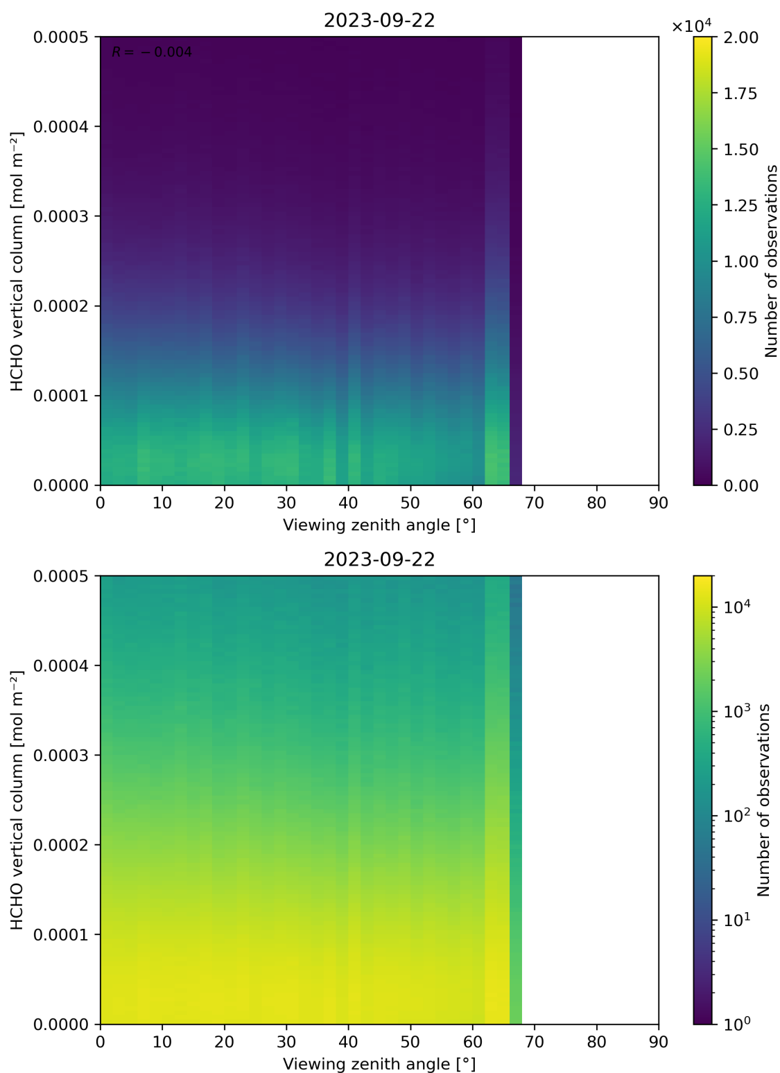
Figure 192: Scatter density plot of “Viewing zenith angle” against “HCHO vertical column” for 2023-09-21 to 2023-09-23.
