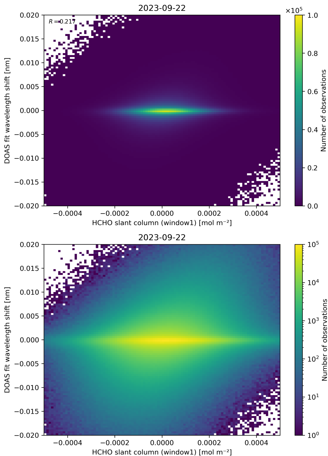
Figure 79: Scatter density plot of “HCHO slant column (window1)” against “DOAS fit wavelength shift” for 2023-09-21 to 2023-09-23.
