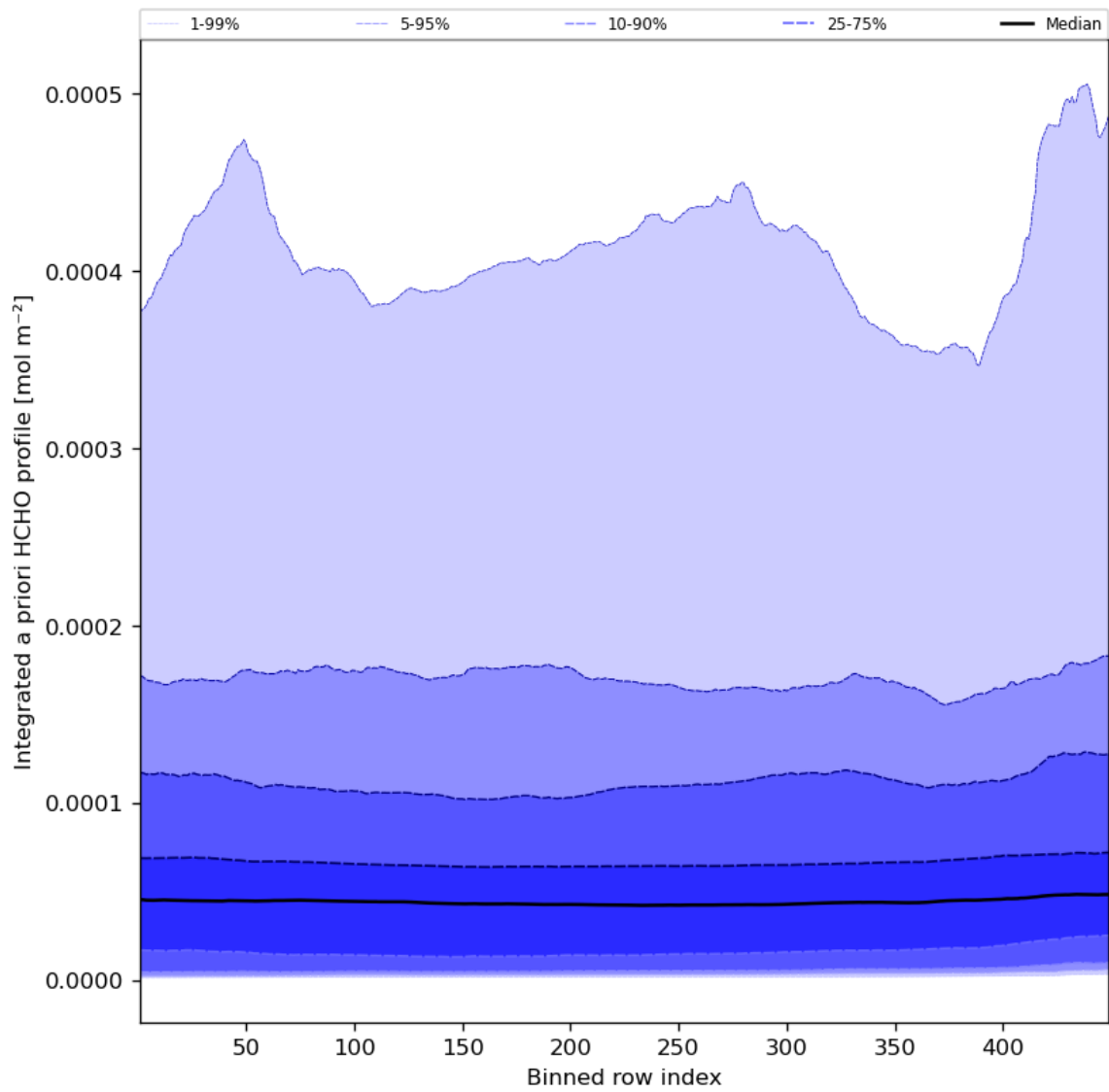
Figure 57: Along track statistics of "Integrated a priori HCHO profile" for 2023-09-21 to 2023-09-23
