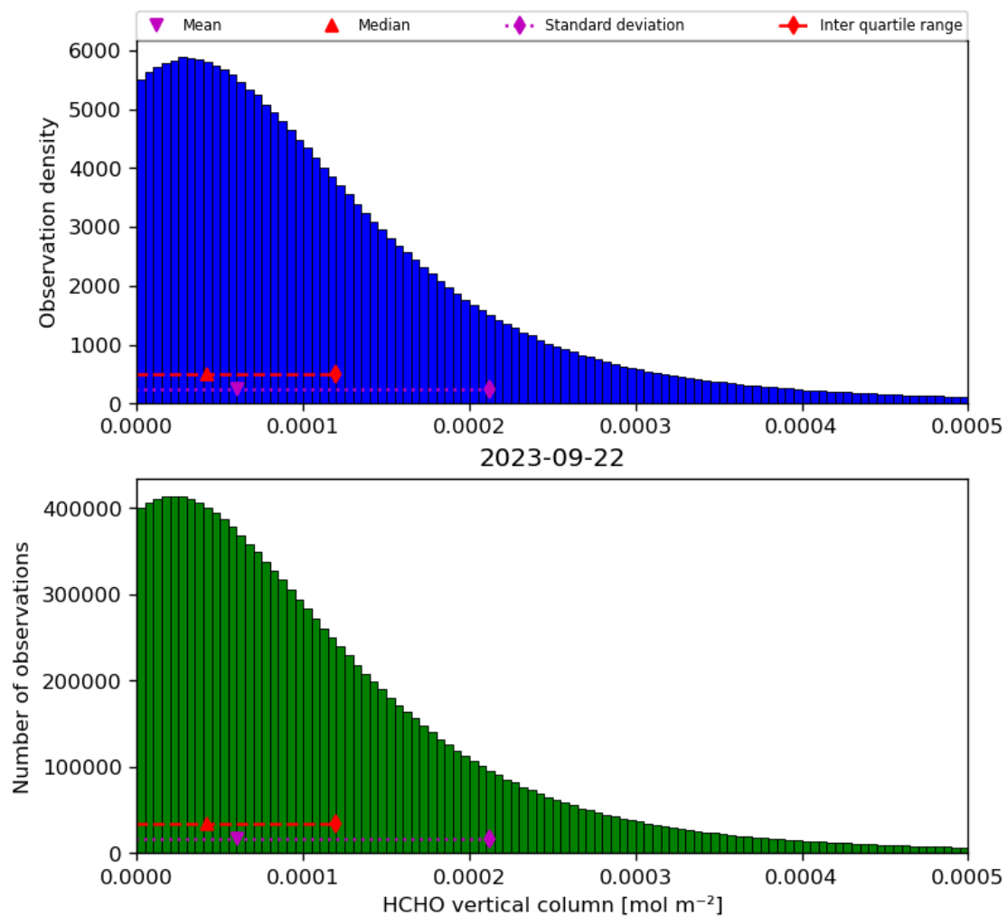
Figure 35: Histogram of “HCHO vertical column” for 2023-09-21 to 2023-09-23
