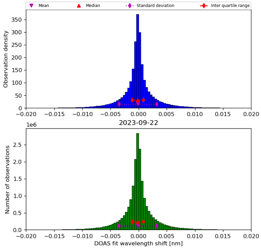
Figure 44: Histogram of “DOAS fit wavelength shift” for 2023-09-21 to 2023-09-23
