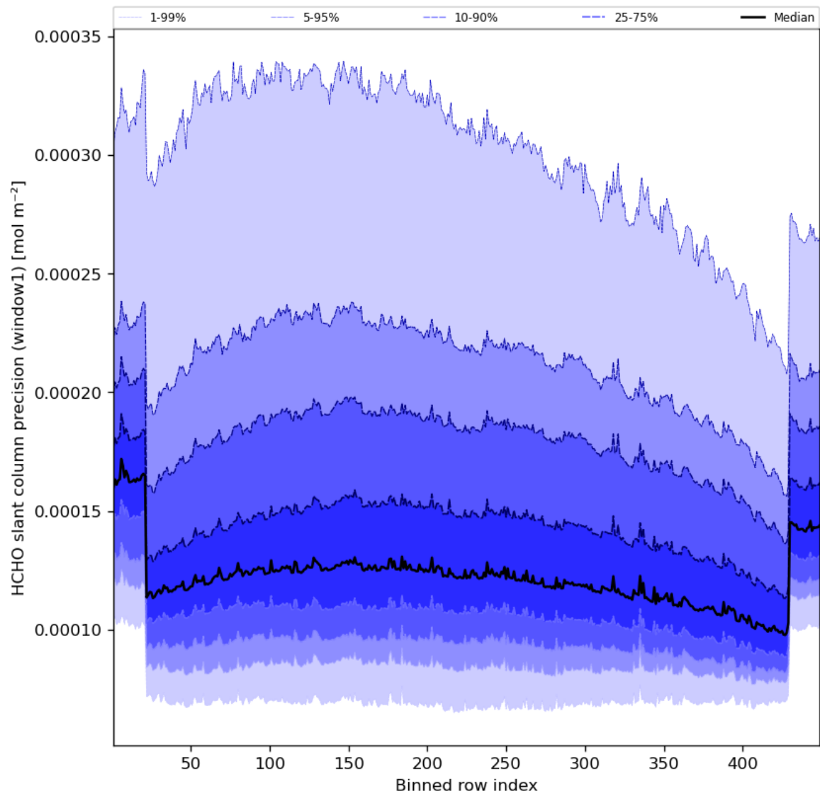
Figure 53: Along track statistics of “HCHO slant column precision (window1)” for 2023-09-21 to 2023-09-23
