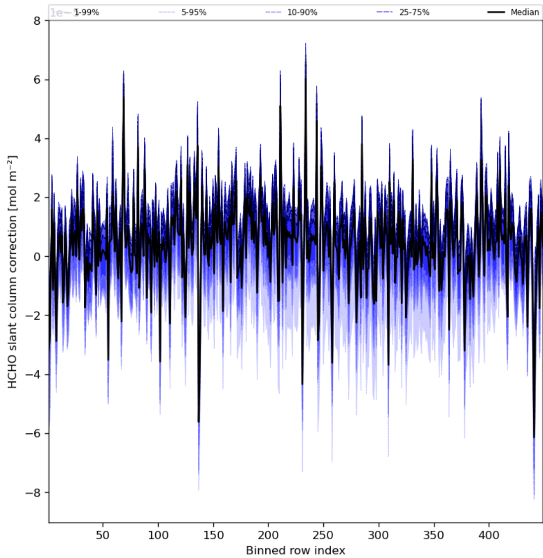
Figure 61: Along track statistics of “HCHO slant column correction” for 2023-09-21 to 2023-09-23
