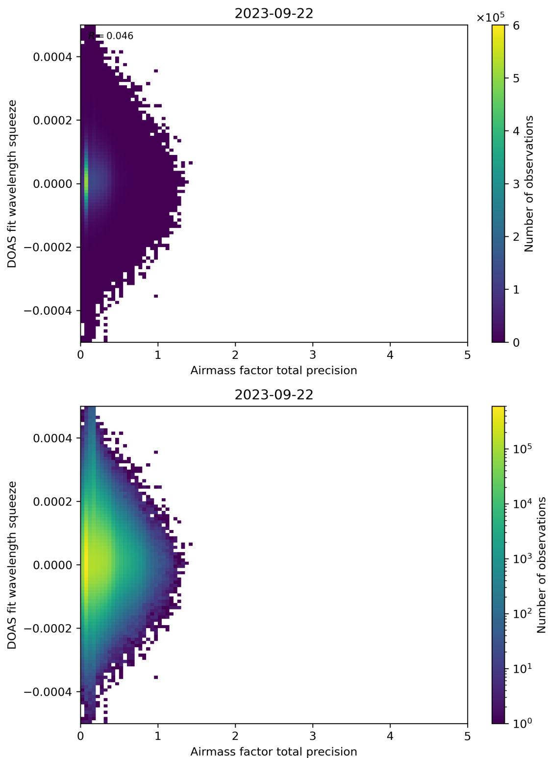
Figure 107: Scatter density plot of “Airmass factor total precision” against “DOAS fit wavelength squeeze” for 2023-09-21 to 2023-09-23.
