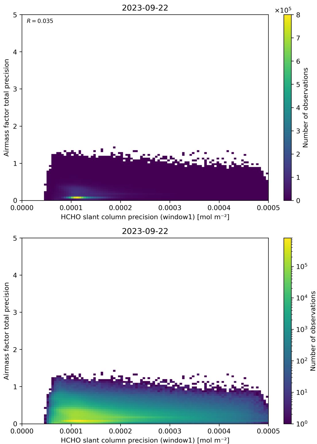
Figure 95: Scatter density plot of “HCHO slant column precision (window1)” against “Airmass factor total precision” for 2023-09-21 to 2023-09-23.
