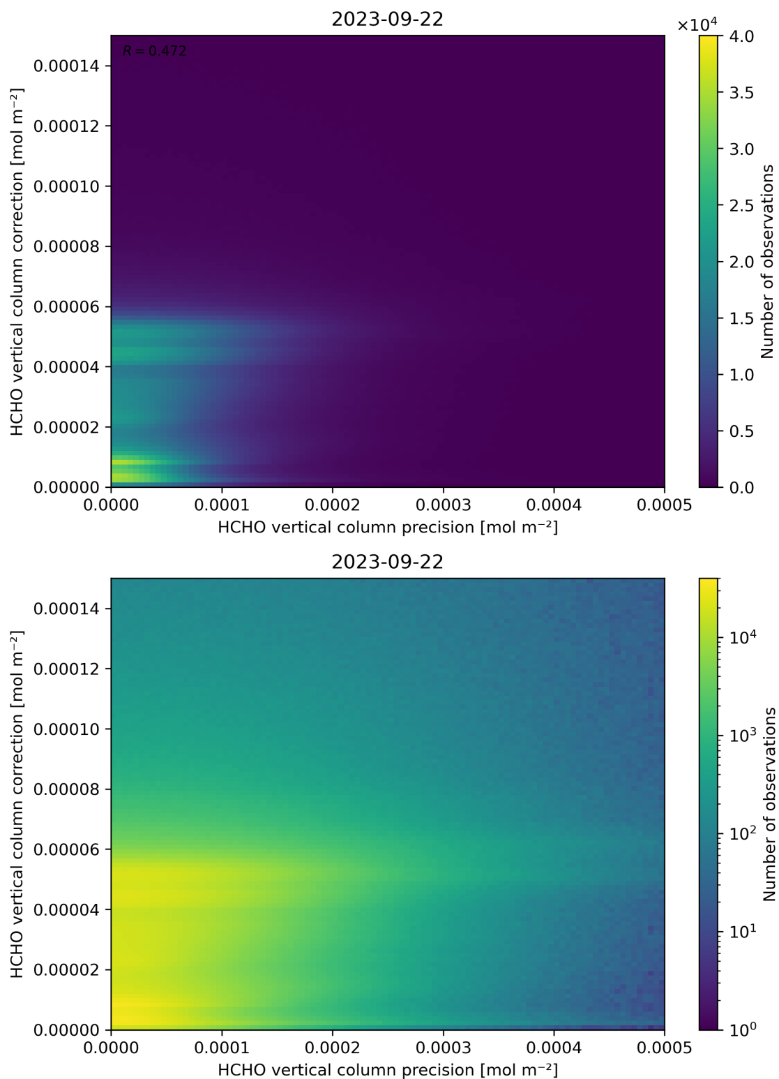
Figure 146: Scatter density plot of “HCHO vertical column precision” against “HCHO vertical column correction” for 2023-09-21 to 2023-09-23.
