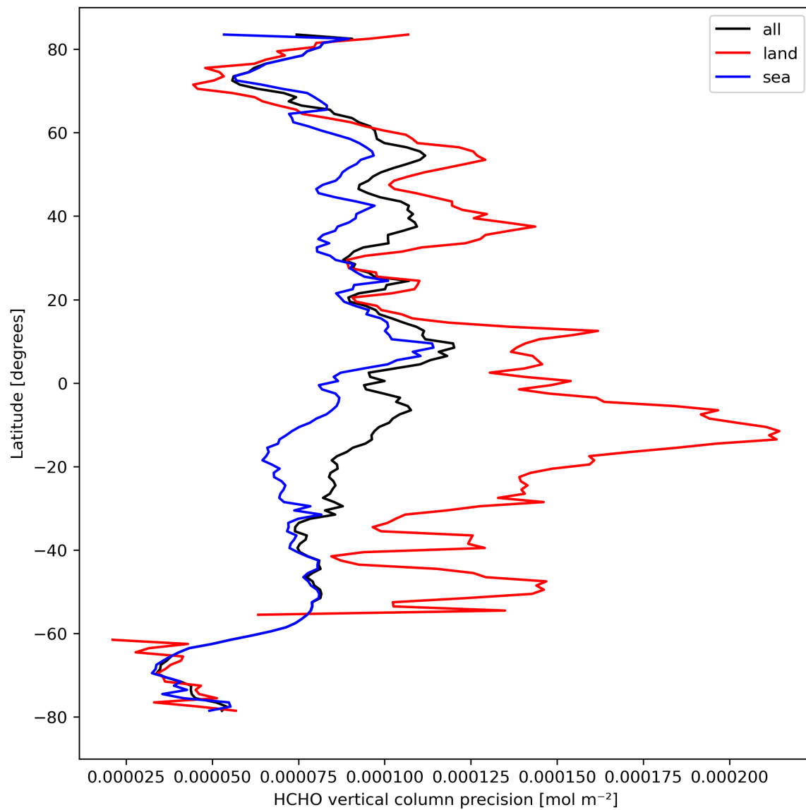
Figure 22: Zonal average of “HCHO vertical column precision” for 2023-09-21 to 2023-09-23.
