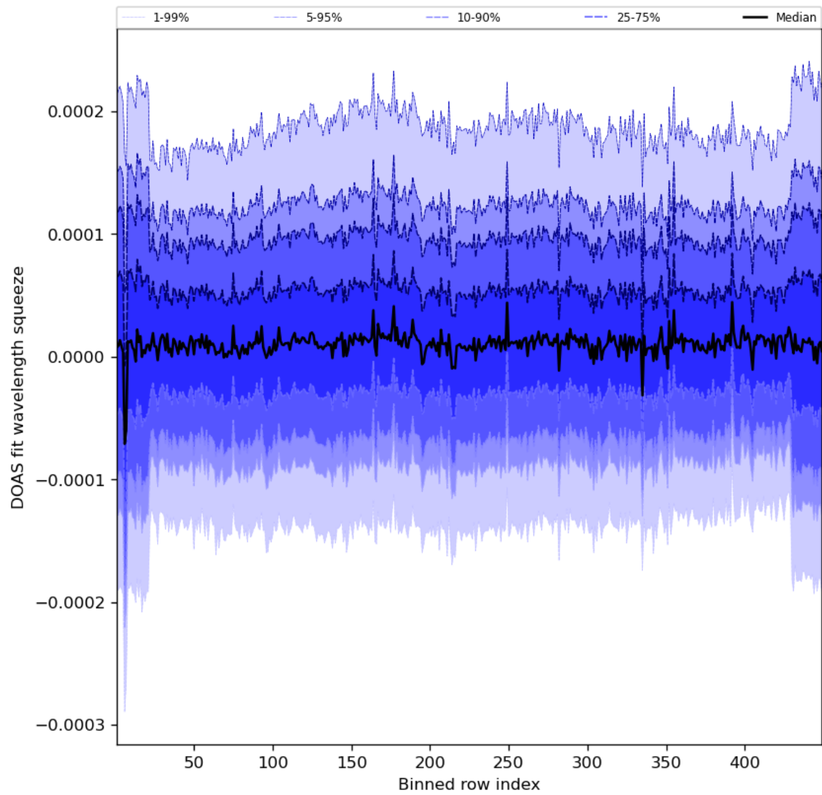
Figure 59: Along track statistics of “DOAS fit wavelength squeeze” for 2023-09-21 to 2023-09-23
