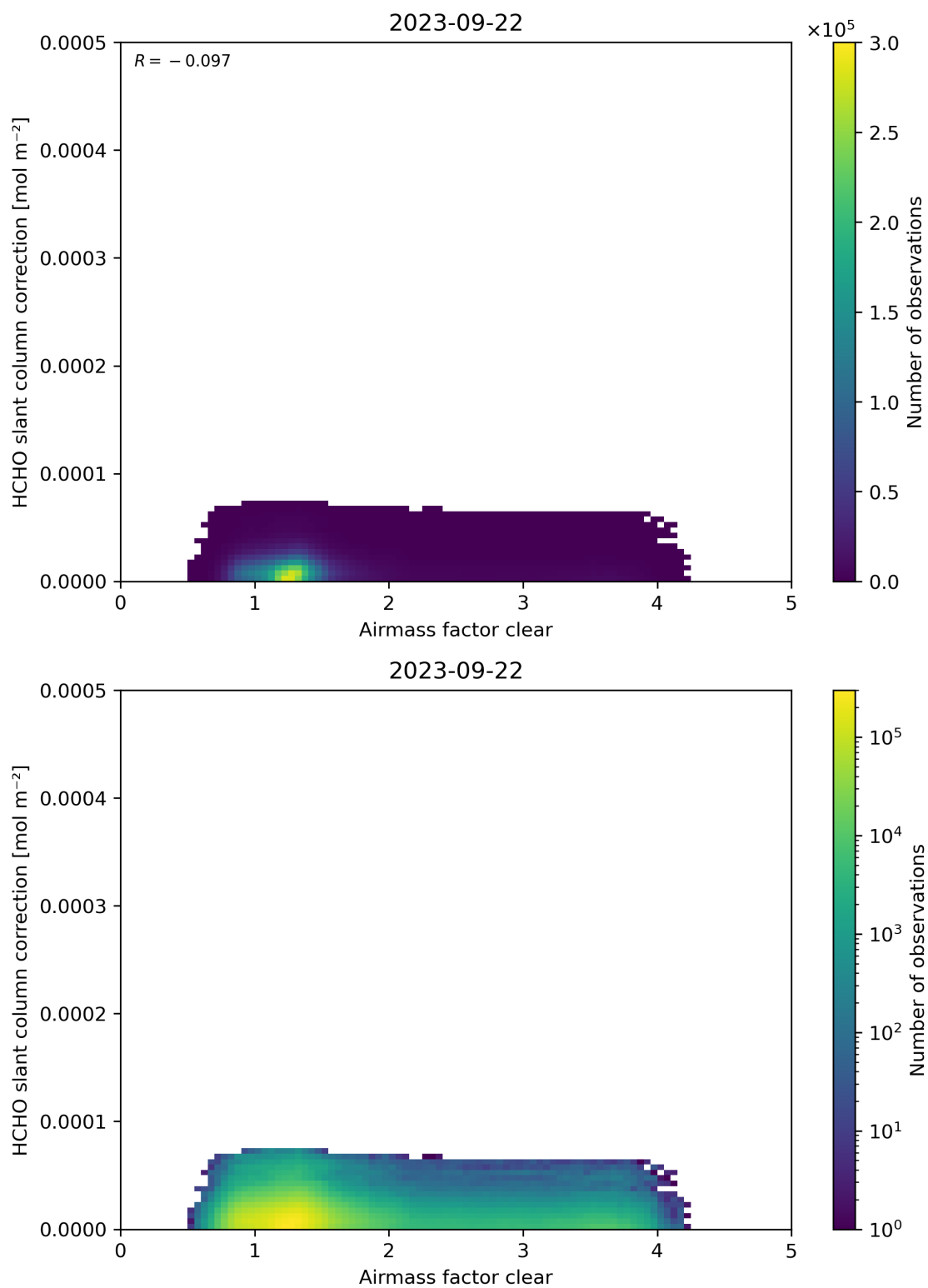
Figure 75: Scatter density plot of “Airmass factor clear” against “HCHO slant column correction” for 2023-09-21 to 2023-09-23.
