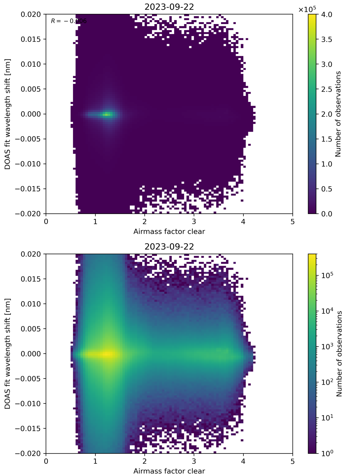
Figure 72: Scatter density plot of “Airmass factor clear” against “DOAS fit wavelength shift” for 2023-09-21 to 2023-09-23.
