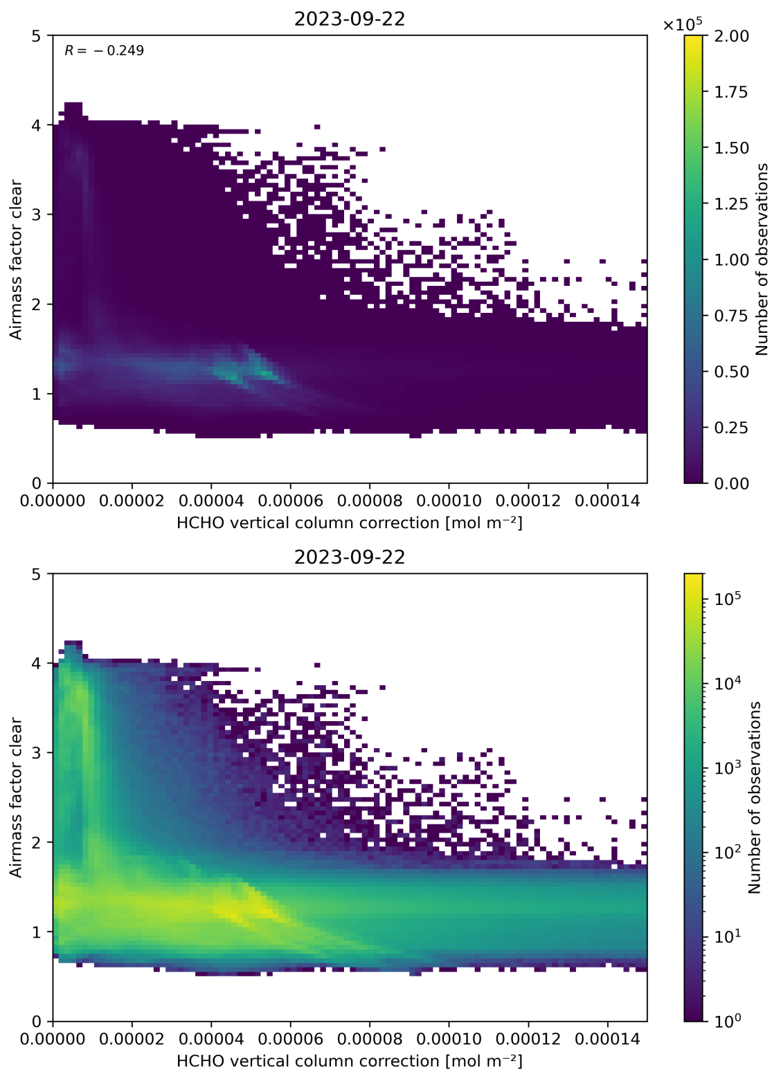
Figure 115: Scatter density plot of “HCHO vertical column correction” against “Airmass factor clear” for 2023-09-21 to 2023-09-23.
