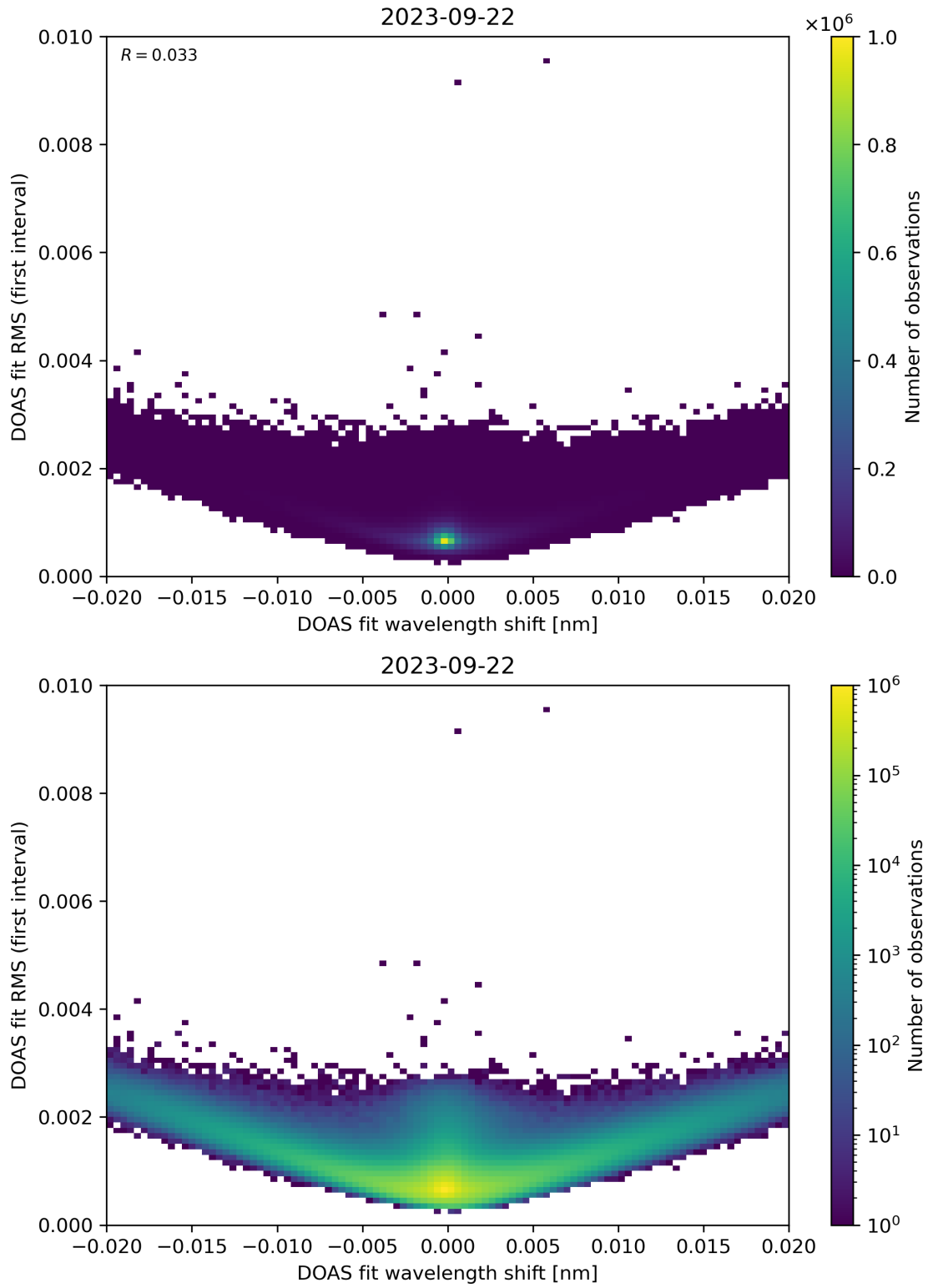
Figure 64: Scatter density plot of “DOAS fit wavelength shift” against “DOAS fit RMS (first interval)” for 2023-09-21 to 2023-09-23.
