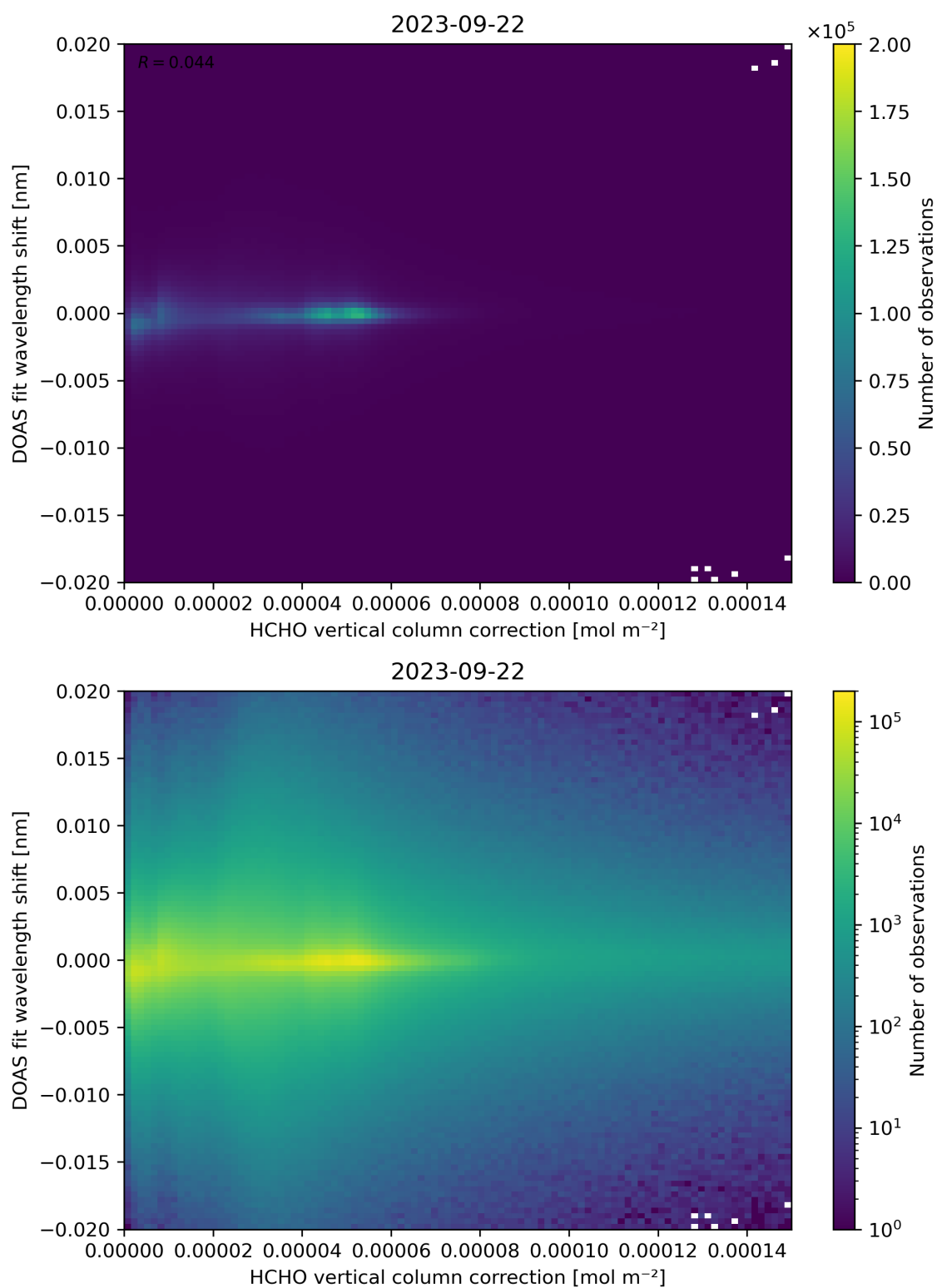
Figure 113: Scatter density plot of “HCHO vertical column correction” against “DOAS fit wavelength shift” for 2023-09-21 to 2023-09-23.
