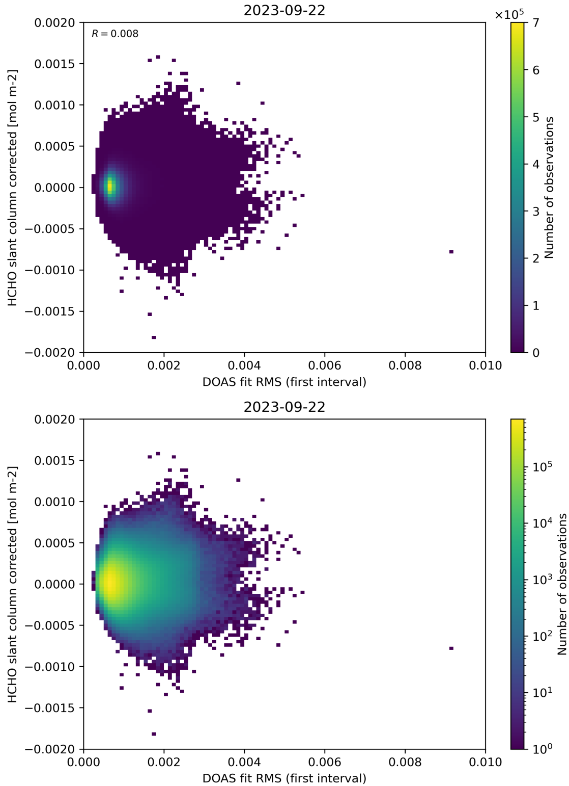
Figure 62: Scatter density plot of “DOAS fit RMS (first interval)” against “HCHO slant column corrected” for 2023-09-21 to 2023-09-23.
