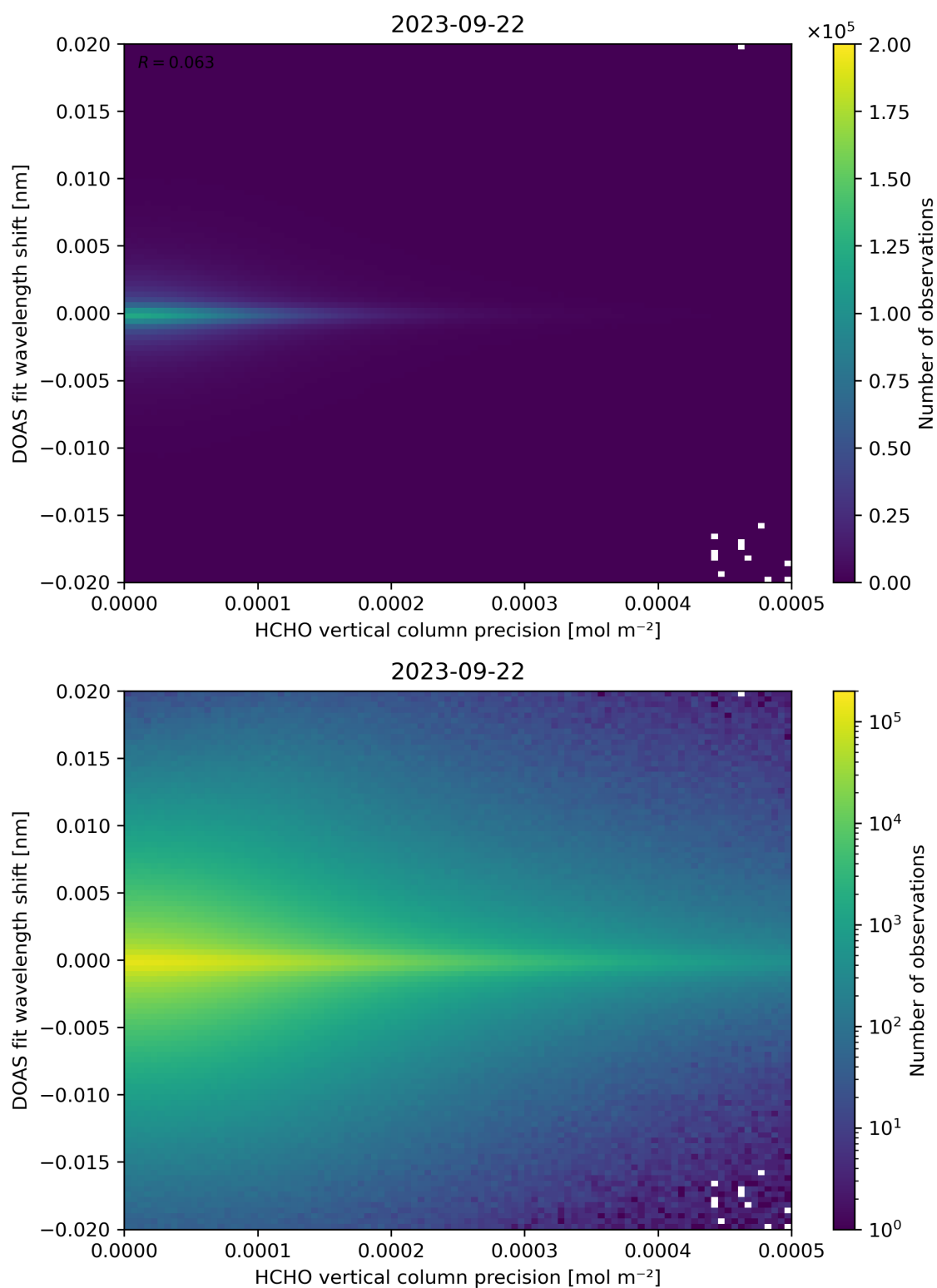
Figure 137: Scatter density plot of “HCHO vertical column precision” against “DOAS fit wavelength shift” for 2023-09-21 to 2023-09-23.
