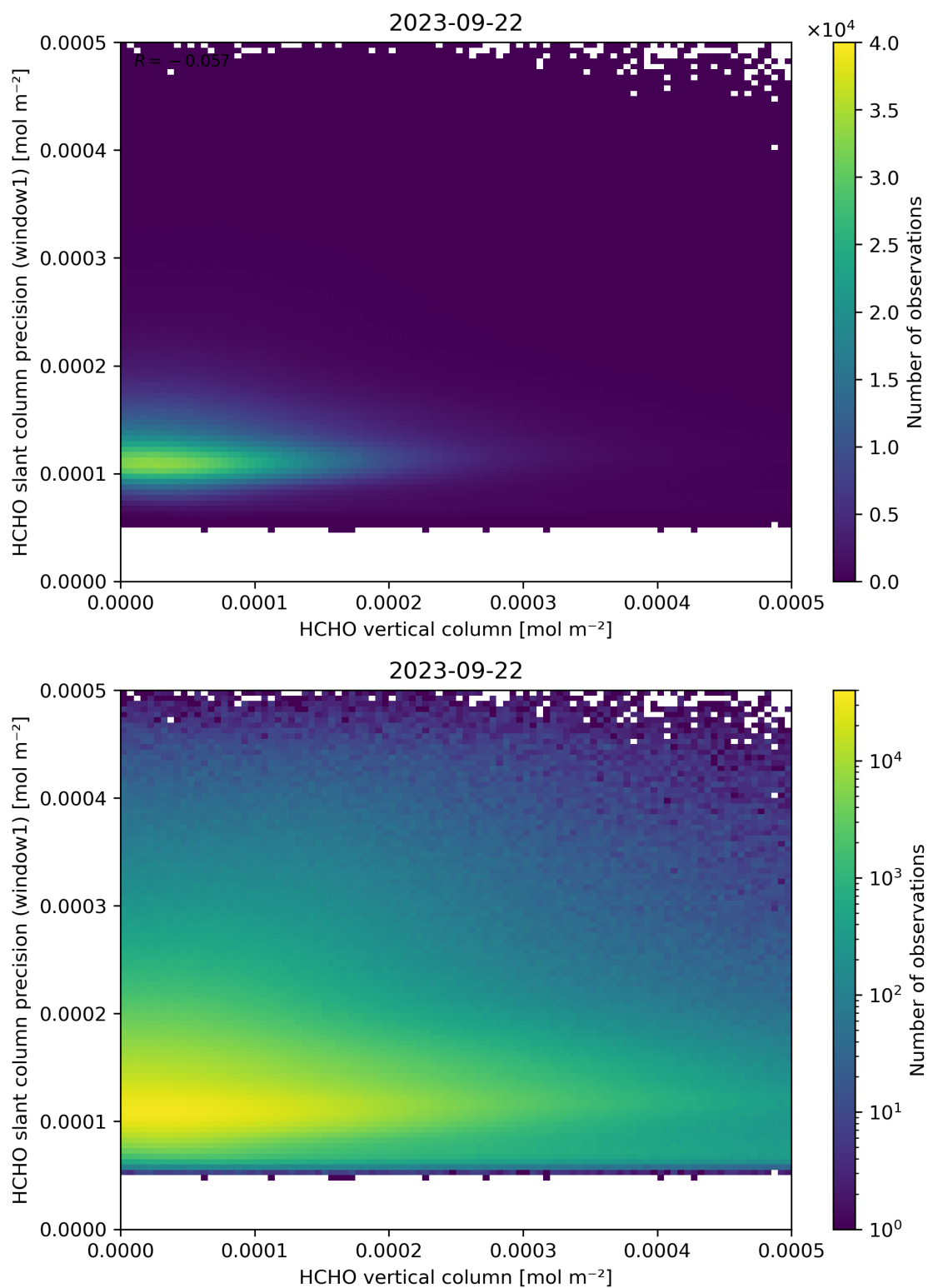
Figure 130: Scatter density plot of “HCHO vertical column” against “HCHO slant column precision (window1)” for 2023-09-21 to 2023-09-23.
