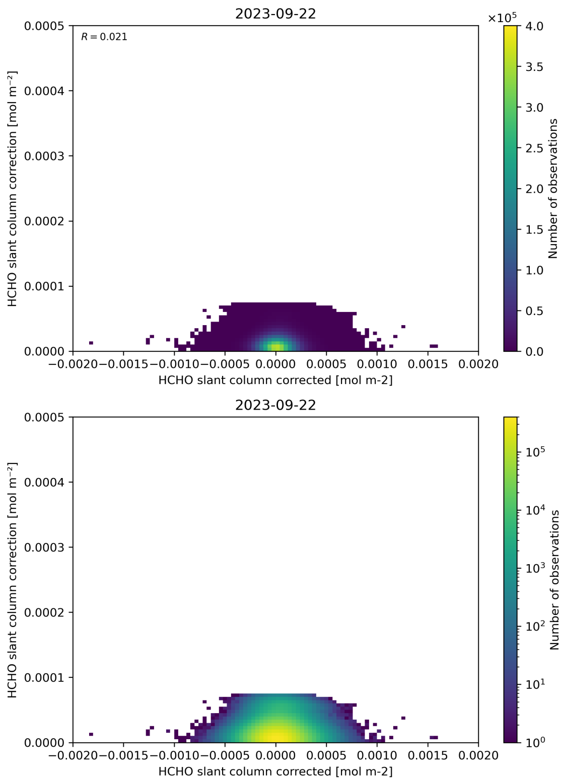
Figure 77: Scatter density plot of “HCHO slant column corrected” against “HCHO slant column correction” for 2023-09-21 to 2023-09-23.
