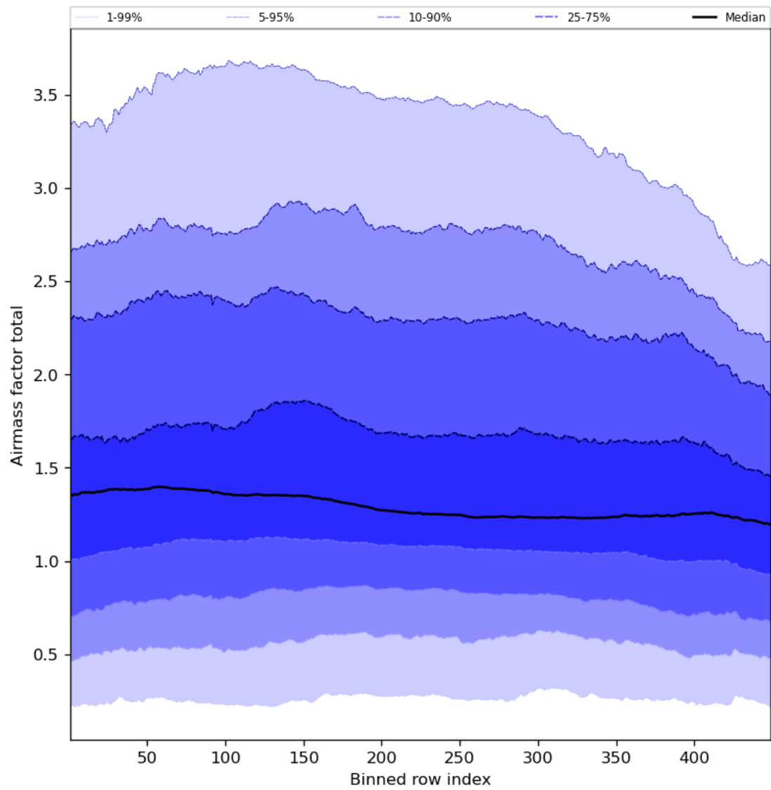
Figure 54: Along track statistics of “Airmass factor total” for 2023-09-21 to 2023-09-23
