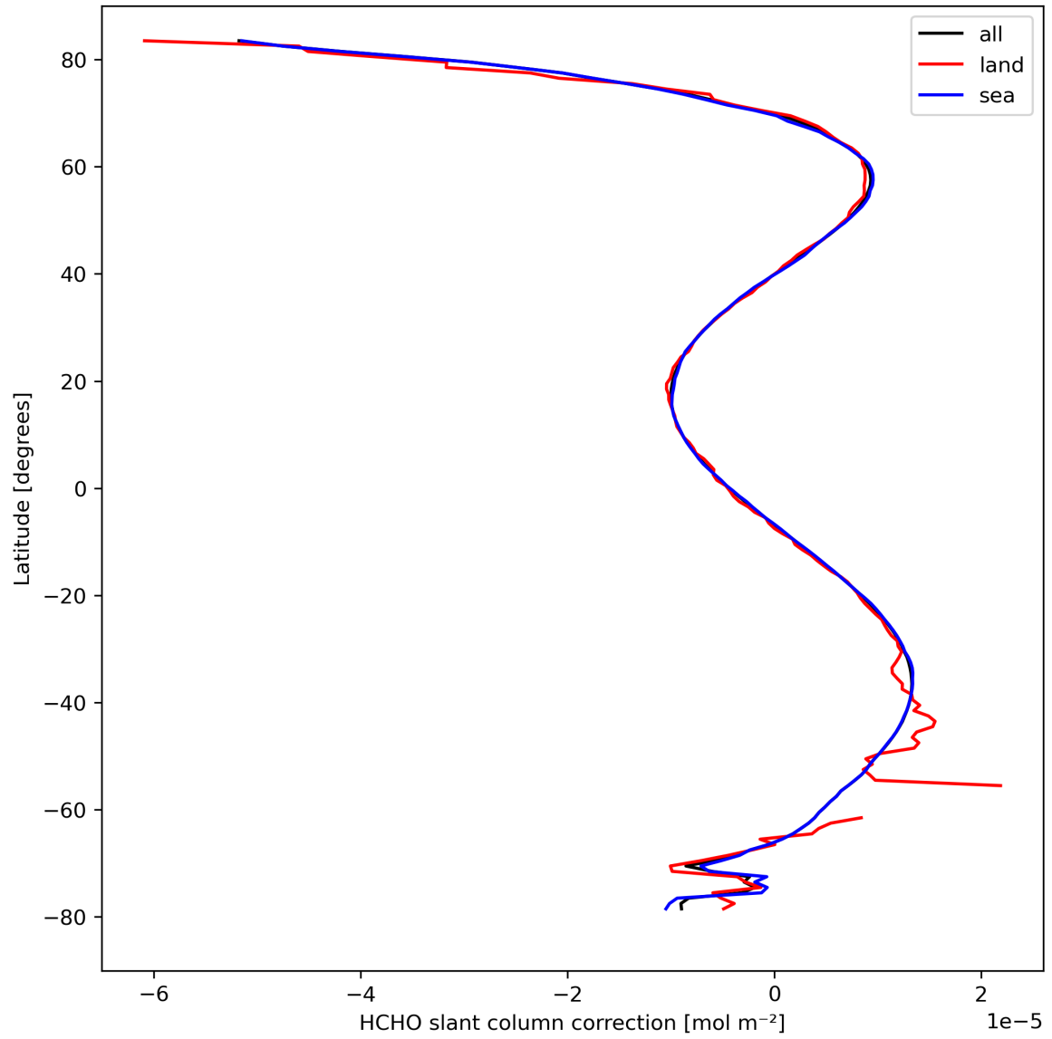
Figure 33: Zonal average of “HCHO slant column correction” for 2023-09-21 to 2023-09-23.
