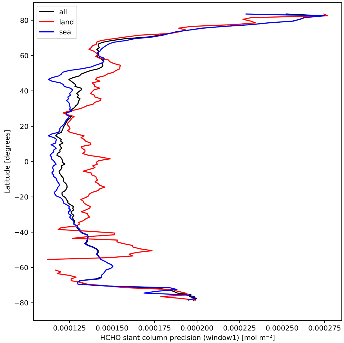
Figure 25: Zonal average of “HCHO slant column precision (window1)” for 2023-09-21 to 2023-09-23.
