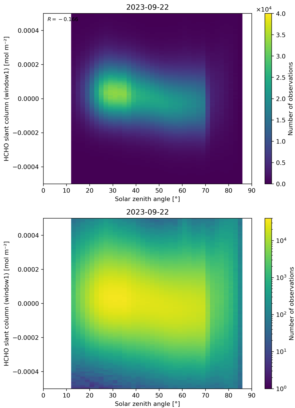
Figure 173: Scatter density plot of “Solar zenith angle” against “HCHO slant column (window1)” for 2023-09-21 to 2023-09-23.
