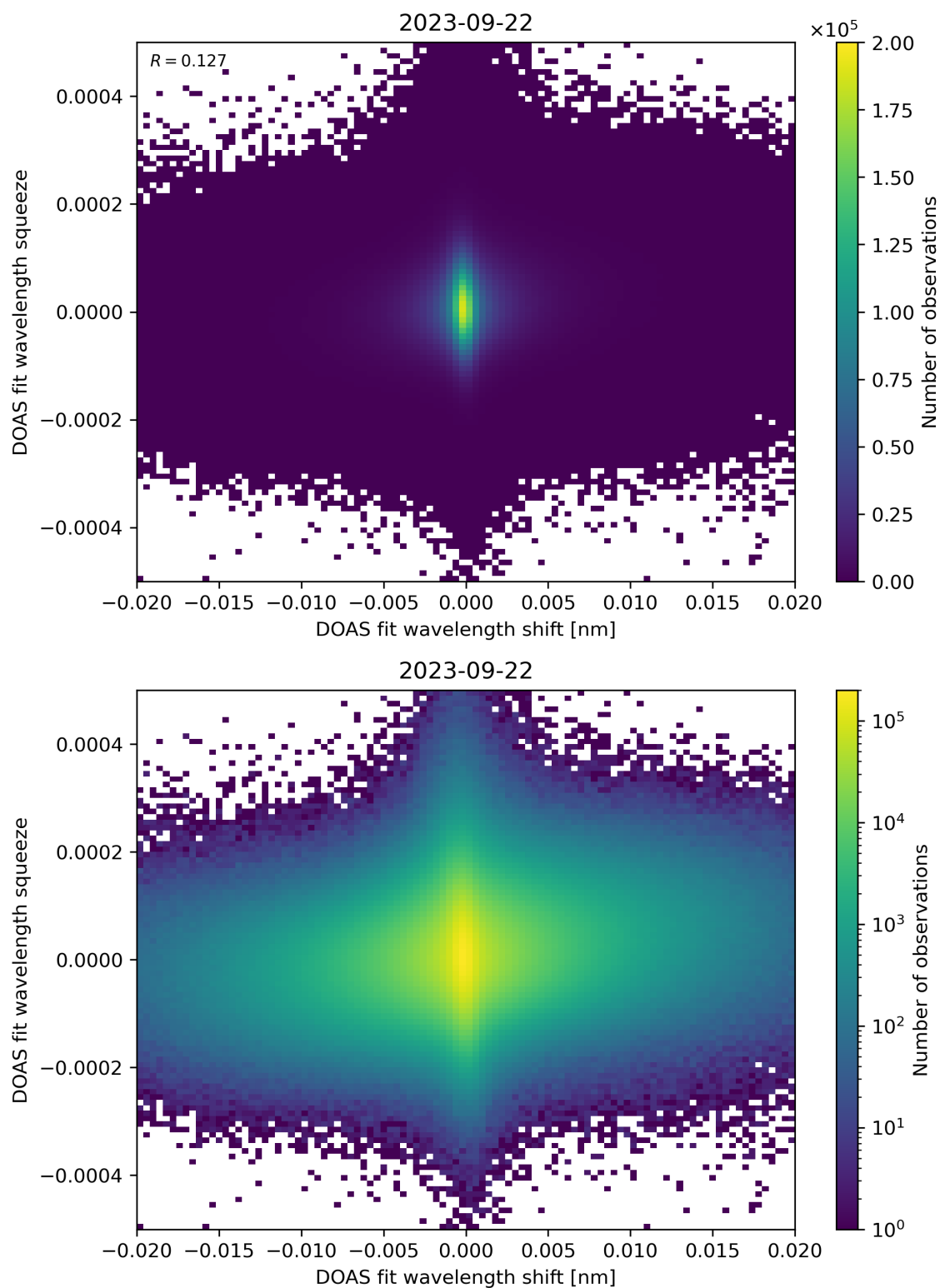
Figure 65: Scatter density plot of “DOAS fit wavelength shift” against “DOAS fit wavelength squeeze” for 2023-09-21 to 2023-09-23.
