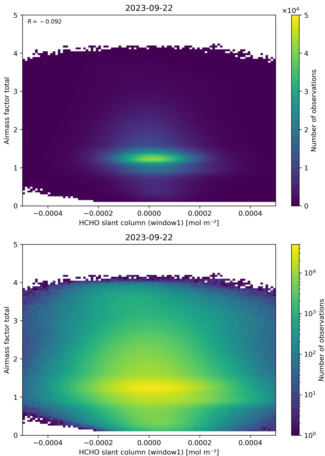
Figure 85: Scatter density plot of “HCHO slant column (window1)” against “Airmass factor total” for 2023-09-21 to 2023-09-23.
