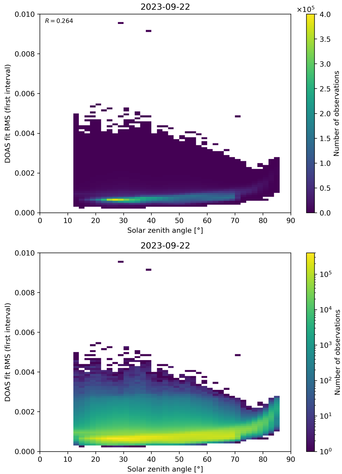
Figure 167: Scatter density plot of “Solar zenith angle” against “DOAS fit RMS (first interval)” for 2023-09-21 to 2023-09-23.
