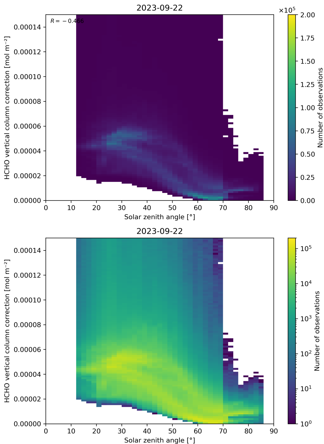
Figure 178: Scatter density plot of “Solar zenith angle” against “HCHO vertical column correction” for 2023-09-21 to 2023-09-23.
