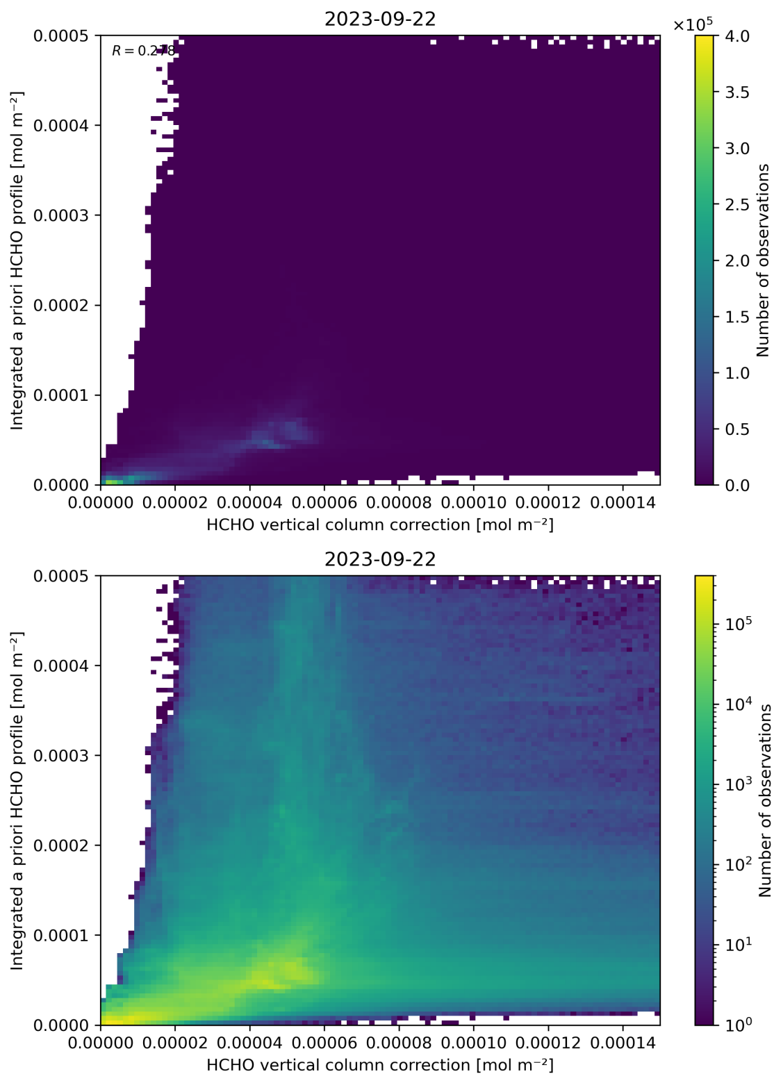
Figure 122: Scatter density plot of “HCHO vertical column correction” against “Integrated a priori HCHO profile” for 2023-09-21 to 2023-09-23.
