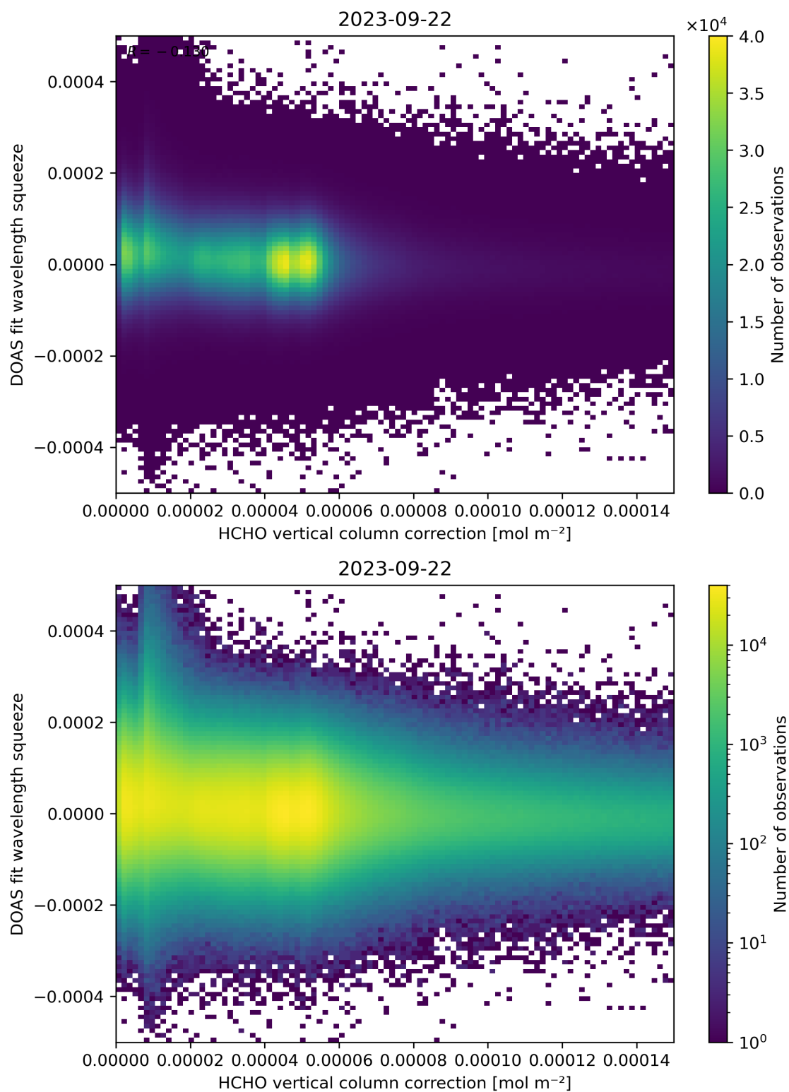
Figure 114: Scatter density plot of “HCHO vertical column correction” against “DOAS fit wavelength squeeze” for 2023-09-21 to 2023-09-23.
