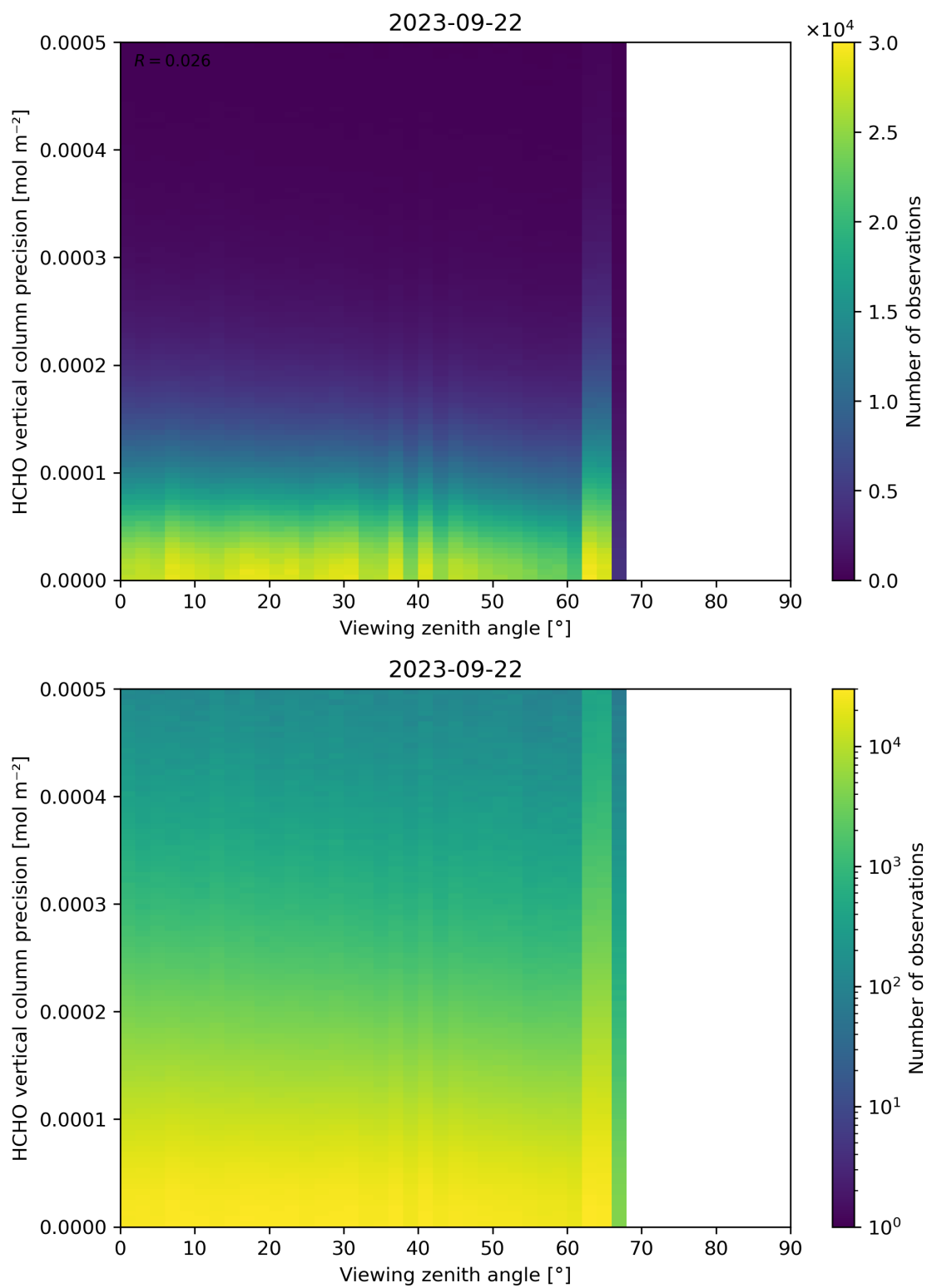
Figure 194: Scatter density plot of “Viewing zenith angle” against “HCHO vertical column precision” for 2023-09-21 to 2023-09-23.
