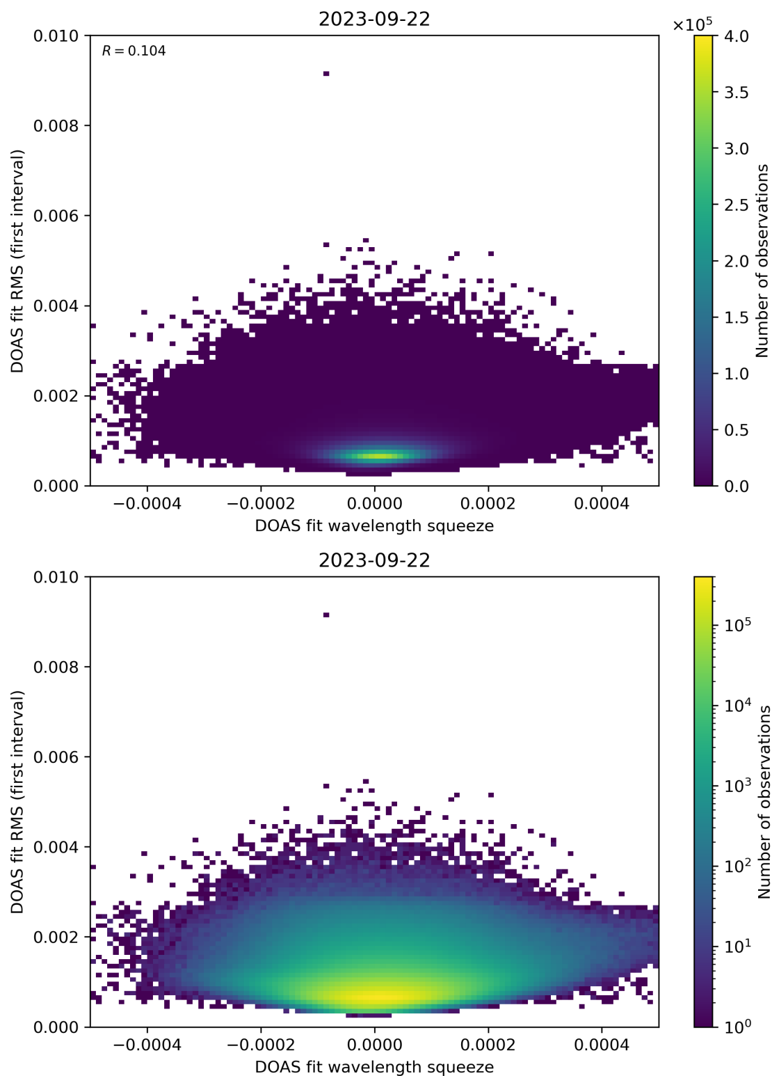
Figure 68: Scatter density plot of “DOAS fit wavelength squeeze” against “DOAS fit RMS (first interval)” for 2023-09-21 to 2023-09-23.
