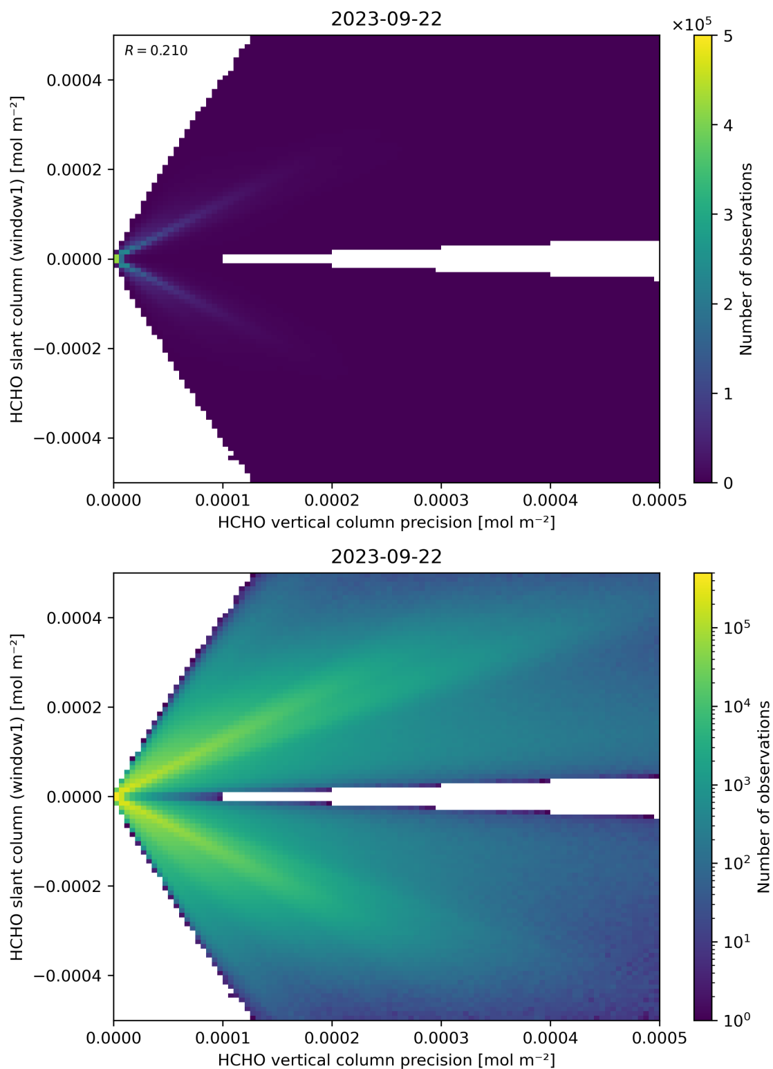
Figure 142: Scatter density plot of “HCHO vertical column precision” against “HCHO slant column (window1)” for 2023-09-21 to 2023-09-23.
