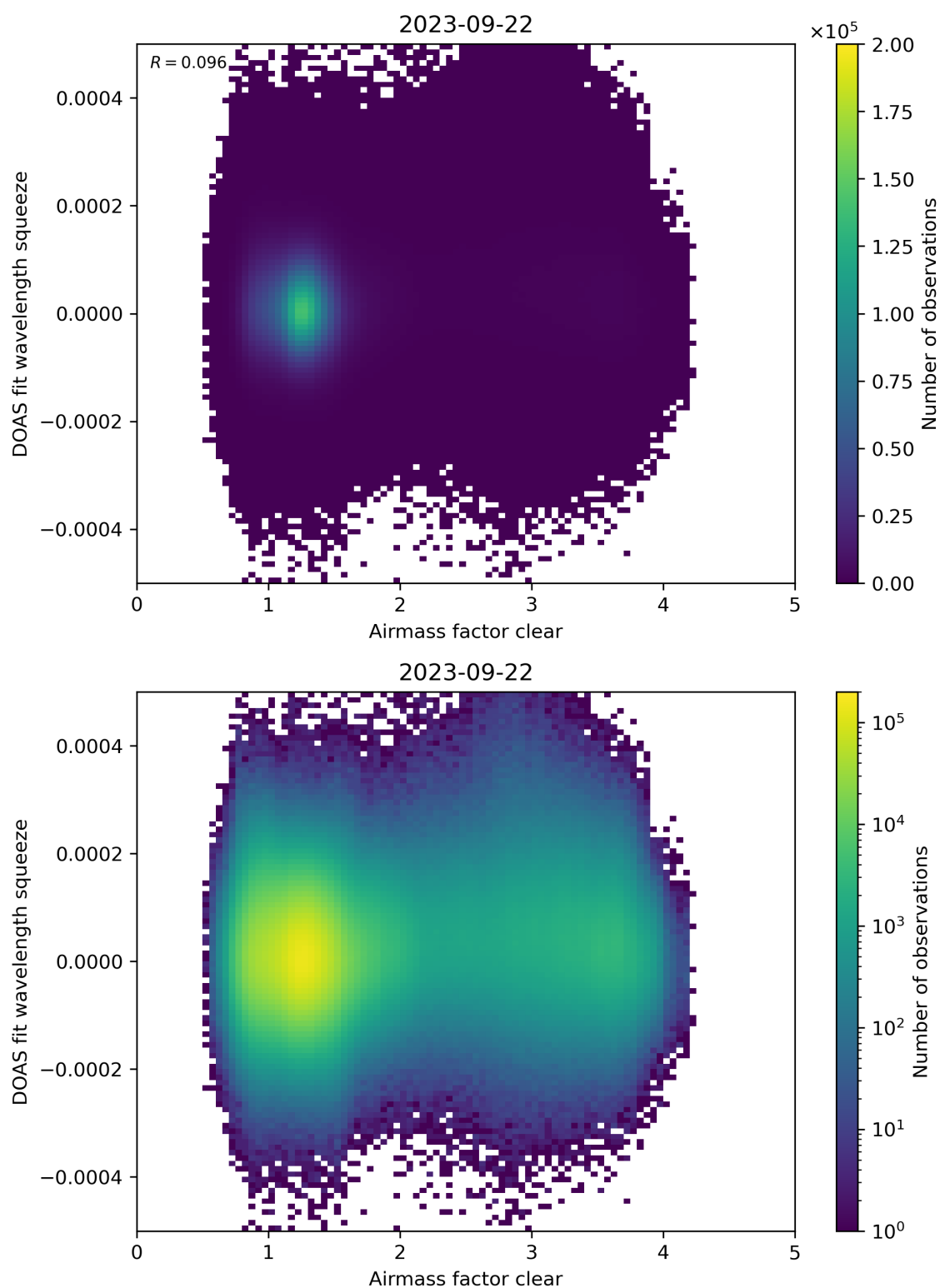
Figure 73: Scatter density plot of “Airmass factor clear” against “DOAS fit wavelength squeeze” for 2023-09-21 to 2023-09-23.
