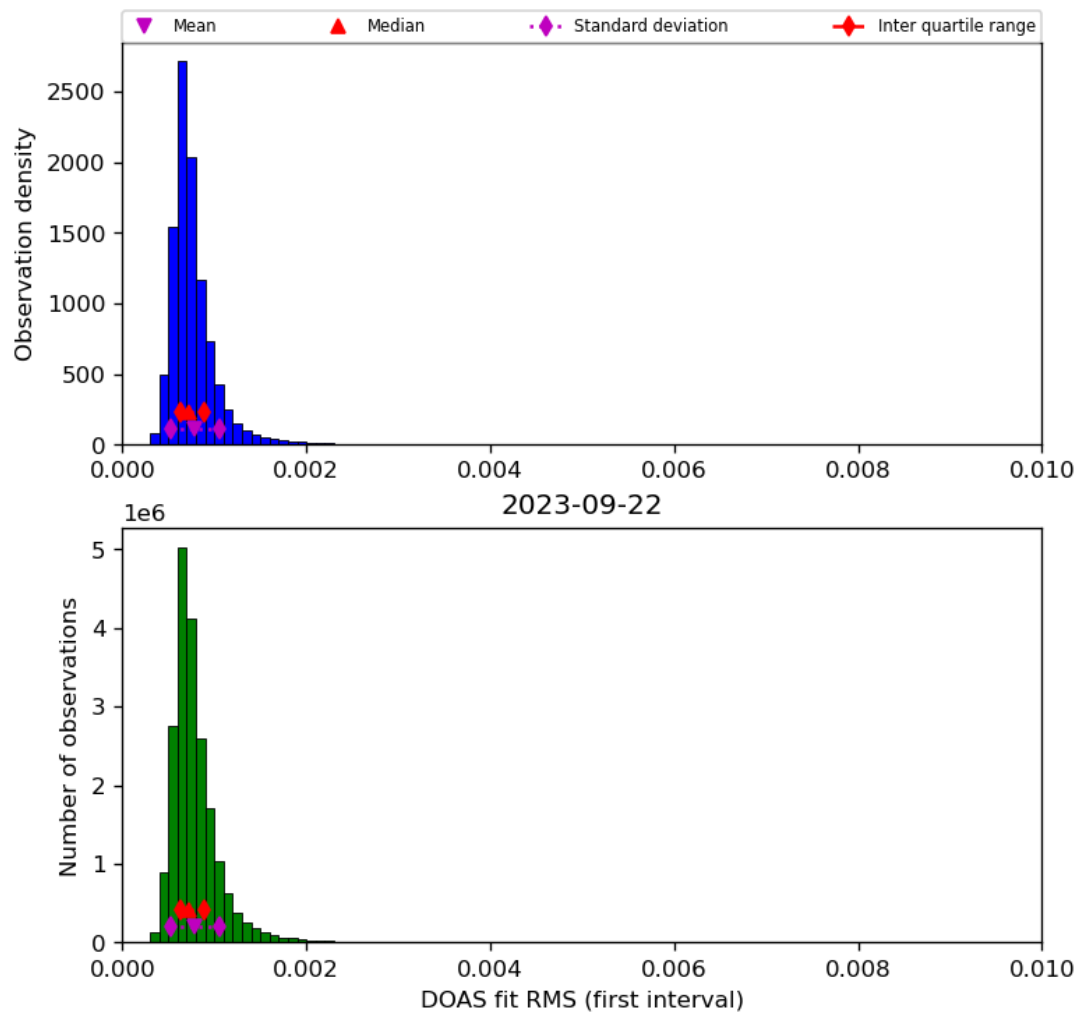
Figure 46: Histogram of “DOAS fit RMS (first interval)” for 2023-09-21 to 2023-09-23
