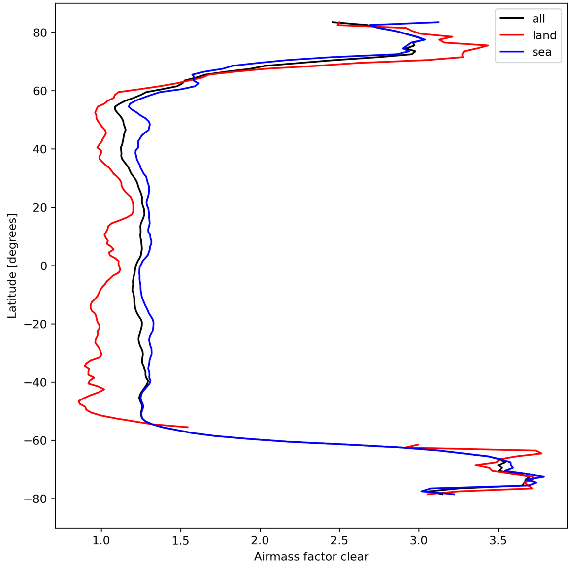
Figure 28: Zonal average of “Airmass factor clear” for 2023-09-21 to 2023-09-23.
