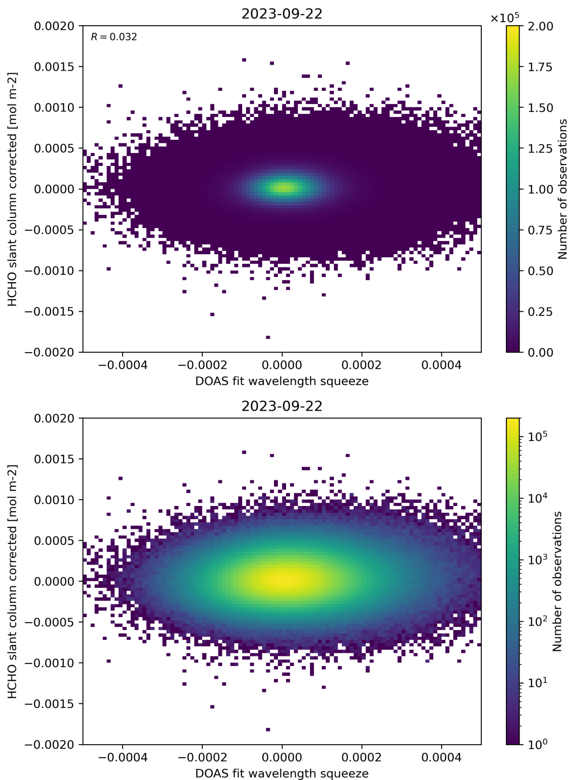
Figure 69: Scatter density plot of “DOAS fit wavelength squeeze” against “HCHO slant column corrected” for 2023-09-21 to 2023-09-23.
