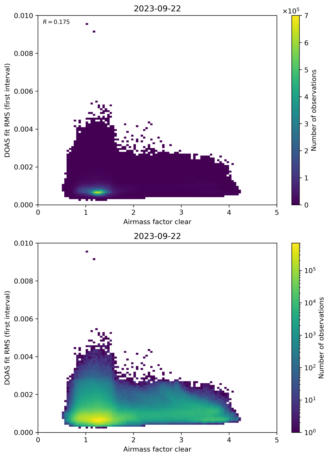
Figure 71: Scatter density plot of “Airmass factor clear” against “DOAS fit RMS (first interval)” for 2023-09-21 to 2023-09-23.
