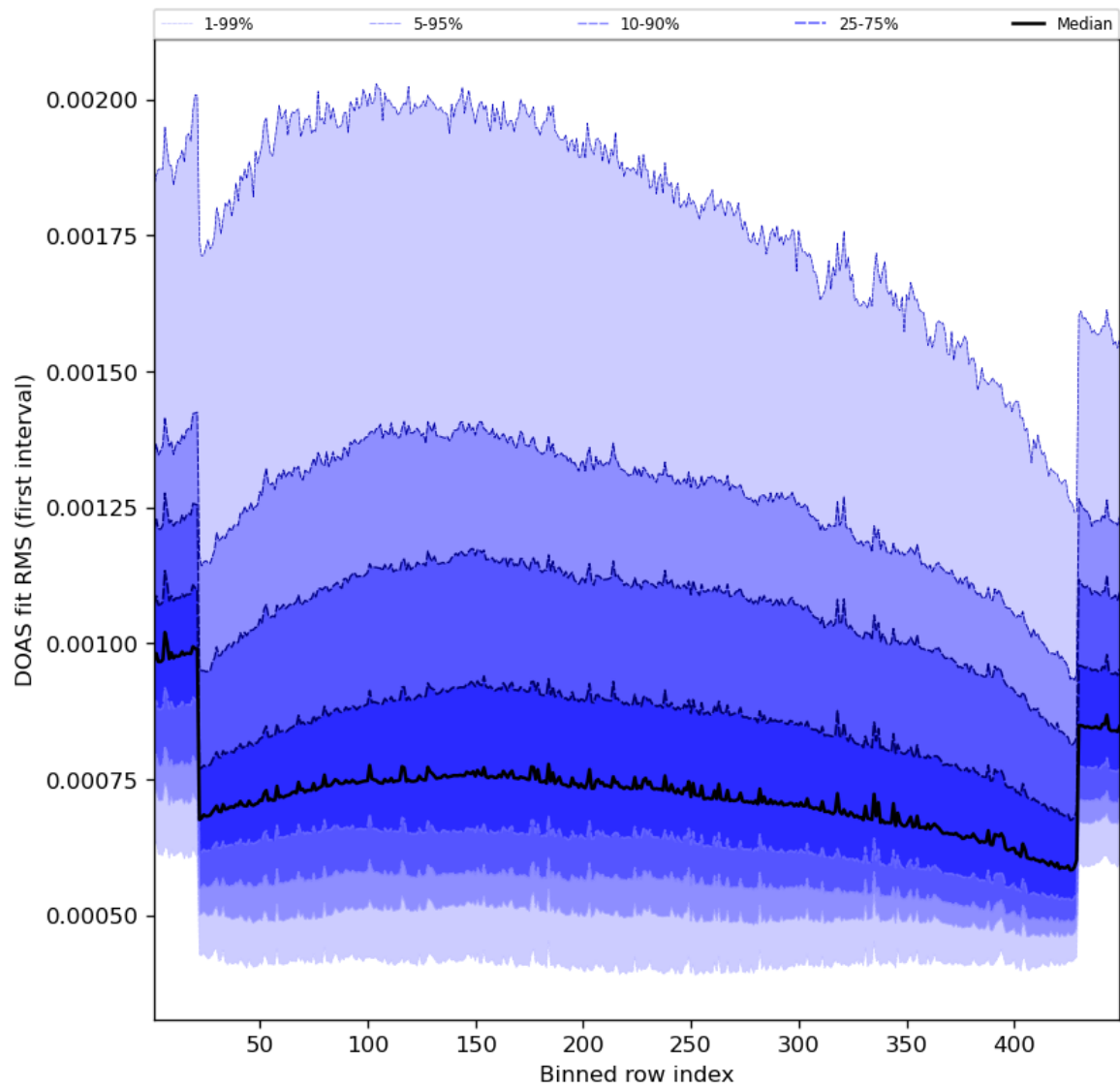
Figure 60: Along track statistics of “DOAS fit RMS (first interval)” for 2023-09-21 to 2023-09-23
