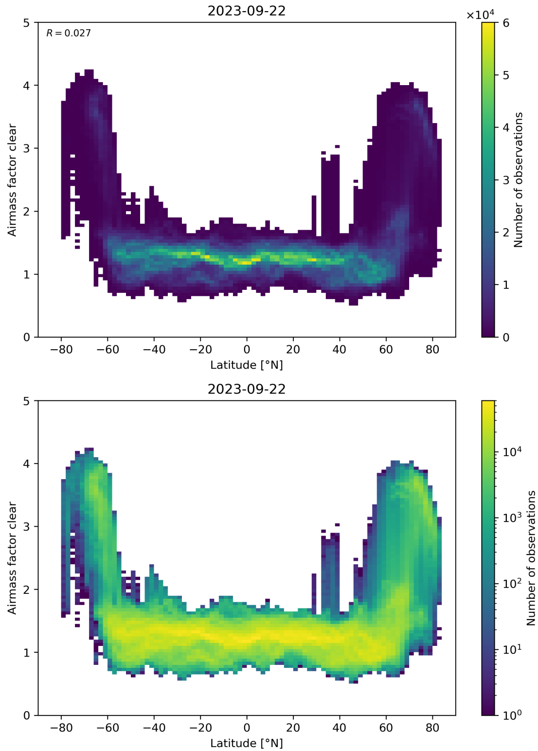
Figure 156: Scatter density plot of “Latitude” against “Airmass factor clear” for 2023-09-21 to 2023-09-23.
