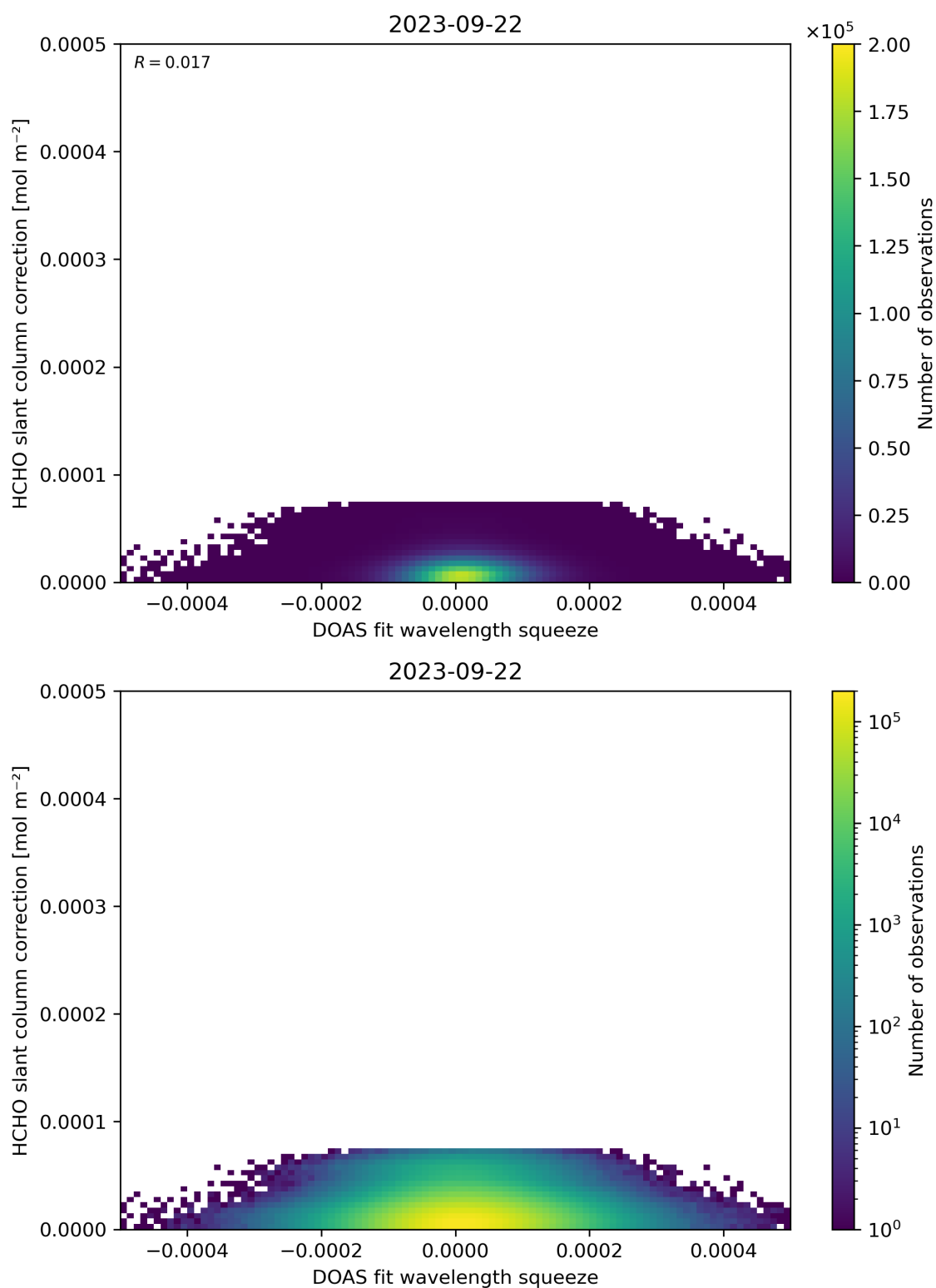
Figure 70: Scatter density plot of “DOAS fit wavelength squeeze” against “HCHO slant column correction” for 2023-09-21 to 2023-09-23.
