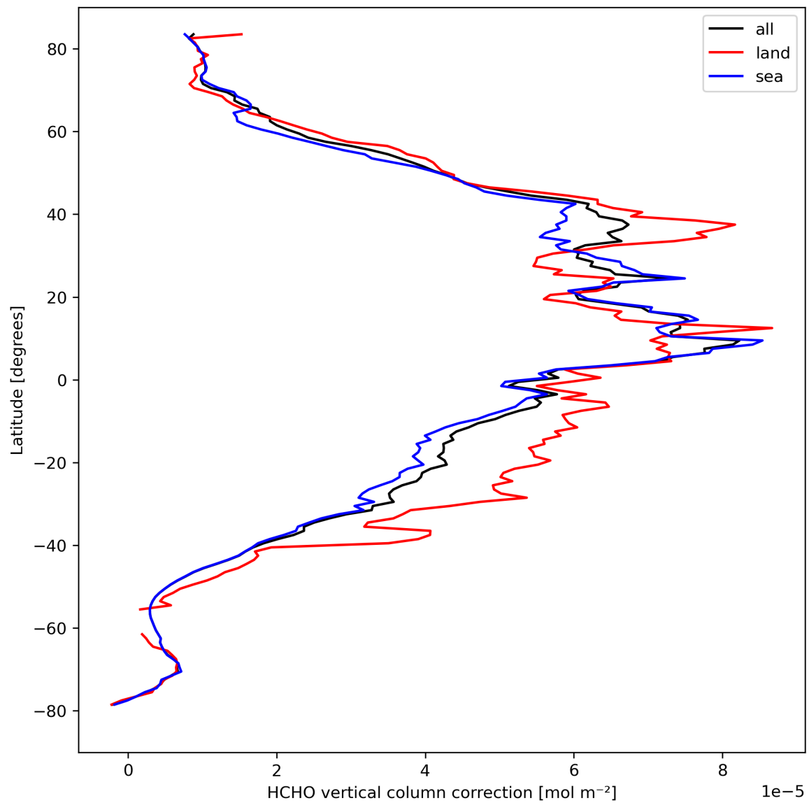
Figure 23: Zonal average of “HCHO vertical column correction” for 2023-09-21 to 2023-09-23.
