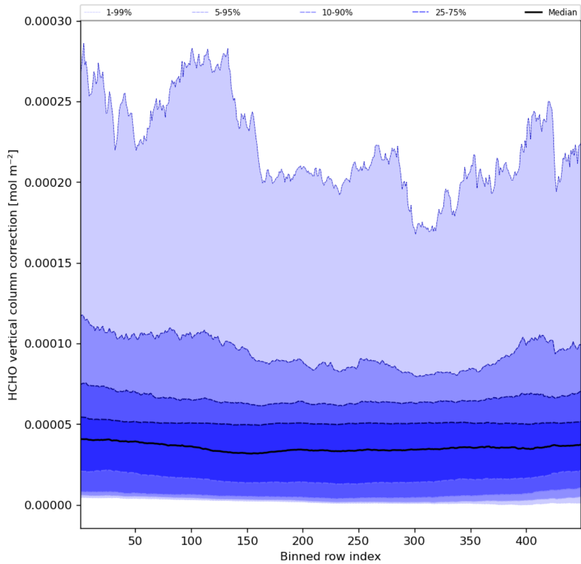
Figure 51: Along track statistics of “HCHO vertical column correction” for 2023-09-21 to 2023-09-23
