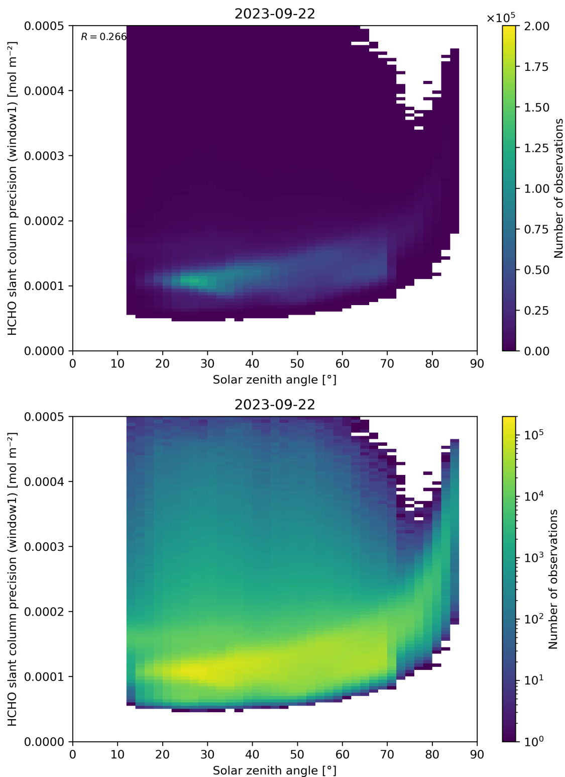
Figure 174: Scatter density plot of “Solar zenith angle” against “HCHO slant column precision (window1)” for 2023-09-21 to 2023-09-23.
