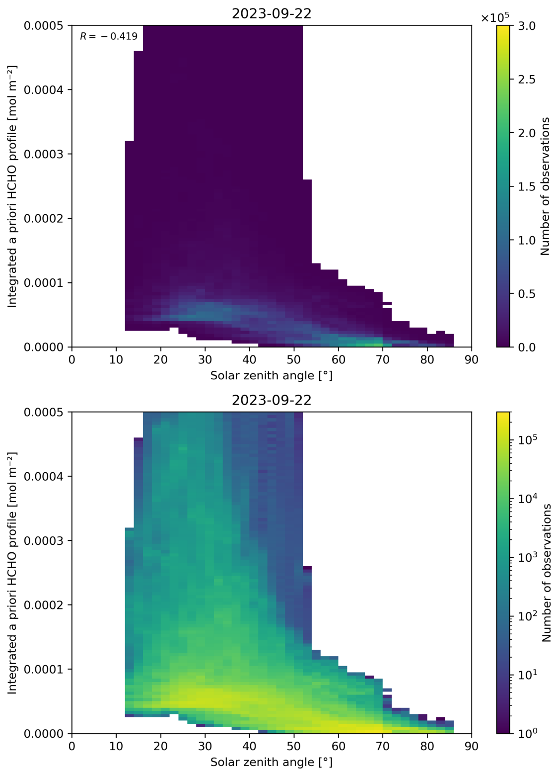
Figure 180: Scatter density plot of “Solar zenith angle” against “Integrated a priori HCHO profile” for 2023-09-21 to 2023-09-23.
