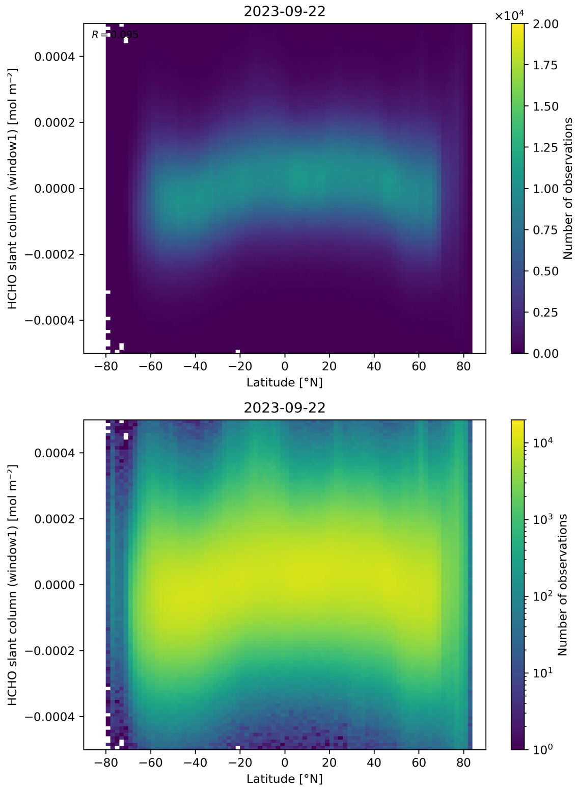
Figure 159: Scatter density plot of “Latitude” against “HCHO slant column (window1)” for 2023-09-21 to 2023-09-23.
