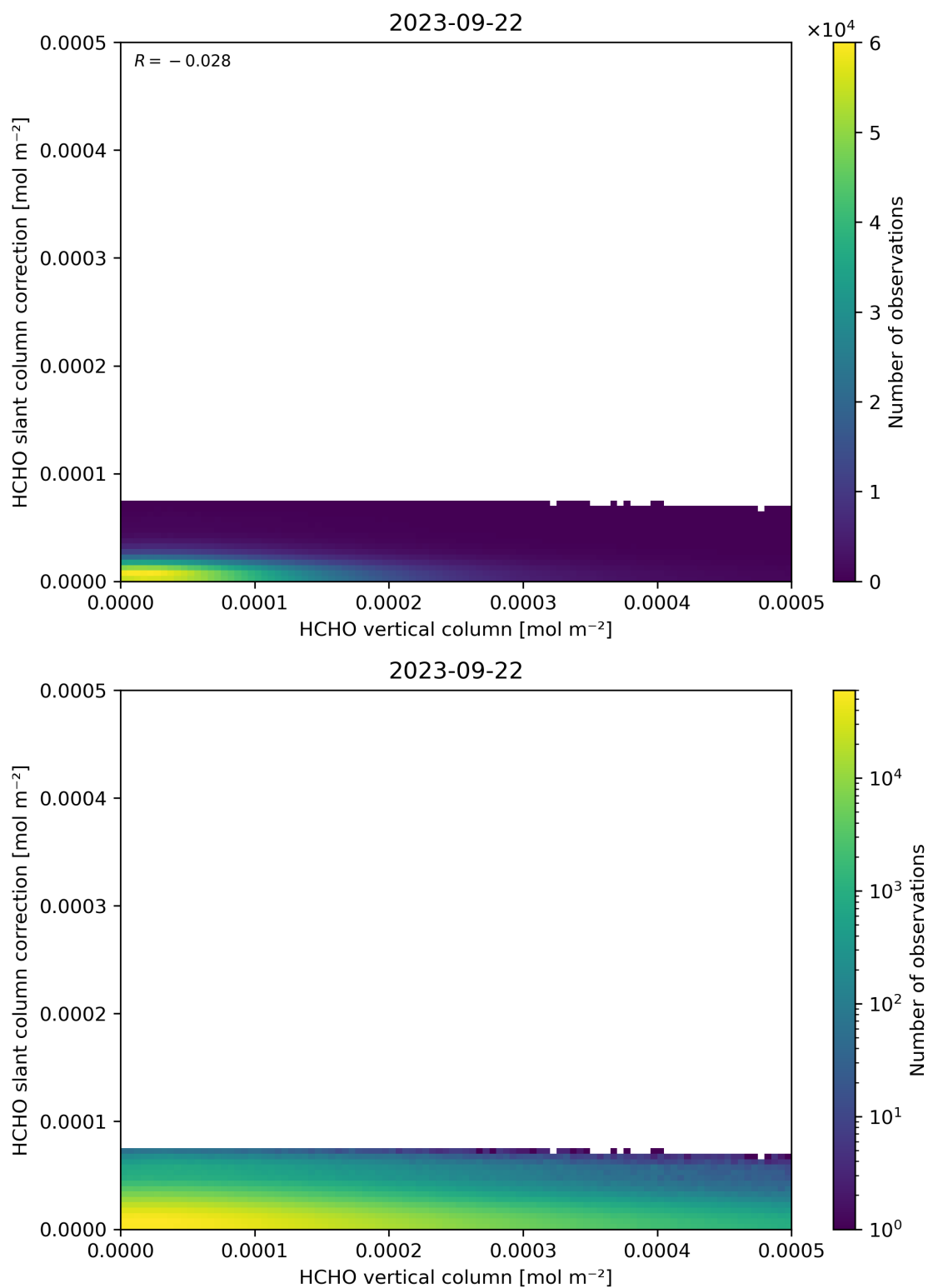
Figure 128: Scatter density plot of “HCHO vertical column” against “HCHO slant column correction” for 2023-09-21 to 2023-09-23.
