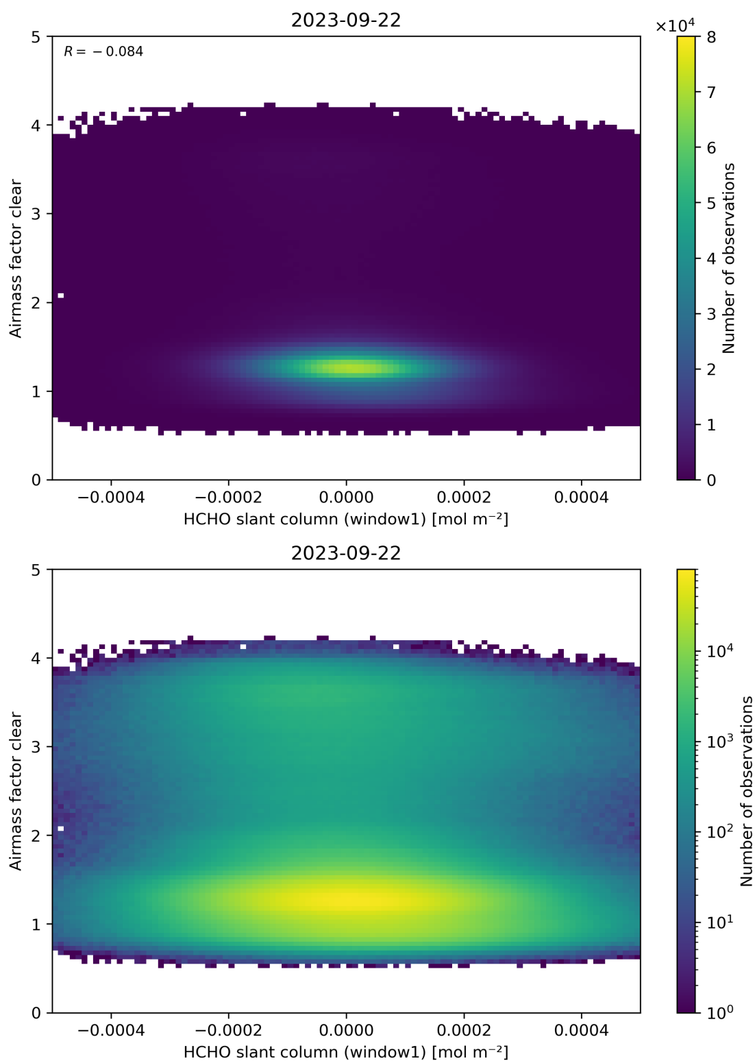
Figure 81: Scatter density plot of “HCHO slant column (window1)” against “Airmass factor clear” for 2023-09-21 to 2023-09-23.
