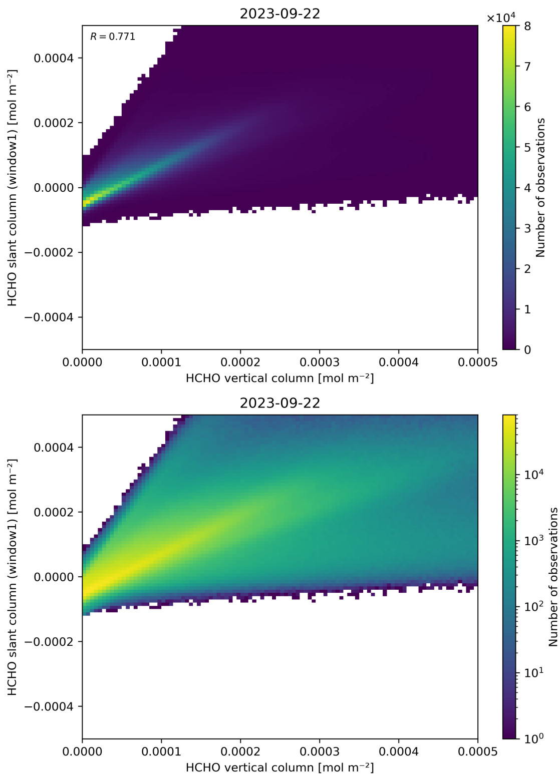
Figure 129: Scatter density plot of “HCHO vertical column” against “HCHO slant column (window1)” for 2023-09-21 to 2023-09-23.
