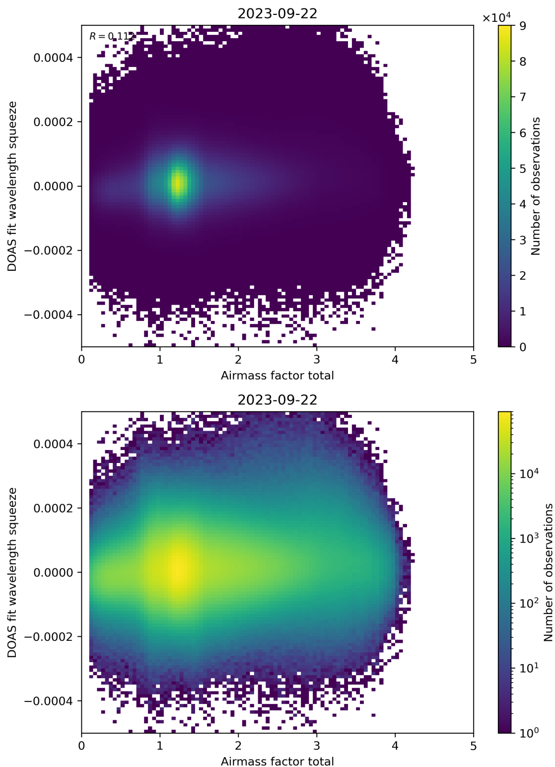
Figure 99: Scatter density plot of “Airmass factor total” against “DOAS fit wavelength squeeze” for 2023-09-21 to 2023-09-23.
