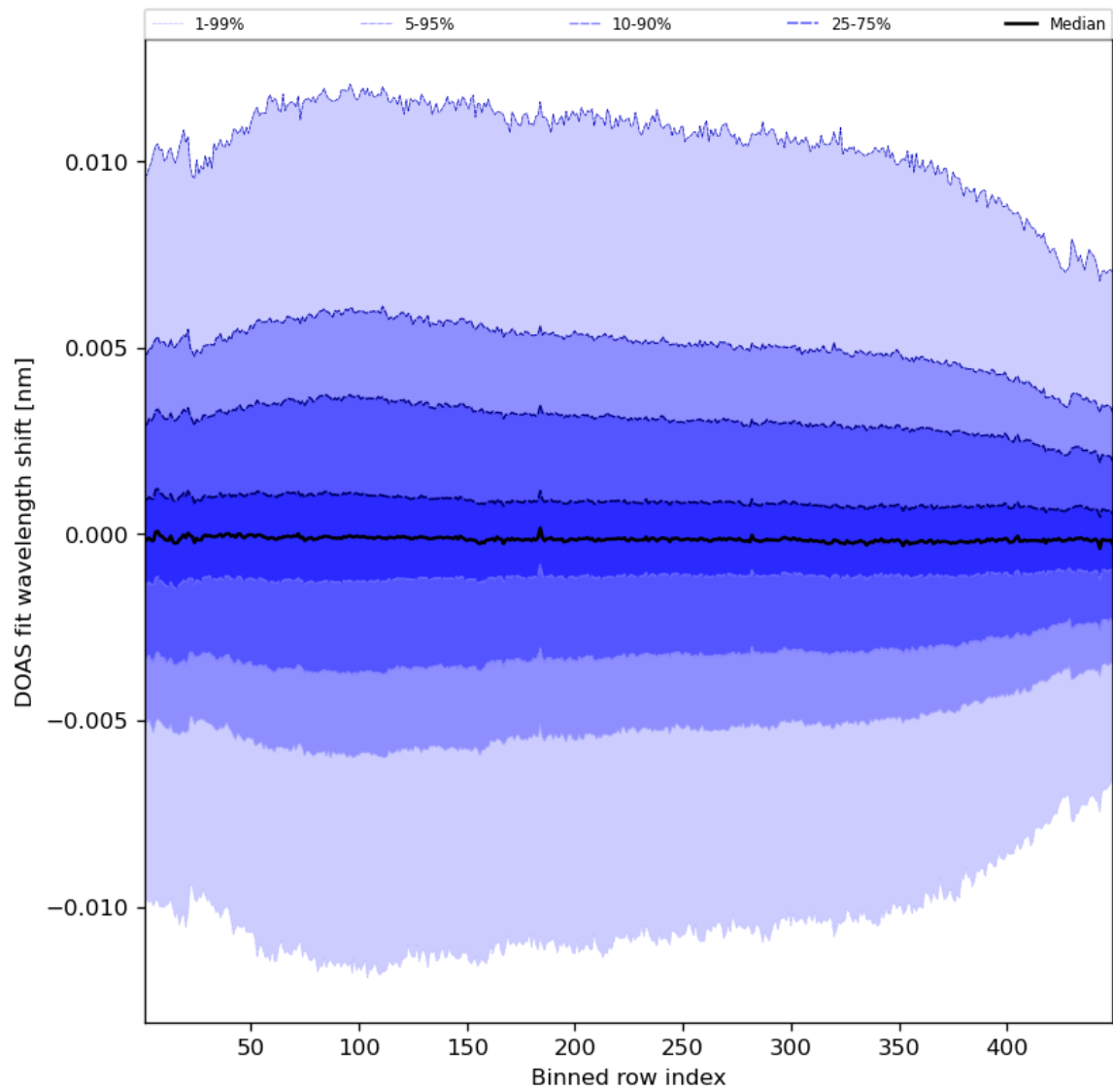
Figure 58: Along track statistics of “DOAS fit wavelength shift” for 2023-09-21 to 2023-09-23
