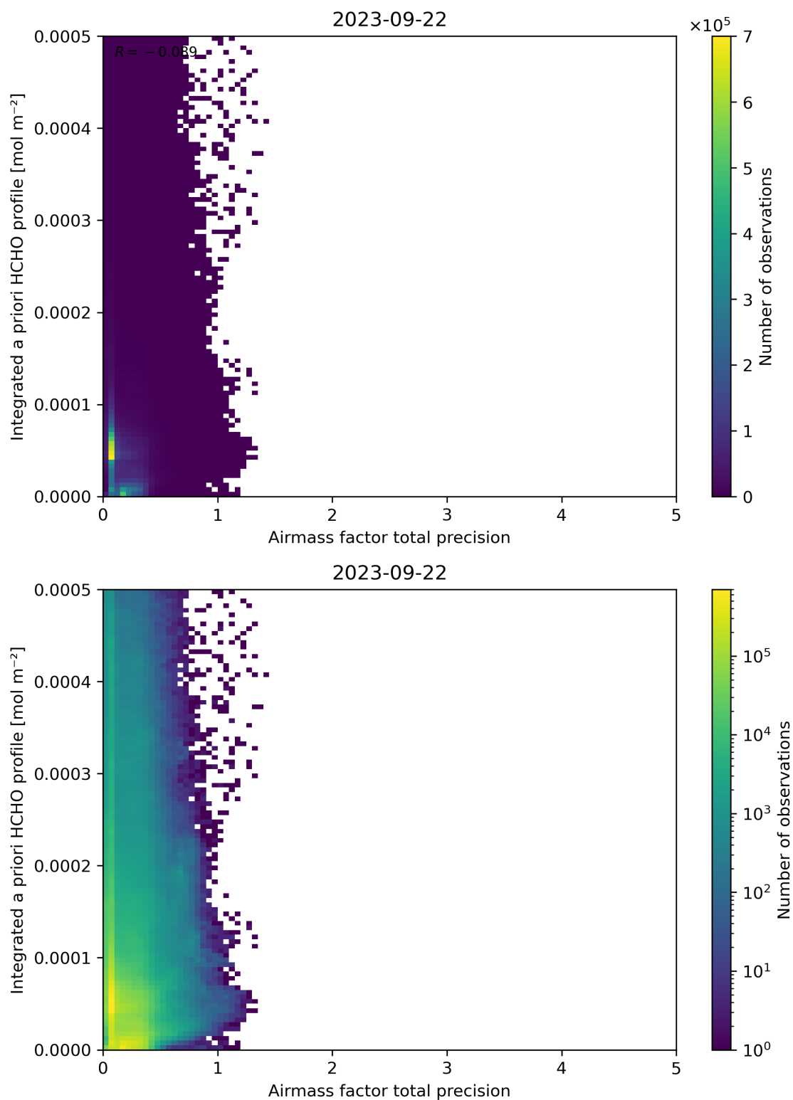
Figure 111: Scatter density plot of “Airmass factor total precision” against “Integrated a priori HCHO profile” for 2023-09-21 to 2023-09-23.
