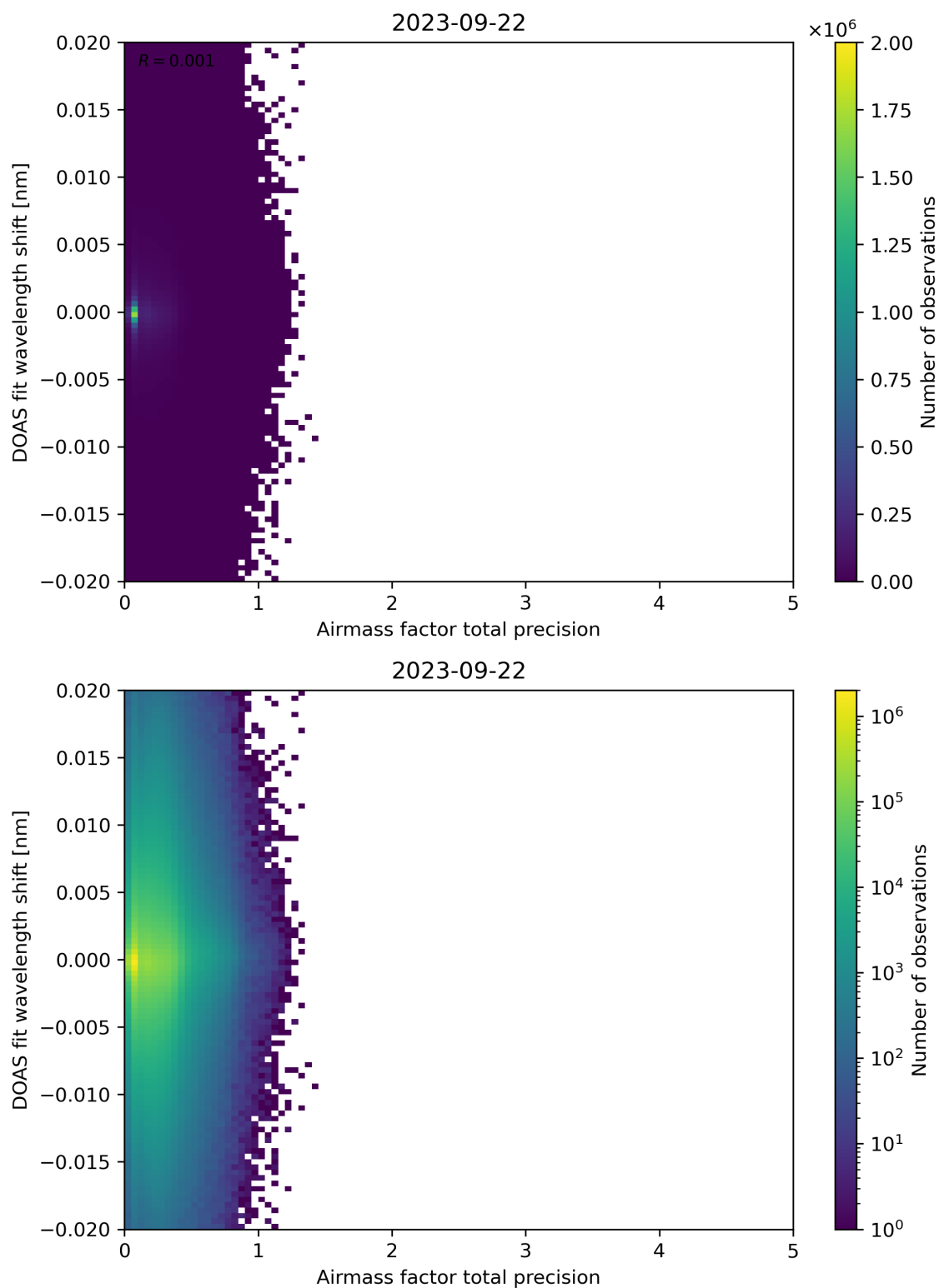
Figure 106: Scatter density plot of “Airmass factor total precision” against “DOAS fit wavelength shift” for 2023-09-21 to 2023-09-23.
