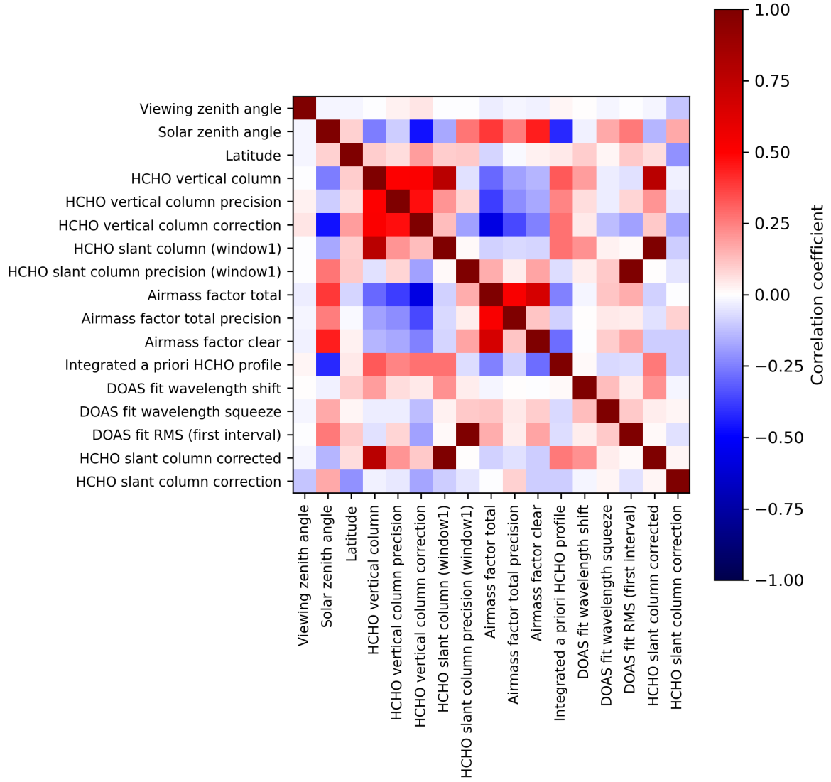
Figure 2: Map of correlation matrix for 2023-09-21 to 2023-09-23.
