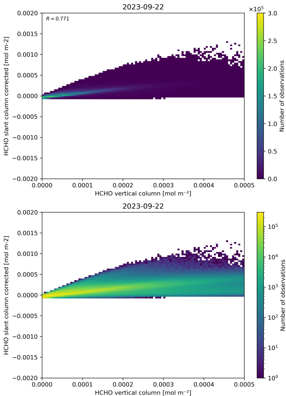
Figure 127: Scatter density plot of “HCHO vertical column” against “HCHO slant column corrected” for 2023-09-21 to 2023-09-23.
