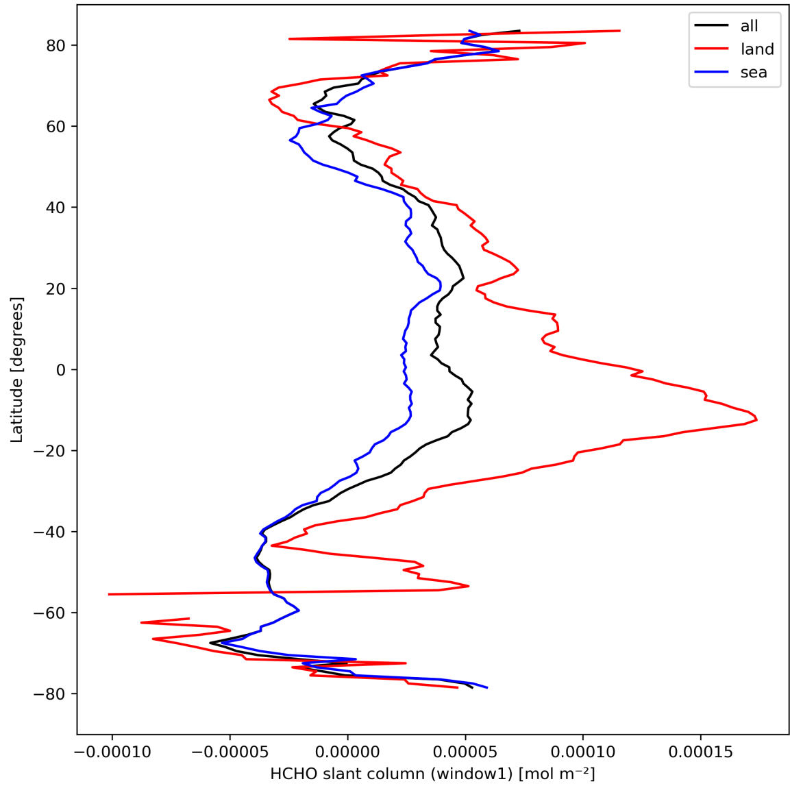
Figure 24: Zonal average of “HCHO slant column (window1)” for 2023-09-21 to 2023-09-23.
