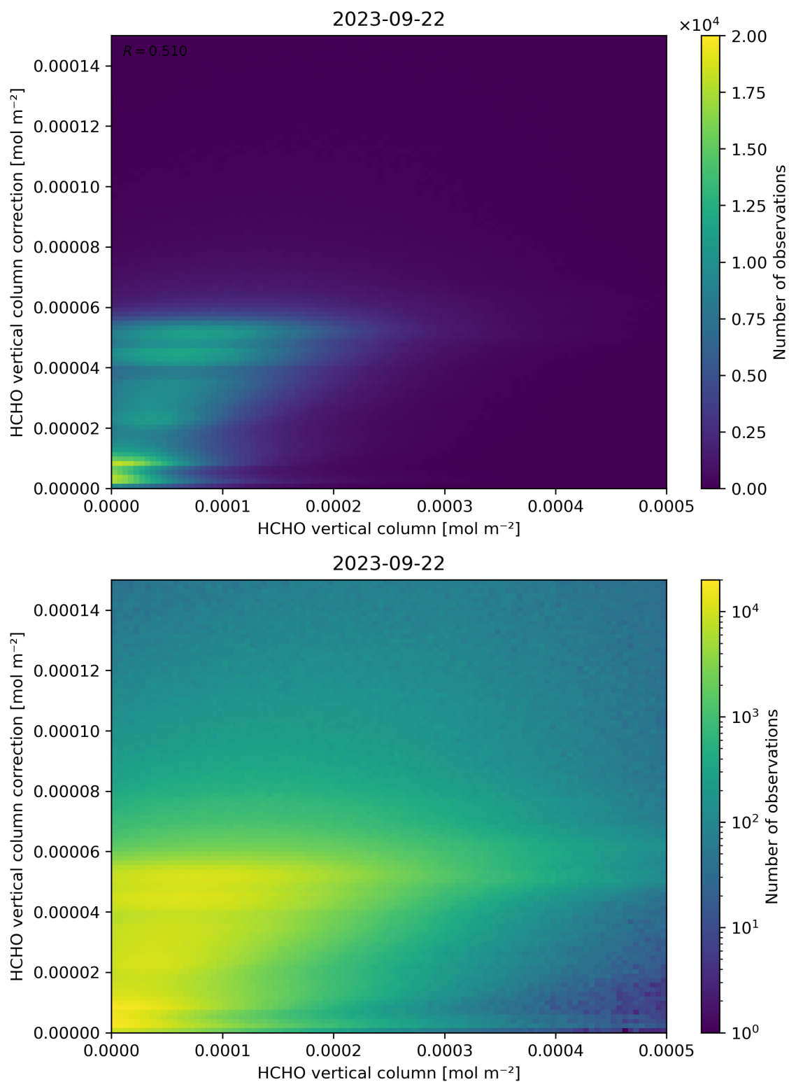
Figure 133: Scatter density plot of “HCHO vertical column” against “HCHO vertical column correction” for 2023-09-21 to 2023-09-23.
