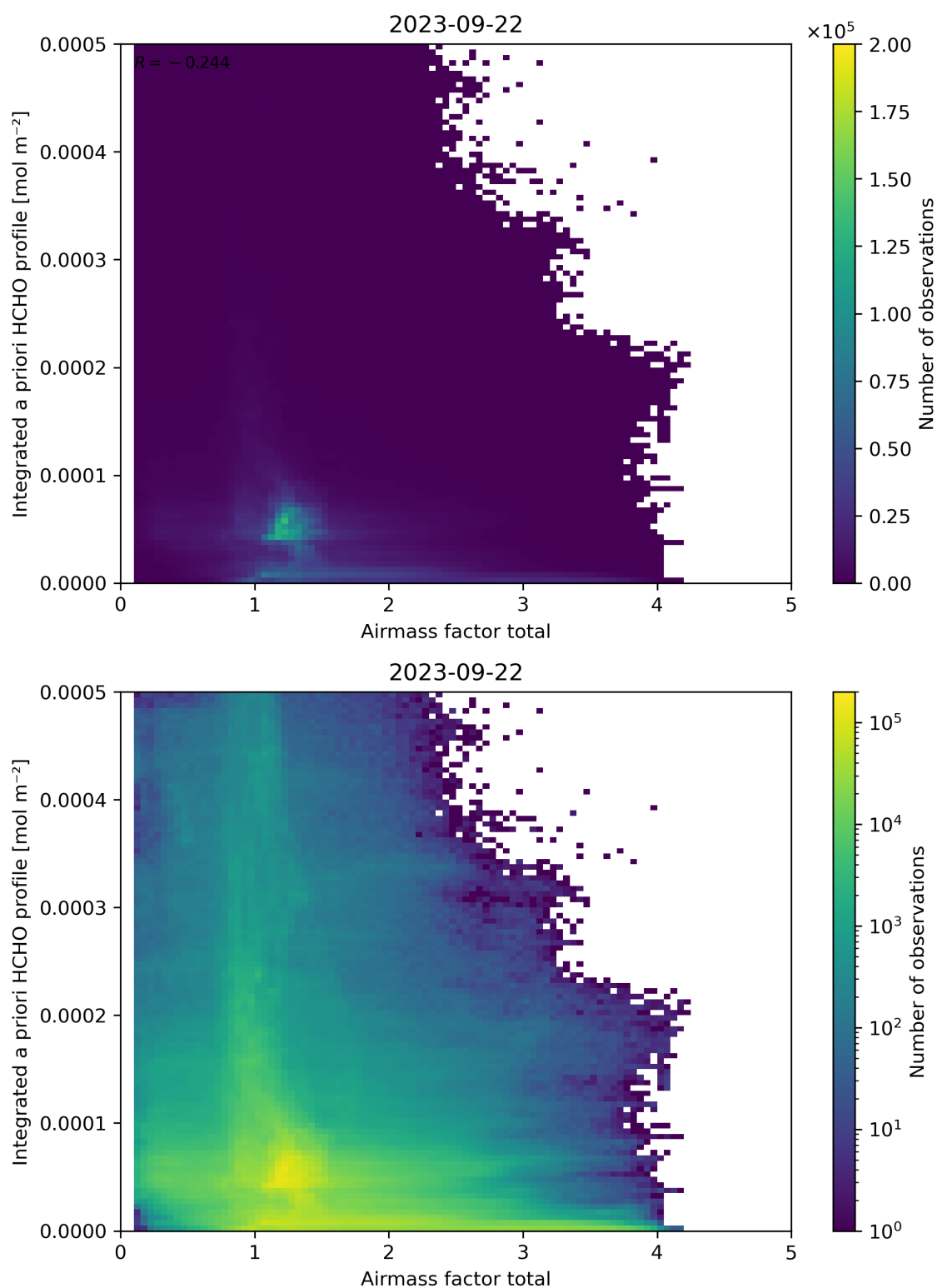
Figure 104: Scatter density plot of “Airmass factor total” against “Integrated a priori HCHO profile” for 2023-09-21 to 2023-09-23.
