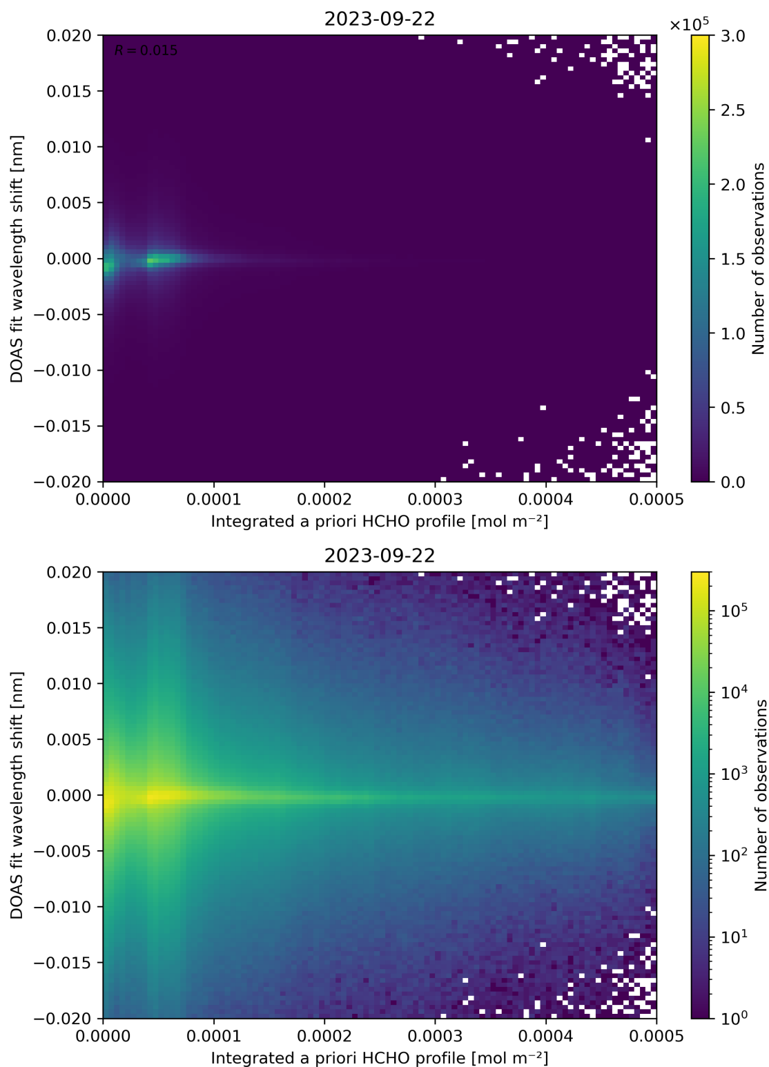
Figure 149: Scatter density plot of “Integrated a priori HCHO profile” against “DOAS fit wavelength shift” for 2023-09-21 to 2023-09-23.
