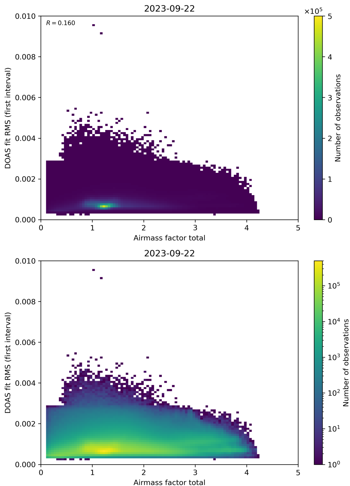
Figure 97: Scatter density plot of “Airmass factor total” against “DOAS fit RMS (first interval)” for 2023-09-21 to 2023-09-23.
