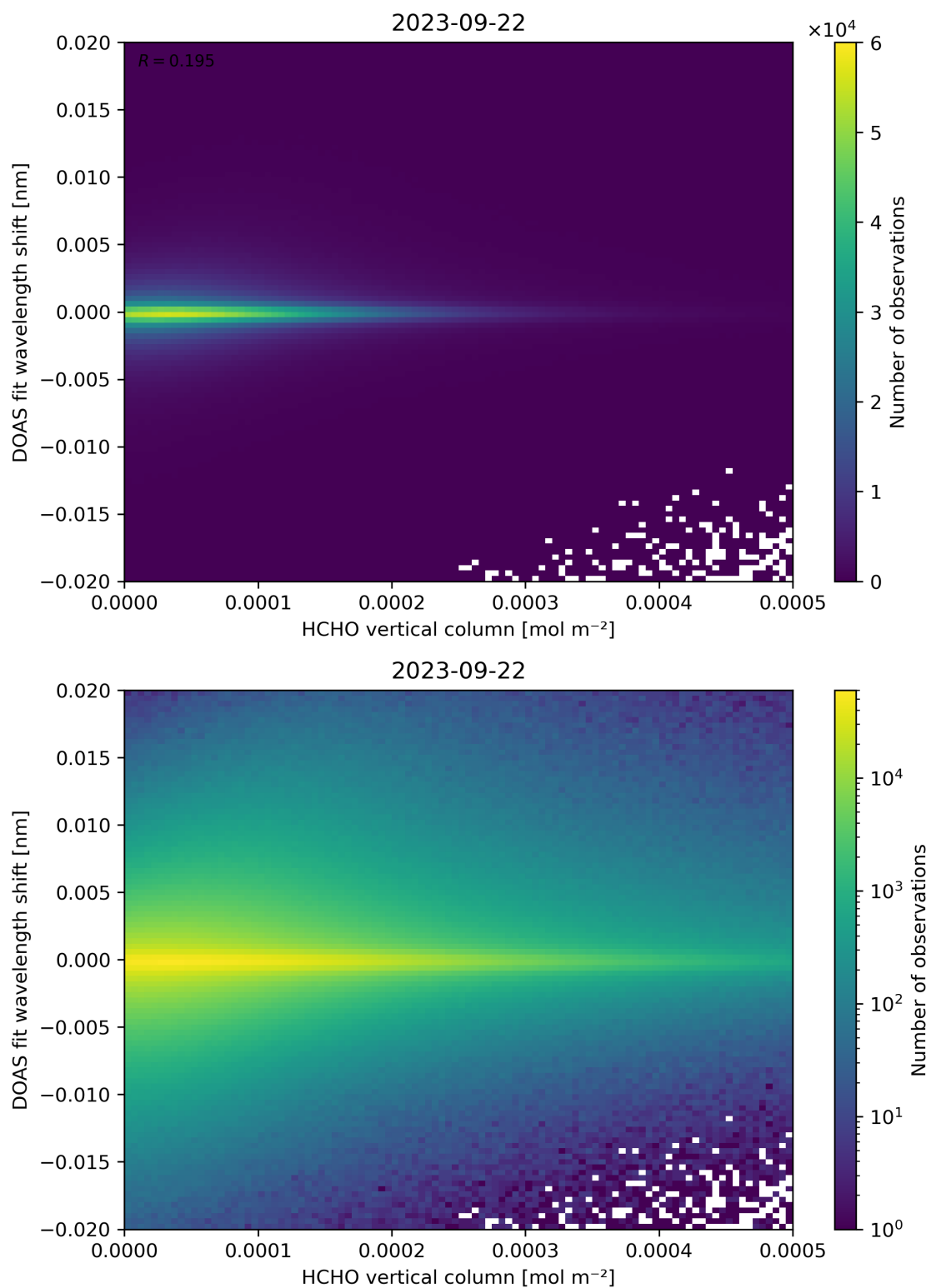
Figure 124: Scatter density plot of “HCHO vertical column” against “DOAS fit wavelength shift” for 2023-09-21 to 2023-09-23.
