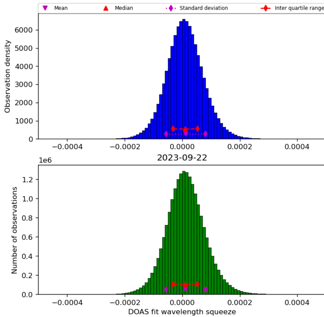
Figure 45: Histogram of “DOAS fit wavelength squeeze” for 2023-09-21 to 2023-09-23
