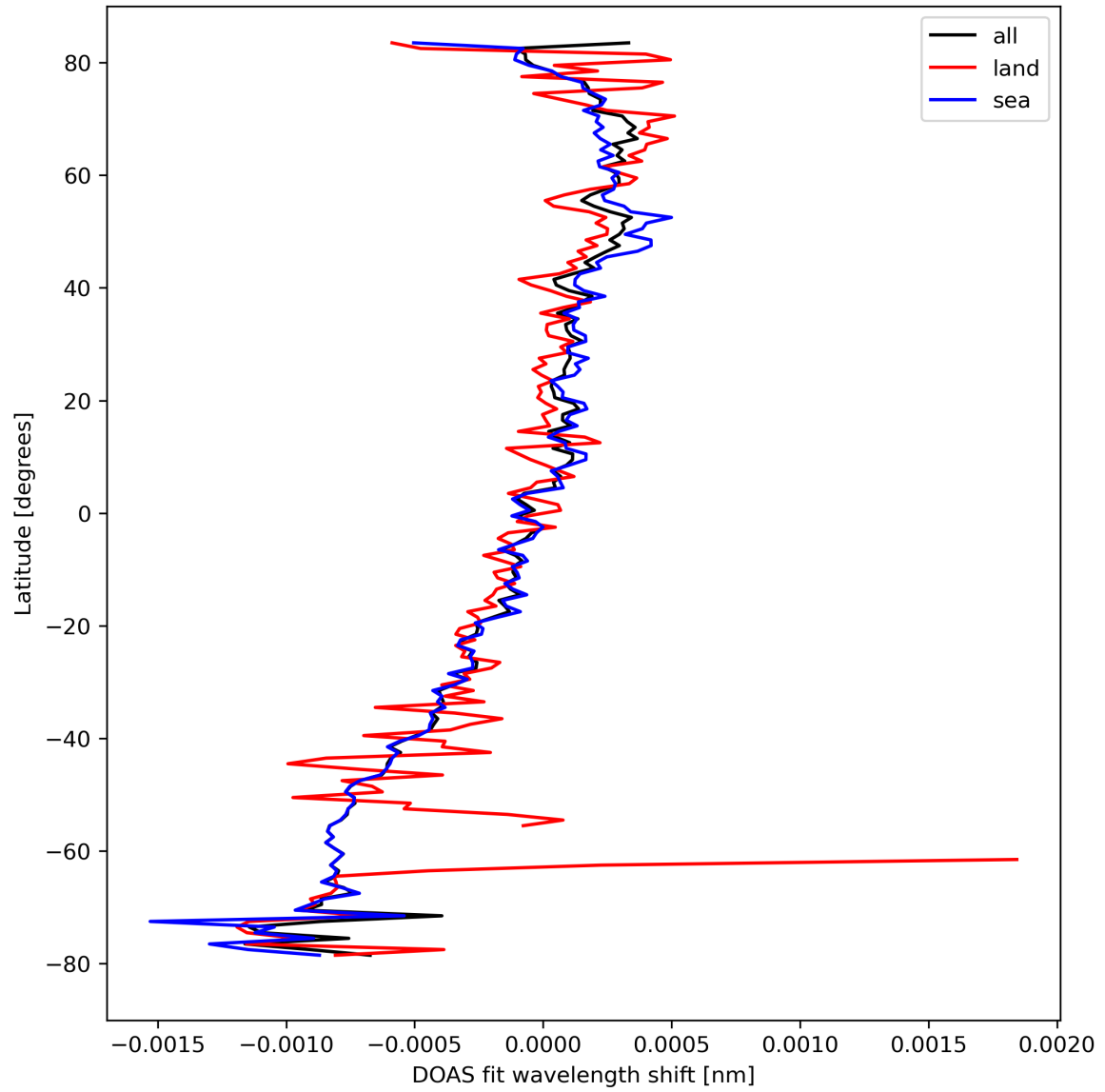
Figure 30: Zonal average of “DOAS fit wavelength shift” for 2023-09-21 to 2023-09-23.
