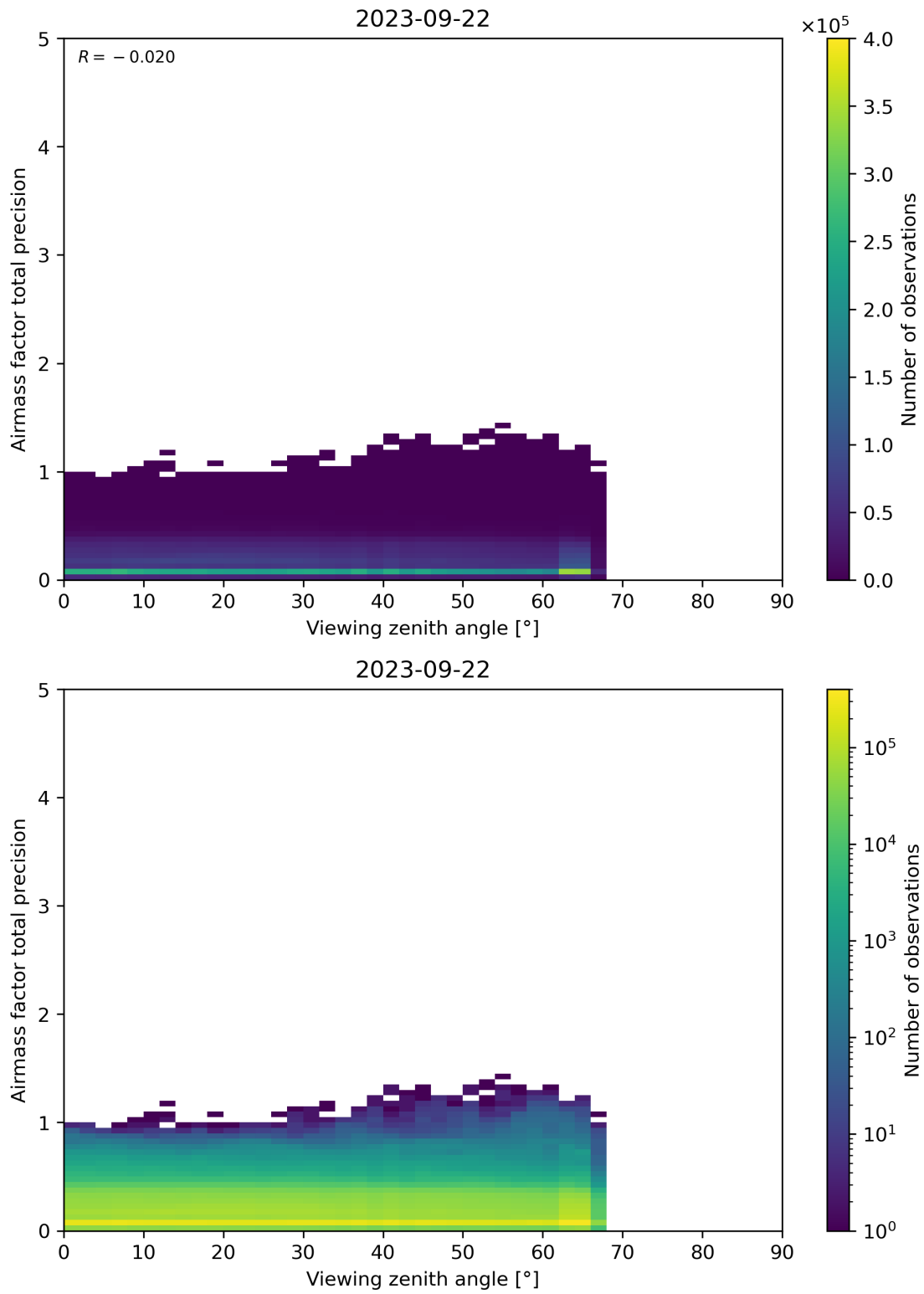
Figure 191: Scatter density plot of “Viewing zenith angle” against “Airmass factor total precision” for 2023-09-21 to 2023-09-23.
