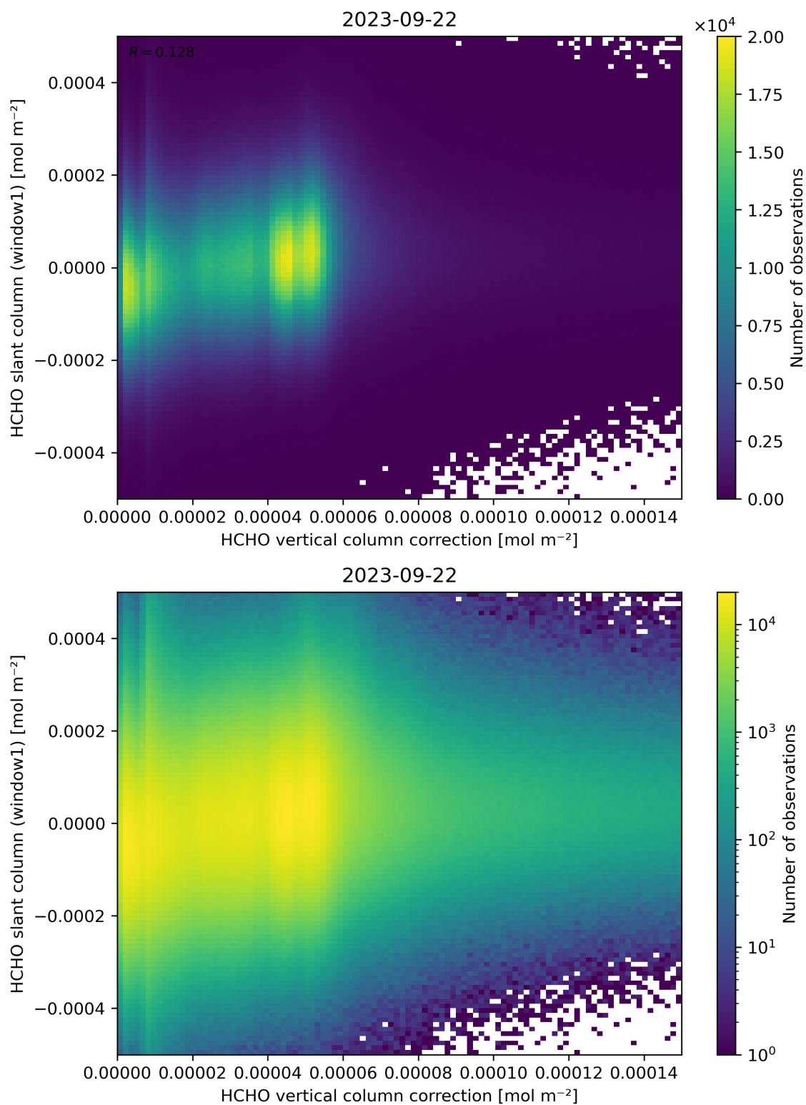
Figure 118: Scatter density plot of “HCHO vertical column correction” against “HCHO slant column (window1)” for 2023-09-21 to 2023-09-23.
