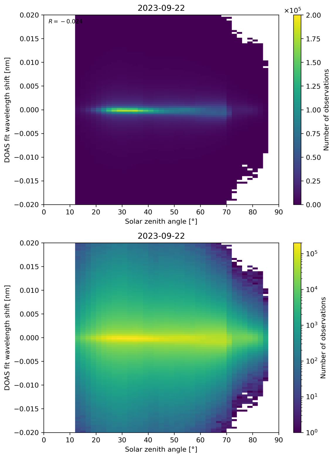
Figure 168: Scatter density plot of “Solar zenith angle” against “DOAS fit wavelength shift” for 2023-09-21 to 2023-09-23.
