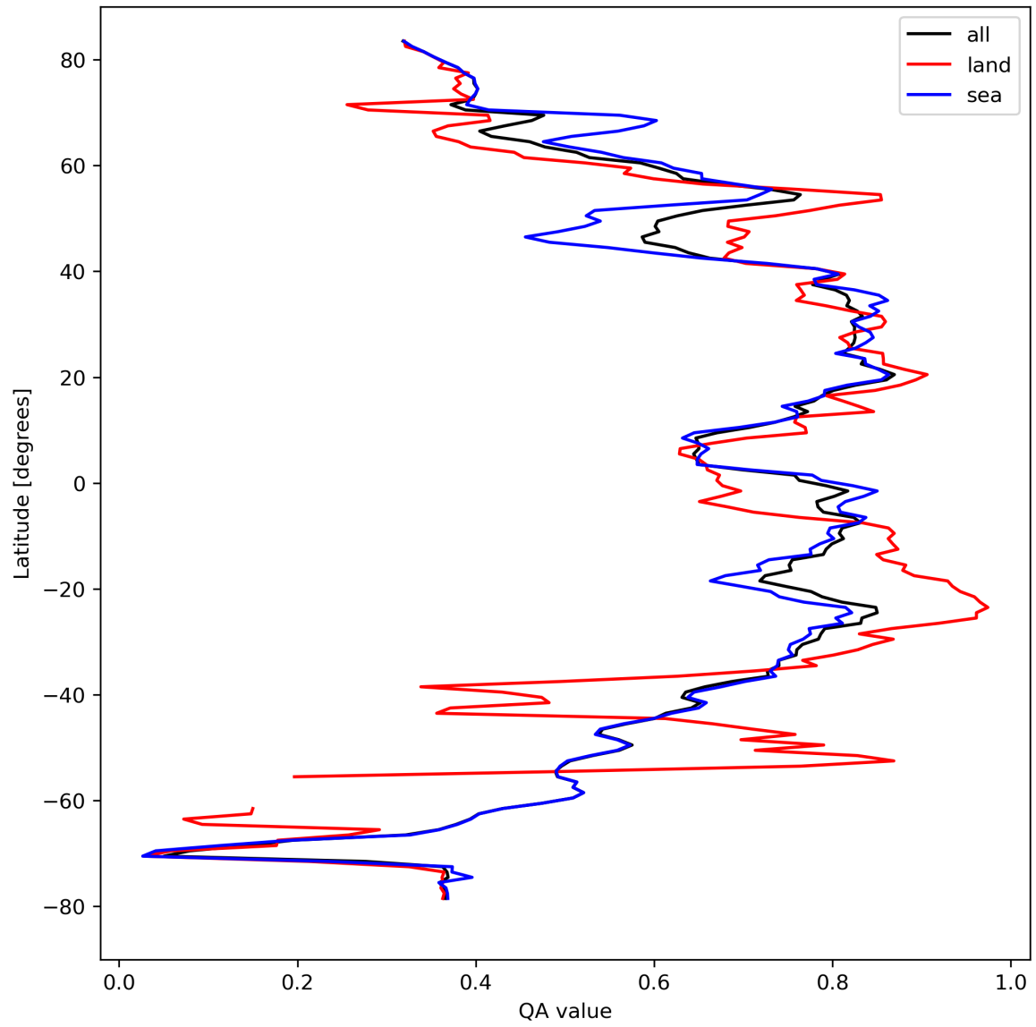
Figure 20: Zonal average of “QA value” for 2023-09-21 to 2023-09-23.
