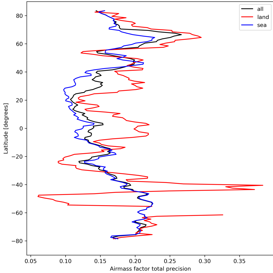
Figure 27: Zonal average of “Airmass factor total precision” for 2023-09-21 to 2023-09-23.
