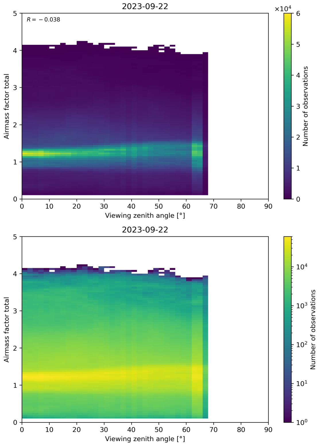
Figure 190: Scatter density plot of “Viewing zenith angle” against “Airmass factor total” for 2023-09-21 to 2023-09-23.
