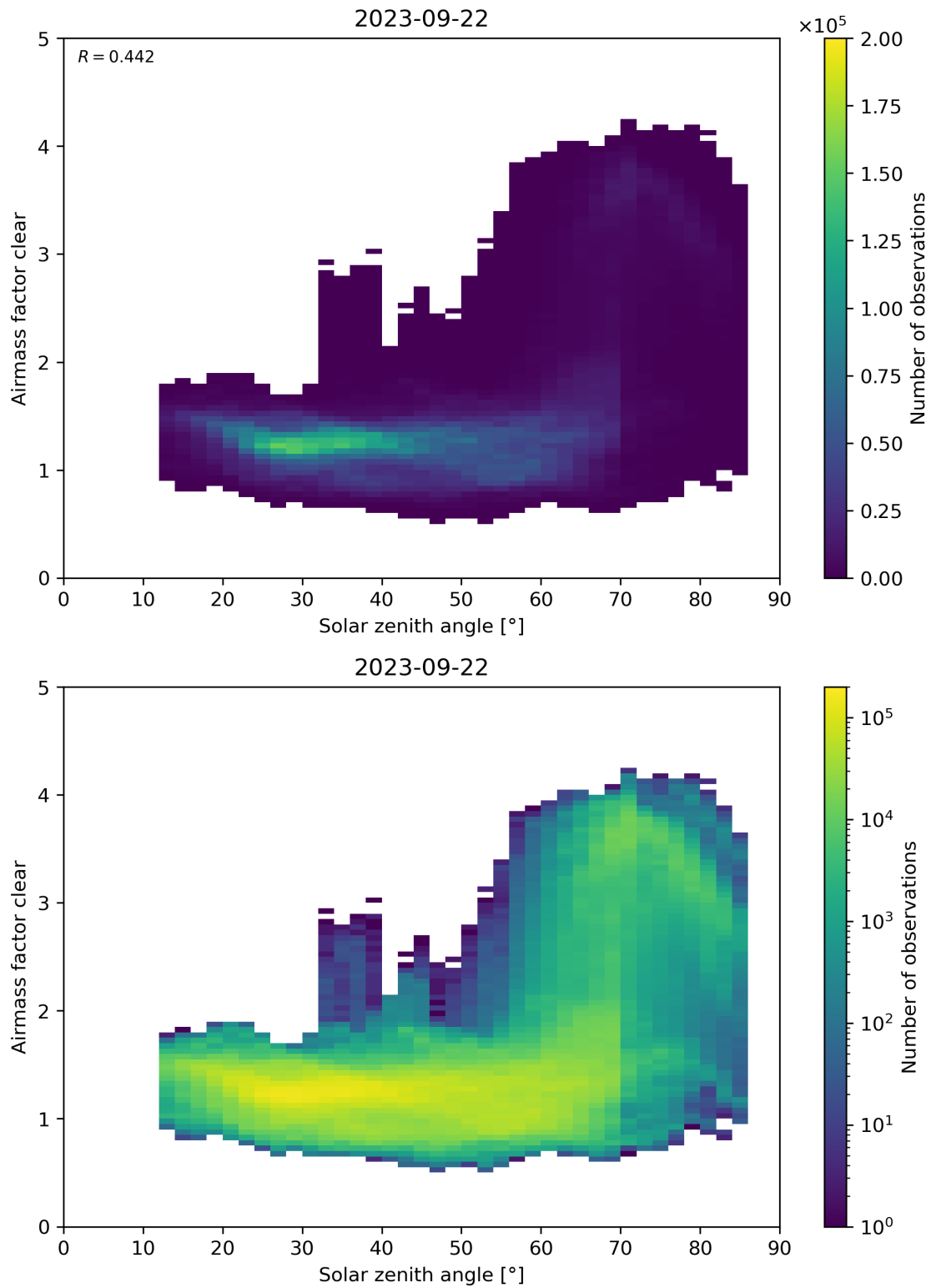
Figure 170: Scatter density plot of “Solar zenith angle” against “Airmass factor clear” for 2023-09-21 to 2023-09-23.
