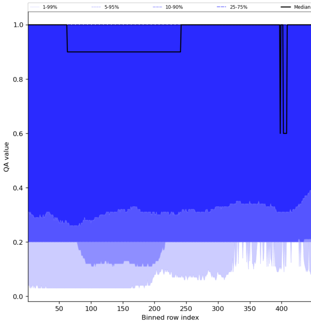
Figure 48: Along track statistics of “QA value” for 2023-09-21 to 2023-09-23
