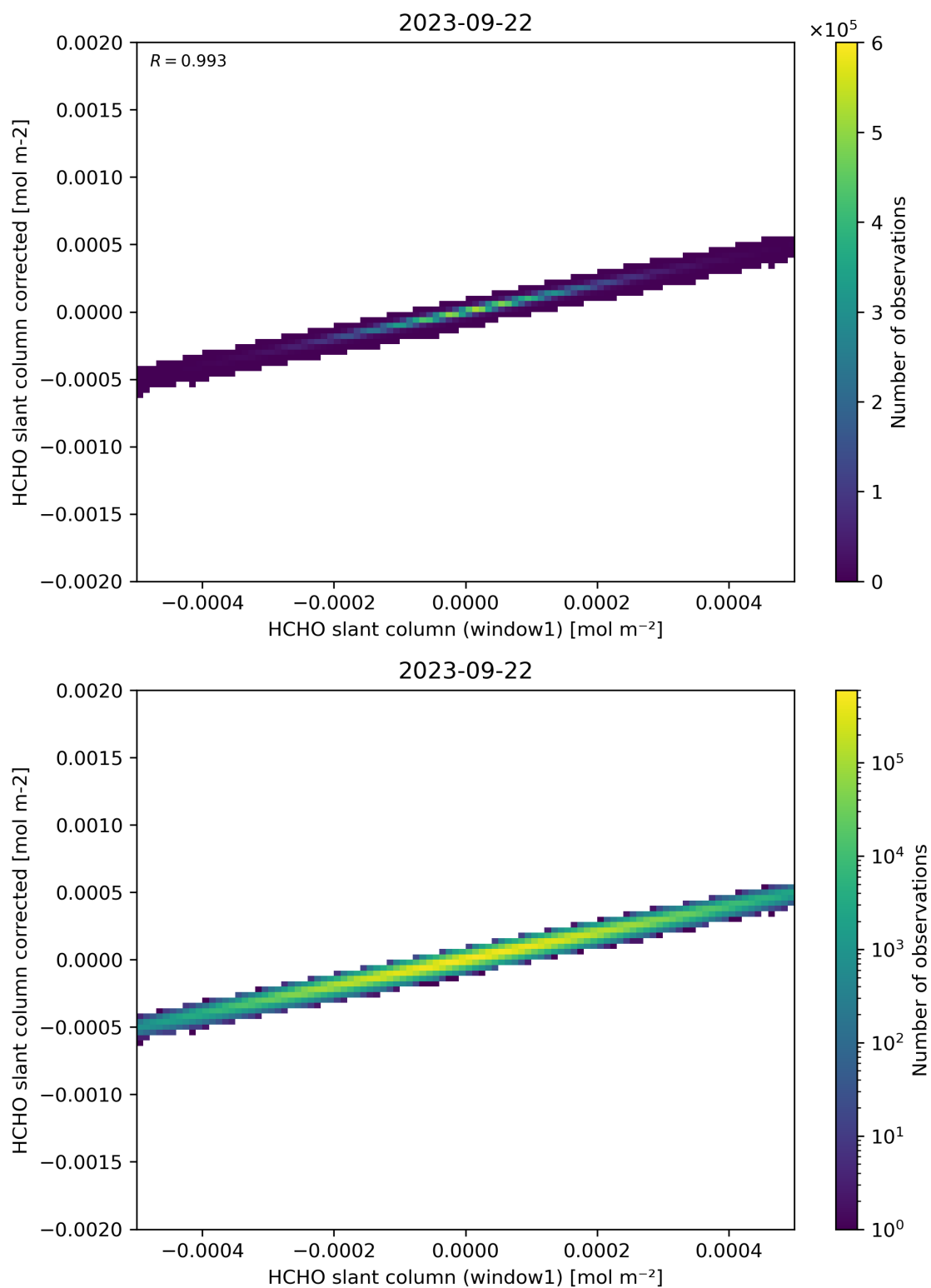
Figure 82: Scatter density plot of “HCHO slant column (window1)” against “HCHO slant column corrected” for 2023-09-21 to 2023-09-23.
