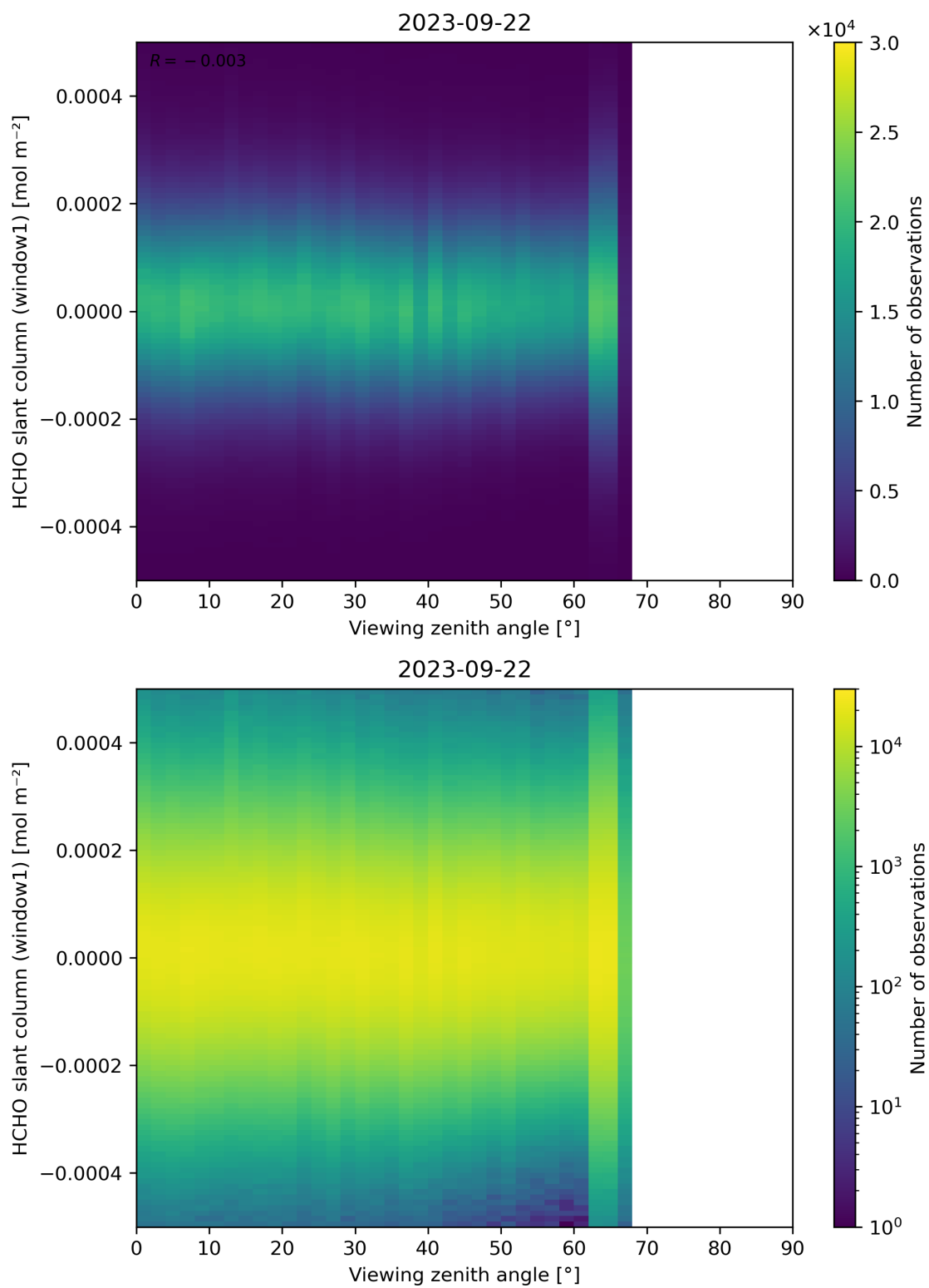
Figure 188: Scatter density plot of “Viewing zenith angle” against “HCHO slant column (window1)” for 2023-09-21 to 2023-09-23.
