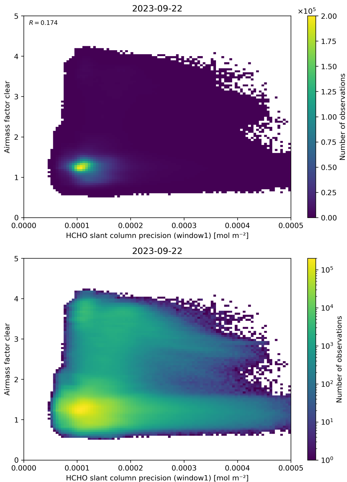
Figure 91: Scatter density plot of “HCHO slant column precision (window1)” against “Airmass factor clear” for 2023-09-21 to 2023-09-23.
