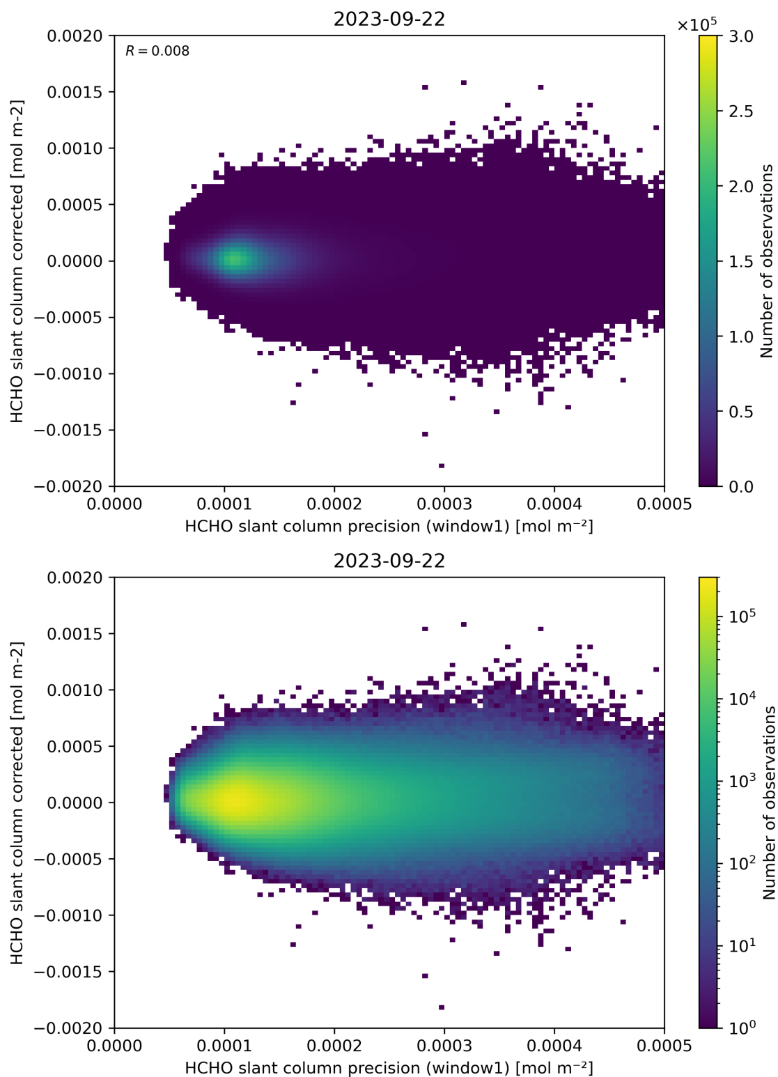
Figure 92: Scatter density plot of “HCHO slant column precision (window1)” against “HCHO slant column corrected” for 2023-09-21 to 2023-09-23.
