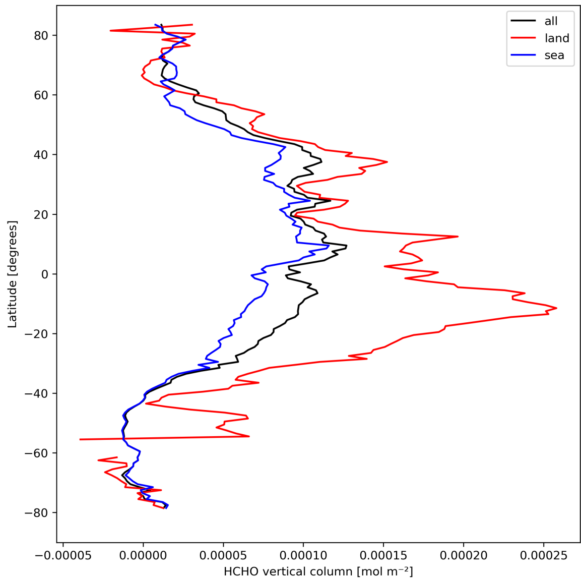
Figure 21: Zonal average of “HCHO vertical column” for 2023-09-21 to 2023-09-23.
