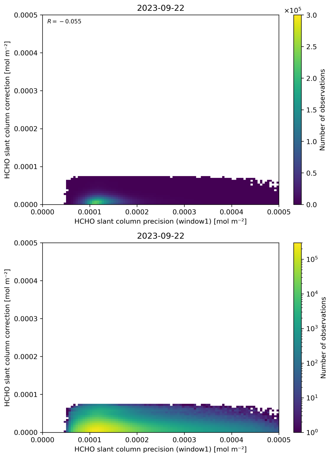
Figure 93: Scatter density plot of “HCHO slant column precision (window1)” against “HCHO slant column correction” for 2023-09-21 to 2023-09-23.
