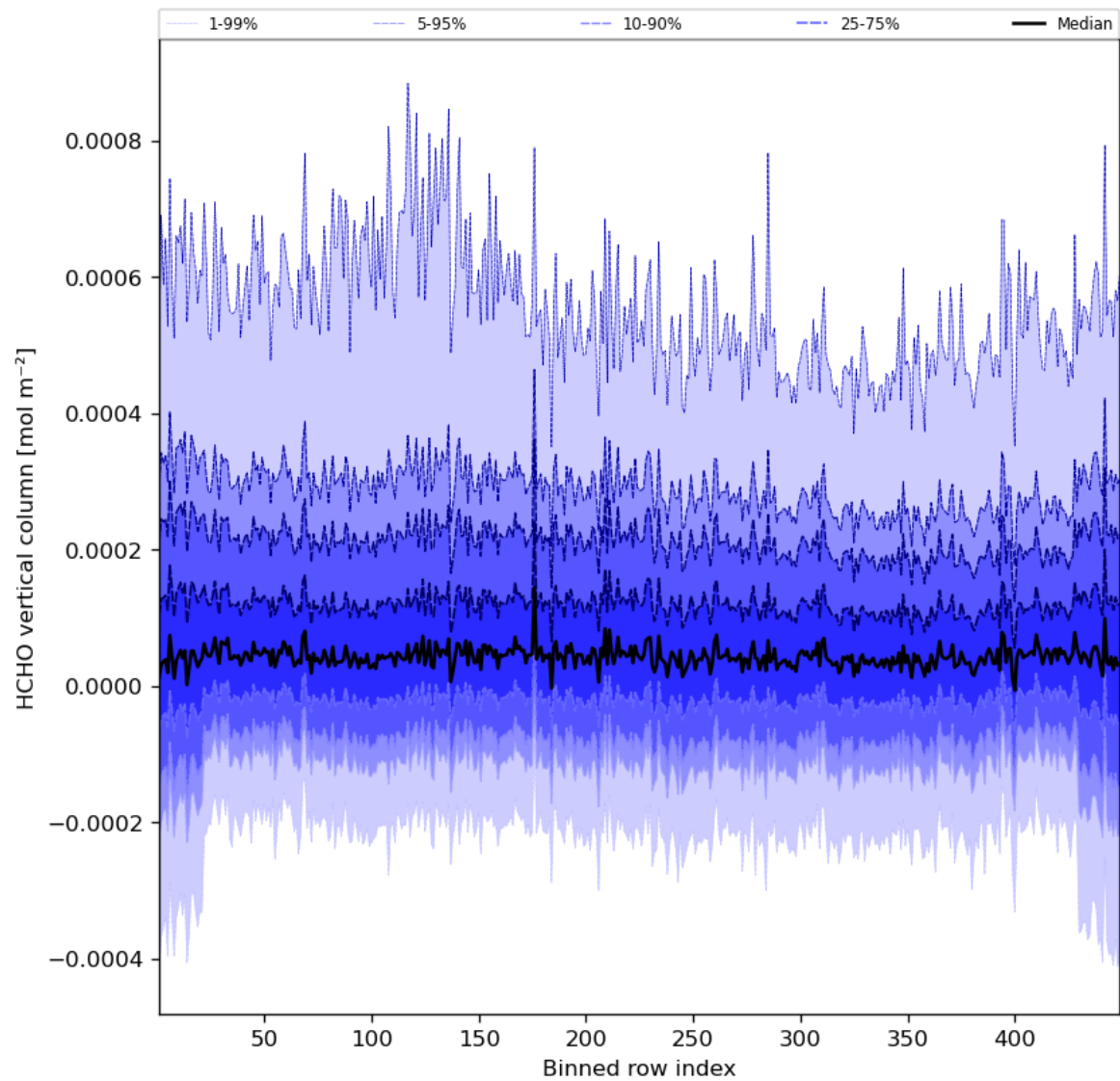
Figure 49: Along track statistics of “HCHO vertical column” for 2023-09-21 to 2023-09-23
