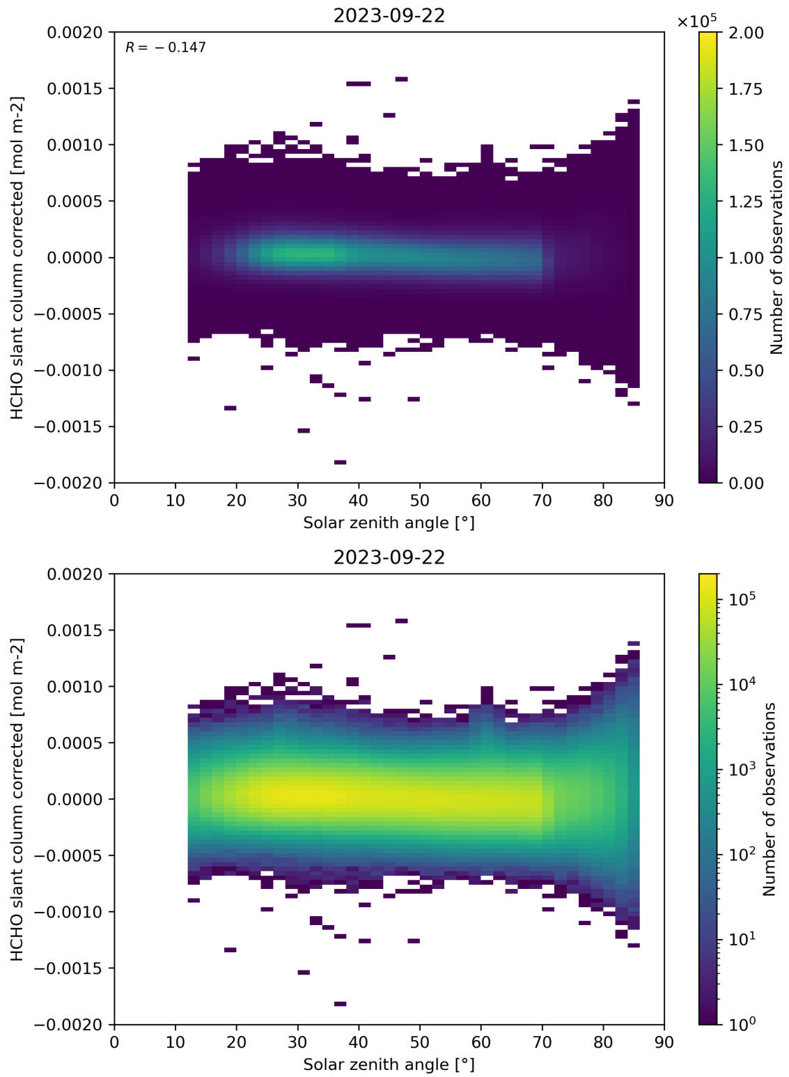
Figure 171: Scatter density plot of “Solar zenith angle” against “HCHO slant column corrected” for 2023-09-21 to 2023-09-23.
