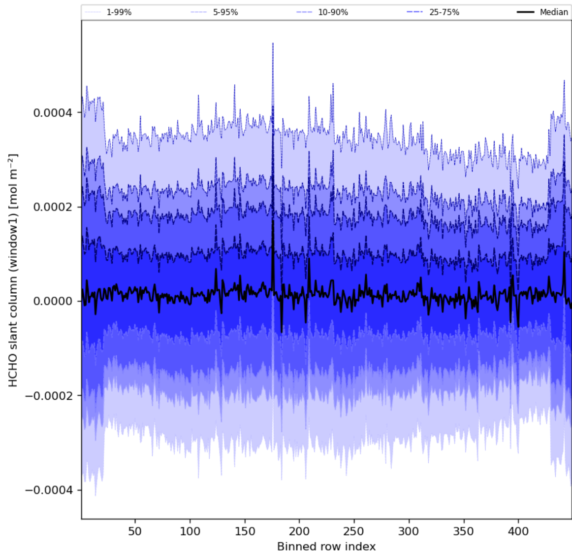
Figure 52: Along track statistics of “HCHO slant column (window1)” for 2023-09-21 to 2023-09-23
