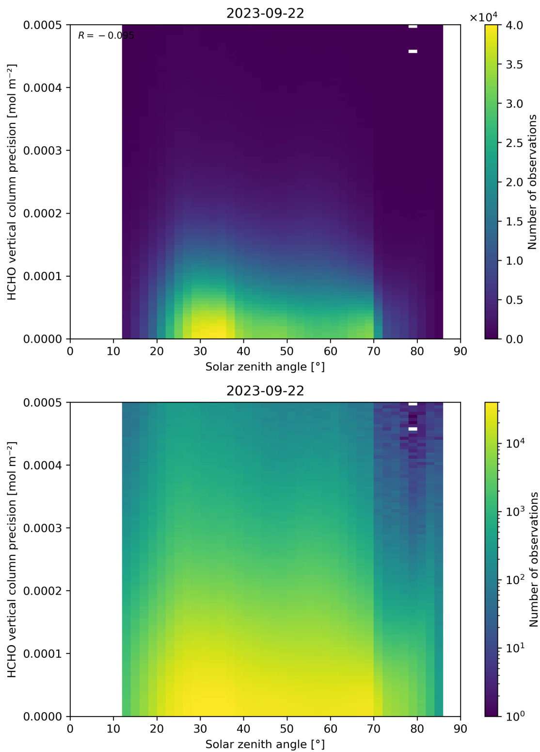
Figure 179: Scatter density plot of “Solar zenith angle” against “HCHO vertical column precision” for 2023-09-21 to 2023-09-23.
