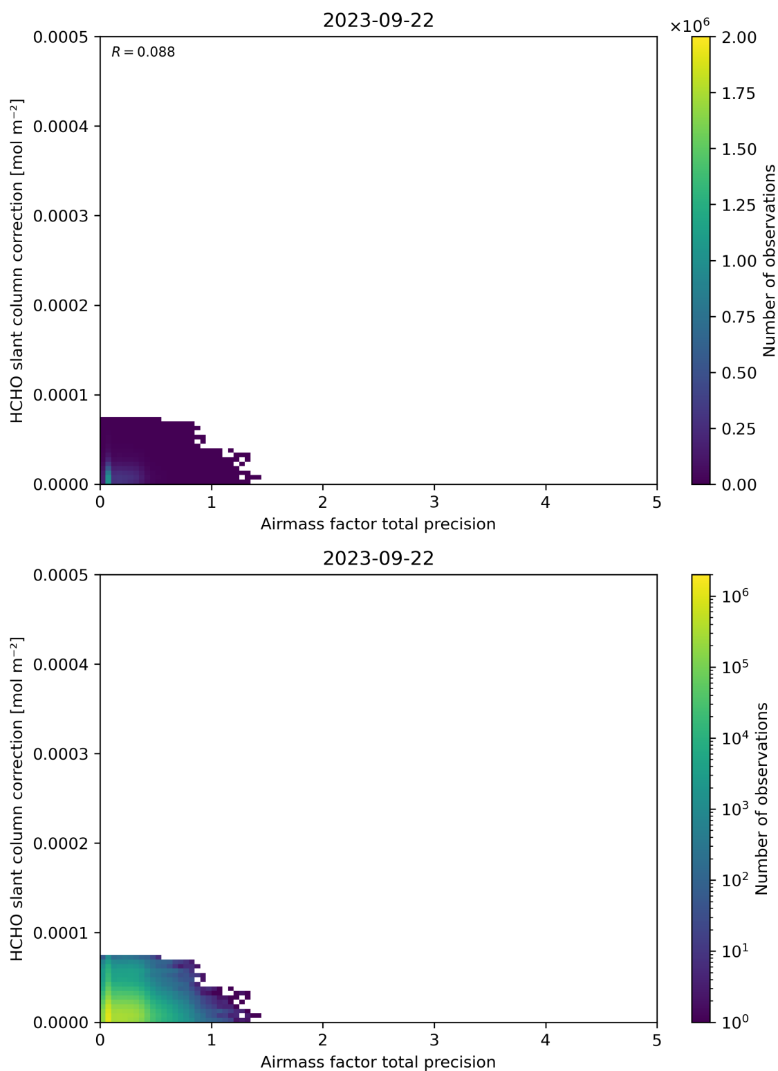
Figure 110: Scatter density plot of “Airmass factor total precision” against “HCHO slant column correction” for 2023-09-21 to 2023-09-23.
