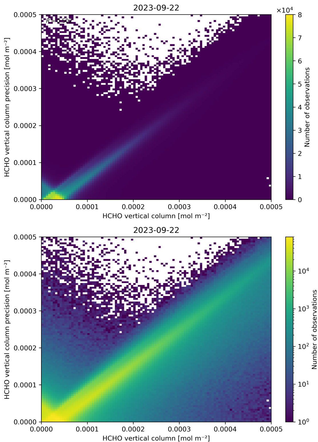
Figure 134: Scatter density plot of “HCHO vertical column” against “HCHO vertical column precision” for 2023-09-21 to 2023-09-23.
