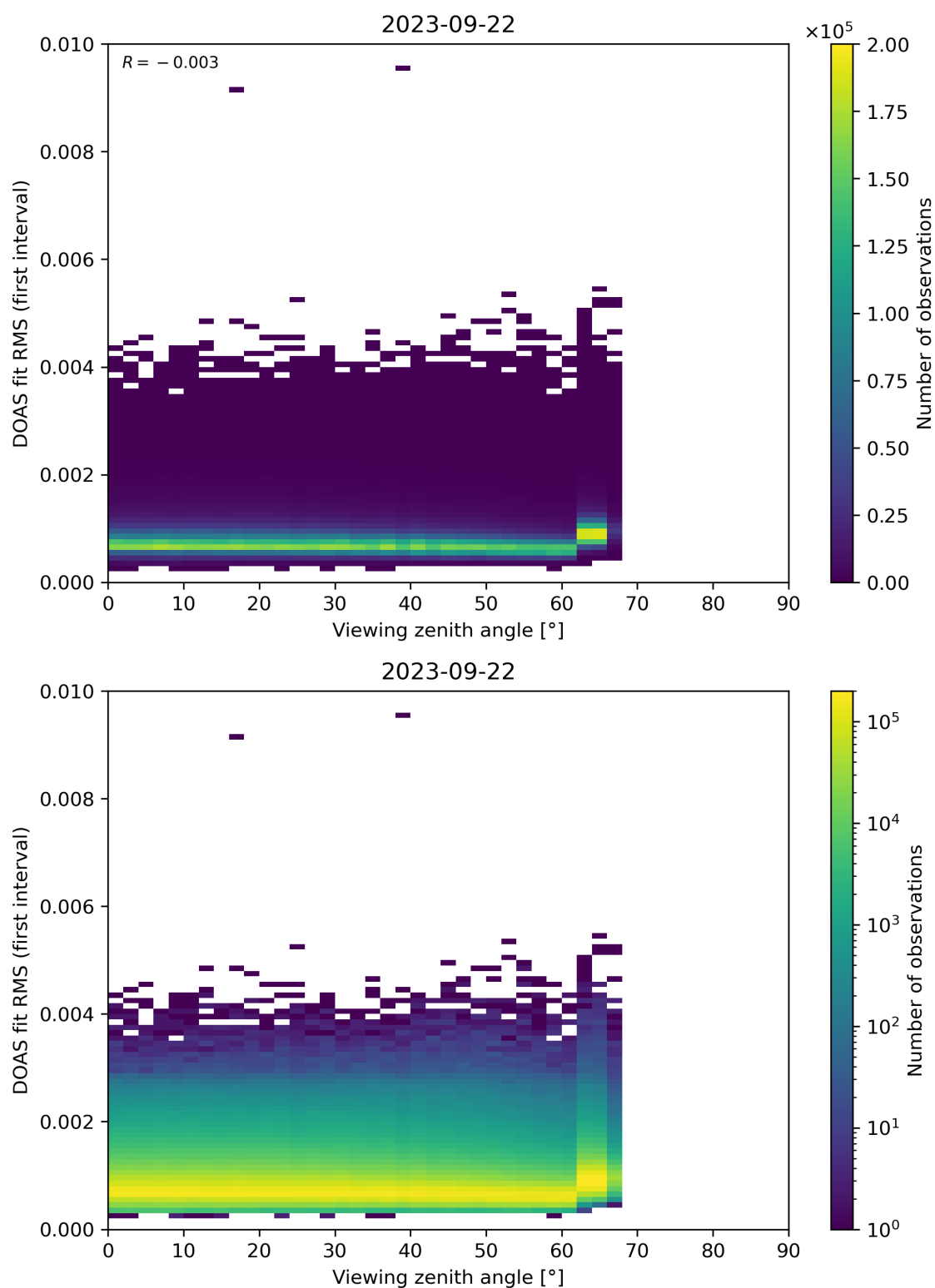
Figure 182: Scatter density plot of “Viewing zenith angle” against “DOAS fit RMS (first interval)” for 2023-09-21 to 2023-09-23.
