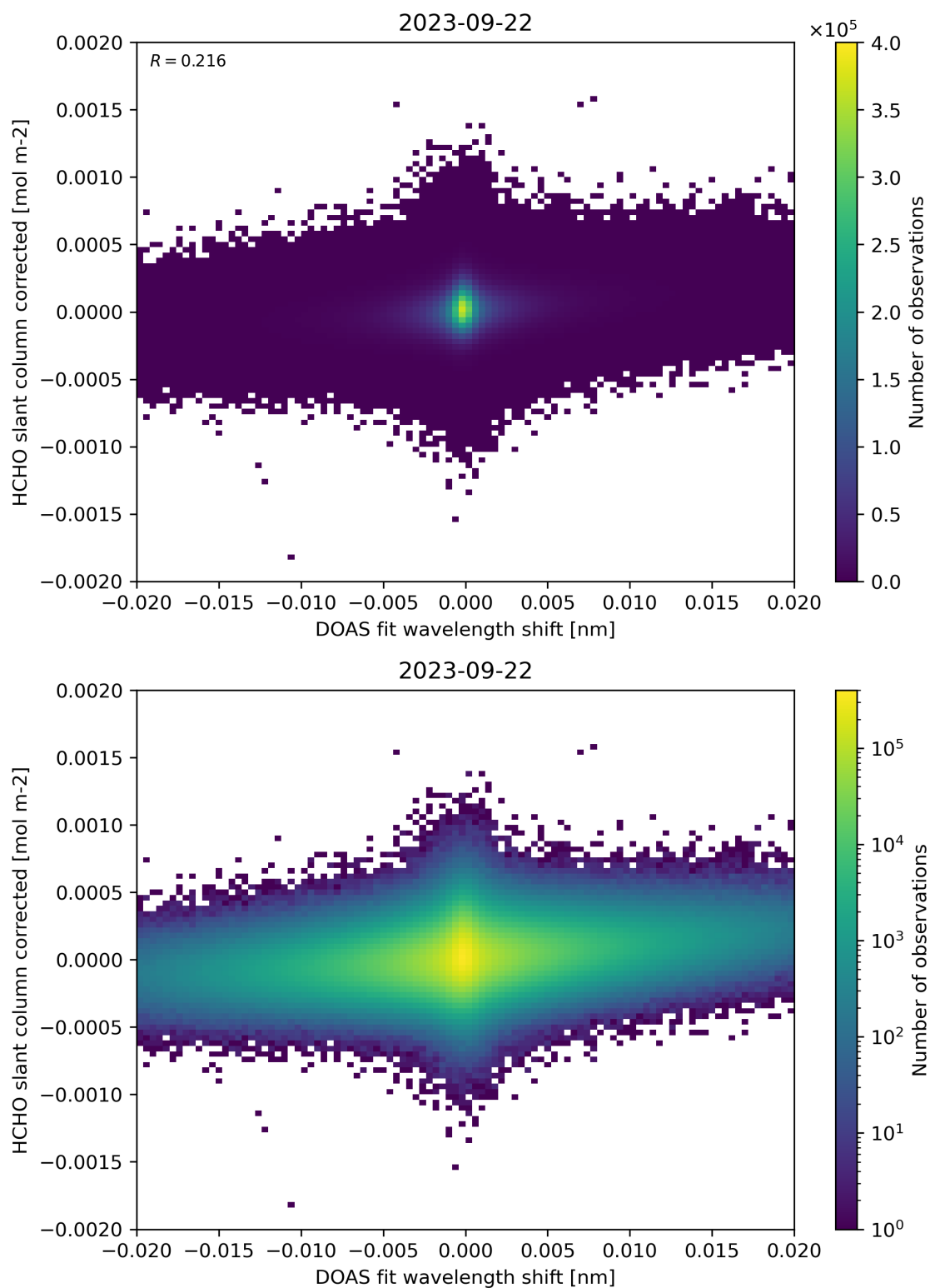
Figure 66: Scatter density plot of “DOAS fit wavelength shift” against “HCHO slant column corrected” for 2023-09-21 to 2023-09-23.
