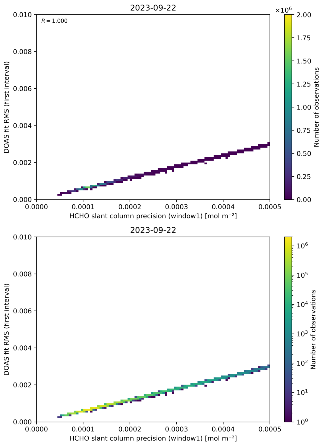
Figure 88: Scatter density plot of “HCHO slant column precision (window1)” against “DOAS fit RMS (first interval)” for 2023-09-21 to 2023-09-23.
