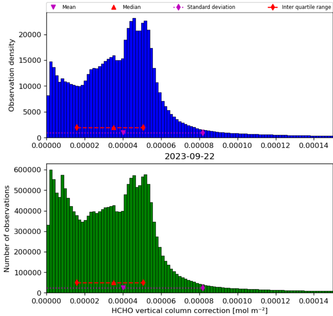
Figure 37: Histogram of “HCHO vertical column correction” for 2023-09-21 to 2023-09-23
