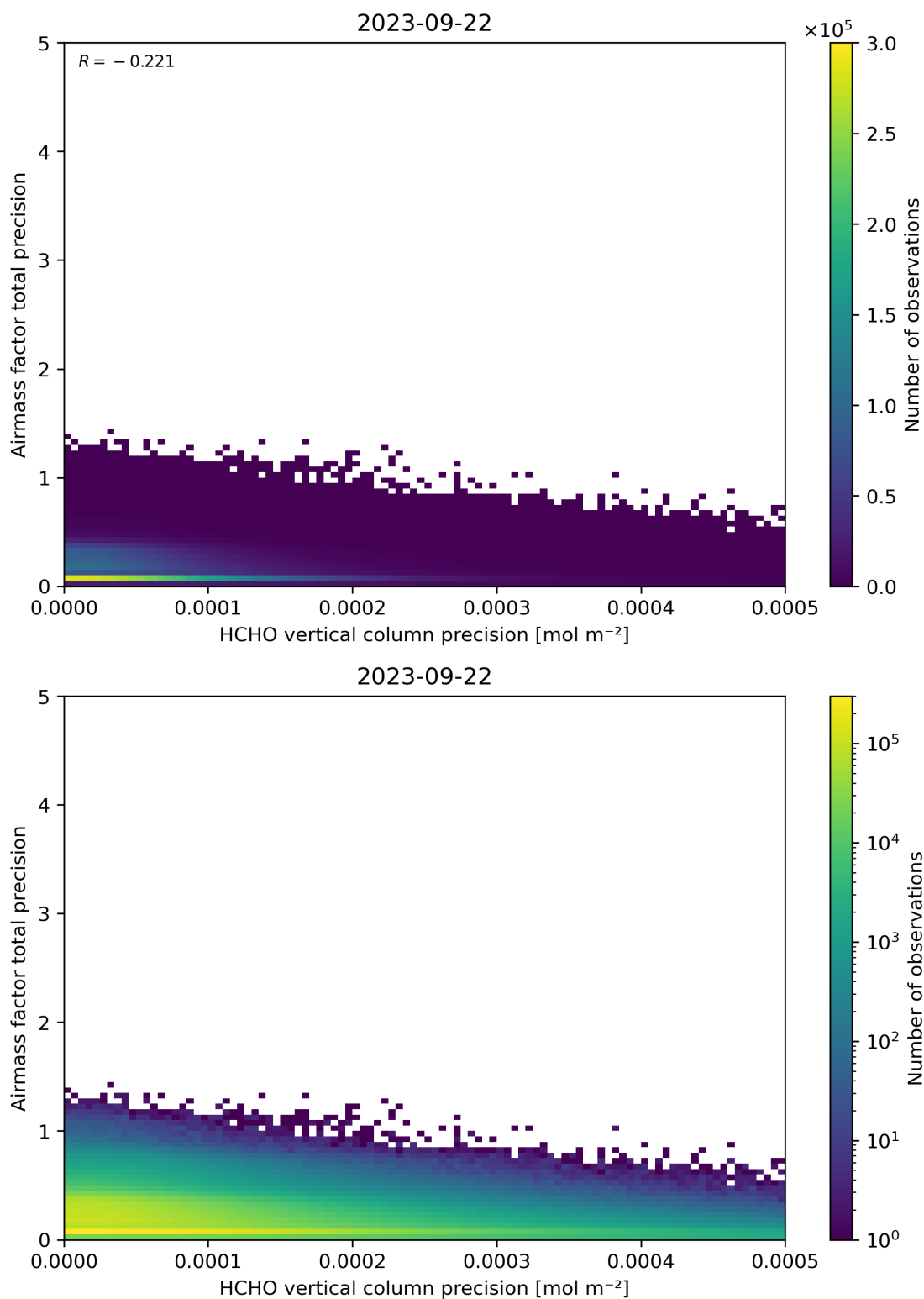
Figure 145: Scatter density plot of “HCHO vertical column precision” against “Airmass factor total precision” for 2023-09-21 to 2023-09-23.
