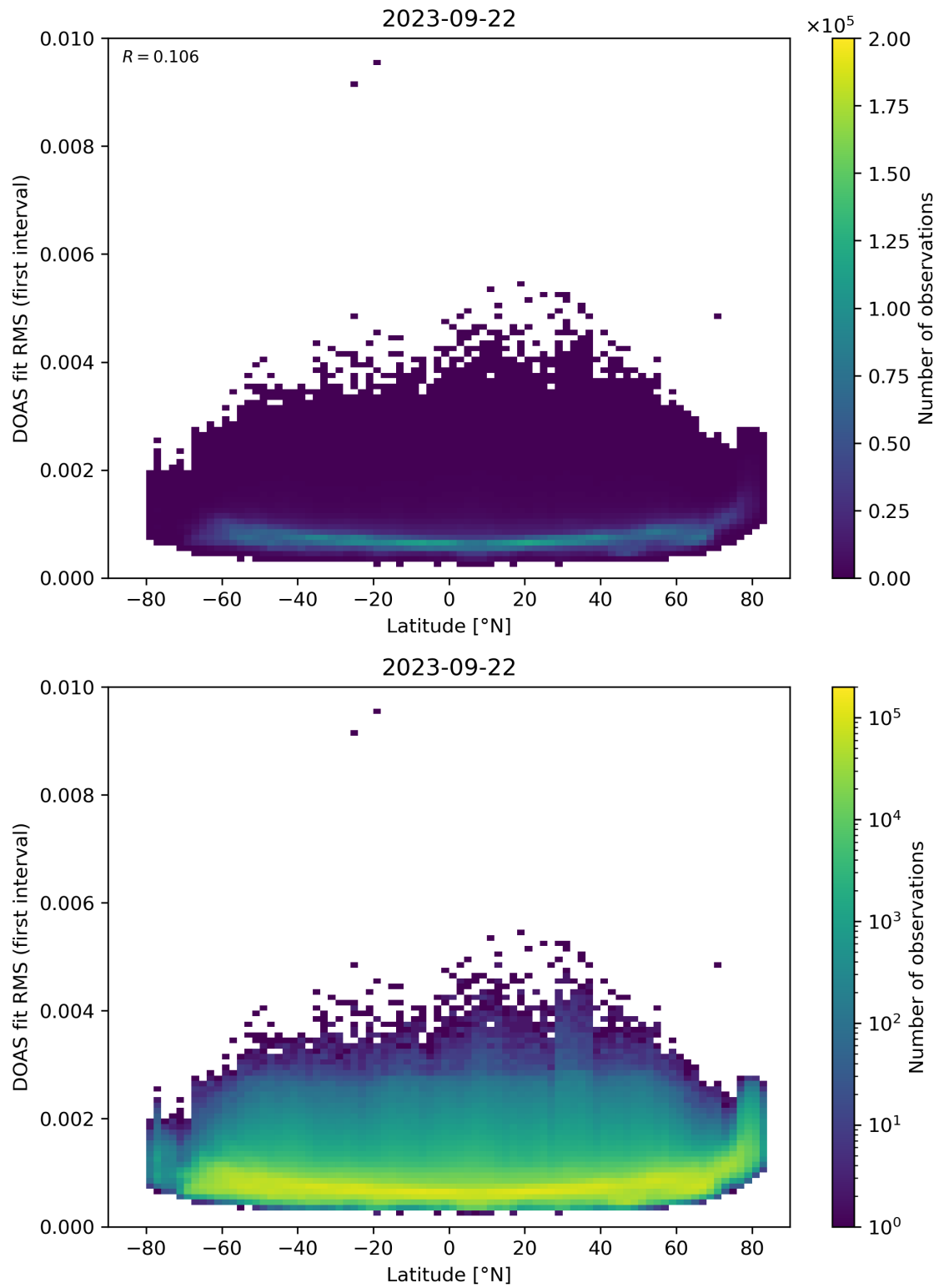
Figure 153: Scatter density plot of “Latitude” against “DOAS fit RMS (first interval)” for 2023-09-21 to 2023-09-23.
