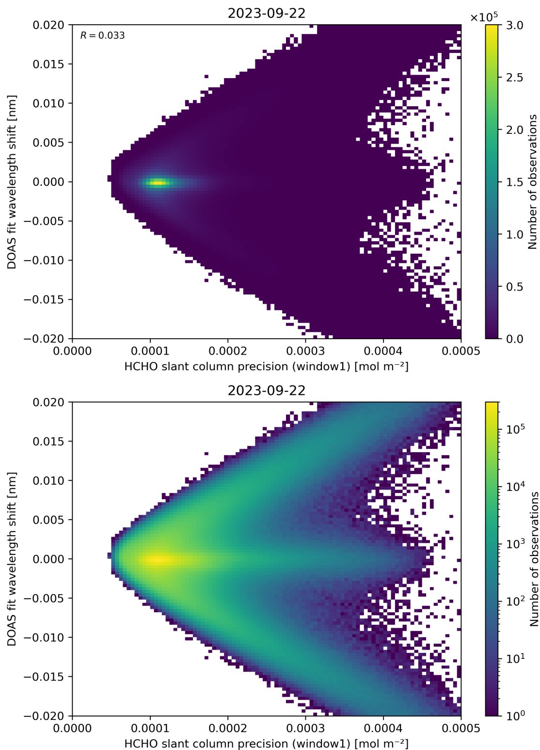
Figure 89: Scatter density plot of “HCHO slant column precision (window1)” against “DOAS fit wavelength shift” for 2023-09-21 to 2023-09-23.
