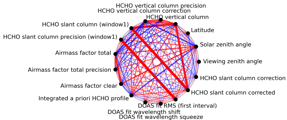
Figure 1: Map of correlation graph for 2023-09-21 to 2023-09-23.
