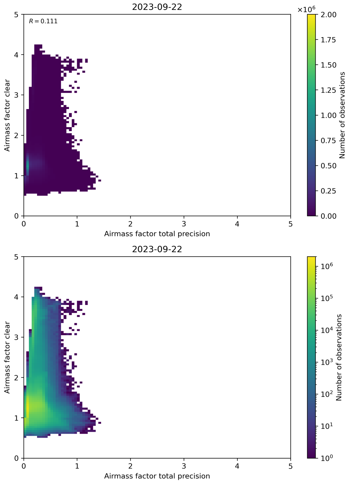
Figure 108: Scatter density plot of “Airmass factor total precision” against “Airmass factor clear” for 2023-09-21 to 2023-09-23.
