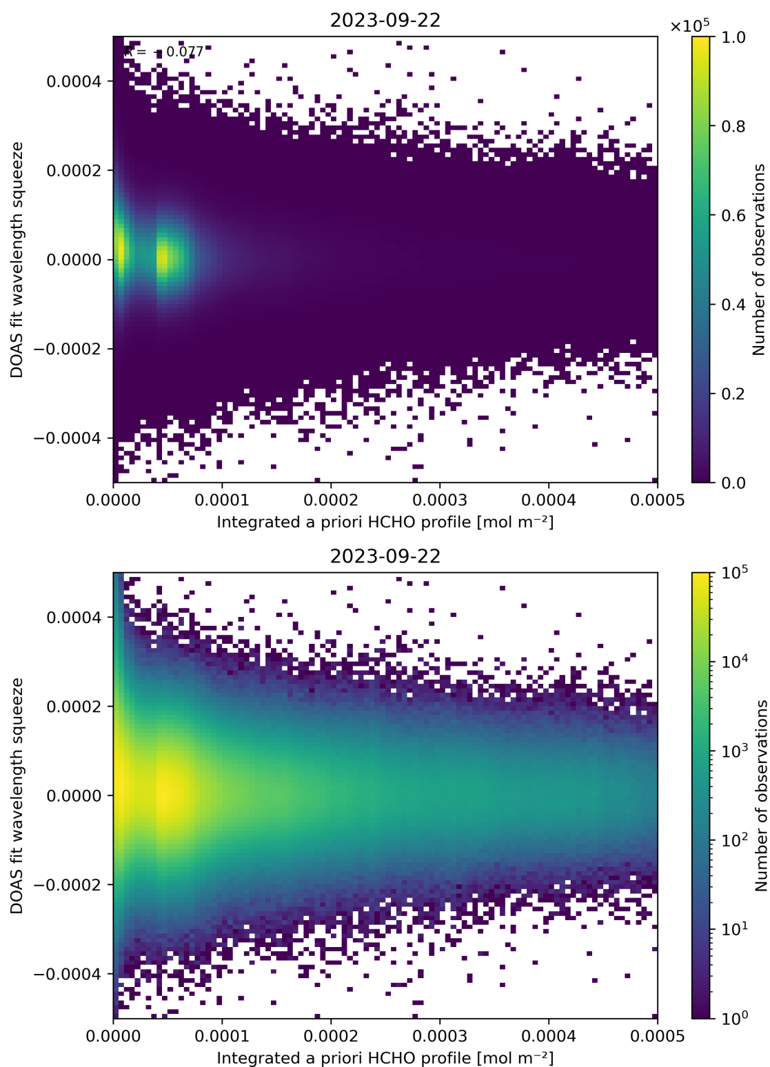
Figure 150: Scatter density plot of “Integrated a priori HCHO profile” against “DOAS fit wavelength squeeze” for 2023-09-21 to 2023-09-23.
