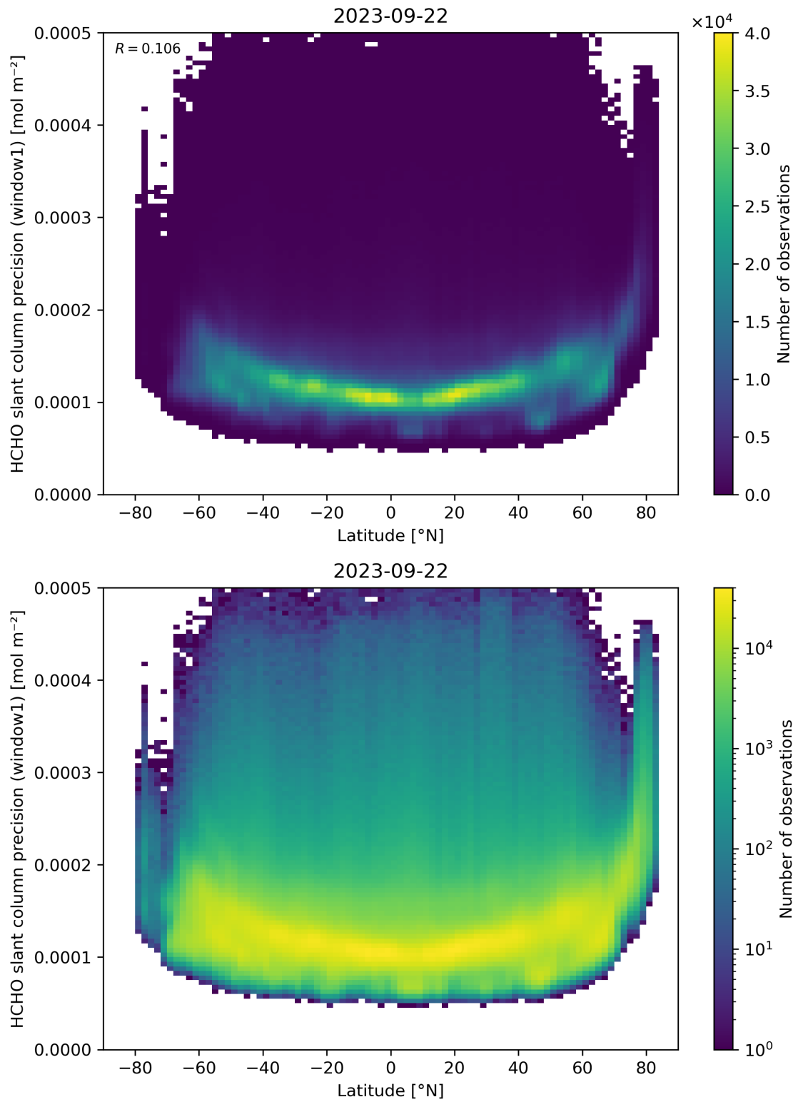
Figure 160: Scatter density plot of “Latitude” against “HCHO slant column precision (window1)” for 2023-09-21 to 2023-09-23.
