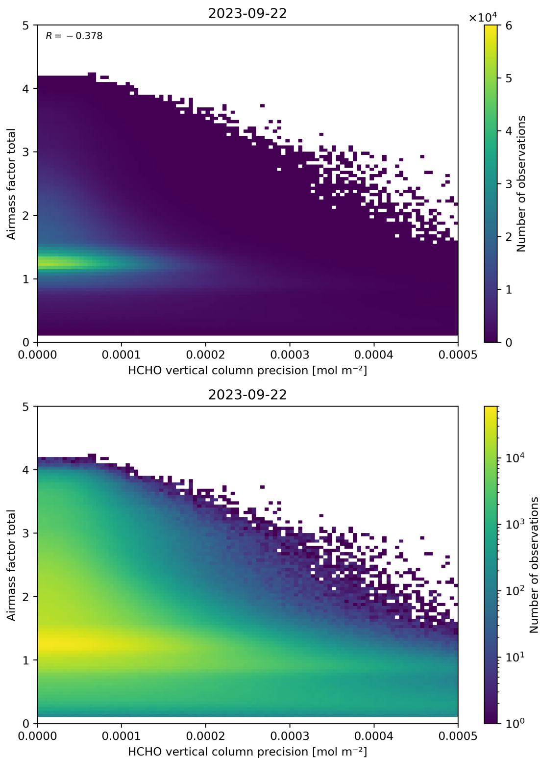
Figure 144: Scatter density plot of “HCHO vertical column precision” against “Airmass factor total” for 2023-09-21 to 2023-09-23.
