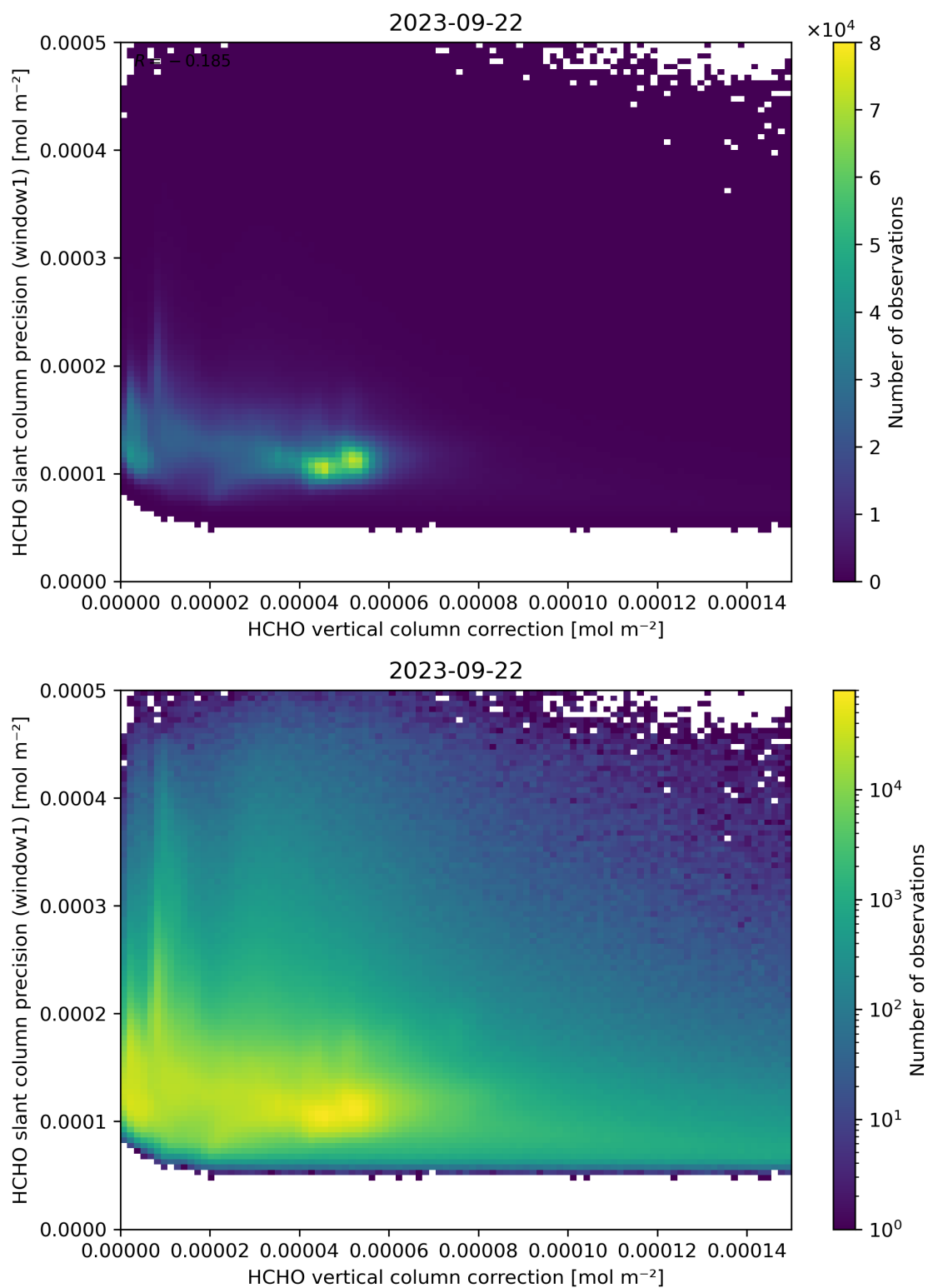
Figure 119: Scatter density plot of “HCHO vertical column correction” against “HCHO slant column precision (window1)” for 2023-09-21 to 2023-09-23.
