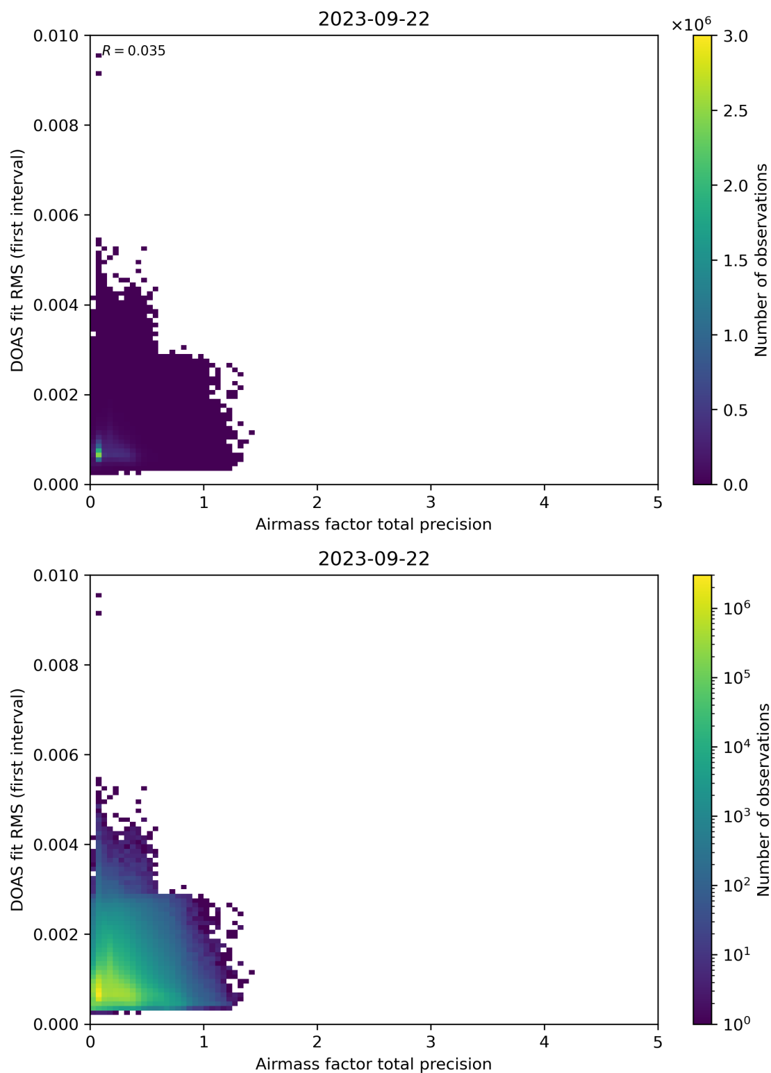
Figure 105: Scatter density plot of “Airmass factor total precision” against “DOAS fit RMS (first interval)” for 2023-09-21 to 2023-09-23.
