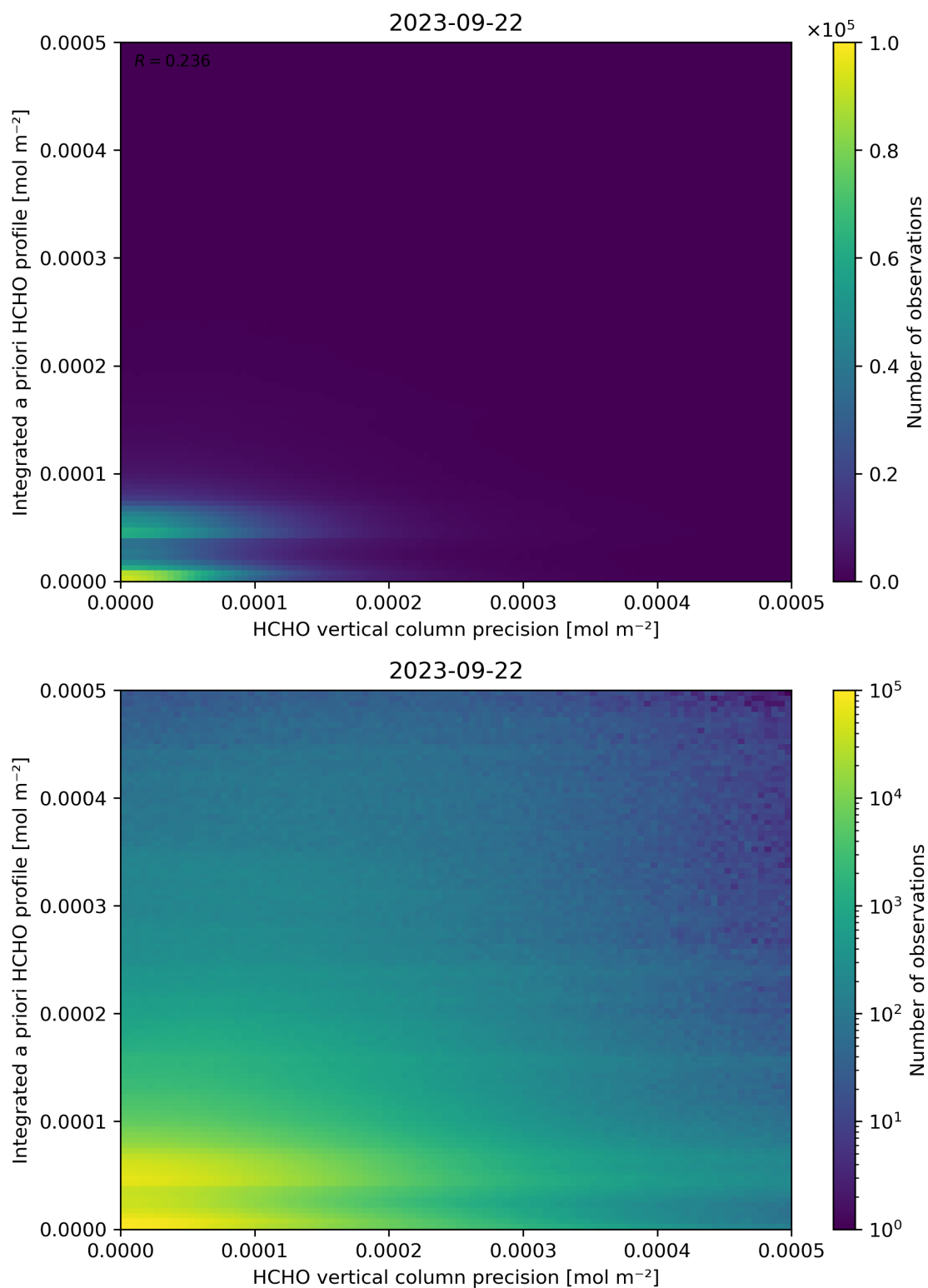
Figure 147: Scatter density plot of “HCHO vertical column precision” against “Integrated a priori HCHO profile” for 2023-09-21 to 2023-09-23.
