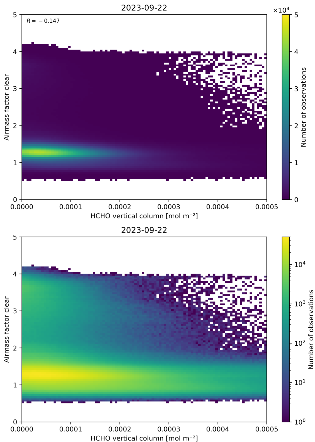
Figure 126: Scatter density plot of “HCHO vertical column” against “Airmass factor clear” for 2023-09-21 to 2023-09-23.
