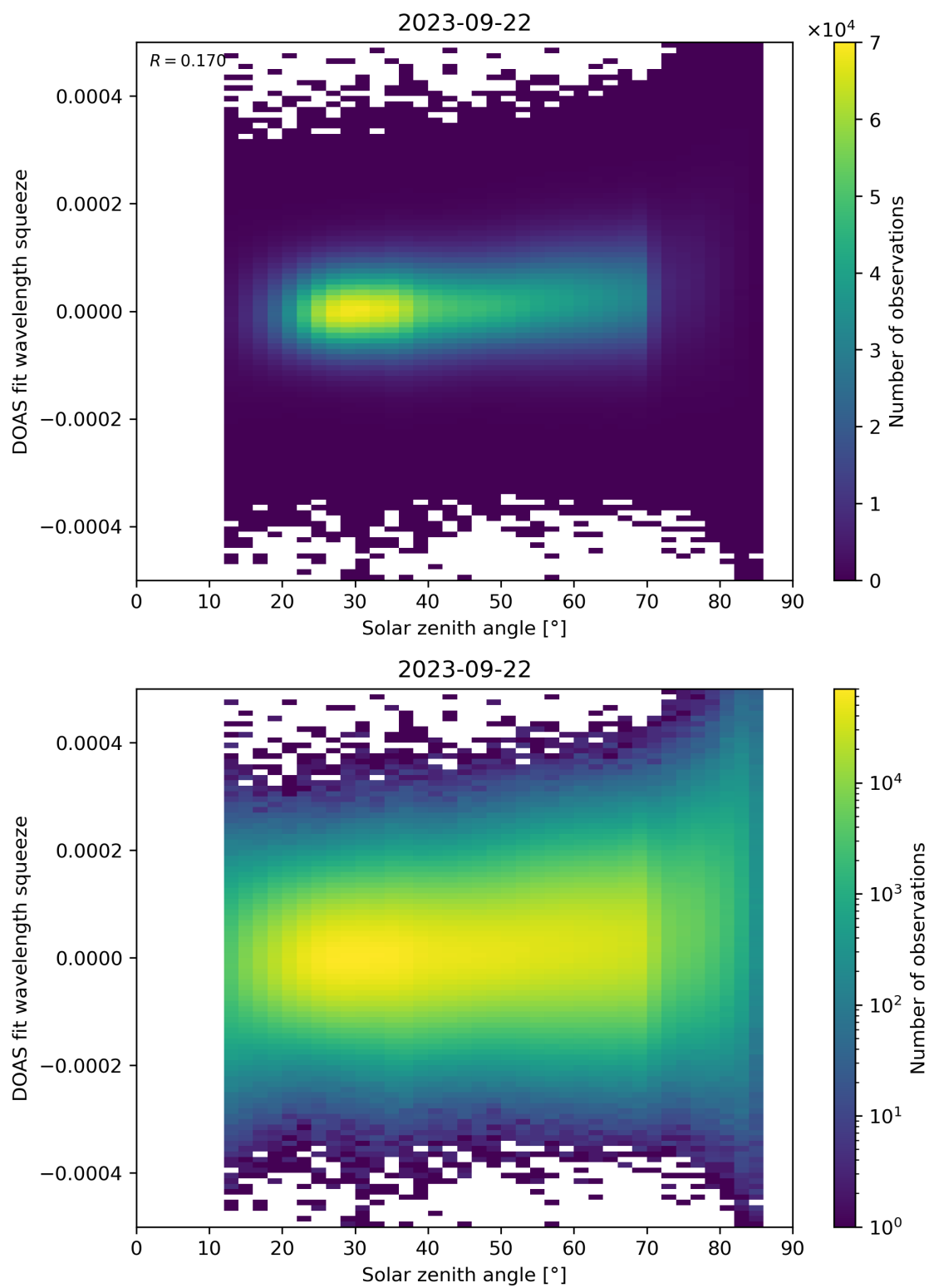
Figure 169: Scatter density plot of “Solar zenith angle” against “DOAS fit wavelength squeeze” for 2023-09-21 to 2023-09-23.
