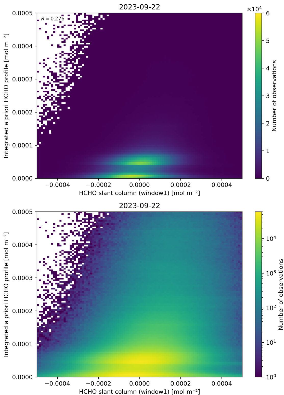
Figure 87: Scatter density plot of “HCHO slant column (window1)” against “Integrated a priori HCHO profile” for 2023-09-21 to 2023-09-23.
