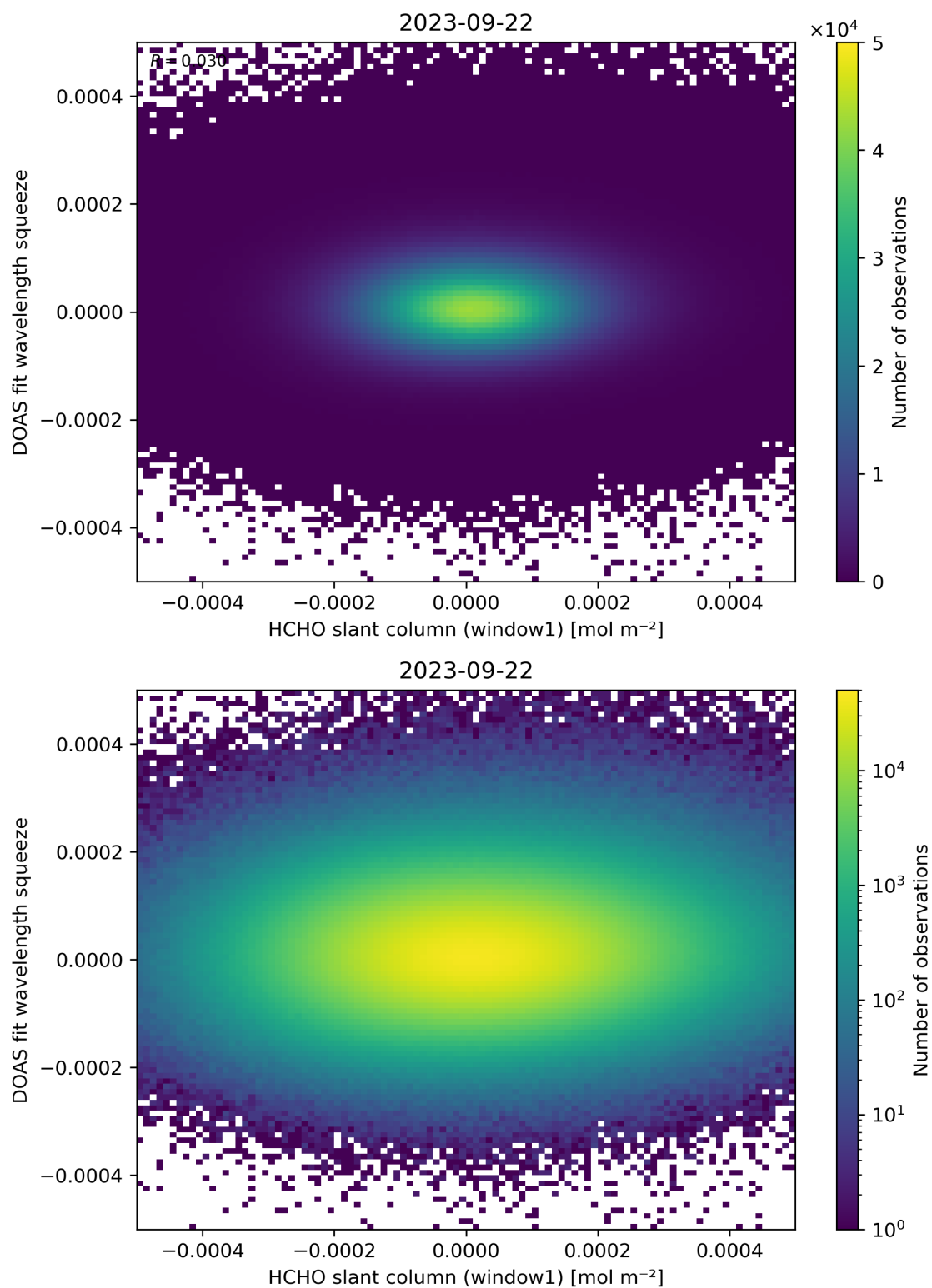
Figure 80: Scatter density plot of “HCHO slant column (window1)” against “DOAS fit wavelength squeeze” for 2023-09-21 to 2023-09-23.
