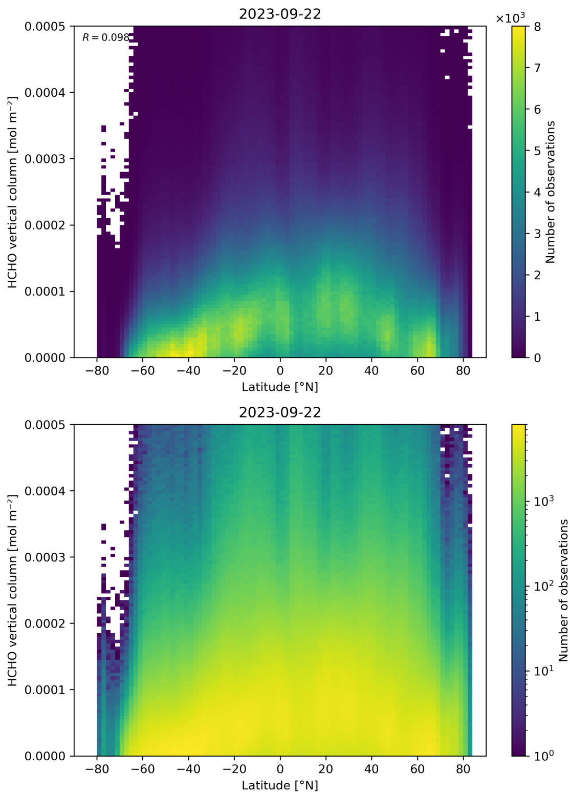
Figure 163: Scatter density plot of “Latitude” against “HCHO vertical column” for 2023-09-21 to 2023-09-23.
