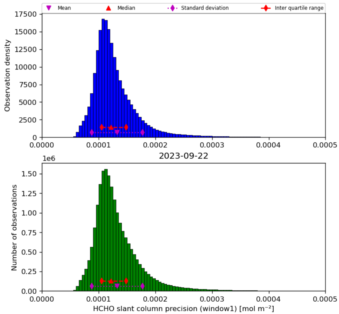
Figure 39: Histogram of “HCHO slant column precision (window1)” for 2023-09-21 to 2023-09-23
