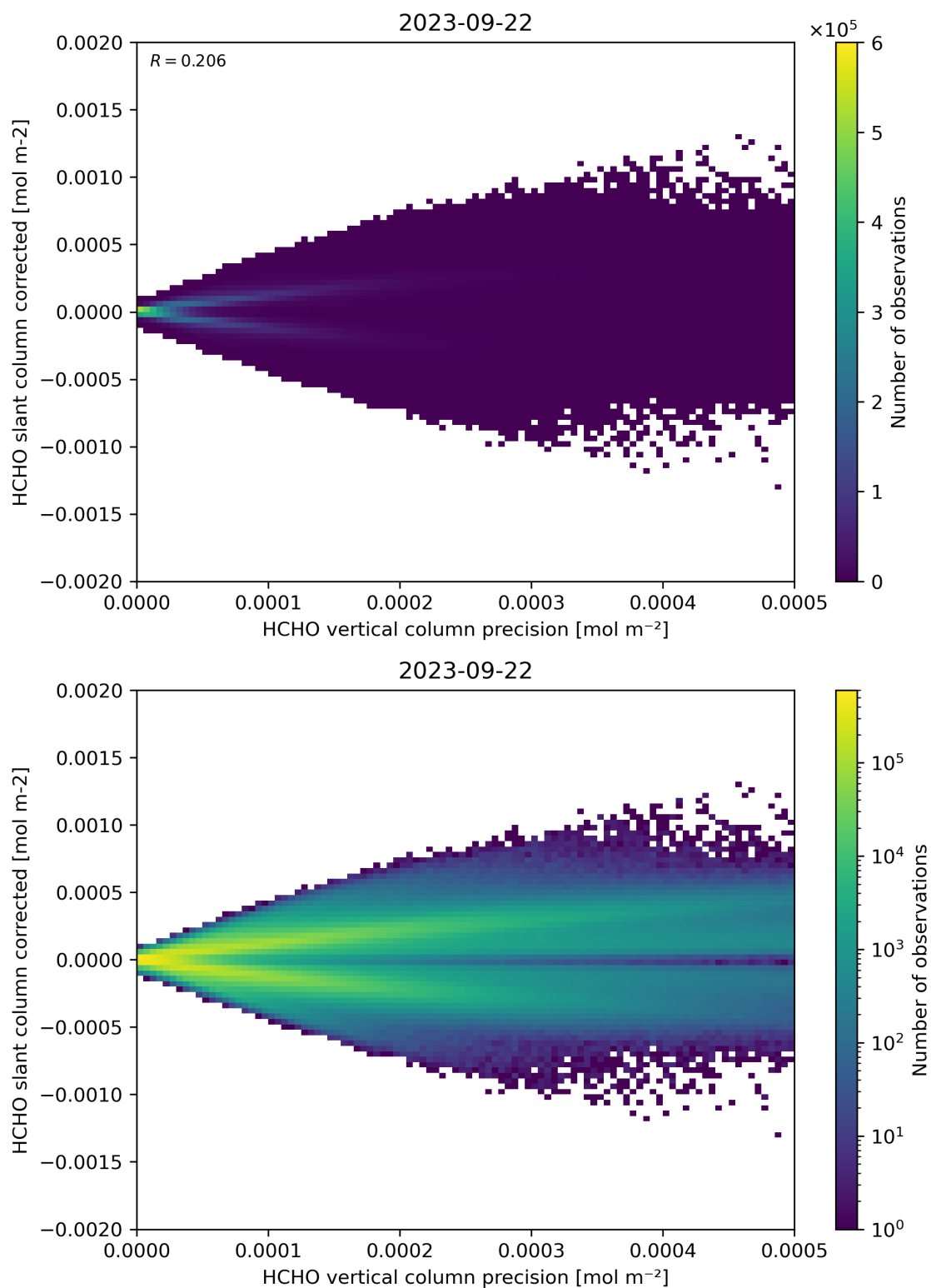
Figure 140: Scatter density plot of “HCHO vertical column precision” against “HCHO slant column corrected” for 2023-09-21 to 2023-09-23.
