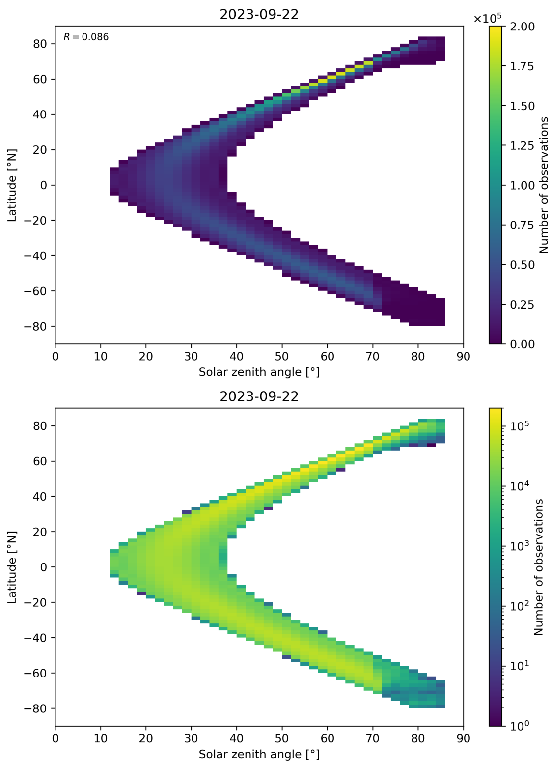
Figure 181: Scatter density plot of “Solar zenith angle” against “Latitude” for 2023-09-21 to 2023-09-23.
