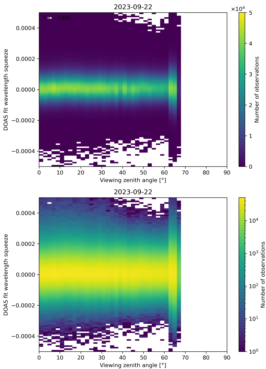
Figure 184: Scatter density plot of “Viewing zenith angle” against “DOAS fit wavelength squeeze” for 2023-09-21 to 2023-09-23.
