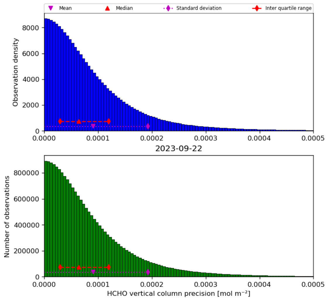
Figure 36: Histogram of “HCHO vertical column precision” for 2023-09-21 to 2023-09-23
