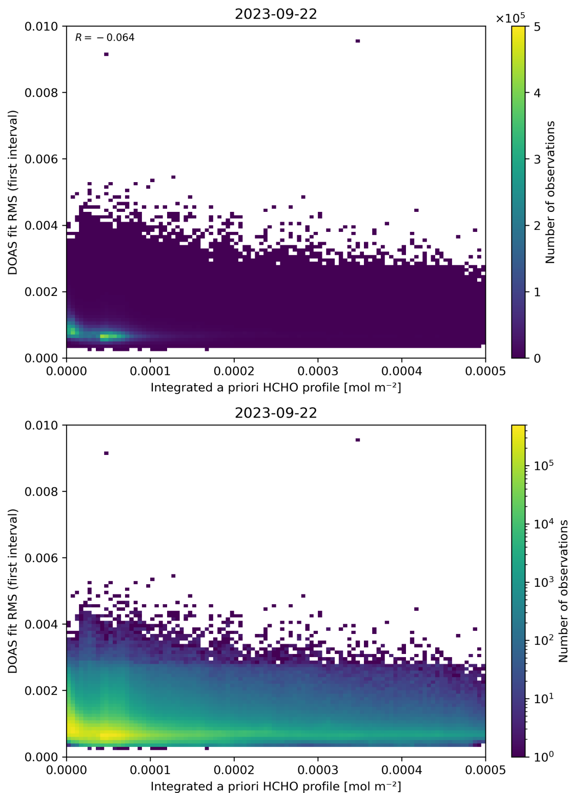
Figure 148: Scatter density plot of “Integrated a priori HCHO profile” against “DOAS fit RMS (first interval)” for 2023-09-21 to 2023-09-23.
