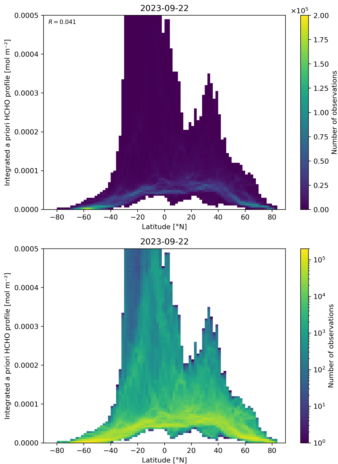
Figure 166: Scatter density plot of “Latitude” against “Integrated a priori HCHO profile” for 2023-09-21 to 2023-09-23.
