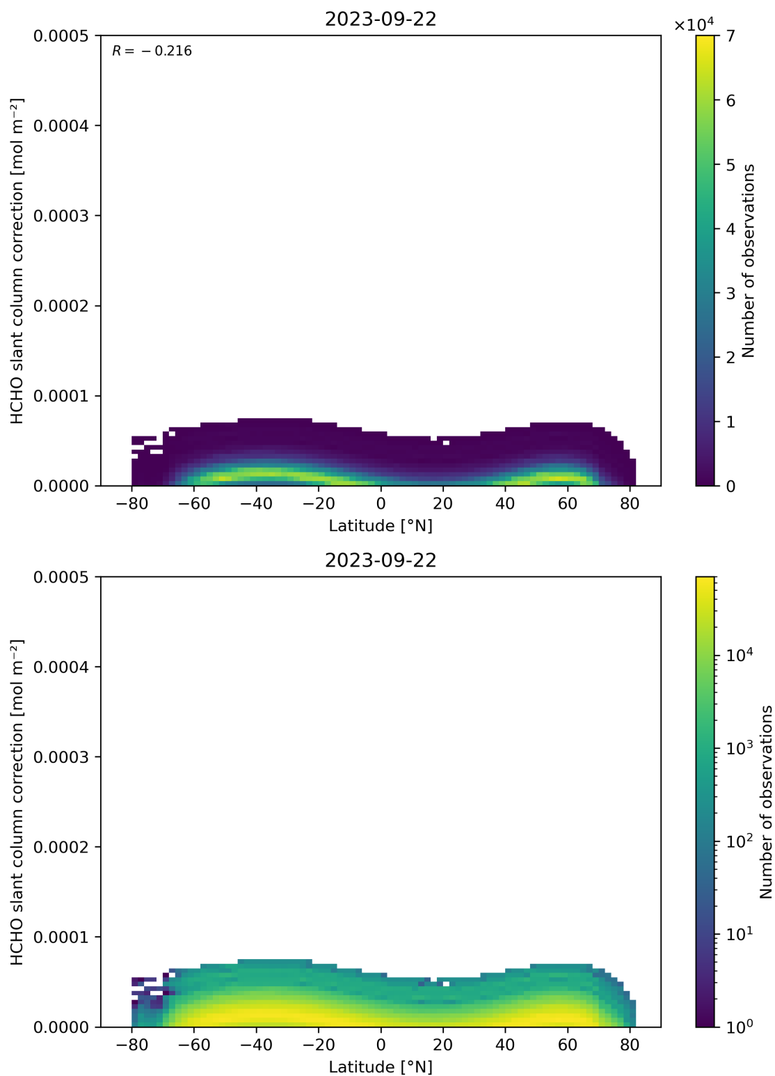
Figure 158: Scatter density plot of “Latitude” against “HCHO slant column correction” for 2023-09-21 to 2023-09-23.
