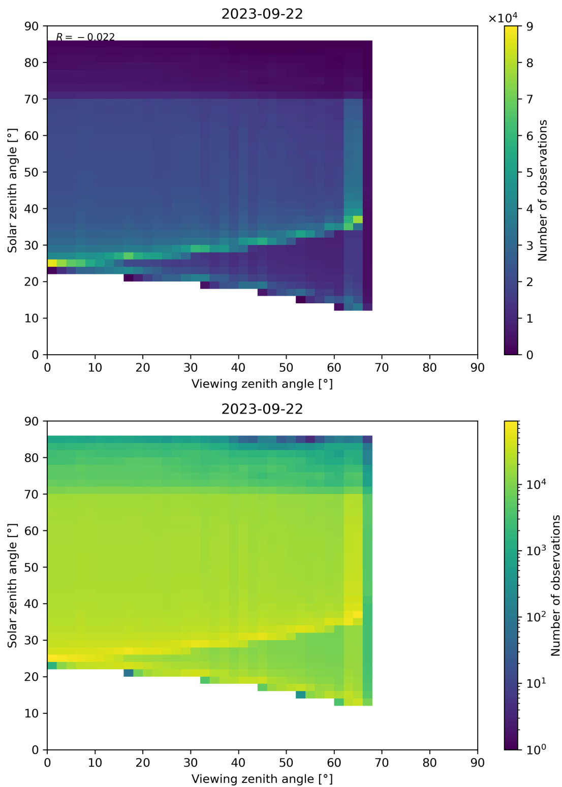
Figure 197: Scatter density plot of “Viewing zenith angle” against “Solar zenith angle” for 2023-09-21 to 2023-09-23.
