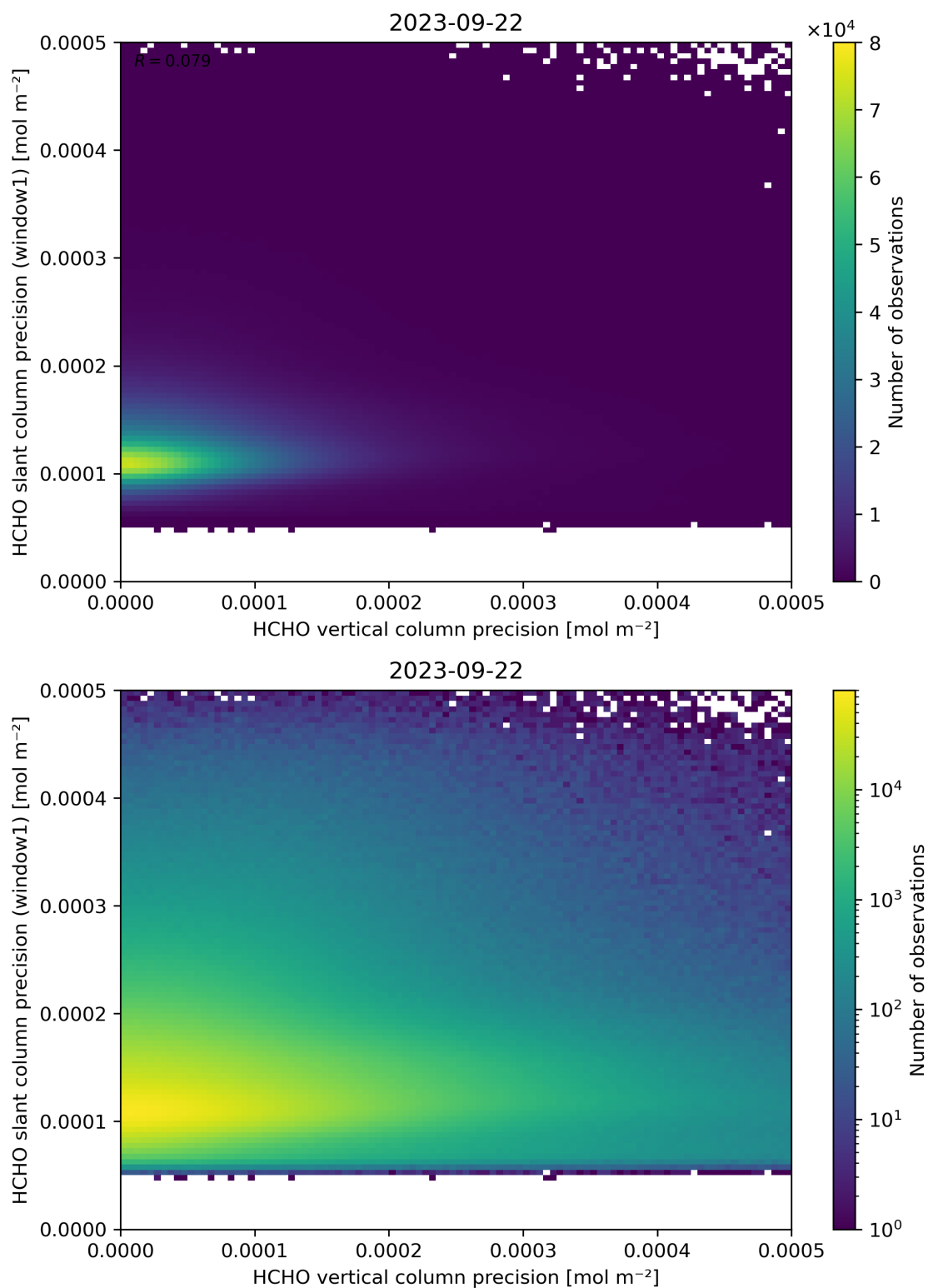
Figure 143: Scatter density plot of “HCHO vertical column precision” against “HCHO slant column precision (window1)” for 2023-09-21 to 2023-09-23.
