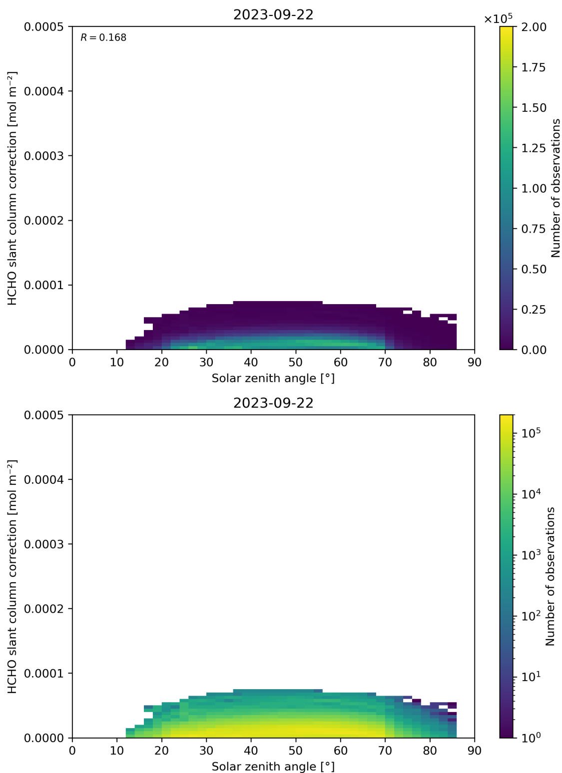
Figure 172: Scatter density plot of “Solar zenith angle” against “HCHO slant column correction” for 2023-09-21 to 2023-09-23.
