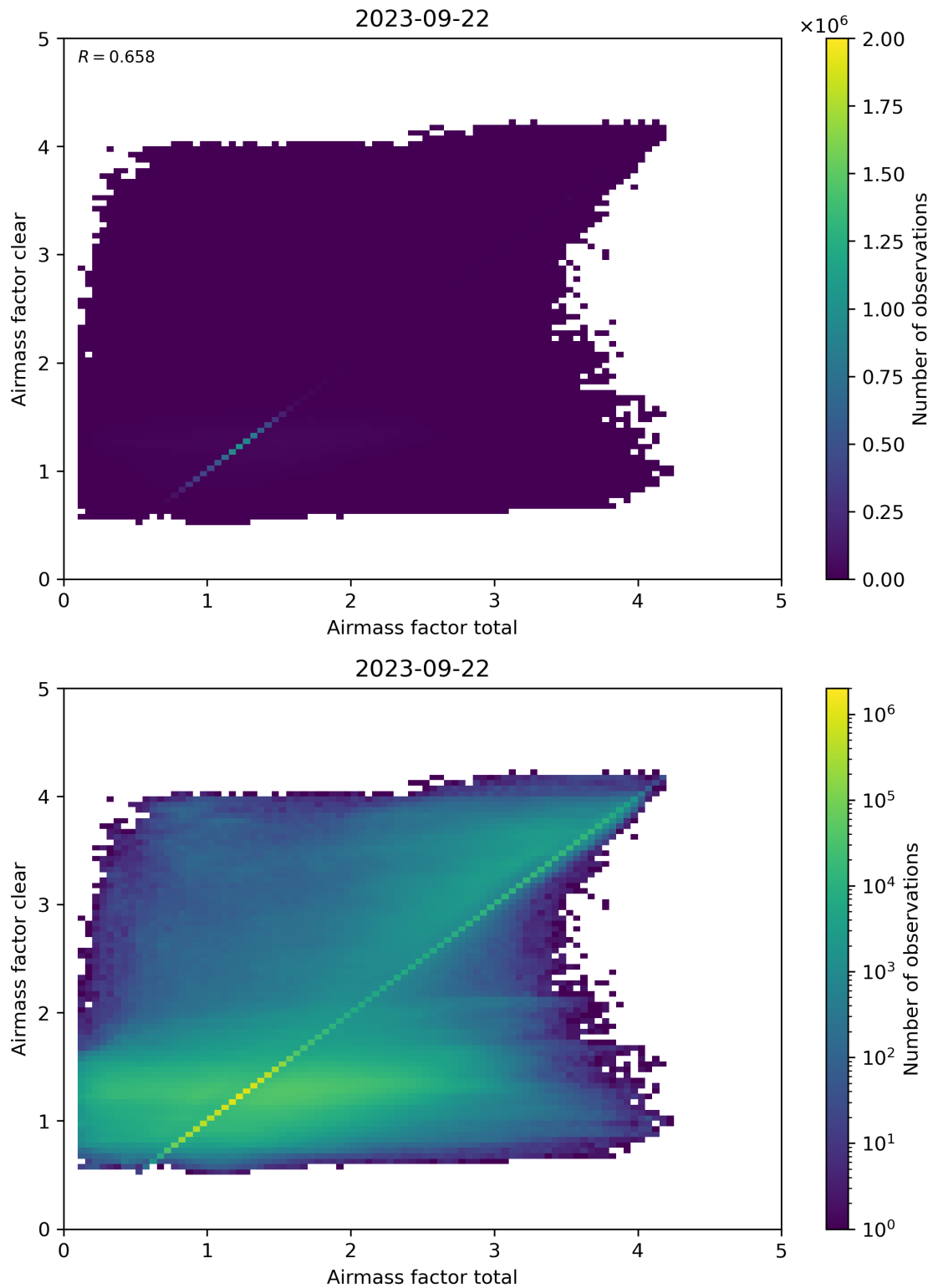
Figure 100: Scatter density plot of “Airmass factor total” against “Airmass factor clear” for 2023-09-21 to 2023-09-23.
