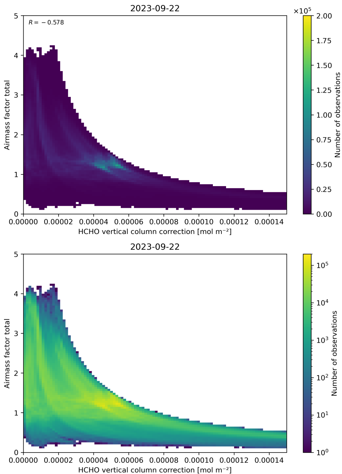
Figure 120: Scatter density plot of “HCHO vertical column correction” against “Airmass factor total” for 2023-09-21 to 2023-09-23.
