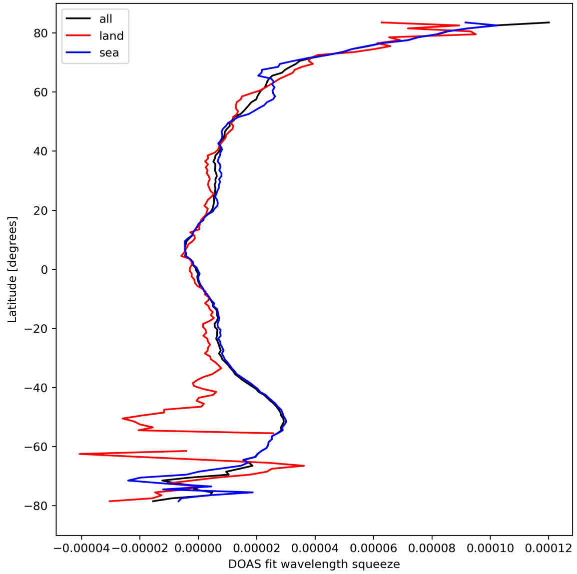
Figure 31: Zonal average of “DOAS fit wavelength squeeze” for 2023-09-21 to 2023-09-23.
