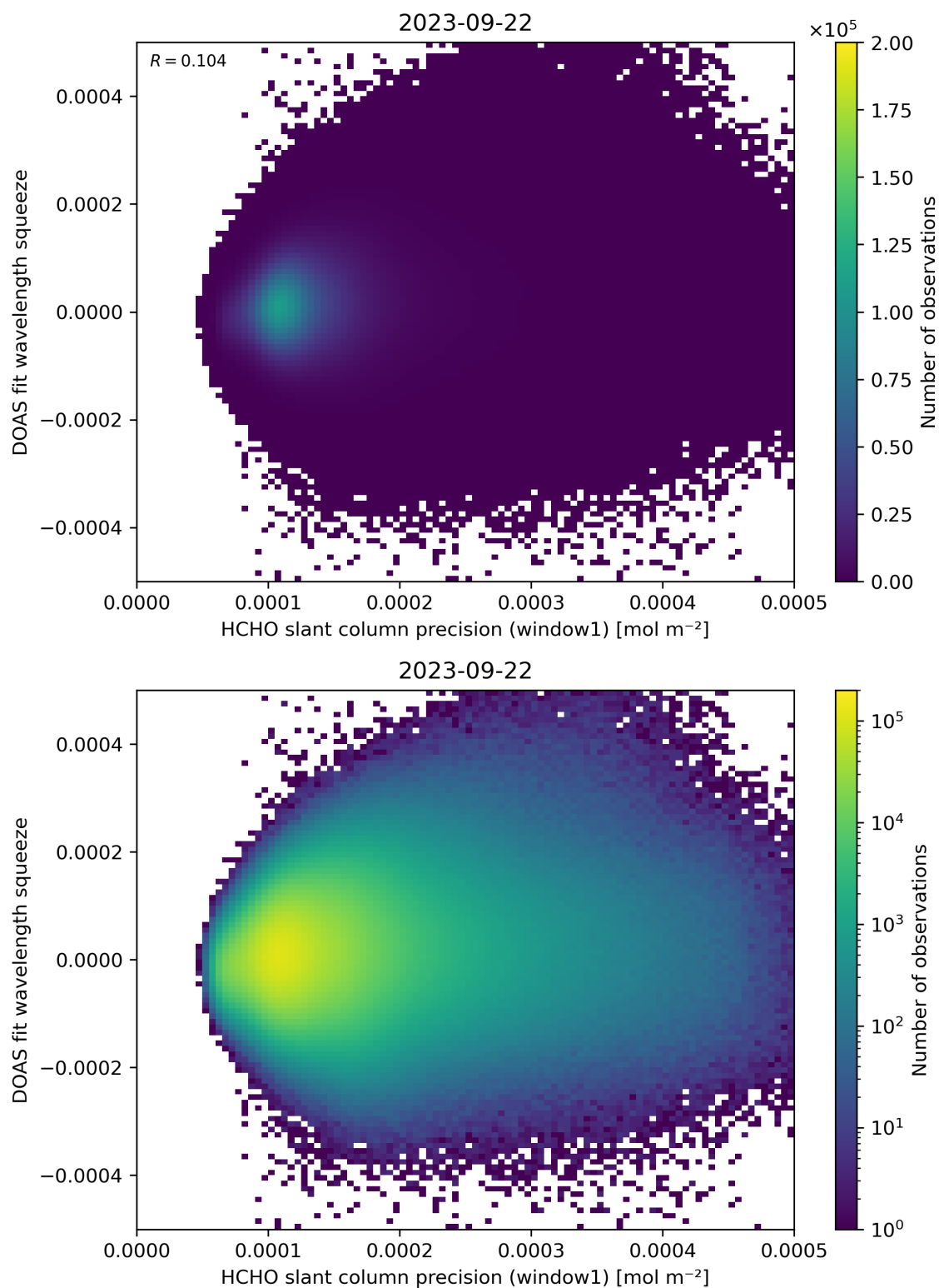
Figure 90: Scatter density plot of “HCHO slant column precision (window1)” against “DOAS fit wavelength squeeze” for 2023-09-21 to 2023-09-23.
