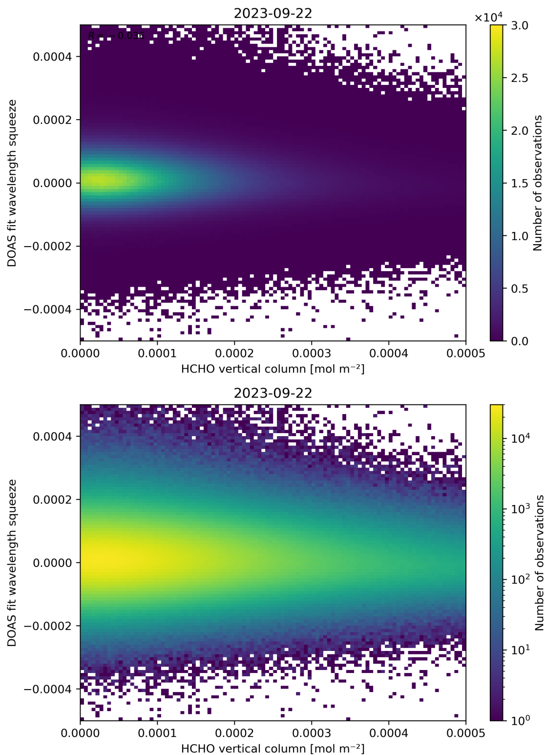
Figure 125: Scatter density plot of “HCHO vertical column” against “DOAS fit wavelength squeeze” for 2023-09-21 to 2023-09-23.
