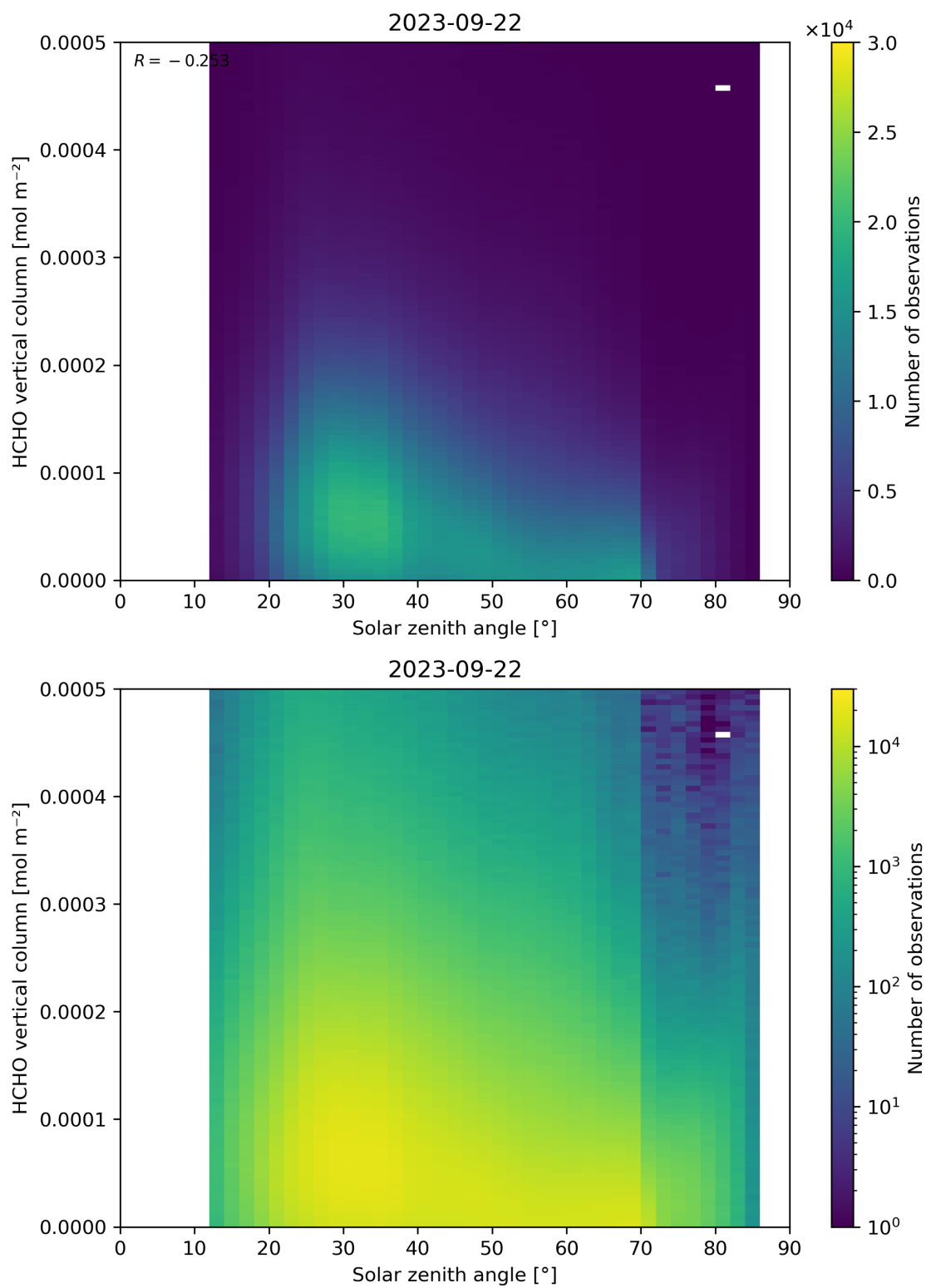
Figure 177: Scatter density plot of “Solar zenith angle” against “HCHO vertical column” for 2023-09-21 to 2023-09-23.
