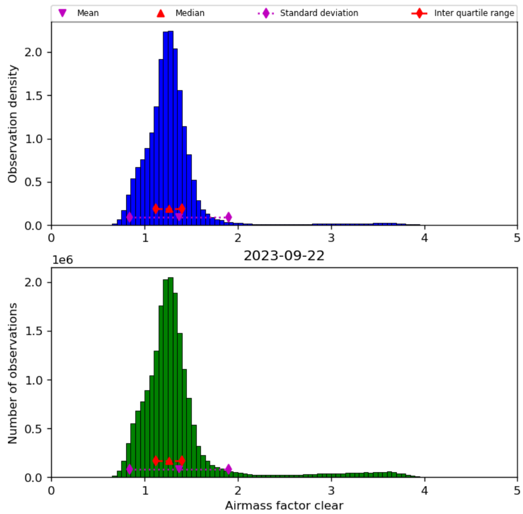
Figure 42: Histogram of “Airmass factor clear” for 2023-09-21 to 2023-09-23
