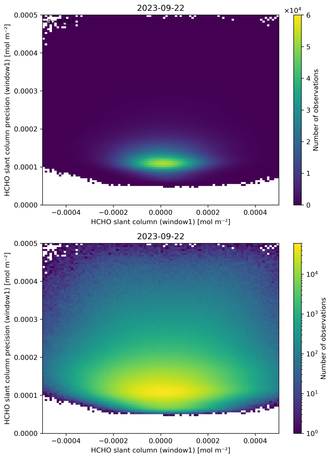
Figure 84: Scatter density plot of “HCHO slant column (window1)” against “HCHO slant column precision (window1)” for 2023-09-21 to 2023-09-23.
