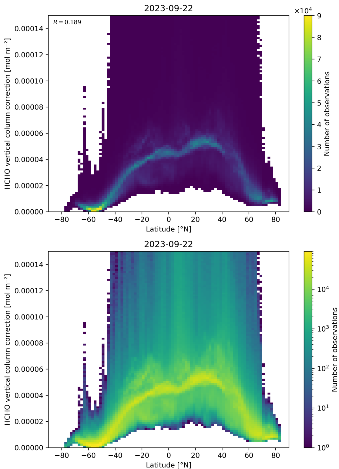
Figure 164: Scatter density plot of “Latitude” against “HCHO vertical column correction” for 2023-09-21 to 2023-09-23.
