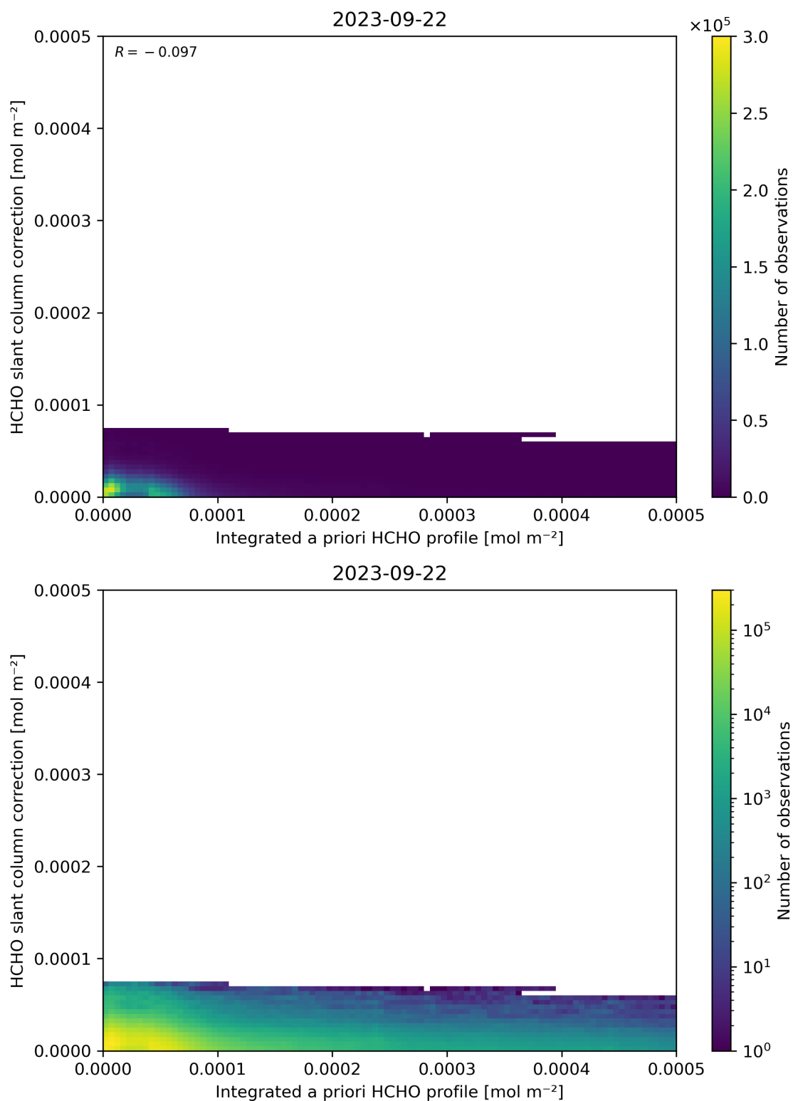
Figure 152: Scatter density plot of “Integrated a priori HCHO profile” against “HCHO slant column correction” for 2023-09-21 to 2023-09-23.
