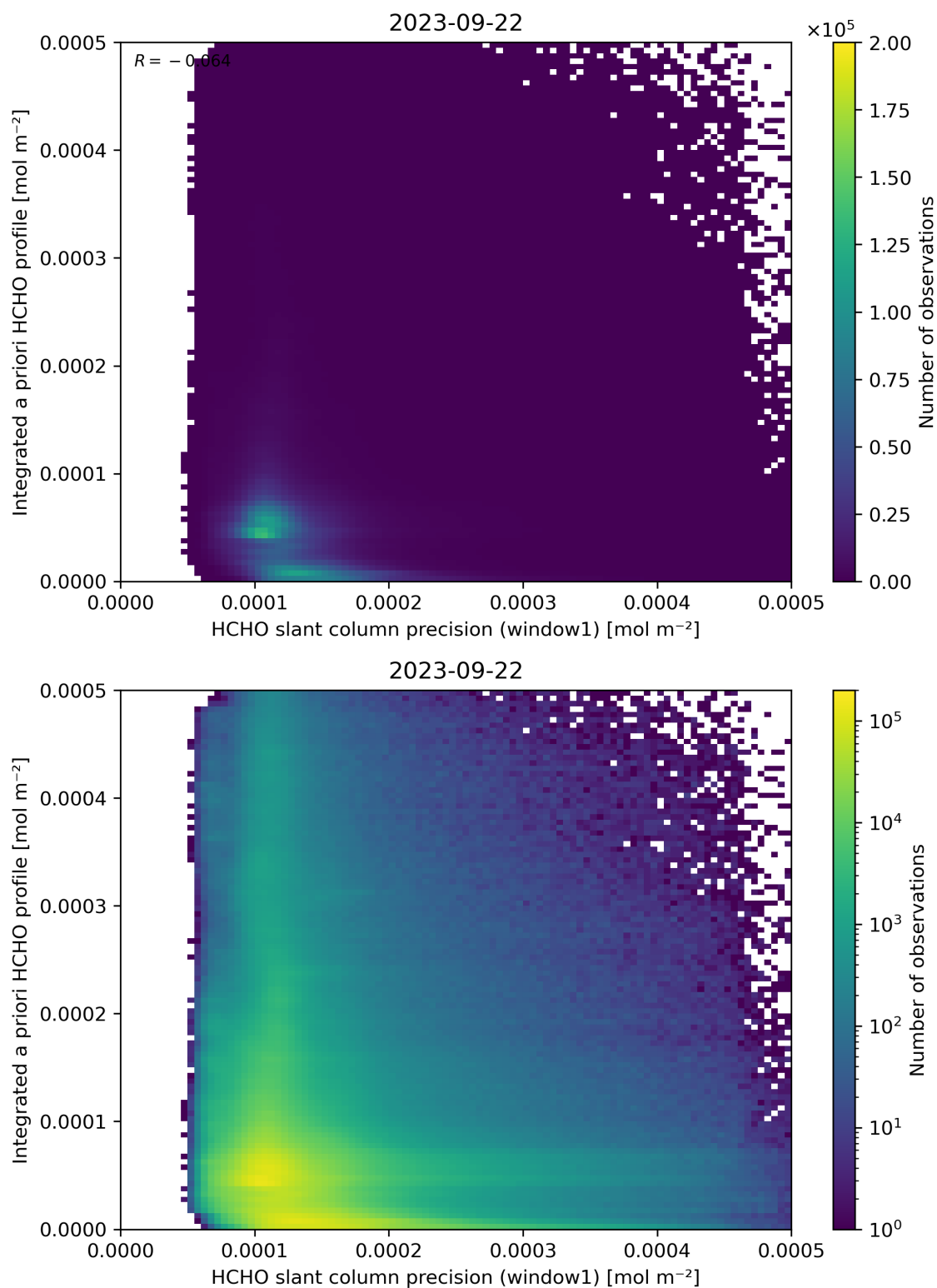
Figure 96: Scatter density plot of “HCHO slant column precision (window1)” against “Integrated a priori HCHO profile” for 2023-09-21 to 2023-09-23.
