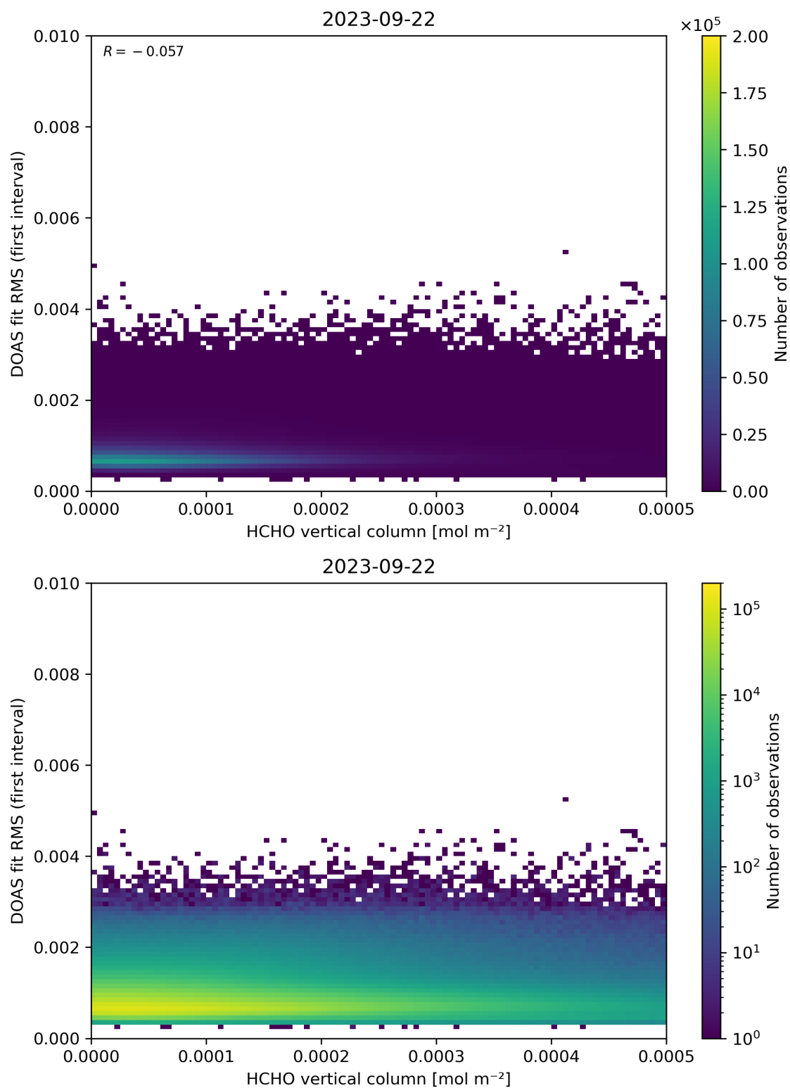
Figure 123: Scatter density plot of “HCHO vertical column” against “DOAS fit RMS (first interval)” for 2023-09-21 to 2023-09-23.
