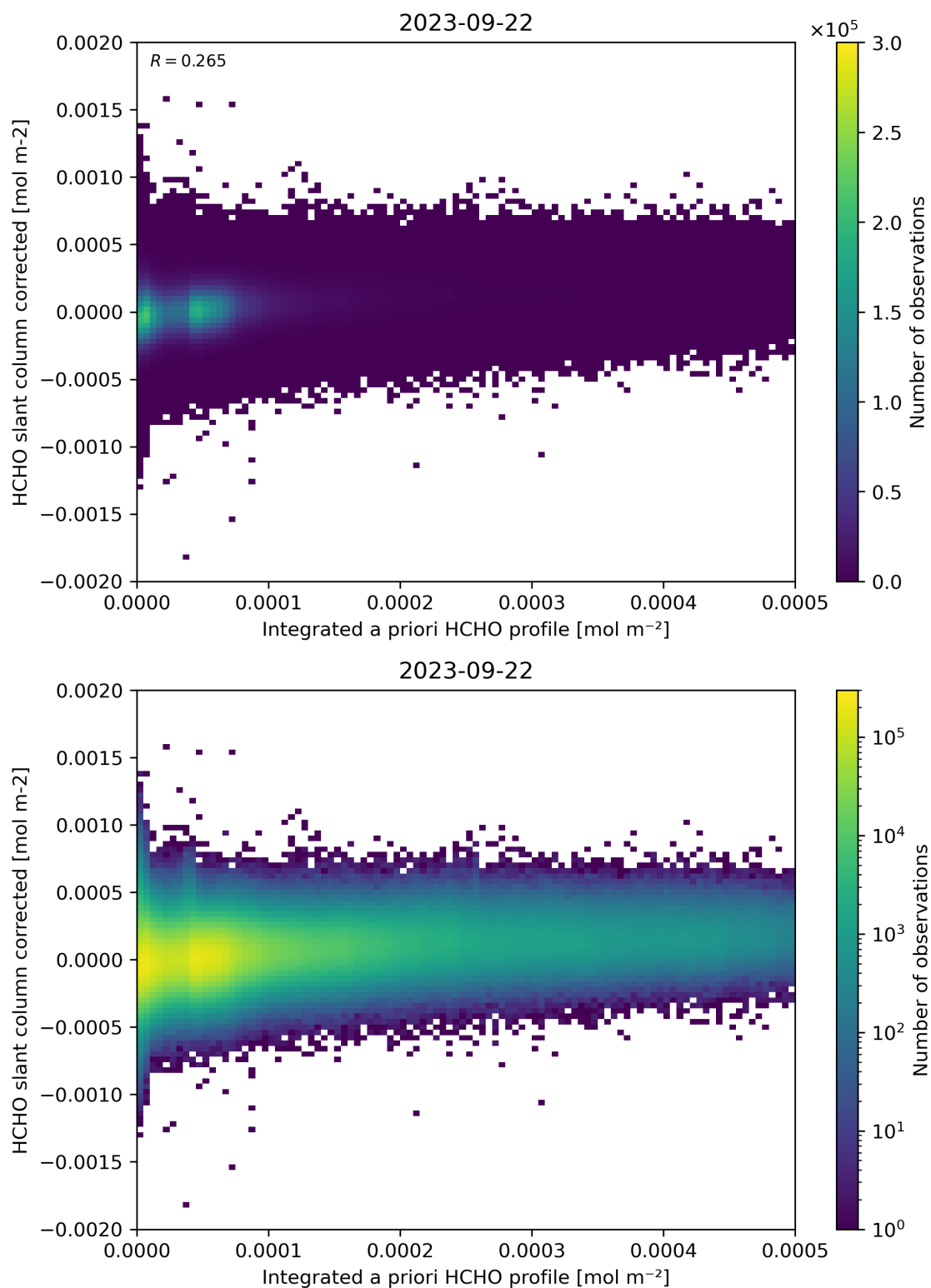
Figure 151: Scatter density plot of “Integrated a priori HCHO profile” against “HCHO slant column corrected” for 2023-09-21 to 2023-09-23.
