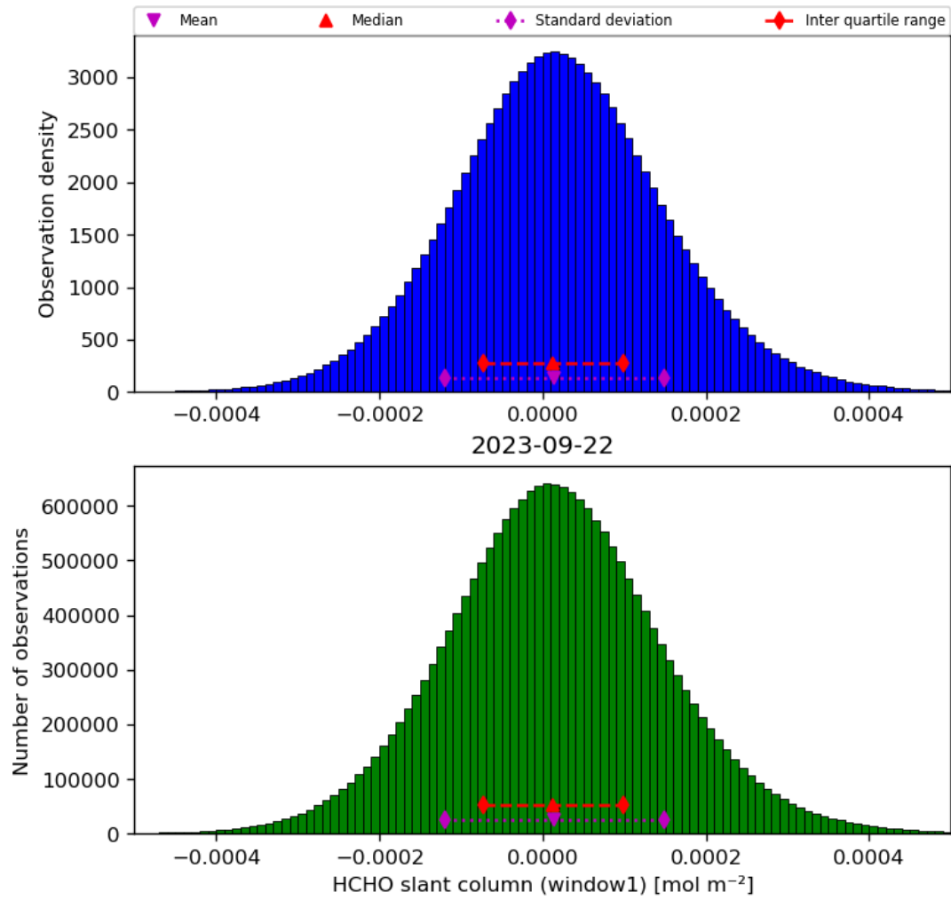
Figure 38: Histogram of “HCHO slant column (window1)” for 2023-09-21 to 2023-09-23
