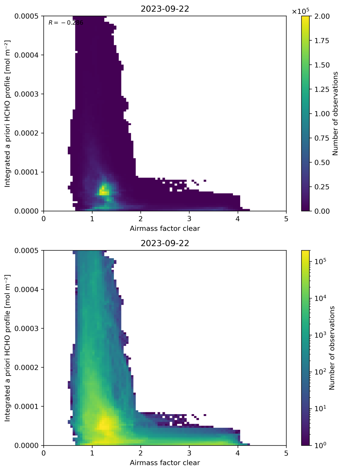
Figure 76: Scatter density plot of “Airmass factor clear” against “Integrated a priori HCHO profile” for 2023-09-21 to 2023-09-23.
