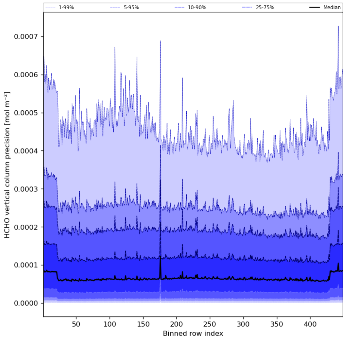
Figure 50: Along track statistics of “HCHO vertical column precision” for 2023-09-21 to 2023-09-23
