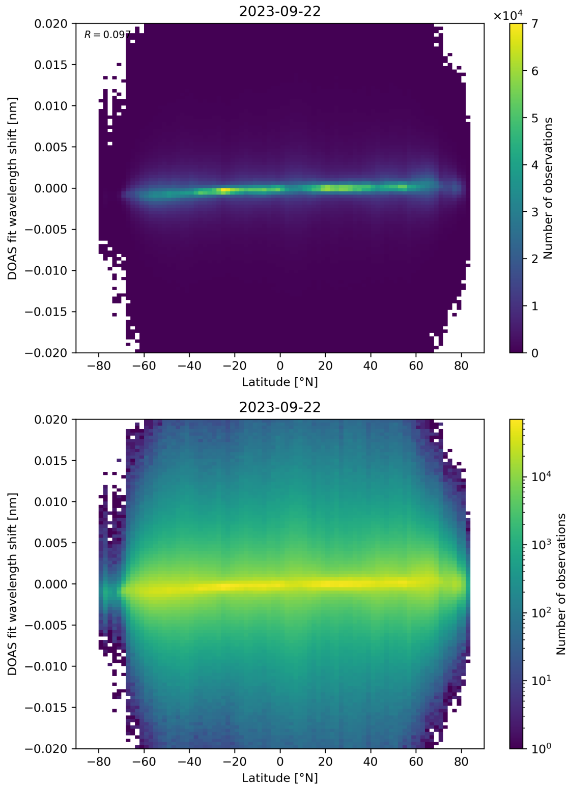
Figure 154: Scatter density plot of “Latitude” against “DOAS fit wavelength shift” for 2023-09-21 to 2023-09-23.
