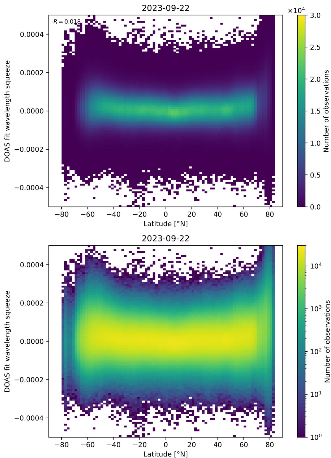
Figure 155: Scatter density plot of “Latitude” against “DOAS fit wavelength squeeze” for 2023-09-21 to 2023-09-23.
