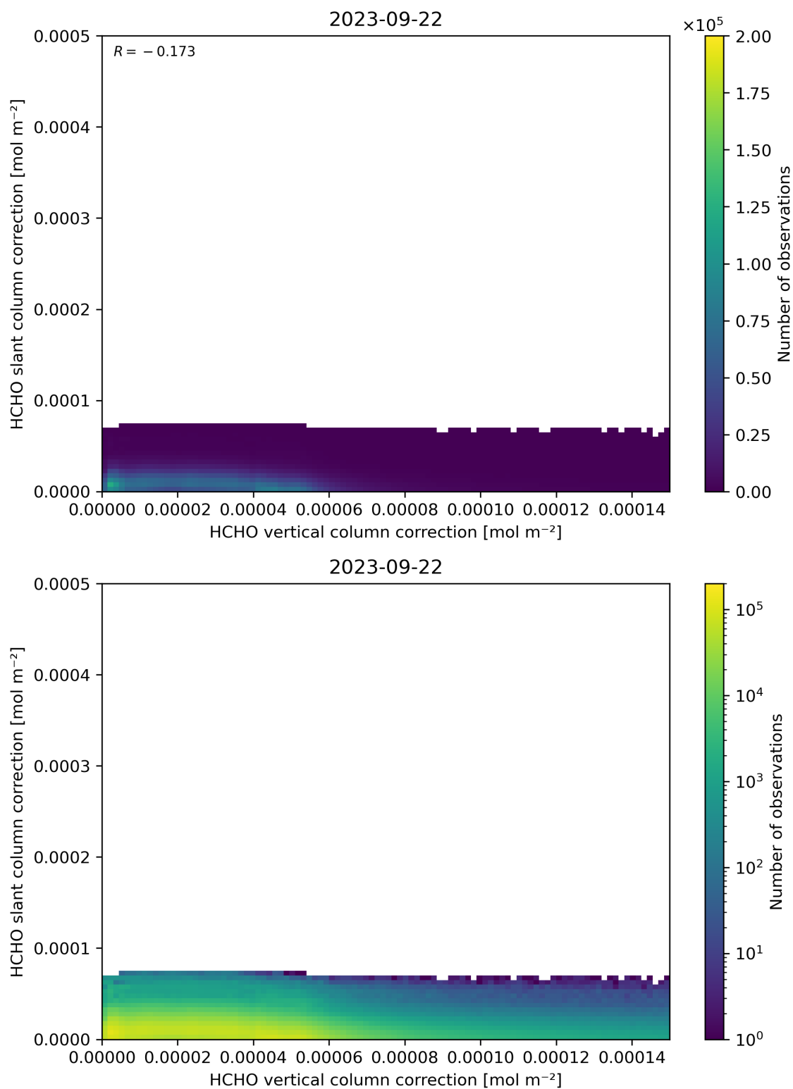
Figure 117: Scatter density plot of “HCHO vertical column correction” against “HCHO slant column correction” for 2023-09-21 to 2023-09-23.
