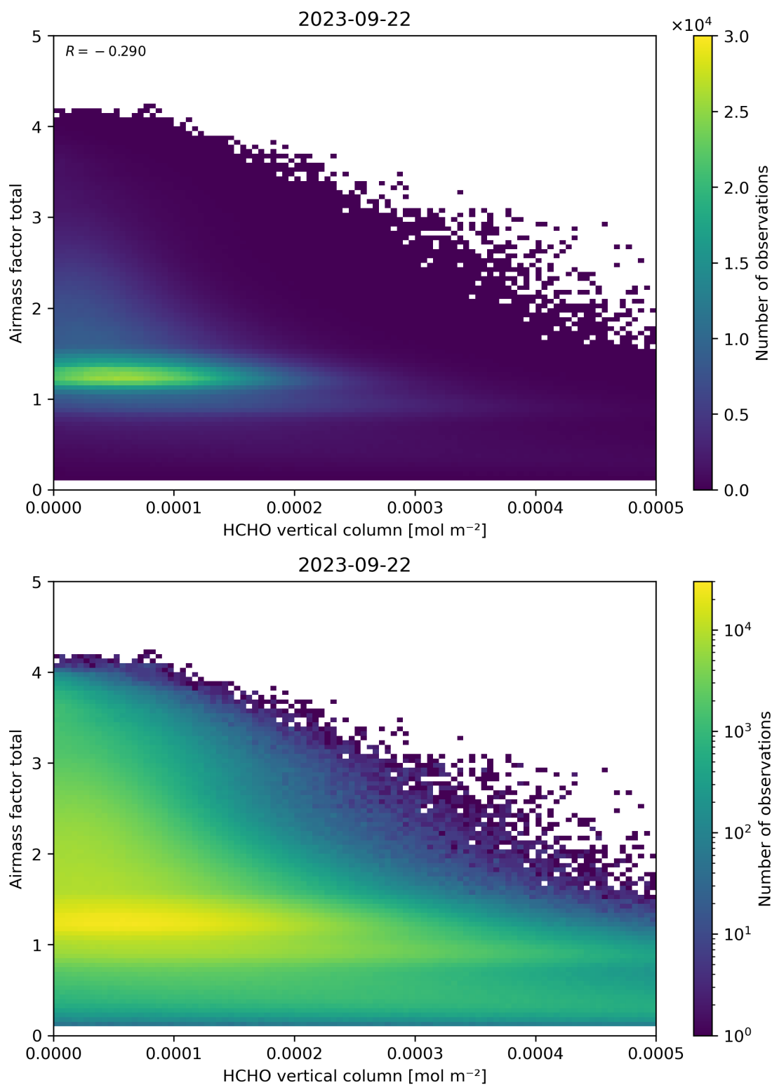
Figure 131: Scatter density plot of “HCHO vertical column” against “Airmass factor total” for 2023-09-21 to 2023-09-23.
