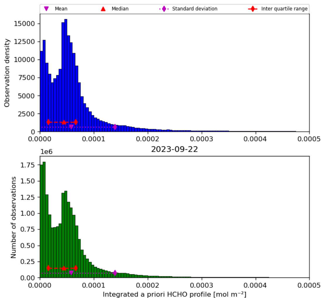
Figure 43: Histogram of “Integrated a priori HCHO profile” for 2023-09-21 to 2023-09-23
