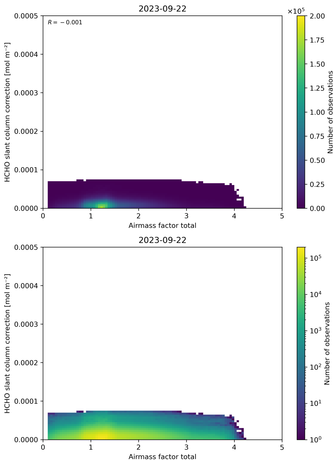
Figure 102: Scatter density plot of “Airmass factor total” against “HCHO slant column correction” for 2023-09-21 to 2023-09-23.
