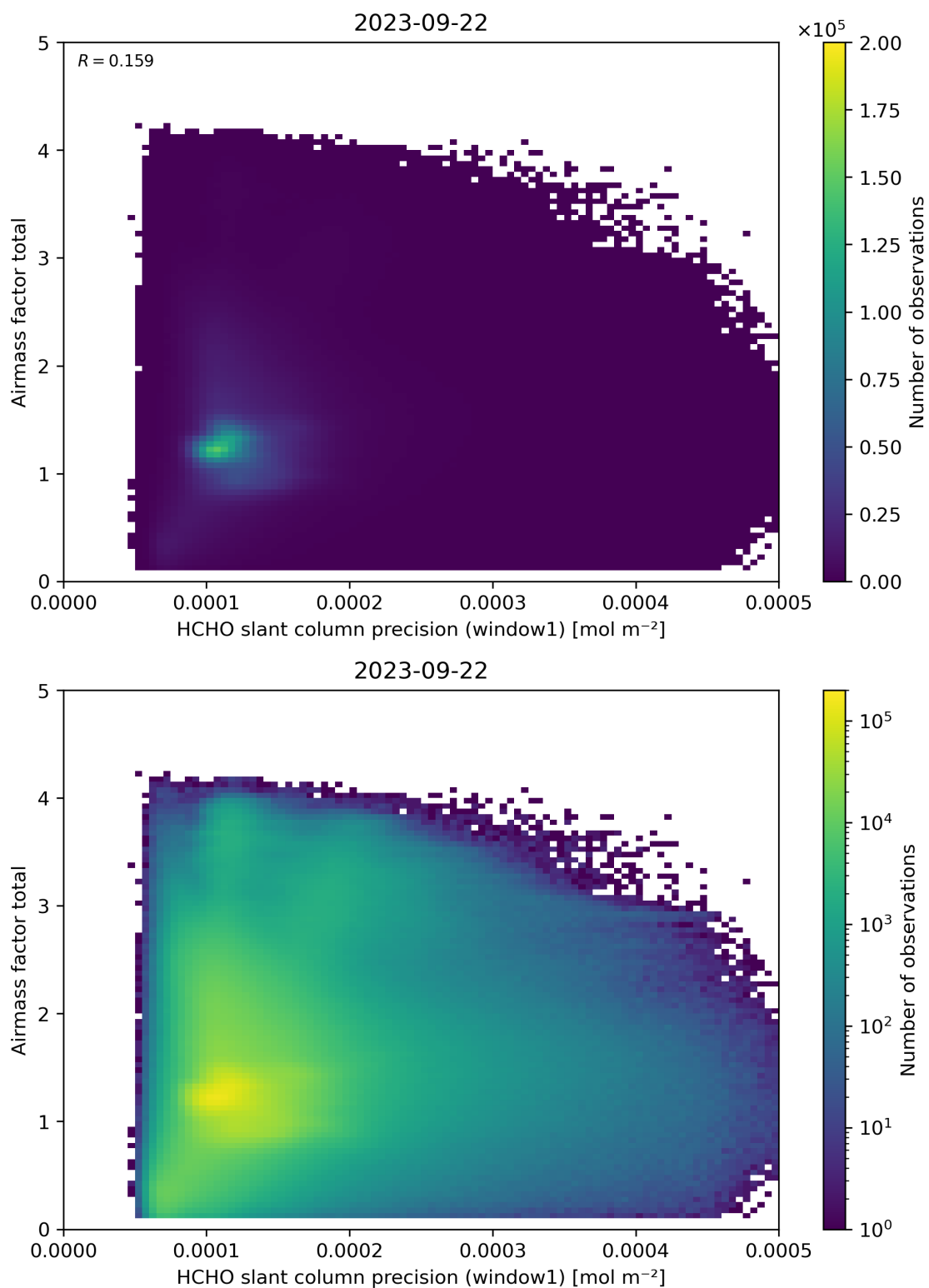
Figure 94: Scatter density plot of “HCHO slant column precision (window1)” against “Airmass factor total” for 2023-09-21 to 2023-09-23.
