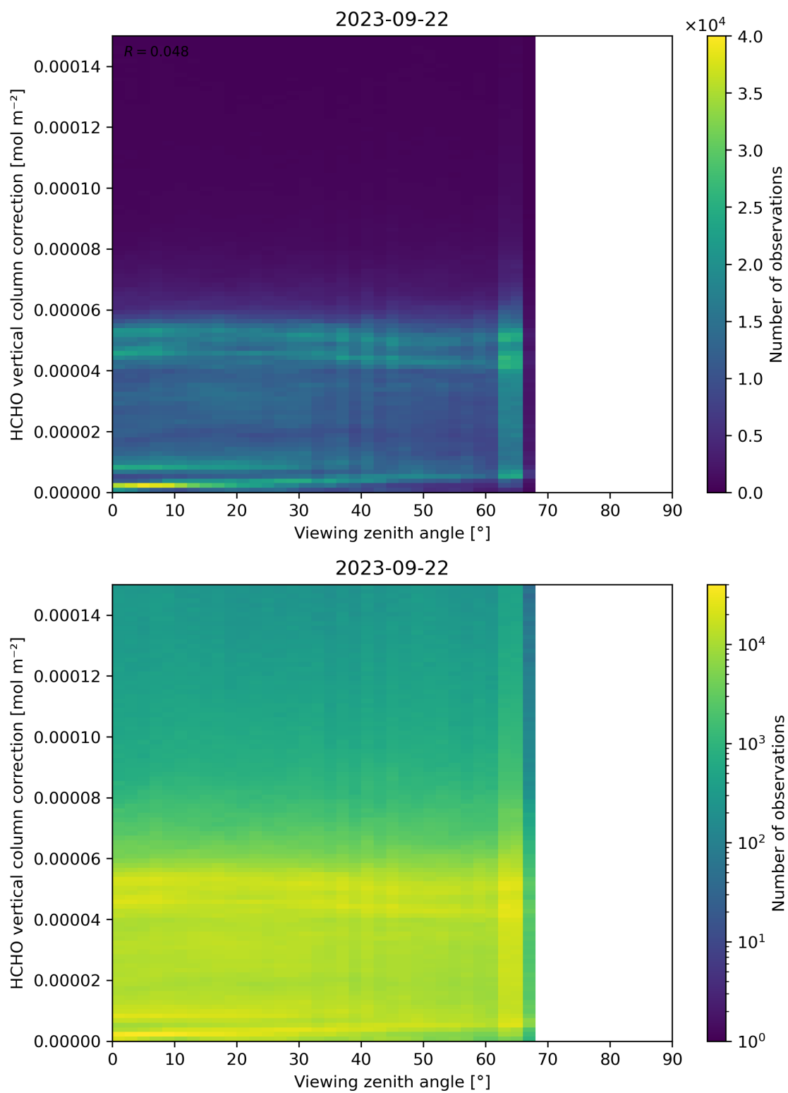
Figure 193: Scatter density plot of “Viewing zenith angle” against “HCHO vertical column correction” for 2023-09-21 to 2023-09-23.
