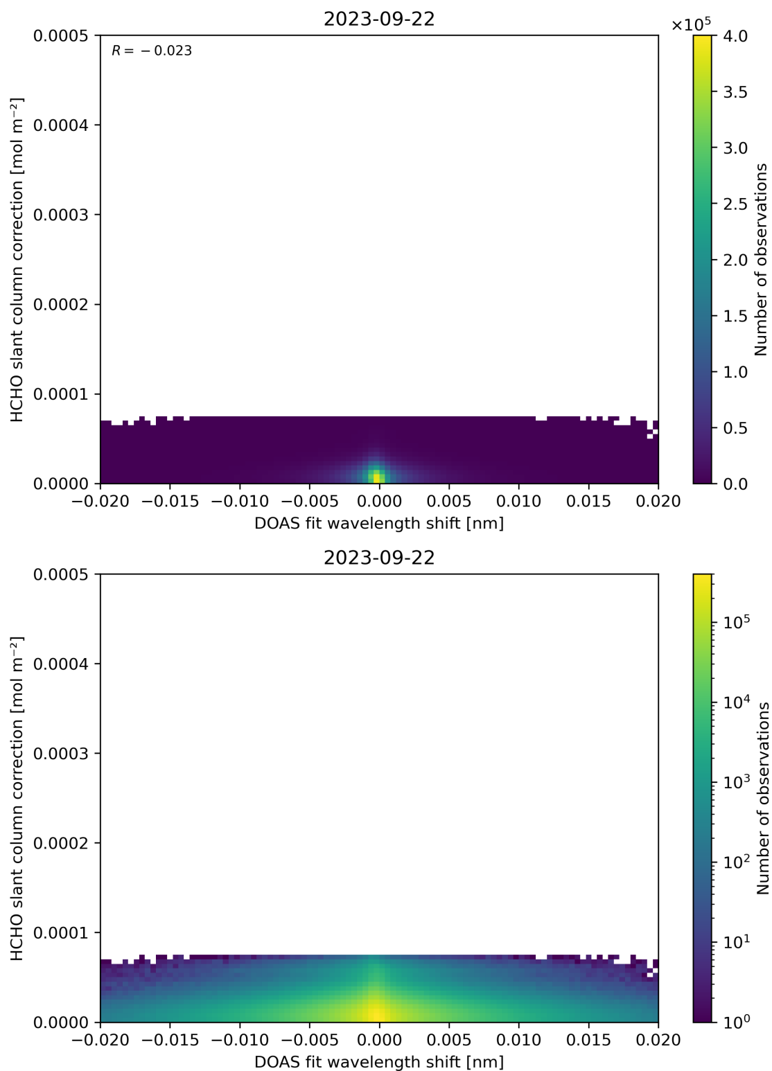
Figure 67: Scatter density plot of “DOAS fit wavelength shift” against “HCHO slant column correction” for 2023-09-21 to 2023-09-23.
