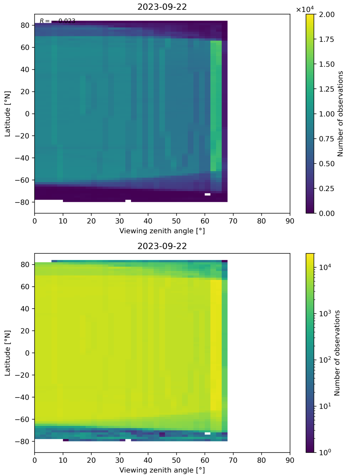
Figure 196: Scatter density plot of “Viewing zenith angle” against “Latitude” for 2023-09-21 to 2023-09-23.
