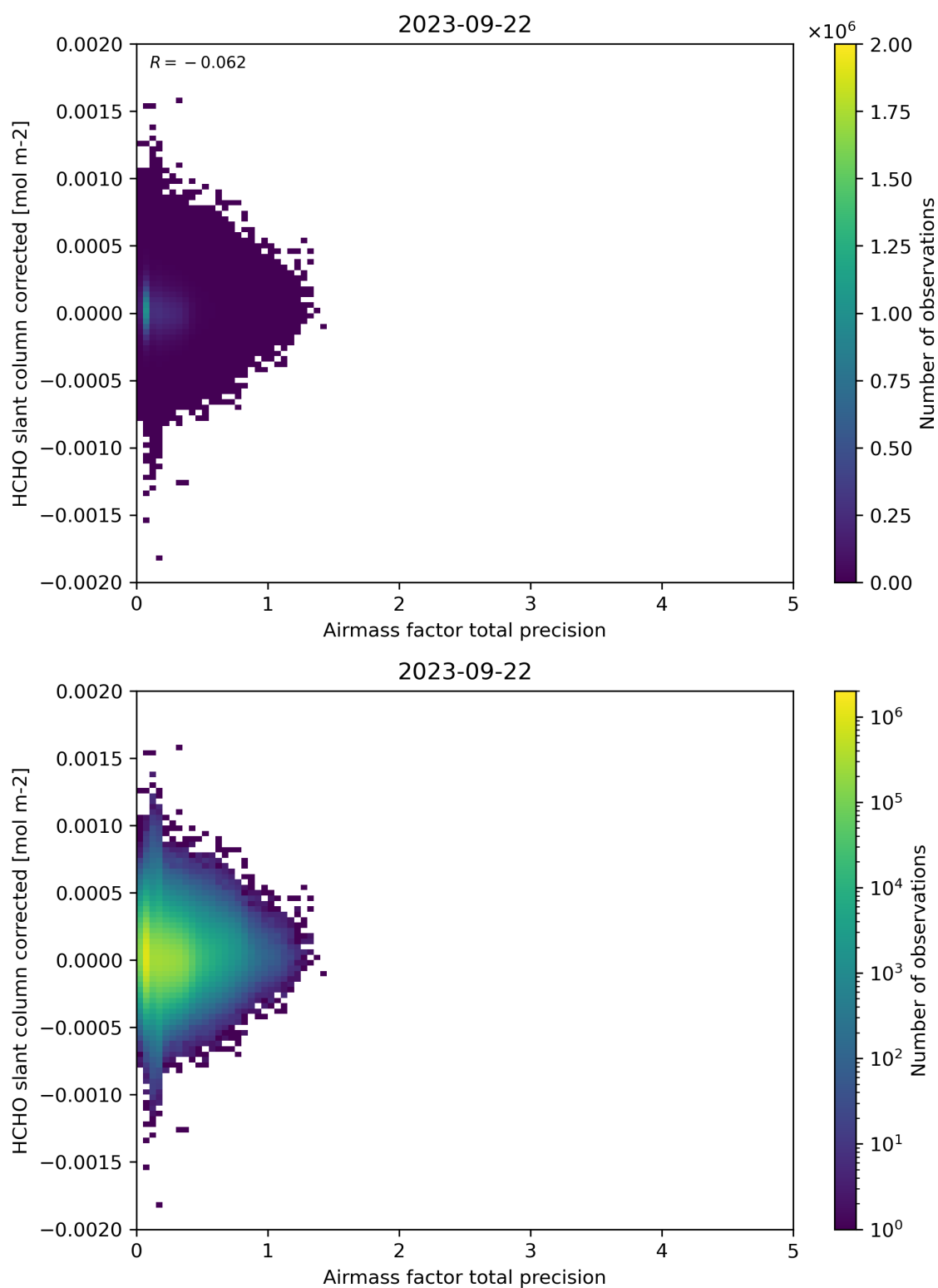
Figure 109: Scatter density plot of “Airmass factor total precision” against “HCHO slant column corrected” for 2023-09-21 to 2023-09-23.
