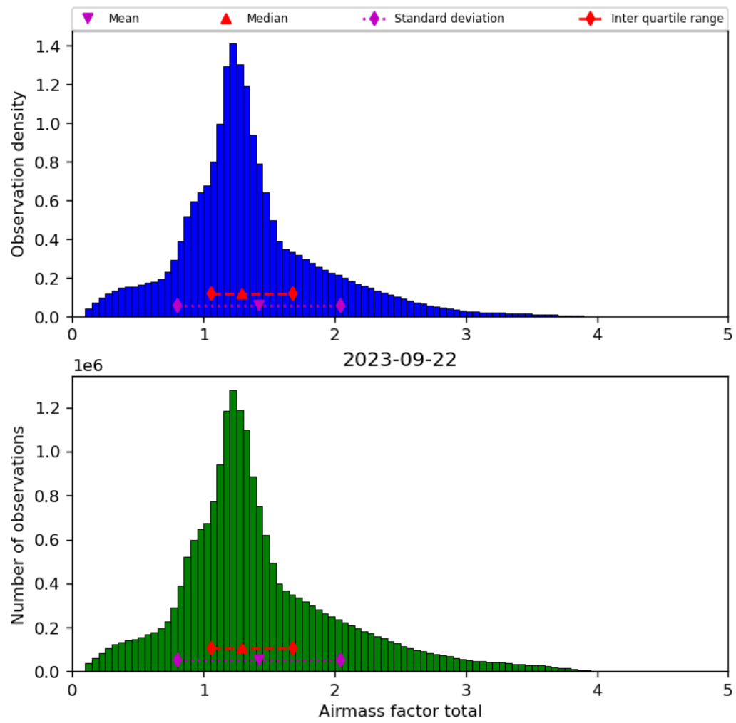
Figure 40: Histogram of “Airmass factor total” for 2023-09-21 to 2023-09-23
