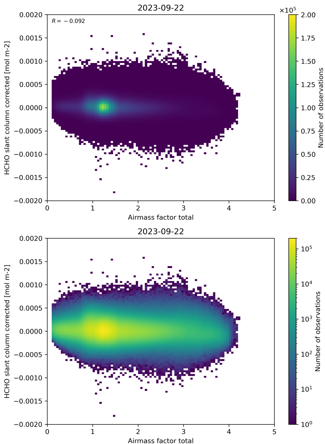
Figure 101: Scatter density plot of “Airmass factor total” against “HCHO slant column corrected” for 2023-09-21 to 2023-09-23.
