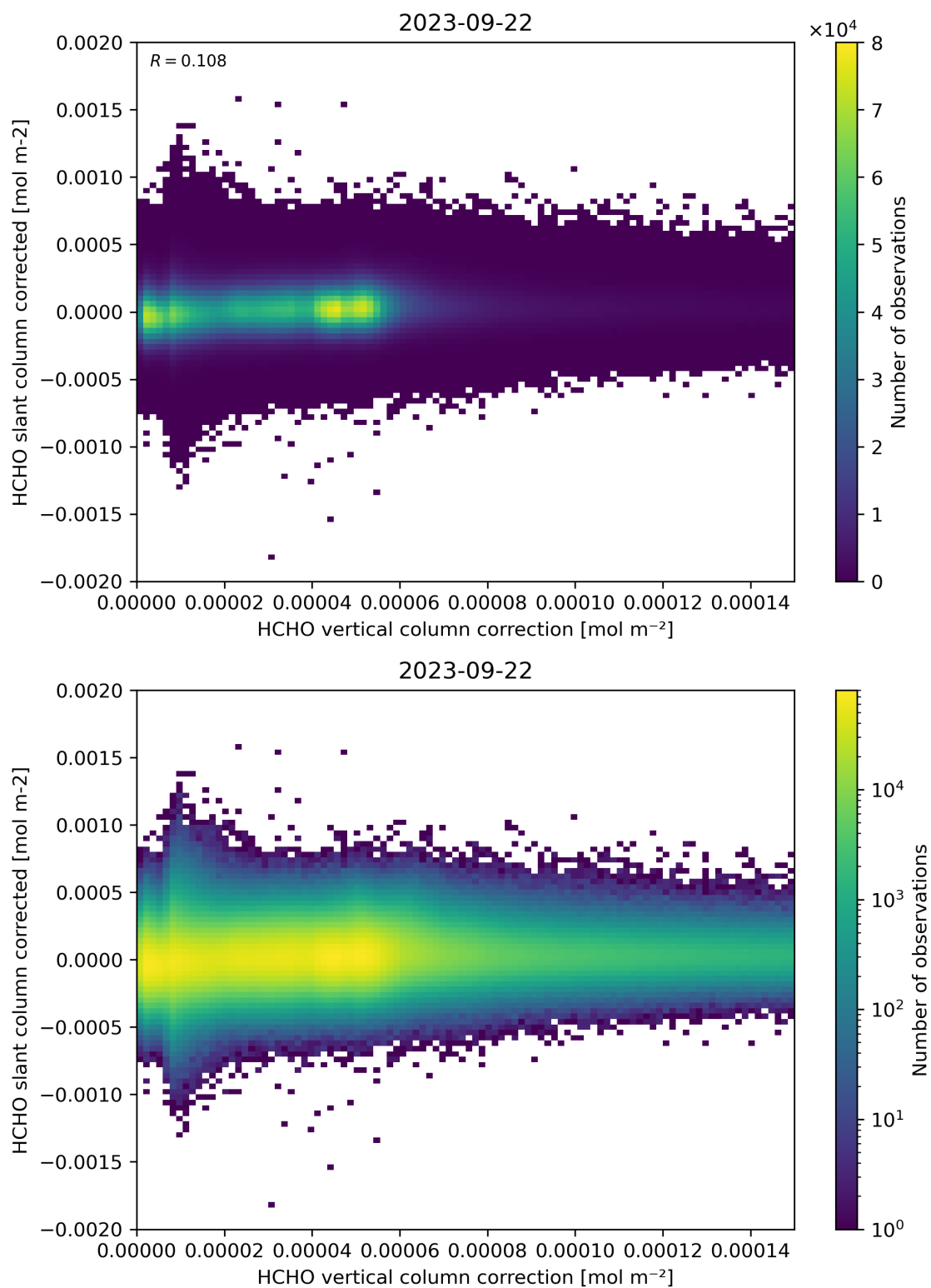
Figure 116: Scatter density plot of “HCHO vertical column correction” against “HCHO slant column corrected” for 2023-09-21 to 2023-09-23.
