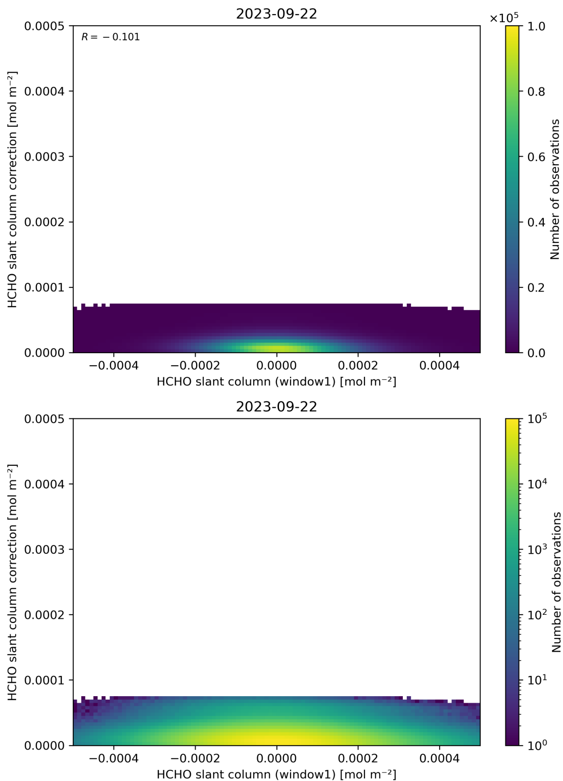
Figure 83: Scatter density plot of “HCHO slant column (window1)” against “HCHO slant column correction” for 2023-09-21 to 2023-09-23.
