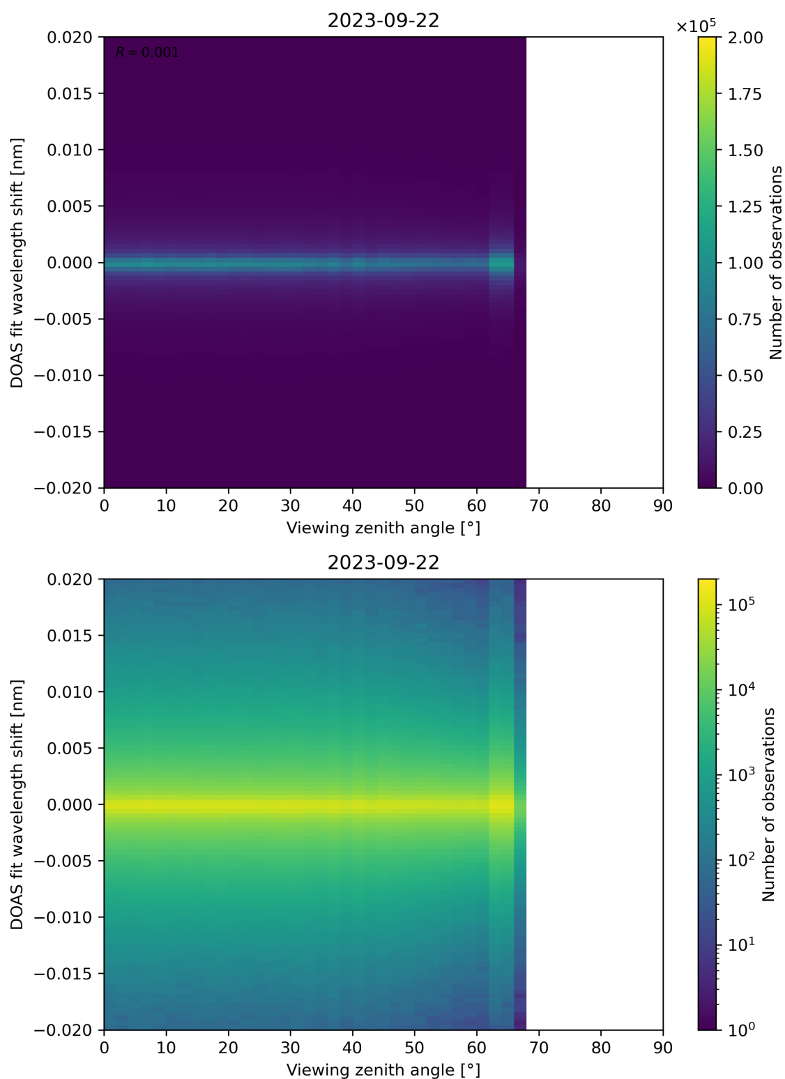
Figure 183: Scatter density plot of “Viewing zenith angle” against “DOAS fit wavelength shift” for 2023-09-21 to 2023-09-23.
