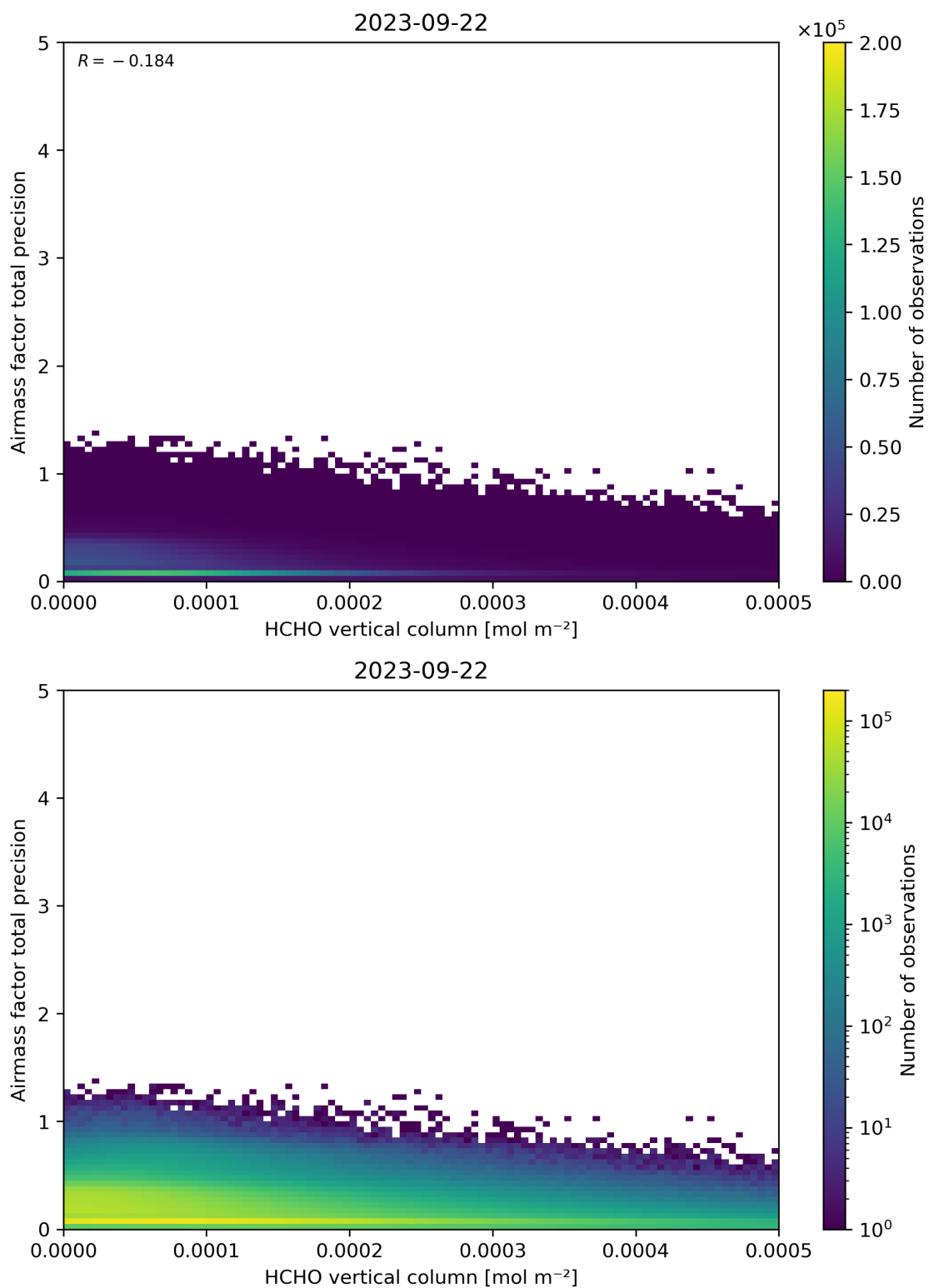
Figure 132: Scatter density plot of “HCHO vertical column” against “Airmass factor total precision” for 2023-09-21 to 2023-09-23.
