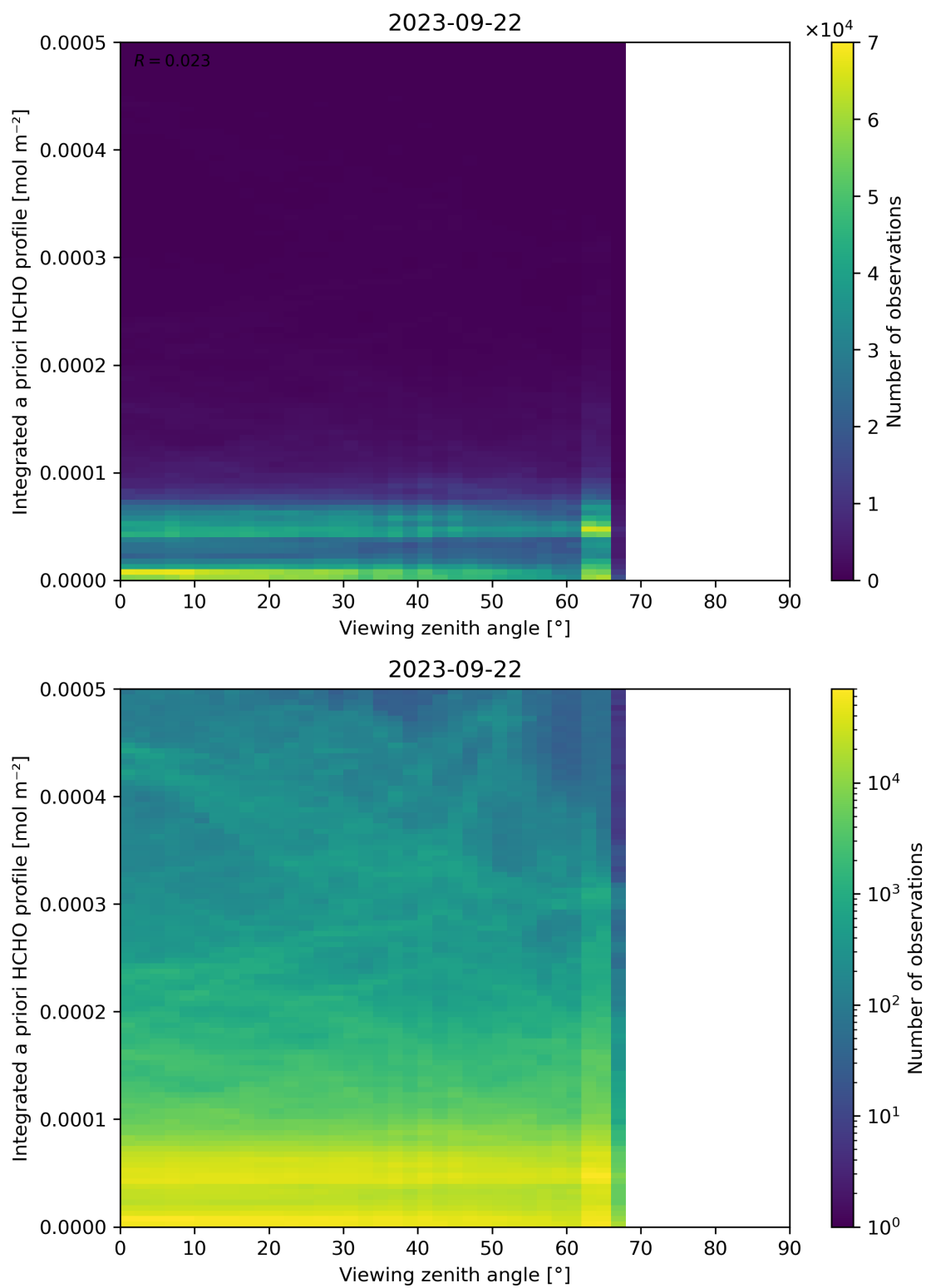
Figure 195: Scatter density plot of “Viewing zenith angle” against “Integrated a priori HCHO profile” for 2023-09-21 to 2023-09-23.
