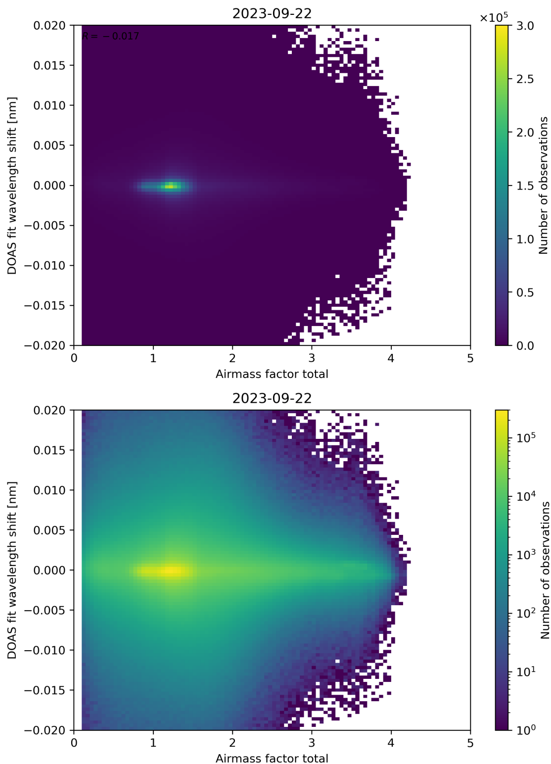
Figure 98: Scatter density plot of “Airmass factor total” against “DOAS fit wavelength shift” for 2023-09-21 to 2023-09-23.
