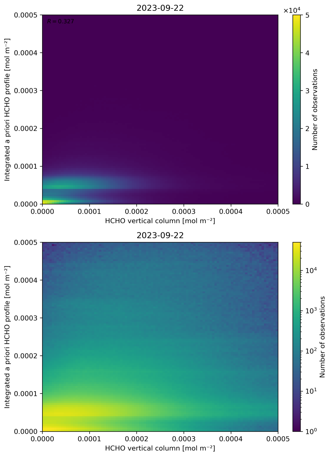
Figure 135: Scatter density plot of “HCHO vertical column” against “Integrated a priori HCHO profile” for 2023-09-21 to 2023-09-23.
