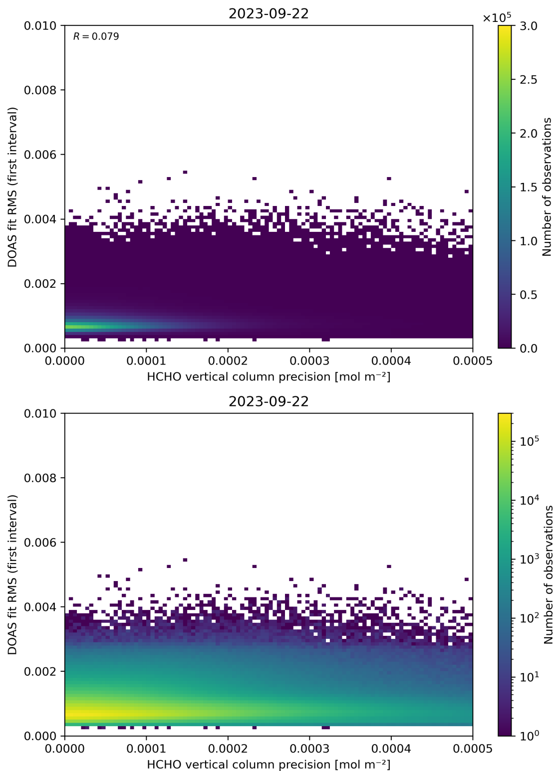
Figure 136: Scatter density plot of “HCHO vertical column precision” against “DOAS fit RMS (first interval)” for 2023-09-21 to 2023-09-23.
