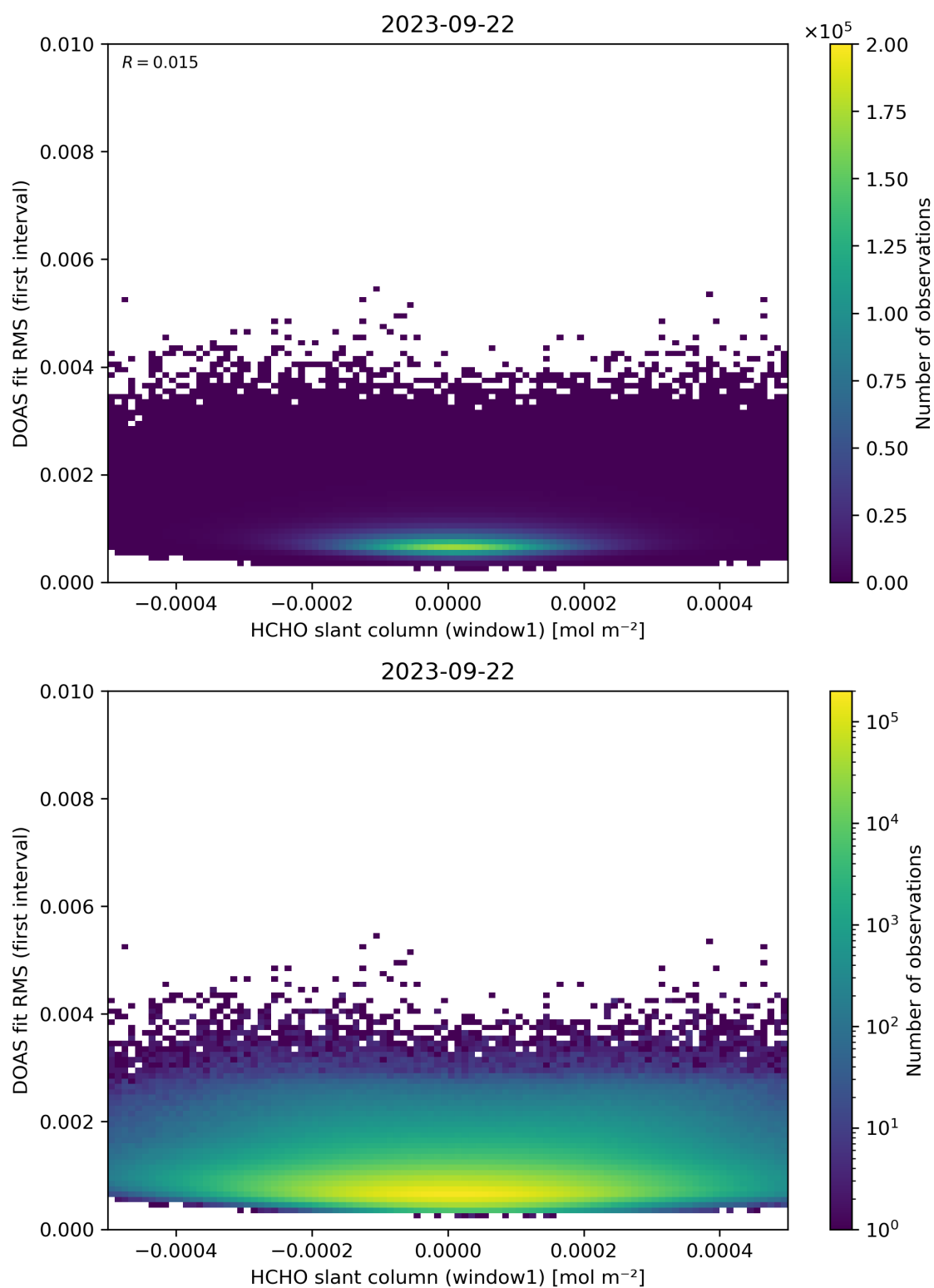
Figure 78: Scatter density plot of “HCHO slant column (window1)” against “DOAS fit RMS (first interval)” for 2023-09-21 to 2023-09-23.
