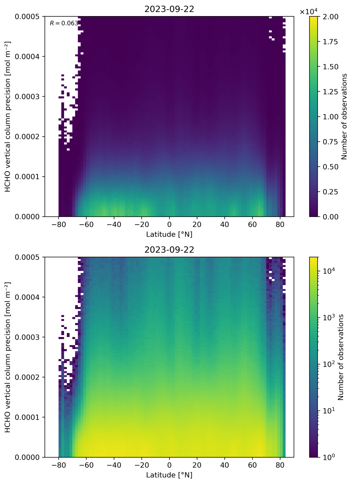
Figure 165: Scatter density plot of “Latitude” against “HCHO vertical column precision” for 2023-09-21 to 2023-09-23.
