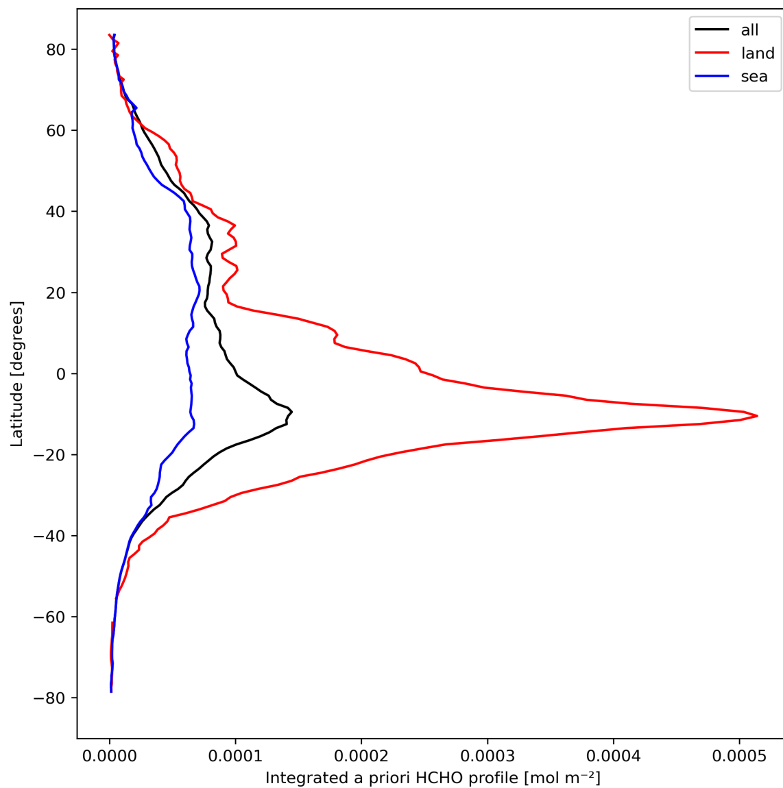
Figure 29: Zonal average of “Integrated a priori HCHO profile” for 2023-09-21 to 2023-09-23.
