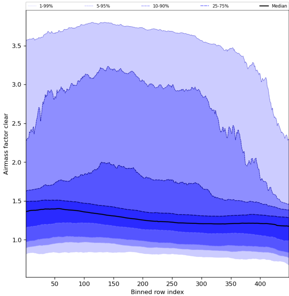
Figure 56: Along track statistics of “Airmass factor clear” for 2023-09-21 to 2023-09-23
