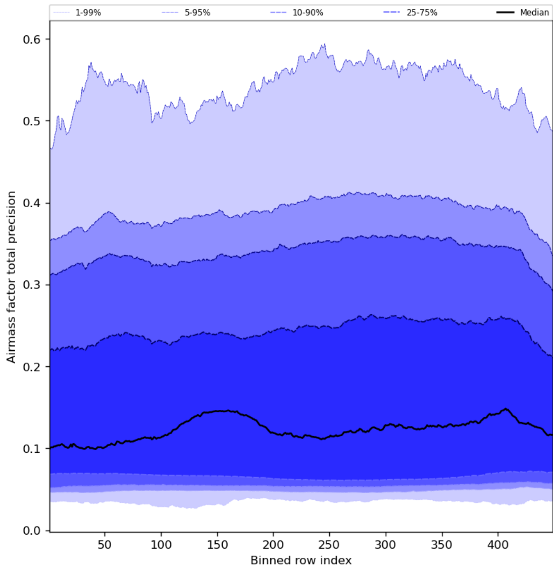
Figure 55: Along track statistics of “Airmass factor total precision” for 2023-09-21 to 2023-09-23
