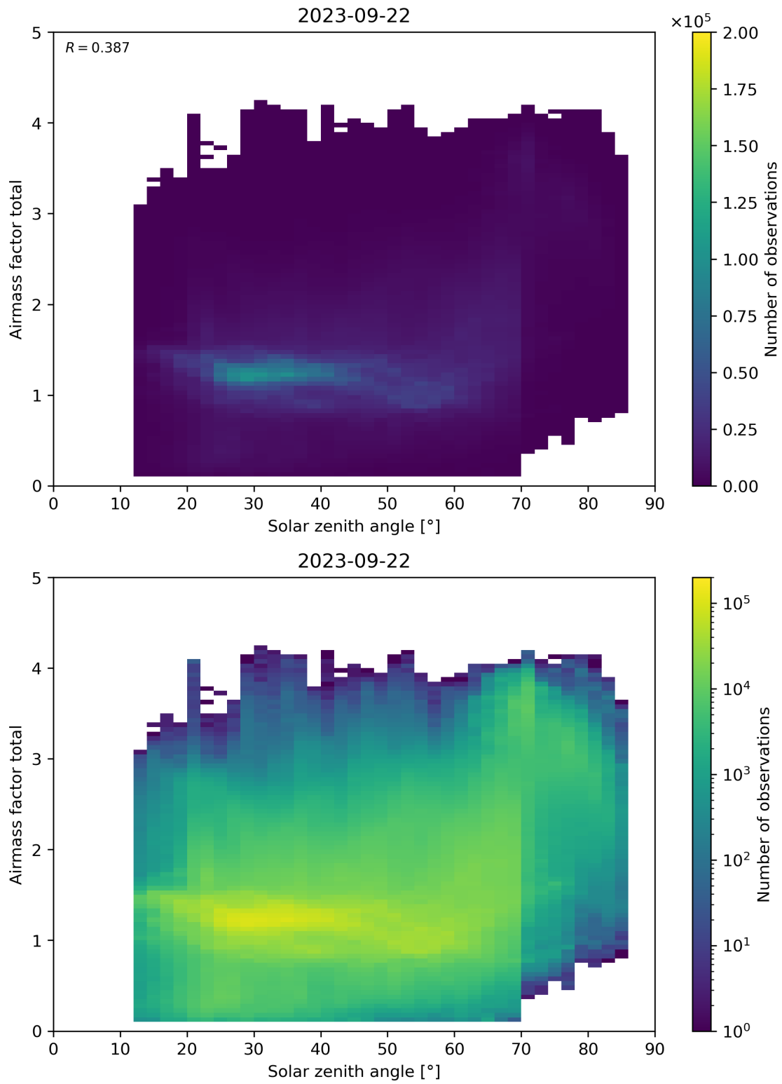
Figure 175: Scatter density plot of “Solar zenith angle” against “Airmass factor total” for 2023-09-21 to 2023-09-23.
