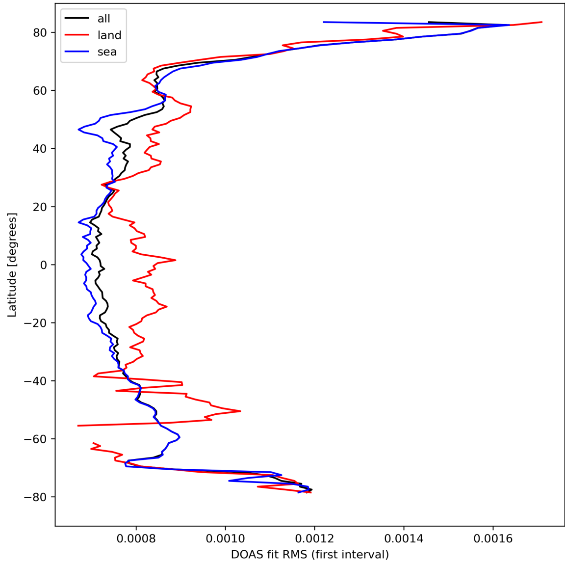
Figure 32: Zonal average of “DOAS fit RMS (first interval)” for 2023-09-21 to 2023-09-23.
