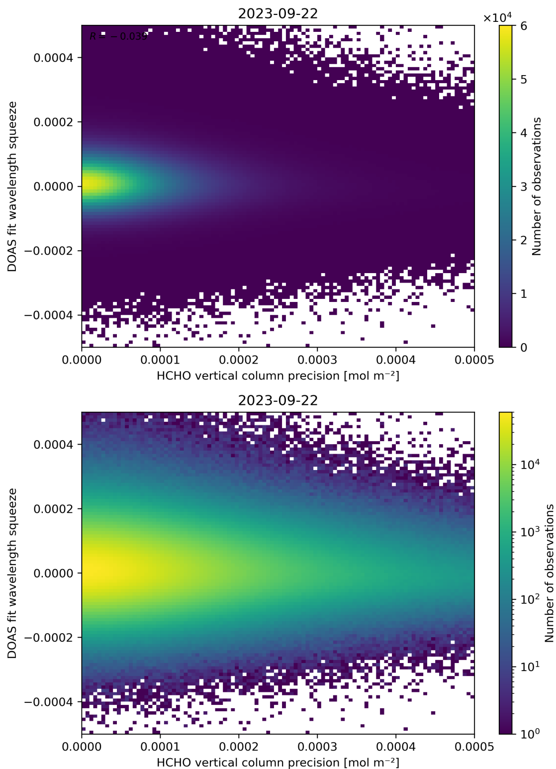
Figure 138: Scatter density plot of “HCHO vertical column precision” against “DOAS fit wavelength squeeze” for 2023-09-21 to 2023-09-23.
