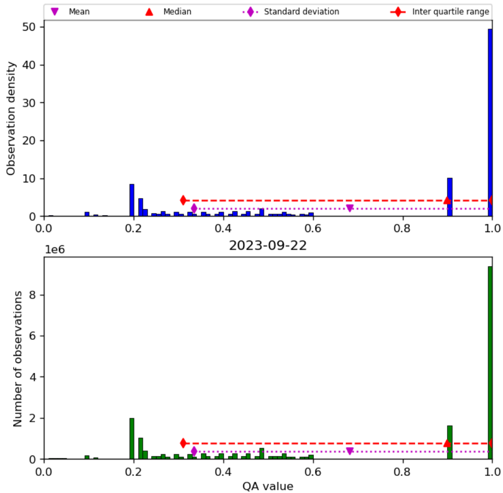
Figure 34: Histogram of “QA value” for 2023-09-21 to 2023-09-23
