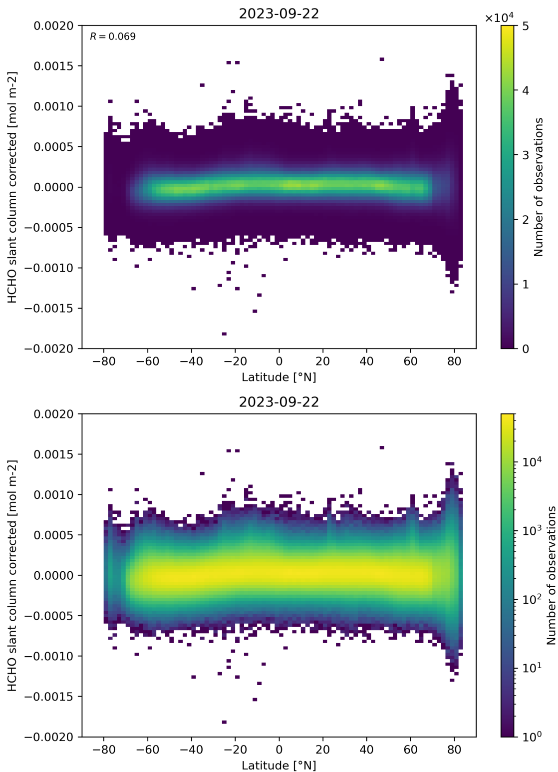
Figure 157: Scatter density plot of “Latitude” against “HCHO slant column corrected” for 2023-09-21 to 2023-09-23.
