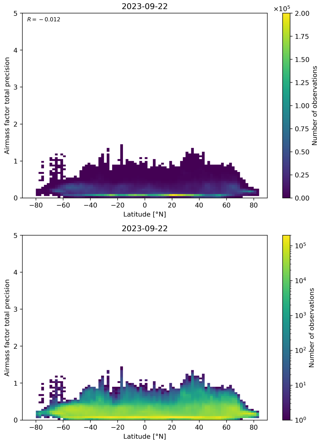
Figure 162: Scatter density plot of “Latitude” against “Airmass factor total precision” for 2023-09-21 to 2023-09-23.
