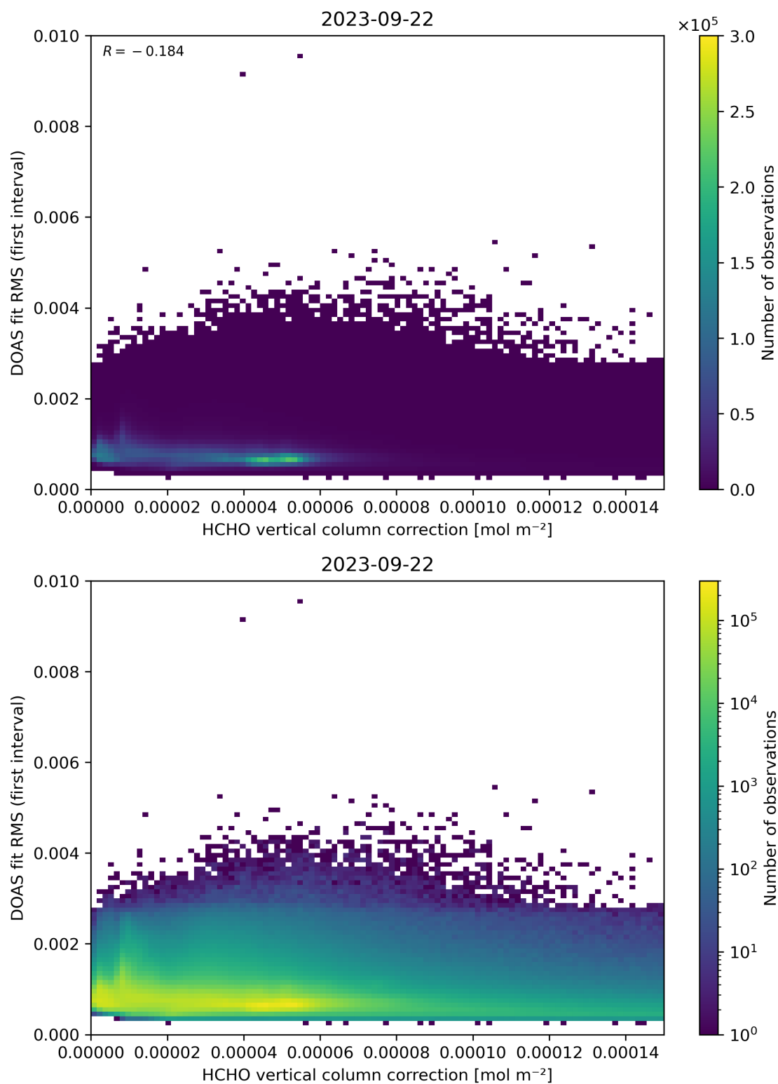
Figure 112: Scatter density plot of “HCHO vertical column correction” against “DOAS fit RMS (first interval)” for 2023-09-21 to 2023-09-23.
