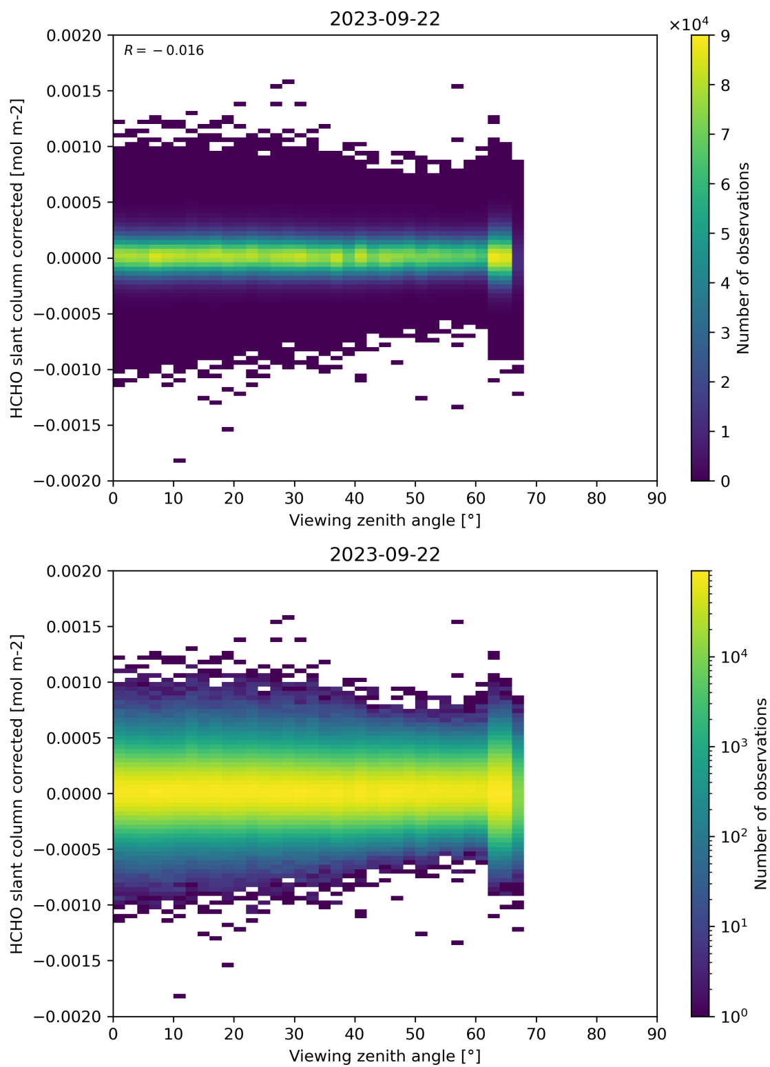
Figure 186: Scatter density plot of “Viewing zenith angle” against “HCHO slant column corrected” for 2023-09-21 to 2023-09-23.
