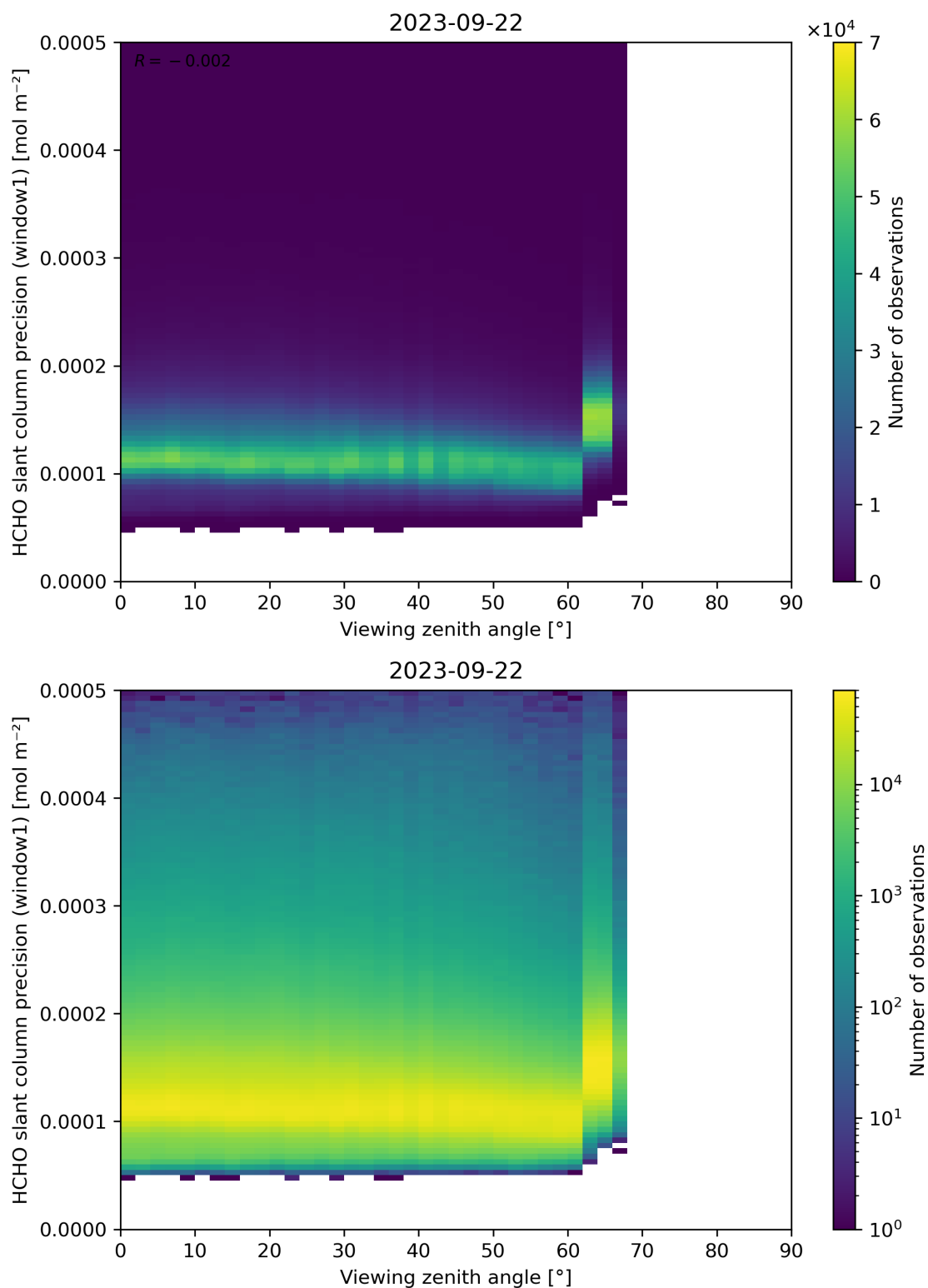
Figure 189: Scatter density plot of “Viewing zenith angle” against “HCHO slant column precision (window1)” for 2023-09-21 to 2023-09-23.
