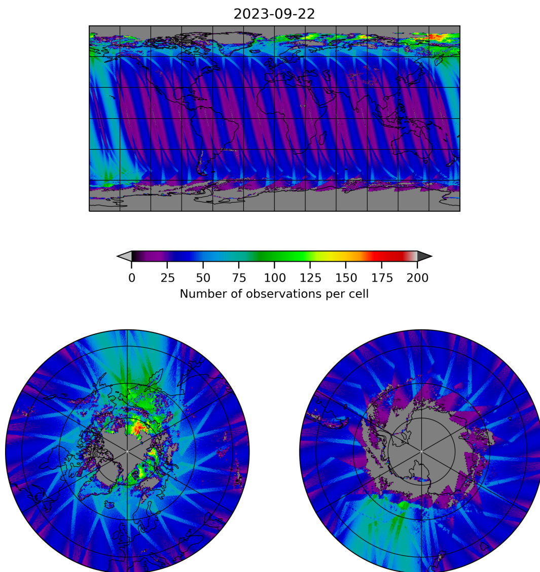
Figure 19: Map of the number of observations for 2023-09-21 to 2023-09-23
