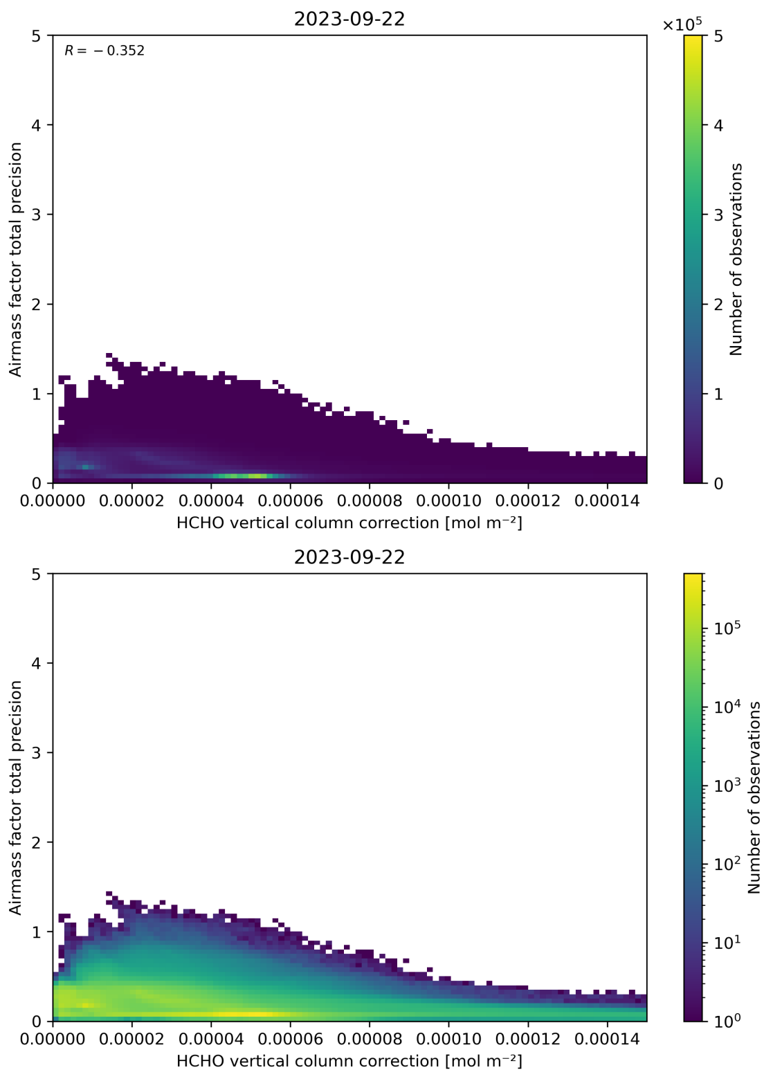
Figure 121: Scatter density plot of “HCHO vertical column correction” against “Airmass factor total precision” for 2023-09-21 to 2023-09-23.
