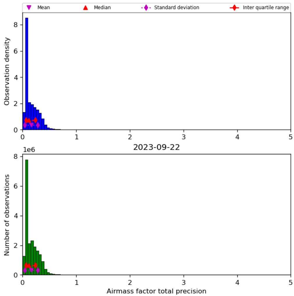
Figure 41: Histogram of “Airmass factor total precision” for 2023-09-21 to 2023-09-23
