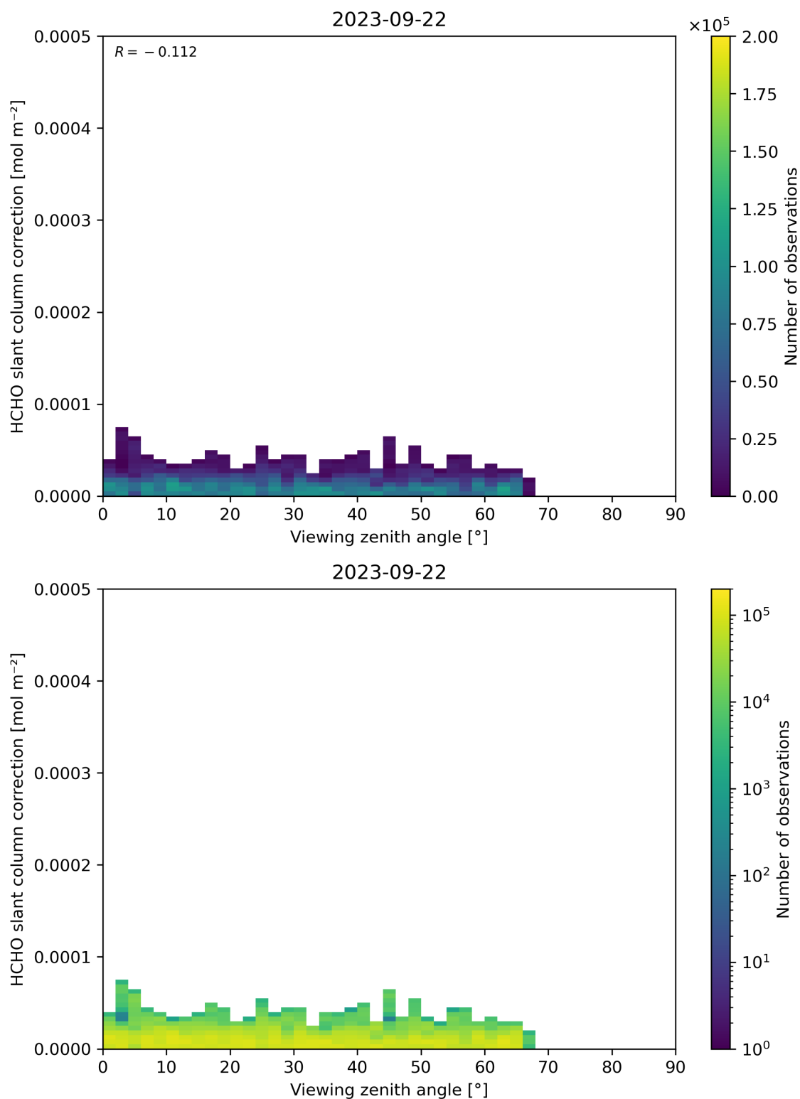
Figure 187: Scatter density plot of “Viewing zenith angle” against “HCHO slant column correction” for 2023-09-21 to 2023-09-23.
