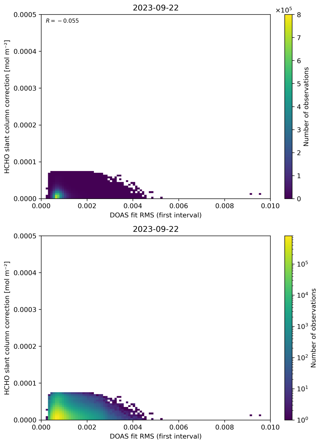
Figure 63: Scatter density plot of “DOAS fit RMS (first interval)” against “HCHO slant column correction” for 2023-09-21 to 2023-09-23.
