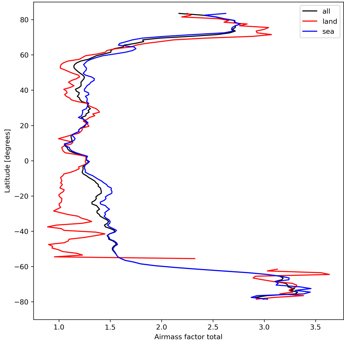
Figure 26: Zonal average of “Airmass factor total” for 2023-09-21 to 2023-09-23.
