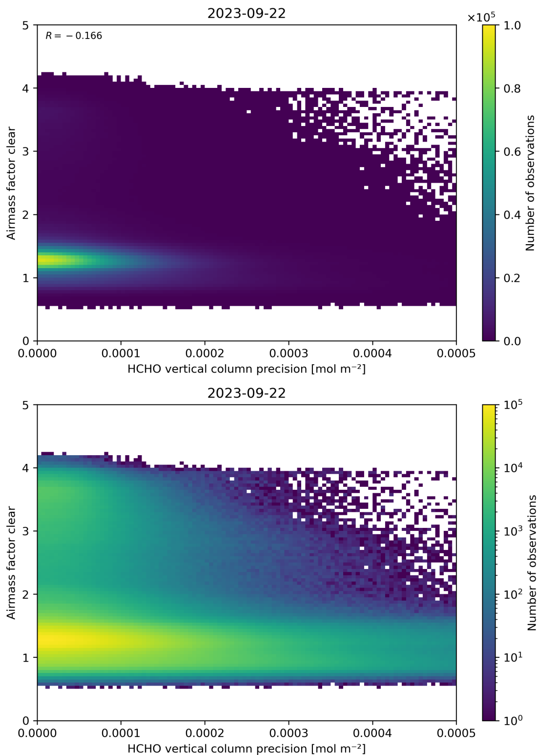
Figure 139: Scatter density plot of “HCHO vertical column precision” against “Airmass factor clear” for 2023-09-21 to 2023-09-23.
