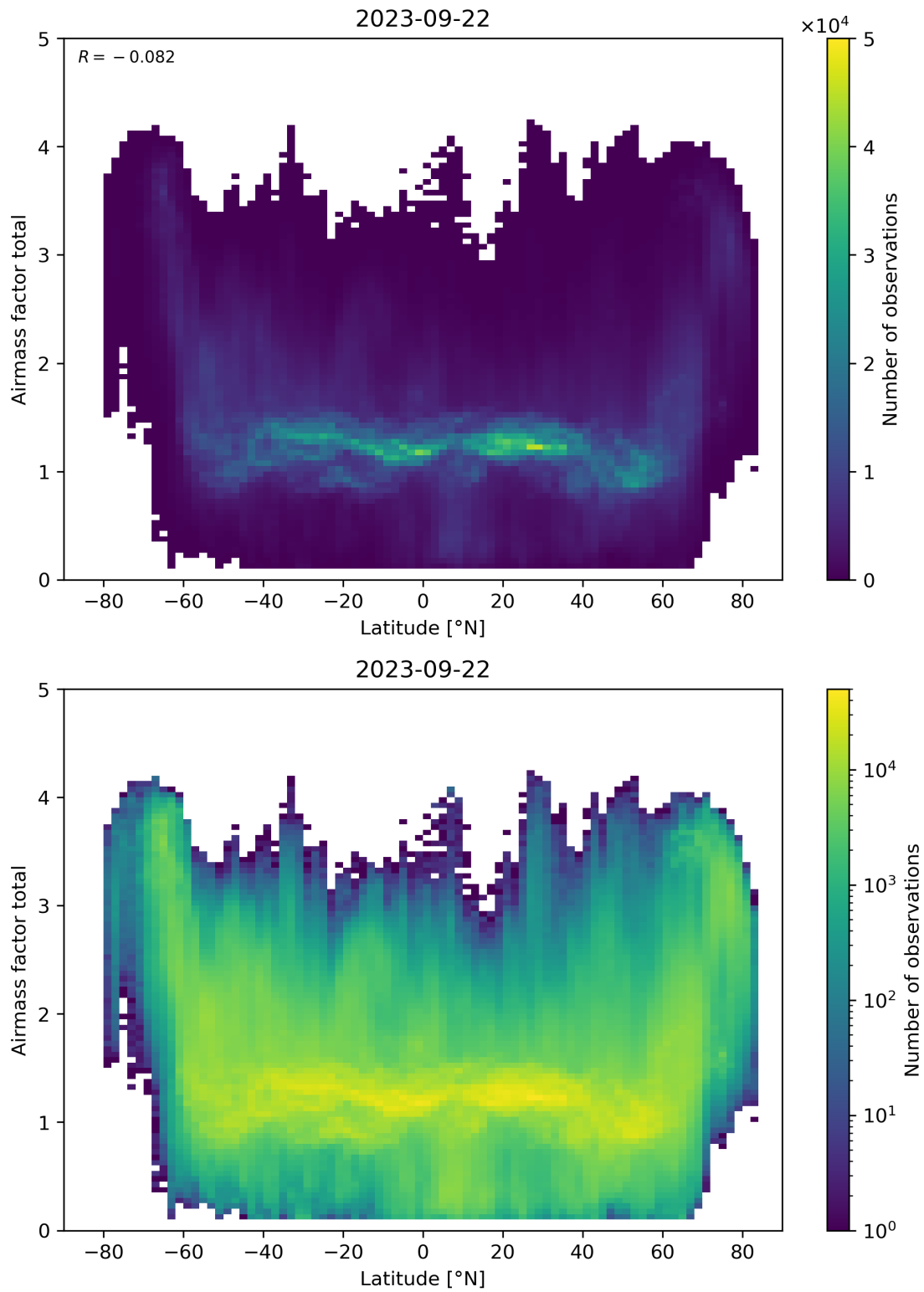
Figure 161: Scatter density plot of “Latitude” against “Airmass factor total” for 2023-09-21 to 2023-09-23.
