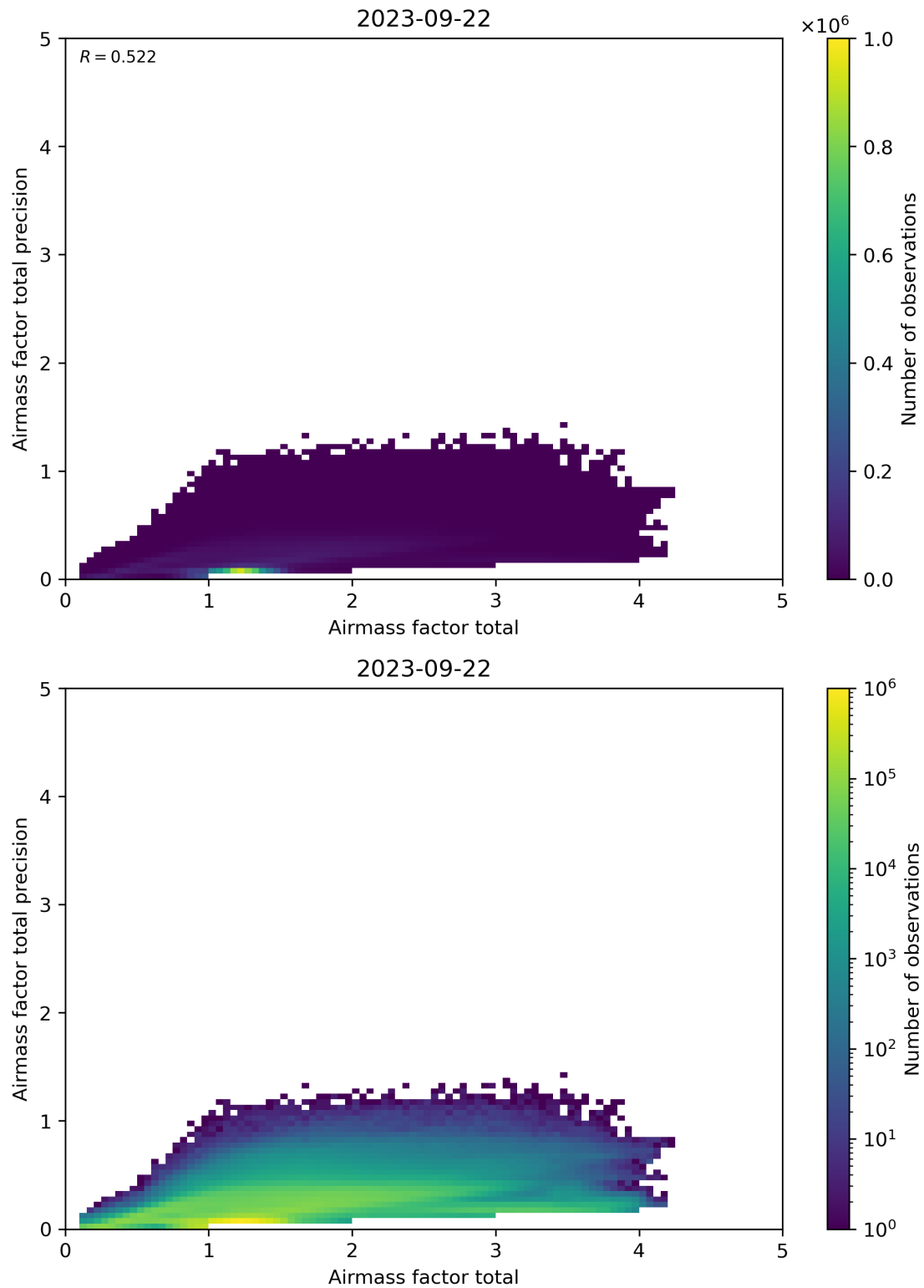
Figure 103: Scatter density plot of “Airmass factor total” against “Airmass factor total precision” for 2023-09-21 to 2023-09-23.
