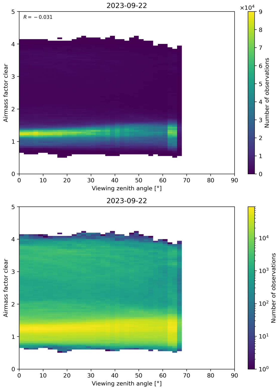
Figure 185: Scatter density plot of “Viewing zenith angle” against “Airmass factor clear” for 2023-09-21 to 2023-09-23.
