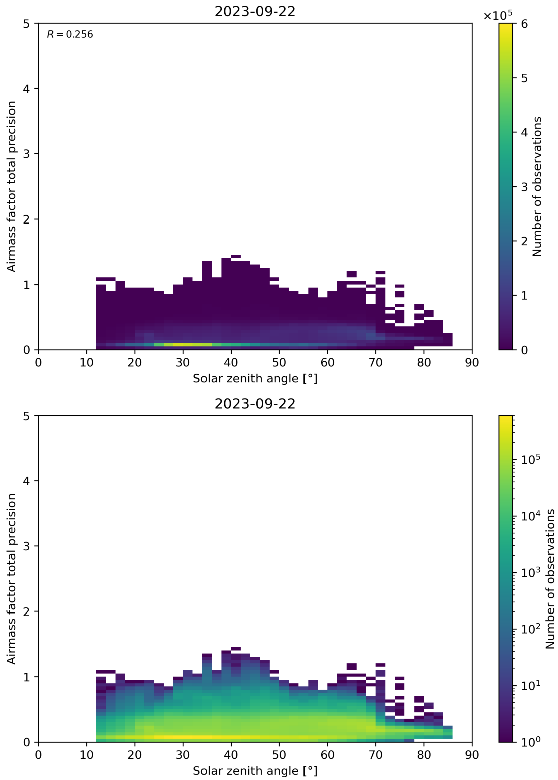
Figure 176: Scatter density plot of “Solar zenith angle” against “Airmass factor total precision” for 2023-09-21 to 2023-09-23.
