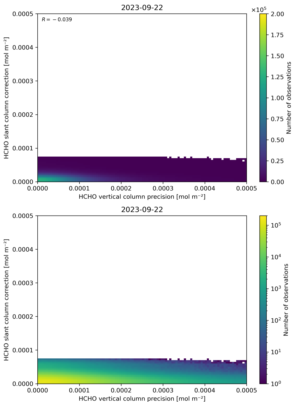
Figure 141: Scatter density plot of “HCHO vertical column precision” against “HCHO slant column correction” for 2023-09-21 to 2023-09-23.
