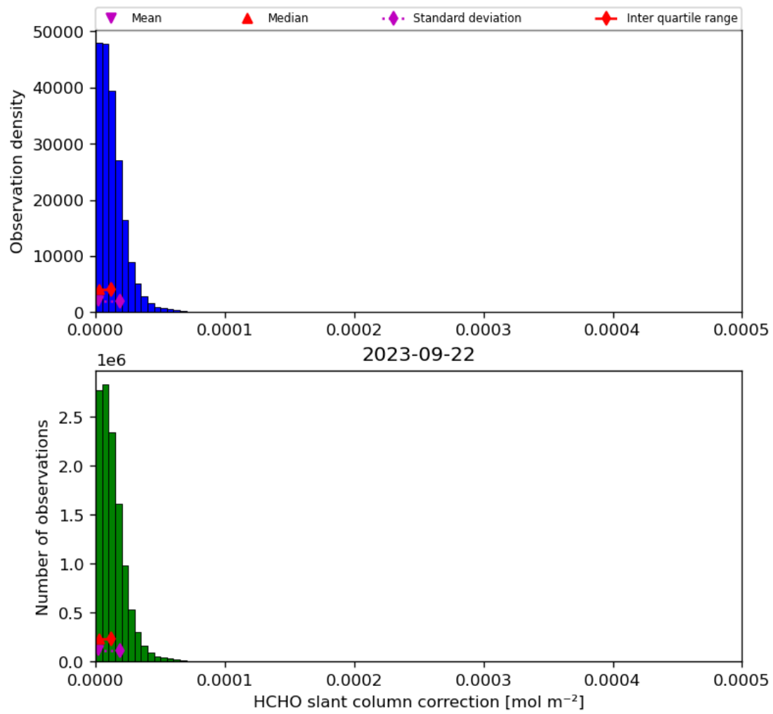
Figure 47: Histogram of “HCHO slant column correction” for 2023-09-21 to 2023-09-23
