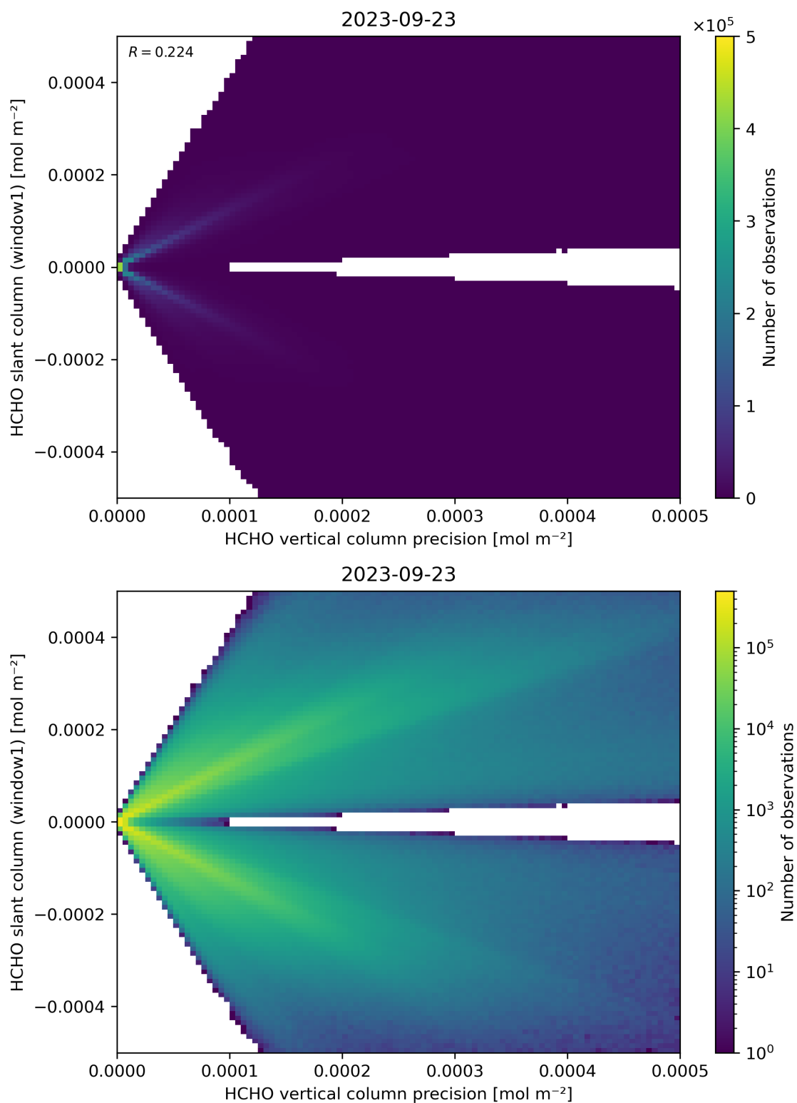
Figure 142: Scatter density plot of “HCHO vertical column precision” against “HCHO slant column (window1)” for 2023-09-22 to 2023-09-24.
