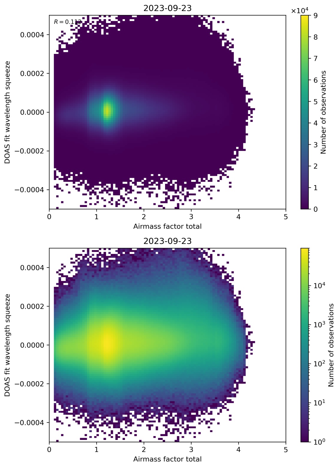
Figure 99: Scatter density plot of “Airmass factor total” against “DOAS fit wavelength squeeze” for 2023-09-22 to 2023-09-24.
