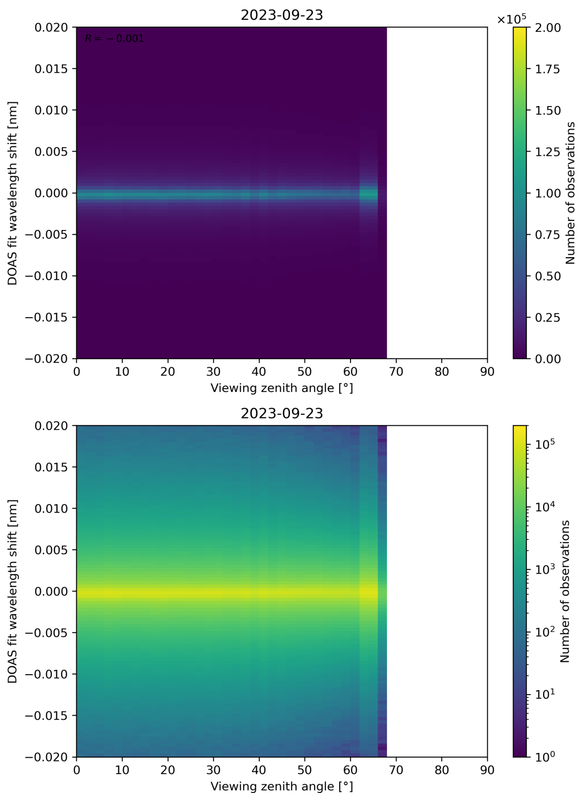
Figure 183: Scatter density plot of “Viewing zenith angle” against “DOAS fit wavelength shift” for 2023-09-22 to 2023-09-24.
