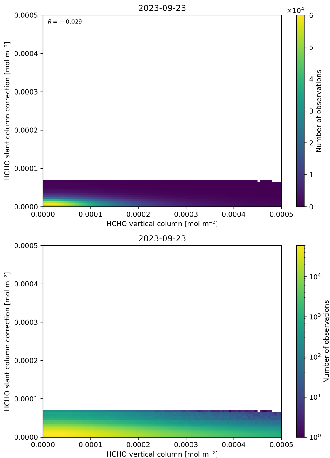
Figure 128: Scatter density plot of “HCHO vertical column” against “HCHO slant column correction” for 2023-09-22 to 2023-09-24.
