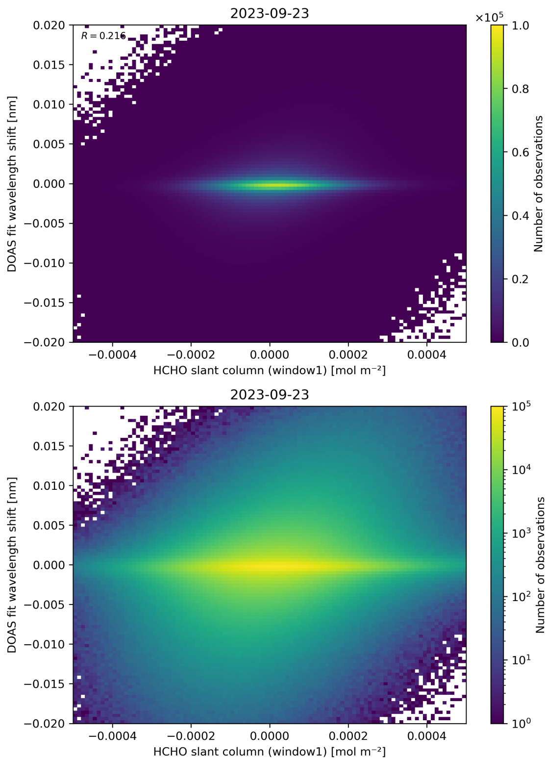
Figure 79: Scatter density plot of “HCHO slant column (window1)” against “DOAS fit wavelength shift” for 2023-09-22 to 2023-09-24.
