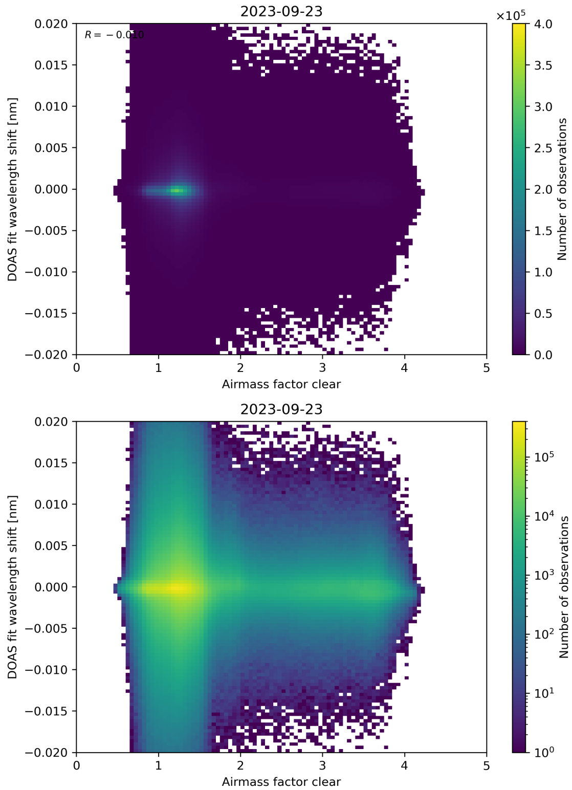
Figure 72: Scatter density plot of “Airmass factor clear” against “DOAS fit wavelength shift” for 2023-09-22 to 2023-09-24.
