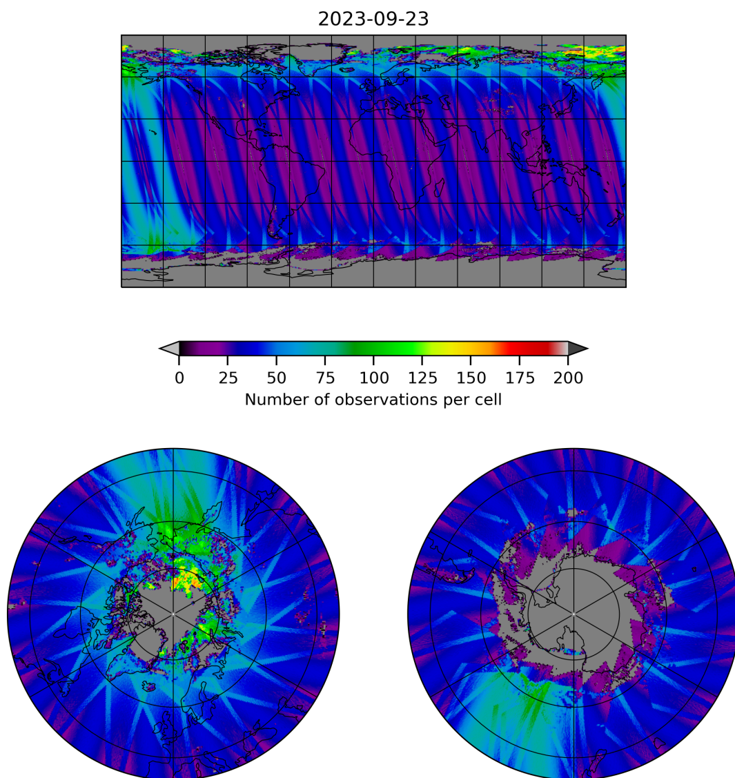
Figure 19: Map of the number of observations for 2023-09-22 to 2023-09-24
