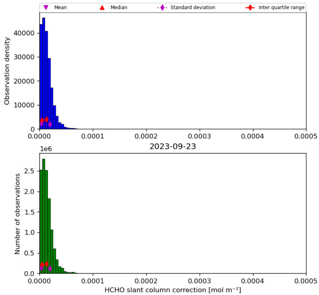
Figure 47: Histogram of “HCHO slant column correction” for 2023-09-22 to 2023-09-24
