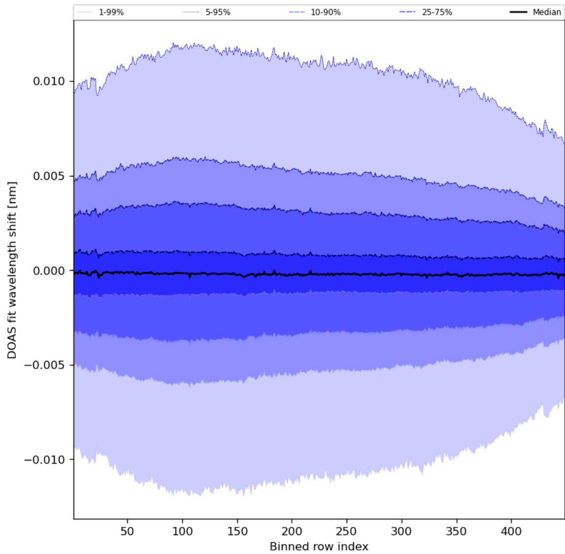
Figure 58: Along track statistics of “DOAS fit wavelength shift” for 2023-09-22 to 2023-09-24
