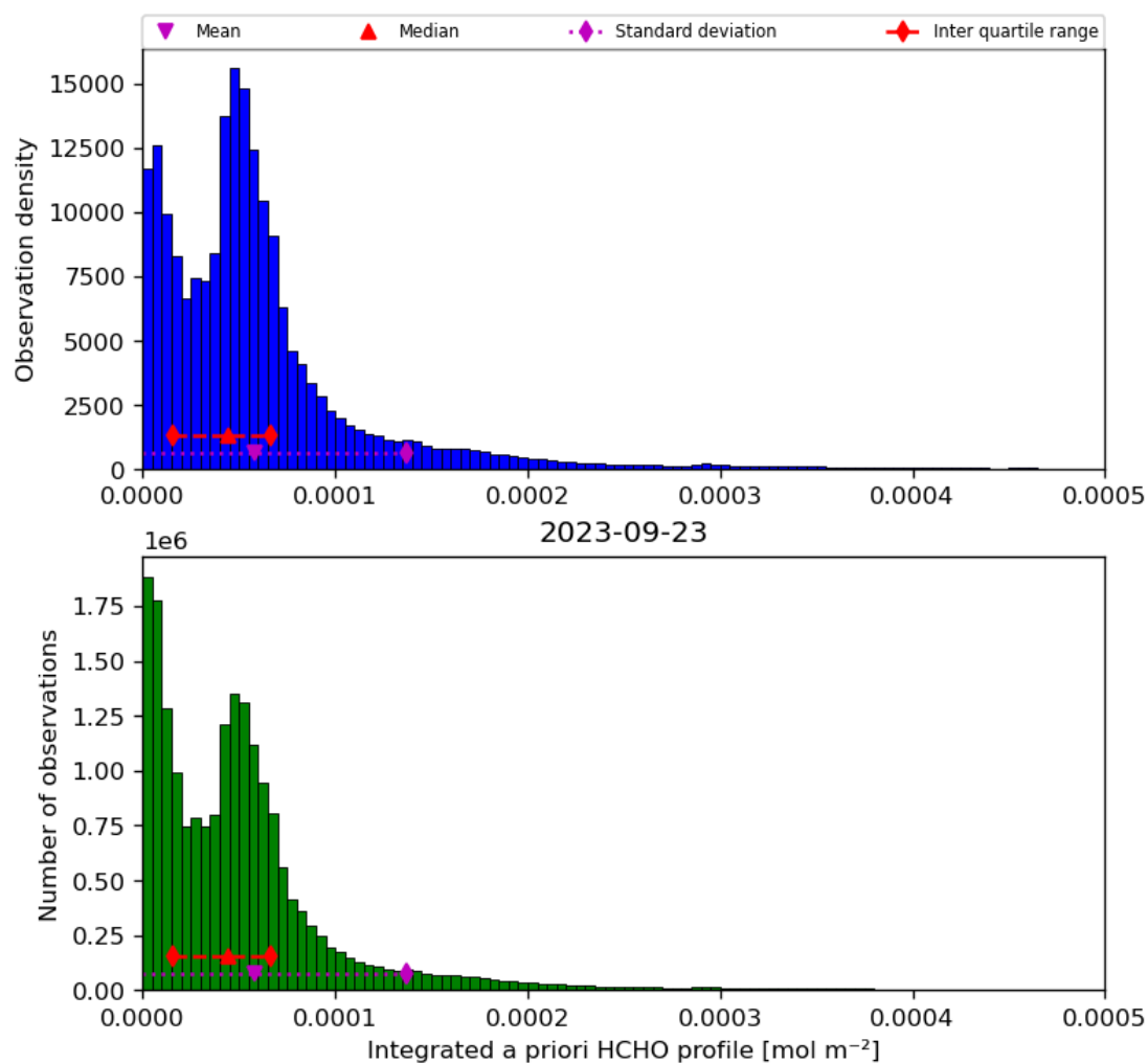
Figure 43: Histogram of “Integrated a priori HCHO profile” for 2023-09-22 to 2023-09-24
