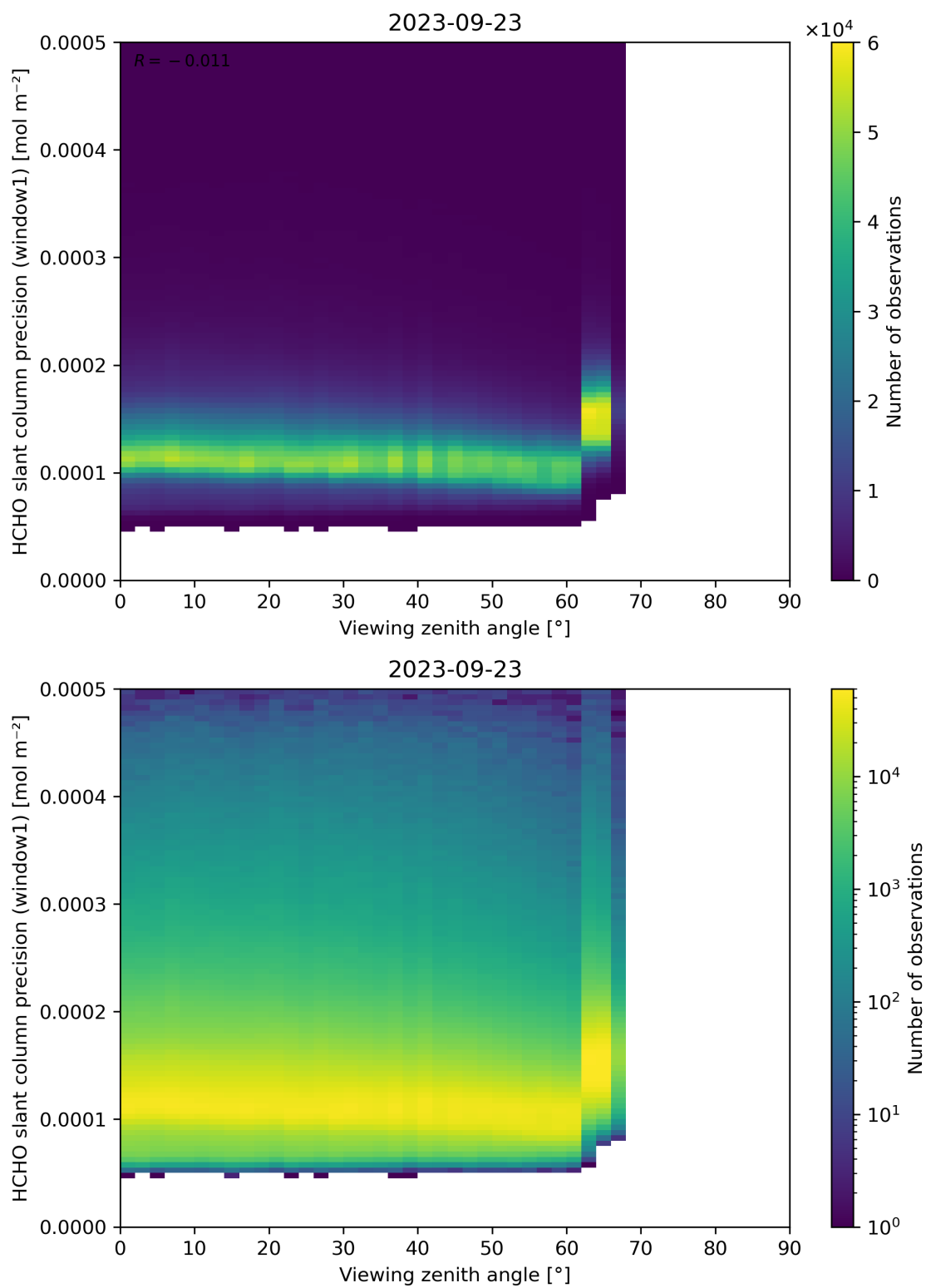
Figure 189: Scatter density plot of “Viewing zenith angle” against “HCHO slant column precision (window1)” for 2023-09-22 to 2023-09-24.
