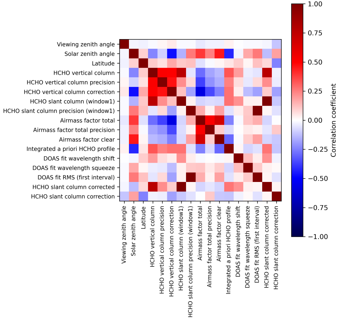
Figure 2: Map of correlation matrix for 2023-09-22 to 2023-09-24.
