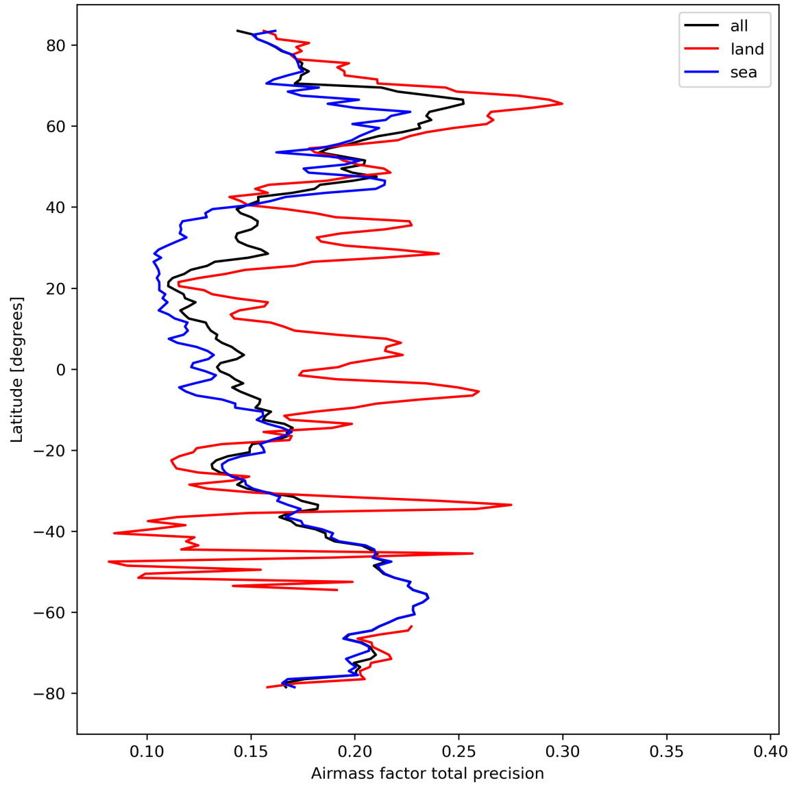
Figure 27: Zonal average of “Airmass factor total precision” for 2023-09-22 to 2023-09-24.
