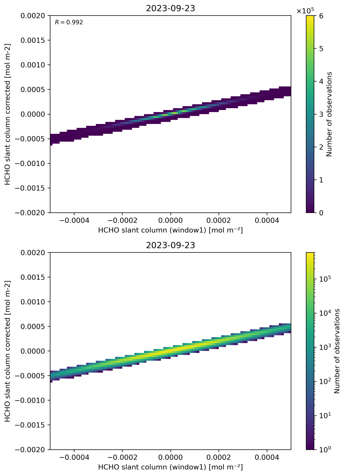
Figure 82: Scatter density plot of “HCHO slant column (window1)” against “HCHO slant column corrected” for 2023-09-22 to 2023-09-24.
