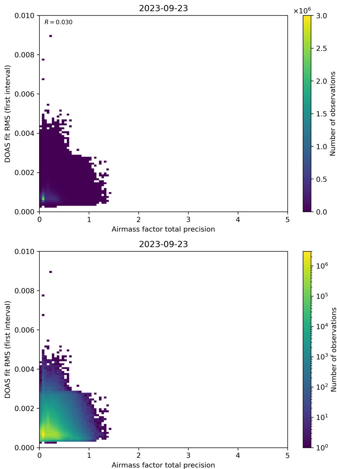
Figure 105: Scatter density plot of “Airmass factor total precision” against “DOAS fit RMS (first interval)” for 2023-09-22 to 2023-09-24.
