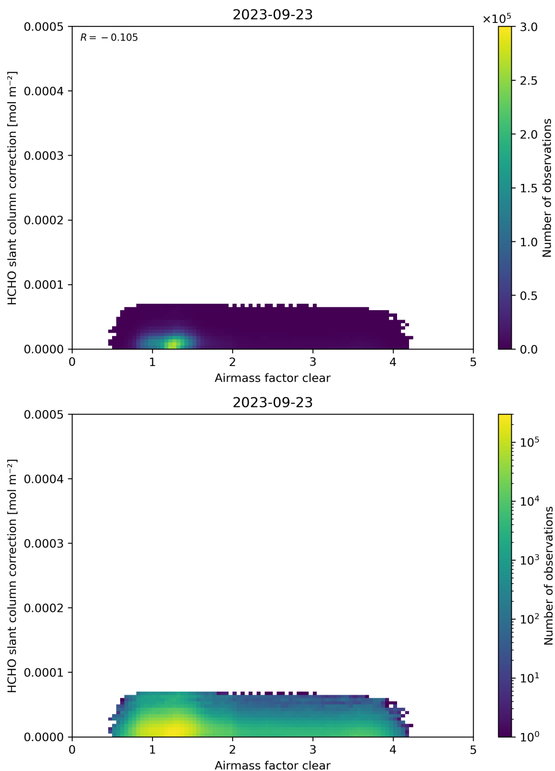
Figure 75: Scatter density plot of “Airmass factor clear” against “HCHO slant column correction” for 2023-09-22 to 2023-09-24.
