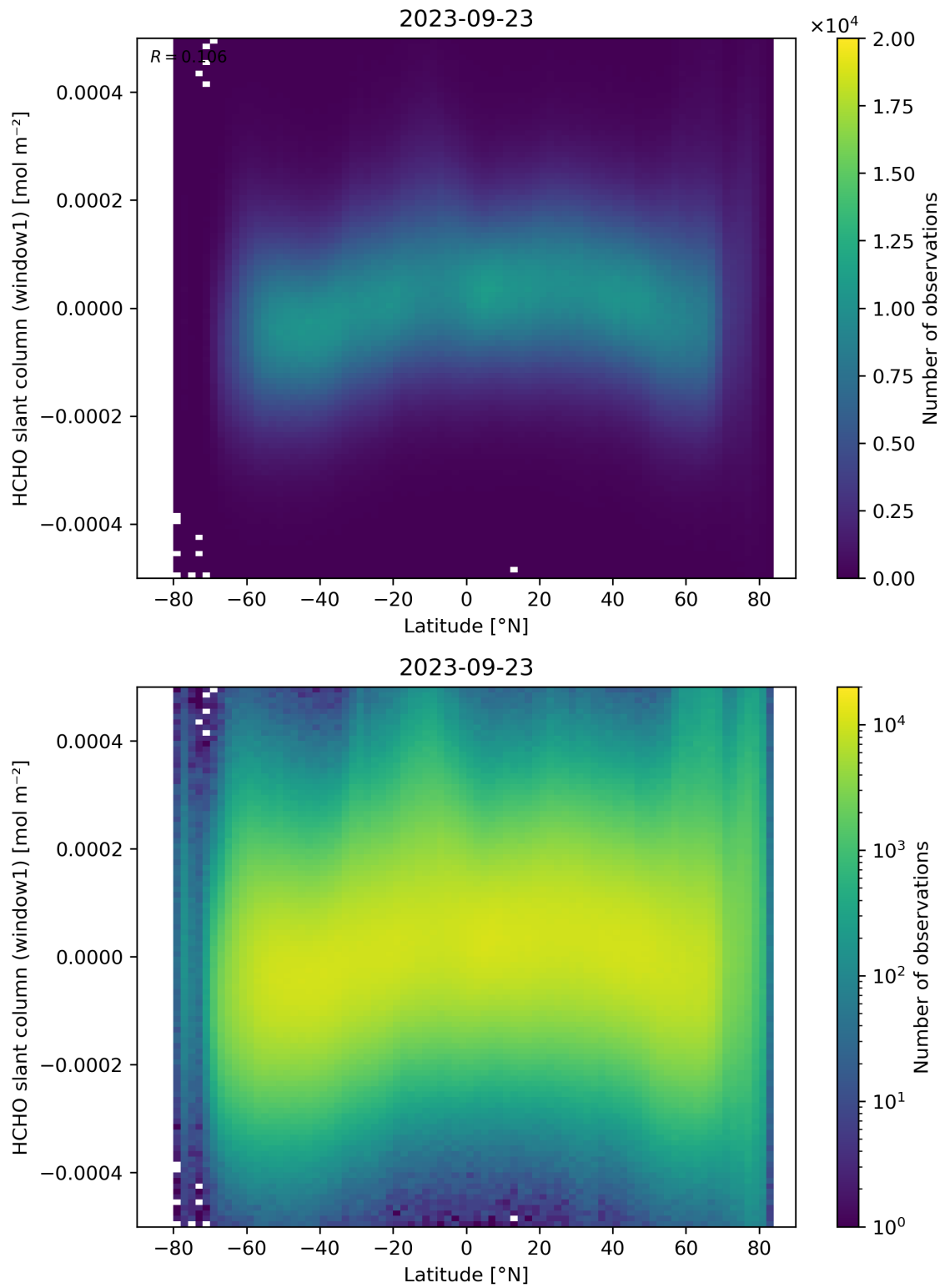
Figure 159: Scatter density plot of “Latitude” against “HCHO slant column (window1)” for 2023-09-22 to 2023-09-24.
