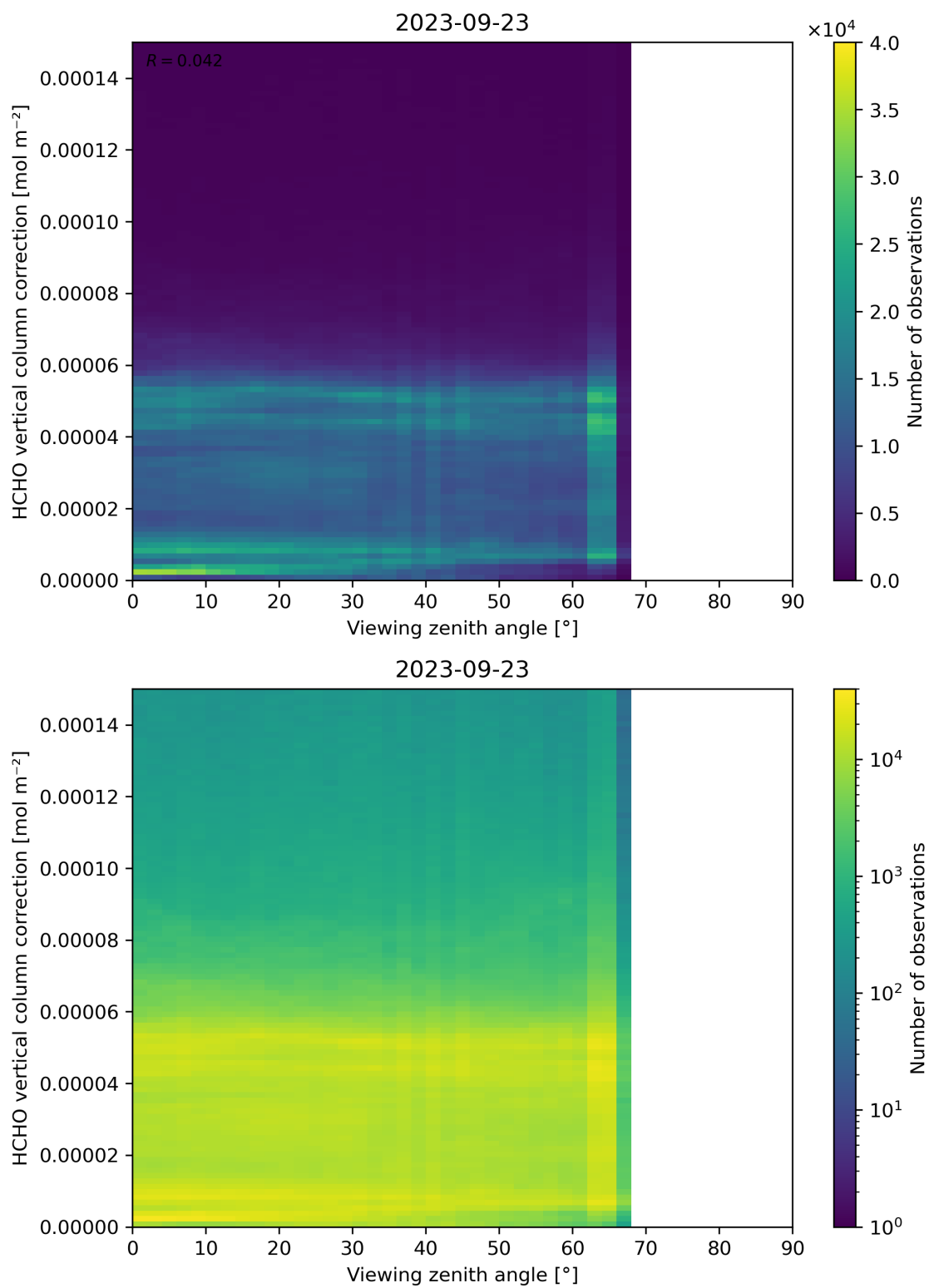
Figure 193: Scatter density plot of “Viewing zenith angle” against “HCHO vertical column correction” for 2023-09-22 to 2023-09-24.
