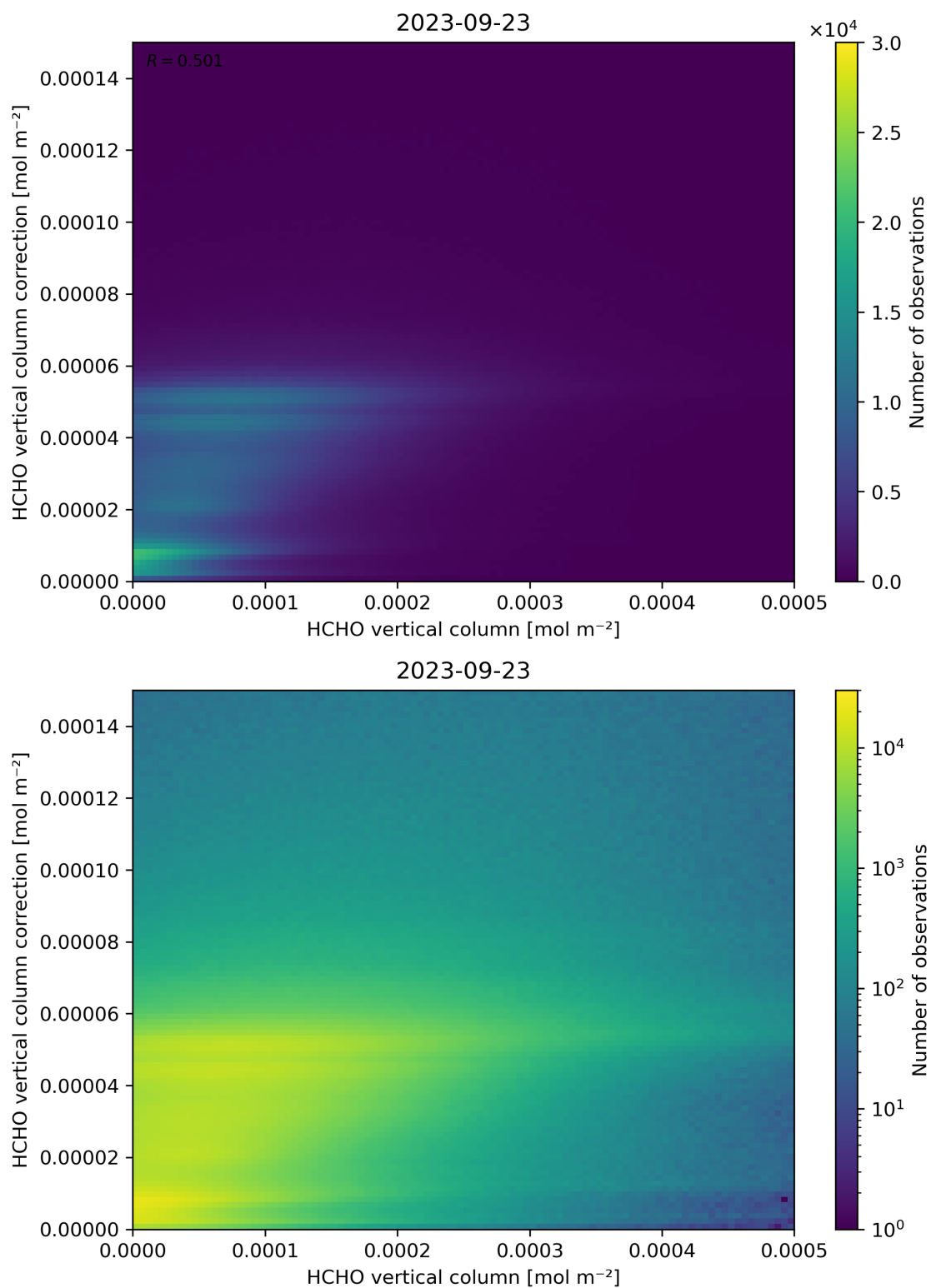
Figure 133: Scatter density plot of “HCHO vertical column” against “HCHO vertical column correction” for 2023-09-22 to 2023-09-24.
