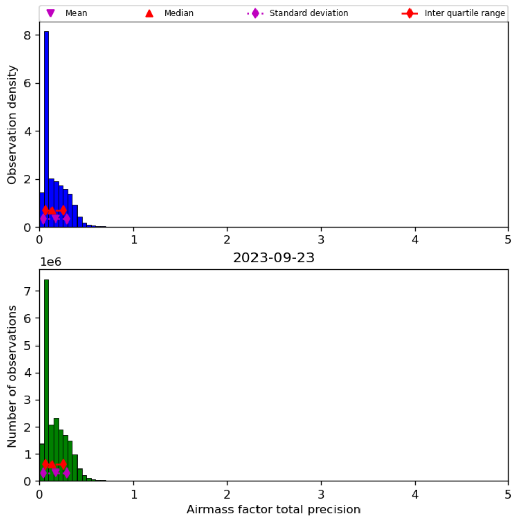
Figure 41: Histogram of “Airmass factor total precision” for 2023-09-22 to 2023-09-24
