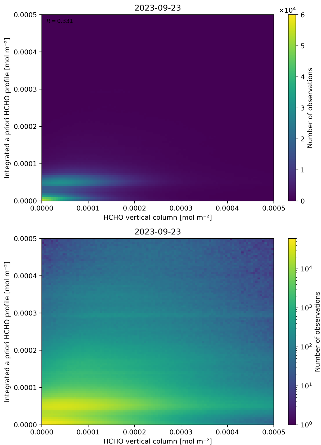
Figure 135: Scatter density plot of “HCHO vertical column” against “Integrated a priori HCHO profile” for 2023-09-22 to 2023-09-24.
