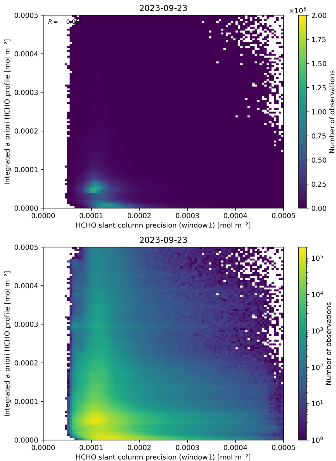
Figure 96: Scatter density plot of “HCHO slant column precision (window1)” against “Integrated a priori HCHO profile” for 2023-09-22 to 2023-09-24.
