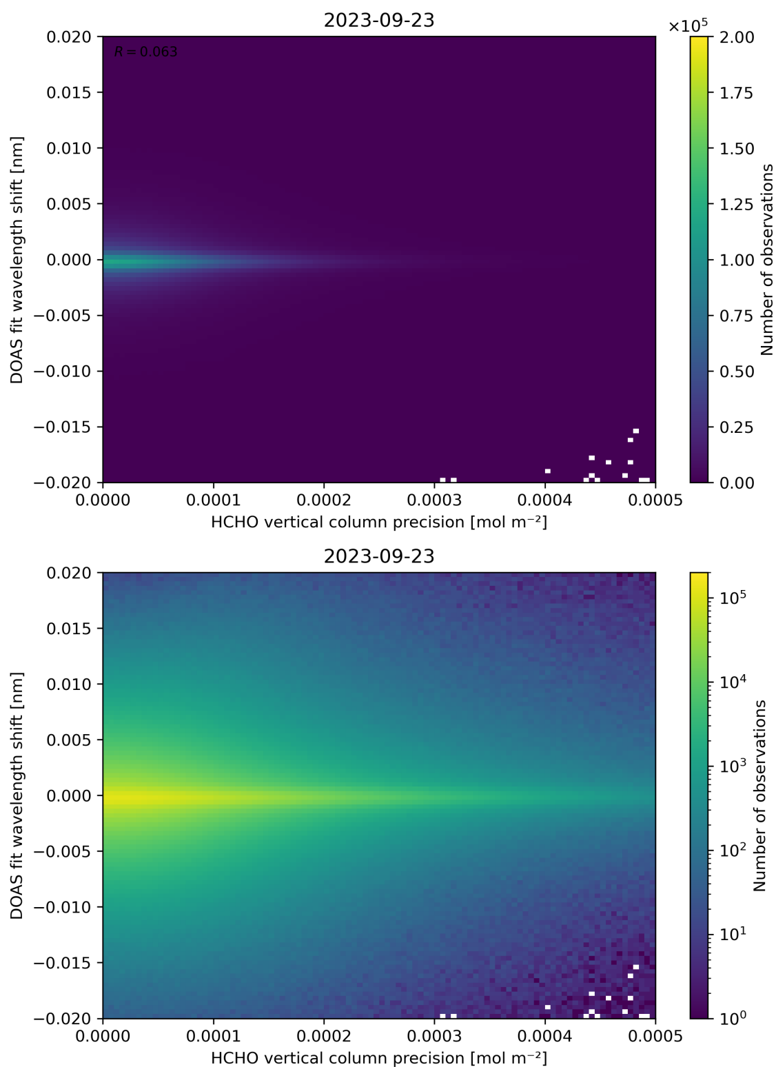
Figure 137: Scatter density plot of “HCHO vertical column precision” against “DOAS fit wavelength shift” for 2023-09-22 to 2023-09-24.
