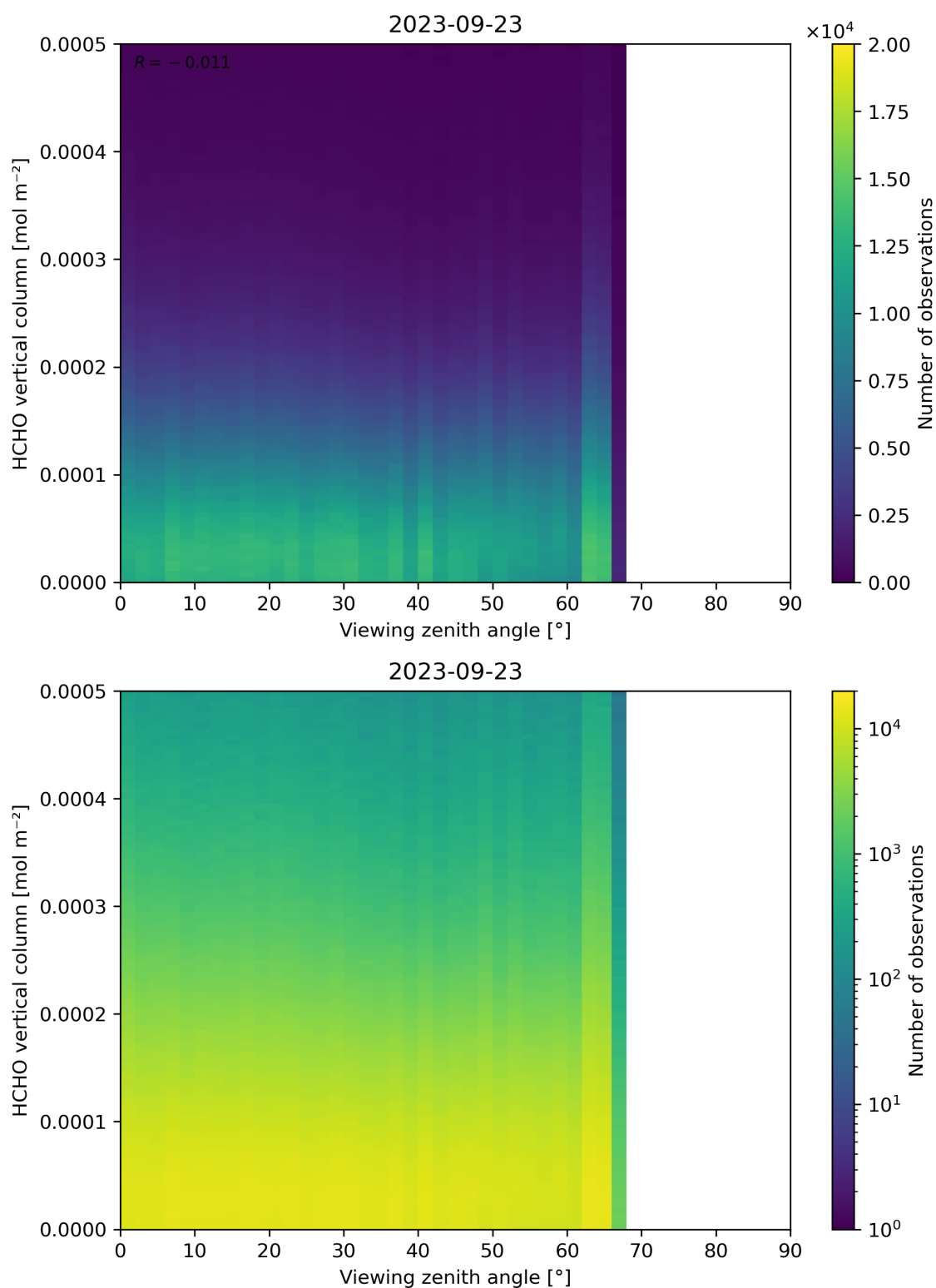
Figure 192: Scatter density plot of “Viewing zenith angle” against “HCHO vertical column” for 2023-09-22 to 2023-09-24.
