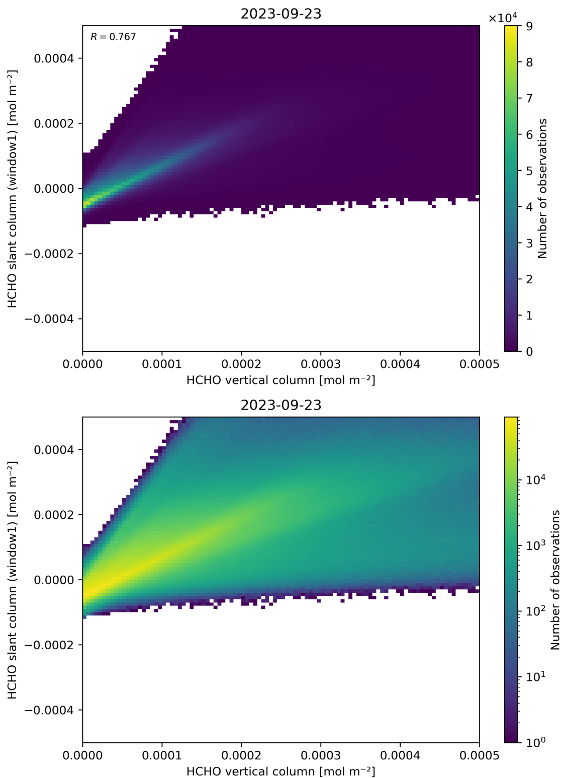
Figure 129: Scatter density plot of “HCHO vertical column” against “HCHO slant column (window1)” for 2023-09-22 to 2023-09-24.
