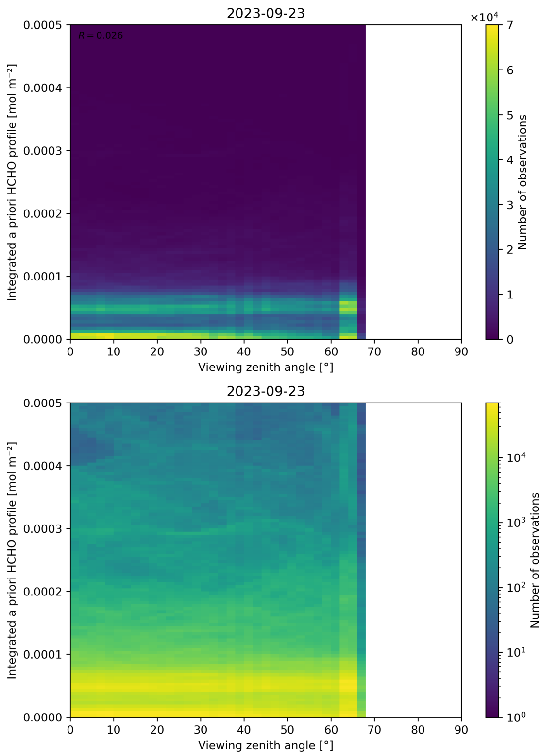
Figure 195: Scatter density plot of “Viewing zenith angle” against “Integrated a priori HCHO profile” for 2023-09-22 to 2023-09-24.
