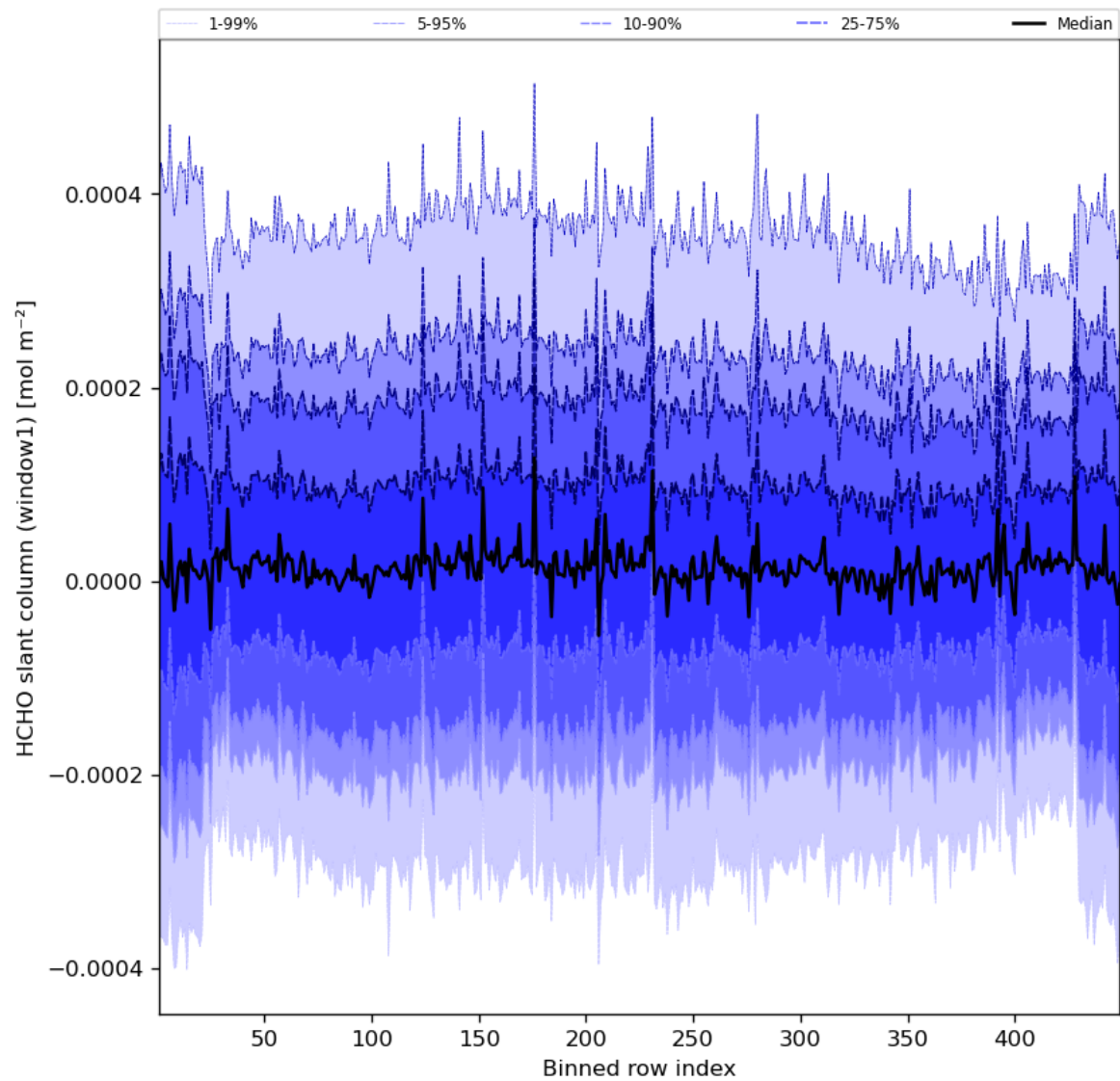
Figure 52: Along track statistics of “HCHO slant column (window1)” for 2023-09-22 to 2023-09-24
