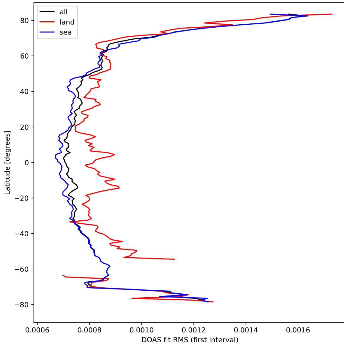
Figure 32: Zonal average of "DOAS fit RMS (first interval)" for 2023-09-22 to 2023-09-24.
