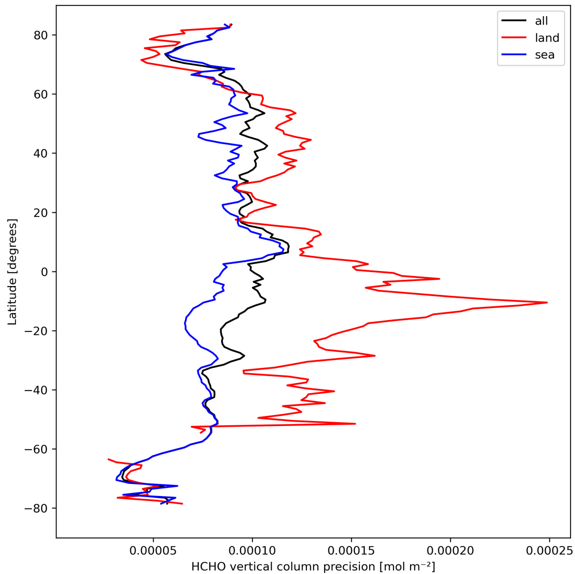
Figure 22: Zonal average of “HCHO vertical column precision” for 2023-09-22 to 2023-09-24.
