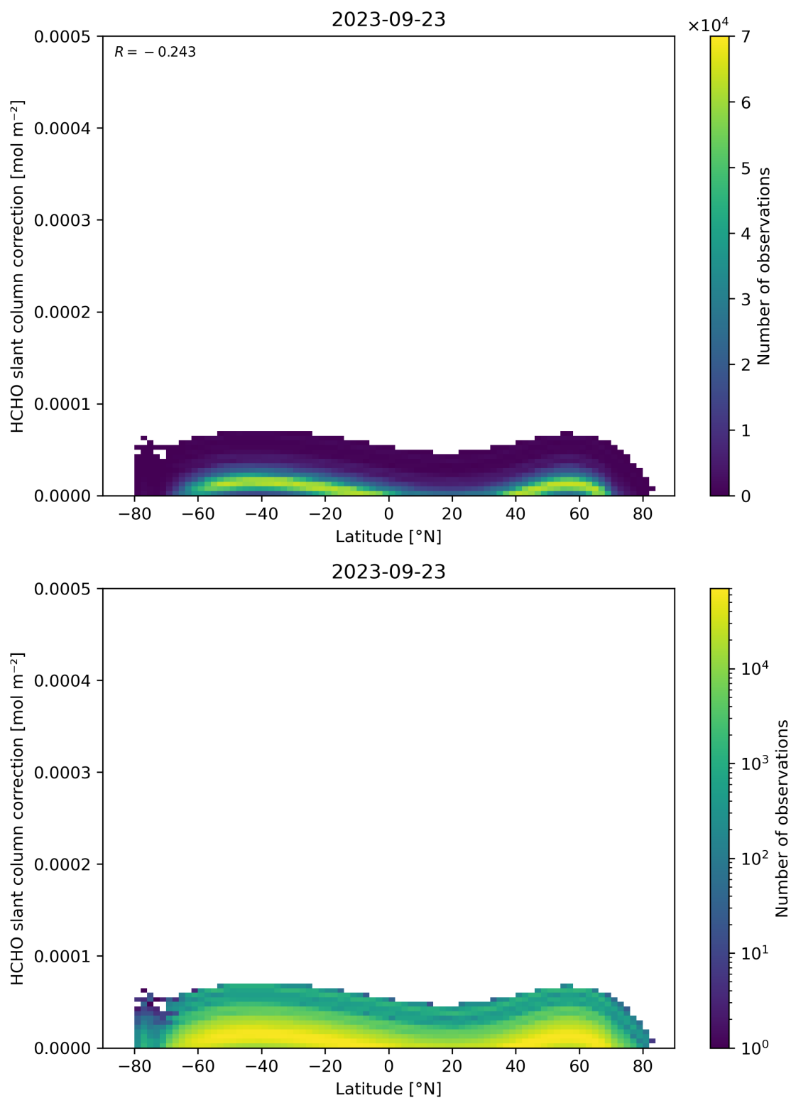
Figure 158: Scatter density plot of “Latitude” against “HCHO slant column correction” for 2023-09-22 to 2023-09-24.
