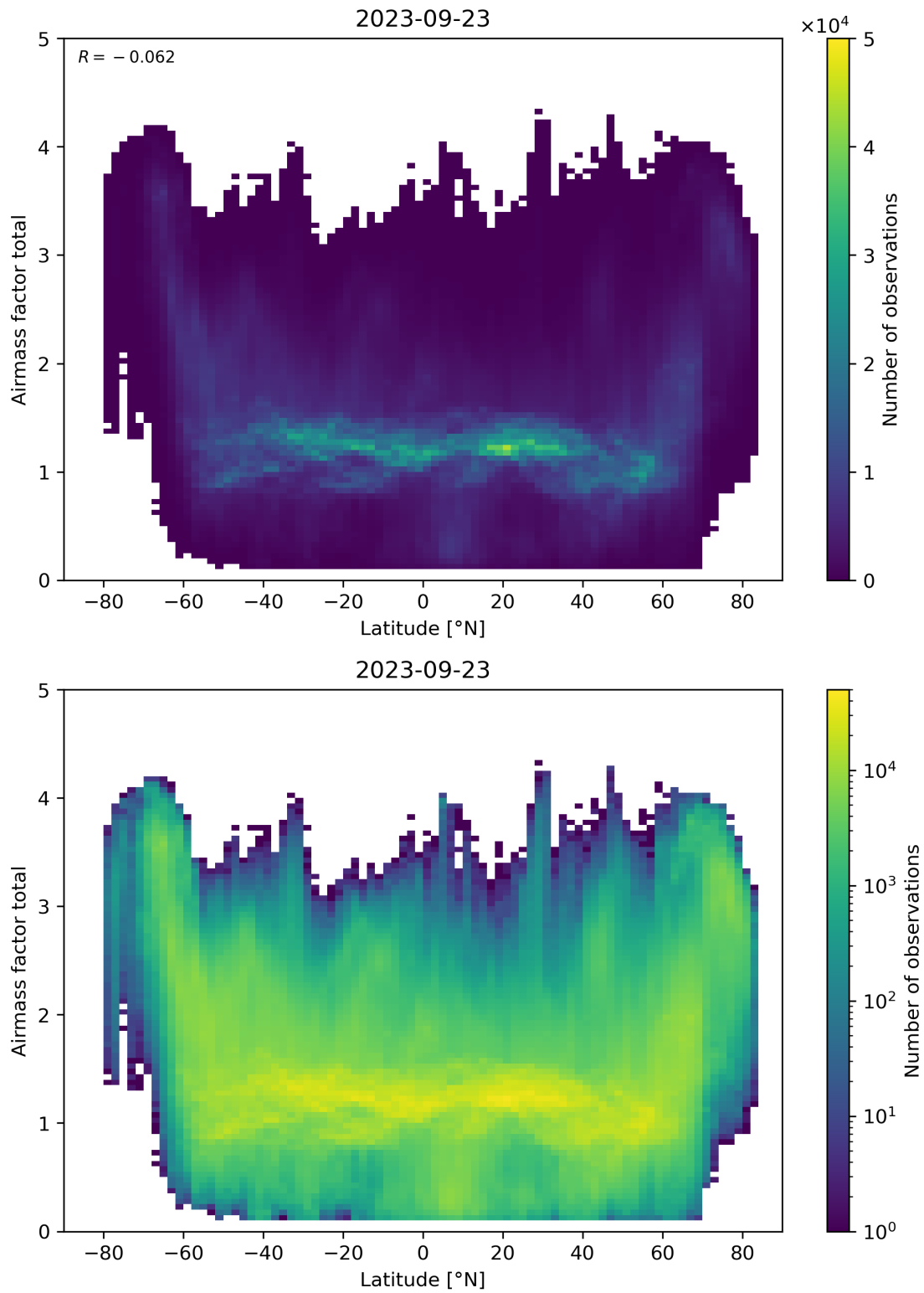
Figure 161: Scatter density plot of “Latitude” against “Airmass factor total” for 2023-09-22 to 2023-09-24.
