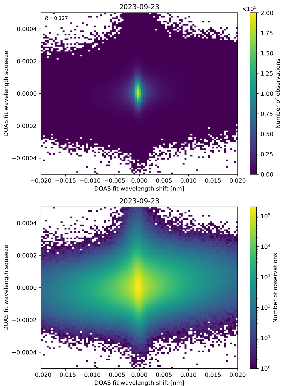
Figure 65: Scatter density plot of “DOAS fit wavelength shift” against “DOAS fit wavelength squeeze” for 2023-09-22 to 2023-09-24.
