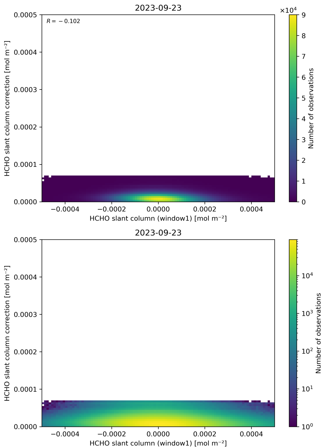
Figure 83: Scatter density plot of “HCHO slant column (window1)” against “HCHO slant column correction” for 2023-09-22 to 2023-09-24.
