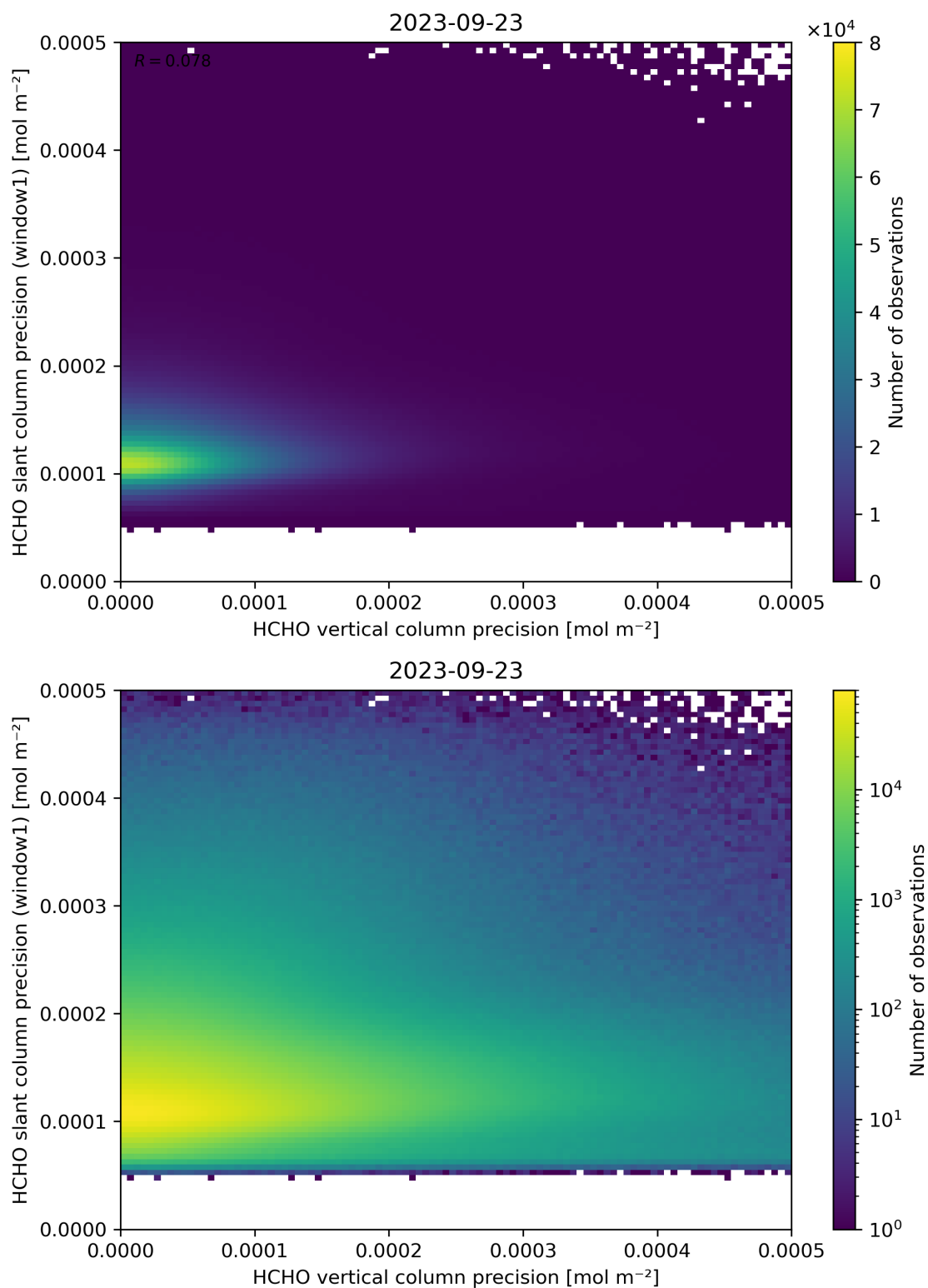
Figure 143: Scatter density plot of “HCHO vertical column precision” against “HCHO slant column precision (window1)” for 2023-09-22 to 2023-09-24.
