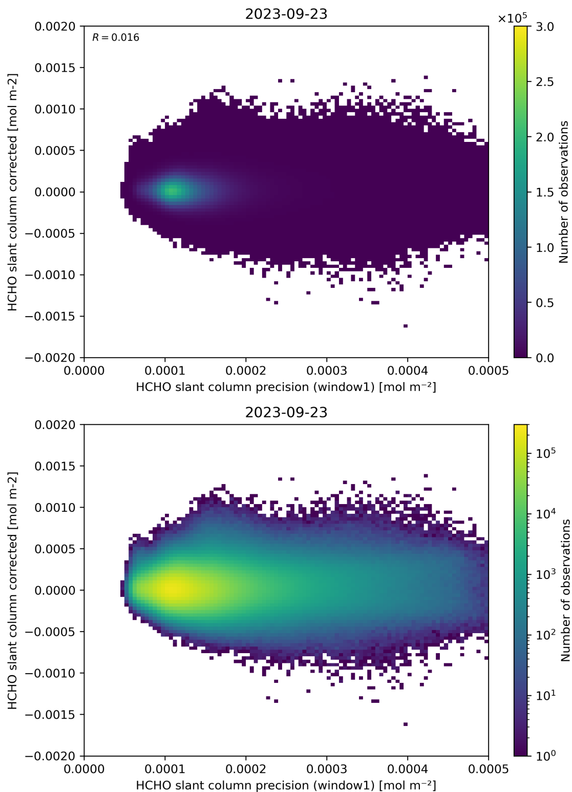
Figure 92: Scatter density plot of “HCHO slant column precision (window1)” against “HCHO slant column corrected” for 2023-09-22 to 2023-09-24.
