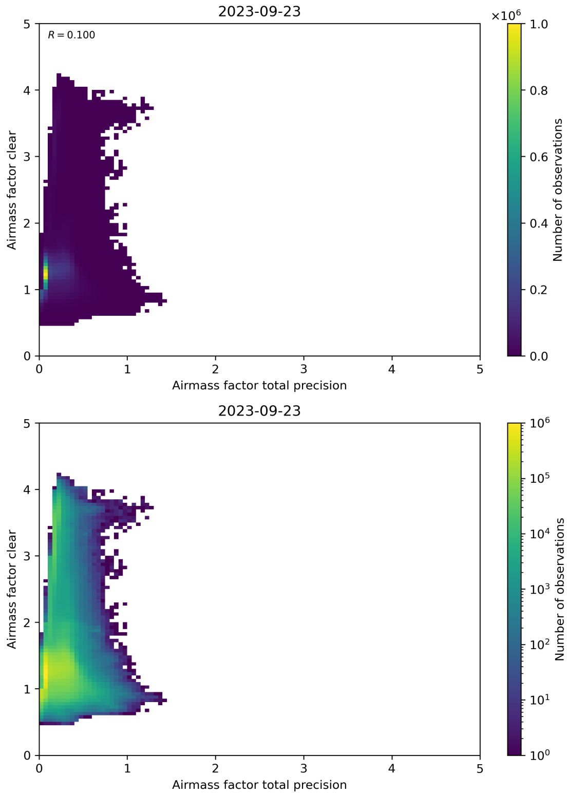
Figure 108: Scatter density plot of “Airmass factor total precision” against “Airmass factor clear” for 2023-09-22 to 2023-09-24.
