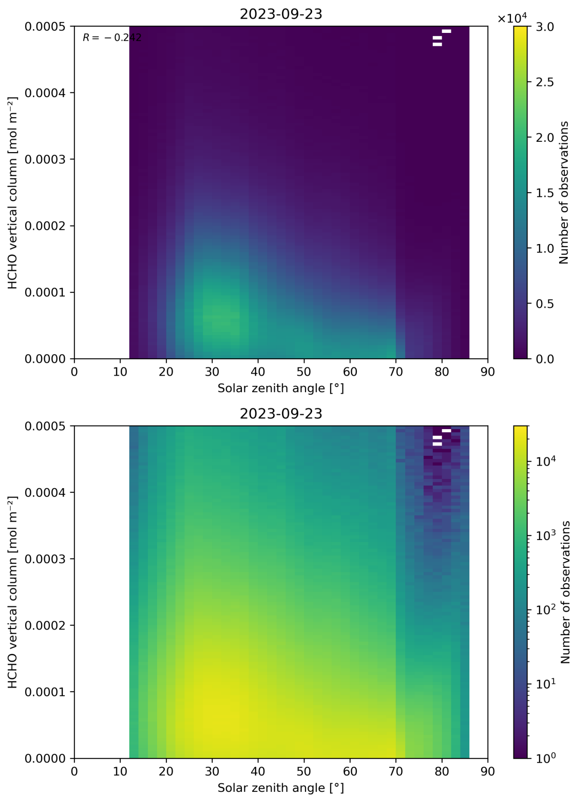
Figure 177: Scatter density plot of “Solar zenith angle” against “HCHO vertical column” for 2023-09-22 to 2023-09-24.
