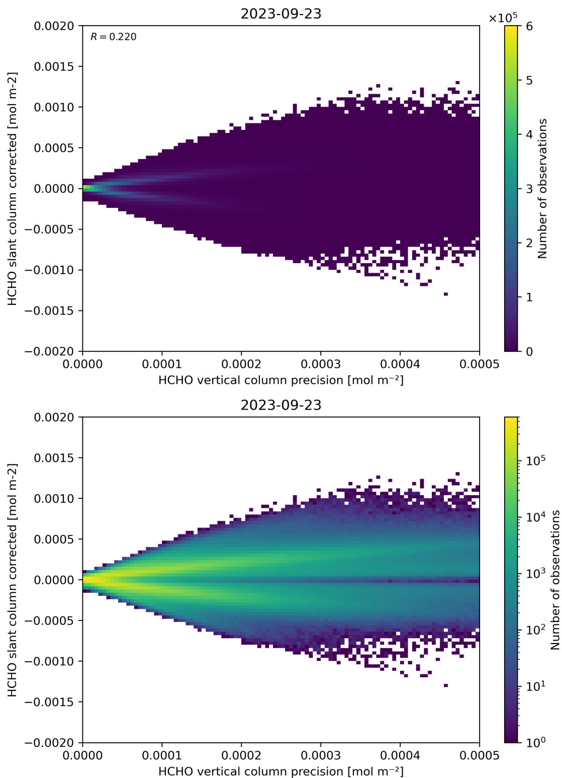
Figure 140: Scatter density plot of “HCHO vertical column precision” against “HCHO slant column corrected” for 2023-09-22 to 2023-09-24.
