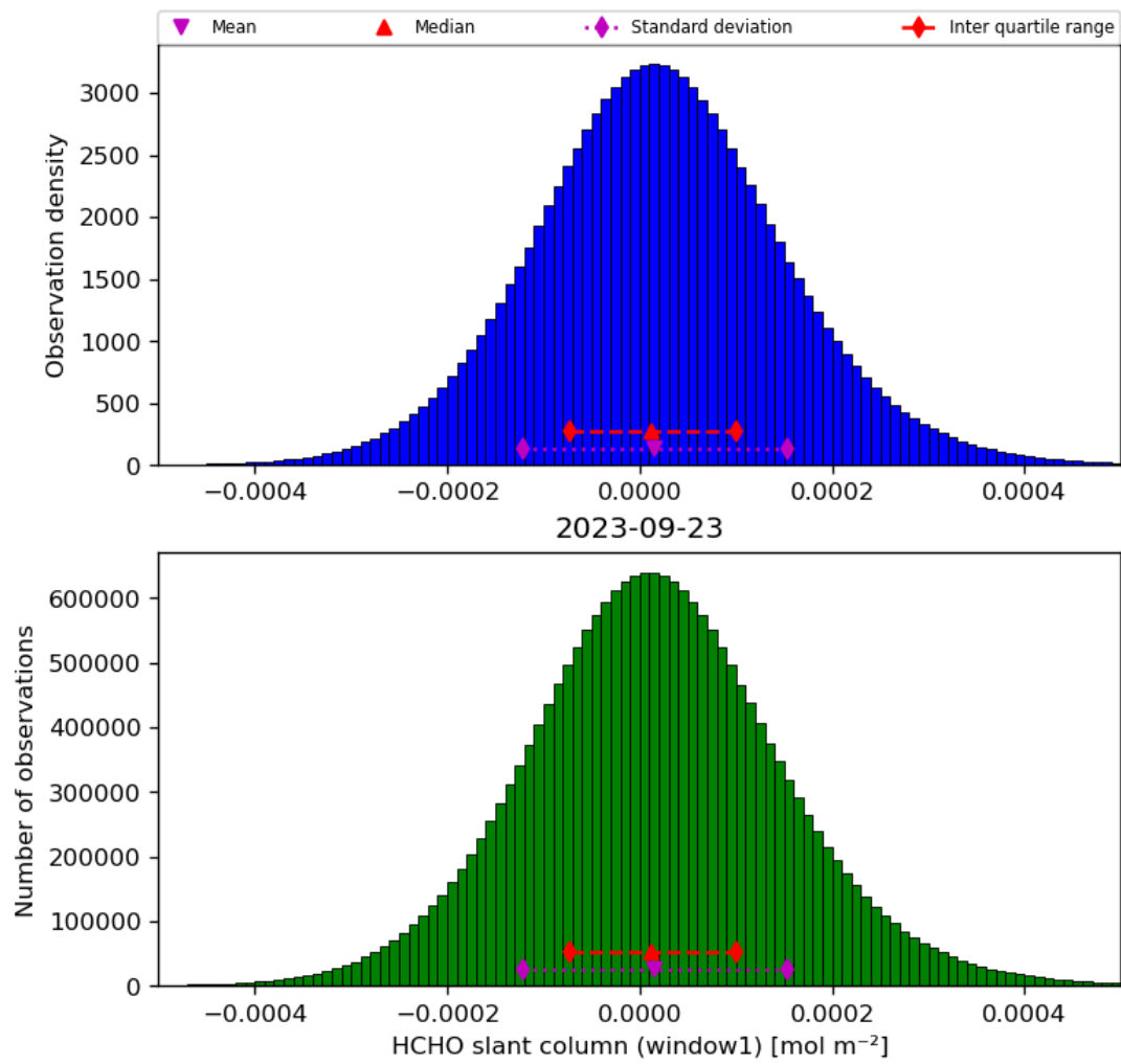
Figure 38: Histogram of “HCHO slant column (window1)” for 2023-09-22 to 2023-09-24
