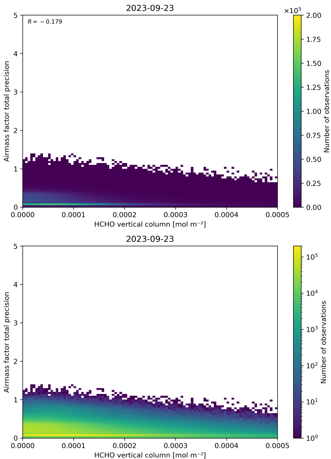
Figure 132: Scatter density plot of “HCHO vertical column” against “Airmass factor total precision” for 2023-09-22 to 2023-09-24.
