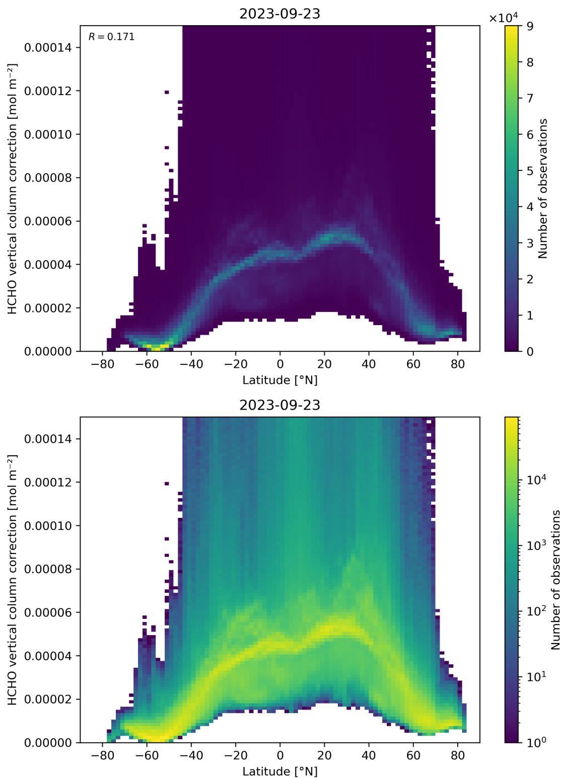
Figure 164: Scatter density plot of “Latitude” against “HCHO vertical column correction” for 2023-09-22 to 2023-09-24.
