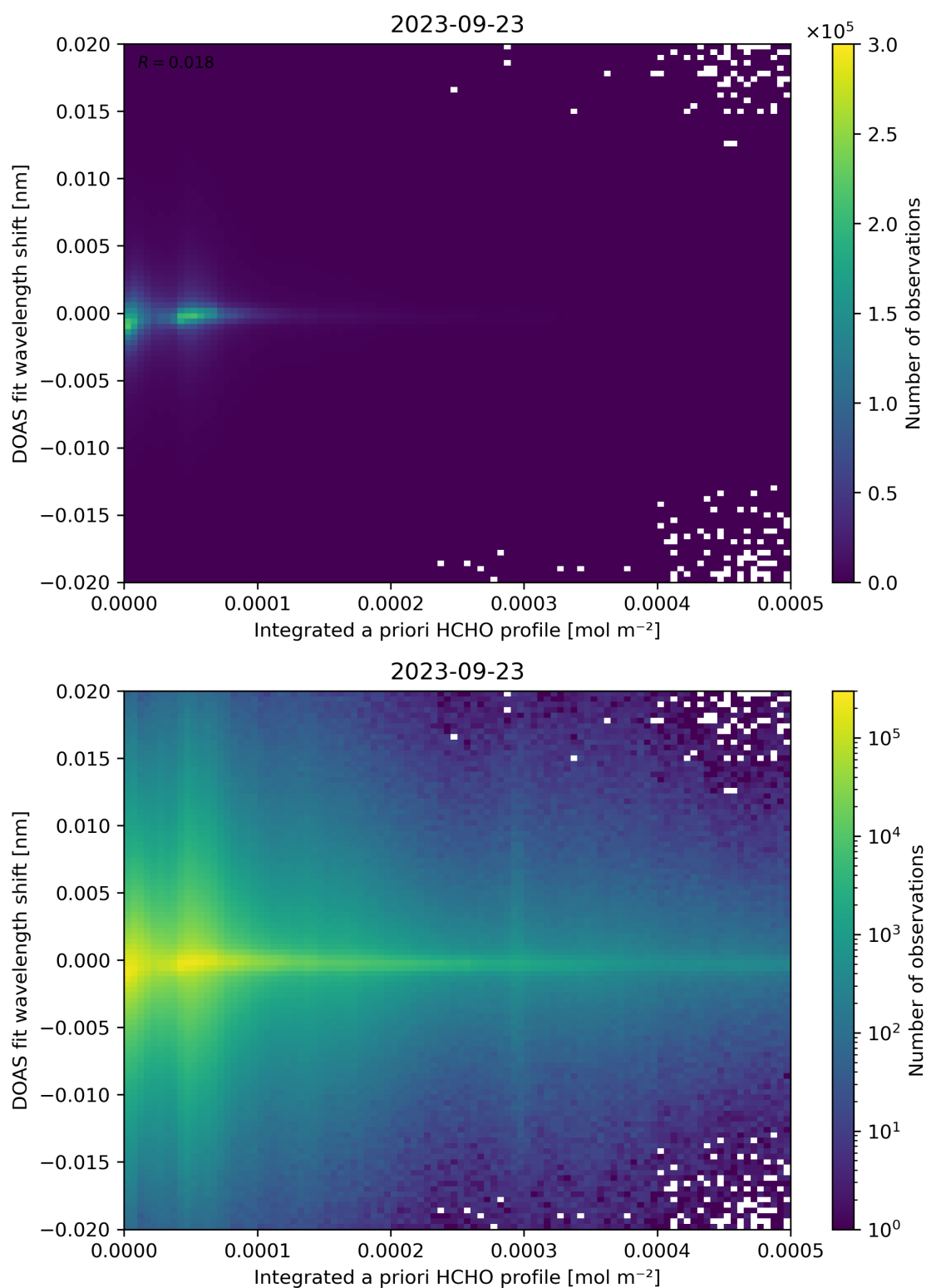
Figure 149: Scatter density plot of “Integrated a priori HCHO profile” against “DOAS fit wavelength shift” for 2023-09-22 to 2023-09-24.
