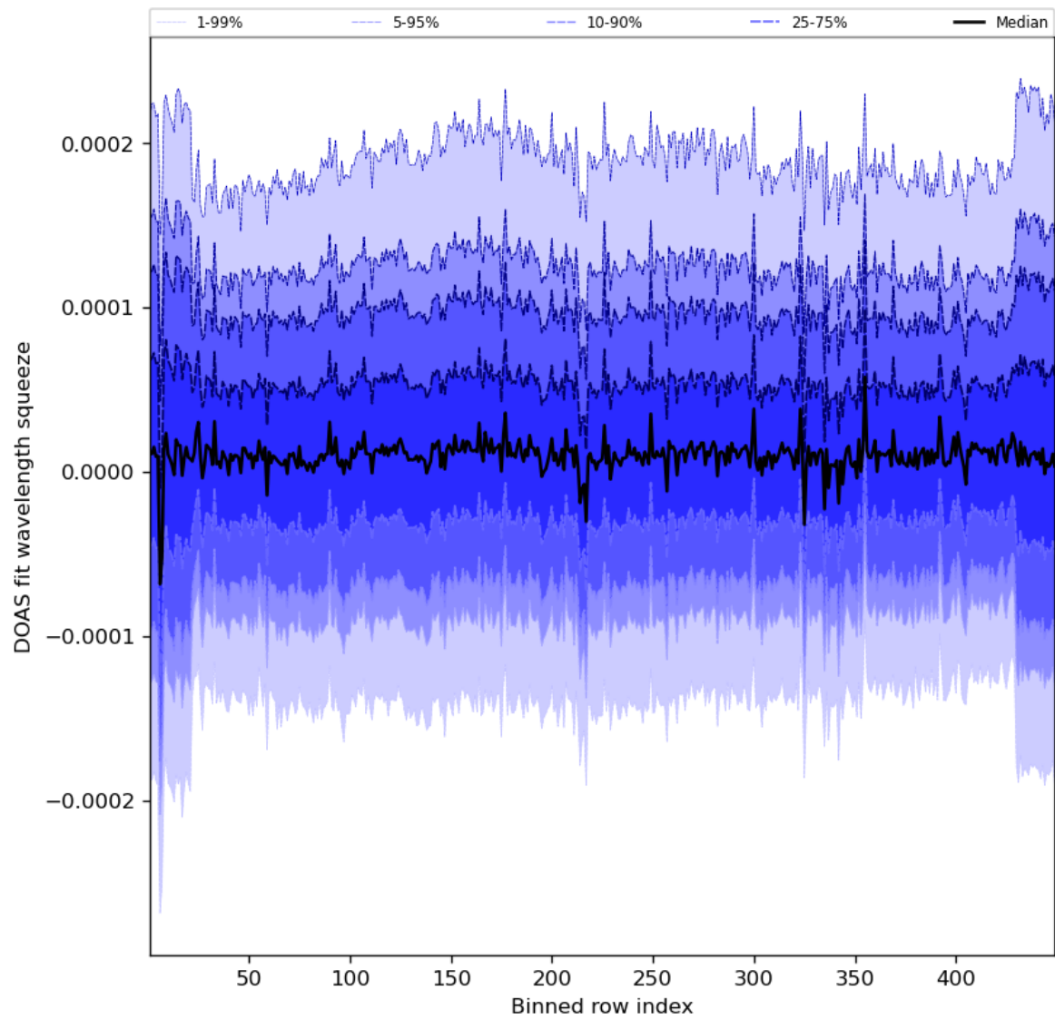
Figure 59: Along track statistics of “DOAS fit wavelength squeeze” for 2023-09-22 to 2023-09-24
