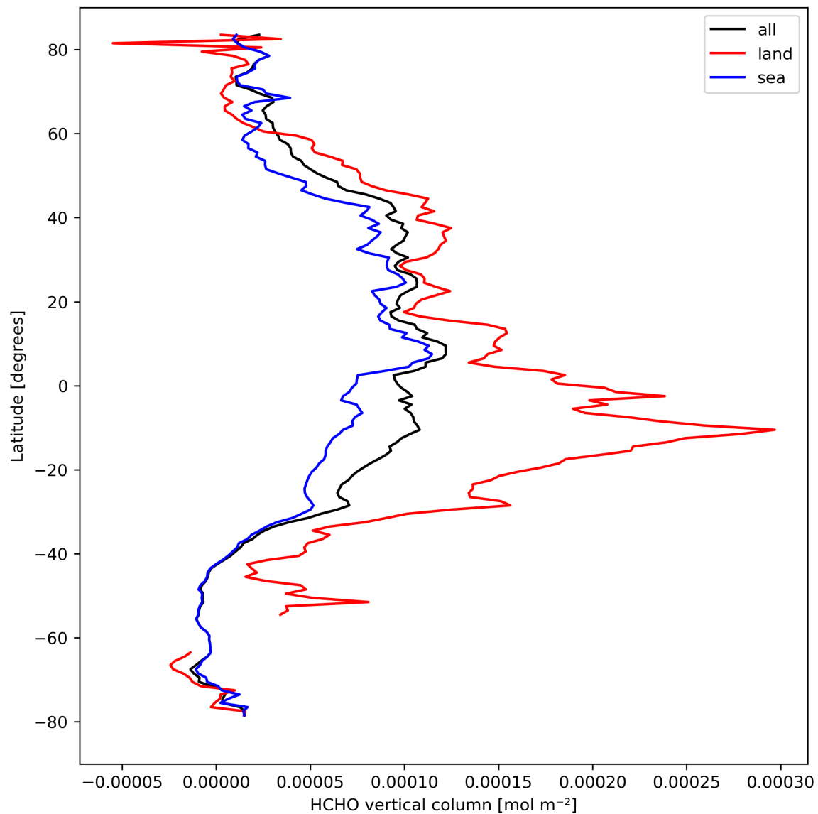
Figure 21: Zonal average of “HCHO vertical column” for 2023-09-22 to 2023-09-24.
