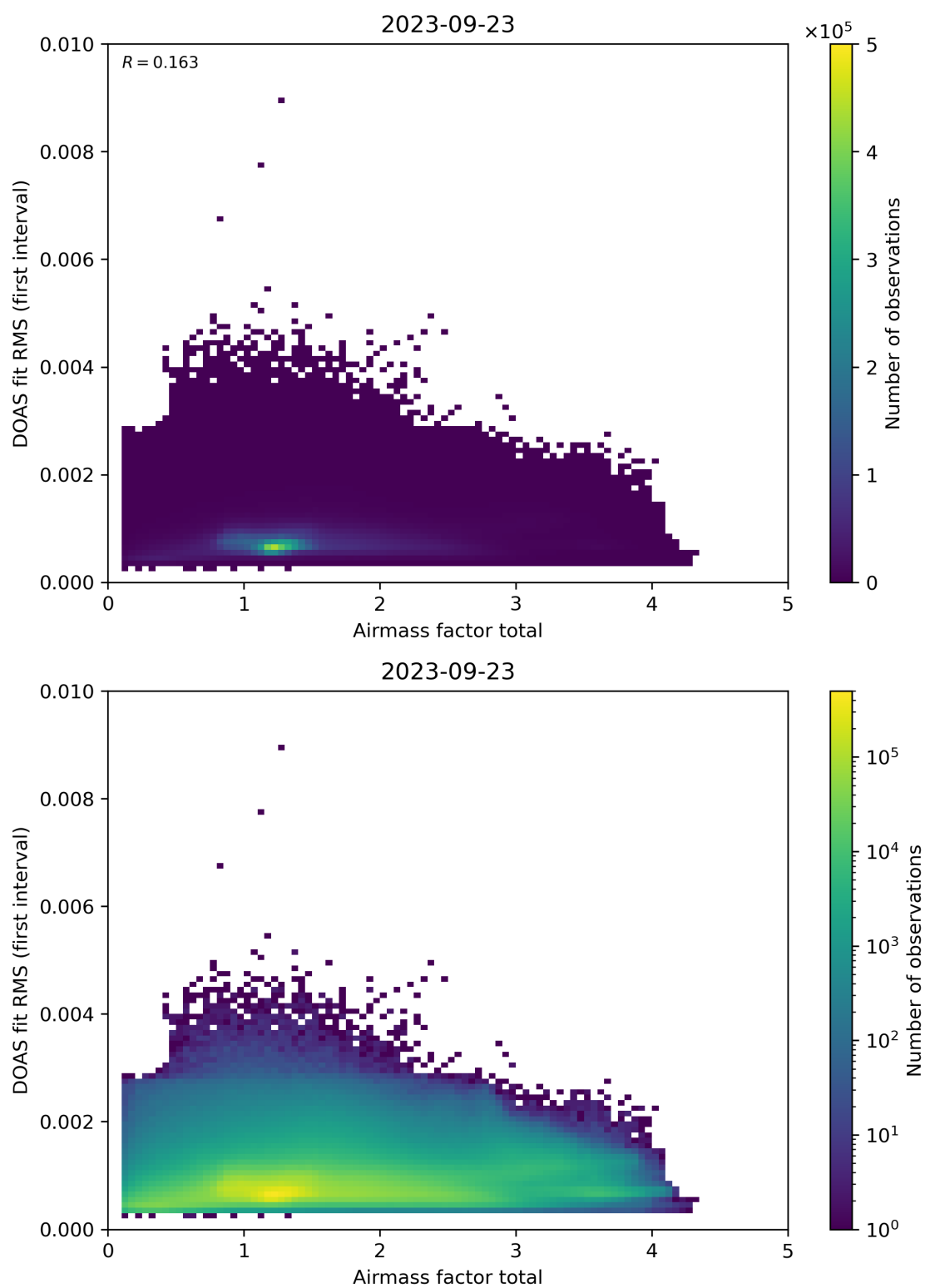
Figure 97: Scatter density plot of “Airmass factor total” against “DOAS fit RMS (first interval)” for 2023-09-22 to 2023-09-24.
