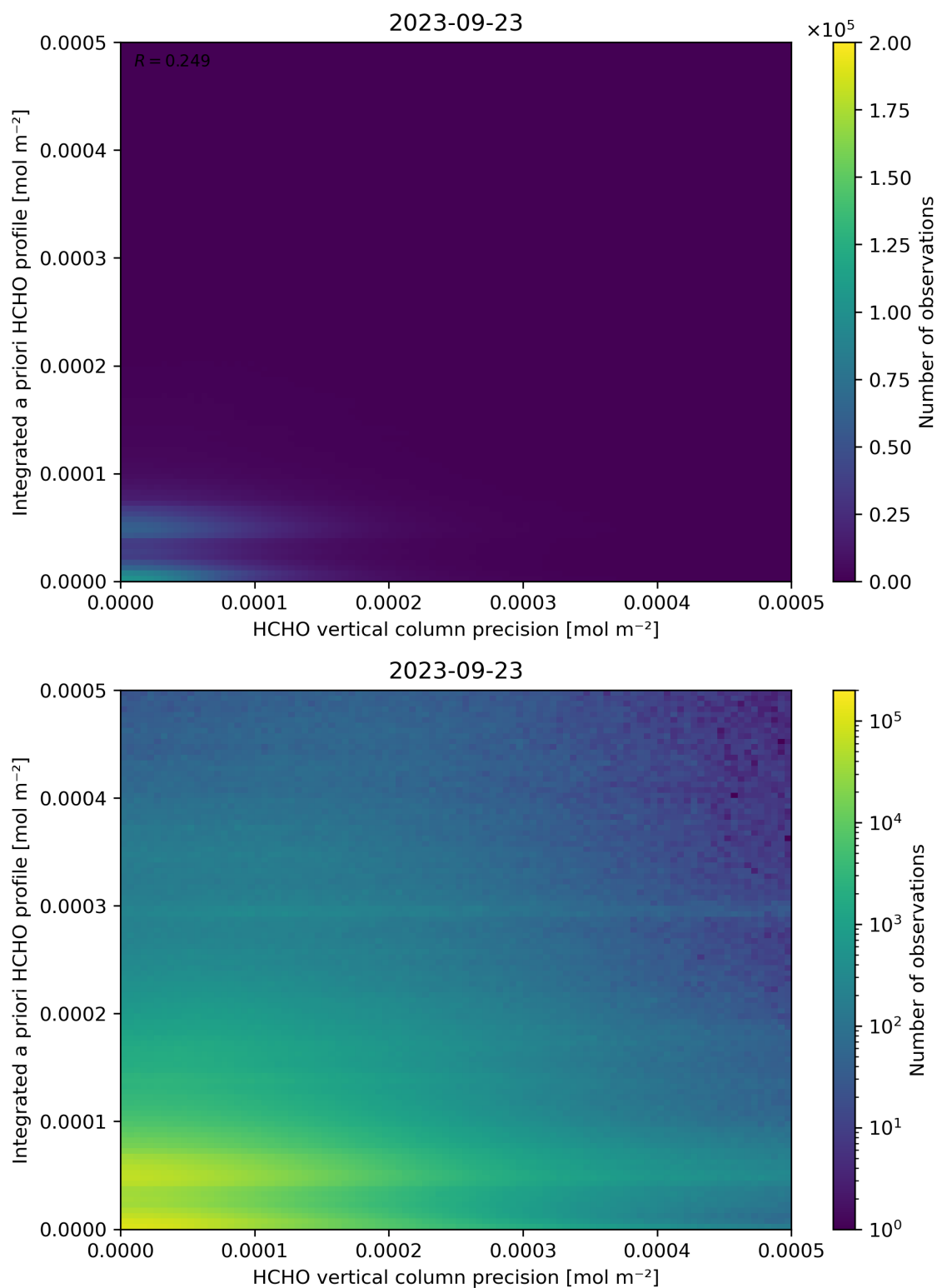
Figure 147: Scatter density plot of “HCHO vertical column precision” against “Integrated a priori HCHO profile” for 2023-09-22 to 2023-09-24.
