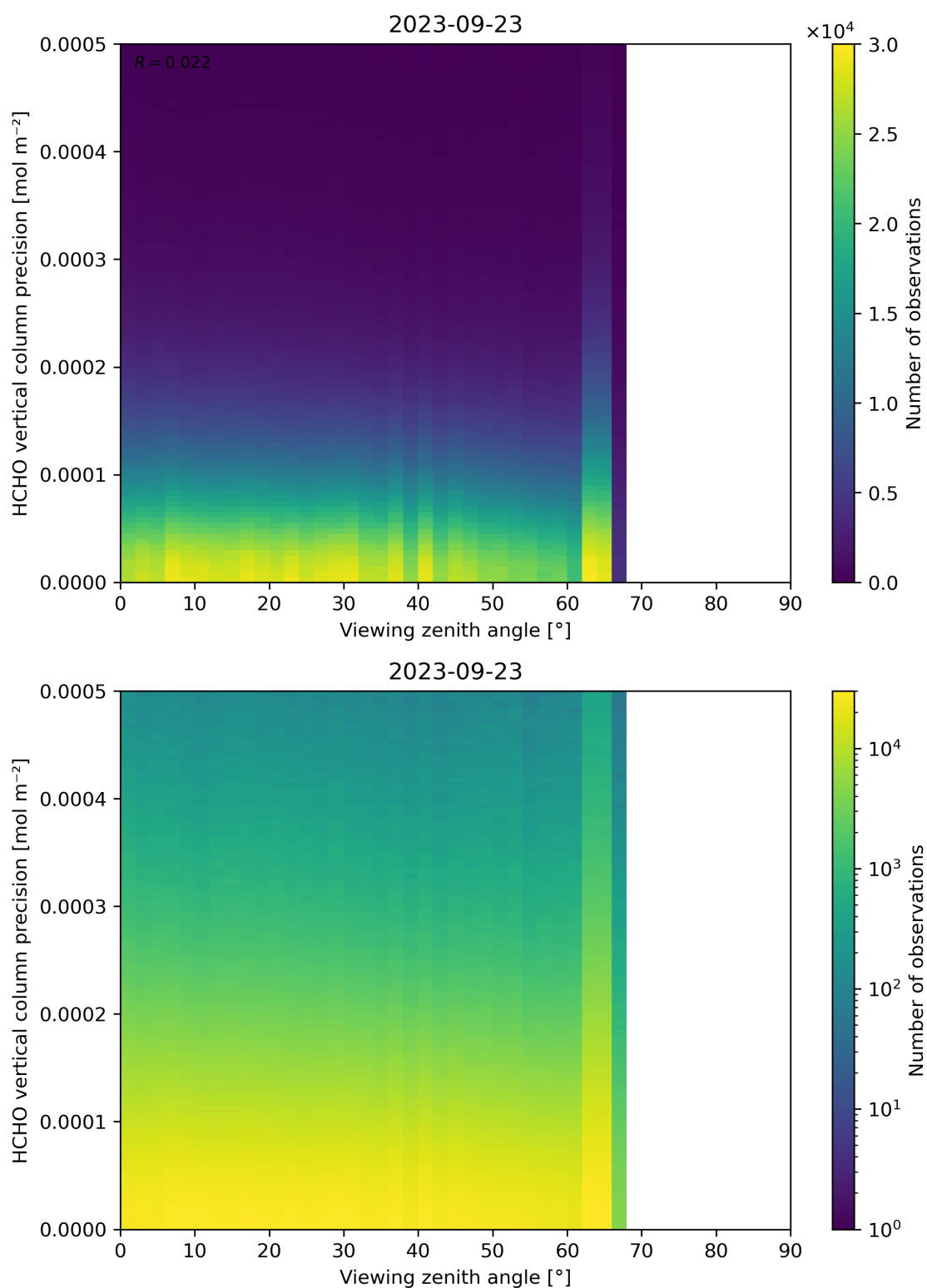
Figure 194: Scatter density plot of “Viewing zenith angle” against “HCHO vertical column precision” for 2023-09-22 to 2023-09-24.
