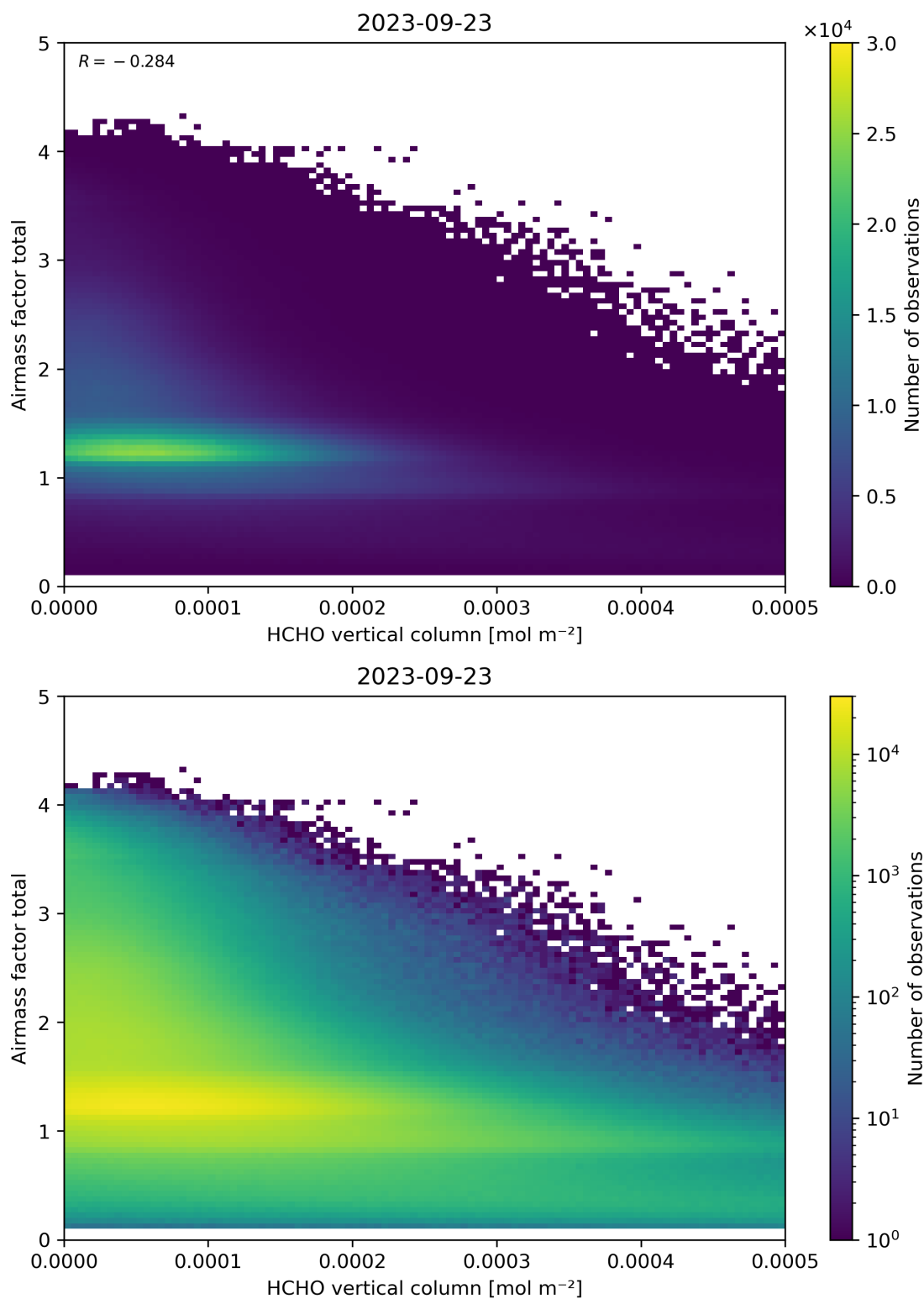
Figure 131: Scatter density plot of “HCHO vertical column” against “Airmass factor total” for 2023-09-22 to 2023-09-24.
