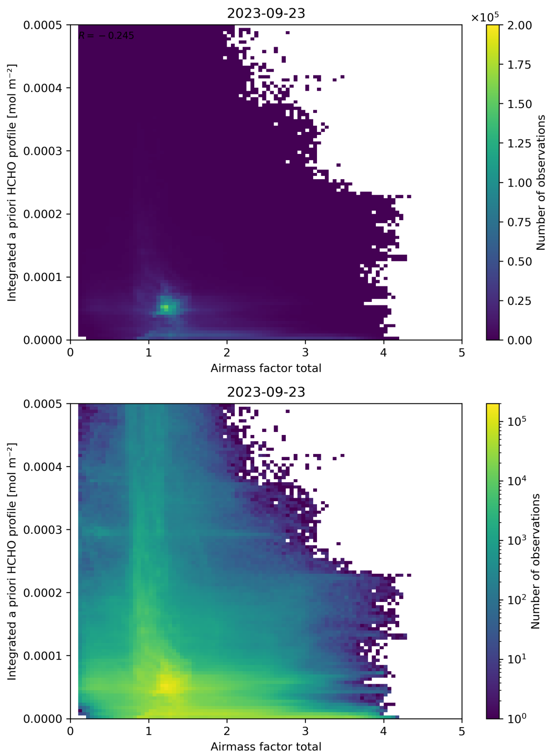
Figure 104: Scatter density plot of “Airmass factor total” against “Integrated a priori HCHO profile” for 2023-09-22 to 2023-09-24.
