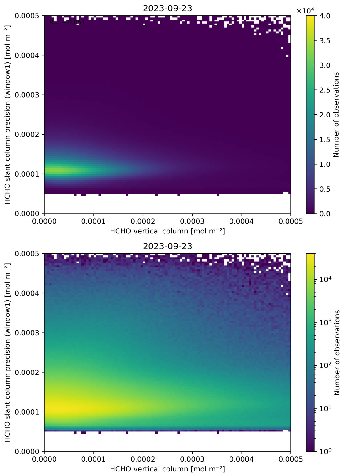
Figure 130: Scatter density plot of “HCHO vertical column” against “HCHO slant column precision (window1)” for 2023-09-22 to 2023-09-24.
