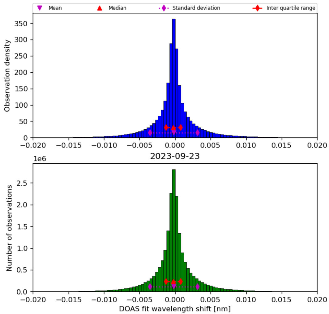
Figure 44: Histogram of “DOAS fit wavelength shift” for 2023-09-22 to 2023-09-24
