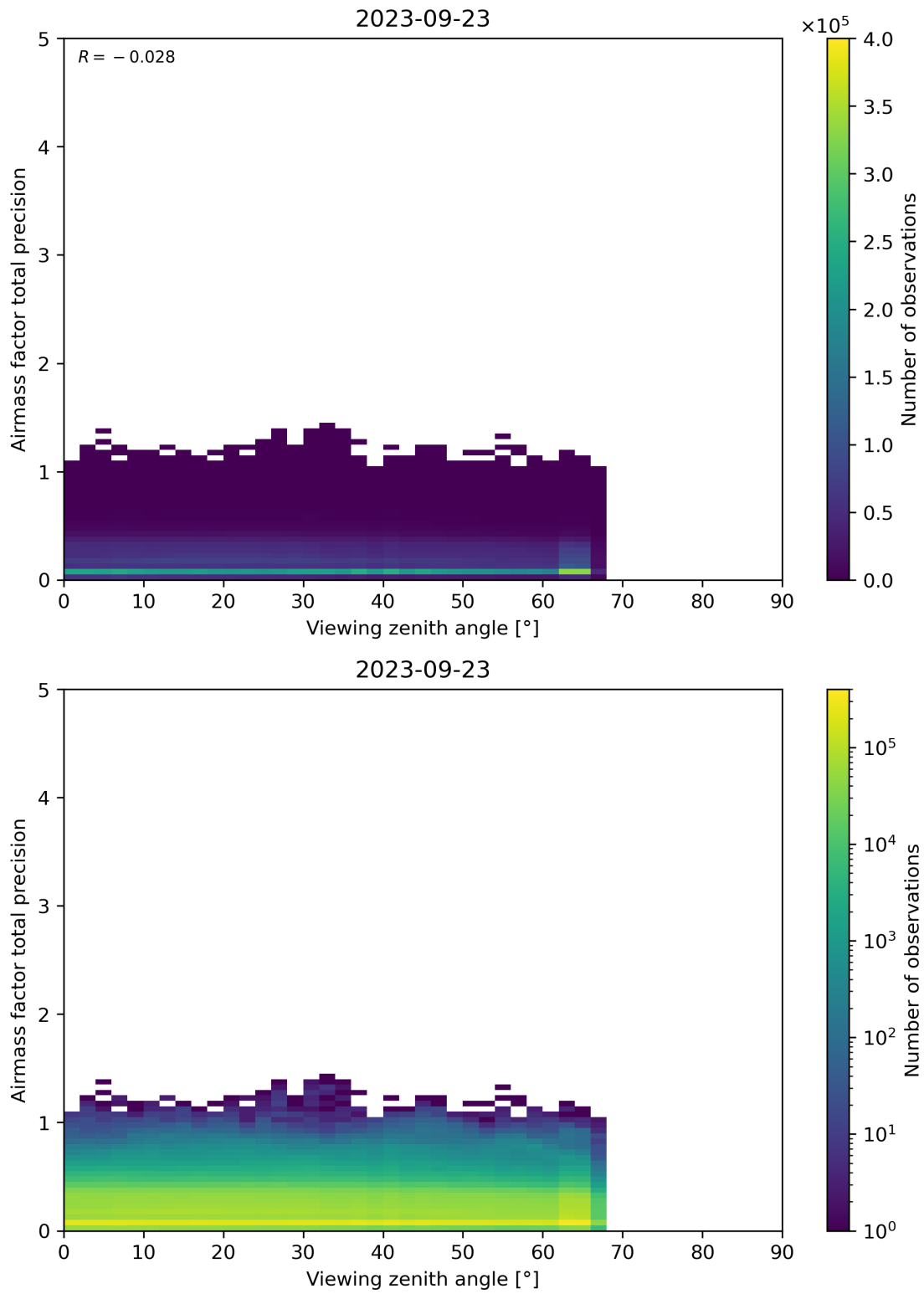
Figure 191: Scatter density plot of “Viewing zenith angle” against “Airmass factor total precision” for 2023-09-22 to 2023-09-24.
