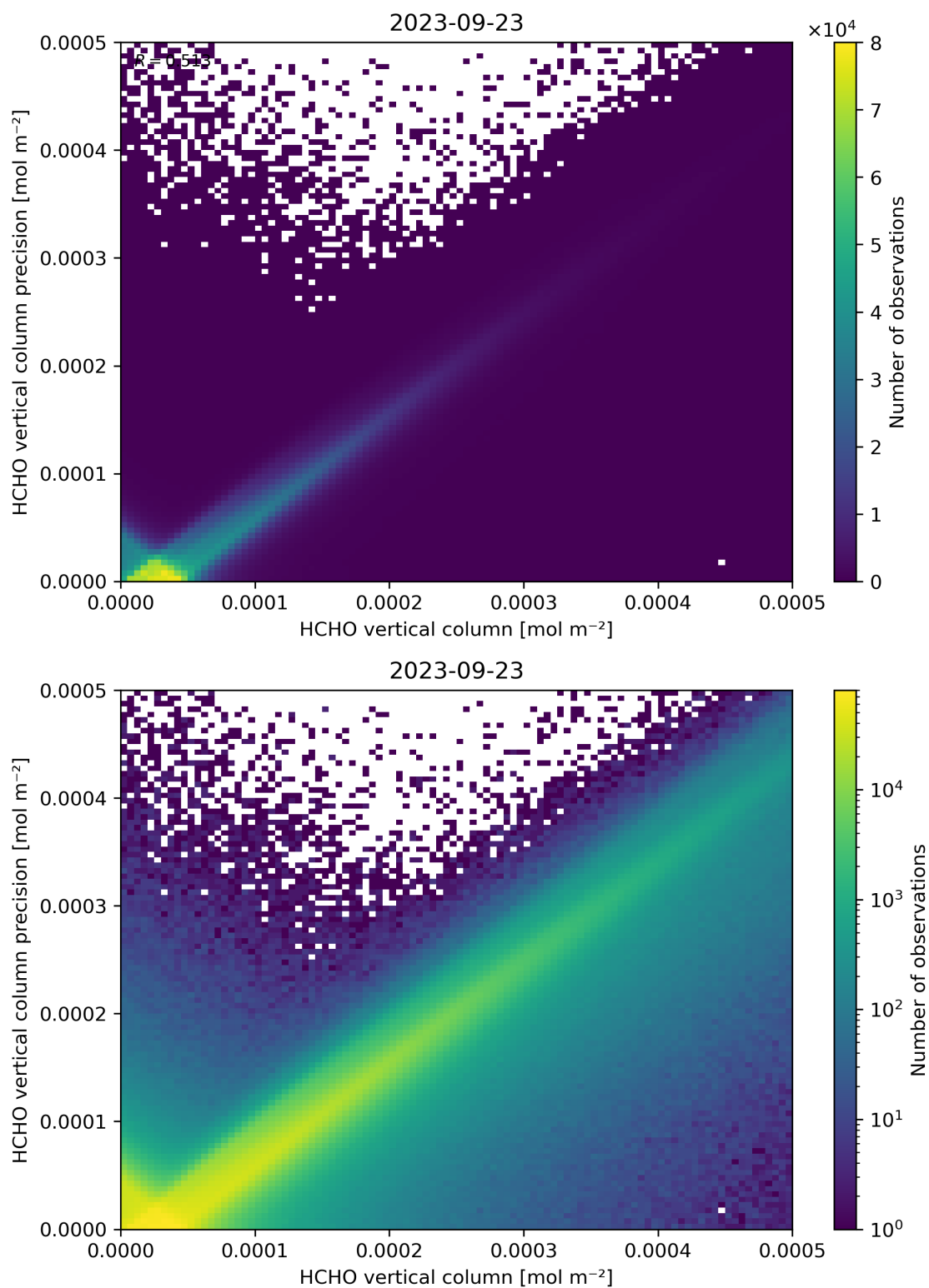
Figure 134: Scatter density plot of “HCHO vertical column” against “HCHO vertical column precision” for 2023-09-22 to 2023-09-24.
