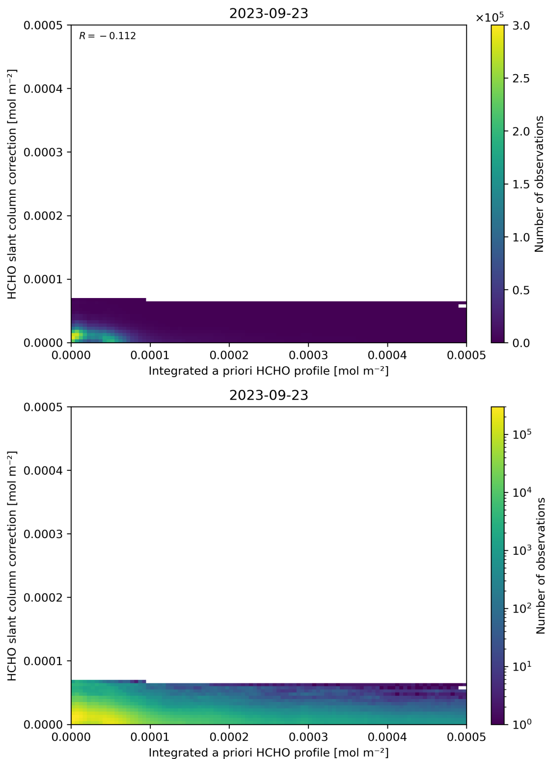
Figure 152: Scatter density plot of “Integrated a priori HCHO profile” against “HCHO slant column correction” for 2023-09-22 to 2023-09-24.
