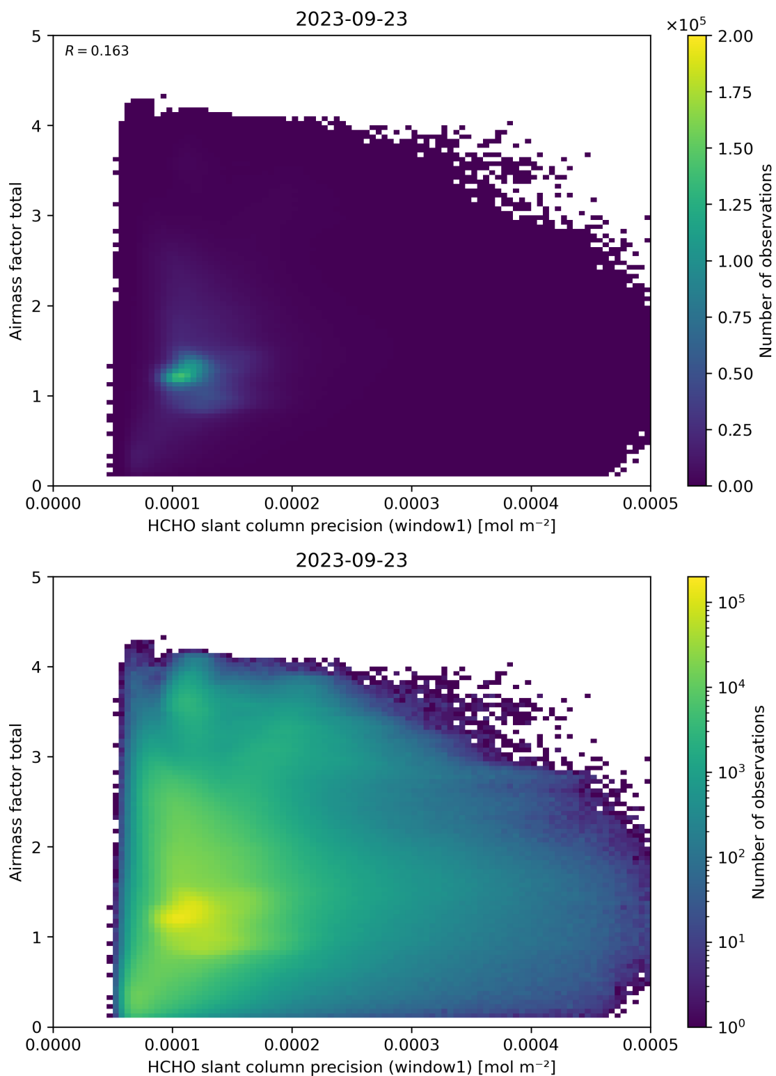
Figure 94: Scatter density plot of “HCHO slant column precision (window1)” against “Airmass factor total” for 2023-09-22 to 2023-09-24.
