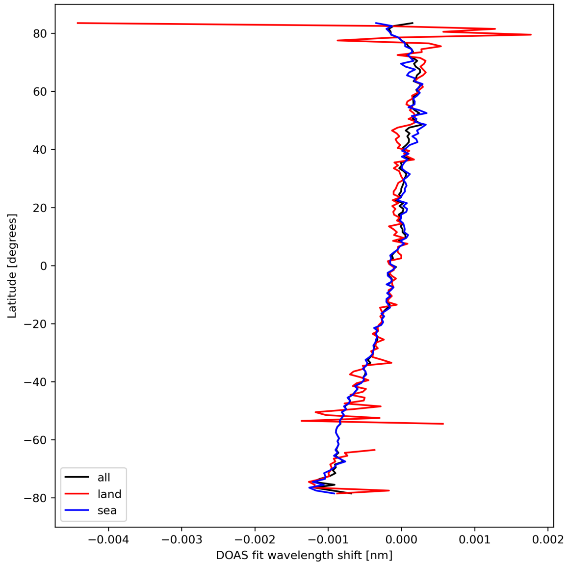
Figure 30: Zonal average of "DOAS fit wavelength shift" for 2023-09-22 to 2023-09-24.
