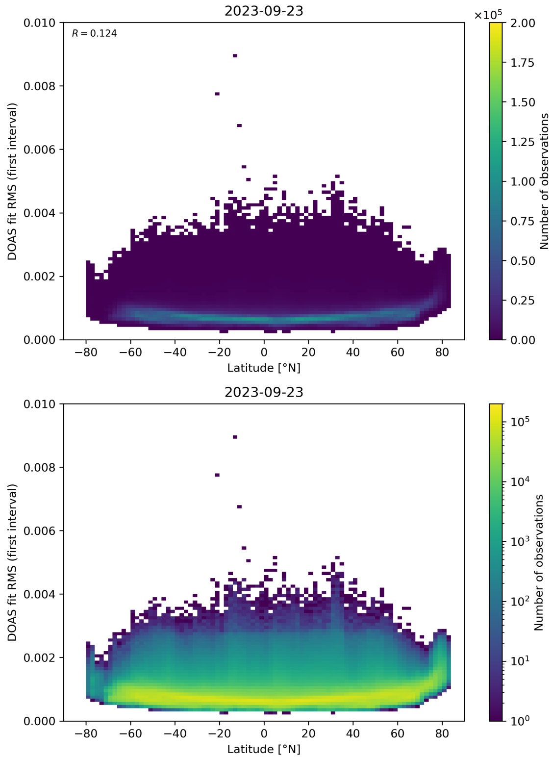
Figure 153: Scatter density plot of “Latitude” against “DOAS fit RMS (first interval)” for 2023-09-22 to 2023-09-24.
