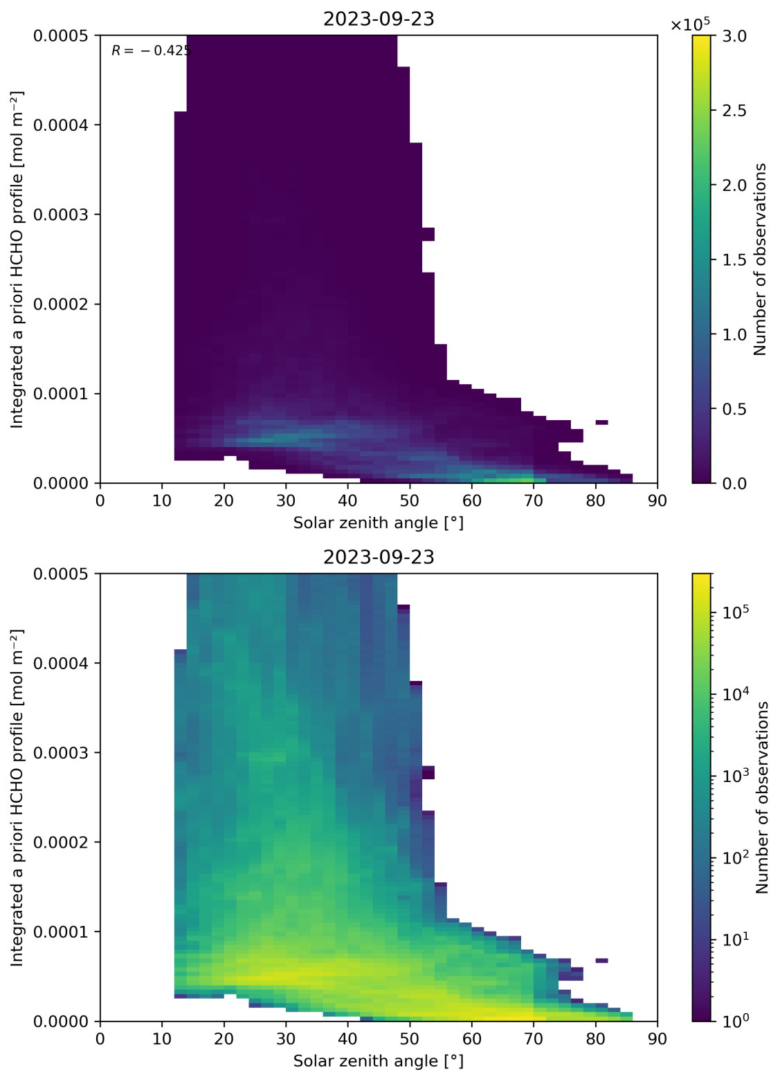
Figure 180: Scatter density plot of “Solar zenith angle” against “Integrated a priori HCHO profile” for 2023-09-22 to 2023-09-24.
