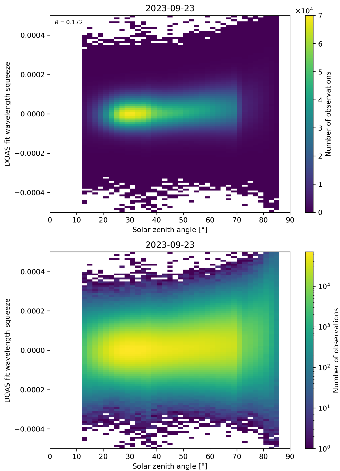
Figure 169: Scatter density plot of “Solar zenith angle” against “DOAS fit wavelength squeeze” for 2023-09-22 to 2023-09-24.
