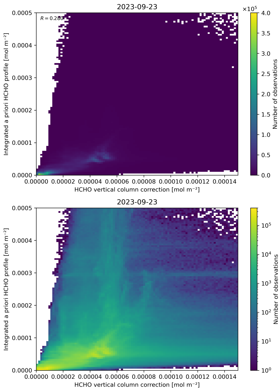
Figure 122: Scatter density plot of “HCHO vertical column correction” against “Integrated a priori HCHO profile” for 2023-09-22 to 2023-09-24.
