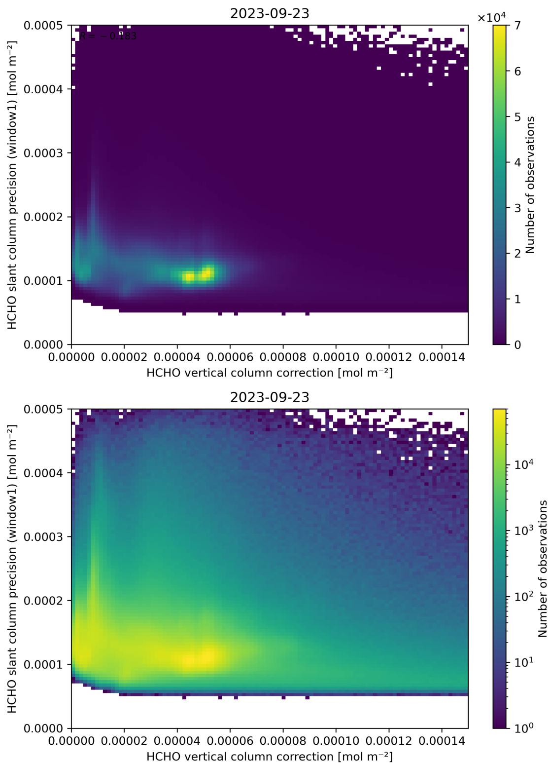
Figure 119: Scatter density plot of “HCHO vertical column correction” against “HCHO slant column precision (window1)” for 2023-09-22 to 2023-09-24.
