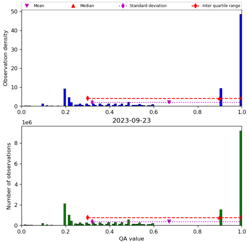
Figure 34: Histogram of “QA value” for 2023-09-22 to 2023-09-24
