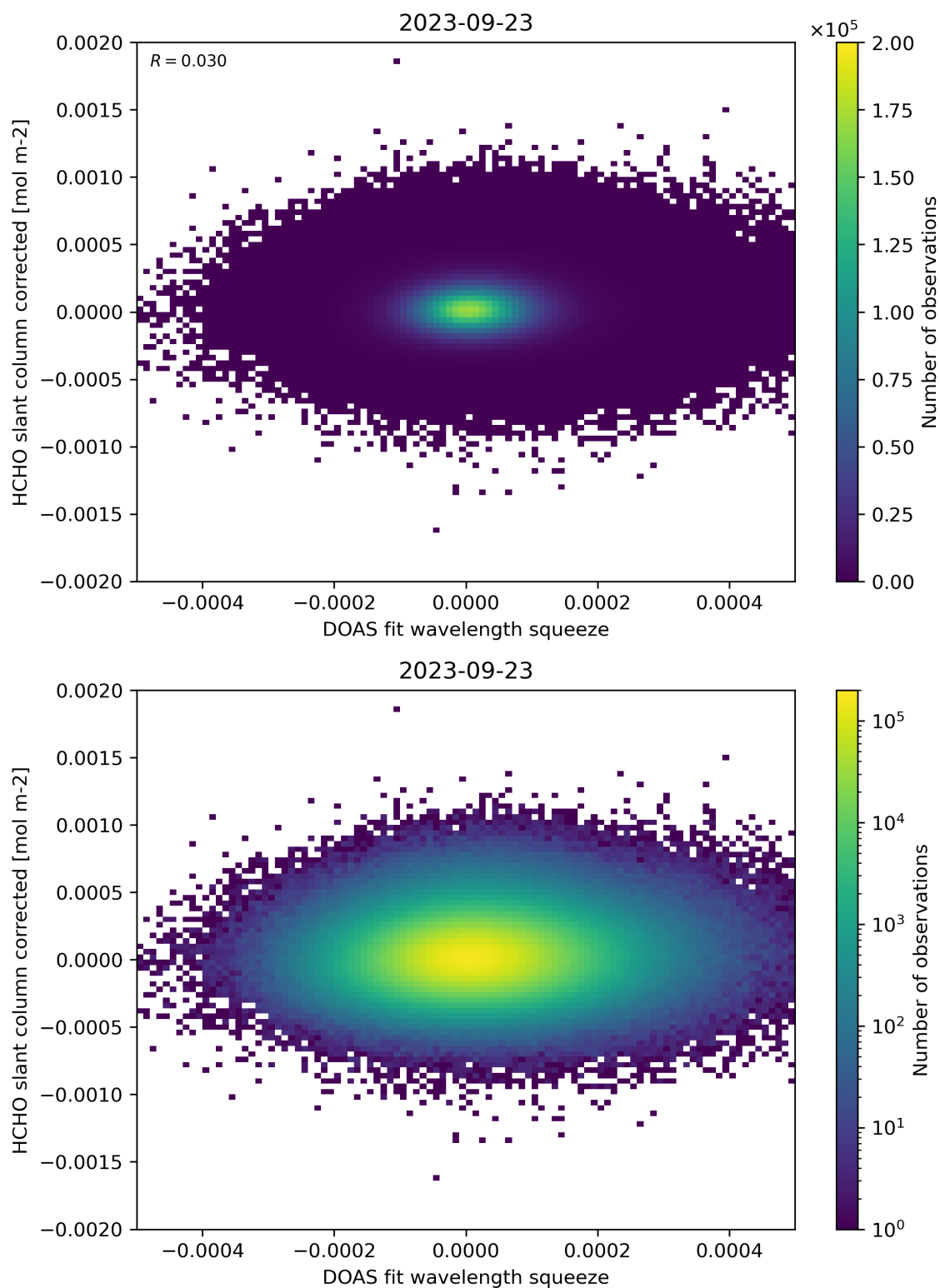
Figure 69: Scatter density plot of “DOAS fit wavelength squeeze” against “HCHO slant column corrected” for 2023-09-22 to 2023-09-24.
