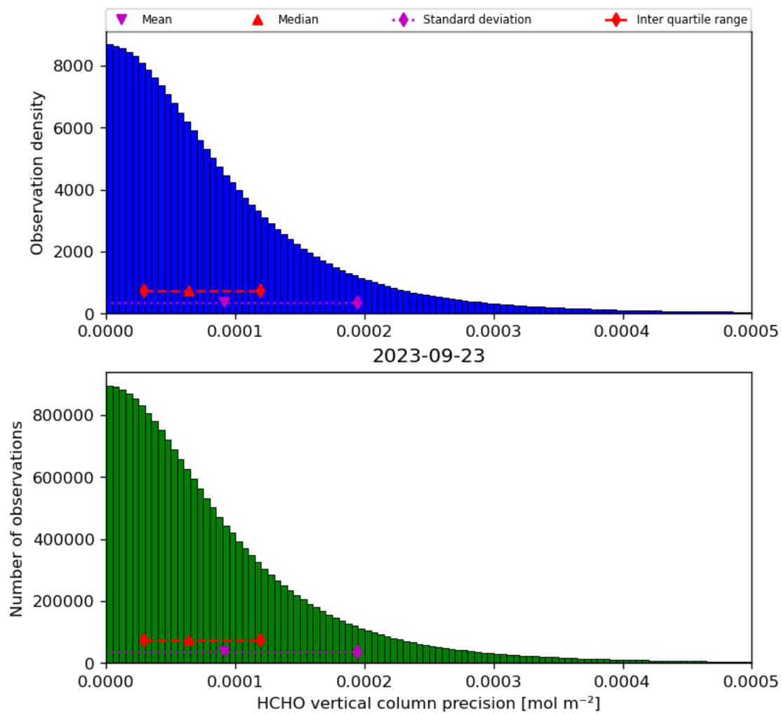
Figure 36: Histogram of “HCHO vertical column precision” for 2023-09-22 to 2023-09-24
