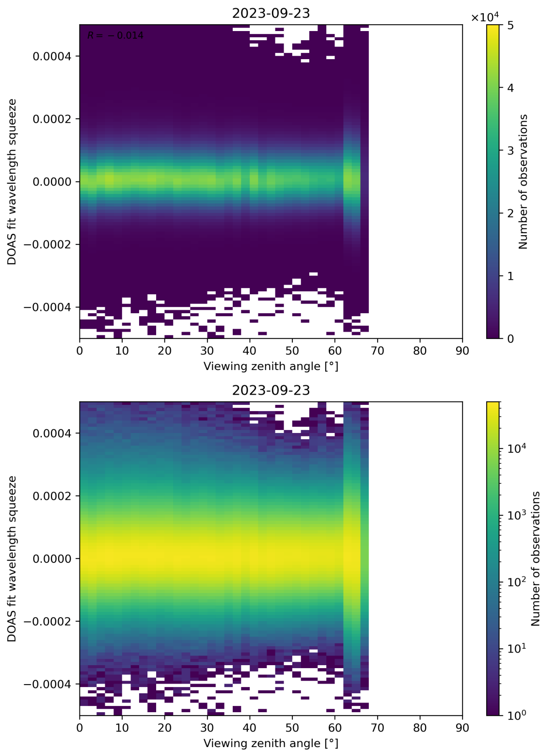
Figure 184: Scatter density plot of “Viewing zenith angle” against “DOAS fit wavelength squeeze” for 2023-09-22 to 2023-09-24.
