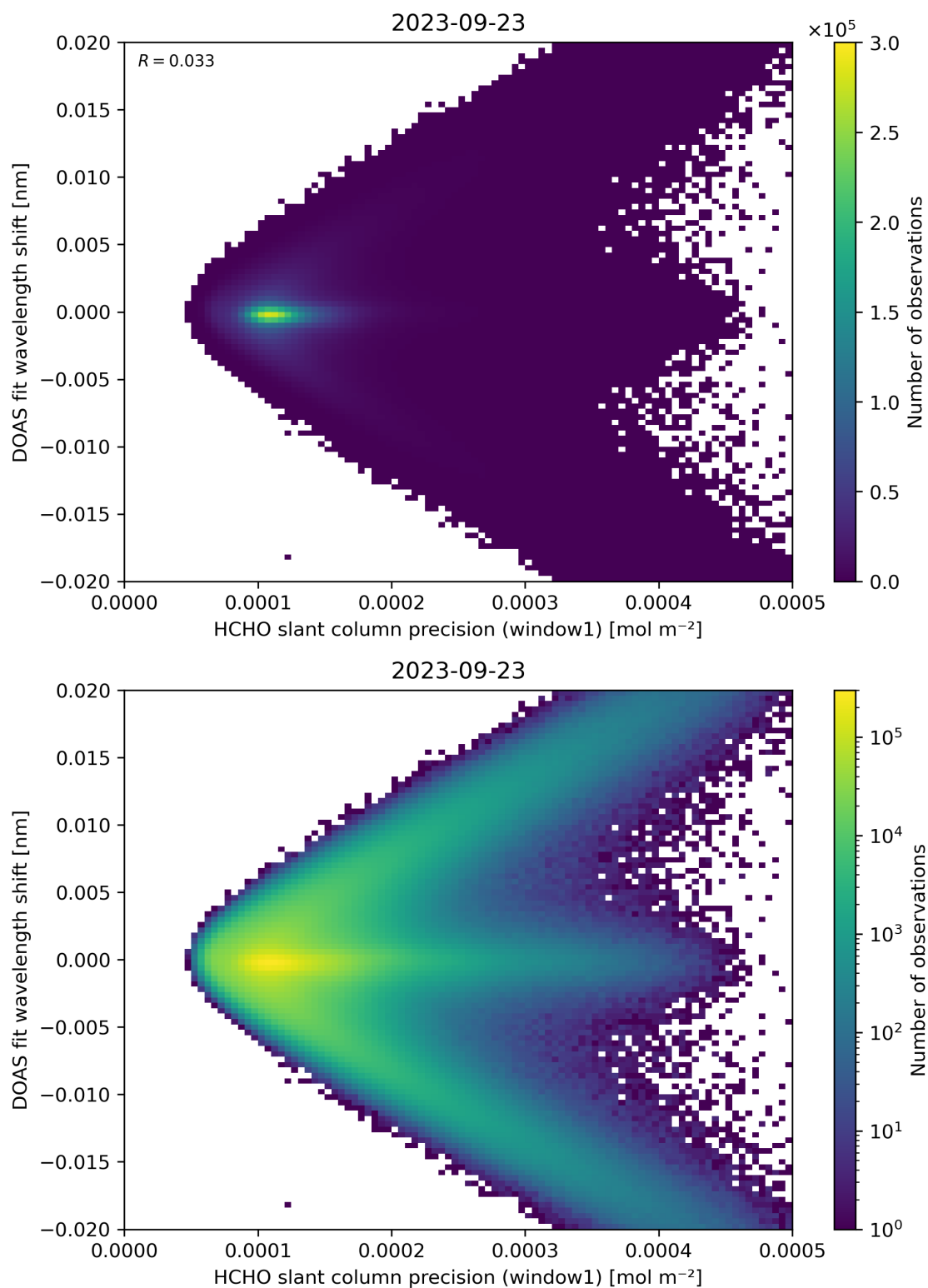
Figure 89: Scatter density plot of “HCHO slant column precision (window1)” against “DOAS fit wavelength shift” for 2023-09-22 to 2023-09-24.
