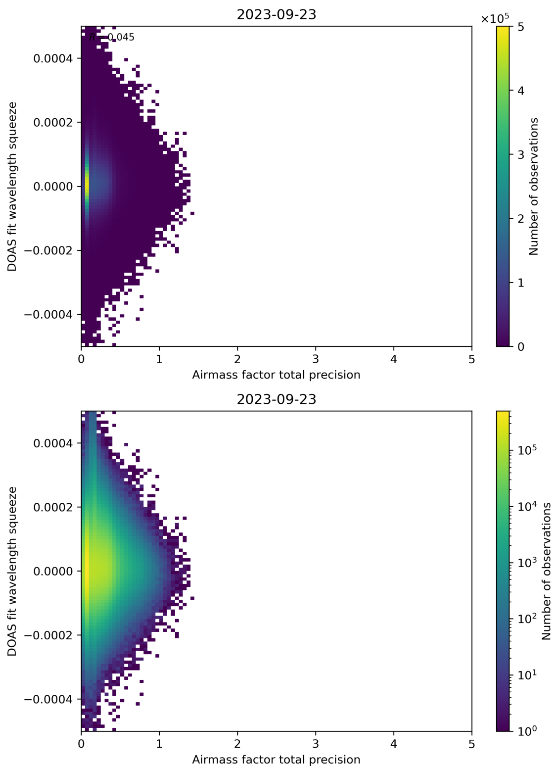
Figure 107: Scatter density plot of “Airmass factor total precision” against “DOAS fit wavelength squeeze” for 2023-09-22 to 2023-09-24.
