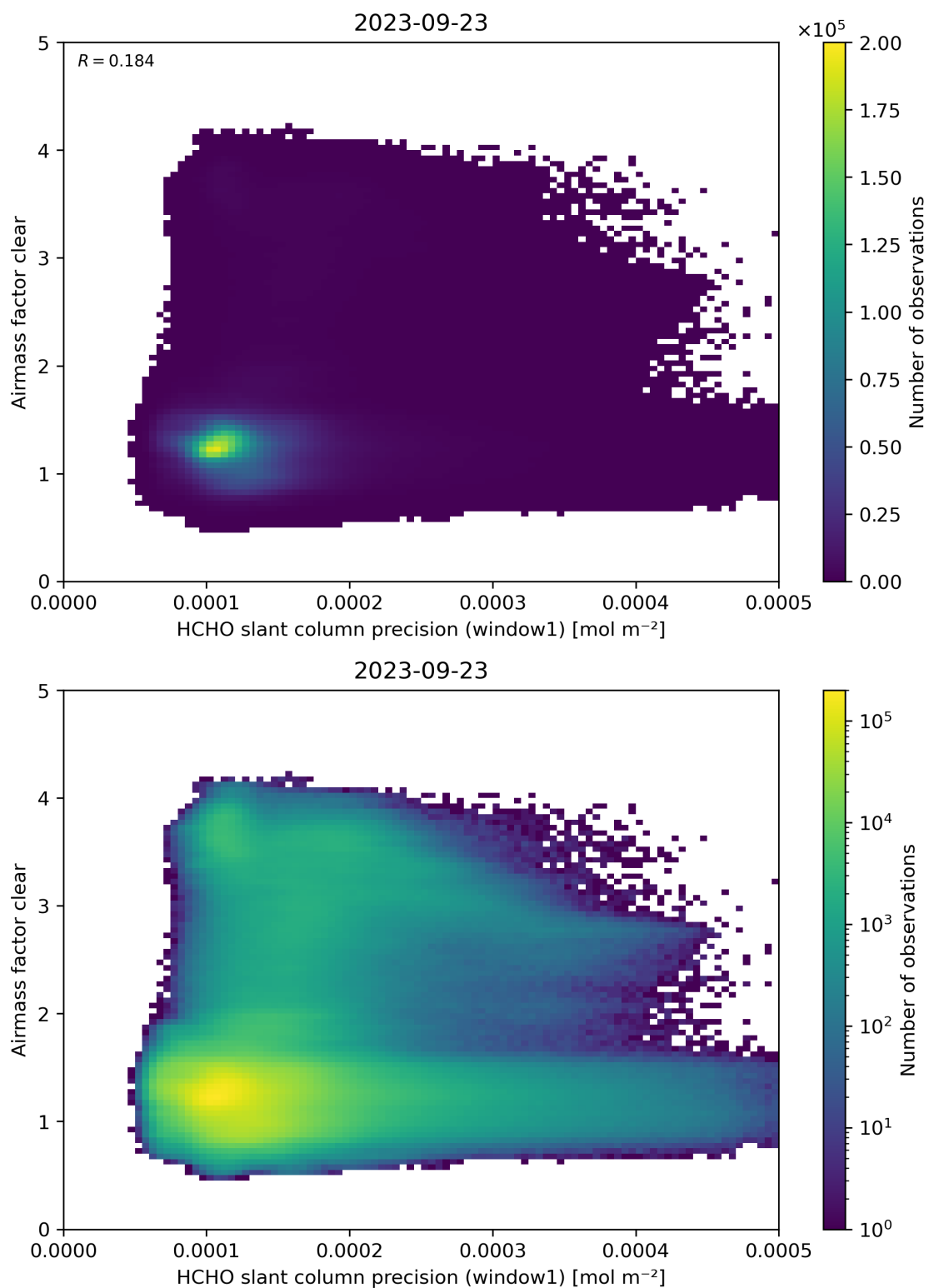
Figure 91: Scatter density plot of “HCHO slant column precision (window1)” against “Airmass factor clear” for 2023-09-22 to 2023-09-24.
