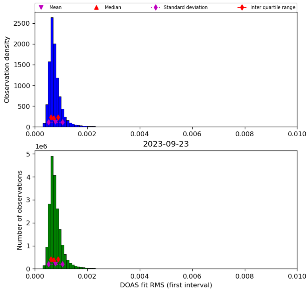
Figure 46: Histogram of “DOAS fit RMS (first interval)” for 2023-09-22 to 2023-09-24
