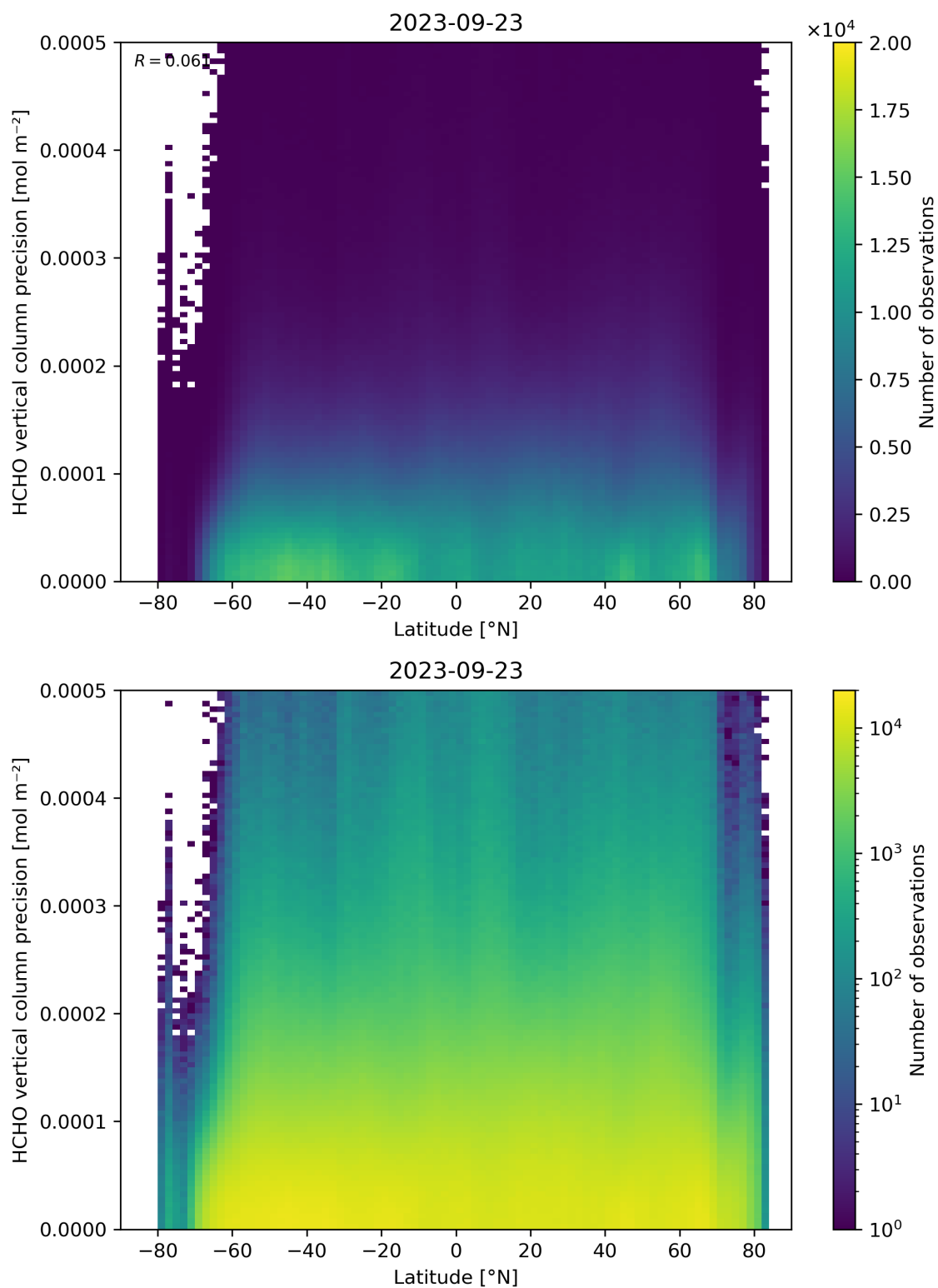
Figure 165: Scatter density plot of “Latitude” against “HCHO vertical column precision” for 2023-09-22 to 2023-09-24.
