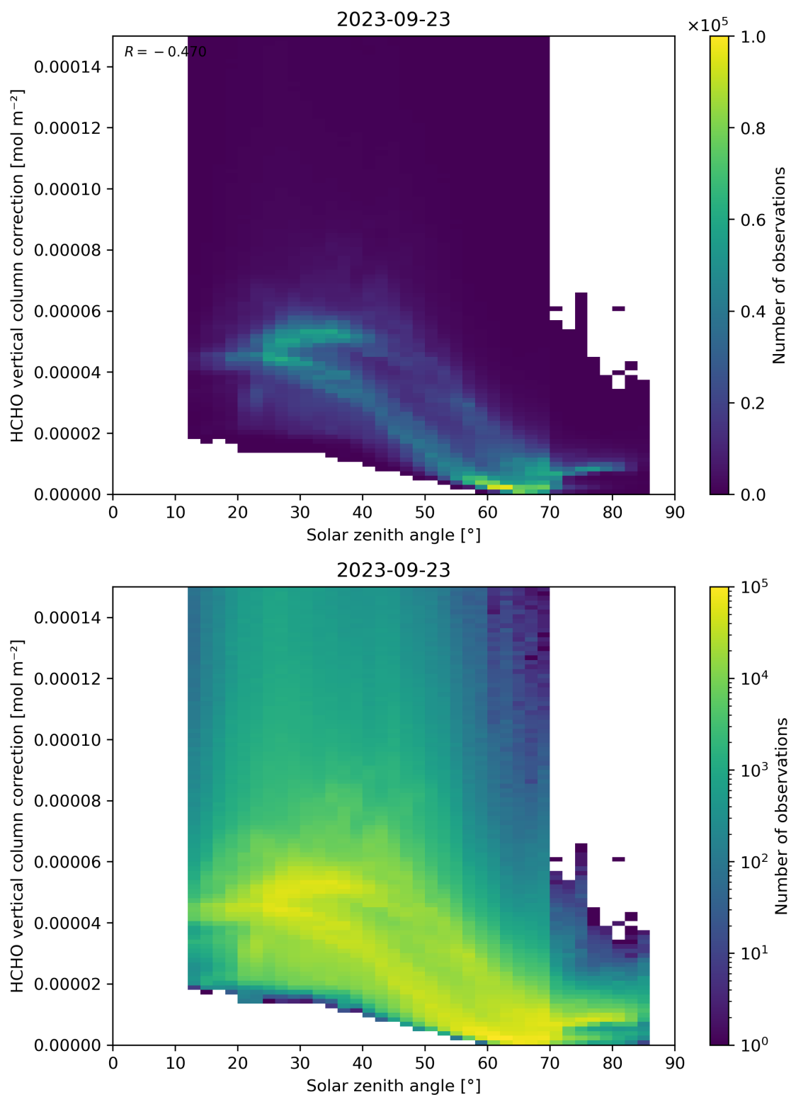
Figure 178: Scatter density plot of “Solar zenith angle” against “HCHO vertical column correction” for 2023-09-22 to 2023-09-24.
