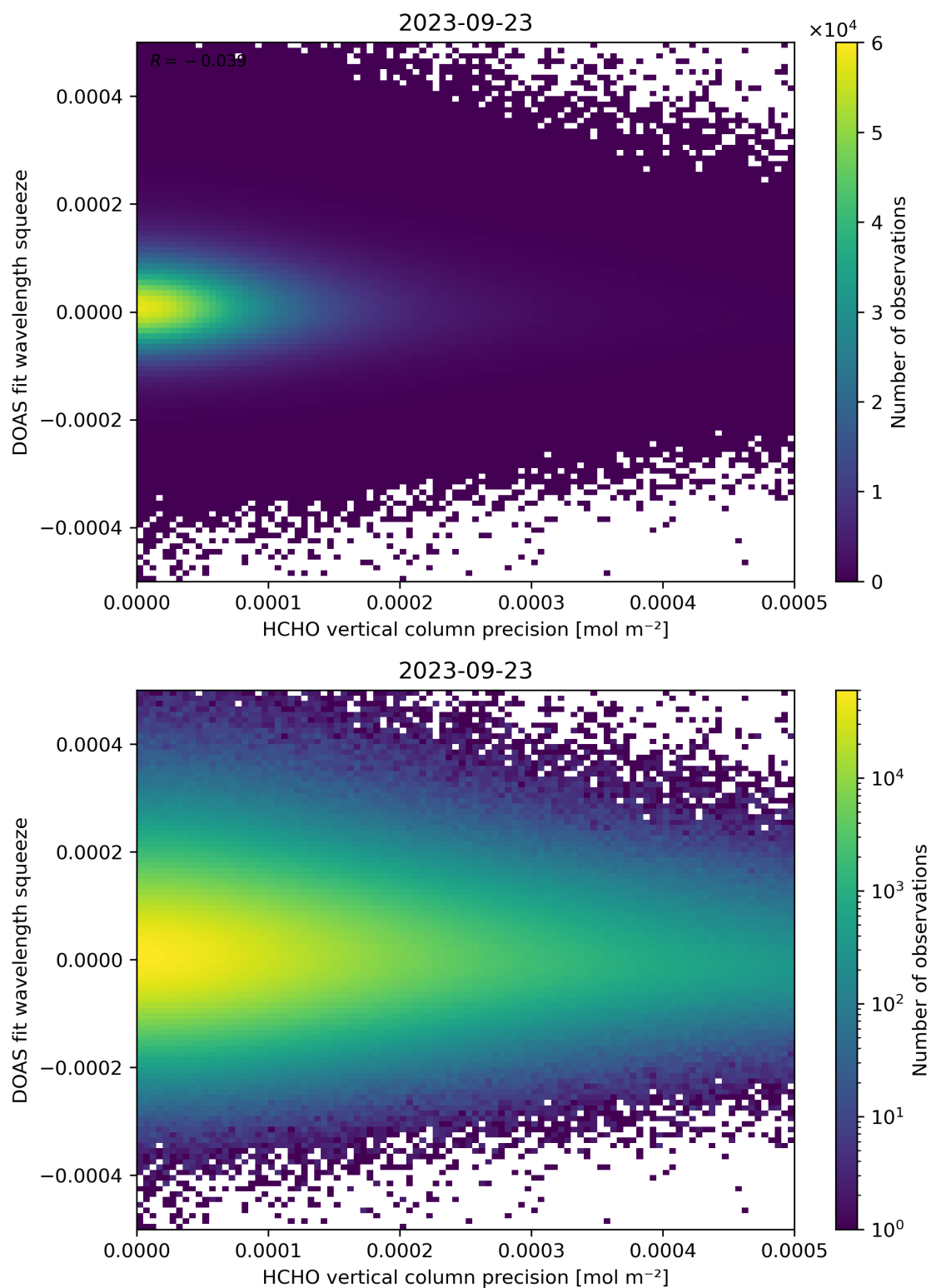
Figure 138: Scatter density plot of “HCHO vertical column precision” against “DOAS fit wavelength squeeze” for 2023-09-22 to 2023-09-24.
