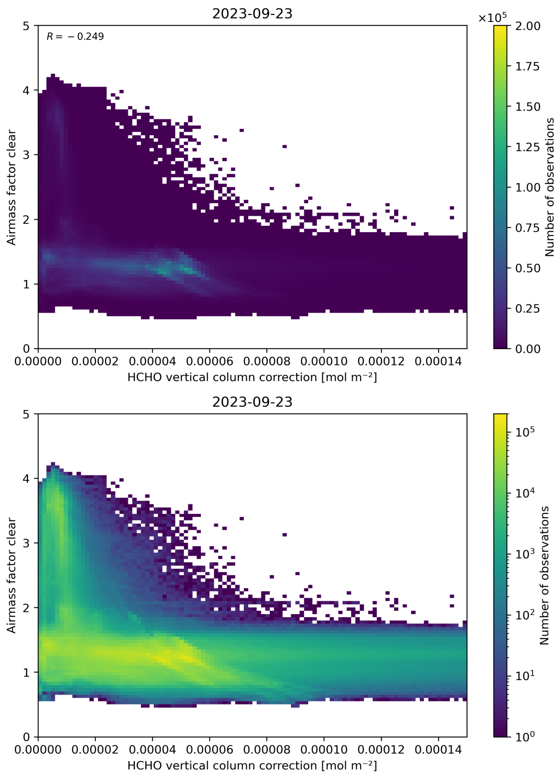
Figure 115: Scatter density plot of “HCHO vertical column correction” against “Airmass factor clear” for 2023-09-22 to 2023-09-24.
