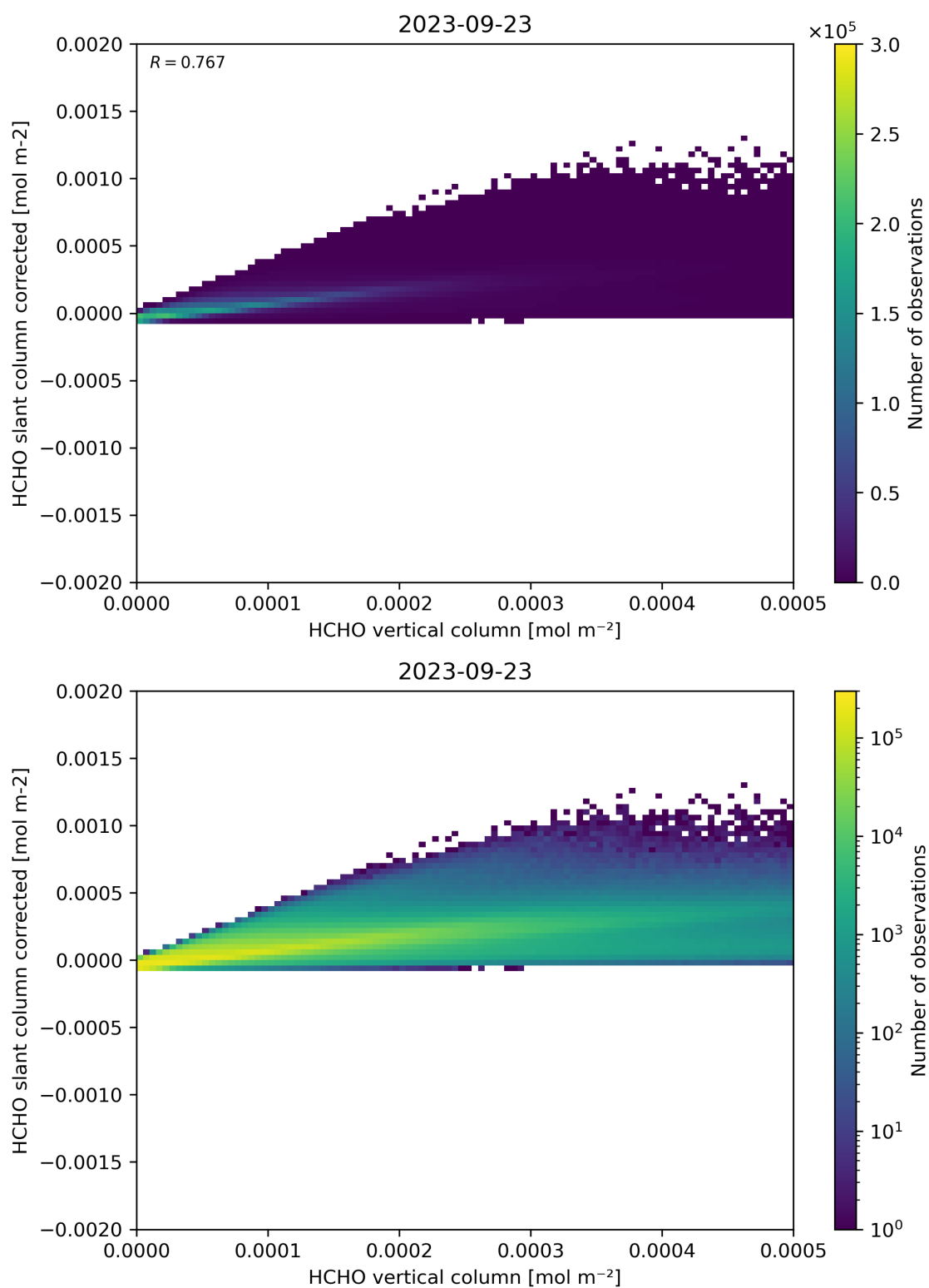
Figure 127: Scatter density plot of “HCHO vertical column” against “HCHO slant column corrected” for 2023-09-22 to 2023-09-24.
