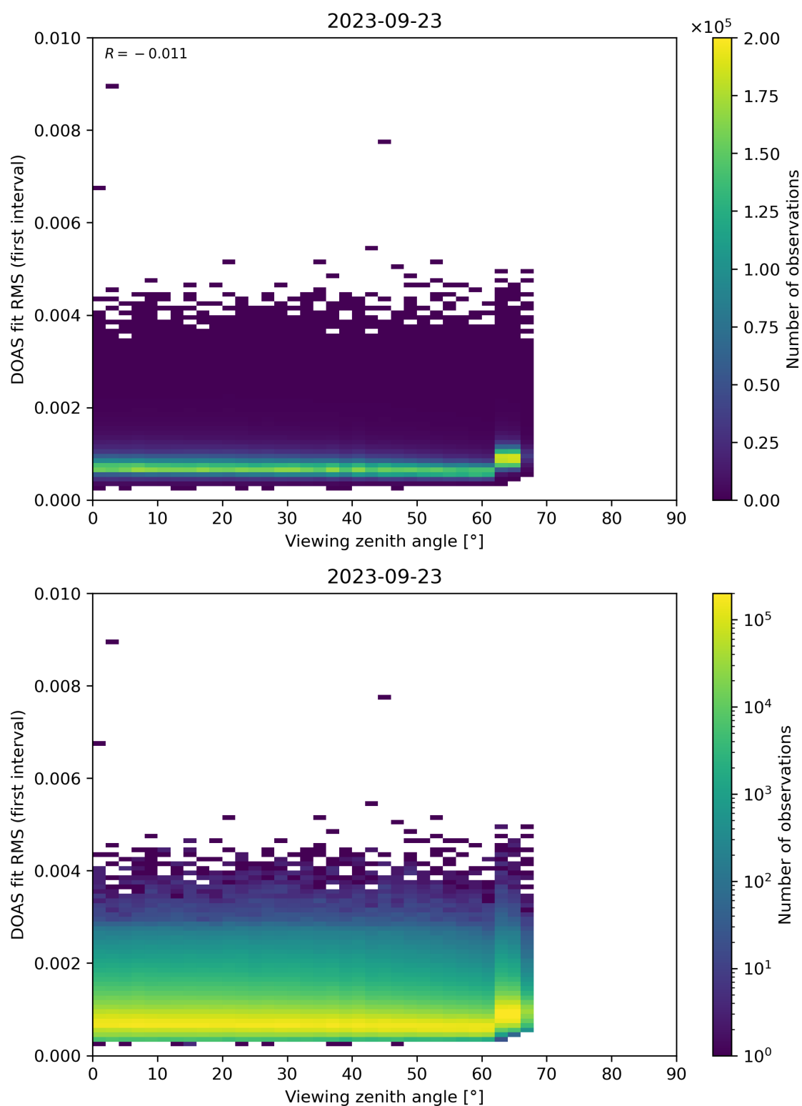
Figure 182: Scatter density plot of “Viewing zenith angle” against “DOAS fit RMS (first interval)” for 2023-09-22 to 2023-09-24.
