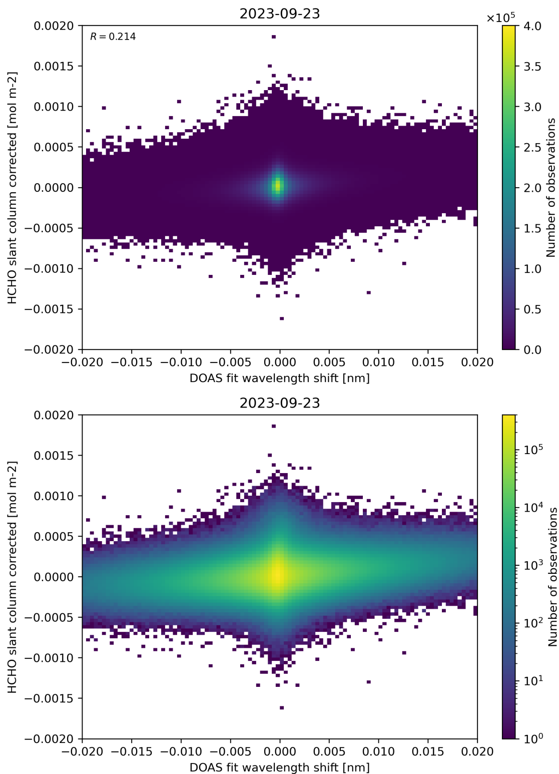
Figure 66: Scatter density plot of “DOAS fit wavelength shift” against “HCHO slant column corrected” for 2023-09-22 to 2023-09-24.
