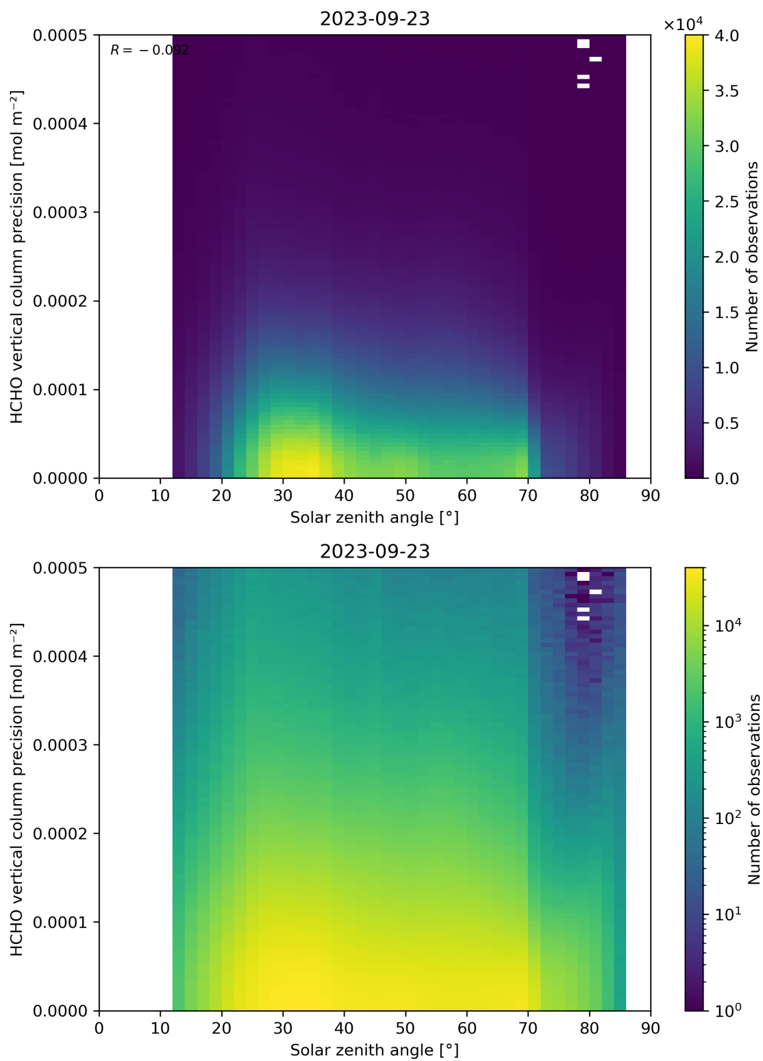
Figure 179: Scatter density plot of “Solar zenith angle” against “HCHO vertical column precision” for 2023-09-22 to 2023-09-24.
