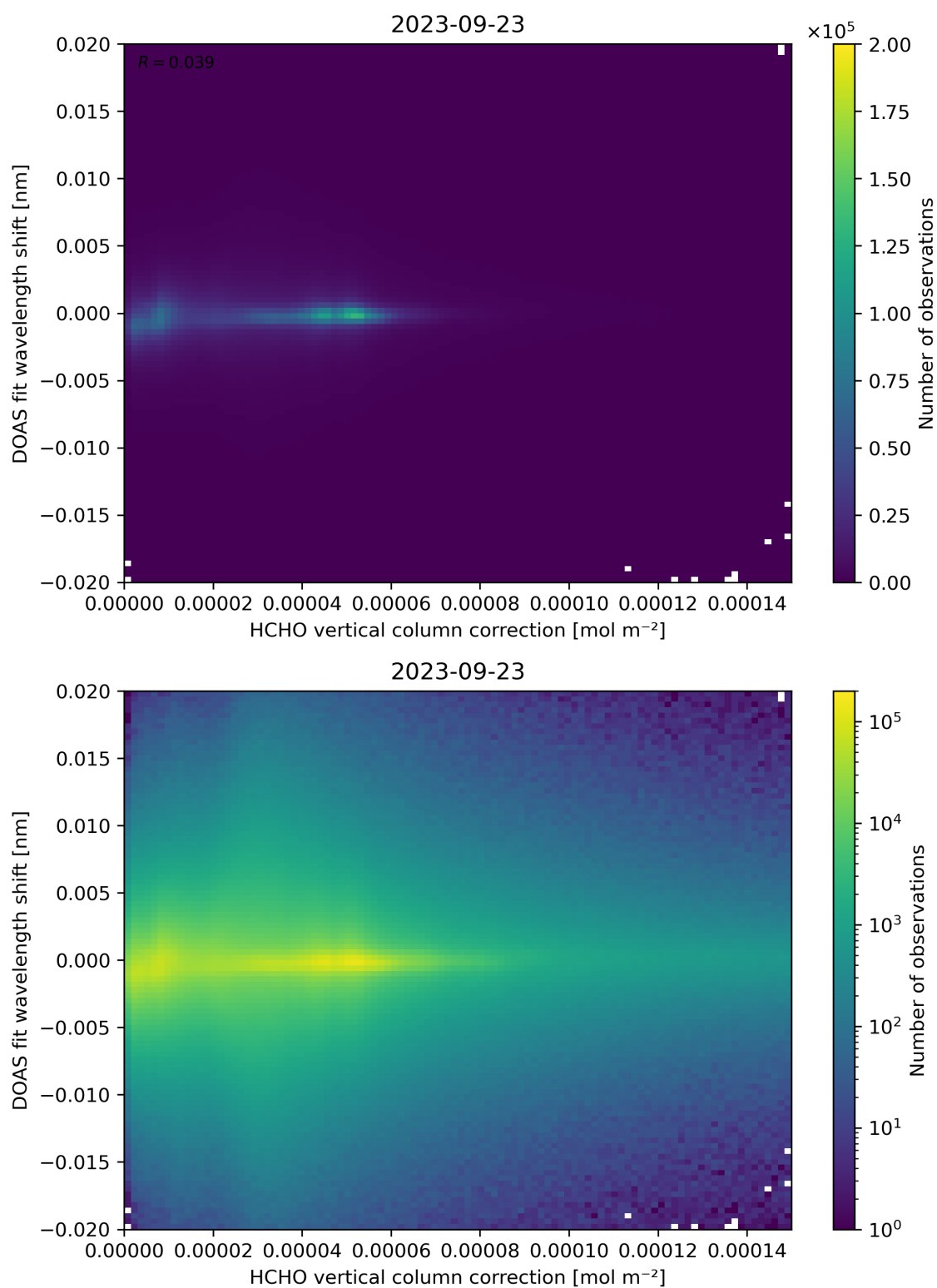
Figure 113: Scatter density plot of “HCHO vertical column correction” against “DOAS fit wavelength shift” for 2023-09-22 to 2023-09-24.
