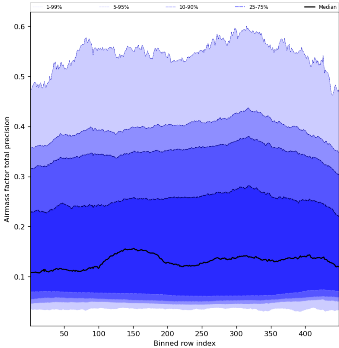
Figure 55: Along track statistics of “Airmass factor total precision” for 2023-09-22 to 2023-09-24
