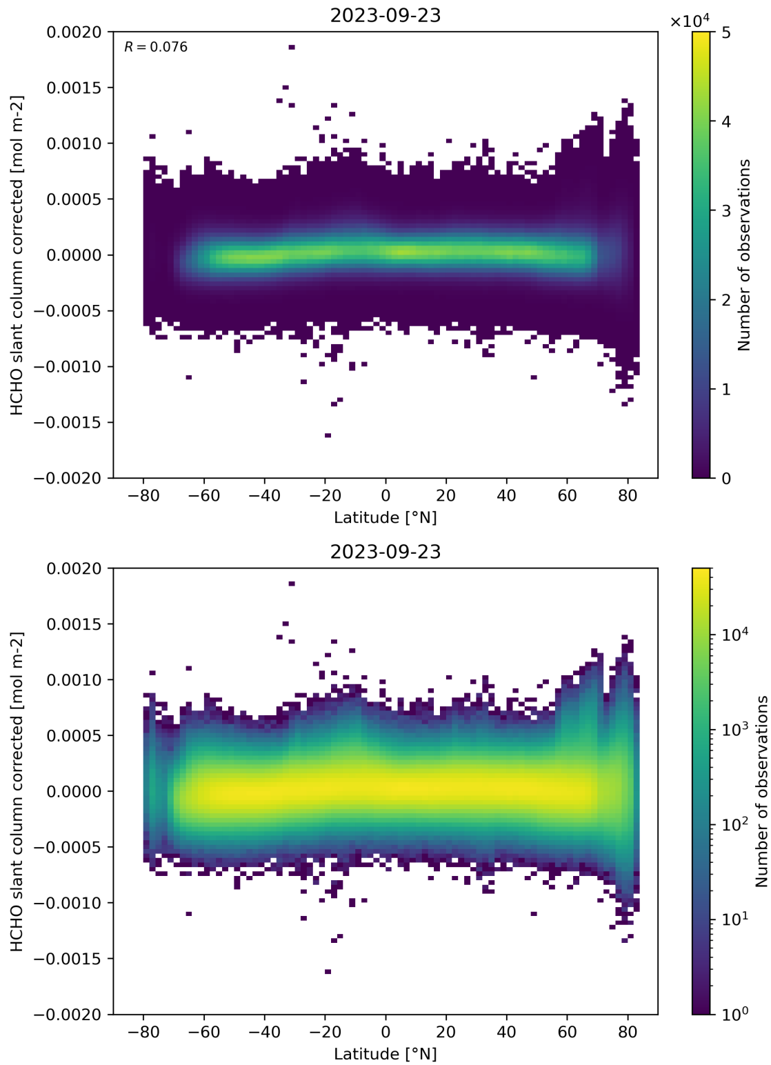
Figure 157: Scatter density plot of “Latitude” against “HCHO slant column corrected” for 2023-09-22 to 2023-09-24.
