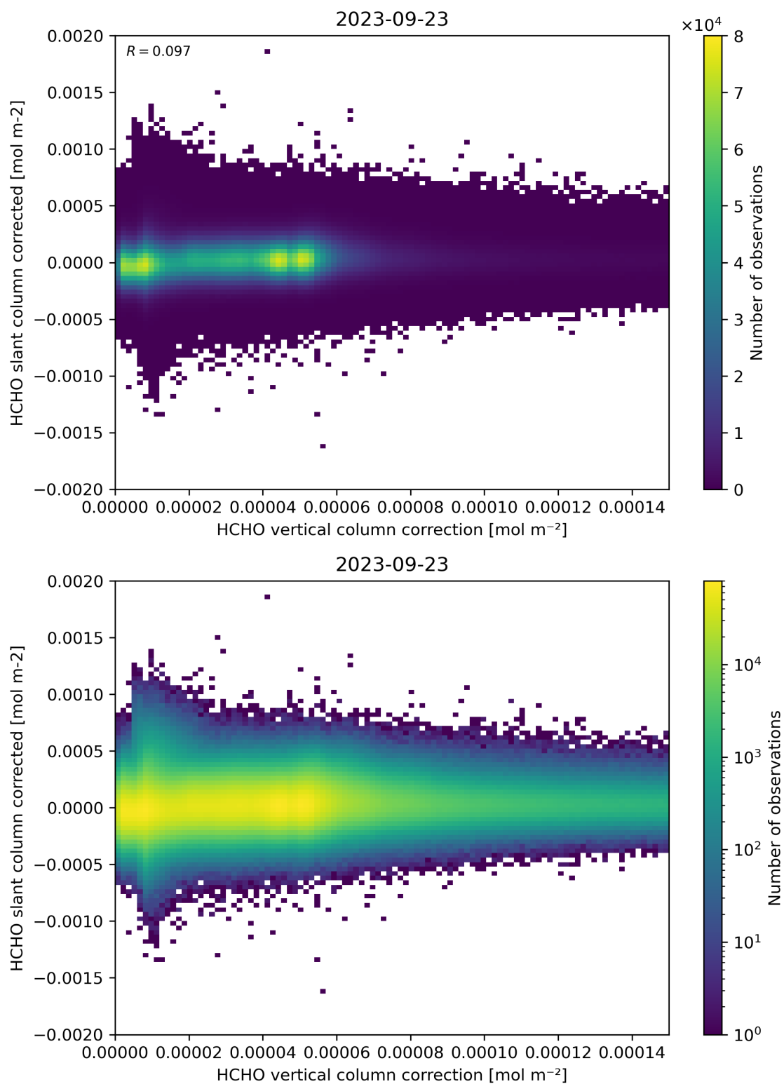
Figure 116: Scatter density plot of “HCHO vertical column correction” against “HCHO slant column corrected” for 2023-09-22 to 2023-09-24.
