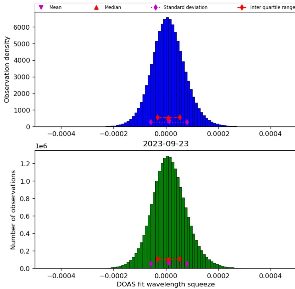
Figure 45: Histogram of “DOAS fit wavelength squeeze” for 2023-09-22 to 2023-09-24
