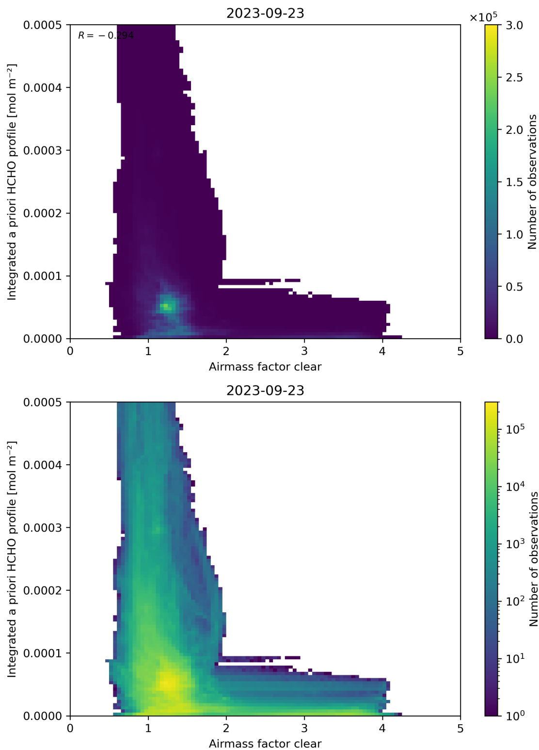
Figure 76: Scatter density plot of “Airmass factor clear” against “Integrated a priori HCHO profile” for 2023-09-22 to 2023-09-24.
