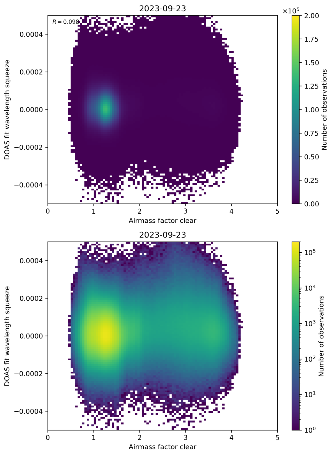
Figure 73: Scatter density plot of “Airmass factor clear” against “DOAS fit wavelength squeeze” for 2023-09-22 to 2023-09-24.
