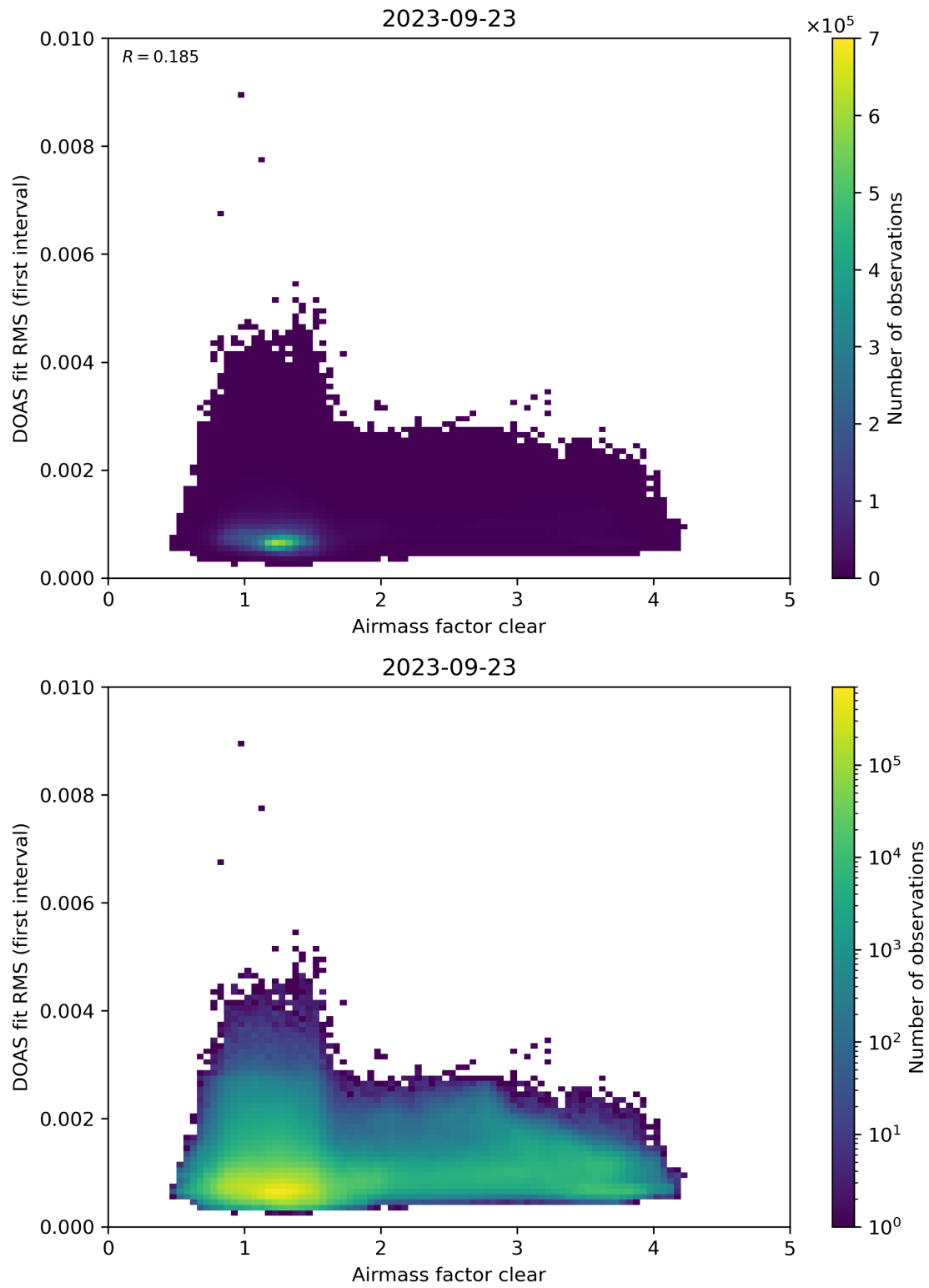
Figure 71: Scatter density plot of “Airmass factor clear” against “DOAS fit RMS (first interval)” for 2023-09-22 to 2023-09-24.
