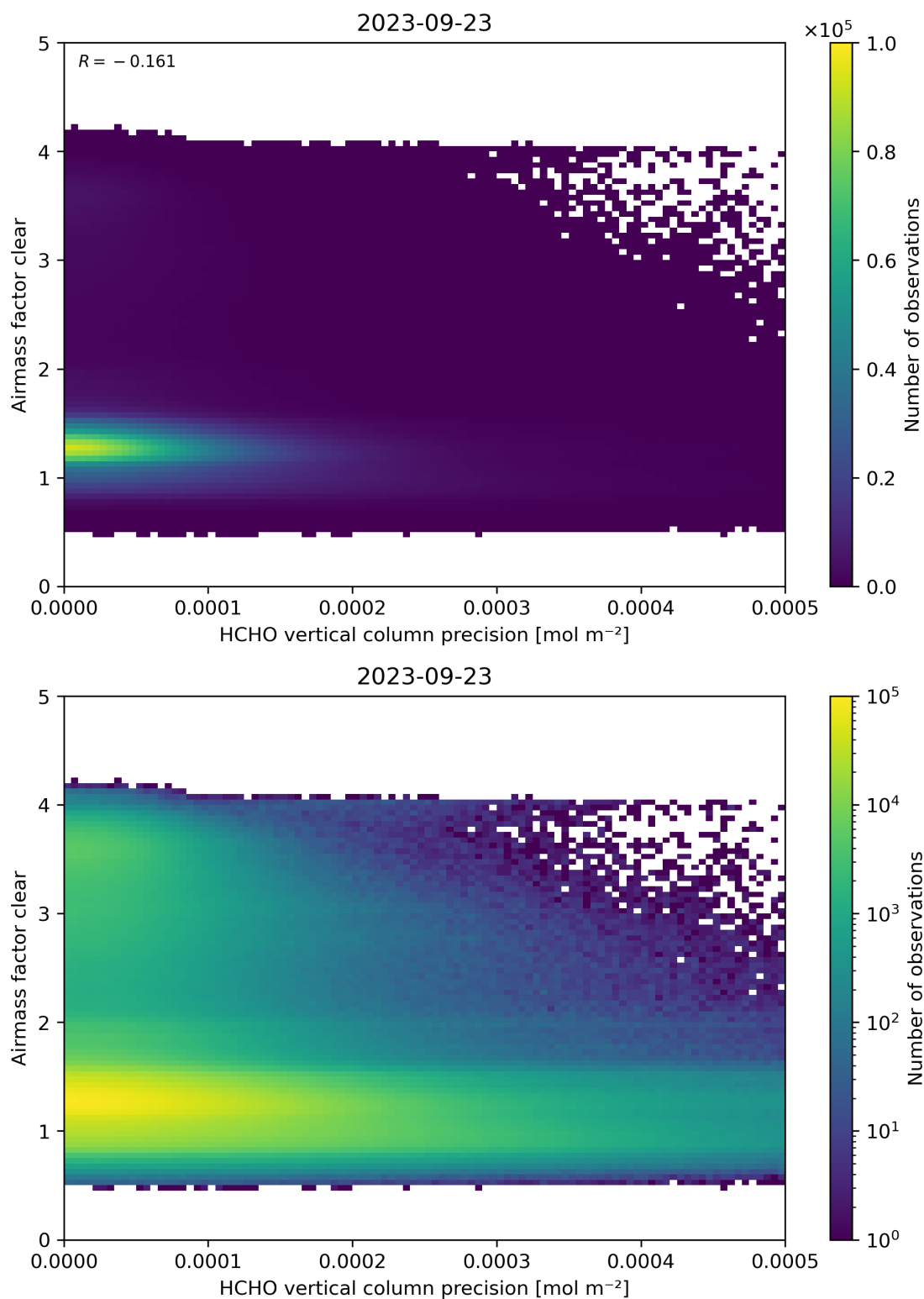
Figure 139: Scatter density plot of “HCHO vertical column precision” against “Airmass factor clear” for 2023-09-22 to 2023-09-24.
