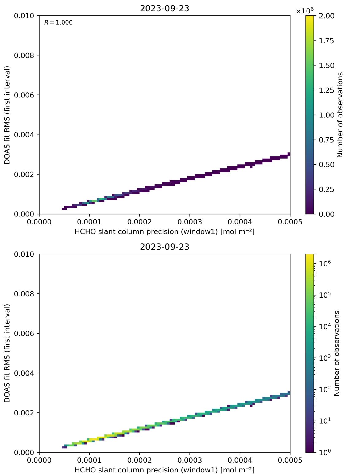
Figure 88: Scatter density plot of “HCHO slant column precision (window1)” against “DOAS fit RMS (first interval)” for 2023-09-22 to 2023-09-24.
