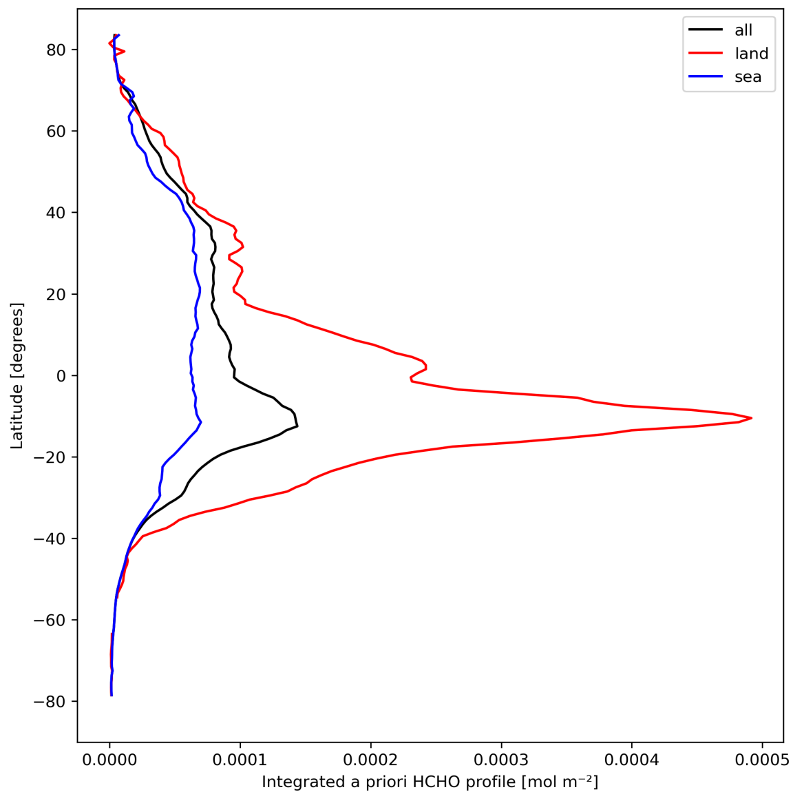
Figure 29: Zonal average of “Integrated a priori HCHO profile” for 2023-09-22 to 2023-09-24.
