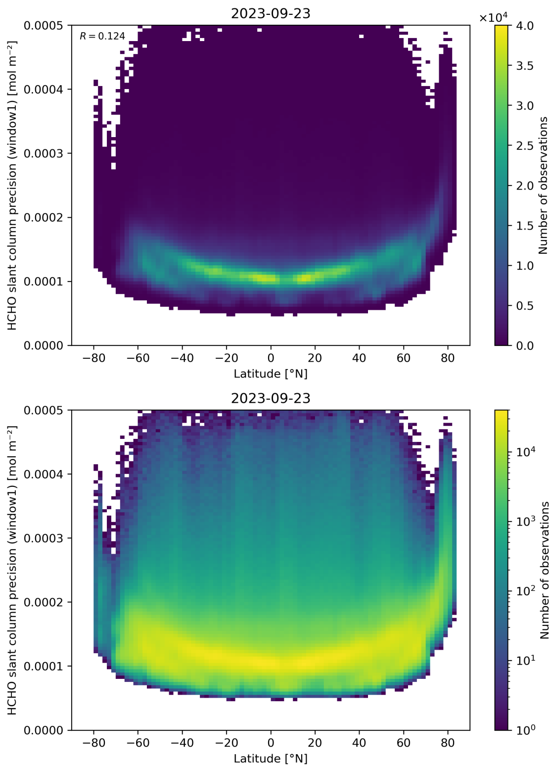
Figure 160: Scatter density plot of “Latitude” against “HCHO slant column precision (window1)” for 2023-09-22 to 2023-09-24.
