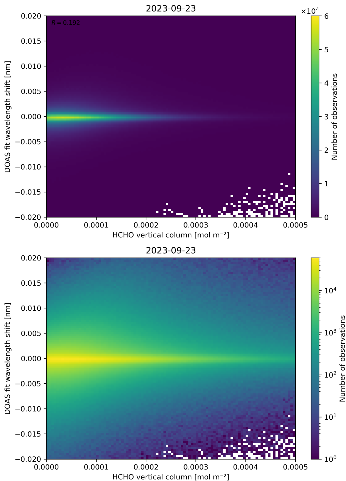
Figure 124: Scatter density plot of “HCHO vertical column” against “DOAS fit wavelength shift” for 2023-09-22 to 2023-09-24.
