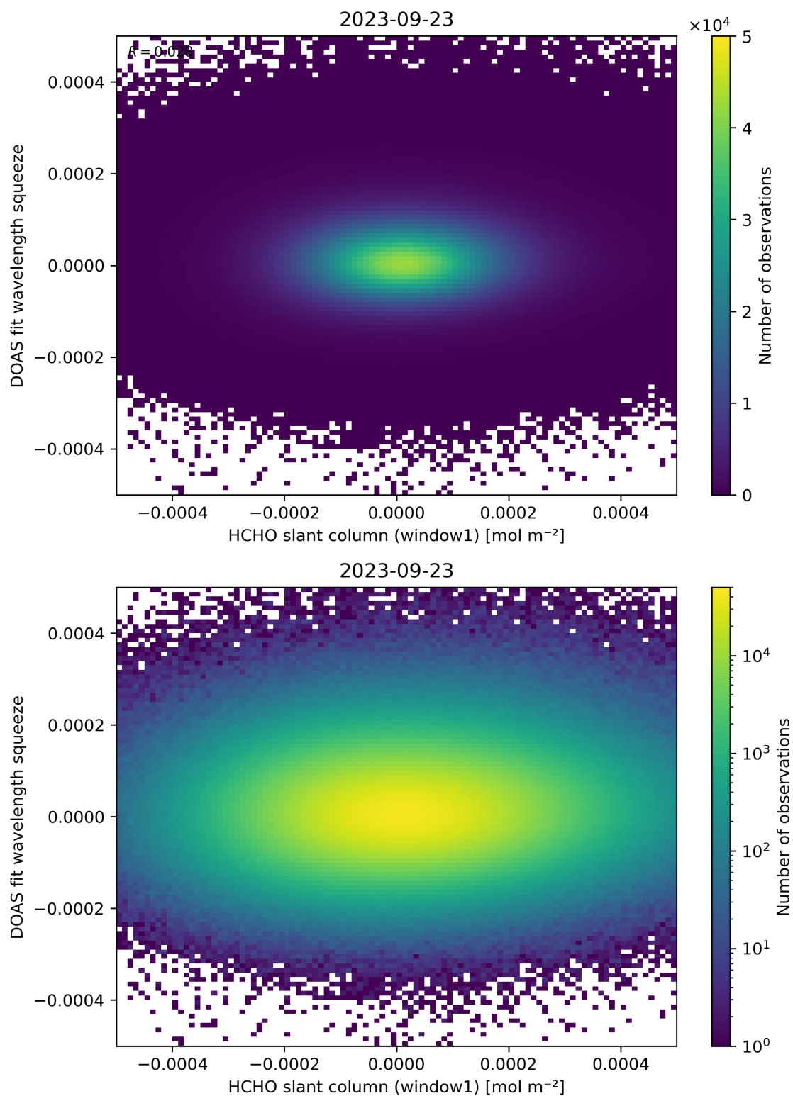
Figure 80: Scatter density plot of “HCHO slant column (window1)” against “DOAS fit wavelength squeeze” for 2023-09-22 to 2023-09-24.
