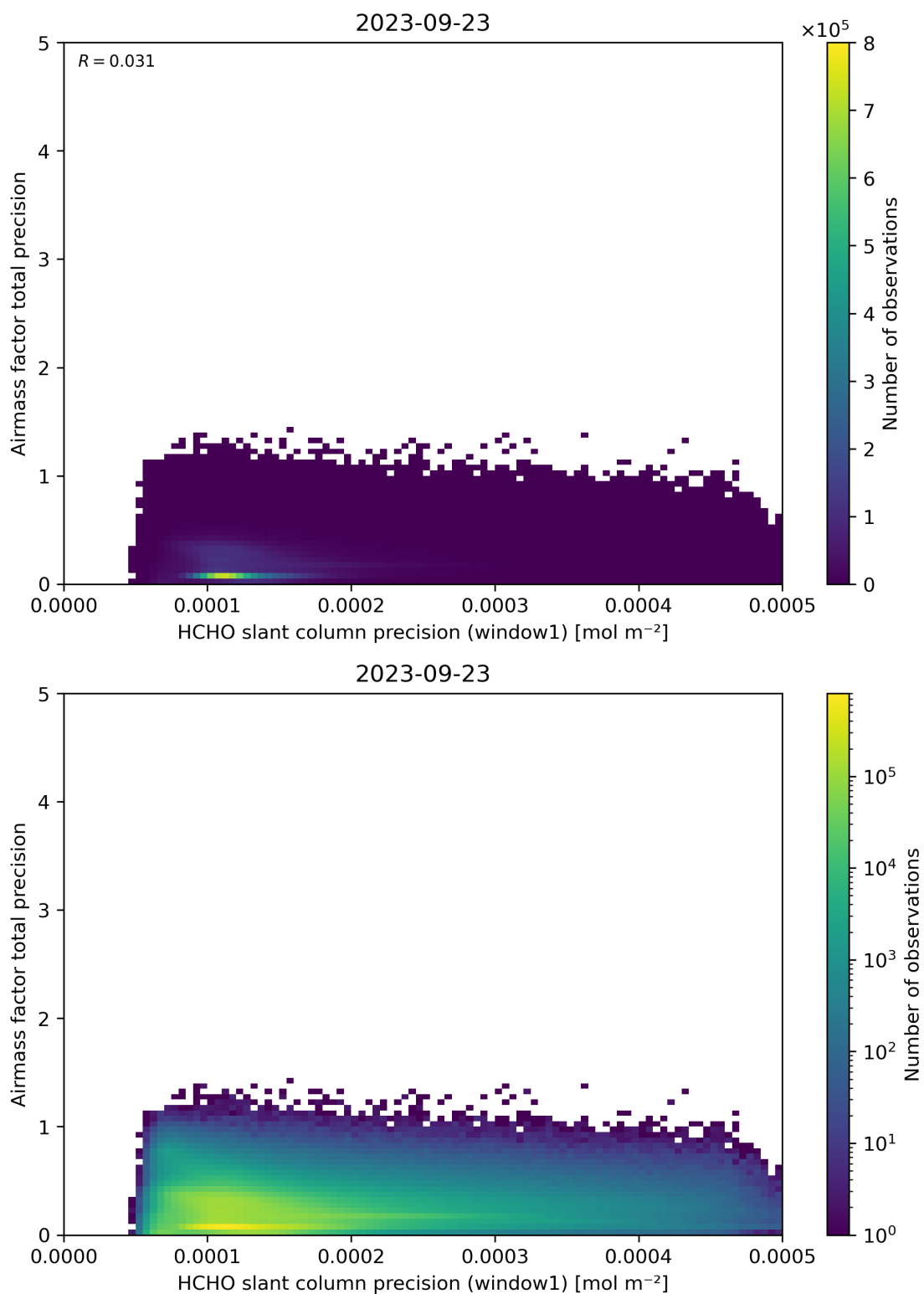
Figure 95: Scatter density plot of “HCHO slant column precision (window1)” against “Airmass factor total precision” for 2023-09-22 to 2023-09-24.
