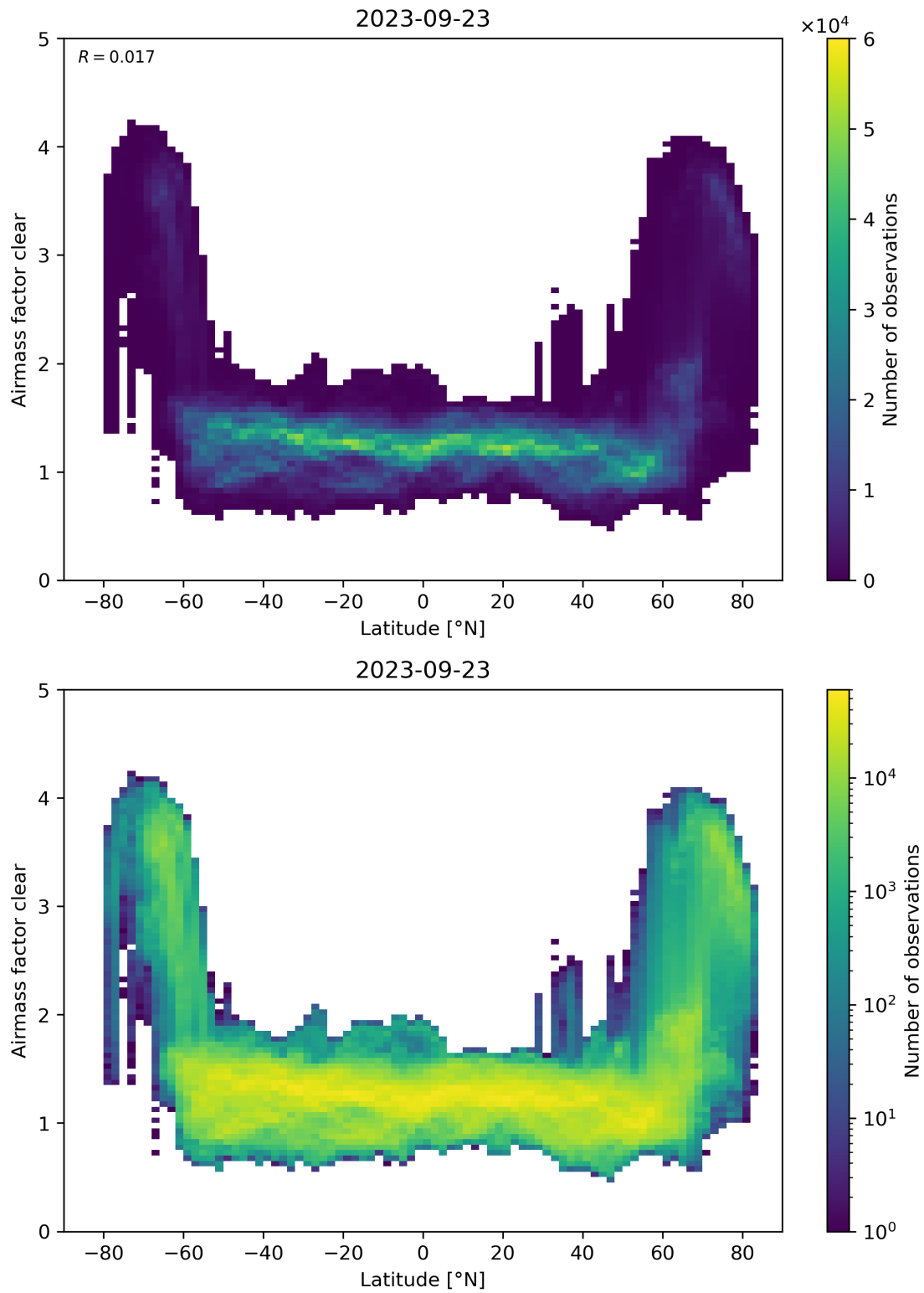
Figure 156: Scatter density plot of “Latitude” against “Airmass factor clear” for 2023-09-22 to 2023-09-24.
