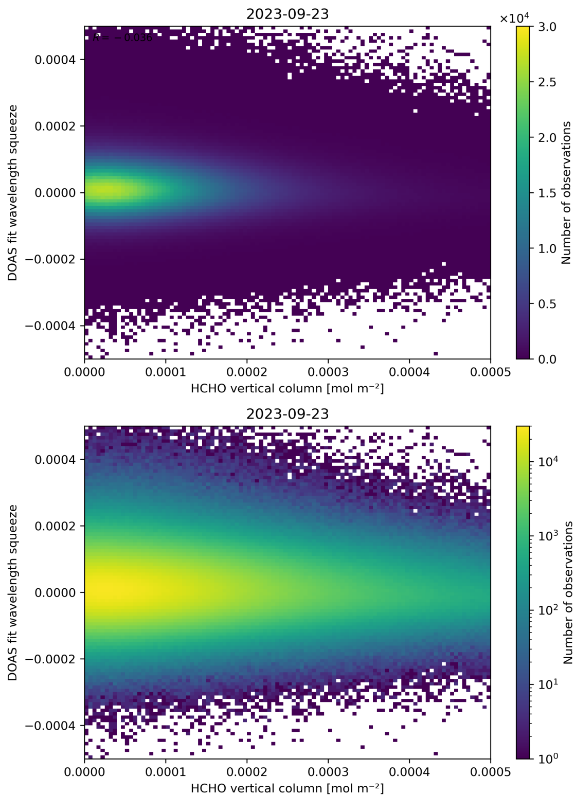
Figure 125: Scatter density plot of “HCHO vertical column” against “DOAS fit wavelength squeeze” for 2023-09-22 to 2023-09-24.
