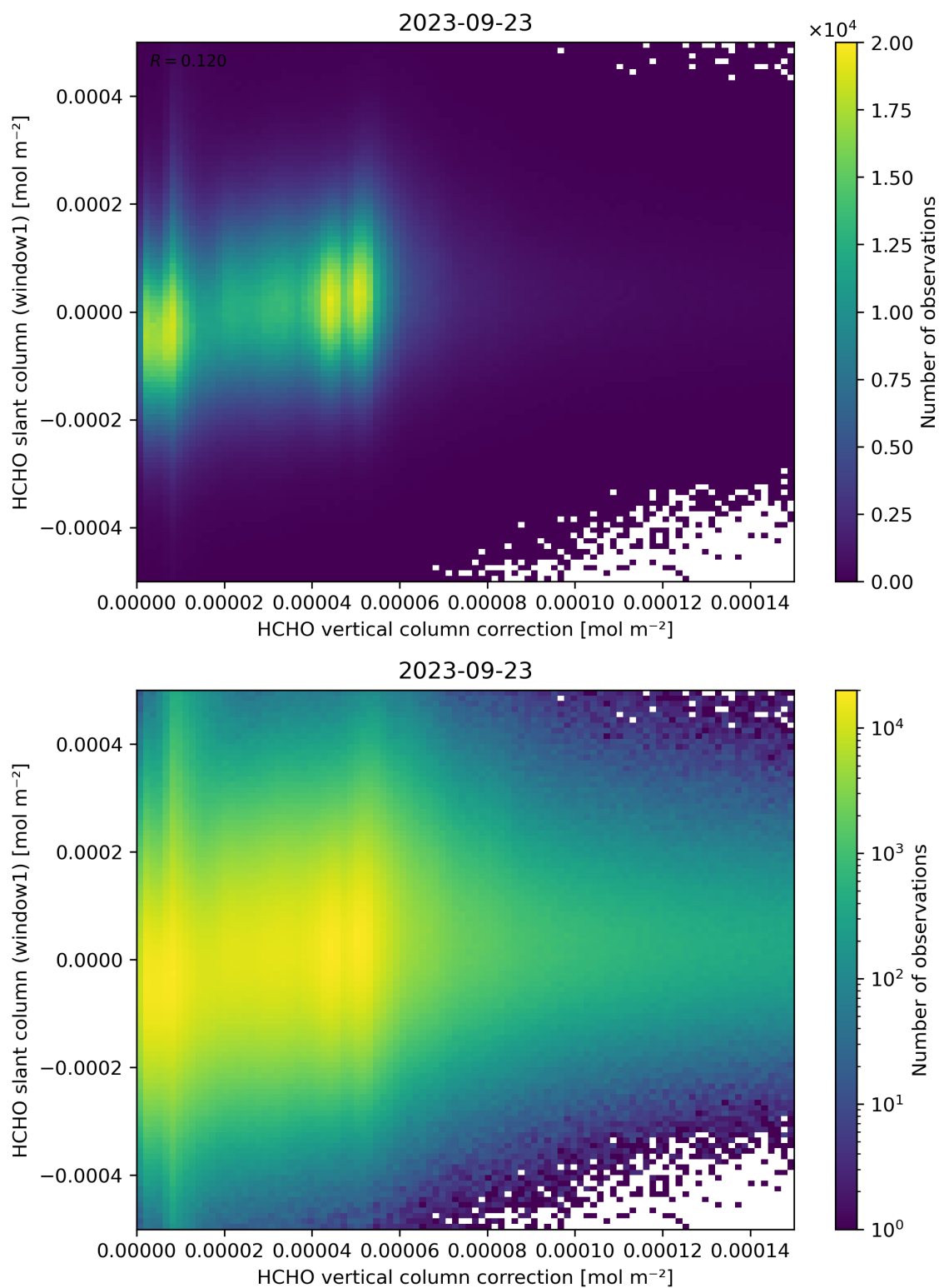
Figure 118: Scatter density plot of “HCHO vertical column correction” against “HCHO slant column (window1)” for 2023-09-22 to 2023-09-24.
