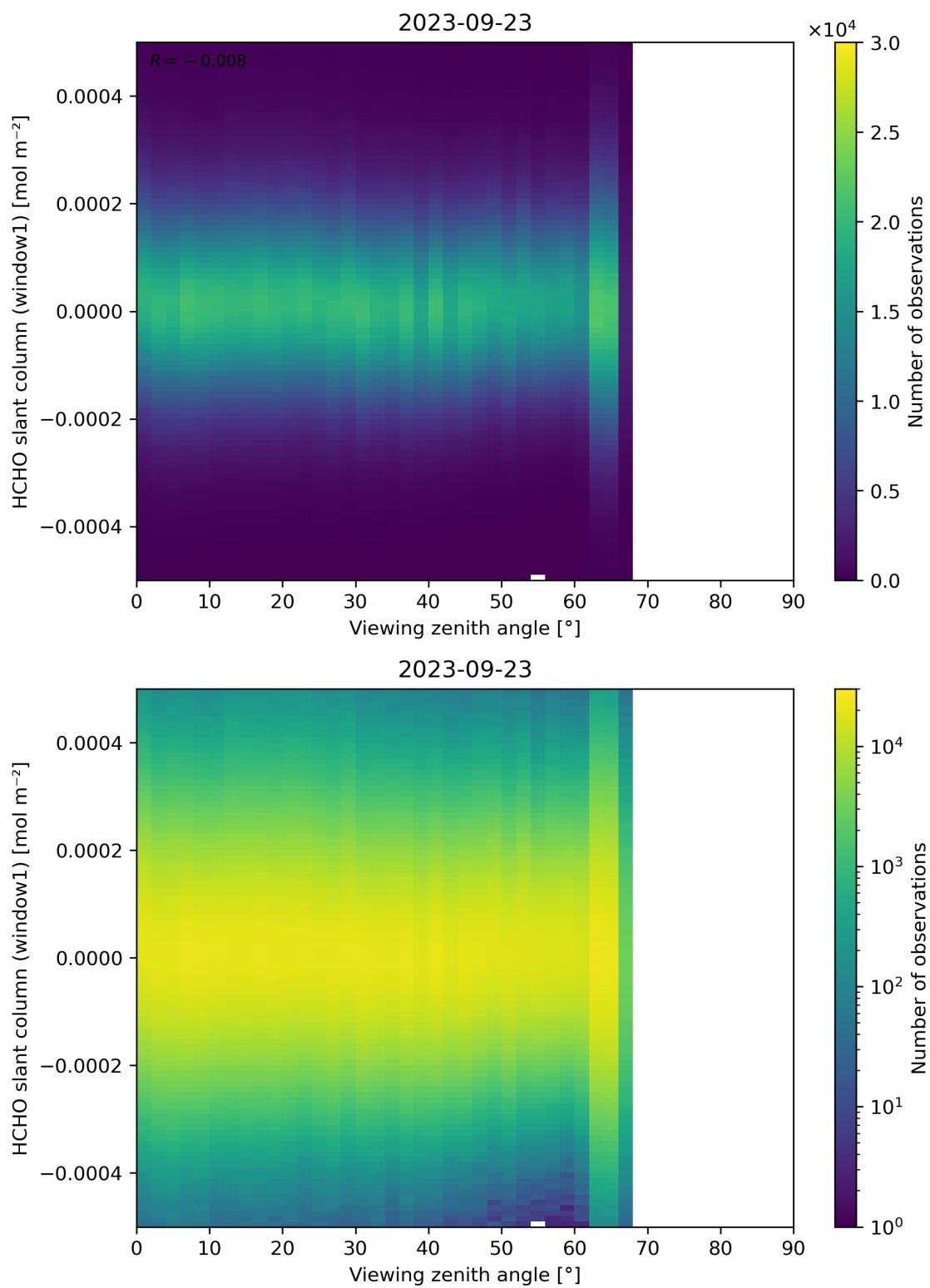
Figure 188: Scatter density plot of “Viewing zenith angle” against “HCHO slant column (window1)” for 2023-09-22 to 2023-09-24.
