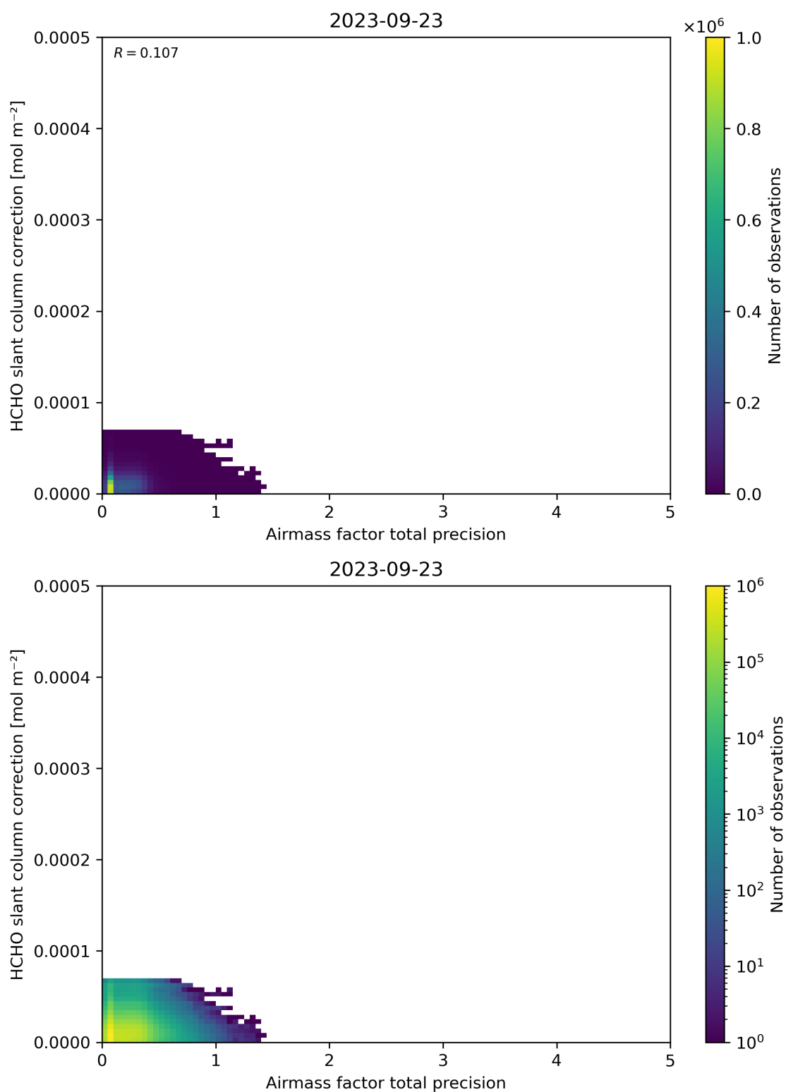
Figure 110: Scatter density plot of “Airmass factor total precision” against “HCHO slant column correction” for 2023-09-22 to 2023-09-24.
