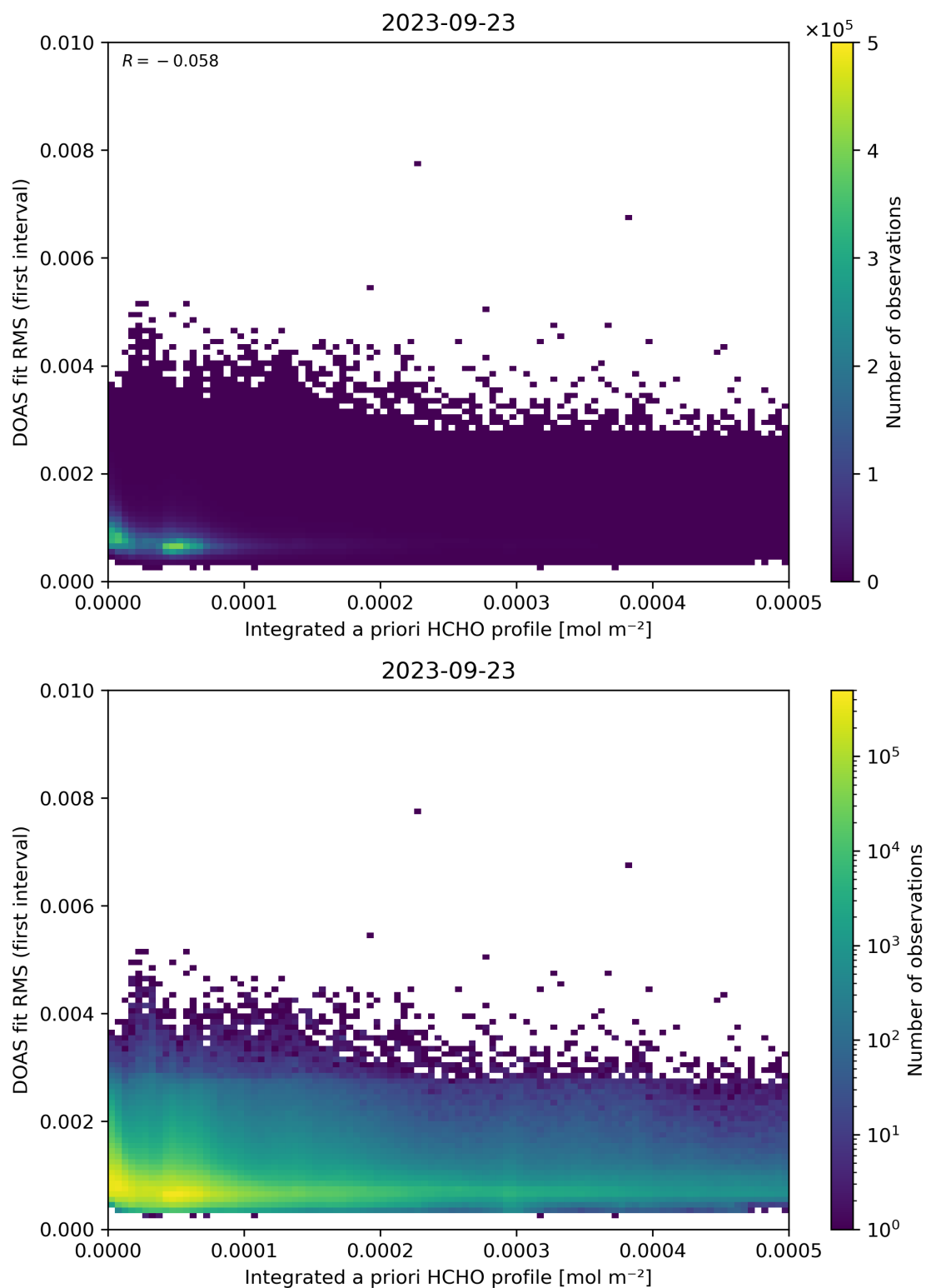
Figure 148: Scatter density plot of “Integrated a priori HCHO profile” against “DOAS fit RMS (first interval)” for 2023-09-22 to 2023-09-24.
