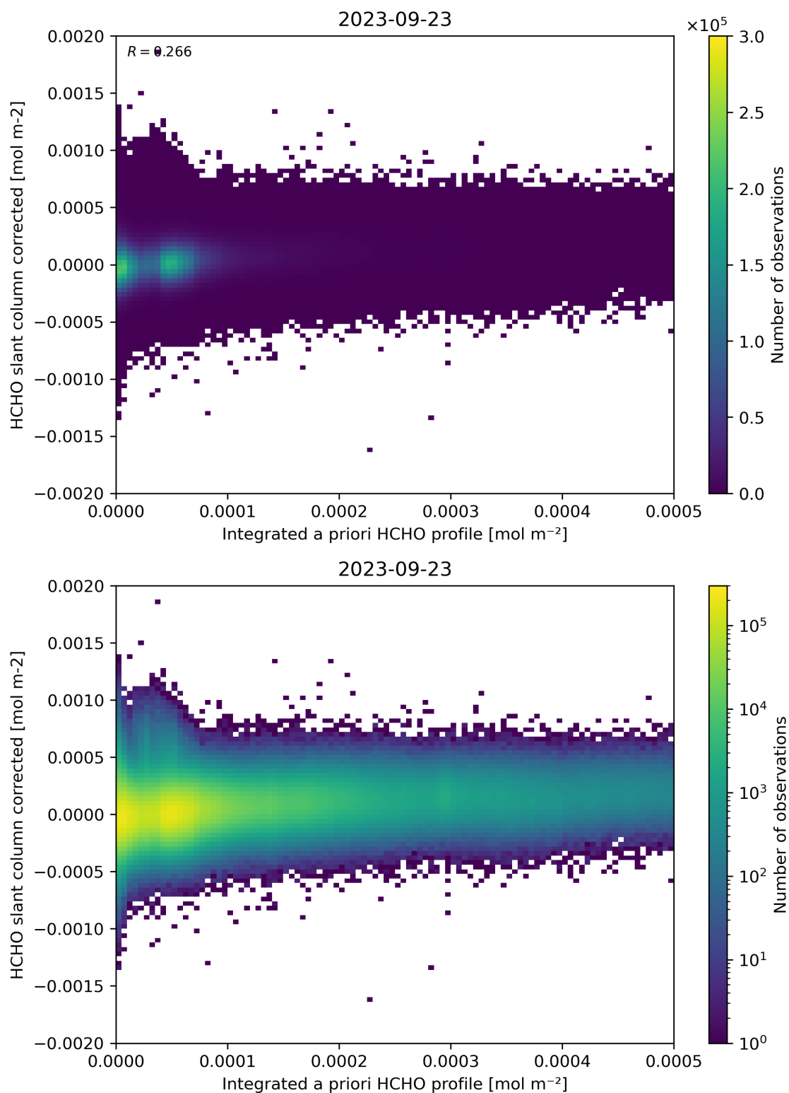
Figure 151: Scatter density plot of “Integrated a priori HCHO profile” against “HCHO slant column corrected” for 2023-09-22 to 2023-09-24.
