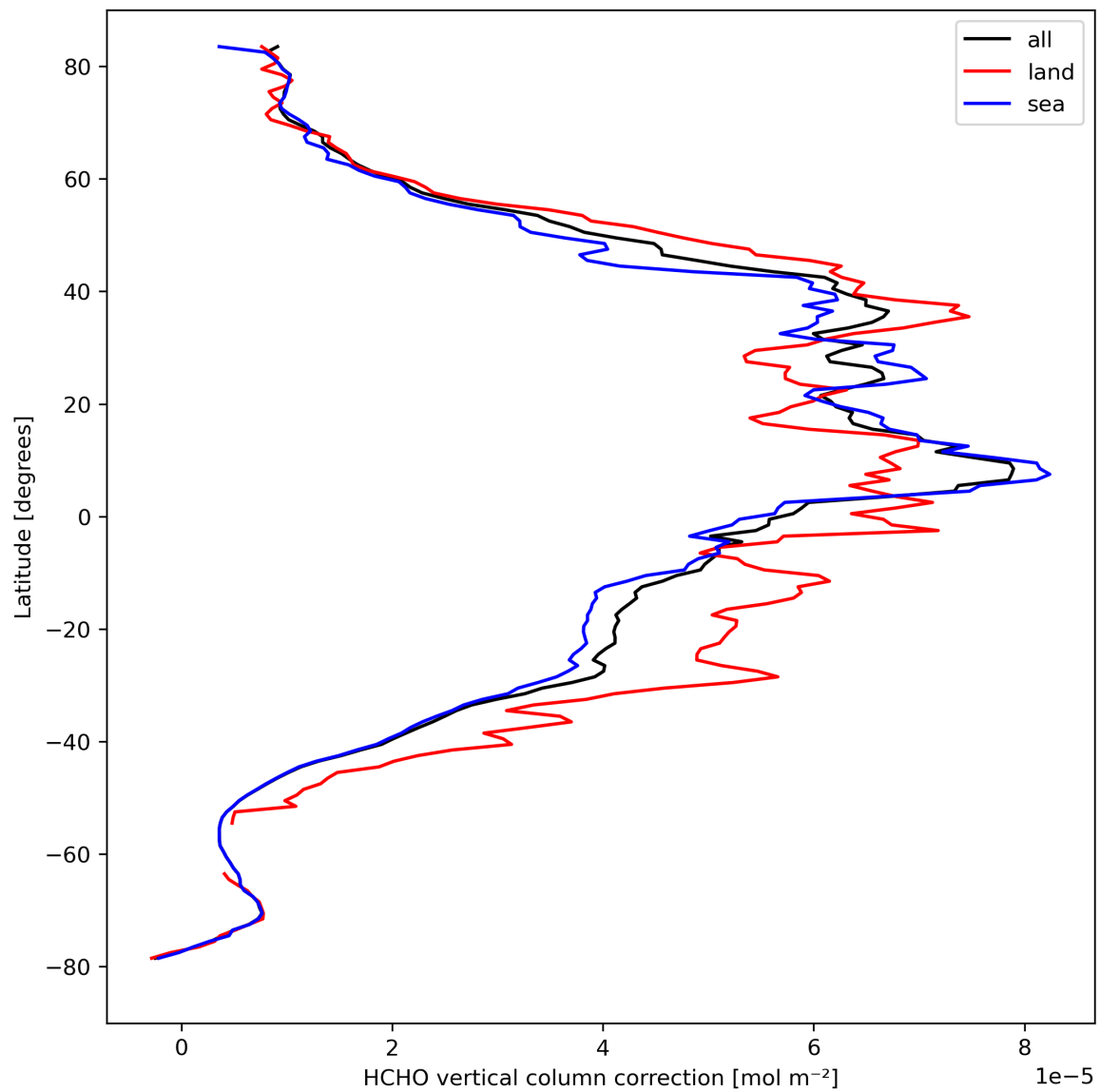
Figure 23: Zonal average of “HCHO vertical column correction” for 2023-09-22 to 2023-09-24.
