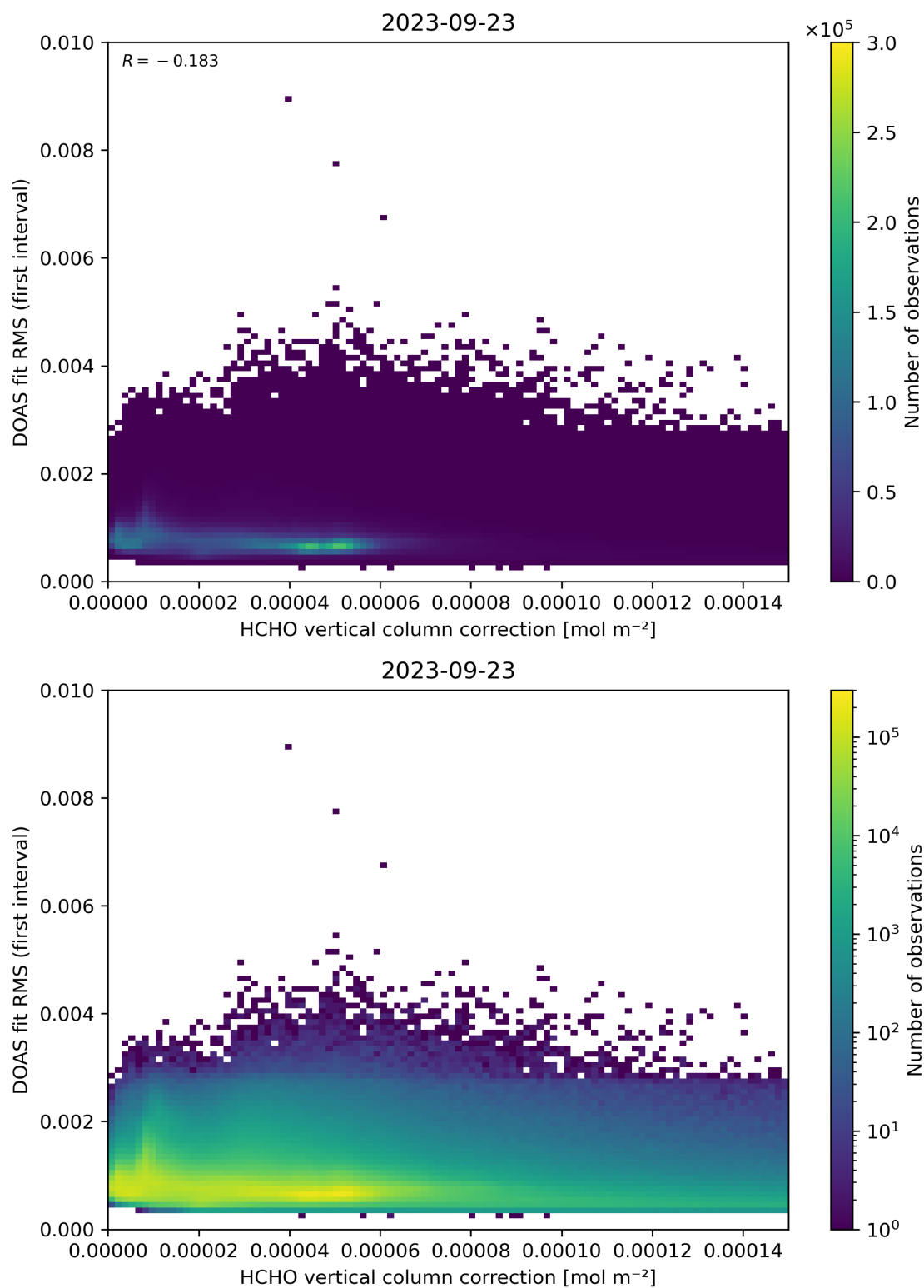
Figure 112: Scatter density plot of “HCHO vertical column correction” against “DOAS fit RMS (first interval)” for 2023-09-22 to 2023-09-24.
