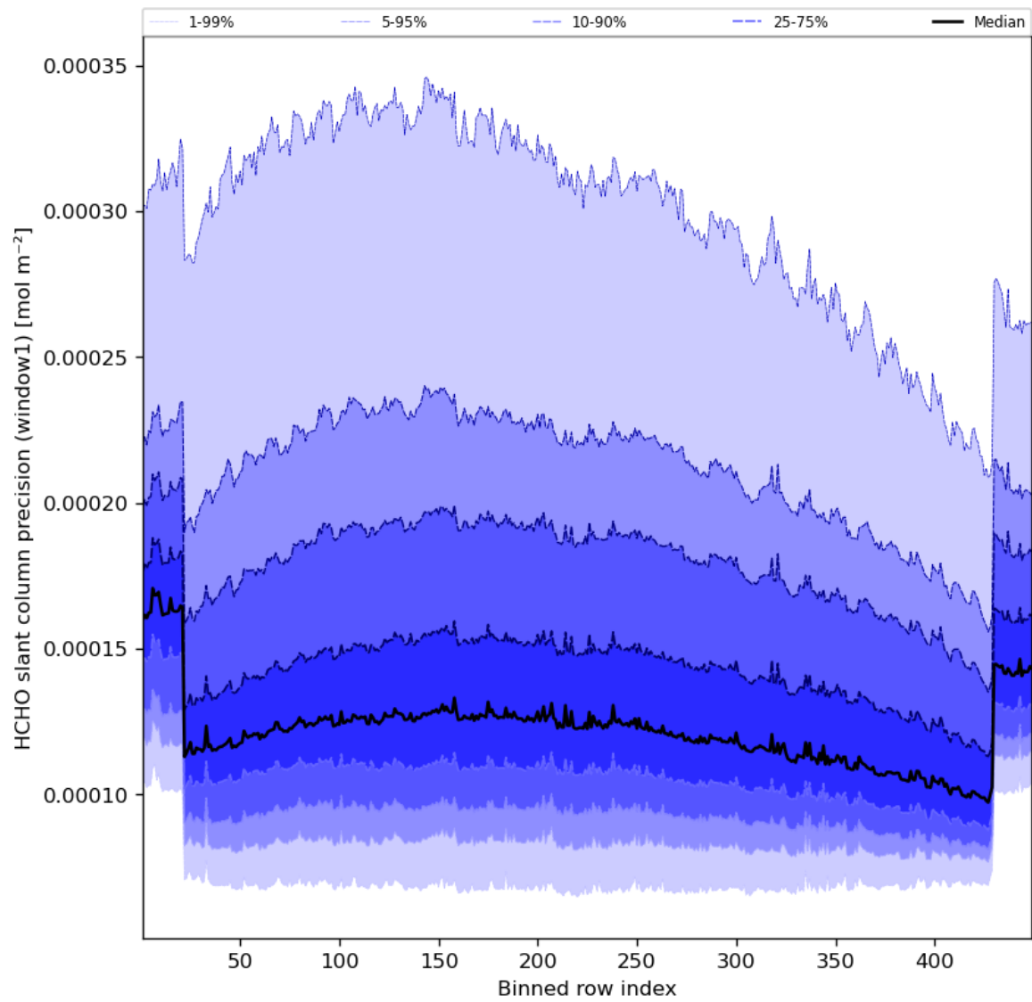
Figure 53: Along track statistics of “HCHO slant column precision (window1)” for 2023-09-22 to 2023-09-24
