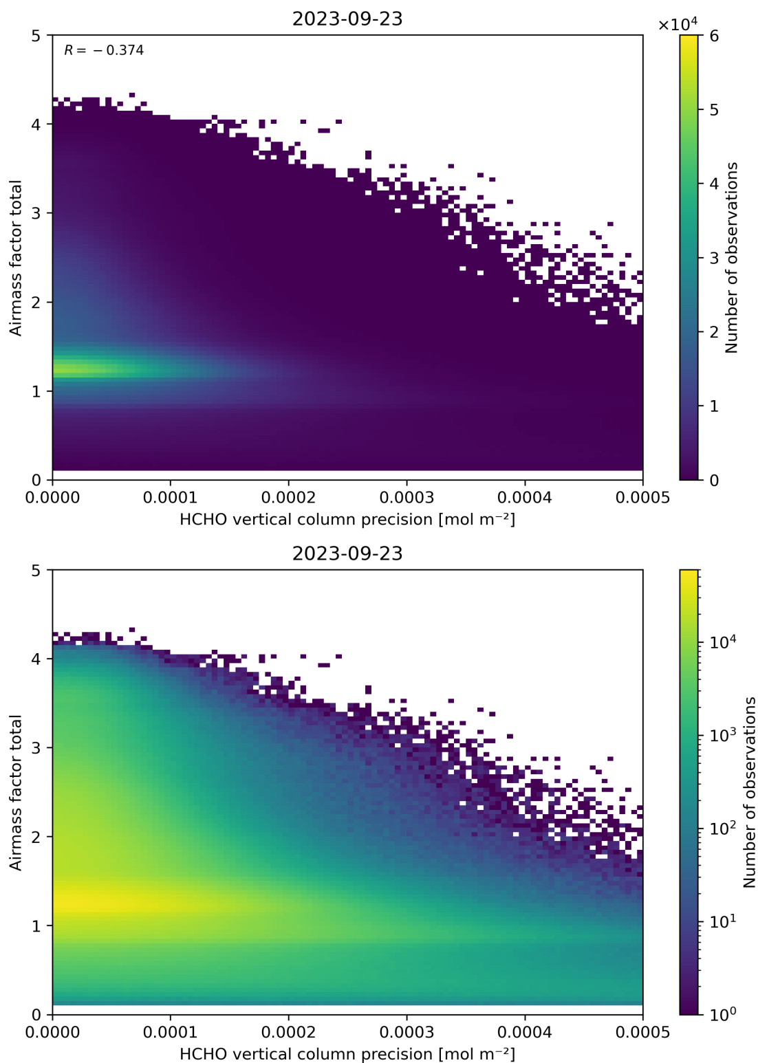
Figure 144: Scatter density plot of “HCHO vertical column precision” against “Airmass factor total” for 2023-09-22 to 2023-09-24.
