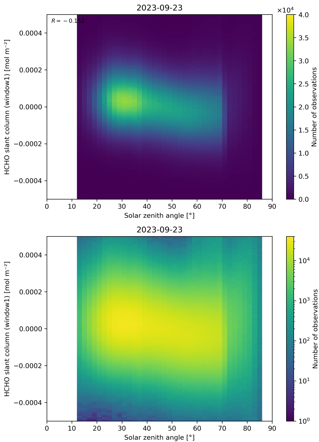
Figure 173: Scatter density plot of “Solar zenith angle” against “HCHO slant column (window1)” for 2023-09-22 to 2023-09-24.
