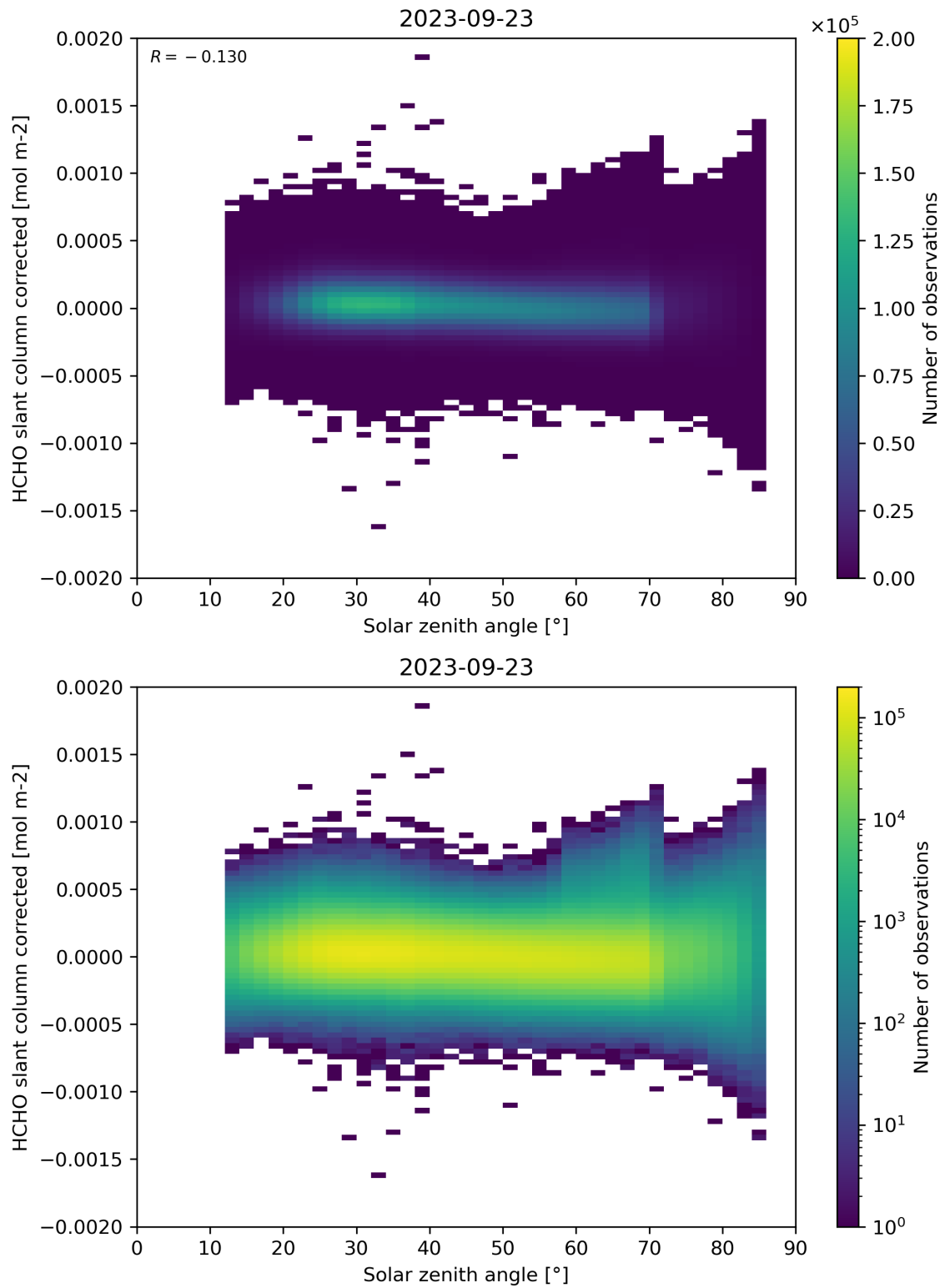
Figure 171: Scatter density plot of “Solar zenith angle” against “HCHO slant column corrected” for 2023-09-22 to 2023-09-24.
