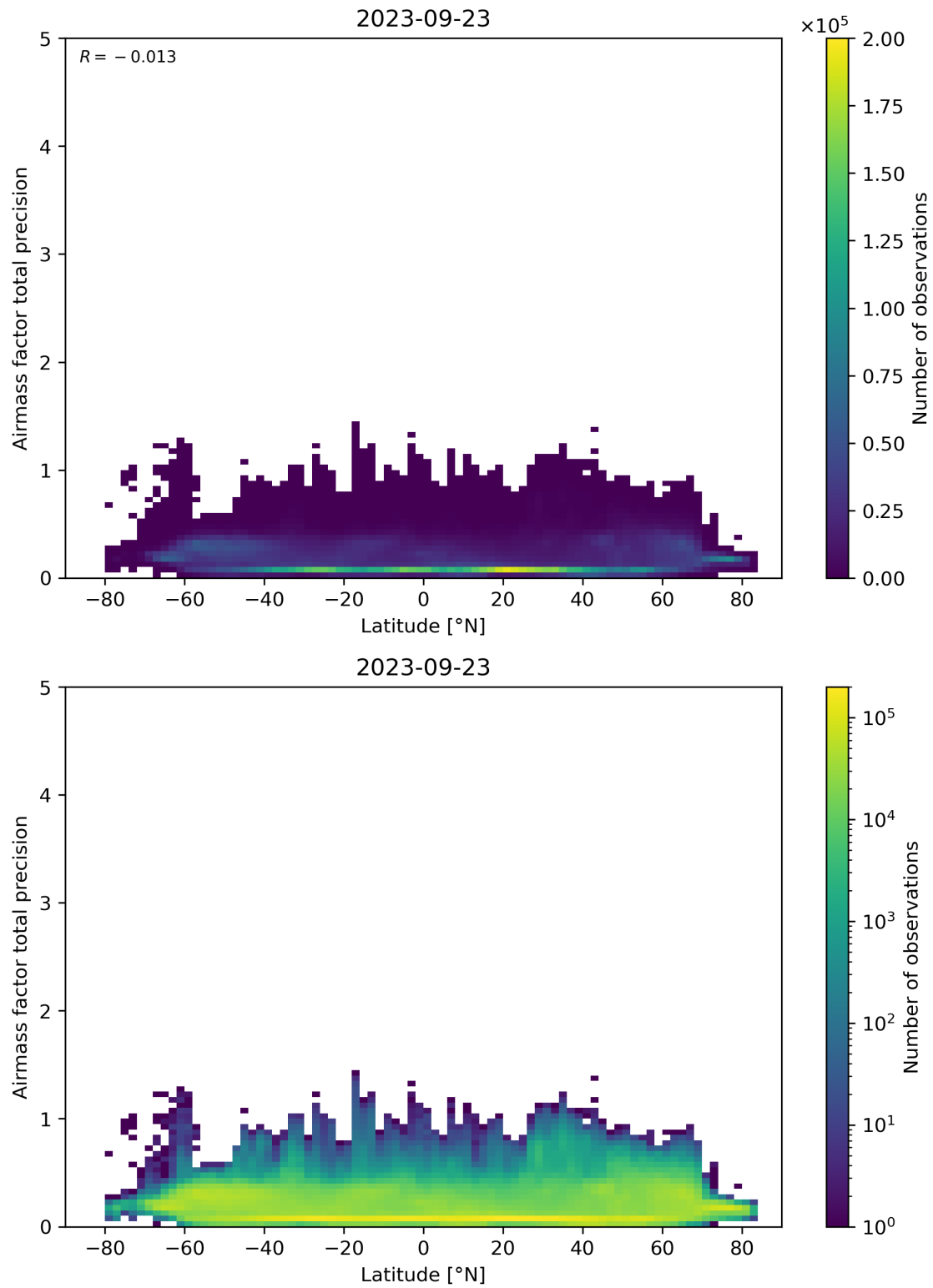
Figure 162: Scatter density plot of “Latitude” against “Airmass factor total precision” for 2023-09-22 to 2023-09-24.
