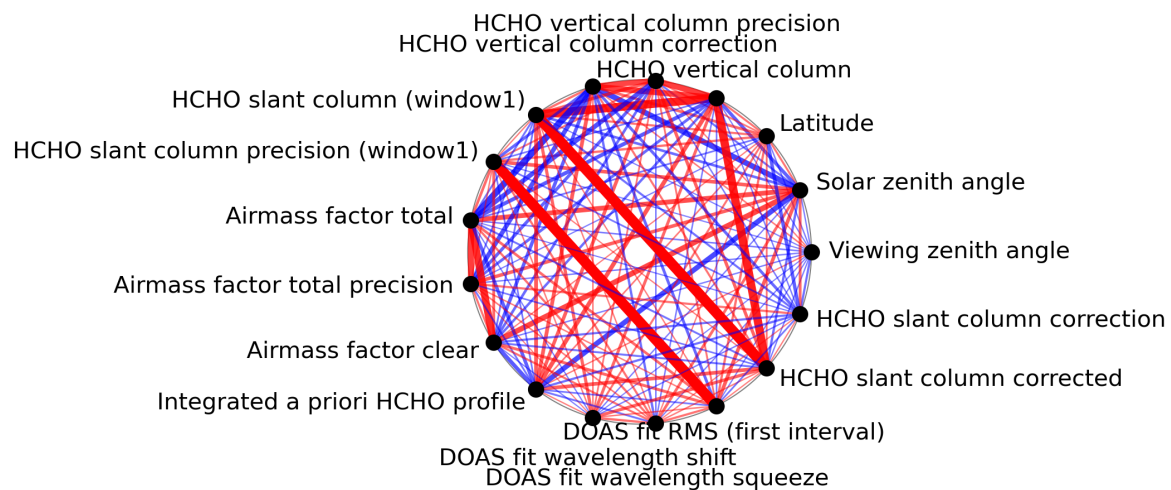
Figure 1: Map of correlation graph for 2023-09-22 to 2023-09-24.
