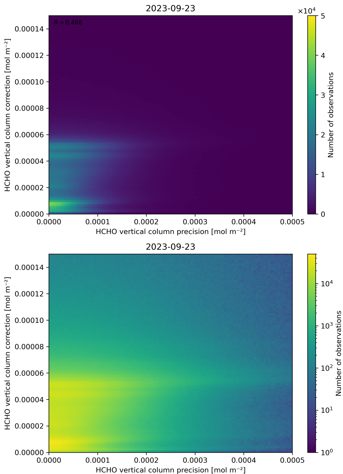
Figure 146: Scatter density plot of “HCHO vertical column precision” against “HCHO vertical column correction” for 2023-09-22 to 2023-09-24.
