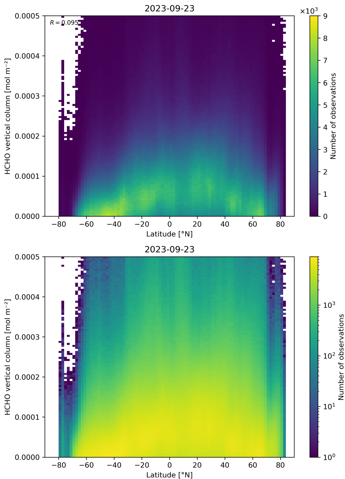
Figure 163: Scatter density plot of “Latitude” against “HCHO vertical column” for 2023-09-22 to 2023-09-24.
