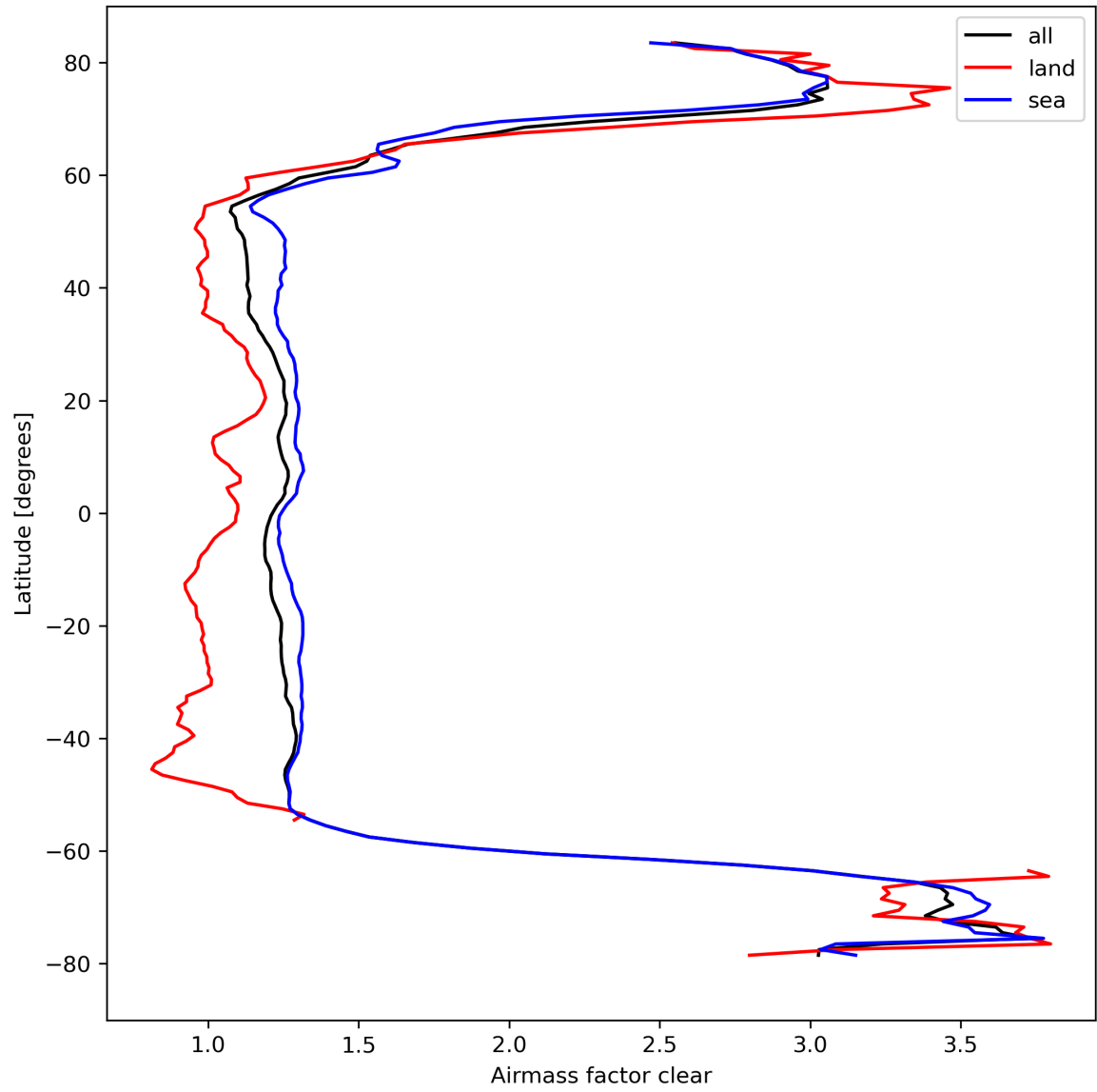
Figure 28: Zonal average of “Airmass factor clear” for 2023-09-22 to 2023-09-24.
