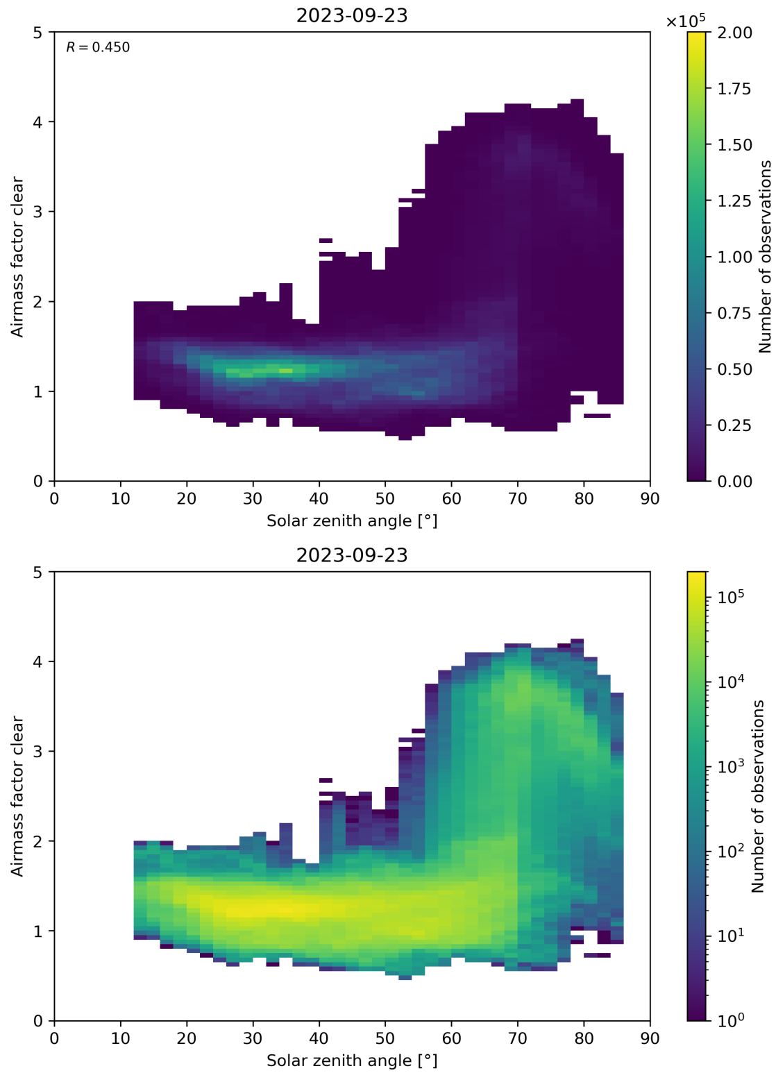
Figure 170: Scatter density plot of “Solar zenith angle” against “Airmass factor clear” for 2023-09-22 to 2023-09-24.
