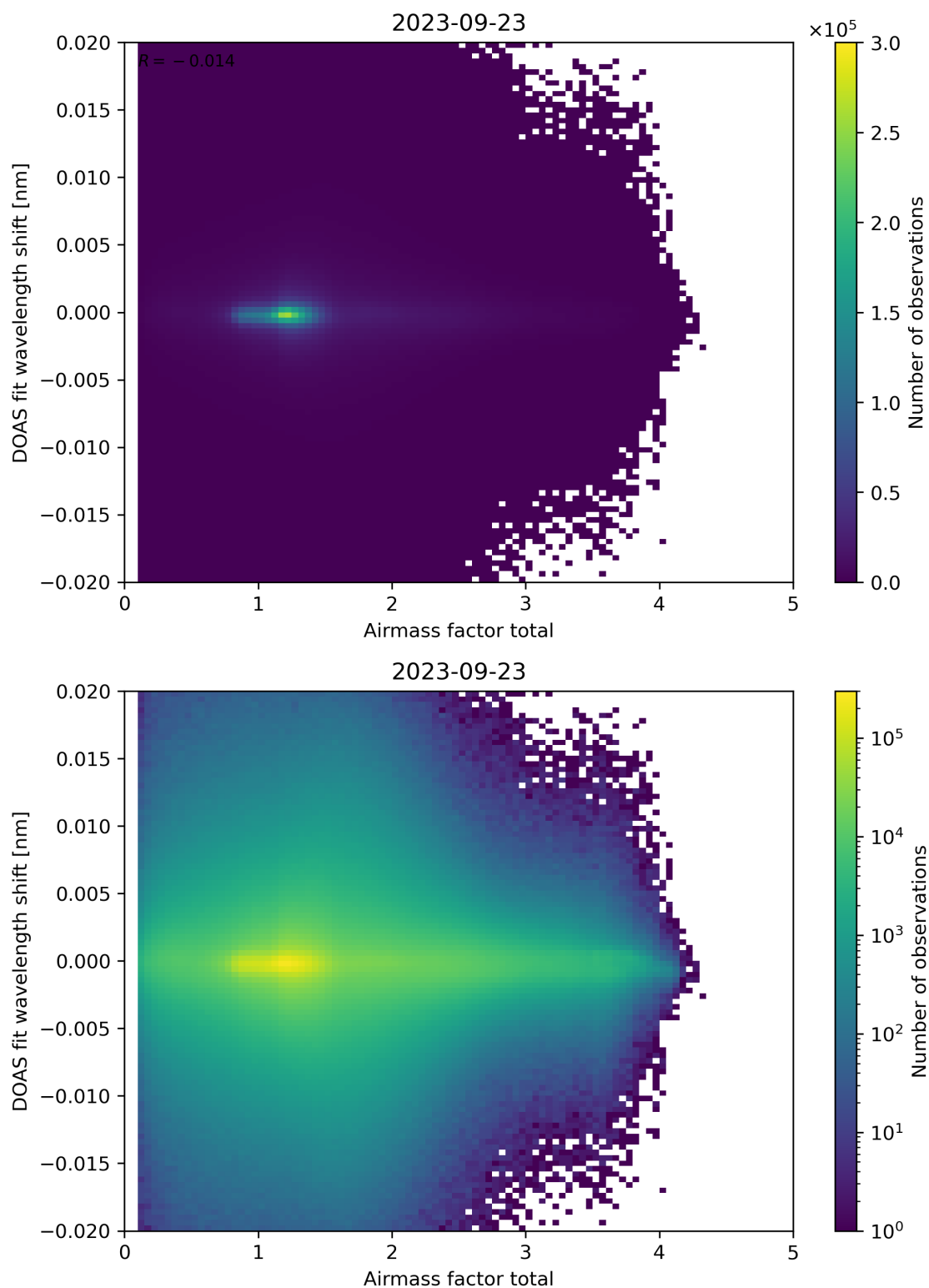
Figure 98: Scatter density plot of “Airmass factor total” against “DOAS fit wavelength shift” for 2023-09-22 to 2023-09-24.
