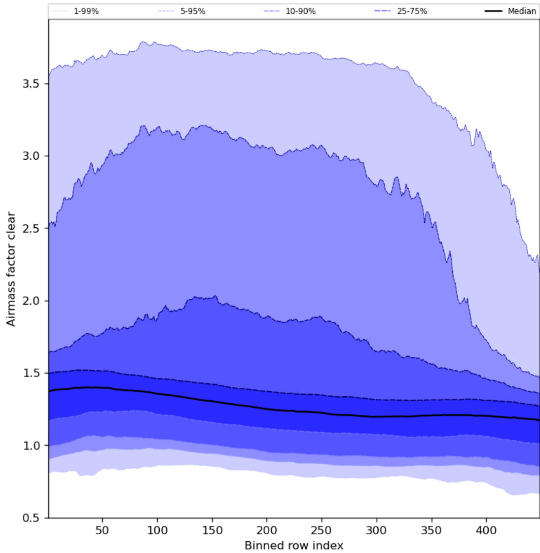
Figure 56: Along track statistics of “Airmass factor clear” for 2023-09-22 to 2023-09-24
