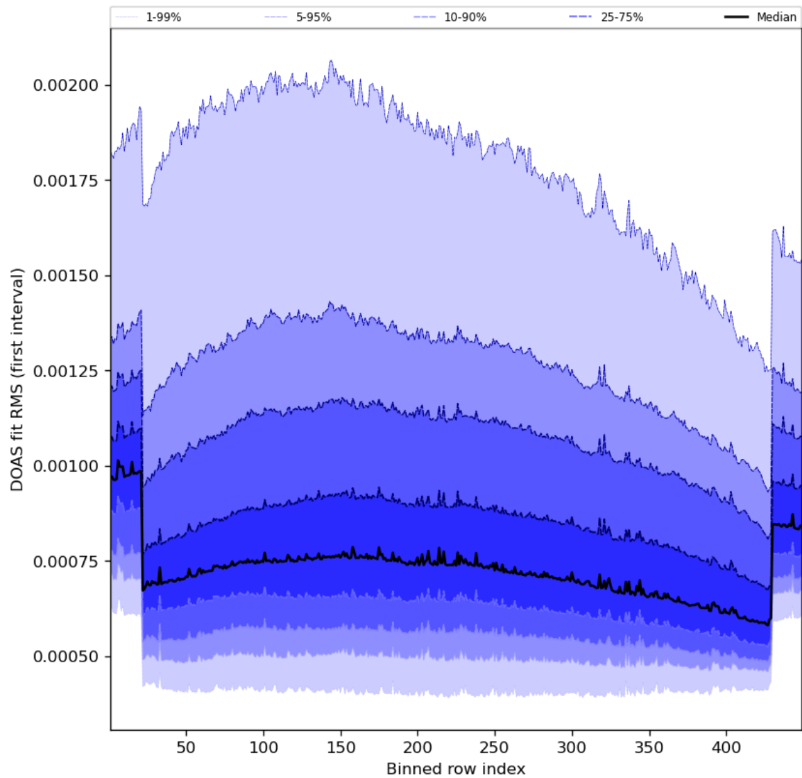
Figure 60: Along track statistics of “DOAS fit RMS (first interval)” for 2023-09-22 to 2023-09-24
