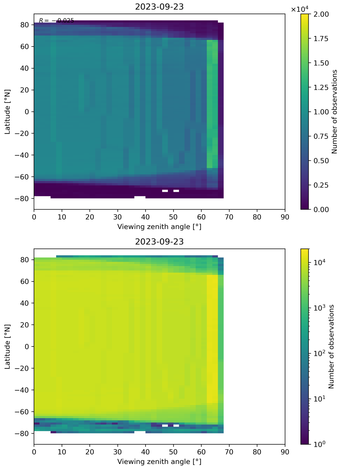
Figure 196: Scatter density plot of “Viewing zenith angle” against “Latitude” for 2023-09-22 to 2023-09-24.
