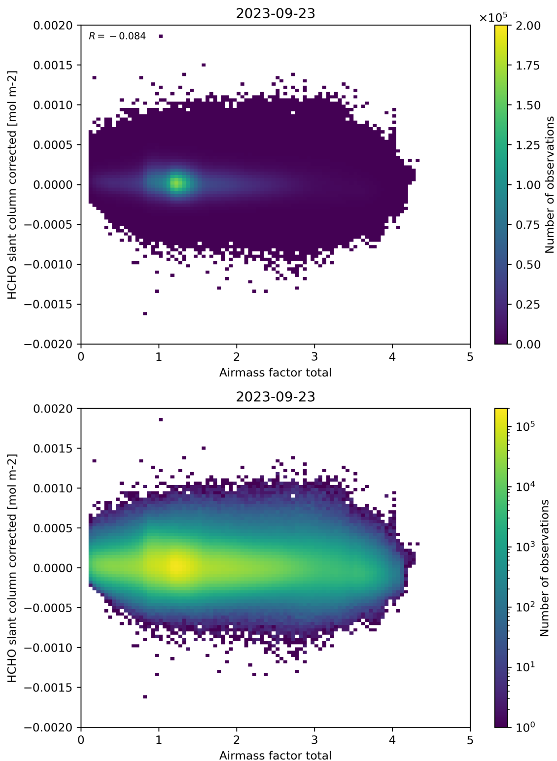
Figure 101: Scatter density plot of “Airmass factor total” against “HCHO slant column corrected” for 2023-09-22 to 2023-09-24.
