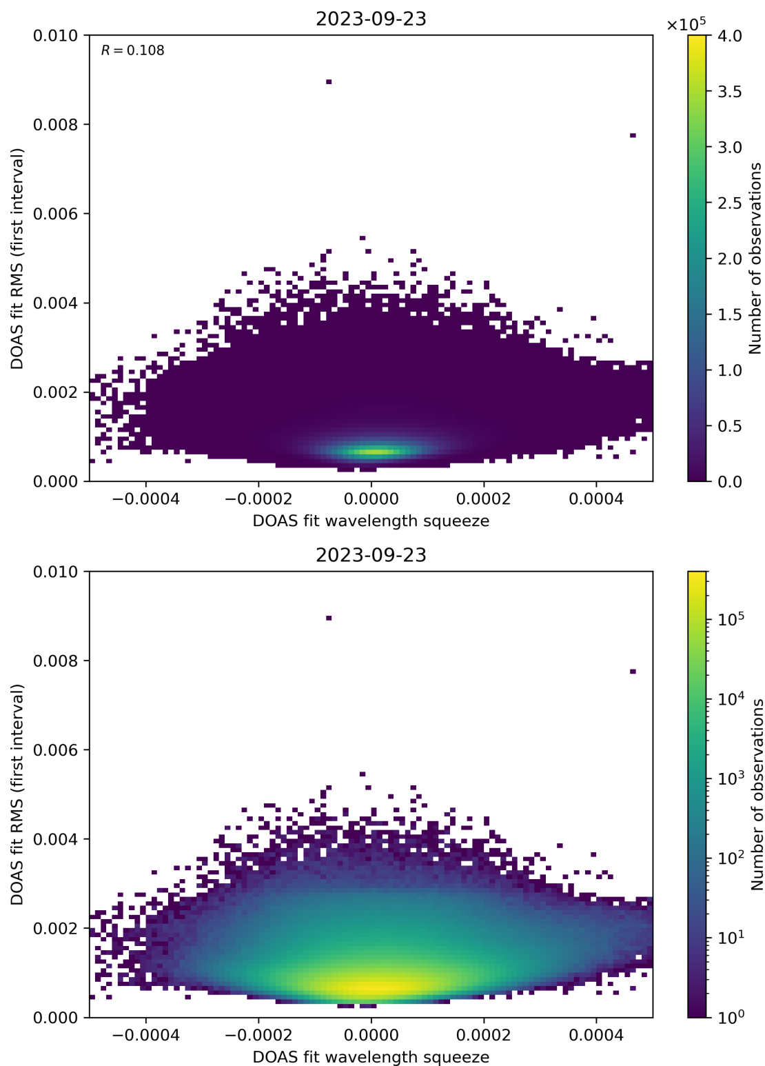
Figure 68: Scatter density plot of “DOAS fit wavelength squeeze” against “DOAS fit RMS (first interval)” for 2023-09-22 to 2023-09-24.
