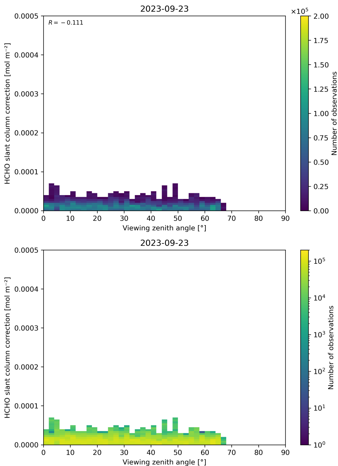
Figure 187: Scatter density plot of “Viewing zenith angle” against “HCHO slant column correction” for 2023-09-22 to 2023-09-24.
