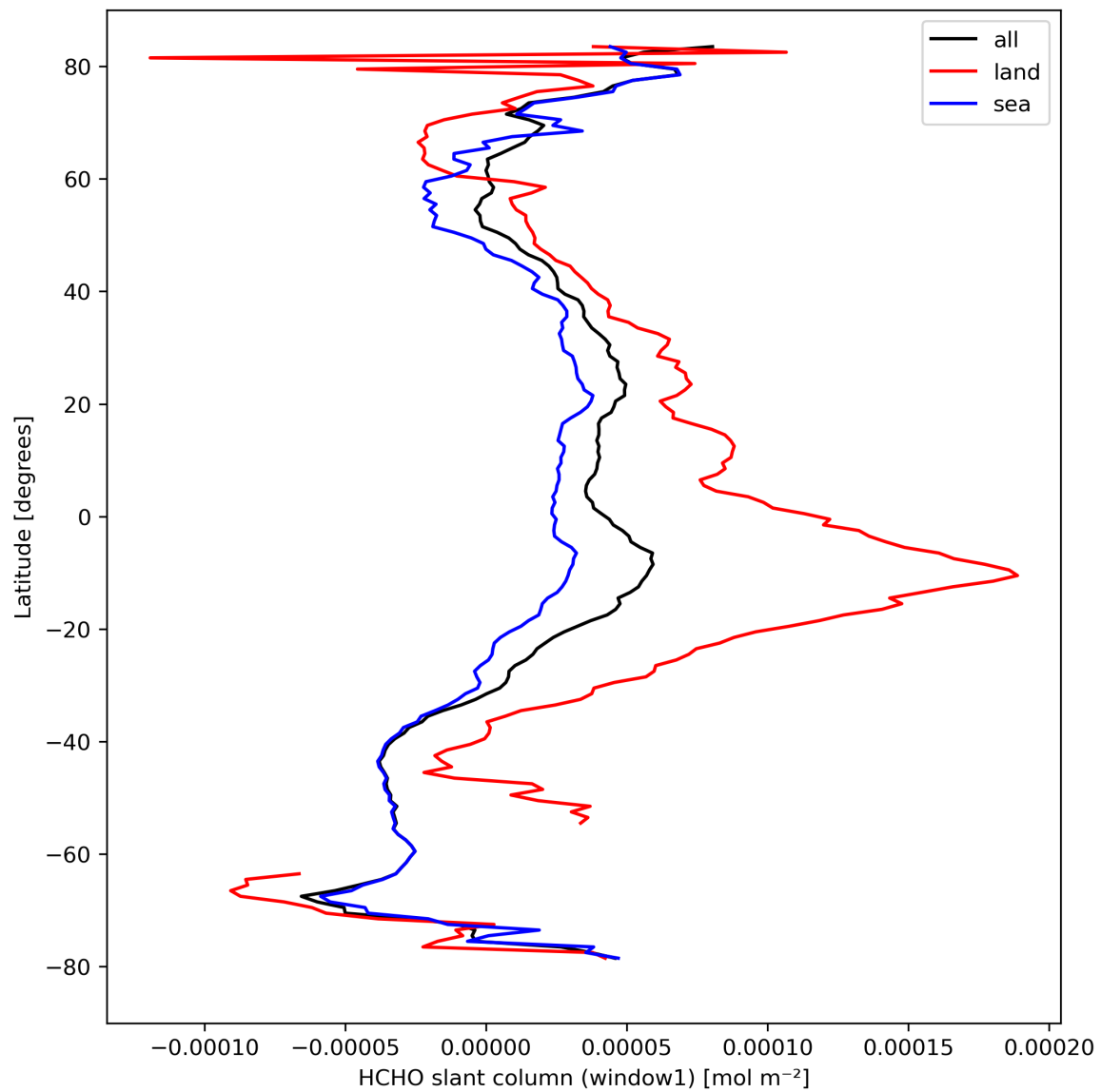
Figure 24: Zonal average of “HCHO slant column (window1)” for 2023-09-22 to 2023-09-24.
