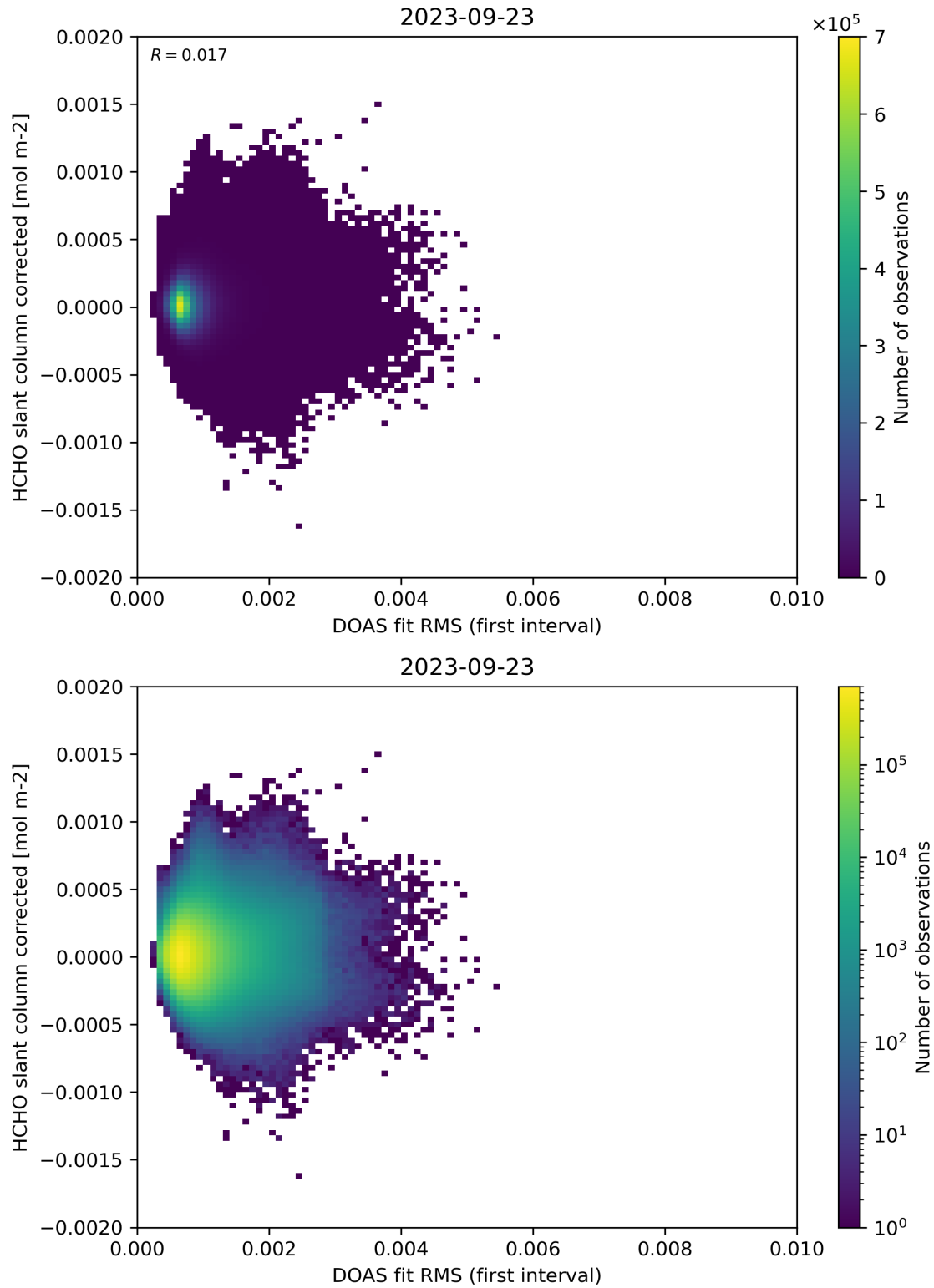
Figure 62: Scatter density plot of “DOAS fit RMS (first interval)” against “HCHO slant column corrected” for 2023-09-22 to 2023-09-24.
