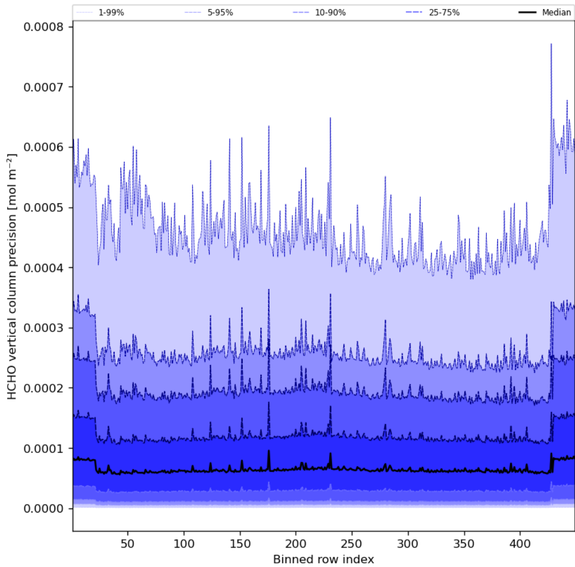
Figure 50: Along track statistics of “HCHO vertical column precision” for 2023-09-22 to 2023-09-24
