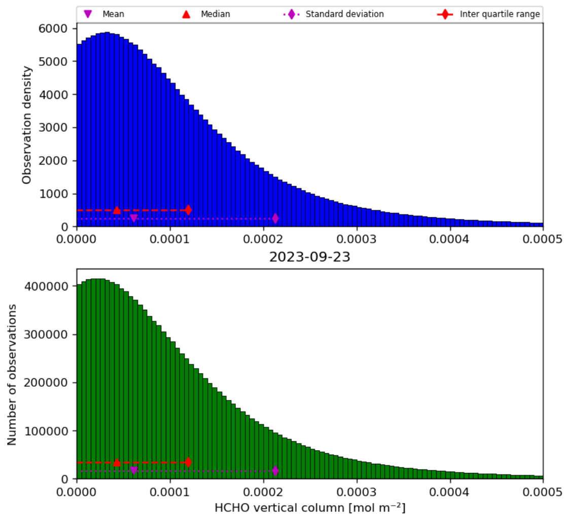
Figure 35: Histogram of “HCHO vertical column” for 2023-09-22 to 2023-09-24
