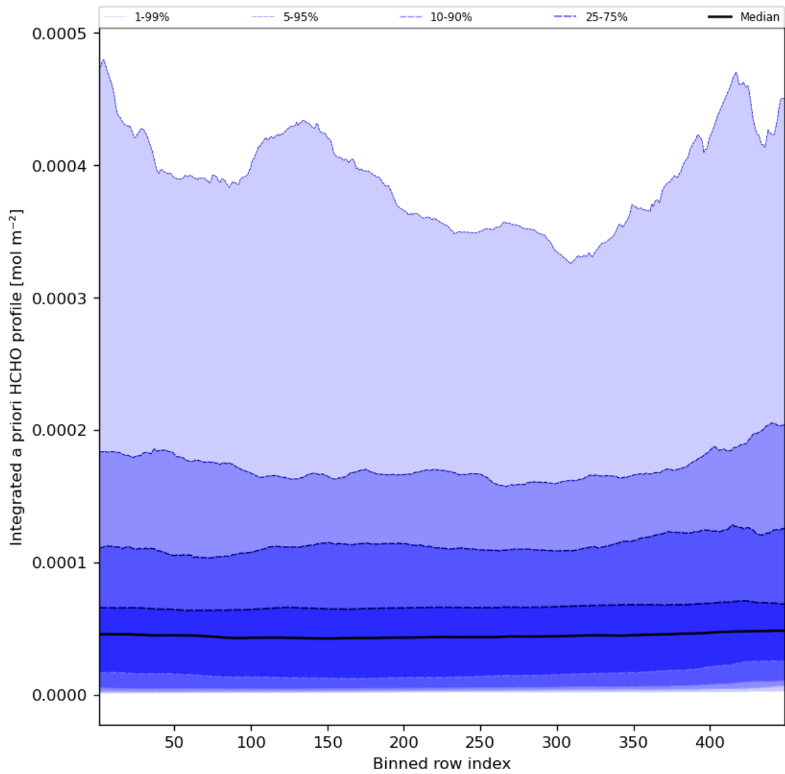
Figure 57: Along track statistics of “Integrated a priori HCHO profile” for 2023-09-22 to 2023-09-24
