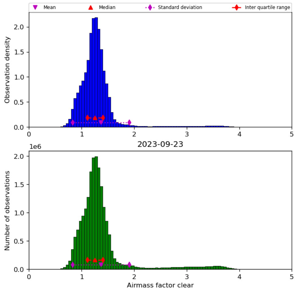
Figure 42: Histogram of “Airmass factor clear” for 2023-09-22 to 2023-09-24
