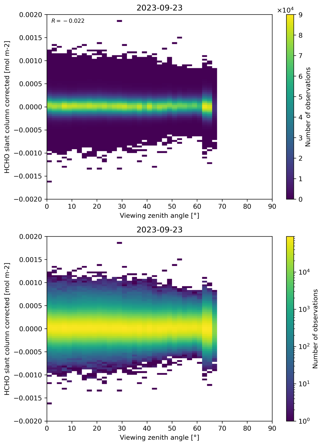
Figure 186: Scatter density plot of “Viewing zenith angle” against “HCHO slant column corrected” for 2023-09-22 to 2023-09-24.
