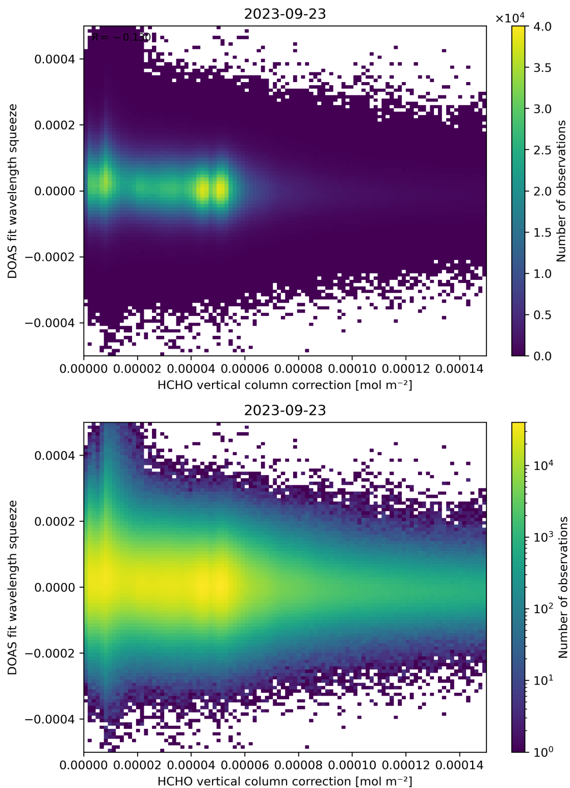
Figure 114: Scatter density plot of “HCHO vertical column correction” against “DOAS fit wavelength squeeze” for 2023-09-22 to 2023-09-24.
