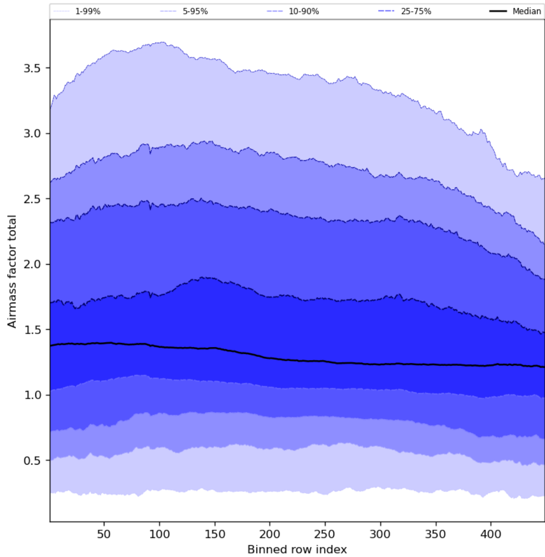
Figure 54: Along track statistics of “Airmass factor total” for 2023-09-22 to 2023-09-24
