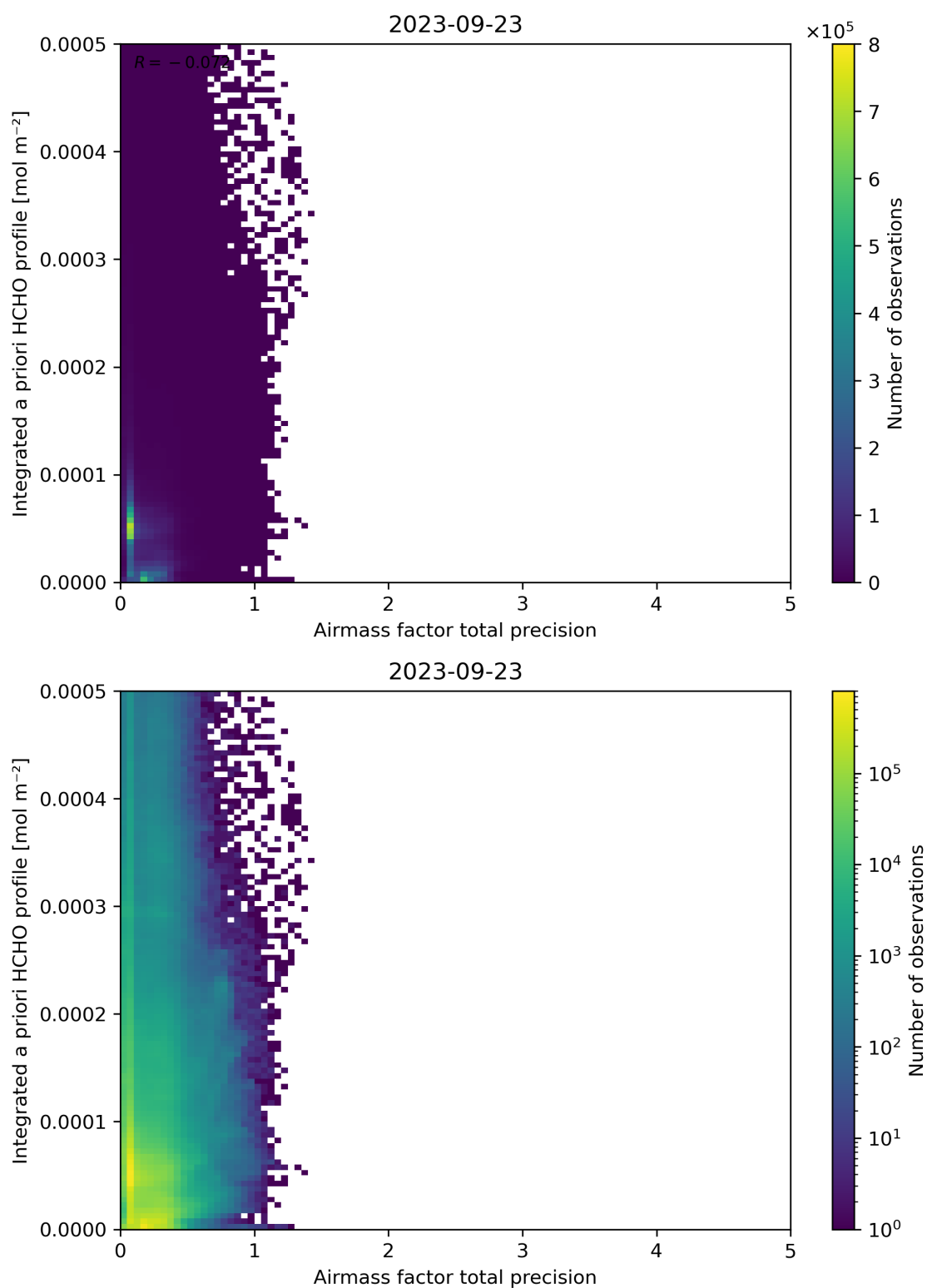
Figure 111: Scatter density plot of “Airmass factor total precision” against “Integrated a priori HCHO profile” for 2023-09-22 to 2023-09-24.
