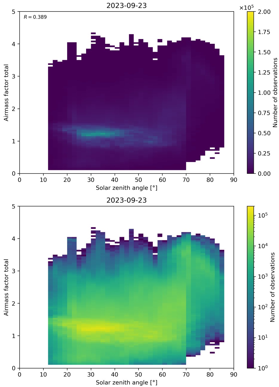
Figure 175: Scatter density plot of “Solar zenith angle” against “Airmass factor total” for 2023-09-22 to 2023-09-24.
