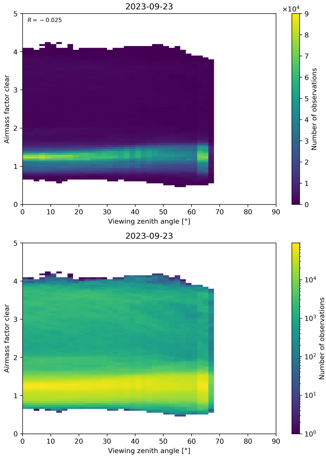
Figure 185: Scatter density plot of “Viewing zenith angle” against “Airmass factor clear” for 2023-09-22 to 2023-09-24.
