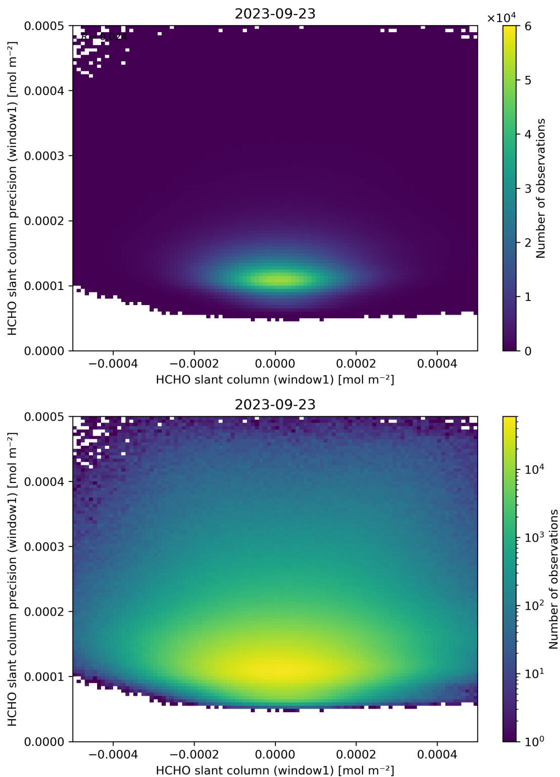
Figure 84: Scatter density plot of “HCHO slant column (window1)” against “HCHO slant column precision (window1)” for 2023-09-22 to 2023-09-24.
