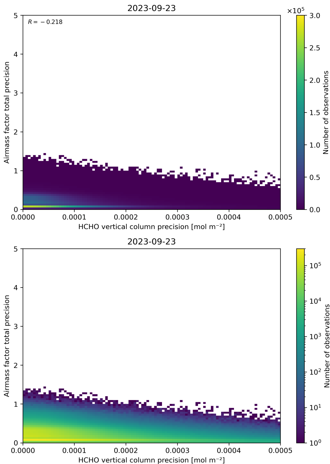
Figure 145: Scatter density plot of “HCHO vertical column precision” against “Airmass factor total precision” for 2023-09-22 to 2023-09-24.
