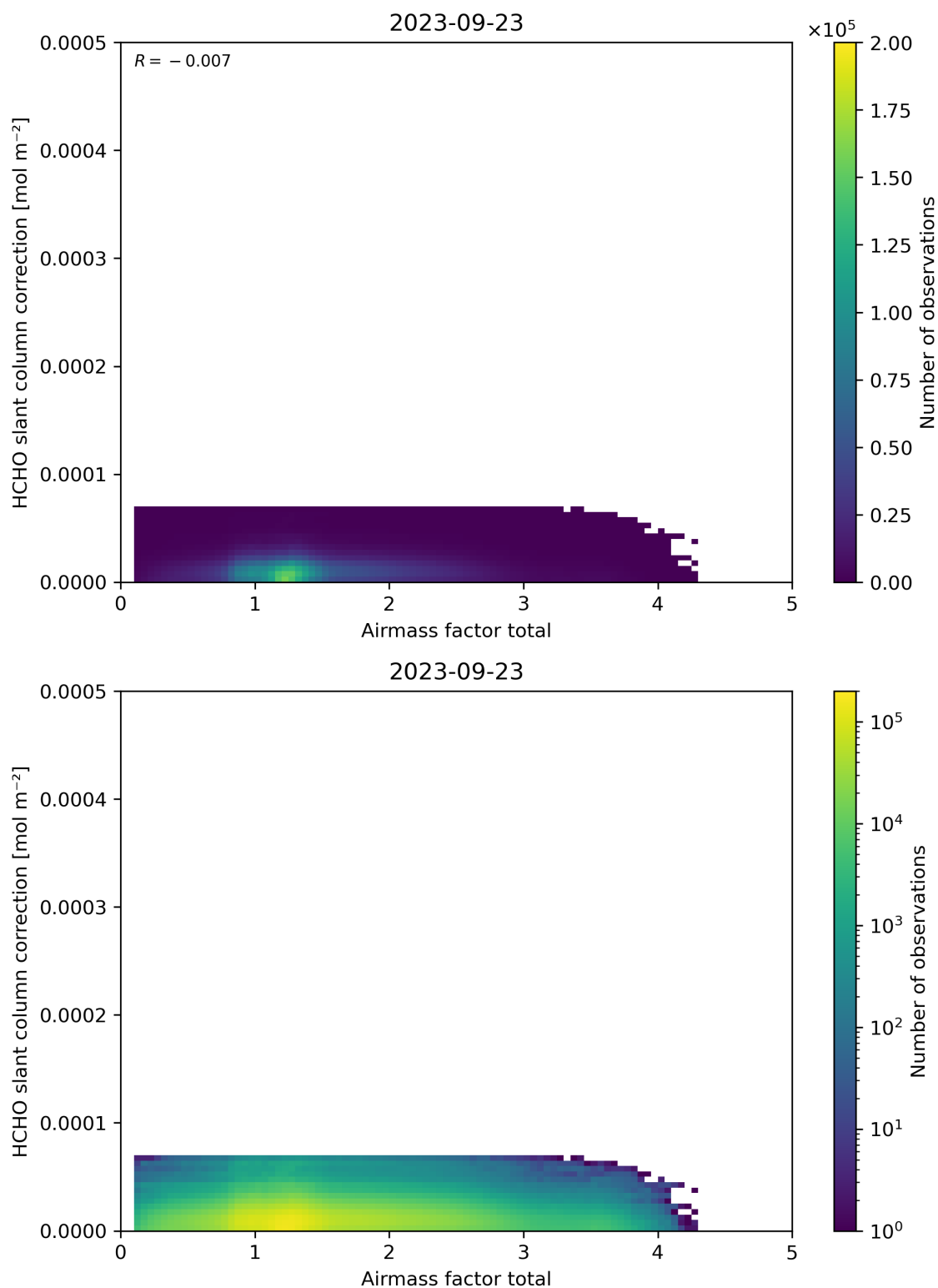
Figure 102: Scatter density plot of “Airmass factor total” against “HCHO slant column correction” for 2023-09-22 to 2023-09-24.
