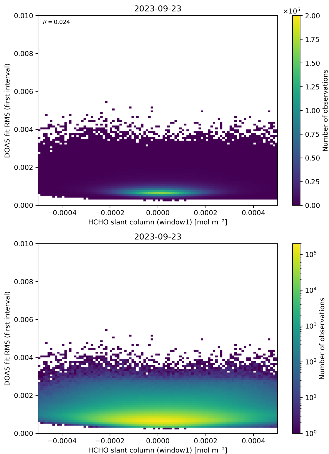
Figure 78: Scatter density plot of “HCHO slant column (window1)” against “DOAS fit RMS (first interval)” for 2023-09-22 to 2023-09-24.
