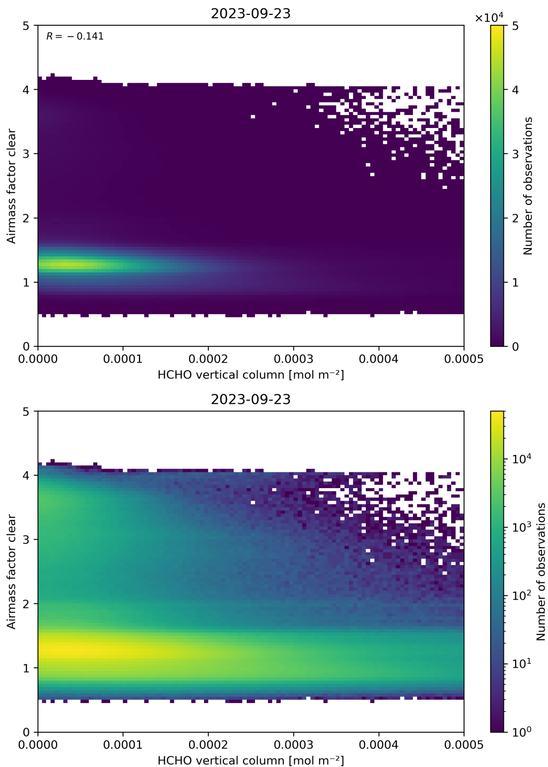
Figure 126: Scatter density plot of “HCHO vertical column” against “Airmass factor clear” for 2023-09-22 to 2023-09-24.
