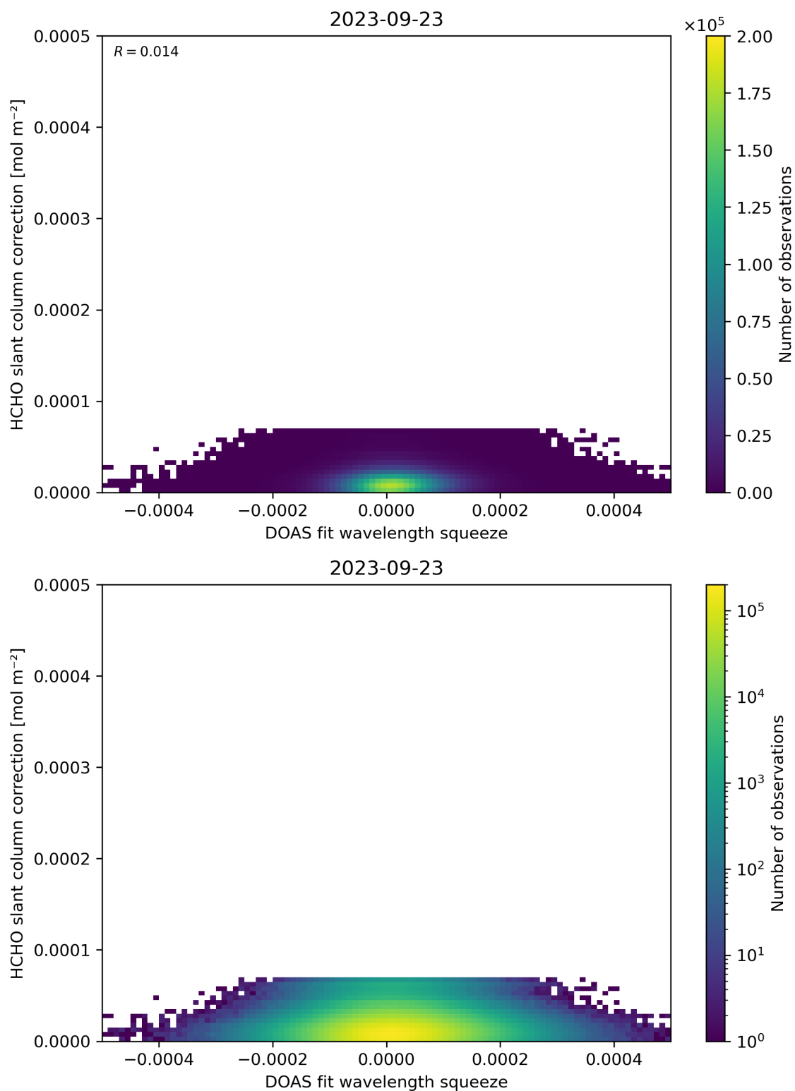
Figure 70: Scatter density plot of “DOAS fit wavelength squeeze” against “HCHO slant column correction” for 2023-09-22 to 2023-09-24.
