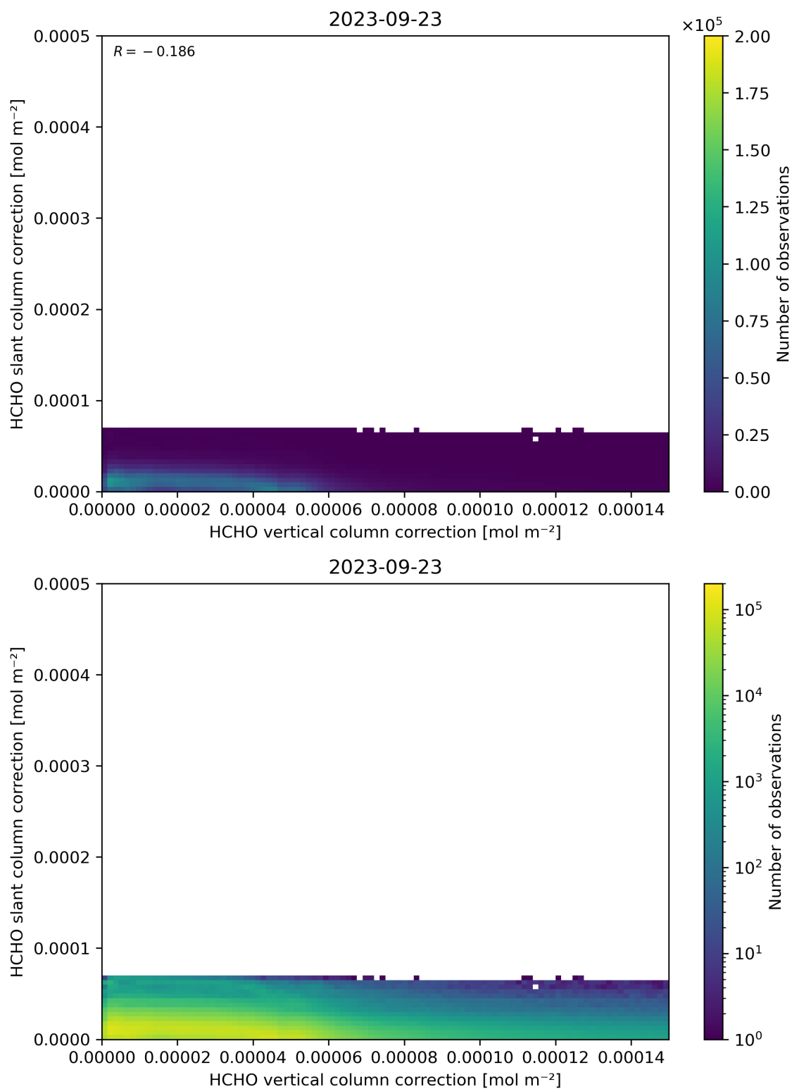
Figure 117: Scatter density plot of “HCHO vertical column correction” against “HCHO slant column correction” for 2023-09-22 to 2023-09-24.
