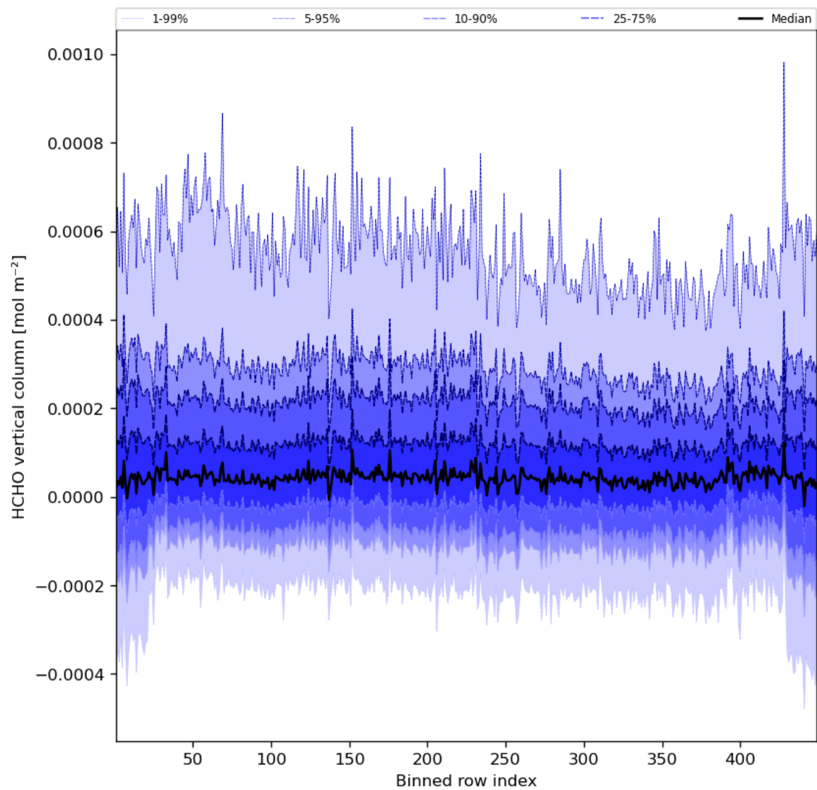
Figure 49: Along track statistics of “HCHO vertical column” for 2023-09-22 to 2023-09-24
