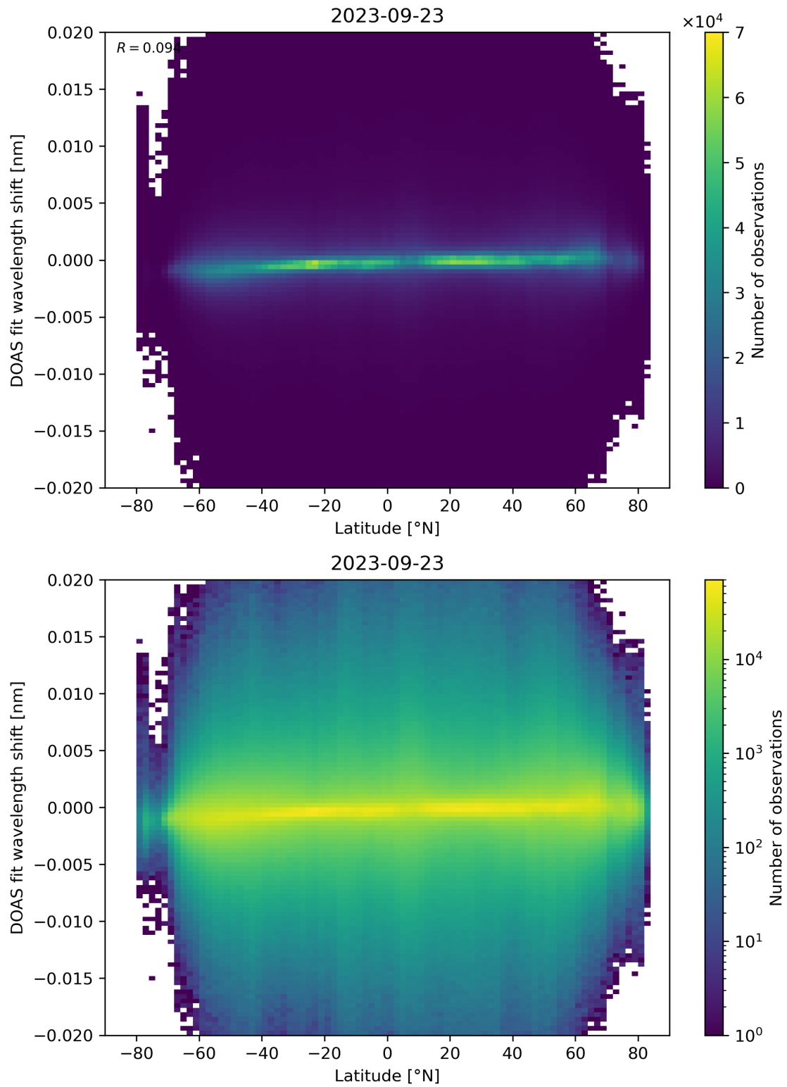
Figure 154: Scatter density plot of “Latitude” against “DOAS fit wavelength shift” for 2023-09-22 to 2023-09-24.
