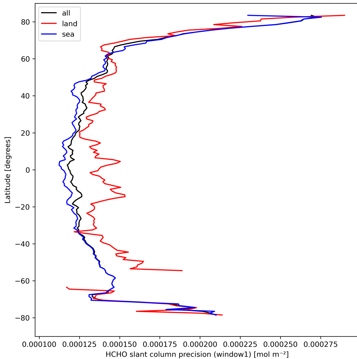
Figure 25: Zonal average of “HCHO slant column precision (window1)” for 2023-09-22 to 2023-09-24.
