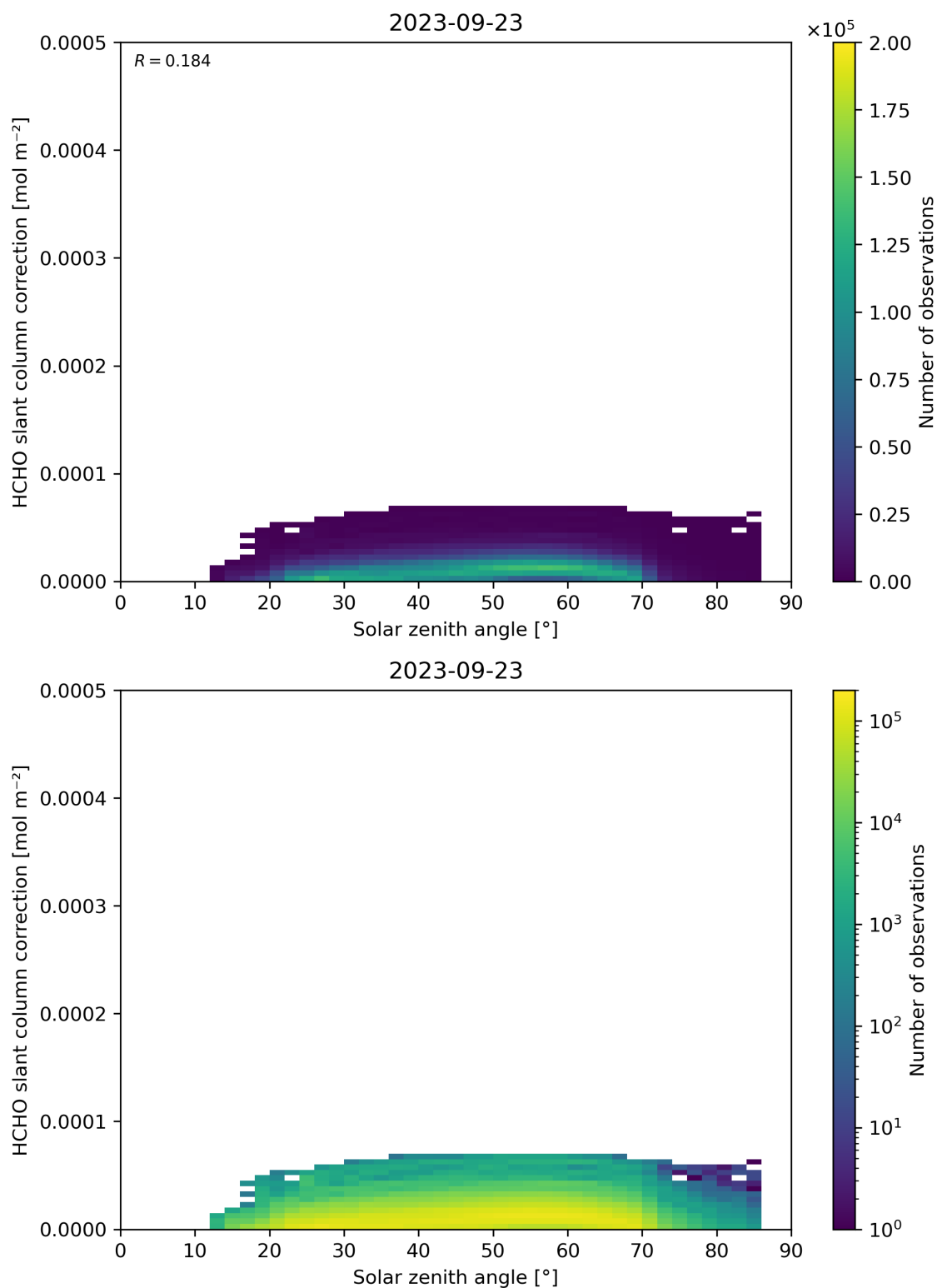
Figure 172: Scatter density plot of “Solar zenith angle” against “HCHO slant column correction” for 2023-09-22 to 2023-09-24.
