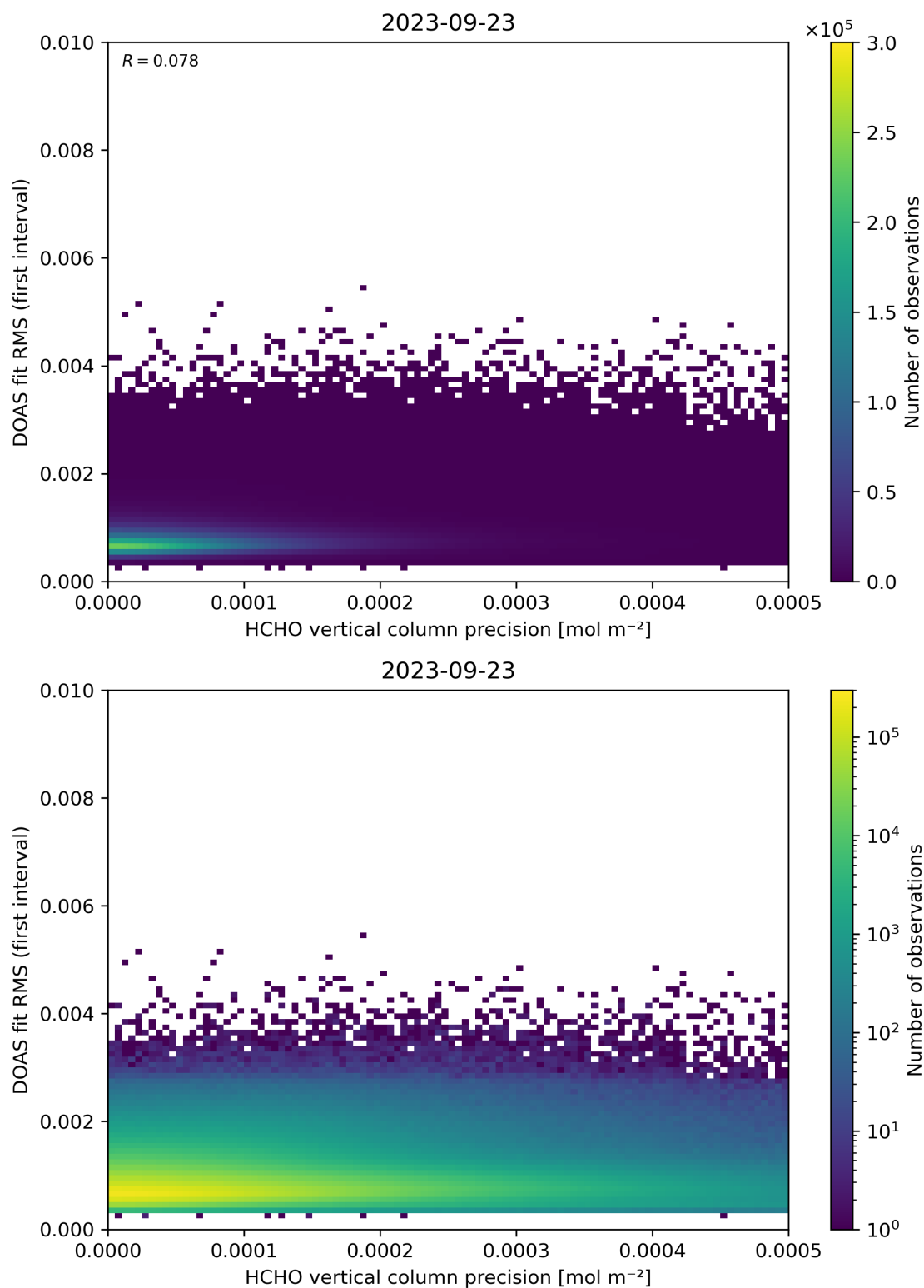
Figure 136: Scatter density plot of “HCHO vertical column precision” against “DOAS fit RMS (first interval)” for 2023-09-22 to 2023-09-24.
