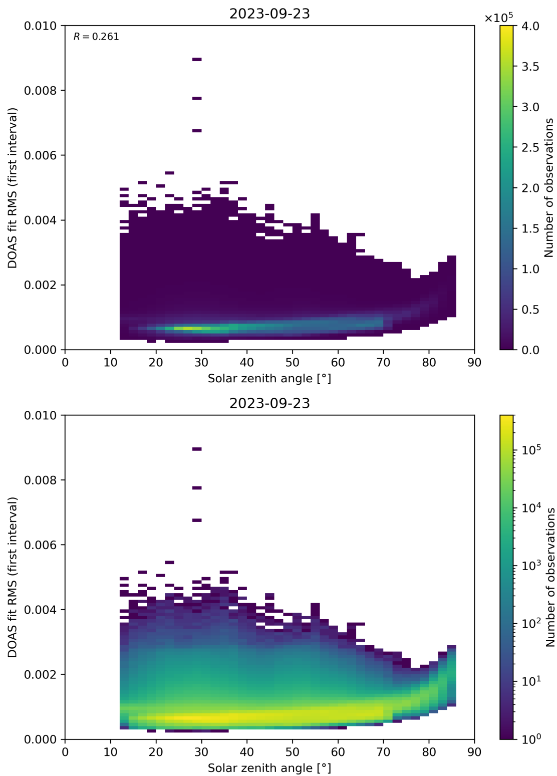
Figure 167: Scatter density plot of “Solar zenith angle” against “DOAS fit RMS (first interval)” for 2023-09-22 to 2023-09-24.
