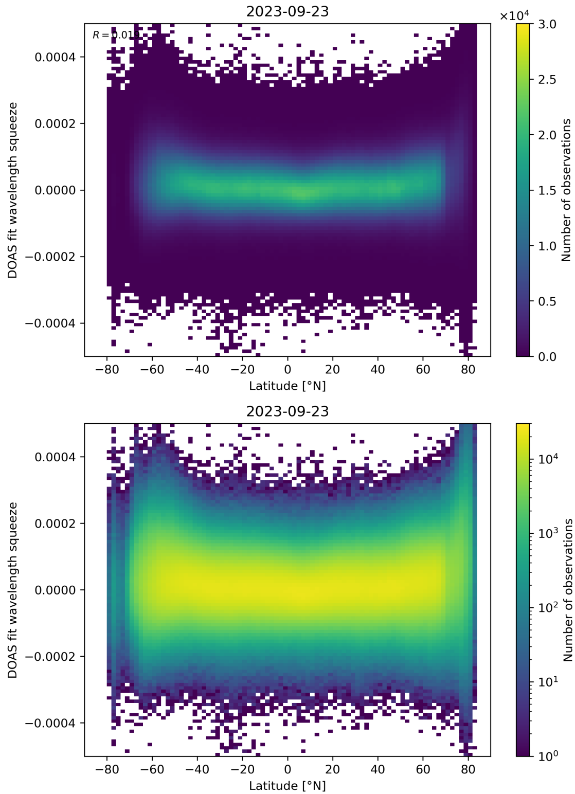
Figure 155: Scatter density plot of “Latitude” against “DOAS fit wavelength squeeze” for 2023-09-22 to 2023-09-24.
