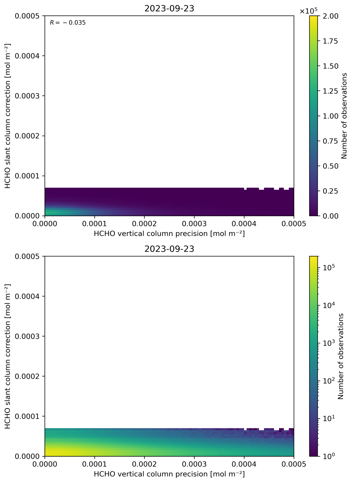
Figure 141: Scatter density plot of “HCHO vertical column precision” against “HCHO slant column correction” for 2023-09-22 to 2023-09-24.
