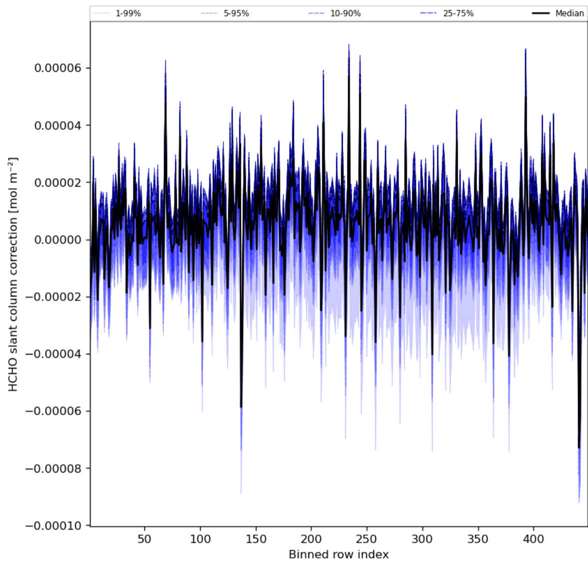
Figure 61: Along track statistics of “HCHO slant column correction” for 2023-09-22 to 2023-09-24
