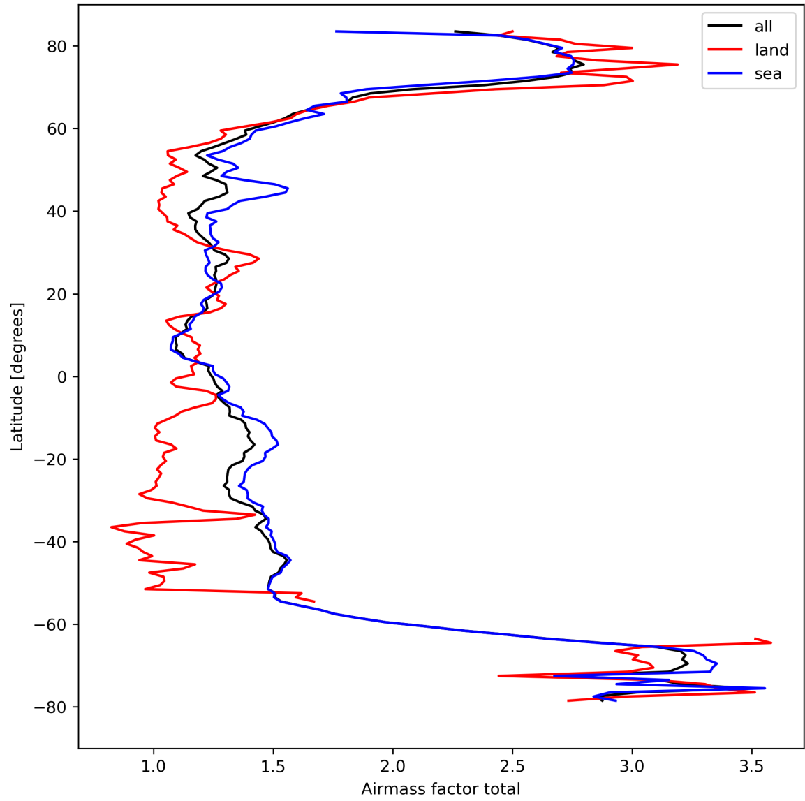
Figure 26: Zonal average of "Airmass factor total" for 2023-09-22 to 2023-09-24.
