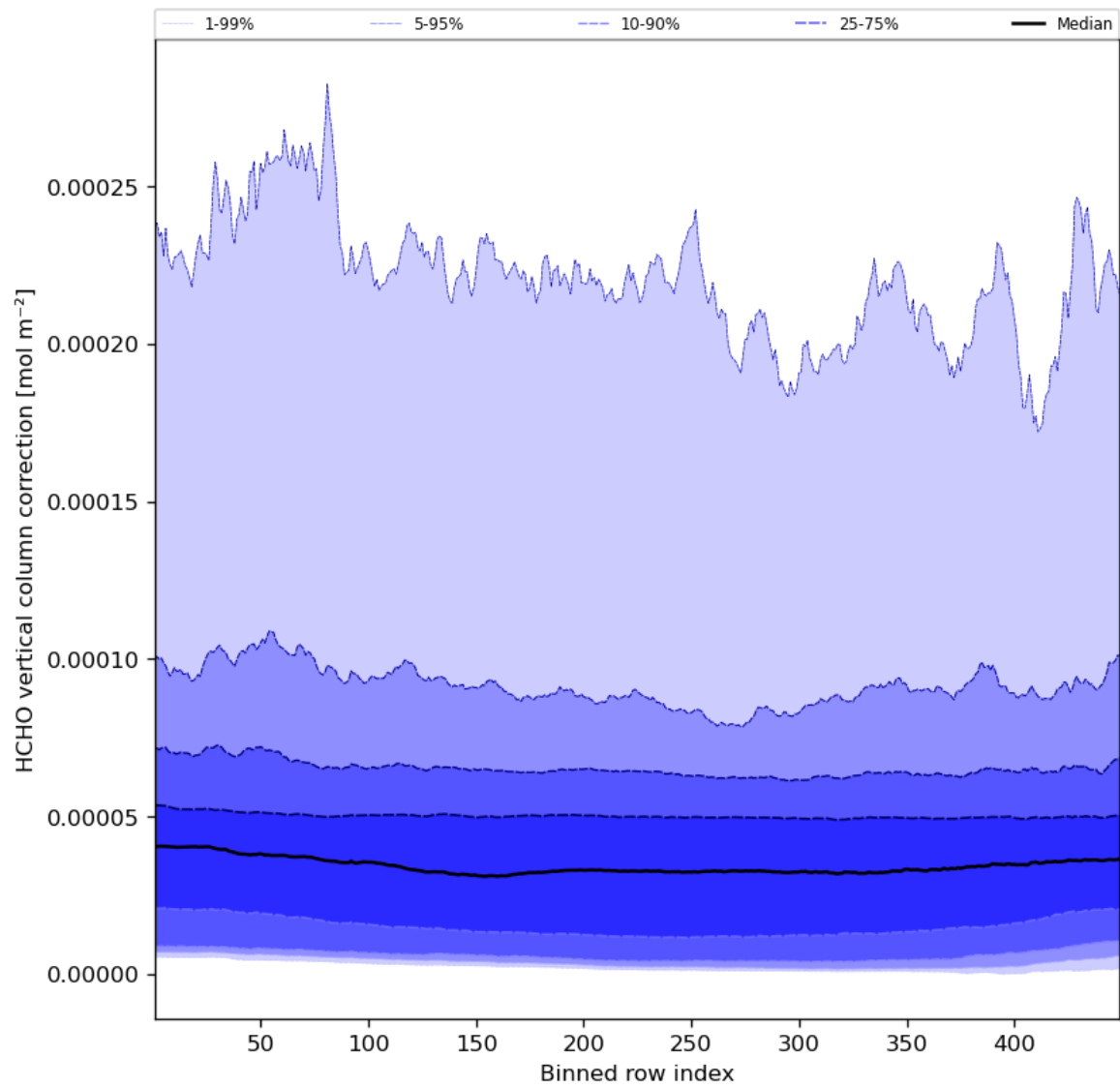
Figure 51: Along track statistics of “HCHO vertical column correction” for 2023-09-22 to 2023-09-24
