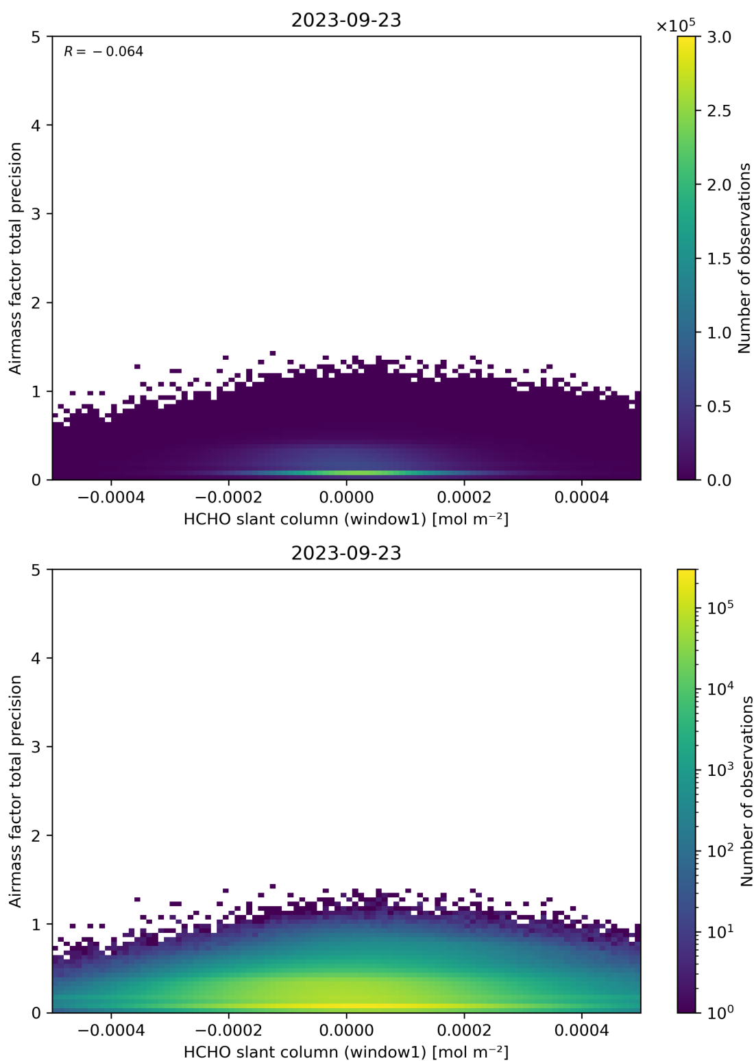
Figure 86: Scatter density plot of “HCHO slant column (window1)” against “Airmass factor total precision” for 2023-09-22 to 2023-09-24.
