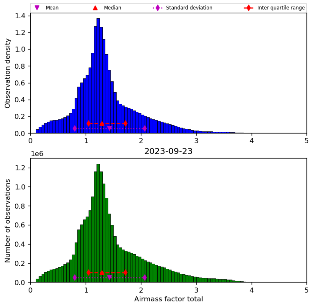
Figure 40: Histogram of “Airmass factor total” for 2023-09-22 to 2023-09-24
