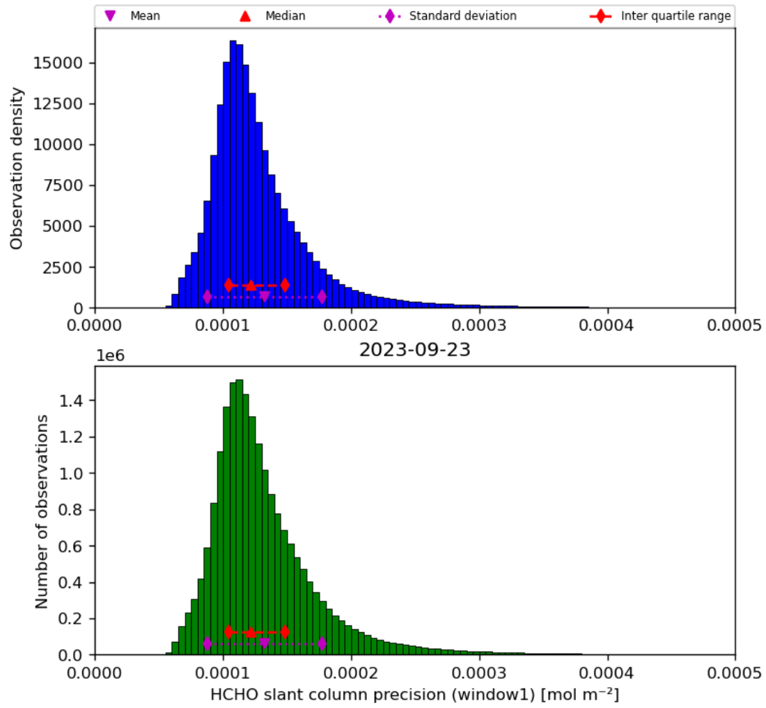
Figure 39: Histogram of “HCHO slant column precision (window1)” for 2023-09-22 to 2023-09-24
