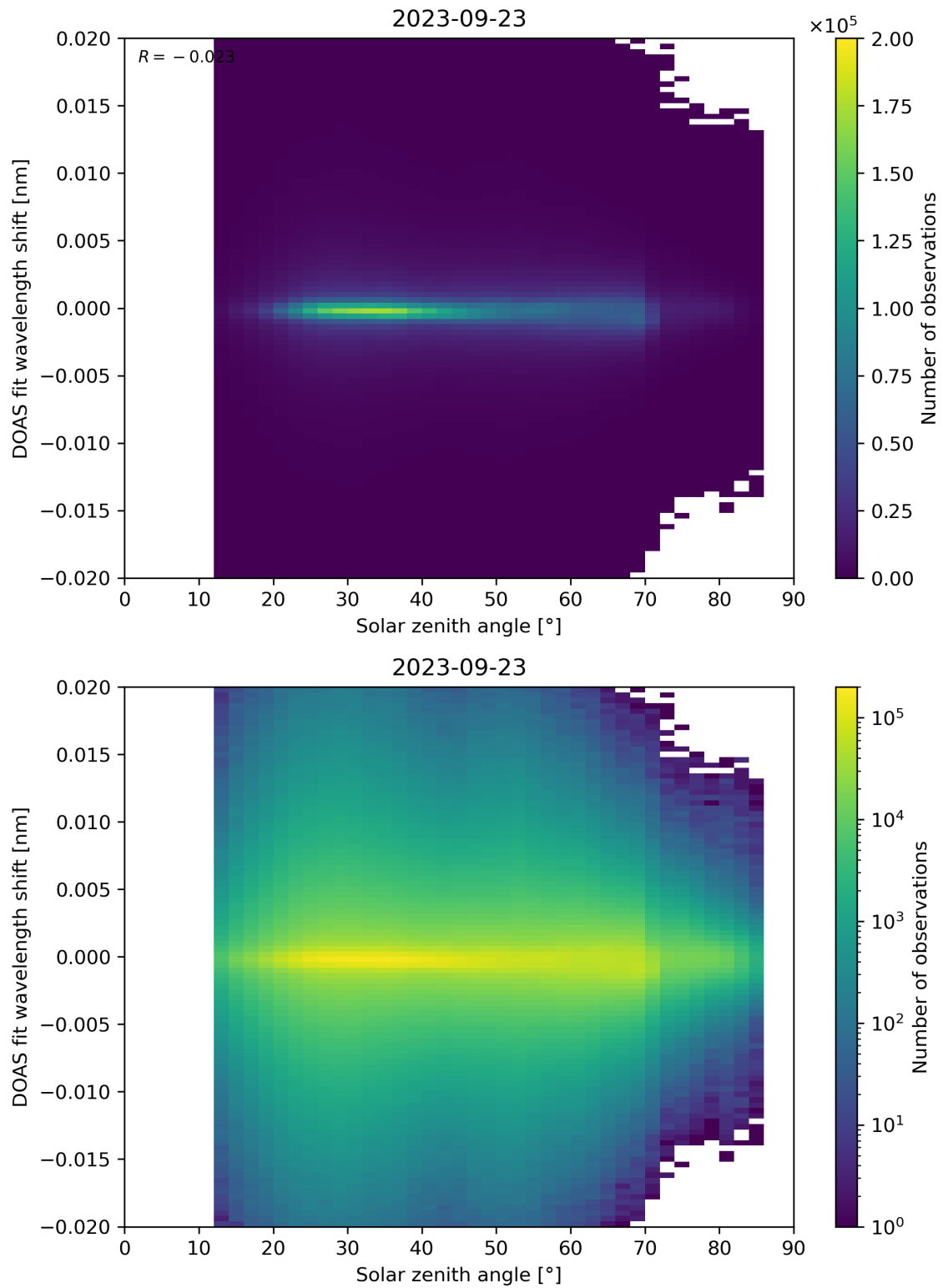
Figure 168: Scatter density plot of “Solar zenith angle” against “DOAS fit wavelength shift” for 2023-09-22 to 2023-09-24.
