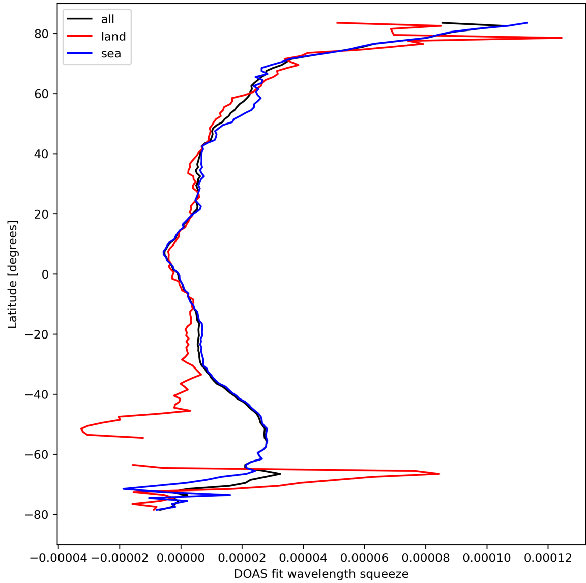
Figure 31: Zonal average of “DOAS fit wavelength squeeze” for 2023-09-22 to 2023-09-24.
