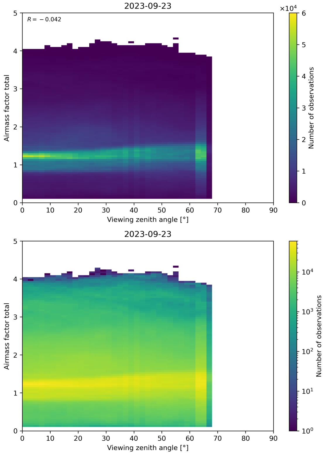
Figure 190: Scatter density plot of “Viewing zenith angle” against “Airmass factor total” for 2023-09-22 to 2023-09-24.
