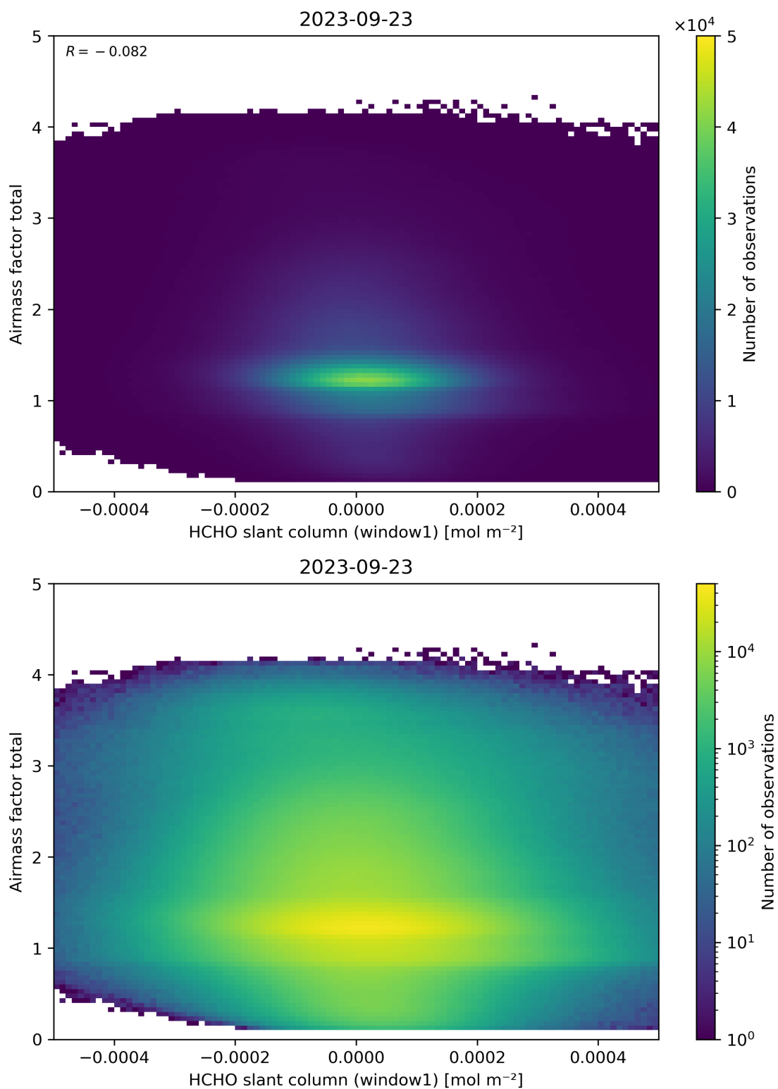
Figure 85: Scatter density plot of “HCHO slant column (window1)” against “Airmass factor total” for 2023-09-22 to 2023-09-24.
