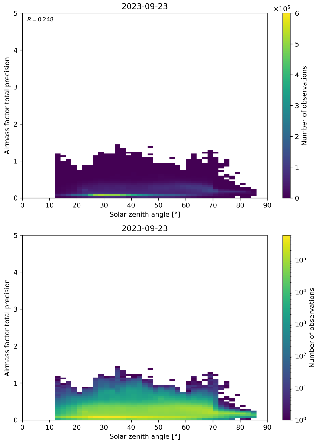
Figure 176: Scatter density plot of “Solar zenith angle” against “Airmass factor total precision” for 2023-09-22 to 2023-09-24.
