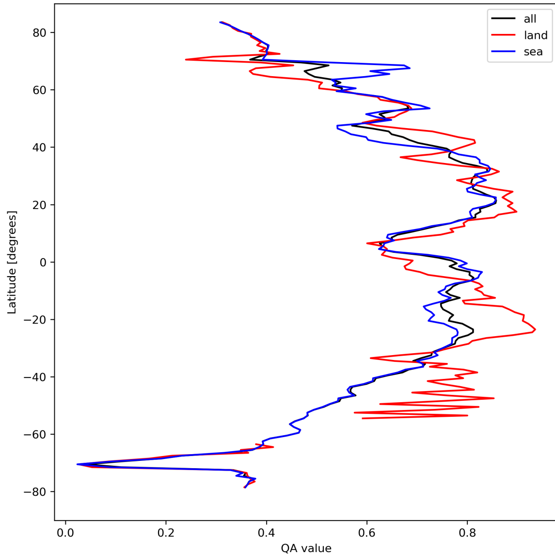
Figure 20: Zonal average of “QA value” for 2023-09-22 to 2023-09-24.
