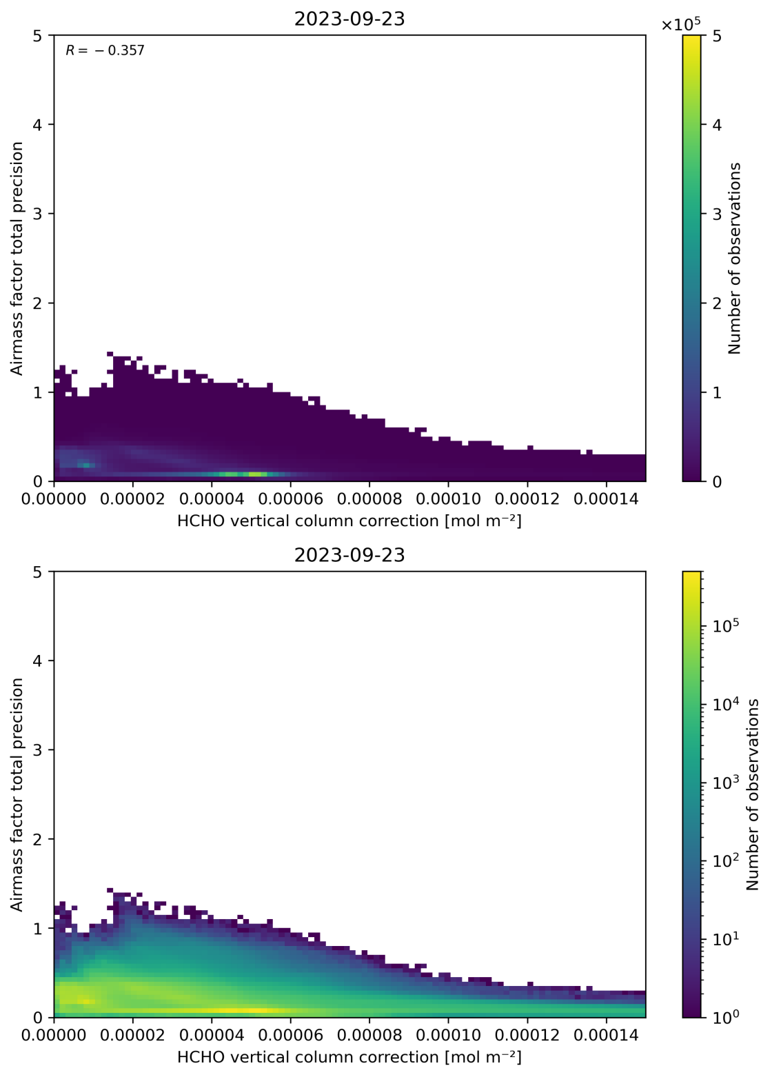
Figure 121: Scatter density plot of “HCHO vertical column correction” against “Airmass factor total precision” for 2023-09-22 to 2023-09-24.
