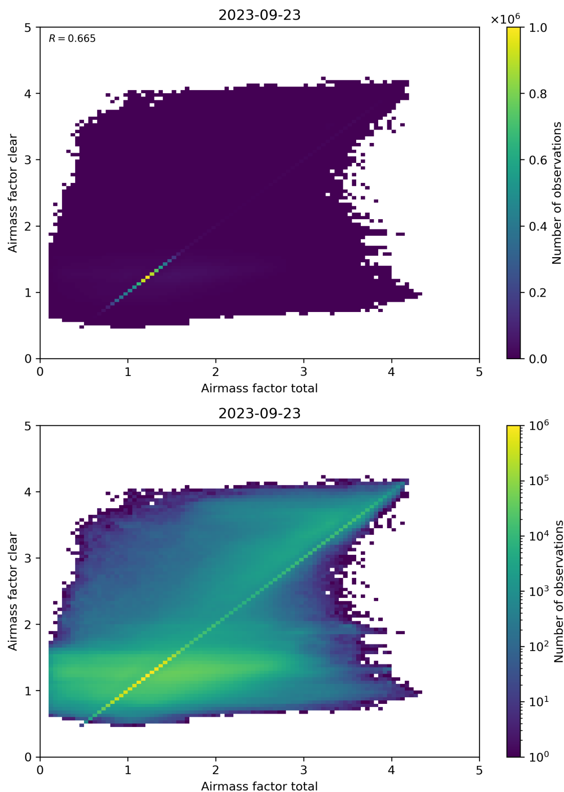
Figure 100: Scatter density plot of “Airmass factor total” against “Airmass factor clear” for 2023-09-22 to 2023-09-24.
