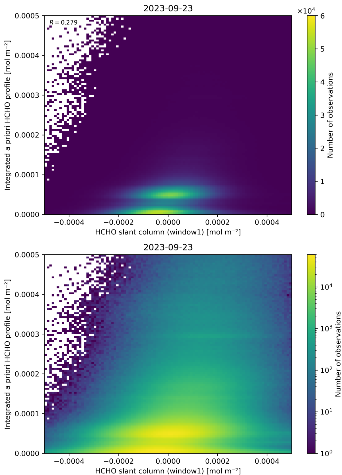
Figure 87: Scatter density plot of “HCHO slant column (window1)” against “Integrated a priori HCHO profile” for 2023-09-22 to 2023-09-24.
