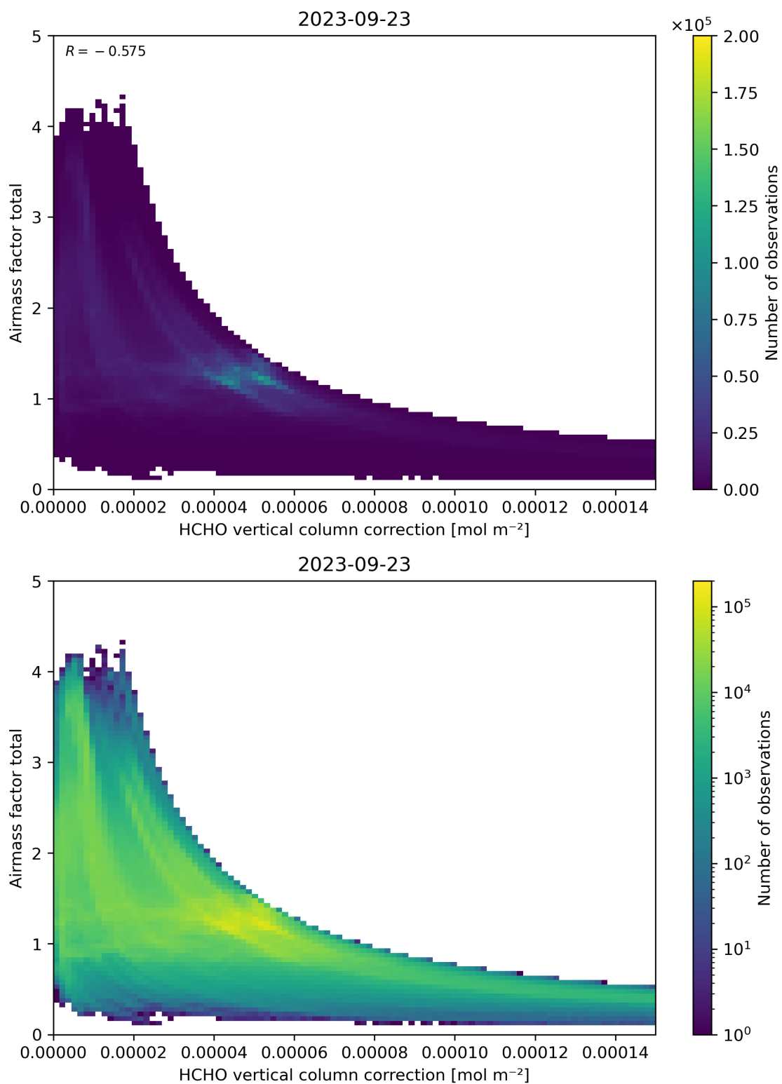
Figure 120: Scatter density plot of “HCHO vertical column correction” against “Airmass factor total” for 2023-09-22 to 2023-09-24.
