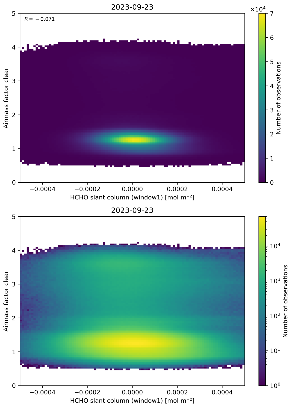
Figure 81: Scatter density plot of “HCHO slant column (window1)” against “Airmass factor clear” for 2023-09-22 to 2023-09-24.
