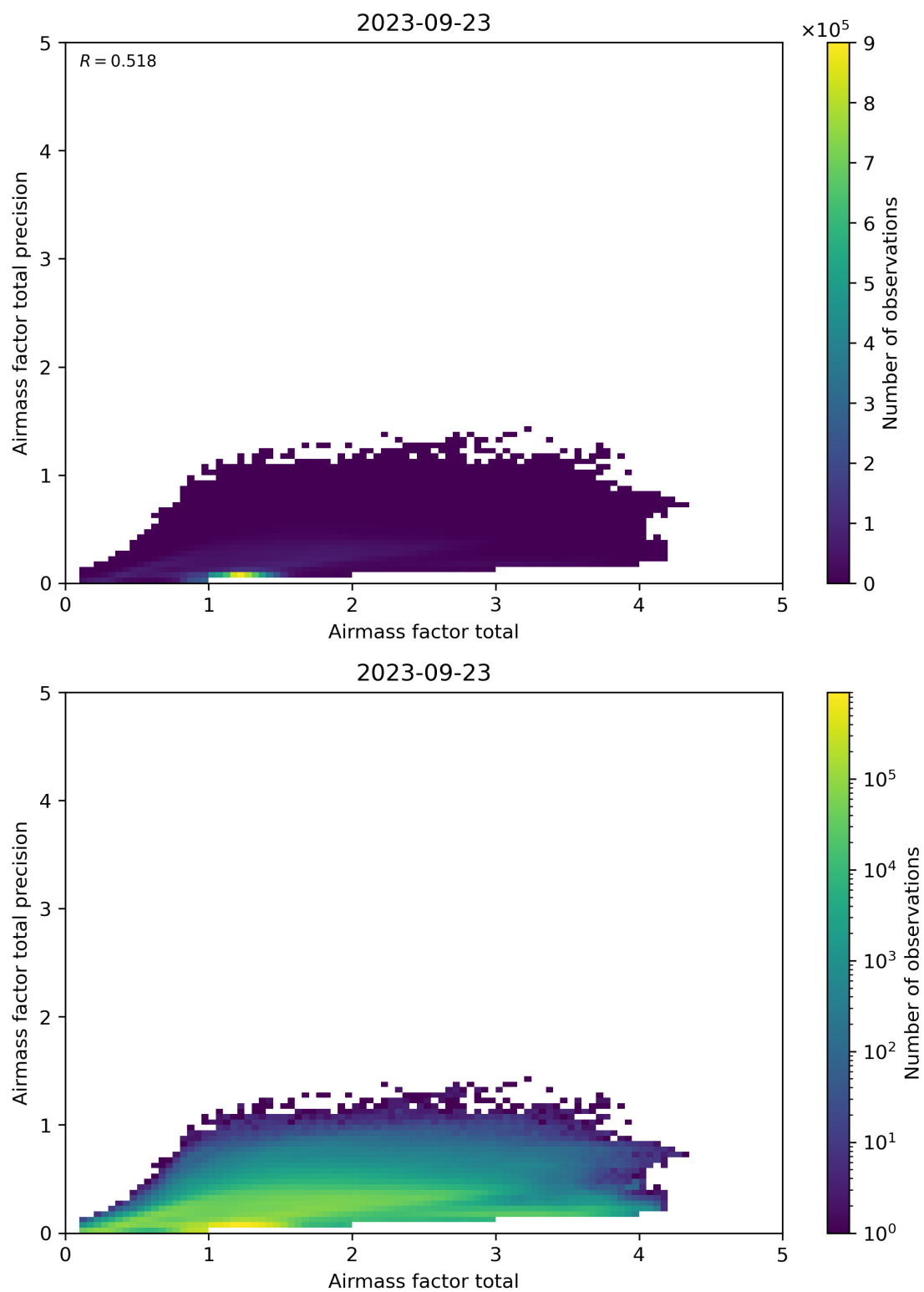
Figure 103: Scatter density plot of “Airmass factor total” against “Airmass factor total precision” for 2023-09-22 to 2023-09-24.
