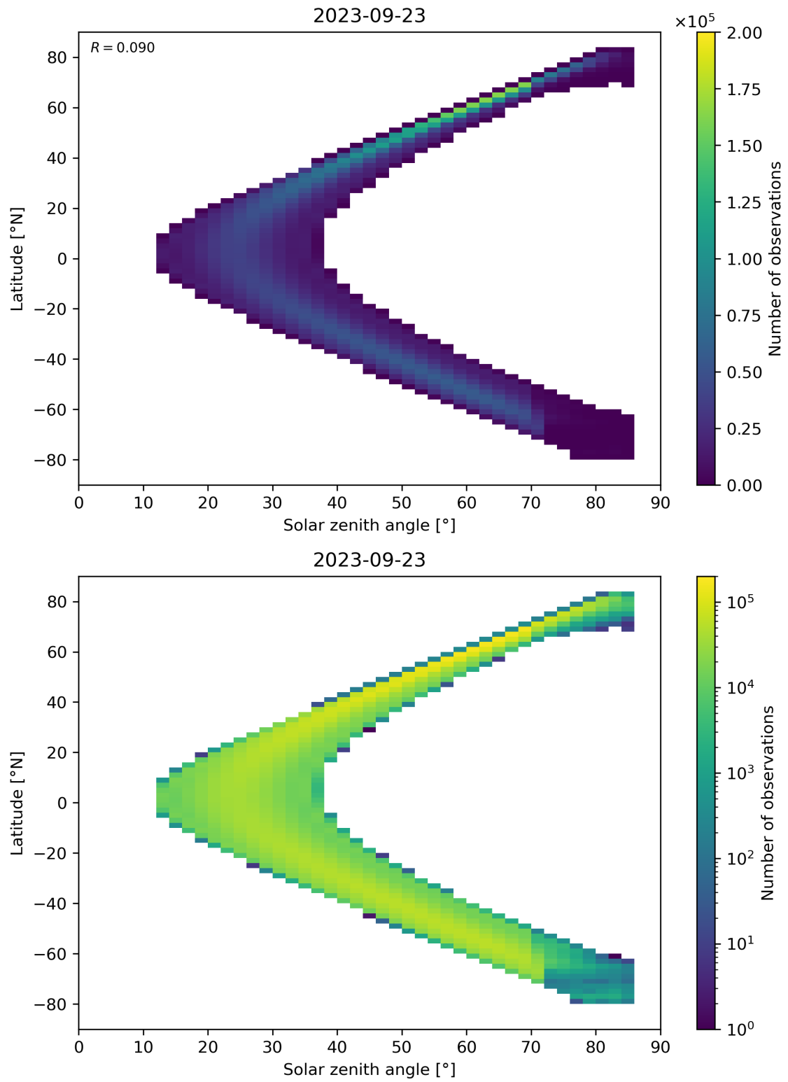
Figure 181: Scatter density plot of “Solar zenith angle” against “Latitude” for 2023-09-22 to 2023-09-24.
