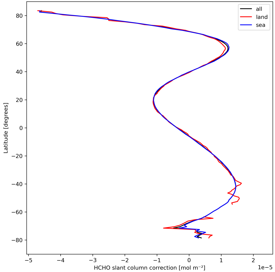
Figure 33: Zonal average of “HCHO slant column correction” for 2023-09-22 to 2023-09-24.
