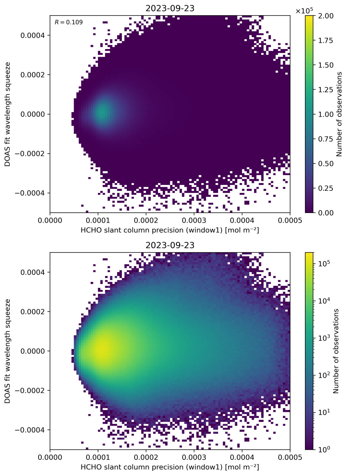
Figure 90: Scatter density plot of “HCHO slant column precision (window1)” against “DOAS fit wavelength squeeze” for 2023-09-22 to 2023-09-24.
