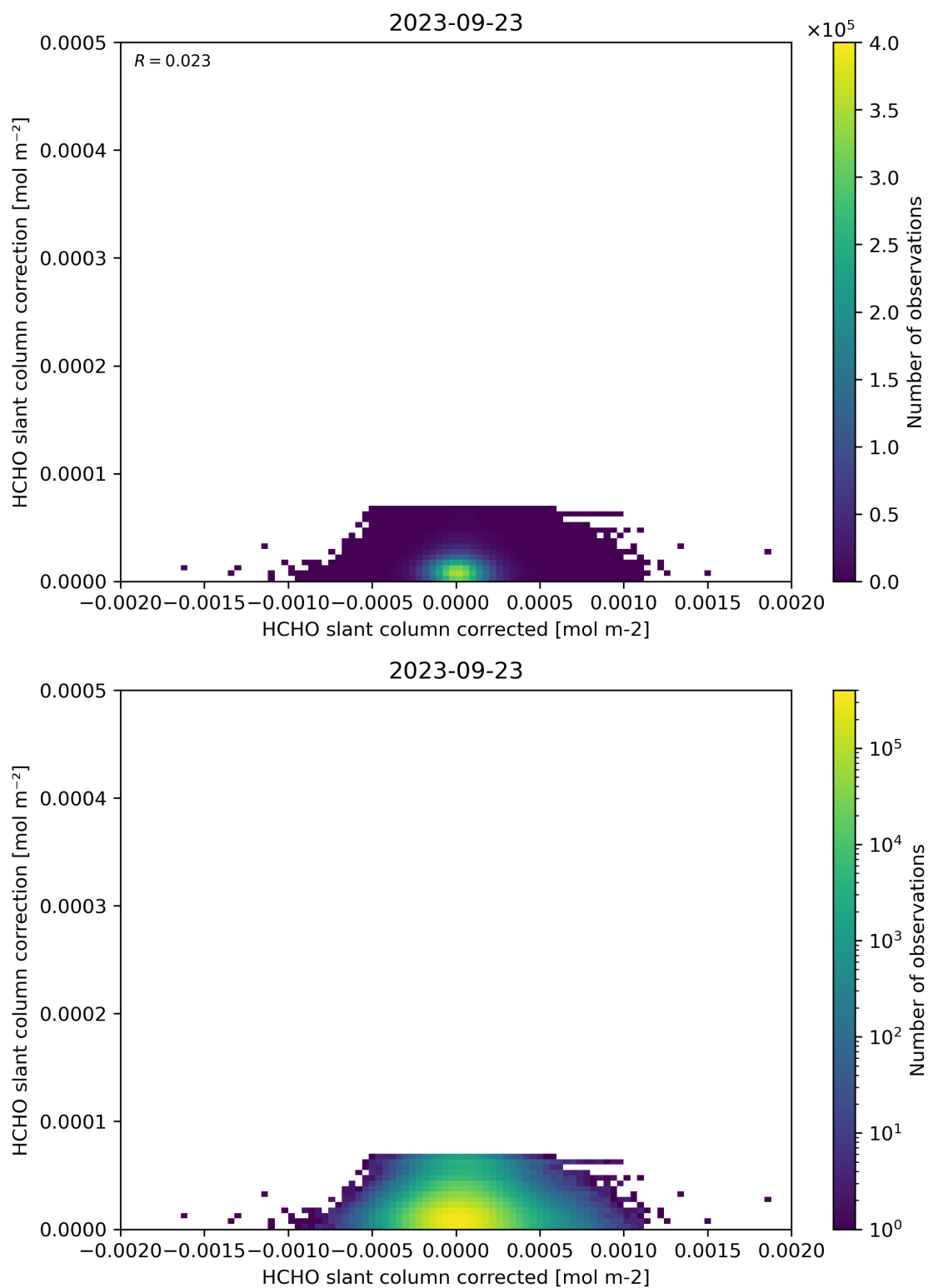
Figure 77: Scatter density plot of “HCHO slant column corrected” against “HCHO slant column correction” for 2023-09-22 to 2023-09-24.
