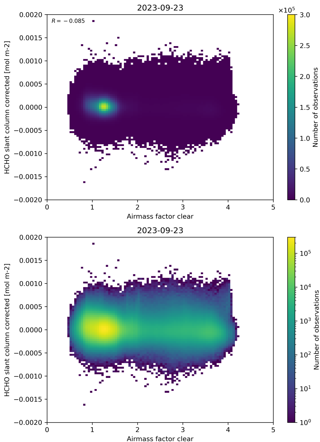
Figure 74: Scatter density plot of “Airmass factor clear” against “HCHO slant column corrected” for 2023-09-22 to 2023-09-24.
