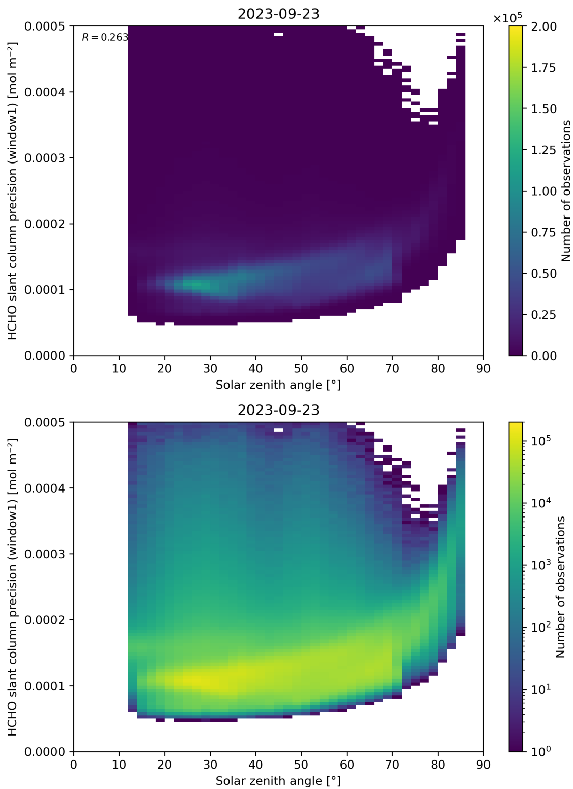
Figure 174: Scatter density plot of “Solar zenith angle” against “HCHO slant column precision (window1)” for 2023-09-22 to 2023-09-24.
