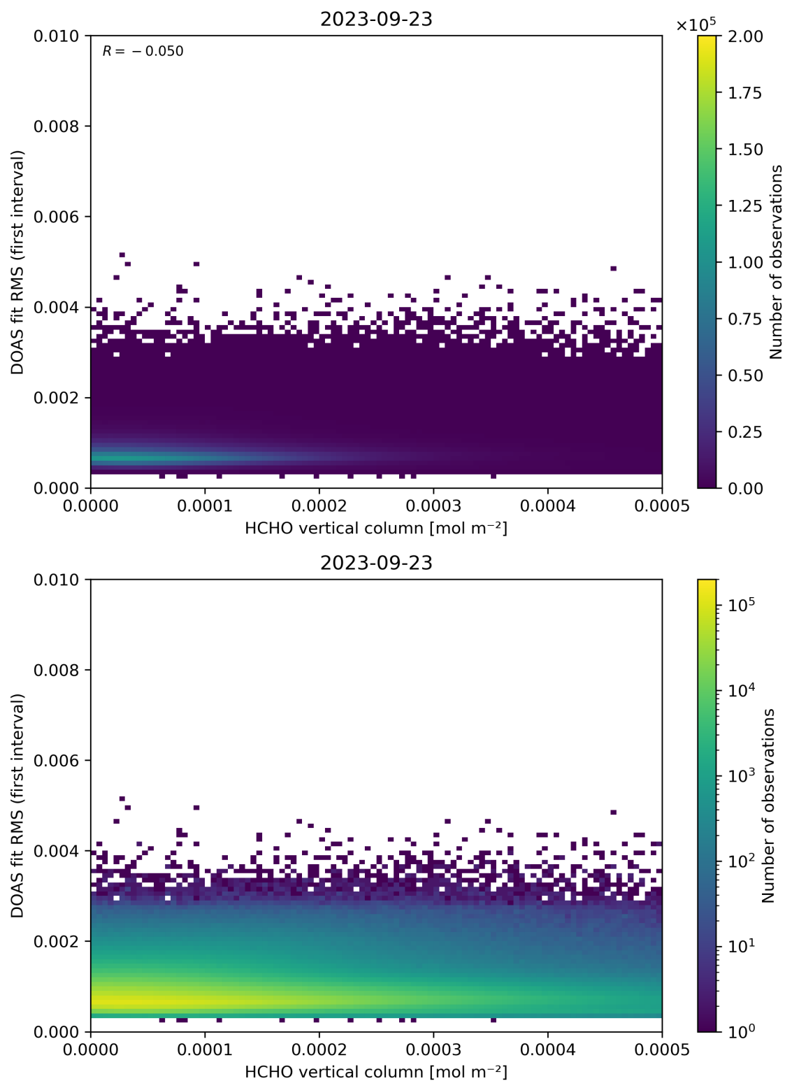
Figure 123: Scatter density plot of “HCHO vertical column” against “DOAS fit RMS (first interval)” for 2023-09-22 to 2023-09-24.
