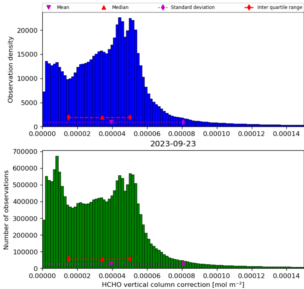
Figure 37: Histogram of “HCHO vertical column correction” for 2023-09-22 to 2023-09-24
