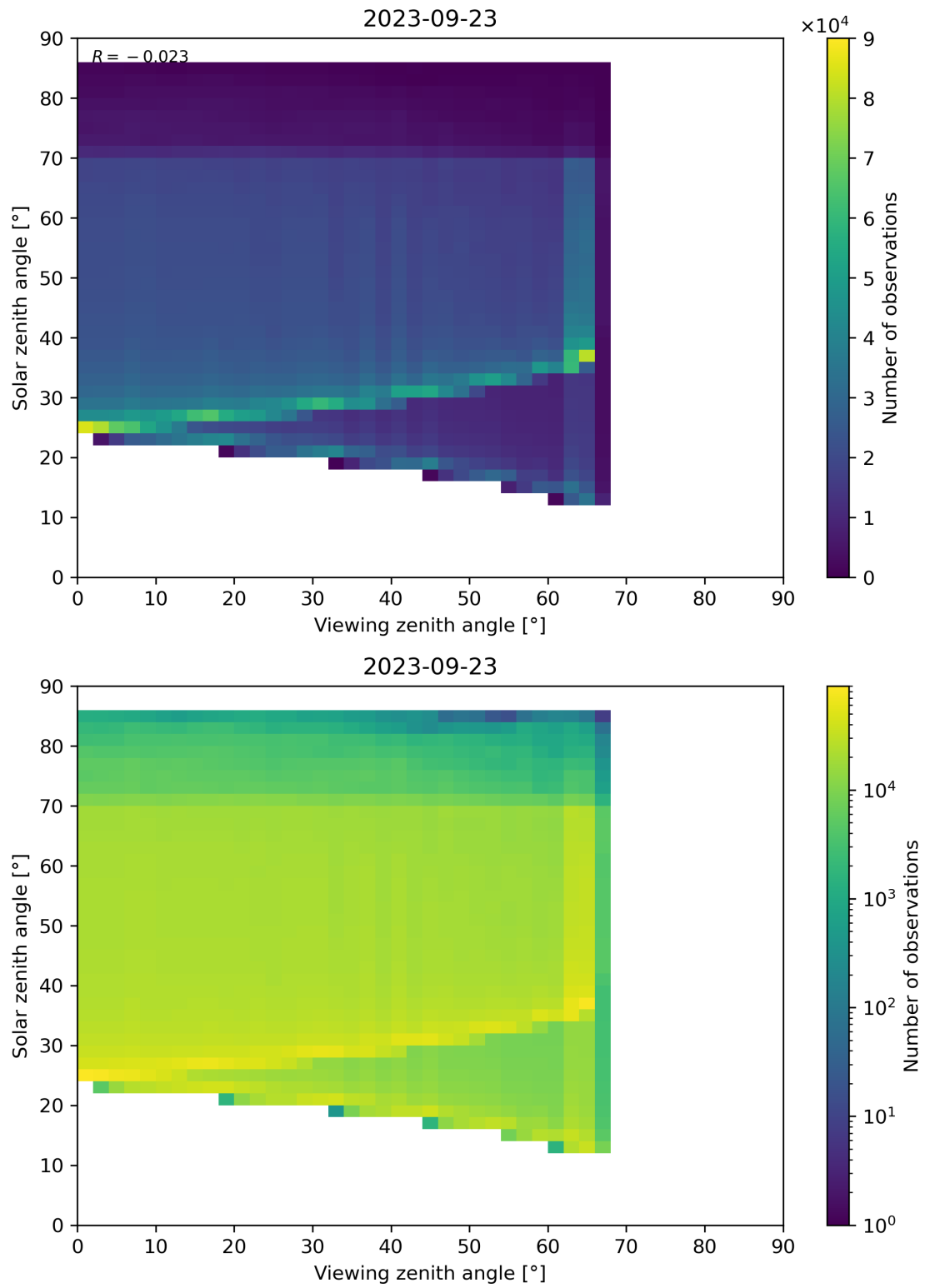
Figure 197: Scatter density plot of “Viewing zenith angle” against “Solar zenith angle” for 2023-09-22 to 2023-09-24.
