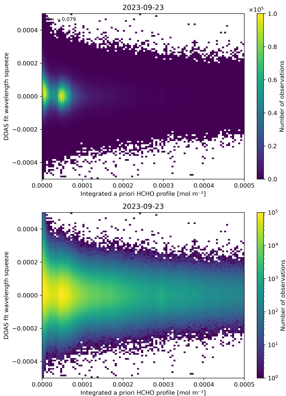
Figure 150: Scatter density plot of “Integrated a priori HCHO profile” against “DOAS fit wavelength squeeze” for 2023-09-22 to 2023-09-24.
