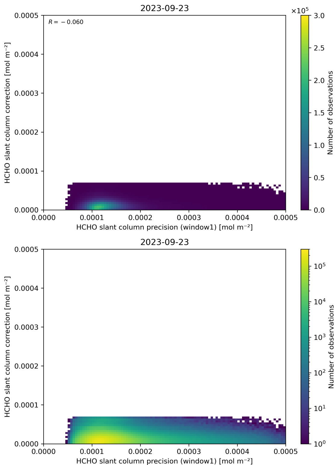
Figure 93: Scatter density plot of “HCHO slant column precision (window1)” against “HCHO slant column correction” for 2023-09-22 to 2023-09-24.
