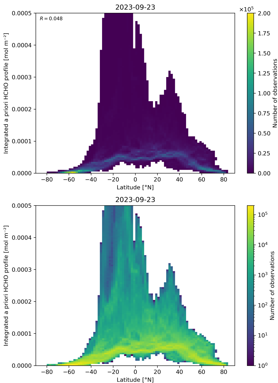
Figure 166: Scatter density plot of “Latitude” against “Integrated a priori HCHO profile” for 2023-09-22 to 2023-09-24.
