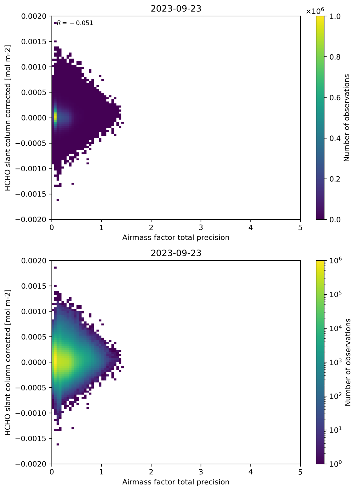
Figure 109: Scatter density plot of “Airmass factor total precision” against “HCHO slant column corrected” for 2023-09-22 to 2023-09-24.
