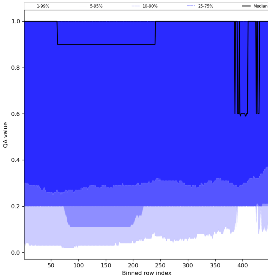
Figure 48: Along track statistics of “QA value” for 2023-09-22 to 2023-09-24
