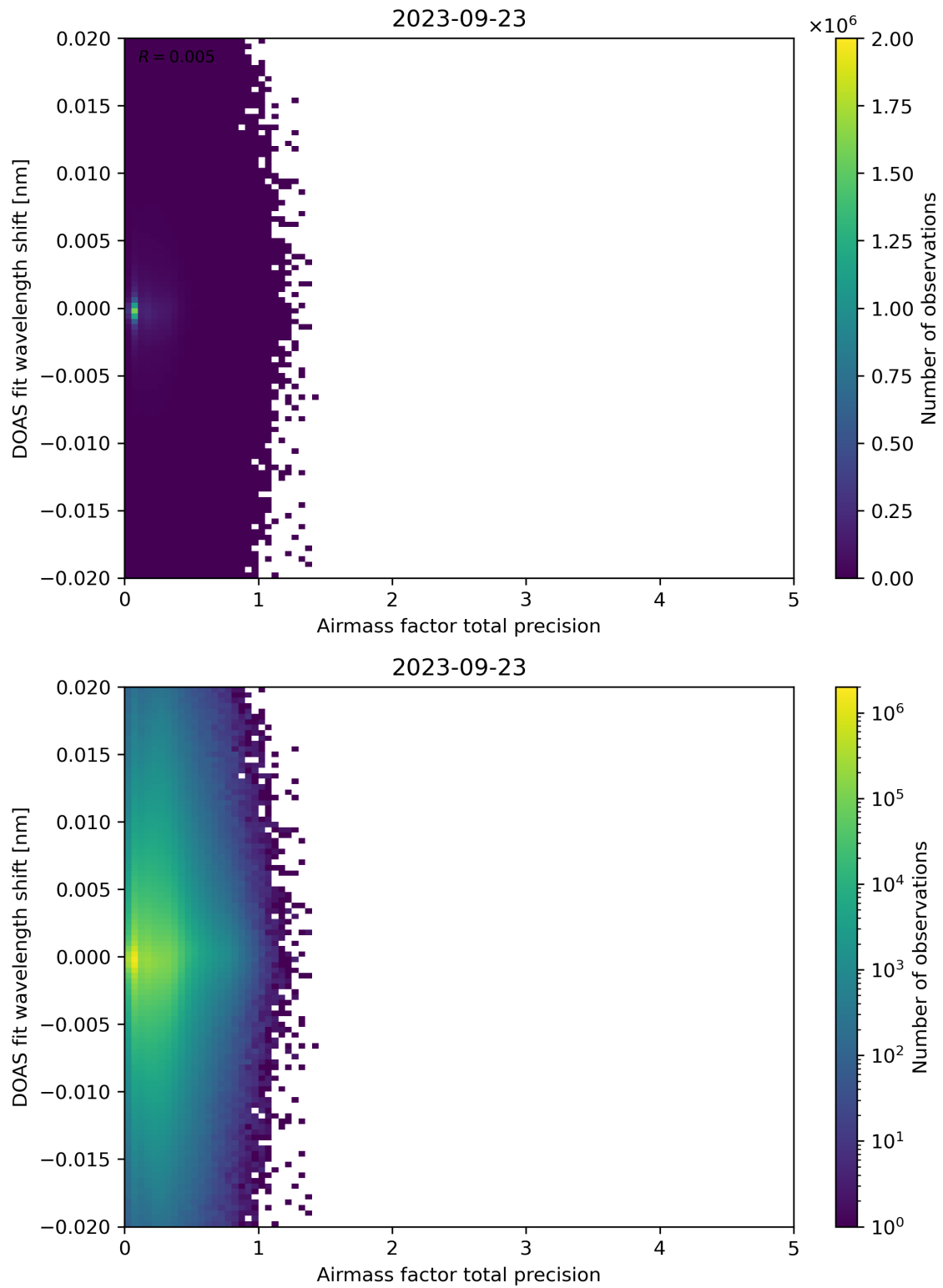
Figure 106: Scatter density plot of “Airmass factor total precision” against “DOAS fit wavelength shift” for 2023-09-22 to 2023-09-24.
