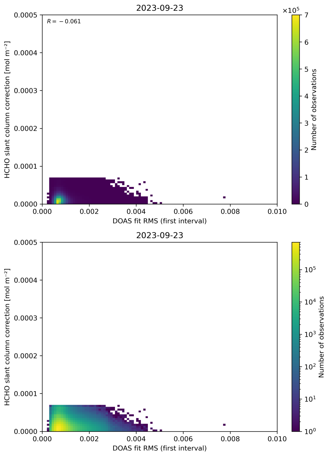
Figure 63: Scatter density plot of “DOAS fit RMS (first interval)” against “HCHO slant column correction” for 2023-09-22 to 2023-09-24.
