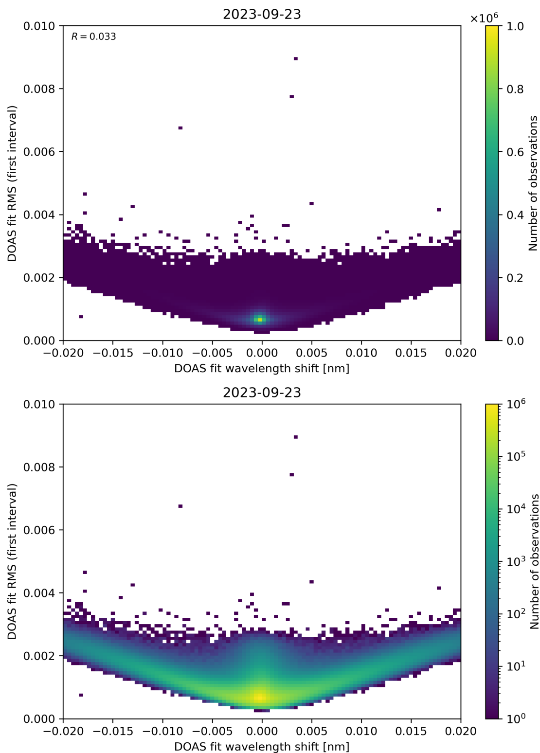
Figure 64: Scatter density plot of “DOAS fit wavelength shift” against “DOAS fit RMS (first interval)” for 2023-09-22 to 2023-09-24.
