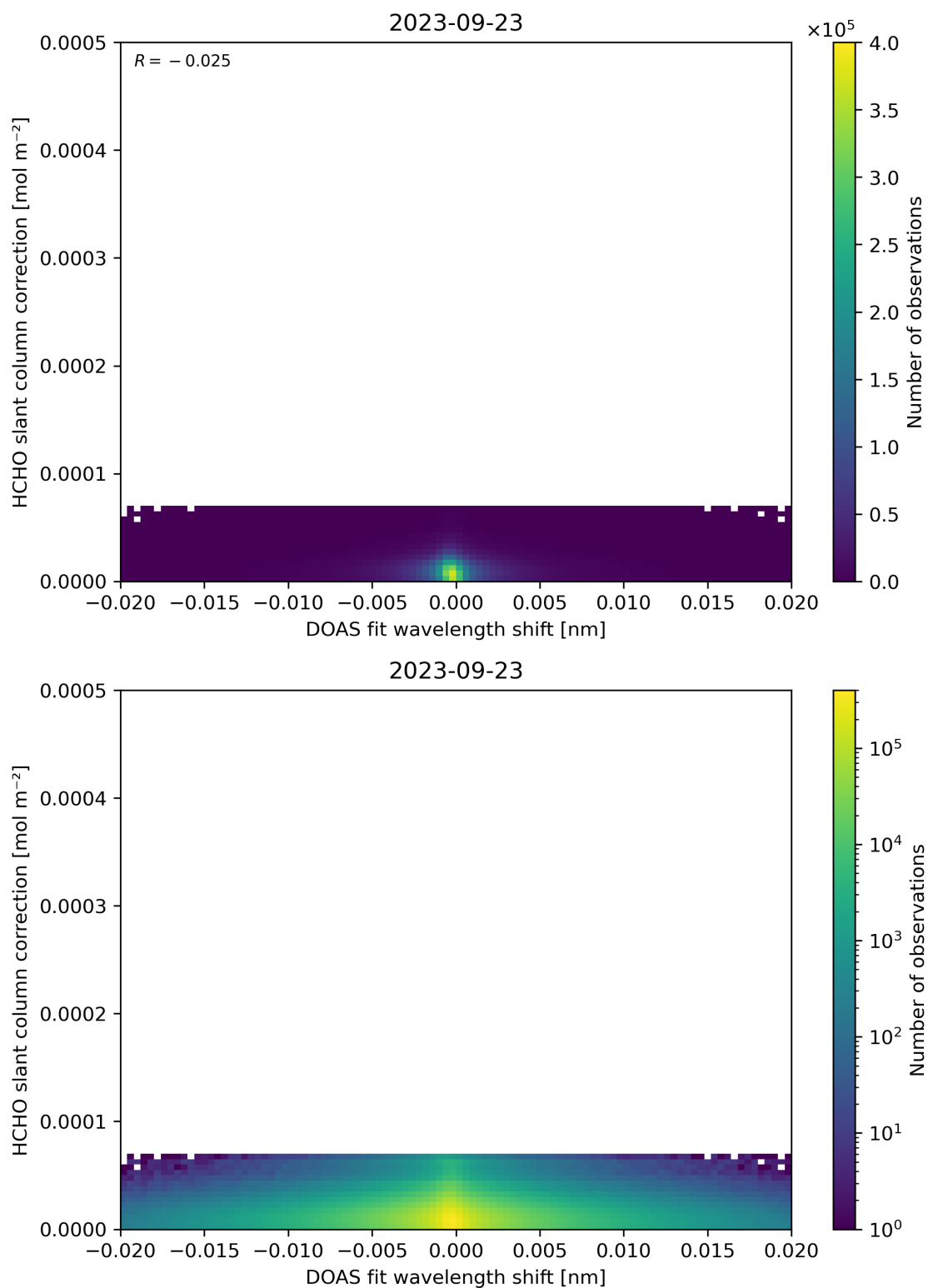
Figure 67: Scatter density plot of “DOAS fit wavelength shift” against “HCHO slant column correction” for 2023-09-22 to 2023-09-24.
