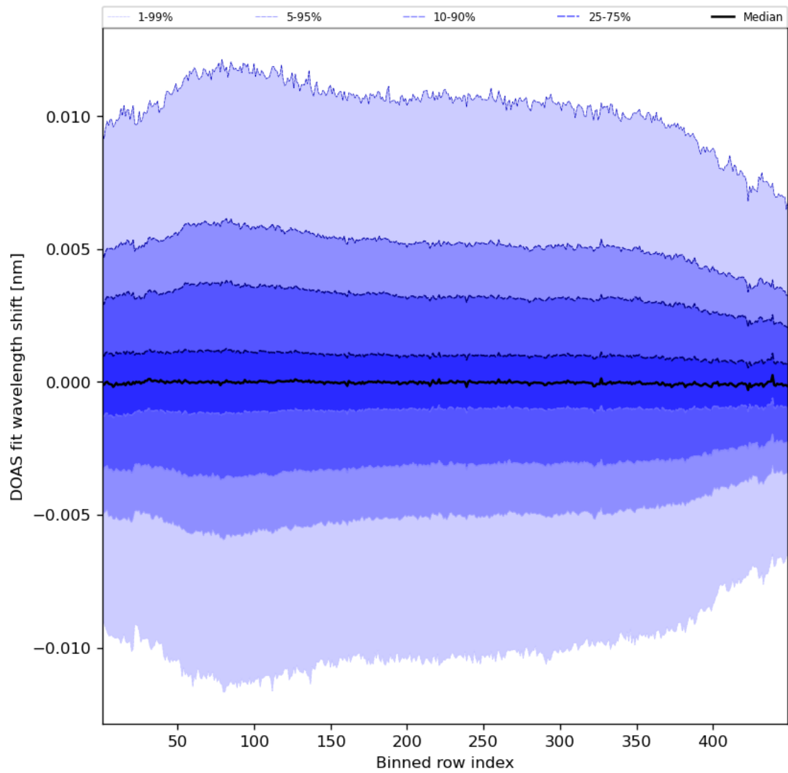
Figure 58: Along track statistics of “DOAS fit wavelength shift” for 2023-09-26 to 2023-09-28
