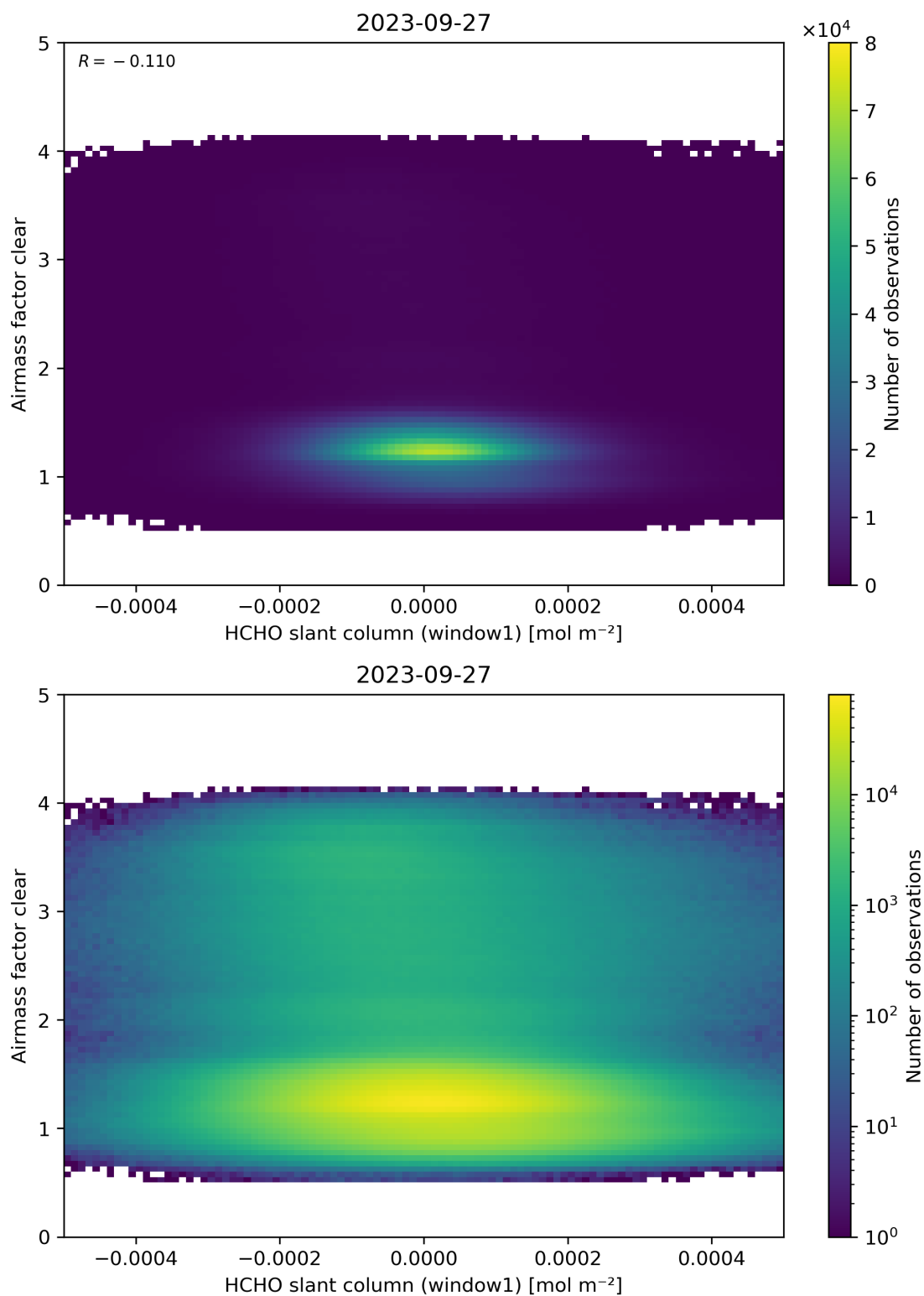
Figure 81: Scatter density plot of “HCHO slant column (window1)” against “Airmass factor clear” for 2023-09-26 to 2023-09-28.
