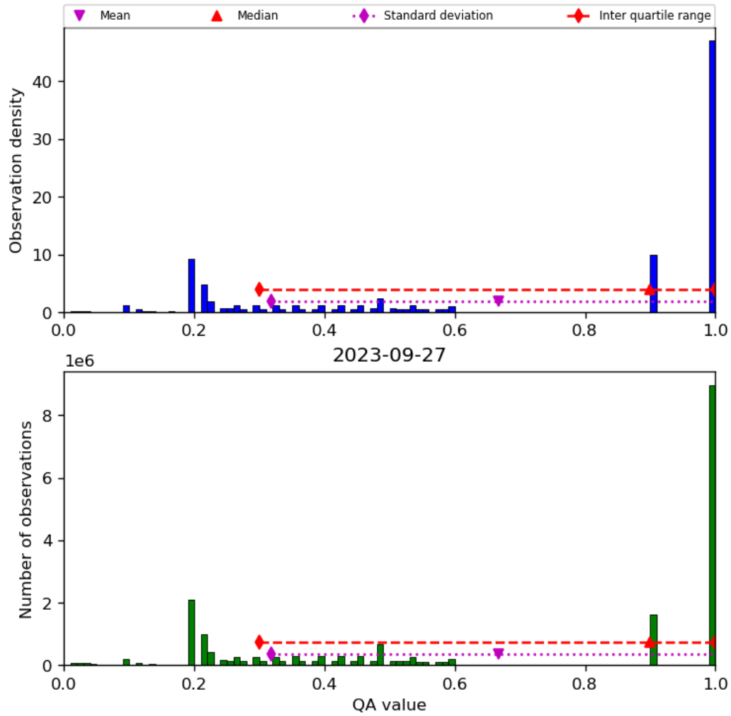
Figure 34: Histogram of “QA value” for 2023-09-26 to 2023-09-28
