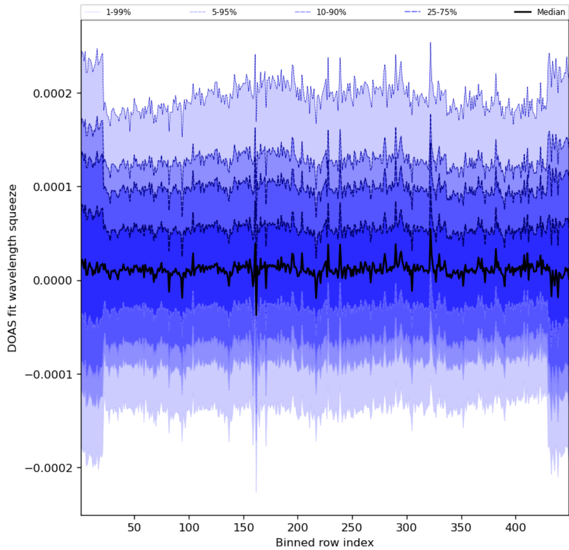
Figure 59: Along track statistics of “DOAS fit wavelength squeeze” for 2023-09-26 to 2023-09-28
