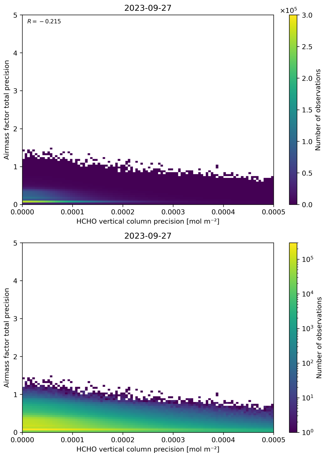
Figure 145: Scatter density plot of “HCHO vertical column precision” against “Airmass factor total precision” for 2023-09-26 to 2023-09-28.
