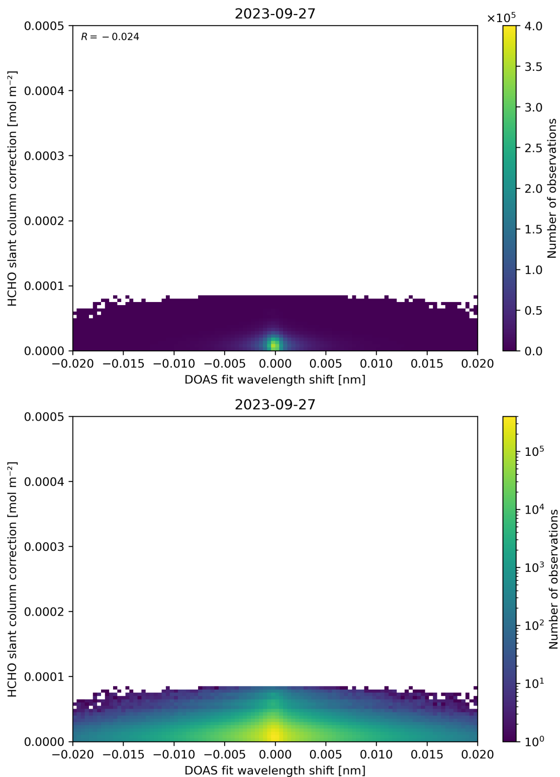
Figure 67: Scatter density plot of “DOAS fit wavelength shift” against “HCHO slant column correction” for 2023-09-26 to 2023-09-28.
