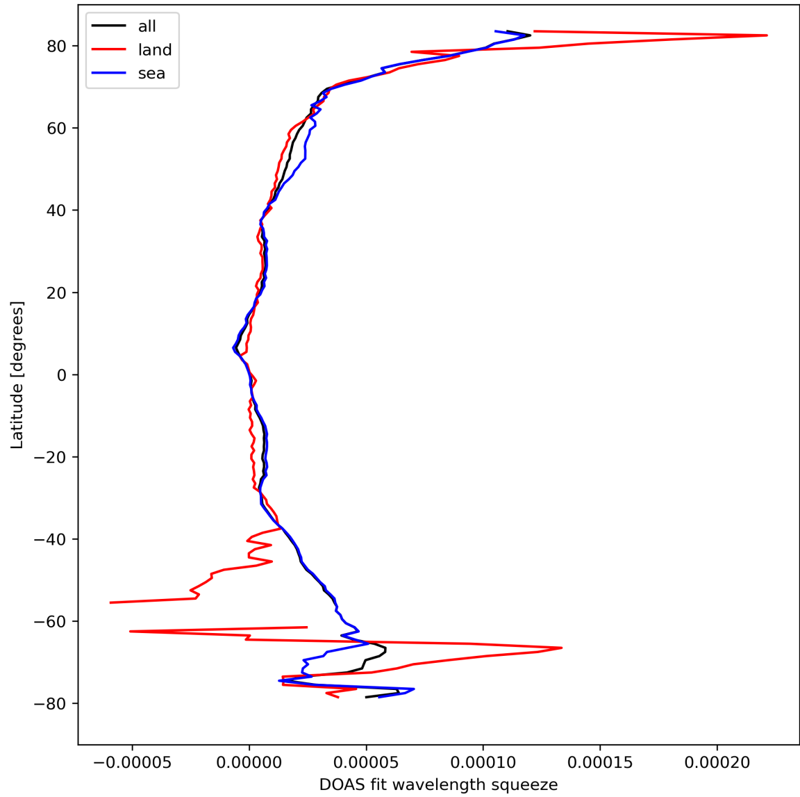
Figure 31: Zonal average of “DOAS fit wavelength squeeze” for 2023-09-26 to 2023-09-28.
