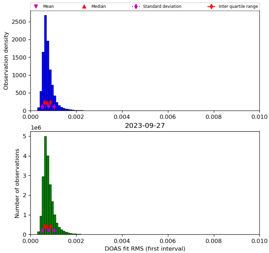
Figure 46: Histogram of “DOAS fit RMS (first interval)” for 2023-09-26 to 2023-09-28
