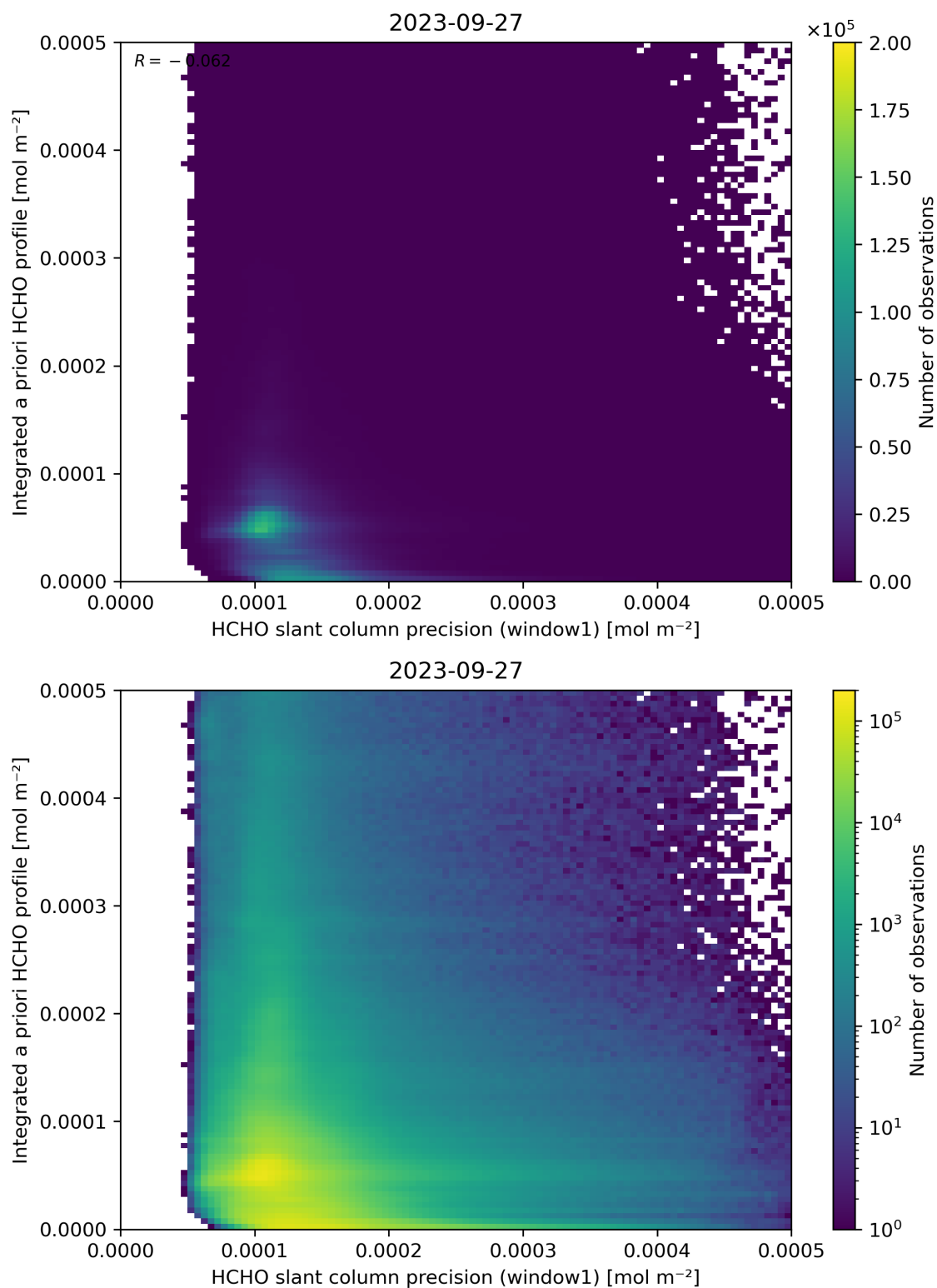
Figure 96: Scatter density plot of “HCHO slant column precision (window1)” against “Integrated a priori HCHO profile” for 2023-09-26 to 2023-09-28.
