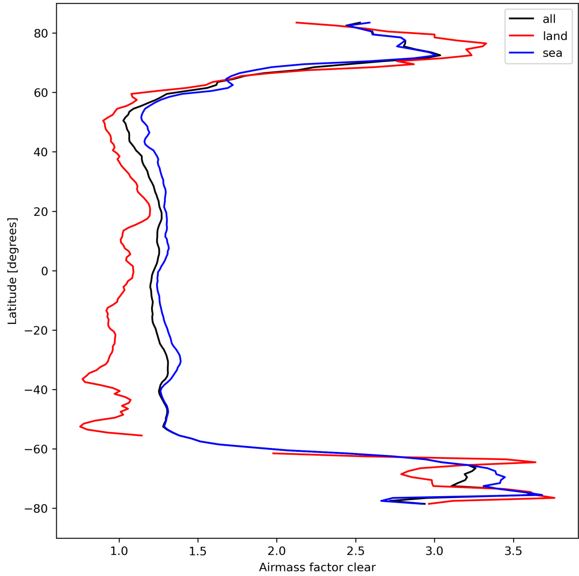
Figure 28: Zonal average of “Airmass factor clear” for 2023-09-26 to 2023-09-28.
