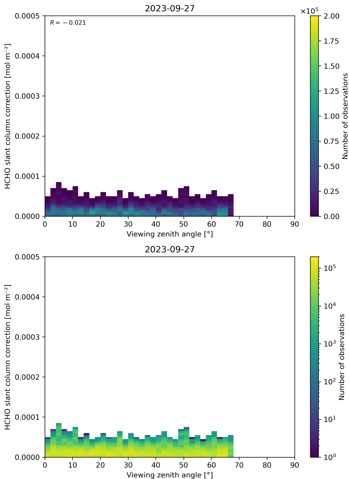
Figure 187: Scatter density plot of “Viewing zenith angle” against “HCHO slant column correction” for 2023-09-26 to 2023-09-28.
