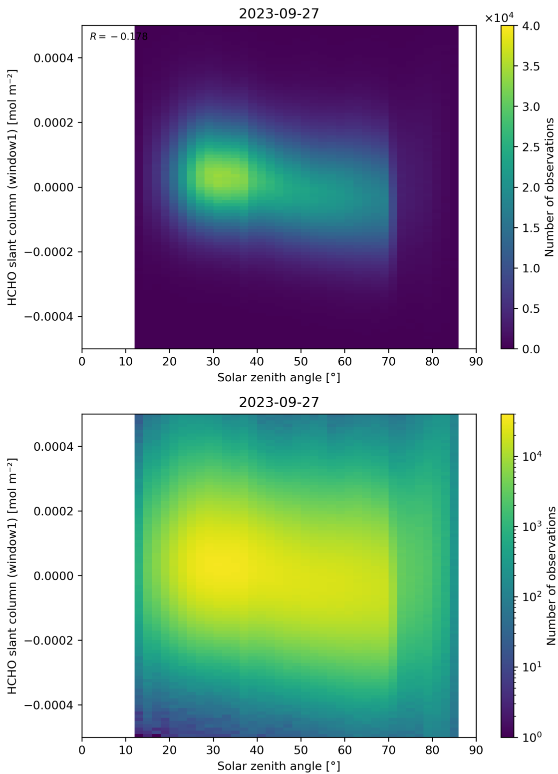
Figure 173: Scatter density plot of “Solar zenith angle” against “HCHO slant column (window1)” for 2023-09-26 to 2023-09-28.
