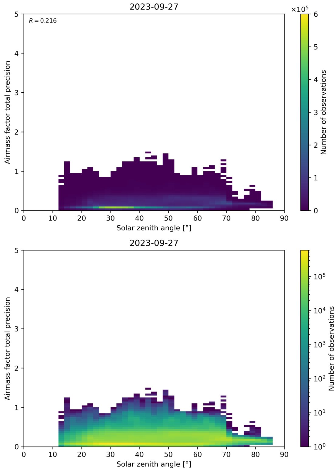
Figure 176: Scatter density plot of “Solar zenith angle” against “Airmass factor total precision” for 2023-09-26 to 2023-09-28.
