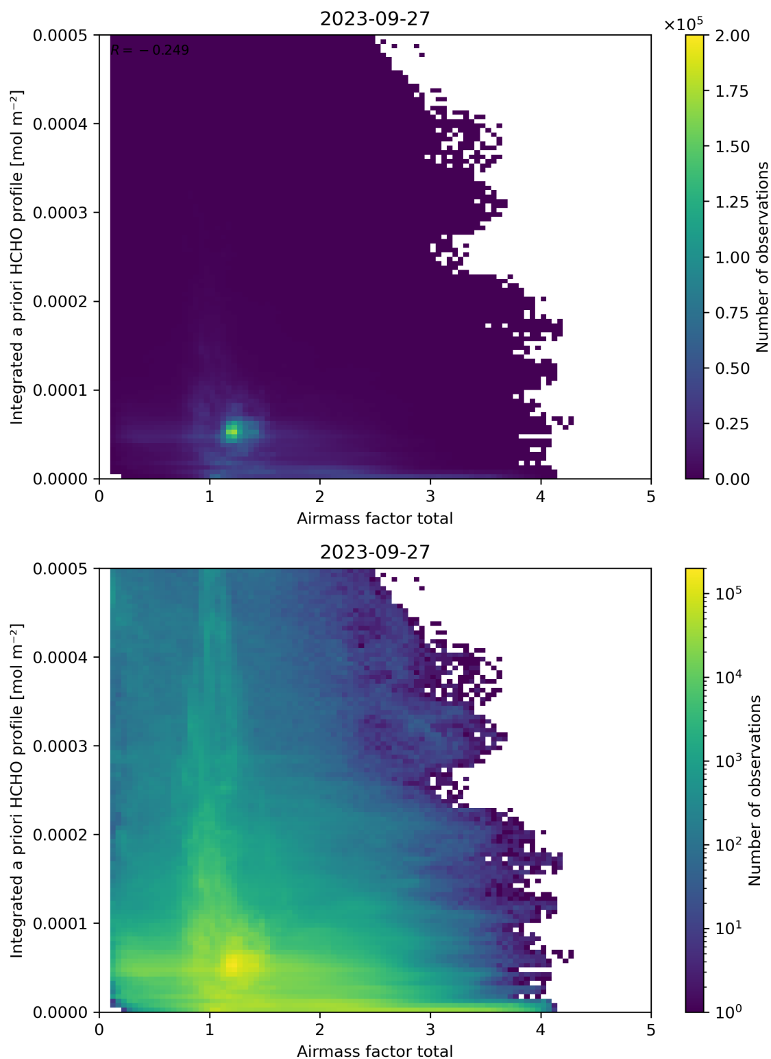
Figure 104: Scatter density plot of “Airmass factor total” against “Integrated a priori HCHO profile” for 2023-09-26 to 2023-09-28.
