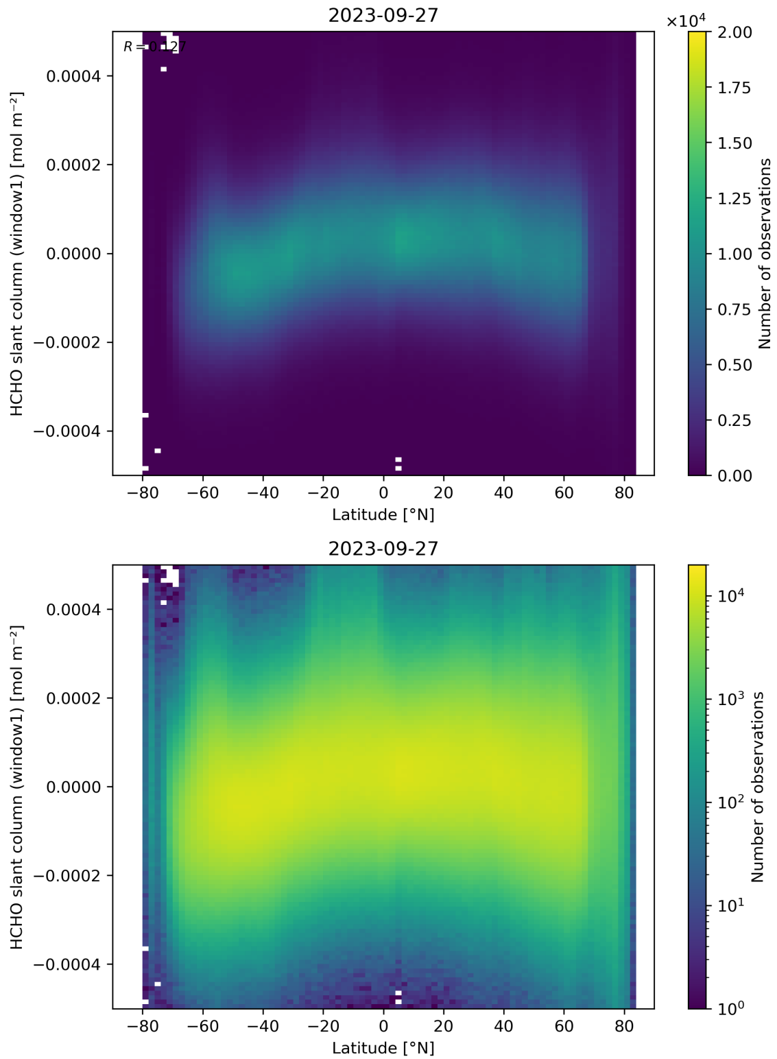
Figure 159: Scatter density plot of “Latitude” against “HCHO slant column (window1)” for 2023-09-26 to 2023-09-28.
