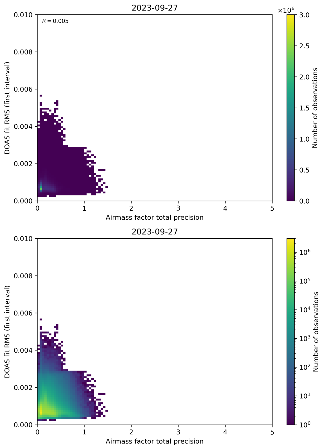
Figure 105: Scatter density plot of “Airmass factor total precision” against “DOAS fit RMS (first interval)” for 2023-09-26 to 2023-09-28.
