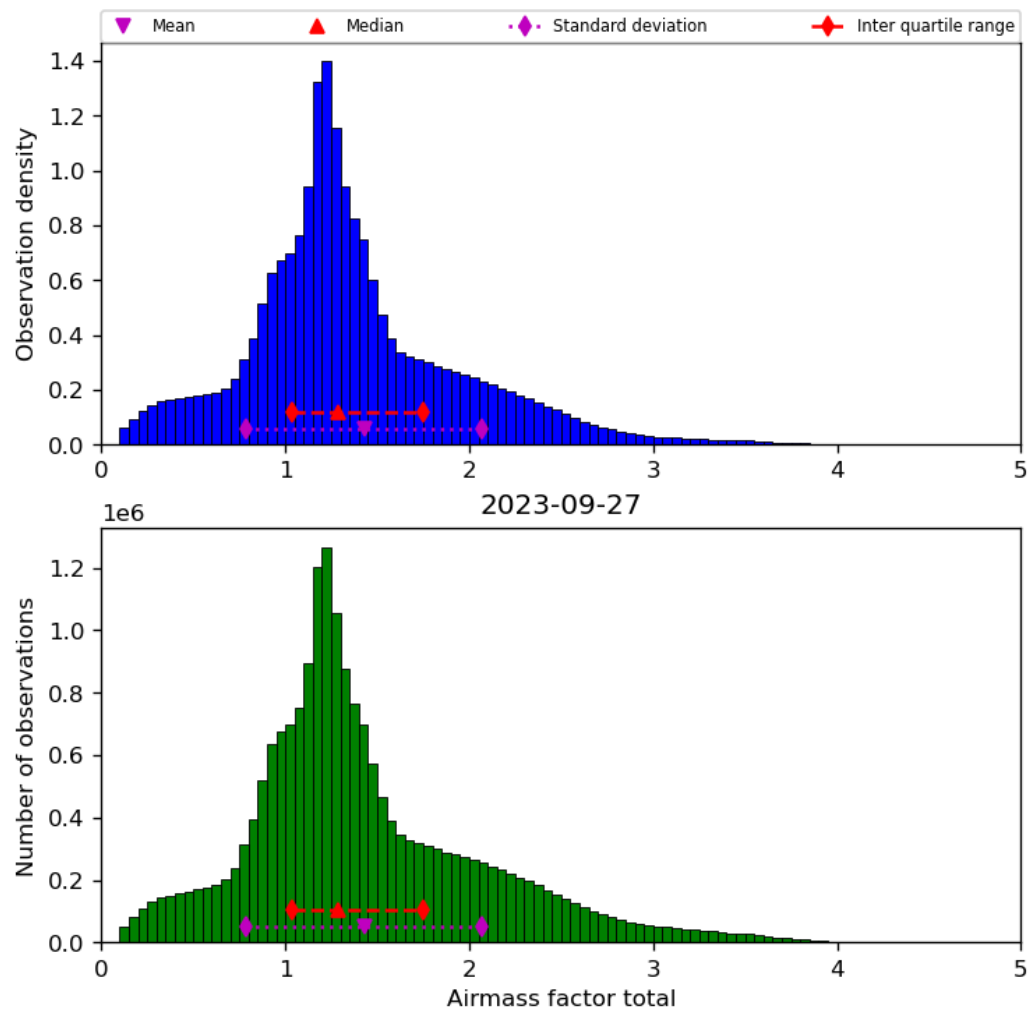
Figure 40: Histogram of “Airmass factor total” for 2023-09-26 to 2023-09-28
