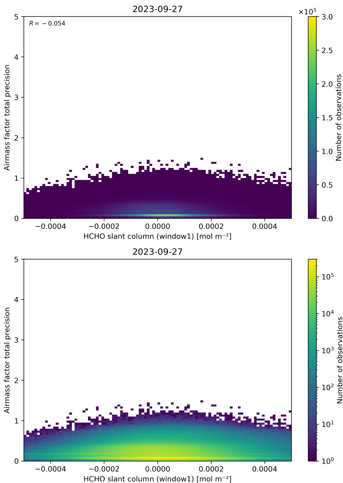
Figure 86: Scatter density plot of “HCHO slant column (window1)” against “Airmass factor total precision” for 2023-09-26 to 2023-09-28.
