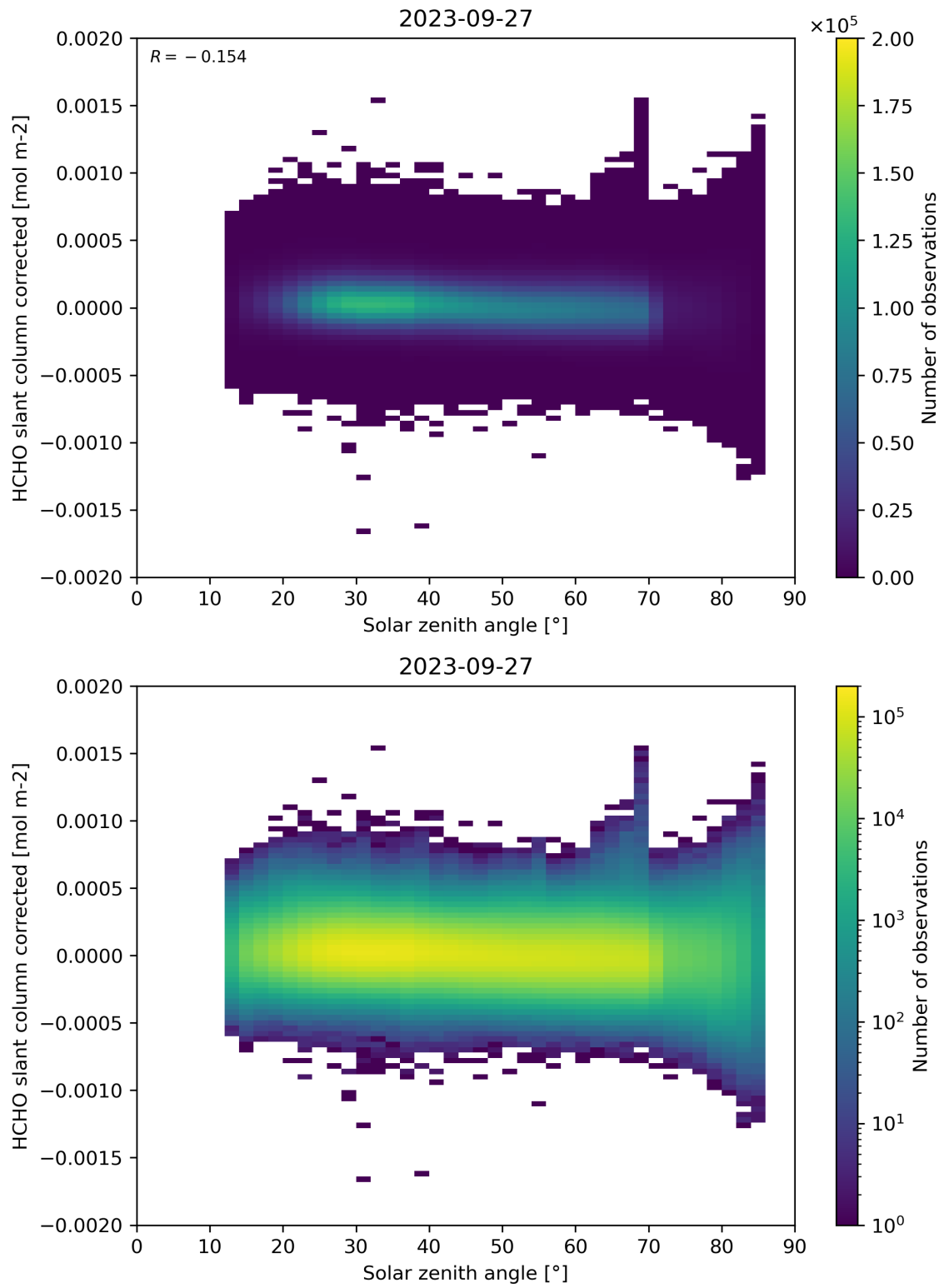
Figure 171: Scatter density plot of “Solar zenith angle” against “HCHO slant column corrected” for 2023-09-26 to 2023-09-28.
