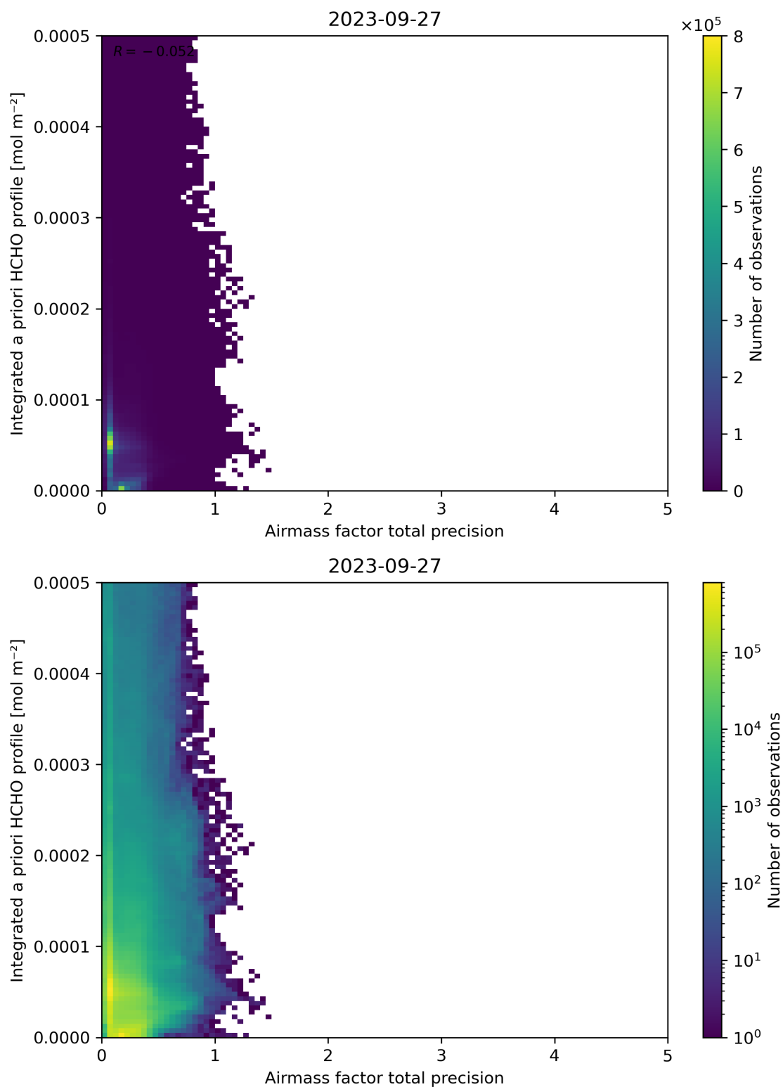
Figure 111: Scatter density plot of “Airmass factor total precision” against “Integrated a priori HCHO profile” for 2023-09-26 to 2023-09-28.
