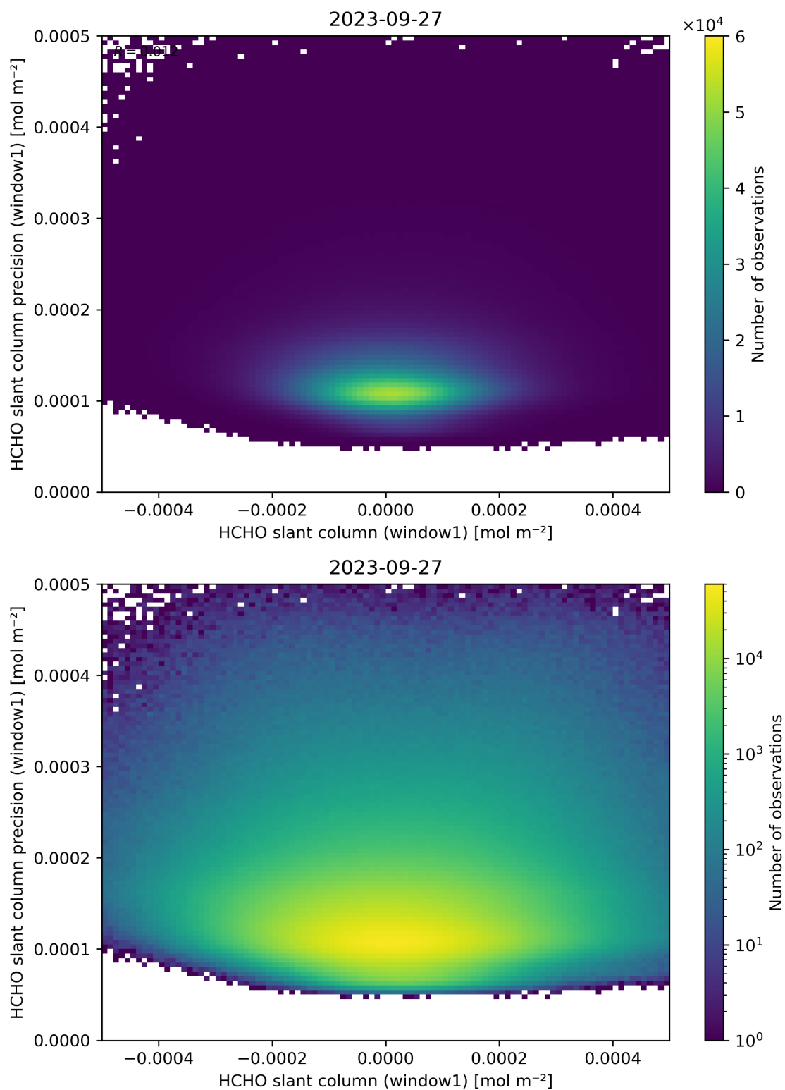
Figure 84: Scatter density plot of “HCHO slant column (window1)” against “HCHO slant column precision (window1)” for 2023-09-26 to 2023-09-28.
