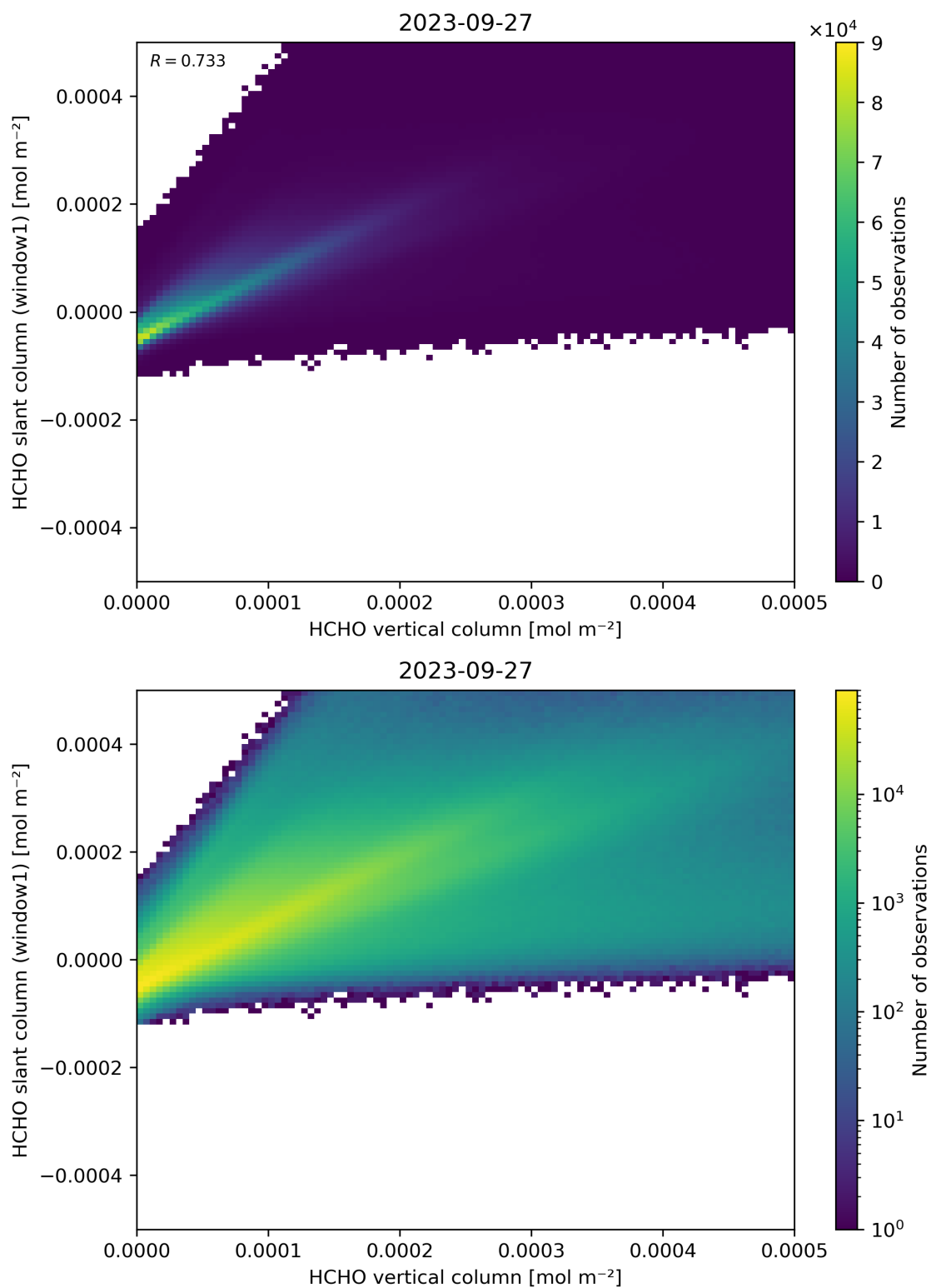
Figure 129: Scatter density plot of “HCHO vertical column” against “HCHO slant column (window1)” for 2023-09-26 to 2023-09-28.
