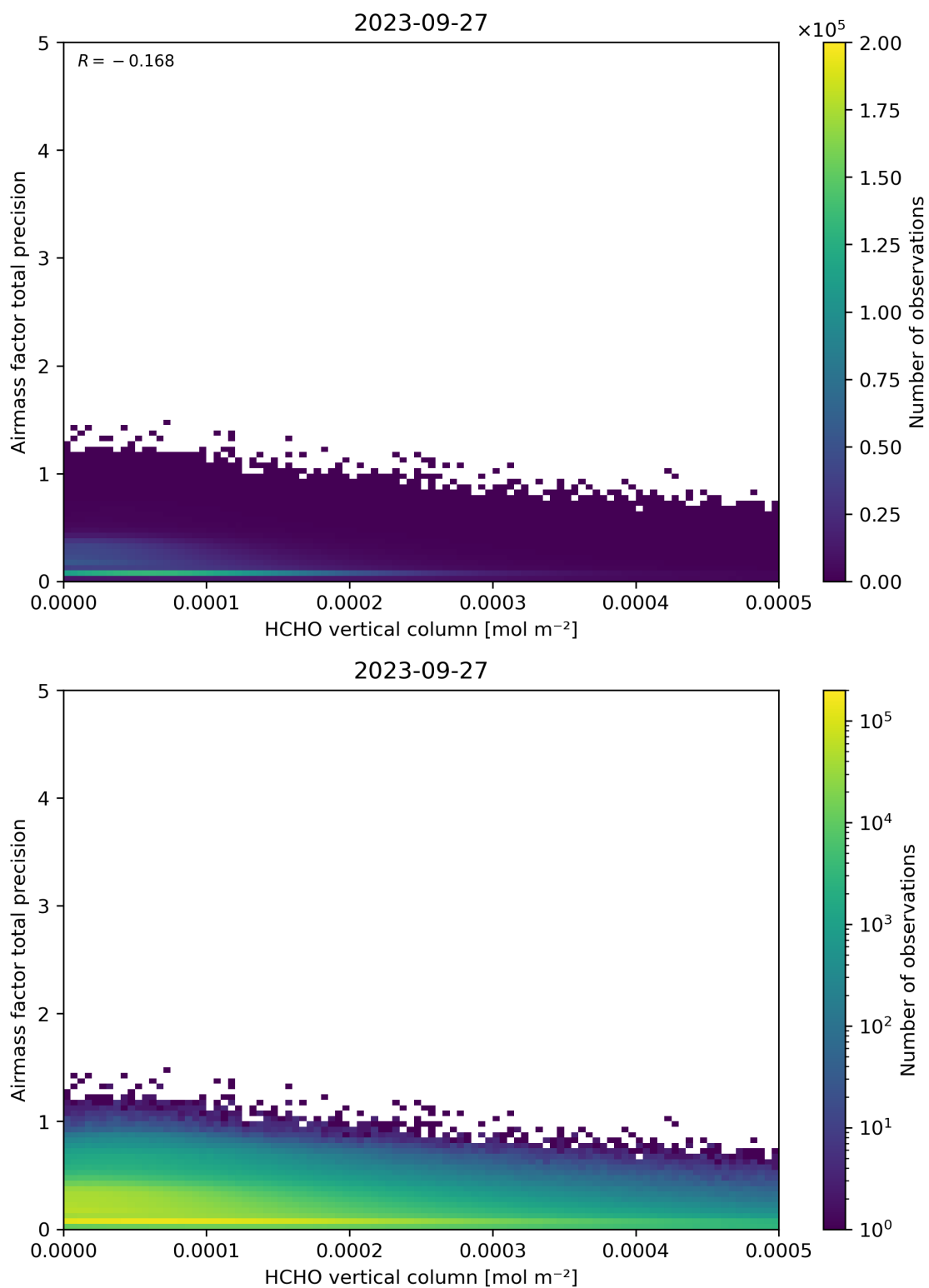
Figure 132: Scatter density plot of “HCHO vertical column” against “Airmass factor total precision” for 2023-09-26 to 2023-09-28.
