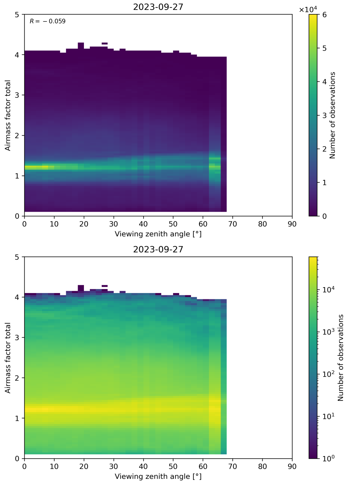
Figure 190: Scatter density plot of “Viewing zenith angle” against “Airmass factor total” for 2023-09-26 to 2023-09-28.
