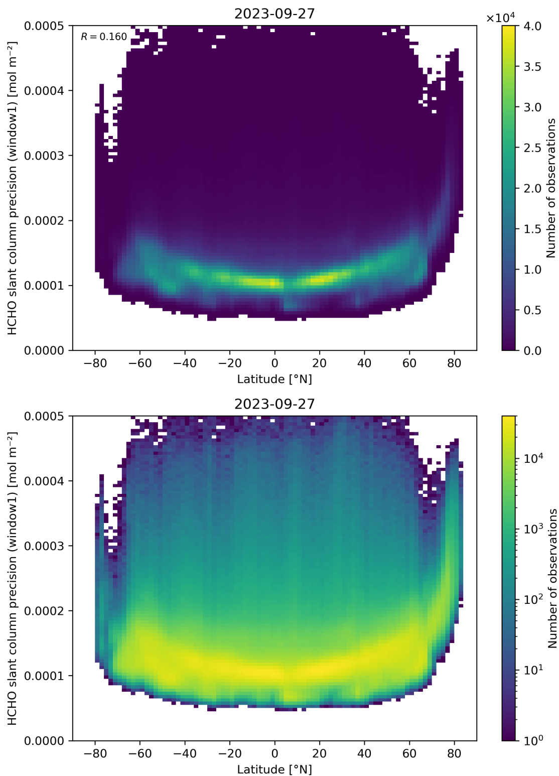
Figure 160: Scatter density plot of “Latitude” against “HCHO slant column precision (window1)” for 2023-09-26 to 2023-09-28.
