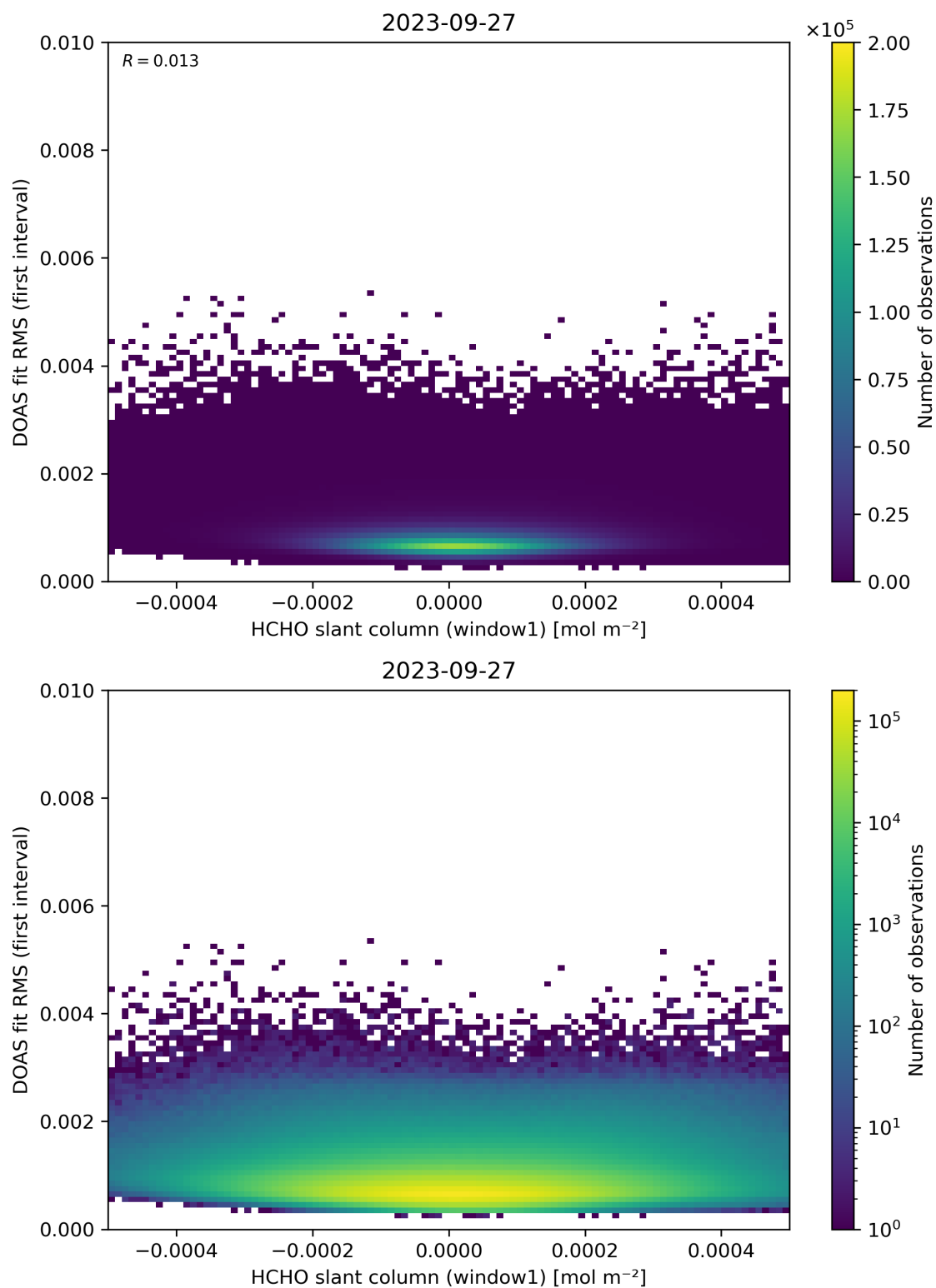
Figure 78: Scatter density plot of “HCHO slant column (window1)” against “DOAS fit RMS (first interval)” for 2023-09-26 to 2023-09-28.
