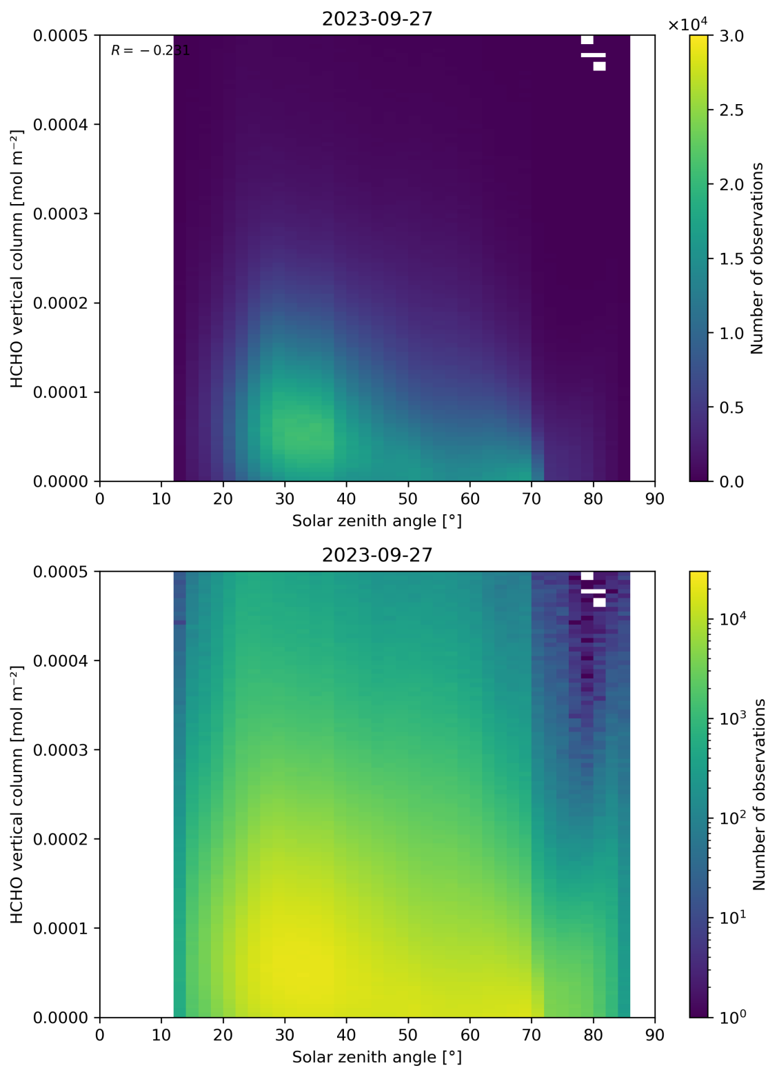
Figure 177: Scatter density plot of “Solar zenith angle” against “HCHO vertical column” for 2023-09-26 to 2023-09-28.
