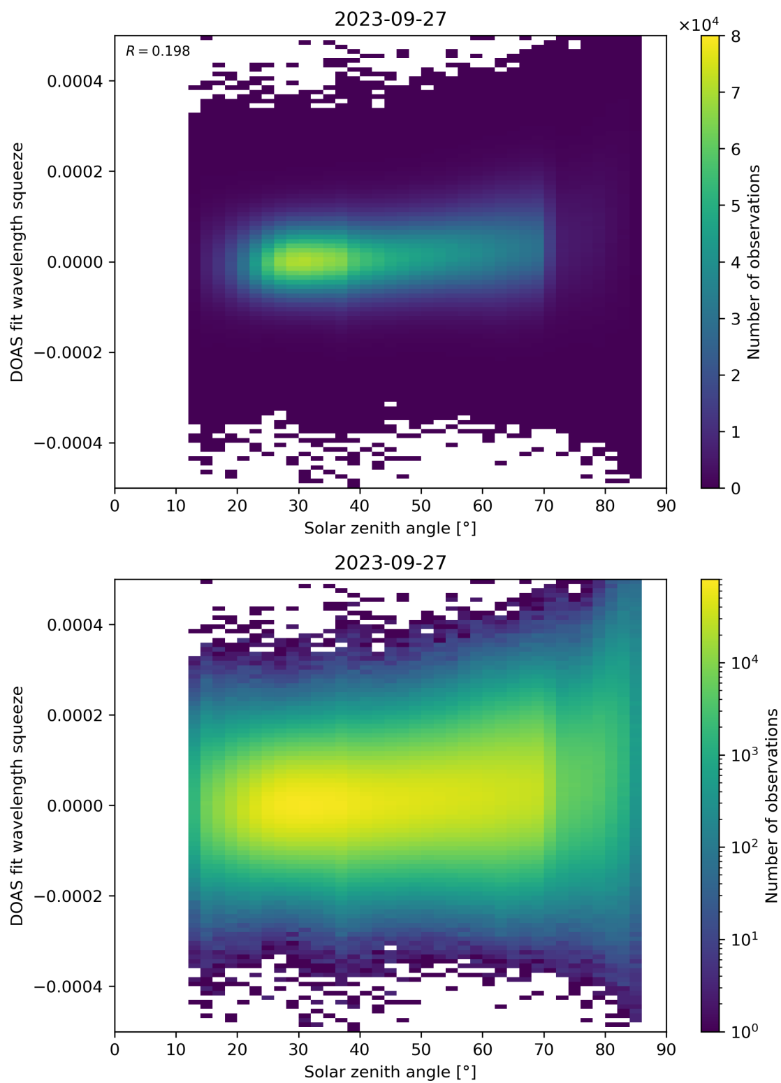
Figure 169: Scatter density plot of “Solar zenith angle” against “DOAS fit wavelength squeeze” for 2023-09-26 to 2023-09-28.
