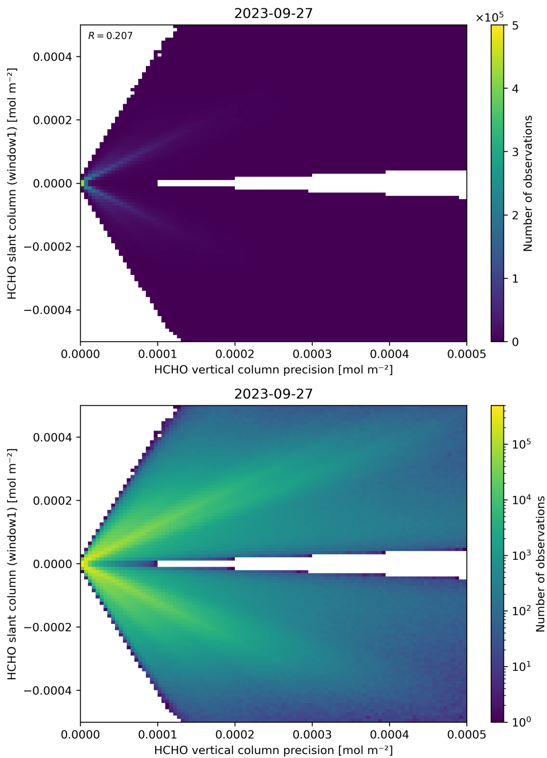
Figure 142: Scatter density plot of “HCHO vertical column precision” against “HCHO slant column (window1)” for 2023-09-26 to 2023-09-28.
