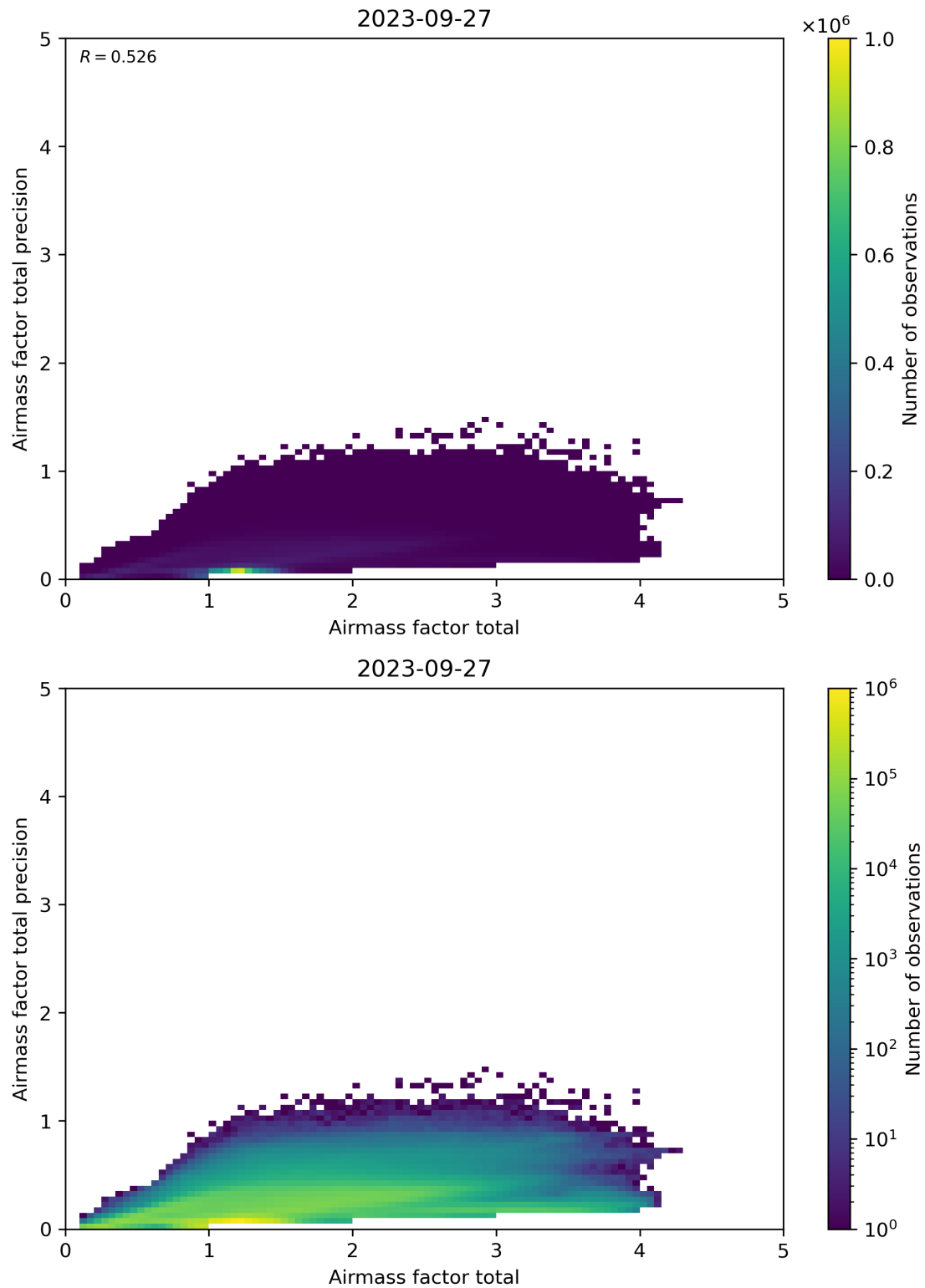
Figure 103: Scatter density plot of “Airmass factor total” against “Airmass factor total precision” for 2023-09-26 to 2023-09-28.
