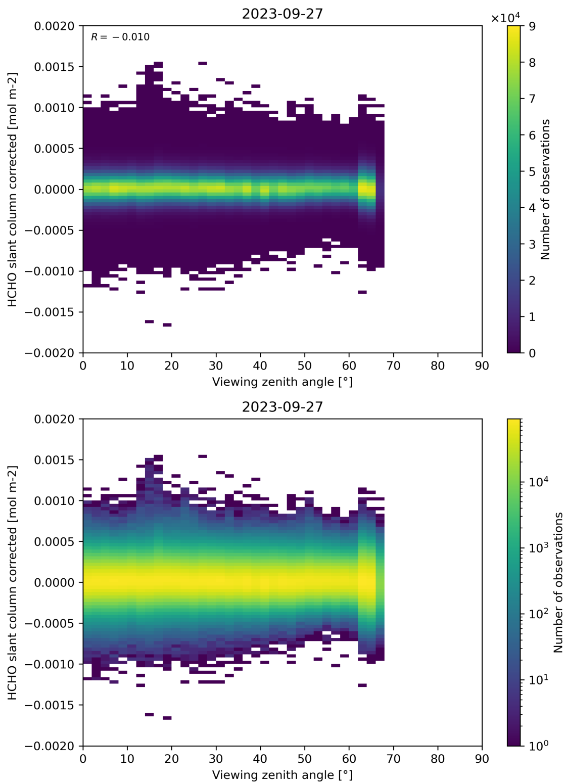
Figure 186: Scatter density plot of “Viewing zenith angle” against “HCHO slant column corrected” for 2023-09-26 to 2023-09-28.
