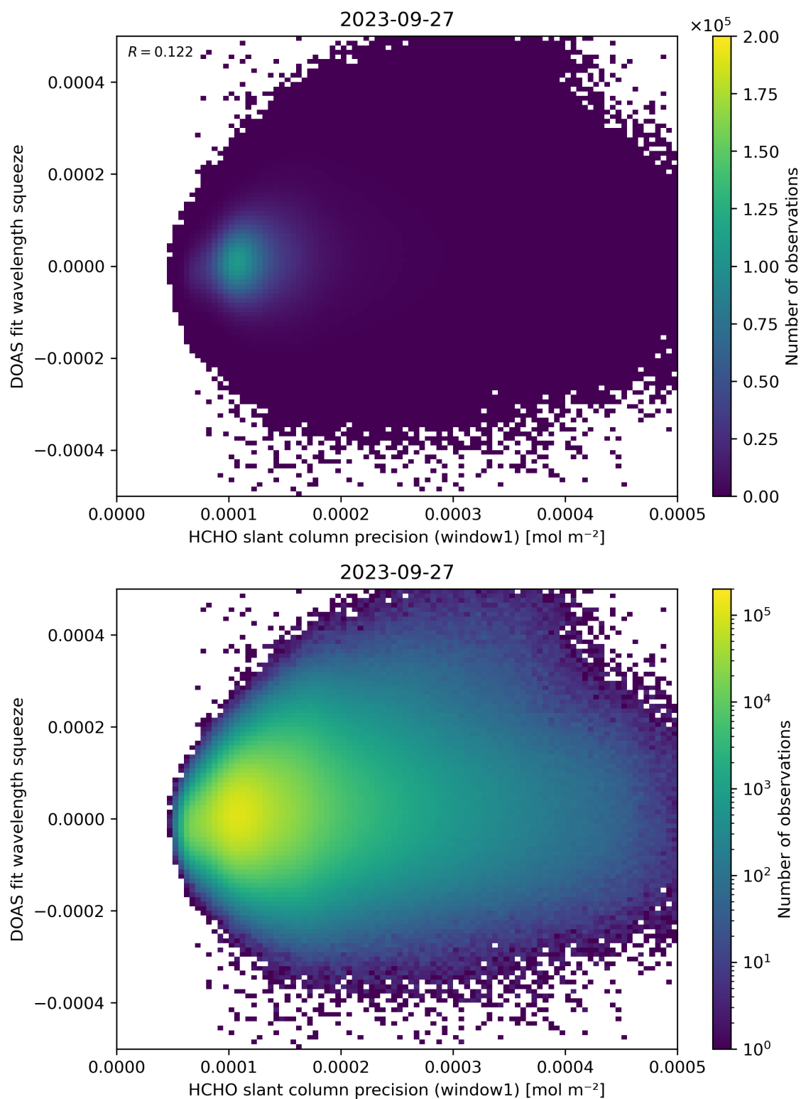
Figure 90: Scatter density plot of “HCHO slant column precision (window1)” against “DOAS fit wavelength squeeze” for 2023-09-26 to 2023-09-28.
