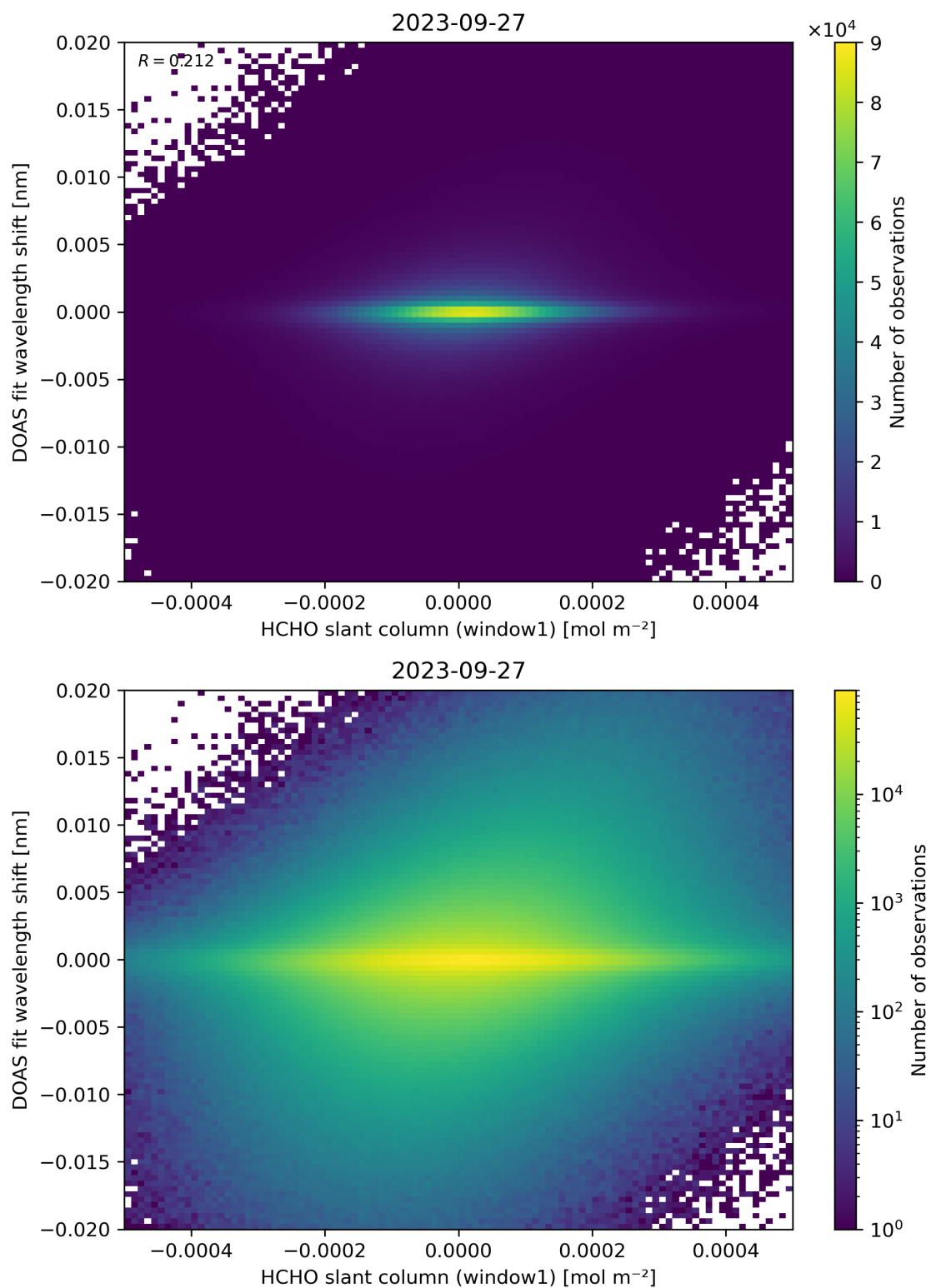
Figure 79: Scatter density plot of “HCHO slant column (window1)” against “DOAS fit wavelength shift” for 2023-09-26 to 2023-09-28.
