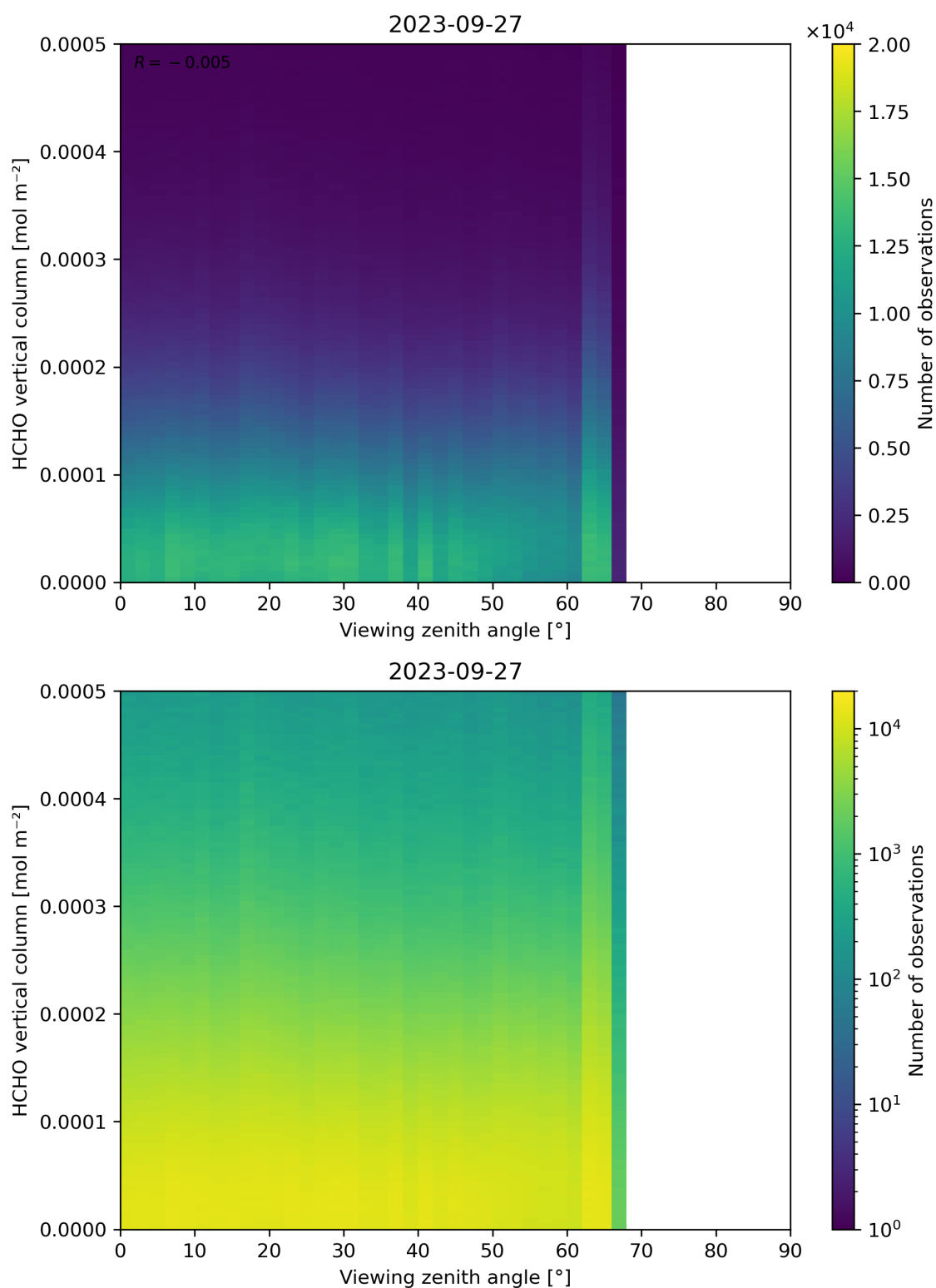
Figure 192: Scatter density plot of “Viewing zenith angle” against “HCHO vertical column” for 2023-09-26 to 2023-09-28.
