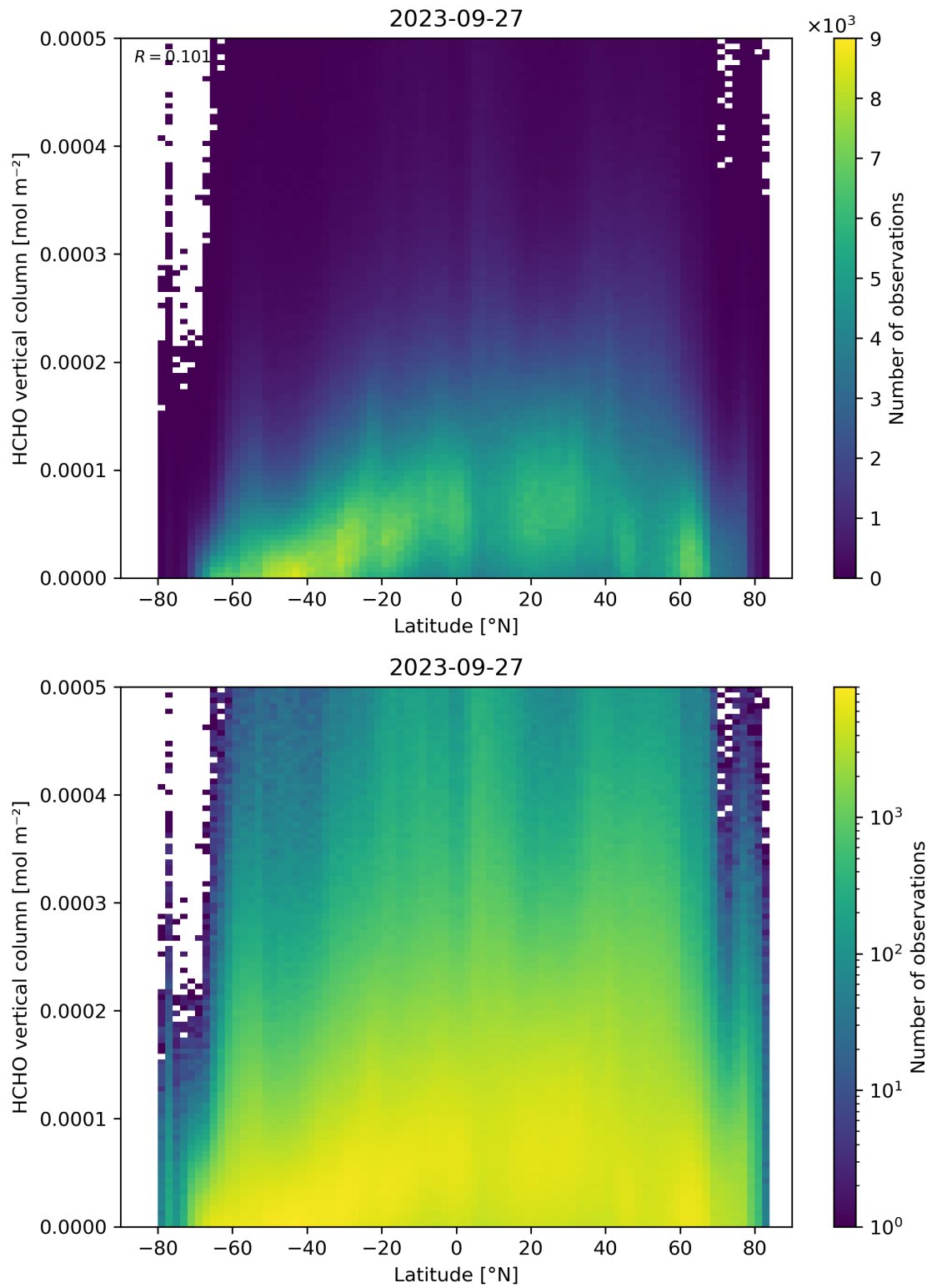
Figure 163: Scatter density plot of “Latitude” against “HCHO vertical column” for 2023-09-26 to 2023-09-28.
