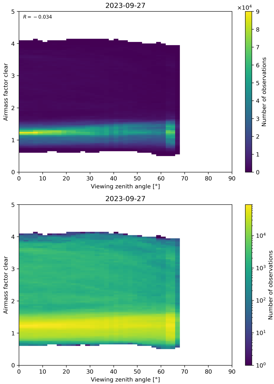
Figure 185: Scatter density plot of “Viewing zenith angle” against “Airmass factor clear” for 2023-09-26 to 2023-09-28.
