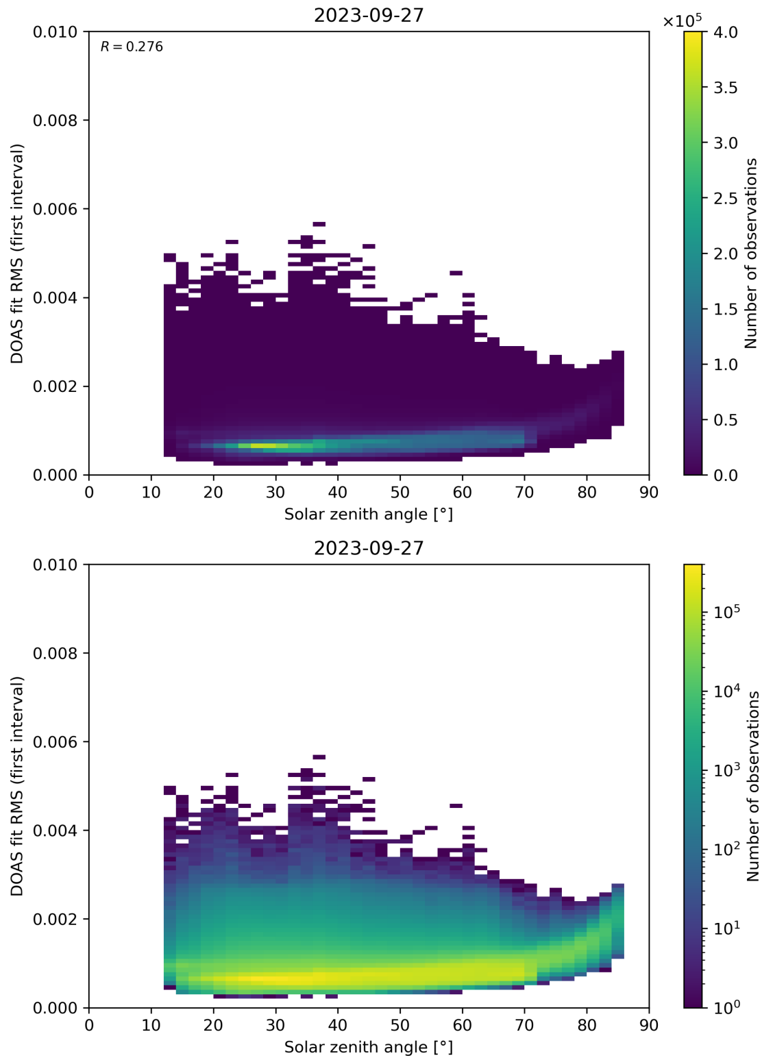
Figure 167: Scatter density plot of “Solar zenith angle” against “DOAS fit RMS (first interval)” for 2023-09-26 to 2023-09-28.
