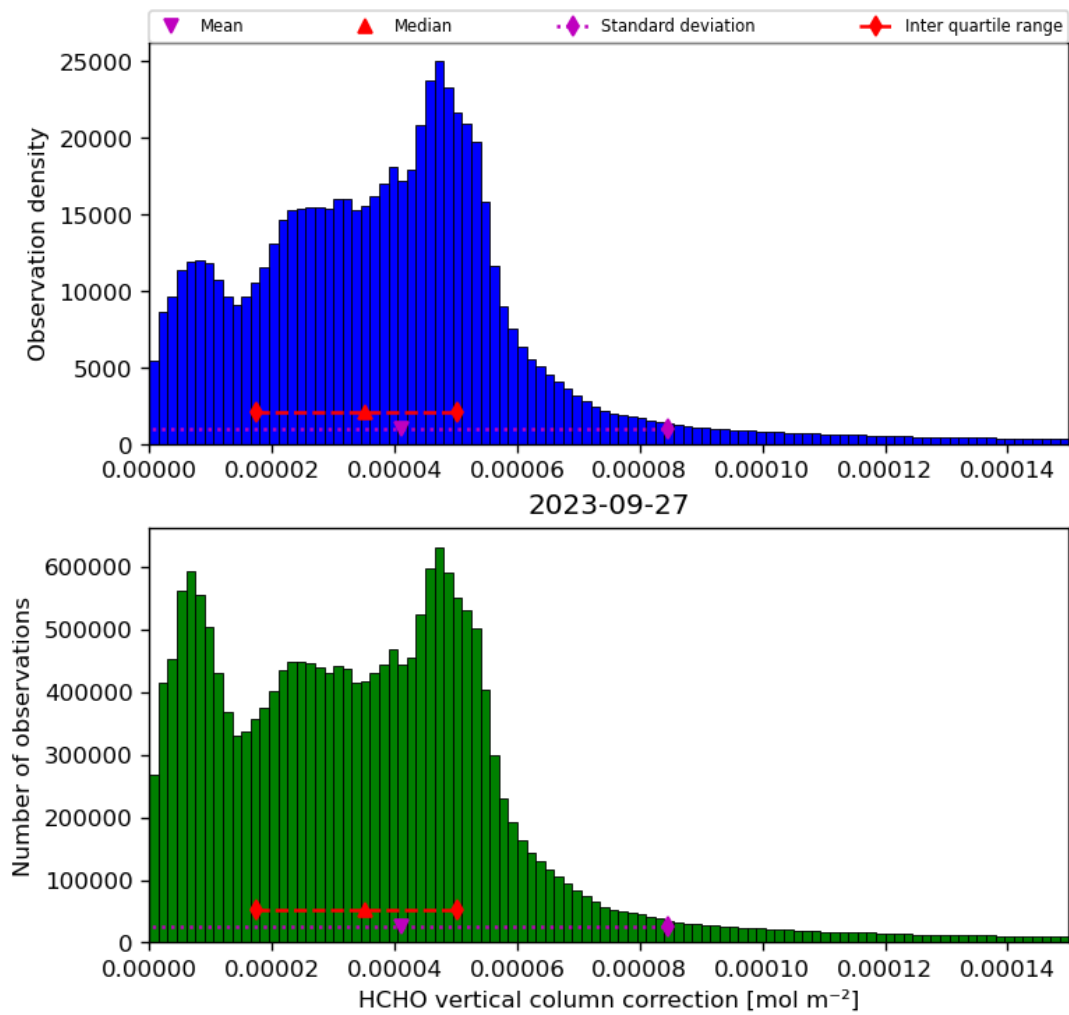
Figure 37: Histogram of “HCHO vertical column correction” for 2023-09-26 to 2023-09-28
