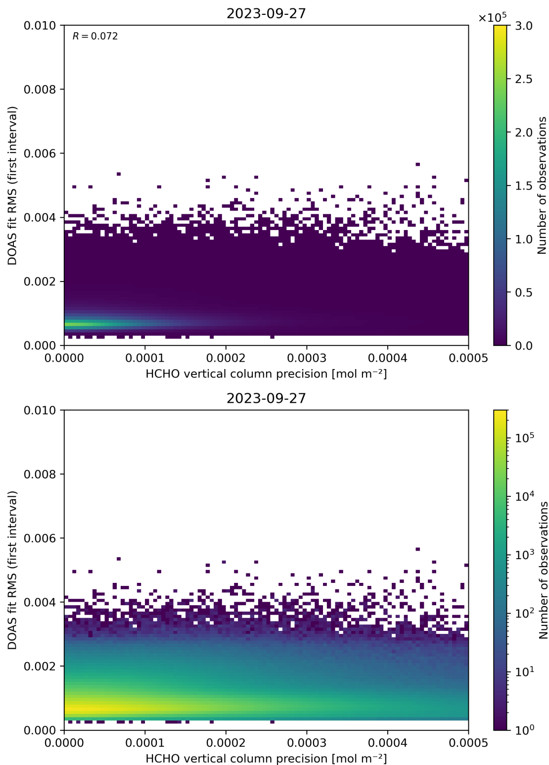
Figure 136: Scatter density plot of “HCHO vertical column precision” against “DOAS fit RMS (first interval)” for 2023-09-26 to 2023-09-28.
