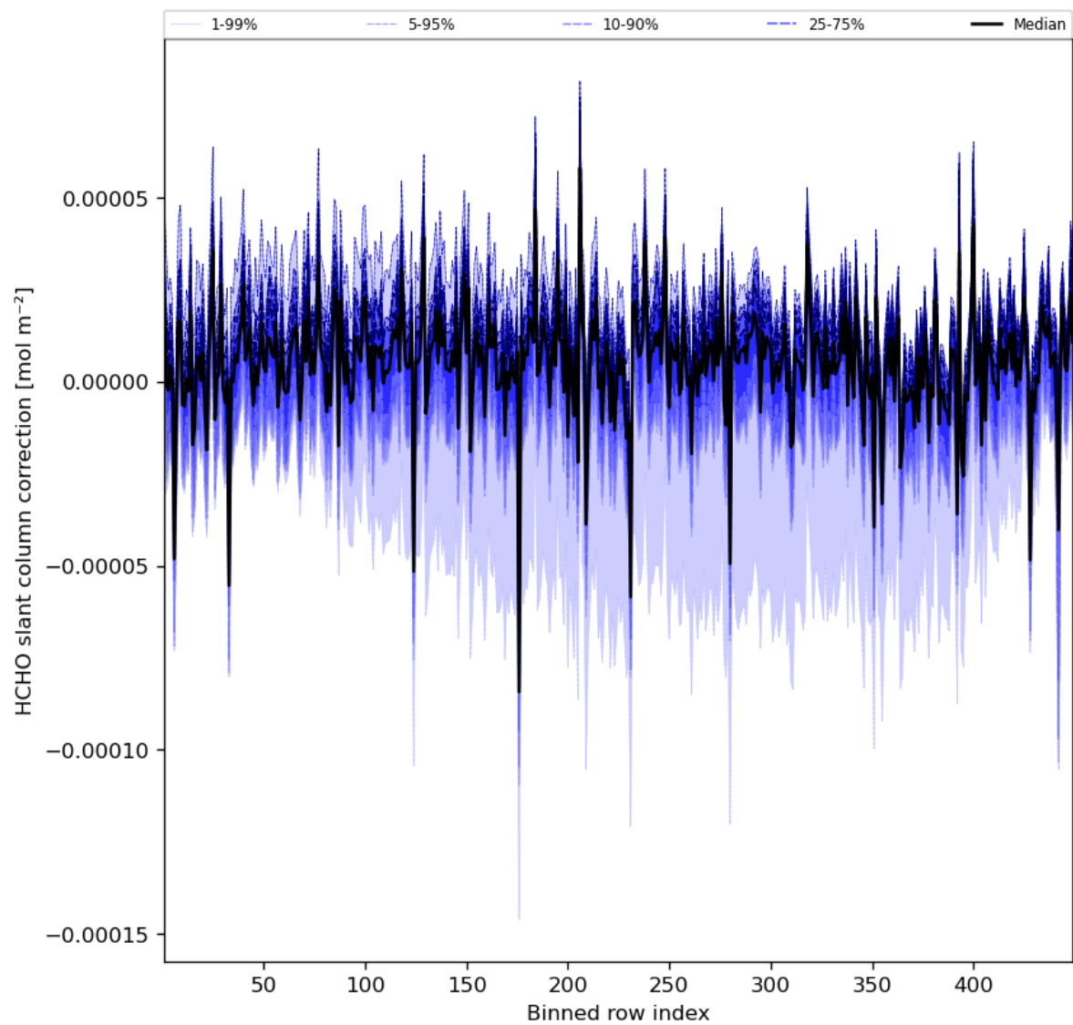
Figure 61: Along track statistics of “HCHO slant column correction” for 2023-09-26 to 2023-09-28
