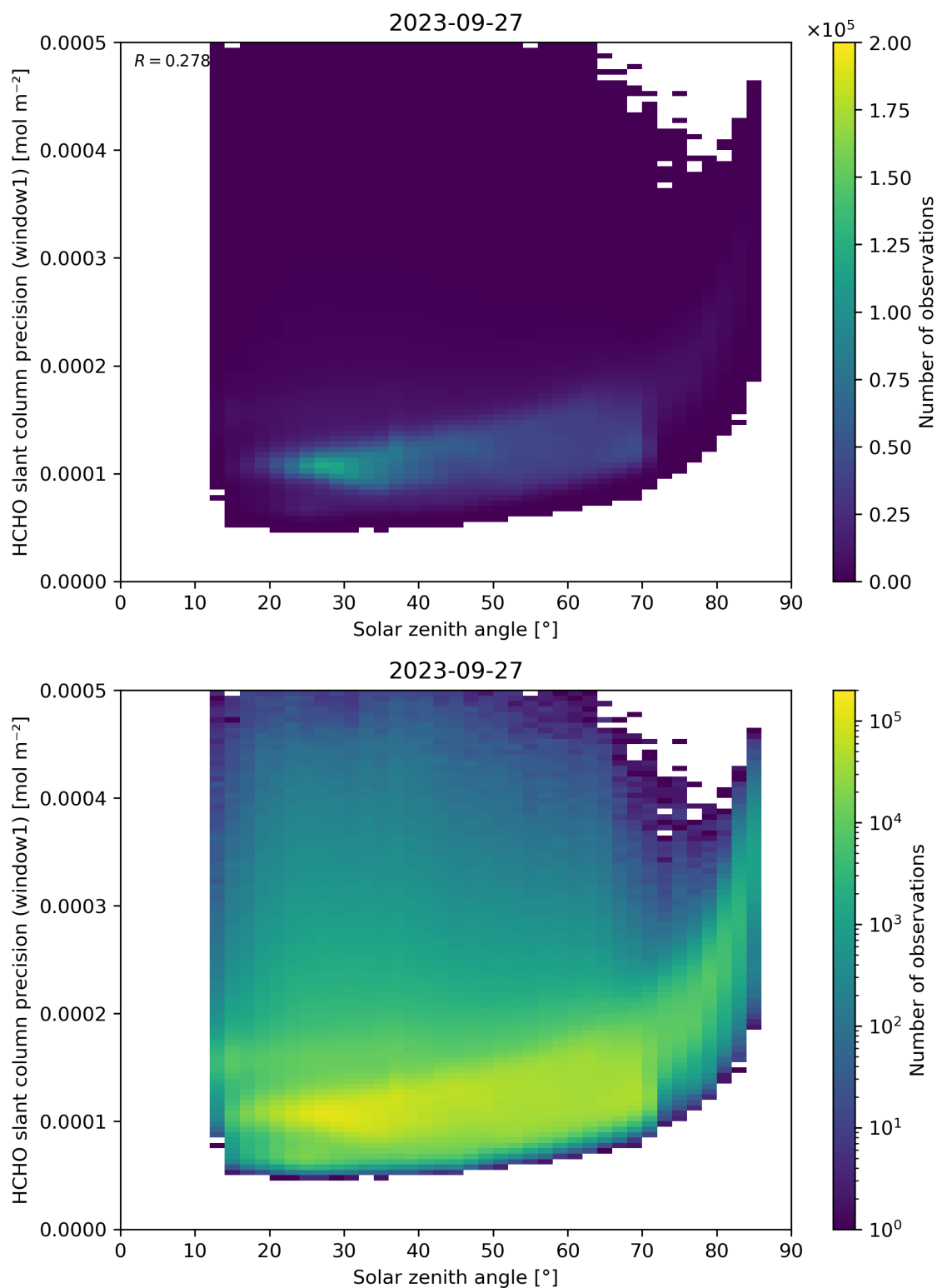
Figure 174: Scatter density plot of “Solar zenith angle” against “HCHO slant column precision (window1)” for 2023-09-26 to 2023-09-28.
