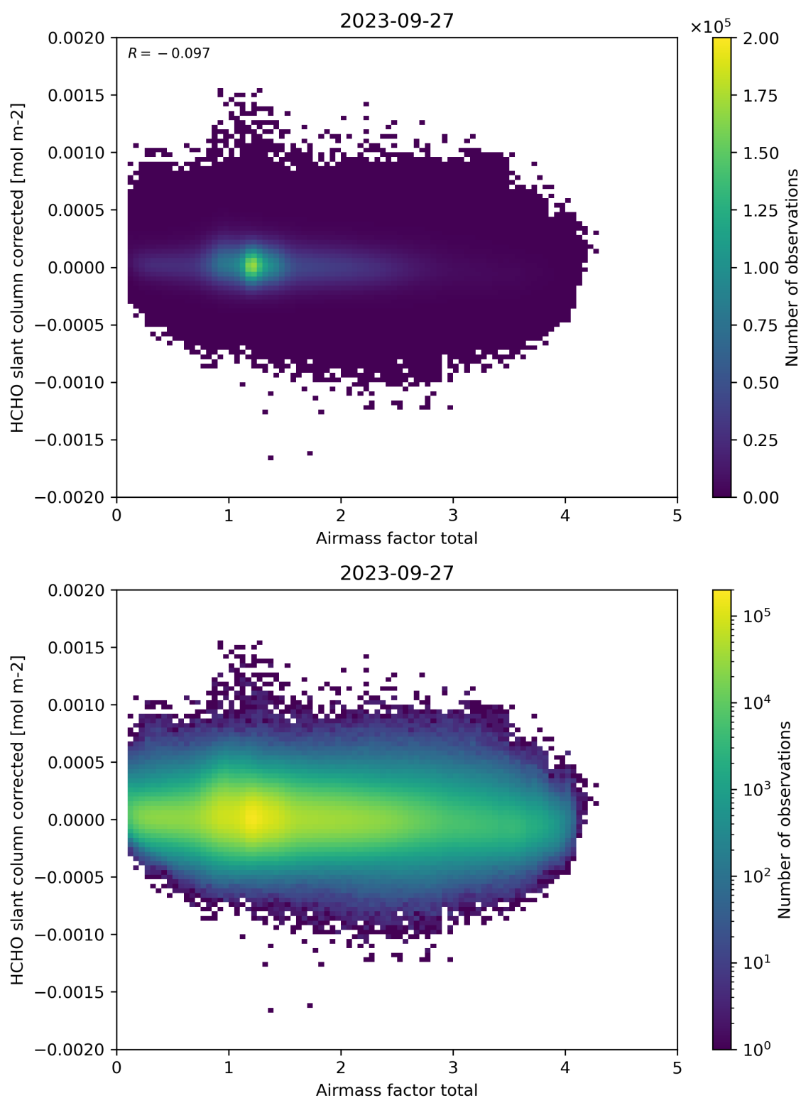
Figure 101: Scatter density plot of “Airmass factor total” against “HCHO slant column corrected” for 2023-09-26 to 2023-09-28.
