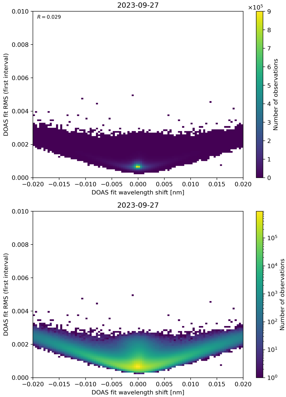
Figure 64: Scatter density plot of “DOAS fit wavelength shift” against “DOAS fit RMS (first interval)” for 2023-09-26 to 2023-09-28.
