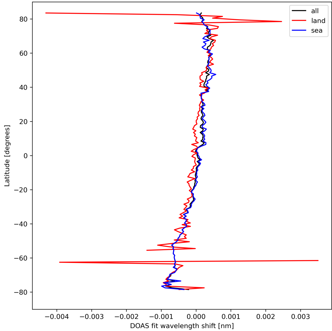
Figure 30: Zonal average of "DOAS fit wavelength shift" for 2023-09-26 to 2023-09-28.
