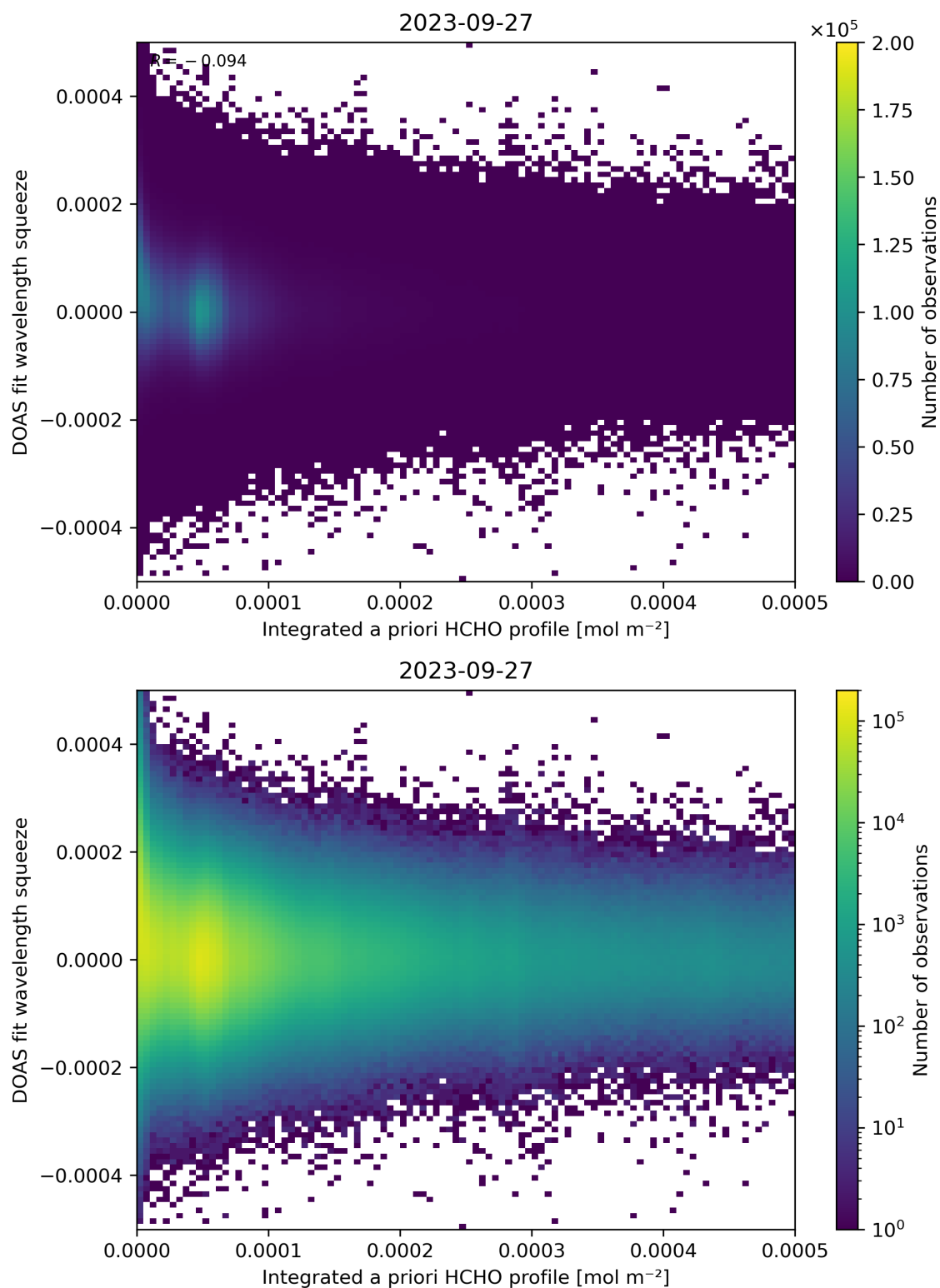
Figure 150: Scatter density plot of “Integrated a priori HCHO profile” against “DOAS fit wavelength squeeze” for 2023-09-26 to 2023-09-28.
