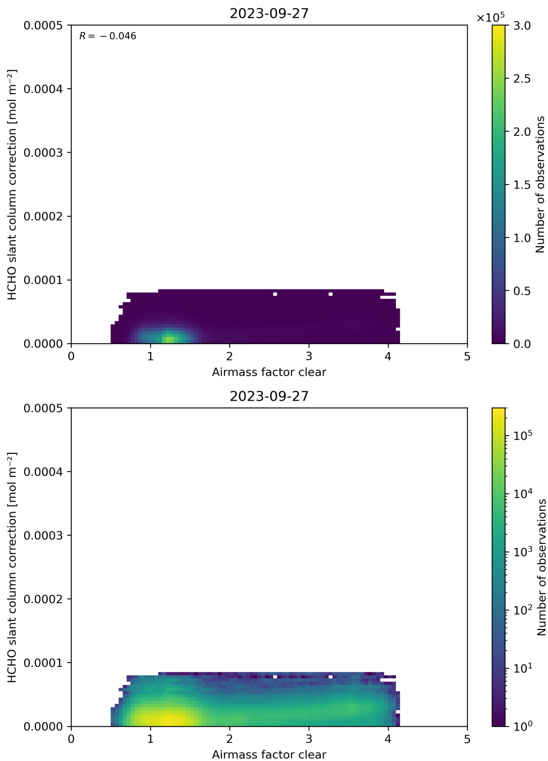
Figure 75: Scatter density plot of “Airmass factor clear” against “HCHO slant column correction” for 2023-09-26 to 2023-09-28.
