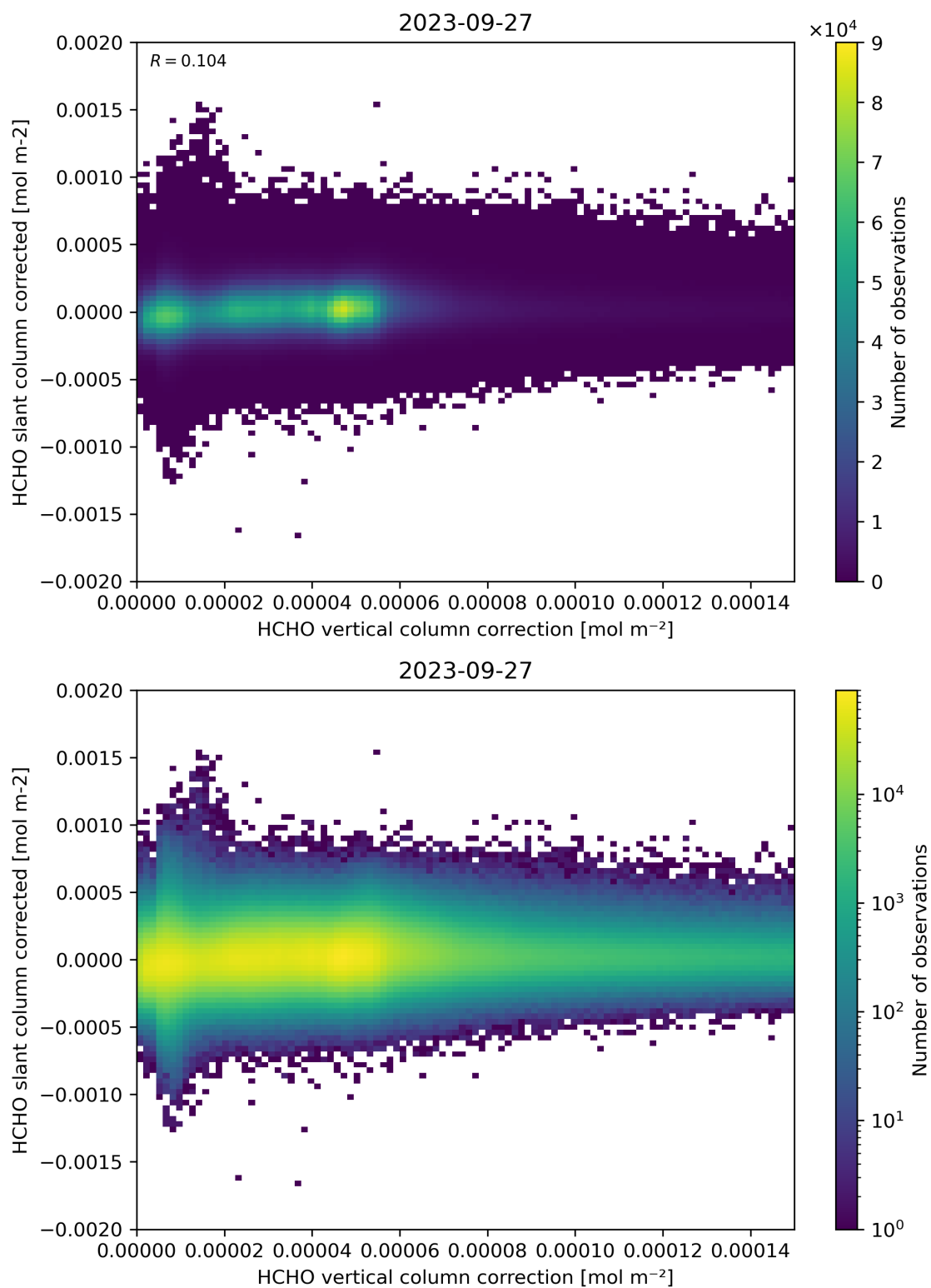
Figure 116: Scatter density plot of “HCHO vertical column correction” against “HCHO slant column corrected” for 2023-09-26 to 2023-09-28.
