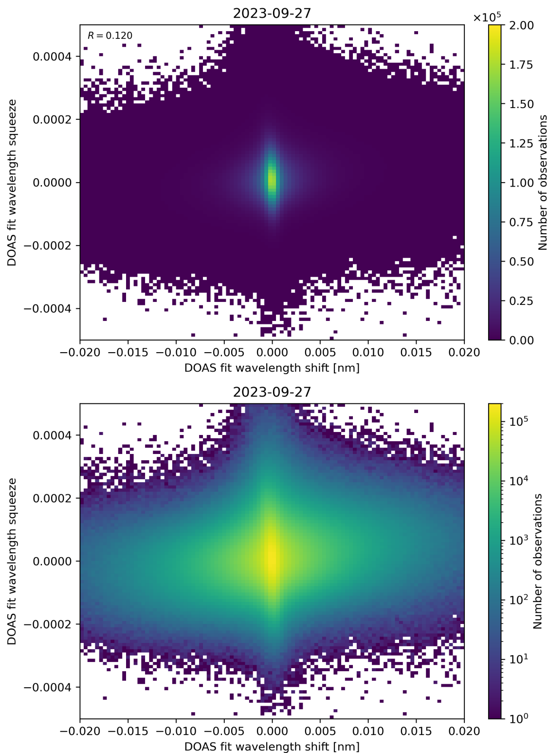
Figure 65: Scatter density plot of “DOAS fit wavelength shift” against “DOAS fit wavelength squeeze” for 2023-09-26 to 2023-09-28.
