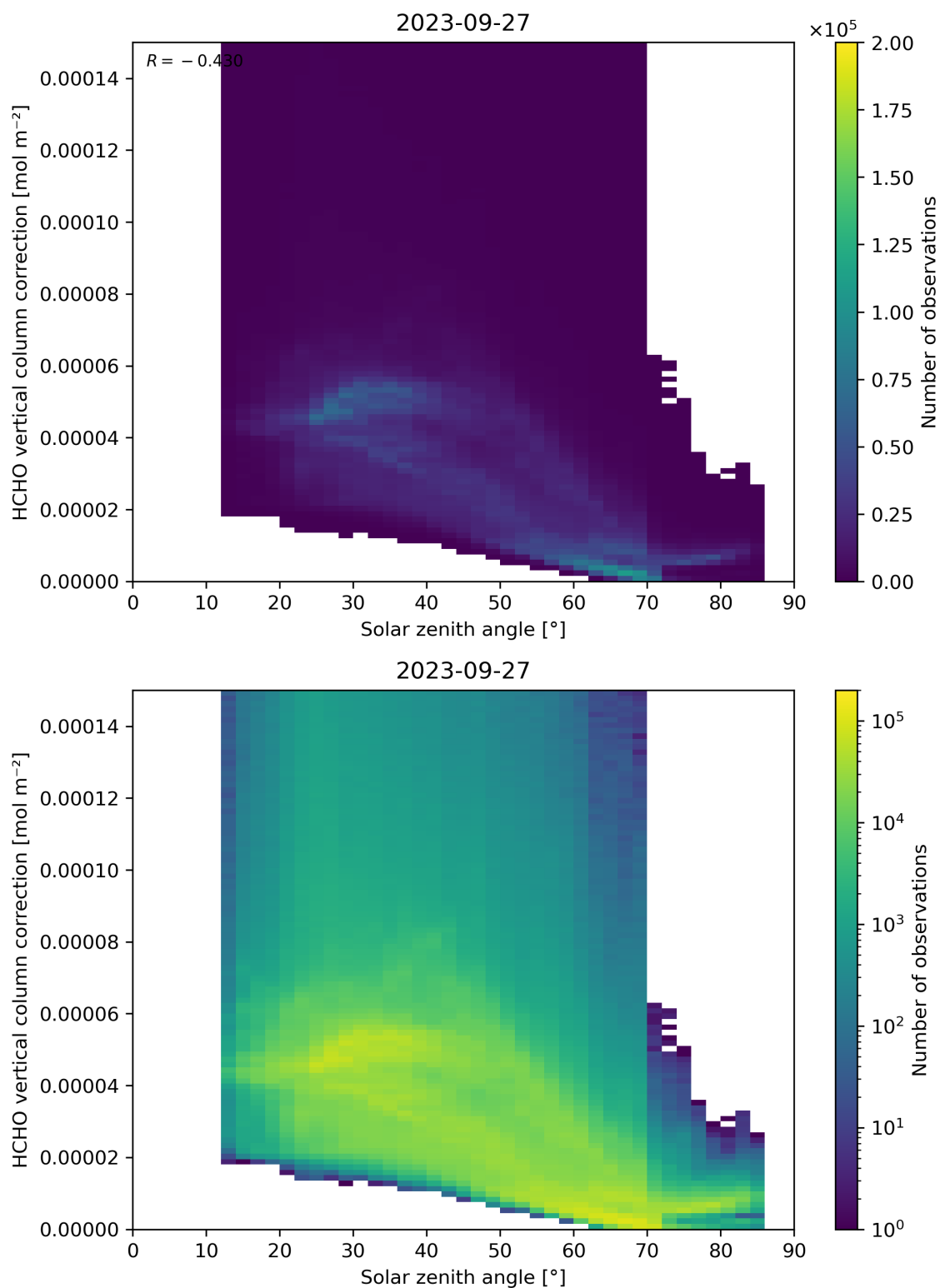
Figure 178: Scatter density plot of “Solar zenith angle” against “HCHO vertical column correction” for 2023-09-26 to 2023-09-28.
