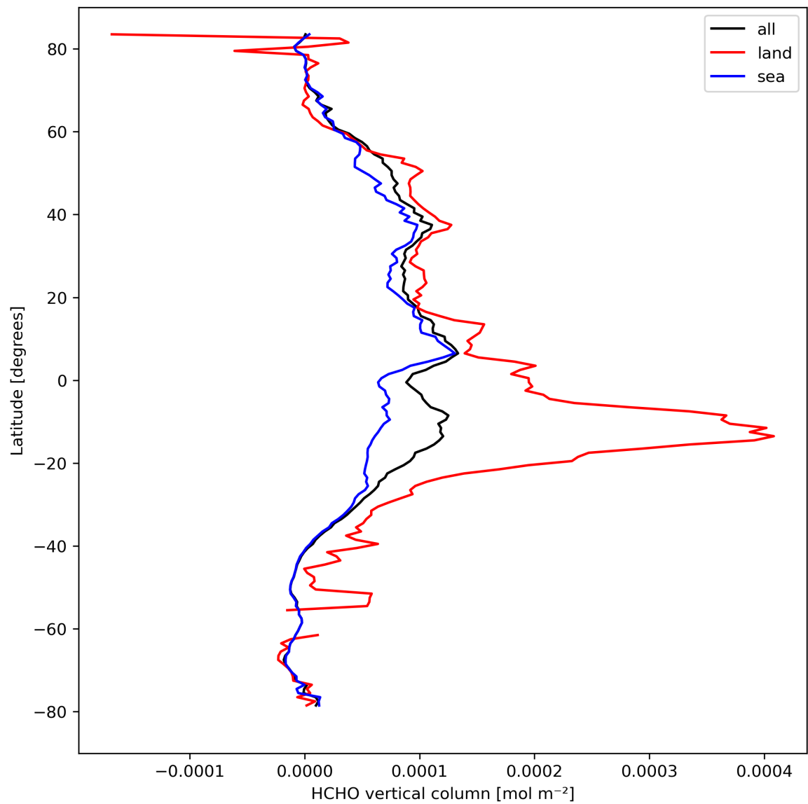
Figure 21: Zonal average of “HCHO vertical column” for 2023-09-26 to 2023-09-28.
