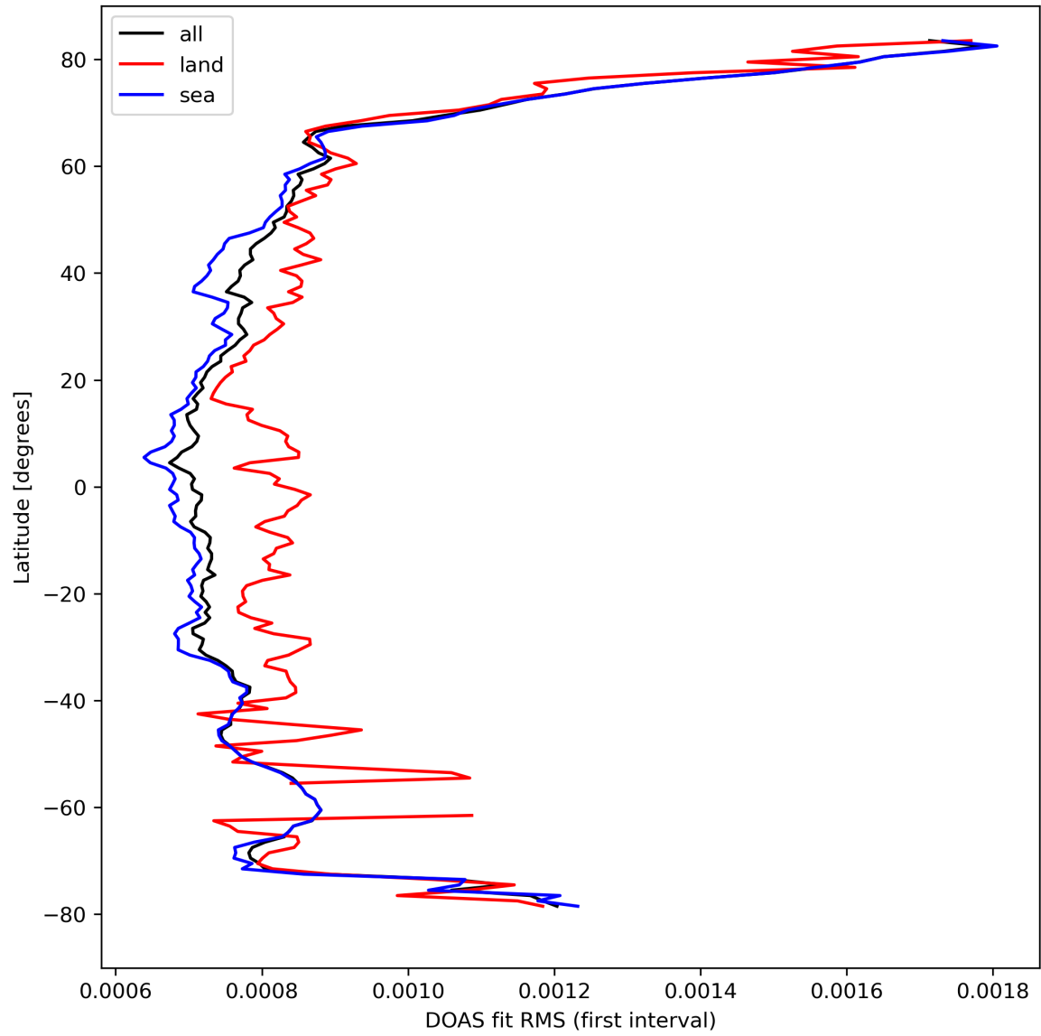
Figure 32: Zonal average of “DOAS fit RMS (first interval)” for 2023-09-26 to 2023-09-28.
