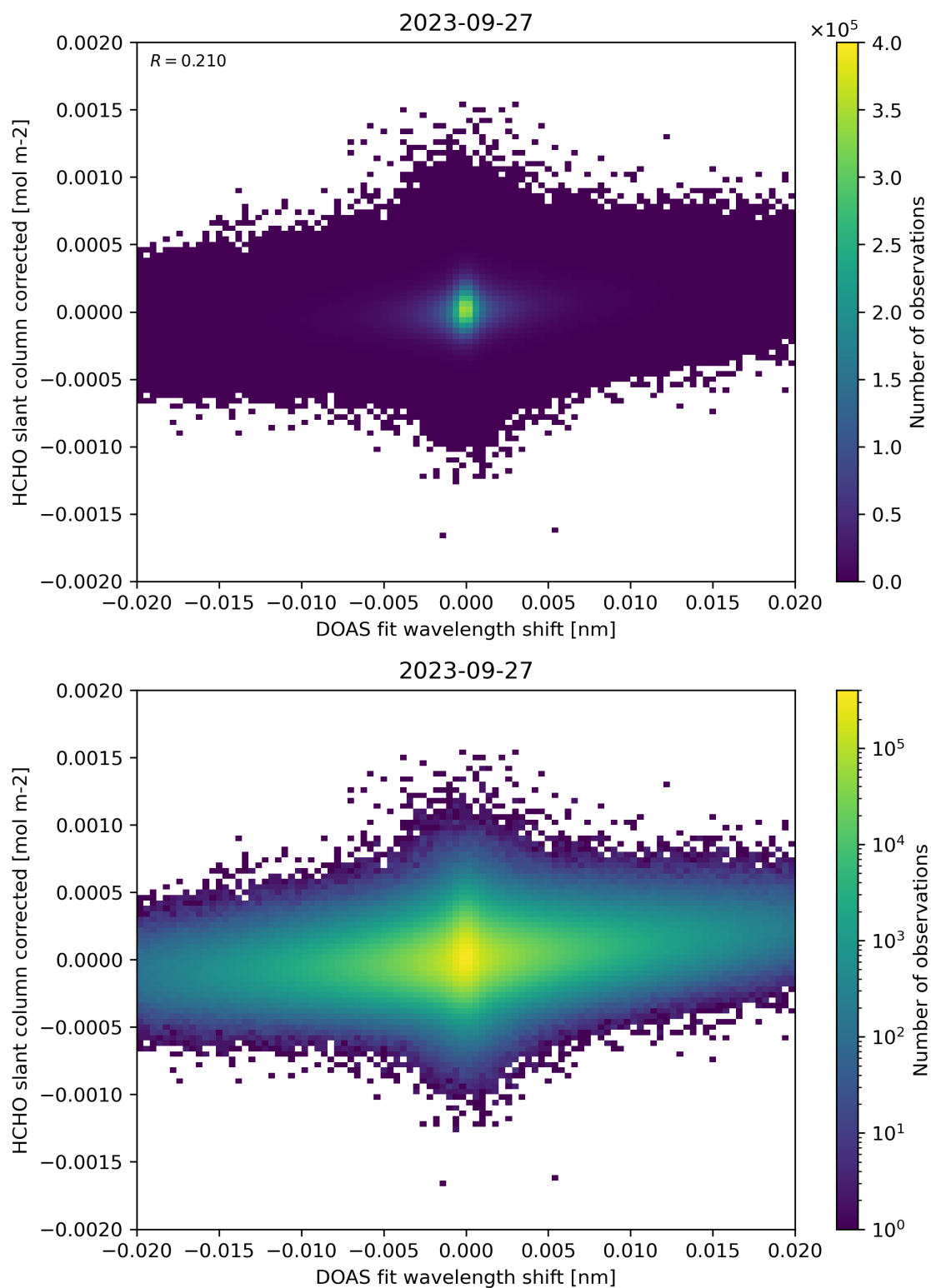
Figure 66: Scatter density plot of “DOAS fit wavelength shift” against “HCHO slant column corrected” for 2023-09-26 to 2023-09-28.
