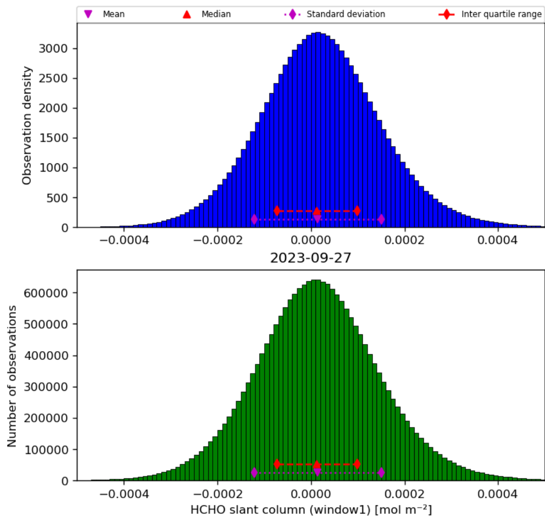
Figure 38: Histogram of “HCHO slant column (window1)” for 2023-09-26 to 2023-09-28
