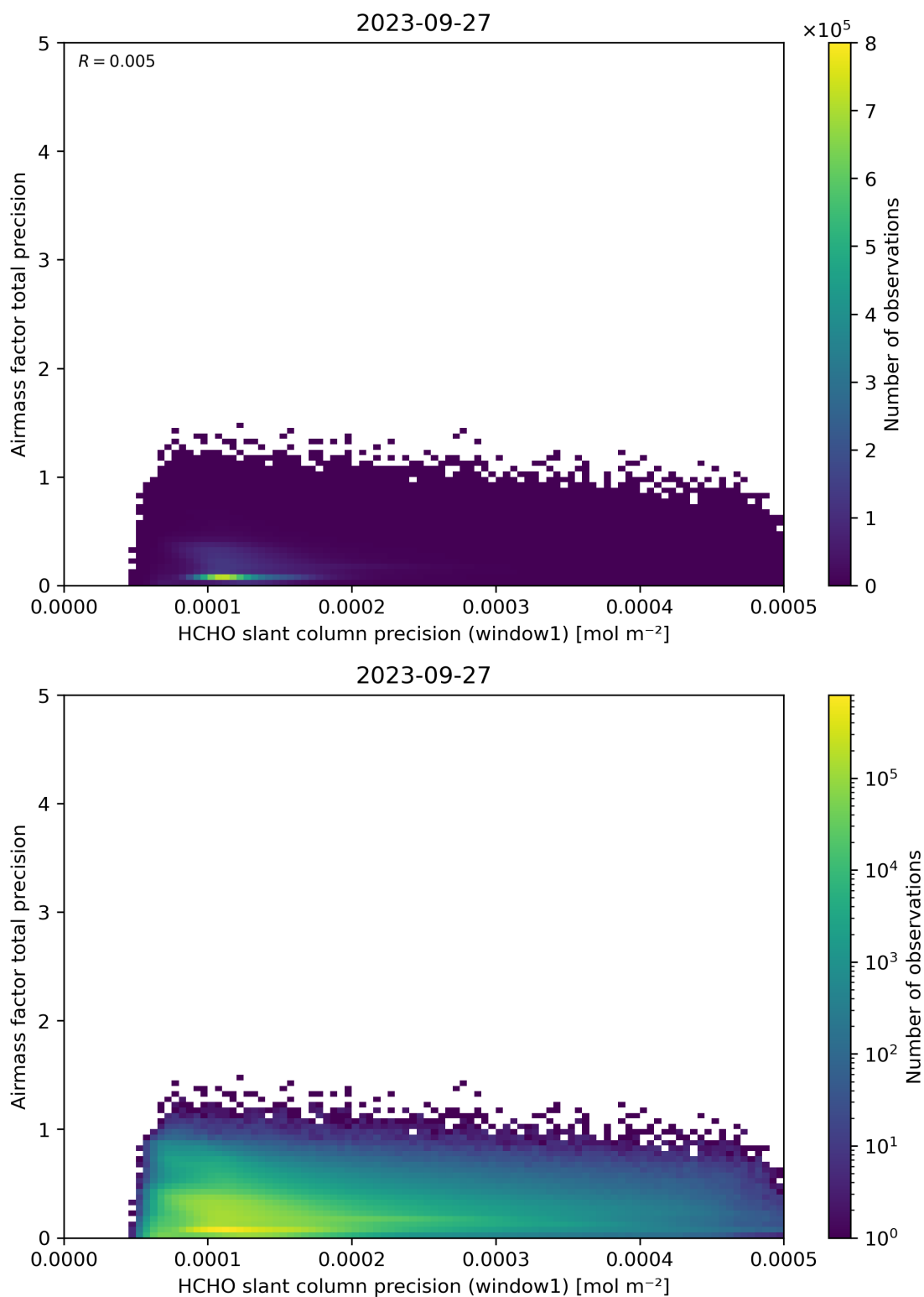
Figure 95: Scatter density plot of “HCHO slant column precision (window1)” against “Airmass factor total precision” for 2023-09-26 to 2023-09-28.
