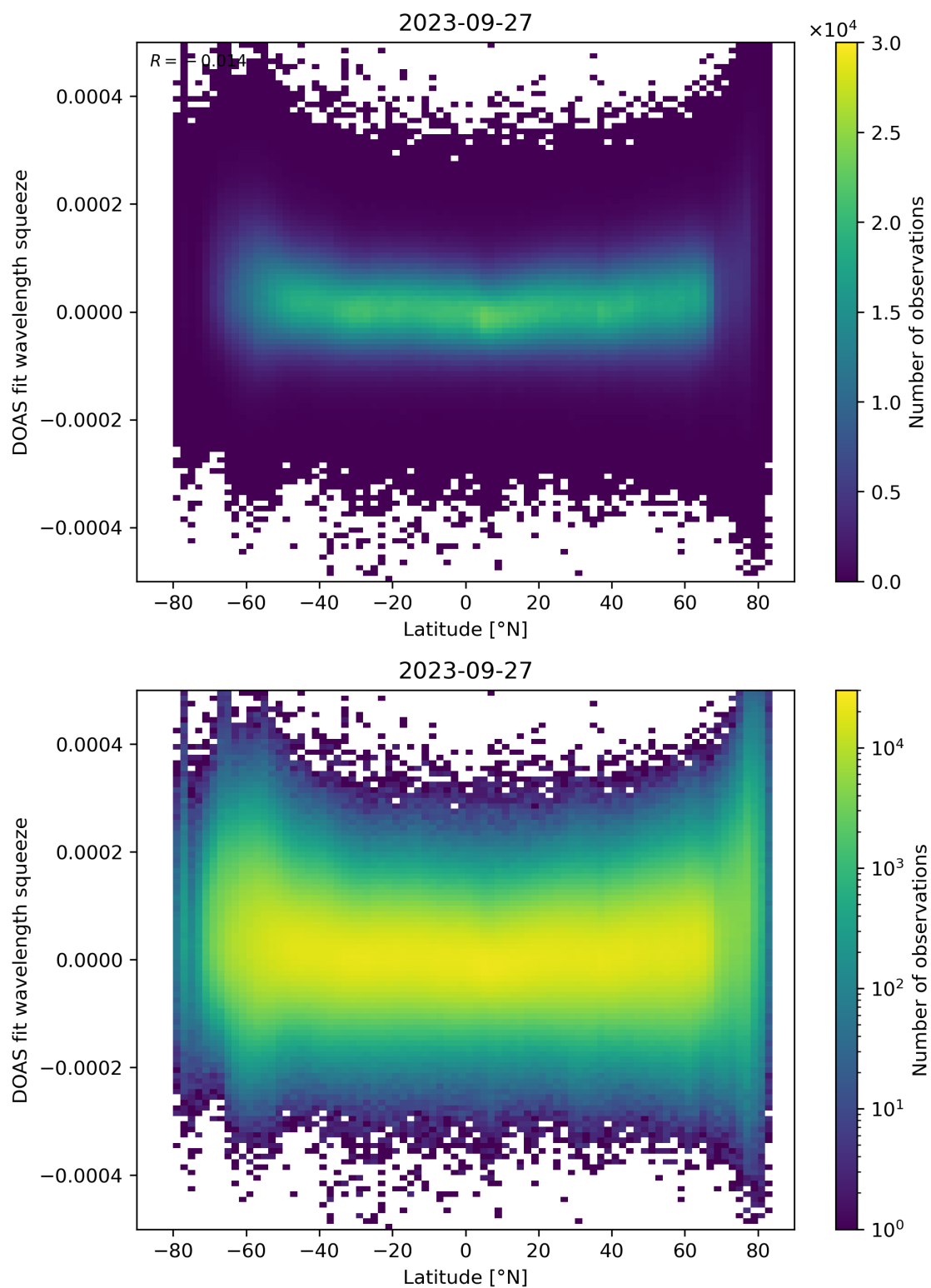
Figure 155: Scatter density plot of “Latitude” against “DOAS fit wavelength squeeze” for 2023-09-26 to 2023-09-28.
