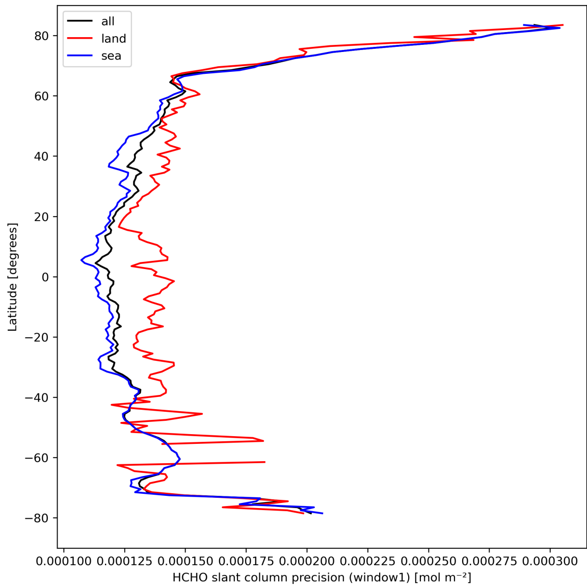
Figure 25: Zonal average of “HCHO slant column precision (window1)” for 2023-09-26 to 2023-09-28.
