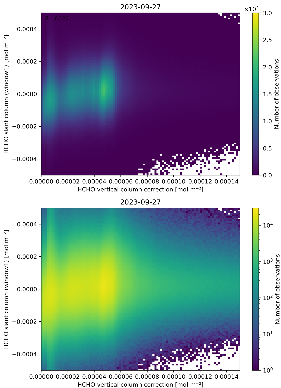
Figure 118: Scatter density plot of “HCHO vertical column correction” against “HCHO slant column (window1)” for 2023-09-26 to 2023-09-28.
