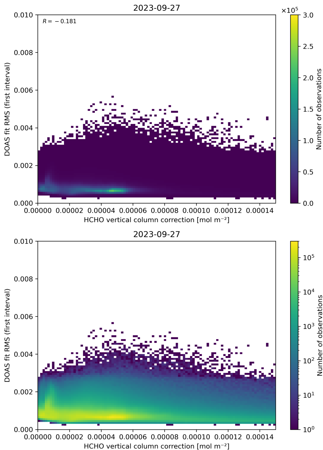
Figure 112: Scatter density plot of “HCHO vertical column correction” against “DOAS fit RMS (first interval)” for 2023-09-26 to 2023-09-28.
