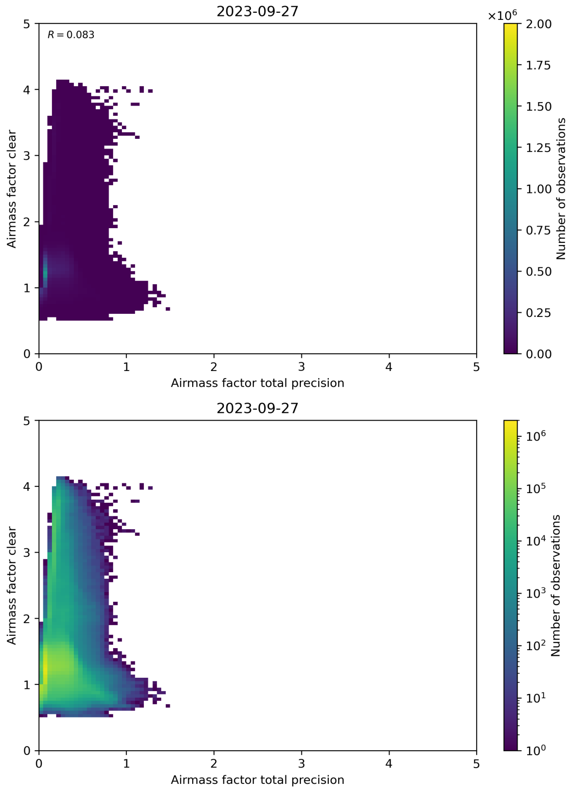
Figure 108: Scatter density plot of “Airmass factor total precision” against “Airmass factor clear” for 2023-09-26 to 2023-09-28.
