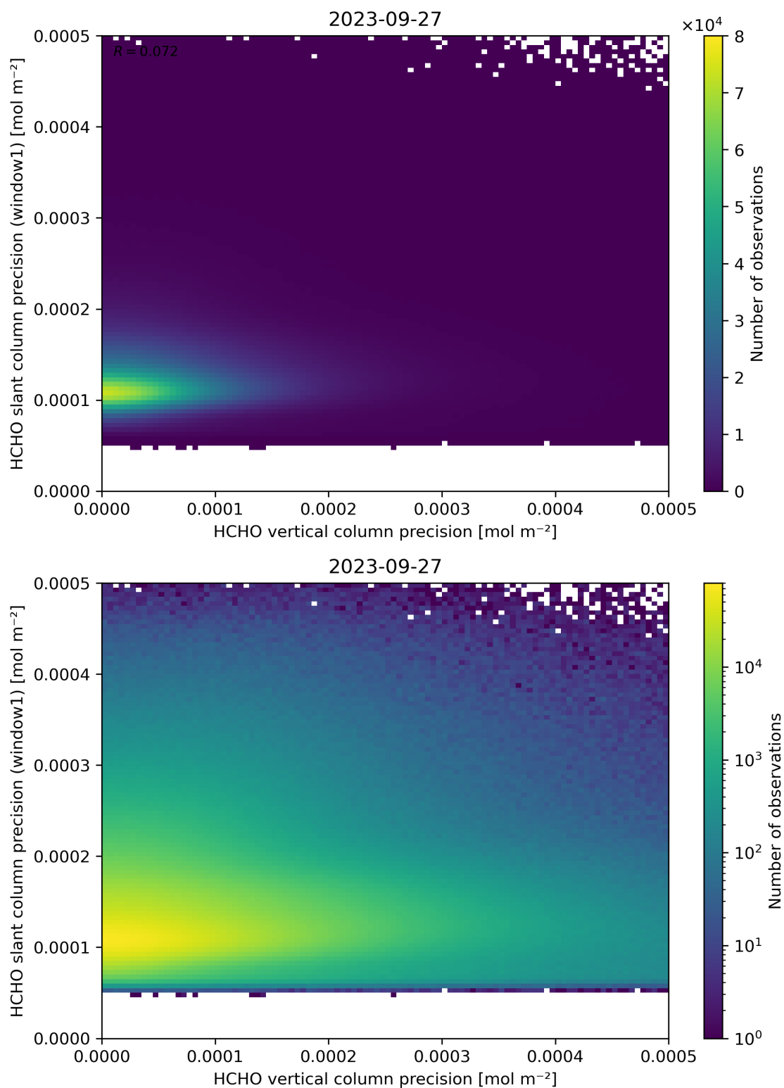
Figure 143: Scatter density plot of “HCHO vertical column precision” against “HCHO slant column precision (window1)” for 2023-09-26 to 2023-09-28.
