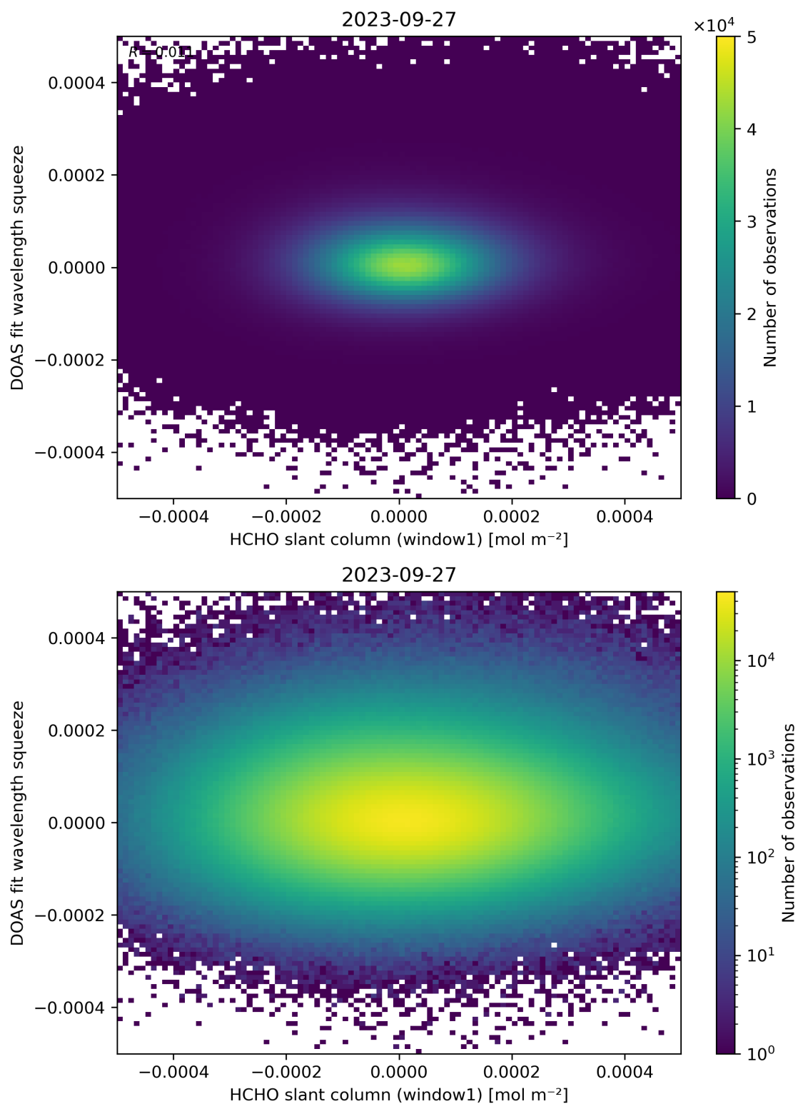
Figure 80: Scatter density plot of “HCHO slant column (window1)” against “DOAS fit wavelength squeeze” for 2023-09-26 to 2023-09-28.
