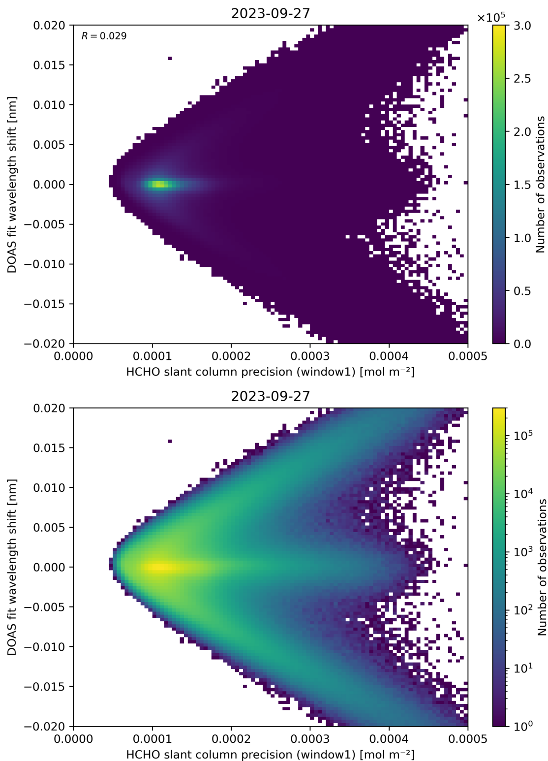
Figure 89: Scatter density plot of “HCHO slant column precision (window1)” against “DOAS fit wavelength shift” for 2023-09-26 to 2023-09-28.
