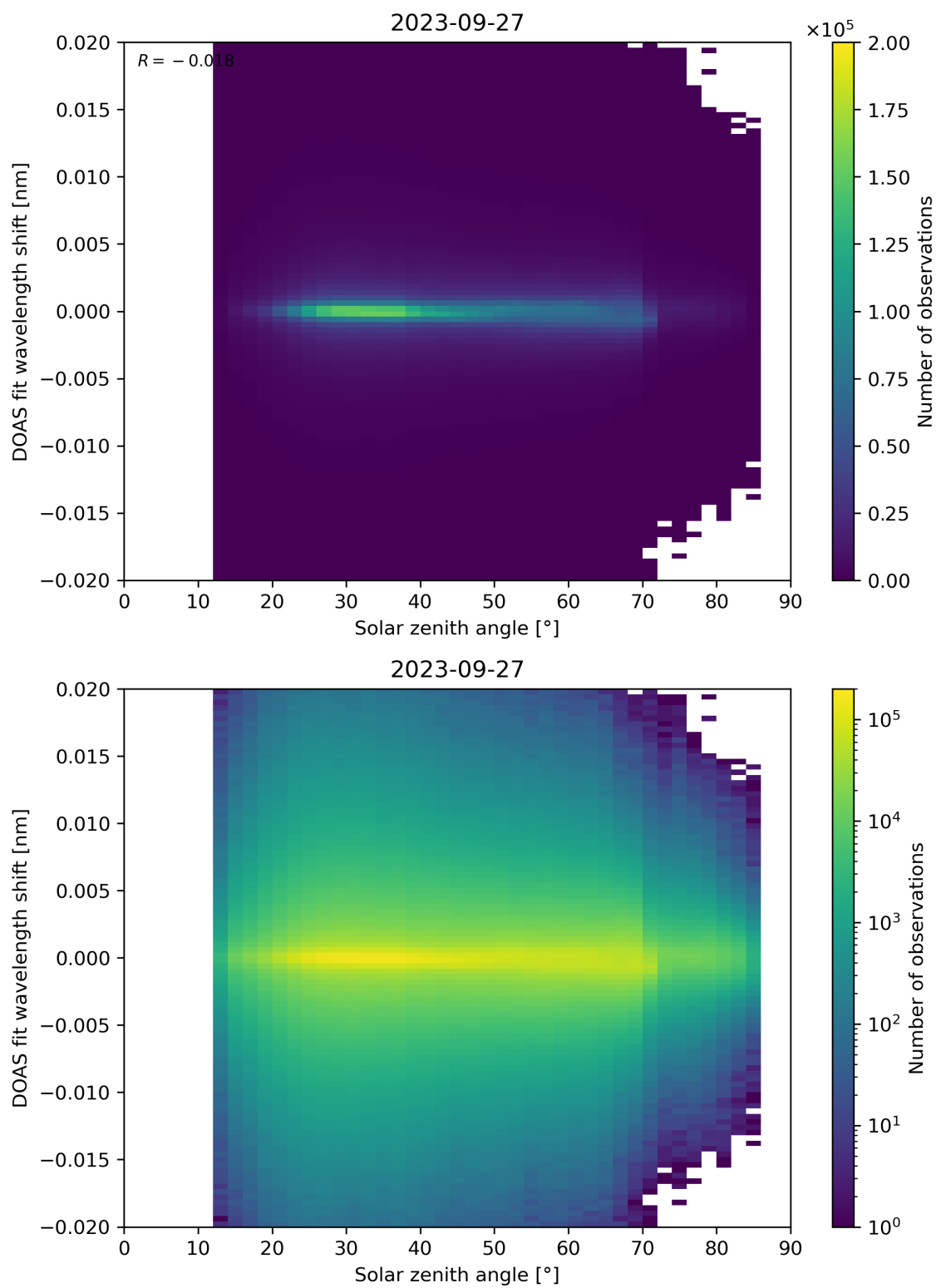
Figure 168: Scatter density plot of “Solar zenith angle” against “DOAS fit wavelength shift” for 2023-09-26 to 2023-09-28.
