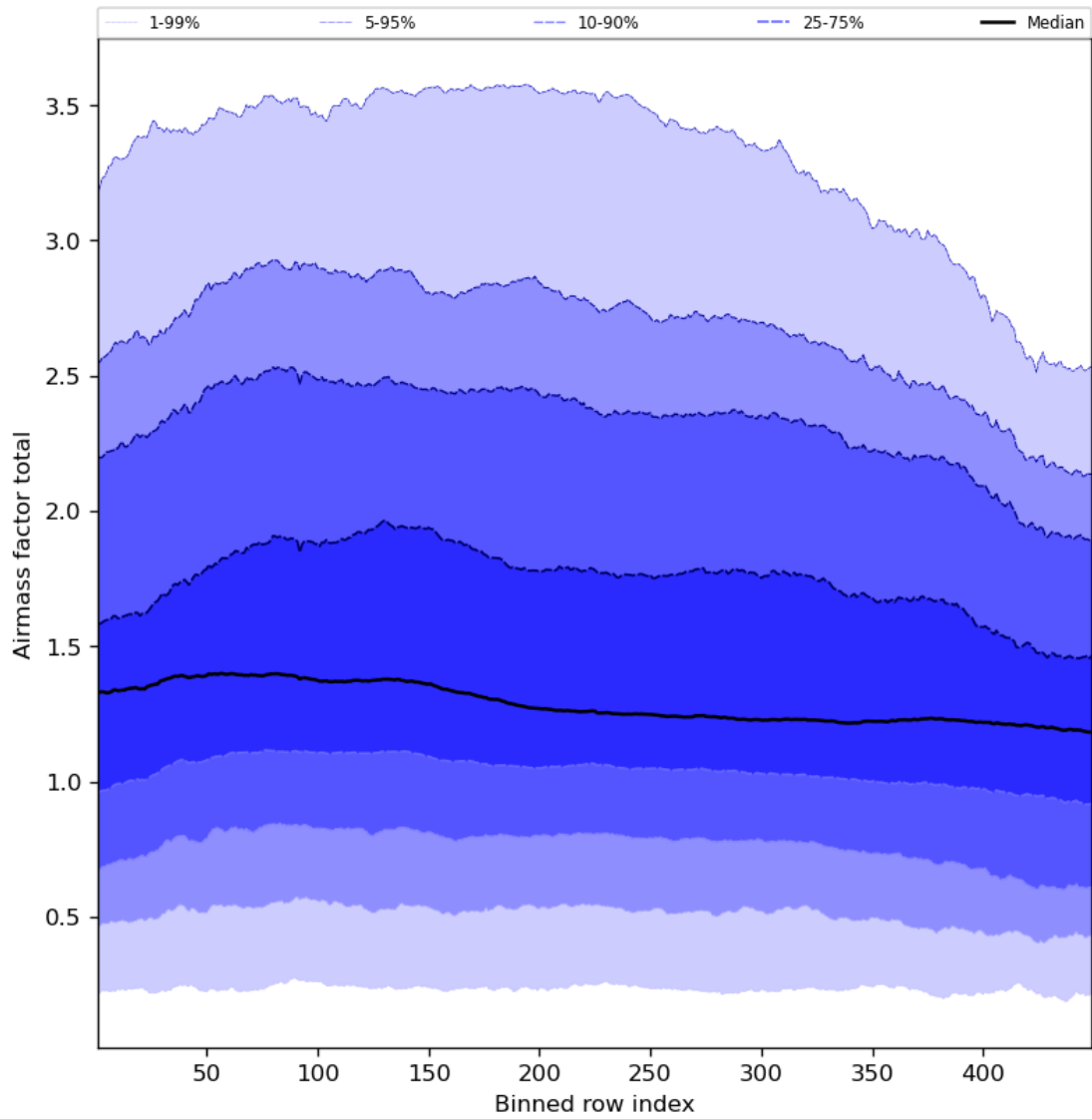
Figure 54: Along track statistics of “Airmass factor total” for 2023-09-26 to 2023-09-28
