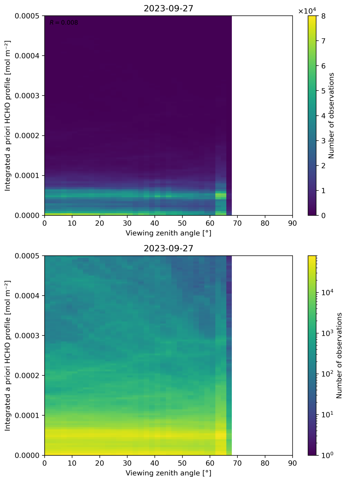
Figure 195: Scatter density plot of “Viewing zenith angle” against “Integrated a priori HCHO profile” for 2023-09-26 to 2023-09-28.
