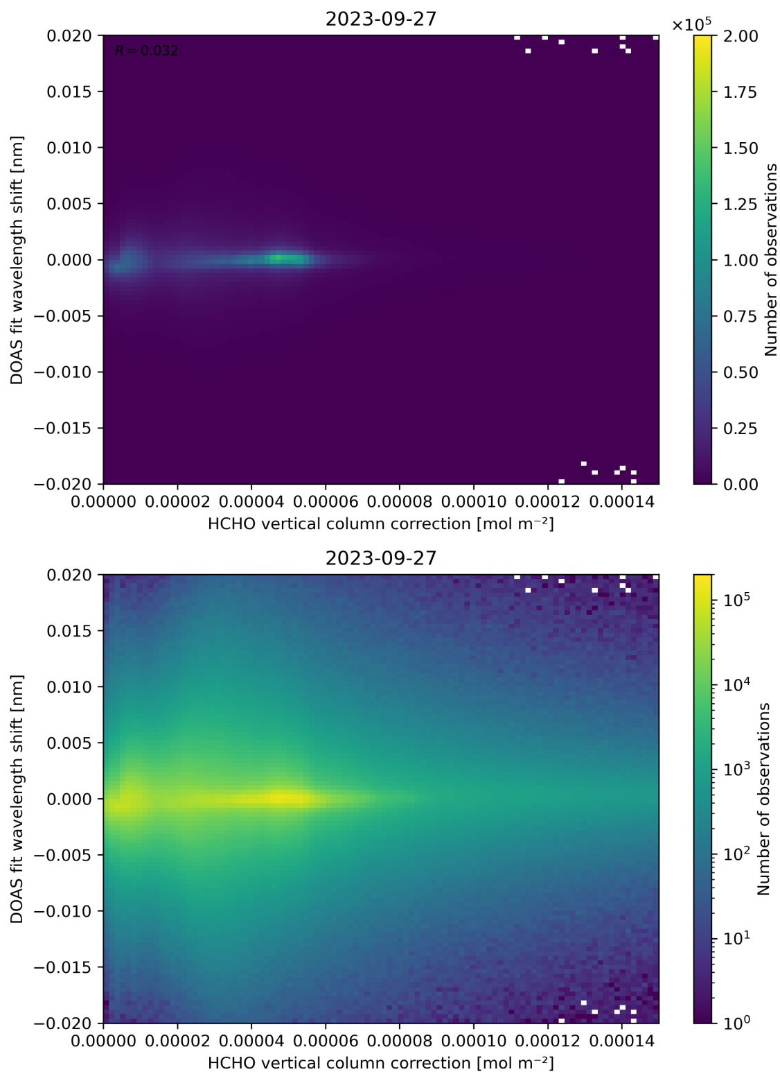
Figure 113: Scatter density plot of “HCHO vertical column correction” against “DOAS fit wavelength shift” for 2023-09-26 to 2023-09-28.
