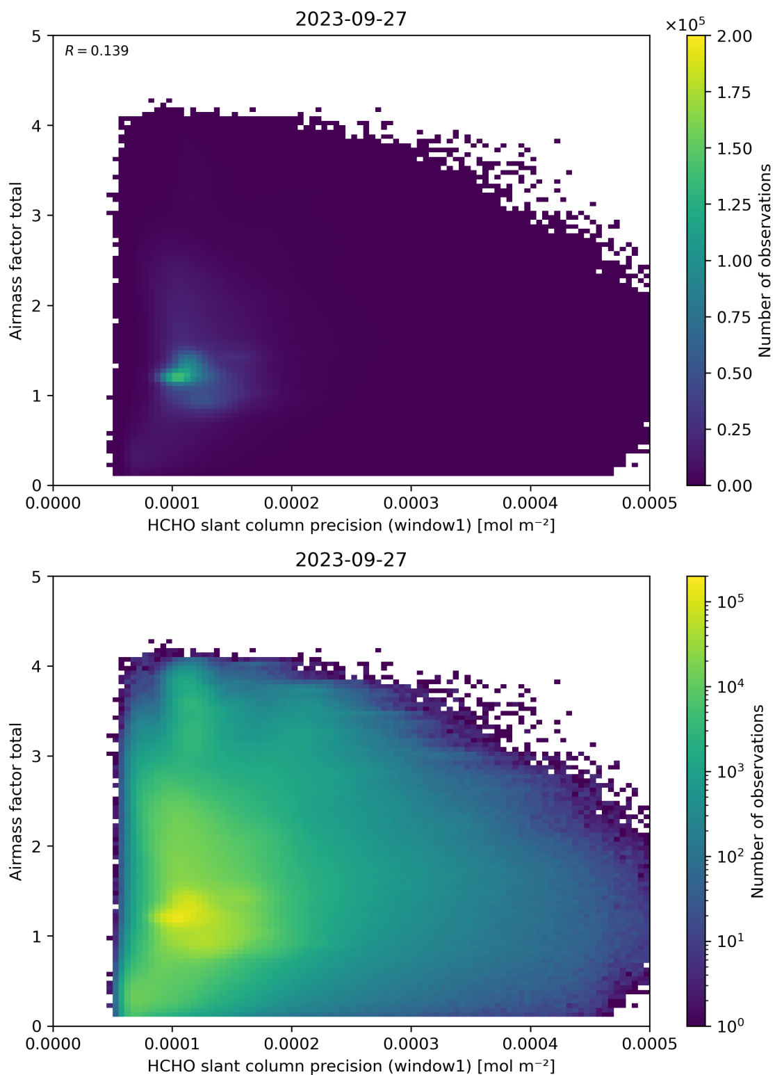
Figure 94: Scatter density plot of “HCHO slant column precision (window1)” against “Airmass factor total” for 2023-09-26 to 2023-09-28.
