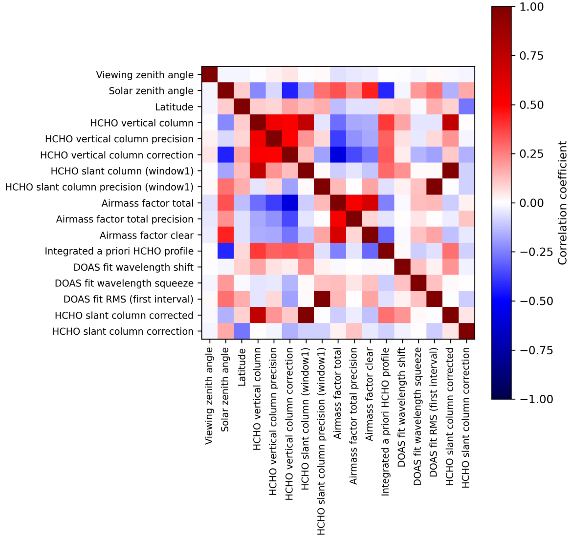
Figure 2: Map of correlation matrix for 2023-09-26 to 2023-09-28.
