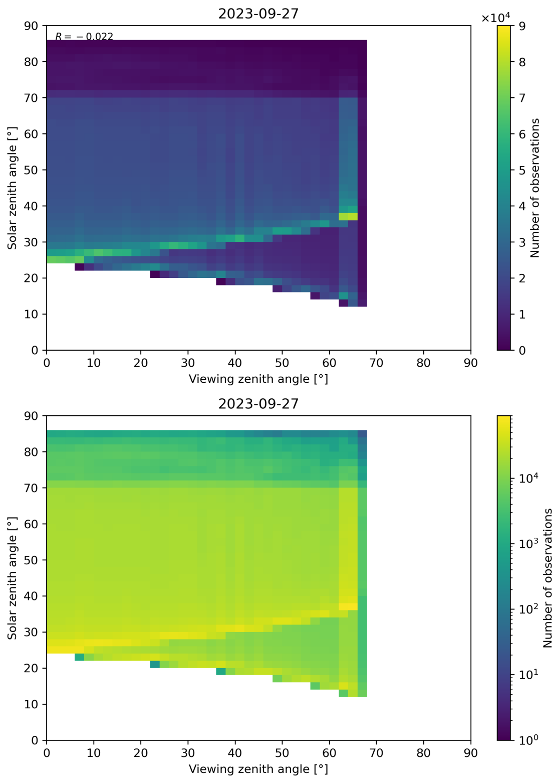
Figure 197: Scatter density plot of “Viewing zenith angle” against “Solar zenith angle” for 2023-09-26 to 2023-09-28.
