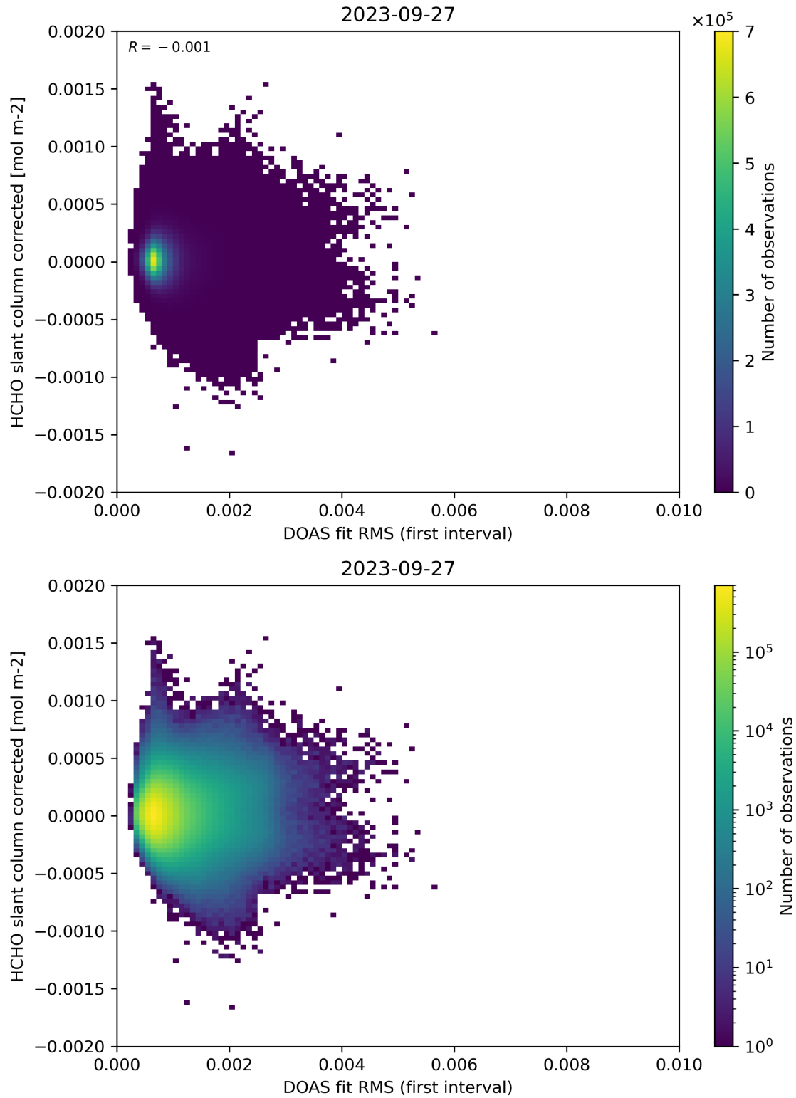
Figure 62: Scatter density plot of “DOAS fit RMS (first interval)” against “HCHO slant column corrected” for 2023-09-26 to 2023-09-28.
