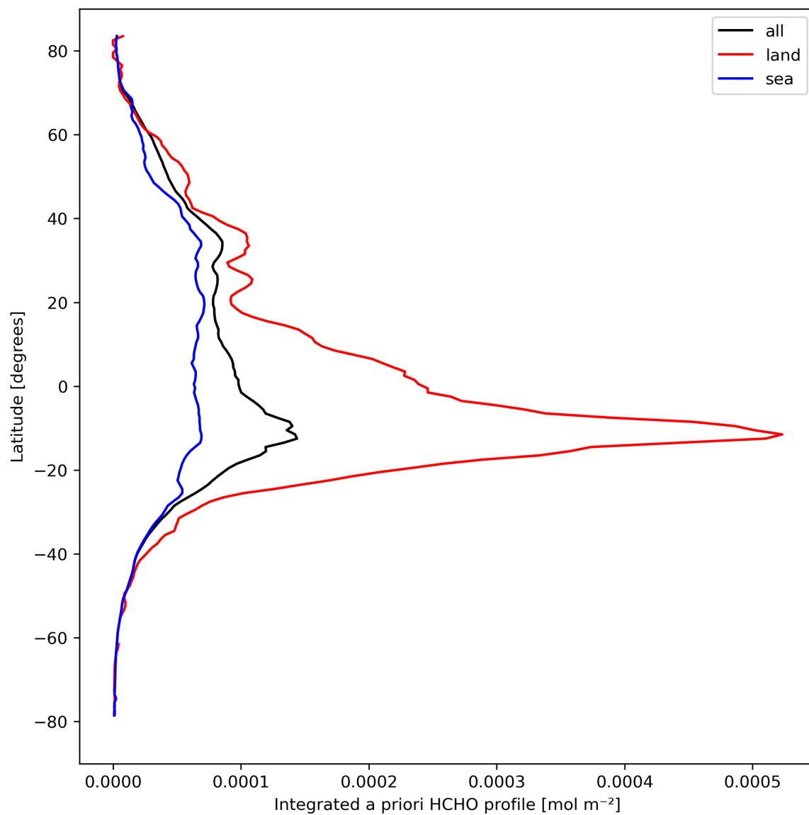
Figure 29: Zonal average of “Integrated a priori HCHO profile” for 2023-09-26 to 2023-09-28.
