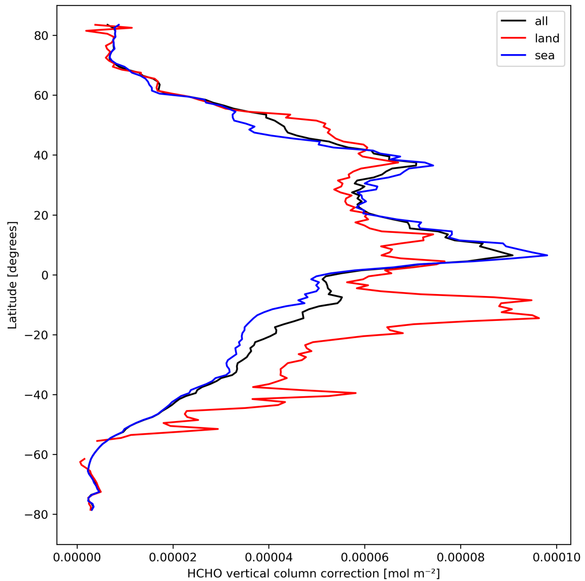
Figure 23: Zonal average of “HCHO vertical column correction” for 2023-09-26 to 2023-09-28.
