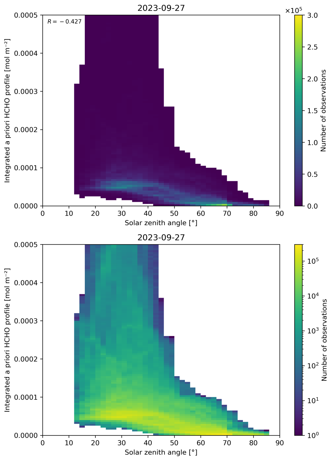
Figure 180: Scatter density plot of “Solar zenith angle” against “Integrated a priori HCHO profile” for 2023-09-26 to 2023-09-28.
