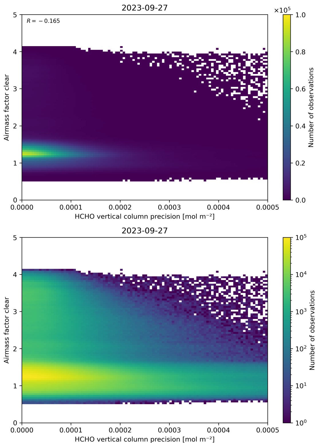
Figure 139: Scatter density plot of “HCHO vertical column precision” against “Airmass factor clear” for 2023-09-26 to 2023-09-28.
