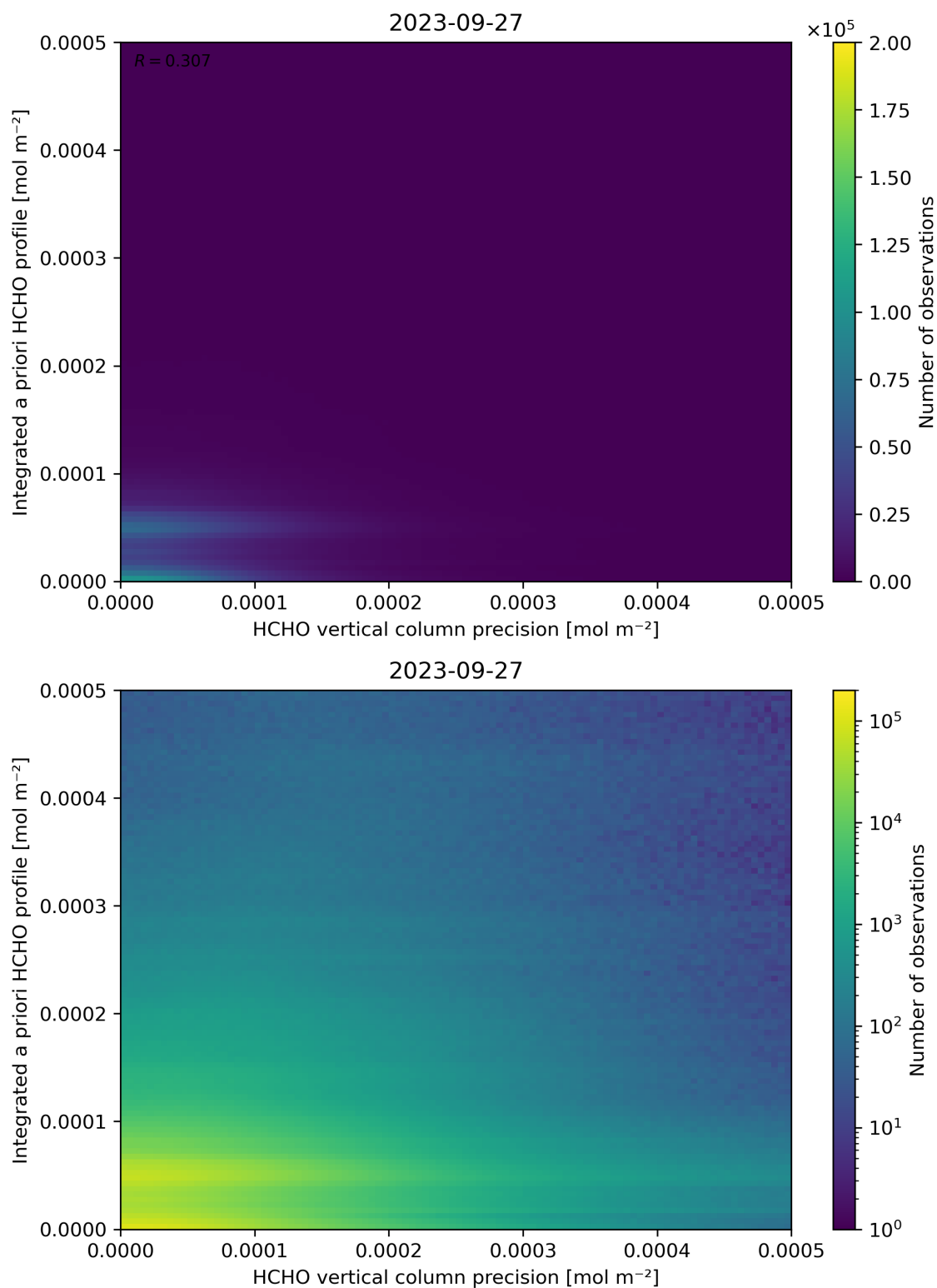
Figure 147: Scatter density plot of “HCHO vertical column precision” against “Integrated a priori HCHO profile” for 2023-09-26 to 2023-09-28.
