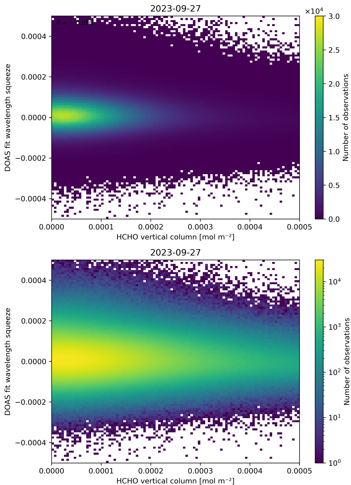
Figure 125: Scatter density plot of “HCHO vertical column” against “DOAS fit wavelength squeeze” for 2023-09-26 to 2023-09-28.
