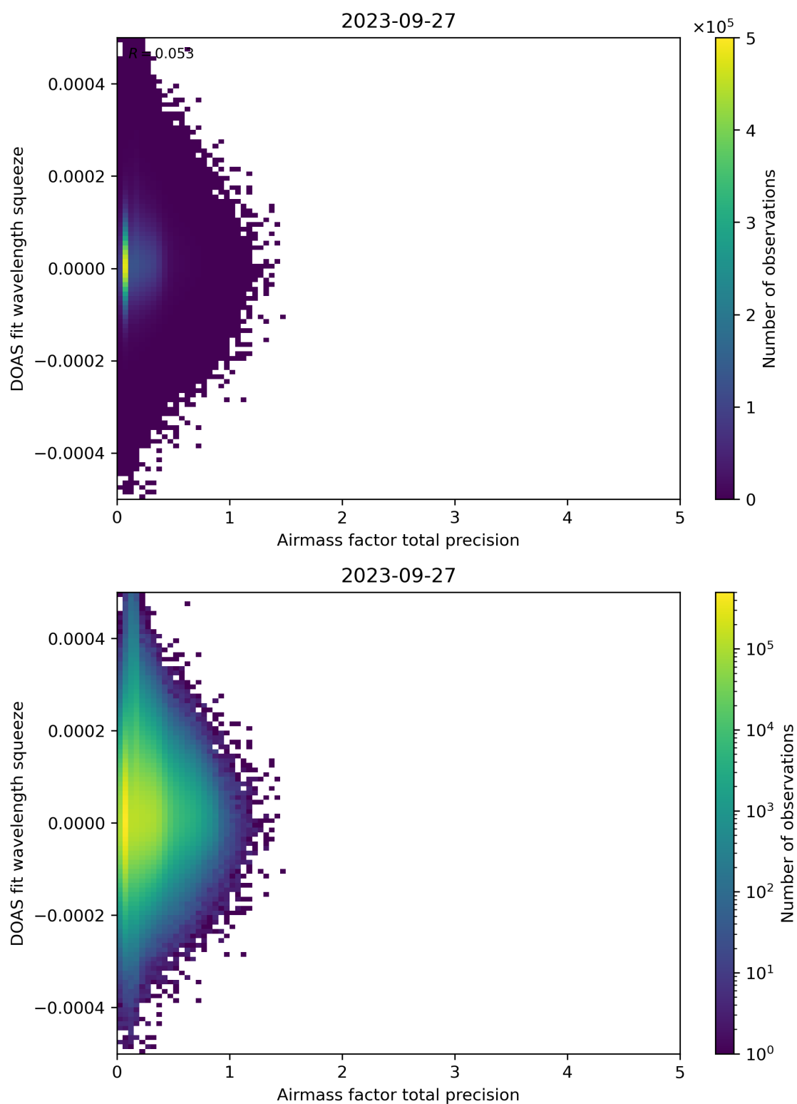
Figure 107: Scatter density plot of “Airmass factor total precision” against “DOAS fit wavelength squeeze” for 2023-09-26 to 2023-09-28.
