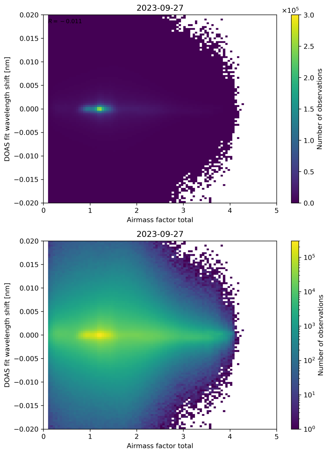
Figure 98: Scatter density plot of “Airmass factor total” against “DOAS fit wavelength shift” for 2023-09-26 to 2023-09-28.
