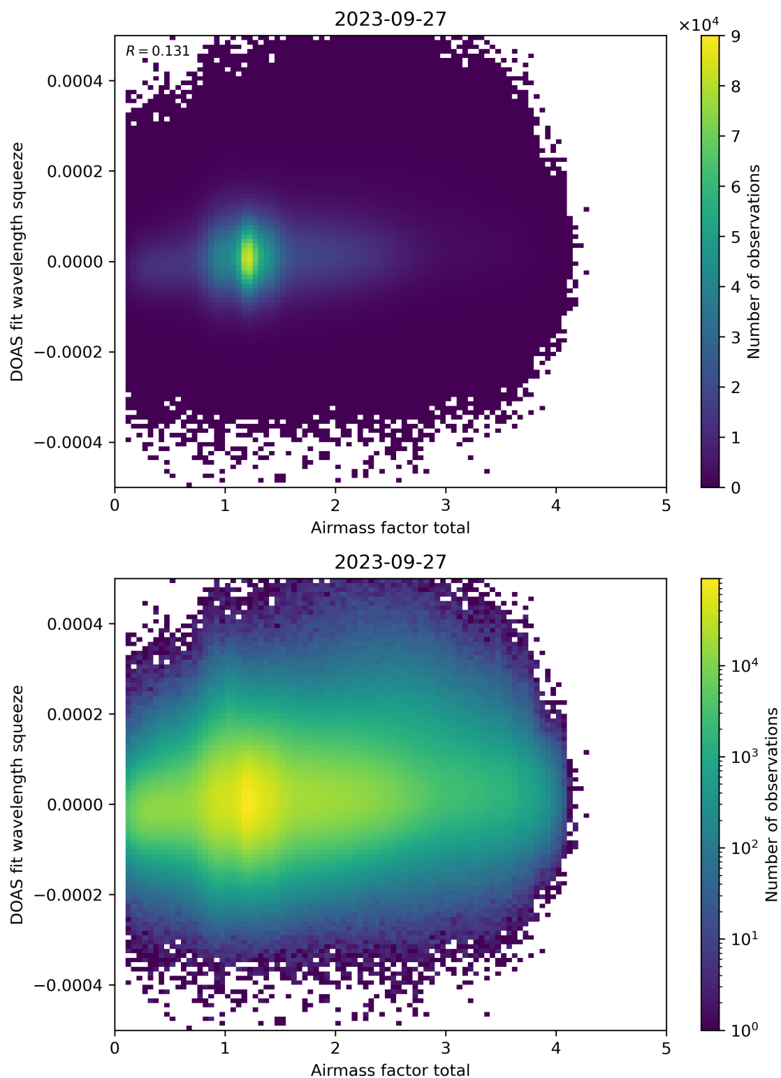
Figure 99: Scatter density plot of “Airmass factor total” against “DOAS fit wavelength squeeze” for 2023-09-26 to 2023-09-28.
