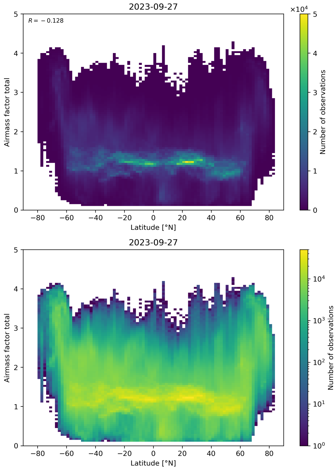
Figure 161: Scatter density plot of “Latitude” against “Airmass factor total” for 2023-09-26 to 2023-09-28.
