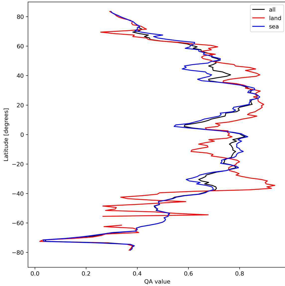
Figure 20: Zonal average of “QA value” for 2023-09-26 to 2023-09-28.
