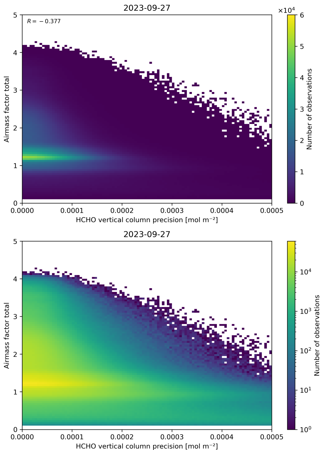
Figure 144: Scatter density plot of “HCHO vertical column precision” against “Airmass factor total” for 2023-09-26 to 2023-09-28.
