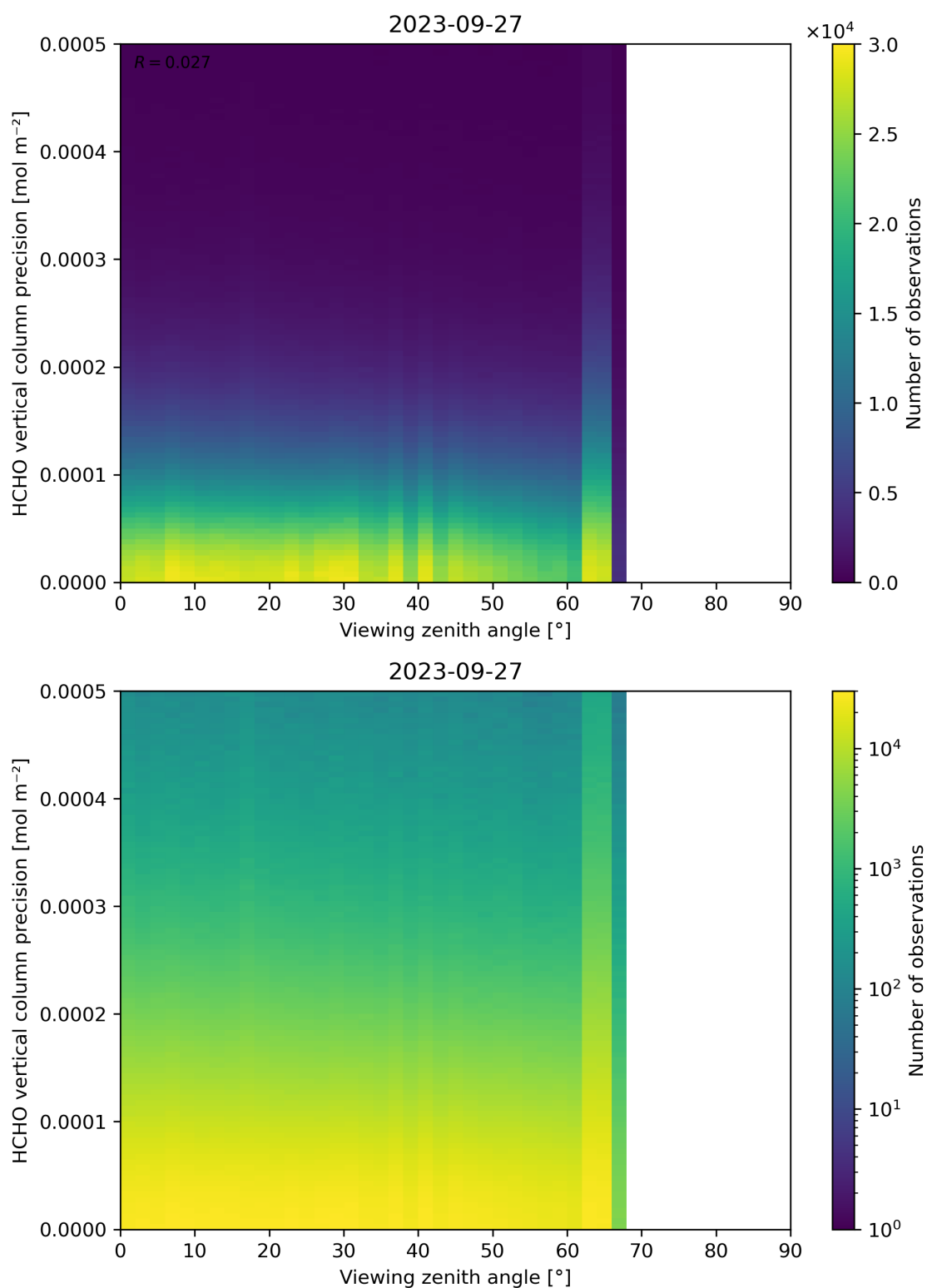
Figure 194: Scatter density plot of “Viewing zenith angle” against “HCHO vertical column precision” for 2023-09-26 to 2023-09-28.
