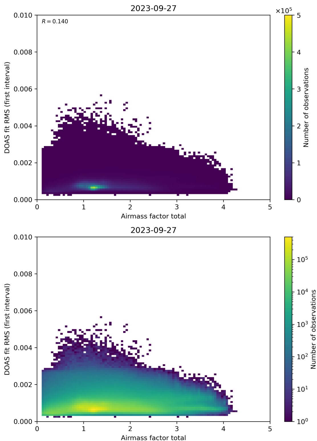
Figure 97: Scatter density plot of “Airmass factor total” against “DOAS fit RMS (first interval)” for 2023-09-26 to 2023-09-28.
