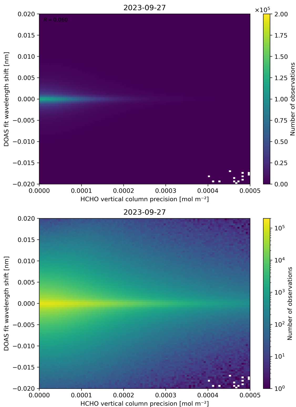
Figure 137: Scatter density plot of “HCHO vertical column precision” against “DOAS fit wavelength shift” for 2023-09-26 to 2023-09-28.
