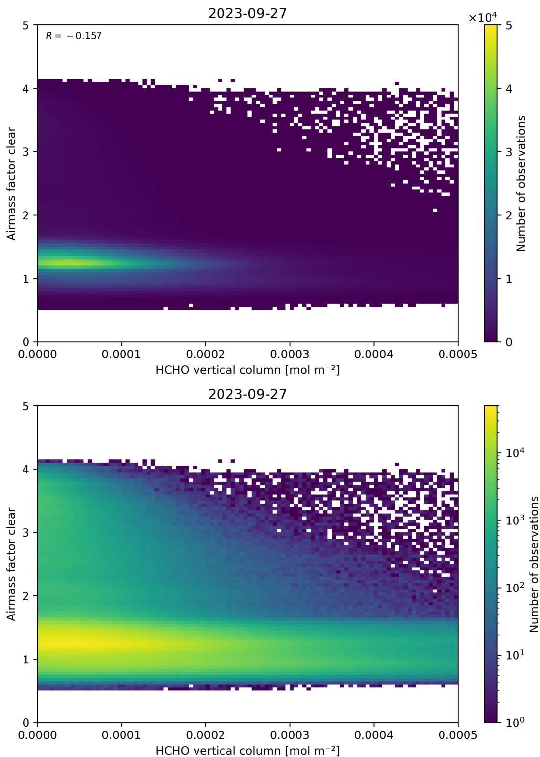
Figure 126: Scatter density plot of “HCHO vertical column” against “Airmass factor clear” for 2023-09-26 to 2023-09-28.
