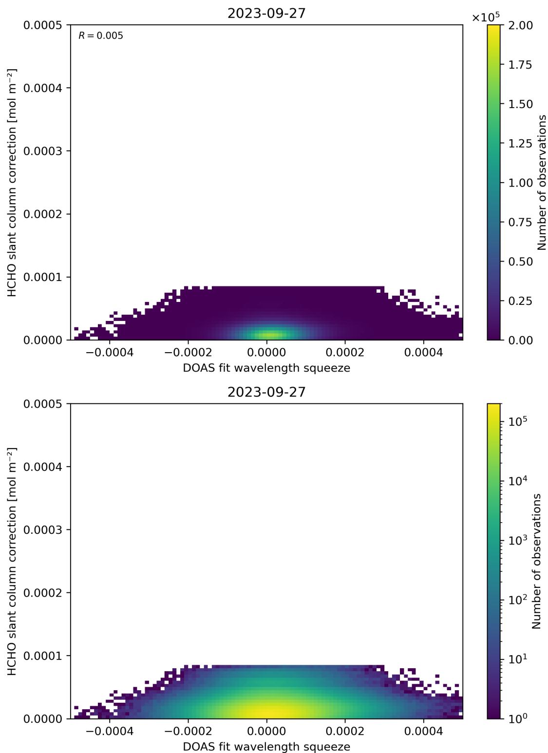
Figure 70: Scatter density plot of “DOAS fit wavelength squeeze” against “HCHO slant column correction” for 2023-09-26 to 2023-09-28.
