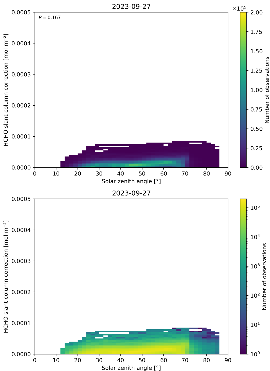
Figure 172: Scatter density plot of “Solar zenith angle” against “HCHO slant column correction” for 2023-09-26 to 2023-09-28.
