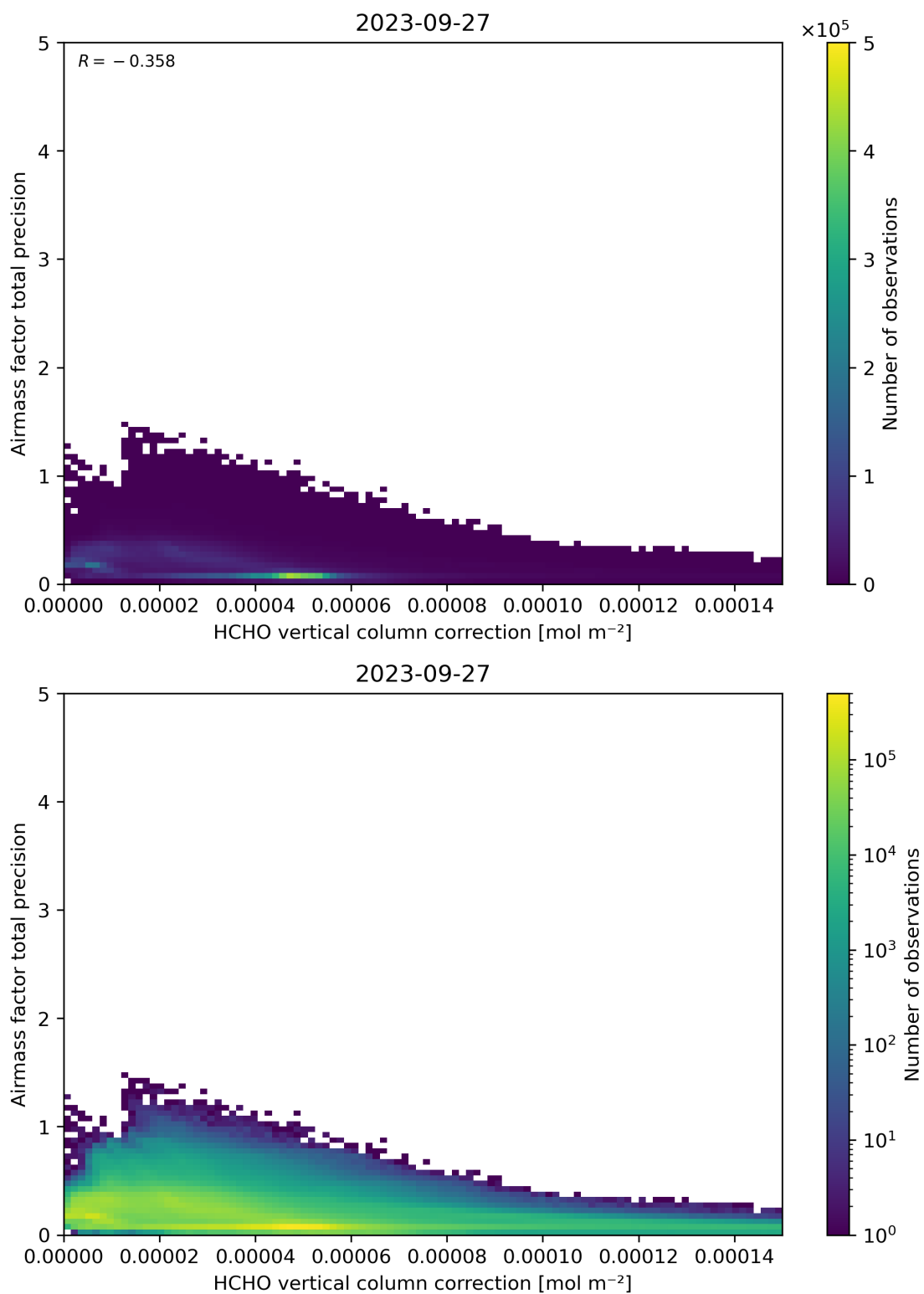
Figure 121: Scatter density plot of “HCHO vertical column correction” against “Airmass factor total precision” for 2023-09-26 to 2023-09-28.
