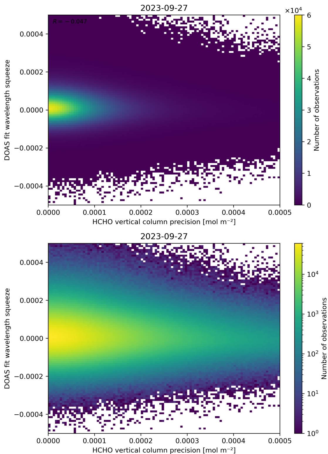
Figure 138: Scatter density plot of “HCHO vertical column precision” against “DOAS fit wavelength squeeze” for 2023-09-26 to 2023-09-28.
