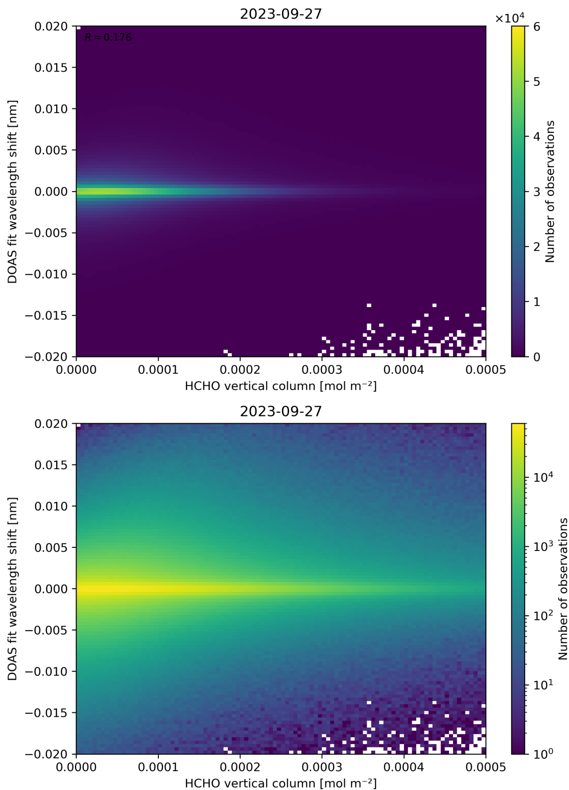
Figure 124: Scatter density plot of “HCHO vertical column” against “DOAS fit wavelength shift” for 2023-09-26 to 2023-09-28.
