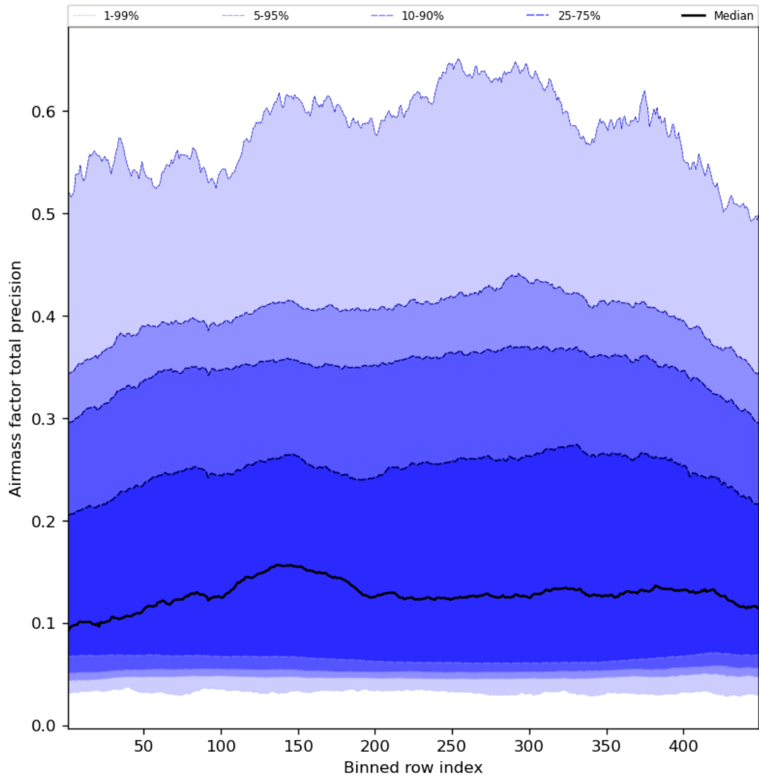
Figure 55: Along track statistics of “Airmass factor total precision” for 2023-09-26 to 2023-09-28
