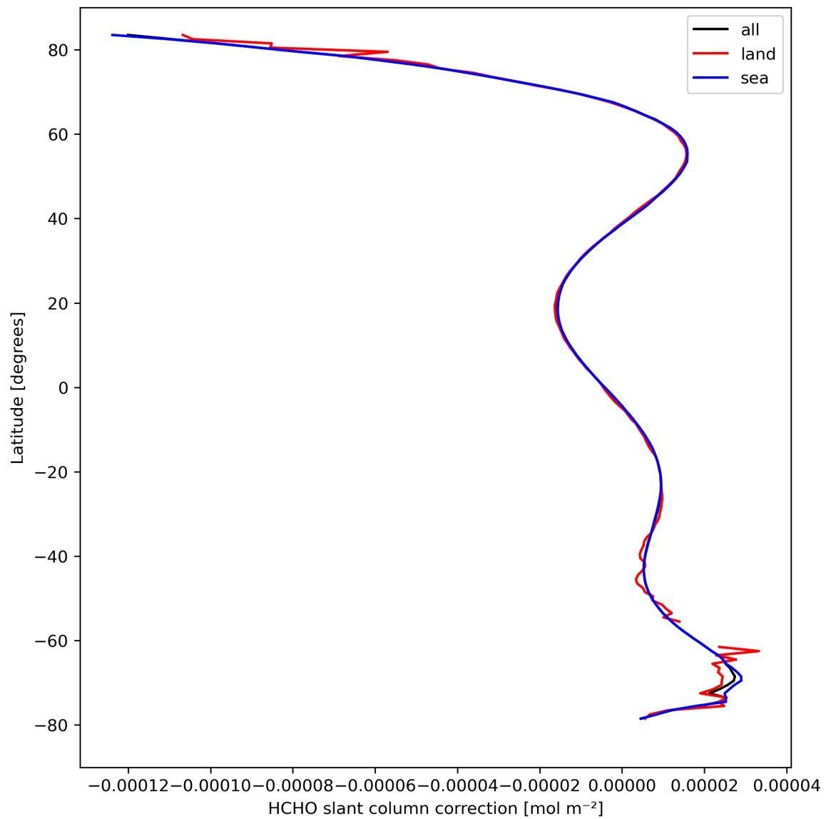
Figure 33: Zonal average of “HCHO slant column correction” for 2023-09-26 to 2023-09-28.
