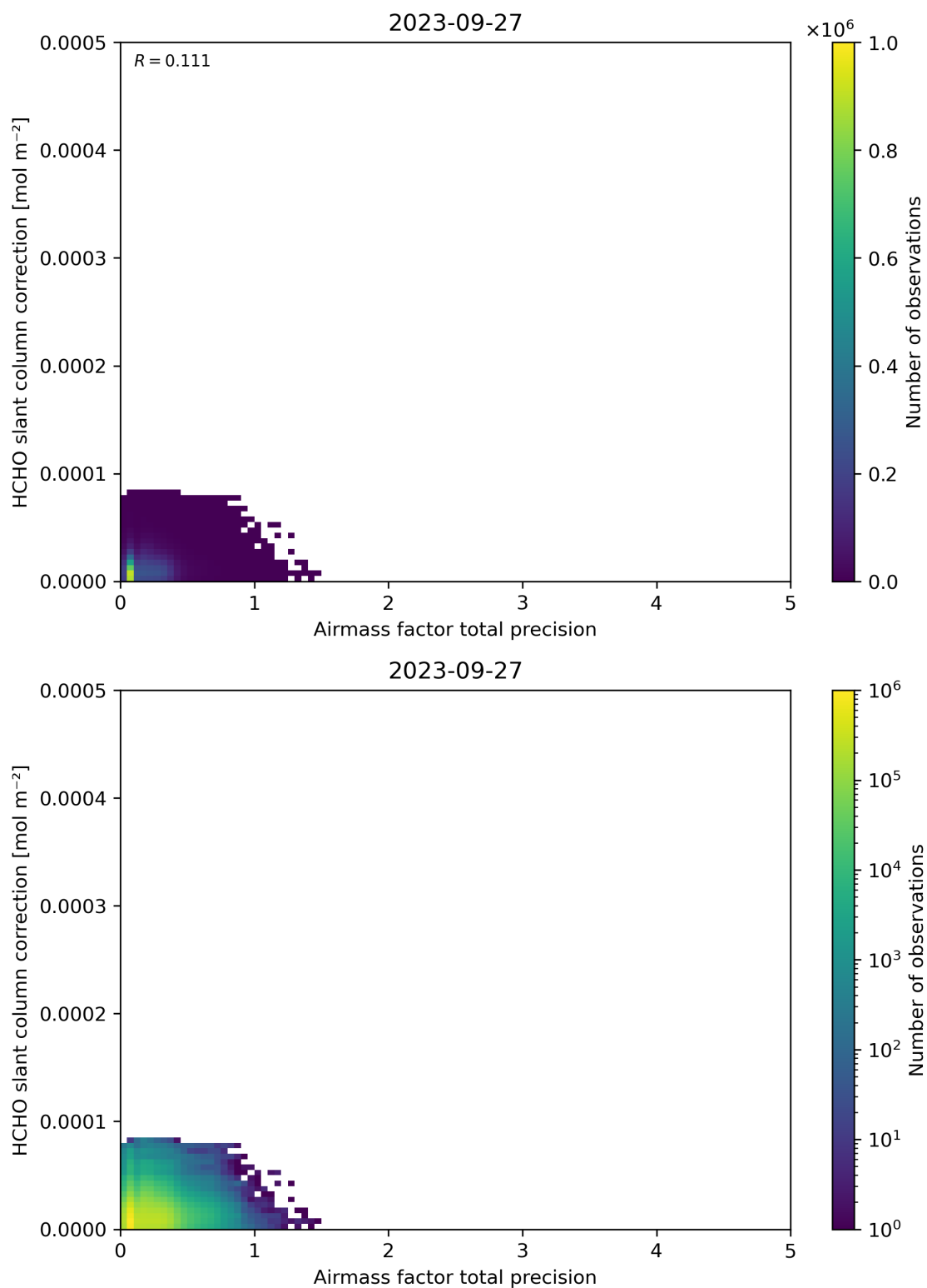
Figure 110: Scatter density plot of “Airmass factor total precision” against “HCHO slant column correction” for 2023-09-26 to 2023-09-28.
