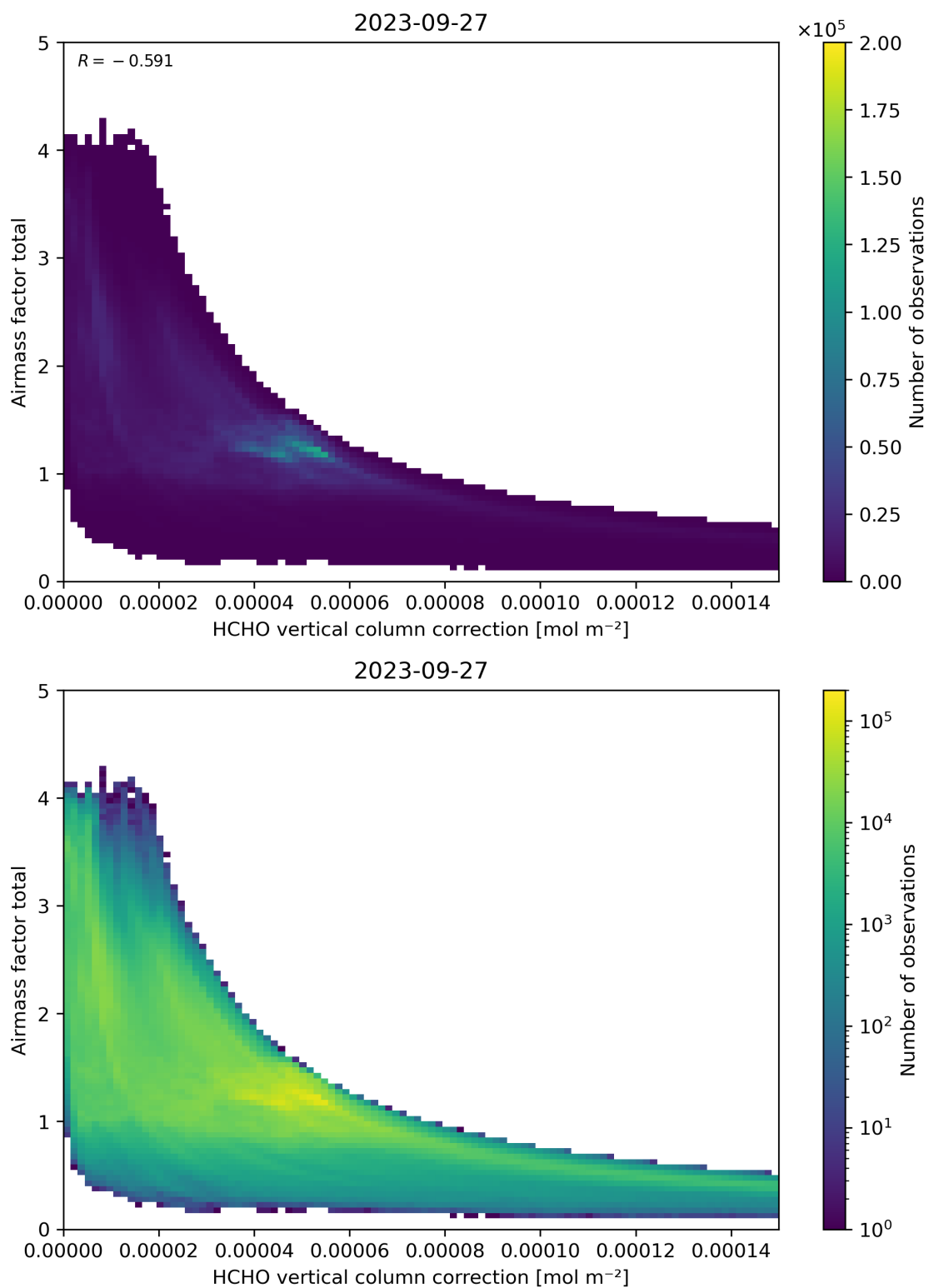
Figure 120: Scatter density plot of “HCHO vertical column correction” against “Airmass factor total” for 2023-09-26 to 2023-09-28.
