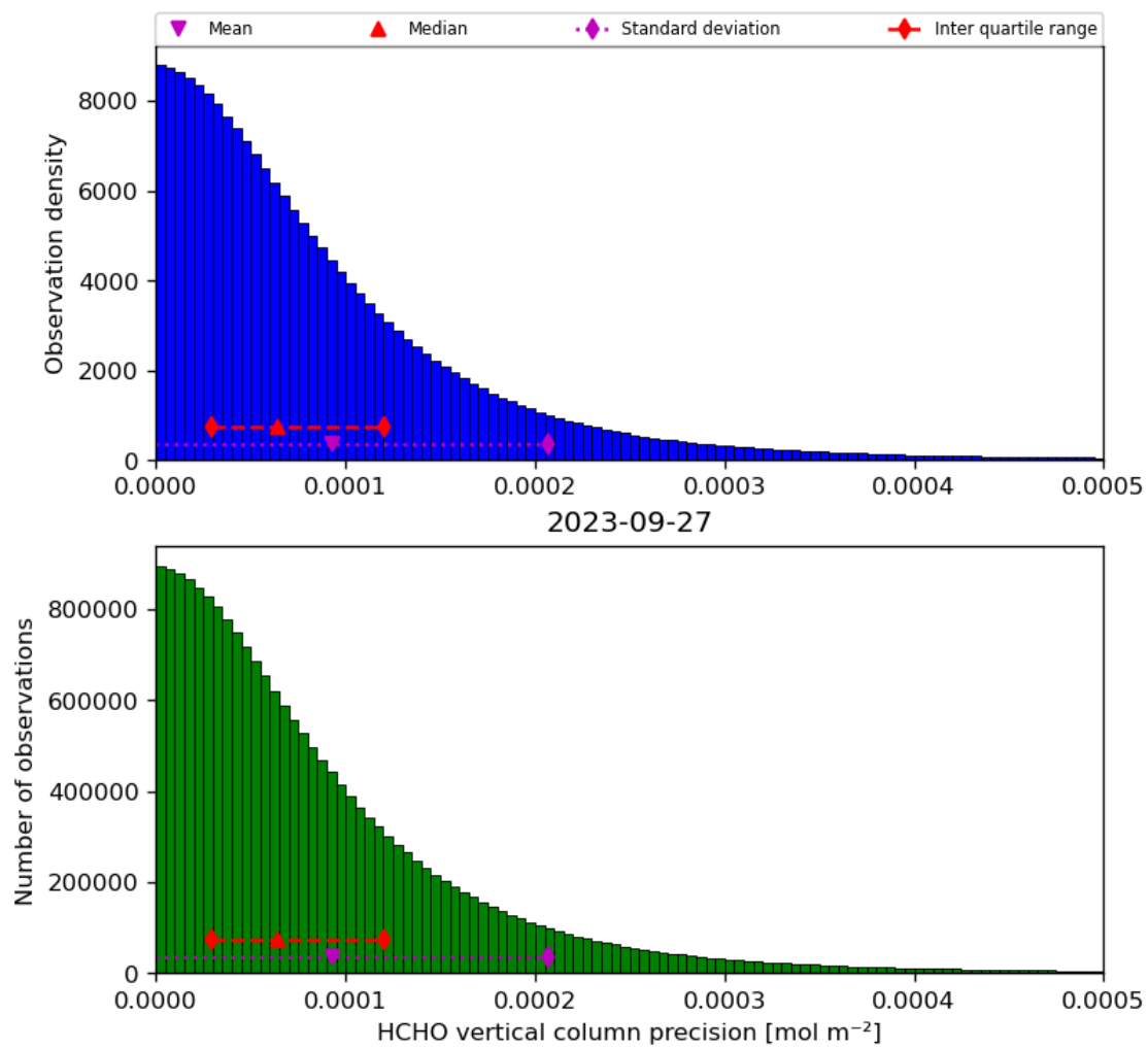
Figure 36: Histogram of “HCHO vertical column precision” for 2023-09-26 to 2023-09-28
