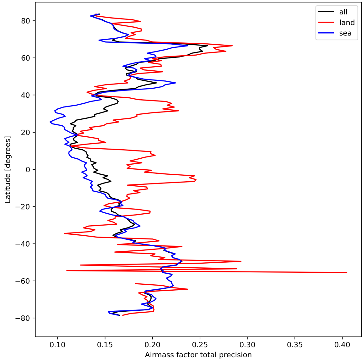
Figure 27: Zonal average of “Airmass factor total precision” for 2023-09-26 to 2023-09-28.
