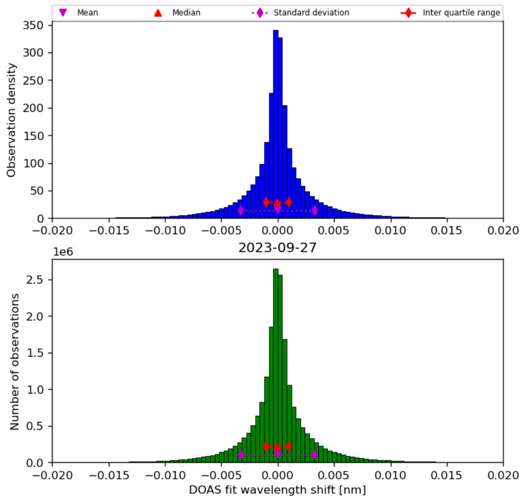
Figure 44: Histogram of “DOAS fit wavelength shift” for 2023-09-26 to 2023-09-28
