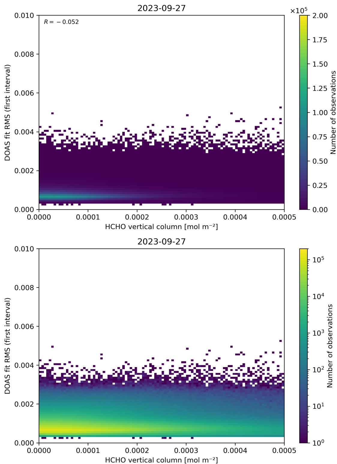
Figure 123: Scatter density plot of “HCHO vertical column” against “DOAS fit RMS (first interval)” for 2023-09-26 to 2023-09-28.
