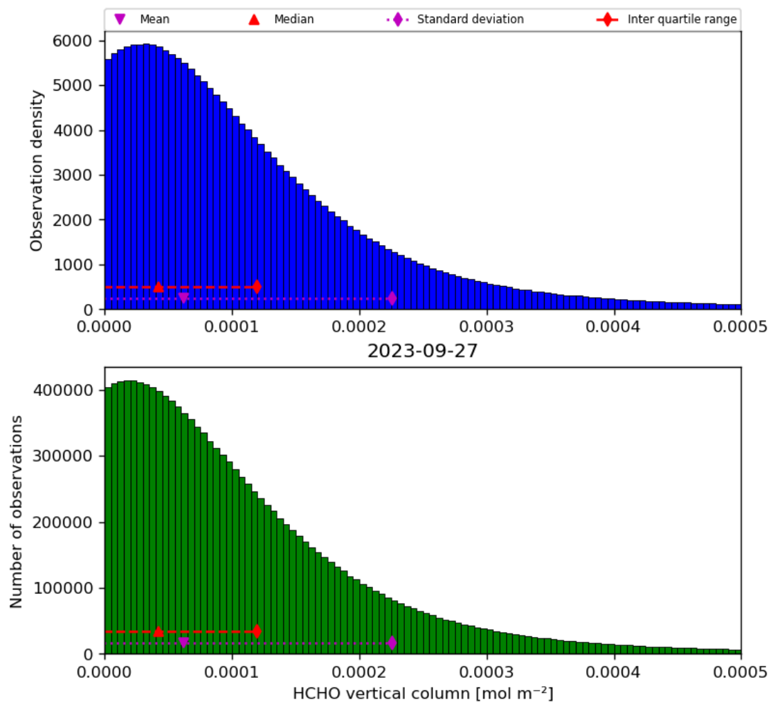
Figure 35: Histogram of “HCHO vertical column” for 2023-09-26 to 2023-09-28
