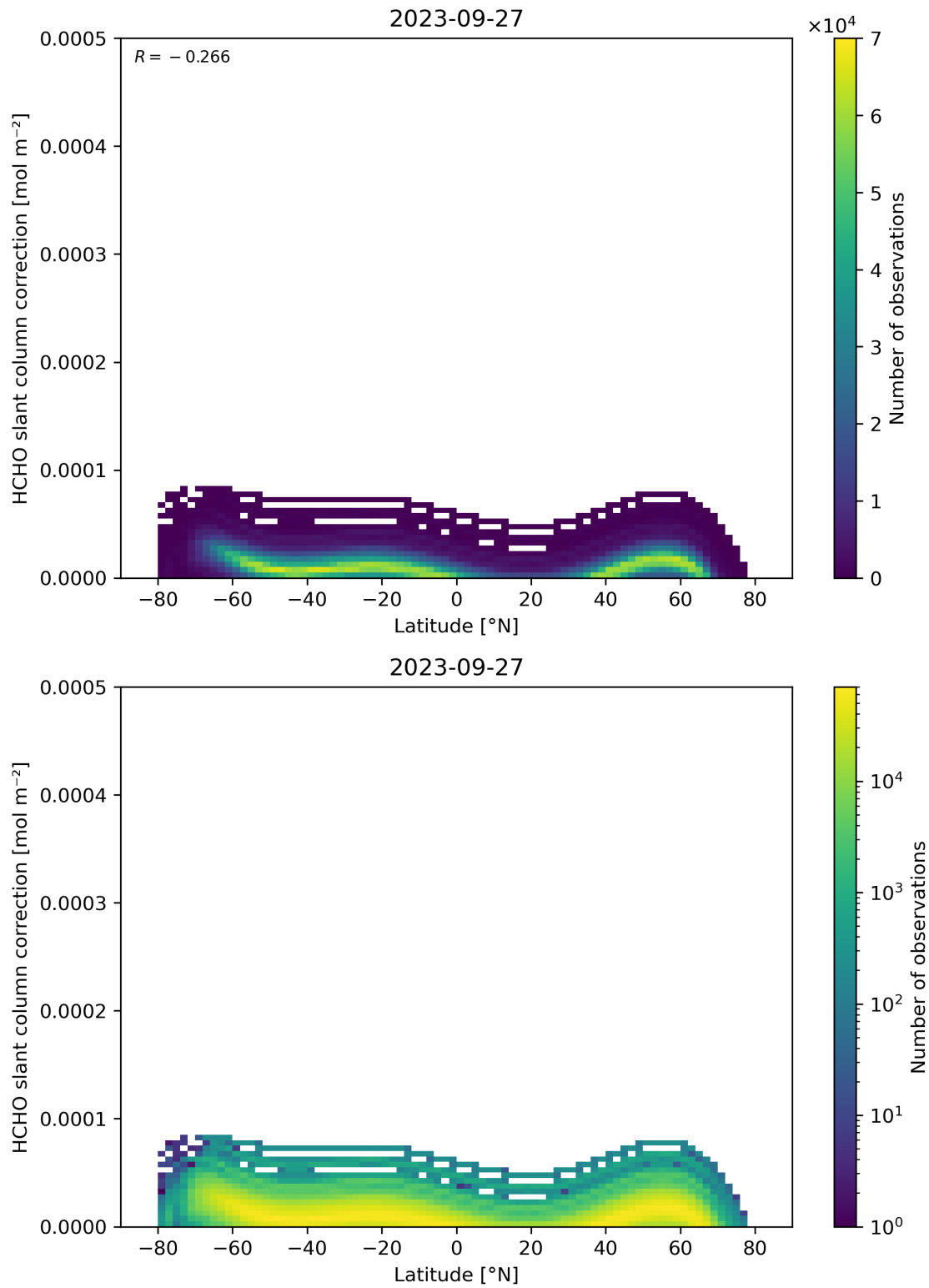
Figure 158: Scatter density plot of “Latitude” against “HCHO slant column correction” for 2023-09-26 to 2023-09-28.
