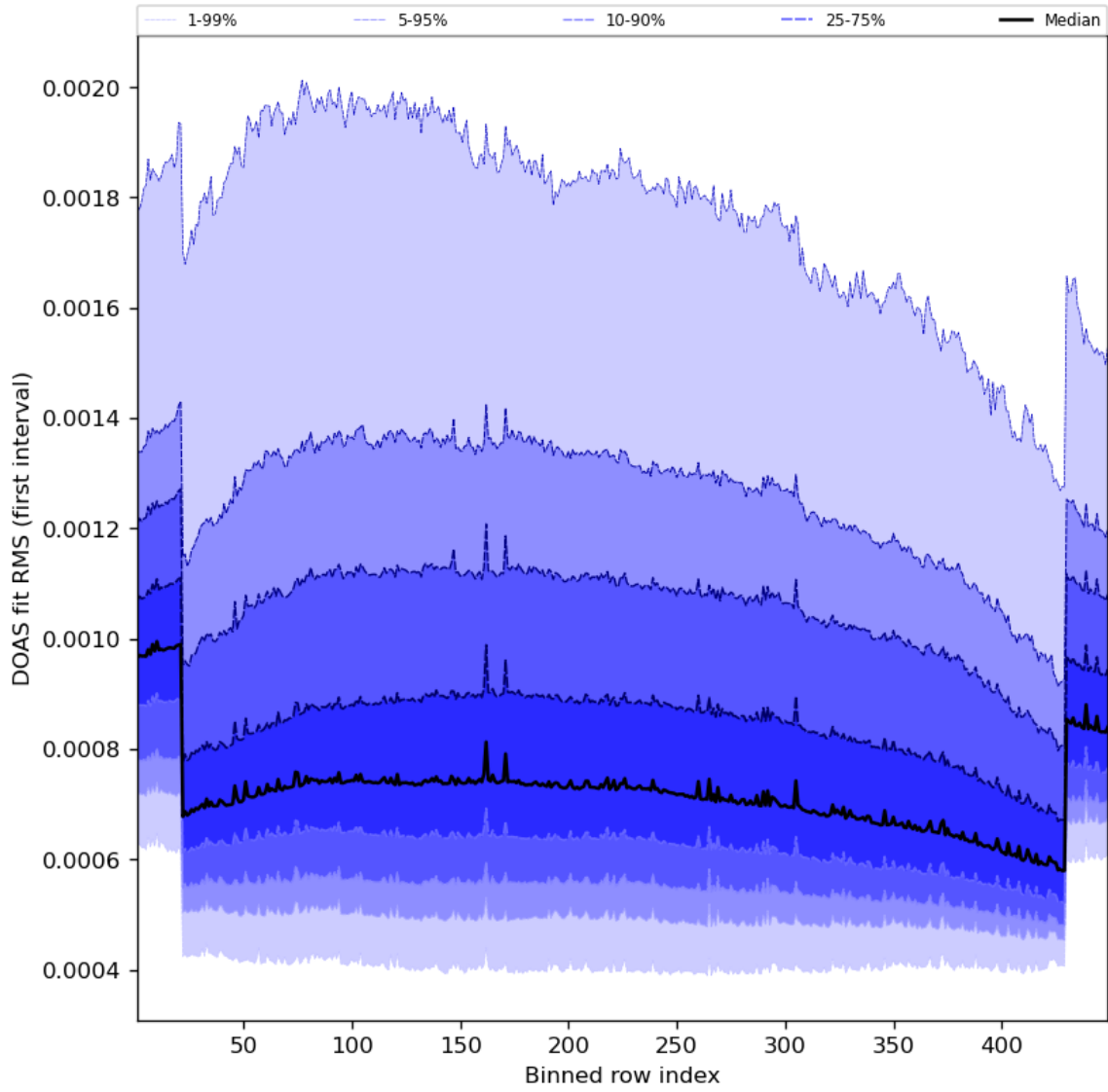
Figure 60: Along track statistics of “DOAS fit RMS (first interval)” for 2023-09-26 to 2023-09-28
