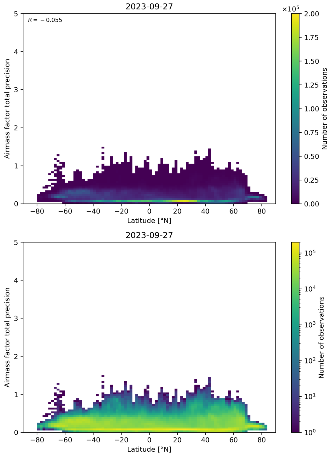
Figure 162: Scatter density plot of “Latitude” against “Airmass factor total precision” for 2023-09-26 to 2023-09-28.
