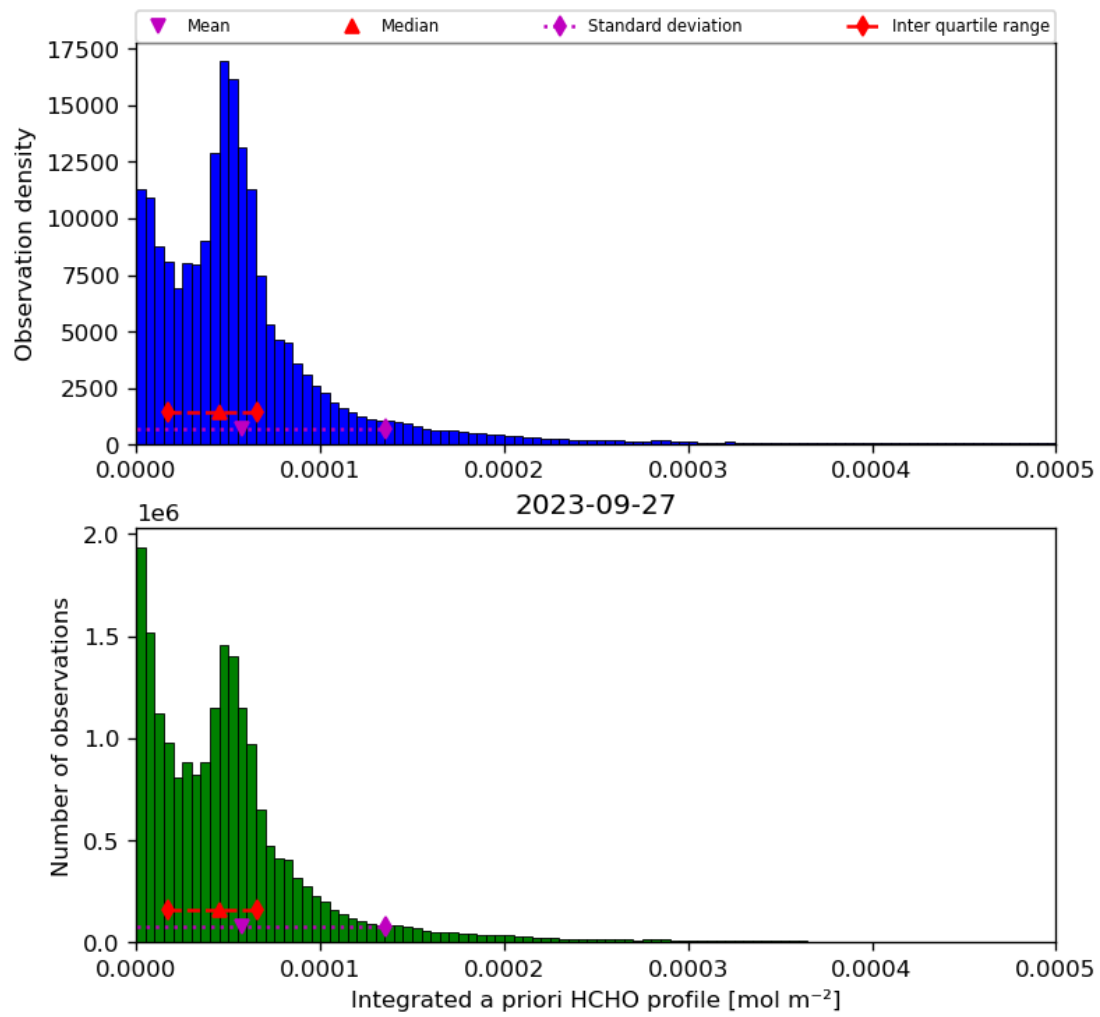
Figure 43: Histogram of “Integrated a priori HCHO profile” for 2023-09-26 to 2023-09-28
