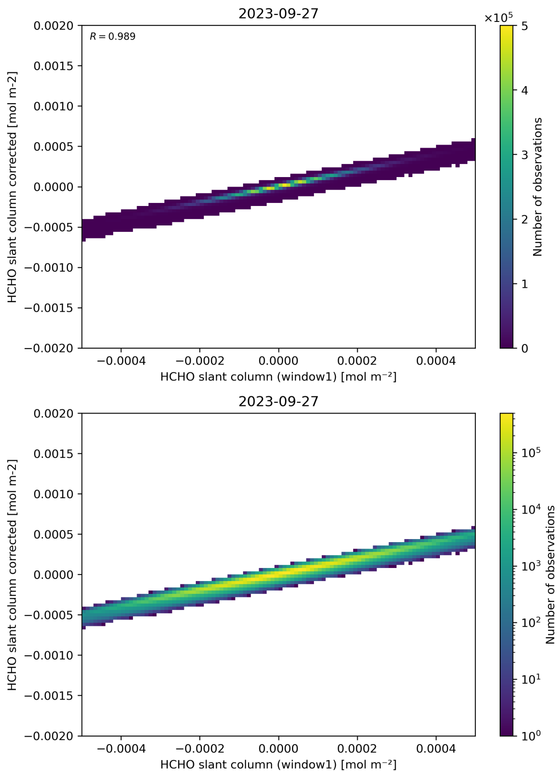
Figure 82: Scatter density plot of “HCHO slant column (window1)” against “HCHO slant column corrected” for 2023-09-26 to 2023-09-28.
