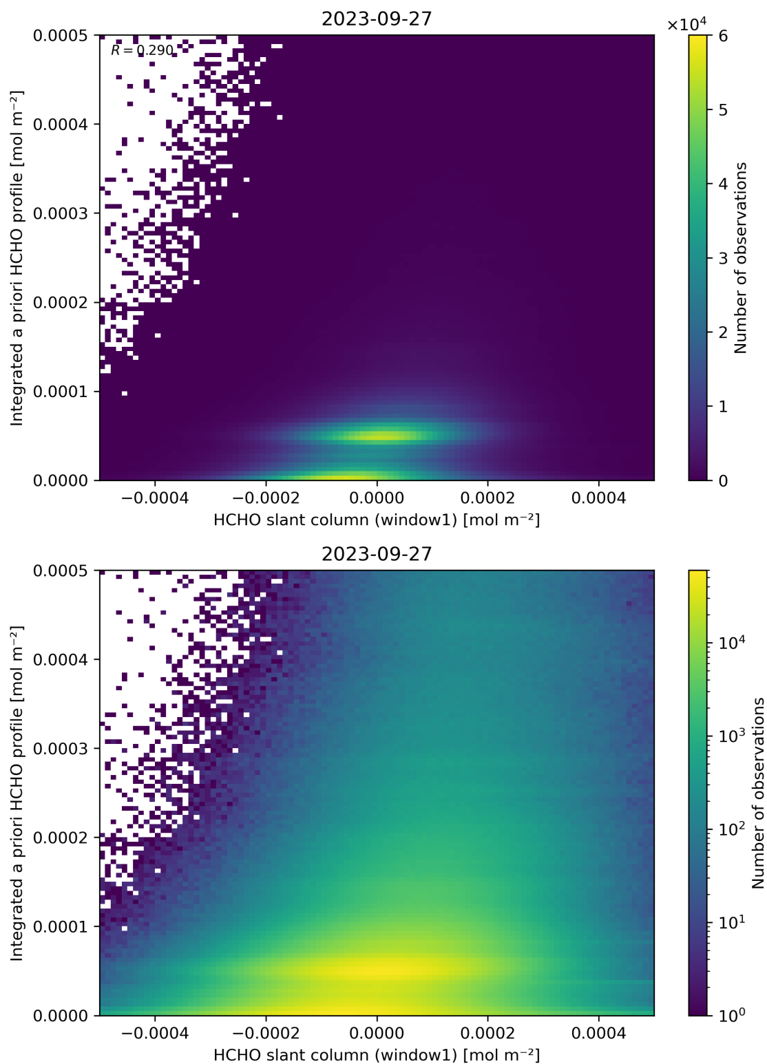
Figure 87: Scatter density plot of “HCHO slant column (window1)” against “Integrated a priori HCHO profile” for 2023-09-26 to 2023-09-28.
