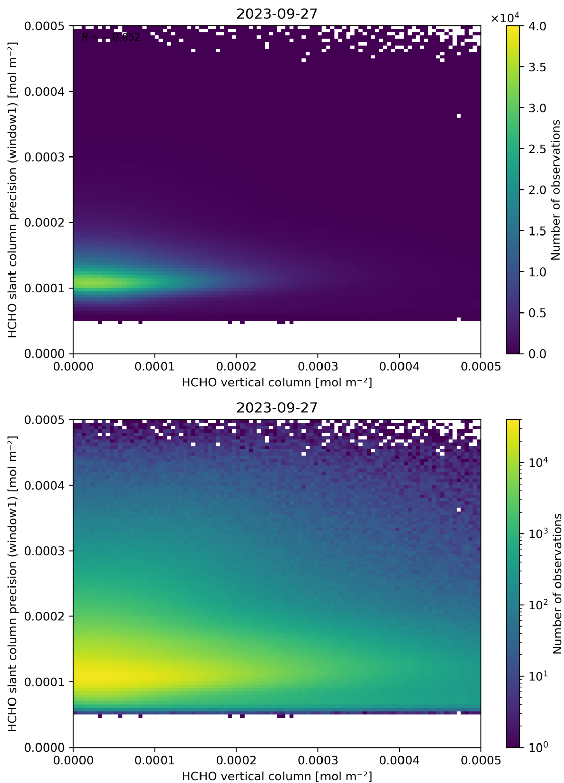
Figure 130: Scatter density plot of “HCHO vertical column” against “HCHO slant column precision (window1)” for 2023-09-26 to 2023-09-28.
