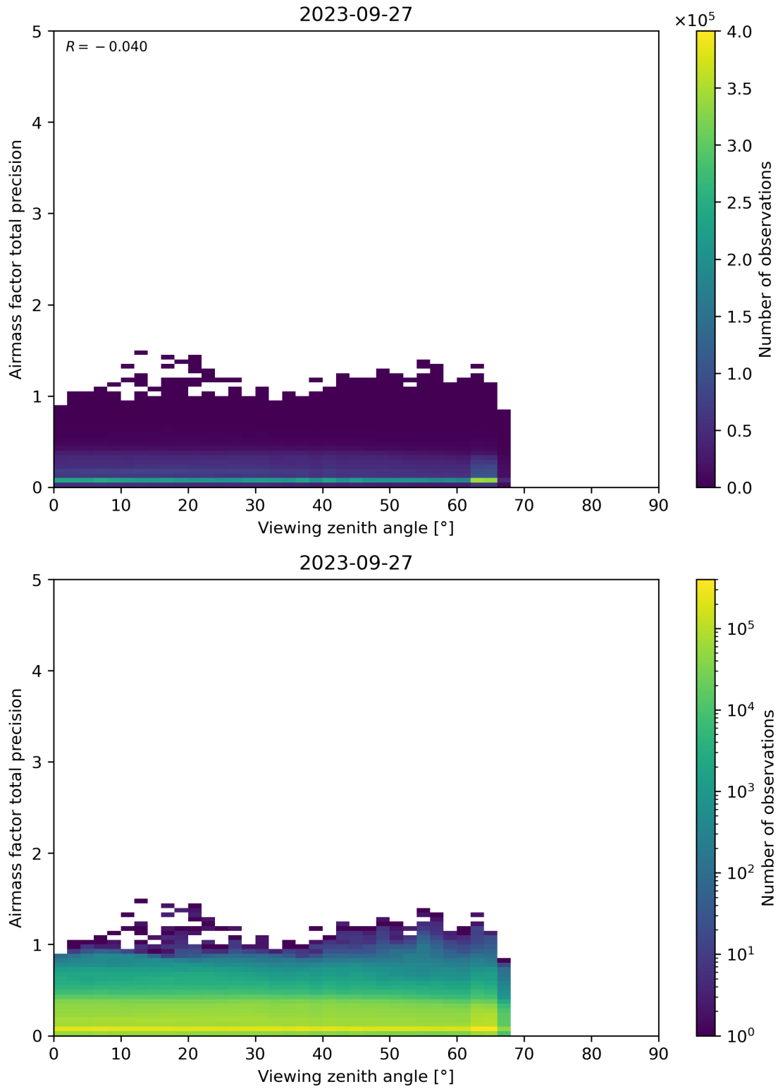
Figure 191: Scatter density plot of “Viewing zenith angle” against “Airmass factor total precision” for 2023-09-26 to 2023-09-28.
