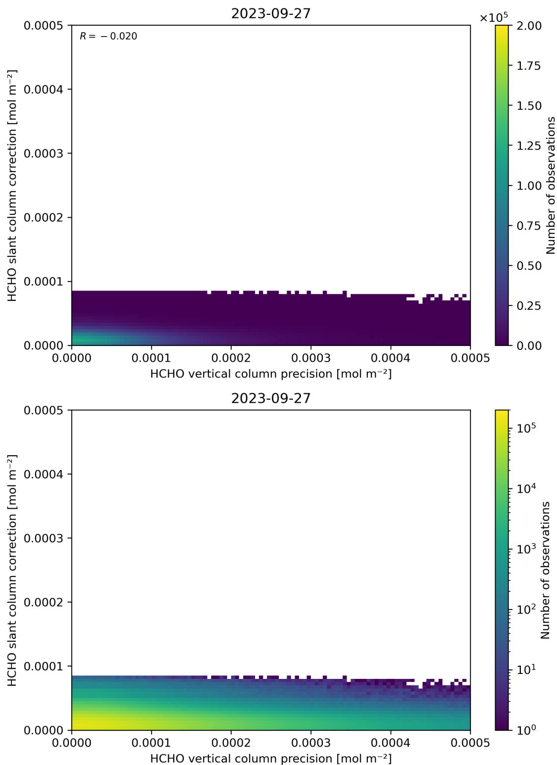
Figure 141: Scatter density plot of “HCHO vertical column precision” against “HCHO slant column correction” for 2023-09-26 to 2023-09-28.
