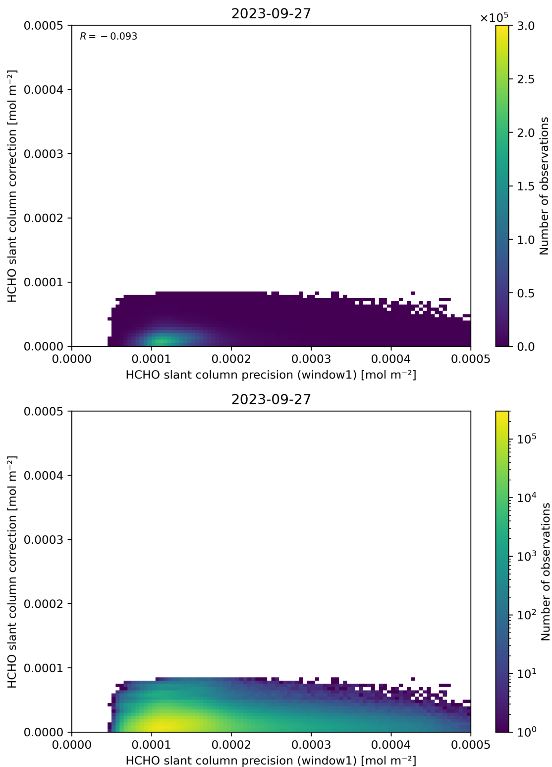
Figure 93: Scatter density plot of “HCHO slant column precision (window1)” against “HCHO slant column correction” for 2023-09-26 to 2023-09-28.
