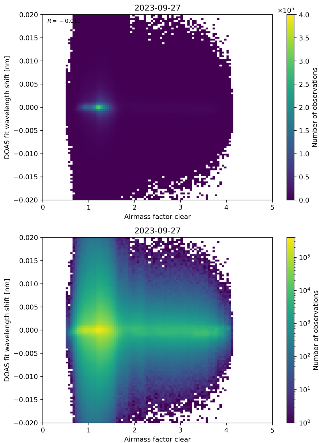
Figure 72: Scatter density plot of “Airmass factor clear” against “DOAS fit wavelength shift” for 2023-09-26 to 2023-09-28.
