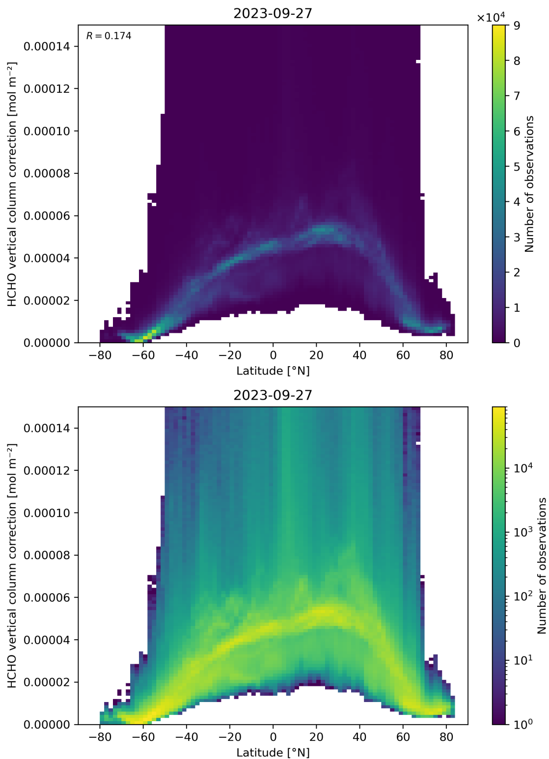
Figure 164: Scatter density plot of “Latitude” against “HCHO vertical column correction” for 2023-09-26 to 2023-09-28.
