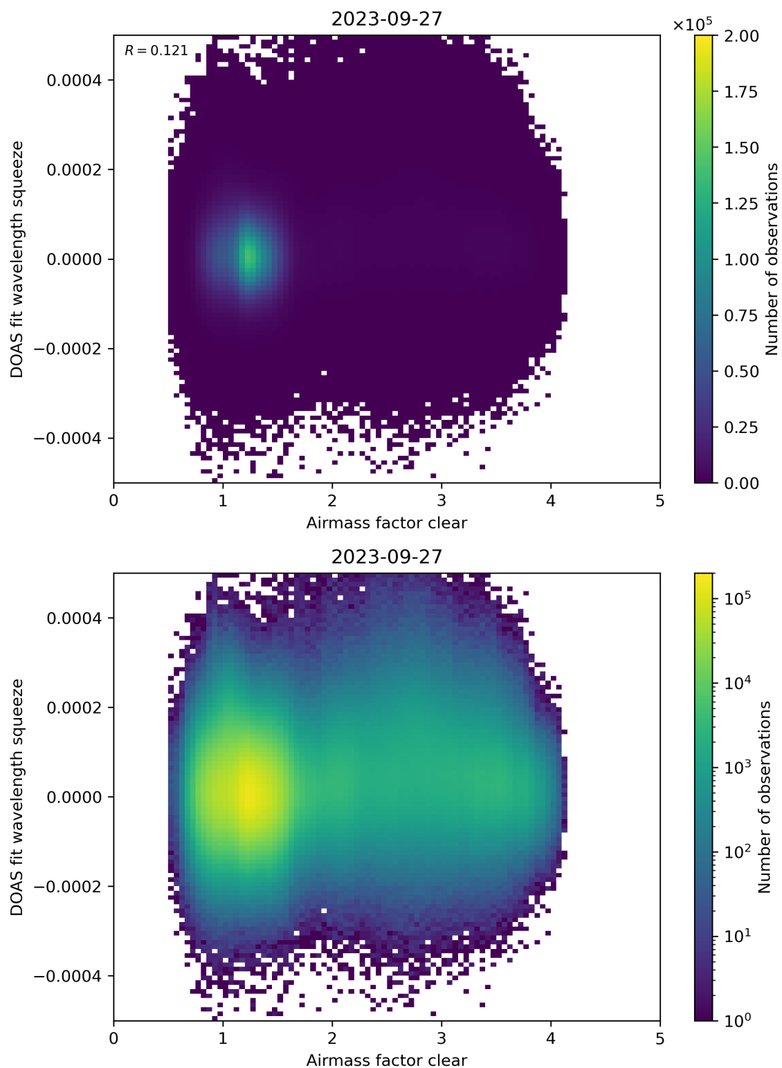
Figure 73: Scatter density plot of “Airmass factor clear” against “DOAS fit wavelength squeeze” for 2023-09-26 to 2023-09-28.
