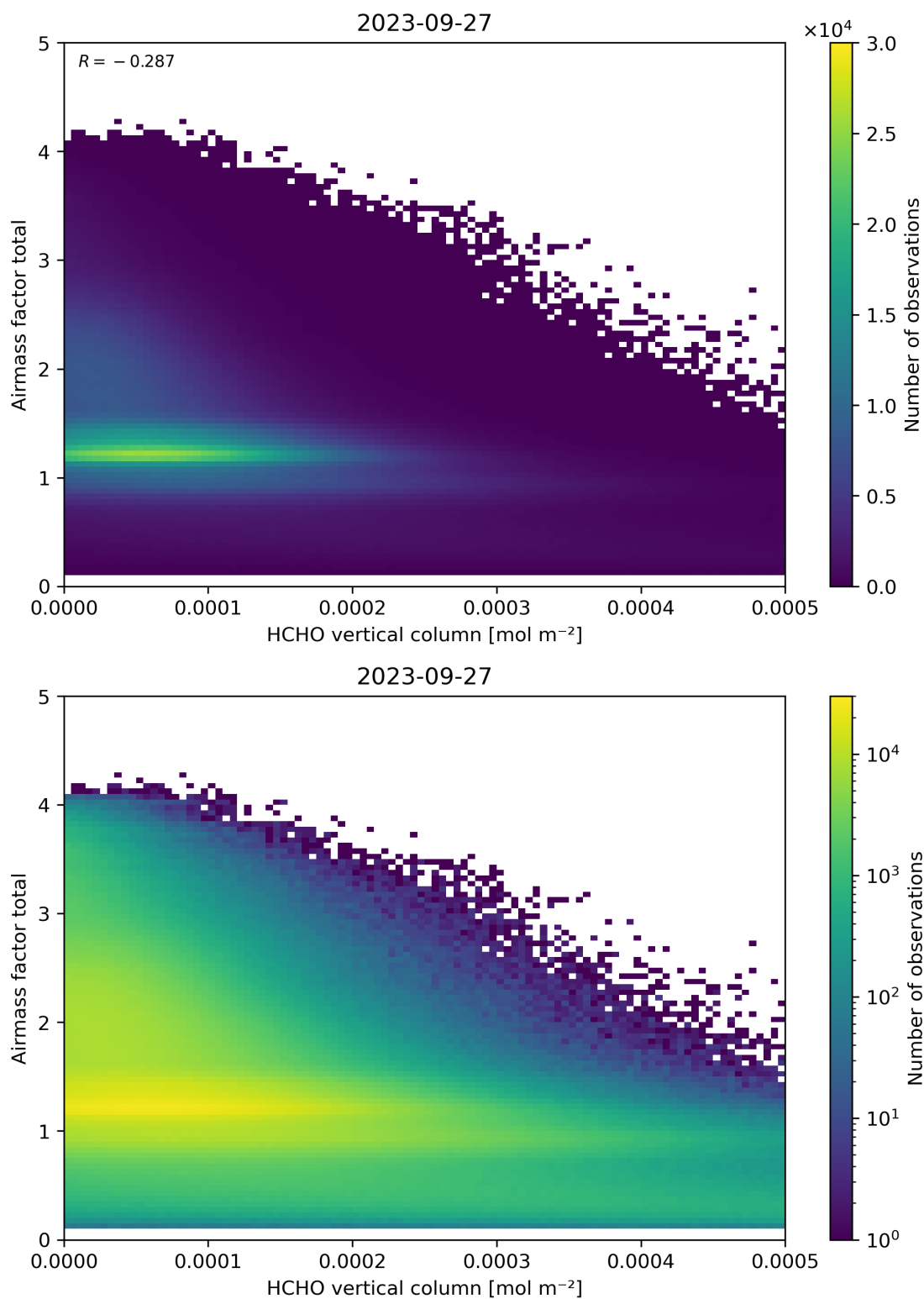
Figure 131: Scatter density plot of “HCHO vertical column” against “Airmass factor total” for 2023-09-26 to 2023-09-28.
