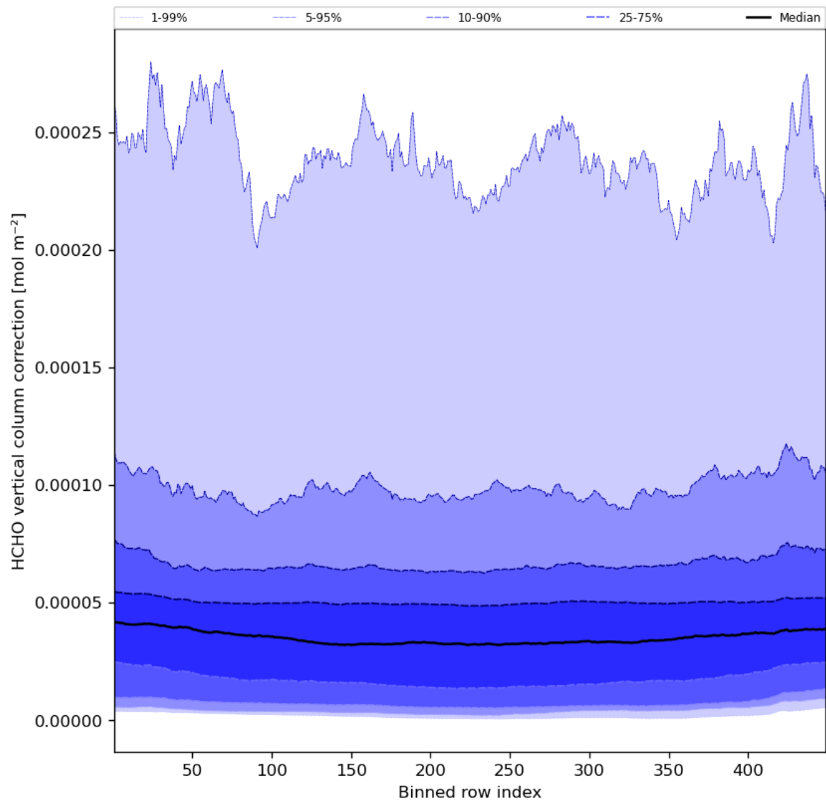
Figure 51: Along track statistics of “HCHO vertical column correction” for 2023-09-26 to 2023-09-28
