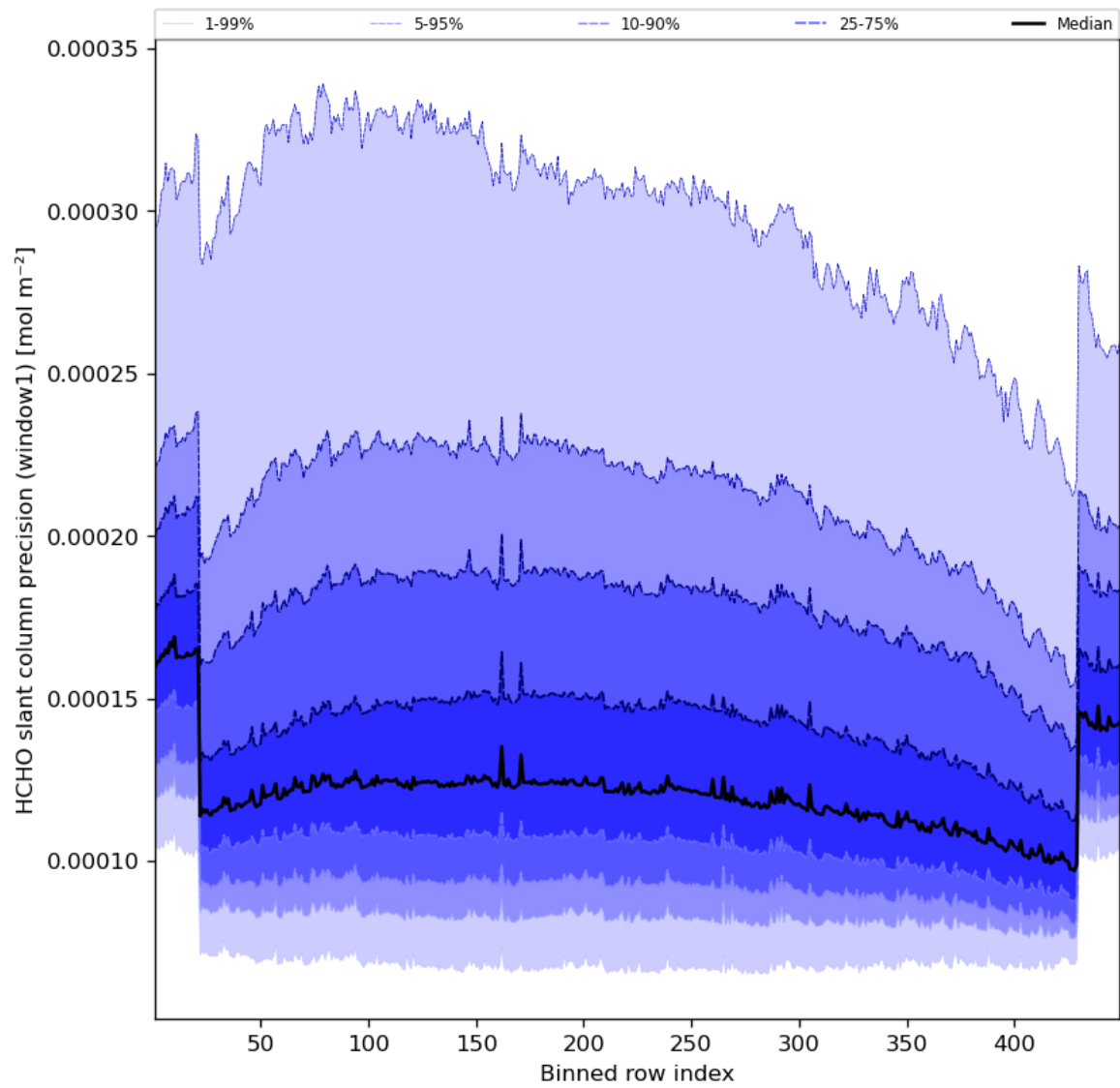
Figure 53: Along track statistics of “HCHO slant column precision (window1)” for 2023-09-26 to 2023-09-28
