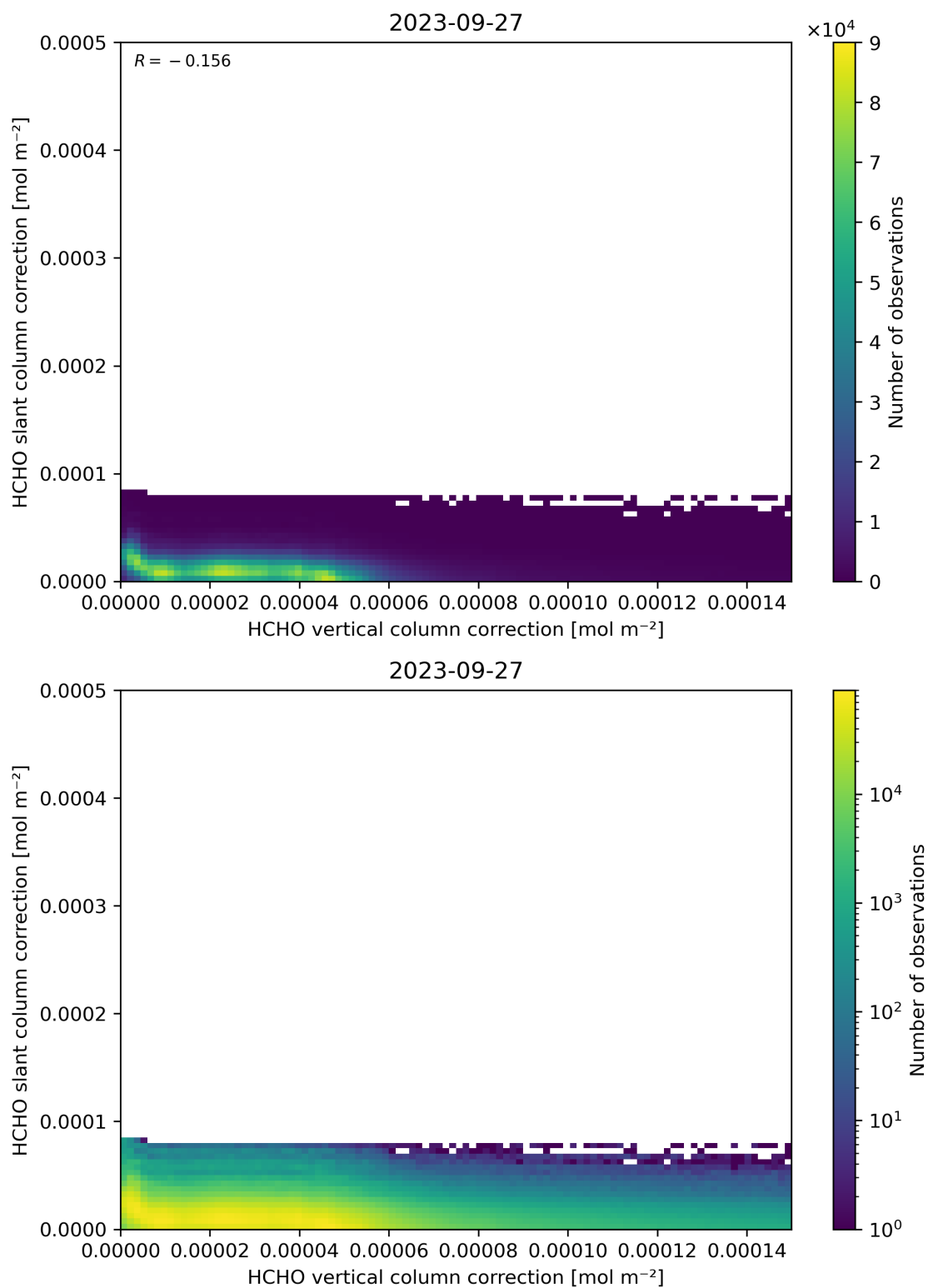
Figure 117: Scatter density plot of “HCHO vertical column correction” against “HCHO slant column correction” for 2023-09-26 to 2023-09-28.
