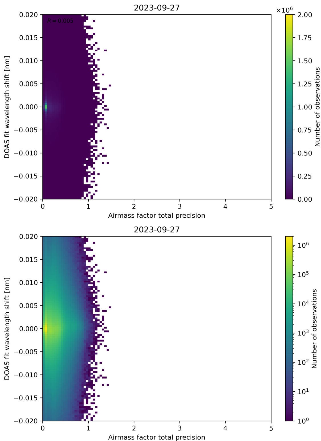
Figure 106: Scatter density plot of “Airmass factor total precision” against “DOAS fit wavelength shift” for 2023-09-26 to 2023-09-28.
