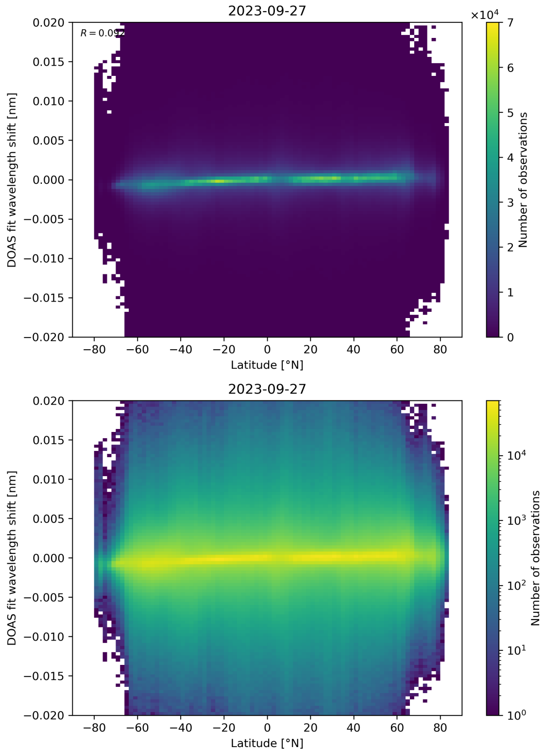
Figure 154: Scatter density plot of “Latitude” against “DOAS fit wavelength shift” for 2023-09-26 to 2023-09-28.
