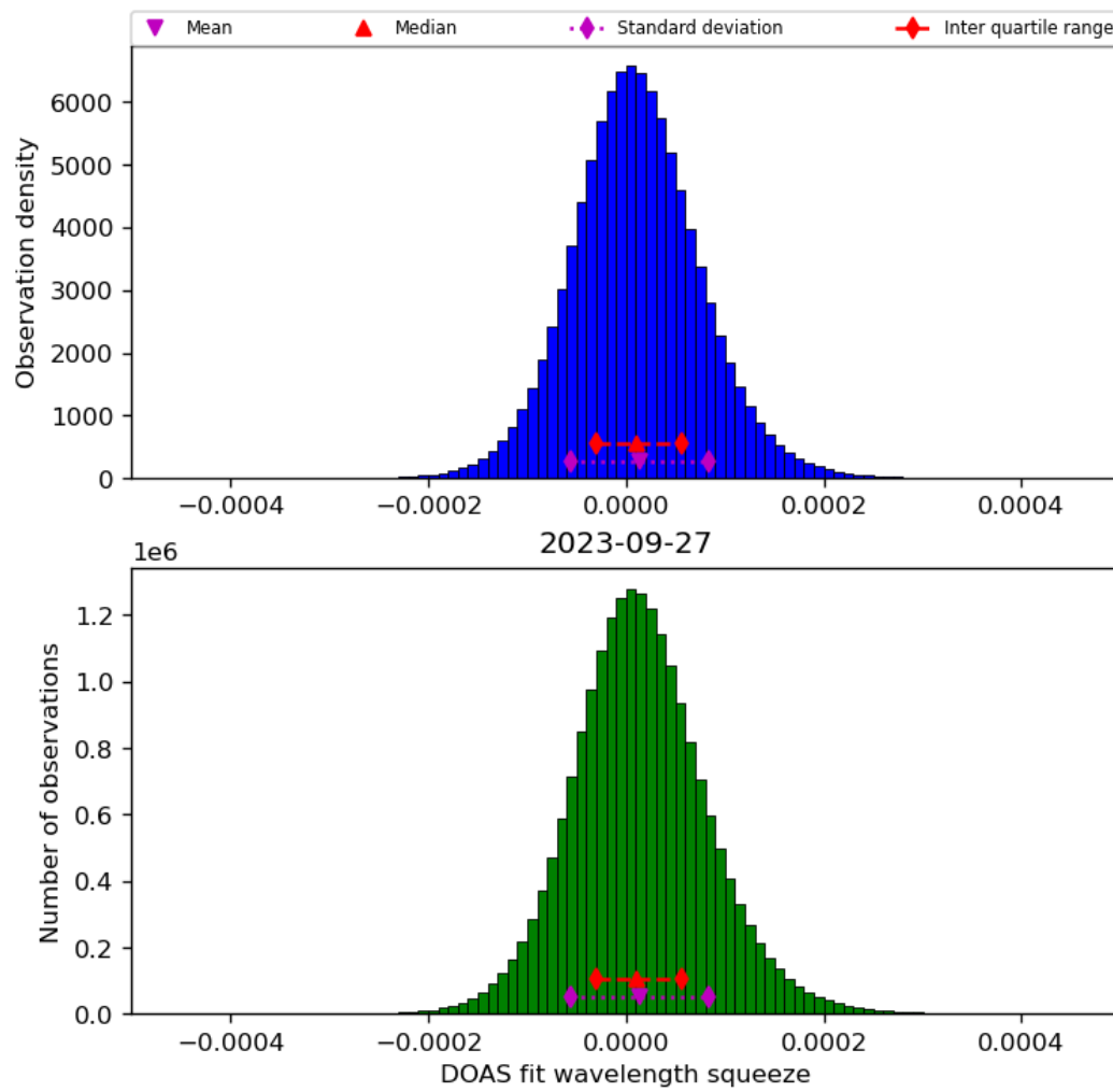
Figure 45: Histogram of “DOAS fit wavelength squeeze” for 2023-09-26 to 2023-09-28
