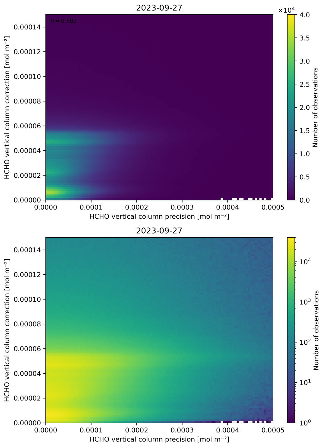
Figure 146: Scatter density plot of “HCHO vertical column precision” against “HCHO vertical column correction” for 2023-09-26 to 2023-09-28.
