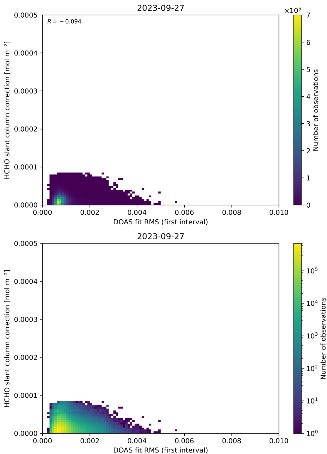
Figure 63: Scatter density plot of “DOAS fit RMS (first interval)” against “HCHO slant column correction” for 2023-09-26 to 2023-09-28.
