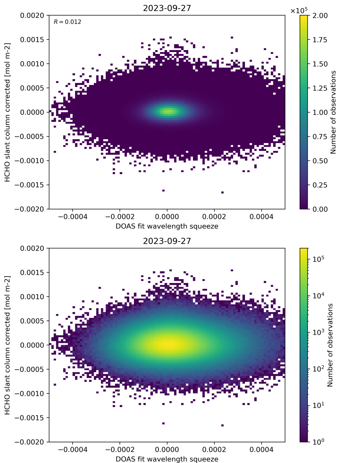
Figure 69: Scatter density plot of “DOAS fit wavelength squeeze” against “HCHO slant column corrected” for 2023-09-26 to 2023-09-28.
