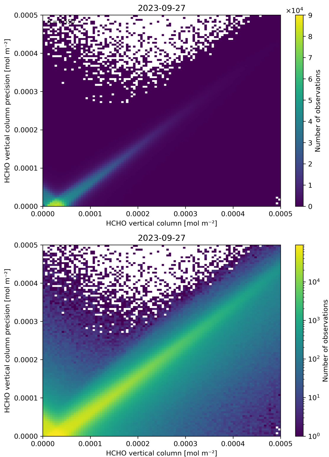
Figure 134: Scatter density plot of “HCHO vertical column” against “HCHO vertical column precision” for 2023-09-26 to 2023-09-28.
