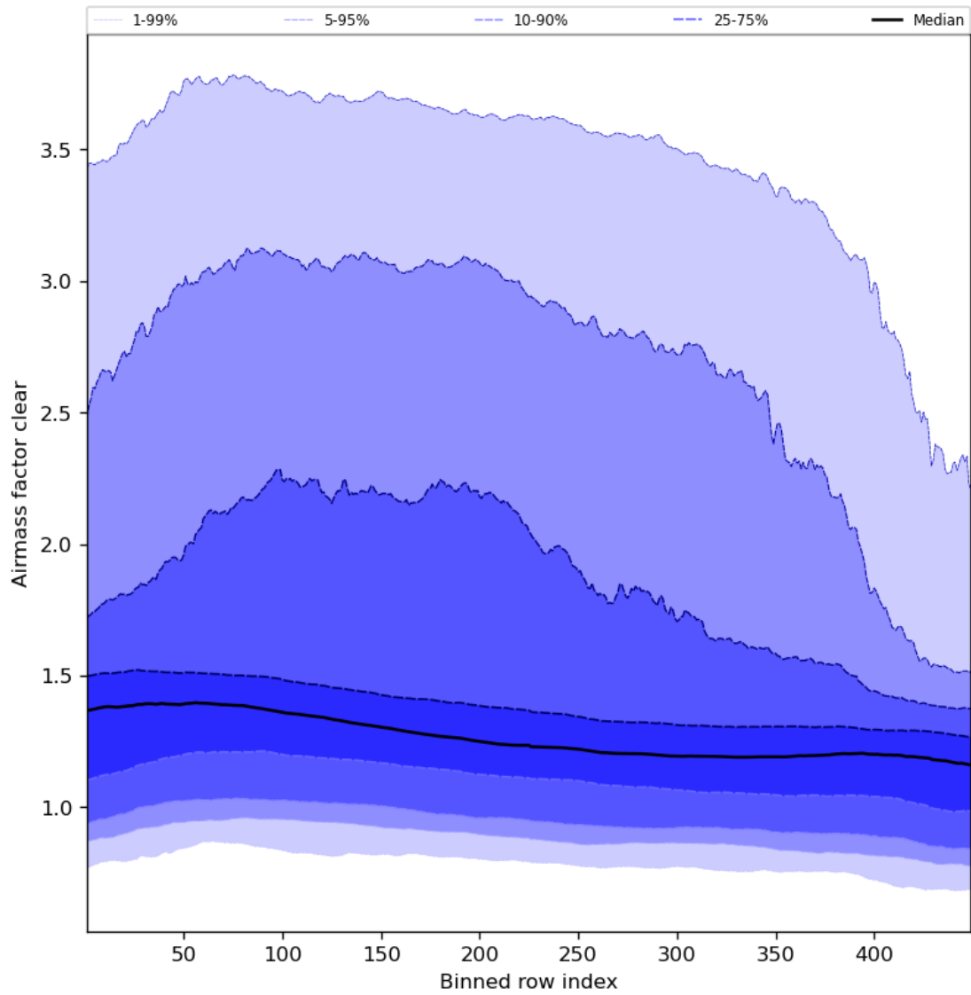
Figure 56: Along track statistics of “Airmass factor clear” for 2023-09-26 to 2023-09-28
