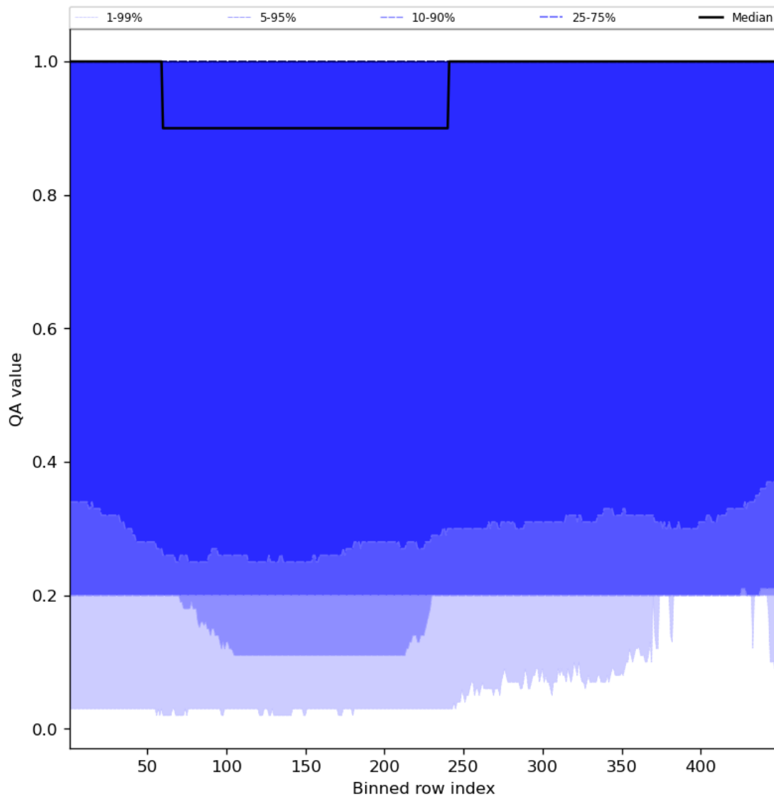
Figure 48: Along track statistics of “QA value” for 2023-09-26 to 2023-09-28
