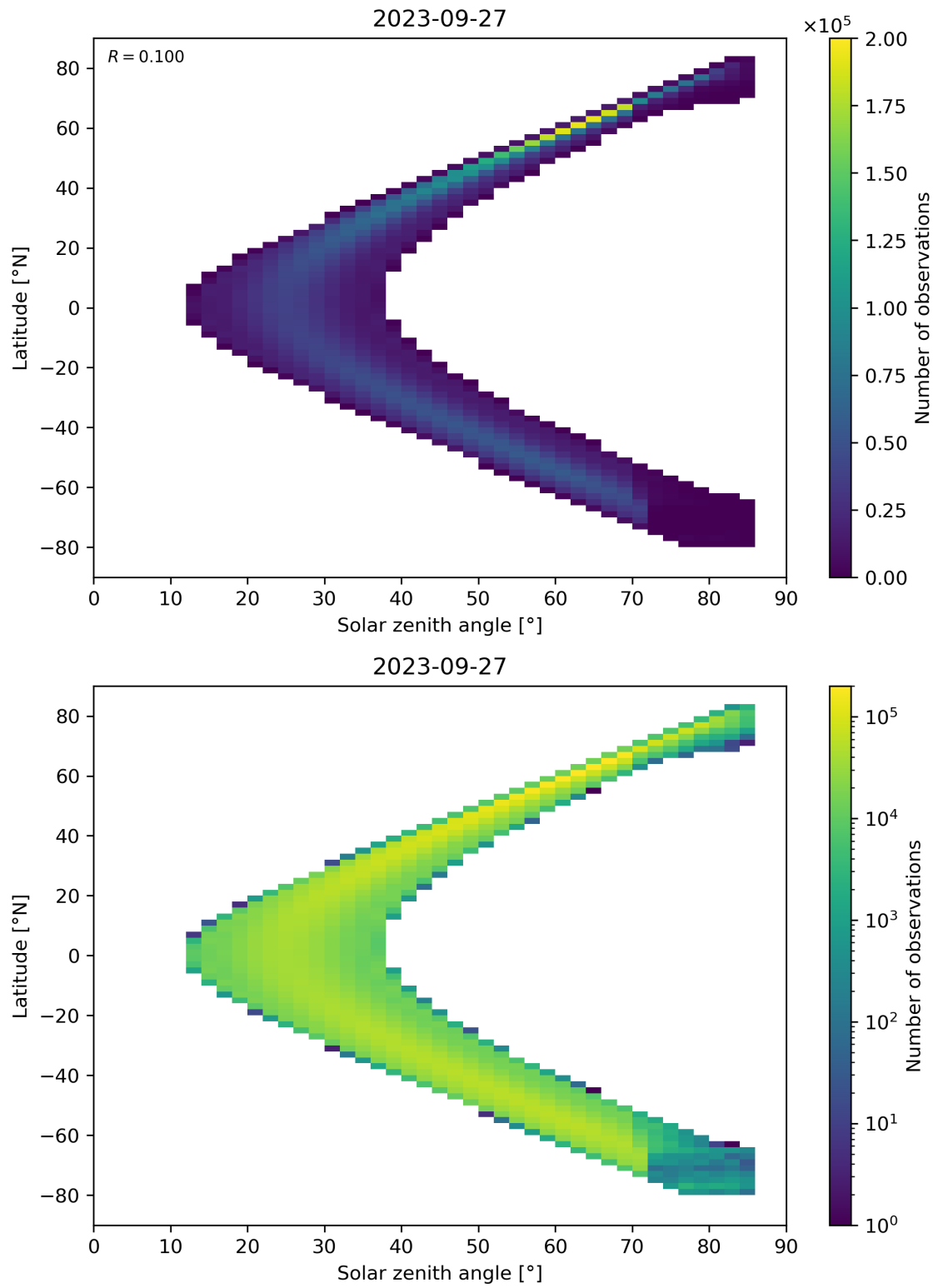
Figure 181: Scatter density plot of “Solar zenith angle” against “Latitude” for 2023-09-26 to 2023-09-28.
