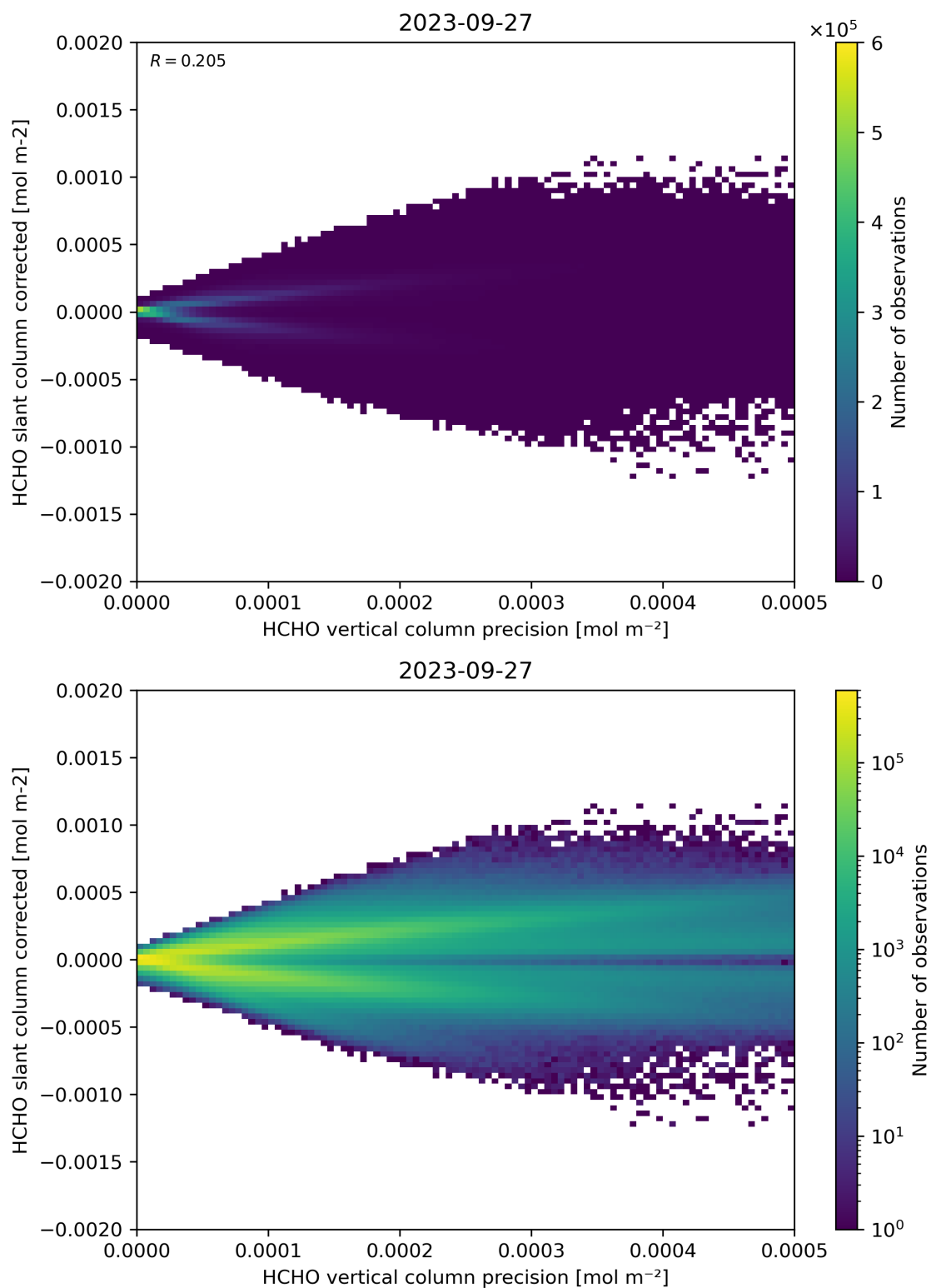
Figure 140: Scatter density plot of “HCHO vertical column precision” against “HCHO slant column corrected” for 2023-09-26 to 2023-09-28.
