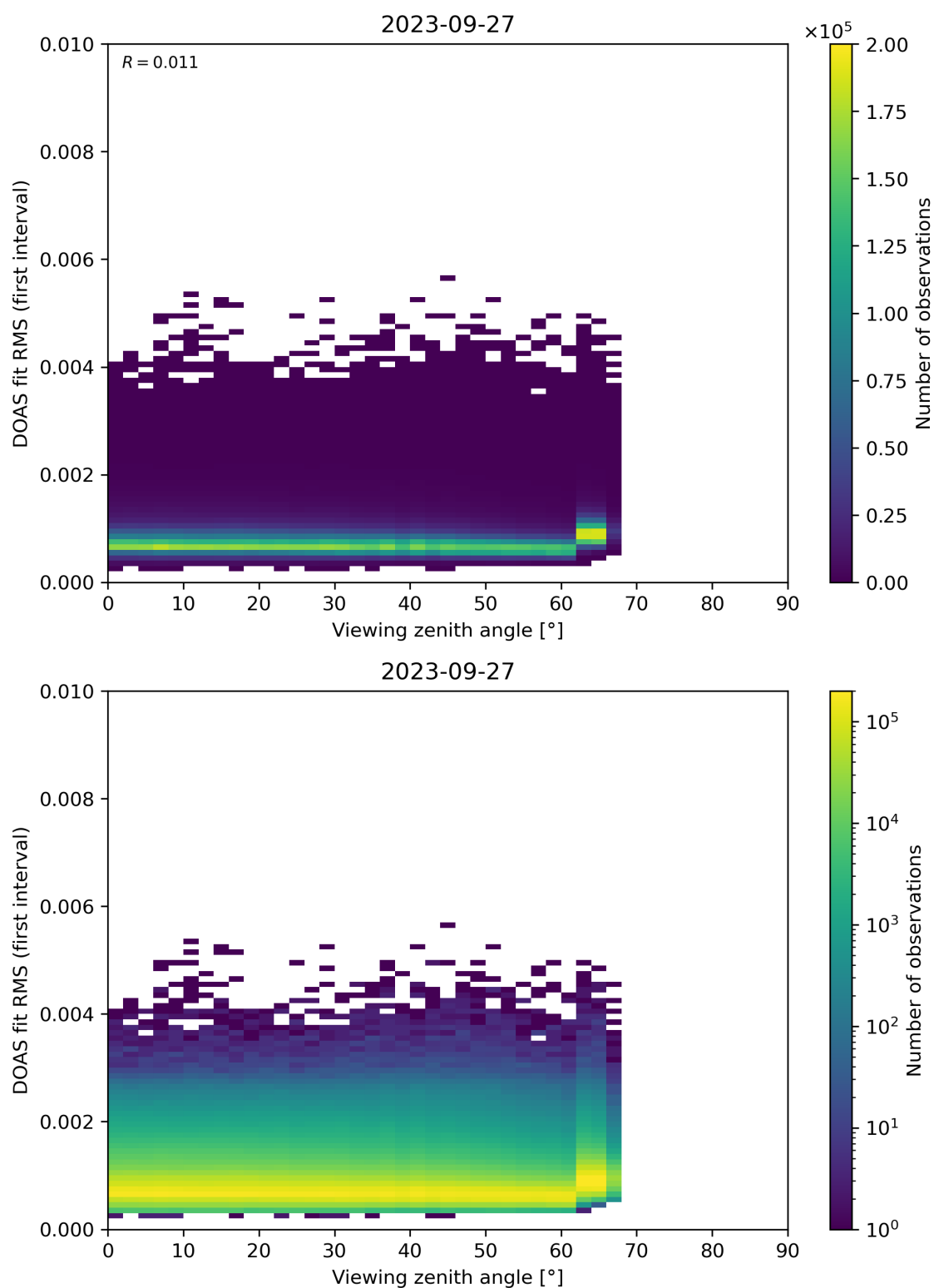
Figure 182: Scatter density plot of “Viewing zenith angle” against “DOAS fit RMS (first interval)” for 2023-09-26 to 2023-09-28.
