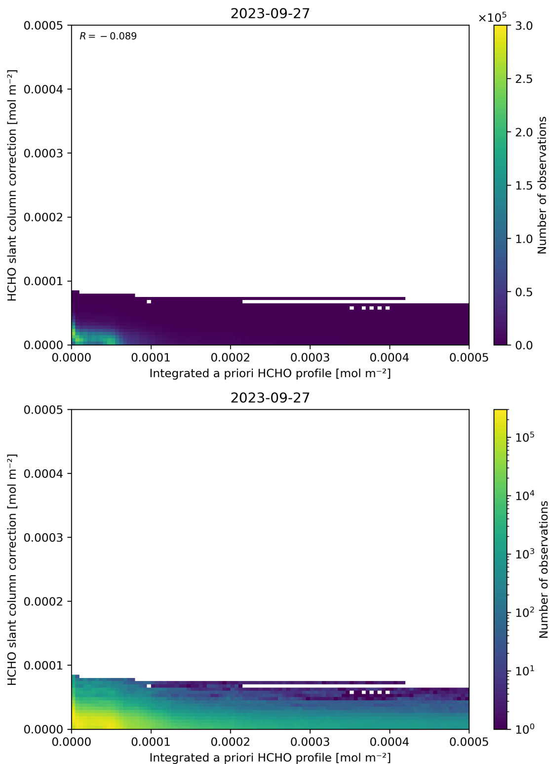
Figure 152: Scatter density plot of “Integrated a priori HCHO profile” against “HCHO slant column correction” for 2023-09-26 to 2023-09-28.
