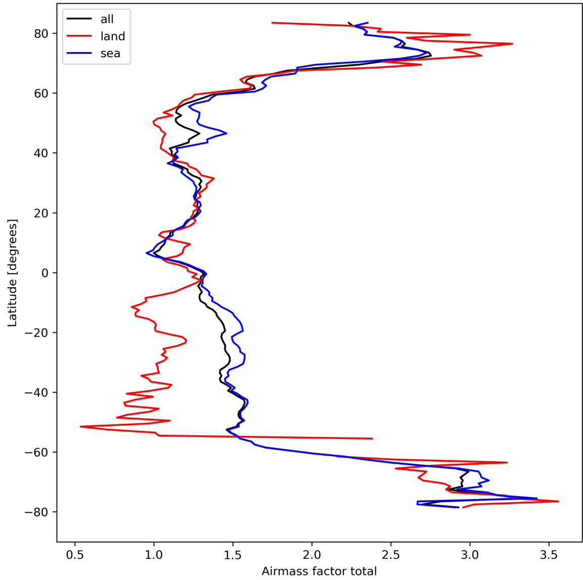
Figure 26: Zonal average of “Airmass factor total” for 2023-09-26 to 2023-09-28.
