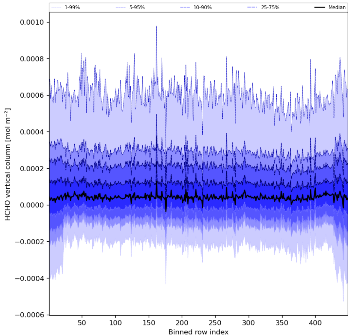
Figure 49: Along track statistics of “HCHO vertical column” for 2023-09-26 to 2023-09-28
