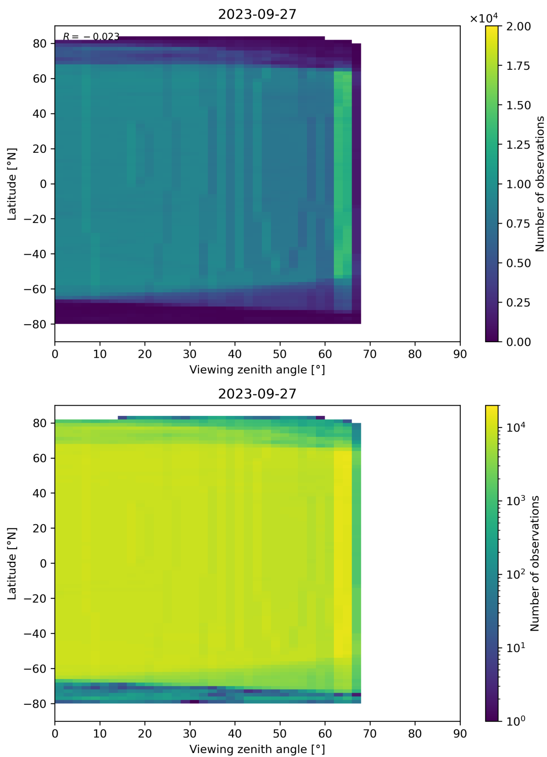
Figure 196: Scatter density plot of “Viewing zenith angle” against “Latitude” for 2023-09-26 to 2023-09-28.
