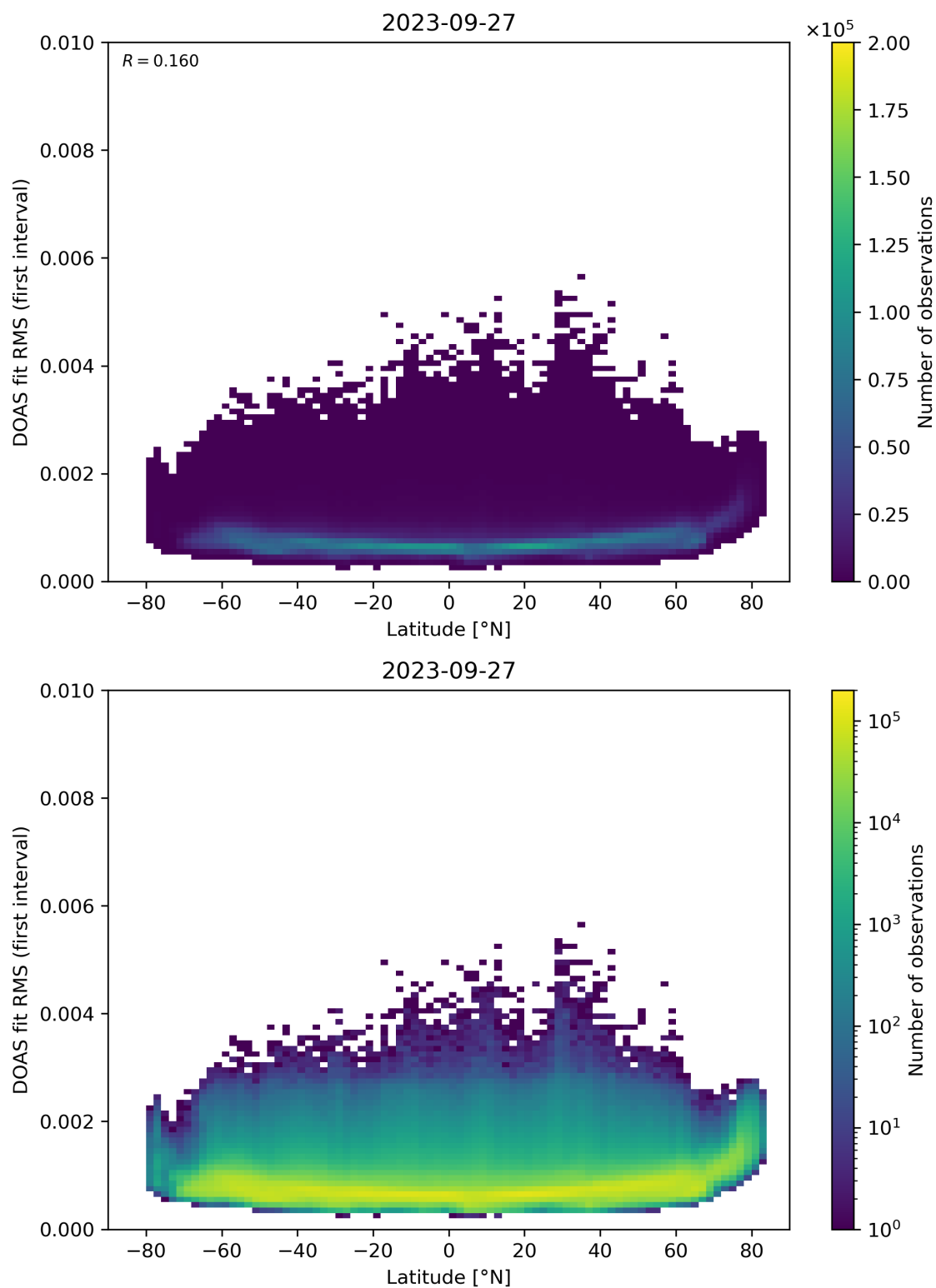
Figure 153: Scatter density plot of “Latitude” against “DOAS fit RMS (first interval)” for 2023-09-26 to 2023-09-28.
