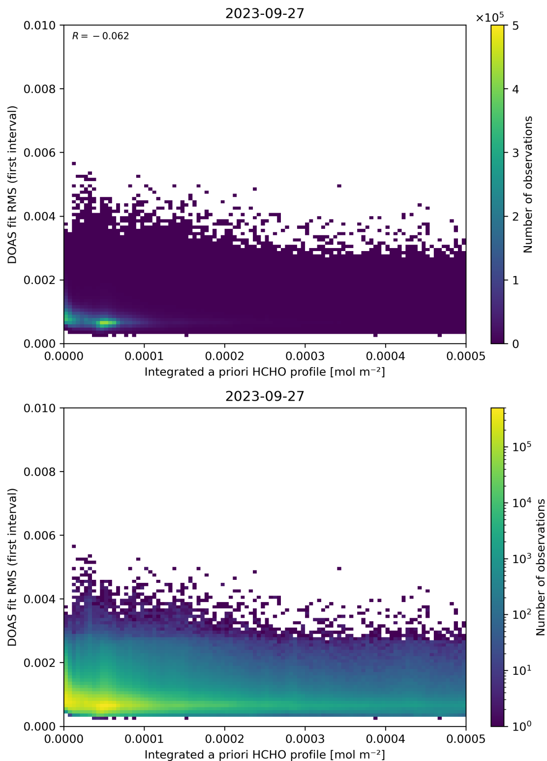
Figure 148: Scatter density plot of “Integrated a priori HCHO profile” against “DOAS fit RMS (first interval)” for 2023-09-26 to 2023-09-28.
