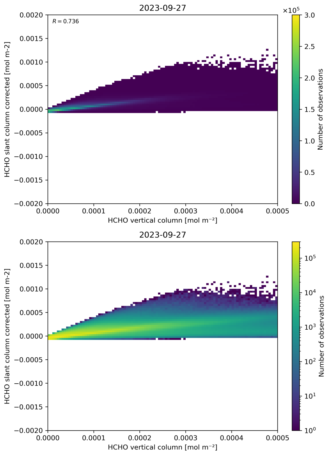
Figure 127: Scatter density plot of “HCHO vertical column” against “HCHO slant column corrected” for 2023-09-26 to 2023-09-28.
