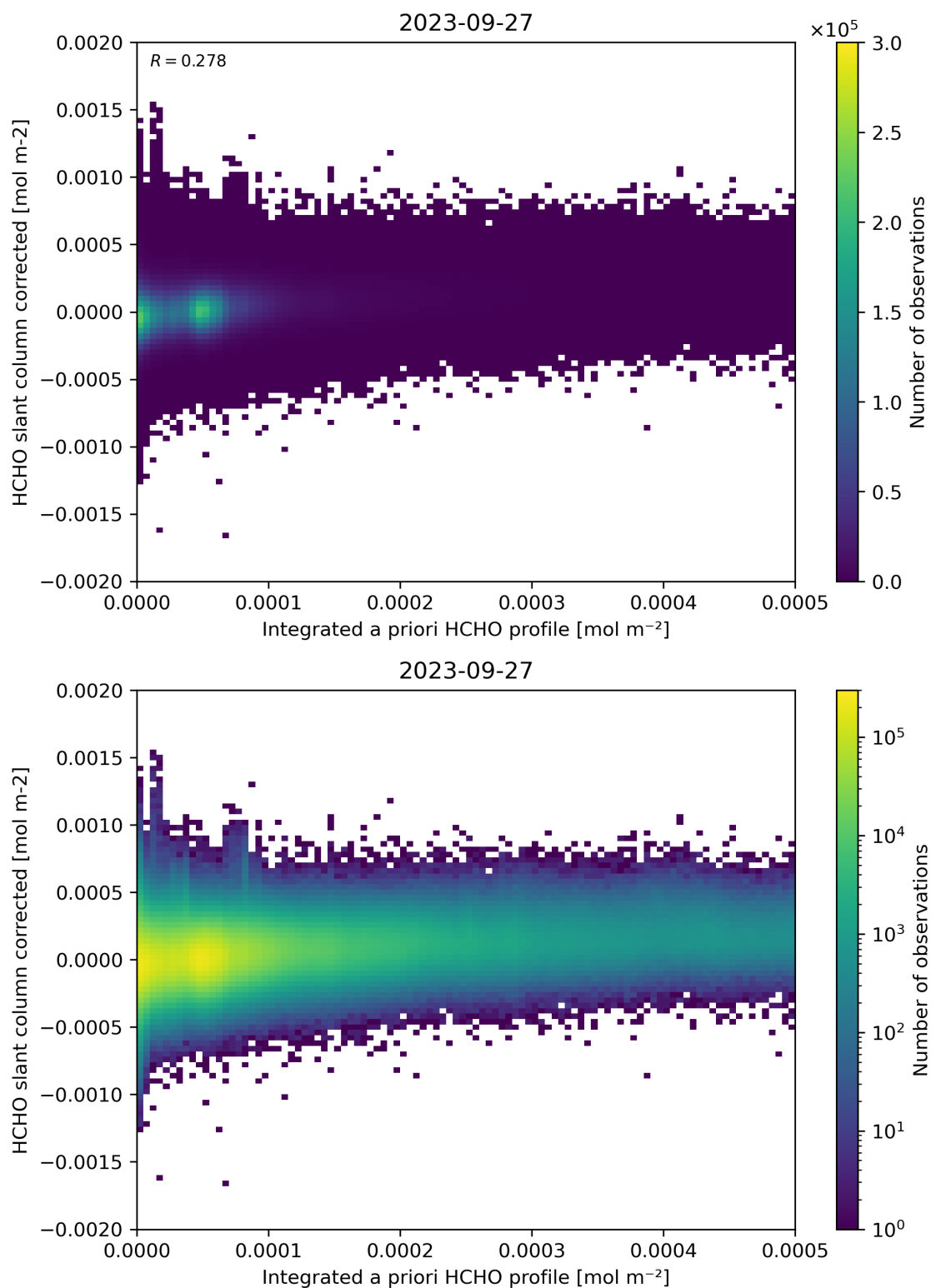
Figure 151: Scatter density plot of “Integrated a priori HCHO profile” against “HCHO slant column corrected” for 2023-09-26 to 2023-09-28.
