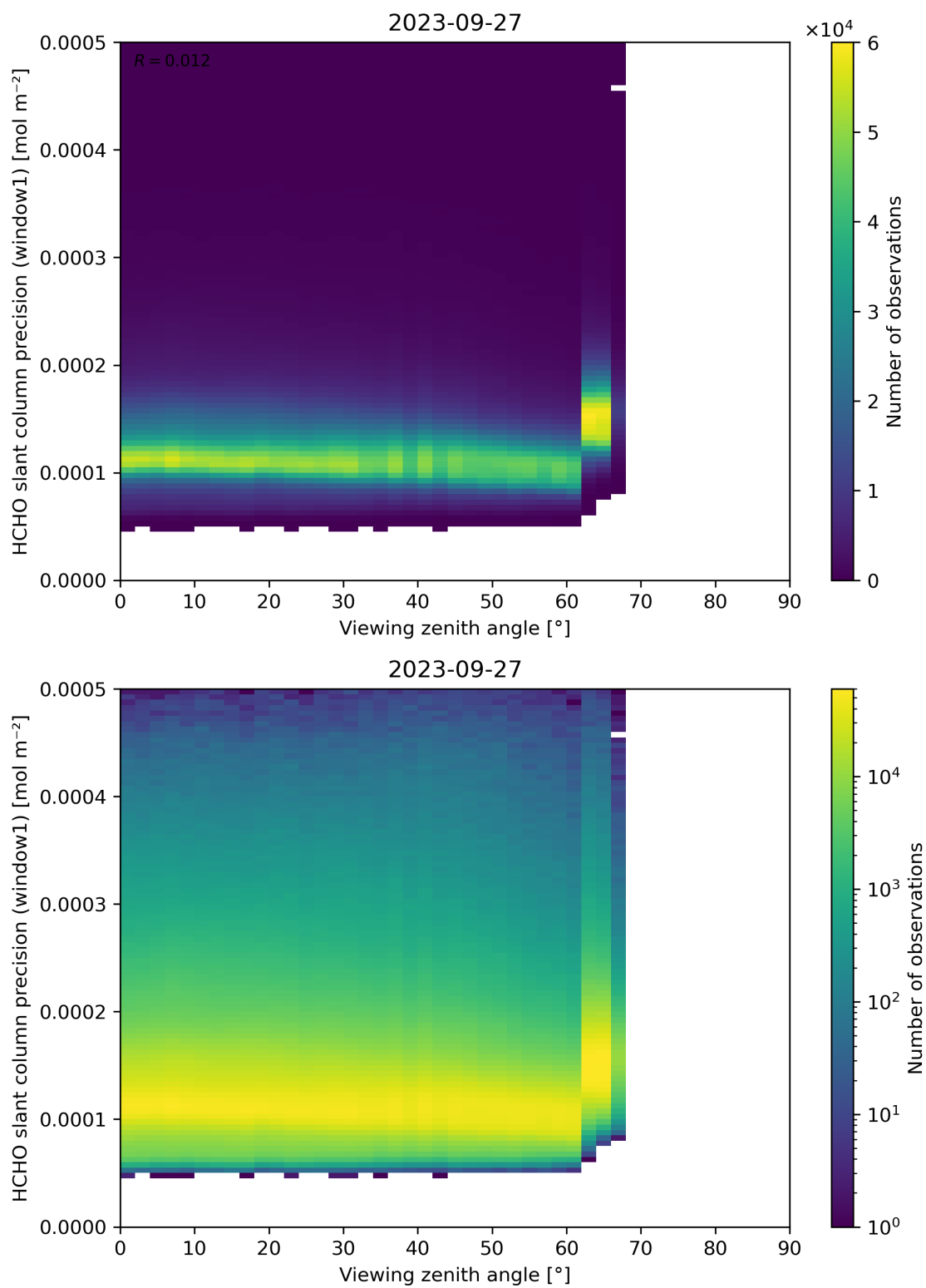
Figure 189: Scatter density plot of “Viewing zenith angle” against “HCHO slant column precision (window1)” for 2023-09-26 to 2023-09-28.
