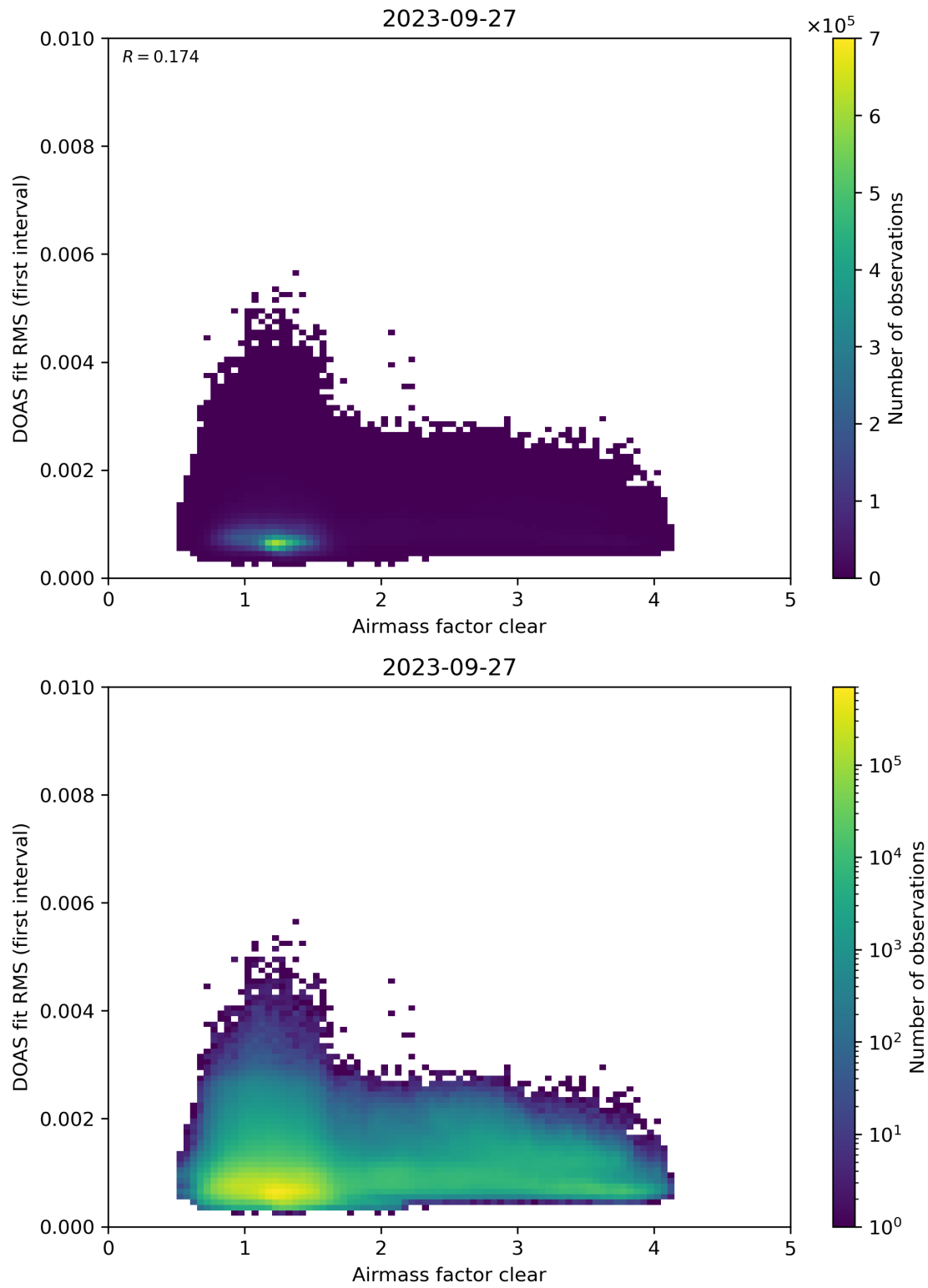
Figure 71: Scatter density plot of “Airmass factor clear” against “DOAS fit RMS (first interval)” for 2023-09-26 to 2023-09-28.
