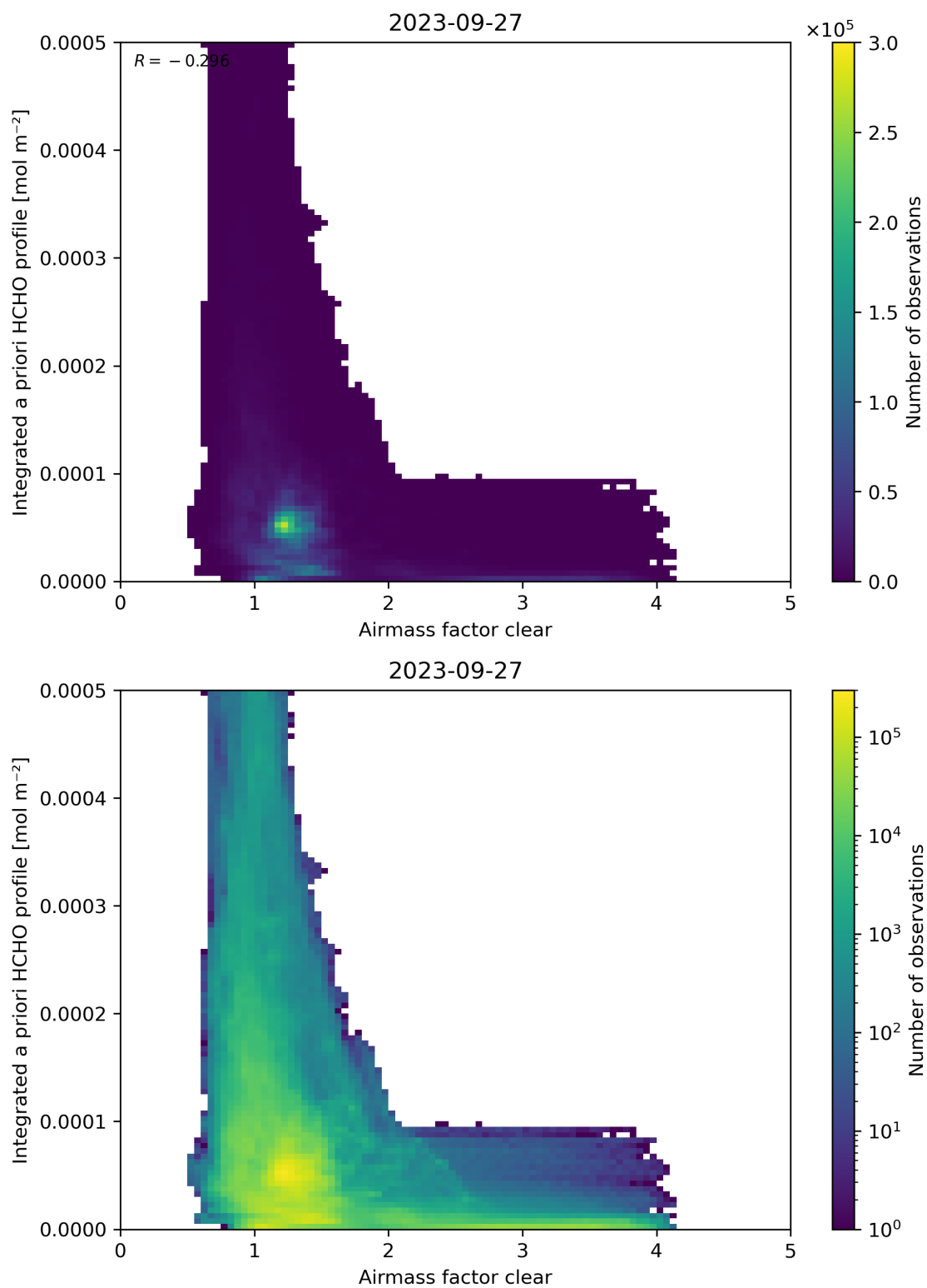
Figure 76: Scatter density plot of “Airmass factor clear” against “Integrated a priori HCHO profile” for 2023-09-26 to 2023-09-28.
