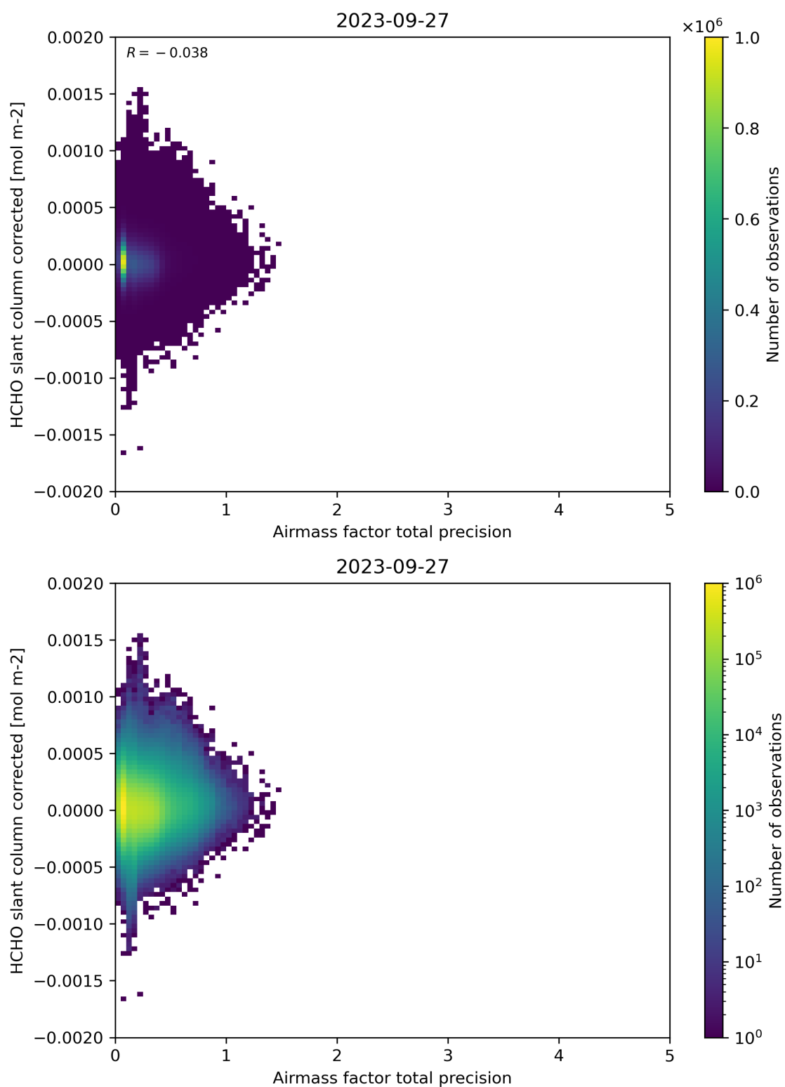
Figure 109: Scatter density plot of “Airmass factor total precision” against “HCHO slant column corrected” for 2023-09-26 to 2023-09-28.
