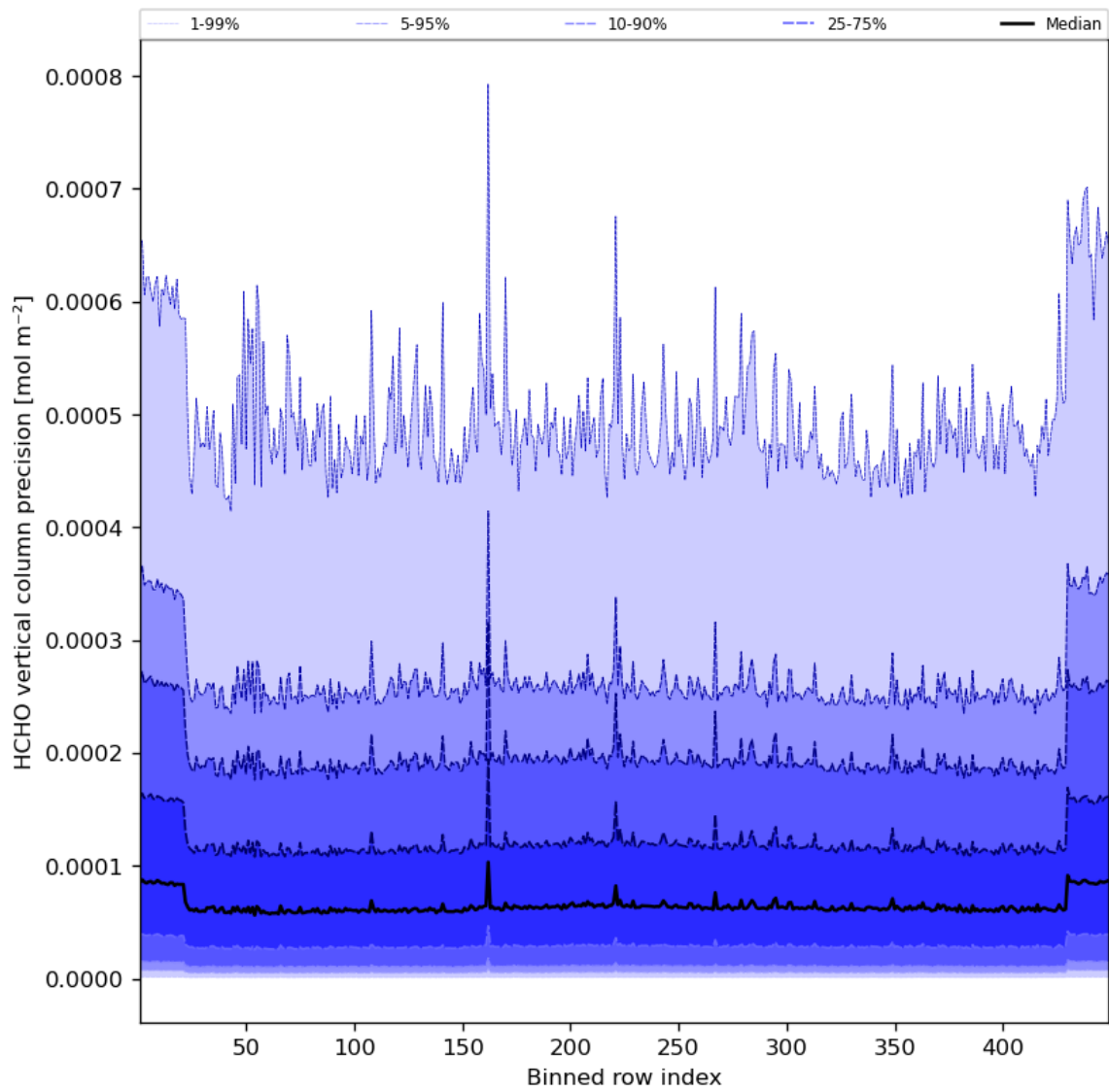
Figure 50: Along track statistics of "HCHO vertical column precision" for 2023-09-26 to 2023-09-28
