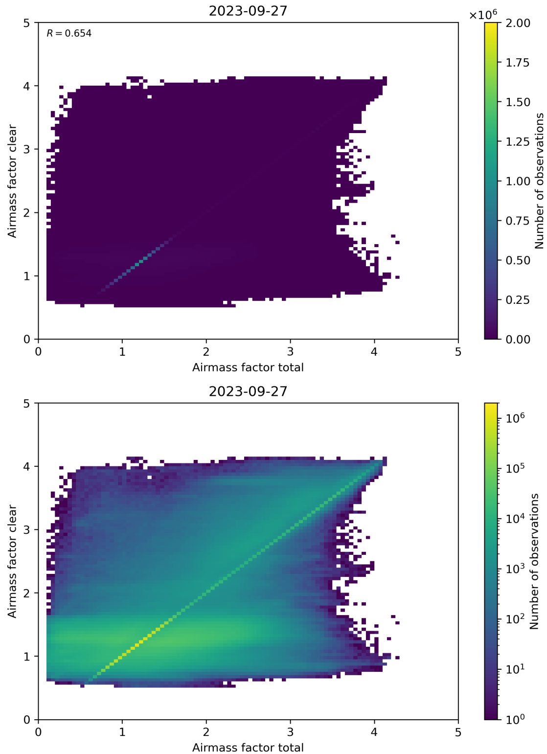
Figure 100: Scatter density plot of “Airmass factor total” against “Airmass factor clear” for 2023-09-26 to 2023-09-28.
