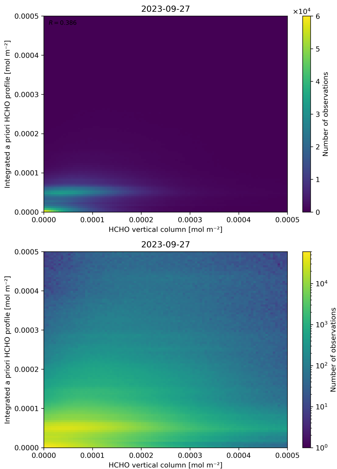
Figure 135: Scatter density plot of “HCHO vertical column” against “Integrated a priori HCHO profile” for 2023-09-26 to 2023-09-28.
