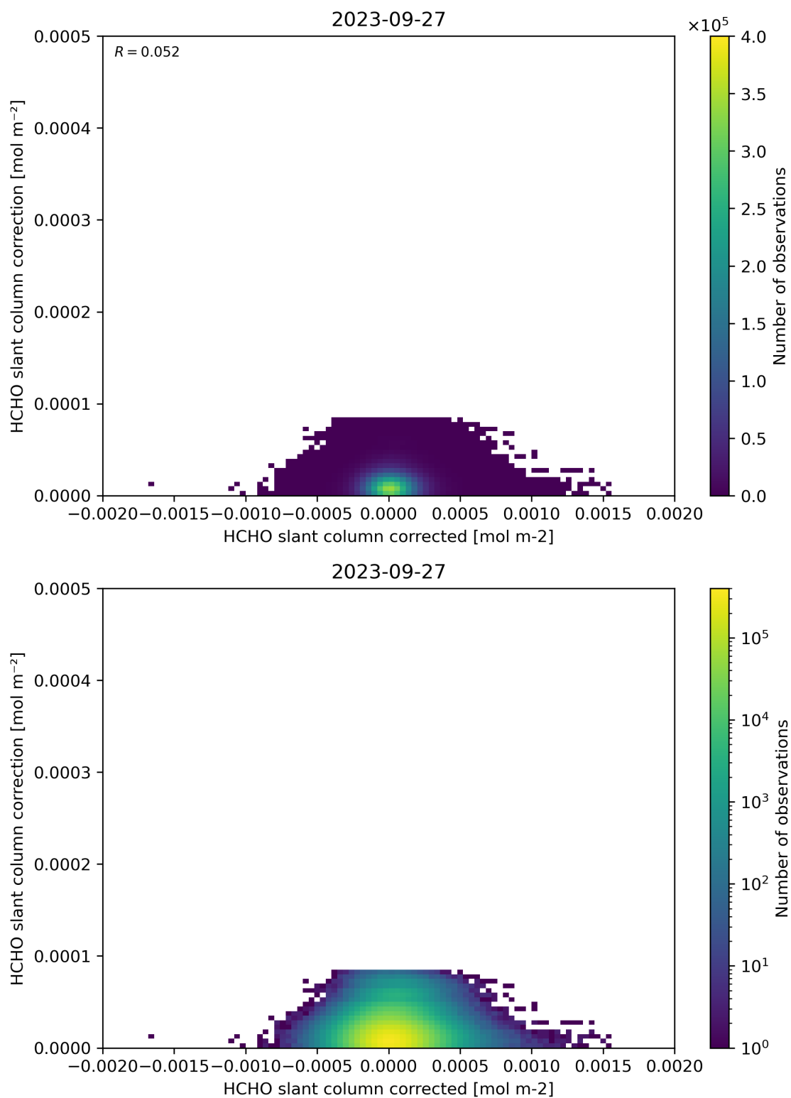
Figure 77: Scatter density plot of “HCHO slant column corrected” against “HCHO slant column correction” for 2023-09-26 to 2023-09-28.
