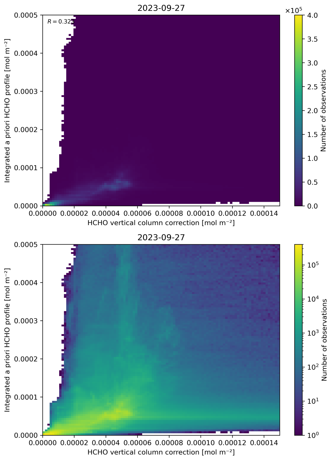
Figure 122: Scatter density plot of “HCHO vertical column correction” against “Integrated a priori HCHO profile” for 2023-09-26 to 2023-09-28.
