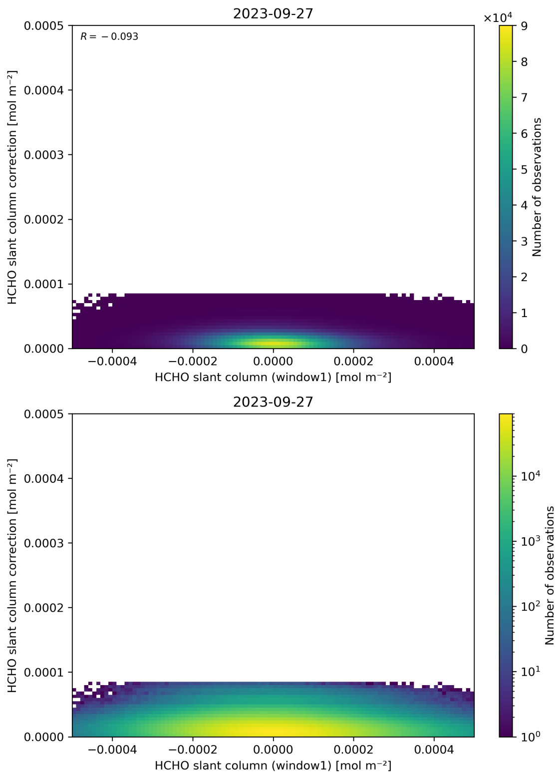
Figure 83: Scatter density plot of “HCHO slant column (window1)” against “HCHO slant column correction” for 2023-09-26 to 2023-09-28.
