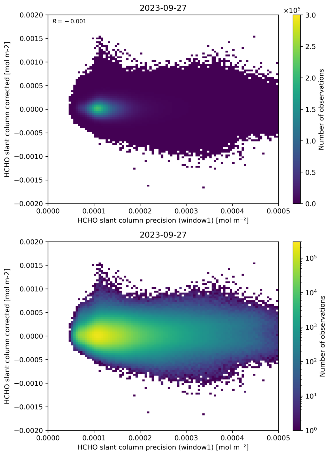
Figure 92: Scatter density plot of “HCHO slant column precision (window1)” against “HCHO slant column corrected” for 2023-09-26 to 2023-09-28.
