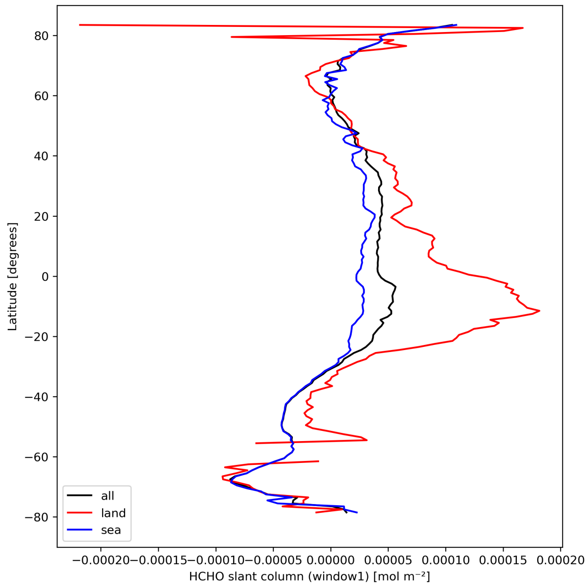
Figure 24: Zonal average of “HCHO slant column (window1)” for 2023-09-26 to 2023-09-28.
