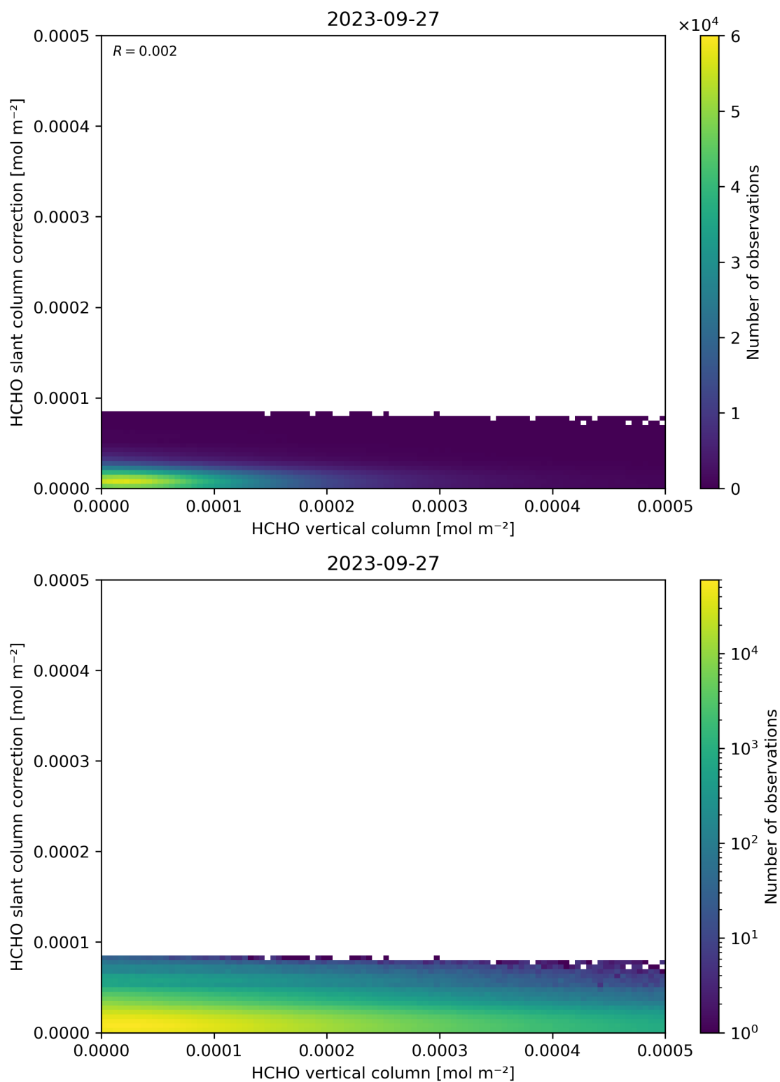
Figure 128: Scatter density plot of “HCHO vertical column” against “HCHO slant column correction” for 2023-09-26 to 2023-09-28.
