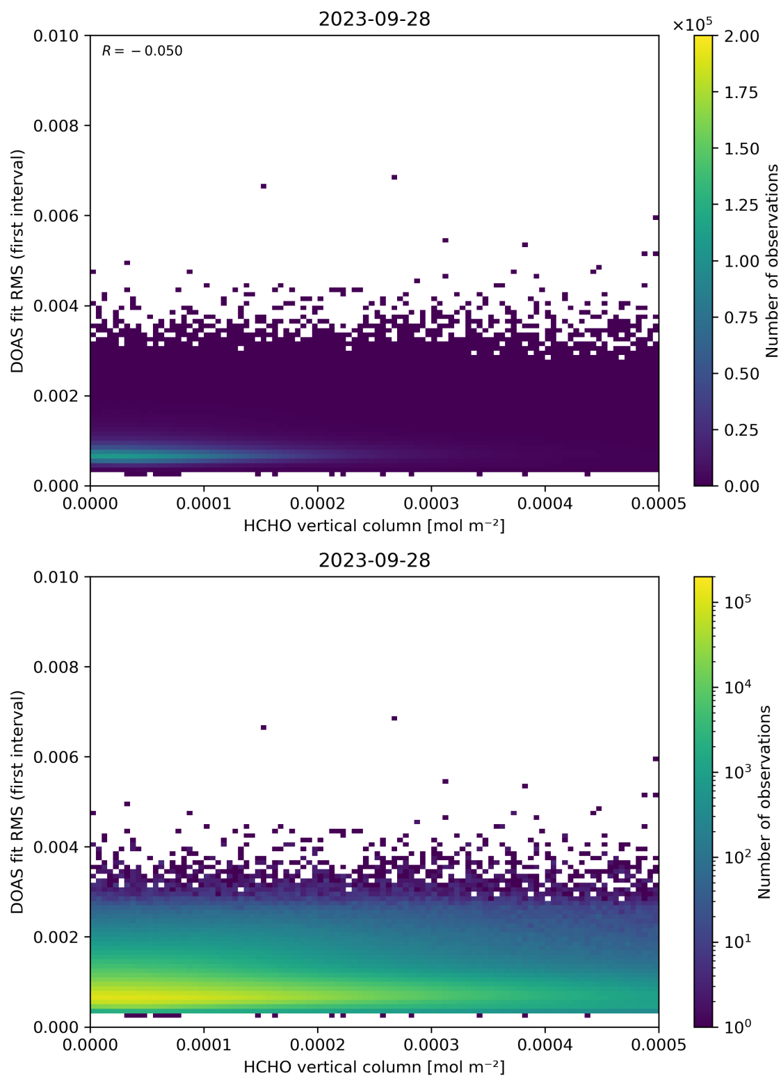
Figure 123: Scatter density plot of “HCHO vertical column” against “DOAS fit RMS (first interval)” for 2023-09-27 to 2023-09-29.
