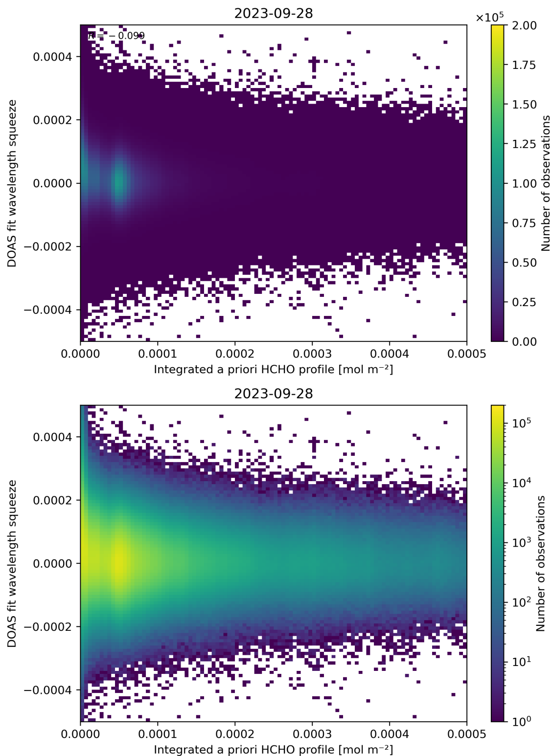
Figure 150: Scatter density plot of “Integrated a priori HCHO profile” against “DOAS fit wavelength squeeze” for 2023-09-27 to 2023-09-29.
