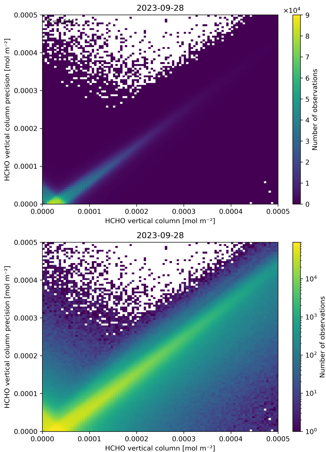
Figure 134: Scatter density plot of “HCHO vertical column” against “HCHO vertical column precision” for 2023-09-27 to 2023-09-29.
