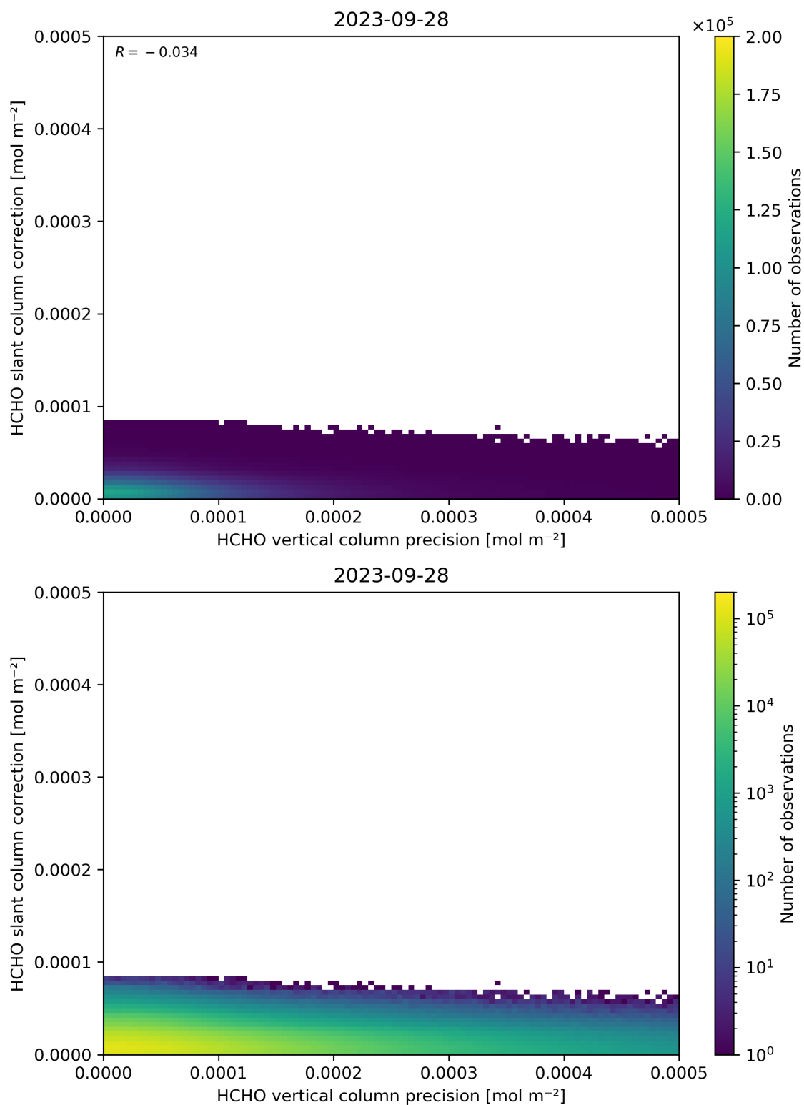
Figure 141: Scatter density plot of “HCHO vertical column precision” against “HCHO slant column correction” for 2023-09-27 to 2023-09-29.
