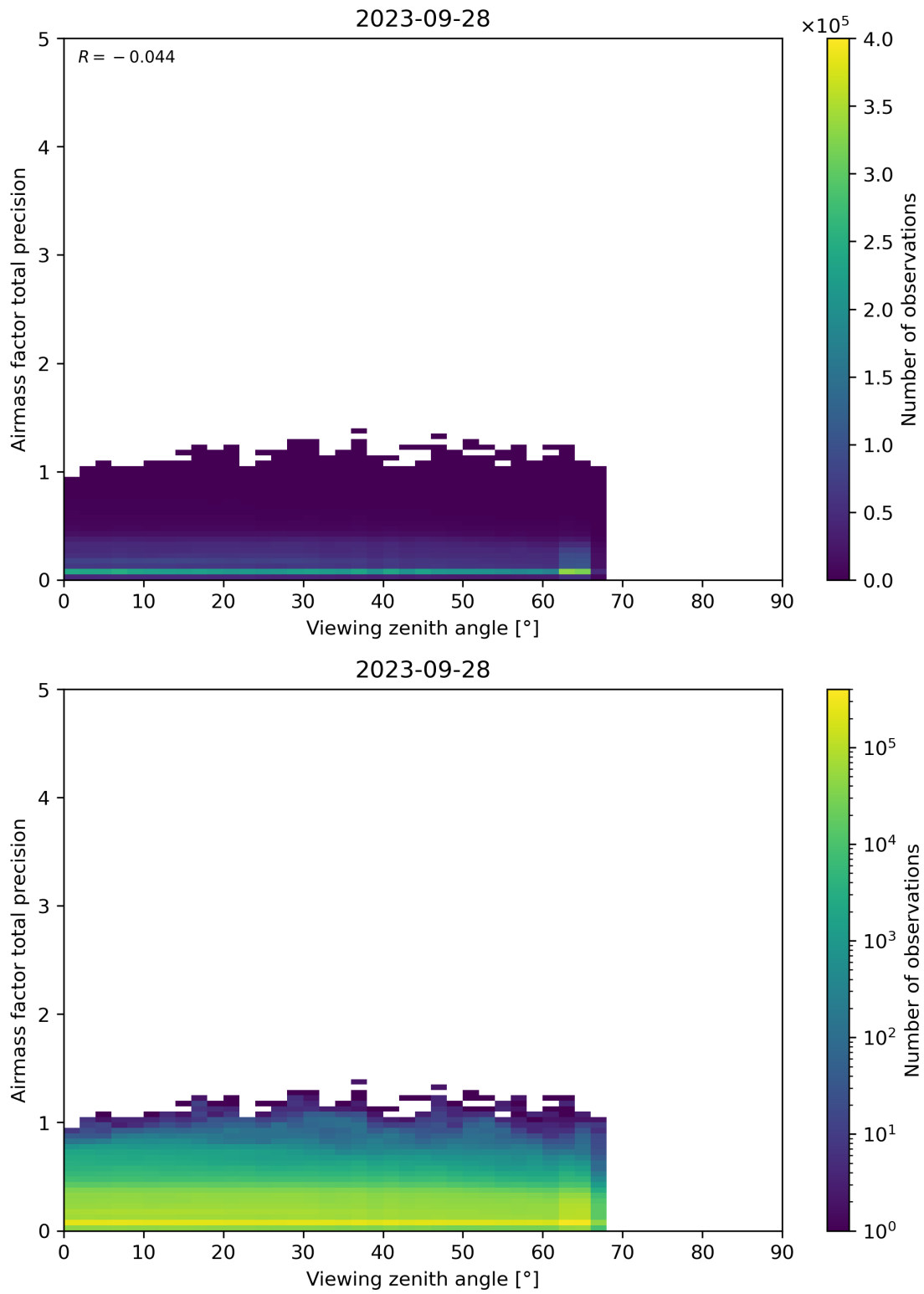
Figure 191: Scatter density plot of “Viewing zenith angle” against “Airmass factor total precision” for 2023-09-27 to 2023-09-29.
