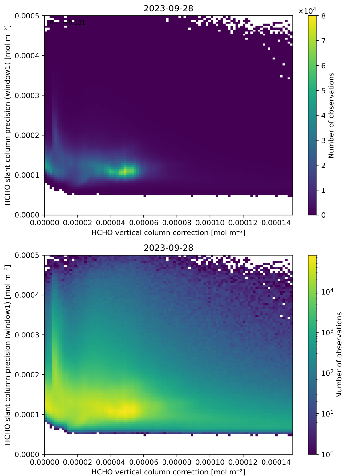
Figure 119: Scatter density plot of “HCHO vertical column correction” against “HCHO slant column precision (window1)” for 2023-09-27 to 2023-09-29.
