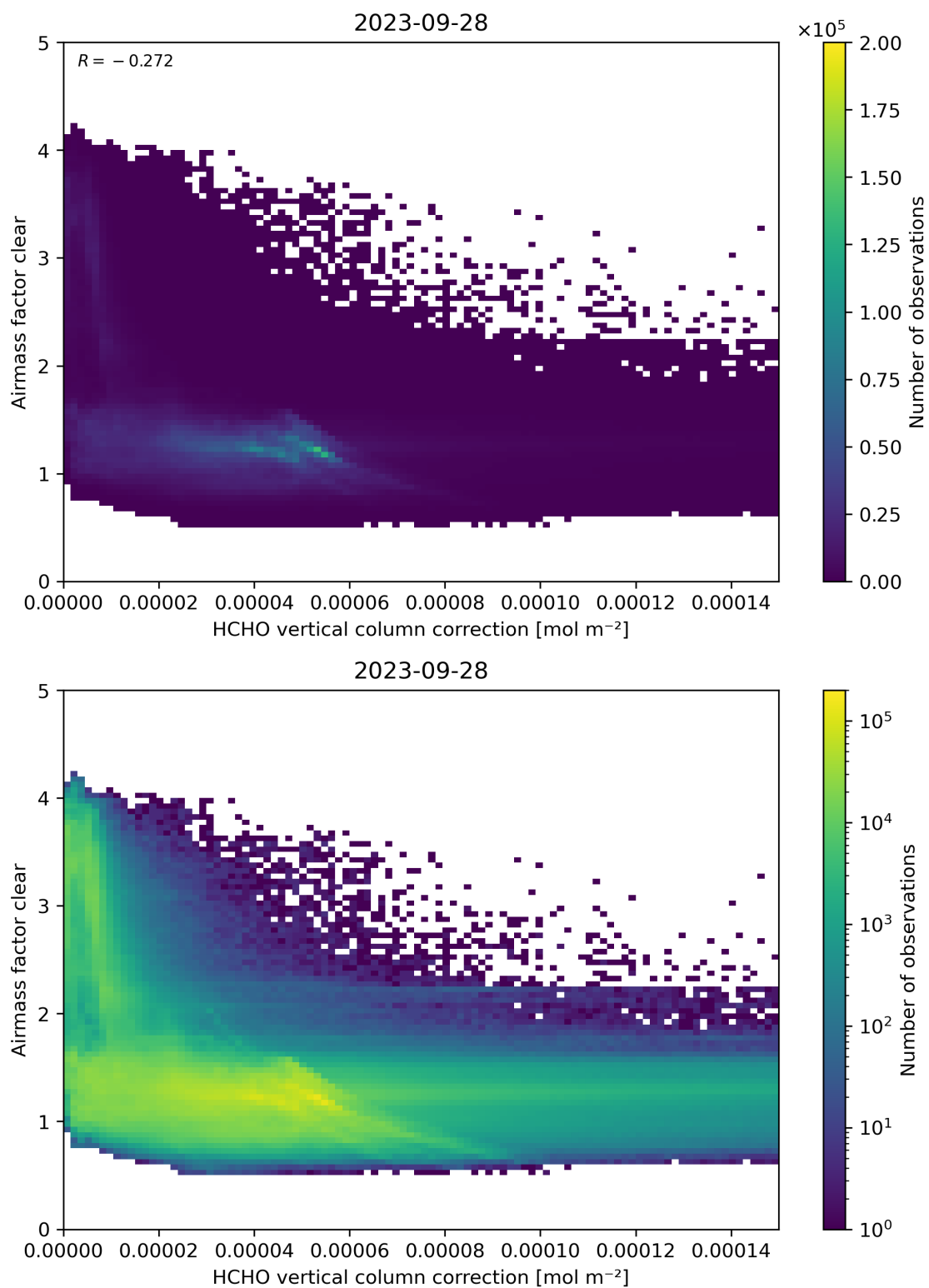
Figure 115: Scatter density plot of “HCHO vertical column correction” against “Airmass factor clear” for 2023-09-27 to 2023-09-29.
