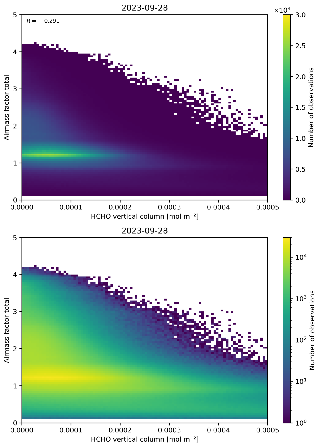
Figure 131: Scatter density plot of “HCHO vertical column” against “Airmass factor total” for 2023-09-27 to 2023-09-29.
