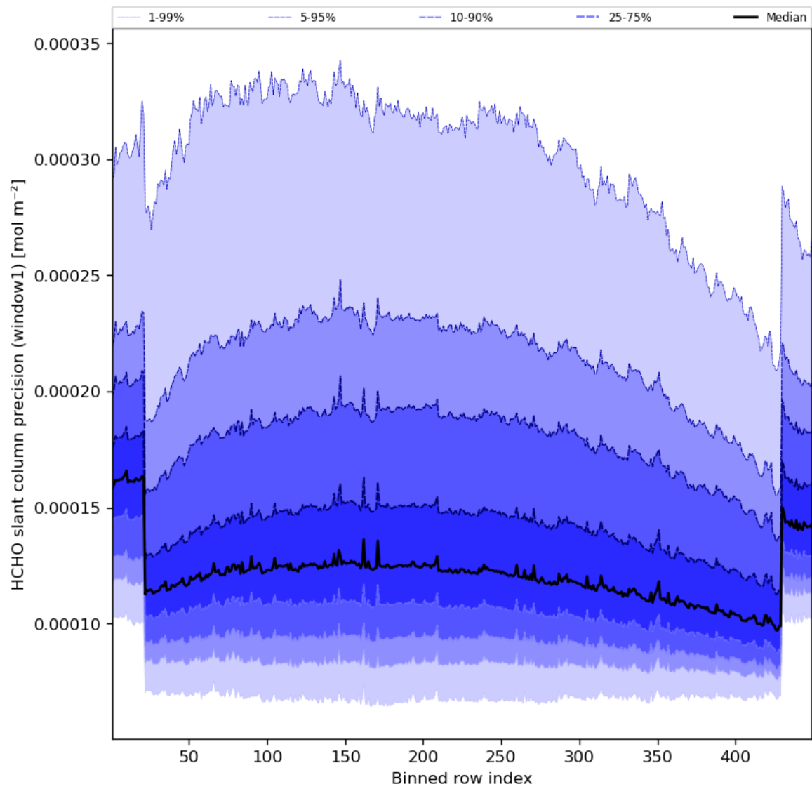
Figure 53: Along track statistics of “HCHO slant column precision (window1)” for 2023-09-27 to 2023-09-29
