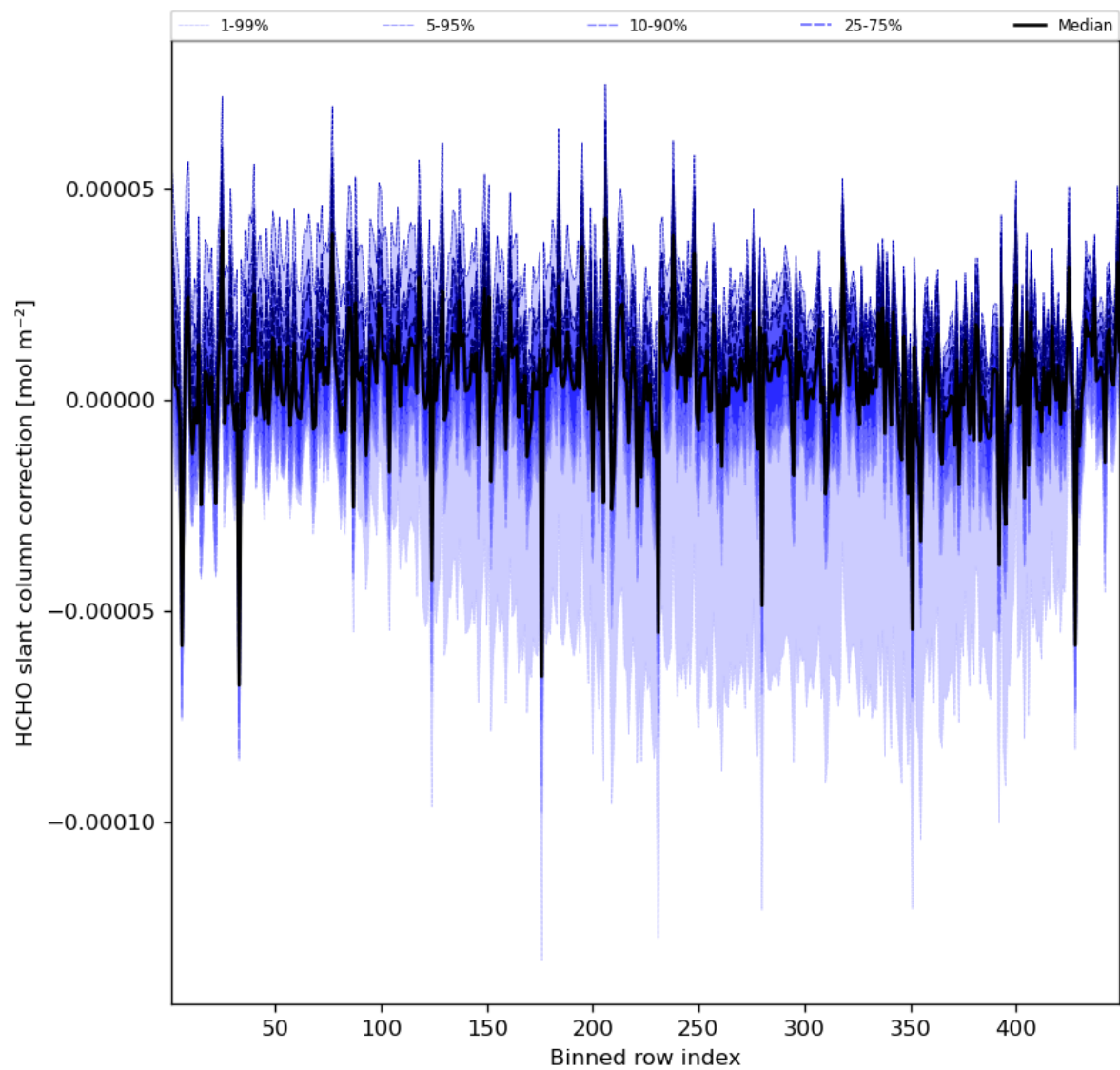
Figure 61: Along track statistics of “HCHO slant column correction” for 2023-09-27 to 2023-09-29
