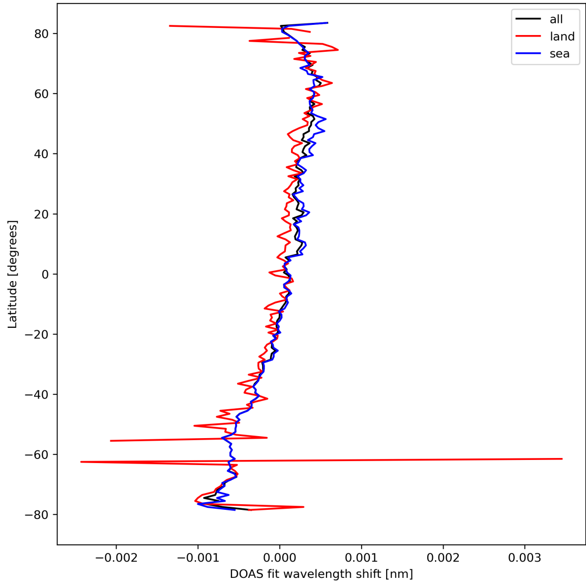
Figure 30: Zonal average of “DOAS fit wavelength shift” for 2023-09-27 to 2023-09-29.
