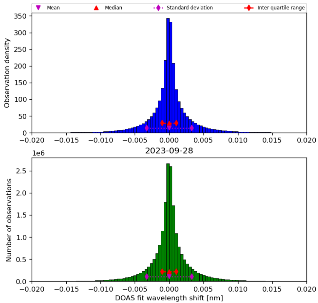
Figure 44: Histogram of “DOAS fit wavelength shift” for 2023-09-27 to 2023-09-29
