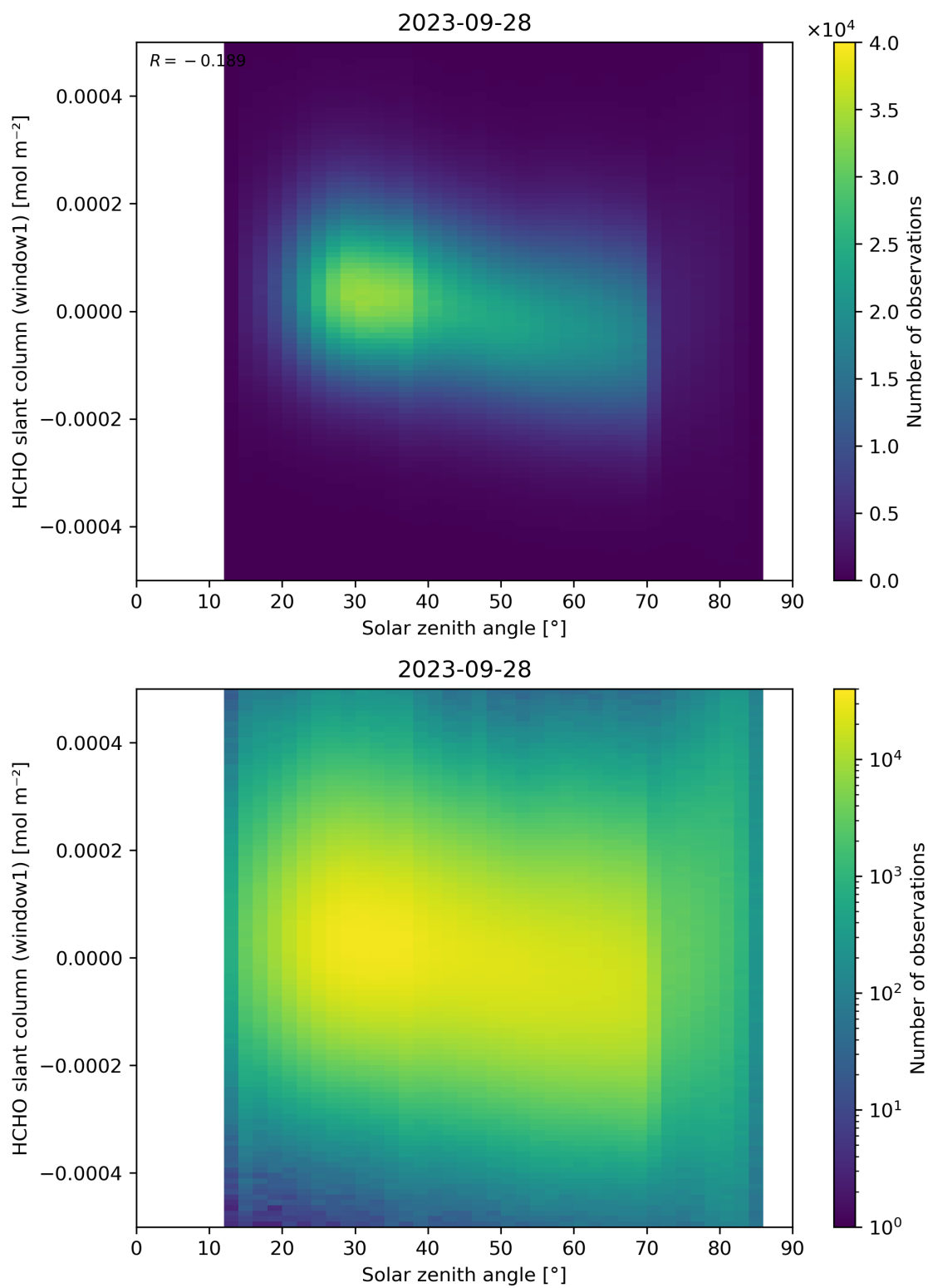
Figure 173: Scatter density plot of “Solar zenith angle” against “HCHO slant column (window1)” for 2023-09-27 to 2023-09-29.
