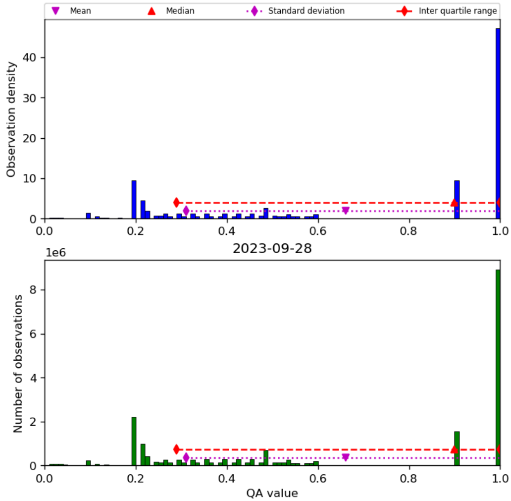
Figure 34: Histogram of “QA value” for 2023-09-27 to 2023-09-29
