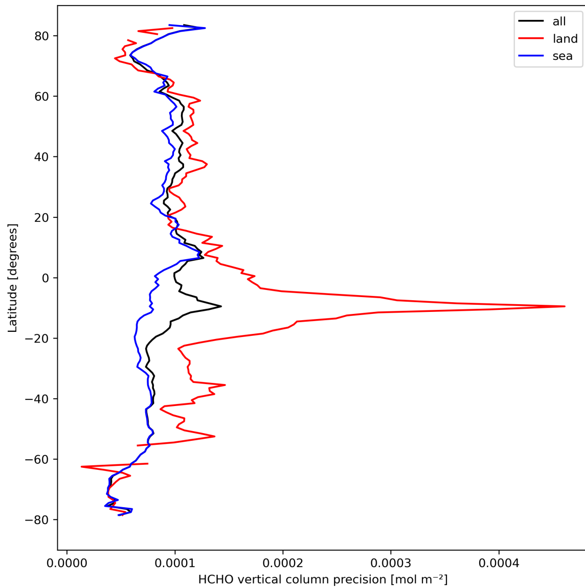
Figure 22: Zonal average of “HCHO vertical column precision” for 2023-09-27 to 2023-09-29.
