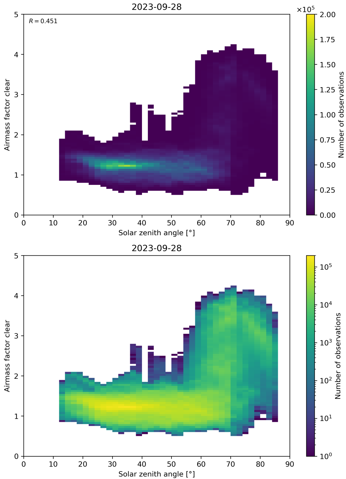
Figure 170: Scatter density plot of “Solar zenith angle” against “Airmass factor clear” for 2023-09-27 to 2023-09-29.
