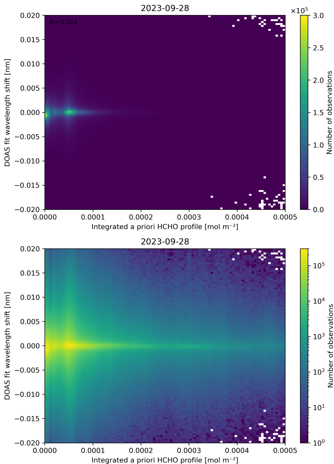
Figure 149: Scatter density plot of “Integrated a priori HCHO profile” against “DOAS fit wavelength shift” for 2023-09-27 to 2023-09-29.
