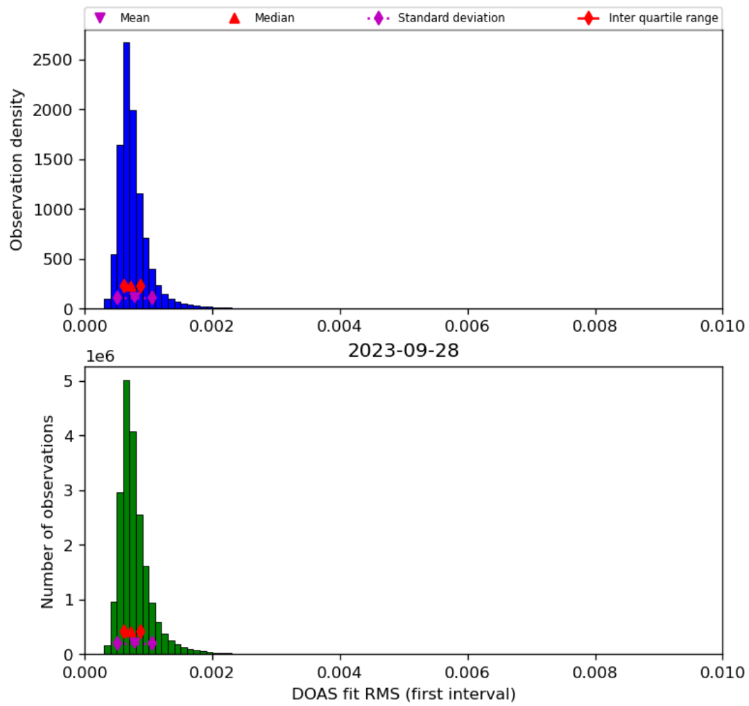
Figure 46: Histogram of “DOAS fit RMS (first interval)” for 2023-09-27 to 2023-09-29
