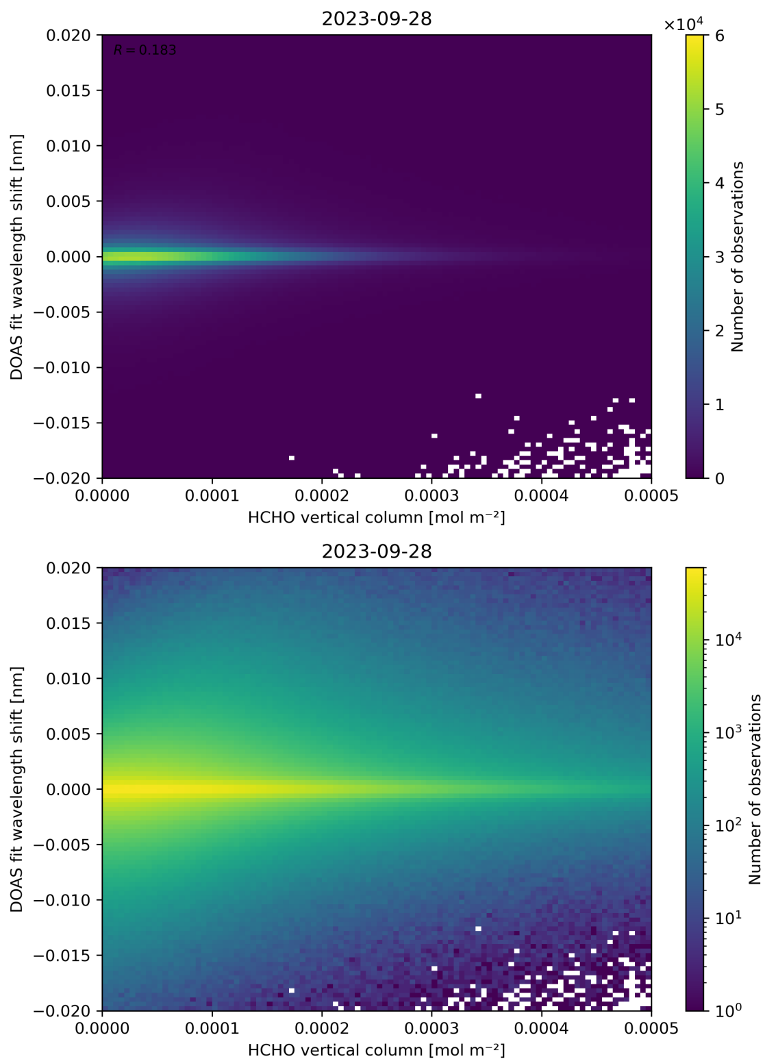
Figure 124: Scatter density plot of “HCHO vertical column” against “DOAS fit wavelength shift” for 2023-09-27 to 2023-09-29.
