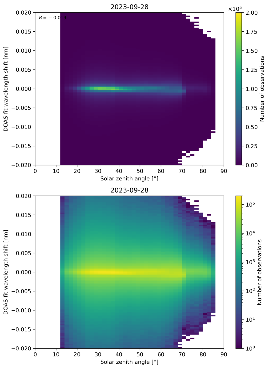
Figure 168: Scatter density plot of “Solar zenith angle” against “DOAS fit wavelength shift” for 2023-09-27 to 2023-09-29.
