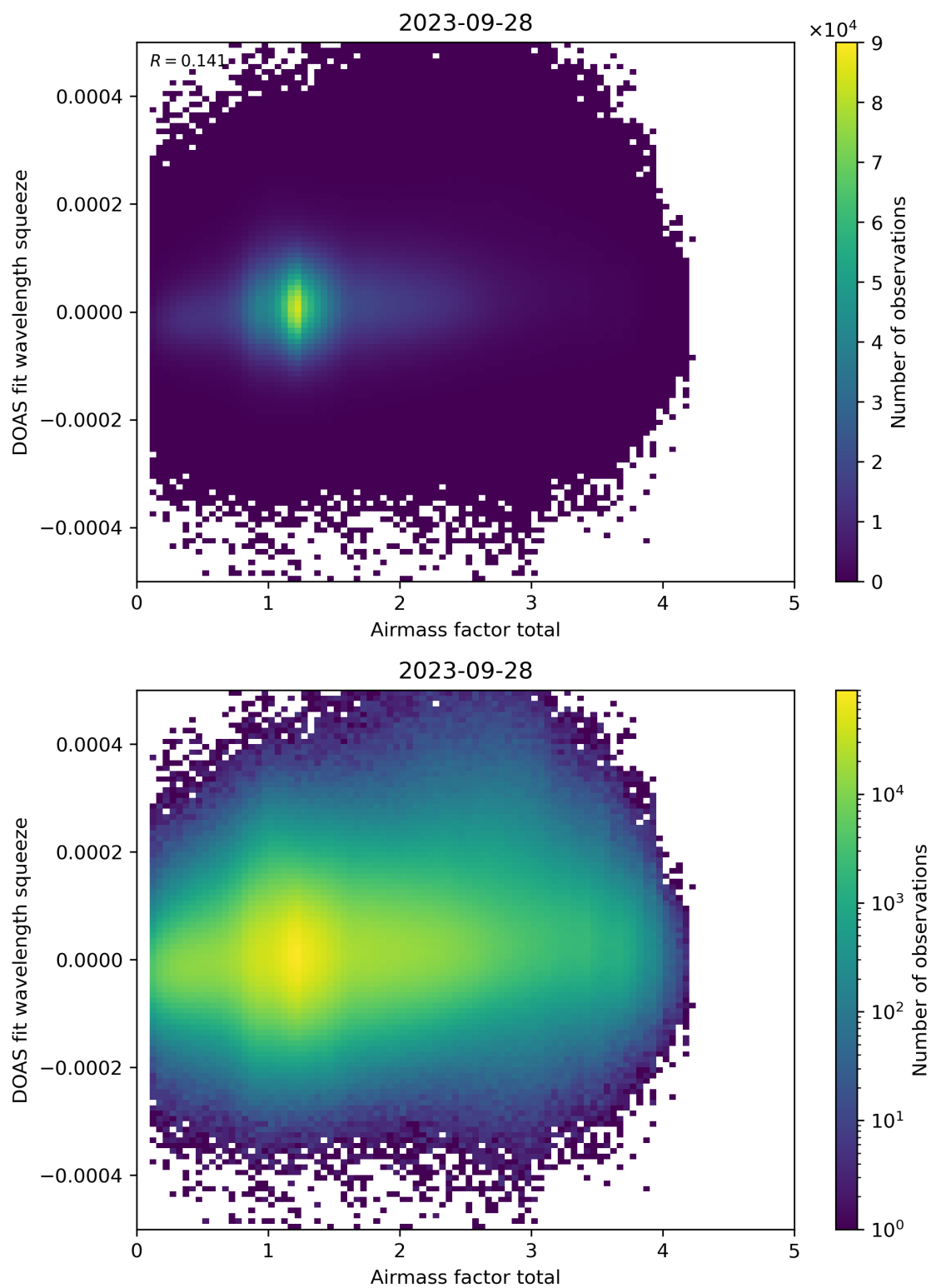
Figure 99: Scatter density plot of “Airmass factor total” against “DOAS fit wavelength squeeze” for 2023-09-27 to 2023-09-29.
