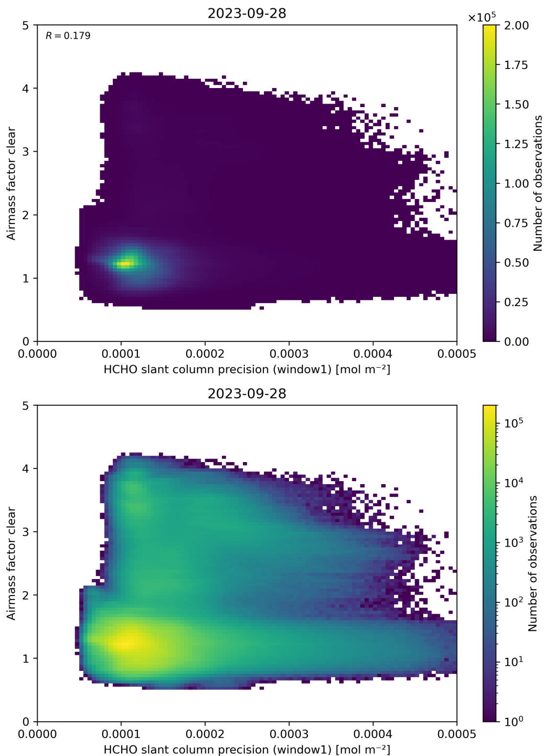
Figure 91: Scatter density plot of “HCHO slant column precision (window1)” against “Airmass factor clear” for 2023-09-27 to 2023-09-29.
