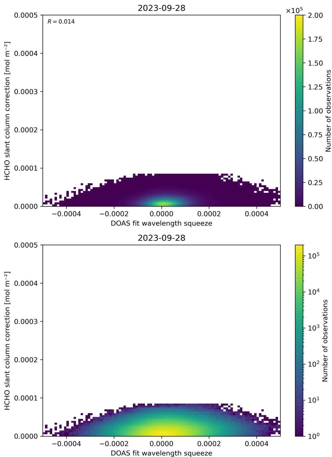
Figure 70: Scatter density plot of “DOAS fit wavelength squeeze” against “HCHO slant column correction” for 2023-09-27 to 2023-09-29.
