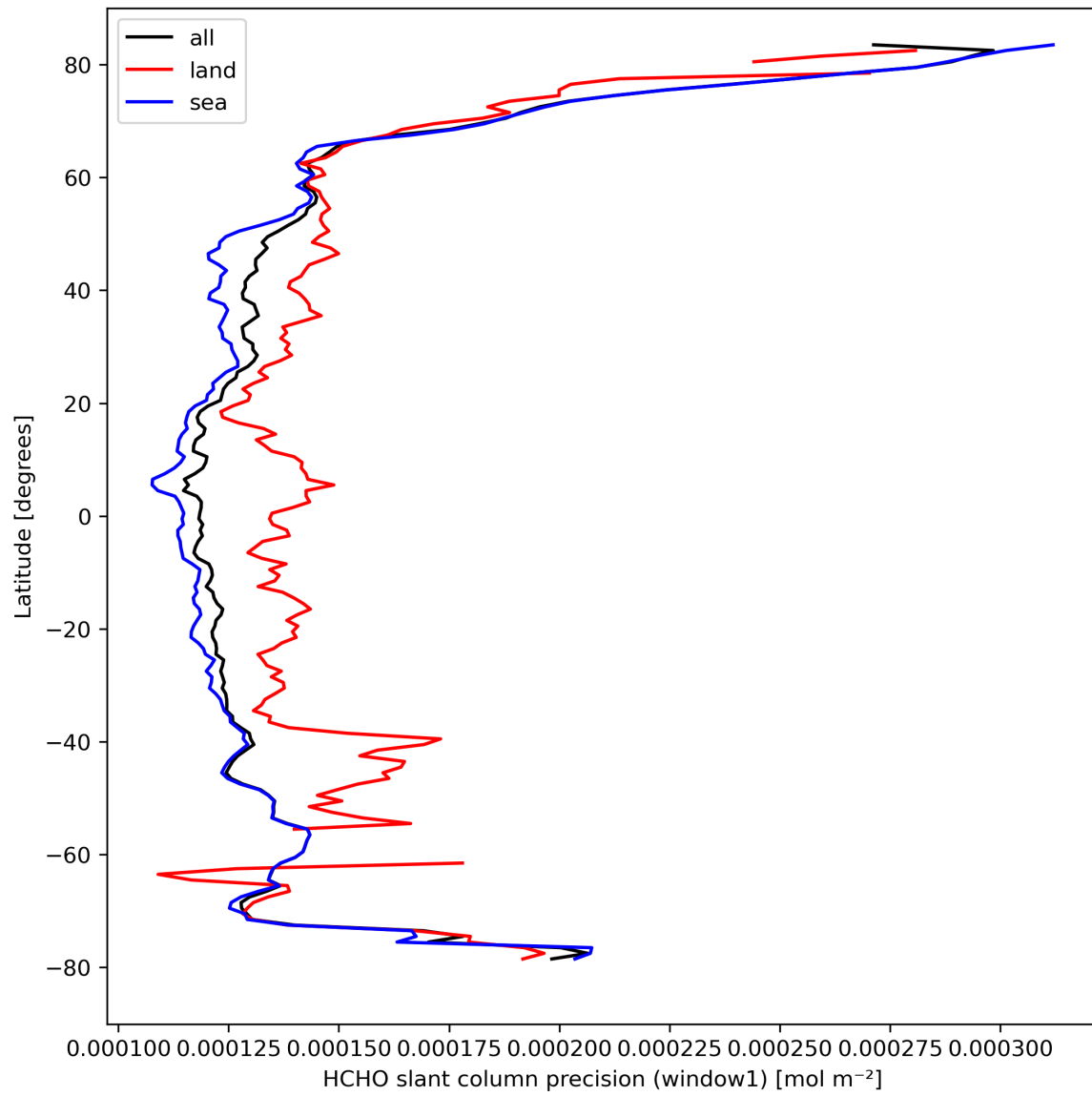
Figure 25: Zonal average of “HCHO slant column precision (window1)” for 2023-09-27 to 2023-09-29.
