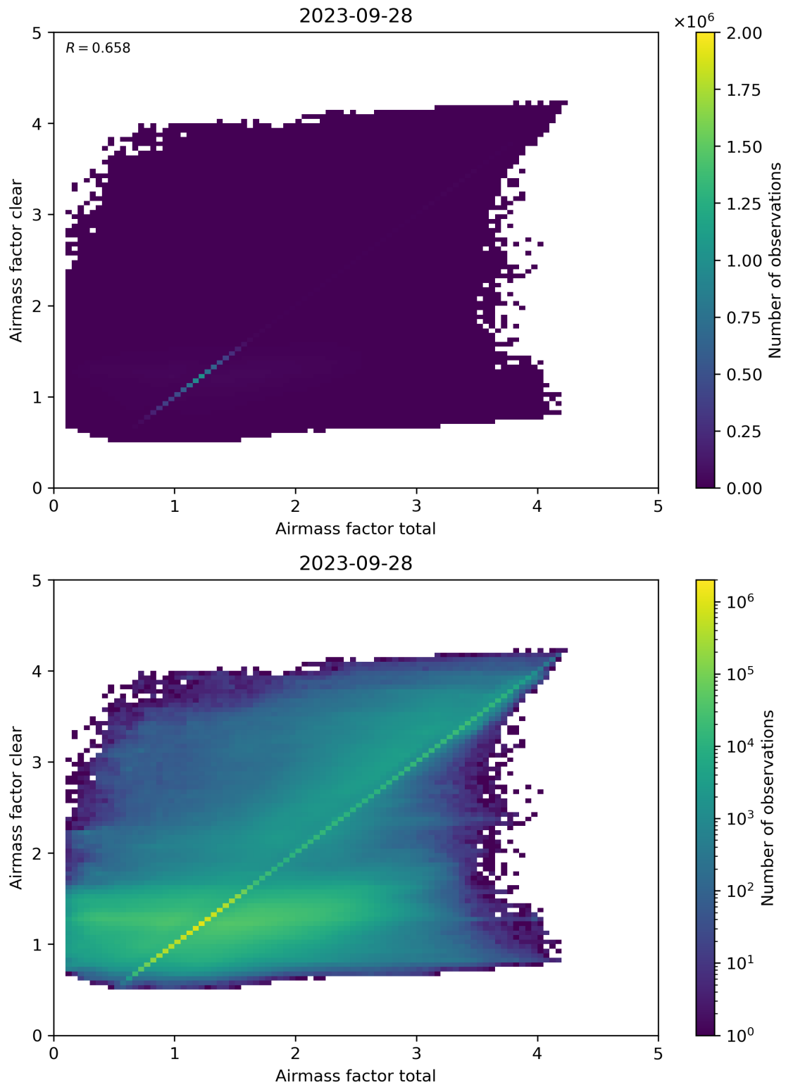
Figure 100: Scatter density plot of “Airmass factor total” against “Airmass factor clear” for 2023-09-27 to 2023-09-29.
