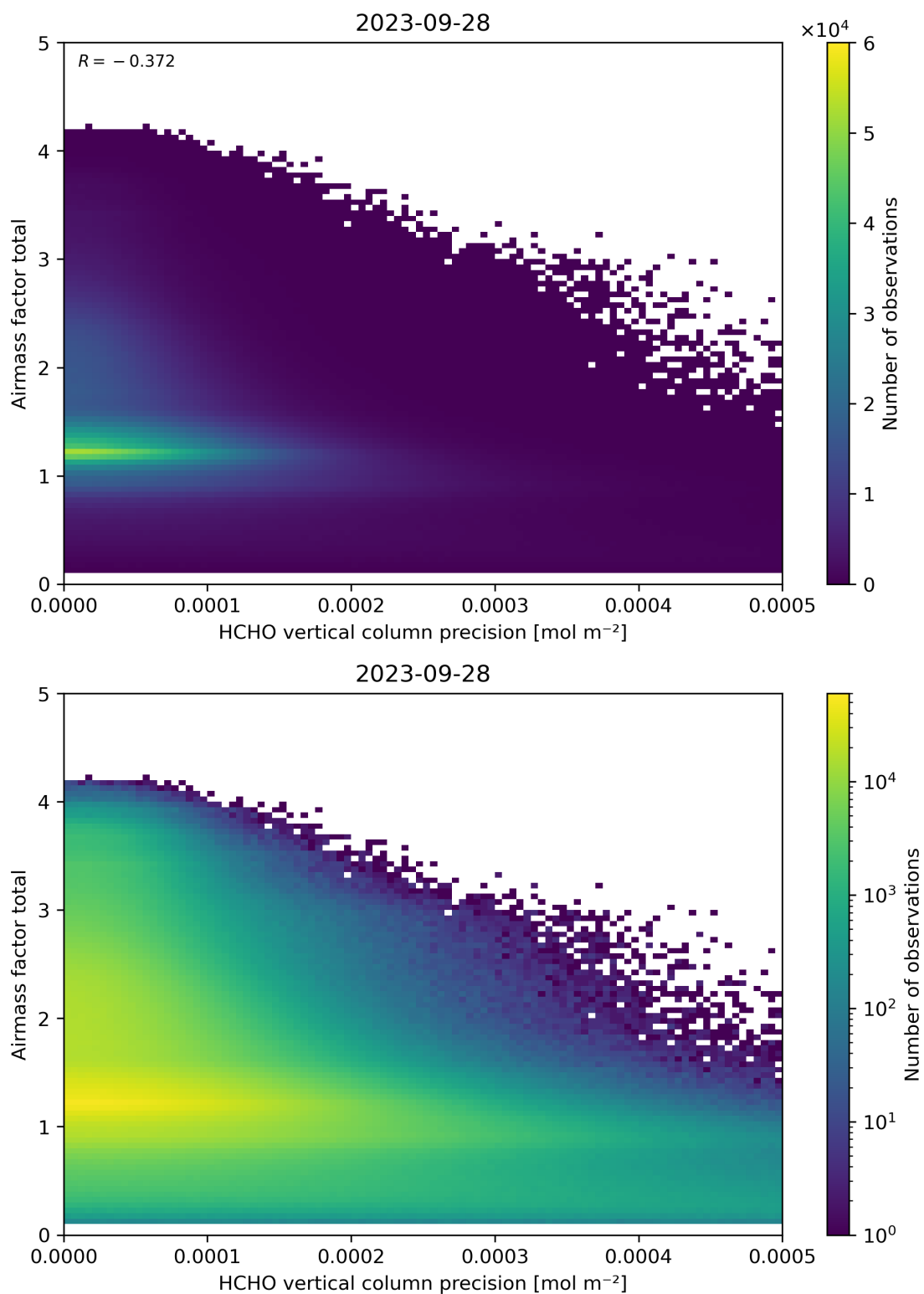
Figure 144: Scatter density plot of “HCHO vertical column precision” against “Airmass factor total” for 2023-09-27 to 2023-09-29.
