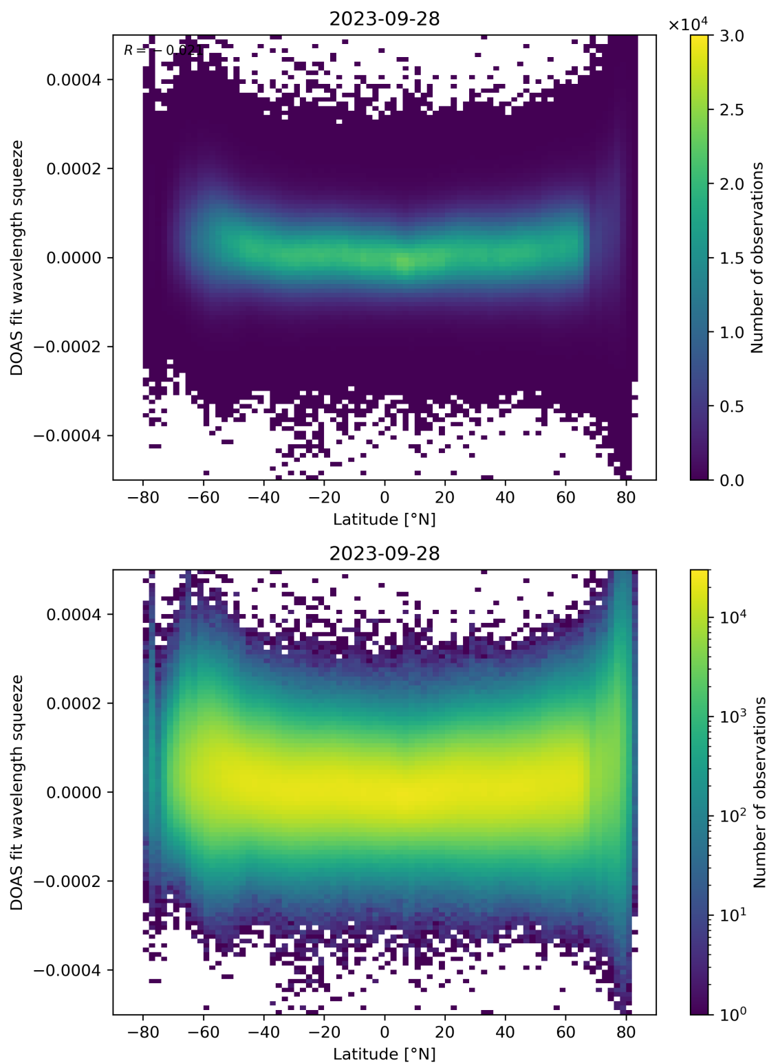
Figure 155: Scatter density plot of “Latitude” against “DOAS fit wavelength squeeze” for 2023-09-27 to 2023-09-29.
