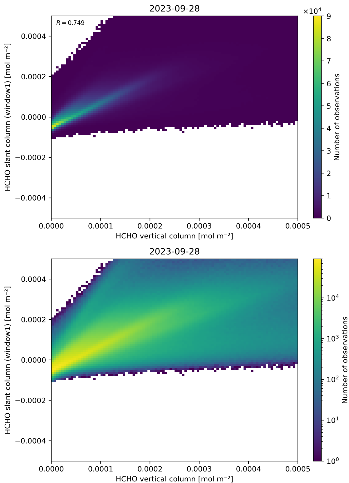
Figure 129: Scatter density plot of “HCHO vertical column” against “HCHO slant column (window1)” for 2023-09-27 to 2023-09-29.
