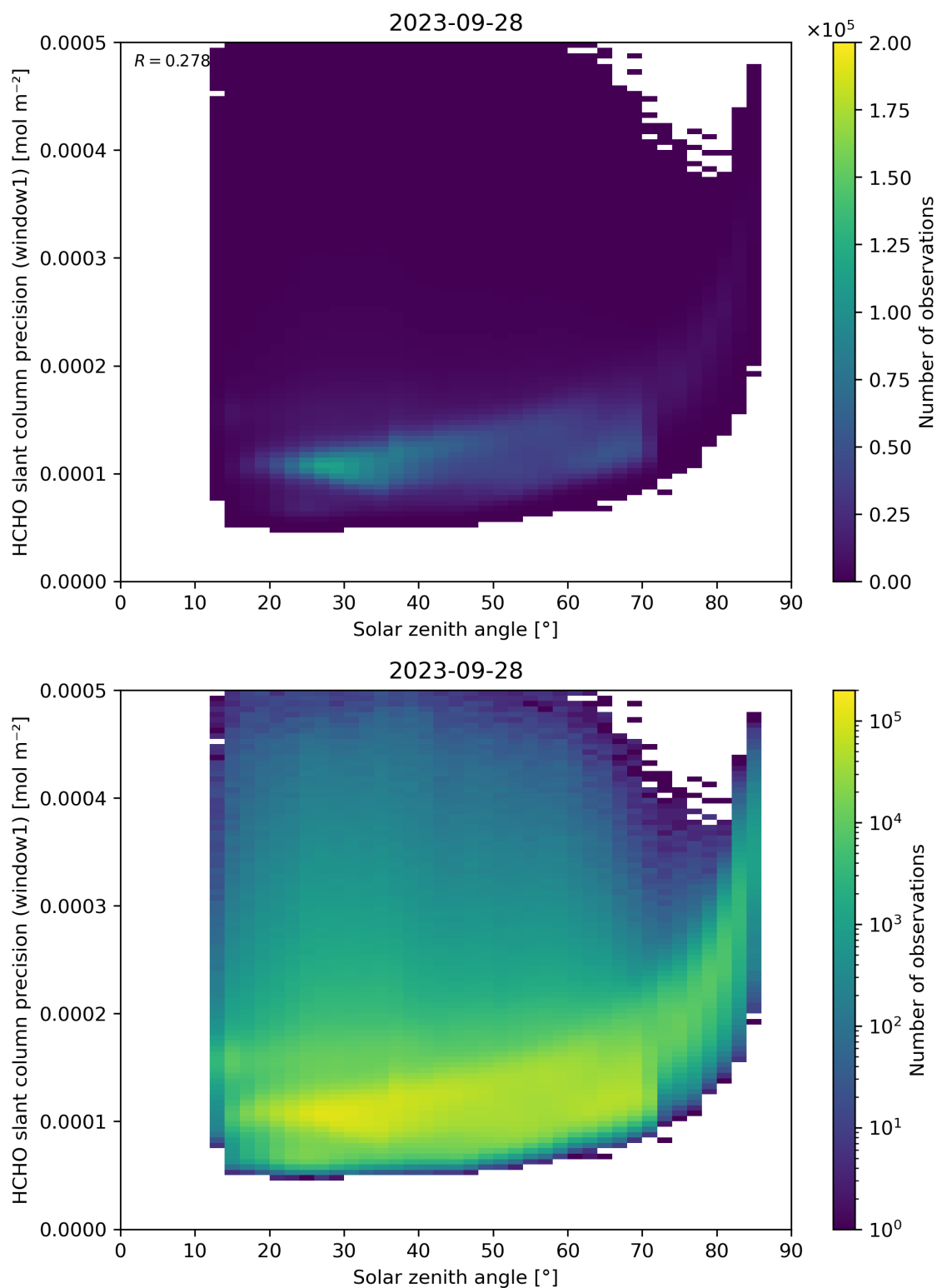
Figure 174: Scatter density plot of “Solar zenith angle” against “HCHO slant column precision (window1)” for 2023-09-27 to 2023-09-29.
