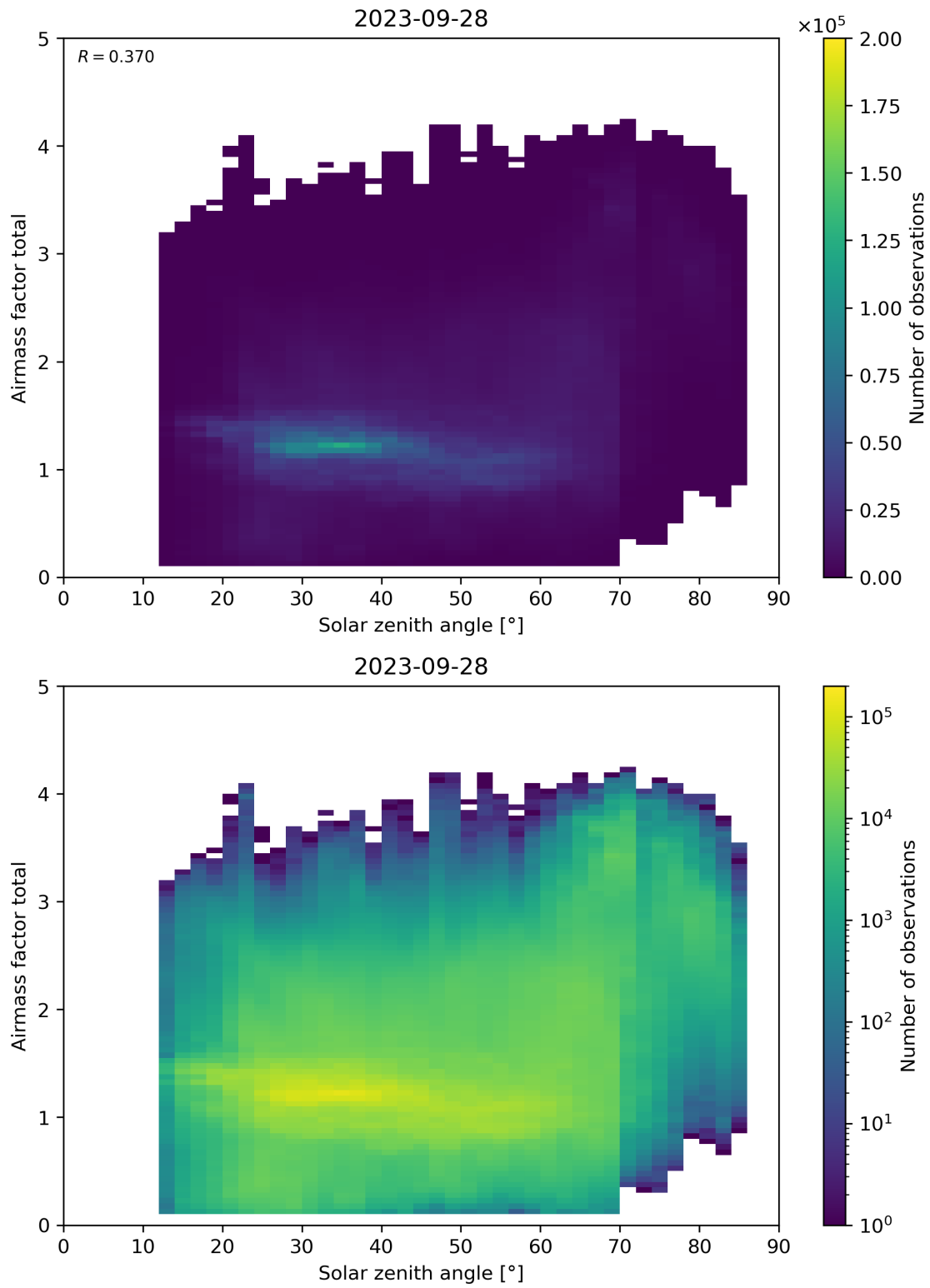
Figure 175: Scatter density plot of “Solar zenith angle” against “Airmass factor total” for 2023-09-27 to 2023-09-29.
