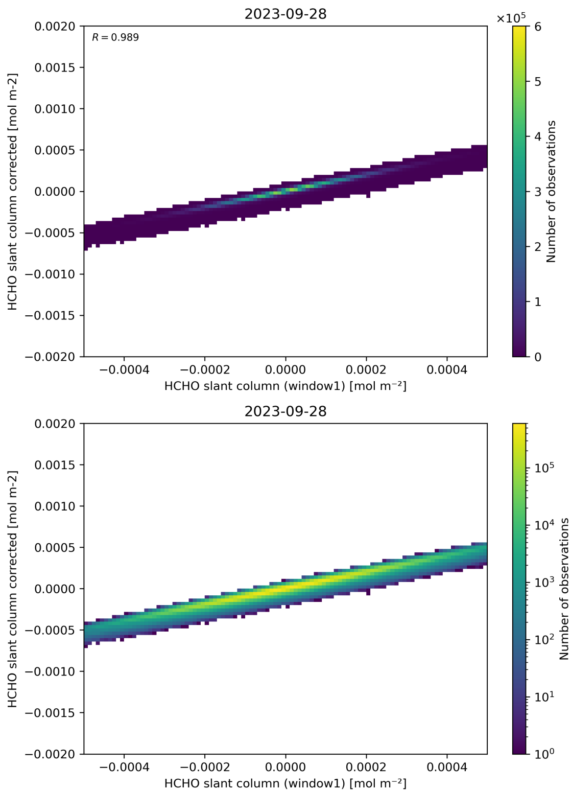
Figure 82: Scatter density plot of “HCHO slant column (window1)” against “HCHO slant column corrected” for 2023-09-27 to 2023-09-29.
