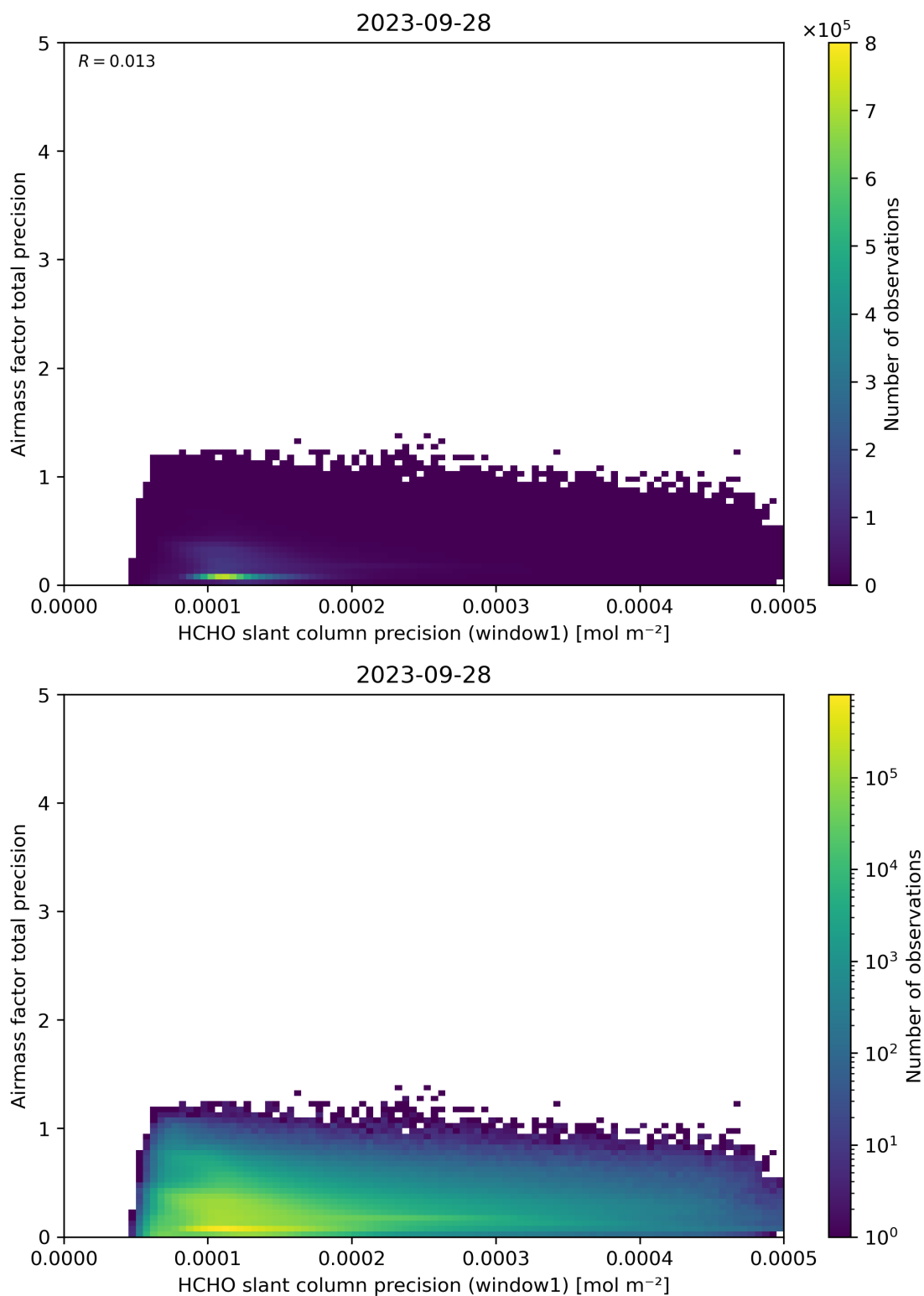
Figure 95: Scatter density plot of “HCHO slant column precision (window1)” against “Airmass factor total precision” for 2023-09-27 to 2023-09-29.
