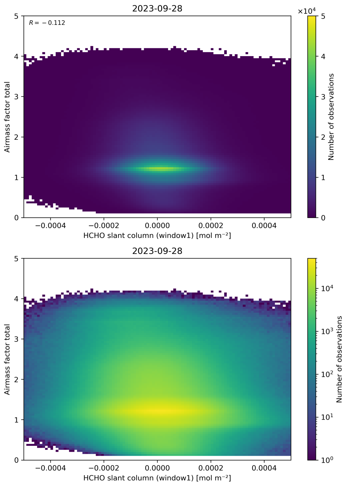
Figure 85: Scatter density plot of “HCHO slant column (window1)” against “Airmass factor total” for 2023-09-27 to 2023-09-29.
