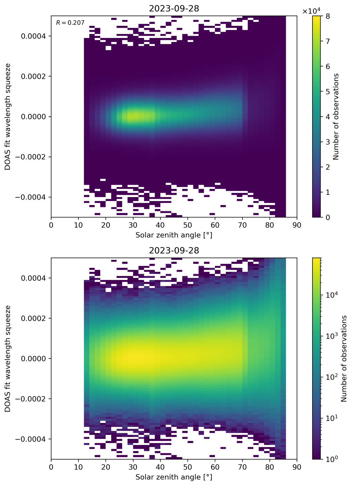
Figure 169: Scatter density plot of “Solar zenith angle” against “DOAS fit wavelength squeeze” for 2023-09-27 to 2023-09-29.
