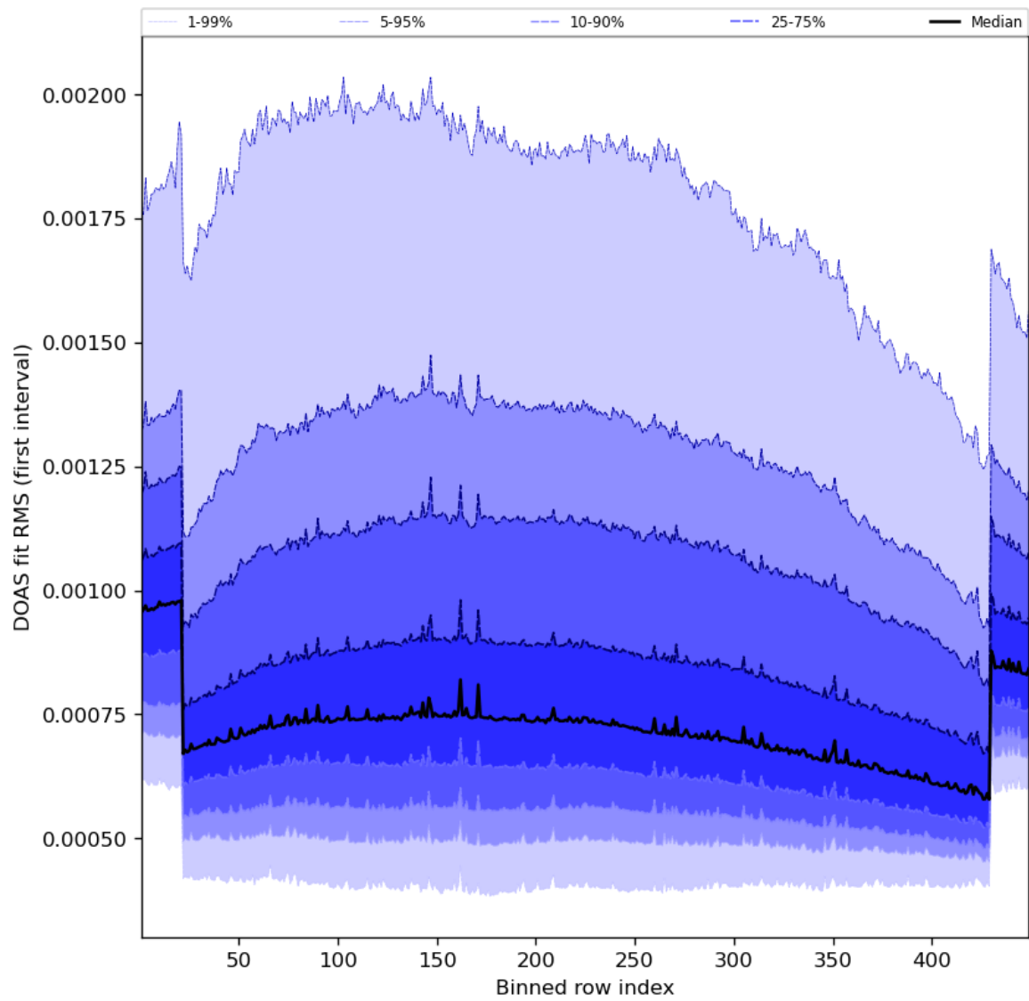
Figure 60: Along track statistics of “DOAS fit RMS (first interval)” for 2023-09-27 to 2023-09-29
