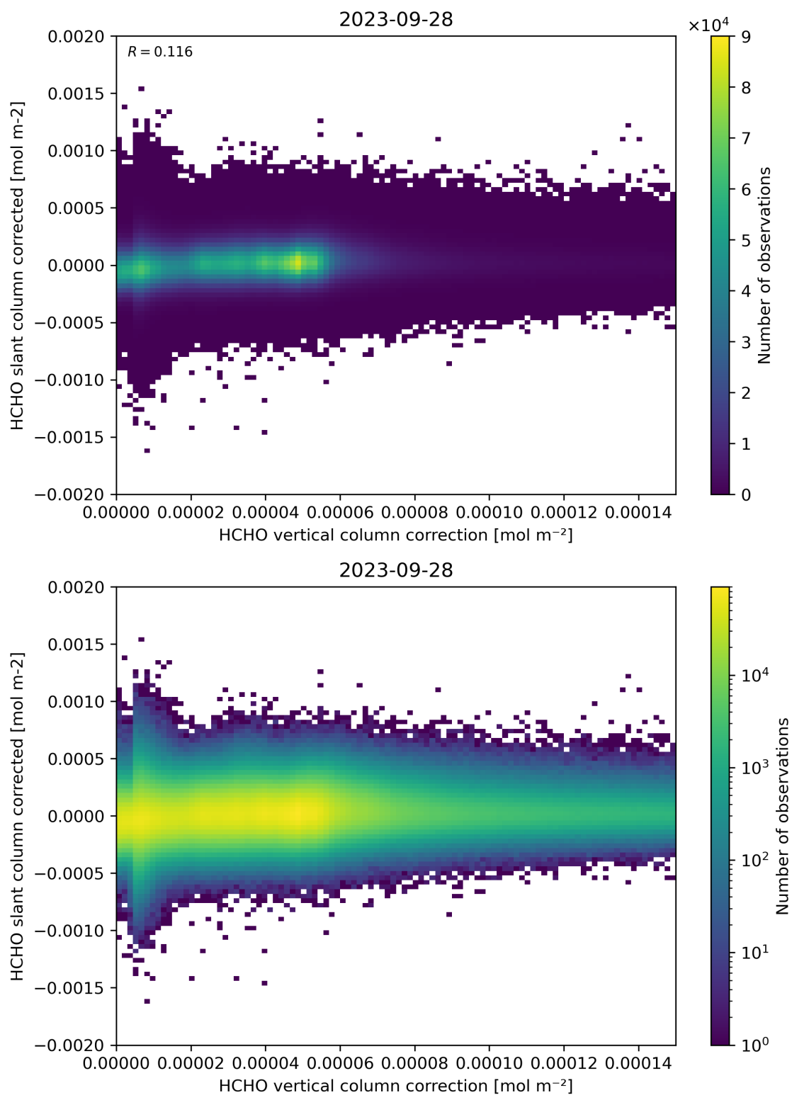
Figure 116: Scatter density plot of “HCHO vertical column correction” against “HCHO slant column corrected” for 2023-09-27 to 2023-09-29.
