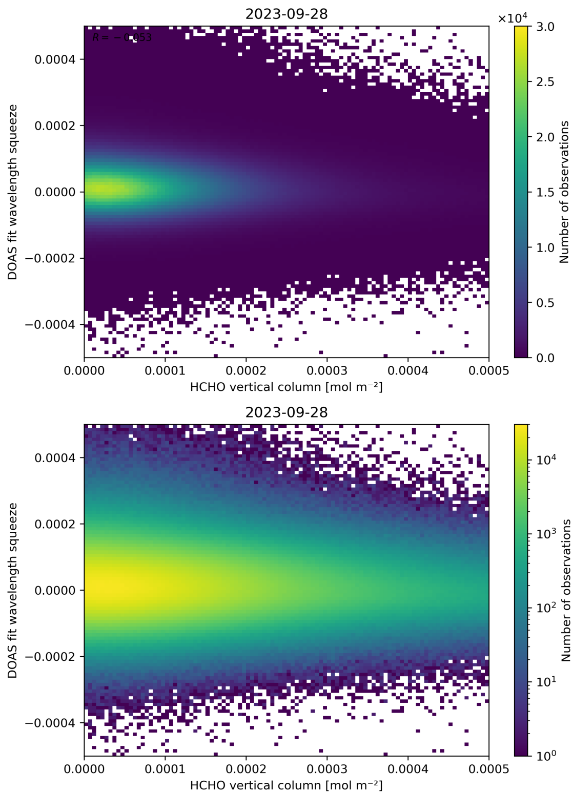
Figure 125: Scatter density plot of “HCHO vertical column” against “DOAS fit wavelength squeeze” for 2023-09-27 to 2023-09-29.
