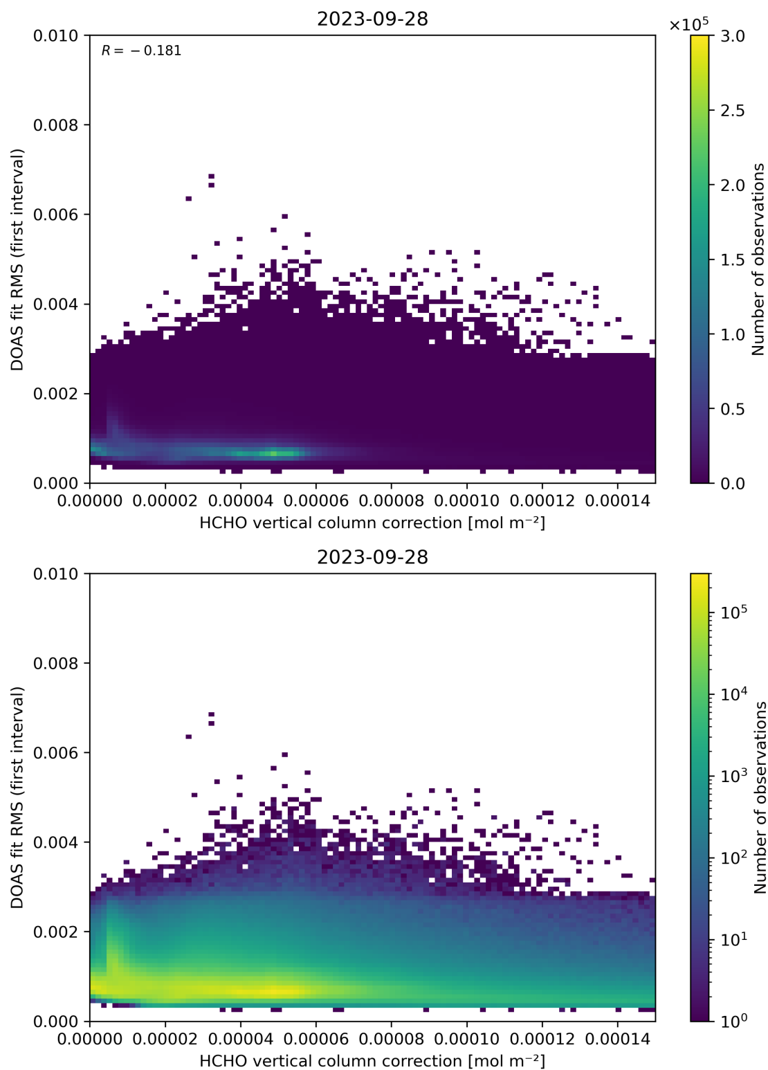
Figure 112: Scatter density plot of “HCHO vertical column correction” against “DOAS fit RMS (first interval)” for 2023-09-27 to 2023-09-29.
