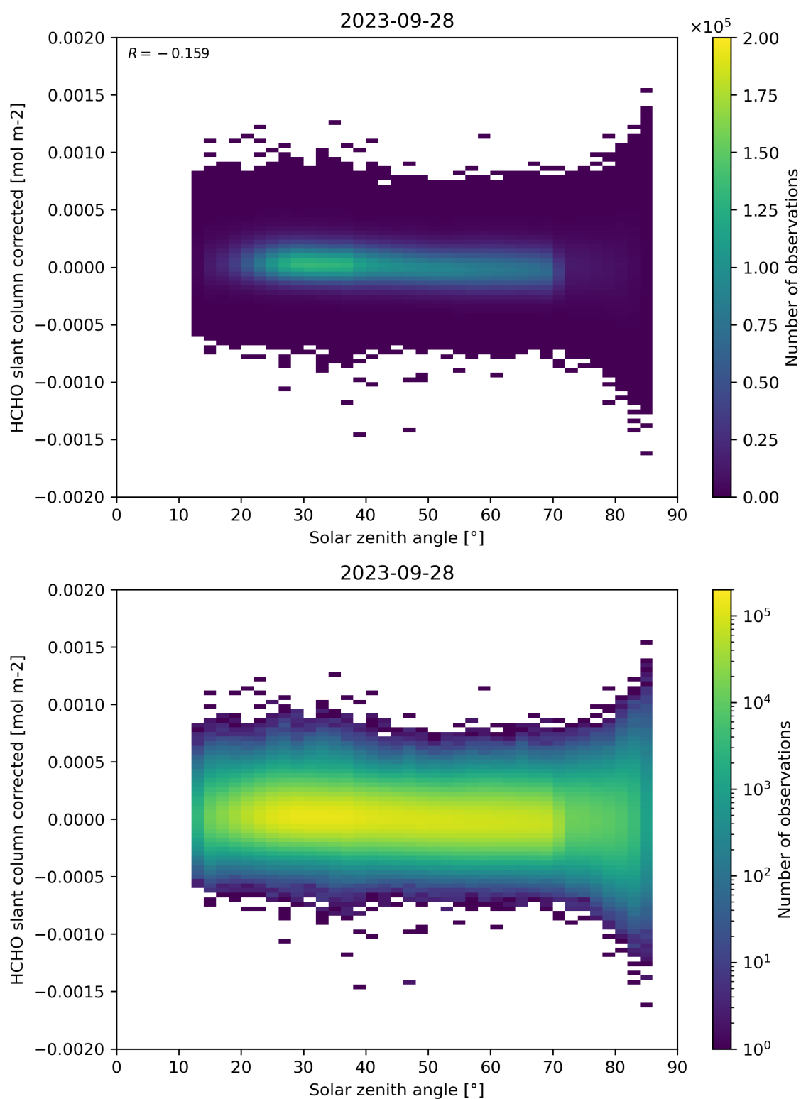
Figure 171: Scatter density plot of “Solar zenith angle” against “HCHO slant column corrected” for 2023-09-27 to 2023-09-29.
