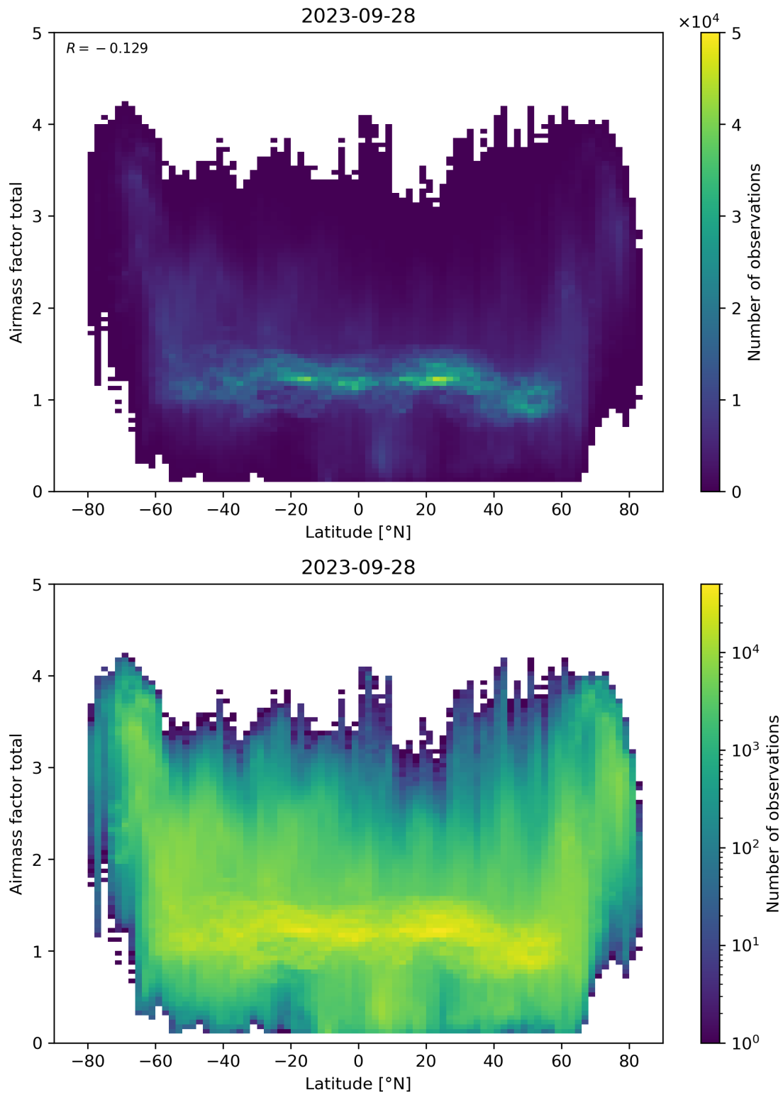
Figure 161: Scatter density plot of “Latitude” against “Airmass factor total” for 2023-09-27 to 2023-09-29.
