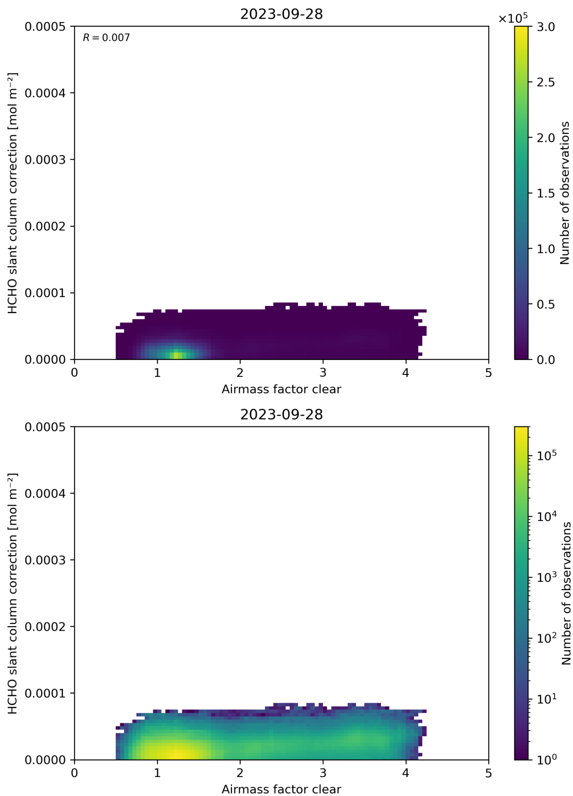
Figure 75: Scatter density plot of “Airmass factor clear” against “HCHO slant column correction” for 2023-09-27 to 2023-09-29.
