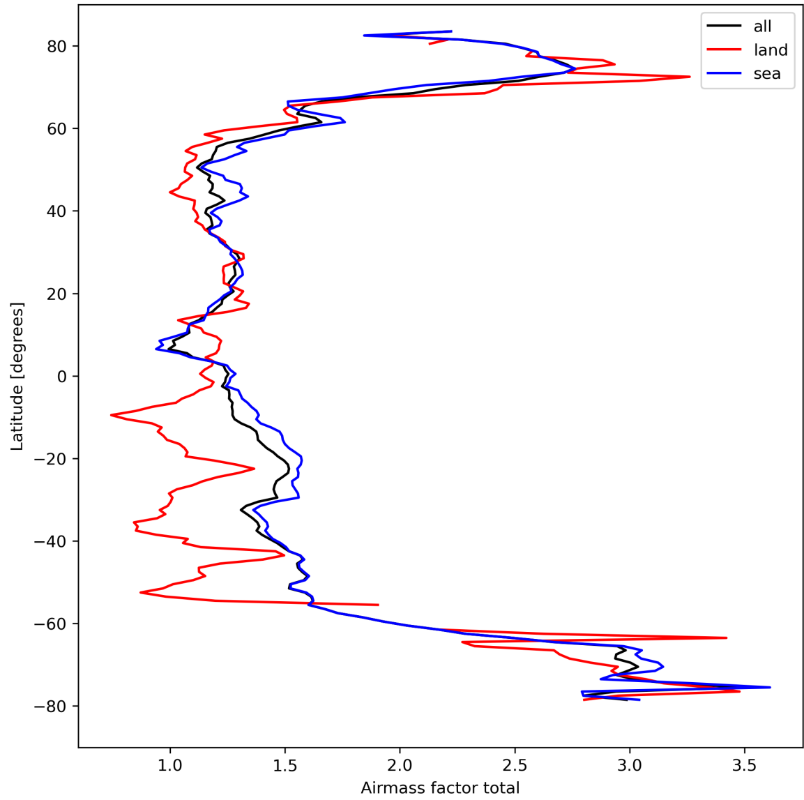
Figure 26: Zonal average of “Airmass factor total” for 2023-09-27 to 2023-09-29.
