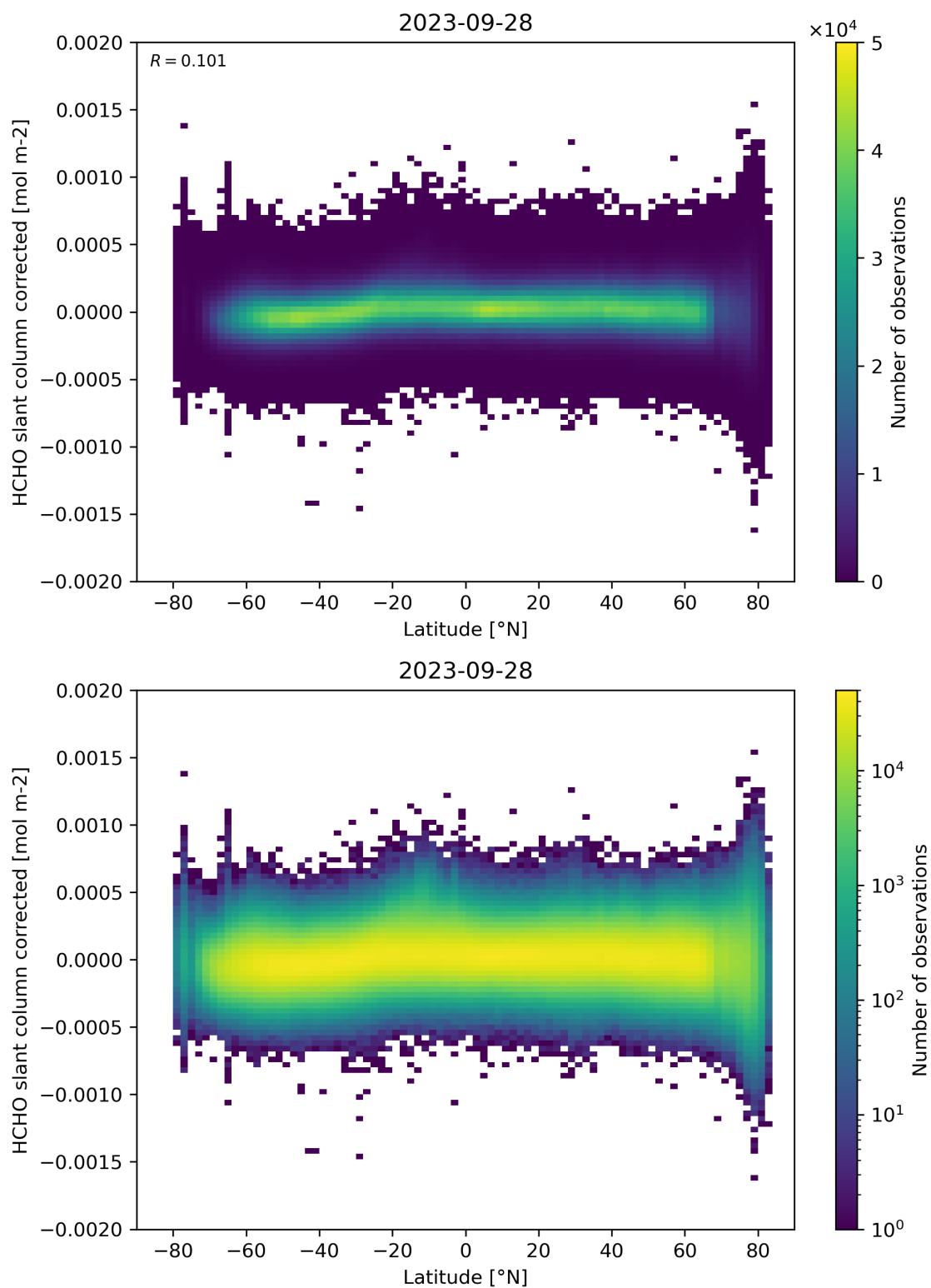
Figure 157: Scatter density plot of “Latitude” against “HCHO slant column corrected” for 2023-09-27 to 2023-09-29.
