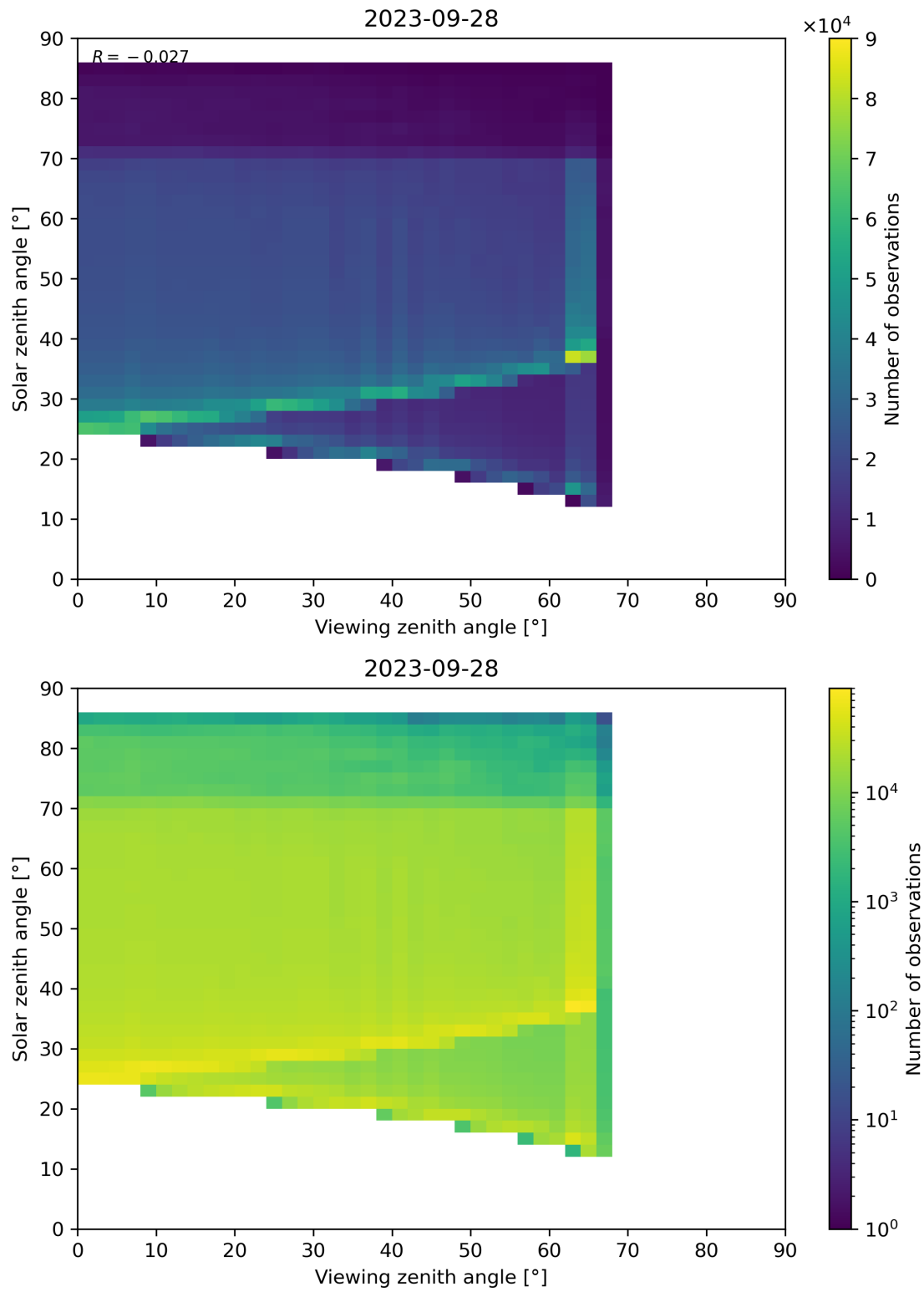
Figure 197: Scatter density plot of “Viewing zenith angle” against “Solar zenith angle” for 2023-09-27 to 2023-09-29.
