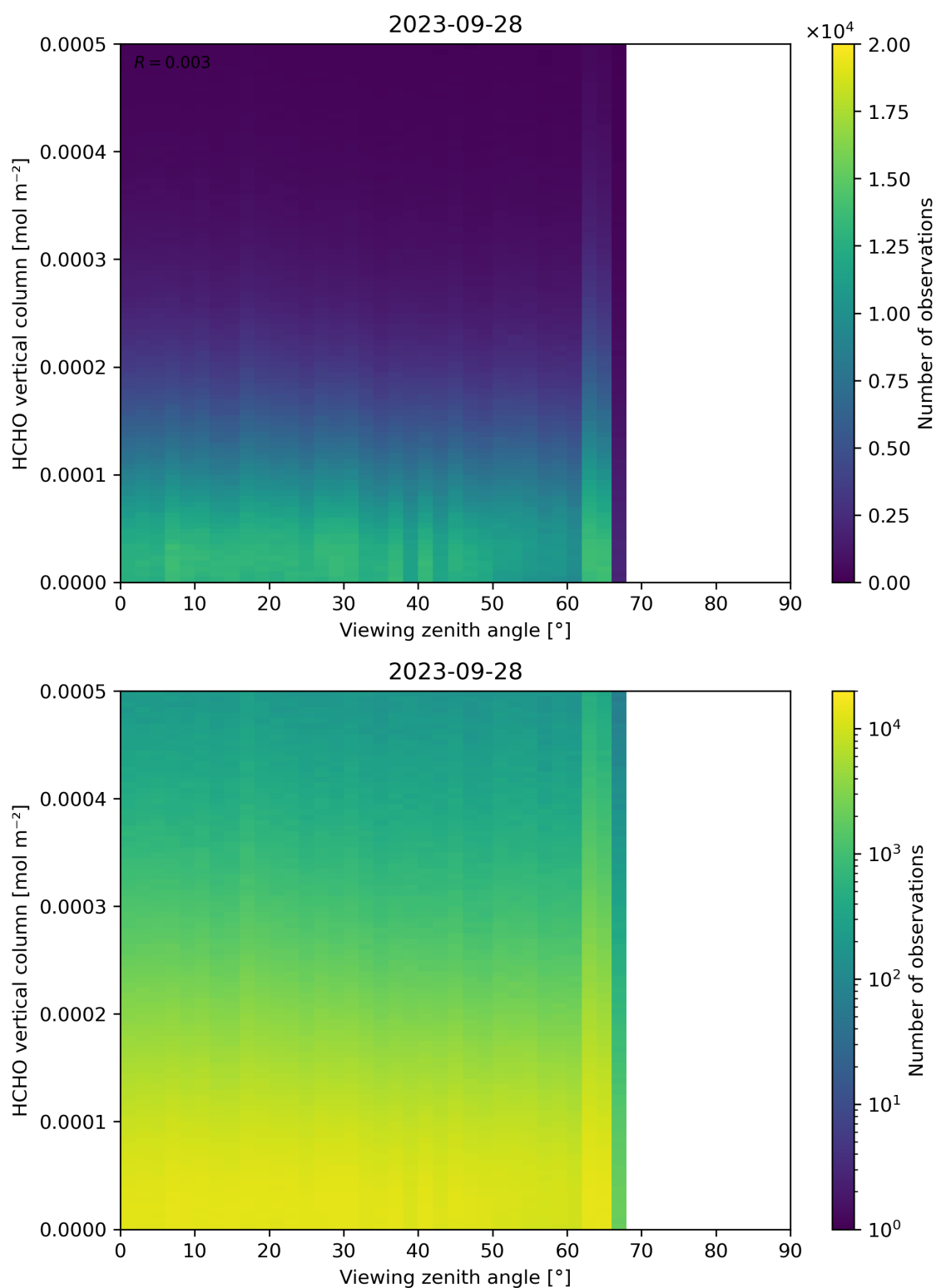
Figure 192: Scatter density plot of “Viewing zenith angle” against “HCHO vertical column” for 2023-09-27 to 2023-09-29.
