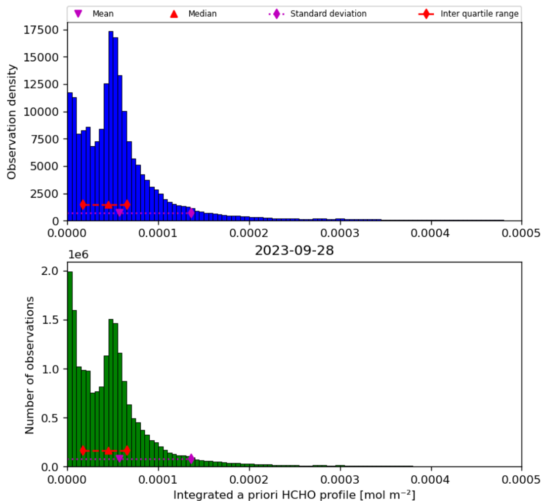
Figure 43: Histogram of “Integrated a priori HCHO profile” for 2023-09-27 to 2023-09-29
