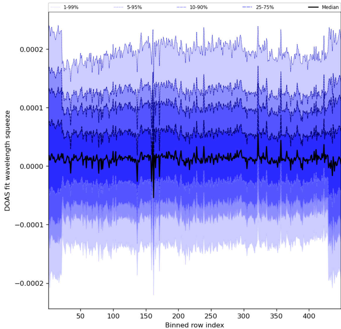
Figure 59: Along track statistics of “DOAS fit wavelength squeeze” for 2023-09-27 to 2023-09-29
