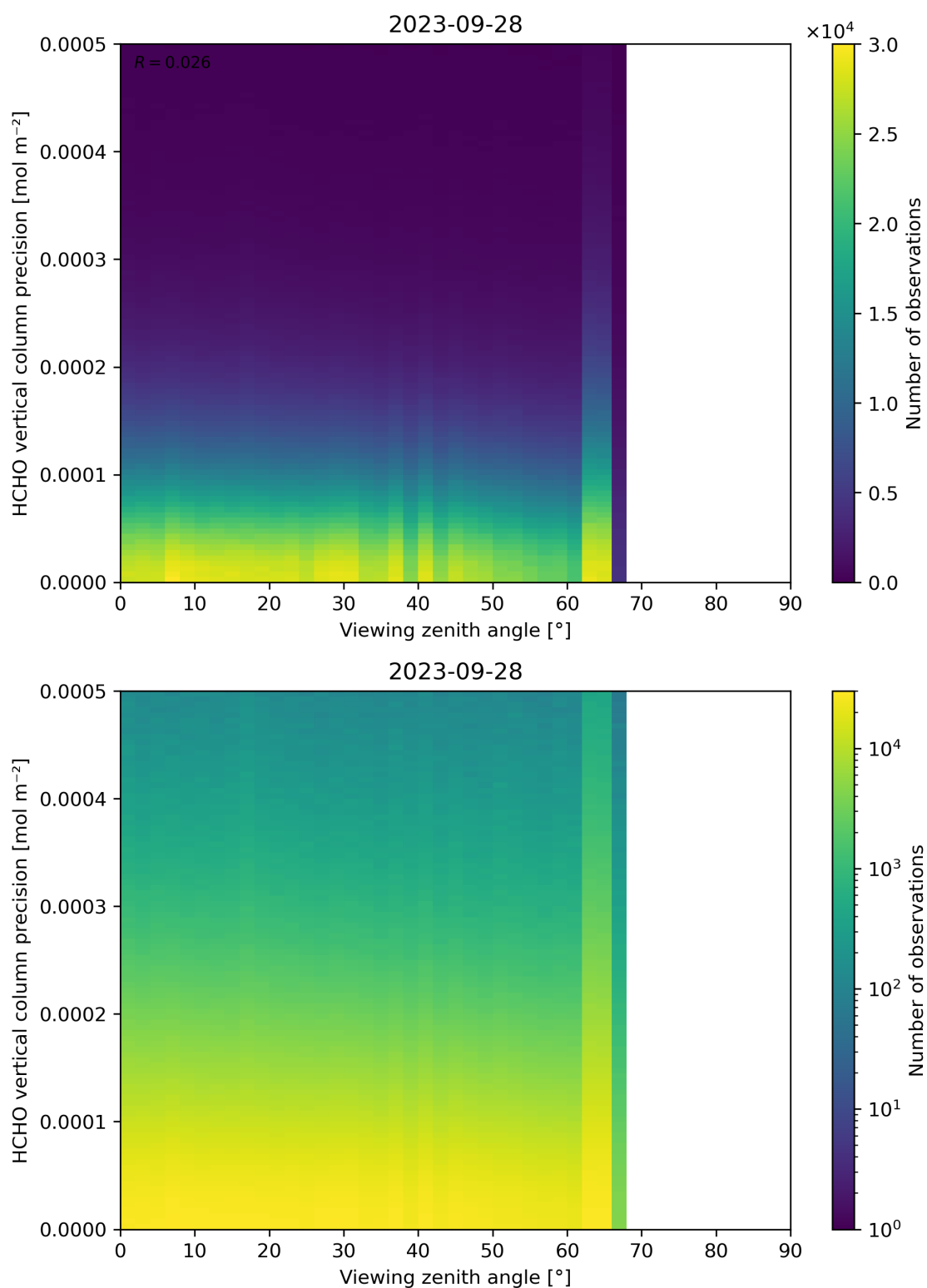
Figure 194: Scatter density plot of “Viewing zenith angle” against “HCHO vertical column precision” for 2023-09-27 to 2023-09-29.
