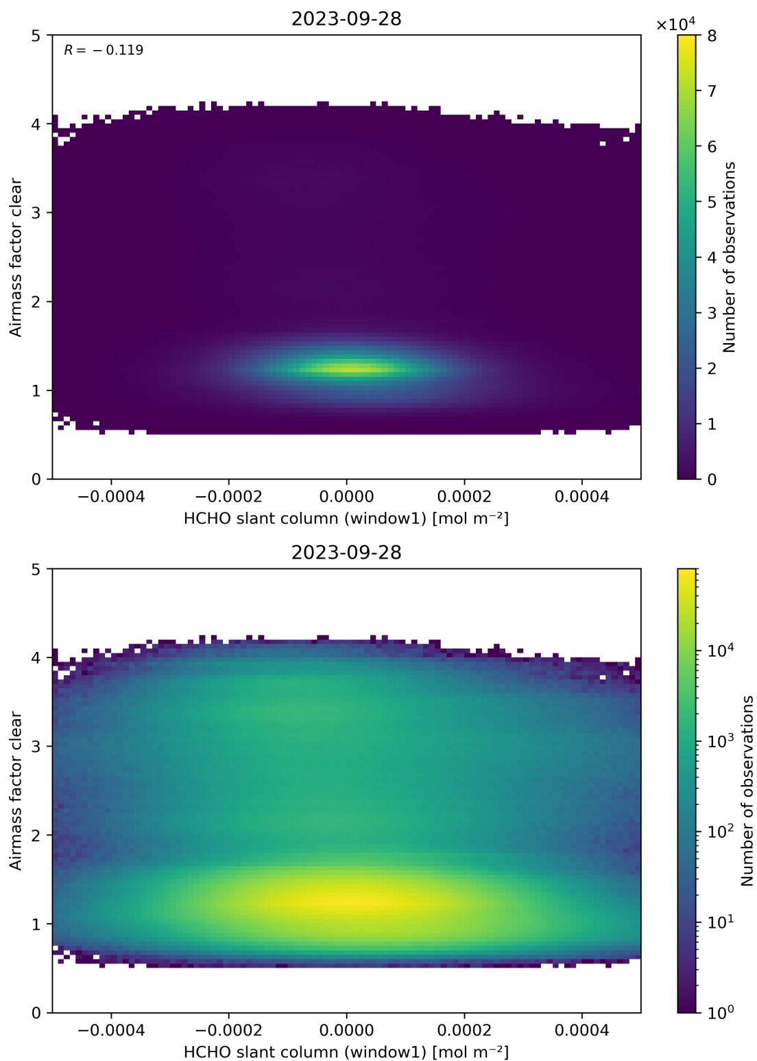
Figure 81: Scatter density plot of “HCHO slant column (window1)” against “Airmass factor clear” for 2023-09-27 to 2023-09-29.
