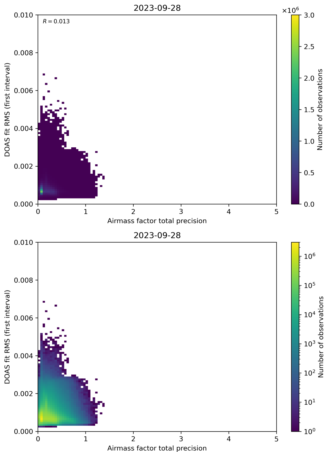
Figure 105: Scatter density plot of “Airmass factor total precision” against “DOAS fit RMS (first interval)” for 2023-09-27 to 2023-09-29.
