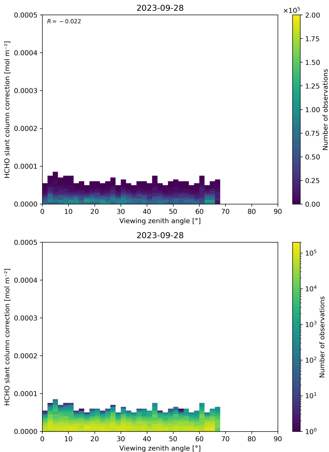
Figure 187: Scatter density plot of “Viewing zenith angle” against “HCHO slant column correction” for 2023-09-27 to 2023-09-29.
