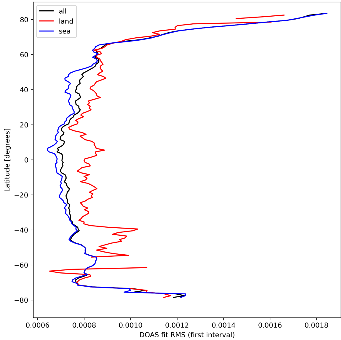
Figure 32: Zonal average of “DOAS fit RMS (first interval)” for 2023-09-27 to 2023-09-29.
