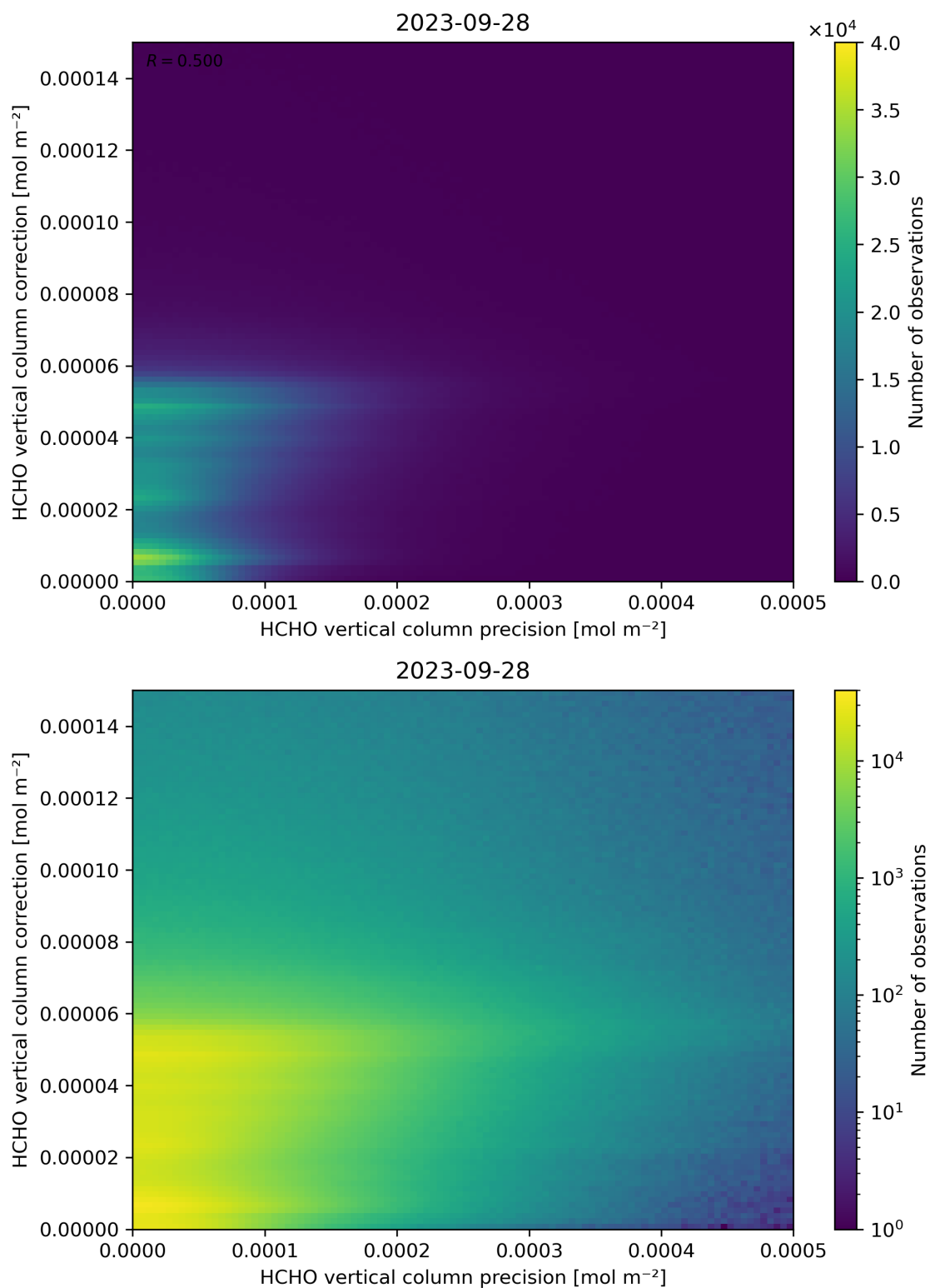
Figure 146: Scatter density plot of “HCHO vertical column precision” against “HCHO vertical column correction” for 2023-09-27 to 2023-09-29.
