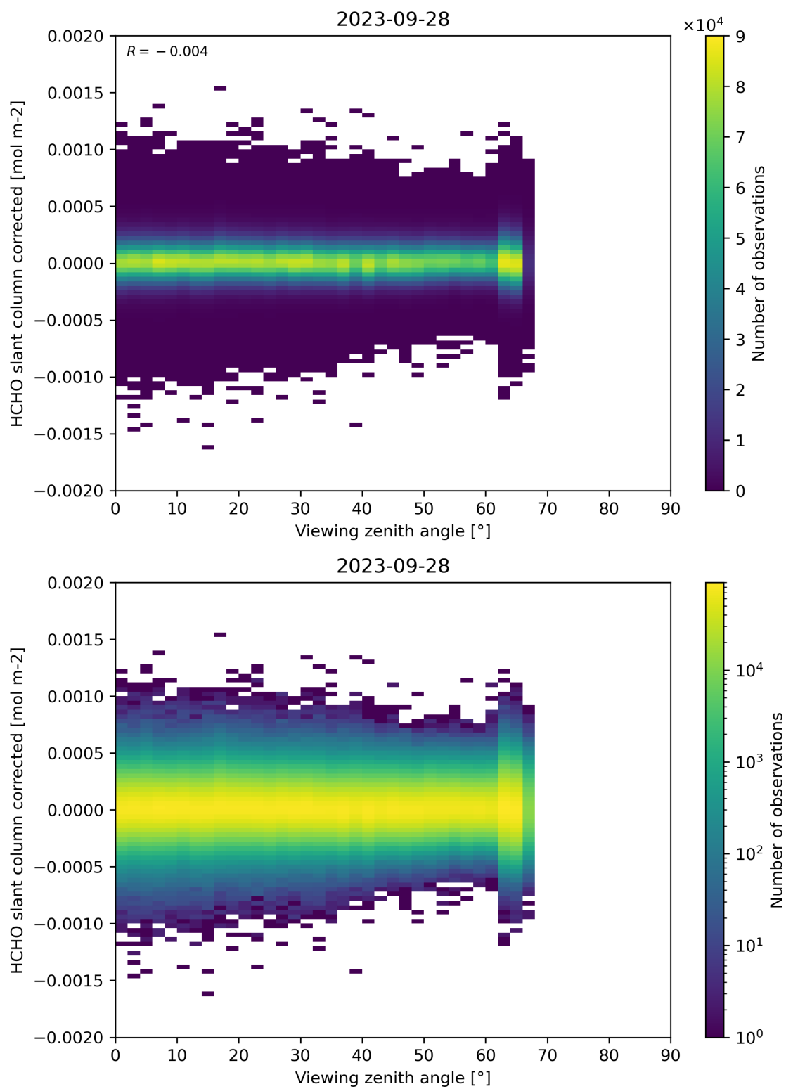
Figure 186: Scatter density plot of “Viewing zenith angle” against “HCHO slant column corrected” for 2023-09-27 to 2023-09-29.
