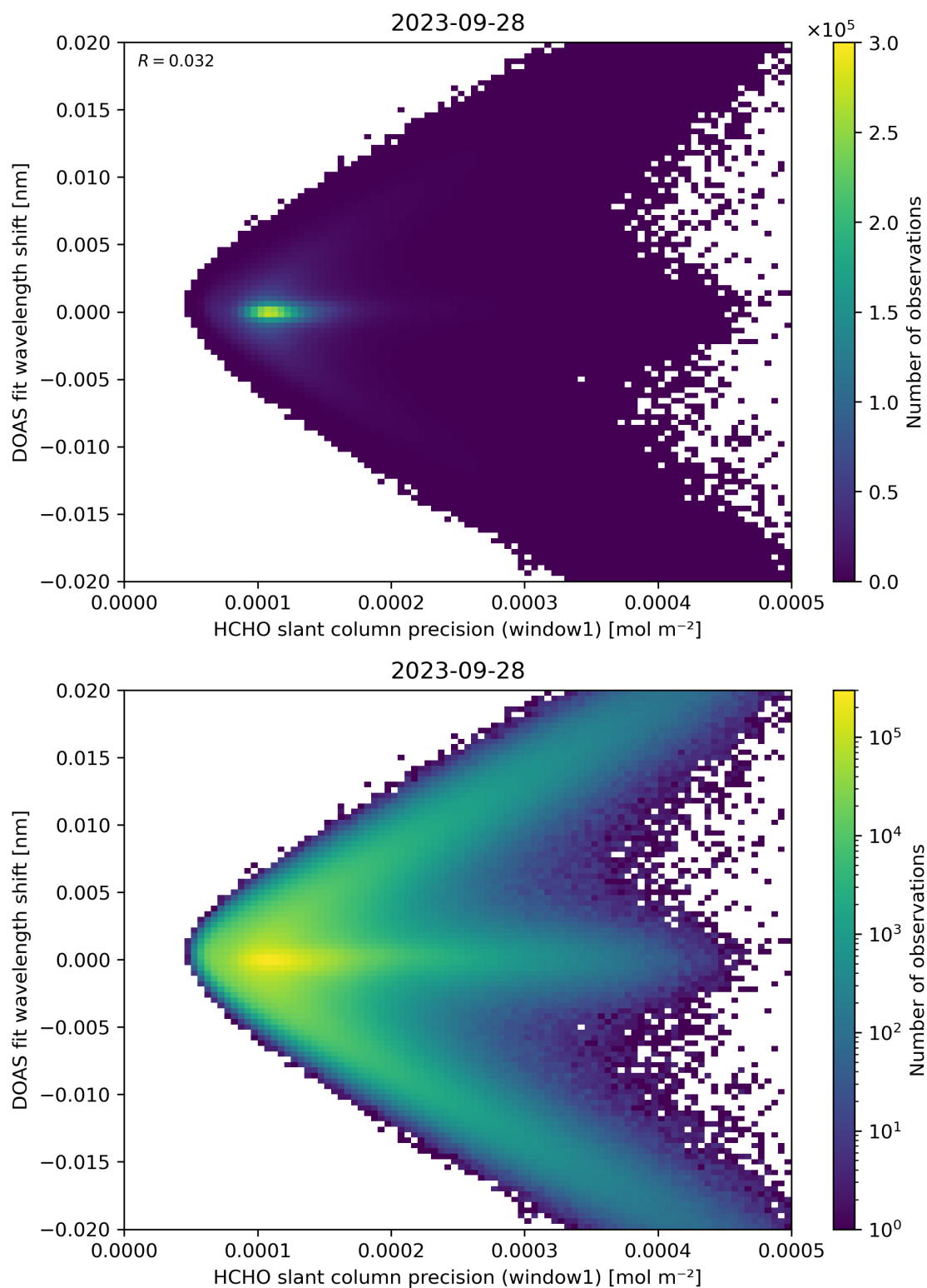
Figure 89: Scatter density plot of “HCHO slant column precision (window1)” against “DOAS fit wavelength shift” for 2023-09-27 to 2023-09-29.
