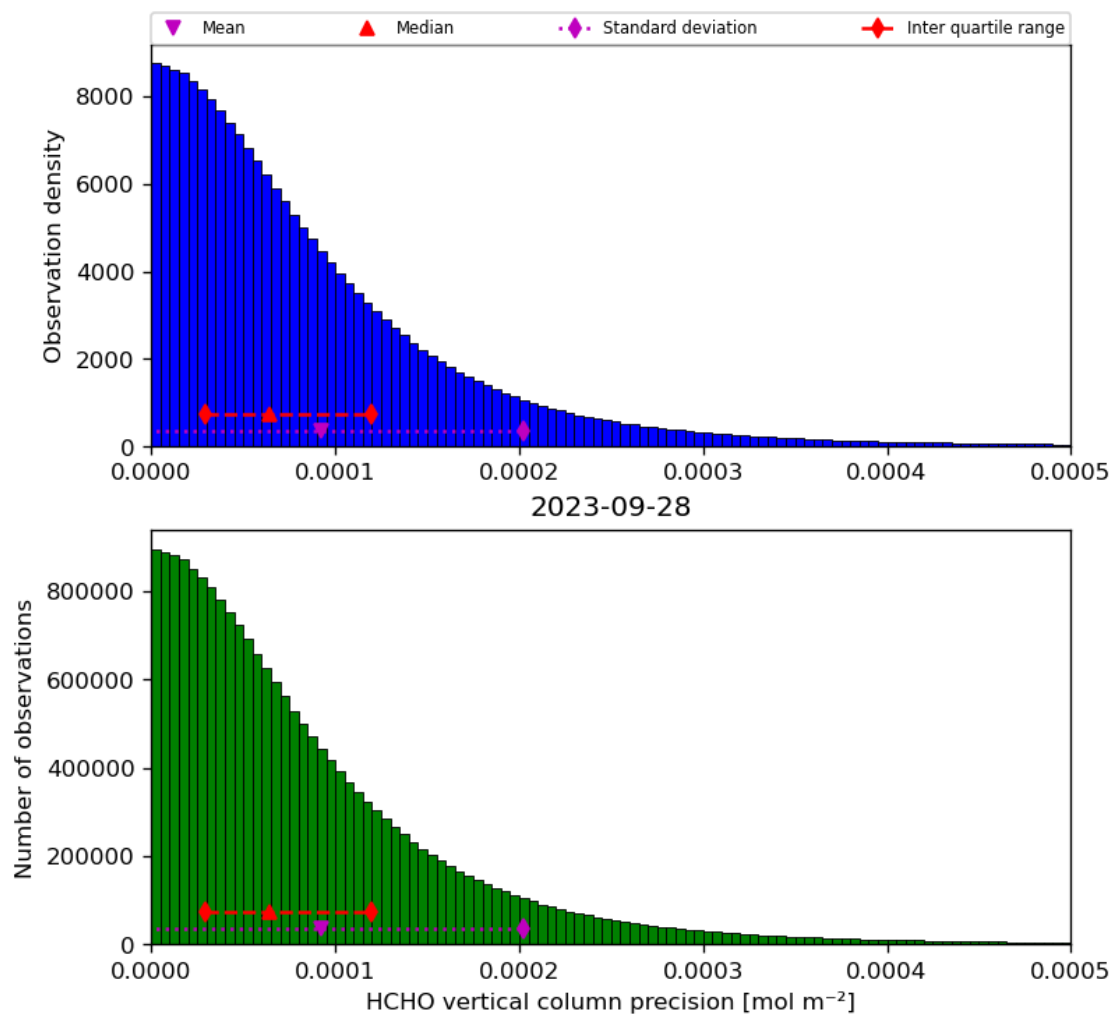
Figure 36: Histogram of “HCHO vertical column precision” for 2023-09-27 to 2023-09-29
