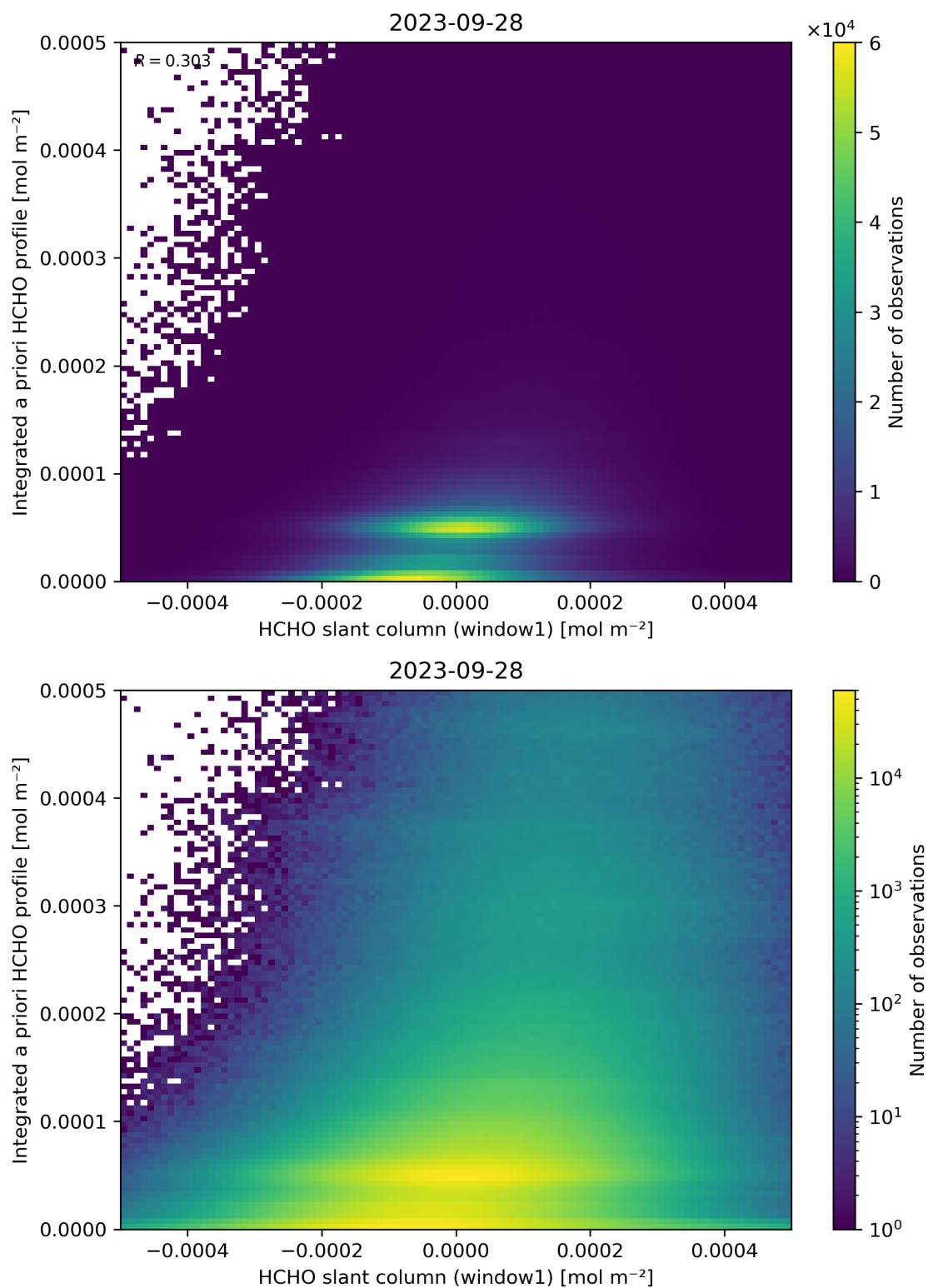
Figure 87: Scatter density plot of “HCHO slant column (window1)” against “Integrated a priori HCHO profile” for 2023-09-27 to 2023-09-29.
