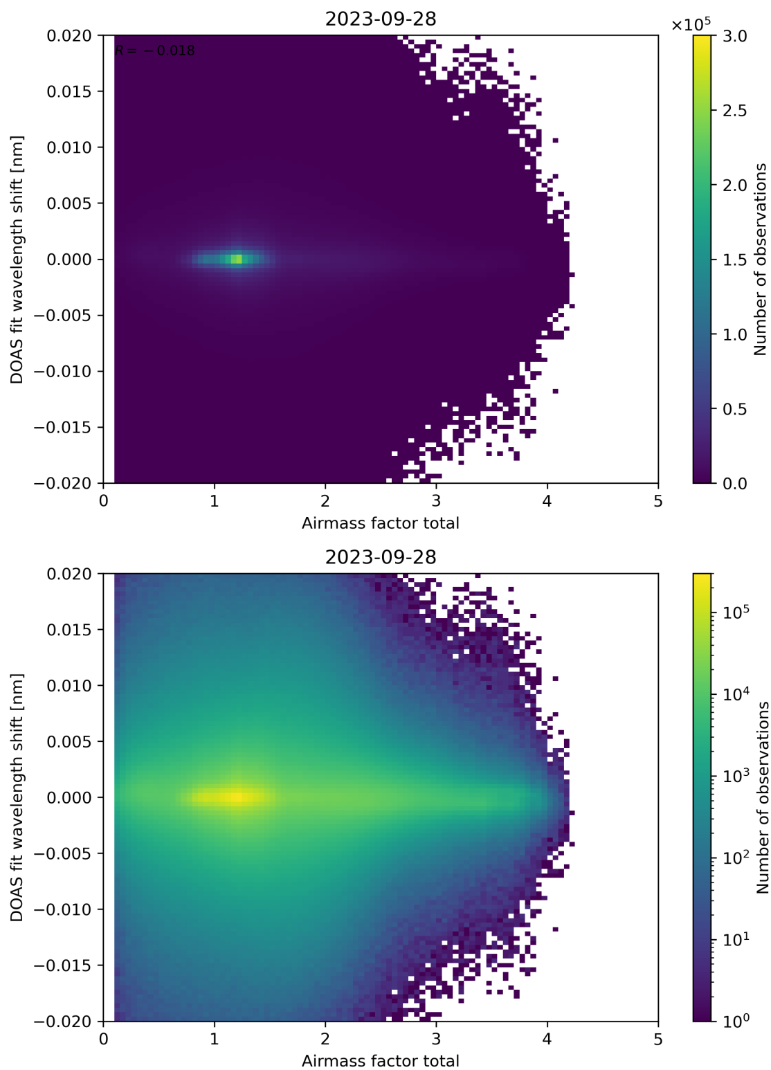
Figure 98: Scatter density plot of “Airmass factor total” against “DOAS fit wavelength shift” for 2023-09-27 to 2023-09-29.
