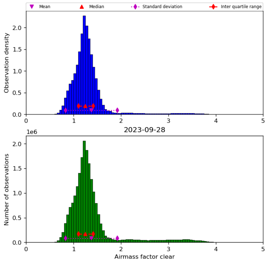
Figure 42: Histogram of “Airmass factor clear” for 2023-09-27 to 2023-09-29
