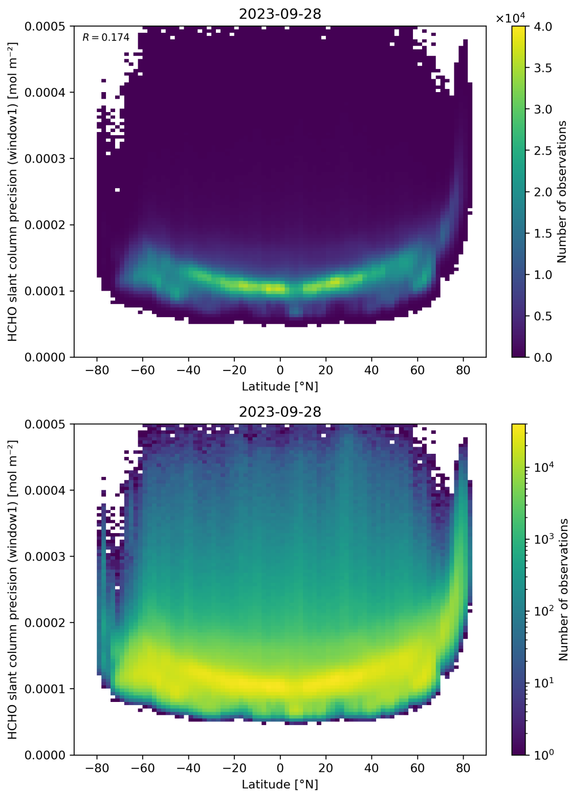
Figure 160: Scatter density plot of “Latitude” against “HCHO slant column precision (window1)” for 2023-09-27 to 2023-09-29.
