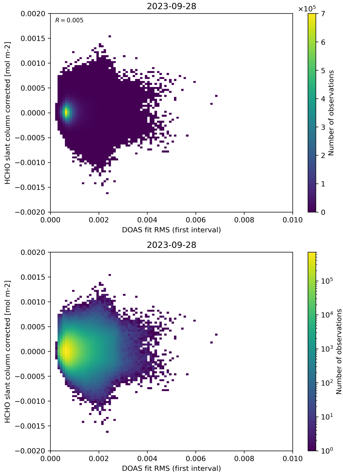
Figure 62: Scatter density plot of “DOAS fit RMS (first interval)” against “HCHO slant column corrected” for 2023-09-27 to 2023-09-29.
