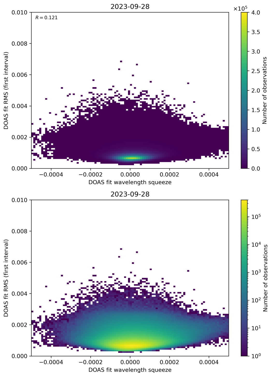
Figure 68: Scatter density plot of “DOAS fit wavelength squeeze” against “DOAS fit RMS (first interval)” for 2023-09-27 to 2023-09-29.
