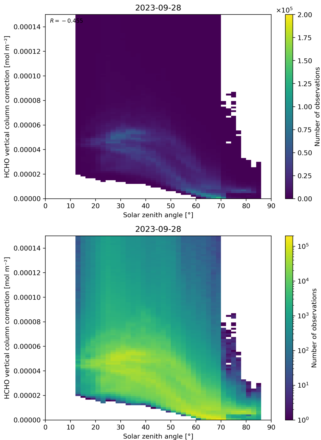
Figure 178: Scatter density plot of “Solar zenith angle” against “HCHO vertical column correction” for 2023-09-27 to 2023-09-29.
