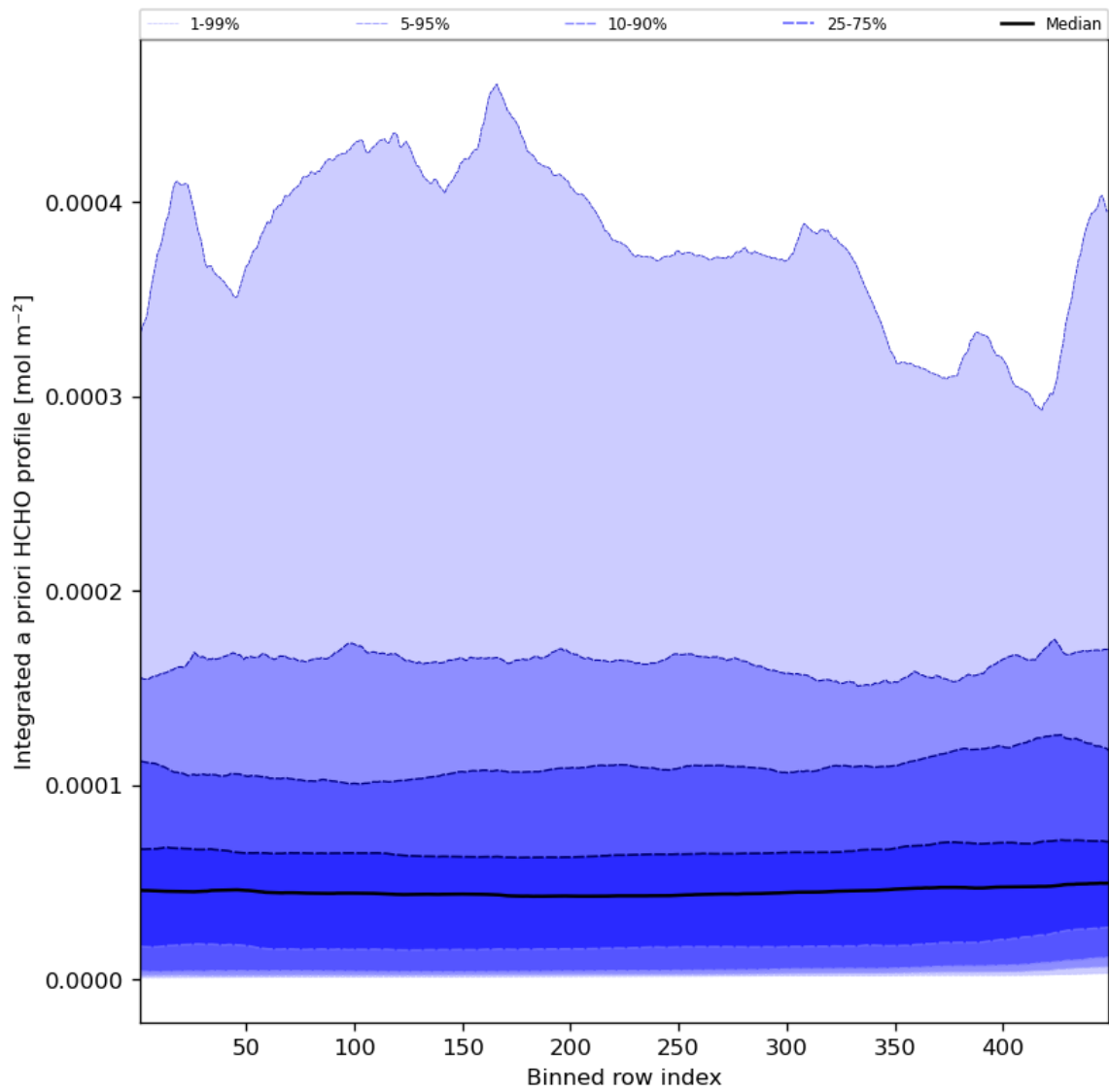
Figure 57: Along track statistics of “Integrated a priori HCHO profile” for 2023-09-27 to 2023-09-29
