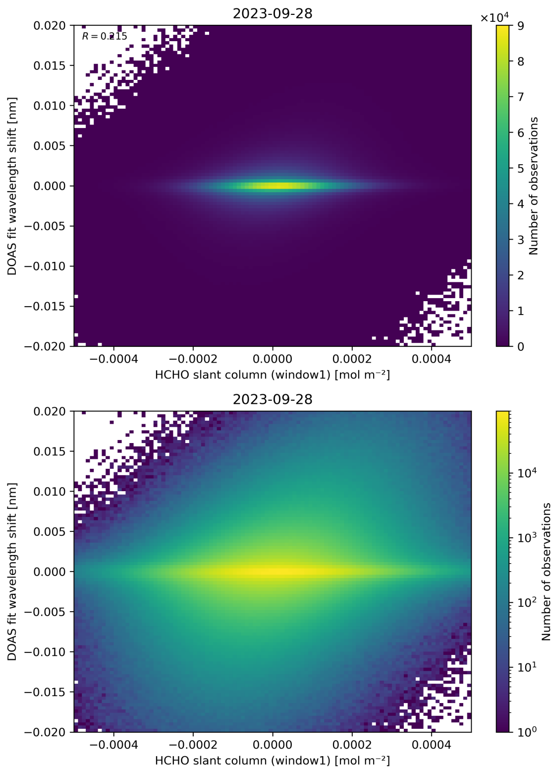
Figure 79: Scatter density plot of “HCHO slant column (window1)” against “DOAS fit wavelength shift” for 2023-09-27 to 2023-09-29.
