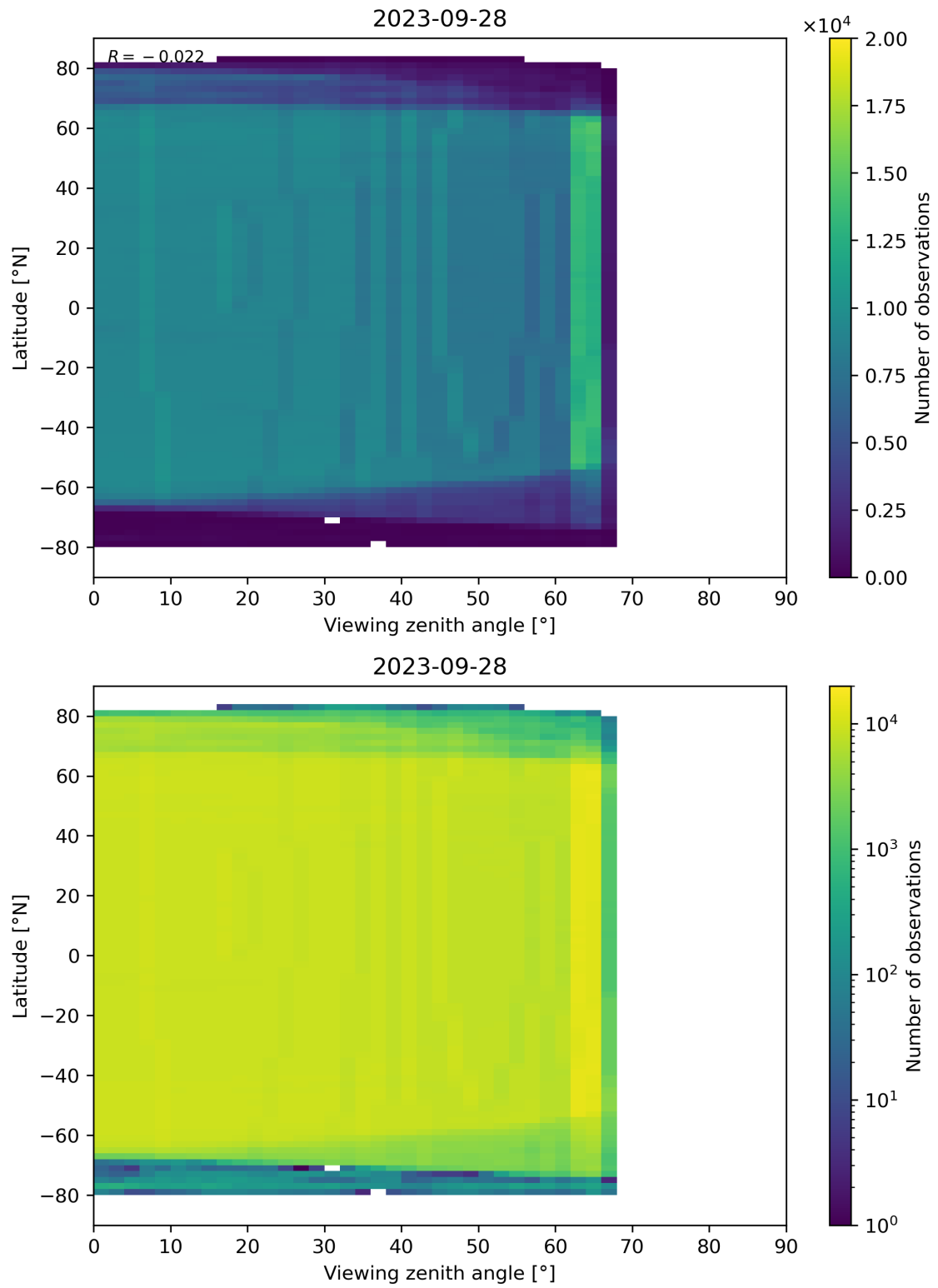
Figure 196: Scatter density plot of “Viewing zenith angle” against “Latitude” for 2023-09-27 to 2023-09-29.
