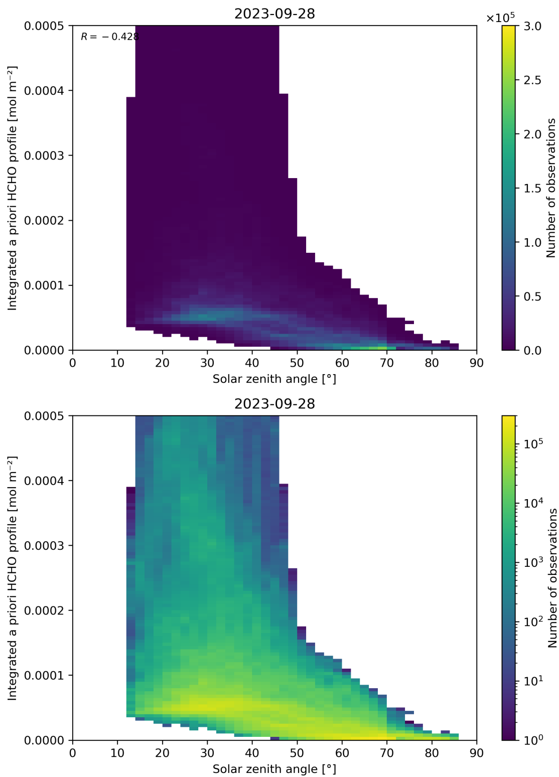
Figure 180: Scatter density plot of “Solar zenith angle” against “Integrated a priori HCHO profile” for 2023-09-27 to 2023-09-29.
