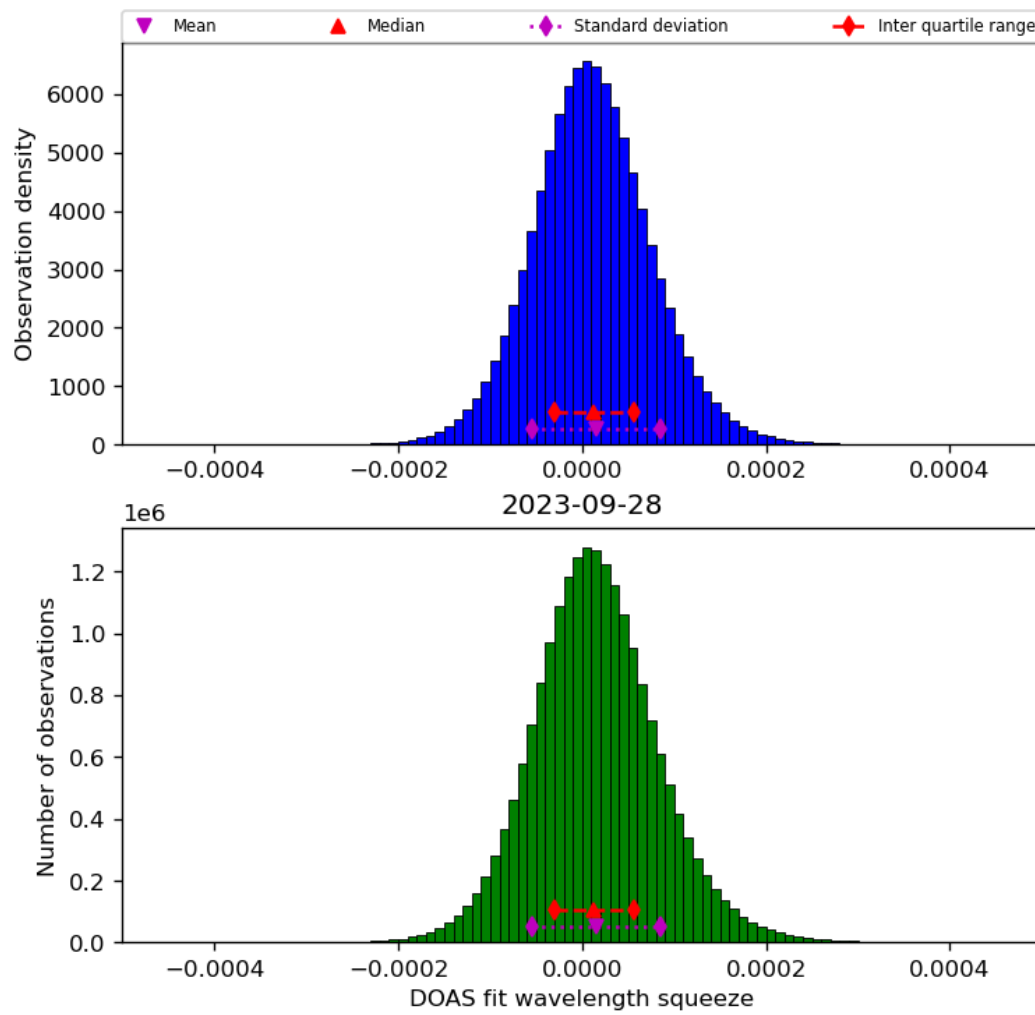
Figure 45: Histogram of “DOAS fit wavelength squeeze” for 2023-09-27 to 2023-09-29
