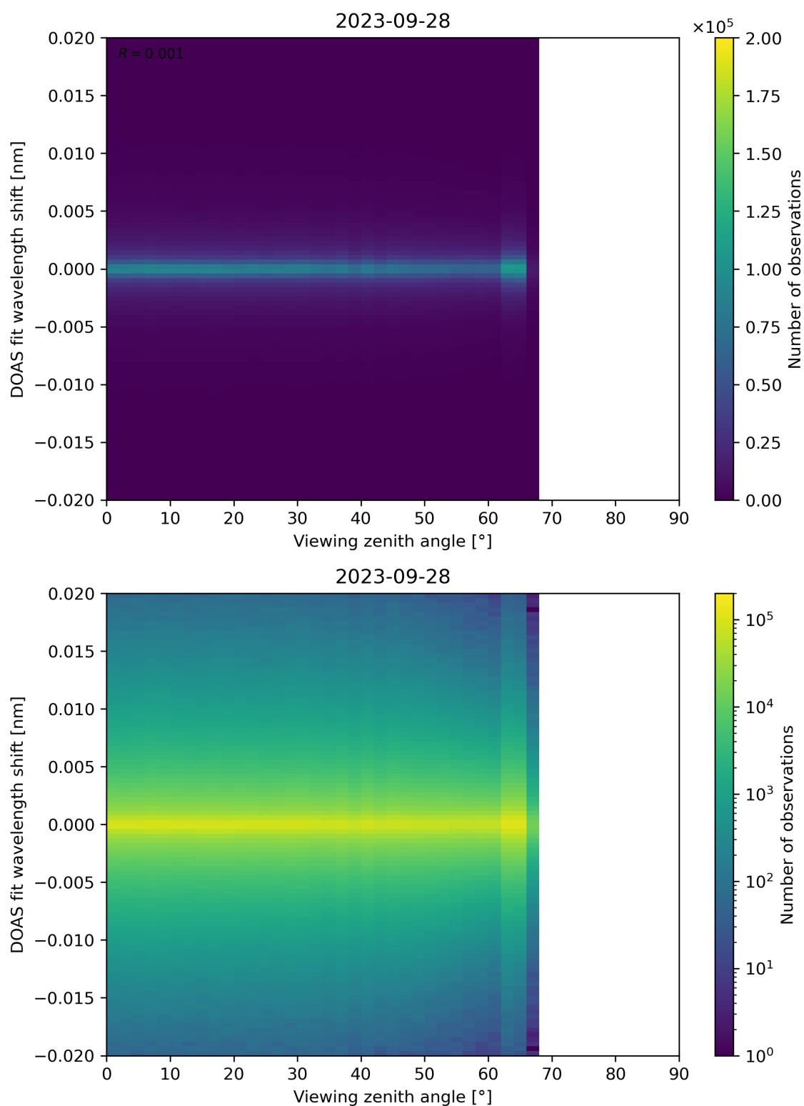
Figure 183: Scatter density plot of “Viewing zenith angle” against “DOAS fit wavelength shift” for 2023-09-27 to 2023-09-29.
