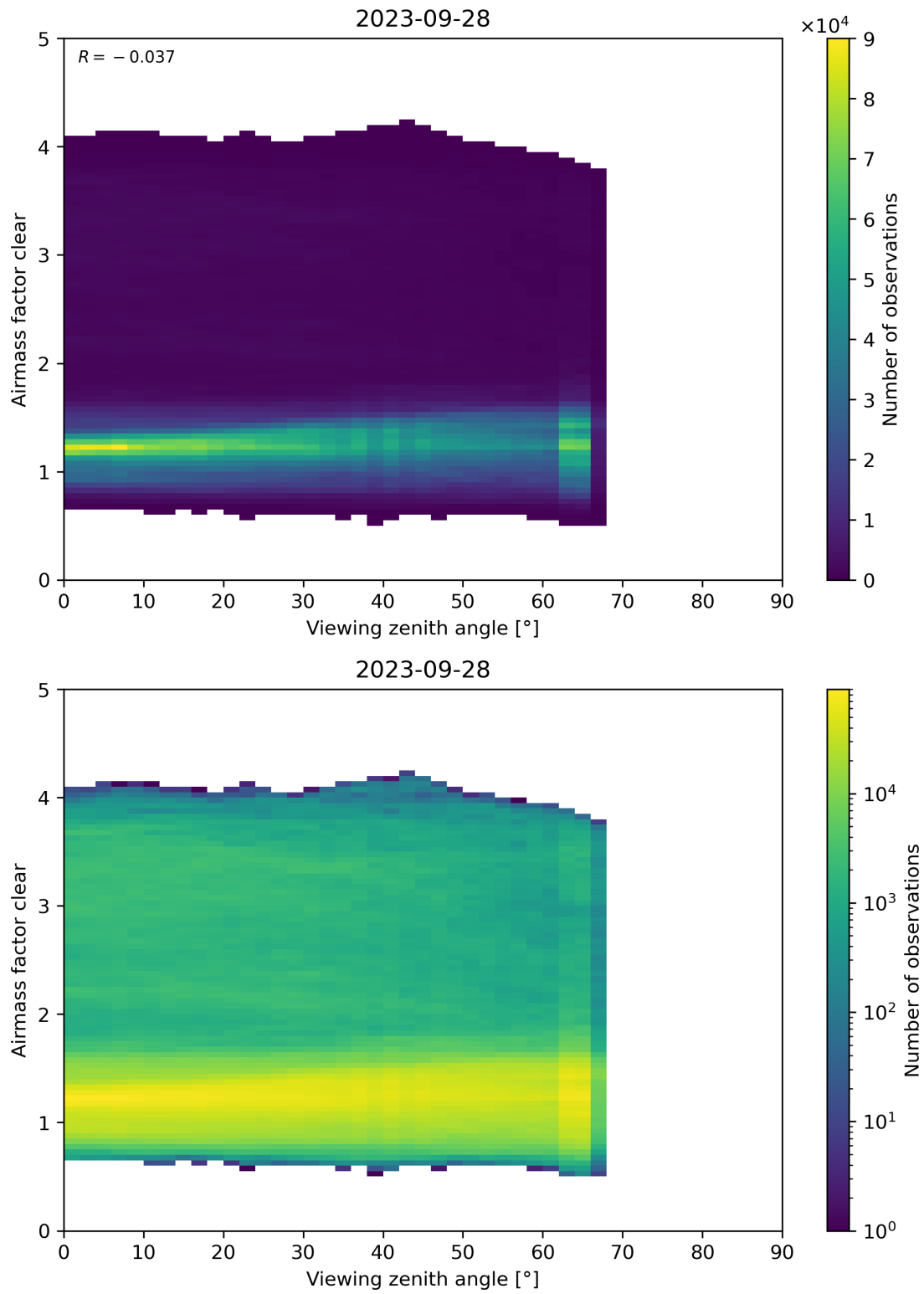
Figure 185: Scatter density plot of “Viewing zenith angle” against “Airmass factor clear” for 2023-09-27 to 2023-09-29.
