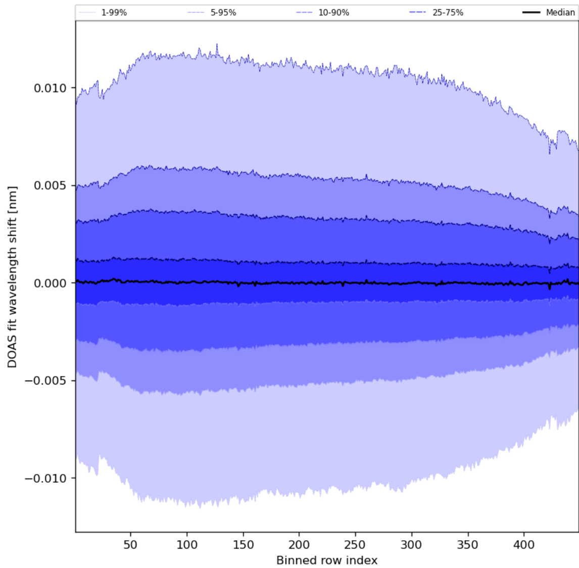
Figure 58: Along track statistics of “DOAS fit wavelength shift” for 2023-09-27 to 2023-09-29
