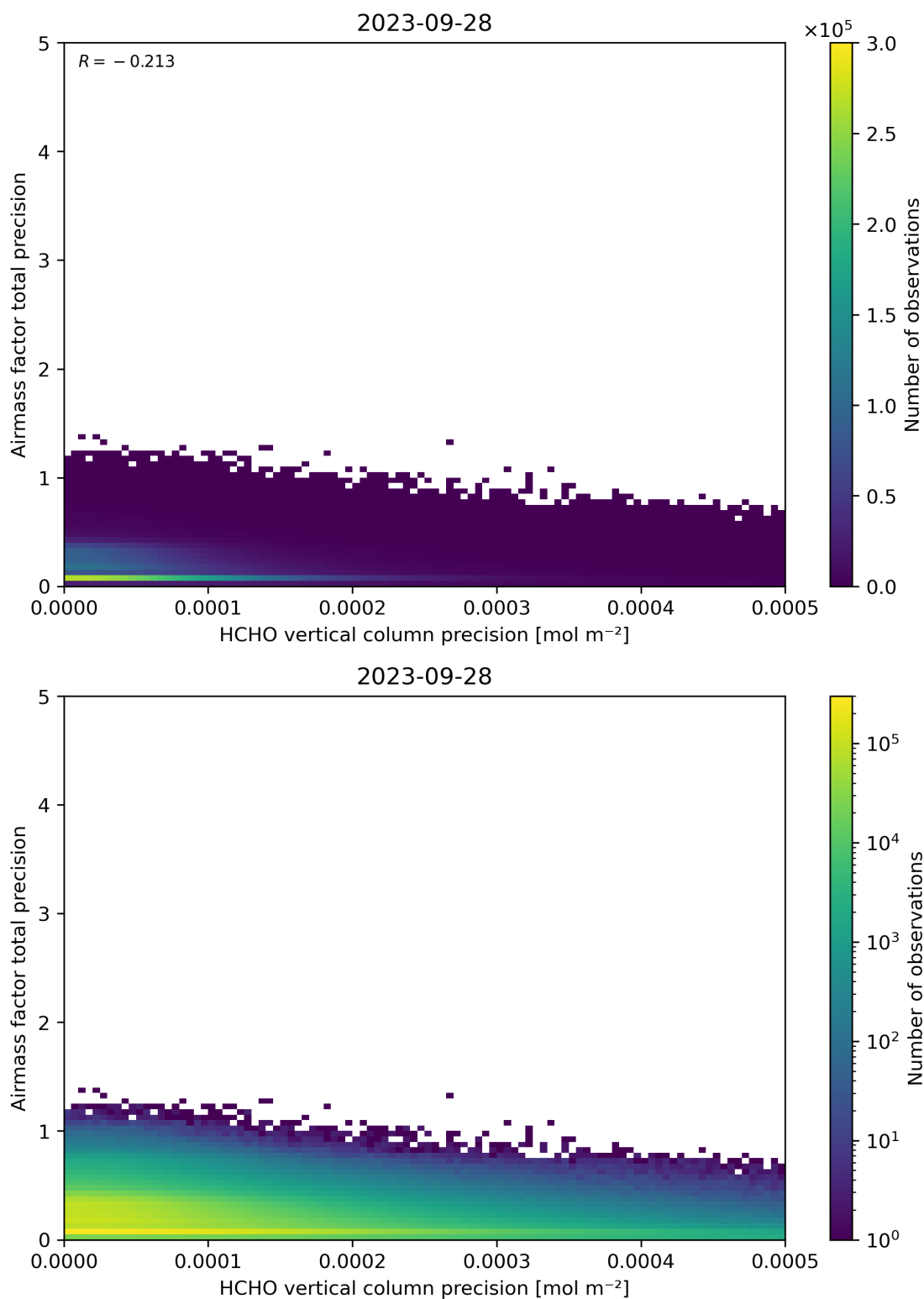
Figure 145: Scatter density plot of “HCHO vertical column precision” against “Airmass factor total precision” for 2023-09-27 to 2023-09-29.
