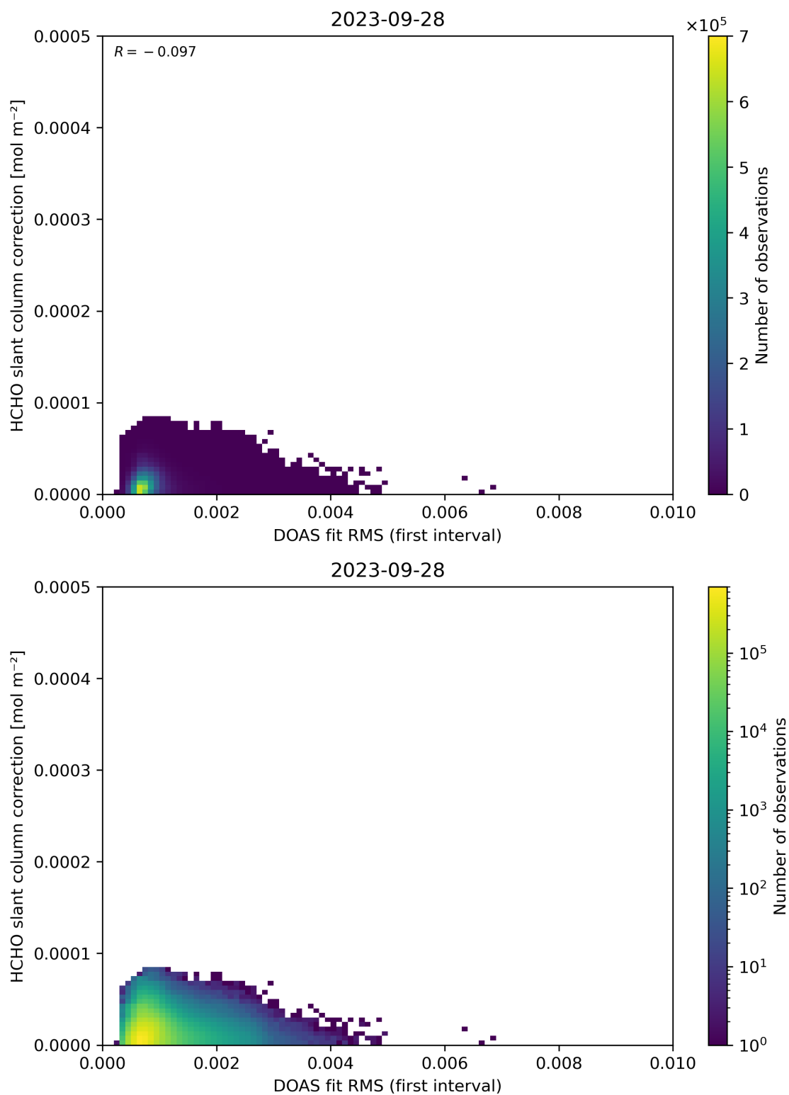
Figure 63: Scatter density plot of “DOAS fit RMS (first interval)” against “HCHO slant column correction” for 2023-09-27 to 2023-09-29.
