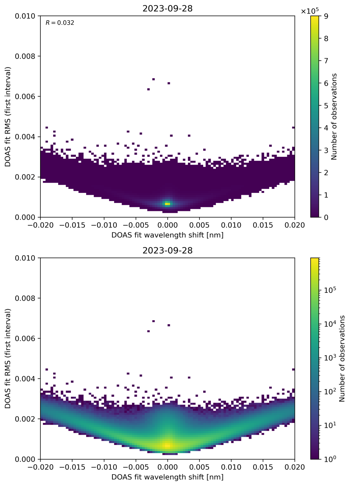
Figure 64: Scatter density plot of “DOAS fit wavelength shift” against “DOAS fit RMS (first interval)” for 2023-09-27 to 2023-09-29.
