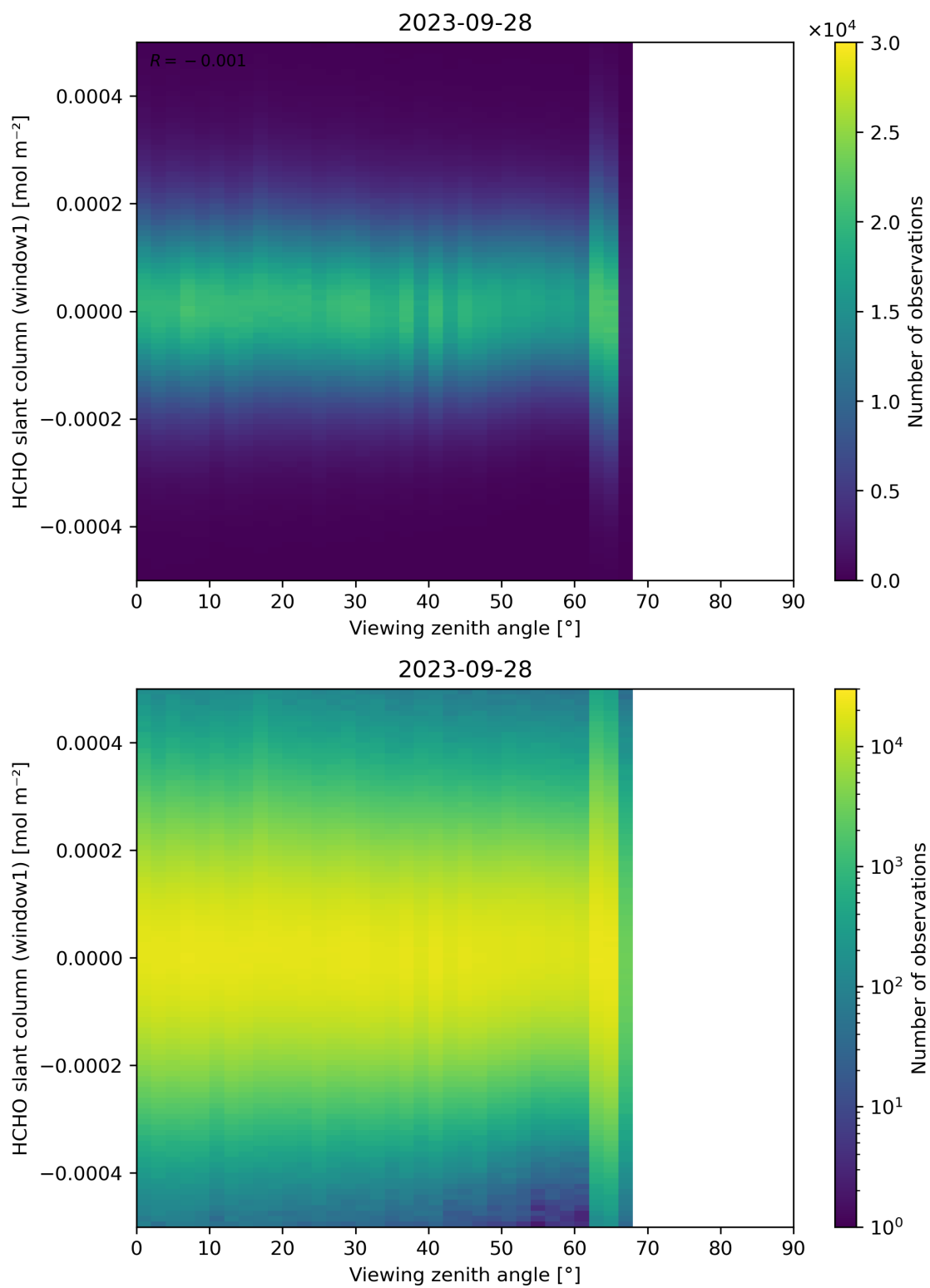
Figure 188: Scatter density plot of “Viewing zenith angle” against “HCHO slant column (window1)” for 2023-09-27 to 2023-09-29.
