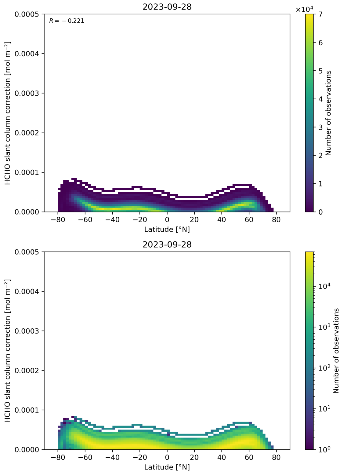
Figure 158: Scatter density plot of “Latitude” against “HCHO slant column correction” for 2023-09-27 to 2023-09-29.
