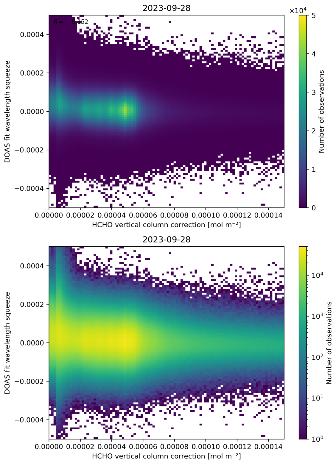
Figure 114: Scatter density plot of “HCHO vertical column correction” against “DOAS fit wavelength squeeze” for 2023-09-27 to 2023-09-29.
