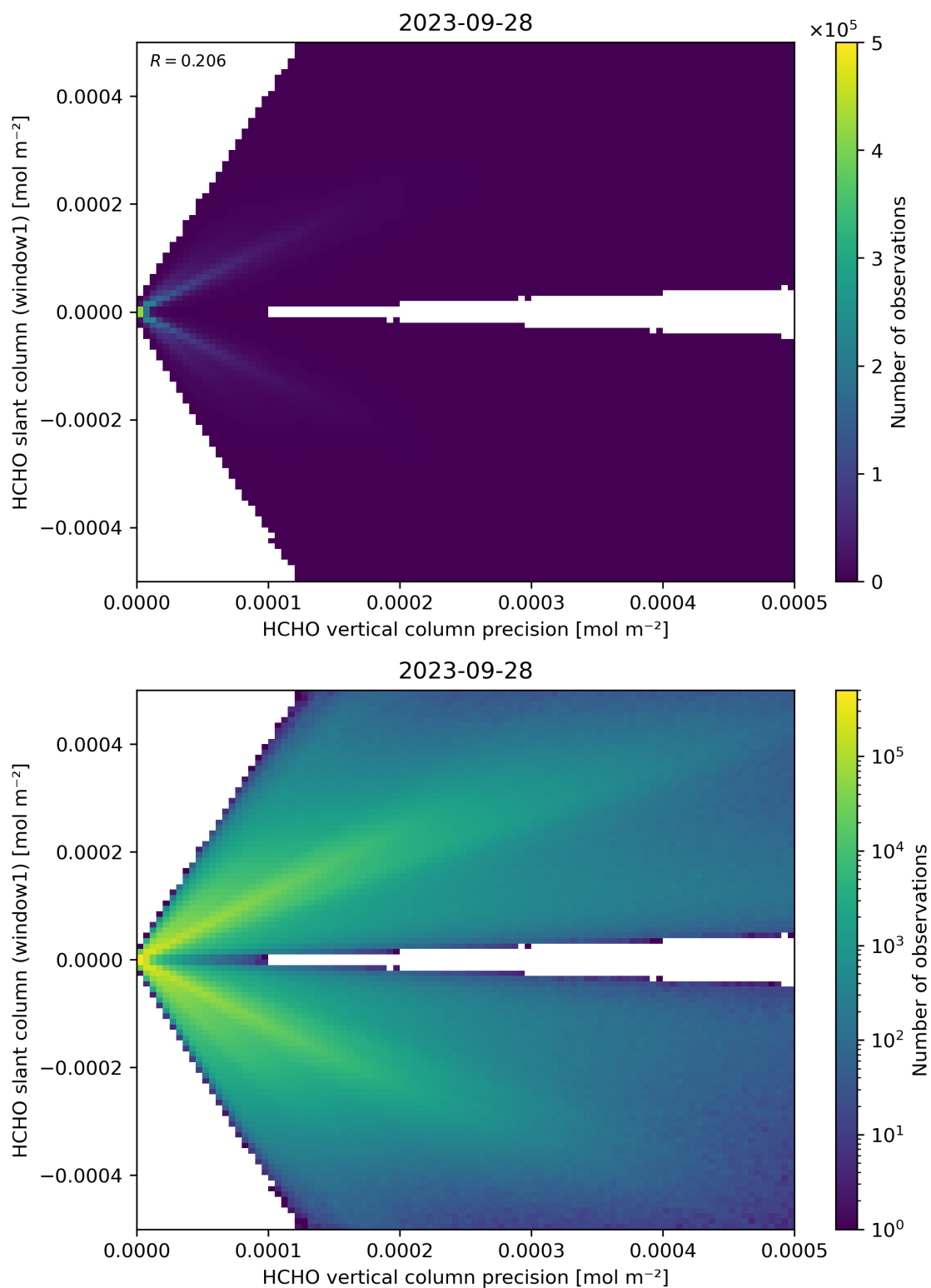
Figure 142: Scatter density plot of “HCHO vertical column precision” against “HCHO slant column (window1)” for 2023-09-27 to 2023-09-29.
