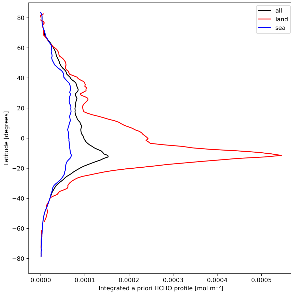
Figure 29: Zonal average of “Integrated a priori HCHO profile” for 2023-09-27 to 2023-09-29.
