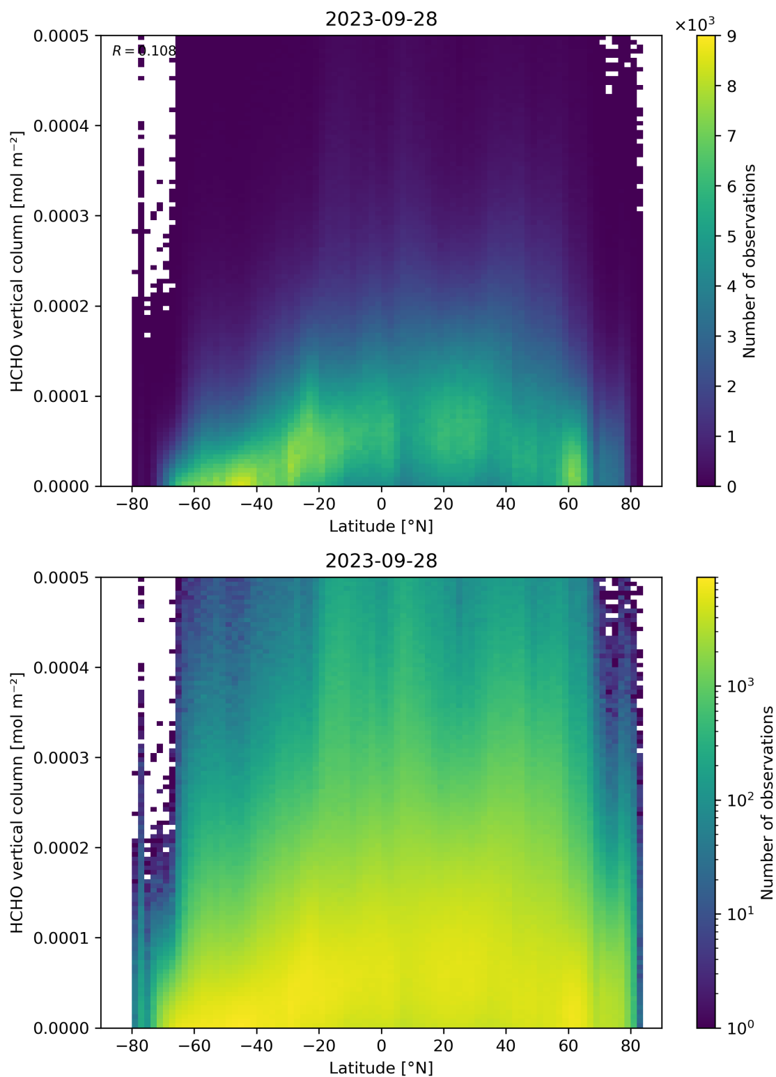
Figure 163: Scatter density plot of “Latitude” against “HCHO vertical column” for 2023-09-27 to 2023-09-29.
