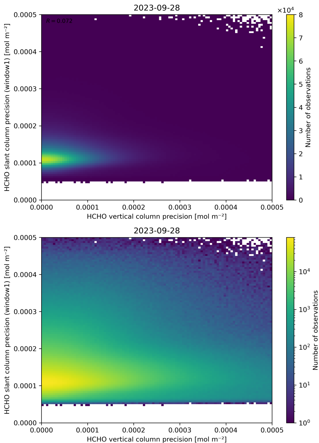
Figure 143: Scatter density plot of “HCHO vertical column precision” against “HCHO slant column precision (window1)” for 2023-09-27 to 2023-09-29.
