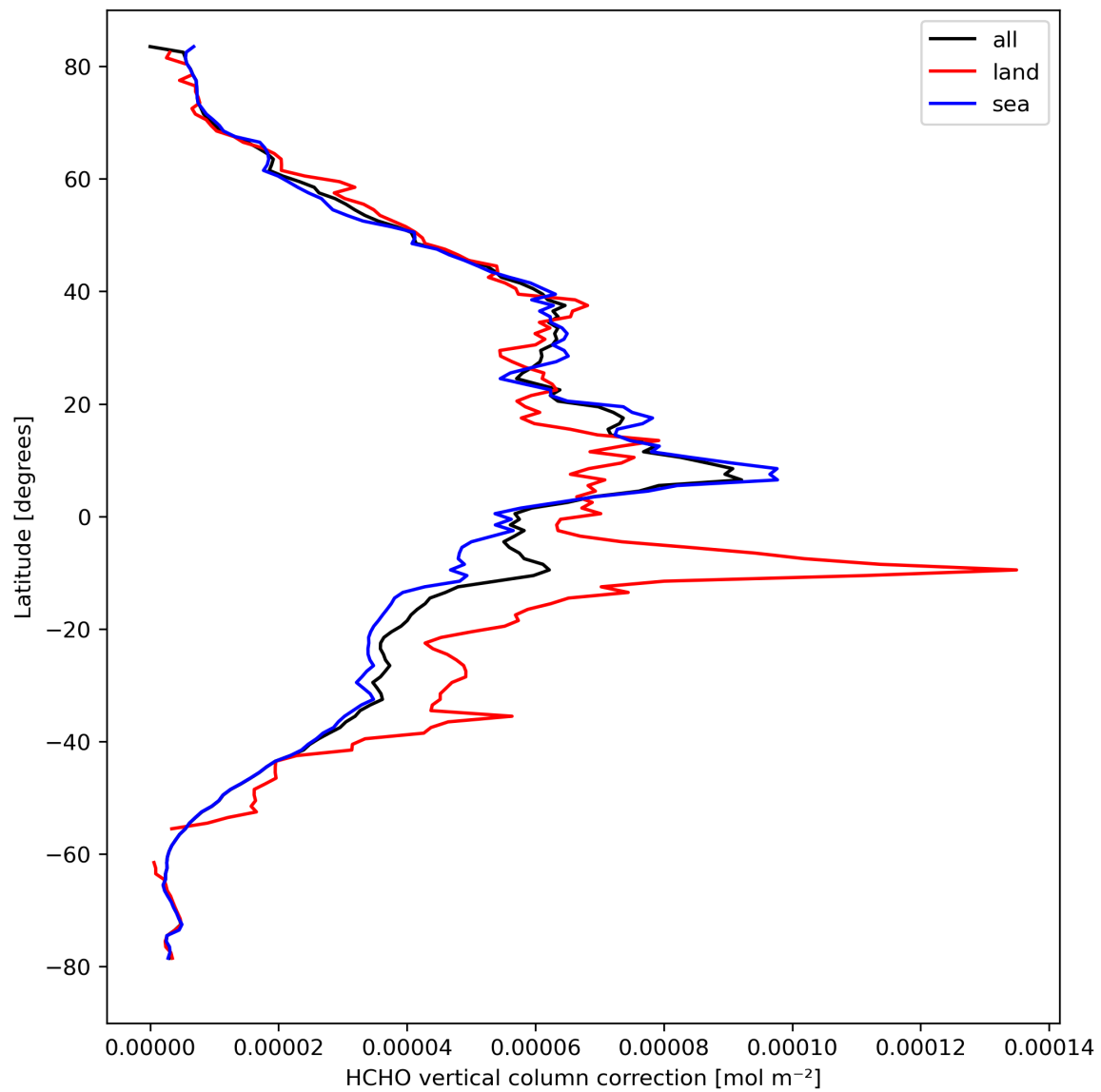
Figure 23: Zonal average of “HCHO vertical column correction” for 2023-09-27 to 2023-09-29.
