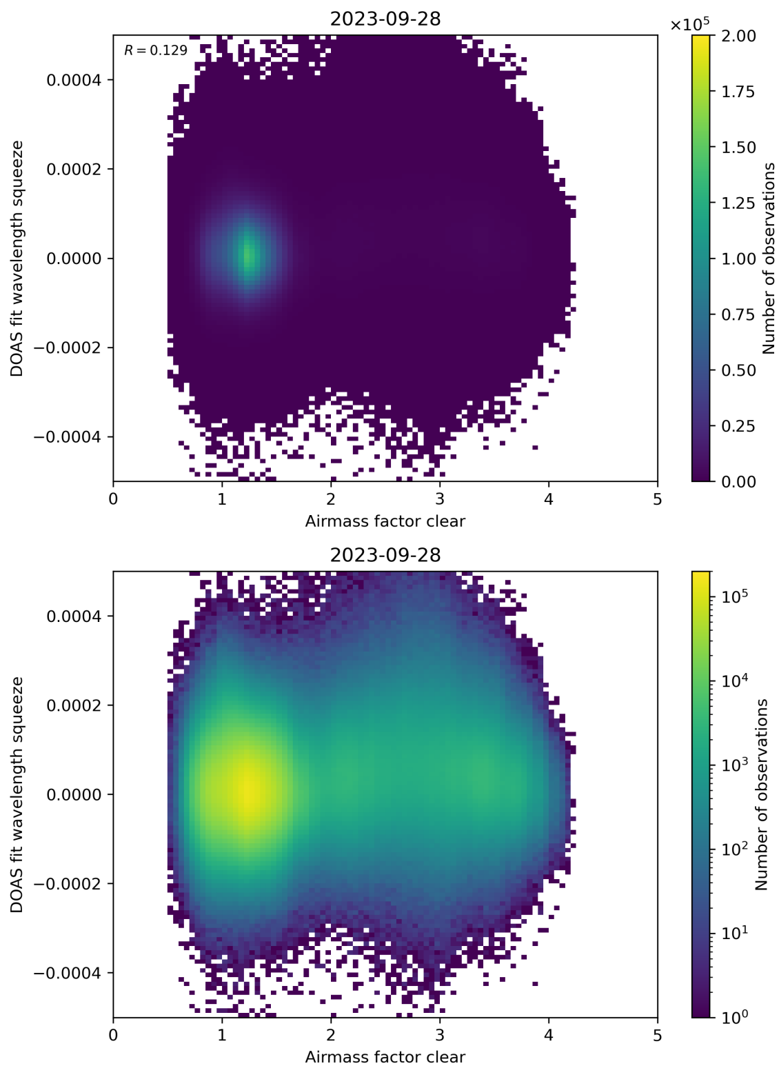
Figure 73: Scatter density plot of “Airmass factor clear” against “DOAS fit wavelength squeeze” for 2023-09-27 to 2023-09-29.
