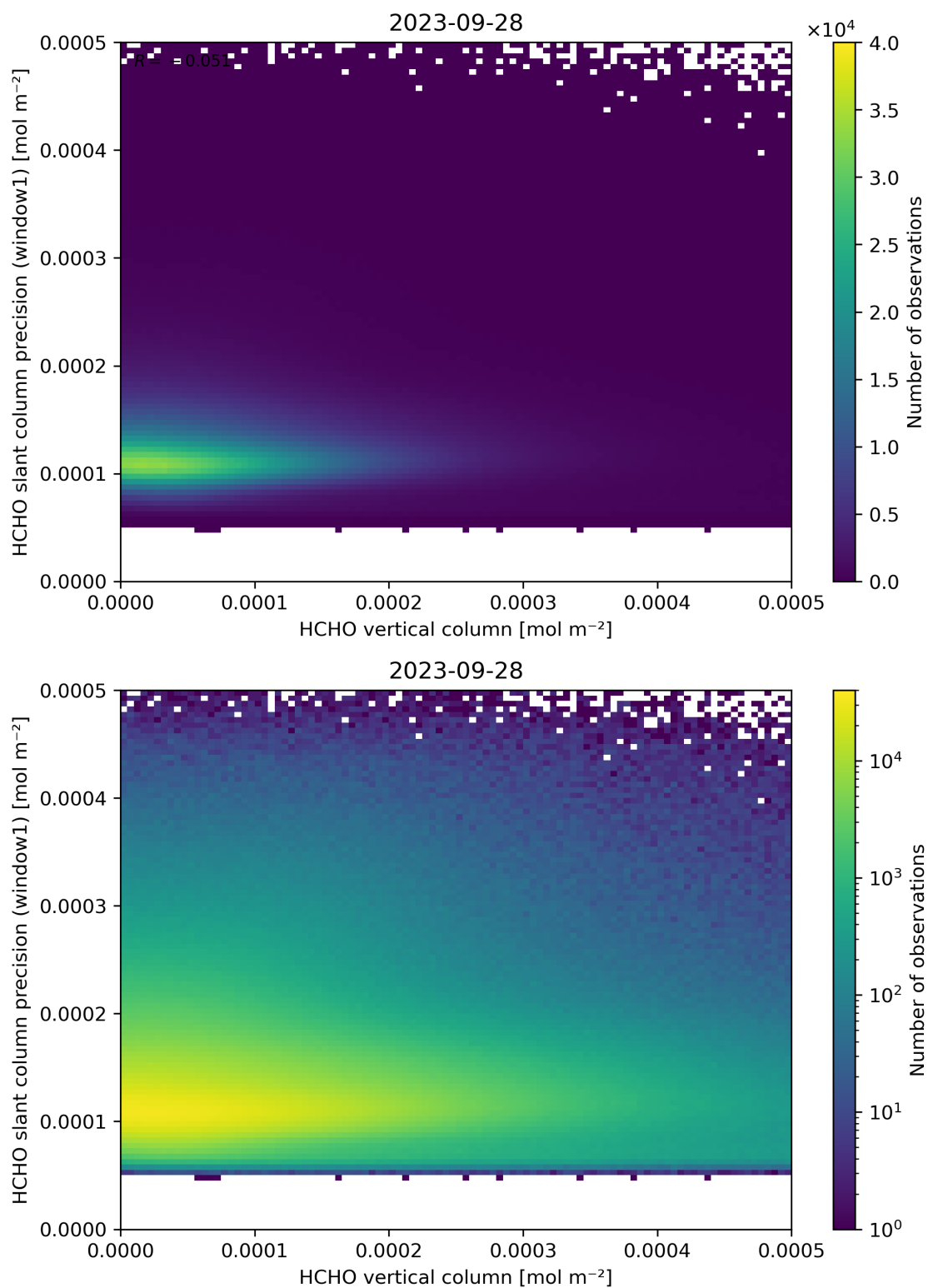
Figure 130: Scatter density plot of “HCHO vertical column” against “HCHO slant column precision (window1)” for 2023-09-27 to 2023-09-29.
