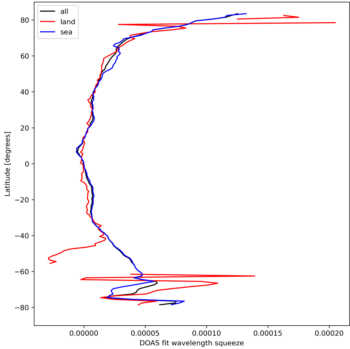
Figure 31: Zonal average of “DOAS fit wavelength squeeze” for 2023-09-27 to 2023-09-29.
