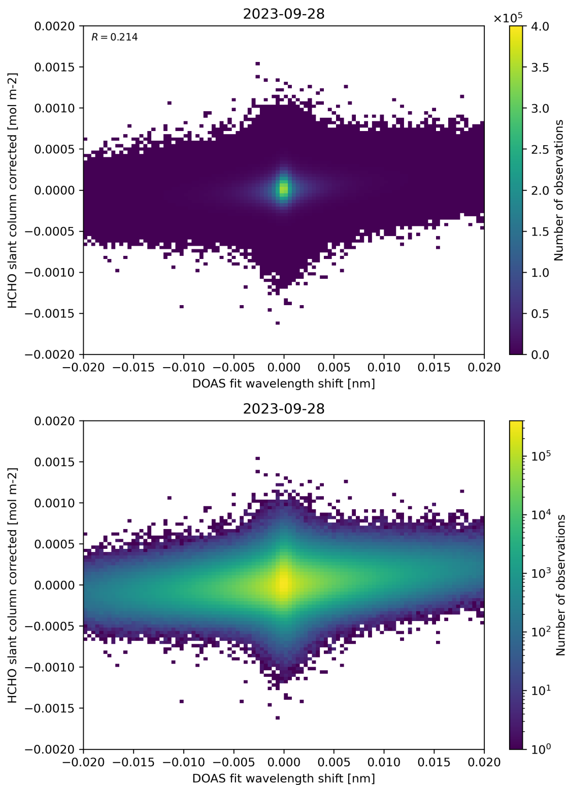
Figure 66: Scatter density plot of “DOAS fit wavelength shift” against “HCHO slant column corrected” for 2023-09-27 to 2023-09-29.
