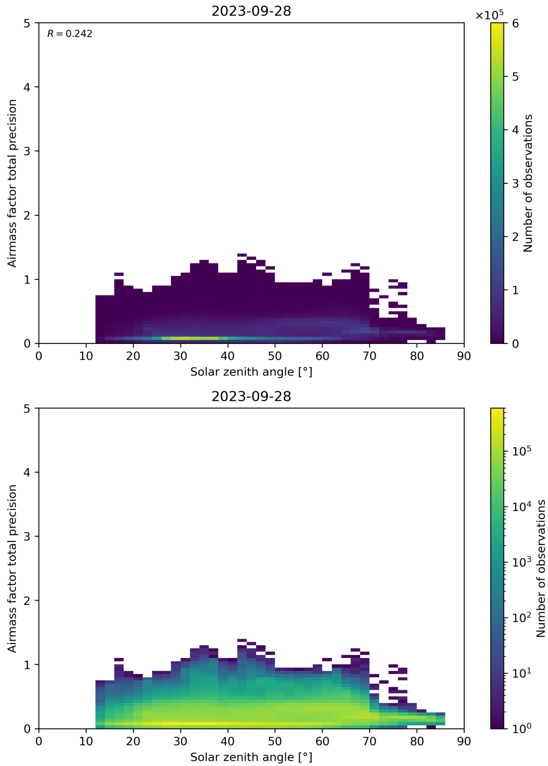
Figure 176: Scatter density plot of “Solar zenith angle” against “Airmass factor total precision” for 2023-09-27 to 2023-09-29.
