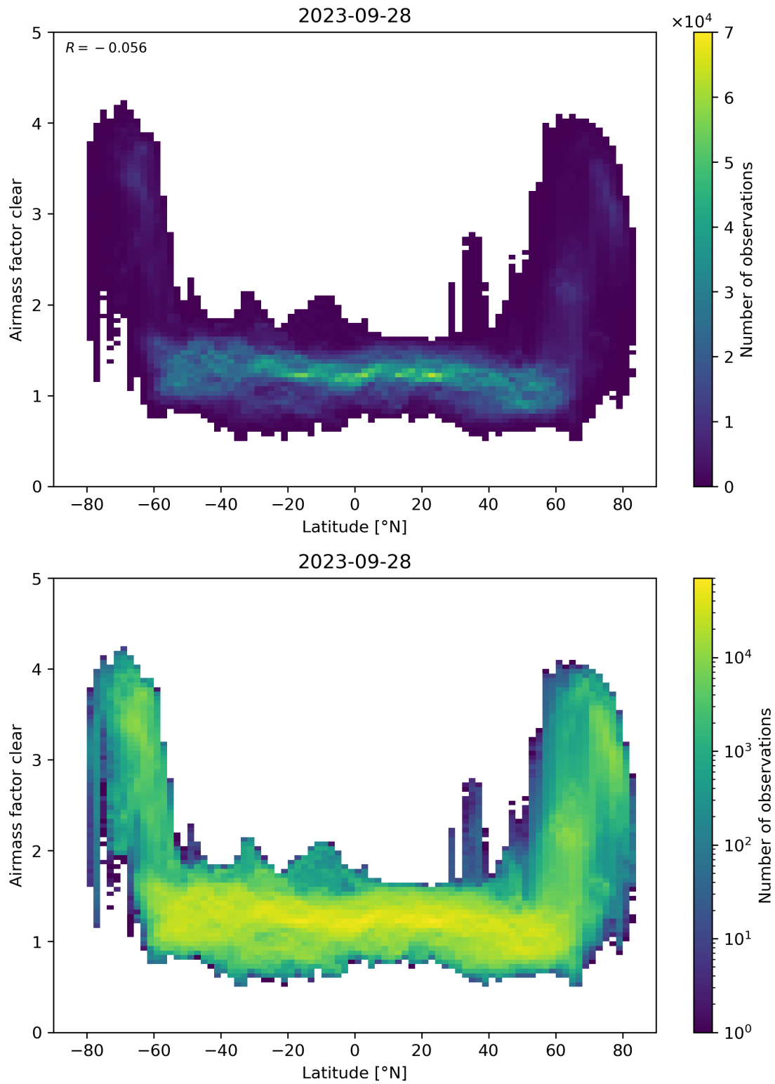
Figure 156: Scatter density plot of “Latitude” against “Airmass factor clear” for 2023-09-27 to 2023-09-29.
