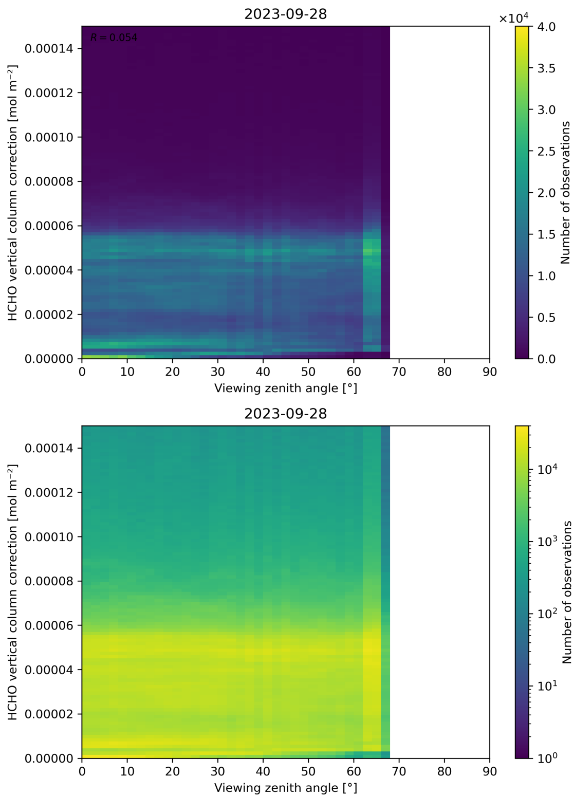
Figure 193: Scatter density plot of “Viewing zenith angle” against “HCHO vertical column correction” for 2023-09-27 to 2023-09-29.
