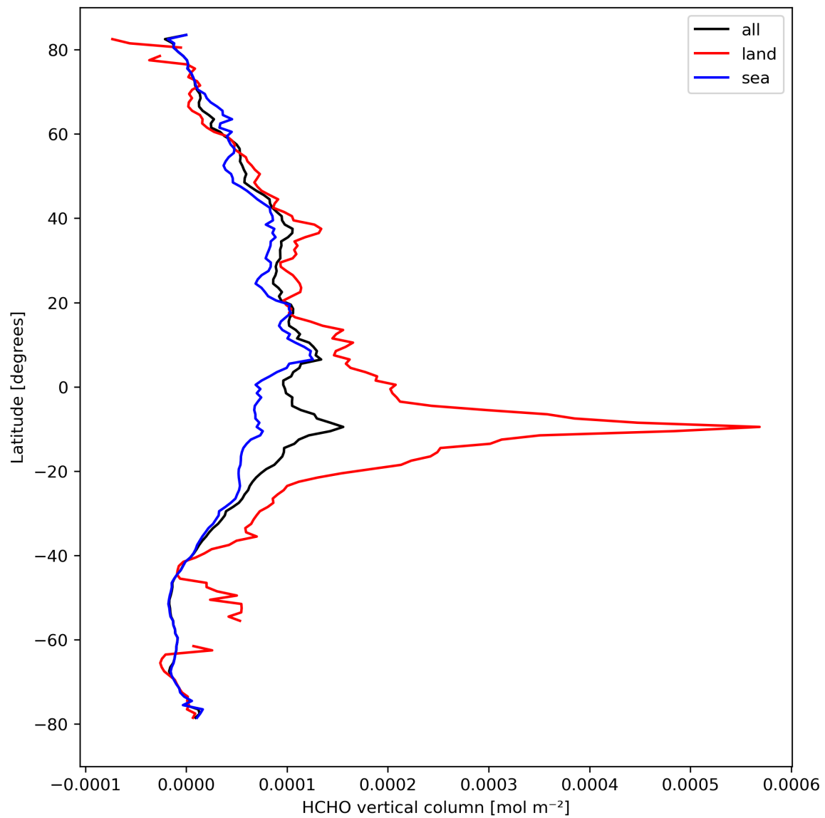
Figure 21: Zonal average of “HCHO vertical column” for 2023-09-27 to 2023-09-29.
