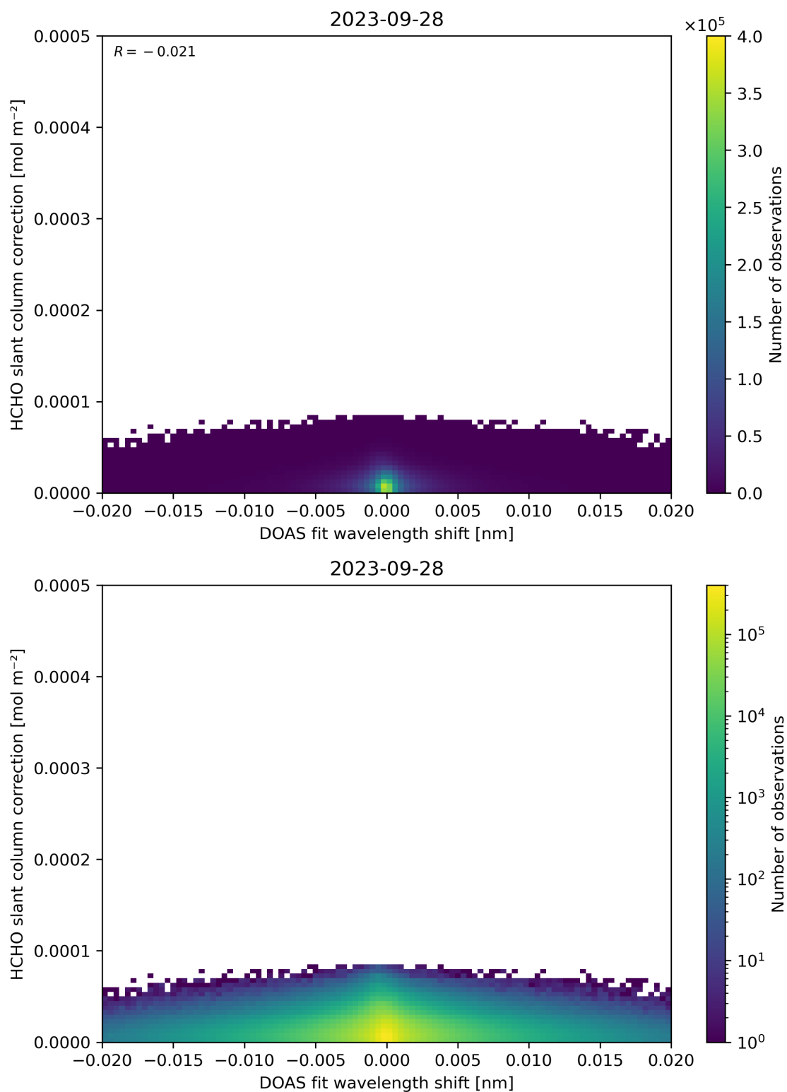
Figure 67: Scatter density plot of “DOAS fit wavelength shift” against “HCHO slant column correction” for 2023-09-27 to 2023-09-29.
