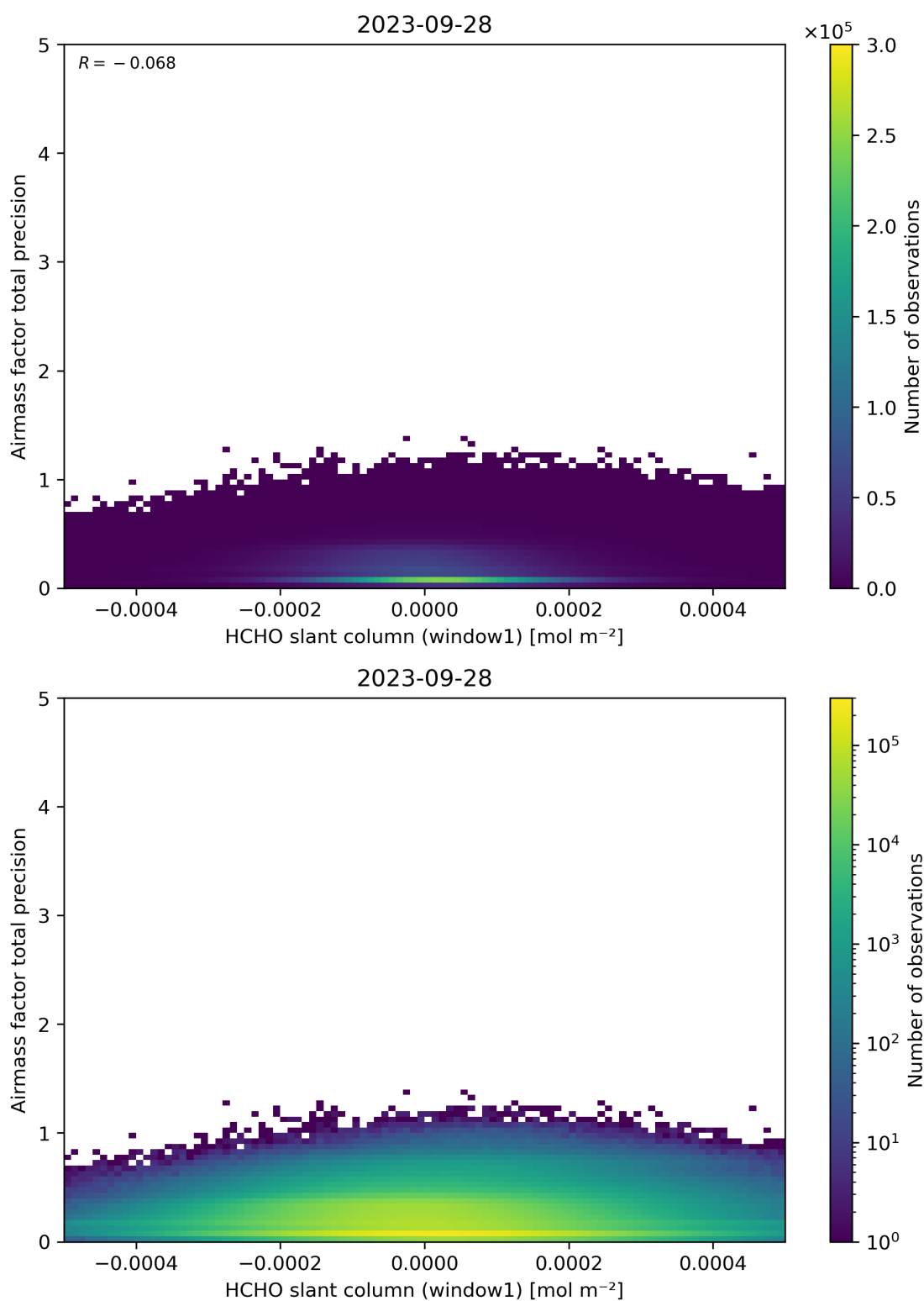
Figure 86: Scatter density plot of “HCHO slant column (window1)” against “Airmass factor total precision” for 2023-09-27 to 2023-09-29.
