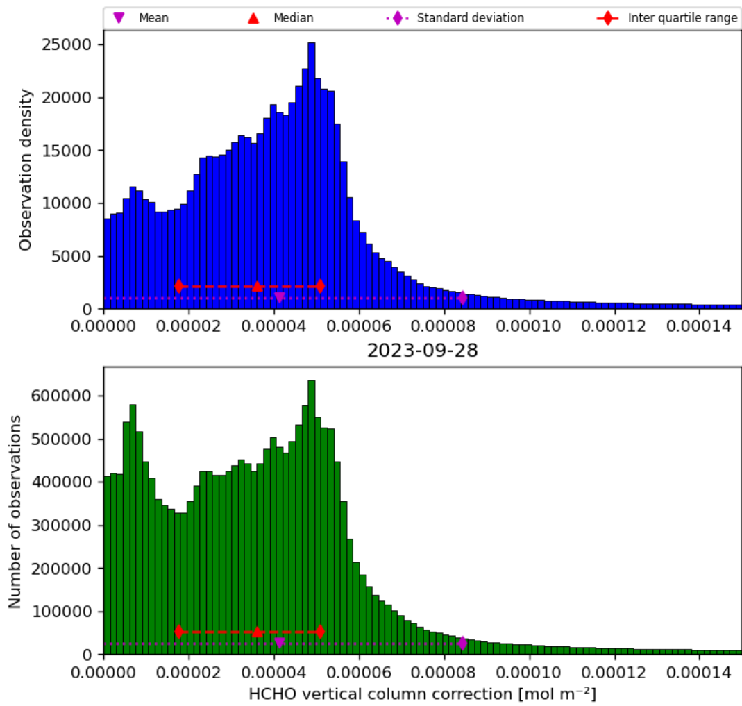
Figure 37: Histogram of “HCHO vertical column correction” for 2023-09-27 to 2023-09-29
