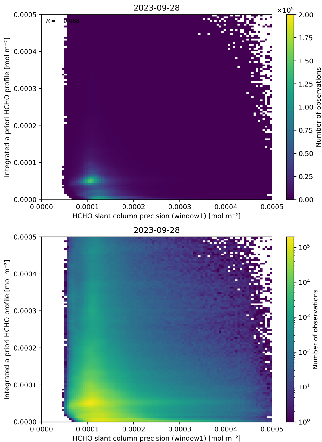
Figure 96: Scatter density plot of “HCHO slant column precision (window1)” against “Integrated a priori HCHO profile” for 2023-09-27 to 2023-09-29.
