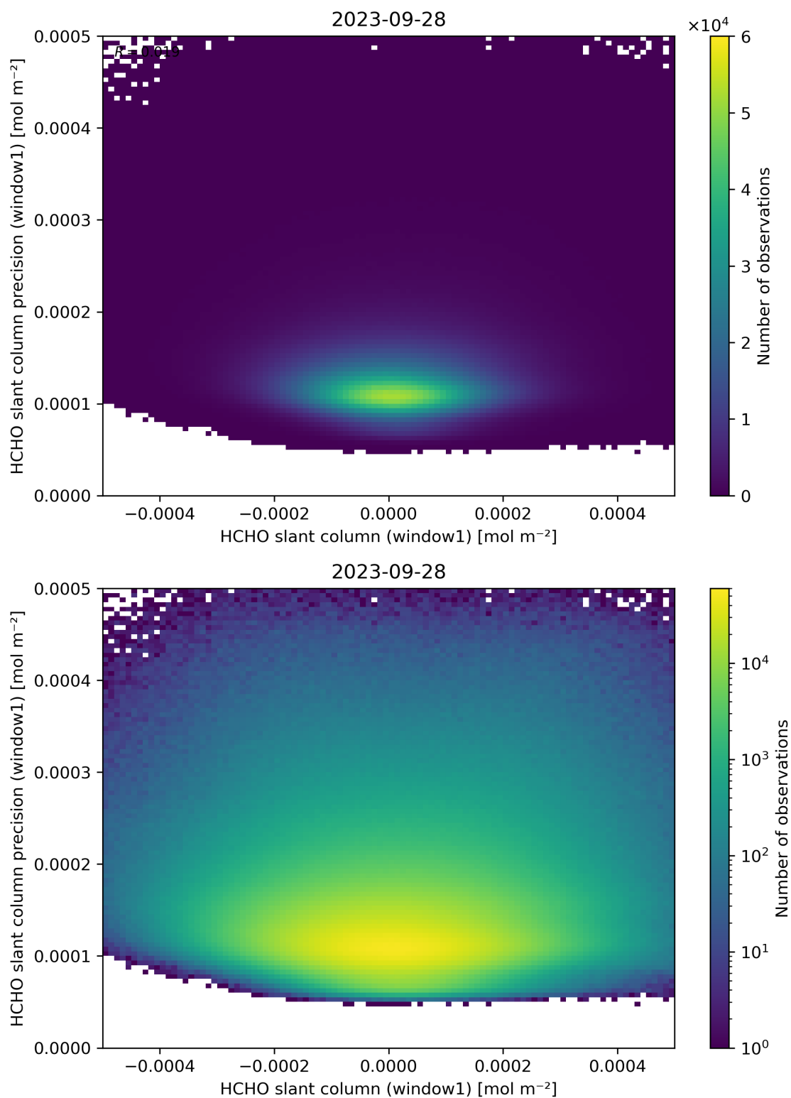
Figure 84: Scatter density plot of “HCHO slant column (window1)” against “HCHO slant column precision (window1)” for 2023-09-27 to 2023-09-29.
