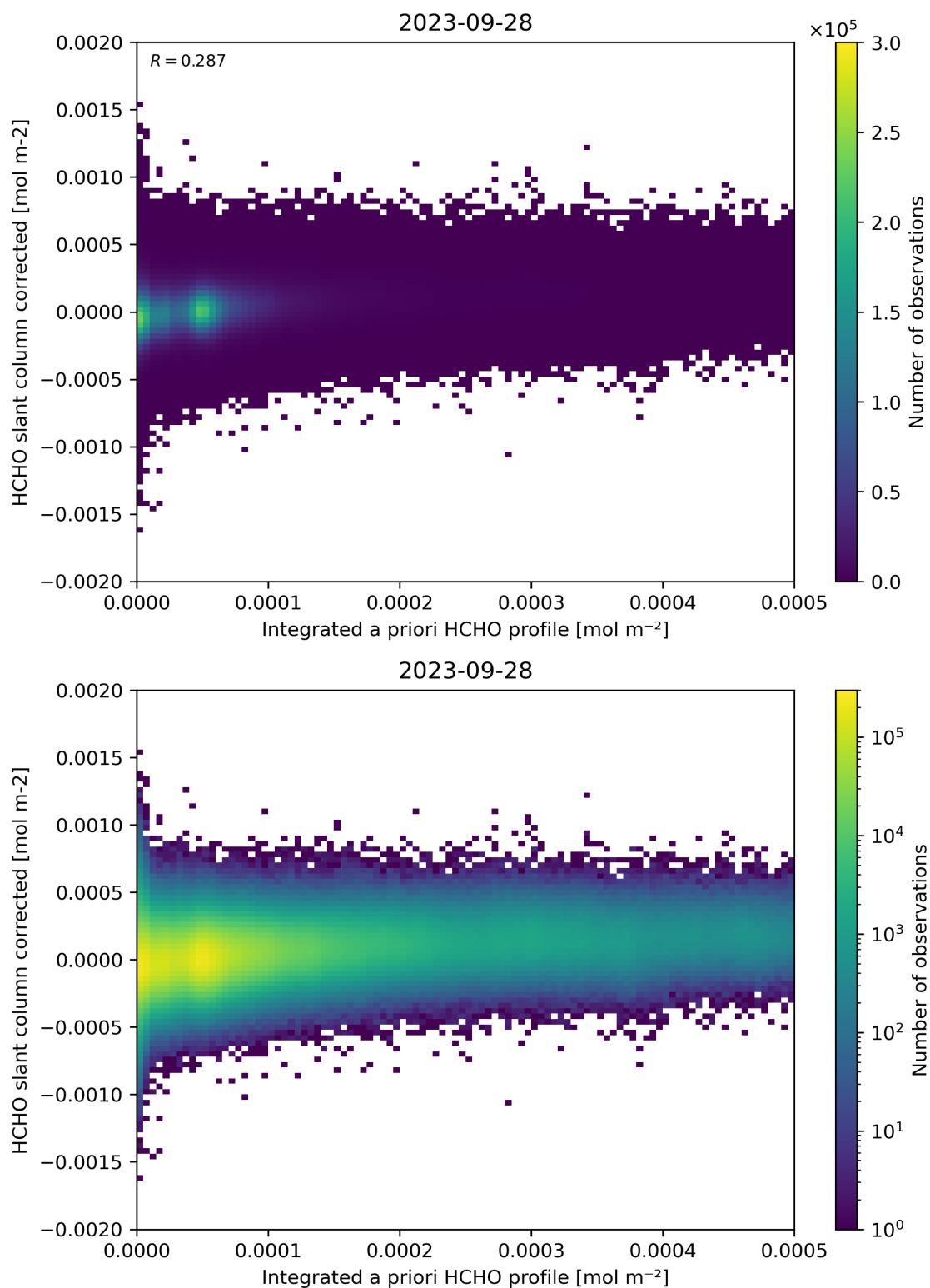
Figure 151: Scatter density plot of “Integrated a priori HCHO profile” against “HCHO slant column corrected” for 2023-09-27 to 2023-09-29.
