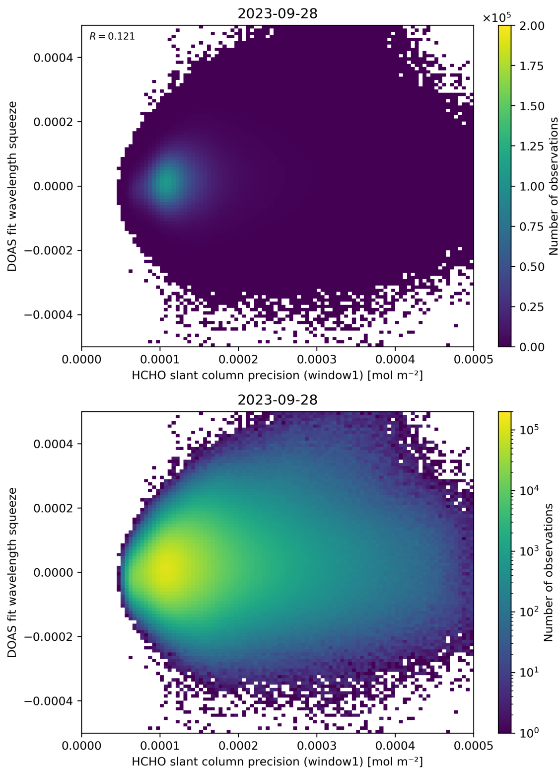
Figure 90: Scatter density plot of “HCHO slant column precision (window1)” against “DOAS fit wavelength squeeze” for 2023-09-27 to 2023-09-29.
