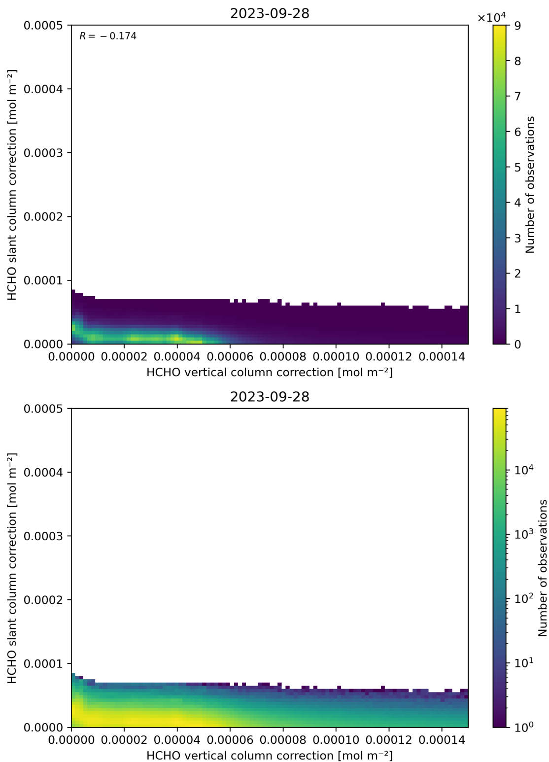
Figure 117: Scatter density plot of “HCHO vertical column correction” against “HCHO slant column correction” for 2023-09-27 to 2023-09-29.
