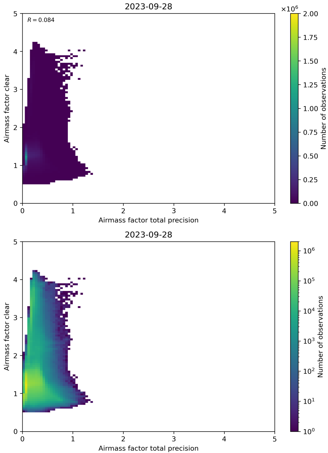
Figure 108: Scatter density plot of “Airmass factor total precision” against “Airmass factor clear” for 2023-09-27 to 2023-09-29.
