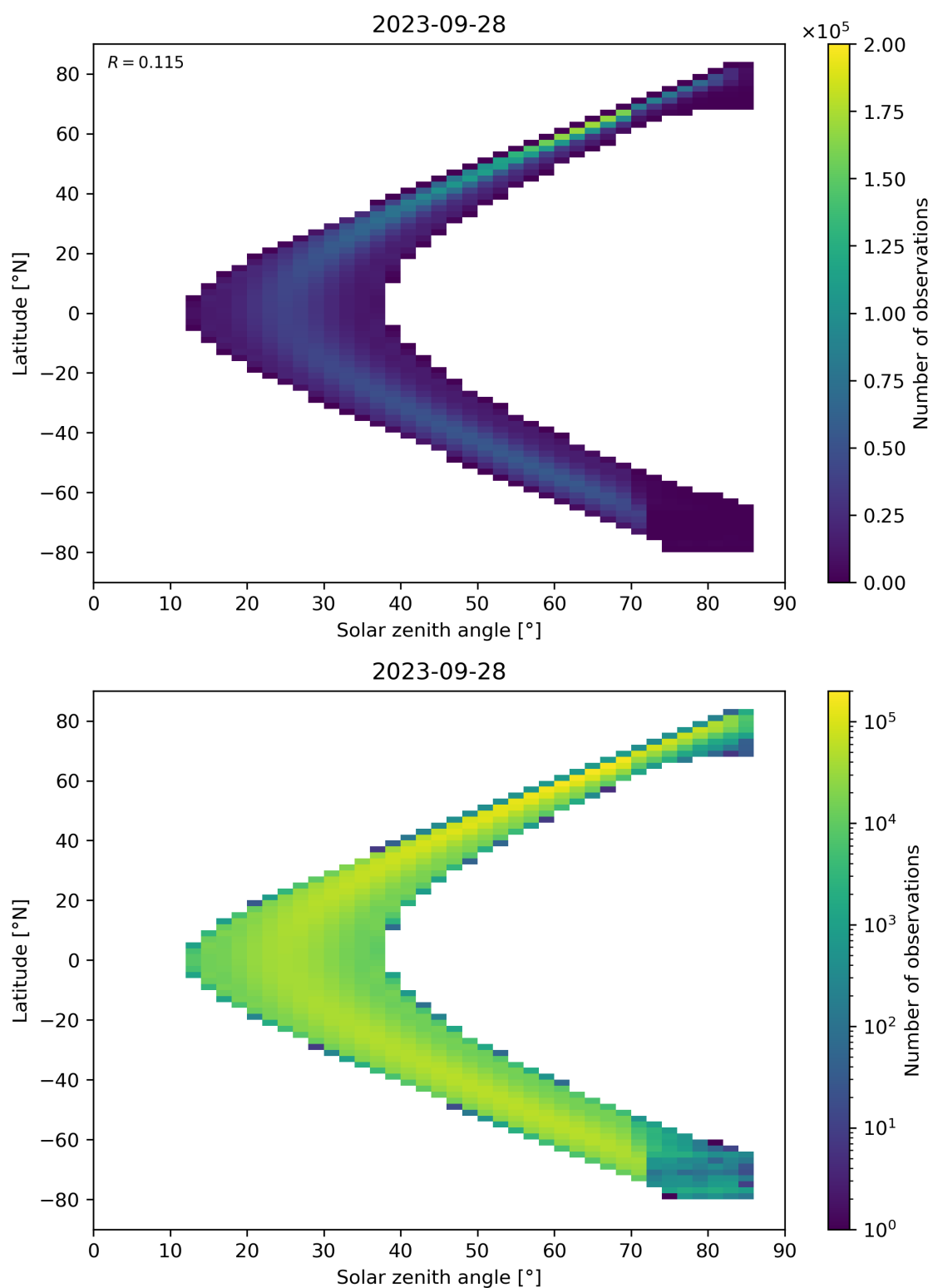
Figure 181: Scatter density plot of “Solar zenith angle” against “Latitude” for 2023-09-27 to 2023-09-29.
