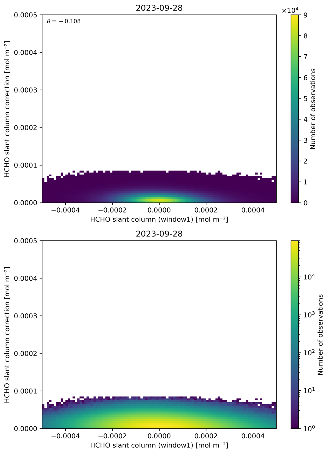
Figure 83: Scatter density plot of “HCHO slant column (window1)” against “HCHO slant column correction” for 2023-09-27 to 2023-09-29.
