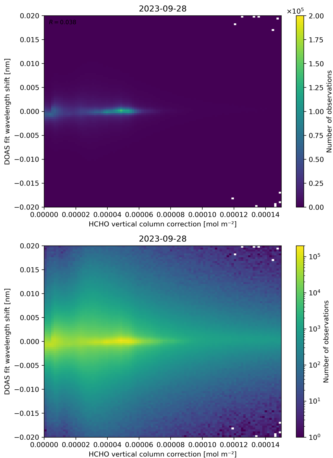
Figure 113: Scatter density plot of “HCHO vertical column correction” against “DOAS fit wavelength shift” for 2023-09-27 to 2023-09-29.
