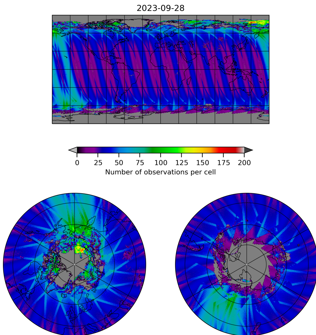
Figure 19: Map of the number of observations for 2023-09-27 to 2023-09-29
