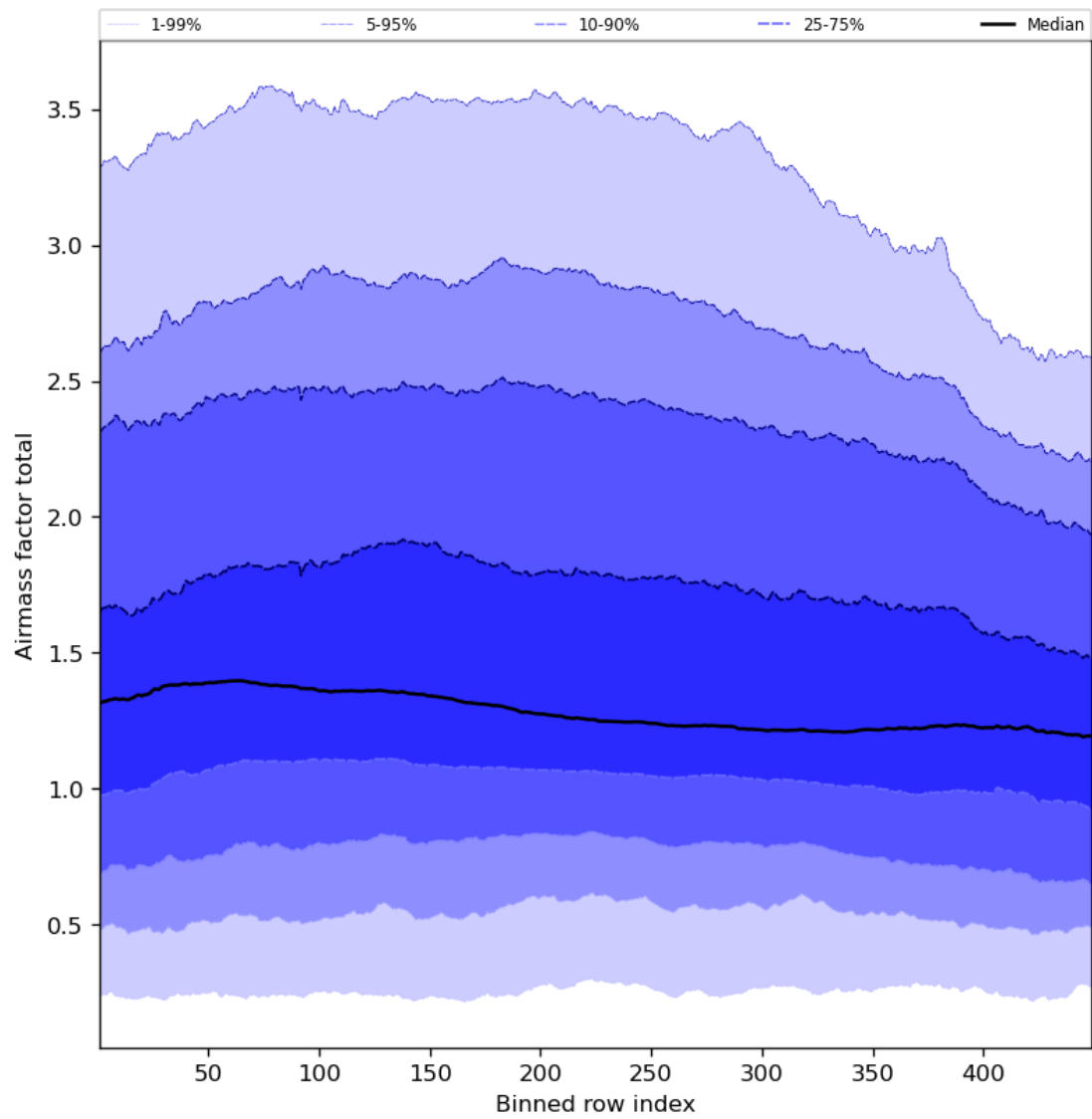
Figure 54: Along track statistics of “Airmass factor total” for 2023-09-27 to 2023-09-29
