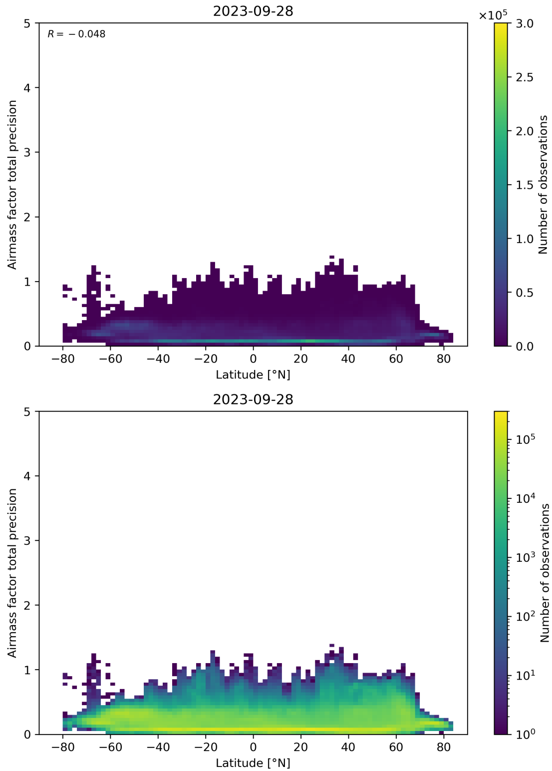
Figure 162: Scatter density plot of “Latitude” against “Airmass factor total precision” for 2023-09-27 to 2023-09-29.
