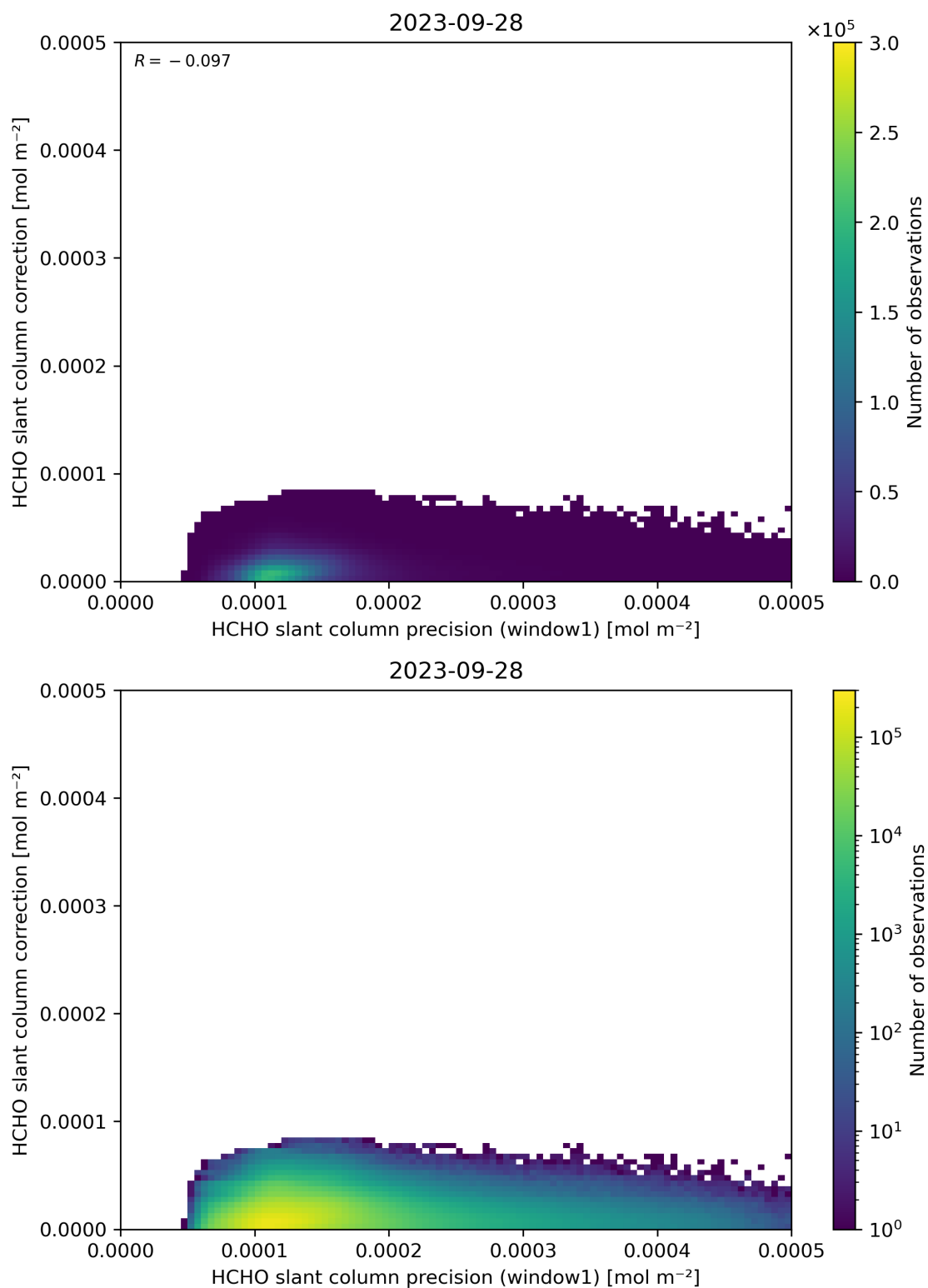
Figure 93: Scatter density plot of “HCHO slant column precision (window1)” against “HCHO slant column correction” for 2023-09-27 to 2023-09-29.
