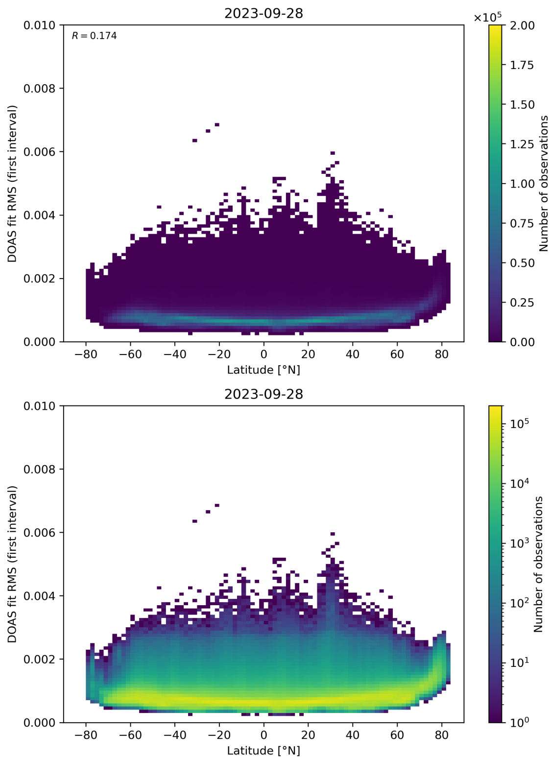
Figure 153: Scatter density plot of “Latitude” against “DOAS fit RMS (first interval)” for 2023-09-27 to 2023-09-29.
