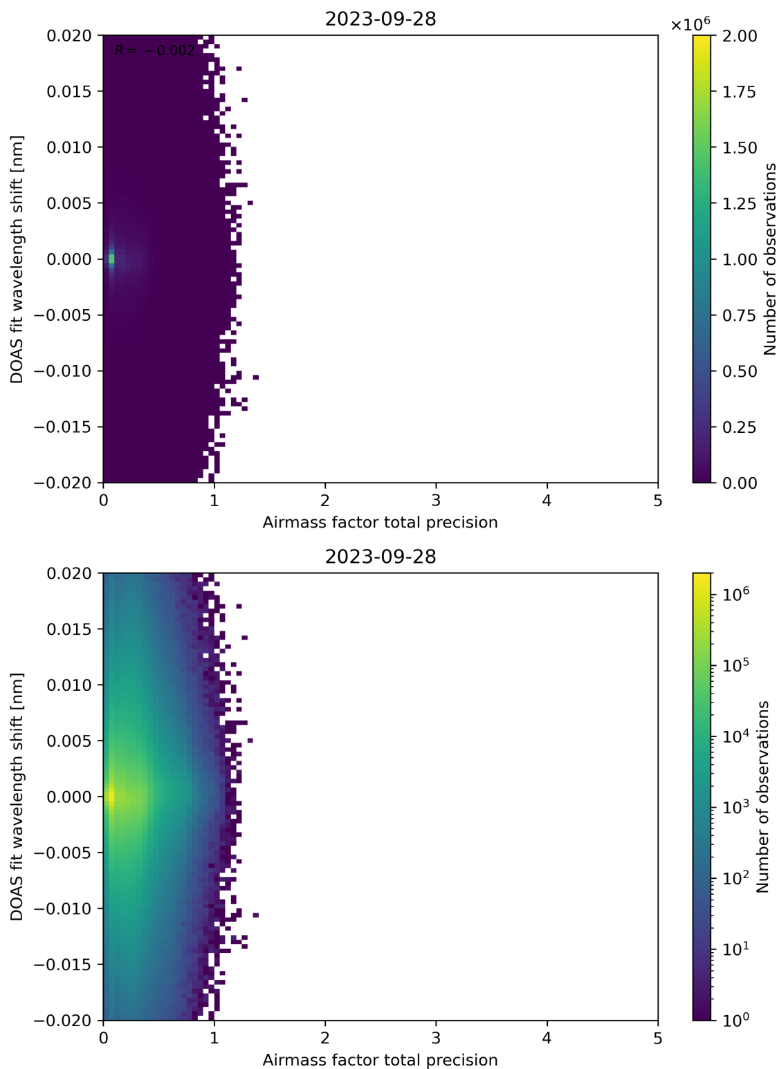
Figure 106: Scatter density plot of “Airmass factor total precision” against “DOAS fit wavelength shift” for 2023-09-27 to 2023-09-29.
