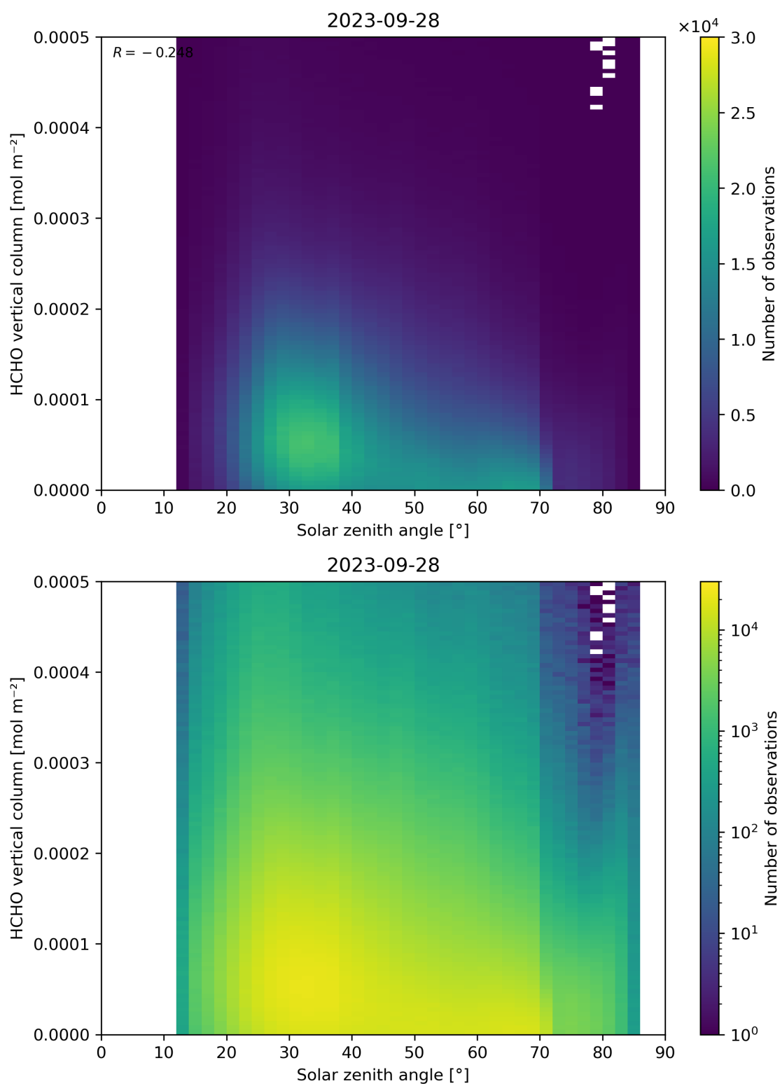
Figure 177: Scatter density plot of “Solar zenith angle” against “HCHO vertical column” for 2023-09-27 to 2023-09-29.
