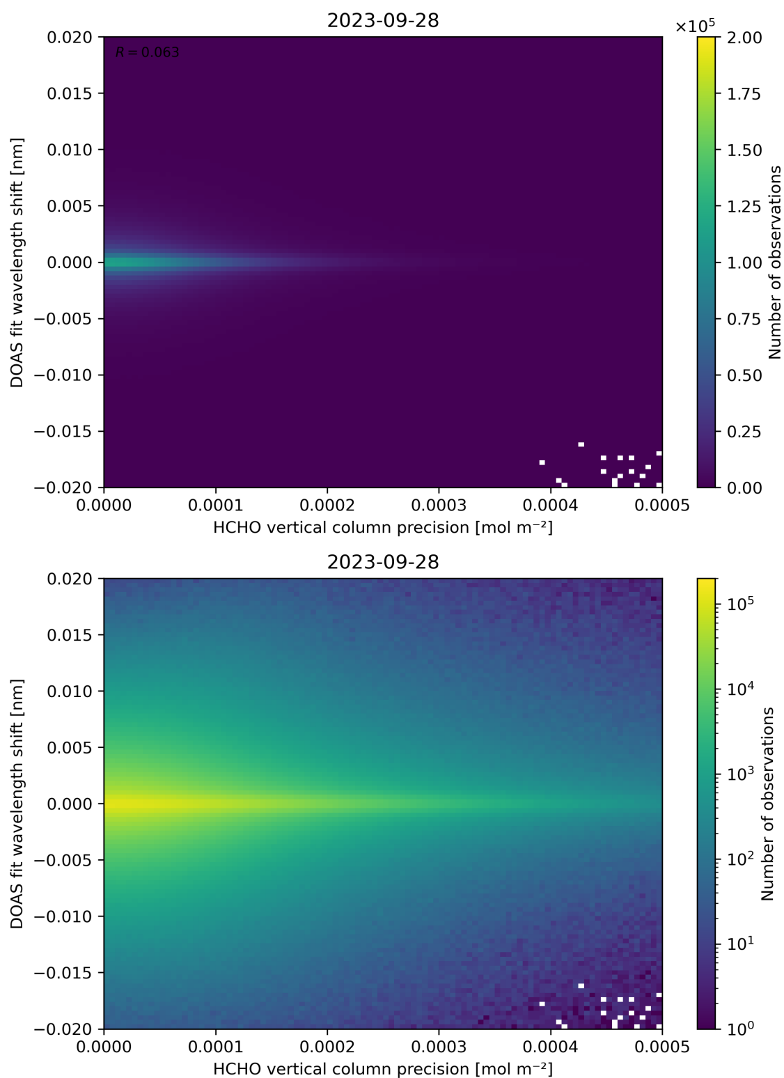
Figure 137: Scatter density plot of “HCHO vertical column precision” against “DOAS fit wavelength shift” for 2023-09-27 to 2023-09-29.
