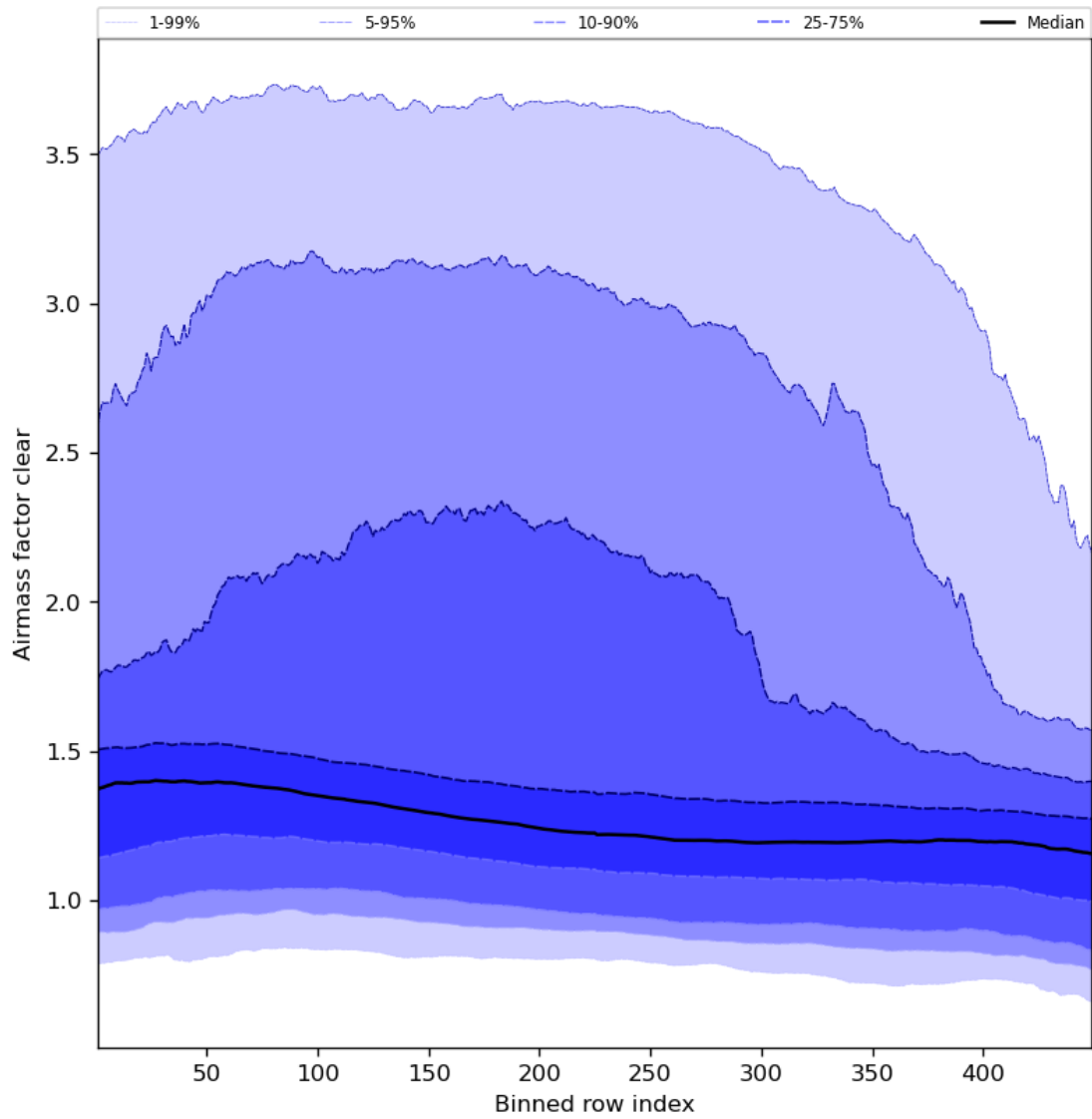
Figure 56: Along track statistics of “Airmass factor clear” for 2023-09-27 to 2023-09-29
