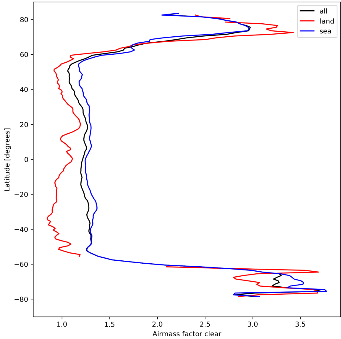
Figure 28: Zonal average of “Airmass factor clear” for 2023-09-27 to 2023-09-29.
