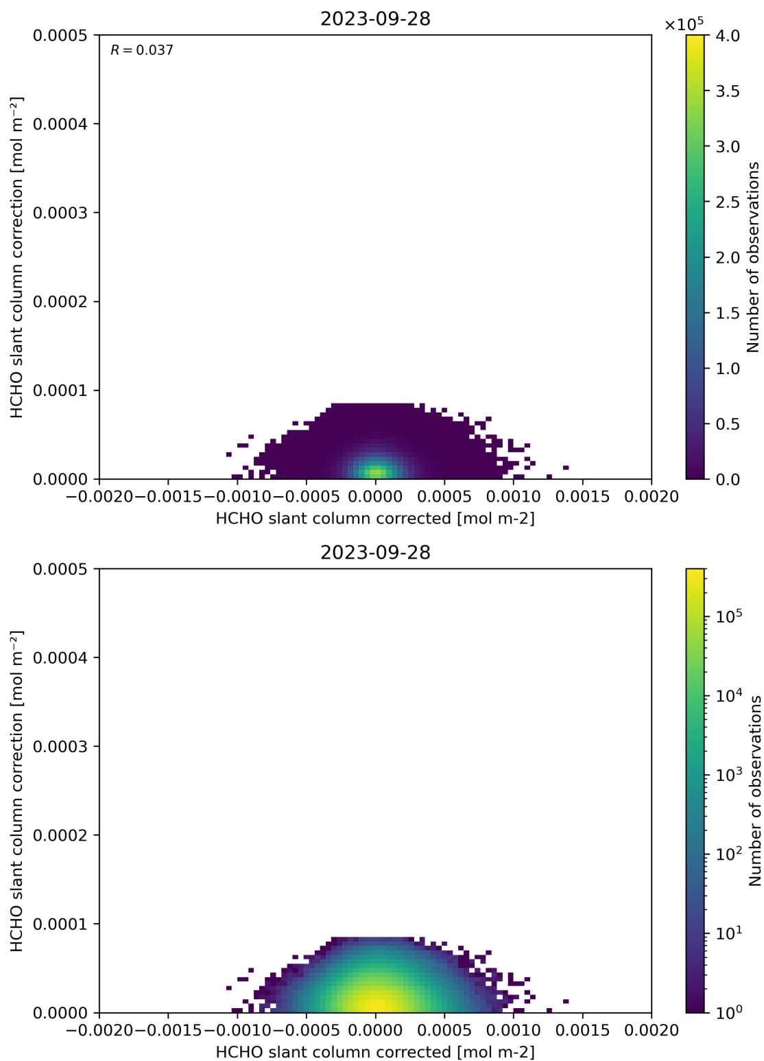
Figure 77: Scatter density plot of “HCHO slant column corrected” against “HCHO slant column correction” for 2023-09-27 to 2023-09-29.
