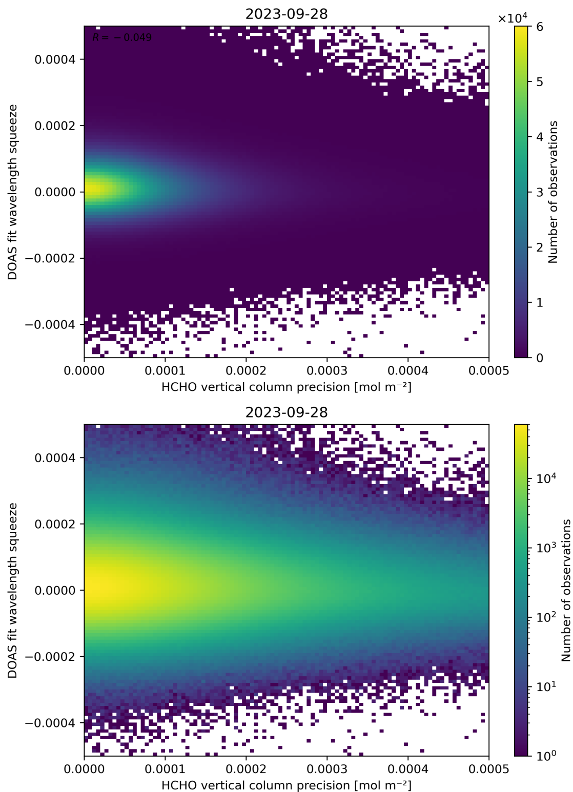
Figure 138: Scatter density plot of “HCHO vertical column precision” against “DOAS fit wavelength squeeze” for 2023-09-27 to 2023-09-29.
