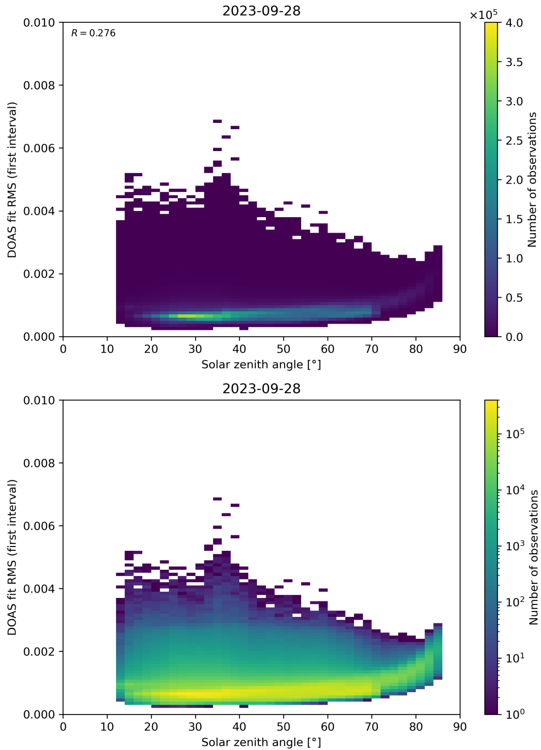
Figure 167: Scatter density plot of “Solar zenith angle” against “DOAS fit RMS (first interval)” for 2023-09-27 to 2023-09-29.
