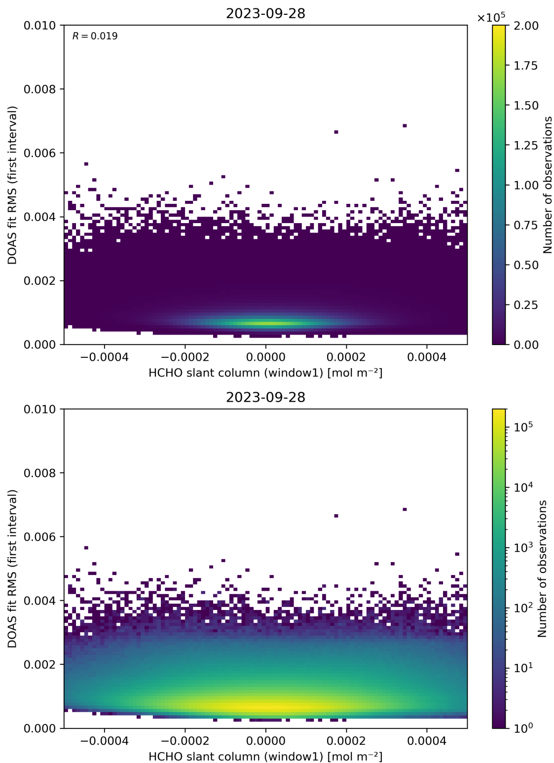
Figure 78: Scatter density plot of “HCHO slant column (window1)” against “DOAS fit RMS (first interval)” for 2023-09-27 to 2023-09-29.
