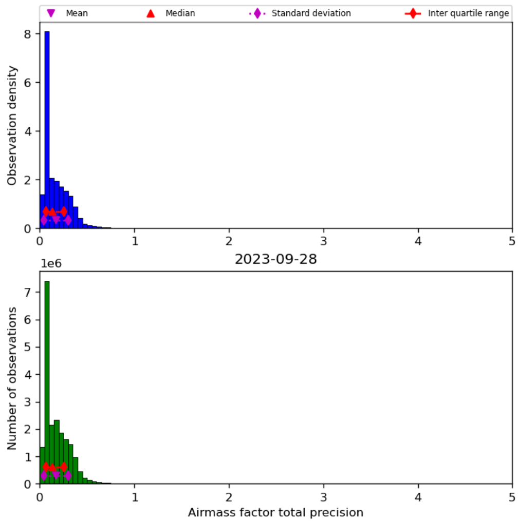
Figure 41: Histogram of "Airmass factor total precision" for 2023-09-27 to 2023-09-29
