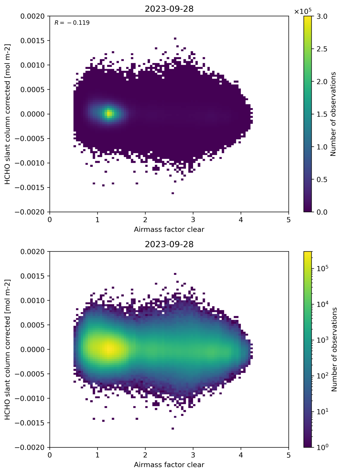
Figure 74: Scatter density plot of “Airmass factor clear” against “HCHO slant column corrected” for 2023-09-27 to 2023-09-29.
