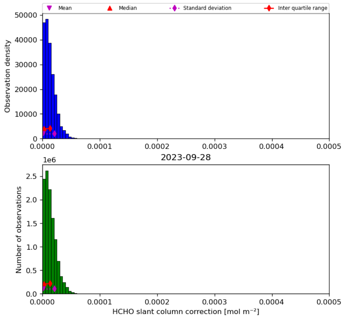
Figure 47: Histogram of “HCHO slant column correction” for 2023-09-27 to 2023-09-29
