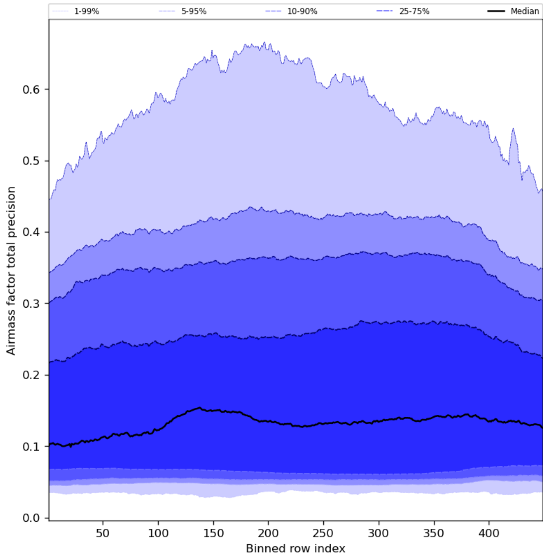
Figure 55: Along track statistics of “Airmass factor total precision” for 2023-09-27 to 2023-09-29
