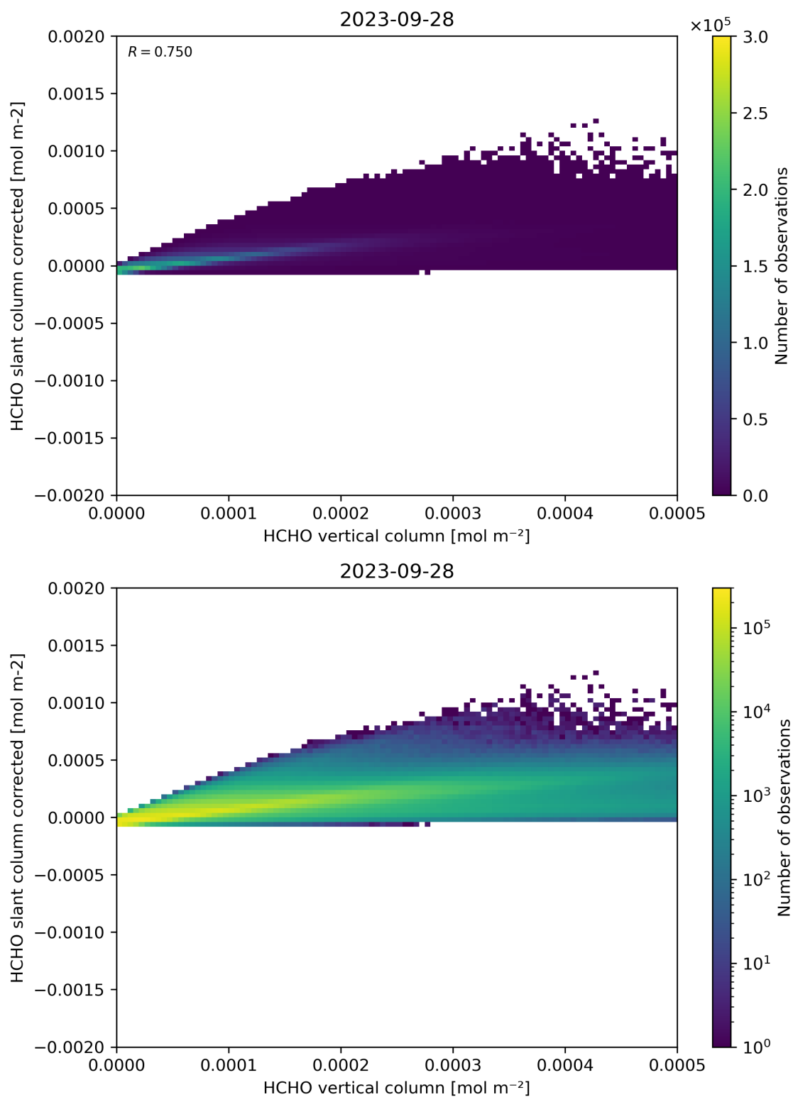
Figure 127: Scatter density plot of “HCHO vertical column” against “HCHO slant column corrected” for 2023-09-27 to 2023-09-29.
