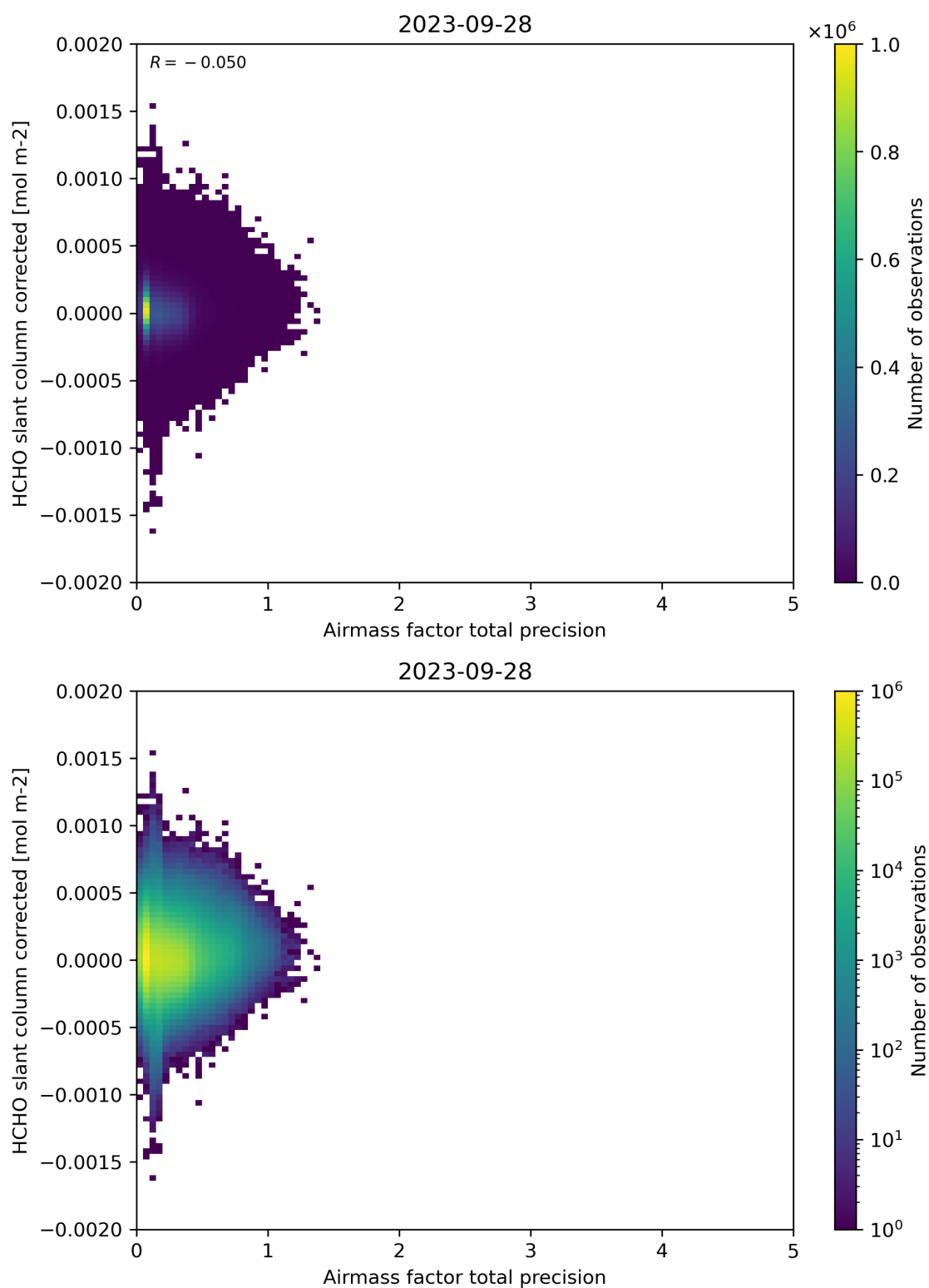
Figure 109: Scatter density plot of “Airmass factor total precision” against “HCHO slant column corrected” for 2023-09-27 to 2023-09-29.
