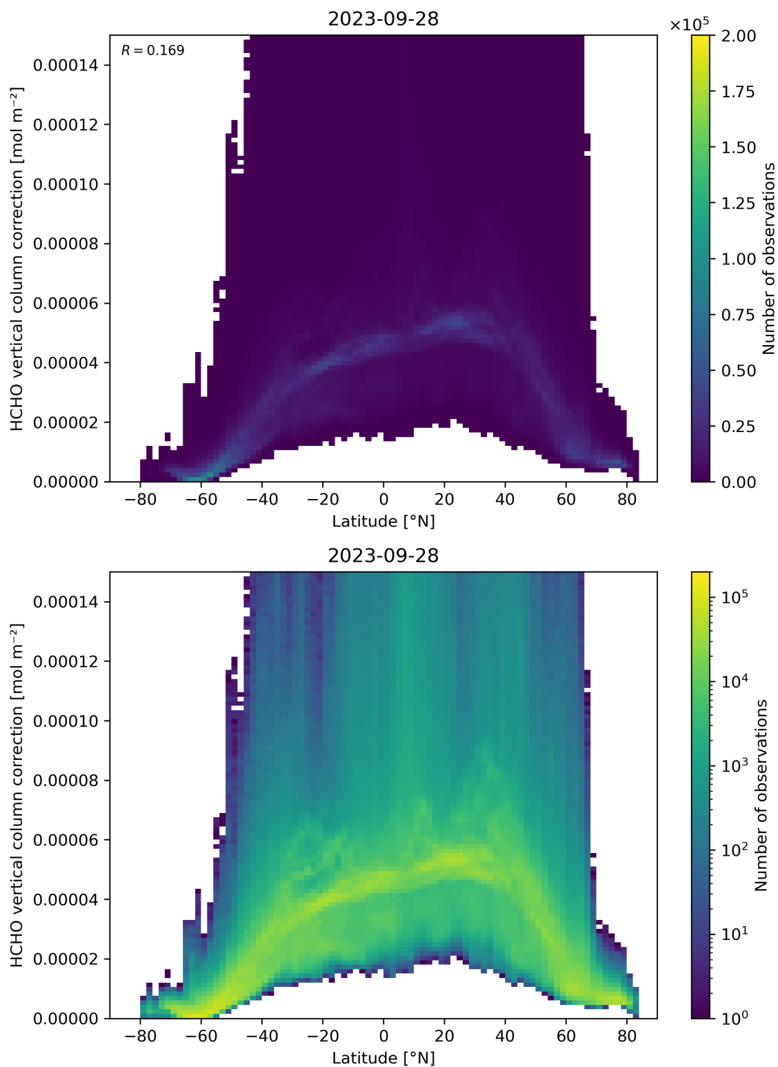
Figure 164: Scatter density plot of “Latitude” against “HCHO vertical column correction” for 2023-09-27 to 2023-09-29.
