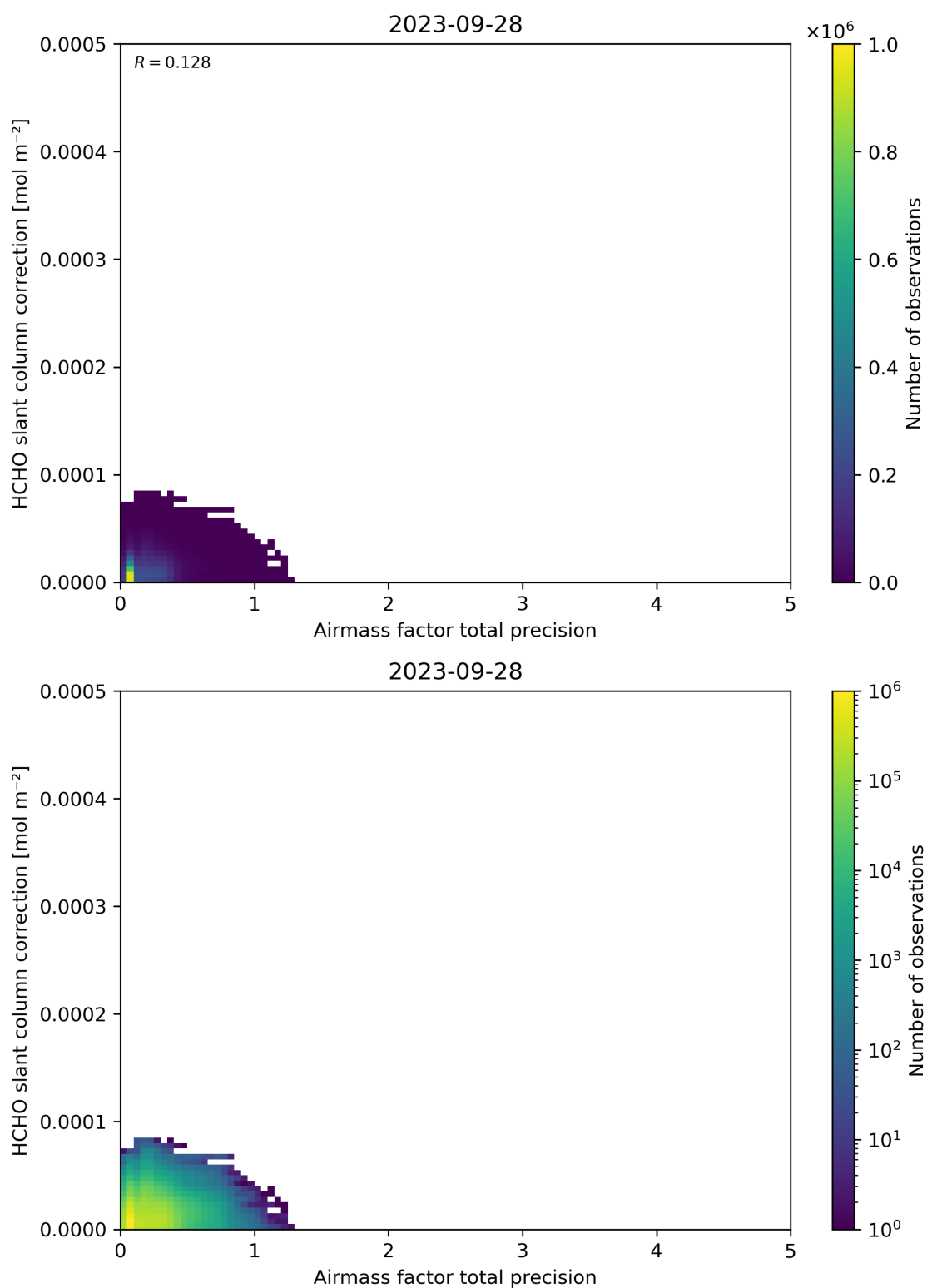
Figure 110: Scatter density plot of “Airmass factor total precision” against “HCHO slant column correction” for 2023-09-27 to 2023-09-29.
