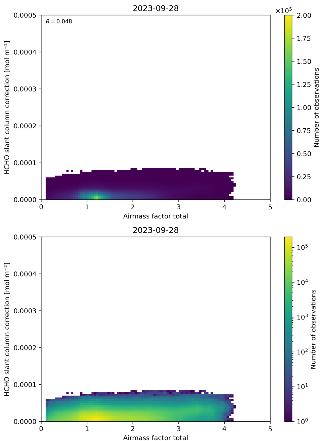
Figure 102: Scatter density plot of “Airmass factor total” against “HCHO slant column correction” for 2023-09-27 to 2023-09-29.
