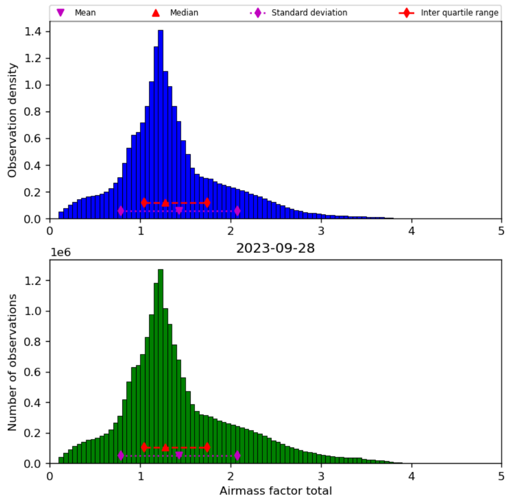
Figure 40: Histogram of “Airmass factor total” for 2023-09-27 to 2023-09-29
