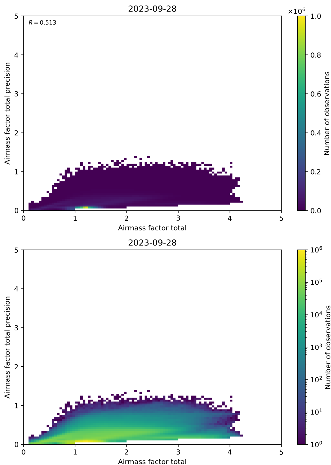
Figure 103: Scatter density plot of “Airmass factor total” against “Airmass factor total precision” for 2023-09-27 to 2023-09-29.
