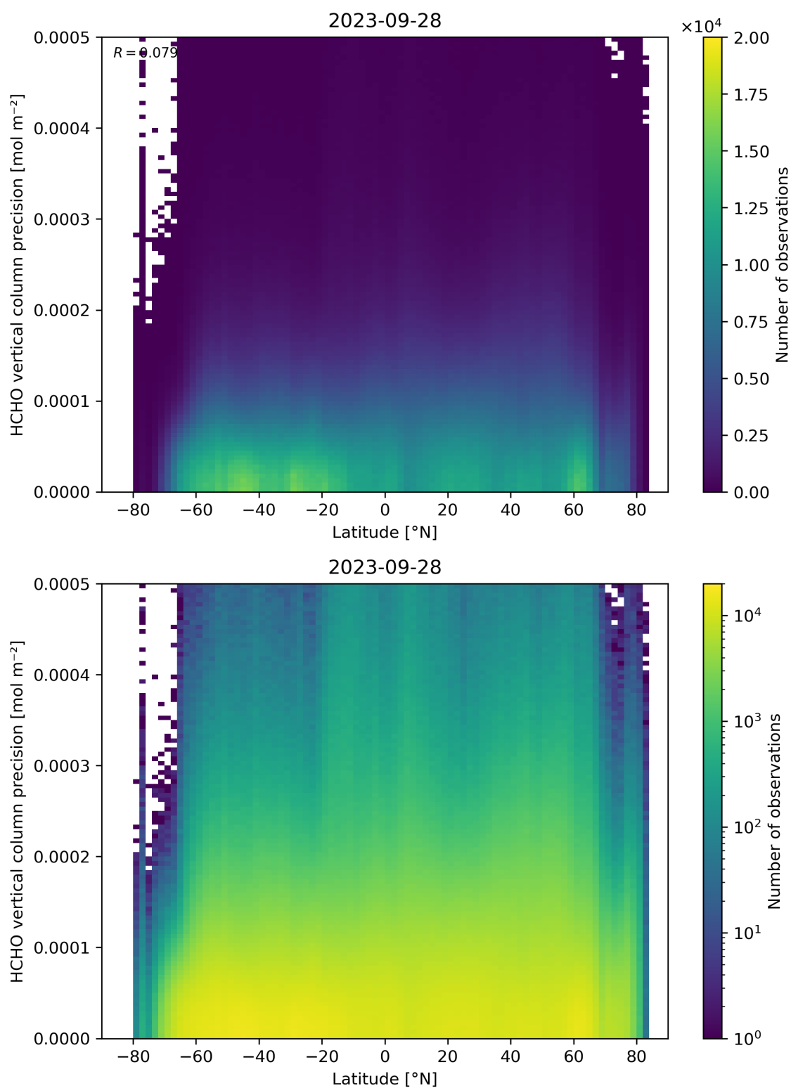
Figure 165: Scatter density plot of “Latitude” against “HCHO vertical column precision” for 2023-09-27 to 2023-09-29.
