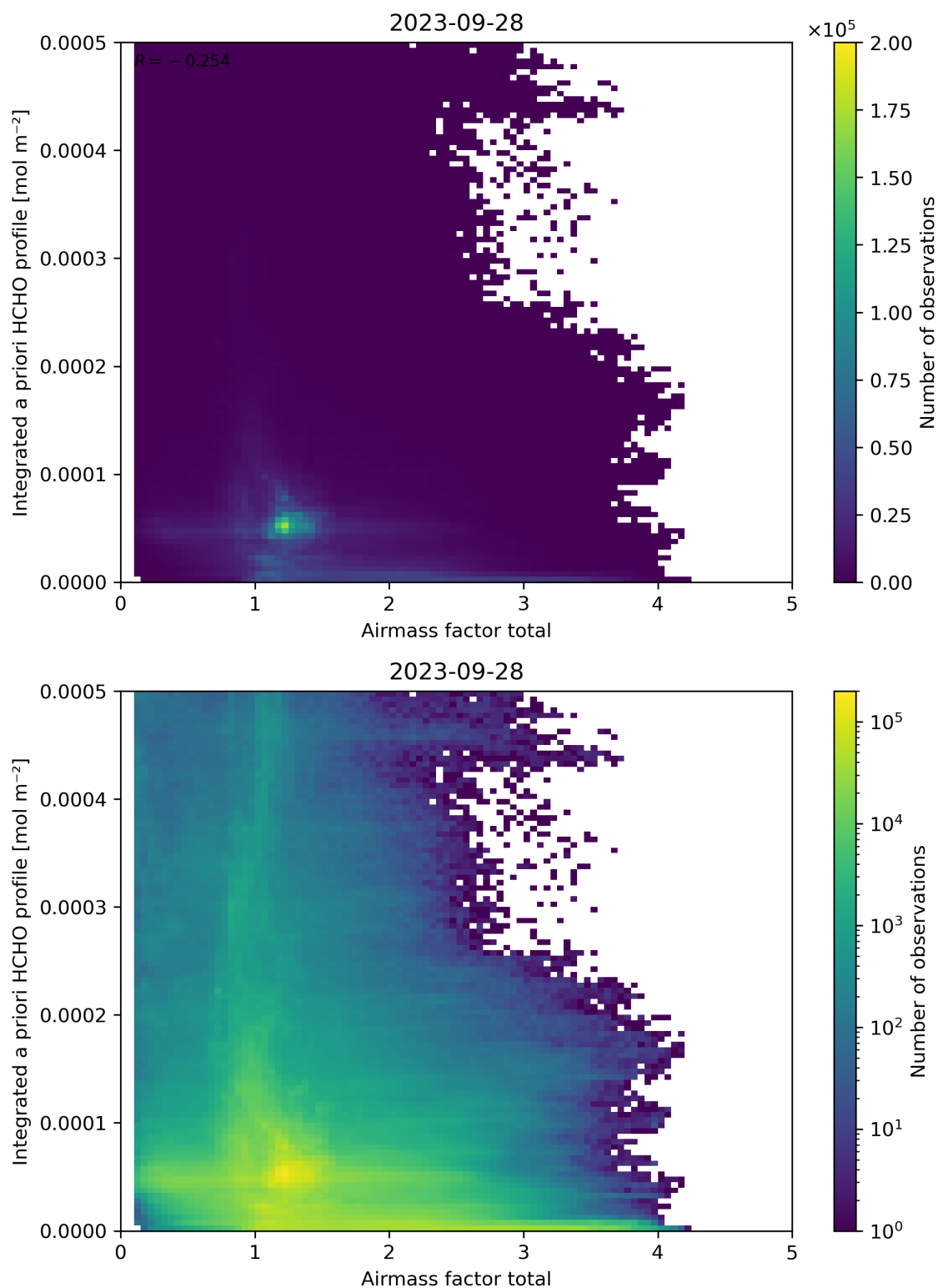
Figure 104: Scatter density plot of “Airmass factor total” against “Integrated a priori HCHO profile” for 2023-09-27 to 2023-09-29.
