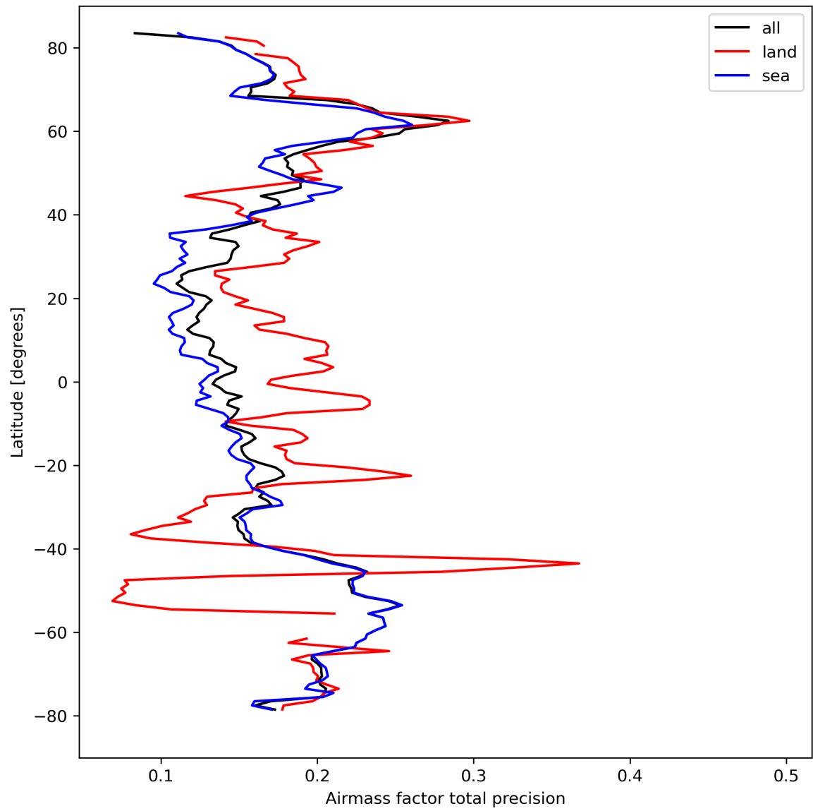
Figure 27: Zonal average of “Airmass factor total precision” for 2023-09-27 to 2023-09-29.
