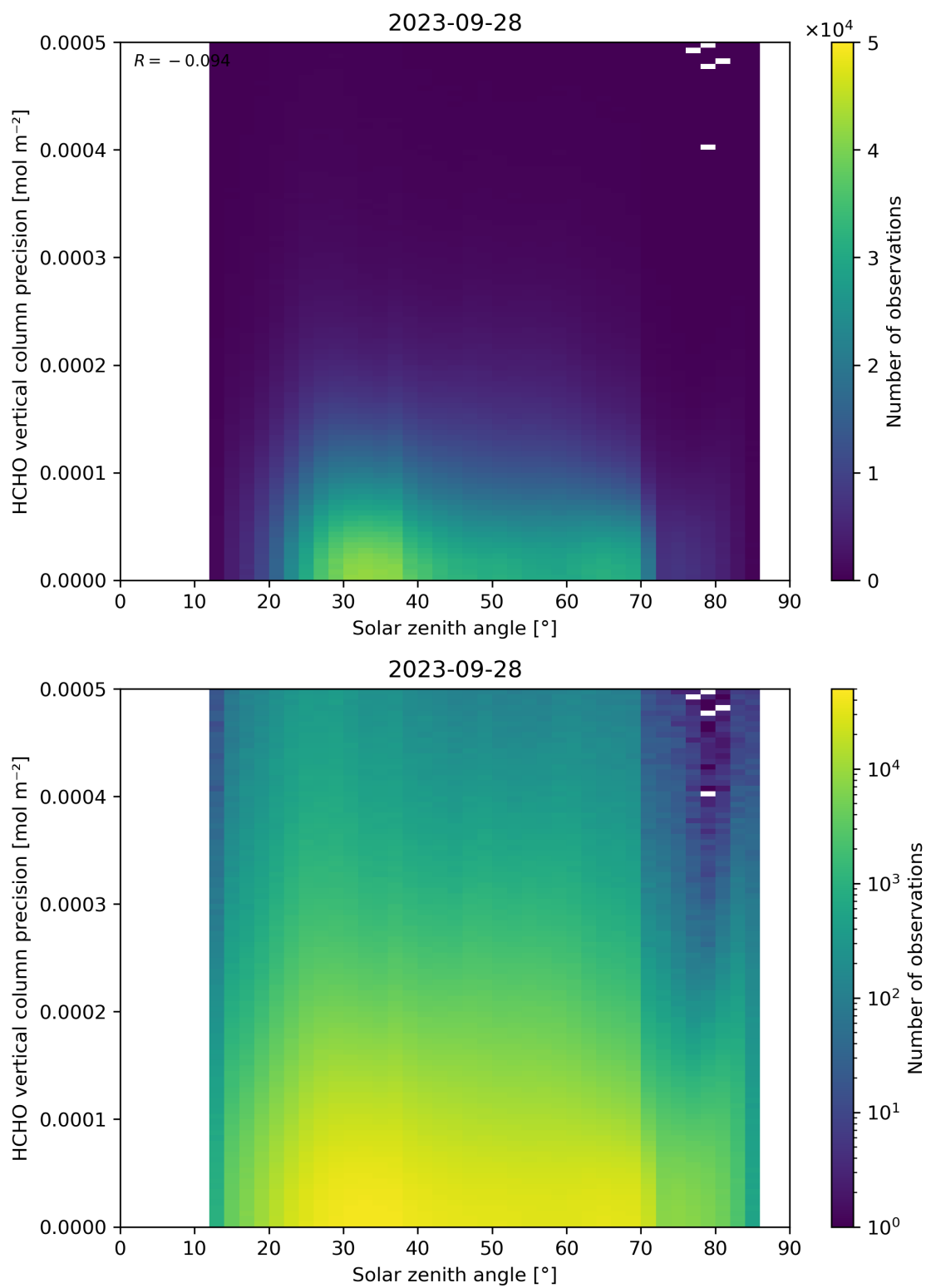
Figure 179: Scatter density plot of “Solar zenith angle” against “HCHO vertical column precision” for 2023-09-27 to 2023-09-29.
