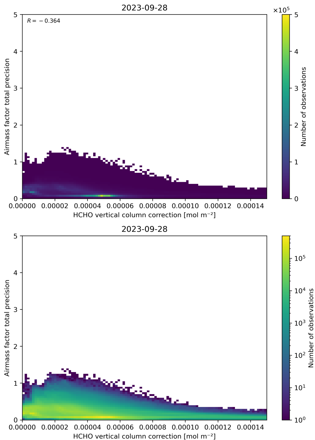
Figure 121: Scatter density plot of “HCHO vertical column correction” against “Airmass factor total precision” for 2023-09-27 to 2023-09-29.
