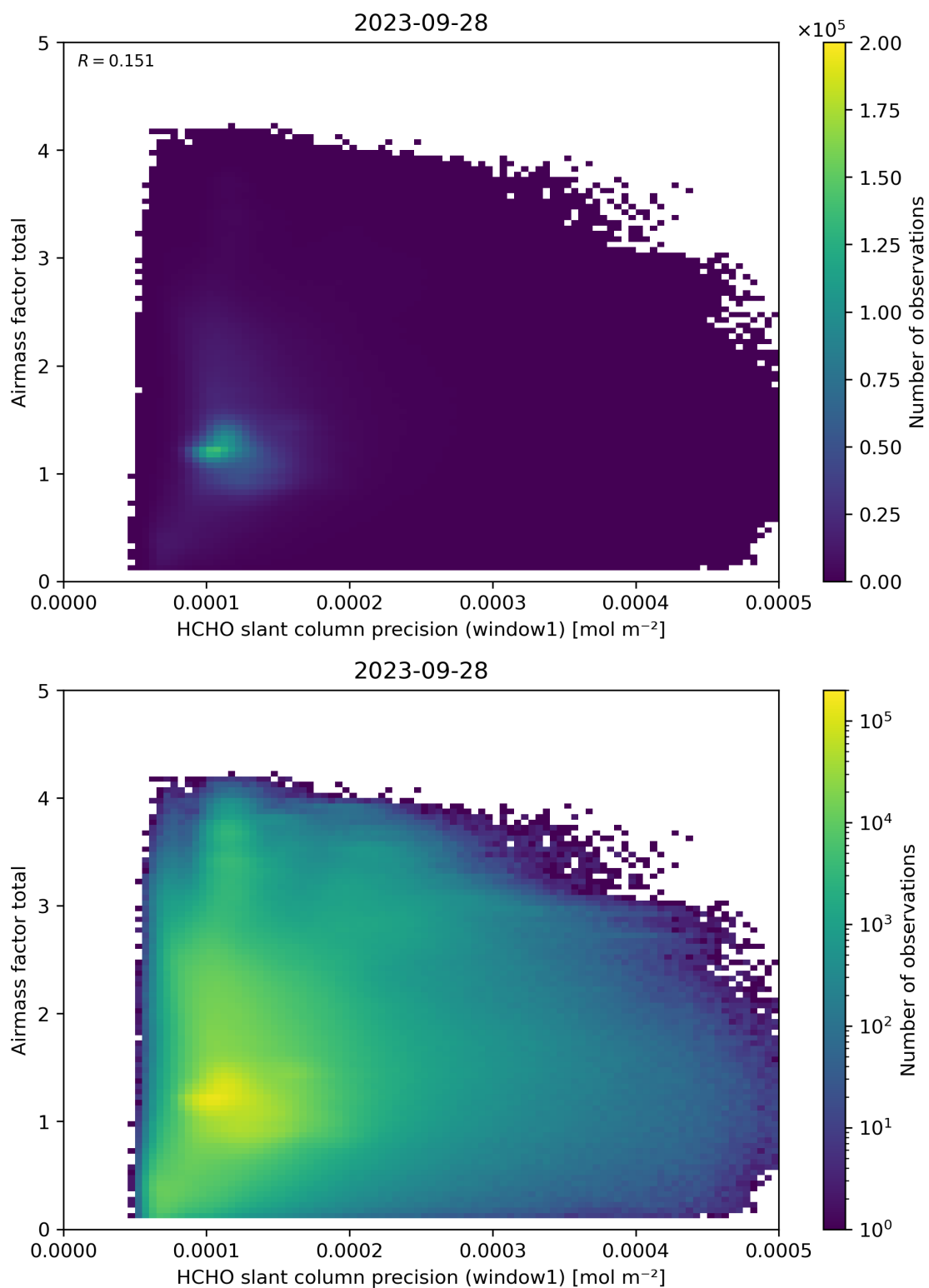
Figure 94: Scatter density plot of “HCHO slant column precision (window1)” against “Airmass factor total” for 2023-09-27 to 2023-09-29.
