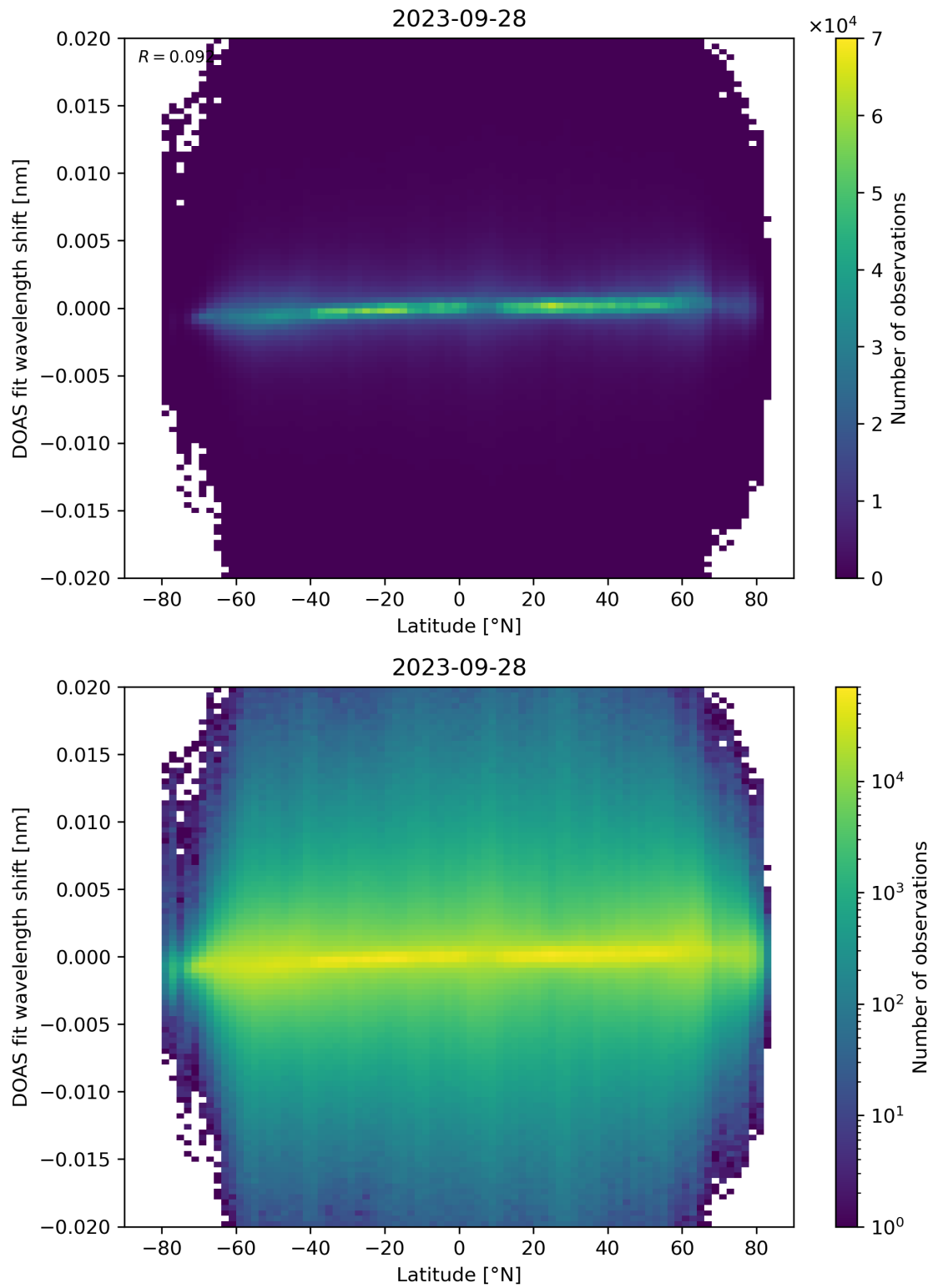
Figure 154: Scatter density plot of “Latitude” against “DOAS fit wavelength shift” for 2023-09-27 to 2023-09-29.
