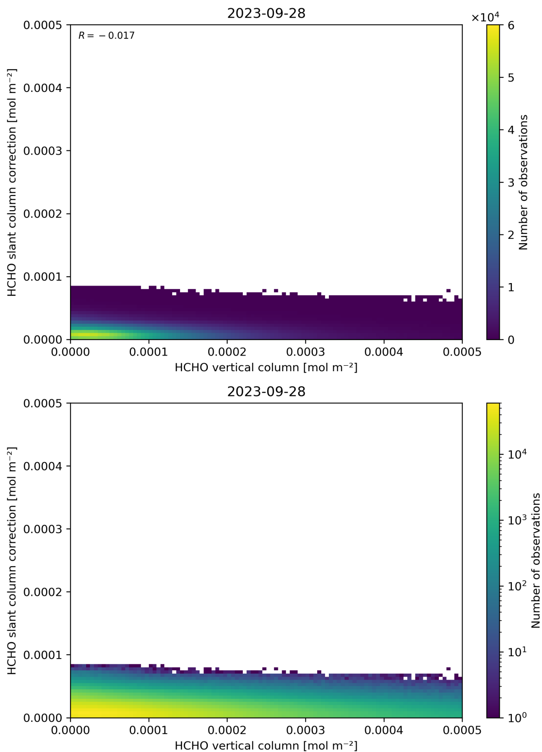
Figure 128: Scatter density plot of “HCHO vertical column” against “HCHO slant column correction” for 2023-09-27 to 2023-09-29.
