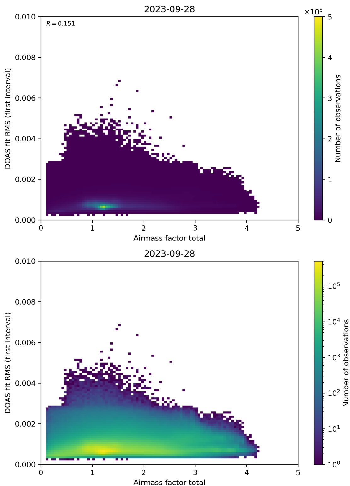
Figure 97: Scatter density plot of “Airmass factor total” against “DOAS fit RMS (first interval)” for 2023-09-27 to 2023-09-29.
