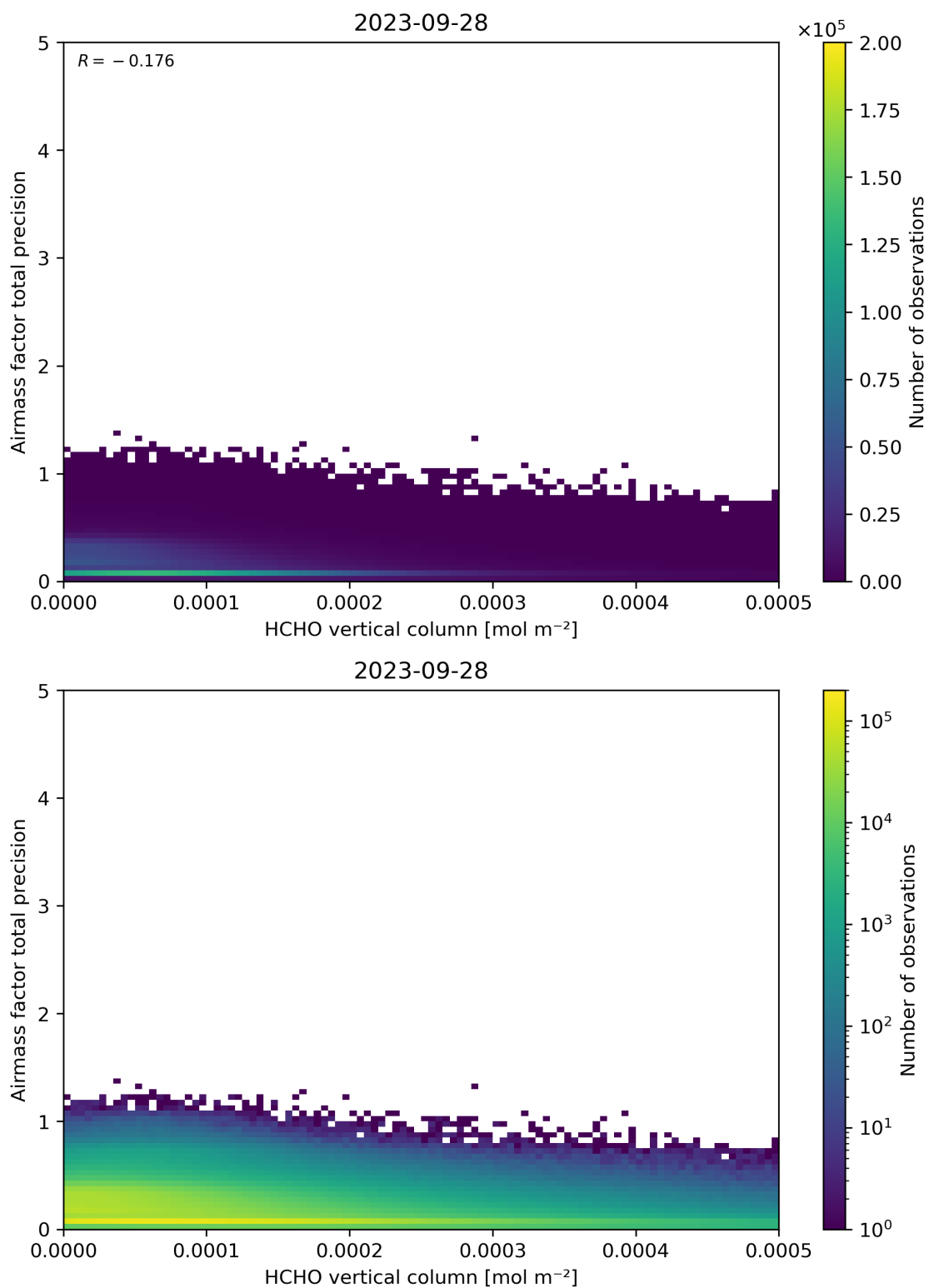
Figure 132: Scatter density plot of “HCHO vertical column” against “Airmass factor total precision” for 2023-09-27 to 2023-09-29.
