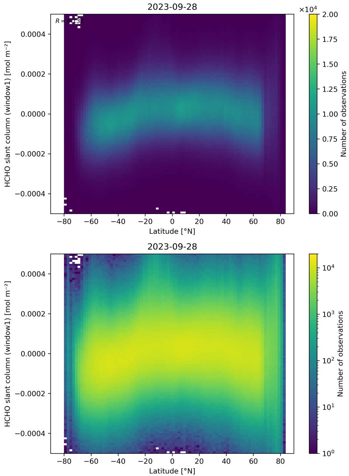
Figure 159: Scatter density plot of “Latitude” against “HCHO slant column (window1)” for 2023-09-27 to 2023-09-29.
