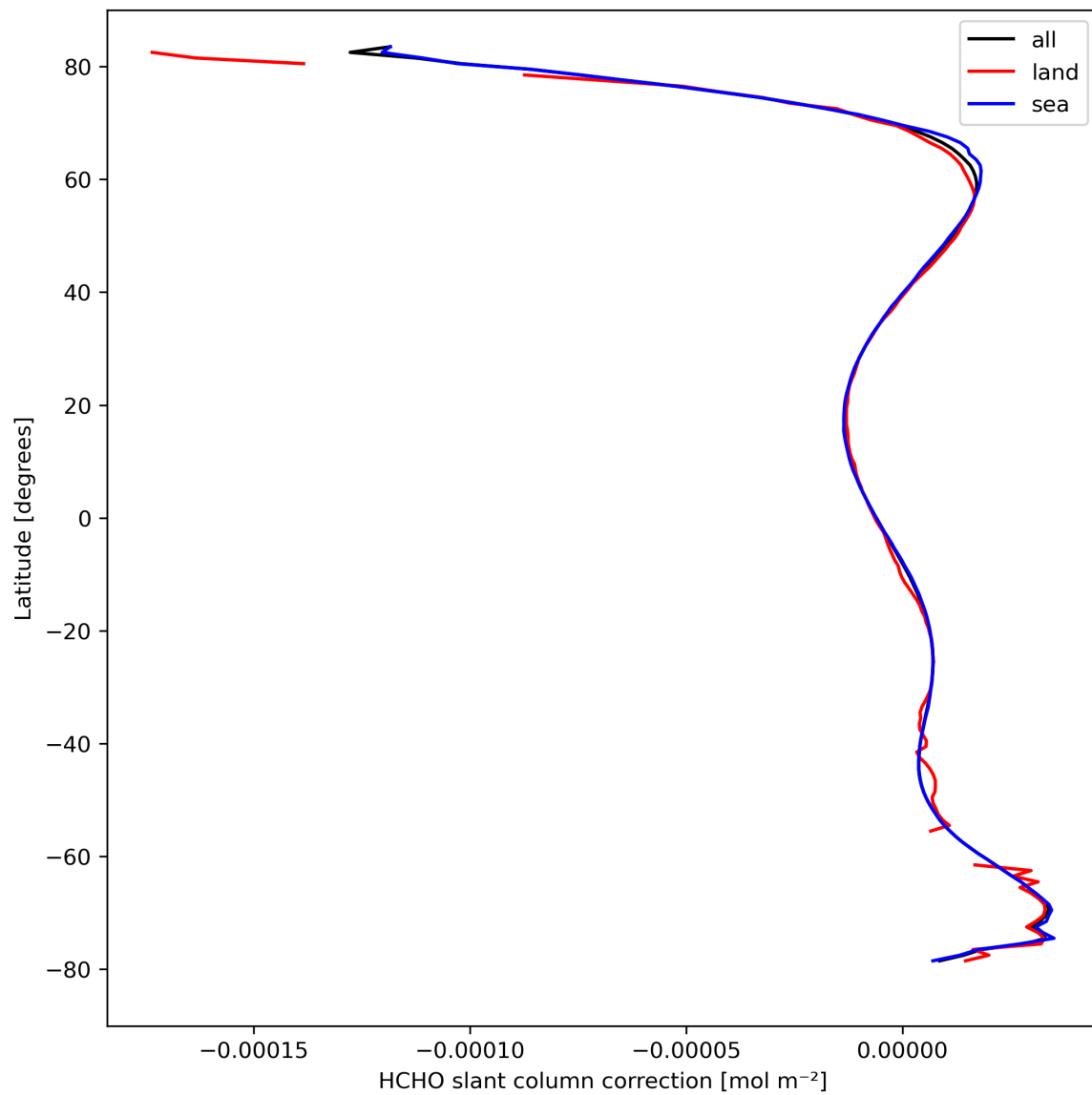
Figure 33: Zonal average of “HCHO slant column correction” for 2023-09-27 to 2023-09-29.
