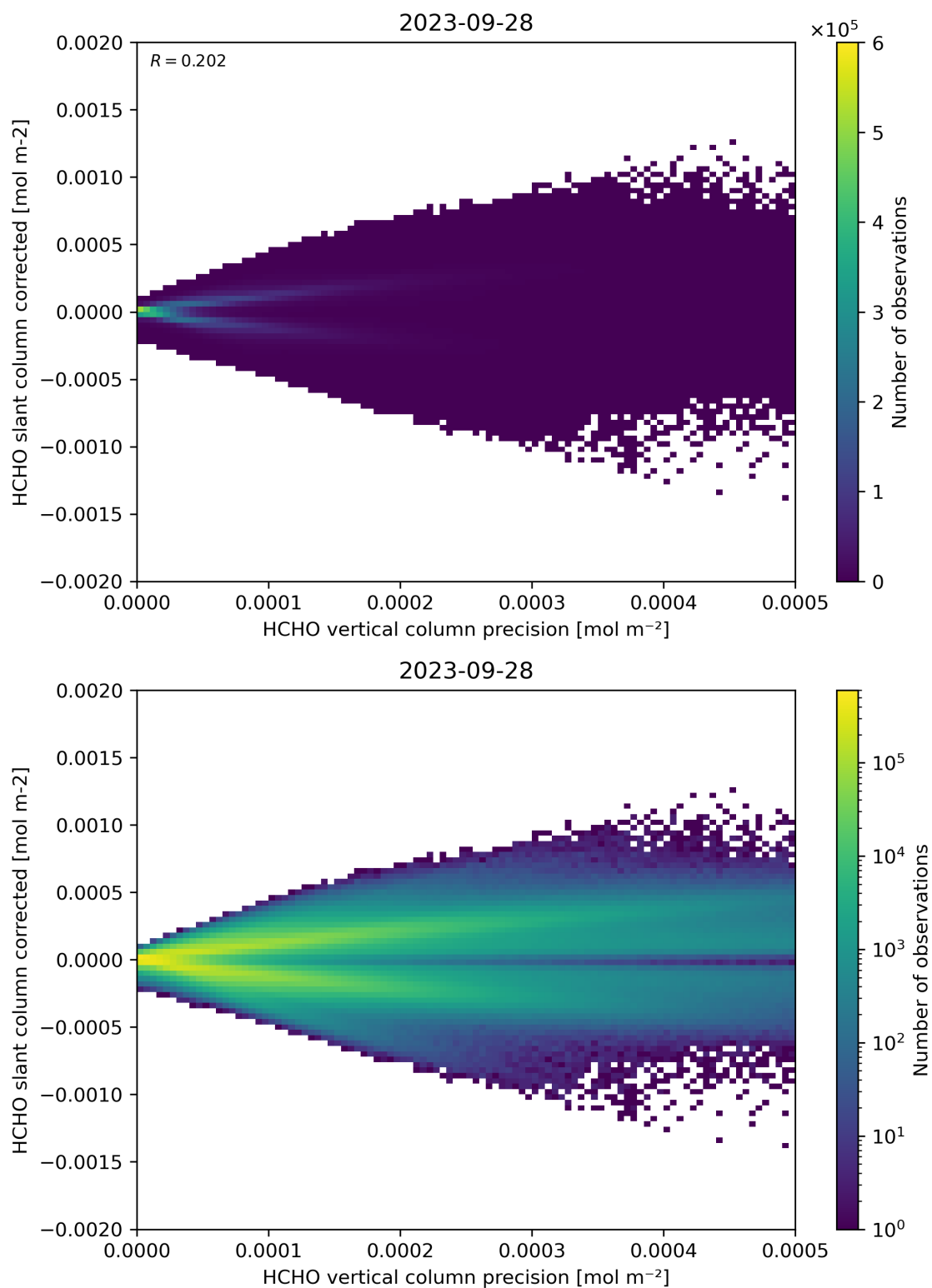
Figure 140: Scatter density plot of “HCHO vertical column precision” against “HCHO slant column corrected” for 2023-09-27 to 2023-09-29.
