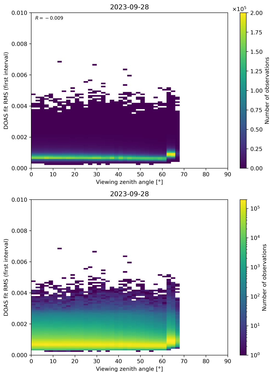
Figure 182: Scatter density plot of “Viewing zenith angle” against “DOAS fit RMS (first interval)” for 2023-09-27 to 2023-09-29.
