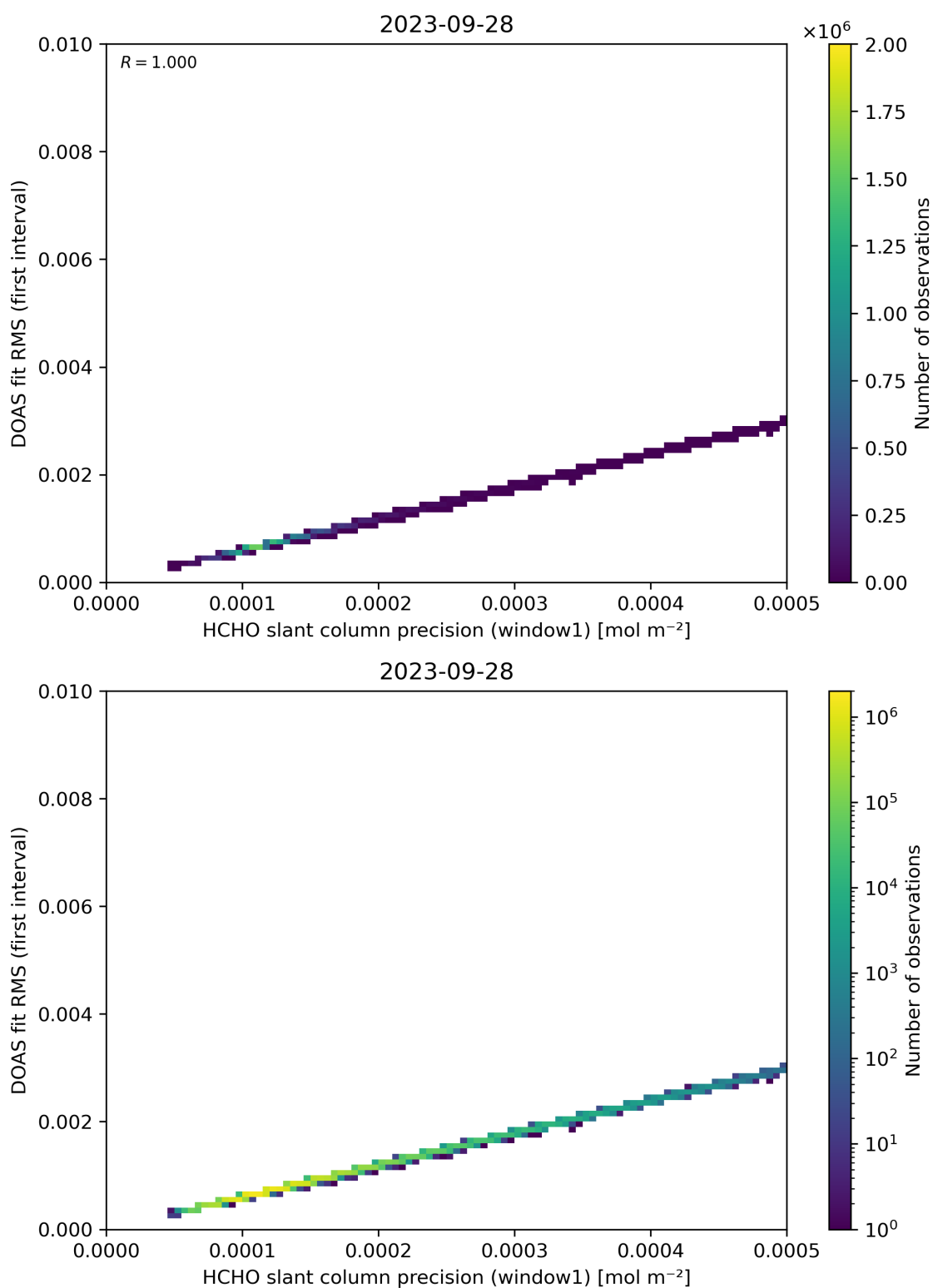
Figure 88: Scatter density plot of “HCHO slant column precision (window1)” against “DOAS fit RMS (first interval)” for 2023-09-27 to 2023-09-29.
