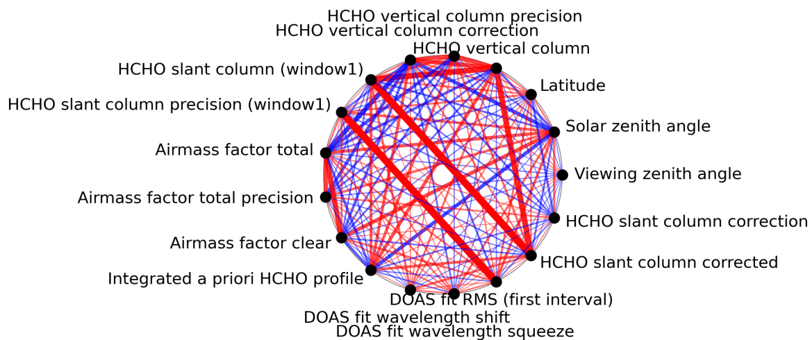
Figure 1: Map of correlation graph for 2023-09-27 to 2023-09-29.
