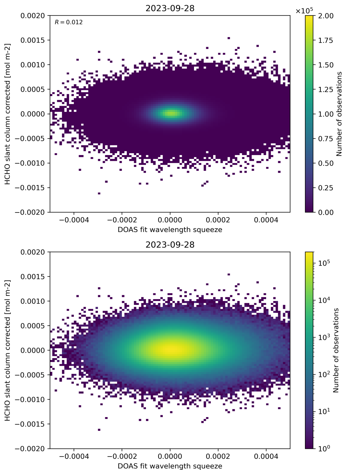
Figure 69: Scatter density plot of “DOAS fit wavelength squeeze” against “HCHO slant column corrected” for 2023-09-27 to 2023-09-29.
