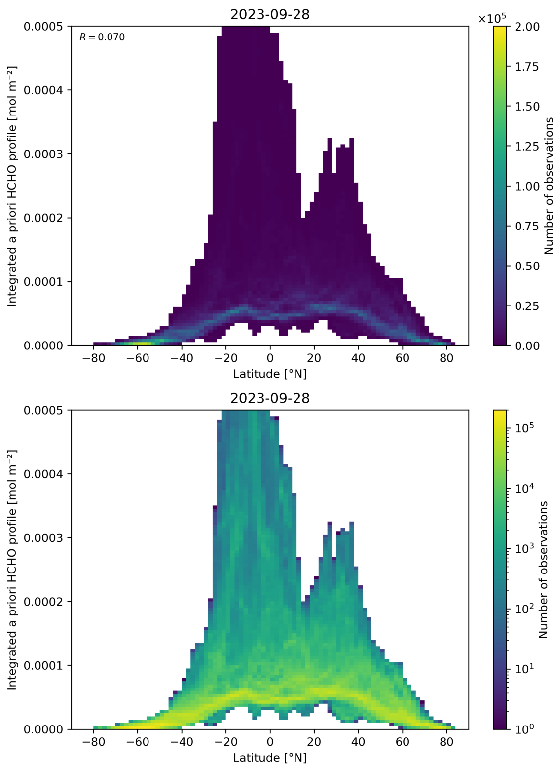
Figure 166: Scatter density plot of “Latitude” against “Integrated a priori HCHO profile” for 2023-09-27 to 2023-09-29.
