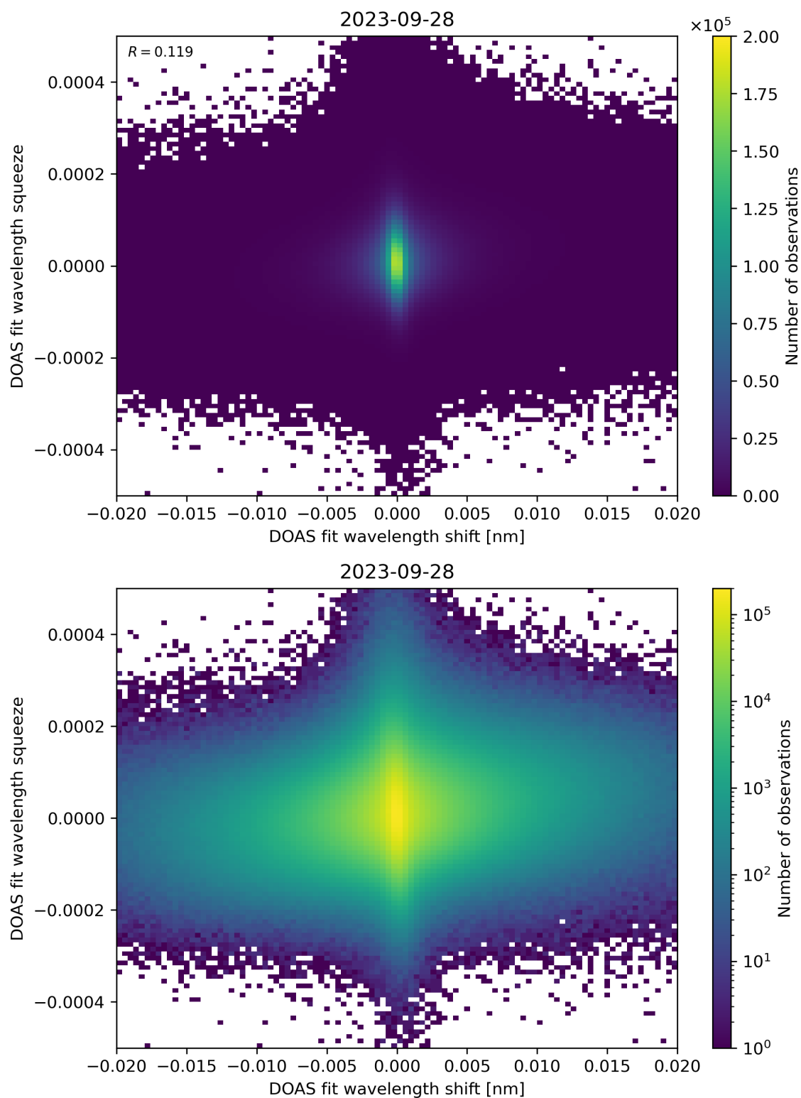
Figure 65: Scatter density plot of “DOAS fit wavelength shift” against “DOAS fit wavelength squeeze” for 2023-09-27 to 2023-09-29.
