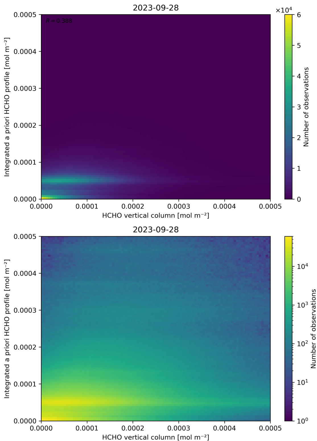
Figure 135: Scatter density plot of “HCHO vertical column” against “Integrated a priori HCHO profile” for 2023-09-27 to 2023-09-29.
