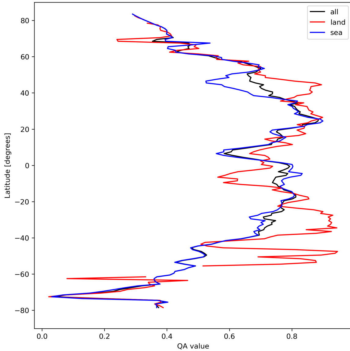
Figure 20: Zonal average of “QA value” for 2023-09-27 to 2023-09-29.
