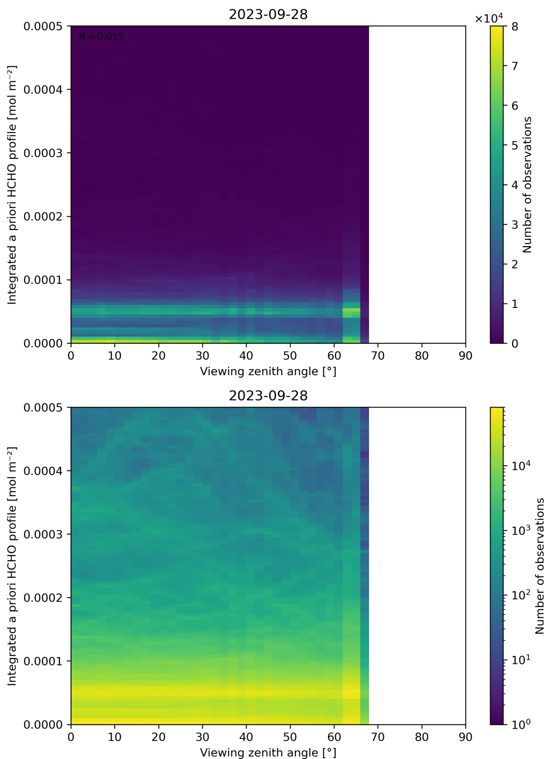
Figure 195: Scatter density plot of “Viewing zenith angle” against “Integrated a priori HCHO profile” for 2023-09-27 to 2023-09-29.
