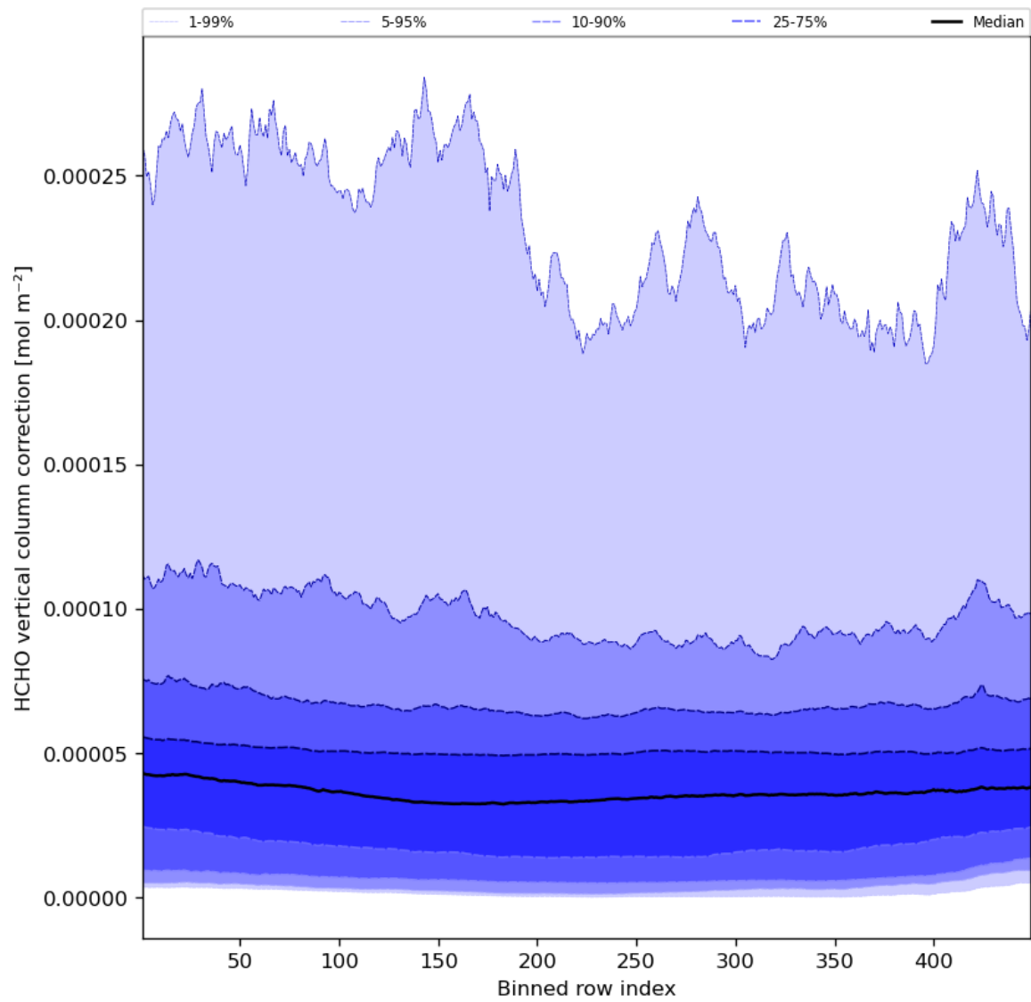
Figure 51: Along track statistics of “HCHO vertical column correction” for 2023-09-27 to 2023-09-29
