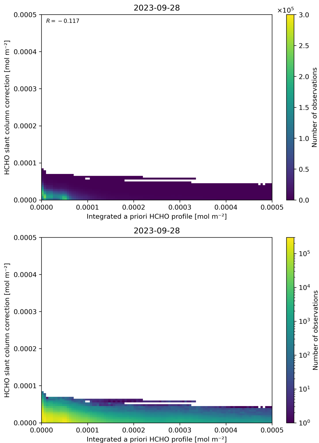
Figure 152: Scatter density plot of “Integrated a priori HCHO profile” against “HCHO slant column correction” for 2023-09-27 to 2023-09-29.
