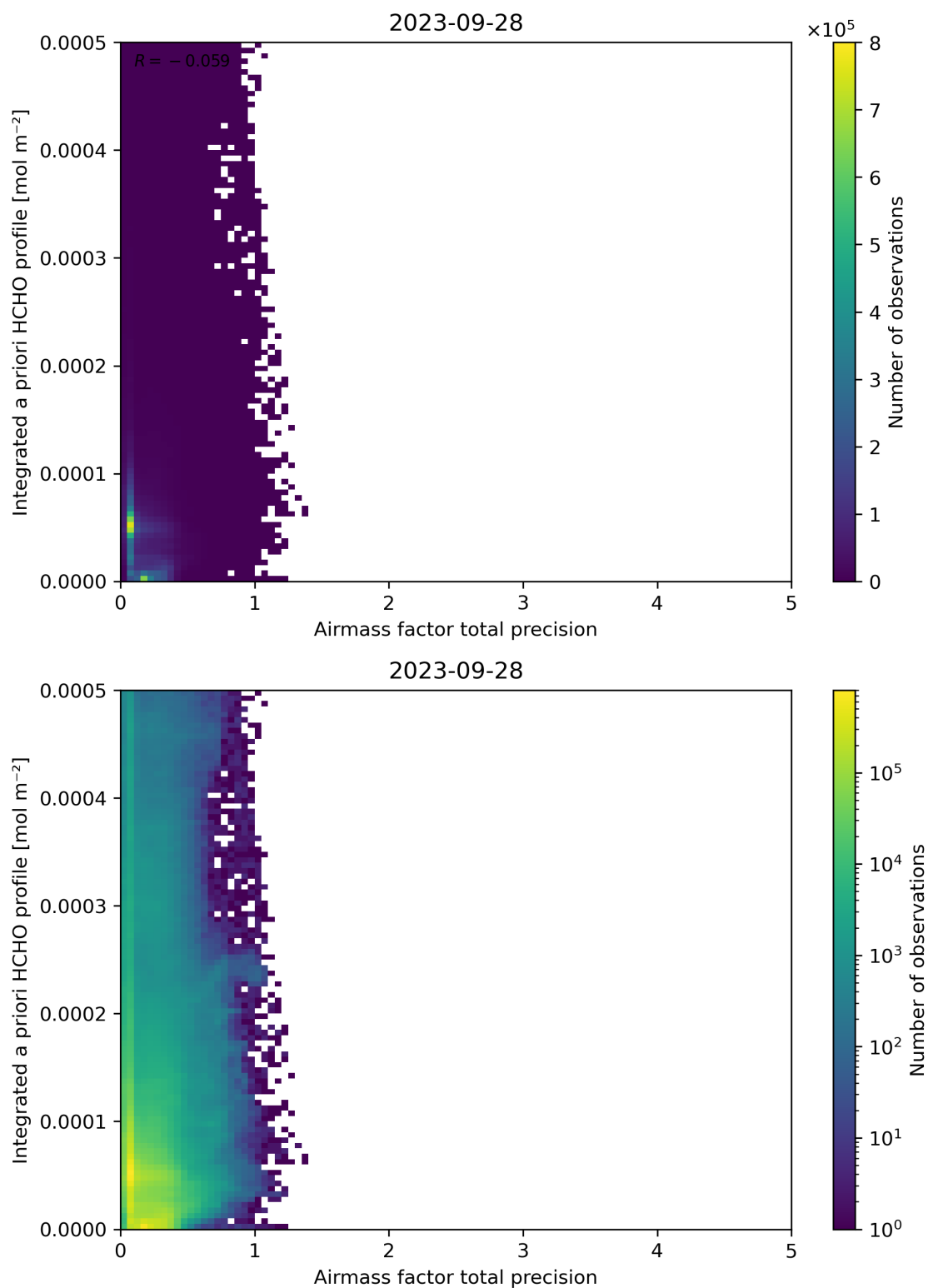
Figure 111: Scatter density plot of “Airmass factor total precision” against “Integrated a priori HCHO profile” for 2023-09-27 to 2023-09-29.
