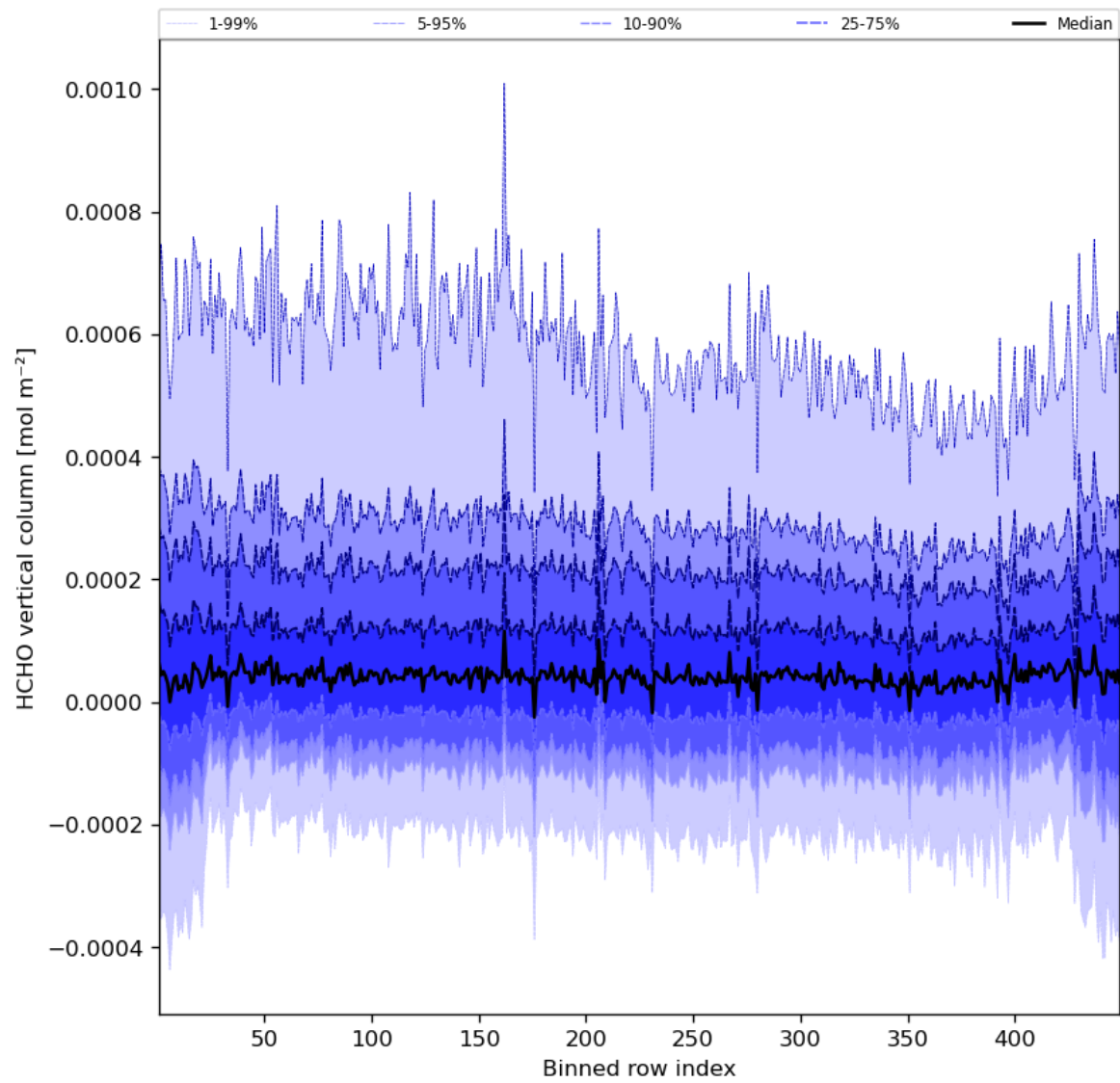
Figure 49: Along track statistics of “HCHO vertical column” for 2023-09-27 to 2023-09-29
