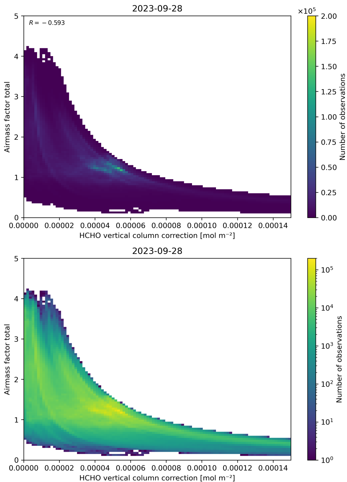
Figure 120: Scatter density plot of “HCHO vertical column correction” against “Airmass factor total” for 2023-09-27 to 2023-09-29.
