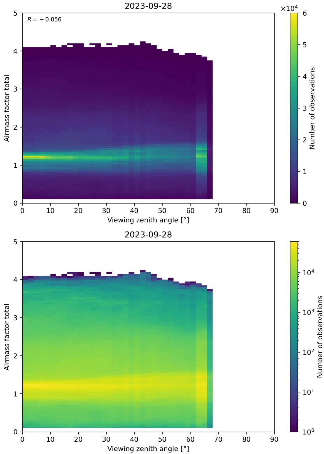
Figure 190: Scatter density plot of “Viewing zenith angle” against “Airmass factor total” for 2023-09-27 to 2023-09-29.
