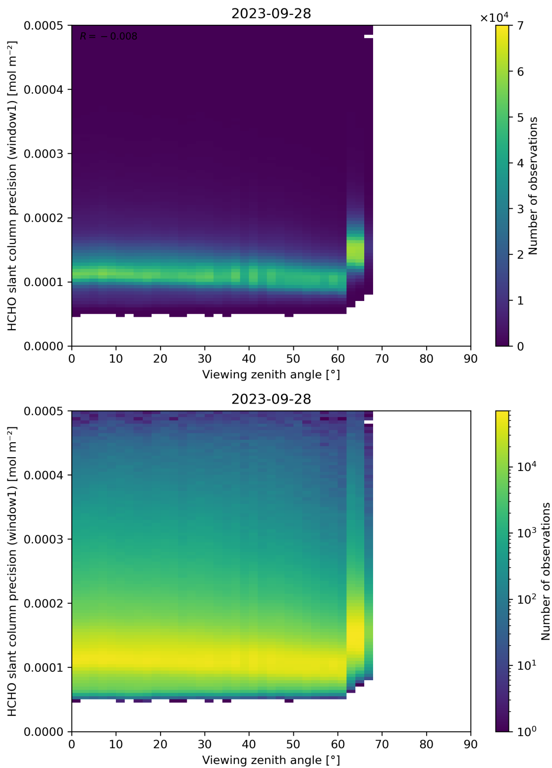
Figure 189: Scatter density plot of “Viewing zenith angle” against “HCHO slant column precision (window1)” for 2023-09-27 to 2023-09-29.
