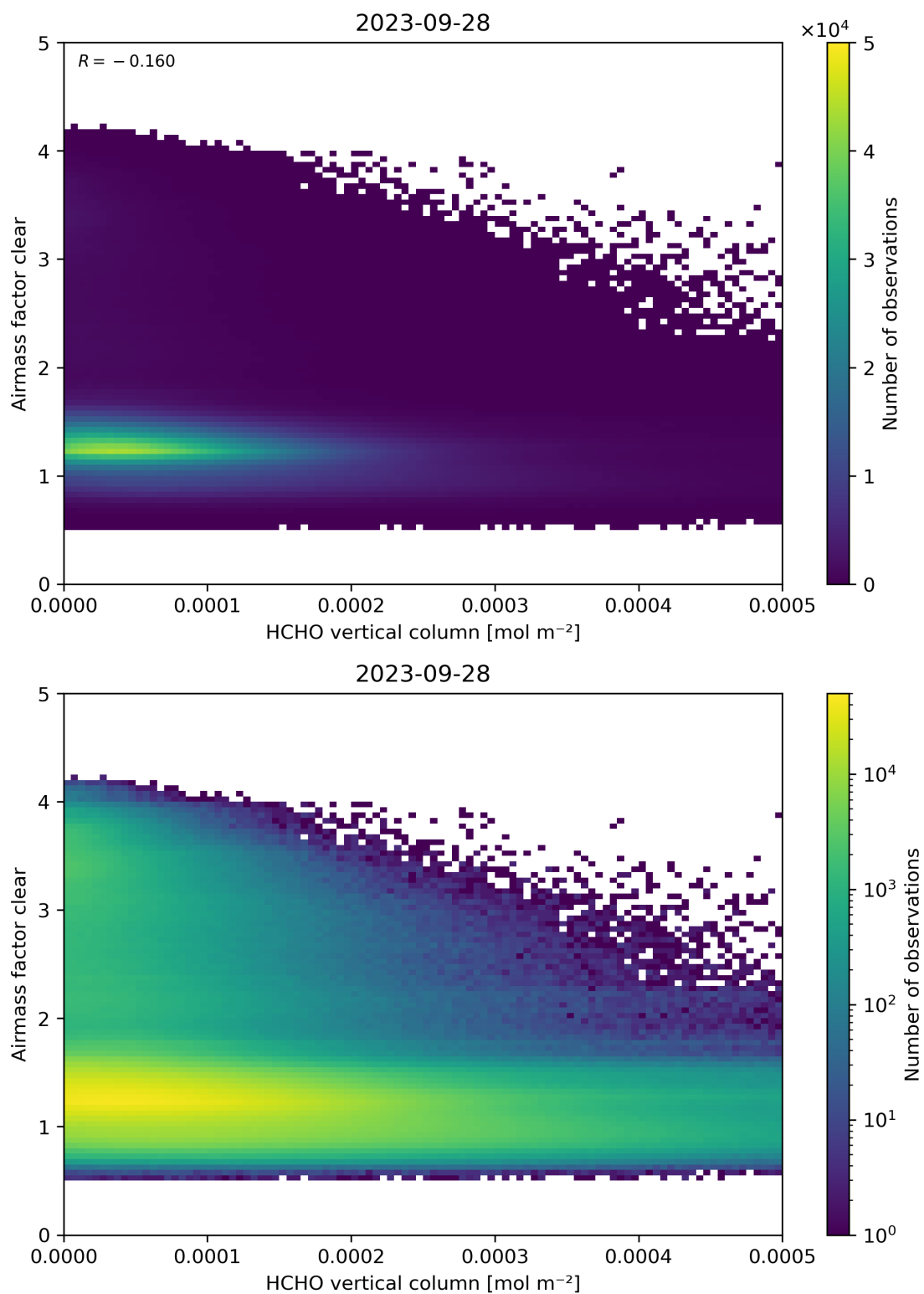
Figure 126: Scatter density plot of “HCHO vertical column” against “Airmass factor clear” for 2023-09-27 to 2023-09-29.
