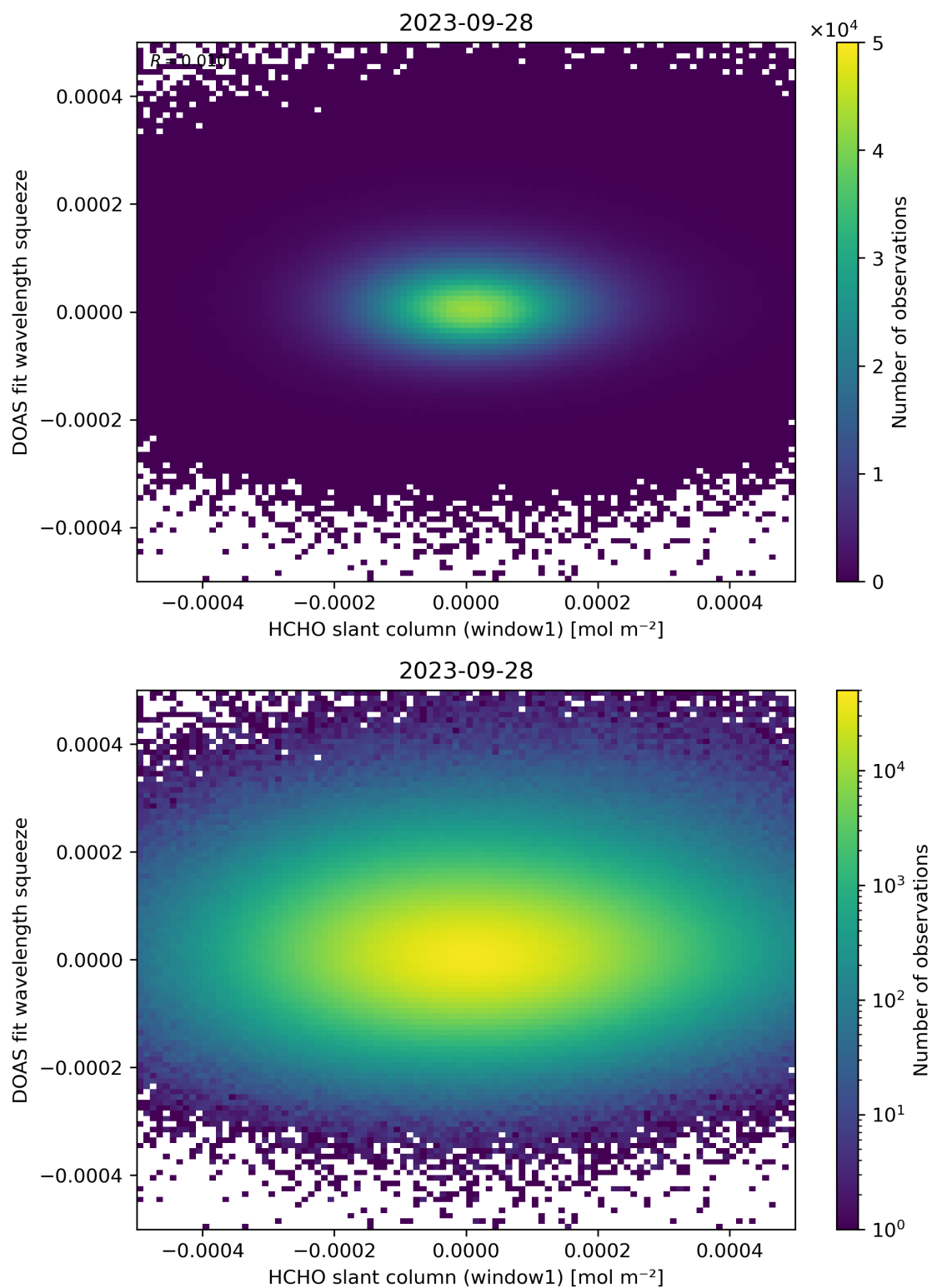
Figure 80: Scatter density plot of “HCHO slant column (window1)” against “DOAS fit wavelength squeeze” for 2023-09-27 to 2023-09-29.
