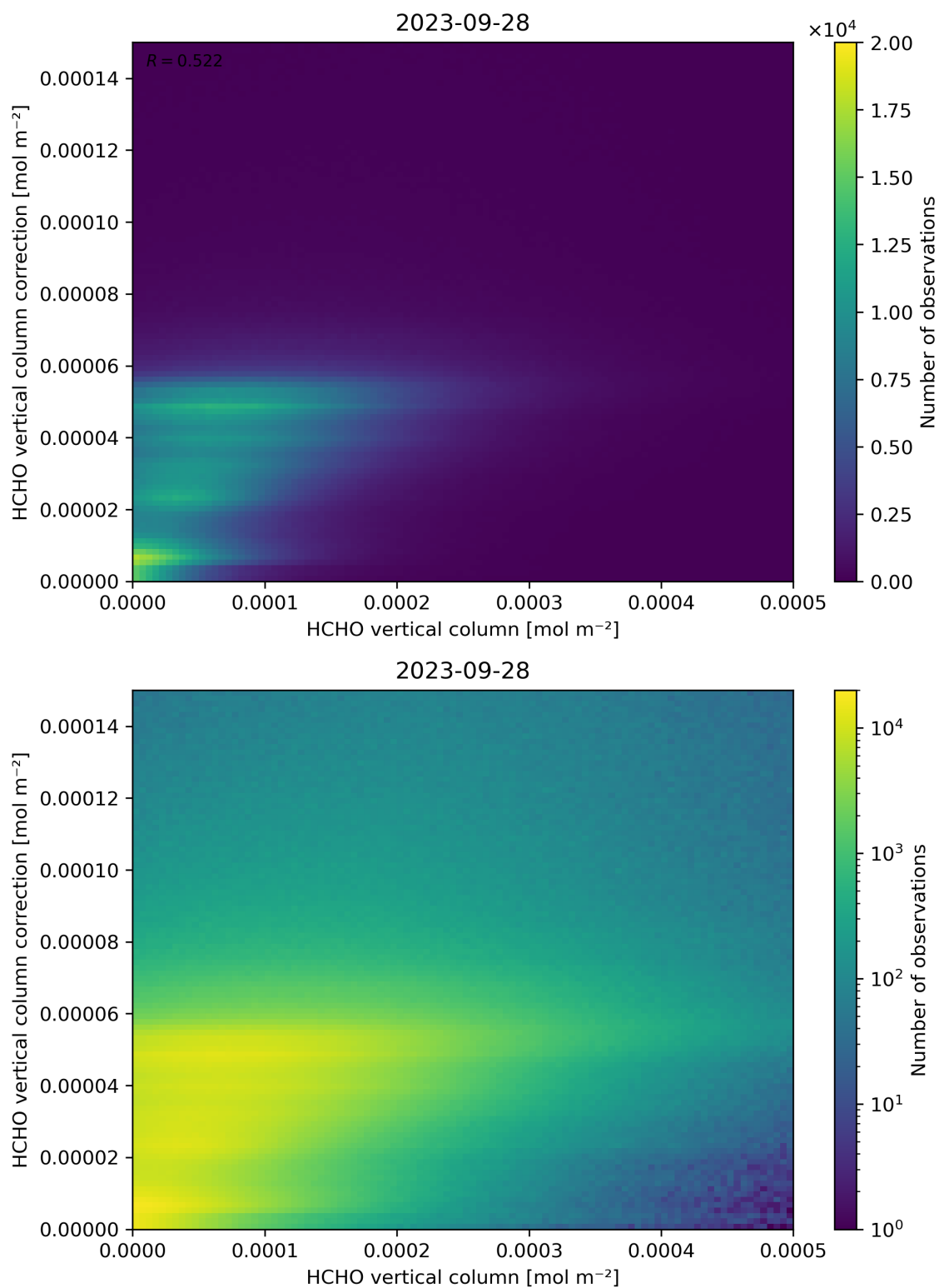
Figure 133: Scatter density plot of “HCHO vertical column” against “HCHO vertical column correction” for 2023-09-27 to 2023-09-29.
