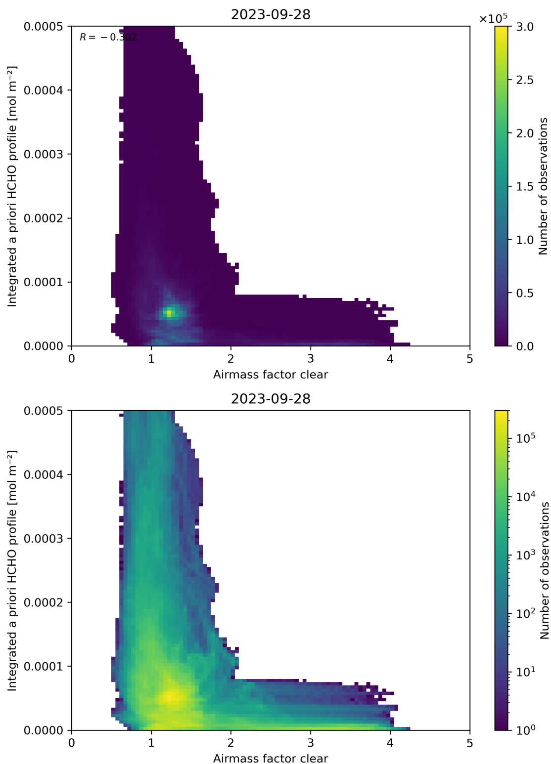
Figure 76: Scatter density plot of “Airmass factor clear” against “Integrated a priori HCHO profile” for 2023-09-27 to 2023-09-29.
