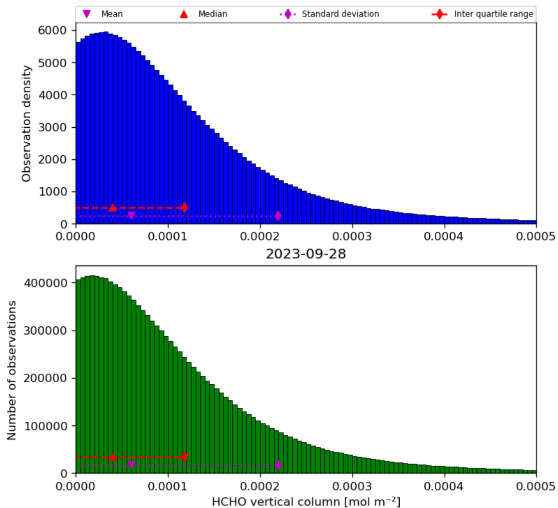
Figure 35: Histogram of “HCHO vertical column” for 2023-09-27 to 2023-09-29
