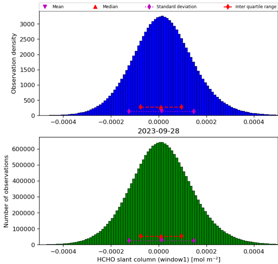
Figure 38: Histogram of “HCHO slant column (window1)” for 2023-09-27 to 2023-09-29
