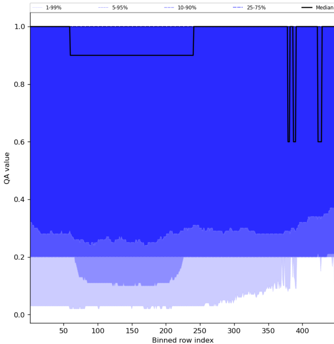
Figure 48: Along track statistics of “QA value” for 2023-09-27 to 2023-09-29
