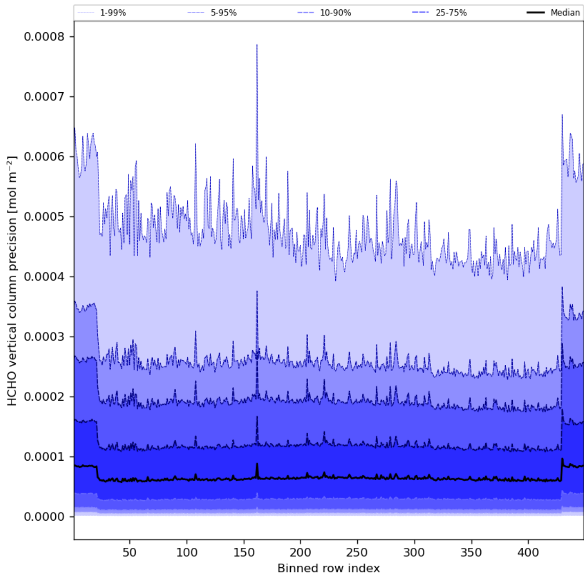
Figure 50: Along track statistics of “HCHO vertical column precision” for 2023-09-27 to 2023-09-29
