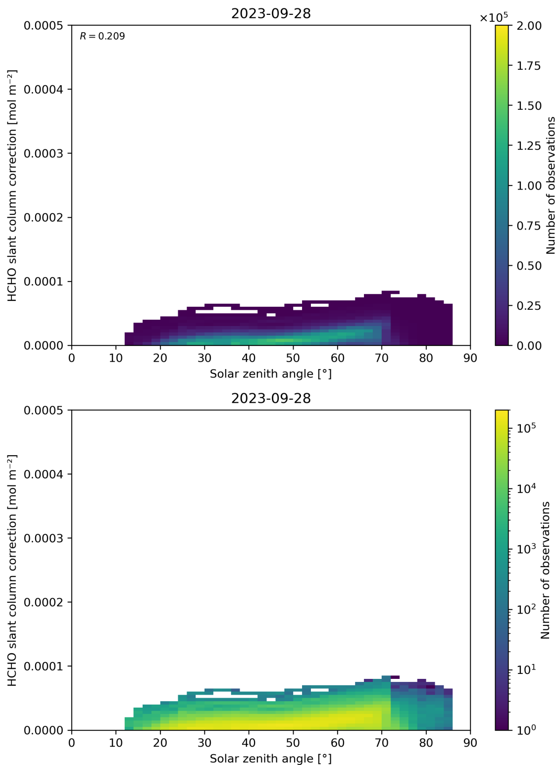
Figure 172: Scatter density plot of “Solar zenith angle” against “HCHO slant column correction” for 2023-09-27 to 2023-09-29.
