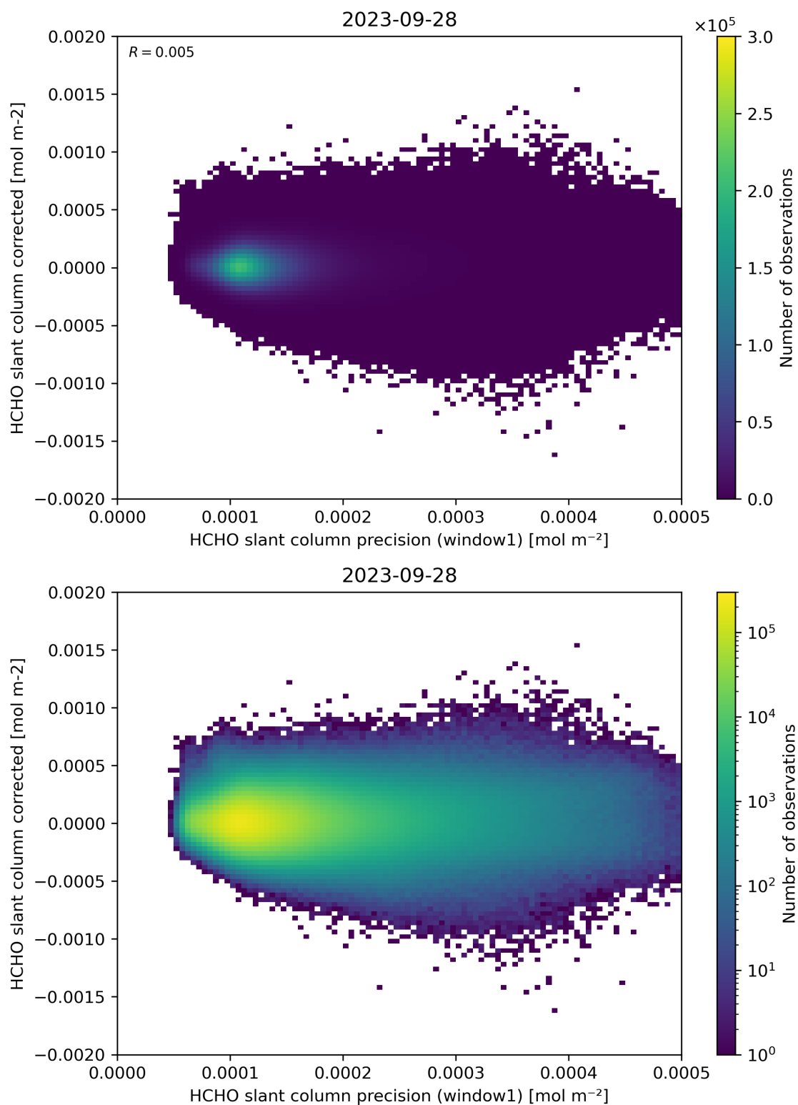
Figure 92: Scatter density plot of “HCHO slant column precision (window1)” against “HCHO slant column corrected” for 2023-09-27 to 2023-09-29.
