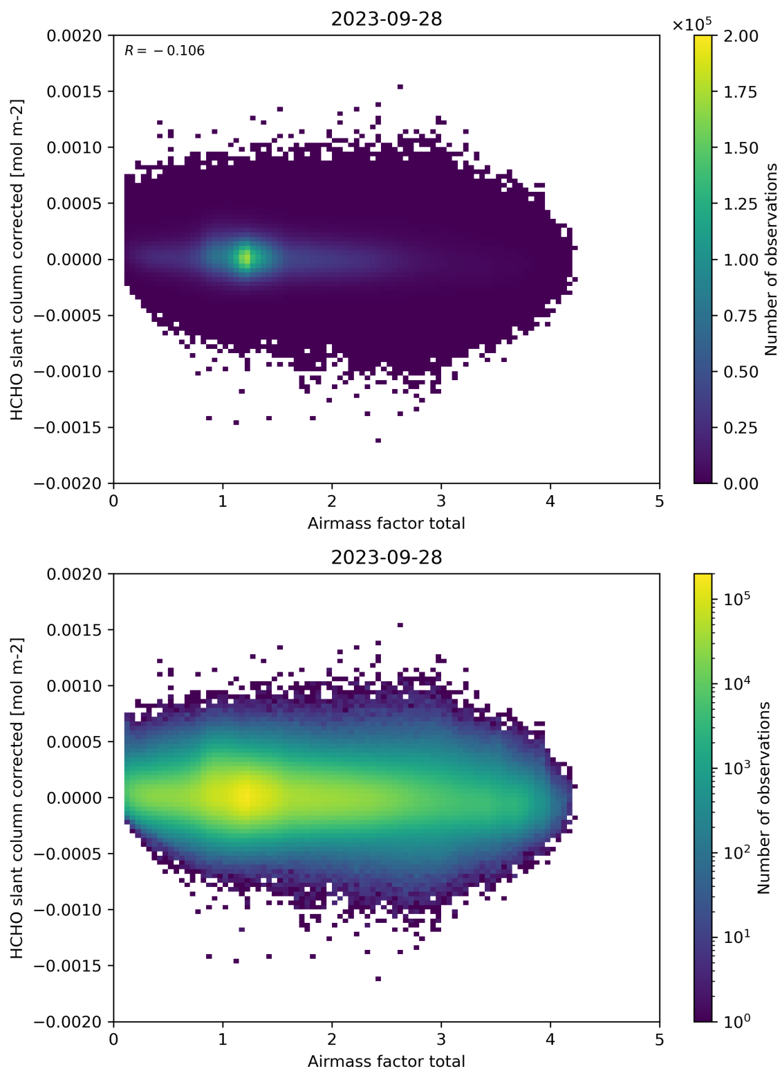
Figure 101: Scatter density plot of “Airmass factor total” against “HCHO slant column corrected” for 2023-09-27 to 2023-09-29.
