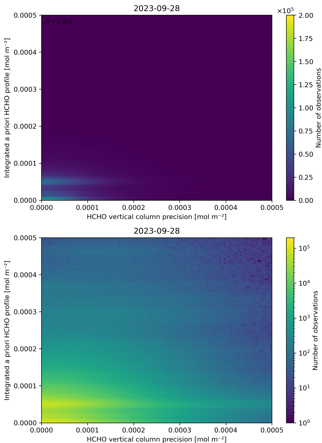
Figure 147: Scatter density plot of “HCHO vertical column precision” against “Integrated a priori HCHO profile” for 2023-09-27 to 2023-09-29.
