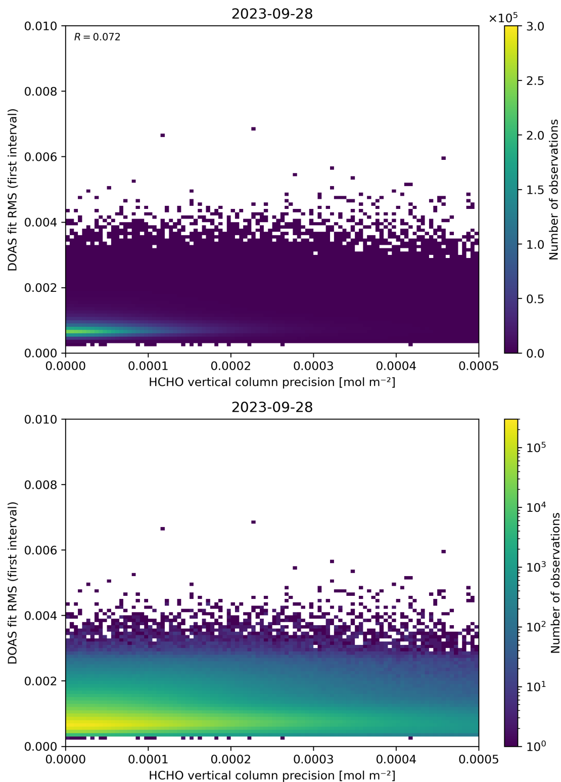
Figure 136: Scatter density plot of “HCHO vertical column precision” against “DOAS fit RMS (first interval)” for 2023-09-27 to 2023-09-29.
