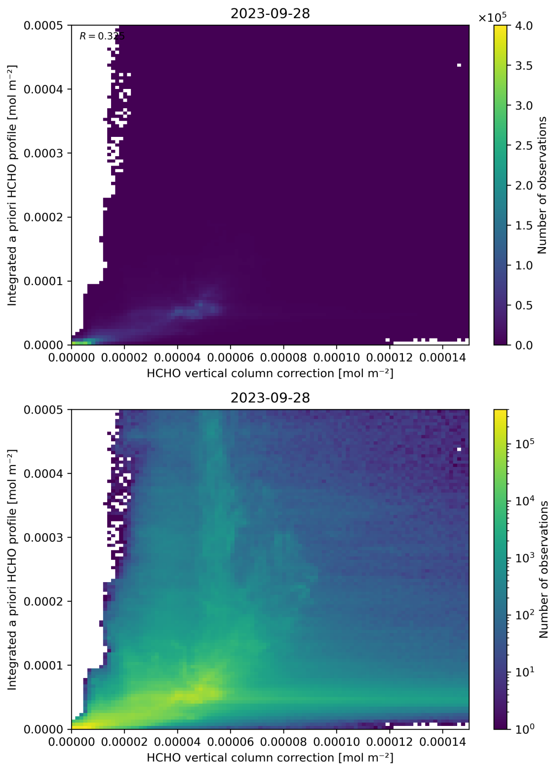
Figure 122: Scatter density plot of “HCHO vertical column correction” against “Integrated a priori HCHO profile” for 2023-09-27 to 2023-09-29.
