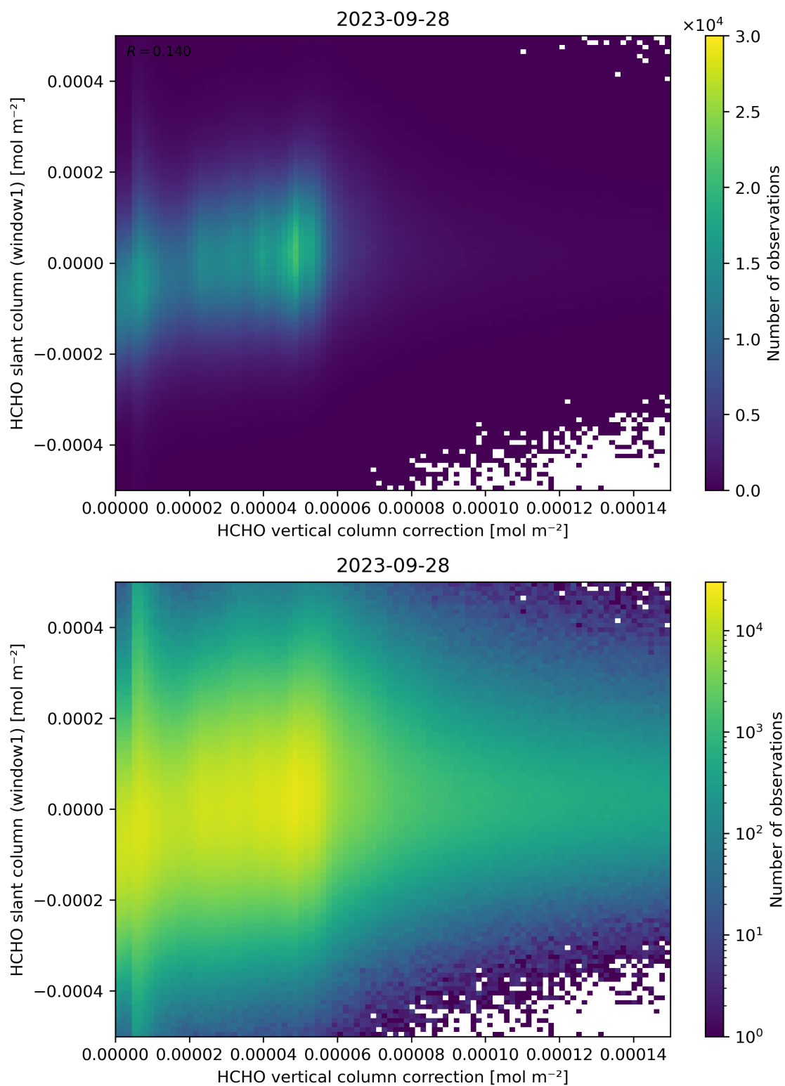
Figure 118: Scatter density plot of “HCHO vertical column correction” against “HCHO slant column (window1)” for 2023-09-27 to 2023-09-29.
