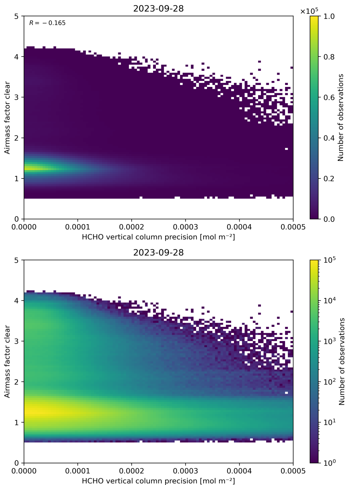
Figure 139: Scatter density plot of “HCHO vertical column precision” against “Airmass factor clear” for 2023-09-27 to 2023-09-29.
