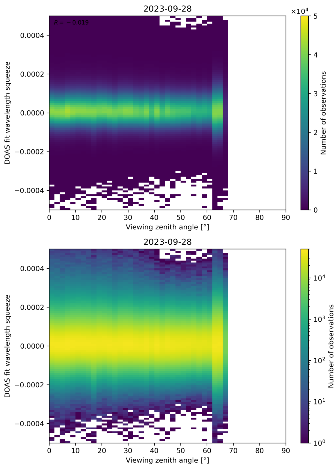
Figure 184: Scatter density plot of “Viewing zenith angle” against “DOAS fit wavelength squeeze” for 2023-09-27 to 2023-09-29.
