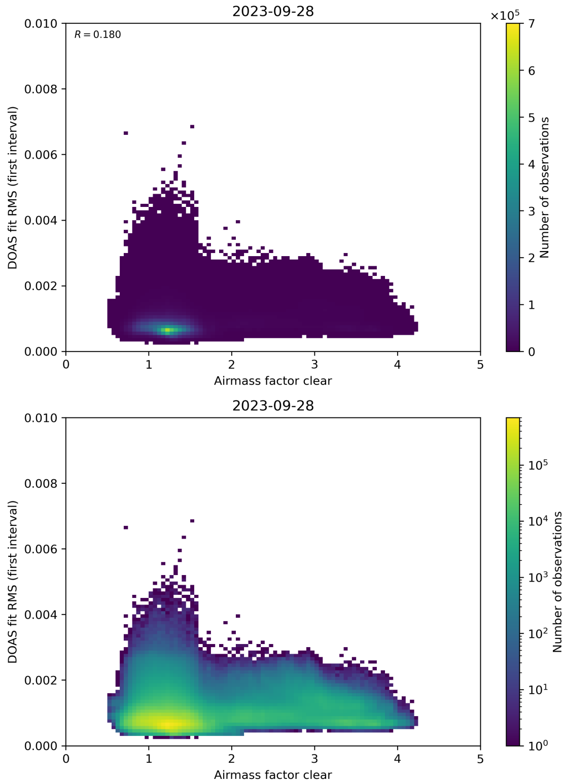
Figure 71: Scatter density plot of “Airmass factor clear” against “DOAS fit RMS (first interval)” for 2023-09-27 to 2023-09-29.
