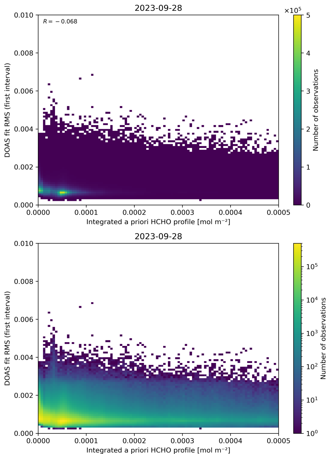
Figure 148: Scatter density plot of “Integrated a priori HCHO profile” against “DOAS fit RMS (first interval)” for 2023-09-27 to 2023-09-29.
