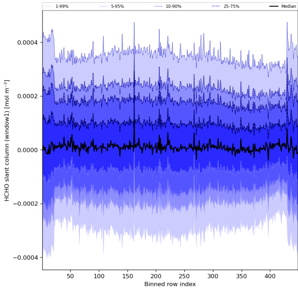
Figure 52: Along track statistics of “HCHO slant column (window1)” for 2023-09-27 to 2023-09-29
