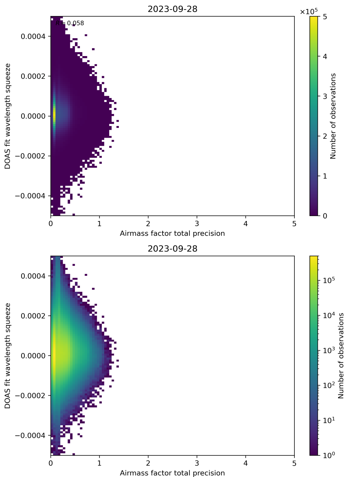
Figure 107: Scatter density plot of “Airmass factor total precision” against “DOAS fit wavelength squeeze” for 2023-09-27 to 2023-09-29.
