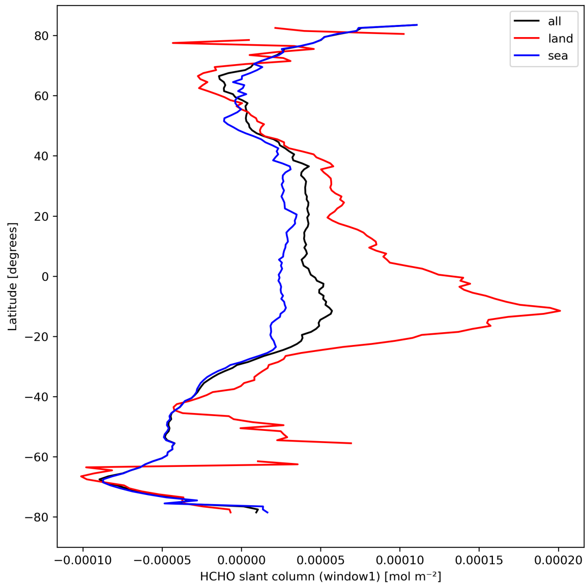
Figure 24: Zonal average of “HCHO slant column (window1)” for 2023-09-27 to 2023-09-29.
