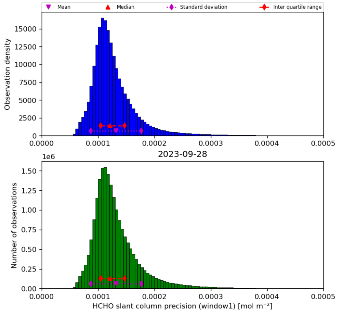
Figure 39: Histogram of “HCHO slant column precision (window1)” for 2023-09-27 to 2023-09-29
