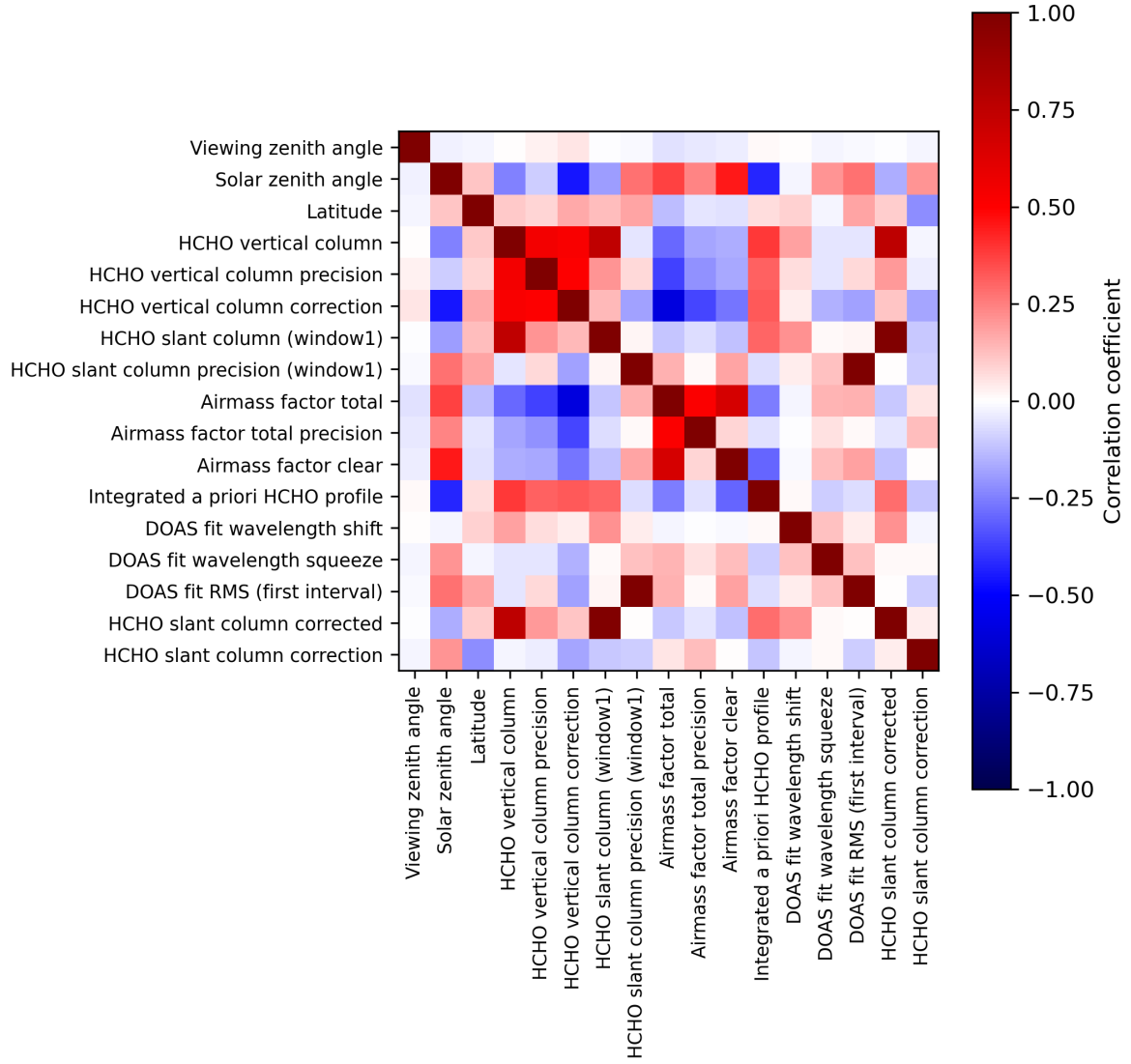
Figure 2: Map of correlation matrix for 2023-09-27 to 2023-09-29.
