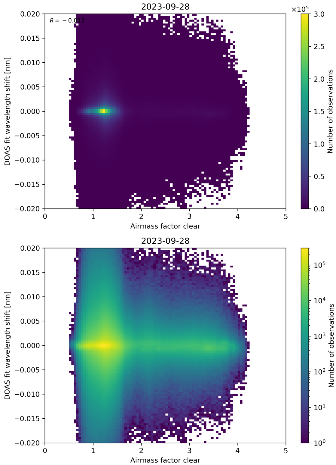
Figure 72: Scatter density plot of “Airmass factor clear” against “DOAS fit wavelength shift” for 2023-09-27 to 2023-09-29.
