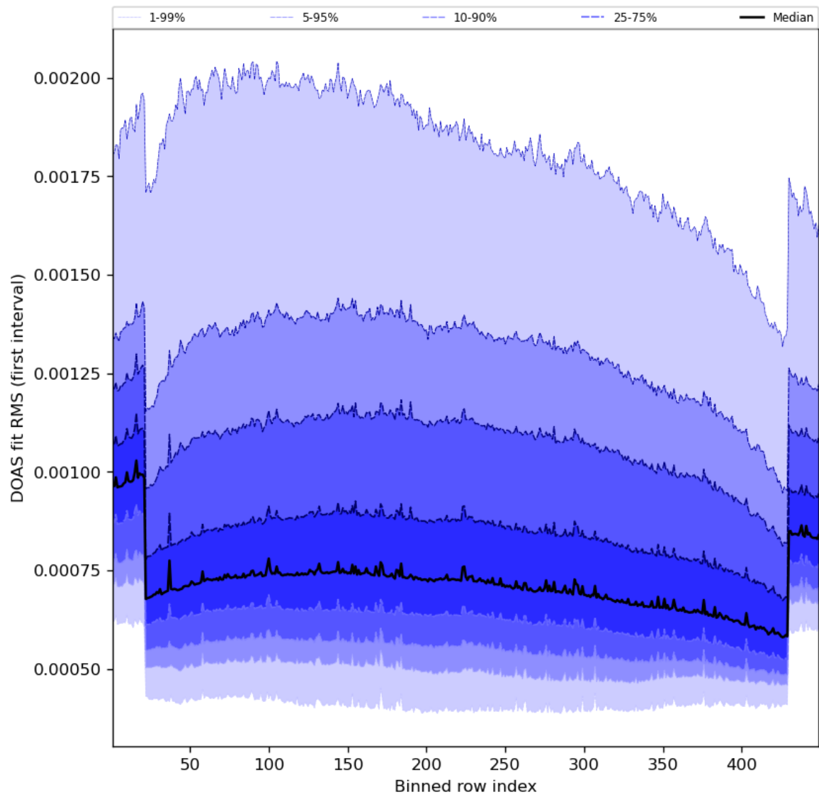
Figure 60: Along track statistics of “DOAS fit RMS (first interval)” for 2023-10-01 to 2023-10-02
