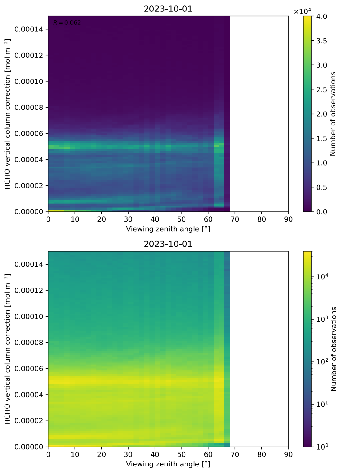
Figure 193: Scatter density plot of “Viewing zenith angle” against “HCHO vertical column correction” for 2023-10-01 to 2023-10-02.
