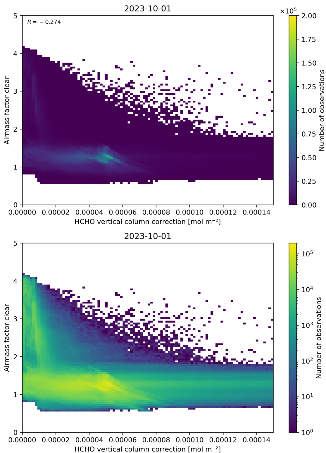
Figure 115: Scatter density plot of “HCHO vertical column correction” against “Airmass factor clear” for 2023-10-01 to 2023-10-02.
