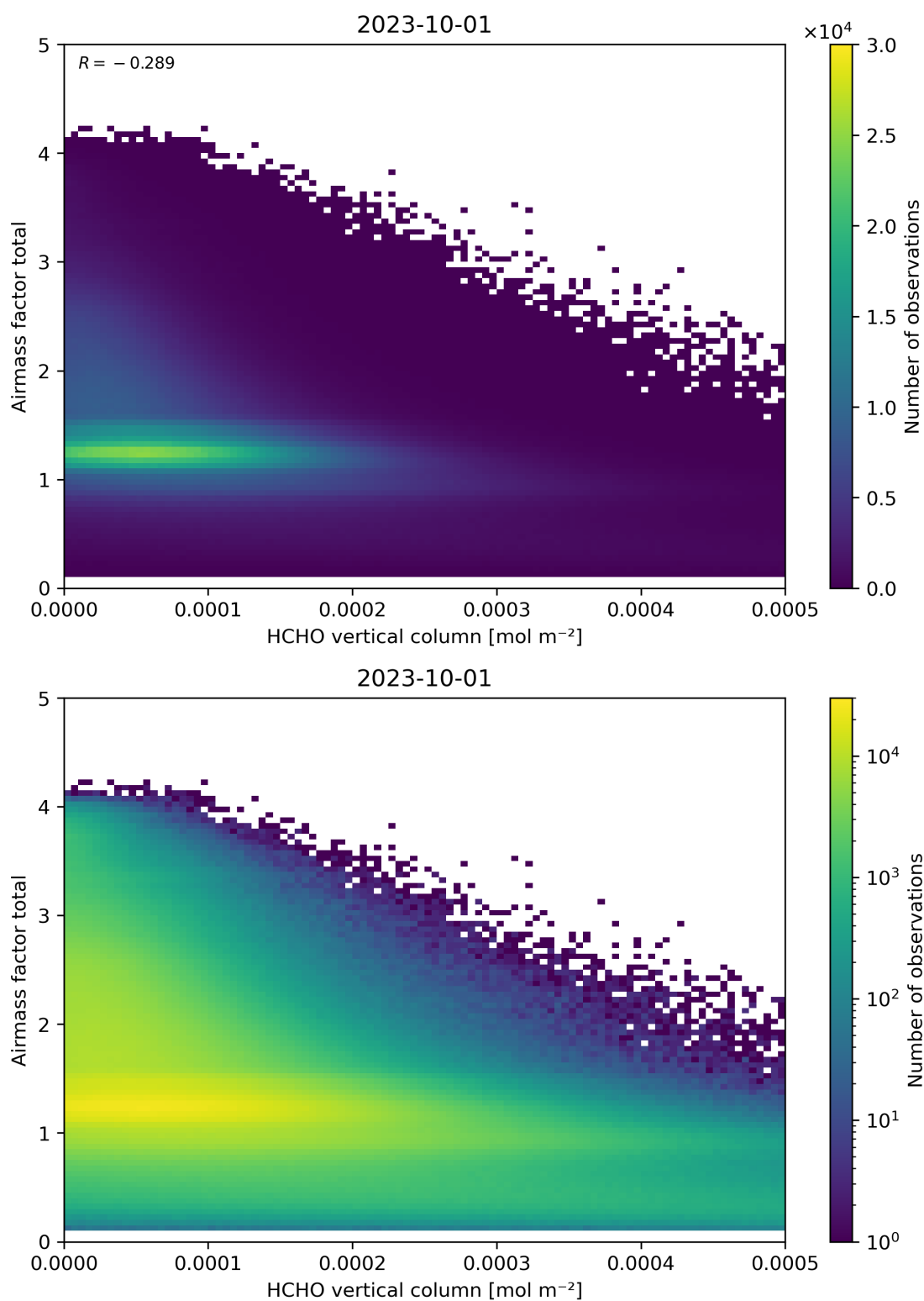
Figure 131: Scatter density plot of “HCHO vertical column” against “Airmass factor total” for 2023-10-01 to 2023-10-02.
