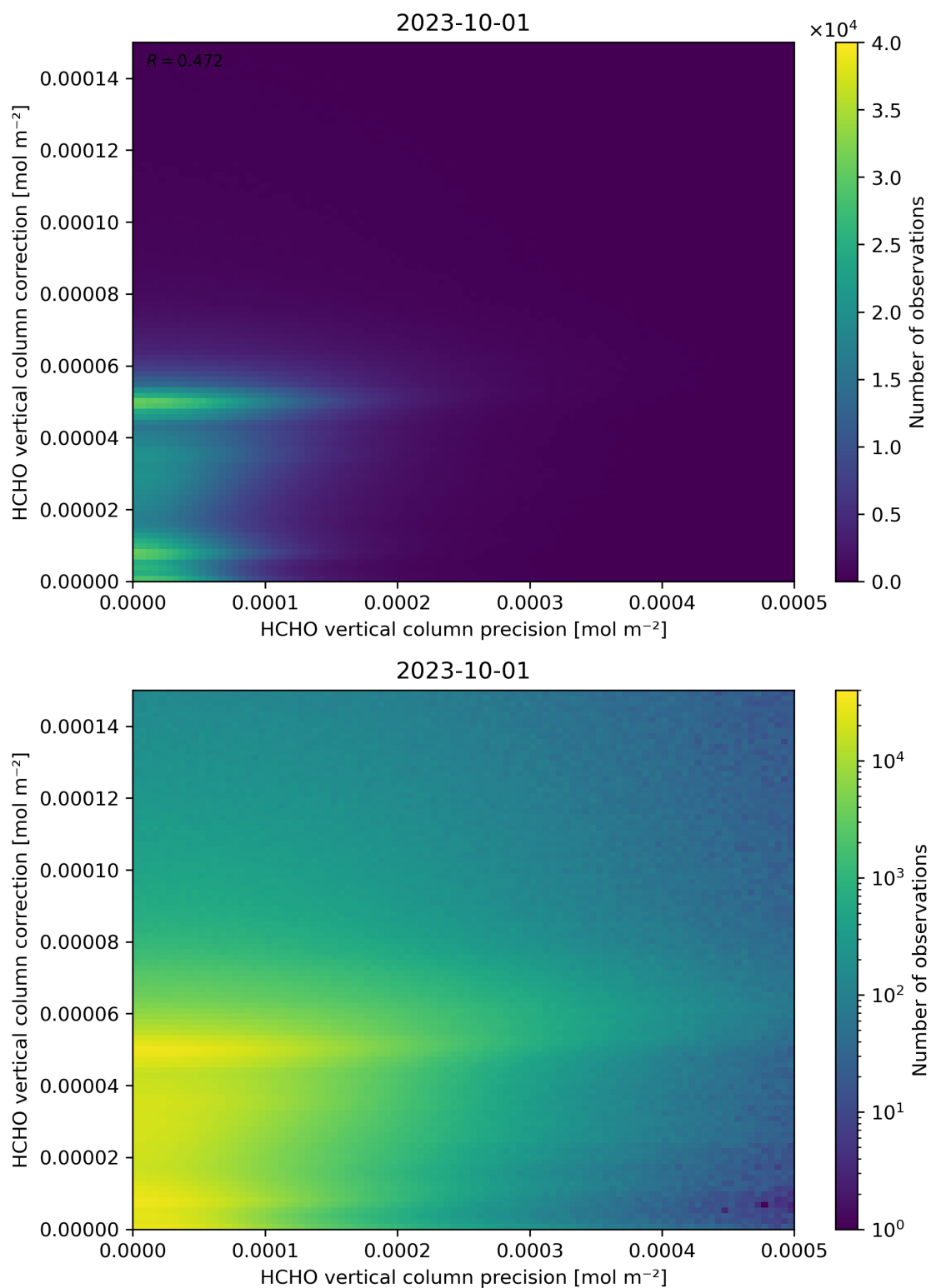
Figure 146: Scatter density plot of “HCHO vertical column precision” against “HCHO vertical column correction” for 2023-10-01 to 2023-10-02.
