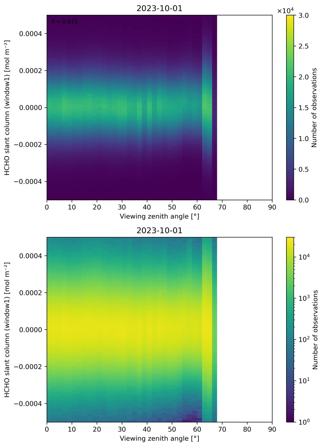
Figure 188: Scatter density plot of “Viewing zenith angle” against “HCHO slant column (window1)” for 2023-10-01 to 2023-10-02.
