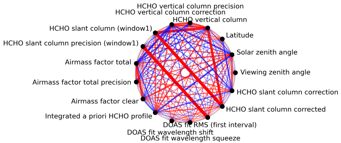
Figure 1: Map of correlation graph for 2023-10-01 to 2023-10-02.
