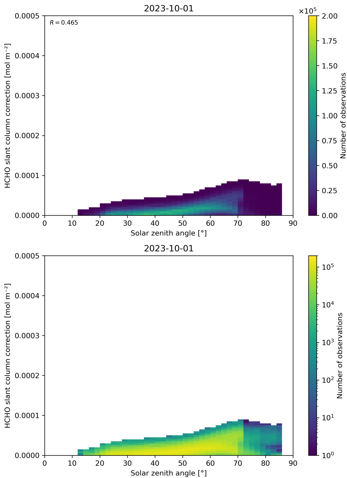
Figure 172: Scatter density plot of “Solar zenith angle” against “HCHO slant column correction” for 2023-10-01 to 2023-10-02.
