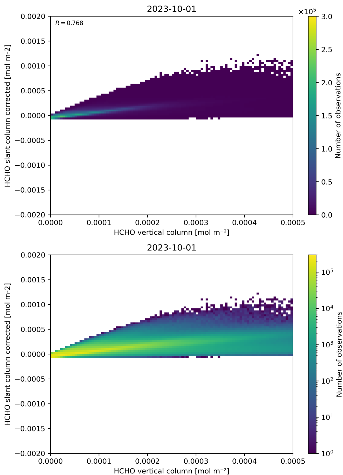
Figure 127: Scatter density plot of “HCHO vertical column” against “HCHO slant column corrected” for 2023-10-01 to 2023-10-02.
