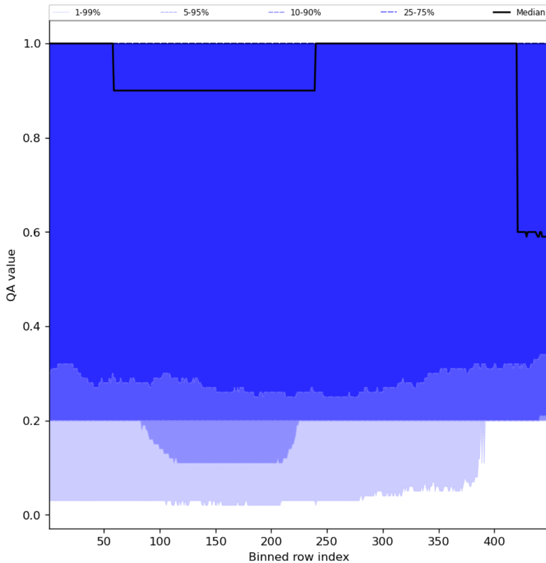
Figure 48: Along track statistics of “QA value” for 2023-10-01 to 2023-10-02
