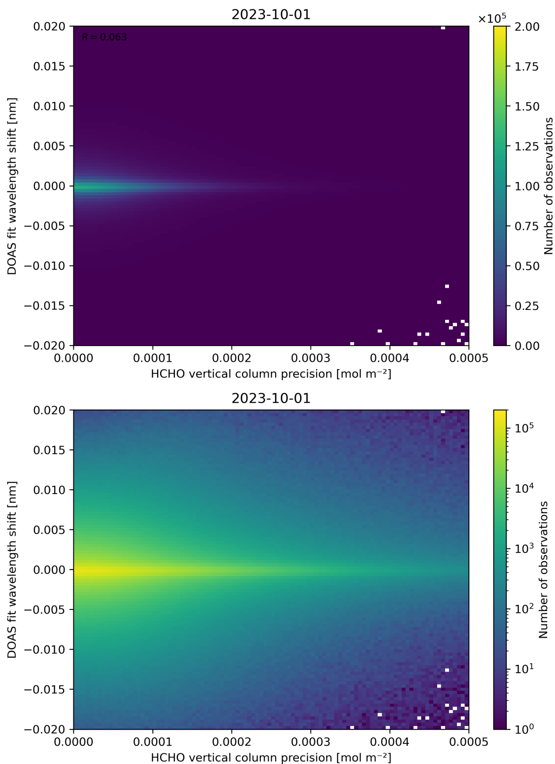
Figure 137: Scatter density plot of “HCHO vertical column precision” against “DOAS fit wavelength shift” for 2023-10-01 to 2023-10-02.
