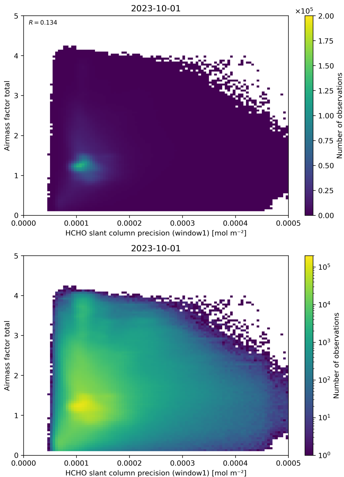
Figure 94: Scatter density plot of “HCHO slant column precision (window1)” against “Airmass factor total” for 2023-10-01 to 2023-10-02.
