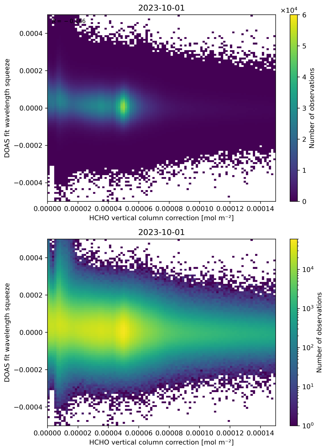
Figure 114: Scatter density plot of “HCHO vertical column correction” against “DOAS fit wavelength squeeze” for 2023-10-01 to 2023-10-02.
