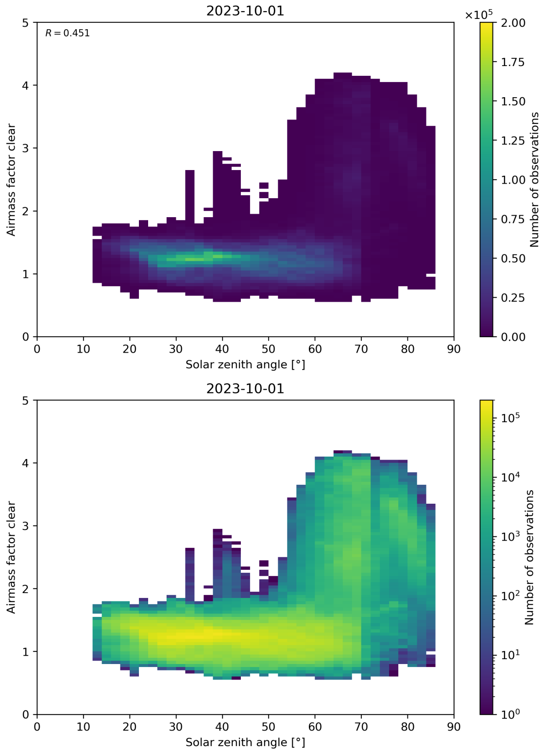
Figure 170: Scatter density plot of “Solar zenith angle” against “Airmass factor clear” for 2023-10-01 to 2023-10-02.
