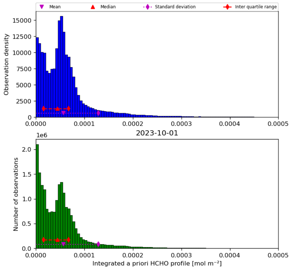
Figure 43: Histogram of “Integrated a priori HCHO profile” for 2023-10-01 to 2023-10-02
