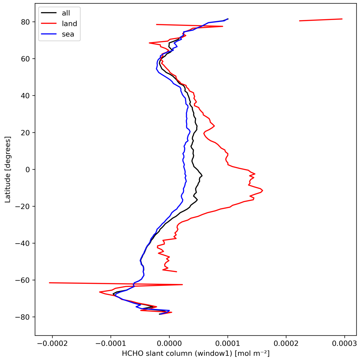
Figure 24: Zonal average of “HCHO slant column (window1)” for 2023-10-01 to 2023-10-02.
