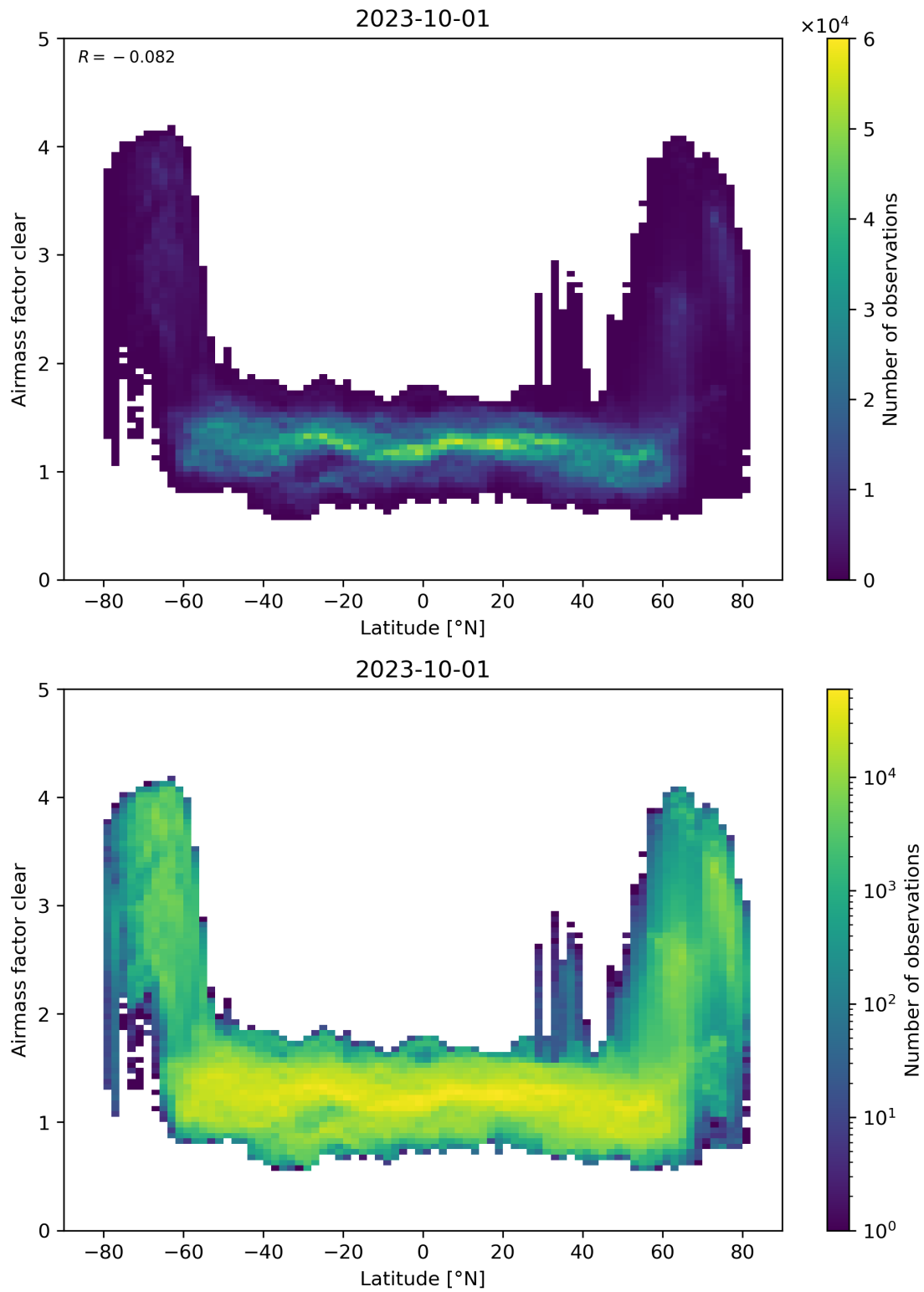
Figure 156: Scatter density plot of “Latitude” against “Airmass factor clear” for 2023-10-01 to 2023-10-02.
