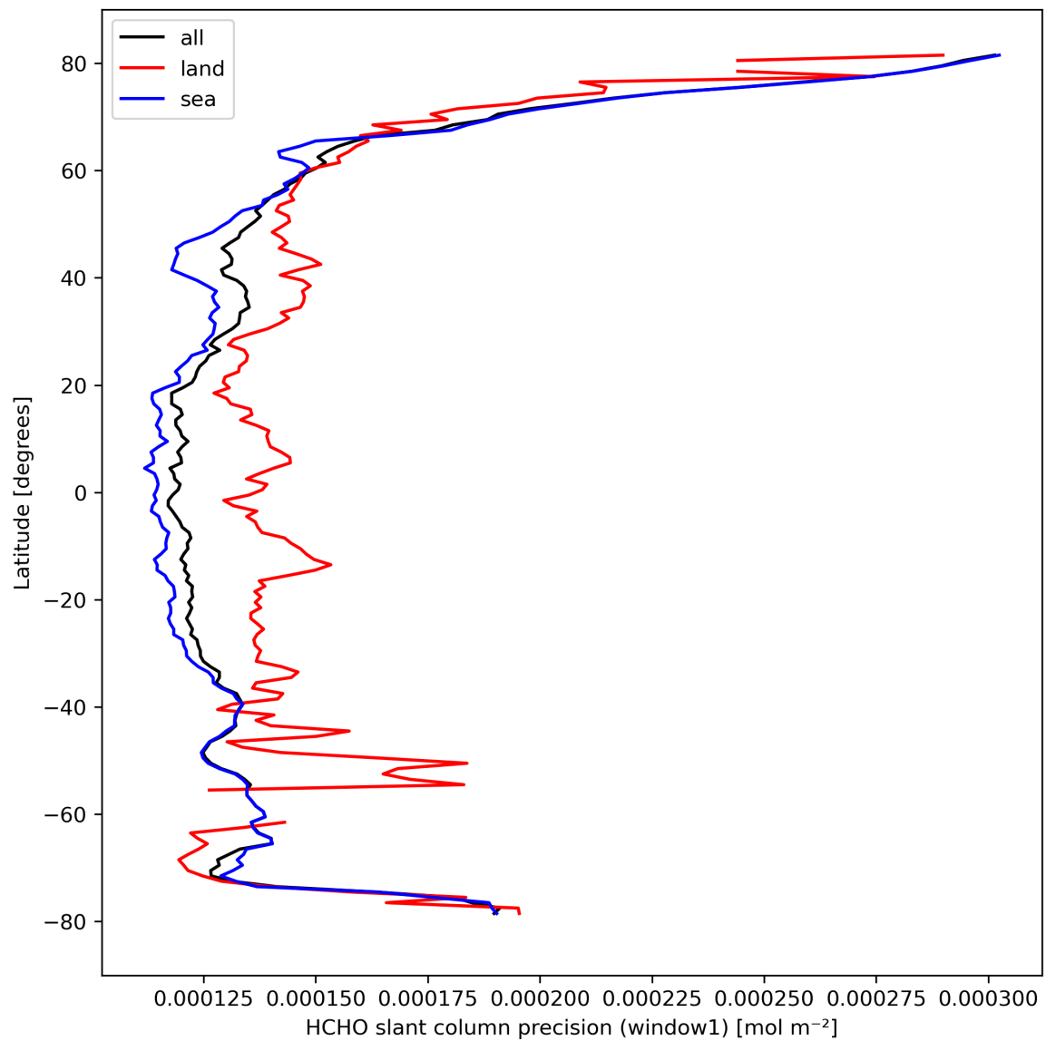
Figure 25: Zonal average of “HCHO slant column precision (window1)” for 2023-10-01 to 2023-10-02.
