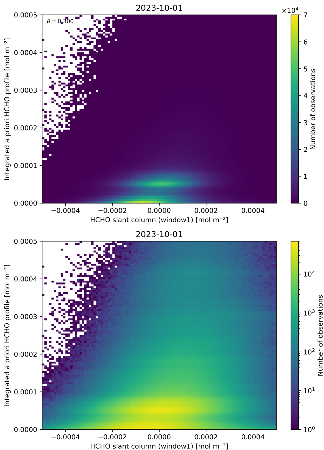
Figure 87: Scatter density plot of “HCHO slant column (window1)” against “Integrated a priori HCHO profile” for 2023-10-01 to 2023-10-02.
