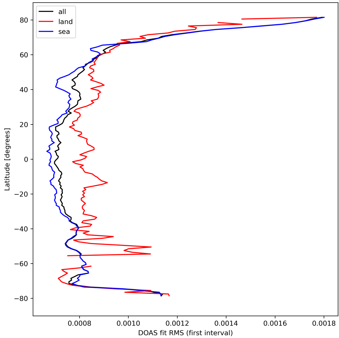
Figure 32: Zonal average of “DOAS fit RMS (first interval)” for 2023-10-01 to 2023-10-02.
