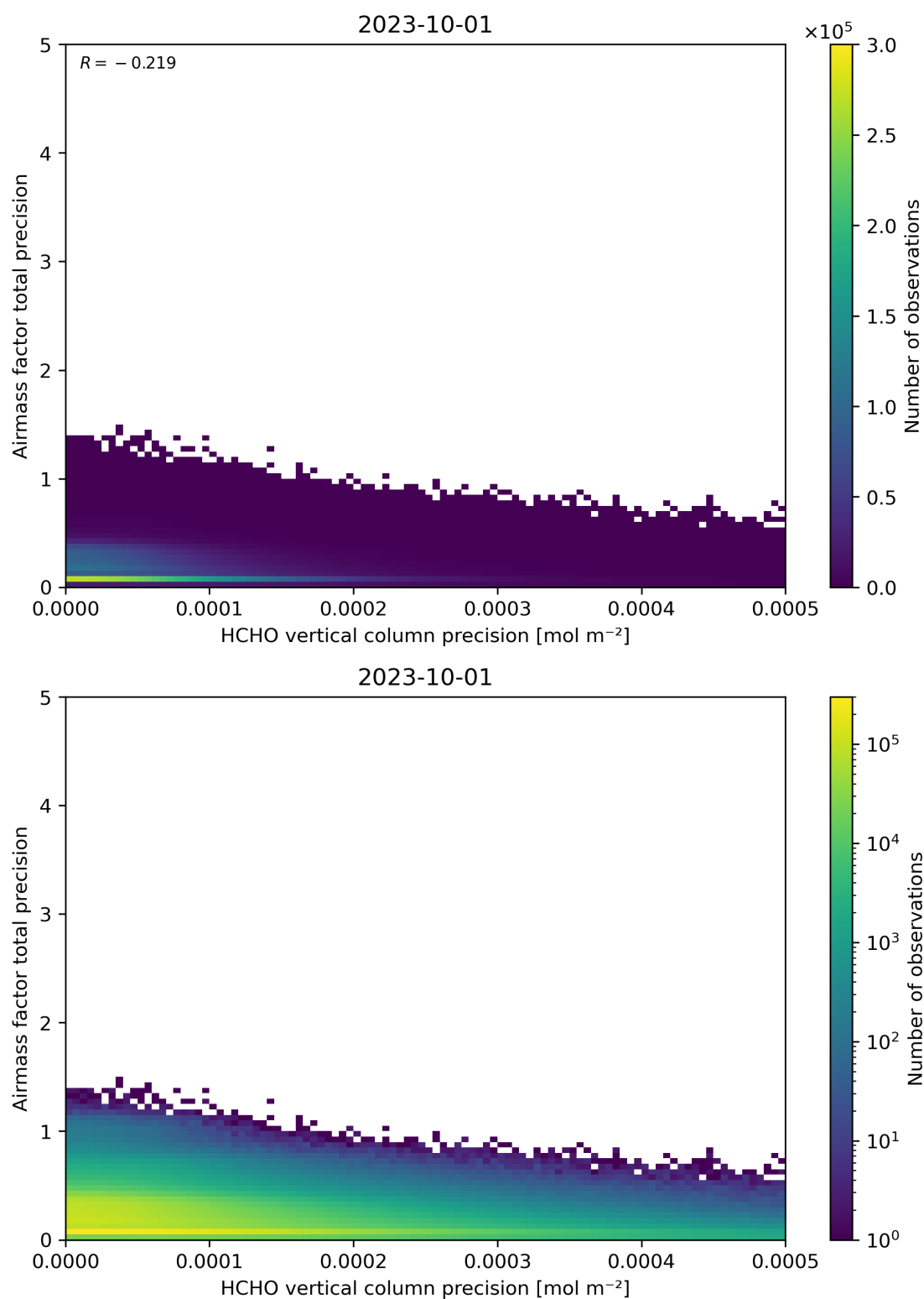
Figure 145: Scatter density plot of “HCHO vertical column precision” against “Airmass factor total precision” for 2023-10-01 to 2023-10-02.
