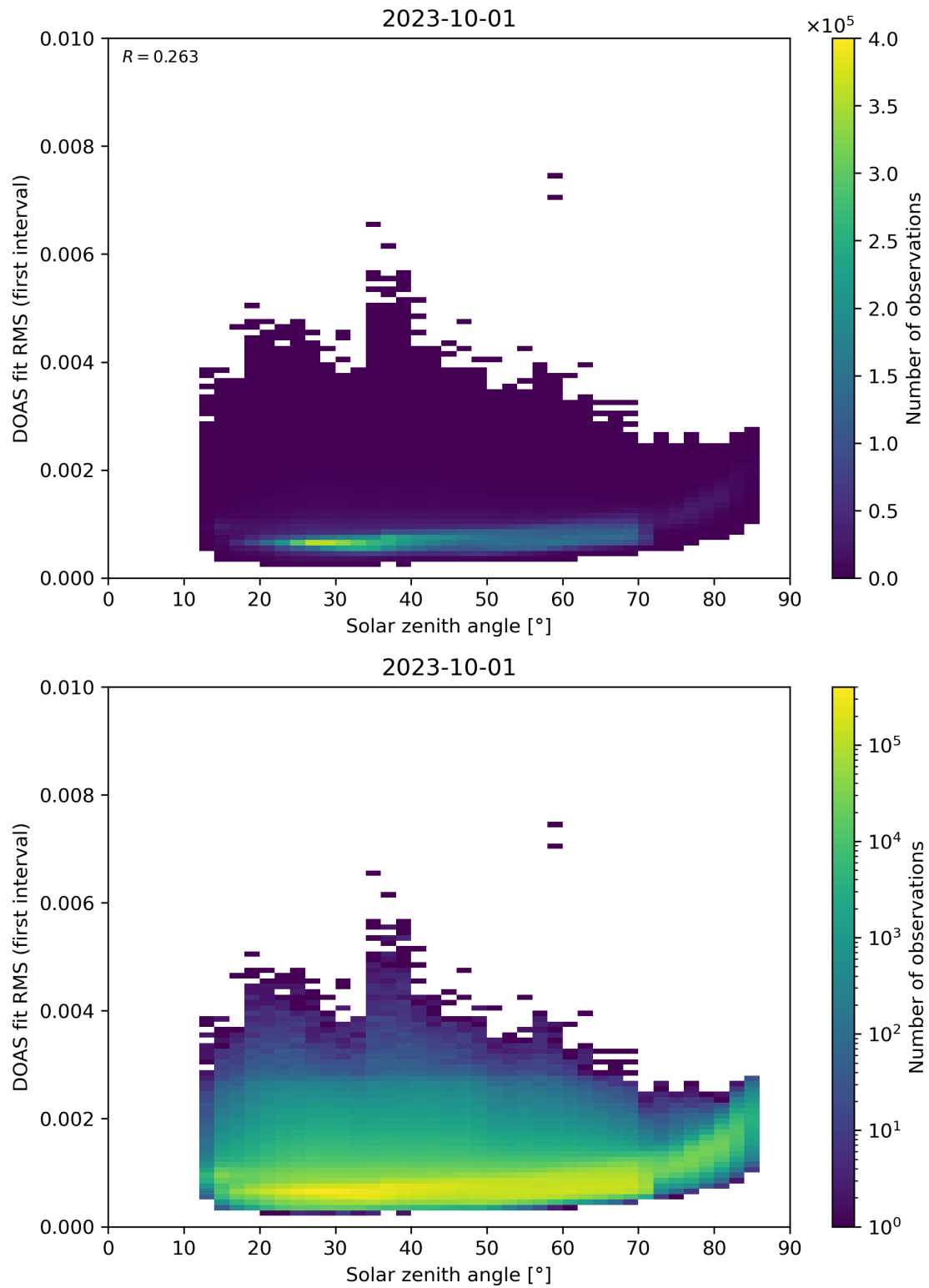
Figure 167: Scatter density plot of “Solar zenith angle” against “DOAS fit RMS (first interval)” for 2023-10-01 to 2023-10-02.
