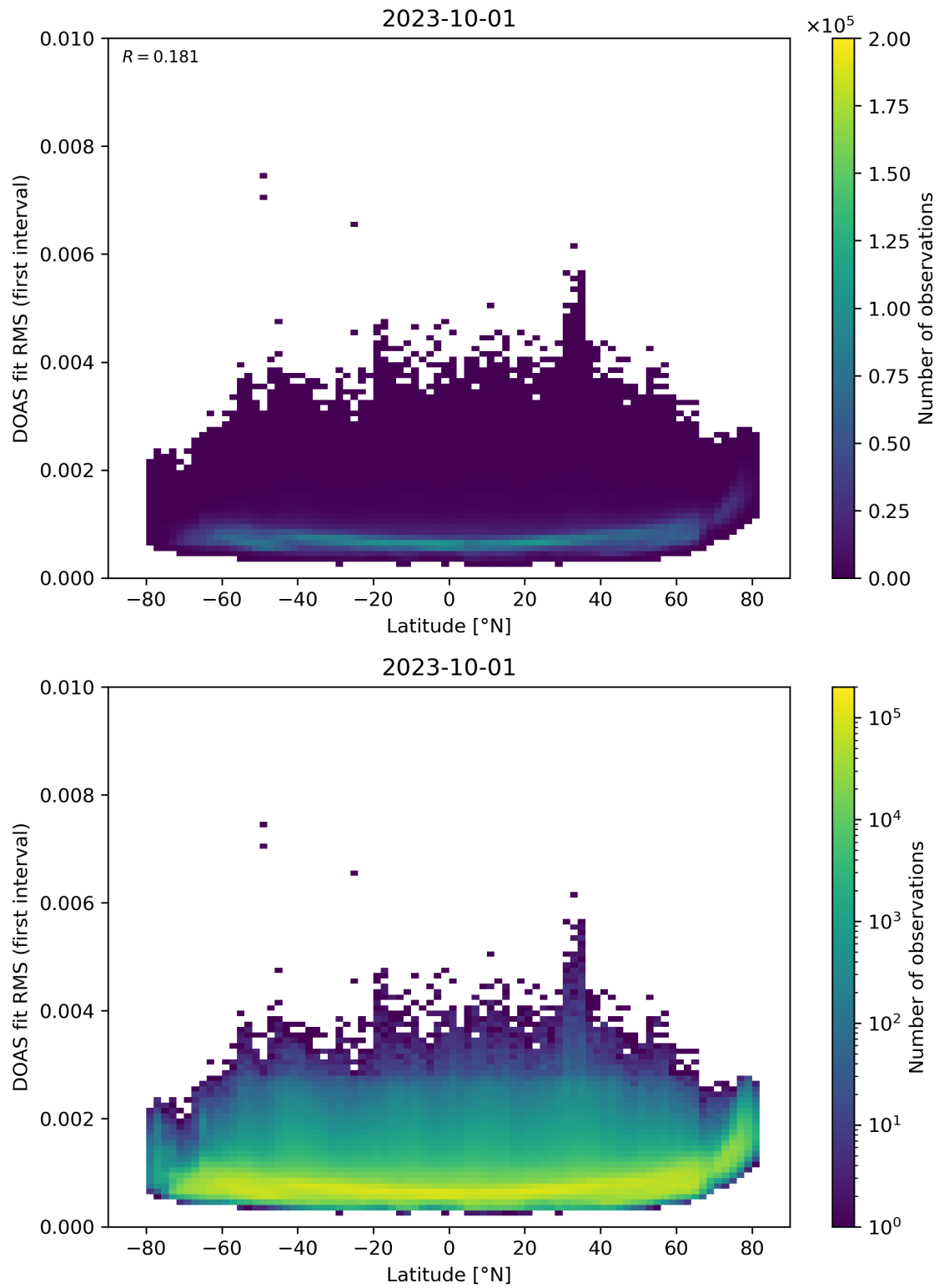
Figure 153: Scatter density plot of “Latitude” against “DOAS fit RMS (first interval)” for 2023-10-01 to 2023-10-02.
