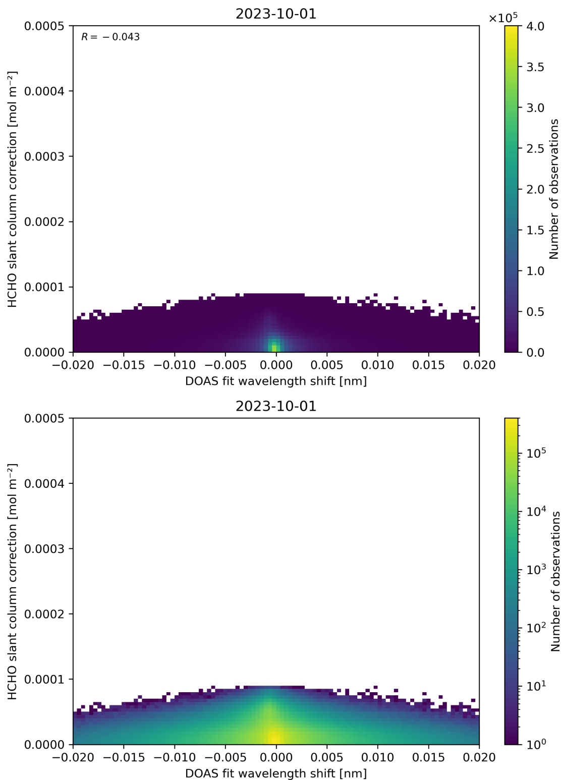
Figure 67: Scatter density plot of “DOAS fit wavelength shift” against “HCHO slant column correction” for 2023-10-01 to 2023-10-02.
