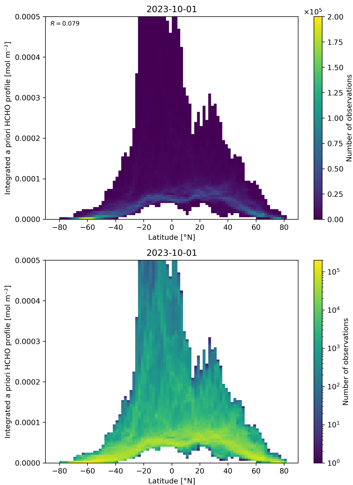
Figure 166: Scatter density plot of “Latitude” against “Integrated a priori HCHO profile” for 2023-10-01 to 2023-10-02.
