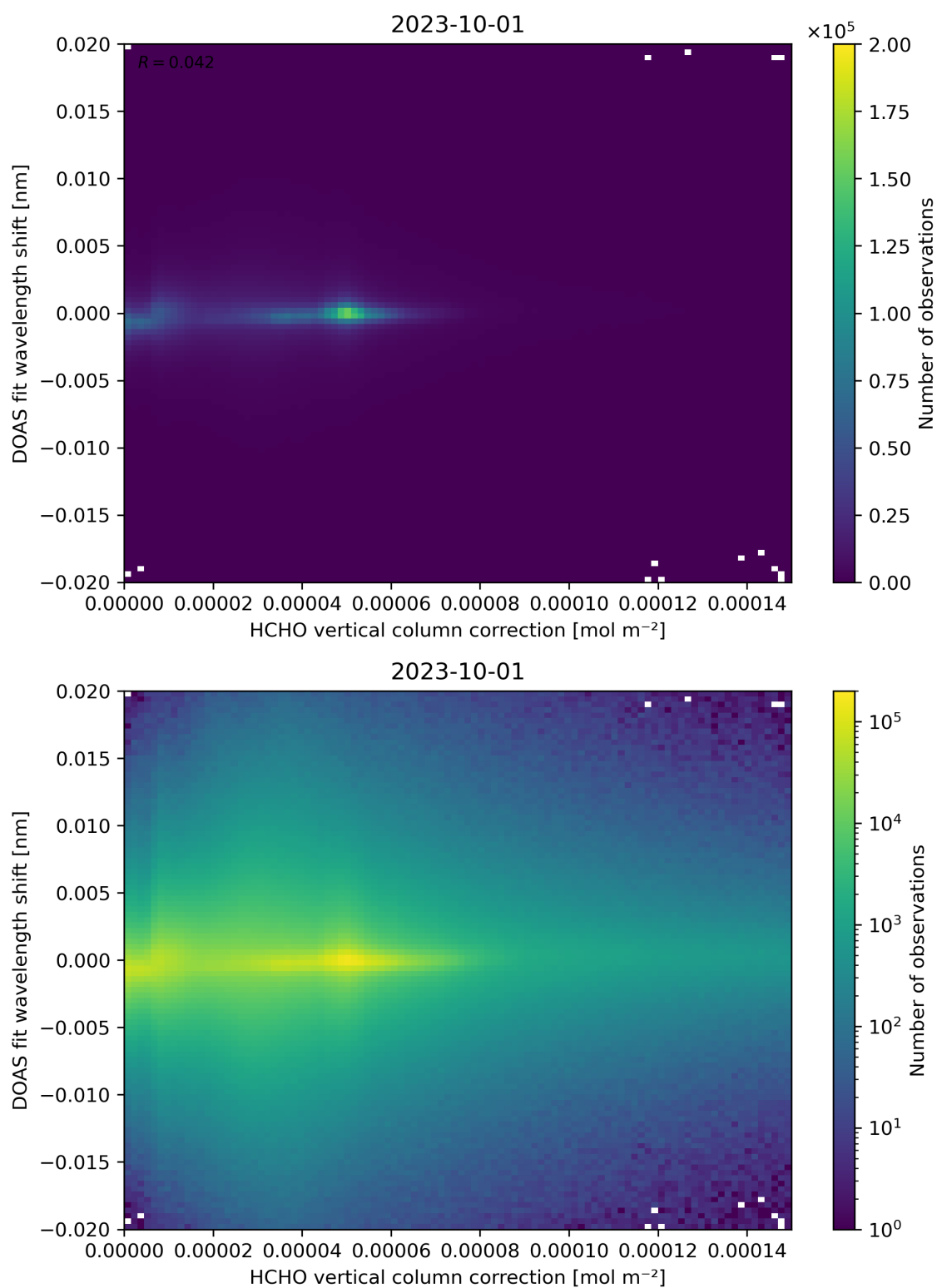
Figure 113: Scatter density plot of “HCHO vertical column correction” against “DOAS fit wavelength shift” for 2023-10-01 to 2023-10-02.
