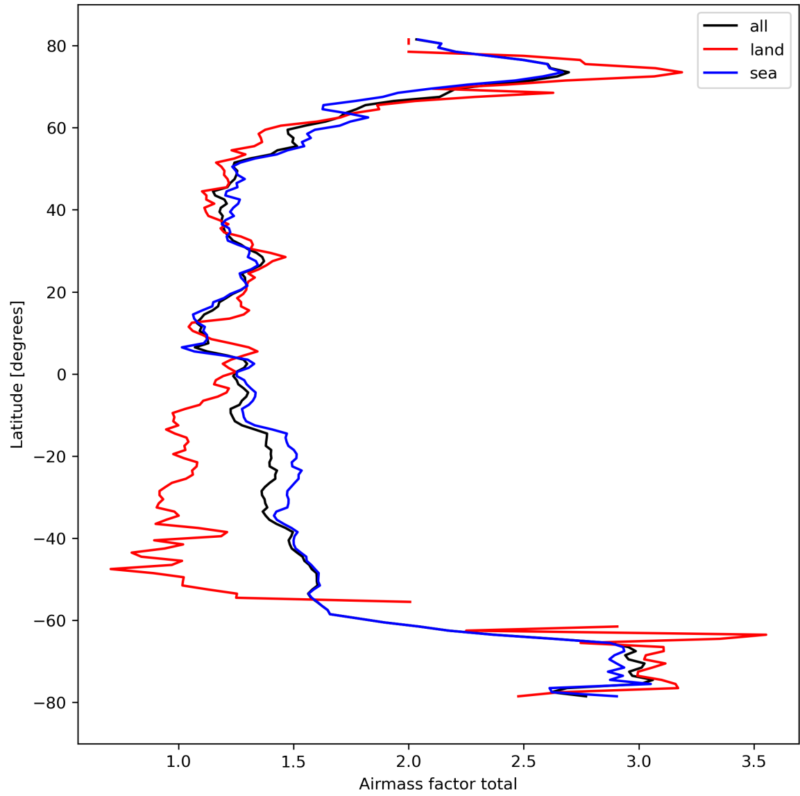
Figure 26: Zonal average of “Airmass factor total” for 2023-10-01 to 2023-10-02.
