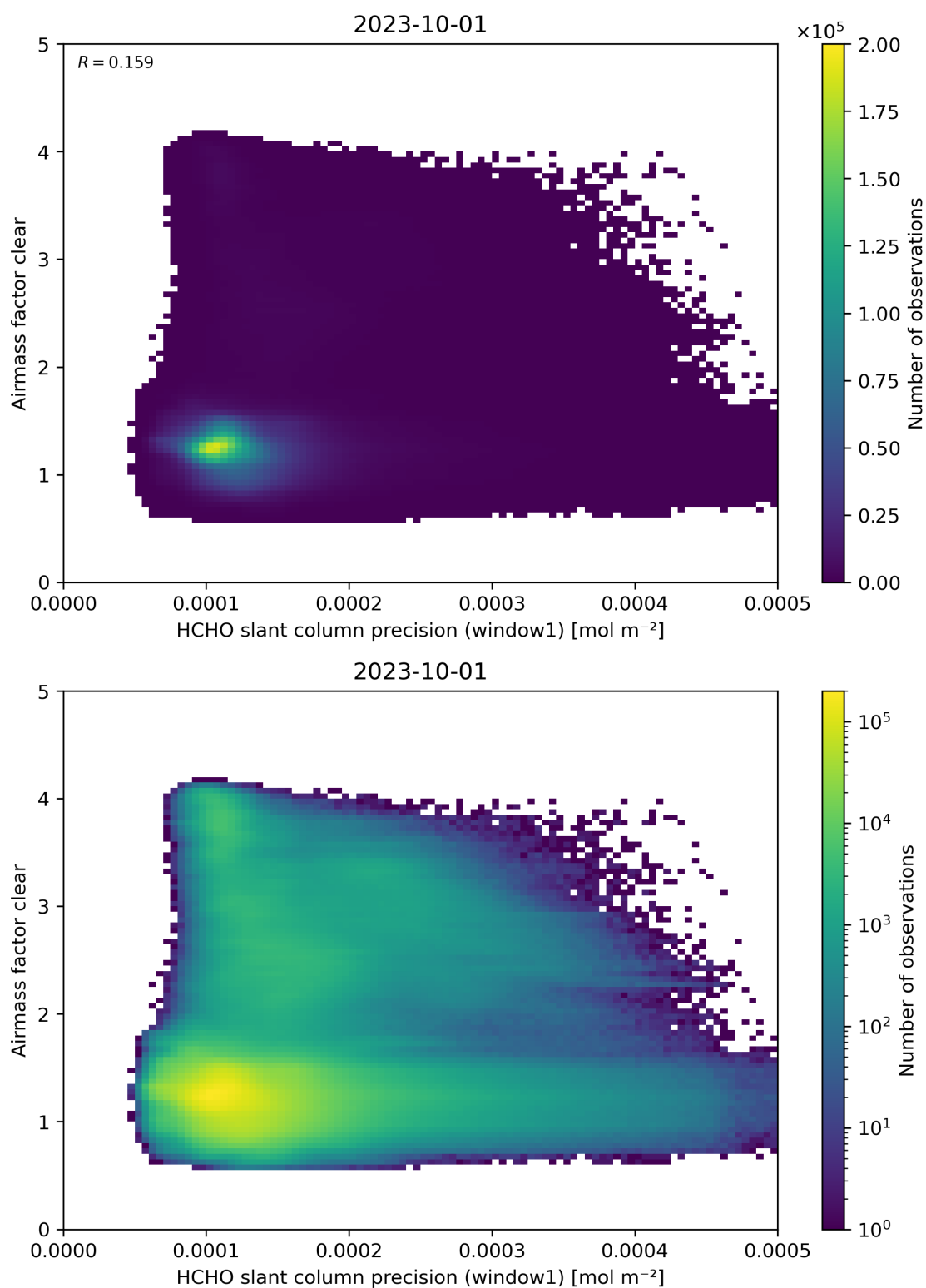
Figure 91: Scatter density plot of “HCHO slant column precision (window1)” against “Airmass factor clear” for 2023-10-01 to 2023-10-02.
