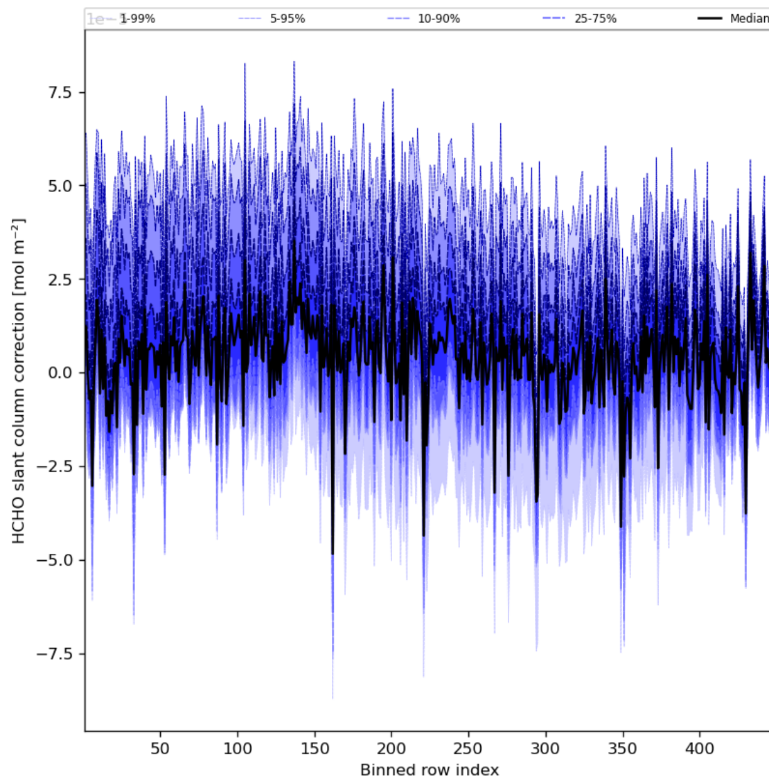
Figure 61: Along track statistics of “HCHO slant column correction” for 2023-10-01 to 2023-10-02
