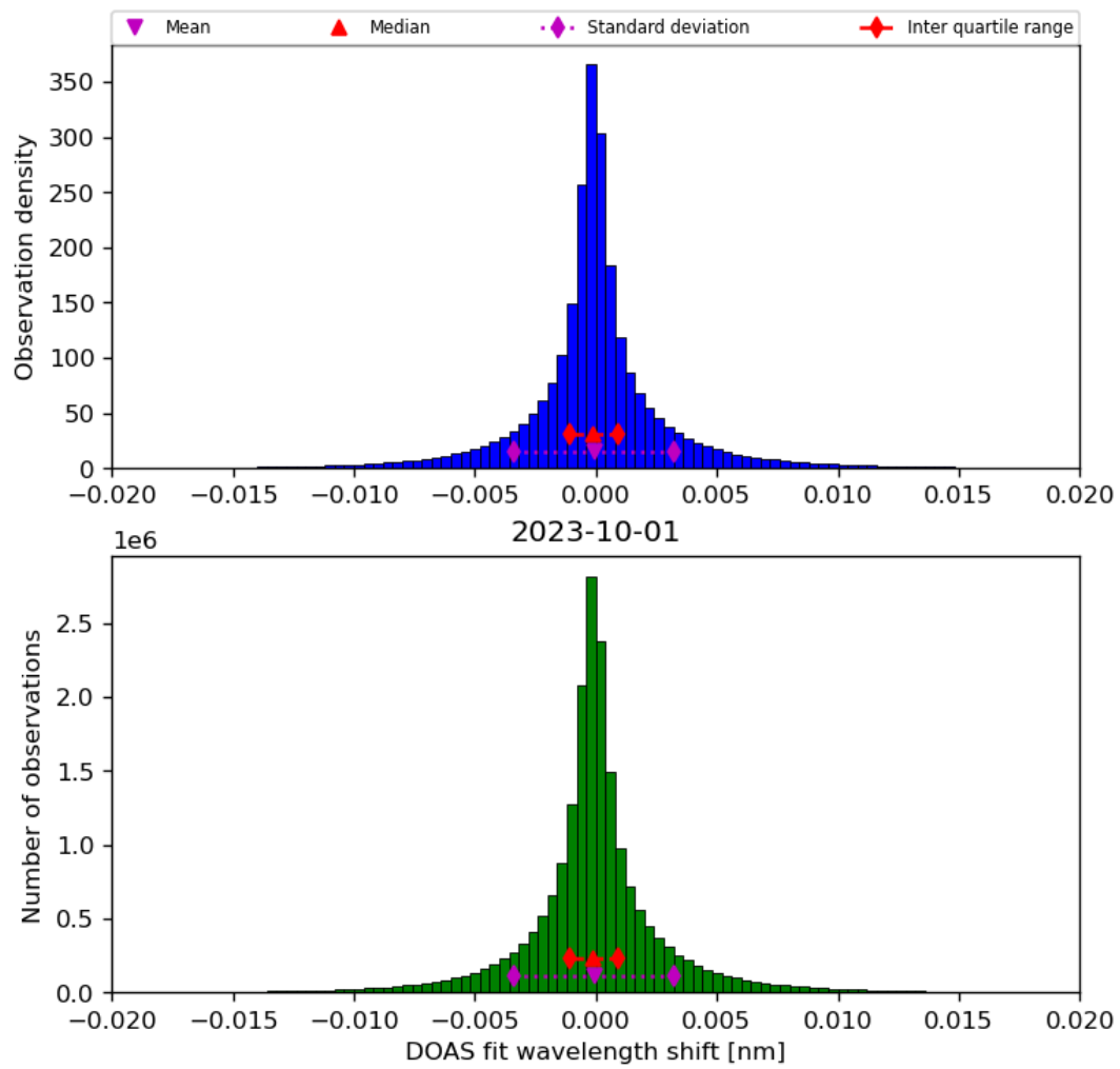
Figure 44: Histogram of “DOAS fit wavelength shift” for 2023-10-01 to 2023-10-02
