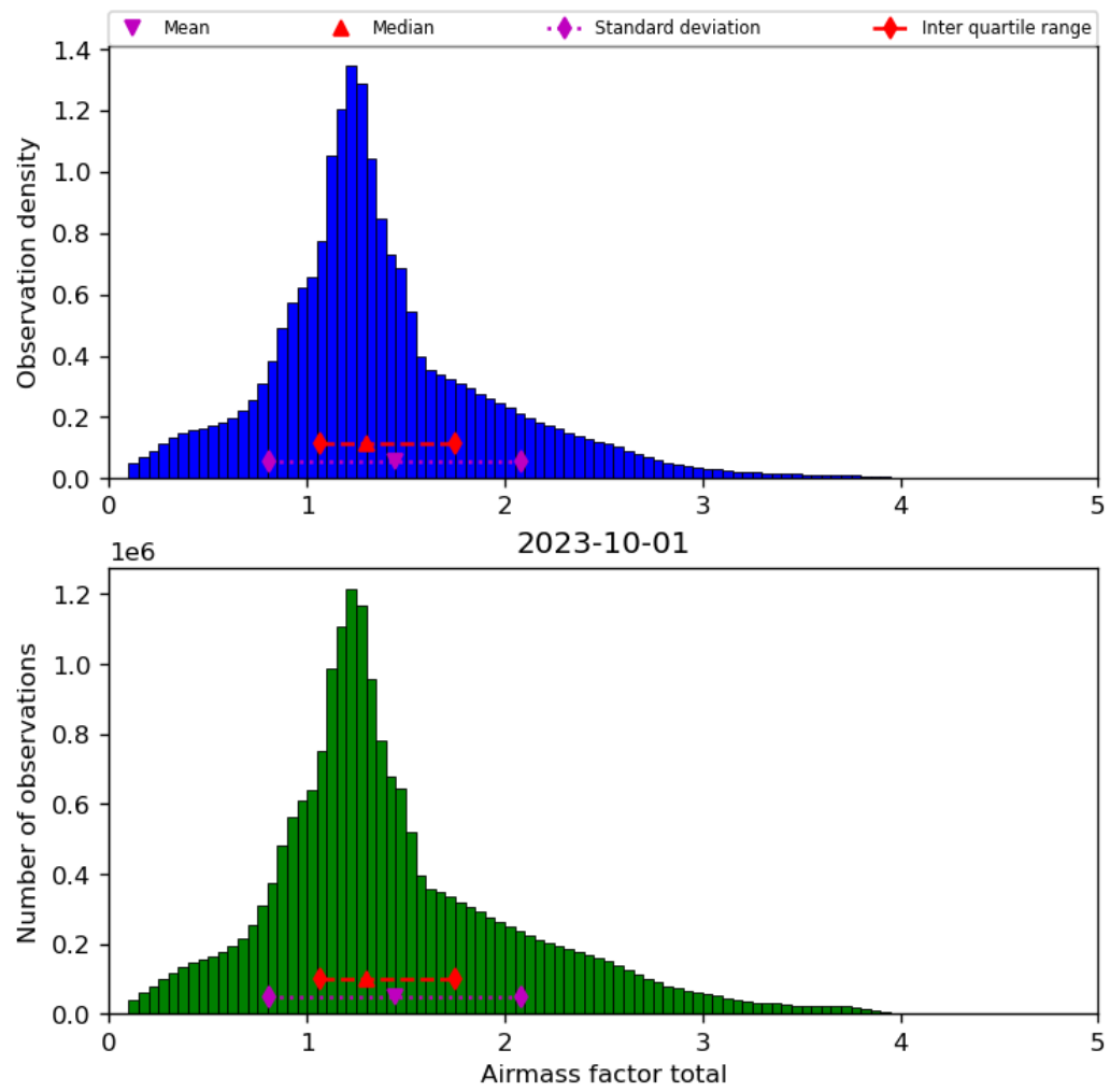
Figure 40: Histogram of “Airmass factor total” for 2023-10-01 to 2023-10-02
