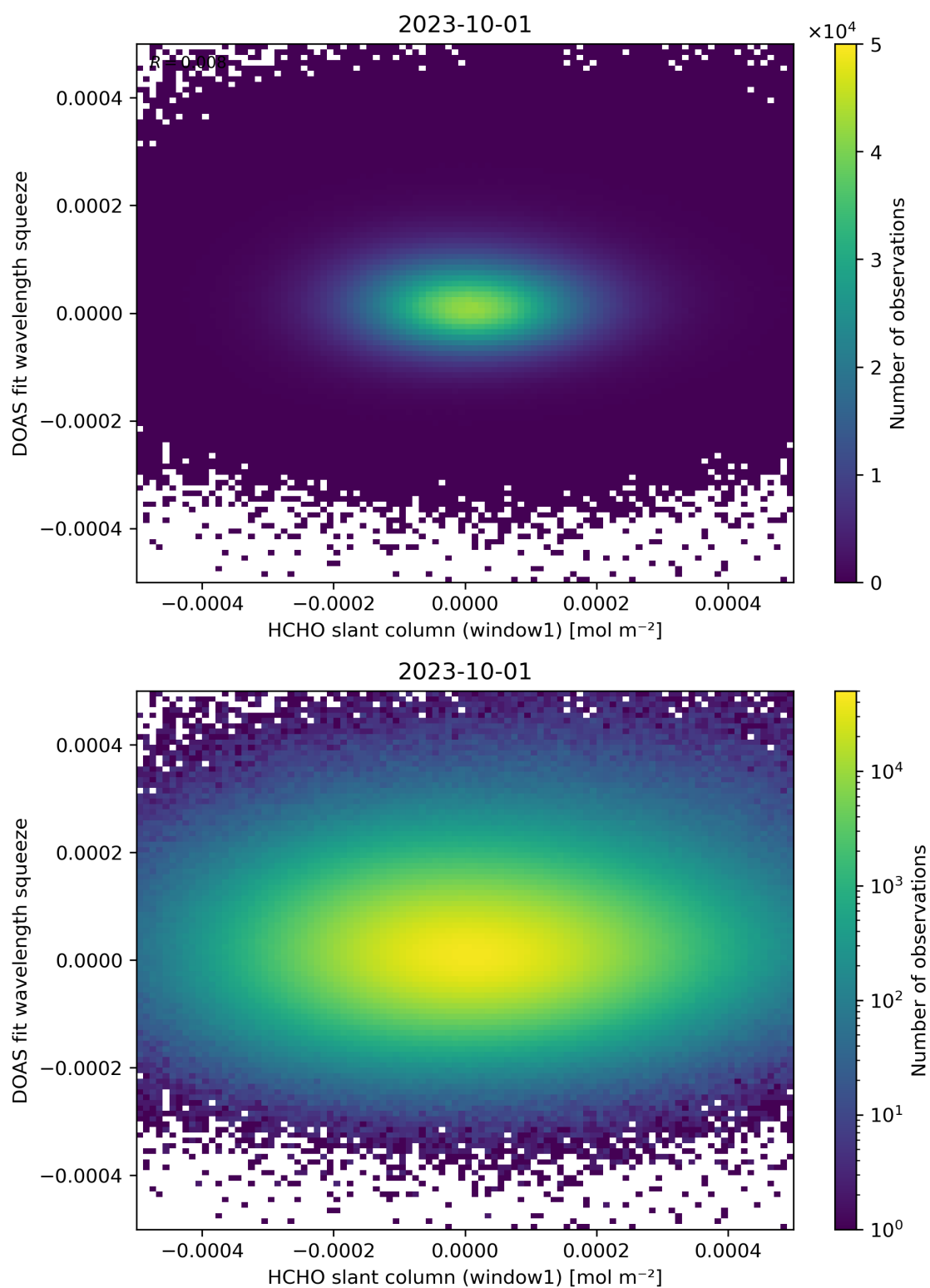
Figure 80: Scatter density plot of “HCHO slant column (window1)” against “DOAS fit wavelength squeeze” for 2023-10-01 to 2023-10-02.
