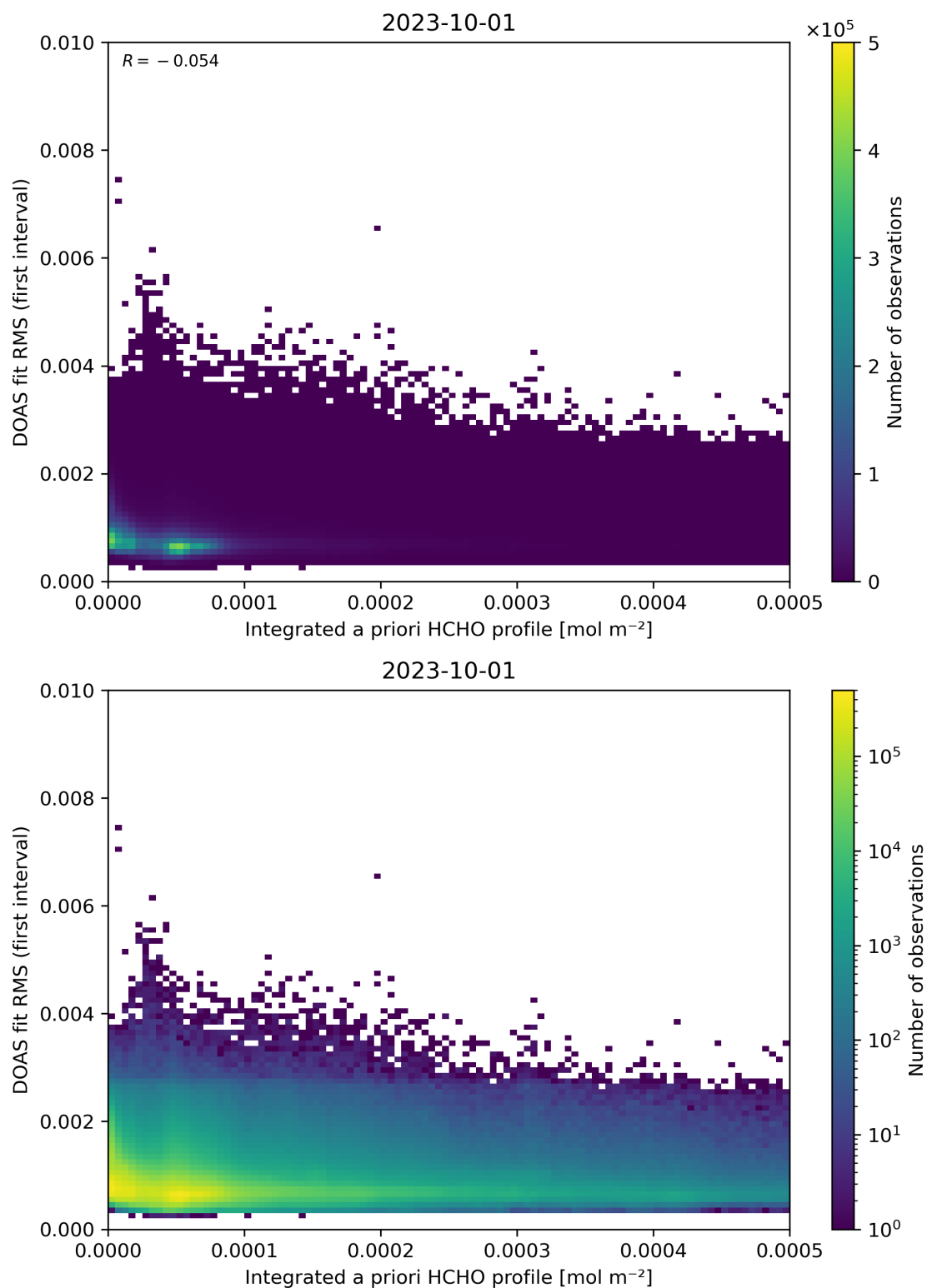
Figure 148: Scatter density plot of “Integrated a priori HCHO profile” against “DOAS fit RMS (first interval)” for 2023-10-01 to 2023-10-02.
