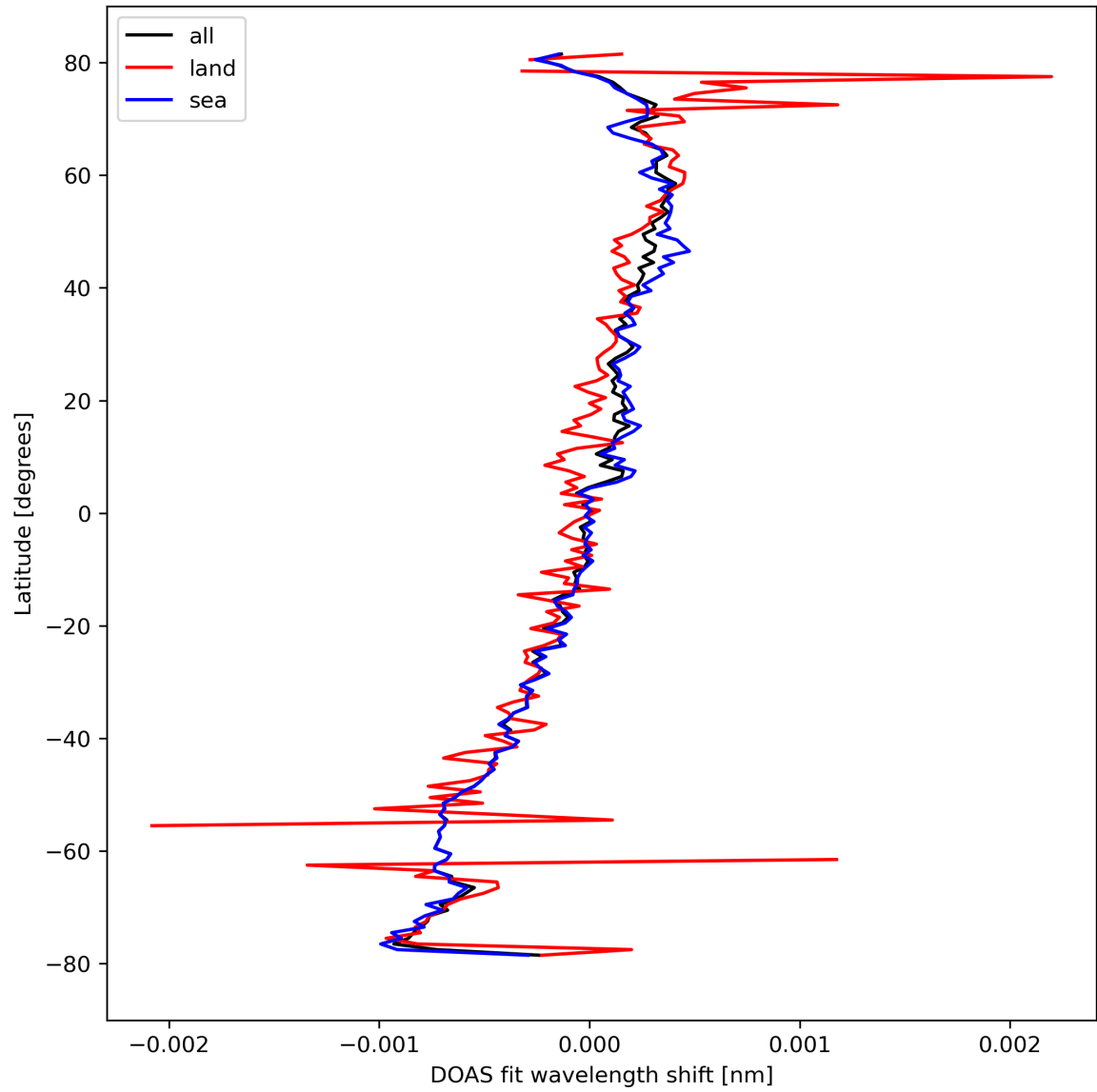
Figure 30: Zonal average of “DOAS fit wavelength shift” for 2023-10-01 to 2023-10-02.
