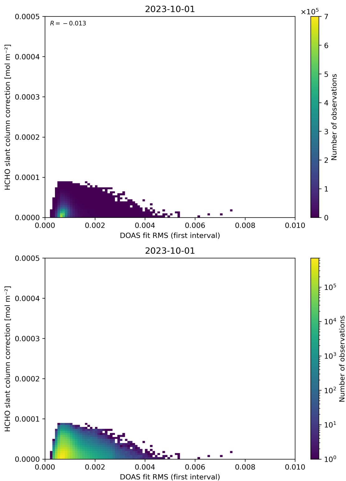
Figure 63: Scatter density plot of “DOAS fit RMS (first interval)” against “HCHO slant column correction” for 2023-10-01 to 2023-10-02.
