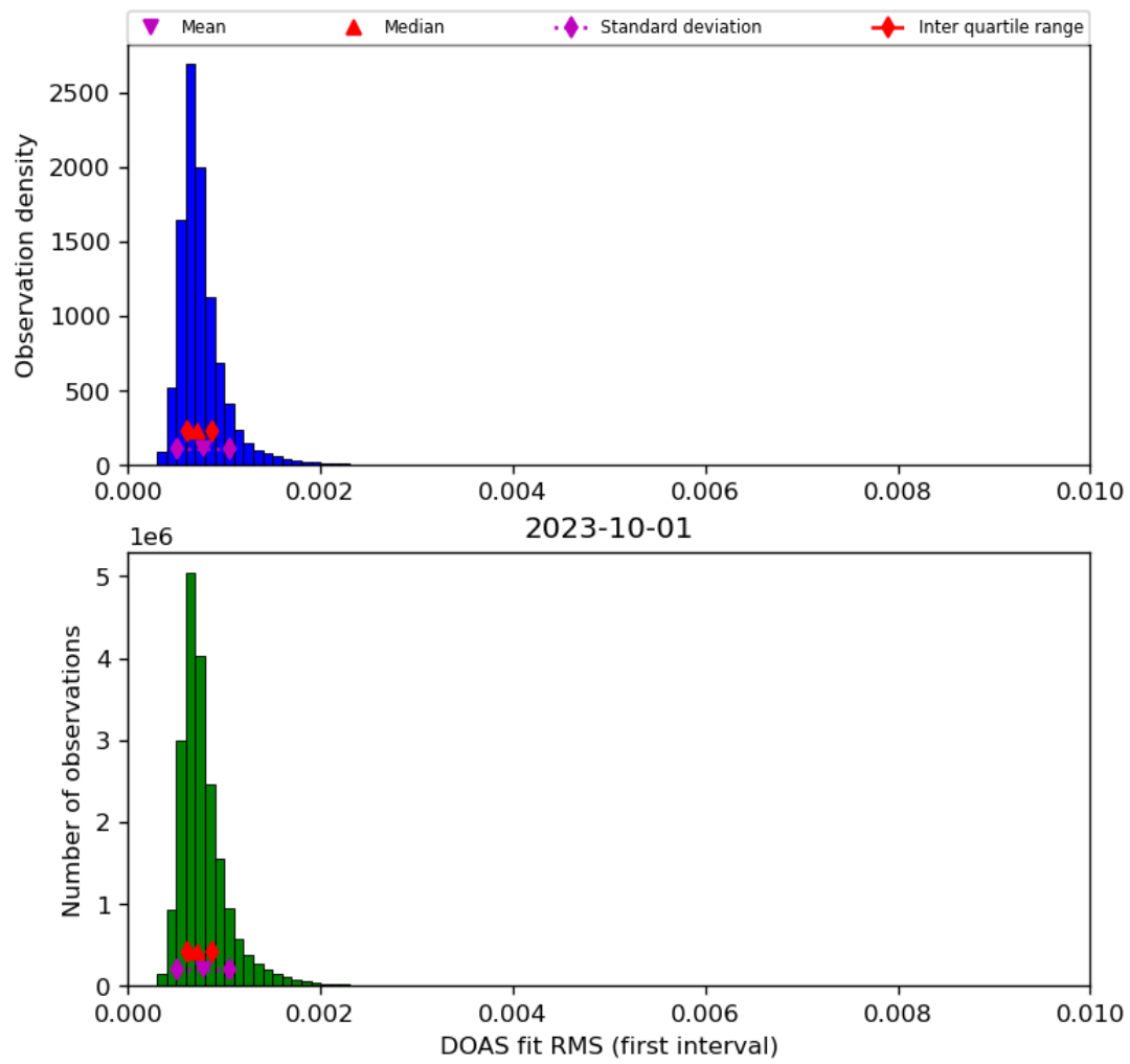
Figure 46: Histogram of “DOAS fit RMS (first interval)” for 2023-10-01 to 2023-10-02
