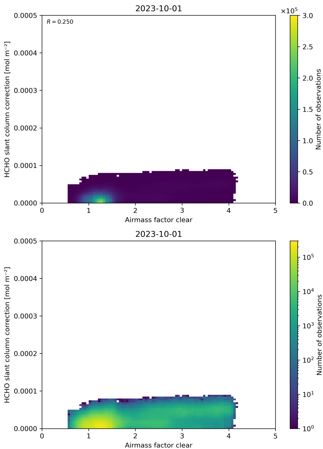
Figure 75: Scatter density plot of “Airmass factor clear” against “HCHO slant column correction” for 2023-10-01 to 2023-10-02.
