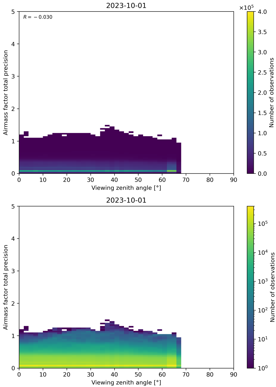
Figure 191: Scatter density plot of “Viewing zenith angle” against “Airmass factor total precision” for 2023-10-01 to 2023-10-02.
