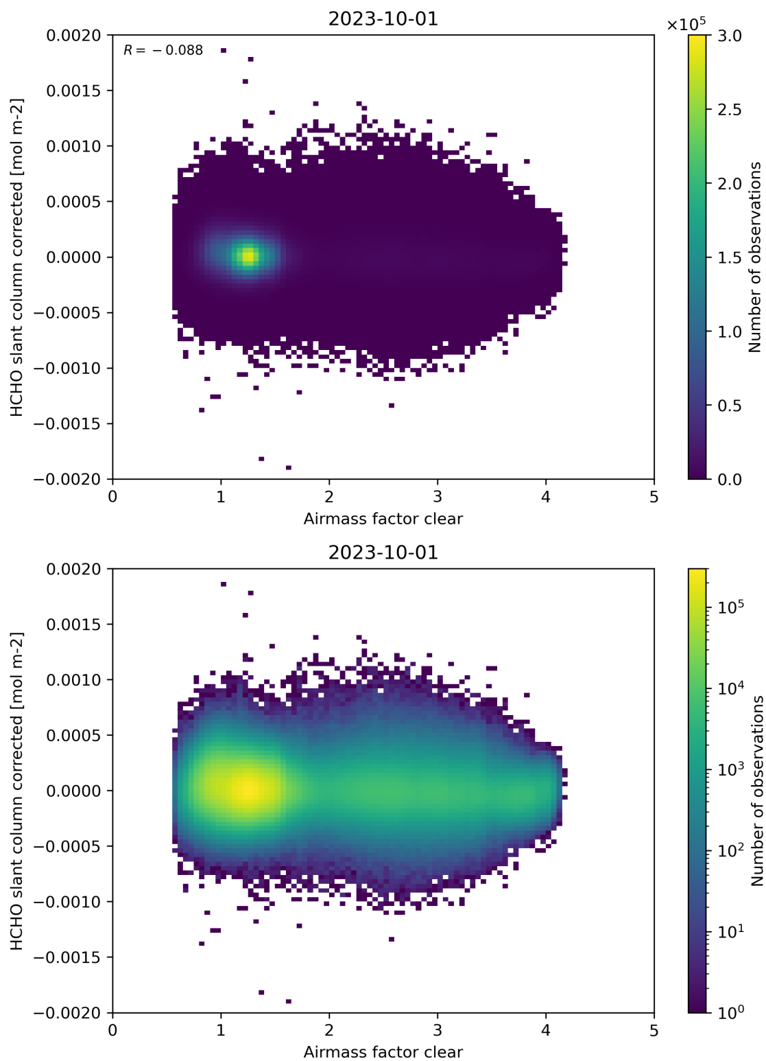
Figure 74: Scatter density plot of “Airmass factor clear” against “HCHO slant column corrected” for 2023-10-01 to 2023-10-02.
