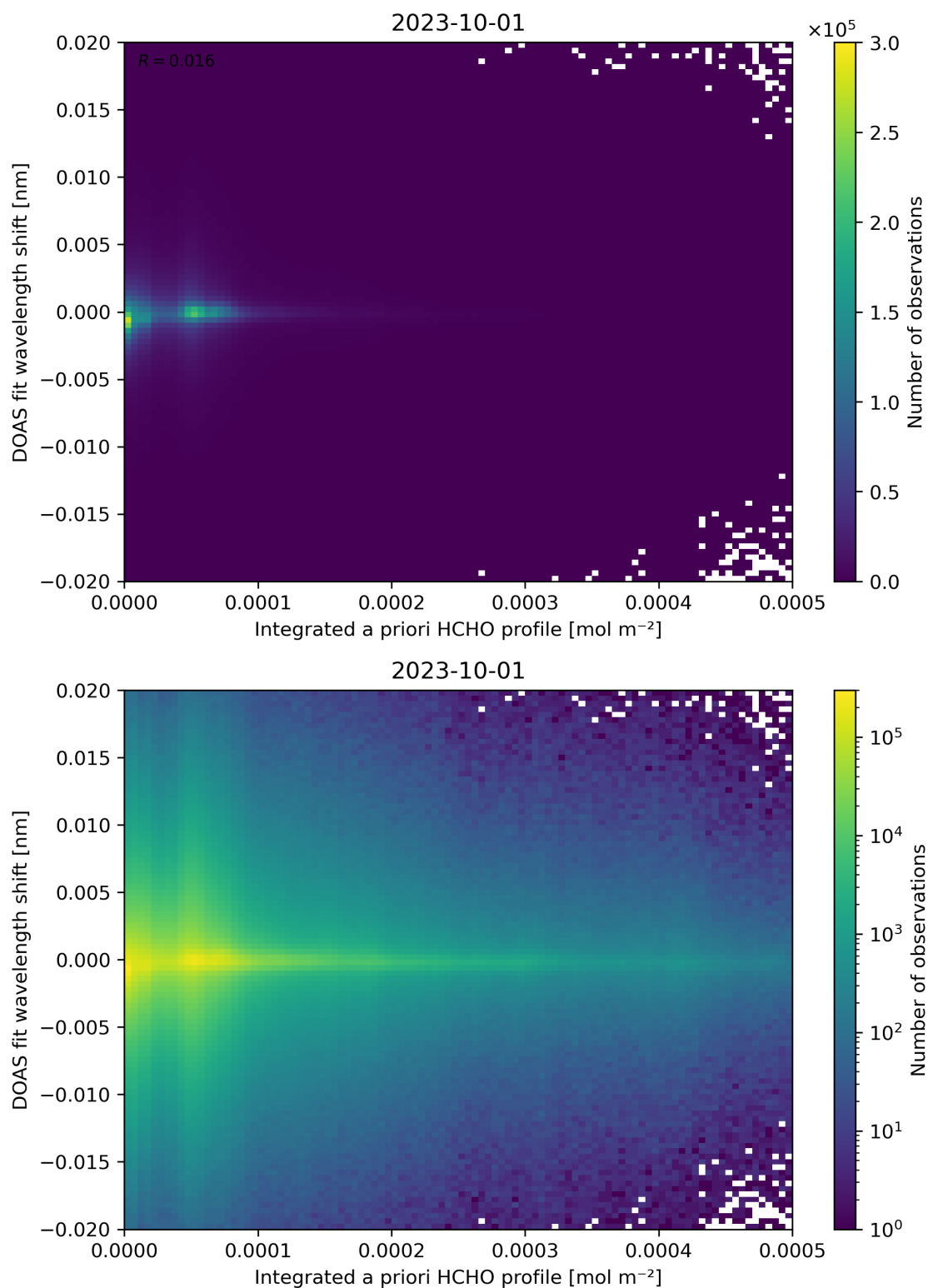
Figure 149: Scatter density plot of “Integrated a priori HCHO profile” against “DOAS fit wavelength shift” for 2023-10-01 to 2023-10-02.
