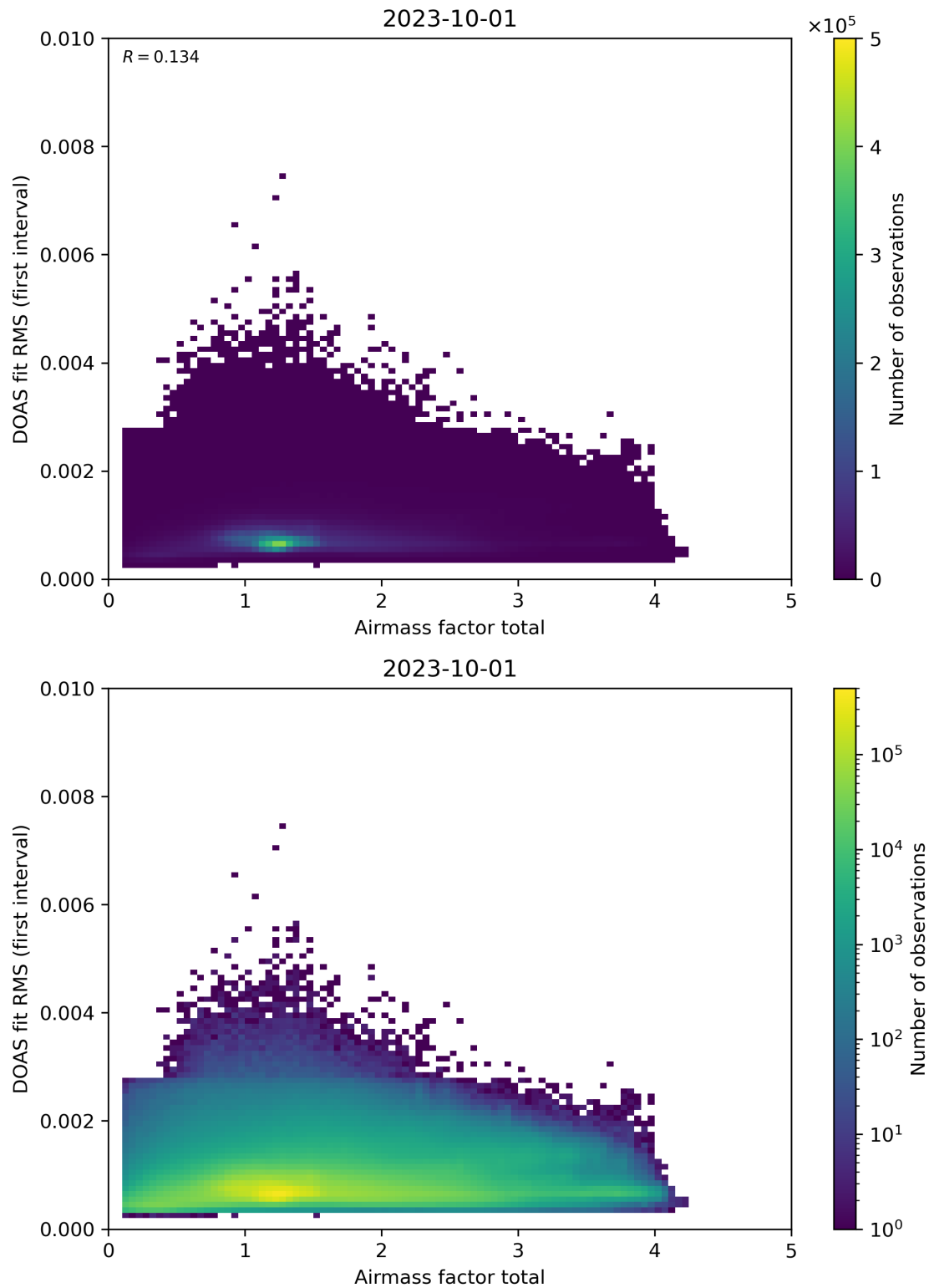
Figure 97: Scatter density plot of “Airmass factor total” against “DOAS fit RMS (first interval)” for 2023-10-01 to 2023-10-02.
