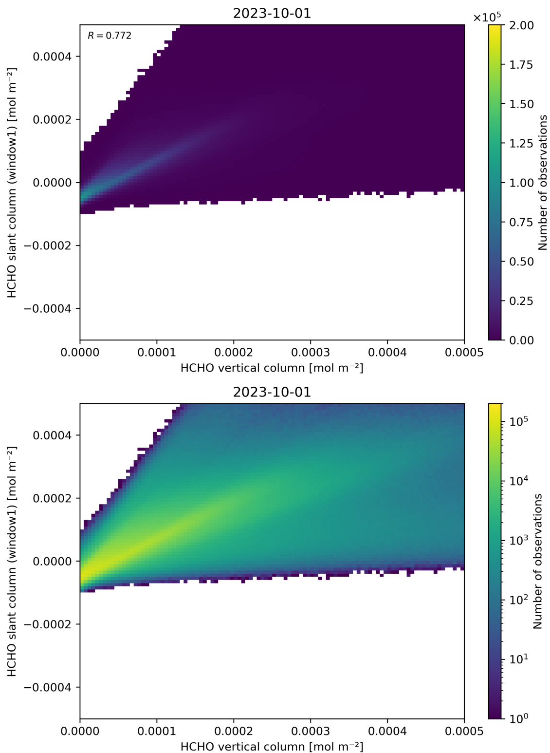
Figure 129: Scatter density plot of “HCHO vertical column” against “HCHO slant column (window1)” for 2023-10-01 to 2023-10-02.
