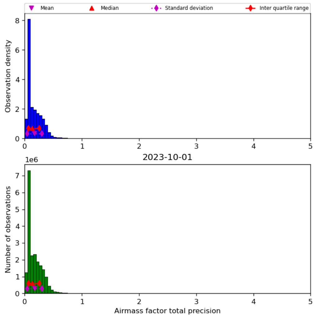
Figure 41: Histogram of “Airmass factor total precision” for 2023-10-01 to 2023-10-02
