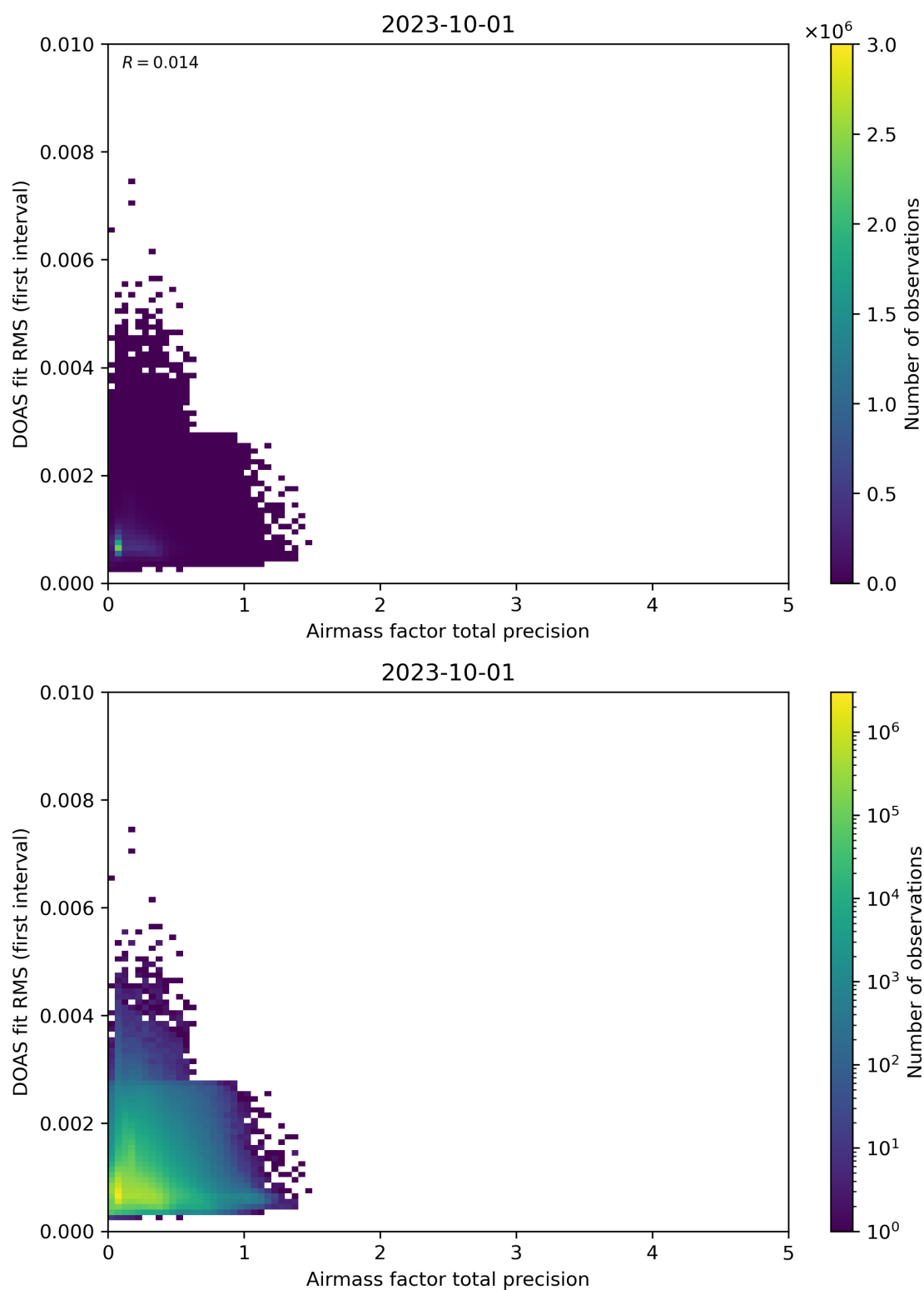
Figure 105: Scatter density plot of “Airmass factor total precision” against “DOAS fit RMS (first interval)” for 2023-10-01 to 2023-10-02.
