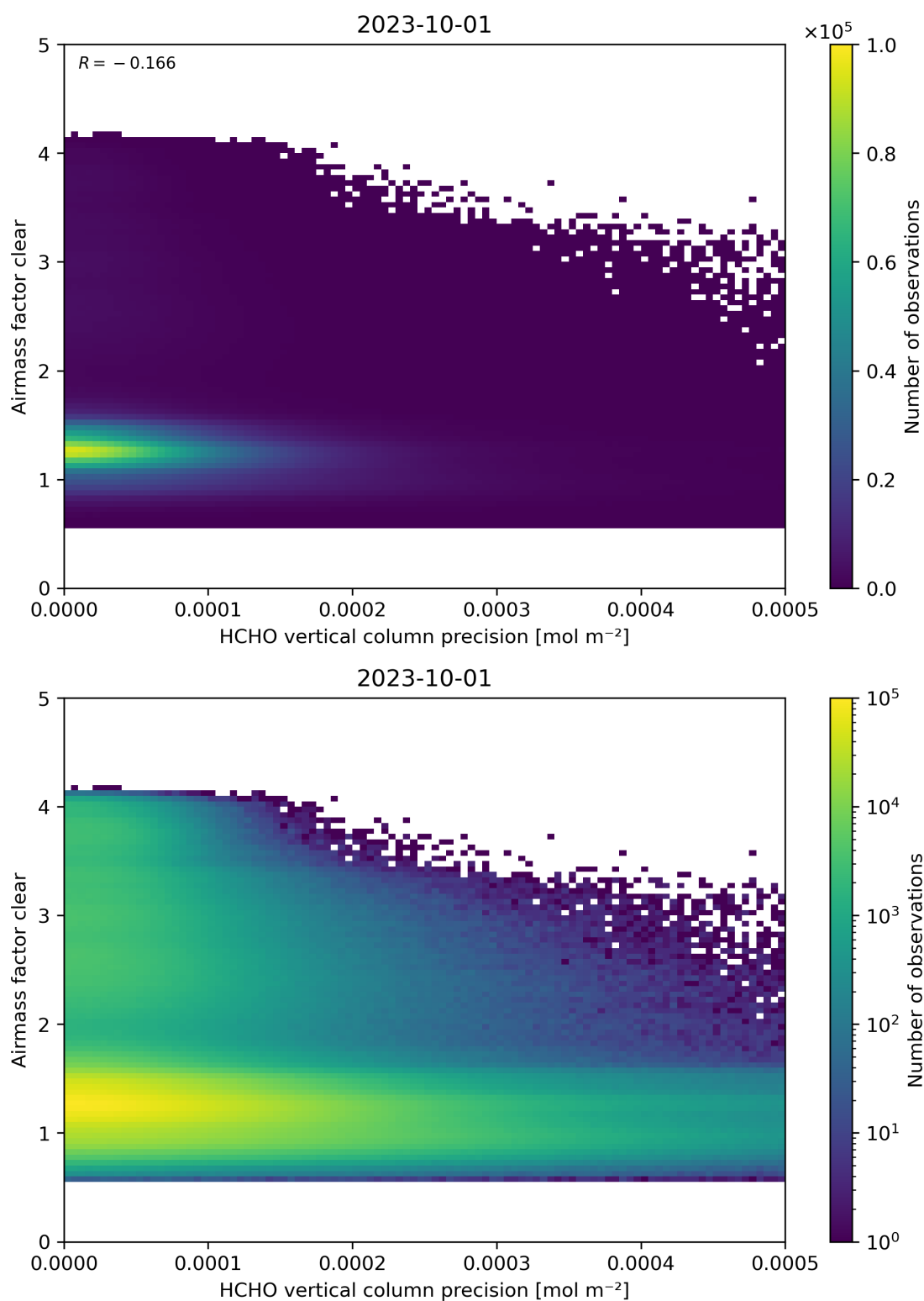
Figure 139: Scatter density plot of “HCHO vertical column precision” against “Airmass factor clear” for 2023-10-01 to 2023-10-02.
