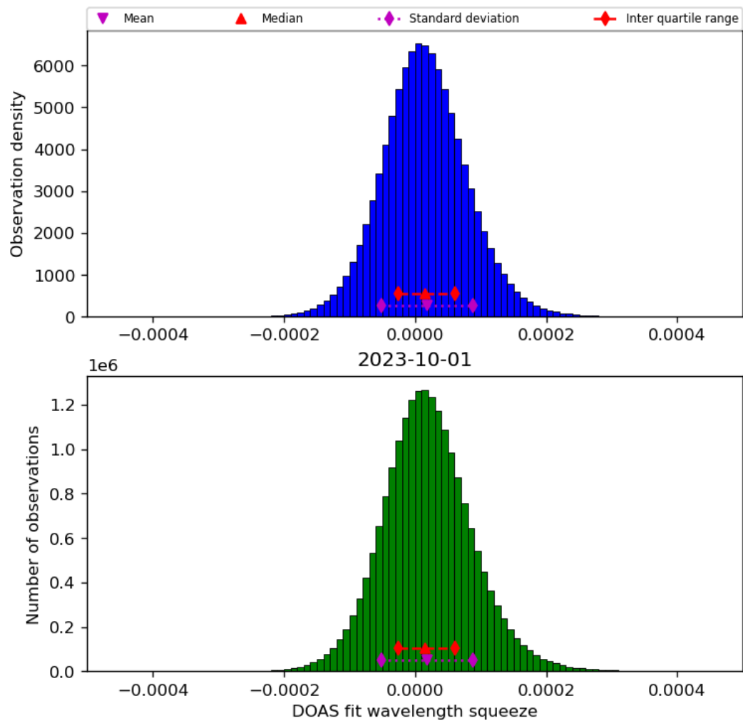
Figure 45: Histogram of “DOAS fit wavelength squeeze” for 2023-10-01 to 2023-10-02
