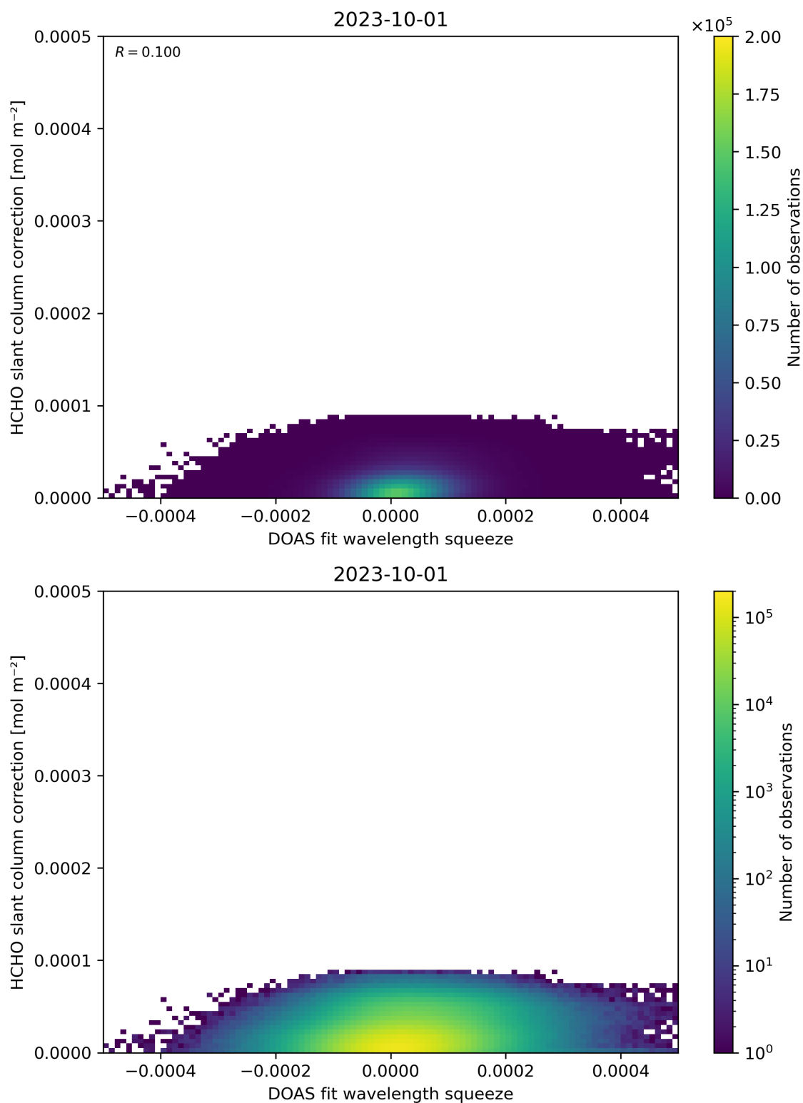
Figure 70: Scatter density plot of “DOAS fit wavelength squeeze” against “HCHO slant column correction” for 2023-10-01 to 2023-10-02.
