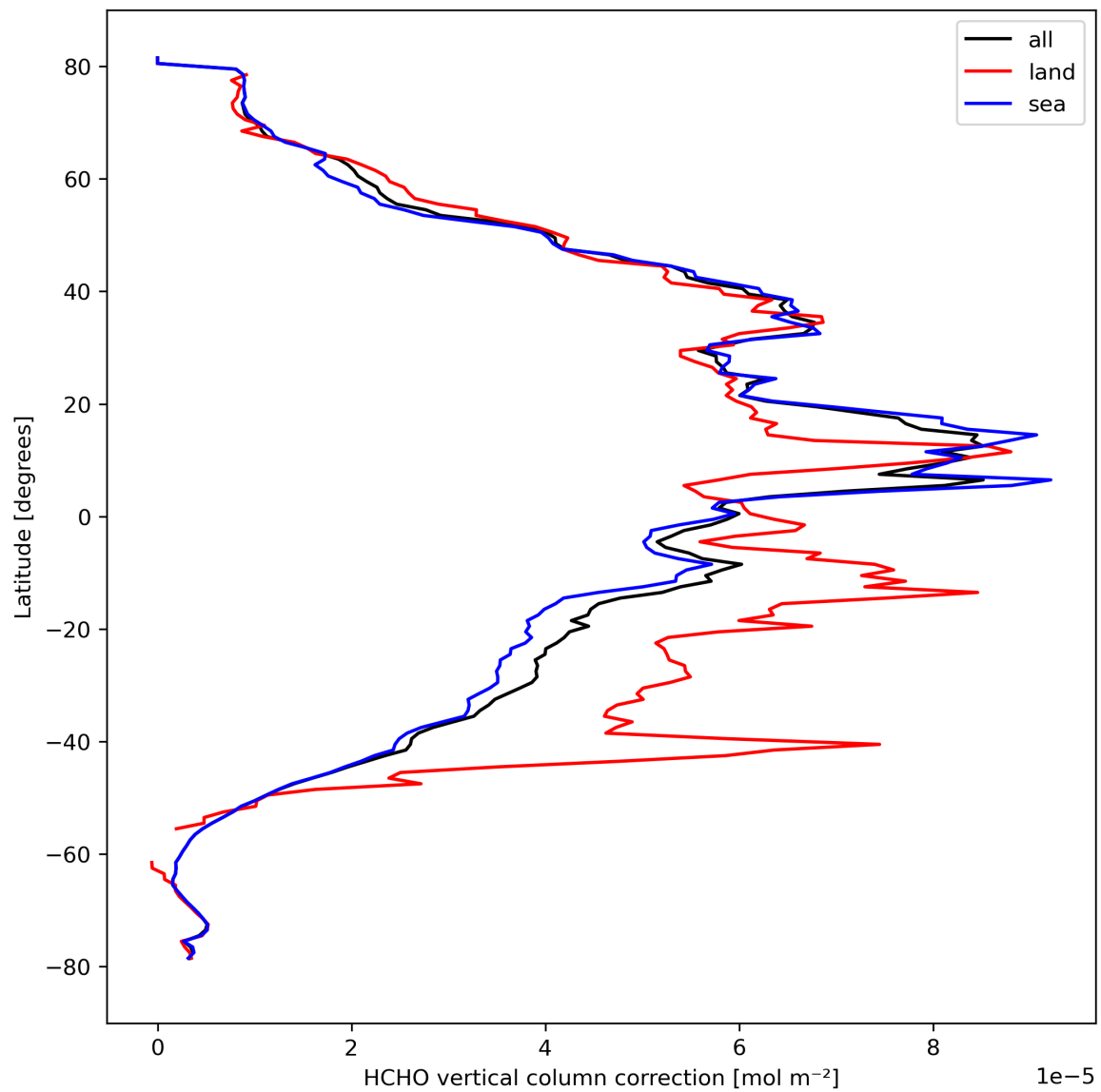
Figure 23: Zonal average of “HCHO vertical column correction” for 2023-10-01 to 2023-10-02.
