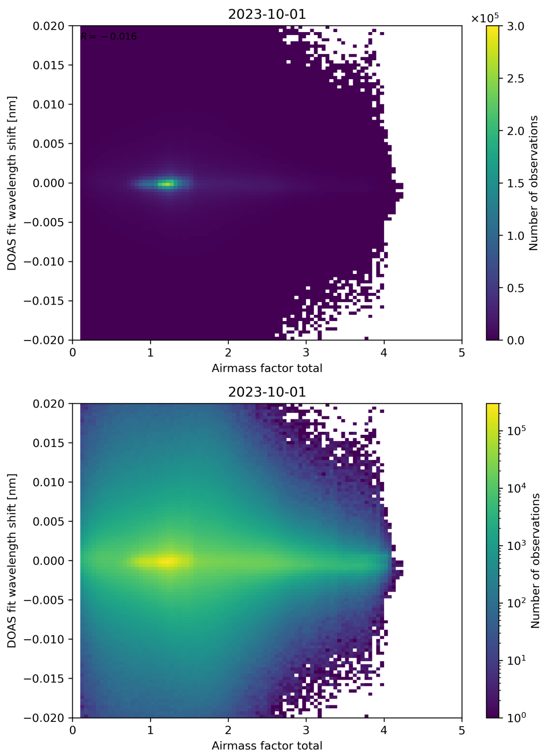
Figure 98: Scatter density plot of “Airmass factor total” against “DOAS fit wavelength shift” for 2023-10-01 to 2023-10-02.
