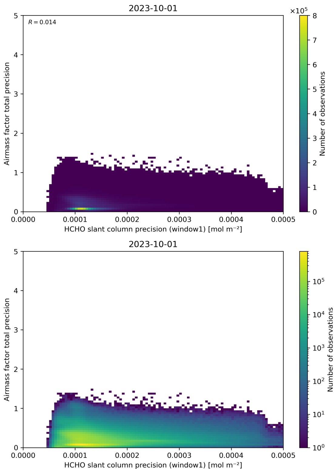
Figure 95: Scatter density plot of “HCHO slant column precision (window1)” against “Airmass factor total precision” for 2023-10-01 to 2023-10-02.
