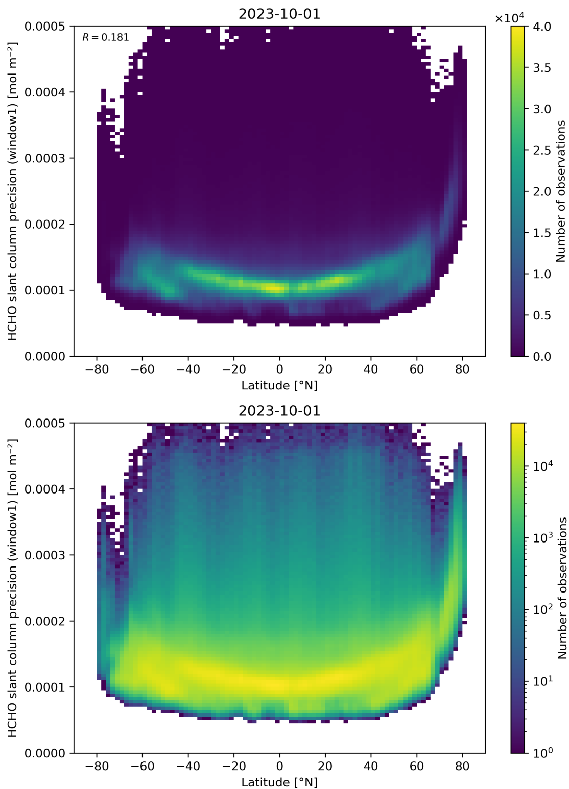
Figure 160: Scatter density plot of “Latitude” against “HCHO slant column precision (window1)” for 2023-10-01 to 2023-10-02.
