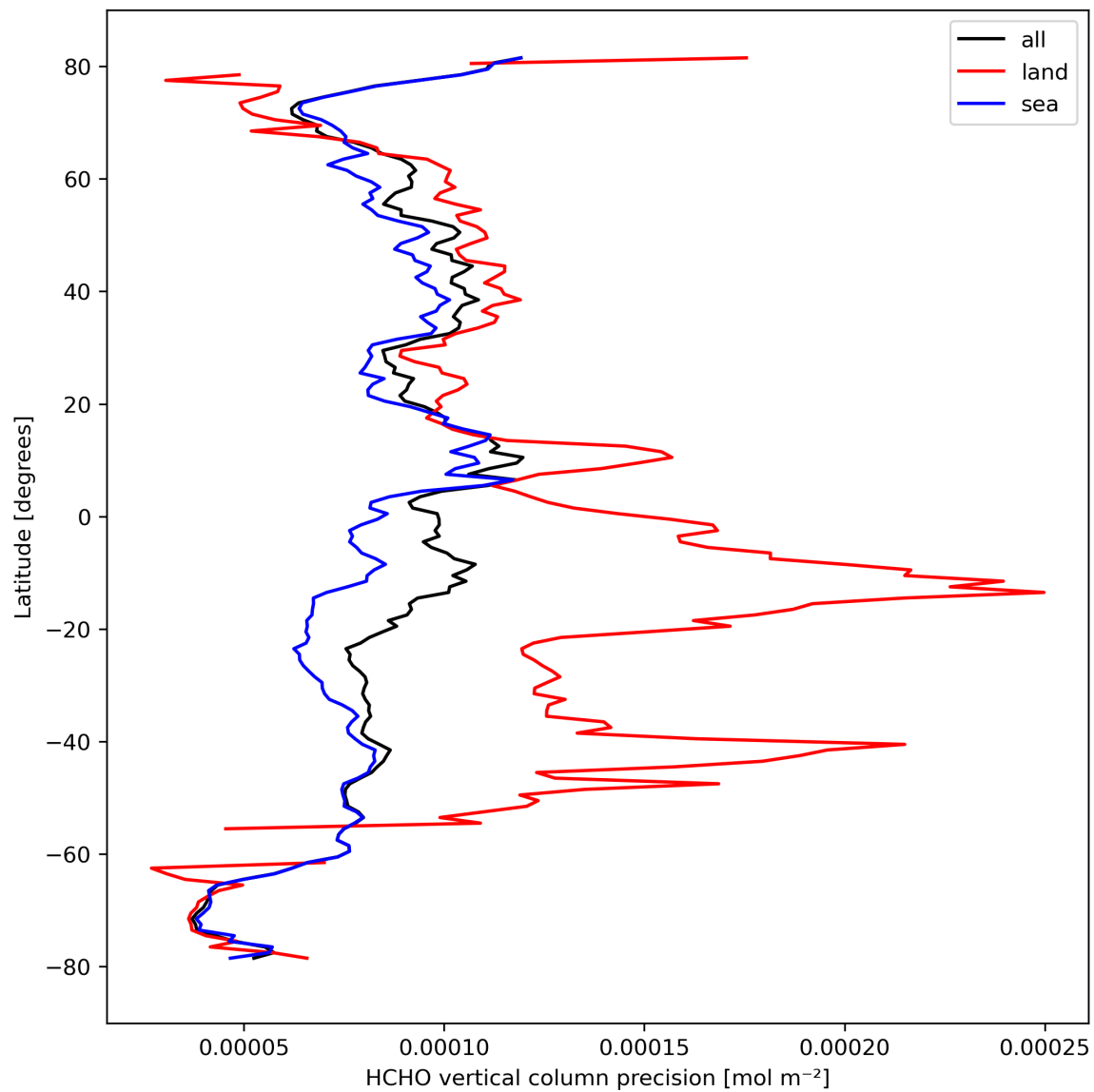
Figure 22: Zonal average of “HCHO vertical column precision” for 2023-10-01 to 2023-10-02.
