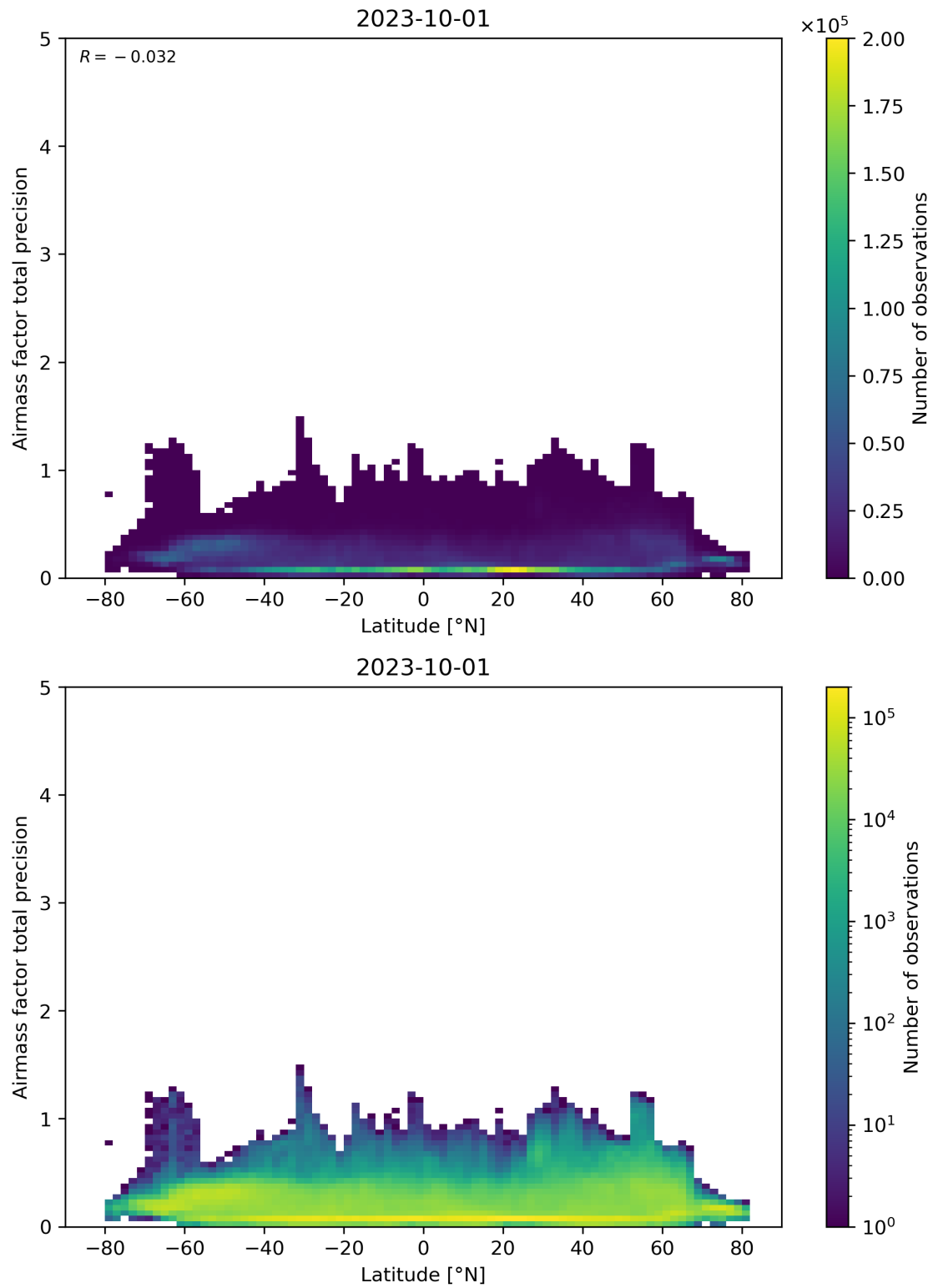
Figure 162: Scatter density plot of “Latitude” against “Airmass factor total precision” for 2023-10-01 to 2023-10-02.
