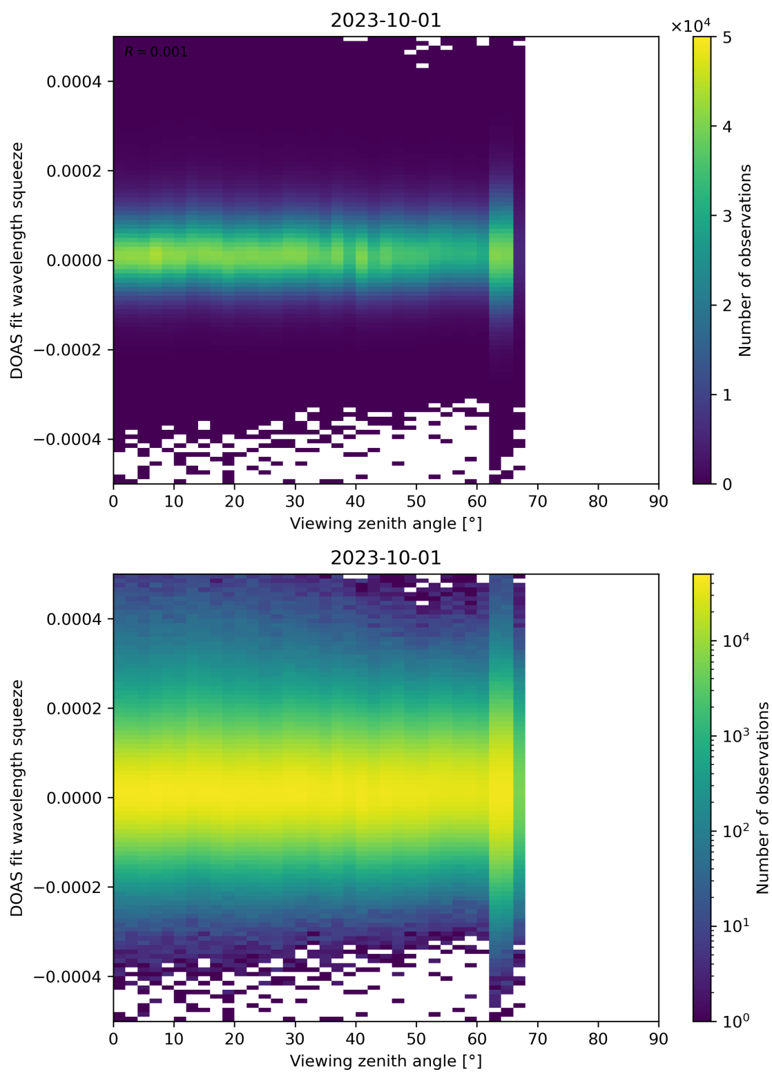
Figure 184: Scatter density plot of “Viewing zenith angle” against “DOAS fit wavelength squeeze” for 2023-10-01 to 2023-10-02.
