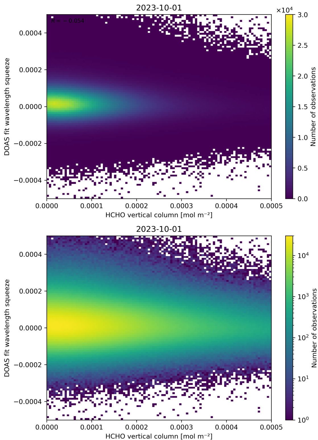
Figure 125: Scatter density plot of “HCHO vertical column” against “DOAS fit wavelength squeeze” for 2023-10-01 to 2023-10-02.
