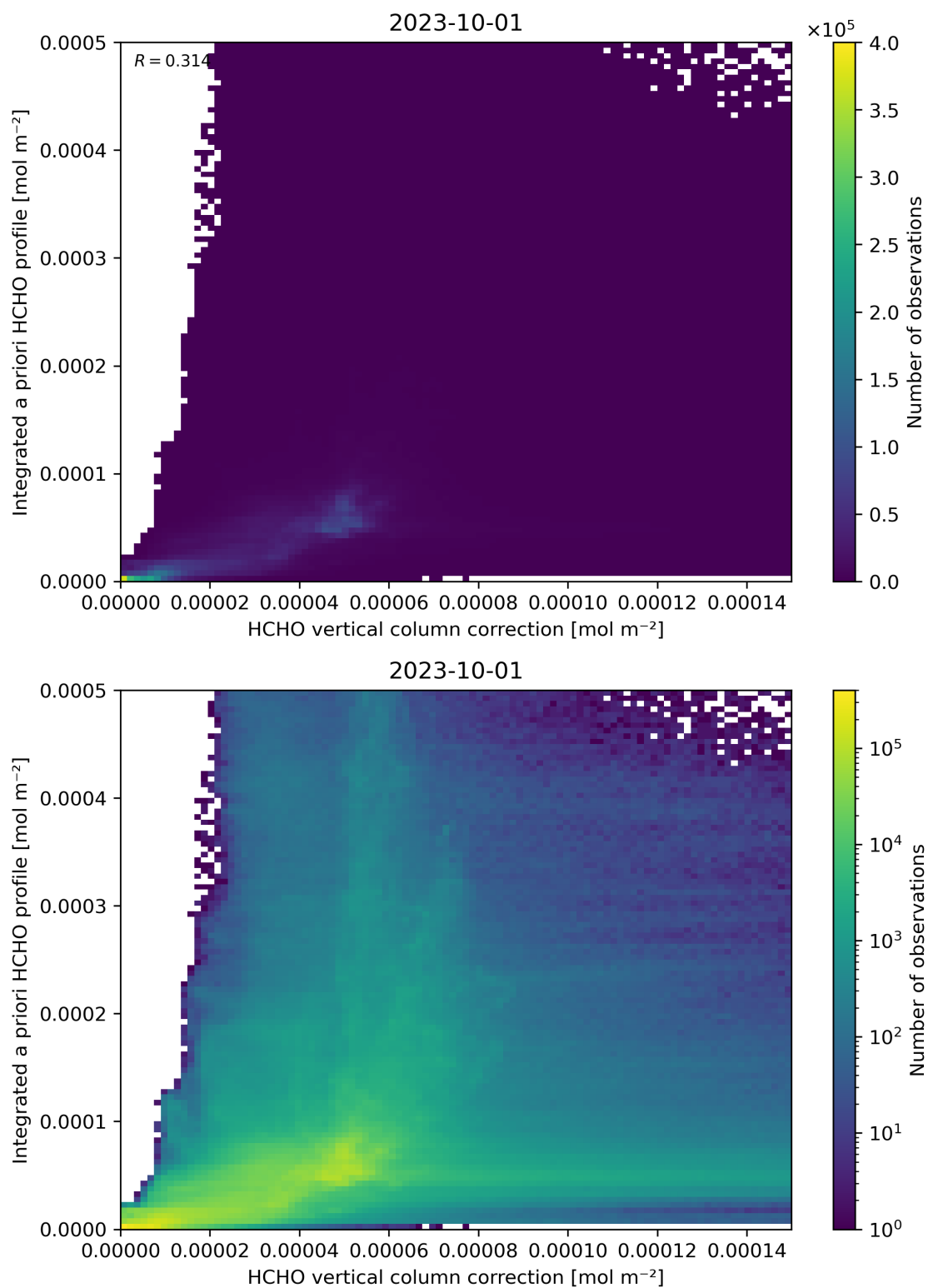
Figure 122: Scatter density plot of “HCHO vertical column correction” against “Integrated a priori HCHO profile” for 2023-10-01 to 2023-10-02.
