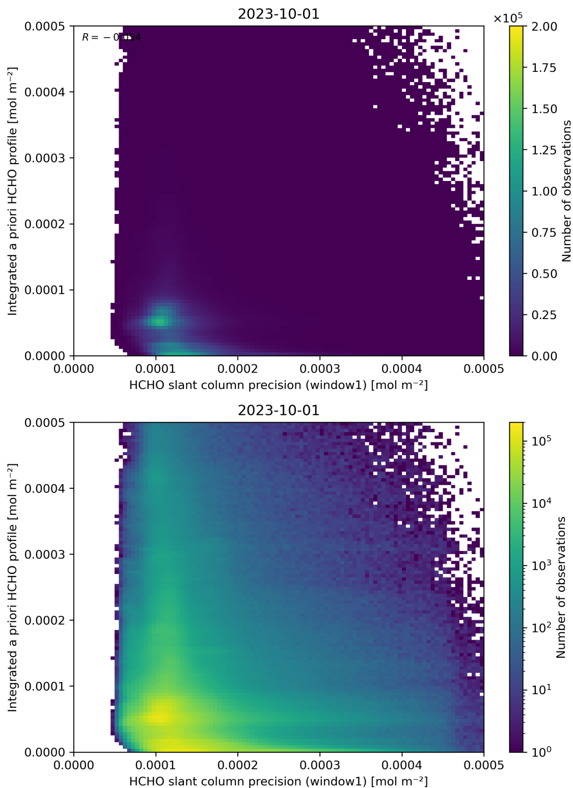
Figure 96: Scatter density plot of “HCHO slant column precision (window1)” against “Integrated a priori HCHO profile” for 2023-10-01 to 2023-10-02.
