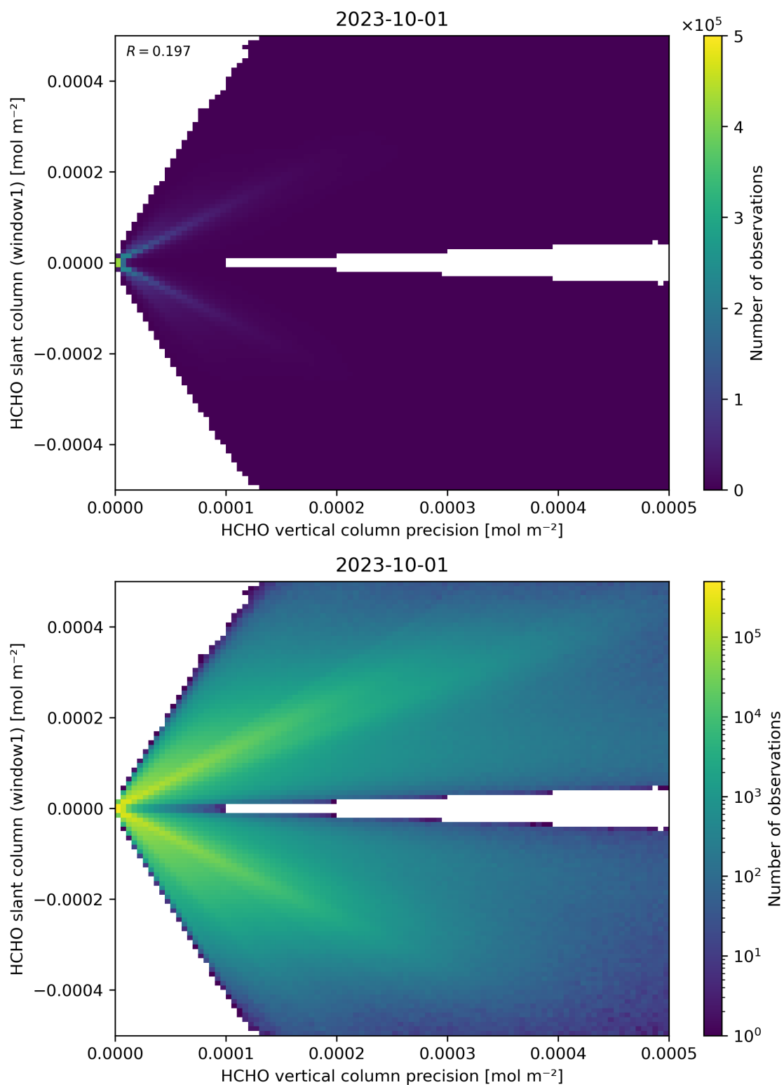
Figure 142: Scatter density plot of “HCHO vertical column precision” against “HCHO slant column (window1)” for 2023-10-01 to 2023-10-02.
