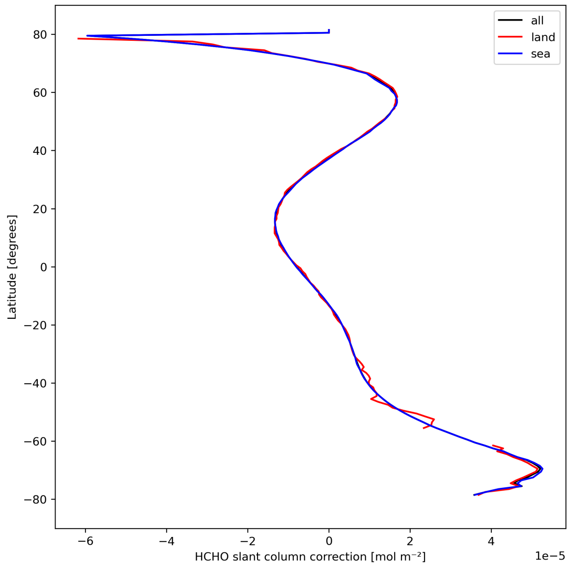
Figure 33: Zonal average of “HCHO slant column correction” for 2023-10-01 to 2023-10-02.
