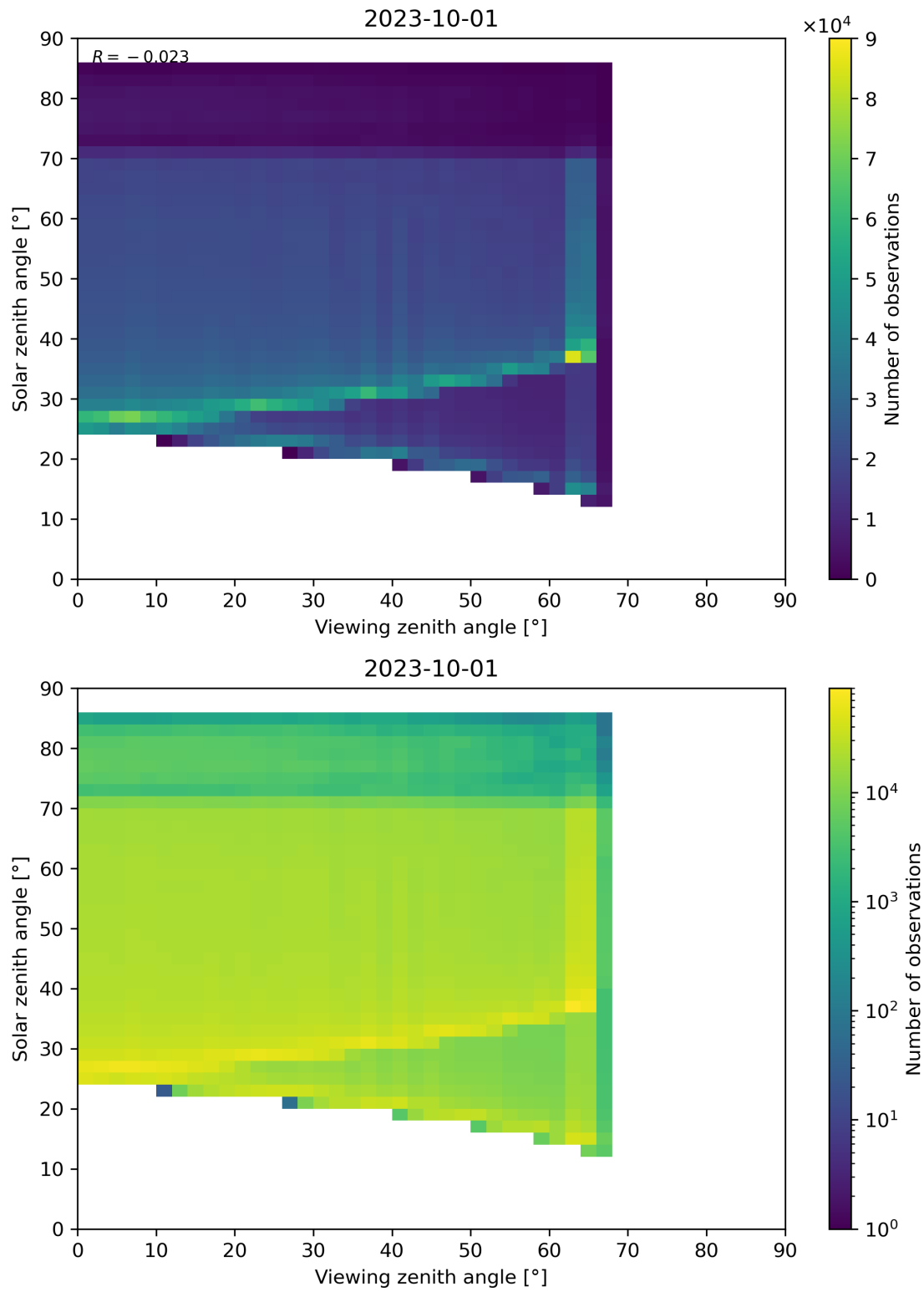
Figure 197: Scatter density plot of “Viewing zenith angle” against “Solar zenith angle” for 2023-10-01 to 2023-10-02.
