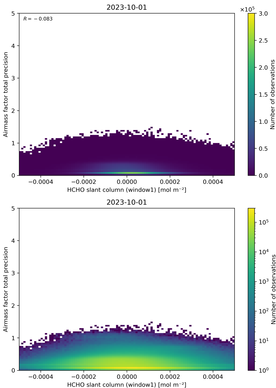
Figure 86: Scatter density plot of “HCHO slant column (window1)” against “Airmass factor total precision” for 2023-10-01 to 2023-10-02.
