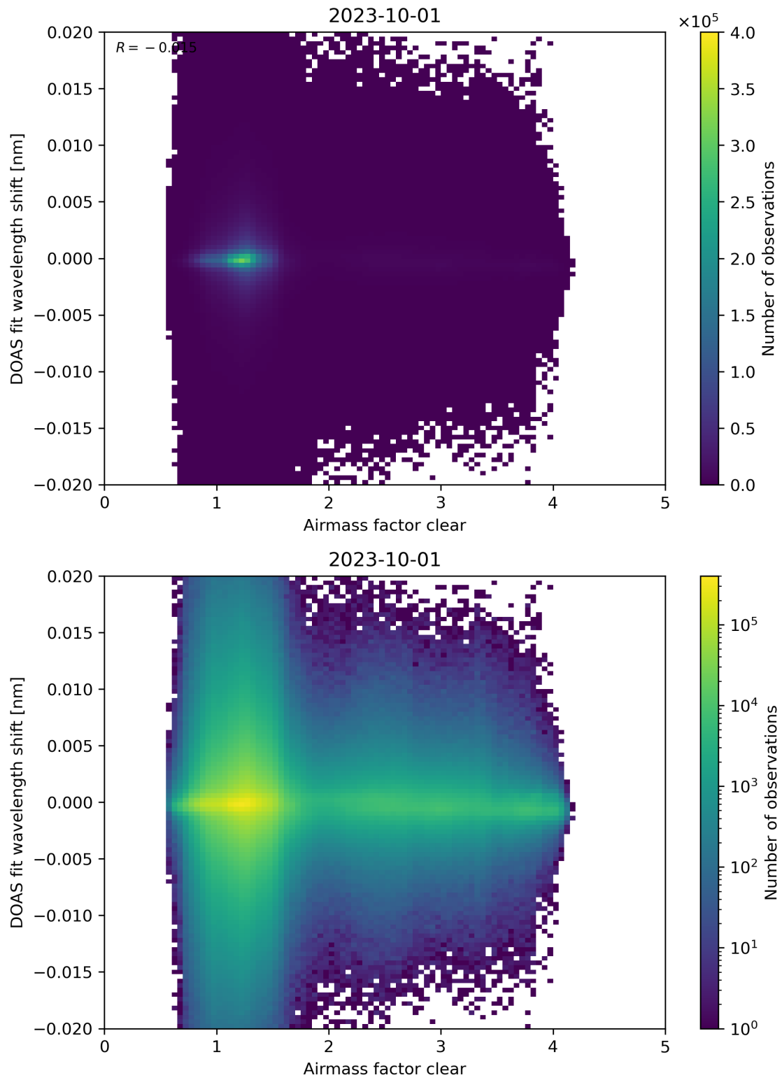
Figure 72: Scatter density plot of “Airmass factor clear” against “DOAS fit wavelength shift” for 2023-10-01 to 2023-10-02.
