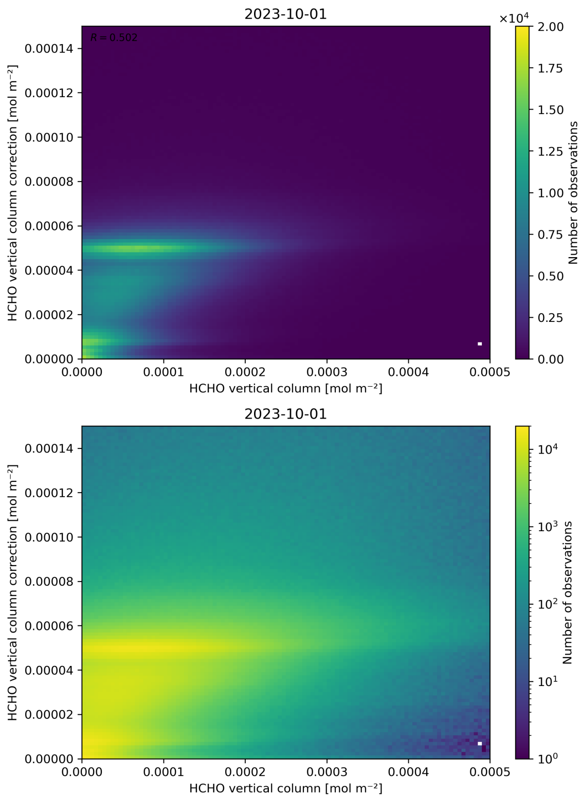
Figure 133: Scatter density plot of “HCHO vertical column” against “HCHO vertical column correction” for 2023-10-01 to 2023-10-02.
