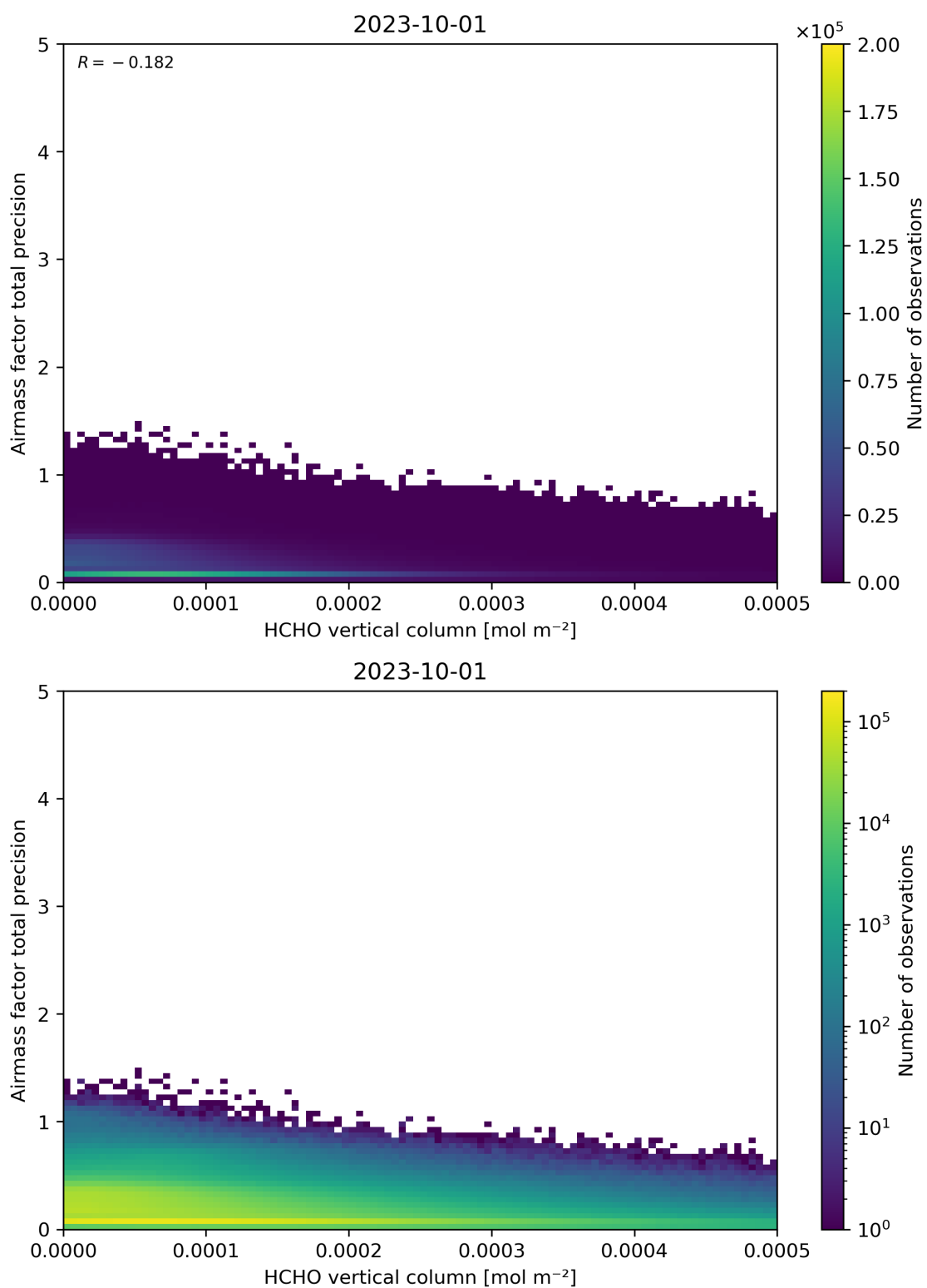
Figure 132: Scatter density plot of “HCHO vertical column” against “Airmass factor total precision” for 2023-10-01 to 2023-10-02.
