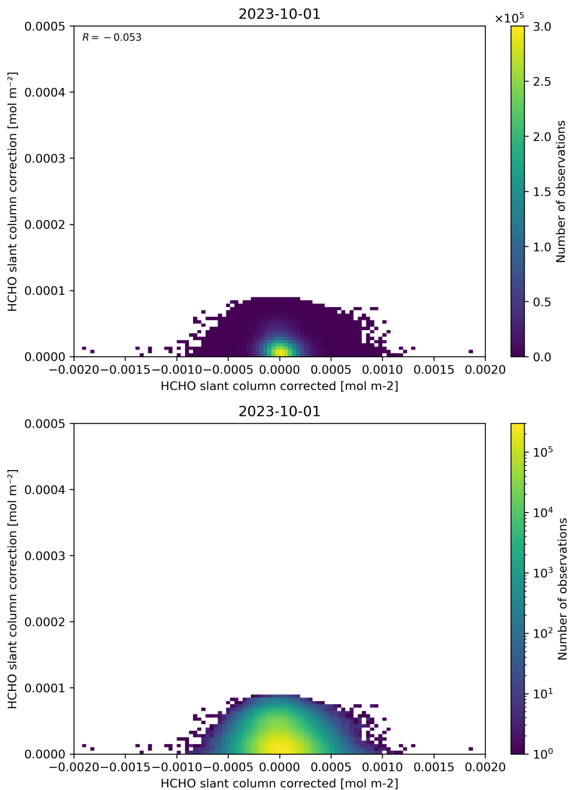
Figure 77: Scatter density plot of “HCHO slant column corrected” against “HCHO slant column correction” for 2023-10-01 to 2023-10-02.
