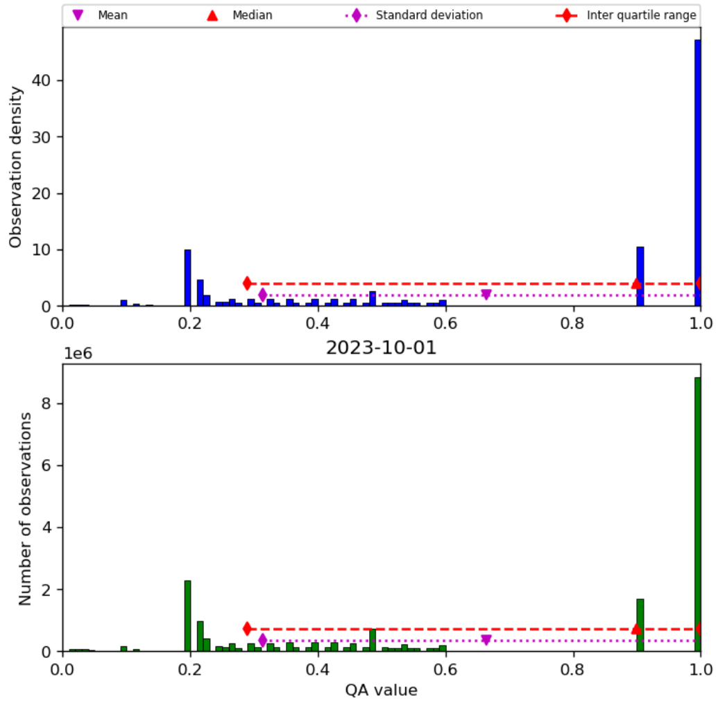
Figure 34: Histogram of “QA value” for 2023-10-01 to 2023-10-02
