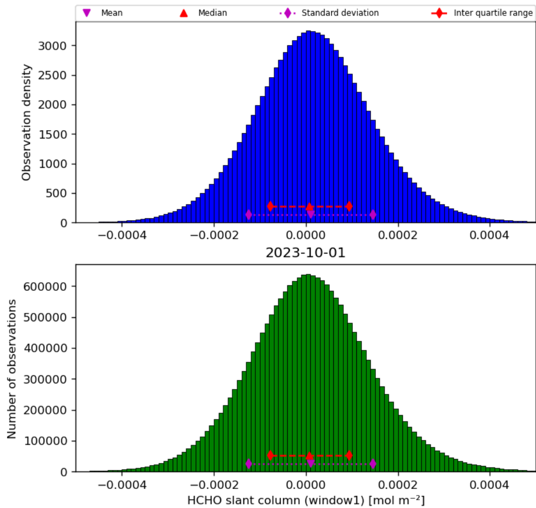
Figure 38: Histogram of “HCHO slant column (window1)” for 2023-10-01 to 2023-10-02
