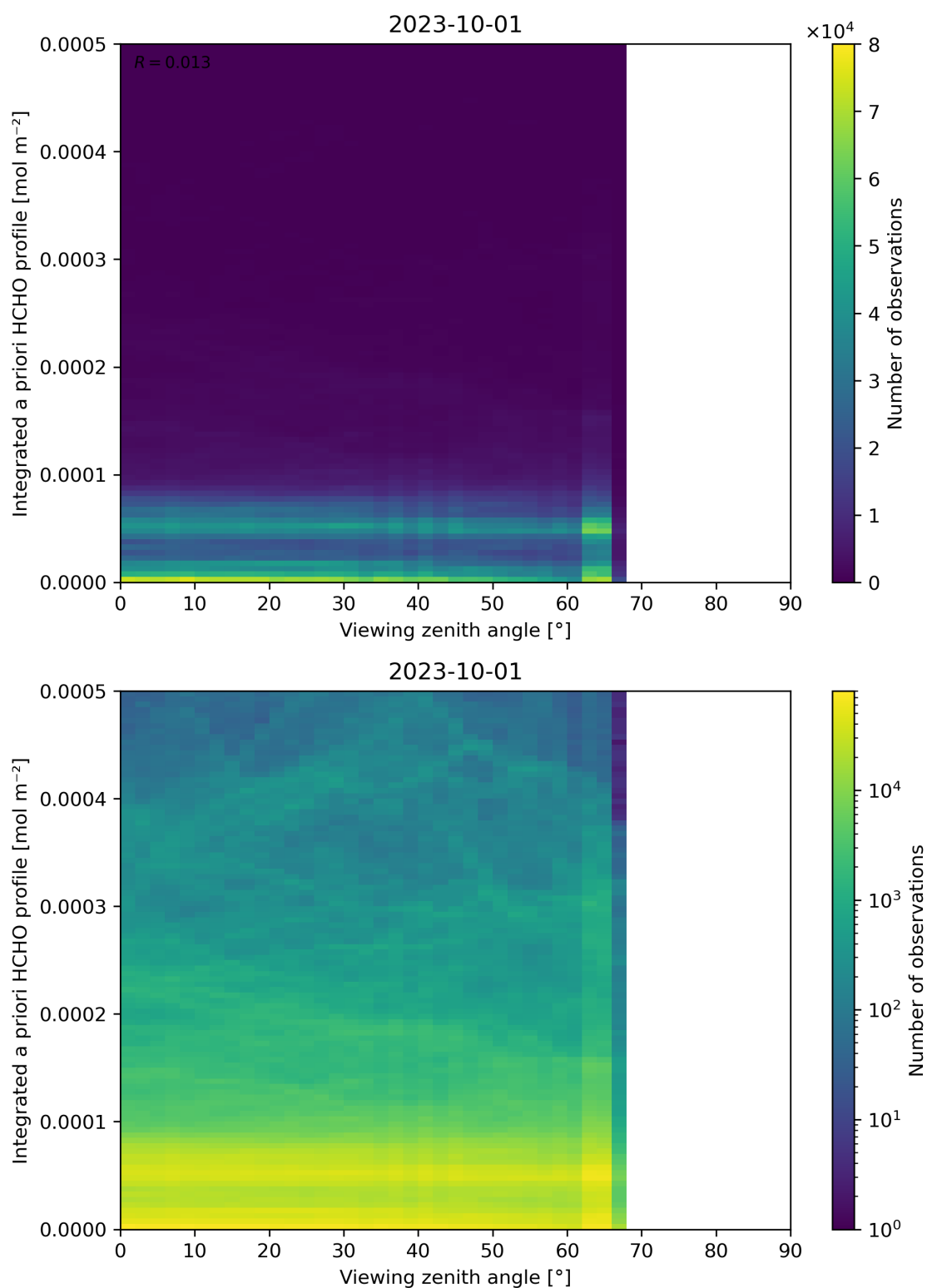
Figure 195: Scatter density plot of “Viewing zenith angle” against “Integrated a priori HCHO profile” for 2023-10-01 to 2023-10-02.
