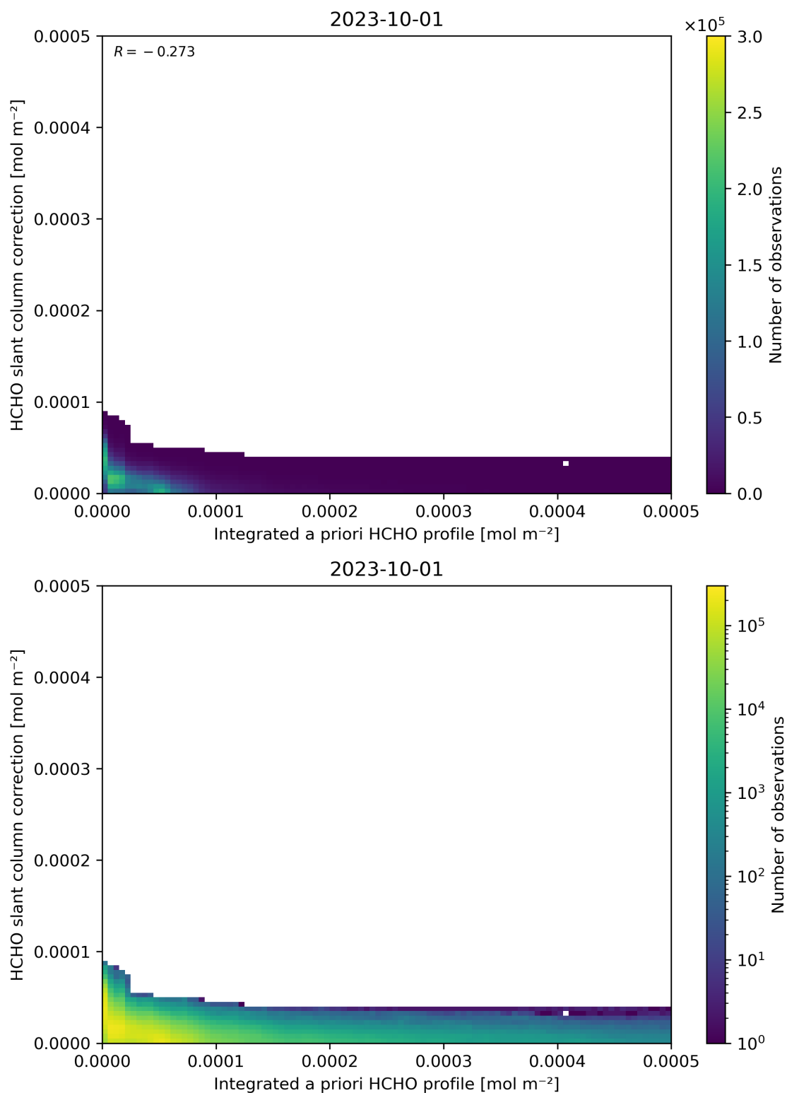
Figure 152: Scatter density plot of “Integrated a priori HCHO profile” against “HCHO slant column correction” for 2023-10-01 to 2023-10-02.
