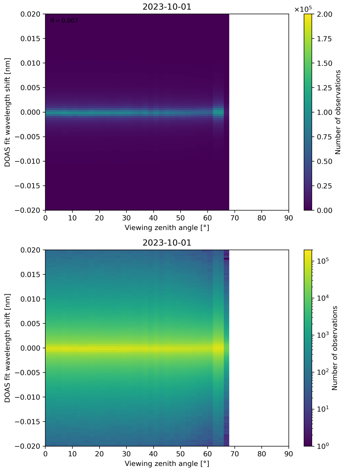
Figure 183: Scatter density plot of “Viewing zenith angle” against “DOAS fit wavelength shift” for 2023-10-01 to 2023-10-02.
