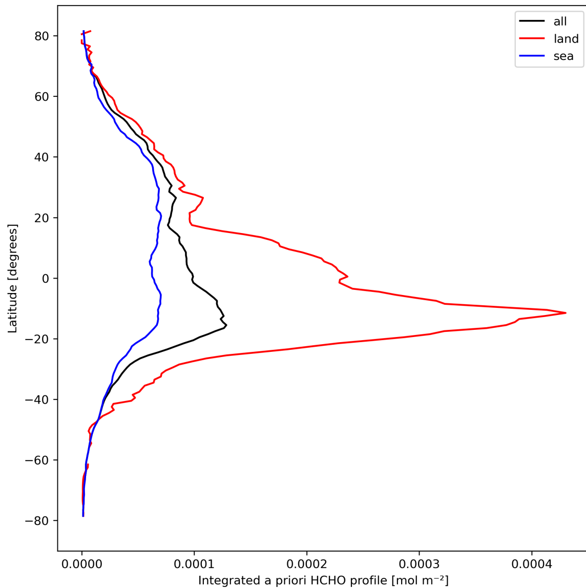
Figure 29: Zonal average of “Integrated a priori HCHO profile” for 2023-10-01 to 2023-10-02.
