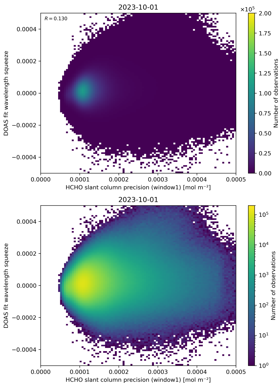
Figure 90: Scatter density plot of “HCHO slant column precision (window1)” against “DOAS fit wavelength squeeze” for 2023-10-01 to 2023-10-02.
