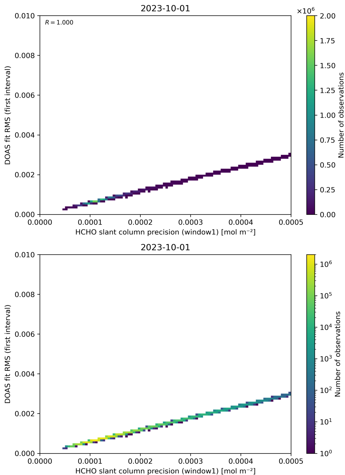
Figure 88: Scatter density plot of “HCHO slant column precision (window1)” against “DOAS fit RMS (first interval)” for 2023-10-01 to 2023-10-02.
