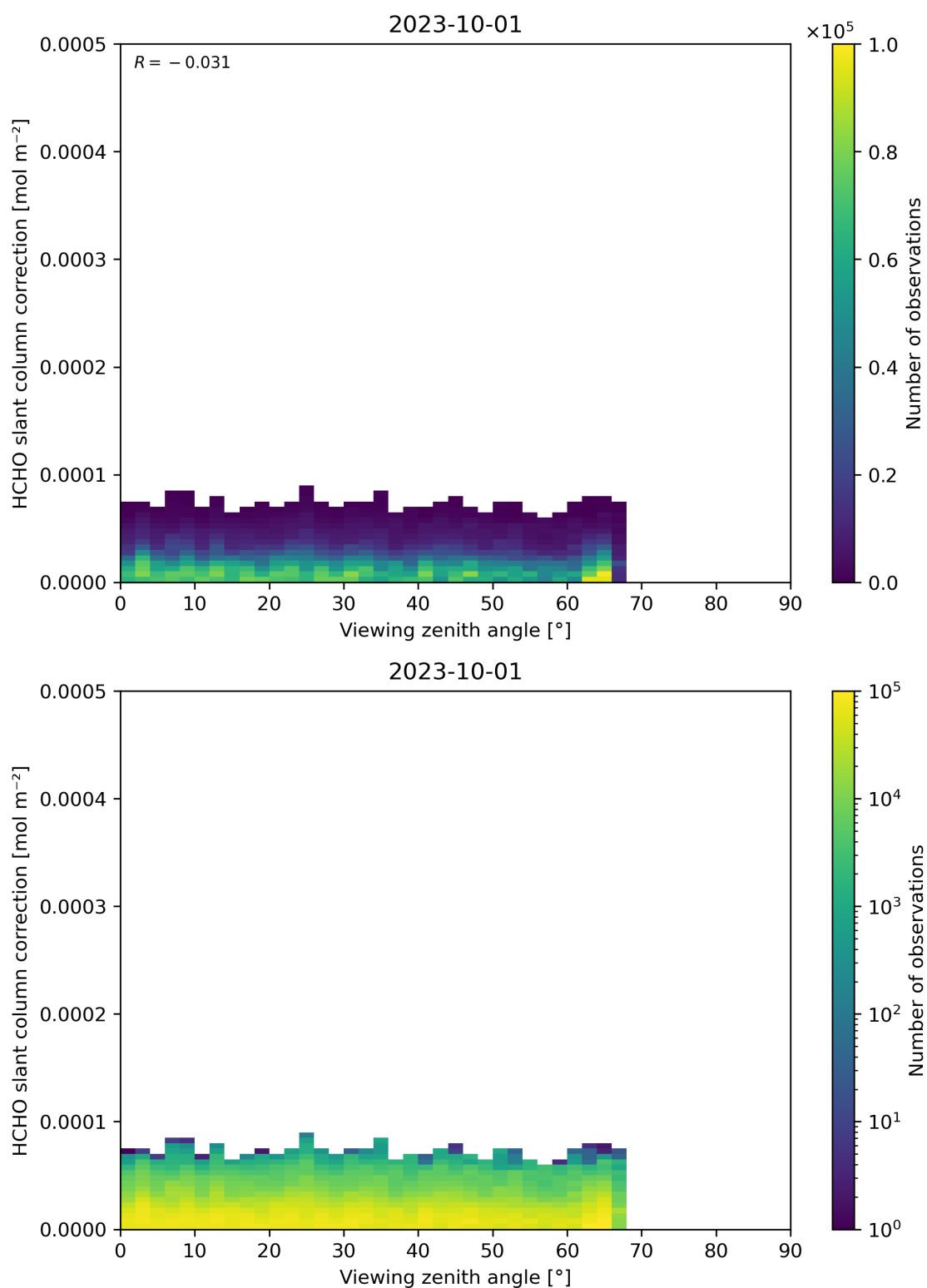
Figure 187: Scatter density plot of “Viewing zenith angle” against “HCHO slant column correction” for 2023-10-01 to 2023-10-02.
