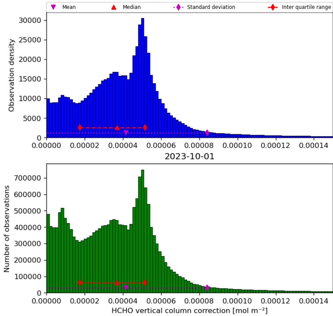
Figure 37: Histogram of “HCHO vertical column correction” for 2023-10-01 to 2023-10-02
