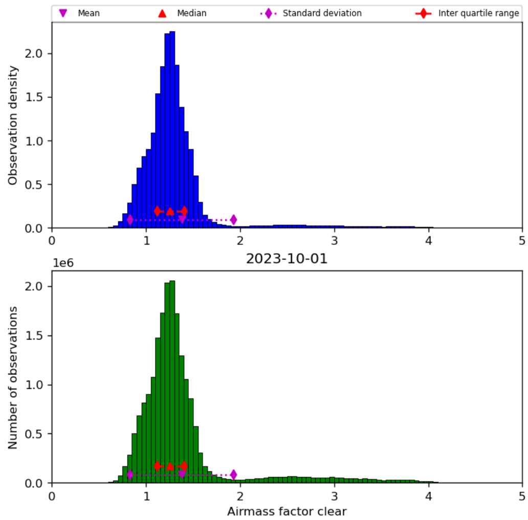
Figure 42: Histogram of “Airmass factor clear” for 2023-10-01 to 2023-10-02
