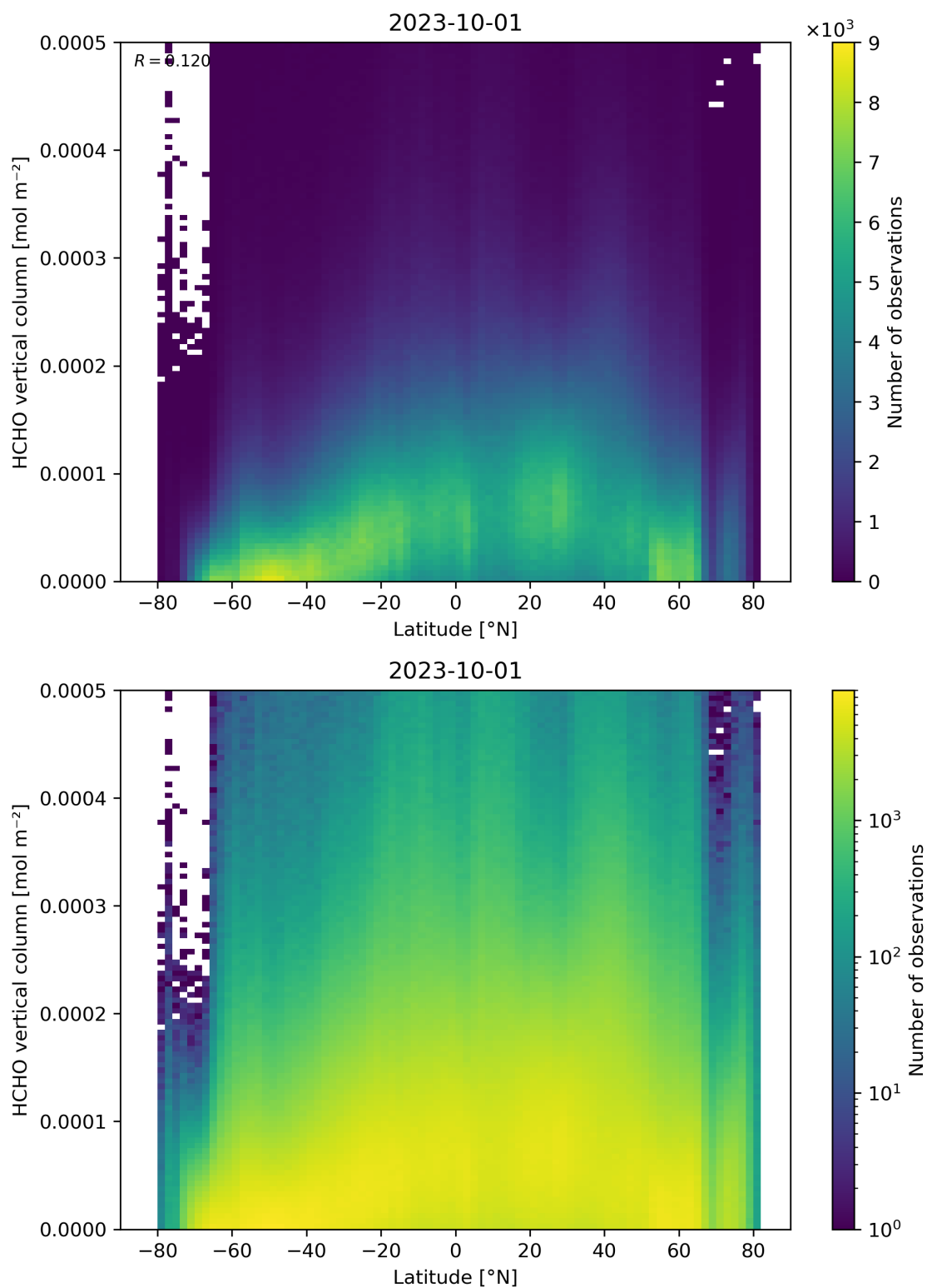
Figure 163: Scatter density plot of “Latitude” against “HCHO vertical column” for 2023-10-01 to 2023-10-02.
