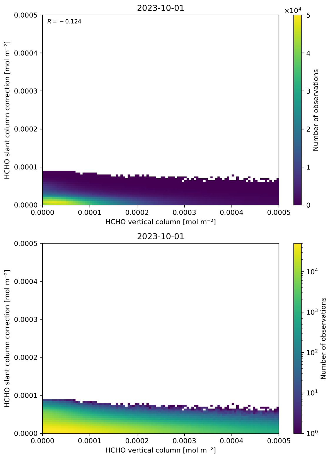
Figure 128: Scatter density plot of “HCHO vertical column” against “HCHO slant column correction” for 2023-10-01 to 2023-10-02.
