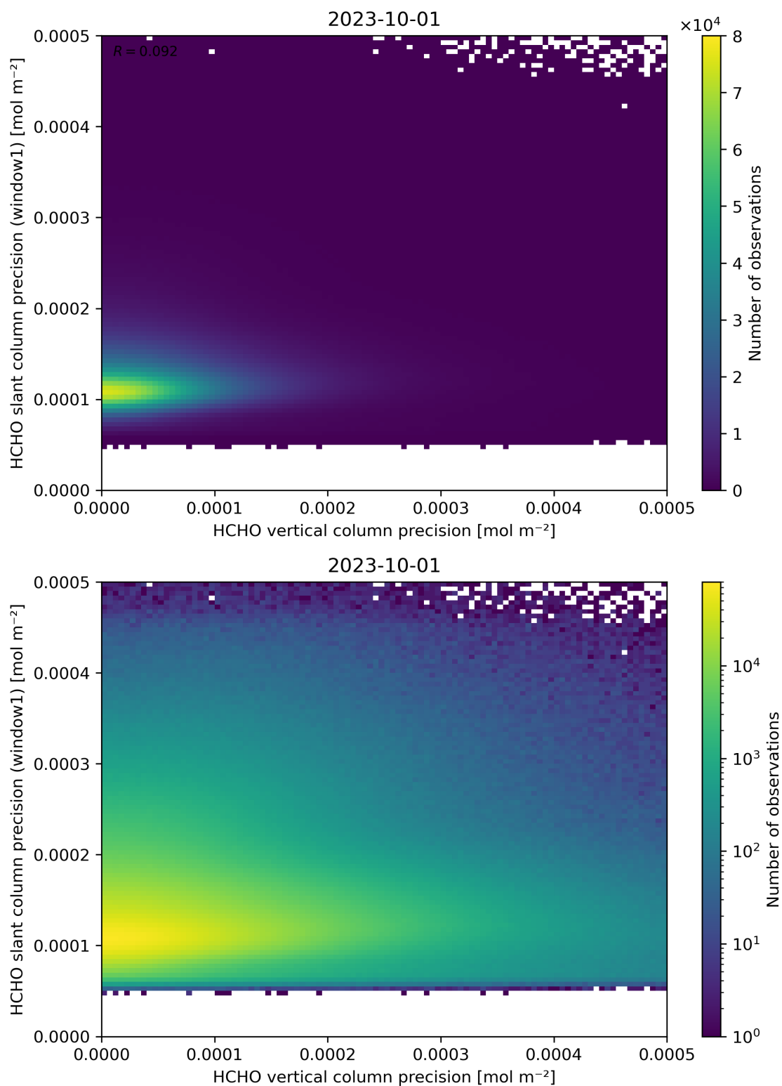
Figure 143: Scatter density plot of “HCHO vertical column precision” against “HCHO slant column precision (window1)” for 2023-10-01 to 2023-10-02.
