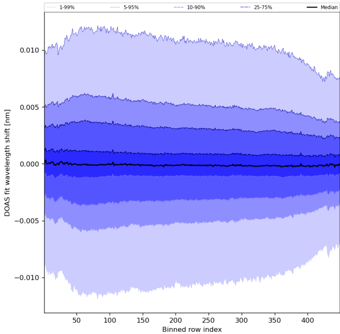
Figure 58: Along track statistics of “DOAS fit wavelength shift” for 2023-10-01 to 2023-10-02
