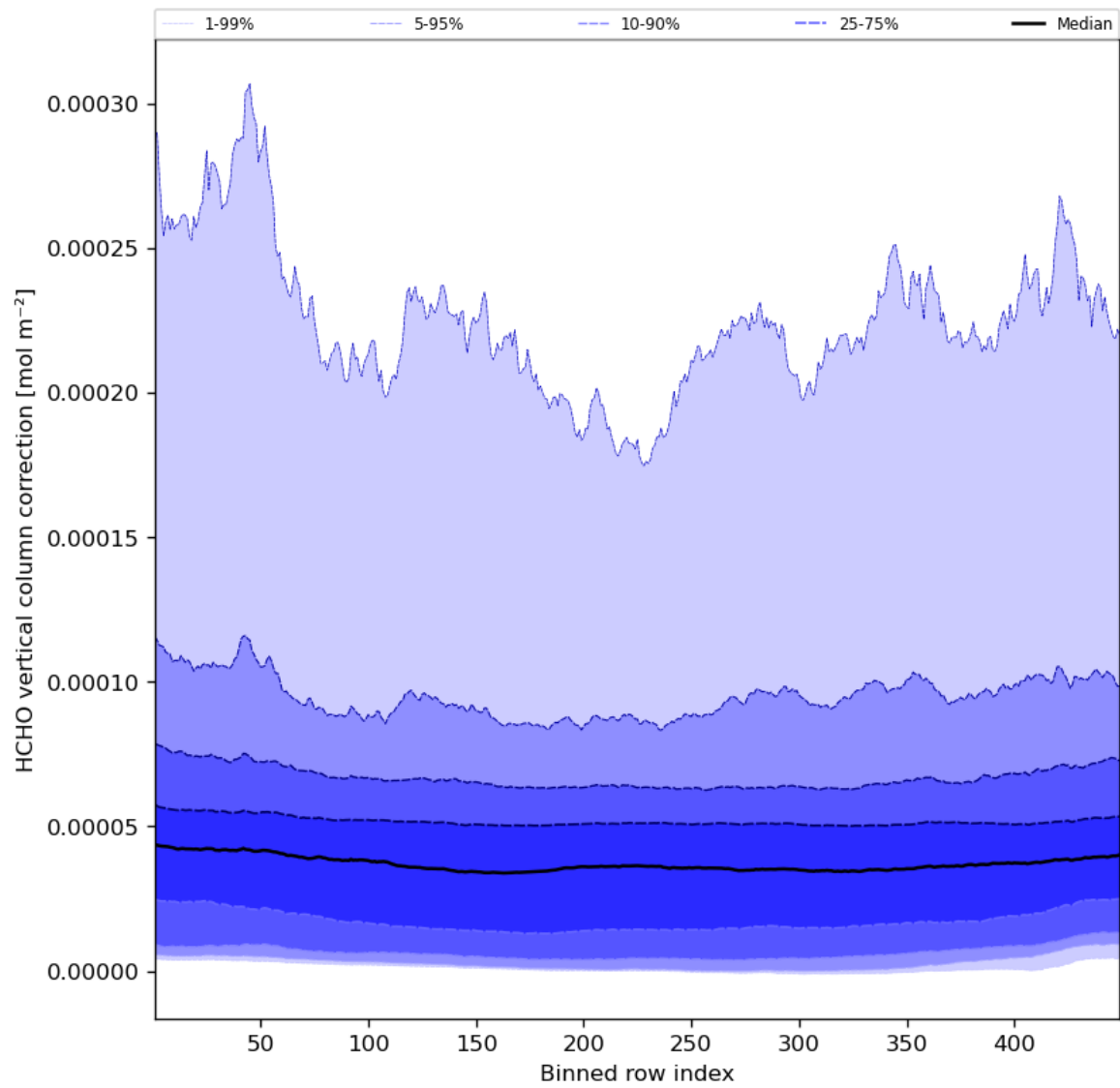
Figure 51: Along track statistics of “HCHO vertical column correction” for 2023-10-01 to 2023-10-02
