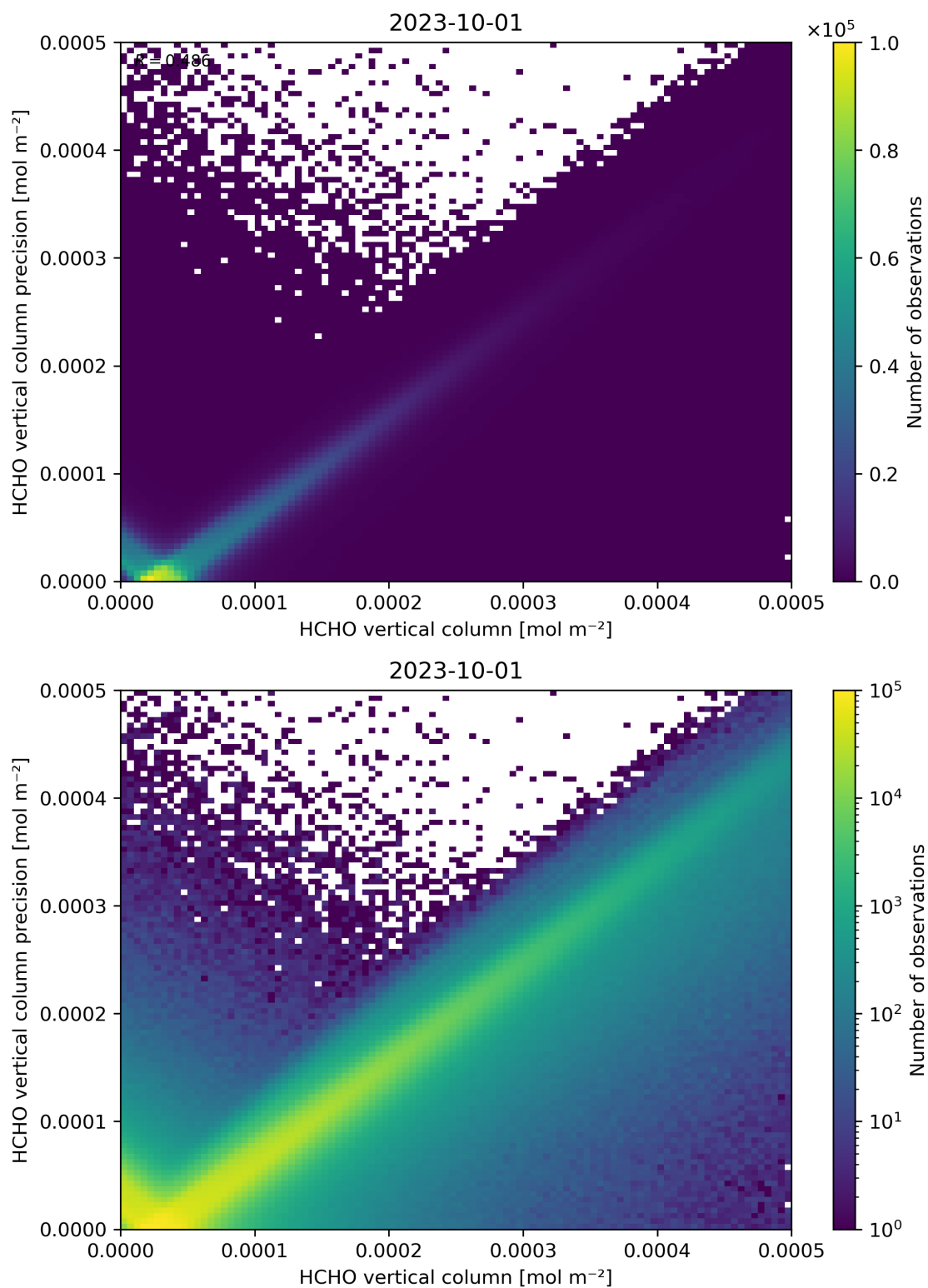
Figure 134: Scatter density plot of “HCHO vertical column” against “HCHO vertical column precision” for 2023-10-01 to 2023-10-02.
