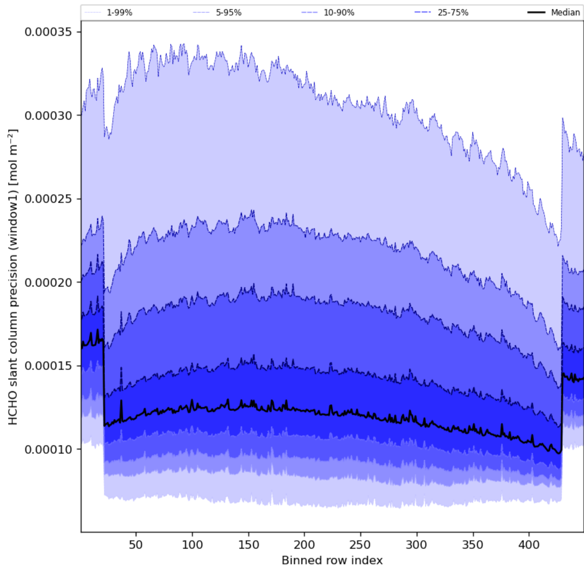
Figure 53: Along track statistics of “HCHO slant column precision (window1)” for 2023-10-01 to 2023-10-02
