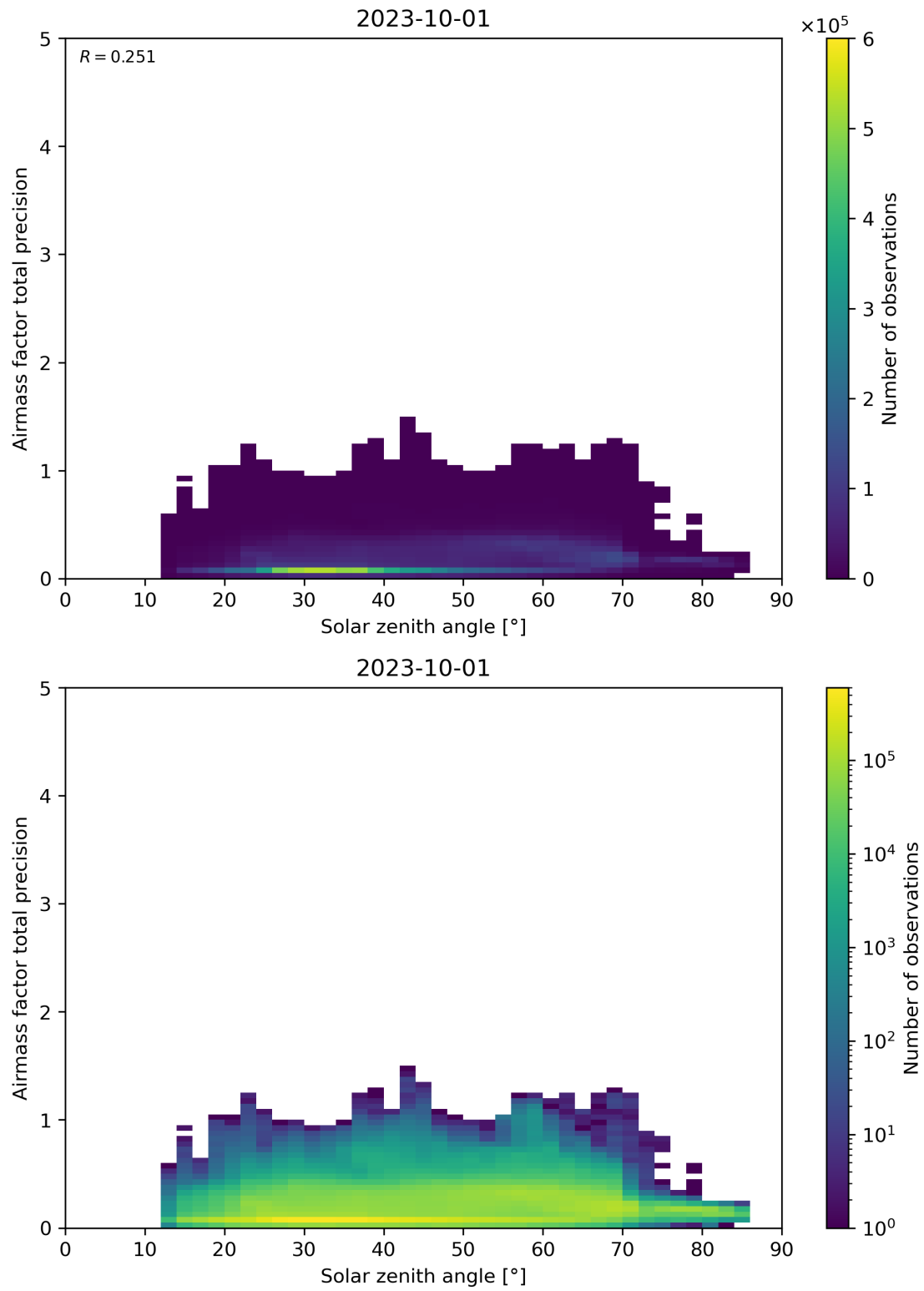
Figure 176: Scatter density plot of “Solar zenith angle” against “Airmass factor total precision” for 2023-10-01 to 2023-10-02.
