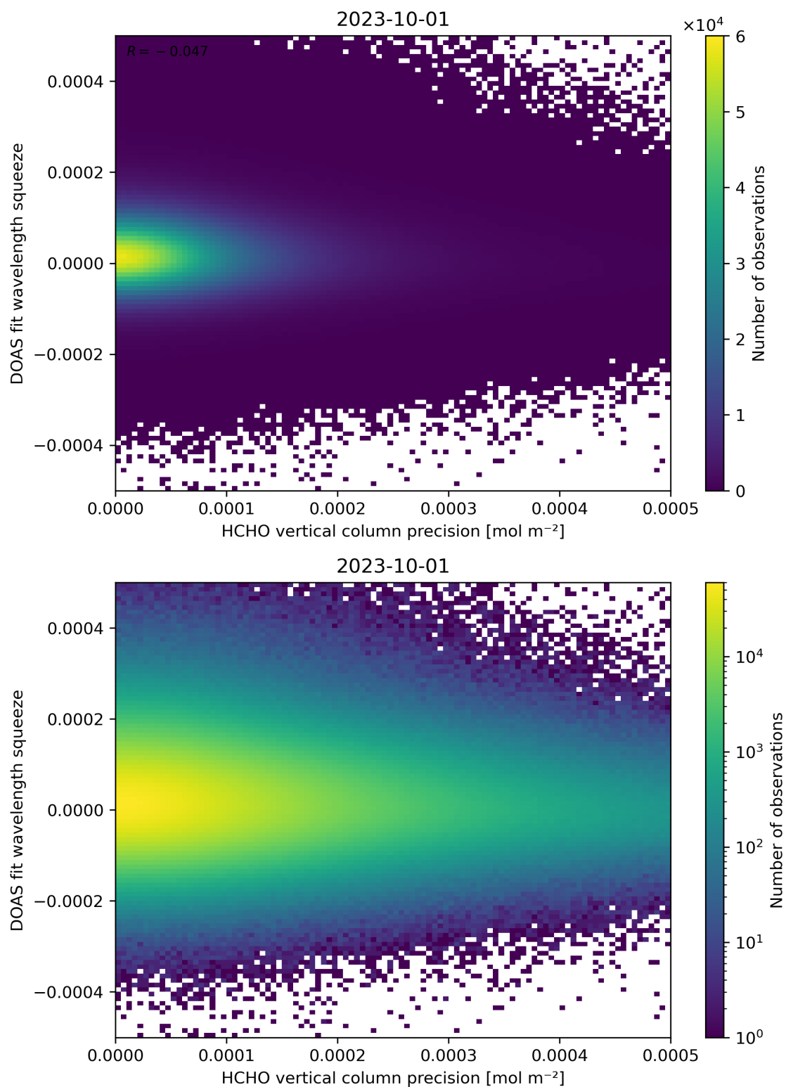
Figure 138: Scatter density plot of “HCHO vertical column precision” against “DOAS fit wavelength squeeze” for 2023-10-01 to 2023-10-02.
