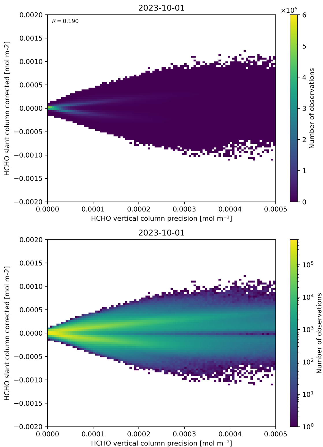
Figure 140: Scatter density plot of “HCHO vertical column precision” against “HCHO slant column corrected” for 2023-10-01 to 2023-10-02.
