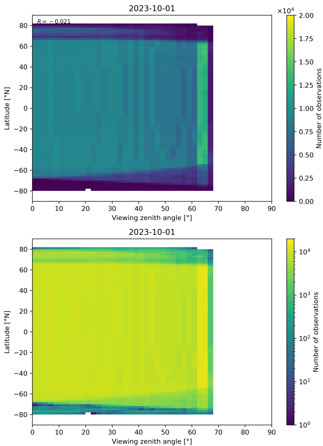
Figure 196: Scatter density plot of “Viewing zenith angle” against “Latitude” for 2023-10-01 to 2023-10-02.
