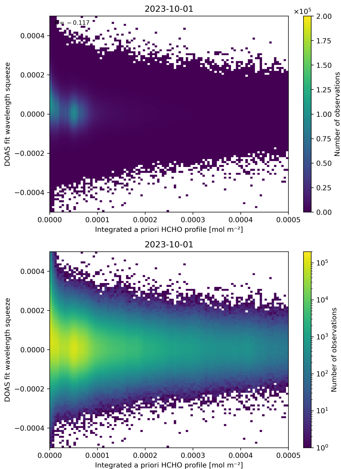
Figure 150: Scatter density plot of “Integrated a priori HCHO profile” against “DOAS fit wavelength squeeze” for 2023-10-01 to 2023-10-02.
