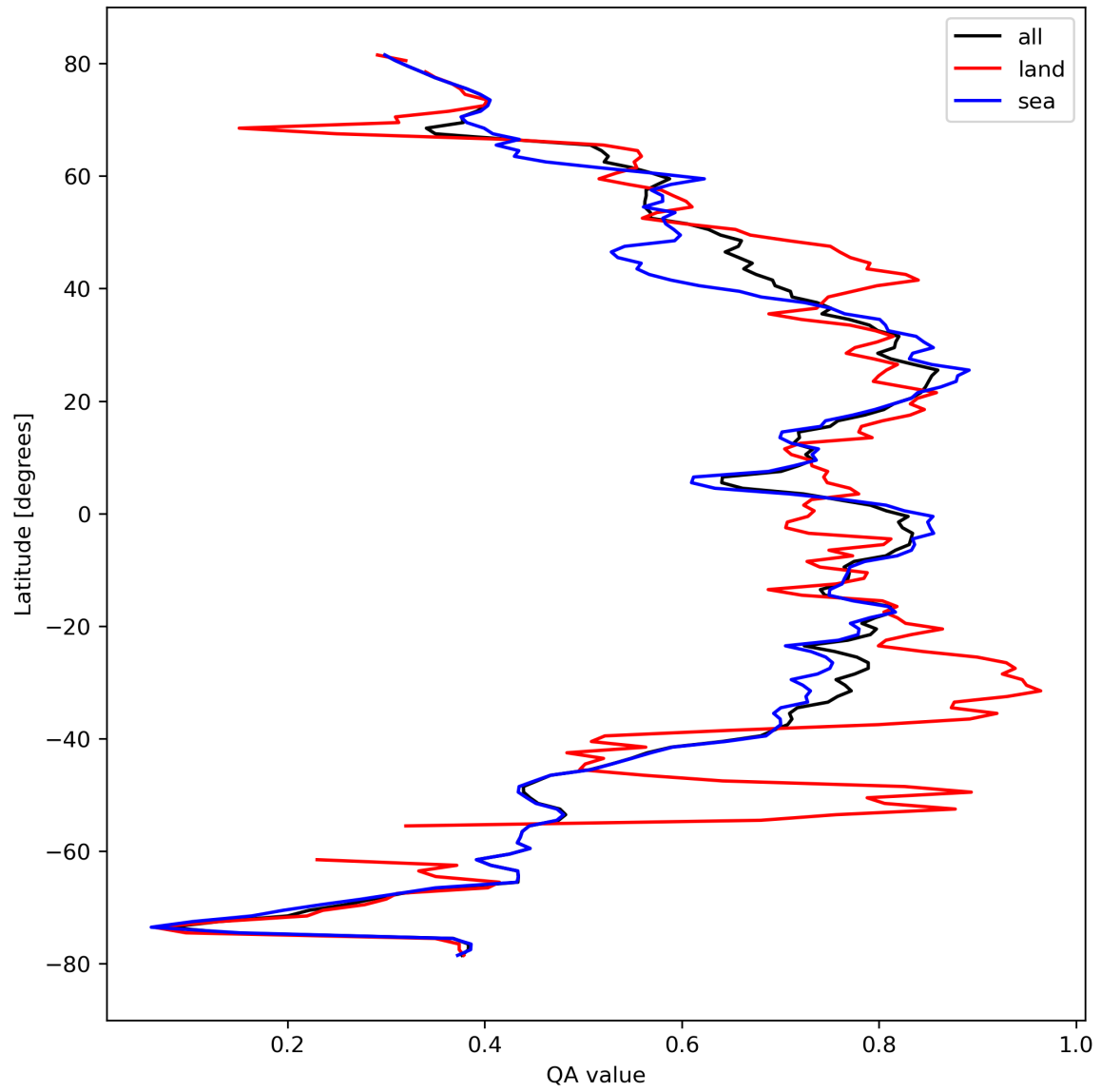
Figure 20: Zonal average of “QA value” for 2023-10-01 to 2023-10-02.
