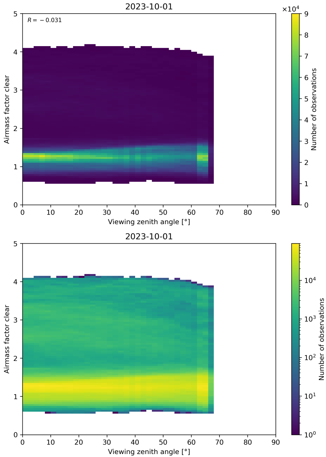
Figure 185: Scatter density plot of “Viewing zenith angle” against “Airmass factor clear” for 2023-10-01 to 2023-10-02.
