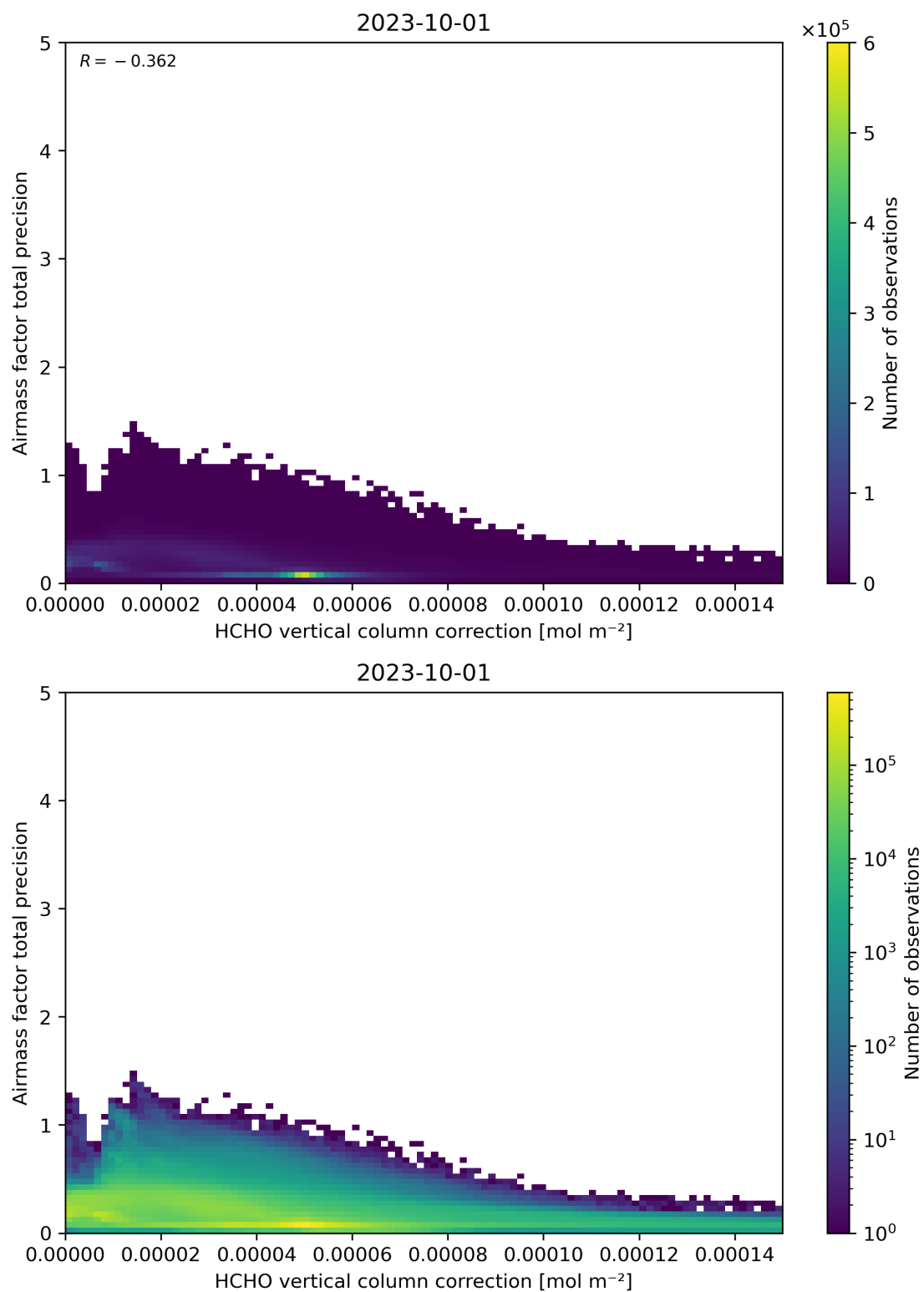
Figure 121: Scatter density plot of “HCHO vertical column correction” against “Airmass factor total precision” for 2023-10-01 to 2023-10-02.
