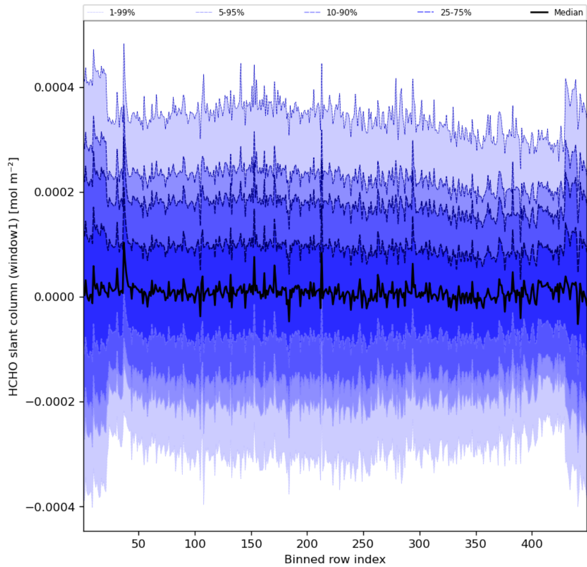
Figure 52: Along track statistics of “HCHO slant column (window1)” for 2023-10-01 to 2023-10-02
