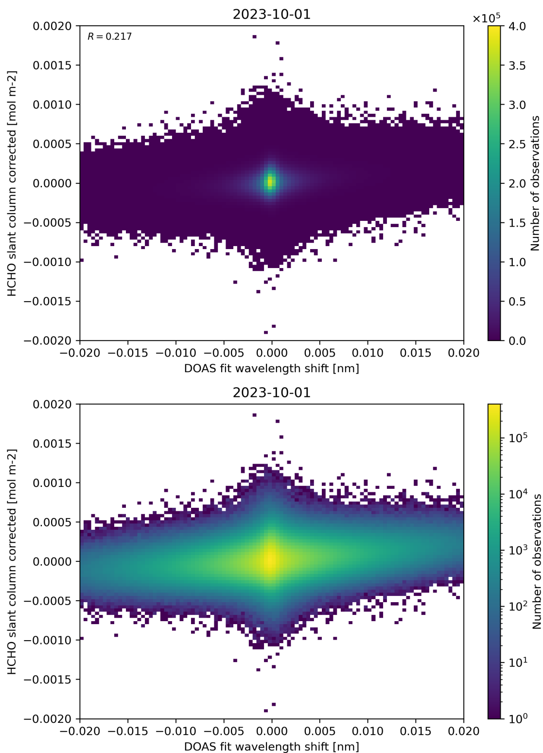
Figure 66: Scatter density plot of “DOAS fit wavelength shift” against “HCHO slant column corrected” for 2023-10-01 to 2023-10-02.
