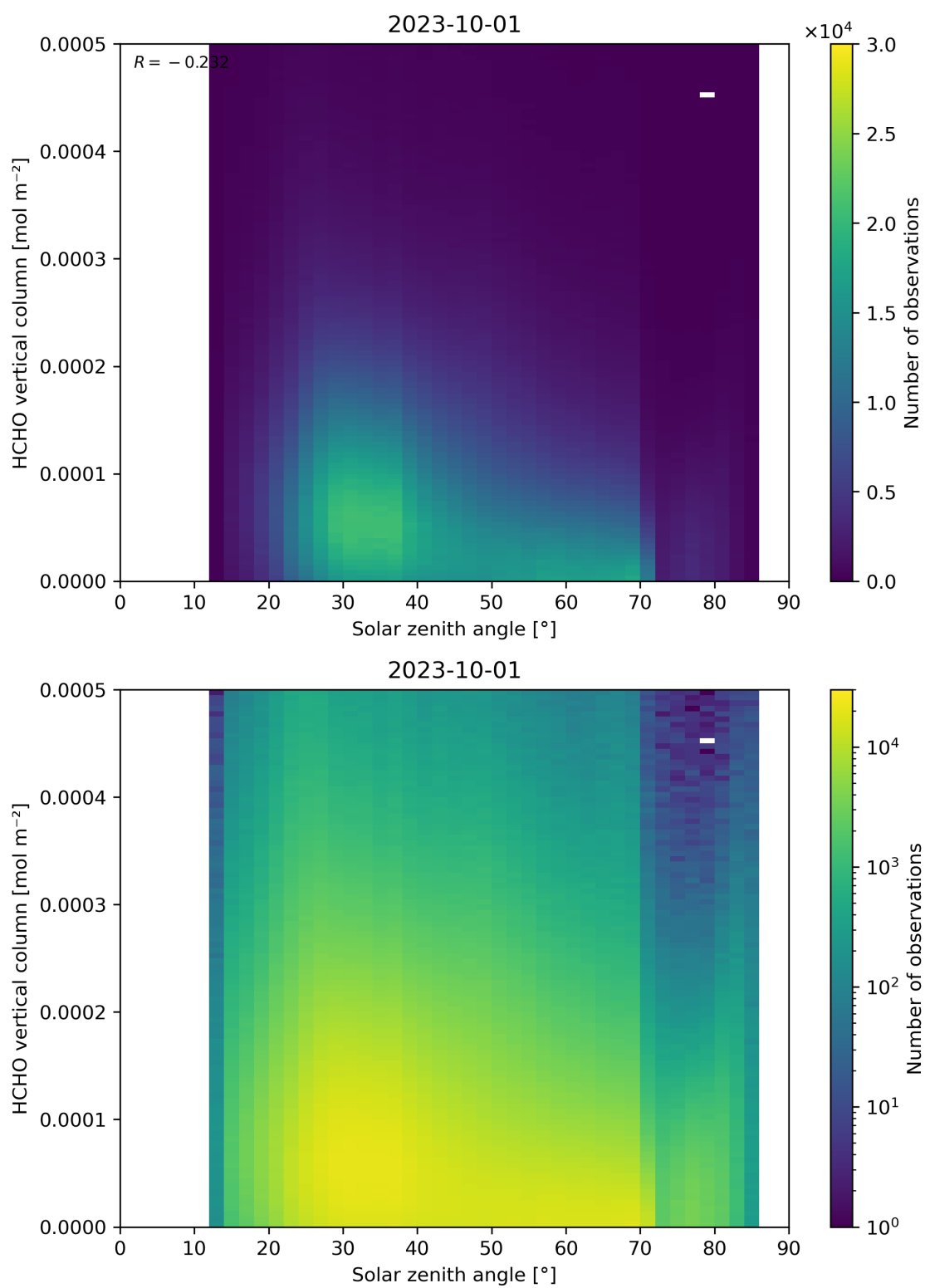
Figure 177: Scatter density plot of “Solar zenith angle” against “HCHO vertical column” for 2023-10-01 to 2023-10-02.
