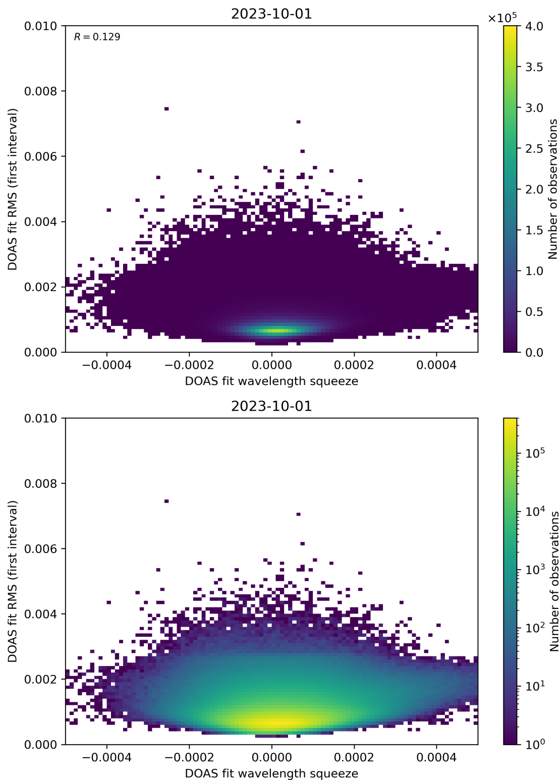
Figure 68: Scatter density plot of “DOAS fit wavelength squeeze” against “DOAS fit RMS (first interval)” for 2023-10-01 to 2023-10-02.
