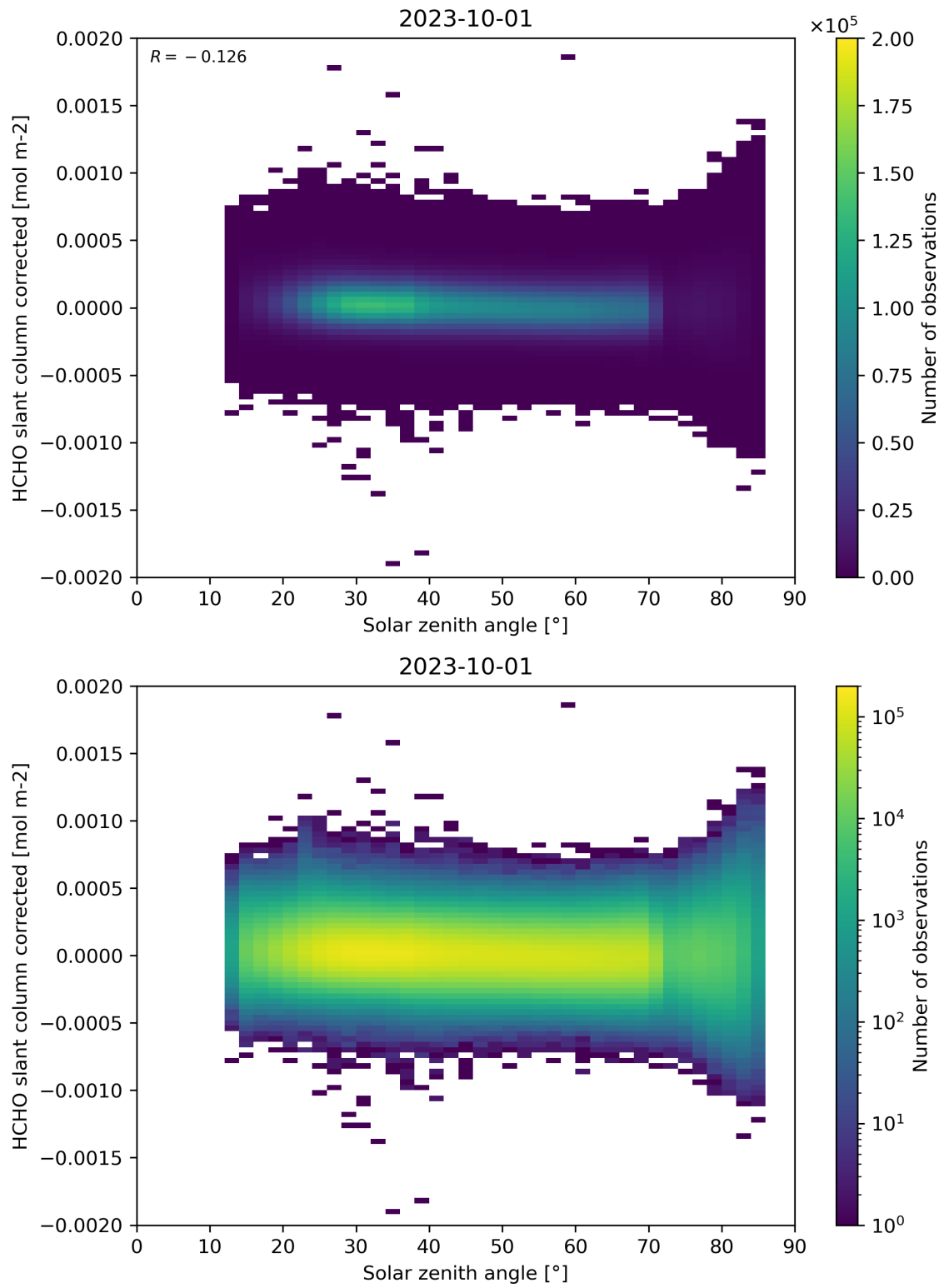
Figure 171: Scatter density plot of “Solar zenith angle” against “HCHO slant column corrected” for 2023-10-01 to 2023-10-02.
