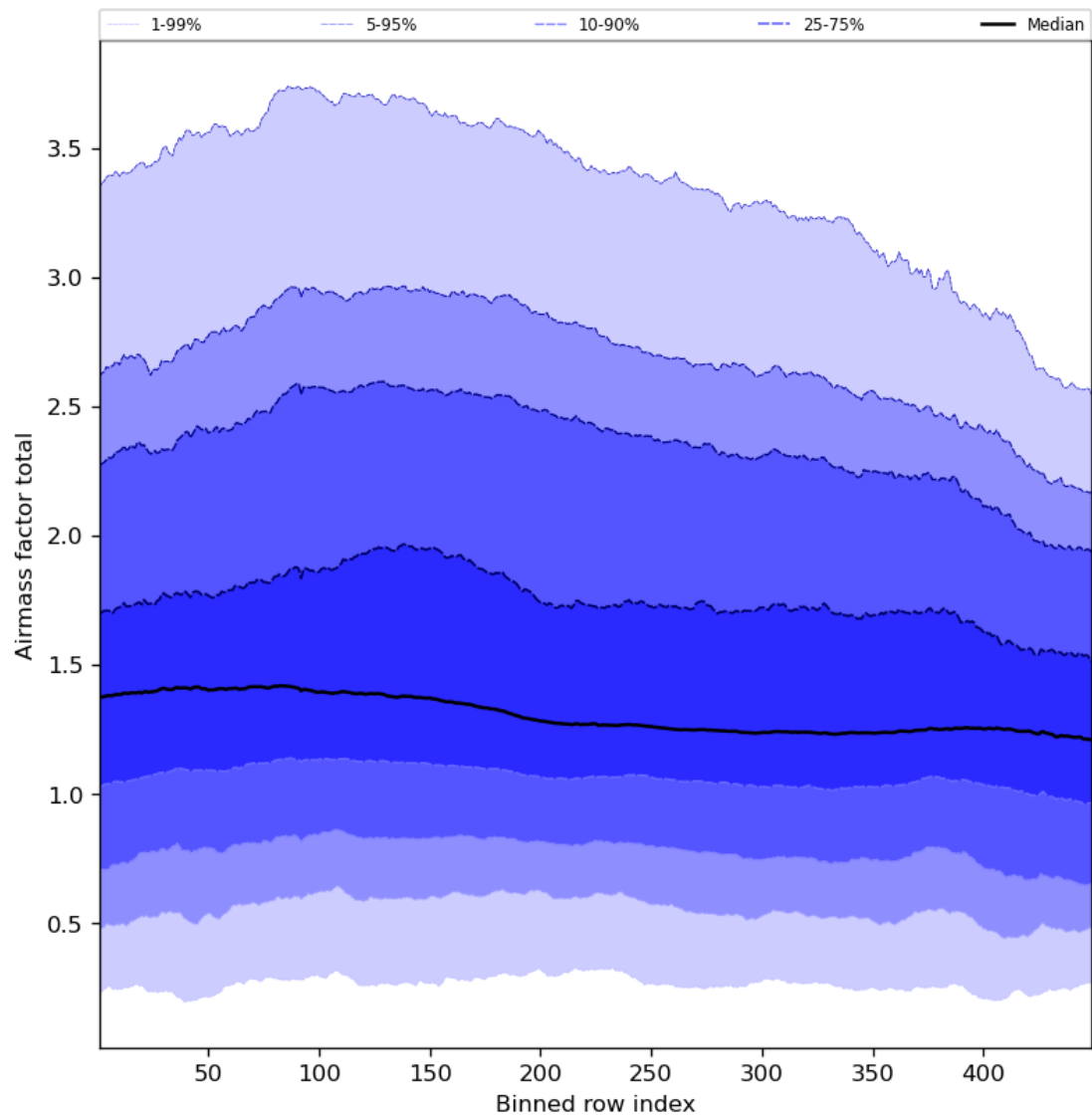
Figure 54: Along track statistics of “Airmass factor total” for 2023-10-01 to 2023-10-02
