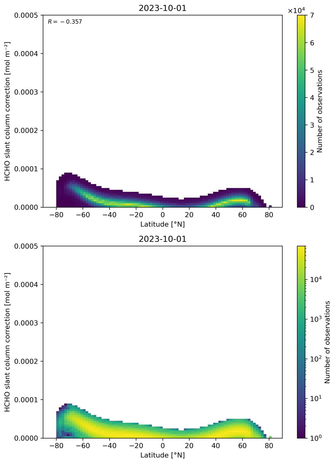
Figure 158: Scatter density plot of “Latitude” against “HCHO slant column correction” for 2023-10-01 to 2023-10-02.
