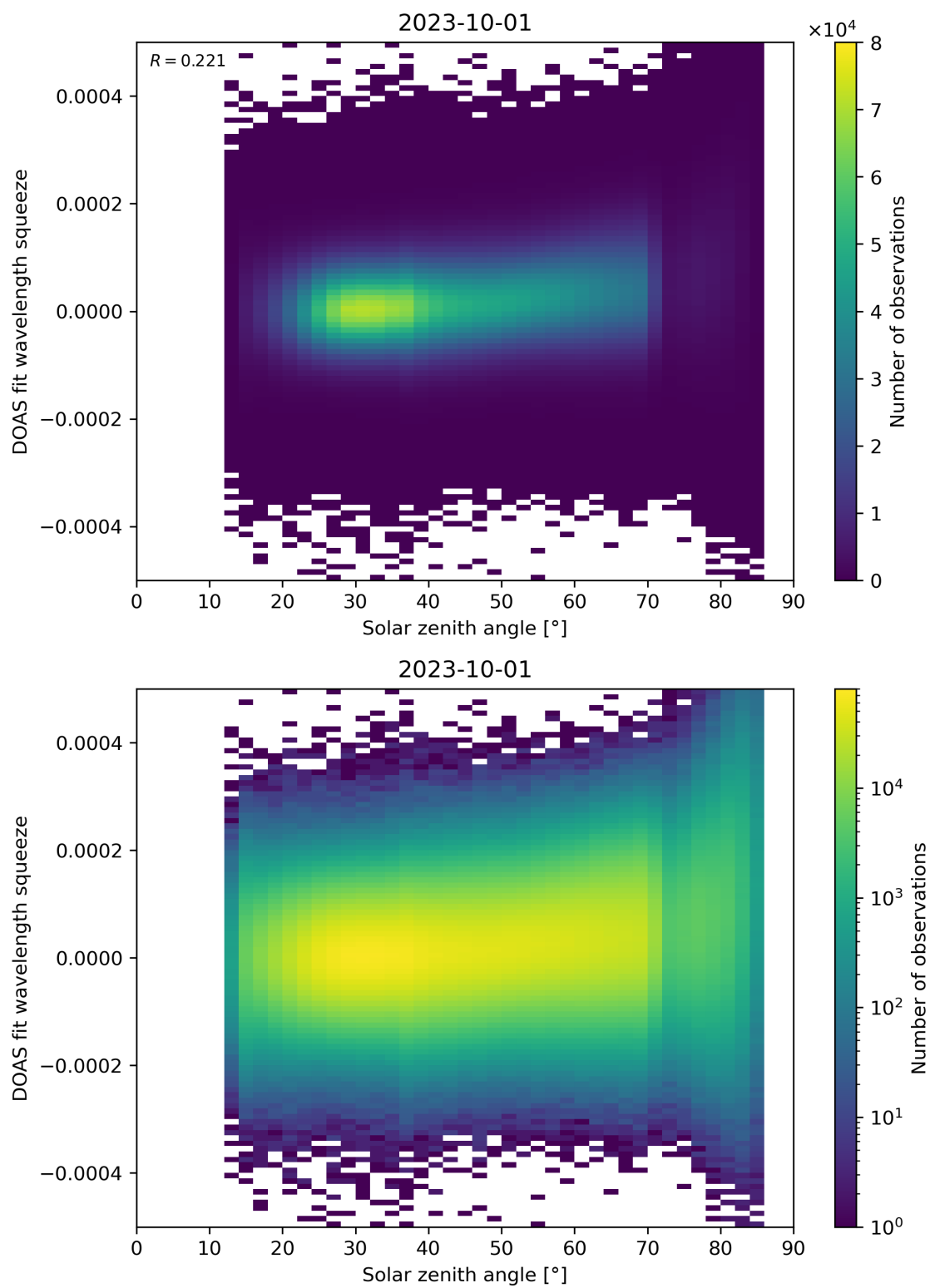
Figure 169: Scatter density plot of “Solar zenith angle” against “DOAS fit wavelength squeeze” for 2023-10-01 to 2023-10-02.
