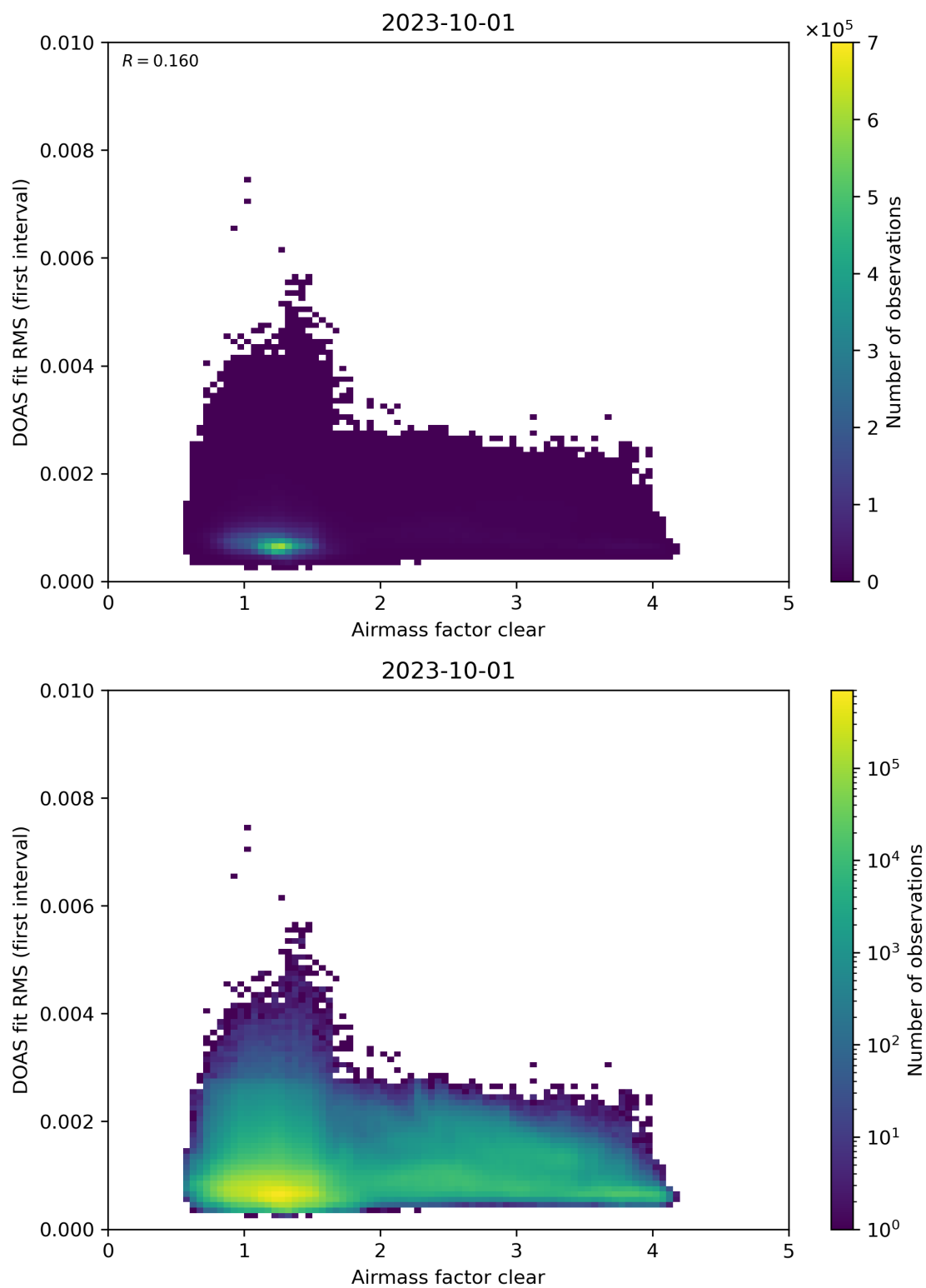
Figure 71: Scatter density plot of “Airmass factor clear” against “DOAS fit RMS (first interval)” for 2023-10-01 to 2023-10-02.
