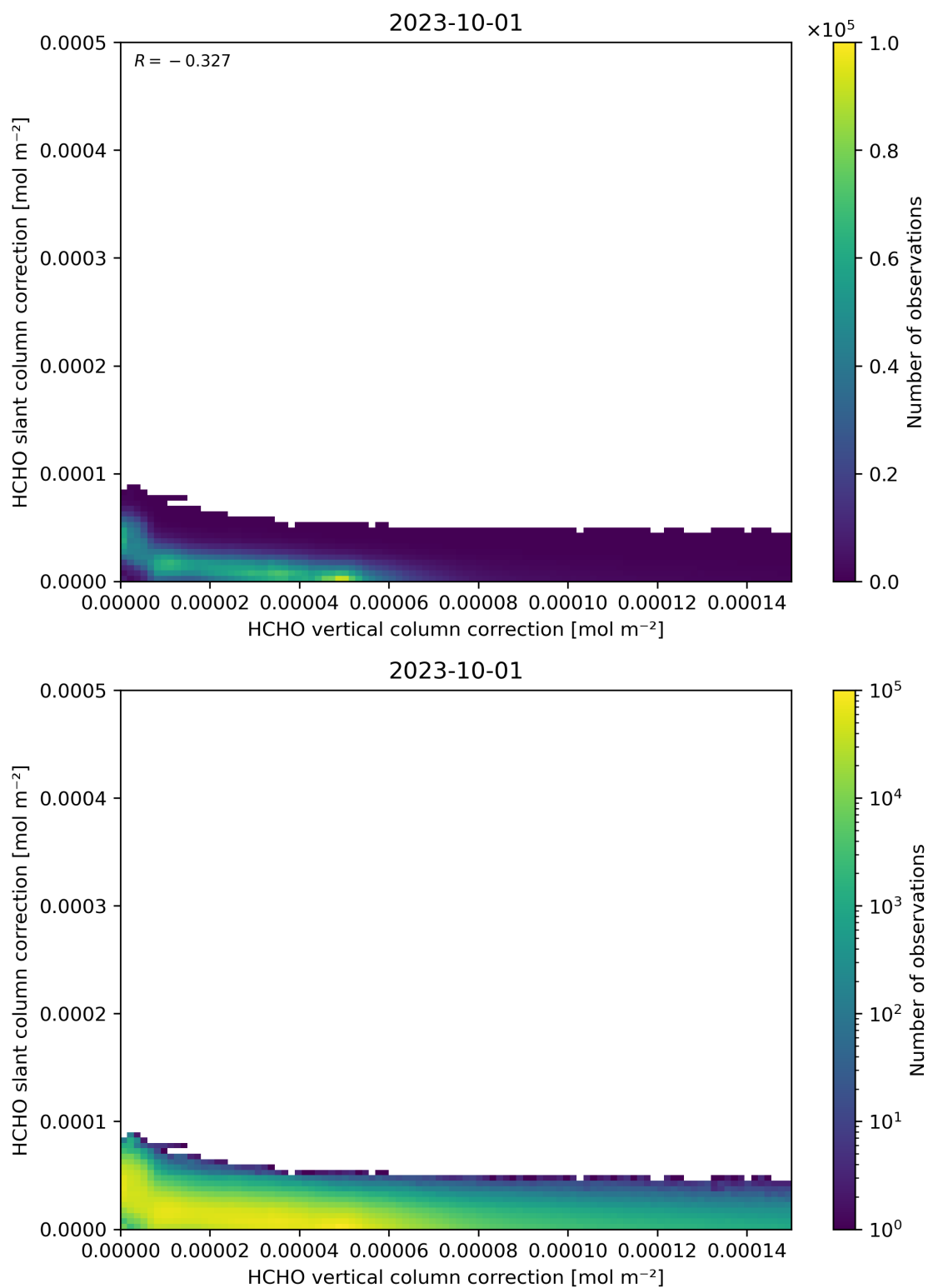
Figure 117: Scatter density plot of “HCHO vertical column correction” against “HCHO slant column correction” for 2023-10-01 to 2023-10-02.
