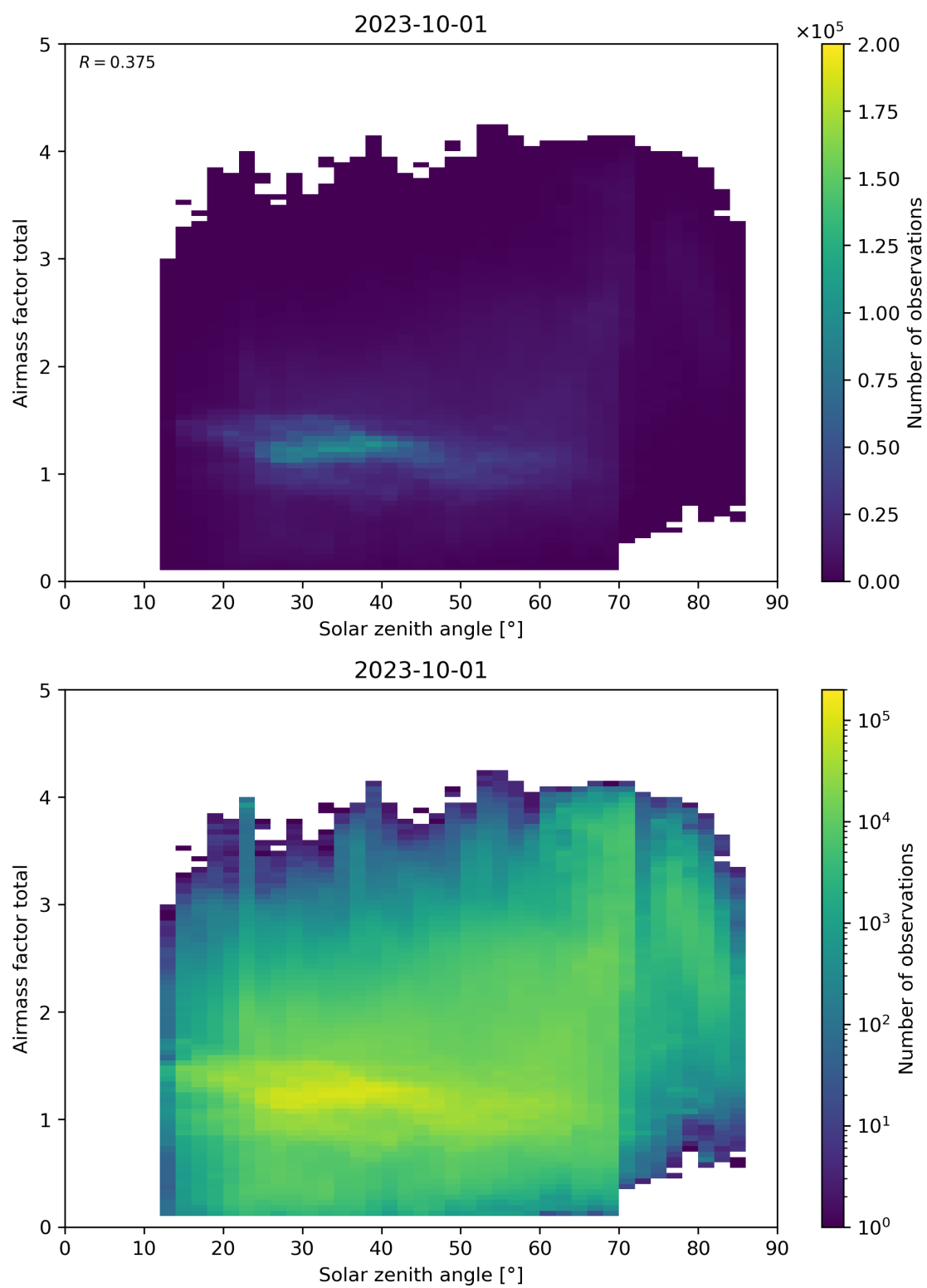
Figure 175: Scatter density plot of “Solar zenith angle” against “Airmass factor total” for 2023-10-01 to 2023-10-02.
