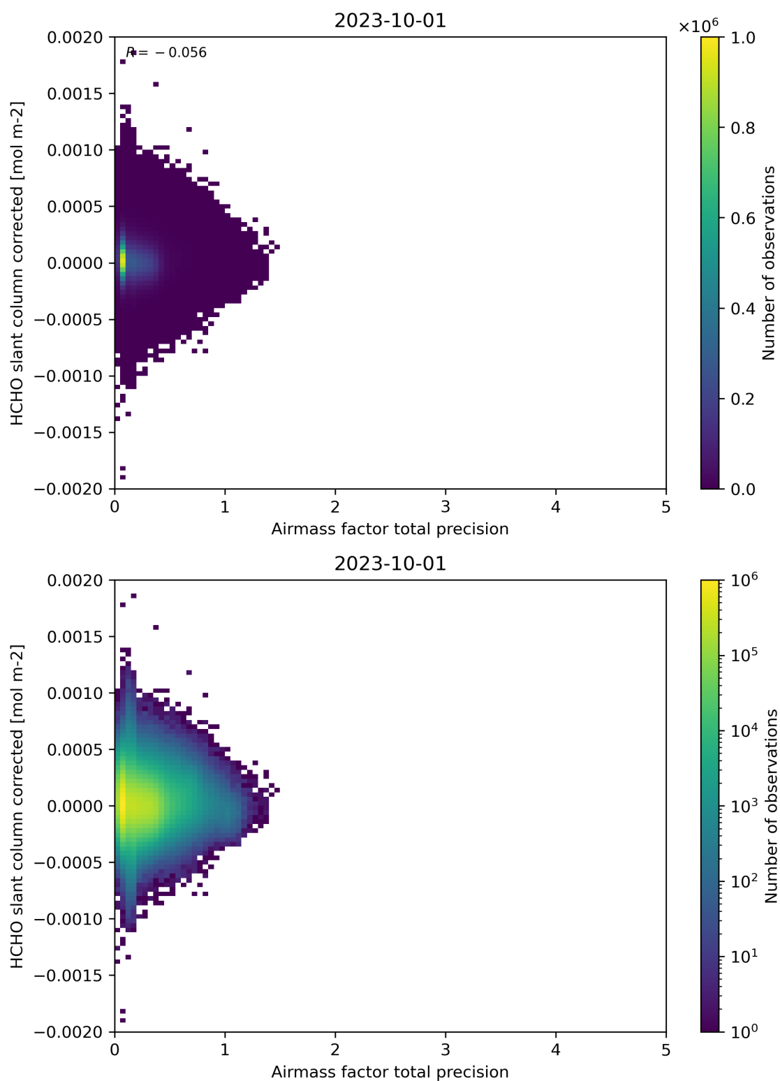
Figure 109: Scatter density plot of “Airmass factor total precision” against “HCHO slant column corrected” for 2023-10-01 to 2023-10-02.
