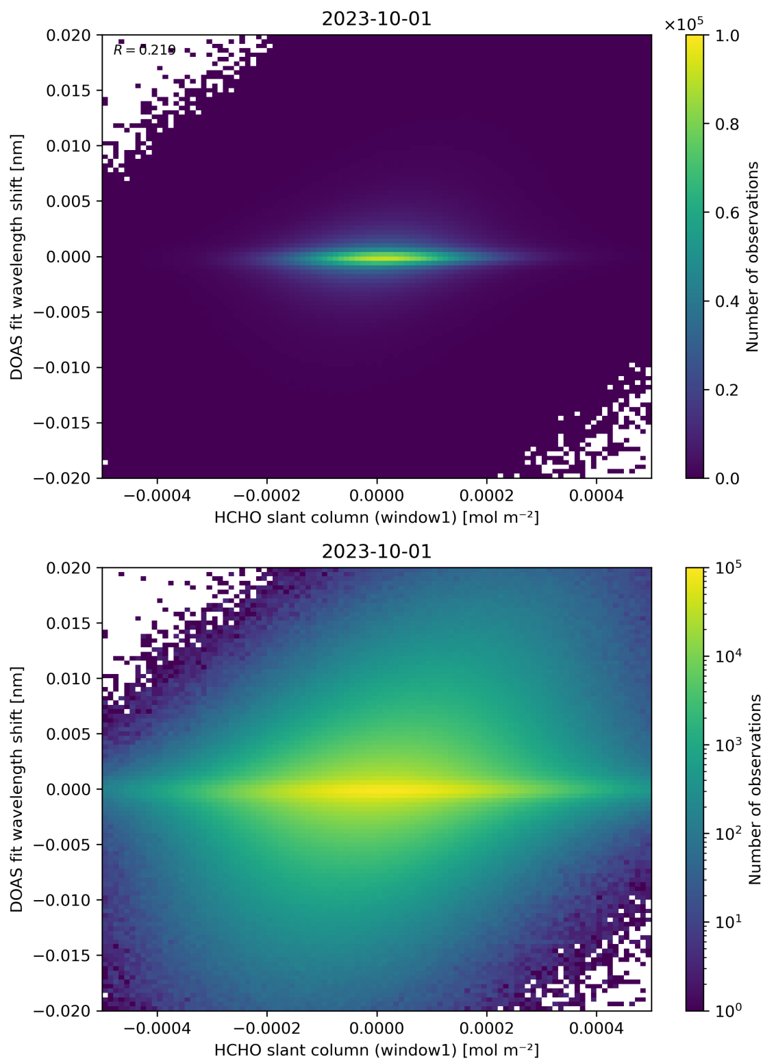
Figure 79: Scatter density plot of “HCHO slant column (window1)” against “DOAS fit wavelength shift” for 2023-10-01 to 2023-10-02.
