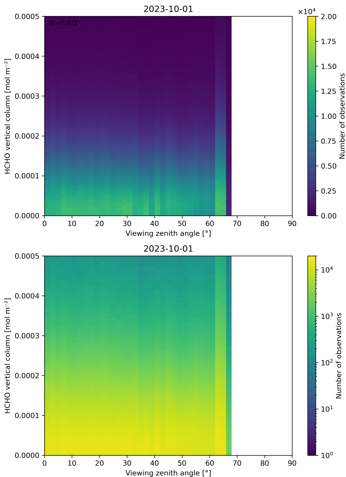
Figure 192: Scatter density plot of “Viewing zenith angle” against “HCHO vertical column” for 2023-10-01 to 2023-10-02.
