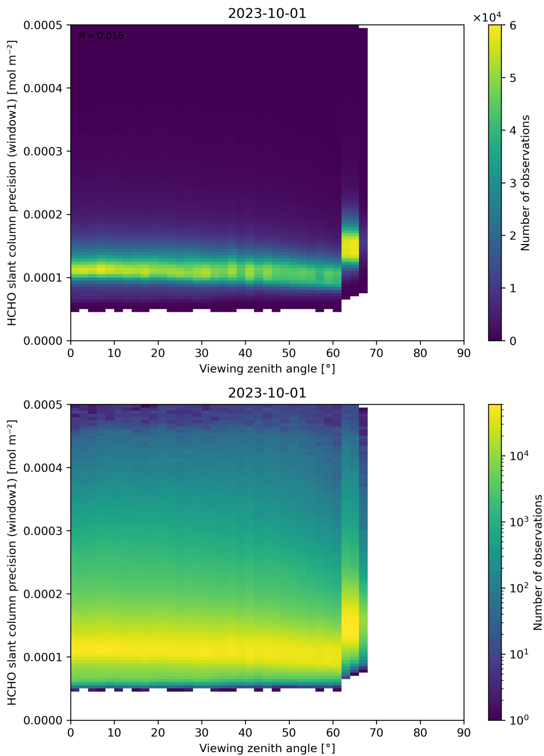
Figure 189: Scatter density plot of “Viewing zenith angle” against “HCHO slant column precision (window1)” for 2023-10-01 to 2023-10-02.
