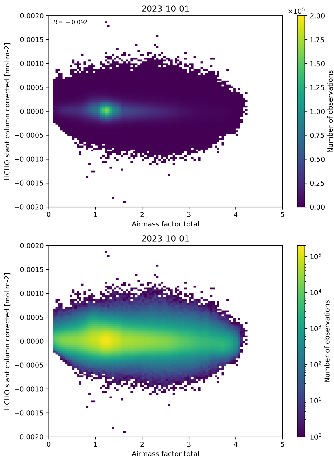
Figure 101: Scatter density plot of “Airmass factor total” against “HCHO slant column corrected” for 2023-10-01 to 2023-10-02.
