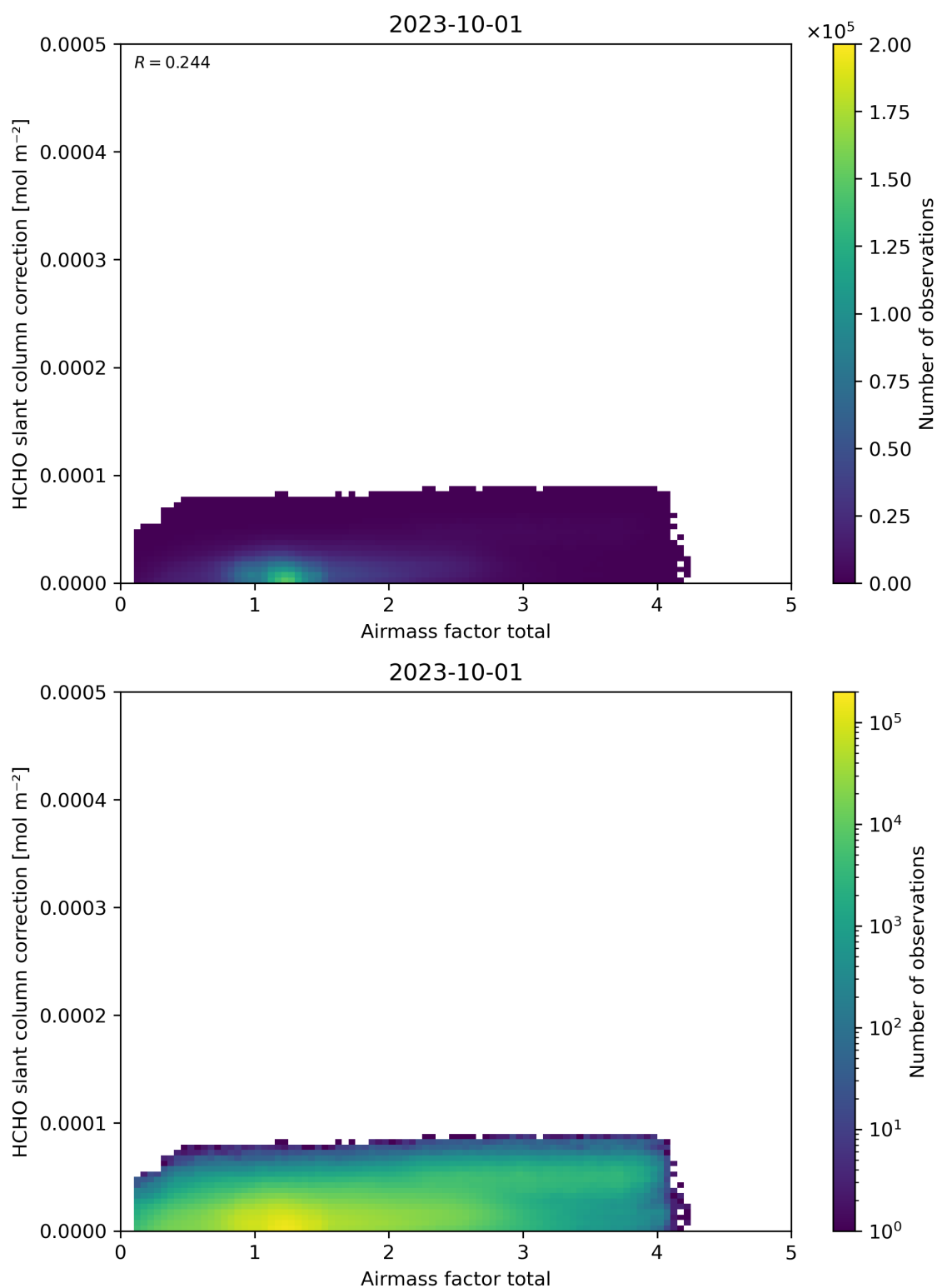
Figure 102: Scatter density plot of “Airmass factor total” against “HCHO slant column correction” for 2023-10-01 to 2023-10-02.
