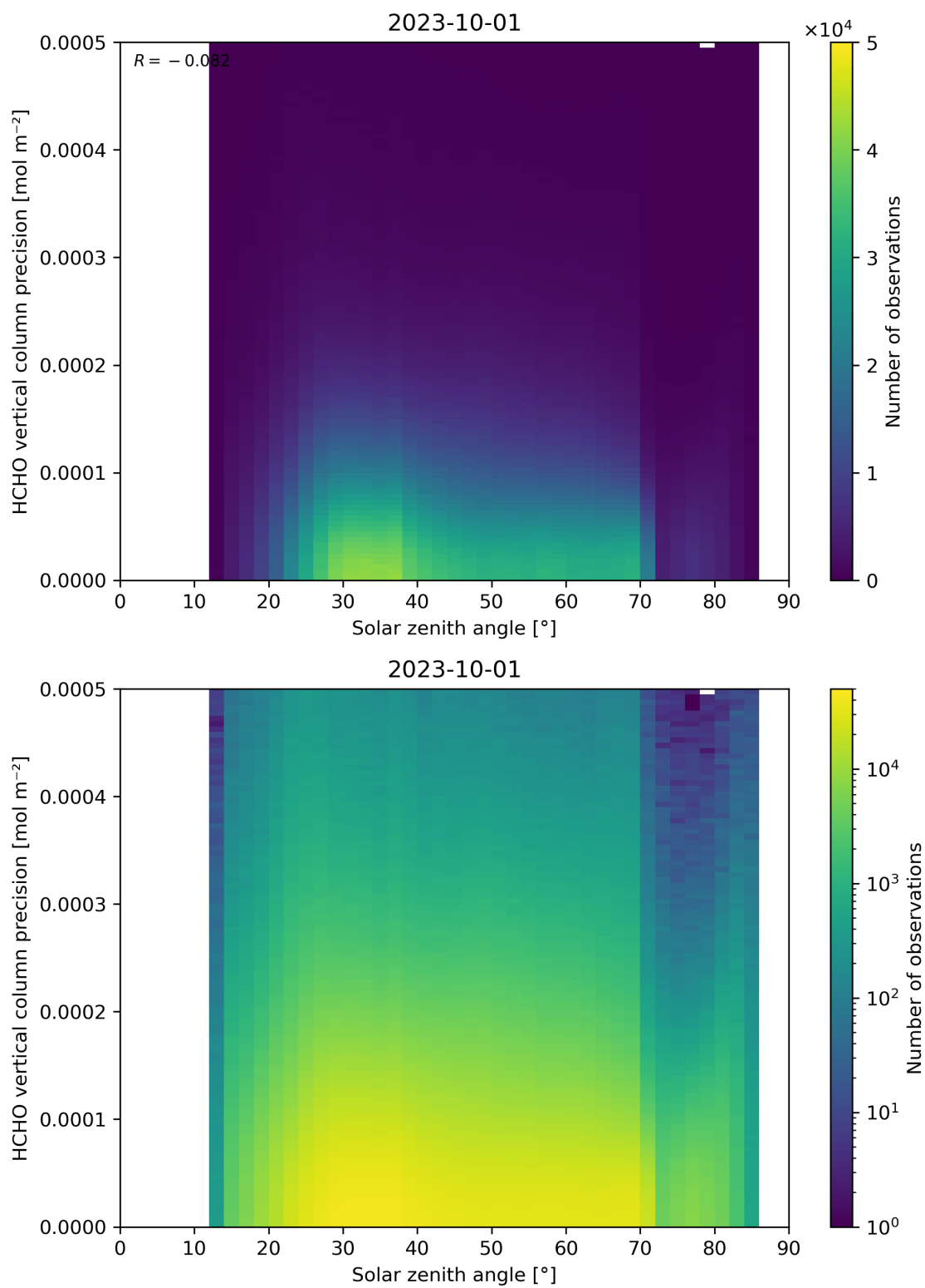
Figure 179: Scatter density plot of “Solar zenith angle” against “HCHO vertical column precision” for 2023-10-01 to 2023-10-02.
