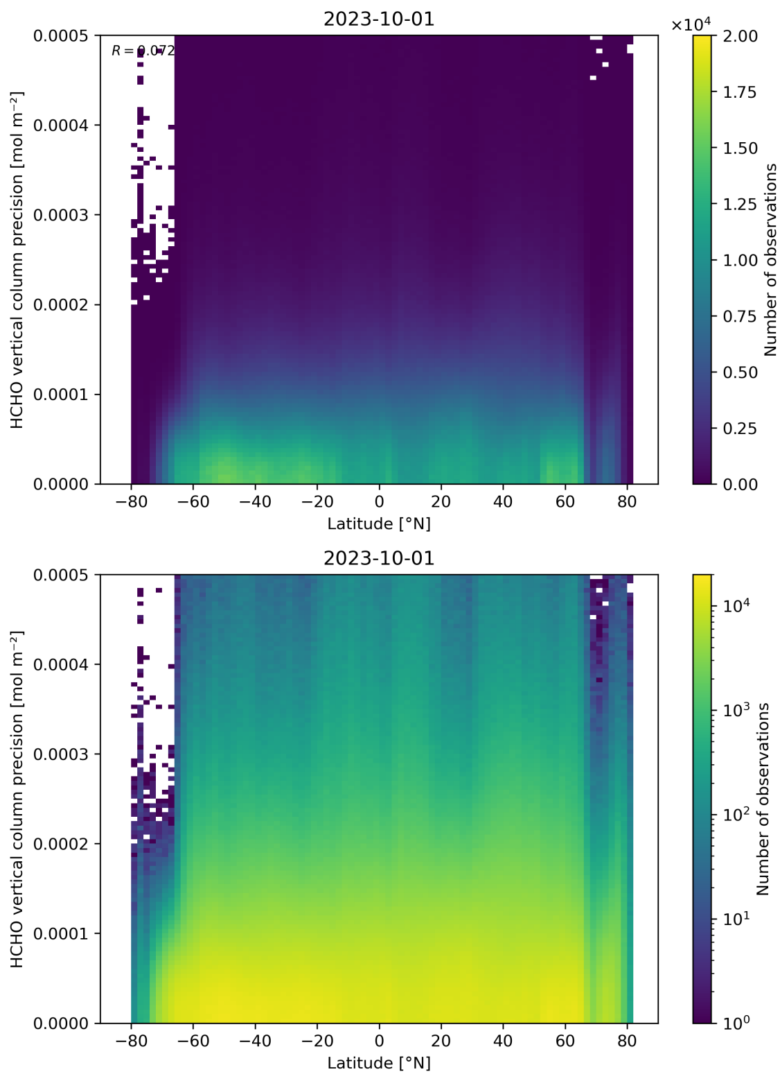
Figure 165: Scatter density plot of “Latitude” against “HCHO vertical column precision” for 2023-10-01 to 2023-10-02.
