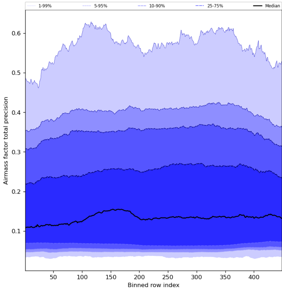
Figure 55: Along track statistics of “Airmass factor total precision” for 2023-10-01 to 2023-10-02
