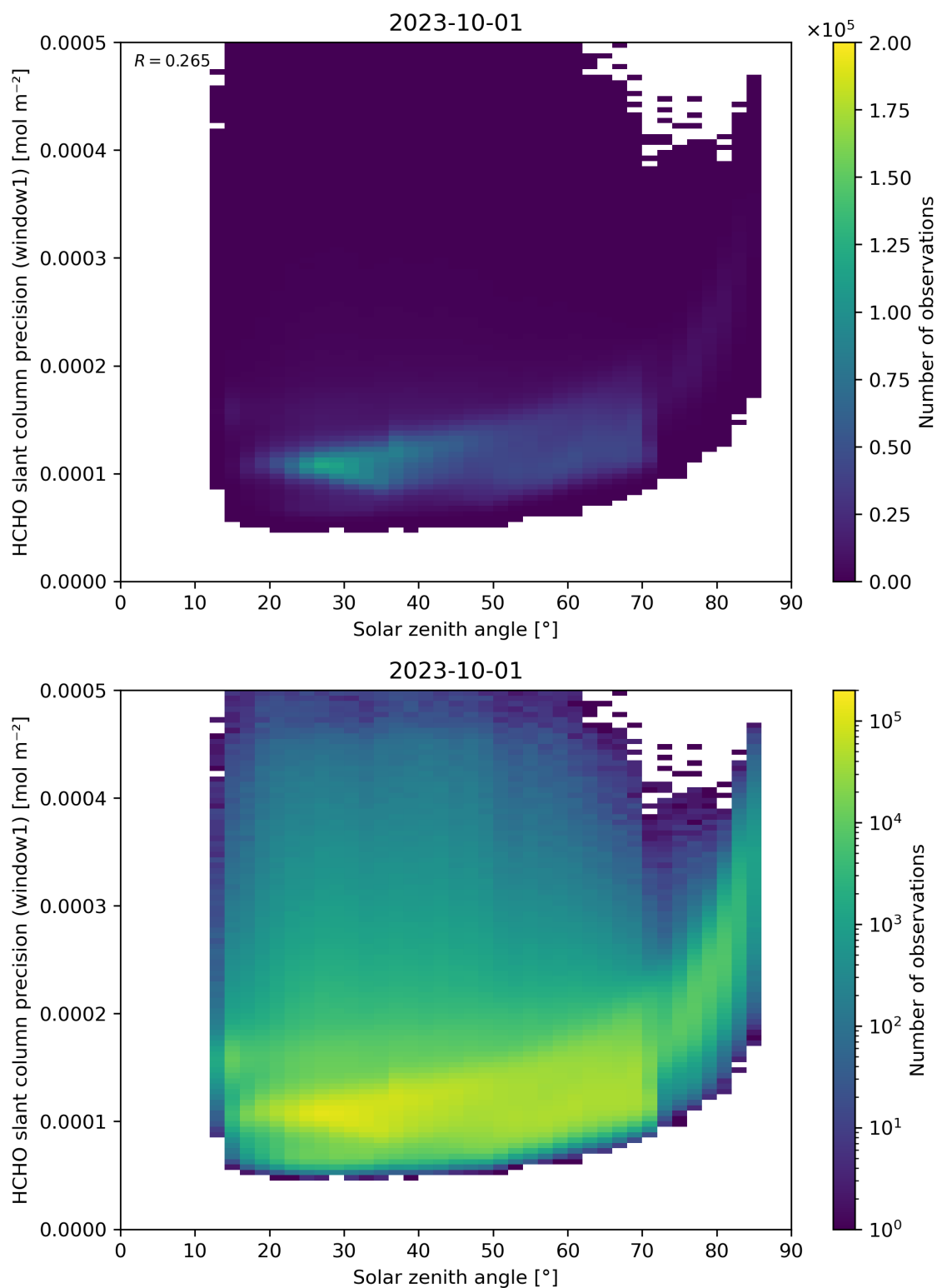
Figure 174: Scatter density plot of “Solar zenith angle” against “HCHO slant column precision (window1)” for 2023-10-01 to 2023-10-02.
