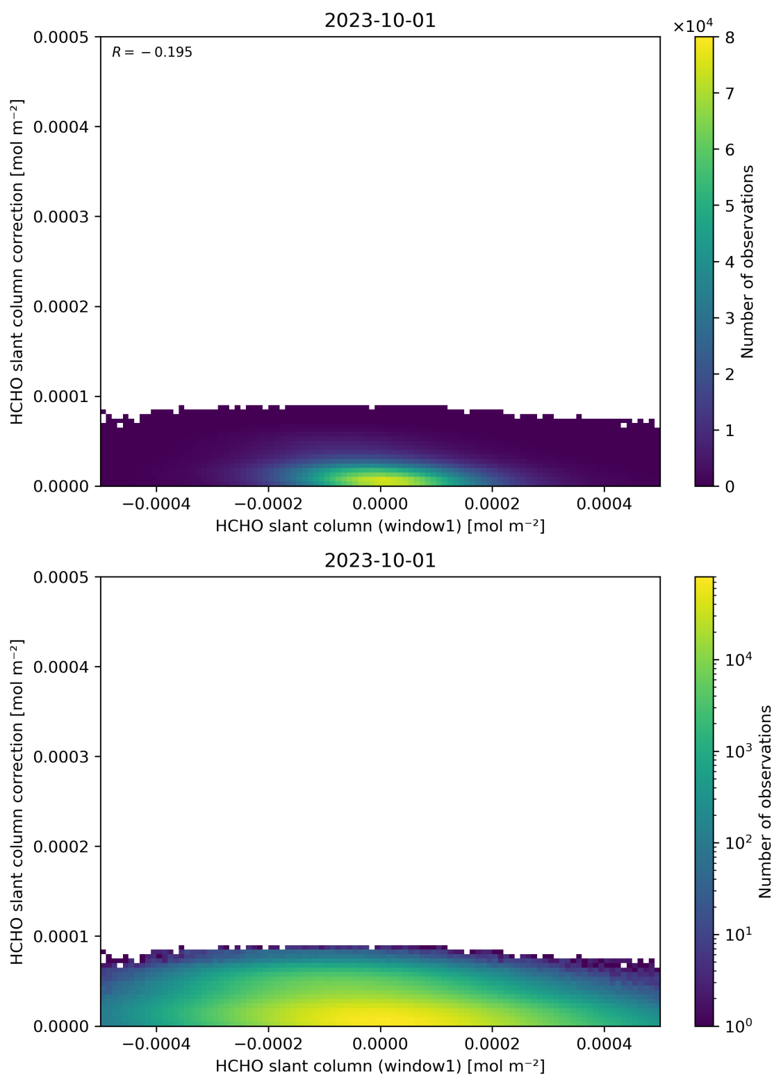
Figure 83: Scatter density plot of “HCHO slant column (window1)” against “HCHO slant column correction” for 2023-10-01 to 2023-10-02.
