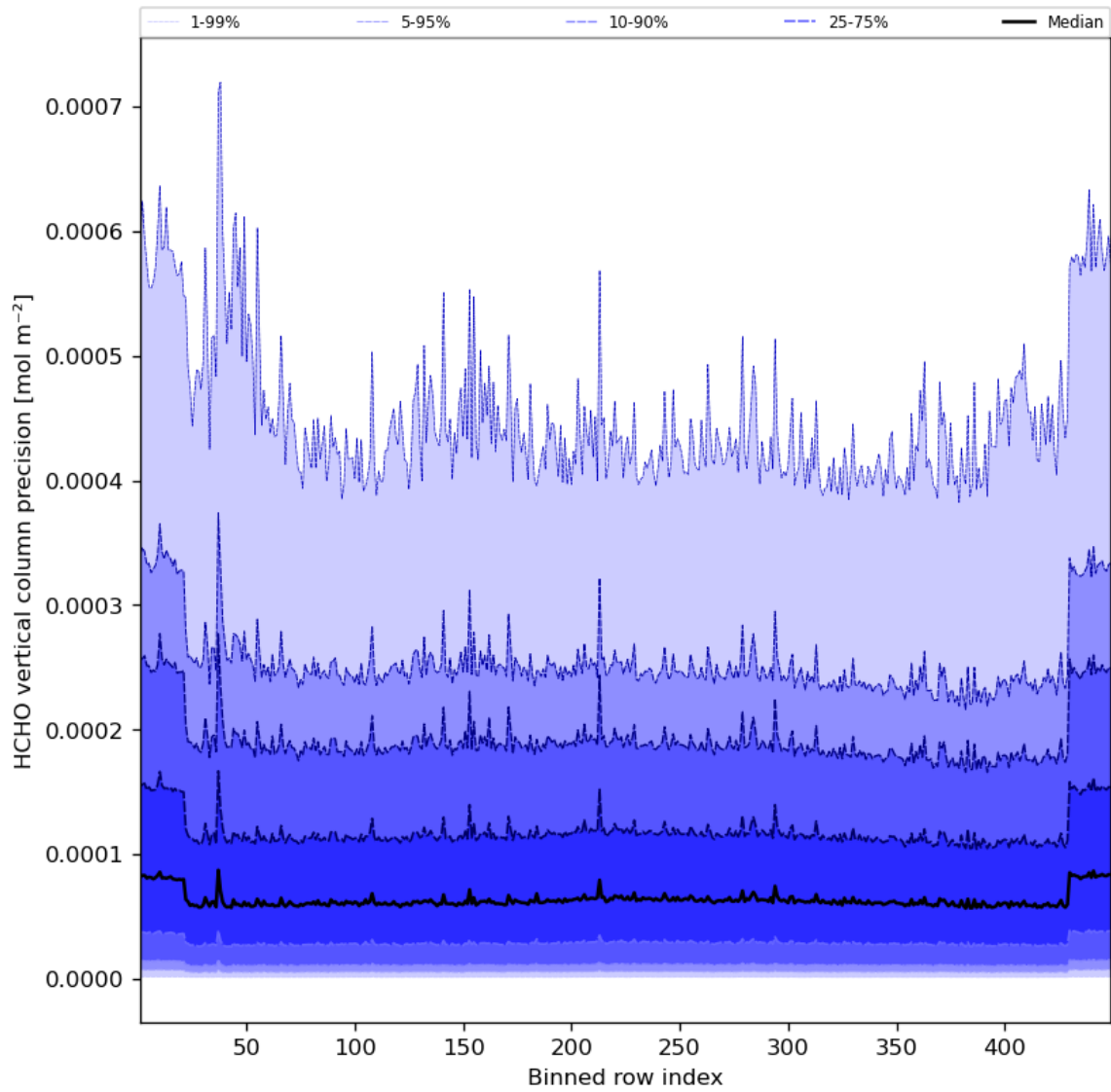
Figure 50: Along track statistics of “HCHO vertical column precision” for 2023-10-01 to 2023-10-02
