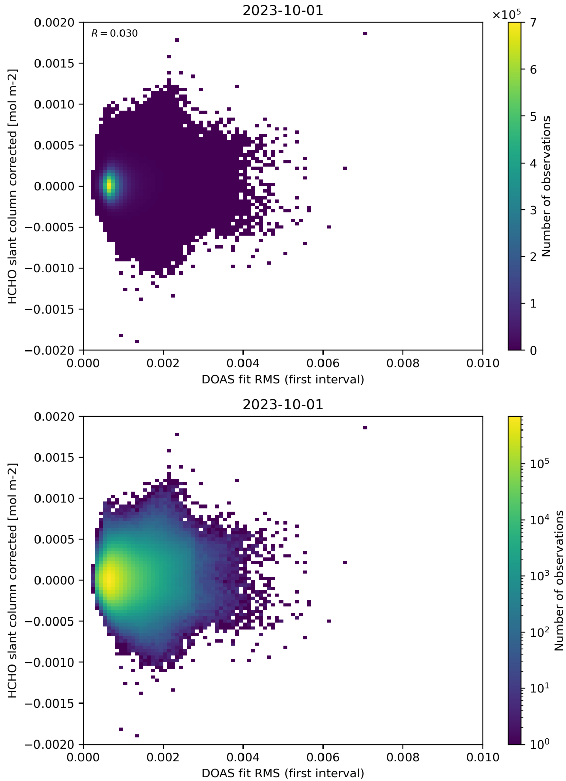
Figure 62: Scatter density plot of “DOAS fit RMS (first interval)” against “HCHO slant column corrected” for 2023-10-01 to 2023-10-02.
