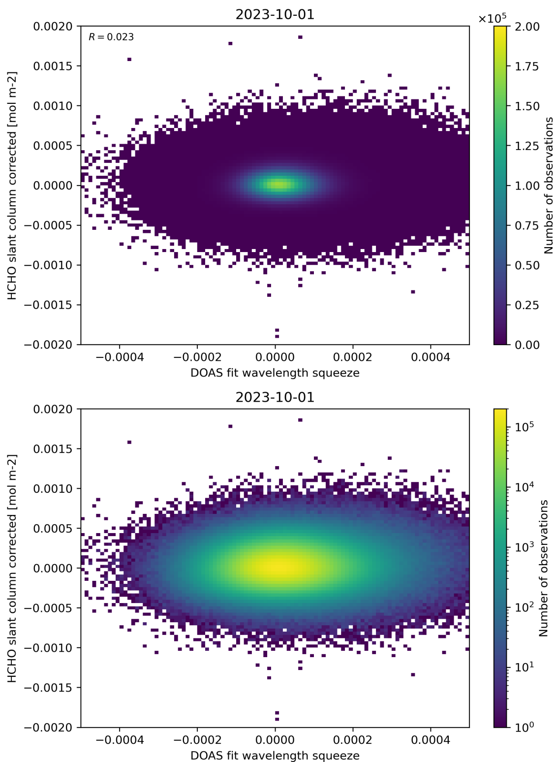
Figure 69: Scatter density plot of “DOAS fit wavelength squeeze” against “HCHO slant column corrected” for 2023-10-01 to 2023-10-02.
