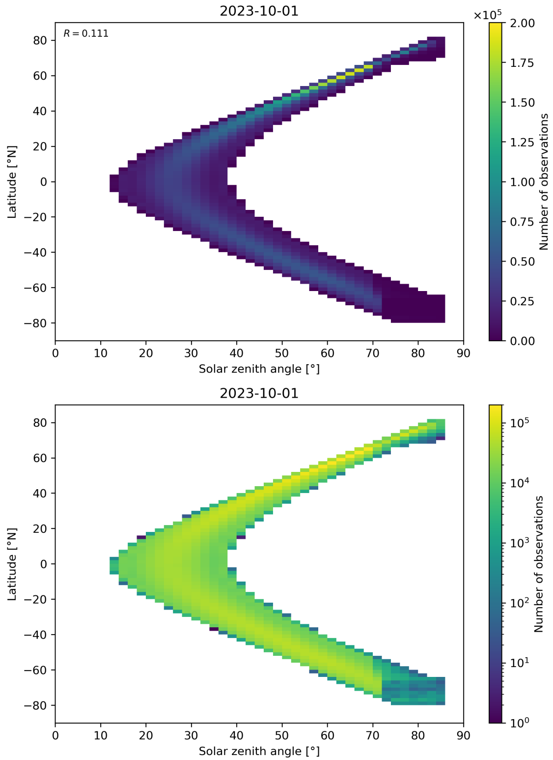
Figure 181: Scatter density plot of “Solar zenith angle” against “Latitude” for 2023-10-01 to 2023-10-02.
