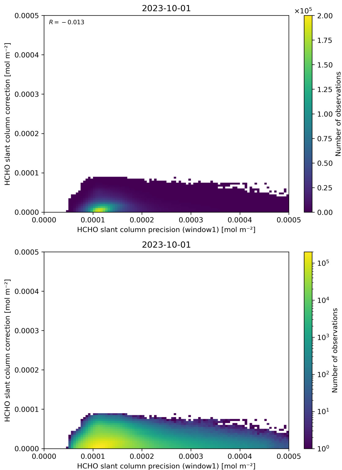
Figure 93: Scatter density plot of “HCHO slant column precision (window1)” against “HCHO slant column correction” for 2023-10-01 to 2023-10-02.
