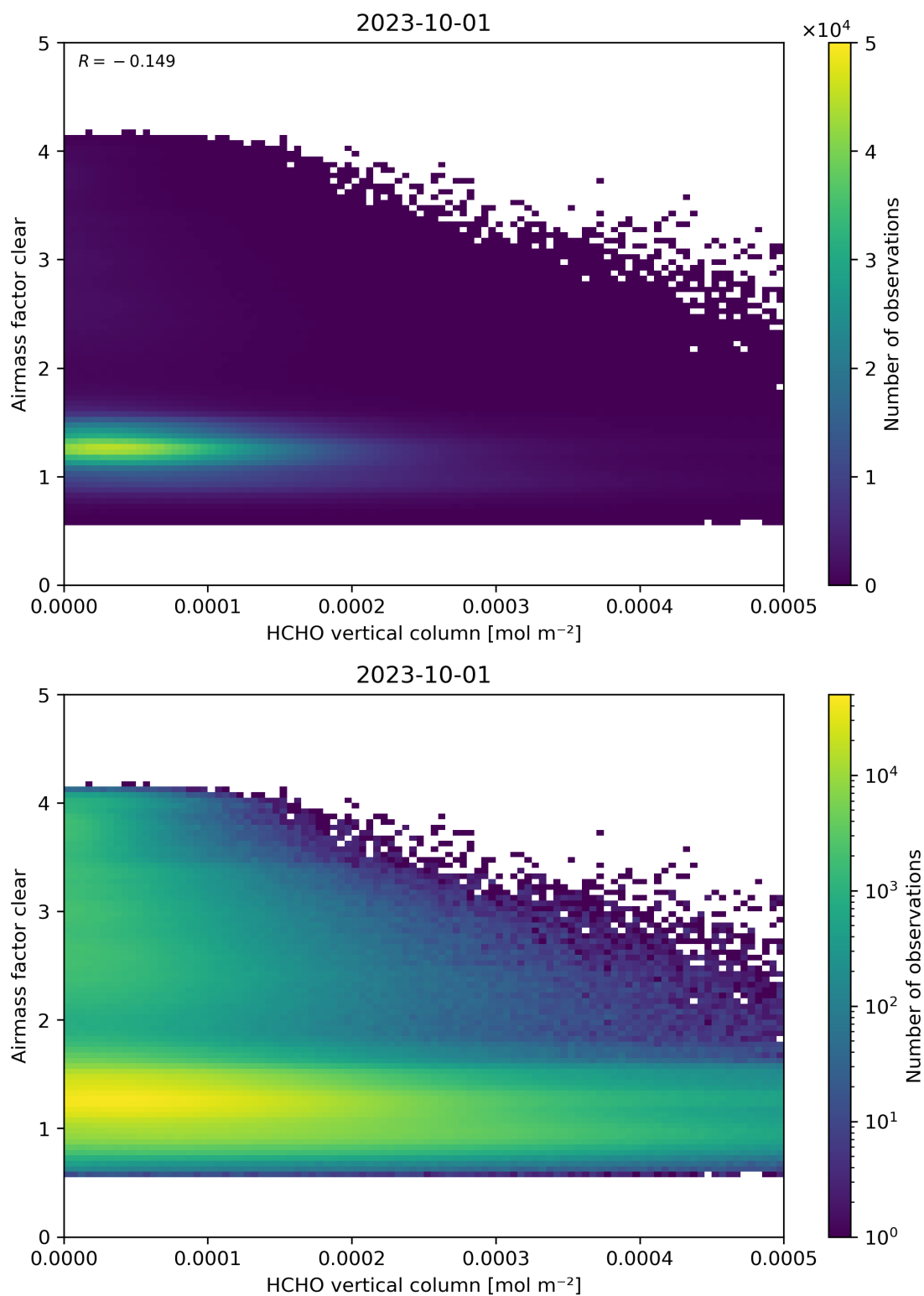
Figure 126: Scatter density plot of “HCHO vertical column” against “Airmass factor clear” for 2023-10-01 to 2023-10-02.
