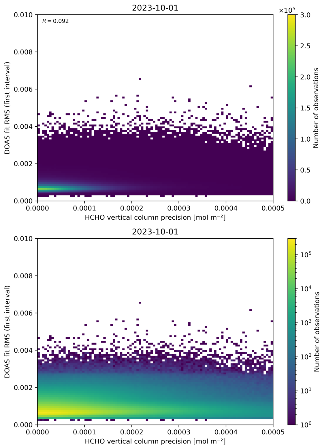
Figure 136: Scatter density plot of “HCHO vertical column precision” against “DOAS fit RMS (first interval)” for 2023-10-01 to 2023-10-02.
