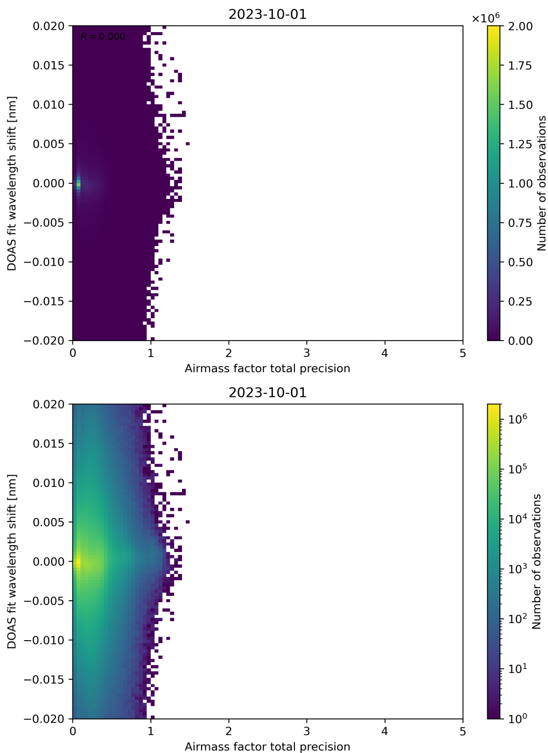
Figure 106: Scatter density plot of “Airmass factor total precision” against “DOAS fit wavelength shift” for 2023-10-01 to 2023-10-02.
