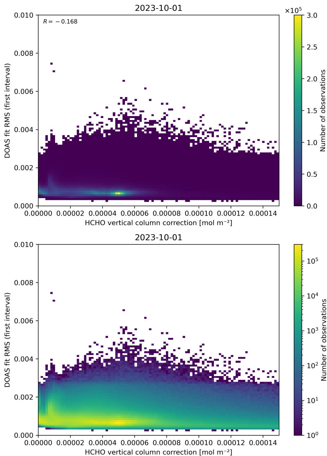
Figure 112: Scatter density plot of “HCHO vertical column correction” against “DOAS fit RMS (first interval)” for 2023-10-01 to 2023-10-02.
