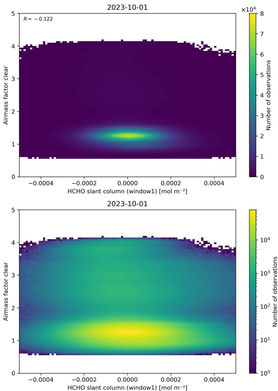
Figure 81: Scatter density plot of “HCHO slant column (window1)” against “Airmass factor clear” for 2023-10-01 to 2023-10-02.
