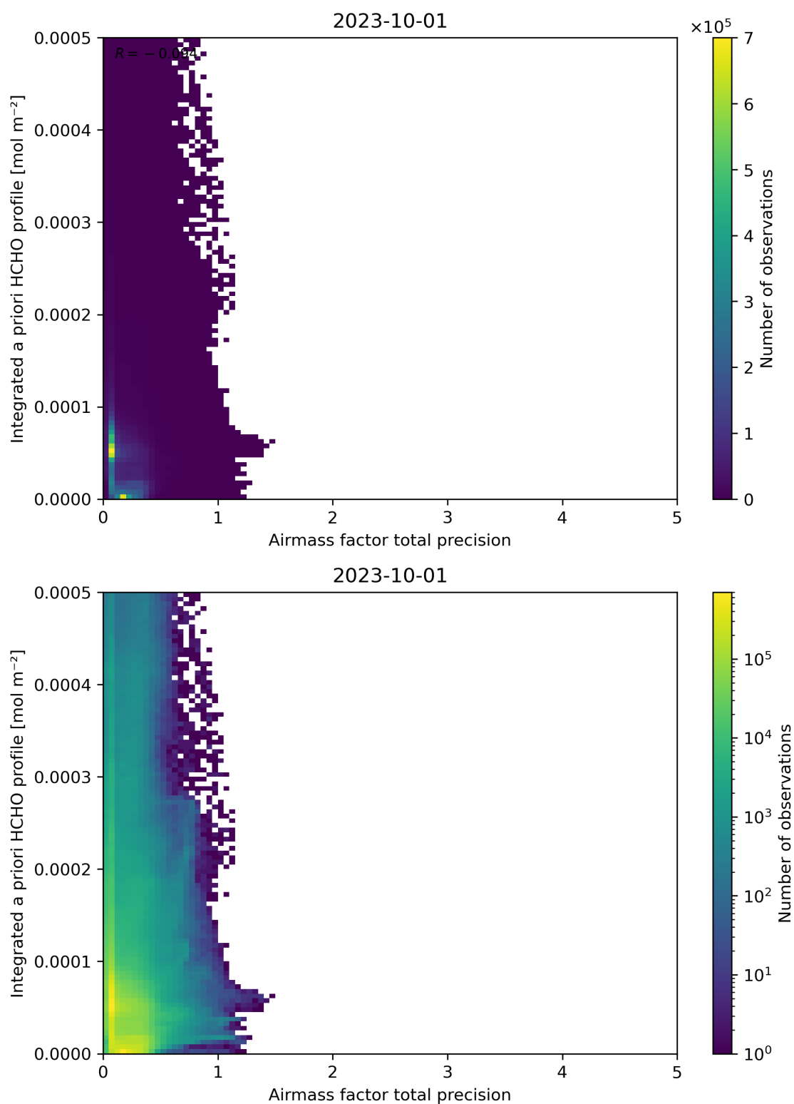
Figure 111: Scatter density plot of “Airmass factor total precision” against “Integrated a priori HCHO profile” for 2023-10-01 to 2023-10-02.
