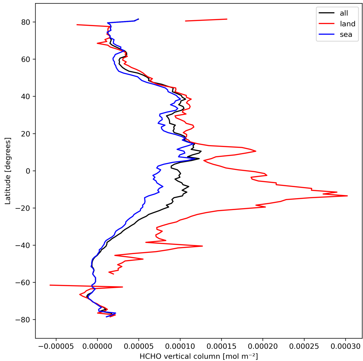
Figure 21: Zonal average of “HCHO vertical column” for 2023-10-01 to 2023-10-02.
