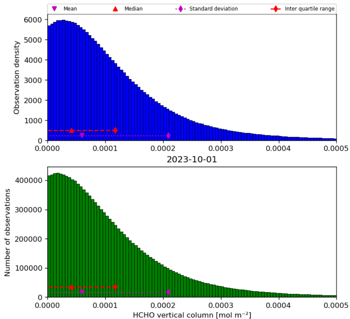
Figure 35: Histogram of “HCHO vertical column” for 2023-10-01 to 2023-10-02
