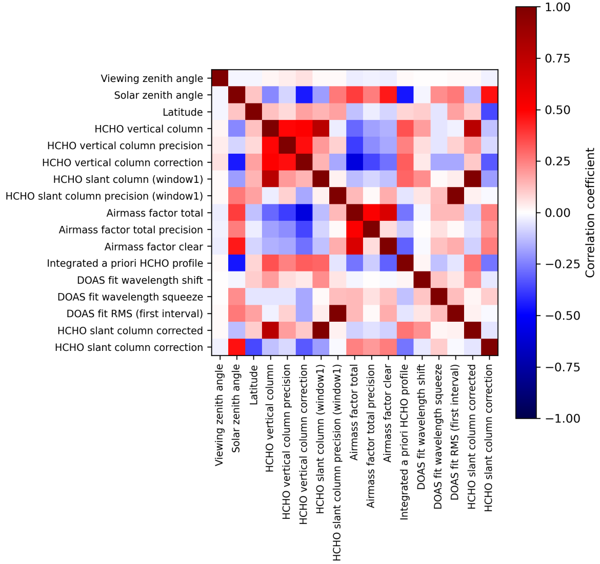
Figure 2: Map of correlation matrix for 2023-10-01 to 2023-10-02.
