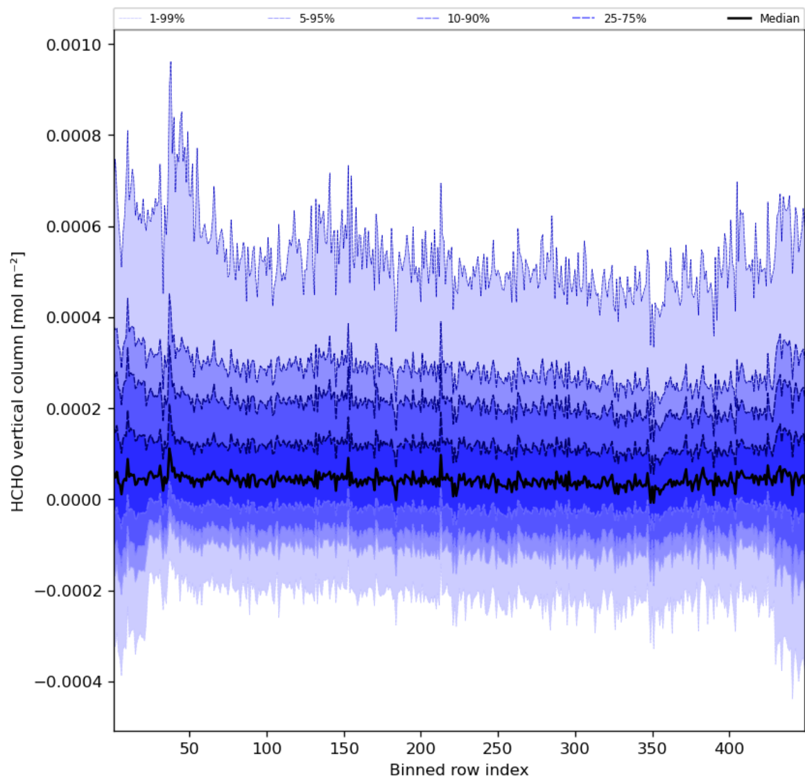
Figure 49: Along track statistics of “HCHO vertical column” for 2023-10-01 to 2023-10-02
