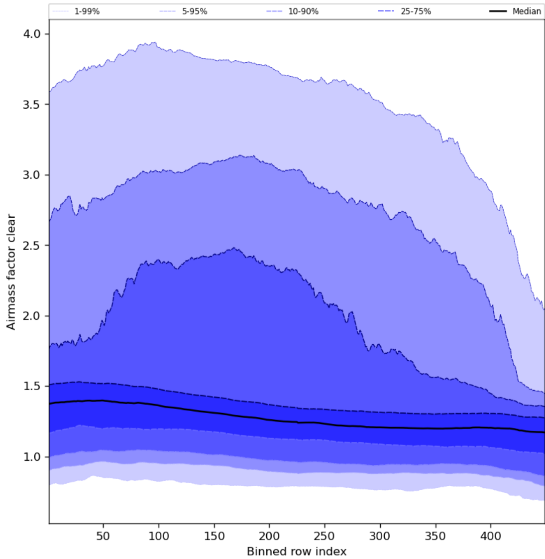
Figure 56: Along track statistics of “Airmass factor clear” for 2023-10-01 to 2023-10-02
