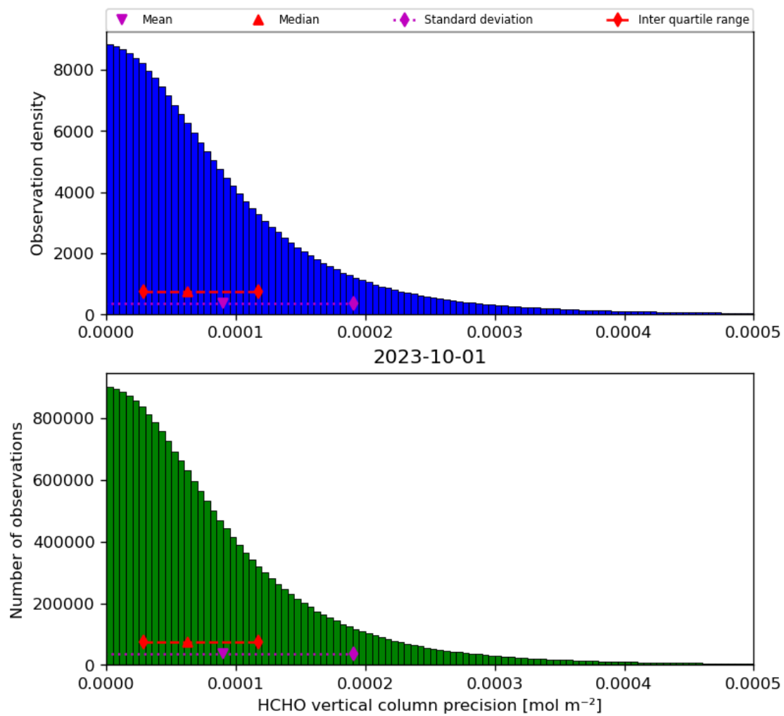
Figure 36: Histogram of “HCHO vertical column precision” for 2023-10-01 to 2023-10-02
