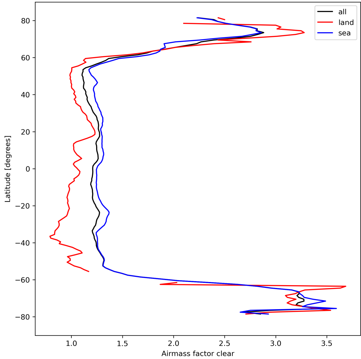
Figure 28: Zonal average of “Airmass factor clear” for 2023-10-01 to 2023-10-02.
