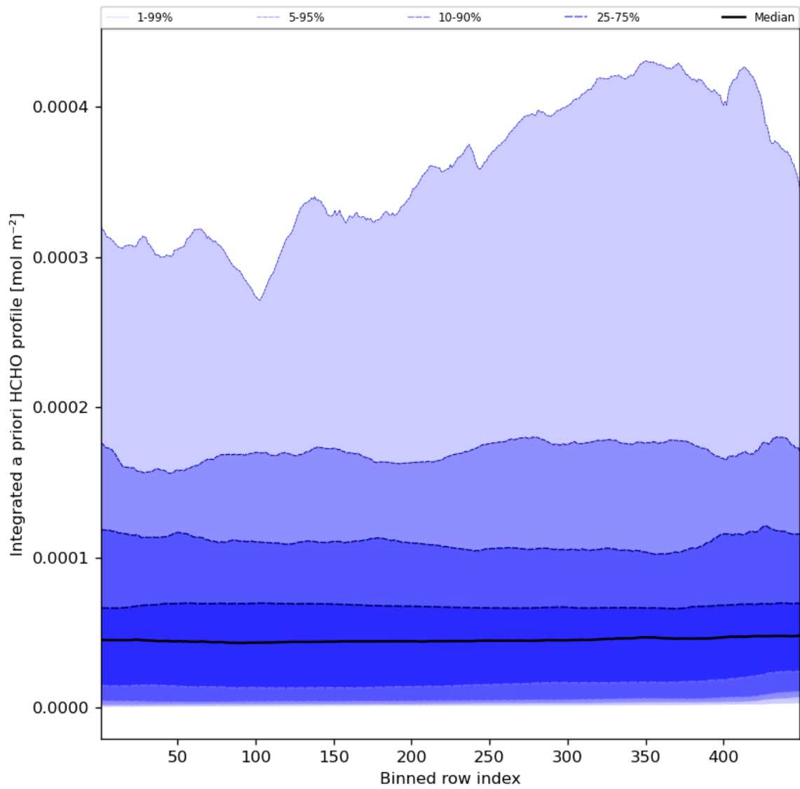
Figure 57: Along track statistics of “Integrated a priori HCHO profile” for 2023-10-01 to 2023-10-02
