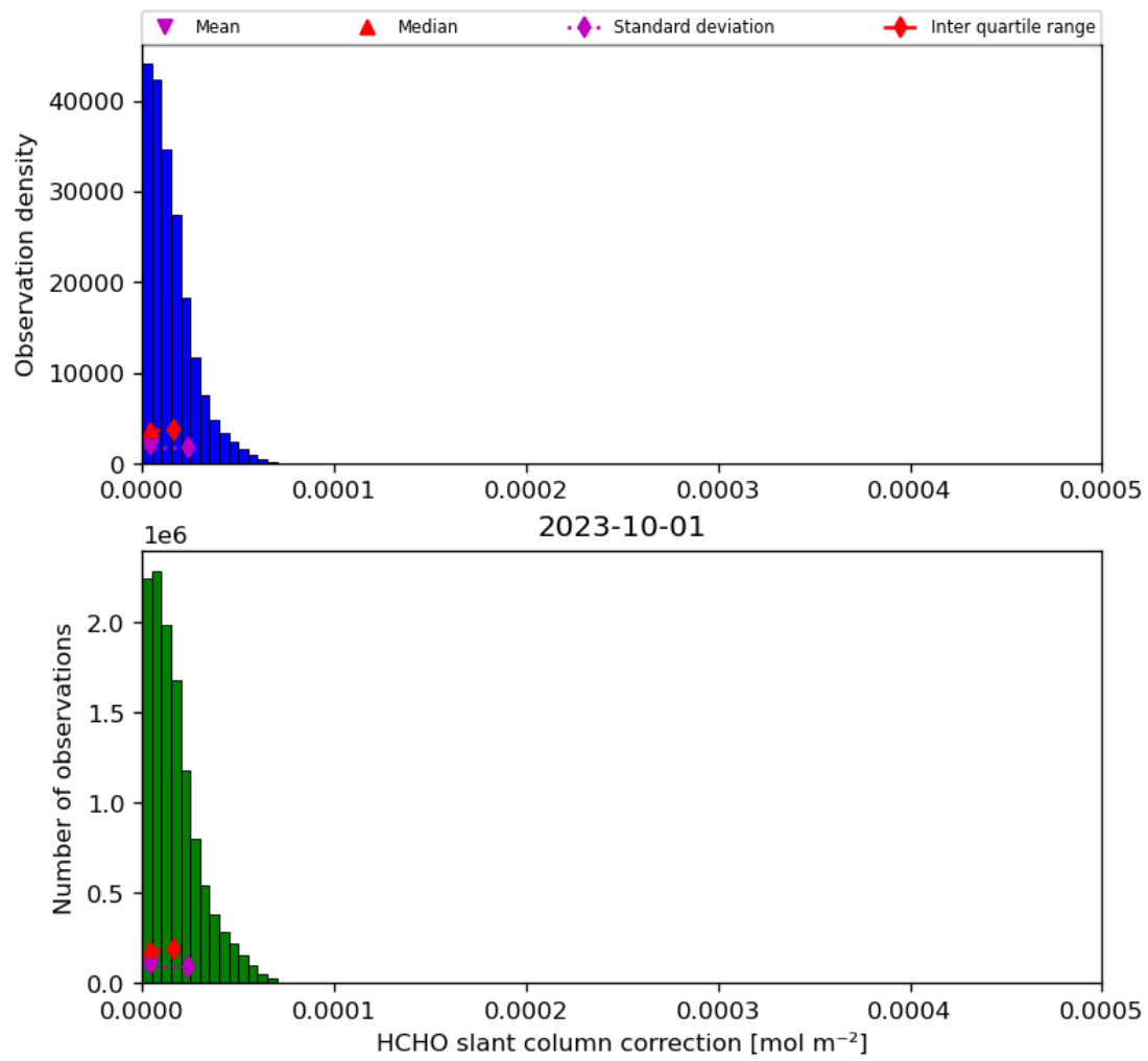
Figure 47: Histogram of “HCHO slant column correction” for 2023-10-01 to 2023-10-02
