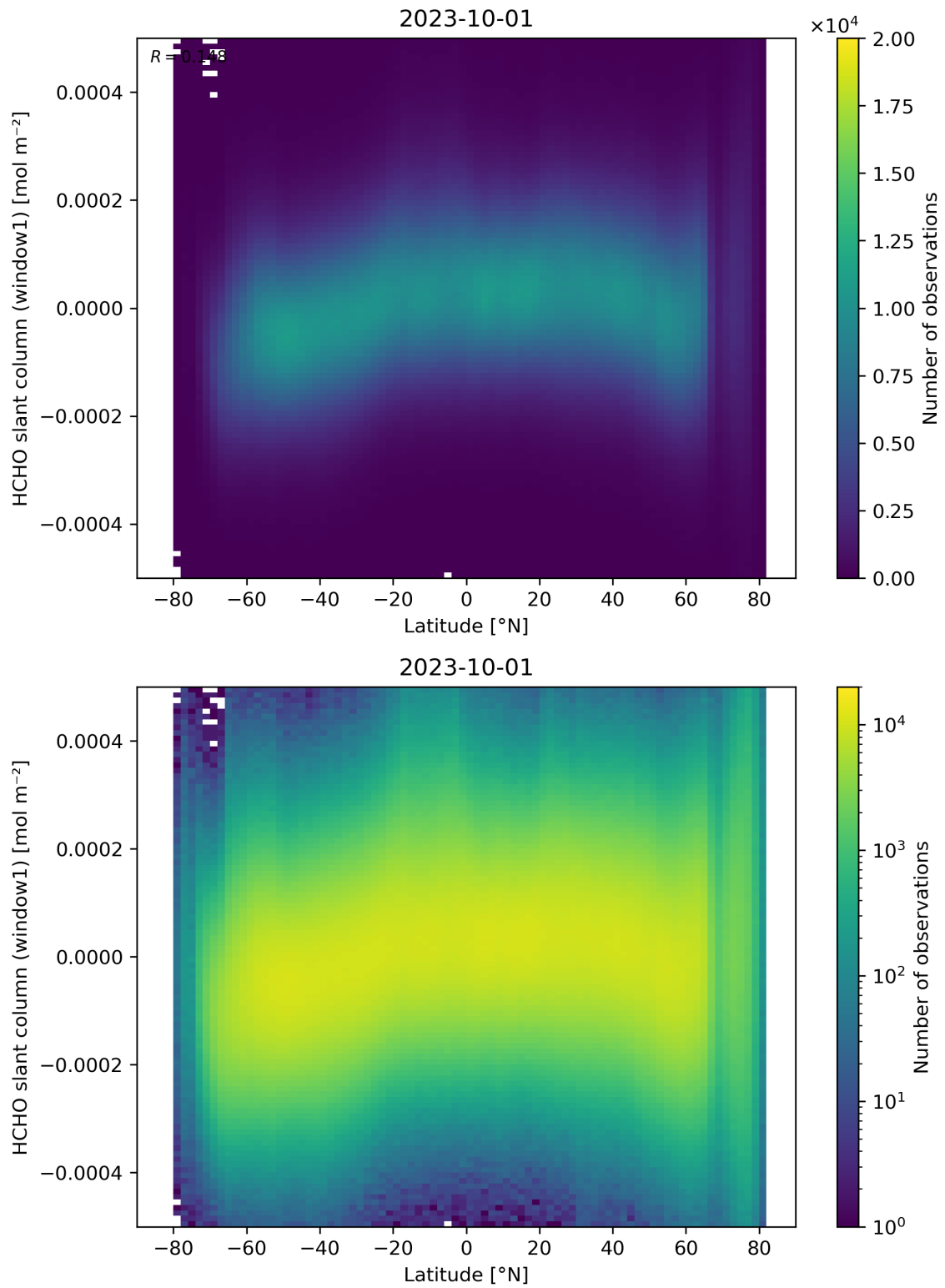
Figure 159: Scatter density plot of “Latitude” against “HCHO slant column (window1)” for 2023-10-01 to 2023-10-02.
