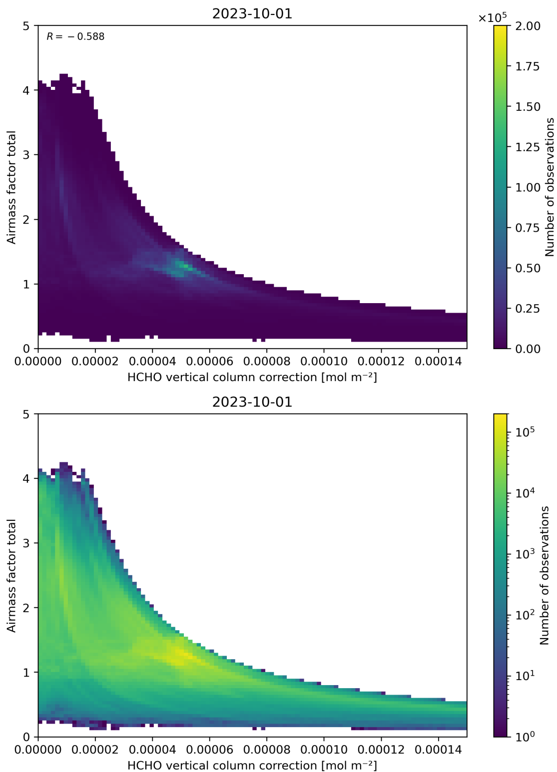
Figure 120: Scatter density plot of “HCHO vertical column correction” against “Airmass factor total” for 2023-10-01 to 2023-10-02.
