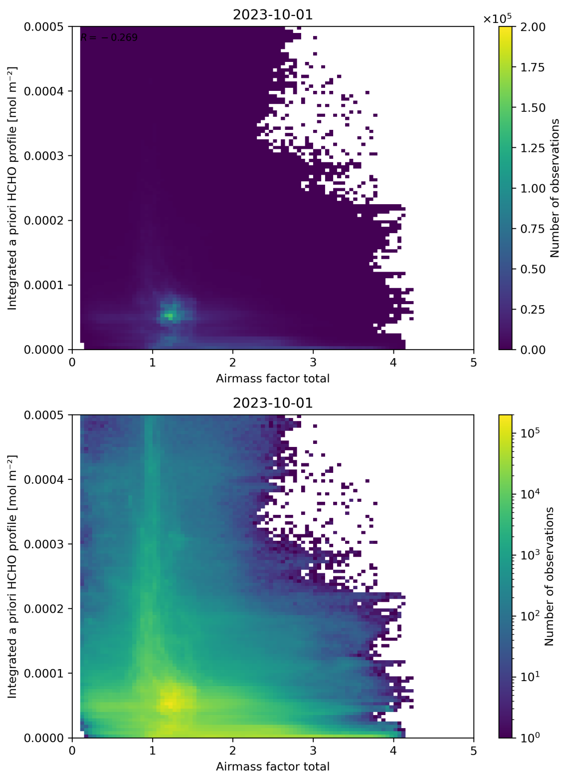
Figure 104: Scatter density plot of “Airmass factor total” against “Integrated a priori HCHO profile” for 2023-10-01 to 2023-10-02.
