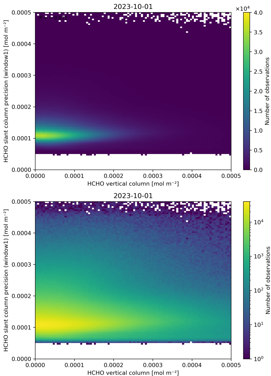
Figure 130: Scatter density plot of “HCHO vertical column” against “HCHO slant column precision (window1)” for 2023-10-01 to 2023-10-02.
