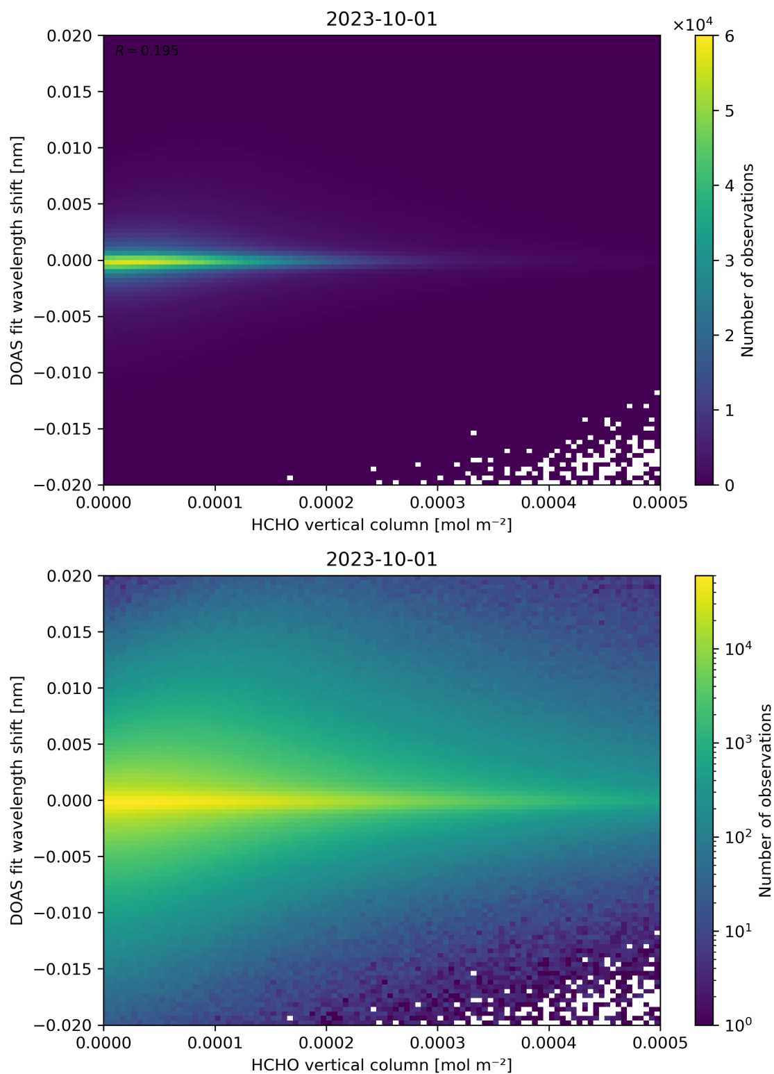
Figure 124: Scatter density plot of “HCHO vertical column” against “DOAS fit wavelength shift” for 2023-10-01 to 2023-10-02.
