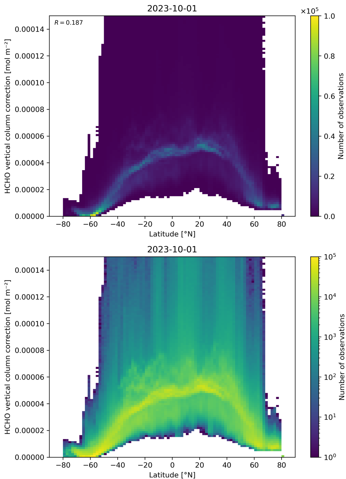
Figure 164: Scatter density plot of “Latitude” against “HCHO vertical column correction” for 2023-10-01 to 2023-10-02.
