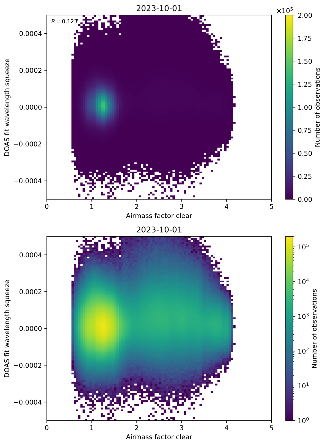
Figure 73: Scatter density plot of “Airmass factor clear” against “DOAS fit wavelength squeeze” for 2023-10-01 to 2023-10-02.
