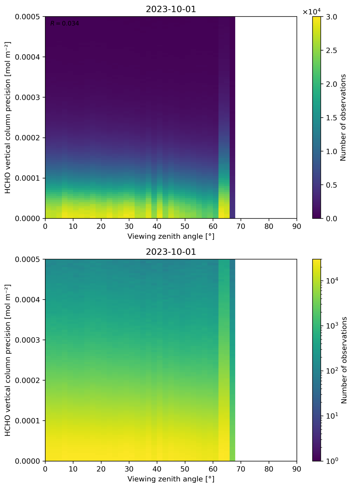
Figure 194: Scatter density plot of “Viewing zenith angle” against “HCHO vertical column precision” for 2023-10-01 to 2023-10-02.
