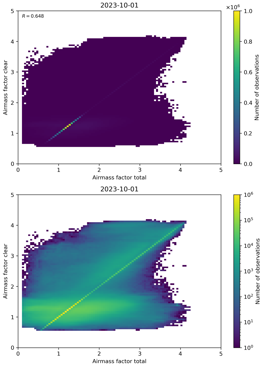
Figure 100: Scatter density plot of “Airmass factor total” against “Airmass factor clear” for 2023-10-01 to 2023-10-02.
