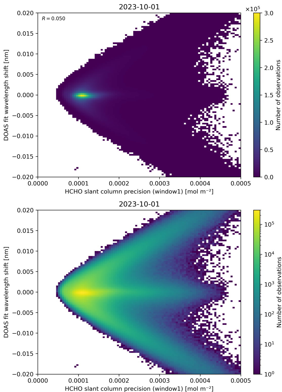
Figure 89: Scatter density plot of “HCHO slant column precision (window1)” against “DOAS fit wavelength shift” for 2023-10-01 to 2023-10-02.
