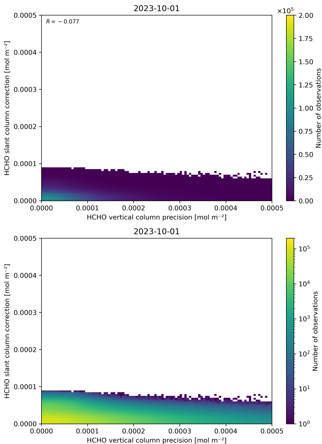
Figure 141: Scatter density plot of “HCHO vertical column precision” against “HCHO slant column correction” for 2023-10-01 to 2023-10-02.
