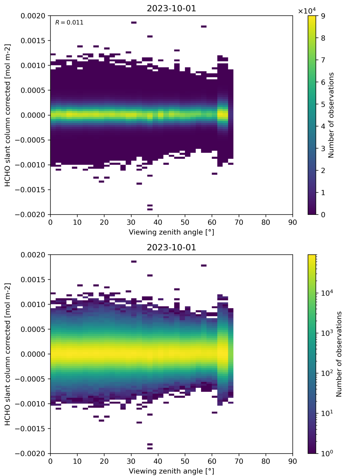
Figure 186: Scatter density plot of “Viewing zenith angle” against “HCHO slant column corrected” for 2023-10-01 to 2023-10-02.
