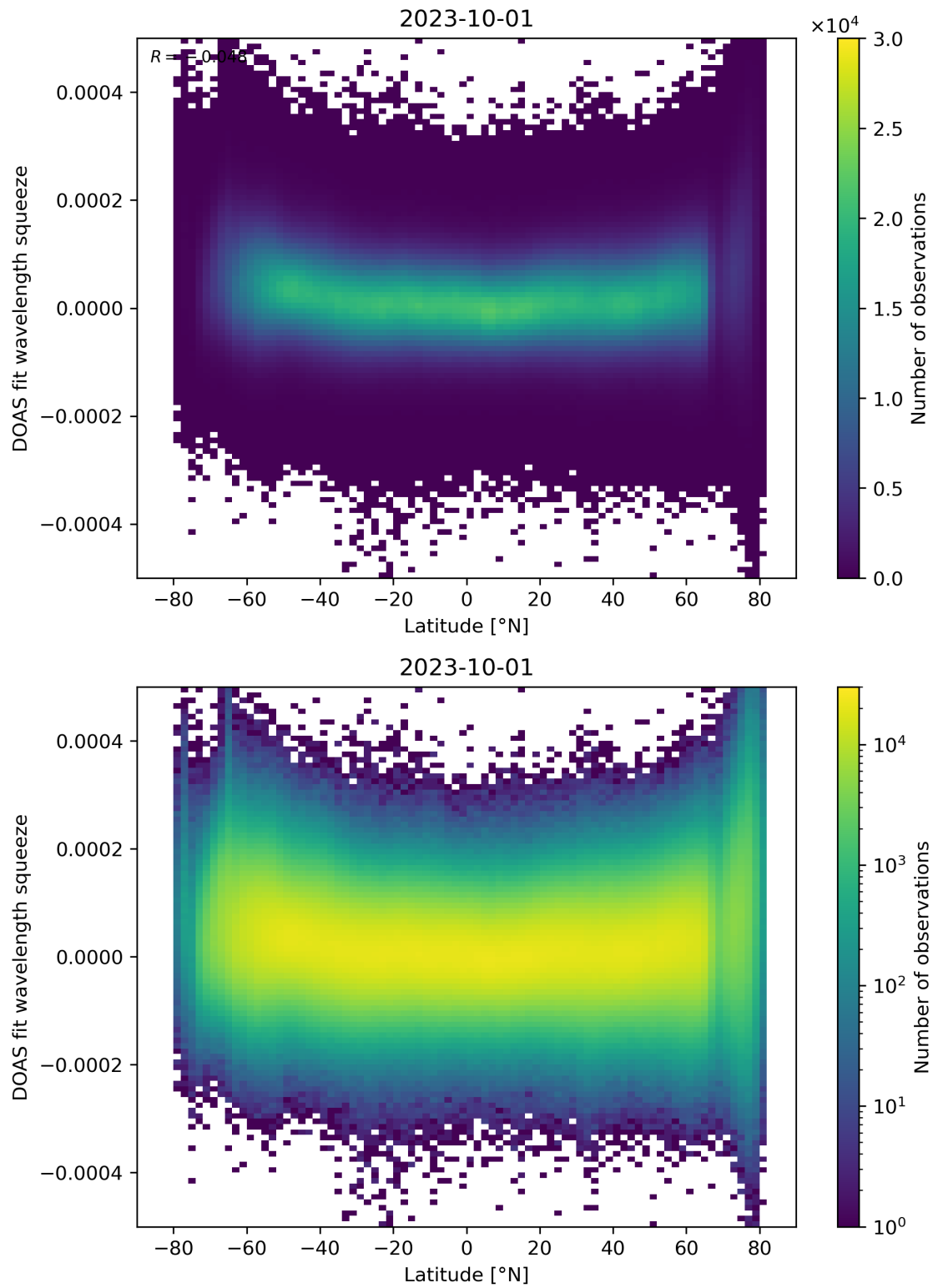
Figure 155: Scatter density plot of “Latitude” against “DOAS fit wavelength squeeze” for 2023-10-01 to 2023-10-02.
