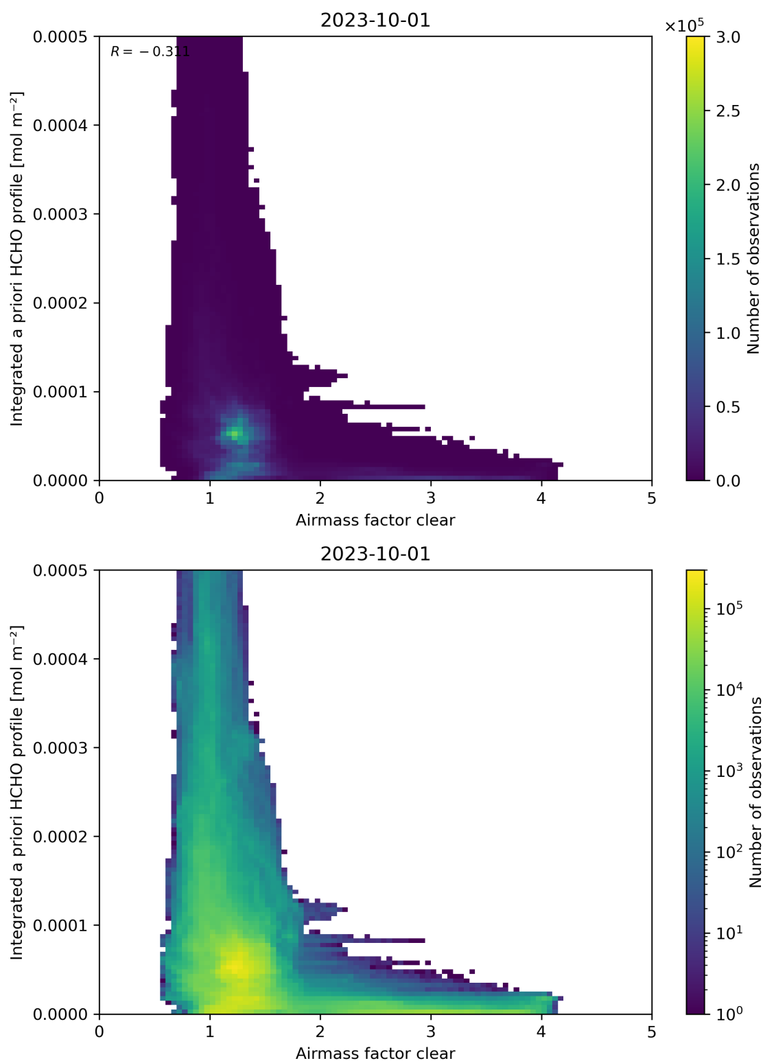
Figure 76: Scatter density plot of “Airmass factor clear” against “Integrated a priori HCHO profile” for 2023-10-01 to 2023-10-02.
