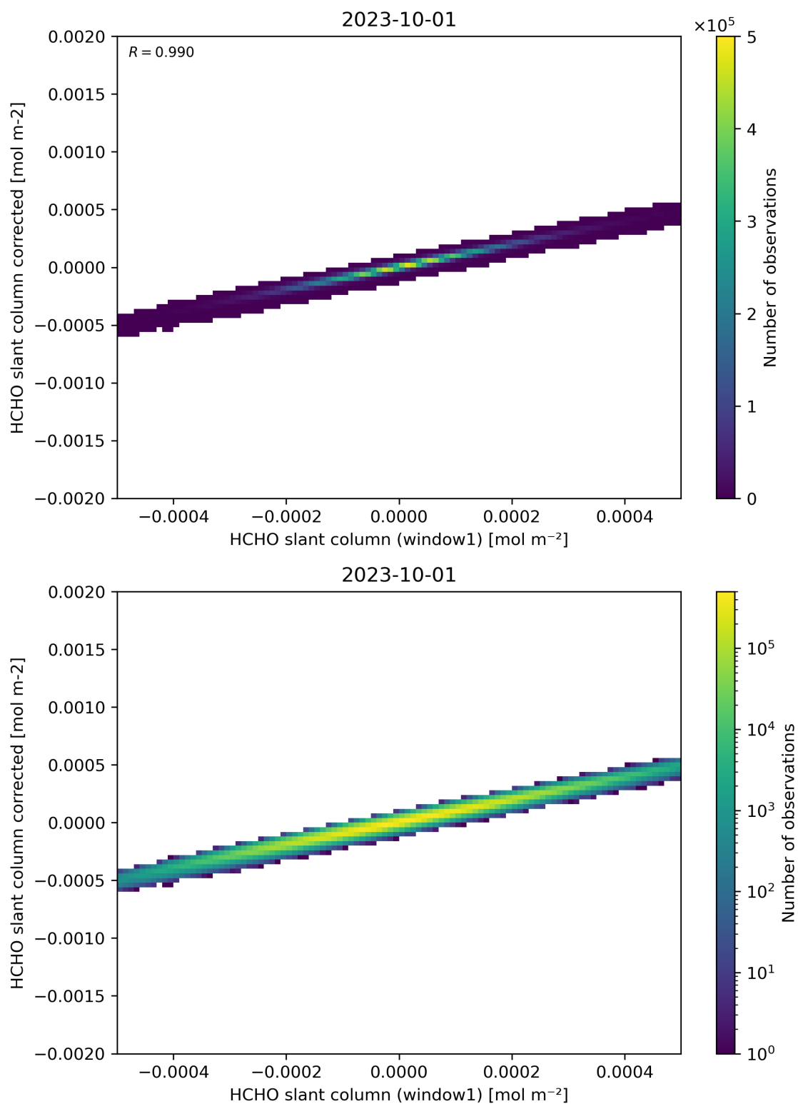
Figure 82: Scatter density plot of “HCHO slant column (window1)” against “HCHO slant column corrected” for 2023-10-01 to 2023-10-02.
