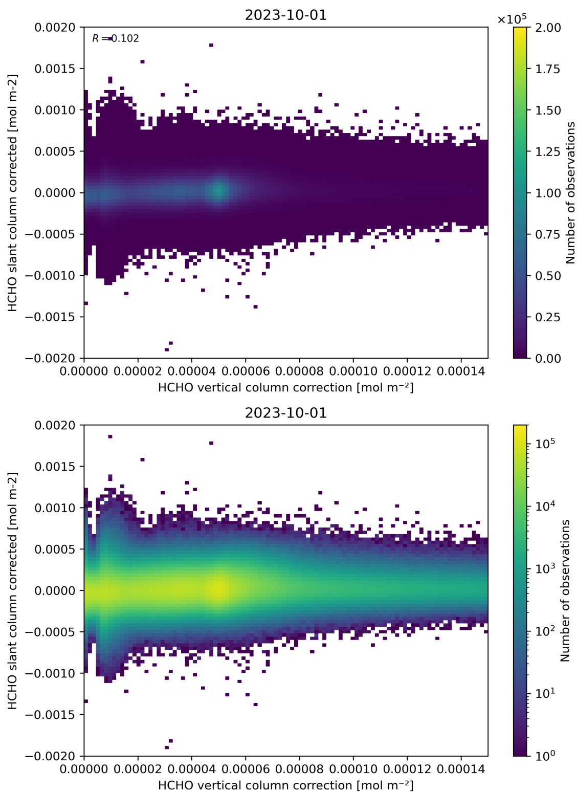
Figure 116: Scatter density plot of “HCHO vertical column correction” against “HCHO slant column corrected” for 2023-10-01 to 2023-10-02.
