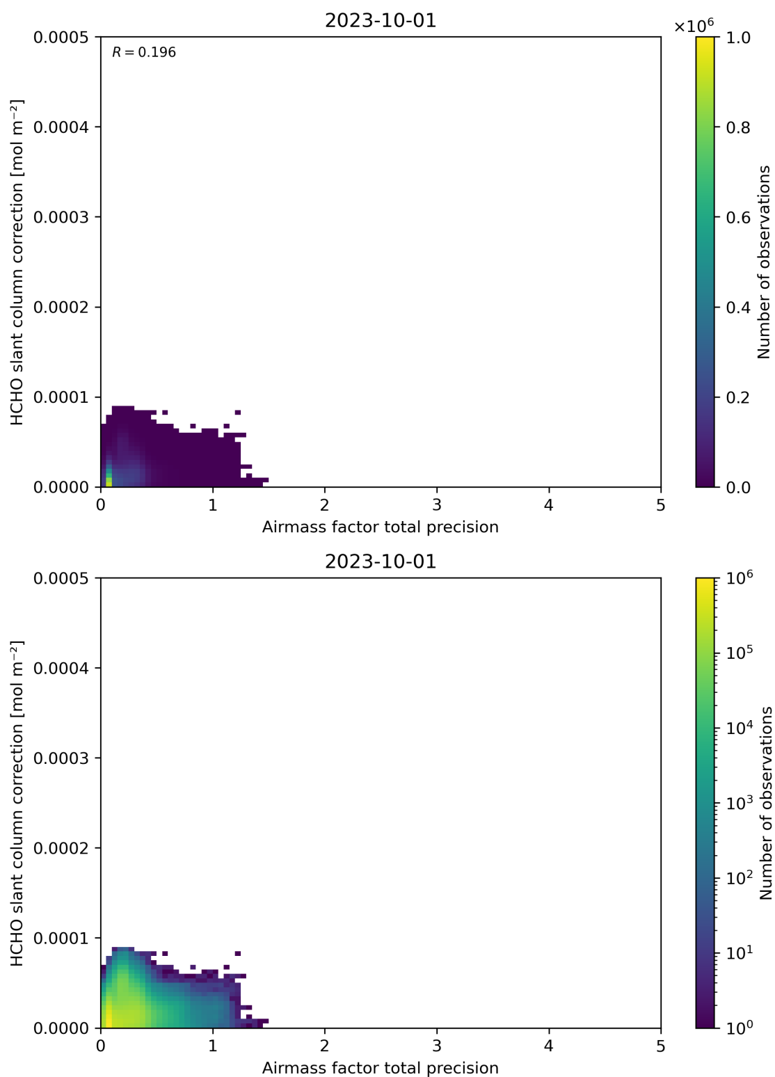
Figure 110: Scatter density plot of “Airmass factor total precision” against “HCHO slant column correction” for 2023-10-01 to 2023-10-02.
