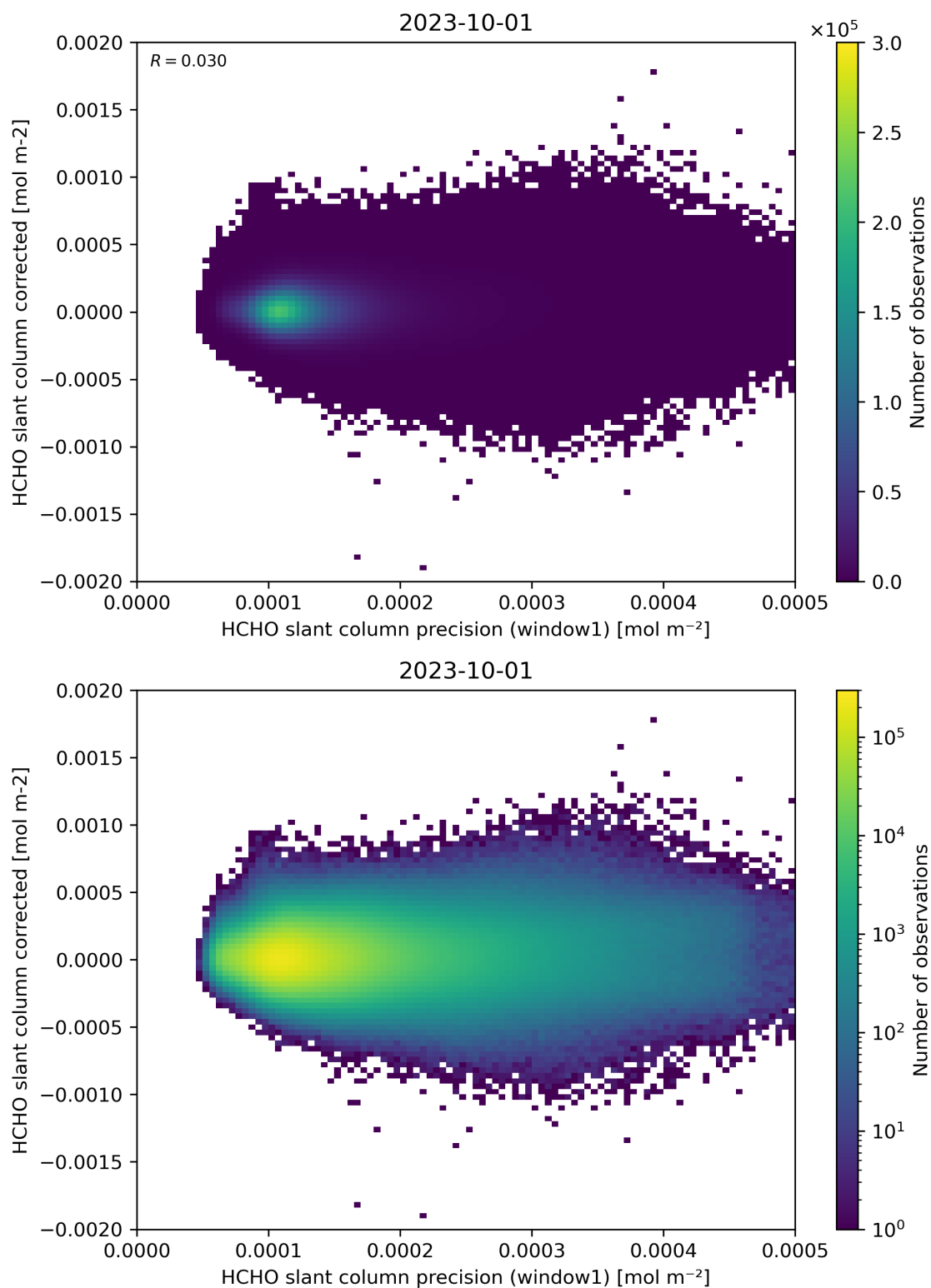
Figure 92: Scatter density plot of “HCHO slant column precision (window1)” against “HCHO slant column corrected” for 2023-10-01 to 2023-10-02.
