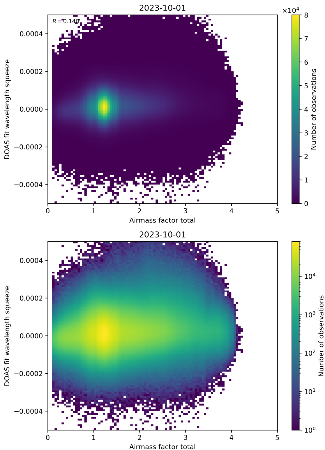
Figure 99: Scatter density plot of “Airmass factor total” against “DOAS fit wavelength squeeze” for 2023-10-01 to 2023-10-02.
