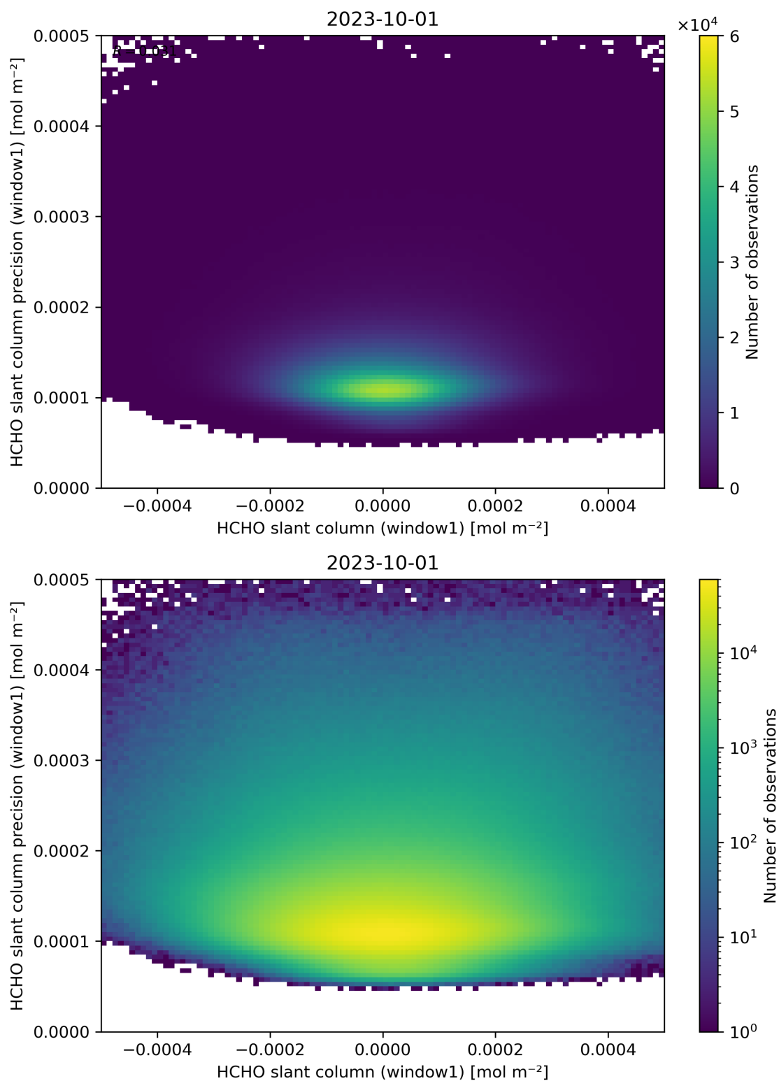
Figure 84: Scatter density plot of “HCHO slant column (window1)” against “HCHO slant column precision (window1)” for 2023-10-01 to 2023-10-02.
