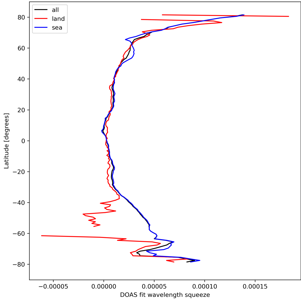
Figure 31: Zonal average of “DOAS fit wavelength squeeze” for 2023-10-01 to 2023-10-02.
