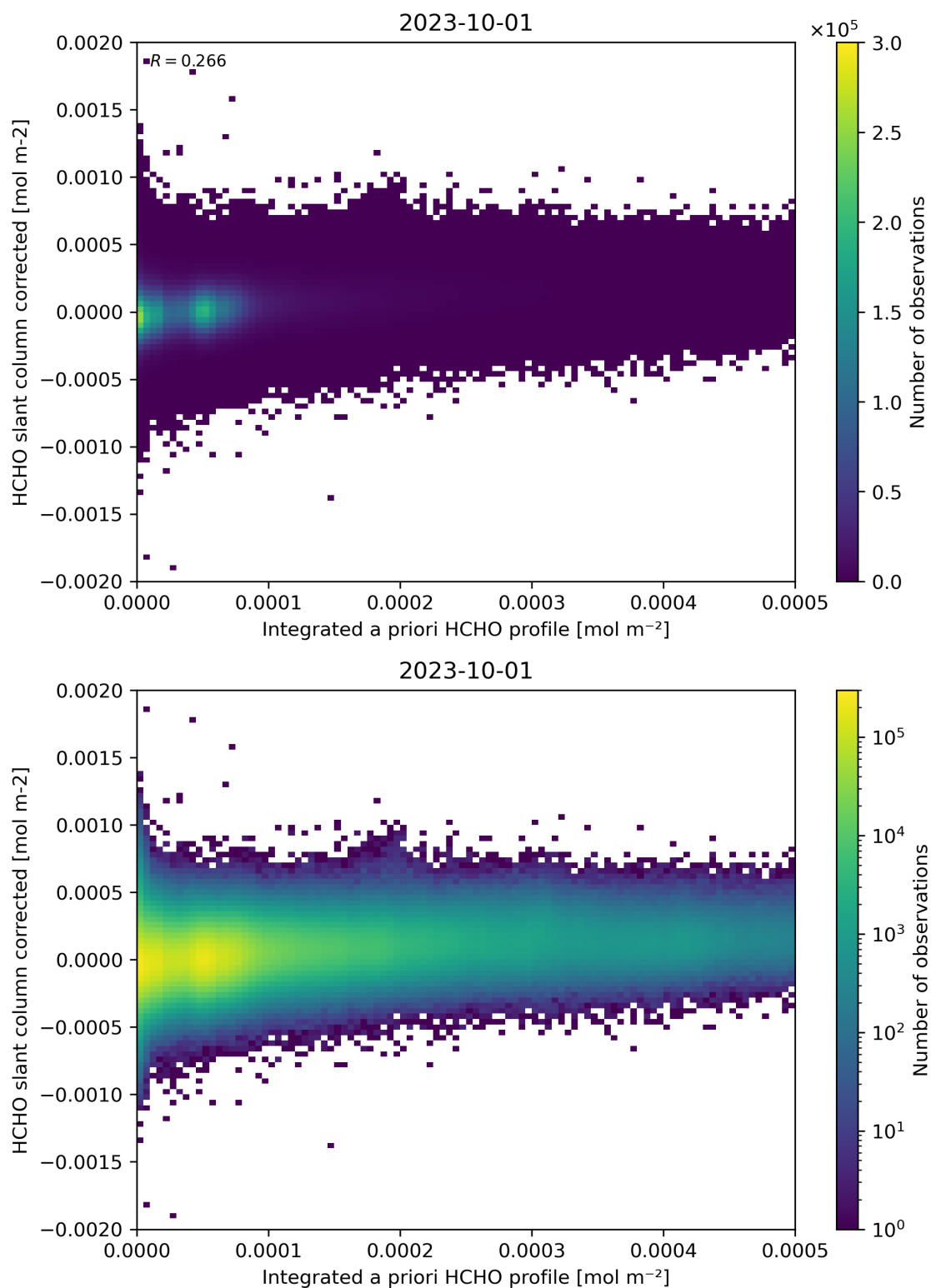
Figure 151: Scatter density plot of “Integrated a priori HCHO profile” against “HCHO slant column corrected” for 2023-10-01 to 2023-10-02.
