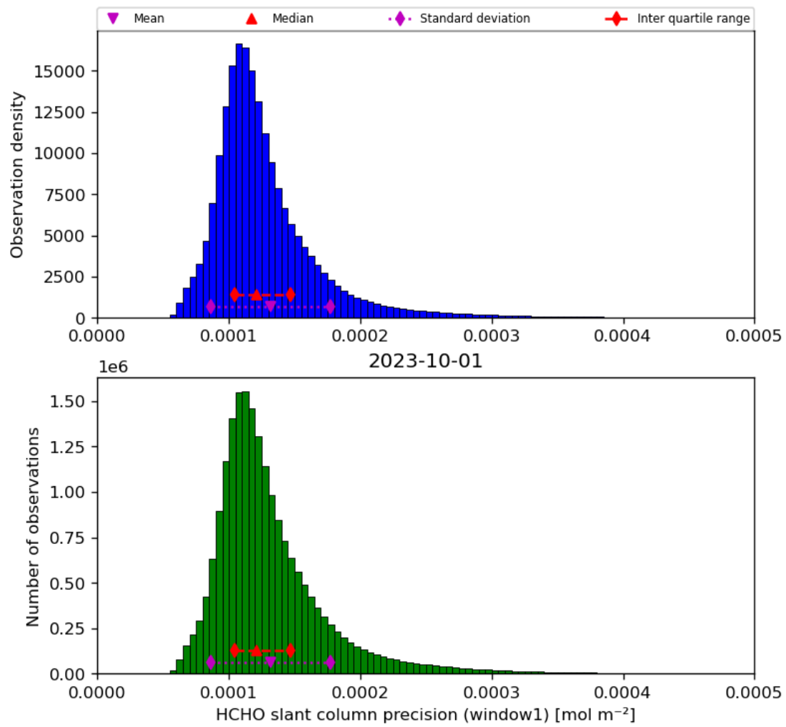
Figure 39: Histogram of “HCHO slant column precision (window1)” for 2023-10-01 to 2023-10-02
