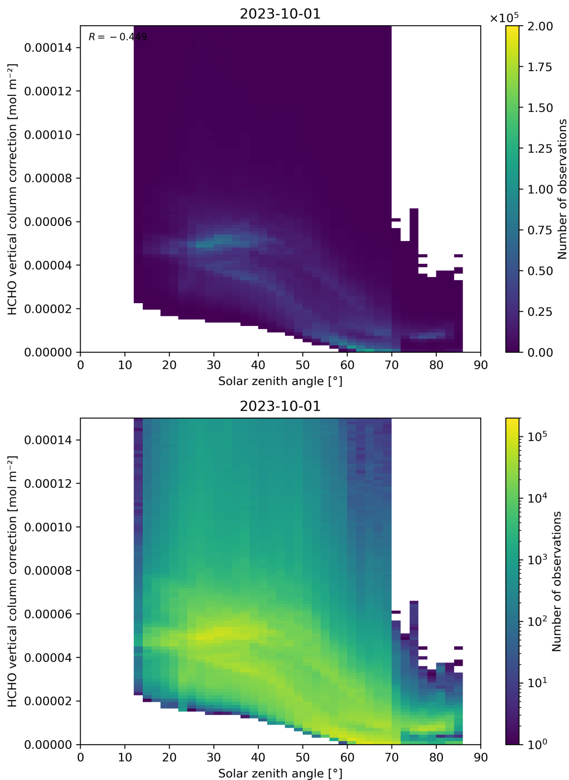
Figure 178: Scatter density plot of “Solar zenith angle” against “HCHO vertical column correction” for 2023-10-01 to 2023-10-02.
