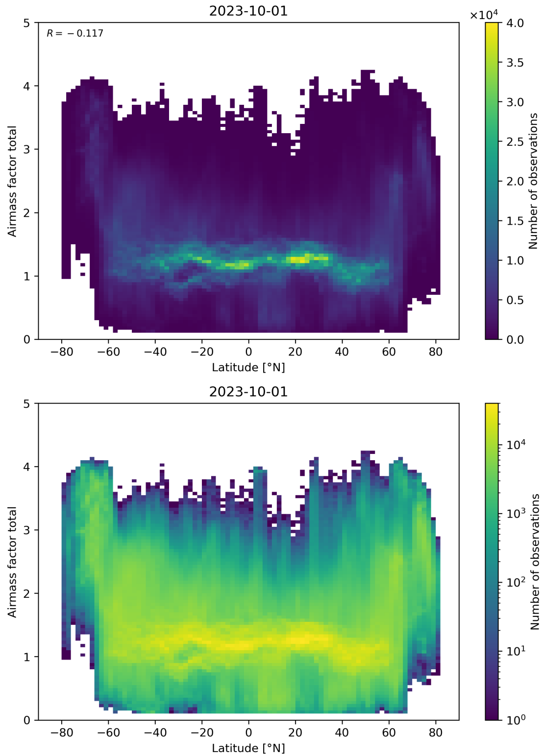
Figure 161: Scatter density plot of “Latitude” against “Airmass factor total” for 2023-10-01 to 2023-10-02.
