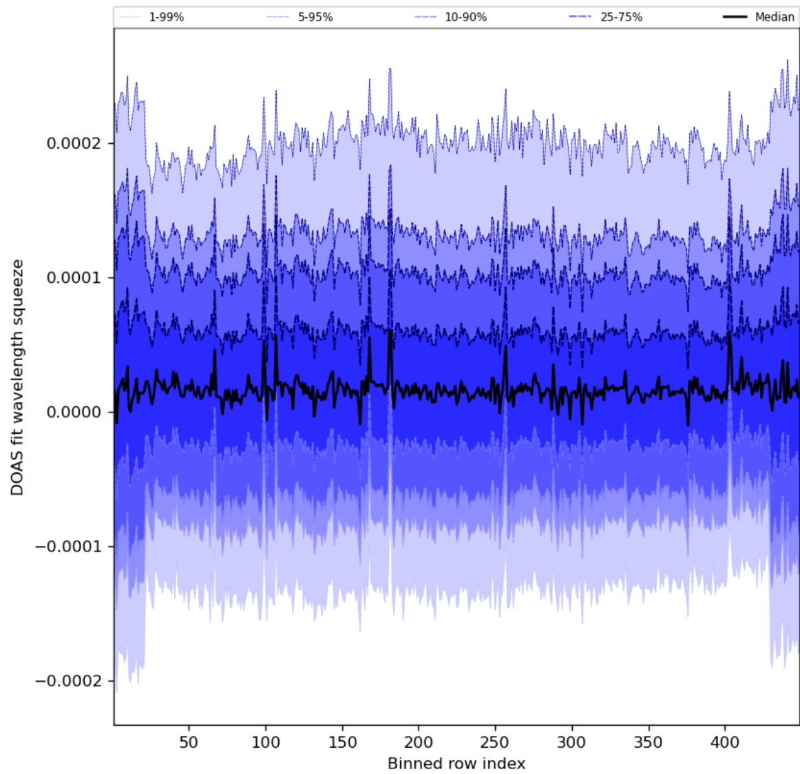
Figure 59: Along track statistics of “DOAS fit wavelength squeeze” for 2023-10-01 to 2023-10-02
