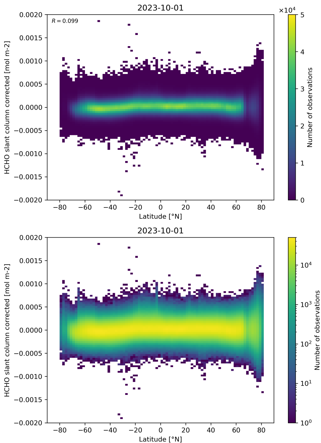
Figure 157: Scatter density plot of “Latitude” against “HCHO slant column corrected” for 2023-10-01 to 2023-10-02.
