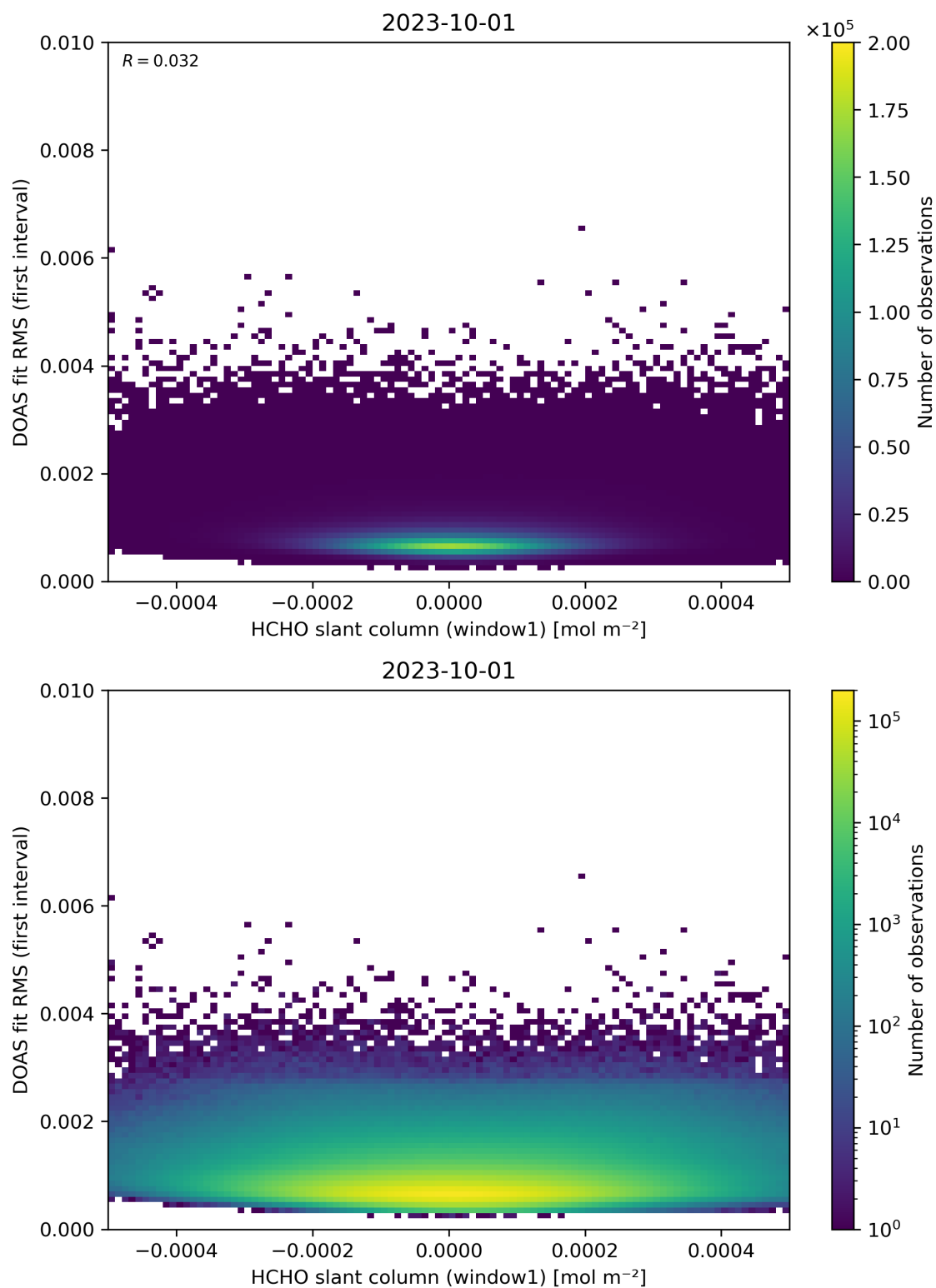
Figure 78: Scatter density plot of “HCHO slant column (window1)” against “DOAS fit RMS (first interval)” for 2023-10-01 to 2023-10-02.
