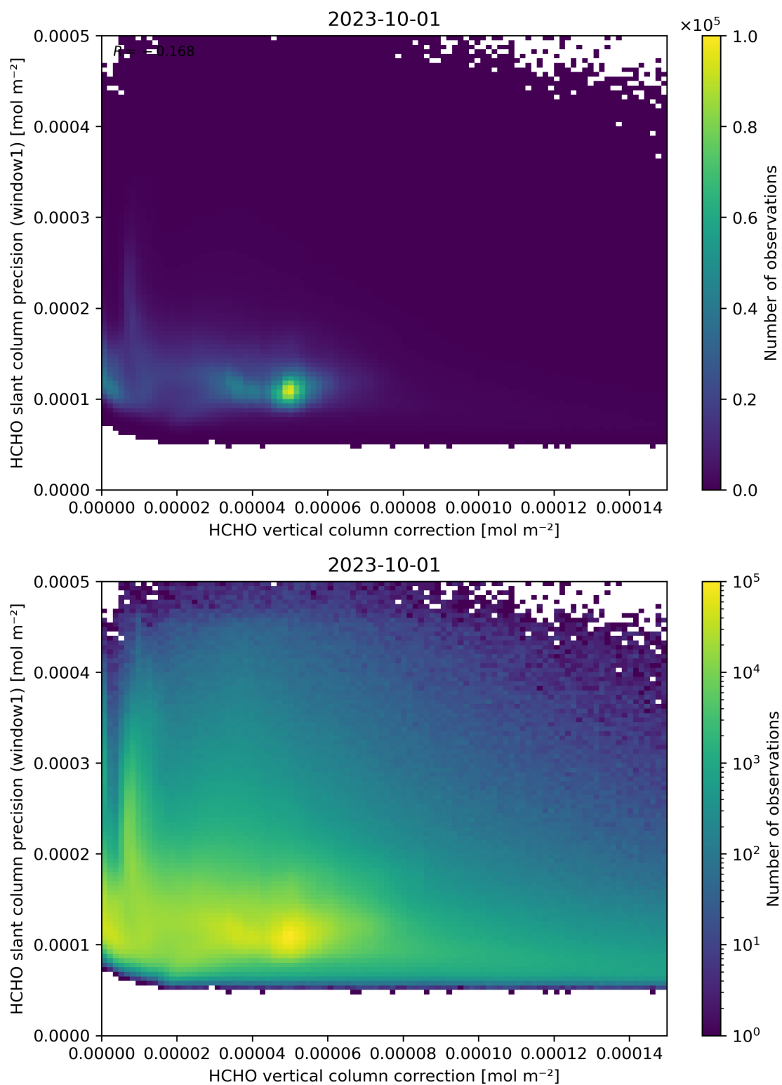
Figure 119: Scatter density plot of “HCHO vertical column correction” against “HCHO slant column precision (window1)” for 2023-10-01 to 2023-10-02.
