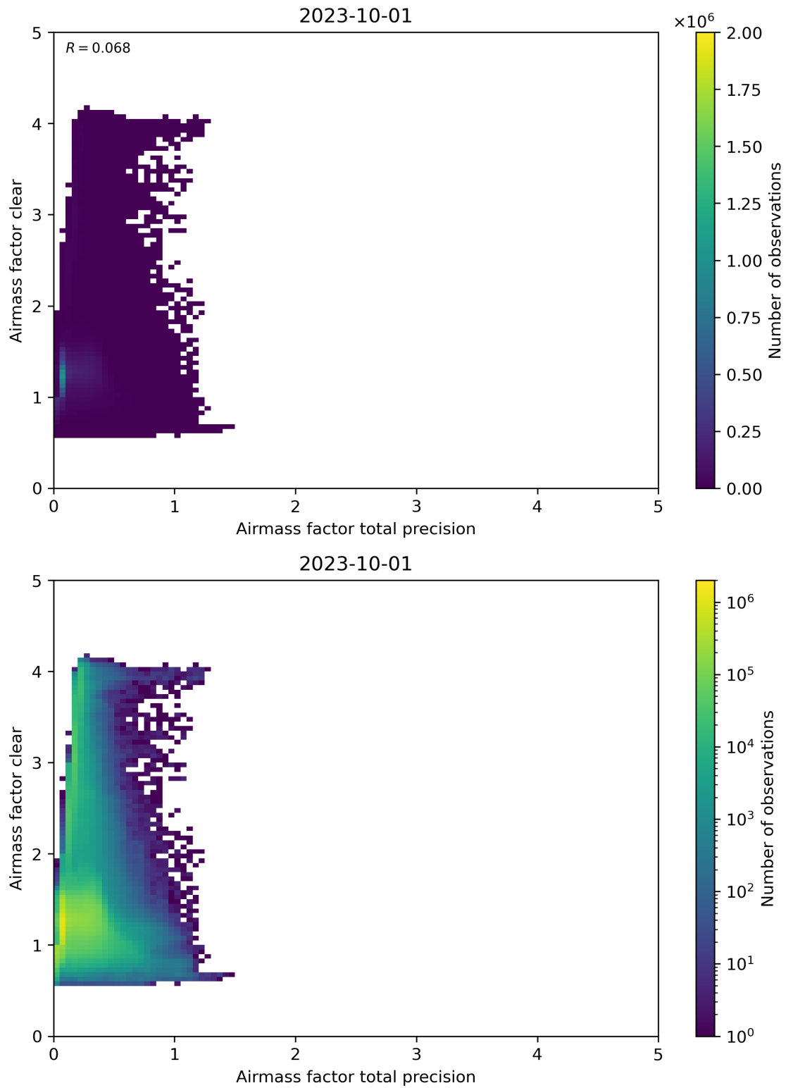
Figure 108: Scatter density plot of “Airmass factor total precision” against “Airmass factor clear” for 2023-10-01 to 2023-10-02.
