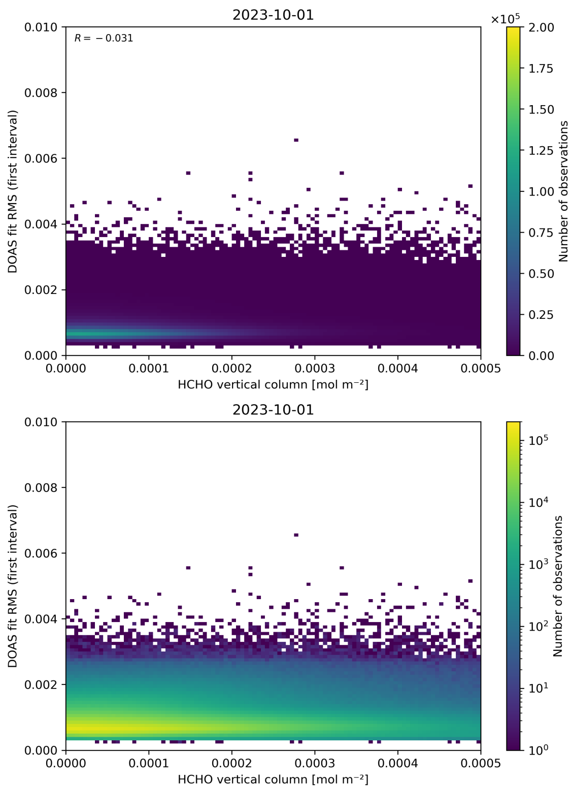
Figure 123: Scatter density plot of “HCHO vertical column” against “DOAS fit RMS (first interval)” for 2023-10-01 to 2023-10-02.
