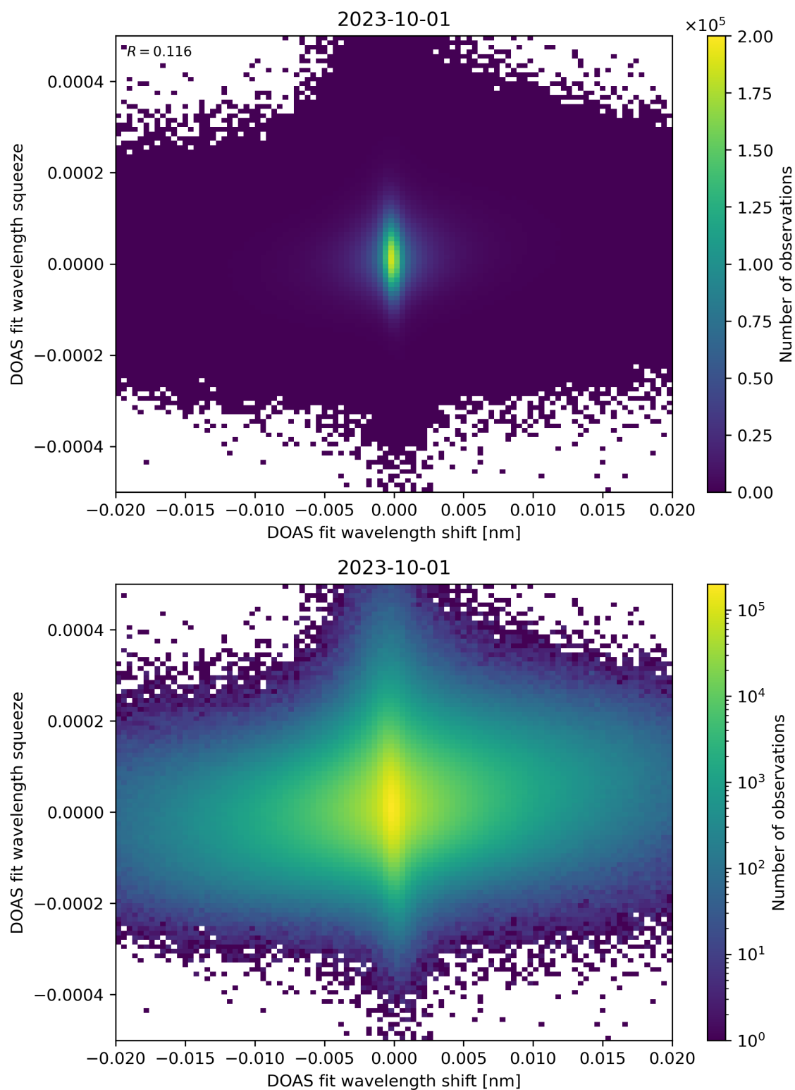
Figure 65: Scatter density plot of “DOAS fit wavelength shift” against “DOAS fit wavelength squeeze” for 2023-10-01 to 2023-10-02.
