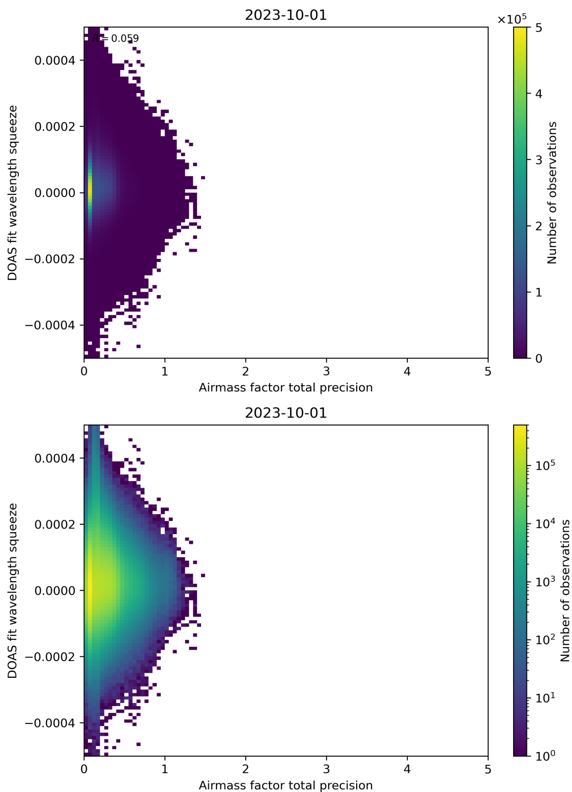
Figure 107: Scatter density plot of “Airmass factor total precision” against “DOAS fit wavelength squeeze” for 2023-10-01 to 2023-10-02.
