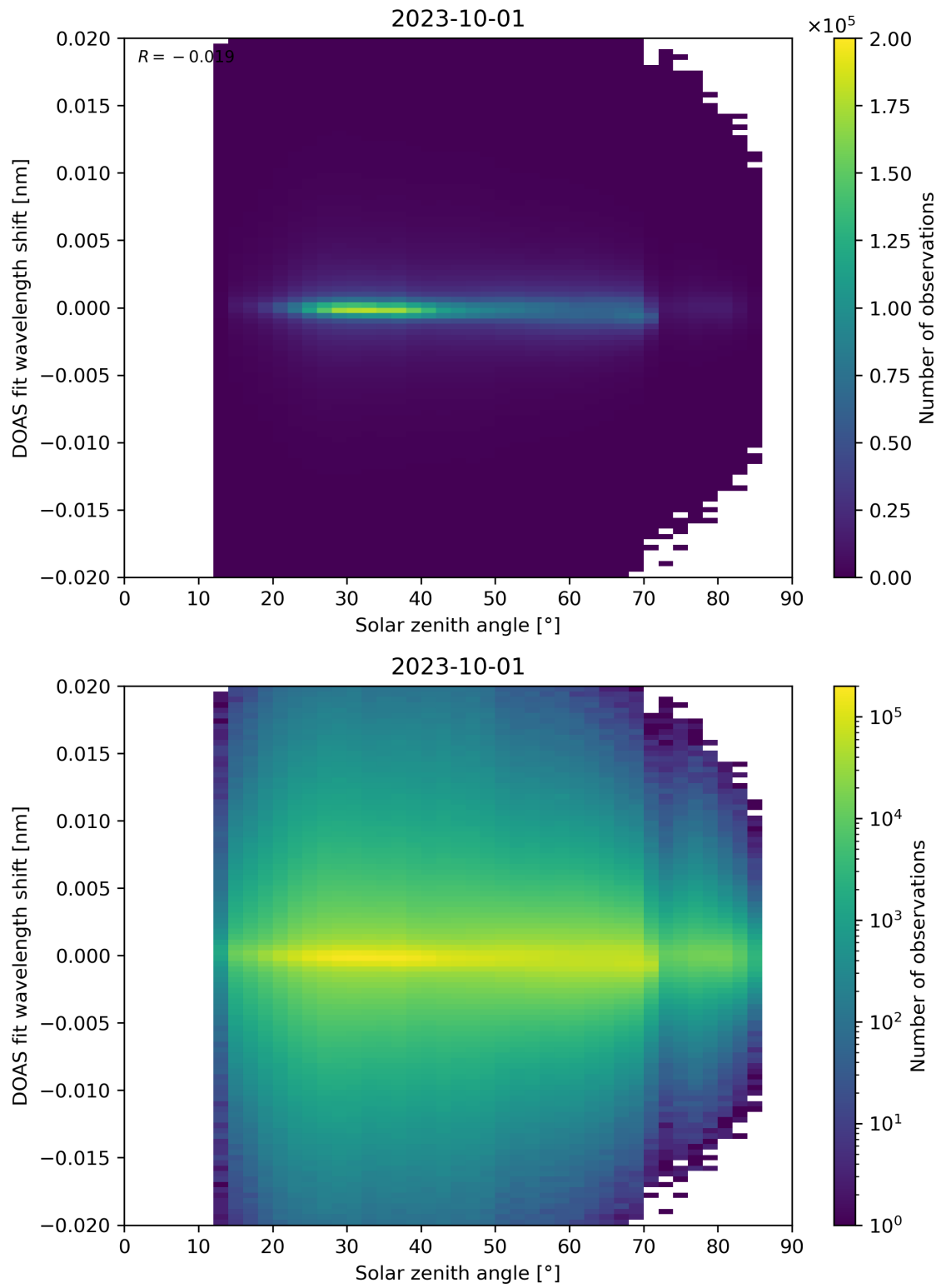
Figure 168: Scatter density plot of “Solar zenith angle” against “DOAS fit wavelength shift” for 2023-10-01 to 2023-10-02.
