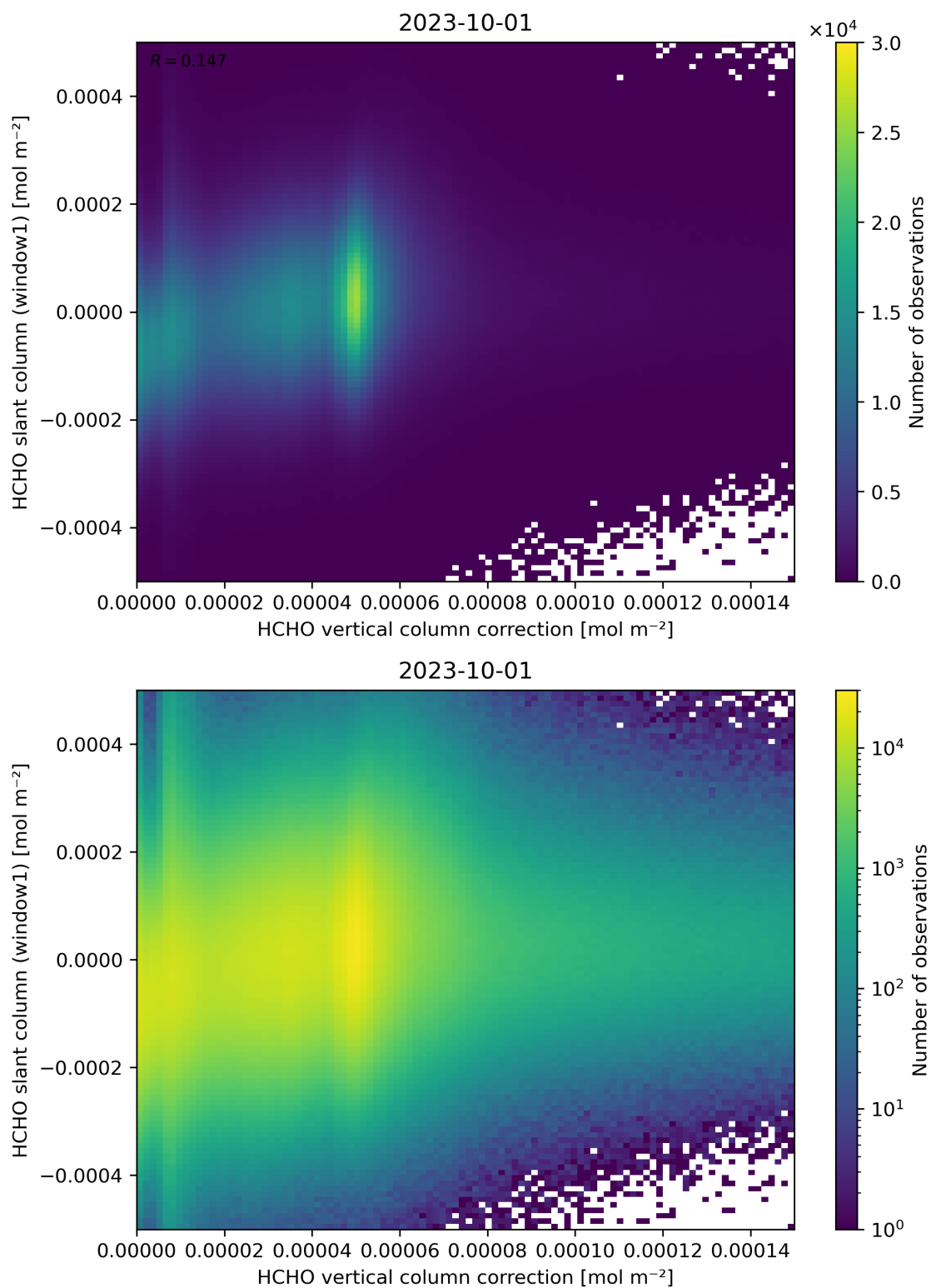
Figure 118: Scatter density plot of “HCHO vertical column correction” against “HCHO slant column (window1)” for 2023-10-01 to 2023-10-02.
