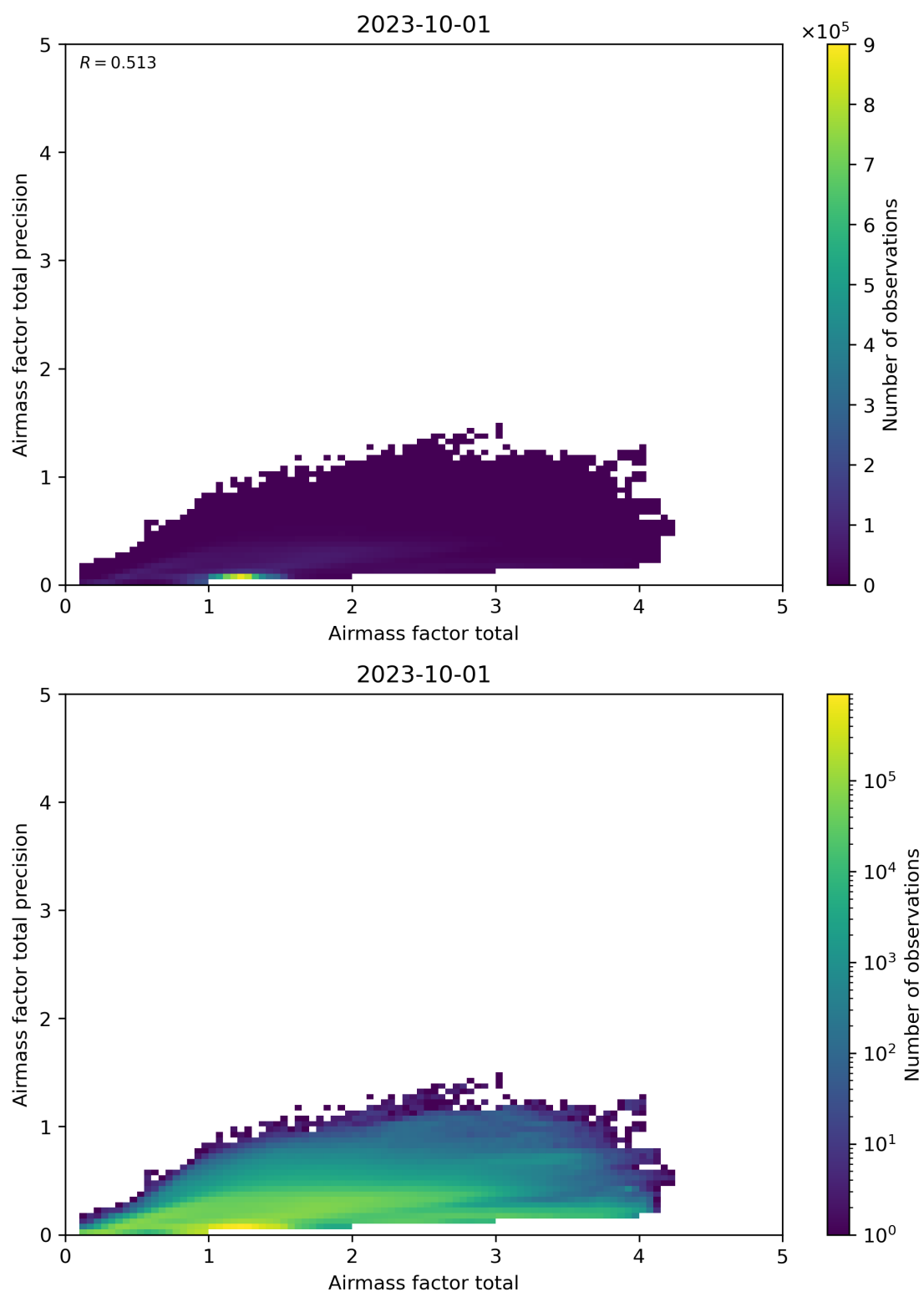
Figure 103: Scatter density plot of “Airmass factor total” against “Airmass factor total precision” for 2023-10-01 to 2023-10-02.
