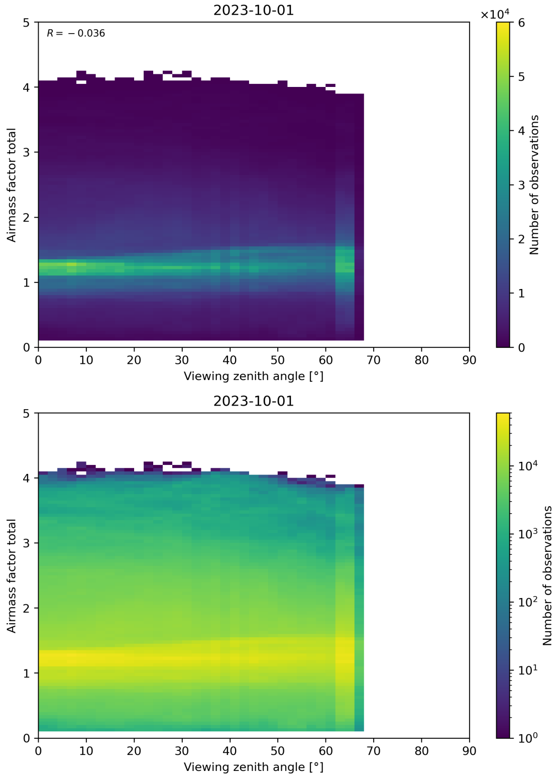
Figure 190: Scatter density plot of “Viewing zenith angle” against “Airmass factor total” for 2023-10-01 to 2023-10-02.
