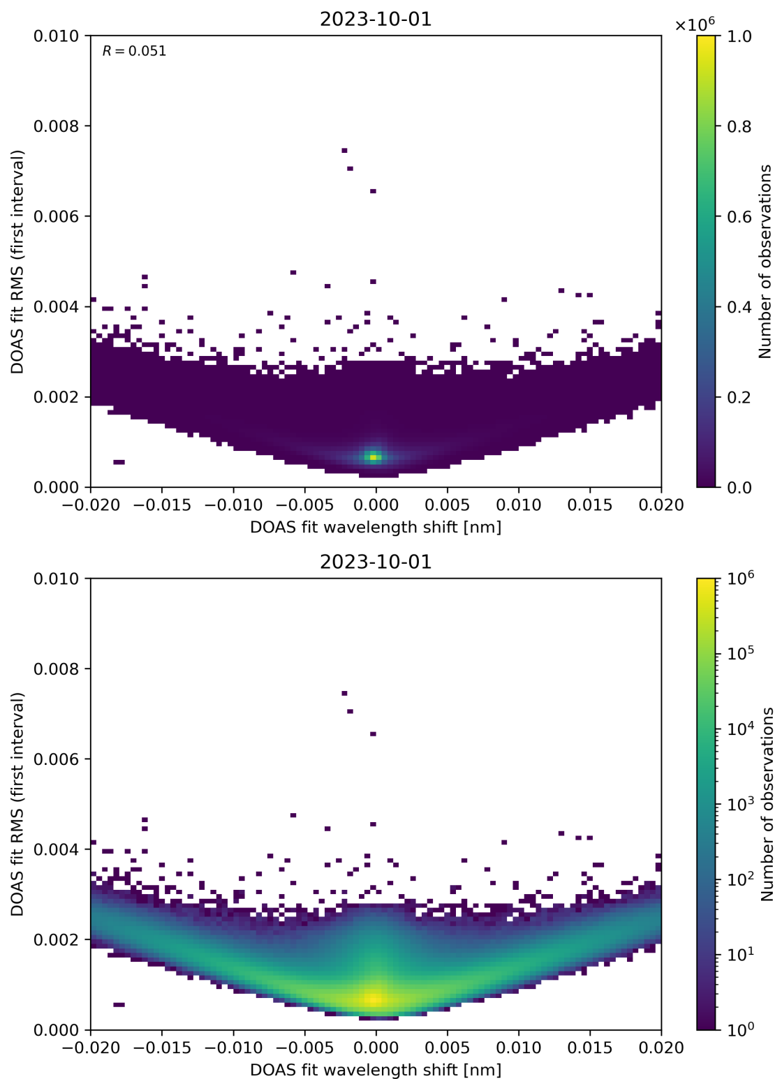
Figure 64: Scatter density plot of “DOAS fit wavelength shift” against “DOAS fit RMS (first interval)” for 2023-10-01 to 2023-10-02.
