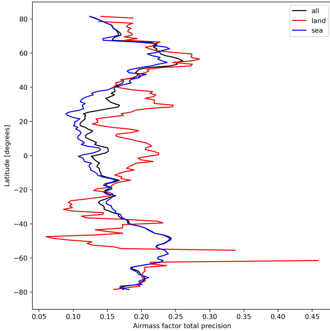
Figure 27: Zonal average of “Airmass factor total precision” for 2023-10-01 to 2023-10-02.
