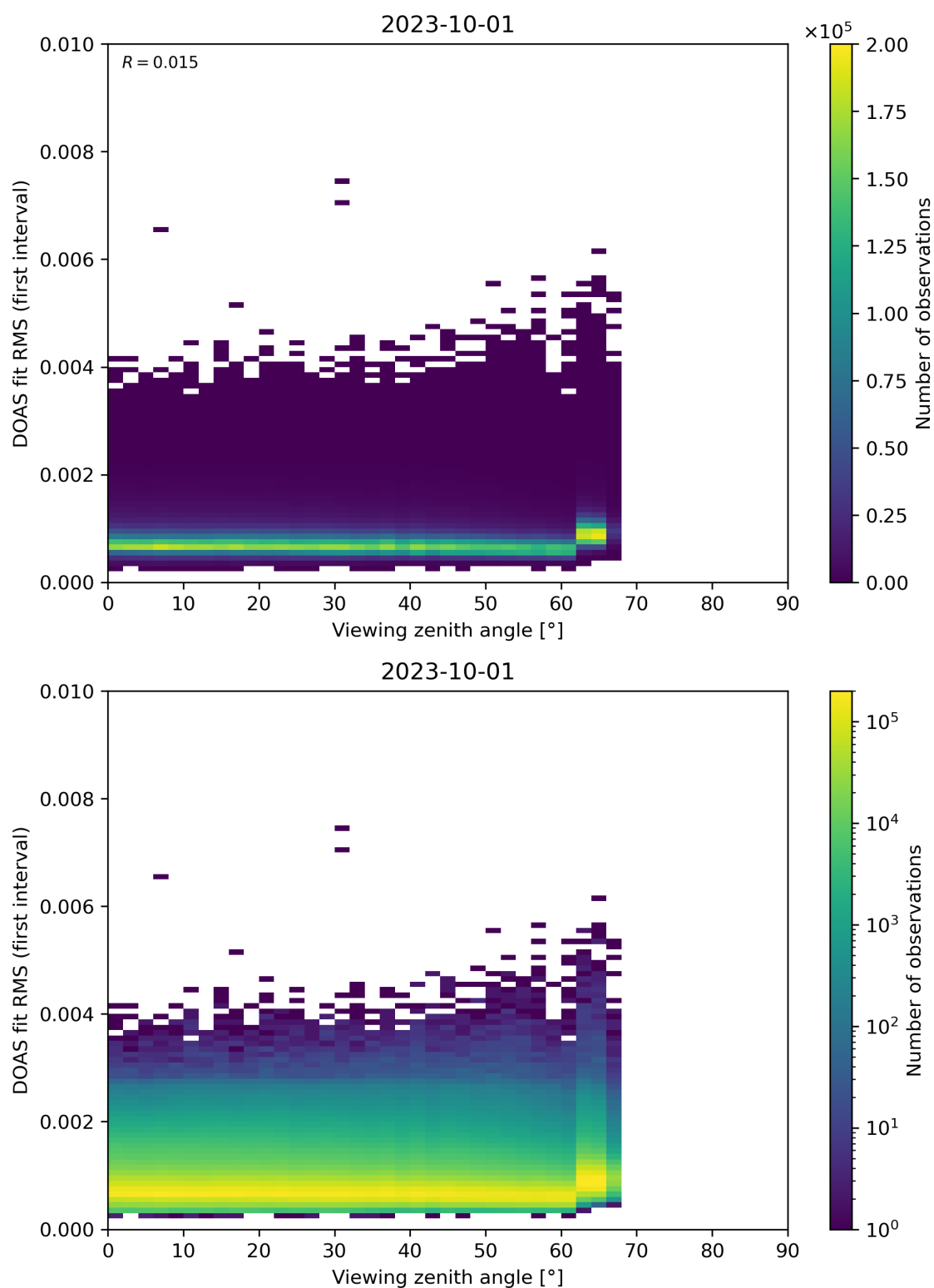
Figure 182: Scatter density plot of “Viewing zenith angle” against “DOAS fit RMS (first interval)” for 2023-10-01 to 2023-10-02.
