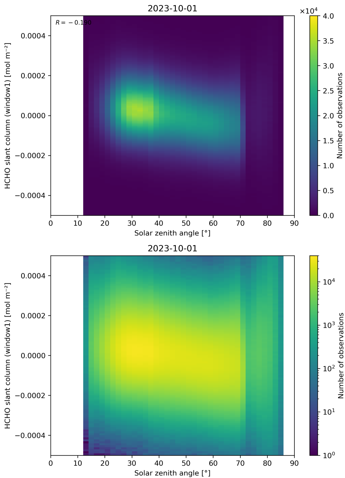
Figure 173: Scatter density plot of “Solar zenith angle” against “HCHO slant column (window1)” for 2023-10-01 to 2023-10-02.
