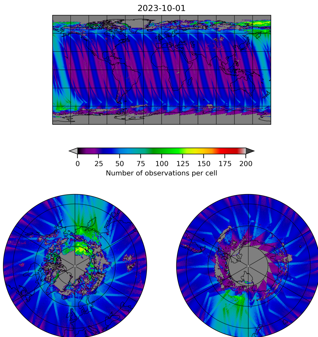
Figure 19: Map of the number of observations for 2023-10-01 to 2023-10-02
