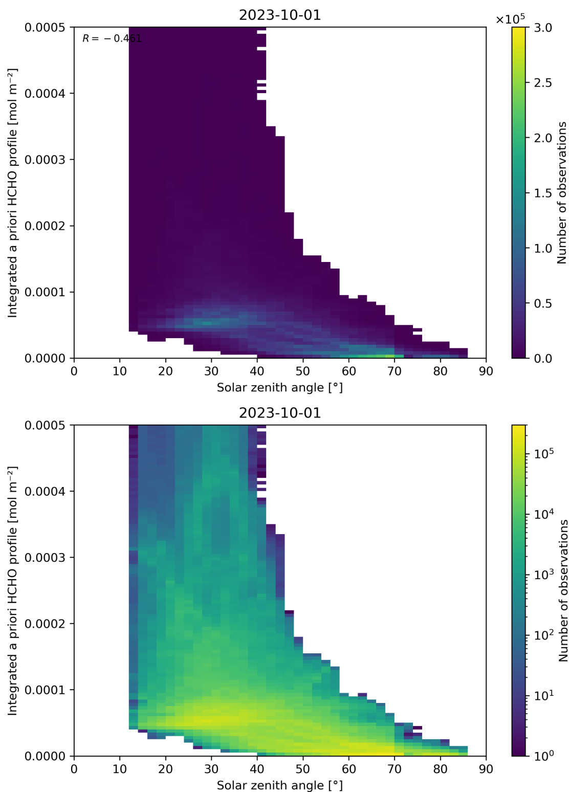
Figure 180: Scatter density plot of “Solar zenith angle” against “Integrated a priori HCHO profile” for 2023-10-01 to 2023-10-02.
