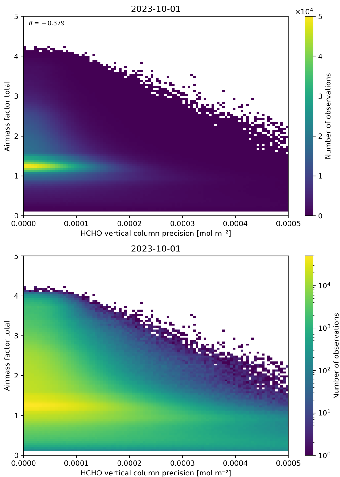
Figure 144: Scatter density plot of “HCHO vertical column precision” against “Airmass factor total” for 2023-10-01 to 2023-10-02.
