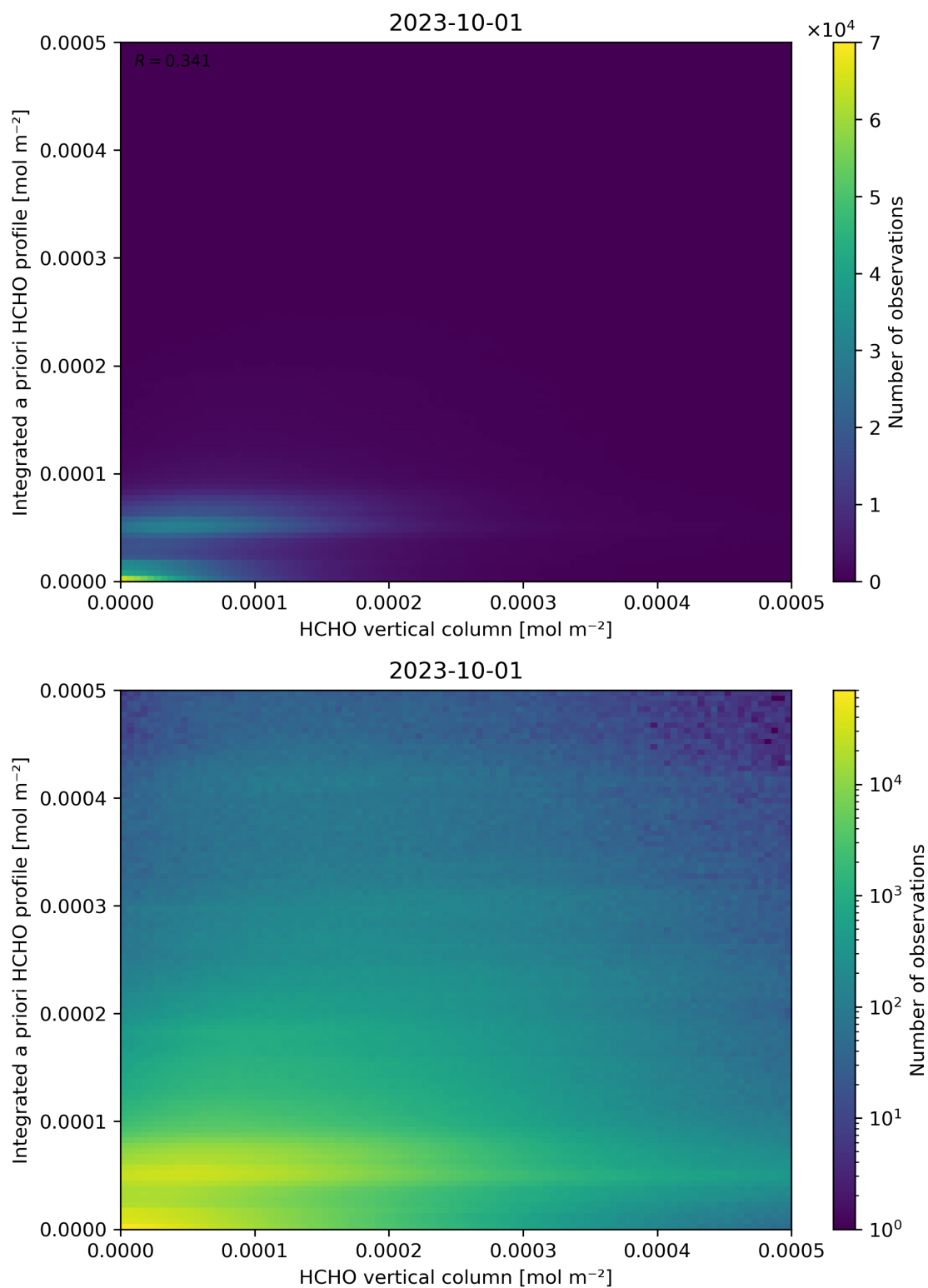
Figure 135: Scatter density plot of “HCHO vertical column” against “Integrated a priori HCHO profile” for 2023-10-01 to 2023-10-02.
