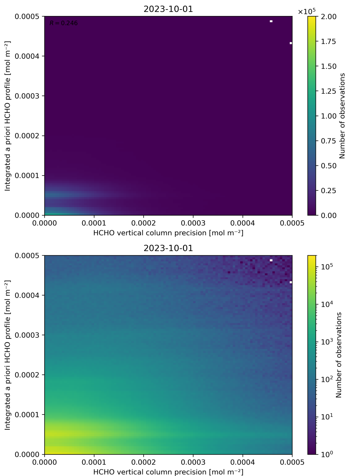
Figure 147: Scatter density plot of “HCHO vertical column precision” against “Integrated a priori HCHO profile” for 2023-10-01 to 2023-10-02.
