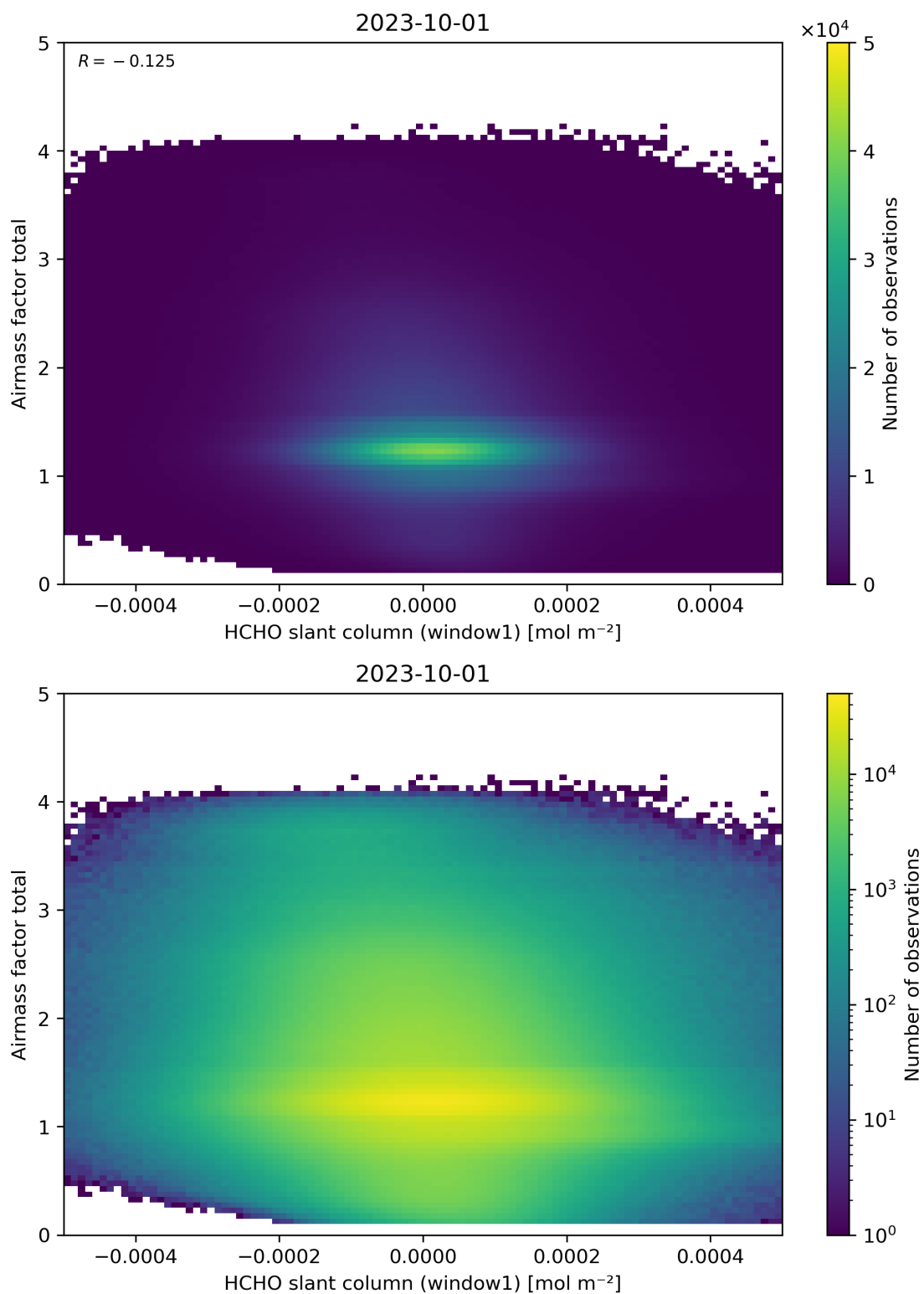
Figure 85: Scatter density plot of “HCHO slant column (window1)” against “Airmass factor total” for 2023-10-01 to 2023-10-02.
