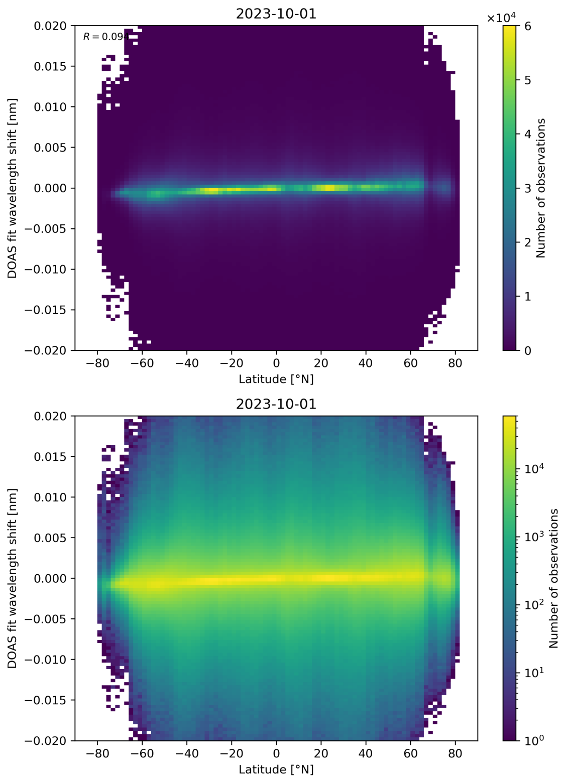
Figure 154: Scatter density plot of “Latitude” against “DOAS fit wavelength shift” for 2023-10-01 to 2023-10-02.
